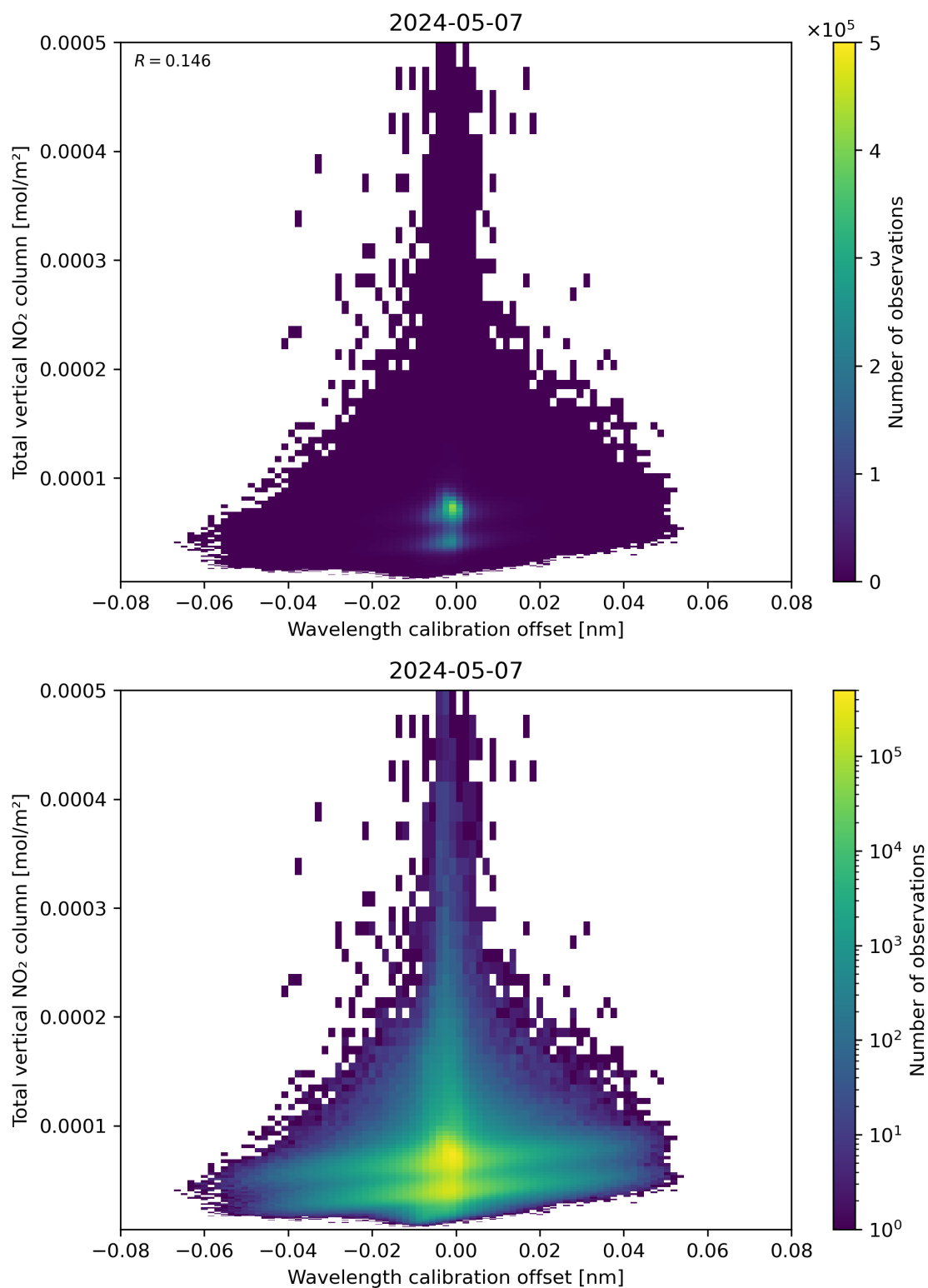
Figure 179: Scatter density plot of “Wavelength calibration offset” against “Total vertical NO 2 column” for 2024-05-07 to 2024-05-08.
