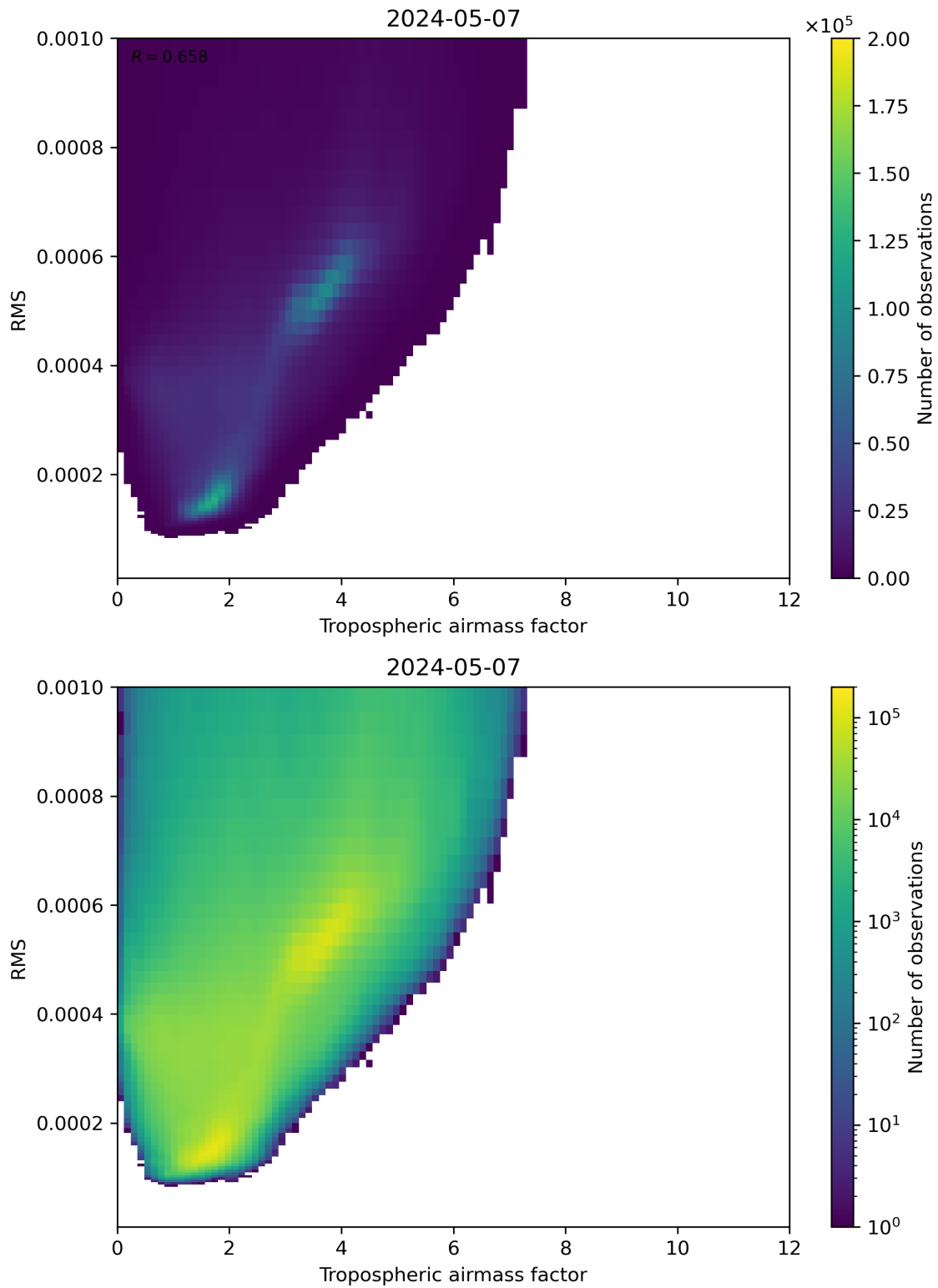
Figure 79: Scatter density plot of “Tropospheric airmass factor” against “RMS” for 2024-05-07 to 2024-05-08.
