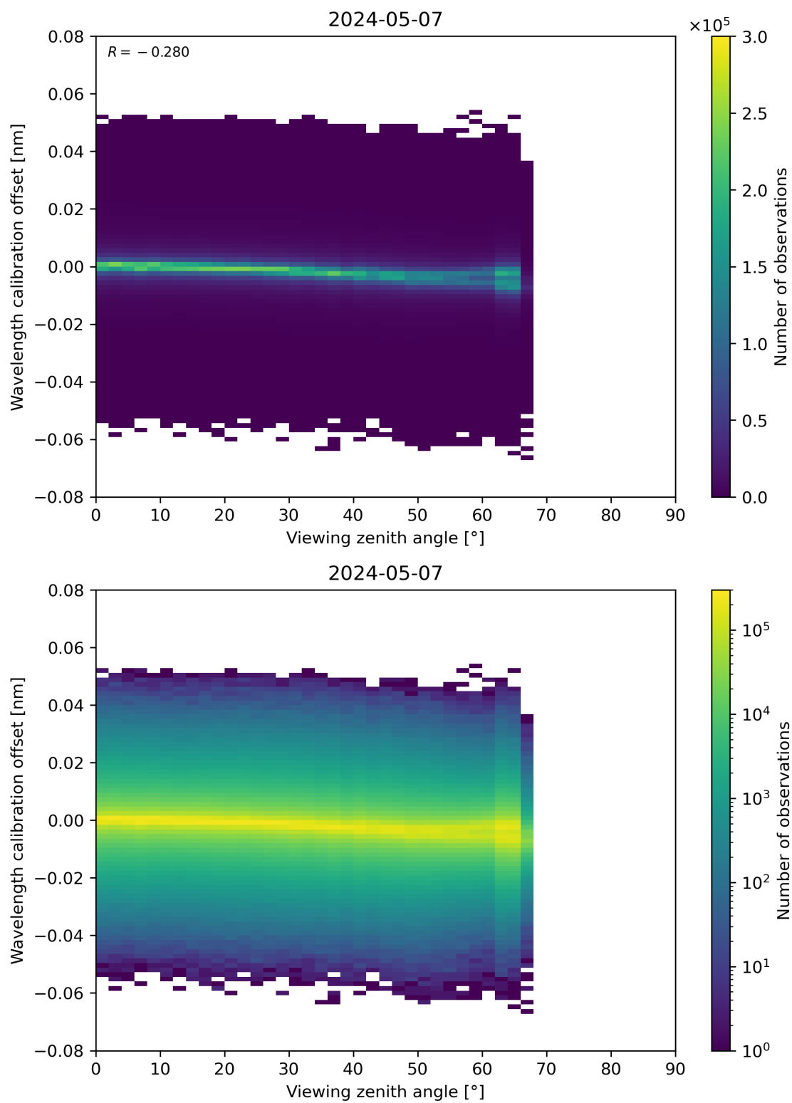
Figure 173: Scatter density plot of “Viewing zenith angle” against “Wavelength calibration offset” for 2024-05-07 to 2024-05-08.
