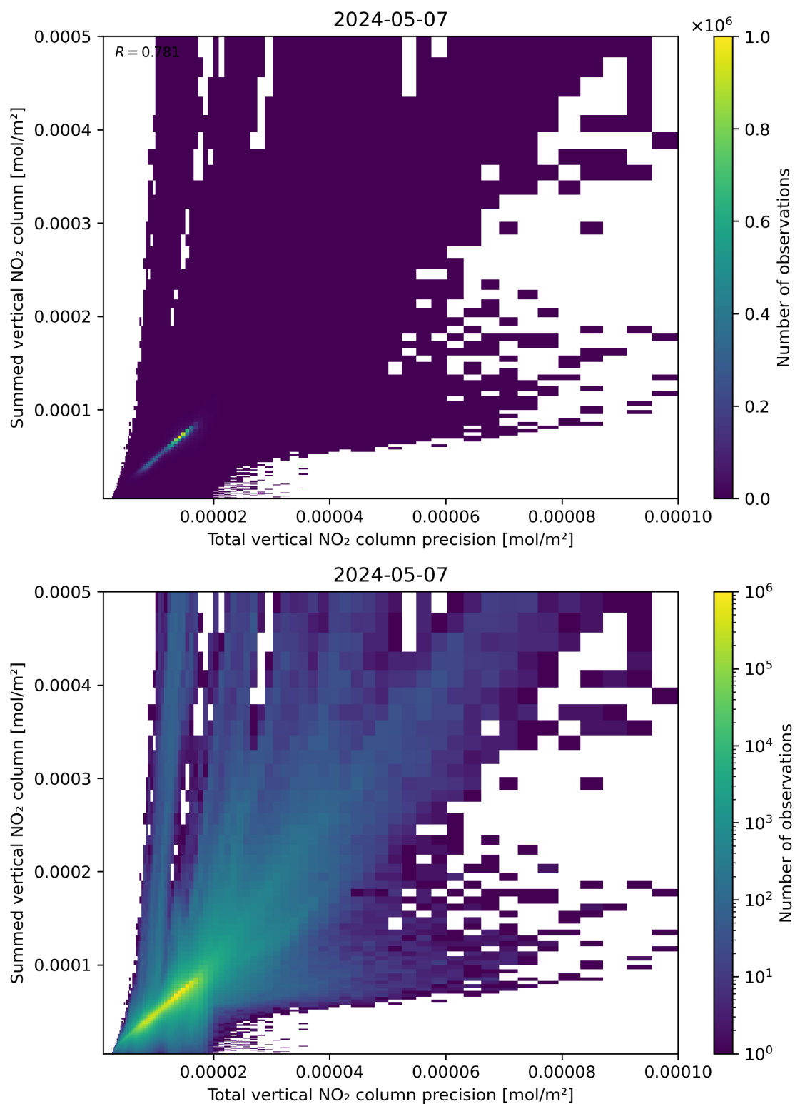
Figure 117: Scatter density plot of “Total vertical NO 2 column precision” against “Summed vertical NO 2 column” for 2024-05-07 to 2024-05-08.
