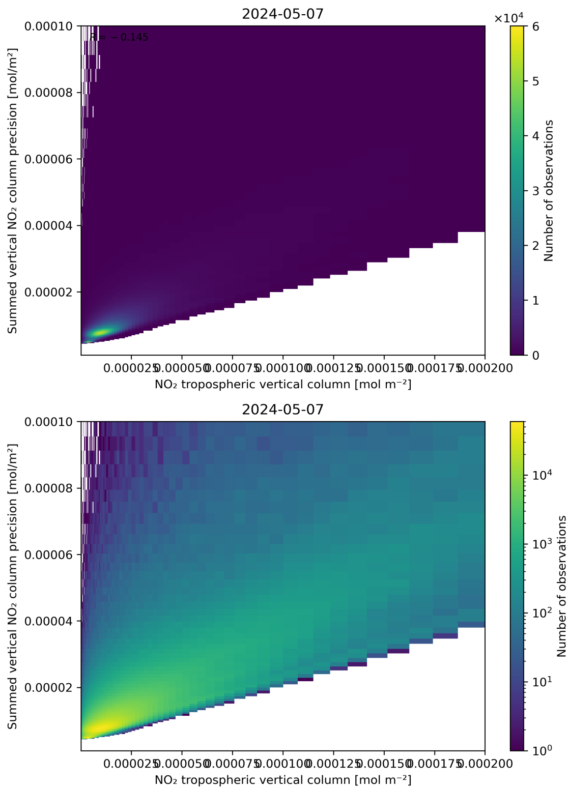
Figure 127: Scatter density plot of “NO 2 tropospheric vertical column” against “Summed vertical NO 2 column precision” for 2024-05-07 to 2024-05-08.
