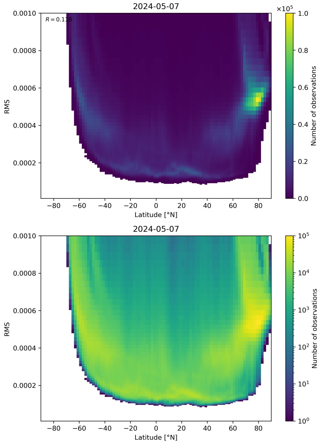
Figure 94: Scatter density plot of “Latitude” against “RMS” for 2024-05-07 to 2024-05-08.
