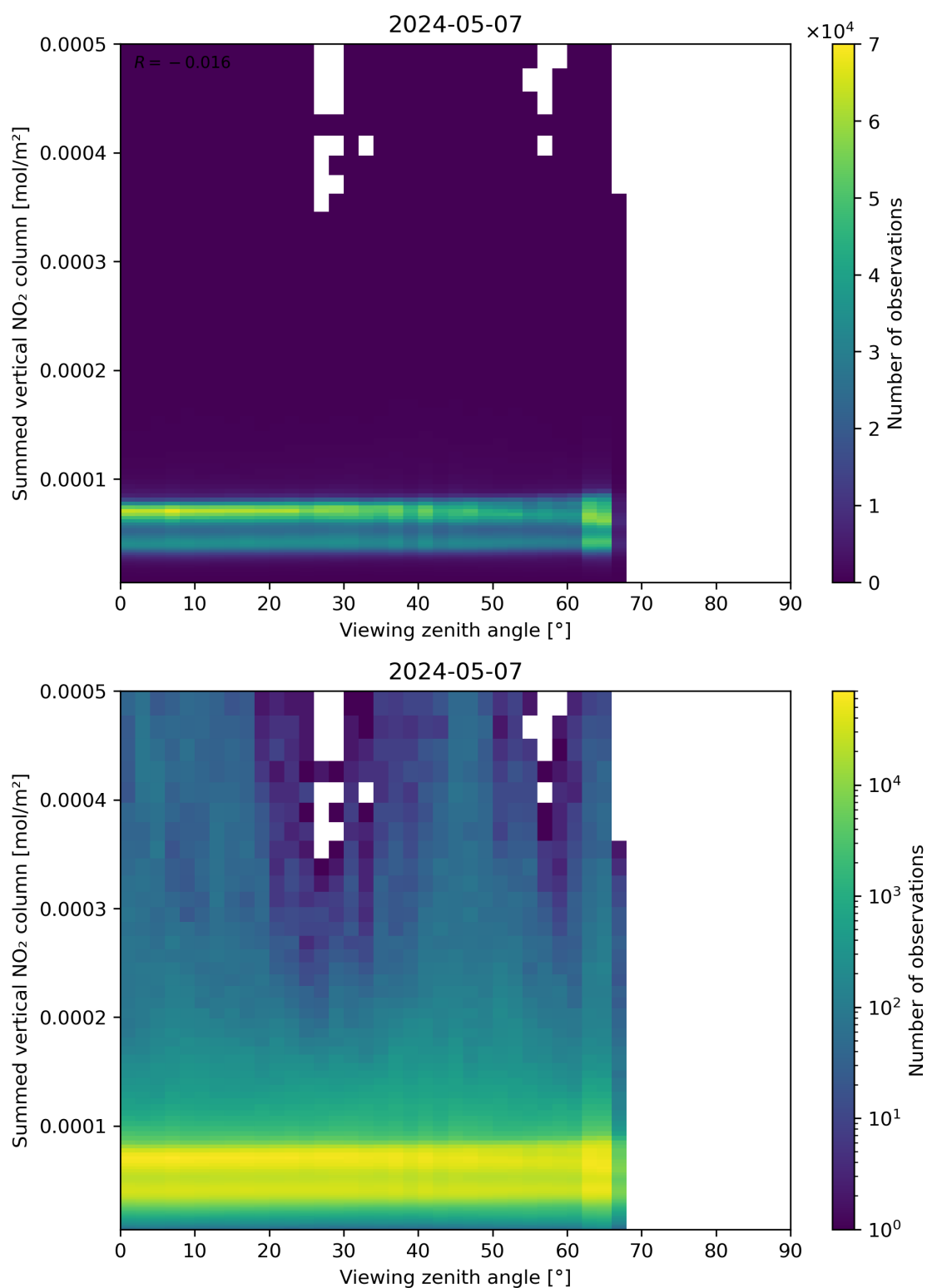
Figure 165: Scatter density plot of “Viewing zenith angle” against “Summed vertical NO 2 column” for 2024-05-07 to 2024-05-08.
