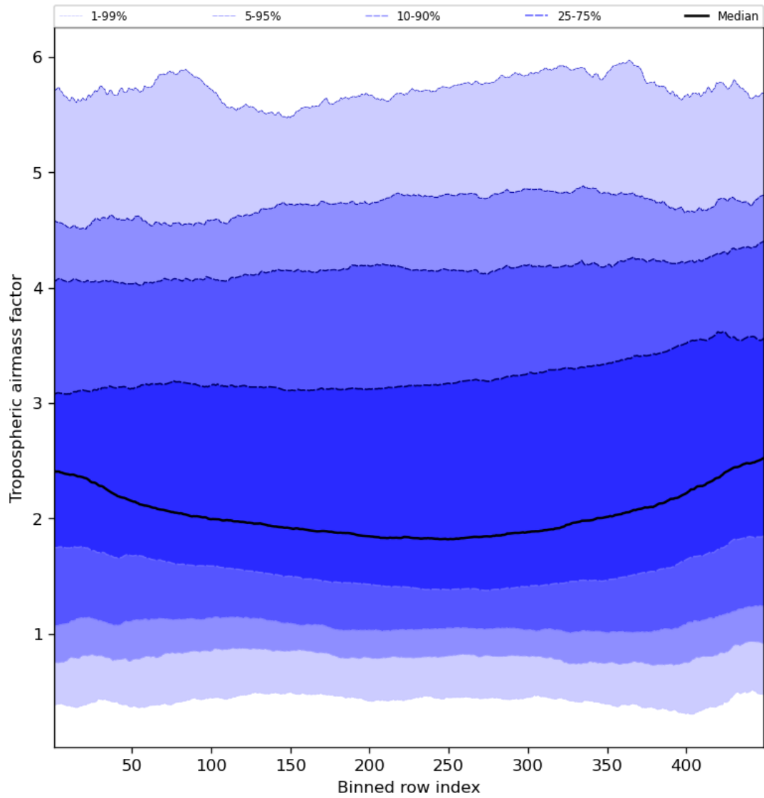
Figure 48: Along track statistics of “Tropospheric airmass factor” for 2024-05-07 to 2024-05-08
