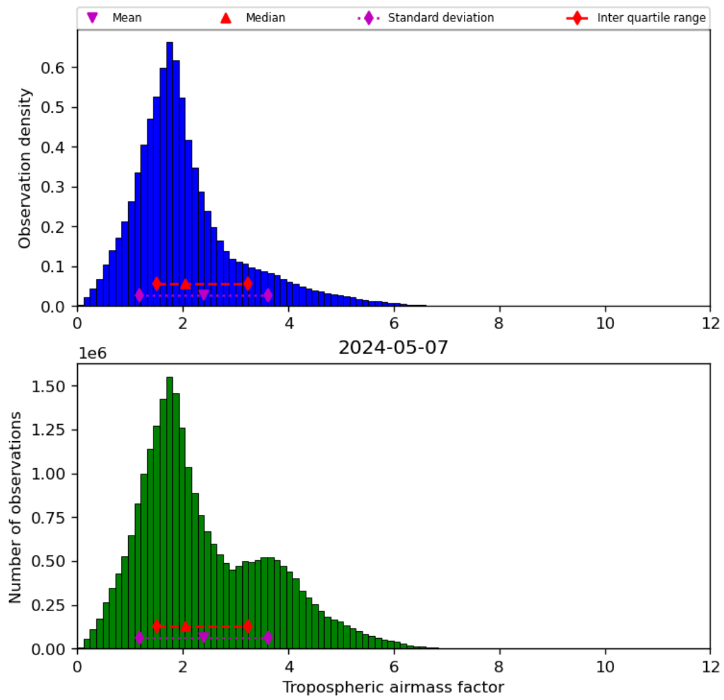
Figure 31: Histogram of “Tropospheric airmass factor” for 2024-05-07 to 2024-05-08
