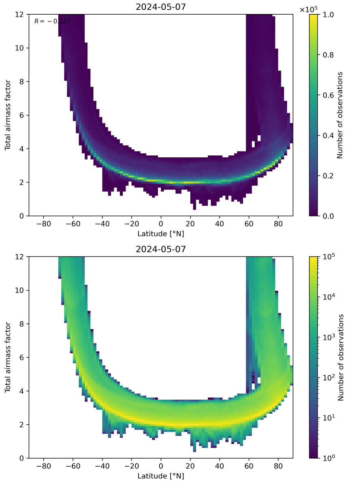
Figure 84: Scatter density plot of “Latitude” against “Total airmass factor” for 2024-05-07 to 2024-05-08.
