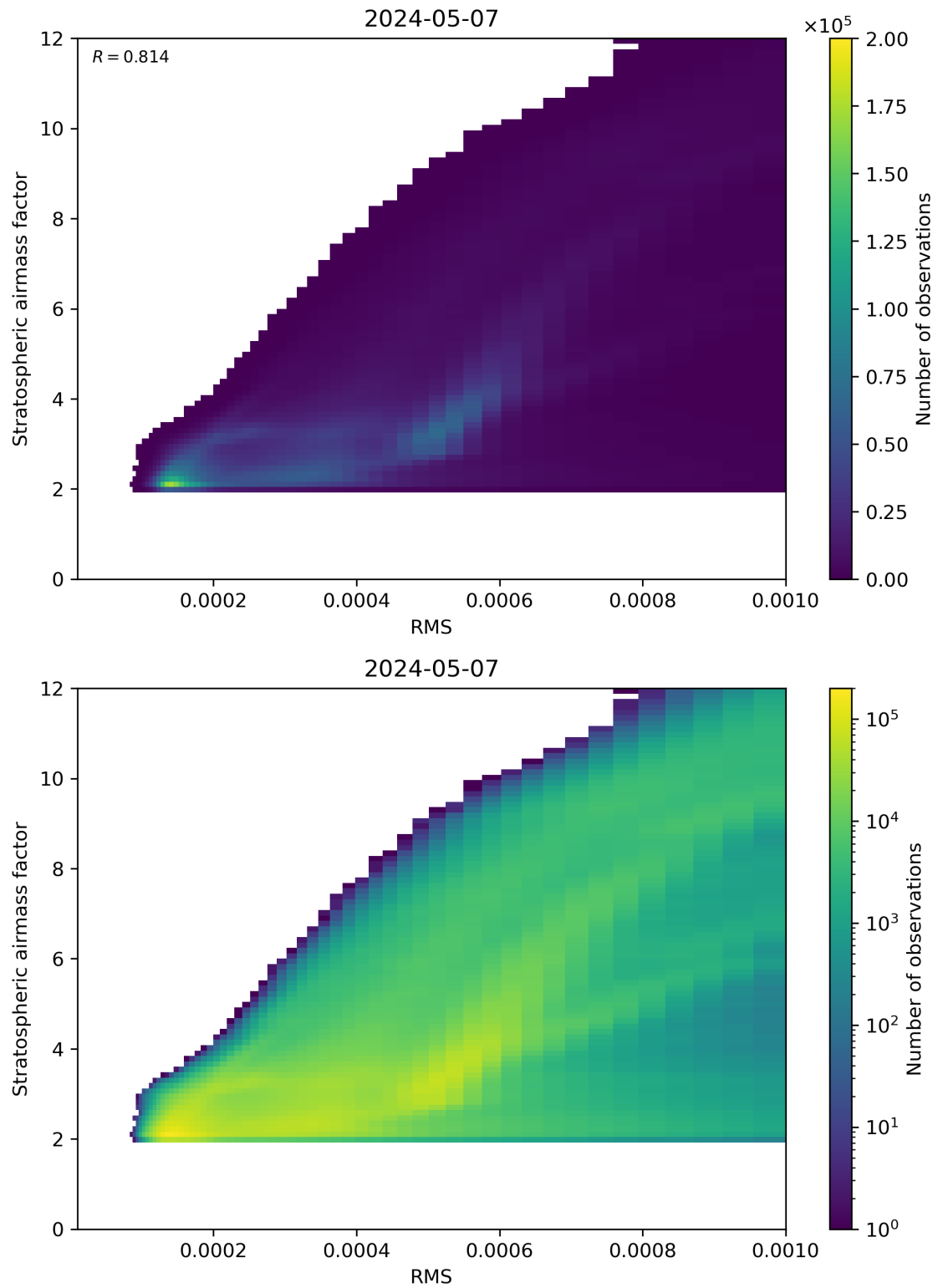
Figure 144: Scatter density plot of “RMS” against “Stratospheric airmass factor” for 2024-05-07 to 2024-05-08.
