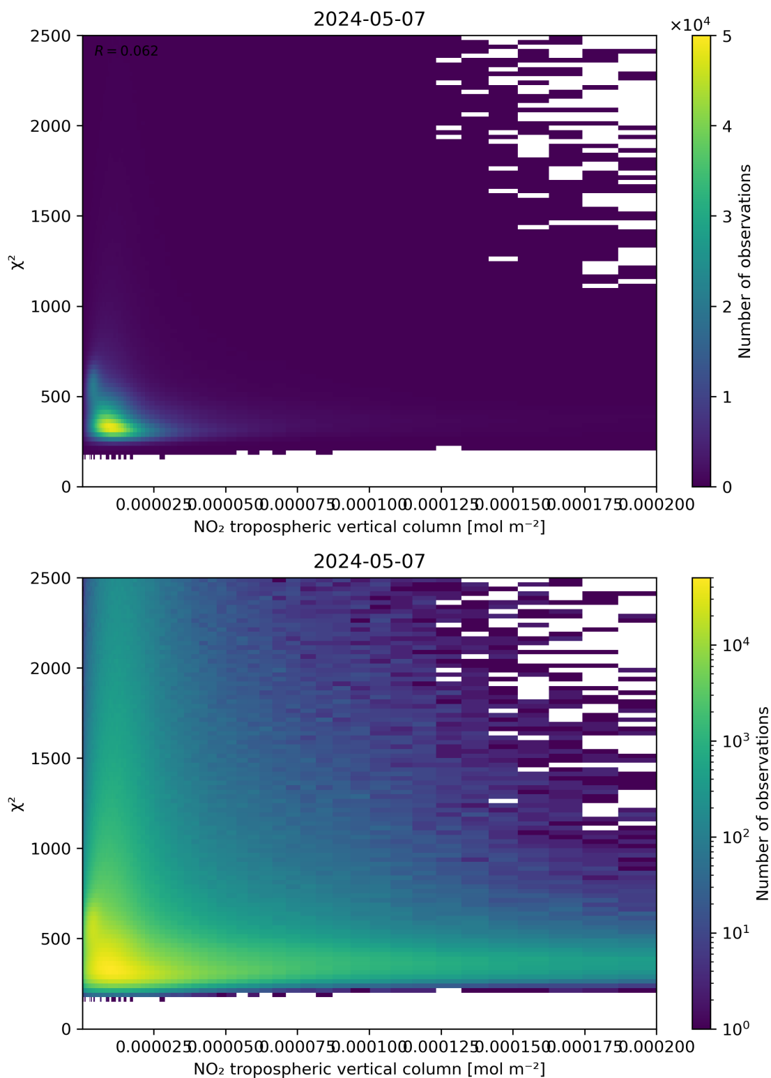
Figure 124: Scatter density plot of “NO 2 tropospheric vertical column” against “ \chi^2 ” for 2024-05-07 to 2024-05-08.
