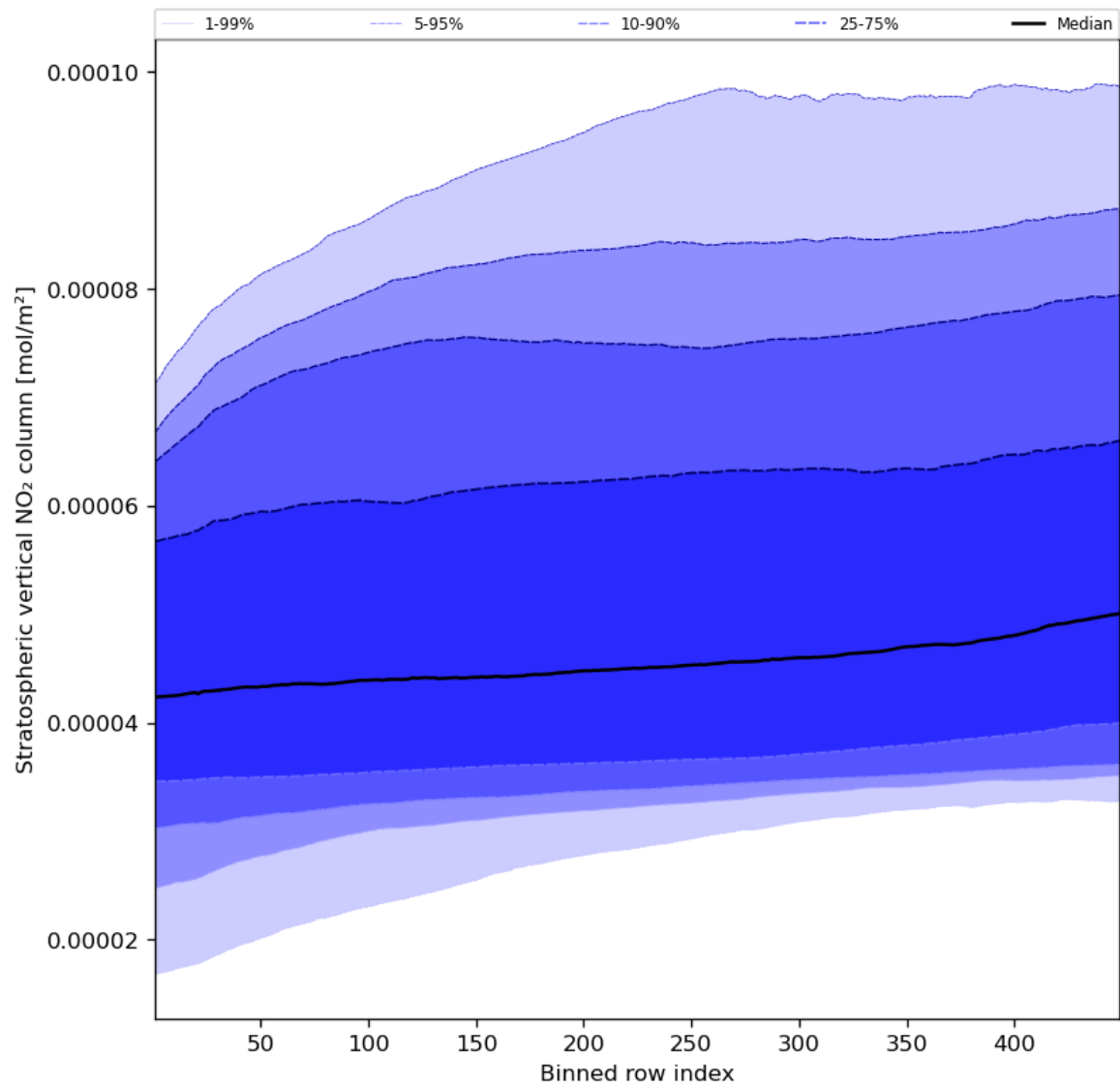
Figure 53: Along track statistics of “Stratospheric vertical NO 2 column” for 2024-05-07 to 2024-05-08
