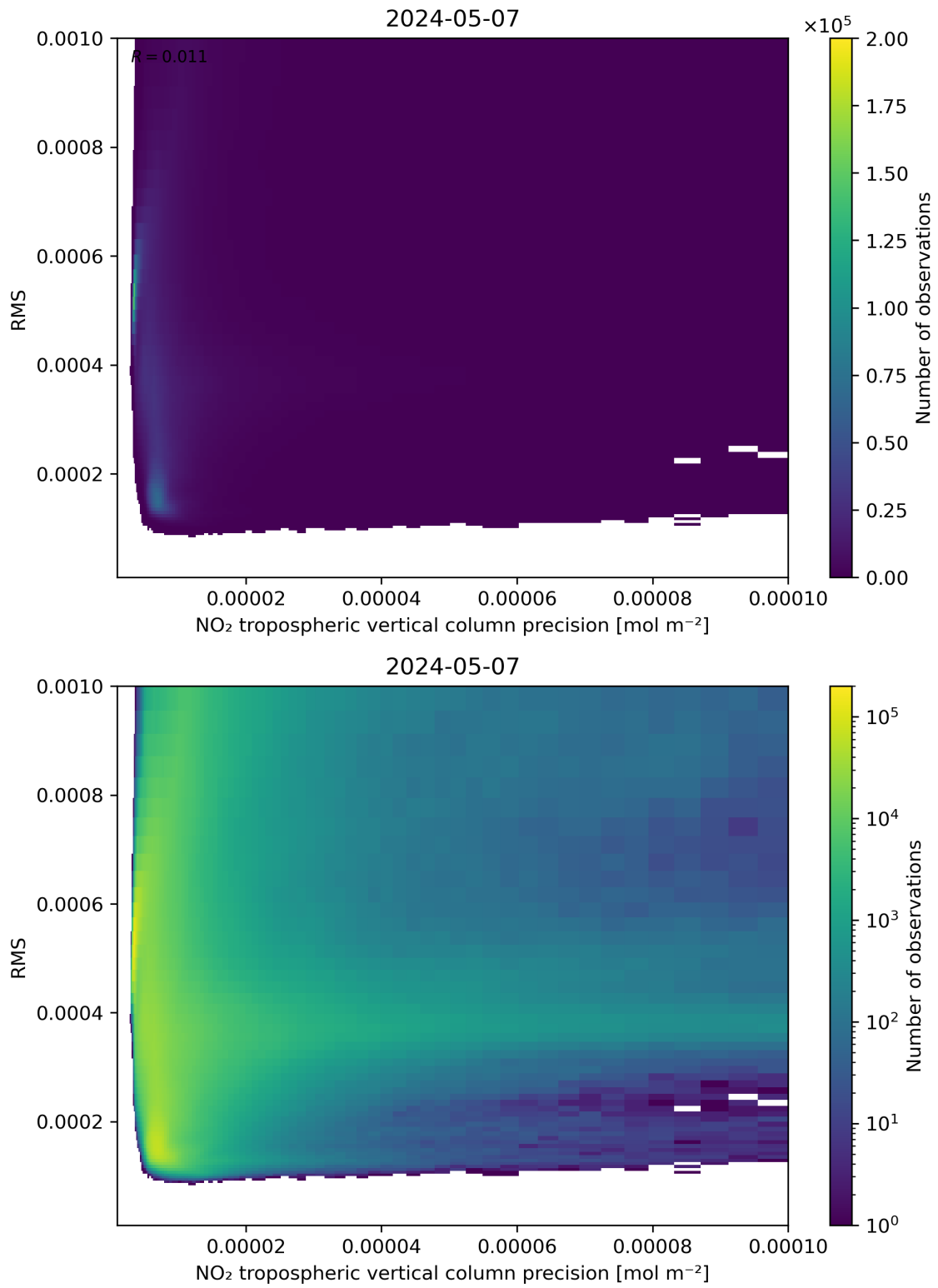
Figure 140: Scatter density plot of “NO 2 tropospheric vertical column precision” against “RMS” for 2024-05-07 to 2024-05-08.
