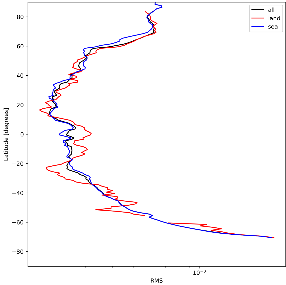
Figure 26: Zonal average of “RMS” for 2024-05-07 to 2024-05-08.
