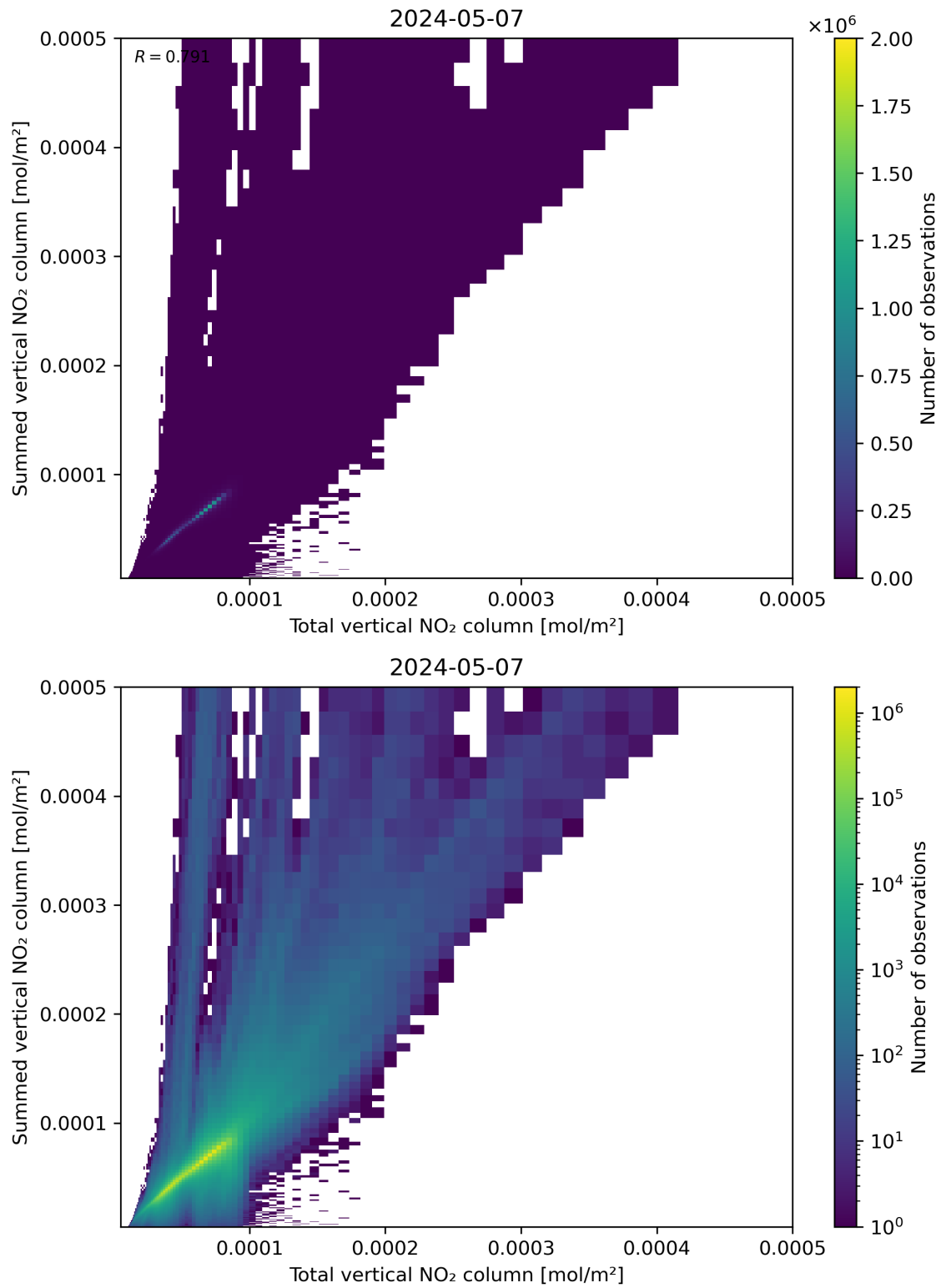
Figure 112: Scatter density plot of “Total vertical NO 2 column” against “Summed vertical NO 2 column” for 2024-05-07 to 2024-05-08.
