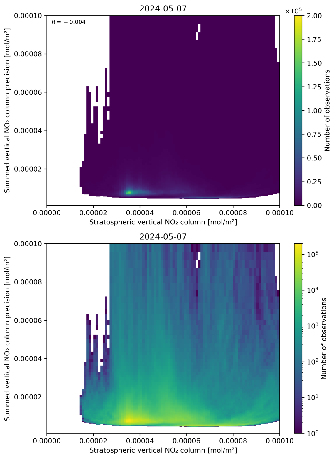
Figure 99: Scatter density plot of “Stratospheric vertical NO 2 column” against “Summed vertical NO 2 column precision” for 2024-05-07 to 2024-05-08.
