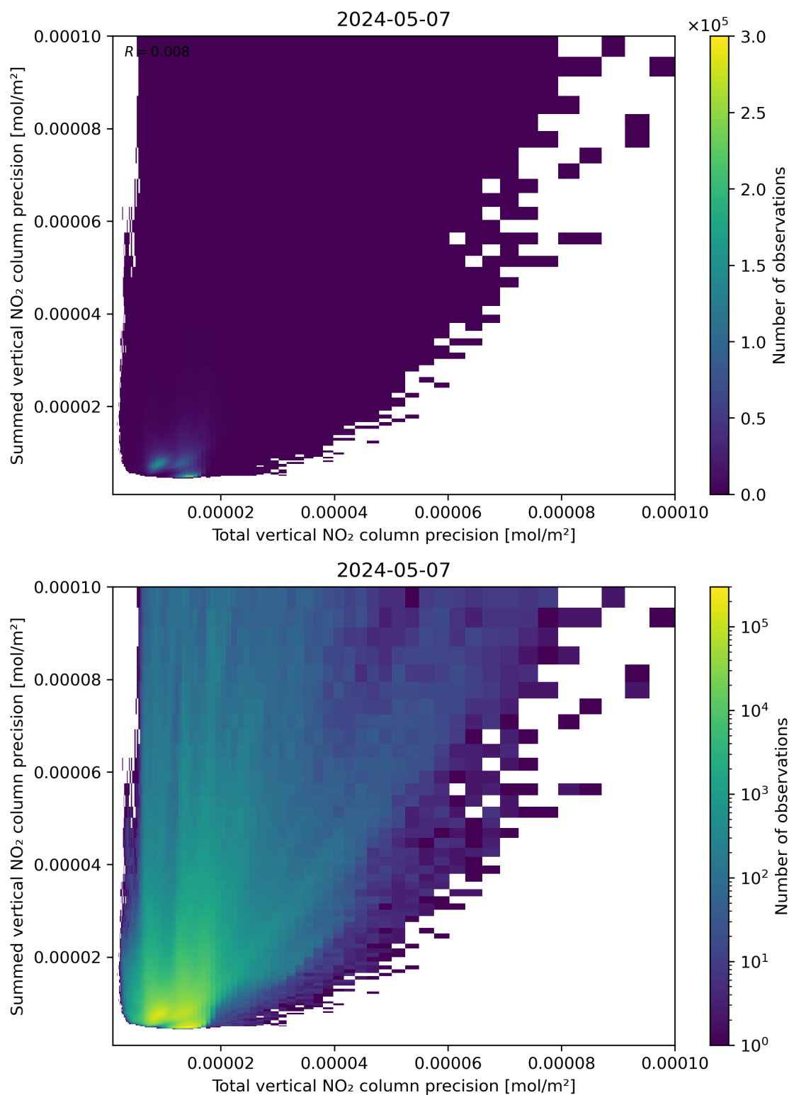
Figure 118: Scatter density plot of “Total vertical NO 2 column precision” against “Summed vertical NO 2 column precision” for 2024-05-07 to 2024-05-08.
