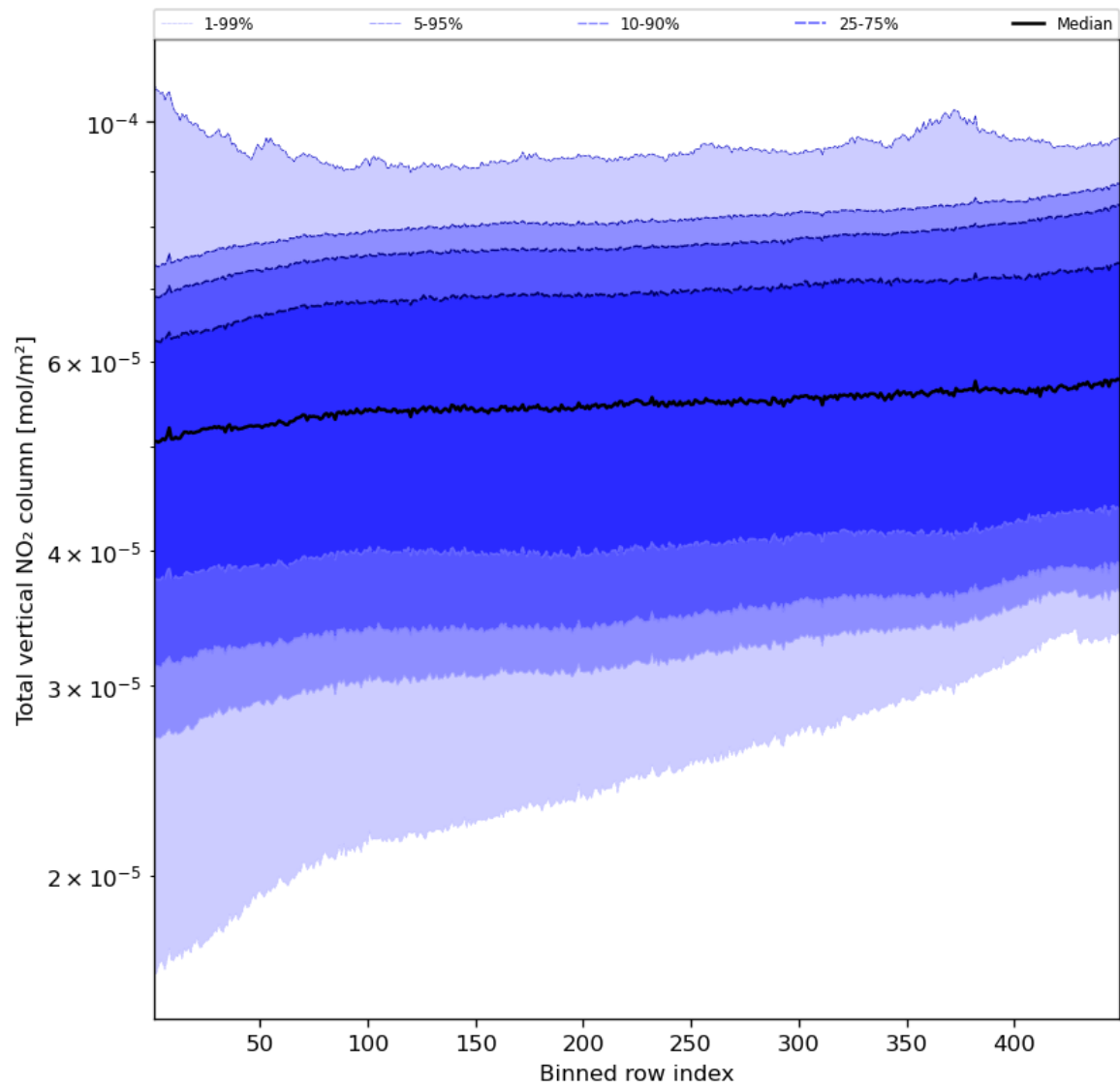
Figure 55: Along track statistics of "Total vertical NO 2 column" for 2024-05-07 to 2024-05-08
