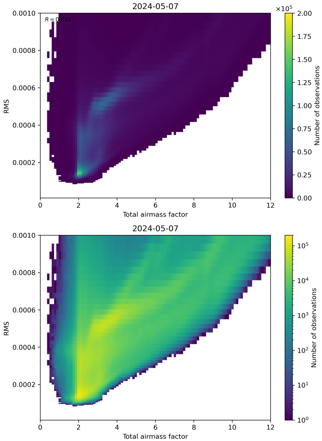
Figure 69: Scatter density plot of “Total airmass factor” against “RMS” for 2024-05-07 to 2024-05-08.
