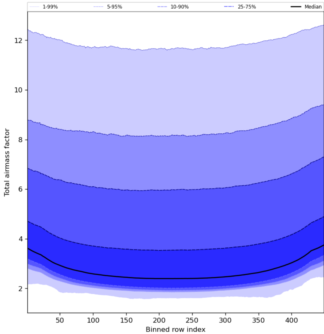
Figure 49: Along track statistics of “Total airmass factor” for 2024-05-07 to 2024-05-08
