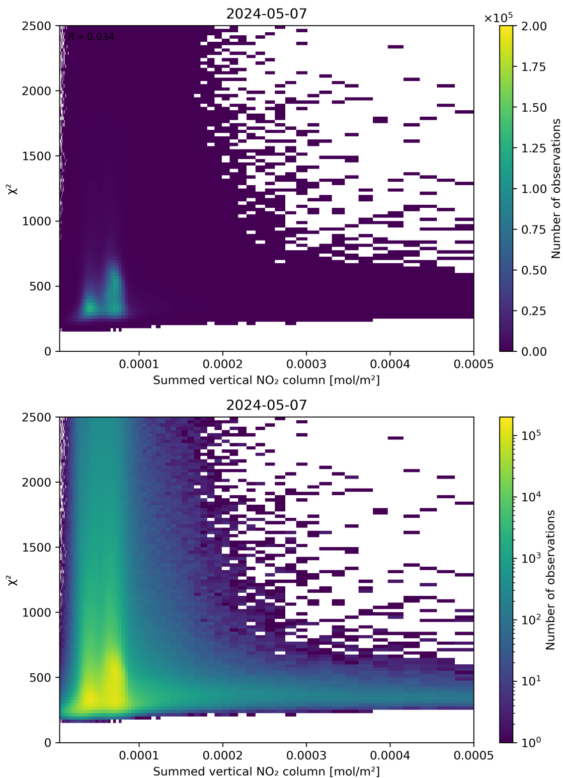
Figure 104: Scatter density plot of “Summed vertical NO 2 column” against “ \chi^2 ” for 2024-05-07 to 2024-05-08.
