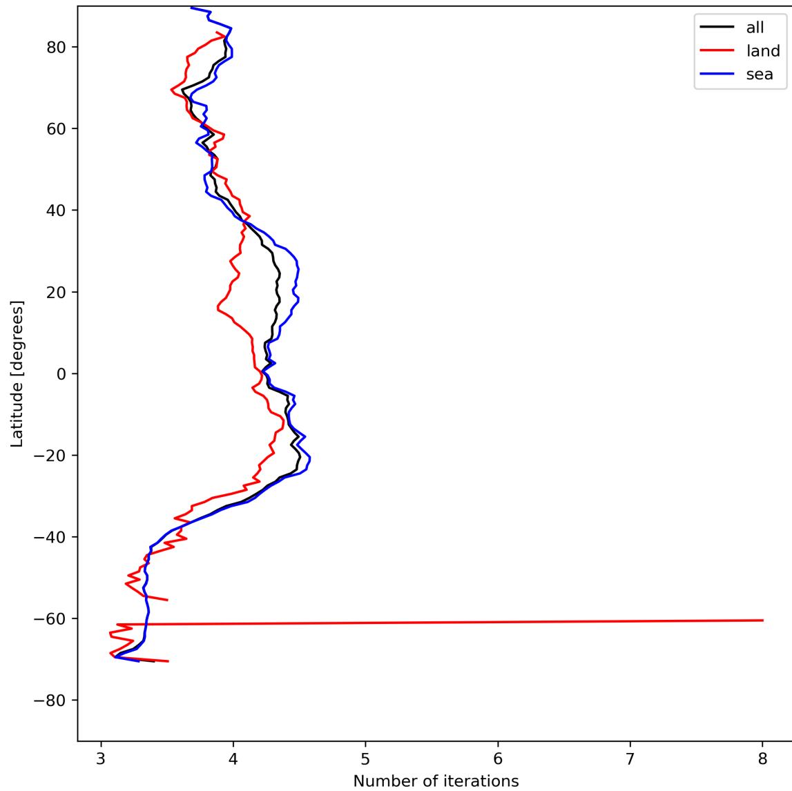
Figure 17: Zonal average of “Number of iterations” for 2024-05-07 to 2024-05-08.
