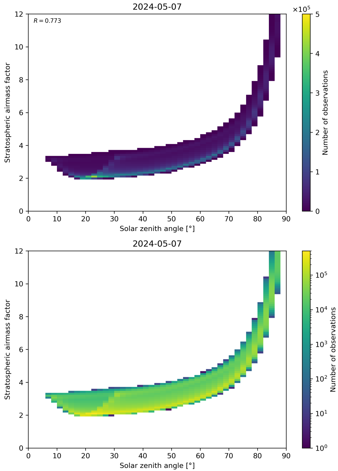
Figure 145: Scatter density plot of “Solar zenith angle” against “Stratospheric airmass factor” for 2024-05-07 to 2024-05-08.
