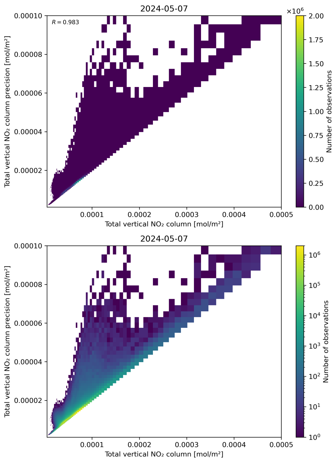
Figure 114: Scatter density plot of “Total vertical NO 2 column” against “Total vertical NO 2 column precision” for 2024-05-07 to 2024-05-08.
