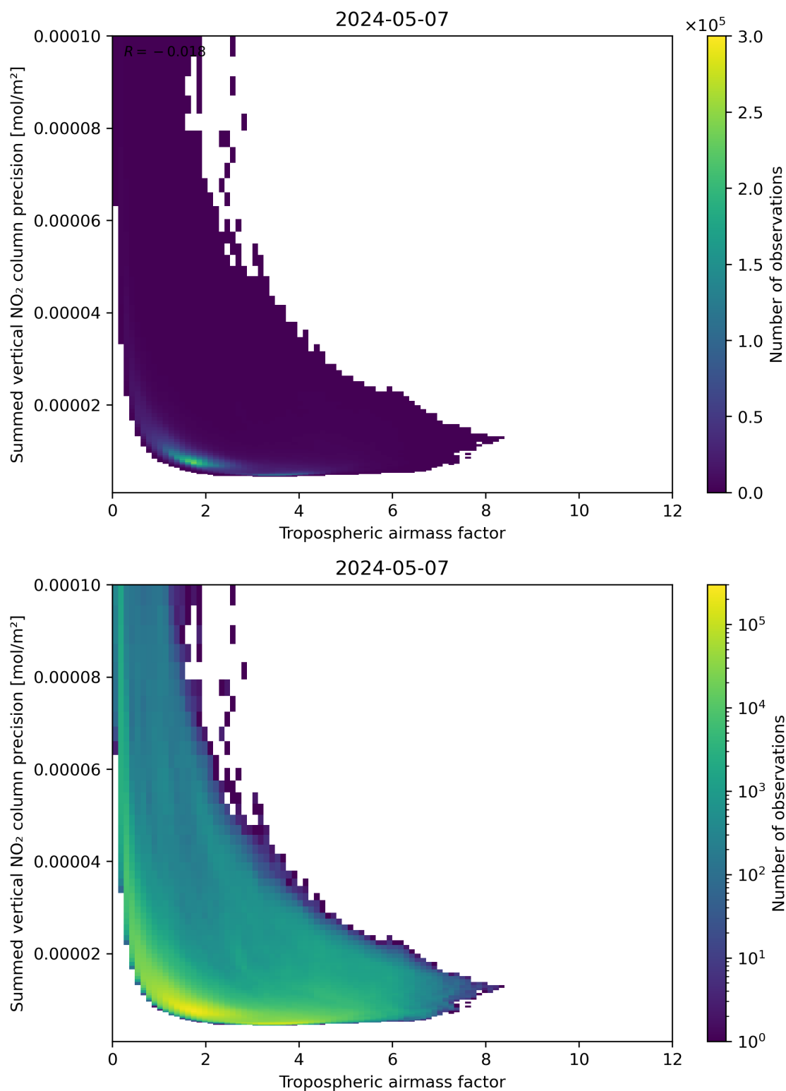
Figure 76: Scatter density plot of “Tropospheric air mass factor” against “Summed vertical NO 2 column precision” for 2024-05-07 to 2024-05-08.
