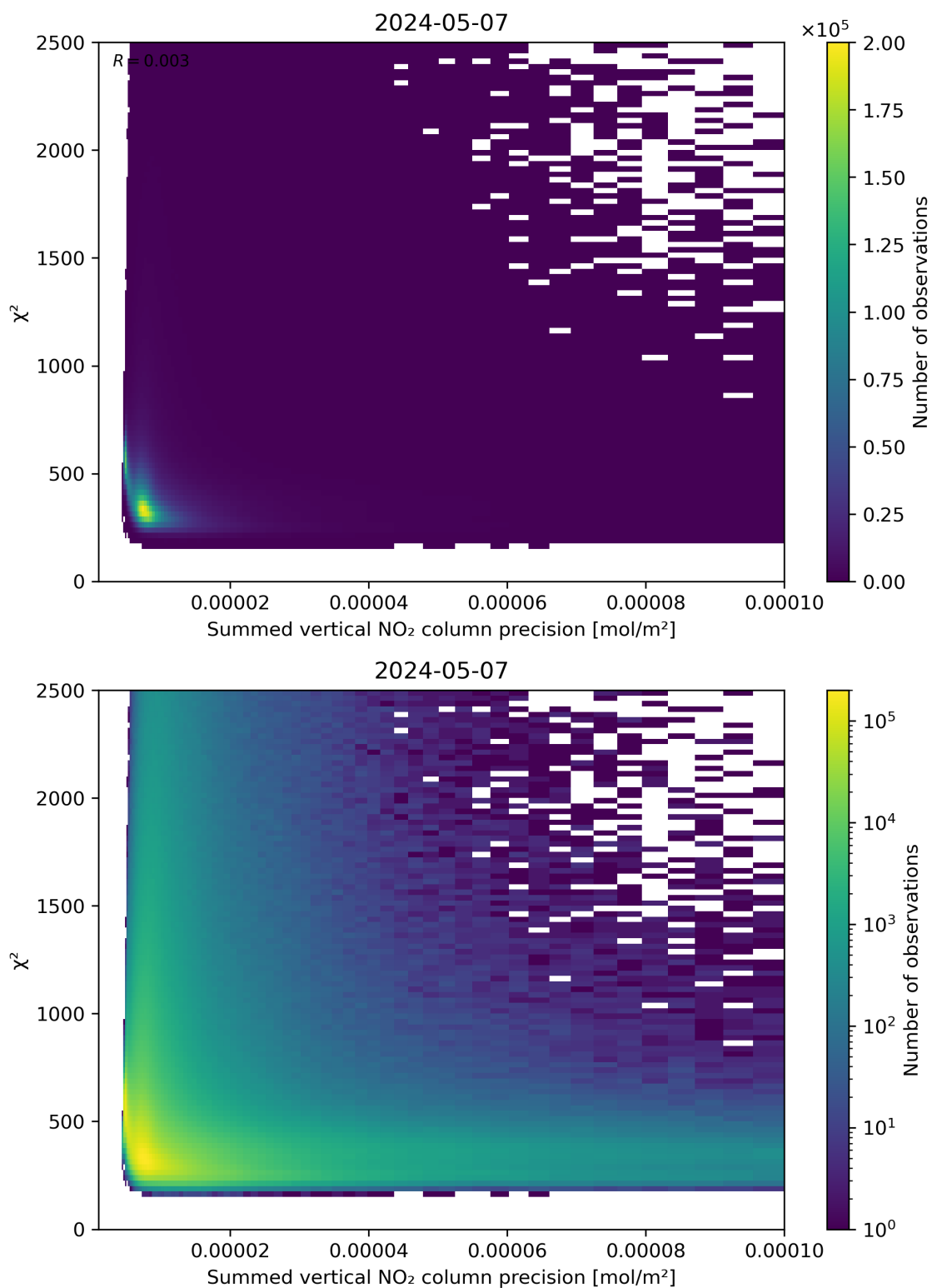
Figure 107: Scatter density plot of “Summed vertical NO 2 column precision” against “ \chi^2 ” for 2024-05-07 to 2024-05-08.
