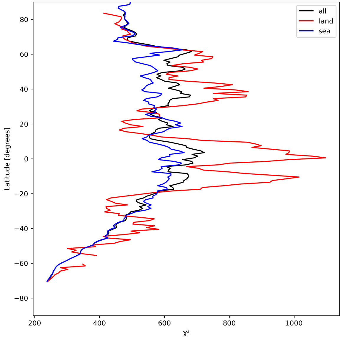
Figure 25: Zonal average of “ \chi^2 ” for 2024-05-07 to 2024-05-08.
