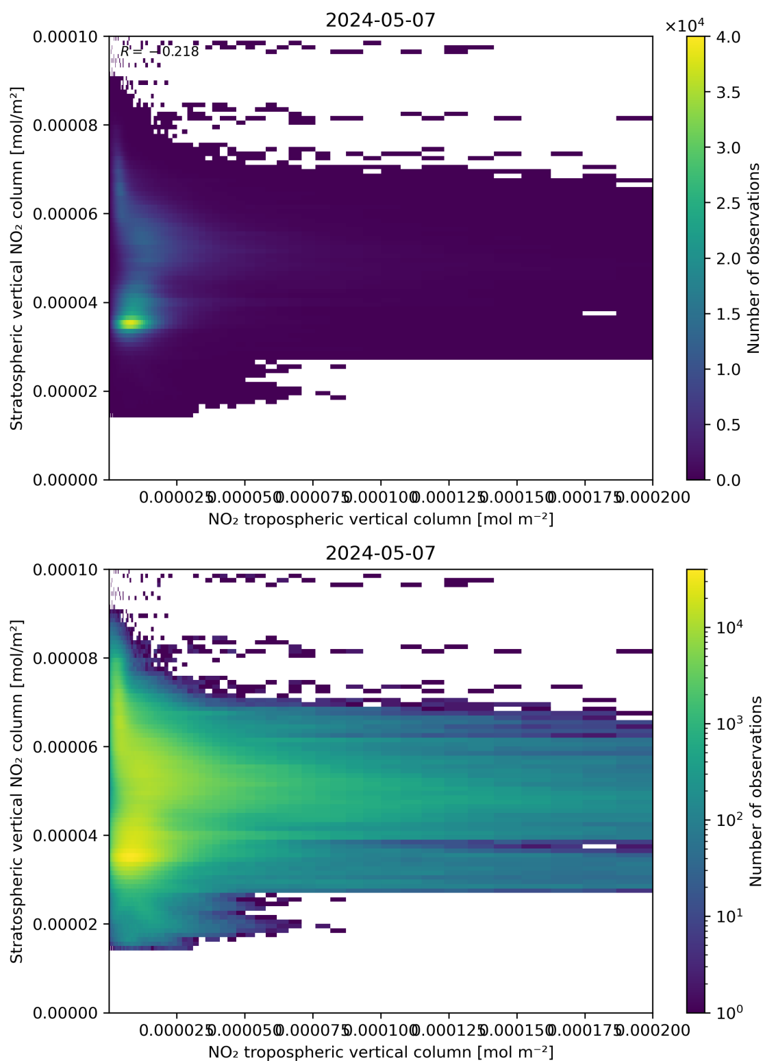
Figure 125: Scatter density plot of “NO 2 tropospheric vertical column” against “Stratospheric vertical NO 2 column” for 2024-05-07 to 2024-05-08.
