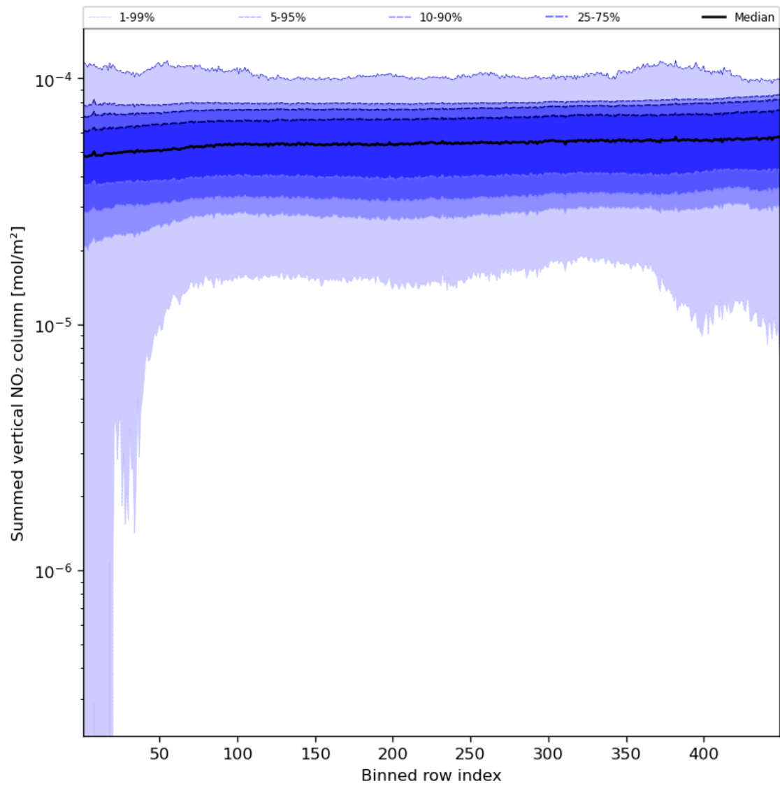
Figure 57: Along track statistics of “Summed vertical NO 2 column” for 2024-05-07 to 2024-05-08
