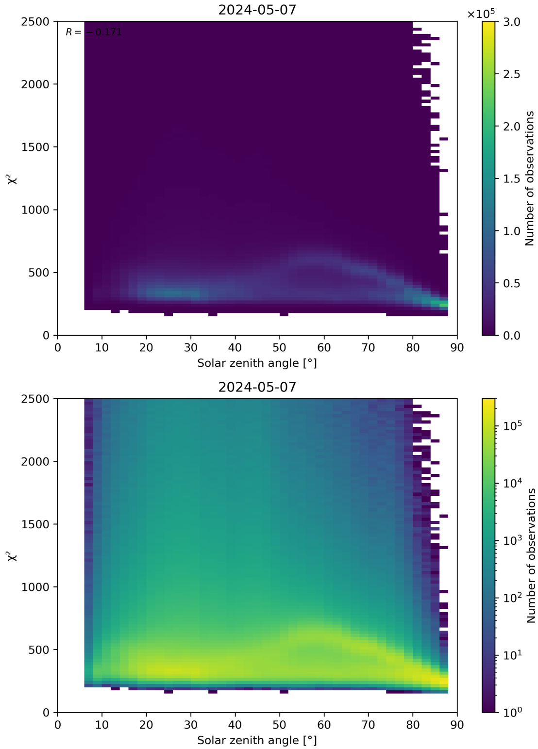
Figure 148: Scatter density plot of “Solar zenith angle” against “ \chi^2 ” for 2024-05-07 to 2024-05-08.
