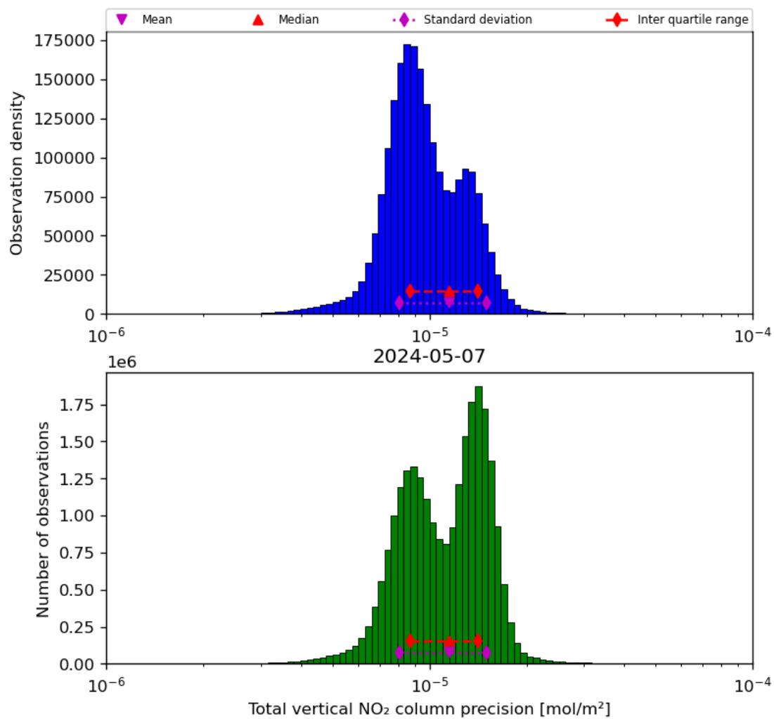
Figure 39: Histogram of “Total vertical NO 2 column precision” for 2024-05-07 to 2024-05-08
