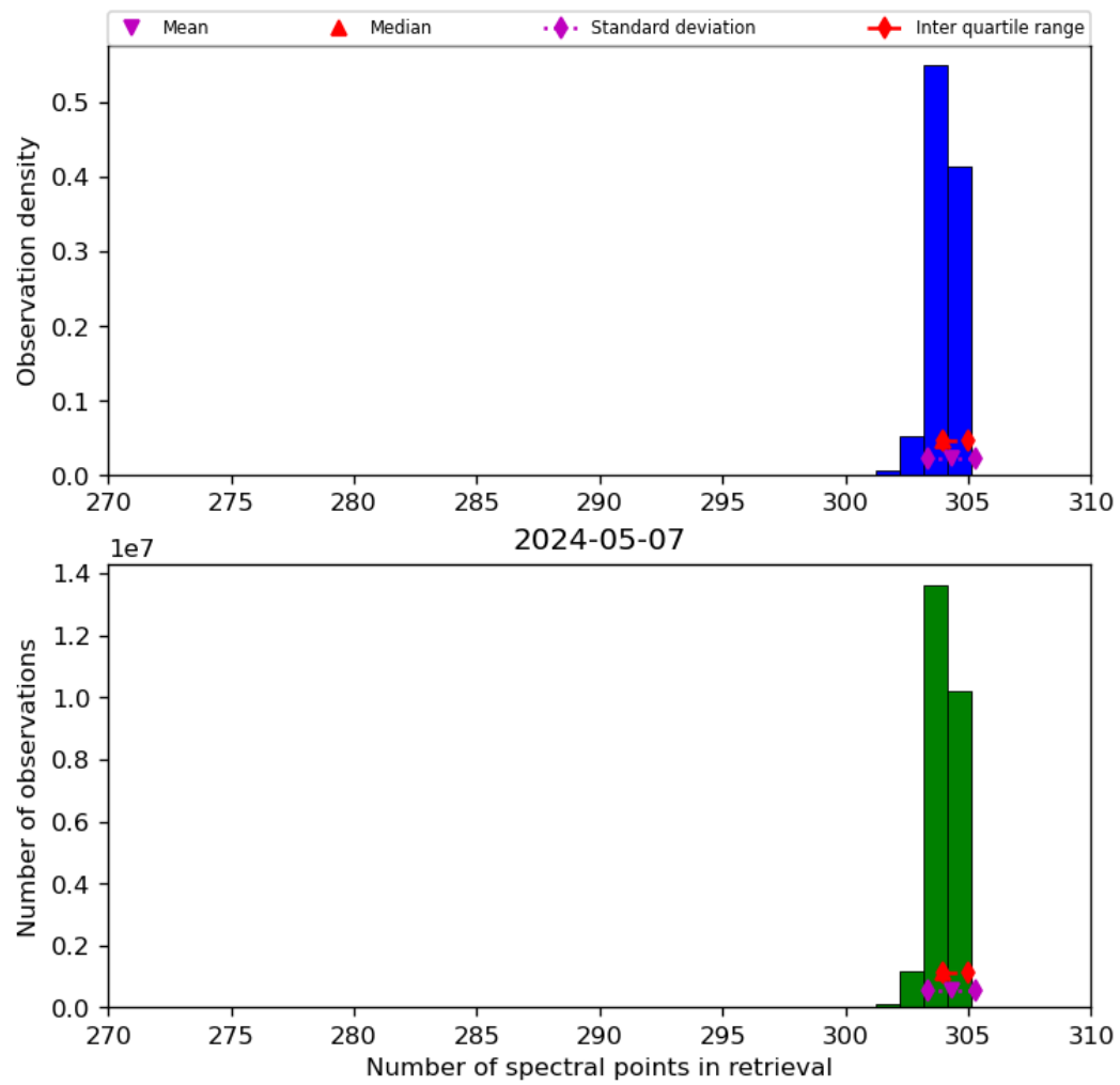
Figure 33: Histogram of “Number of spectral points in retrieval” for 2024-05-07 to 2024-05-08
