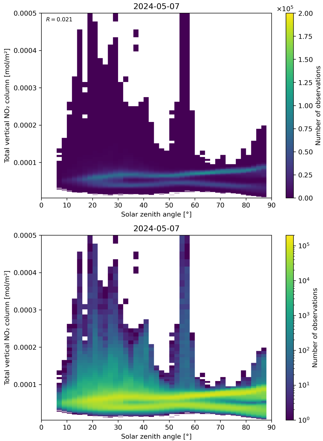
Figure 153: Scatter density plot of “Solar zenith angle” against “Total vertical NO 2 column” for 2024-05-07 to 2024-05-08.
