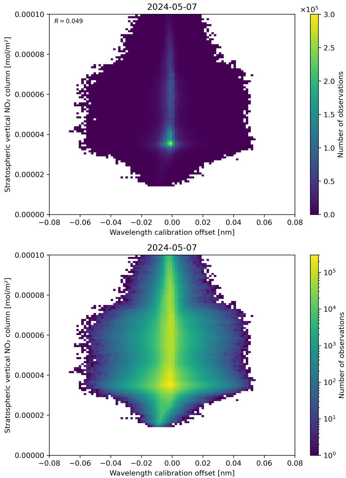
Figure 176: Scatter density plot of “Wavelength calibration offset” against “Stratospheric vertical NO 2 column” for 2024-05-07 to 2024-05-08.
