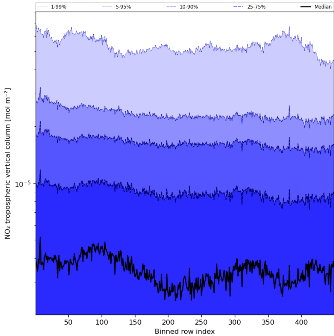
Figure 46: Along track statistics of “NO 2 tropospheric vertical column” for 2024-05-07 to 2024-05-08
