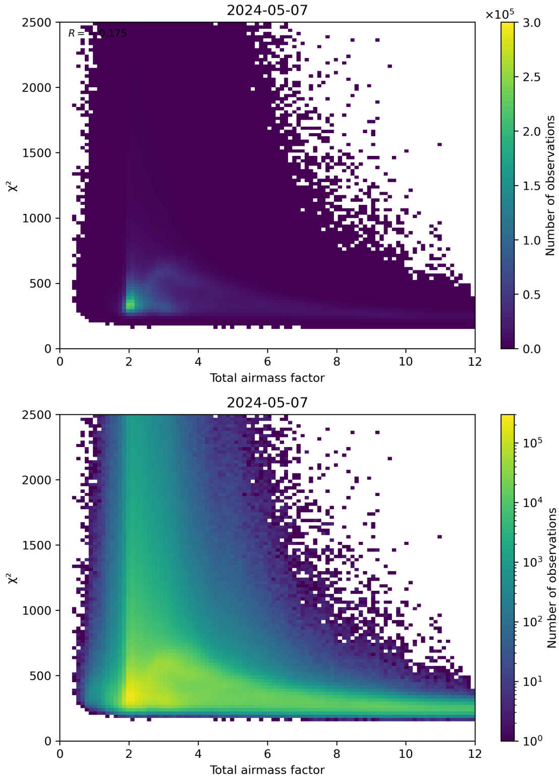
Figure 63: Scatter density plot of “Total airmass factor” against “ \chi^2 ” for 2024-05-07 to 2024-05-08.
