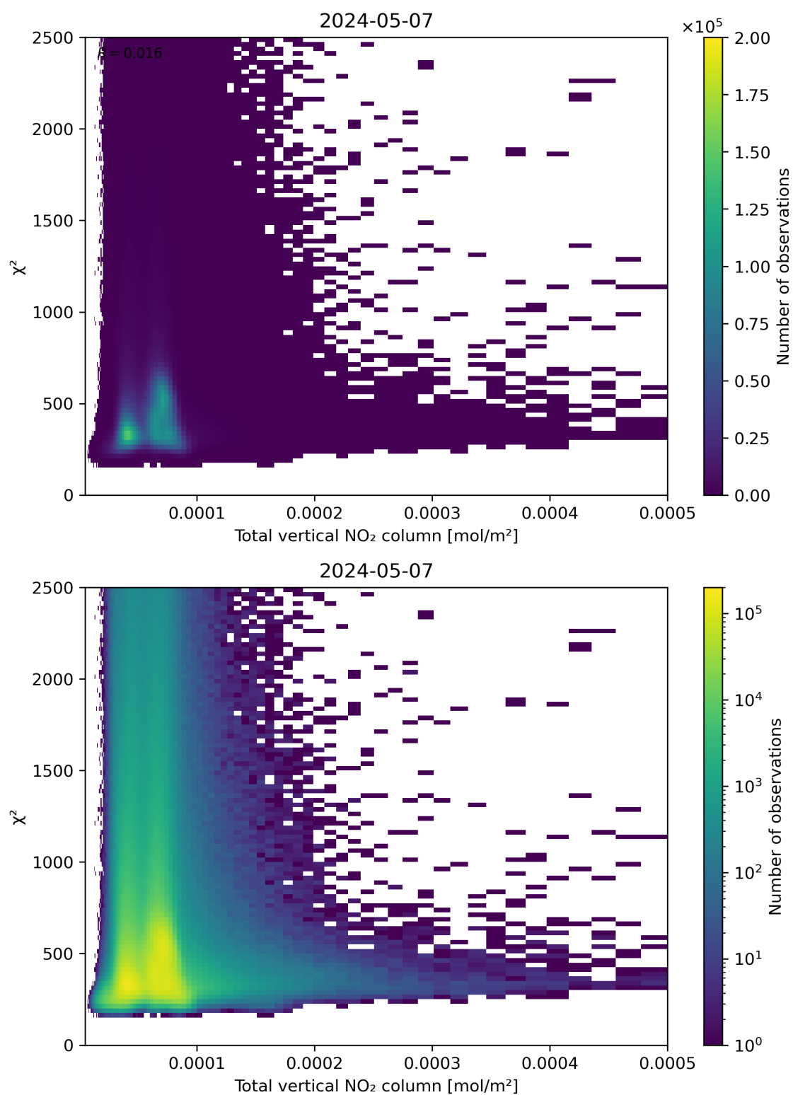
Figure 111: Scatter density plot of “Total vertical NO 2 column” against “ \chi^2 ” for 2024-05-07 to 2024-05-08.
