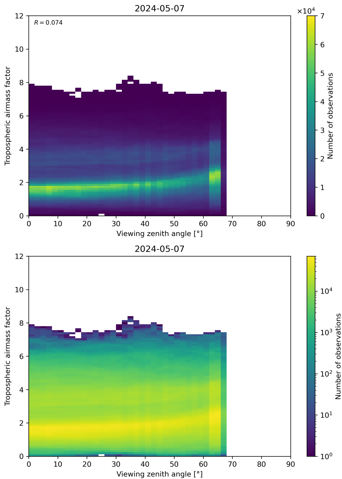
Figure 161: Scatter density plot of “Viewing zenith angle” against “Tropospheric airmass factor” for 2024-05-07 to 2024-05-08.
