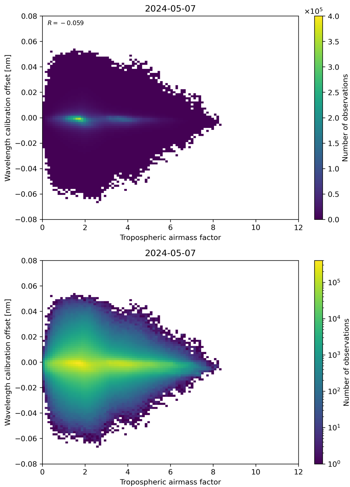
Figure 80: Scatter density plot of “Tropospheric air mass factor” against “Wavelength calibration offset” for 2024-05-07 to 2024-05-08.
