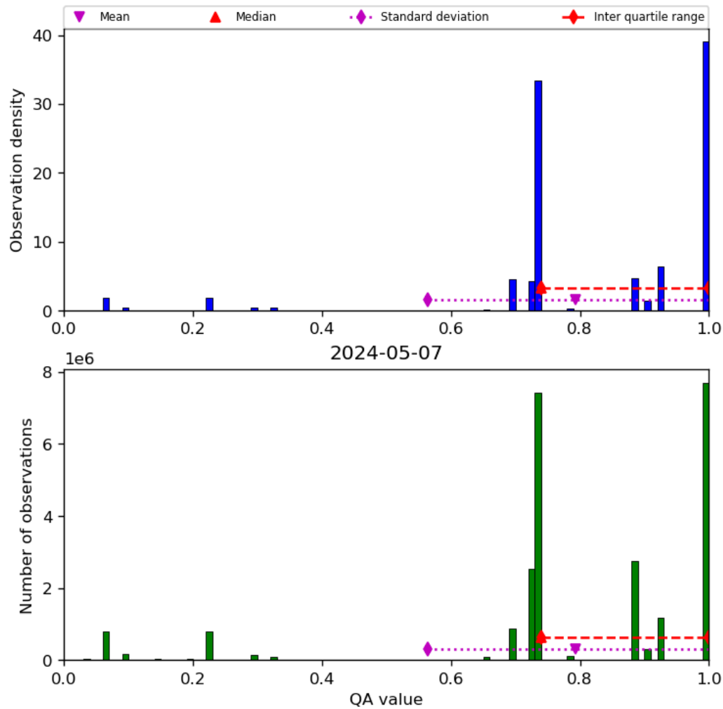
Figure 28: Histogram of “QA value” for 2024-05-07 to 2024-05-08
