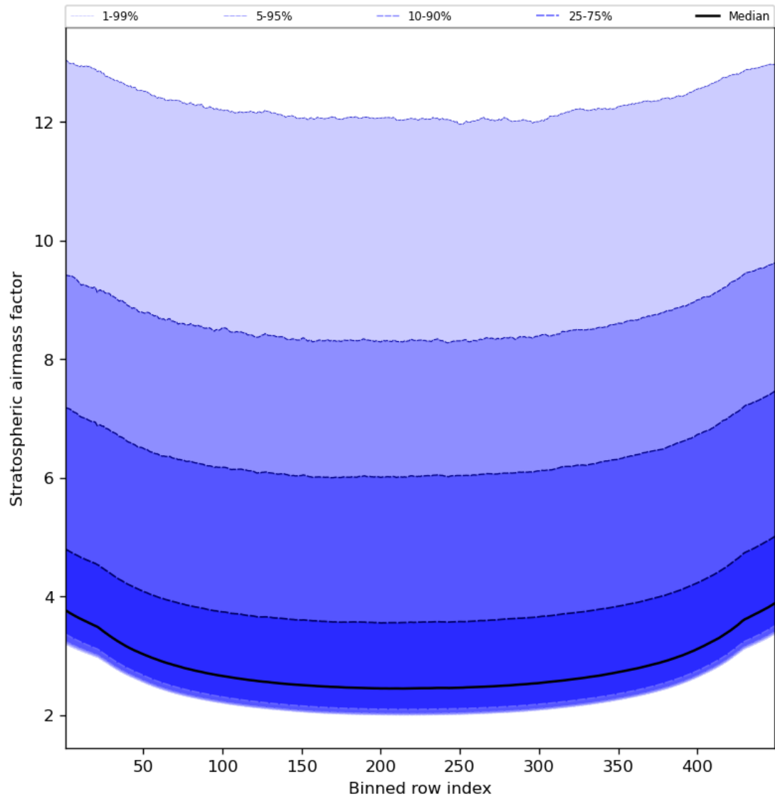
Figure 61: Along track statistics of “Stratospheric airmass factor” for 2024-05-07 to 2024-05-08
