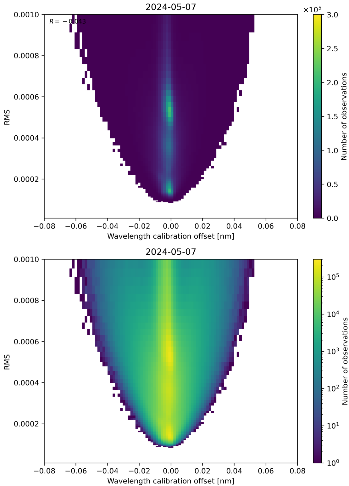
Figure 181: Scatter density plot of “Wavelength calibration offset” against “RMS” for 2024-05-07 to 2024-05-08.
