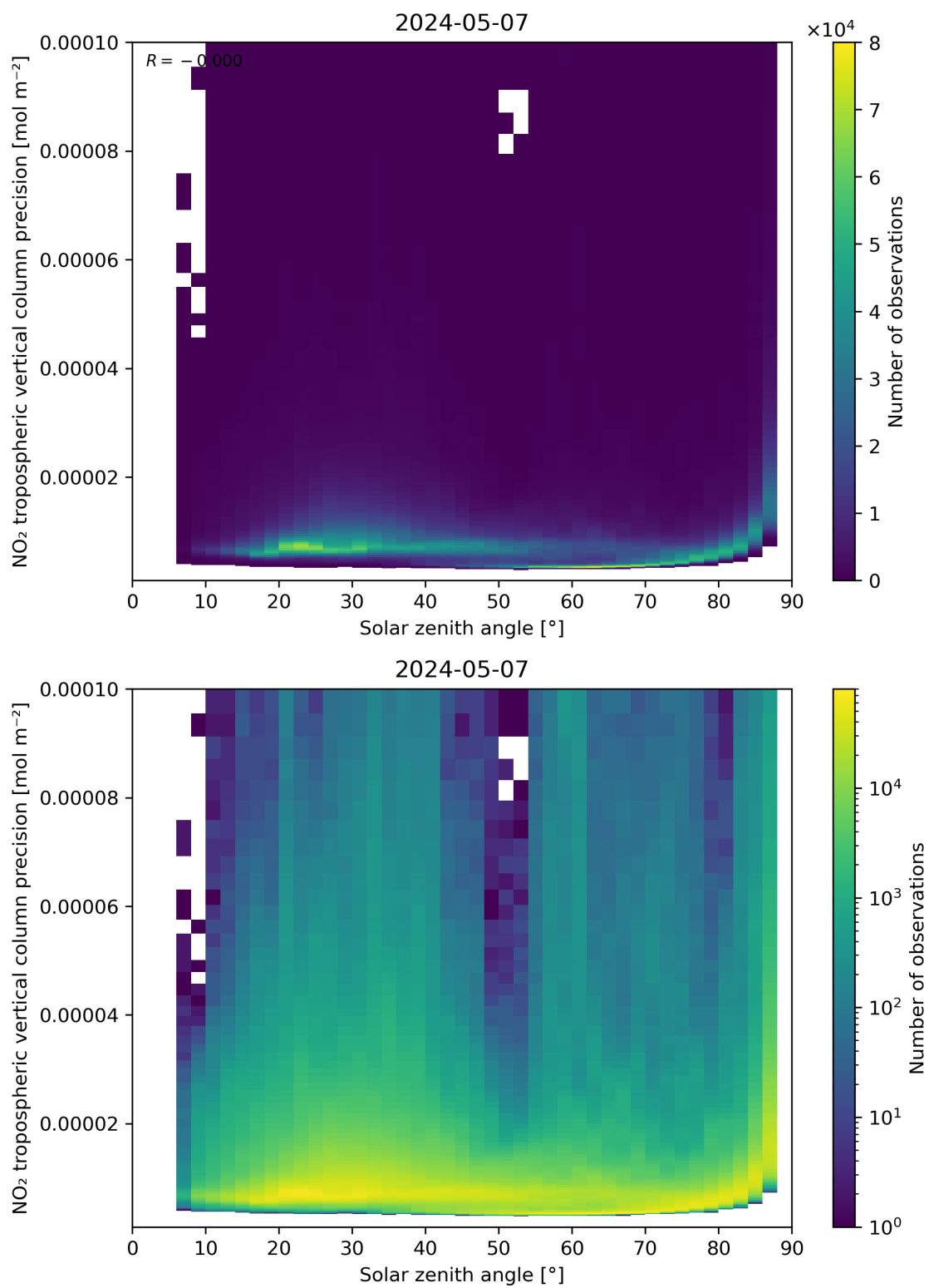
Figure 156: Scatter density plot of “Solar zenith angle” against “NO 2 tropospheric vertical column precision” for 2024-05-07 to 2024-05-08.
