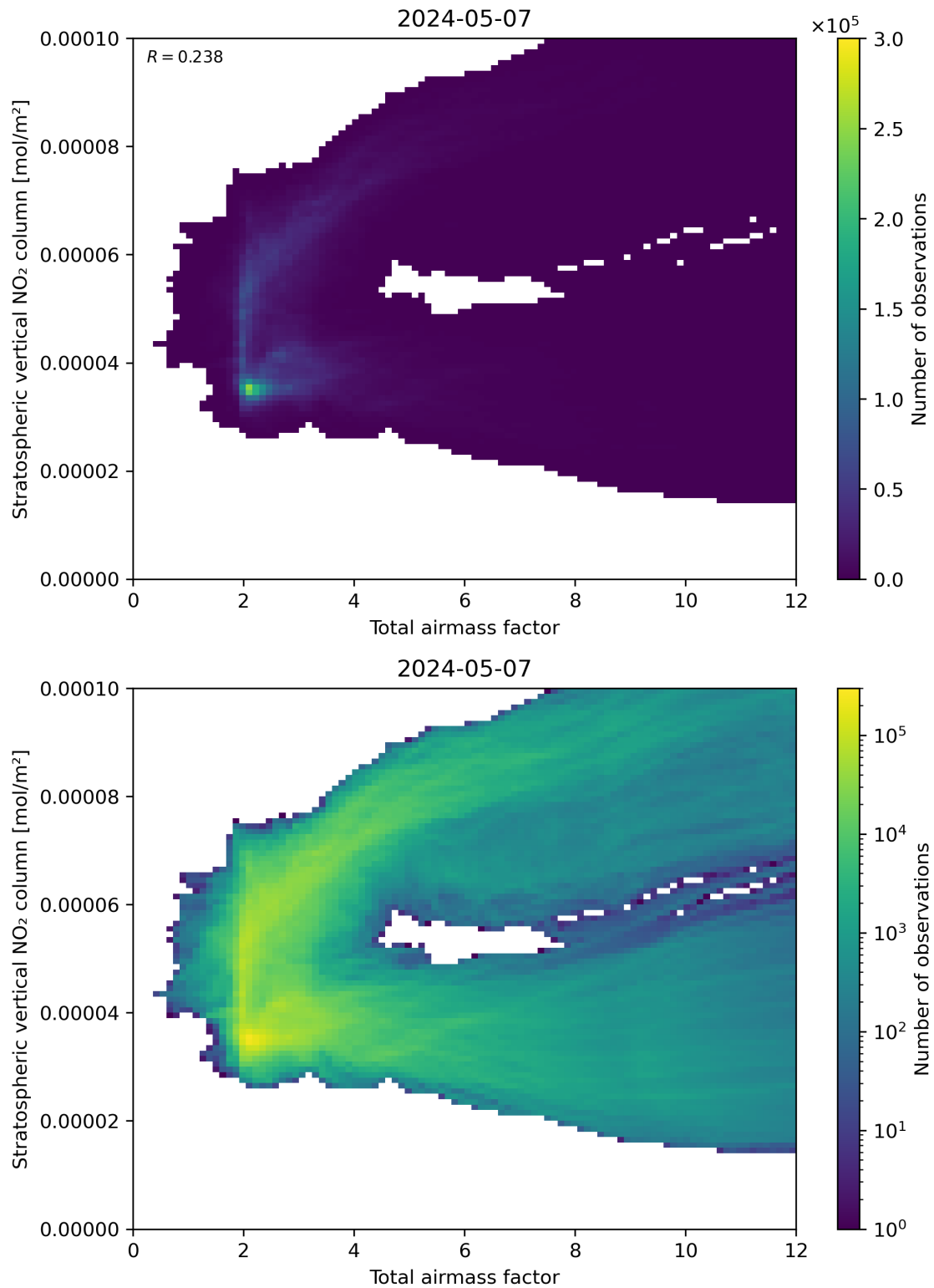
Figure 64: Scatter density plot of “Total airmass factor” against “Stratospheric vertical \text{NO}_2 column” for 2024-05-07 to 2024-05-08.
