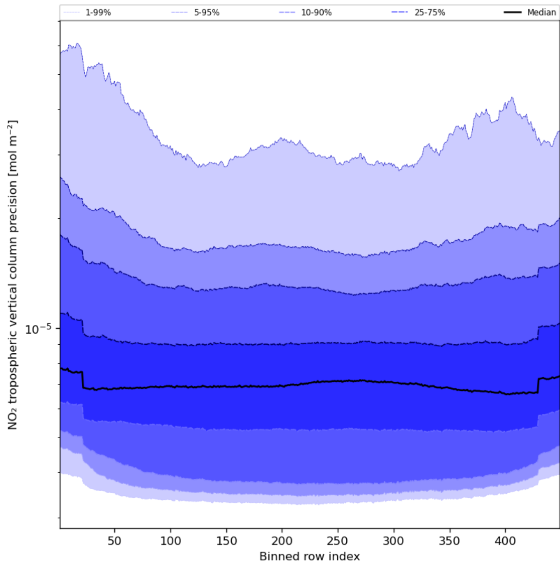
Figure 47: Along track statistics of “NO 2 tropospheric vertical column precision” for 2024-05-07 to 2024-05-08
