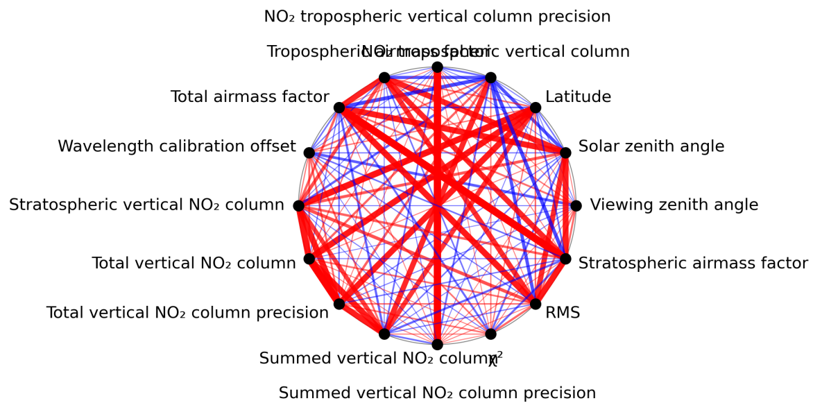
Figure 1: Map of correlation graph for 2024-05-07 to 2024-05-08.
