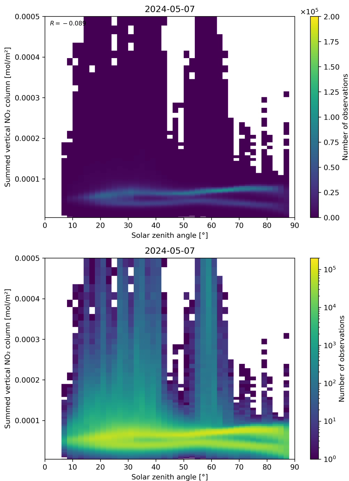
Figure 151: Scatter density plot of “Solar zenith angle” against “Summed vertical NO 2 column” for 2024-05-07 to 2024-05-08.
