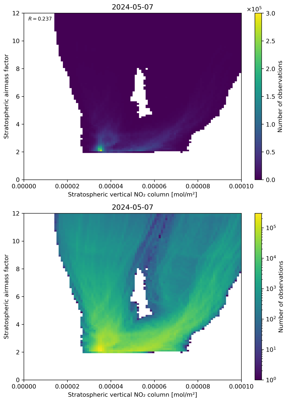
Figure 96: Scatter density plot of “Stratospheric vertical NO 2 column” against “Stratospheric airmass factor” for 2024-05-07 to 2024-05-08.
