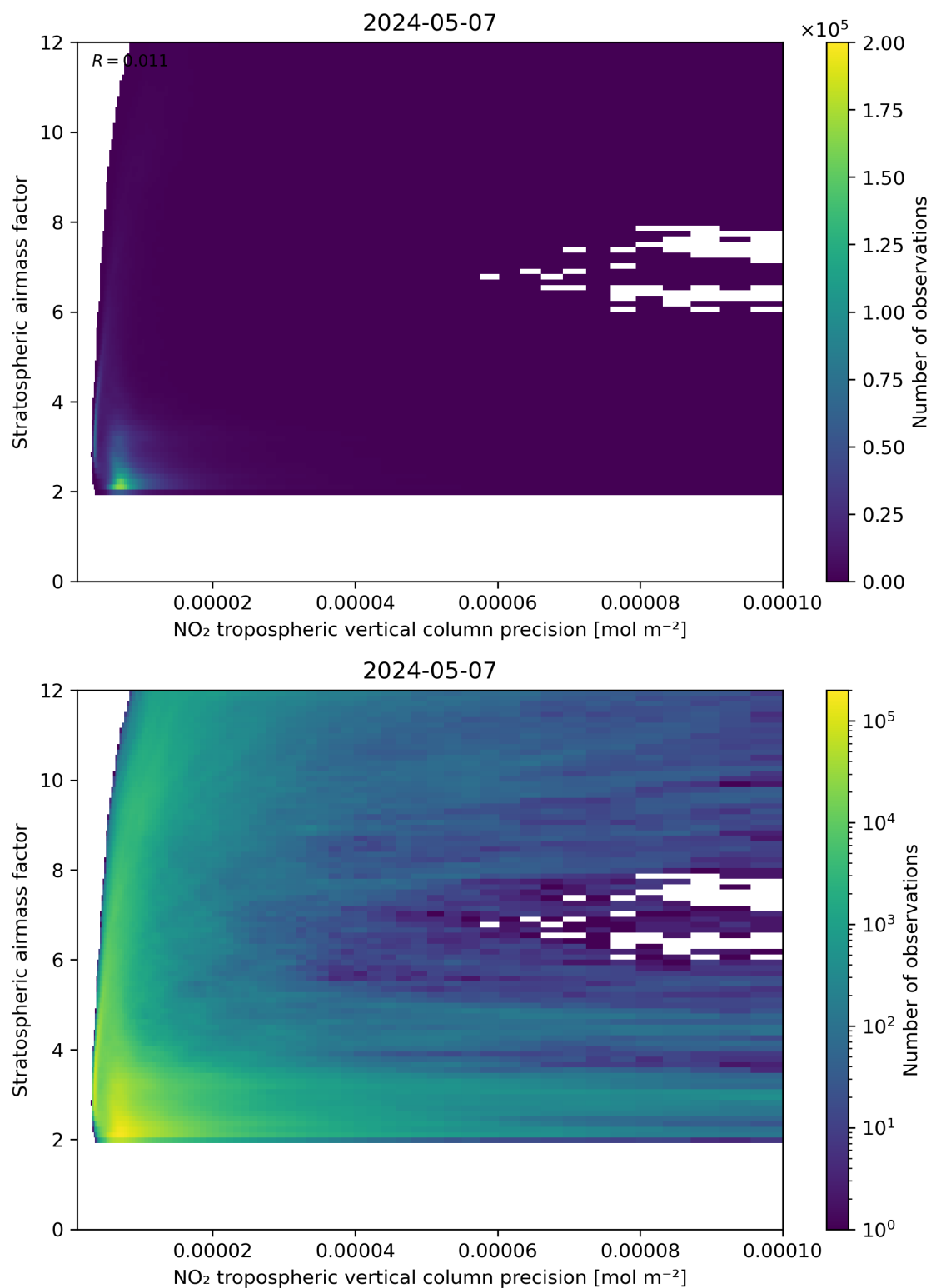
Figure 131: Scatter density plot of “NO 2 tropospheric vertical column precision” against “Stratospheric airmass factor” for 2024-05-07 to 2024-05-08.
