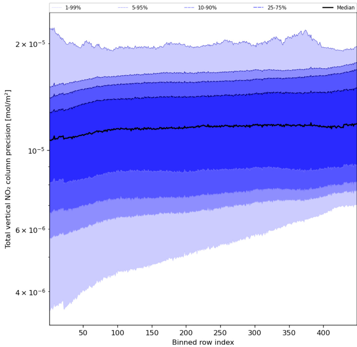
Figure 56: Along track statistics of “Total vertical NO 2 column precision” for 2024-05-07 to 2024-05-08
