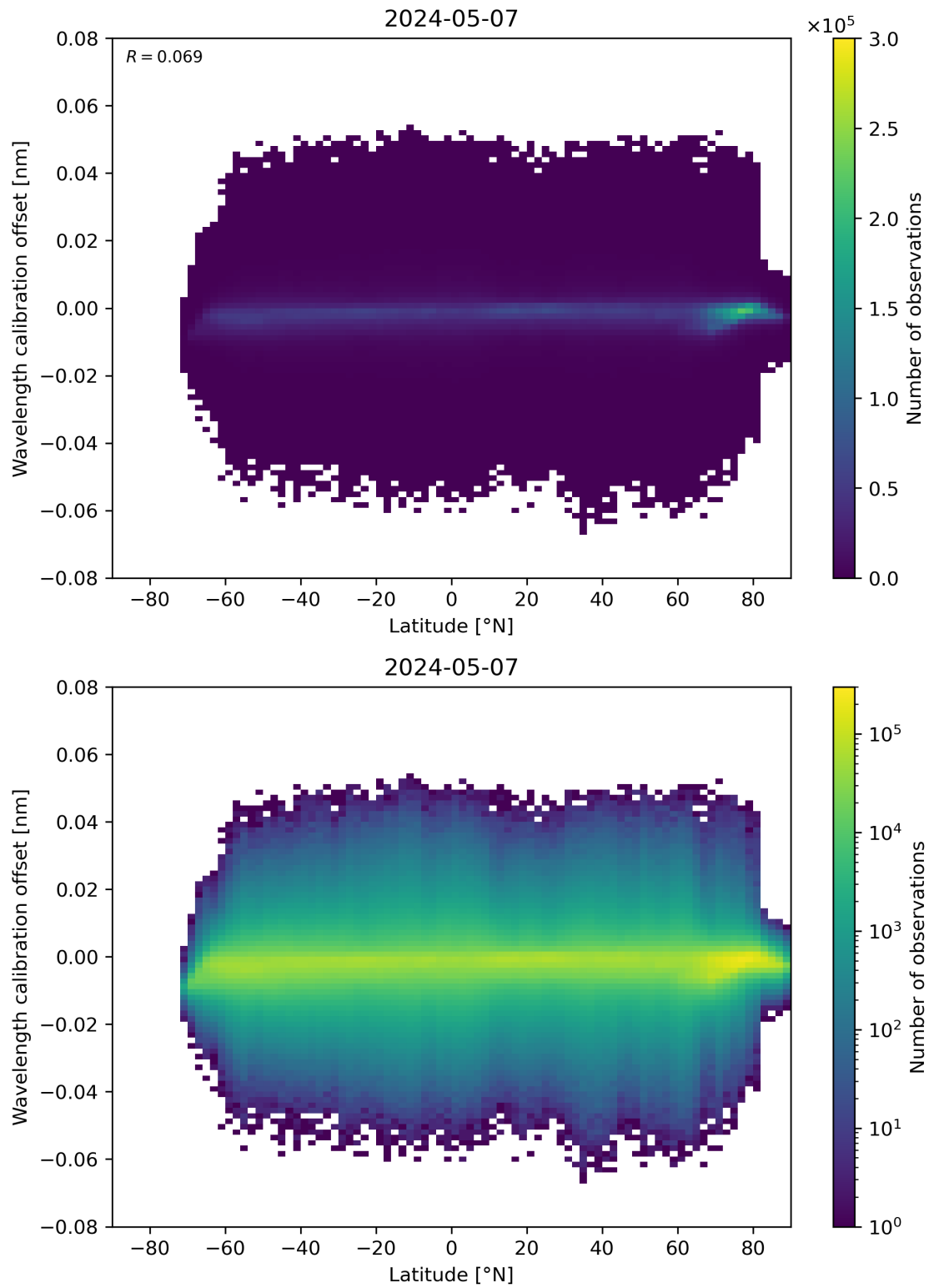
Figure 95: Scatter density plot of “Latitude” against “Wavelength calibration offset” for 2024-05-07 to 2024-05-08.
