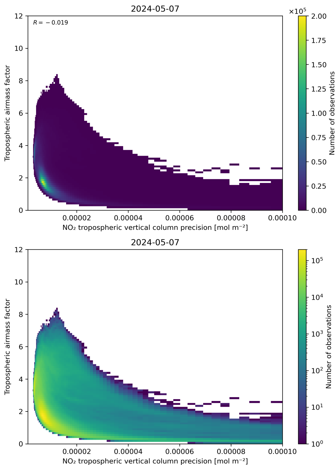
Figure 133: Scatter density plot of “NO 2 tropospheric vertical column precision” against “Tropospheric airmass factor” for 2024-05-07 to 2024-05-08.
