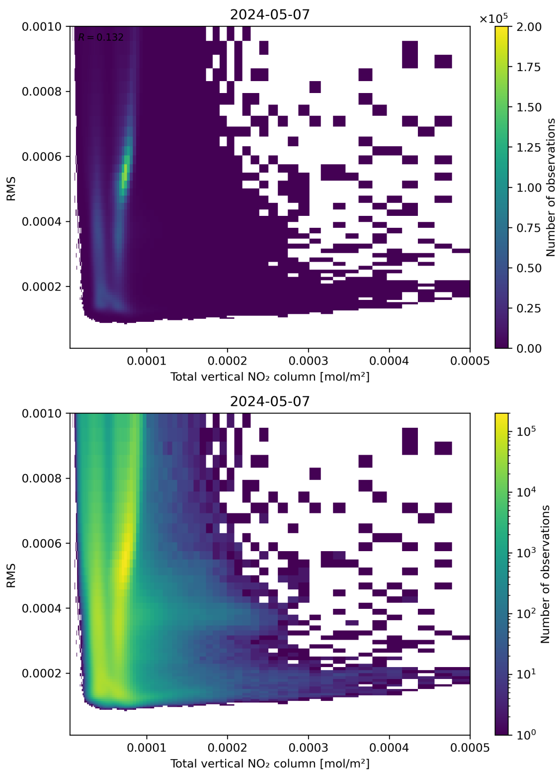
Figure 120: Scatter density plot of “Total vertical NO 2 column” against “RMS” for 2024-05-07 to 2024-05-08.
