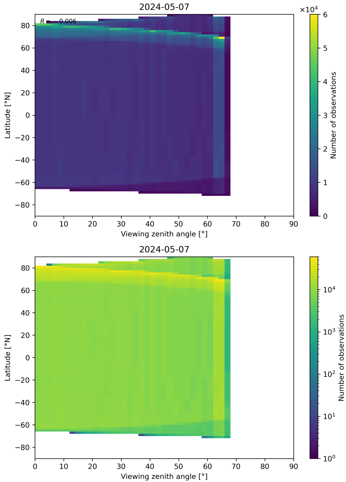
Figure 163: Scatter density plot of “Viewing zenith angle” against “Latitude” for 2024-05-07 to 2024-05-08.
