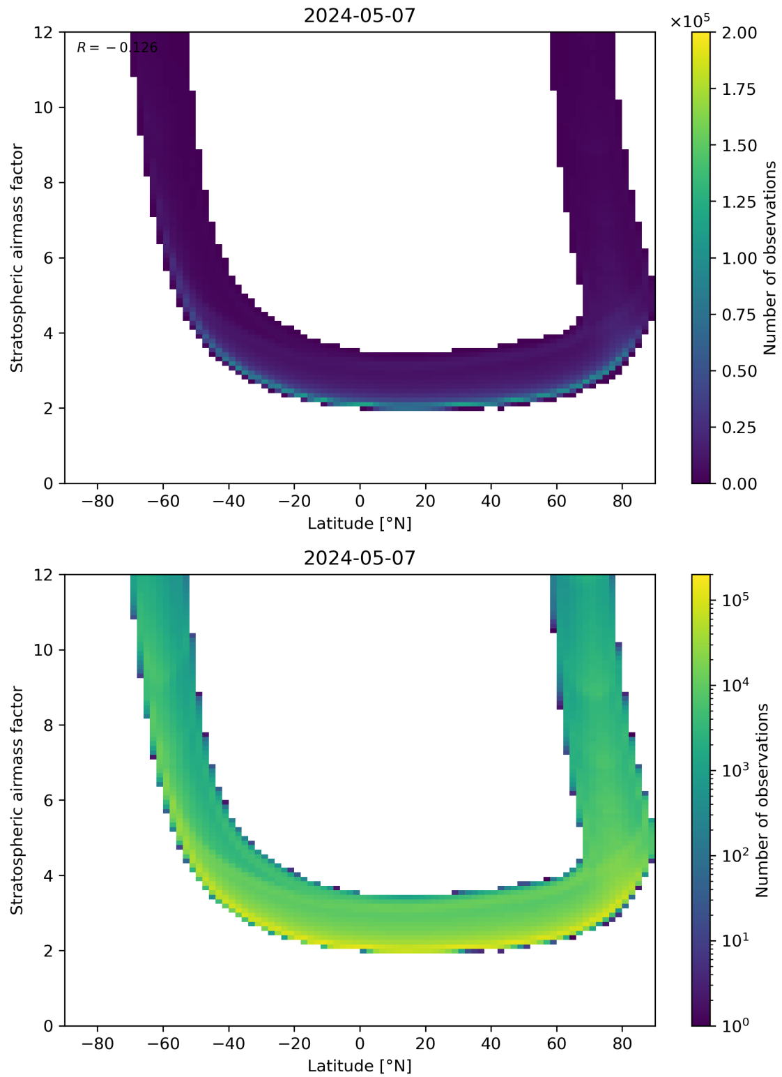
Figure 83: Scatter density plot of “Latitude” against “Stratospheric air mass factor” for 2024-05-07 to 2024-05-08.
