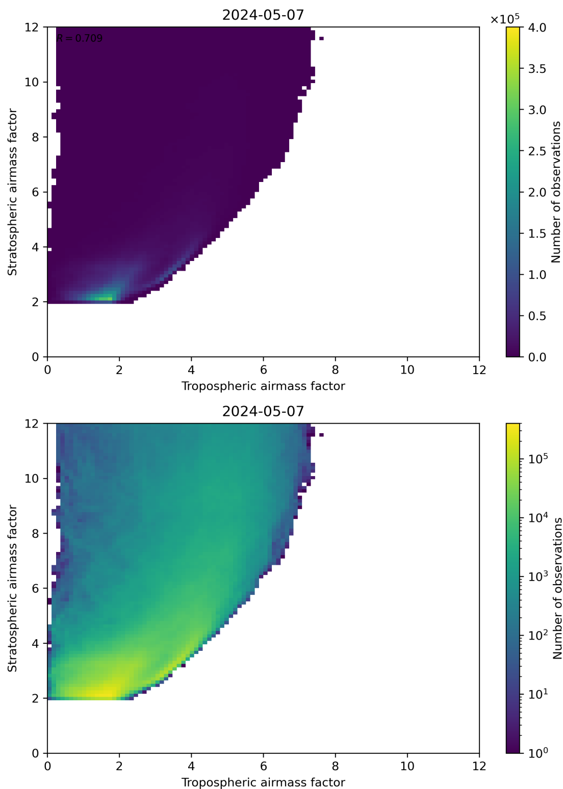
Figure 71: Scatter density plot of “Tropospheric airmass factor” against “Stratospheric airmass factor” for 2024-05-07 to 2024-05-08.
