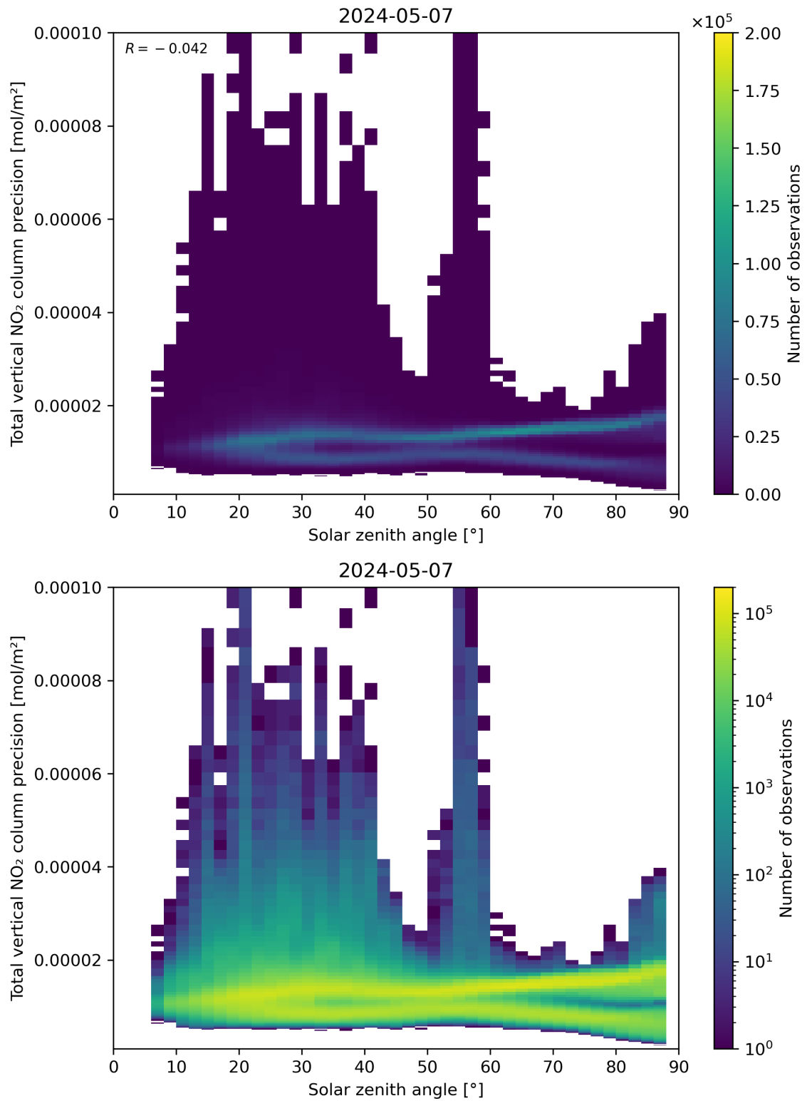
Figure 154: Scatter density plot of “Solar zenith angle” against “Total vertical NO 2 column precision” for 2024-05-07 to 2024-05-08.
