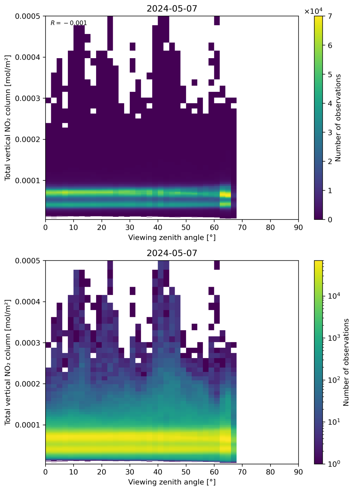
Figure 167: Scatter density plot of “Viewing zenith angle” against “Total vertical NO 2 column” for 2024-05-07 to 2024-05-08.
