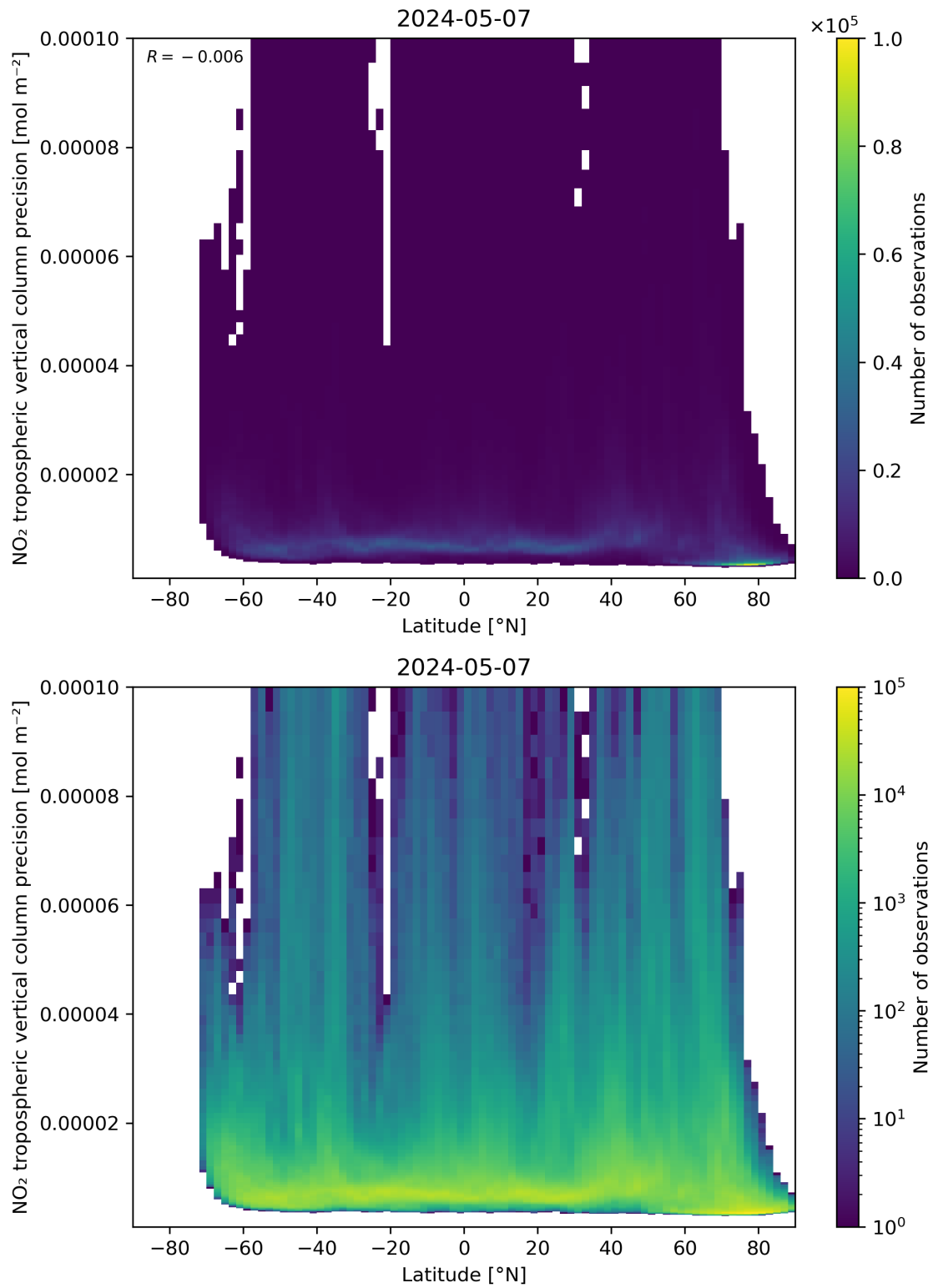
Figure 93: Scatter density plot of “Latitude” against “NO 2 tropospheric vertical column precision” for 2024-05-07 to 2024-05-08.
