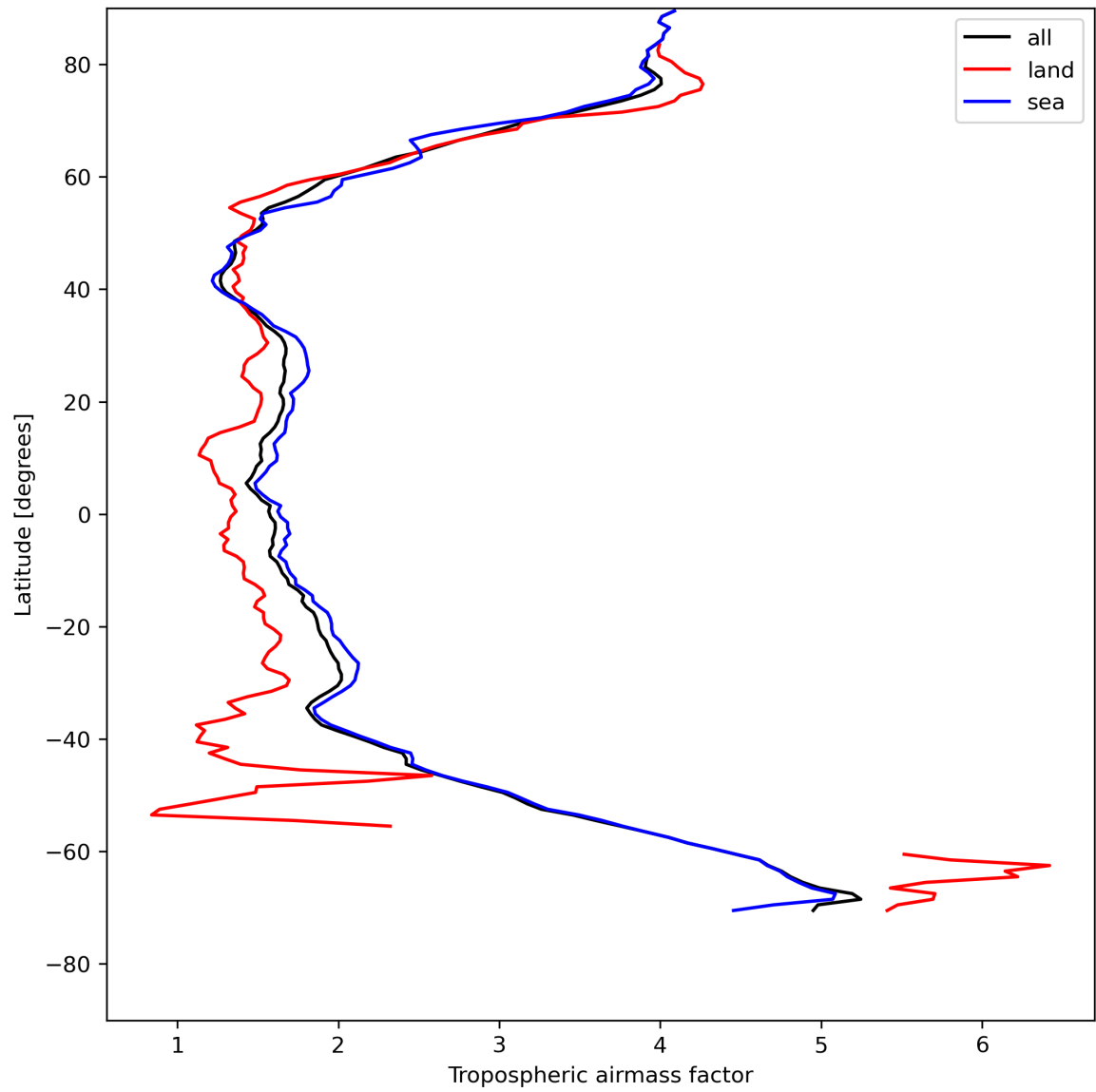
Figure 14: Zonal average of “Tropospheric airmass factor” for 2024-05-07 to 2024-05-08.
