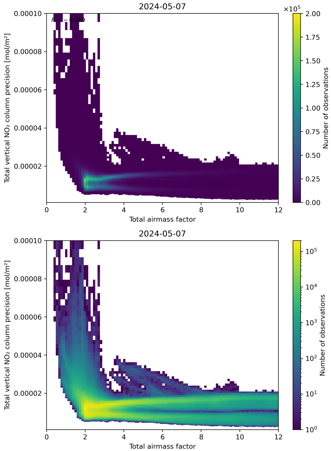
Figure 68: Scatter density plot of “Total airmass factor” against “Total vertical NO 2 column precision” for 2024-05-07 to 2024-05-08.
