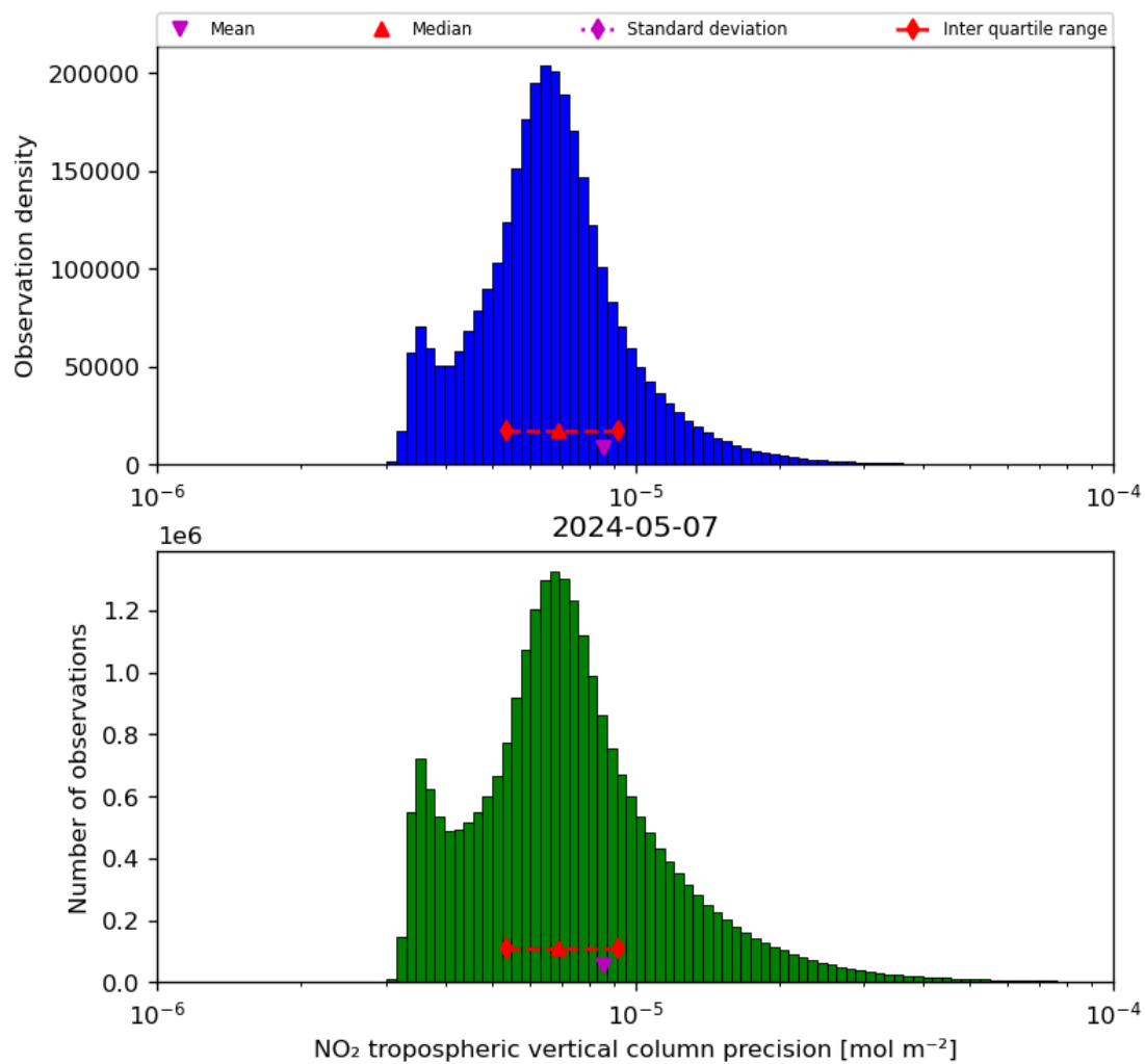
Figure 30: Histogram of “NO 2 tropospheric vertical column precision” for 2024-05-07 to 2024-05-08
