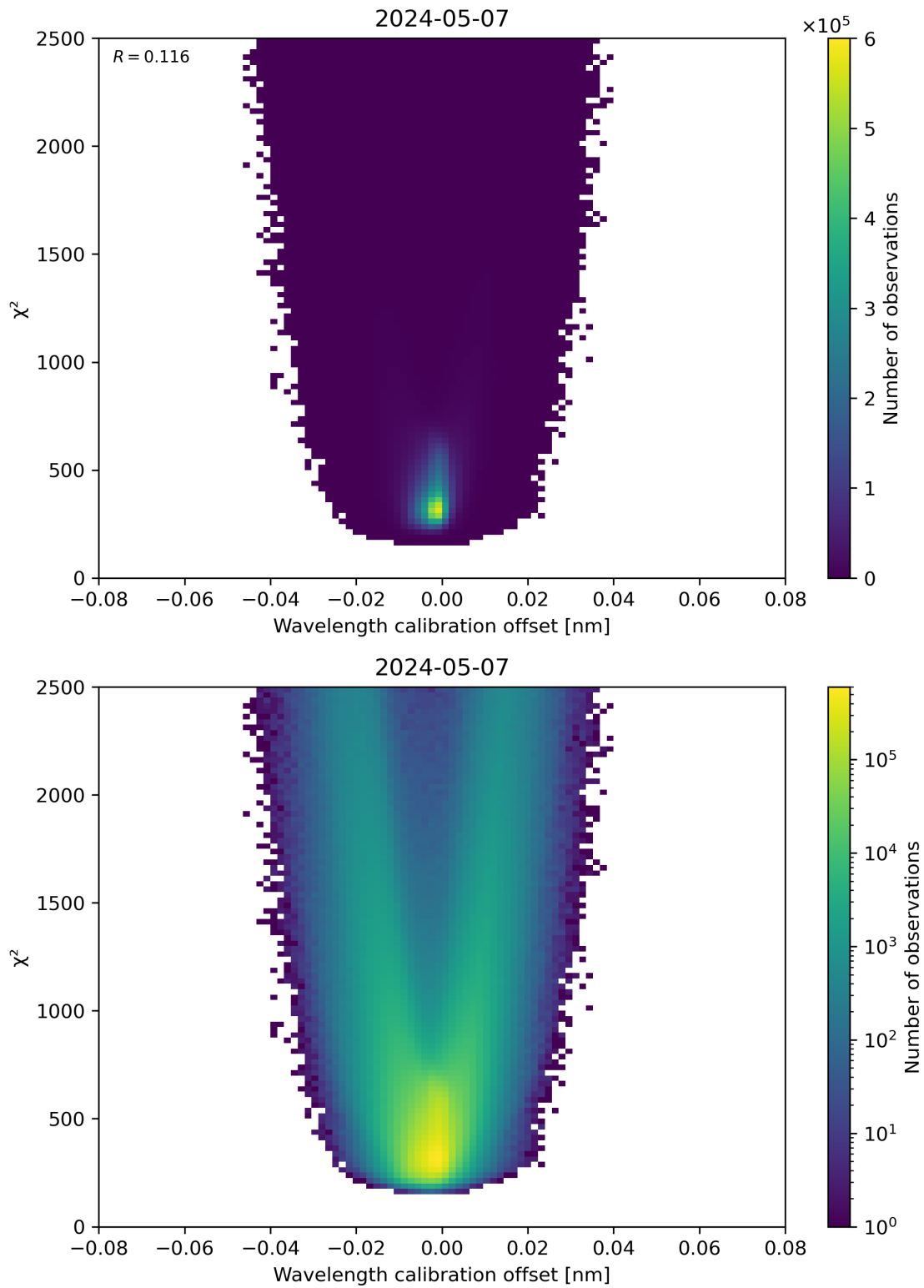
Figure 175: Scatter density plot of “Wavelength calibration offset” against “ \chi^2 ” for 2024-05-07 to 2024-05-08.
