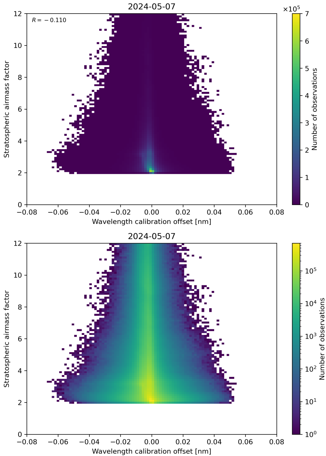
Figure 174: Scatter density plot of “Wavelength calibration offset” against “Stratospheric airmass factor” for 2024-05-07 to 2024-05-08.
