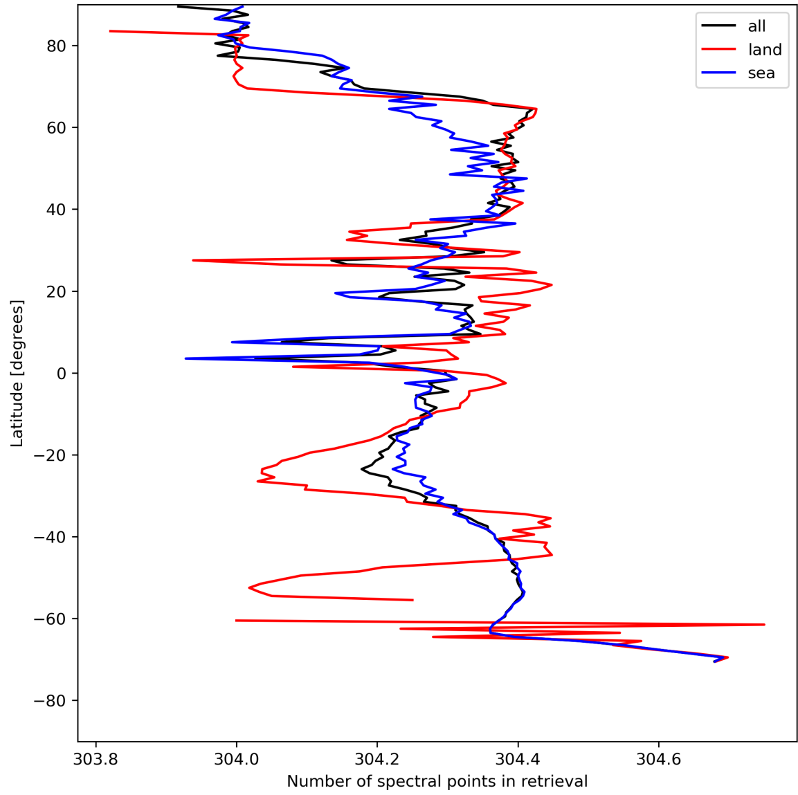
Figure 16: Zonal average of “Number of spectral points in retrieval” for 2024-05-07 to 2024-05-08.
