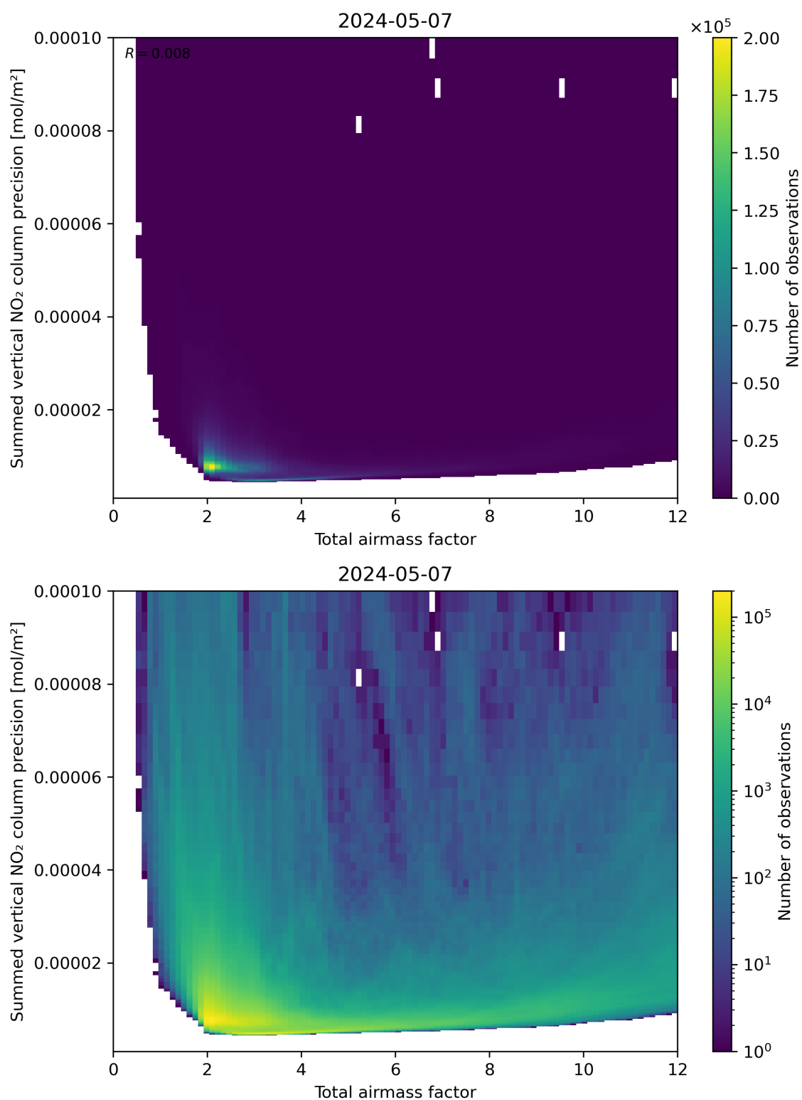
Figure 66: Scatter density plot of “Total airmass factor” against “Summed vertical NO 2 column precision” for 2024-05-07 to 2024-05-08.
