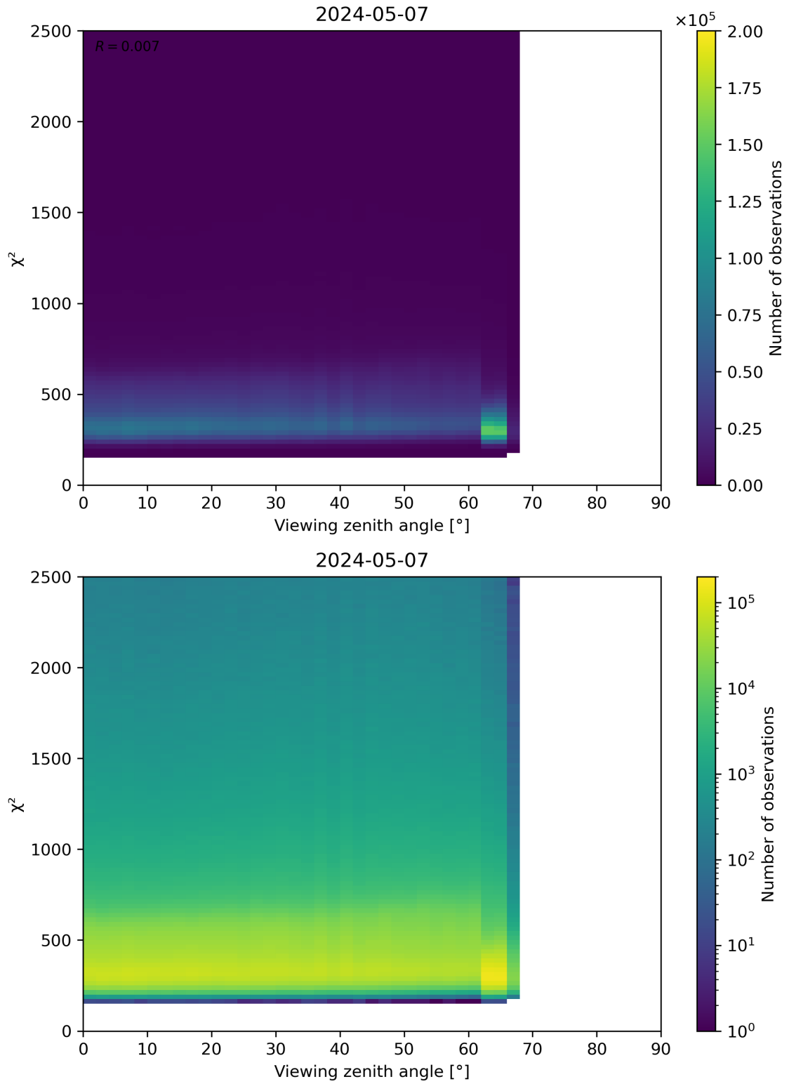
Figure 162: Scatter density plot of “Viewing zenith angle” against “ \chi^2 ” for 2024-05-07 to 2024-05-08.
