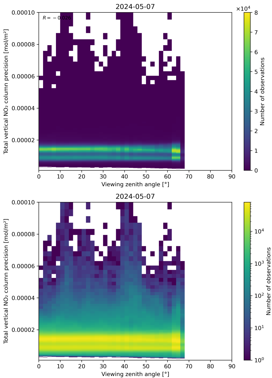
Figure 168: Scatter density plot of “Viewing zenith angle” against “Total vertical NO 2 column precision” for 2024-05-07 to 2024-05-08.
