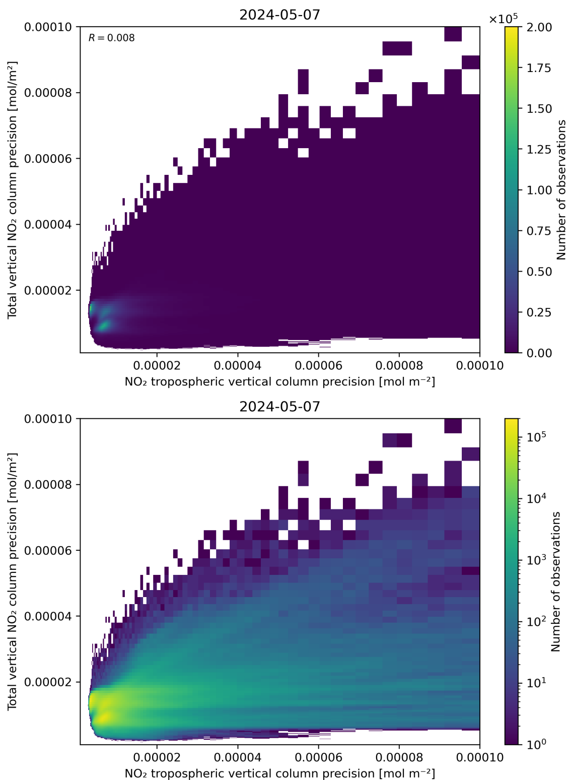
Figure 139: Scatter density plot of “NO 2 tropospheric vertical column precision” against “Total vertical NO 2 column precision” for 2024-05-07 to 2024-05-08.
