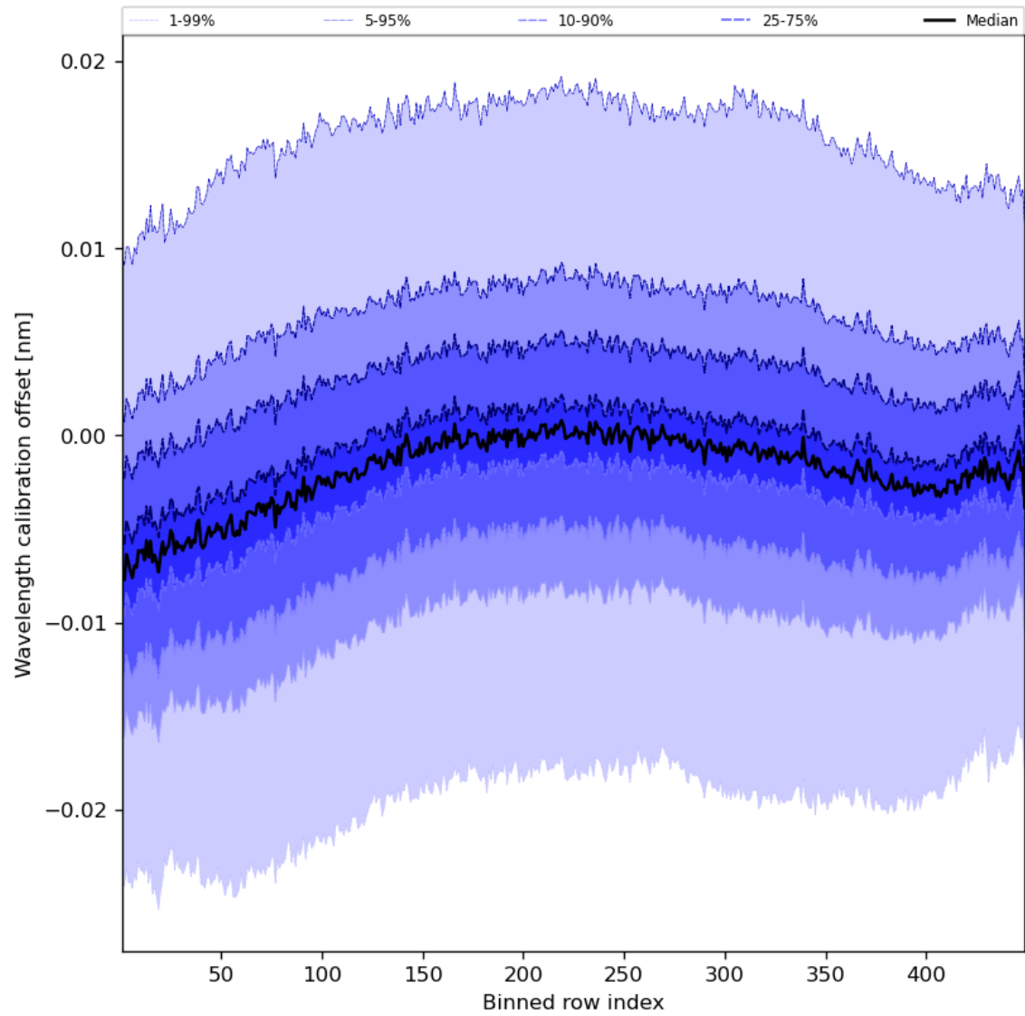
Figure 52: Along track statistics of “Wavelength calibration offset” for 2024-05-07 to 2024-05-08
