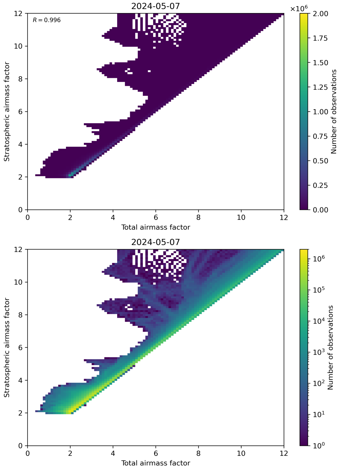
Figure 62: Scatter density plot of “Total airmass factor” against “Stratospheric airmass factor” for 2024-05-07 to 2024-05-08.
