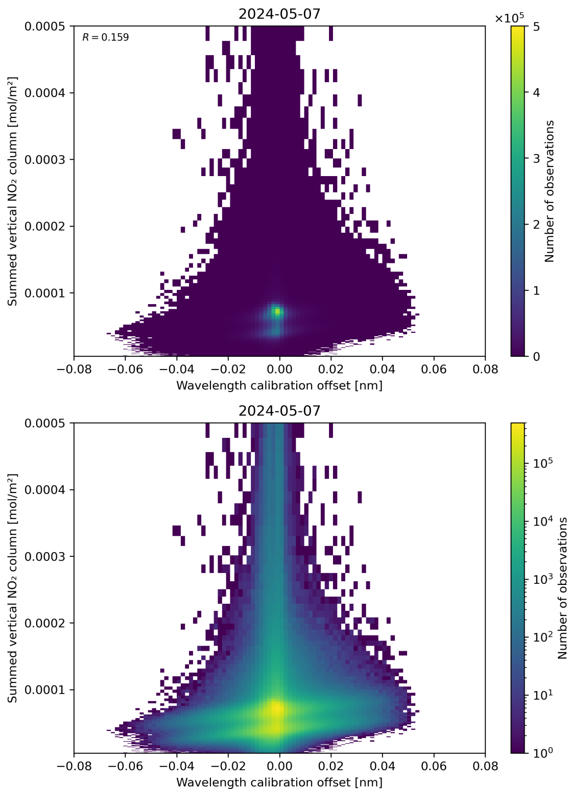
Figure 177: Scatter density plot of “Wavelength calibration offset” against “Summed vertical NO 2 column” for 2024-05-07 to 2024-05-08.
