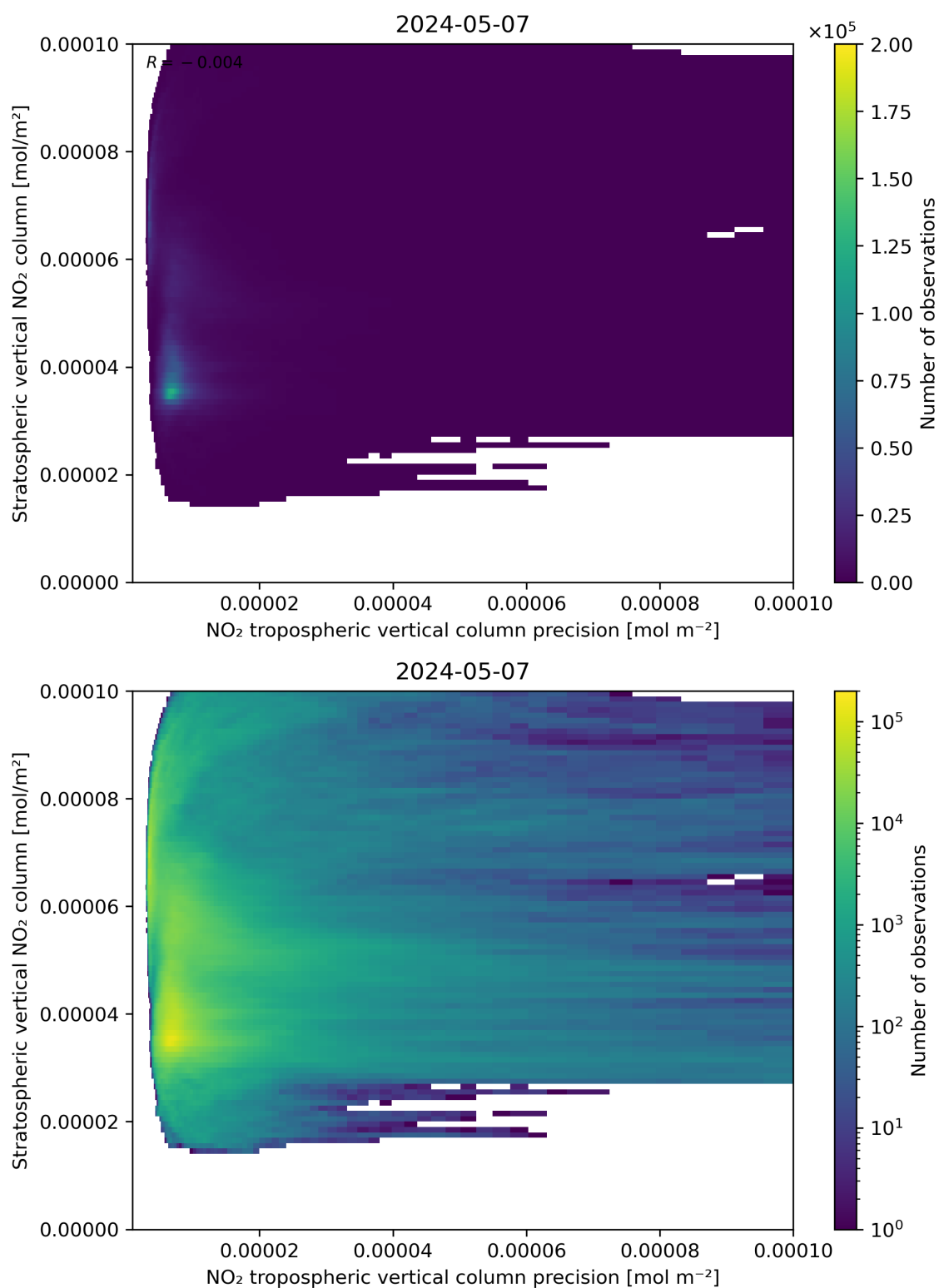
Figure 135: Scatter density plot of “NO 2 tropospheric vertical column precision” against “Stratospheric vertical NO 2 column” for 2024-05-07 to 2024-05-08.
