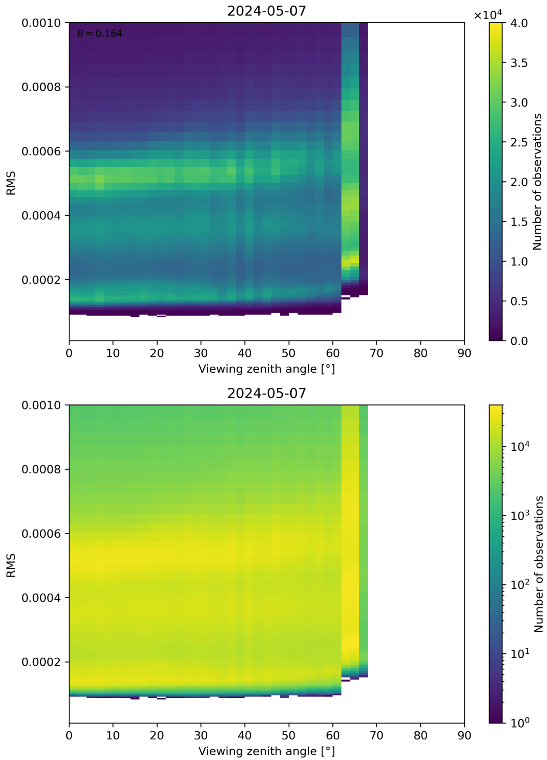
Figure 171: Scatter density plot of “Viewing zenith angle” against “RMS” for 2024-05-07 to 2024-05-08.
