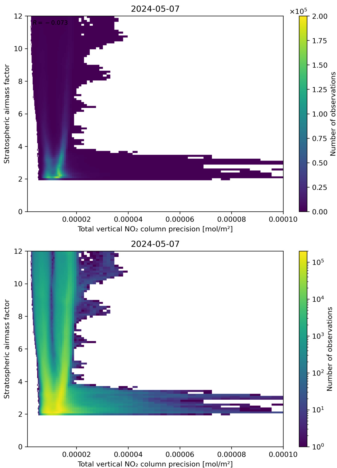
Figure 115: Scatter density plot of “Total vertical NO 2 column precision” against “Stratospheric air mass factor” for 2024-05-07 to 2024-05-08.
