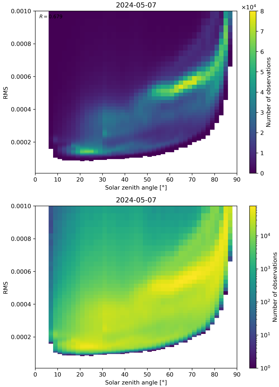
Figure 157: Scatter density plot of “Solar zenith angle” against “RMS” for 2024-05-07 to 2024-05-08.
