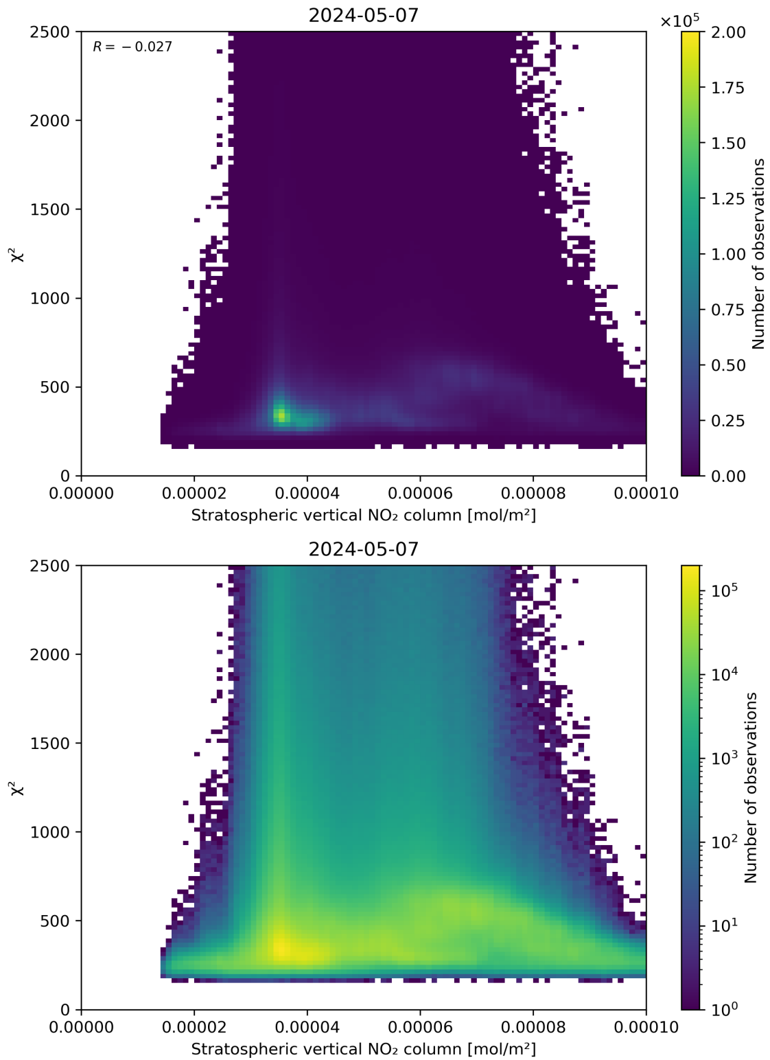
Figure 97: Scatter density plot of “Stratospheric vertical NO 2 column” against “ \chi^2 ” for 2024-05-07 to 2024-05-08.
