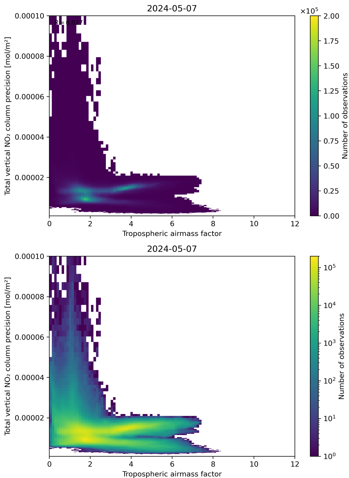
Figure 78: Scatter density plot of “Tropospheric air mass factor” against “Total vertical NO 2 column precision” for 2024-05-07 to 2024-05-08.
