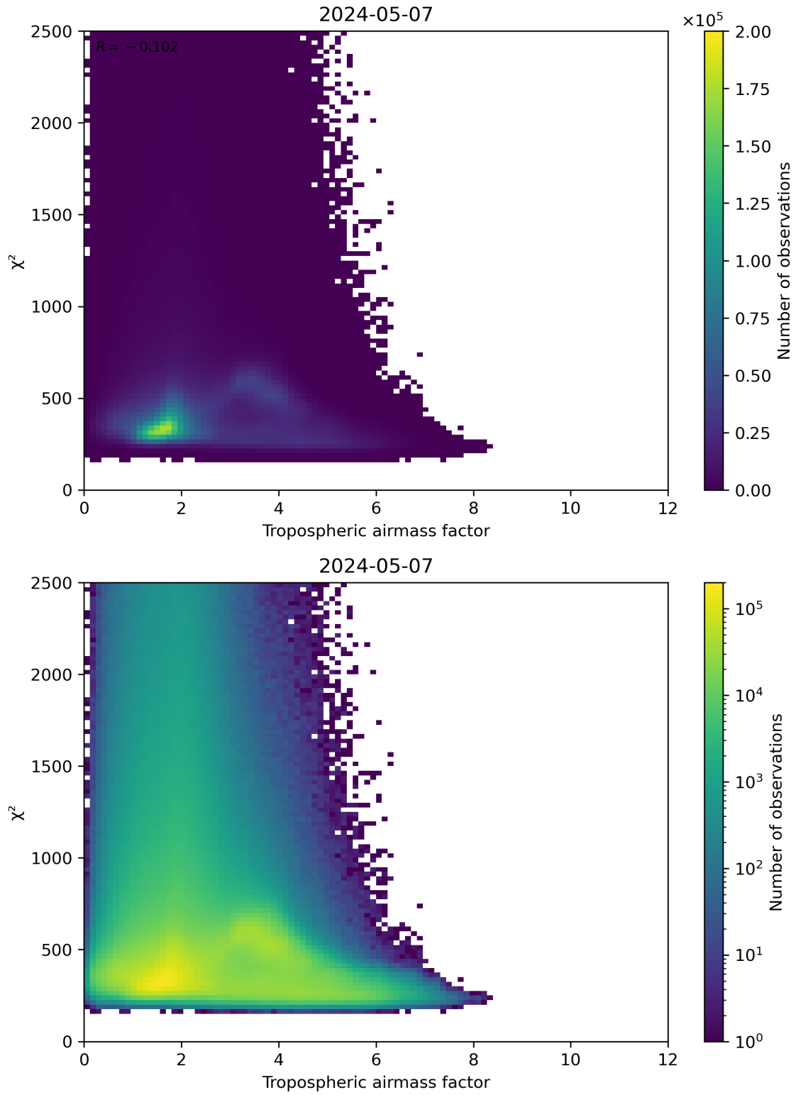
Figure 73: Scatter density plot of “Tropospheric airmass factor” against “ \chi^2 ” for 2024-05-07 to 2024-05-08.
