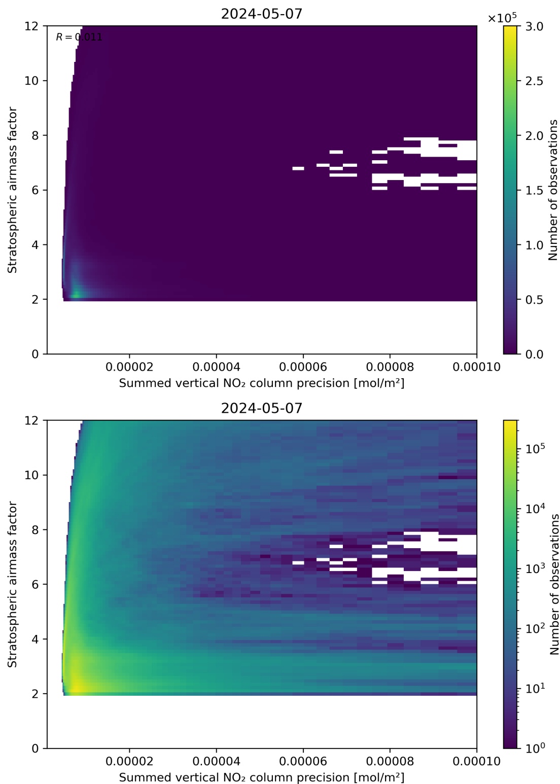
Figure 106: Scatter density plot of “Summed vertical NO 2 column precision” against “Stratospheric airmass factor” for 2024-05-07 to 2024-05-08.
