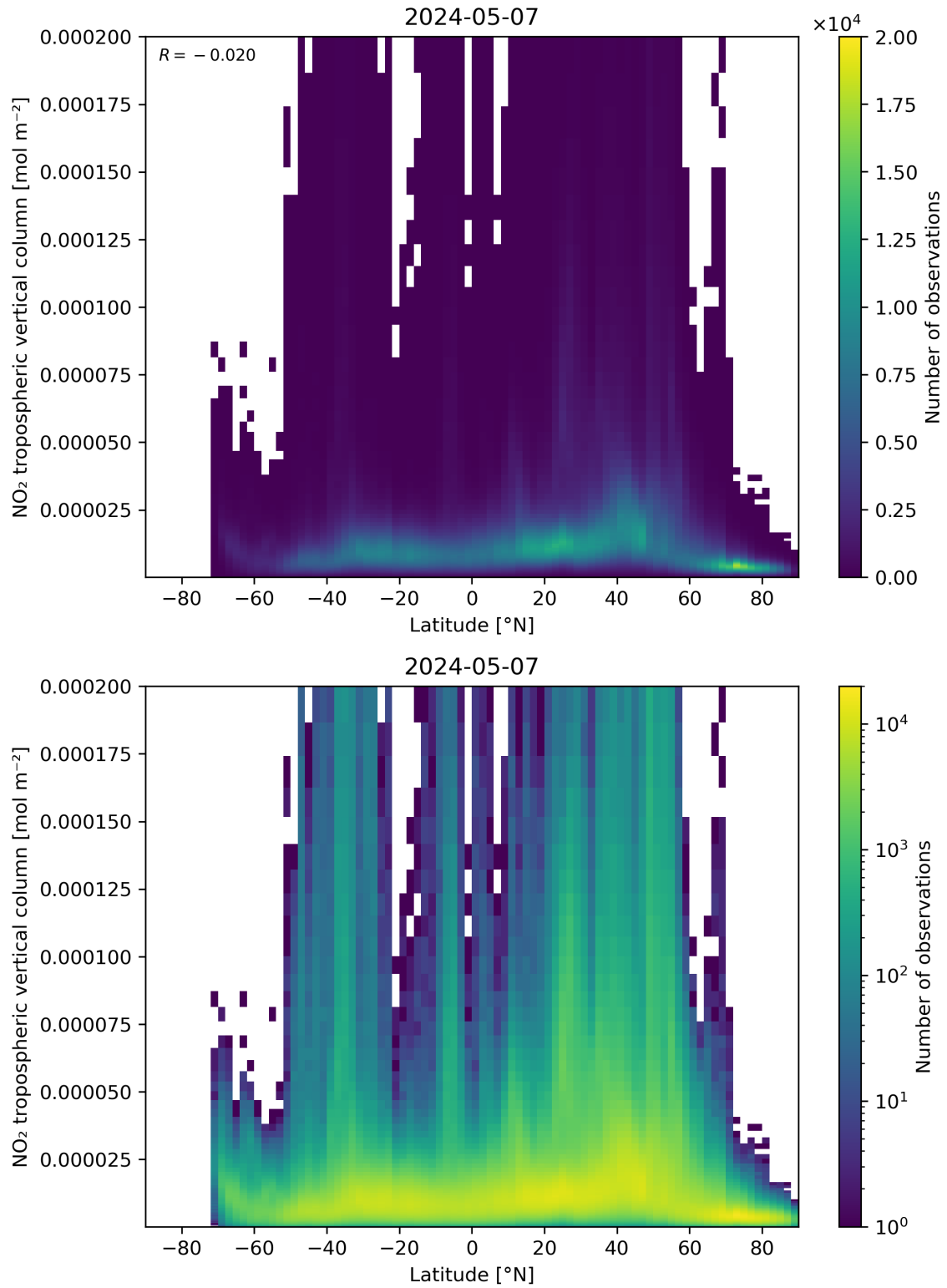
Figure 92: Scatter density plot of “Latitude” against “NO 2 tropospheric vertical column” for 2024-05-07 to 2024-05-08.
