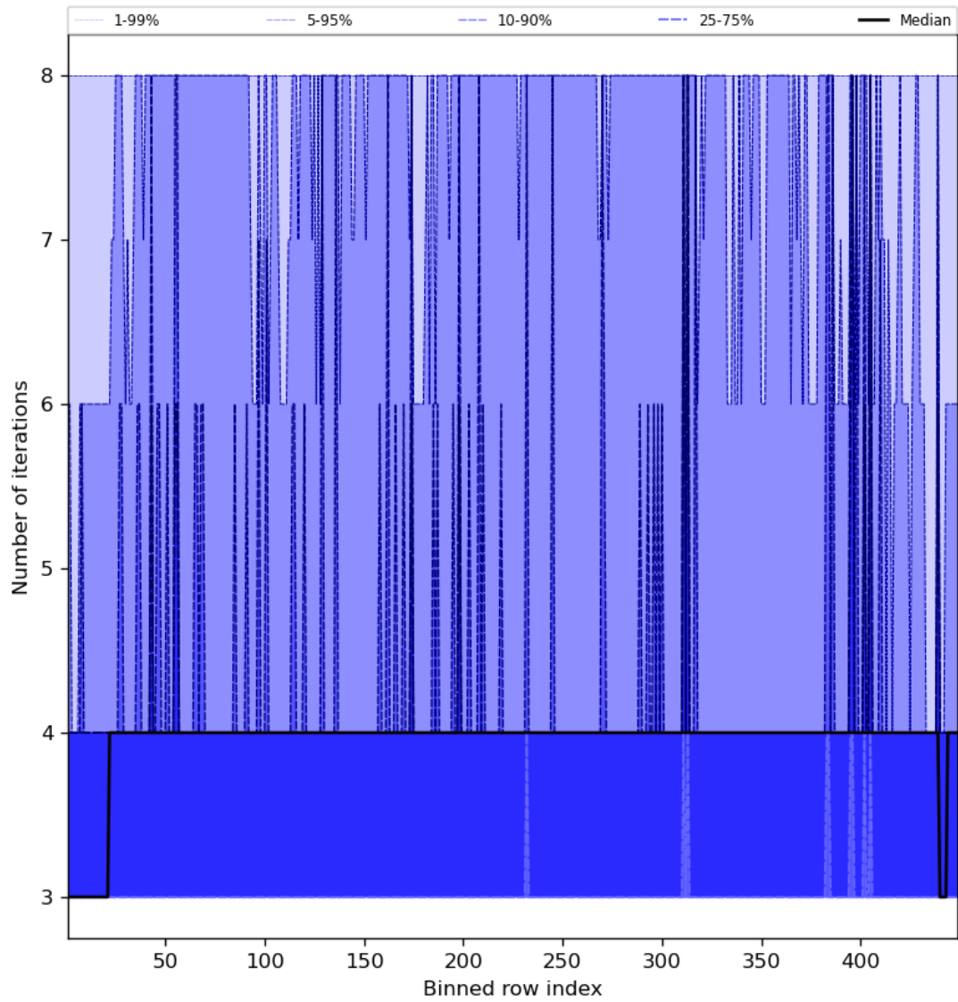
Figure 51: Along track statistics of “Number of iterations” for 2024-05-07 to 2024-05-08
