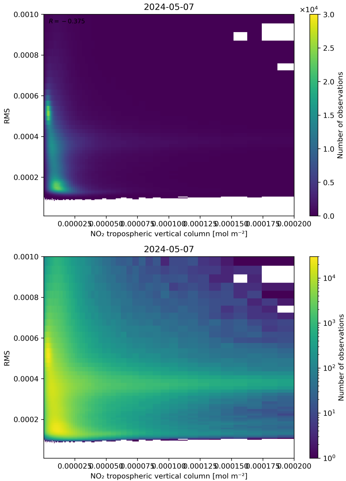
Figure 142: Scatter density plot of “NO 2 tropospheric vertical column” against “RMS” for 2024-05-07 to 2024-05-08.
