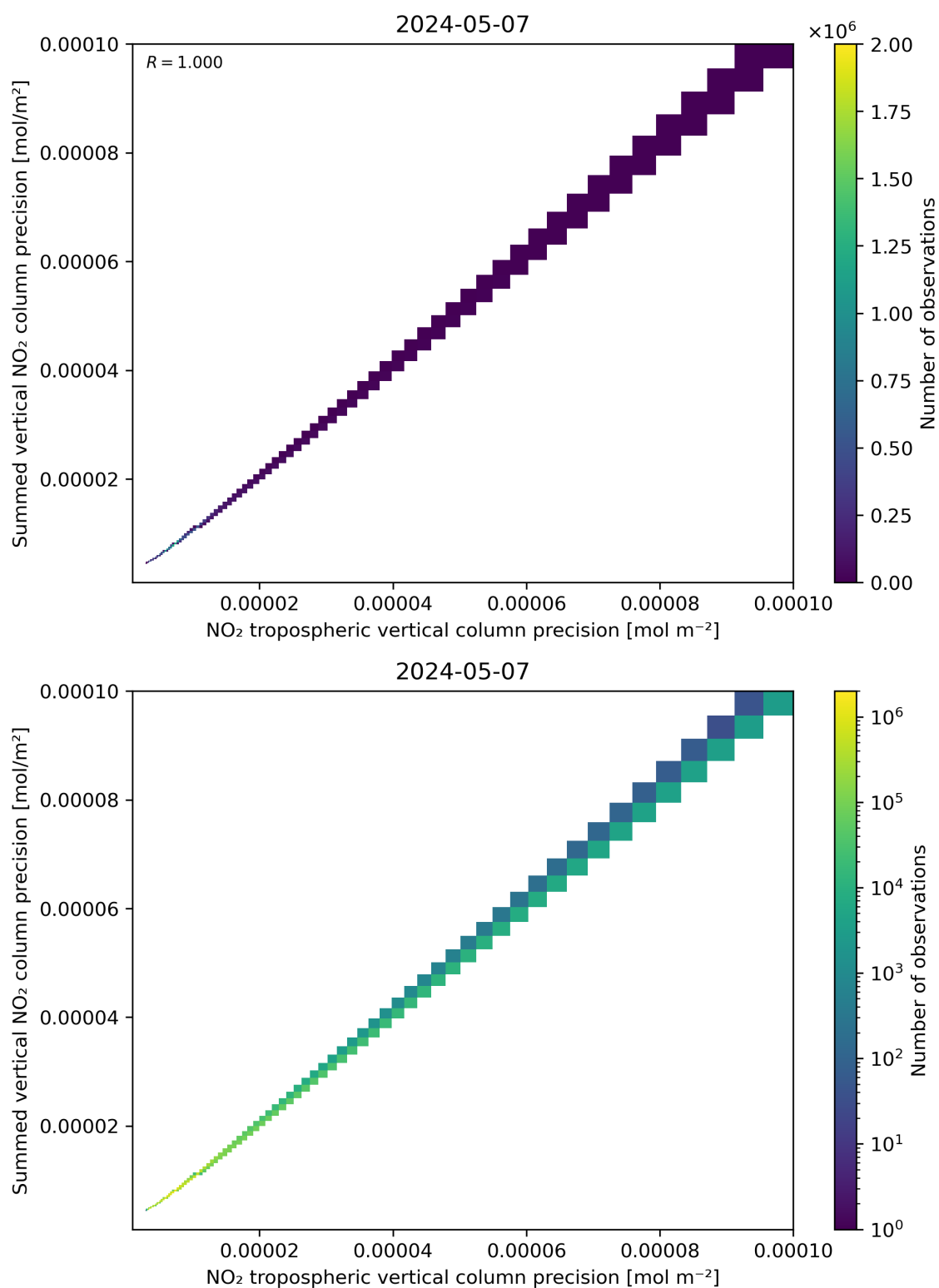
Figure 137: Scatter density plot of “NO 2 tropospheric vertical column precision” against “Summed vertical NO 2 column precision” for 2024-05-07 to 2024-05-08.
