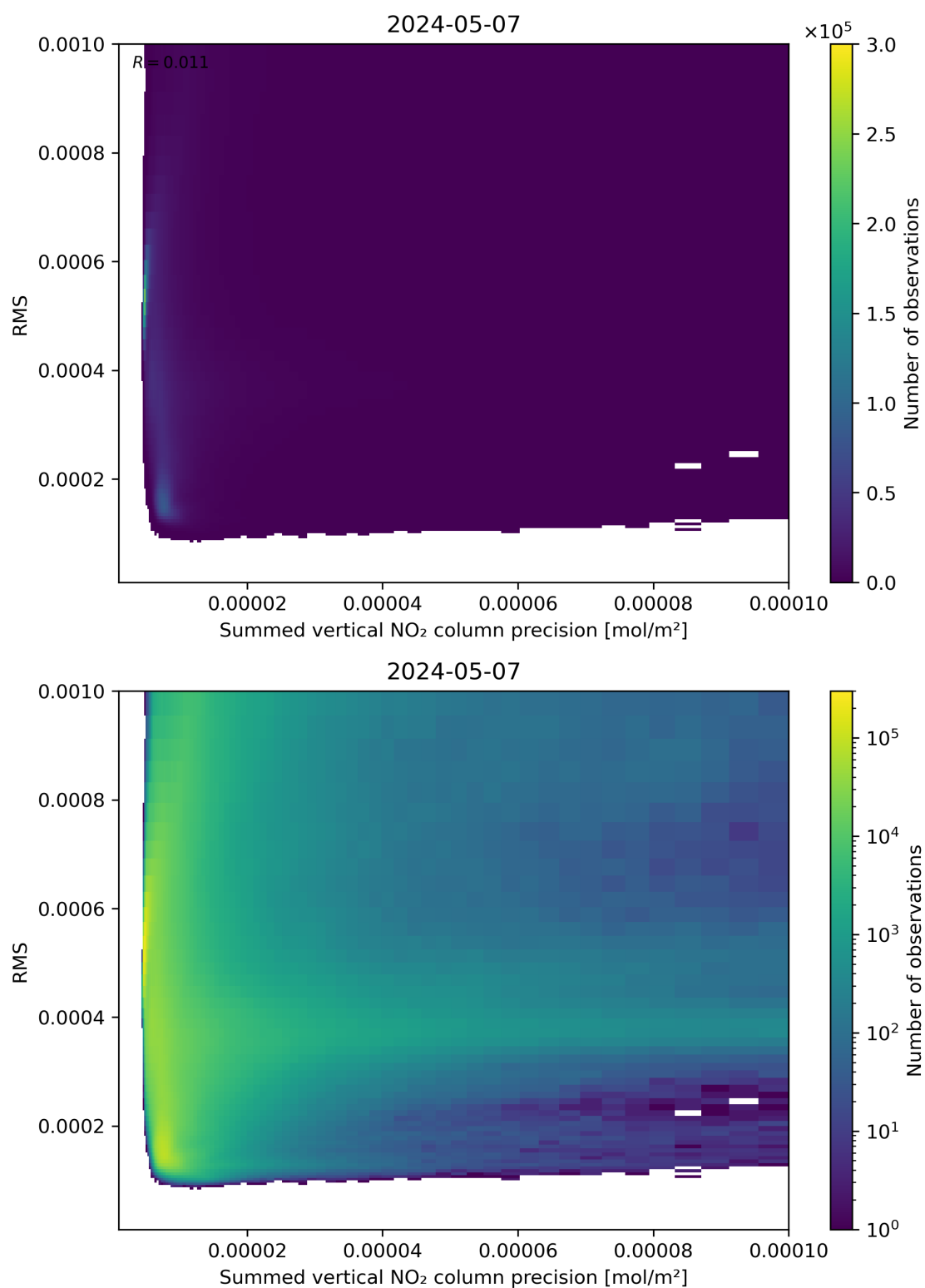
Figure 108: Scatter density plot of “Summed vertical NO 2 column precision” against “RMS” for 2024-05-07 to 2024-05-08.
