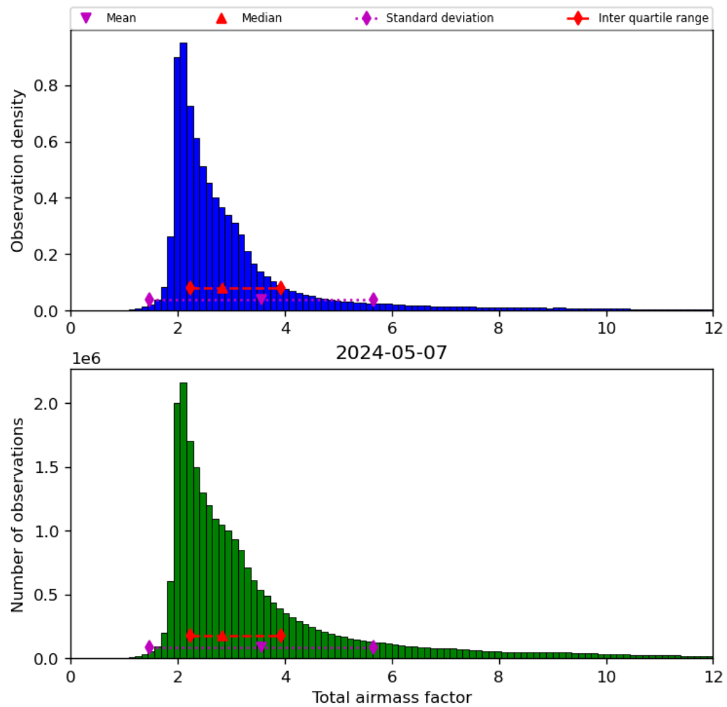
Figure 32: Histogram of “Total airmass factor” for 2024-05-07 to 2024-05-08
