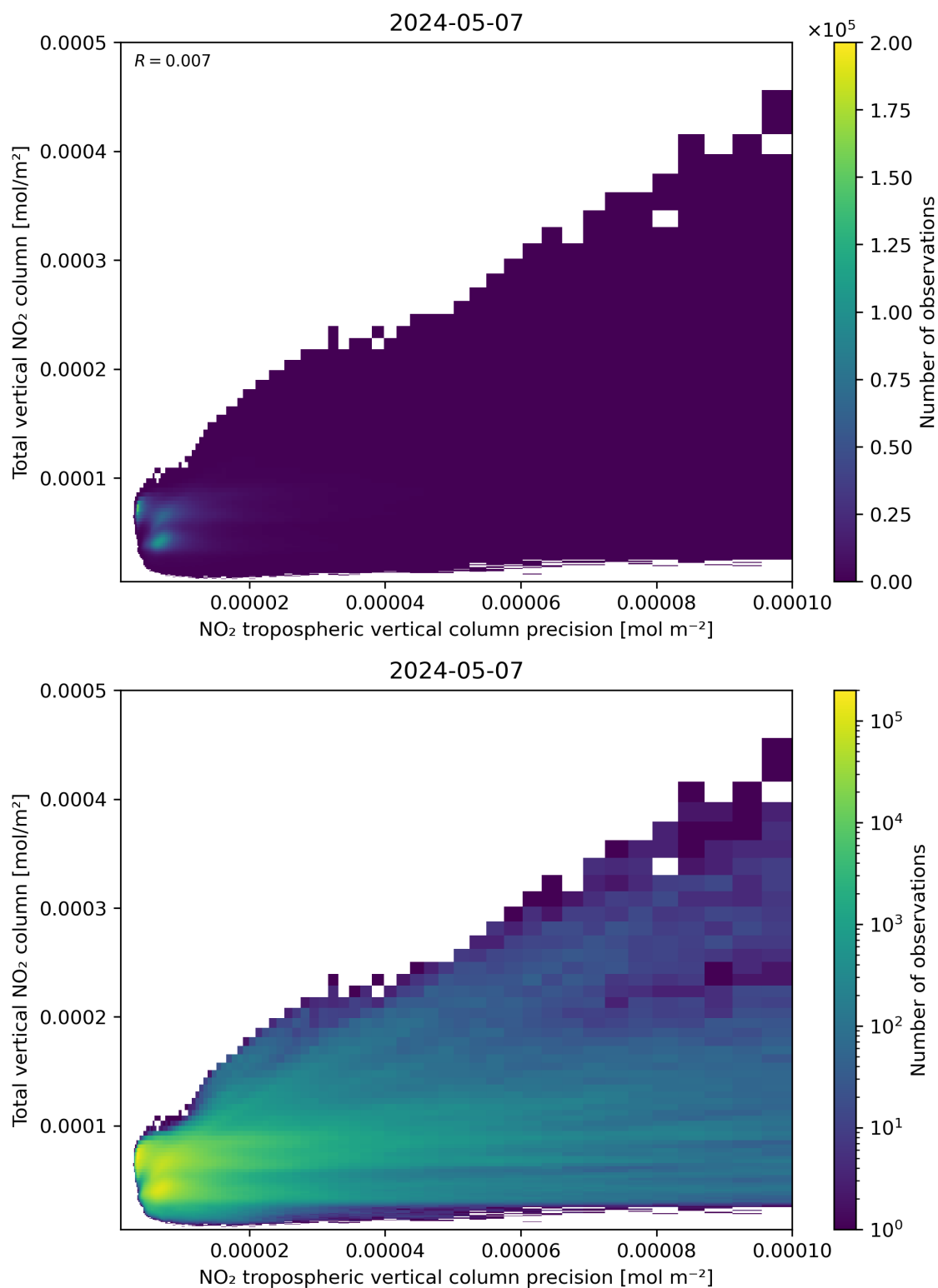
Figure 138: Scatter density plot of “NO 2 tropospheric vertical column precision” against “Total vertical NO 2 column” for 2024-05-07 to 2024-05-08.
