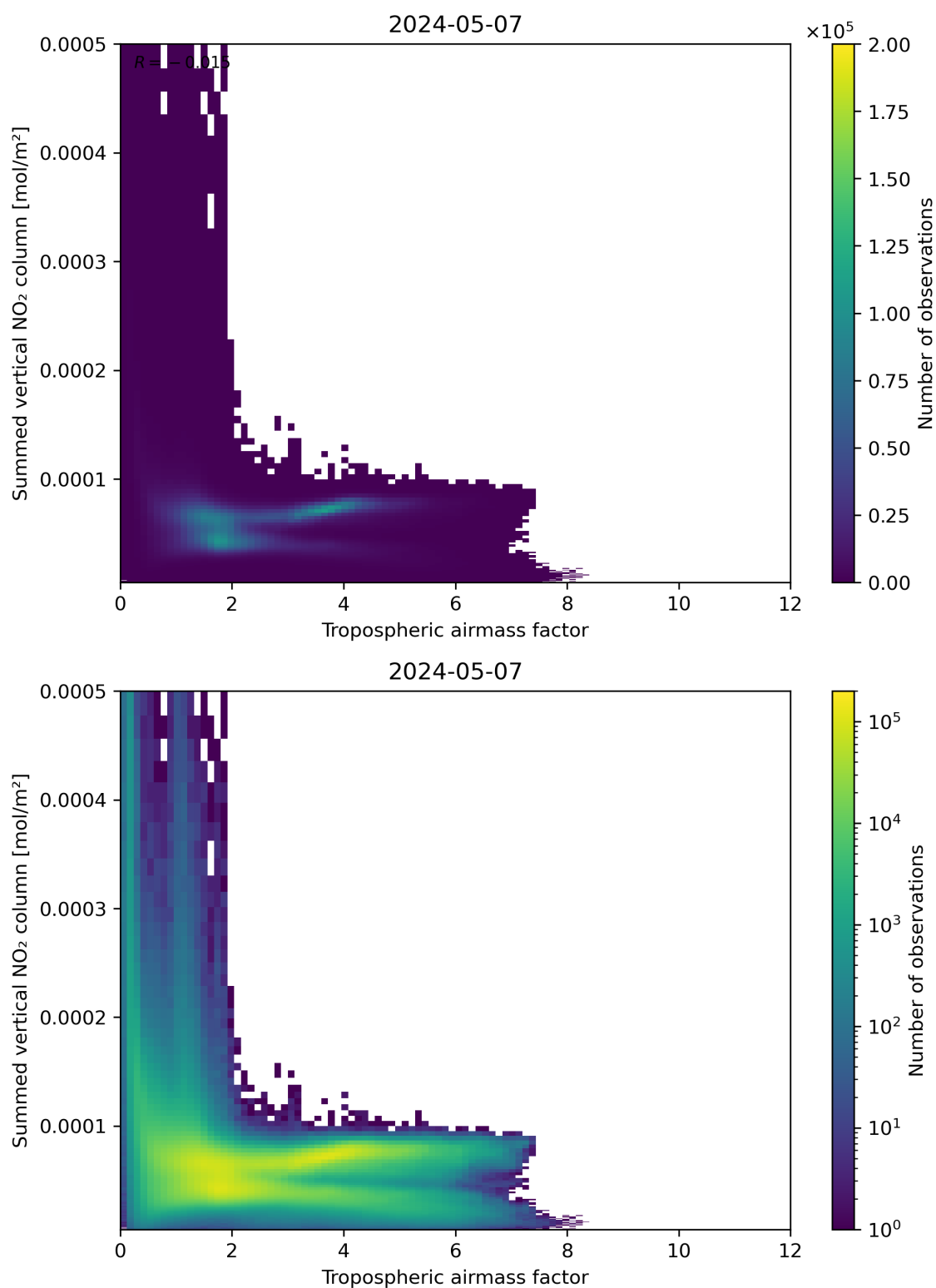
Figure 75: Scatter density plot of “Tropospheric air mass factor” against “Summed vertical NO 2 column” for 2024-05-07 to 2024-05-08.
