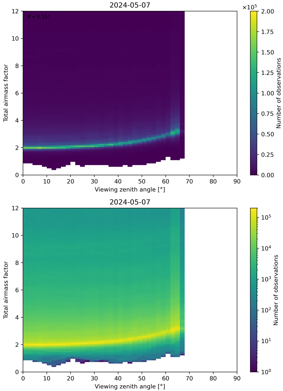
Figure 160: Scatter density plot of “Viewing zenith angle” against “Total airmass factor” for 2024-05-07 to 2024-05-08.
