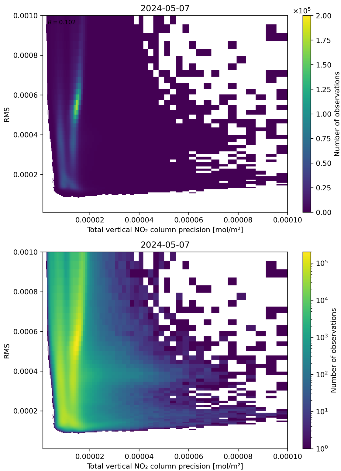
Figure 119: Scatter density plot of “Total vertical NO 2 column precision” against “RMS” for 2024-05-07 to 2024-05-08.
