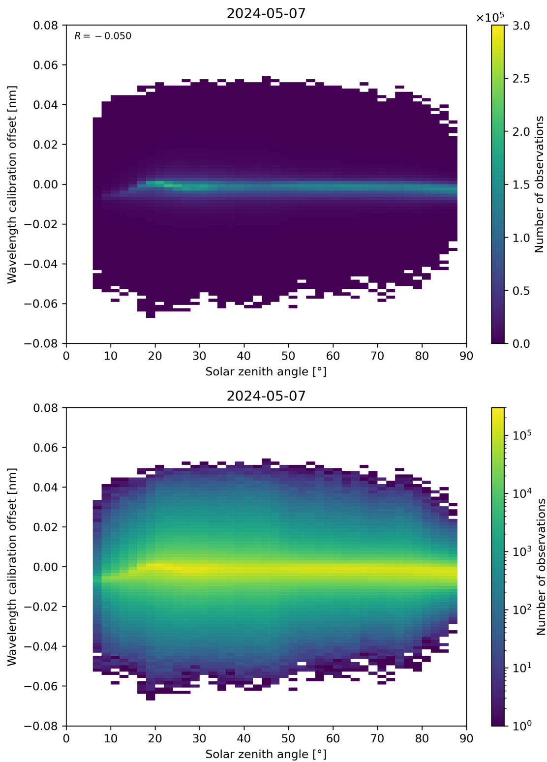
Figure 158: Scatter density plot of “Solar zenith angle” against “Wavelength calibration offset” for 2024-05-07 to 2024-05-08.
