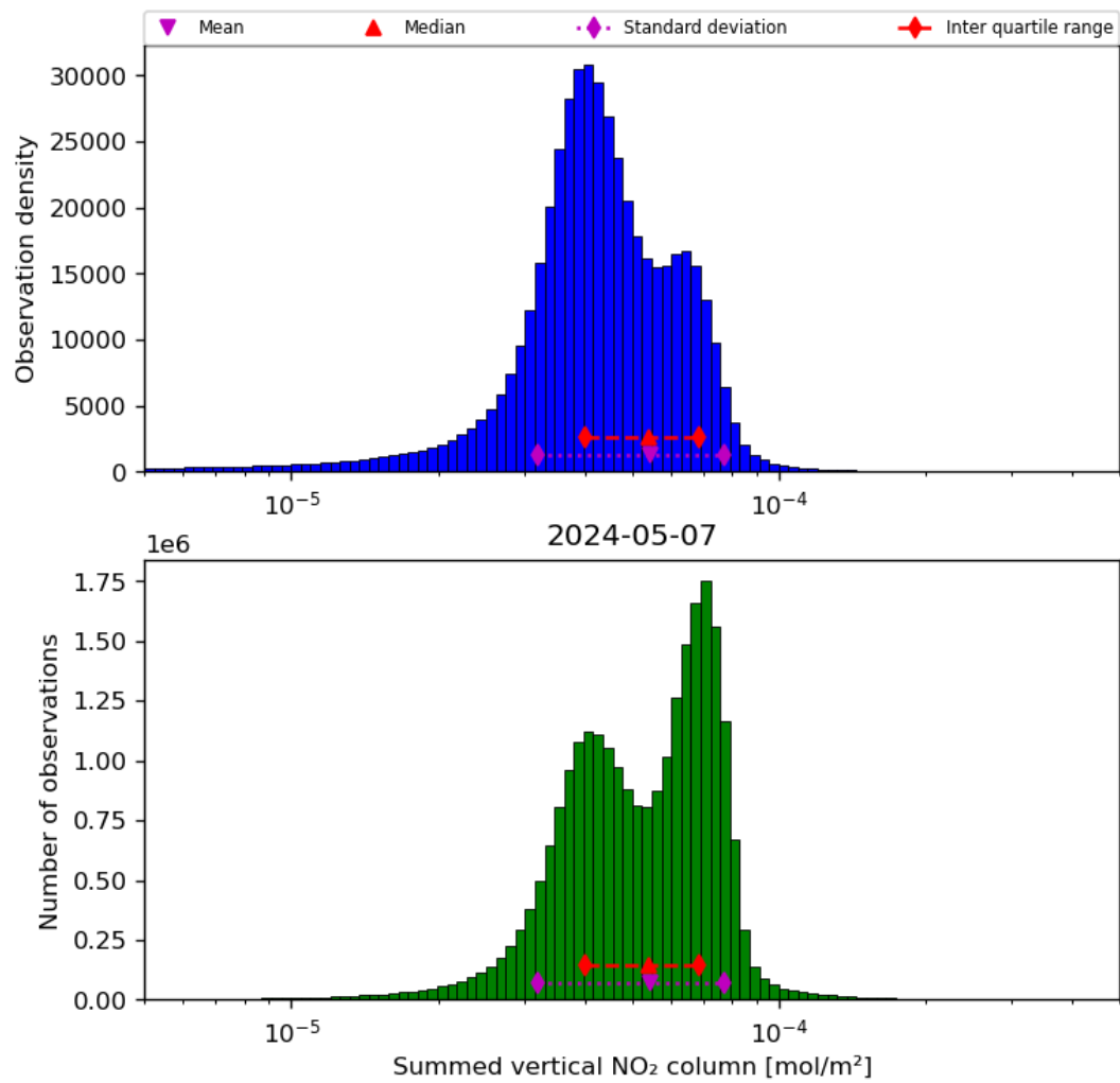
Figure 40: Histogram of "Summed vertical NO 2 column" for 2024-05-07 to 2024-05-08
