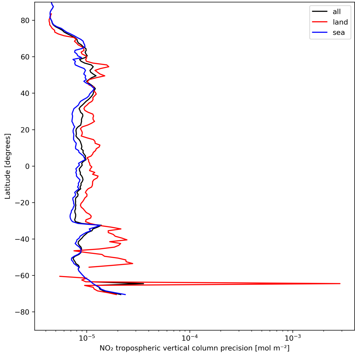
Figure 13: Zonal average of “NO 2 tropospheric vertical column precision” for 2024-05-07 to 2024-05-08.
