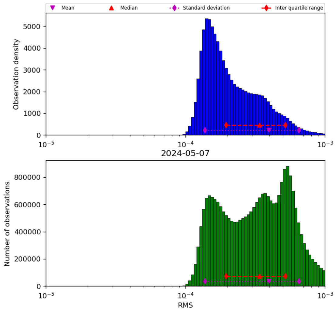
Figure 43: Histogram of “RMS” for 2024-05-07 to 2024-05-08
