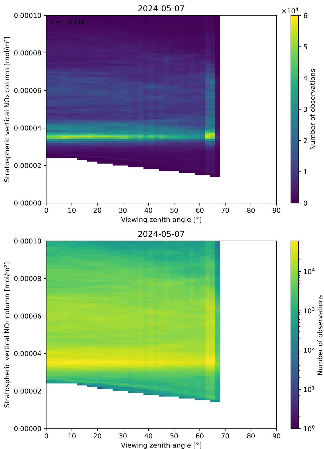
Figure 164: Scatter density plot of “Viewing zenith angle” against “Stratospheric vertical NO 2 column” for 2024-05-07 to 2024-05-08.
