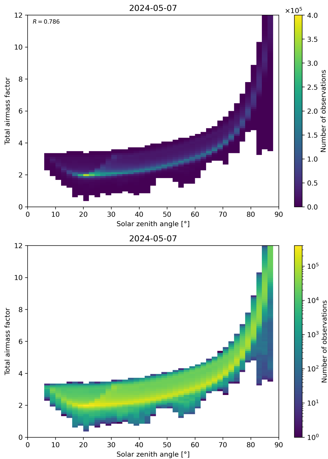
Figure 146: Scatter density plot of “Solar zenith angle” against “Total air mass factor” for 2024-05-07 to 2024-05-08.
