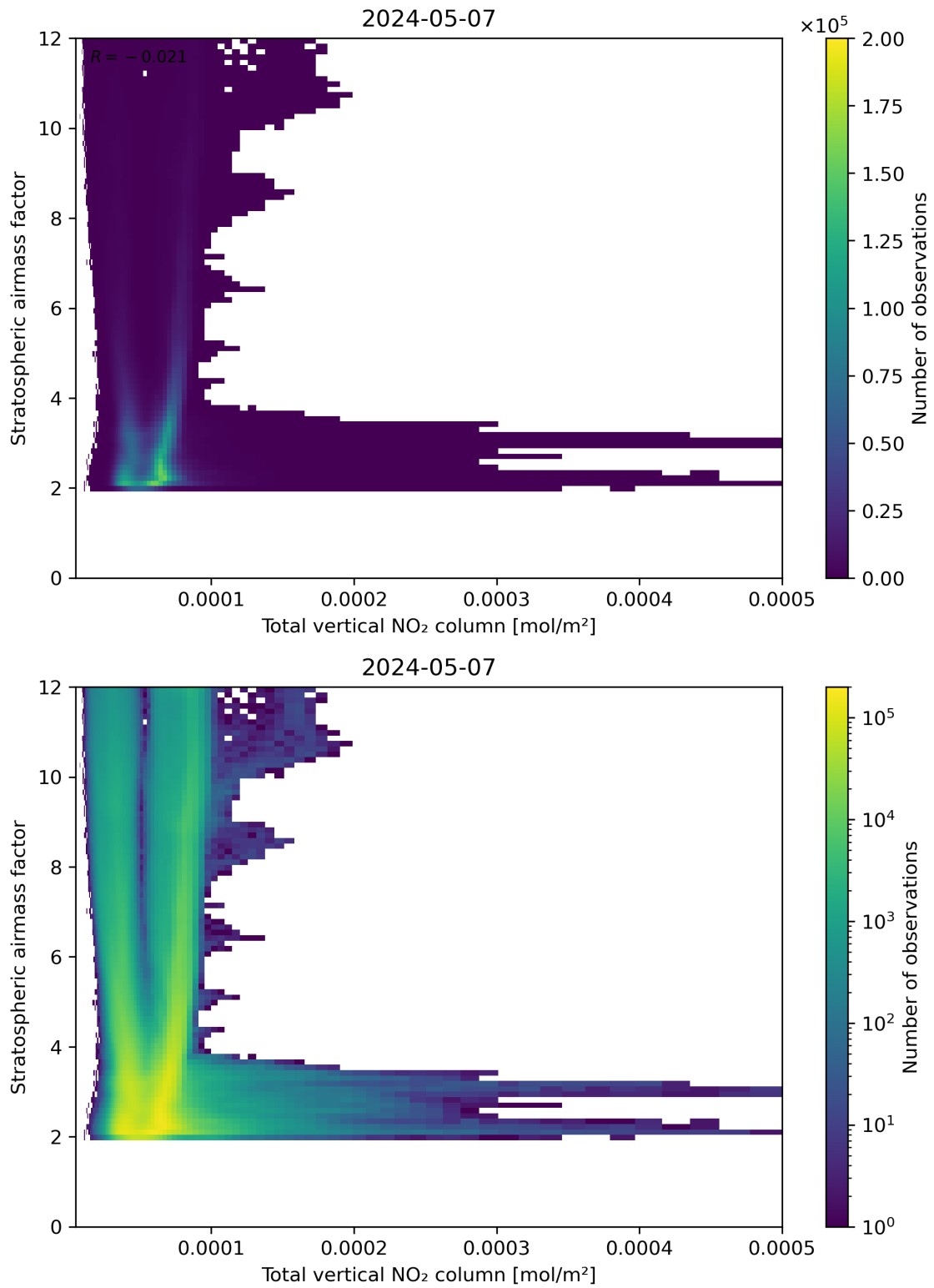
Figure 110: Scatter density plot of “Total vertical NO 2 column” against “Stratospheric airmass factor” for 2024-05-07 to 2024-05-08.
