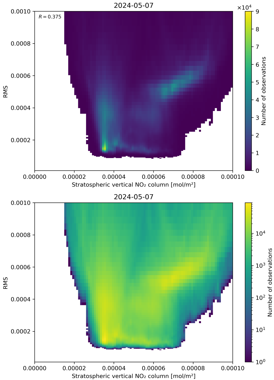
Figure 102: Scatter density plot of “Stratospheric vertical NO 2 column” against “RMS” for 2024-05-07 to 2024-05-08.
