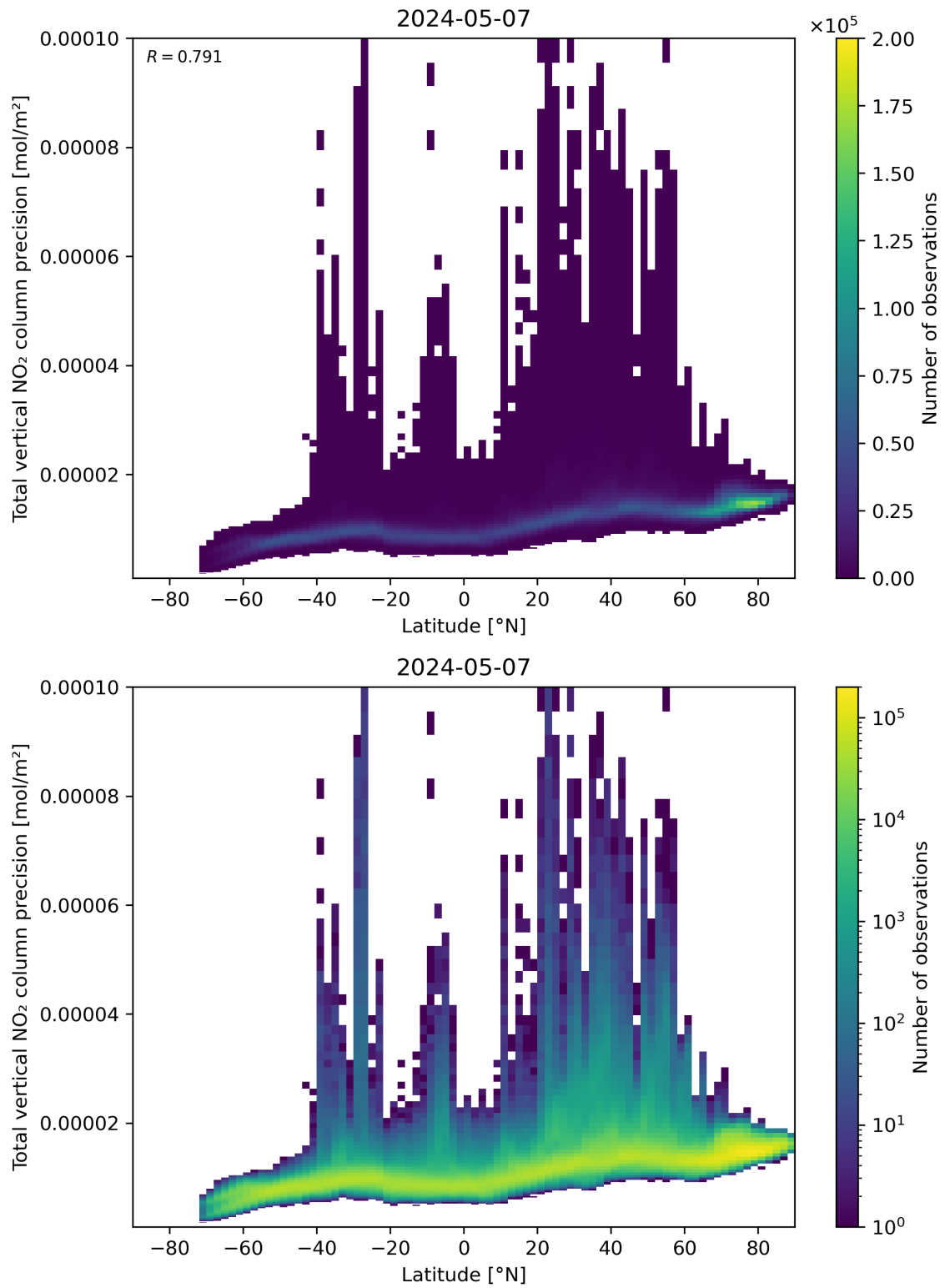
Figure 91: Scatter density plot of “Latitude” against “Total vertical NO 2 column precision” for 2024-05-07 to 2024-05-08.
