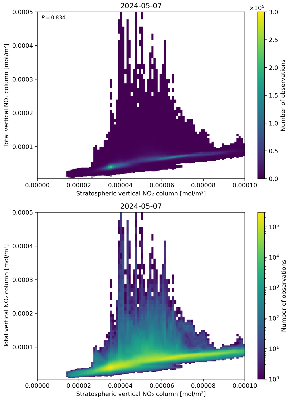
Figure 100: Scatter density plot of “Stratospheric vertical NO 2 column” against “Total vertical NO 2 column” for 2024-05-07 to 2024-05-08.
