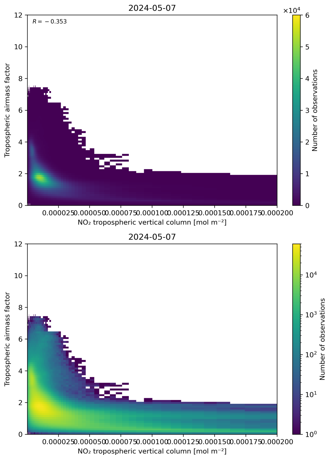
Figure 123: Scatter density plot of “NO 2 tropospheric vertical column” against “Tropospheric air mass factor” for 2024-05-07 to 2024-05-08.
