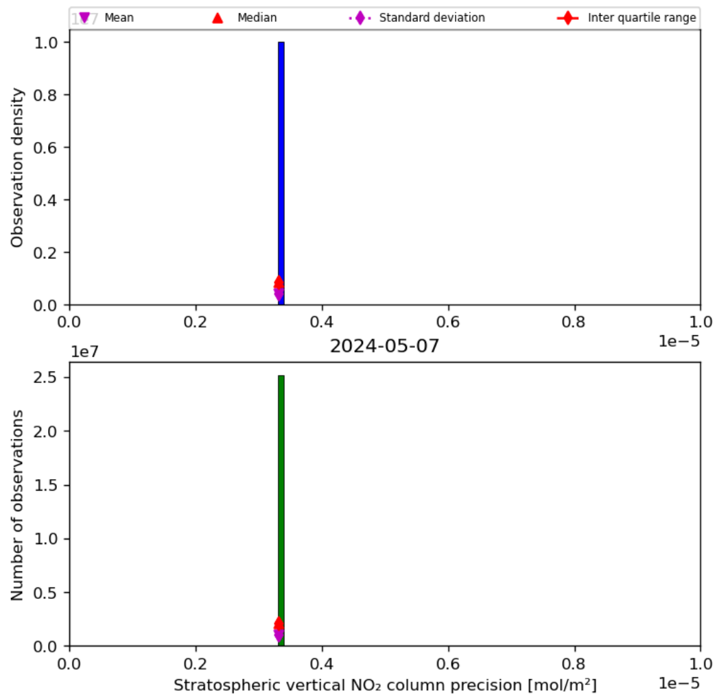
Figure 37: Histogram of “Stratospheric vertical NO 2 column precision” for 2024-05-07 to 2024-05-08
