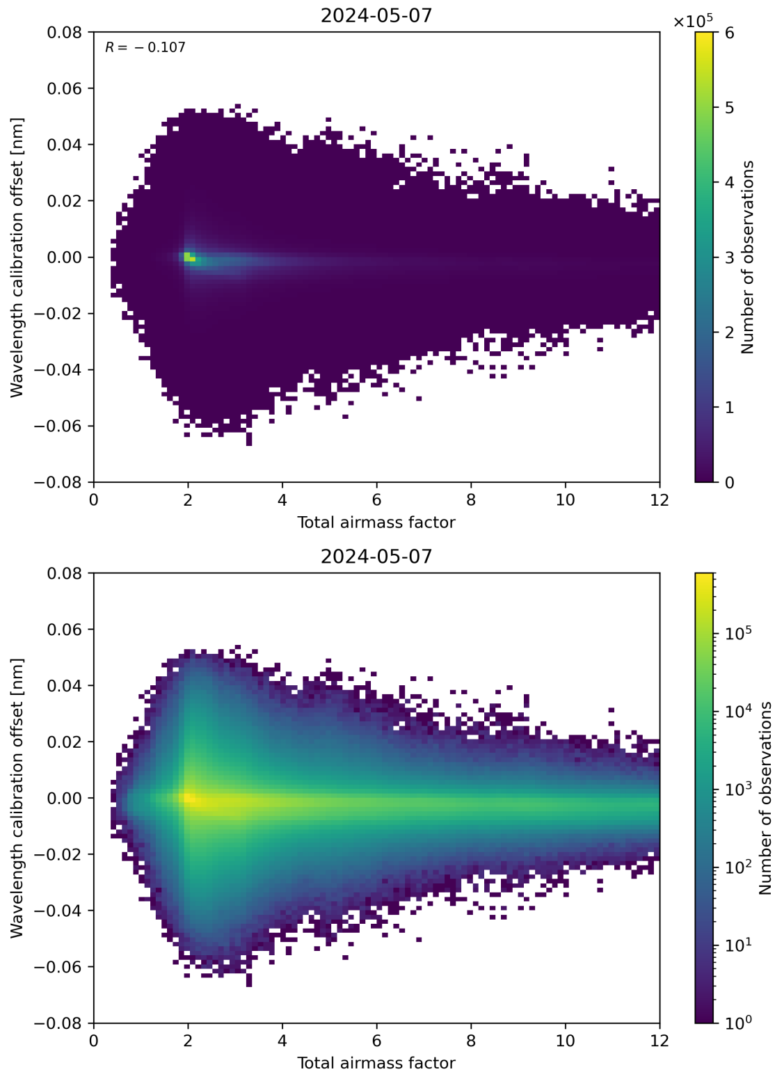
Figure 70: Scatter density plot of “Total airmass factor” against “Wavelength calibration offset” for 2024-05-07 to 2024-05-08.
