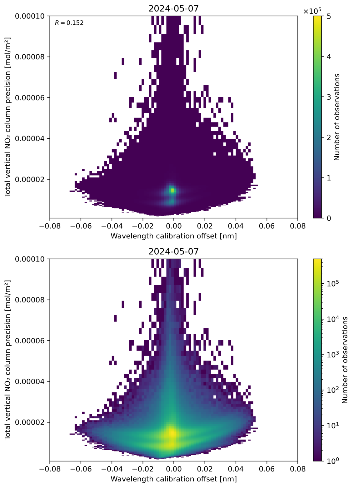
Figure 180: Scatter density plot of “Wavelength calibration offset” against “Total vertical NO 2 column precision” for 2024-05-07 to 2024-05-08.
