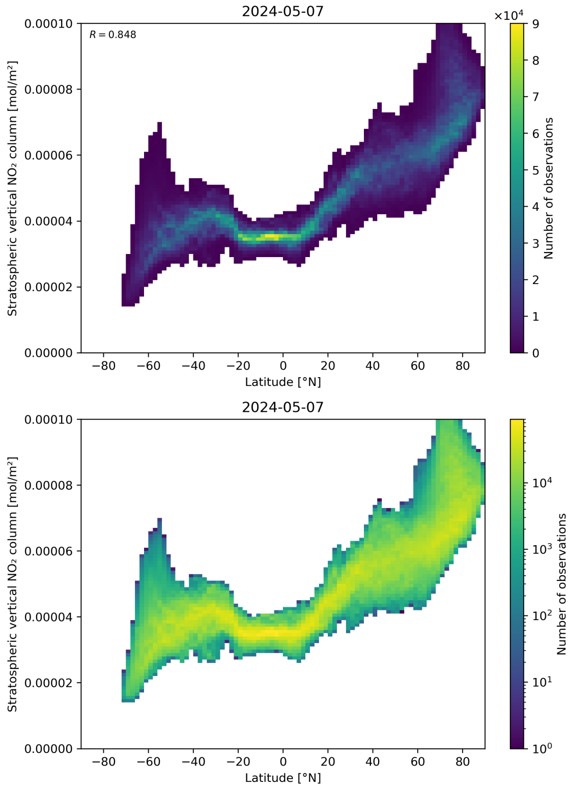
Figure 87: Scatter density plot of “Latitude” against “Stratospheric vertical \text{NO}_2 column” for 2024-05-07 to 2024-05-08.
