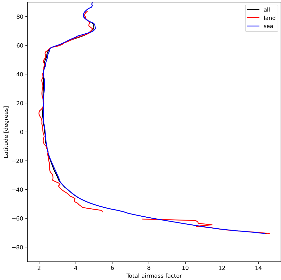
Figure 15: Zonal average of “Total airmass factor” for 2024-05-07 to 2024-05-08.
