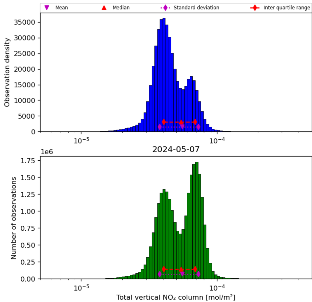
Figure 38: Histogram of "Total vertical NO 2 column" for 2024-05-07 to 2024-05-08
