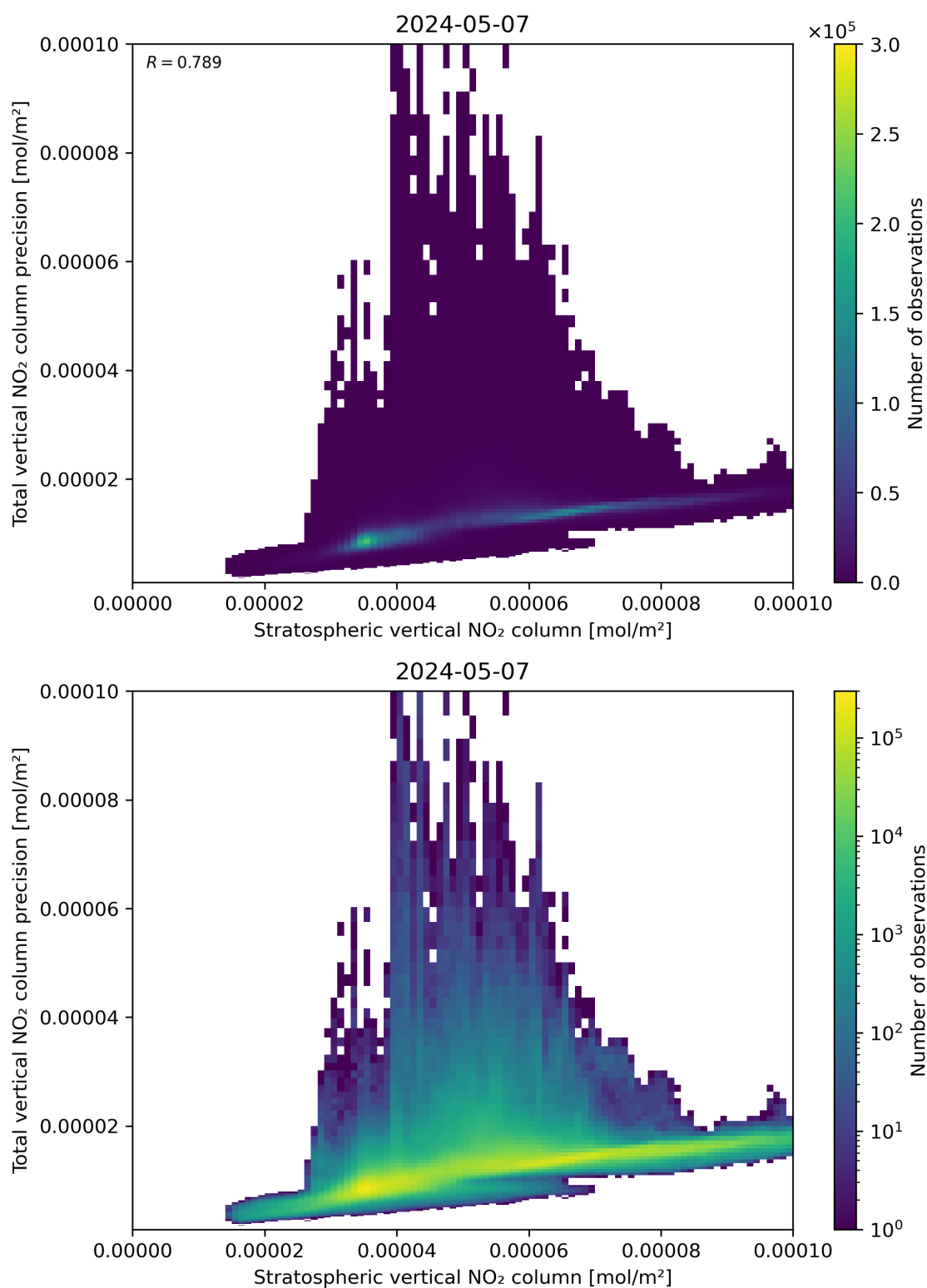
Figure 101: Scatter density plot of “Stratospheric vertical NO 2 column” against “Total vertical NO 2 column precision” for 2024-05-07 to 2024-05-08.
