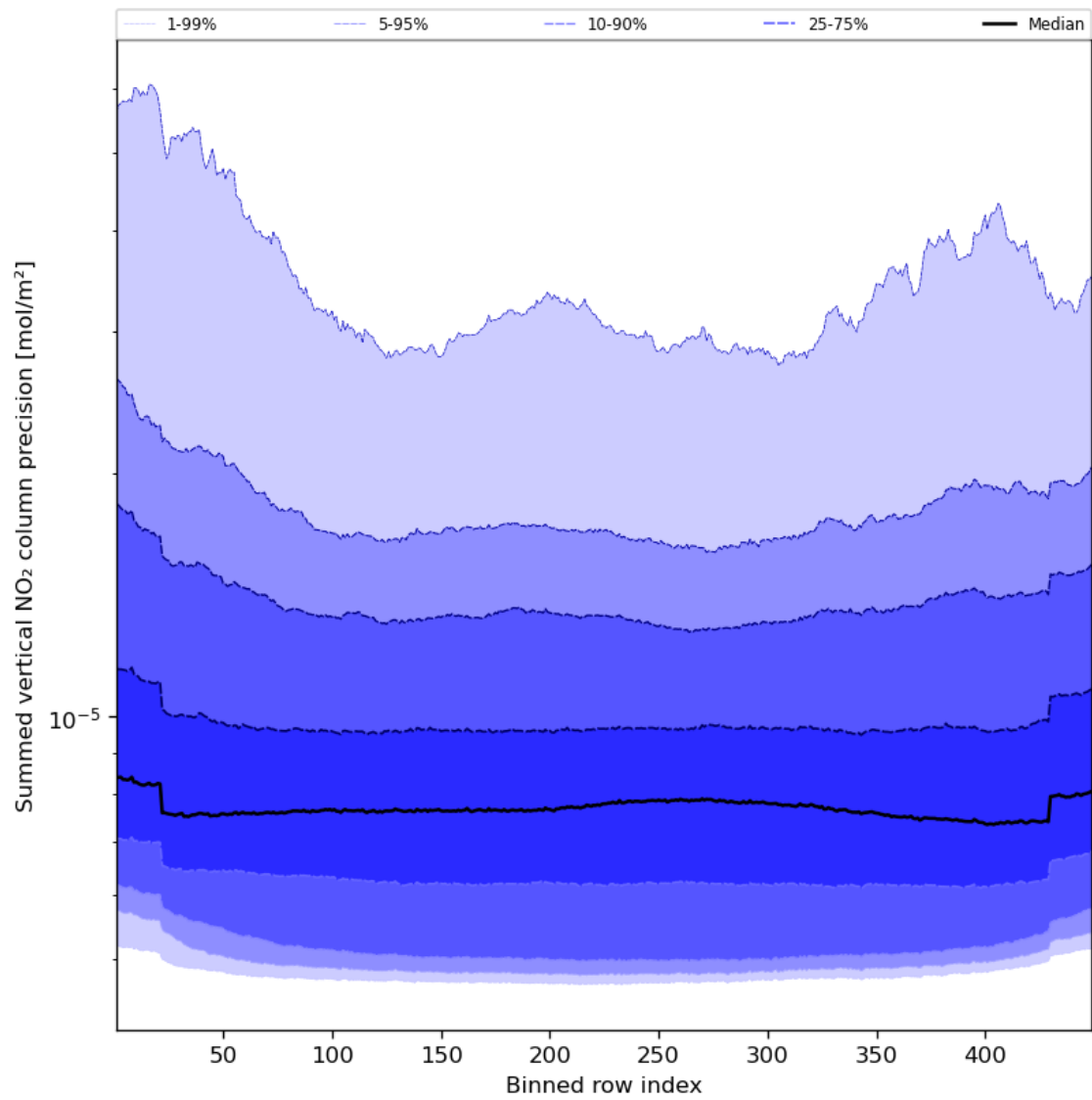
Figure 58: Along track statistics of “Summed vertical NO 2 column precision” for 2024-05-07 to 2024-05-08
