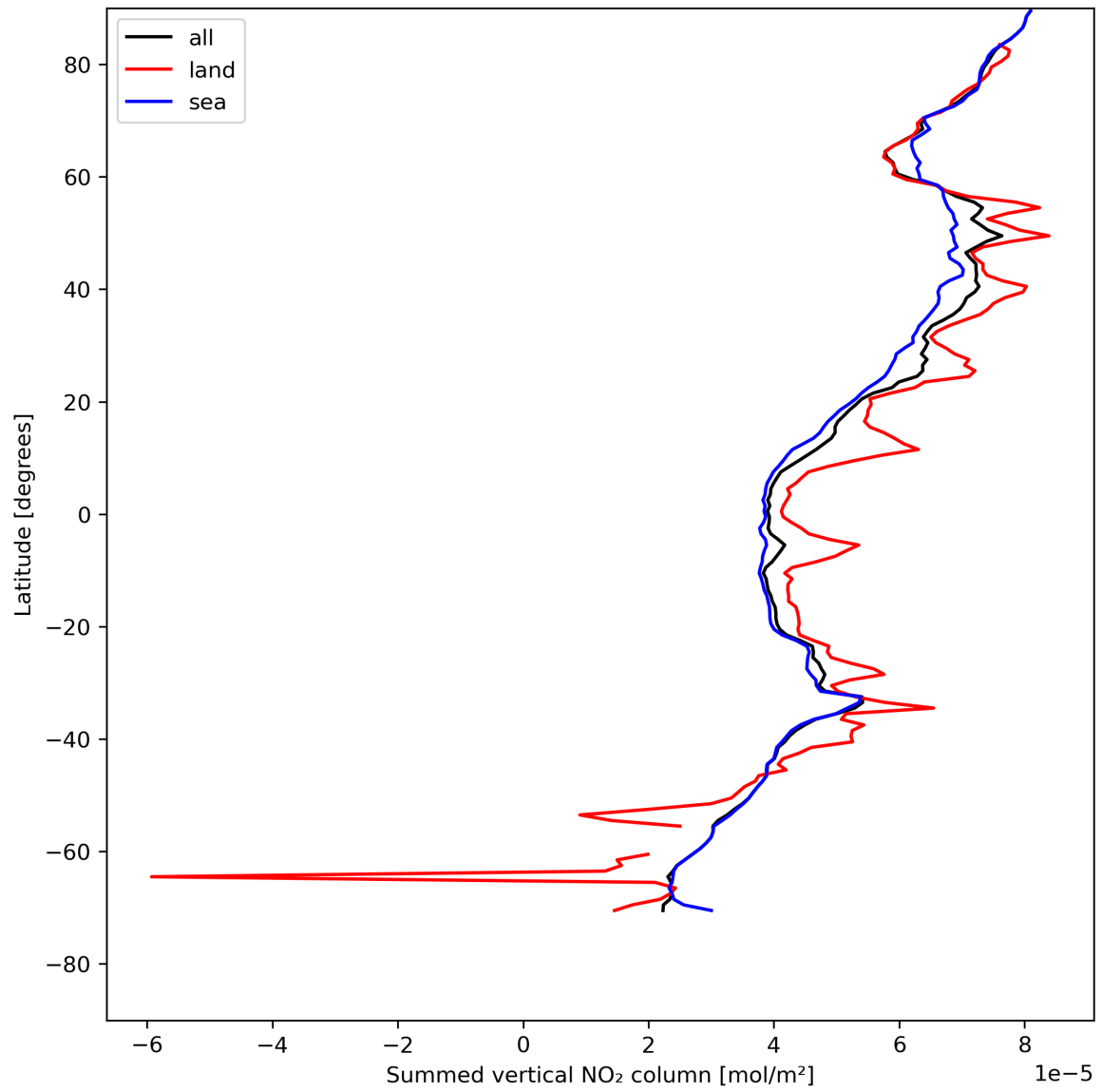
Figure 23: Zonal average of “Summed vertical NO 2 column” for 2024-05-07 to 2024-05-08.
