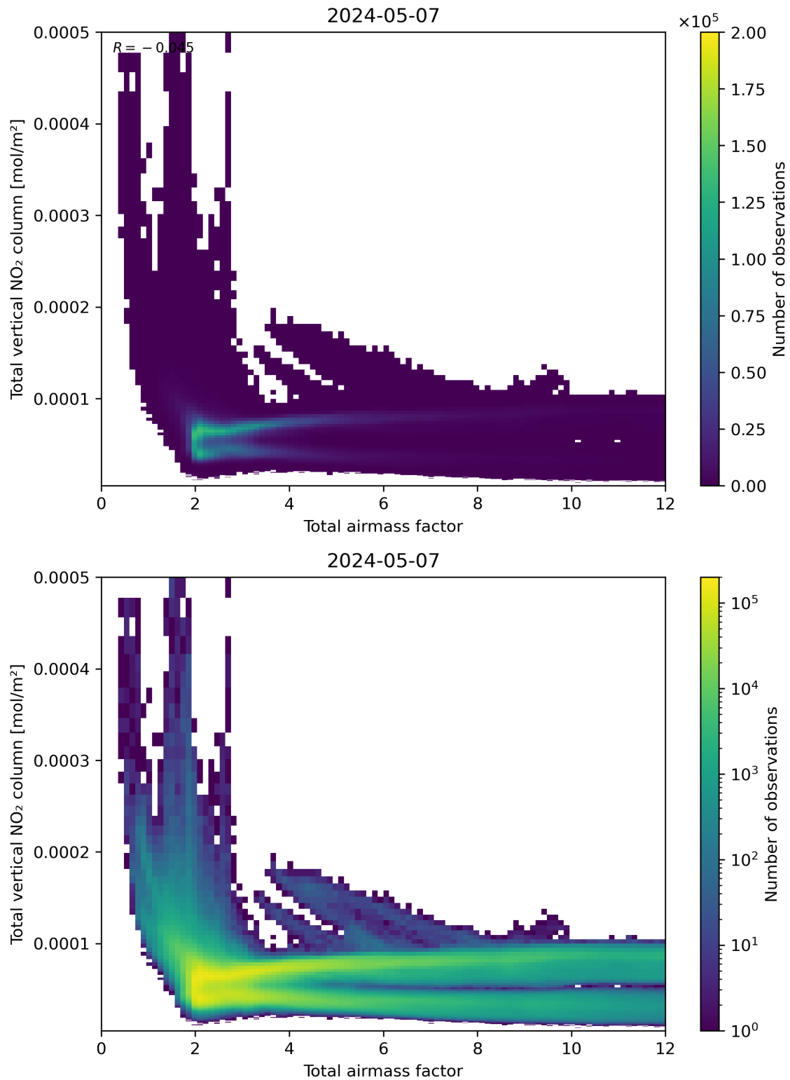
Figure 67: Scatter density plot of “Total airmass factor” against “Total vertical NO 2 column” for 2024-05-07 to 2024-05-08.
