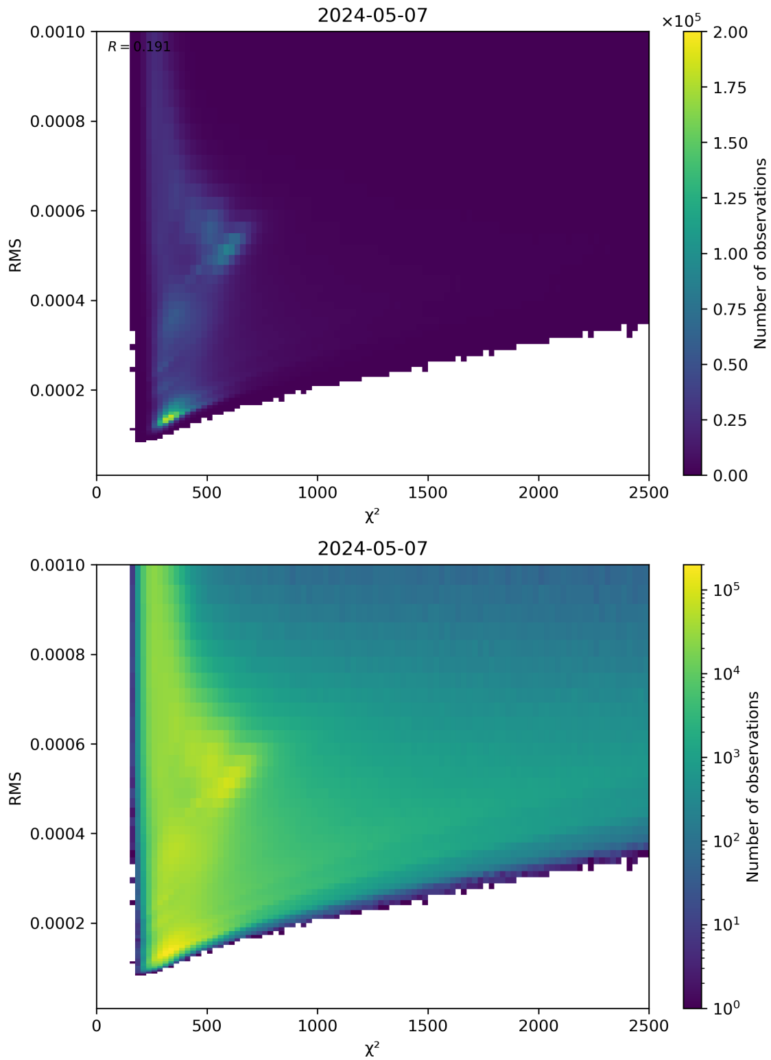
Figure 82: Scatter density plot of “ \chi^2 ” against “RMS” for 2024-05-07 to 2024-05-08.
