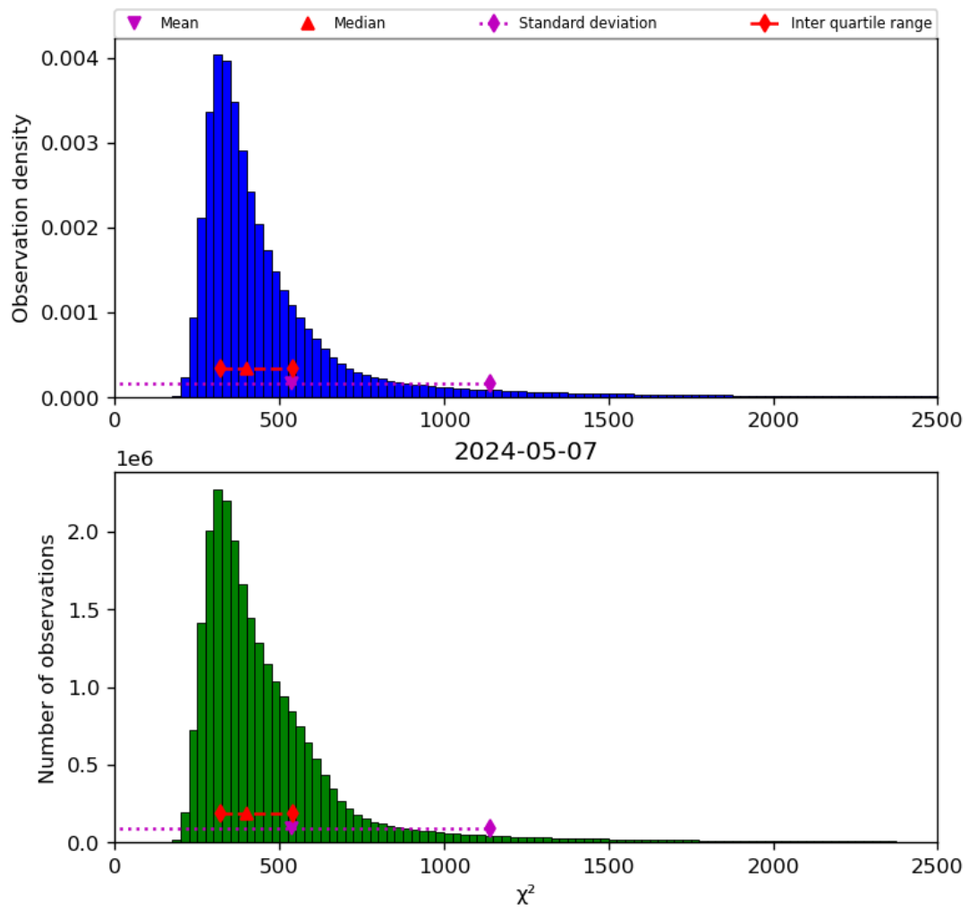
Figure 42: Histogram of “ \chi^2 ” for 2024-05-07 to 2024-05-08
