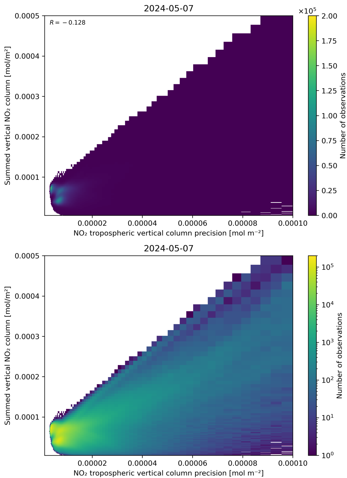
Figure 136: Scatter density plot of “NO 2 tropospheric vertical column precision” against “Summed vertical NO 2 column” for 2024-05-07 to 2024-05-08.
