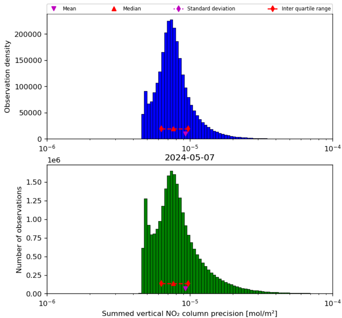
Figure 41: Histogram of “Summed vertical NO 2 column precision” for 2024-05-07 to 2024-05-08
