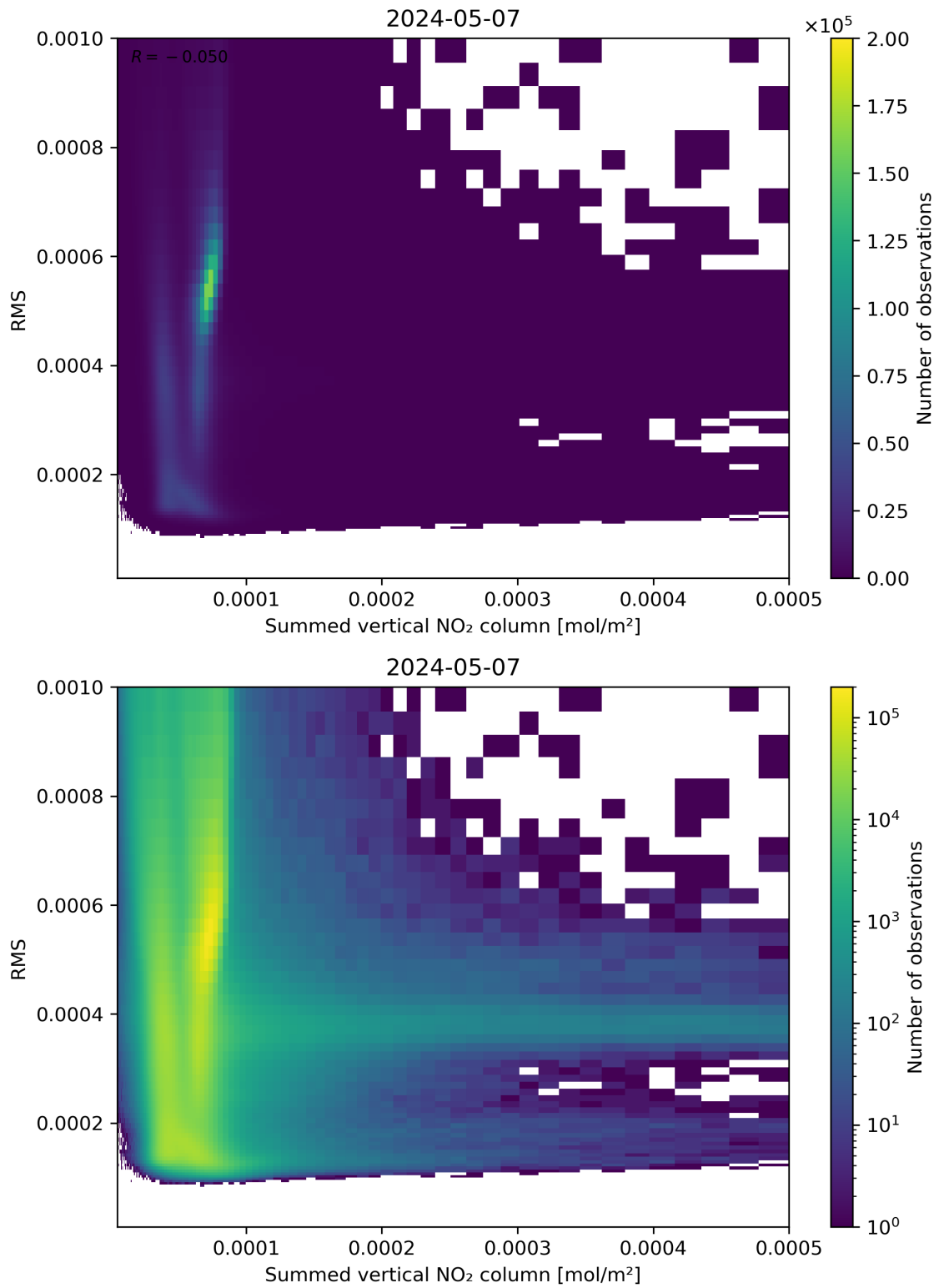
Figure 109: Scatter density plot of “Summed vertical NO 2 column” against “RMS” for 2024-05-07 to 2024-05-08.
