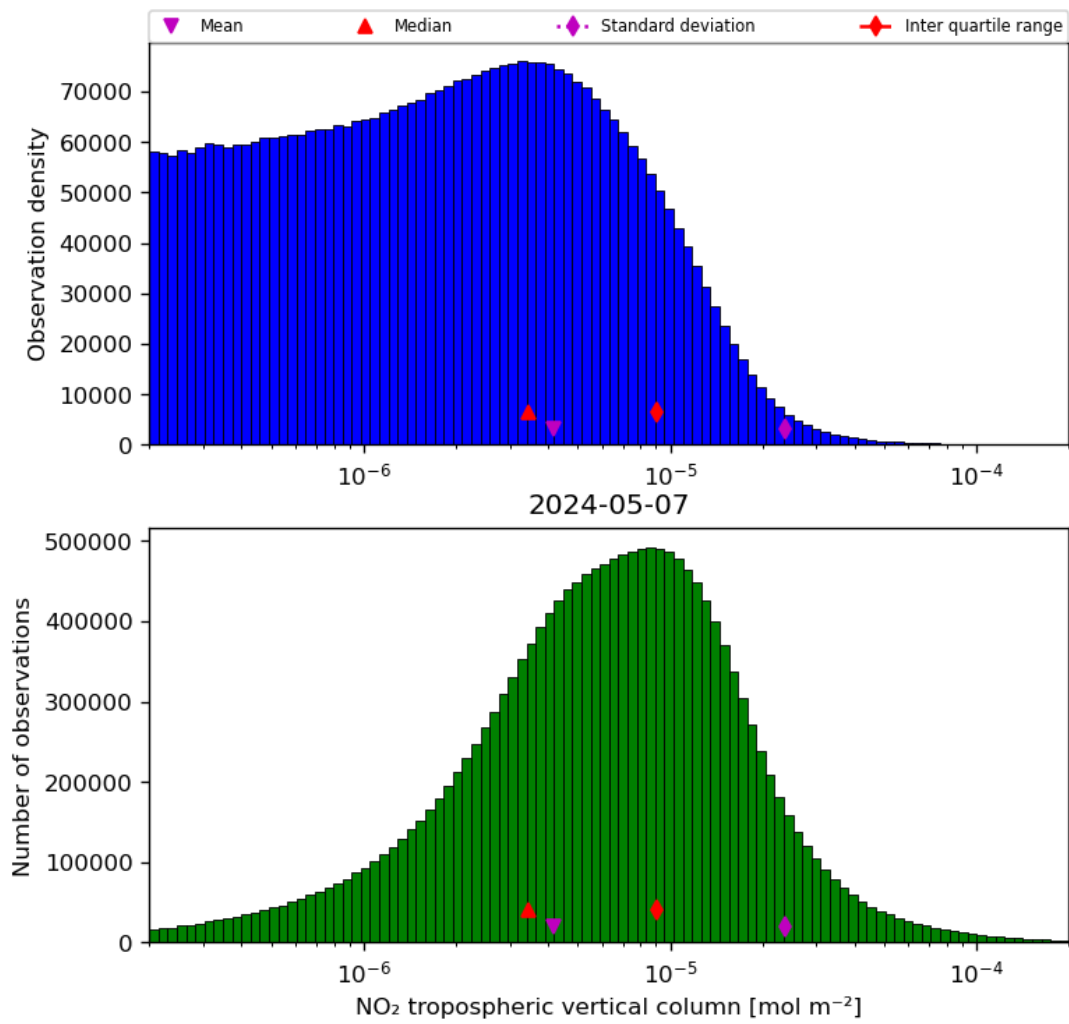
Figure 29: Histogram of “NO 2 tropospheric vertical column” for 2024-05-07 to 2024-05-08
