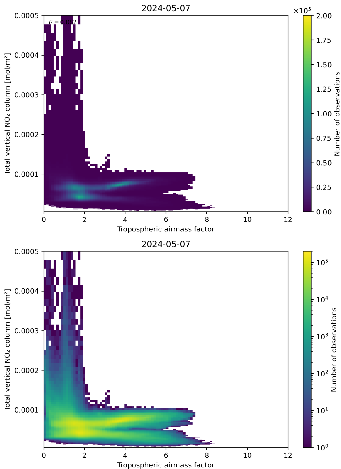
Figure 77: Scatter density plot of “Tropospheric airmass factor” against “Total vertical NO 2 column” for 2024-05-07 to 2024-05-08.
