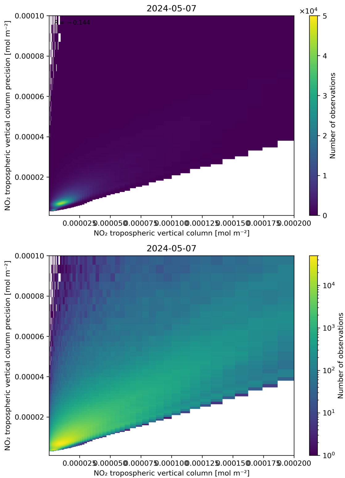
Figure 130: Scatter density plot of “NO 2 tropospheric vertical column” against “NO 2 tropospheric vertical column precision” for 2024-05-07 to 2024-05-08.
