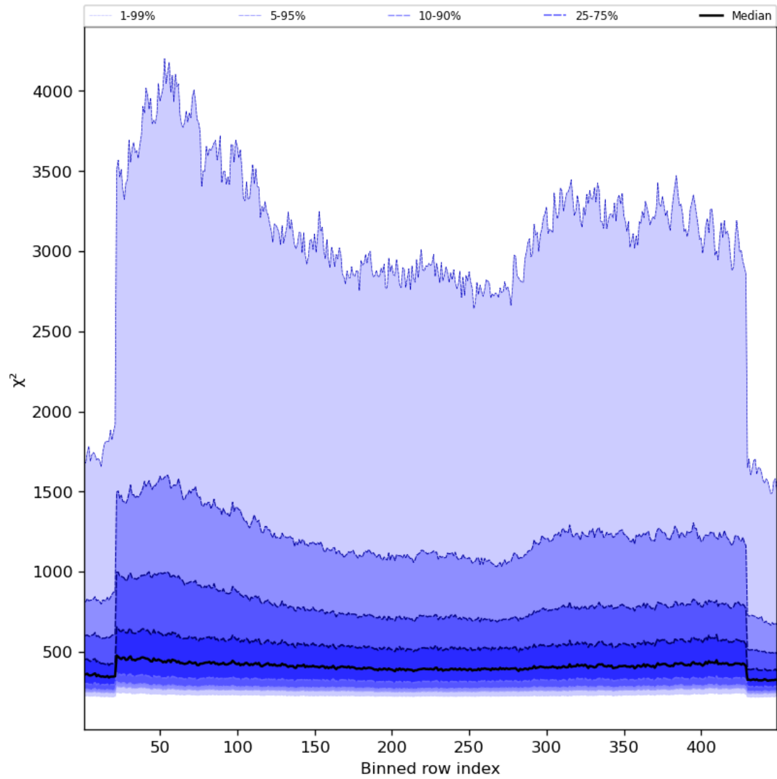
Figure 59: Along track statistics of “ \chi^2 ” for 2024-05-07 to 2024-05-08
