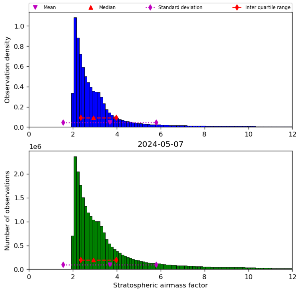
Figure 44: Histogram of “Stratospheric airmass factor” for 2024-05-07 to 2024-05-08
