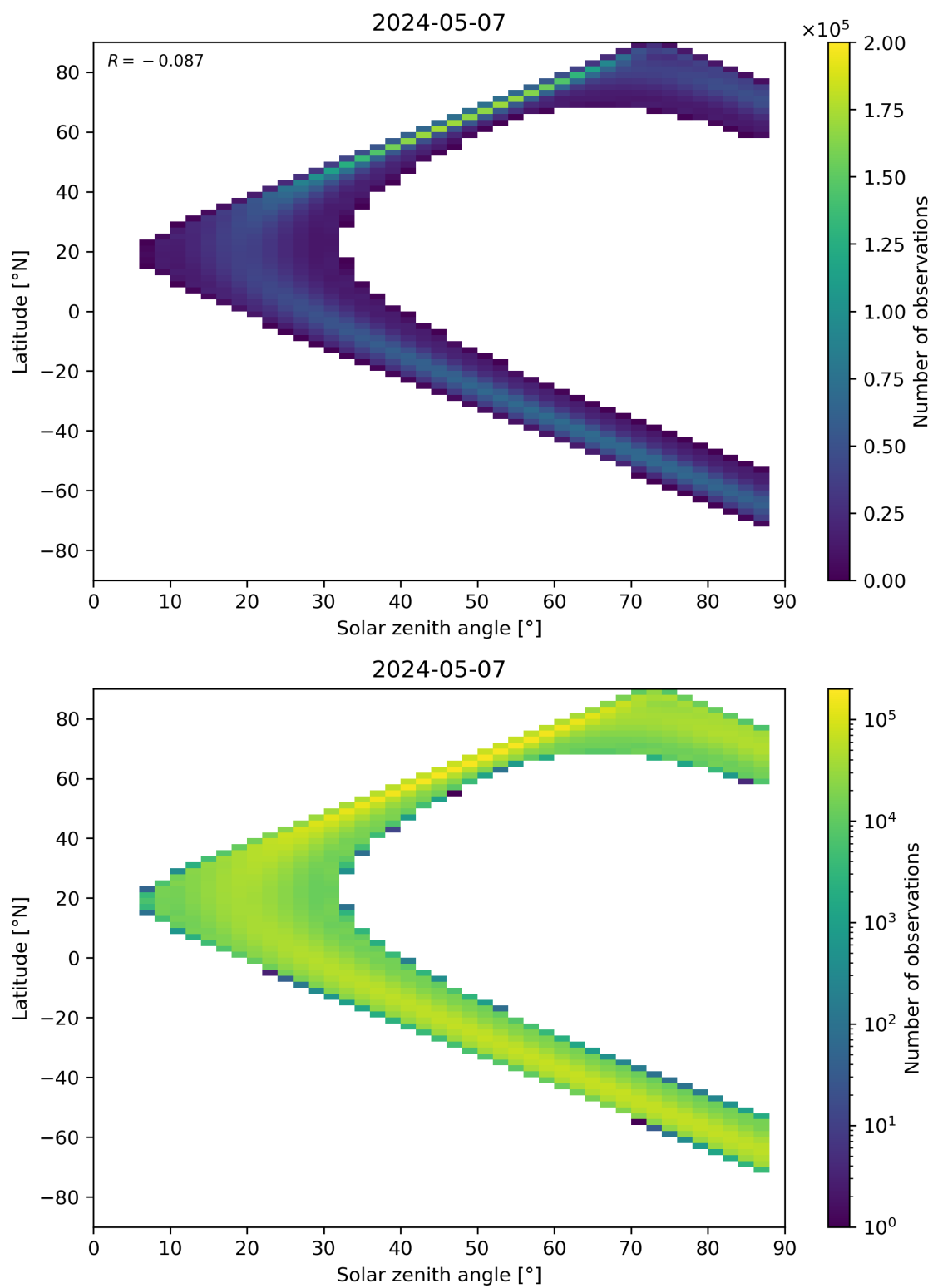
Figure 149: Scatter density plot of “Solar zenith angle” against “Latitude” for 2024-05-07 to 2024-05-08.
