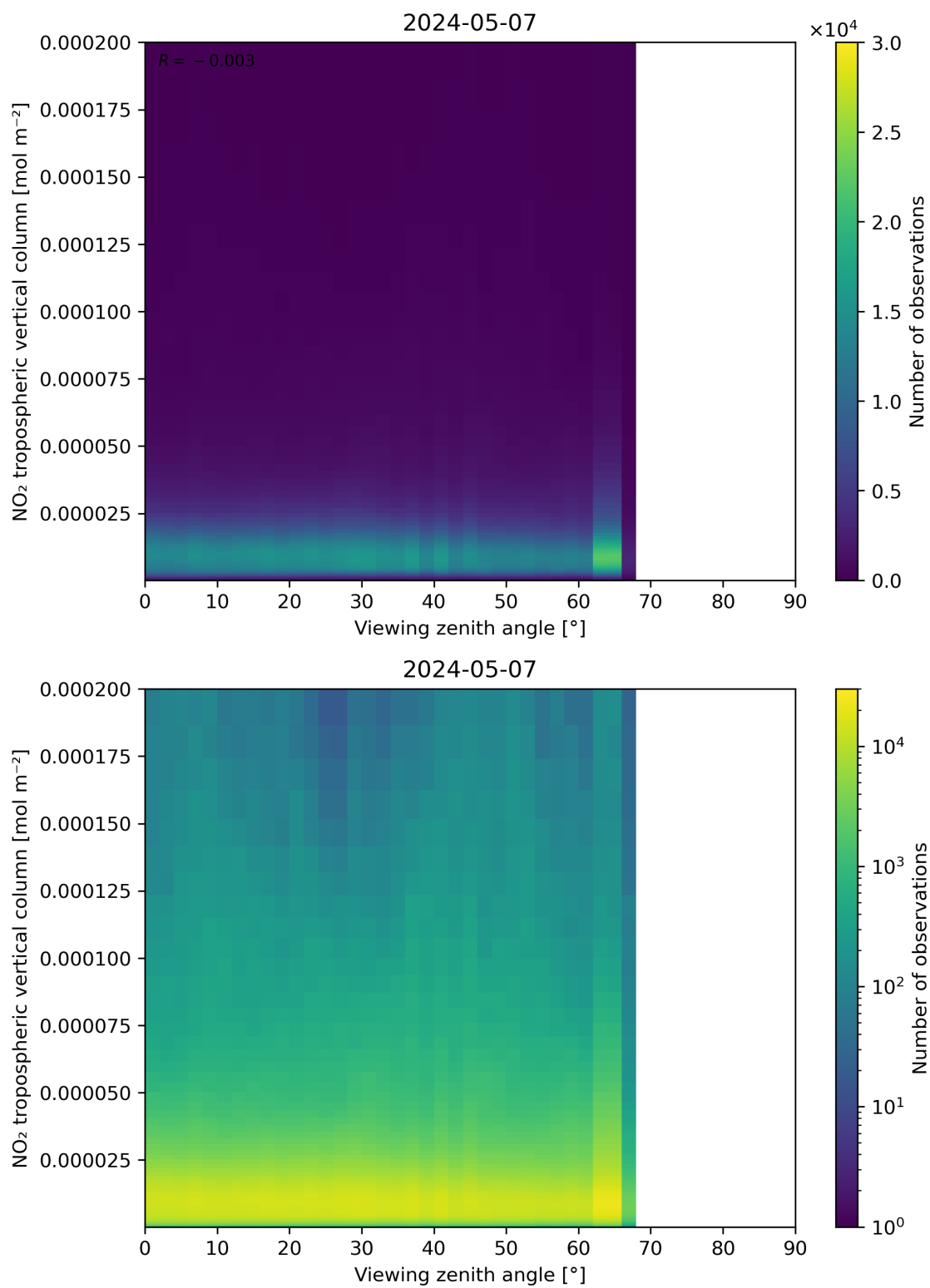
Figure 169: Scatter density plot of “Viewing zenith angle” against “NO 2 tropospheric vertical column” for 2024-05-07 to 2024-05-08.
