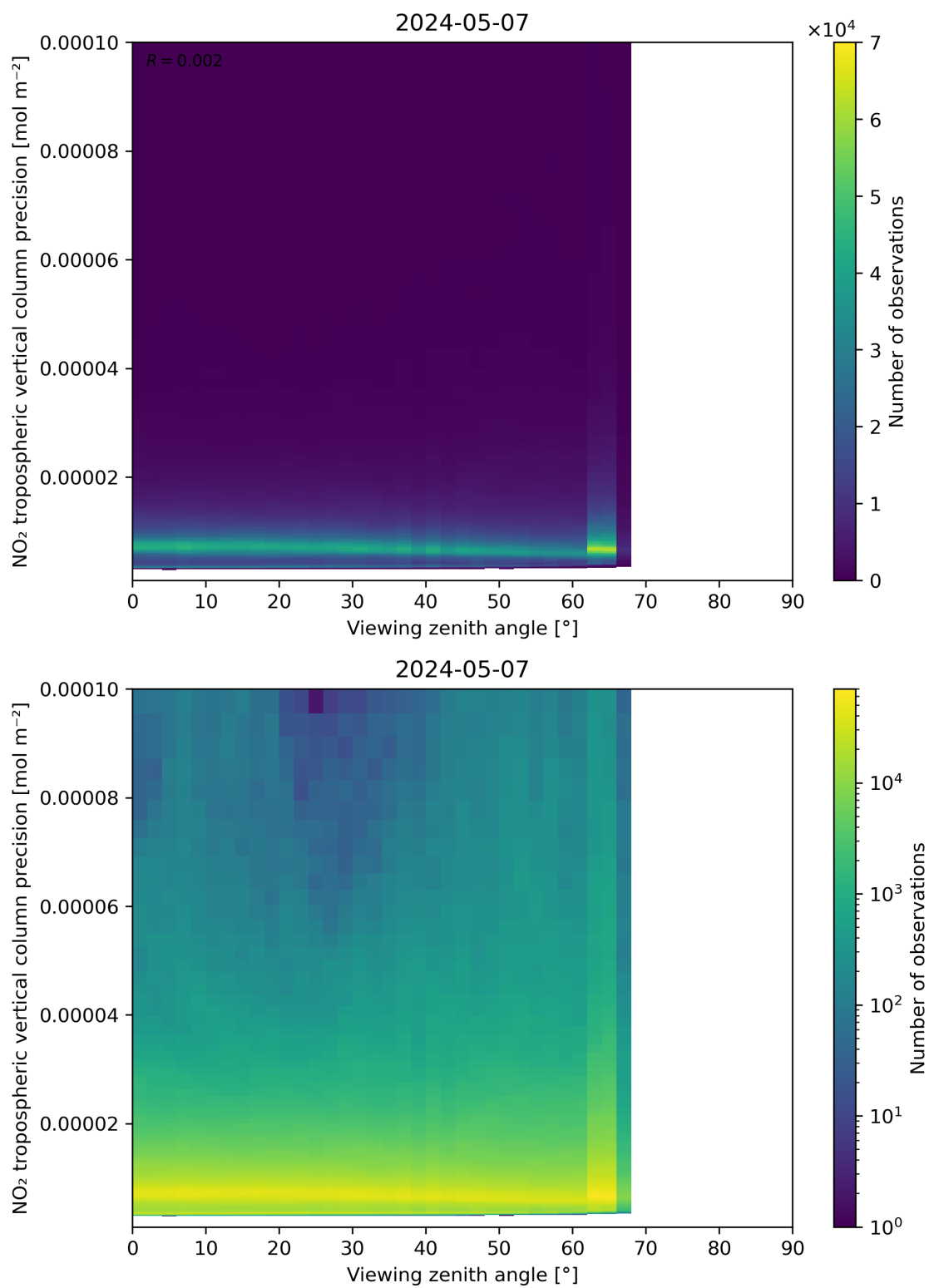
Figure 170: Scatter density plot of “Viewing zenith angle” against “NO 2 tropospheric vertical column precision” for 2024-05-07 to 2024-05-08.
