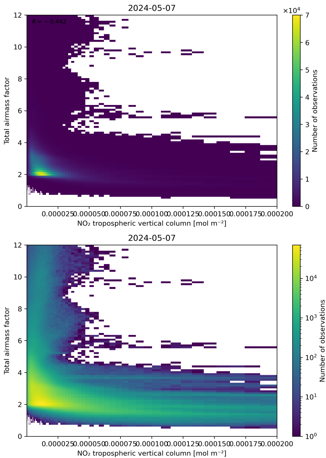
Figure 122: Scatter density plot of “NO 2 tropospheric vertical column” against “Total air mass factor” for 2024-05-07 to 2024-05-08.
