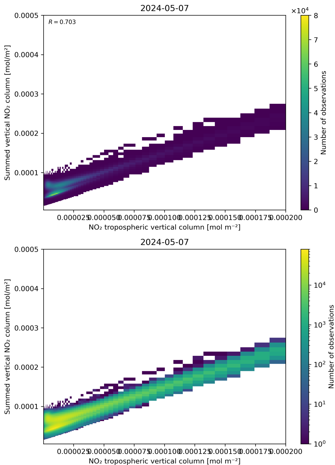
Figure 126: Scatter density plot of “NO 2 tropospheric vertical column” against “Summed vertical NO 2 column” for 2024-05-07 to 2024-05-08.
