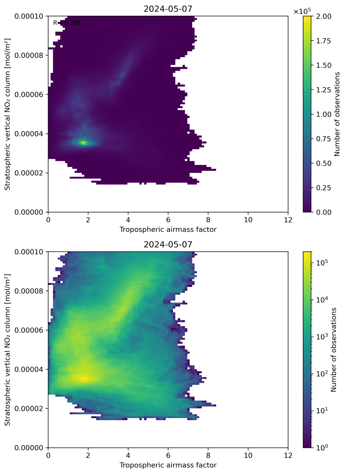
Figure 74: Scatter density plot of “Tropospheric airmass factor” against “Stratospheric vertical NO 2 column” for 2024-05-07 to 2024-05-08.
