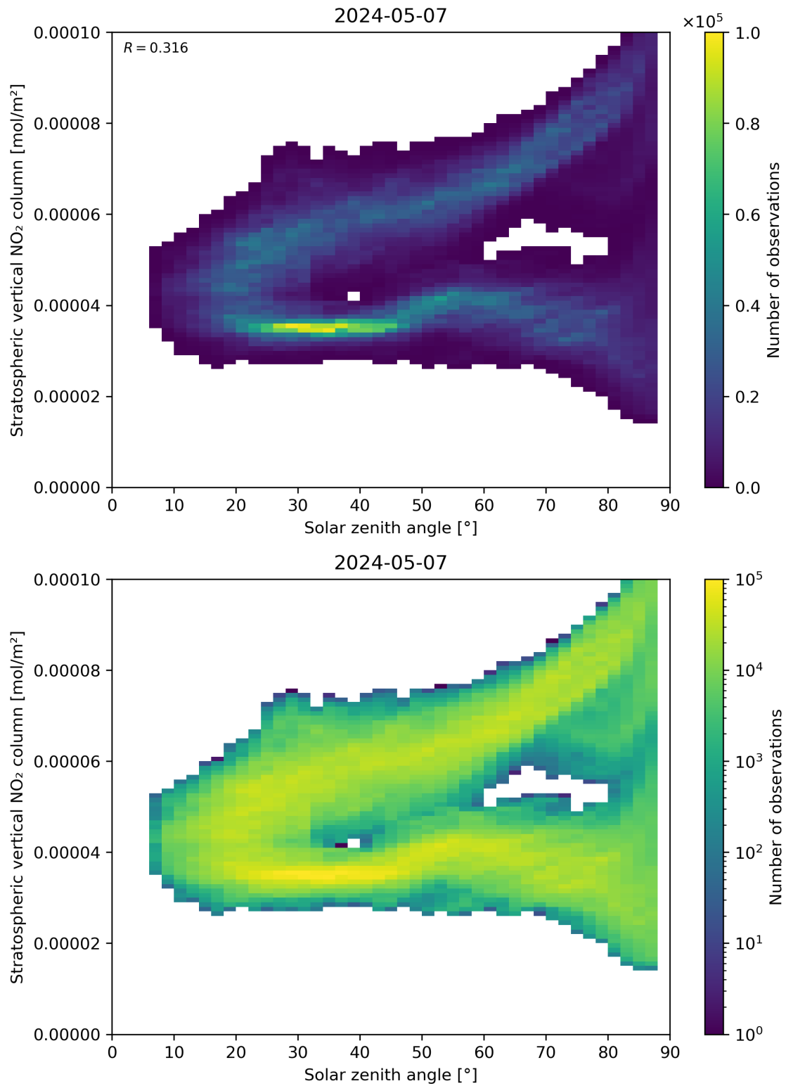
Figure 150: Scatter density plot of “Solar zenith angle” against “Stratospheric vertical NO 2 column” for 2024-05-07 to 2024-05-08.
