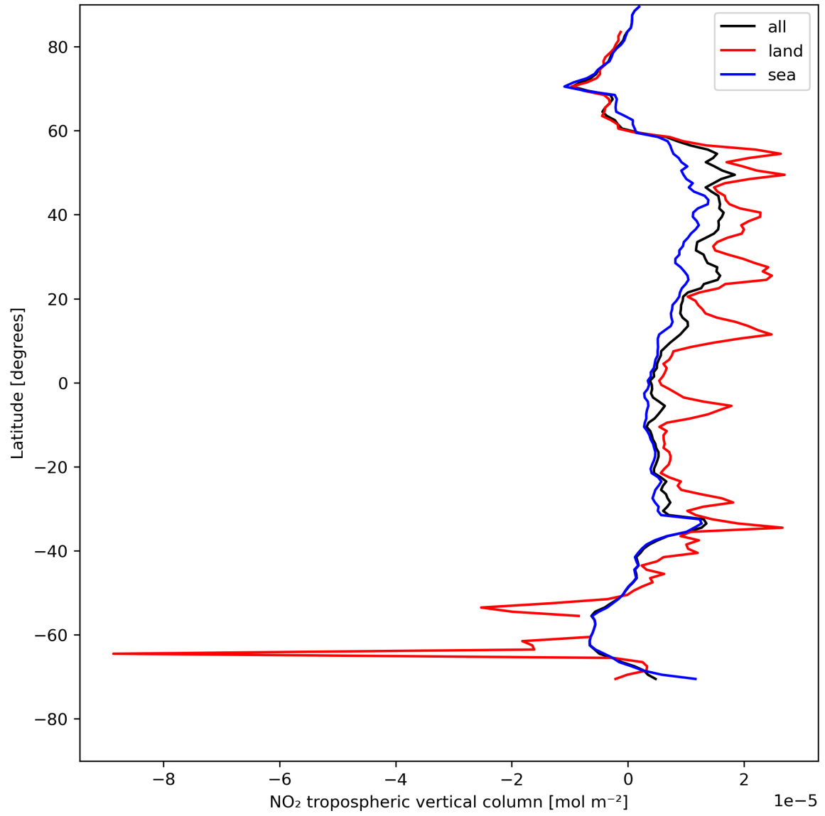
Figure 12: Zonal average of “NO 2 tropospheric vertical column” for 2024-05-07 to 2024-05-08.
