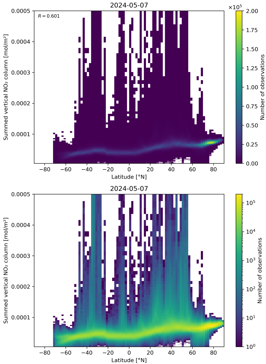
Figure 88: Scatter density plot of “Latitude” against “Summed vertical NO 2 column” for 2024-05-07 to 2024-05-08.
