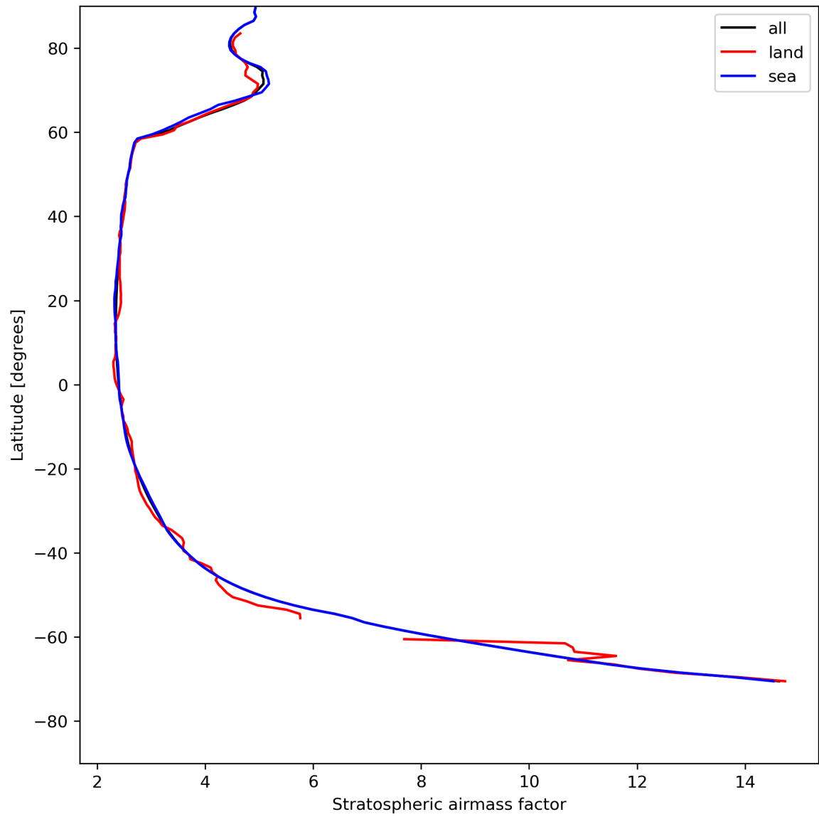
Figure 27: Zonal average of “Stratospheric air mass factor” for 2024-05-07 to 2024-05-08.
