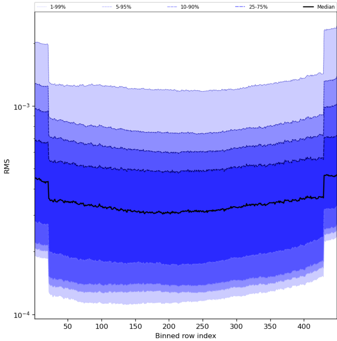
Figure 60: Along track statistics of “RMS” for 2024-05-07 to 2024-05-08
