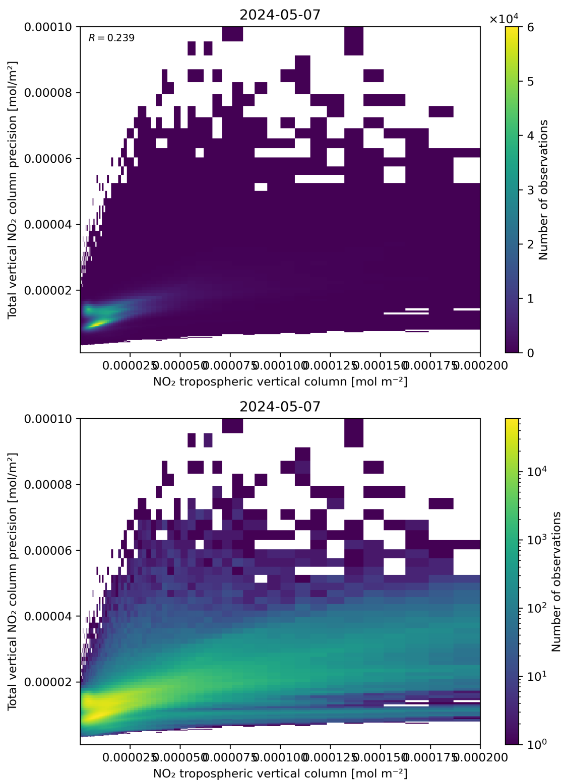
Figure 129: Scatter density plot of “NO 2 tropospheric vertical column” against “Total vertical NO 2 column precision” for 2024-05-07 to 2024-05-08.
