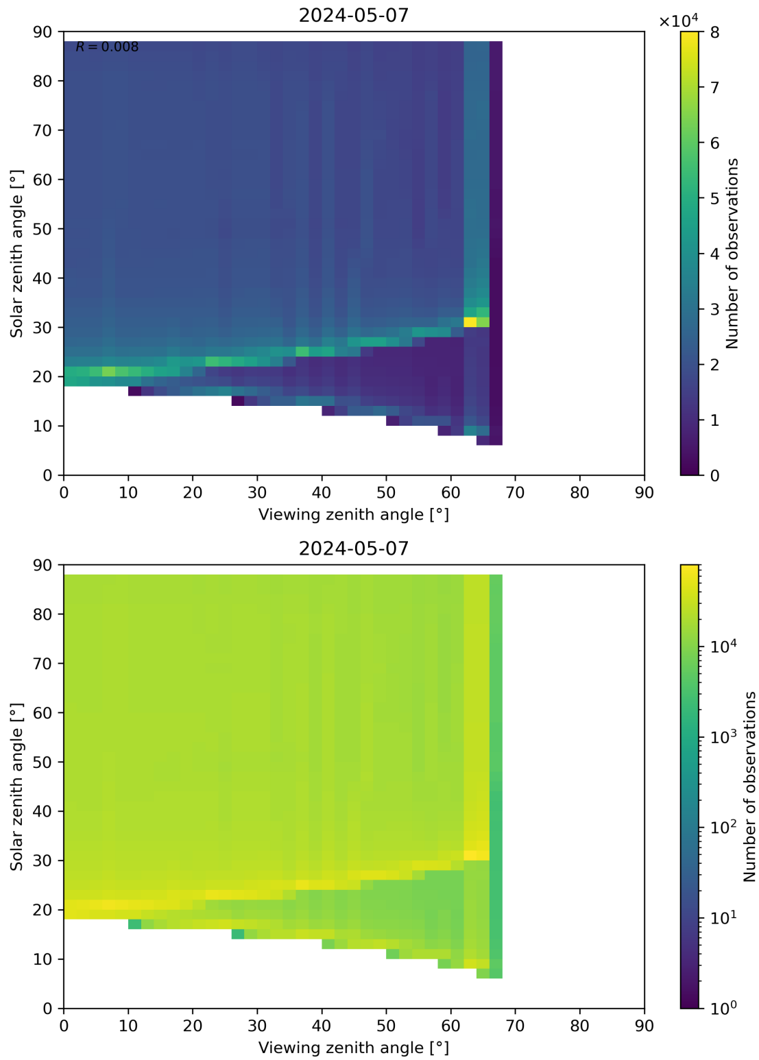
Figure 172: Scatter density plot of “Viewing zenith angle” against “Solar zenith angle” for 2024-05-07 to 2024-05-08.
