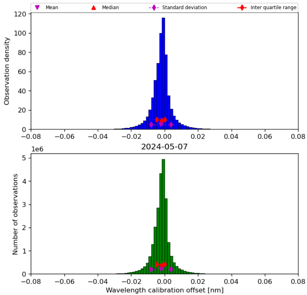
Figure 35: Histogram of “Wavelength calibration offset” for 2024-05-07 to 2024-05-08
