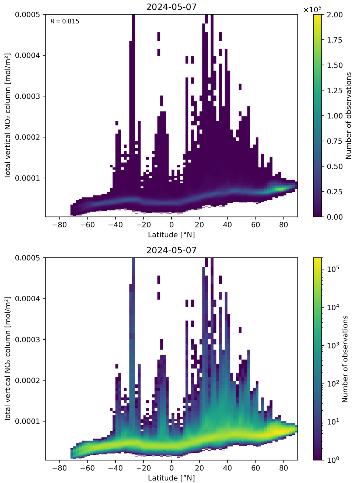
Figure 90: Scatter density plot of “Latitude” against “Total vertical NO 2 column” for 2024-05-07 to 2024-05-08.
