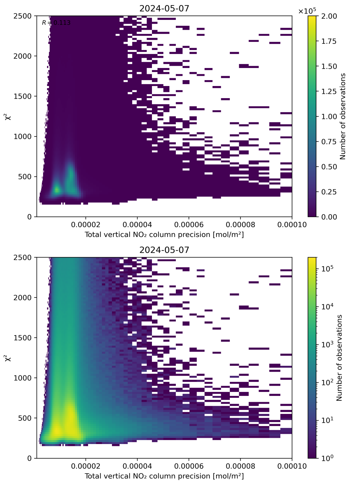
Figure 116: Scatter density plot of “Total vertical NO 2 column precision” against “ \chi^2 ” for 2024-05-07 to 2024-05-08.
