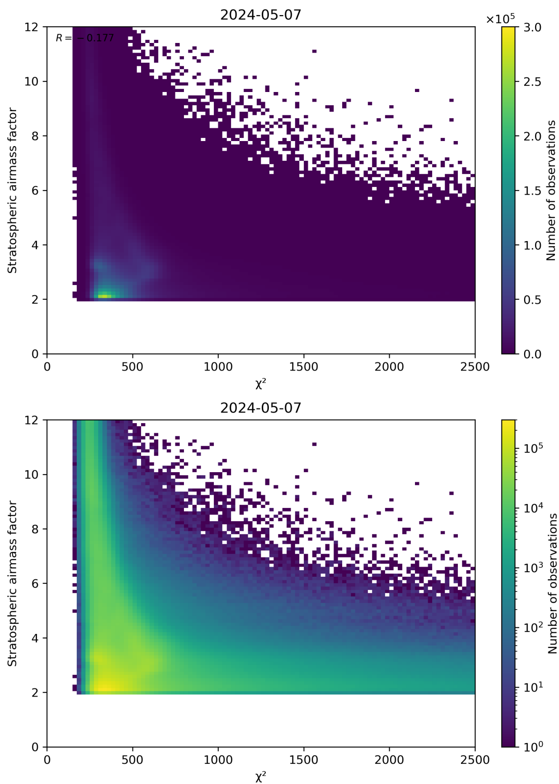
Figure 81: Scatter density plot of “ \chi^2 ” against “Stratospheric airmass factor” for 2024-05-07 to 2024-05-08.
