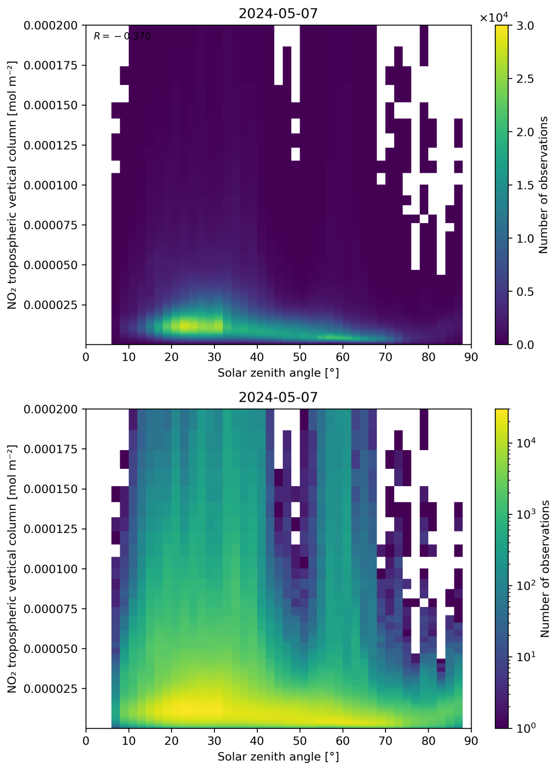
Figure 155: Scatter density plot of “Solar zenith angle” against “NO 2 tropospheric vertical column” for 2024-05-07 to 2024-05-08.
