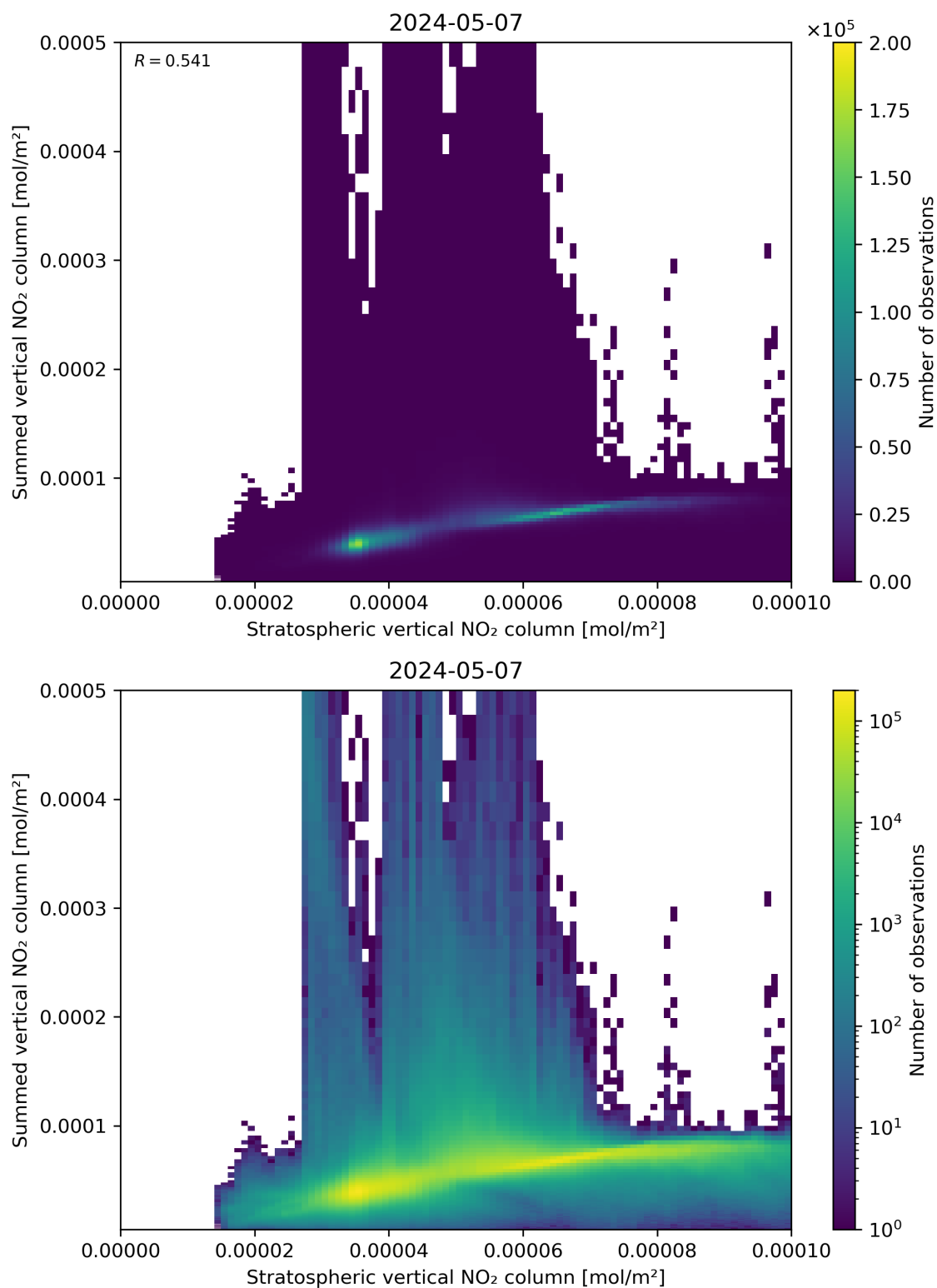
Figure 98: Scatter density plot of “Stratospheric vertical NO 2 column” against “Summed vertical NO 2 column” for 2024-05-07 to 2024-05-08.
