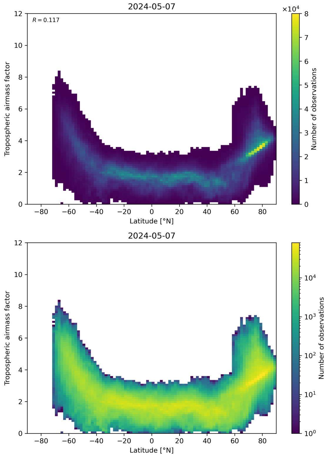
Figure 85: Scatter density plot of “Latitude” against “Tropospheric airmass factor” for 2024-05-07 to 2024-05-08.
