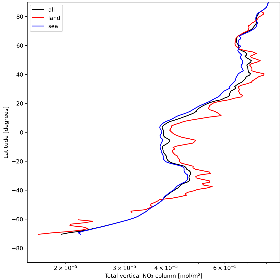
Figure 21: Zonal average of “Total vertical NO 2 column” for 2024-05-07 to 2024-05-08.
