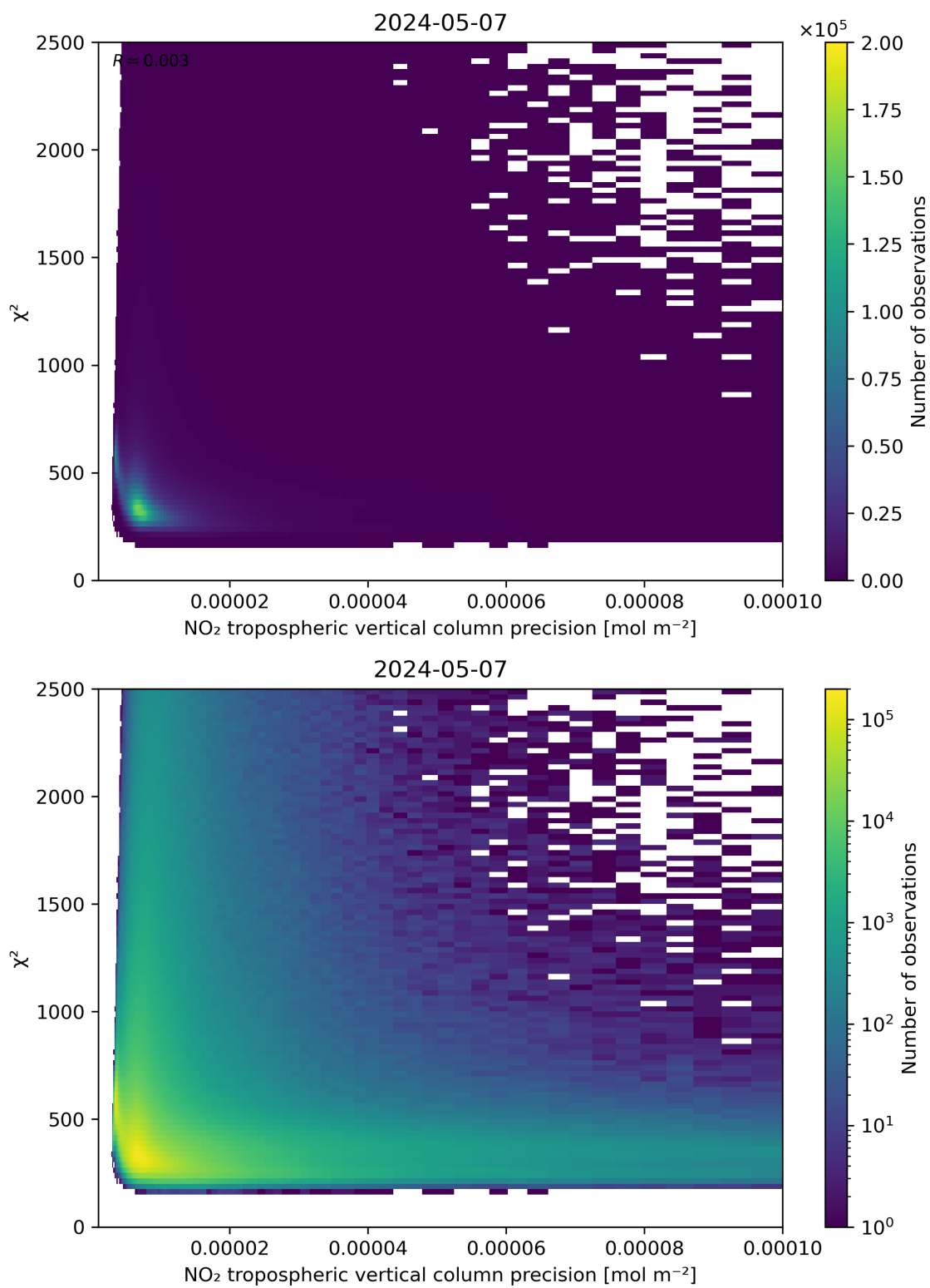
Figure 134: Scatter density plot of “NO 2 tropospheric vertical column precision” against “ \chi^2 ” for 2024-05-07 to 2024-05-08.
