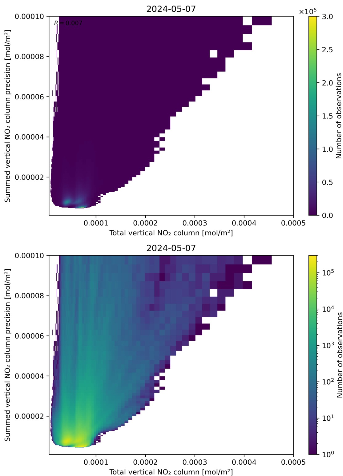
Figure 113: Scatter density plot of “Total vertical NO 2 column” against “Summed vertical NO 2 column precision” for 2024-05-07 to 2024-05-08.
