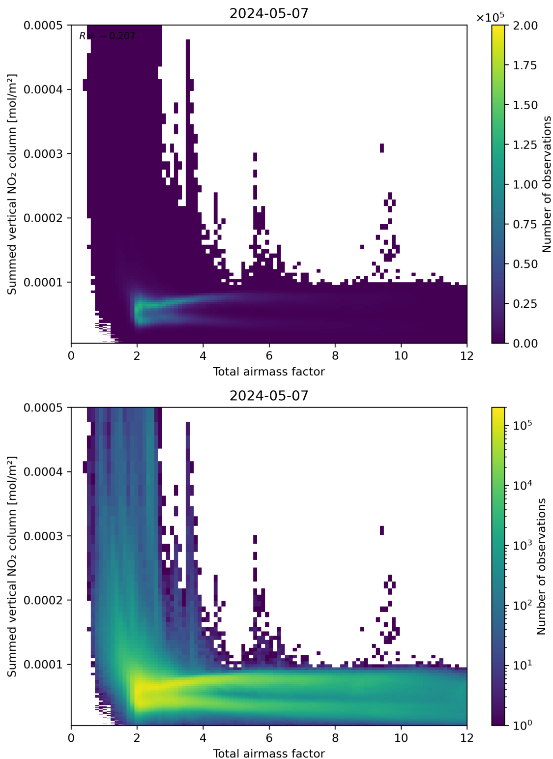
Figure 65: Scatter density plot of “Total airmass factor” against “Summed vertical NO 2 column” for 2024-05-07 to 2024-05-08.
