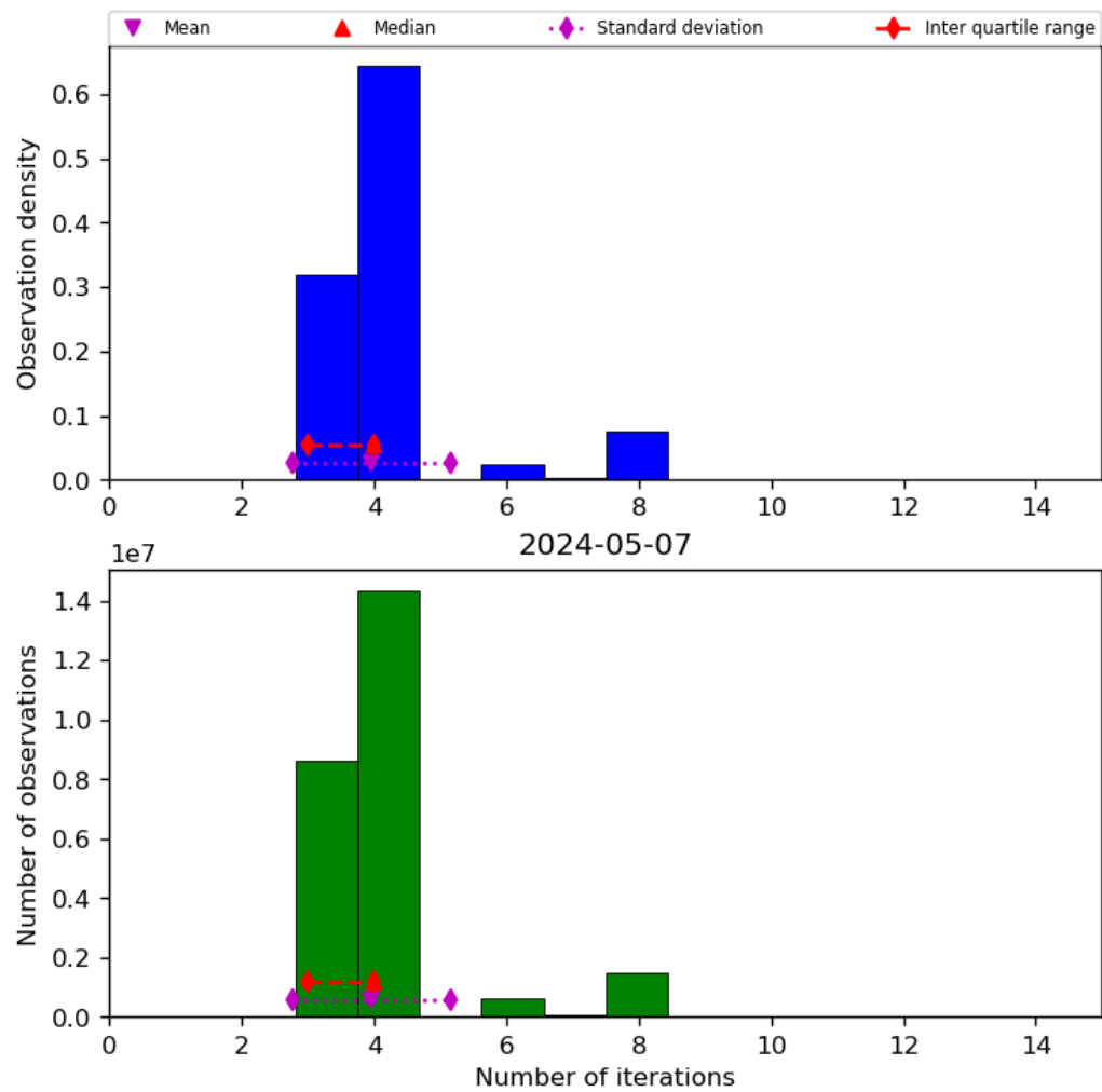
Figure 34: Histogram of “Number of iterations” for 2024-05-07 to 2024-05-08
