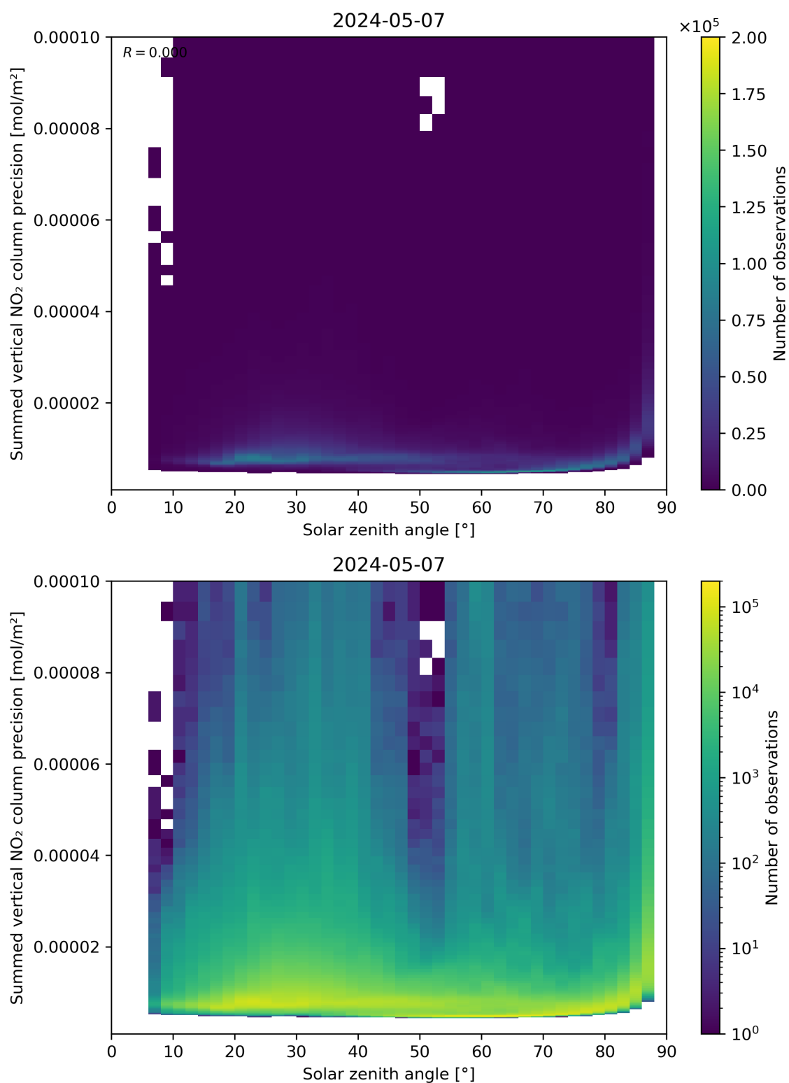
Figure 152: Scatter density plot of “Solar zenith angle” against “Summed vertical NO 2 column precision” for 2024-05-07 to 2024-05-08.
