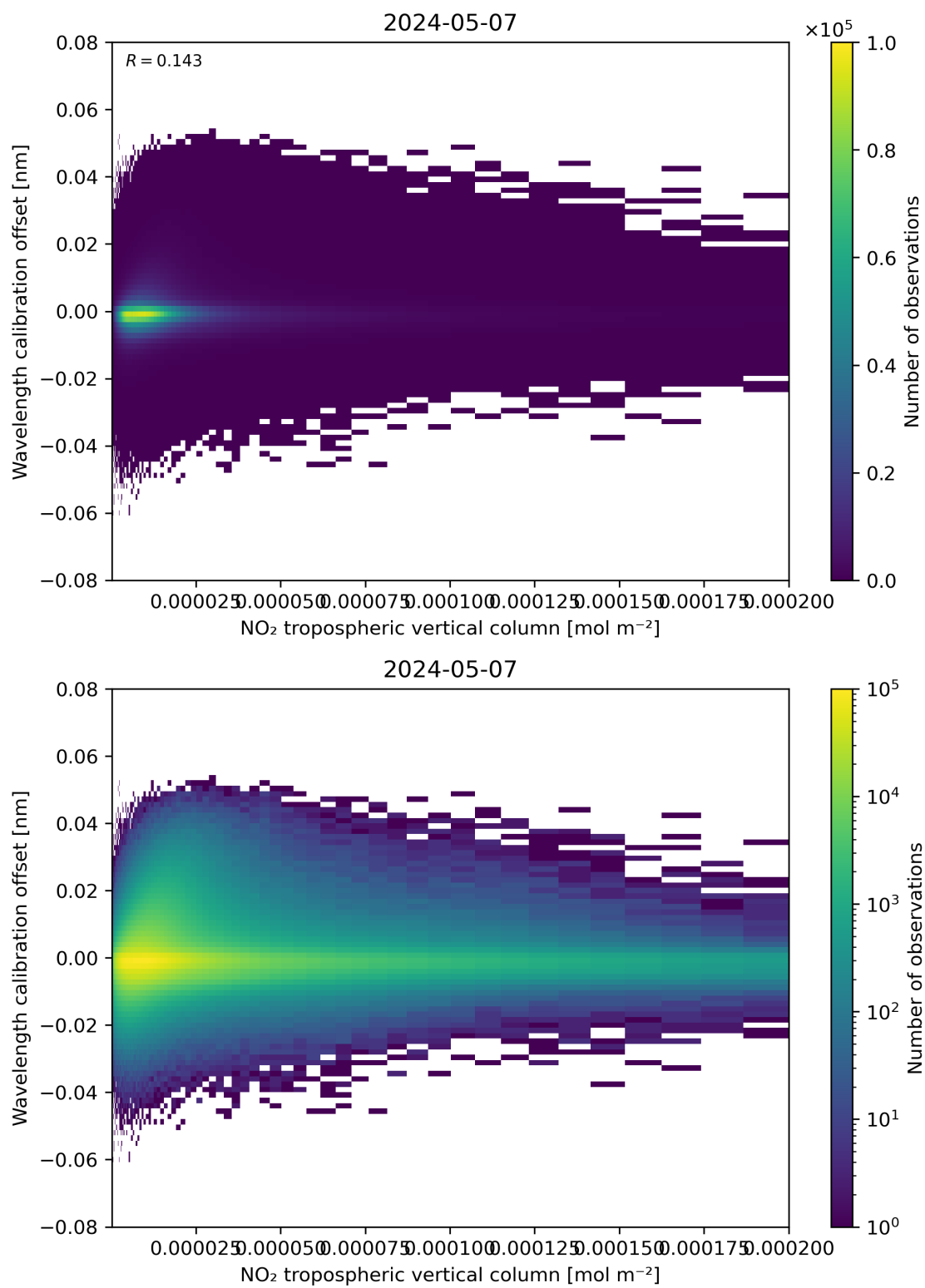
Figure 143: Scatter density plot of “NO 2 tropospheric vertical column” against “Wavelength calibration offset” for 2024-05-07 to 2024-05-08.
