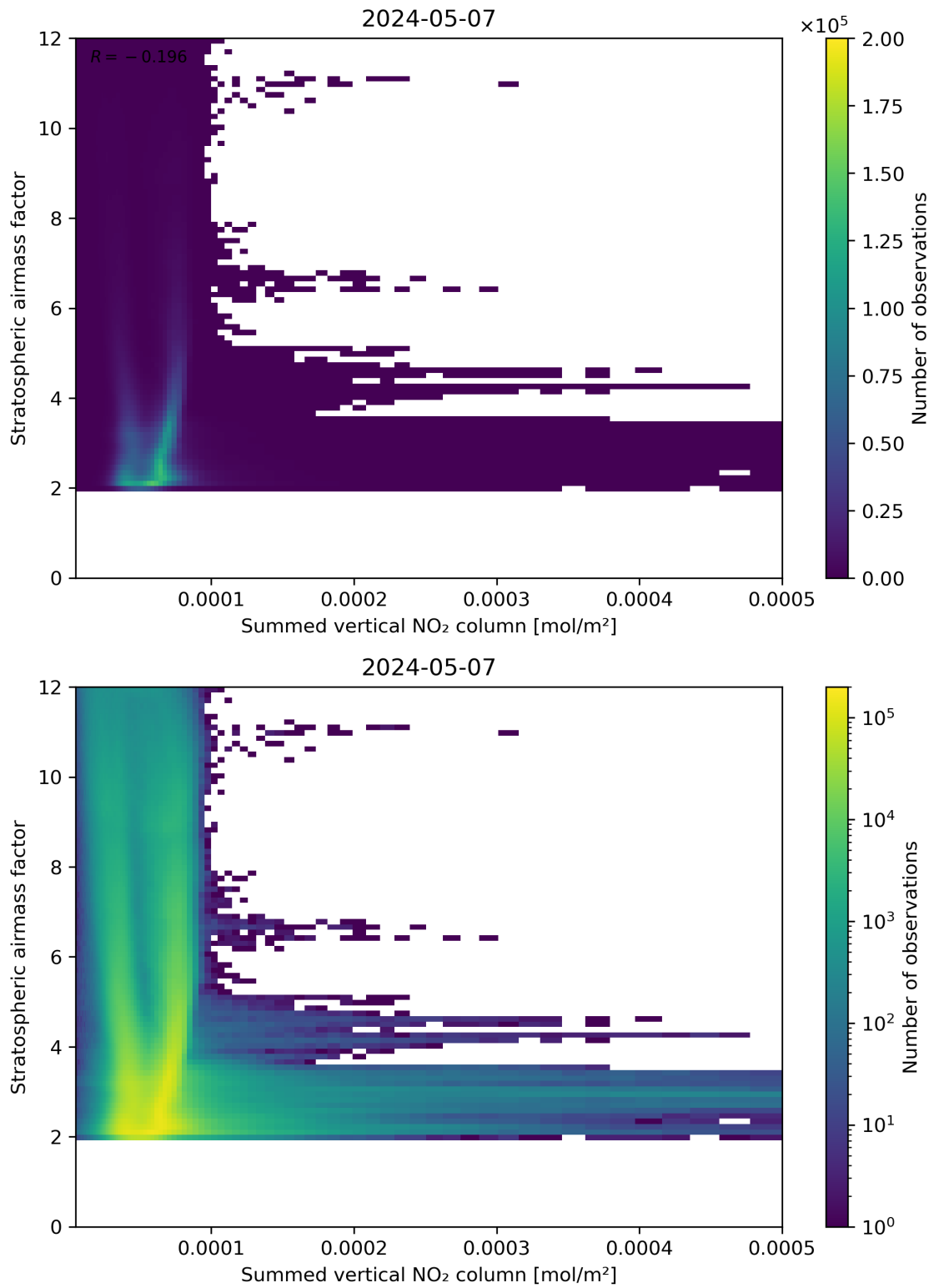
Figure 103: Scatter density plot of “Summed vertical NO 2 column” against “Stratospheric airmass factor” for 2024-05-07 to 2024-05-08.
