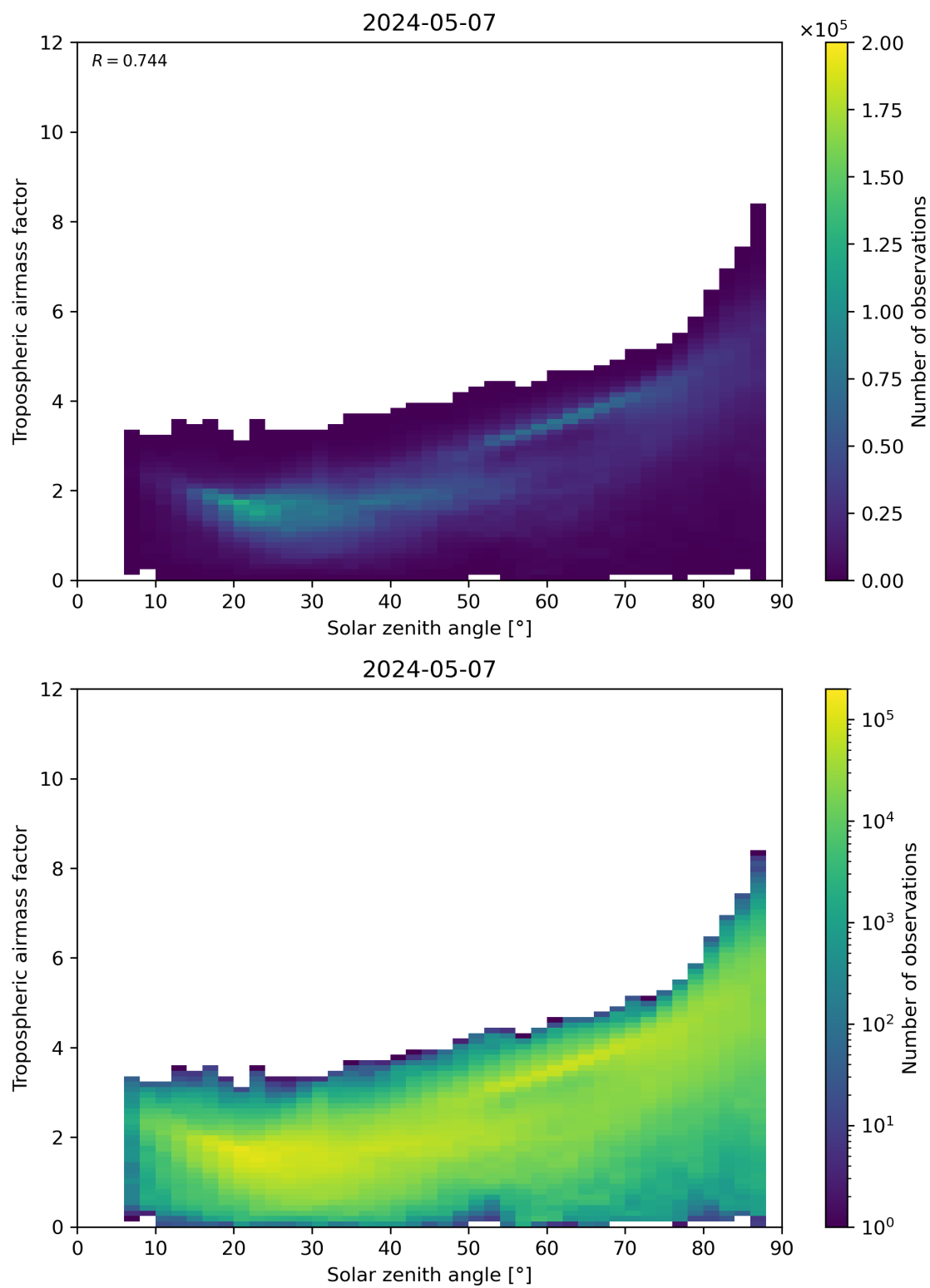
Figure 147: Scatter density plot of “Solar zenith angle” against “Tropospheric airmass factor” for 2024-05-07 to 2024-05-08.
