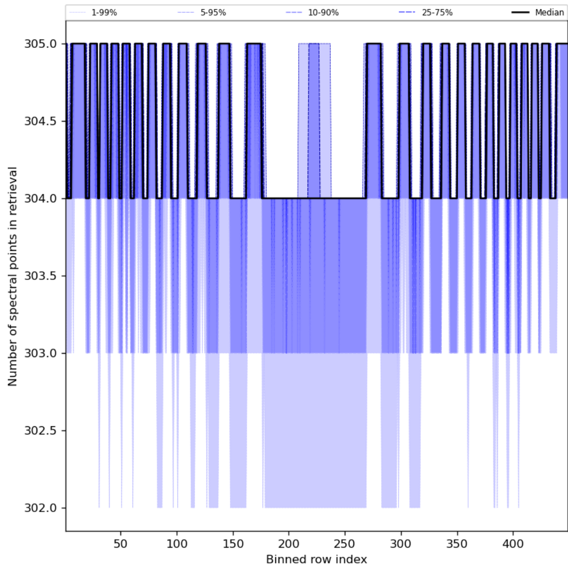
Figure 50: Along track statistics of “Number of spectral points in retrieval” for 2024-05-07 to 2024-05-08
