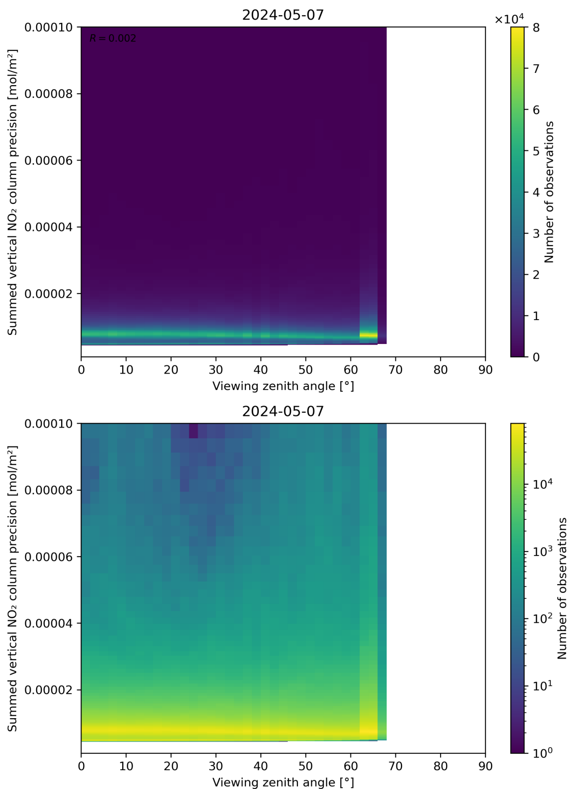
Figure 166: Scatter density plot of “Viewing zenith angle” against “Summed vertical NO 2 column precision” for 2024-05-07 to 2024-05-08.
