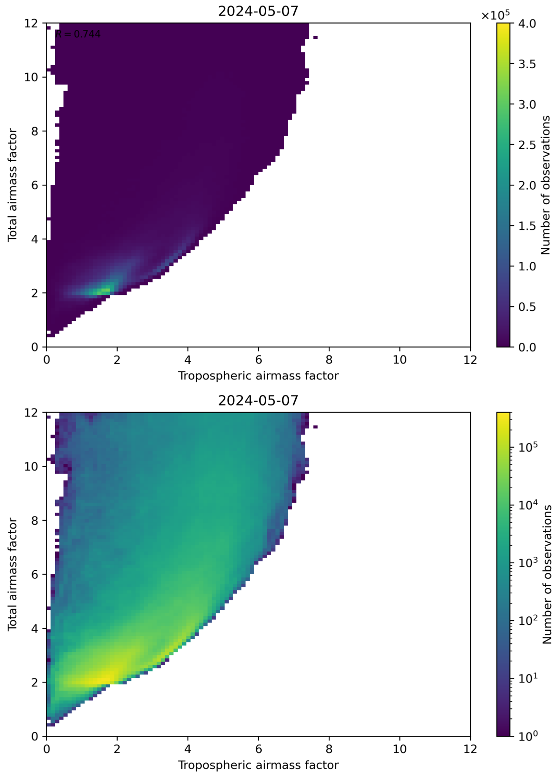
Figure 72: Scatter density plot of “Tropospheric airmass factor” against “Total airmass factor” for 2024-05-07 to 2024-05-08.
