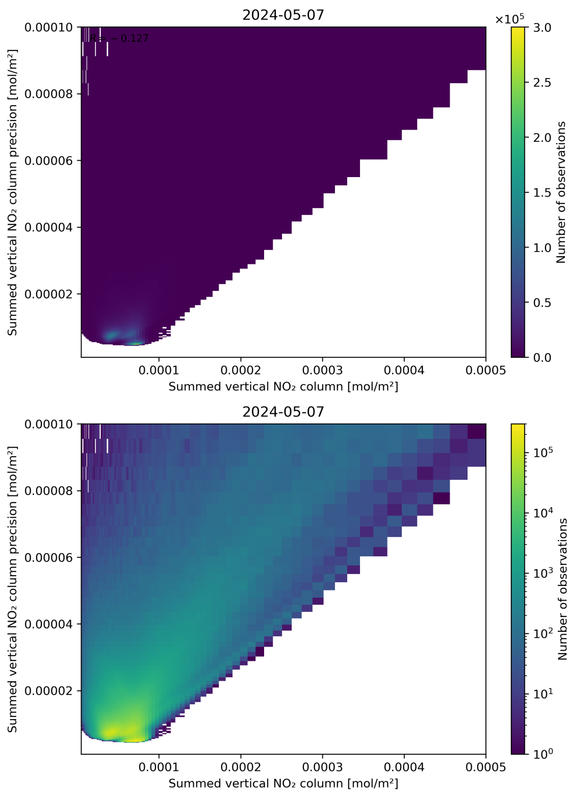
Figure 105: Scatter density plot of “Summed vertical NO 2 column” against “Summed vertical NO 2 column precision” for 2024-05-07 to 2024-05-08.
