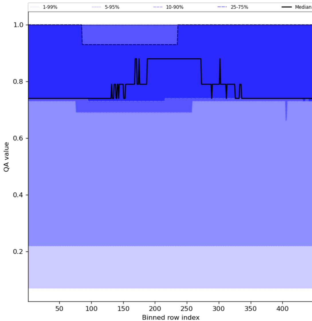
Figure 45: Along track statistics of “QA value” for 2024-05-07 to 2024-05-08
