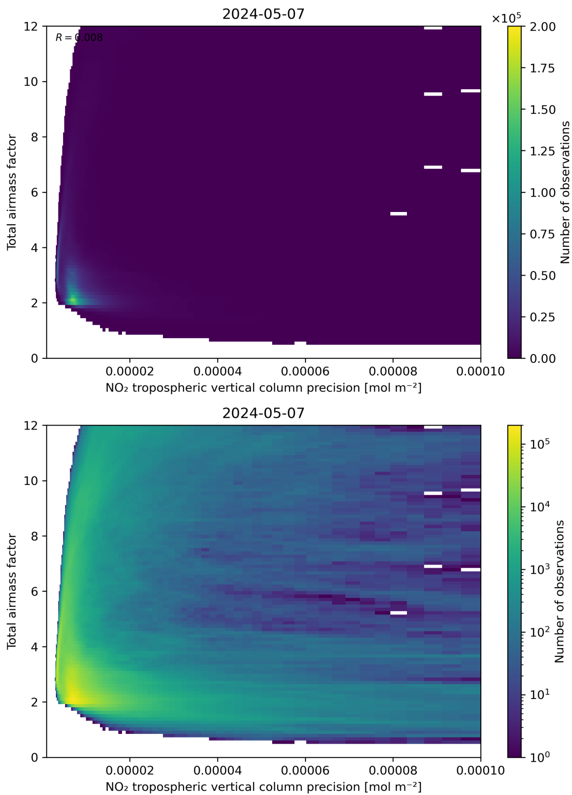
Figure 132: Scatter density plot of “NO 2 tropospheric vertical column precision” against “Total air mass factor” for 2024-05-07 to 2024-05-08.
