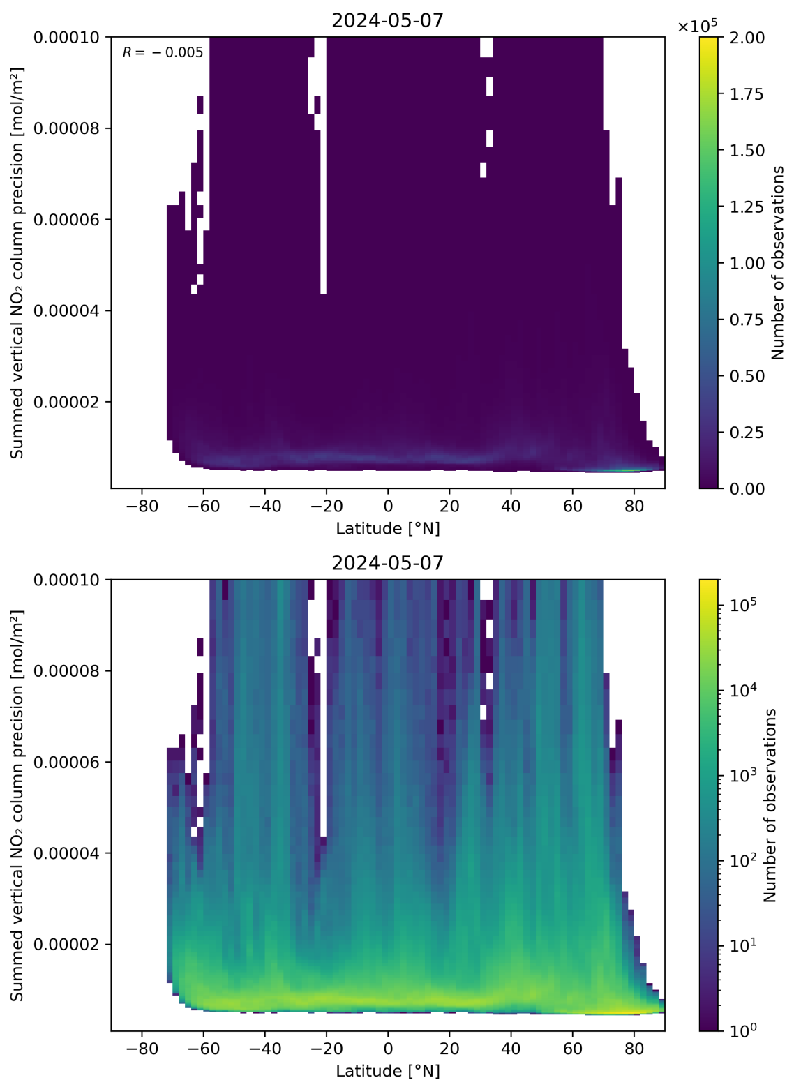
Figure 89: Scatter density plot of “Latitude” against “Summed vertical NO 2 column precision” for 2024-05-07 to 2024-05-08.
