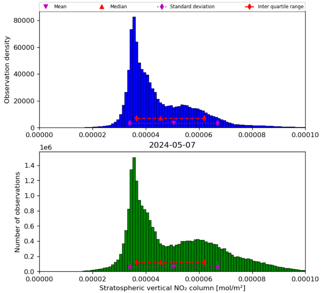
Figure 36: Histogram of “Stratospheric vertical NO 2 column” for 2024-05-07 to 2024-05-08
