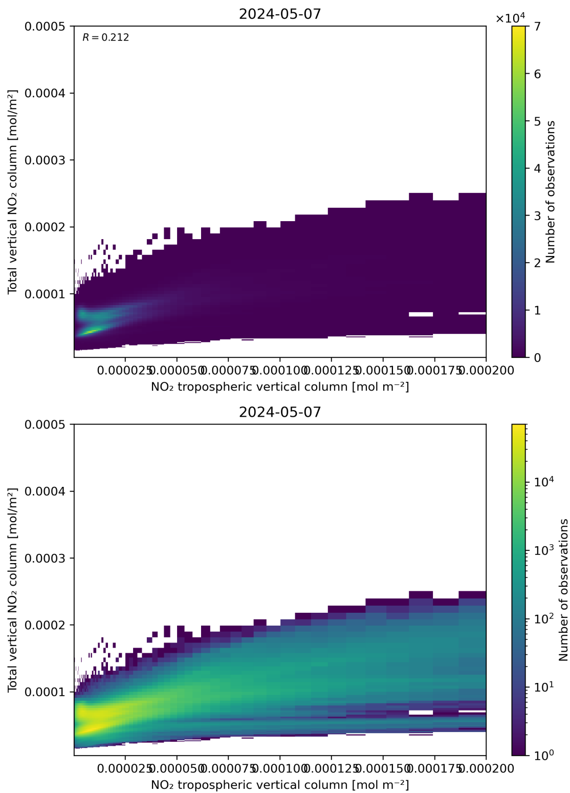
Figure 128: Scatter density plot of “NO 2 tropospheric vertical column” against “Total vertical NO 2 column” for 2024-05-07 to 2024-05-08.
