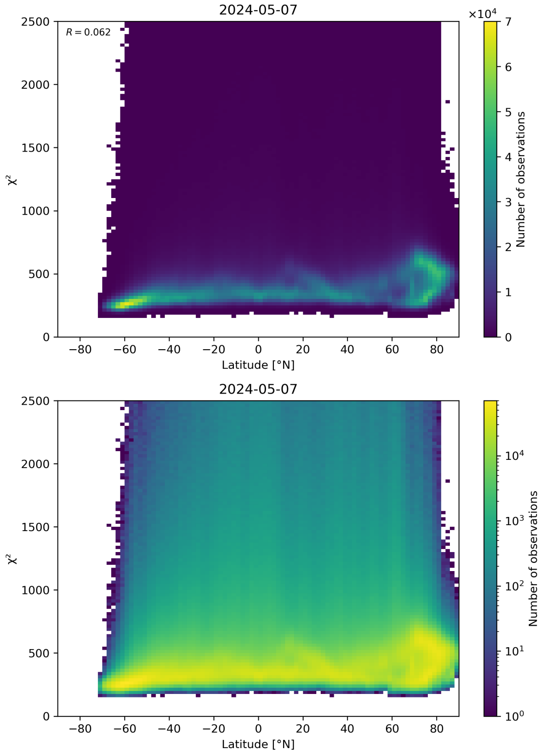
Figure 86: Scatter density plot of “Latitude” against “ \chi^2 ” for 2024-05-07 to 2024-05-08.
