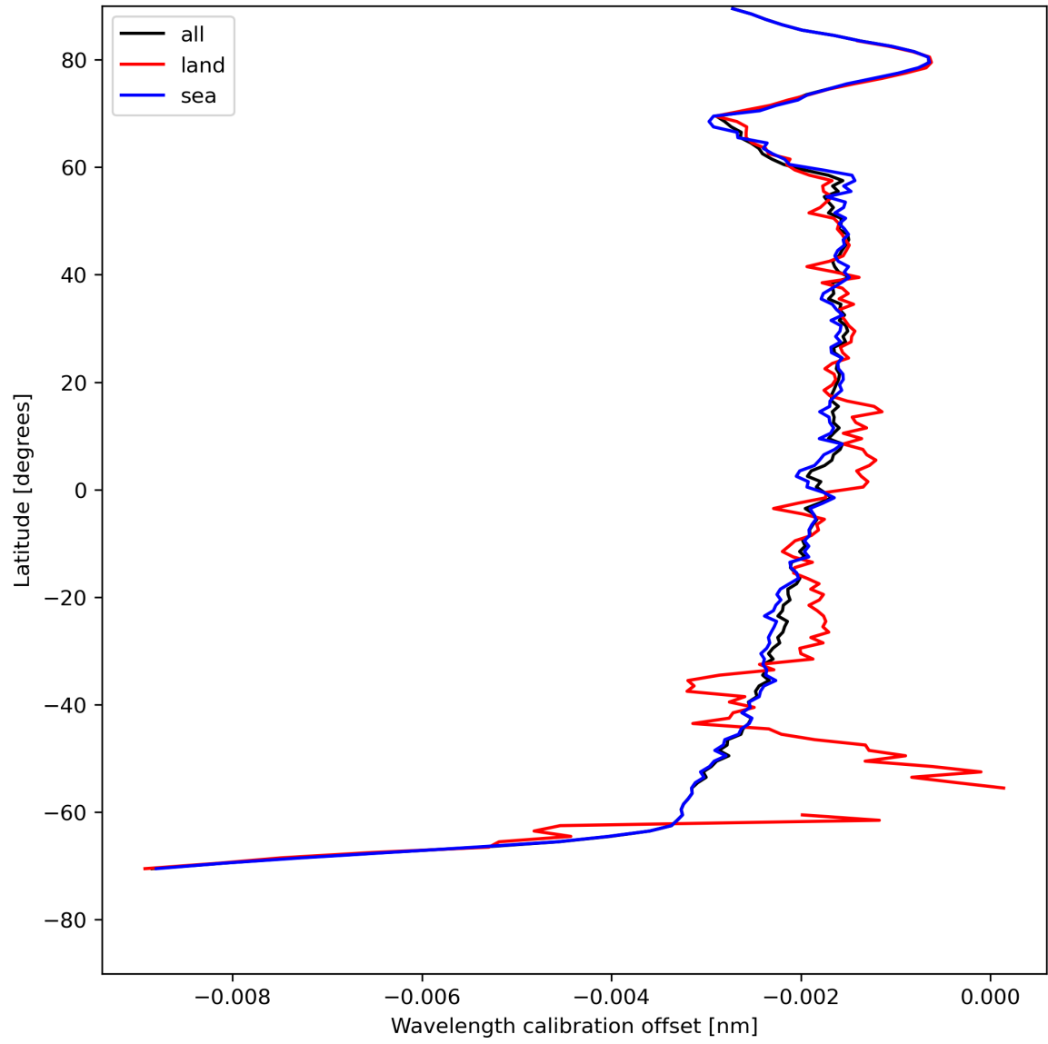
Figure 18: Zonal average of “Wavelength calibration offset” for 2024-05-07 to 2024-05-08.
