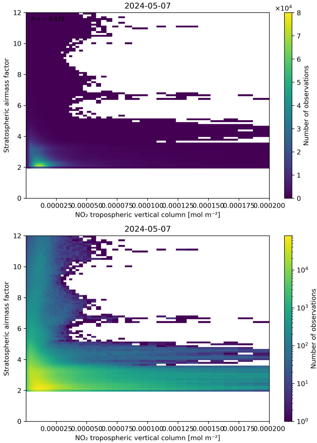
Figure 121: Scatter density plot of “NO 2 tropospheric vertical column” against “Stratospheric air mass factor” for 2024-05-07 to 2024-05-08.
