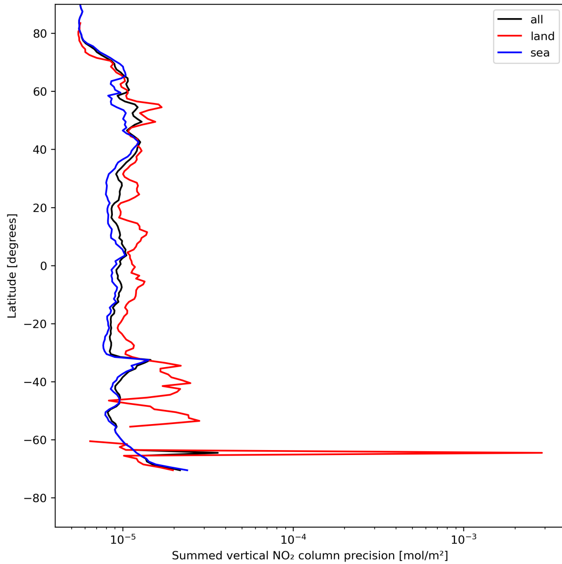
Figure 24: Zonal average of “Summed vertical NO 2 column precision” for 2024-05-07 to 2024-05-08.
