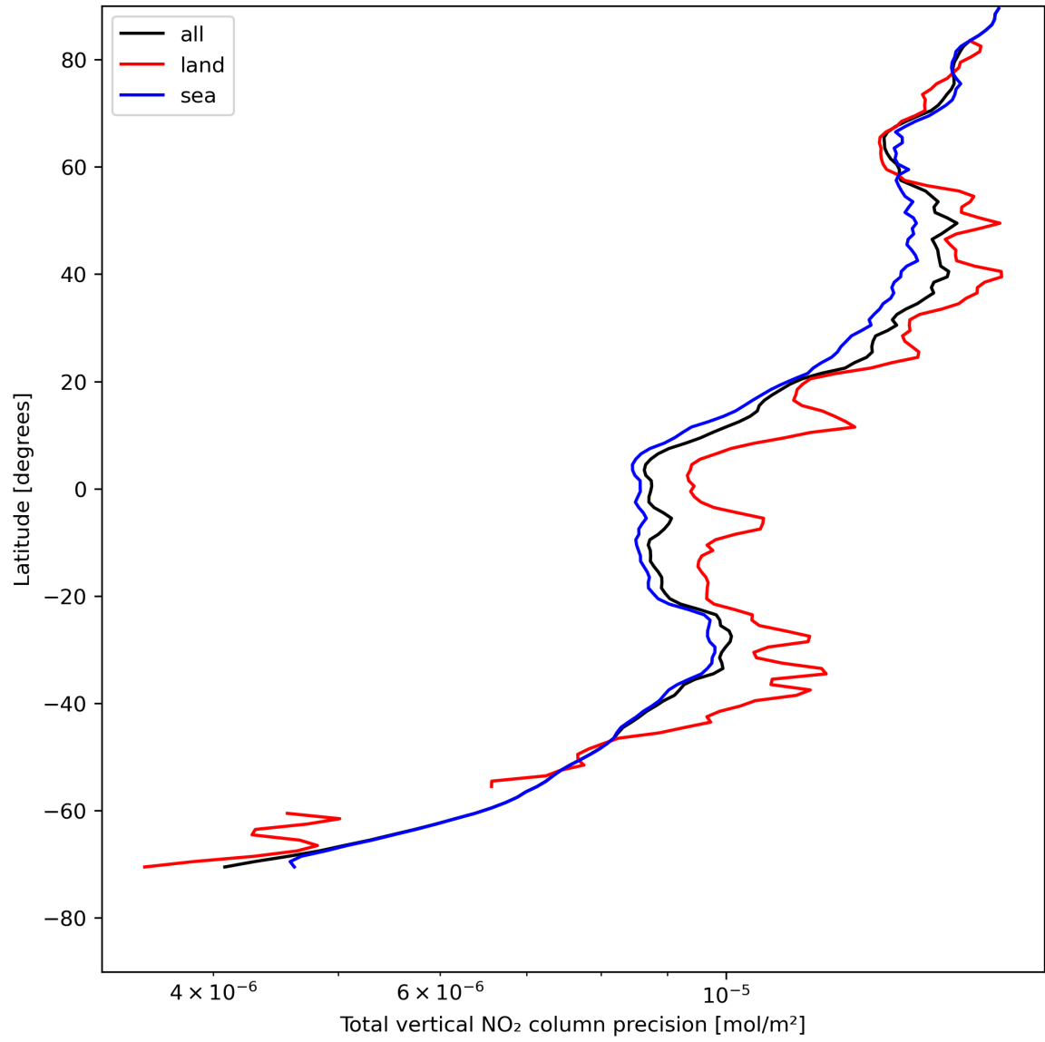
Figure 22: Zonal average of “Total vertical NO 2 column precision” for 2024-05-07 to 2024-05-08.
