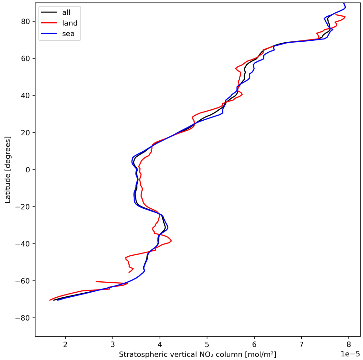
Figure 19: Zonal average of “Stratospheric vertical NO 2 column” for 2024-05-07 to 2024-05-08.
