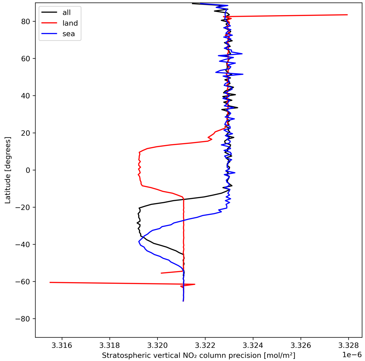
Figure 20: Zonal average of “Stratospheric vertical NO 2 column precision” for 2024-05-07 to 2024-05-08.
