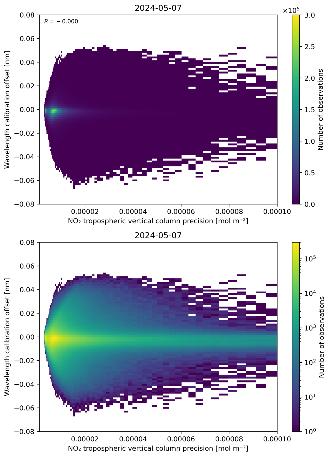
Figure 141: Scatter density plot of “NO 2 tropospheric vertical column precision” against “Wavelength calibration offset” for 2024-05-07 to 2024-05-08.
