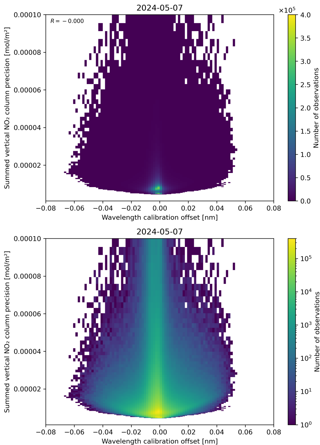
Figure 178: Scatter density plot of “Wavelength calibration offset” against “Summed vertical NO 2 column precision” for 2024-05-07 to 2024-05-08.
