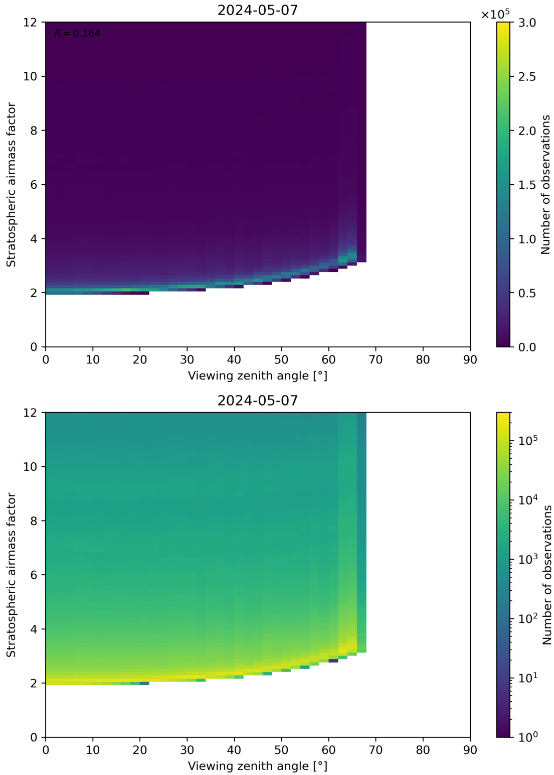
Figure 159: Scatter density plot of “Viewing zenith angle” against “Stratospheric airmass factor” for 2024-05-07 to 2024-05-08.
