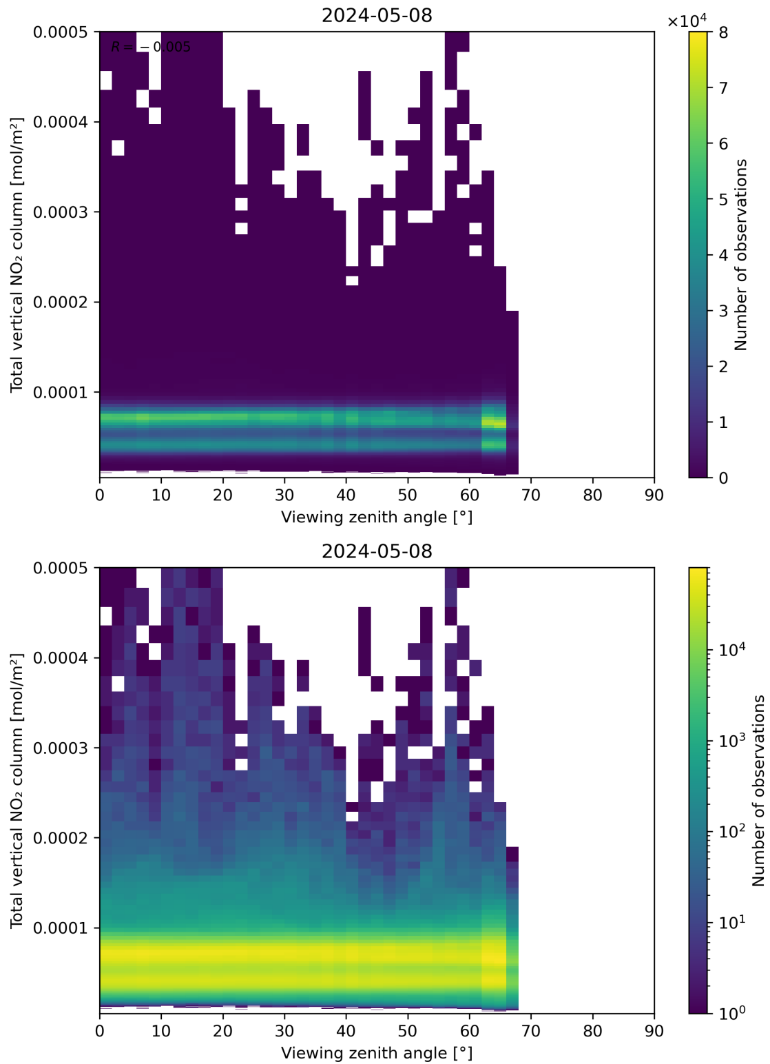
Figure 167: Scatter density plot of “Viewing zenith angle” against “Total vertical NO 2 column” for 2024-05-07 to 2024-05-09.
