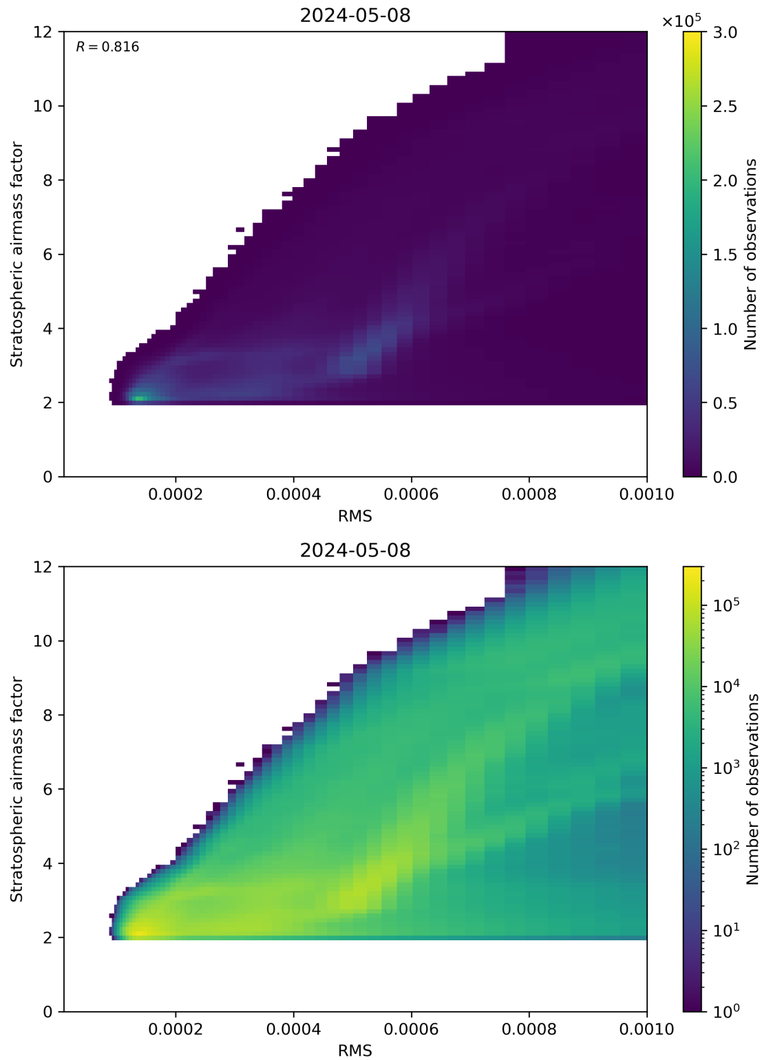
Figure 144: Scatter density plot of “RMS” against “Stratospheric airmass factor” for 2024-05-07 to 2024-05-09.
