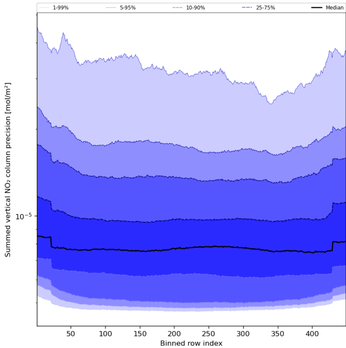
Figure 58: Along track statistics of “Summed vertical NO 2 column precision” for 2024-05-07 to 2024-05-09
