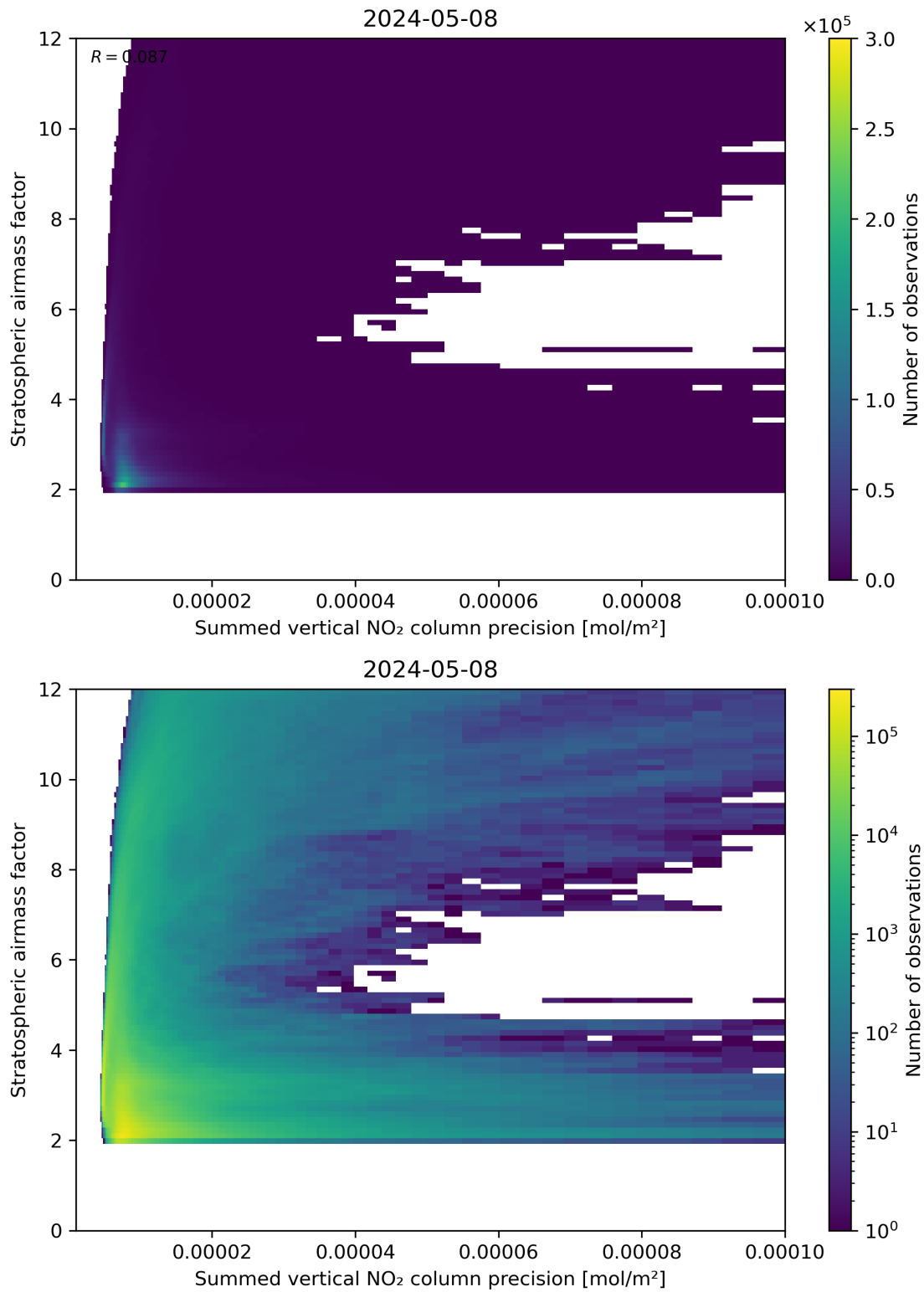
Figure 106: Scatter density plot of “Summed vertical NO 2 column precision” against “Stratospheric airmass factor” for 2024-05-07 to 2024-05-09.
