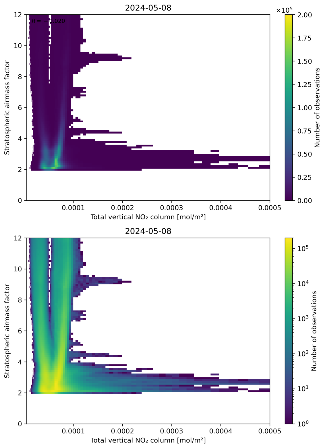
Figure 110: Scatter density plot of “Total vertical NO 2 column” against “Stratospheric airmass factor” for 2024-05-07 to 2024-05-09.
