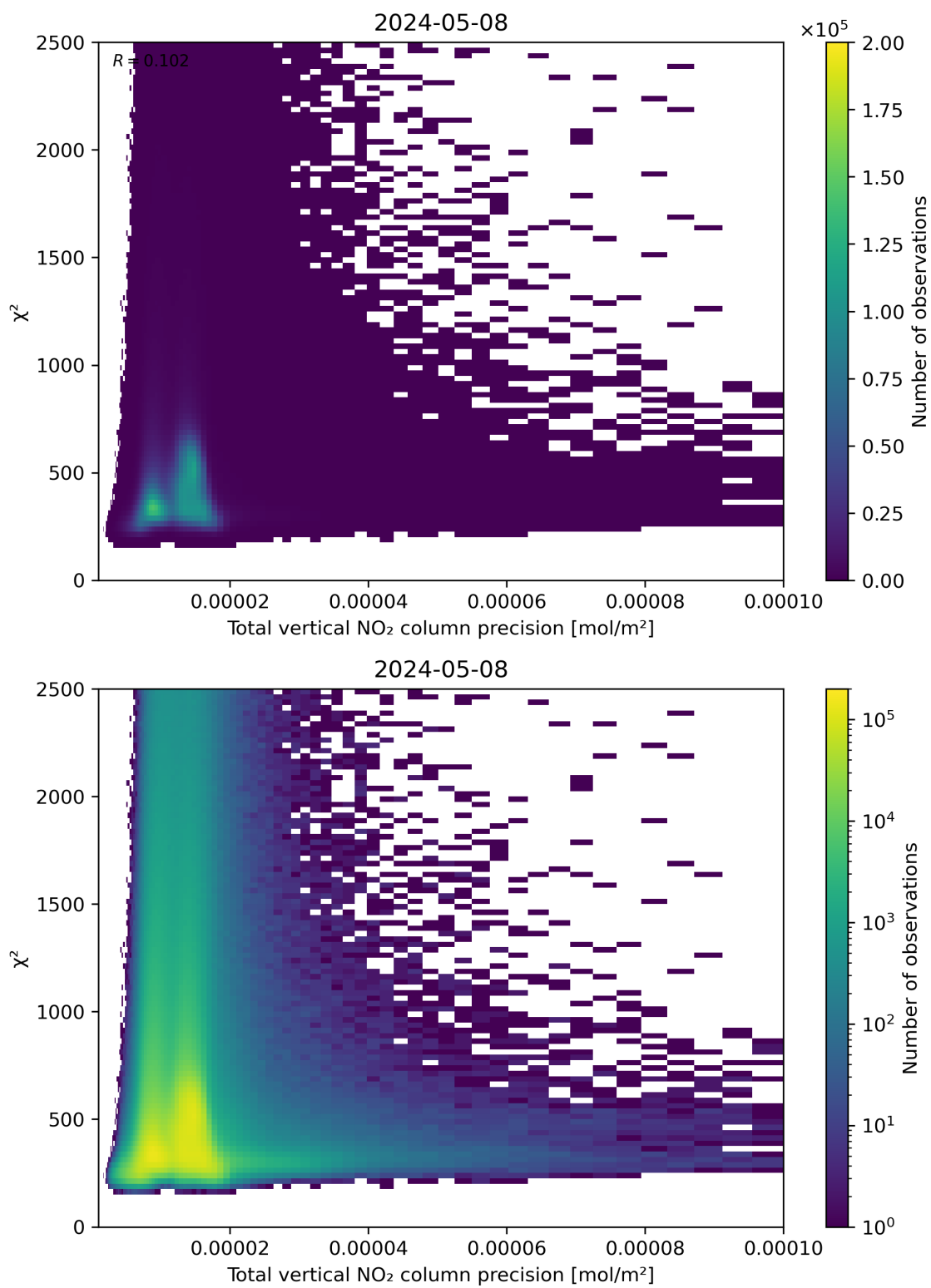
Figure 116: Scatter density plot of “Total vertical NO 2 column precision” against “ \chi^2 ” for 2024-05-07 to 2024-05-09.
