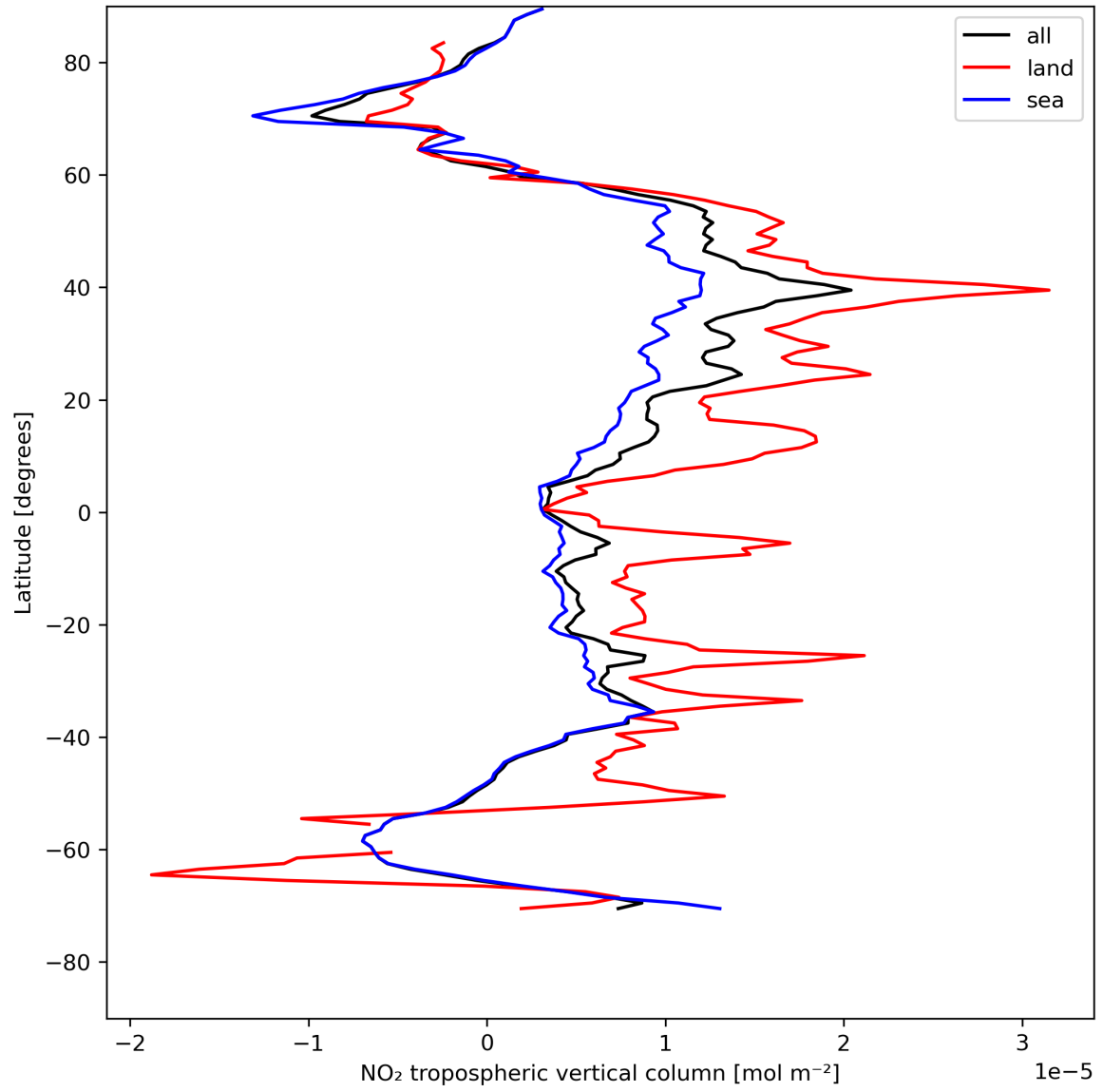
Figure 12: Zonal average of “NO 2 tropospheric vertical column” for 2024-05-07 to 2024-05-09.
