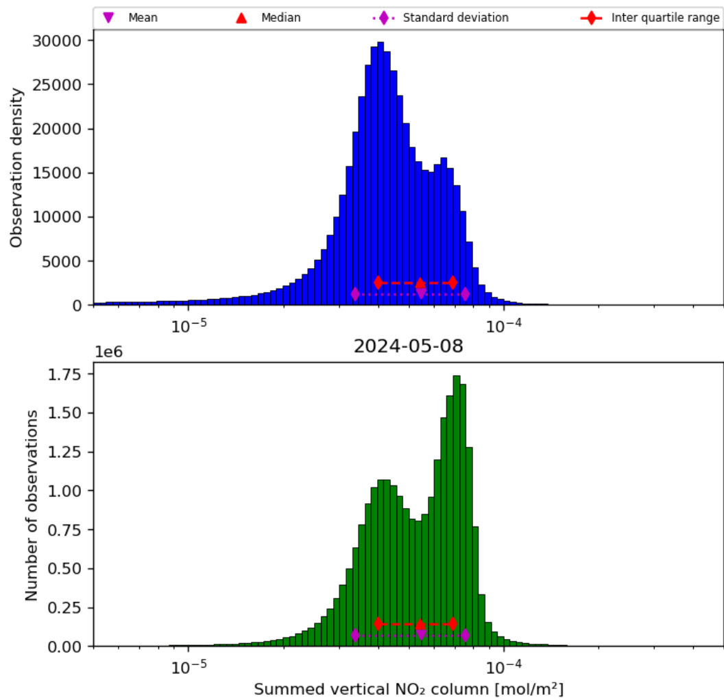
Figure 40: Histogram of “Summed vertical NO 2 column” for 2024-05-07 to 2024-05-09
