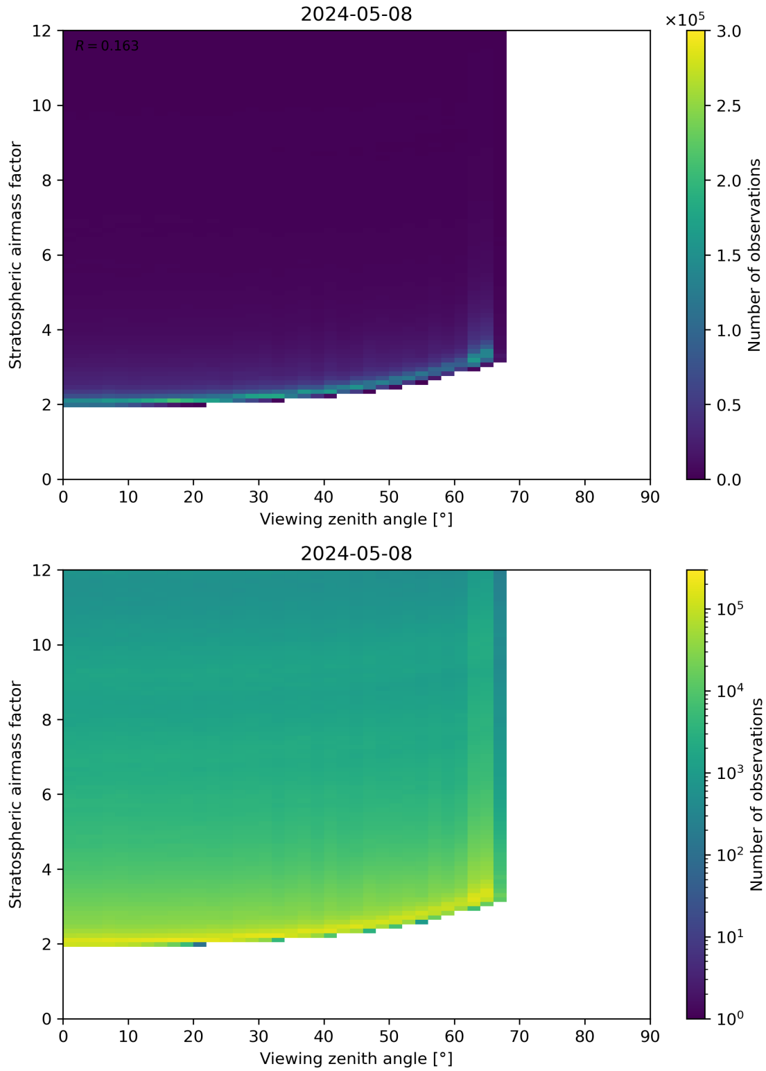
Figure 159: Scatter density plot of “Viewing zenith angle” against “Stratospheric airmass factor” for 2024-05-07 to 2024-05-09.
