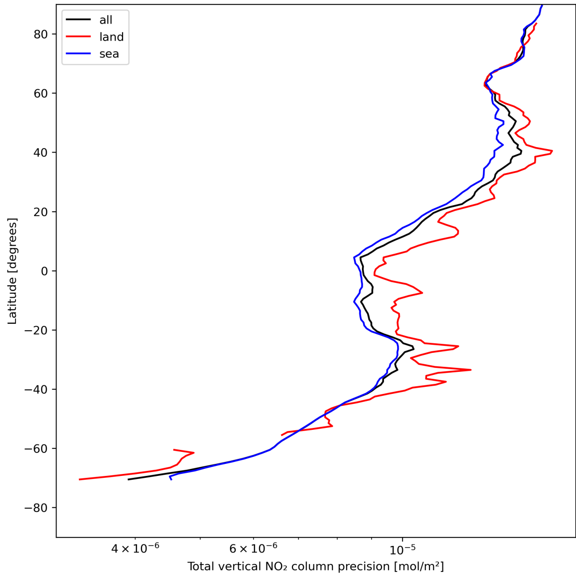
Figure 22: Zonal average of “Total vertical NO 2 column precision” for 2024-05-07 to 2024-05-09.
