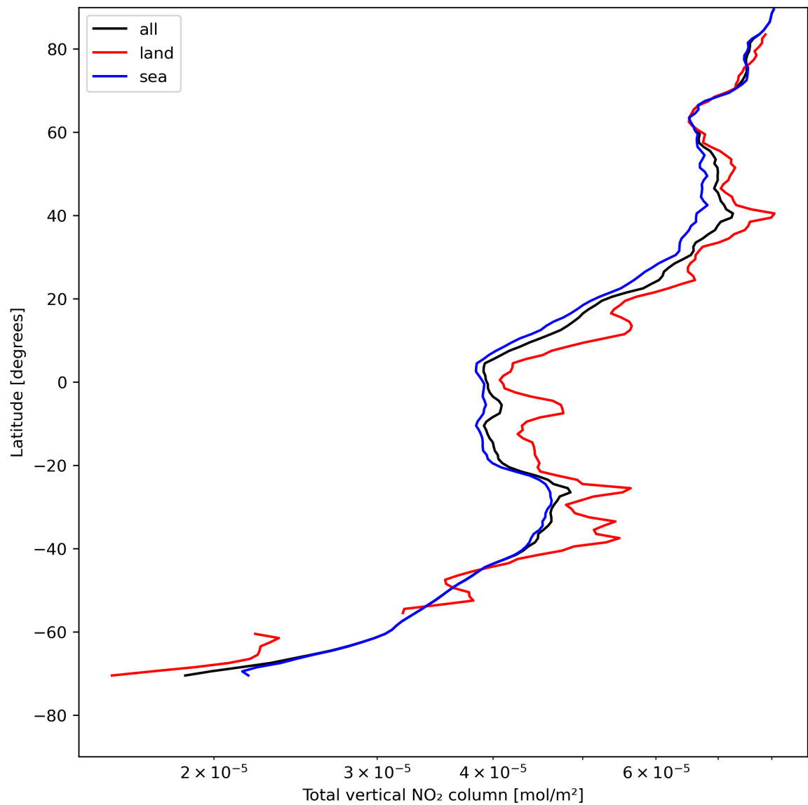
Figure 21: Zonal average of “Total vertical NO 2 column” for 2024-05-07 to 2024-05-09.
