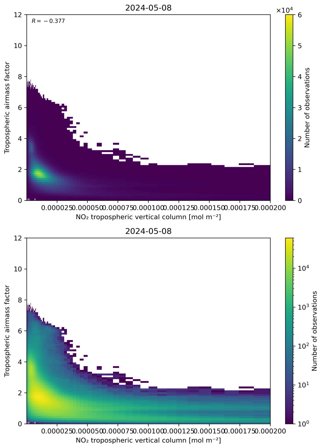
Figure 123: Scatter density plot of “NO 2 tropospheric vertical column” against “Tropospheric air mass factor” for 2024-05-07 to 2024-05-09.
