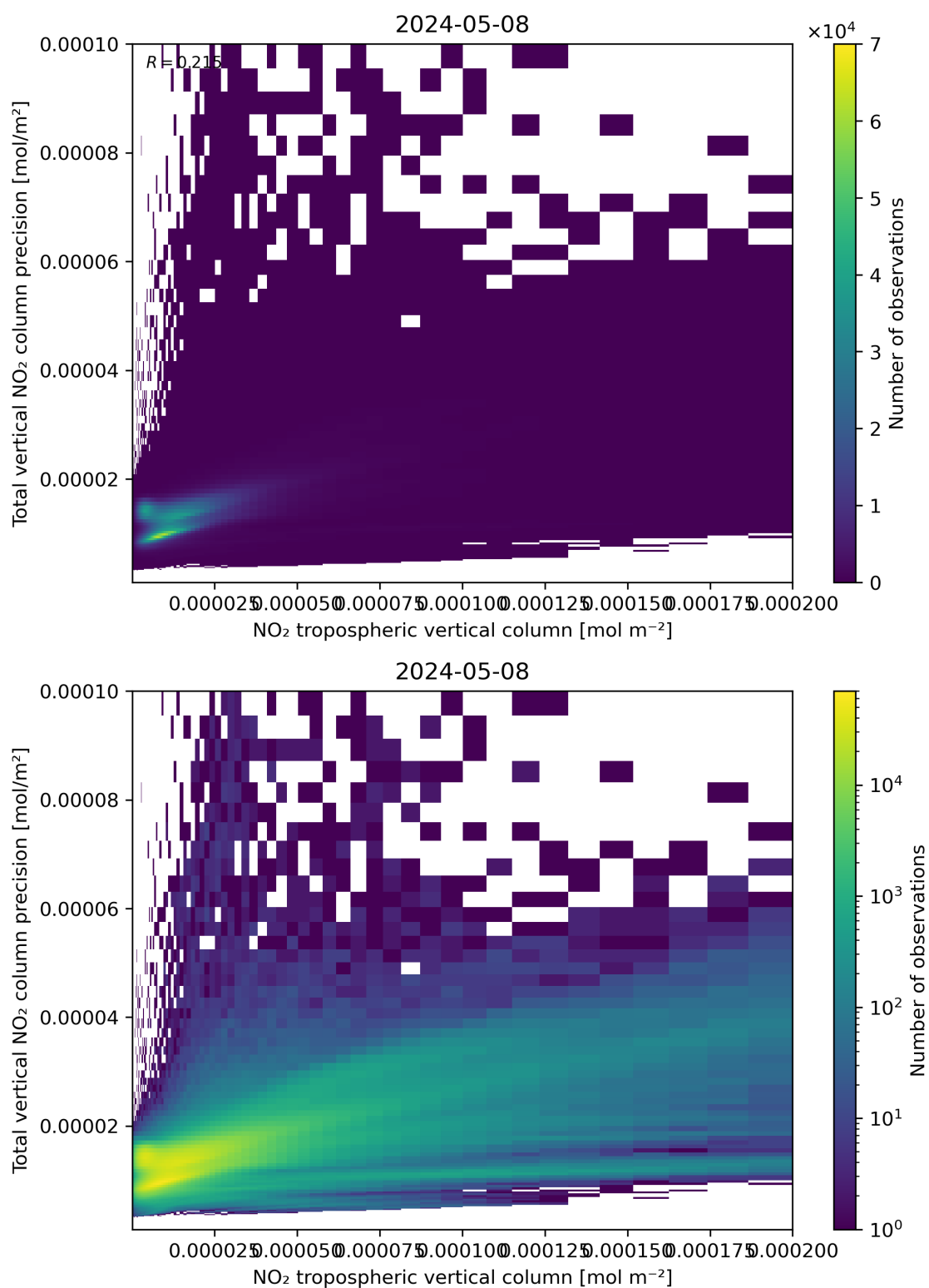
Figure 129: Scatter density plot of “NO 2 tropospheric vertical column” against “Total vertical NO 2 column precision” for 2024-05-07 to 2024-05-09.
