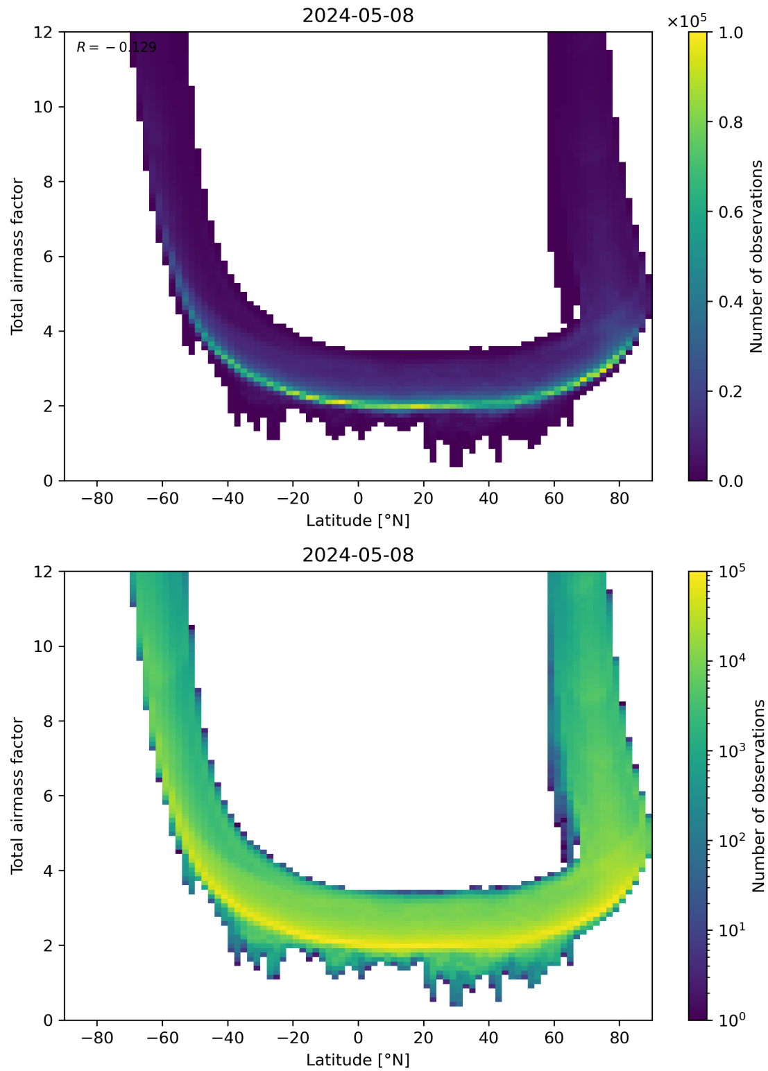
Figure 84: Scatter density plot of “Latitude” against “Total airmass factor” for 2024-05-07 to 2024-05-09.
