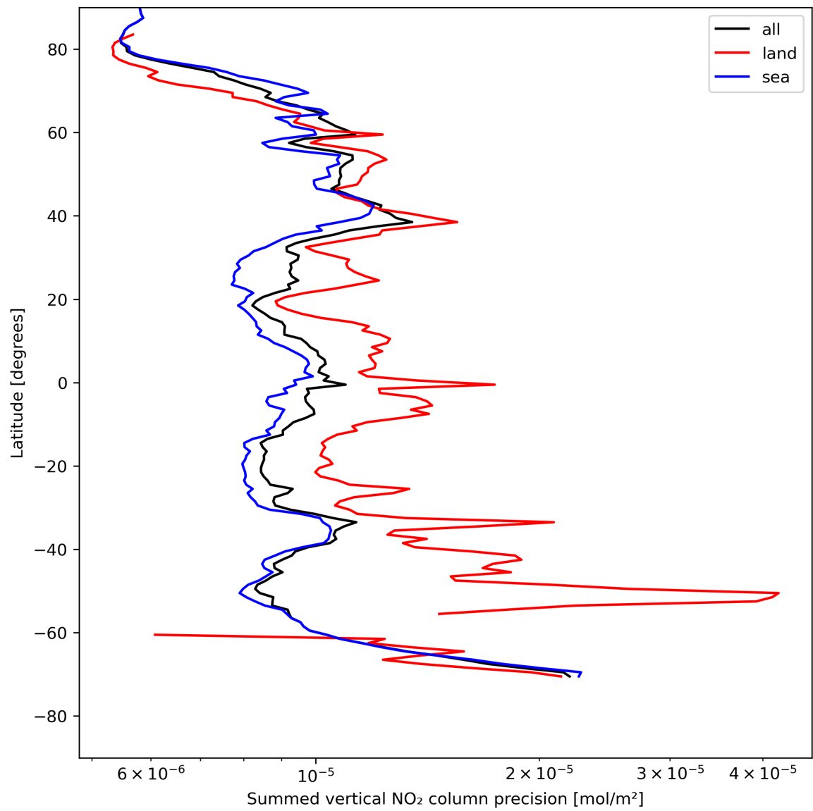
Figure 24: Zonal average of “Summed vertical NO 2 column precision” for 2024-05-07 to 2024-05-09.
