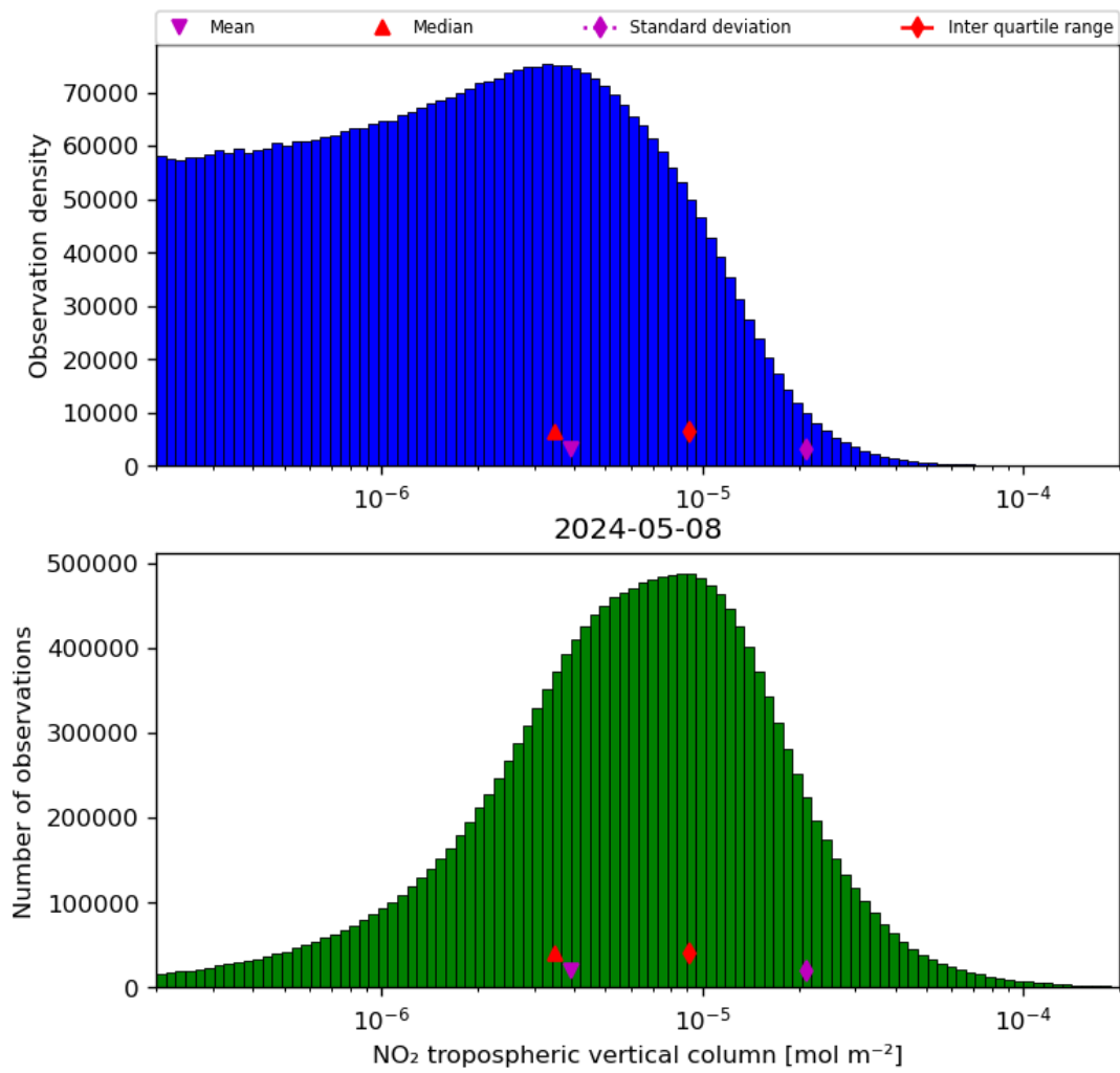
Figure 29: Histogram of “NO 2 tropospheric vertical column” for 2024-05-07 to 2024-05-09
