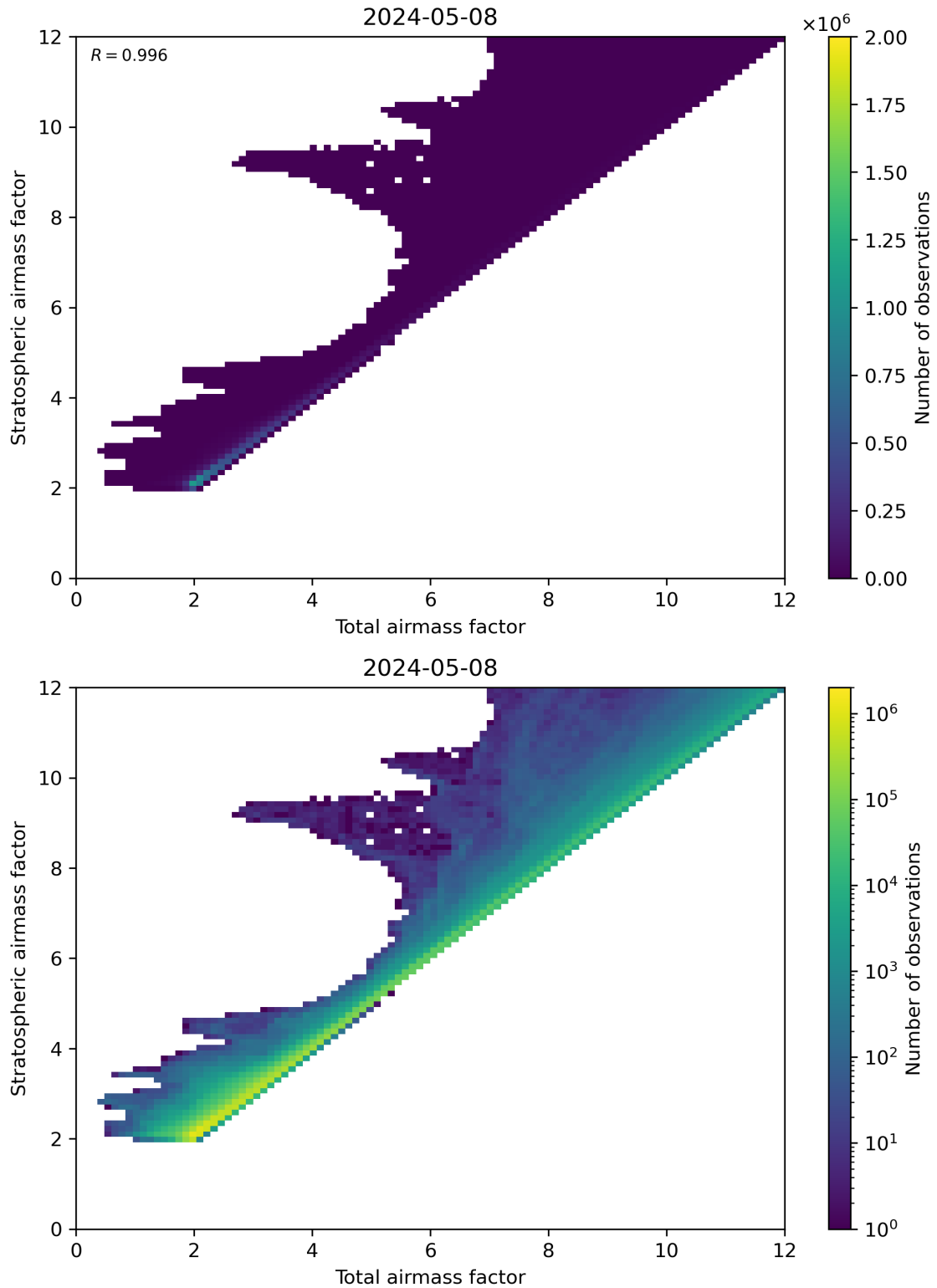
Figure 62: Scatter density plot of “Total airmass factor” against “Stratospheric airmass factor” for 2024-05-07 to 2024-05-09.
