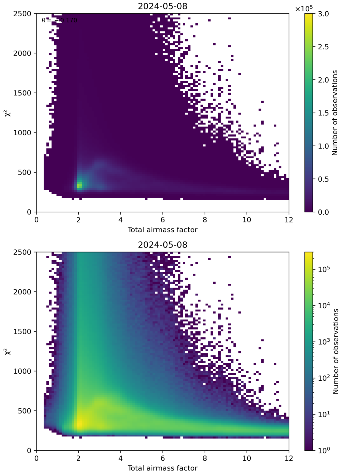
Figure 63: Scatter density plot of “Total airmass factor” against “ \chi^2 ” for 2024-05-07 to 2024-05-09.
