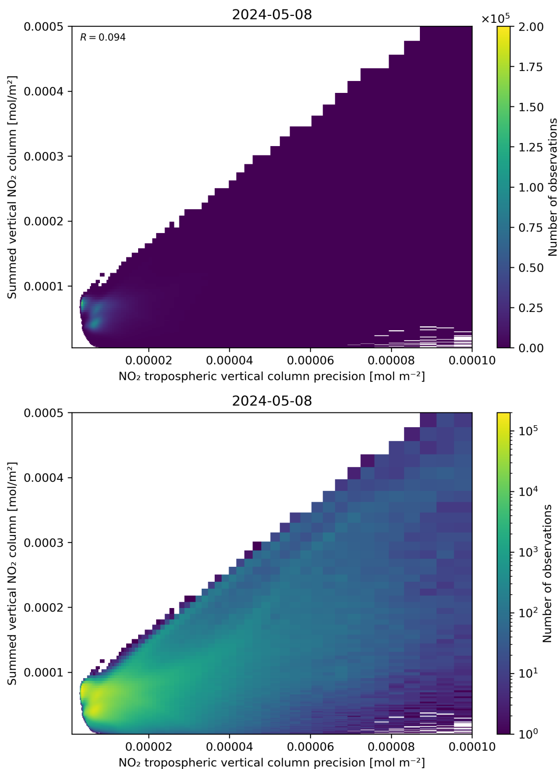
Figure 136: Scatter density plot of “NO 2 tropospheric vertical column precision” against “Summed vertical NO 2 column” for 2024-05-07 to 2024-05-09.
