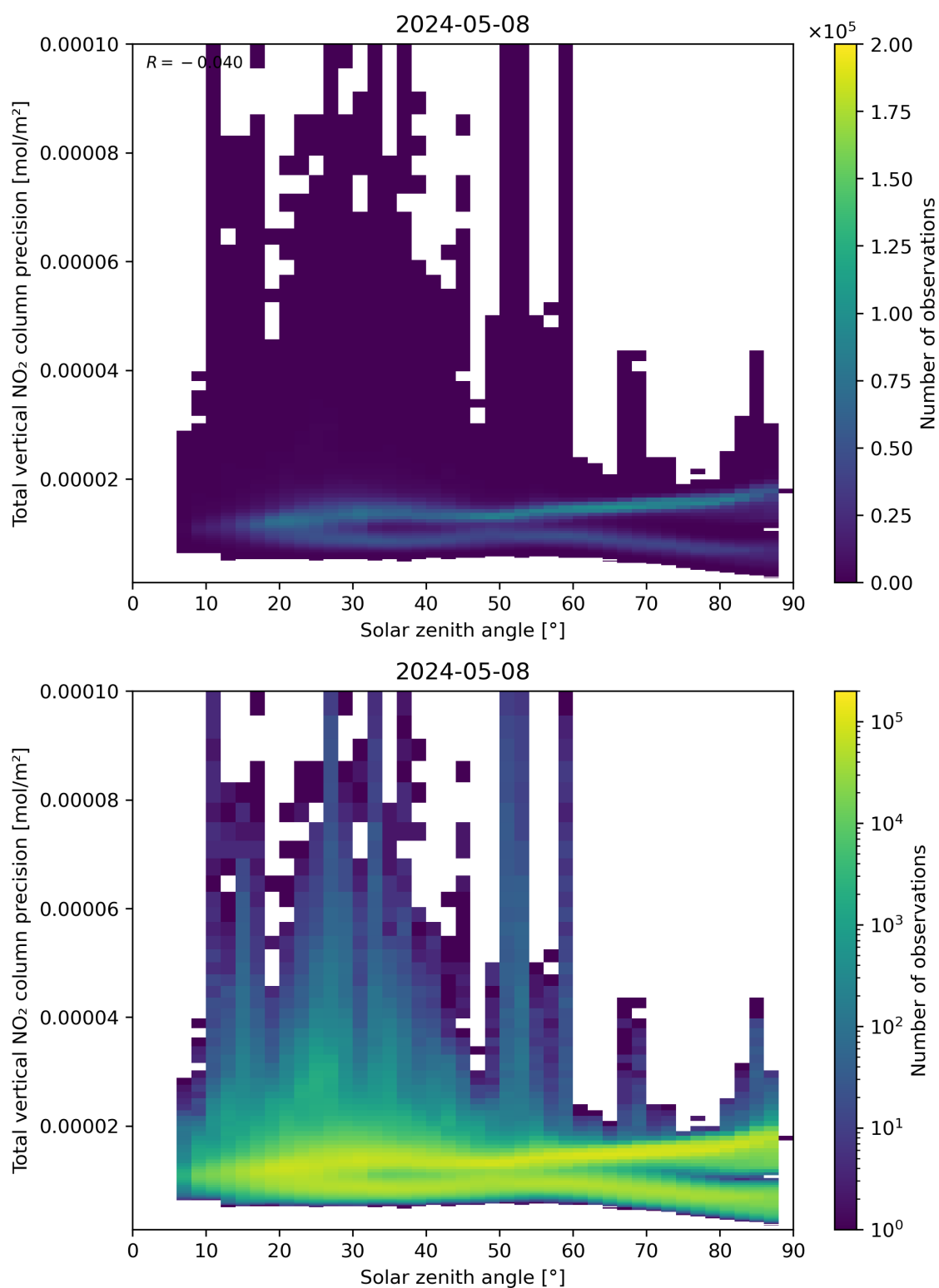
Figure 154: Scatter density plot of “Solar zenith angle” against “Total vertical NO 2 column precision” for 2024-05-07 to 2024-05-09.
