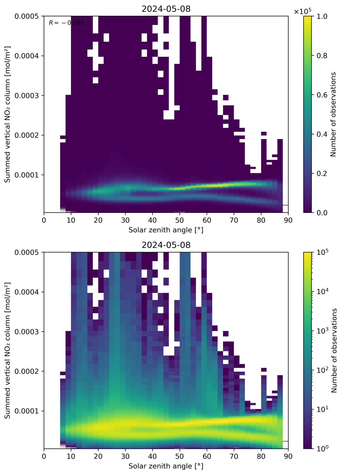
Figure 151: Scatter density plot of “Solar zenith angle” against “Summed vertical NO 2 column” for 2024-05-07 to 2024-05-09.
