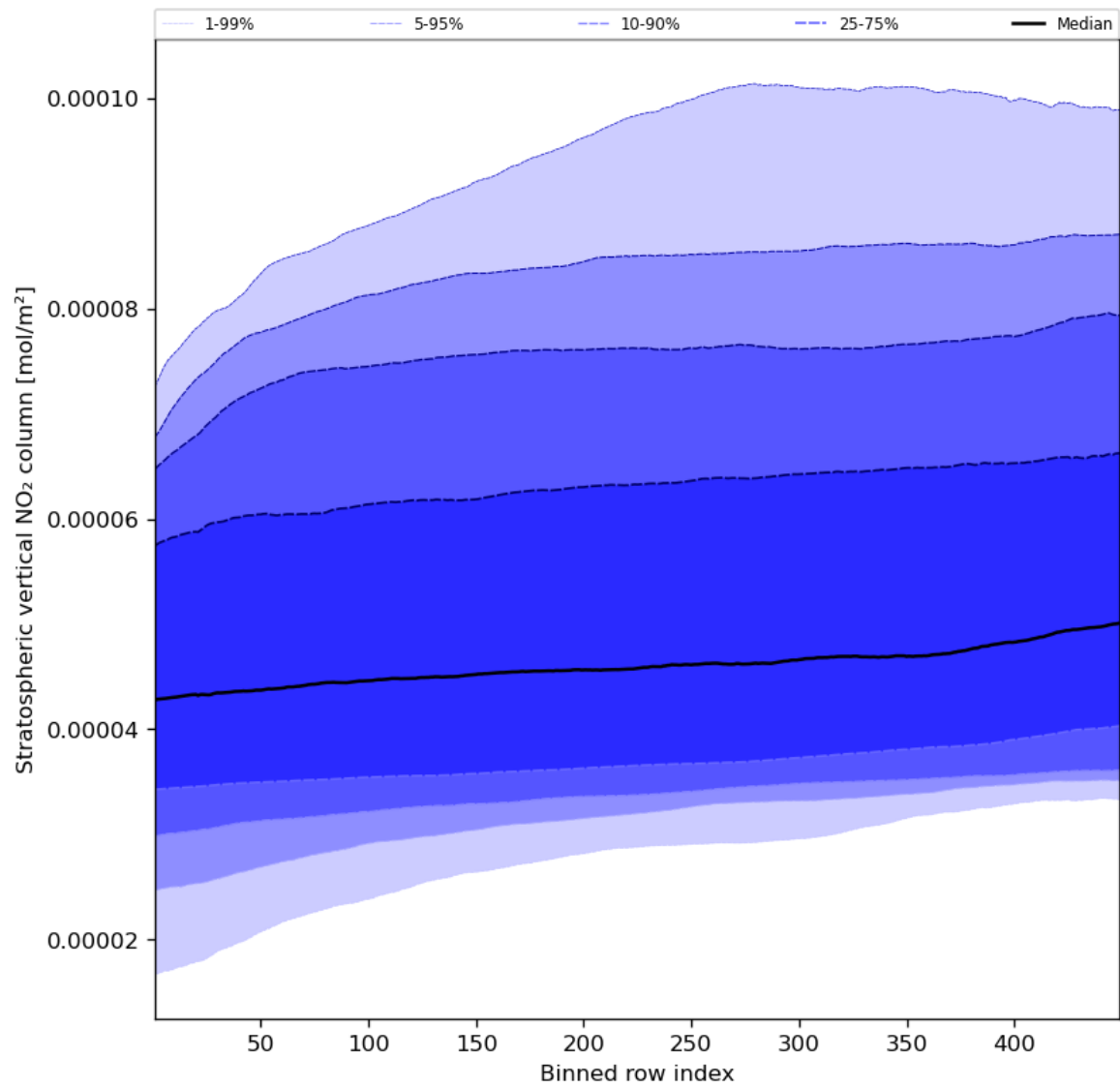
Figure 53: Along track statistics of “Stratospheric vertical NO 2 column” for 2024-05-07 to 2024-05-09
