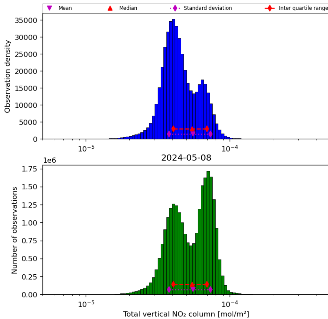
Figure 38: Histogram of “Total vertical NO 2 column” for 2024-05-07 to 2024-05-09
