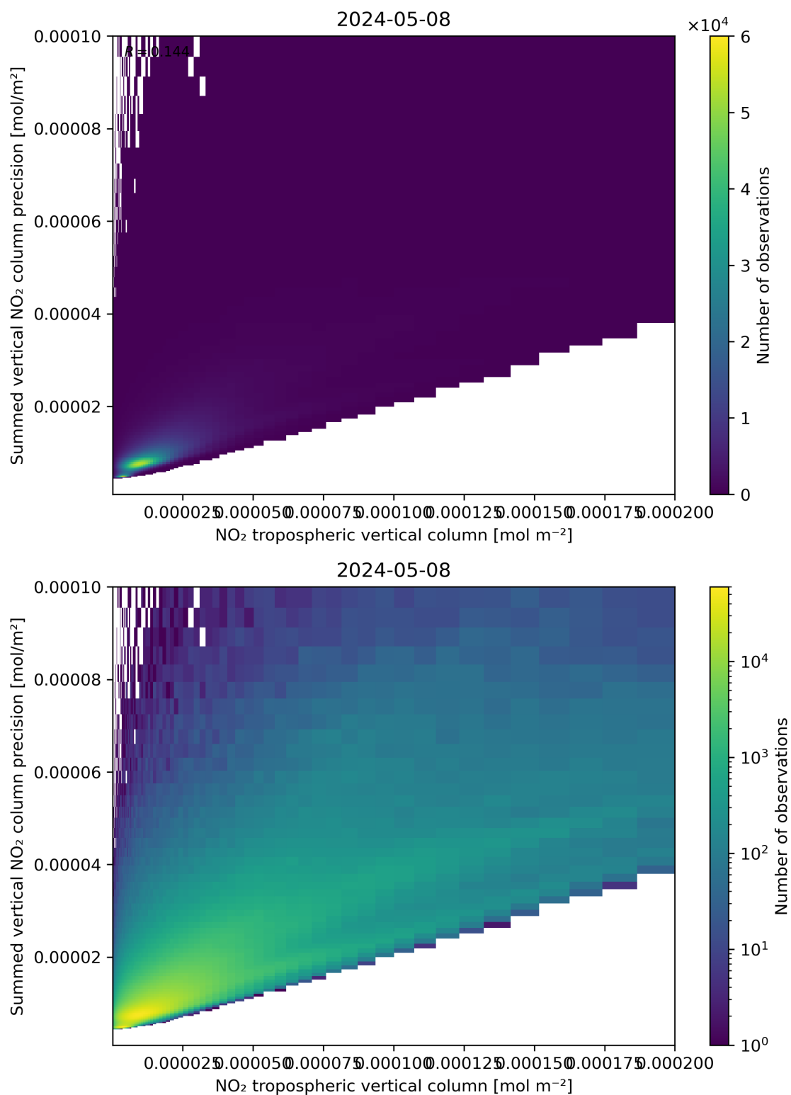
Figure 127: Scatter density plot of “NO 2 tropospheric vertical column” against “Summed vertical NO 2 column precision” for 2024-05-07 to 2024-05-09.
