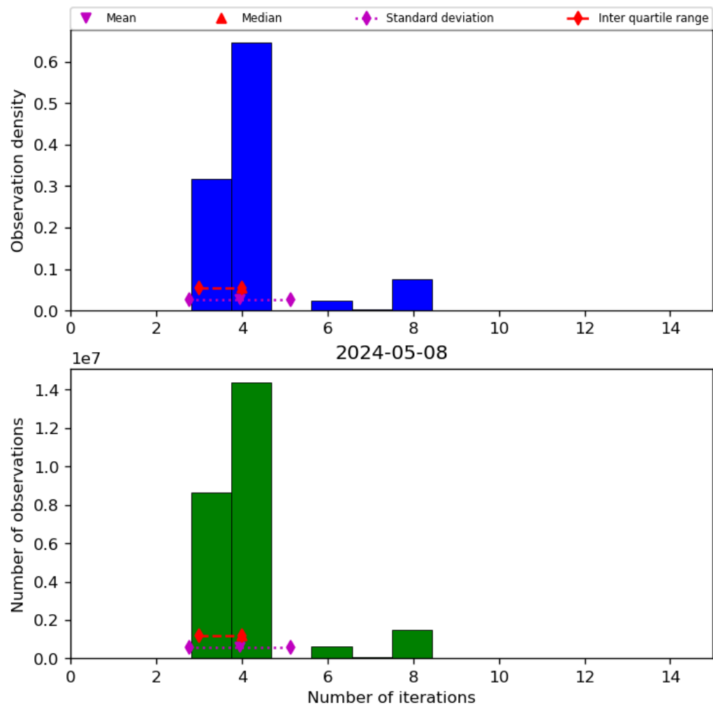
Figure 34: Histogram of “Number of iterations” for 2024-05-07 to 2024-05-09
