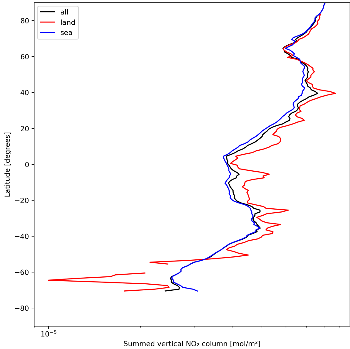
Figure 23: Zonal average of “Summed vertical NO 2 column” for 2024-05-07 to 2024-05-09.
