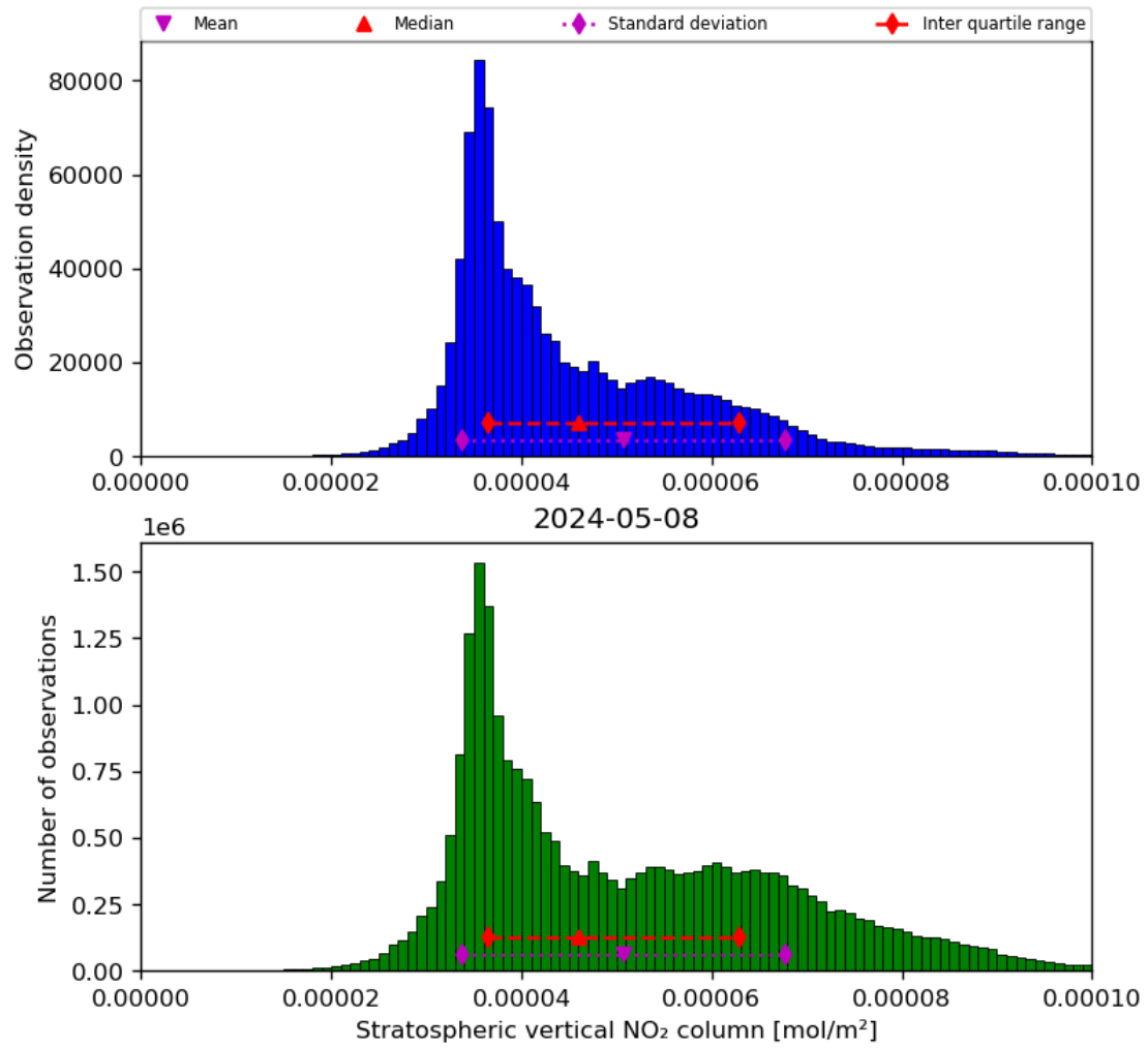
Figure 36: Histogram of “Stratospheric vertical NO 2 column” for 2024-05-07 to 2024-05-09
