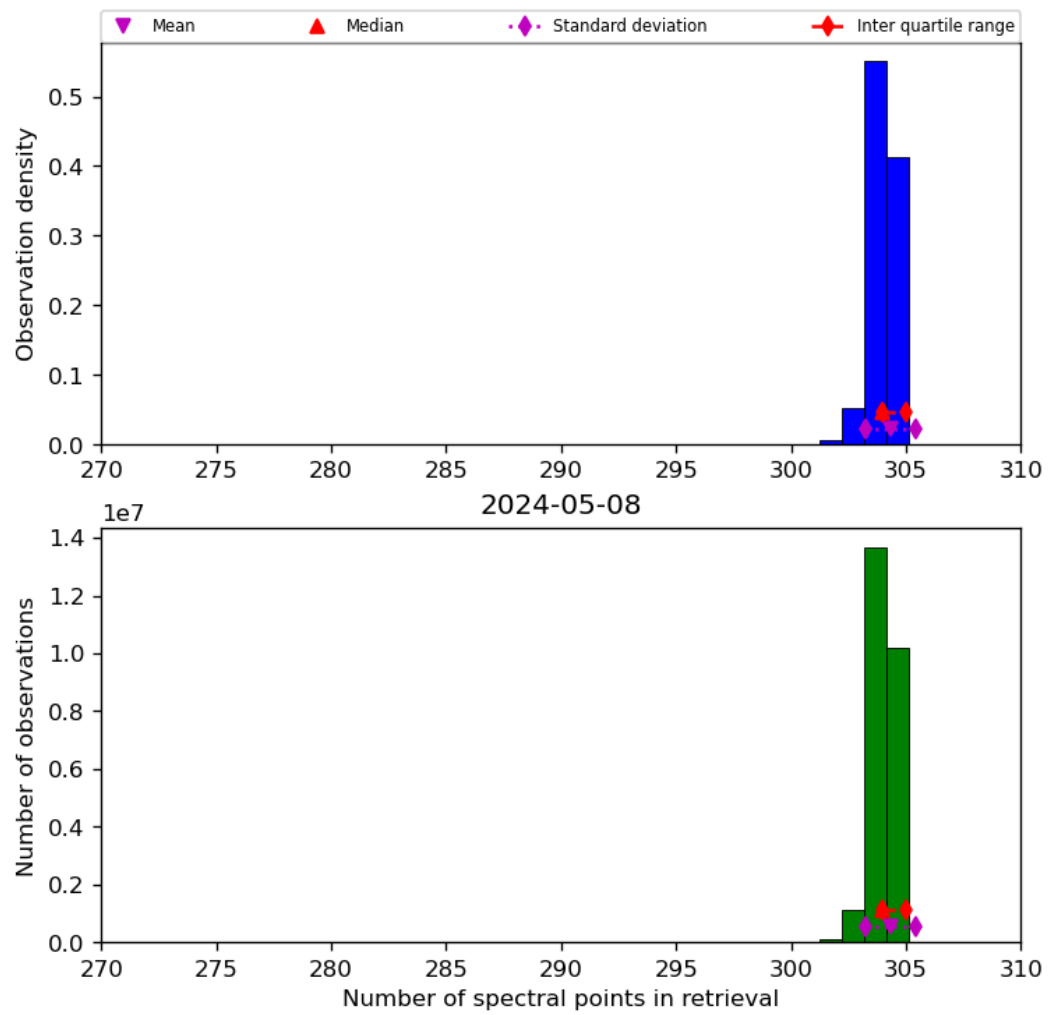
Figure 33: Histogram of “Number of spectral points in retrieval” for 2024-05-07 to 2024-05-09
