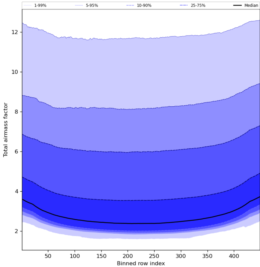
Figure 49: Along track statistics of “Total airmass factor” for 2024-05-07 to 2024-05-09
