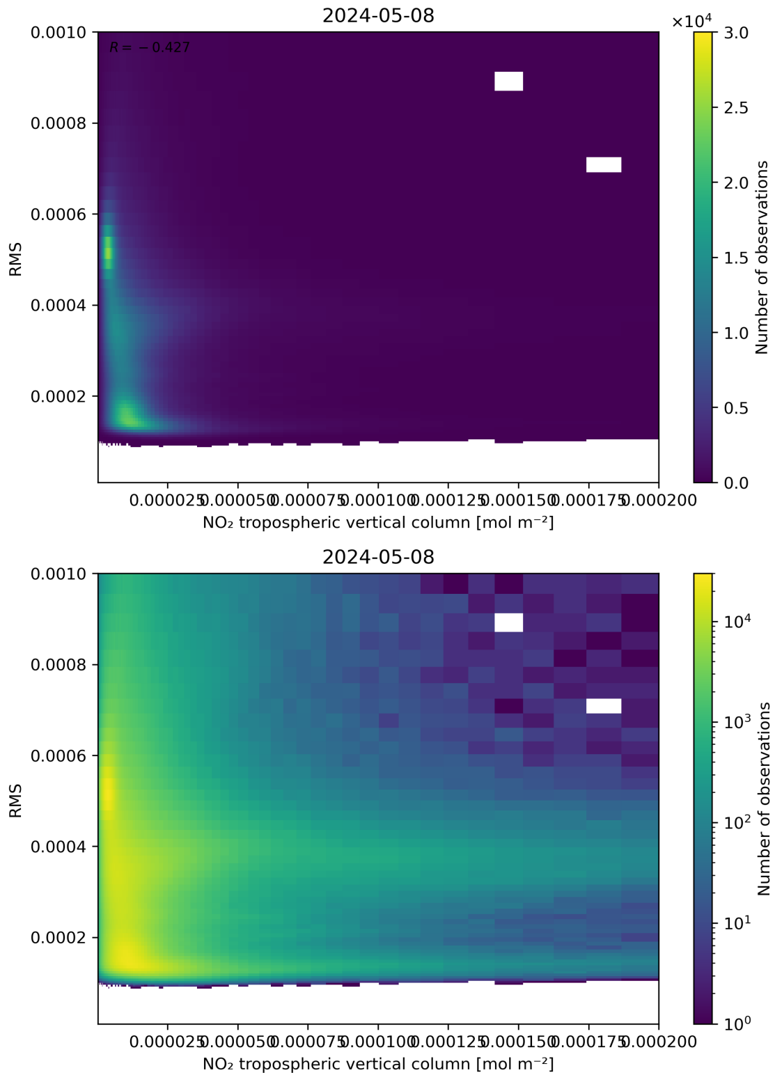
Figure 142: Scatter density plot of “NO 2 tropospheric vertical column” against “RMS” for 2024-05-07 to 2024-05-09.
