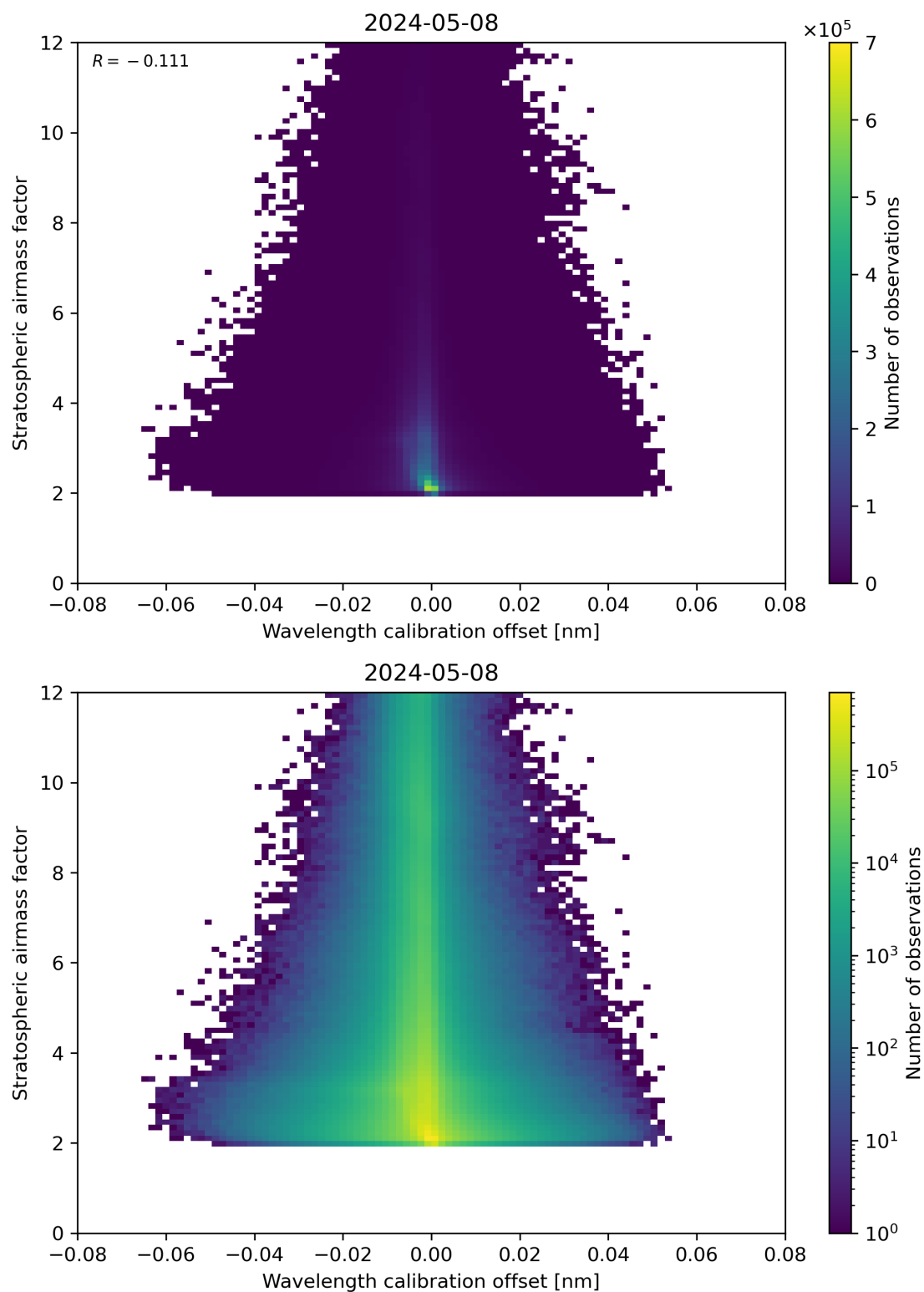
Figure 174: Scatter density plot of “Wavelength calibration offset” against “Stratospheric airmass factor” for 2024-05-07 to 2024-05-09.
