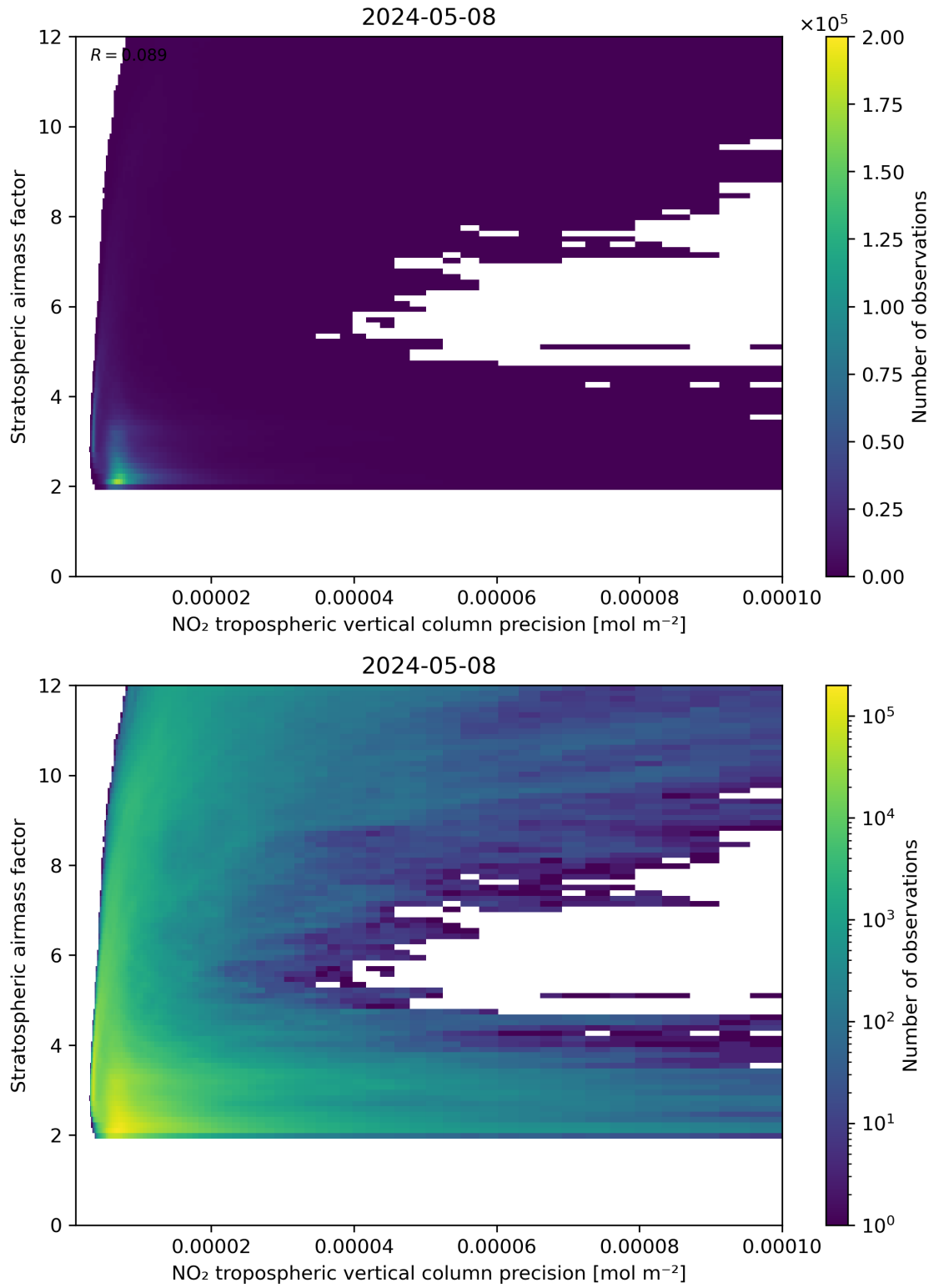
Figure 131: Scatter density plot of “NO 2 tropospheric vertical column precision” against “Stratospheric airmass factor” for 2024-05-07 to 2024-05-09.
