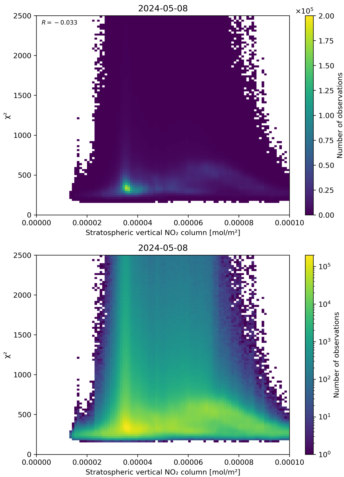
Figure 97: Scatter density plot of “Stratospheric vertical NO 2 column” against “ \chi^2 ” for 2024-05-07 to 2024-05-09.
