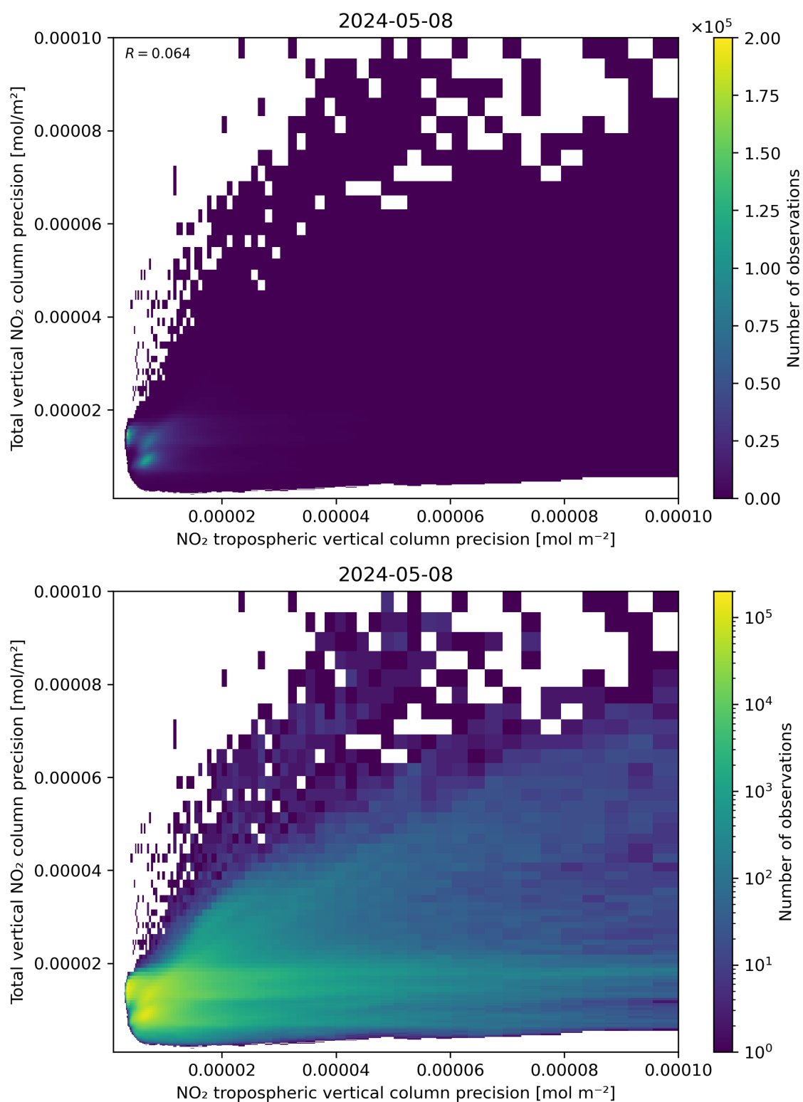
Figure 139: Scatter density plot of “NO 2 tropospheric vertical column precision” against “Total vertical NO 2 column precision” for 2024-05-07 to 2024-05-09.
