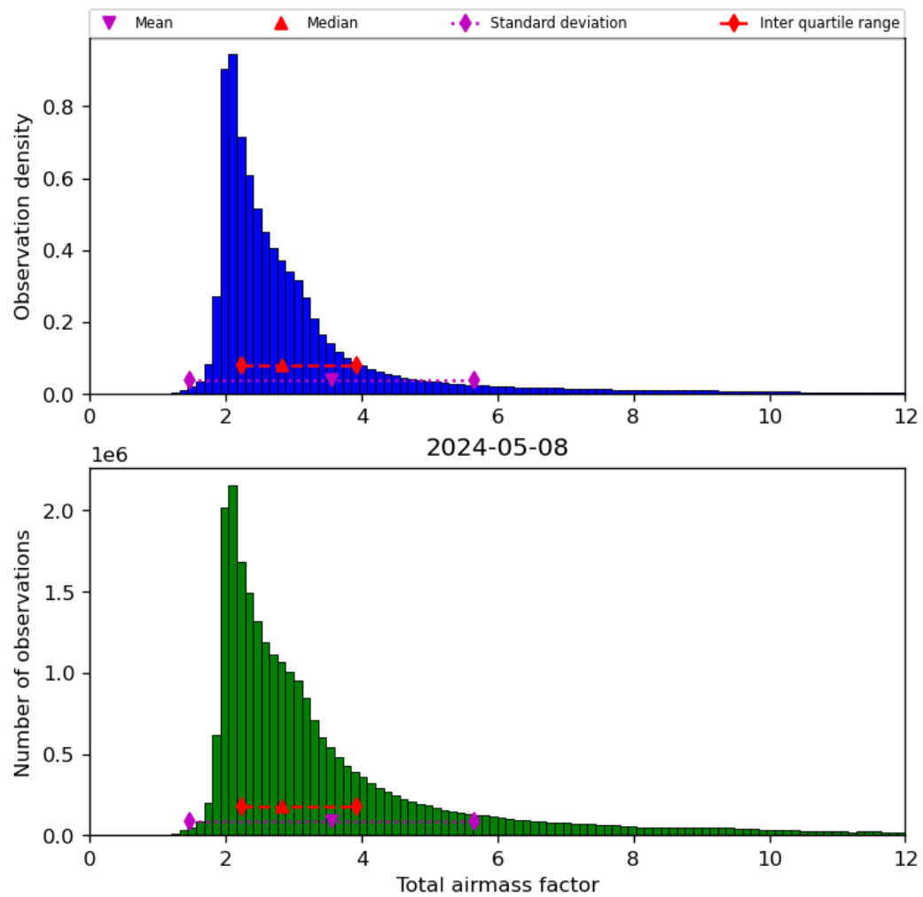
Figure 32: Histogram of “Total airmass factor” for 2024-05-07 to 2024-05-09
