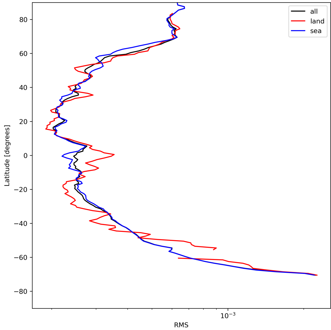
Figure 26: Zonal average of “RMS” for 2024-05-07 to 2024-05-09.
