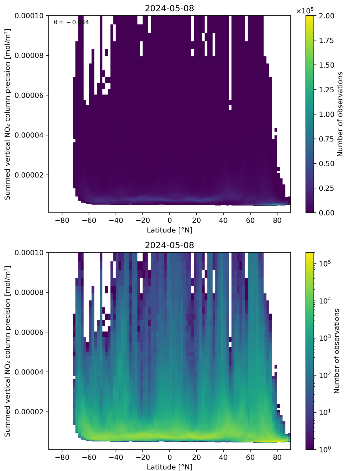
Figure 89: Scatter density plot of “Latitude” against “Summed vertical NO 2 column precision” for 2024-05-07 to 2024-05-09.
