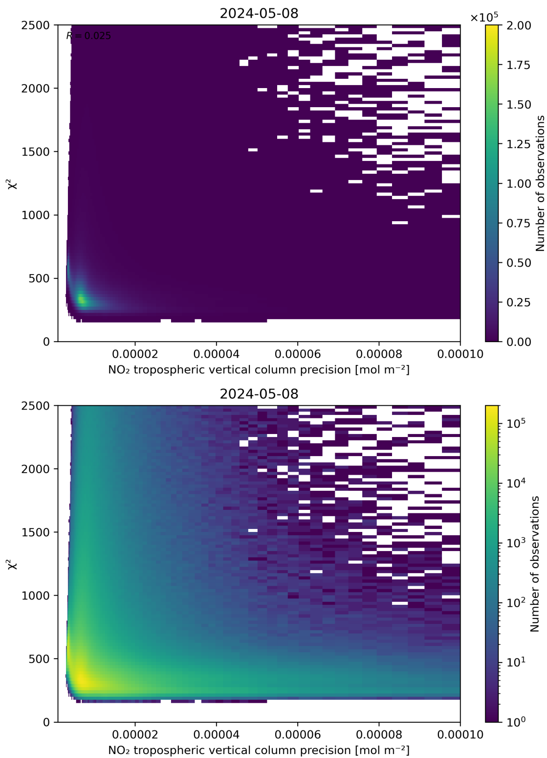
Figure 134: Scatter density plot of “NO 2 tropospheric vertical column precision” against “ \chi^2 ” for 2024-05-07 to 2024-05-09.
