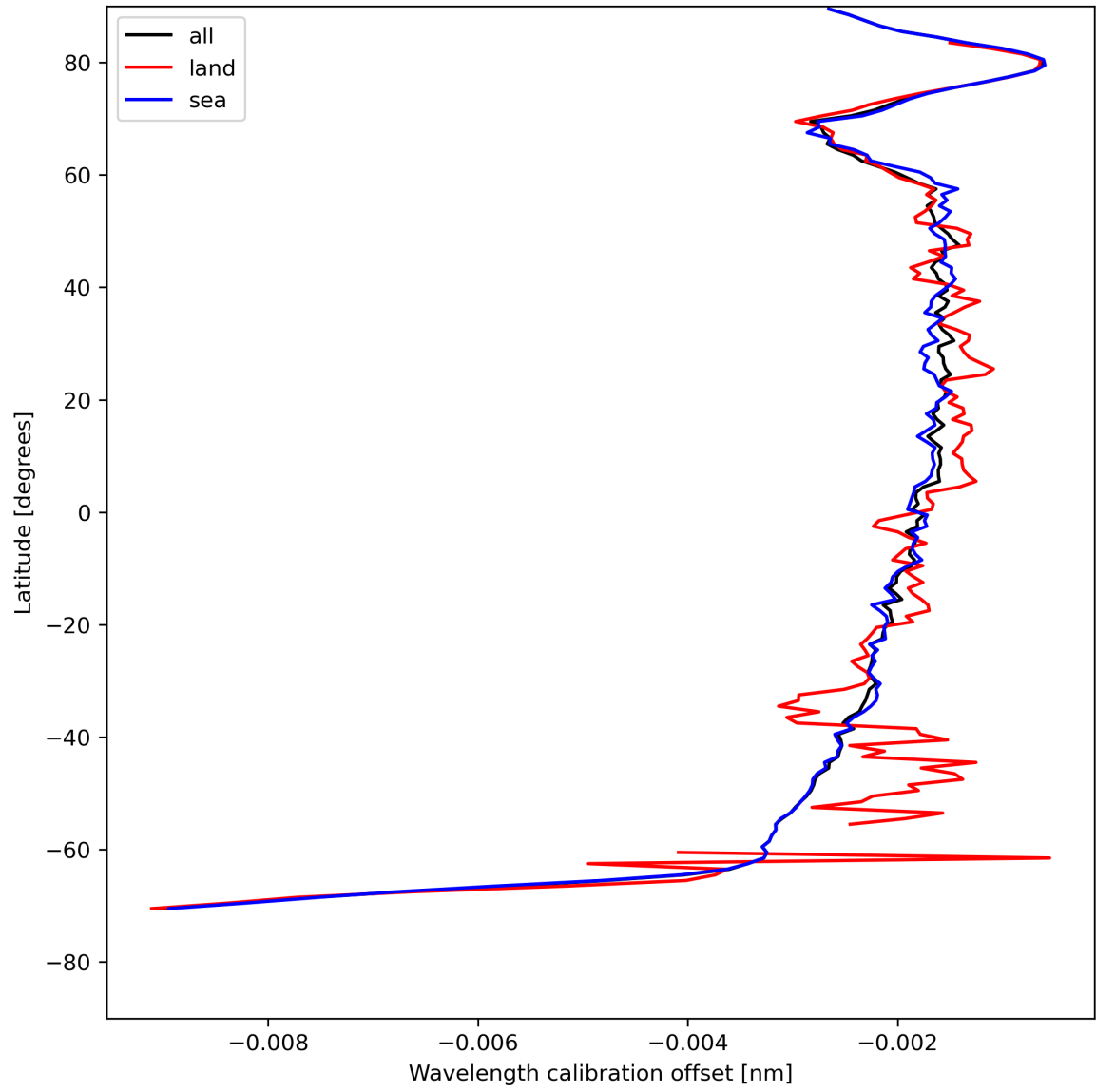
Figure 18: Zonal average of “Wavelength calibration offset” for 2024-05-07 to 2024-05-09.
