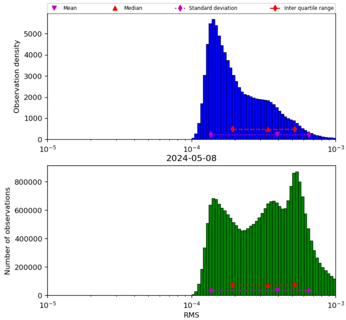
Figure 43: Histogram of “RMS” for 2024-05-07 to 2024-05-09
