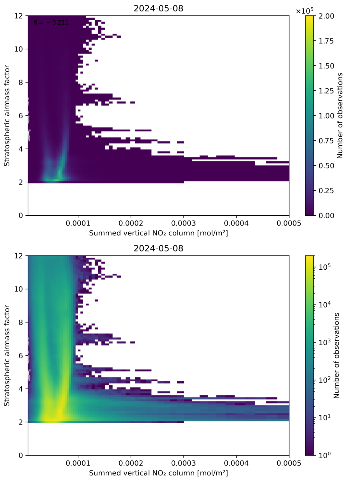
Figure 103: Scatter density plot of “Summed vertical NO 2 column” against “Stratospheric airmass factor” for 2024-05-07 to 2024-05-09.
