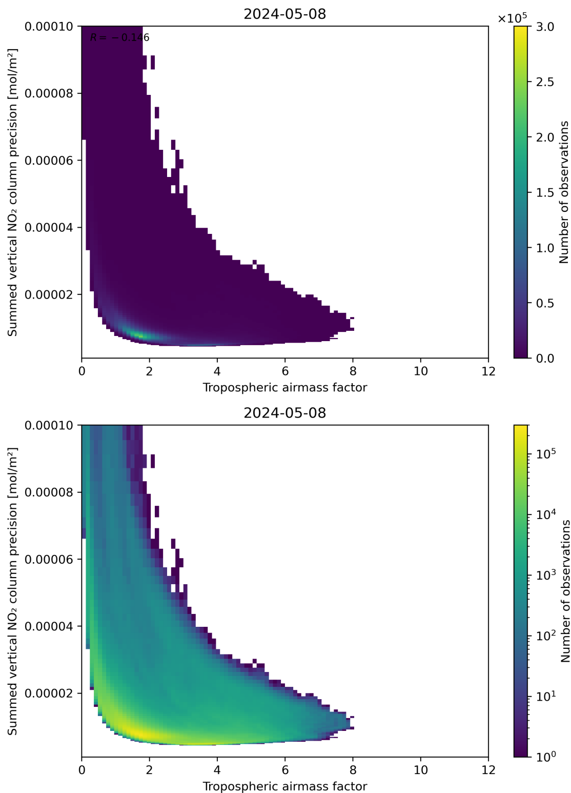
Figure 76: Scatter density plot of “Tropospheric air mass factor” against “Summed vertical NO 2 column precision” for 2024-05-07 to 2024-05-09.
