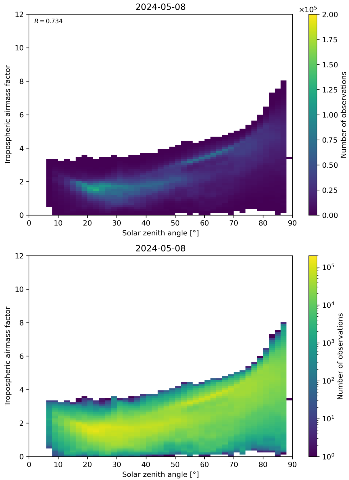
Figure 147: Scatter density plot of “Solar zenith angle” against “Tropospheric airmass factor” for 2024-05-07 to 2024-05-09.
