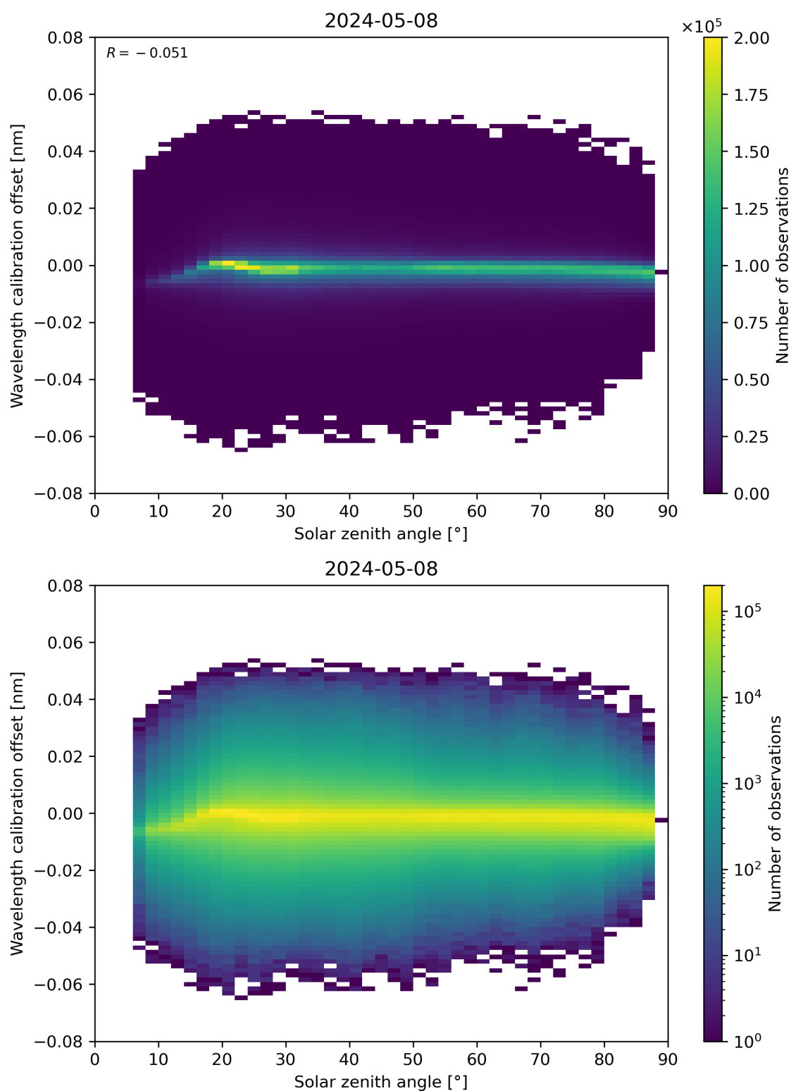
Figure 158: Scatter density plot of “Solar zenith angle” against “Wavelength calibration offset” for 2024-05-07 to 2024-05-09.
