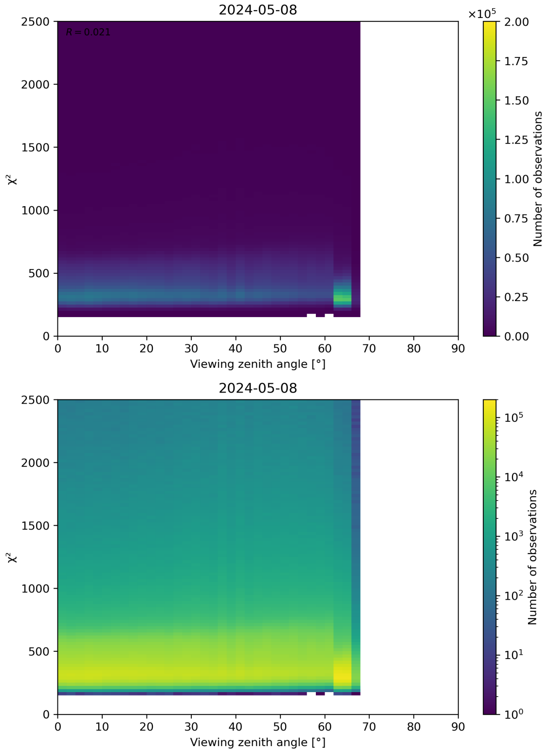
Figure 162: Scatter density plot of “Viewing zenith angle” against “ \chi^2 ” for 2024-05-07 to 2024-05-09.
