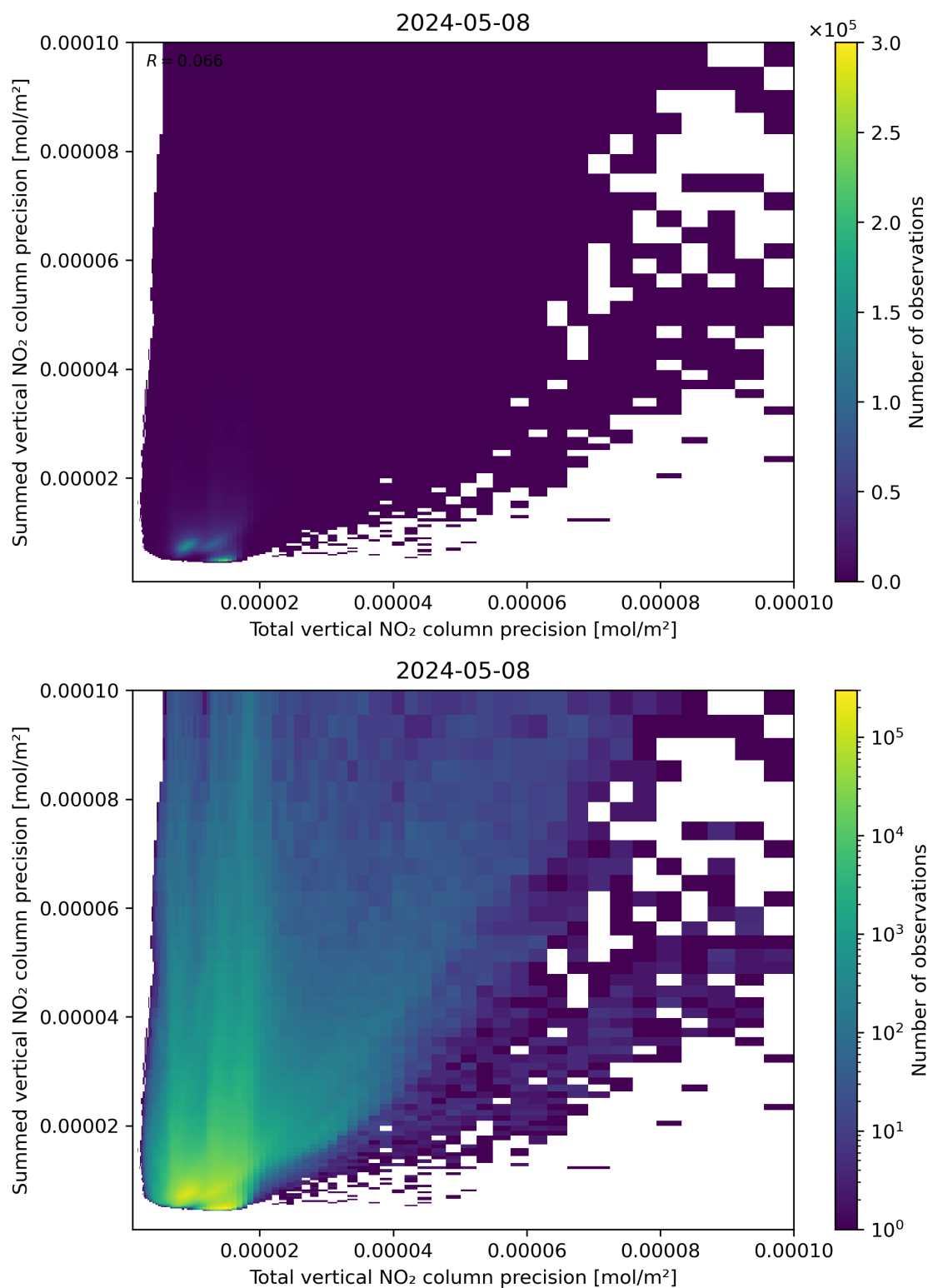
Figure 118: Scatter density plot of “Total vertical NO 2 column precision” against “Summed vertical NO 2 column precision” for 2024-05-07 to 2024-05-09.
