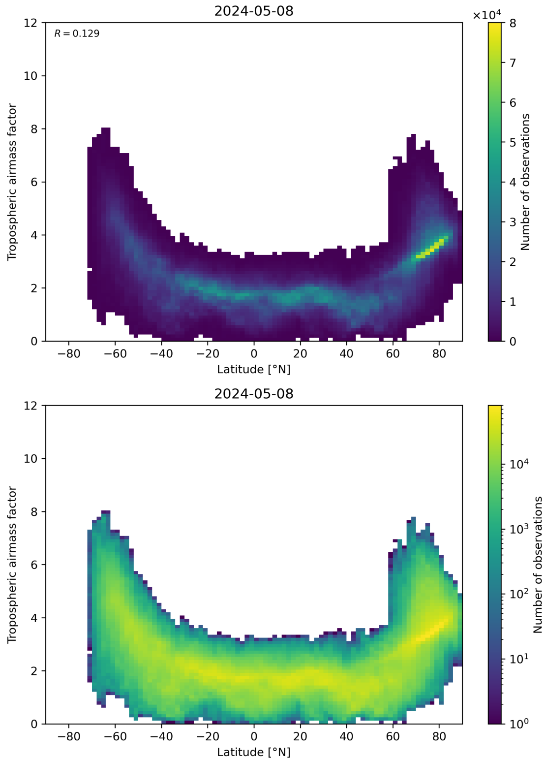
Figure 85: Scatter density plot of “Latitude” against “Tropospheric air mass factor” for 2024-05-07 to 2024-05-09.
