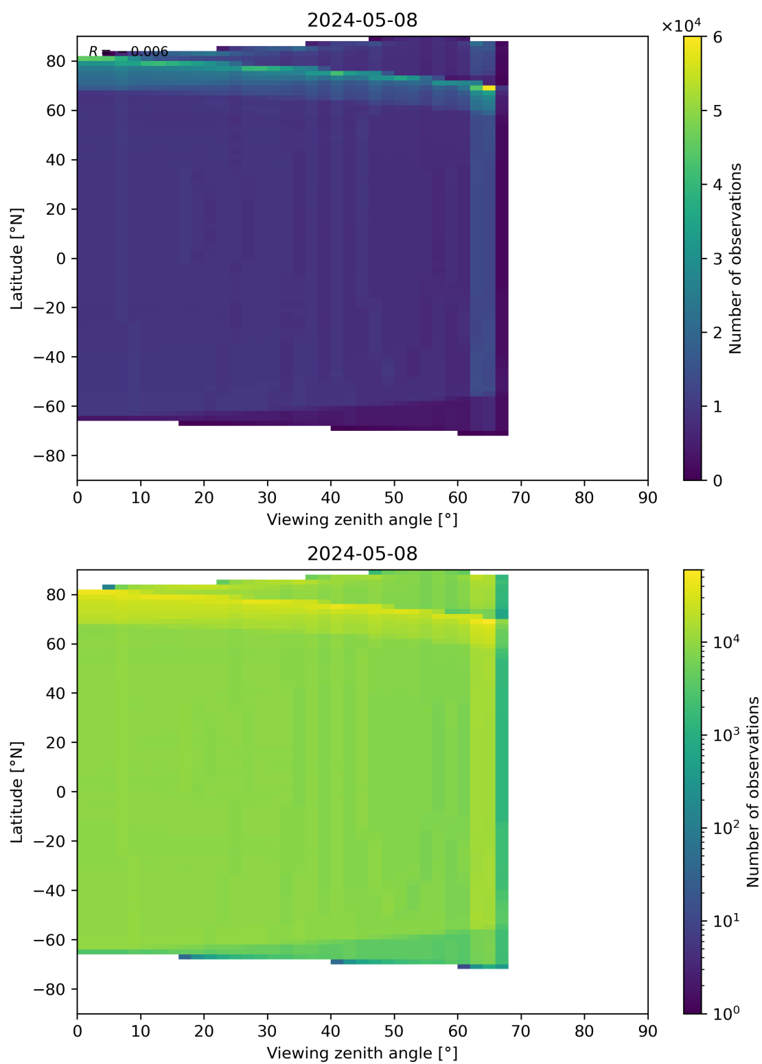
Figure 163: Scatter density plot of “Viewing zenith angle” against “Latitude” for 2024-05-07 to 2024-05-09.
