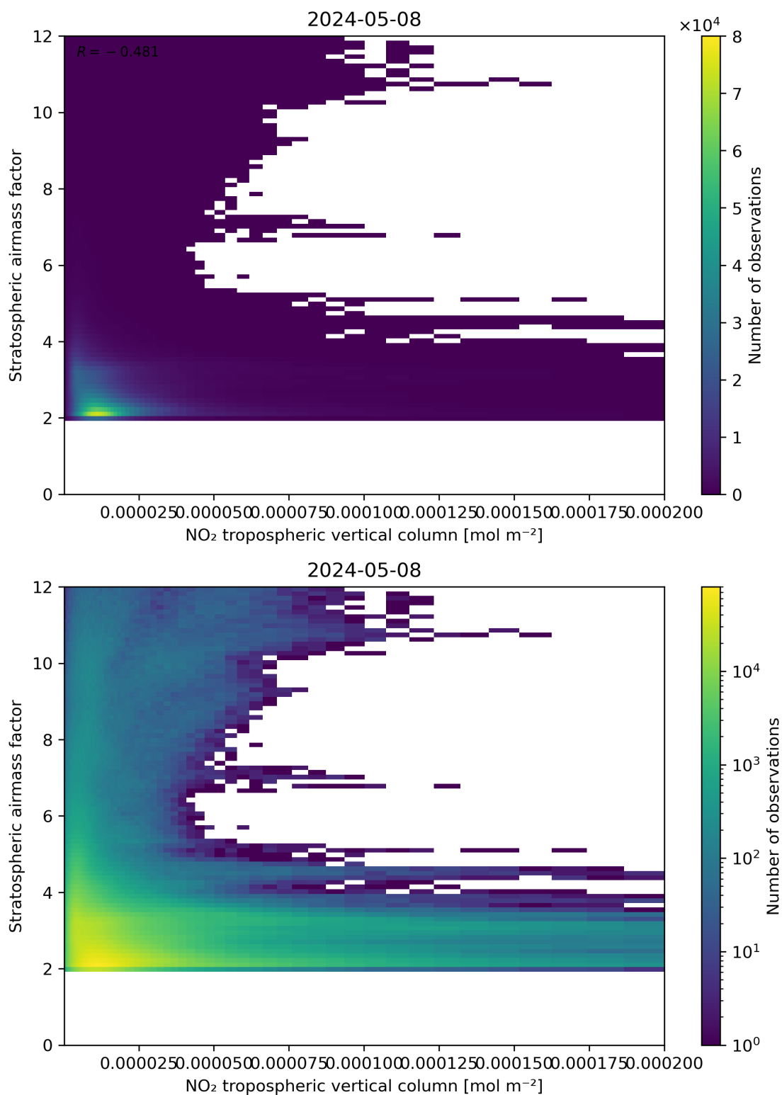
Figure 121: Scatter density plot of “NO 2 tropospheric vertical column” against “Stratospheric air mass factor” for 2024-05-07 to 2024-05-09.
