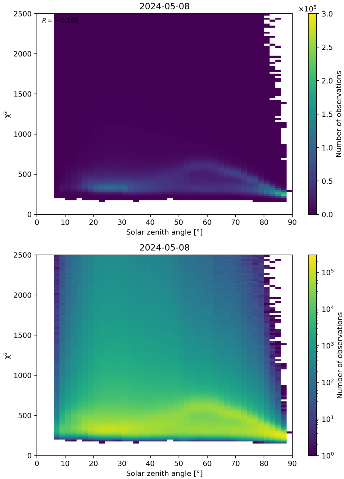
Figure 148: Scatter density plot of “Solar zenith angle” against “ \chi^2 ” for 2024-05-07 to 2024-05-09.
