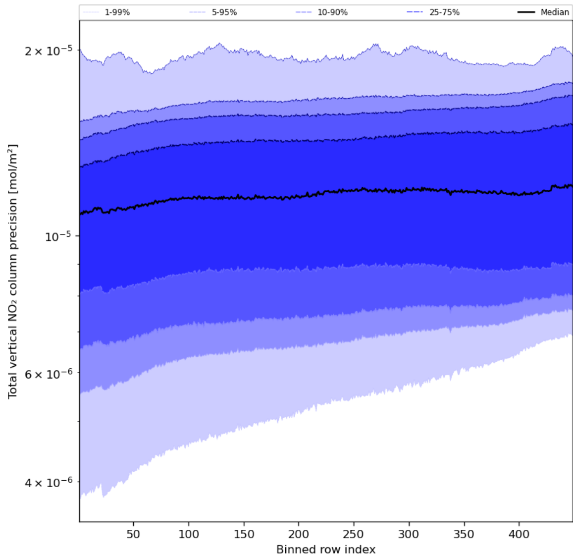
Figure 56: Along track statistics of “Total vertical NO 2 column precision” for 2024-05-07 to 2024-05-09
