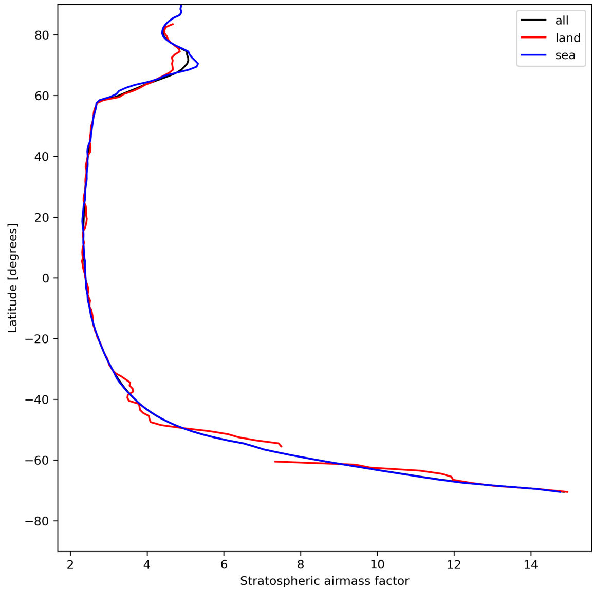
Figure 27: Zonal average of “Stratospheric air mass factor” for 2024-05-07 to 2024-05-09.
