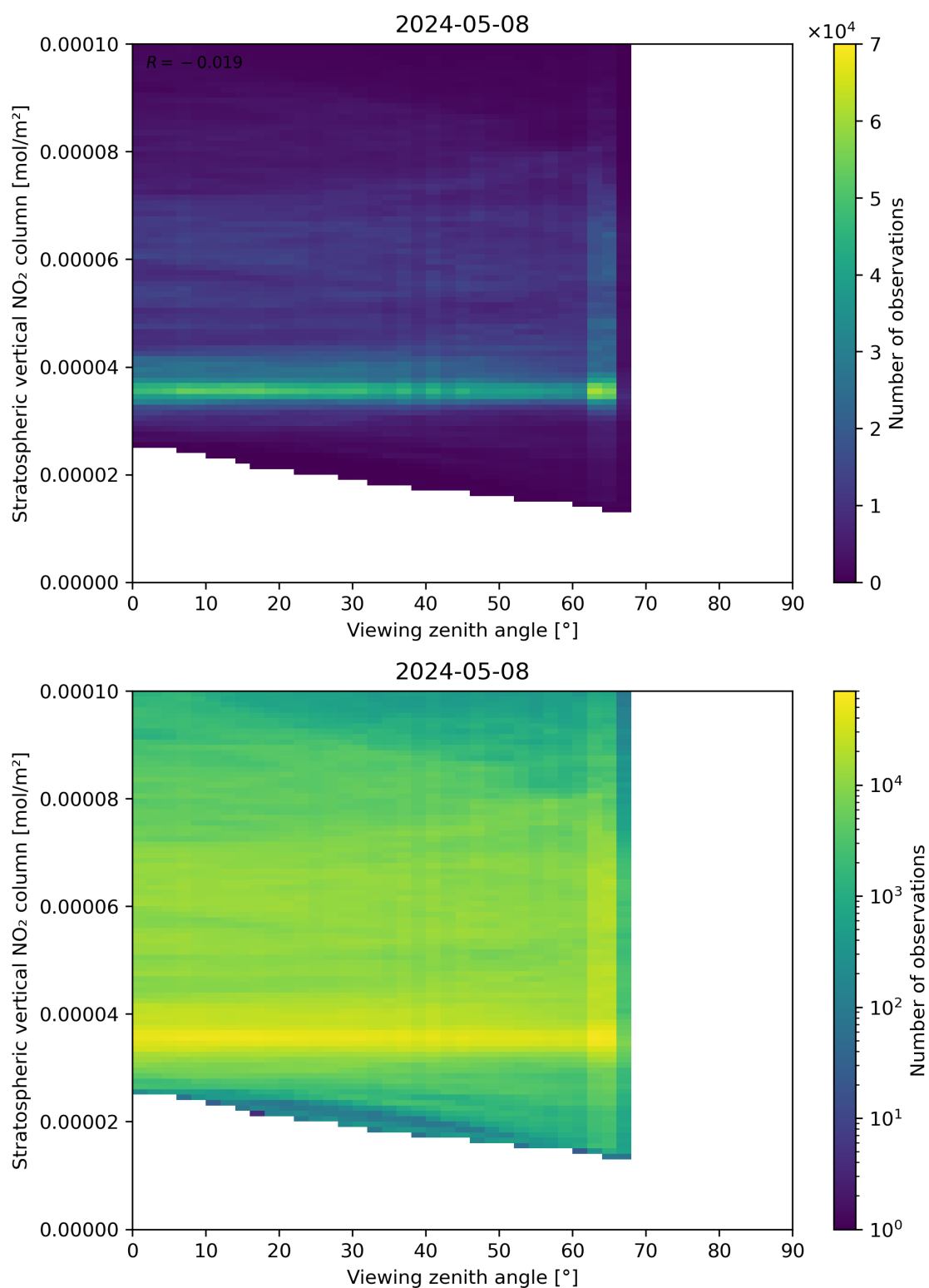
Figure 164: Scatter density plot of “Viewing zenith angle” against “Stratospheric vertical NO 2 column” for 2024-05-07 to 2024-05-09.
