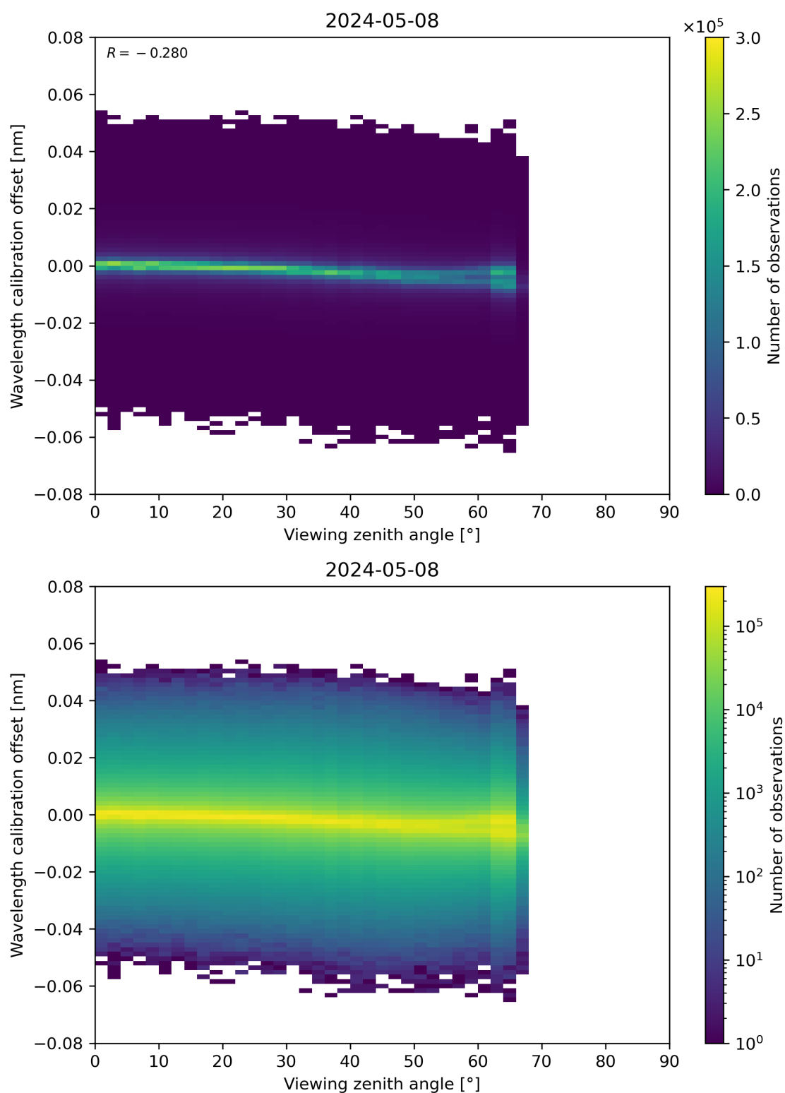
Figure 173: Scatter density plot of “Viewing zenith angle” against “Wavelength calibration offset” for 2024-05-07 to 2024-05-09.
