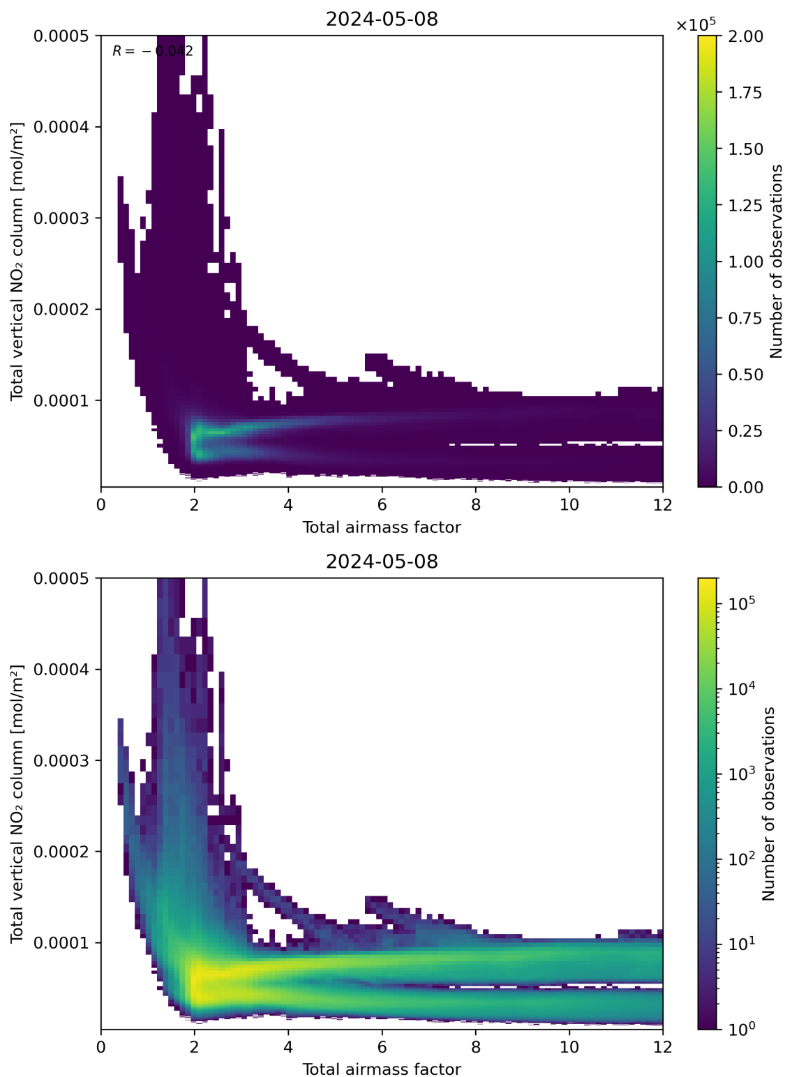
Figure 67: Scatter density plot of “Total airmass factor” against “Total vertical NO 2 column” for 2024-05-07 to 2024-05-09.
