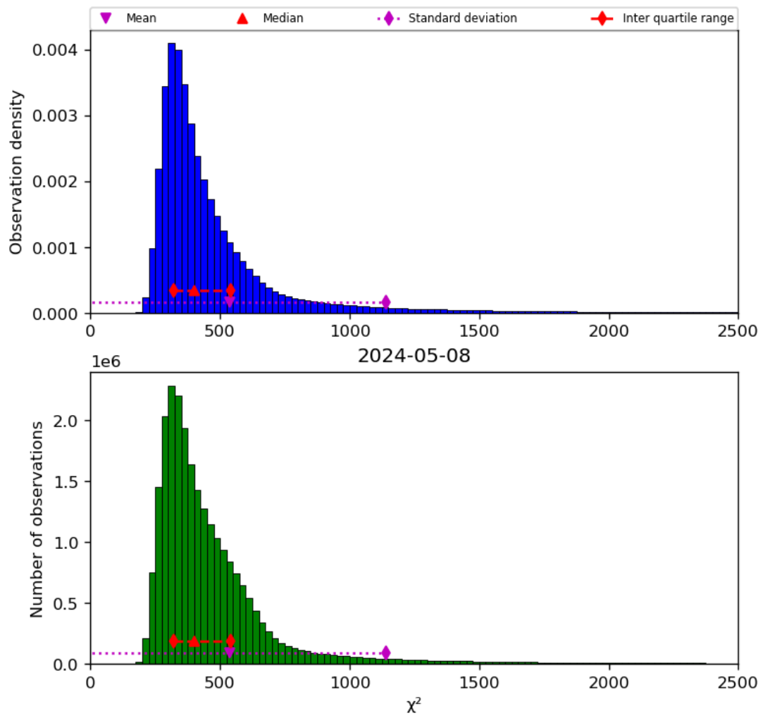
Figure 42: Histogram of “ \chi^2 ” for 2024-05-07 to 2024-05-09
