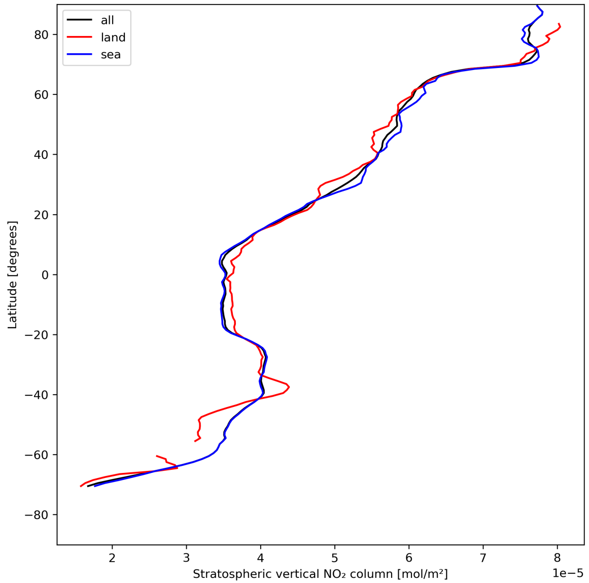
Figure 19: Zonal average of “Stratospheric vertical NO 2 column” for 2024-05-07 to 2024-05-09.
