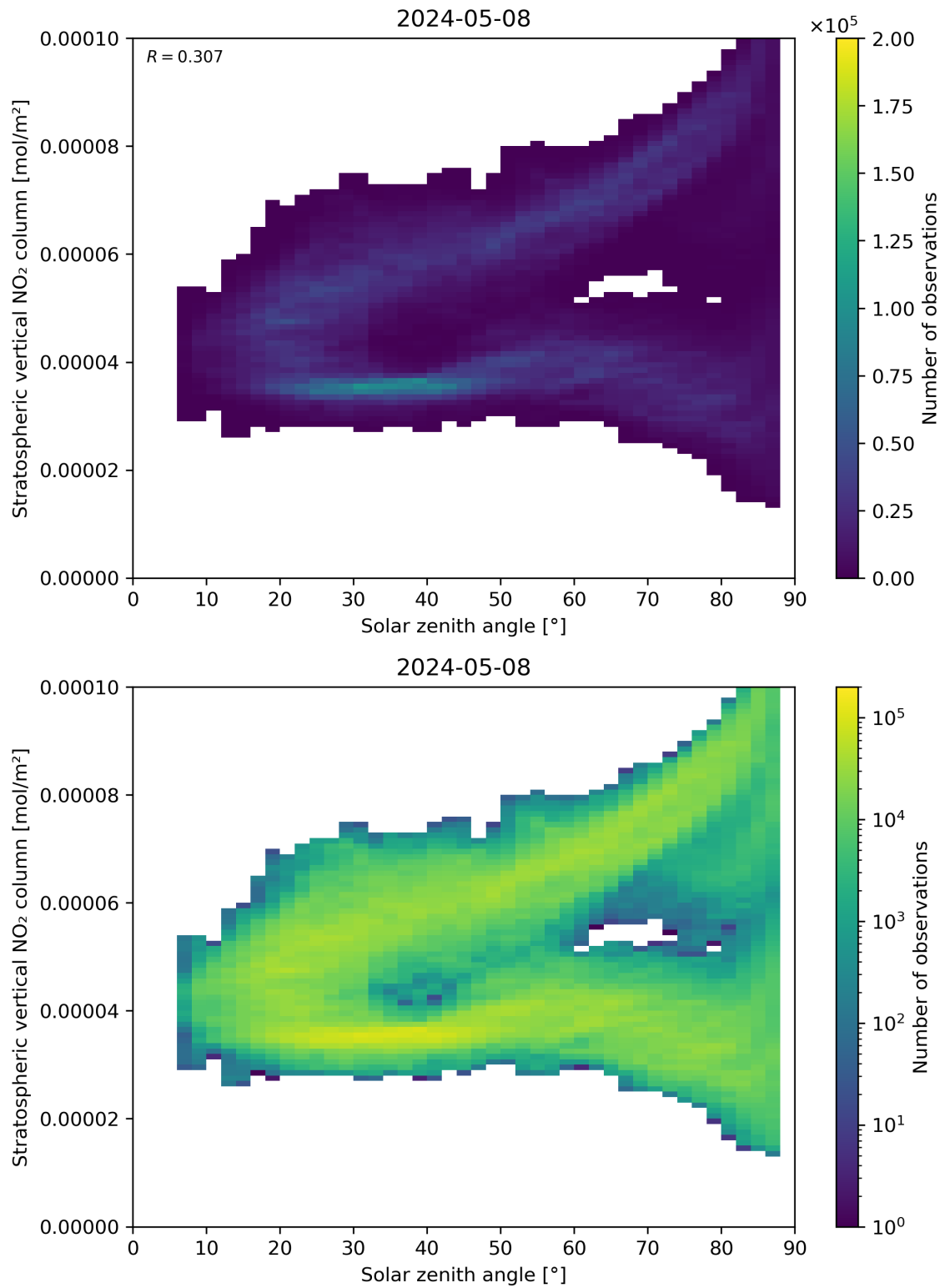
Figure 150: Scatter density plot of “Solar zenith angle” against “Stratospheric vertical NO 2 column” for 2024-05-07 to 2024-05-09.
