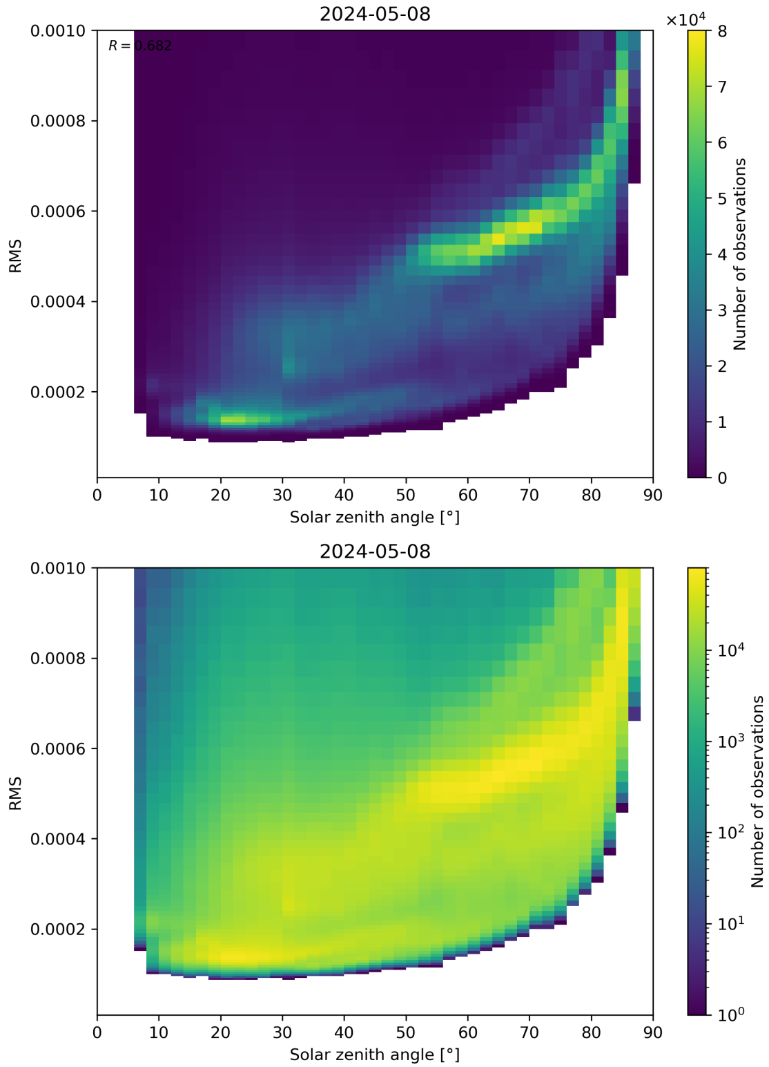
Figure 157: Scatter density plot of “Solar zenith angle” against “RMS” for 2024-05-07 to 2024-05-09.
