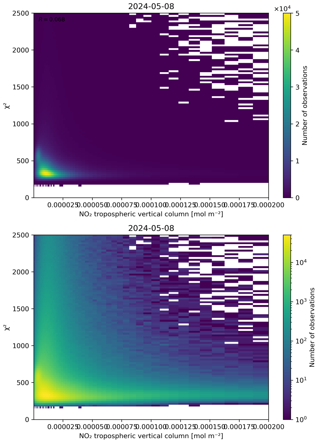
Figure 124: Scatter density plot of “NO 2 tropospheric vertical column” against “ \chi^2 ” for 2024-05-07 to 2024-05-09.
