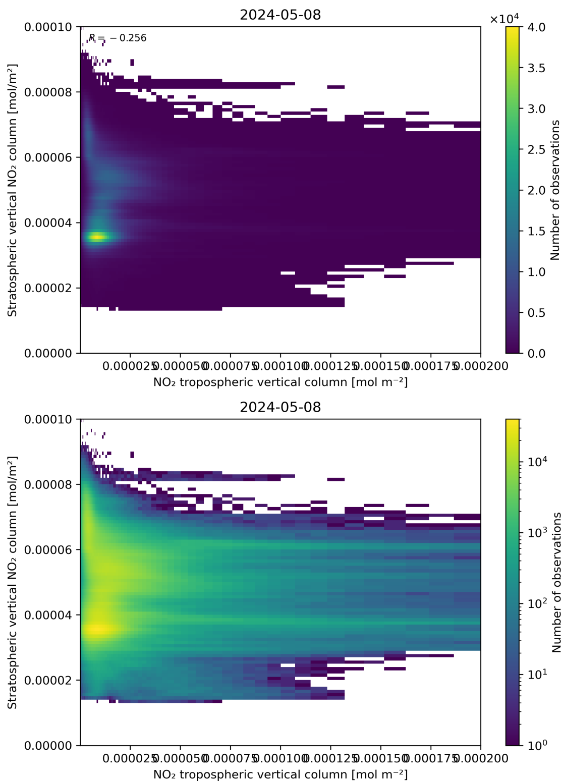
Figure 125: Scatter density plot of “NO 2 tropospheric vertical column” against “Stratospheric vertical NO 2 column” for 2024-05-07 to 2024-05-09.
