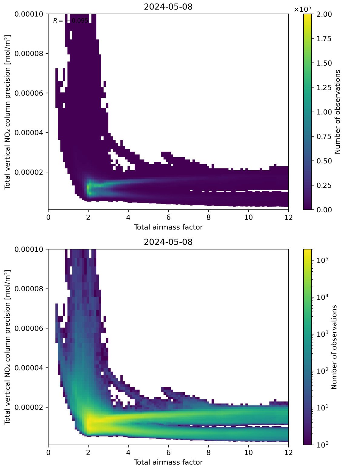
Figure 68: Scatter density plot of “Total airmass factor” against “Total vertical NO 2 column precision” for 2024-05-07 to 2024-05-09.
