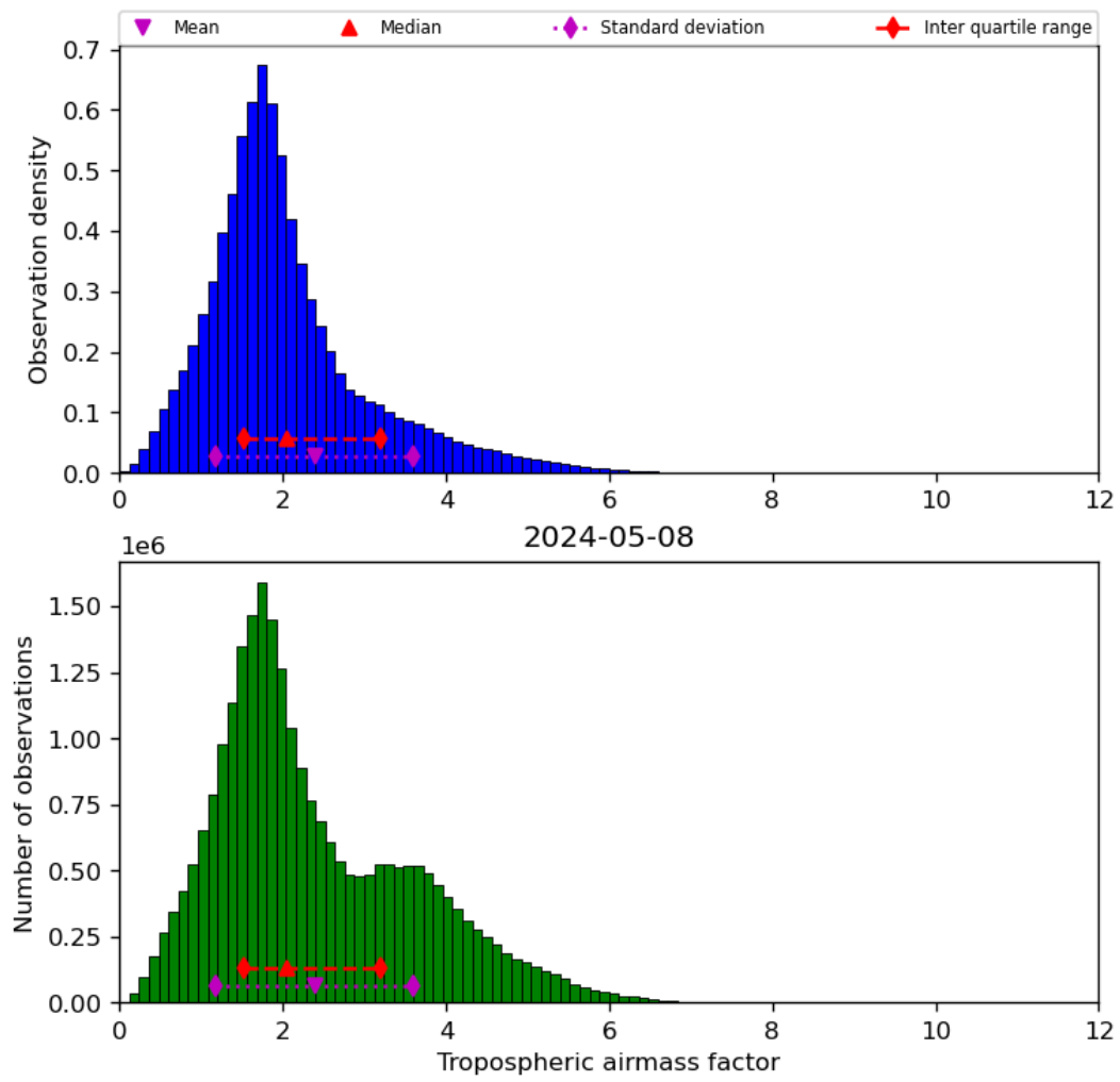
Figure 31: Histogram of “Tropospheric airmass factor” for 2024-05-07 to 2024-05-09
