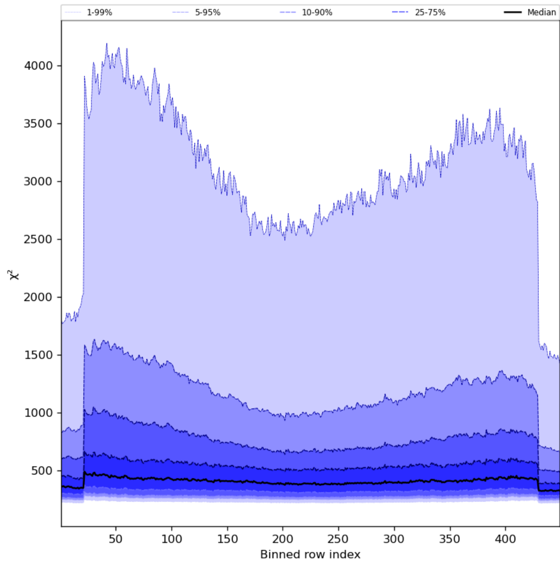
Figure 59: Along track statistics of “ \chi^2 ” for 2024-05-07 to 2024-05-09
