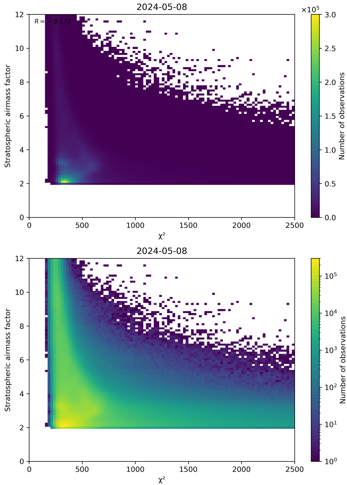
Figure 81: Scatter density plot of “ \chi^2 ” against “Stratospheric airmass factor” for 2024-05-07 to 2024-05-09.
