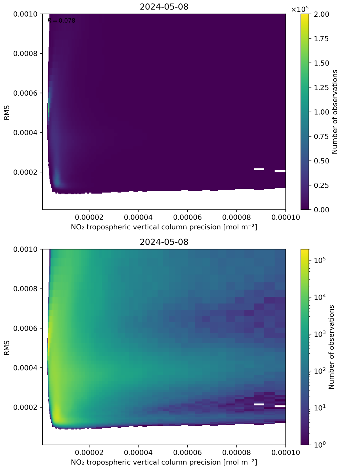
Figure 140: Scatter density plot of “NO 2 tropospheric vertical column precision” against “RMS” for 2024-05-07 to 2024-05-09.
