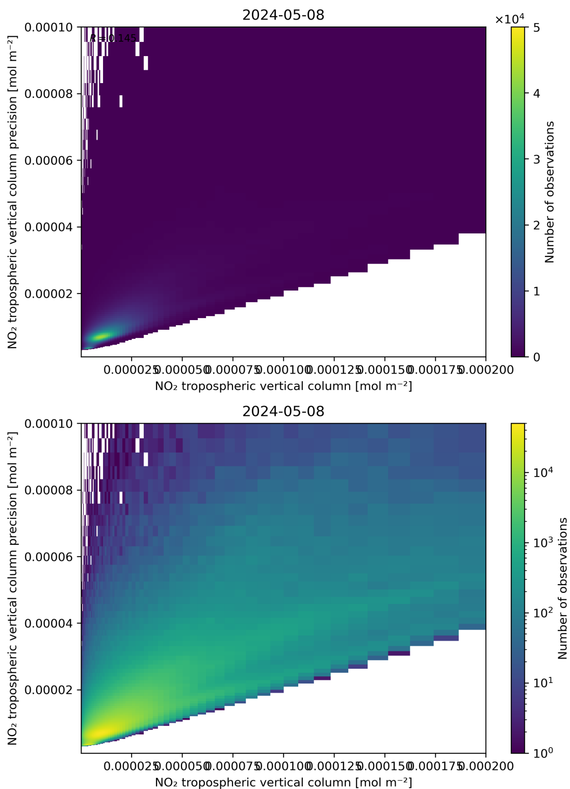
Figure 130: Scatter density plot of “NO 2 tropospheric vertical column” against “NO 2 tropospheric vertical column precision” for 2024-05-07 to 2024-05-09.
