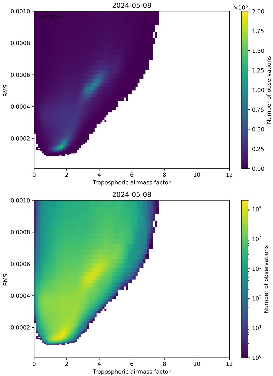
Figure 79: Scatter density plot of “Tropospheric airmass factor” against “RMS” for 2024-05-07 to 2024-05-09.
