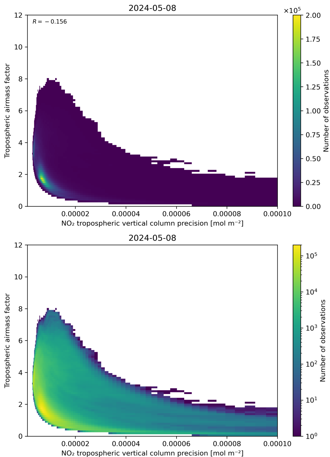
Figure 133: Scatter density plot of “NO 2 tropospheric vertical column precision” against “Tropospheric airmass factor” for 2024-05-07 to 2024-05-09.
