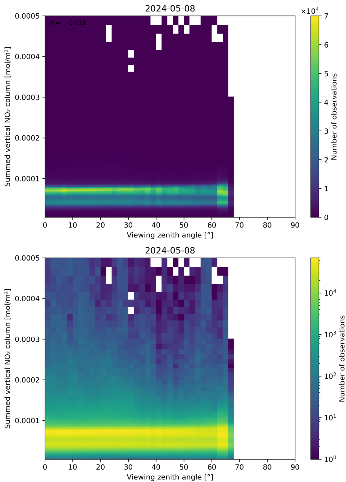
Figure 165: Scatter density plot of “Viewing zenith angle” against “Summed vertical NO 2 column” for 2024-05-07 to 2024-05-09.
