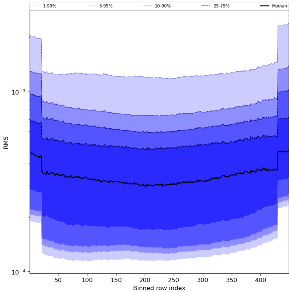
Figure 60: Along track statistics of “RMS” for 2024-05-07 to 2024-05-09
