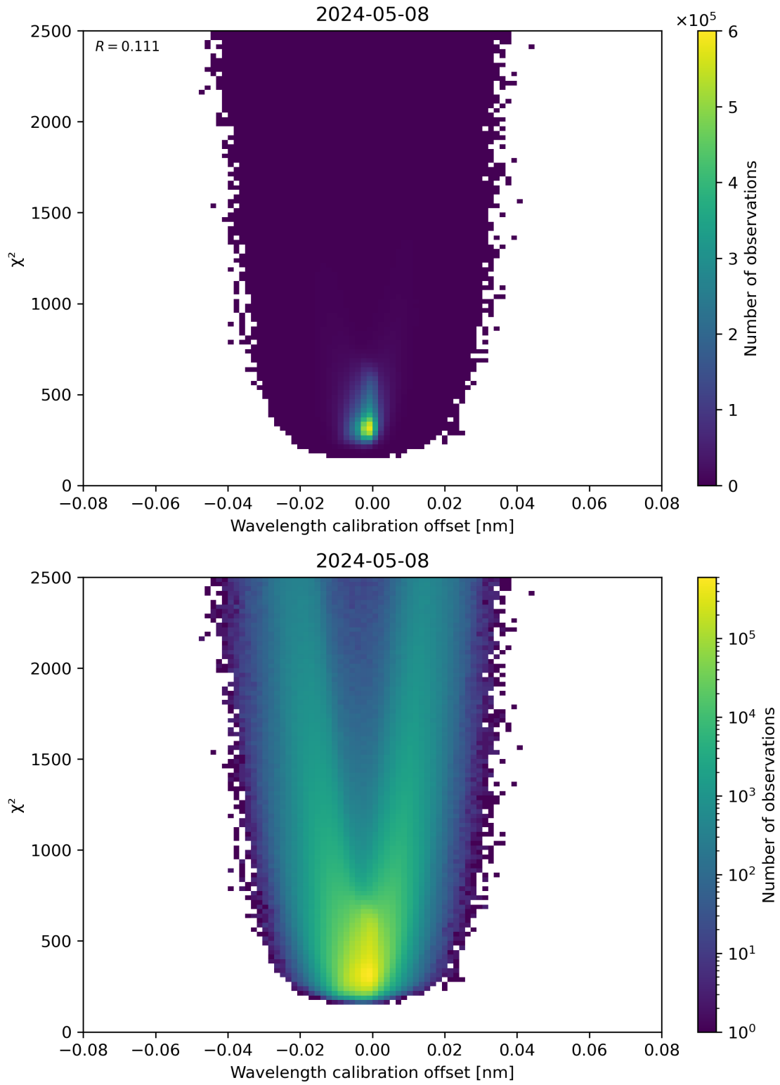
Figure 175: Scatter density plot of “Wavelength calibration offset” against “ \chi^2 ” for 2024-05-07 to 2024-05-09.
