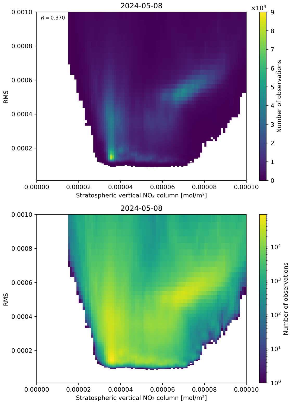
Figure 102: Scatter density plot of “Stratospheric vertical NO 2 column” against “RMS” for 2024-05-07 to 2024-05-09.
