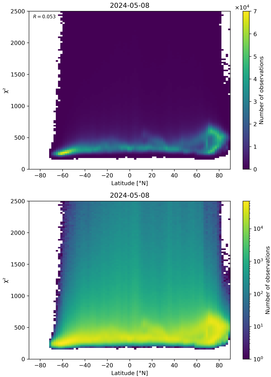
Figure 86: Scatter density plot of “Latitude” against “ \chi^2 ” for 2024-05-07 to 2024-05-09.
