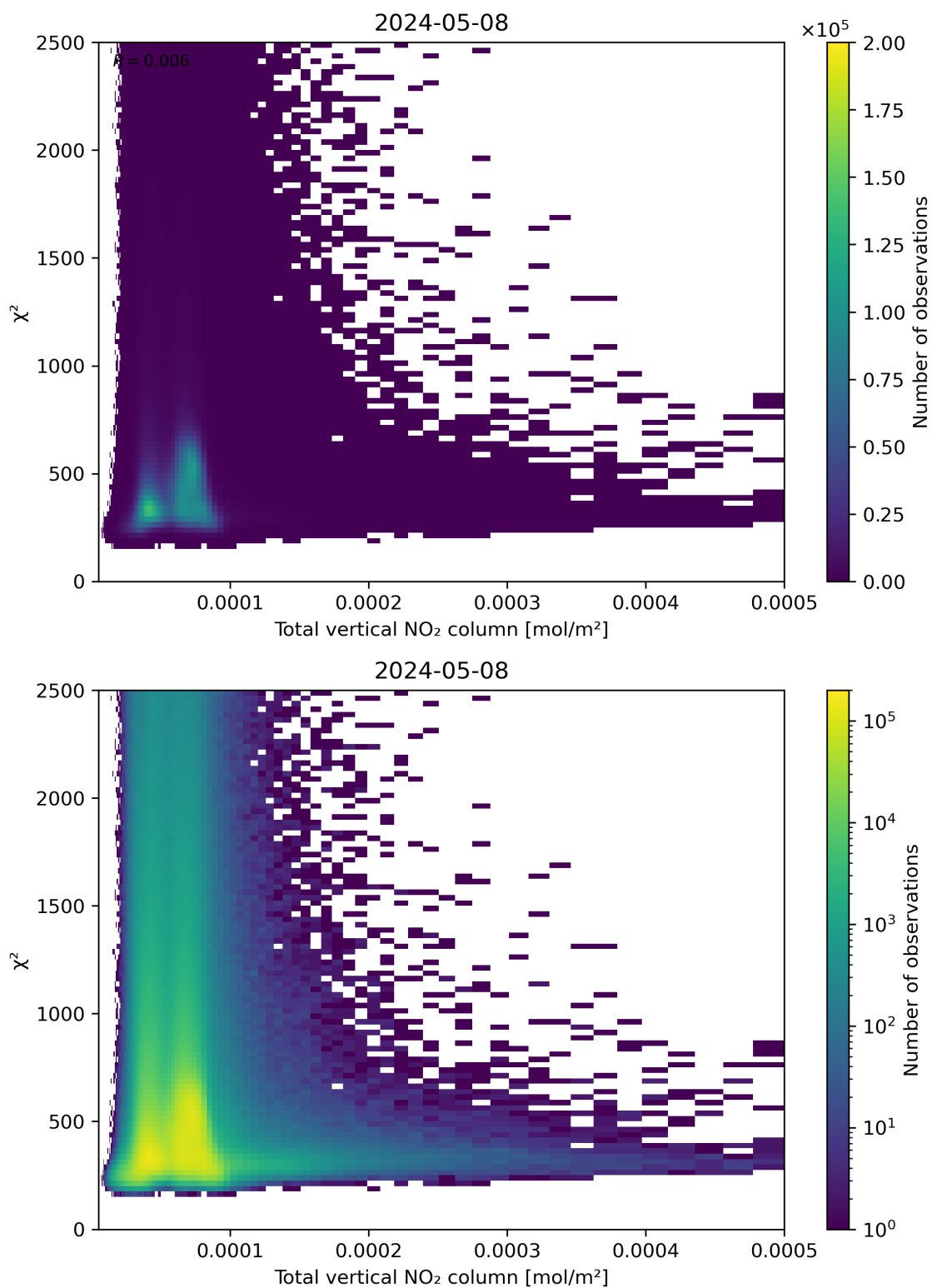
Figure 111: Scatter density plot of “Total vertical NO 2 column” against “ \chi^2 ” for 2024-05-07 to 2024-05-09.
