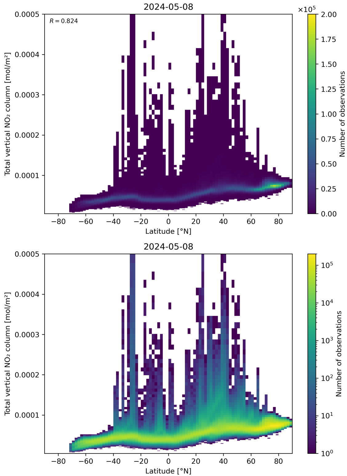
Figure 90: Scatter density plot of “Latitude” against “Total vertical NO 2 column” for 2024-05-07 to 2024-05-09.
