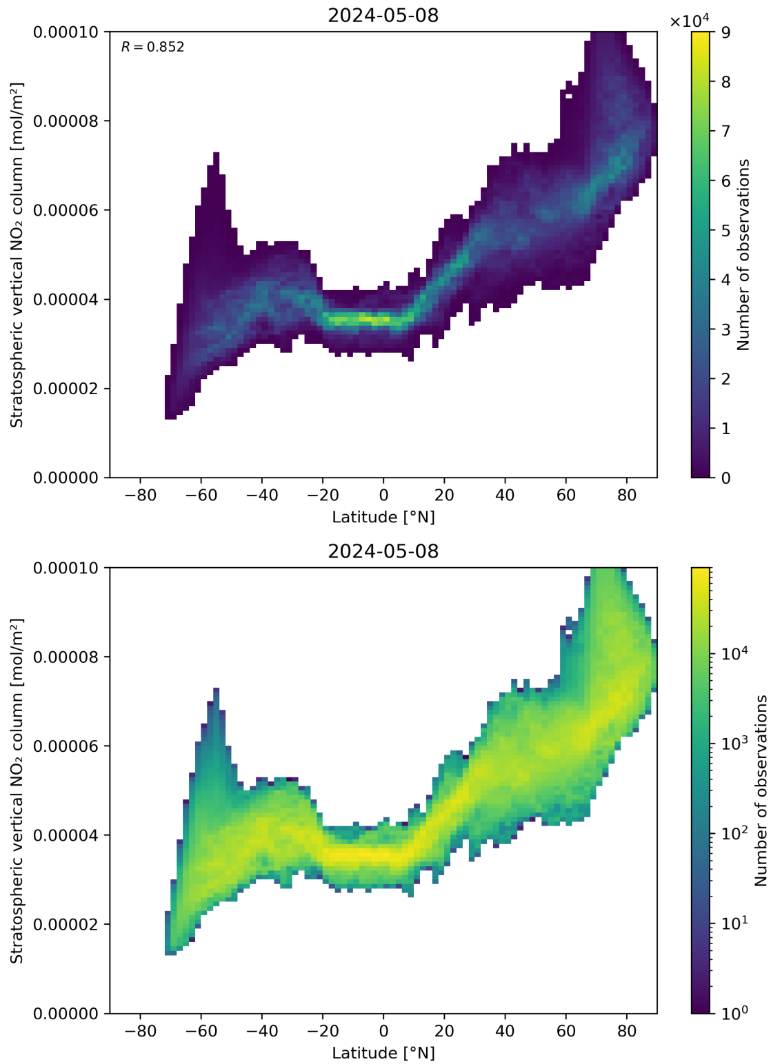
Figure 87: Scatter density plot of “Latitude” against “Stratospheric vertical NO 2 column” for 2024-05-07 to 2024-05-09.
