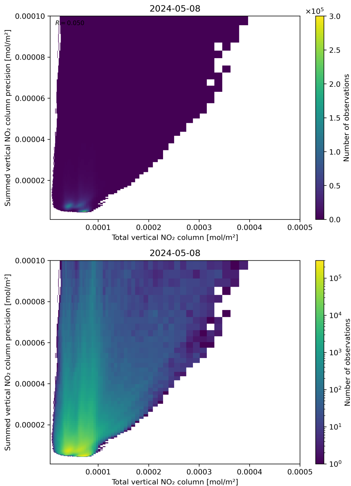
Figure 113: Scatter density plot of “Total vertical NO 2 column” against “Summed vertical NO 2 column precision” for 2024-05-07 to 2024-05-09.
