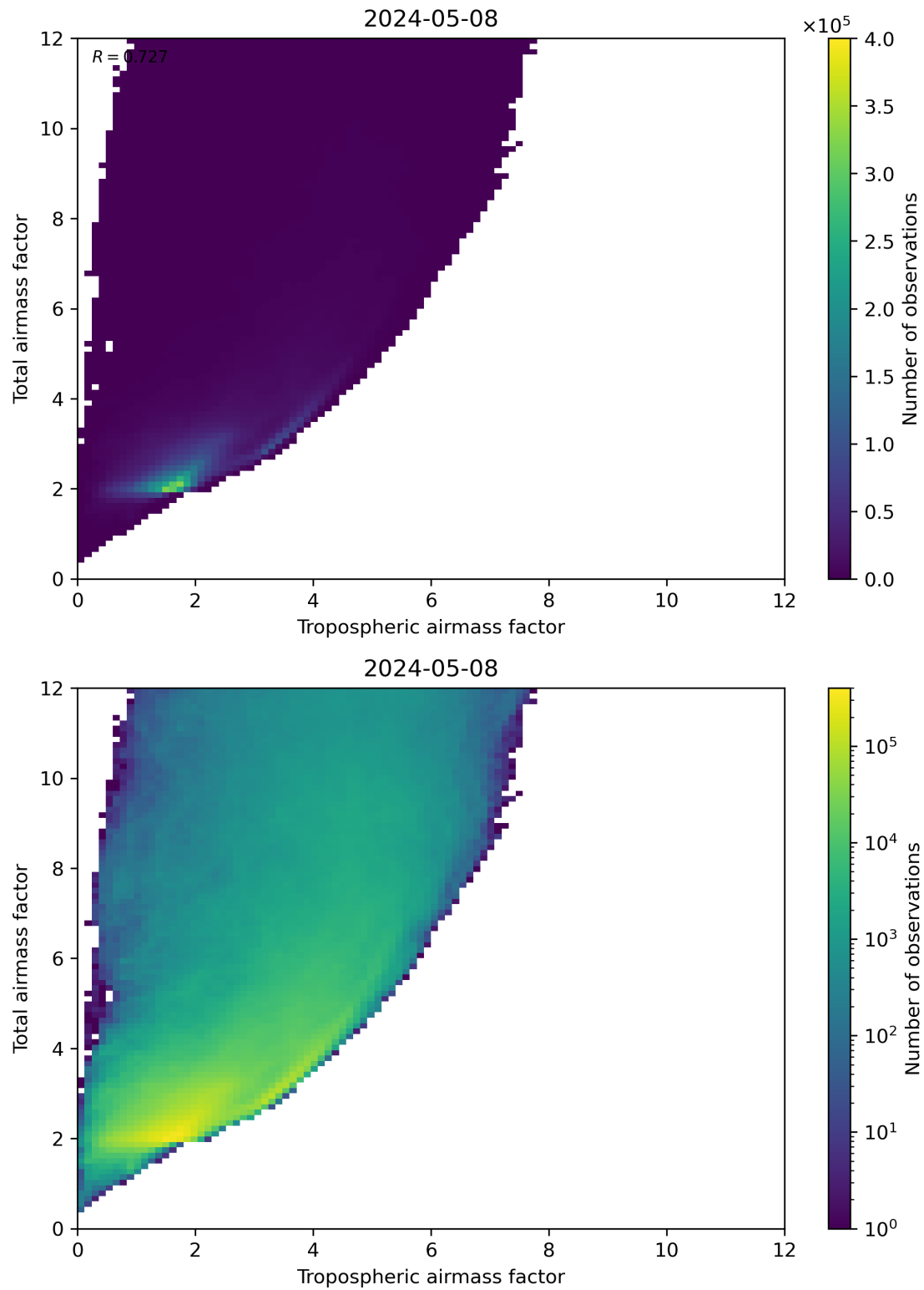
Figure 72: Scatter density plot of “Tropospheric airmass factor” against “Total airmass factor” for 2024-05-07 to 2024-05-09.
