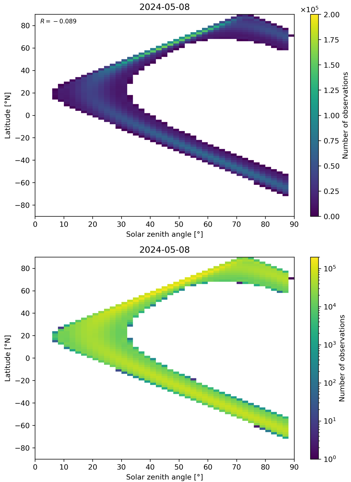
Figure 149: Scatter density plot of “Solar zenith angle” against “Latitude” for 2024-05-07 to 2024-05-09.
