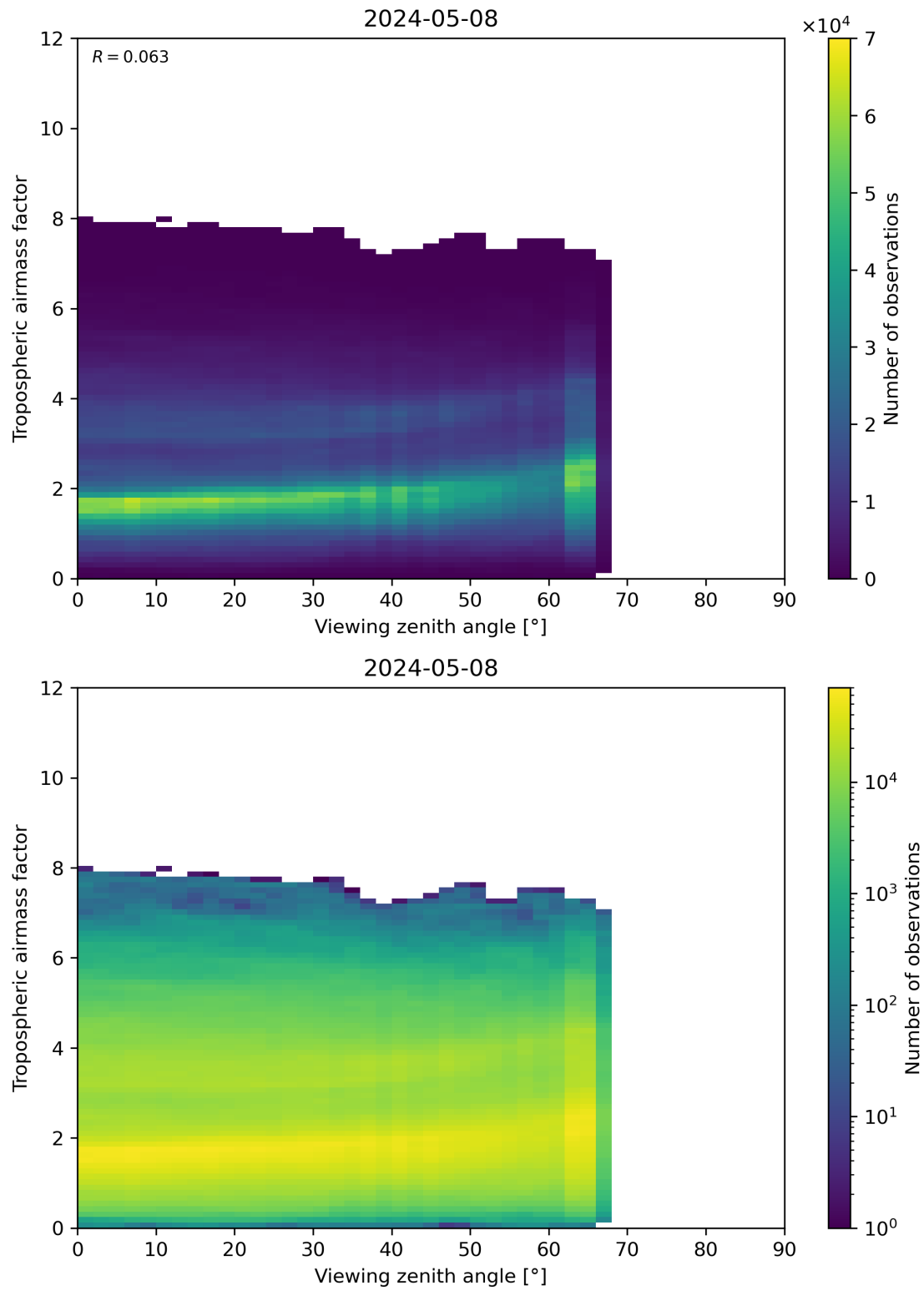
Figure 161: Scatter density plot of “Viewing zenith angle” against “Tropospheric airmass factor” for 2024-05-07 to 2024-05-09.
