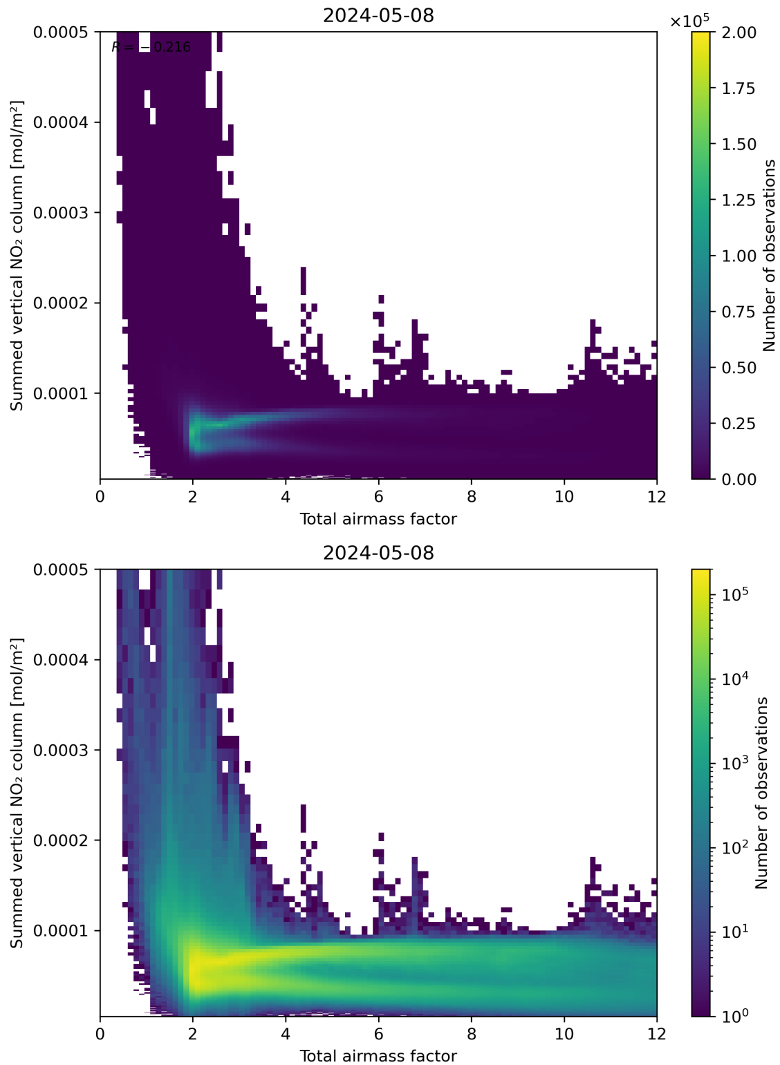
Figure 65: Scatter density plot of “Total airmass factor” against “Summed vertical NO 2 column” for 2024-05-07 to 2024-05-09.
