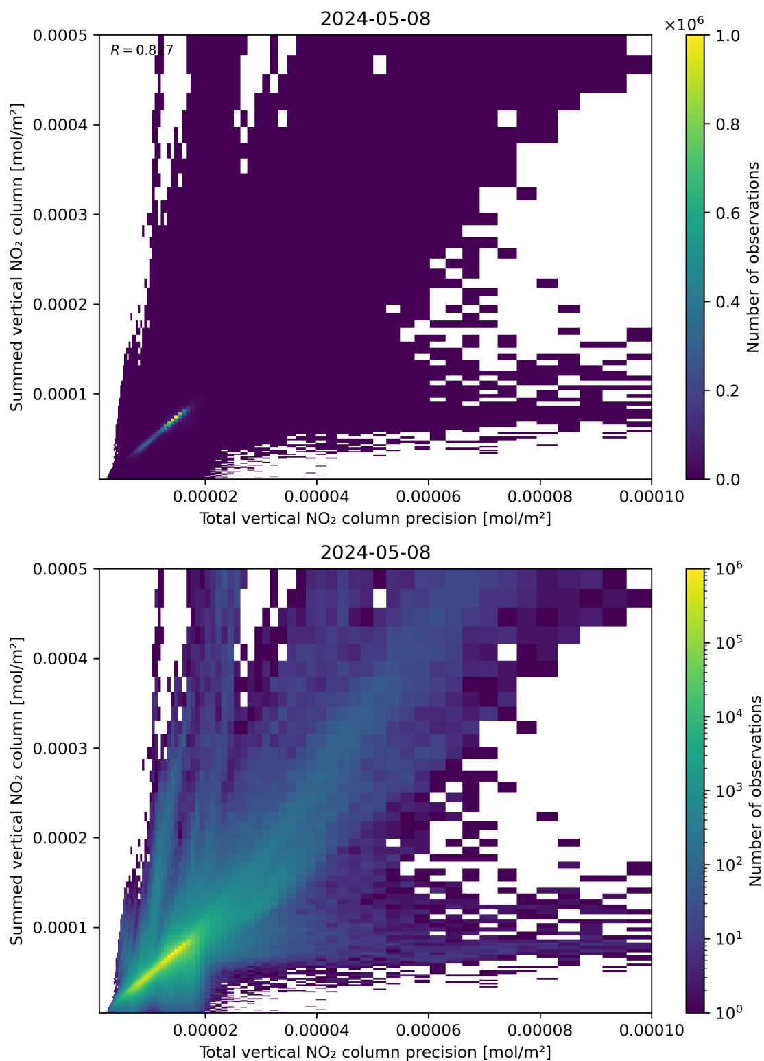
Figure 117: Scatter density plot of “Total vertical NO 2 column precision” against “Summed vertical NO 2 column” for 2024-05-07 to 2024-05-09.
