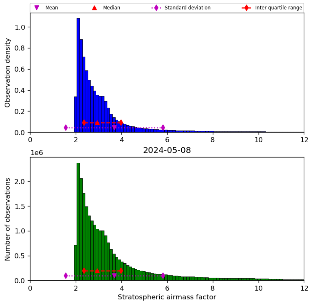
Figure 44: Histogram of “Stratospheric airmass factor” for 2024-05-07 to 2024-05-09
