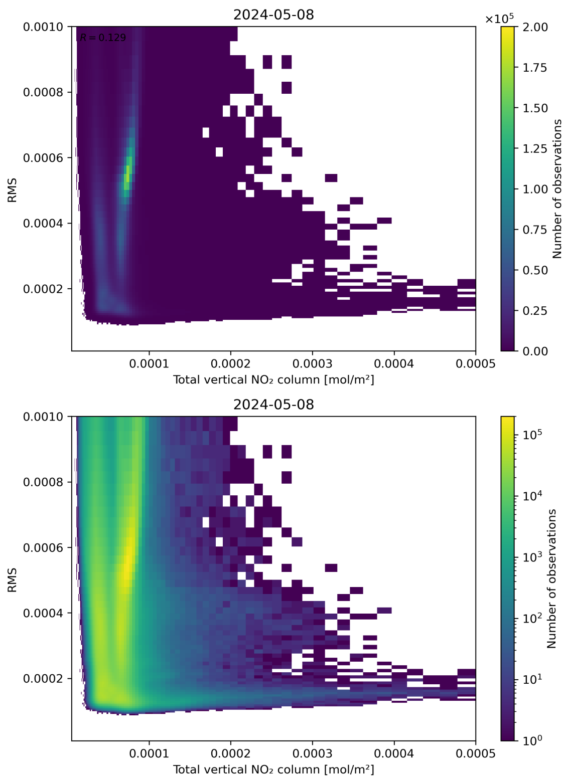
Figure 120: Scatter density plot of “Total vertical NO 2 column” against “RMS” for 2024-05-07 to 2024-05-09.
