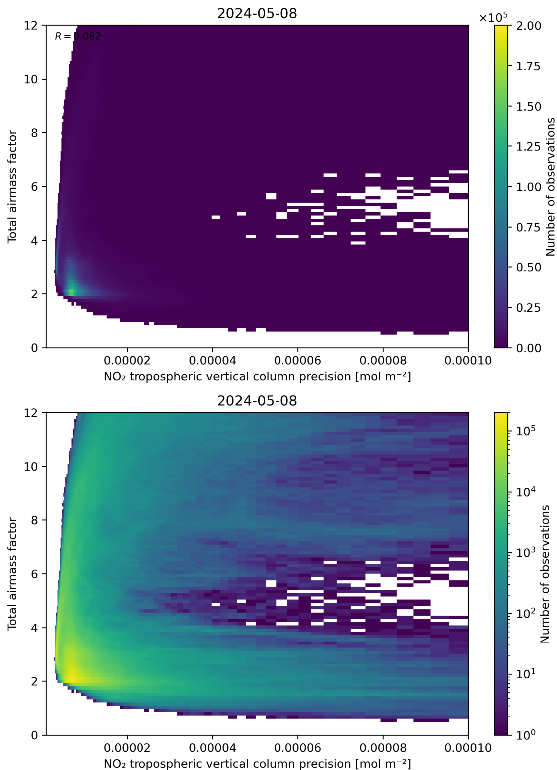
Figure 132: Scatter density plot of “NO 2 tropospheric vertical column precision” against “Total air mass factor” for 2024-05-07 to 2024-05-09.
