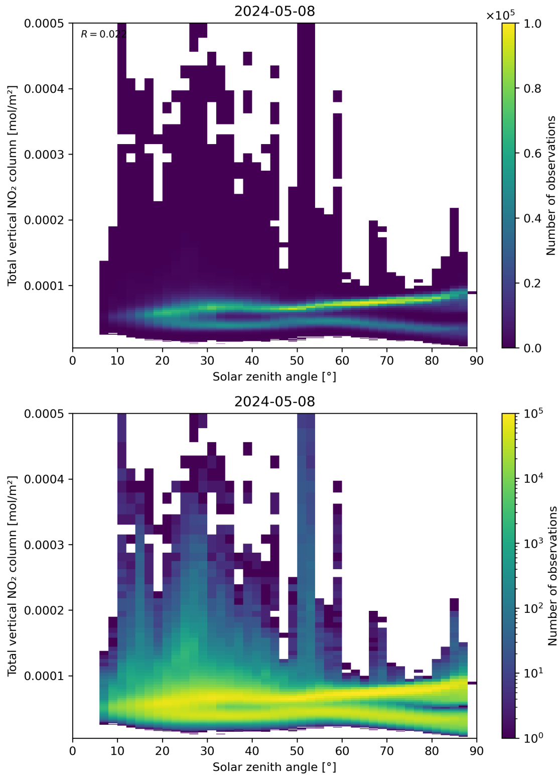
Figure 153: Scatter density plot of “Solar zenith angle” against “Total vertical NO 2 column” for 2024-05-07 to 2024-05-09.
