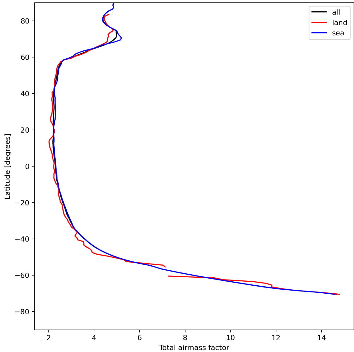
Figure 15: Zonal average of “Total airmass factor” for 2024-05-07 to 2024-05-09.
