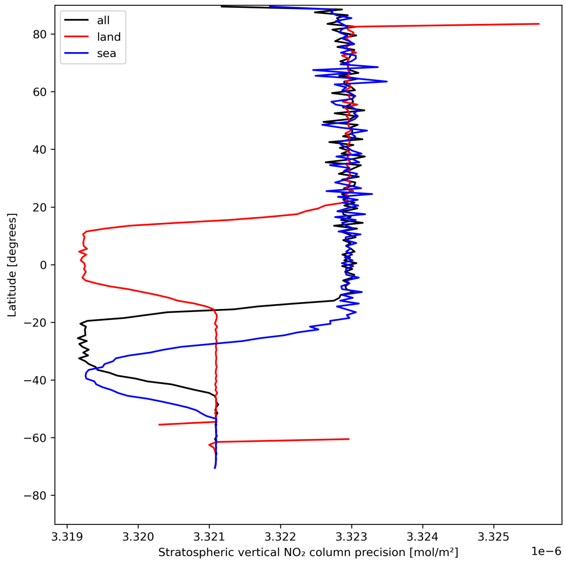
Figure 20: Zonal average of “Stratospheric vertical NO 2 column precision” for 2024-05-07 to 2024-05-09.
