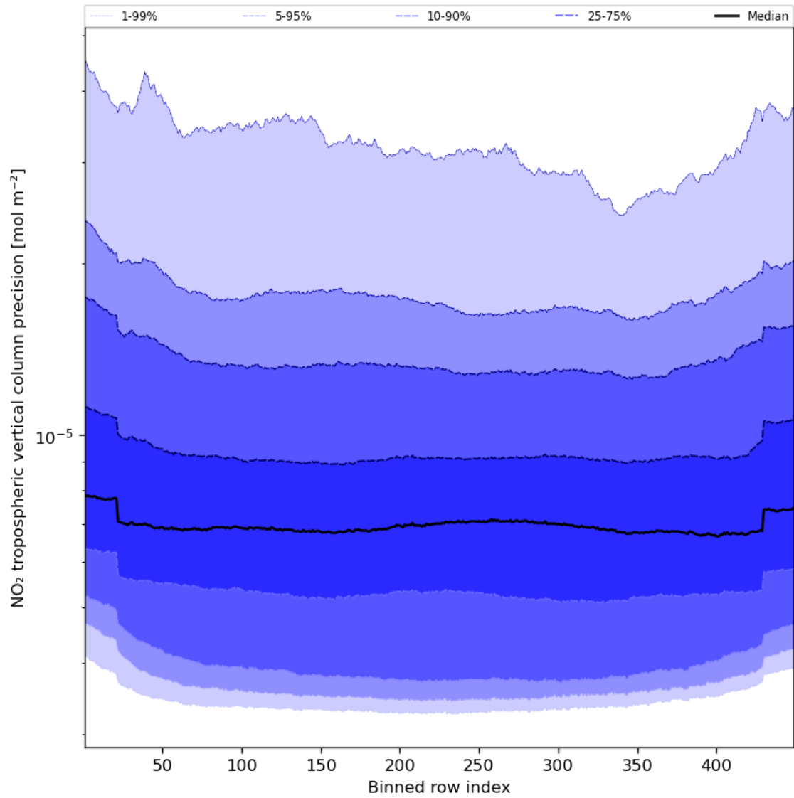
Figure 47: Along track statistics of “NO 2 tropospheric vertical column precision” for 2024-05-07 to 2024-05-09
