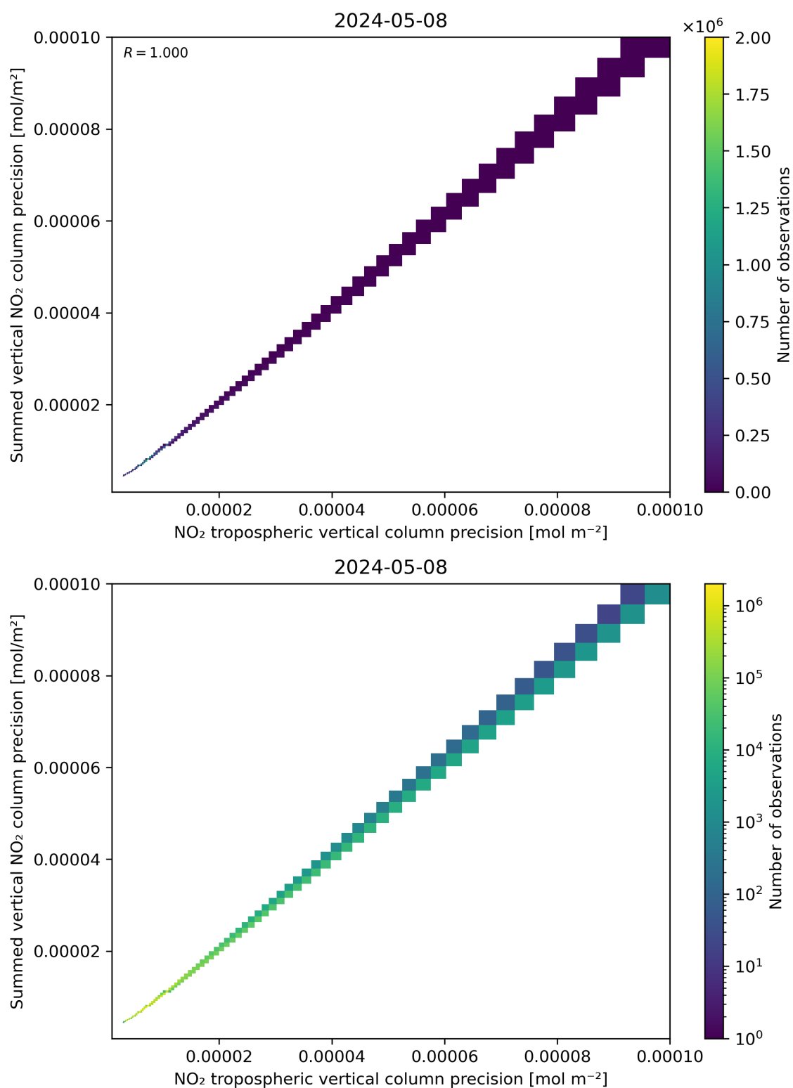
Figure 137: Scatter density plot of “NO 2 tropospheric vertical column precision” against “Summed vertical NO 2 column precision” for 2024-05-07 to 2024-05-09.
