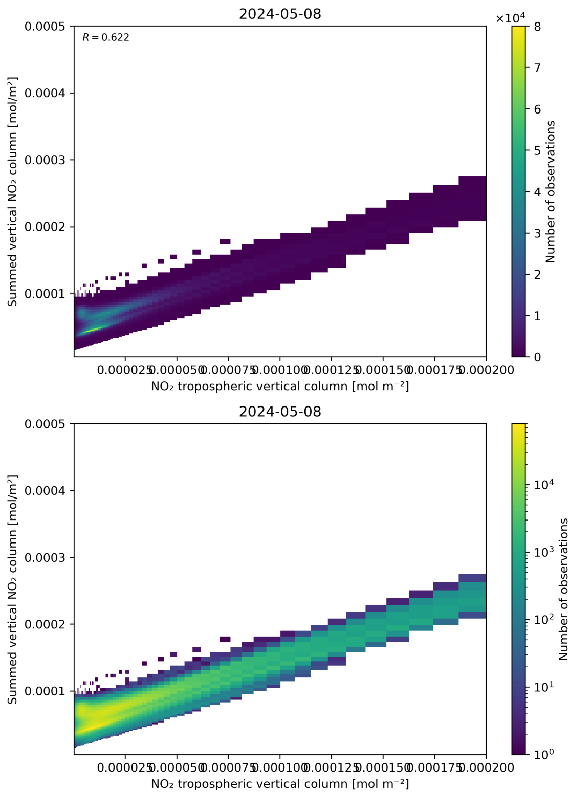
Figure 126: Scatter density plot of “NO 2 tropospheric vertical column” against “Summed vertical NO 2 column” for 2024-05-07 to 2024-05-09.
