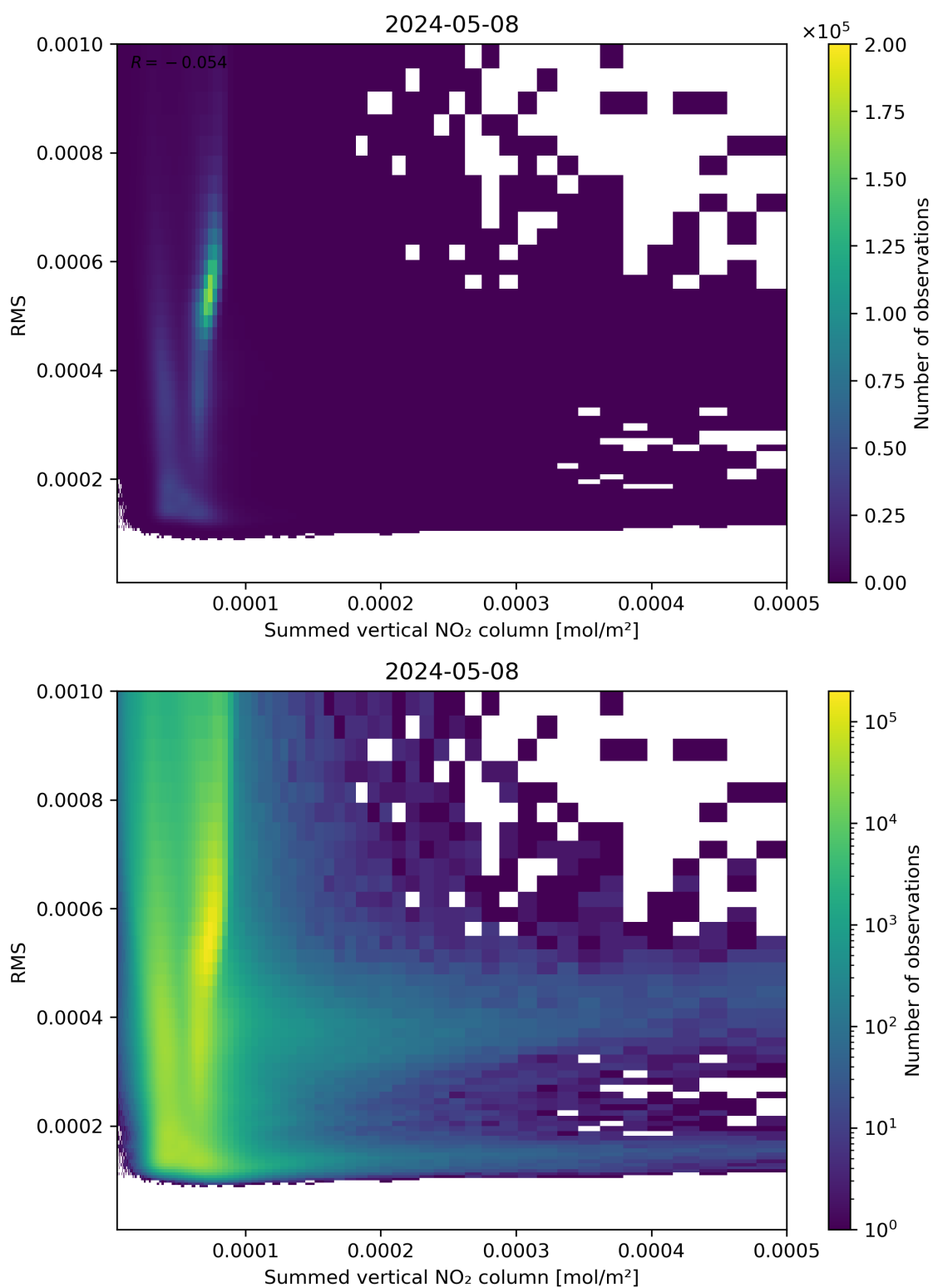
Figure 109: Scatter density plot of “Summed vertical NO 2 column” against “RMS” for 2024-05-07 to 2024-05-09.
