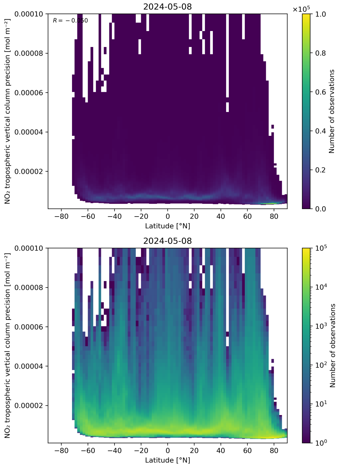
Figure 93: Scatter density plot of “Latitude” against “NO 2 tropospheric vertical column precision” for 2024-05-07 to 2024-05-09.
