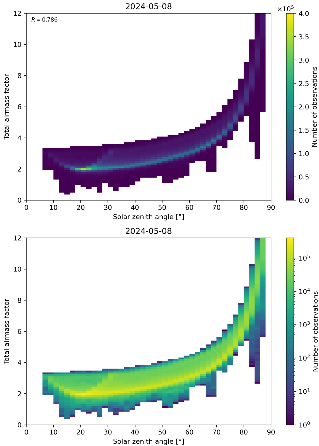
Figure 146: Scatter density plot of “Solar zenith angle” against “Total air mass factor” for 2024-05-07 to 2024-05-09.
