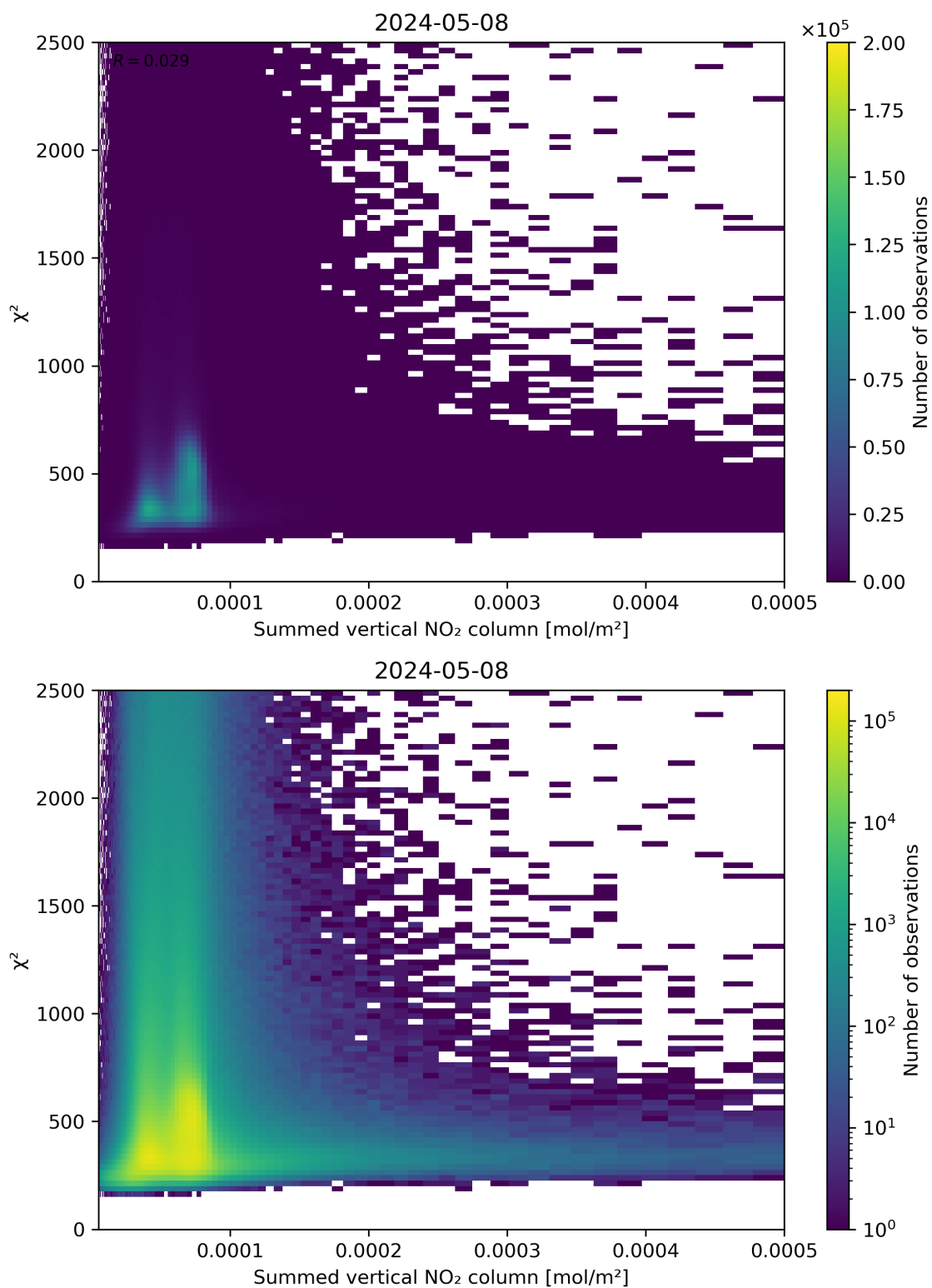
Figure 104: Scatter density plot of “Summed vertical NO 2 column” against “ \chi^2 ” for 2024-05-07 to 2024-05-09.
