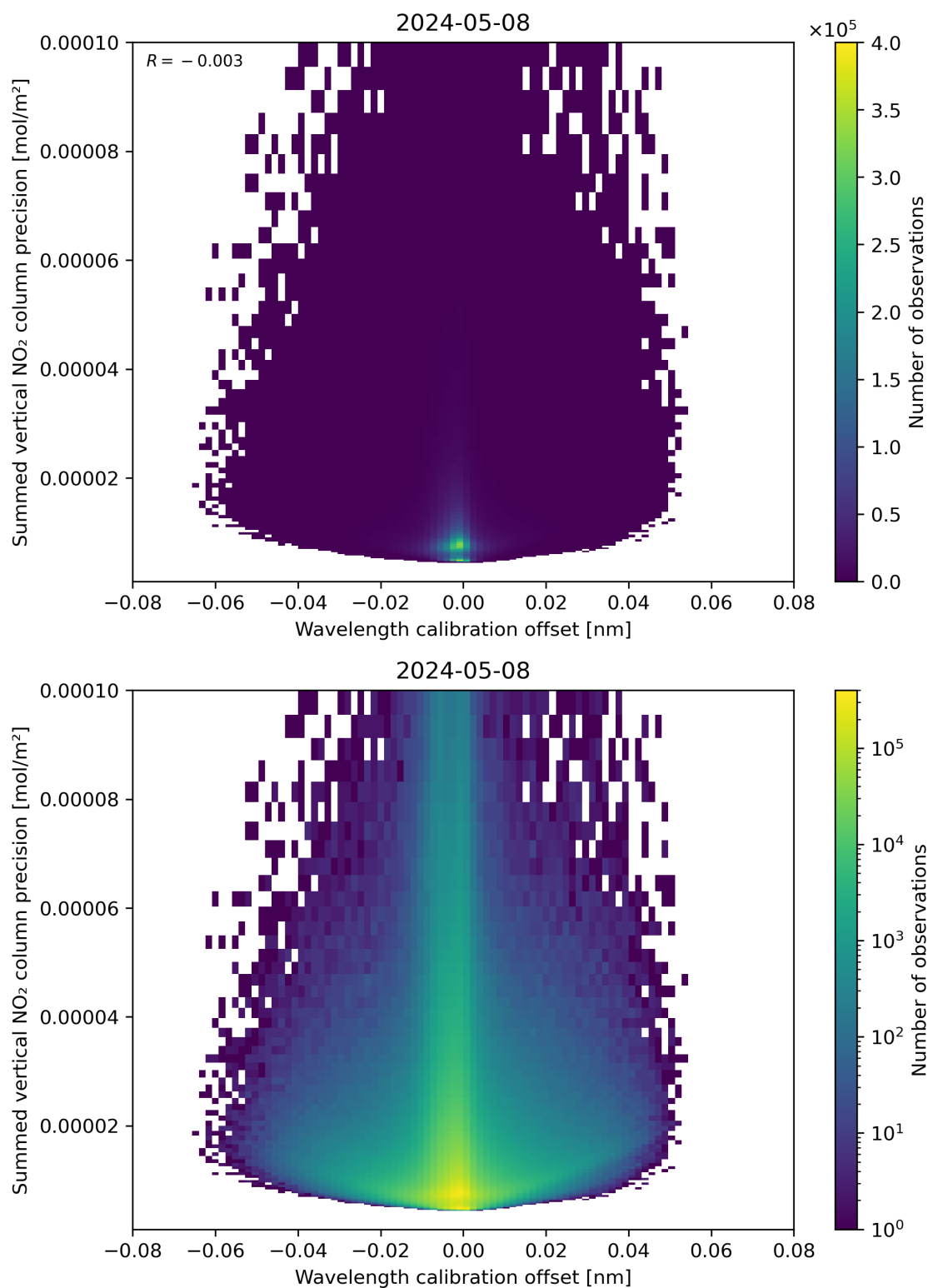
Figure 178: Scatter density plot of “Wavelength calibration offset” against “Summed vertical NO 2 column precision” for 2024-05-07 to 2024-05-09.
