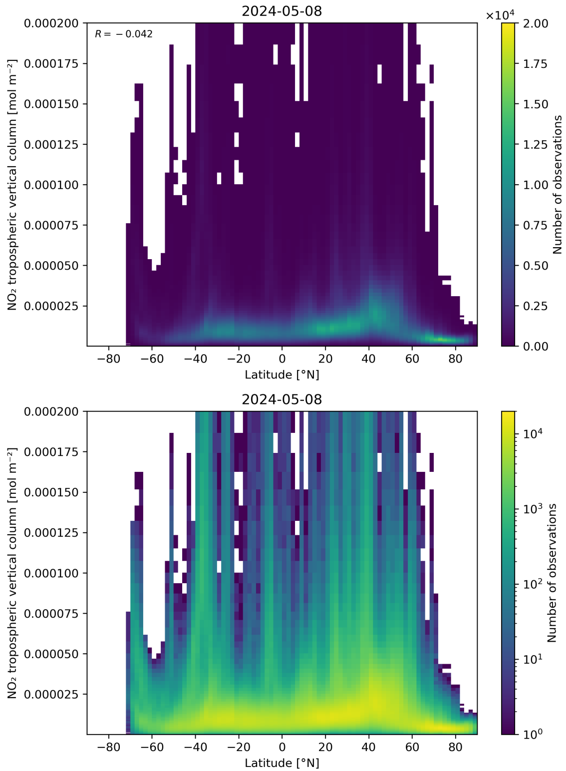
Figure 92: Scatter density plot of “Latitude” against “NO 2 tropospheric vertical column” for 2024-05-07 to 2024-05-09.
