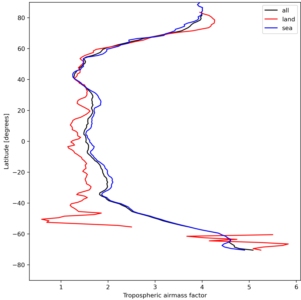
Figure 14: Zonal average of “Tropospheric airmass factor” for 2024-05-07 to 2024-05-09.
