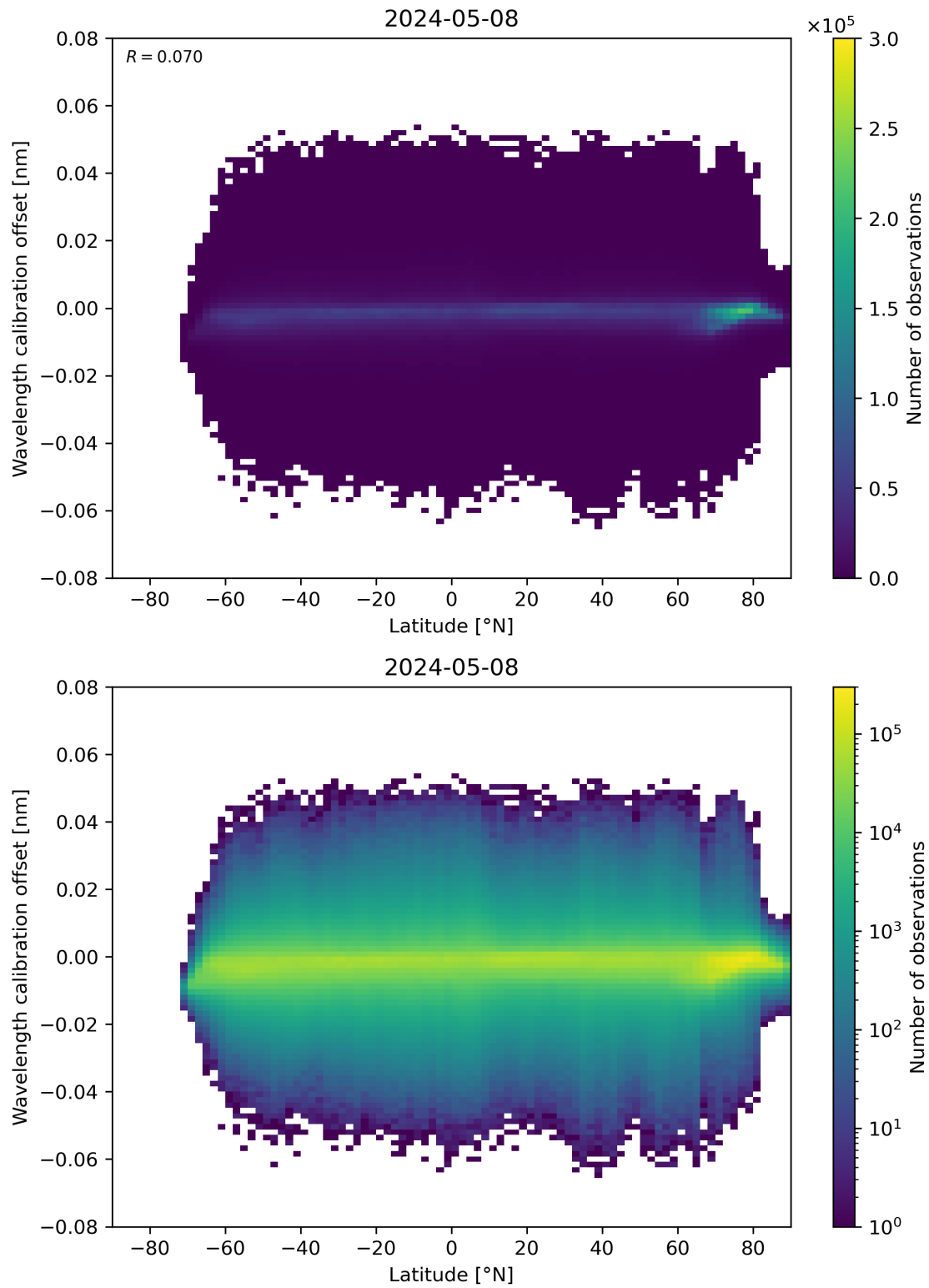
Figure 95: Scatter density plot of “Latitude” against “Wavelength calibration offset” for 2024-05-07 to 2024-05-09.
