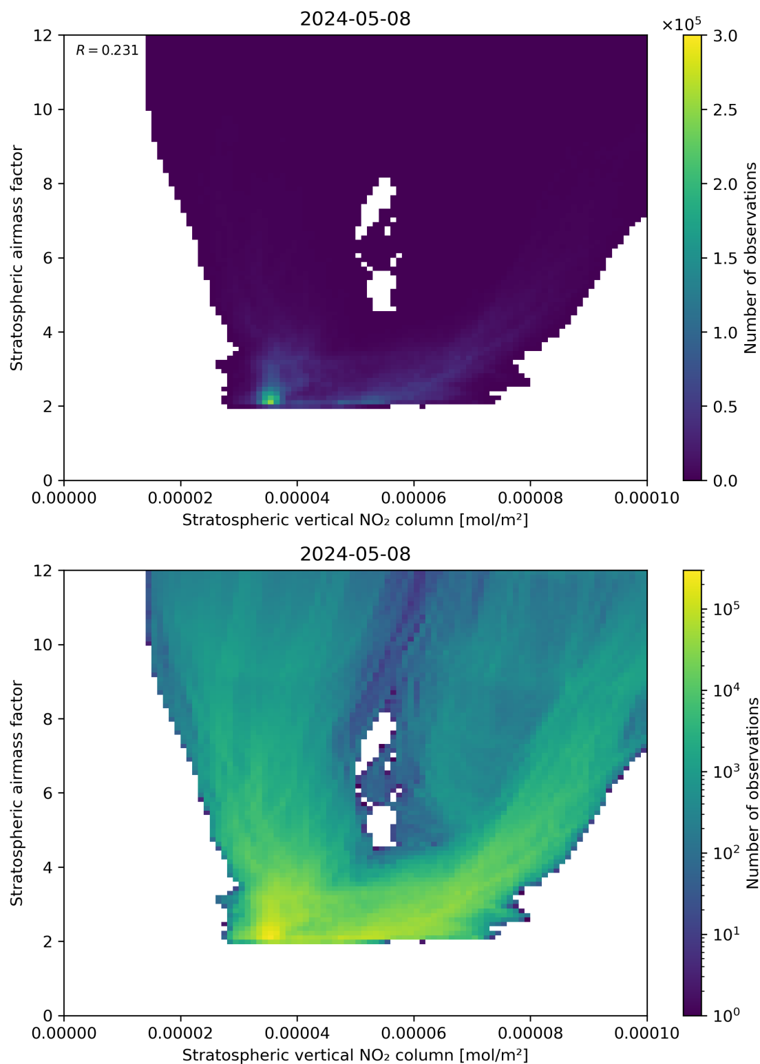
Figure 96: Scatter density plot of “Stratospheric vertical NO 2 column” against “Stratospheric airmass factor” for 2024-05-07 to 2024-05-09.
