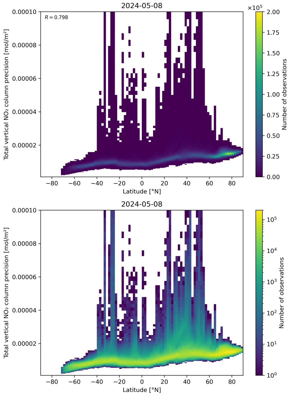
Figure 91: Scatter density plot of “Latitude” against “Total vertical NO 2 column precision” for 2024-05-07 to 2024-05-09.
