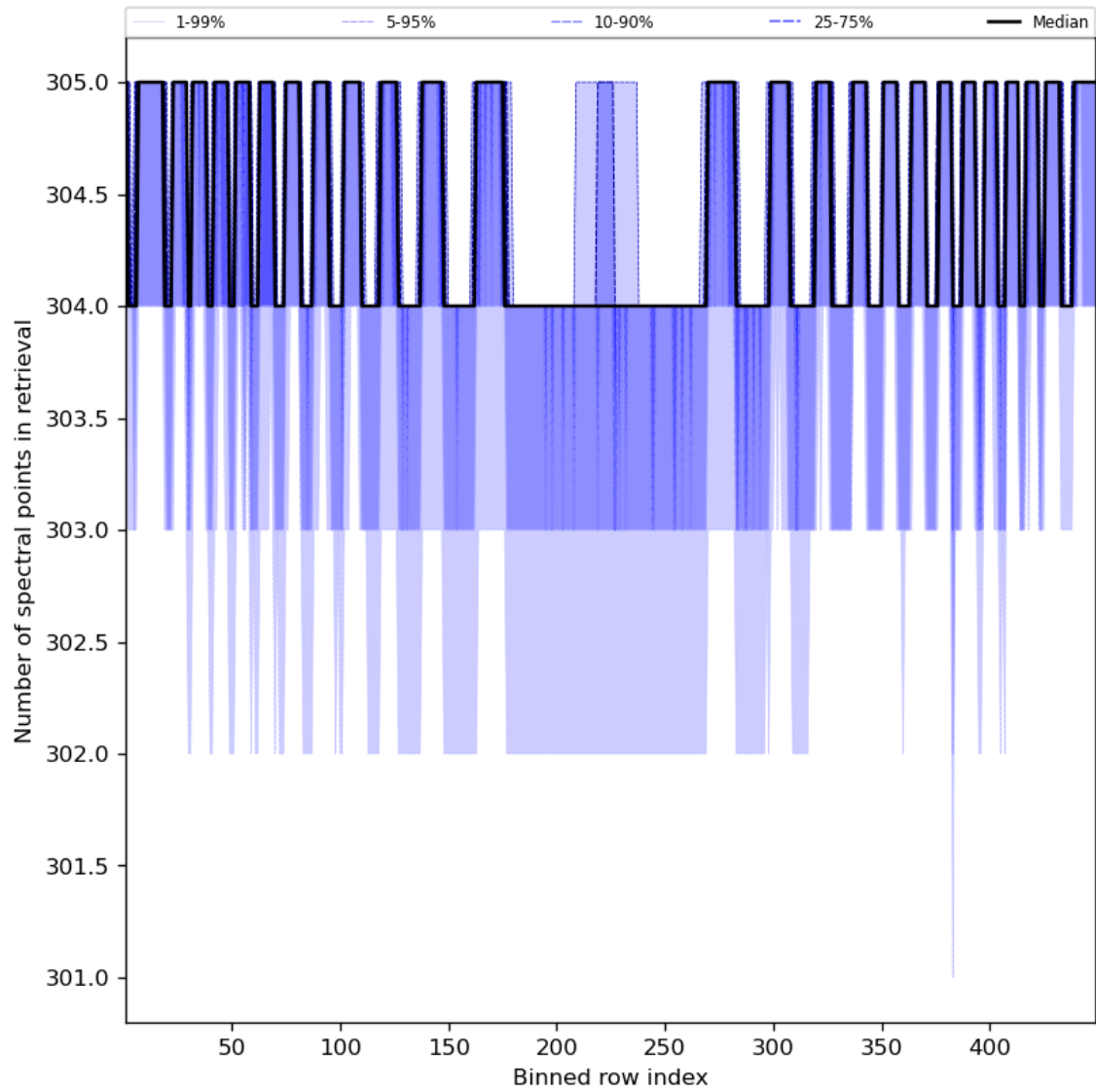
Figure 50: Along track statistics of “Number of spectral points in retrieval” for 2024-05-07 to 2024-05-09
