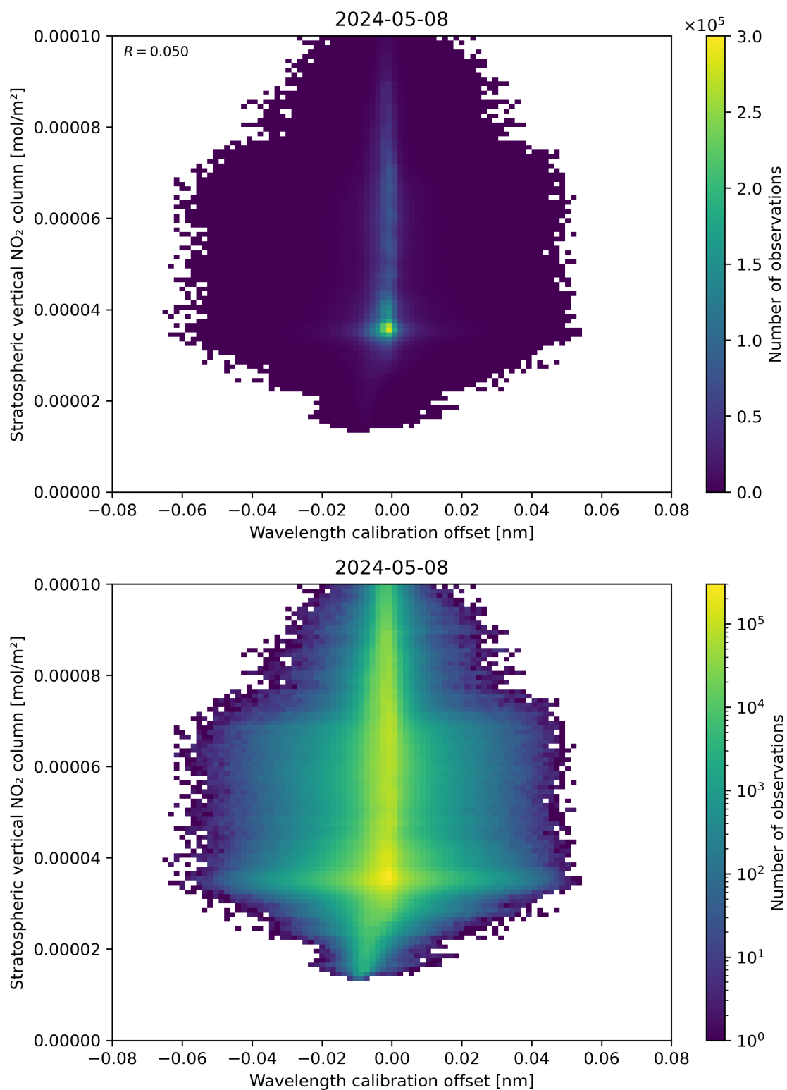
Figure 176: Scatter density plot of “Wavelength calibration offset” against “Stratospheric vertical NO 2 column” for 2024-05-07 to 2024-05-09.
