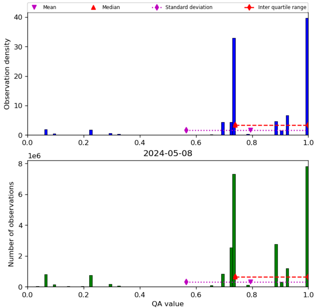
Figure 28: Histogram of “QA value” for 2024-05-07 to 2024-05-09
