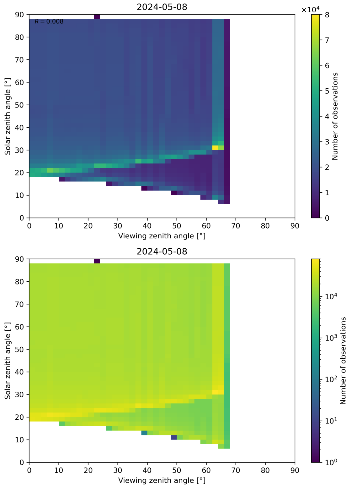
Figure 172: Scatter density plot of “Viewing zenith angle” against “Solar zenith angle” for 2024-05-07 to 2024-05-09.
