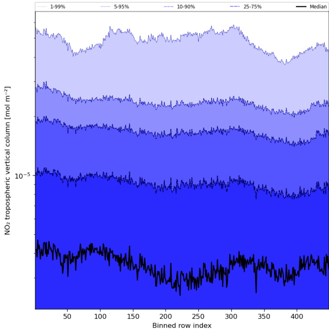
Figure 46: Along track statistics of “NO 2 tropospheric vertical column” for 2024-05-07 to 2024-05-09
