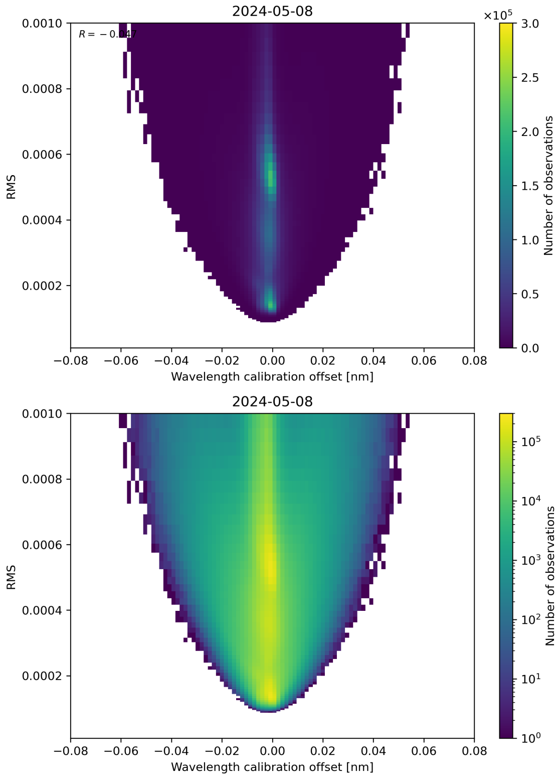
Figure 181: Scatter density plot of “Wavelength calibration offset” against “RMS” for 2024-05-07 to 2024-05-09.
