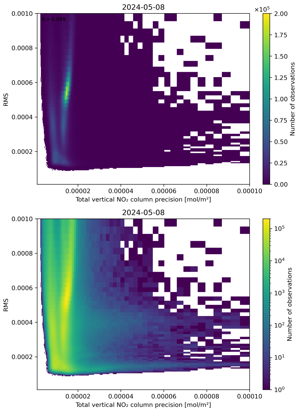
Figure 119: Scatter density plot of “Total vertical NO 2 column precision” against “RMS” for 2024-05-07 to 2024-05-09.
