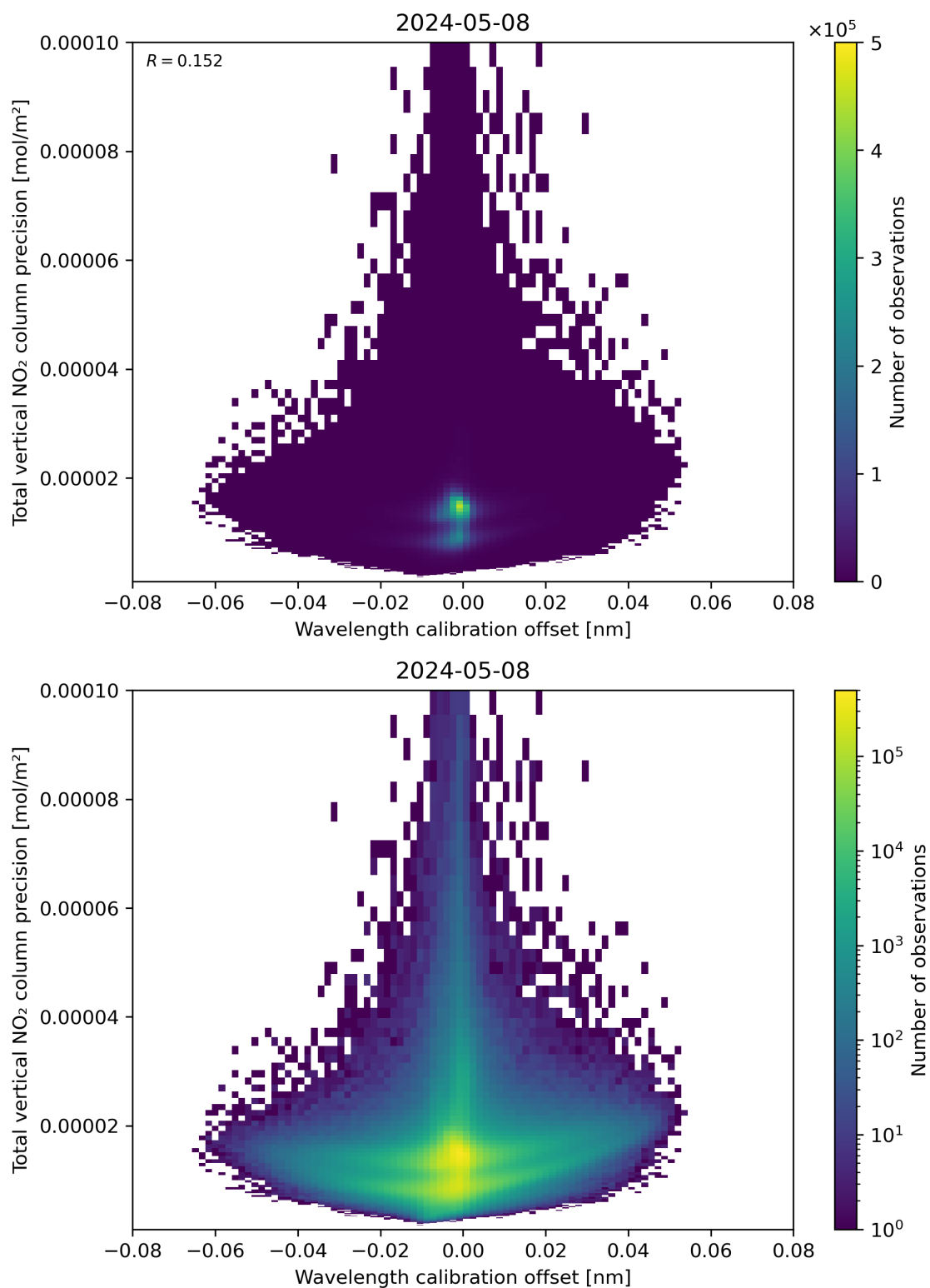
Figure 180: Scatter density plot of “Wavelength calibration offset” against “Total vertical NO 2 column precision” for 2024-05-07 to 2024-05-09.
