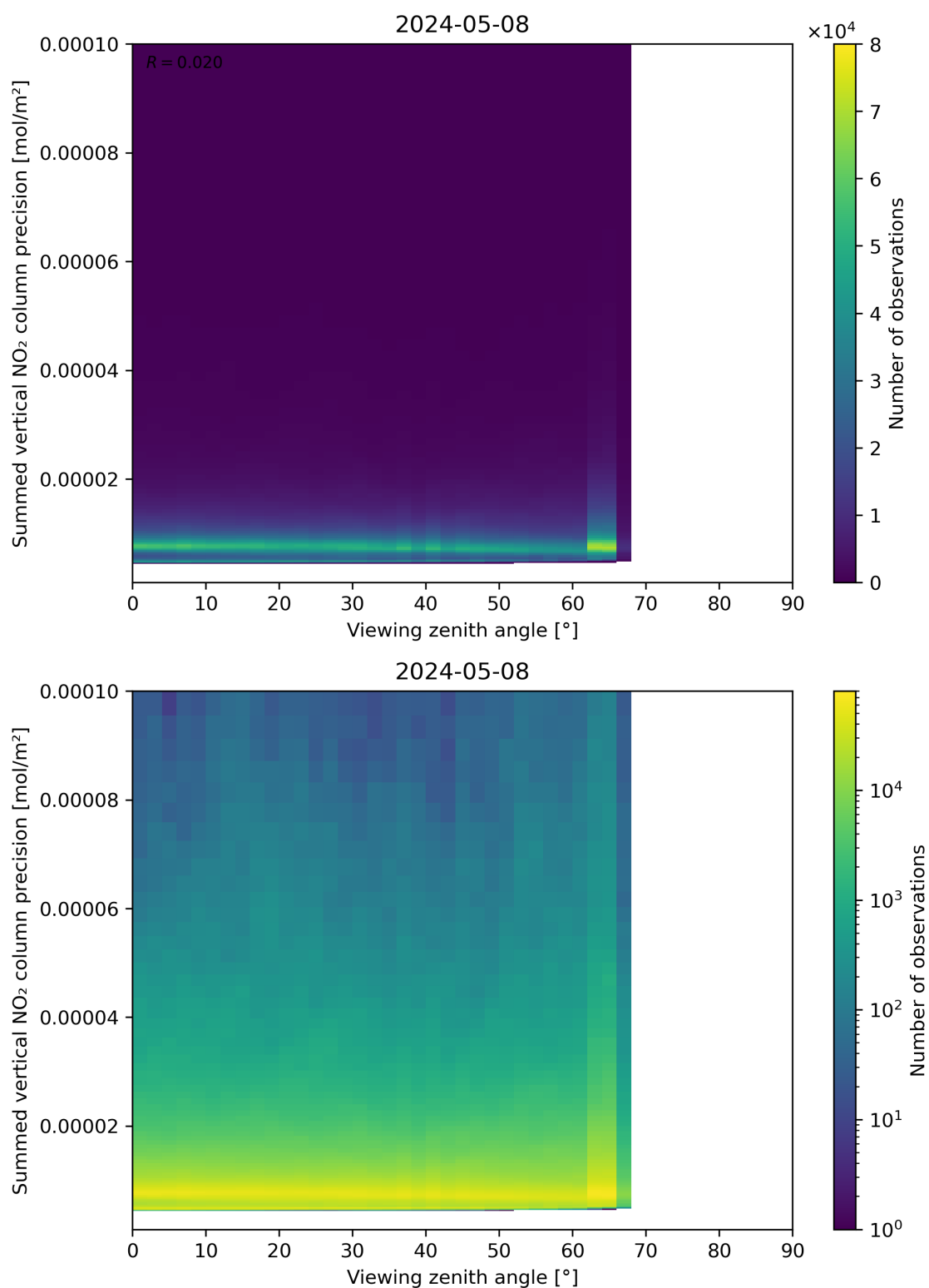
Figure 166: Scatter density plot of “Viewing zenith angle” against “Summed vertical NO 2 column precision” for 2024-05-07 to 2024-05-09.
