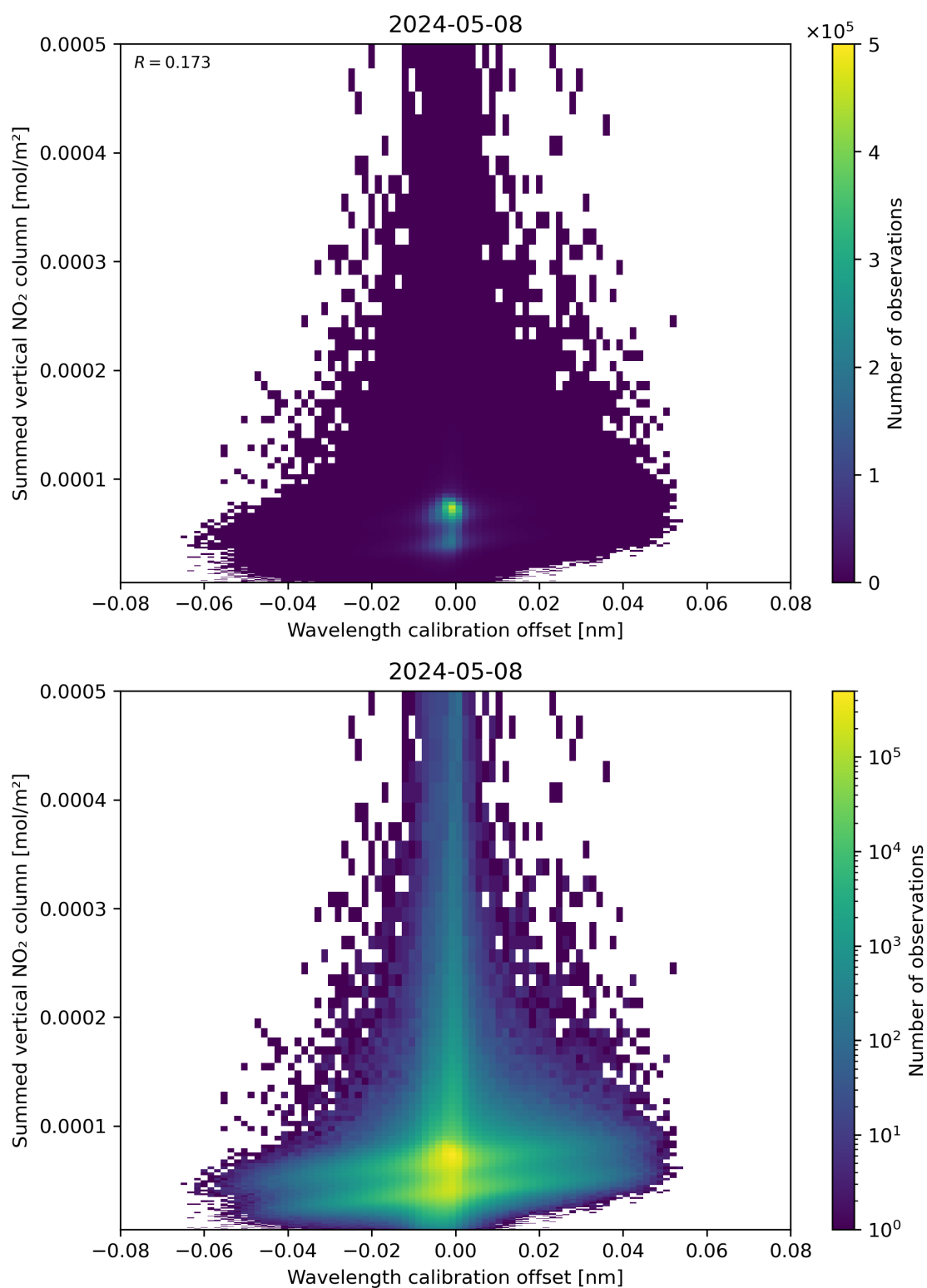
Figure 177: Scatter density plot of “Wavelength calibration offset” against “Summed vertical NO 2 column” for 2024-05-07 to 2024-05-09.
