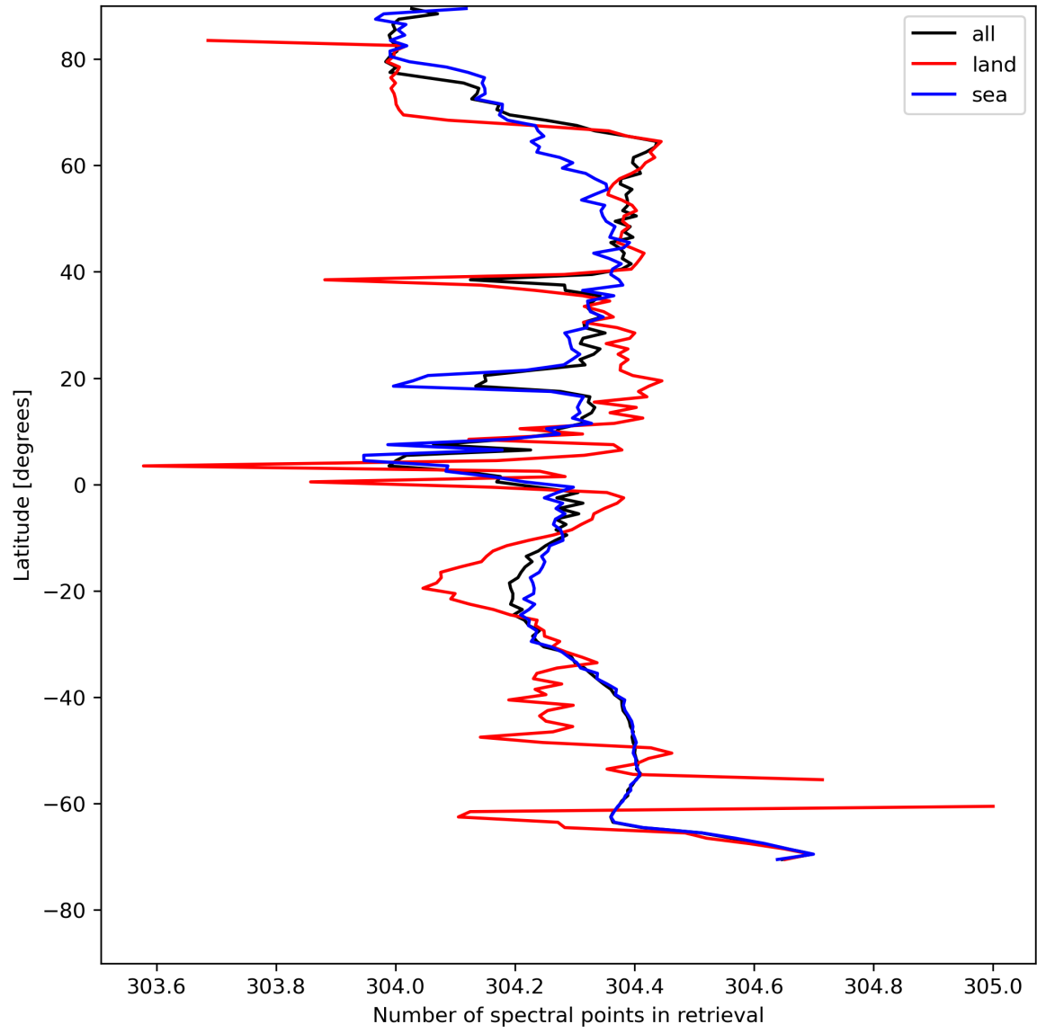
Figure 16: Zonal average of “Number of spectral points in retrieval” for 2024-05-07 to 2024-05-09.
