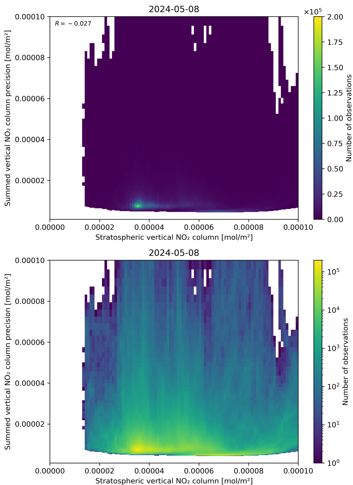
Figure 99: Scatter density plot of “Stratospheric vertical NO 2 column” against “Summed vertical NO 2 column precision” for 2024-05-07 to 2024-05-09.
