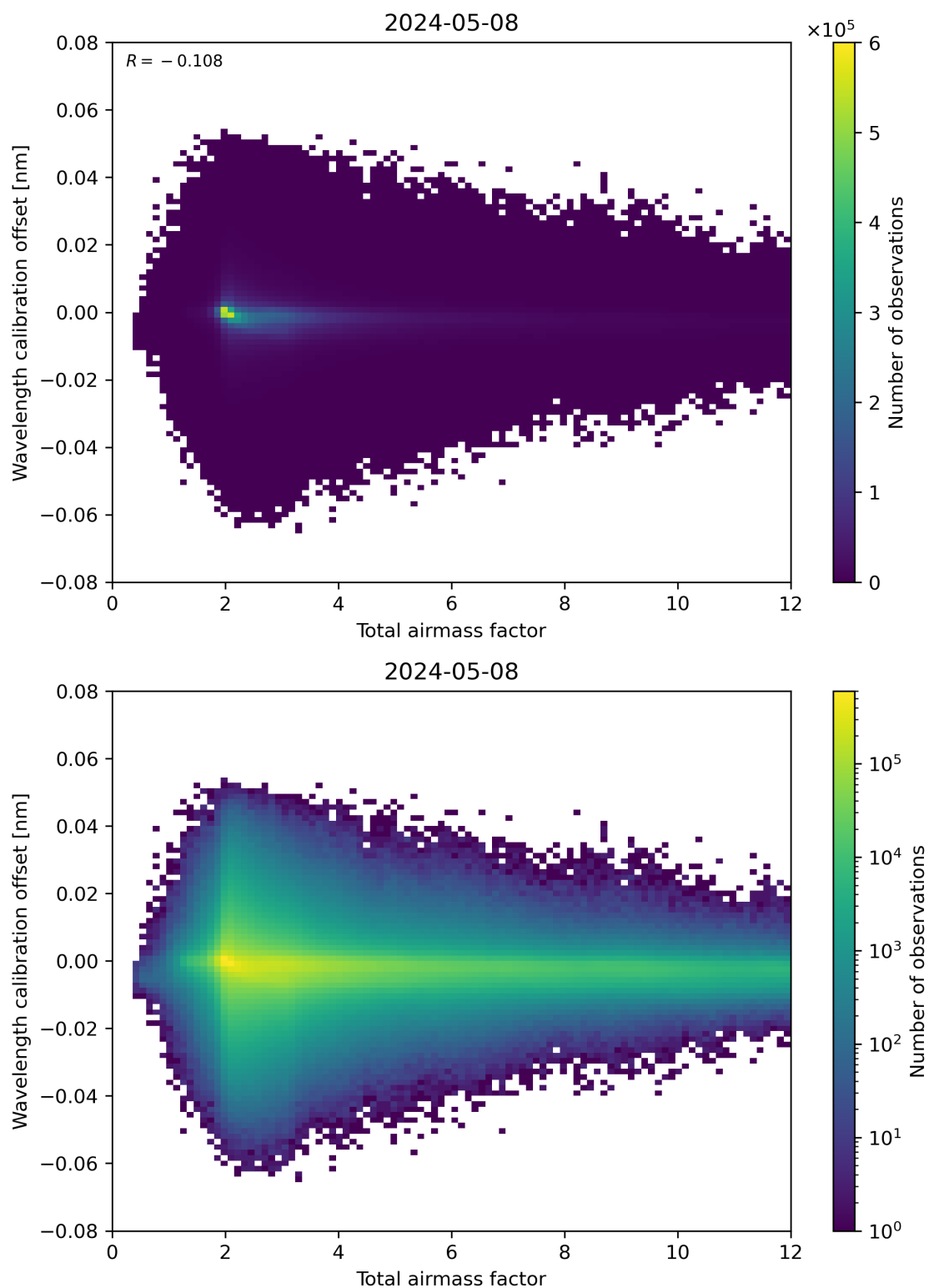
Figure 70: Scatter density plot of “Total airmass factor” against “Wavelength calibration offset” for 2024-05-07 to 2024-05-09.
