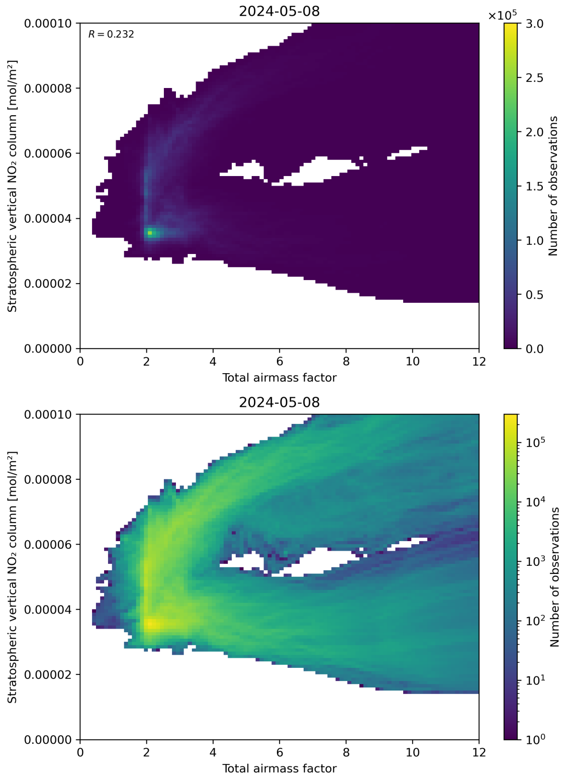
Figure 64: Scatter density plot of “Total airmass factor” against “Stratospheric vertical NO 2 column” for 2024-05-07 to 2024-05-09.
