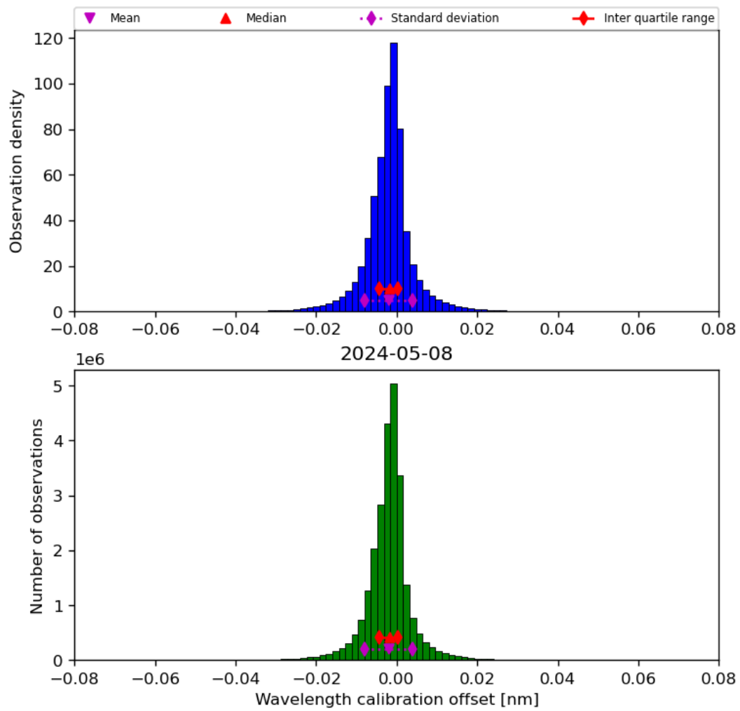
Figure 35: Histogram of “Wavelength calibration offset” for 2024-05-07 to 2024-05-09
