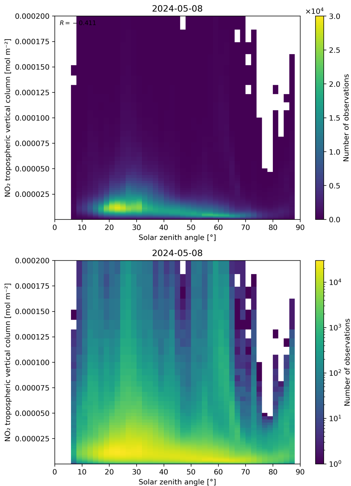
Figure 155: Scatter density plot of “Solar zenith angle” against “NO 2 tropospheric vertical column” for 2024-05-07 to 2024-05-09.
