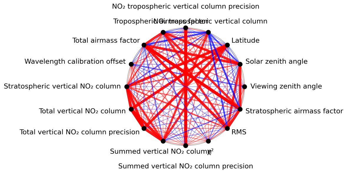
Figure 1: Map of correlation graph for 2024-05-07 to 2024-05-09.
