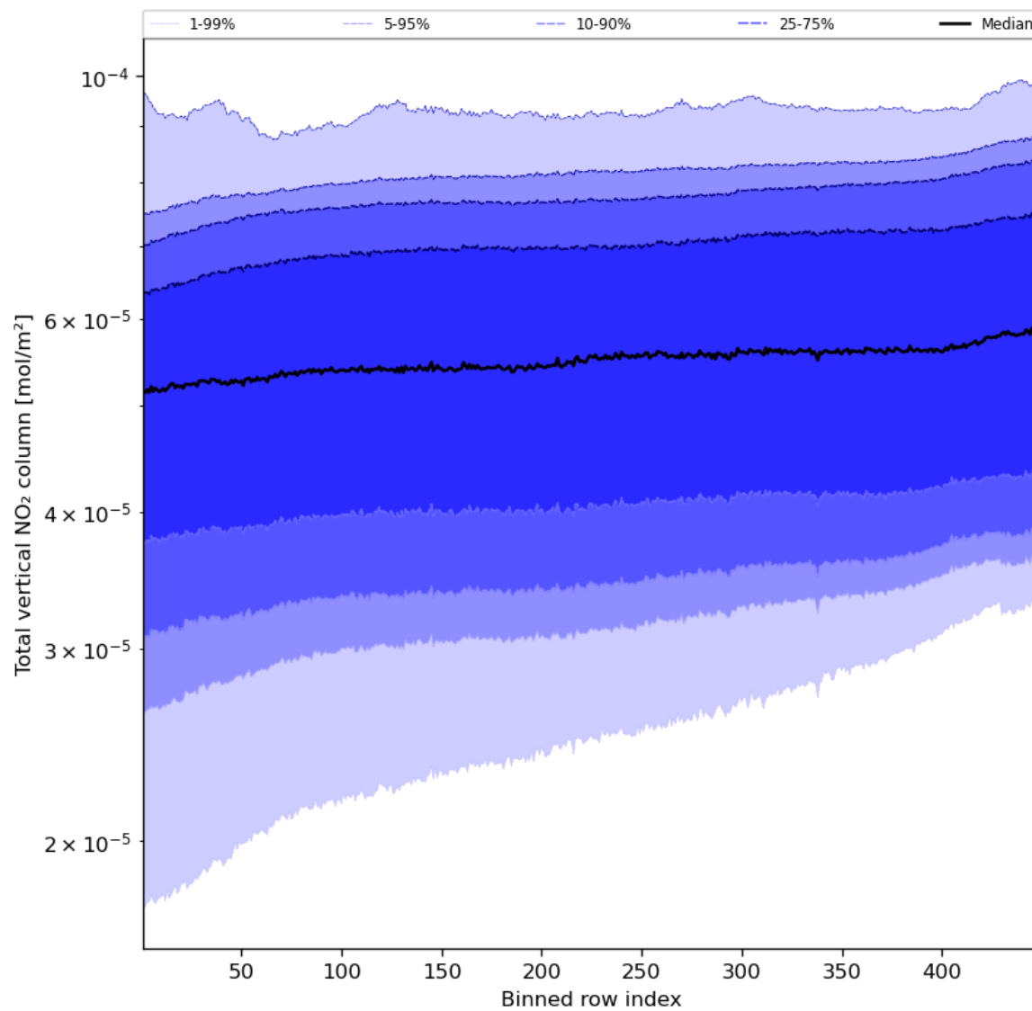
Figure 55: Along track statistics of “Total vertical NO 2 column” for 2024-05-07 to 2024-05-09
