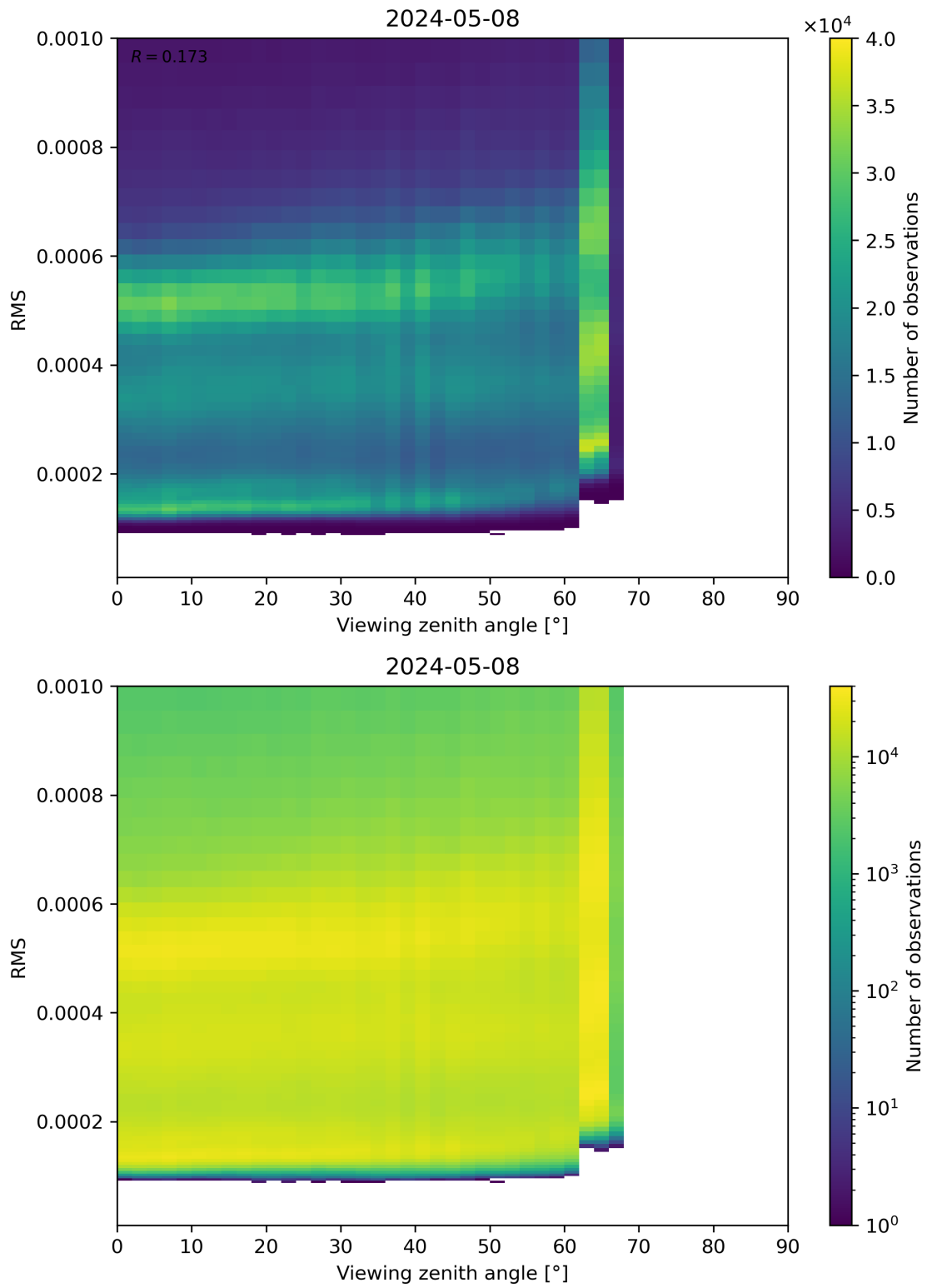
Figure 171: Scatter density plot of “Viewing zenith angle” against “RMS” for 2024-05-07 to 2024-05-09.
