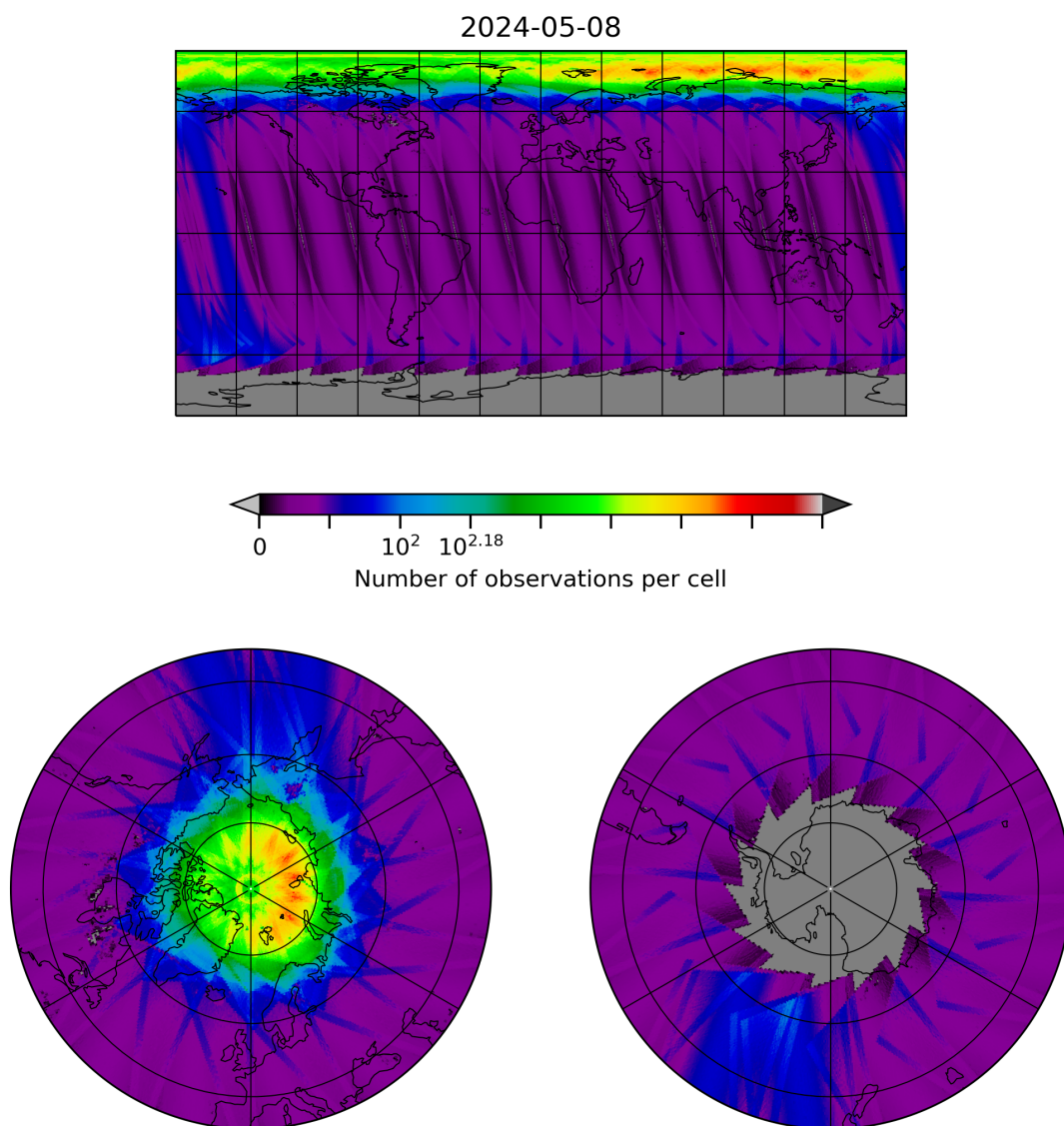
Figure 10: Map of the number of observations for 2024-05-07 to 2024-05-09
