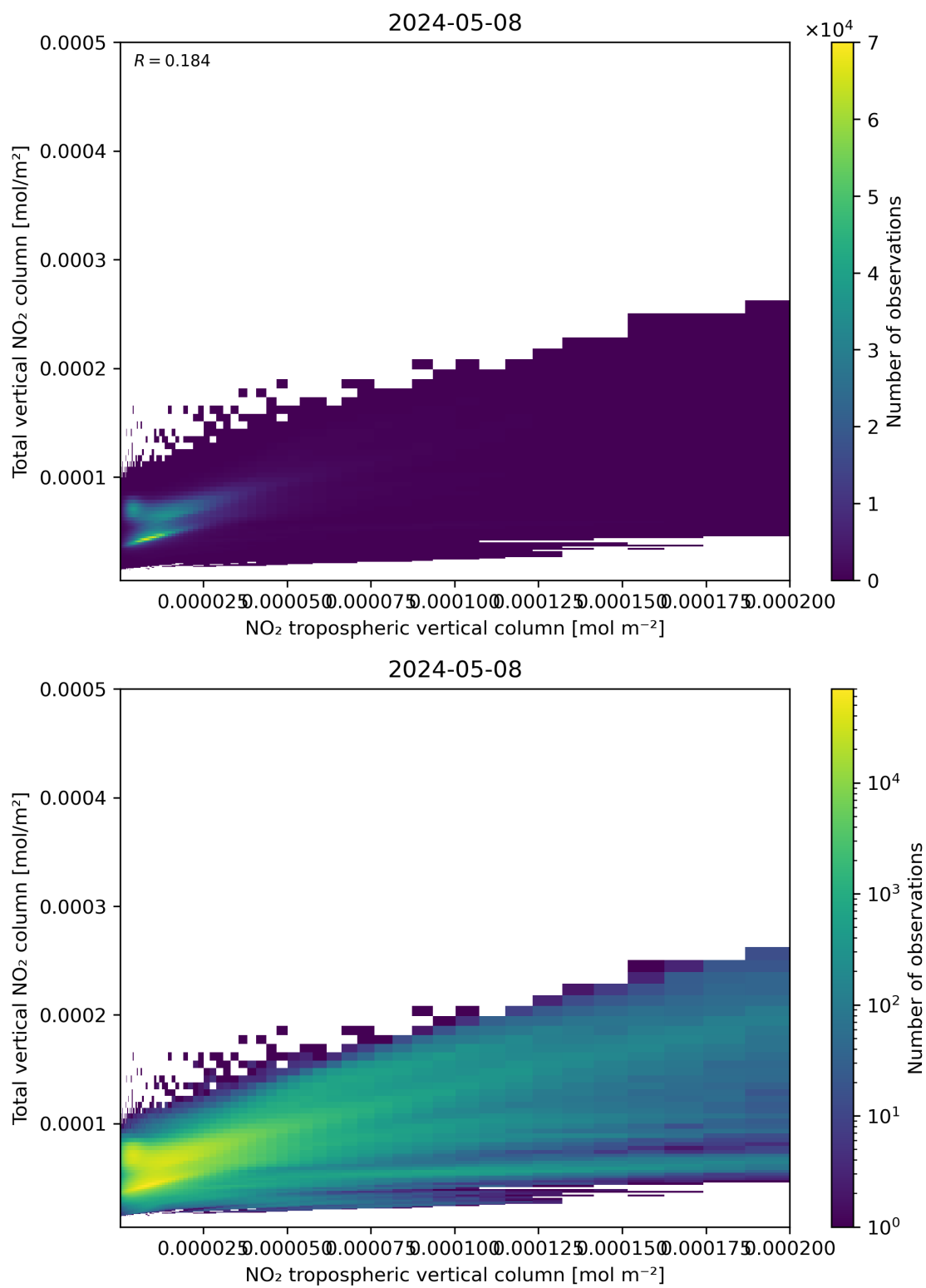
Figure 128: Scatter density plot of “NO 2 tropospheric vertical column” against “Total vertical NO 2 column” for 2024-05-07 to 2024-05-09.
