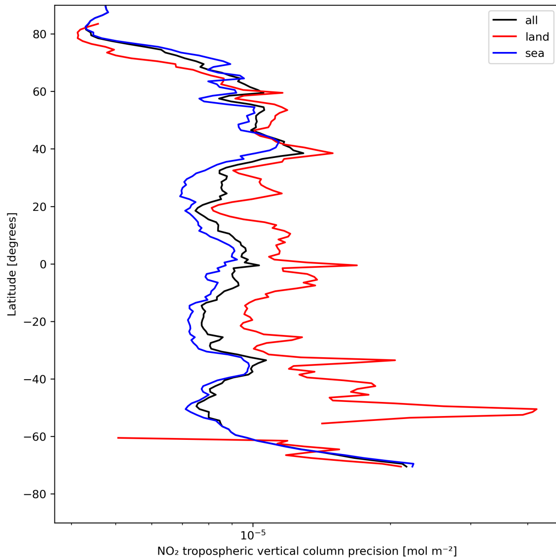
Figure 13: Zonal average of “NO 2 tropospheric vertical column precision” for 2024-05-07 to 2024-05-09.
