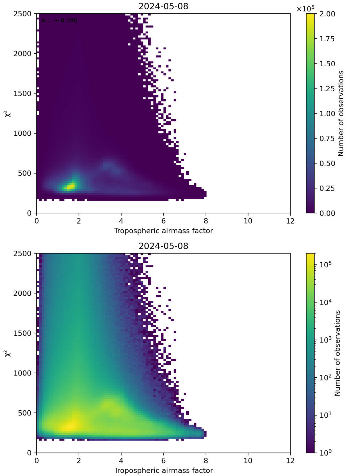
Figure 73: Scatter density plot of “Tropospheric airmass factor” against “ \chi^2 ” for 2024-05-07 to 2024-05-09.
