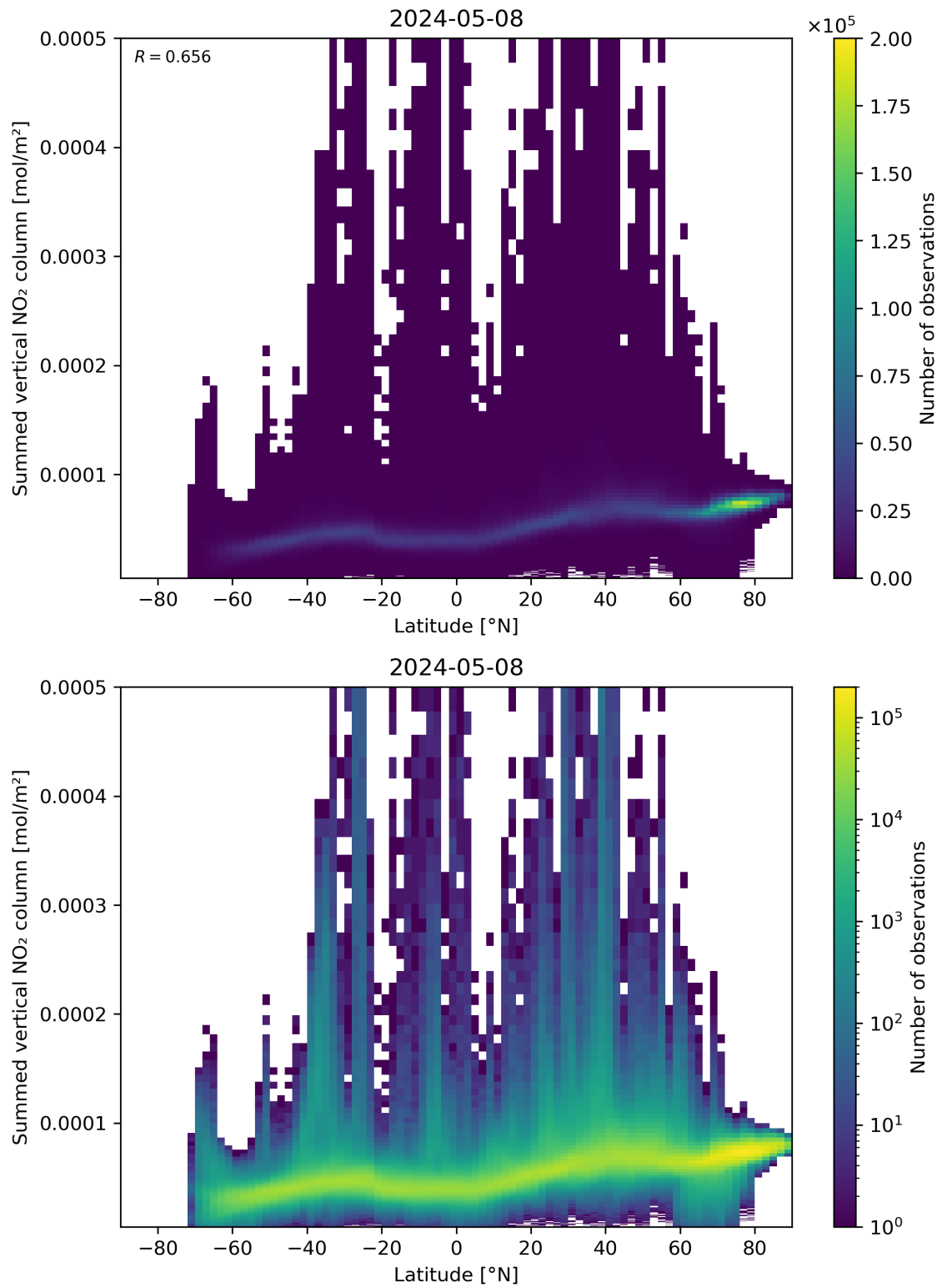
Figure 88: Scatter density plot of “Latitude” against “Summed vertical NO 2 column” for 2024-05-07 to 2024-05-09.
