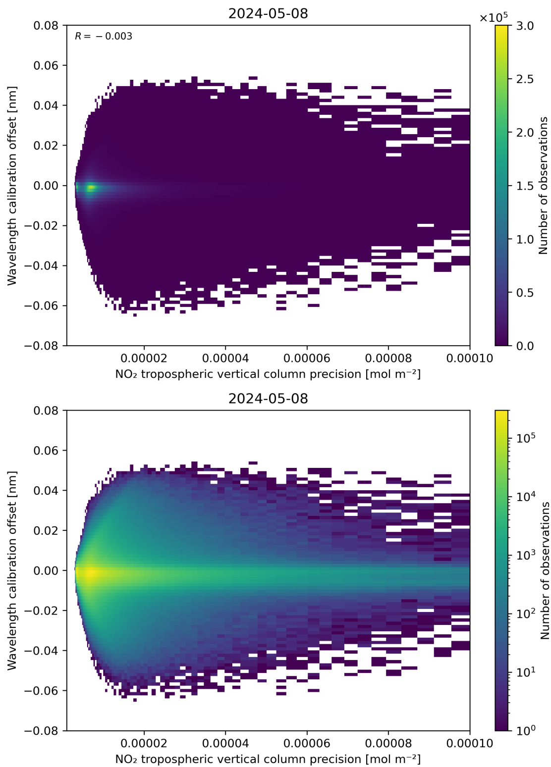
Figure 141: Scatter density plot of “NO 2 tropospheric vertical column precision” against “Wavelength calibration offset” for 2024-05-07 to 2024-05-09.
