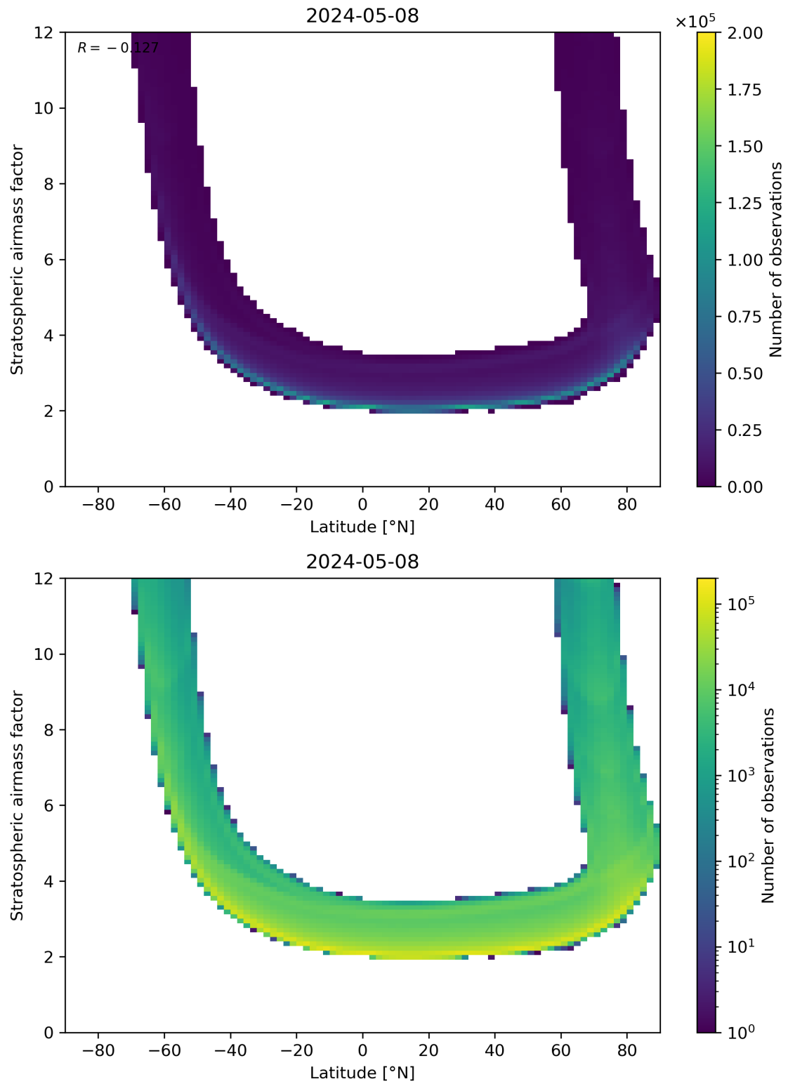
Figure 83: Scatter density plot of “Latitude” against “Stratospheric air mass factor” for 2024-05-07 to 2024-05-09.
