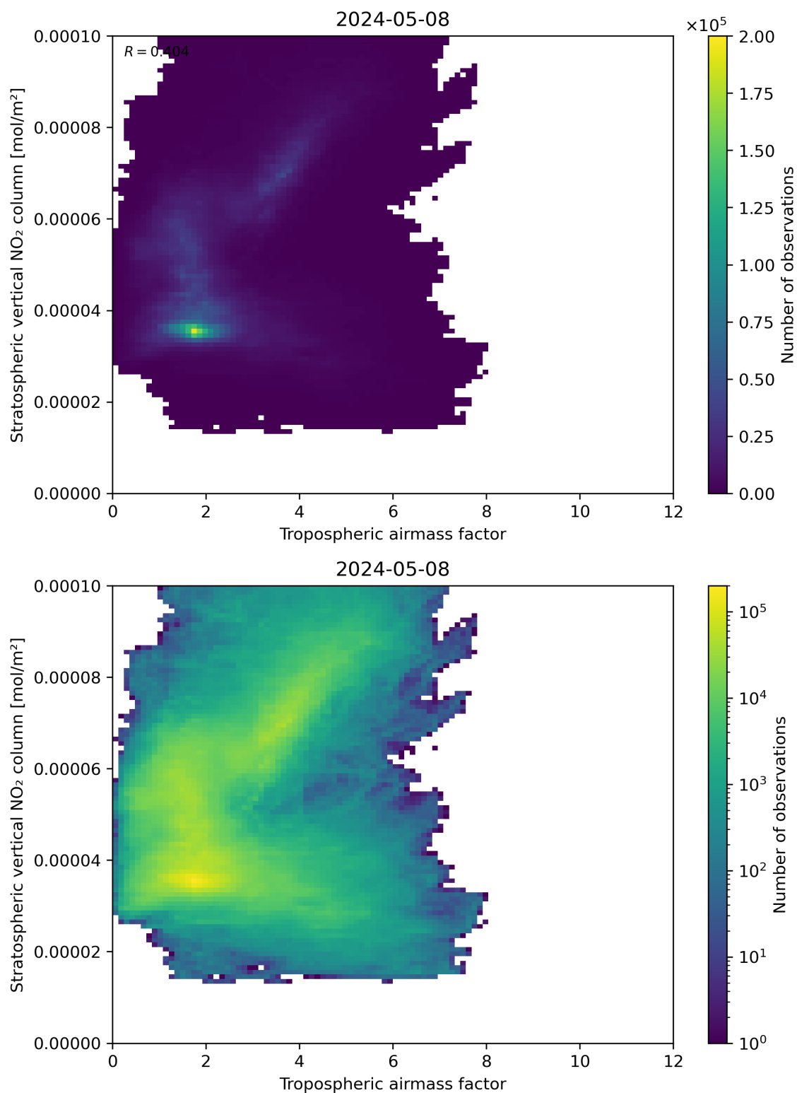
Figure 74: Scatter density plot of “Tropospheric airmass factor” against “Stratospheric vertical NO 2 column” for 2024-05-07 to 2024-05-09.
