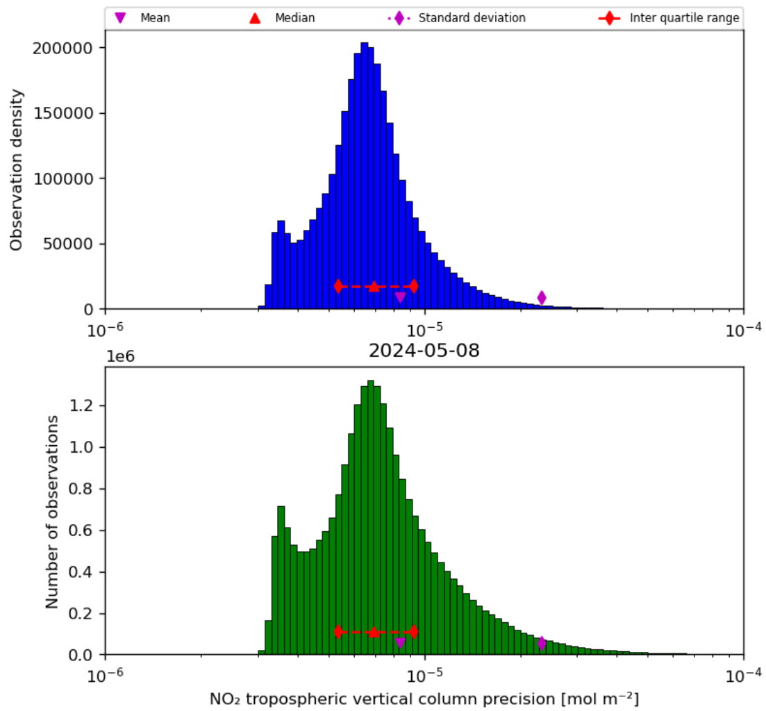
Figure 30: Histogram of “NO 2 tropospheric vertical column precision” for 2024-05-07 to 2024-05-09
