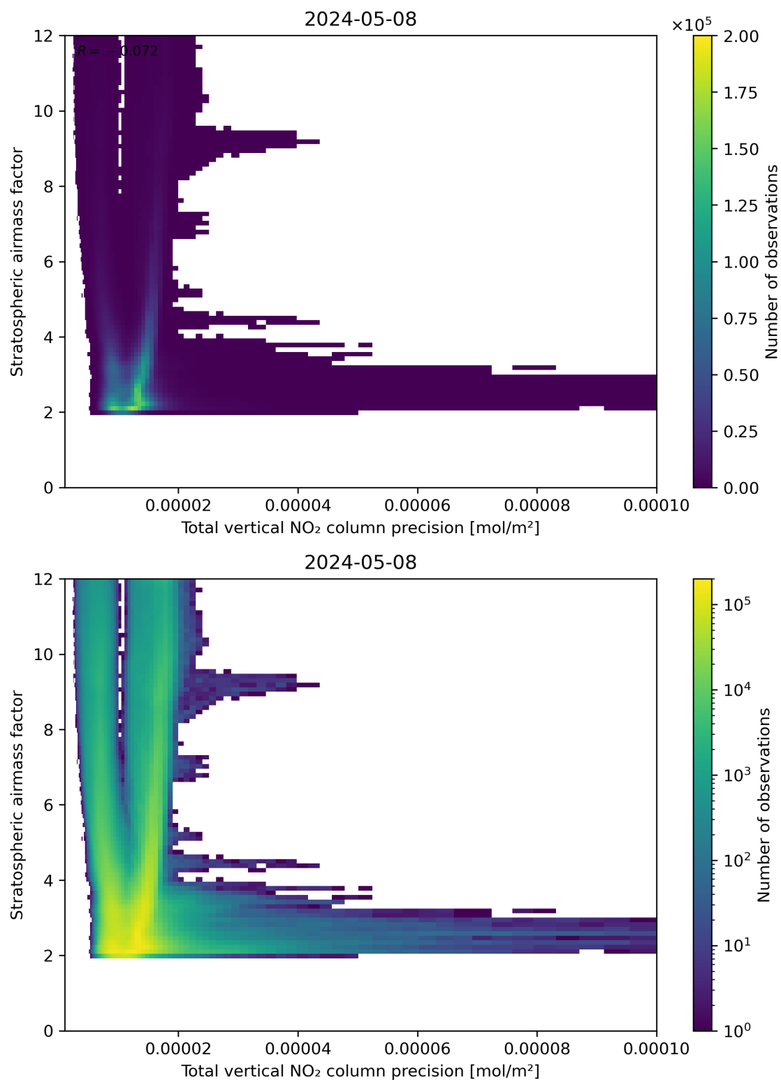
Figure 115: Scatter density plot of “Total vertical NO 2 column precision” against “Stratospheric air mass factor” for 2024-05-07 to 2024-05-09.
