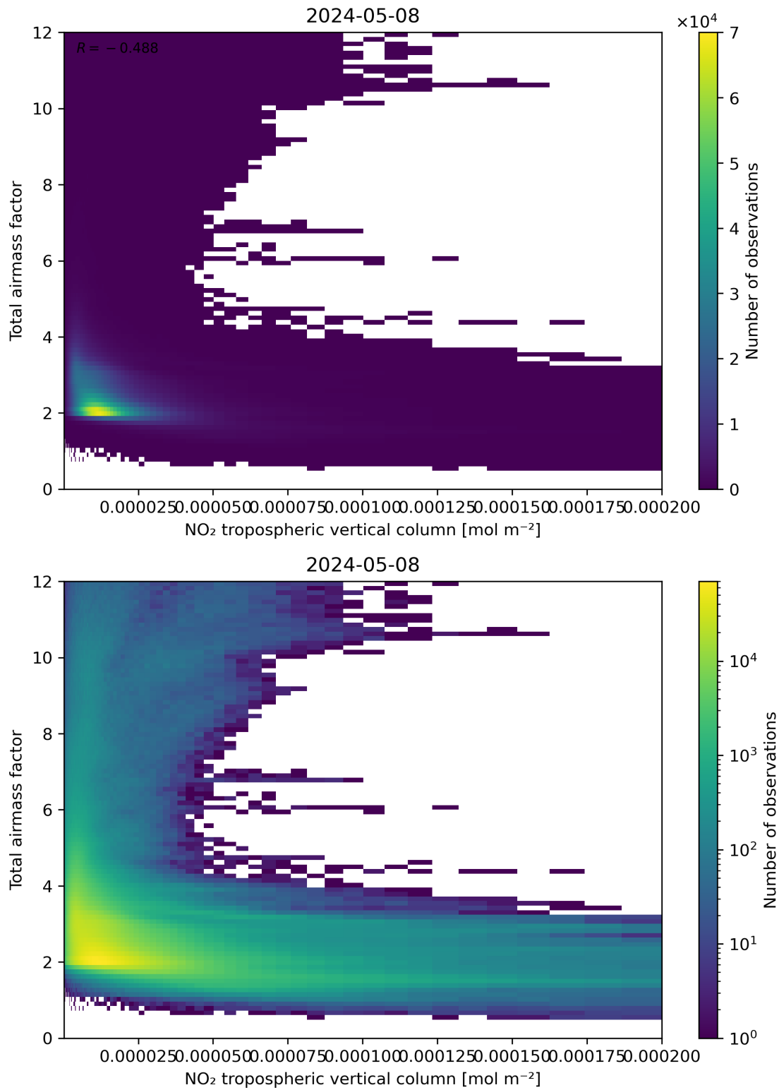
Figure 122: Scatter density plot of “NO 2 tropospheric vertical column” against “Total airmass factor” for 2024-05-07 to 2024-05-09.
