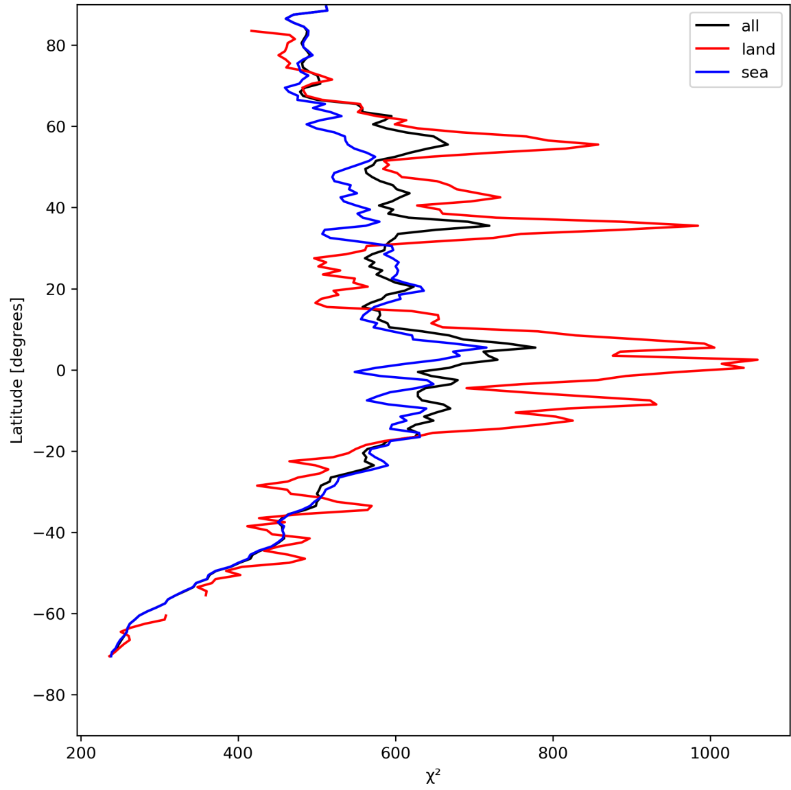
Figure 25: Zonal average of “ \chi^2 ” for 2024-05-07 to 2024-05-09.
