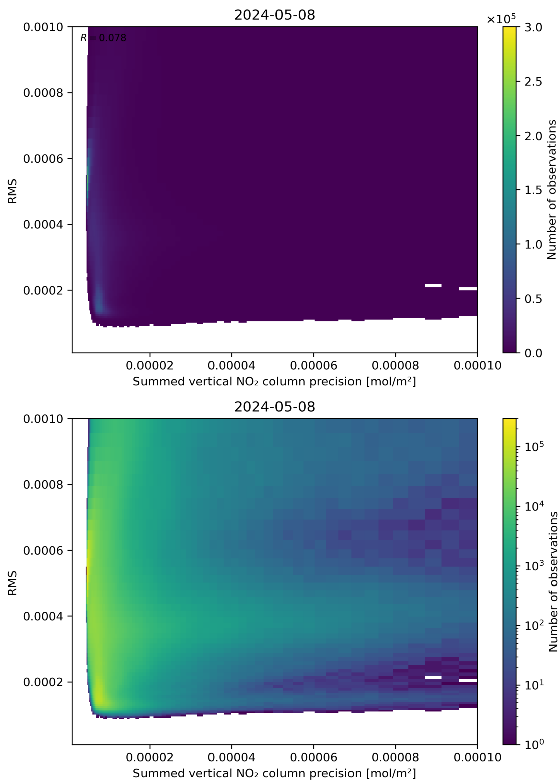
Figure 108: Scatter density plot of “Summed vertical NO 2 column precision” against “RMS” for 2024-05-07 to 2024-05-09.
