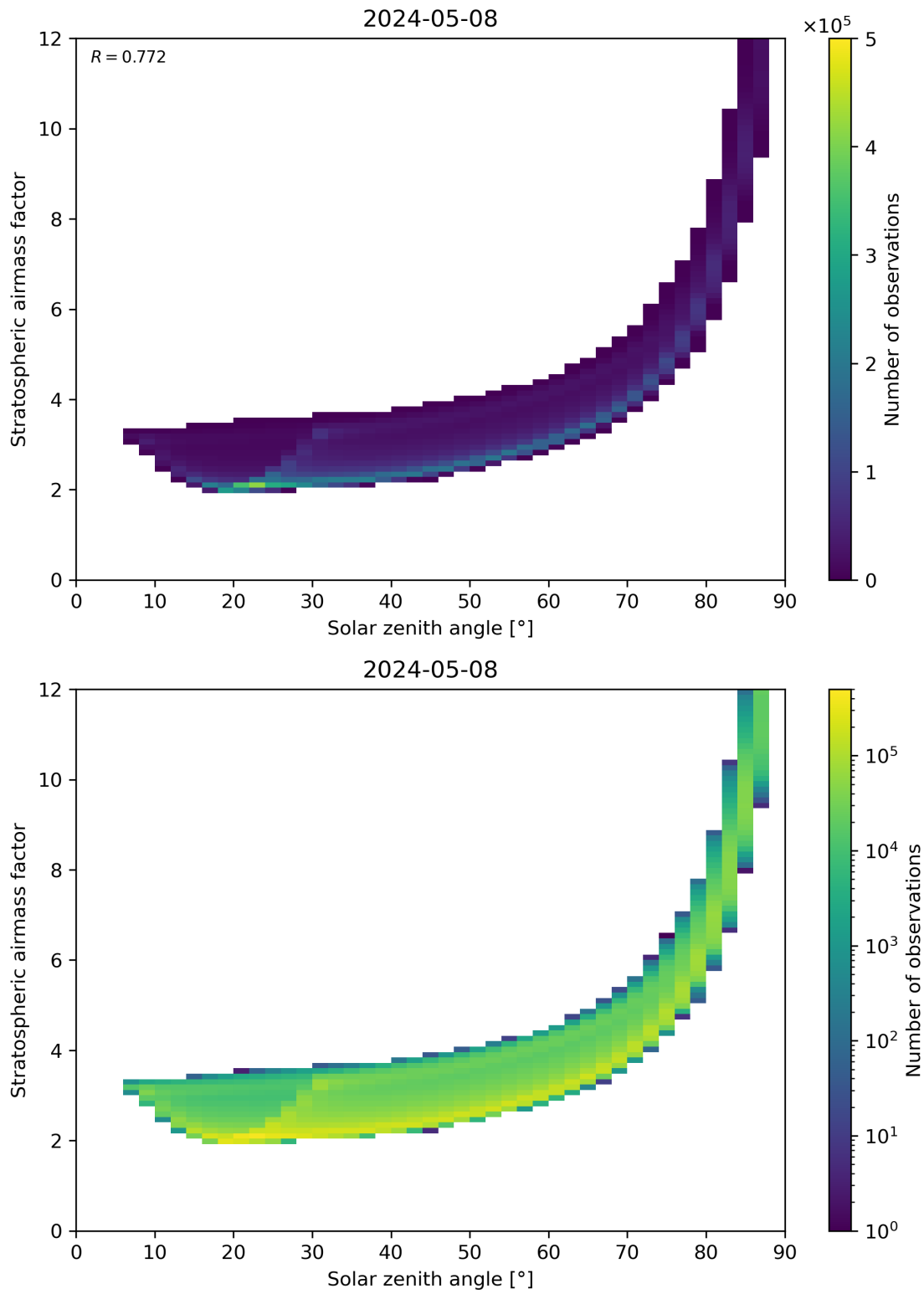
Figure 145: Scatter density plot of “Solar zenith angle” against “Stratospheric airmass factor” for 2024-05-07 to 2024-05-09.
