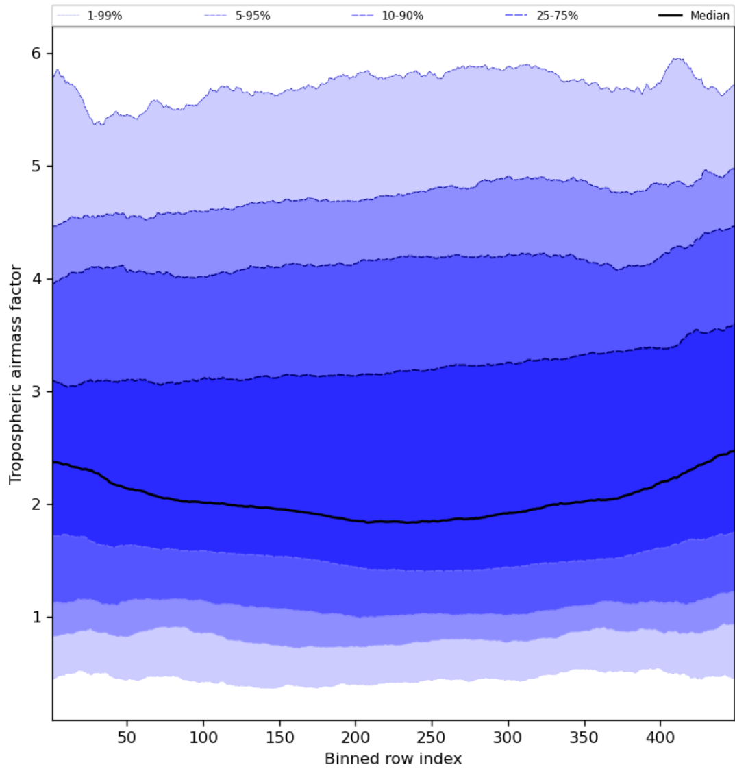
Figure 48: Along track statistics of “Tropospheric airmass factor” for 2024-05-07 to 2024-05-09
