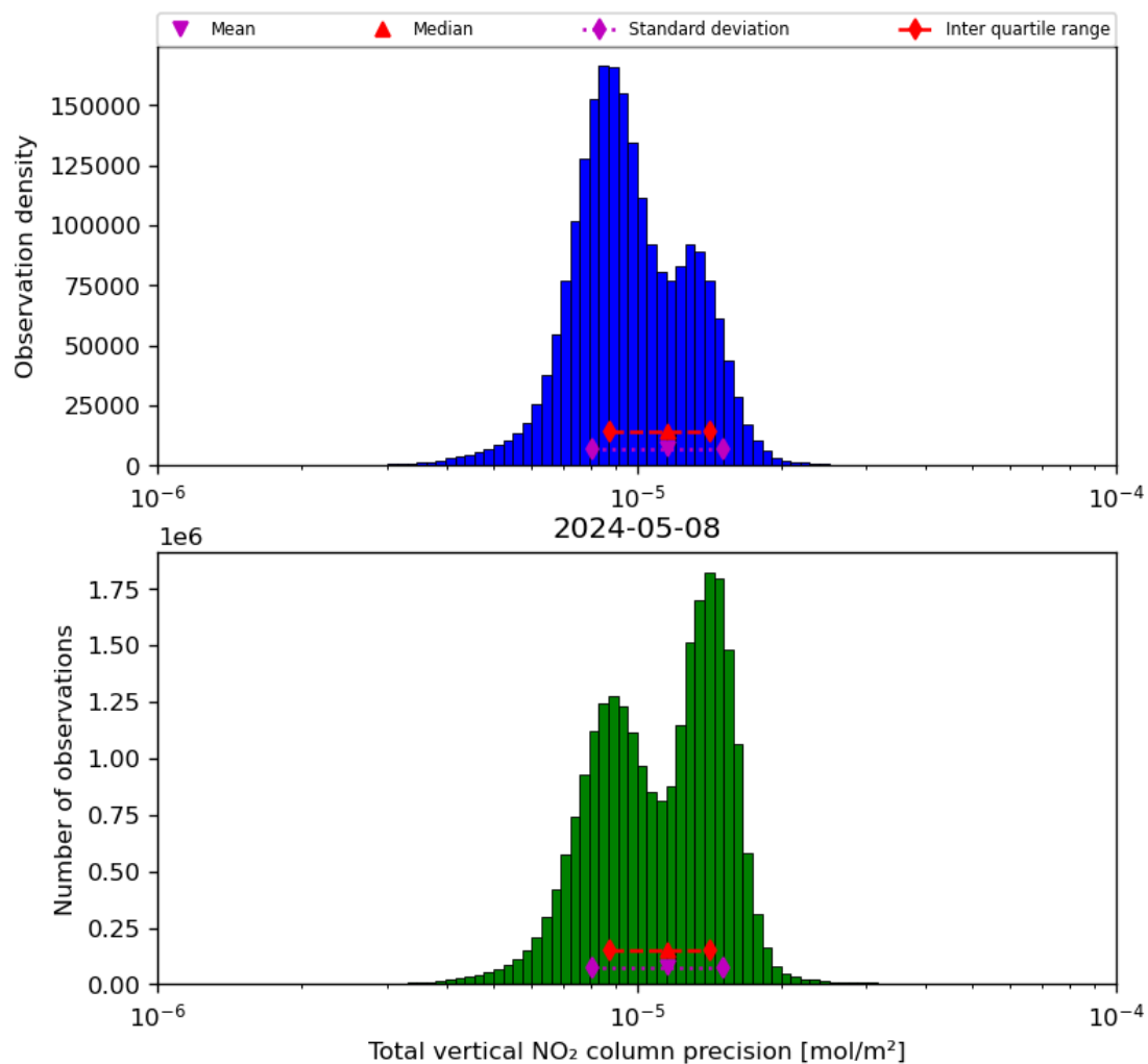
Figure 39: Histogram of “Total vertical NO 2 column precision” for 2024-05-07 to 2024-05-09
