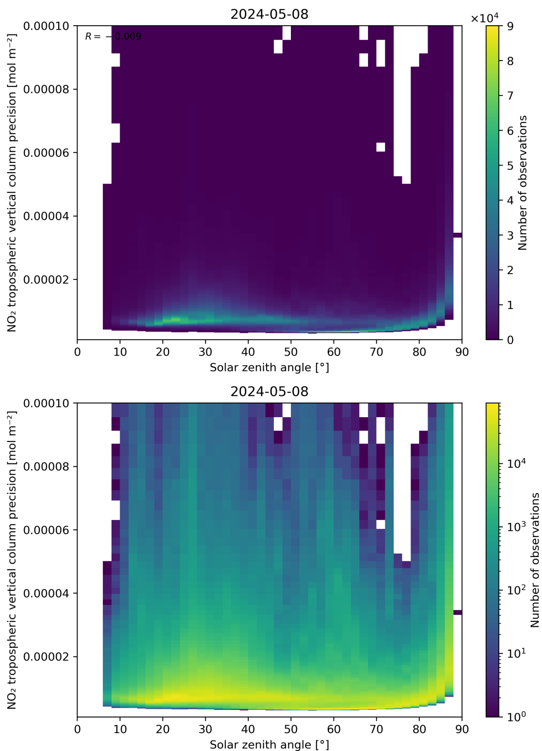
Figure 156: Scatter density plot of “Solar zenith angle” against “NO 2 tropospheric vertical column precision” for 2024-05-07 to 2024-05-09.
