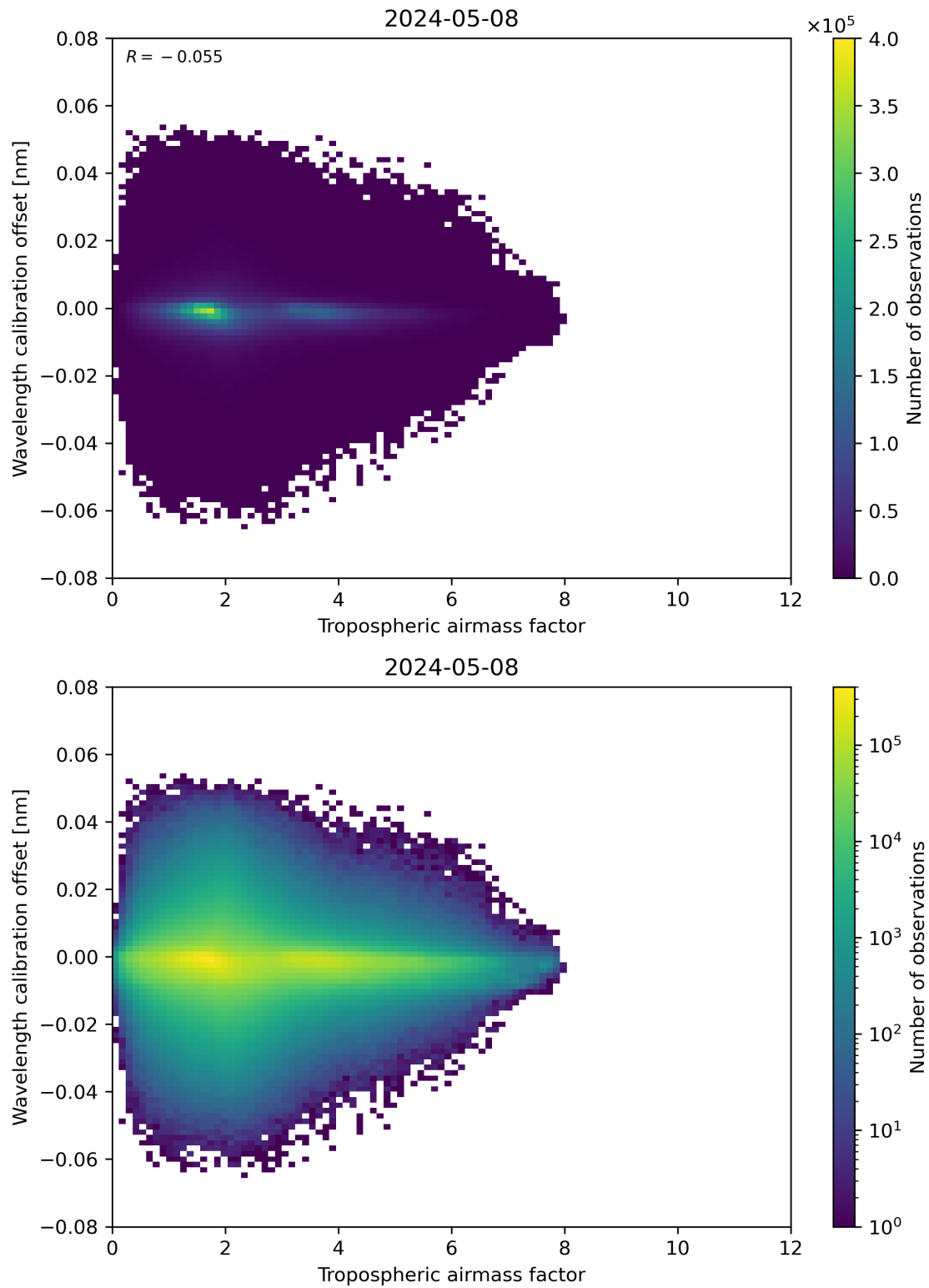
Figure 80: Scatter density plot of “Tropospheric airmass factor” against “Wavelength calibration offset” for 2024-05-07 to 2024-05-09.
