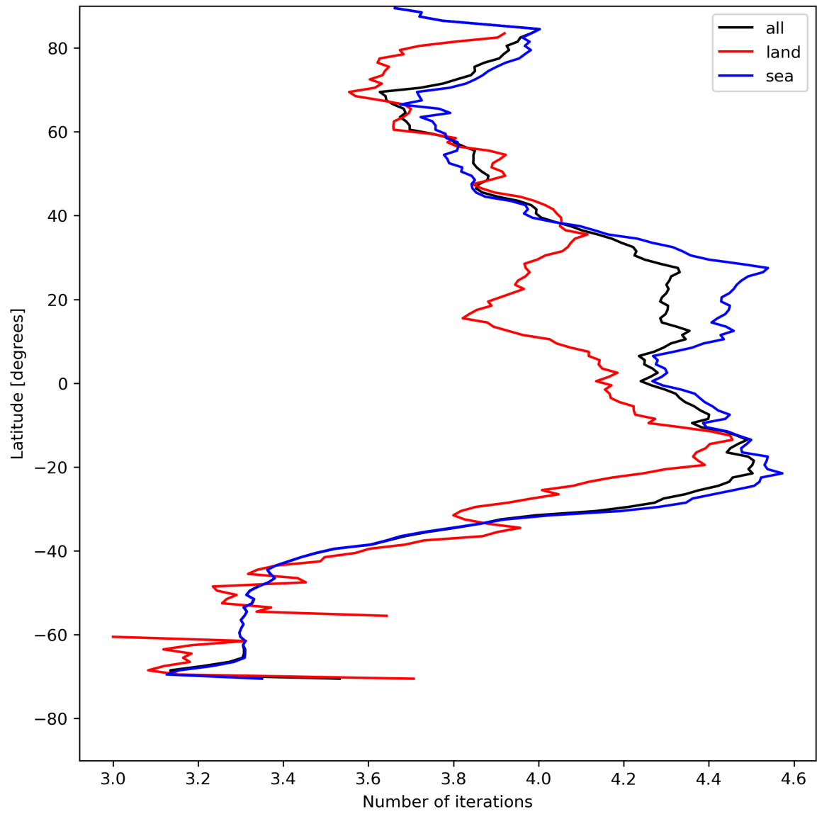
Figure 17: Zonal average of “Number of iterations” for 2024-05-07 to 2024-05-09.
