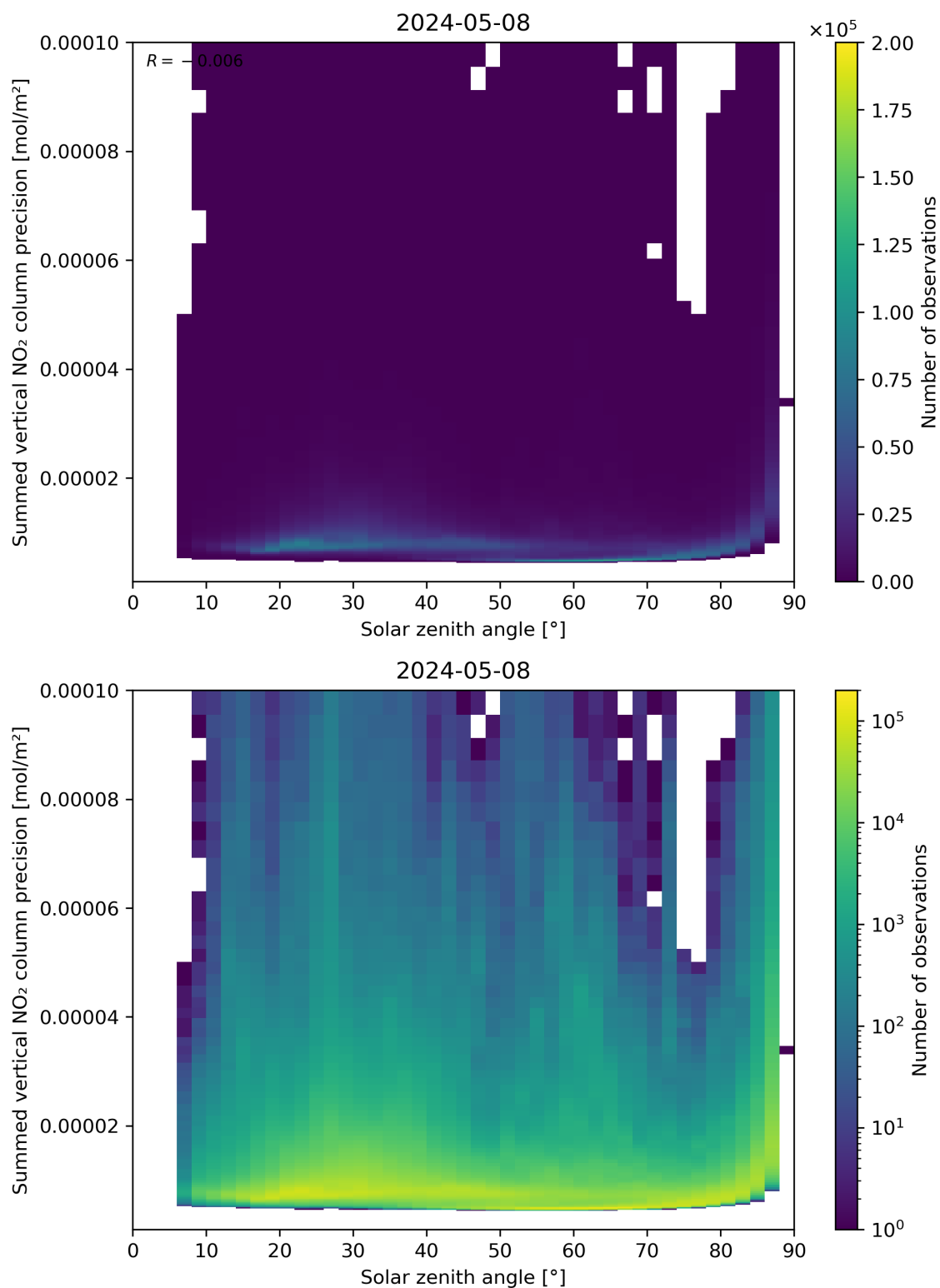
Figure 152: Scatter density plot of “Solar zenith angle” against “Summed vertical NO 2 column precision” for 2024-05-07 to 2024-05-09.
