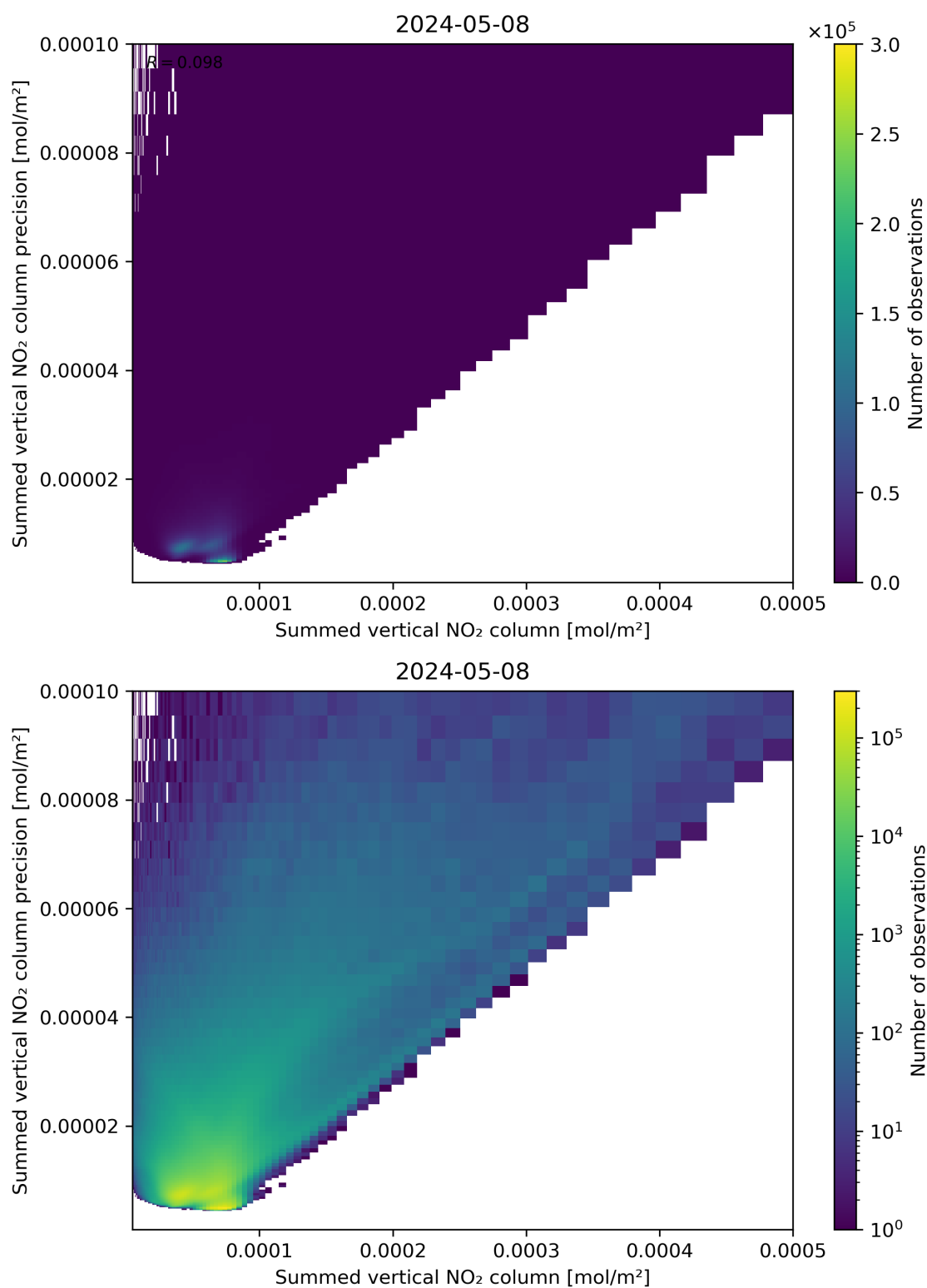
Figure 105: Scatter density plot of “Summed vertical NO 2 column” against “Summed vertical NO 2 column precision” for 2024-05-07 to 2024-05-09.
