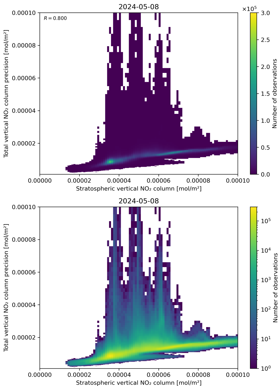
Figure 101: Scatter density plot of “Stratospheric vertical NO 2 column” against “Total vertical NO 2 column precision” for 2024-05-07 to 2024-05-09.
