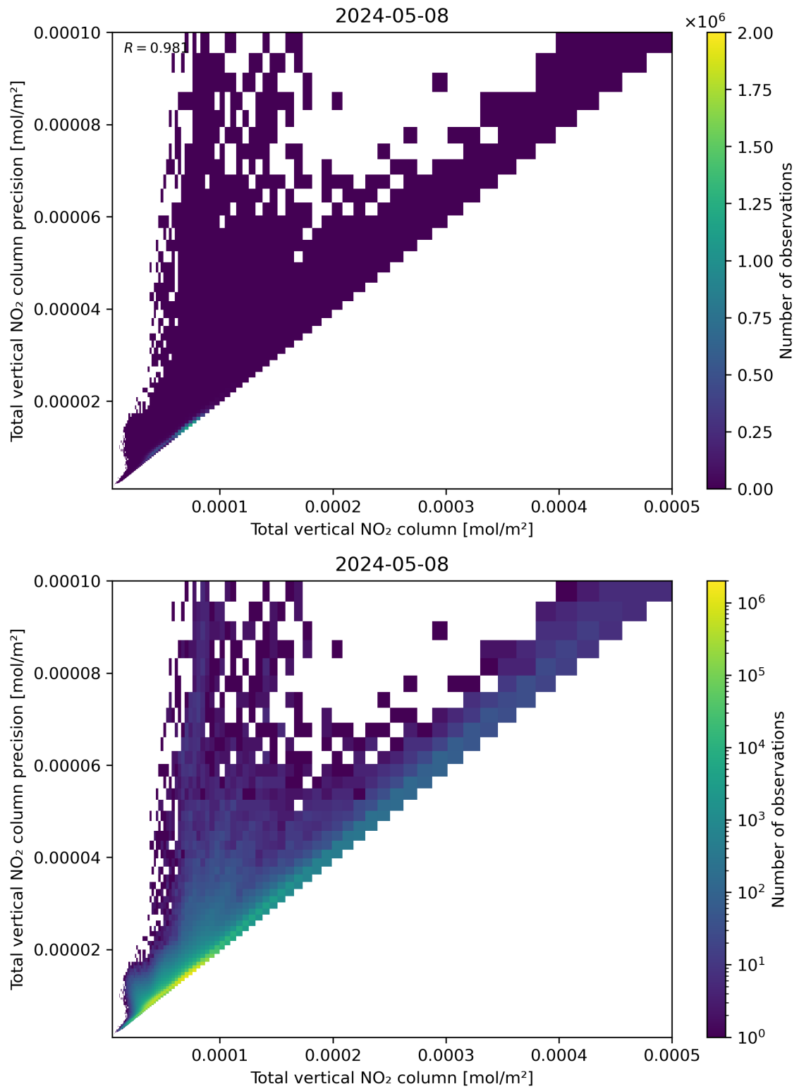
Figure 114: Scatter density plot of “Total vertical NO 2 column” against “Total vertical NO 2 column precision” for 2024-05-07 to 2024-05-09.
