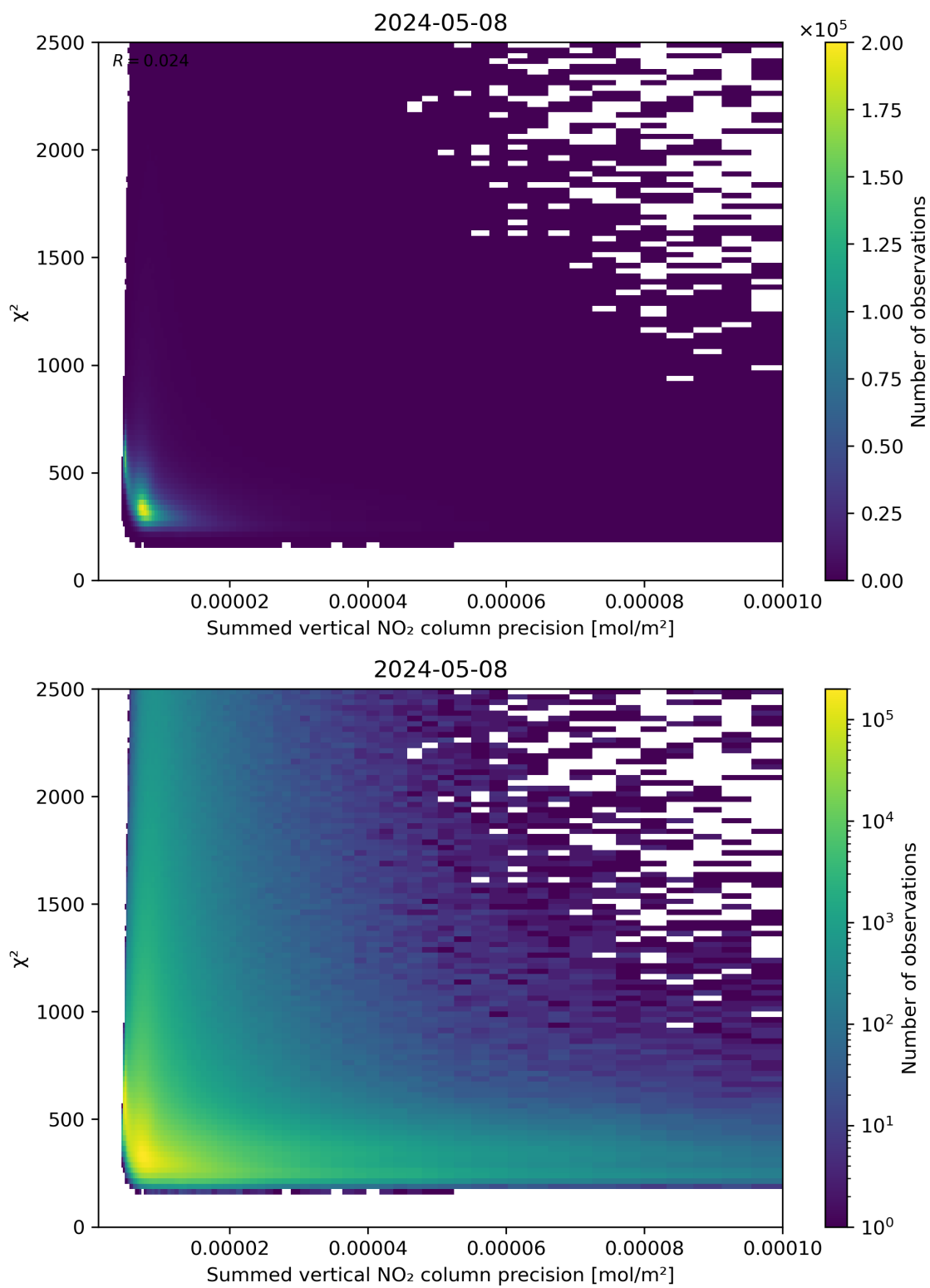
Figure 107: Scatter density plot of “Summed vertical NO 2 column precision” against “ \chi^2 ” for 2024-05-07 to 2024-05-09.
