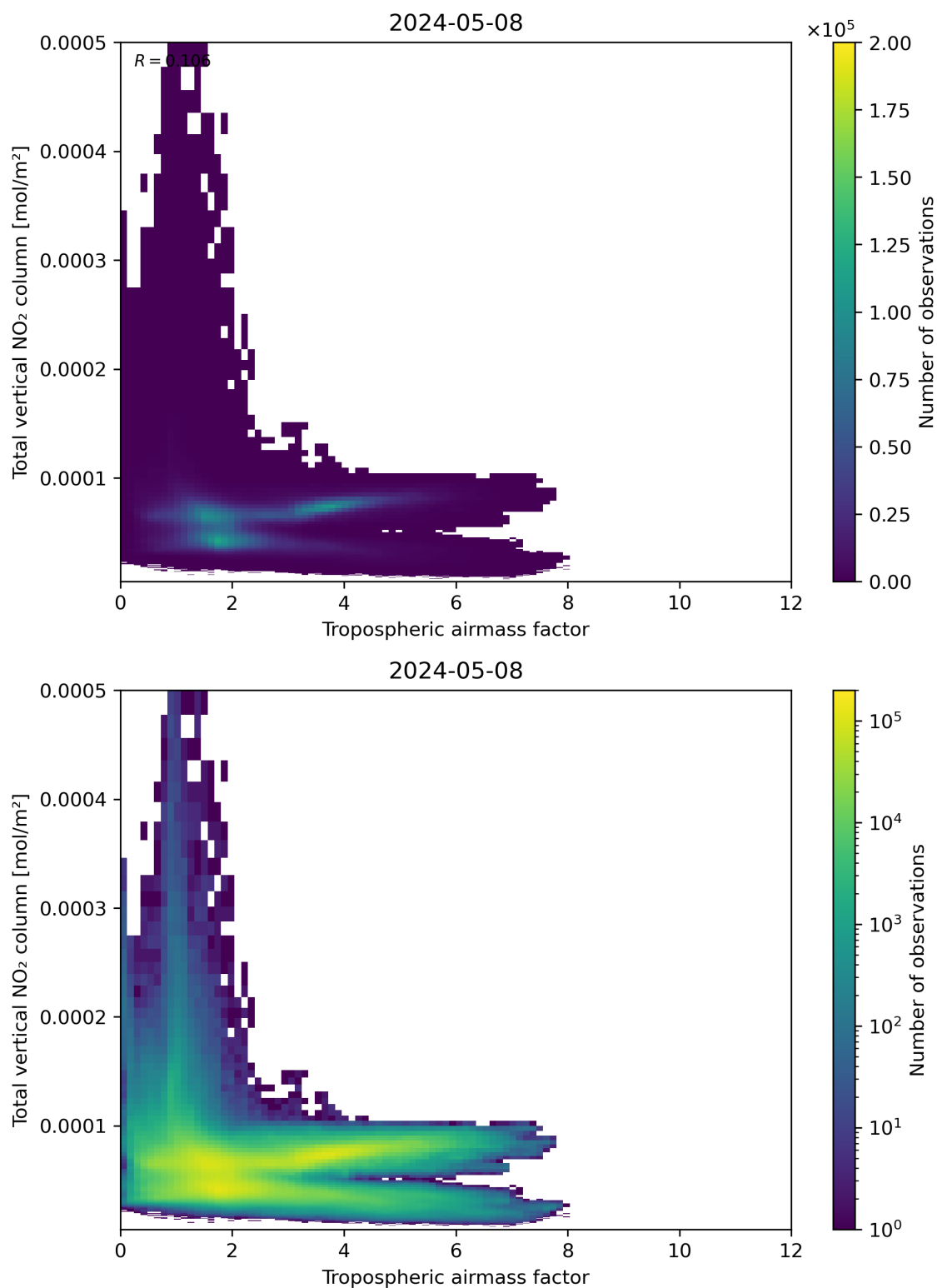
Figure 77: Scatter density plot of “Tropospheric airmass factor” against “Total vertical NO 2 column” for 2024-05-07 to 2024-05-09.
