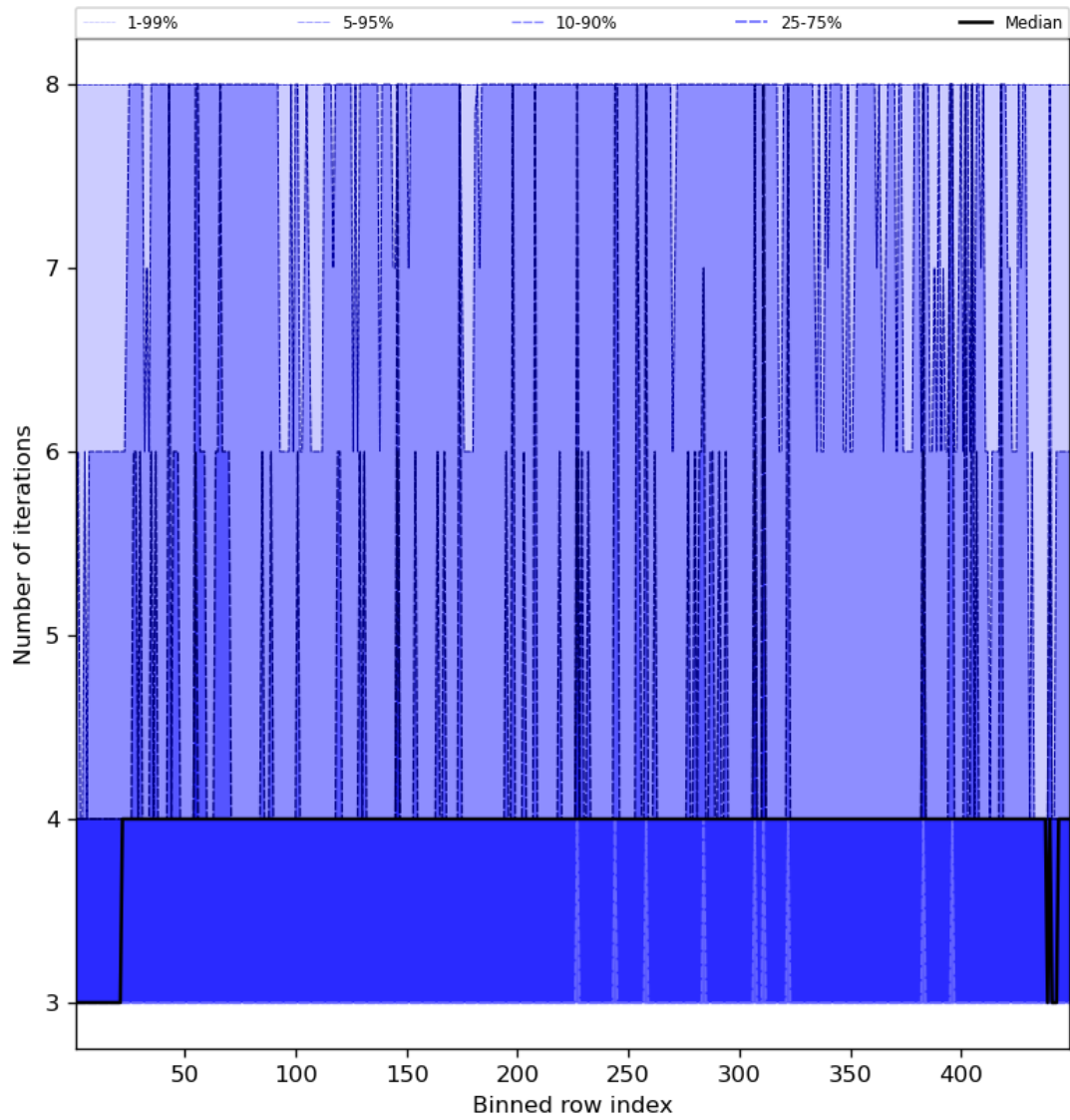
Figure 51: Along track statistics of “Number of iterations” for 2024-05-07 to 2024-05-09
