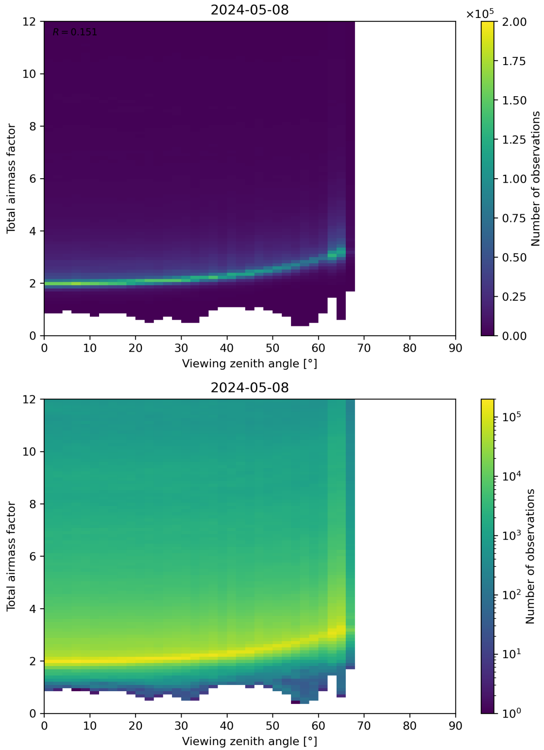
Figure 160: Scatter density plot of “Viewing zenith angle” against “Total airmass factor” for 2024-05-07 to 2024-05-09.
