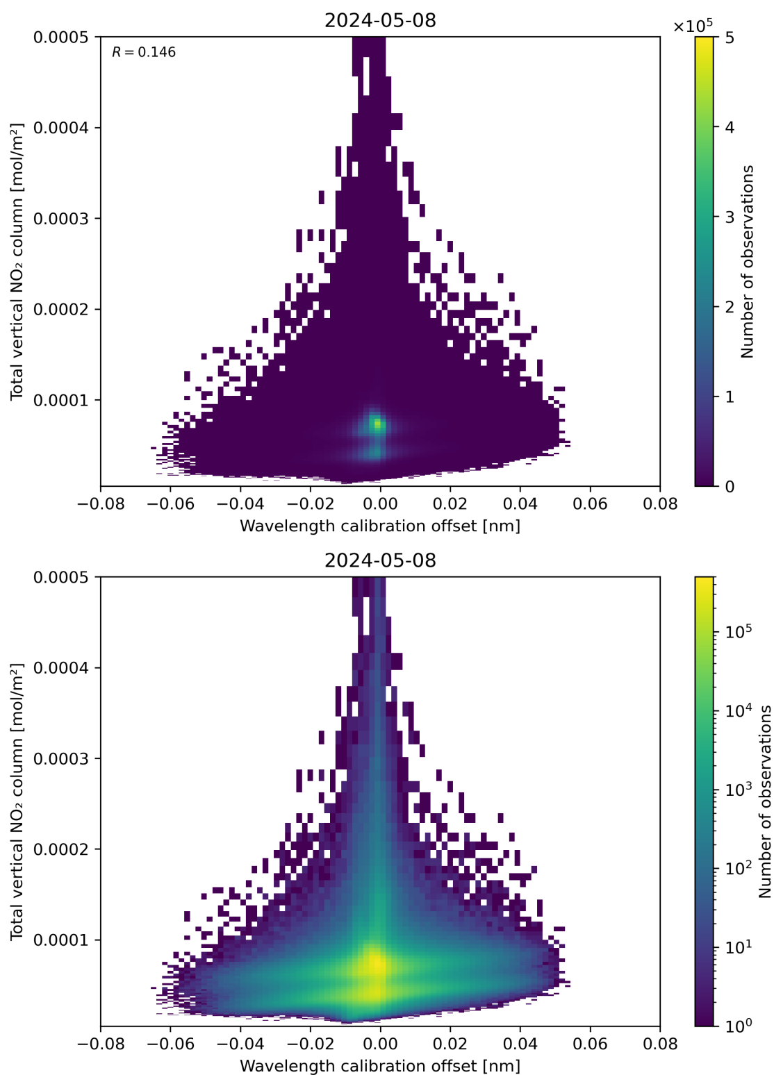
Figure 179: Scatter density plot of “Wavelength calibration offset” against “Total vertical NO 2 column” for 2024-05-07 to 2024-05-09.
