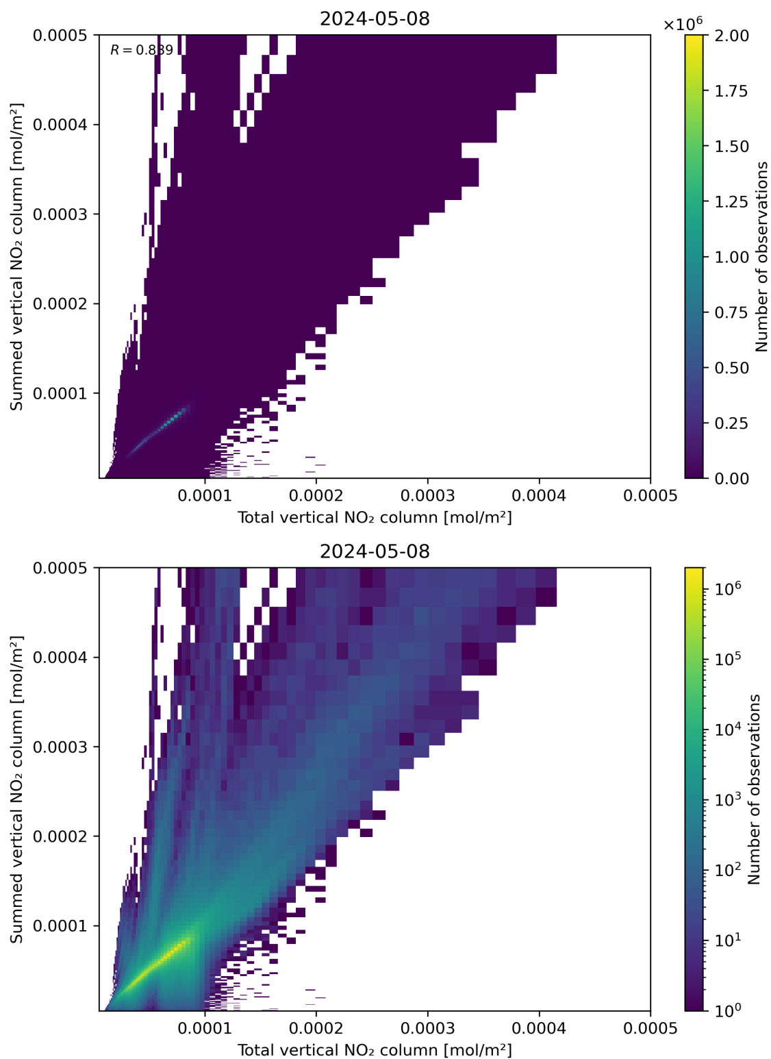
Figure 112: Scatter density plot of “Total vertical NO 2 column” against “Summed vertical NO 2 column” for 2024-05-07 to 2024-05-09.
