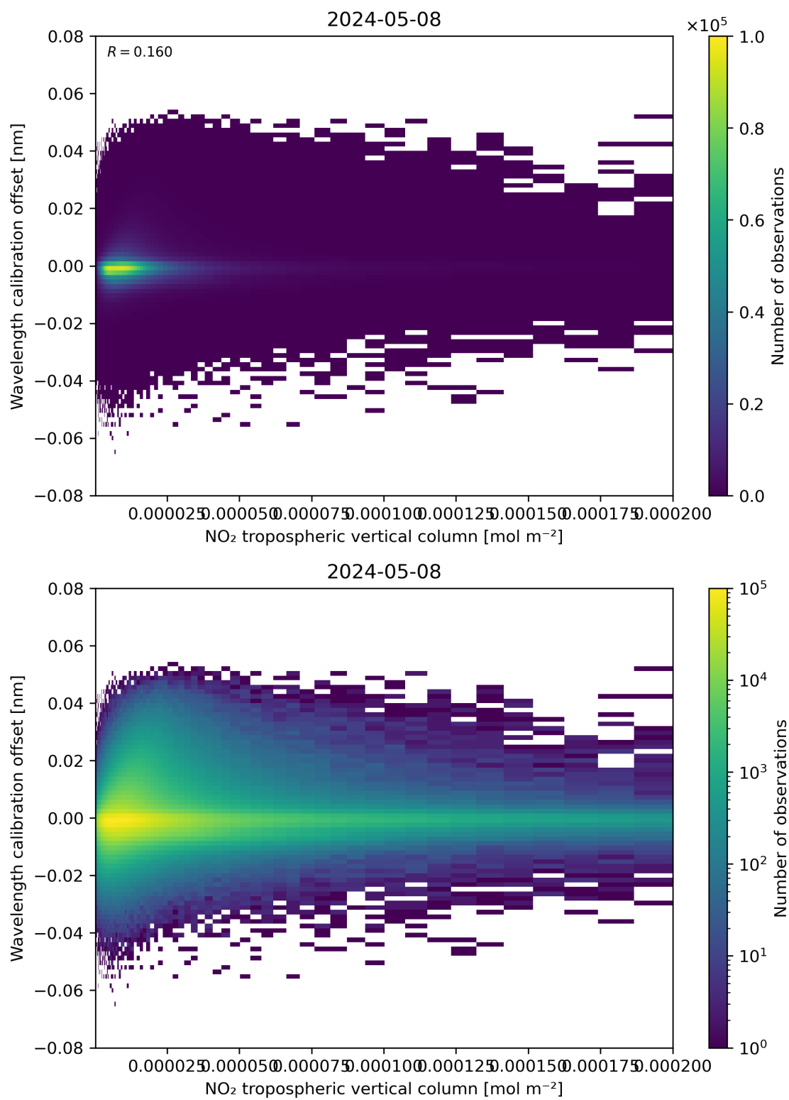
Figure 143: Scatter density plot of “NO 2 tropospheric vertical column” against “Wavelength calibration offset” for 2024-05-07 to 2024-05-09.
