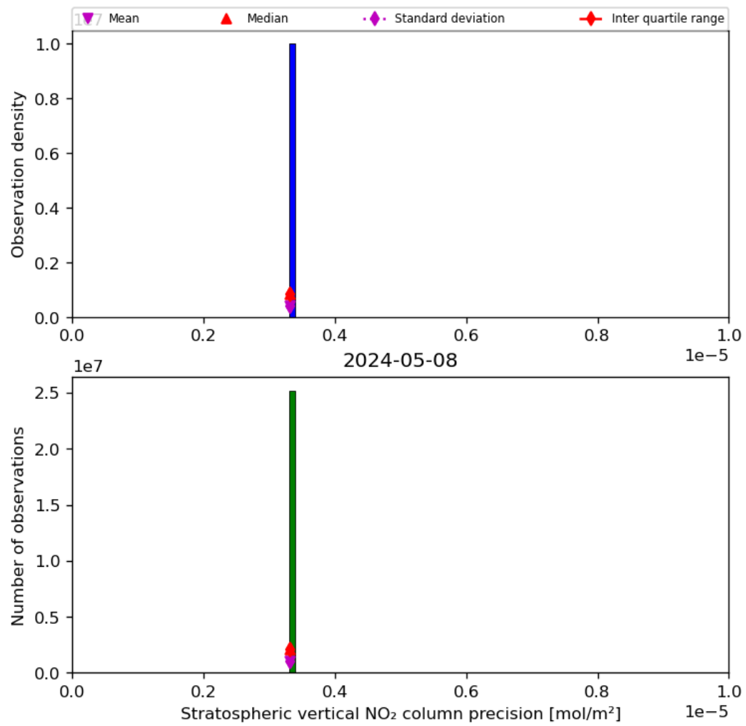
Figure 37: Histogram of “Stratospheric vertical NO 2 column precision” for 2024-05-07 to 2024-05-09
