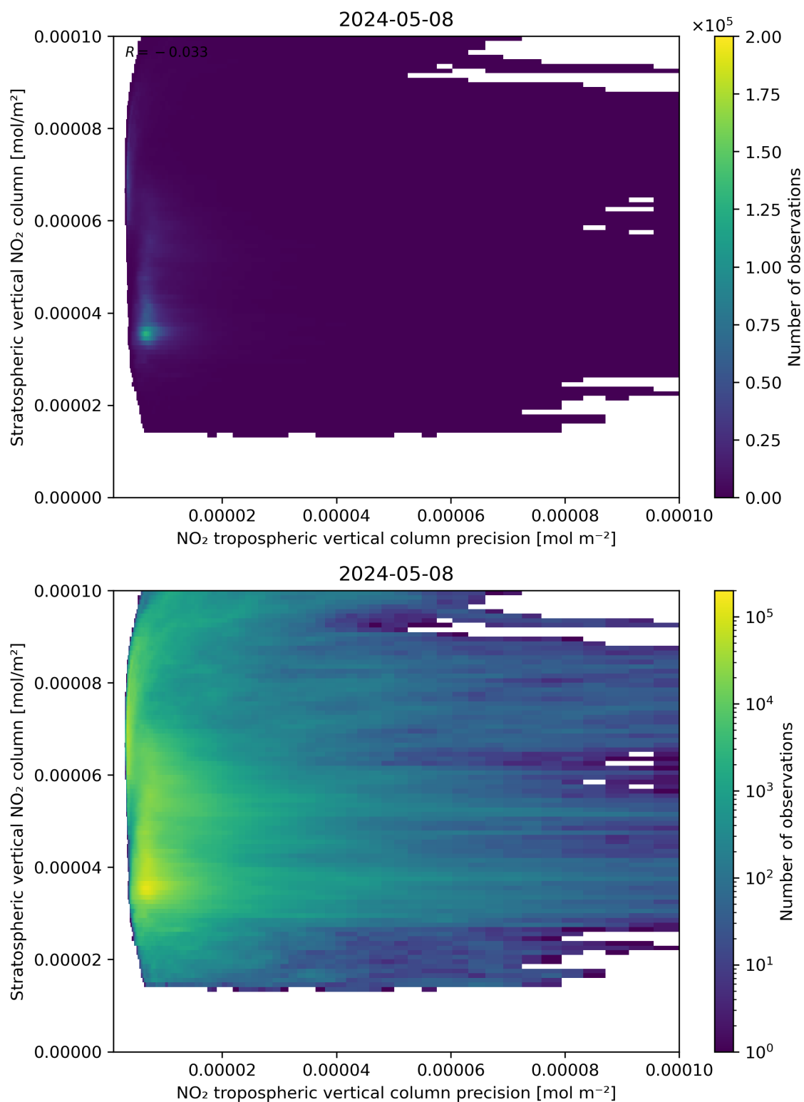
Figure 135: Scatter density plot of “NO 2 tropospheric vertical column precision” against “Stratospheric vertical NO 2 column” for 2024-05-07 to 2024-05-09.
