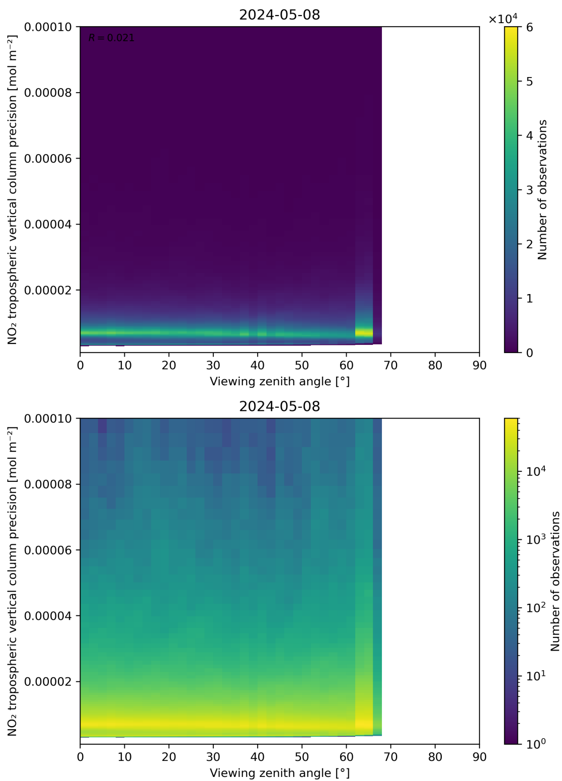
Figure 170: Scatter density plot of “Viewing zenith angle” against “NO 2 tropospheric vertical column precision” for 2024-05-07 to 2024-05-09.
