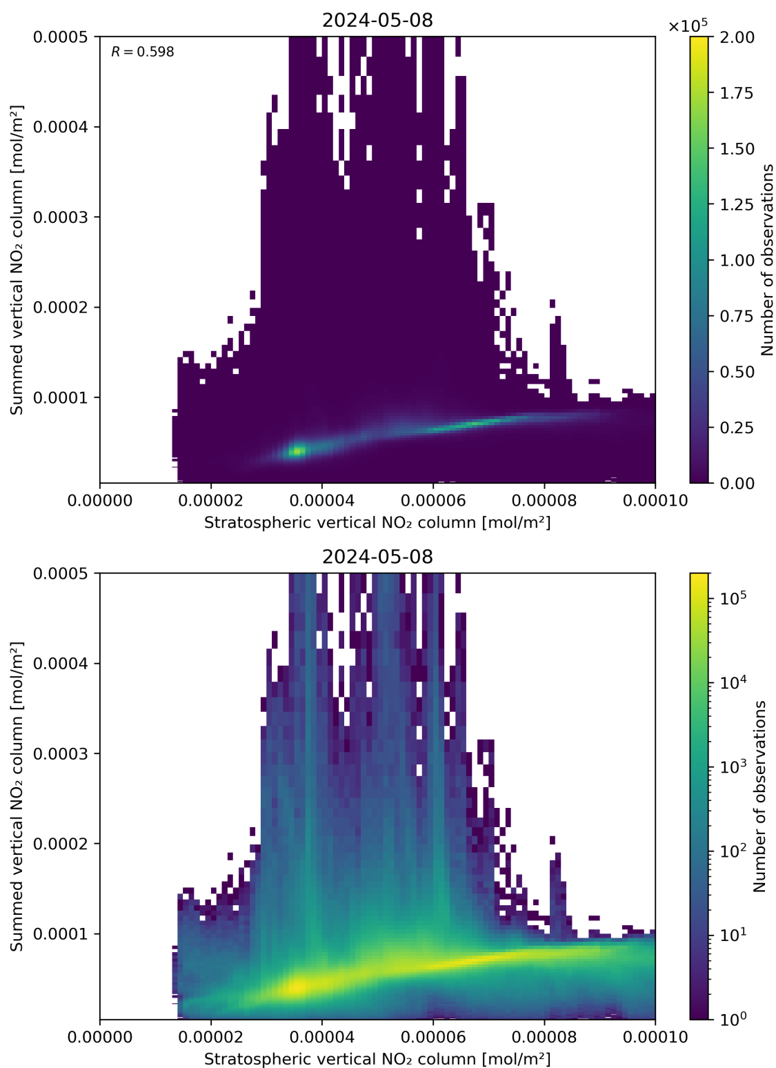
Figure 98: Scatter density plot of “Stratospheric vertical NO 2 column” against “Summed vertical NO 2 column” for 2024-05-07 to 2024-05-09.
