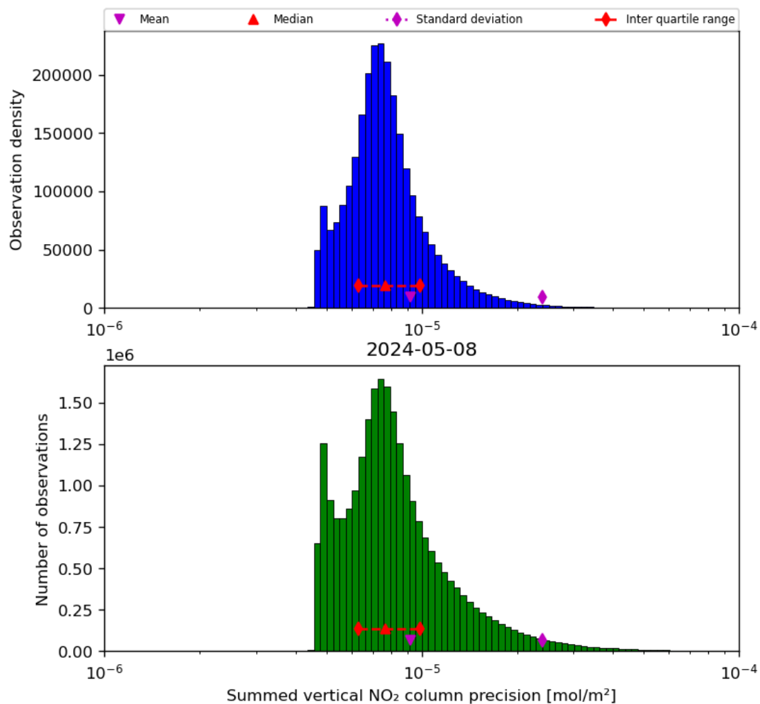
Figure 41: Histogram of “Summed vertical NO 2 column precision” for 2024-05-07 to 2024-05-09
