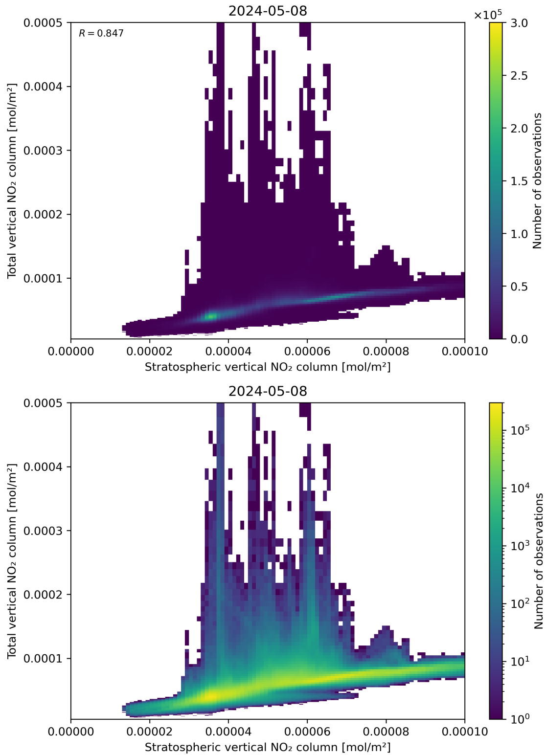
Figure 100: Scatter density plot of “Stratospheric vertical NO 2 column” against “Total vertical NO 2 column” for 2024-05-07 to 2024-05-09.
