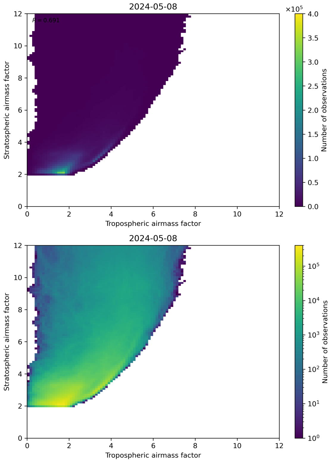
Figure 71: Scatter density plot of “Tropospheric airmass factor” against “Stratospheric airmass factor” for 2024-05-07 to 2024-05-09.
