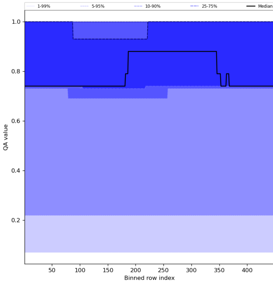
Figure 45: Along track statistics of “QA value” for 2024-05-07 to 2024-05-09
