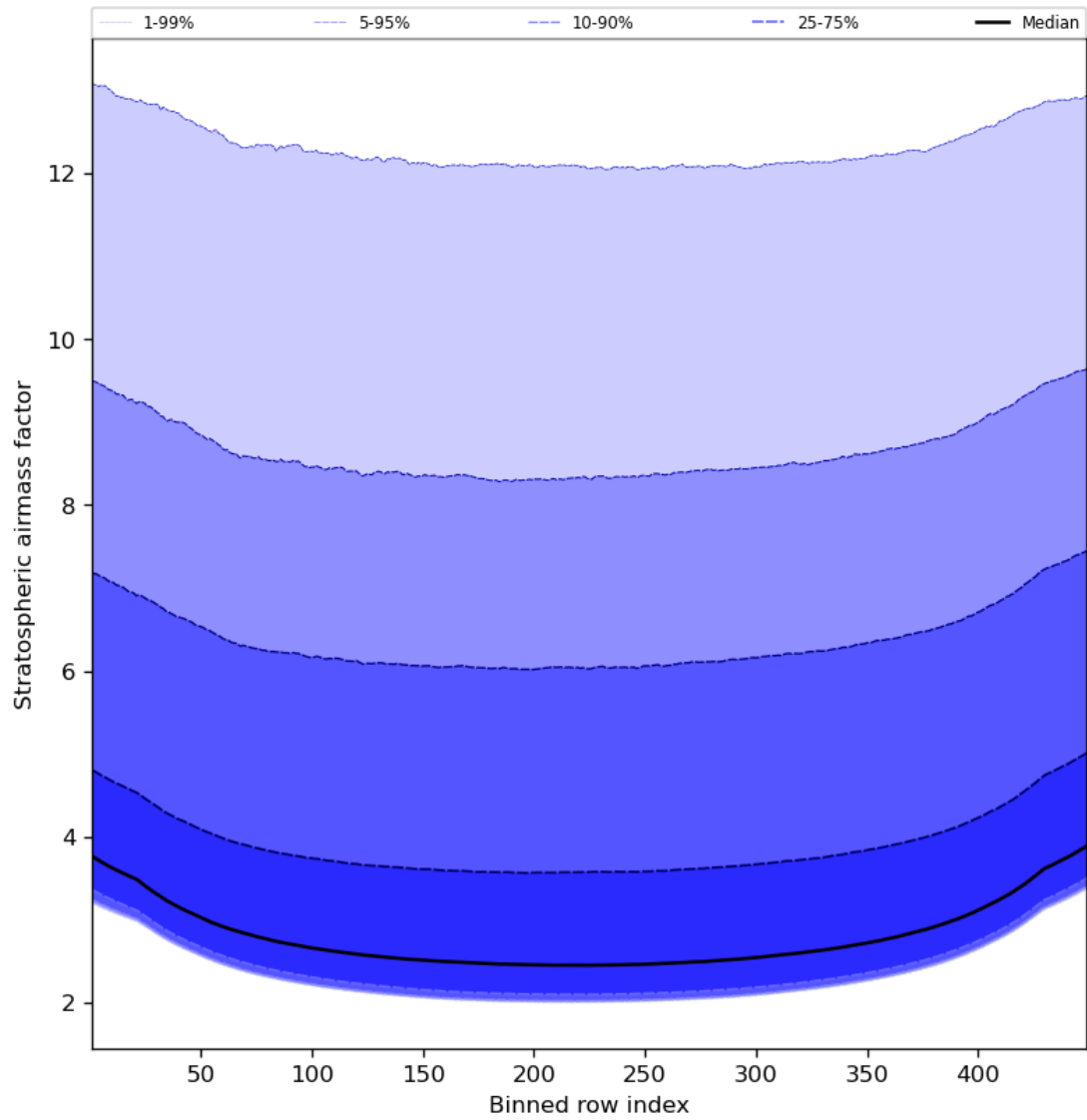
Figure 61: Along track statistics of “Stratospheric airmass factor” for 2024-05-07 to 2024-05-09
