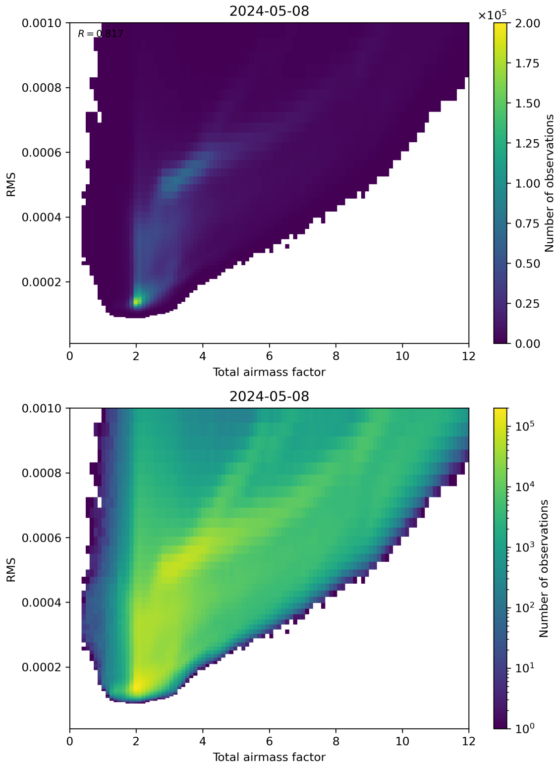
Figure 69: Scatter density plot of “Total airmass factor” against “RMS” for 2024-05-07 to 2024-05-09.
