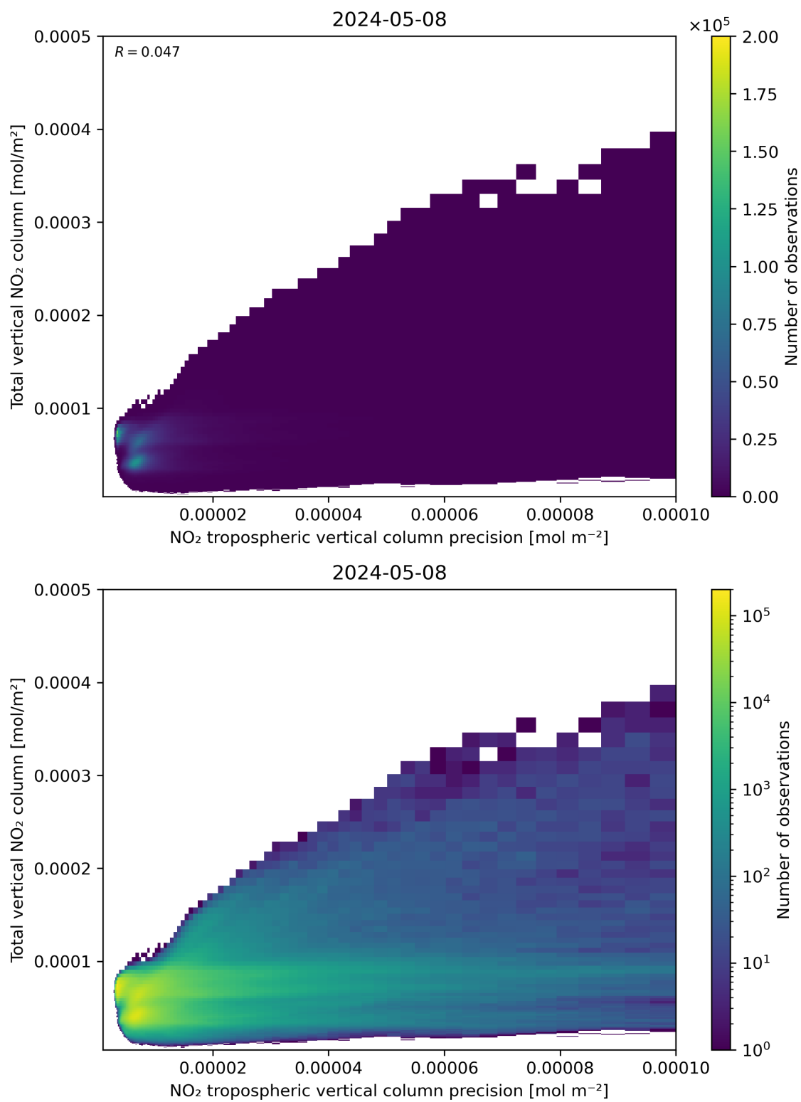
Figure 138: Scatter density plot of “NO 2 tropospheric vertical column precision” against “Total vertical NO 2 column” for 2024-05-07 to 2024-05-09.
