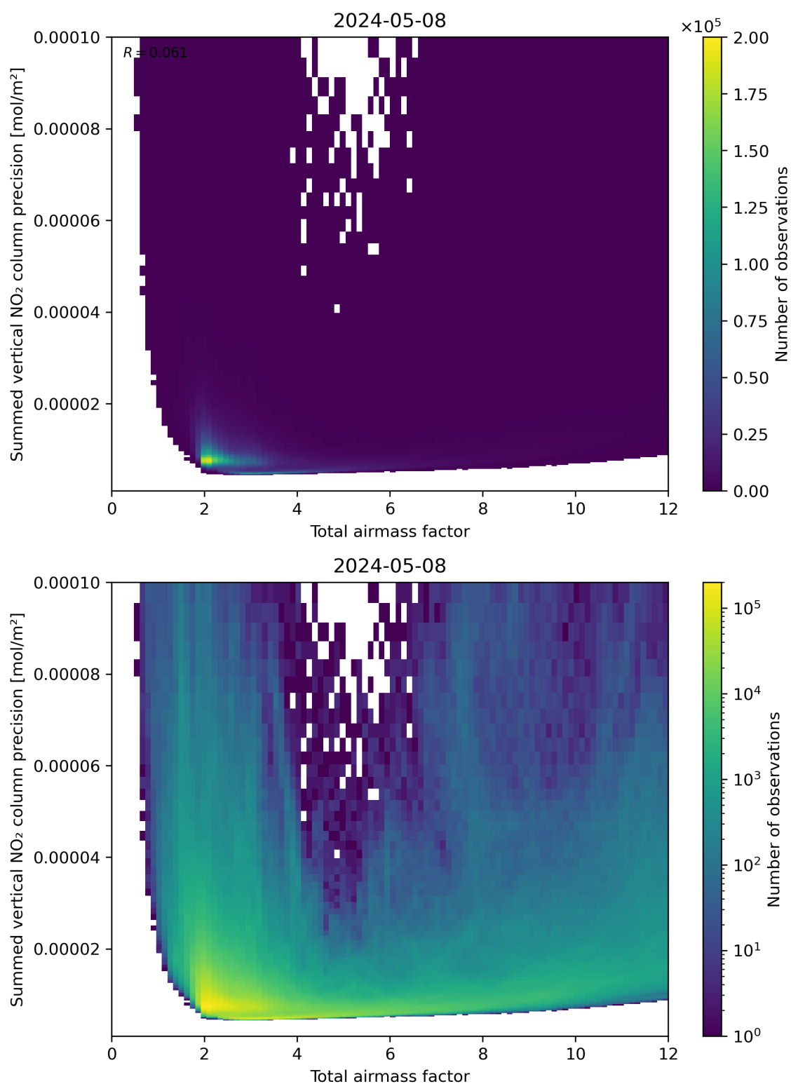
Figure 66: Scatter density plot of “Total airmass factor” against “Summed vertical NO 2 column precision” for 2024-05-07 to 2024-05-09.
