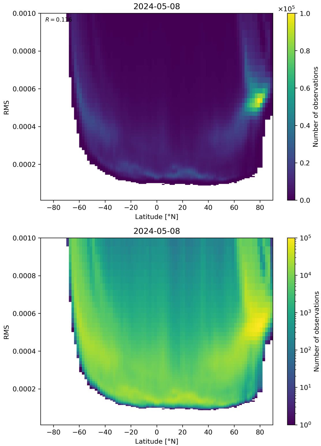
Figure 94: Scatter density plot of “Latitude” against “RMS” for 2024-05-07 to 2024-05-09.
