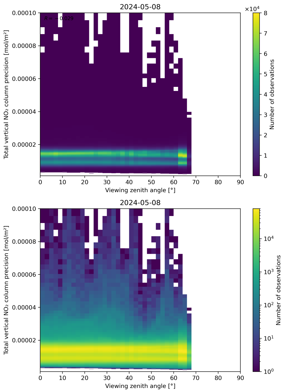
Figure 168: Scatter density plot of “Viewing zenith angle” against “Total vertical NO 2 column precision” for 2024-05-07 to 2024-05-09.
