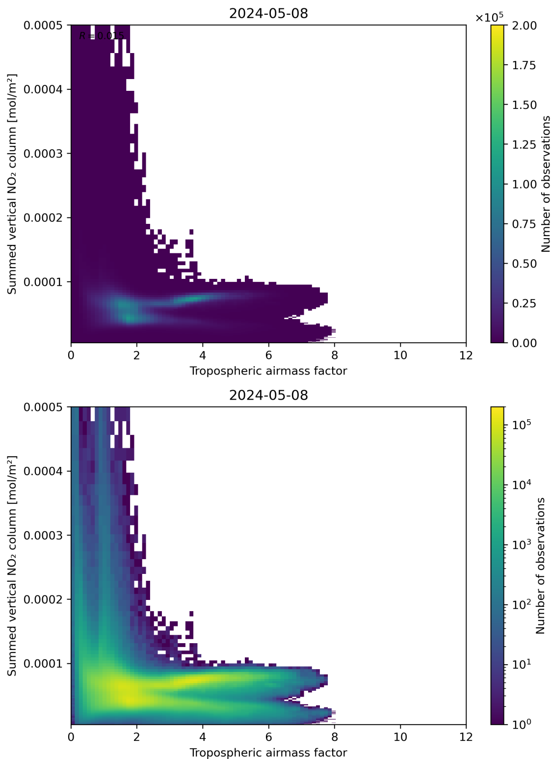
Figure 75: Scatter density plot of “Tropospheric airmass factor” against “Summed vertical NO 2 column” for 2024-05-07 to 2024-05-09.
