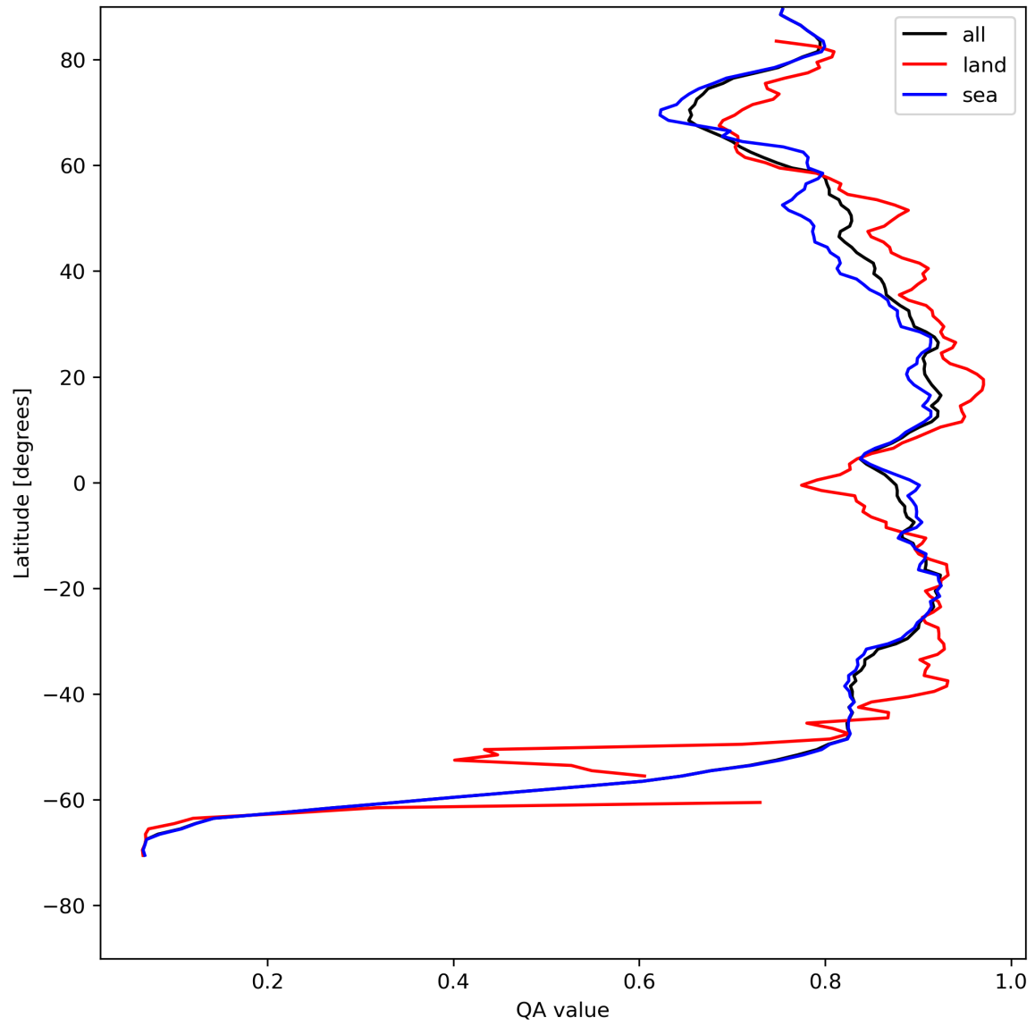
Figure 11: Zonal average of “QA value” for 2024-05-07 to 2024-05-09.
