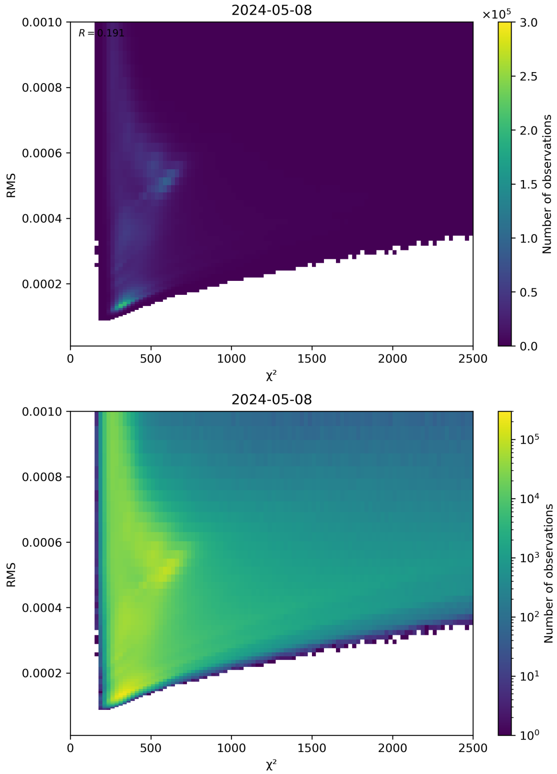
Figure 82: Scatter density plot of “ \chi^2 ” against “RMS” for 2024-05-07 to 2024-05-09.
