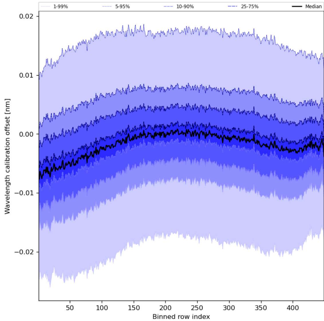
Figure 52: Along track statistics of “Wavelength calibration offset” for 2024-05-07 to 2024-05-09
