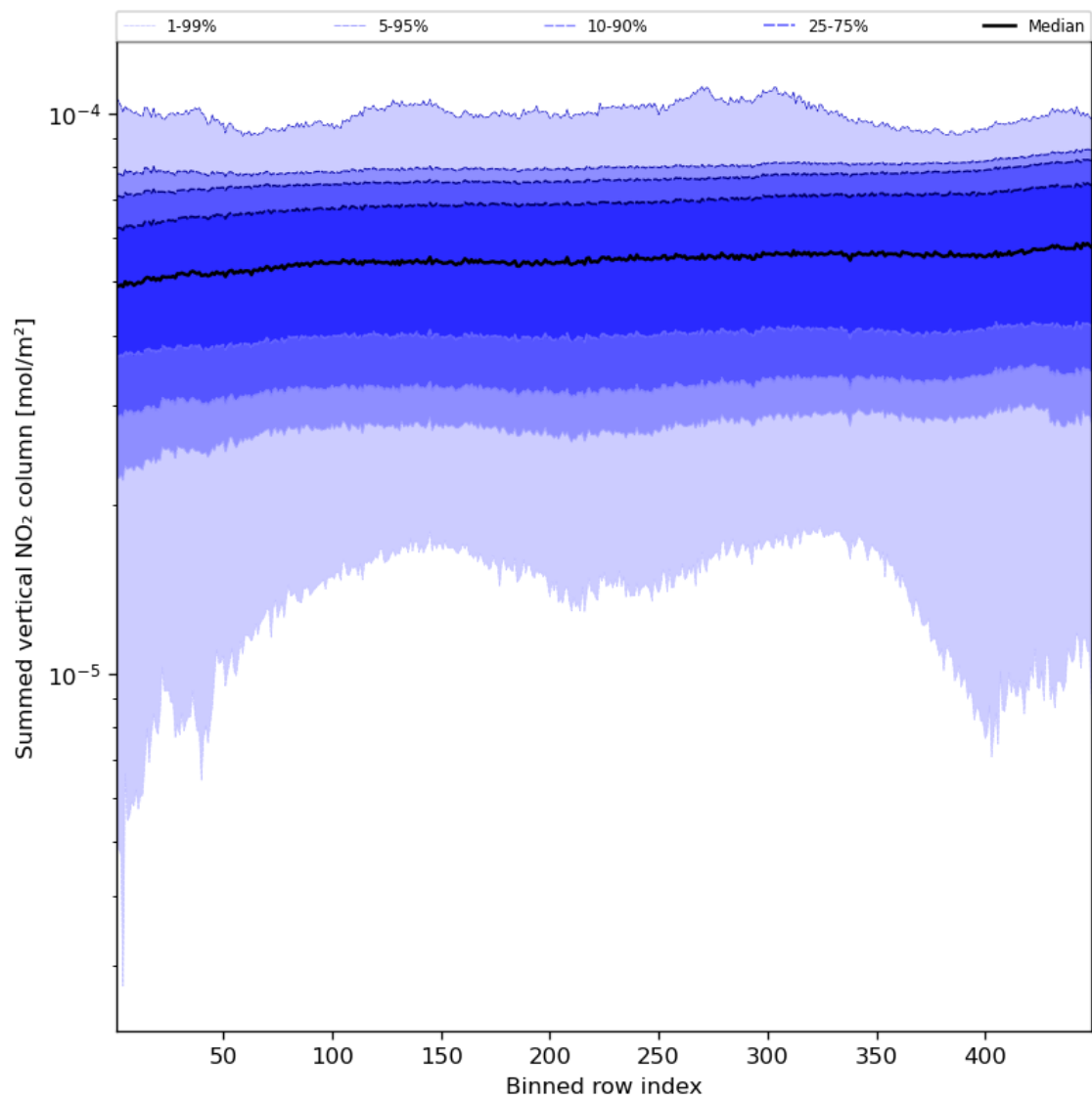
Figure 57: Along track statistics of “Summed vertical NO 2 column” for 2024-05-07 to 2024-05-09
