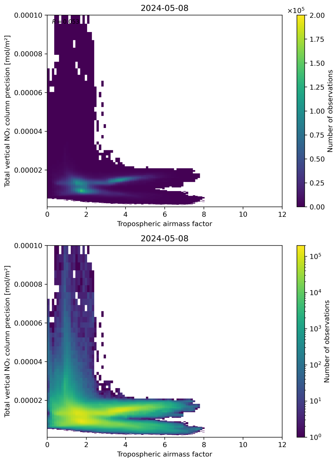
Figure 78: Scatter density plot of “Tropospheric air mass factor” against “Total vertical NO 2 column precision” for 2024-05-07 to 2024-05-09.
