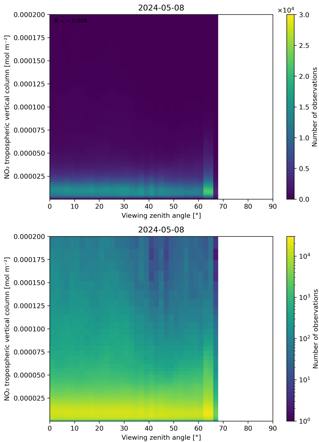
Figure 169: Scatter density plot of “Viewing zenith angle” against “NO 2 tropospheric vertical column” for 2024-05-07 to 2024-05-09.
