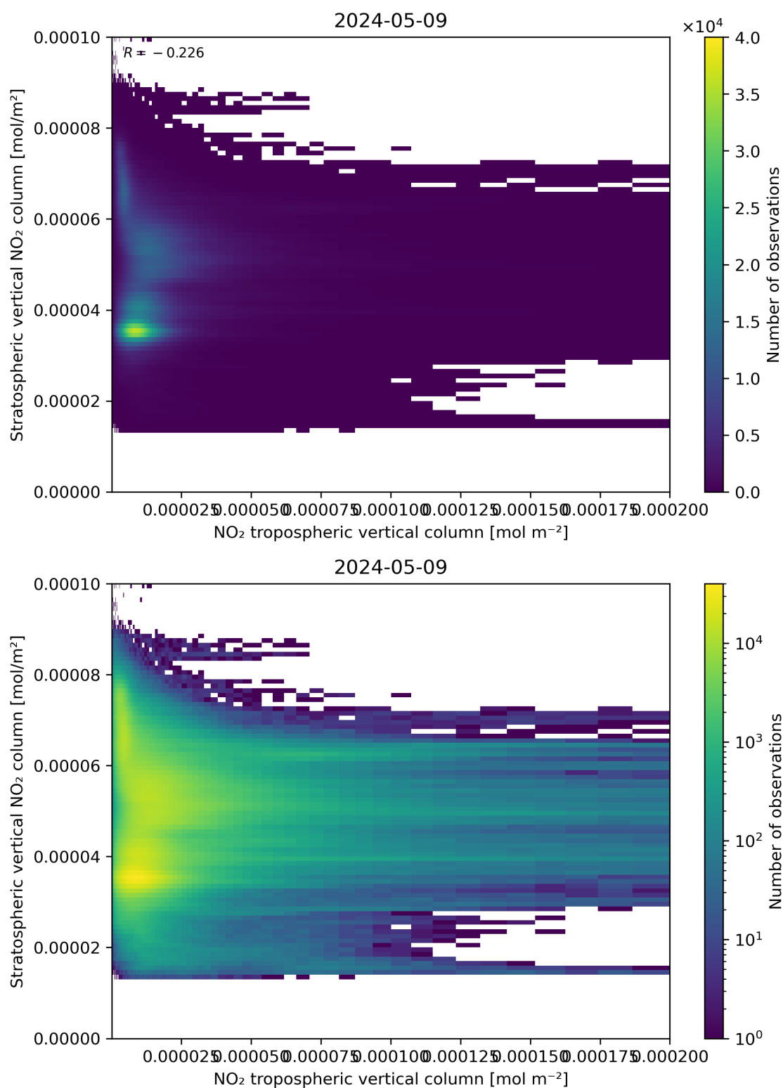
Figure 125: Scatter density plot of “NO 2 tropospheric vertical column” against “Stratospheric vertical NO 2 column” for 2024-05-08 to 2024-05-10.
