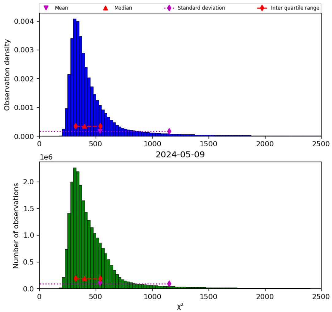
Figure 42: Histogram of “ \chi^2 ” for 2024-05-08 to 2024-05-10
