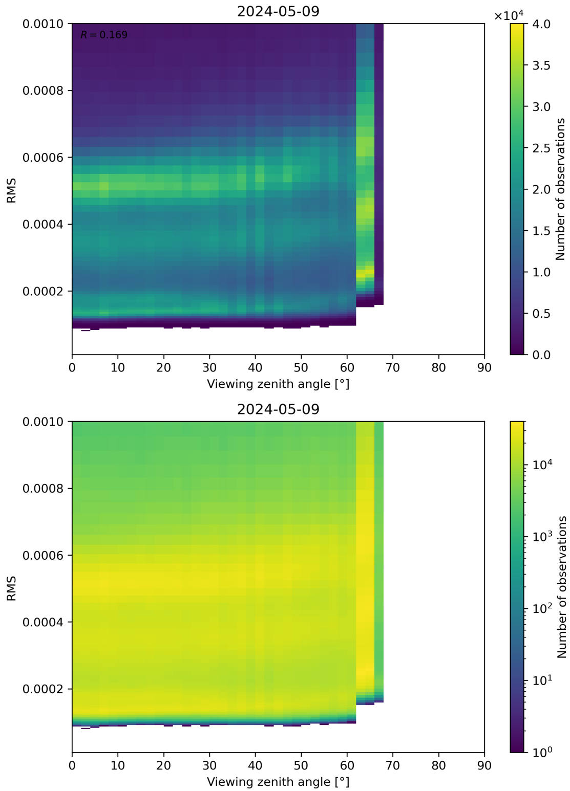
Figure 171: Scatter density plot of “Viewing zenith angle” against “RMS” for 2024-05-08 to 2024-05-10.
