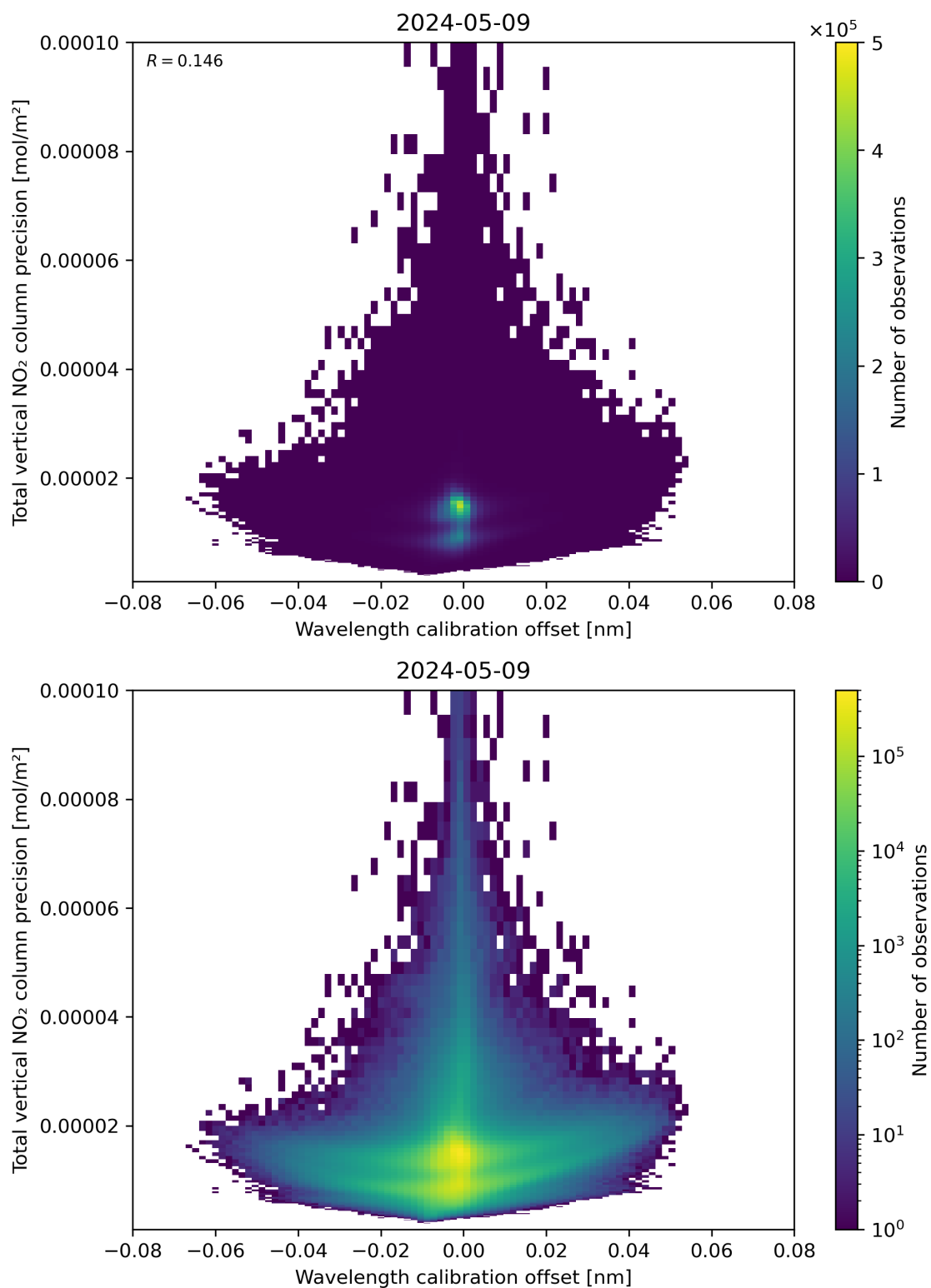
Figure 180: Scatter density plot of “Wavelength calibration offset” against “Total vertical NO 2 column precision” for 2024-05-08 to 2024-05-10.
