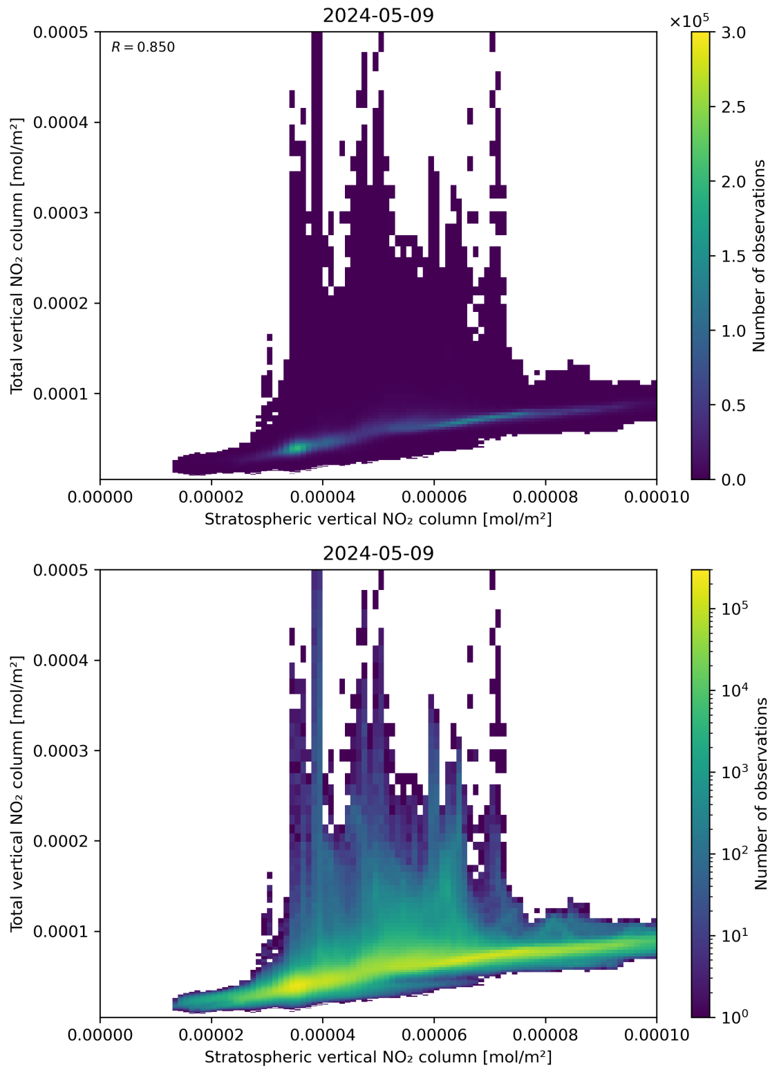
Figure 100: Scatter density plot of “Stratospheric vertical NO 2 column” against “Total vertical NO 2 column” for 2024-05-08 to 2024-05-10.
