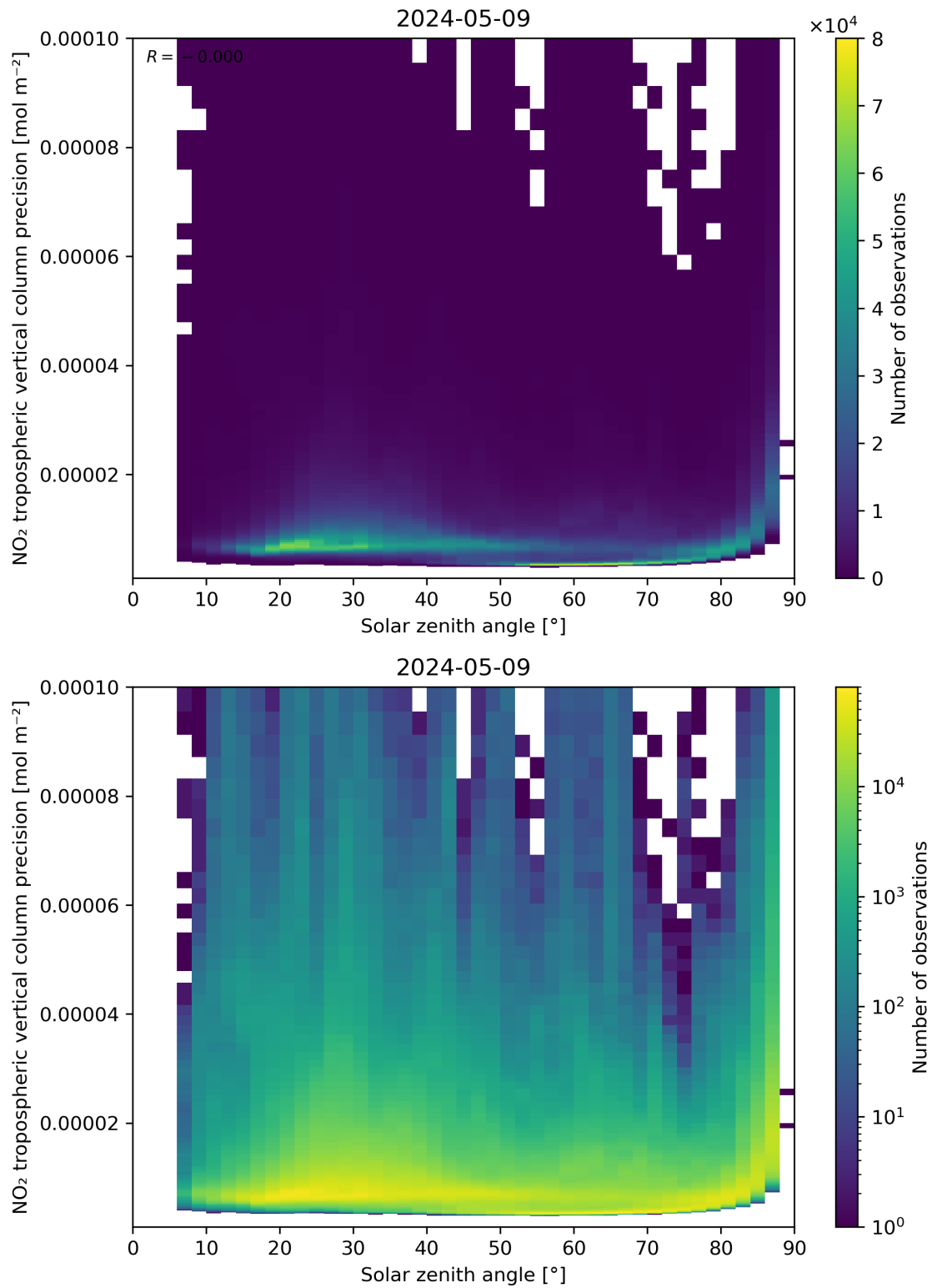
Figure 156: Scatter density plot of “Solar zenith angle” against “NO 2 tropospheric vertical column precision” for 2024-05-08 to 2024-05-10.
