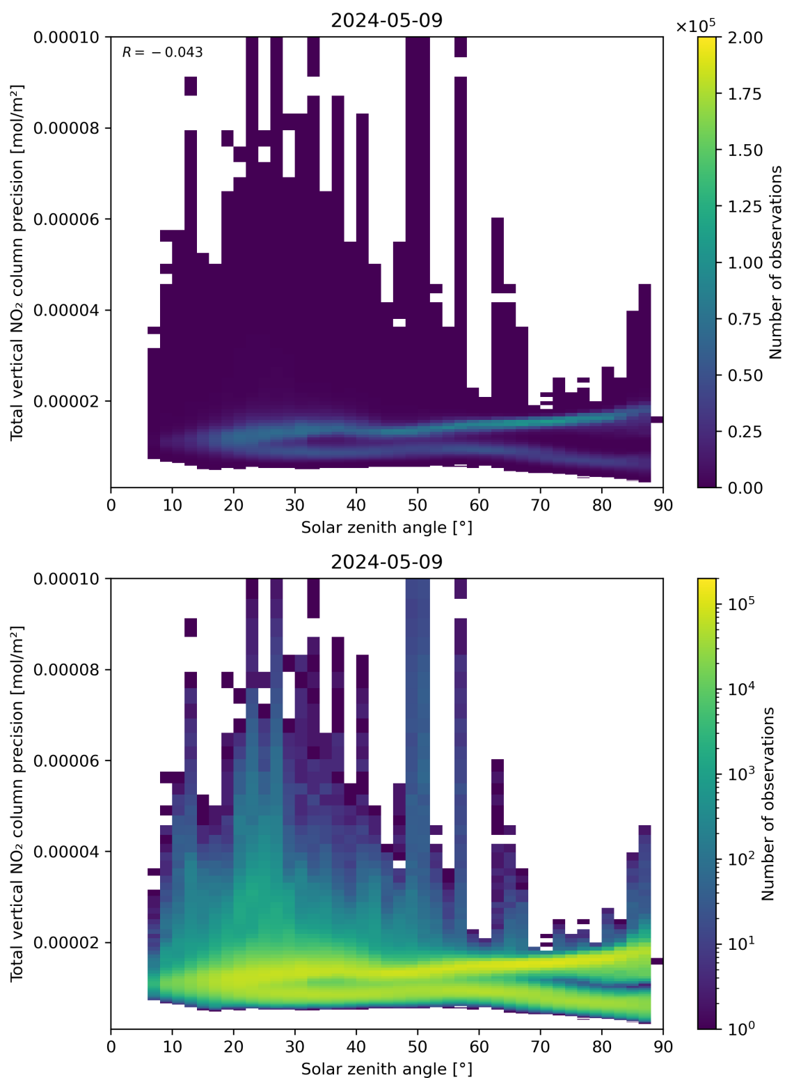
Figure 154: Scatter density plot of “Solar zenith angle” against “Total vertical NO 2 column precision” for 2024-05-08 to 2024-05-10.
