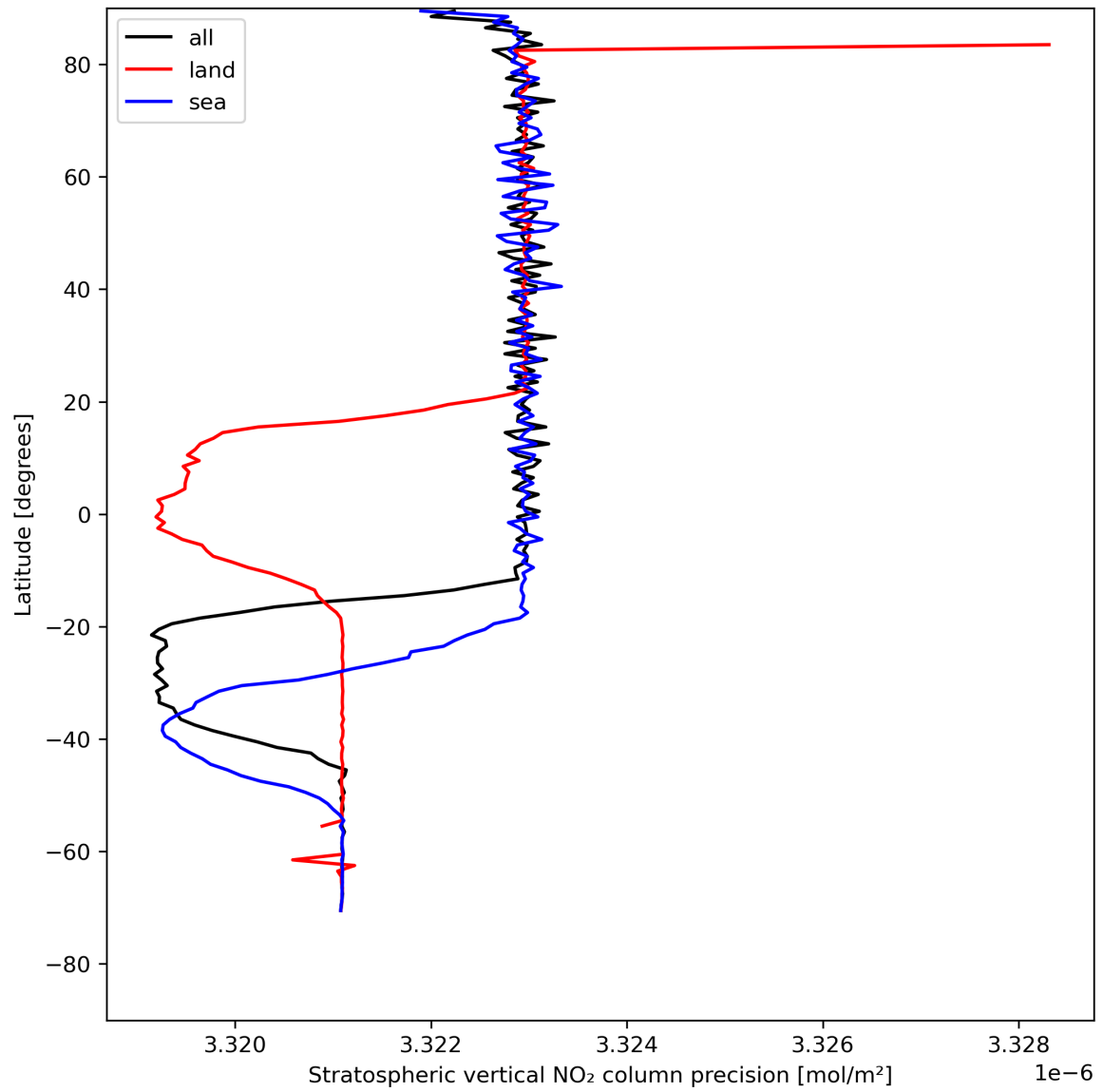
Figure 20: Zonal average of “Stratospheric vertical NO 2 column precision” for 2024-05-08 to 2024-05-10.
