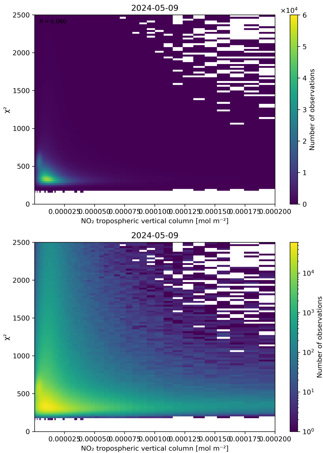
Figure 124: Scatter density plot of “NO 2 tropospheric vertical column” against “ \chi^2 ” for 2024-05-08 to 2024-05-10.
