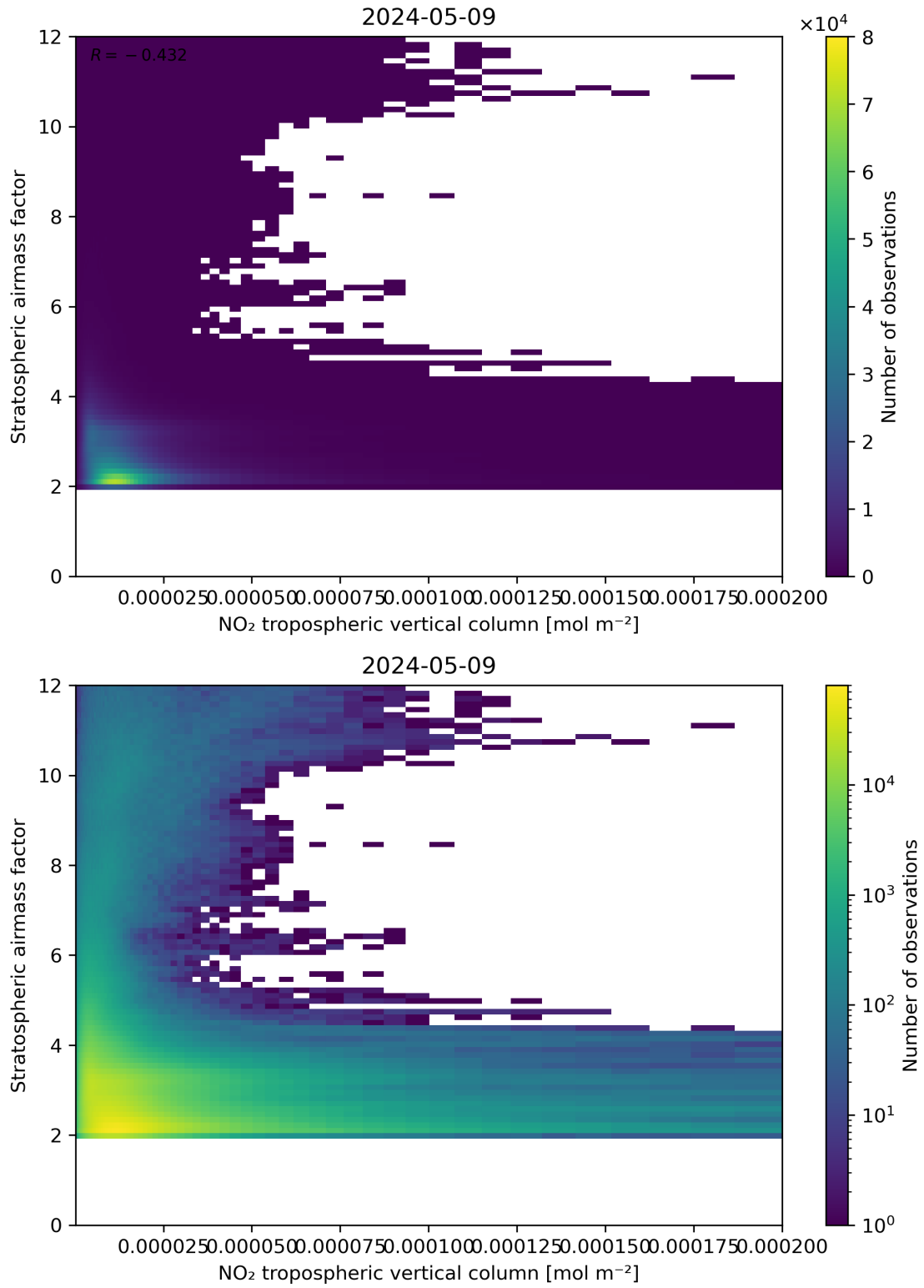
Figure 121: Scatter density plot of “NO 2 tropospheric vertical column” against “Stratospheric airmass factor” for 2024-05-08 to 2024-05-10.
