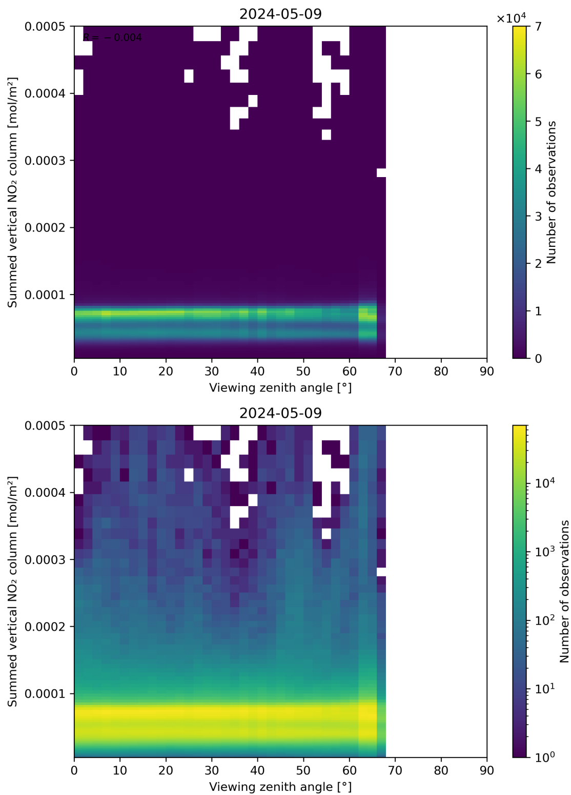
Figure 165: Scatter density plot of “Viewing zenith angle” against “Summed vertical NO 2 column” for 2024-05-08 to 2024-05-10.
