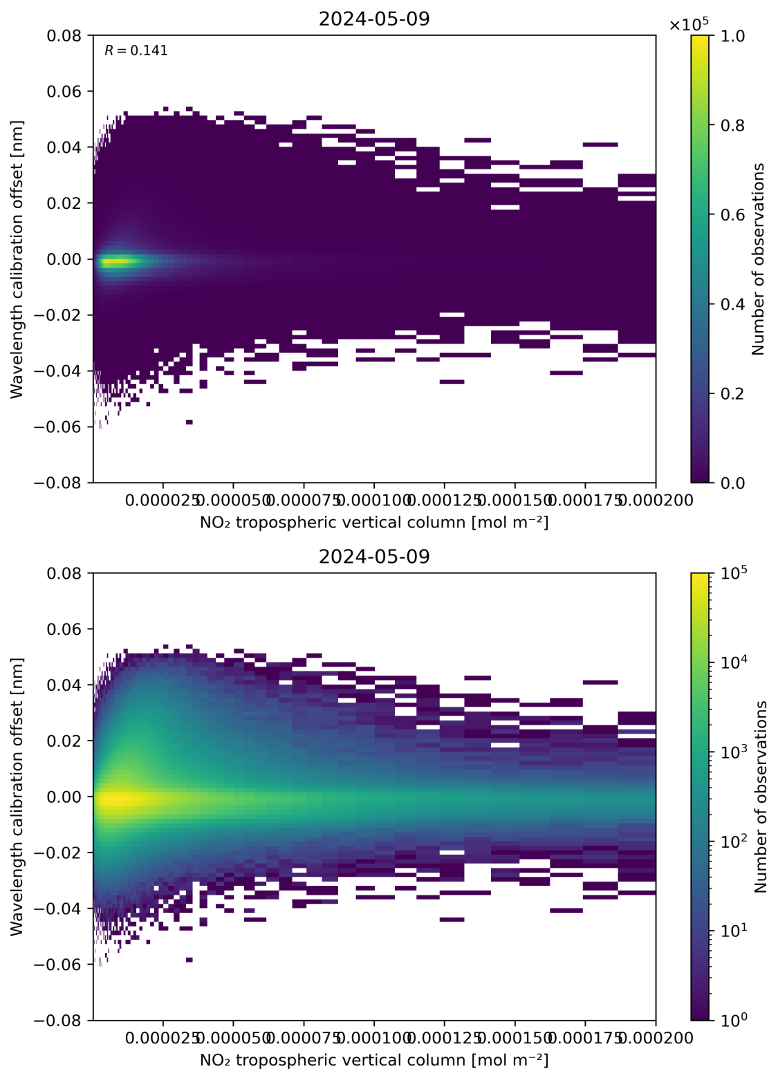
Figure 143: Scatter density plot of “NO 2 tropospheric vertical column” against “Wavelength calibration offset” for 2024-05-08 to 2024-05-10.
