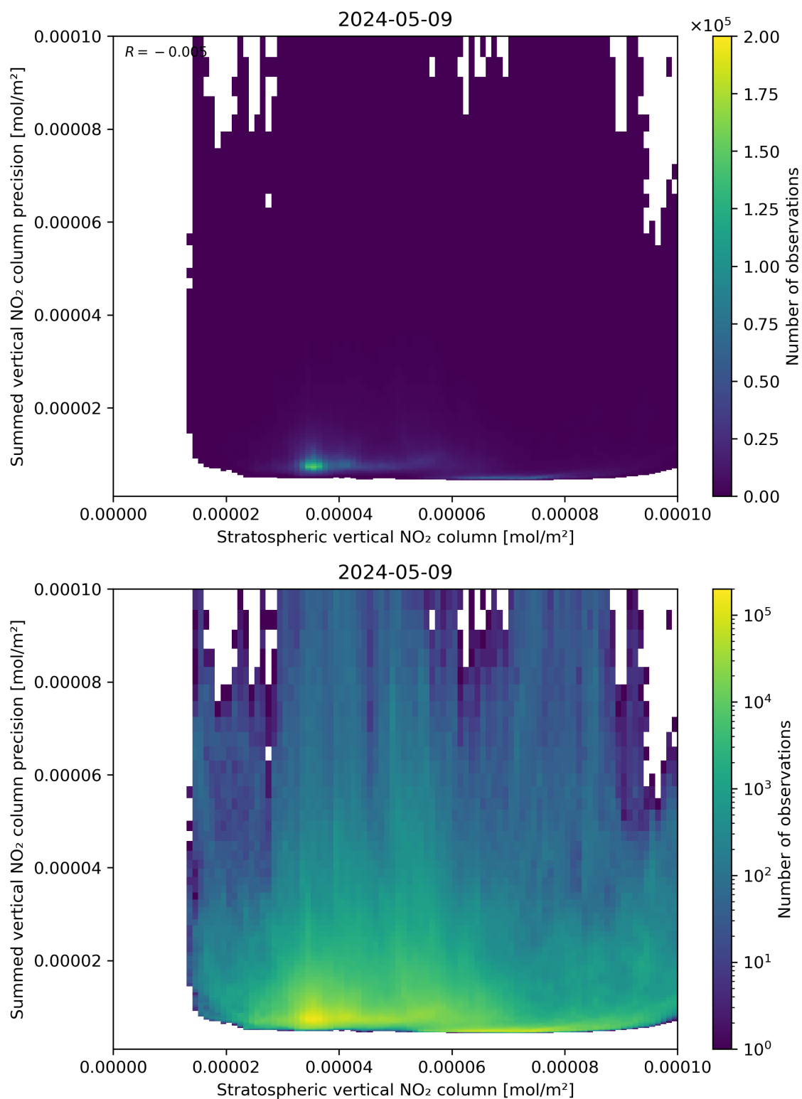
Figure 99: Scatter density plot of “Stratospheric vertical NO 2 column” against “Summed vertical NO 2 column precision” for 2024-05-08 to 2024-05-10.
