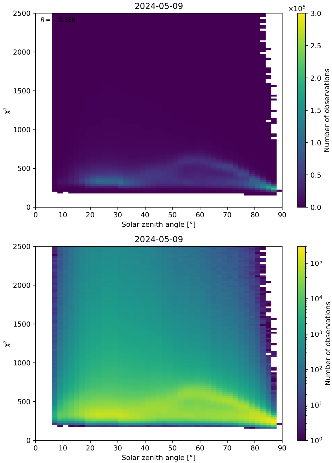
Figure 148: Scatter density plot of “Solar zenith angle” against “ \chi^2 ” for 2024-05-08 to 2024-05-10.
