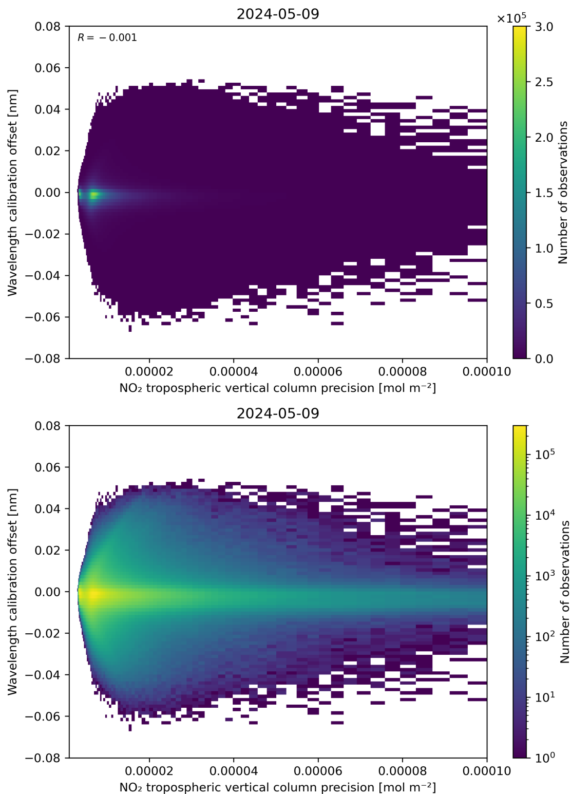
Figure 141: Scatter density plot of “NO 2 tropospheric vertical column precision” against “Wavelength calibration offset” for 2024-05-08 to 2024-05-10.
