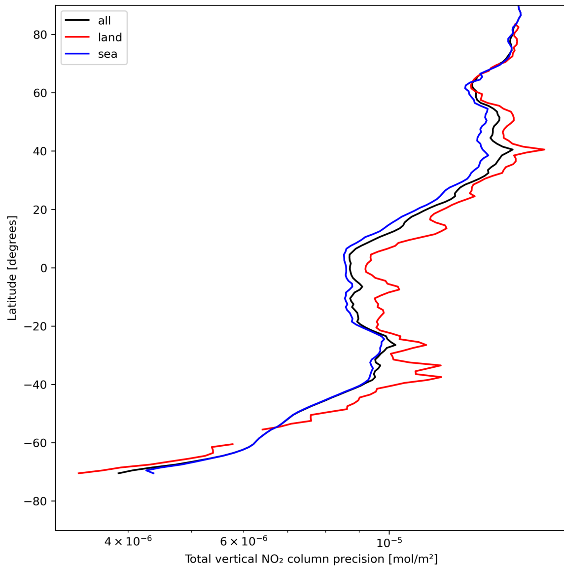
Figure 22: Zonal average of “Total vertical NO 2 column precision” for 2024-05-08 to 2024-05-10.
