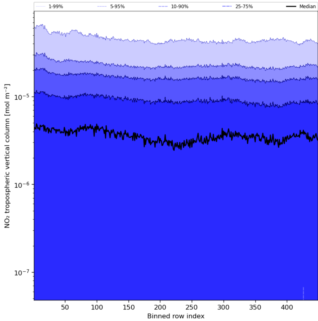
Figure 46: Along track statistics of “NO 2 tropospheric vertical column” for 2024-05-08 to 2024-05-10
