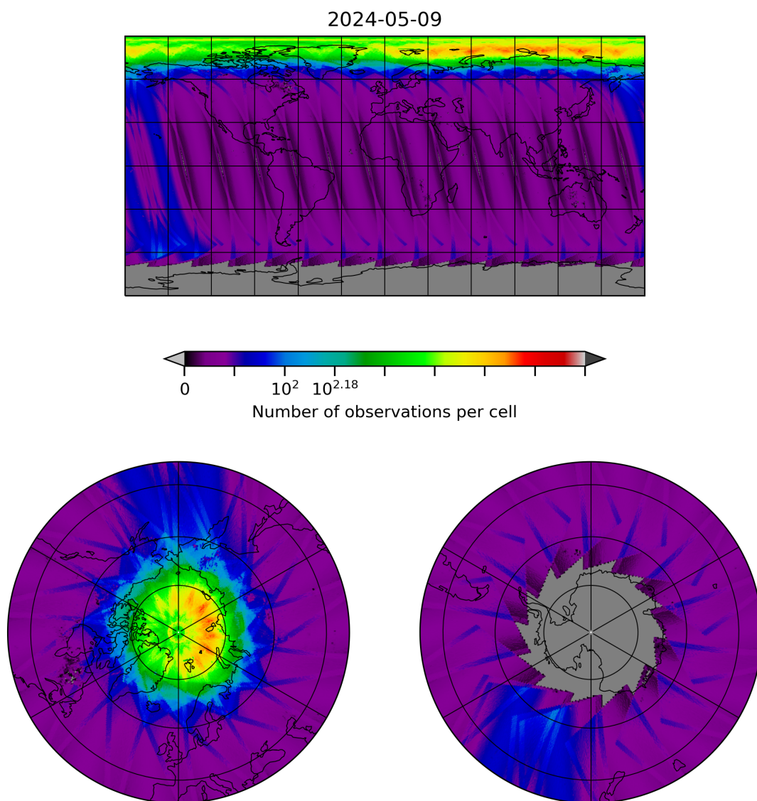
Figure 10: Map of the number of observations for 2024-05-08 to 2024-05-10
