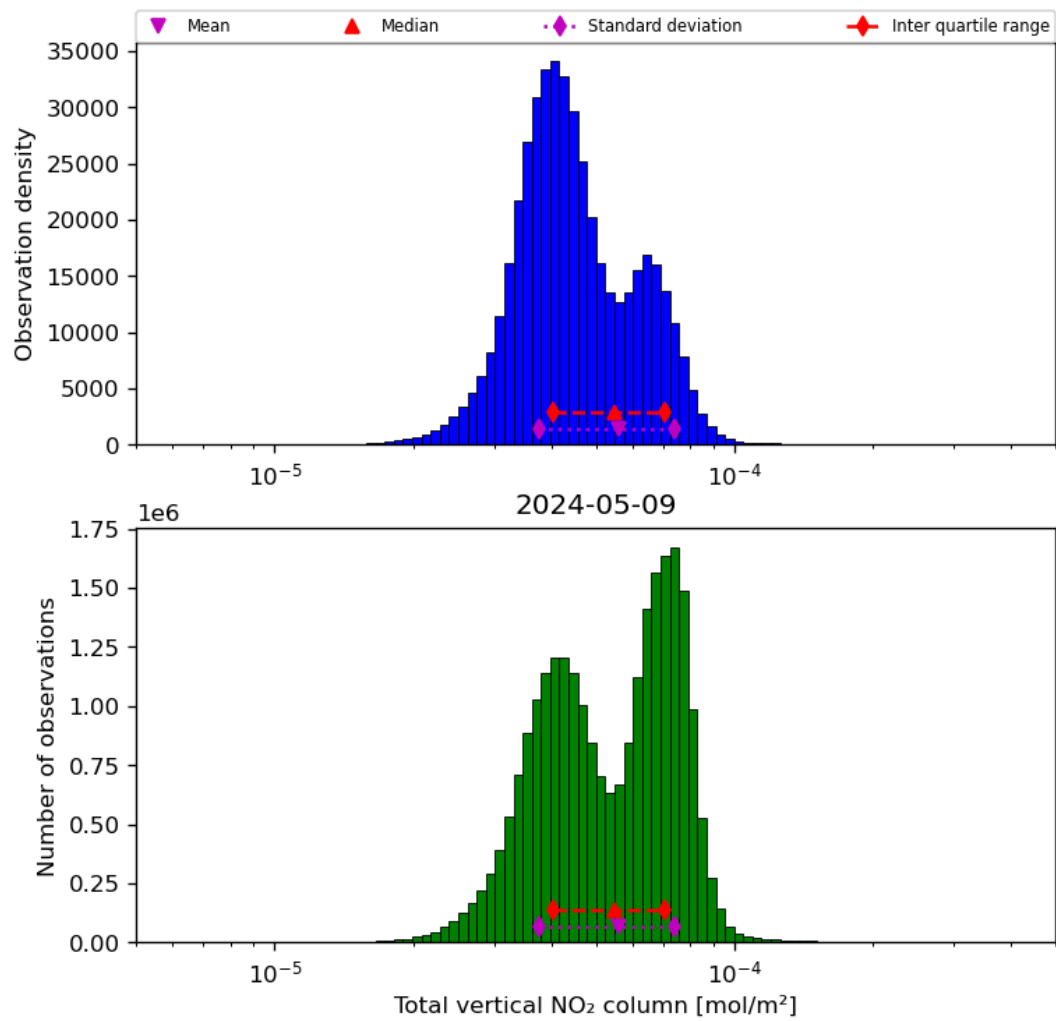
Figure 38: Histogram of “Total vertical NO 2 column” for 2024-05-08 to 2024-05-10
