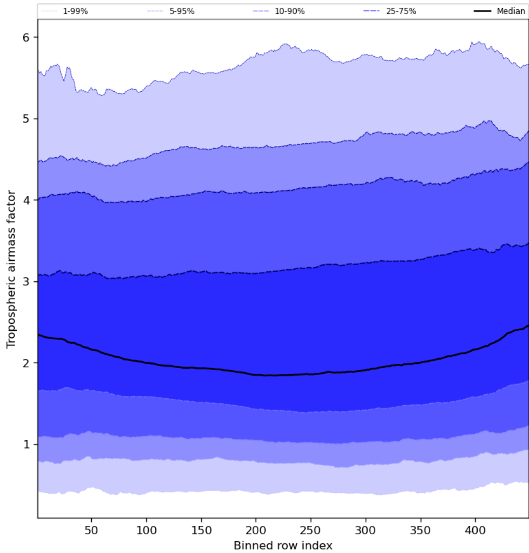
Figure 48: Along track statistics of “Tropospheric airmass factor” for 2024-05-08 to 2024-05-10
