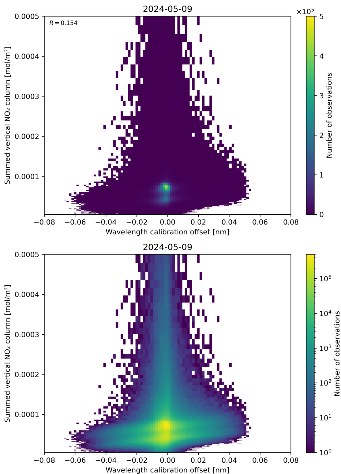
Figure 177: Scatter density plot of “Wavelength calibration offset” against “Summed vertical NO 2 column” for 2024-05-08 to 2024-05-10.
