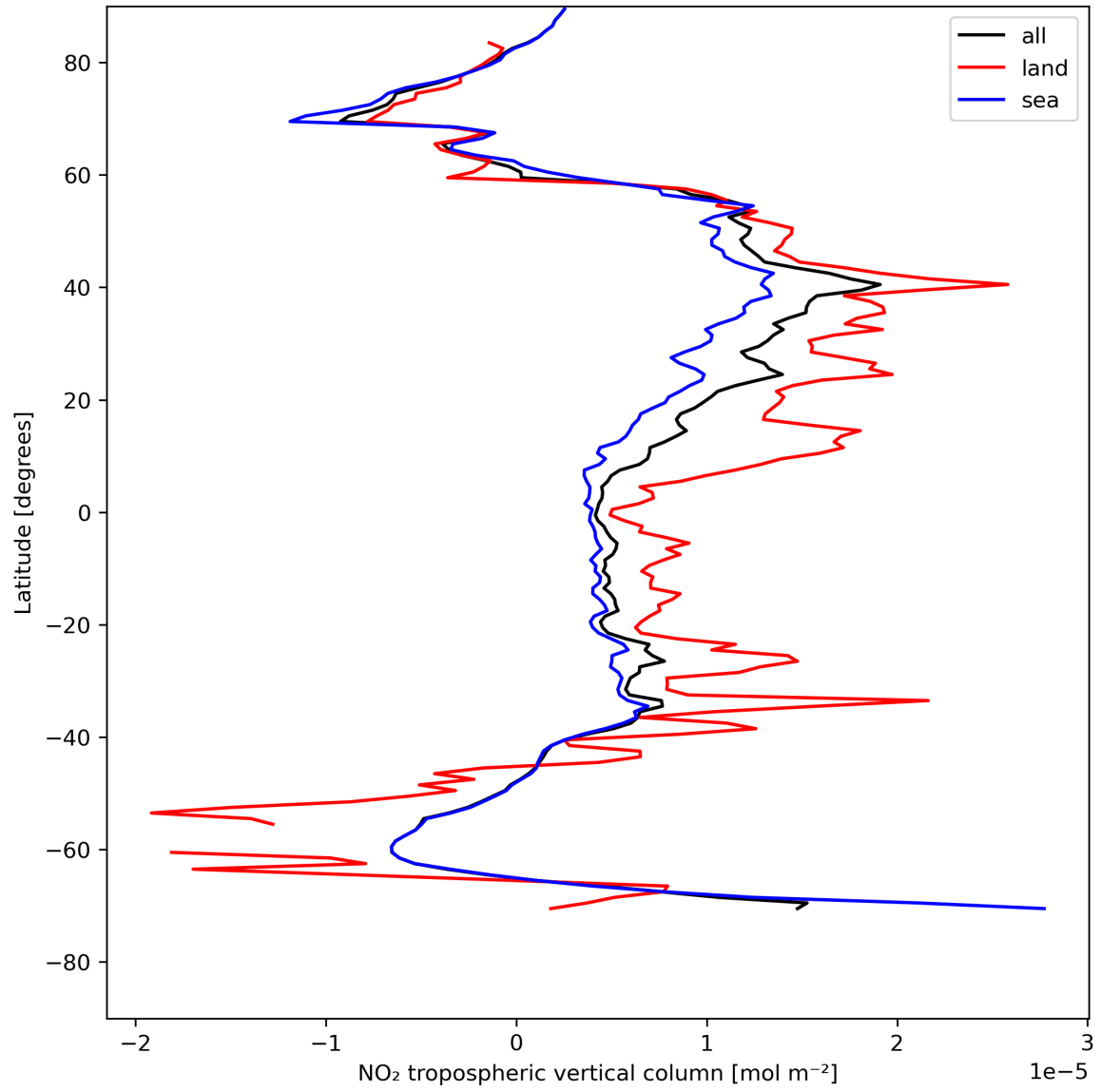
Figure 12: Zonal average of “NO 2 tropospheric vertical column” for 2024-05-08 to 2024-05-10.
