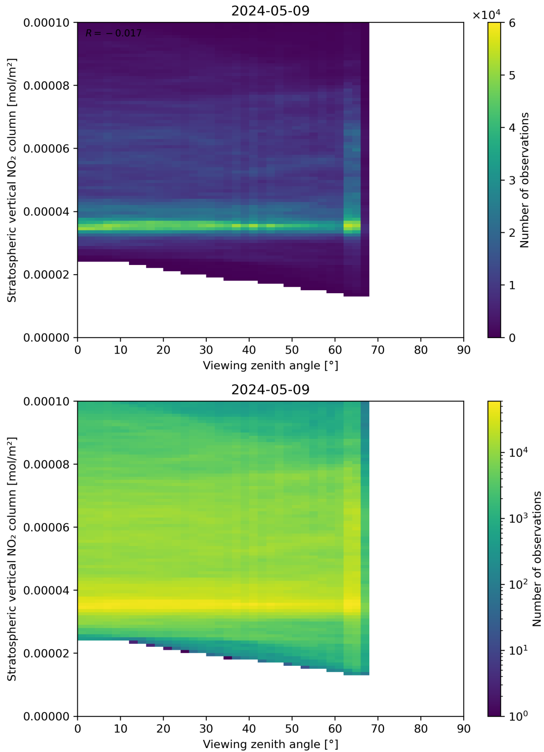
Figure 164: Scatter density plot of “Viewing zenith angle” against “Stratospheric vertical NO 2 column” for 2024-05-08 to 2024-05-10.
