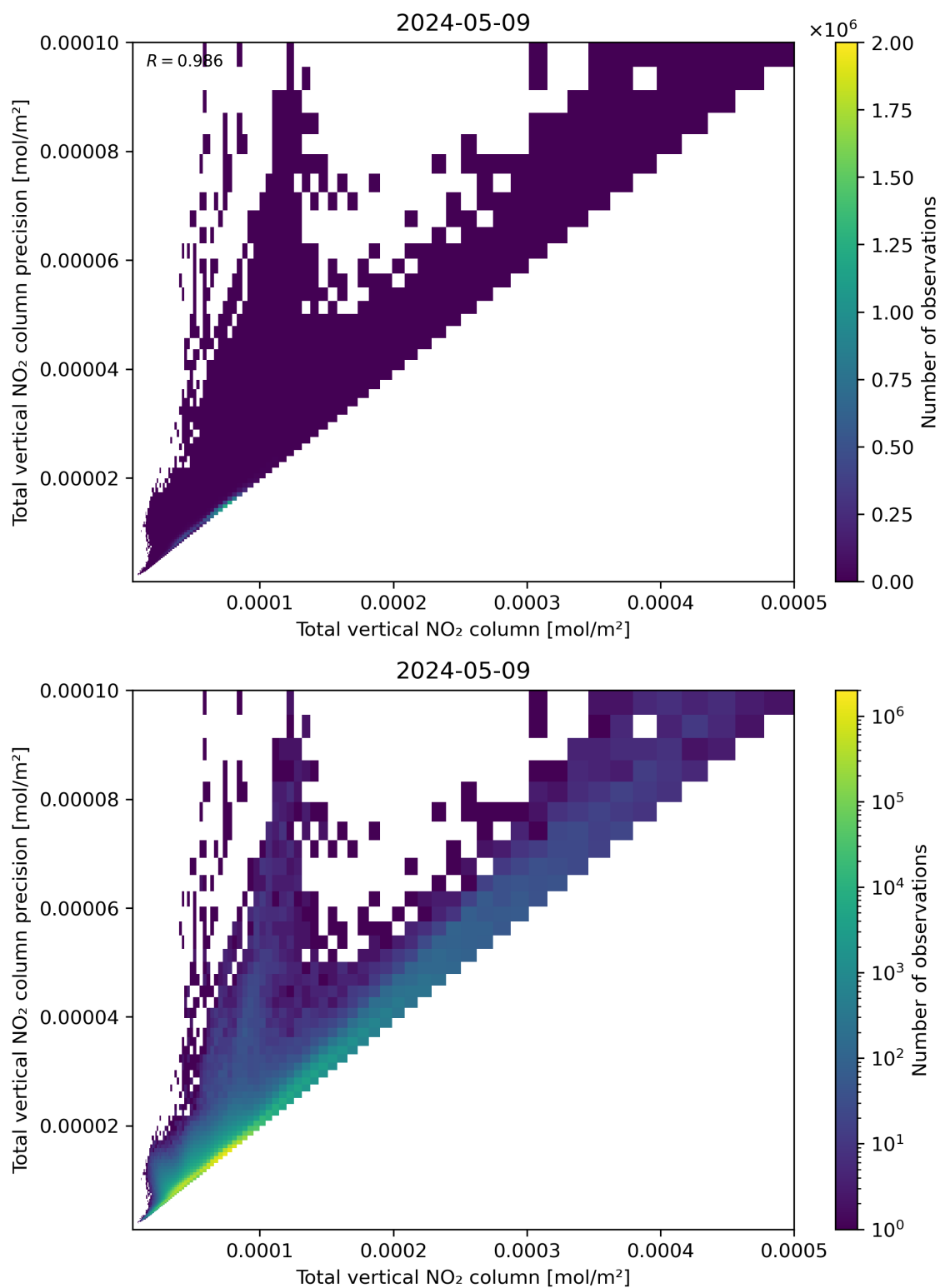
Figure 114: Scatter density plot of “Total vertical NO 2 column” against “Total vertical NO 2 column precision” for 2024-05-08 to 2024-05-10.
