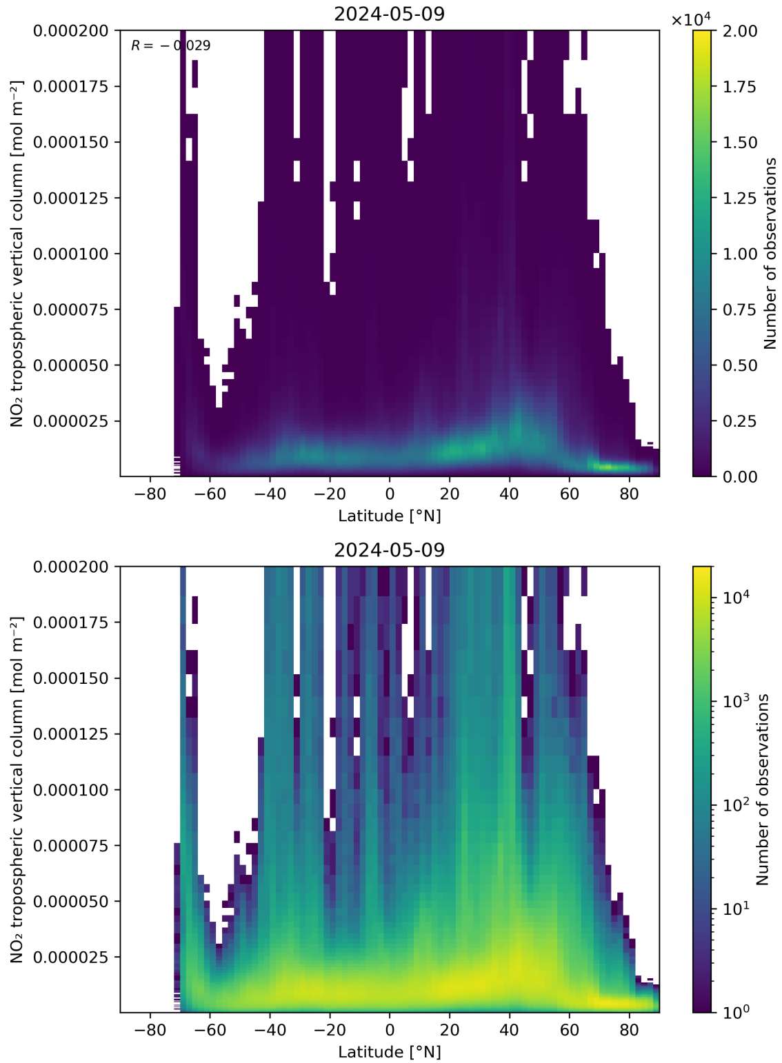
Figure 92: Scatter density plot of “Latitude” against “NO 2 tropospheric vertical column” for 2024-05-08 to 2024-05-10.
