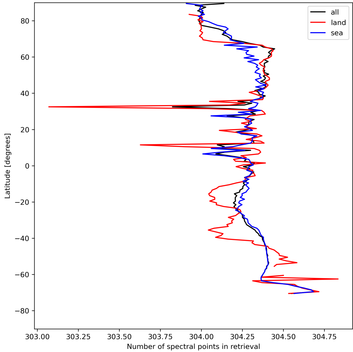
Figure 16: Zonal average of “Number of spectral points in retrieval” for 2024-05-08 to 2024-05-10.
