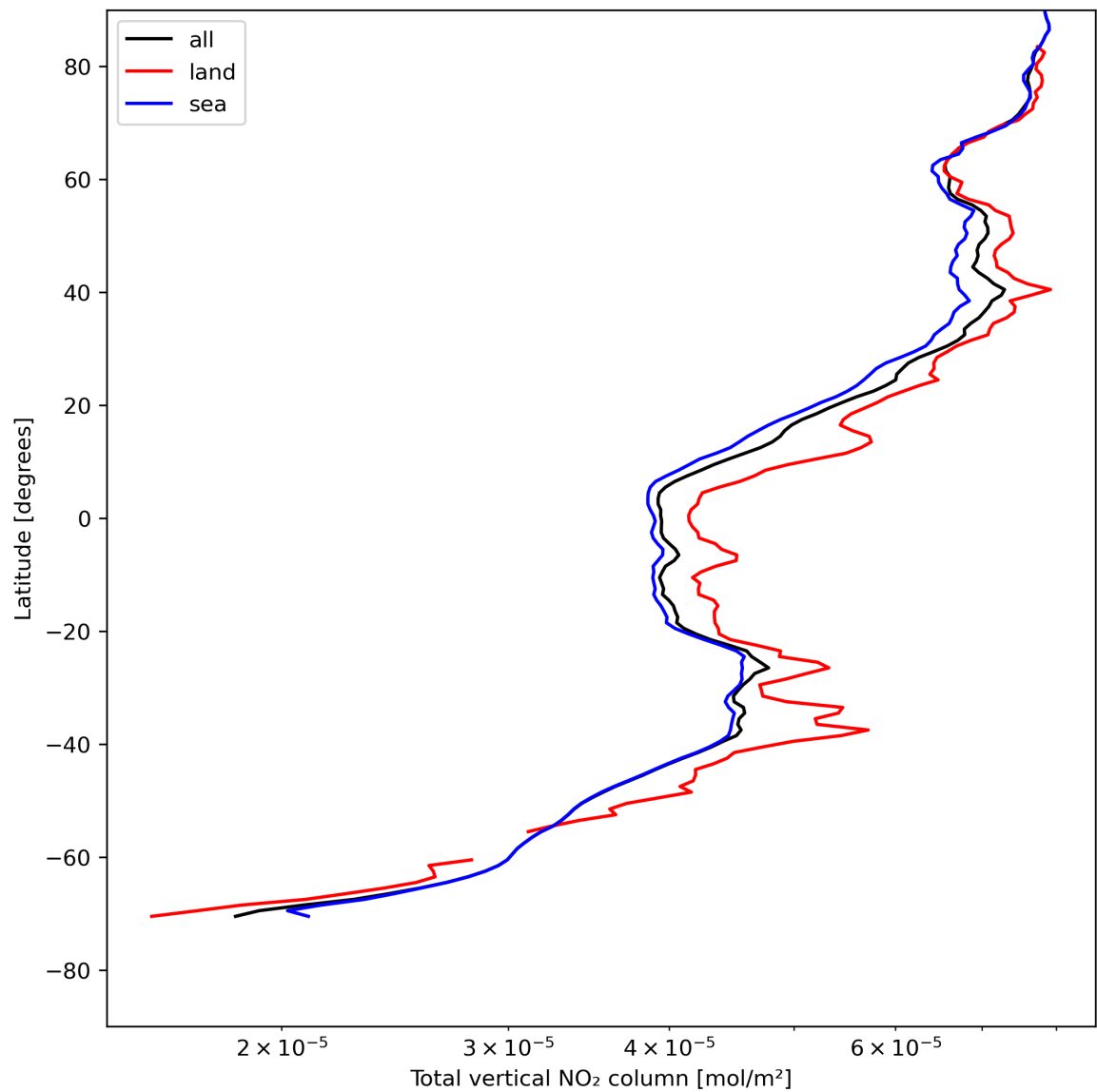
Figure 21: Zonal average of “Total vertical NO 2 column” for 2024-05-08 to 2024-05-10.
