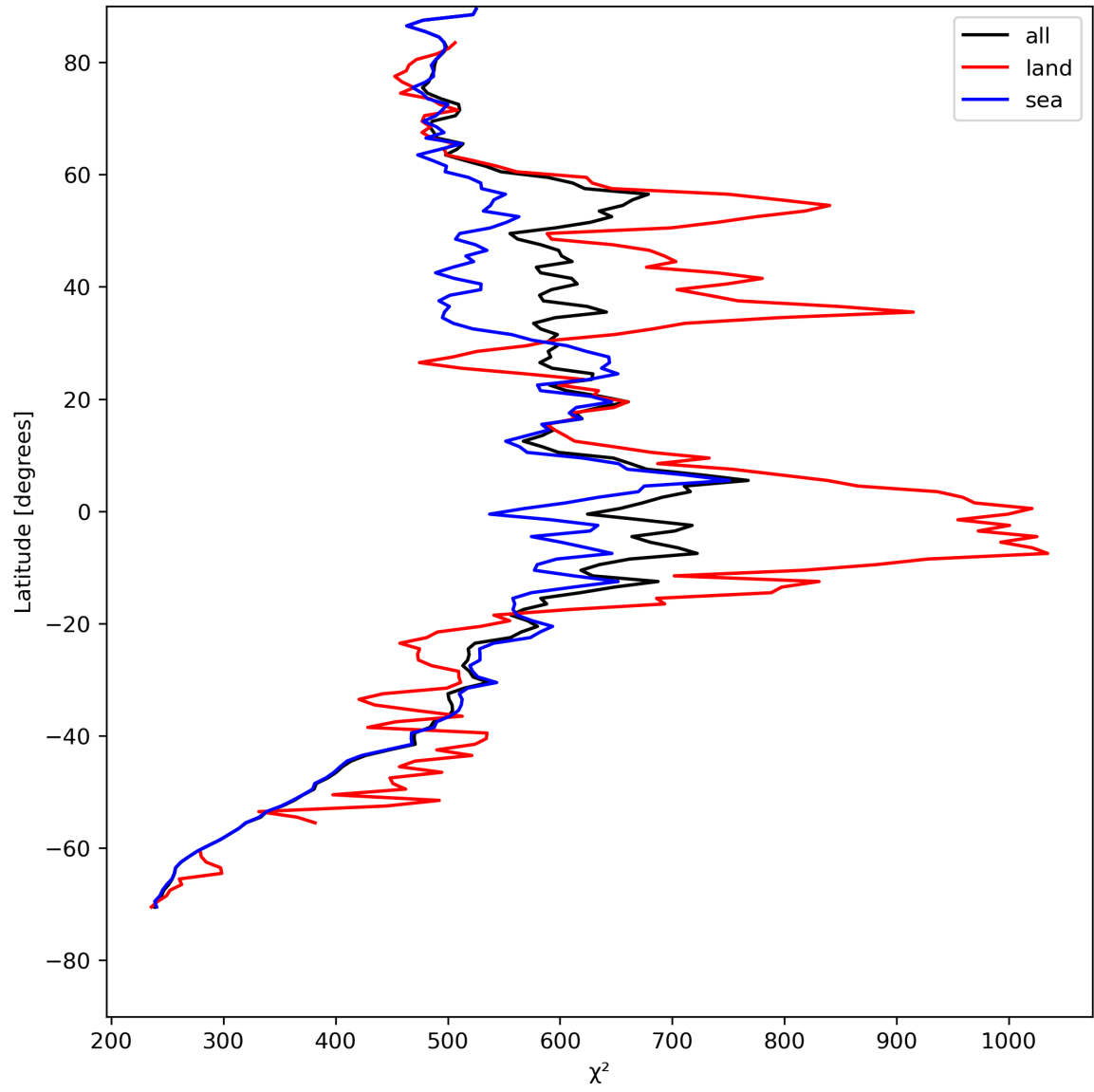
Figure 25: Zonal average of “ \chi^2 ” for 2024-05-08 to 2024-05-10.
