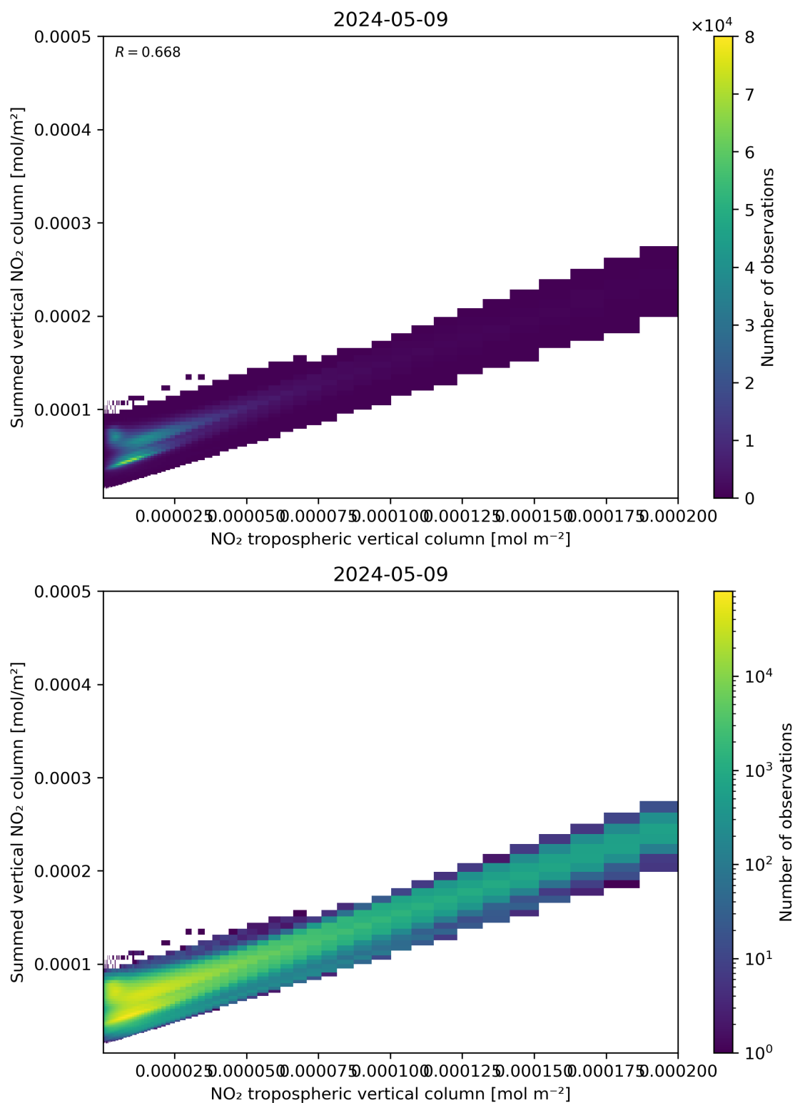
Figure 126: Scatter density plot of “NO 2 tropospheric vertical column” against “Summed vertical NO 2 column” for 2024-05-08 to 2024-05-10.
