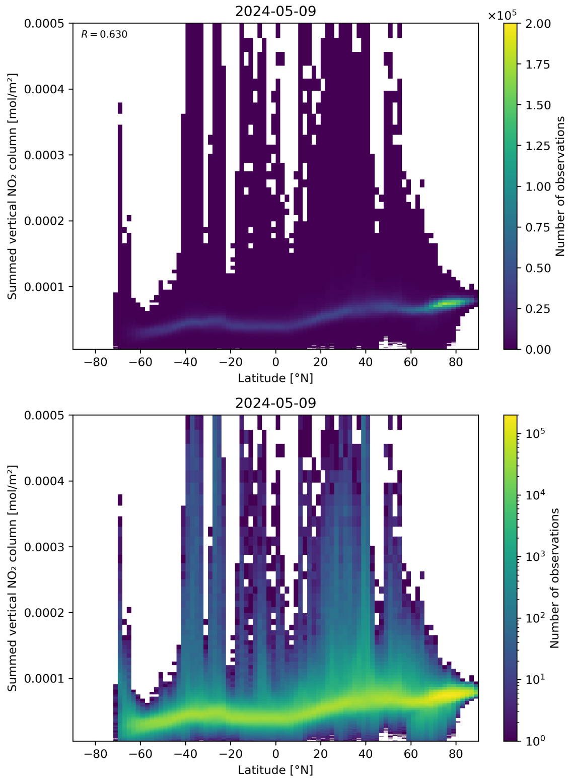
Figure 88: Scatter density plot of “Latitude” against “Summed vertical NO 2 column” for 2024-05-08 to 2024-05-10.
