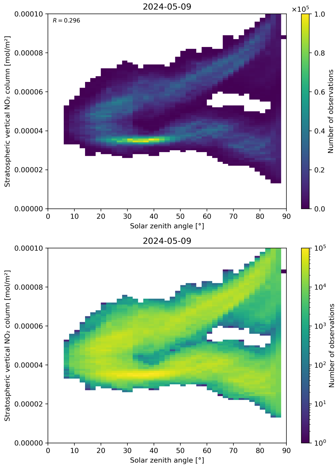
Figure 150: Scatter density plot of “Solar zenith angle” against “Stratospheric vertical NO 2 column” for 2024-05-08 to 2024-05-10.
