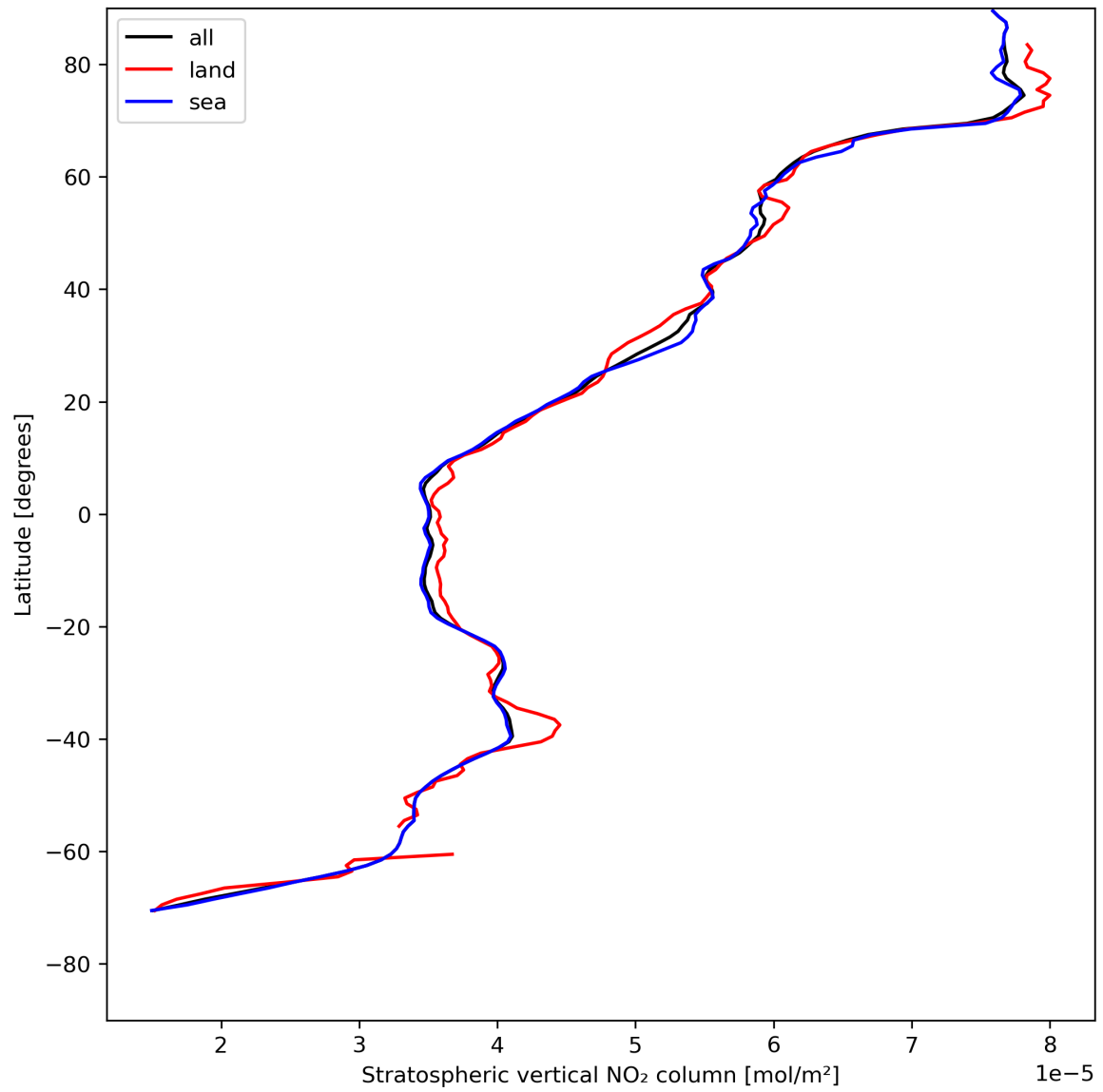
Figure 19: Zonal average of “Stratospheric vertical NO 2 column” for 2024-05-08 to 2024-05-10.
