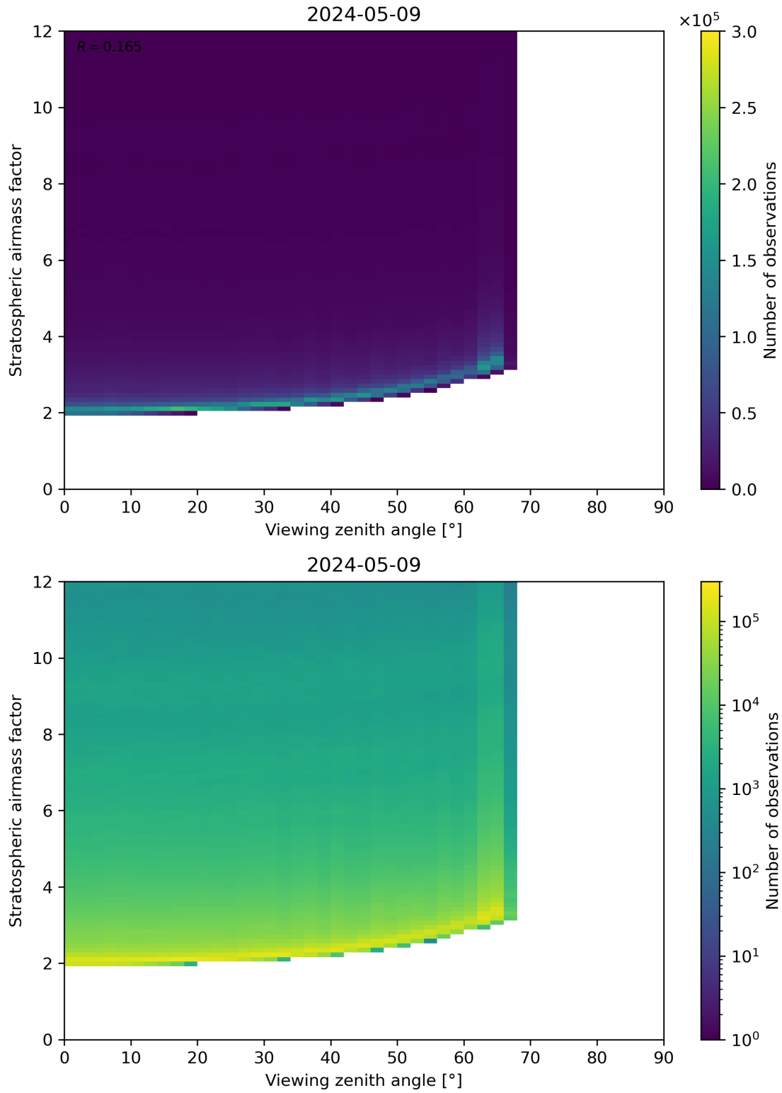
Figure 159: Scatter density plot of “Viewing zenith angle” against “Stratospheric airmass factor” for 2024-05-08 to 2024-05-10.
