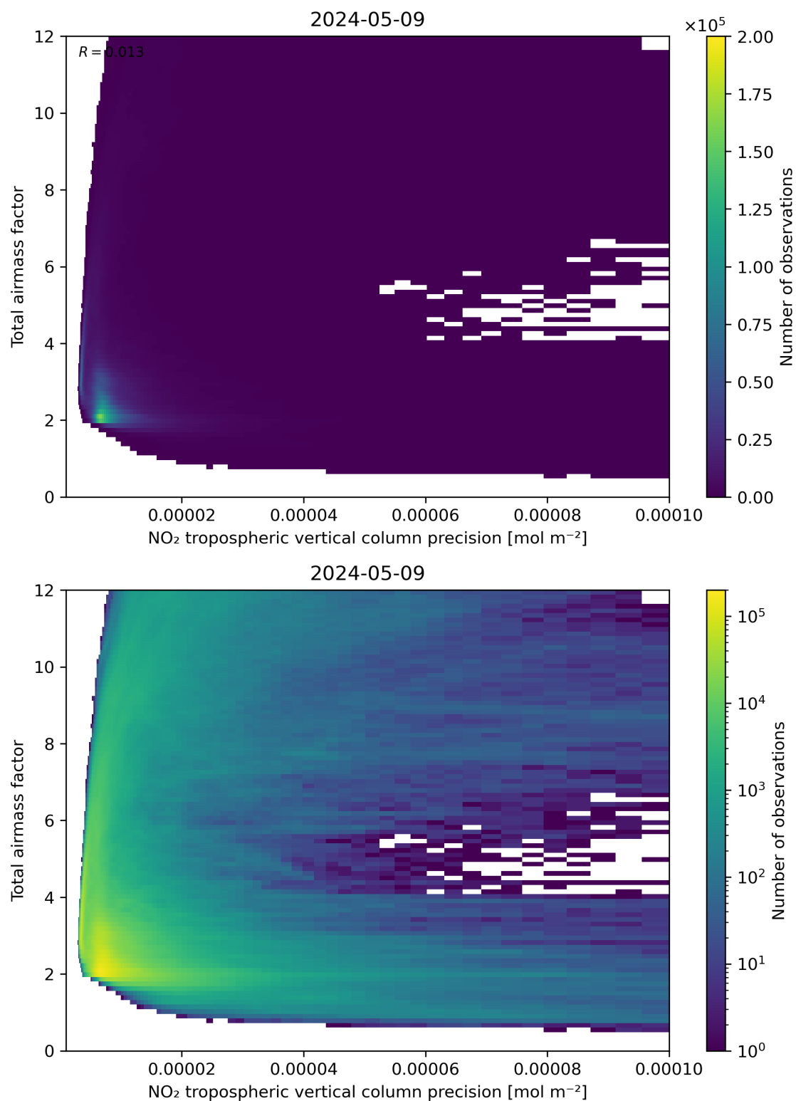
Figure 132: Scatter density plot of “NO 2 tropospheric vertical column precision” against “Total air mass factor” for 2024-05-08 to 2024-05-10.
