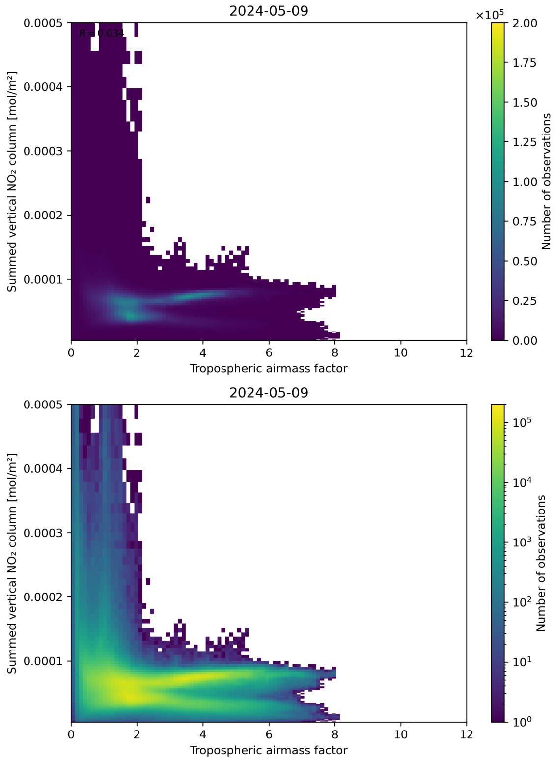
Figure 75: Scatter density plot of “Tropospheric airmass factor” against “Summed vertical NO 2 column” for 2024-05-08 to 2024-05-10.
