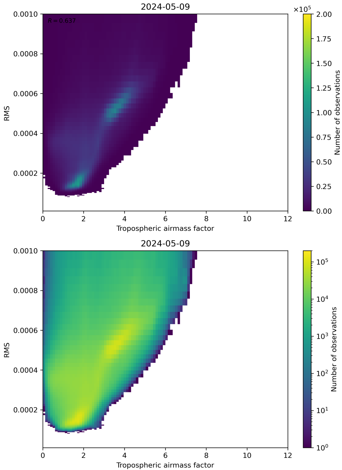
Figure 79: Scatter density plot of “Tropospheric airmass factor” against “RMS” for 2024-05-08 to 2024-05-10.
