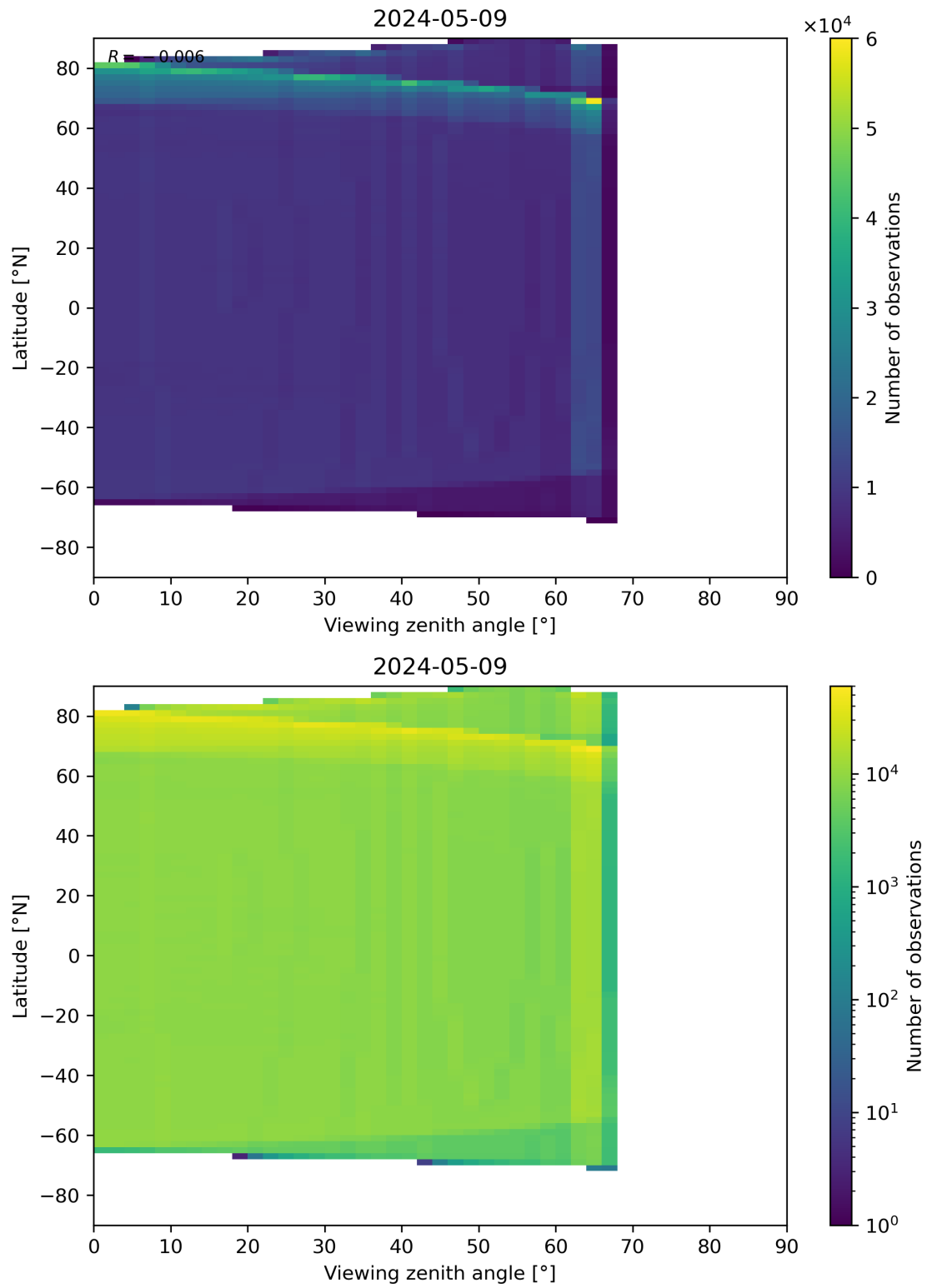
Figure 163: Scatter density plot of “Viewing zenith angle” against “Latitude” for 2024-05-08 to 2024-05-10.
