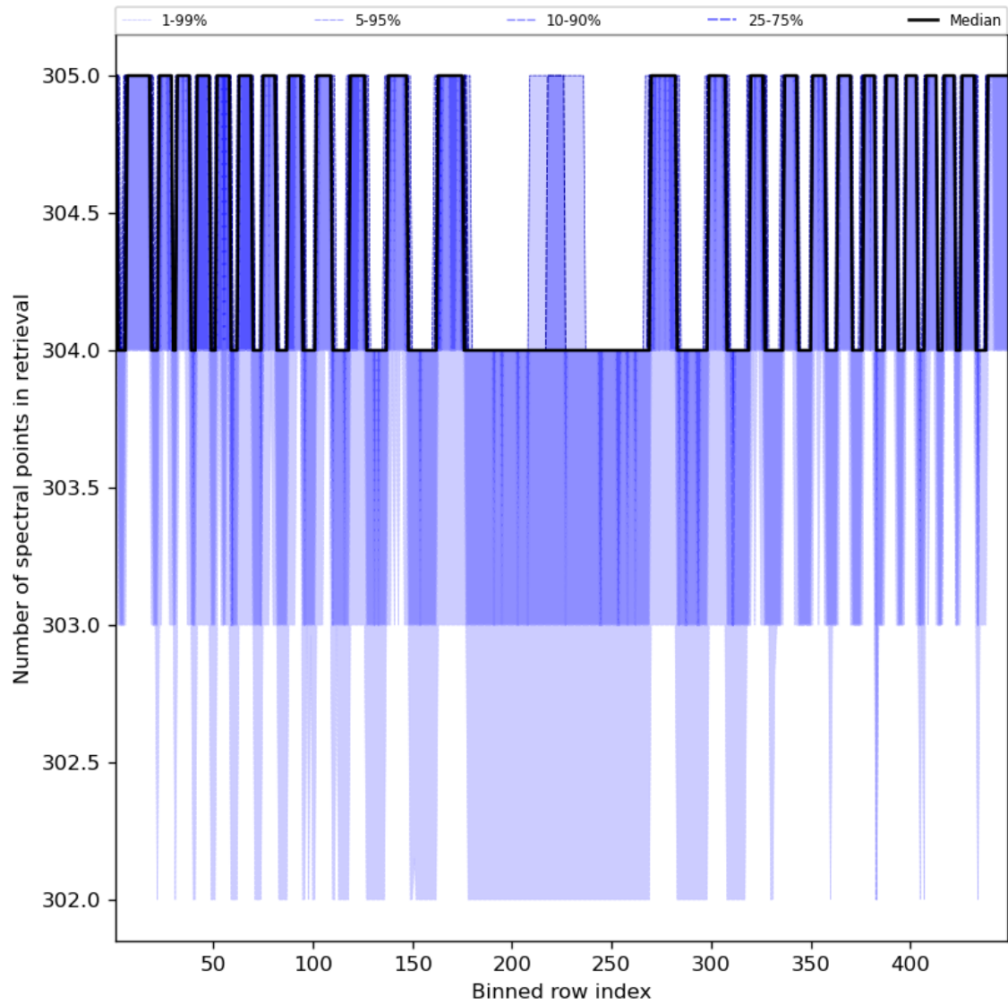
Figure 50: Along track statistics of “Number of spectral points in retrieval” for 2024-05-08 to 2024-05-10
