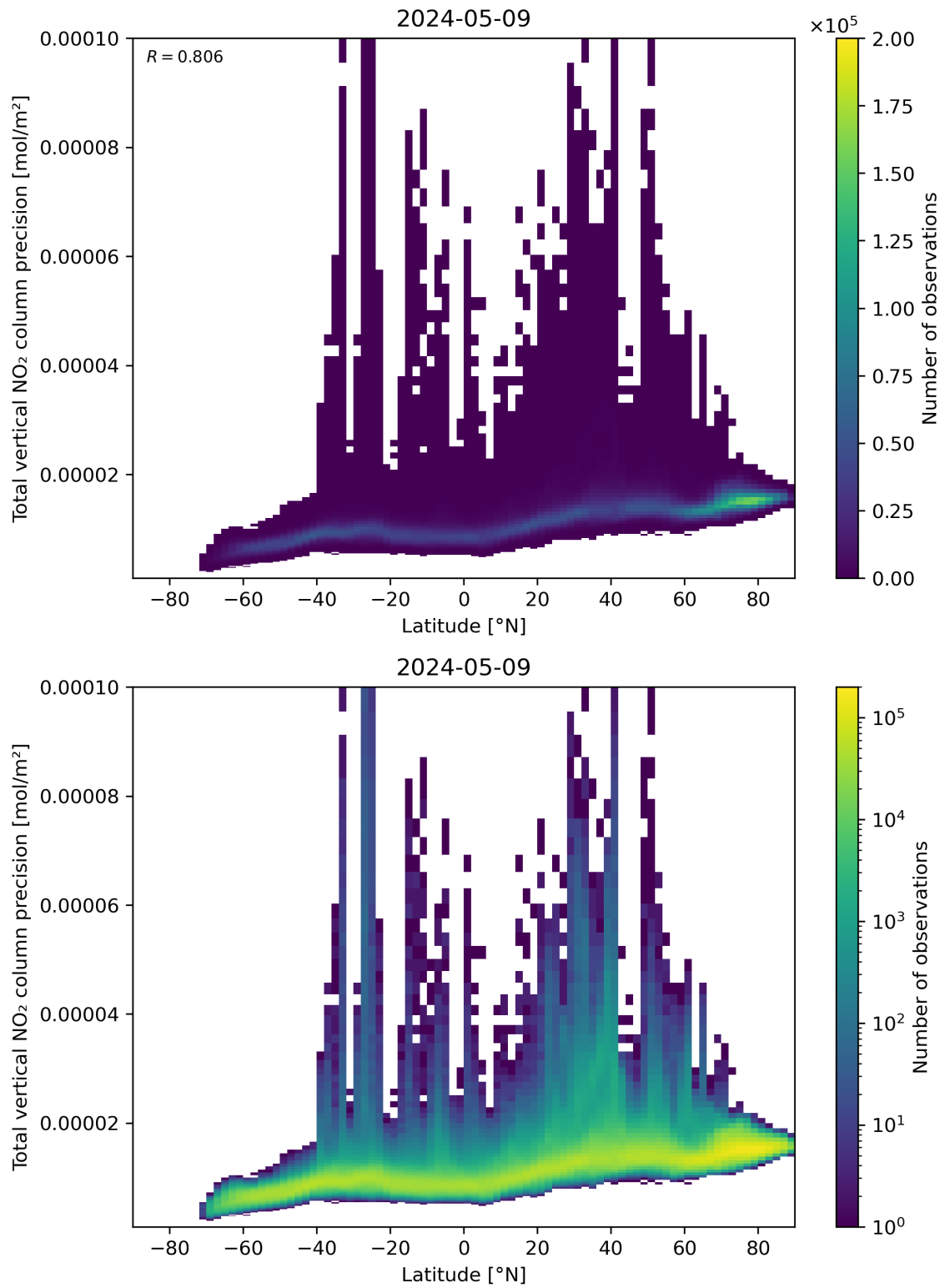
Figure 91: Scatter density plot of “Latitude” against “Total vertical NO 2 column precision” for 2024-05-08 to 2024-05-10.
