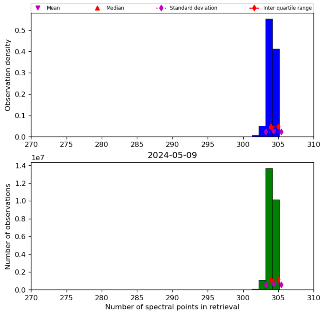
Figure 33: Histogram of “Number of spectral points in retrieval” for 2024-05-08 to 2024-05-10
