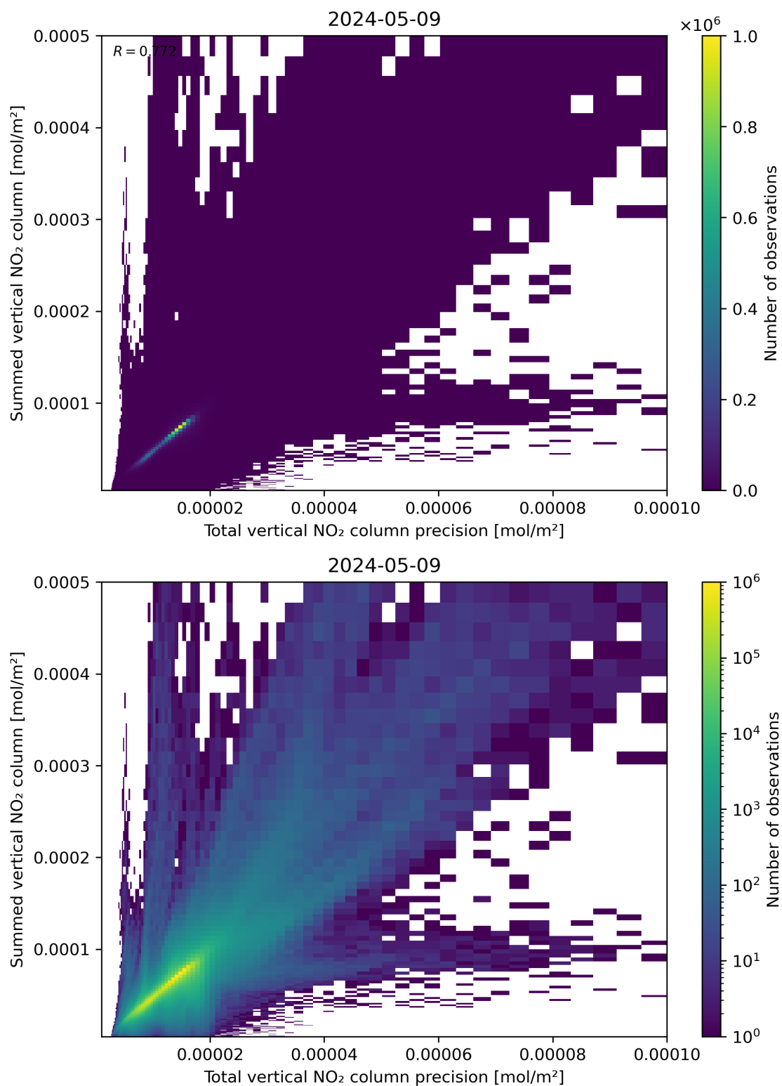
Figure 117: Scatter density plot of “Total vertical NO 2 column precision” against “Summed vertical NO 2 column” for 2024-05-08 to 2024-05-10.
