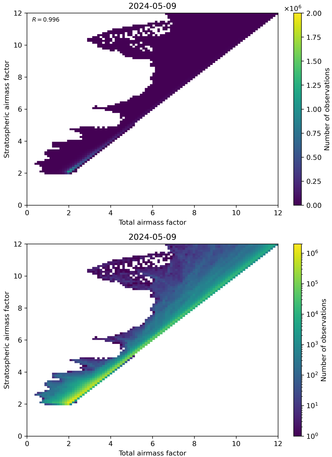
Figure 62: Scatter density plot of “Total airmass factor” against “Stratospheric airmass factor” for 2024-05-08 to 2024-05-10.
