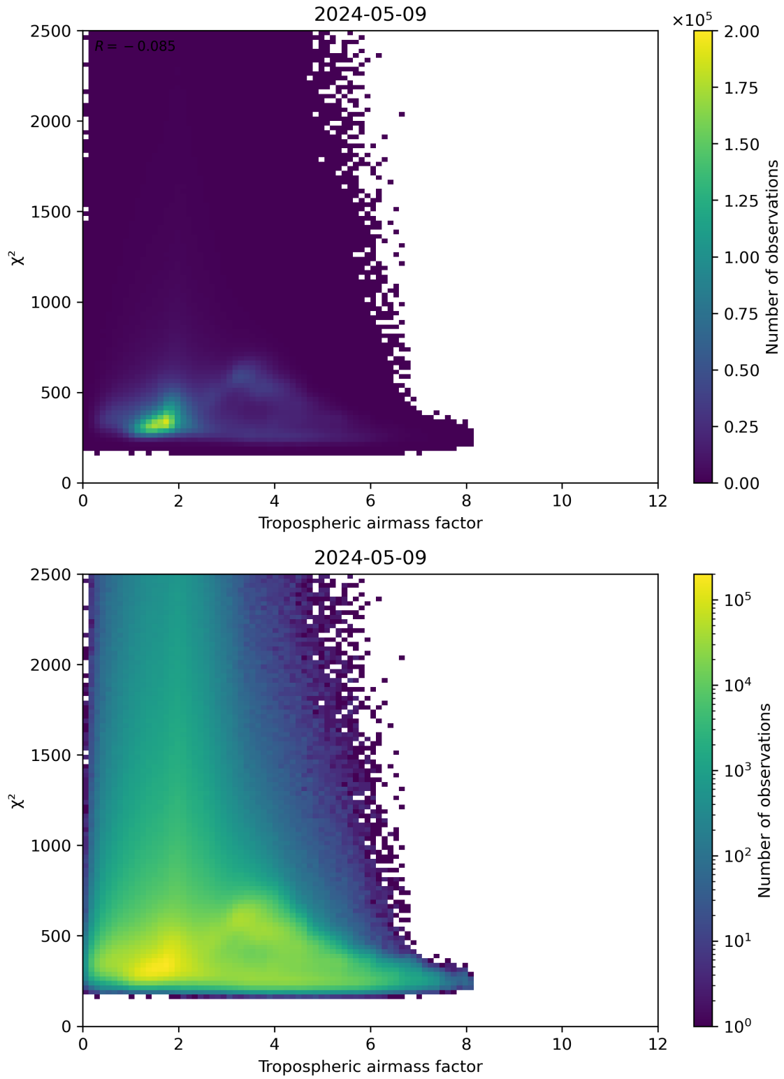
Figure 73: Scatter density plot of “Tropospheric airmass factor” against “ \chi^2 ” for 2024-05-08 to 2024-05-10.
