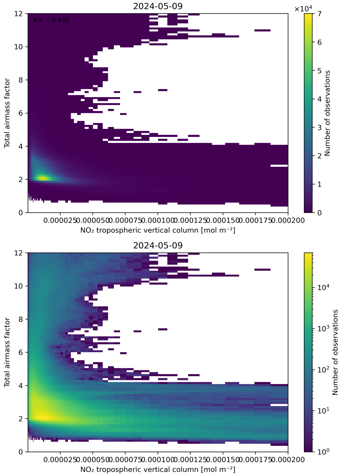
Figure 122: Scatter density plot of “NO 2 tropospheric vertical column” against “Total air mass factor” for 2024-05-08 to 2024-05-10.
