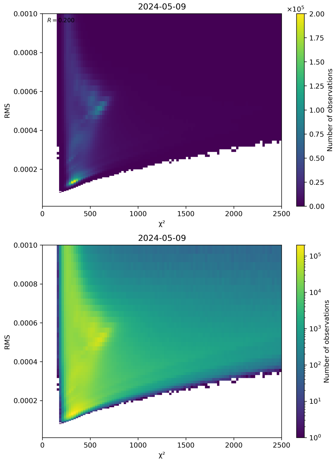
Figure 82: Scatter density plot of “ \chi^2 ” against “RMS” for 2024-05-08 to 2024-05-10.
