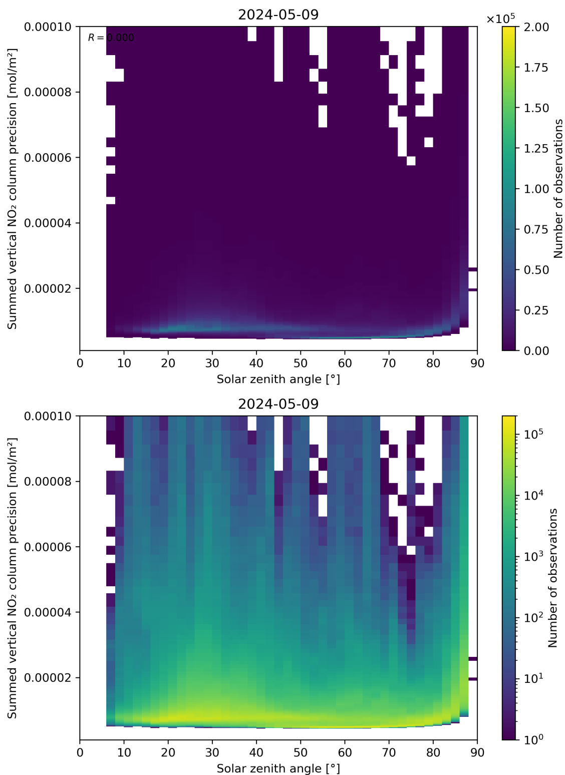
Figure 152: Scatter density plot of “Solar zenith angle” against “Summed vertical NO 2 column precision” for 2024-05-08 to 2024-05-10.
