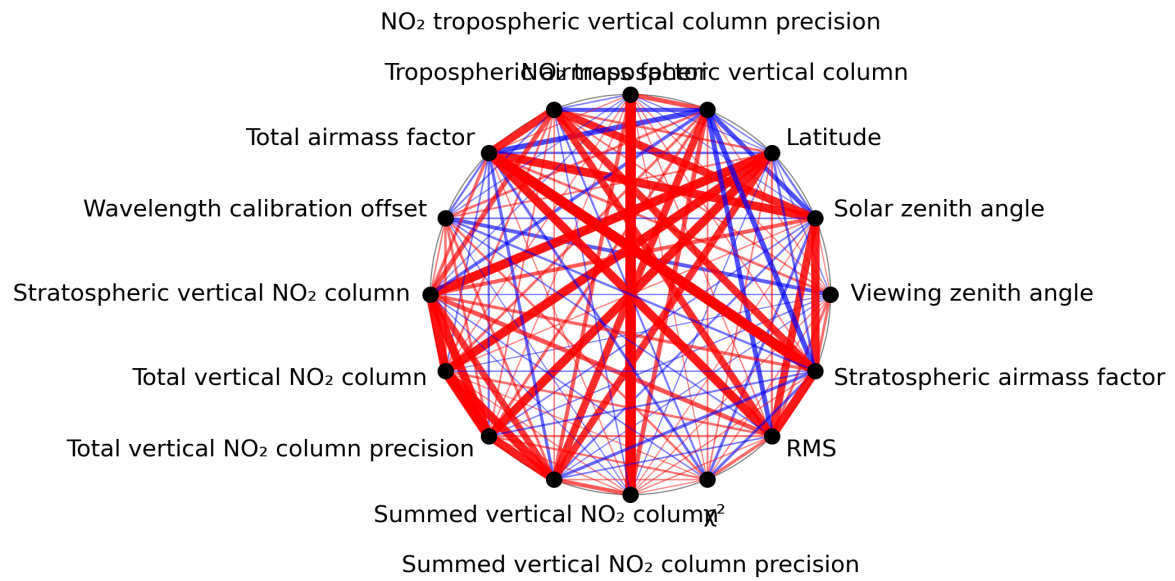
Figure 1: Map of correlation graph for 2024-05-08 to 2024-05-10.
