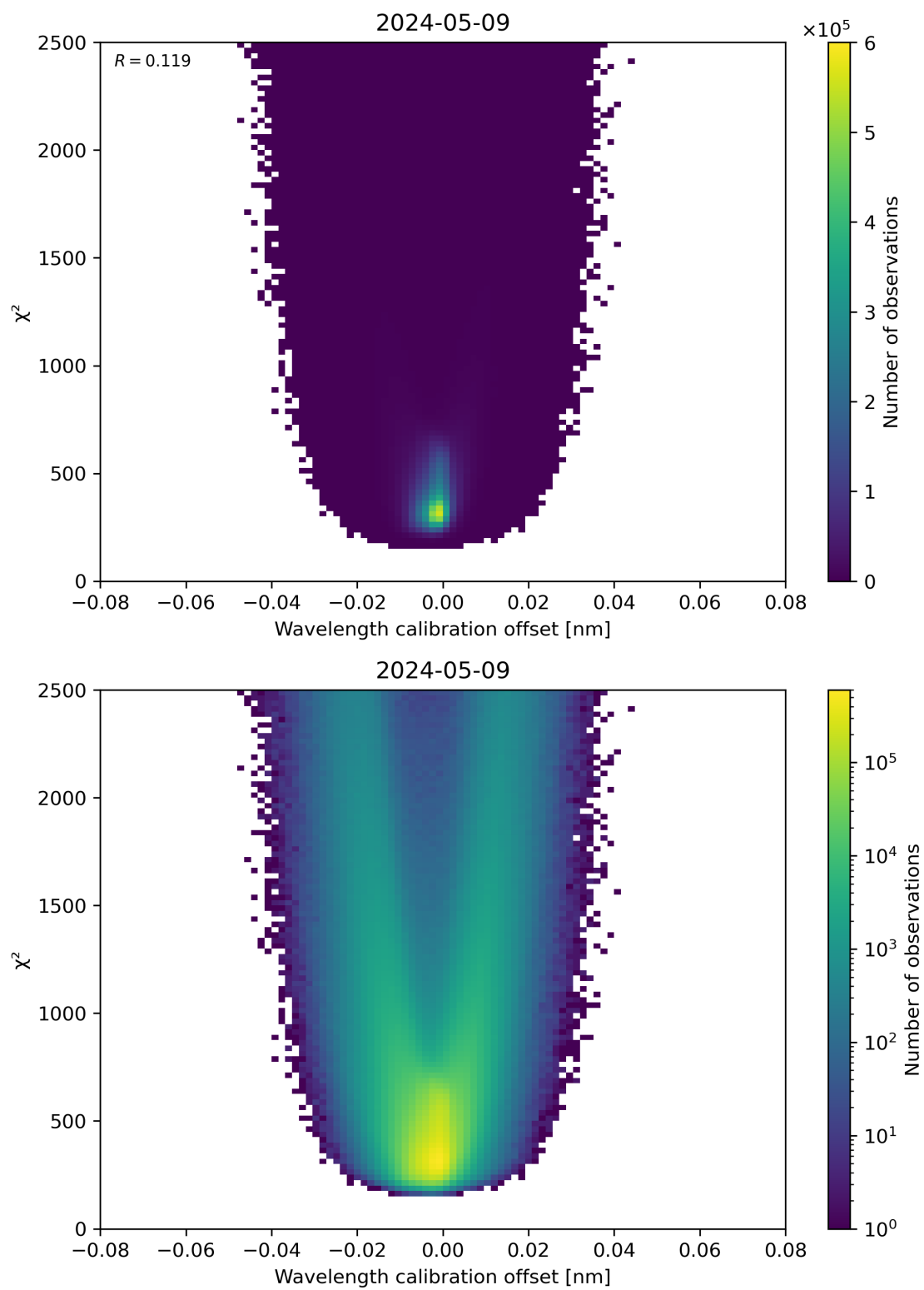
Figure 175: Scatter density plot of “Wavelength calibration offset” against “ \chi^2 ” for 2024-05-08 to 2024-05-10.
