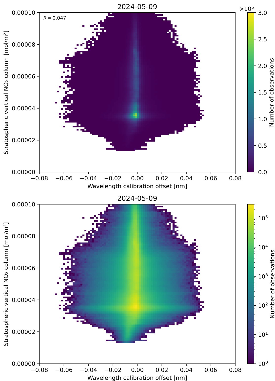
Figure 176: Scatter density plot of “Wavelength calibration offset” against “Stratospheric vertical NO 2 column” for 2024-05-08 to 2024-05-10.
