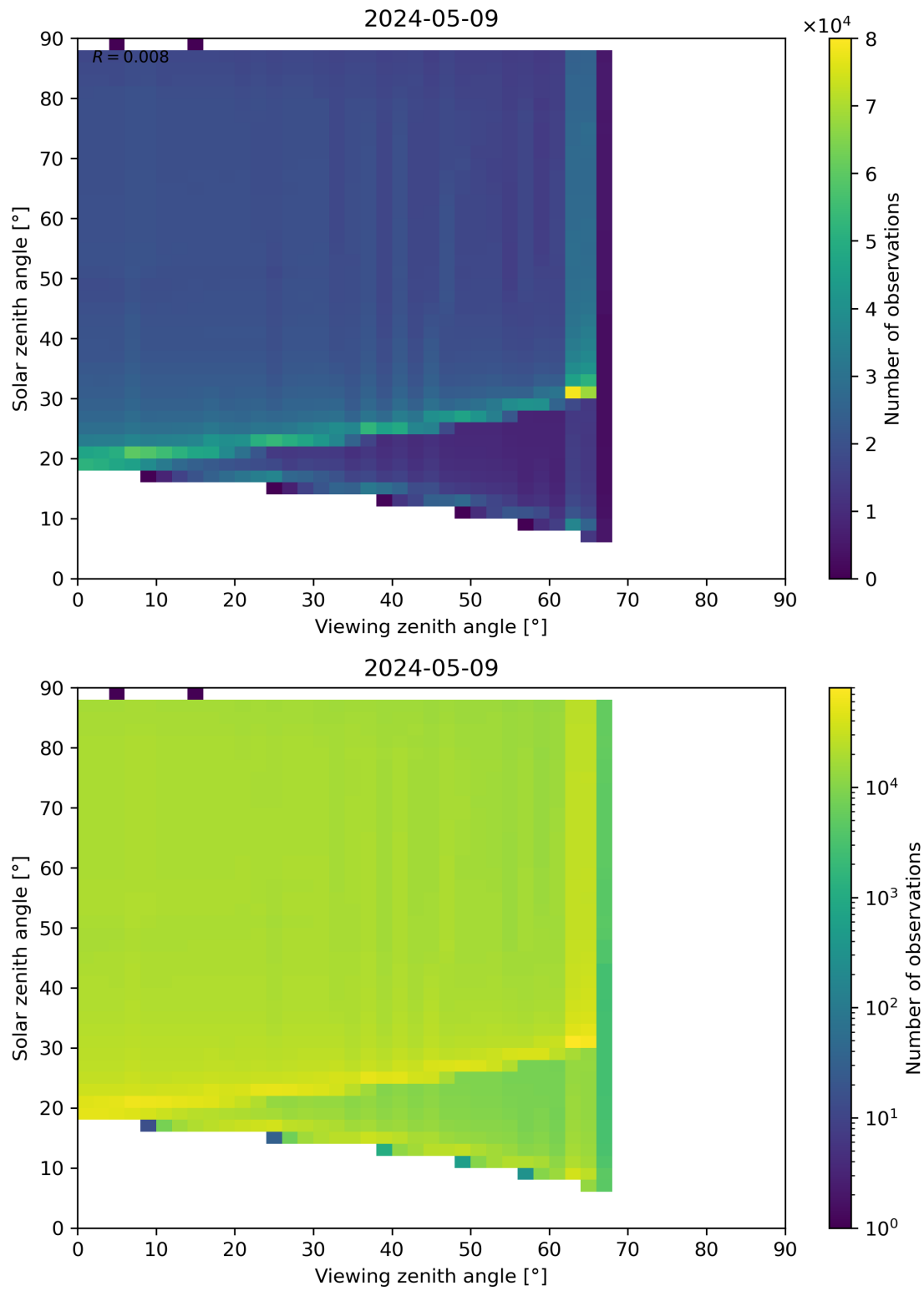
Figure 172: Scatter density plot of “Viewing zenith angle” against “Solar zenith angle” for 2024-05-08 to 2024-05-10.
