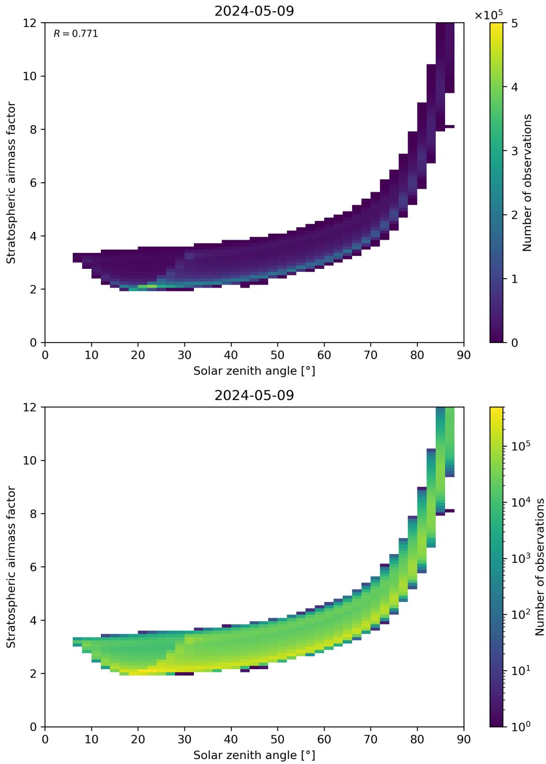
Figure 145: Scatter density plot of “Solar zenith angle” against “Stratospheric airmass factor” for 2024-05-08 to 2024-05-10.
