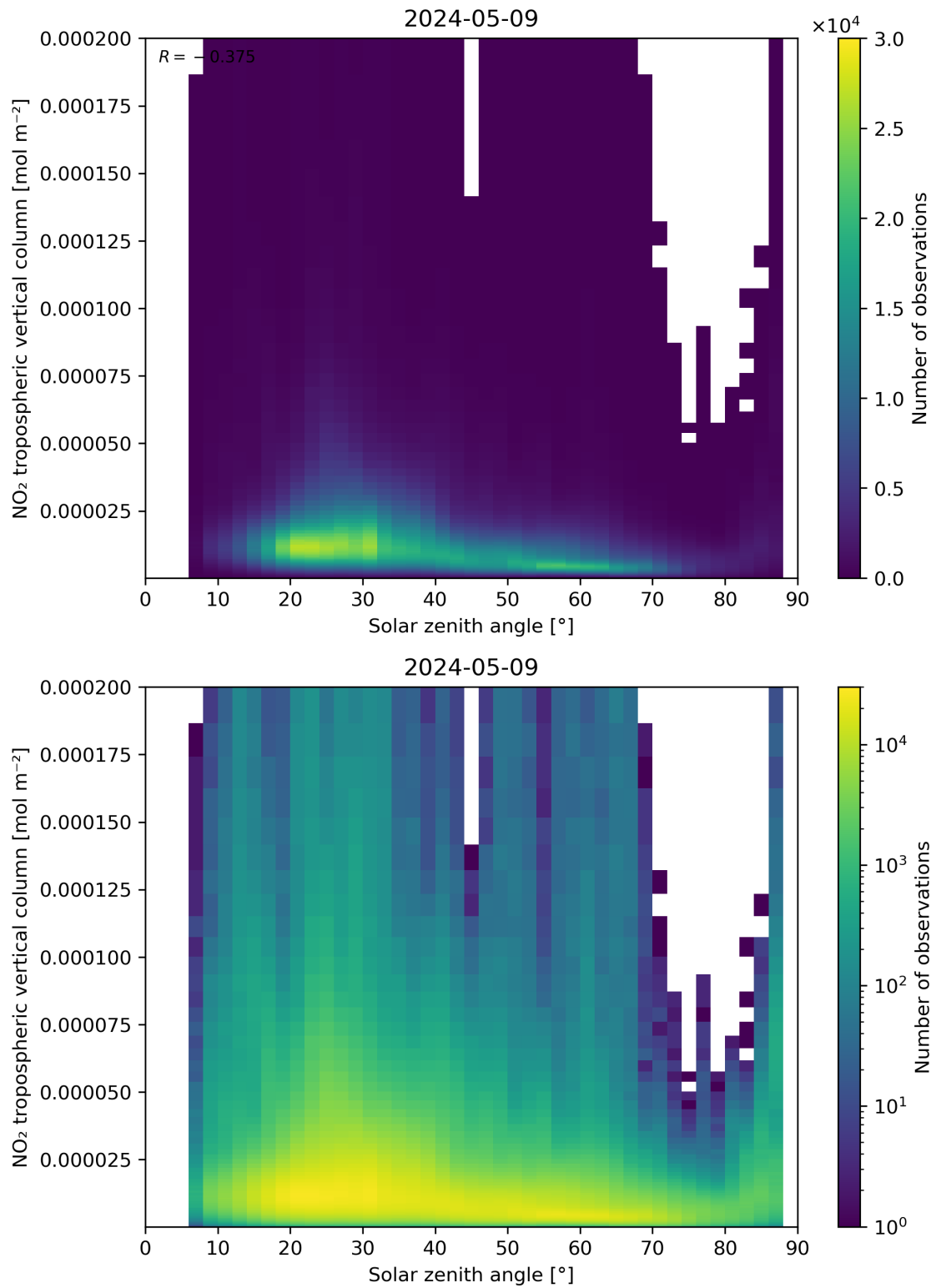
Figure 155: Scatter density plot of “Solar zenith angle” against “NO 2 tropospheric vertical column” for 2024-05-08 to 2024-05-10.
