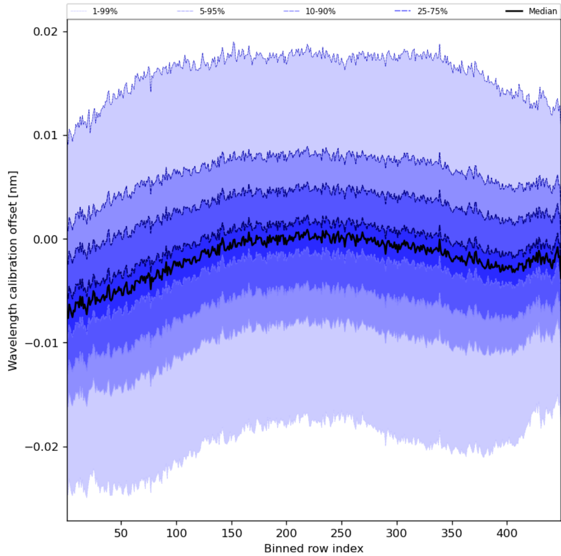
Figure 52: Along track statistics of “Wavelength calibration offset” for 2024-05-08 to 2024-05-10
