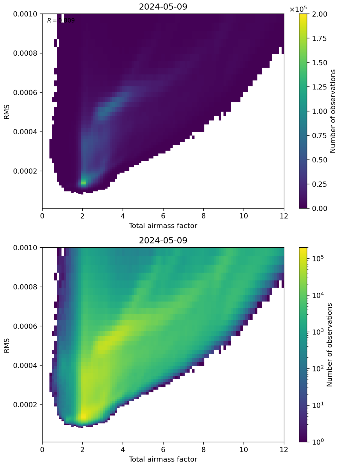
Figure 69: Scatter density plot of “Total airmass factor” against “RMS” for 2024-05-08 to 2024-05-10.
