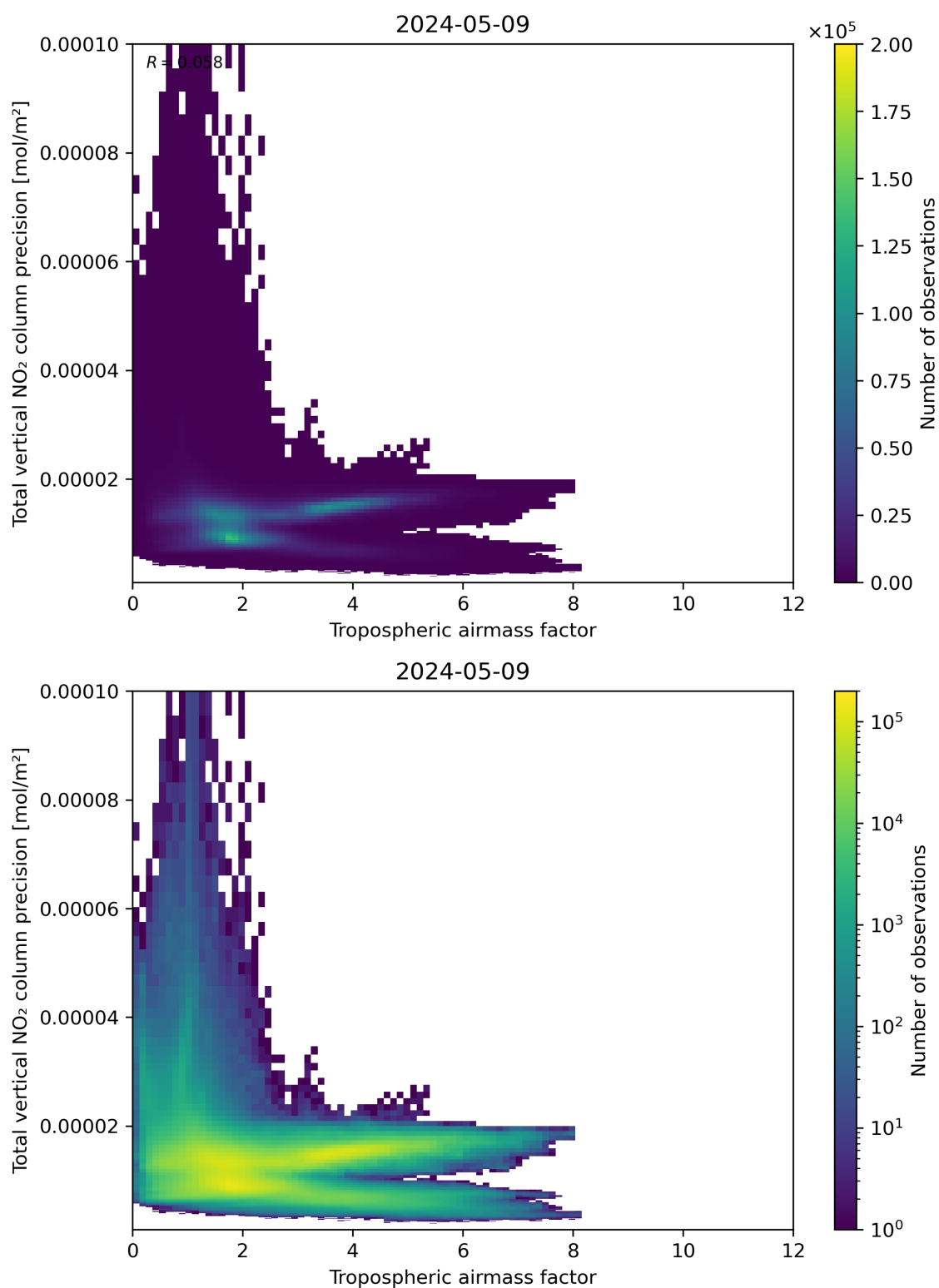
Figure 78: Scatter density plot of “Tropospheric air mass factor” against “Total vertical NO 2 column precision” for 2024-05-08 to 2024-05-10.
