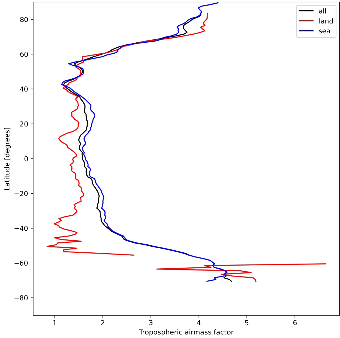
Figure 14: Zonal average of “Tropospheric airmass factor” for 2024-05-08 to 2024-05-10.
