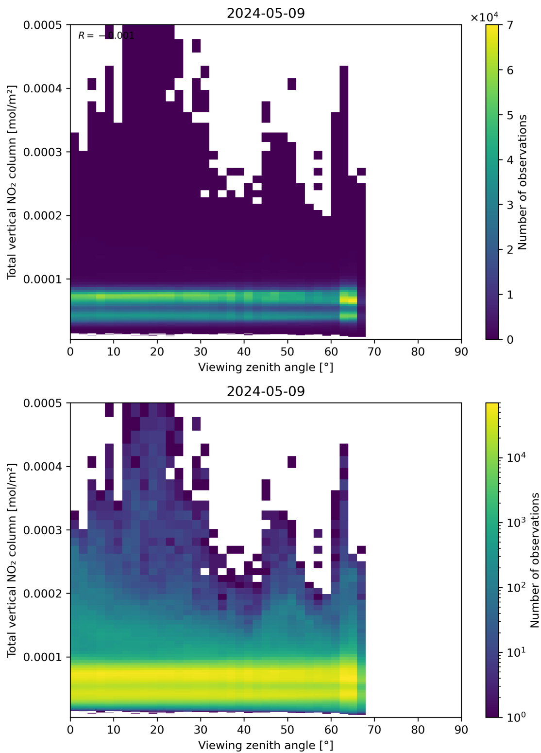
Figure 167: Scatter density plot of “Viewing zenith angle” against “Total vertical NO 2 column” for 2024-05-08 to 2024-05-10.
