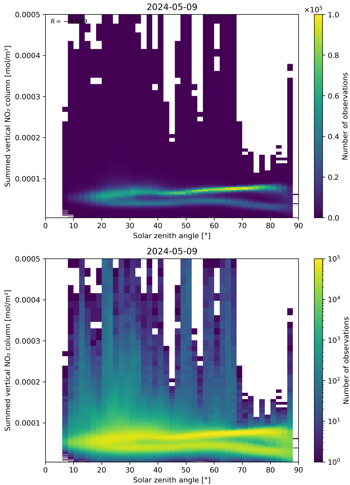
Figure 151: Scatter density plot of “Solar zenith angle” against “Summed vertical NO 2 column” for 2024-05-08 to 2024-05-10.
