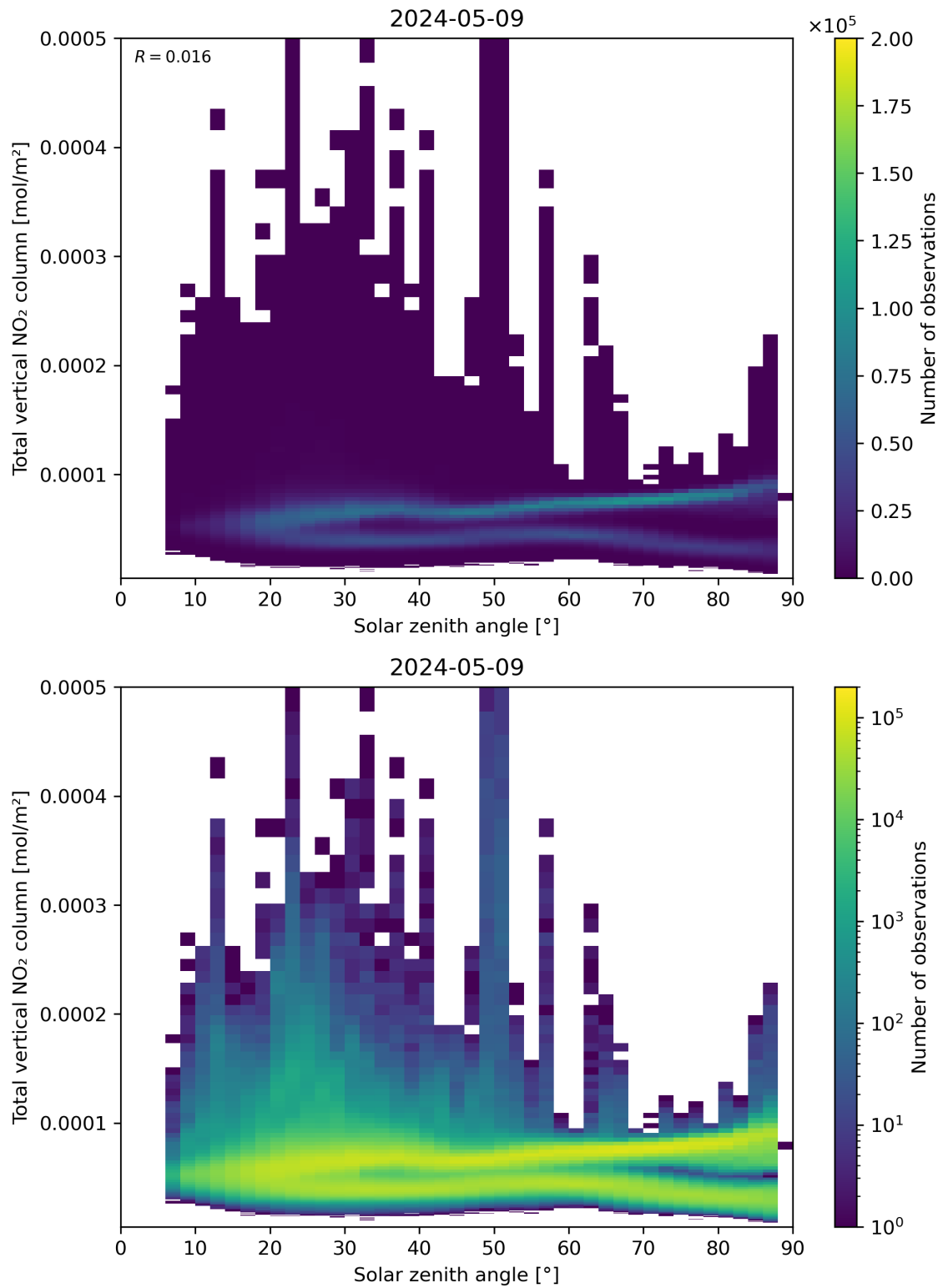
Figure 153: Scatter density plot of “Solar zenith angle” against “Total vertical NO 2 column” for 2024-05-08 to 2024-05-10.
