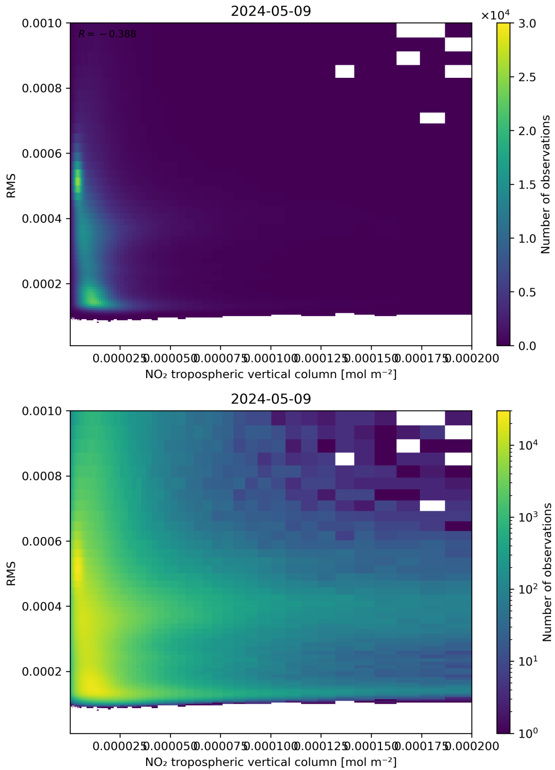
Figure 142: Scatter density plot of “NO 2 tropospheric vertical column” against “RMS” for 2024-05-08 to 2024-05-10.
