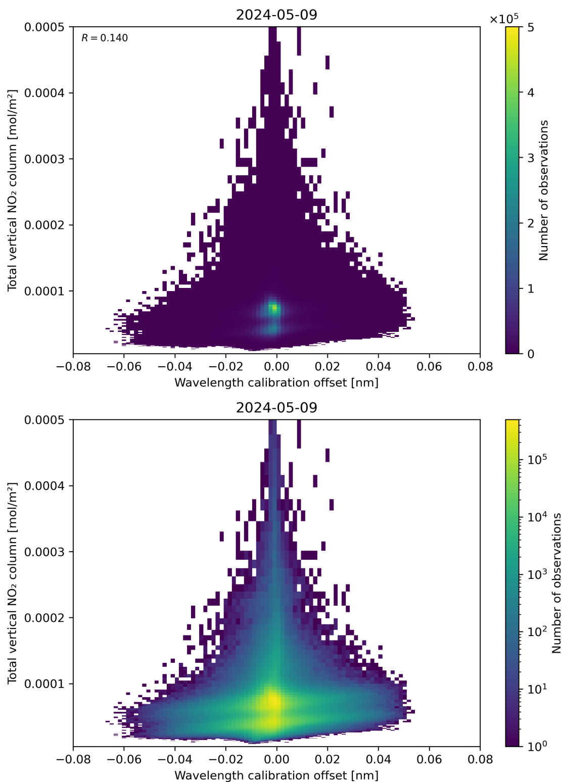
Figure 179: Scatter density plot of “Wavelength calibration offset” against “Total vertical NO 2 column” for 2024-05-08 to 2024-05-10.
