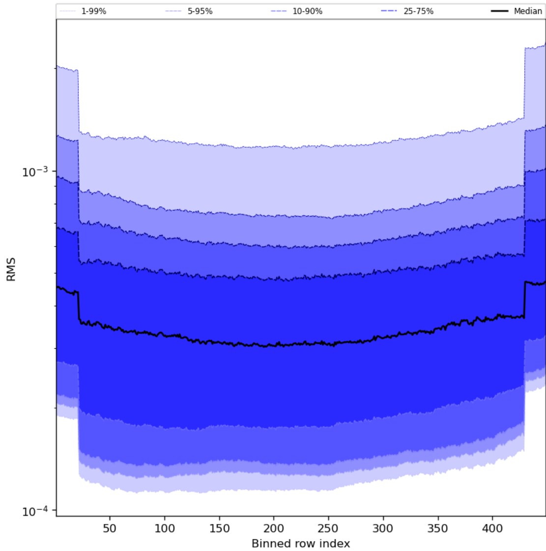
Figure 60: Along track statistics of “RMS” for 2024-05-08 to 2024-05-10
