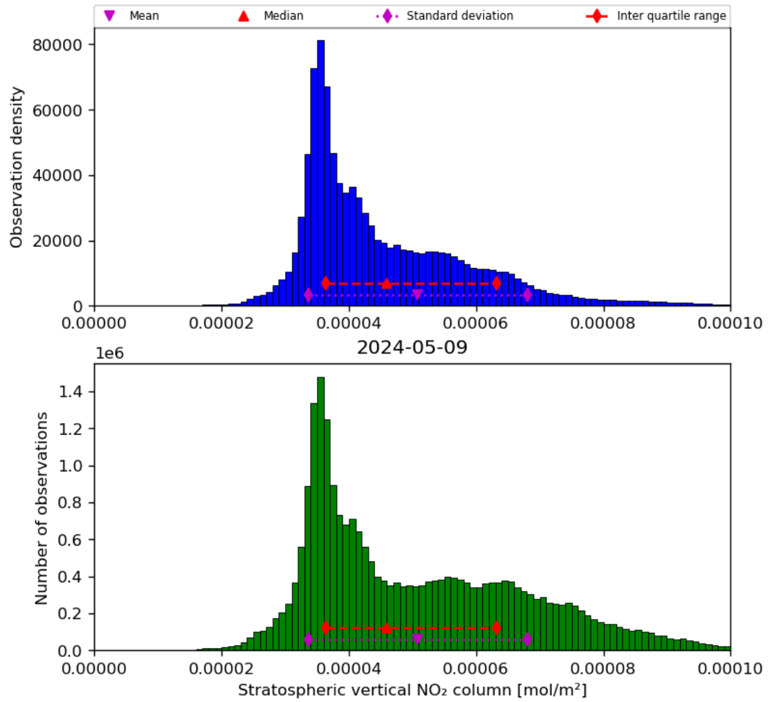
Figure 36: Histogram of “Stratospheric vertical NO 2 column” for 2024-05-08 to 2024-05-10
