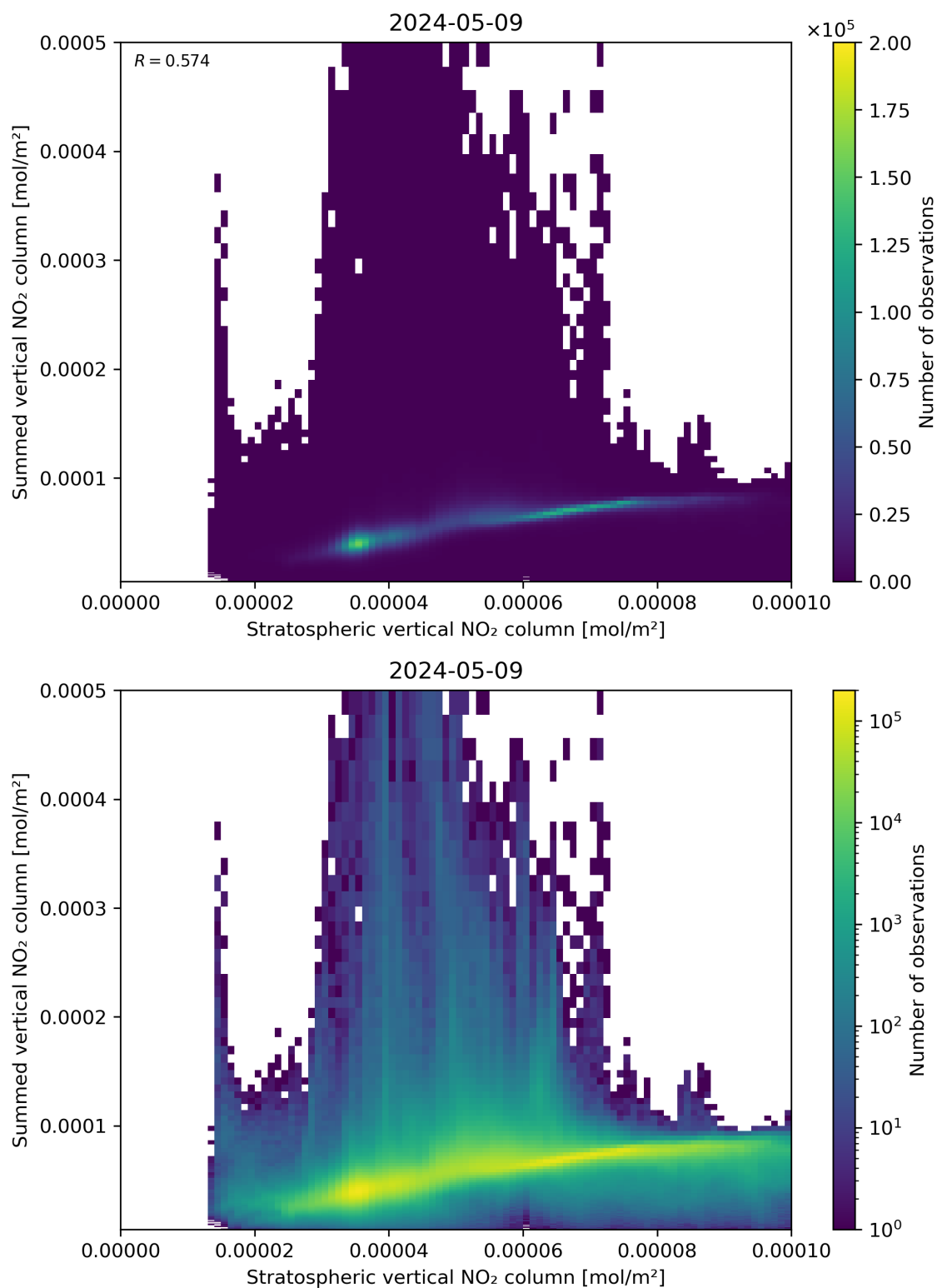
Figure 98: Scatter density plot of “Stratospheric vertical NO 2 column” against “Summed vertical NO 2 column” for 2024-05-08 to 2024-05-10.
