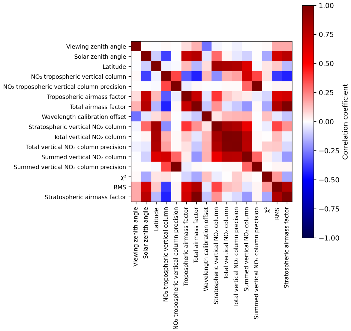
Figure 2: Map of correlation matrix for 2024-05-08 to 2024-05-10.
