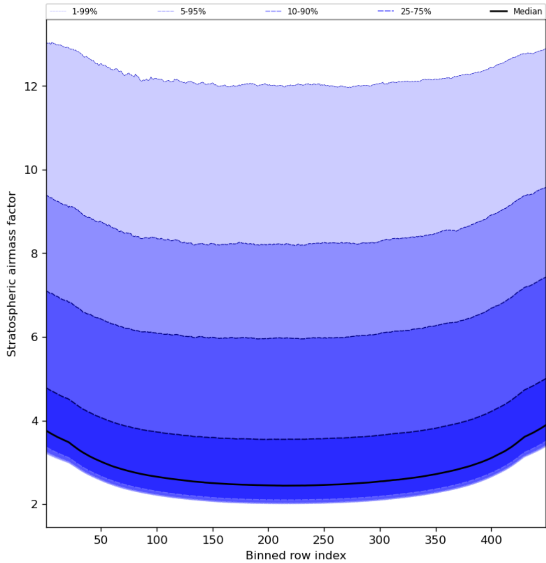
Figure 61: Along track statistics of “Stratospheric airmass factor” for 2024-05-08 to 2024-05-10
