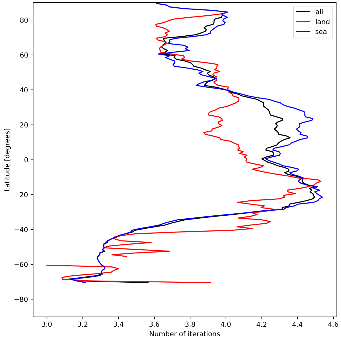
Figure 17: Zonal average of “Number of iterations” for 2024-05-08 to 2024-05-10.
