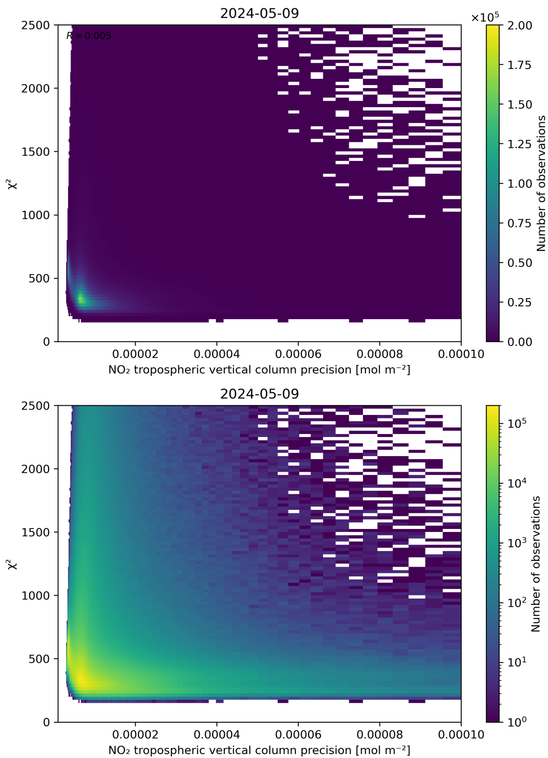
Figure 134: Scatter density plot of “NO 2 tropospheric vertical column precision” against “ \chi^2 ” for 2024-05-08 to 2024-05-10.
