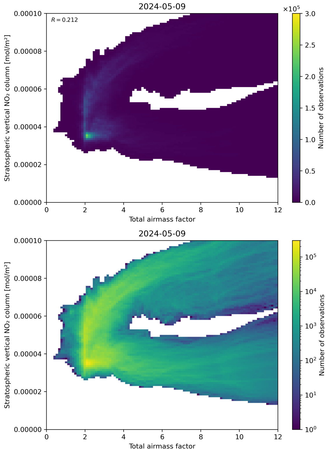
Figure 64: Scatter density plot of “Total airmass factor” against “Stratospheric vertical \text{NO}_2 column” for 2024-05-08 to 2024-05-10.
