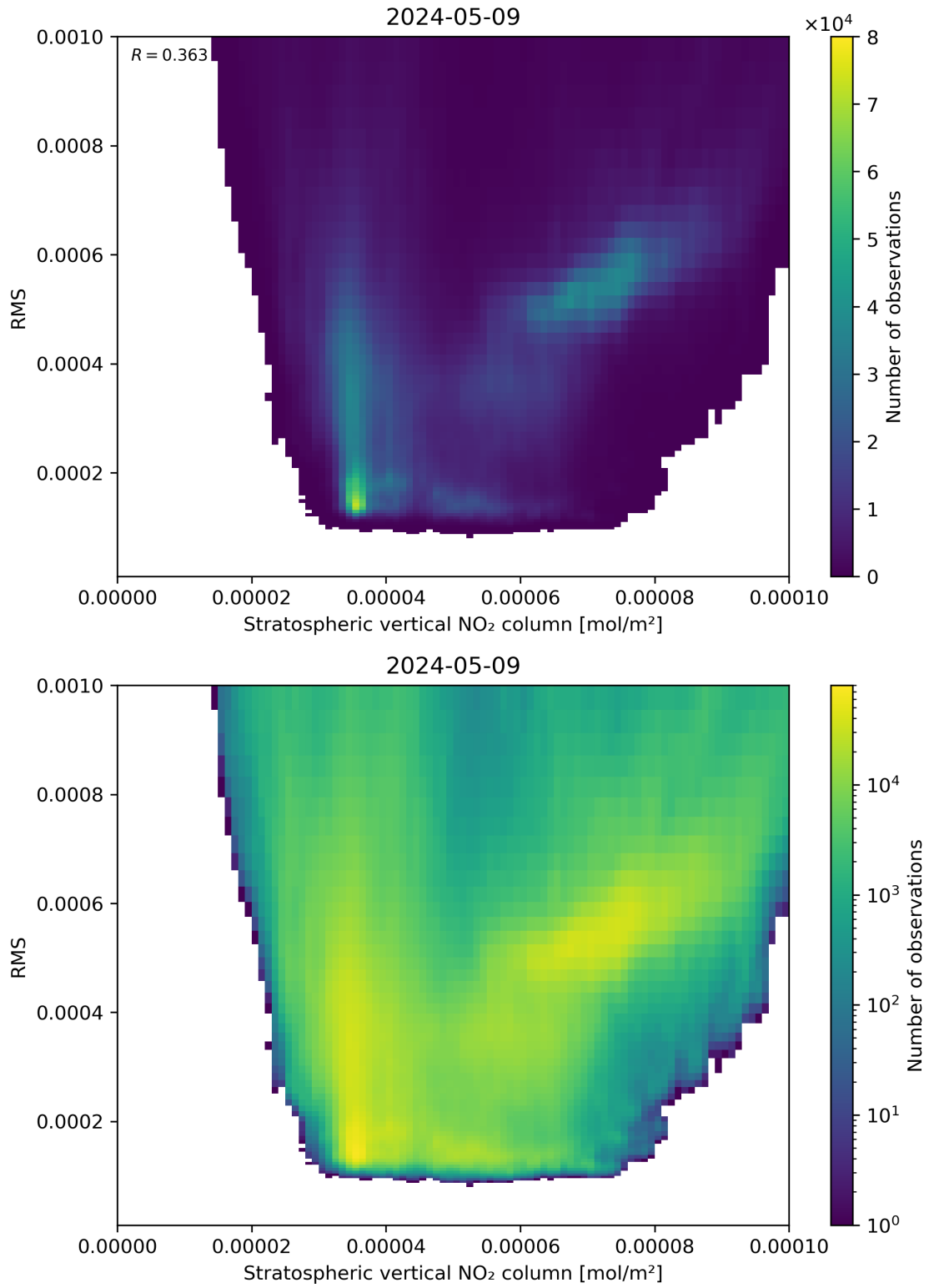
Figure 102: Scatter density plot of “Stratospheric vertical NO 2 column” against “RMS” for 2024-05-08 to 2024-05-10.
