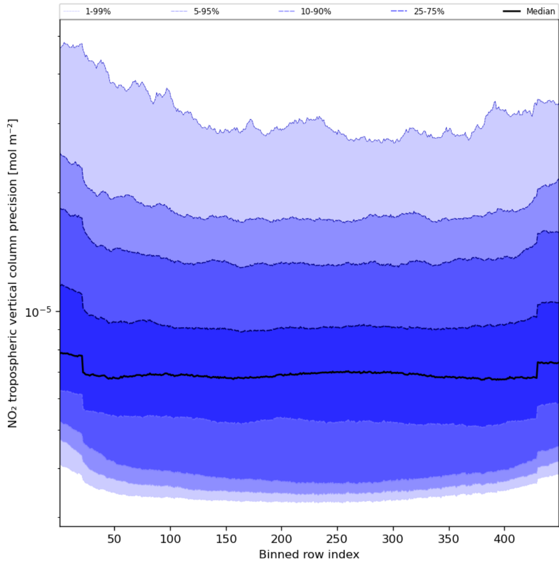
Figure 47: Along track statistics of “NO 2 tropospheric vertical column precision” for 2024-05-08 to 2024-05-10
