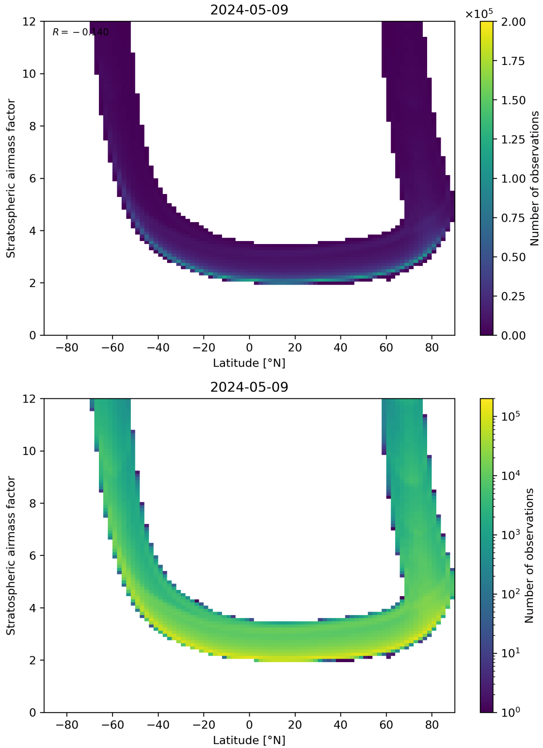
Figure 83: Scatter density plot of “Latitude” against “Stratospheric air mass factor” for 2024-05-08 to 2024-05-10.
