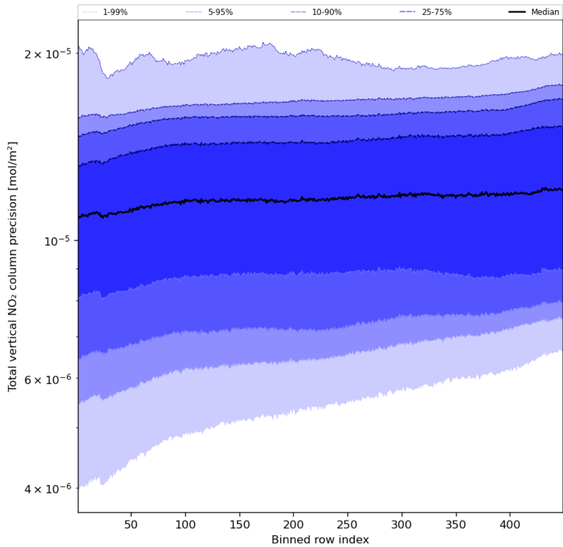
Figure 56: Along track statistics of “Total vertical NO 2 column precision” for 2024-05-08 to 2024-05-10
