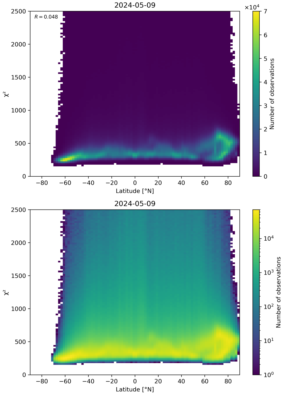
Figure 86: Scatter density plot of “Latitude” against “ \chi^2 ” for 2024-05-08 to 2024-05-10.
