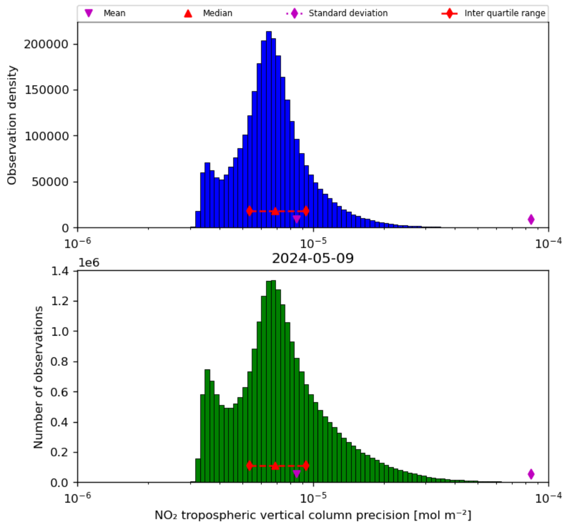
Figure 30: Histogram of “NO 2 tropospheric vertical column precision” for 2024-05-08 to 2024-05-10
