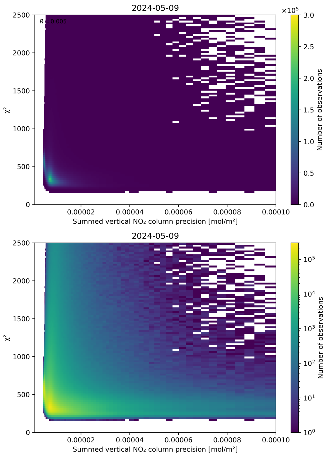
Figure 107: Scatter density plot of “Summed vertical NO 2 column precision” against “ \chi^2 ” for 2024-05-08 to 2024-05-10.
