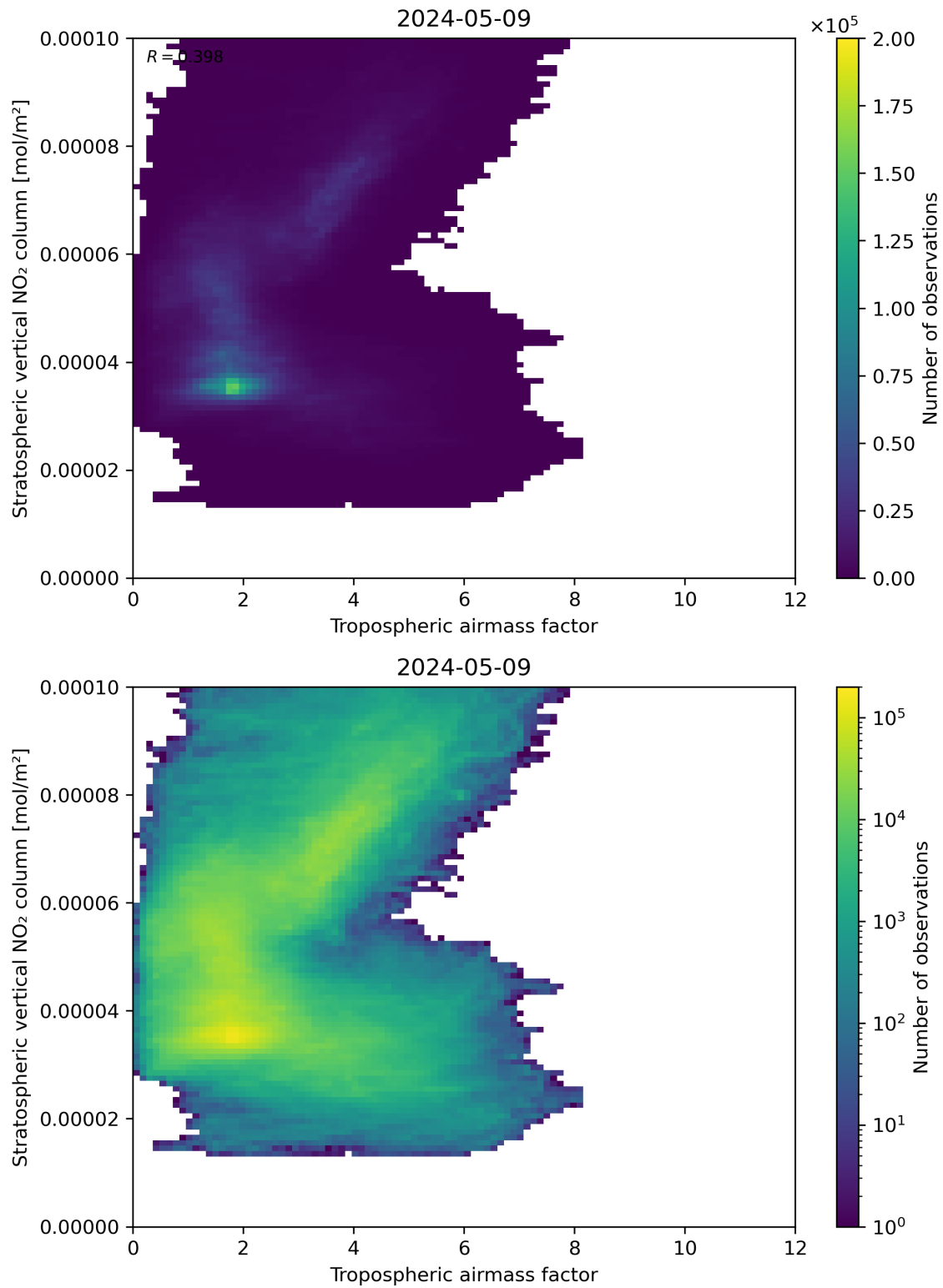
Figure 74: Scatter density plot of “Tropospheric air mass factor” against “Stratospheric vertical NO 2 column” for 2024-05-08 to 2024-05-10.
