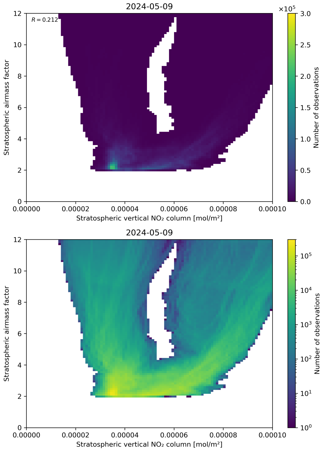
Figure 96: Scatter density plot of “Stratospheric vertical NO 2 column” against “Stratospheric airmass factor” for 2024-05-08 to 2024-05-10.
