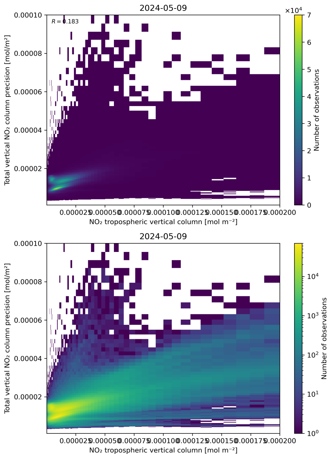
Figure 129: Scatter density plot of “NO 2 tropospheric vertical column” against “Total vertical NO 2 column precision” for 2024-05-08 to 2024-05-10.
