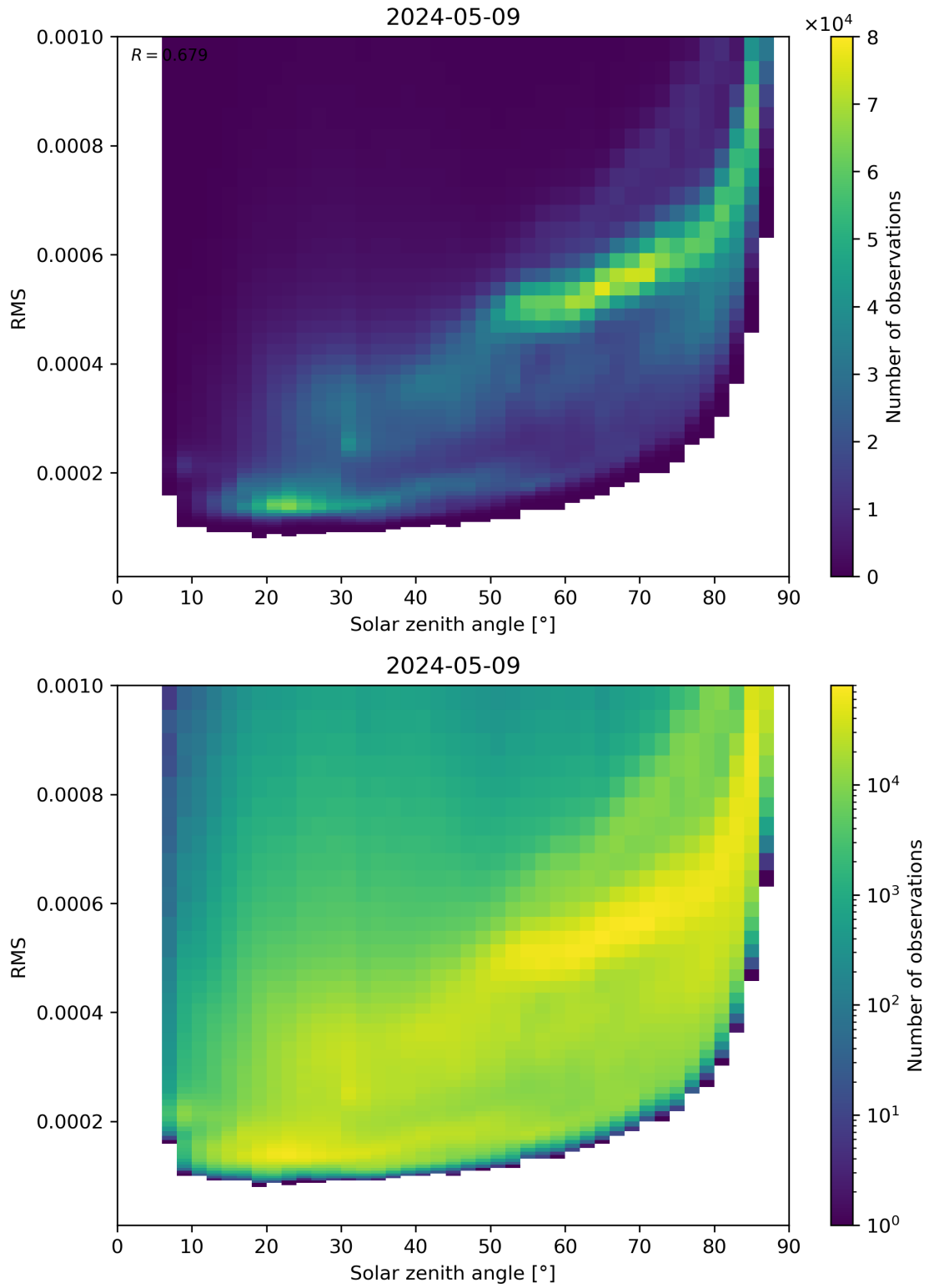
Figure 157: Scatter density plot of “Solar zenith angle” against “RMS” for 2024-05-08 to 2024-05-10.
