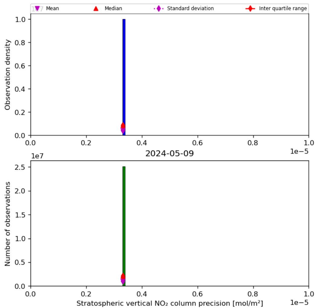
Figure 37: Histogram of “Stratospheric vertical NO 2 column precision” for 2024-05-08 to 2024-05-10
