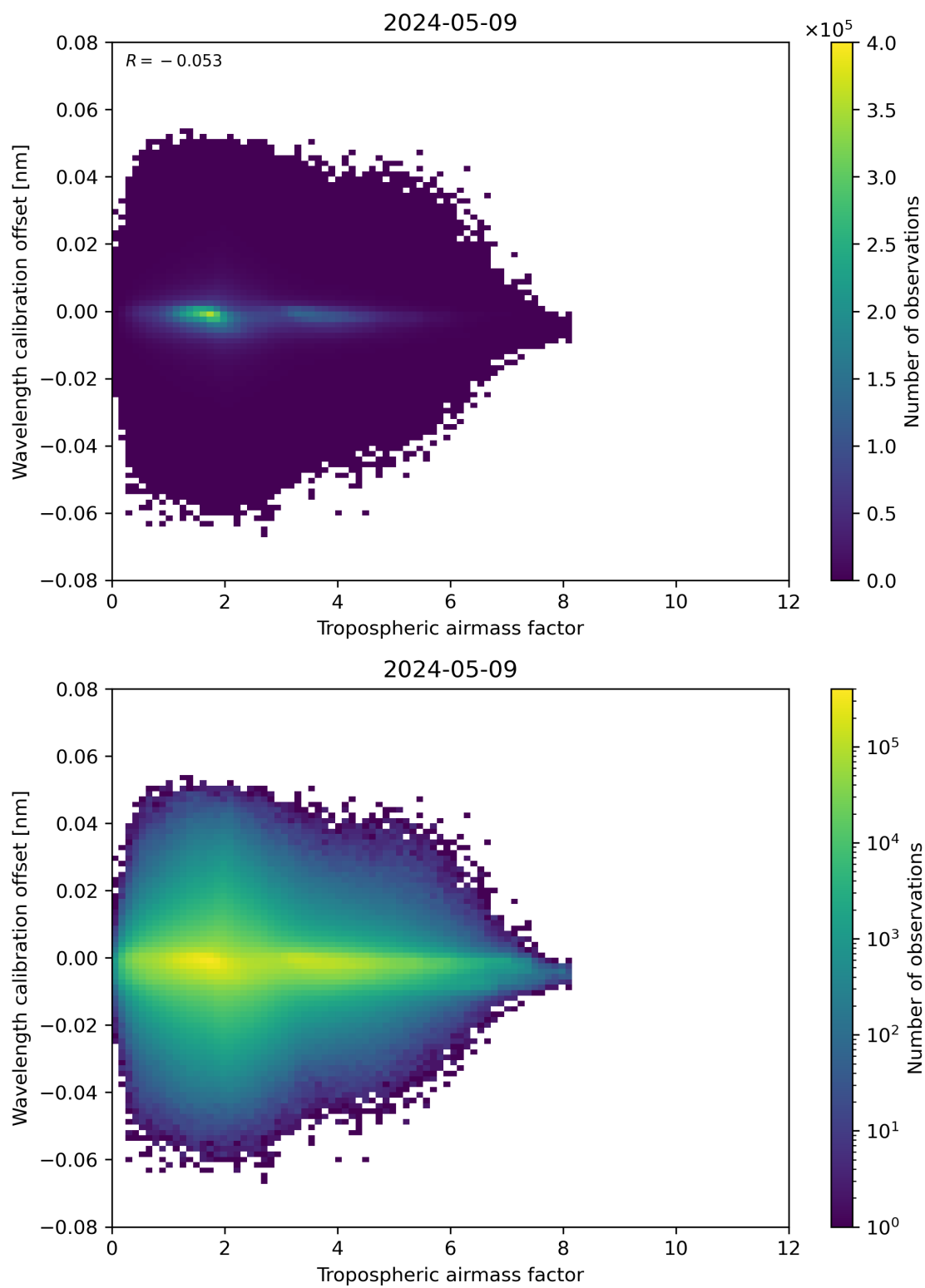
Figure 80: Scatter density plot of “Tropospheric airmass factor” against “Wavelength calibration offset” for 2024-05-08 to 2024-05-10.
