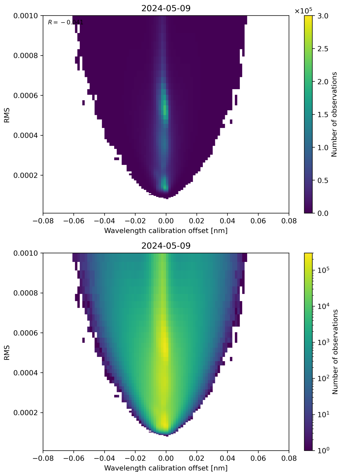
Figure 181: Scatter density plot of “Wavelength calibration offset” against “RMS” for 2024-05-08 to 2024-05-10.
