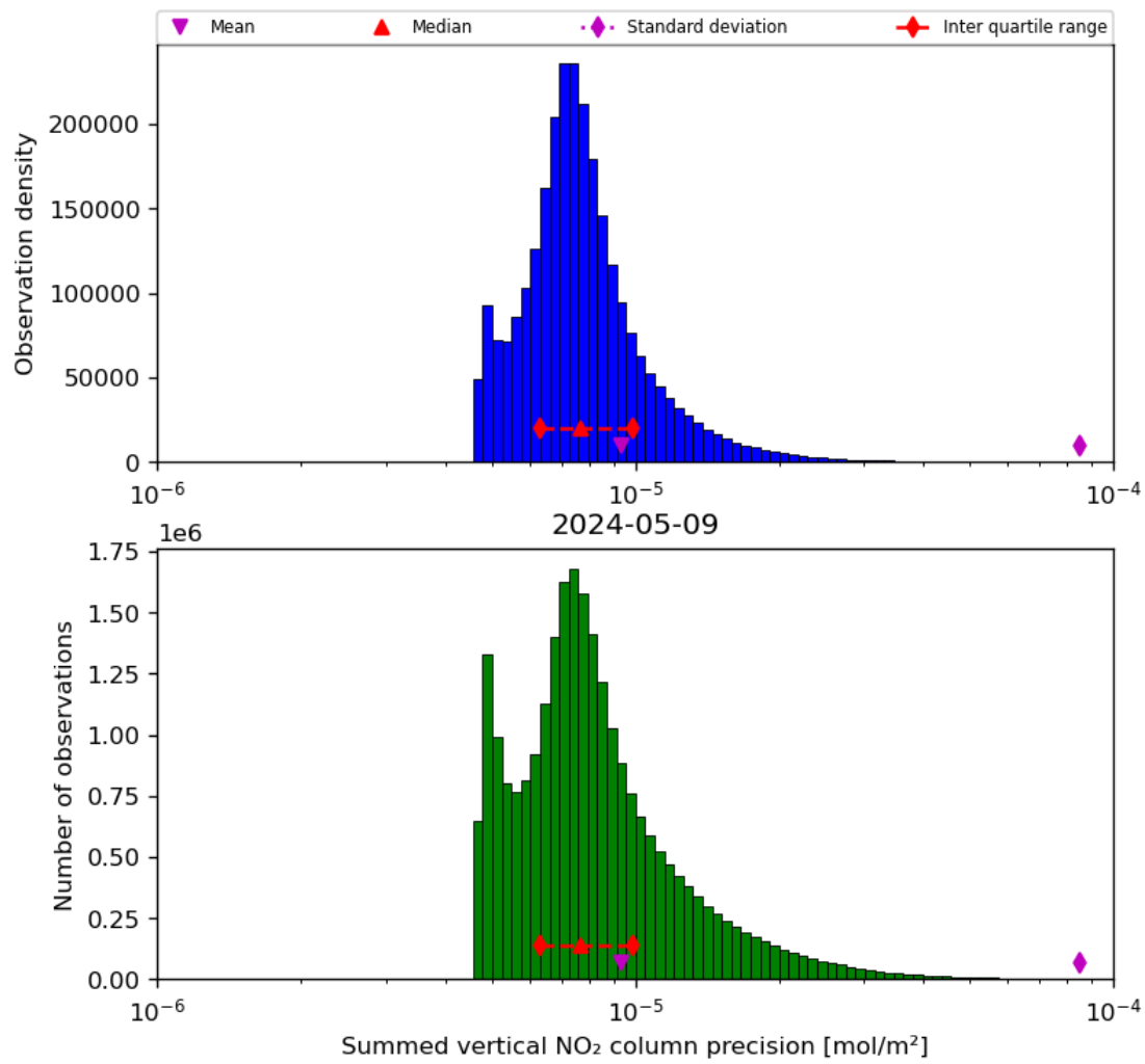
Figure 41: Histogram of "Summed vertical NO 2 column precision" for 2024-05-08 to 2024-05-10
