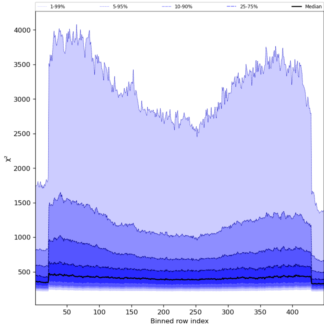
Figure 59: Along track statistics of “ \chi^2 ” for 2024-05-08 to 2024-05-10
