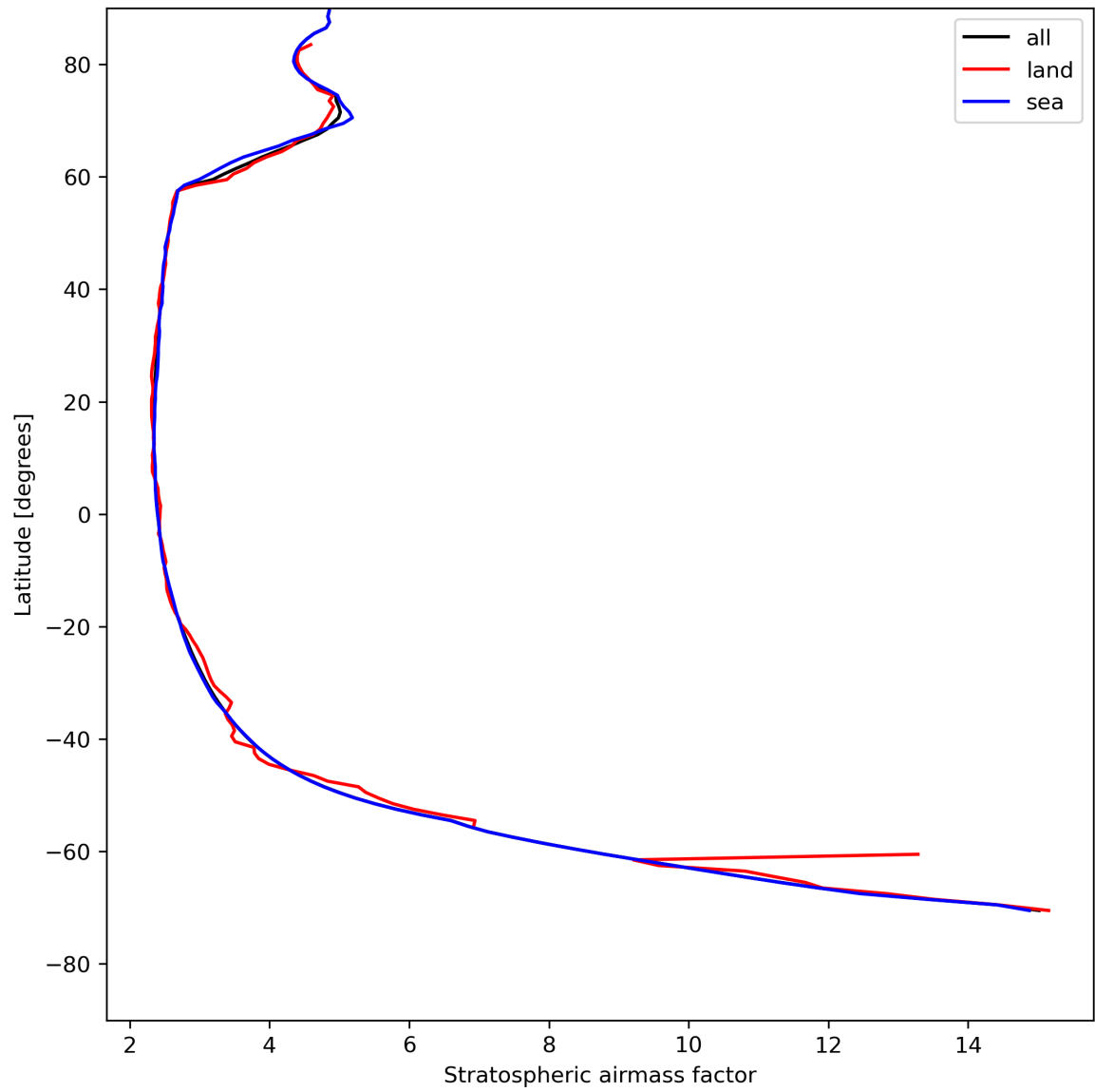
Figure 27: Zonal average of “Stratospheric air mass factor” for 2024-05-08 to 2024-05-10.
