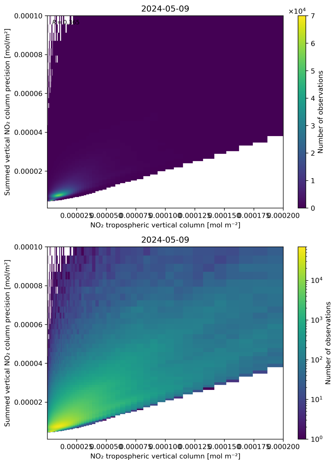
Figure 127: Scatter density plot of “NO 2 tropospheric vertical column” against “Summed vertical NO 2 column precision” for 2024-05-08 to 2024-05-10.
