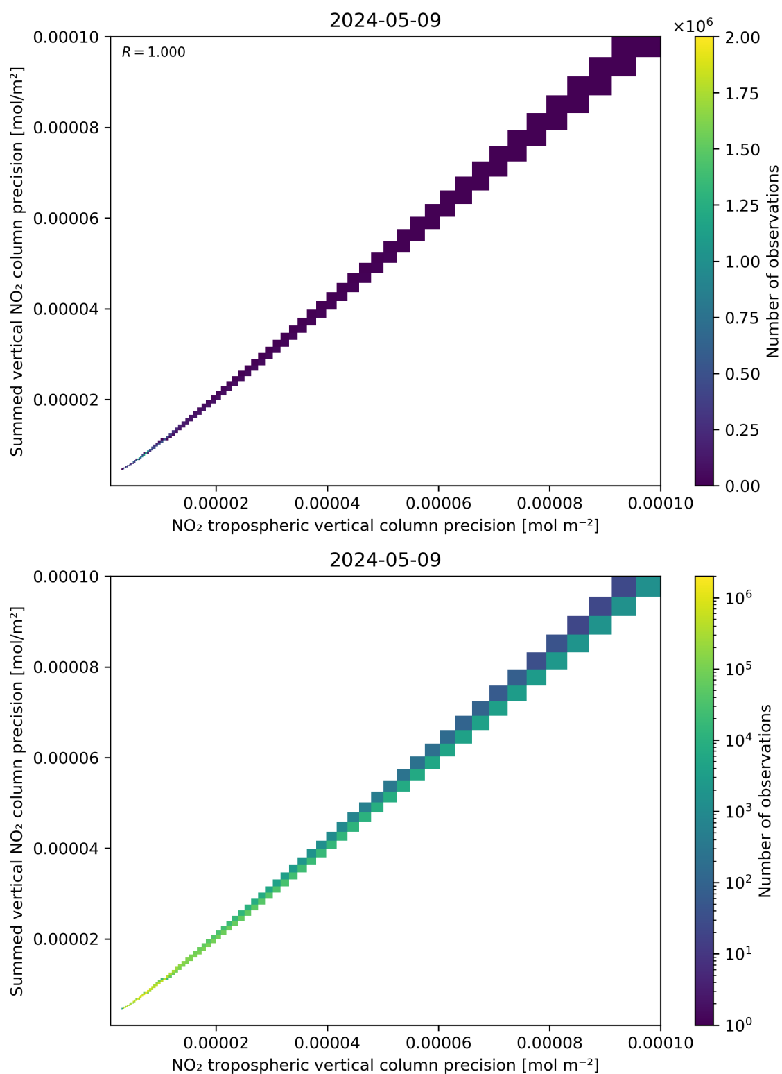
Figure 137: Scatter density plot of “NO 2 tropospheric vertical column precision” against “Summed vertical NO 2 column precision” for 2024-05-08 to 2024-05-10.
