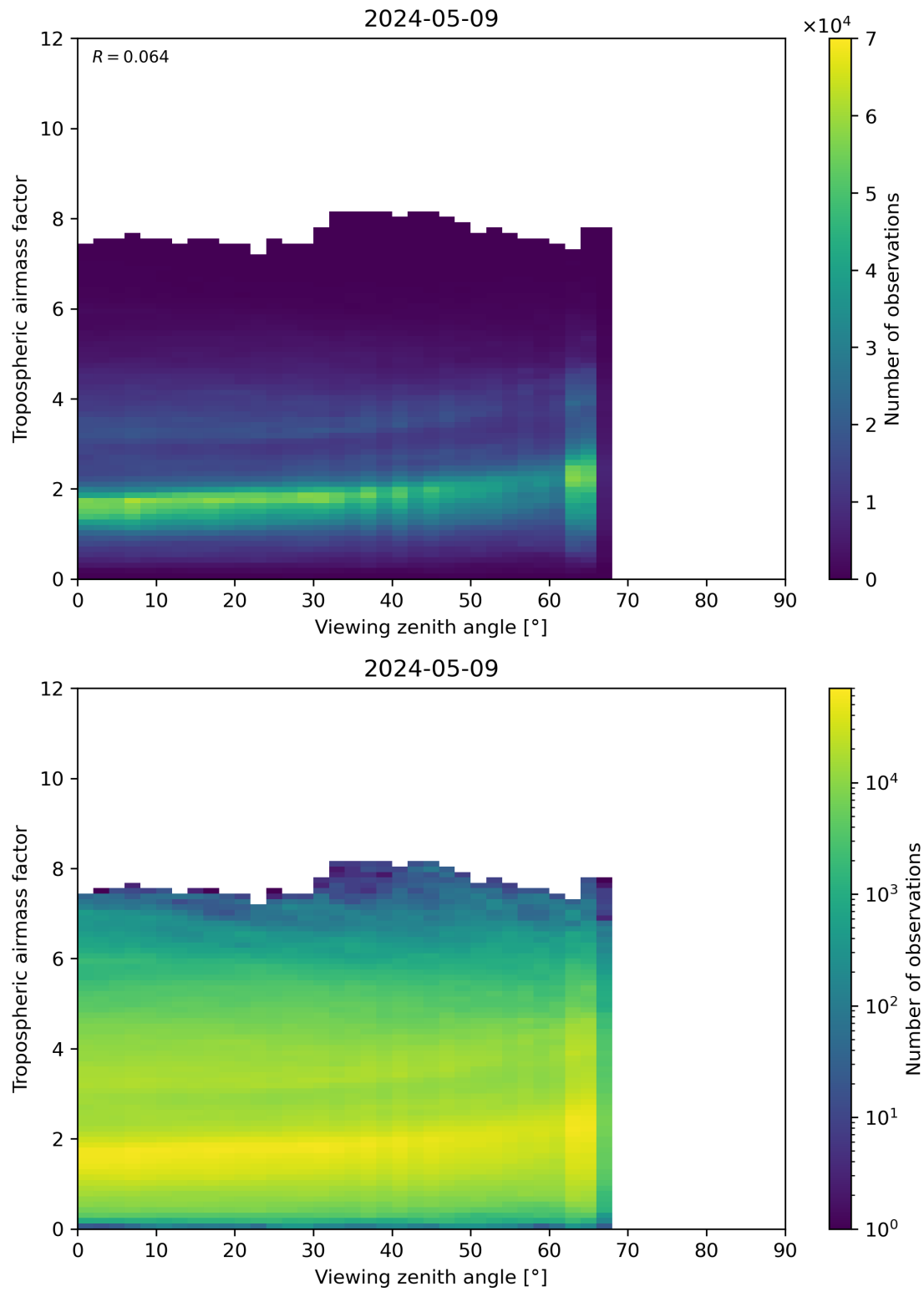
Figure 161: Scatter density plot of “Viewing zenith angle” against “Tropospheric airmass factor” for 2024-05-08 to 2024-05-10.
