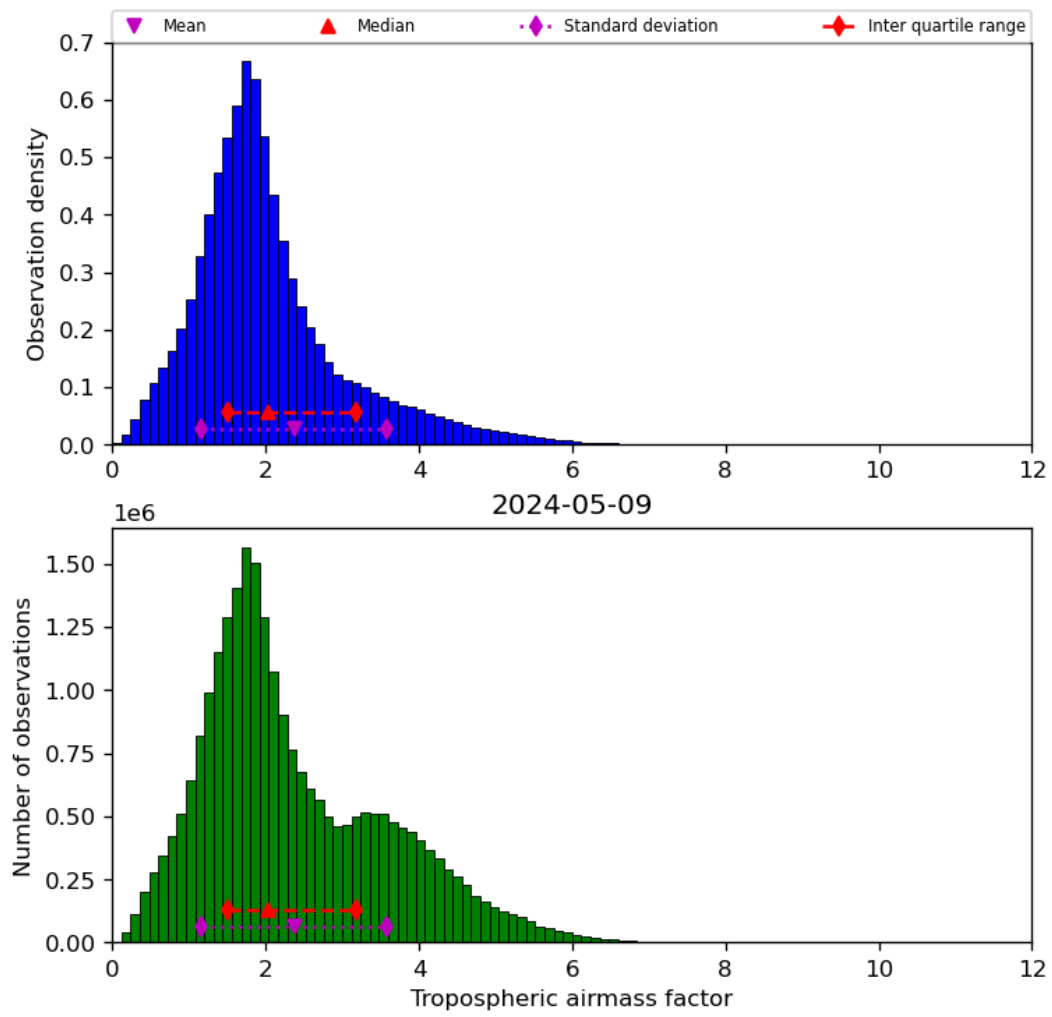
Figure 31: Histogram of “Tropospheric airmass factor” for 2024-05-08 to 2024-05-10
