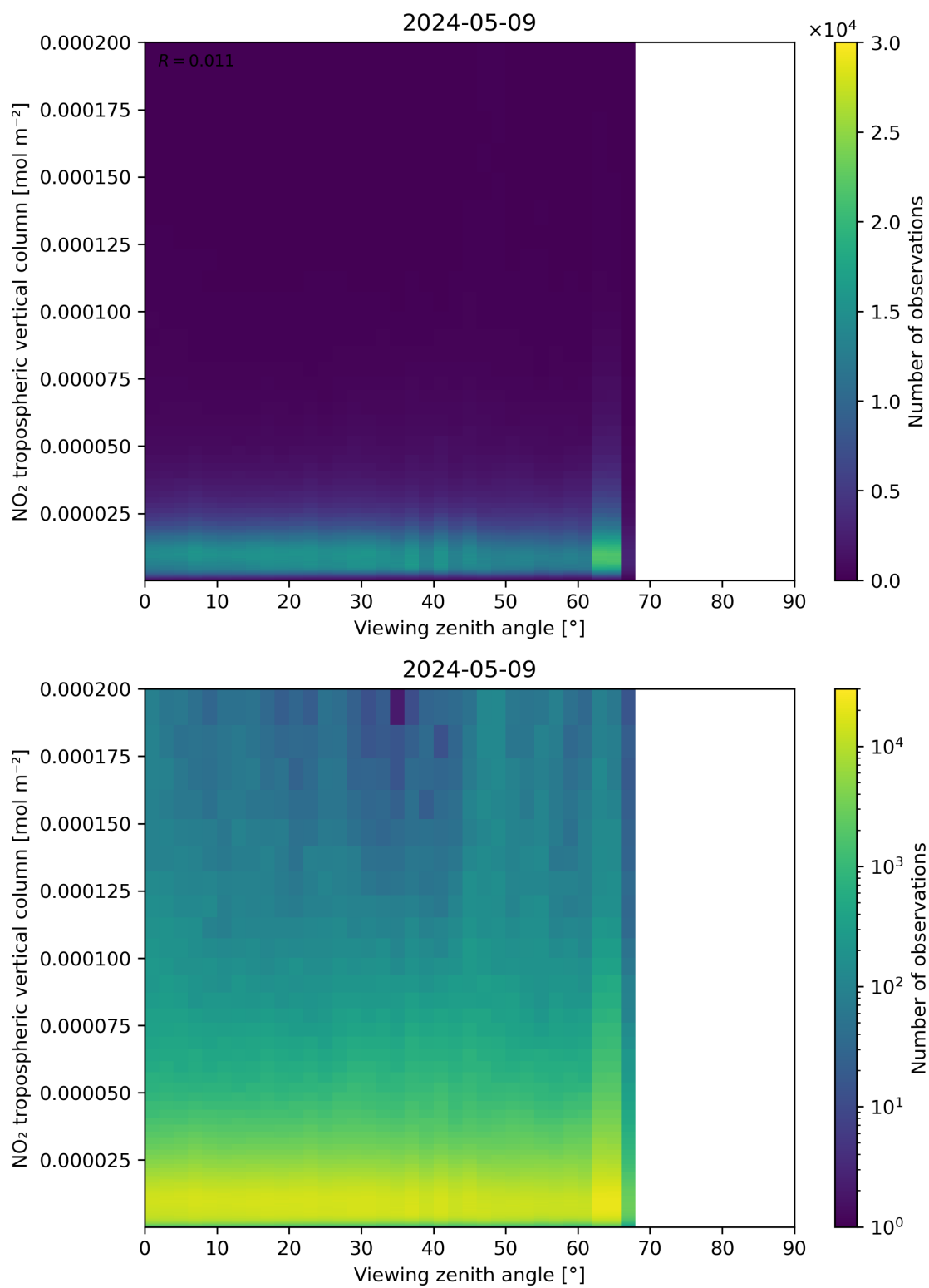
Figure 169: Scatter density plot of “Viewing zenith angle” against “NO 2 tropospheric vertical column” for 2024-05-08 to 2024-05-10.
