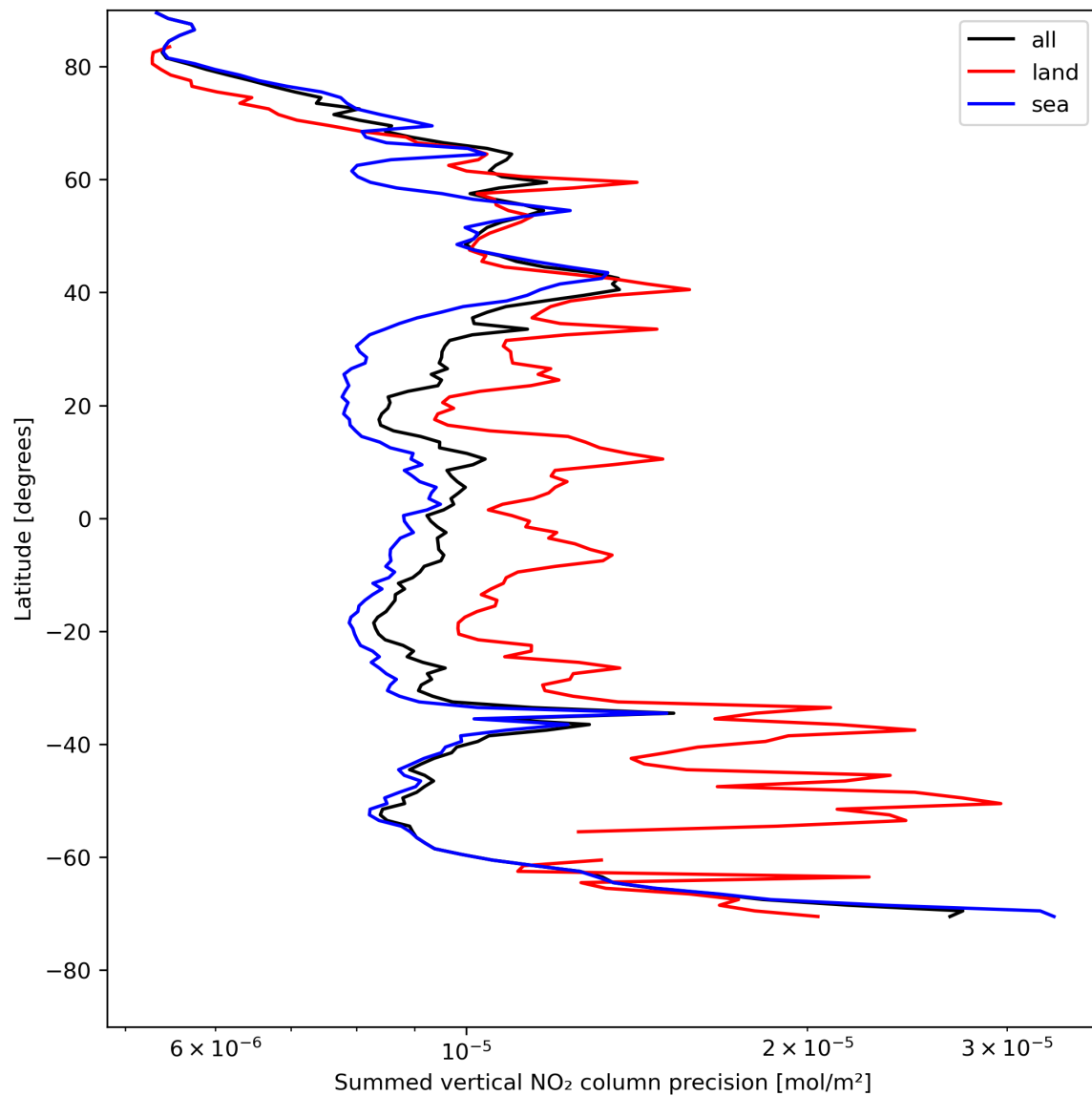
Figure 24: Zonal average of “Summed vertical NO 2 column precision” for 2024-05-08 to 2024-05-10.
