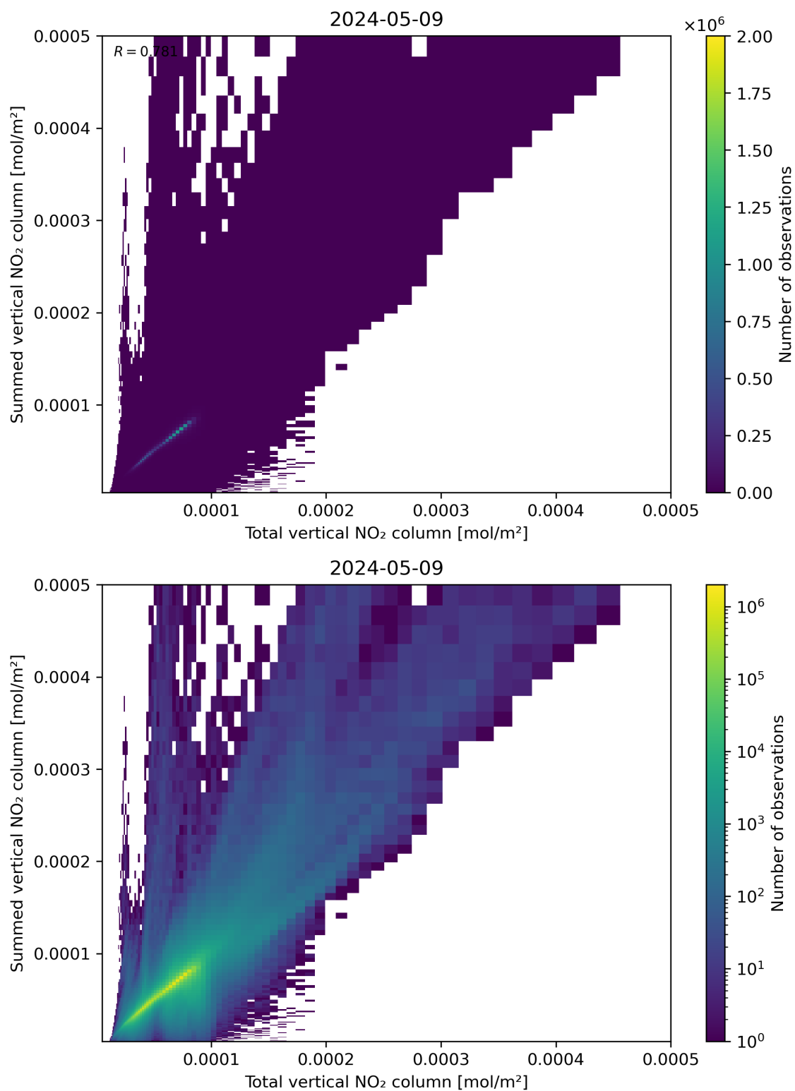
Figure 112: Scatter density plot of “Total vertical NO 2 column” against “Summed vertical NO 2 column” for 2024-05-08 to 2024-05-10.
