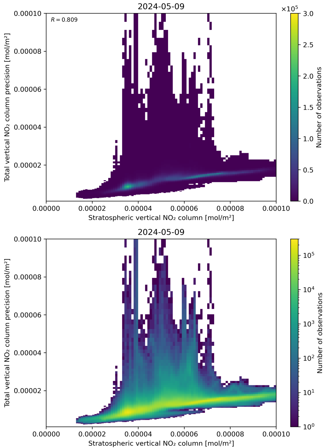
Figure 101: Scatter density plot of “Stratospheric vertical NO 2 column” against “Total vertical NO 2 column precision” for 2024-05-08 to 2024-05-10.
