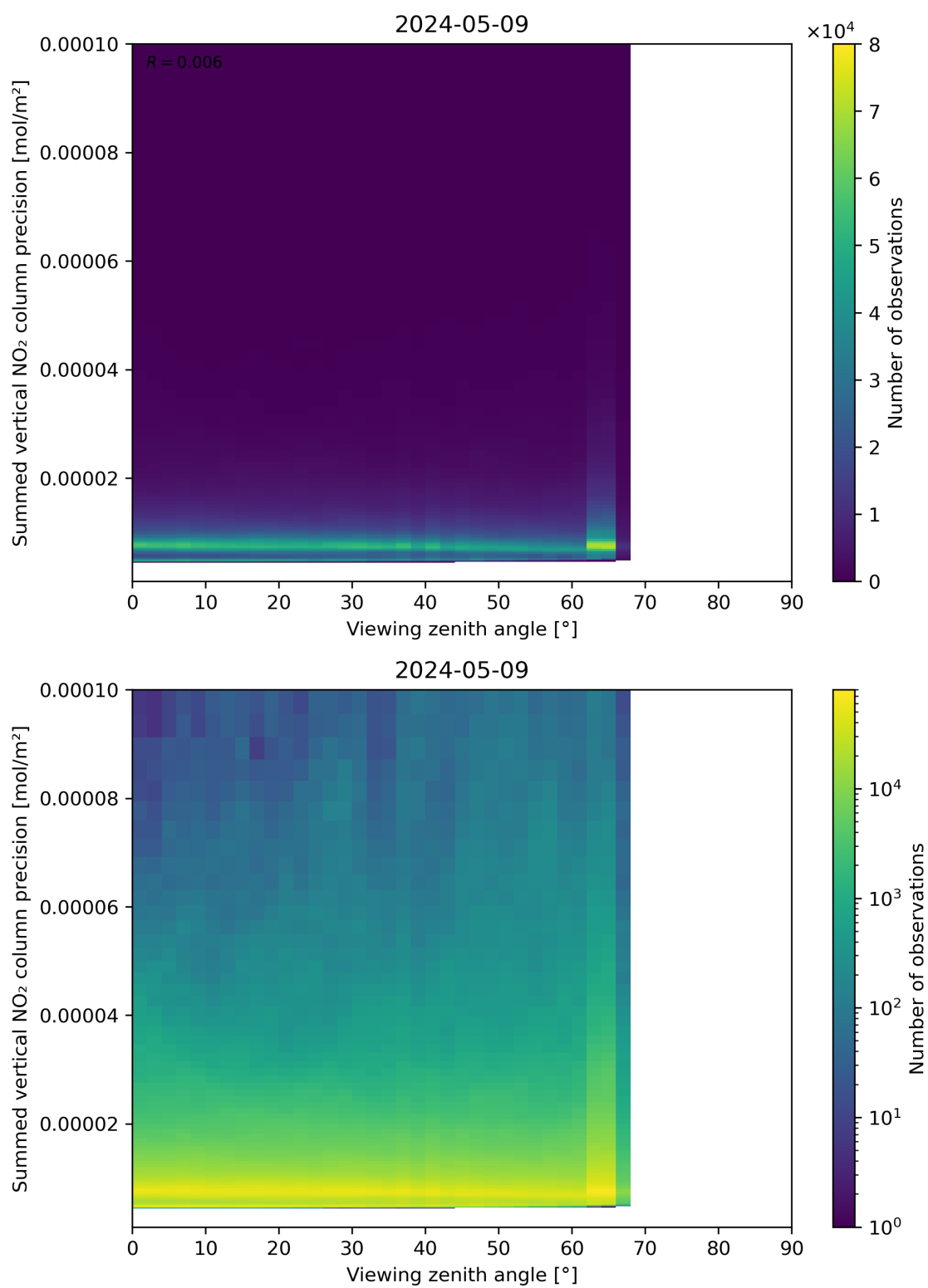
Figure 166: Scatter density plot of “Viewing zenith angle” against “Summed vertical NO 2 column precision” for 2024-05-08 to 2024-05-10.
