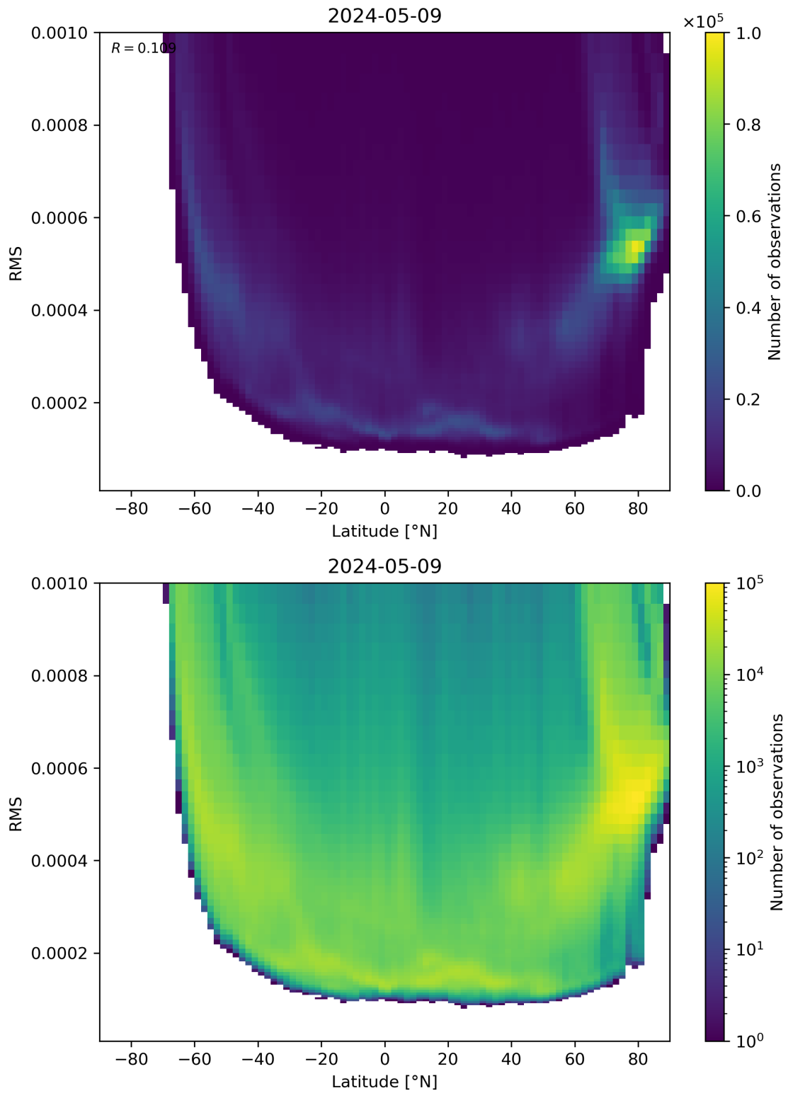
Figure 94: Scatter density plot of “Latitude” against “RMS” for 2024-05-08 to 2024-05-10.
