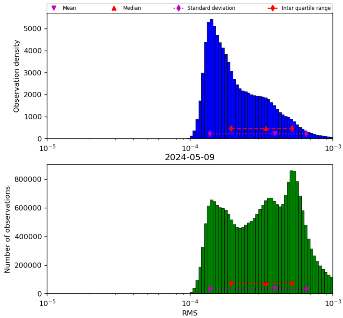
Figure 43: Histogram of “RMS” for 2024-05-08 to 2024-05-10
