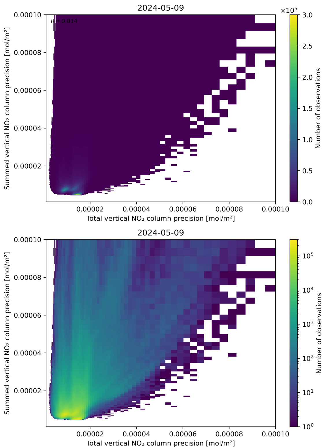
Figure 118: Scatter density plot of “Total vertical NO 2 column precision” against “Summed vertical NO 2 column precision” for 2024-05-08 to 2024-05-10.
