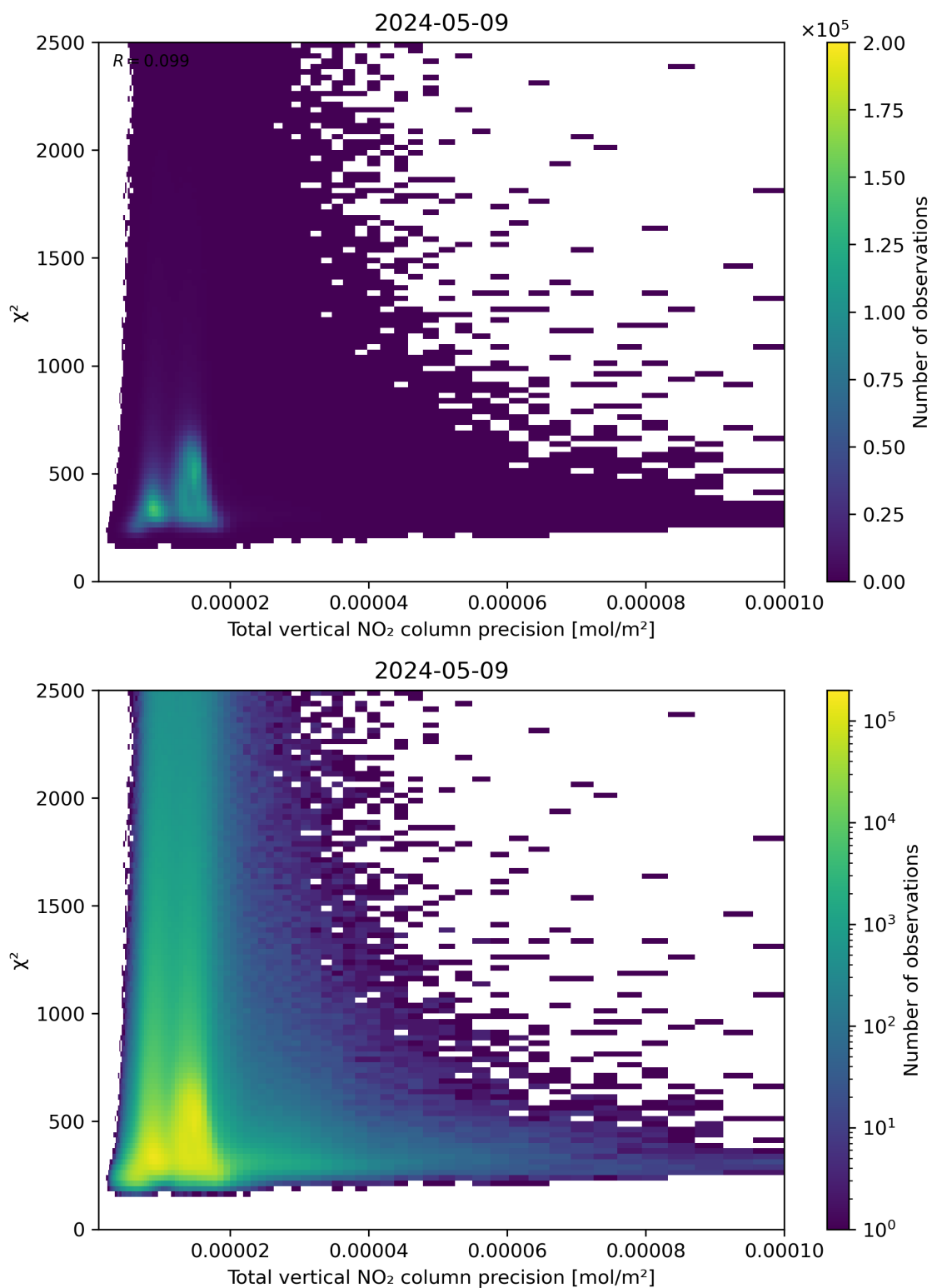
Figure 116: Scatter density plot of “Total vertical NO 2 column precision” against “ \chi^2 ” for 2024-05-08 to 2024-05-10.
