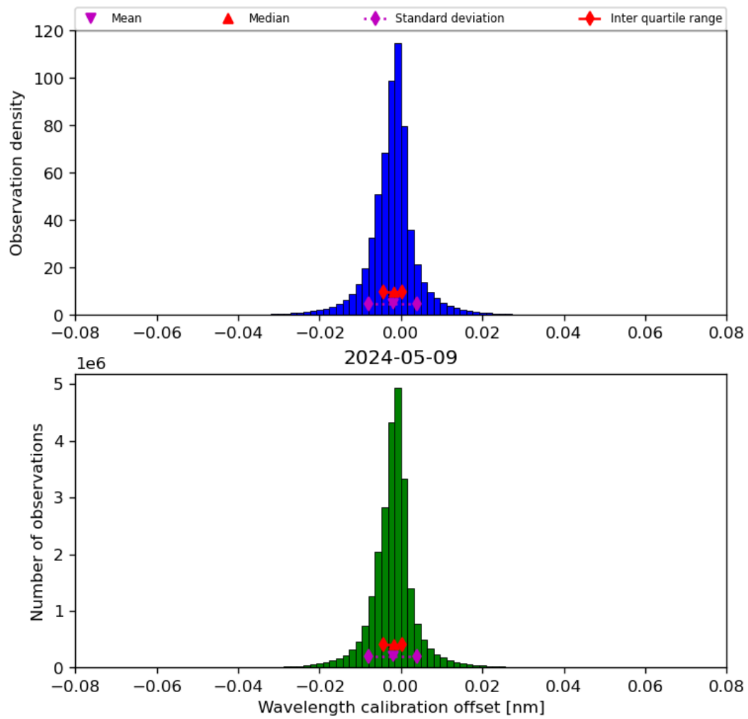
Figure 35: Histogram of “Wavelength calibration offset” for 2024-05-08 to 2024-05-10
