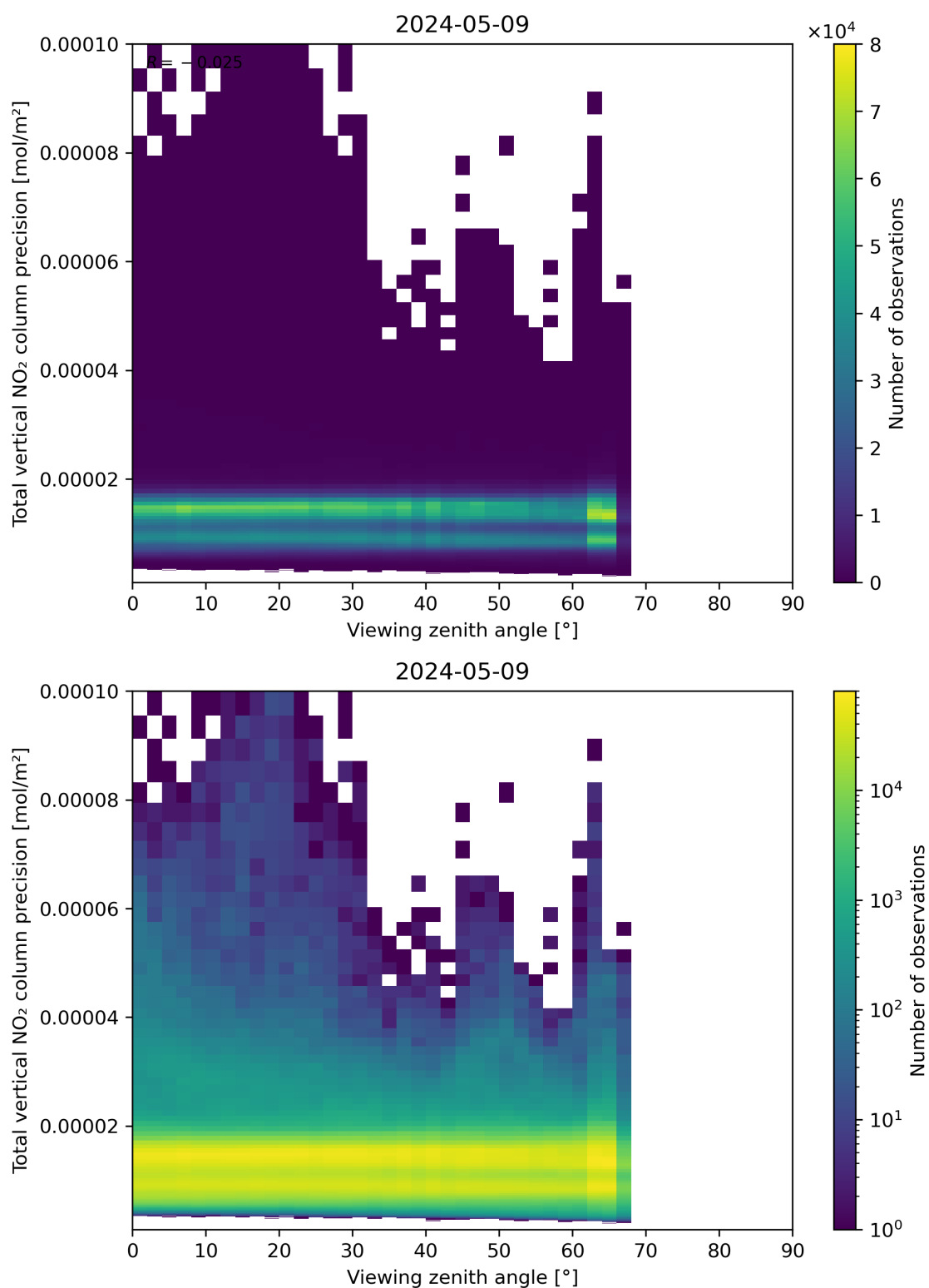
Figure 168: Scatter density plot of “Viewing zenith angle” against “Total vertical NO 2 column precision” for 2024-05-08 to 2024-05-10.
