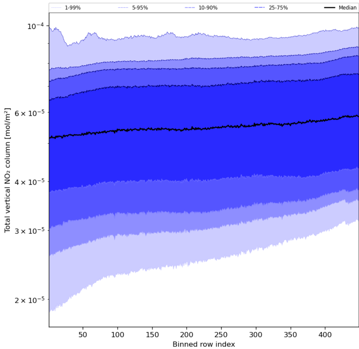
Figure 55: Along track statistics of “Total vertical NO 2 column” for 2024-05-08 to 2024-05-10
