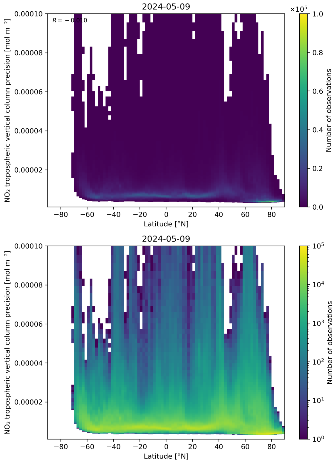
Figure 93: Scatter density plot of “Latitude” against “NO 2 tropospheric vertical column precision” for 2024-05-08 to 2024-05-10.
