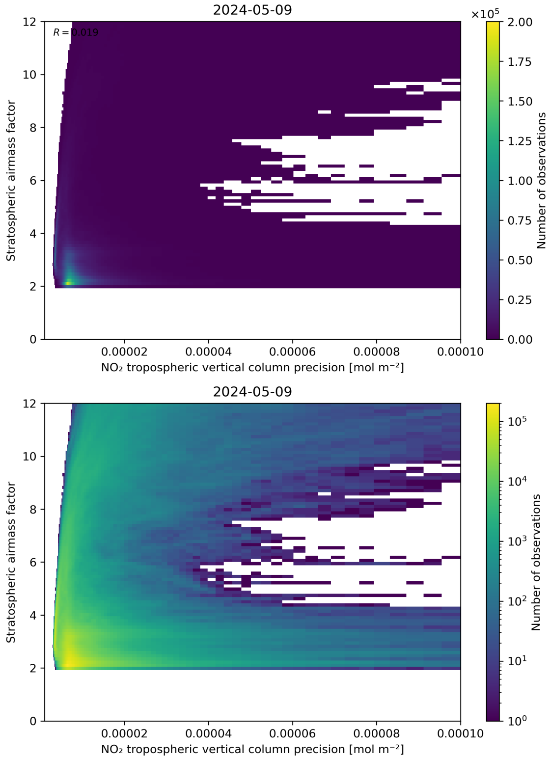
Figure 131: Scatter density plot of “NO 2 tropospheric vertical column precision” against “Stratospheric airmass factor” for 2024-05-08 to 2024-05-10.
