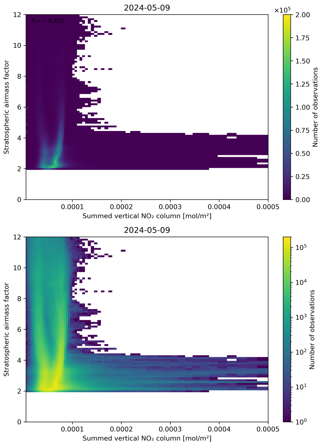
Figure 103: Scatter density plot of “Summed vertical NO 2 column” against “Stratospheric air mass factor” for 2024-05-08 to 2024-05-10.
