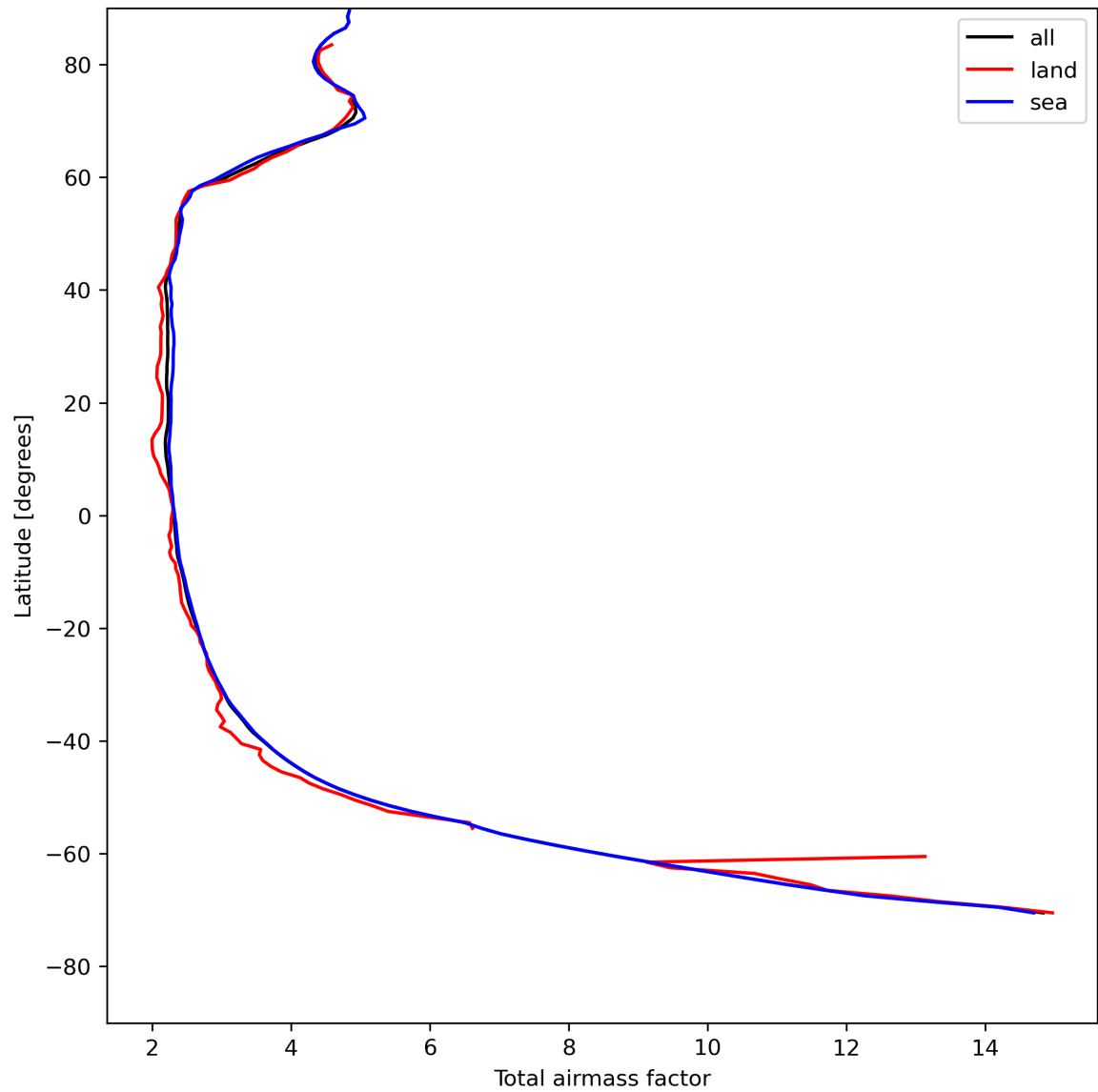
Figure 15: Zonal average of “Total airmass factor” for 2024-05-08 to 2024-05-10.
