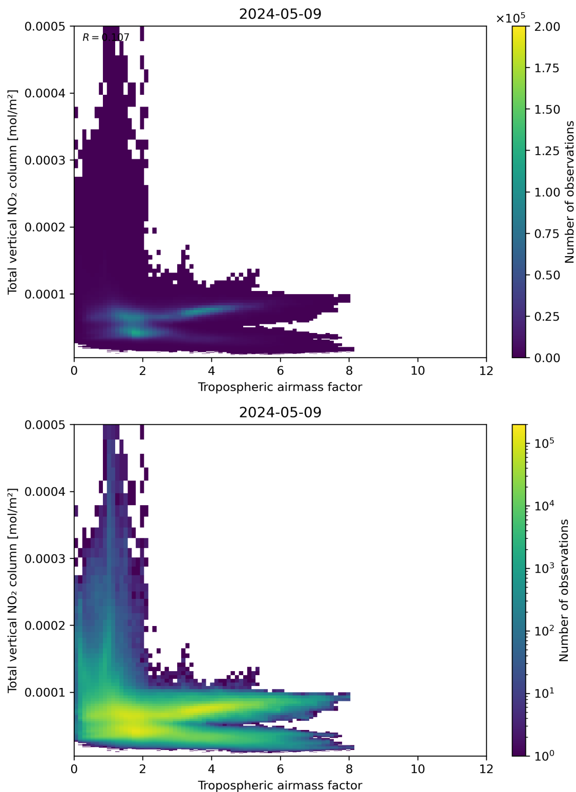
Figure 77: Scatter density plot of “Tropospheric airmass factor” against “Total vertical NO 2 column” for 2024-05-08 to 2024-05-10.
