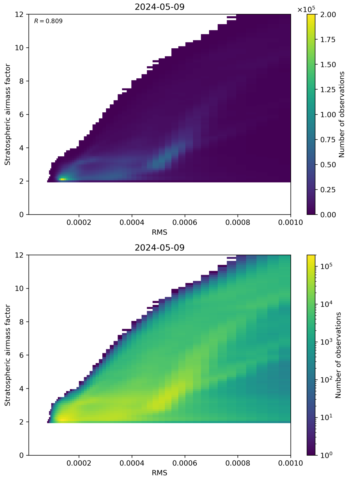
Figure 144: Scatter density plot of “RMS” against “Stratospheric airmass factor” for 2024-05-08 to 2024-05-10.
