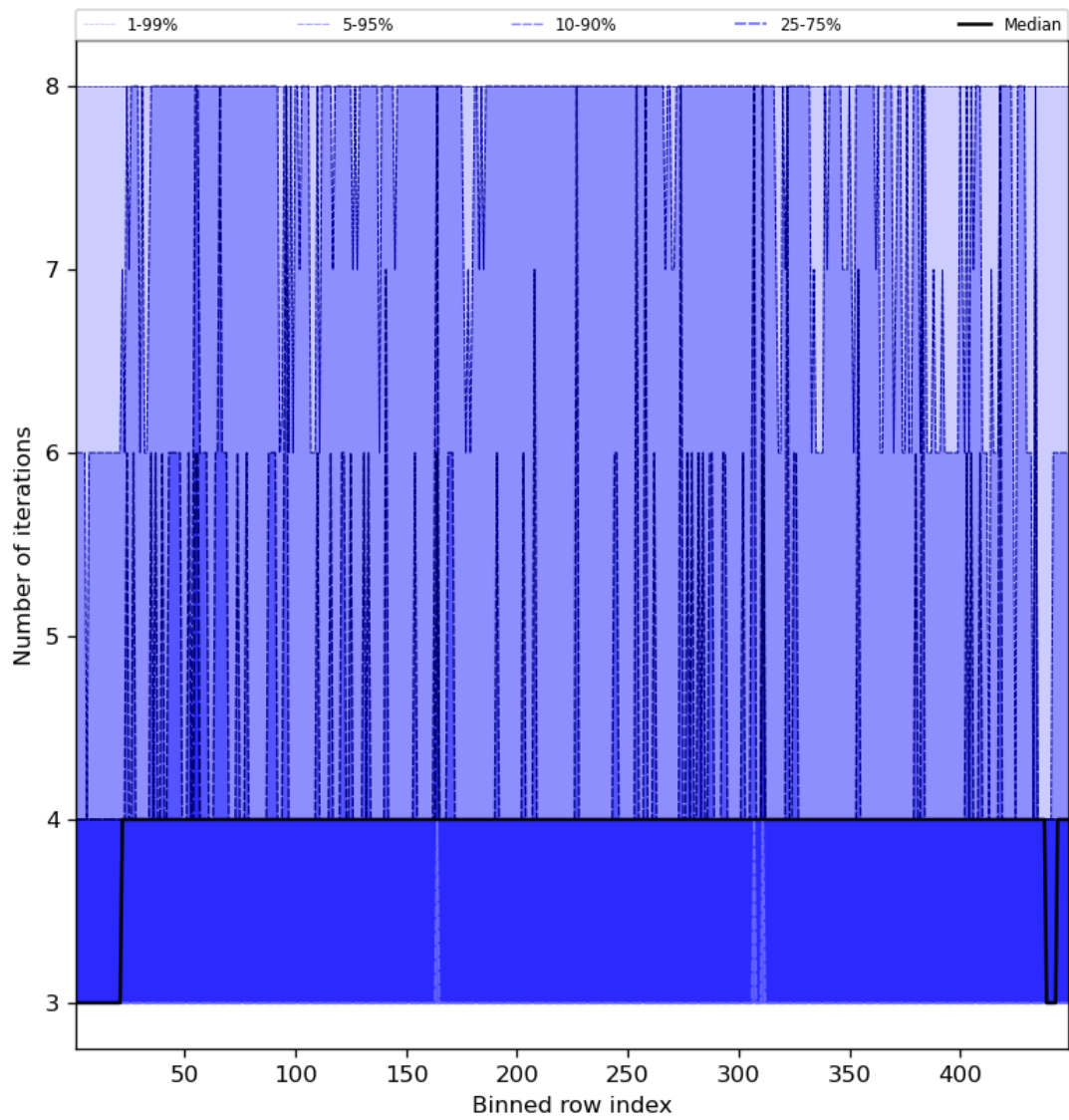
Figure 51: Along track statistics of “Number of iterations” for 2024-05-08 to 2024-05-10
