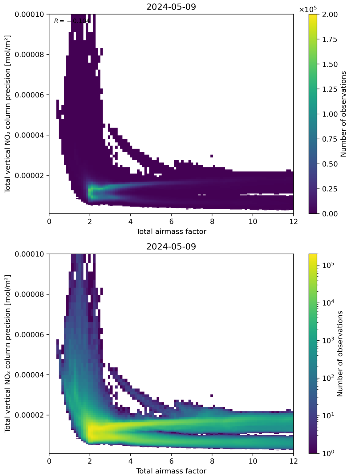
Figure 68: Scatter density plot of “Total airmass factor” against “Total vertical NO 2 column precision” for 2024-05-08 to 2024-05-10.
