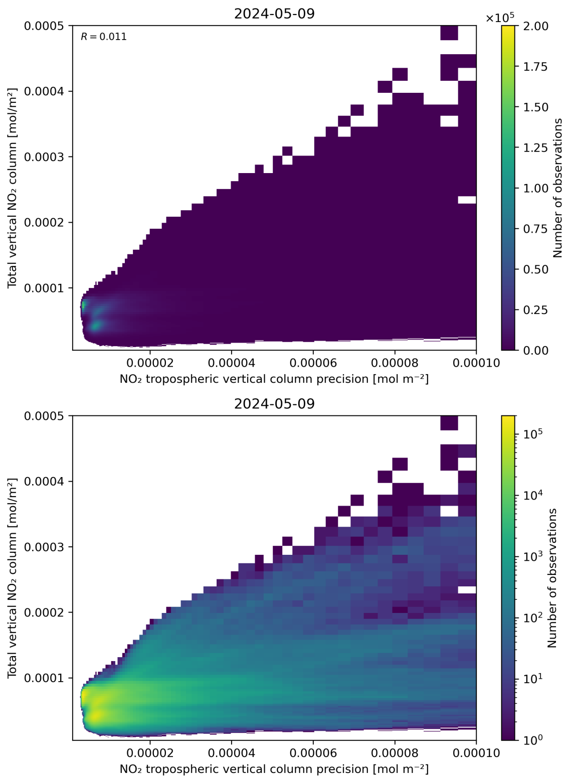
Figure 138: Scatter density plot of “NO 2 tropospheric vertical column precision” against “Total vertical NO 2 column” for 2024-05-08 to 2024-05-10.
