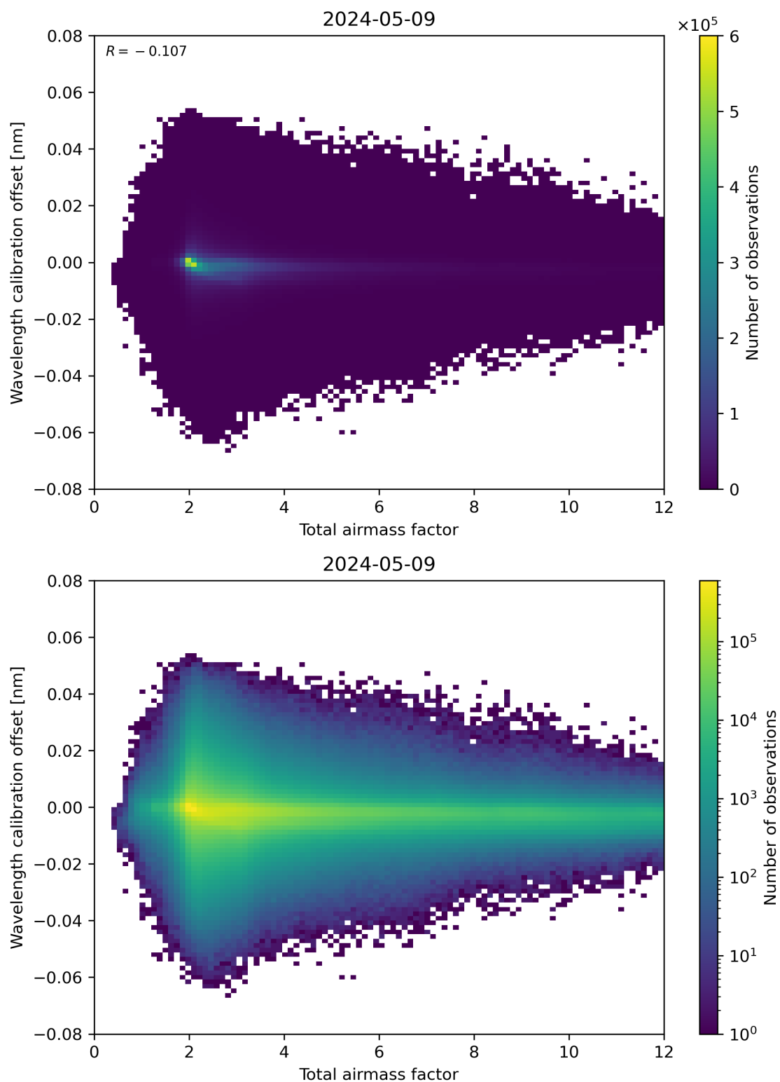
Figure 70: Scatter density plot of “Total airmass factor” against “Wavelength calibration offset” for 2024-05-08 to 2024-05-10.
