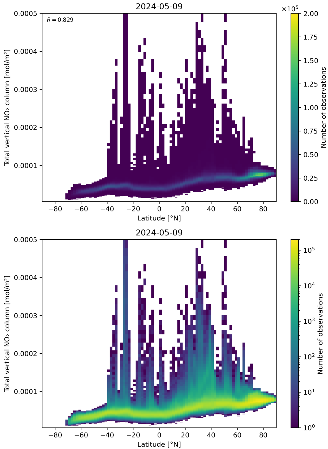
Figure 90: Scatter density plot of “Latitude” against “Total vertical NO 2 column” for 2024-05-08 to 2024-05-10.
