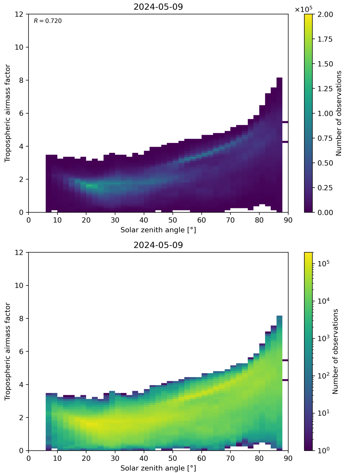
Figure 147: Scatter density plot of “Solar zenith angle” against “Tropospheric airmass factor” for 2024-05-08 to 2024-05-10.
