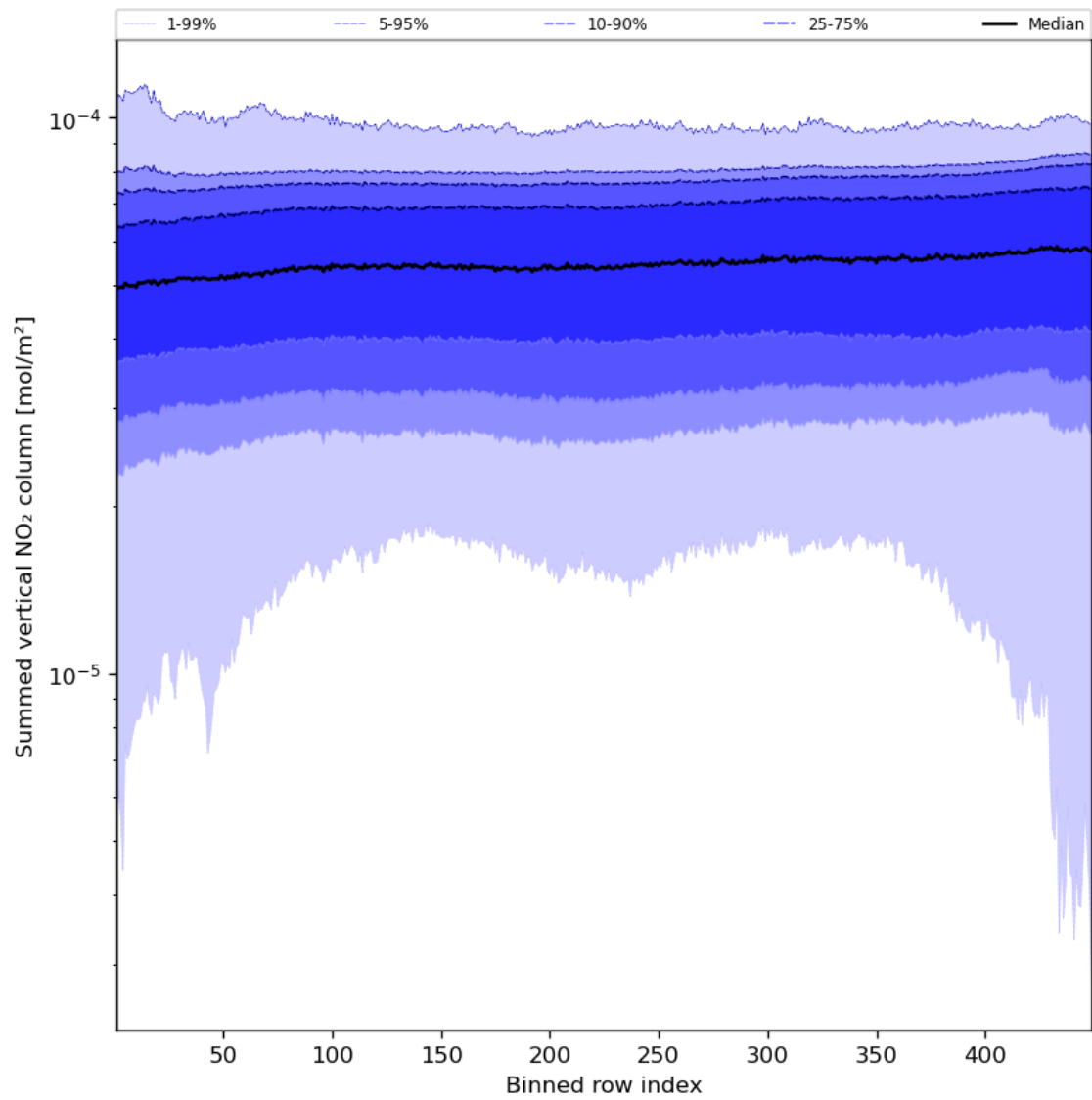
Figure 57: Along track statistics of “Summed vertical NO 2 column” for 2024-05-08 to 2024-05-10
