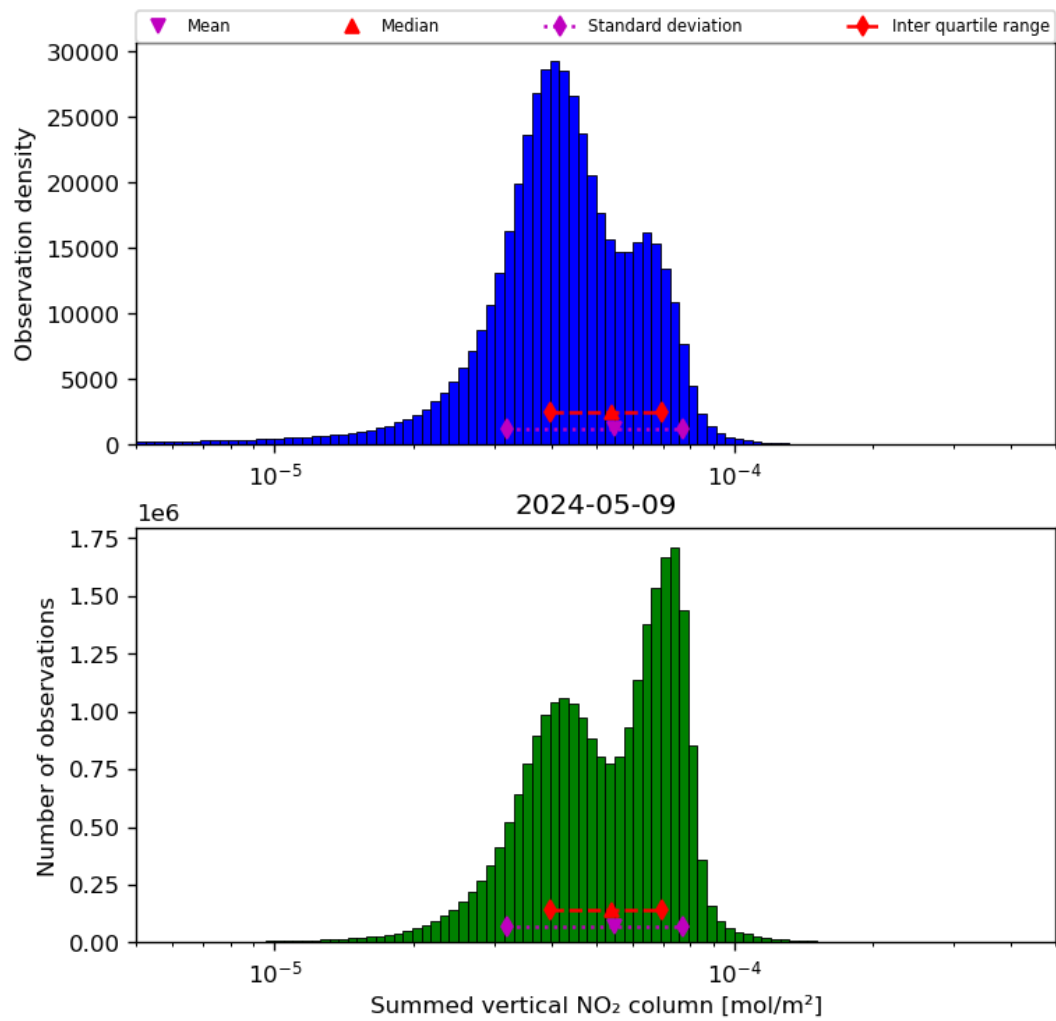
Figure 40: Histogram of “Summed vertical NO 2 column” for 2024-05-08 to 2024-05-10
