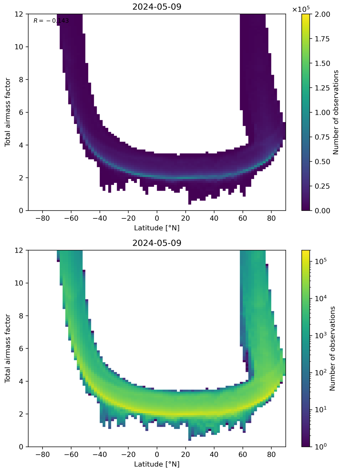
Figure 84: Scatter density plot of “Latitude” against “Total airmass factor” for 2024-05-08 to 2024-05-10.
