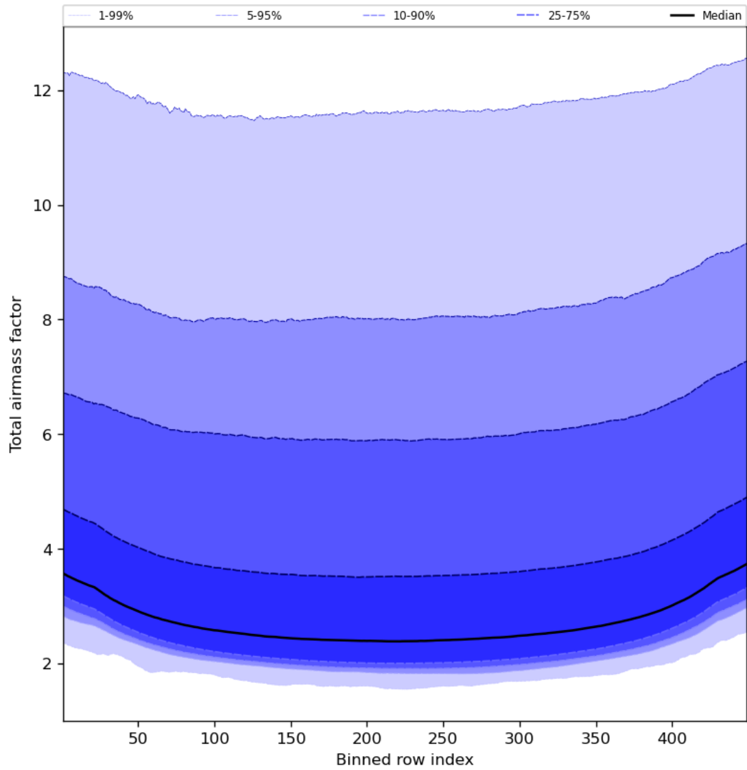
Figure 49: Along track statistics of “Total airmass factor” for 2024-05-08 to 2024-05-10
