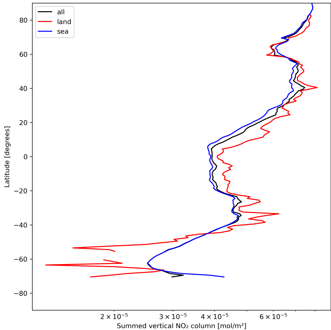
Figure 23: Zonal average of “Summed vertical NO 2 column” for 2024-05-08 to 2024-05-10.
