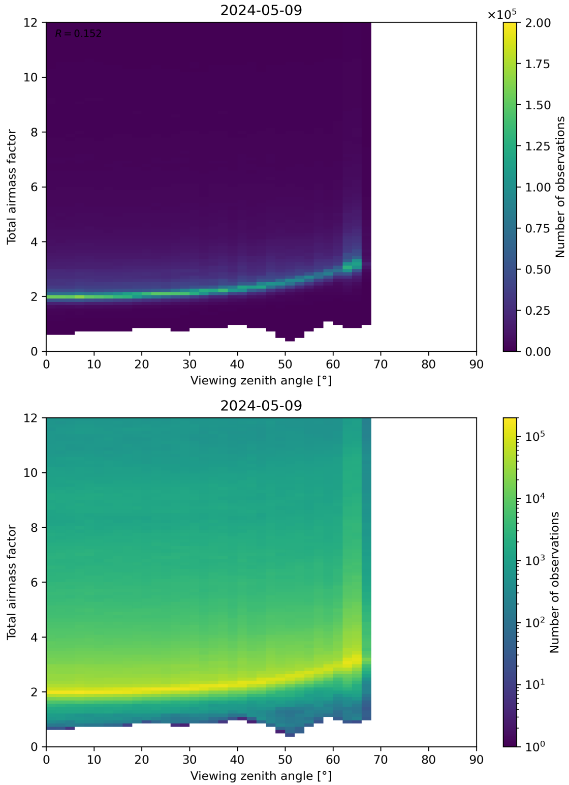
Figure 160: Scatter density plot of “Viewing zenith angle” against “Total airmass factor” for 2024-05-08 to 2024-05-10.
