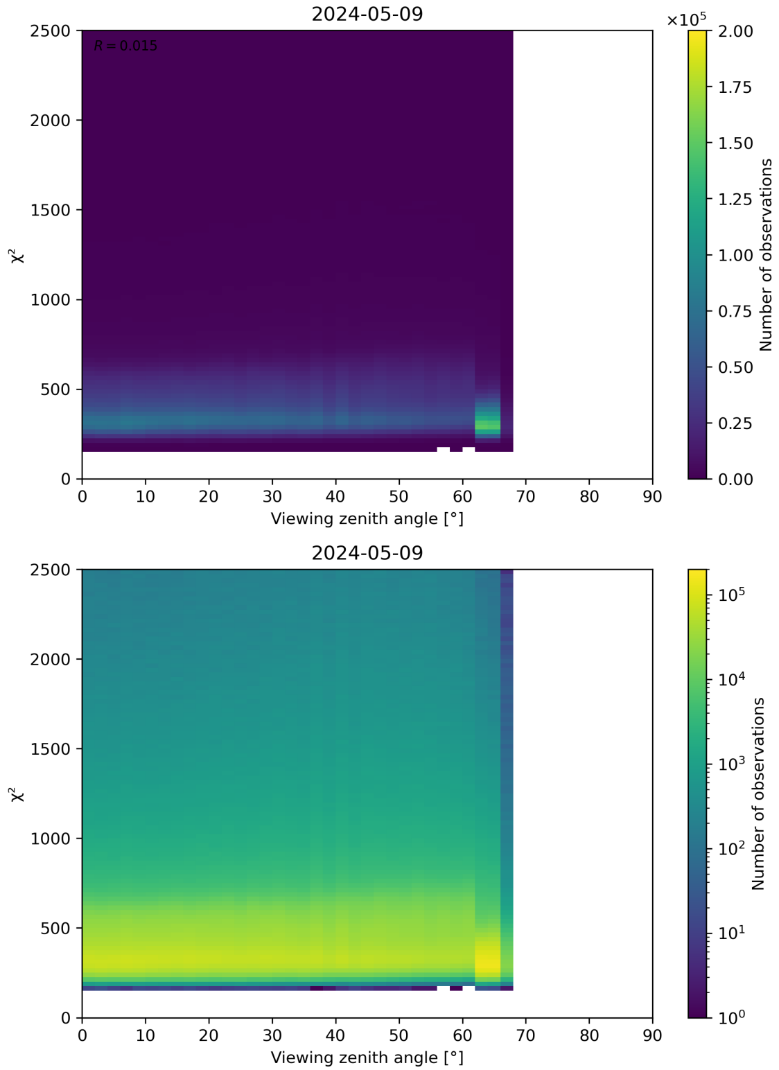
Figure 162: Scatter density plot of “Viewing zenith angle” against “ \chi^2 ” for 2024-05-08 to 2024-05-10.
