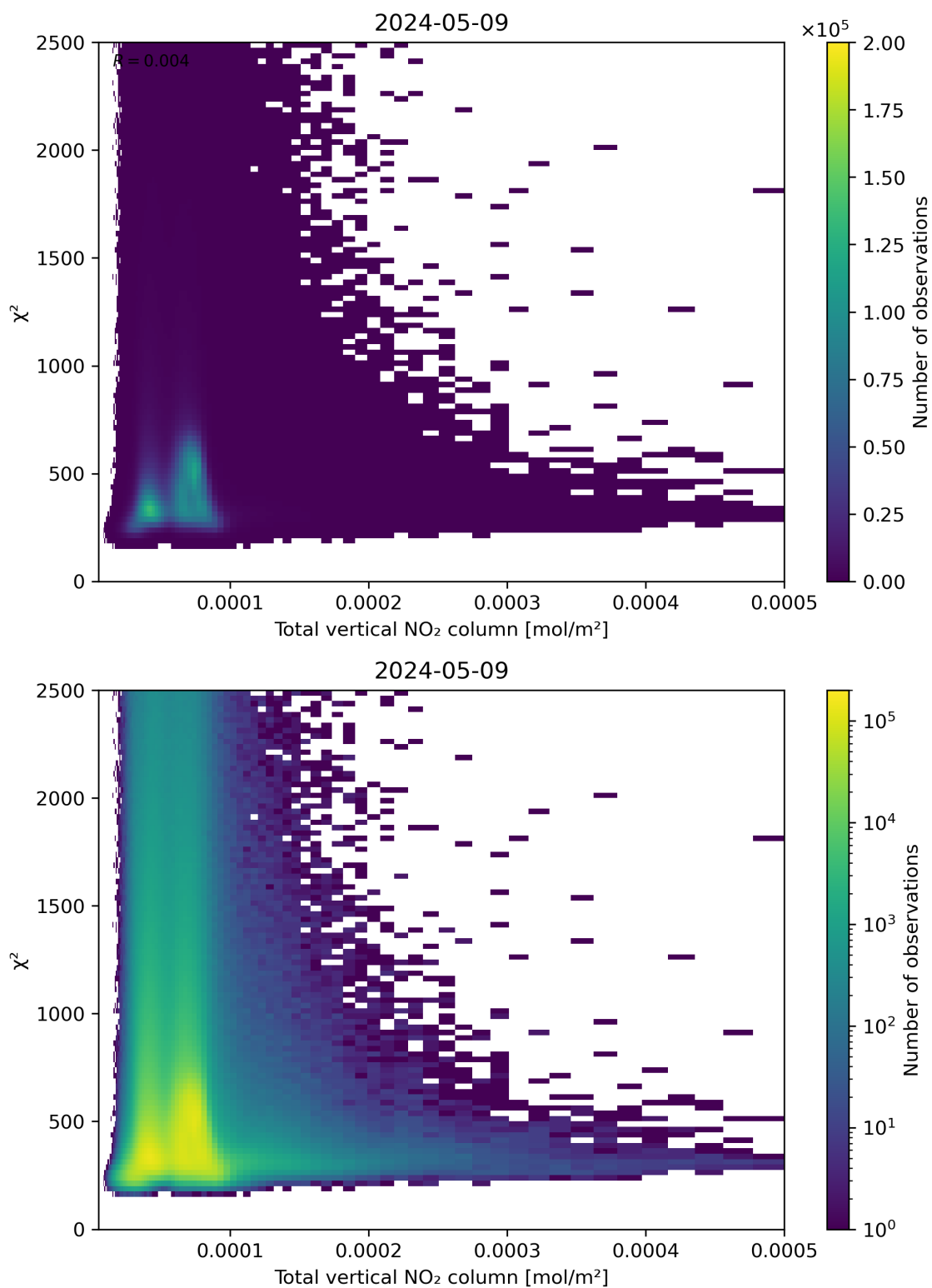
Figure 111: Scatter density plot of “Total vertical NO 2 column” against “ \chi^2 ” for 2024-05-08 to 2024-05-10.
