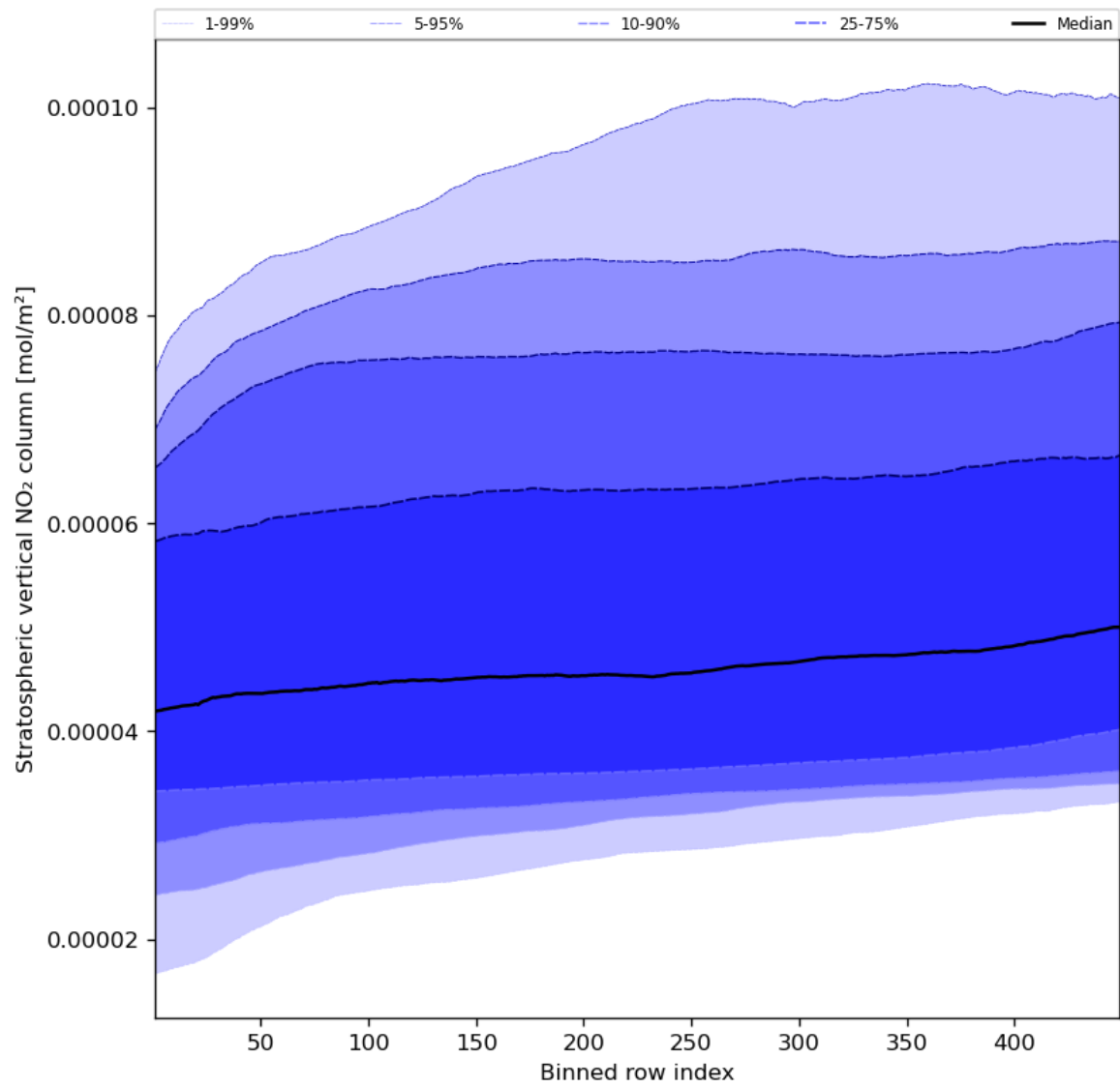
Figure 53: Along track statistics of “Stratospheric vertical NO 2 column” for 2024-05-08 to 2024-05-10
