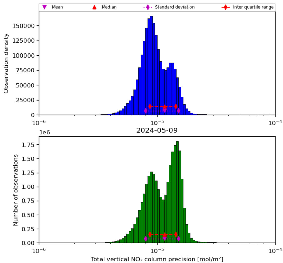
Figure 39: Histogram of "Total vertical NO 2 column precision" for 2024-05-08 to 2024-05-10
