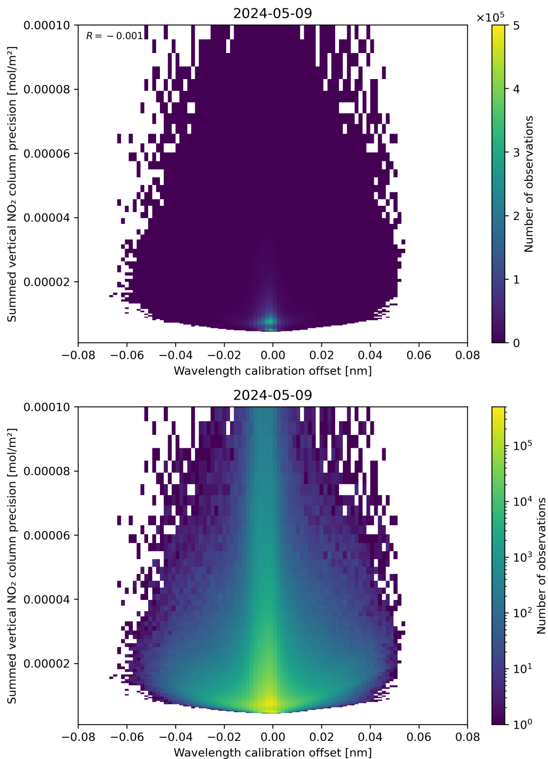
Figure 178: Scatter density plot of “Wavelength calibration offset” against “Summed vertical NO 2 column precision” for 2024-05-08 to 2024-05-10.
