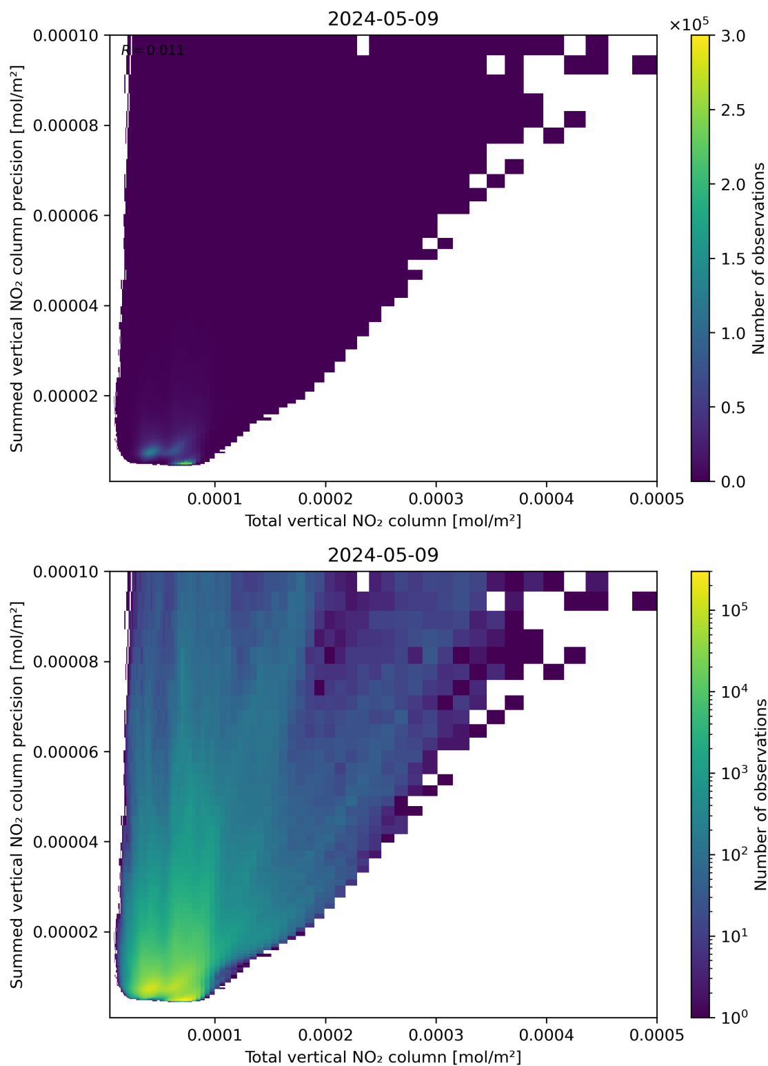
Figure 113: Scatter density plot of “Total vertical NO 2 column” against “Summed vertical NO 2 column precision” for 2024-05-08 to 2024-05-10.
