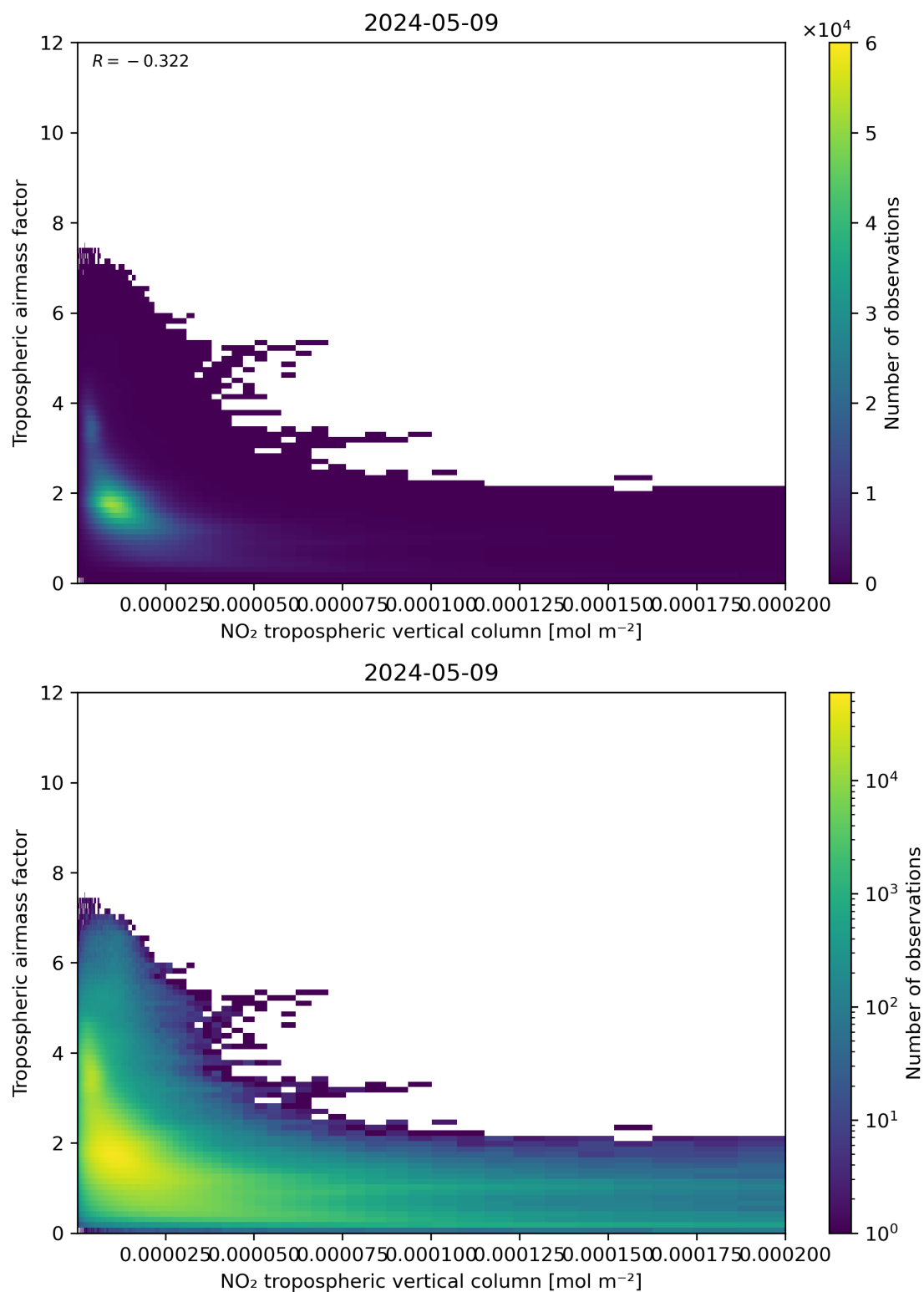
Figure 123: Scatter density plot of “NO 2 tropospheric vertical column” against “Tropospheric airmass factor” for 2024-05-08 to 2024-05-10.
