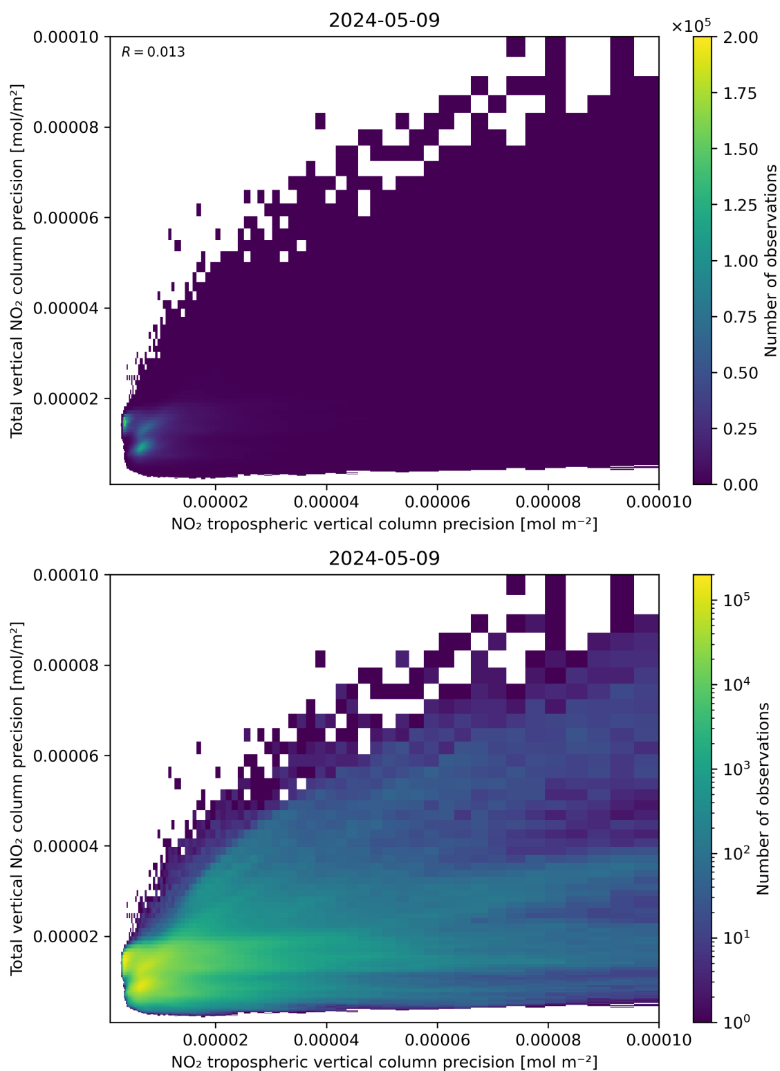
Figure 139: Scatter density plot of “NO 2 tropospheric vertical column precision” against “Total vertical NO 2 column precision” for 2024-05-08 to 2024-05-10.
