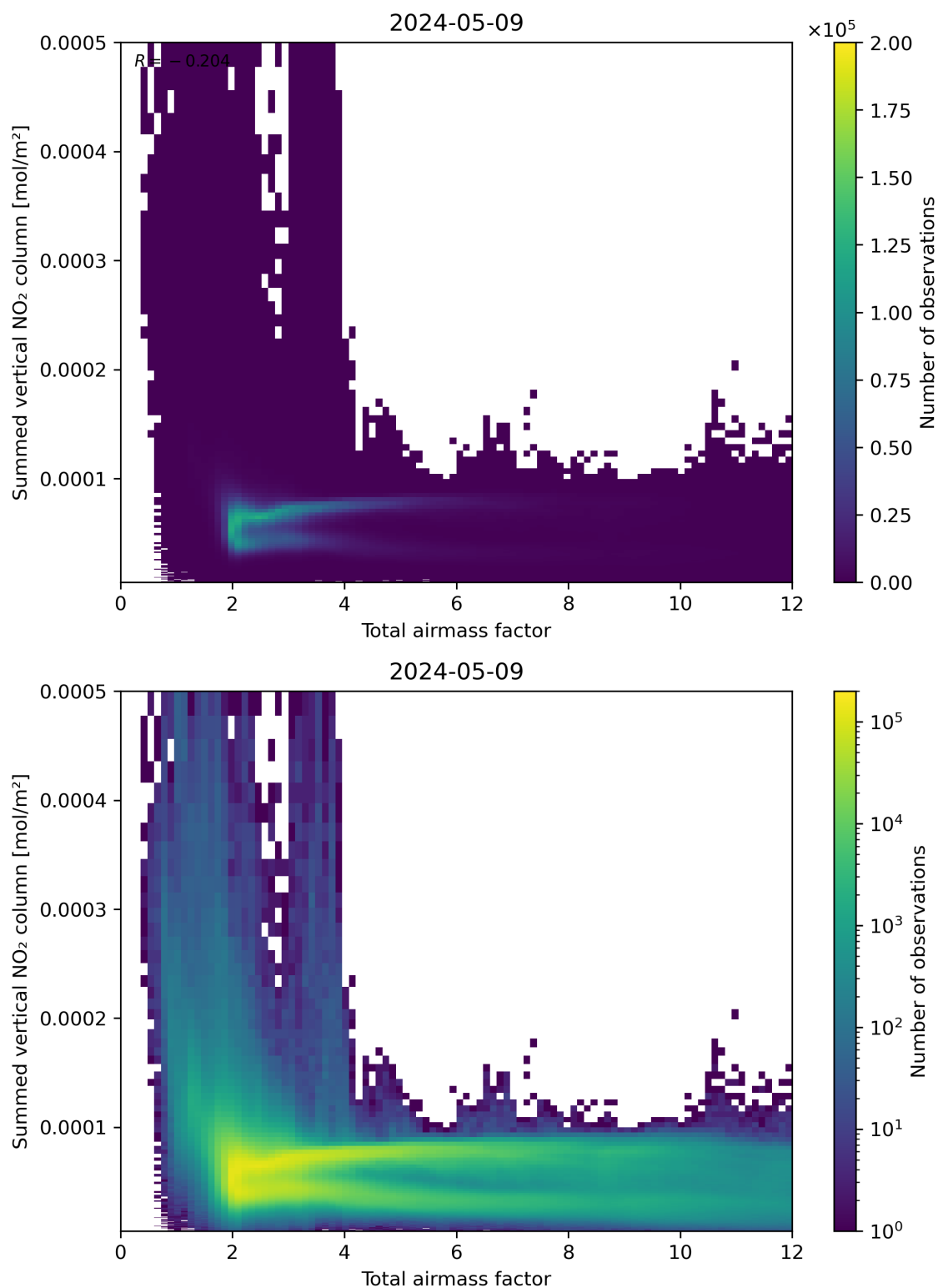
Figure 65: Scatter density plot of “Total airmass factor” against “Summed vertical NO 2 column” for 2024-05-08 to 2024-05-10.
