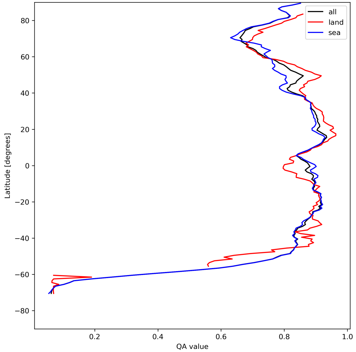
Figure 11: Zonal average of “QA value” for 2024-05-08 to 2024-05-10.
