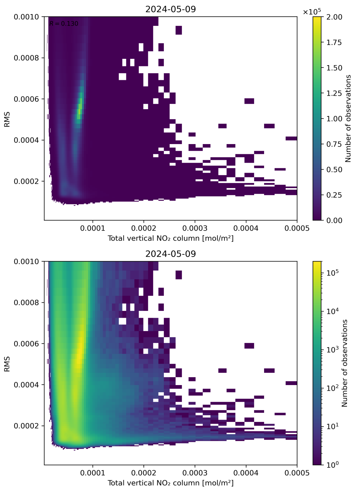
Figure 120: Scatter density plot of “Total vertical NO 2 column” against “RMS” for 2024-05-08 to 2024-05-10.
