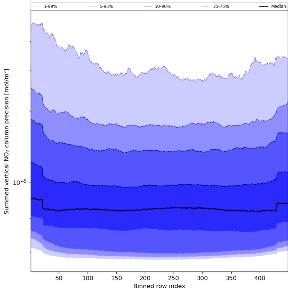
Figure 58: Along track statistics of “Summed vertical NO 2 column precision” for 2024-05-08 to 2024-05-10
