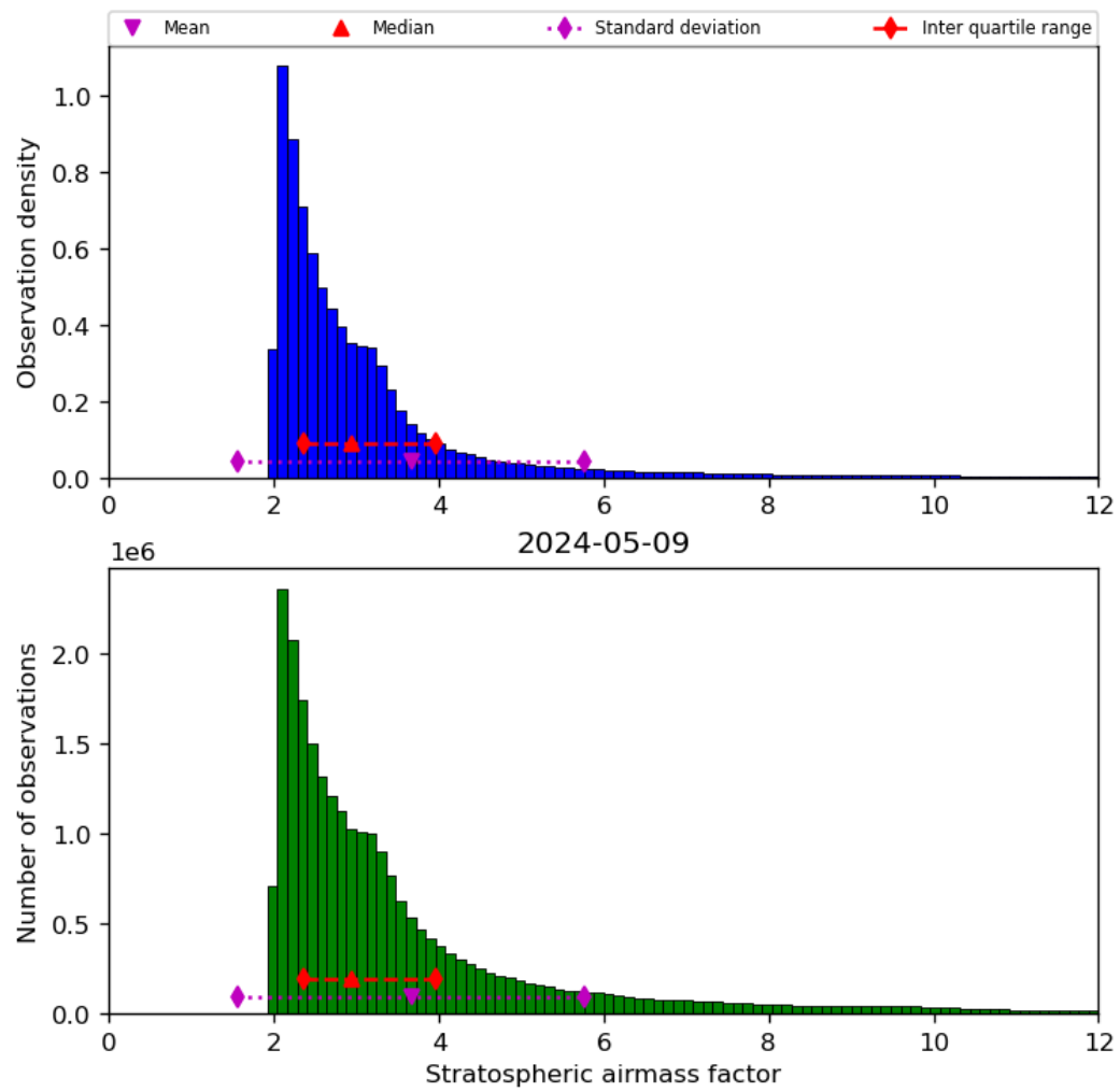
Figure 44: Histogram of “Stratospheric airmass factor” for 2024-05-08 to 2024-05-10
