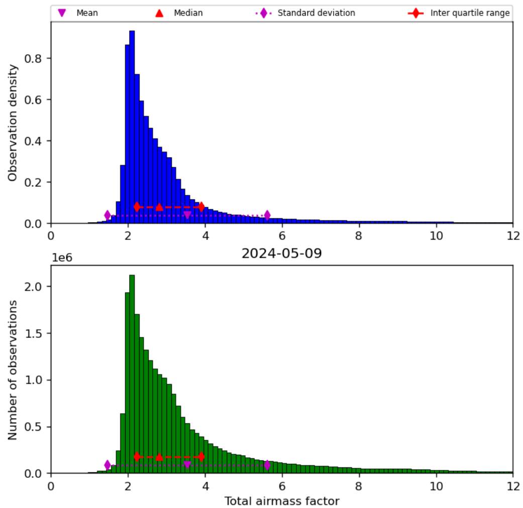
Figure 32: Histogram of “Total airmass factor” for 2024-05-08 to 2024-05-10
