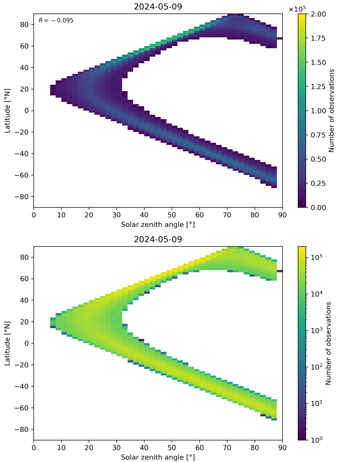
Figure 149: Scatter density plot of “Solar zenith angle” against “Latitude” for 2024-05-08 to 2024-05-10.
