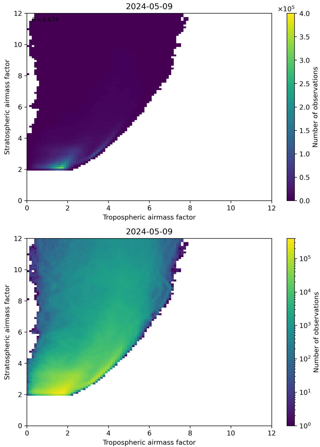
Figure 71: Scatter density plot of “Tropospheric airmass factor” against “Stratospheric airmass factor” for 2024-05-08 to 2024-05-10.
