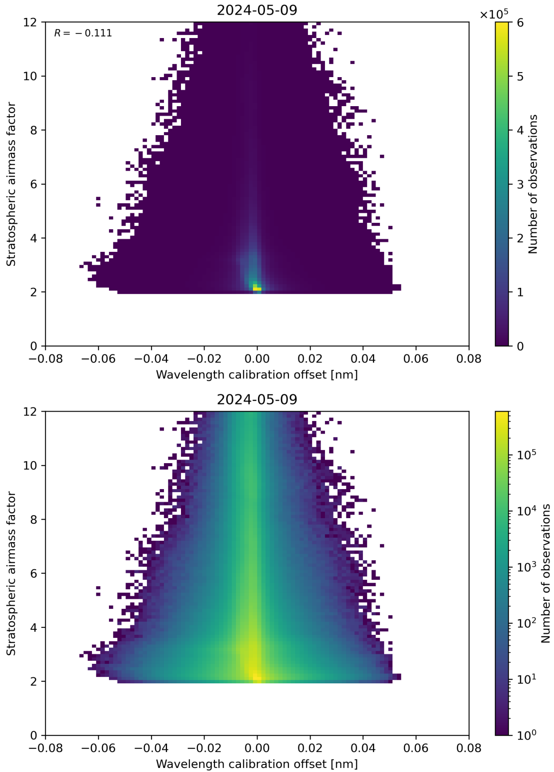
Figure 174: Scatter density plot of “Wavelength calibration offset” against “Stratospheric airmass factor” for 2024-05-08 to 2024-05-10.
