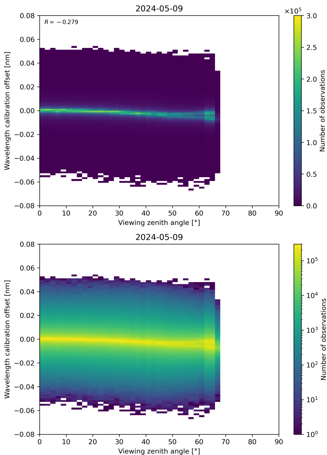
Figure 173: Scatter density plot of “Viewing zenith angle” against “Wavelength calibration offset” for 2024-05-08 to 2024-05-10.
