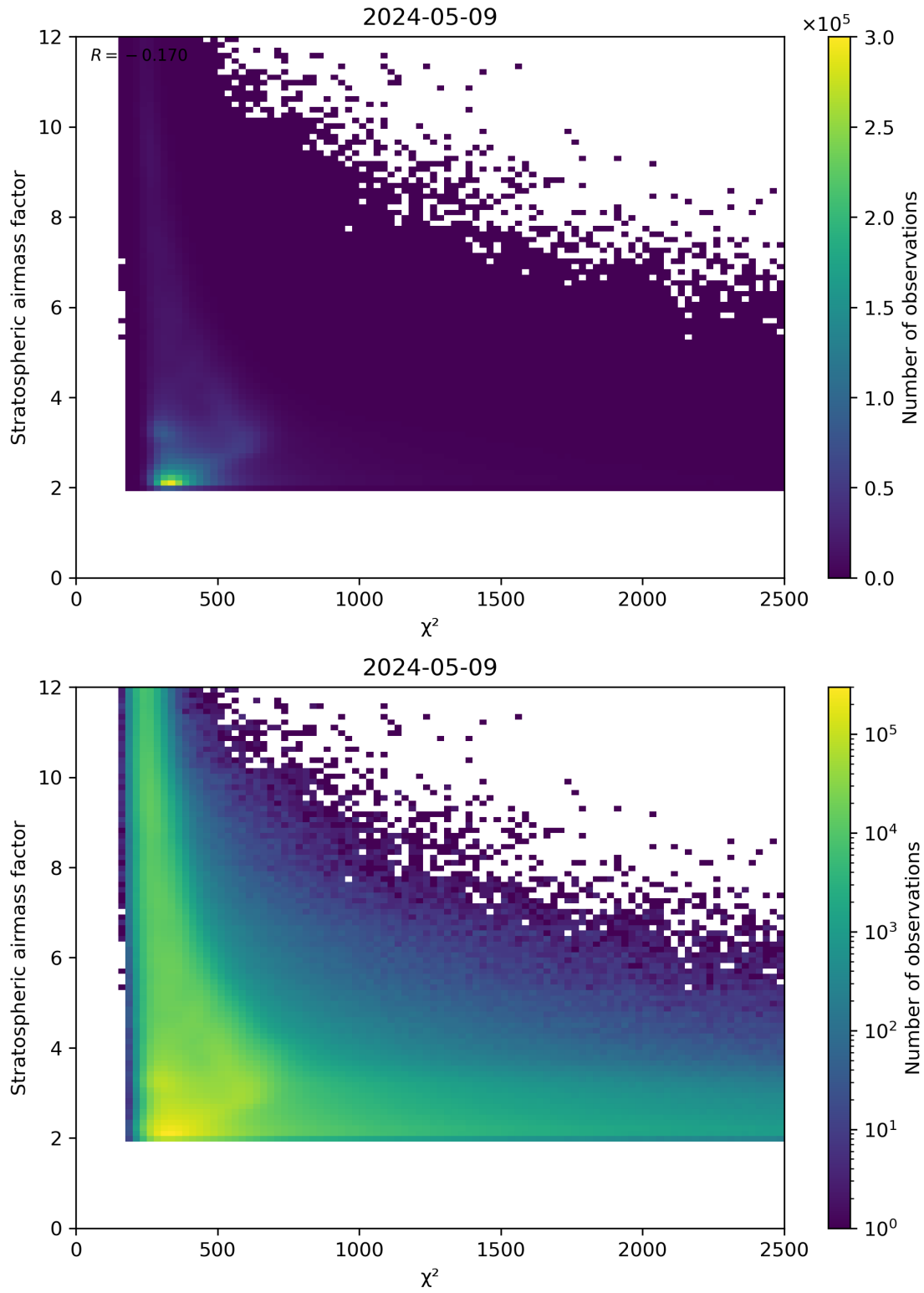
Figure 81: Scatter density plot of “ \chi^2 ” against “Stratospheric airmass factor” for 2024-05-08 to 2024-05-10.
