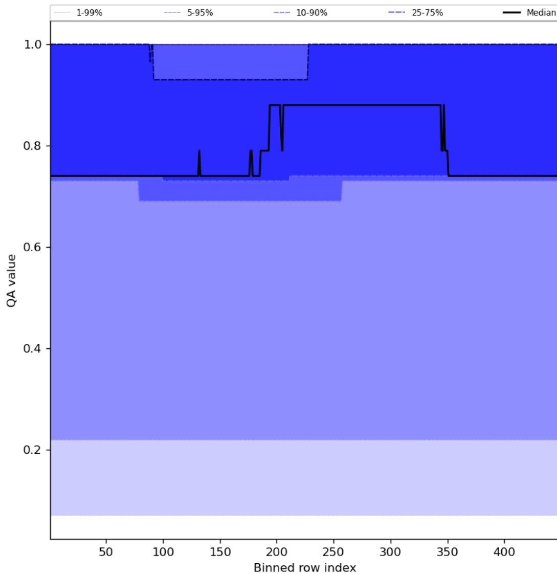
Figure 45: Along track statistics of “QA value” for 2024-05-08 to 2024-05-10
