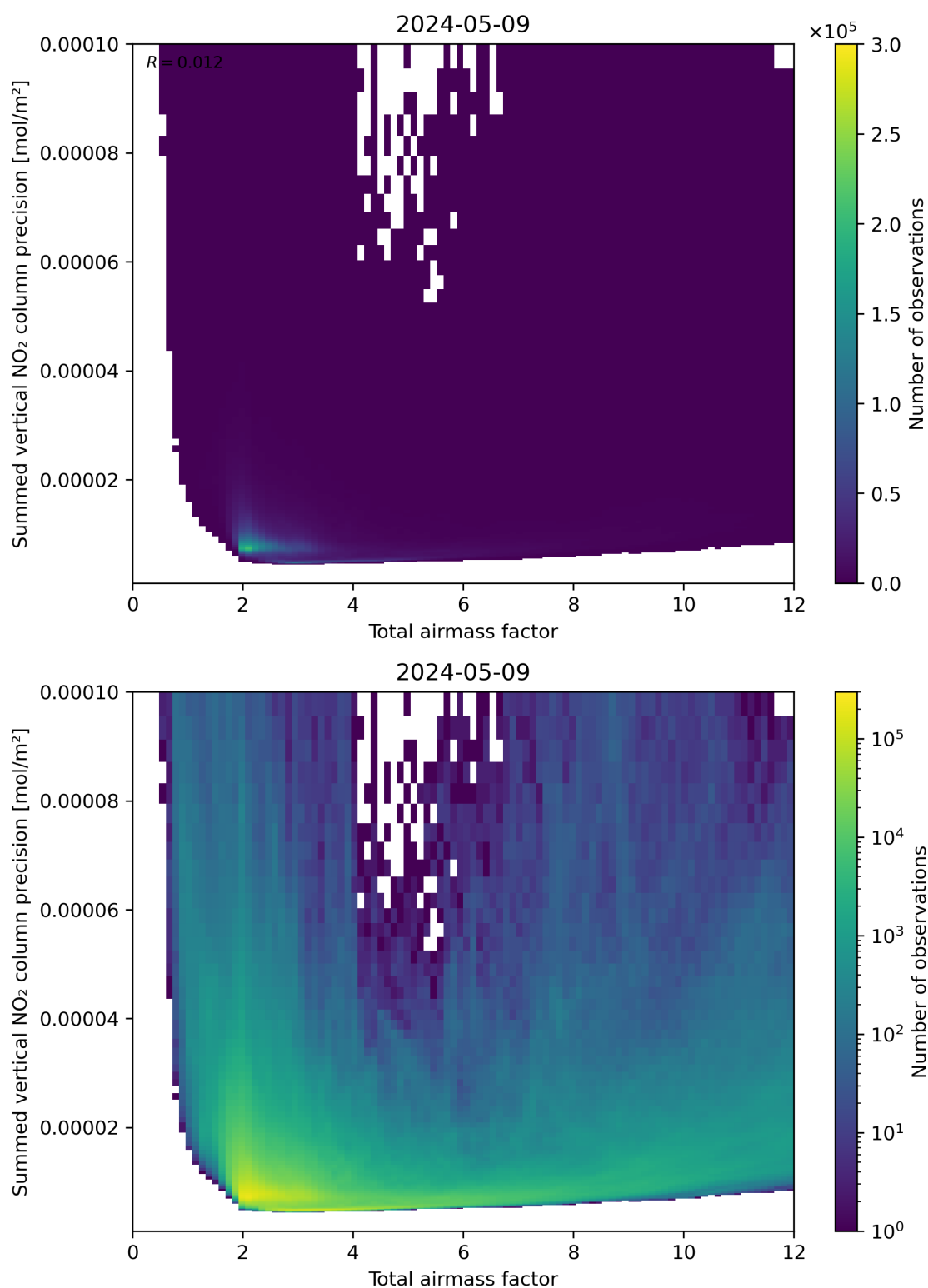
Figure 66: Scatter density plot of “Total airmass factor” against “Summed vertical NO 2 column precision” for 2024-05-08 to 2024-05-10.
