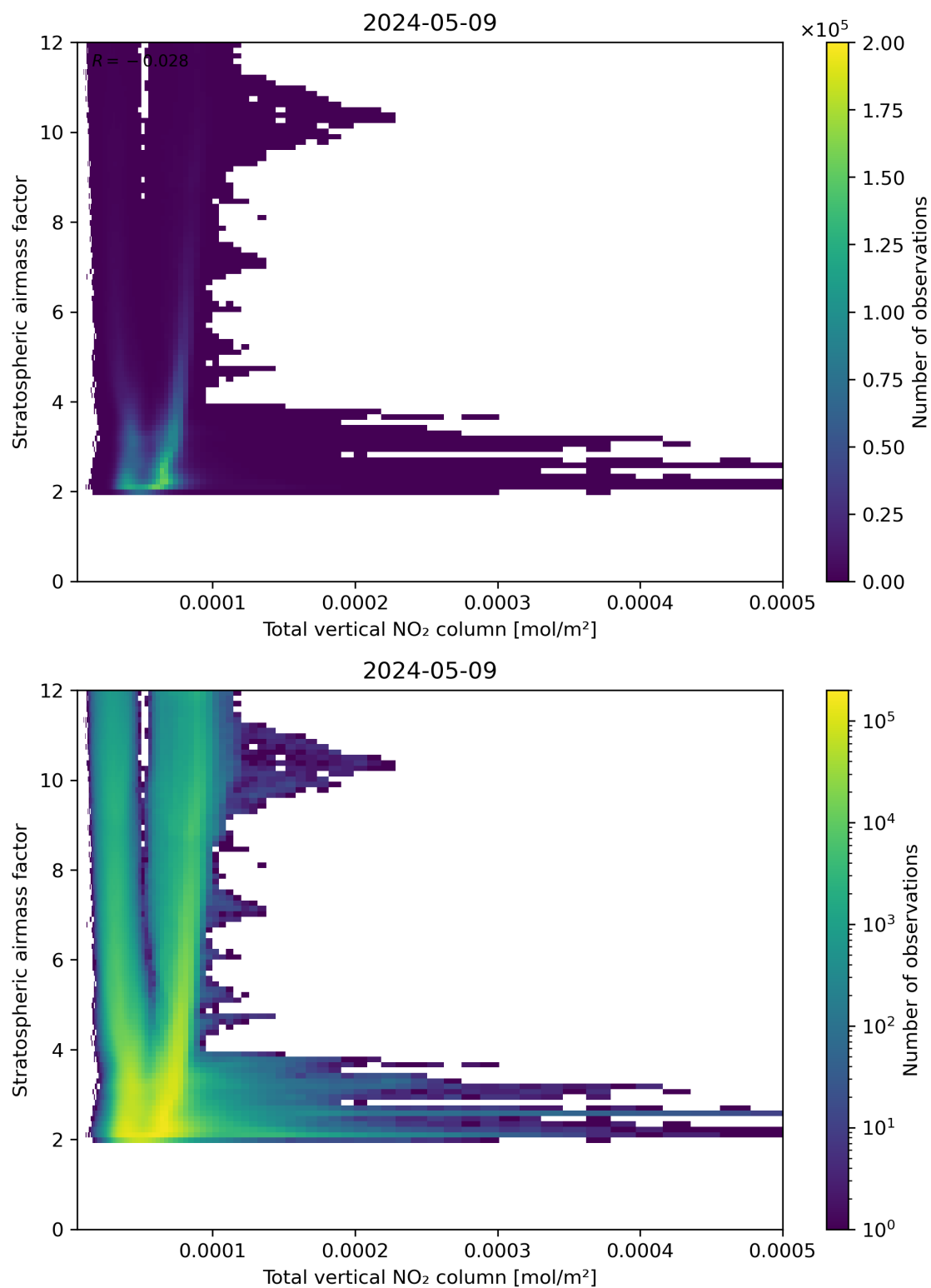
Figure 110: Scatter density plot of “Total vertical NO 2 column” against “Stratospheric airmass factor” for 2024-05-08 to 2024-05-10.
