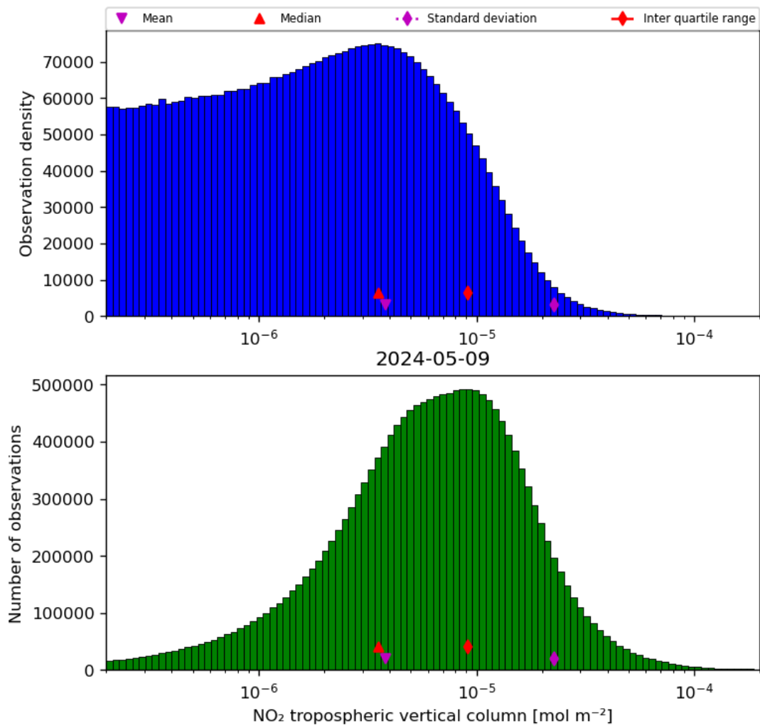
Figure 29: Histogram of “NO 2 tropospheric vertical column” for 2024-05-08 to 2024-05-10
