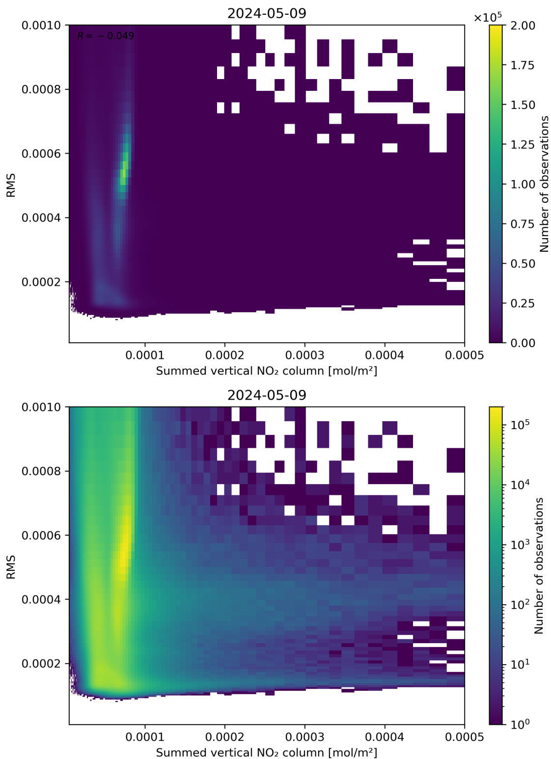
Figure 109: Scatter density plot of “Summed vertical NO 2 column” against “RMS” for 2024-05-08 to 2024-05-10.
