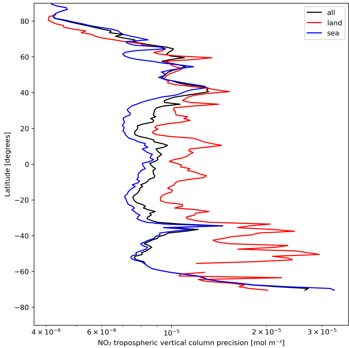
Figure 13: Zonal average of “NO 2 tropospheric vertical column precision” for 2024-05-08 to 2024-05-10.
