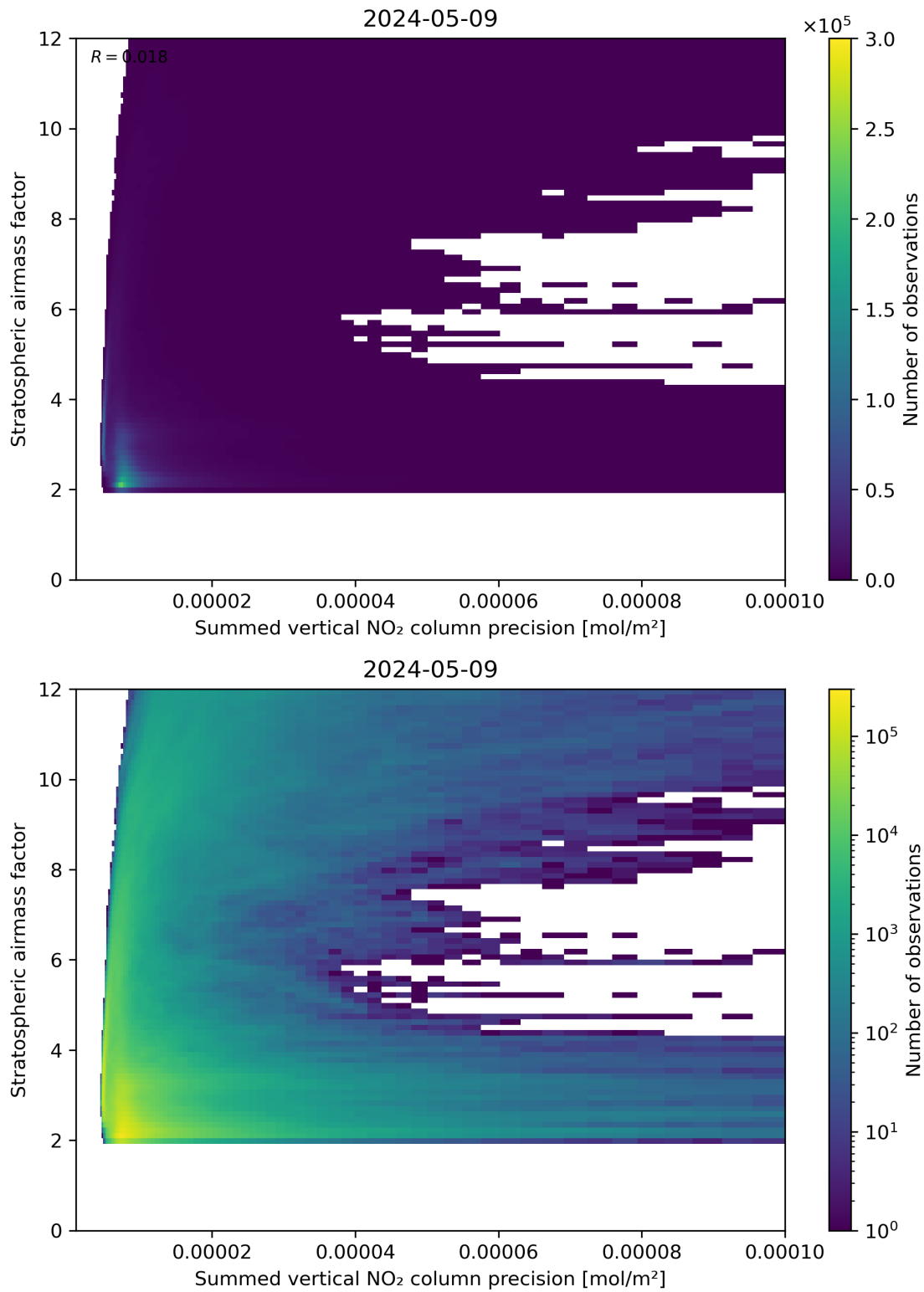
Figure 106: Scatter density plot of “Summed vertical NO 2 column precision” against “Stratospheric airmass factor” for 2024-05-08 to 2024-05-10.
