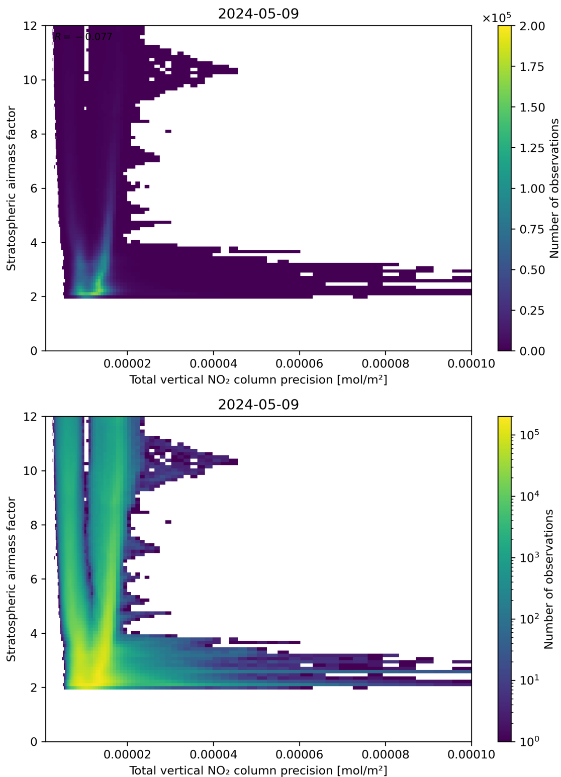
Figure 115: Scatter density plot of “Total vertical NO 2 column precision” against “Stratospheric airmass factor” for 2024-05-08 to 2024-05-10.
