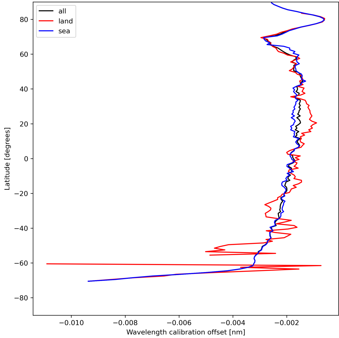
Figure 18: Zonal average of “Wavelength calibration offset” for 2024-05-08 to 2024-05-10.
