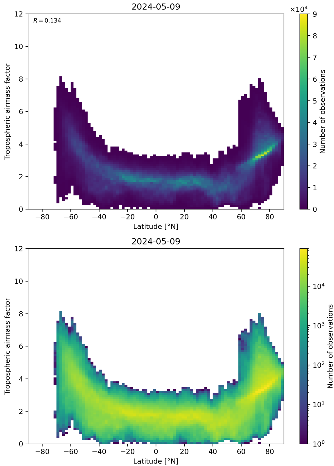
Figure 85: Scatter density plot of “Latitude” against “Tropospheric airmass factor” for 2024-05-08 to 2024-05-10.
