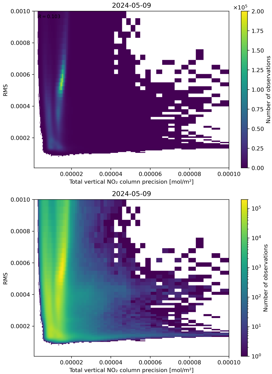
Figure 119: Scatter density plot of “Total vertical NO 2 column precision” against “RMS” for 2024-05-08 to 2024-05-10.
