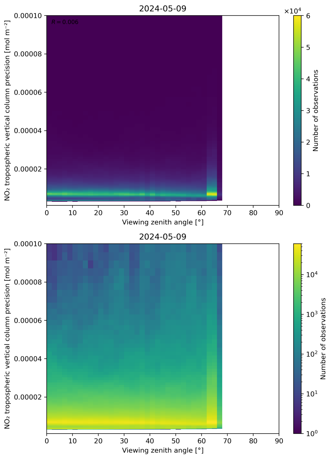
Figure 170: Scatter density plot of “Viewing zenith angle” against “NO 2 tropospheric vertical column precision” for 2024-05-08 to 2024-05-10.
