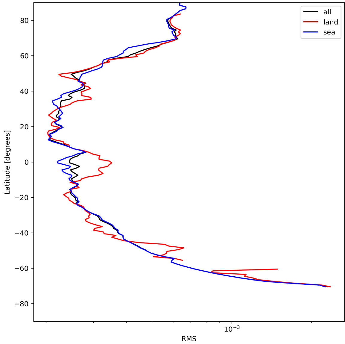
Figure 26: Zonal average of “RMS” for 2024-05-08 to 2024-05-10.
