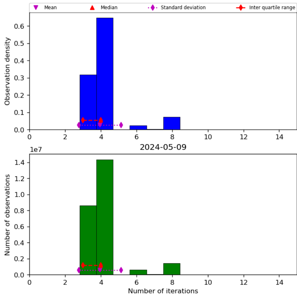
Figure 34: Histogram of “Number of iterations” for 2024-05-08 to 2024-05-10
