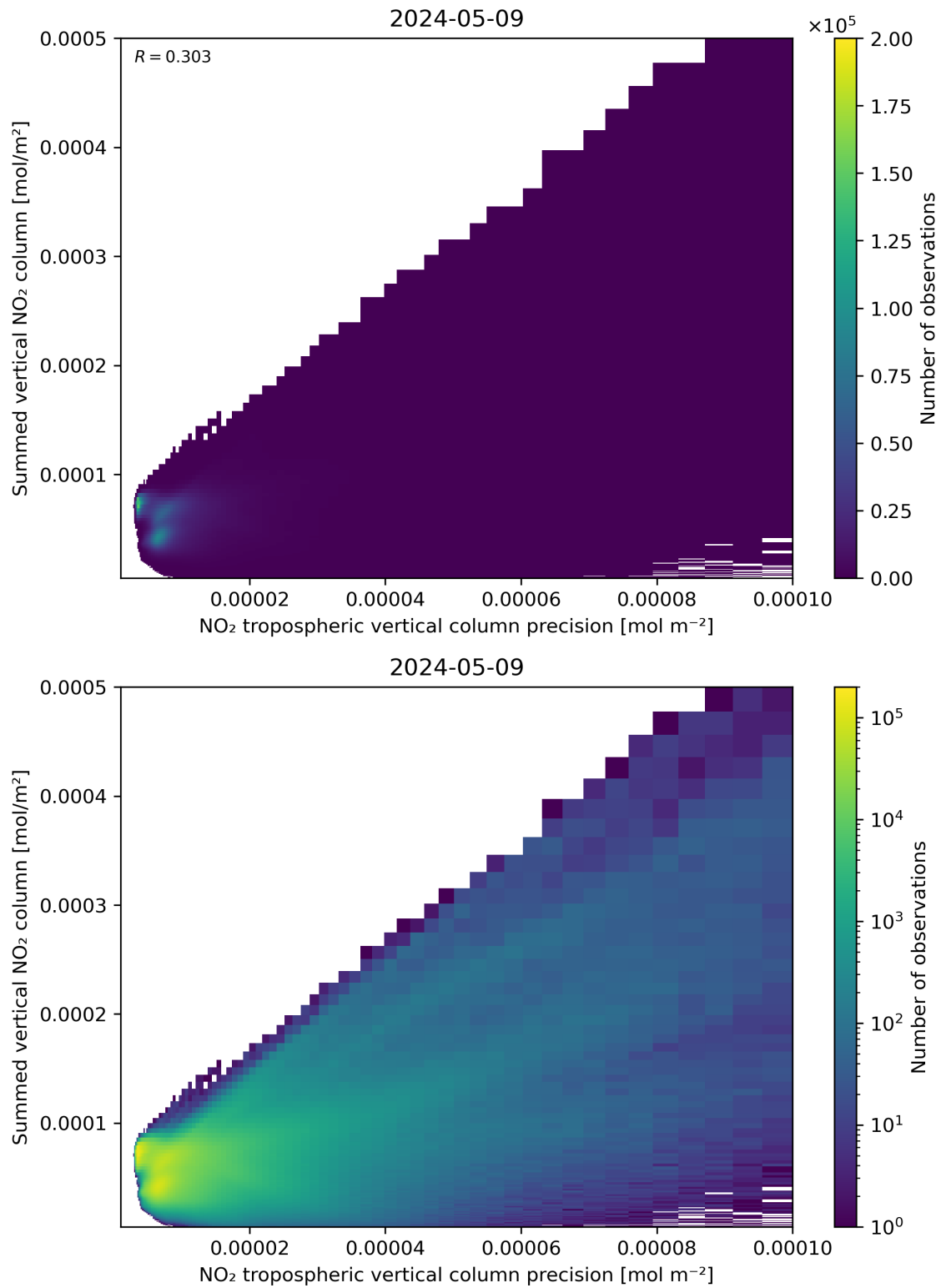
Figure 136: Scatter density plot of “NO 2 tropospheric vertical column precision” against “Summed vertical NO 2 column” for 2024-05-08 to 2024-05-10.
