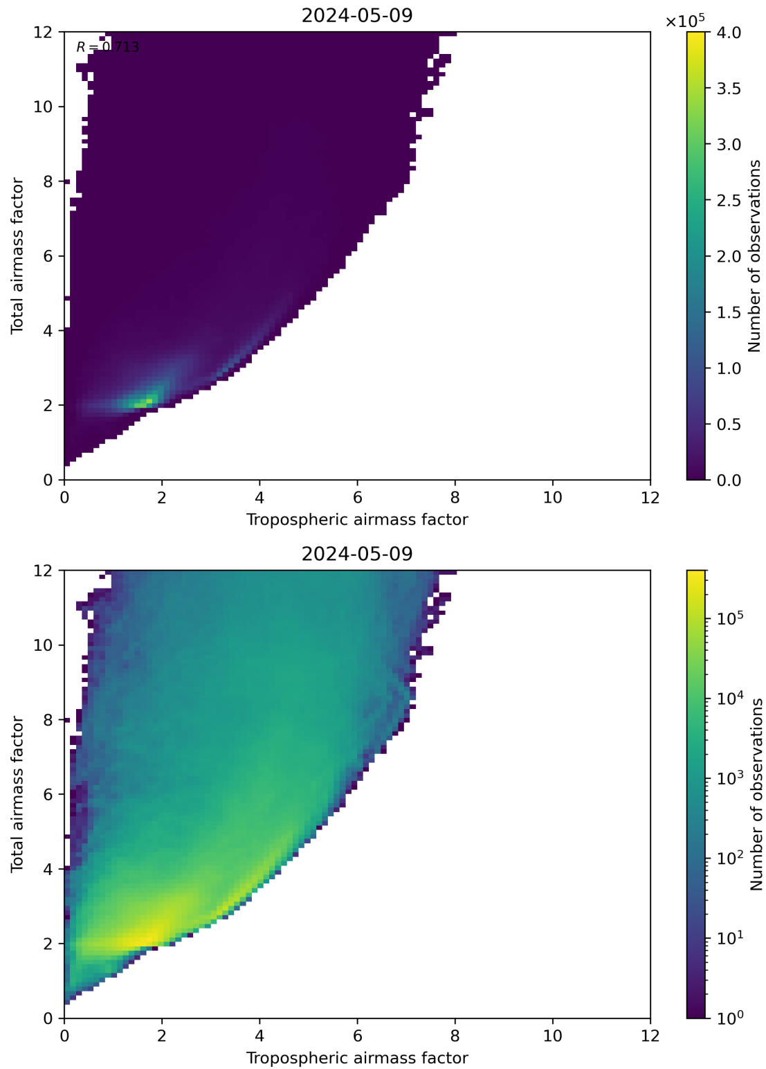
Figure 72: Scatter density plot of “Tropospheric airmass factor” against “Total airmass factor” for 2024-05-08 to 2024-05-10.
