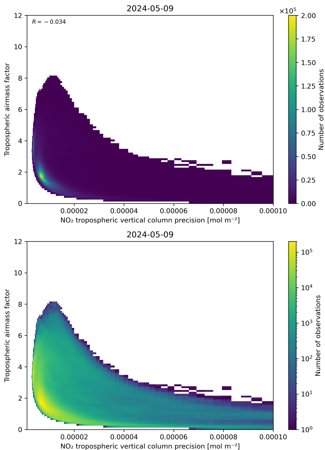
Figure 133: Scatter density plot of “NO 2 tropospheric vertical column precision” against “Tropospheric airmass factor” for 2024-05-08 to 2024-05-10.
