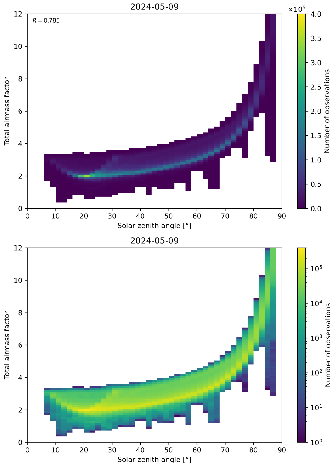
Figure 146: Scatter density plot of “Solar zenith angle” against “Total air mass factor” for 2024-05-08 to 2024-05-10.
