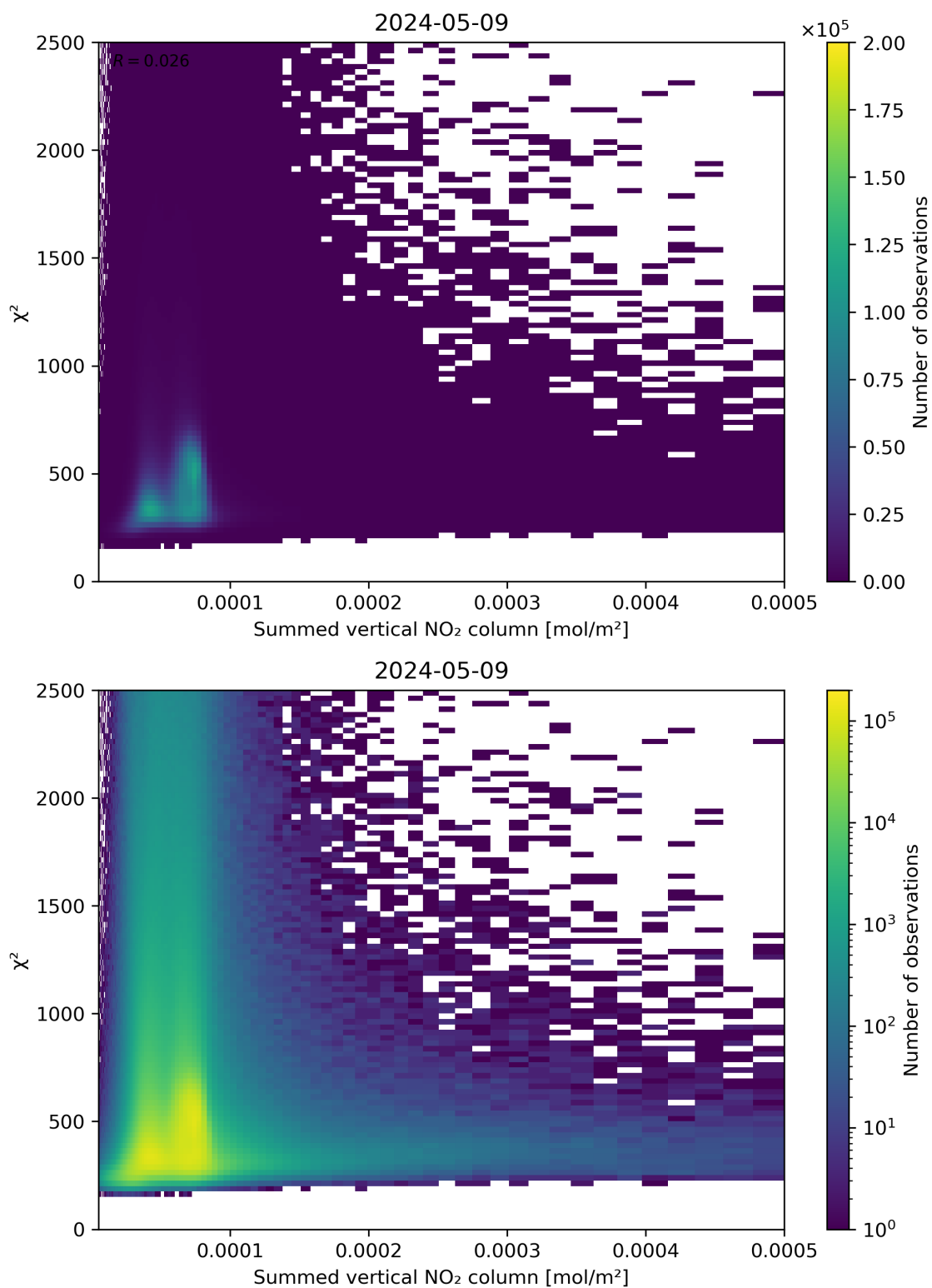
Figure 104: Scatter density plot of “Summed vertical NO 2 column” against “ \chi^2 ” for 2024-05-08 to 2024-05-10.
