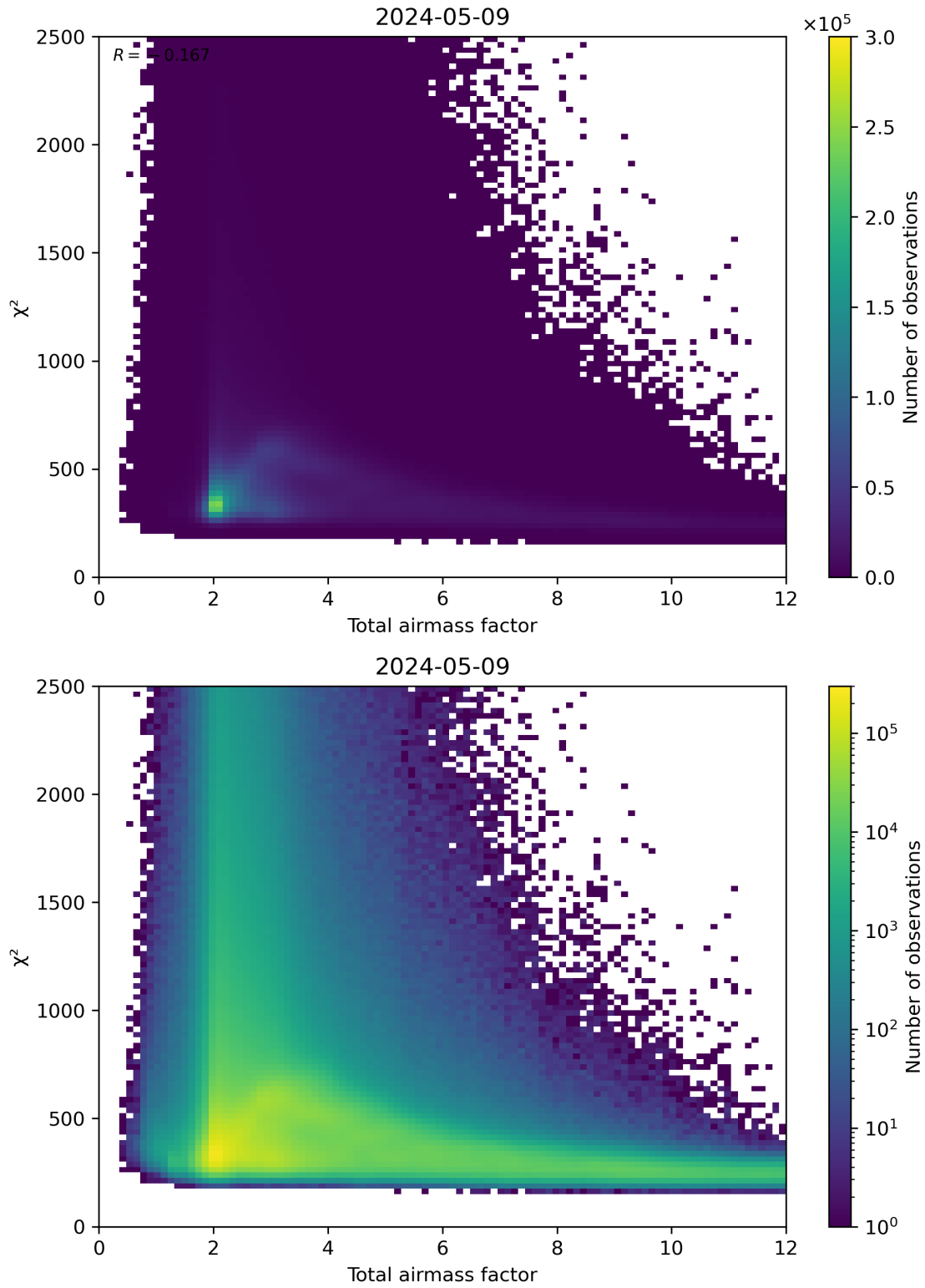
Figure 63: Scatter density plot of “Total airmass factor” against “ \chi^2 ” for 2024-05-08 to 2024-05-10.
