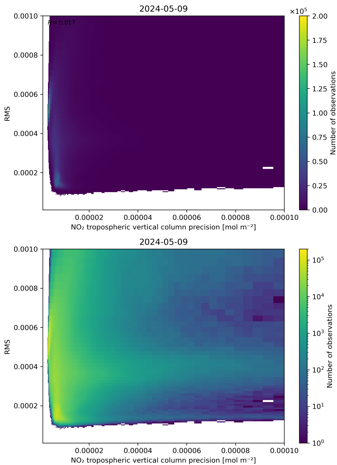
Figure 140: Scatter density plot of “NO 2 tropospheric vertical column precision” against “RMS” for 2024-05-08 to 2024-05-10.
