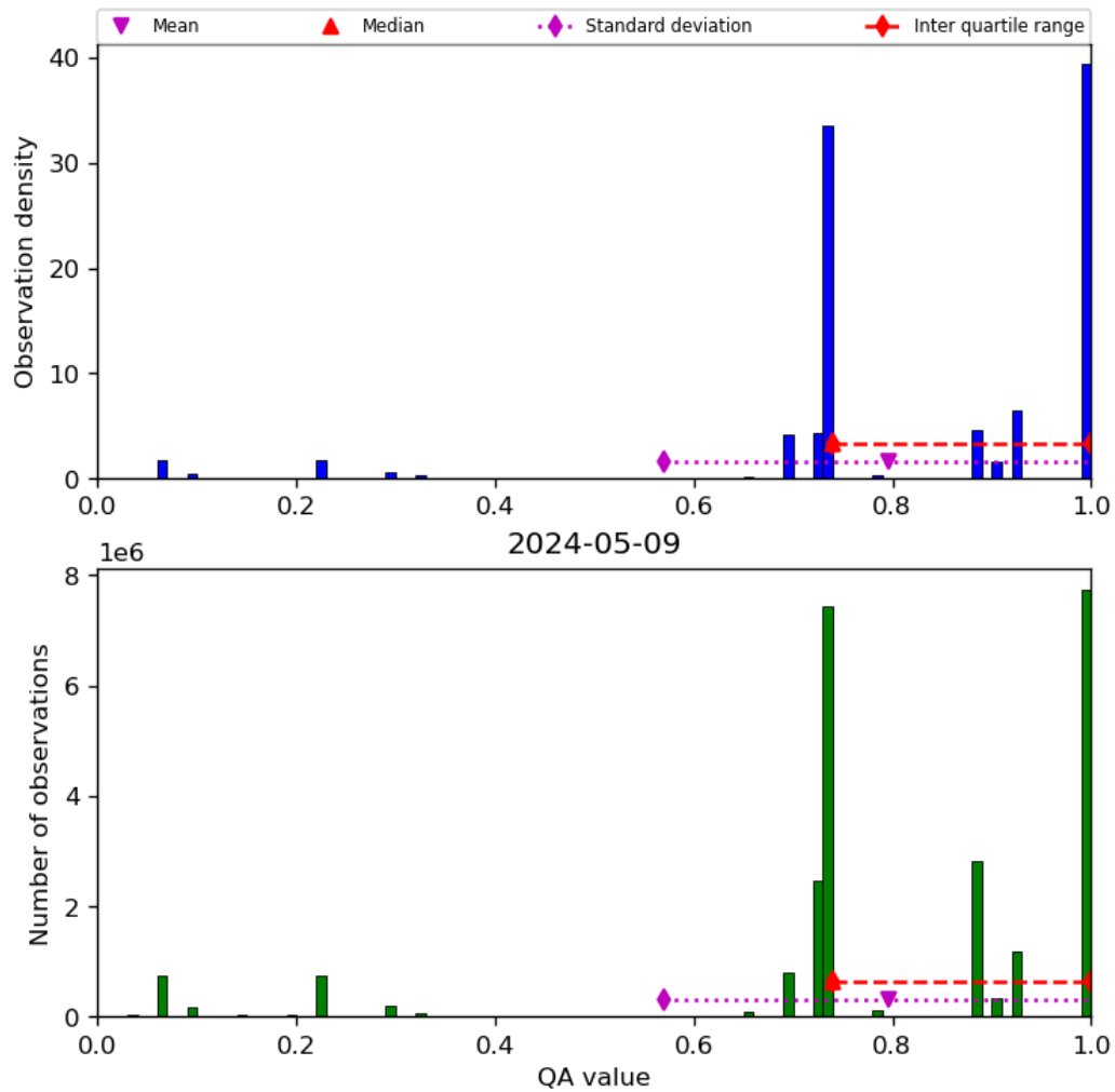
Figure 28: Histogram of “QA value” for 2024-05-08 to 2024-05-10
