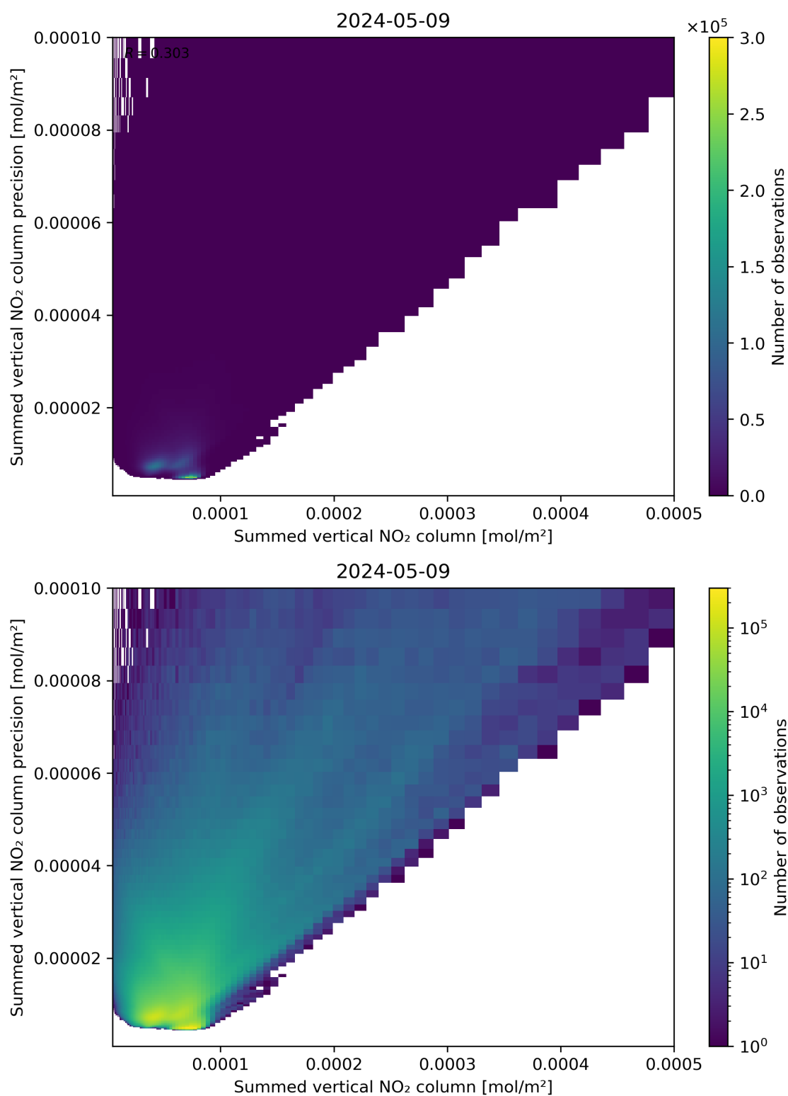
Figure 105: Scatter density plot of “Summed vertical NO 2 column” against “Summed vertical NO 2 column precision” for 2024-05-08 to 2024-05-10.
