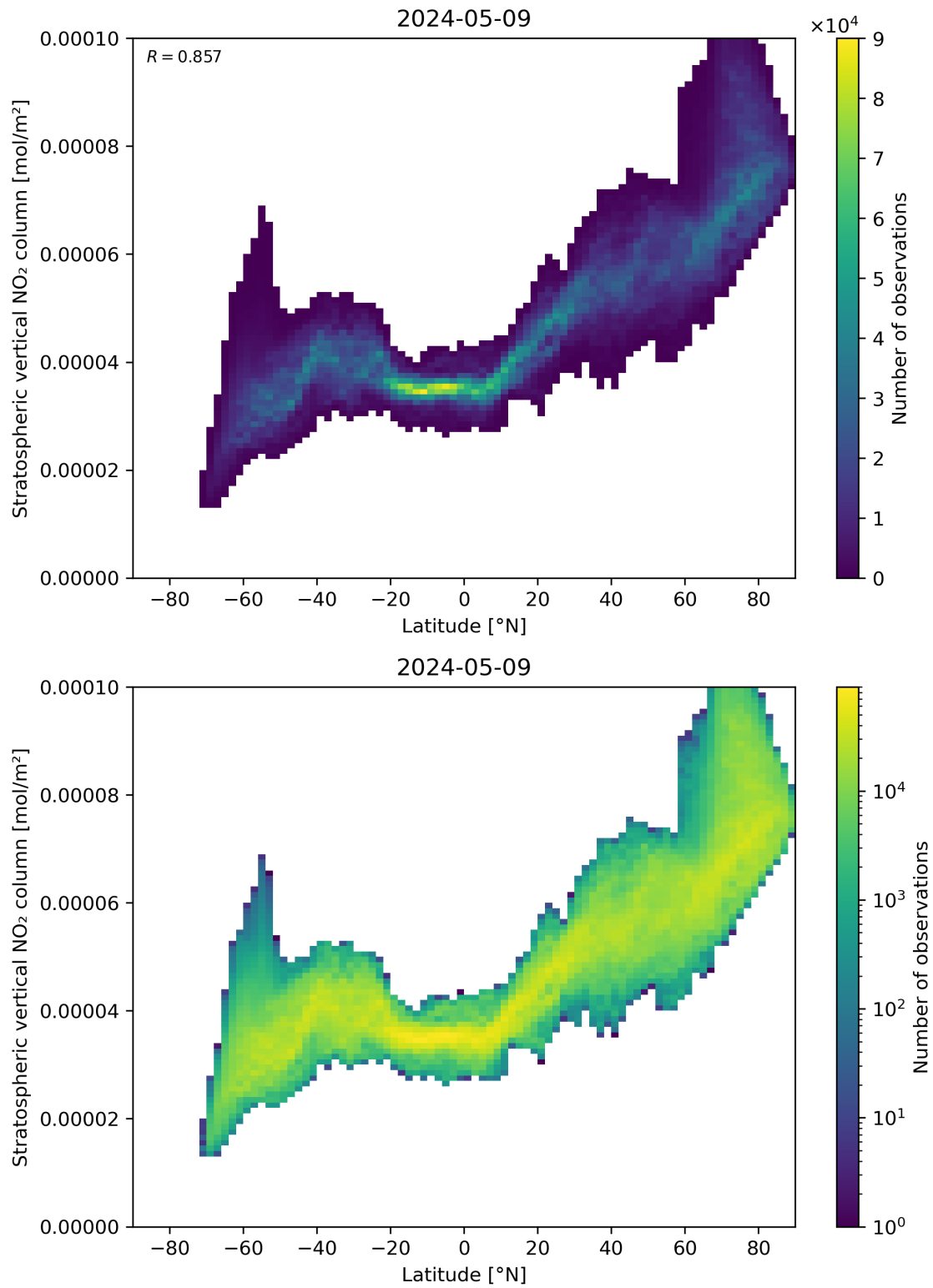
Figure 87: Scatter density plot of “Latitude” against “Stratospheric vertical NO 2 column” for 2024-05-08 to 2024-05-10.
