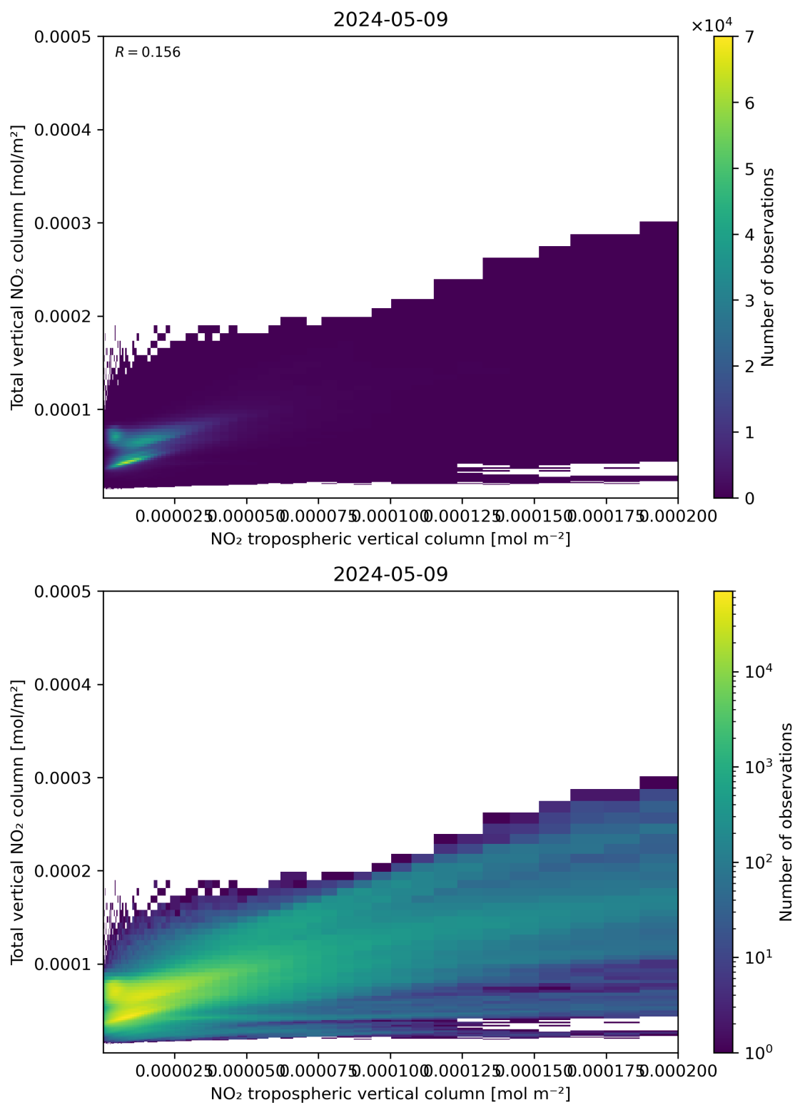
Figure 128: Scatter density plot of “NO 2 tropospheric vertical column” against “Total vertical NO 2 column” for 2024-05-08 to 2024-05-10.
