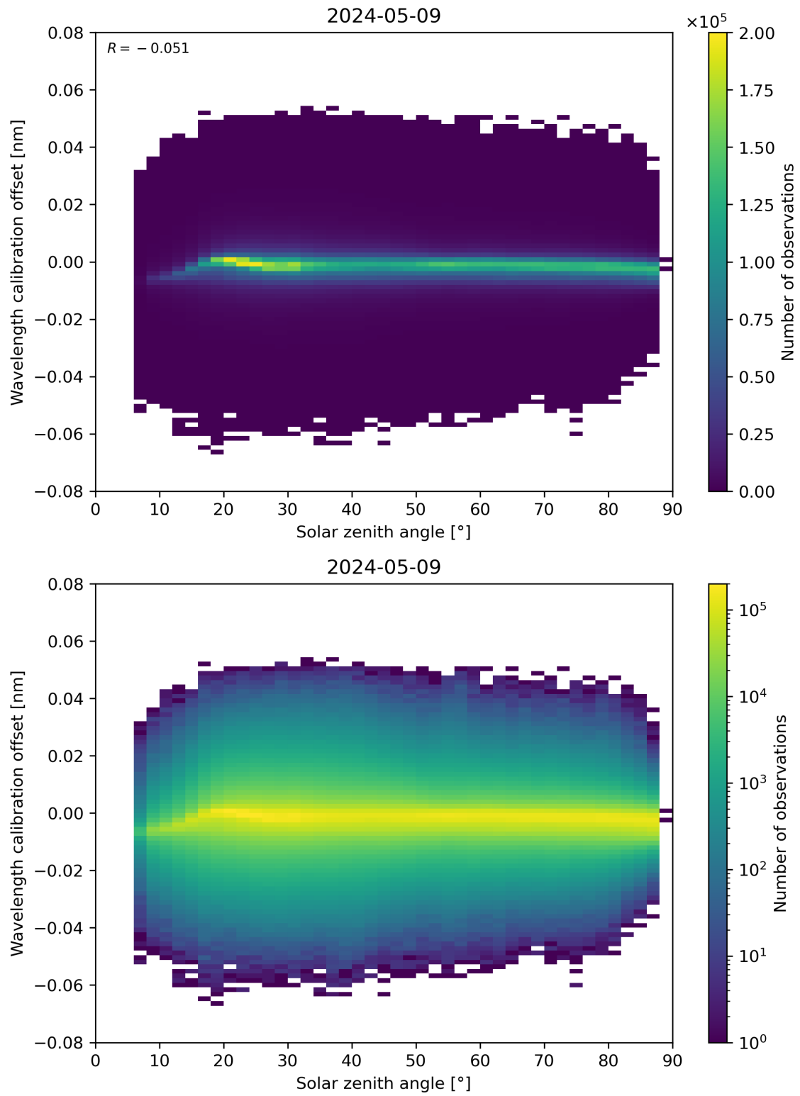
Figure 158: Scatter density plot of “Solar zenith angle” against “Wavelength calibration offset” for 2024-05-08 to 2024-05-10.
