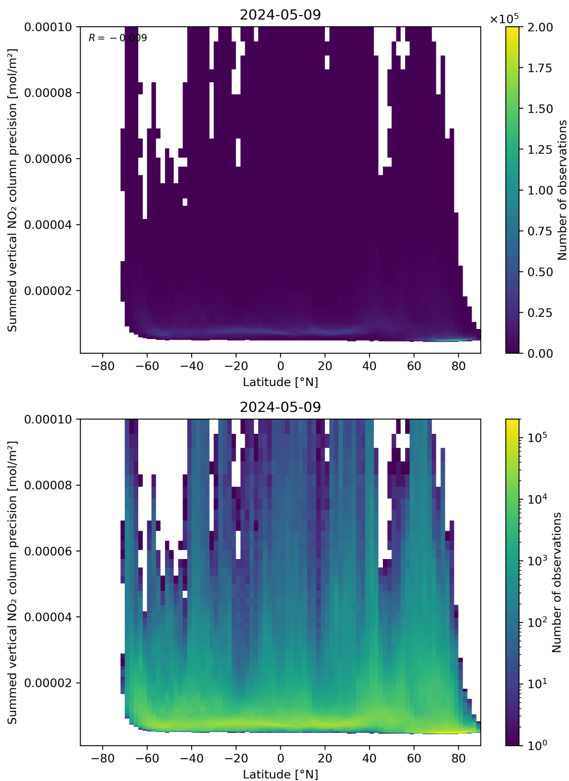
Figure 89: Scatter density plot of “Latitude” against “Summed vertical NO 2 column precision” for 2024-05-08 to 2024-05-10.
