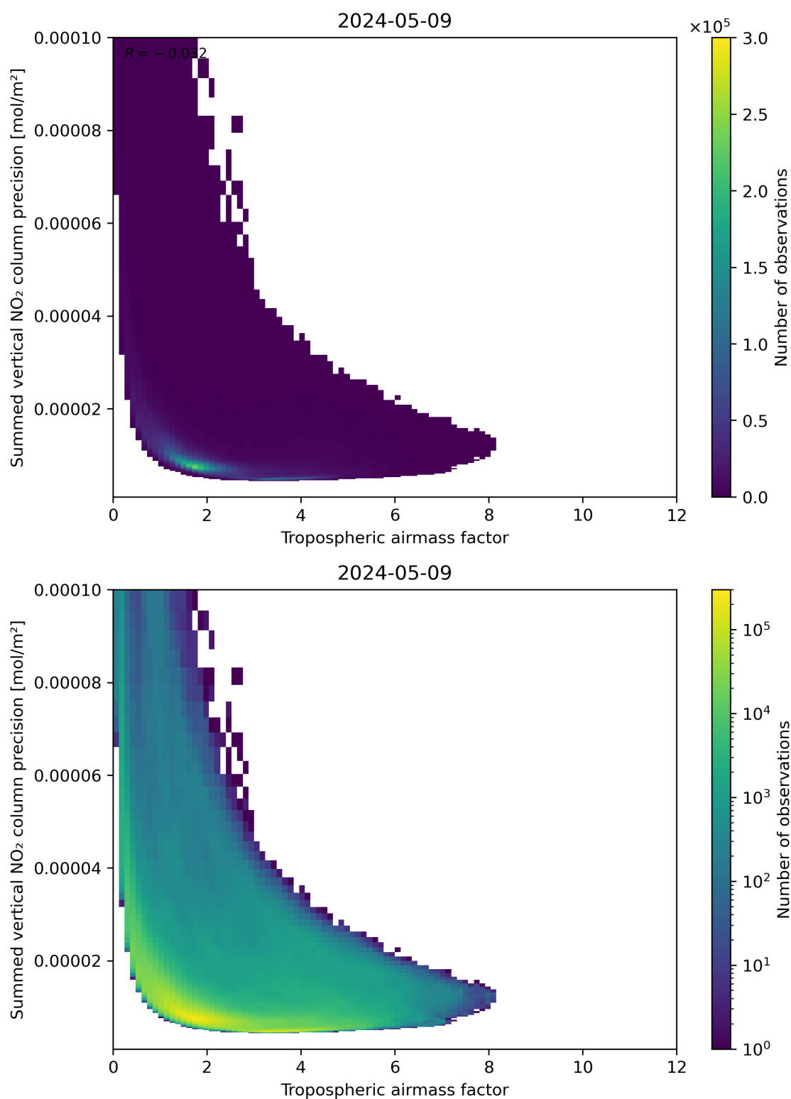
Figure 76: Scatter density plot of “Tropospheric air mass factor” against “Summed vertical NO 2 column precision” for 2024-05-08 to 2024-05-10.
