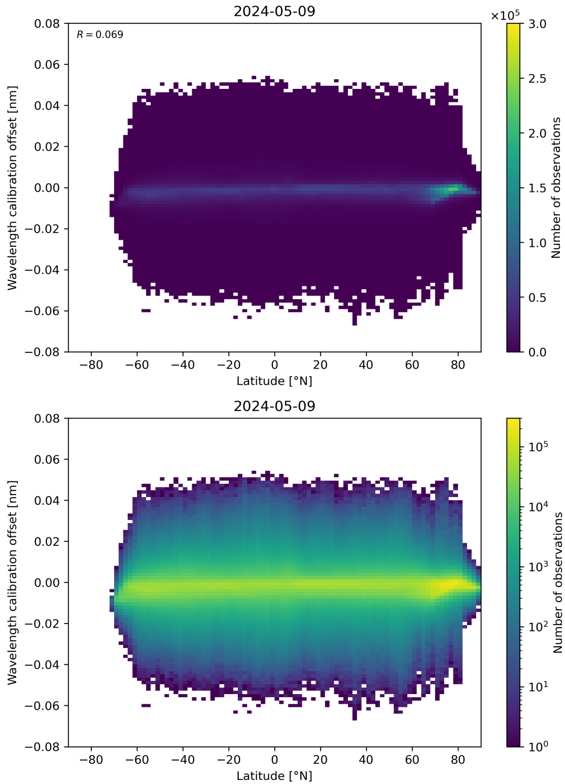
Figure 95: Scatter density plot of “Latitude” against “Wavelength calibration offset” for 2024-05-08 to 2024-05-10.
