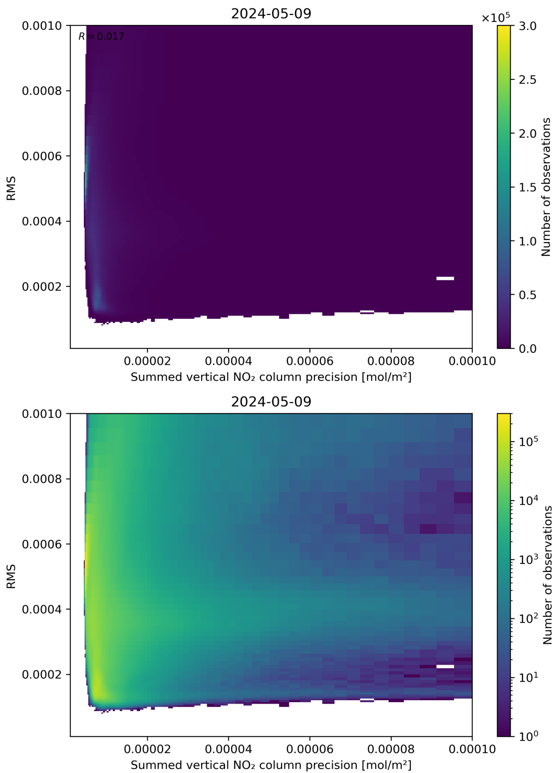
Figure 108: Scatter density plot of “Summed vertical NO 2 column precision” against “RMS” for 2024-05-08 to 2024-05-10.
