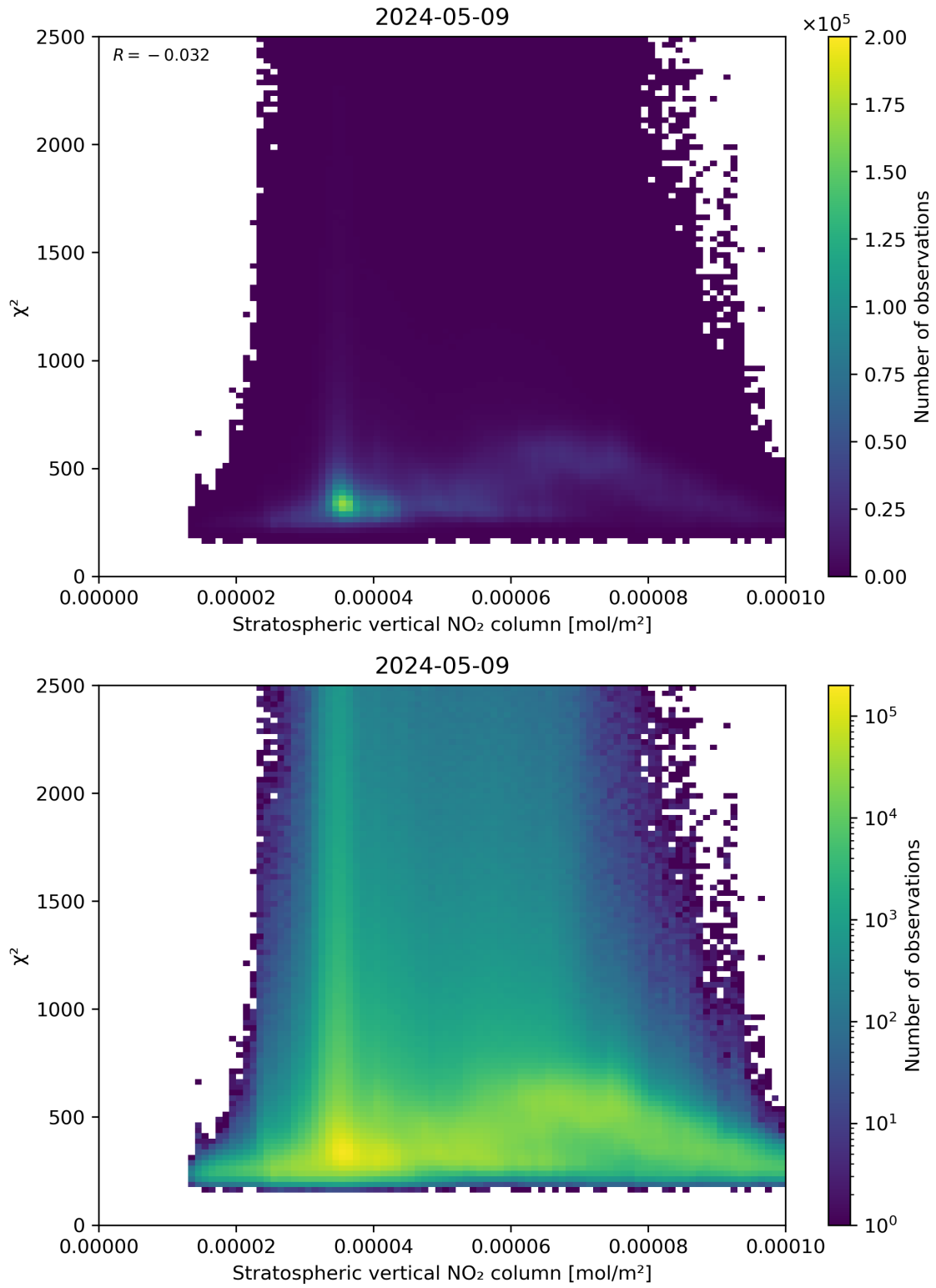
Figure 97: Scatter density plot of “Stratospheric vertical NO 2 column” against “ \chi^2 ” for 2024-05-08 to 2024-05-10.
