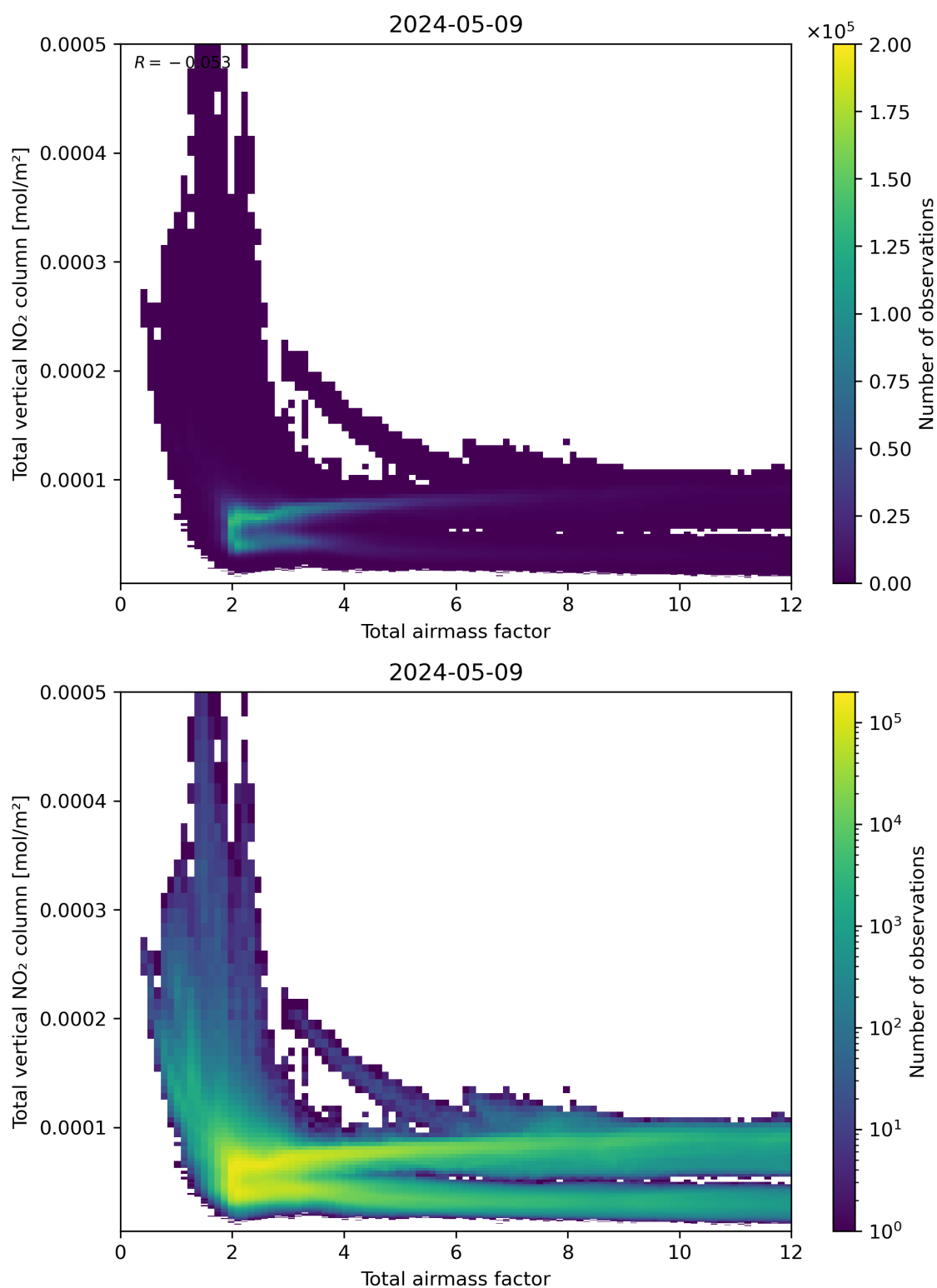
Figure 67: Scatter density plot of “Total airmass factor” against “Total vertical NO 2 column” for 2024-05-08 to 2024-05-10.
