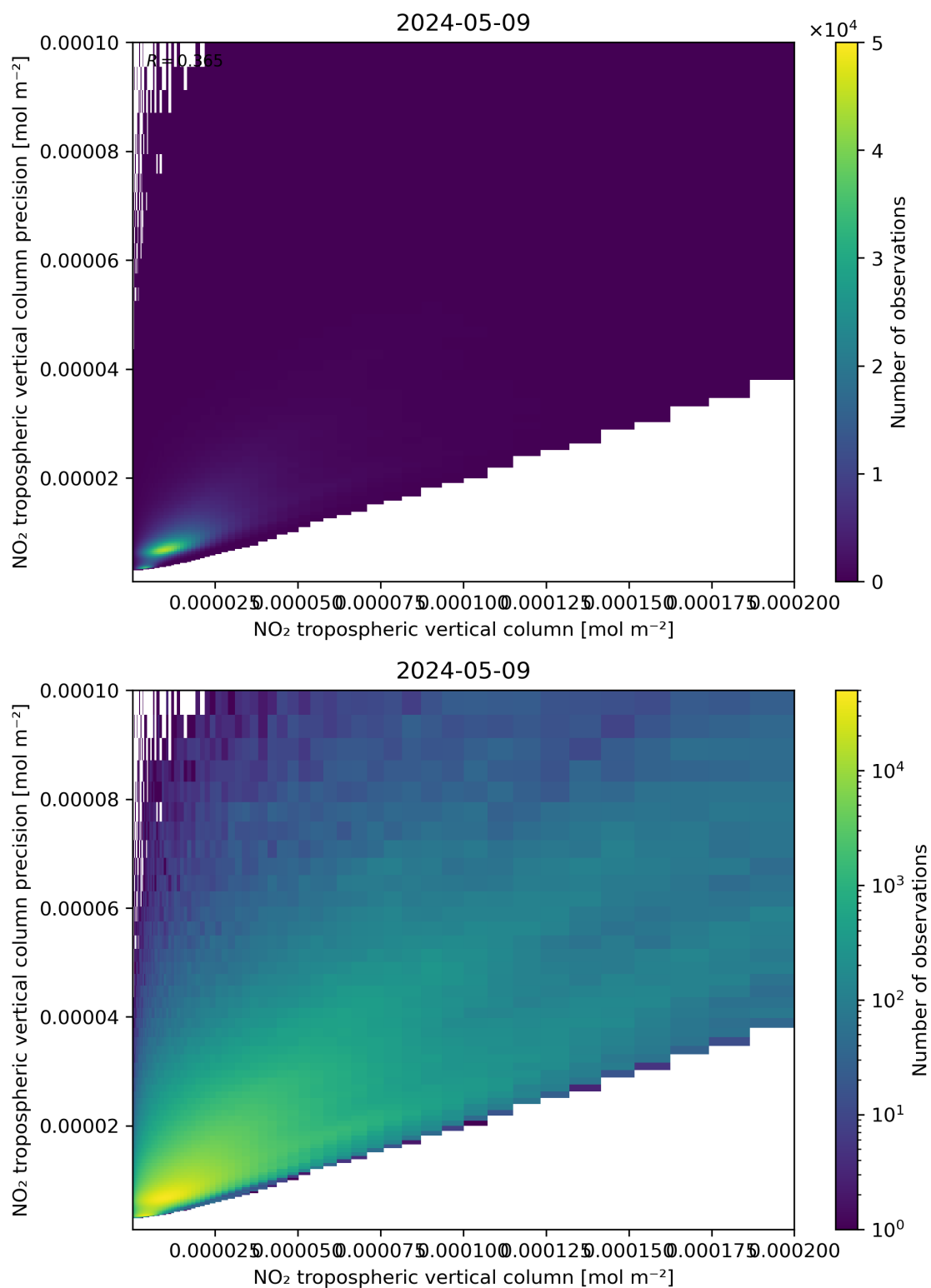
Figure 130: Scatter density plot of “NO 2 tropospheric vertical column” against “NO 2 tropospheric vertical column precision” for 2024-05-08 to 2024-05-10.
