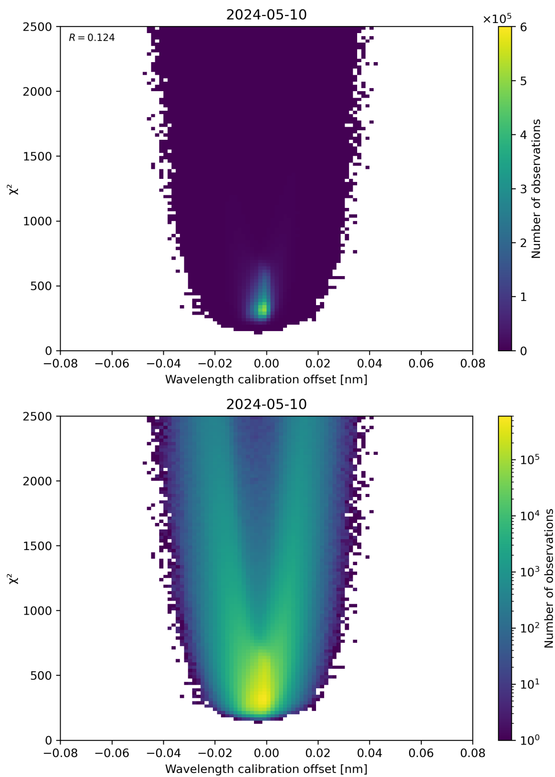
Figure 175: Scatter density plot of “Wavelength calibration offset” against “ \chi^2 ” for 2024-05-09 to 2024-05-11.
