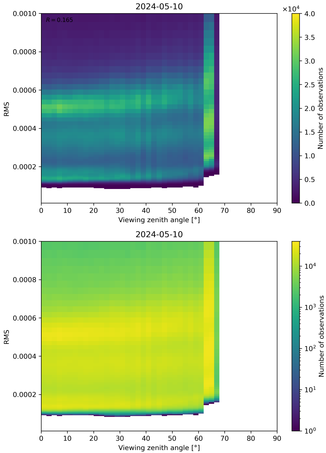
Figure 171: Scatter density plot of “Viewing zenith angle” against “RMS” for 2024-05-09 to 2024-05-11.
