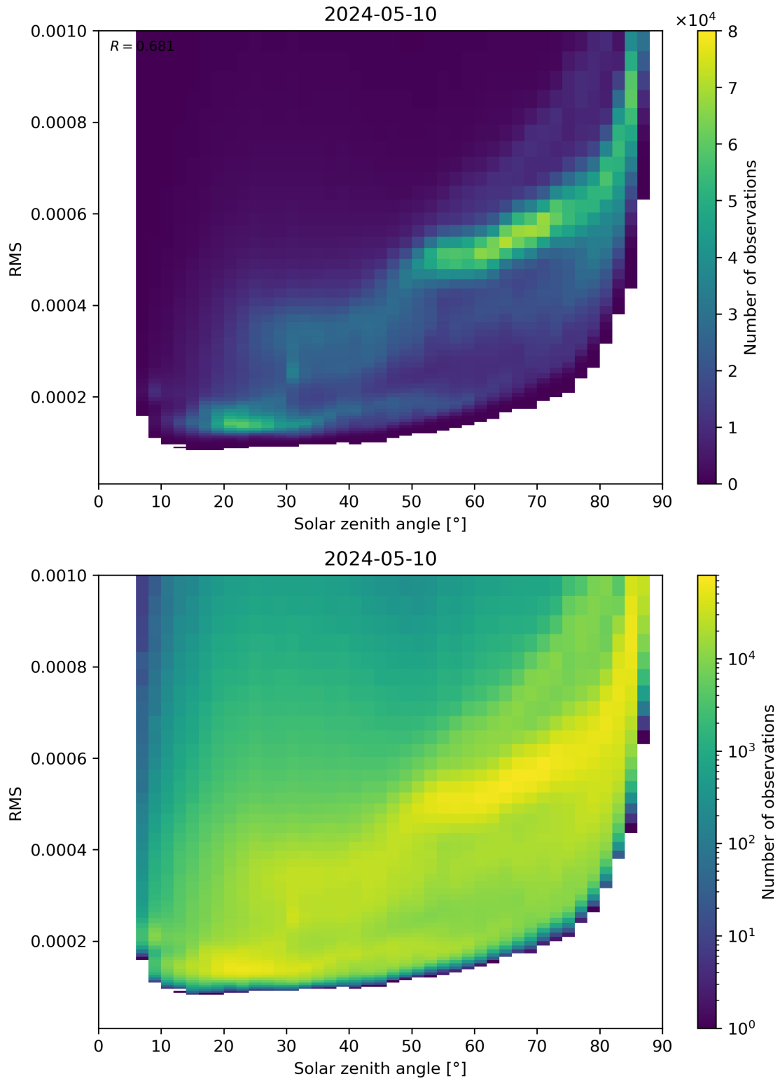
Figure 157: Scatter density plot of “Solar zenith angle” against “RMS” for 2024-05-09 to 2024-05-11.
