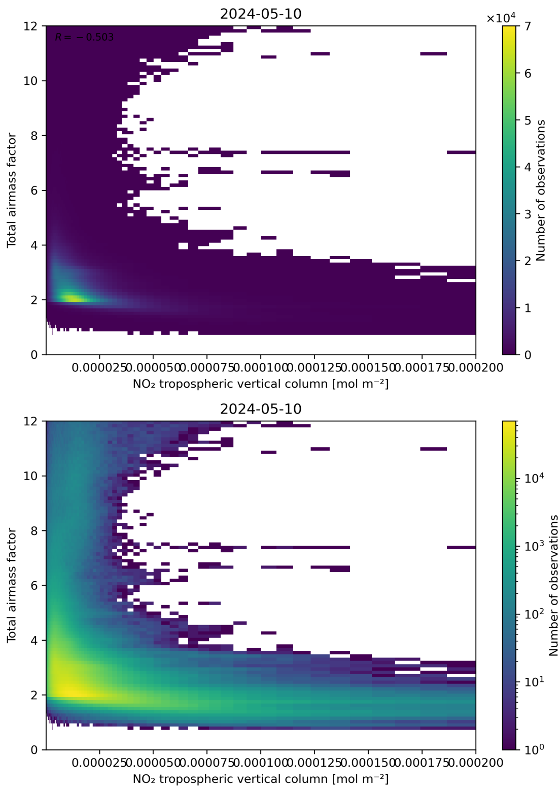
Figure 122: Scatter density plot of “NO 2 tropospheric vertical column” against “Total air mass factor” for 2024-05-09 to 2024-05-11.
