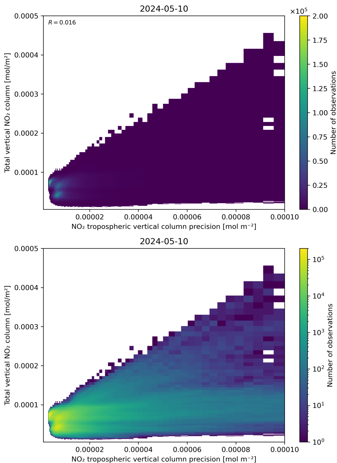
Figure 138: Scatter density plot of “NO 2 tropospheric vertical column precision” against “Total vertical NO 2 column” for 2024-05-09 to 2024-05-11.
