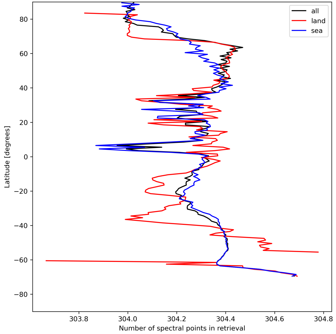
Figure 16: Zonal average of “Number of spectral points in retrieval” for 2024-05-09 to 2024-05-11.
