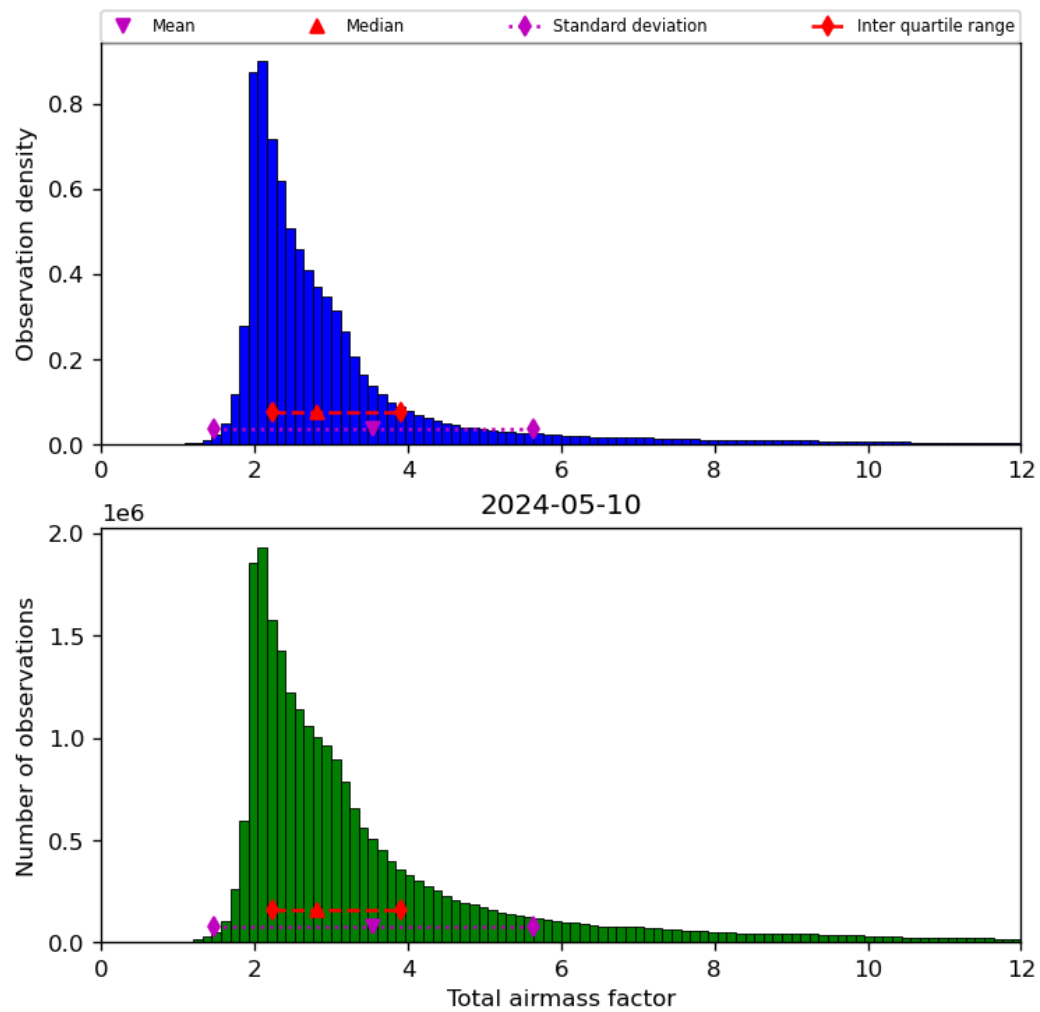
Figure 32: Histogram of “Total airmass factor” for 2024-05-09 to 2024-05-11
