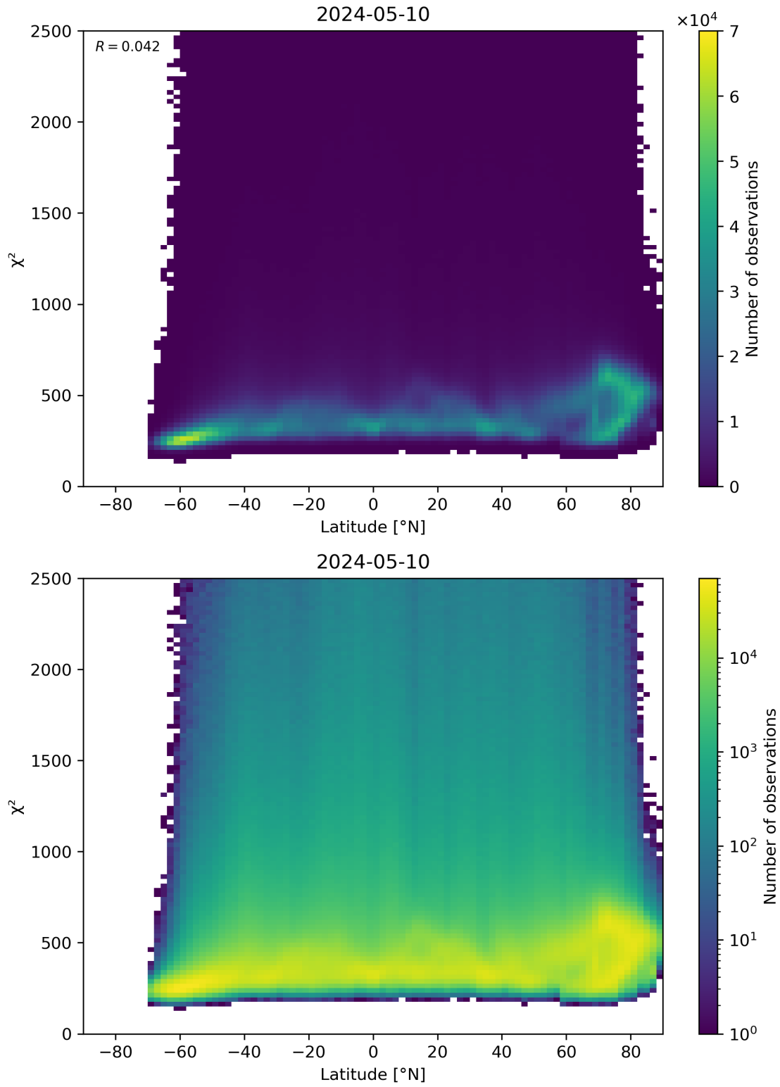
Figure 86: Scatter density plot of “Latitude” against “ \chi^2 ” for 2024-05-09 to 2024-05-11.
