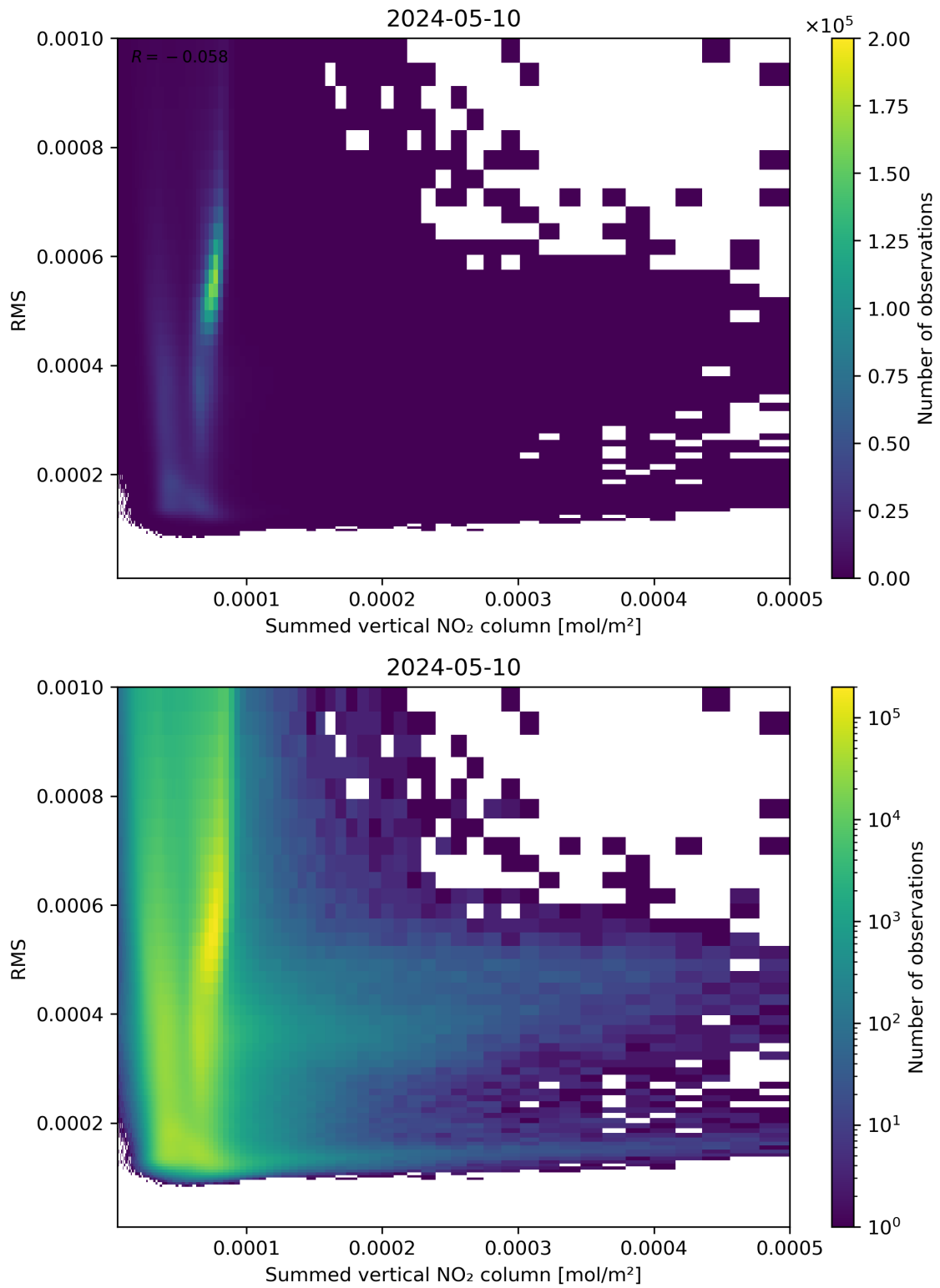
Figure 109: Scatter density plot of “Summed vertical NO 2 column” against “RMS” for 2024-05-09 to 2024-05-11.
