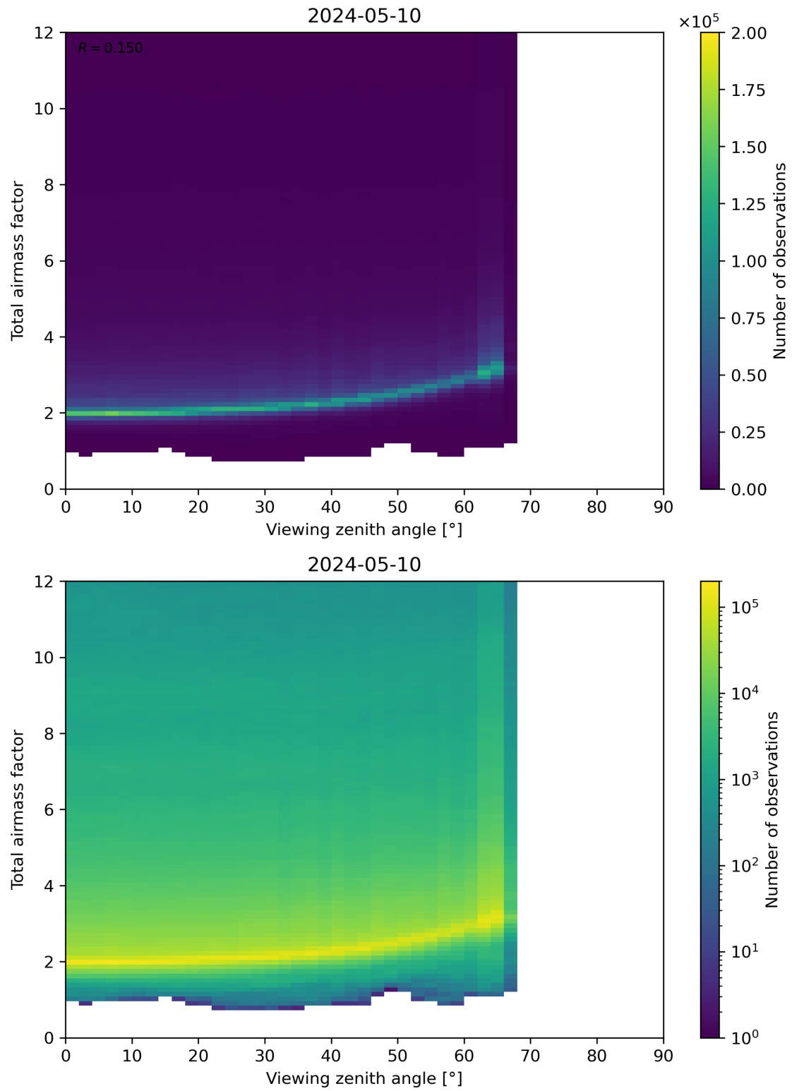
Figure 160: Scatter density plot of “Viewing zenith angle” against “Total airmass factor” for 2024-05-09 to 2024-05-11.
