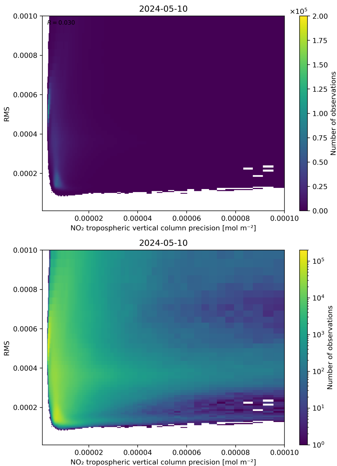
Figure 140: Scatter density plot of “NO 2 tropospheric vertical column precision” against “RMS” for 2024-05-09 to 2024-05-11.
