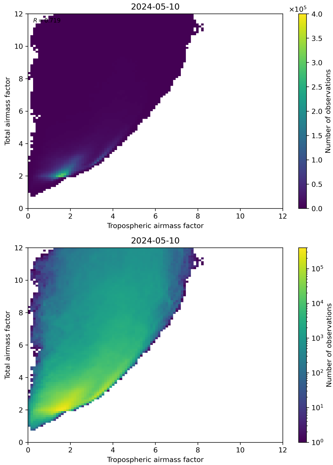
Figure 72: Scatter density plot of “Tropospheric airmass factor” against “Total airmass factor” for 2024-05-09 to 2024-05-11.
