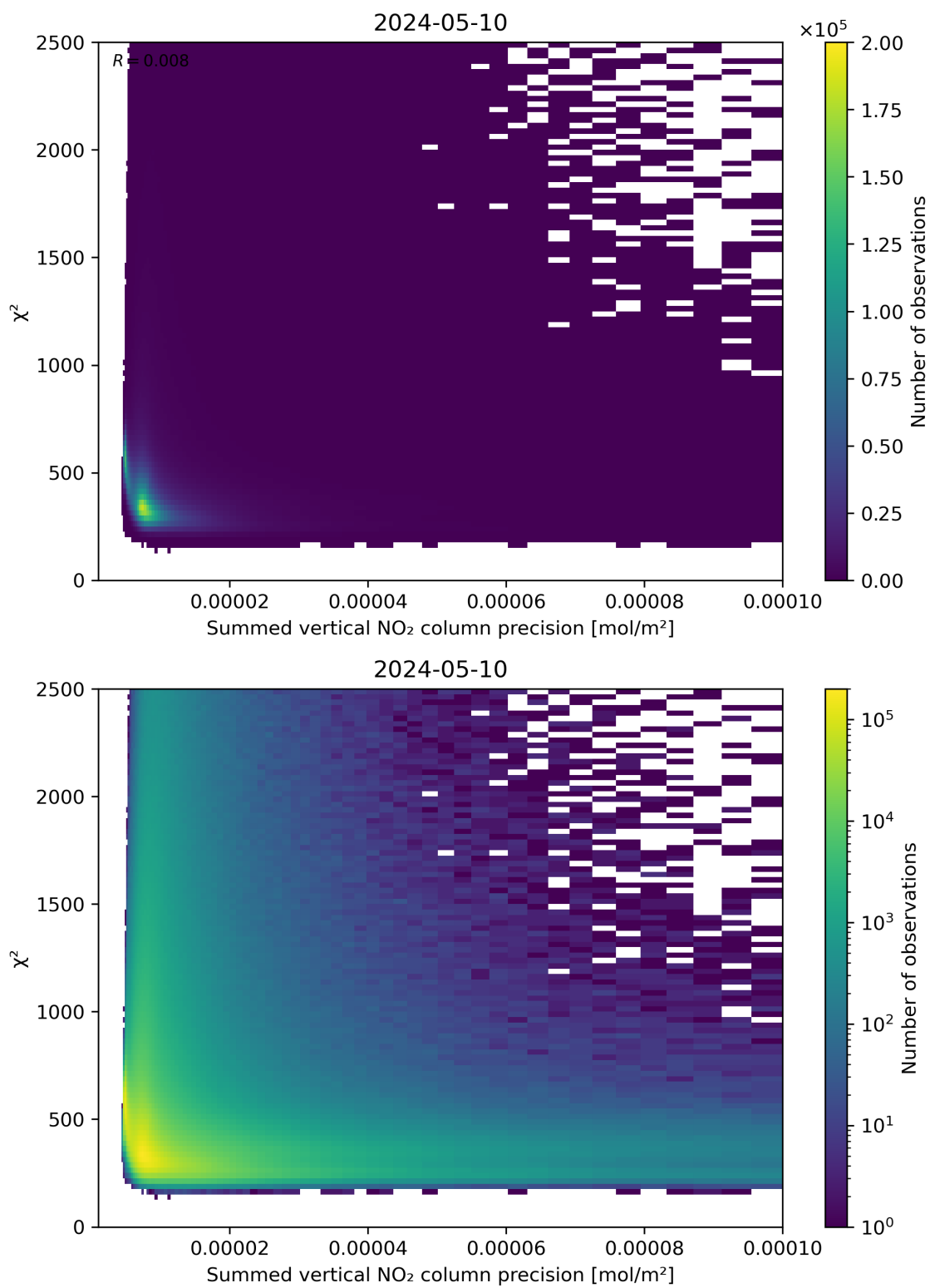
Figure 107: Scatter density plot of “Summed vertical NO 2 column precision” against “ \chi^2 ” for 2024-05-09 to 2024-05-11.
