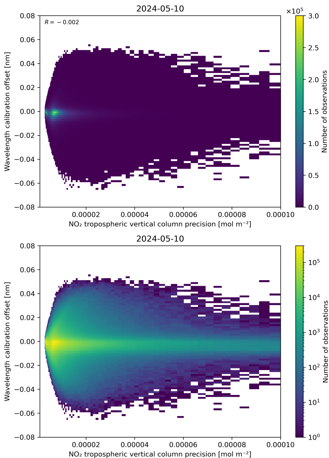
Figure 141: Scatter density plot of “NO 2 tropospheric vertical column precision” against “Wavelength calibration offset” for 2024-05-09 to 2024-05-11.
