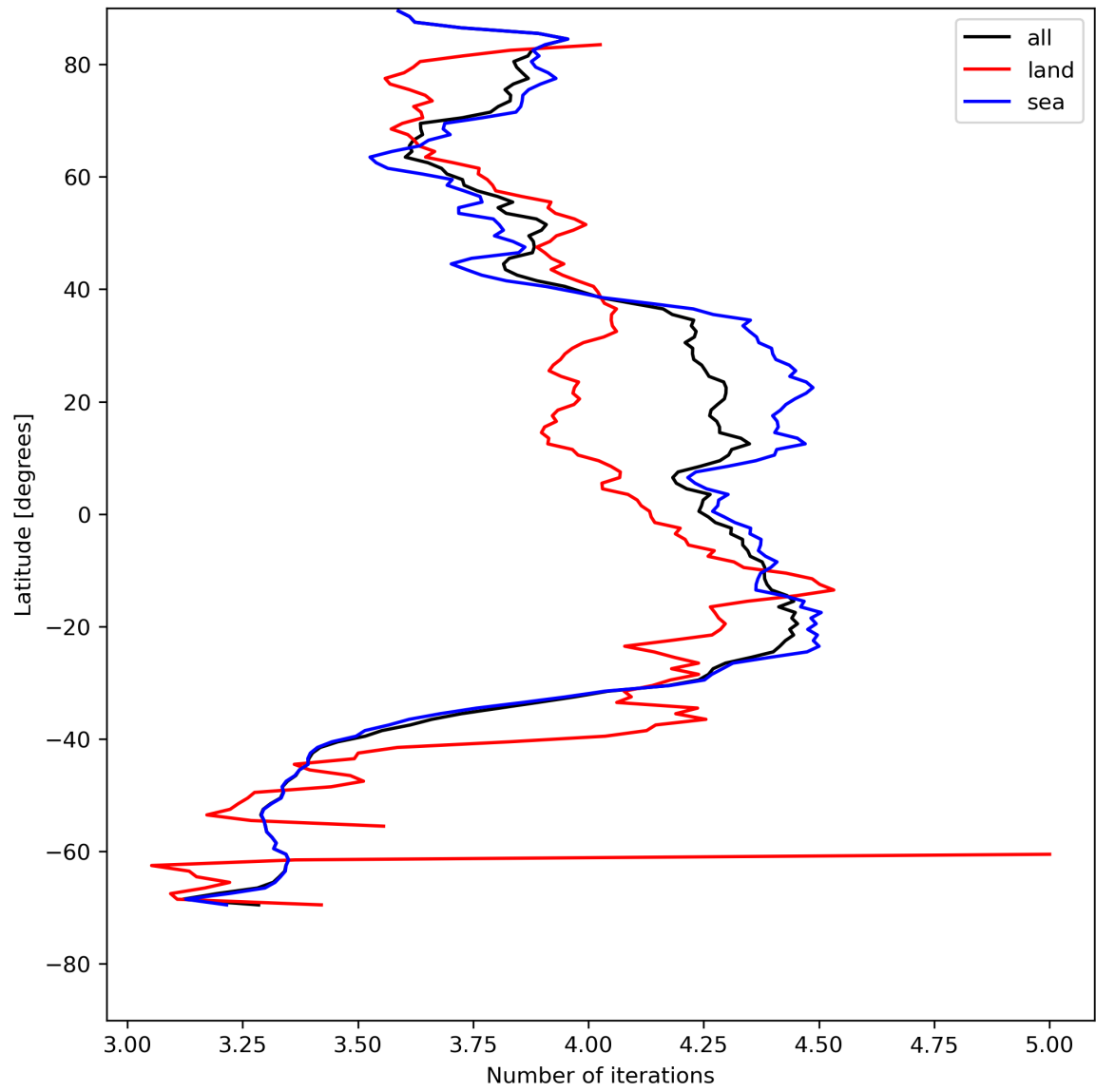
Figure 17: Zonal average of “Number of iterations” for 2024-05-09 to 2024-05-11.
