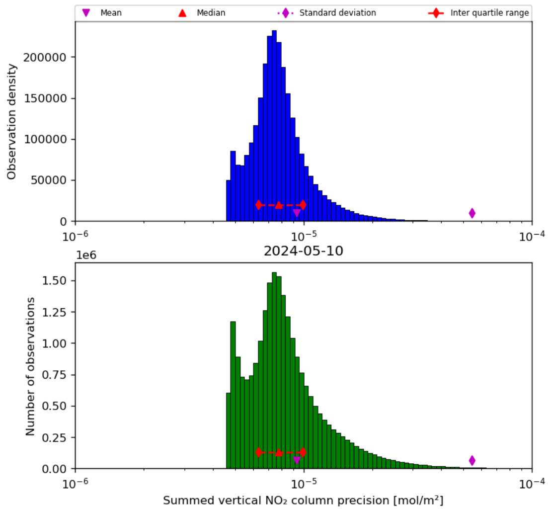
Figure 41: Histogram of “Summed vertical NO 2 column precision” for 2024-05-09 to 2024-05-11
