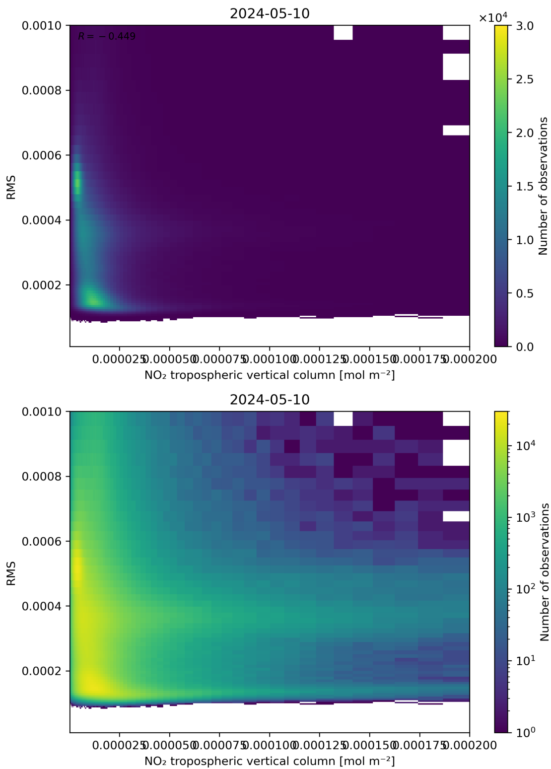
Figure 142: Scatter density plot of “NO 2 tropospheric vertical column” against “RMS” for 2024-05-09 to 2024-05-11.
