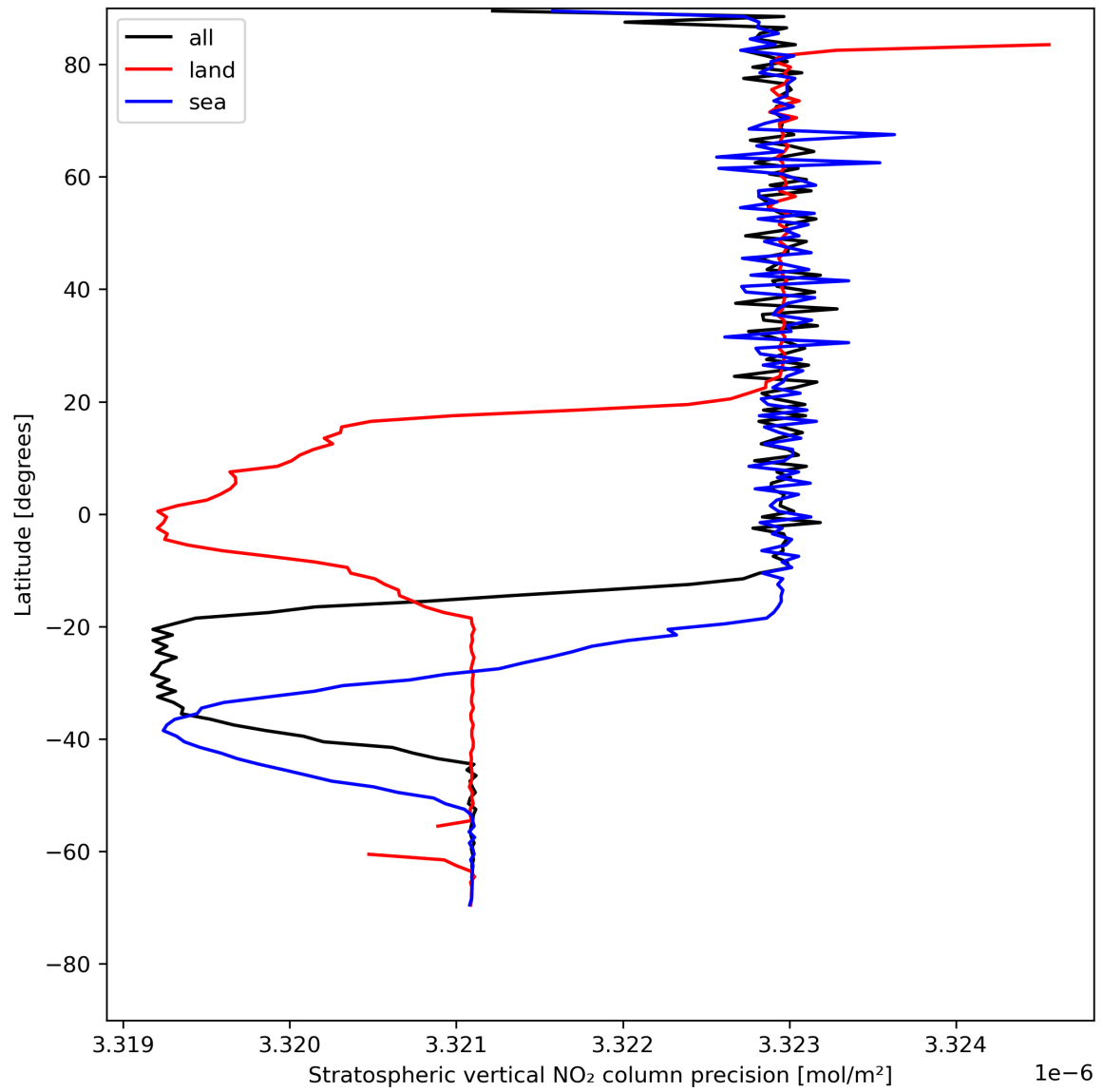
Figure 20: Zonal average of “Stratospheric vertical NO 2 column precision” for 2024-05-09 to 2024-05-11.
