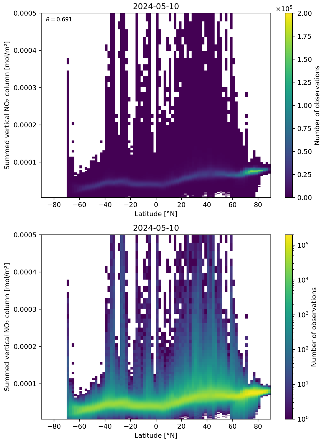
Figure 88: Scatter density plot of “Latitude” against “Summed vertical NO 2 column” for 2024-05-09 to 2024-05-11.
