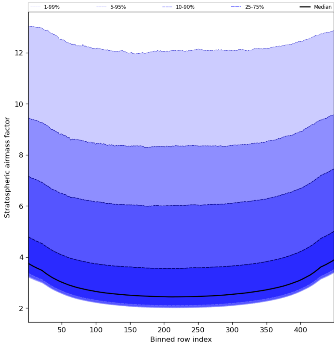
Figure 61: Along track statistics of “Stratospheric air mass factor” for 2024-05-09 to 2024-05-11
