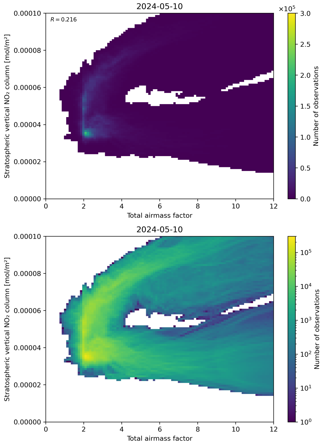
Figure 64: Scatter density plot of “Total airmass factor” against “Stratospheric vertical \text{NO}_2 column” for 2024-05-09 to 2024-05-11.
