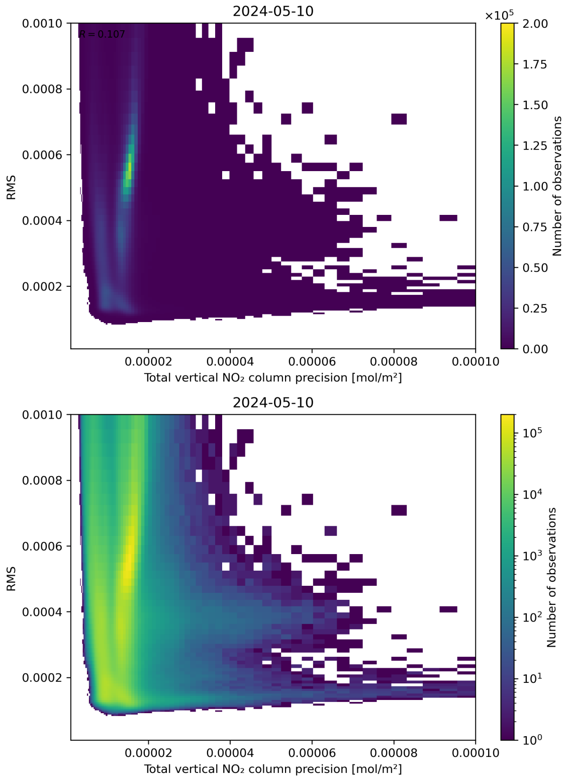
Figure 119: Scatter density plot of “Total vertical NO 2 column precision” against “RMS” for 2024-05-09 to 2024-05-11.
