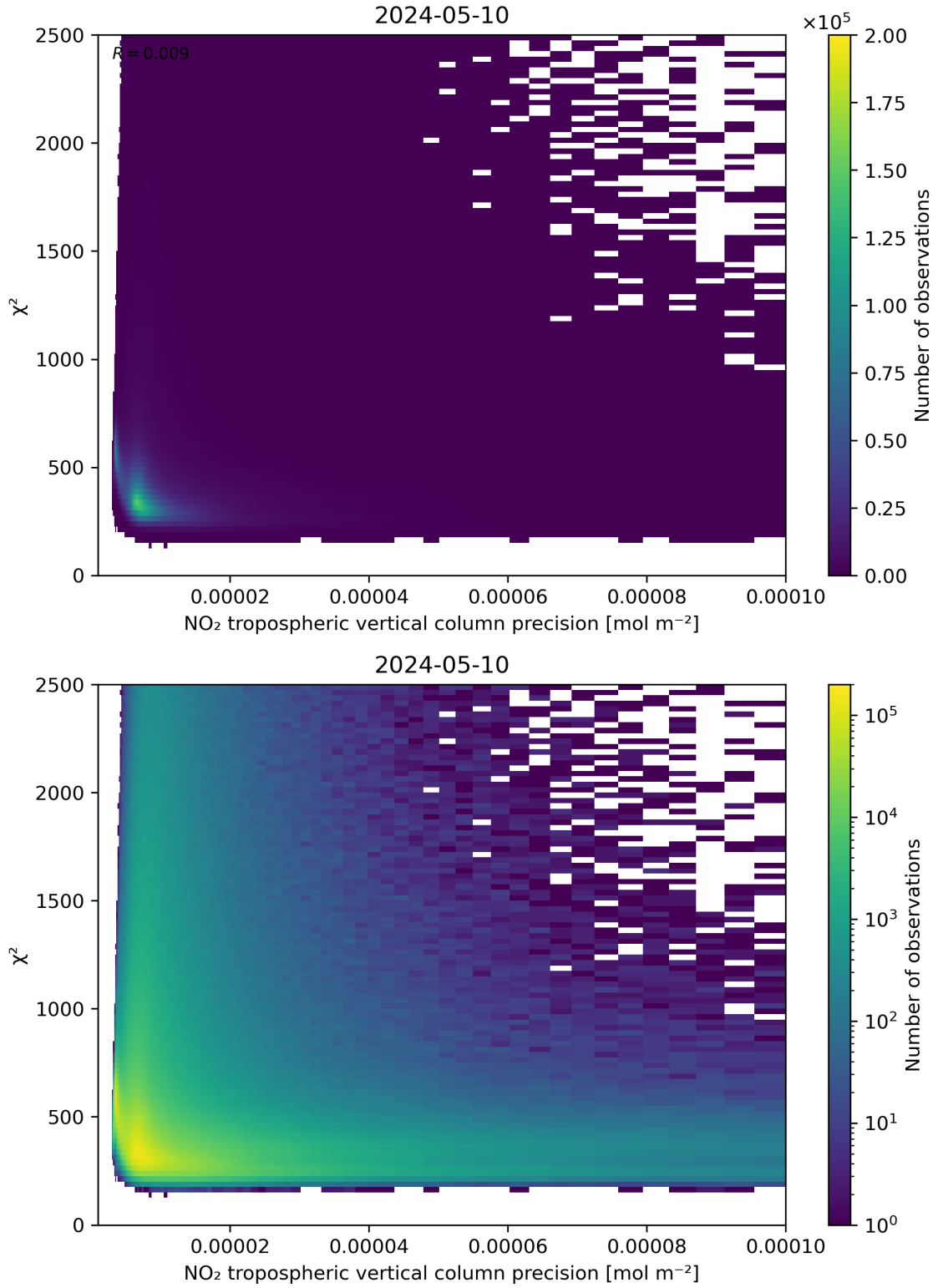
Figure 134: Scatter density plot of “NO 2 tropospheric vertical column precision” against “ \chi^2 ” for 2024-05-09 to 2024-05-11.
