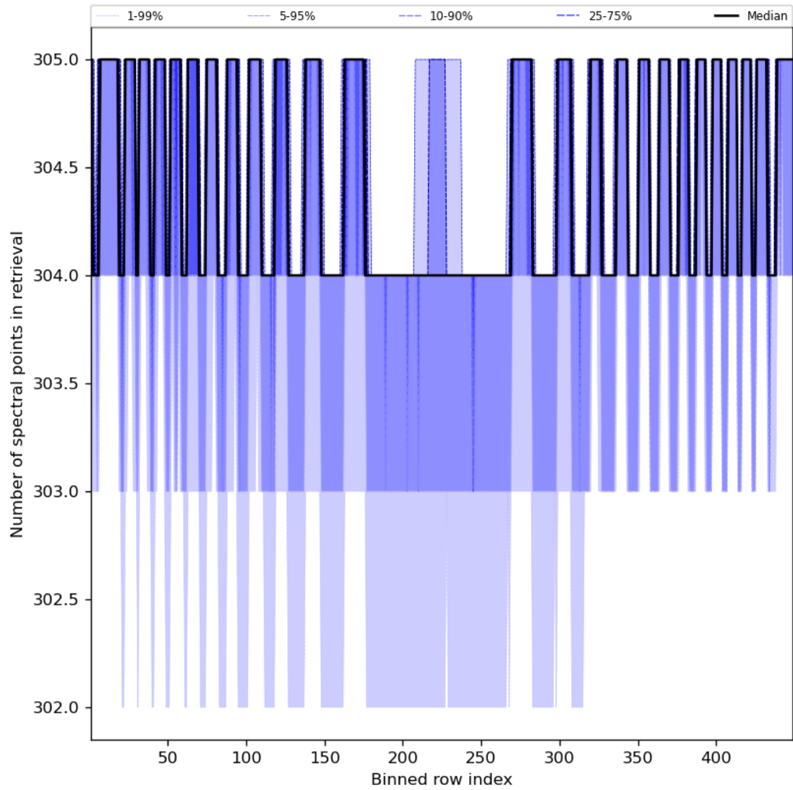
Figure 50: Along track statistics of “Number of spectral points in retrieval” for 2024-05-09 to 2024-05-11
