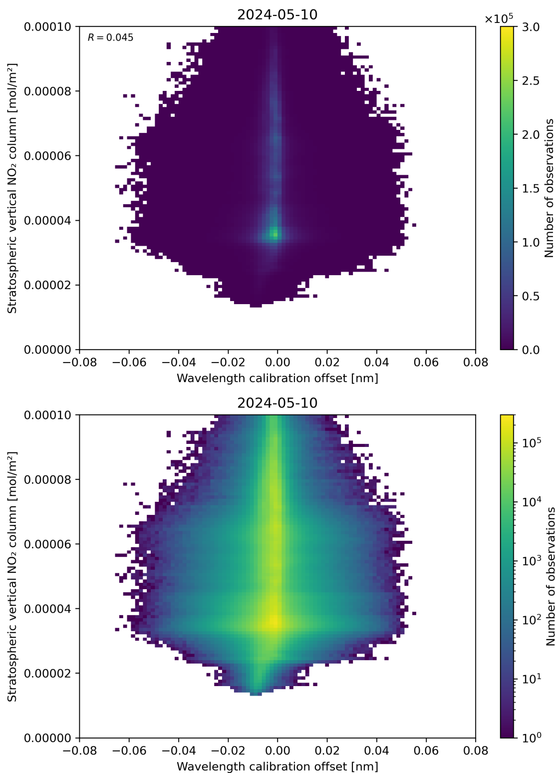
Figure 176: Scatter density plot of “Wavelength calibration offset” against “Stratospheric vertical NO 2 column” for 2024-05-09 to 2024-05-11.
