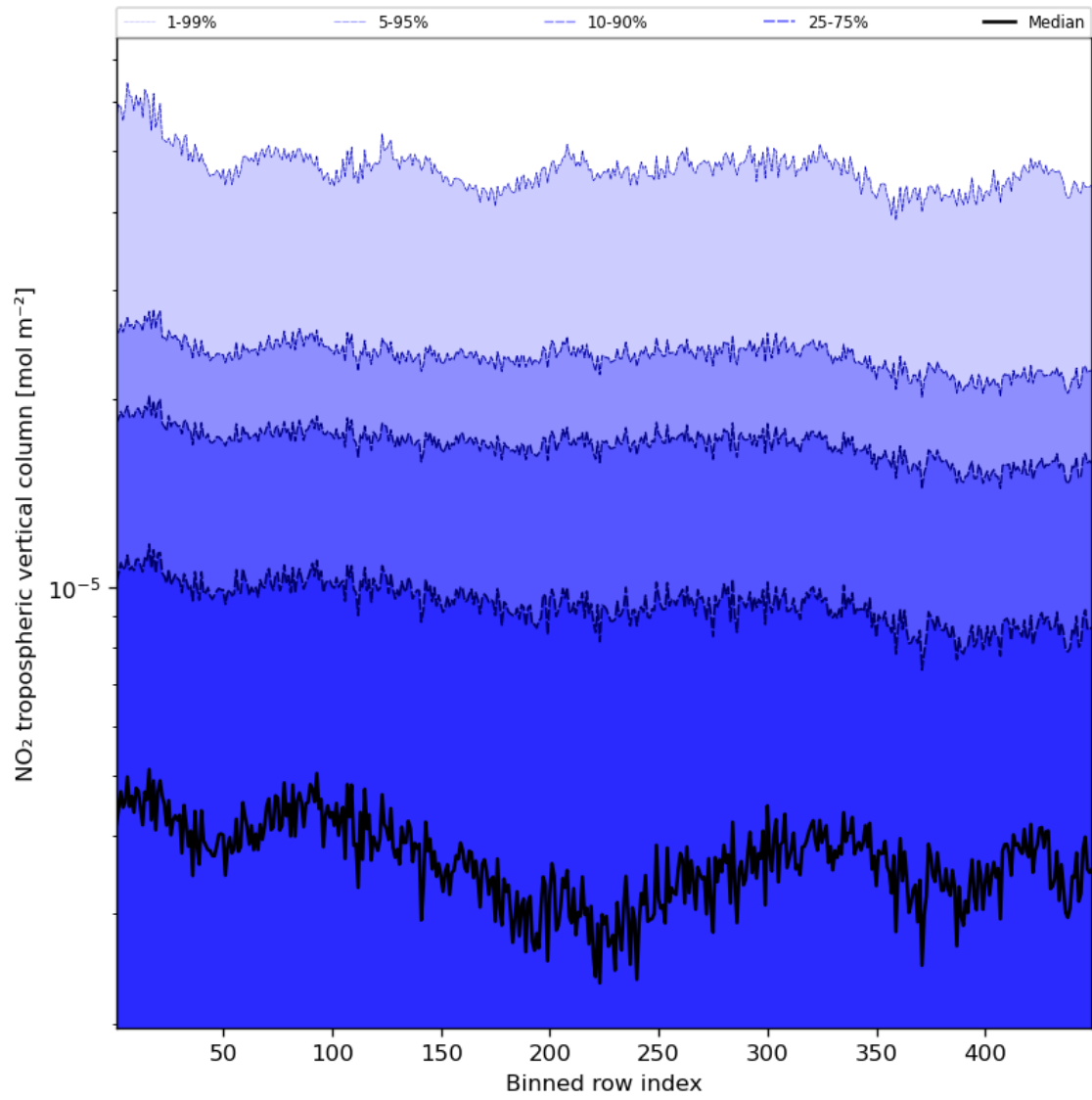
Figure 46: Along track statistics of “NO 2 tropospheric vertical column” for 2024-05-09 to 2024-05-11
