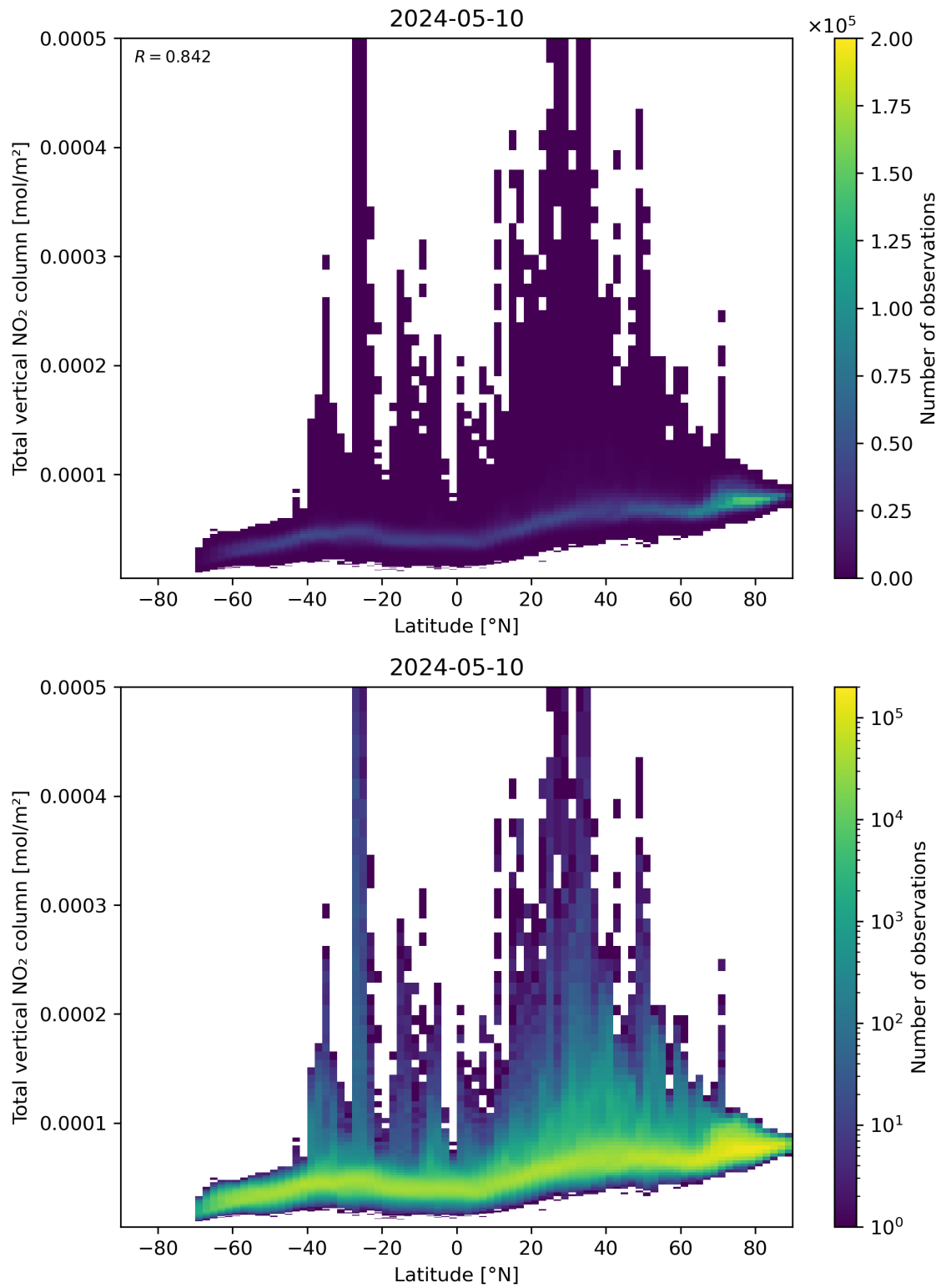
Figure 90: Scatter density plot of “Latitude” against “Total vertical NO 2 column” for 2024-05-09 to 2024-05-11.
