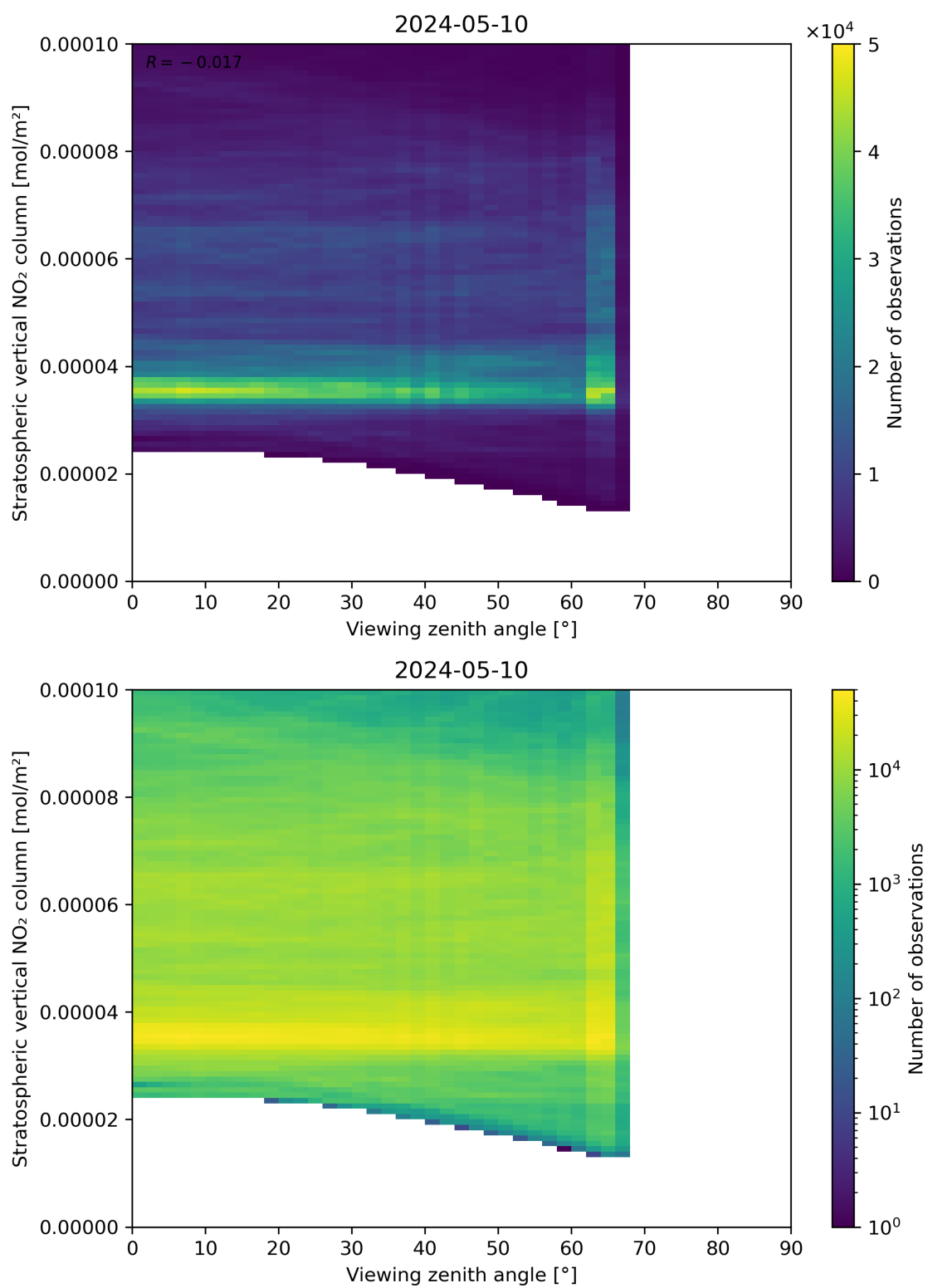
Figure 164: Scatter density plot of “Viewing zenith angle” against “Stratospheric vertical NO 2 column” for 2024-05-09 to 2024-05-11.
