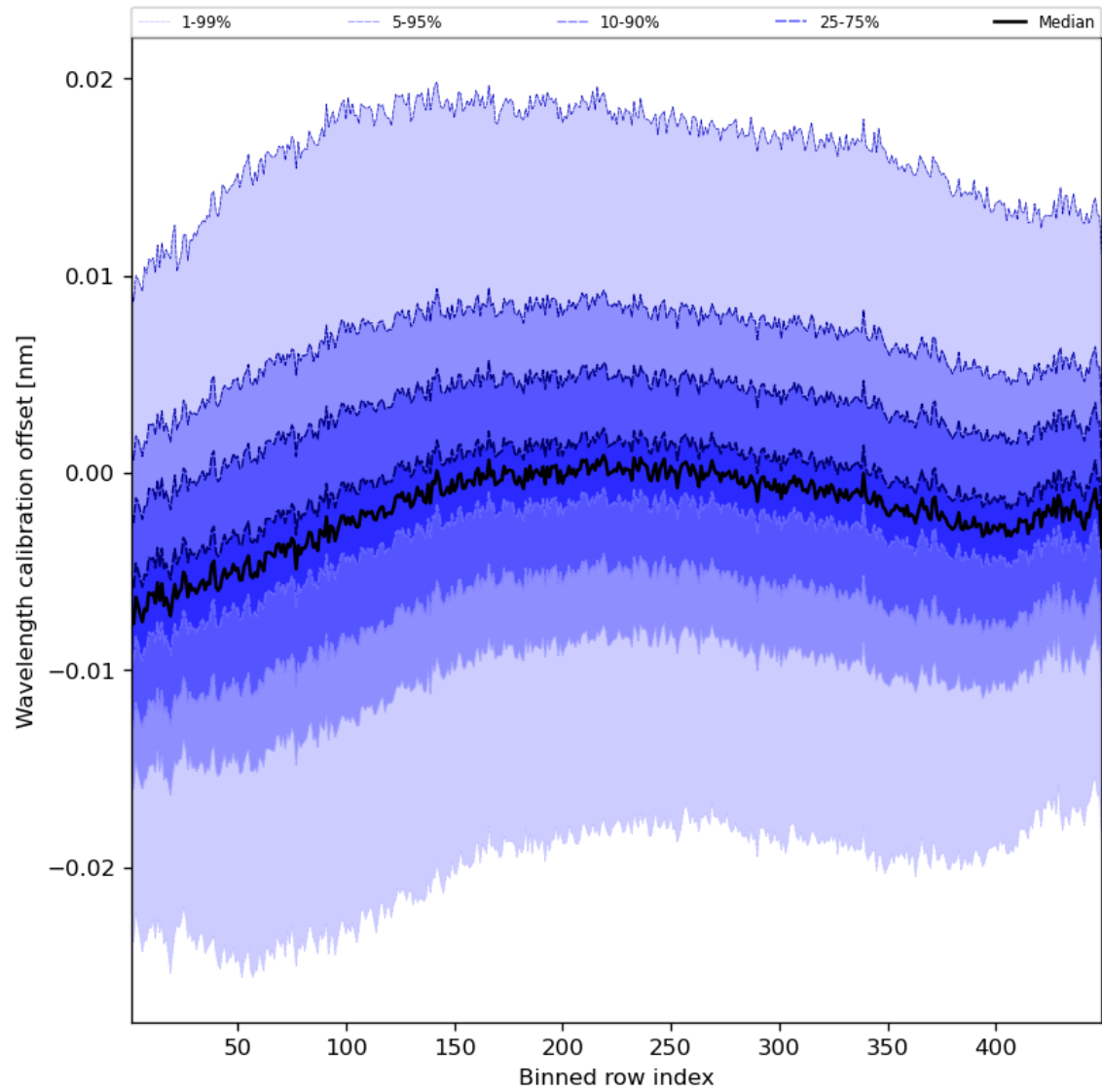
Figure 52: Along track statistics of “Wavelength calibration offset” for 2024-05-09 to 2024-05-11
