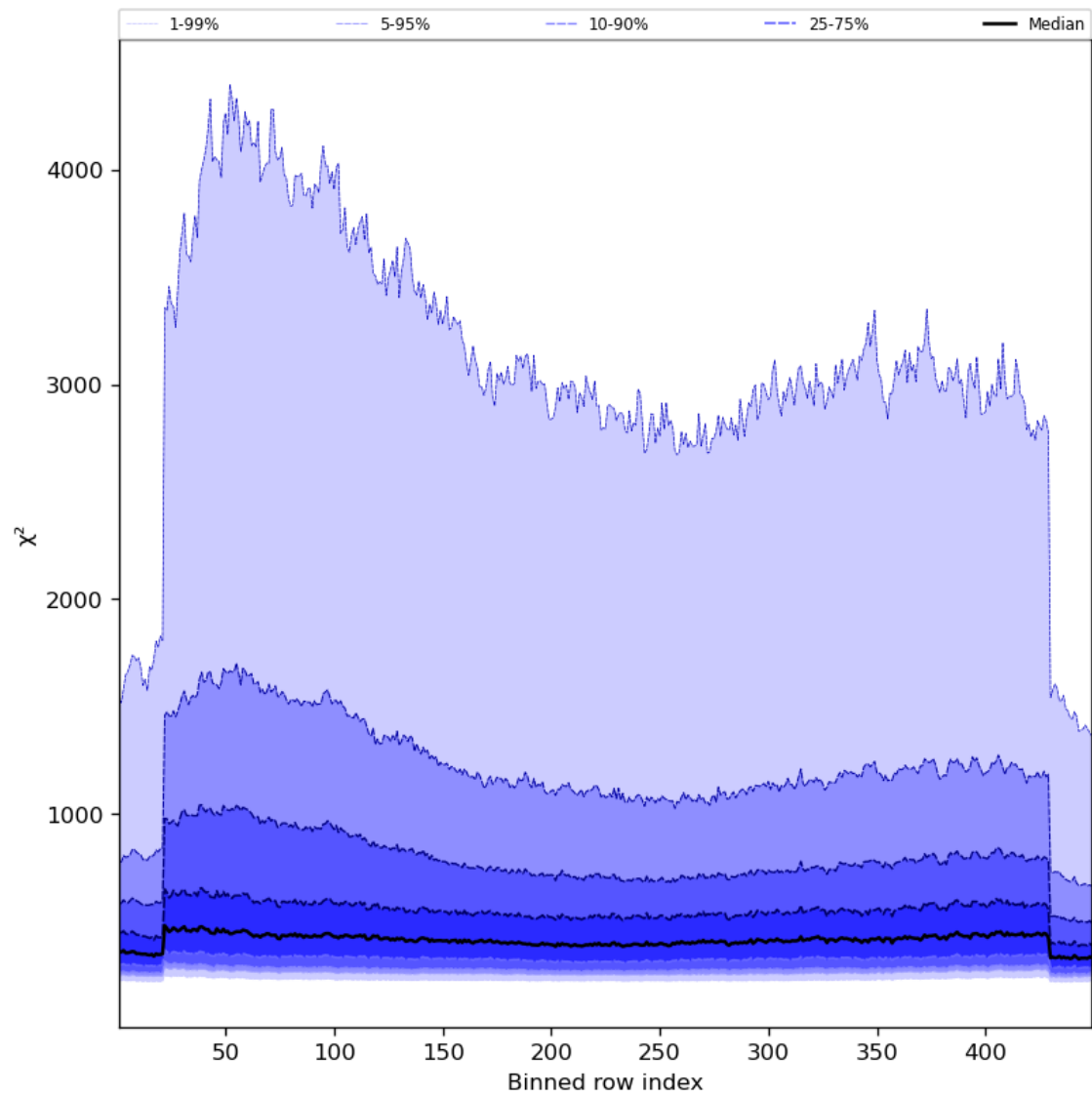
Figure 59: Along track statistics of “ \chi^2 ” for 2024-05-09 to 2024-05-11
