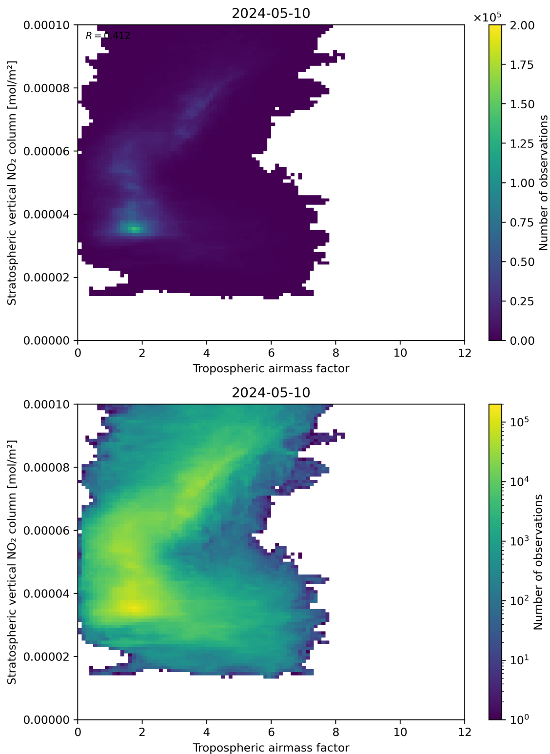
Figure 74: Scatter density plot of “Tropospheric airmass factor” against “Stratospheric vertical NO 2 column” for 2024-05-09 to 2024-05-11.
