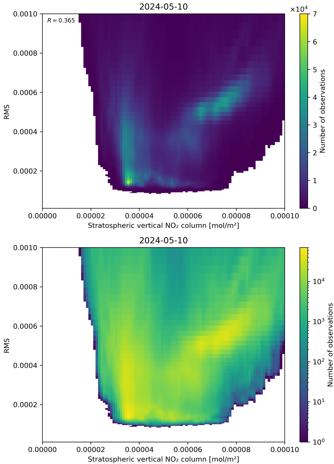
Figure 102: Scatter density plot of “Stratospheric vertical NO 2 column” against “RMS” for 2024-05-09 to 2024-05-11.
