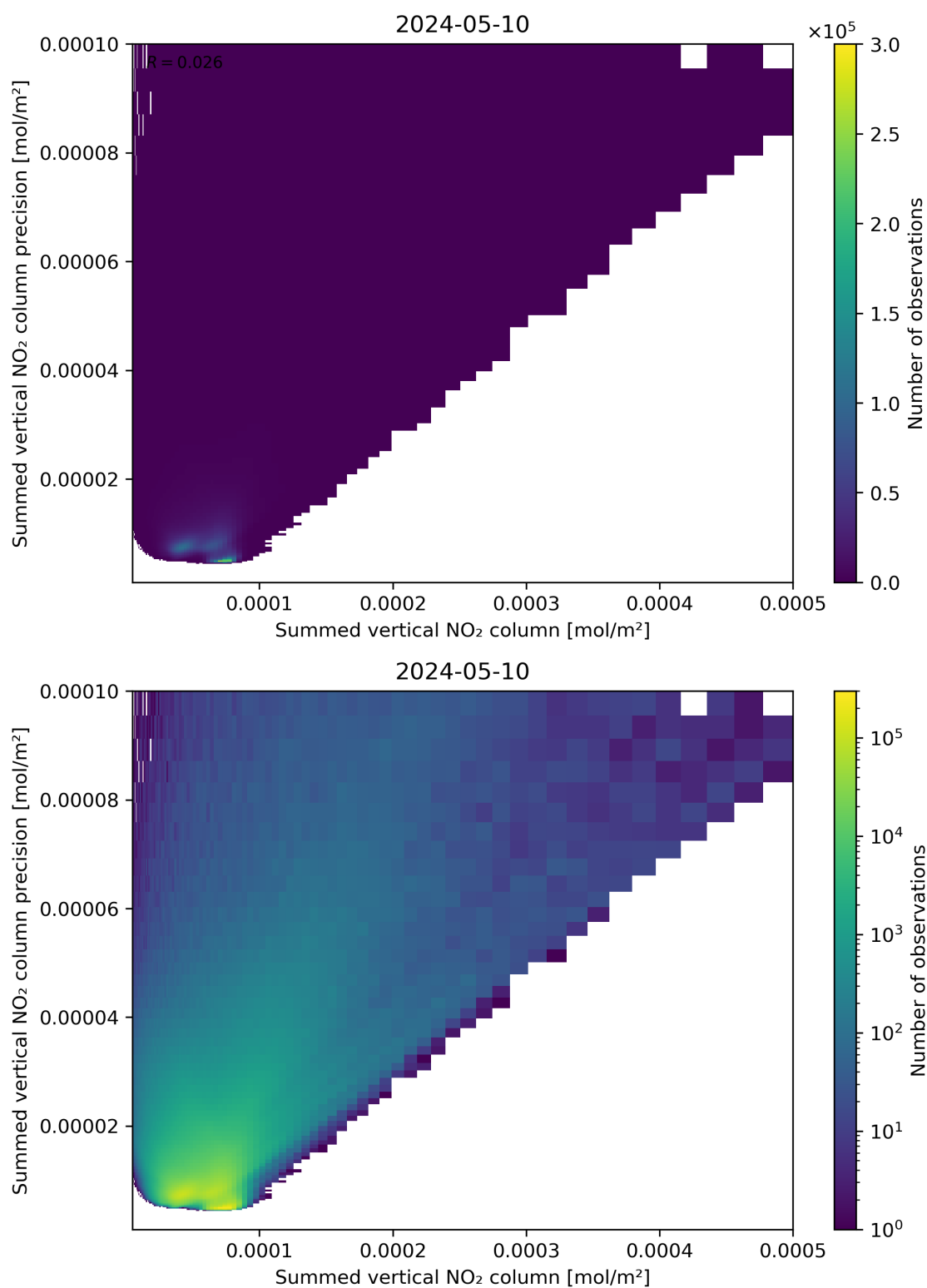
Figure 105: Scatter density plot of “Summed vertical NO 2 column” against “Summed vertical NO 2 column precision” for 2024-05-09 to 2024-05-11.
