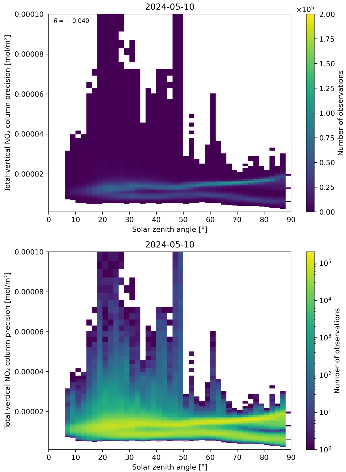
Figure 154: Scatter density plot of “Solar zenith angle” against “Total vertical NO 2 column precision” for 2024-05-09 to 2024-05-11.
