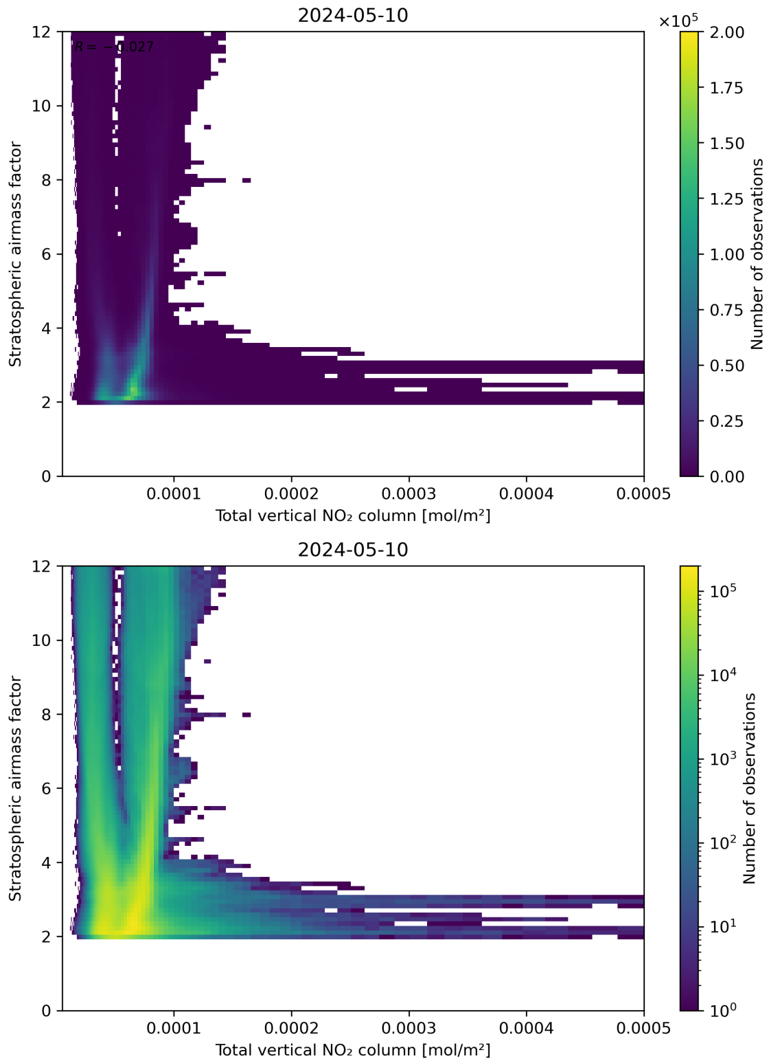
Figure 110: Scatter density plot of “Total vertical NO 2 column” against “Stratospheric airmass factor” for 2024-05-09 to 2024-05-11.
