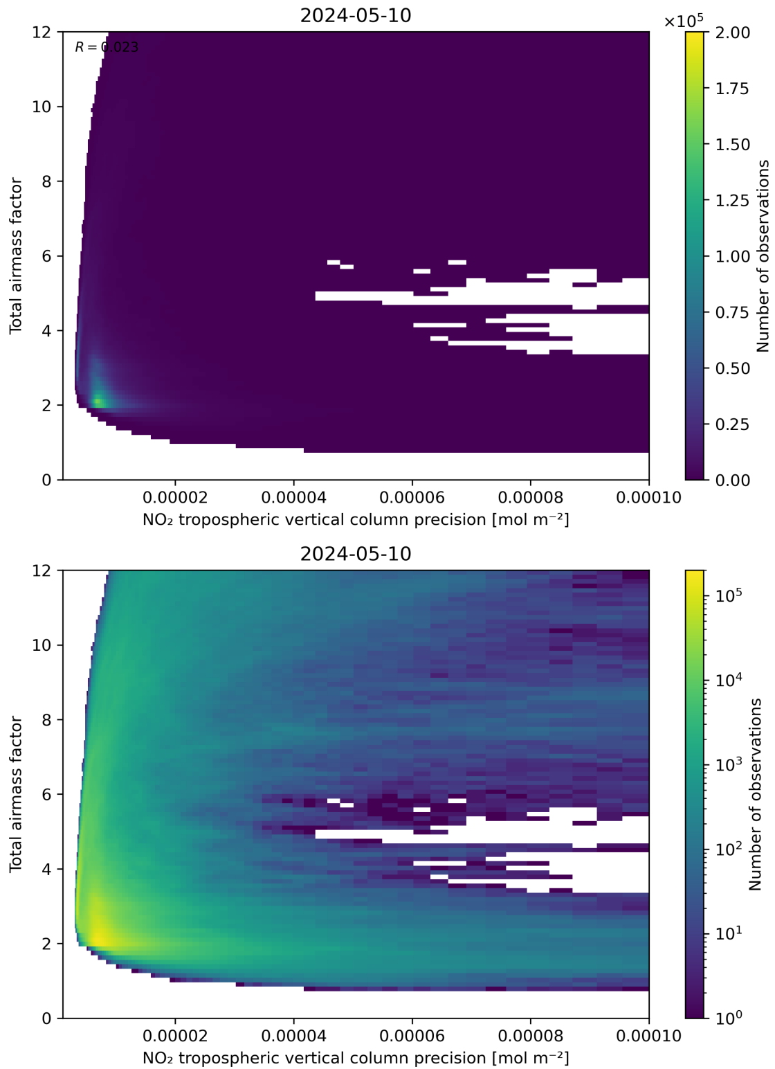
Figure 132: Scatter density plot of “NO 2 tropospheric vertical column precision” against “Total air mass factor” for 2024-05-09 to 2024-05-11.
