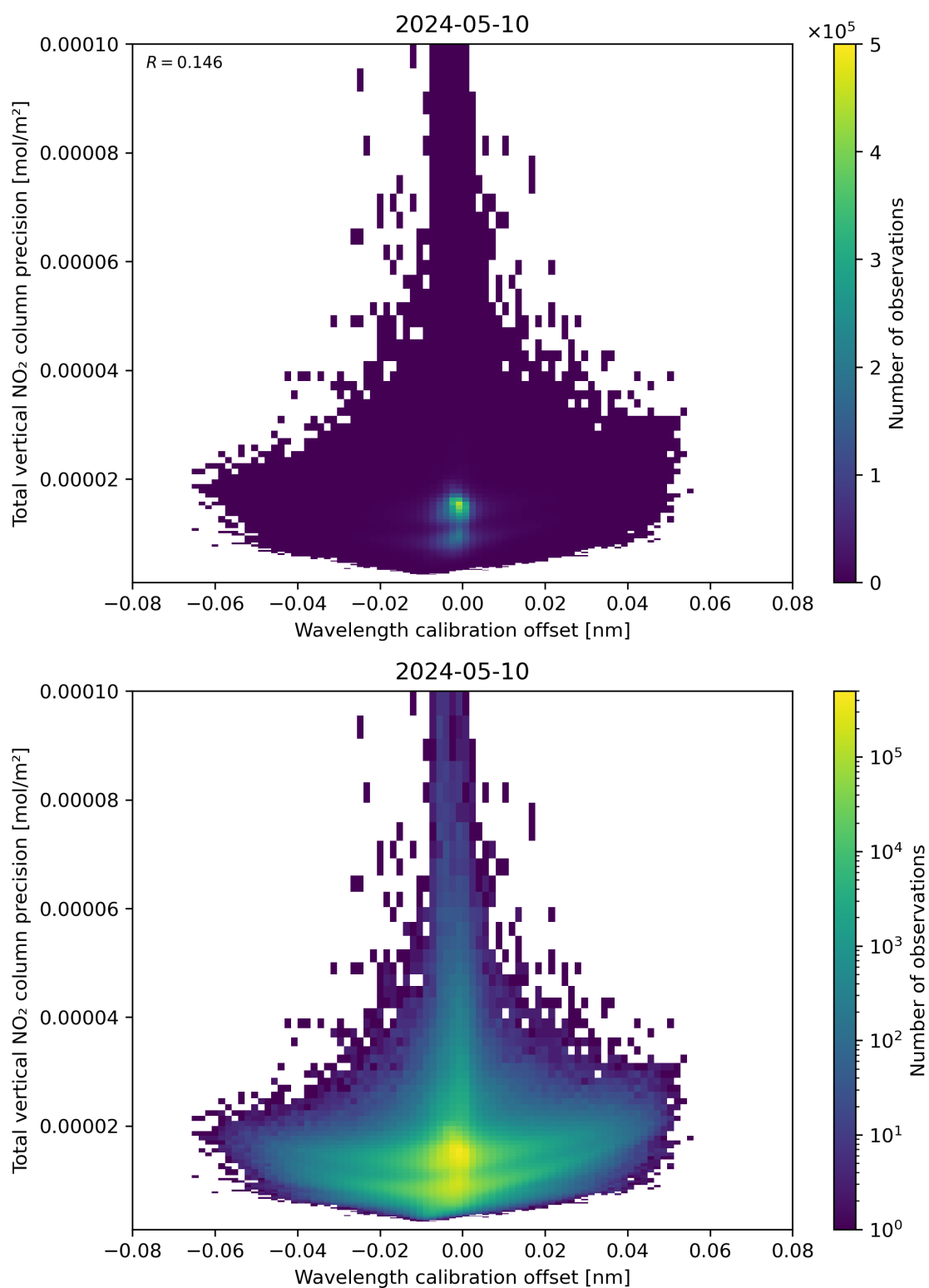
Figure 180: Scatter density plot of “Wavelength calibration offset” against “Total vertical NO 2 column precision” for 2024-05-09 to 2024-05-11.
