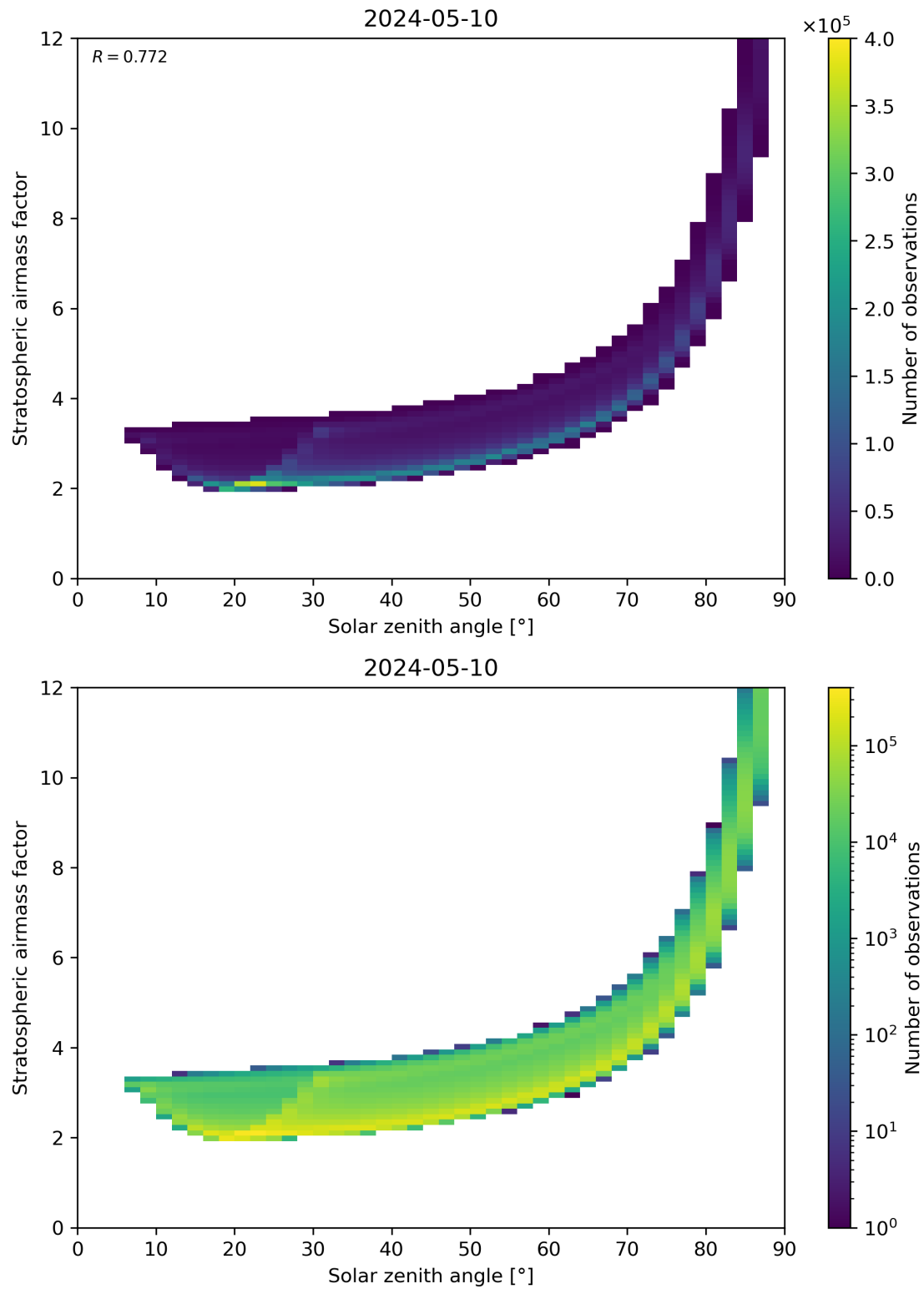
Figure 145: Scatter density plot of “Solar zenith angle” against “Stratospheric airmass factor” for 2024-05-09 to 2024-05-11.
