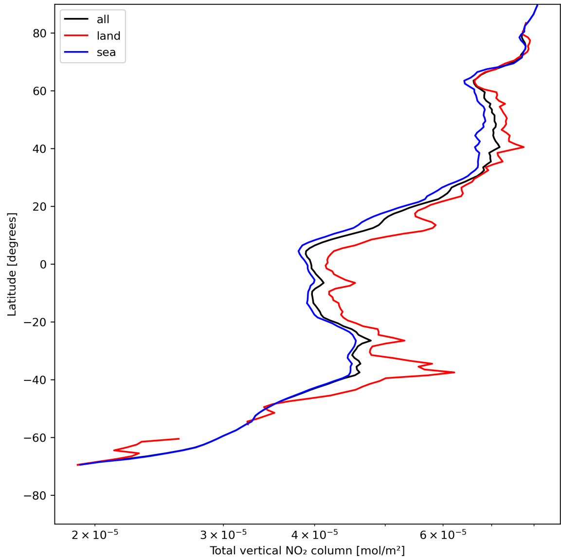
Figure 21: Zonal average of “Total vertical NO 2 column” for 2024-05-09 to 2024-05-11.
