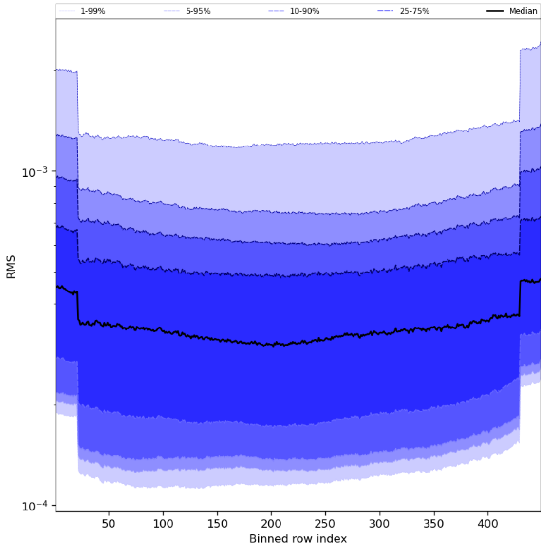
Figure 60: Along track statistics of “RMS” for 2024-05-09 to 2024-05-11
