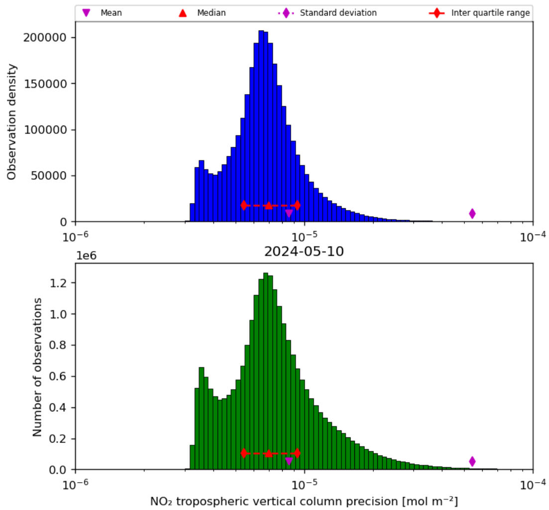
Figure 30: Histogram of “NO 2 tropospheric vertical column precision” for 2024-05-09 to 2024-05-11
