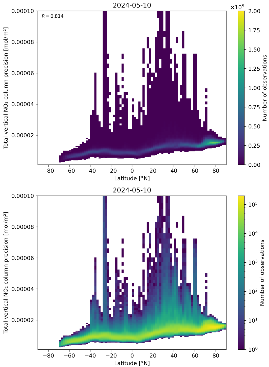
Figure 91: Scatter density plot of “Latitude” against “Total vertical NO 2 column precision” for 2024-05-09 to 2024-05-11.
