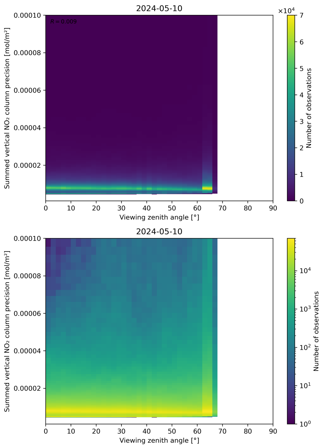
Figure 166: Scatter density plot of “Viewing zenith angle” against “Summed vertical NO 2 column precision” for 2024-05-09 to 2024-05-11.
