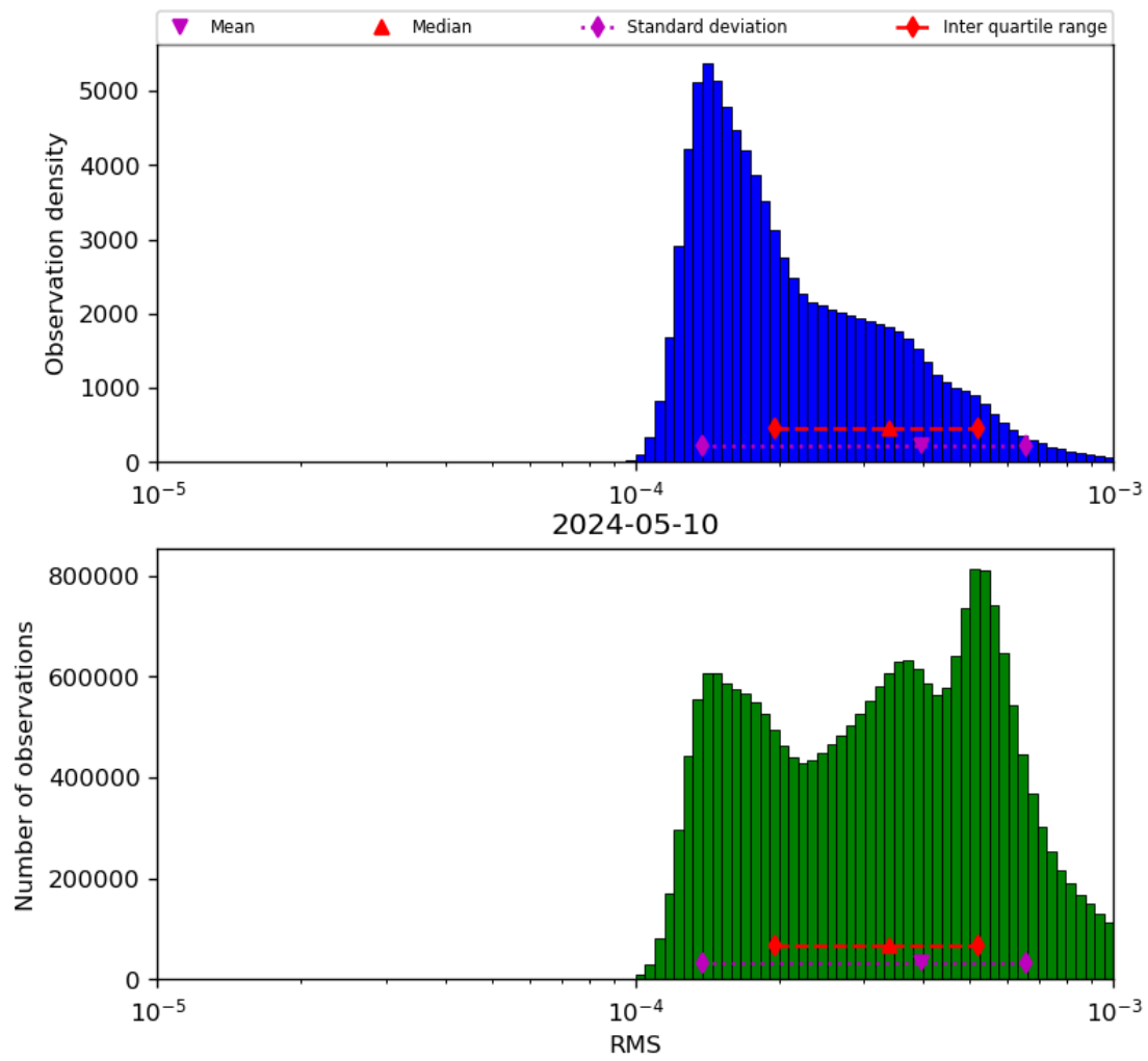
Figure 43: Histogram of “RMS” for 2024-05-09 to 2024-05-11
