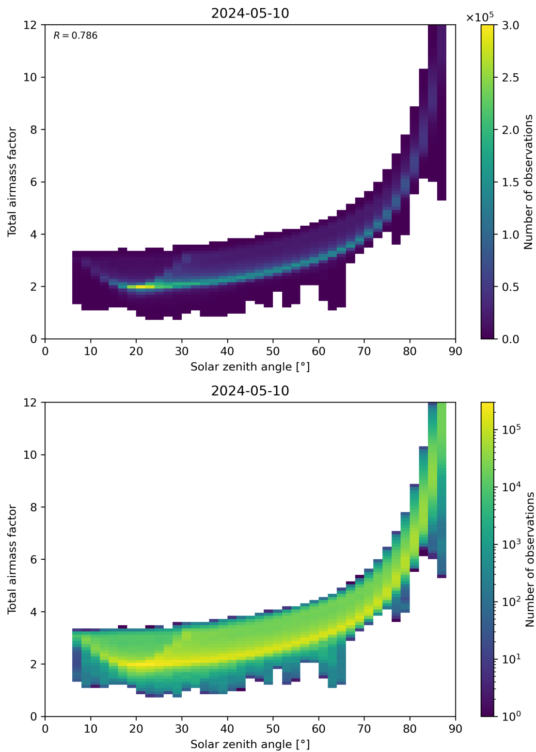
Figure 146: Scatter density plot of “Solar zenith angle” against “Total air mass factor” for 2024-05-09 to 2024-05-11.
