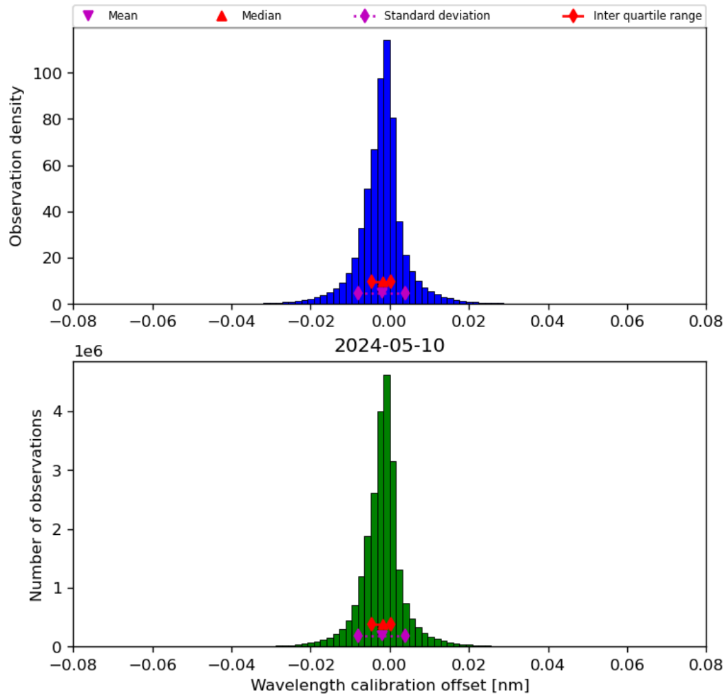
Figure 35: Histogram of “Wavelength calibration offset” for 2024-05-09 to 2024-05-11
