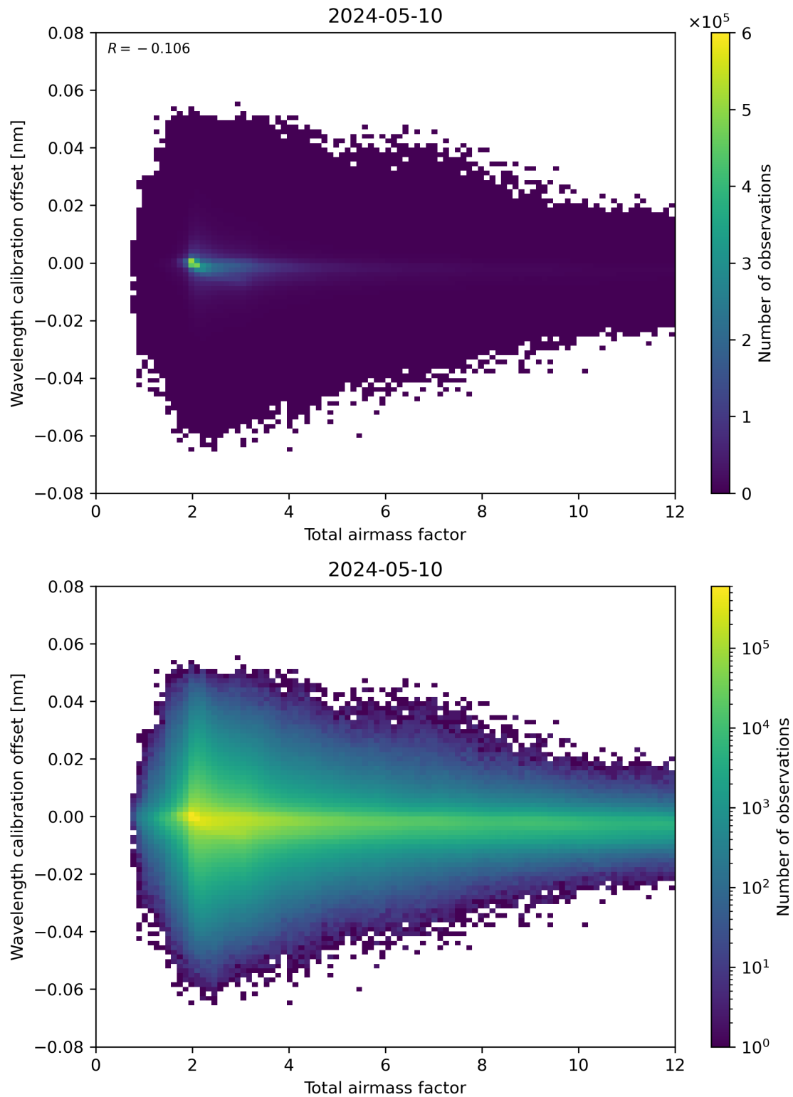
Figure 70: Scatter density plot of “Total airmass factor” against “Wavelength calibration offset” for 2024-05-09 to 2024-05-11.
