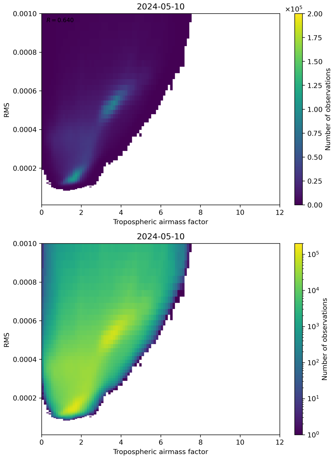
Figure 79: Scatter density plot of “Tropospheric airmass factor” against “RMS” for 2024-05-09 to 2024-05-11.
