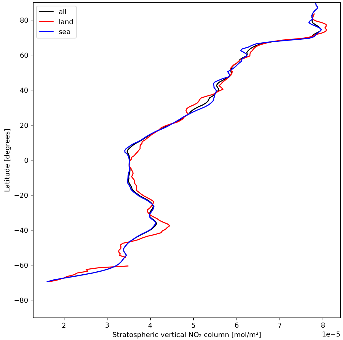
Figure 19: Zonal average of “Stratospheric vertical NO 2 column” for 2024-05-09 to 2024-05-11.
