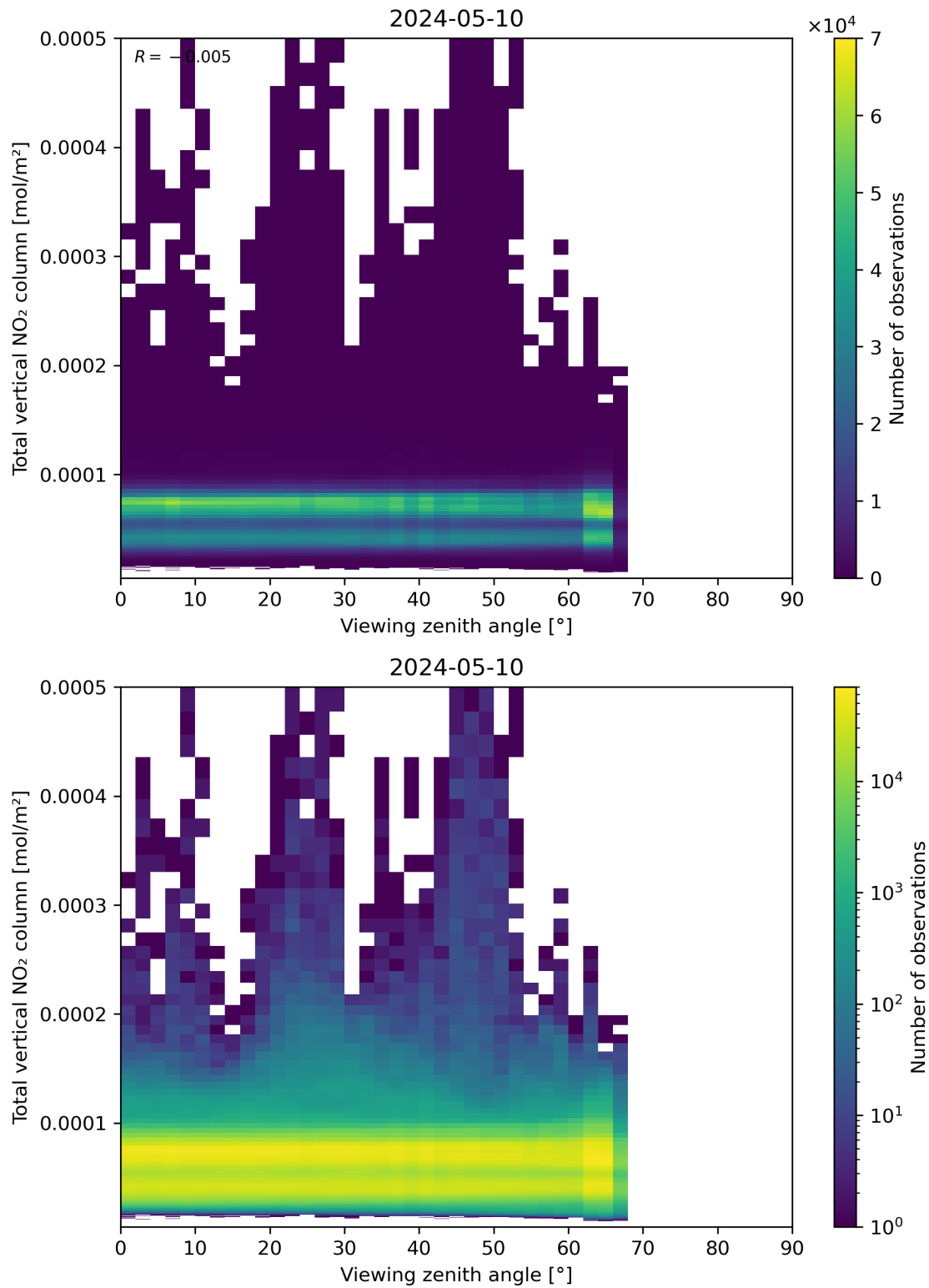
Figure 167: Scatter density plot of “Viewing zenith angle” against “Total vertical NO 2 column” for 2024-05-09 to 2024-05-11.
