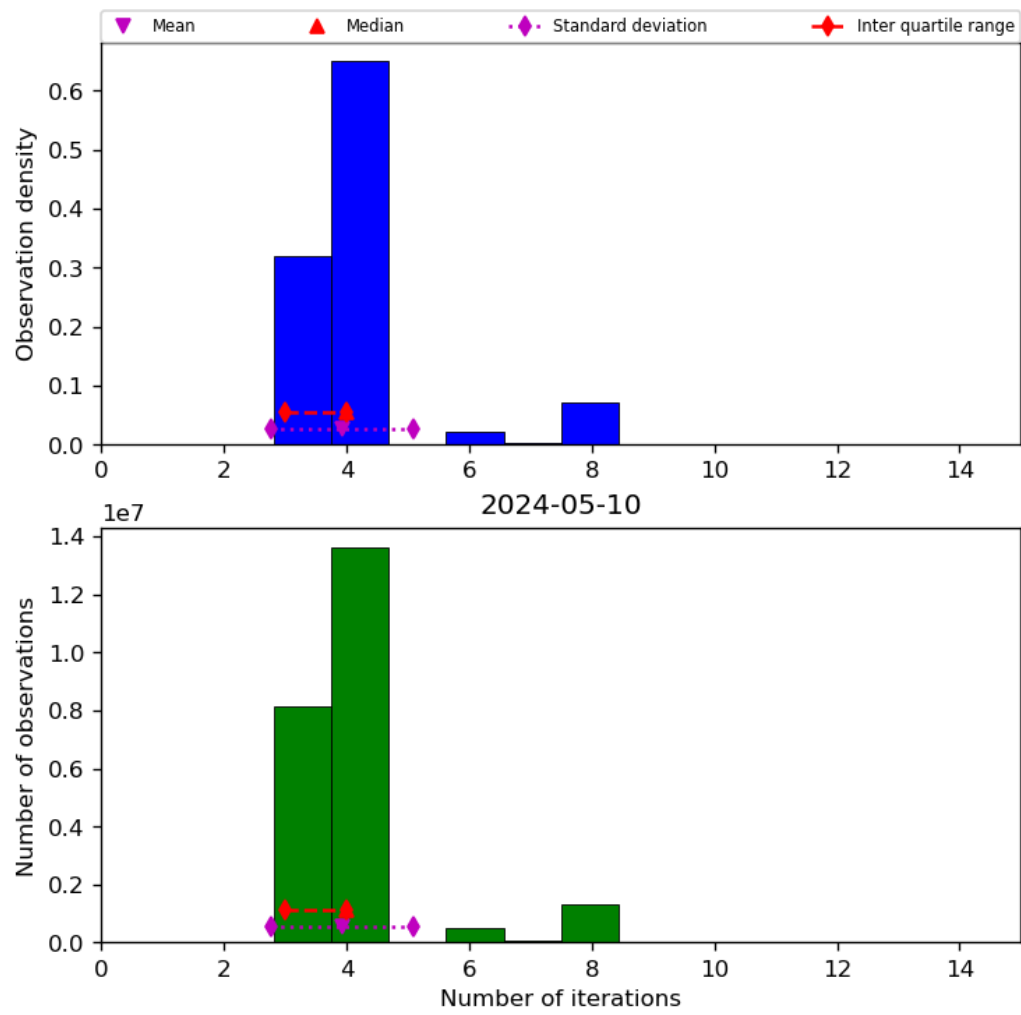
Figure 34: Histogram of "Number of iterations" for 2024-05-09 to 2024-05-11
