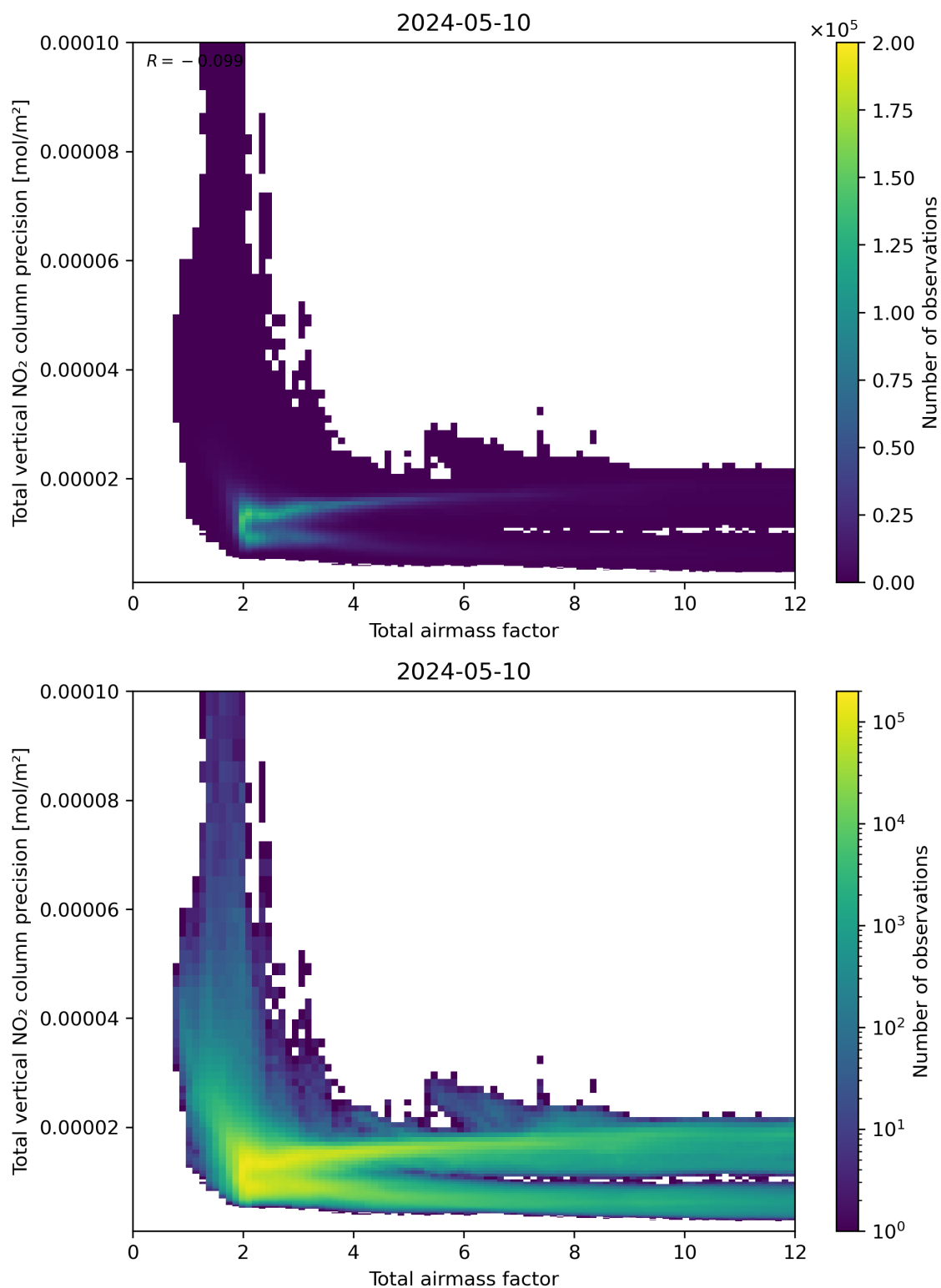
Figure 68: Scatter density plot of “Total airmass factor” against “Total vertical NO 2 column precision” for 2024-05-09 to 2024-05-11.
