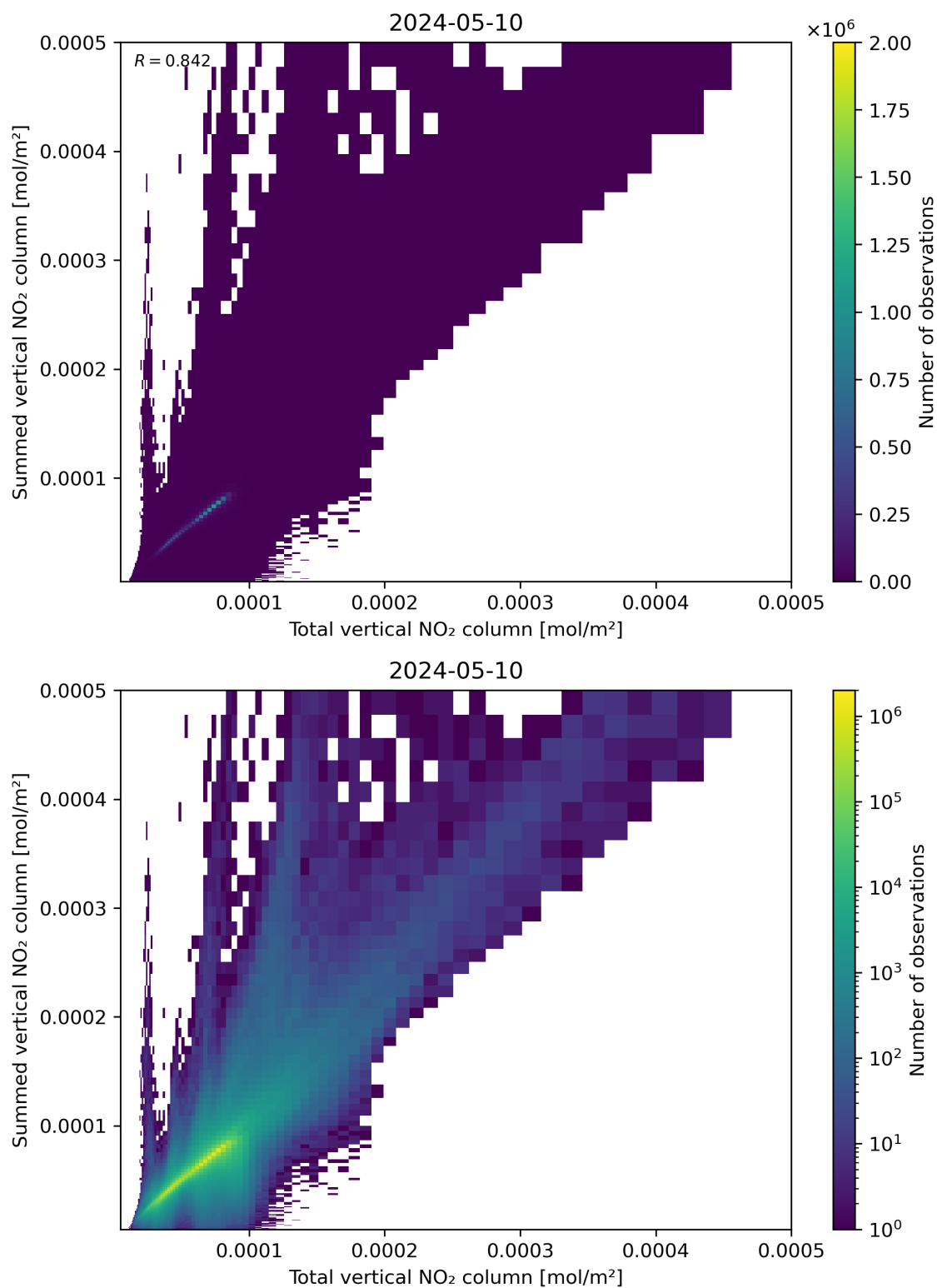
Figure 112: Scatter density plot of “Total vertical NO 2 column” against “Summed vertical NO 2 column” for 2024-05-09 to 2024-05-11.
