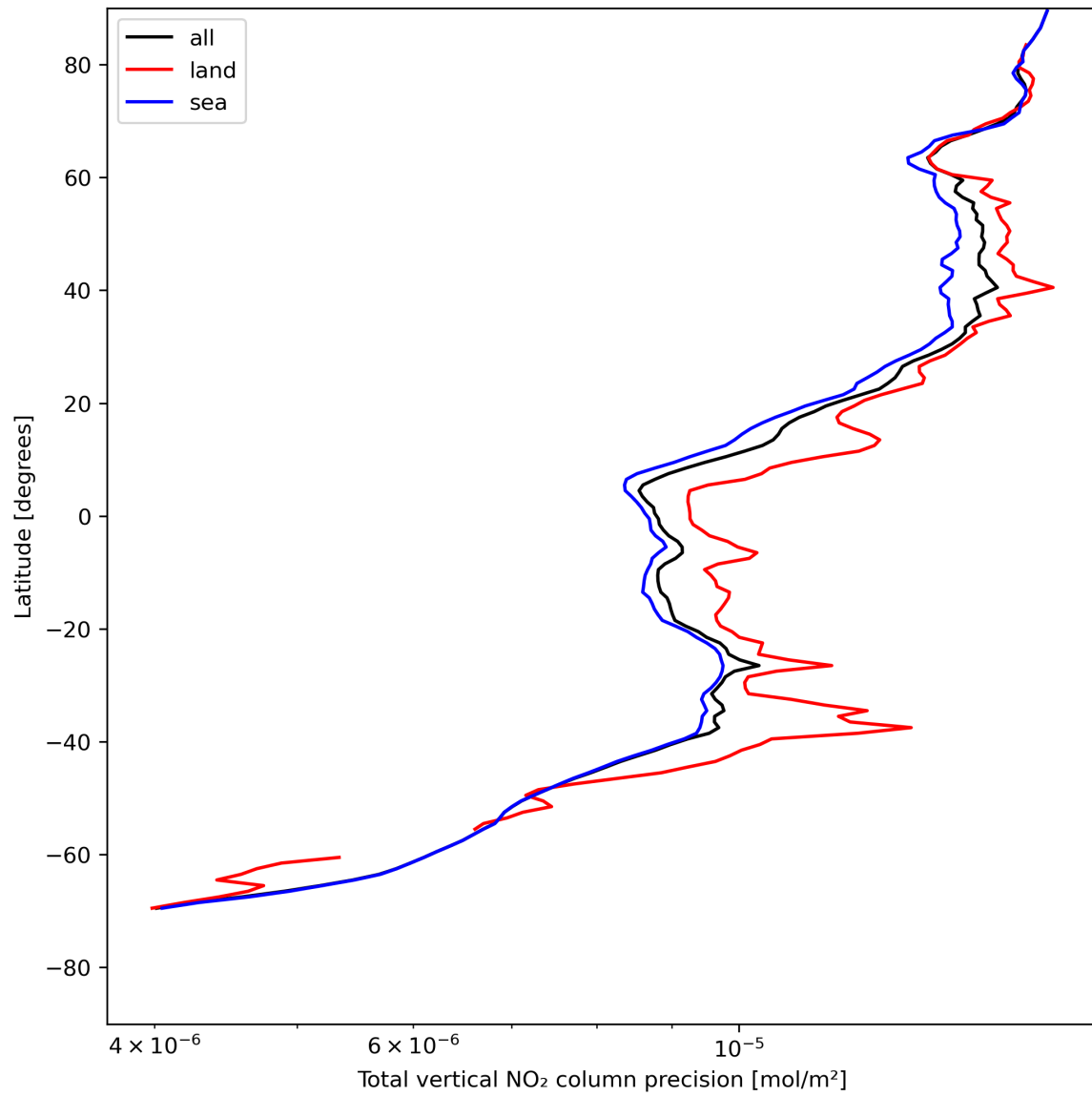
Figure 22: Zonal average of “Total vertical NO 2 column precision” for 2024-05-09 to 2024-05-11.
