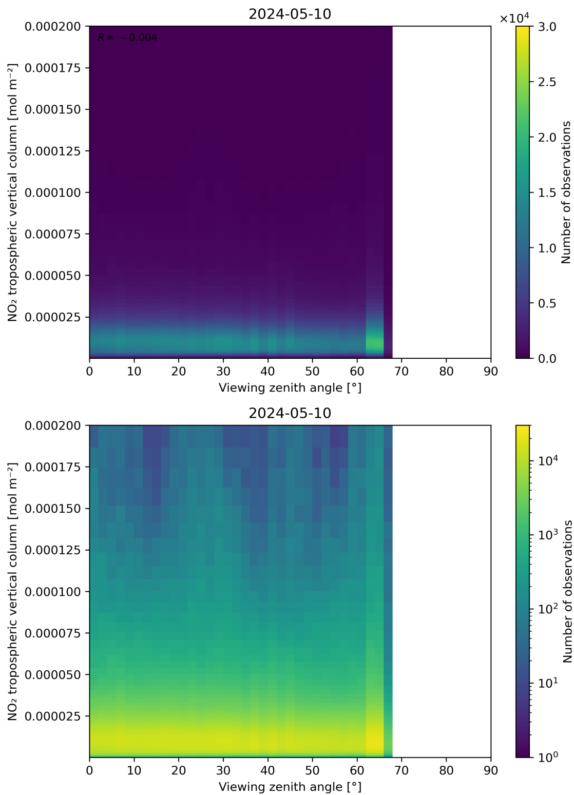
Figure 169: Scatter density plot of “Viewing zenith angle” against “NO 2 tropospheric vertical column” for 2024-05-09 to 2024-05-11.
