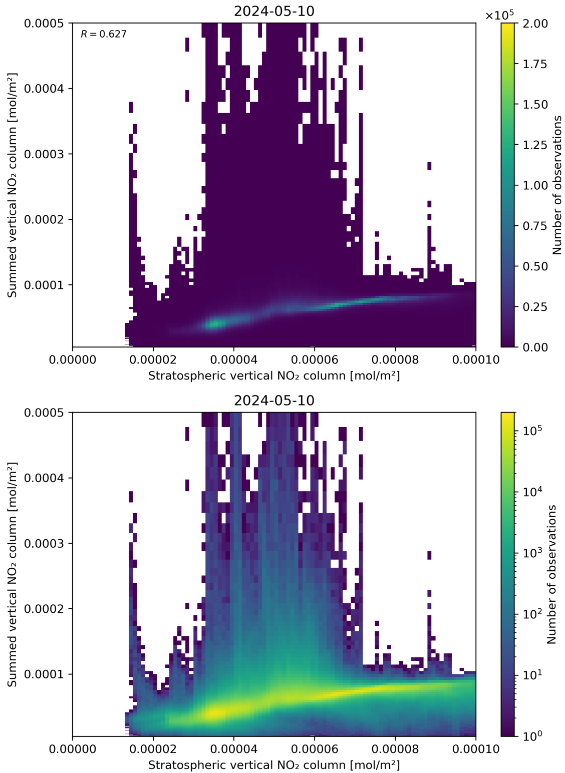
Figure 98: Scatter density plot of “Stratospheric vertical NO 2 column” against “Summed vertical NO 2 column” for 2024-05-09 to 2024-05-11.
