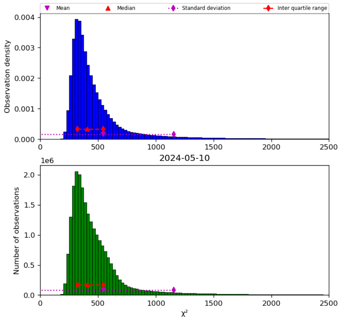
Figure 42: Histogram of “ \chi^2 ” for 2024-05-09 to 2024-05-11
