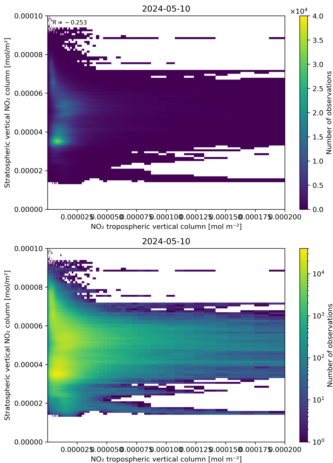
Figure 125: Scatter density plot of “NO 2 tropospheric vertical column” against “Stratospheric vertical NO 2 column” for 2024-05-09 to 2024-05-11.
