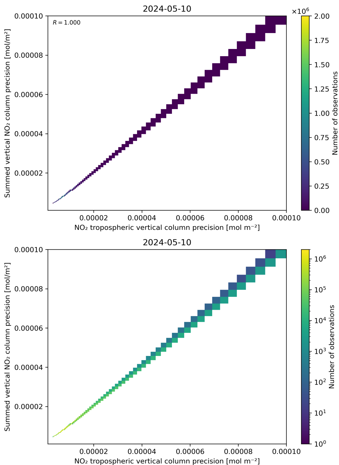
Figure 137: Scatter density plot of “NO 2 tropospheric vertical column precision” against “Summed vertical NO 2 column precision” for 2024-05-09 to 2024-05-11.
