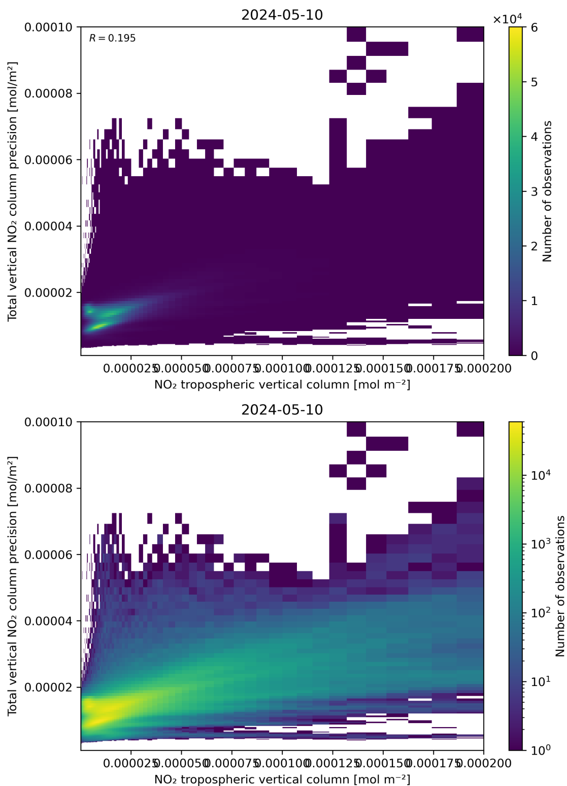
Figure 129: Scatter density plot of “NO 2 tropospheric vertical column” against “Total vertical NO 2 column precision” for 2024-05-09 to 2024-05-11.
