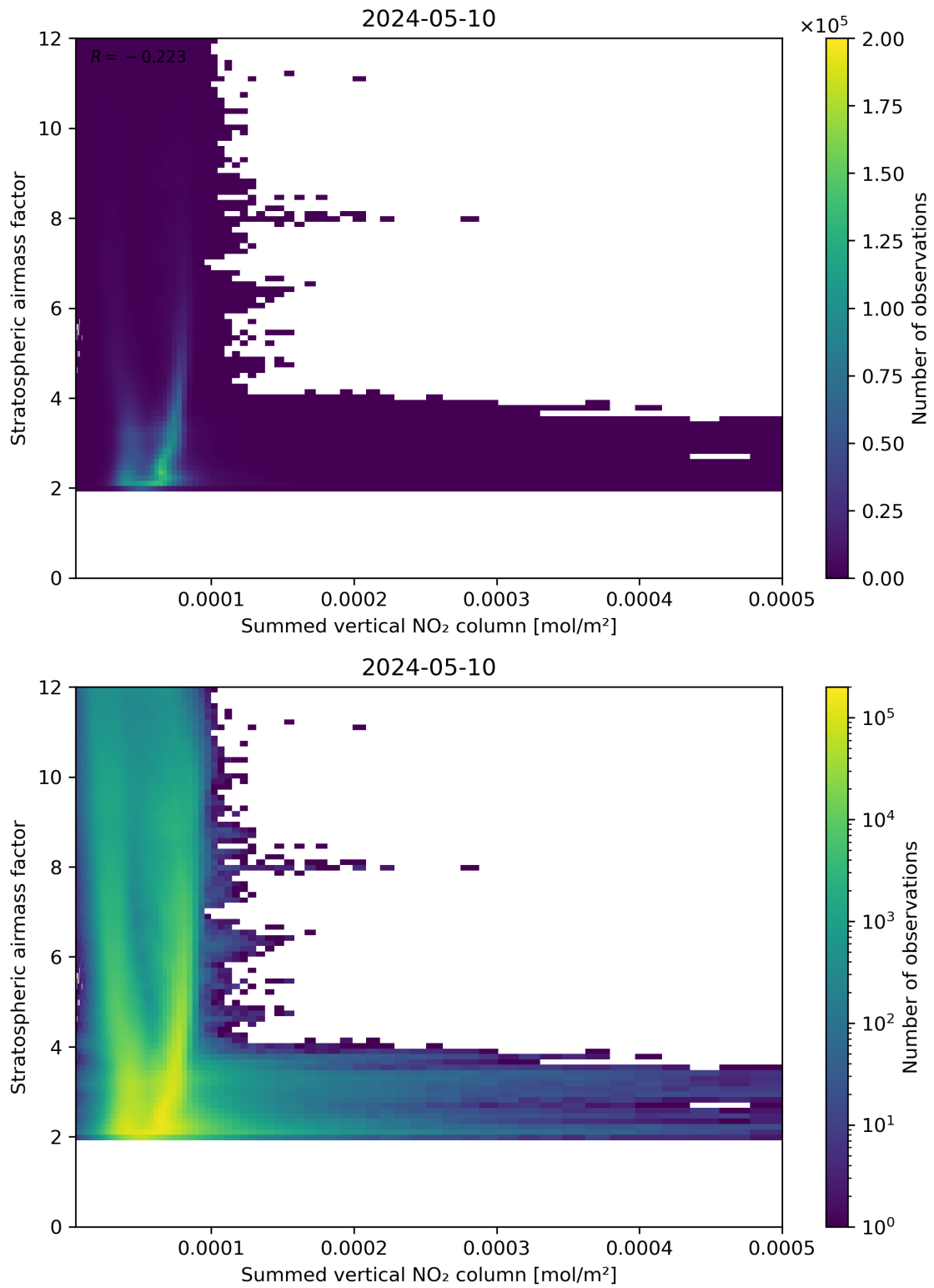
Figure 103: Scatter density plot of “Summed vertical NO 2 column” against “Stratospheric air mass factor” for 2024-05-09 to 2024-05-11.
