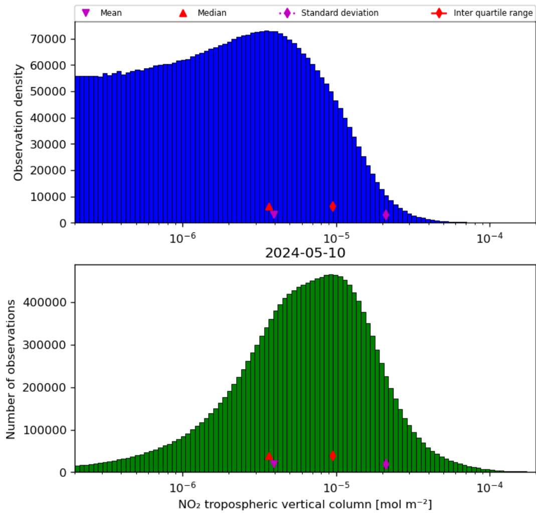
Figure 29: Histogram of “NO 2 tropospheric vertical column” for 2024-05-09 to 2024-05-11
