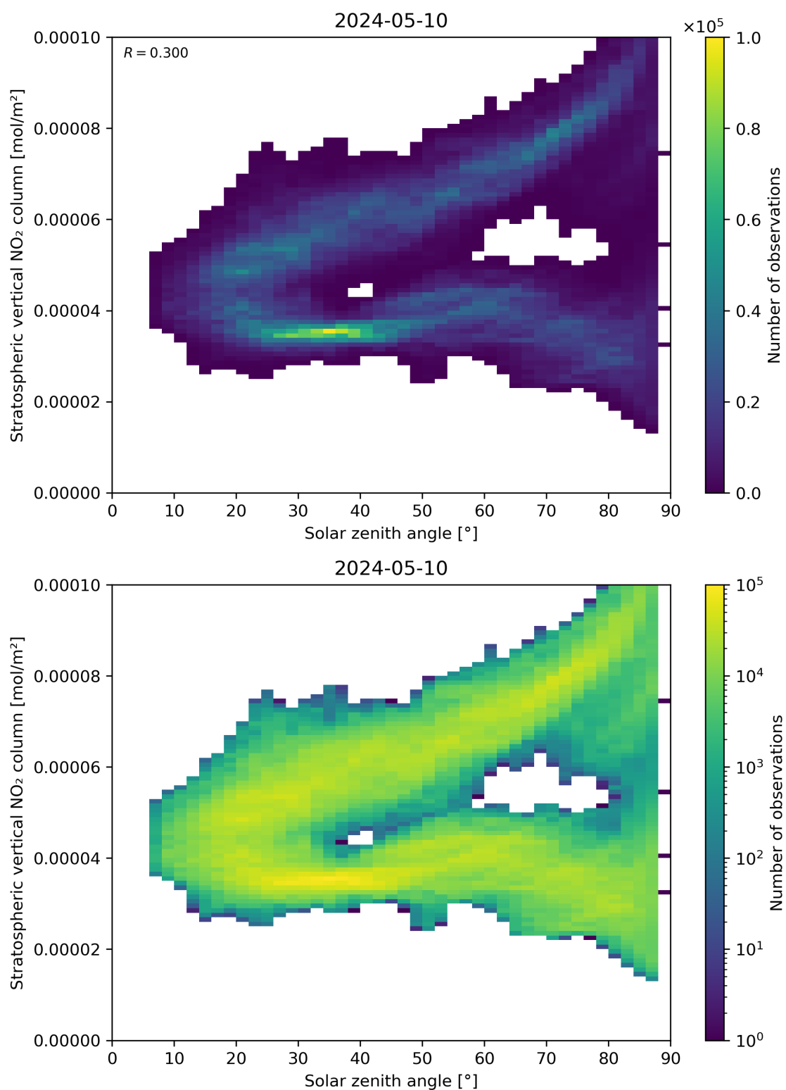
Figure 150: Scatter density plot of “Solar zenith angle” against “Stratospheric vertical NO 2 column” for 2024-05-09 to 2024-05-11.
