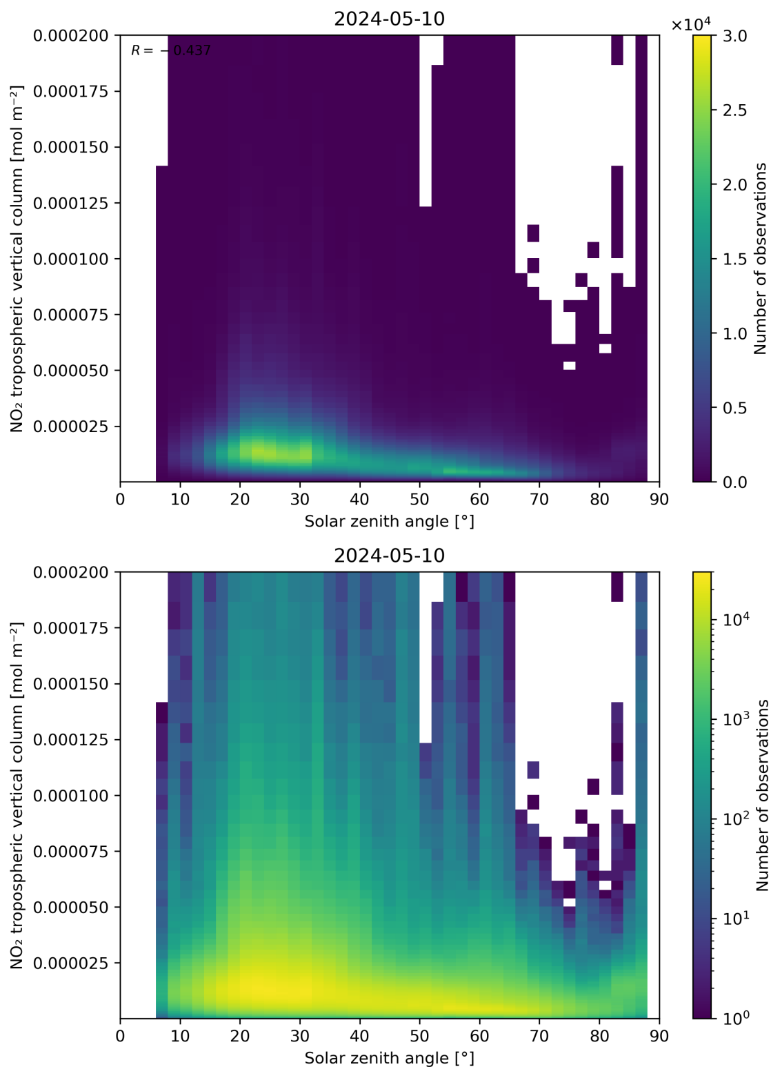
Figure 155: Scatter density plot of “Solar zenith angle” against “NO 2 tropospheric vertical column” for 2024-05-09 to 2024-05-11.
