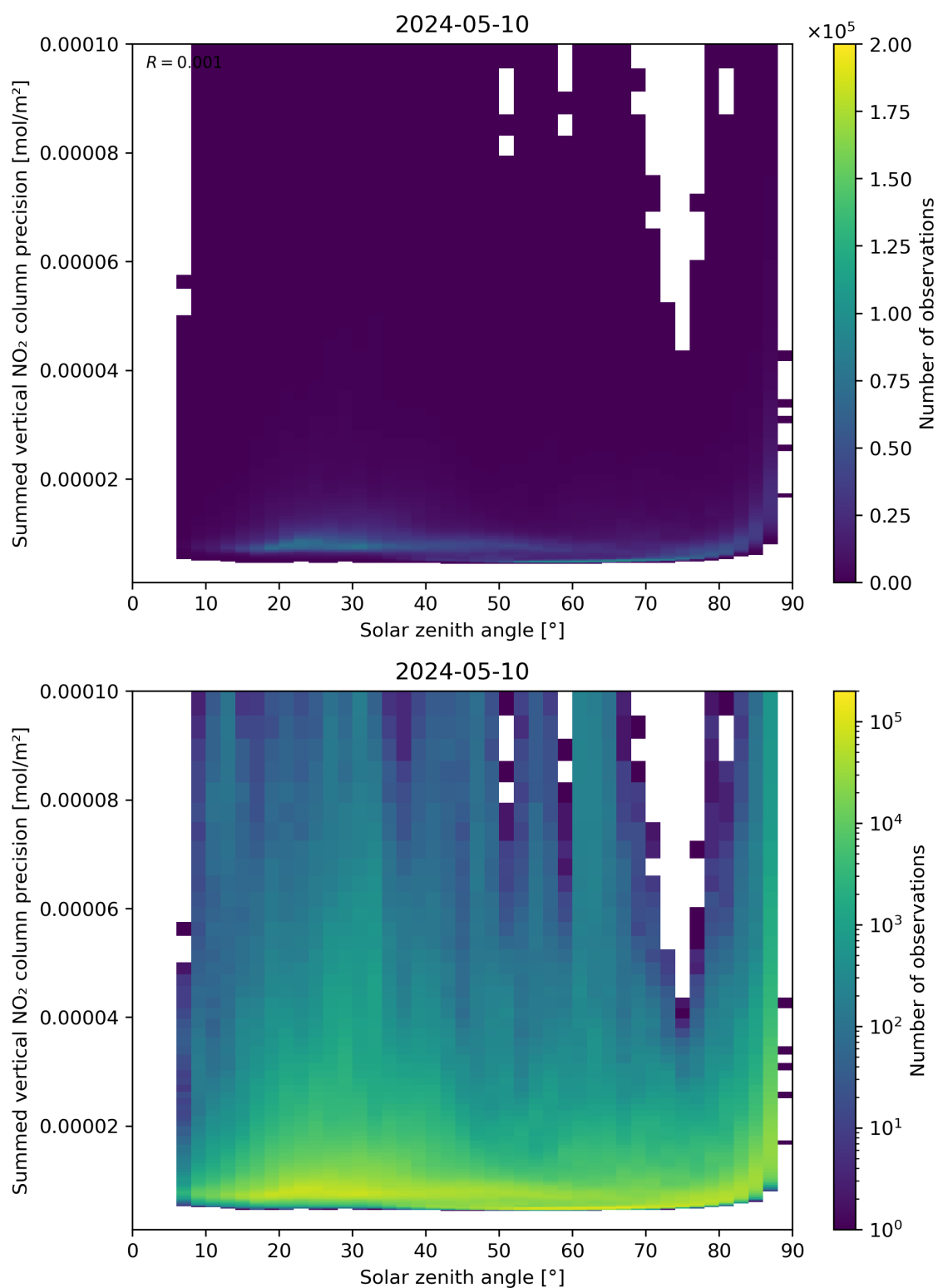
Figure 152: Scatter density plot of “Solar zenith angle” against “Summed vertical NO 2 column precision” for 2024-05-09 to 2024-05-11.
