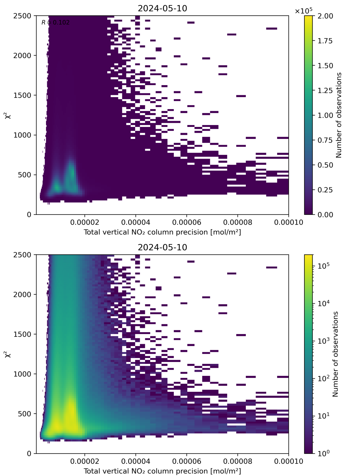
Figure 116: Scatter density plot of “Total vertical NO 2 column precision” against “ \chi^2 ” for 2024-05-09 to 2024-05-11.
