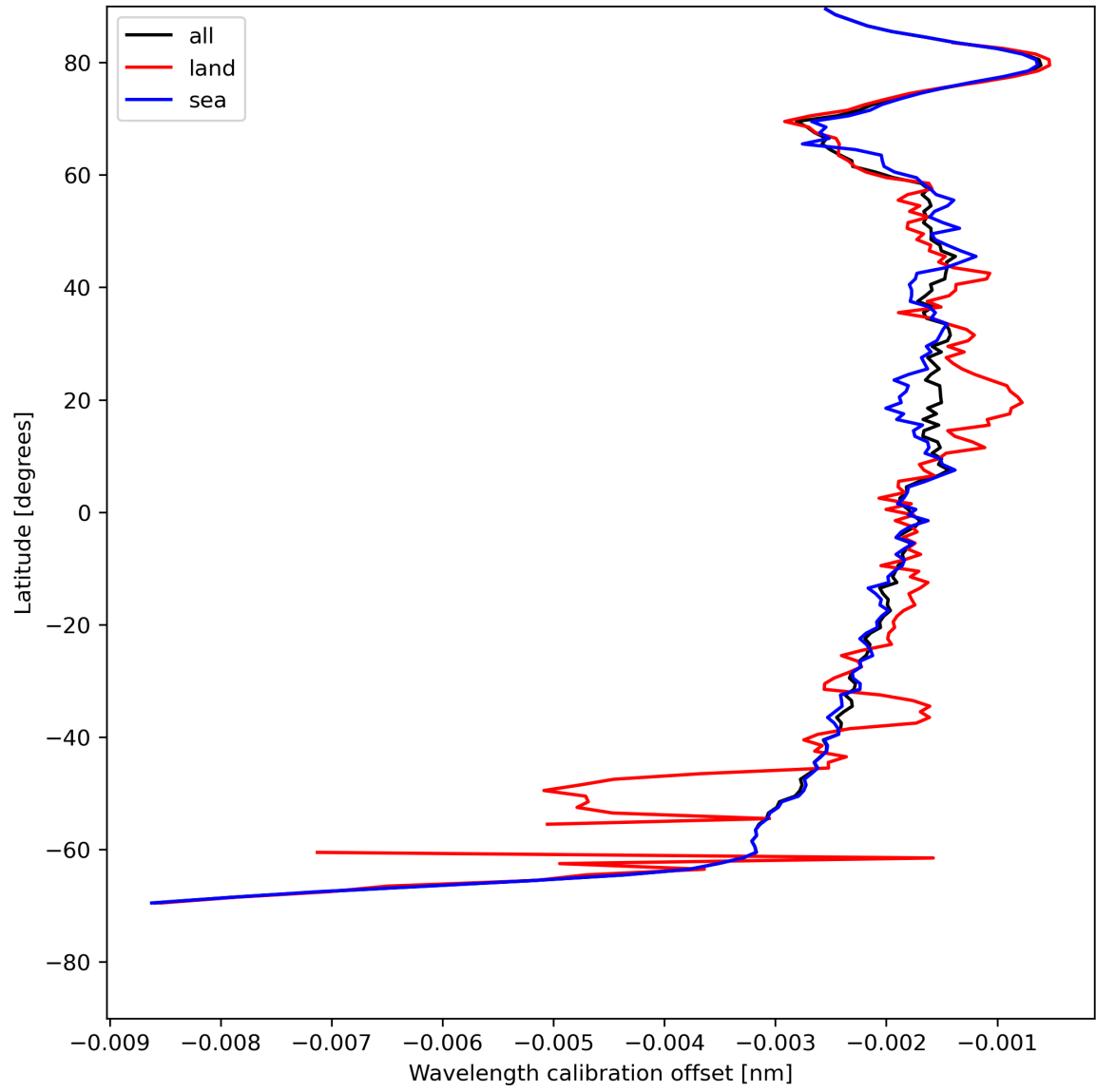
Figure 18: Zonal average of “Wavelength calibration offset” for 2024-05-09 to 2024-05-11.
