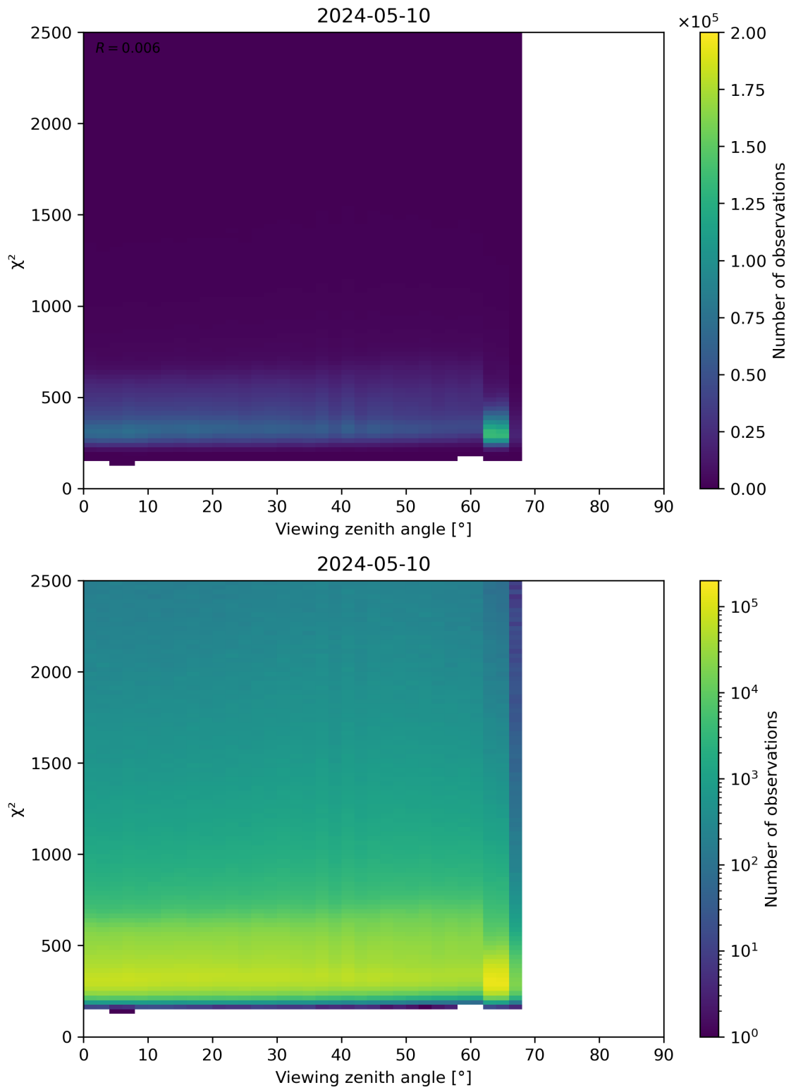
Figure 162: Scatter density plot of “Viewing zenith angle” against “ \chi^2 ” for 2024-05-09 to 2024-05-11.
