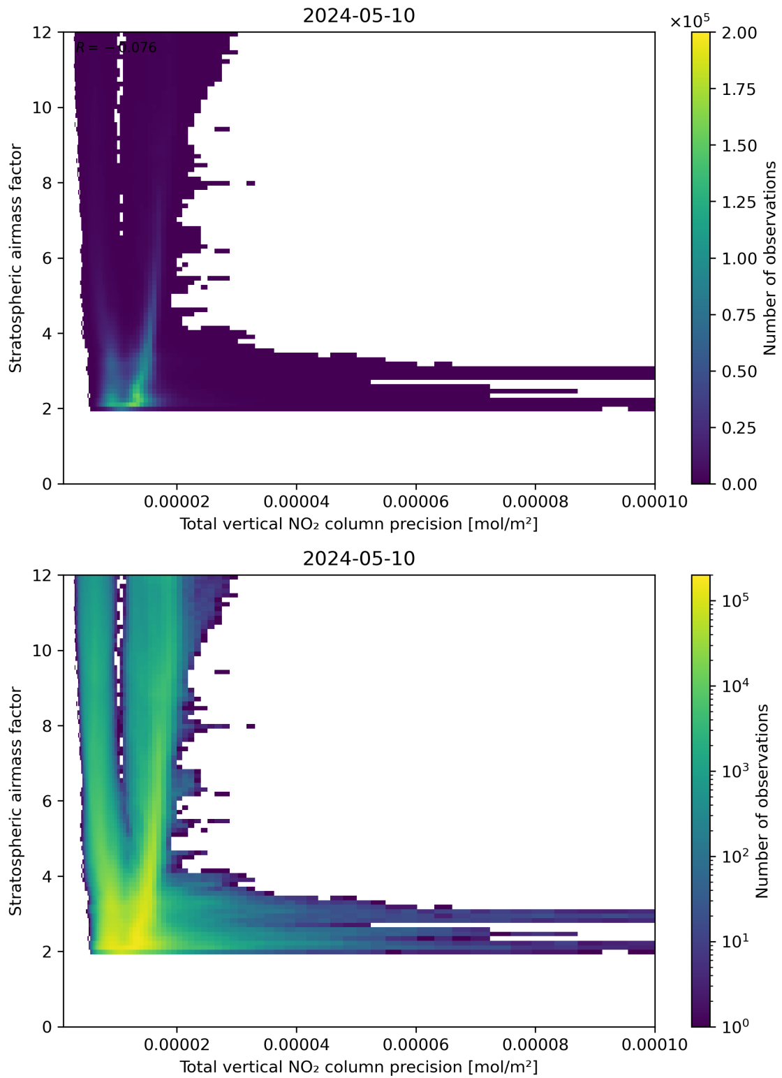
Figure 115: Scatter density plot of “Total vertical NO 2 column precision” against “Stratospheric airmass factor” for 2024-05-09 to 2024-05-11.
