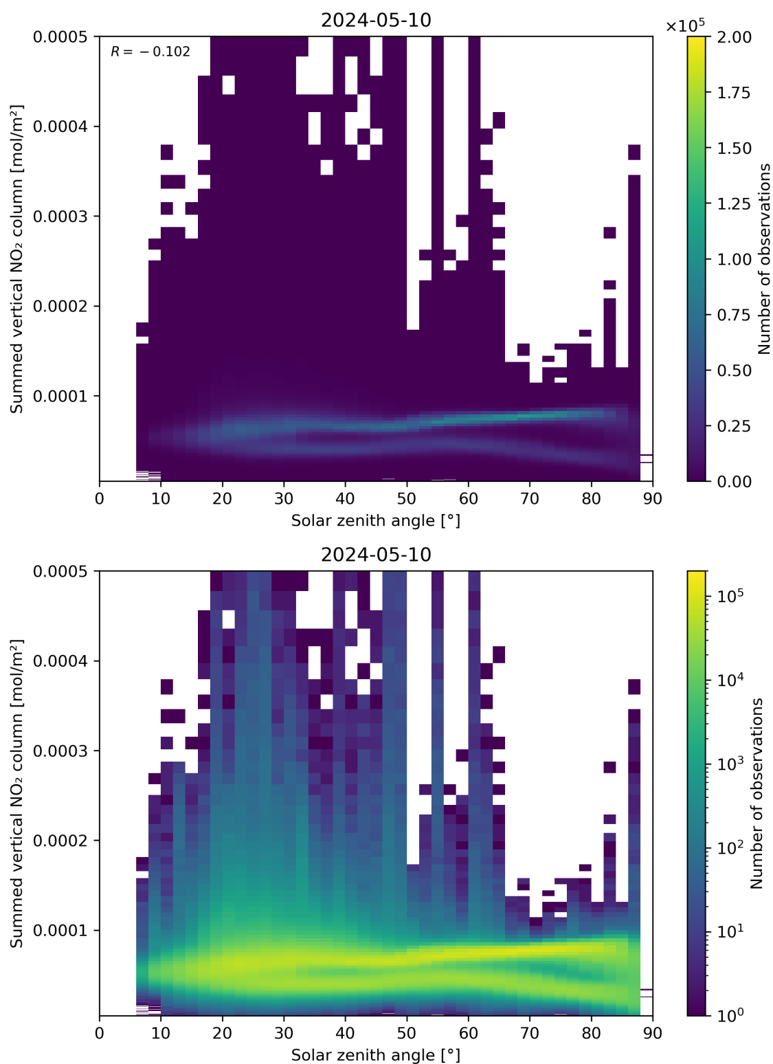
Figure 151: Scatter density plot of “Solar zenith angle” against “Summed vertical NO 2 column” for 2024-05-09 to 2024-05-11.
