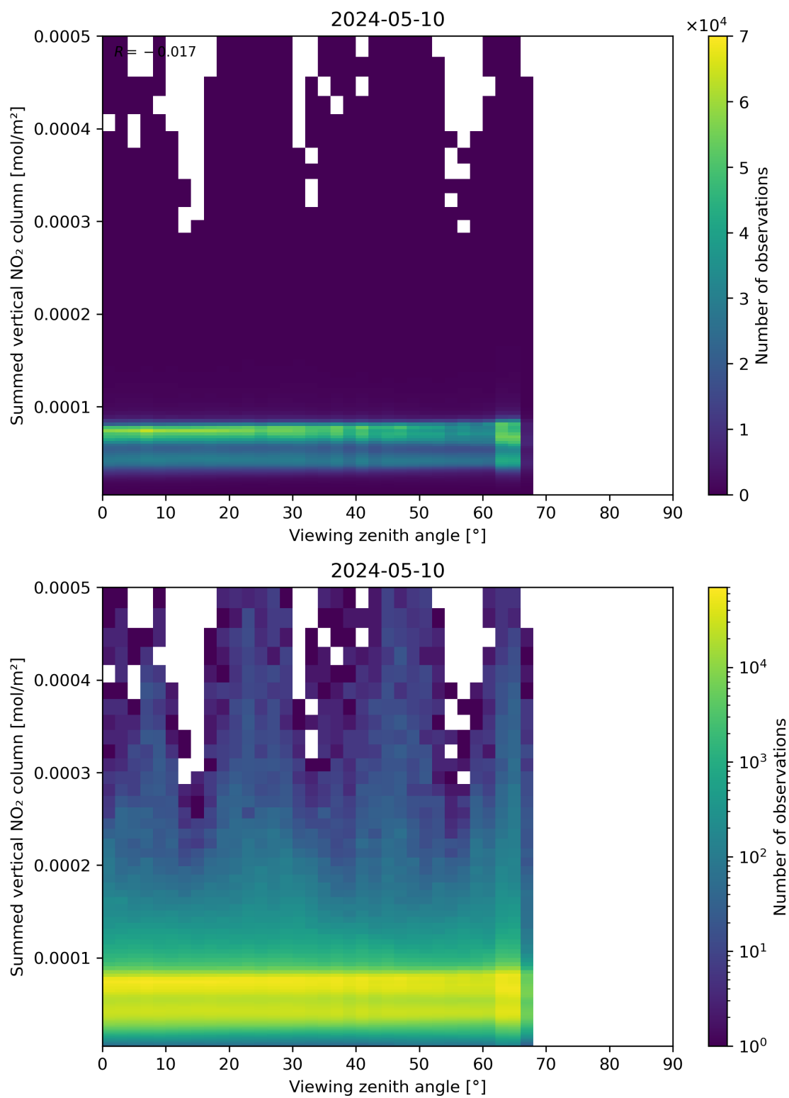
Figure 165: Scatter density plot of “Viewing zenith angle” against “Summed vertical NO 2 column” for 2024-05-09 to 2024-05-11.
