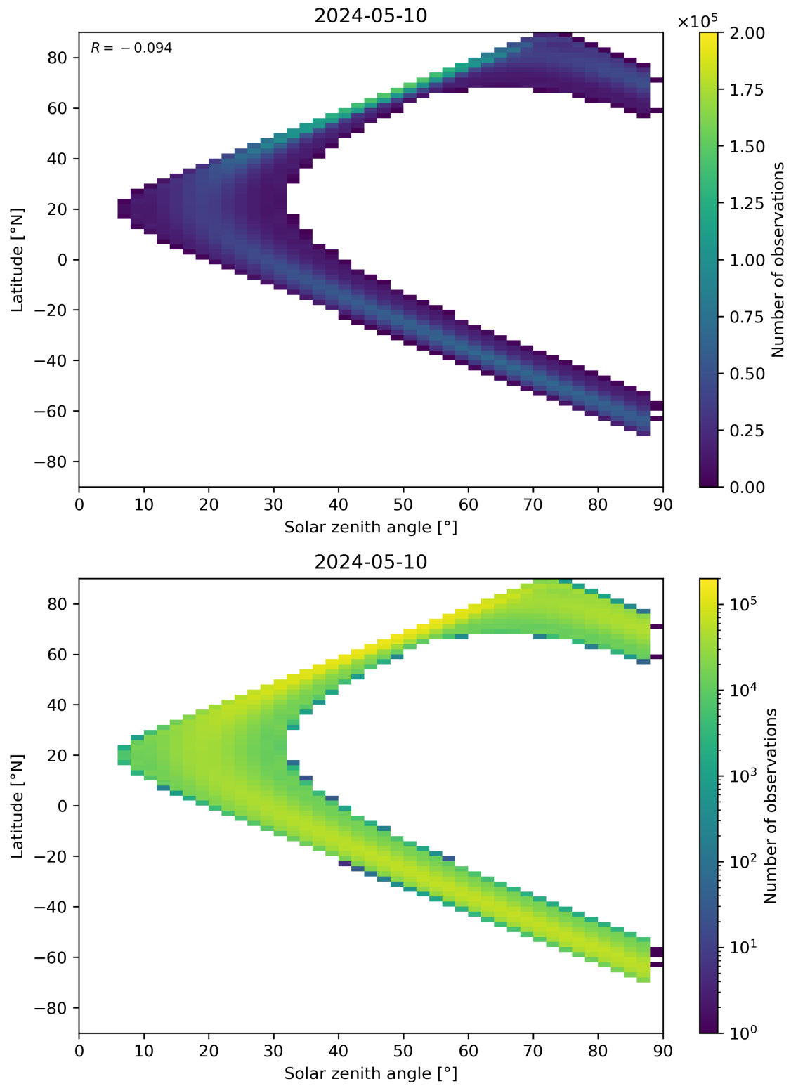
Figure 149: Scatter density plot of “Solar zenith angle” against “Latitude” for 2024-05-09 to 2024-05-11.
