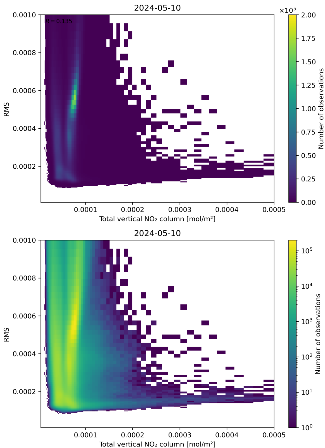
Figure 120: Scatter density plot of “Total vertical NO 2 column” against “RMS” for 2024-05-09 to 2024-05-11.
