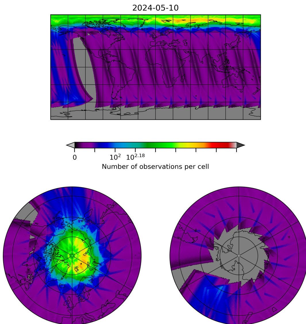
Figure 10: Map of the number of observations for 2024-05-09 to 2024-05-11
