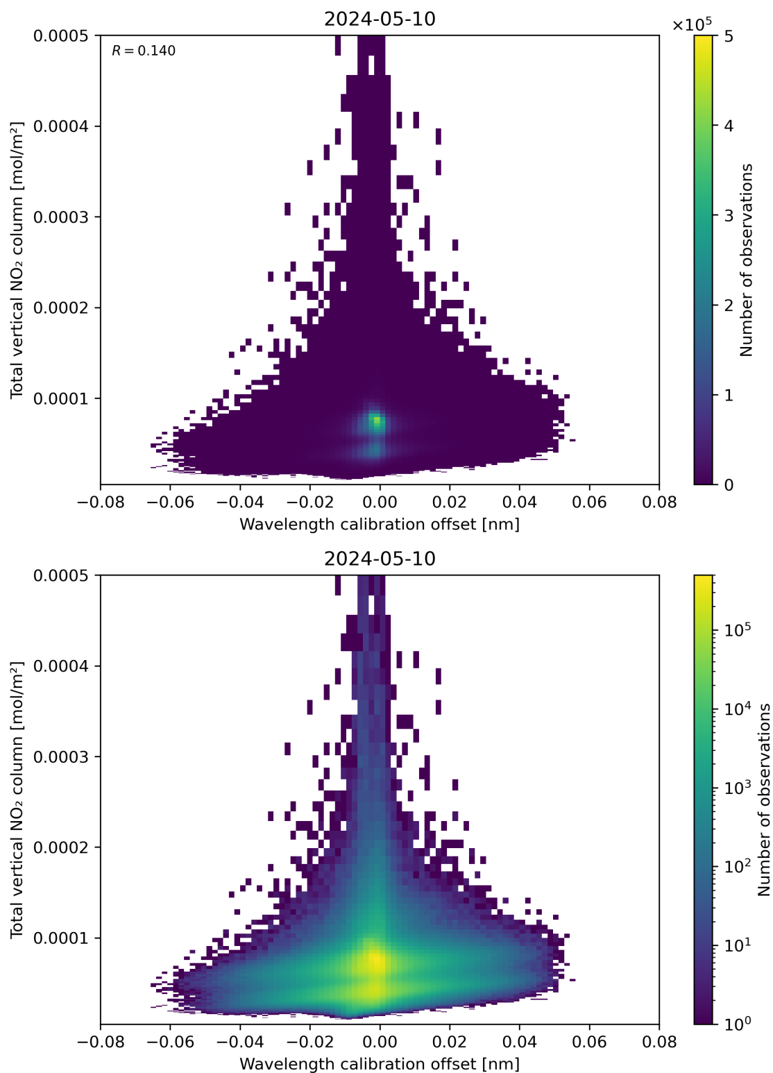
Figure 179: Scatter density plot of “Wavelength calibration offset” against “Total vertical NO 2 column” for 2024-05-09 to 2024-05-11.
