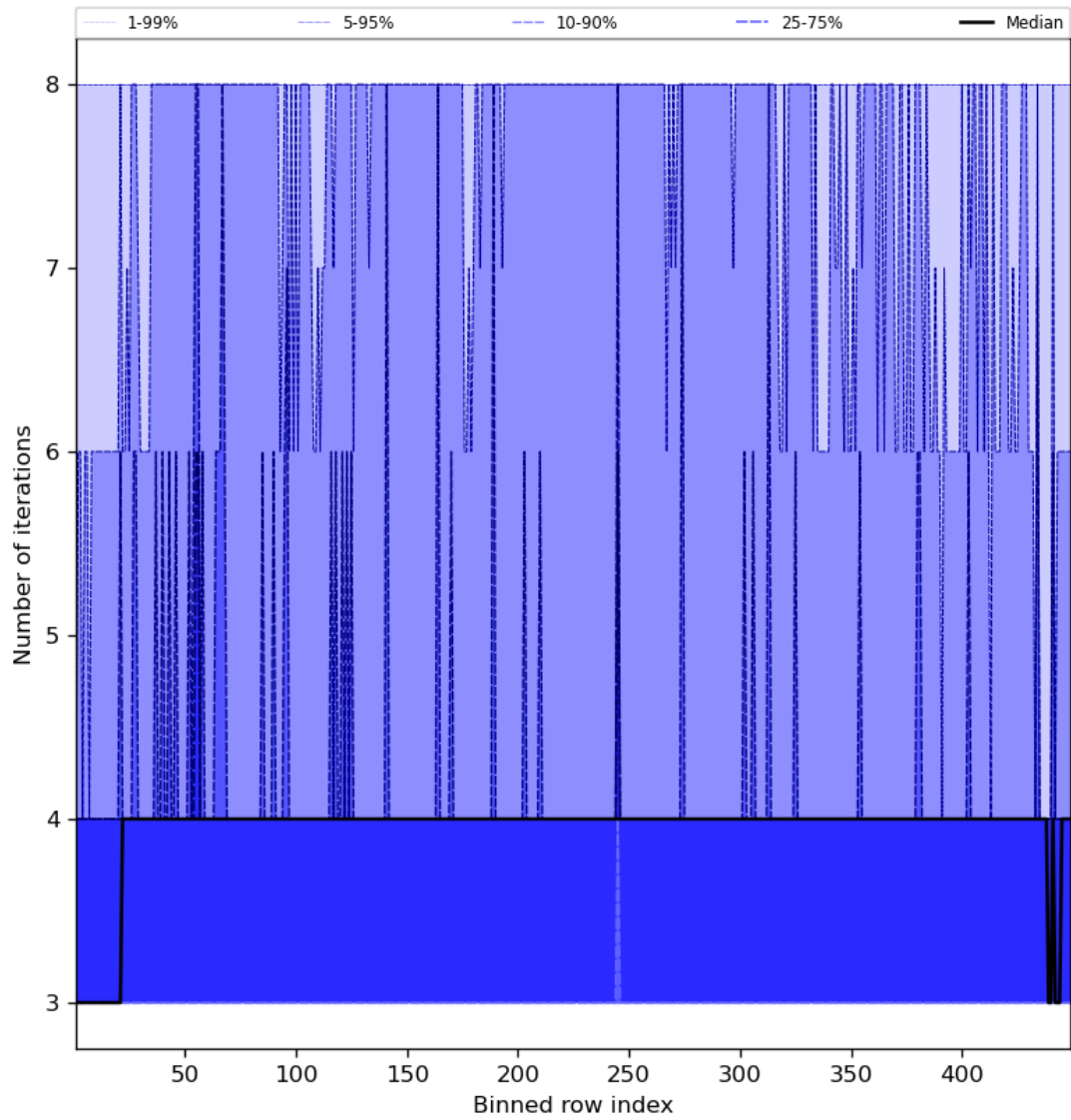
Figure 51: Along track statistics of “Number of iterations” for 2024-05-09 to 2024-05-11
