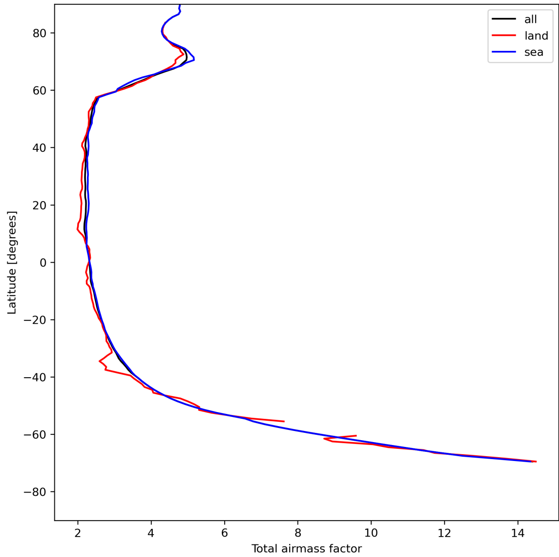
Figure 15: Zonal average of “Total airmass factor” for 2024-05-09 to 2024-05-11.
