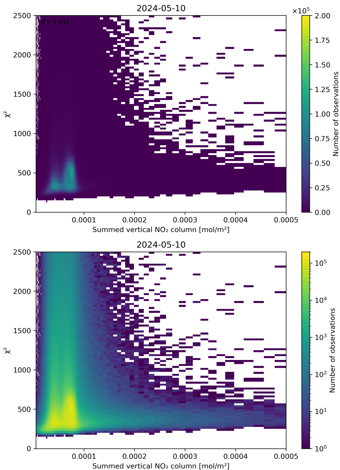
Figure 104: Scatter density plot of “Summed vertical NO 2 column” against “ \chi^2 ” for 2024-05-09 to 2024-05-11.
