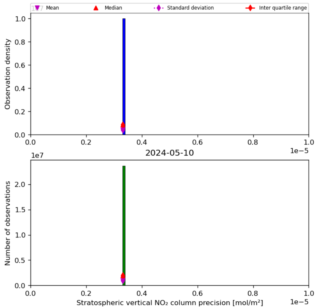
Figure 37: Histogram of “Stratospheric vertical NO 2 column precision” for 2024-05-09 to 2024-05-11
