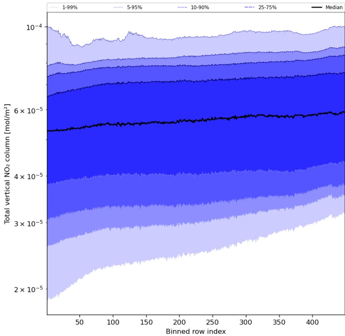
Figure 55: Along track statistics of "Total vertical NO 2 column" for 2024-05-09 to 2024-05-11
