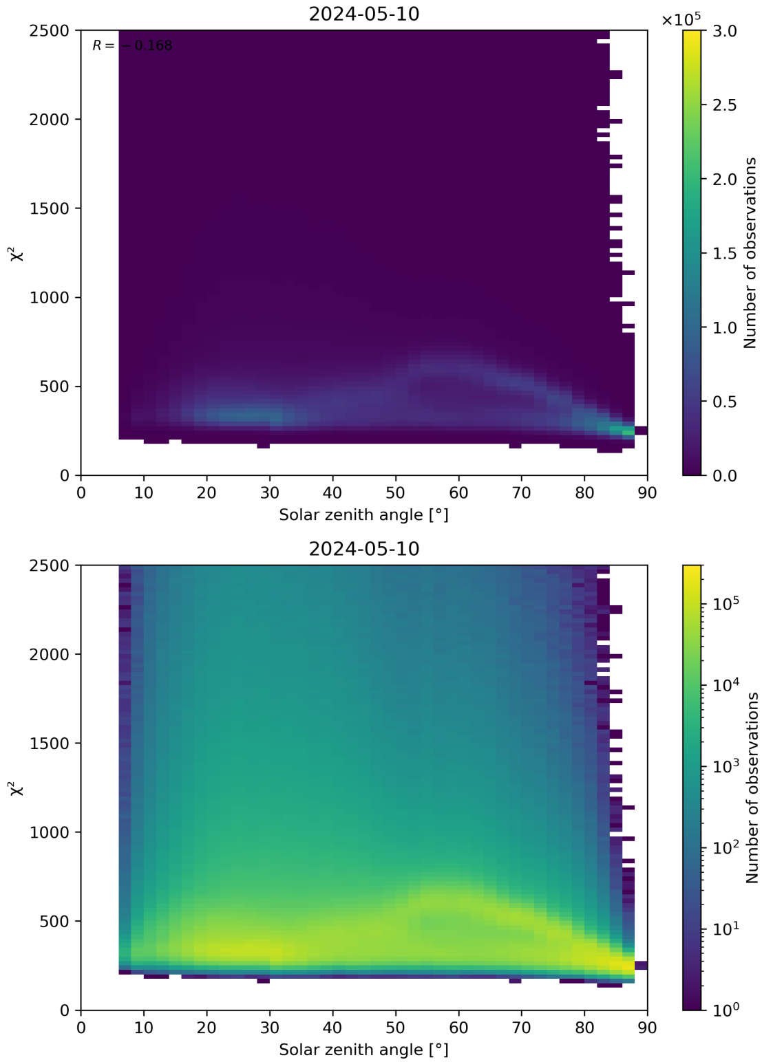
Figure 148: Scatter density plot of “Solar zenith angle” against “ \chi^2 ” for 2024-05-09 to 2024-05-11.
