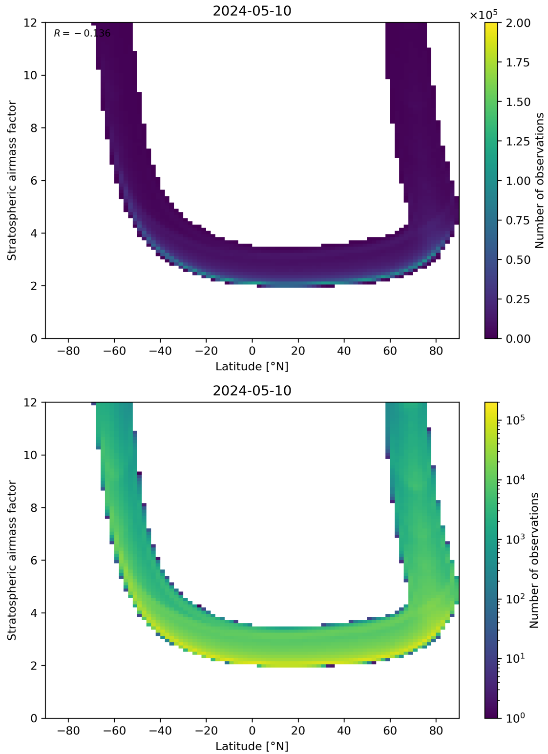
Figure 83: Scatter density plot of “Latitude” against “Stratospheric air mass factor” for 2024-05-09 to 2024-05-11.
