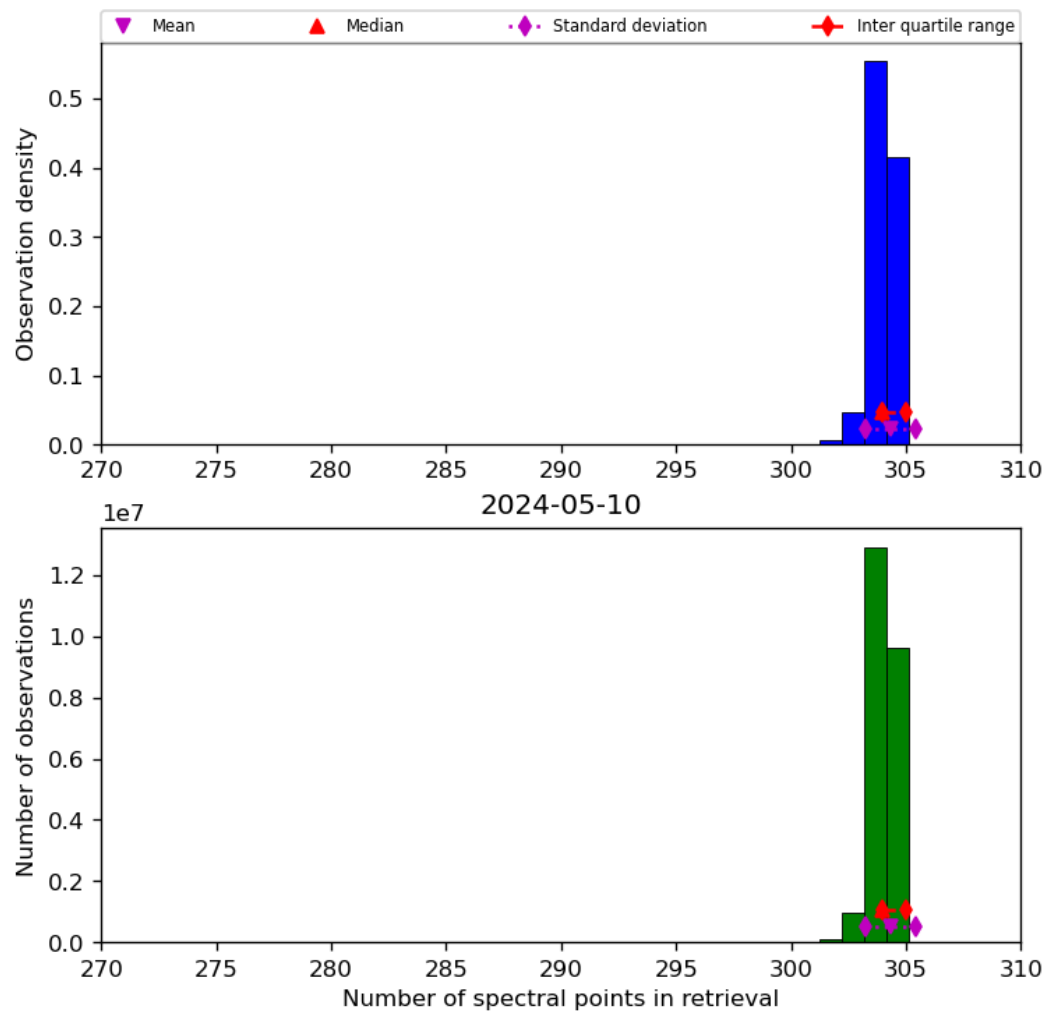
Figure 33: Histogram of “Number of spectral points in retrieval” for 2024-05-09 to 2024-05-11
