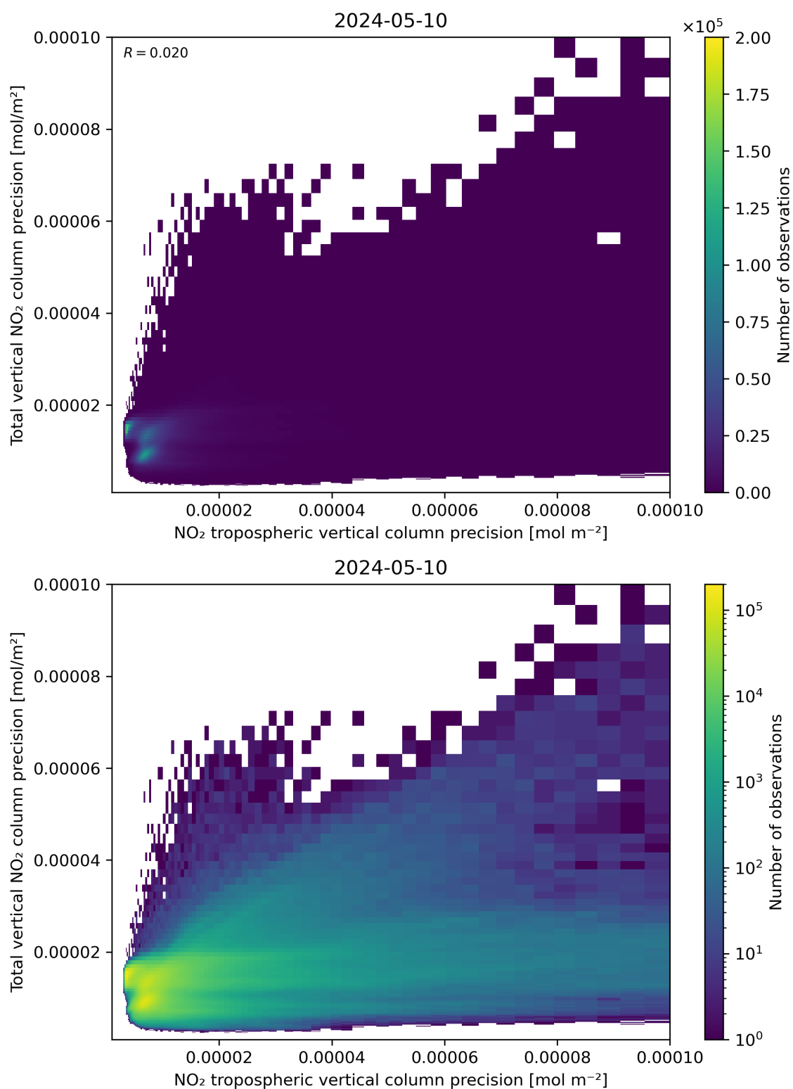
Figure 139: Scatter density plot of “NO 2 tropospheric vertical column precision” against “Total vertical NO 2 column precision” for 2024-05-09 to 2024-05-11.
