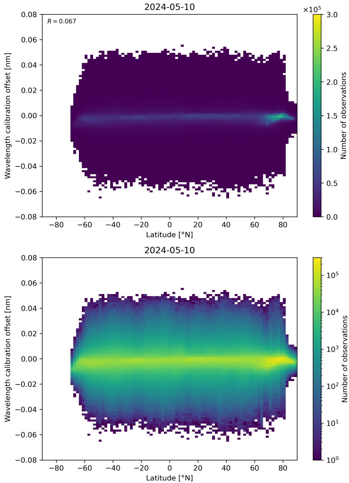
Figure 95: Scatter density plot of “Latitude” against “Wavelength calibration offset” for 2024-05-09 to 2024-05-11.
