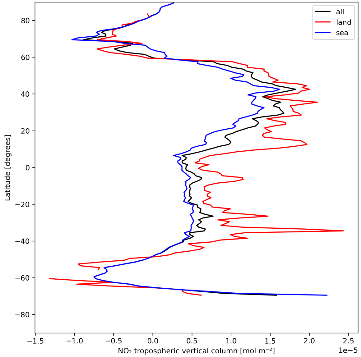
Figure 12: Zonal average of “NO 2 tropospheric vertical column” for 2024-05-09 to 2024-05-11.
