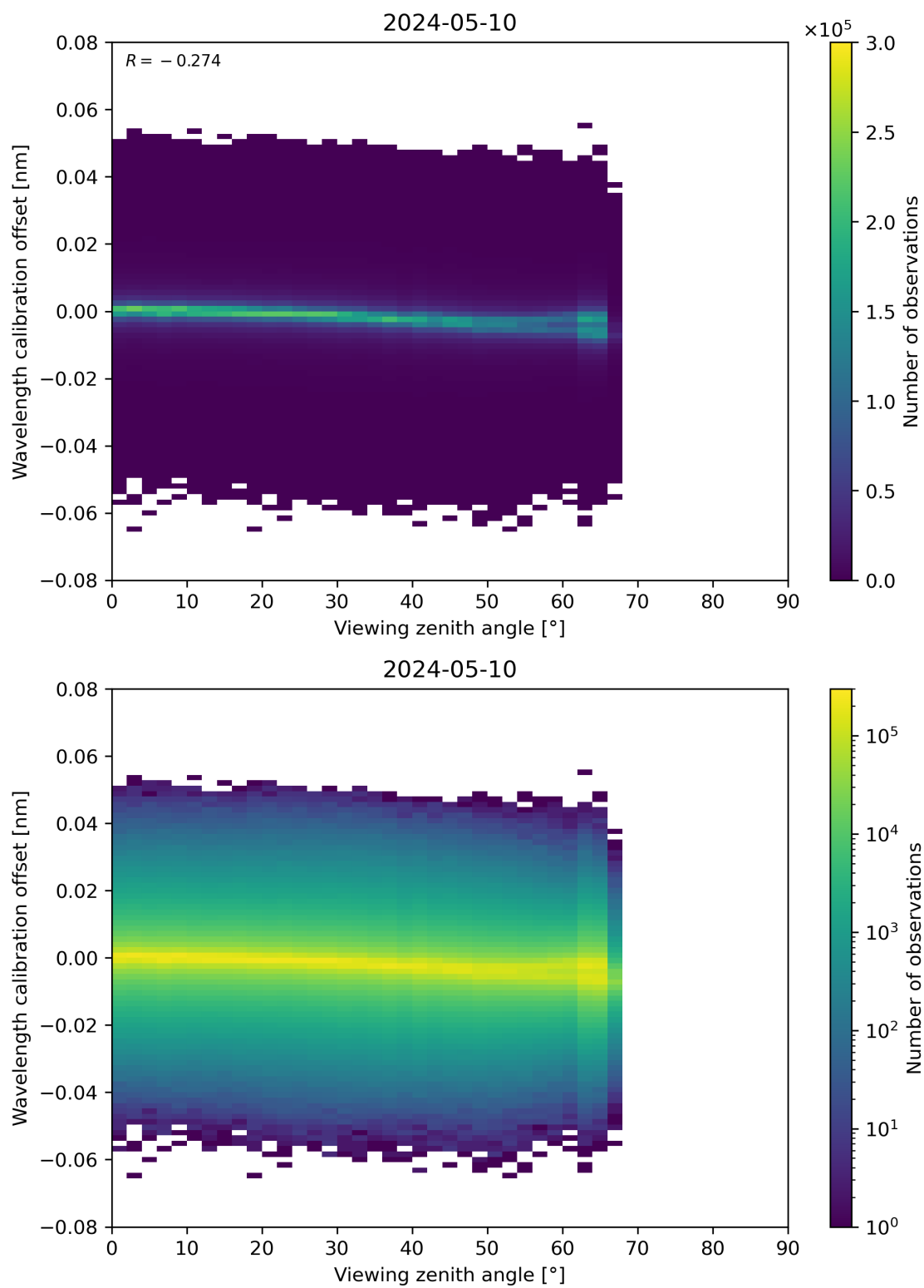
Figure 173: Scatter density plot of “Viewing zenith angle” against “Wavelength calibration offset” for 2024-05-09 to 2024-05-11.
