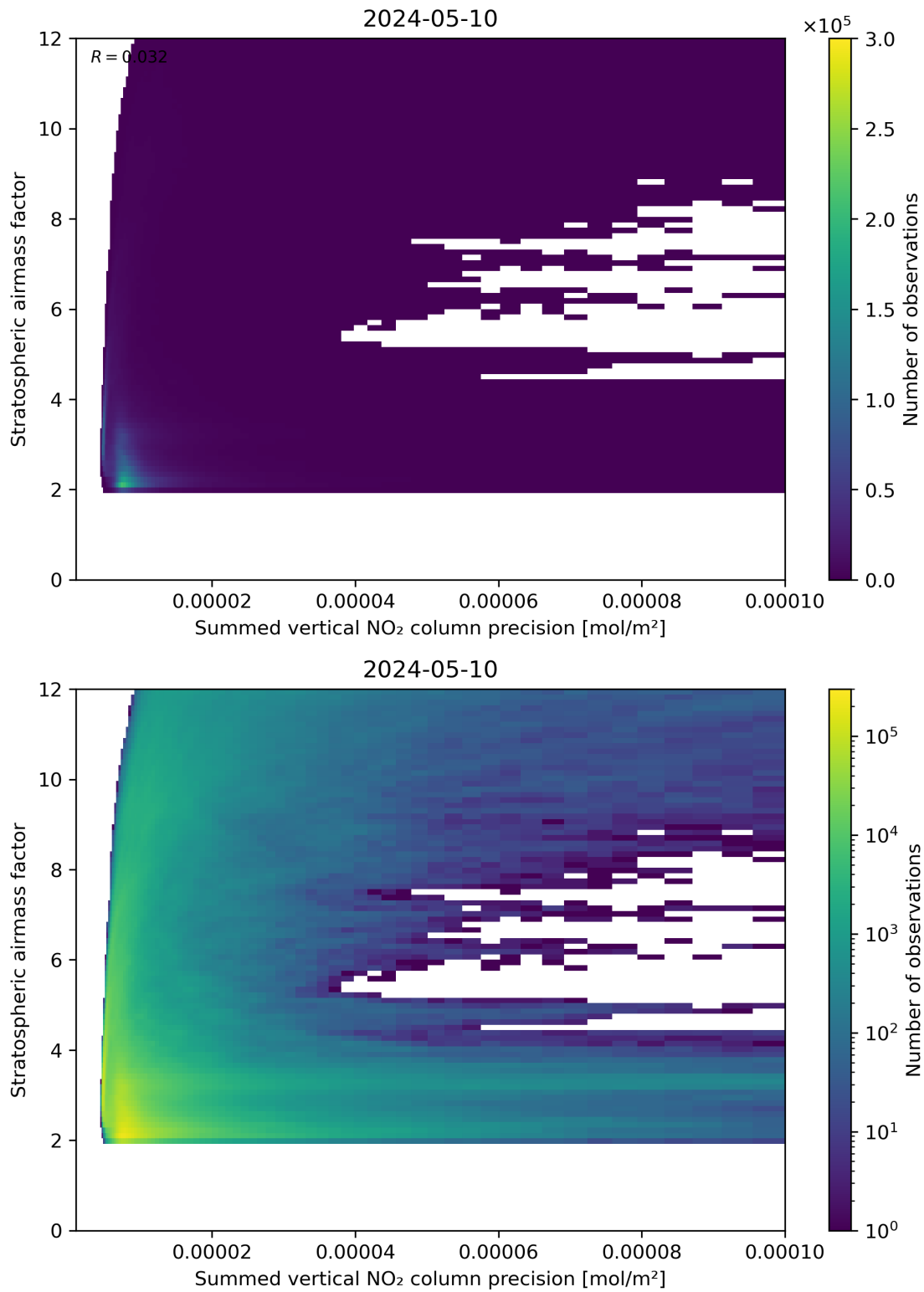
Figure 106: Scatter density plot of “Summed vertical NO 2 column precision” against “Stratospheric airmass factor” for 2024-05-09 to 2024-05-11.
