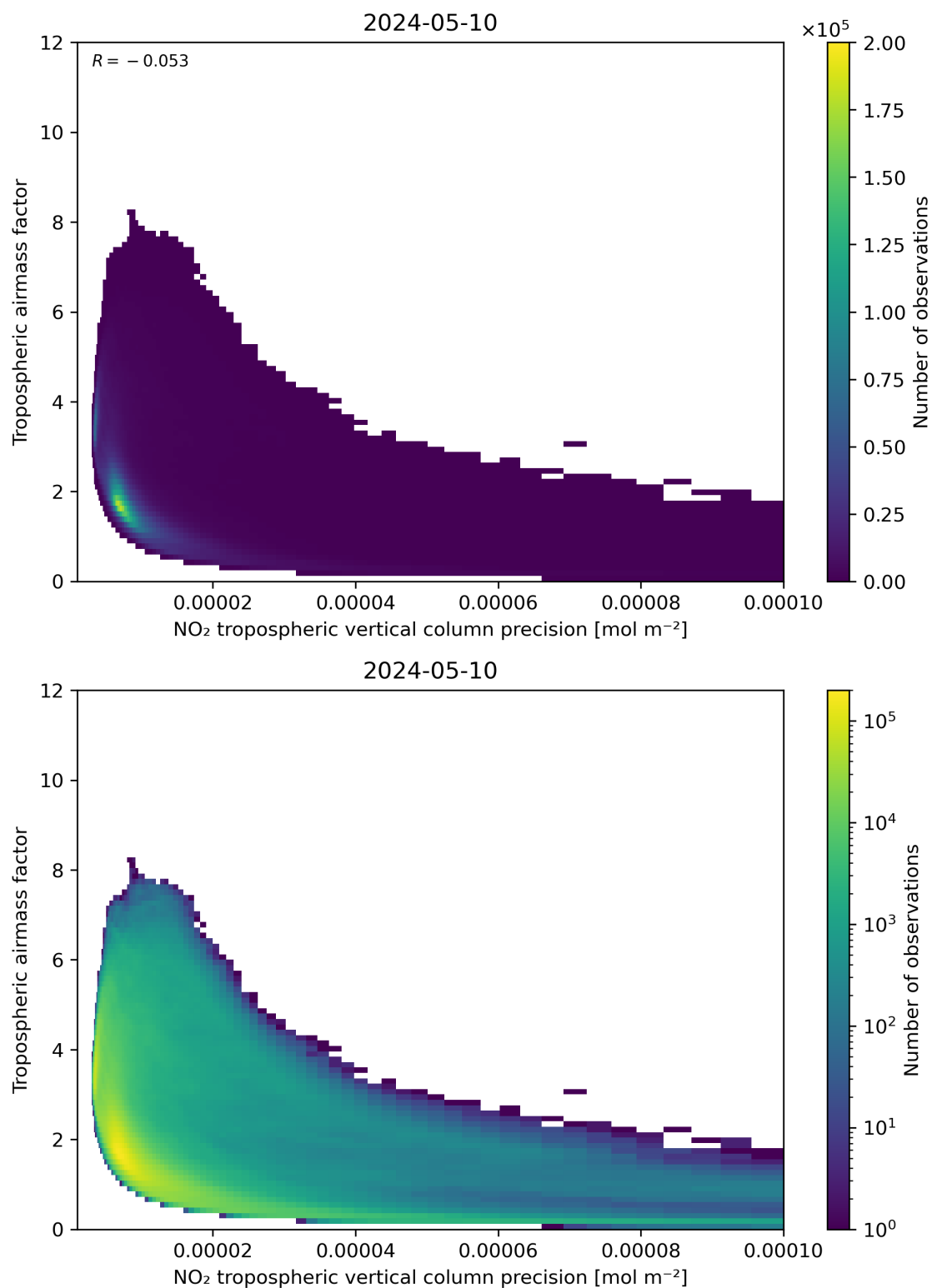
Figure 133: Scatter density plot of “NO 2 tropospheric vertical column precision” against “Tropospheric airmass factor” for 2024-05-09 to 2024-05-11.
