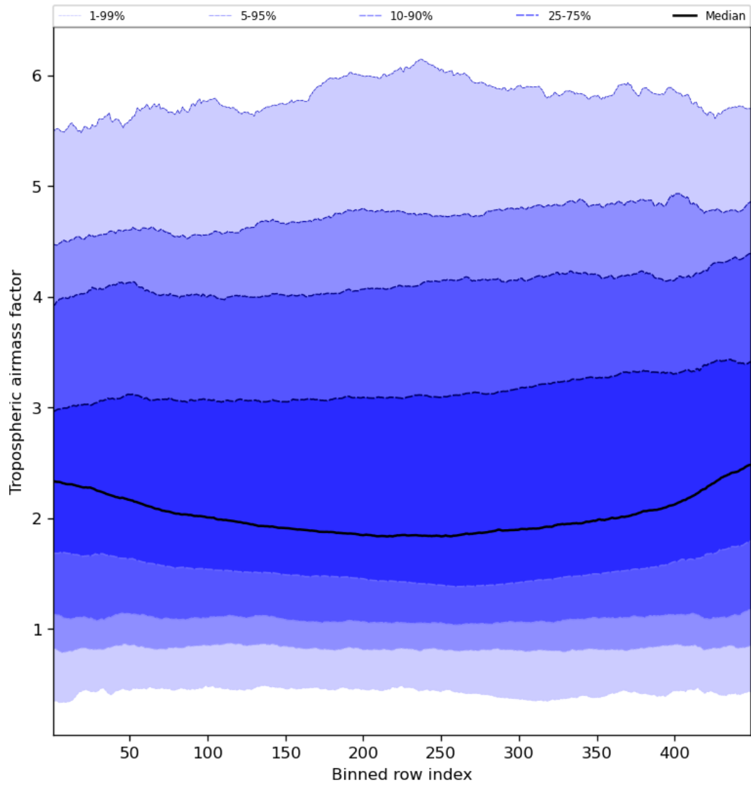
Figure 48: Along track statistics of “Tropospheric airmass factor” for 2024-05-09 to 2024-05-11
