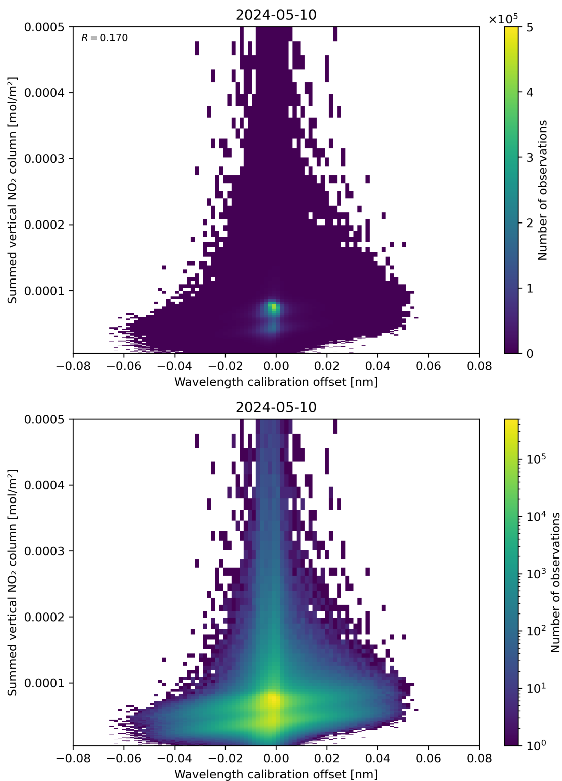
Figure 177: Scatter density plot of “Wavelength calibration offset” against “Summed vertical NO 2 column” for 2024-05-09 to 2024-05-11.
