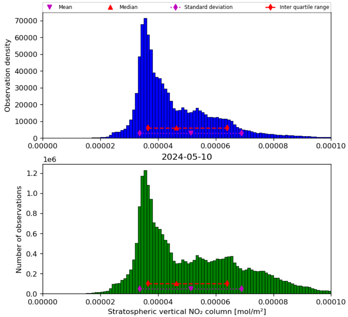
Figure 36: Histogram of “Stratospheric vertical NO 2 column” for 2024-05-09 to 2024-05-11
