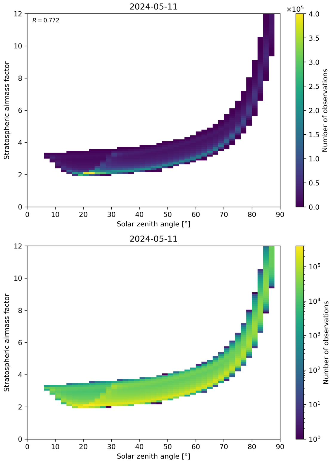
Figure 145: Scatter density plot of “Solar zenith angle” against “Stratospheric airmass factor” for 2024-05-10 to 2024-05-12.
