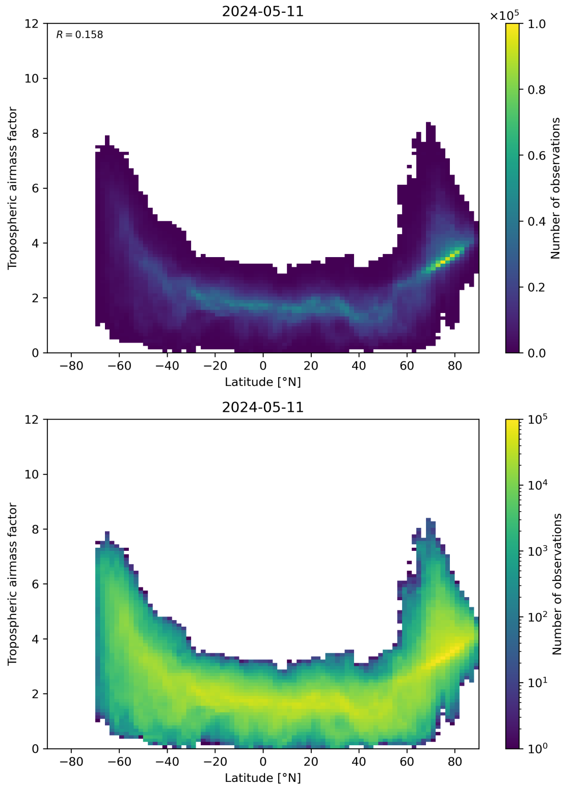
Figure 85: Scatter density plot of “Latitude” against “Tropospheric air mass factor” for 2024-05-10 to 2024-05-12.
