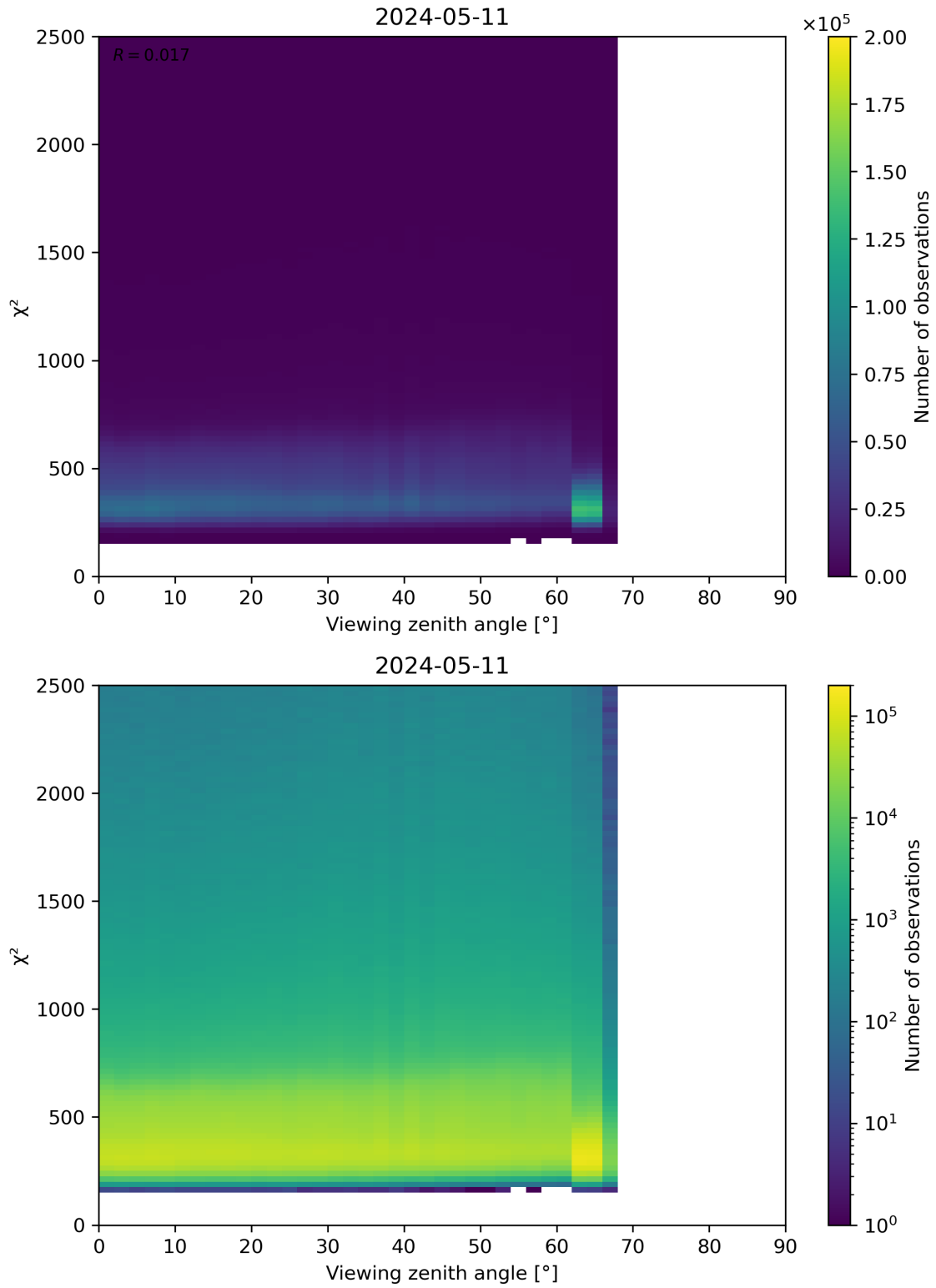
Figure 162: Scatter density plot of “Viewing zenith angle” against “ \chi^2 ” for 2024-05-10 to 2024-05-12.
