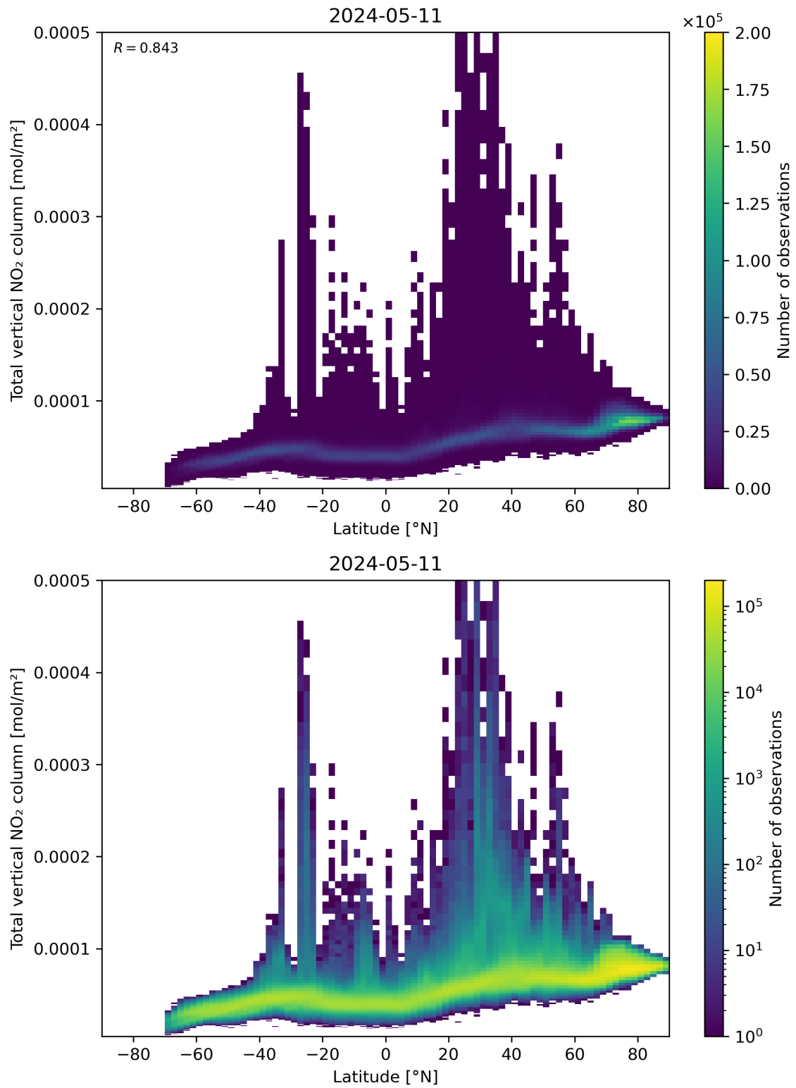
Figure 90: Scatter density plot of “Latitude” against “Total vertical NO 2 column” for 2024-05-10 to 2024-05-12.
