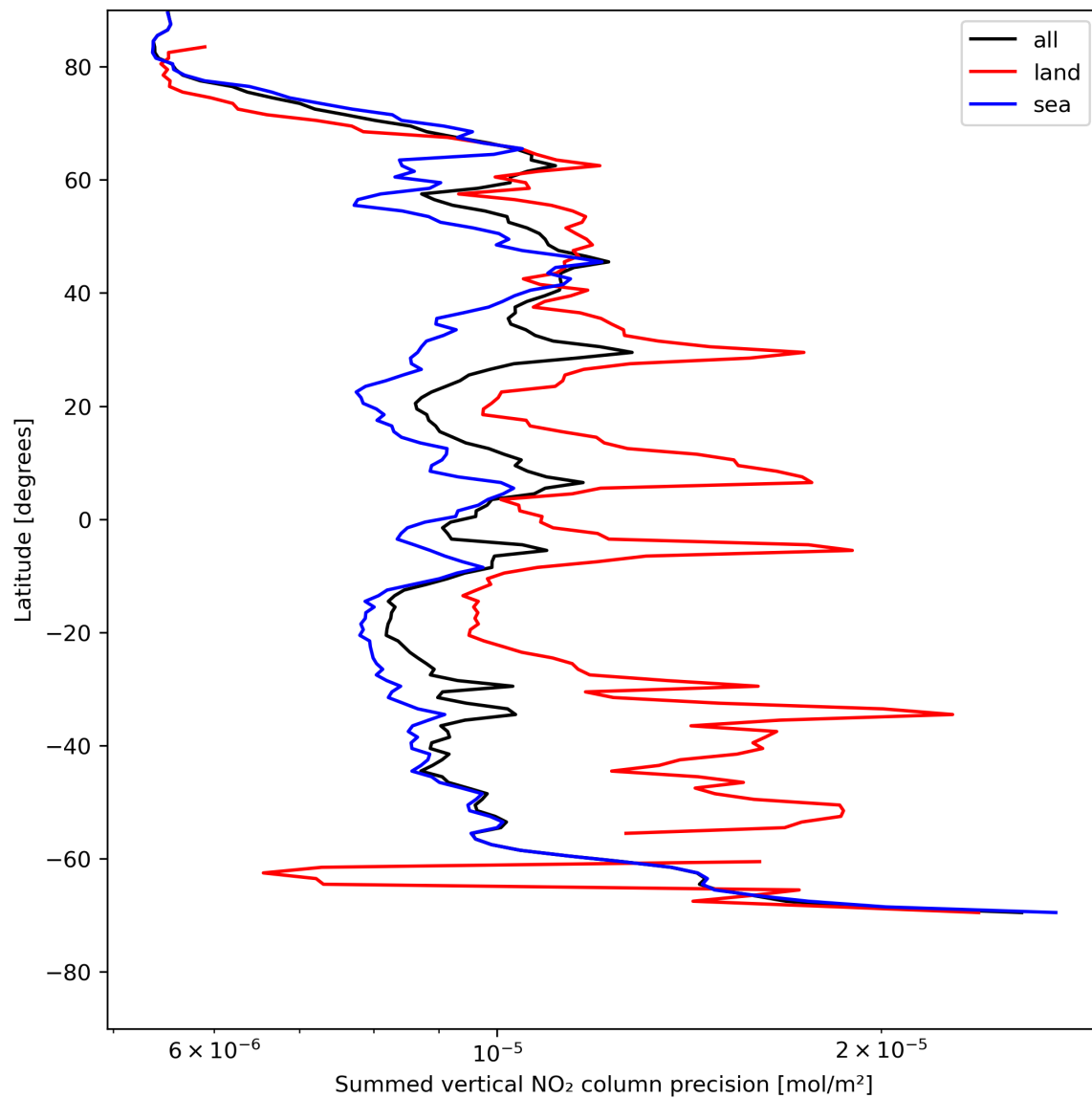
Figure 24: Zonal average of “Summed vertical NO 2 column precision” for 2024-05-10 to 2024-05-12.
