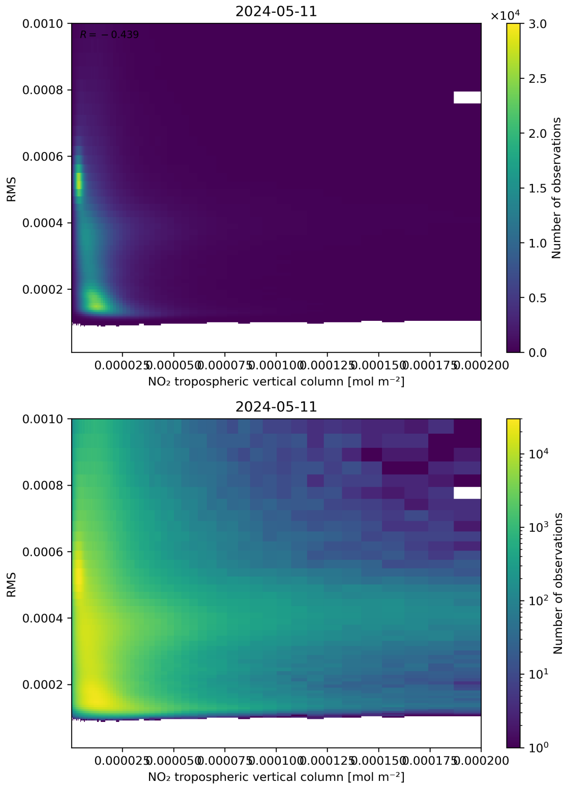
Figure 142: Scatter density plot of “NO 2 tropospheric vertical column” against “RMS” for 2024-05-10 to 2024-05-12.
