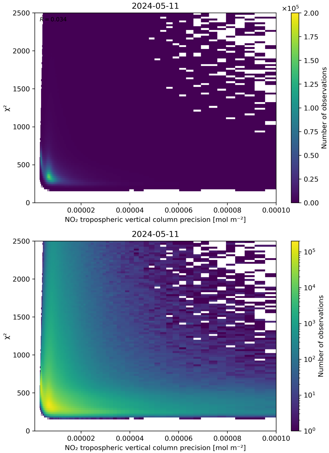
Figure 134: Scatter density plot of “NO 2 tropospheric vertical column precision” against “ \chi^2 ” for 2024-05-10 to 2024-05-12.
