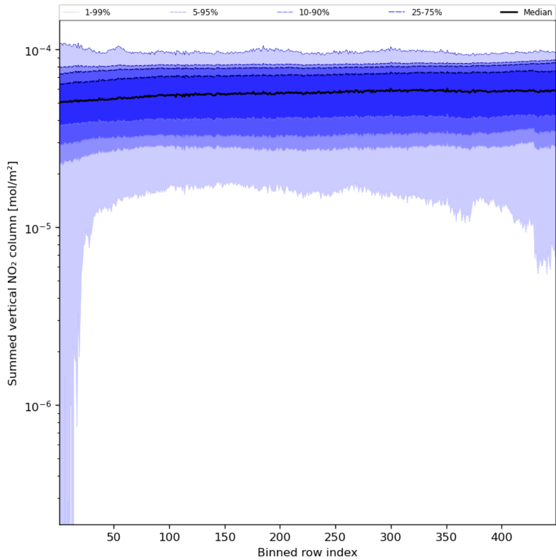
Figure 57: Along track statistics of “Summed vertical NO 2 column” for 2024-05-10 to 2024-05-12
