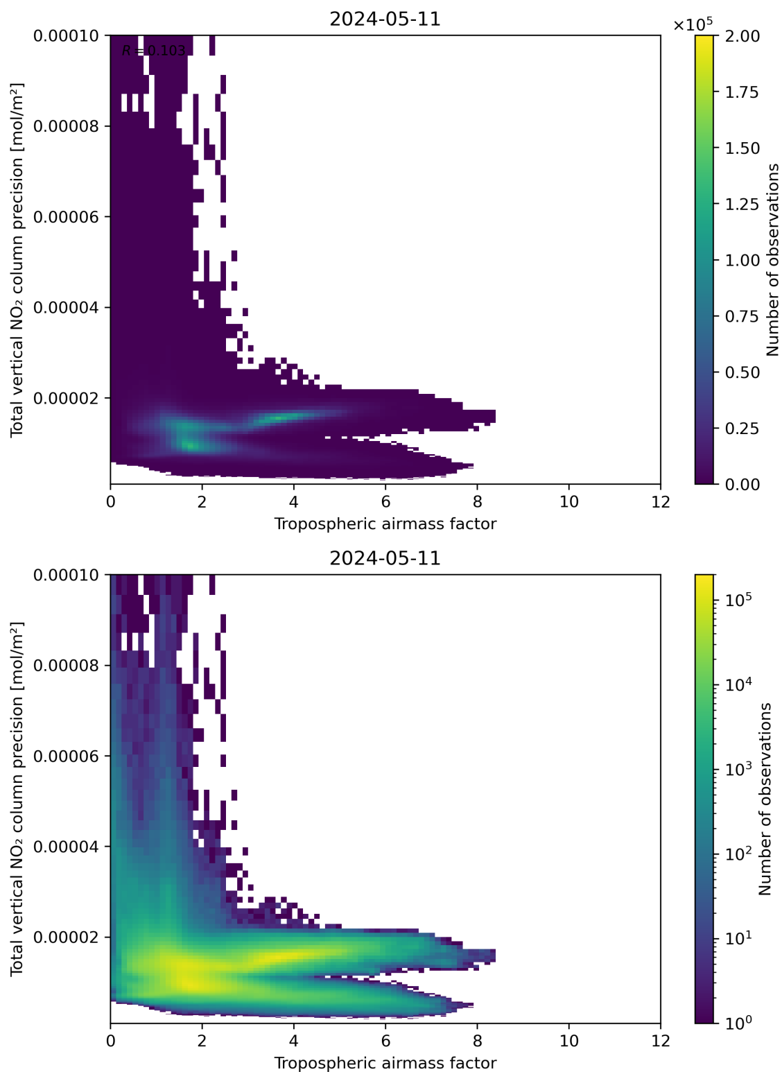
Figure 78: Scatter density plot of “Tropospheric air mass factor” against “Total vertical NO 2 column precision” for 2024-05-10 to 2024-05-12.
