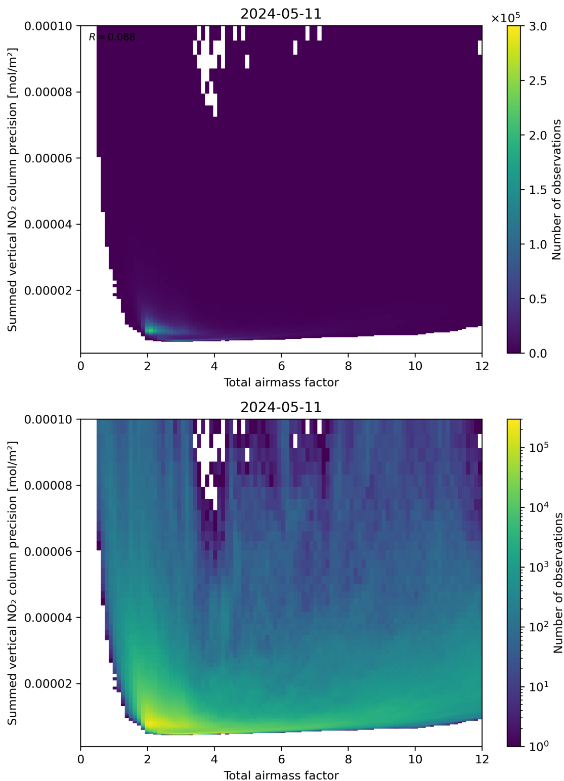
Figure 66: Scatter density plot of “Total airmass factor” against “Summed vertical NO 2 column precision” for 2024-05-10 to 2024-05-12.
