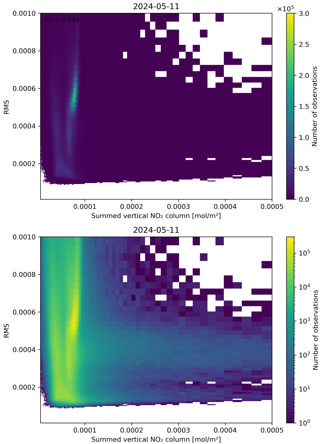
Figure 109: Scatter density plot of “Summed vertical NO 2 column” against “RMS” for 2024-05-10 to 2024-05-12.
