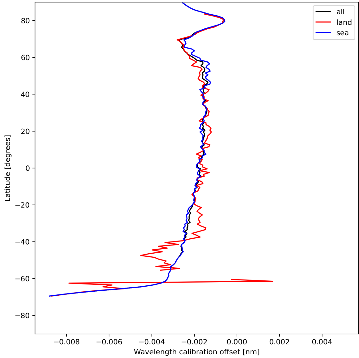
Figure 18: Zonal average of “Wavelength calibration offset” for 2024-05-10 to 2024-05-12.
