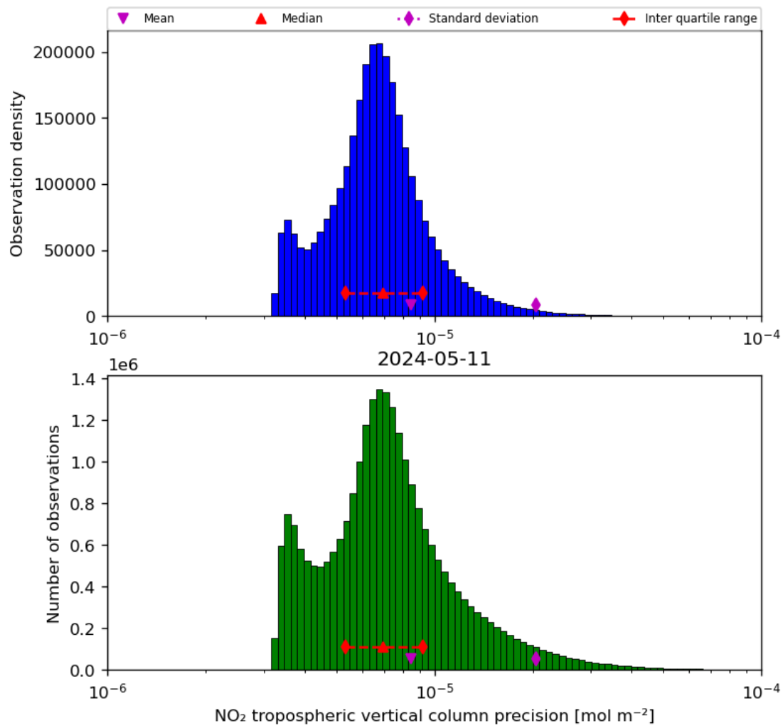
Figure 30: Histogram of “NO 2 tropospheric vertical column precision” for 2024-05-10 to 2024-05-12
