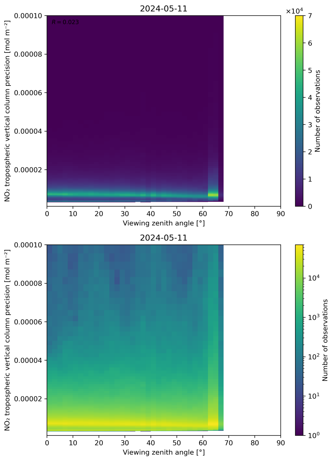
Figure 170: Scatter density plot of “Viewing zenith angle” against “NO 2 tropospheric vertical column precision” for 2024-05-10 to 2024-05-12.
