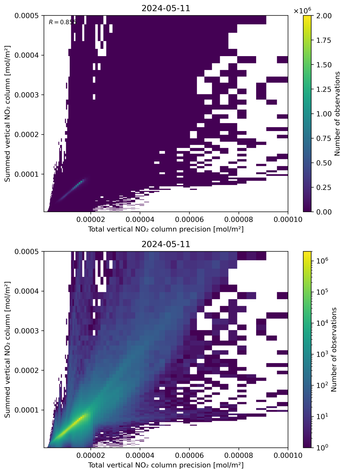
Figure 117: Scatter density plot of “Total vertical NO 2 column precision” against “Summed vertical NO 2 column” for 2024-05-10 to 2024-05-12.
