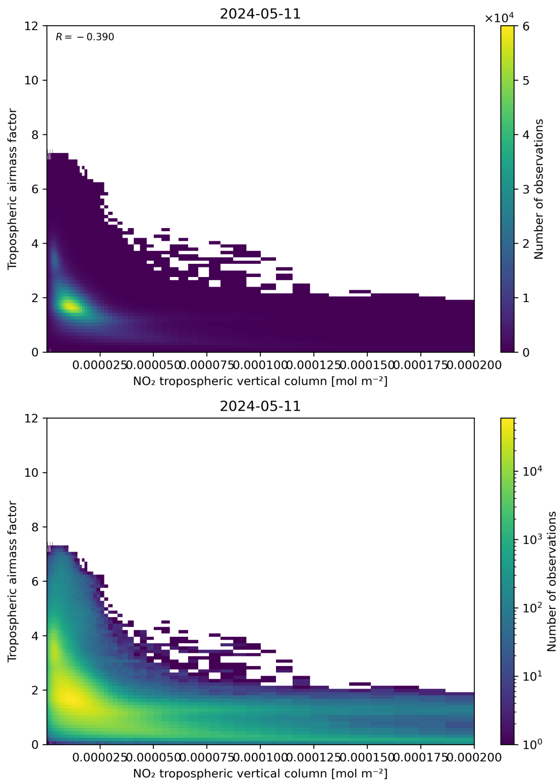
Figure 123: Scatter density plot of “NO 2 tropospheric vertical column” against “Tropospheric airmass factor” for 2024-05-10 to 2024-05-12.
