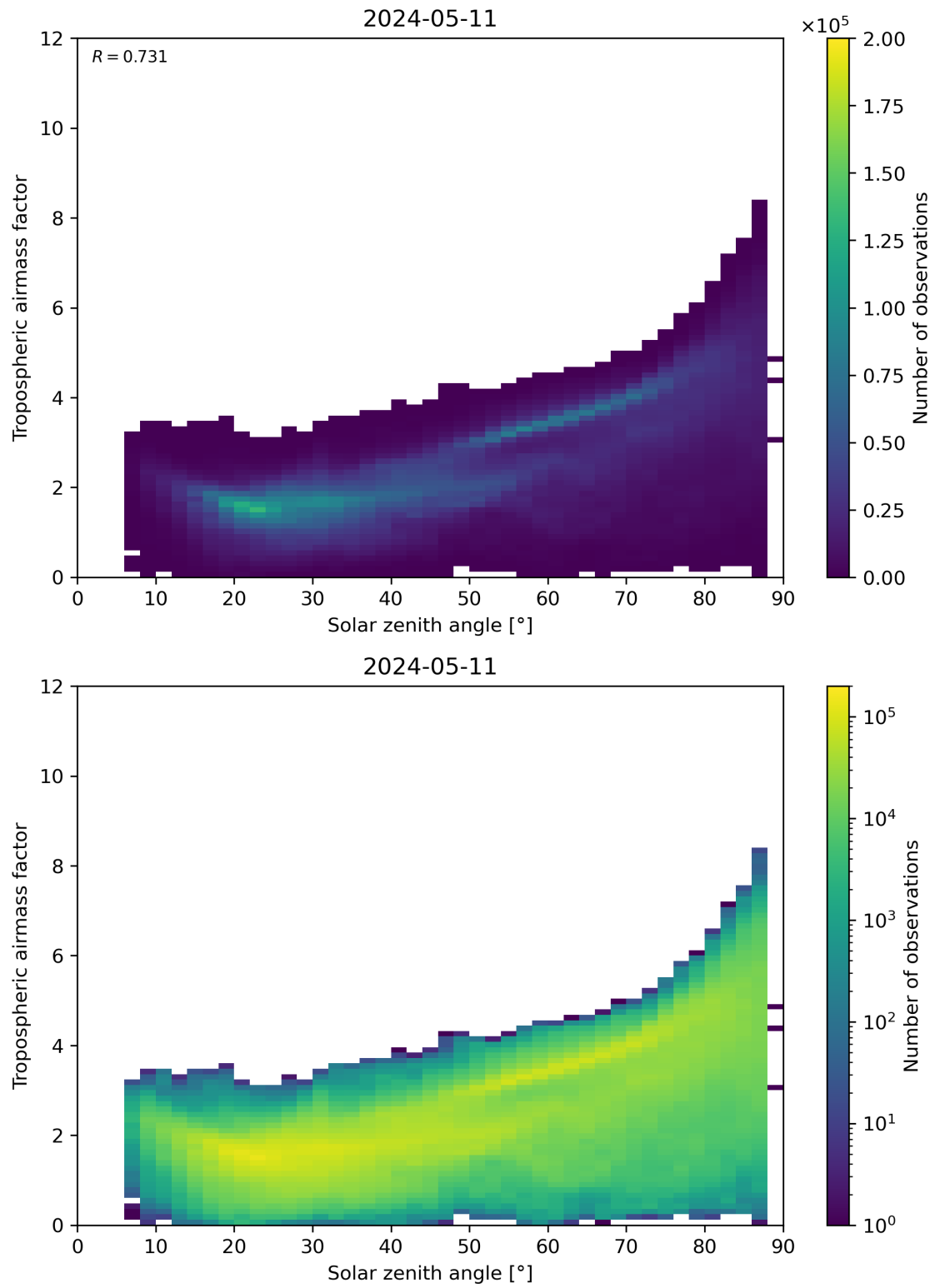
Figure 147: Scatter density plot of “Solar zenith angle” against “Tropospheric airmass factor” for 2024-05-10 to 2024-05-12.
