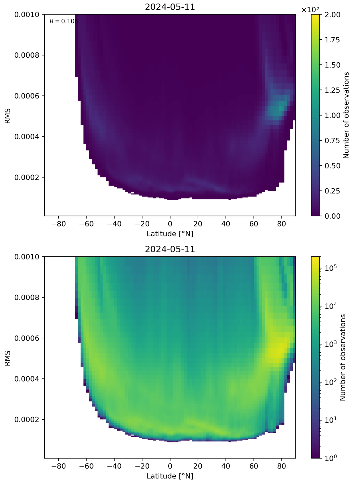
Figure 94: Scatter density plot of “Latitude” against “RMS” for 2024-05-10 to 2024-05-12.
