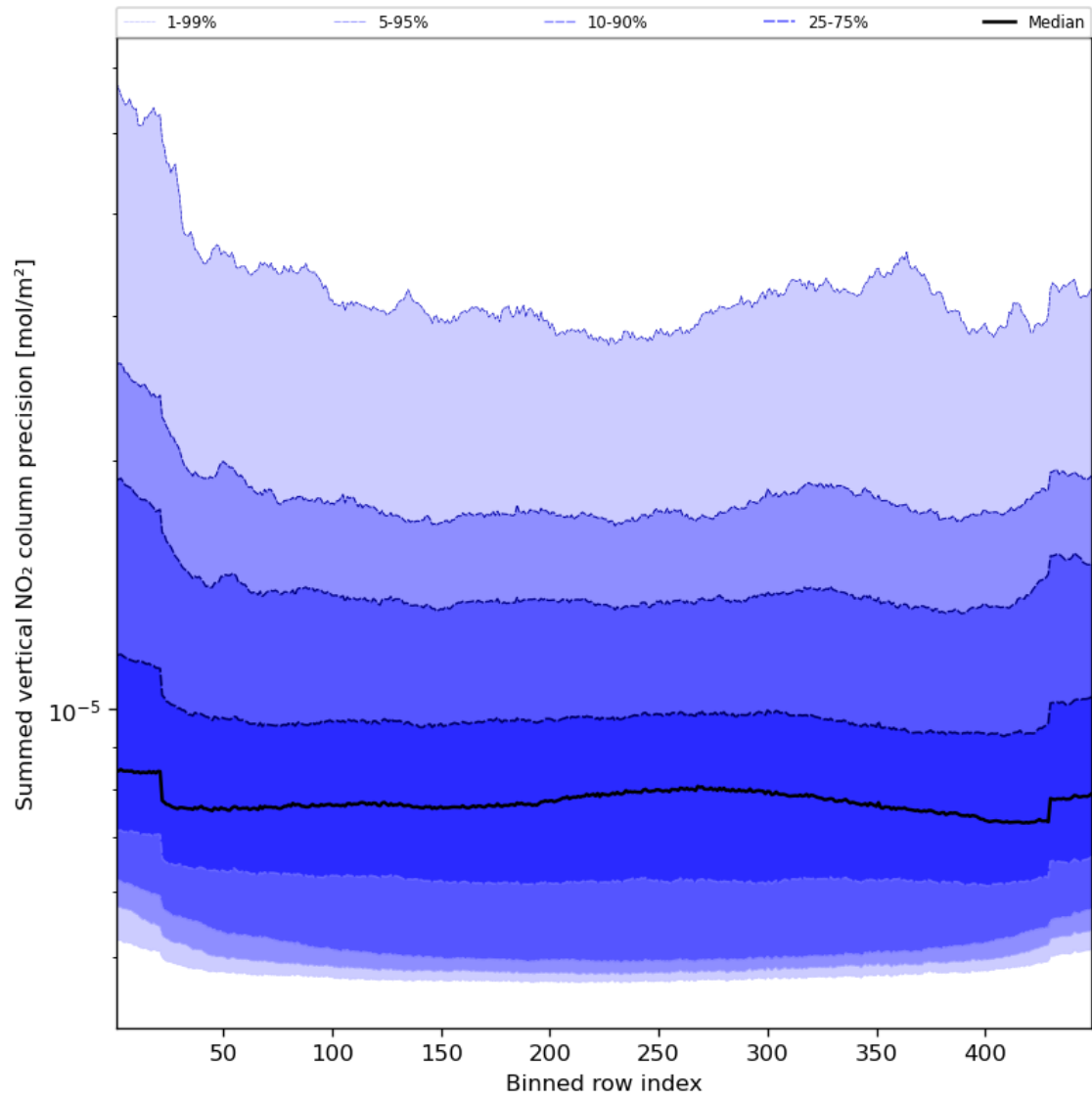
Figure 58: Along track statistics of “Summed vertical NO 2 column precision” for 2024-05-10 to 2024-05-12
