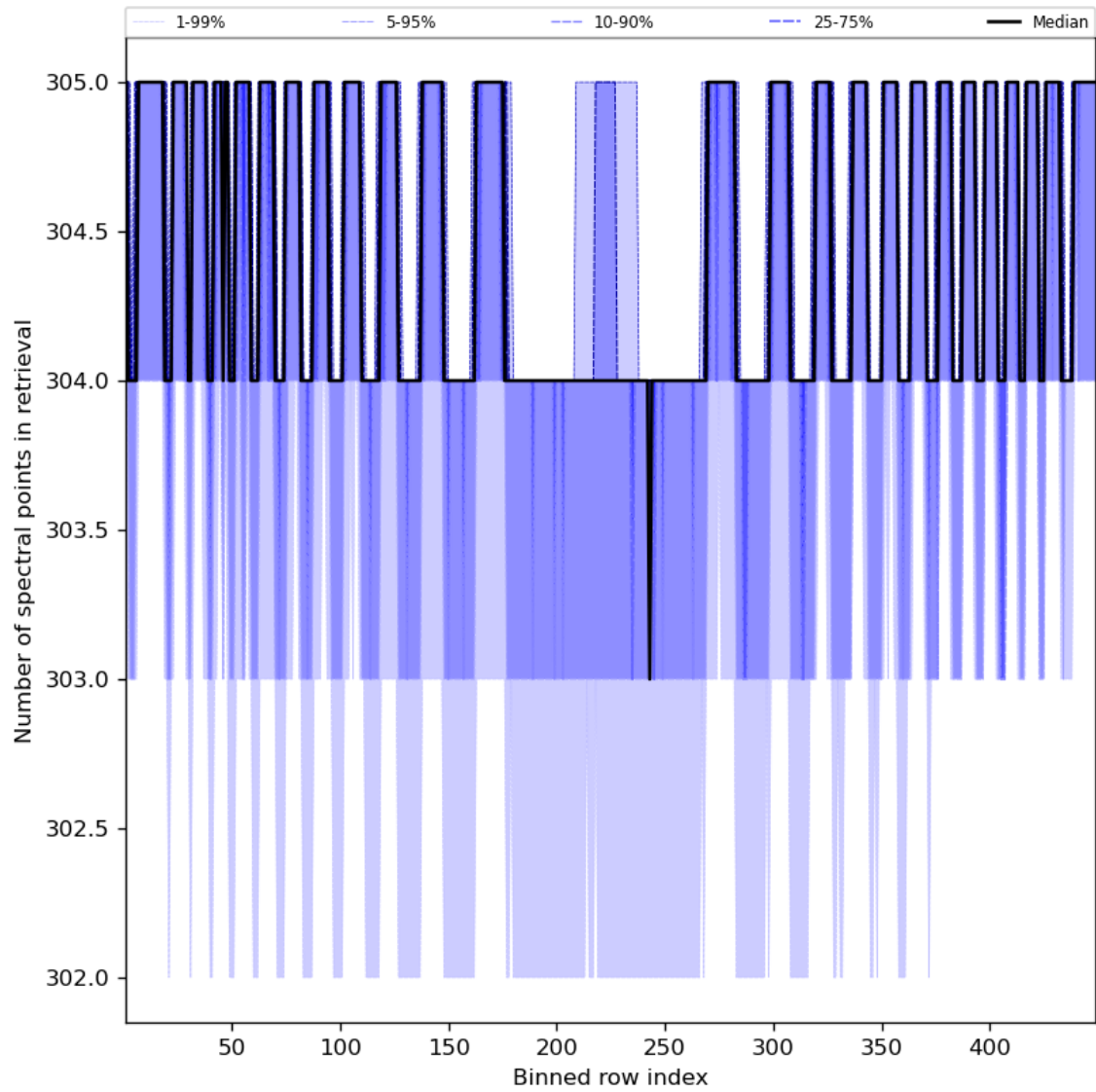
Figure 50: Along track statistics of “Number of spectral points in retrieval” for 2024-05-10 to 2024-05-12
