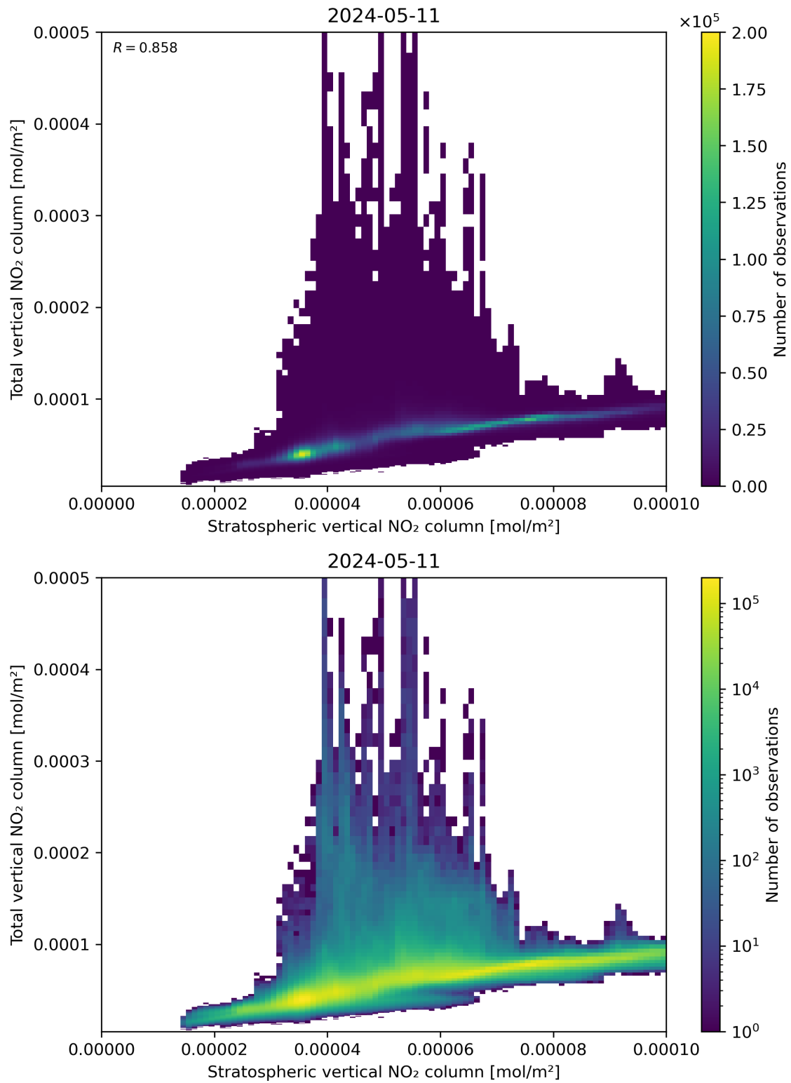
Figure 100: Scatter density plot of “Stratospheric vertical NO 2 column” against “Total vertical NO 2 column” for 2024-05-10 to 2024-05-12.
