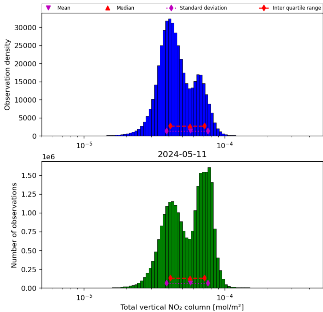
Figure 38: Histogram of “Total vertical NO 2 column” for 2024-05-10 to 2024-05-12
