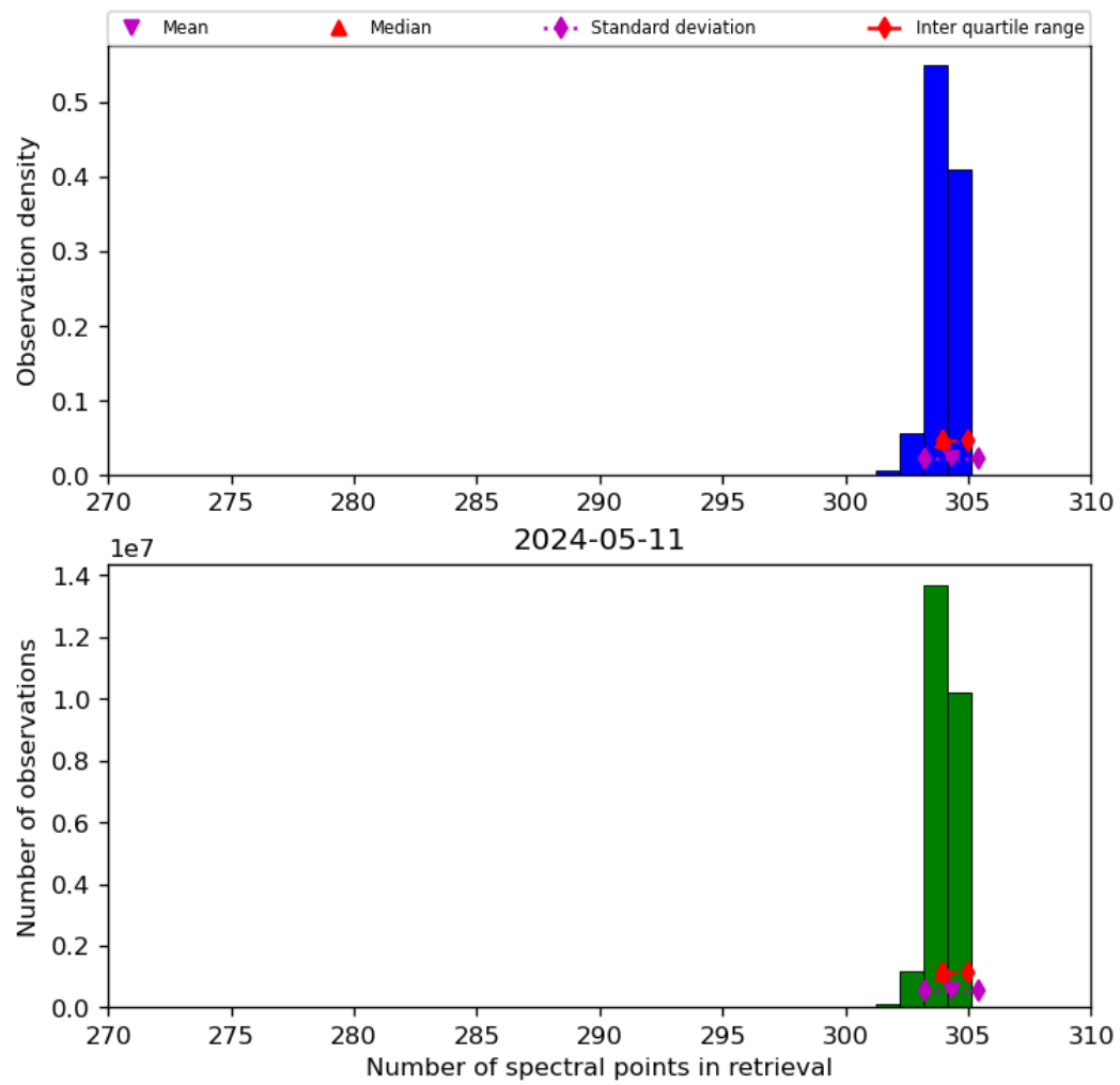
Figure 33: Histogram of “Number of spectral points in retrieval” for 2024-05-10 to 2024-05-12
