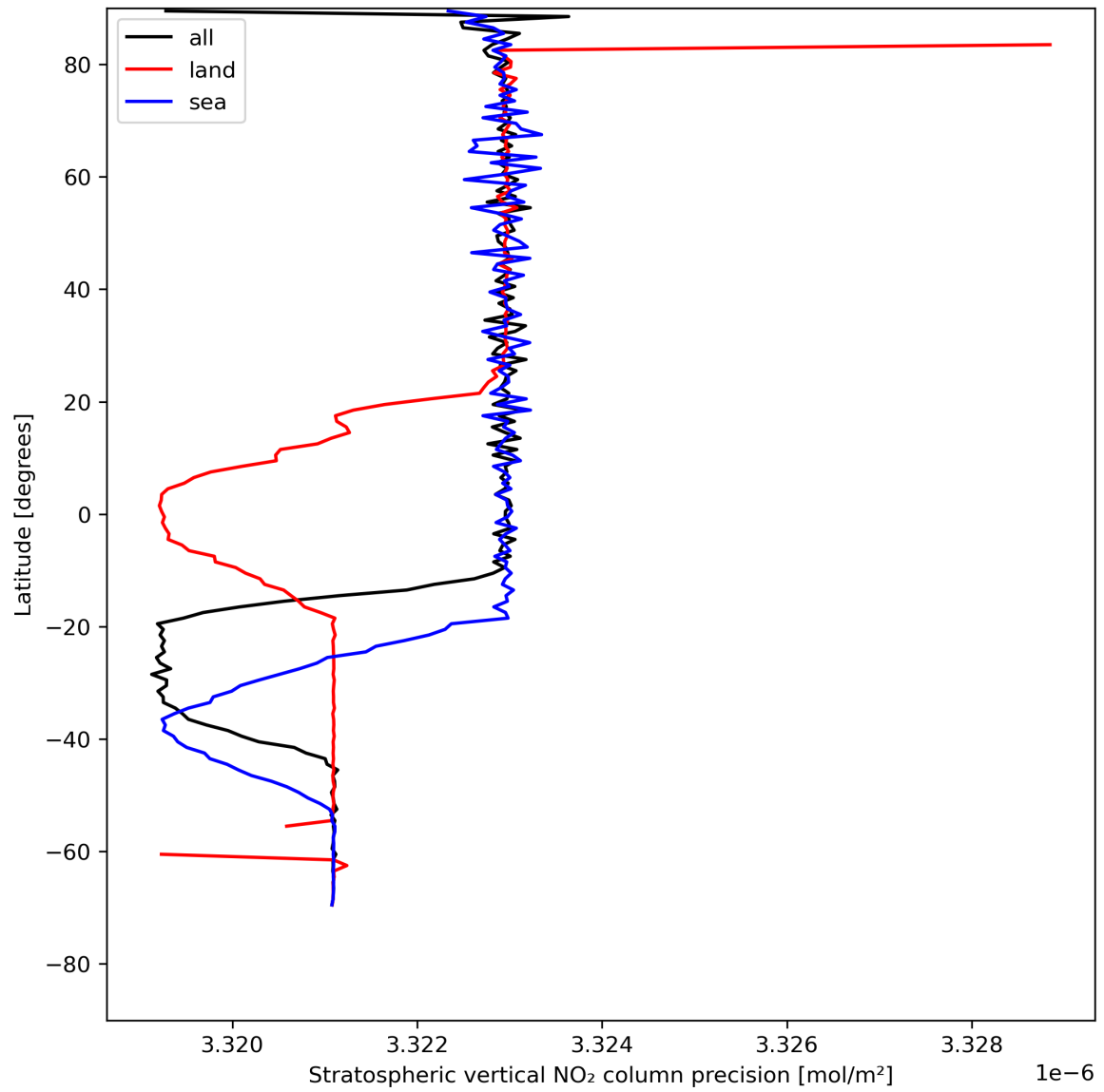
Figure 20: Zonal average of “Stratospheric vertical NO 2 column precision” for 2024-05-10 to 2024-05-12.
