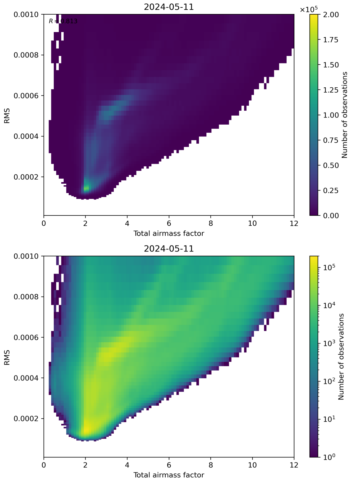
Figure 69: Scatter density plot of “Total airmass factor” against “RMS” for 2024-05-10 to 2024-05-12.
