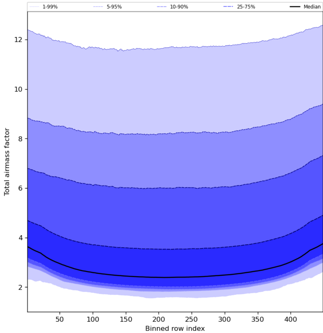
Figure 49: Along track statistics of “Total airmass factor” for 2024-05-10 to 2024-05-12
