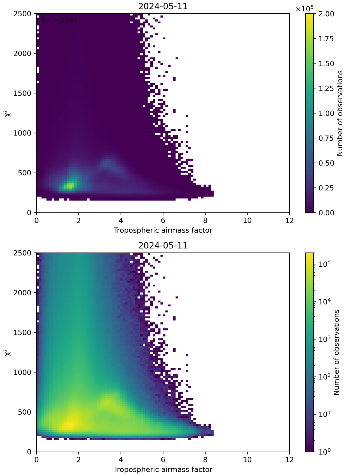
Figure 73: Scatter density plot of “Tropospheric airmass factor” against “ \chi^2 ” for 2024-05-10 to 2024-05-12.
