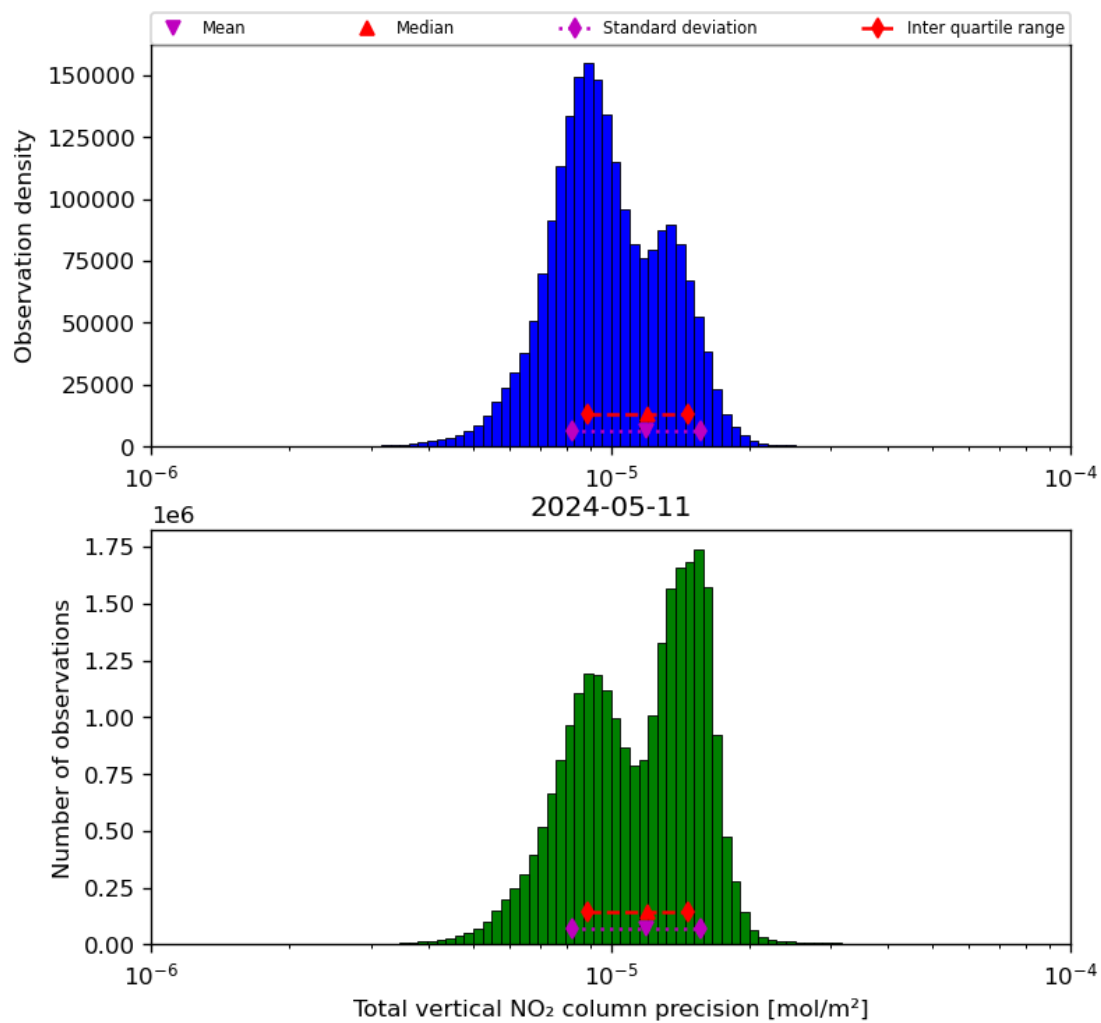
Figure 39: Histogram of “Total vertical NO 2 column precision” for 2024-05-10 to 2024-05-12
