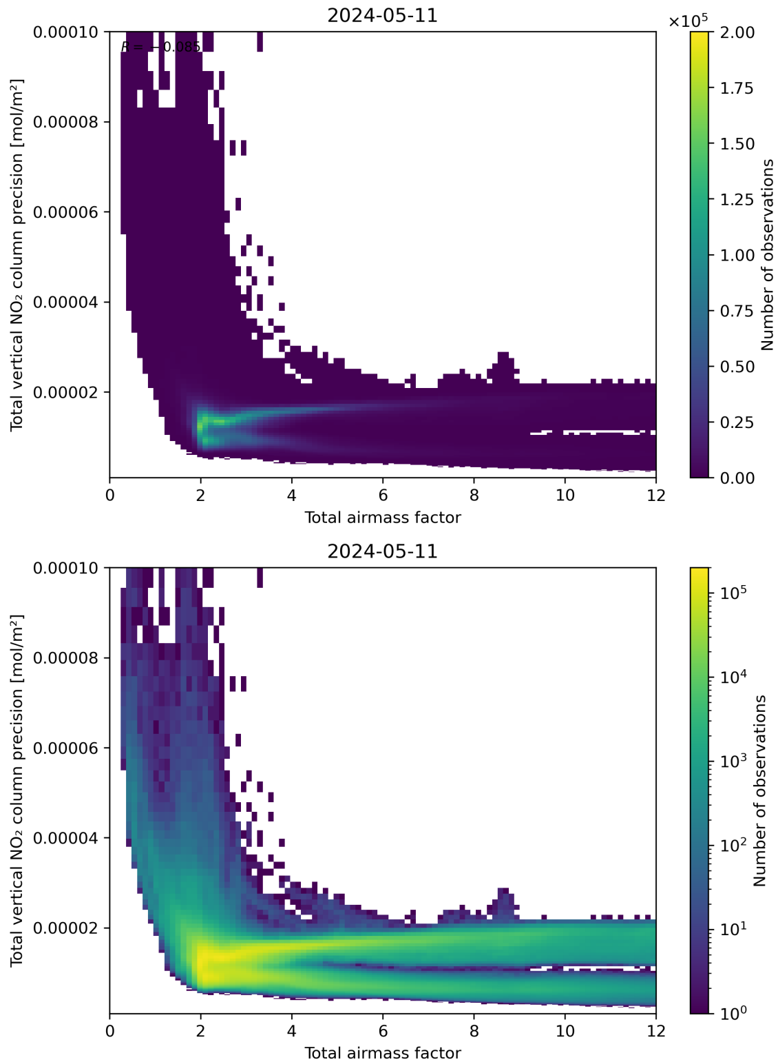
Figure 68: Scatter density plot of “Total airmass factor” against “Total vertical NO 2 column precision” for 2024-05-10 to 2024-05-12.
