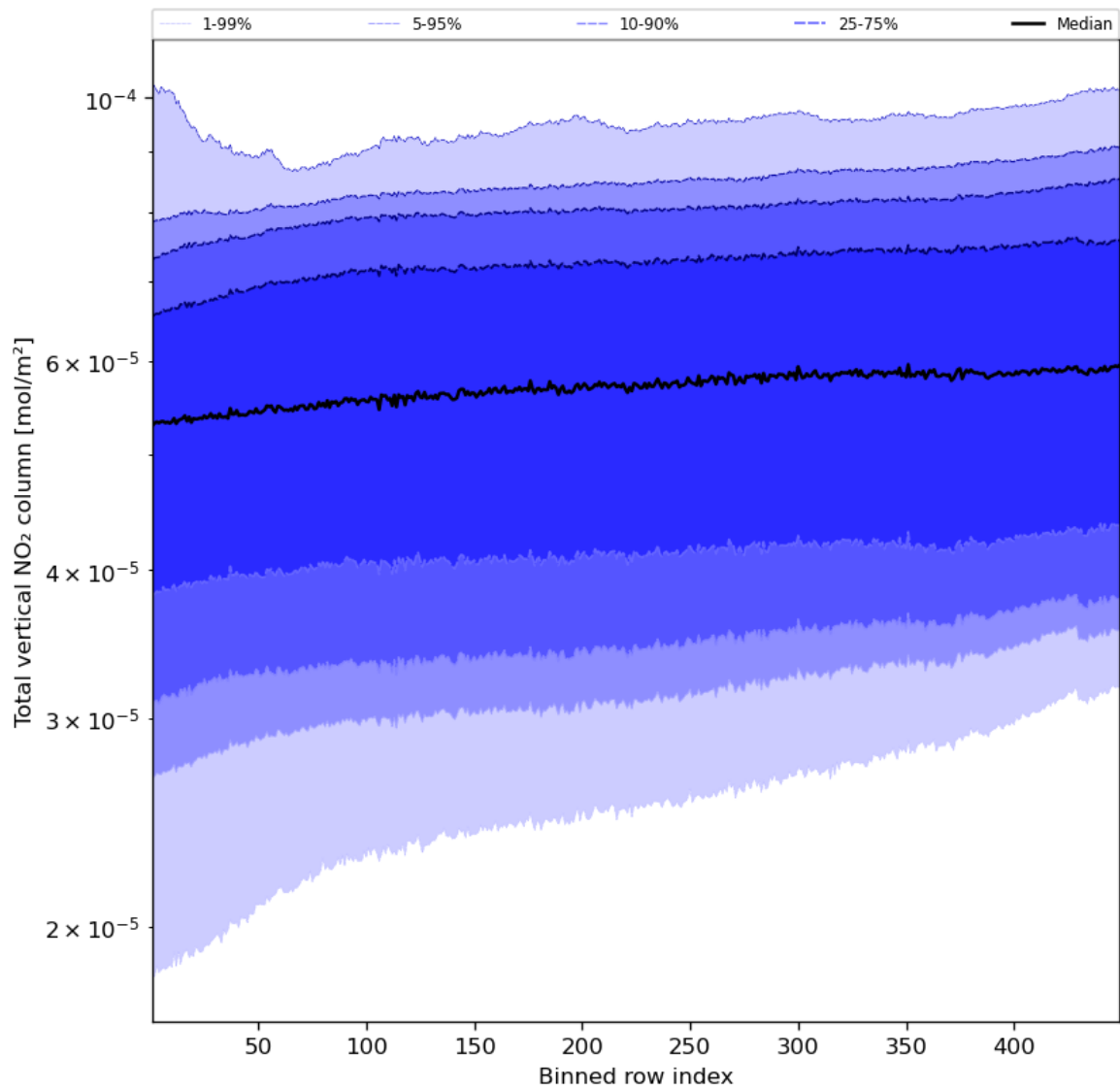
Figure 55: Along track statistics of “Total vertical NO 2 column” for 2024-05-10 to 2024-05-12
