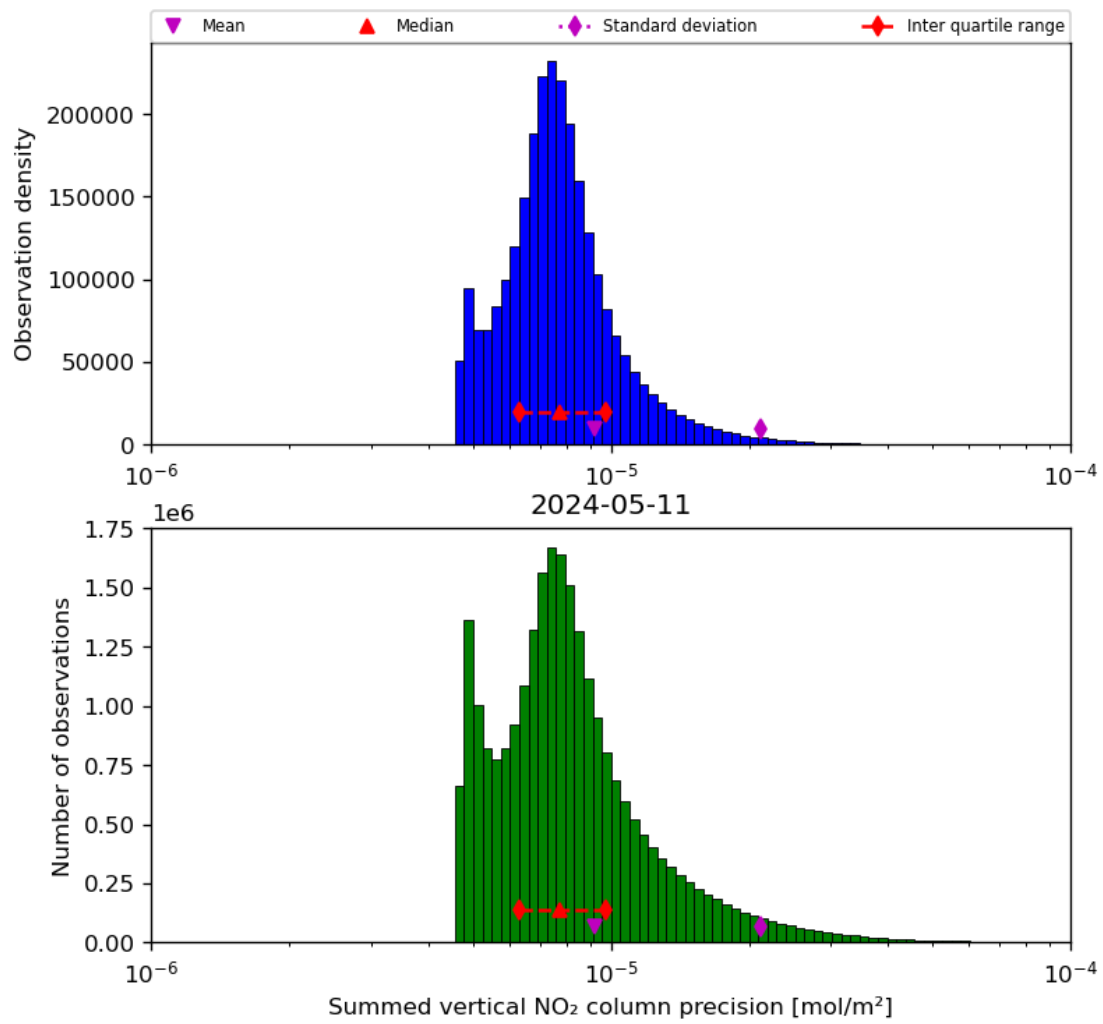
Figure 41: Histogram of “Summed vertical NO 2 column precision” for 2024-05-10 to 2024-05-12
