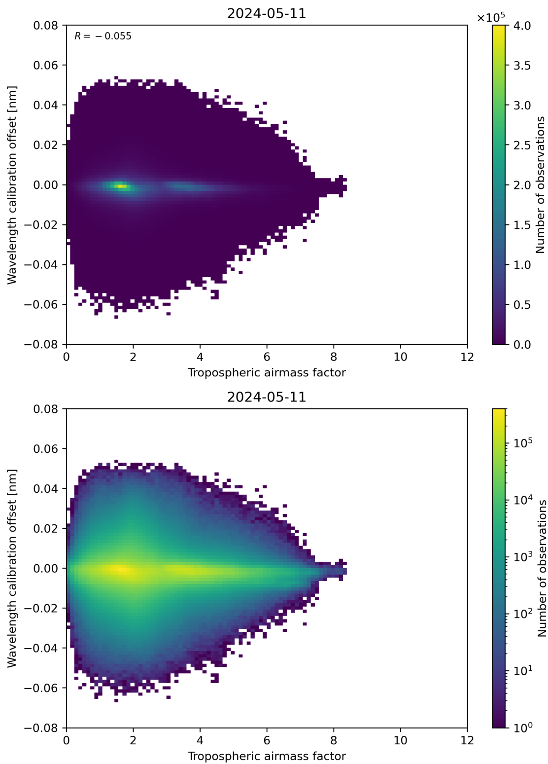
Figure 80: Scatter density plot of “Tropospheric airmass factor” against “Wavelength calibration offset” for 2024-05-10 to 2024-05-12.
