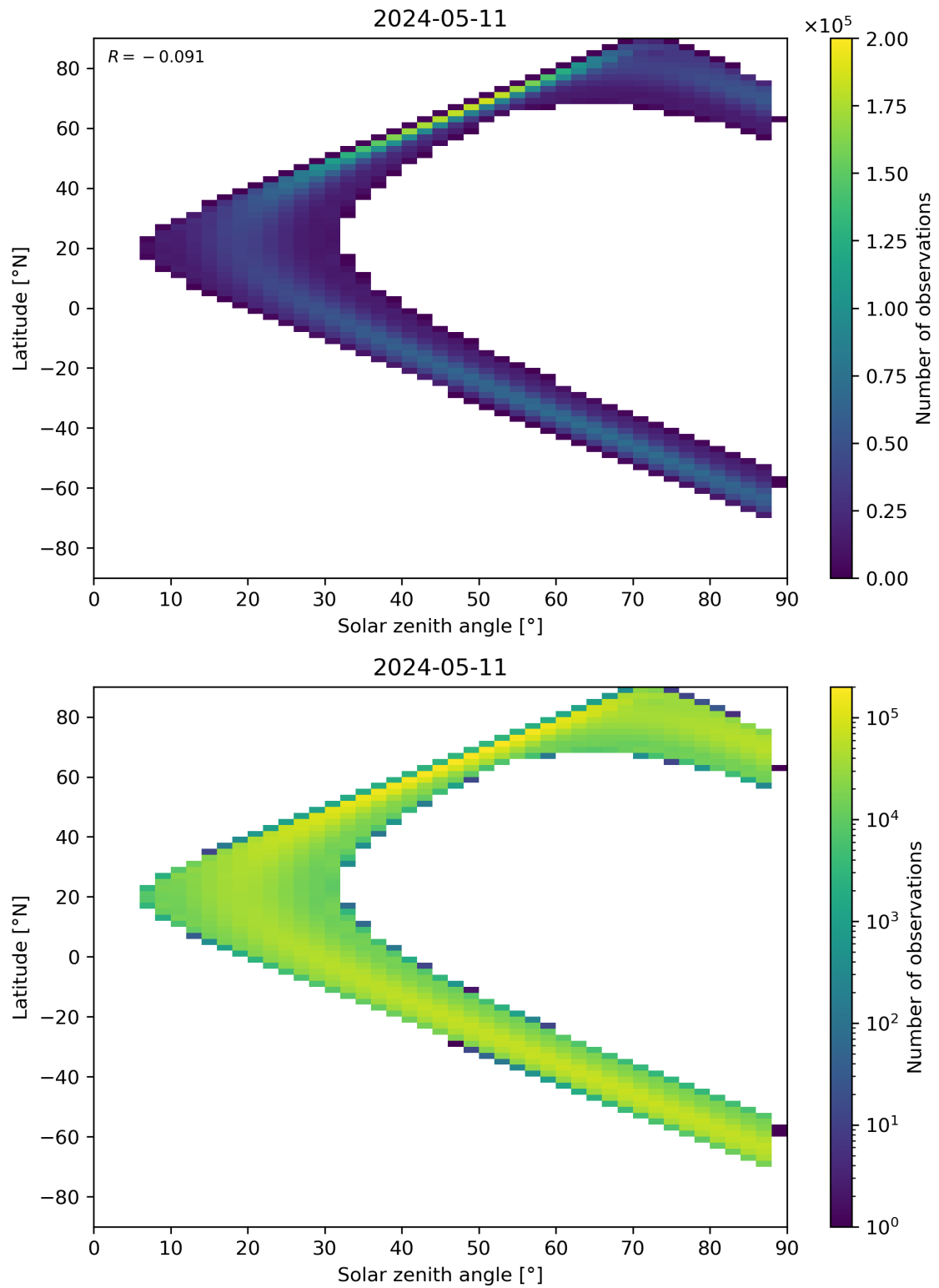
Figure 149: Scatter density plot of “Solar zenith angle” against “Latitude” for 2024-05-10 to 2024-05-12.
