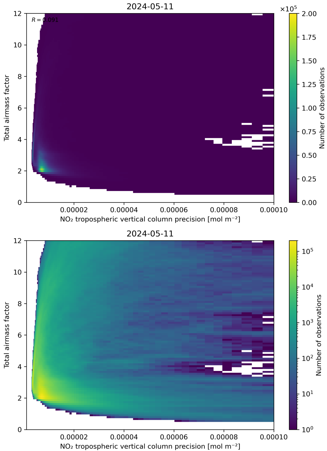
Figure 132: Scatter density plot of “NO 2 tropospheric vertical column precision” against “Total air mass factor” for 2024-05-10 to 2024-05-12.
