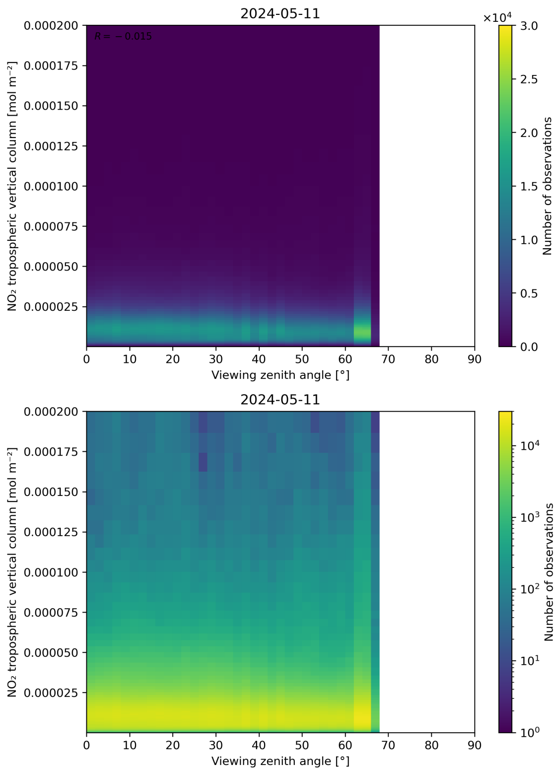
Figure 169: Scatter density plot of “Viewing zenith angle” against “NO 2 tropospheric vertical column” for 2024-05-10 to 2024-05-12.
