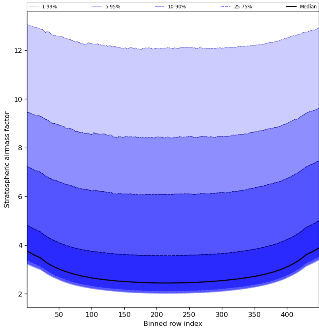
Figure 61: Along track statistics of “Stratospheric airmass factor” for 2024-05-10 to 2024-05-12
