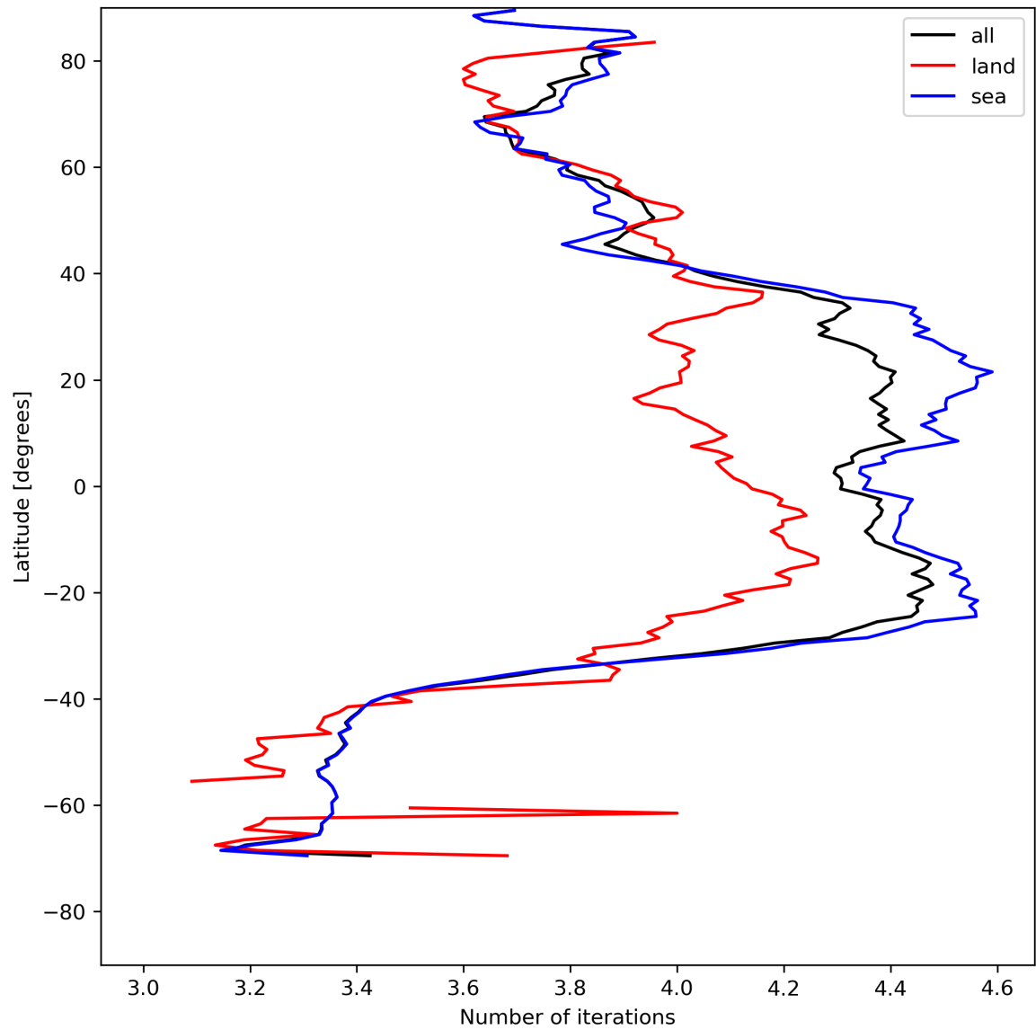
Figure 17: Zonal average of “Number of iterations” for 2024-05-10 to 2024-05-12.
