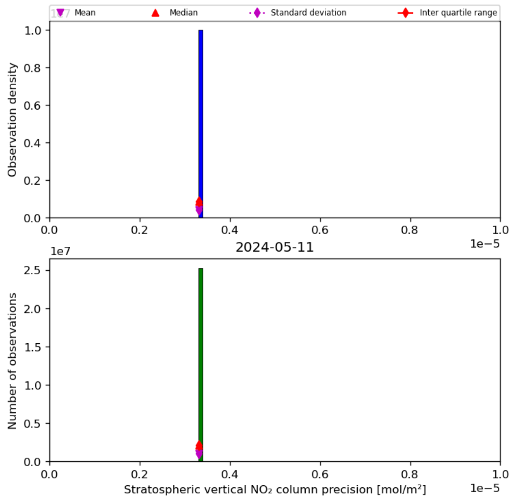
Figure 37: Histogram of “Stratospheric vertical NO 2 column precision” for 2024-05-10 to 2024-05-12
