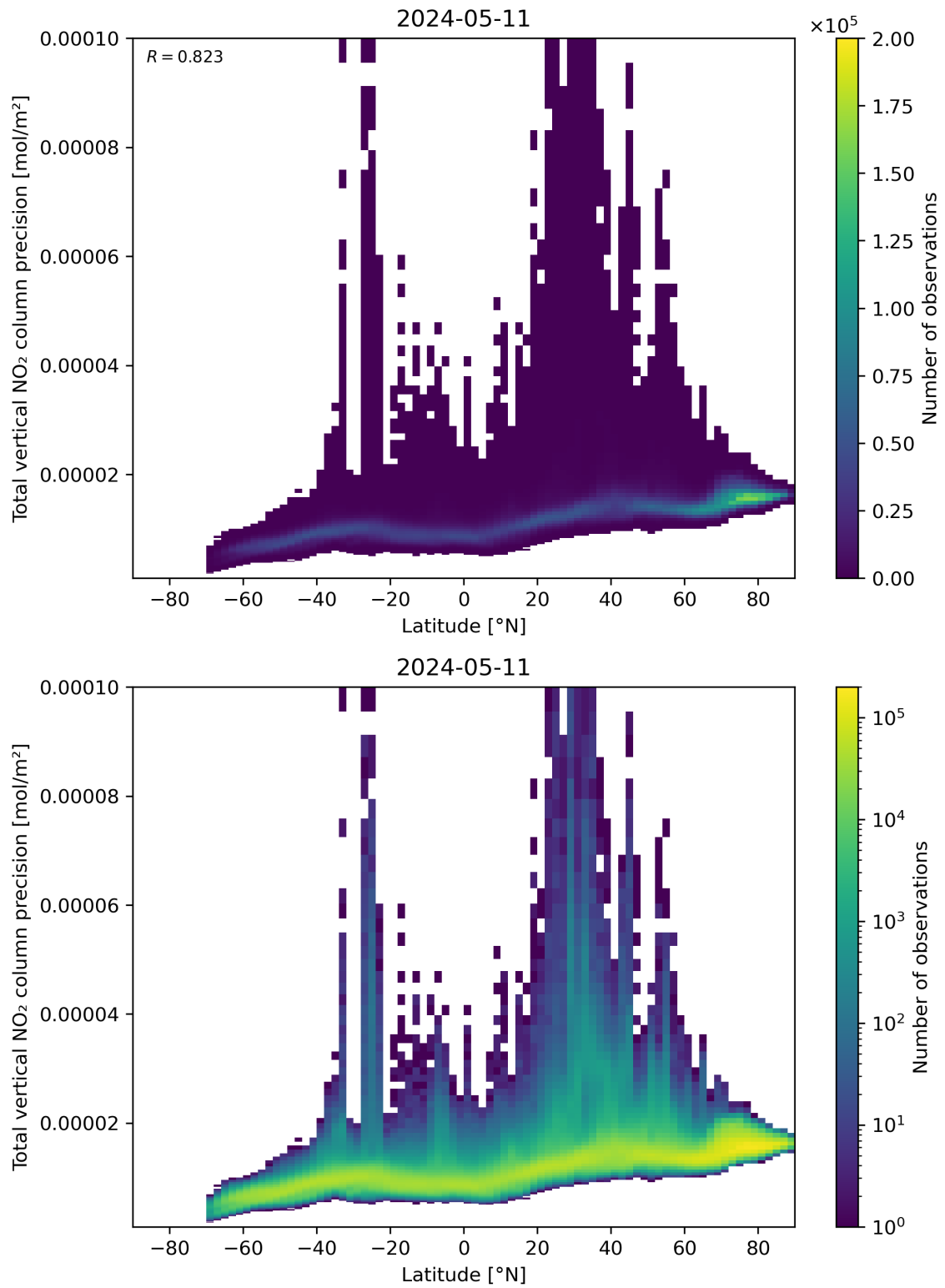
Figure 91: Scatter density plot of “Latitude” against “Total vertical NO 2 column precision” for 2024-05-10 to 2024-05-12.
