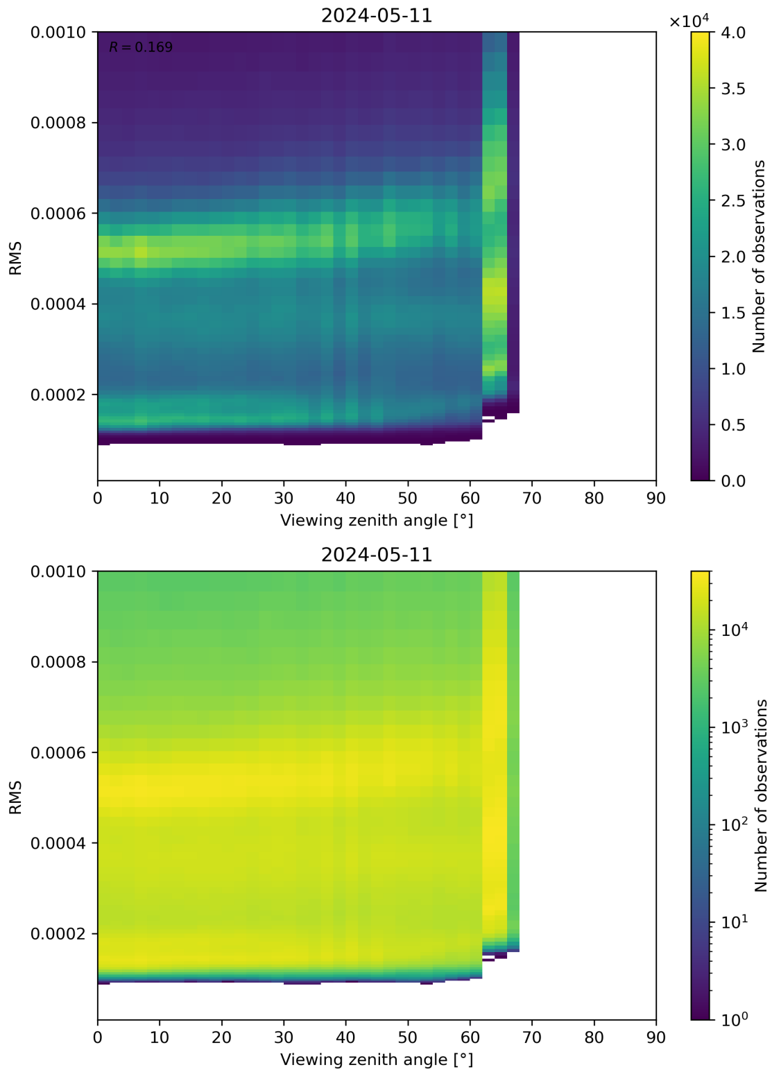
Figure 171: Scatter density plot of “Viewing zenith angle” against “RMS” for 2024-05-10 to 2024-05-12.
