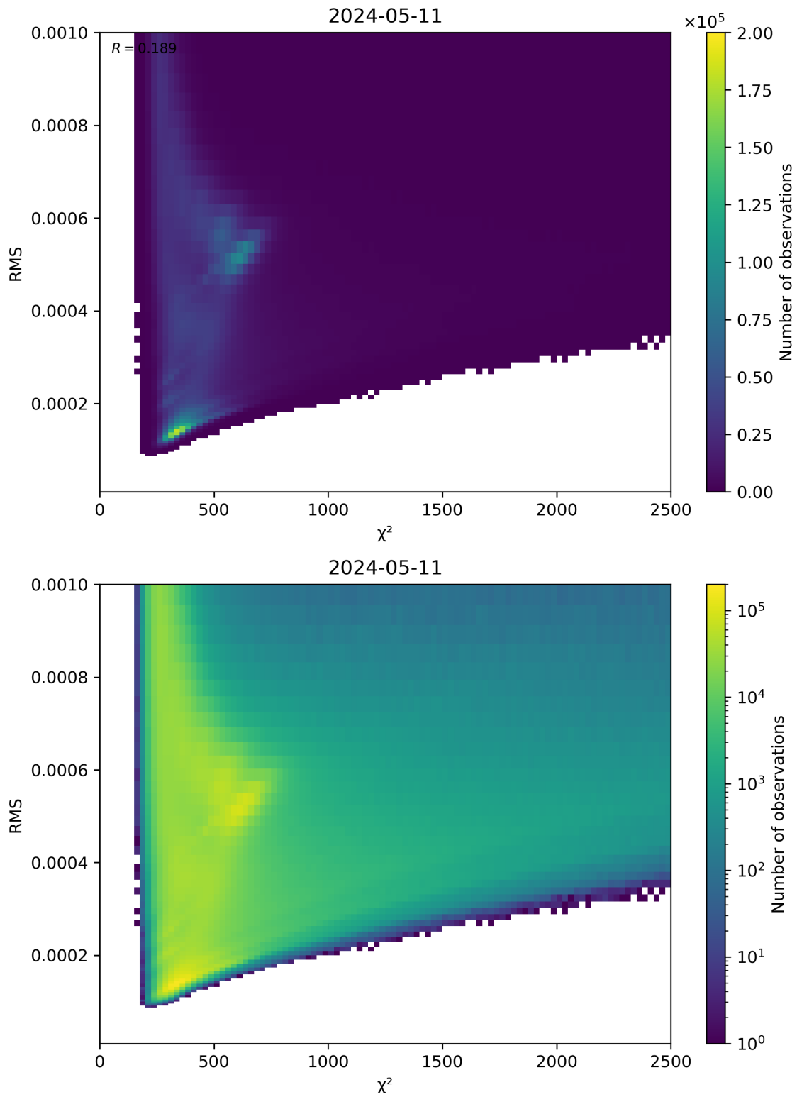
Figure 82: Scatter density plot of “ \chi^2 ” against “RMS” for 2024-05-10 to 2024-05-12.
