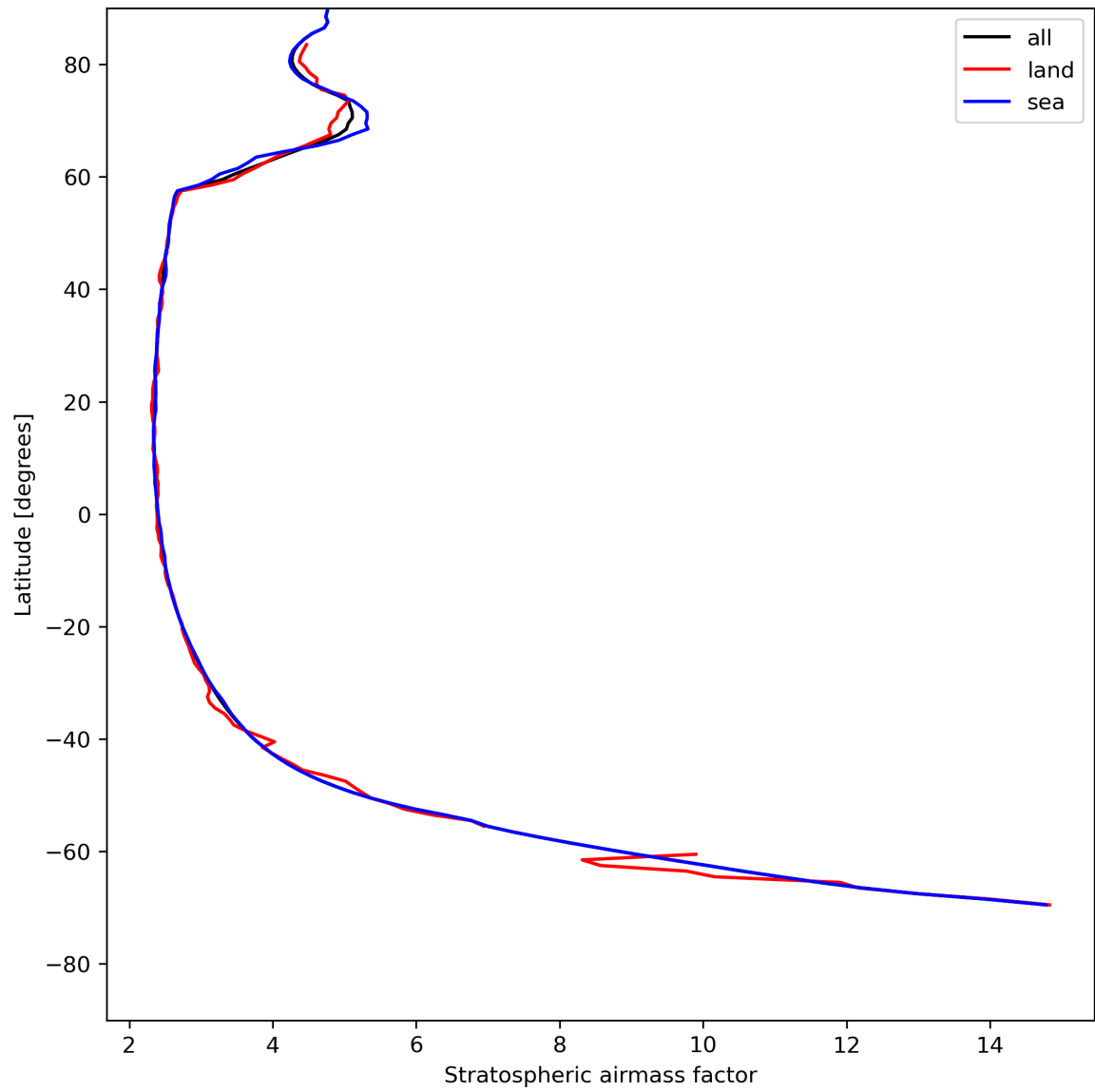
Figure 27: Zonal average of “Stratospheric air mass factor” for 2024-05-10 to 2024-05-12.
