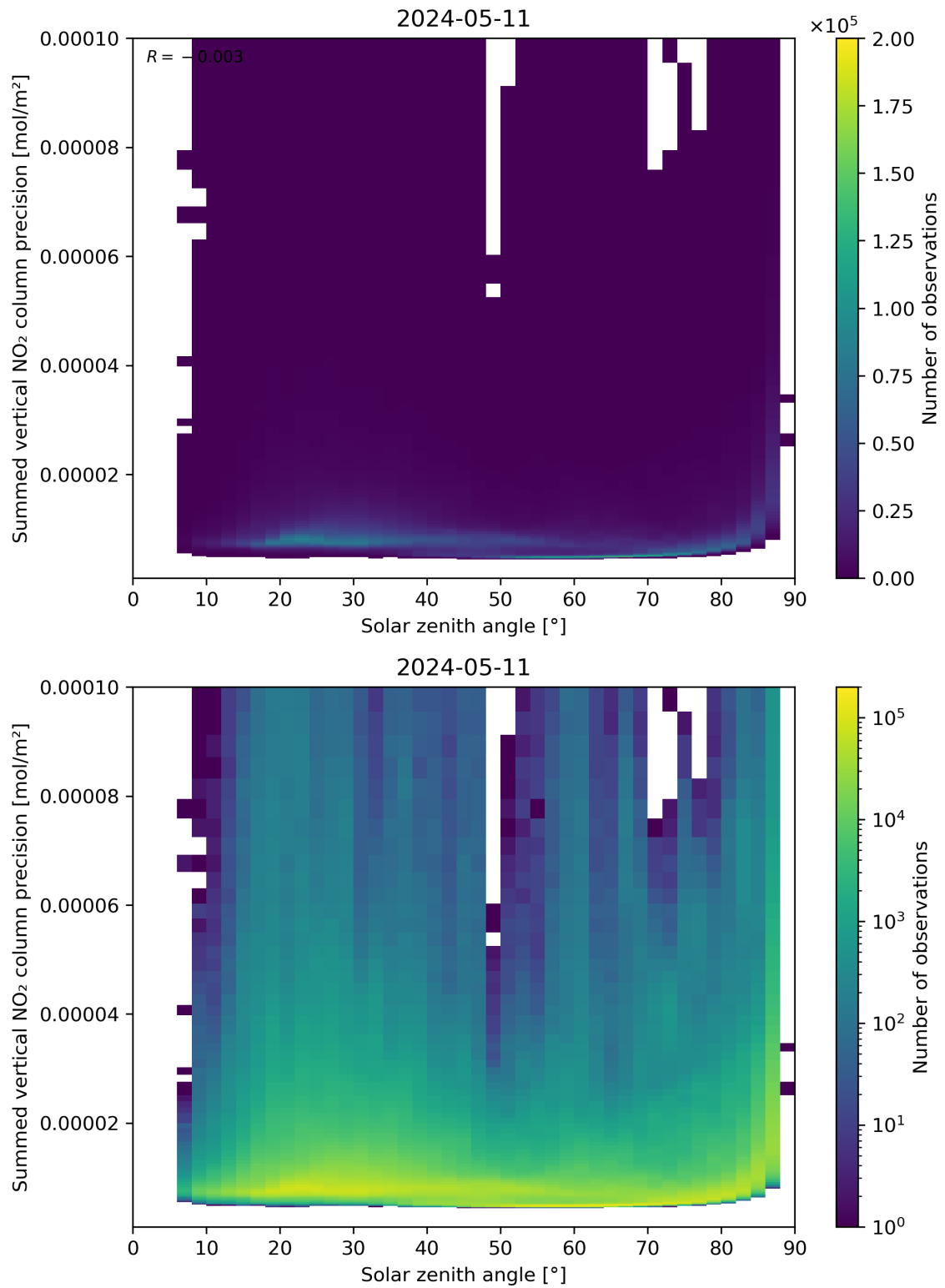
Figure 152: Scatter density plot of “Solar zenith angle” against “Summed vertical NO 2 column precision” for 2024-05-10 to 2024-05-12.
