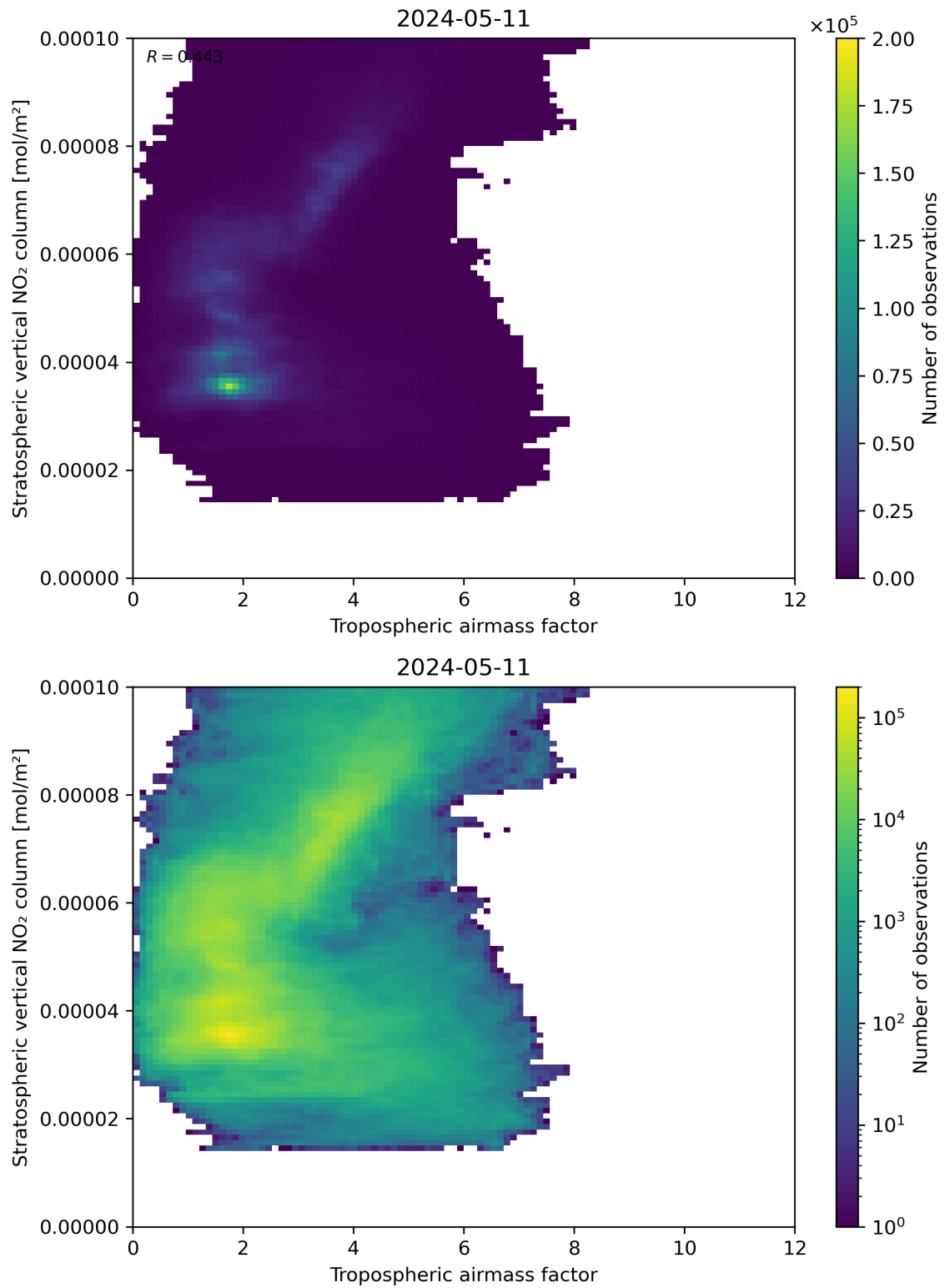
Figure 74: Scatter density plot of “Tropospheric air mass factor” against “Stratospheric vertical NO 2 column” for 2024-05-10 to 2024-05-12.
