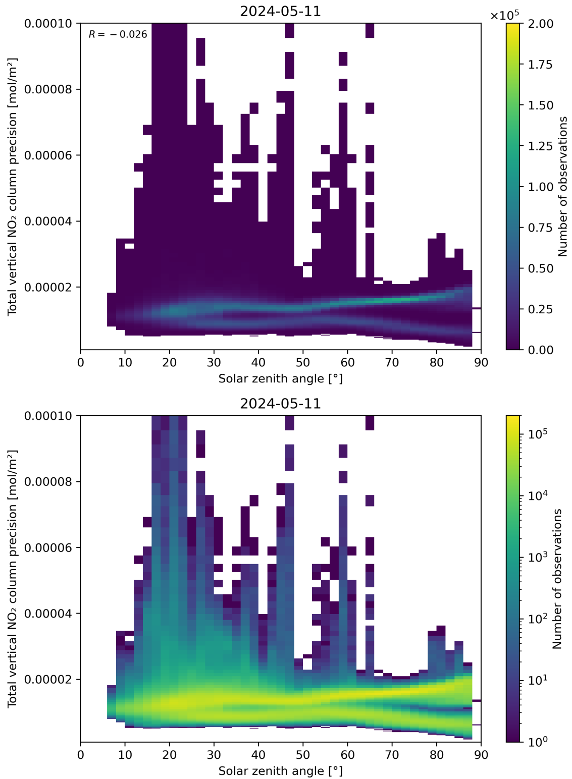
Figure 154: Scatter density plot of “Solar zenith angle” against “Total vertical NO 2 column precision” for 2024-05-10 to 2024-05-12.
