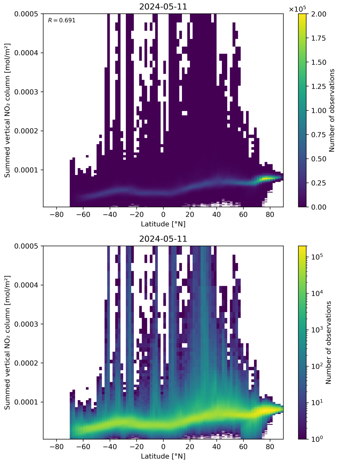
Figure 88: Scatter density plot of “Latitude” against “Summed vertical NO 2 column” for 2024-05-10 to 2024-05-12.
