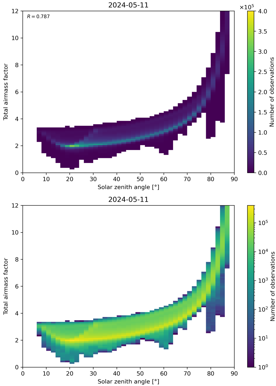
Figure 146: Scatter density plot of “Solar zenith angle” against “Total air mass factor” for 2024-05-10 to 2024-05-12.
