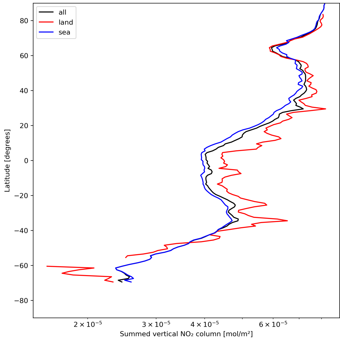
Figure 23: Zonal average of “Summed vertical NO 2 column” for 2024-05-10 to 2024-05-12.
