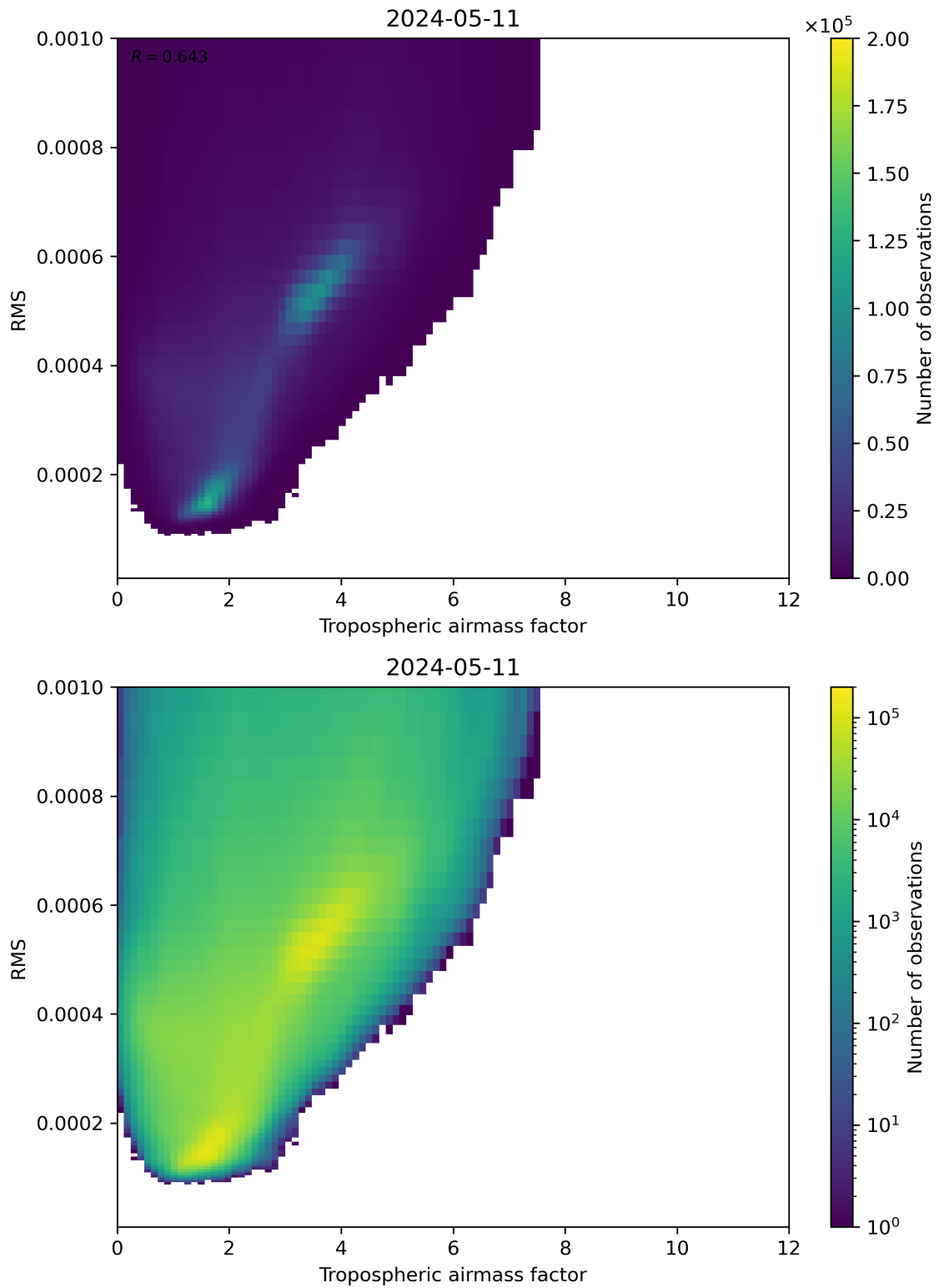
Figure 79: Scatter density plot of “Tropospheric airmass factor” against “RMS” for 2024-05-10 to 2024-05-12.
