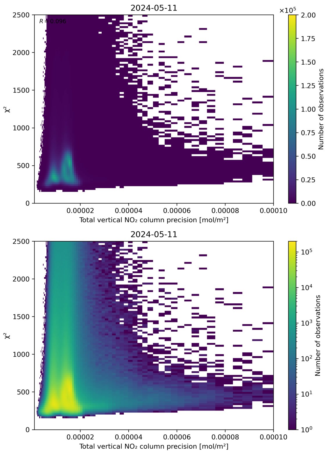
Figure 116: Scatter density plot of “Total vertical NO 2 column precision” against “ \chi^2 ” for 2024-05-10 to 2024-05-12.
