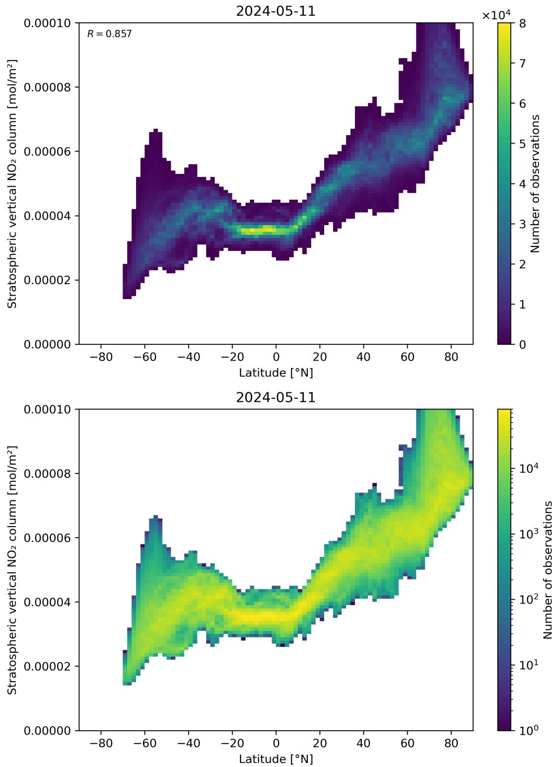
Figure 87: Scatter density plot of “Latitude” against “Stratospheric vertical NO 2 column” for 2024-05-10 to 2024-05-12.
