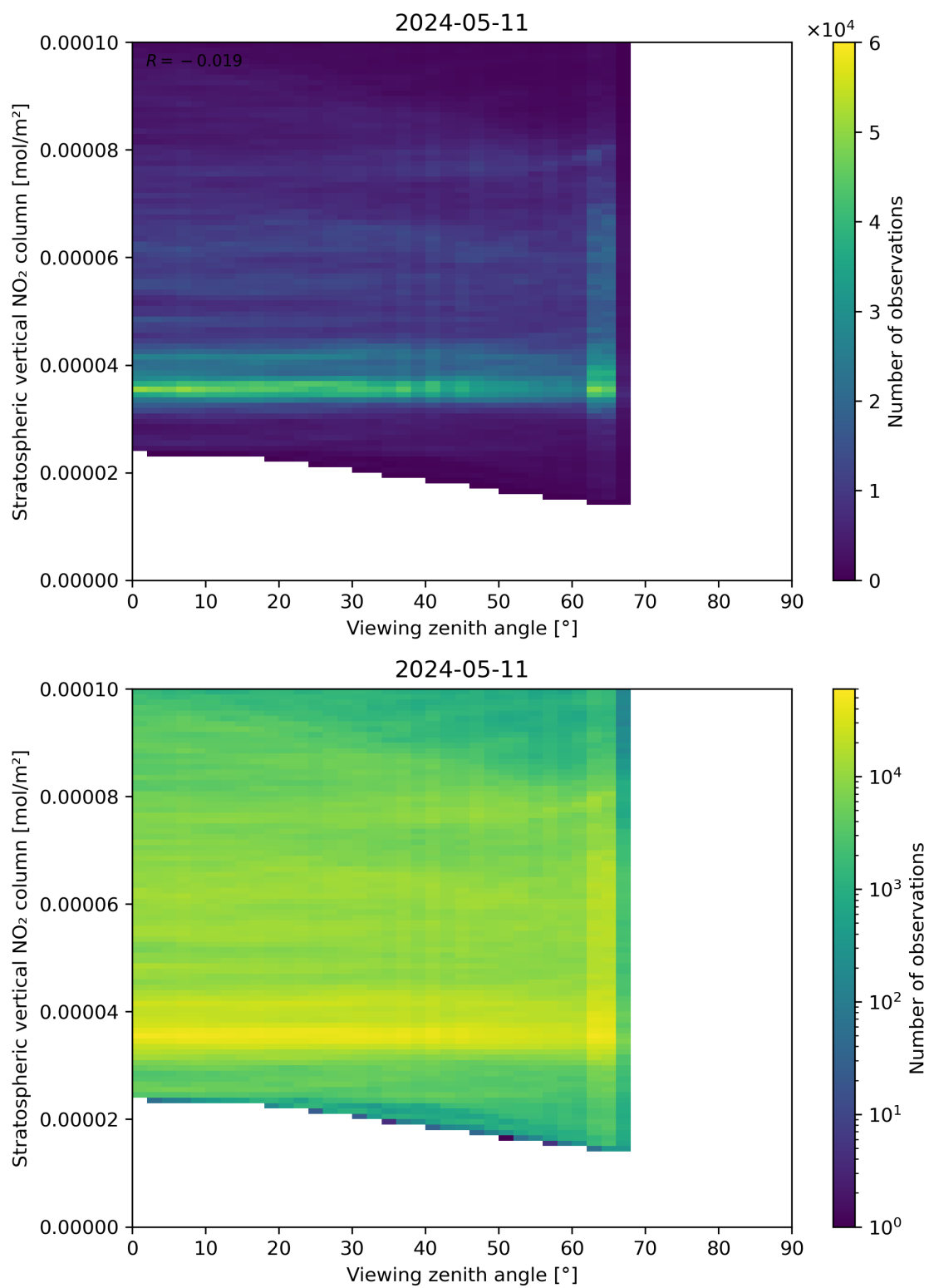
Figure 164: Scatter density plot of “Viewing zenith angle” against “Stratospheric vertical NO 2 column” for 2024-05-10 to 2024-05-12.
