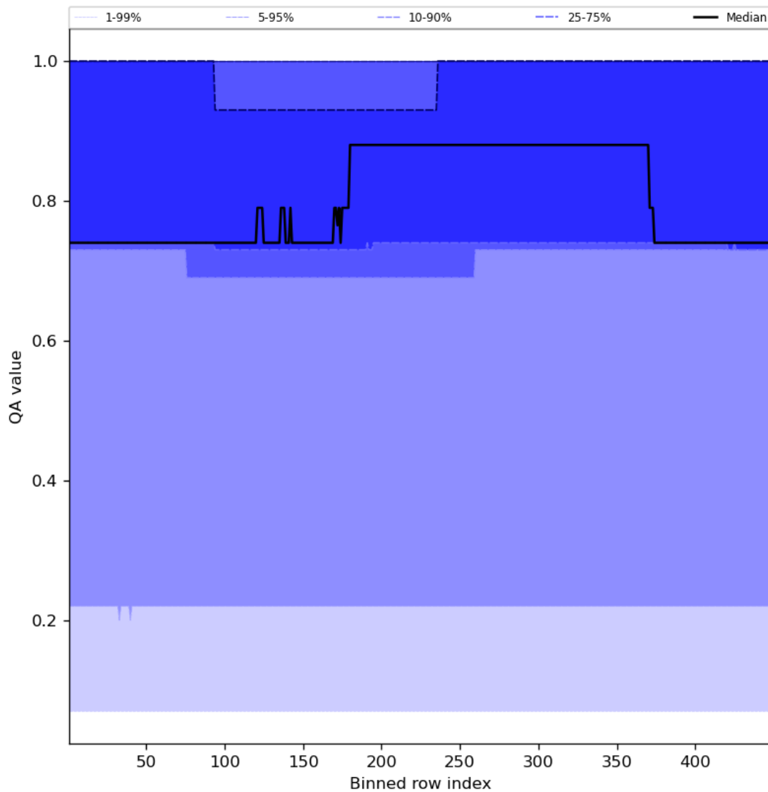
Figure 45: Along track statistics of “QA value” for 2024-05-10 to 2024-05-12
