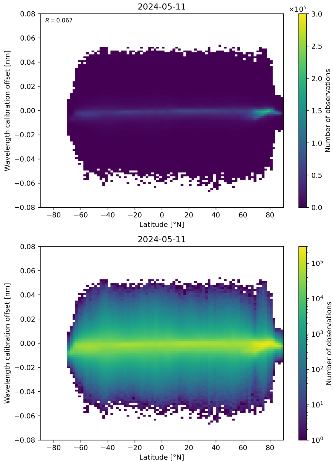
Figure 95: Scatter density plot of “Latitude” against “Wavelength calibration offset” for 2024-05-10 to 2024-05-12.
