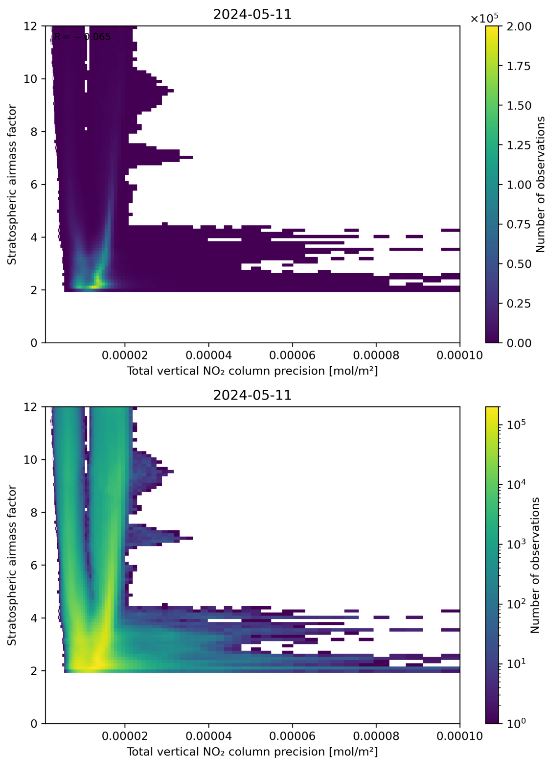
Figure 115: Scatter density plot of “Total vertical NO 2 column precision” against “Stratospheric air mass factor” for 2024-05-10 to 2024-05-12.
