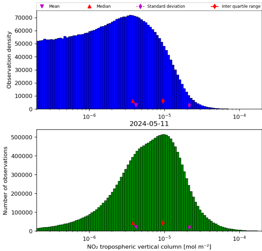
Figure 29: Histogram of “NO 2 tropospheric vertical column” for 2024-05-10 to 2024-05-12
