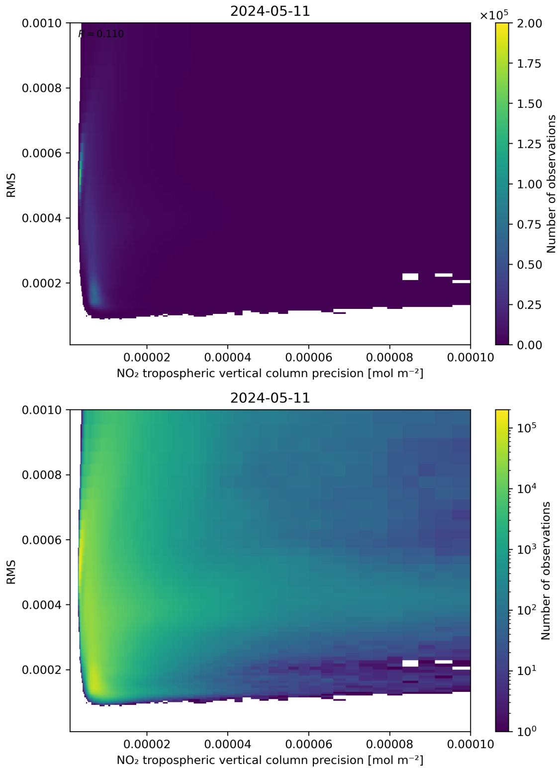
Figure 140: Scatter density plot of “NO 2 tropospheric vertical column precision” against “RMS” for 2024-05-10 to 2024-05-12.
