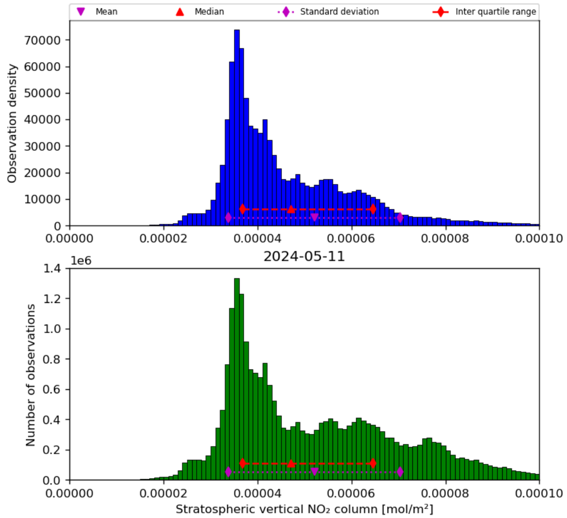
Figure 36: Histogram of “Stratospheric vertical NO 2 column” for 2024-05-10 to 2024-05-12
