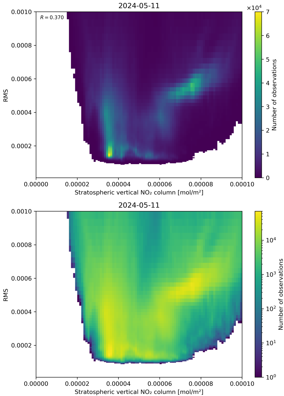
Figure 102: Scatter density plot of “Stratospheric vertical NO 2 column” against “RMS” for 2024-05-10 to 2024-05-12.
