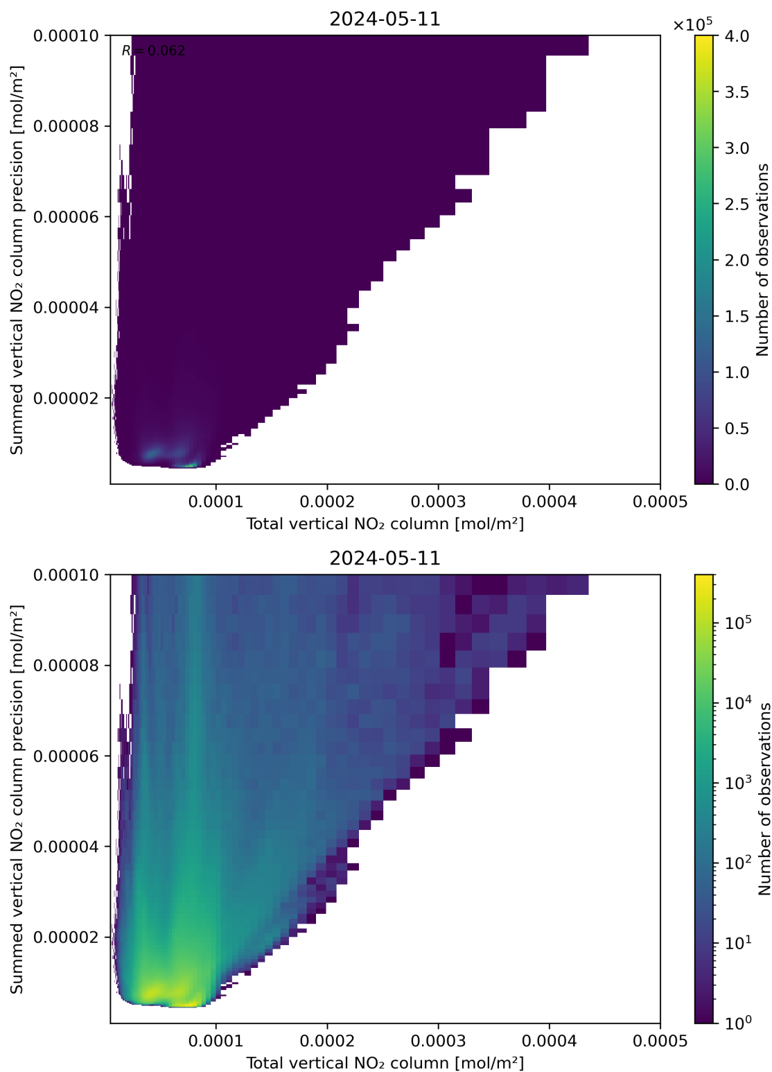
Figure 113: Scatter density plot of “Total vertical NO 2 column” against “Summed vertical NO 2 column precision” for 2024-05-10 to 2024-05-12.
