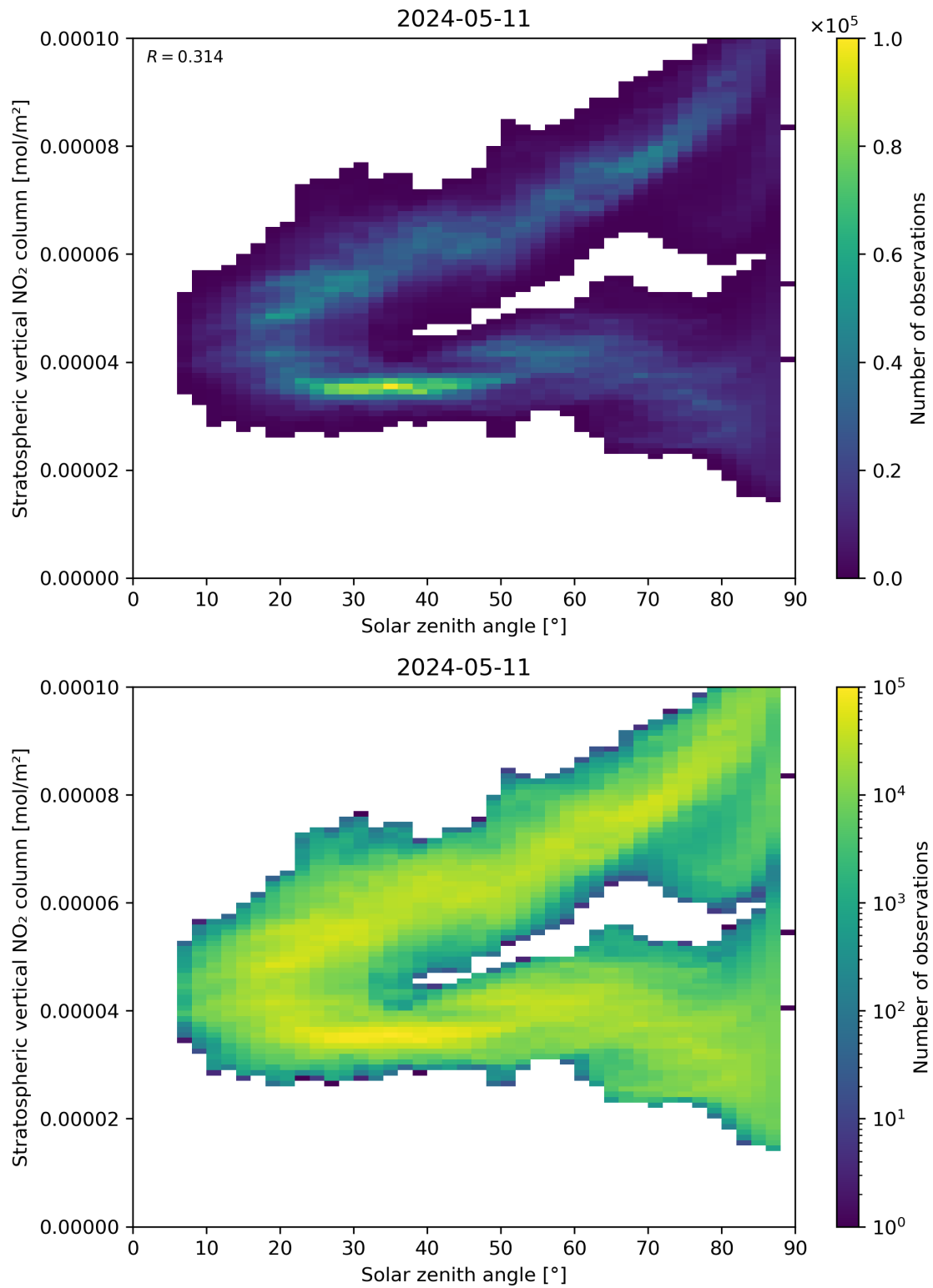
Figure 150: Scatter density plot of “Solar zenith angle” against “Stratospheric vertical NO 2 column” for 2024-05-10 to 2024-05-12.
