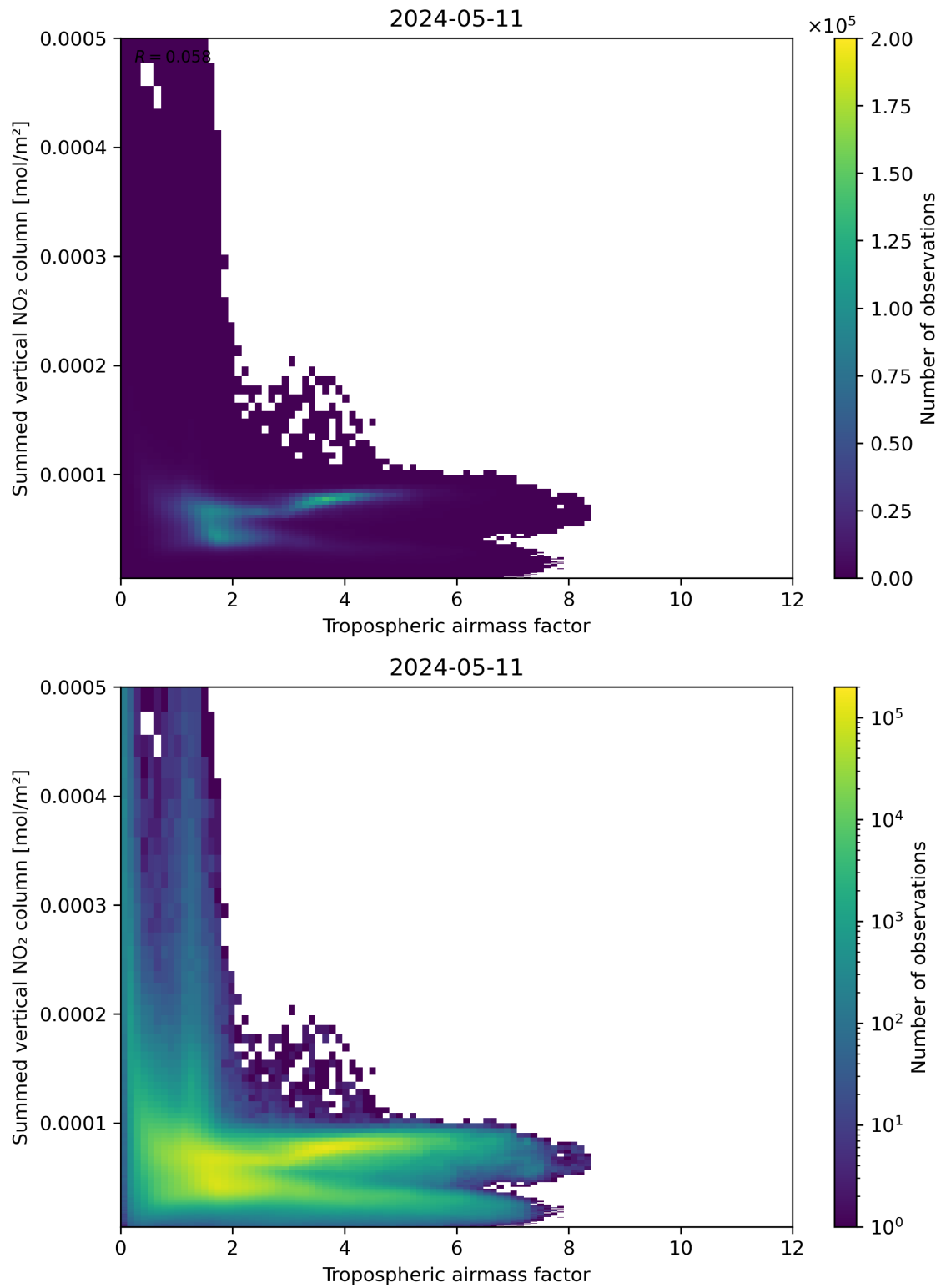
Figure 75: Scatter density plot of “Tropospheric air mass factor” against “Summed vertical NO 2 column” for 2024-05-10 to 2024-05-12.
