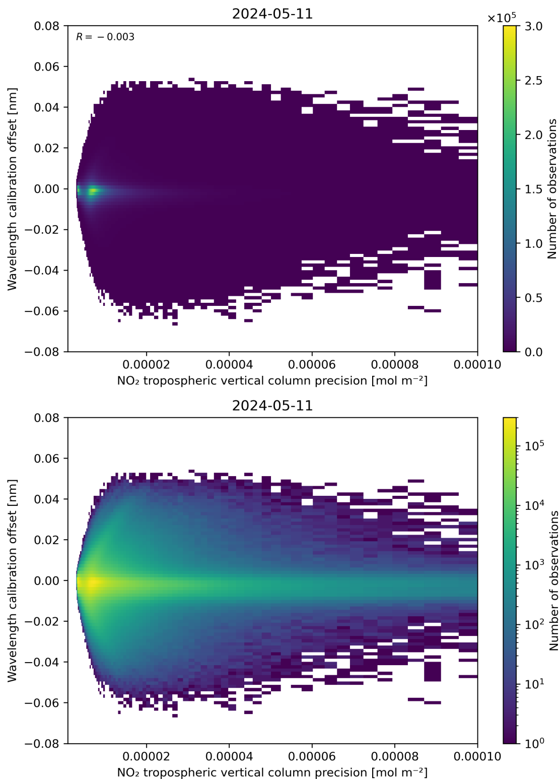
Figure 141: Scatter density plot of “NO 2 tropospheric vertical column precision” against “Wavelength calibration offset” for 2024-05-10 to 2024-05-12.
