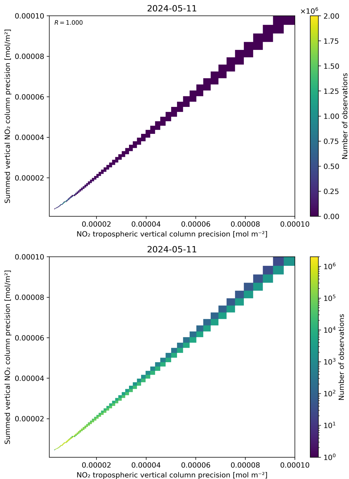
Figure 137: Scatter density plot of “NO 2 tropospheric vertical column precision” against “Summed vertical NO 2 column precision” for 2024-05-10 to 2024-05-12.
