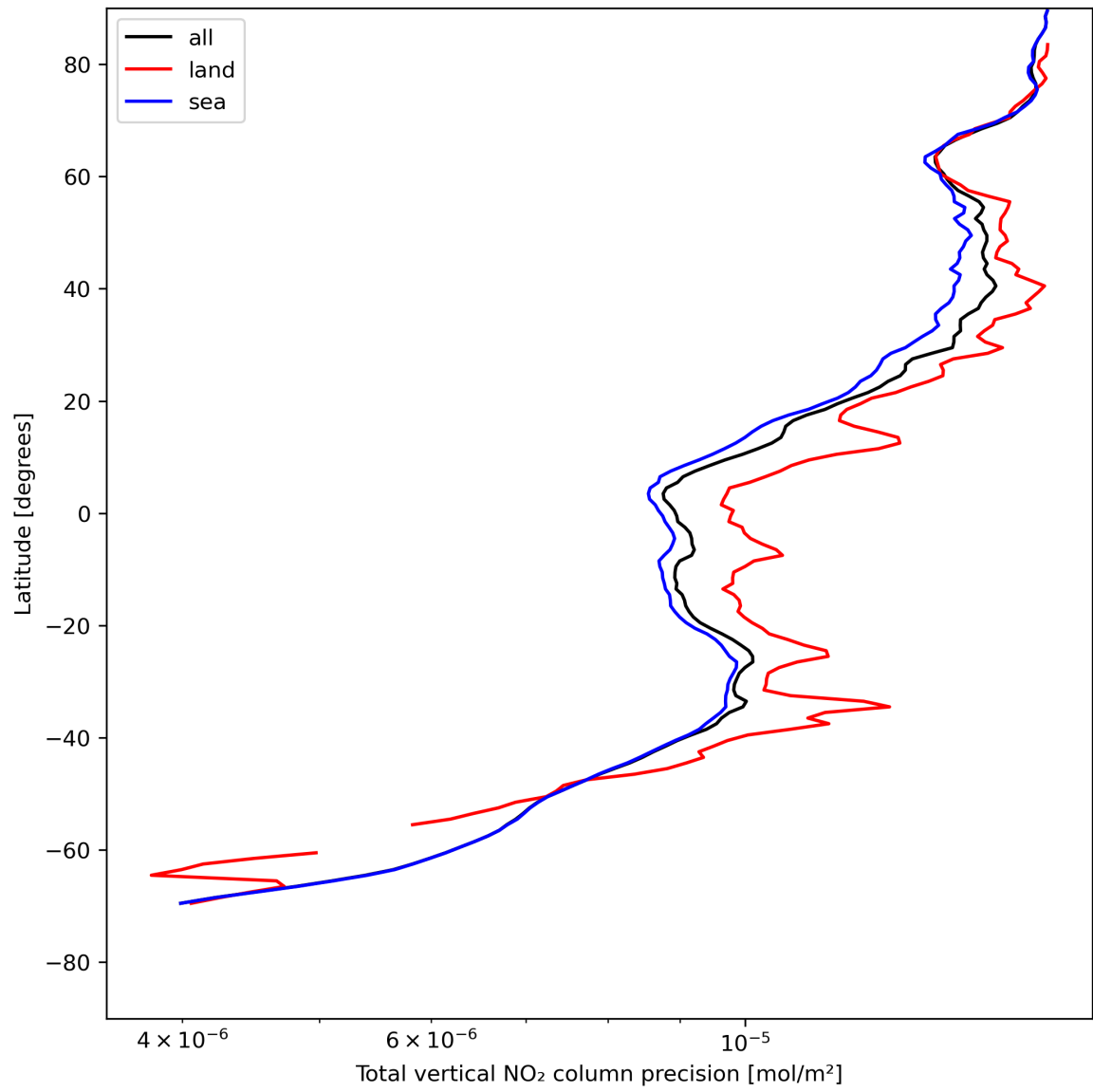
Figure 22: Zonal average of “Total vertical NO 2 column precision” for 2024-05-10 to 2024-05-12.
