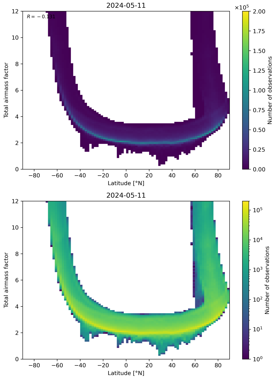
Figure 84: Scatter density plot of “Latitude” against “Total airmass factor” for 2024-05-10 to 2024-05-12.
