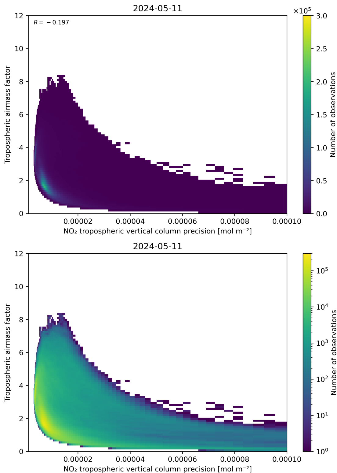
Figure 133: Scatter density plot of “NO 2 tropospheric vertical column precision” against “Tropospheric air mass factor” for 2024-05-10 to 2024-05-12.
