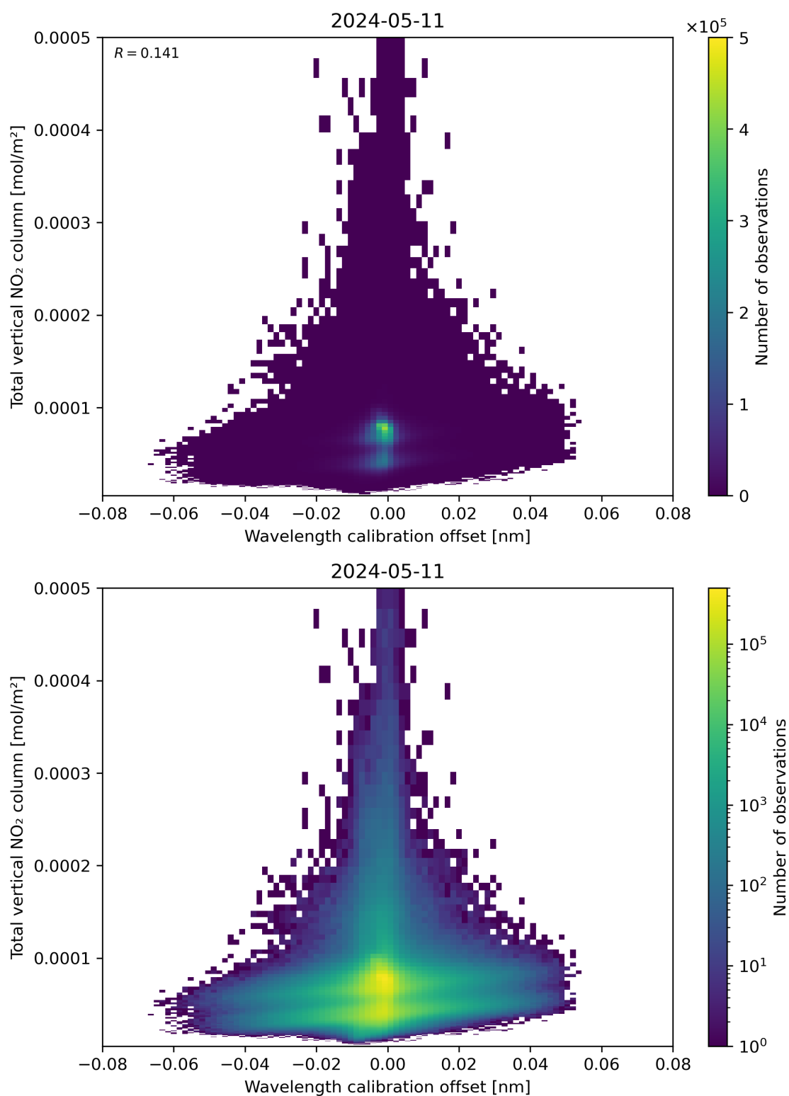
Figure 179: Scatter density plot of “Wavelength calibration offset” against “Total vertical NO 2 column” for 2024-05-10 to 2024-05-12.
