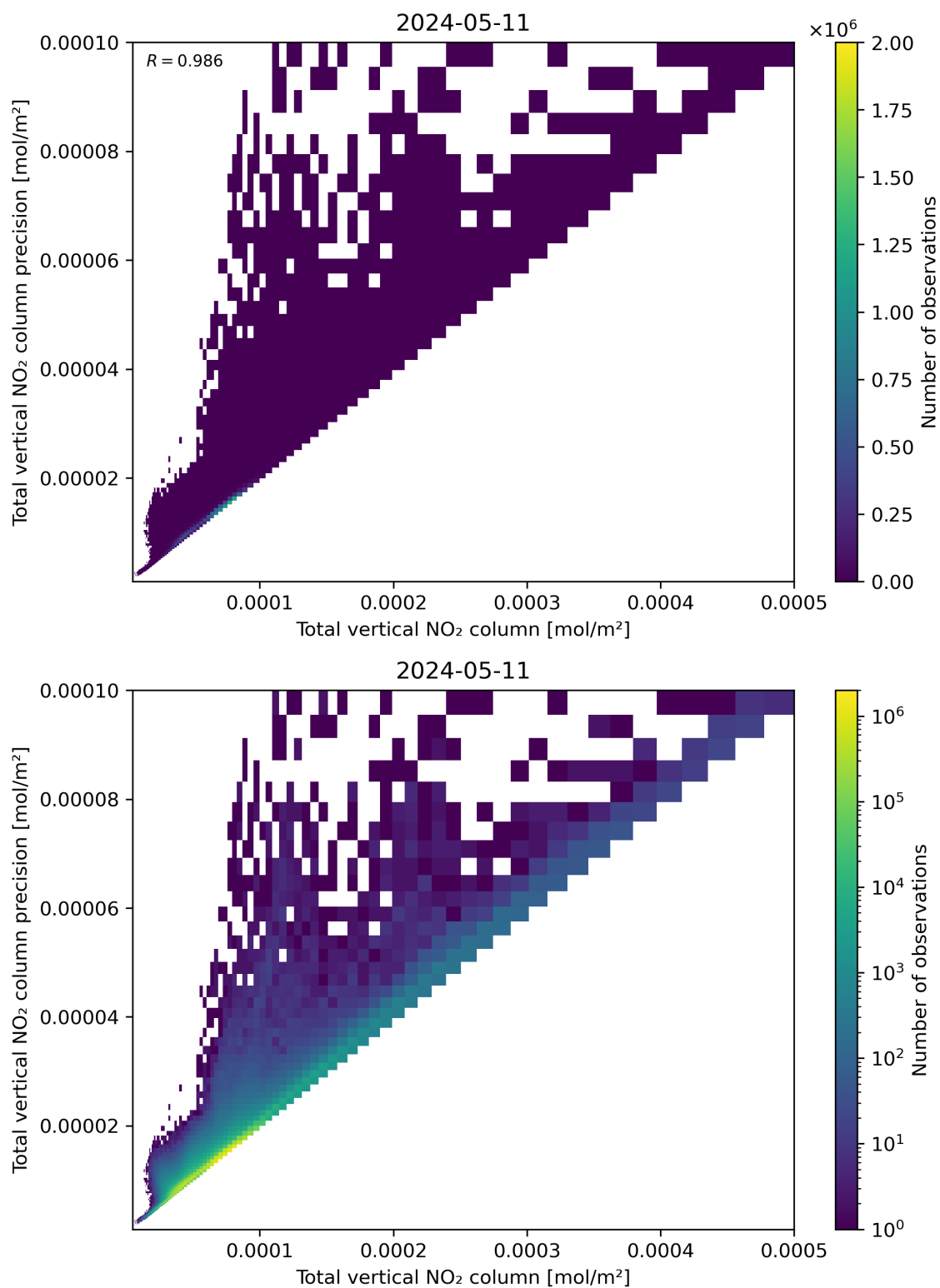
Figure 114: Scatter density plot of “Total vertical NO 2 column” against “Total vertical NO 2 column precision” for 2024-05-10 to 2024-05-12.
