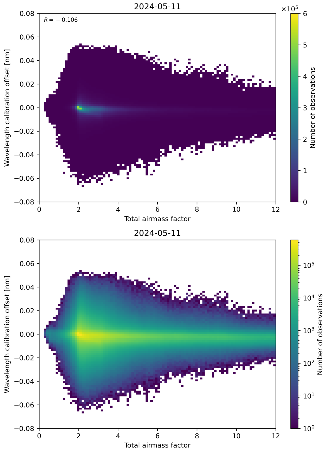
Figure 70: Scatter density plot of “Total airmass factor” against “Wavelength calibration offset” for 2024-05-10 to 2024-05-12.
