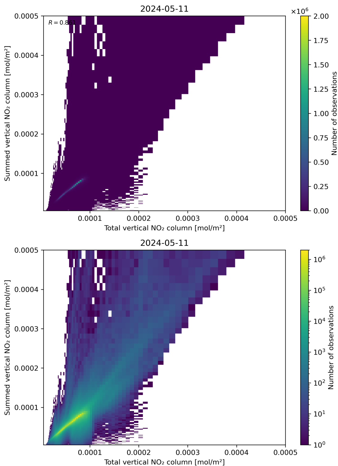
Figure 112: Scatter density plot of “Total vertical NO 2 column” against “Summed vertical NO 2 column” for 2024-05-10 to 2024-05-12.
