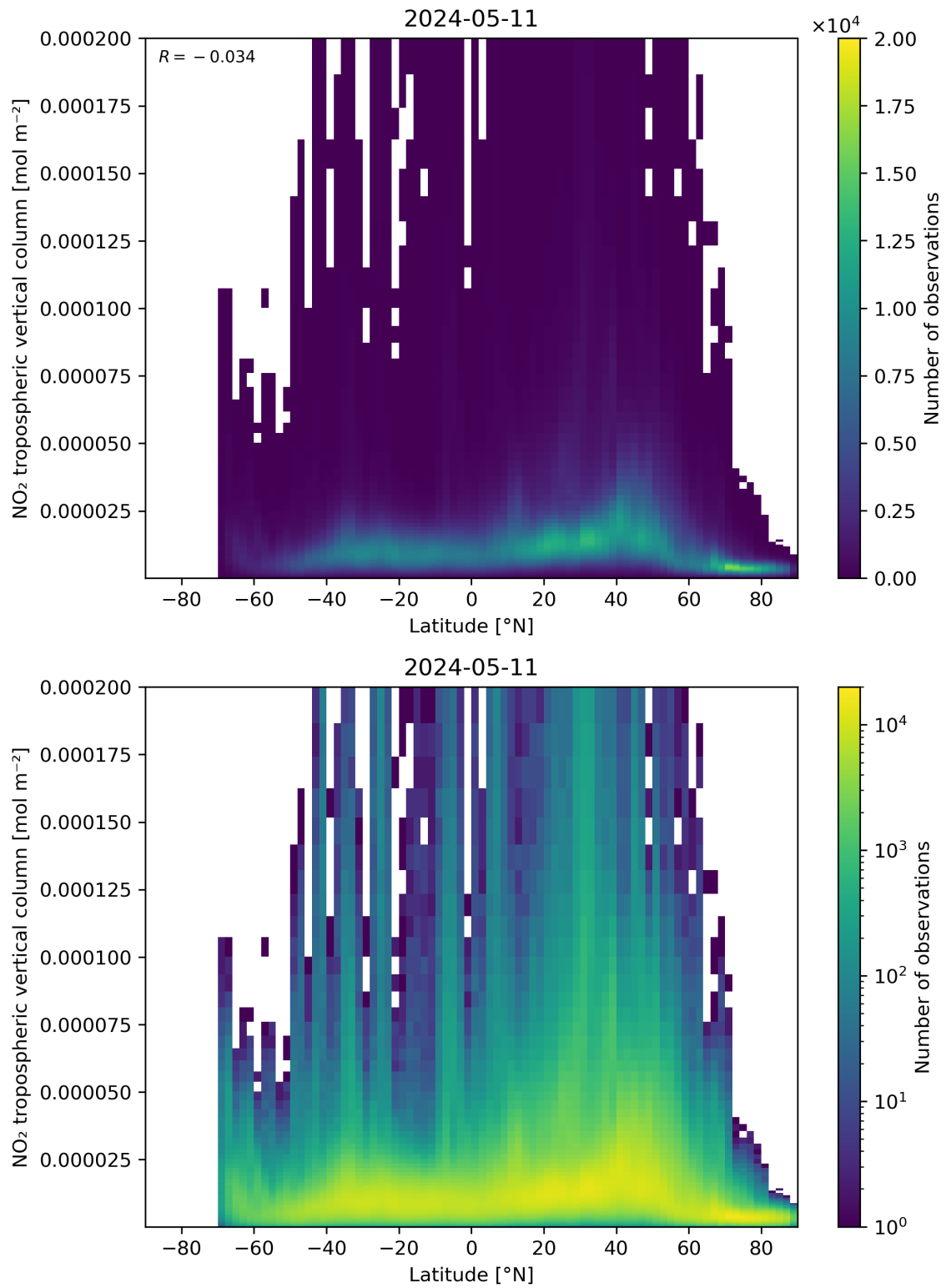
Figure 92: Scatter density plot of “Latitude” against “NO 2 tropospheric vertical column” for 2024-05-10 to 2024-05-12.
