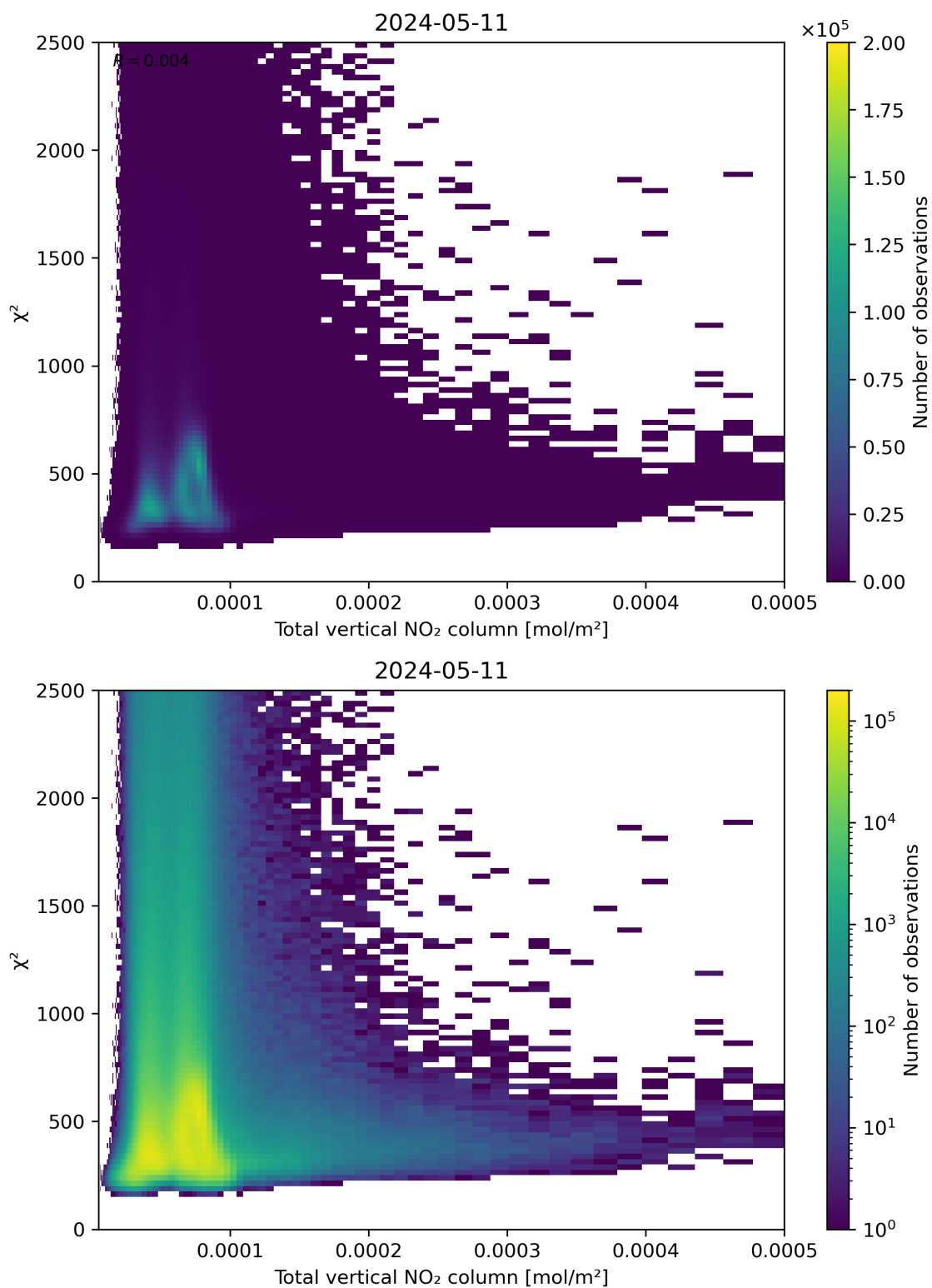
Figure 111: Scatter density plot of “Total vertical NO 2 column” against “ \chi^2 ” for 2024-05-10 to 2024-05-12.
