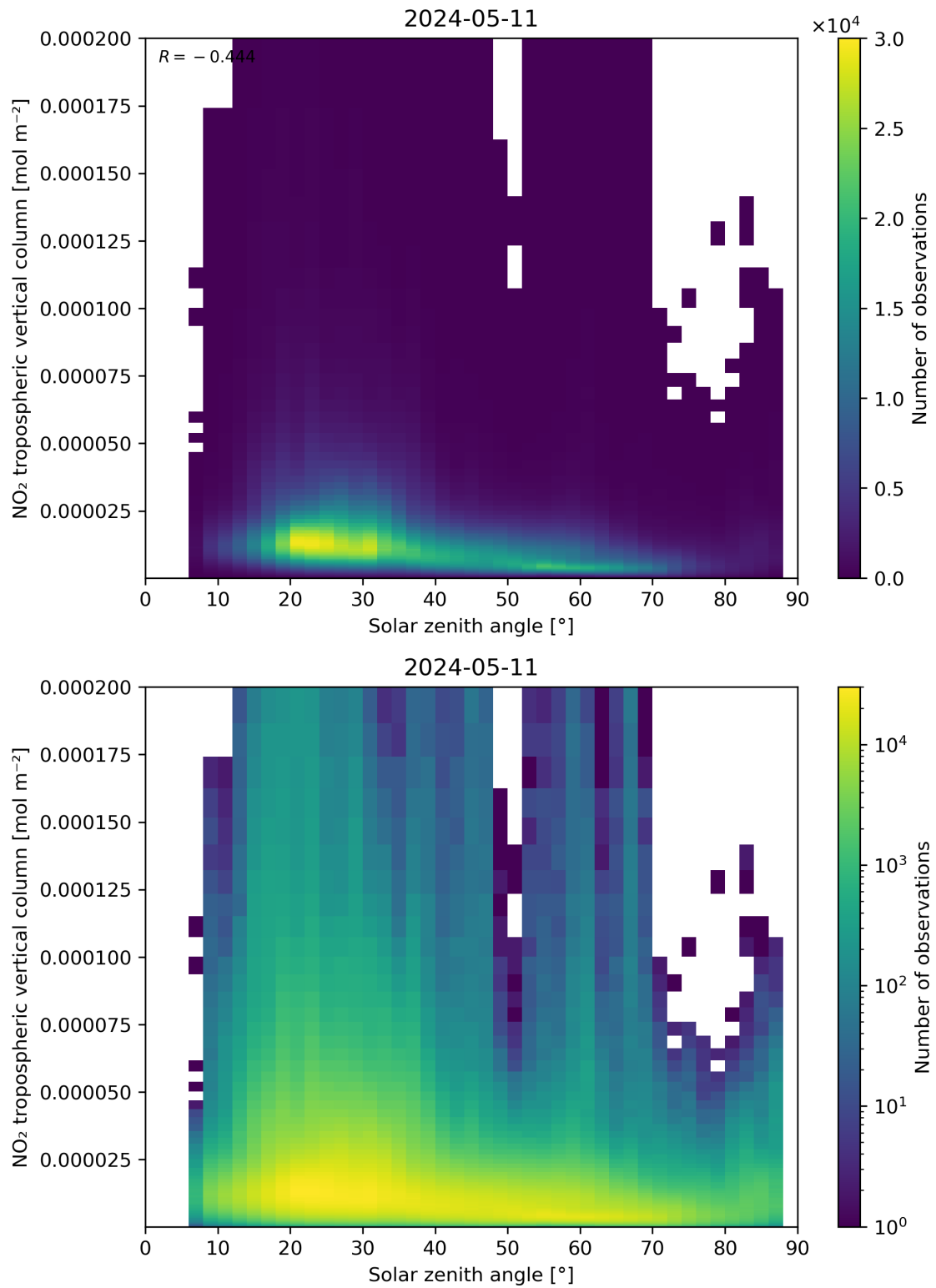
Figure 155: Scatter density plot of “Solar zenith angle” against “NO 2 tropospheric vertical column” for 2024-05-10 to 2024-05-12.
