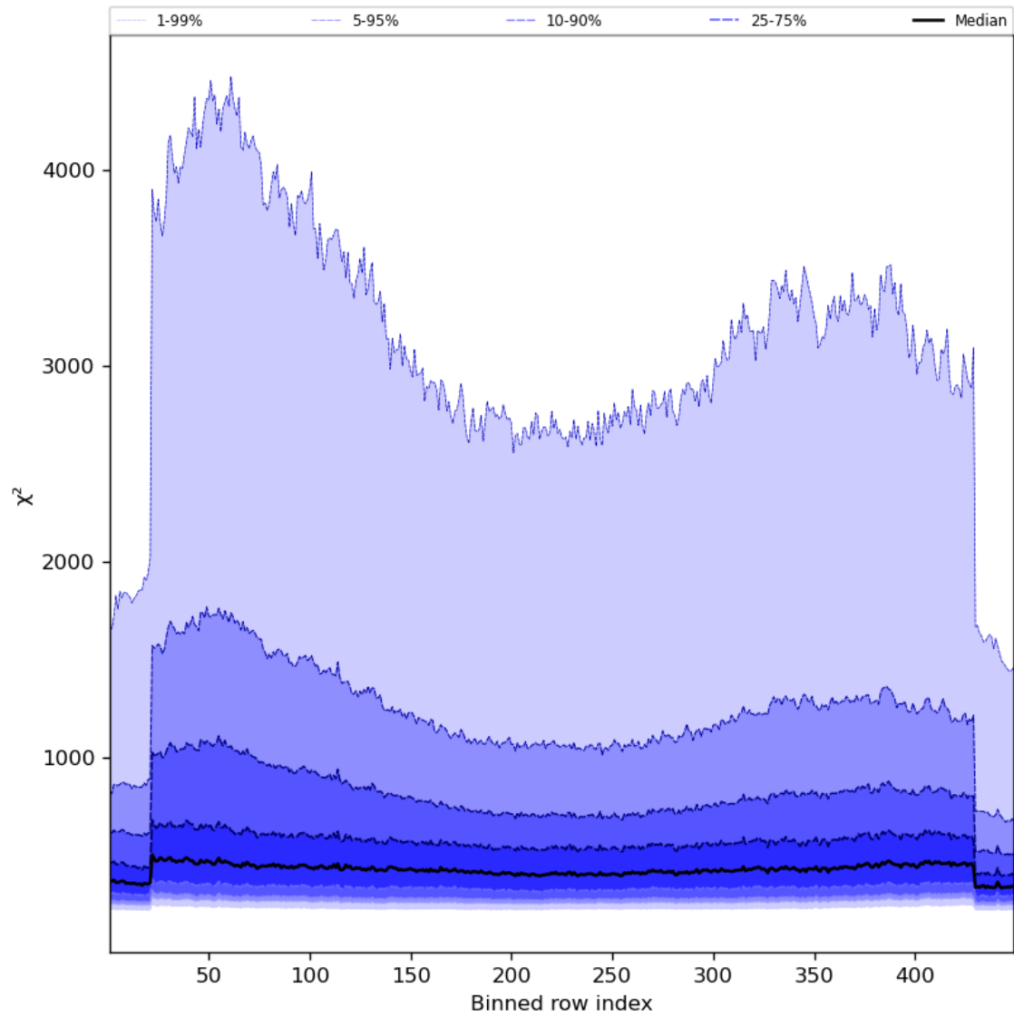
Figure 59: Along track statistics of “ \chi^2 ” for 2024-05-10 to 2024-05-12
