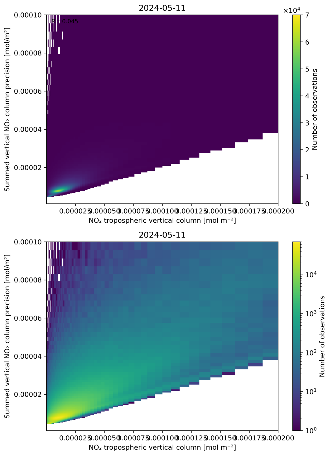
Figure 127: Scatter density plot of “NO 2 tropospheric vertical column” against “Summed vertical NO 2 column precision” for 2024-05-10 to 2024-05-12.
