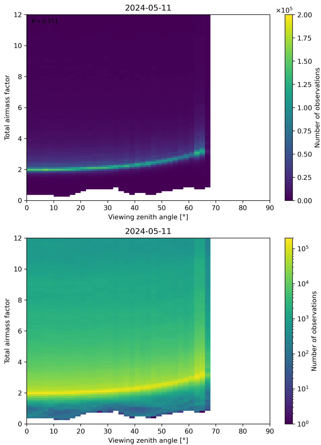
Figure 160: Scatter density plot of “Viewing zenith angle” against “Total airmass factor” for 2024-05-10 to 2024-05-12.
