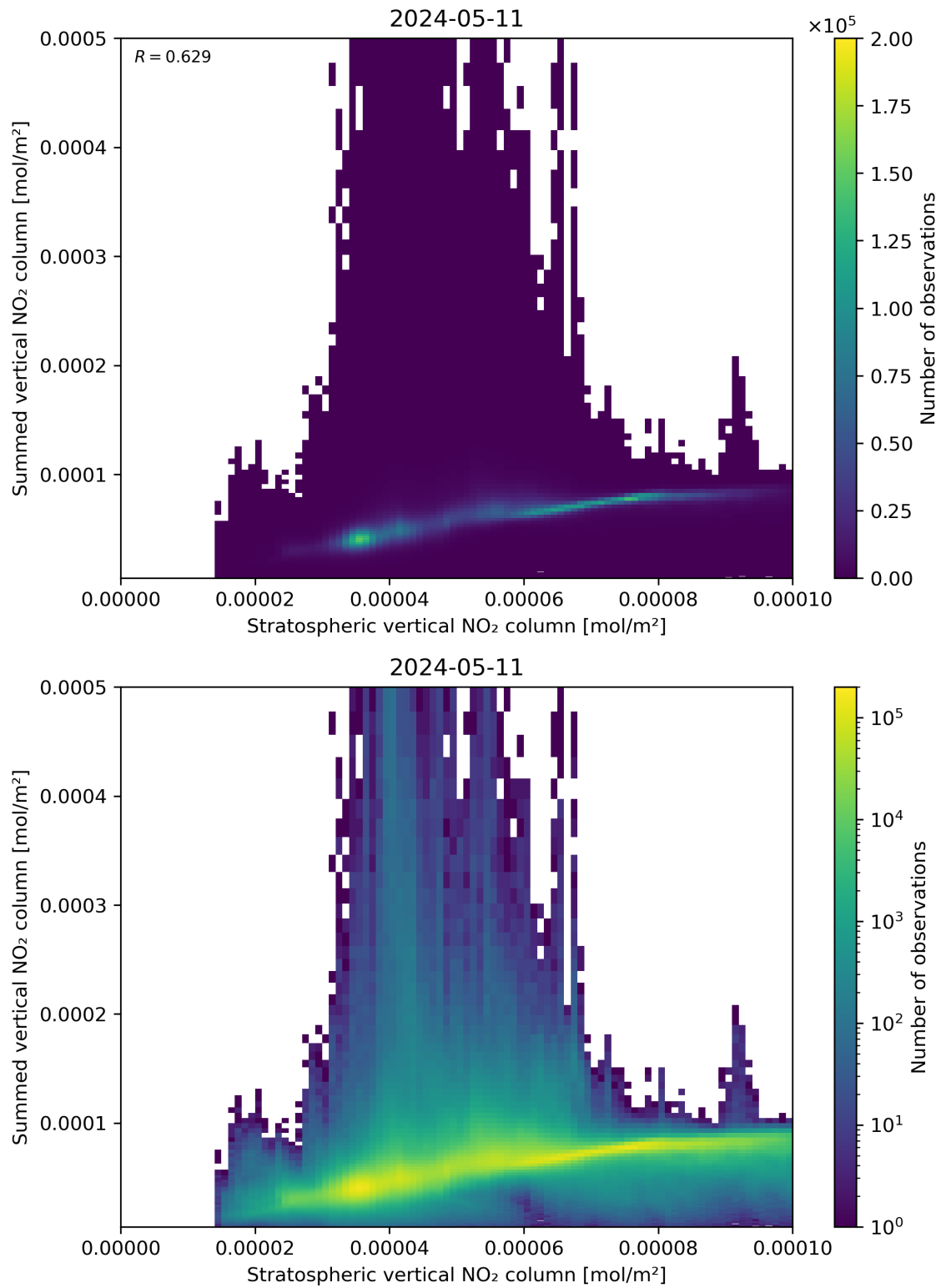
Figure 98: Scatter density plot of “Stratospheric vertical NO 2 column” against “Summed vertical NO 2 column” for 2024-05-10 to 2024-05-12.
