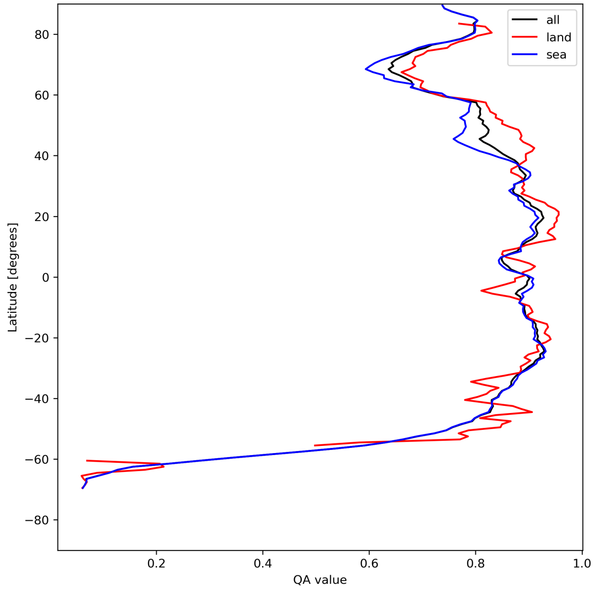
Figure 11: Zonal average of “QA value” for 2024-05-10 to 2024-05-12.
