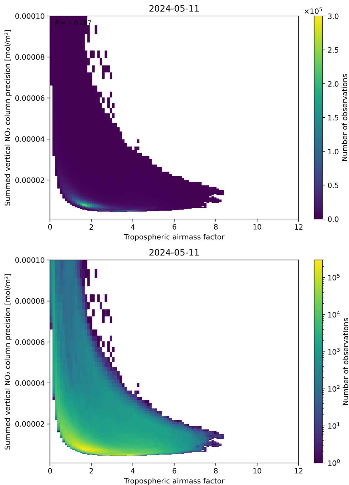
Figure 76: Scatter density plot of “Tropospheric air mass factor” against “Summed vertical NO 2 column precision” for 2024-05-10 to 2024-05-12.
