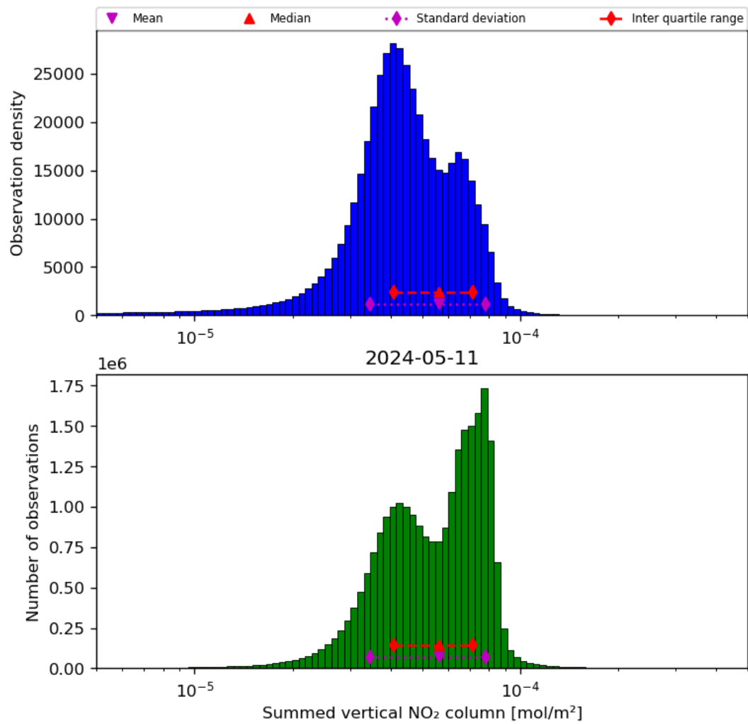
Figure 40: Histogram of “Summed vertical NO 2 column” for 2024-05-10 to 2024-05-12
