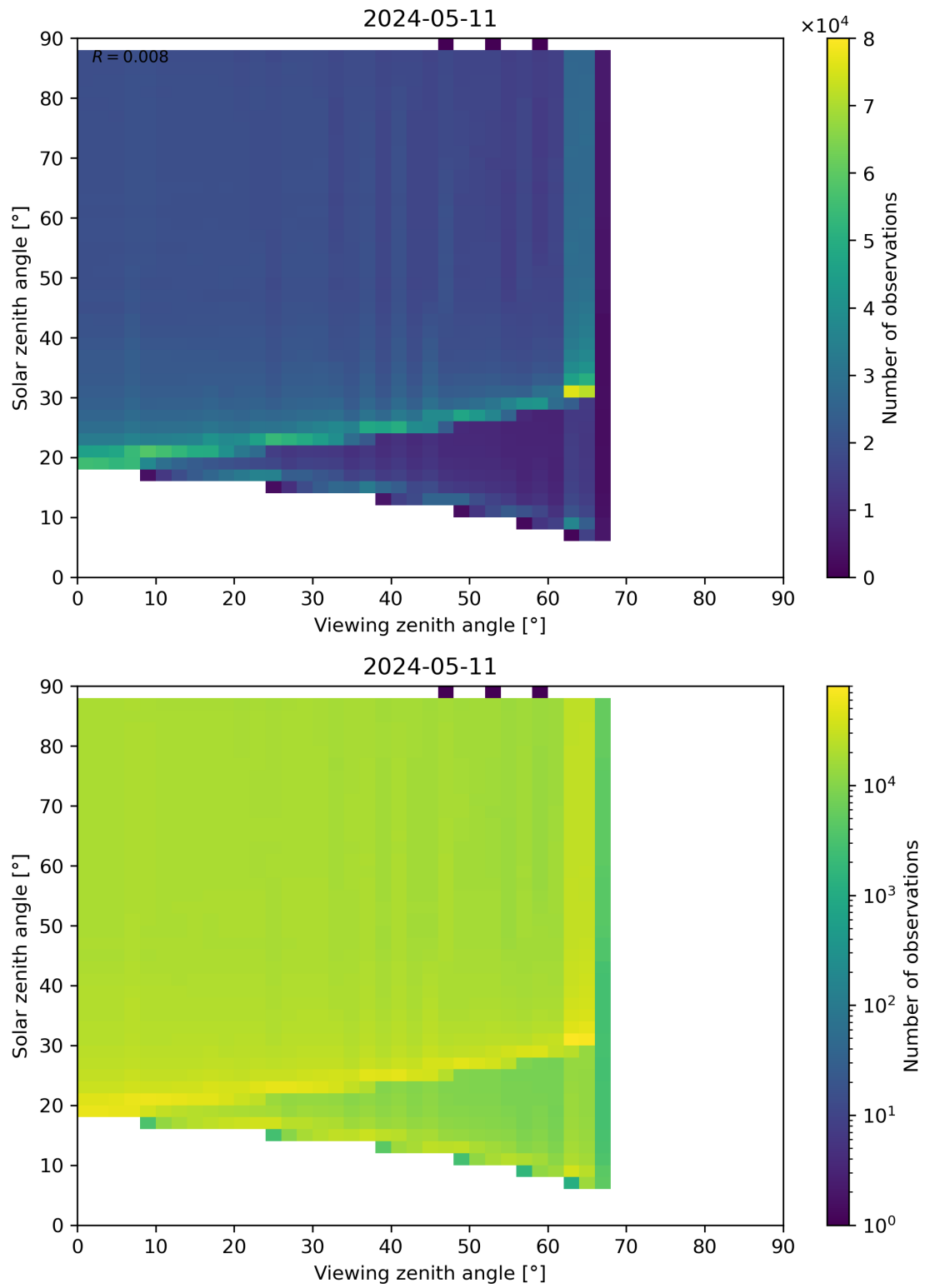
Figure 172: Scatter density plot of “Viewing zenith angle” against “Solar zenith angle” for 2024-05-10 to 2024-05-12.
