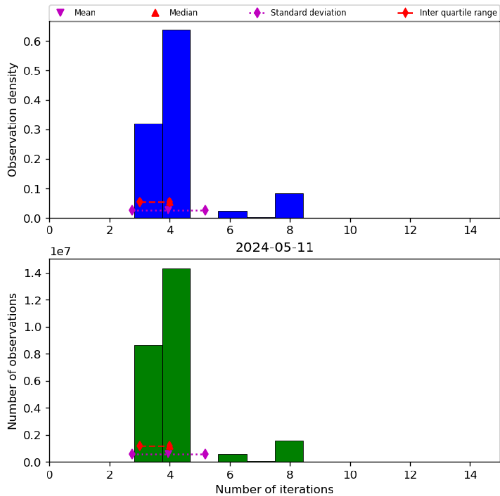
Figure 34: Histogram of “Number of iterations” for 2024-05-10 to 2024-05-12
