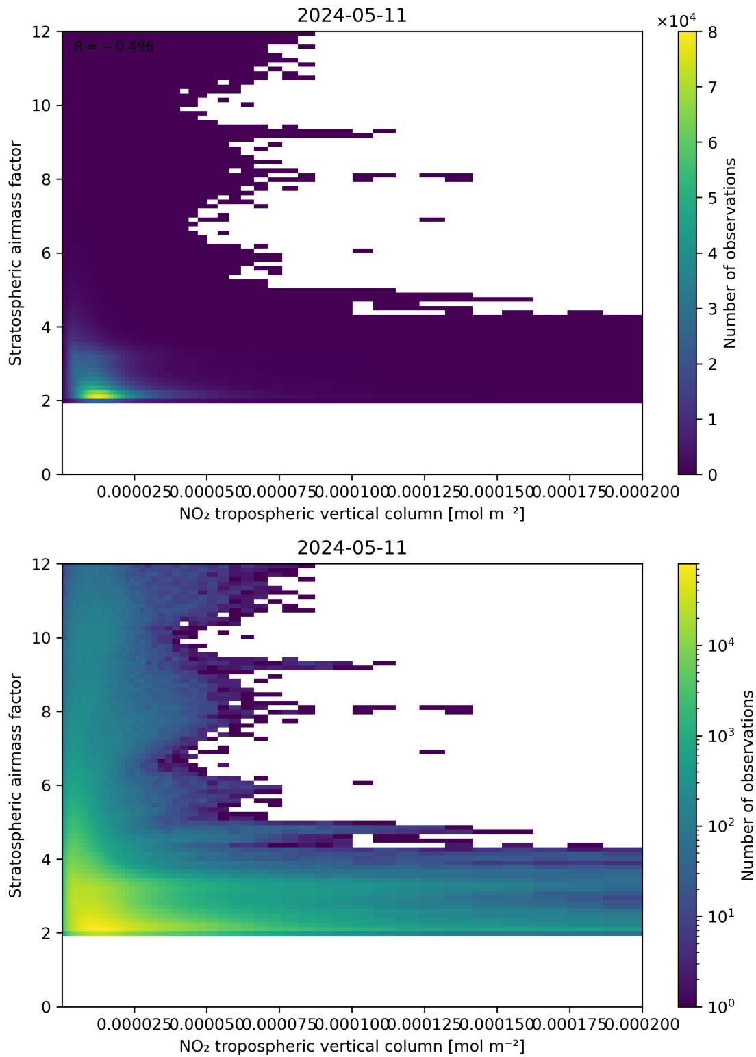
Figure 121: Scatter density plot of “NO 2 tropospheric vertical column” against “Stratospheric air mass factor” for 2024-05-10 to 2024-05-12.
