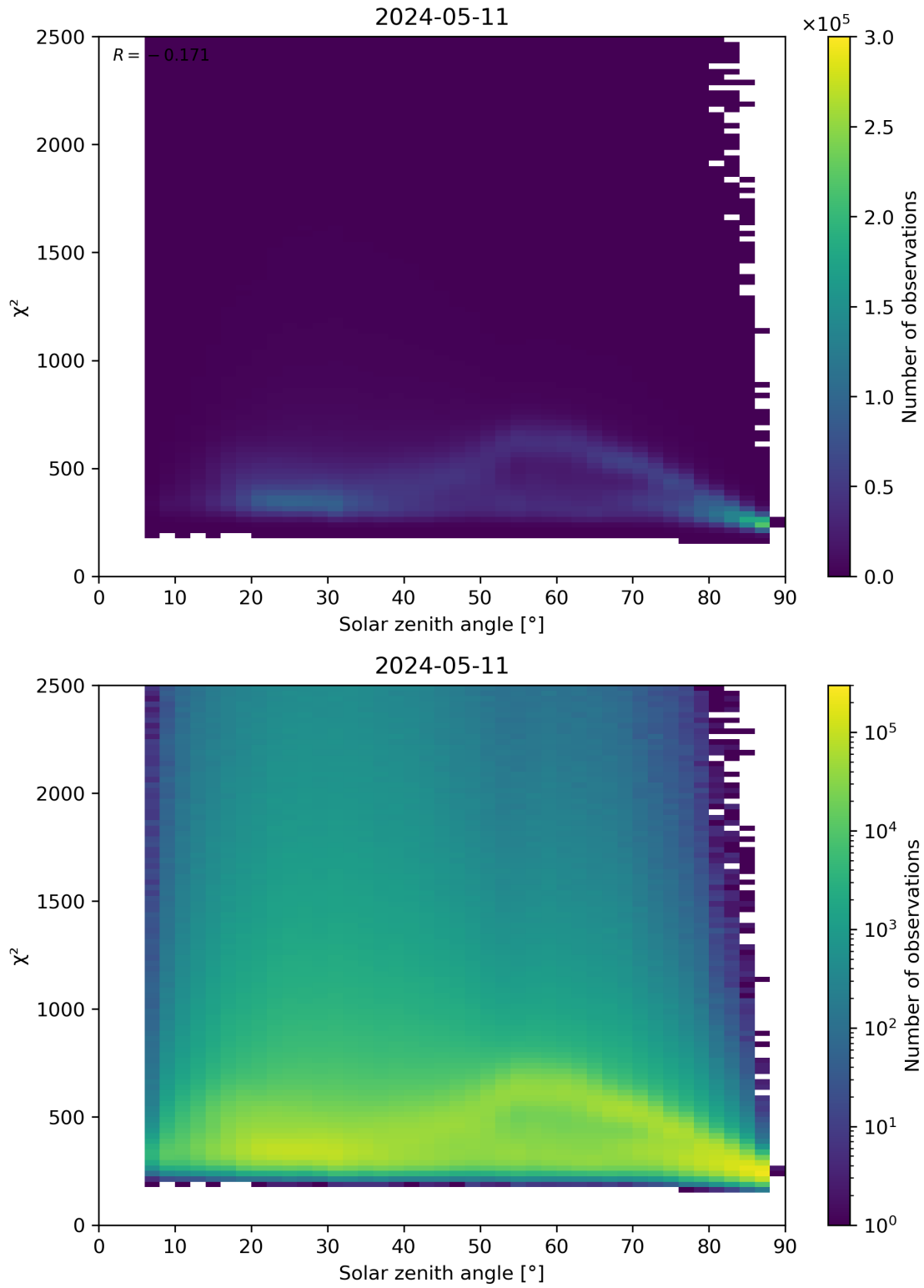
Figure 148: Scatter density plot of “Solar zenith angle” against “ \chi^2 ” for 2024-05-10 to 2024-05-12.
