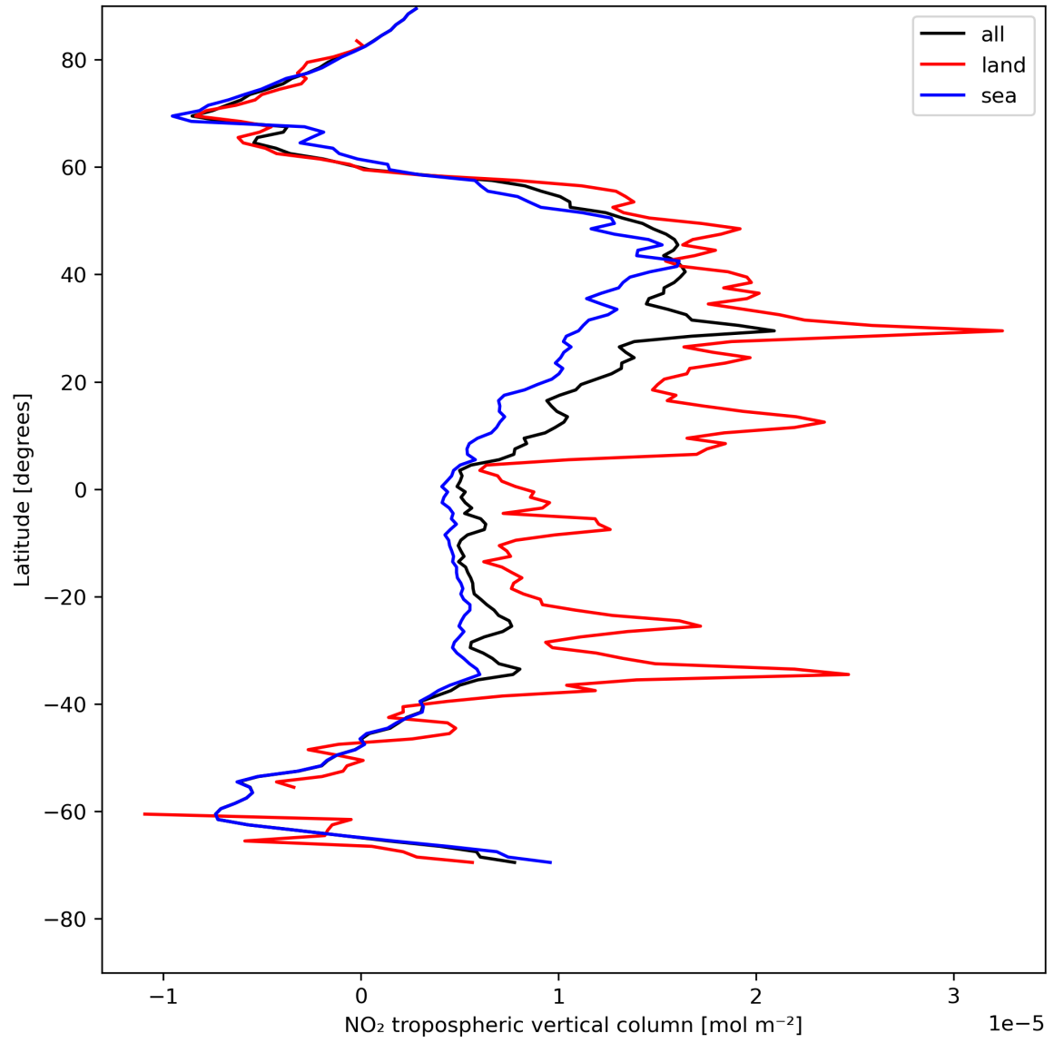
Figure 12: Zonal average of “NO 2 tropospheric vertical column” for 2024-05-10 to 2024-05-12.
