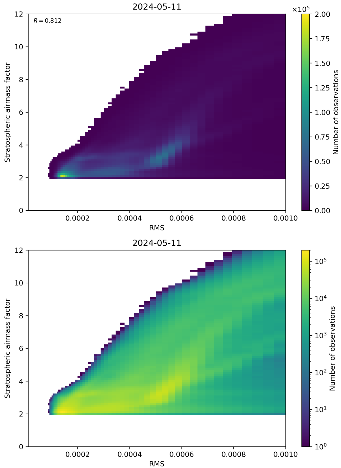
Figure 144: Scatter density plot of “RMS” against “Stratospheric airmass factor” for 2024-05-10 to 2024-05-12.
