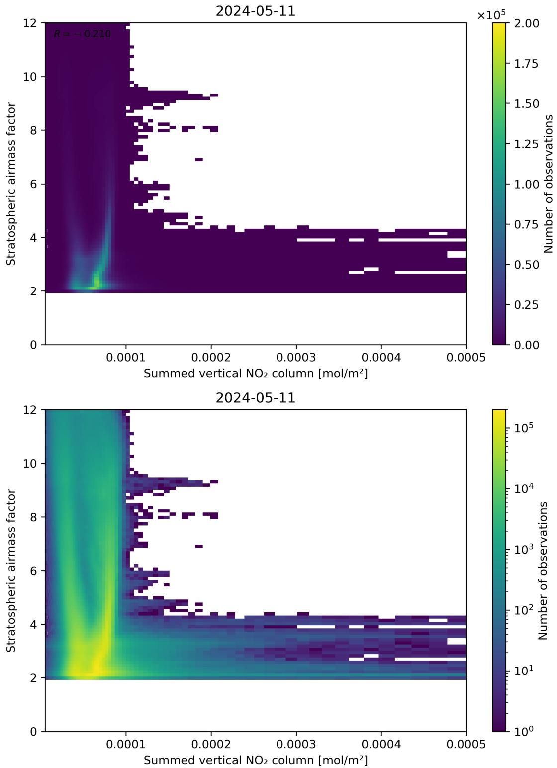
Figure 103: Scatter density plot of “Summed vertical NO 2 column” against “Stratospheric air mass factor” for 2024-05-10 to 2024-05-12.
