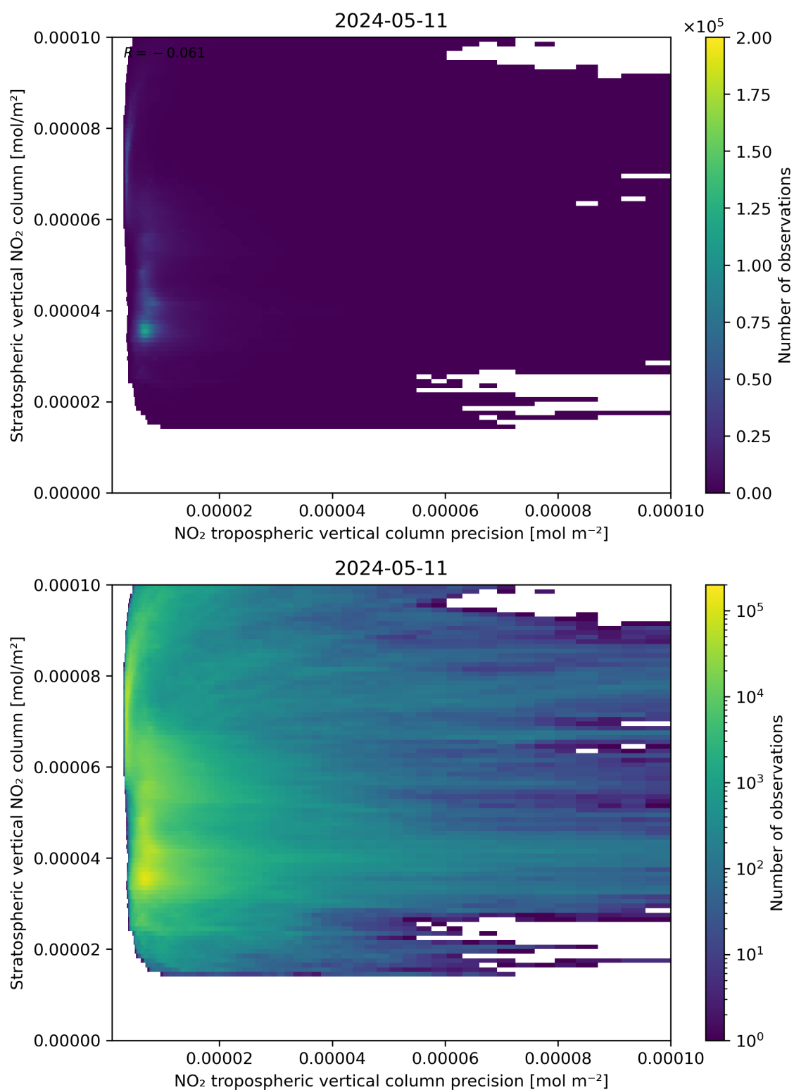
Figure 135: Scatter density plot of “NO 2 tropospheric vertical column precision” against “Stratospheric vertical NO 2 column” for 2024-05-10 to 2024-05-12.
