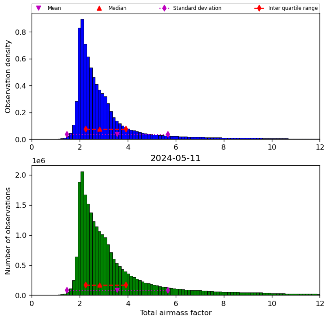
Figure 32: Histogram of “Total airmass factor” for 2024-05-10 to 2024-05-12
