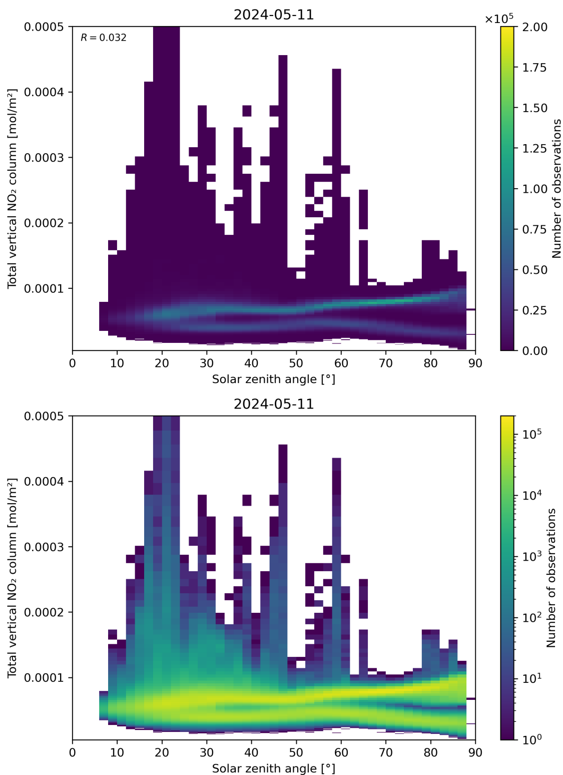
Figure 153: Scatter density plot of “Solar zenith angle” against “Total vertical NO 2 column” for 2024-05-10 to 2024-05-12.
