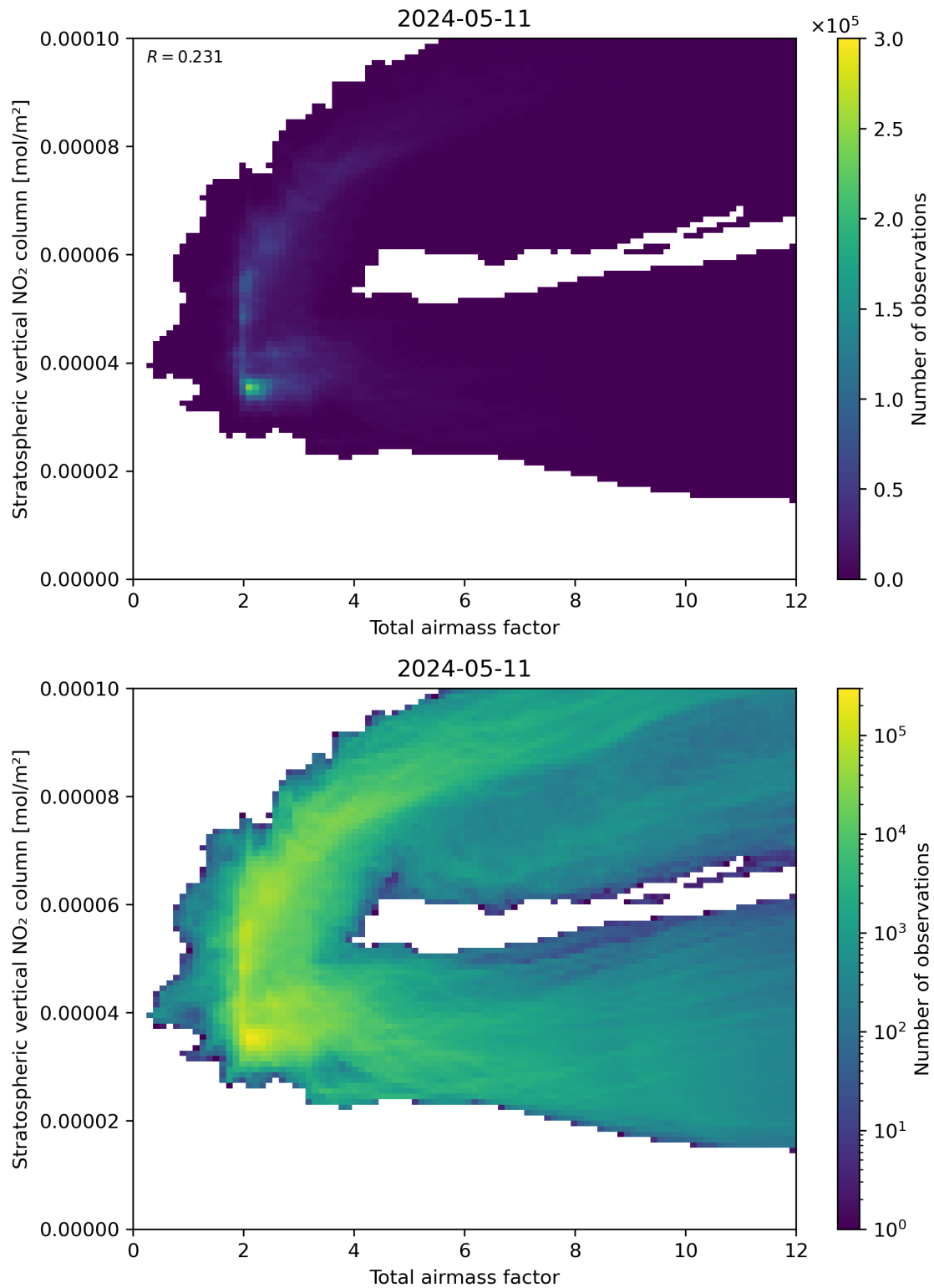
Figure 64: Scatter density plot of “Total airmass factor” against “Stratospheric vertical \text{NO}_2 column” for 2024-05-10 to 2024-05-12.
