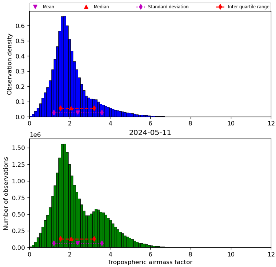
Figure 31: Histogram of “Tropospheric airmass factor” for 2024-05-10 to 2024-05-12
