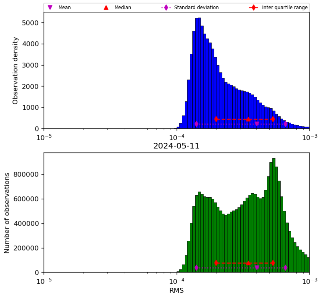
Figure 43: Histogram of “RMS” for 2024-05-10 to 2024-05-12
