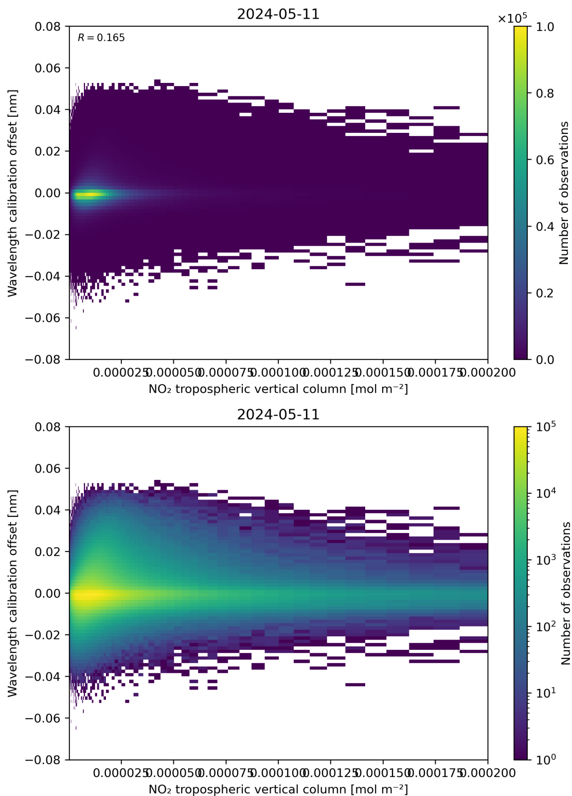
Figure 143: Scatter density plot of “NO 2 tropospheric vertical column” against “Wavelength calibration offset” for 2024-05-10 to 2024-05-12.
