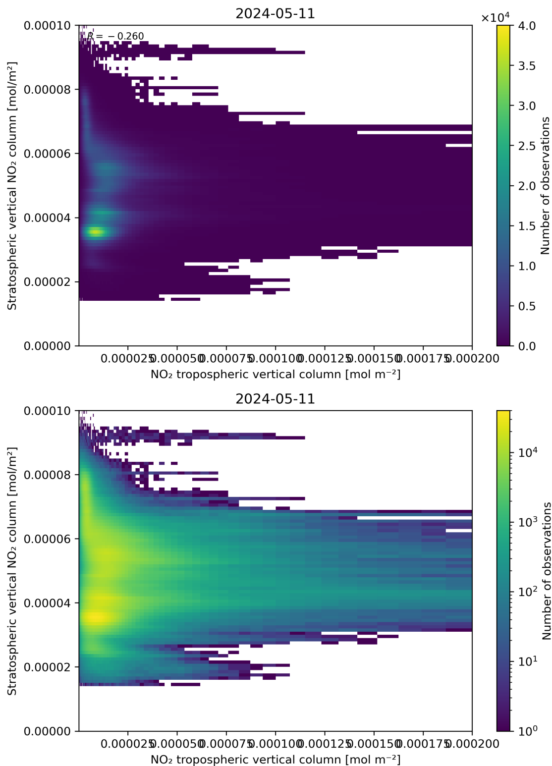
Figure 125: Scatter density plot of “NO 2 tropospheric vertical column” against “Stratospheric vertical NO 2 column” for 2024-05-10 to 2024-05-12.
