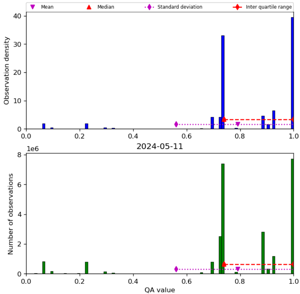
Figure 28: Histogram of “QA value” for 2024-05-10 to 2024-05-12
