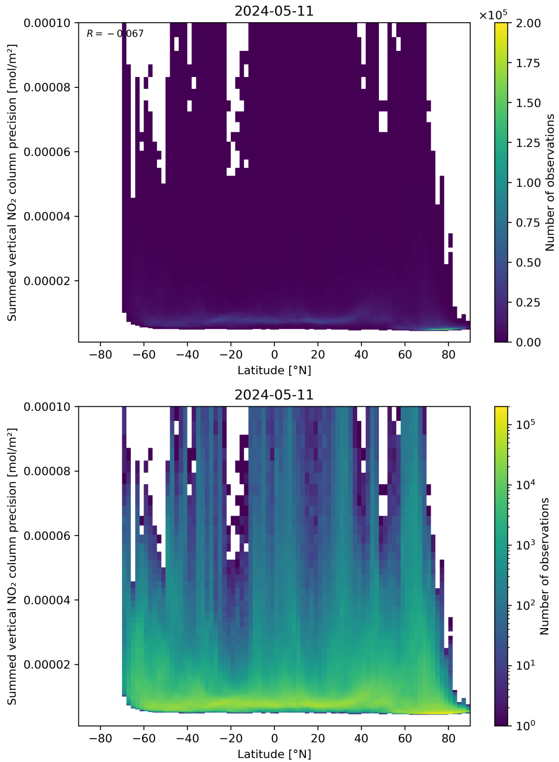
Figure 89: Scatter density plot of “Latitude” against “Summed vertical NO 2 column precision” for 2024-05-10 to 2024-05-12.
