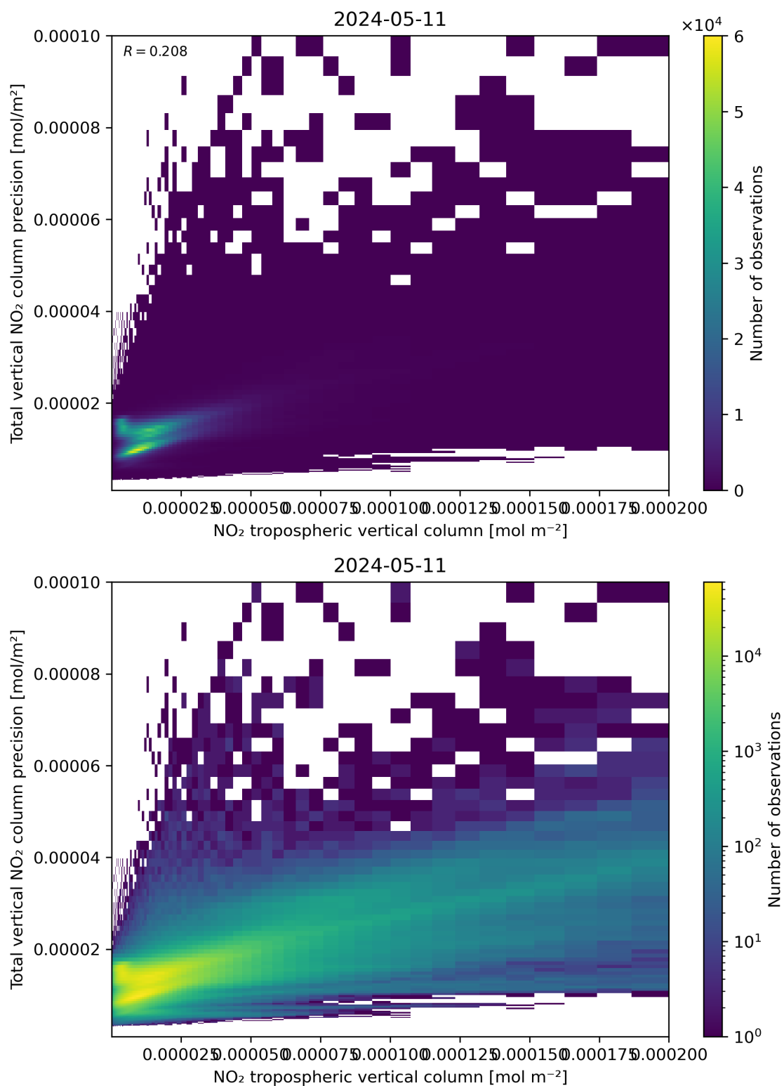
Figure 129: Scatter density plot of “NO 2 tropospheric vertical column” against “Total vertical NO 2 column precision” for 2024-05-10 to 2024-05-12.
