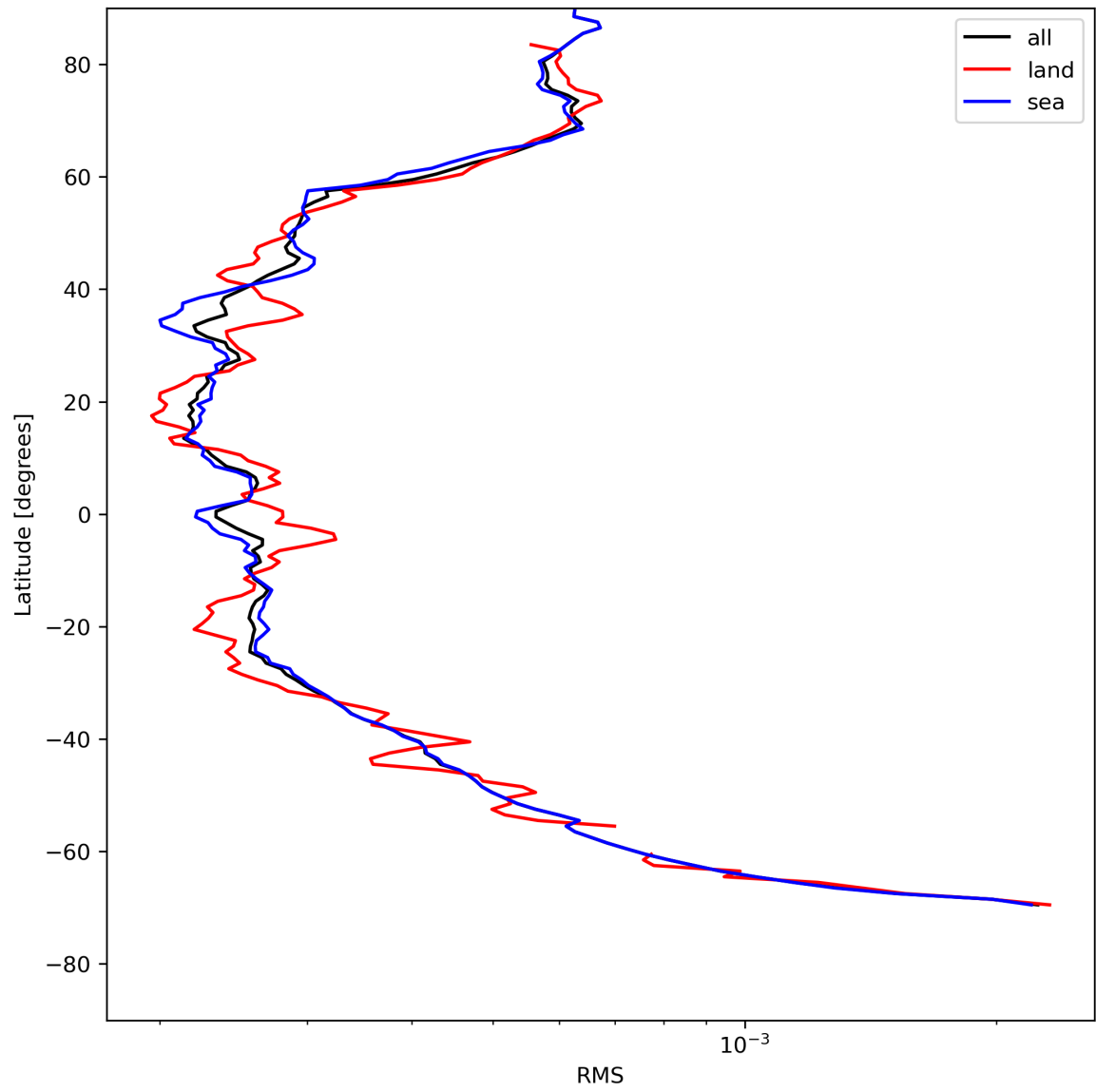
Figure 26: Zonal average of “RMS” for 2024-05-10 to 2024-05-12.
