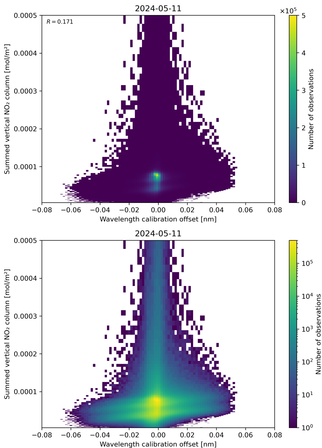
Figure 177: Scatter density plot of “Wavelength calibration offset” against “Summed vertical NO 2 column” for 2024-05-10 to 2024-05-12.
