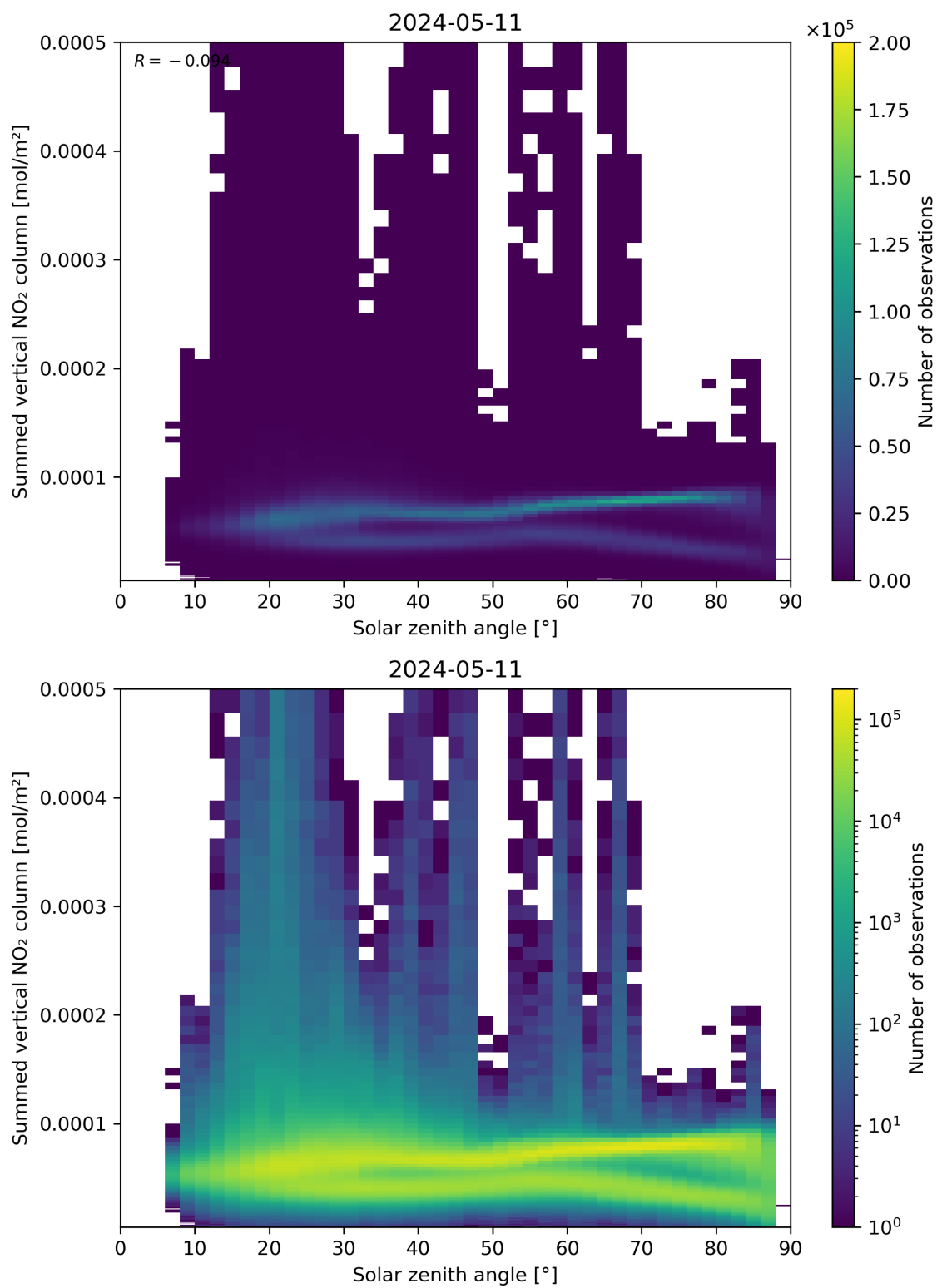
Figure 151: Scatter density plot of “Solar zenith angle” against “Summed vertical NO 2 column” for 2024-05-10 to 2024-05-12.
