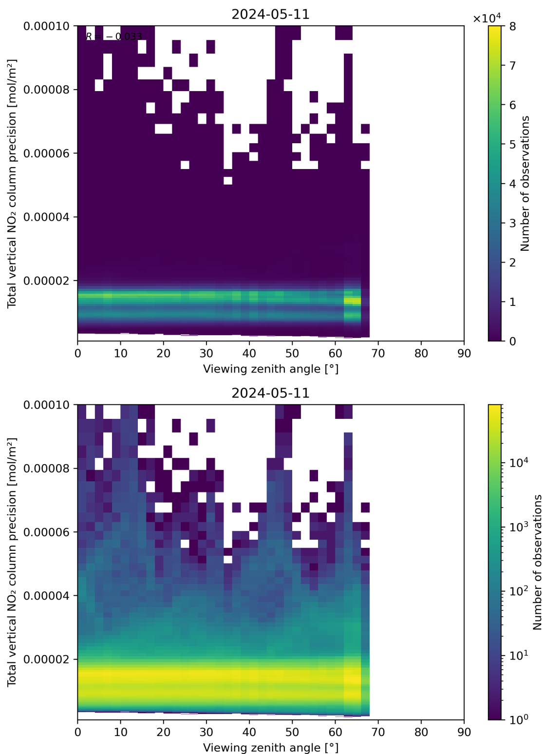
Figure 168: Scatter density plot of “Viewing zenith angle” against “Total vertical NO 2 column precision” for 2024-05-10 to 2024-05-12.
