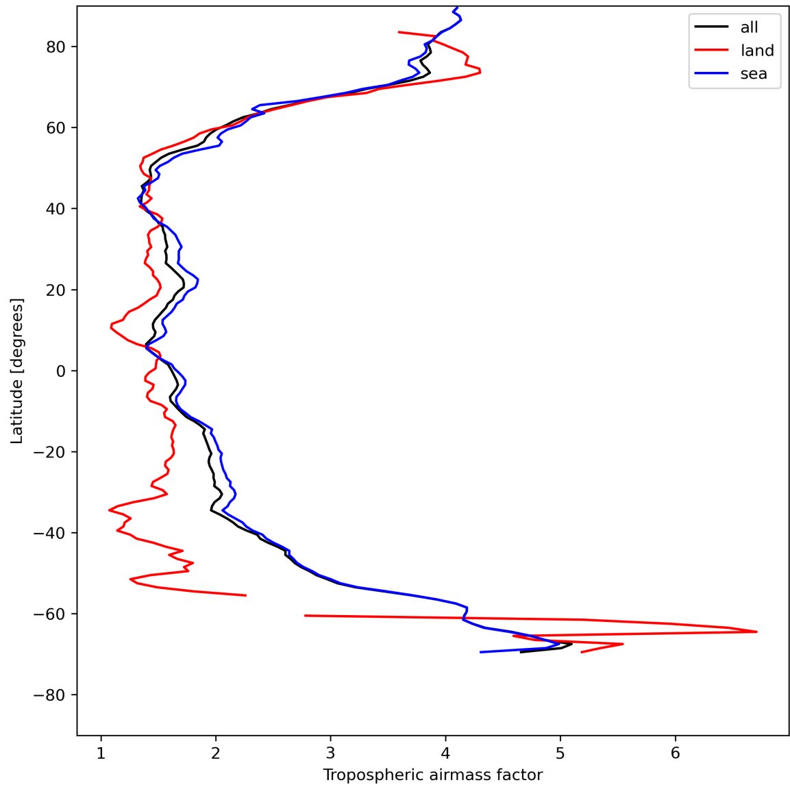
Figure 14: Zonal average of “Tropospheric air mass factor” for 2024-05-10 to 2024-05-12.
