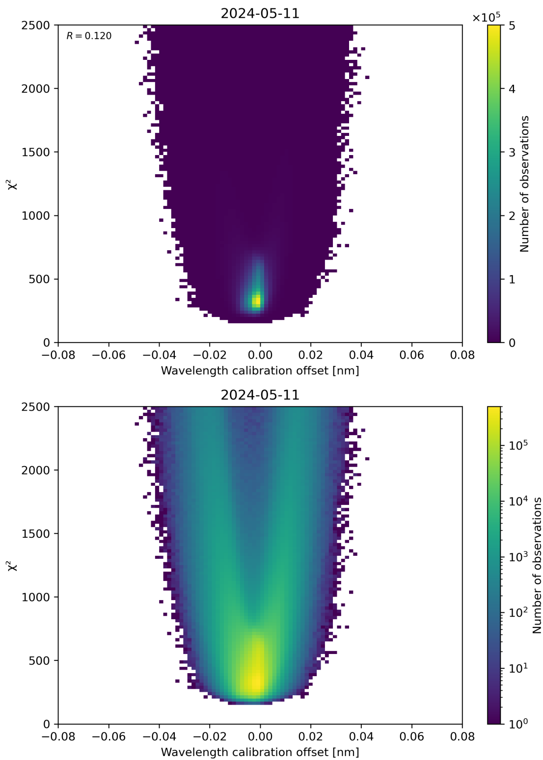
Figure 175: Scatter density plot of “Wavelength calibration offset” against “ \chi^2 ” for 2024-05-10 to 2024-05-12.
