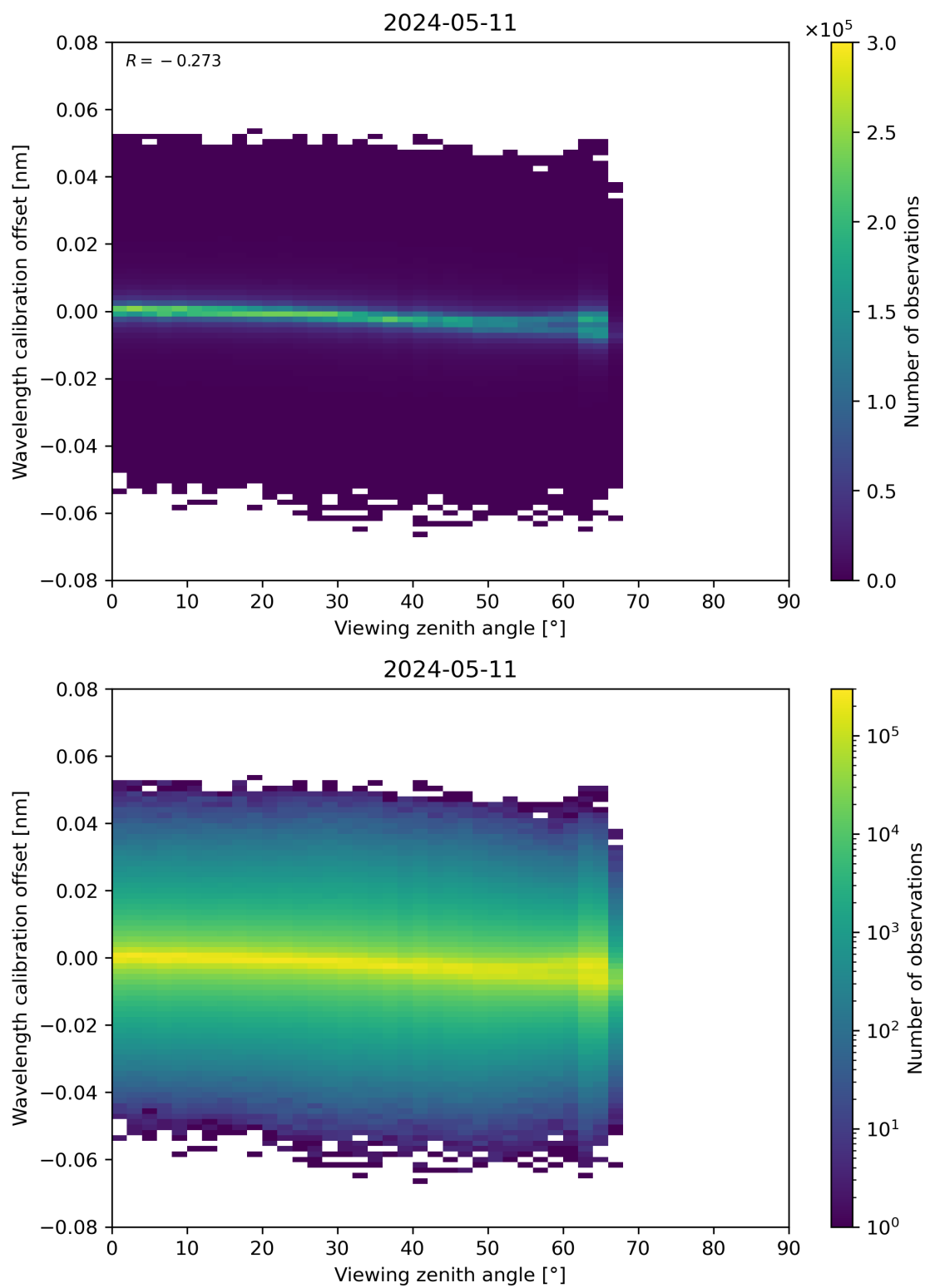
Figure 173: Scatter density plot of “Viewing zenith angle” against “Wavelength calibration offset” for 2024-05-10 to 2024-05-12.
