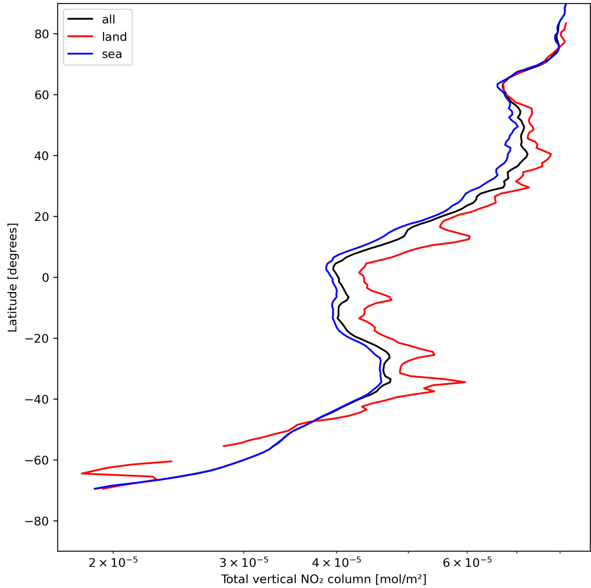
Figure 21: Zonal average of “Total vertical NO 2 column” for 2024-05-10 to 2024-05-12.
