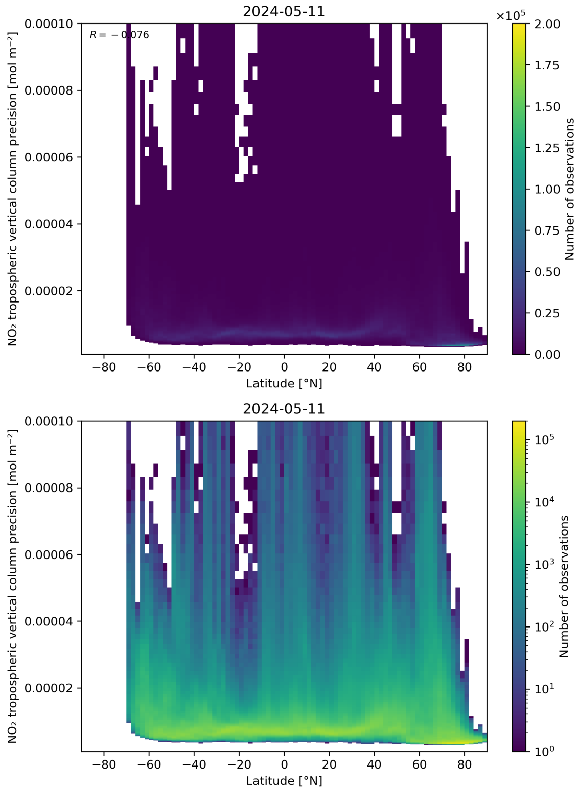
Figure 93: Scatter density plot of “Latitude” against “NO 2 tropospheric vertical column precision” for 2024-05-10 to 2024-05-12.
