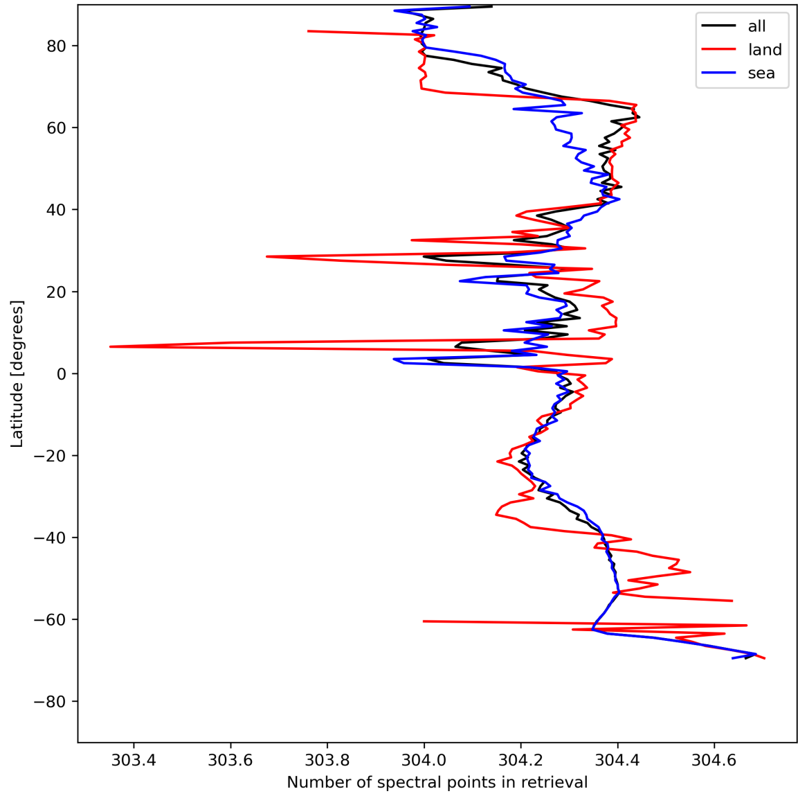
Figure 16: Zonal average of “Number of spectral points in retrieval” for 2024-05-10 to 2024-05-12.
