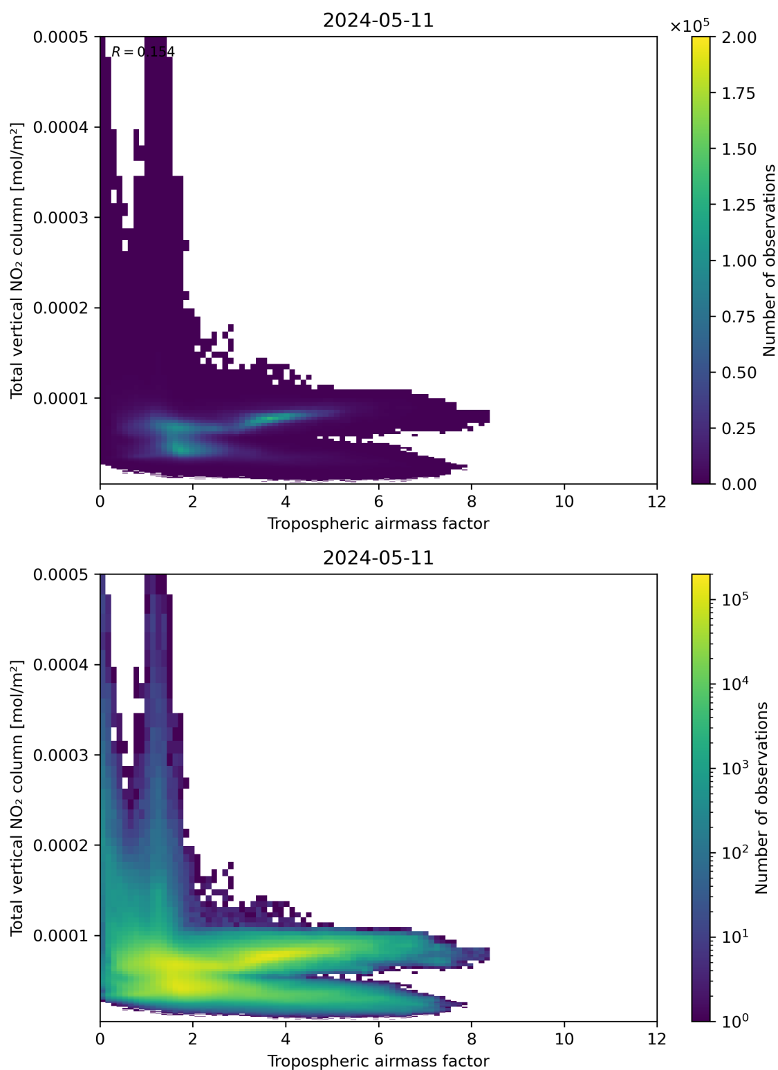
Figure 77: Scatter density plot of “Tropospheric airmass factor” against “Total vertical NO 2 column” for 2024-05-10 to 2024-05-12.
