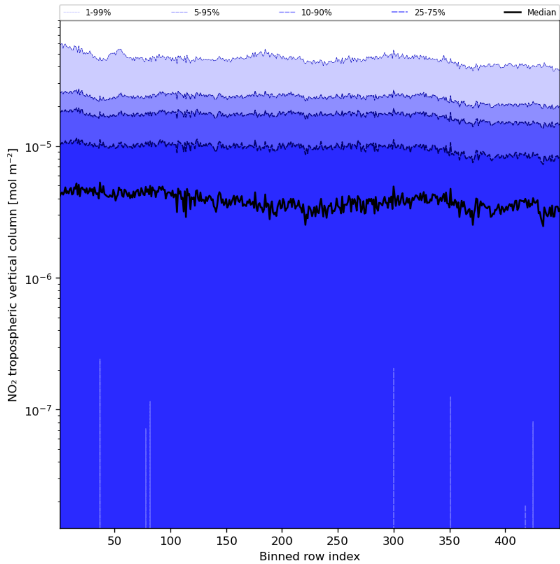
Figure 46: Along track statistics of “NO 2 tropospheric vertical column” for 2024-05-10 to 2024-05-12
