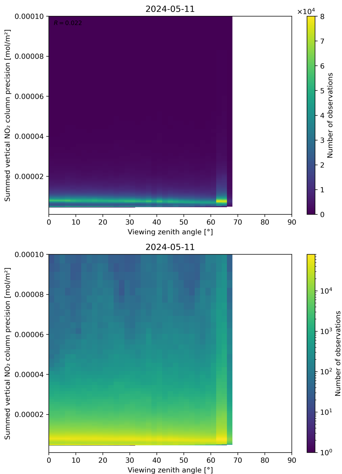
Figure 166: Scatter density plot of “Viewing zenith angle” against “Summed vertical NO 2 column precision” for 2024-05-10 to 2024-05-12.
