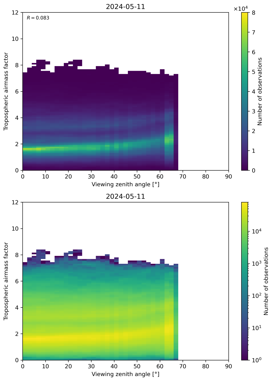
Figure 161: Scatter density plot of “Viewing zenith angle” against “Tropospheric airmass factor” for 2024-05-10 to 2024-05-12.
