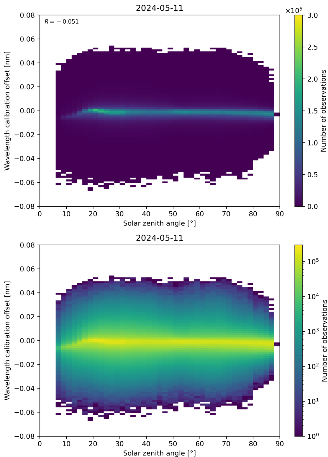
Figure 158: Scatter density plot of “Solar zenith angle” against “Wavelength calibration offset” for 2024-05-10 to 2024-05-12.
