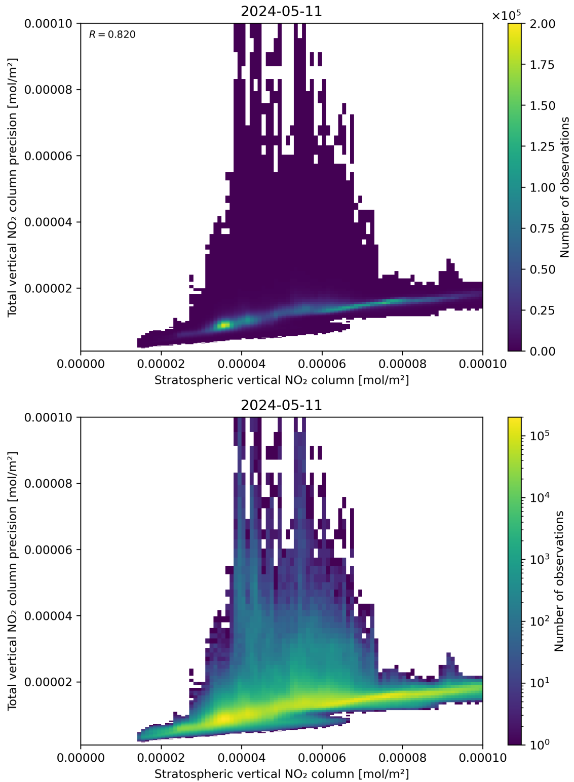
Figure 101: Scatter density plot of “Stratospheric vertical NO 2 column” against “Total vertical NO 2 column precision” for 2024-05-10 to 2024-05-12.
