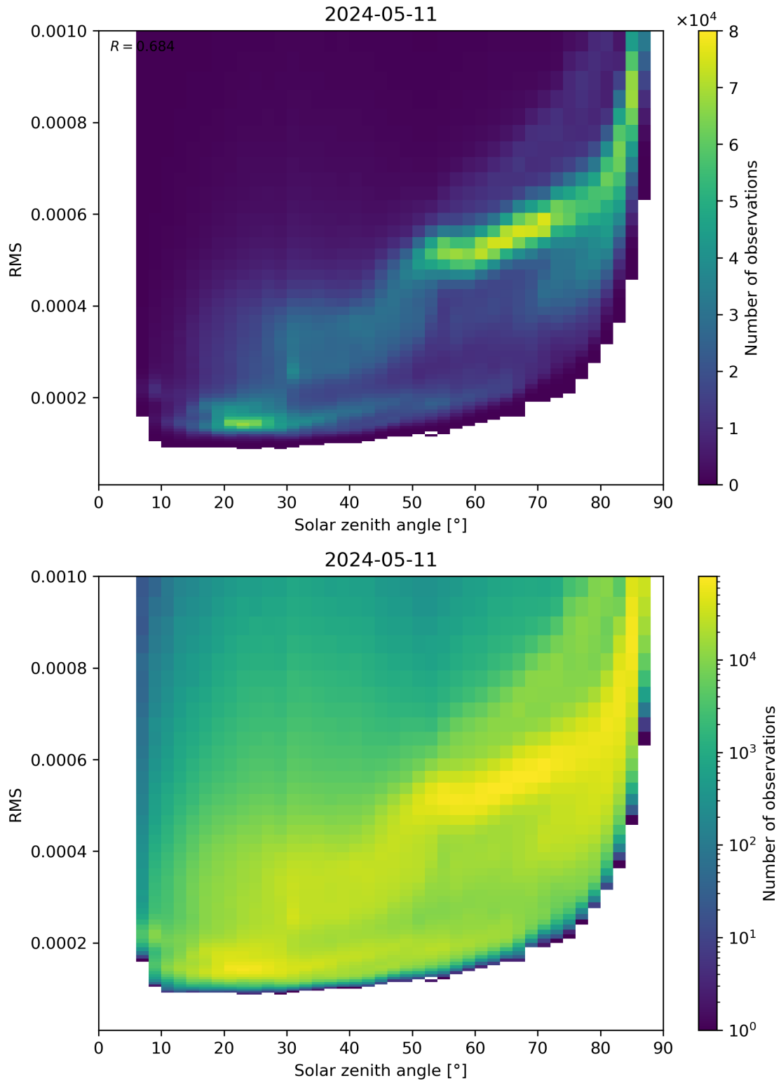
Figure 157: Scatter density plot of “Solar zenith angle” against “RMS” for 2024-05-10 to 2024-05-12.
