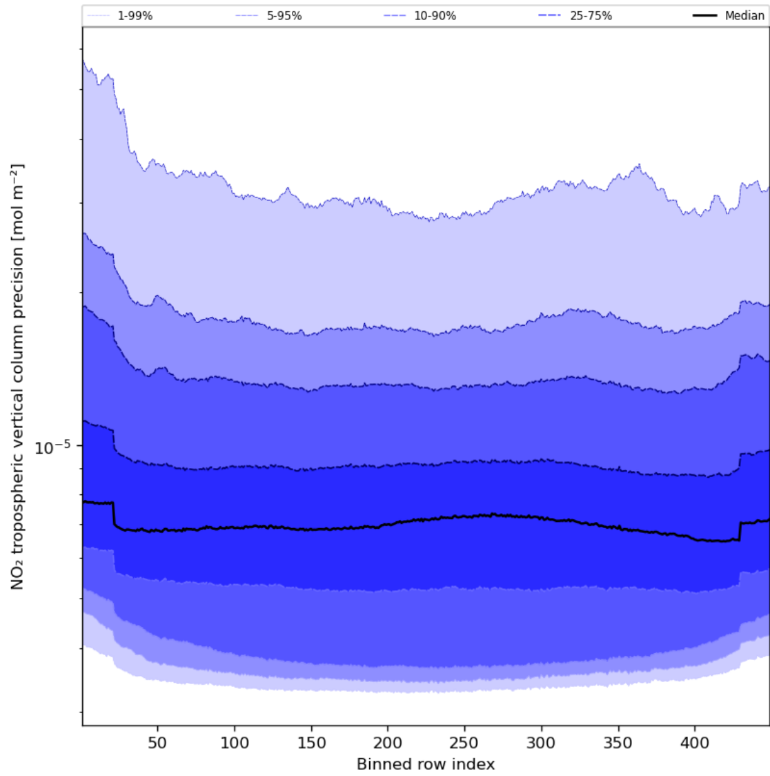
Figure 47: Along track statistics of “NO 2 tropospheric vertical column precision” for 2024-05-10 to 2024-05-12
