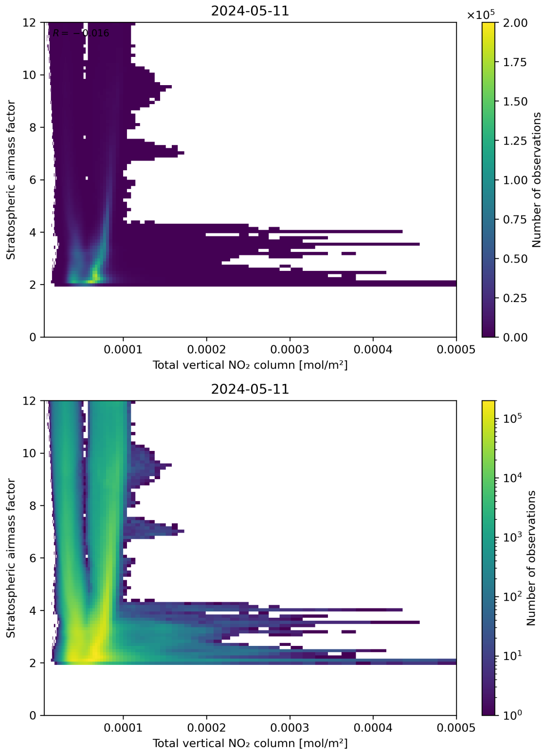
Figure 110: Scatter density plot of “Total vertical NO 2 column” against “Stratospheric airmass factor” for 2024-05-10 to 2024-05-12.
