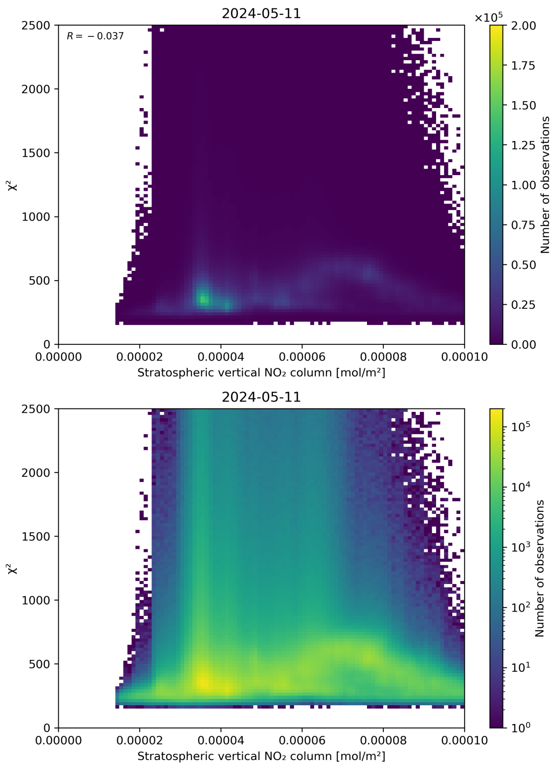
Figure 97: Scatter density plot of “Stratospheric vertical NO 2 column” against “ \chi^2 ” for 2024-05-10 to 2024-05-12.
