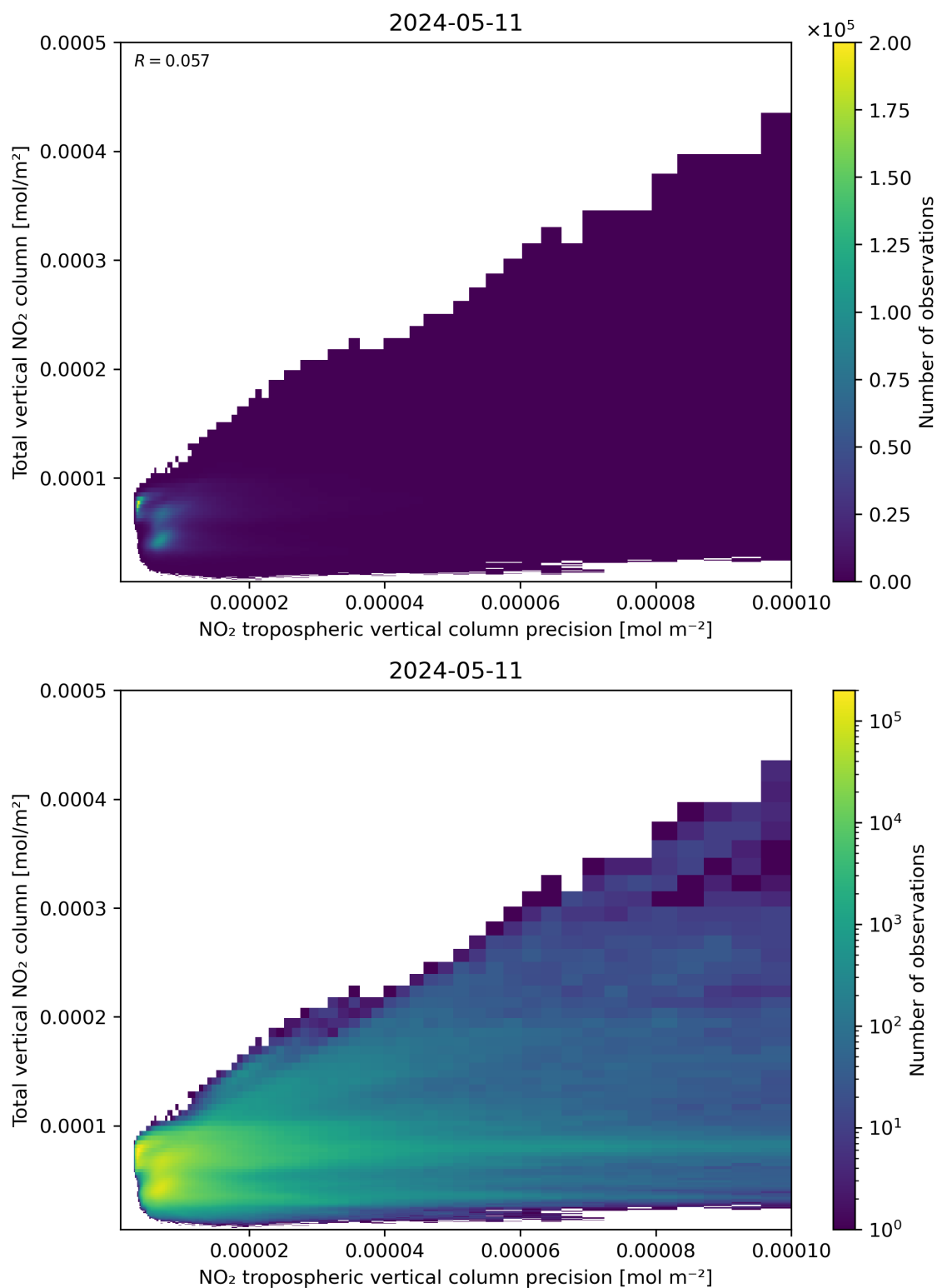
Figure 138: Scatter density plot of “NO 2 tropospheric vertical column precision” against “Total vertical NO 2 column” for 2024-05-10 to 2024-05-12.
