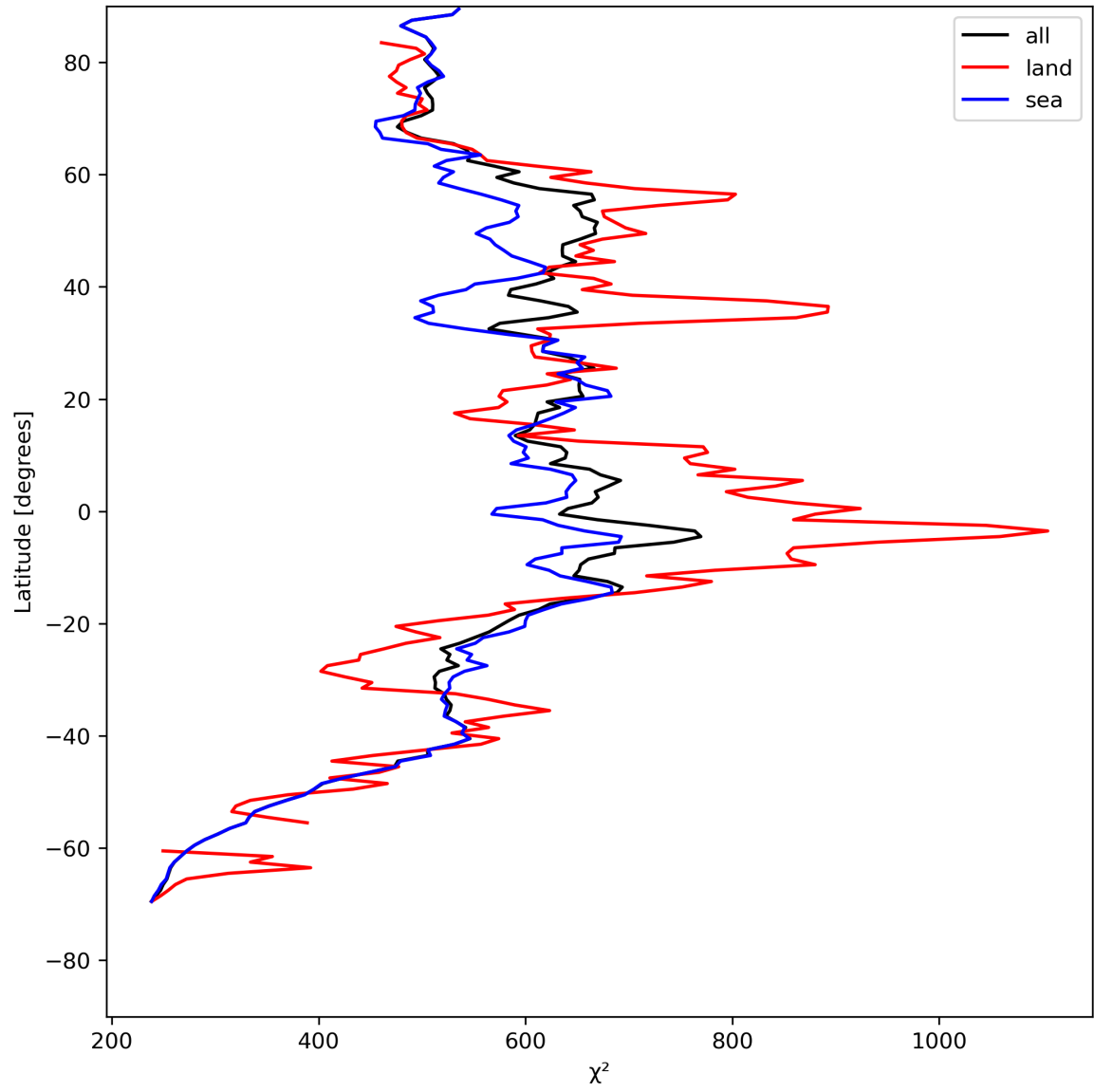
Figure 25: Zonal average of “ \chi^2 ” for 2024-05-10 to 2024-05-12.
