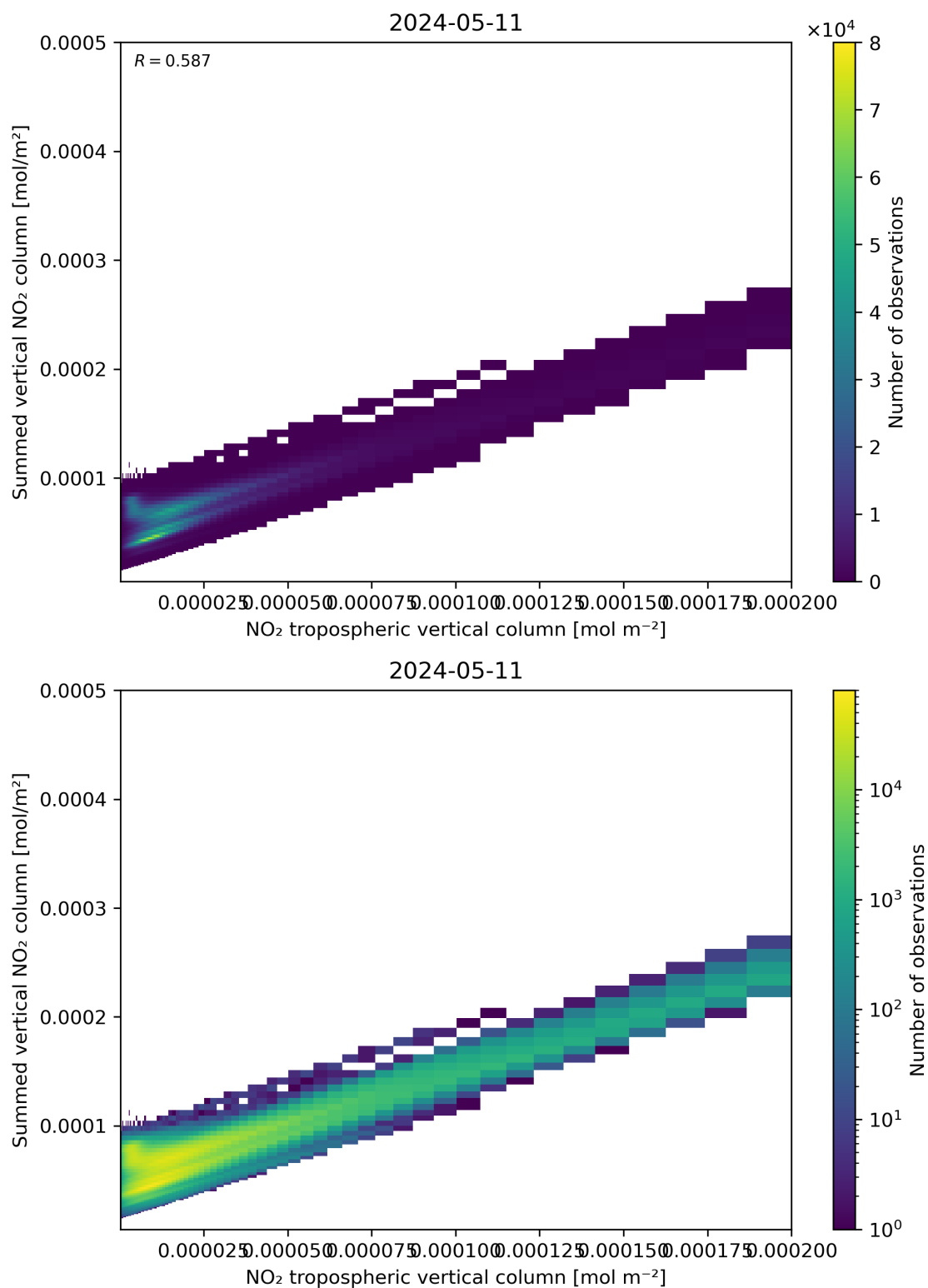
Figure 126: Scatter density plot of “NO 2 tropospheric vertical column” against “Summed vertical NO 2 column” for 2024-05-10 to 2024-05-12.
