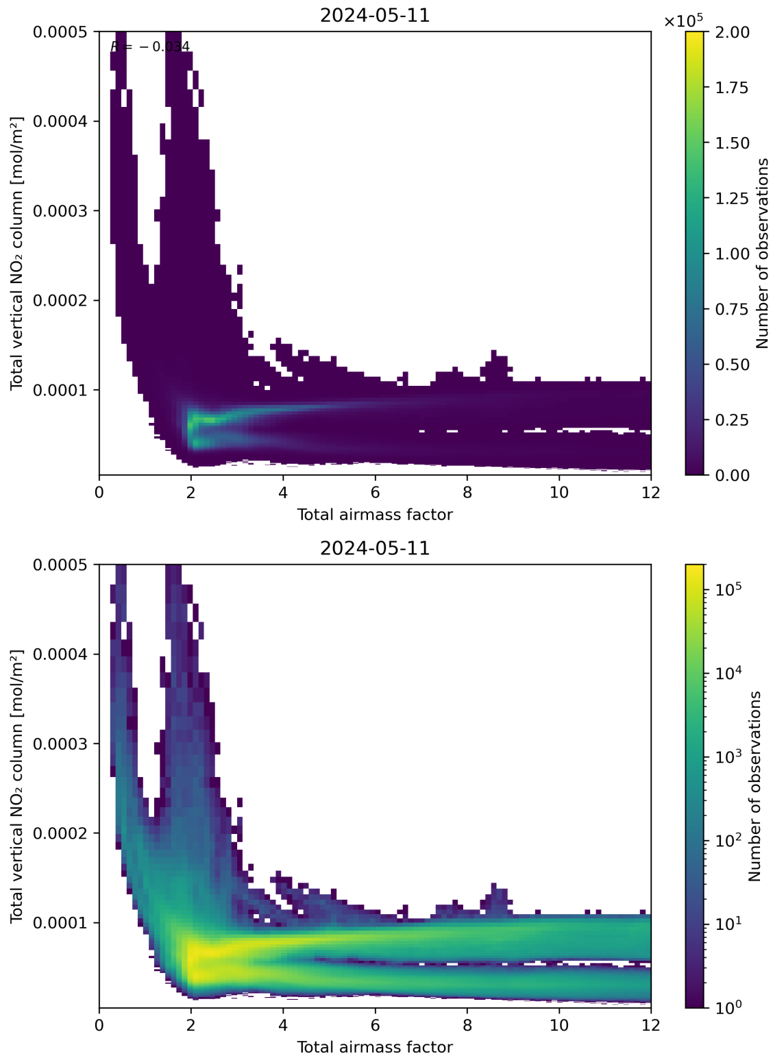
Figure 67: Scatter density plot of “Total airmass factor” against “Total vertical NO 2 column” for 2024-05-10 to 2024-05-12.
