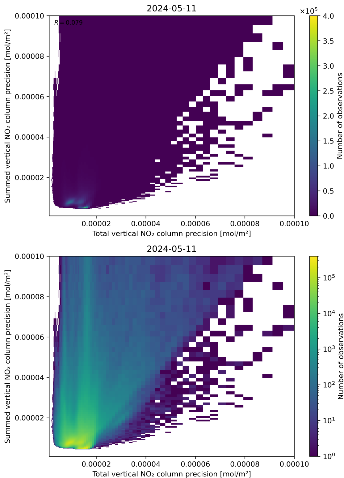
Figure 118: Scatter density plot of “Total vertical NO 2 column precision” against “Summed vertical NO 2 column precision” for 2024-05-10 to 2024-05-12.
