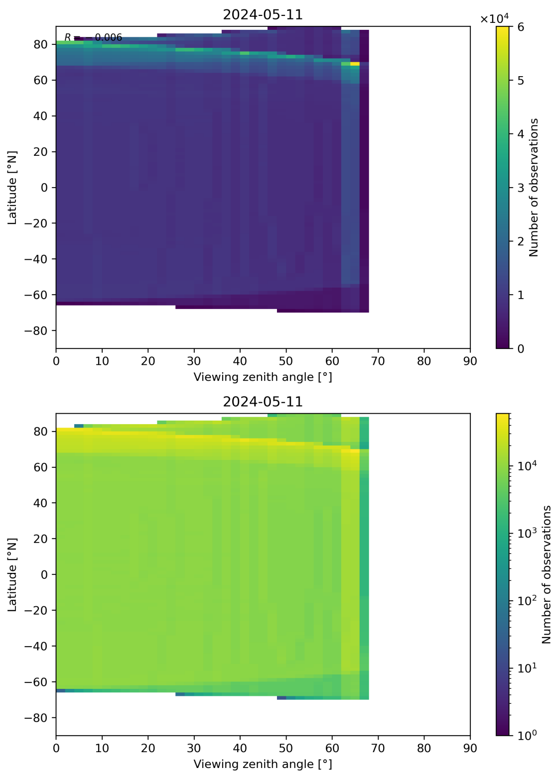
Figure 163: Scatter density plot of “Viewing zenith angle” against “Latitude” for 2024-05-10 to 2024-05-12.
