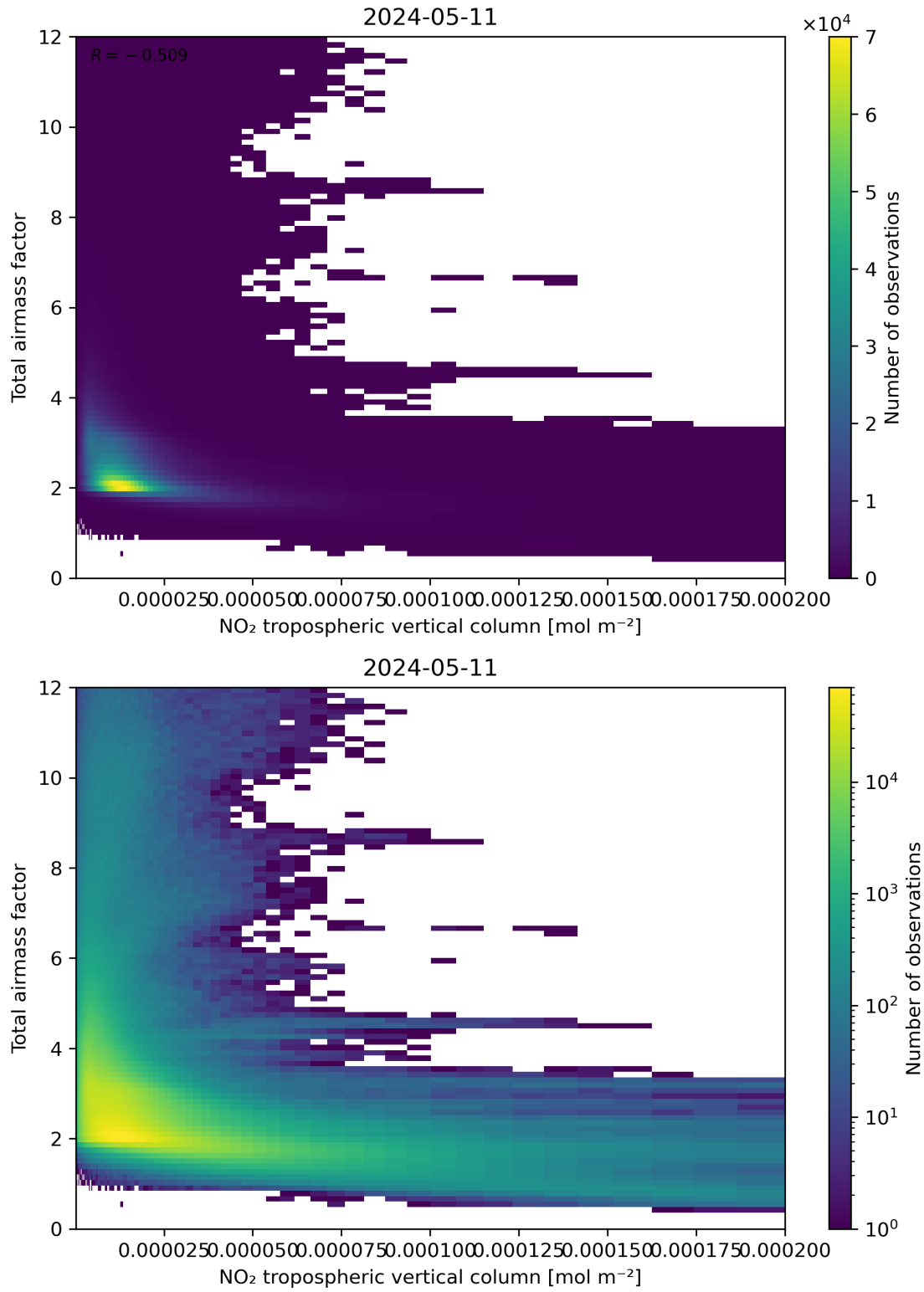
Figure 122: Scatter density plot of “NO 2 tropospheric vertical column” against “Total airmass factor” for 2024-05-10 to 2024-05-12.
