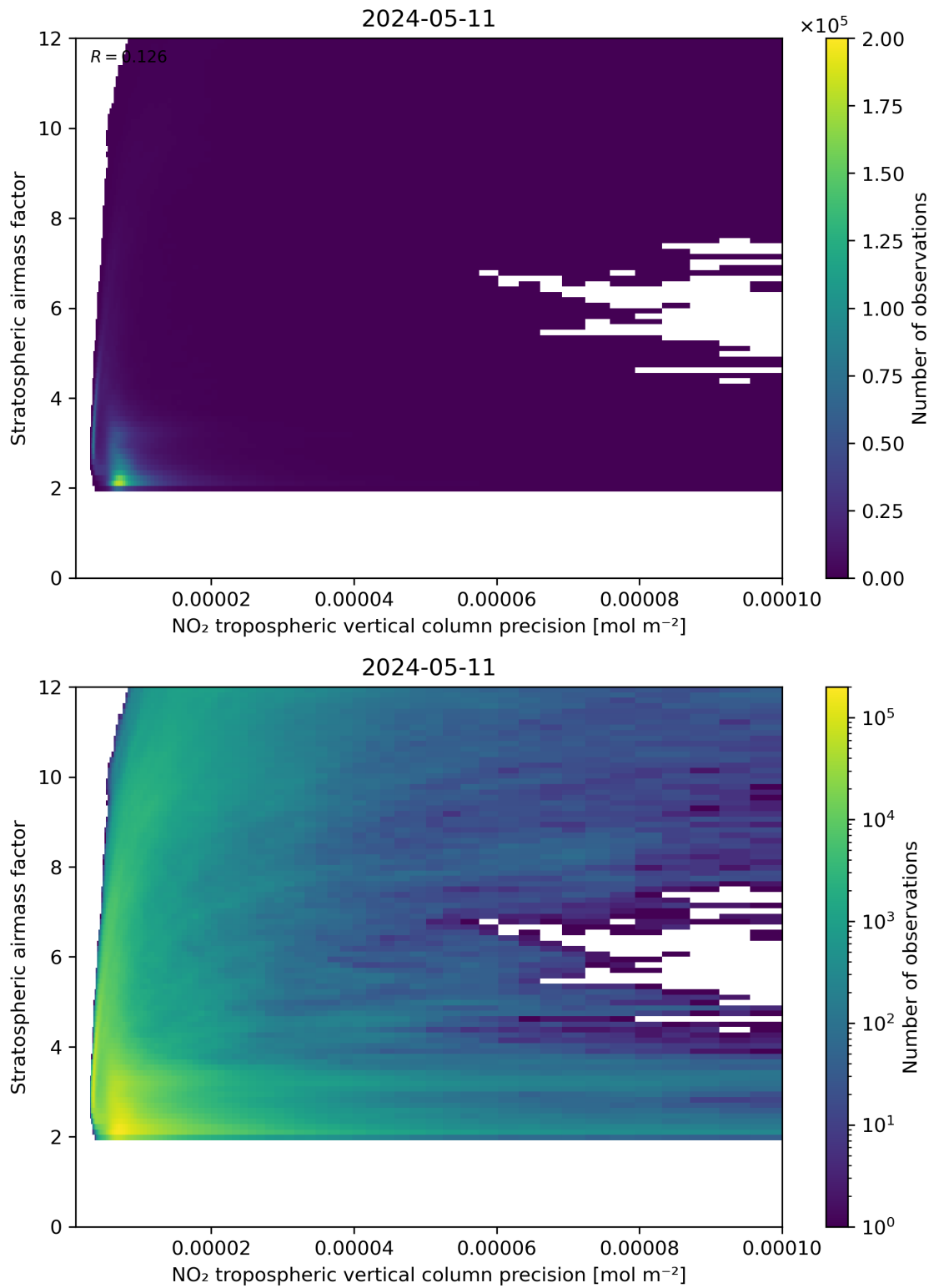
Figure 131: Scatter density plot of “NO 2 tropospheric vertical column precision” against “Stratospheric airmass factor” for 2024-05-10 to 2024-05-12.
