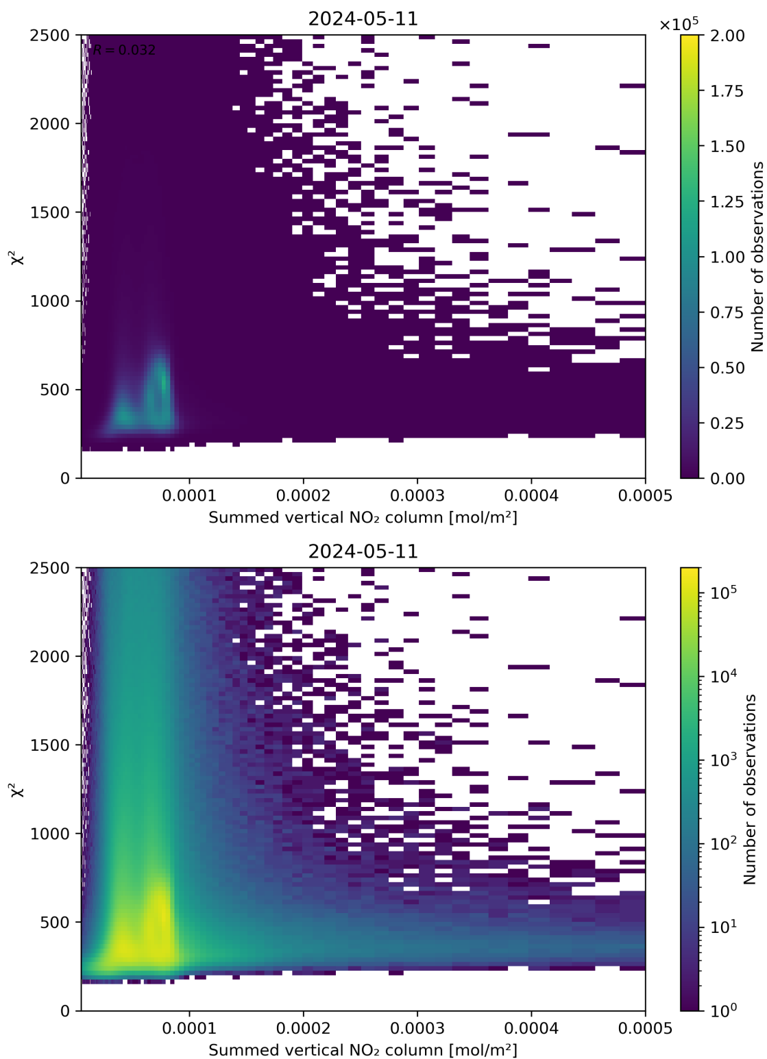
Figure 104: Scatter density plot of “Summed vertical NO 2 column” against “ \chi^2 ” for 2024-05-10 to 2024-05-12.
