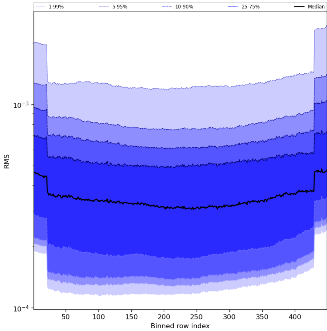
Figure 60: Along track statistics of “RMS” for 2024-05-10 to 2024-05-12
