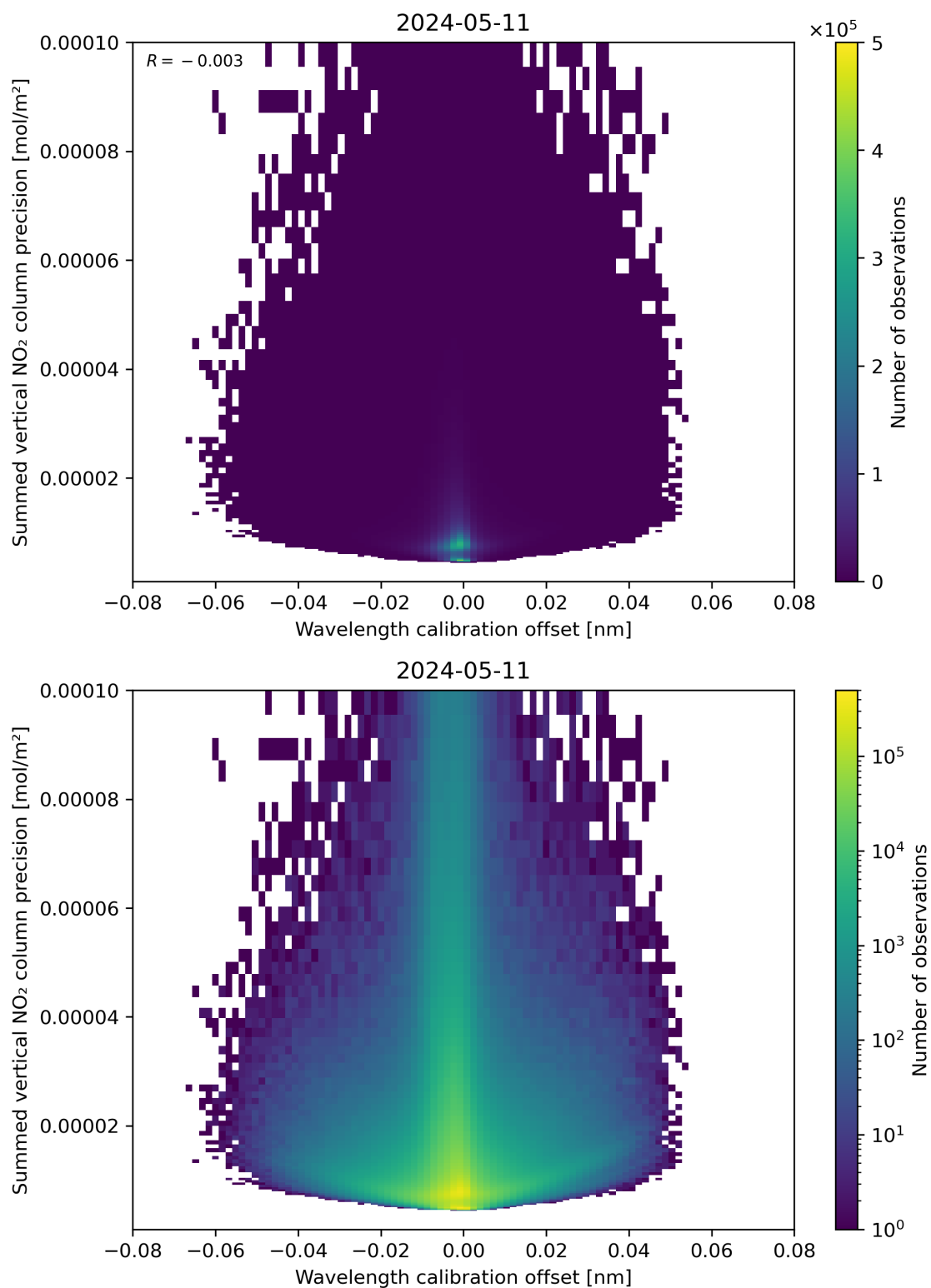
Figure 178: Scatter density plot of “Wavelength calibration offset” against “Summed vertical NO 2 column precision” for 2024-05-10 to 2024-05-12.
