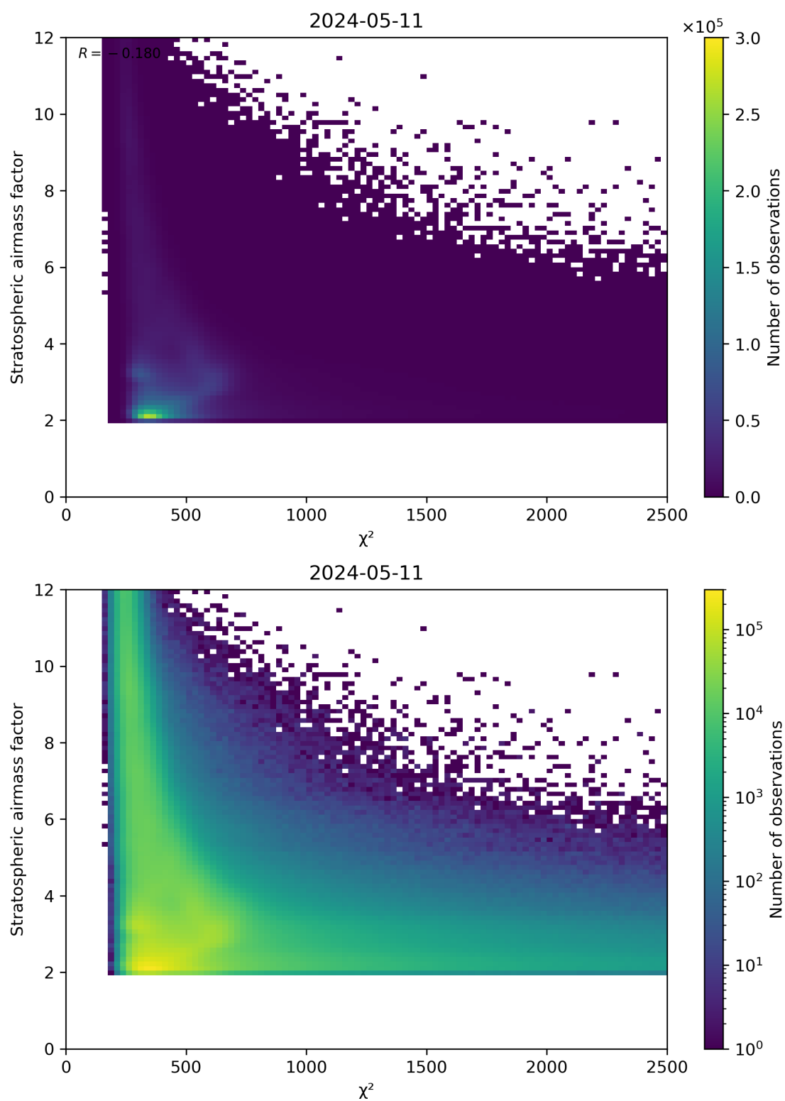
Figure 81: Scatter density plot of “ \chi^2 ” against “Stratospheric airmass factor” for 2024-05-10 to 2024-05-12.
