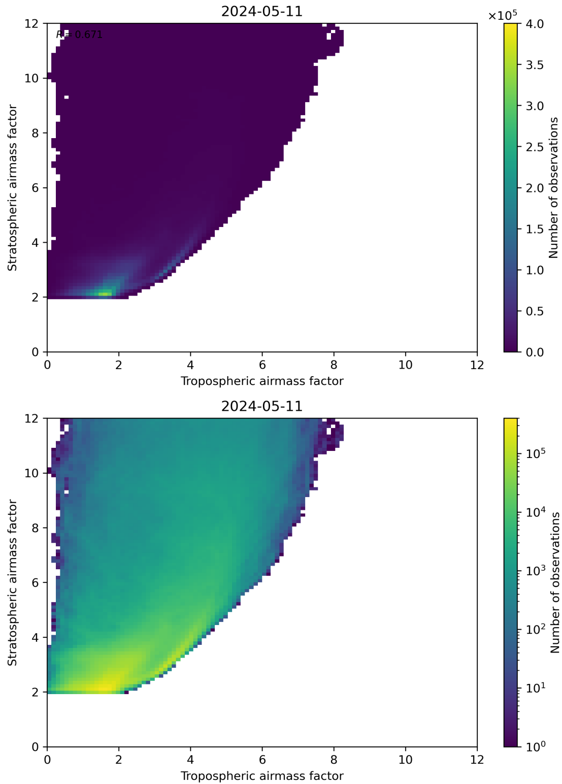
Figure 71: Scatter density plot of “Tropospheric airmass factor” against “Stratospheric airmass factor” for 2024-05-10 to 2024-05-12.
