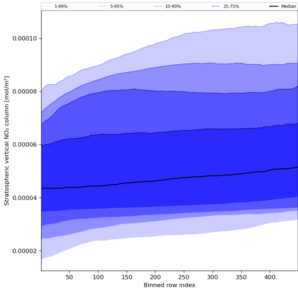
Figure 53: Along track statistics of “Stratospheric vertical NO 2 column” for 2024-05-10 to 2024-05-12
