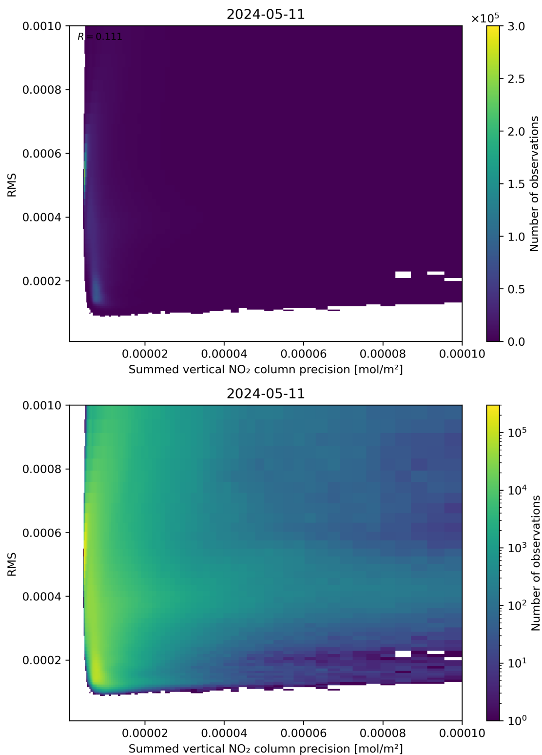
Figure 108: Scatter density plot of “Summed vertical NO 2 column precision” against “RMS” for 2024-05-10 to 2024-05-12.
