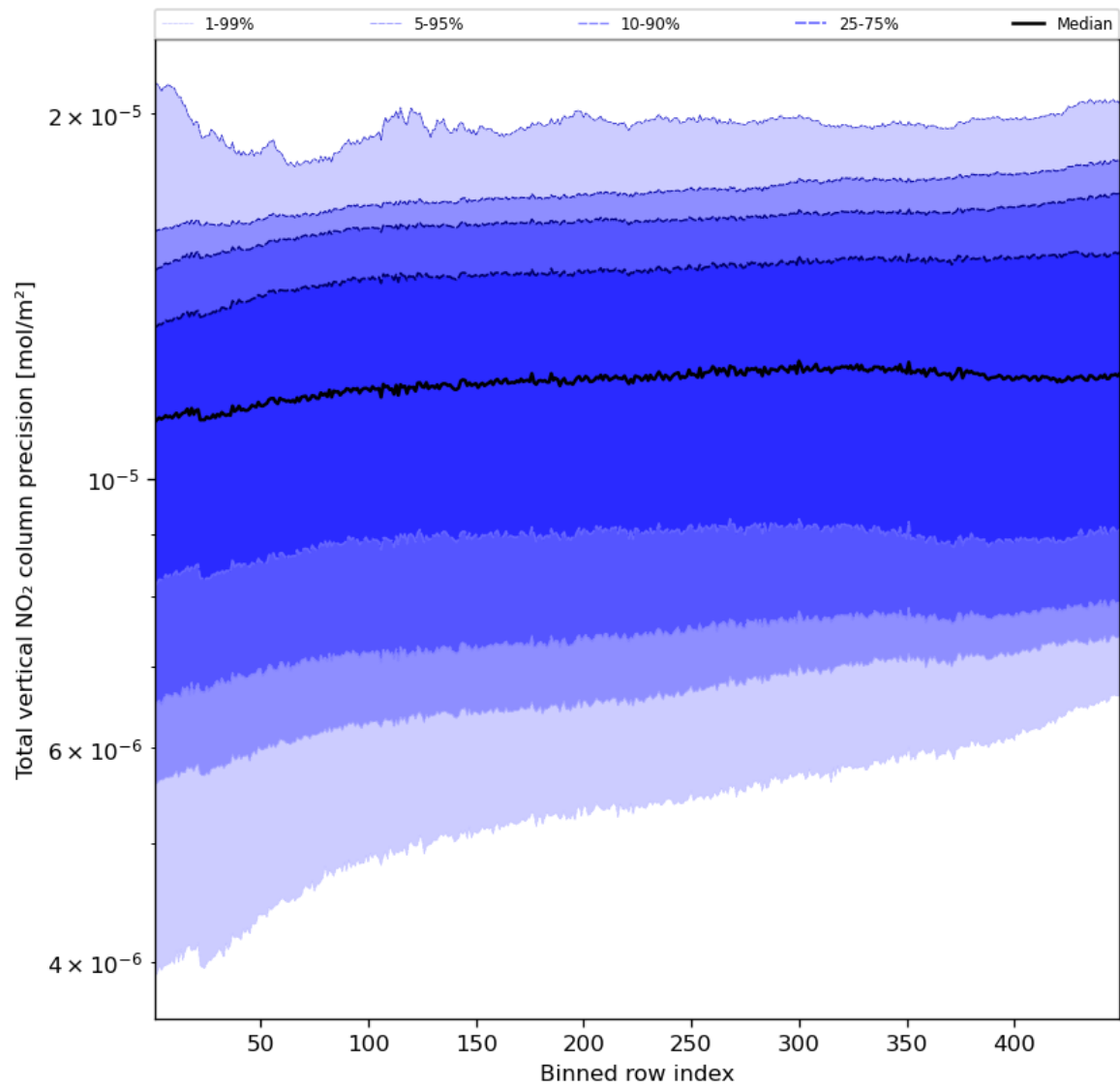
Figure 56: Along track statistics of “Total vertical NO 2 column precision” for 2024-05-10 to 2024-05-12
