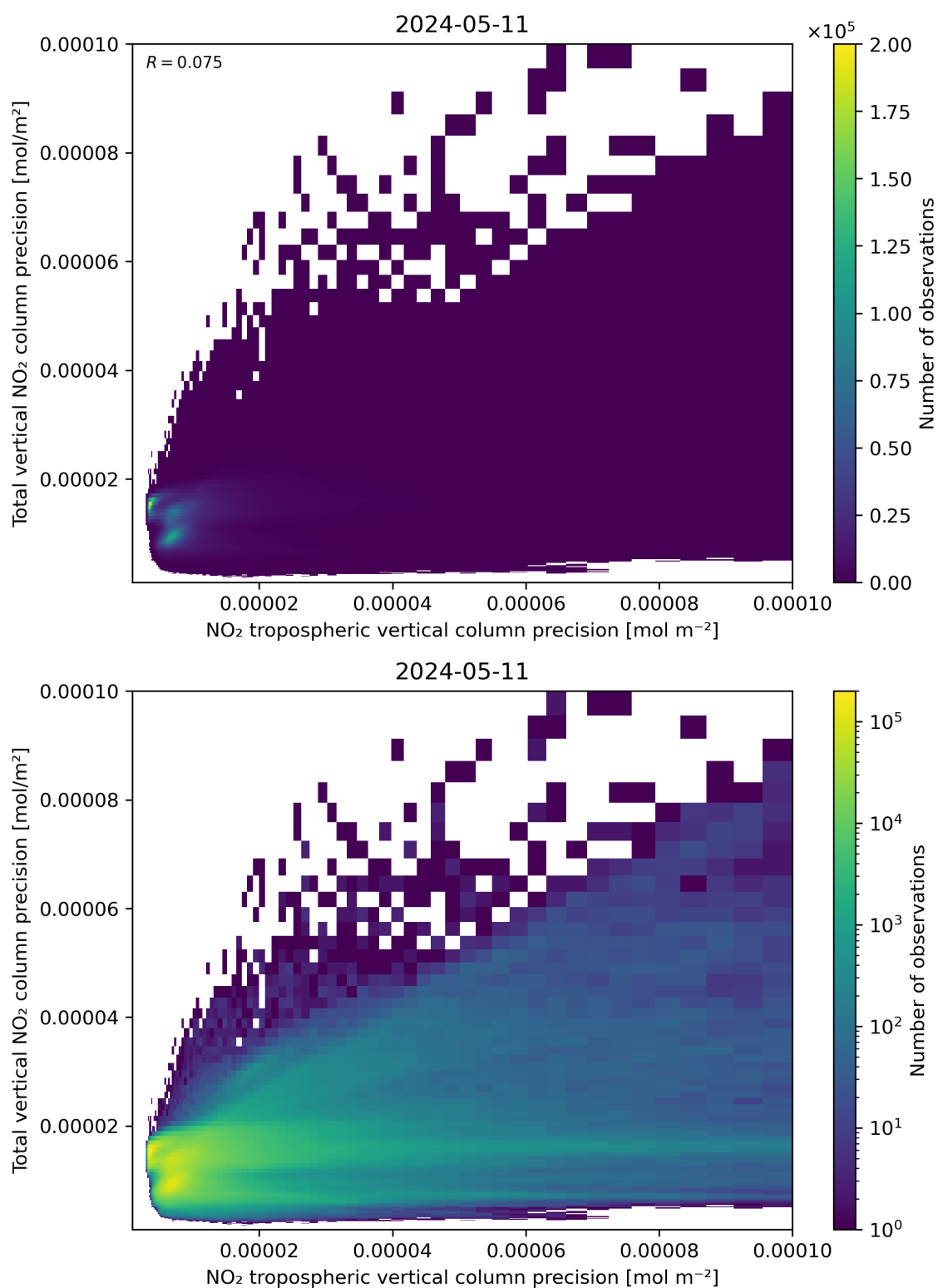
Figure 139: Scatter density plot of “NO 2 tropospheric vertical column precision” against “Total vertical NO 2 column precision” for 2024-05-10 to 2024-05-12.
