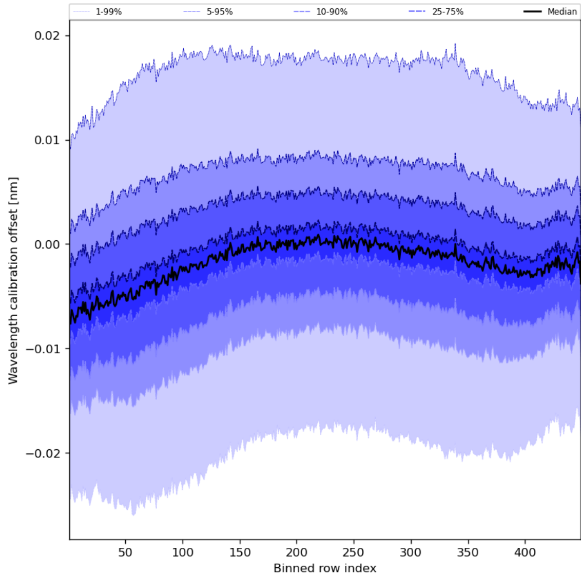
Figure 52: Along track statistics of “Wavelength calibration offset” for 2024-05-10 to 2024-05-12
