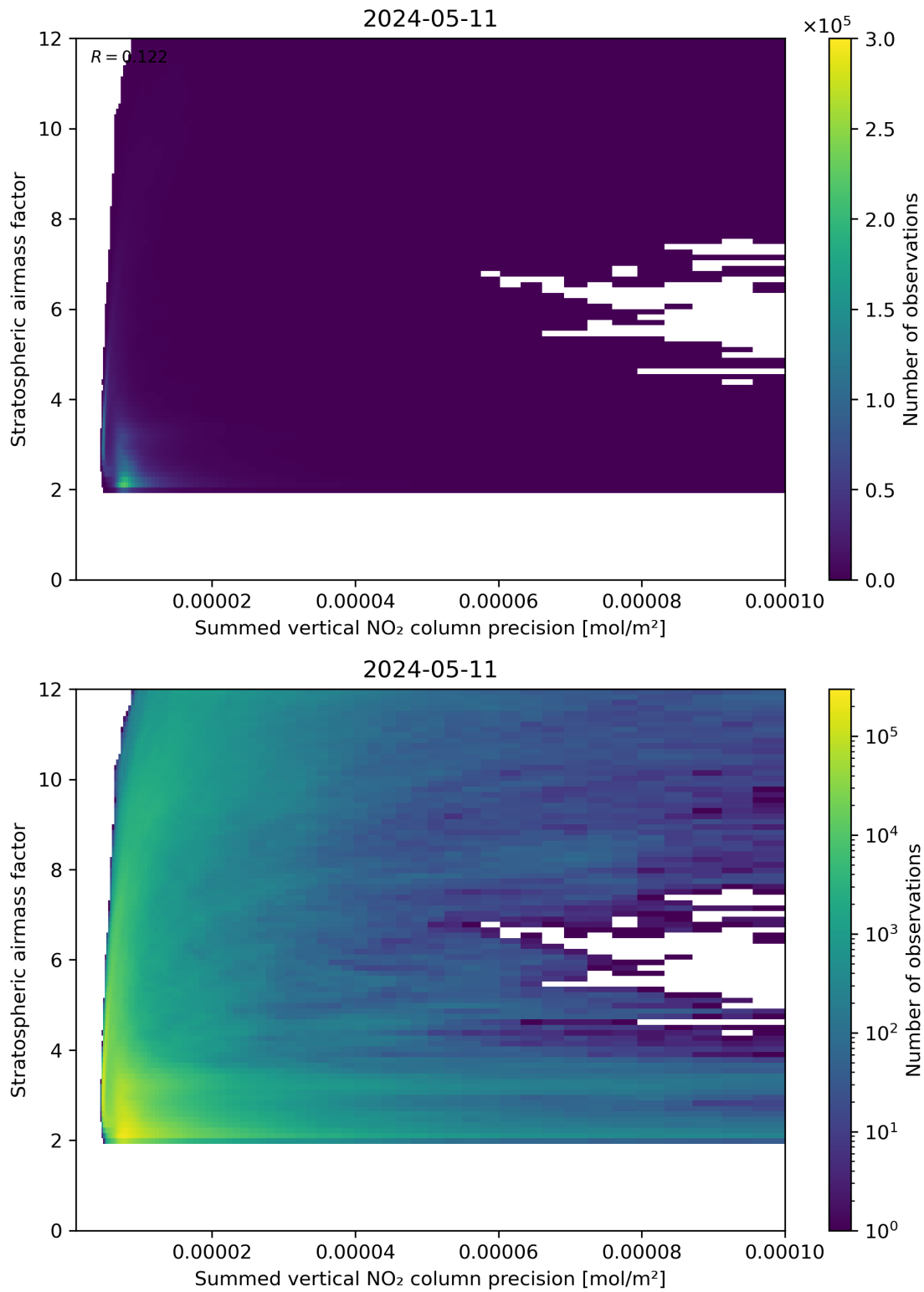
Figure 106: Scatter density plot of “Summed vertical NO 2 column precision” against “Stratospheric airmass factor” for 2024-05-10 to 2024-05-12.
