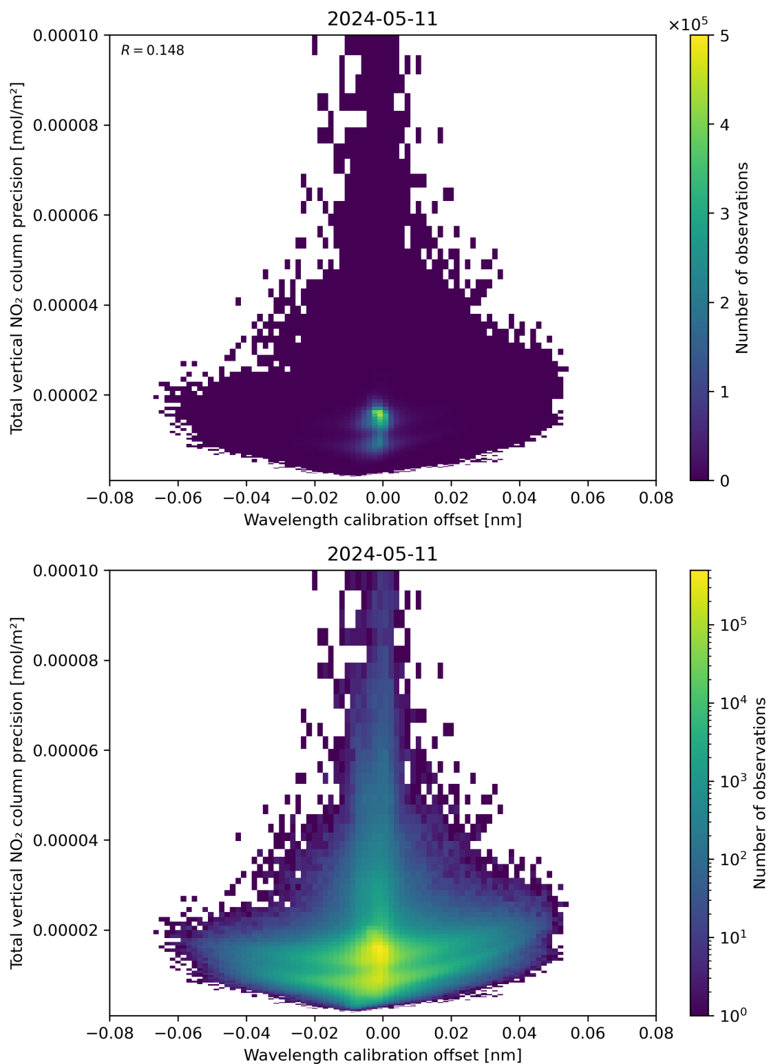
Figure 180: Scatter density plot of “Wavelength calibration offset” against “Total vertical NO 2 column precision” for 2024-05-10 to 2024-05-12.
