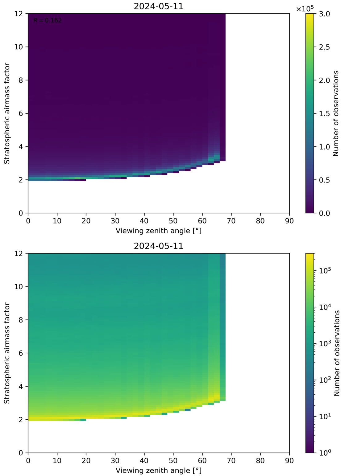
Figure 159: Scatter density plot of “Viewing zenith angle” against “Stratospheric airmass factor” for 2024-05-10 to 2024-05-12.
