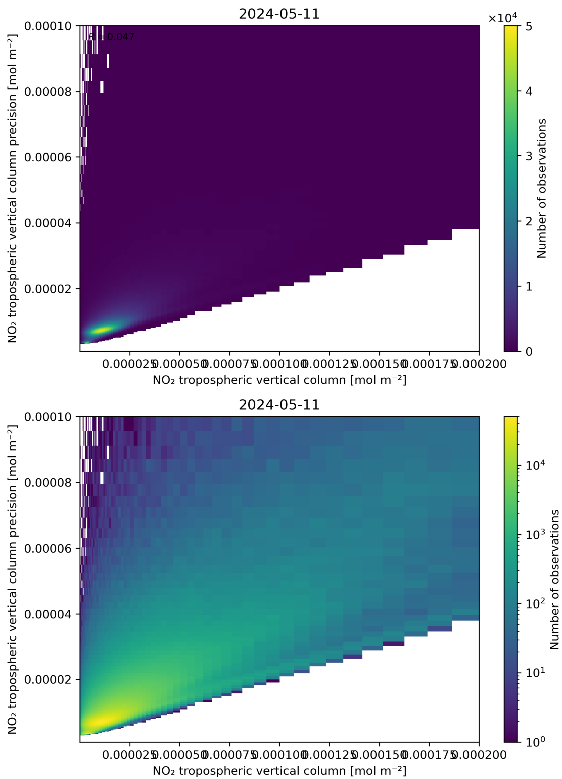
Figure 130: Scatter density plot of “NO 2 tropospheric vertical column” against “NO 2 tropospheric vertical column precision” for 2024-05-10 to 2024-05-12.
