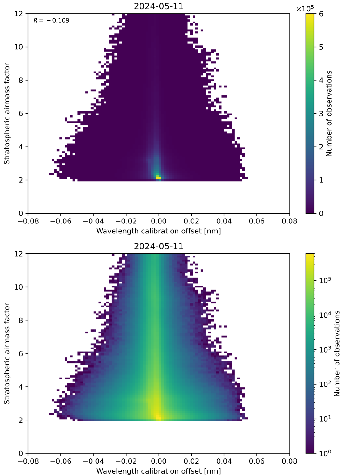
Figure 174: Scatter density plot of “Wavelength calibration offset” against “Stratospheric airmass factor” for 2024-05-10 to 2024-05-12.
