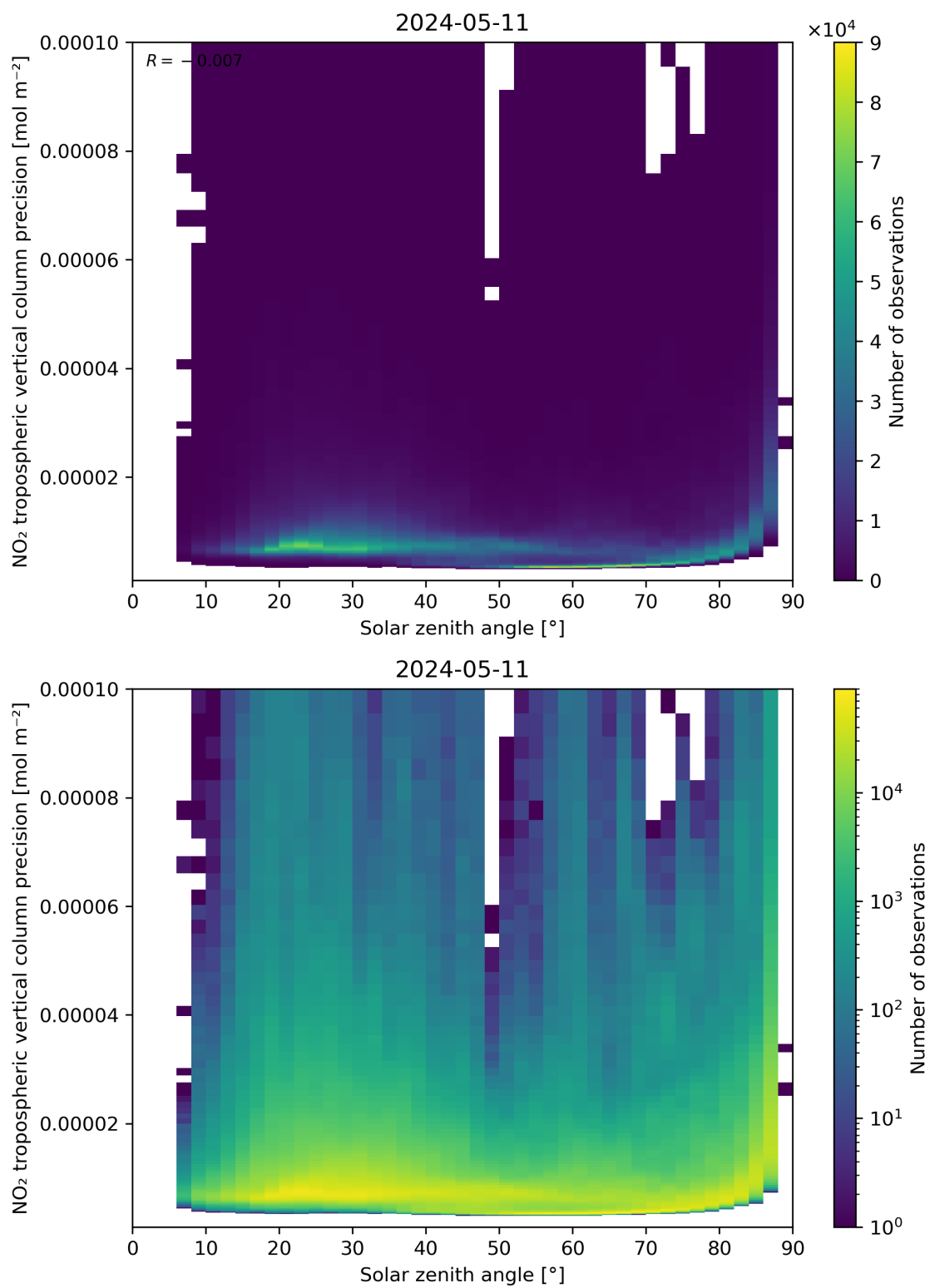
Figure 156: Scatter density plot of “Solar zenith angle” against “NO 2 tropospheric vertical column precision” for 2024-05-10 to 2024-05-12.
