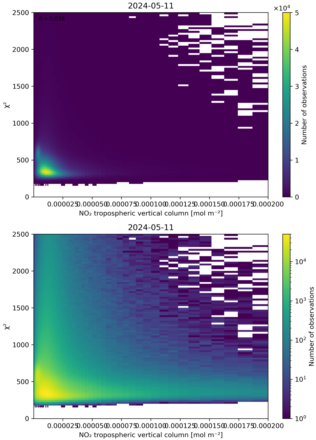
Figure 124: Scatter density plot of “NO 2 tropospheric vertical column” against “ \chi^2 ” for 2024-05-10 to 2024-05-12.
