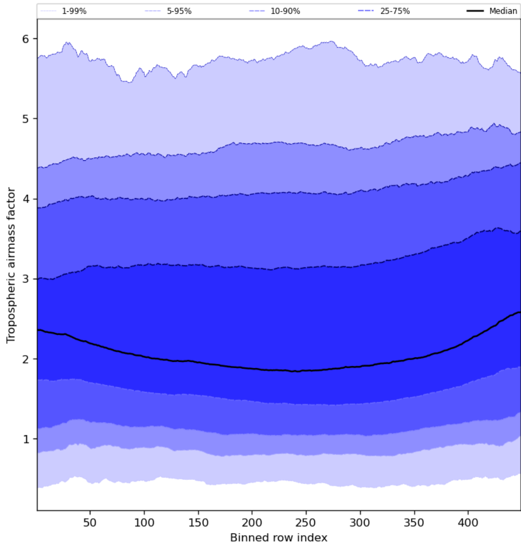
Figure 48: Along track statistics of “Tropospheric airmass factor” for 2024-05-10 to 2024-05-12
