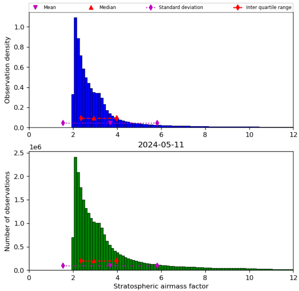
Figure 44: Histogram of “Stratospheric airmass factor” for 2024-05-10 to 2024-05-12
