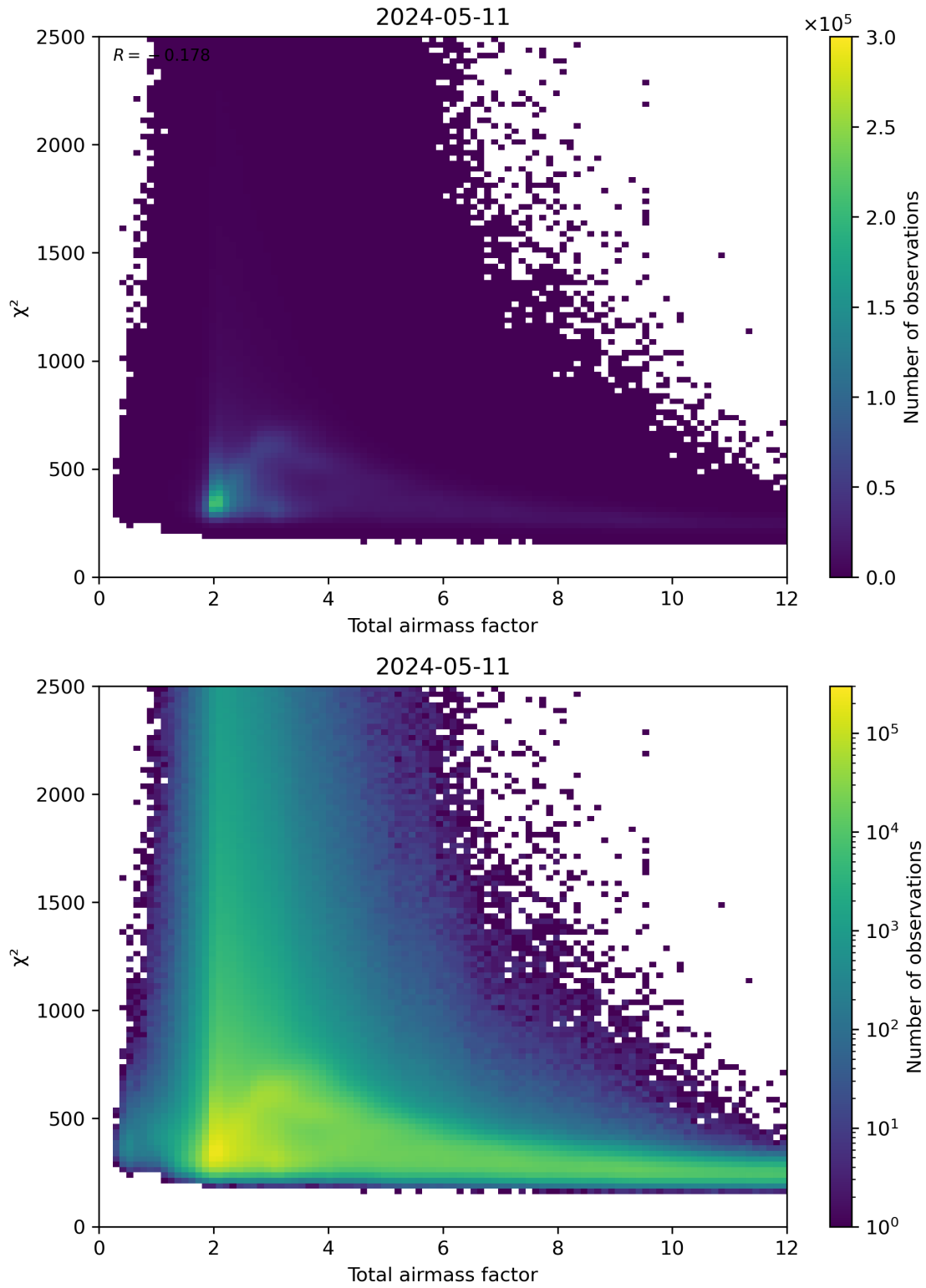
Figure 63: Scatter density plot of “Total airmass factor” against “ \chi^2 ” for 2024-05-10 to 2024-05-12.
