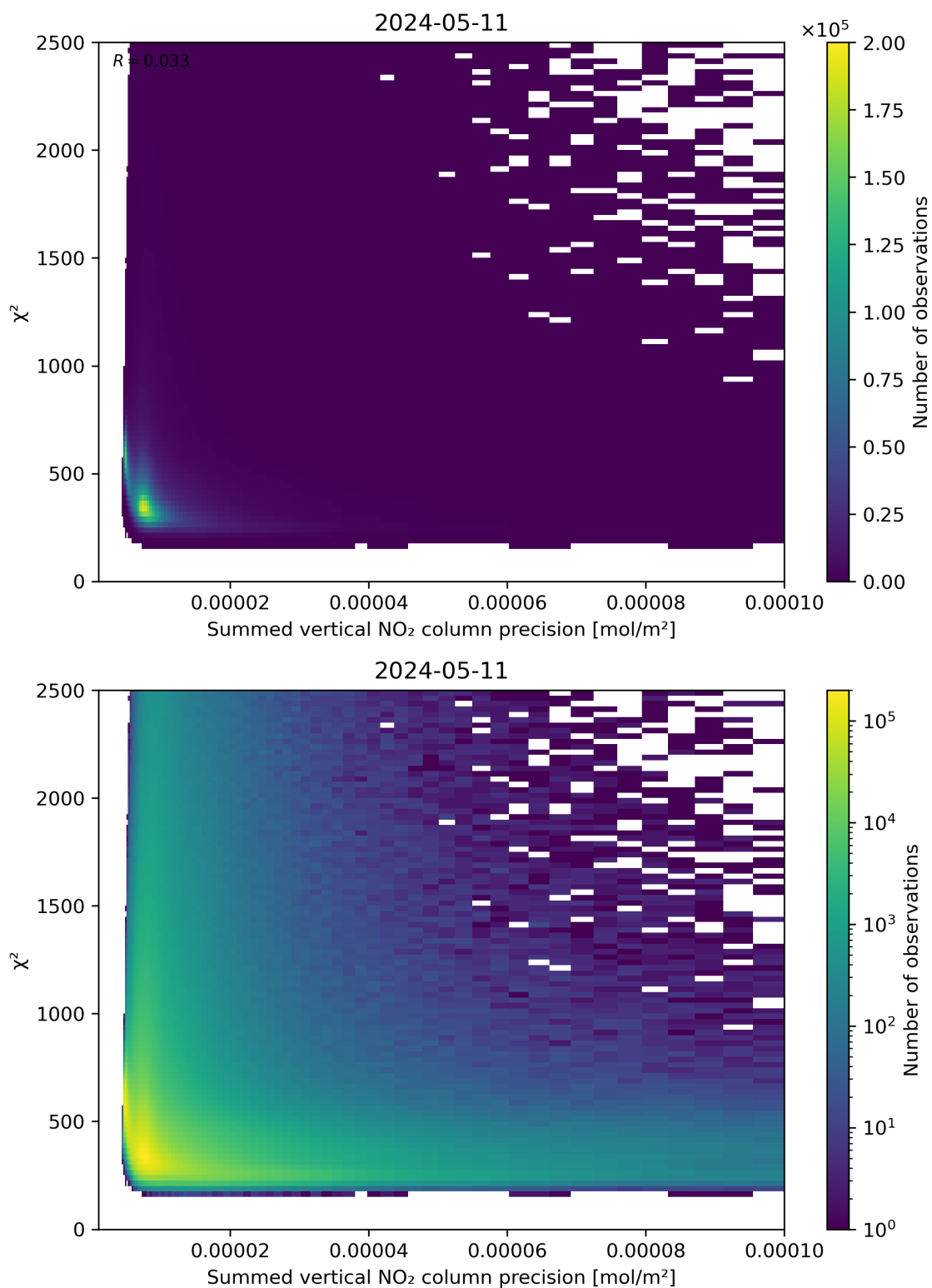
Figure 107: Scatter density plot of “Summed vertical NO 2 column precision” against “ \chi^2 ” for 2024-05-10 to 2024-05-12.
