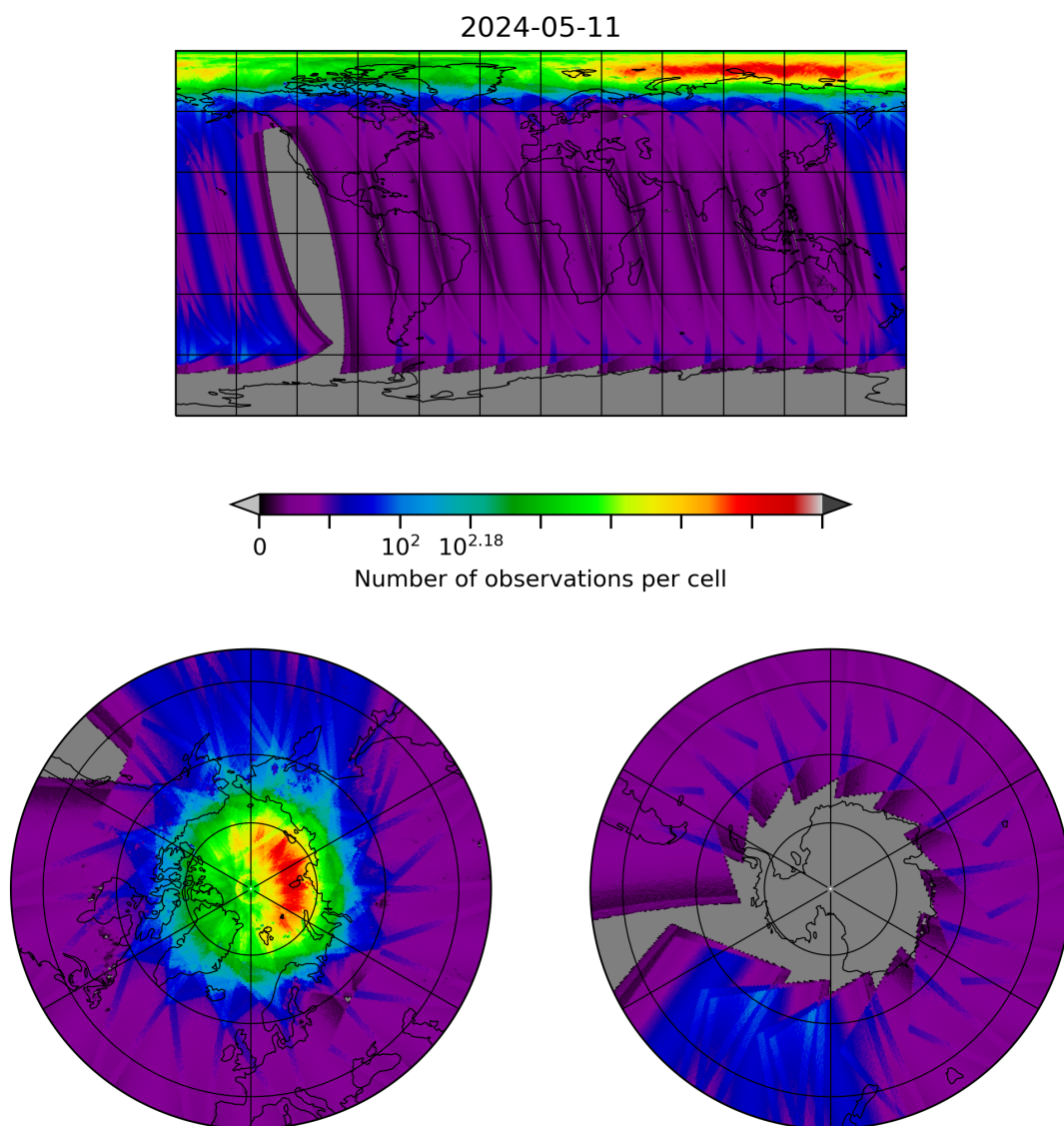
Figure 10: Map of the number of observations for 2024-05-10 to 2024-05-12
