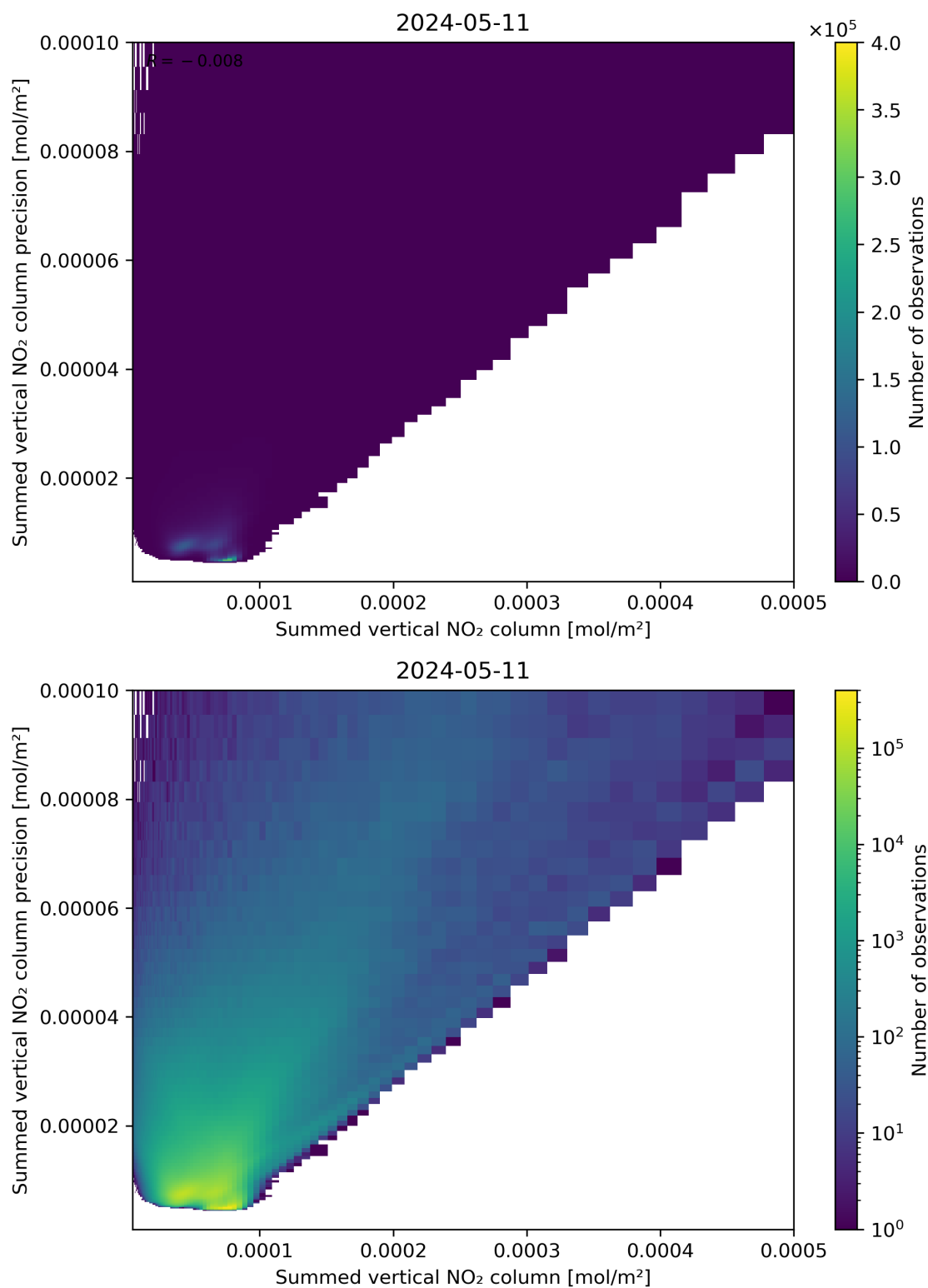
Figure 105: Scatter density plot of “Summed vertical NO 2 column” against “Summed vertical NO 2 column precision” for 2024-05-10 to 2024-05-12.
