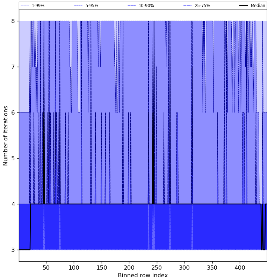
Figure 51: Along track statistics of “Number of iterations” for 2024-05-10 to 2024-05-12
