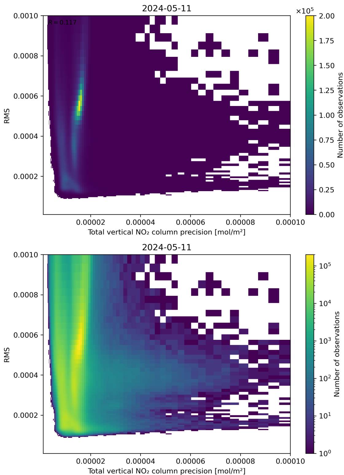
Figure 119: Scatter density plot of “Total vertical NO 2 column precision” against “RMS” for 2024-05-10 to 2024-05-12.
