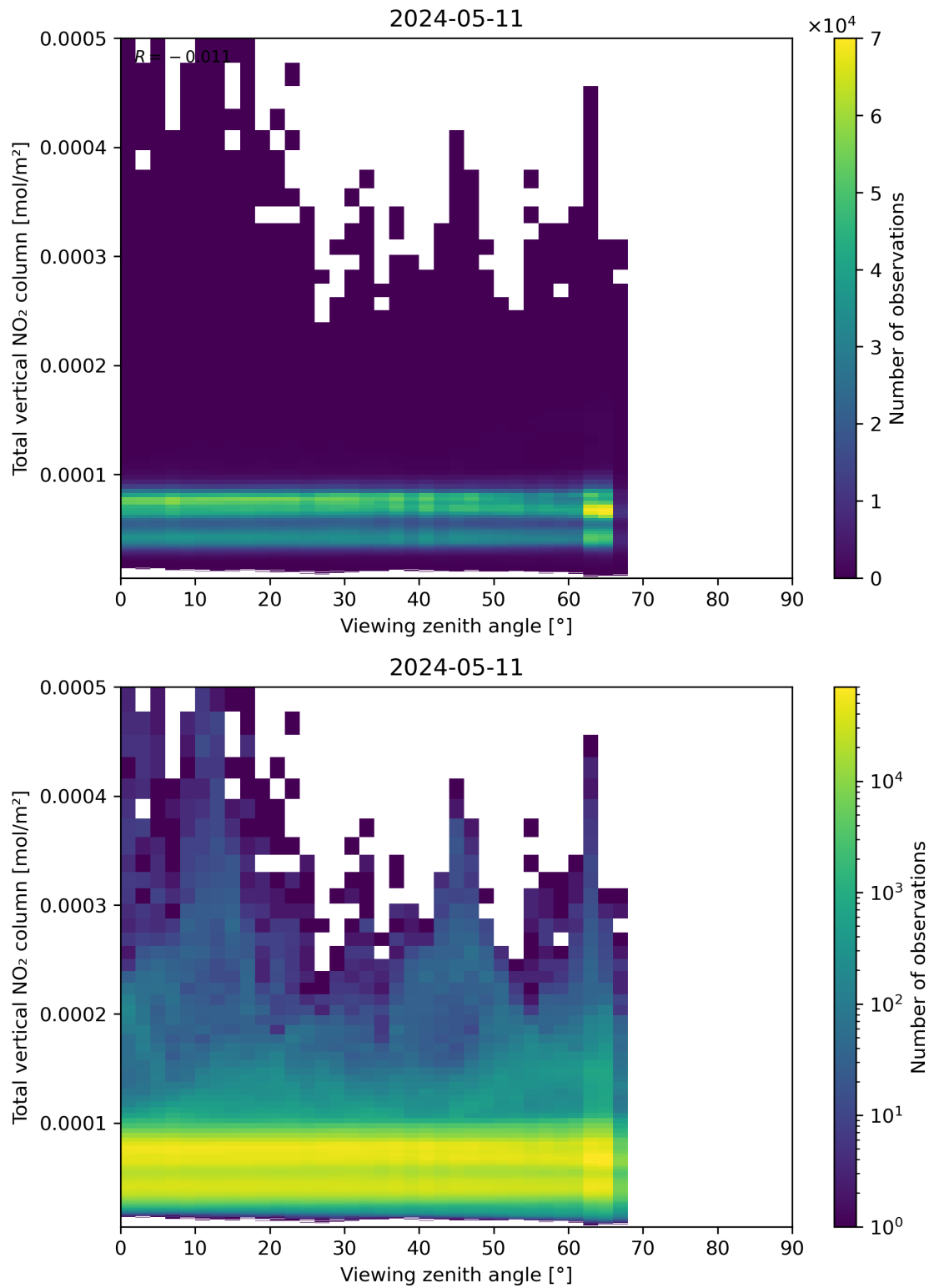
Figure 167: Scatter density plot of “Viewing zenith angle” against “Total vertical NO 2 column” for 2024-05-10 to 2024-05-12.
