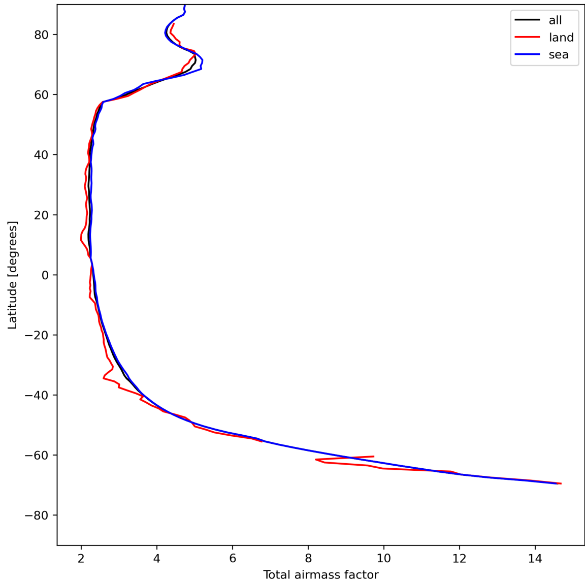
Figure 15: Zonal average of “Total airmass factor” for 2024-05-10 to 2024-05-12.
