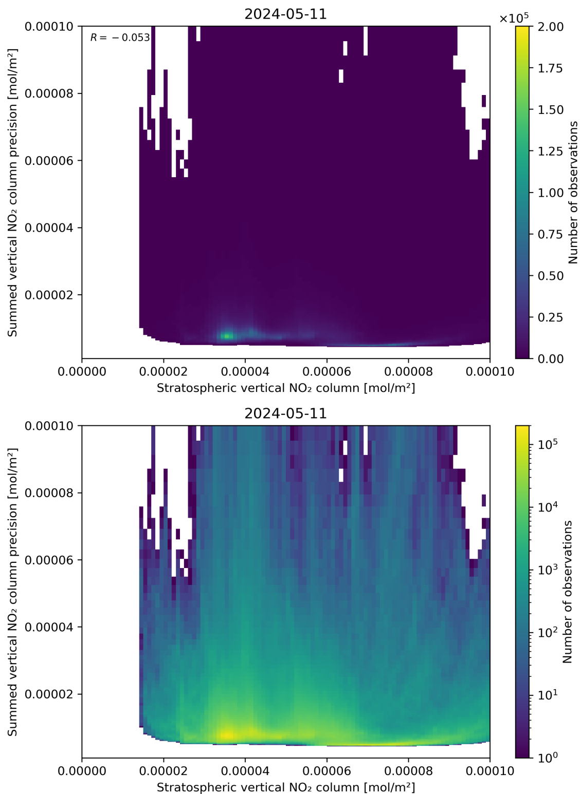
Figure 99: Scatter density plot of “Stratospheric vertical NO 2 column” against “Summed vertical NO 2 column precision” for 2024-05-10 to 2024-05-12.
