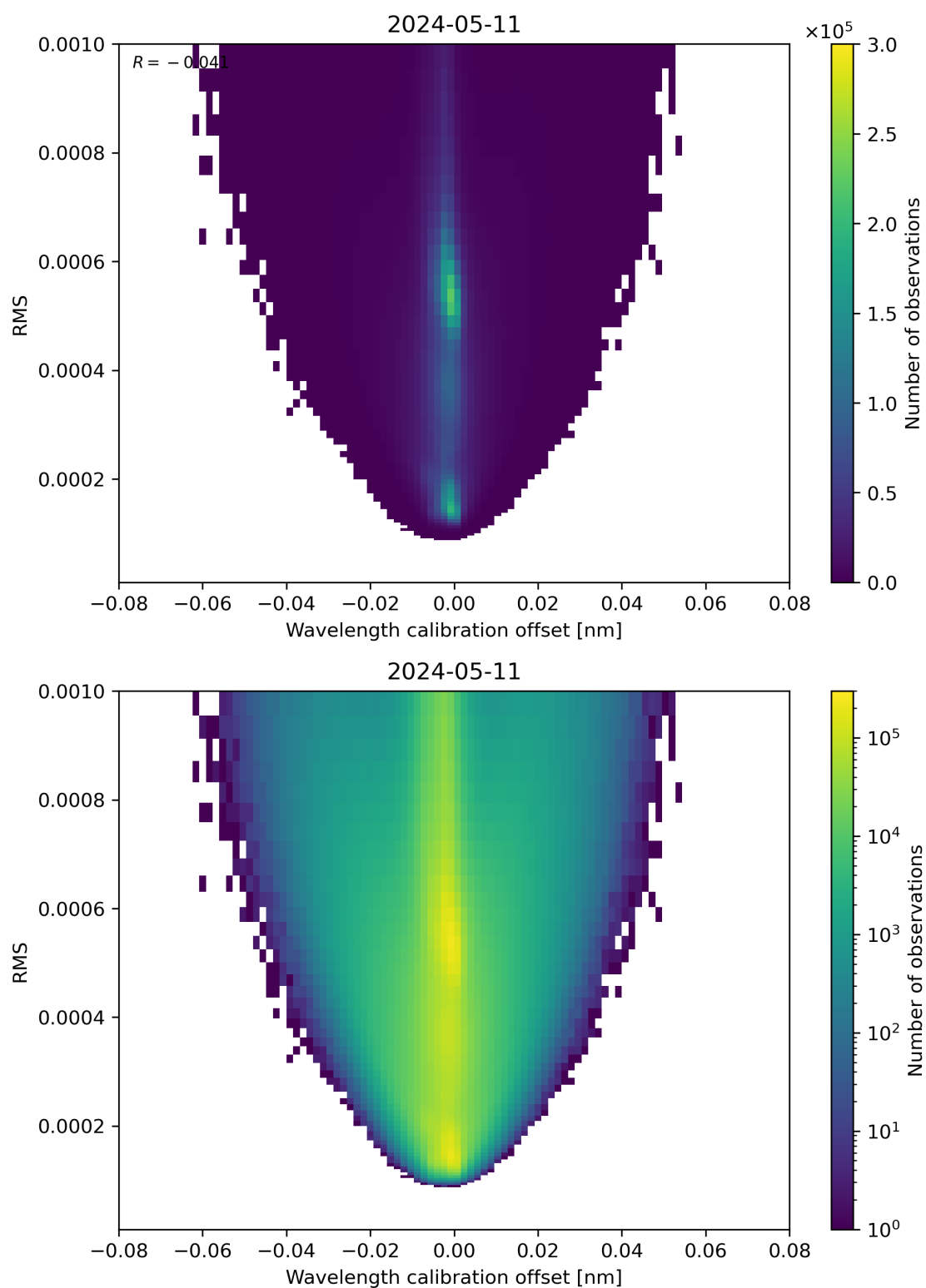
Figure 181: Scatter density plot of “Wavelength calibration offset” against “RMS” for 2024-05-10 to 2024-05-12.
