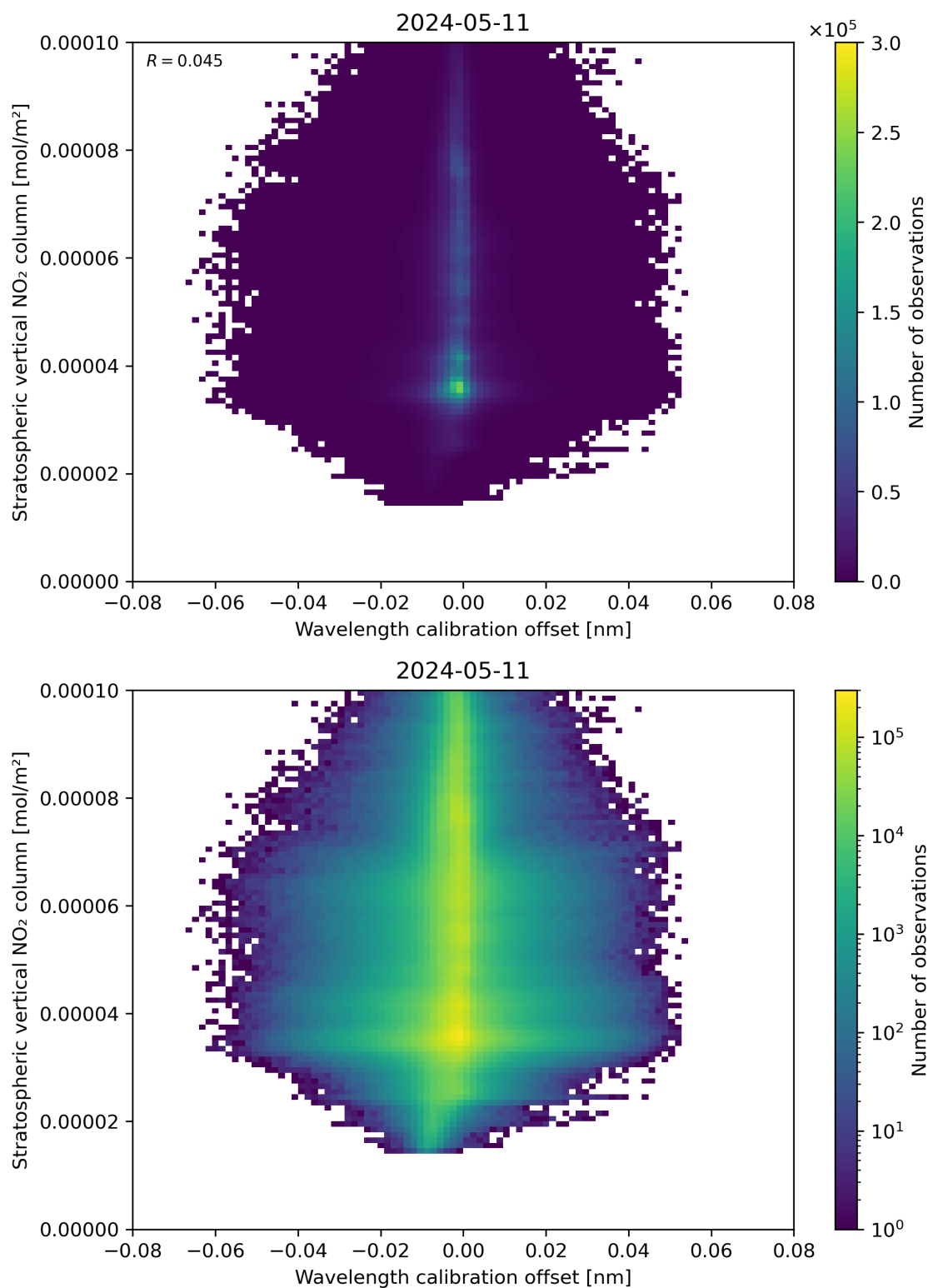
Figure 176: Scatter density plot of “Wavelength calibration offset” against “Stratospheric vertical NO 2 column” for 2024-05-10 to 2024-05-12.
