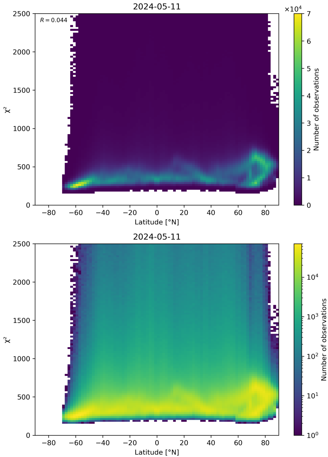
Figure 86: Scatter density plot of “Latitude” against “ \chi^2 ” for 2024-05-10 to 2024-05-12.
