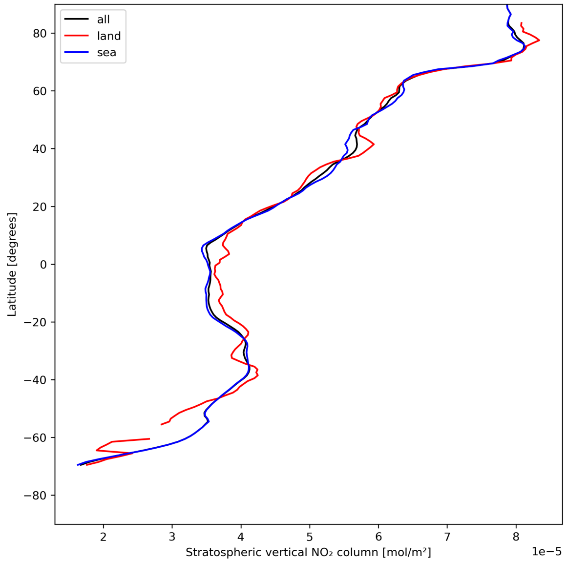
Figure 19: Zonal average of “Stratospheric vertical NO 2 column” for 2024-05-10 to 2024-05-12.
