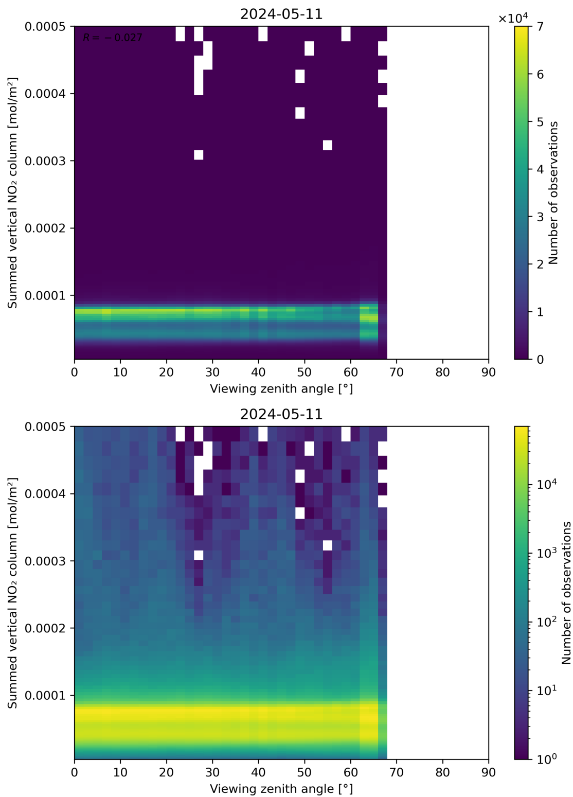
Figure 165: Scatter density plot of “Viewing zenith angle” against “Summed vertical NO 2 column” for 2024-05-10 to 2024-05-12.
