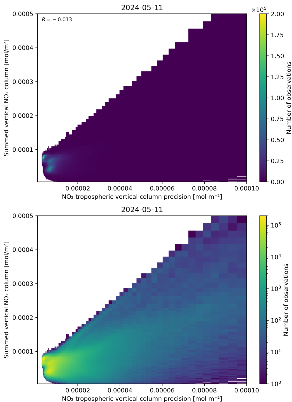
Figure 136: Scatter density plot of “NO 2 tropospheric vertical column precision” against “Summed vertical NO 2 column” for 2024-05-10 to 2024-05-12.
