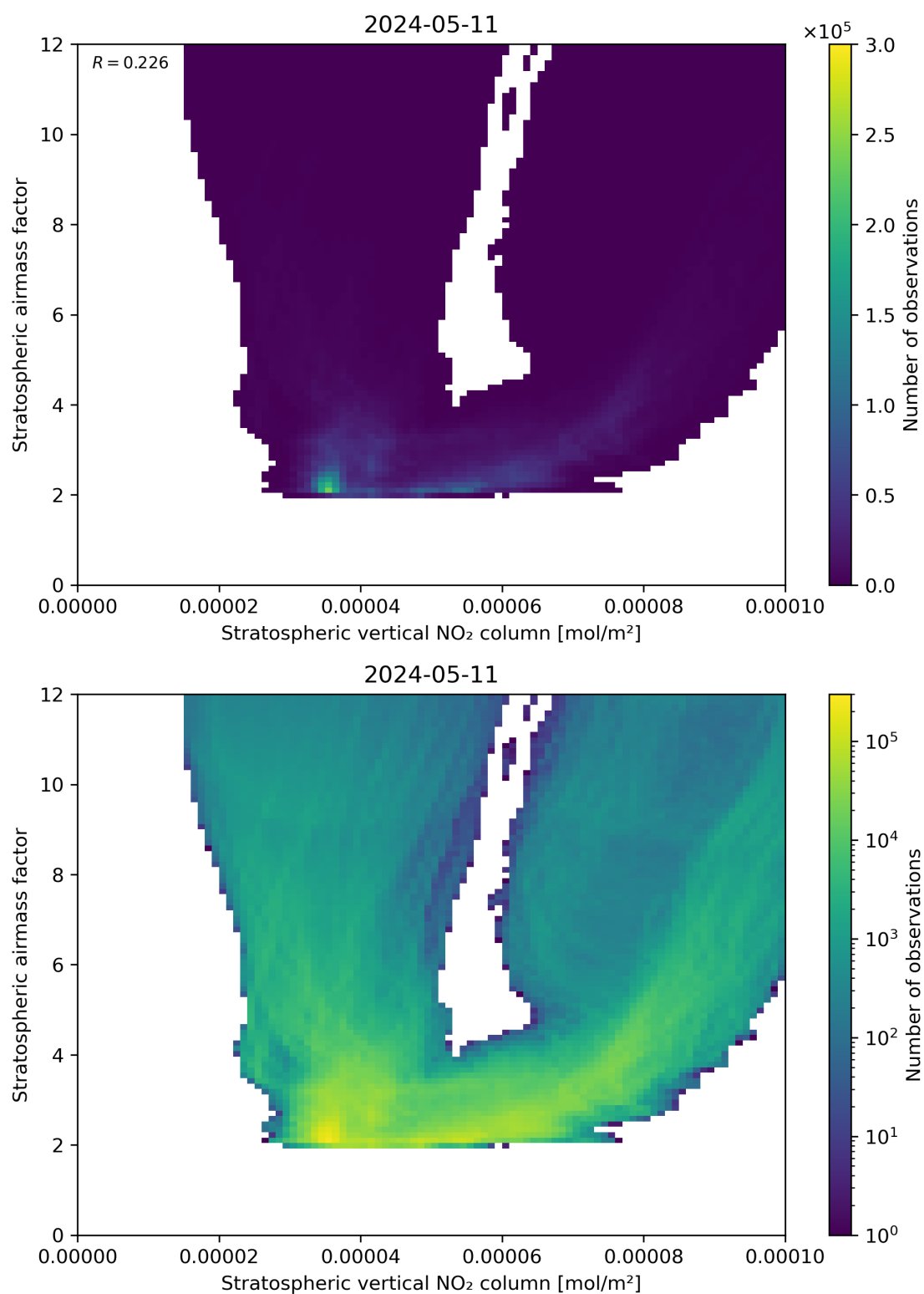
Figure 96: Scatter density plot of “Stratospheric vertical NO 2 column” against “Stratospheric airmass factor” for 2024-05-10 to 2024-05-12.
