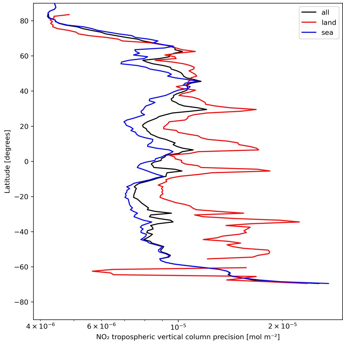
Figure 13: Zonal average of “NO 2 tropospheric vertical column precision” for 2024-05-10 to 2024-05-12.
