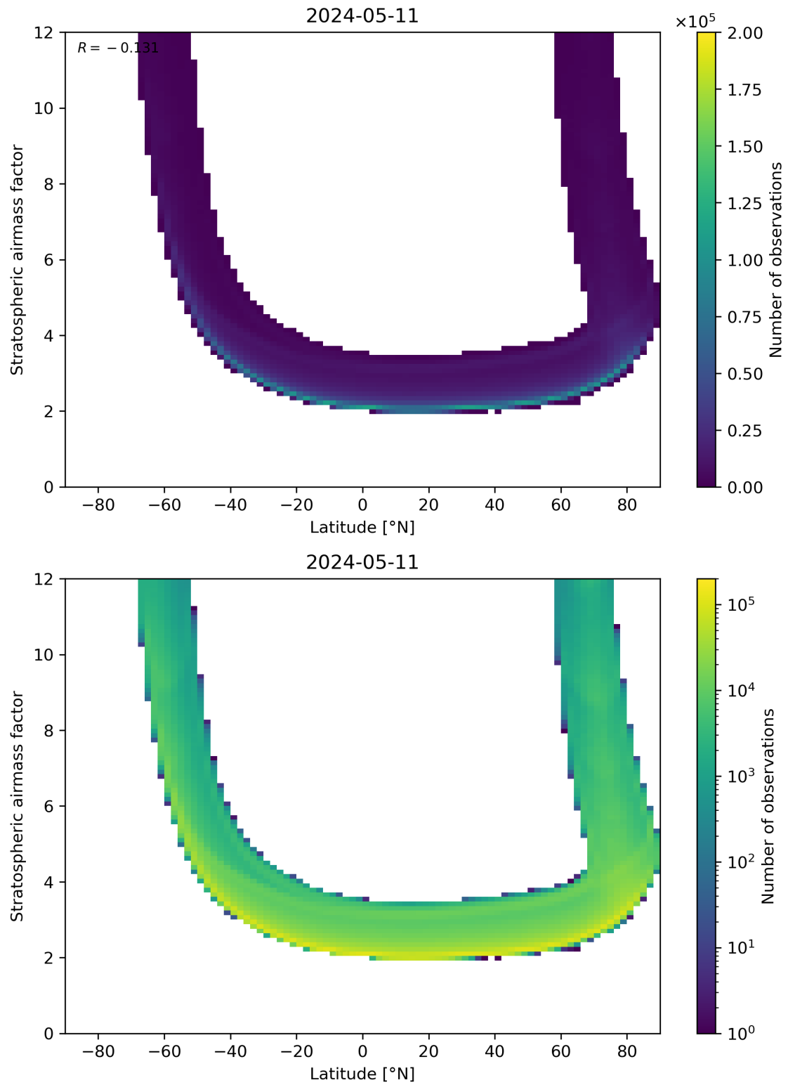
Figure 83: Scatter density plot of “Latitude” against “Stratospheric airmass factor” for 2024-05-10 to 2024-05-12.
