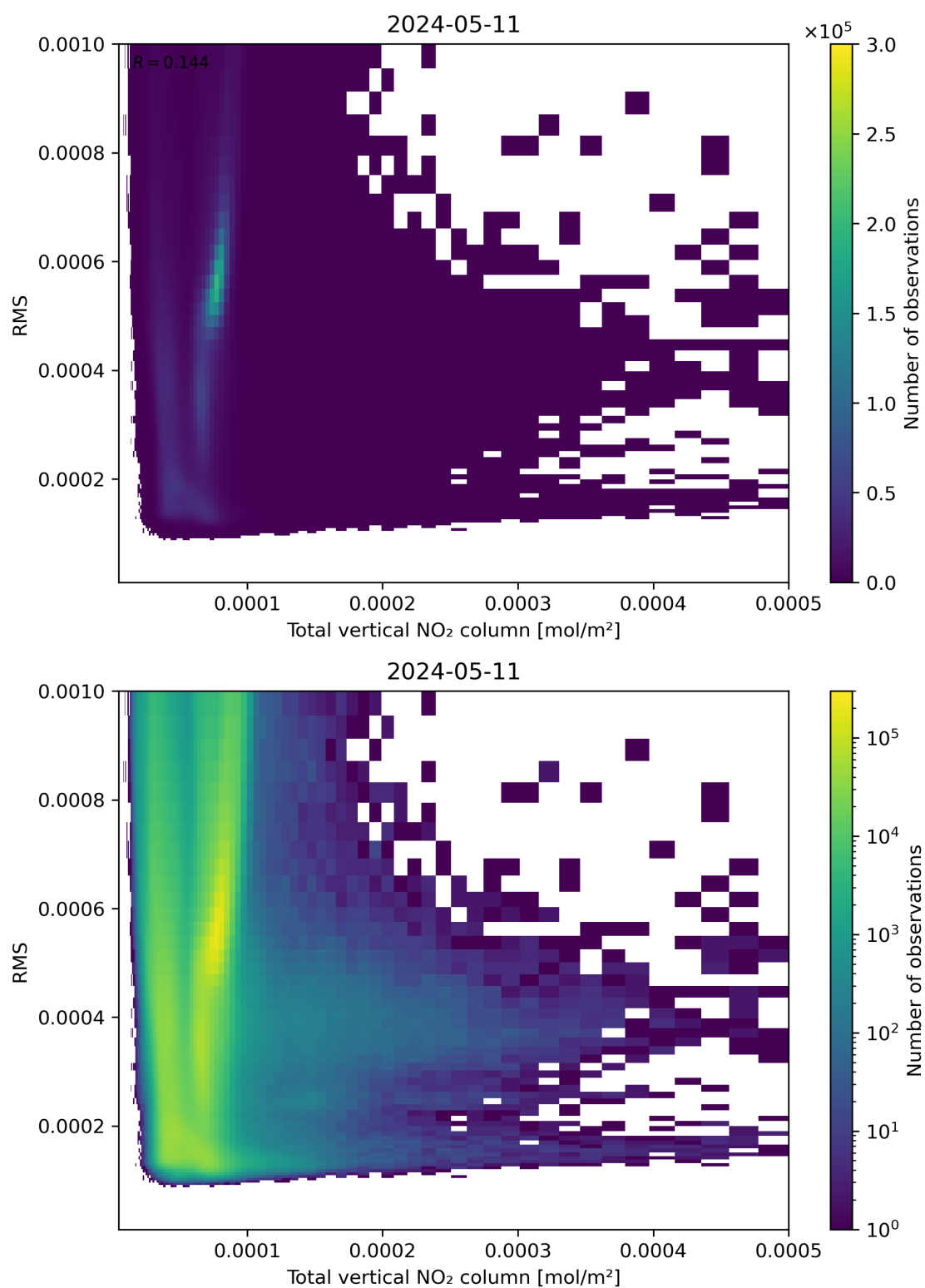
Figure 120: Scatter density plot of “Total vertical NO 2 column” against “RMS” for 2024-05-10 to 2024-05-12.
