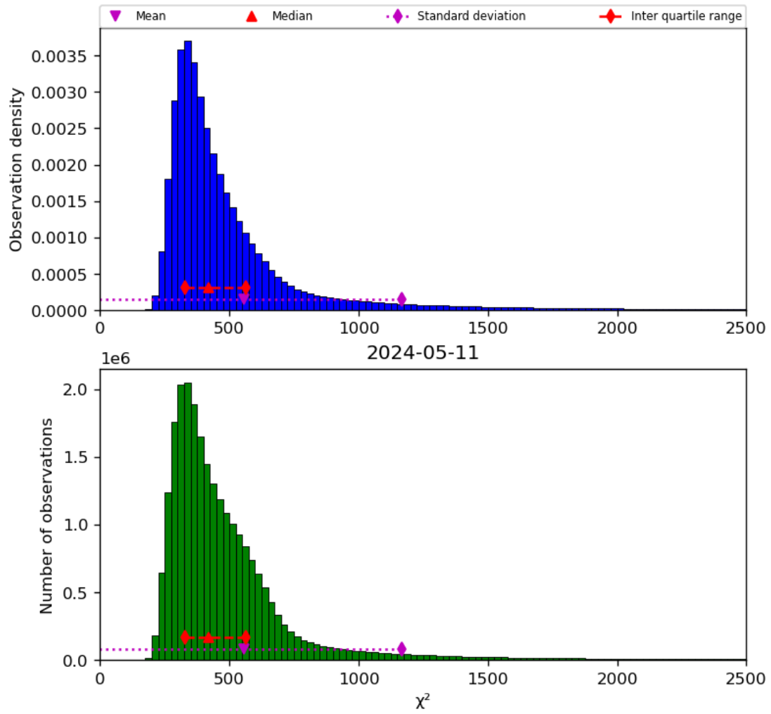
Figure 42: Histogram of " \chi^2 " for 2024-05-10 to 2024-05-12
