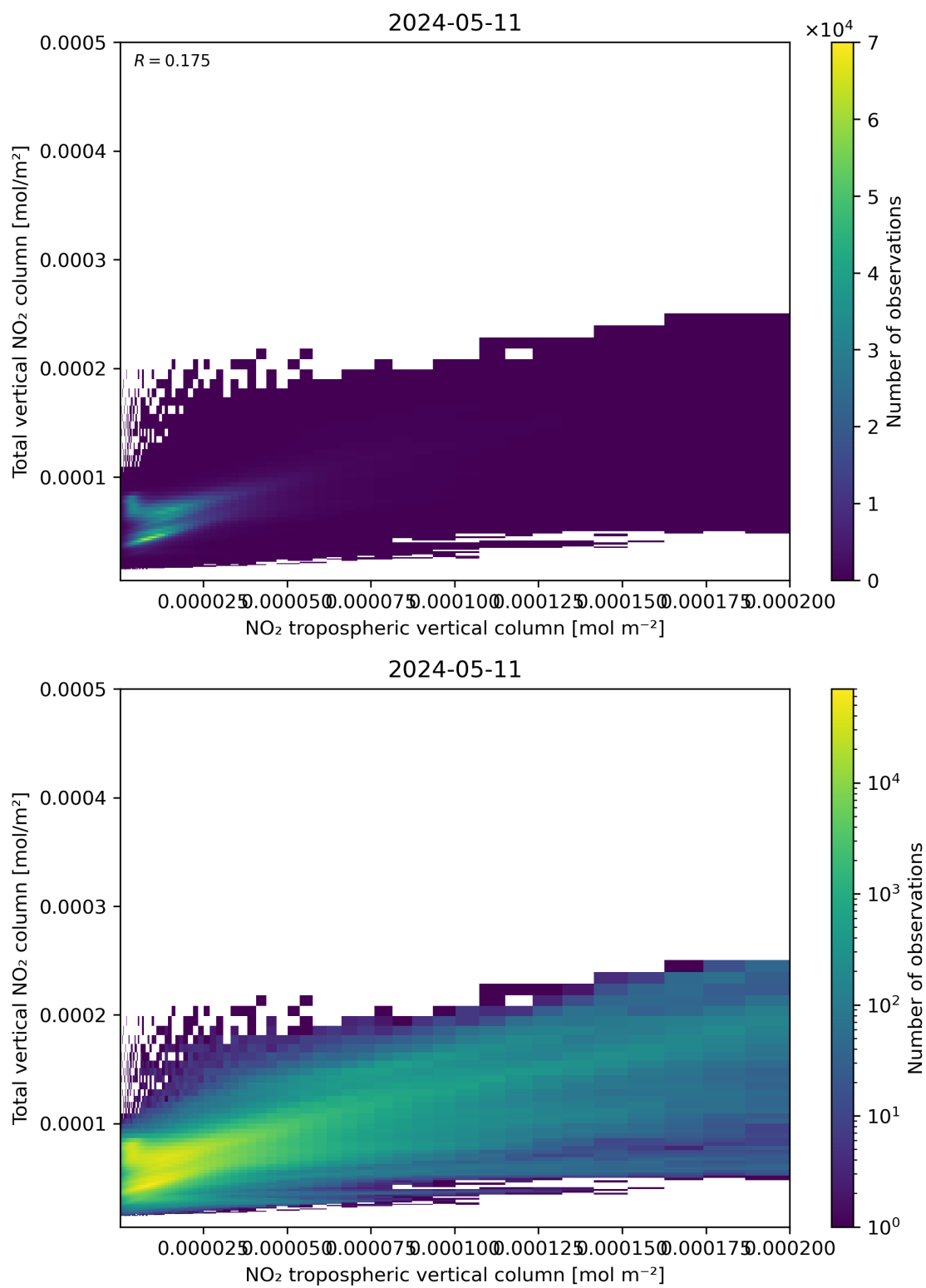
Figure 128: Scatter density plot of “NO 2 tropospheric vertical column” against “Total vertical NO 2 column” for 2024-05-10 to 2024-05-12.
