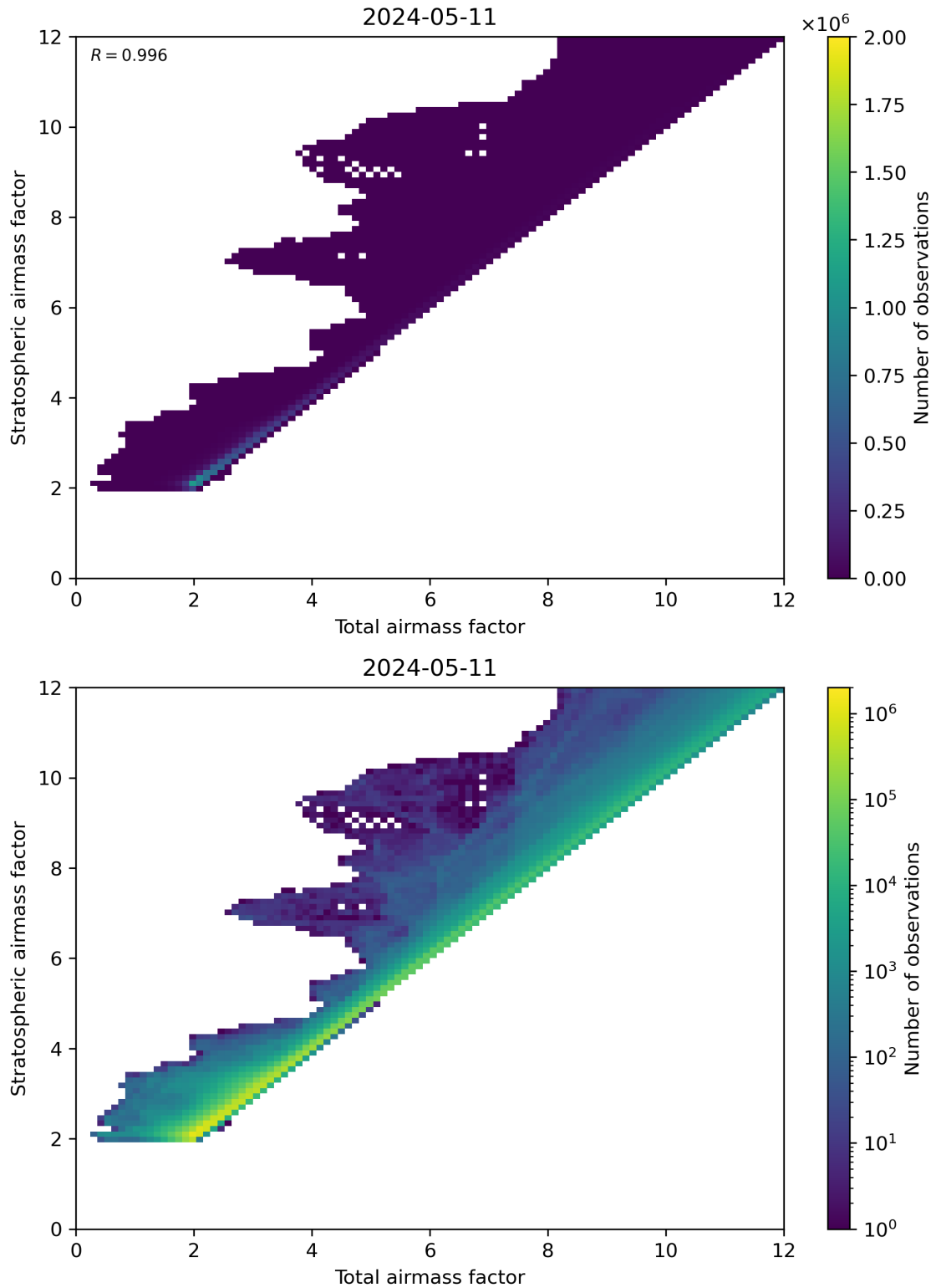
Figure 62: Scatter density plot of “Total airmass factor” against “Stratospheric airmass factor” for 2024-05-10 to 2024-05-12.
