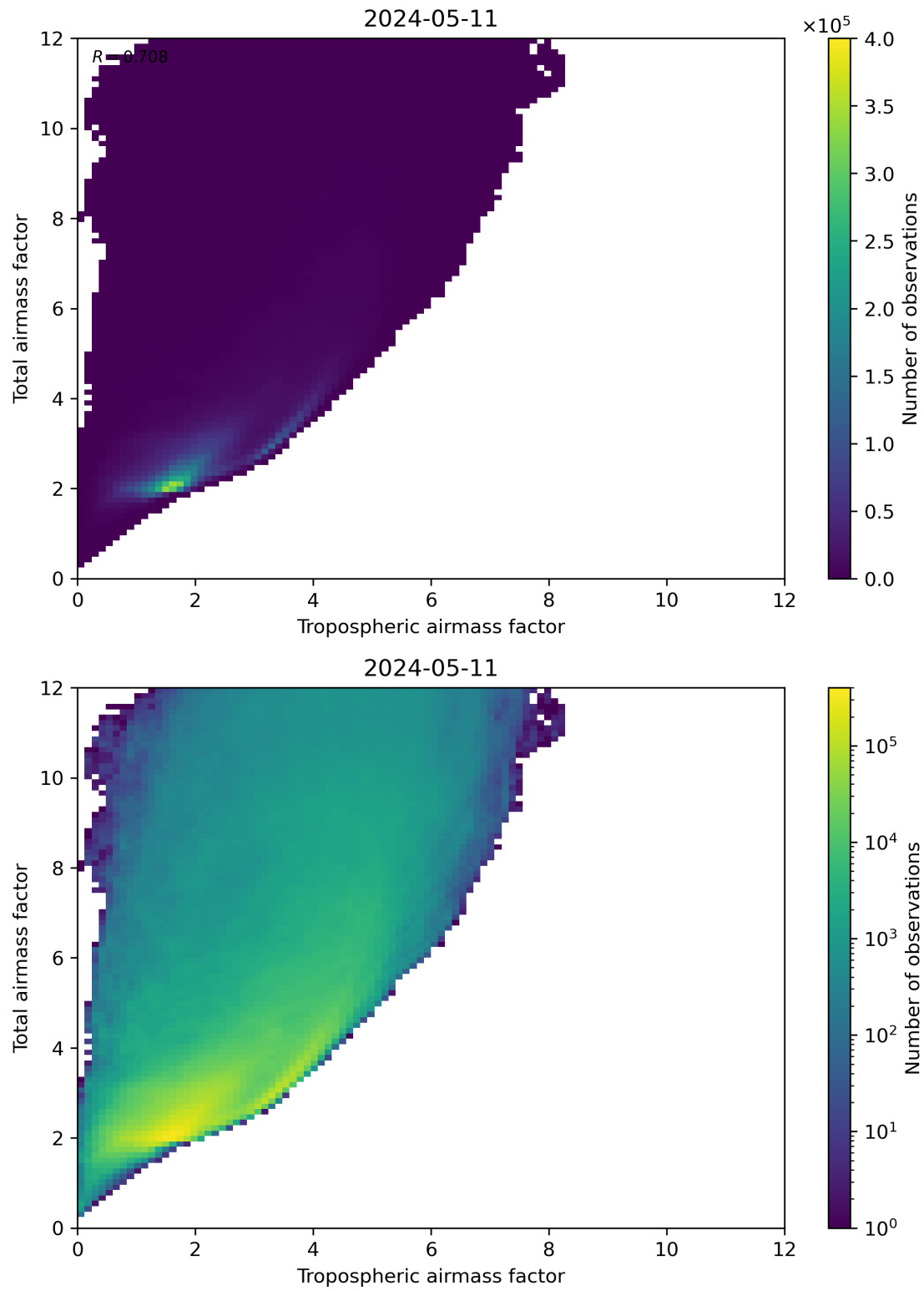
Figure 72: Scatter density plot of “Tropospheric airmass factor” against “Total airmass factor” for 2024-05-10 to 2024-05-12.
