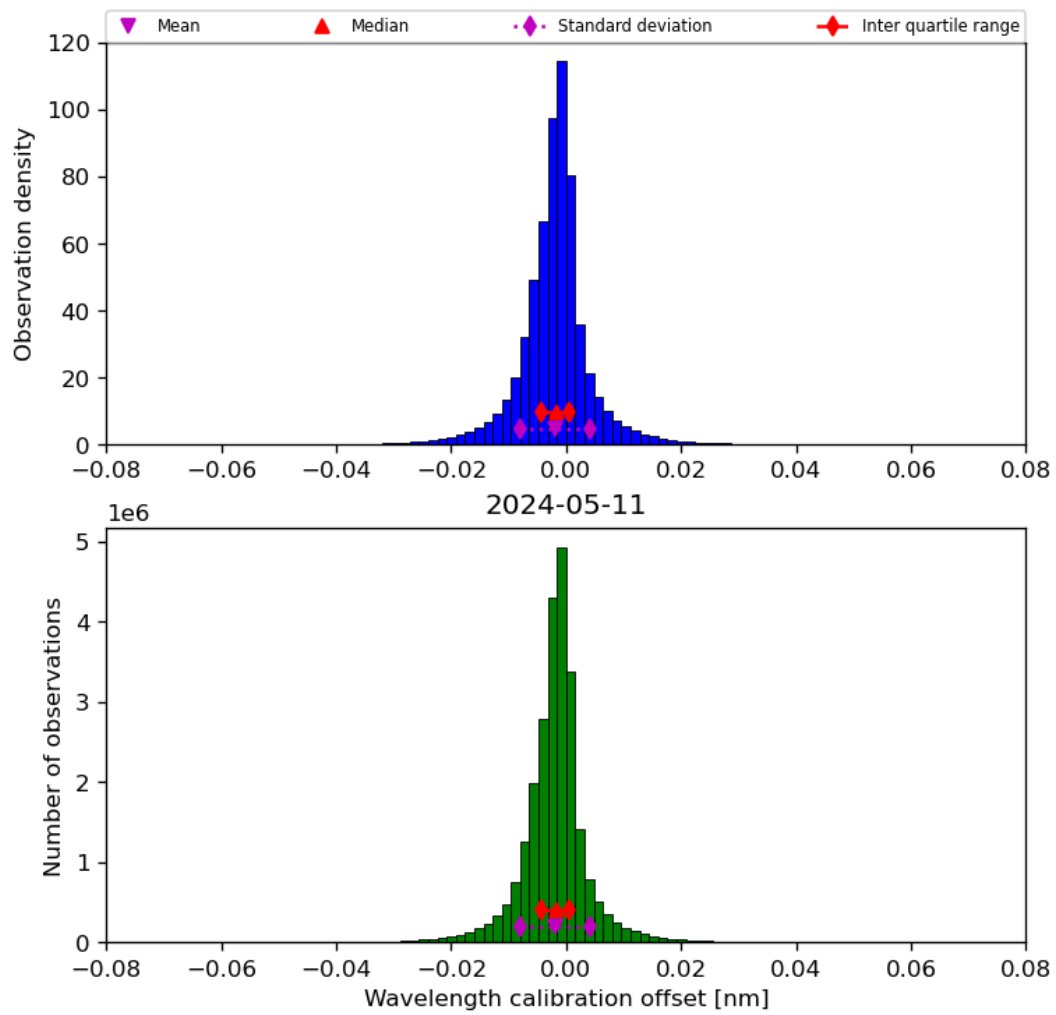
Figure 35: Histogram of “Wavelength calibration offset” for 2024-05-10 to 2024-05-12
