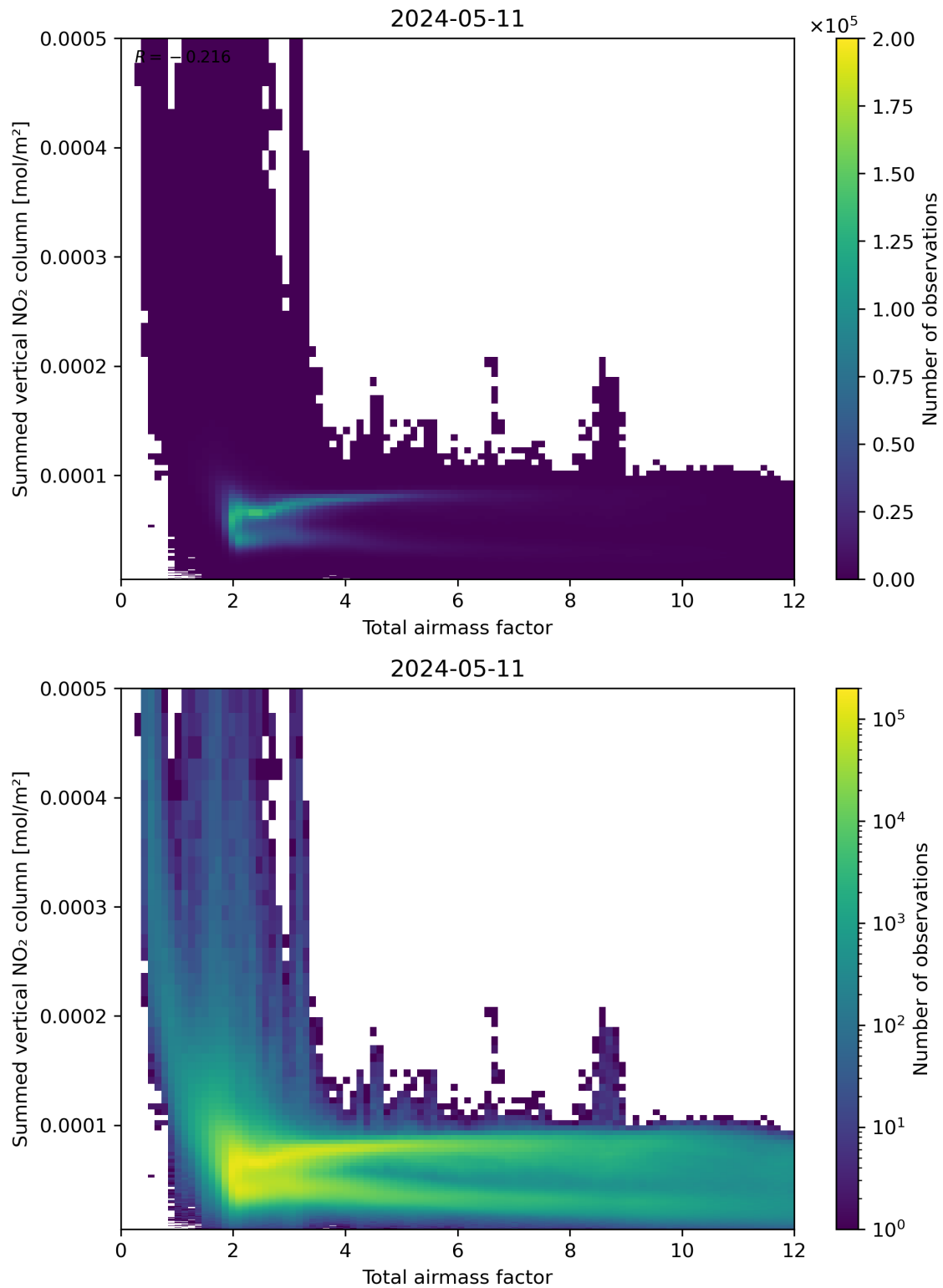
Figure 65: Scatter density plot of “Total airmass factor” against “Summed vertical NO 2 column” for 2024-05-10 to 2024-05-12.
