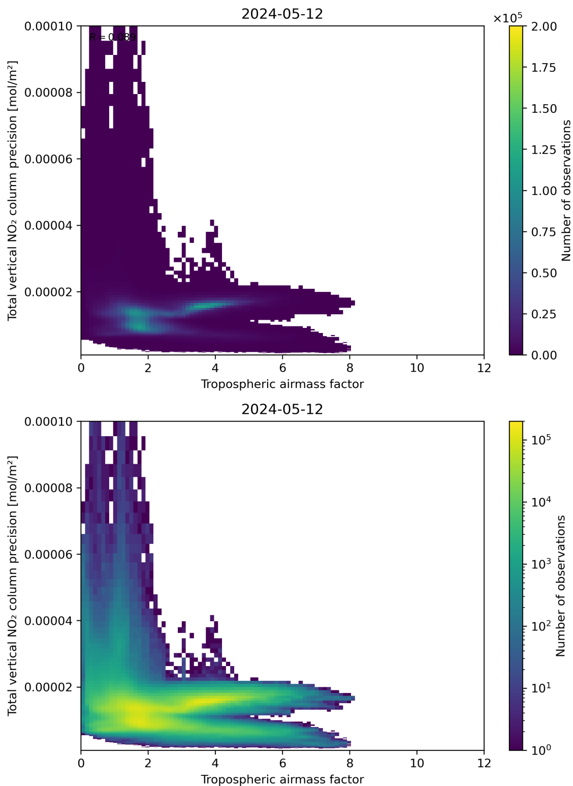
Figure 78: Scatter density plot of “Tropospheric air mass factor” against “Total vertical NO 2 column precision” for 2024-05-12 to 2024-05-13.
