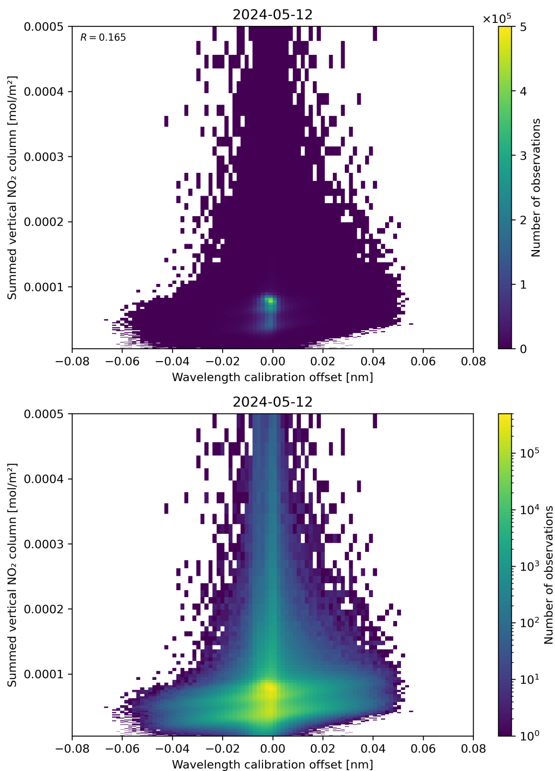
Figure 177: Scatter density plot of “Wavelength calibration offset” against “Summed vertical NO 2 column” for 2024-05-12 to 2024-05-13.
