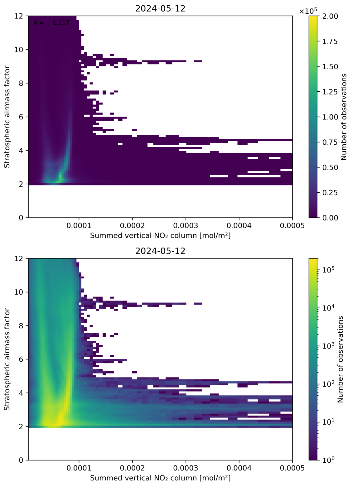
Figure 103: Scatter density plot of “Summed vertical NO 2 column” against “Stratospheric air mass factor” for 2024-05-12 to 2024-05-13.
