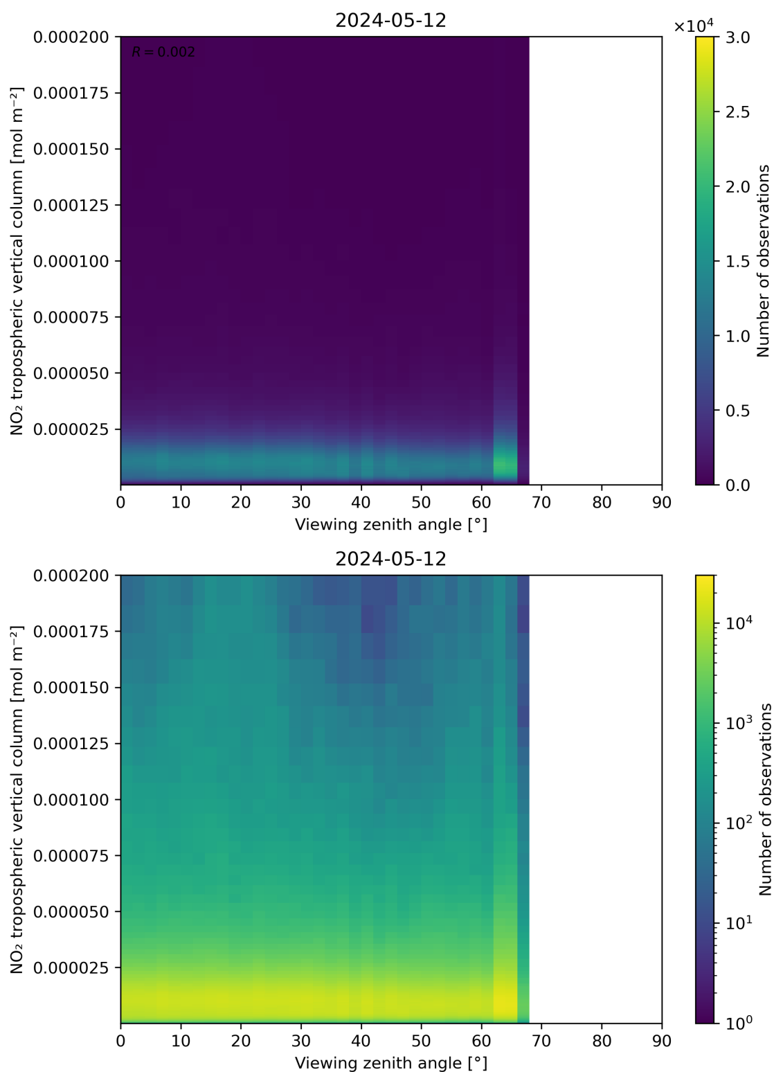
Figure 169: Scatter density plot of “Viewing zenith angle” against “NO 2 tropospheric vertical column” for 2024-05-12 to 2024-05-13.
