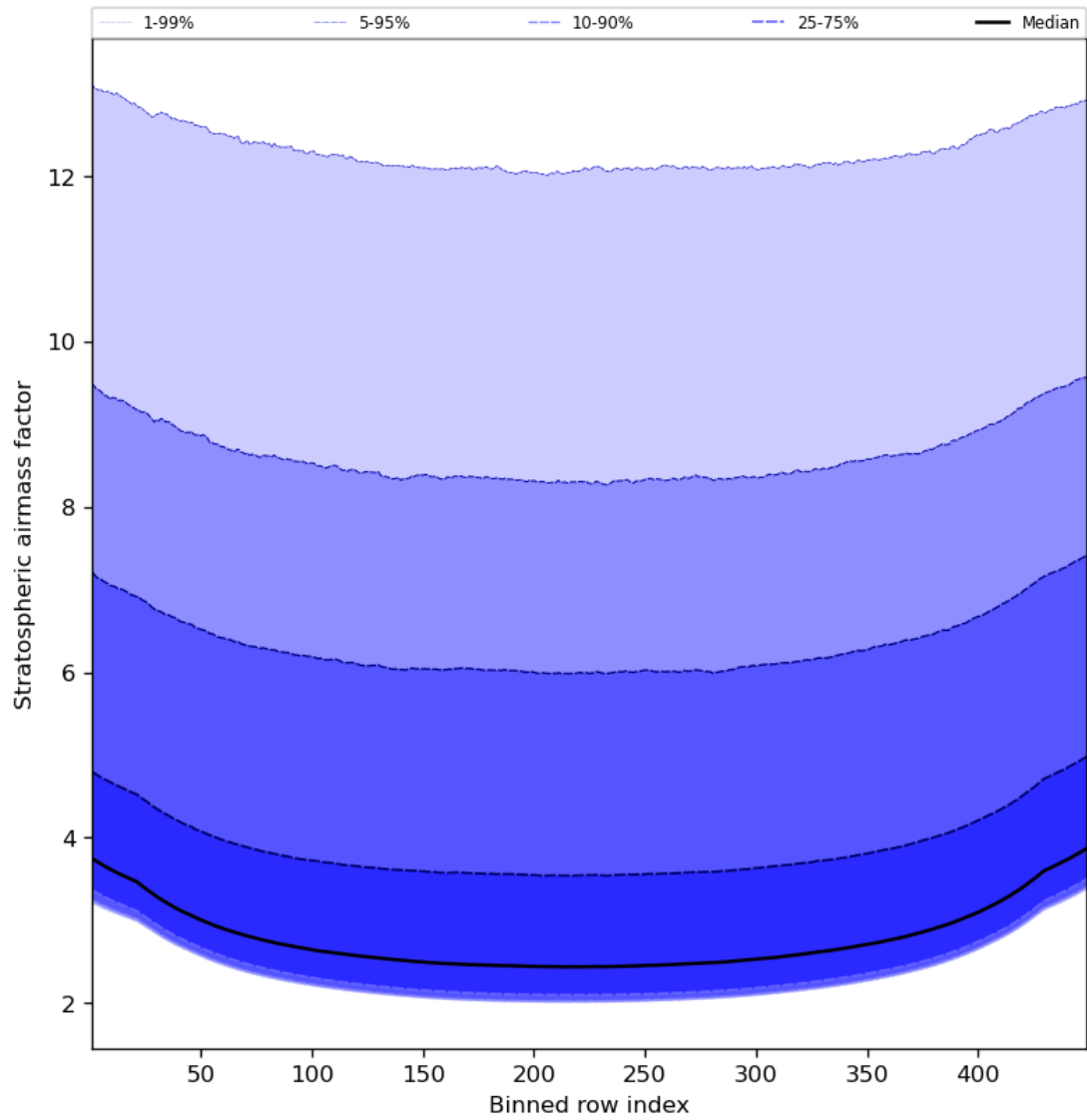
Figure 61: Along track statistics of “Stratospheric airmass factor” for 2024-05-12 to 2024-05-13
