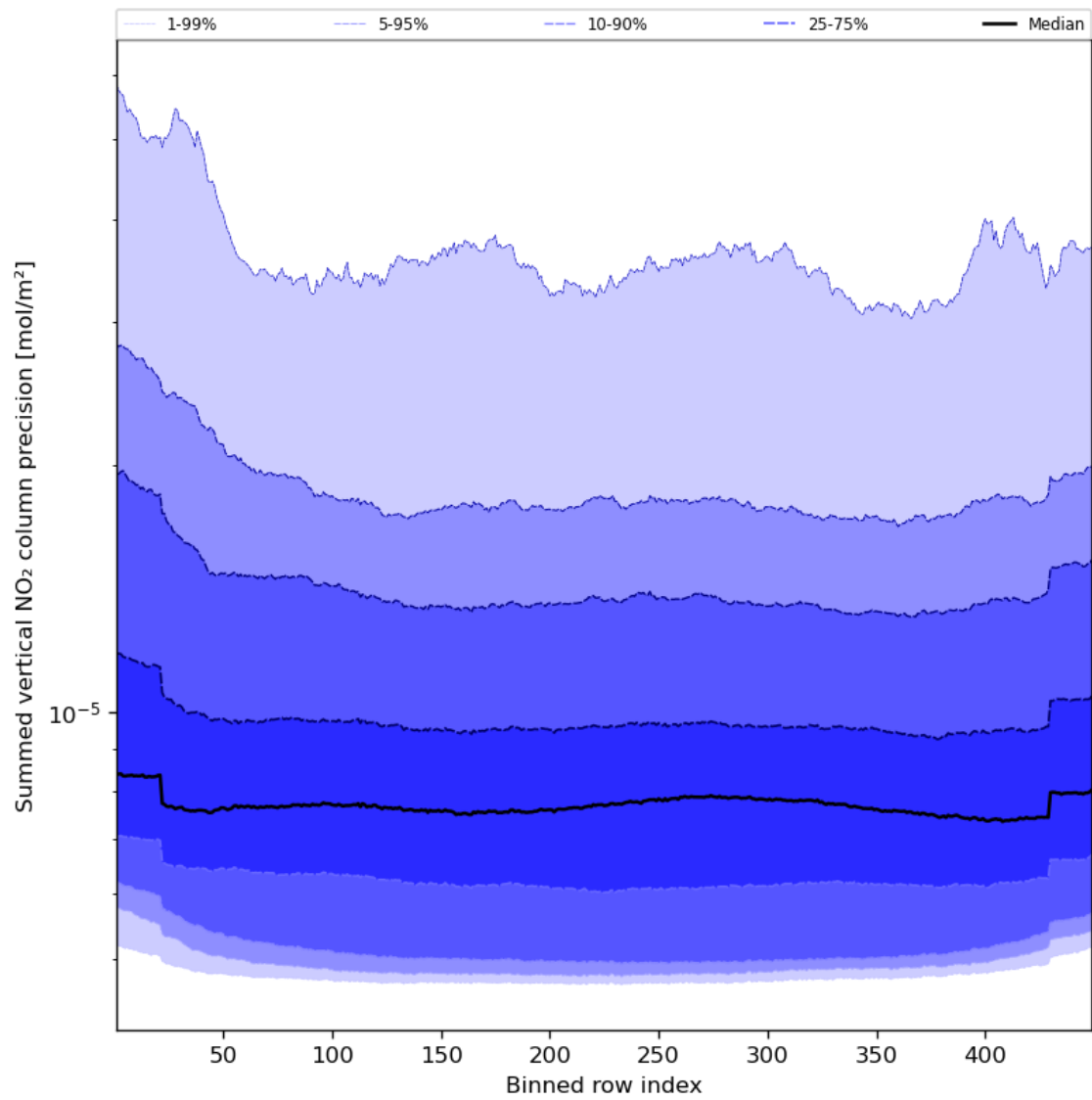
Figure 58: Along track statistics of “Summed vertical NO 2 column precision” for 2024-05-12 to 2024-05-13
