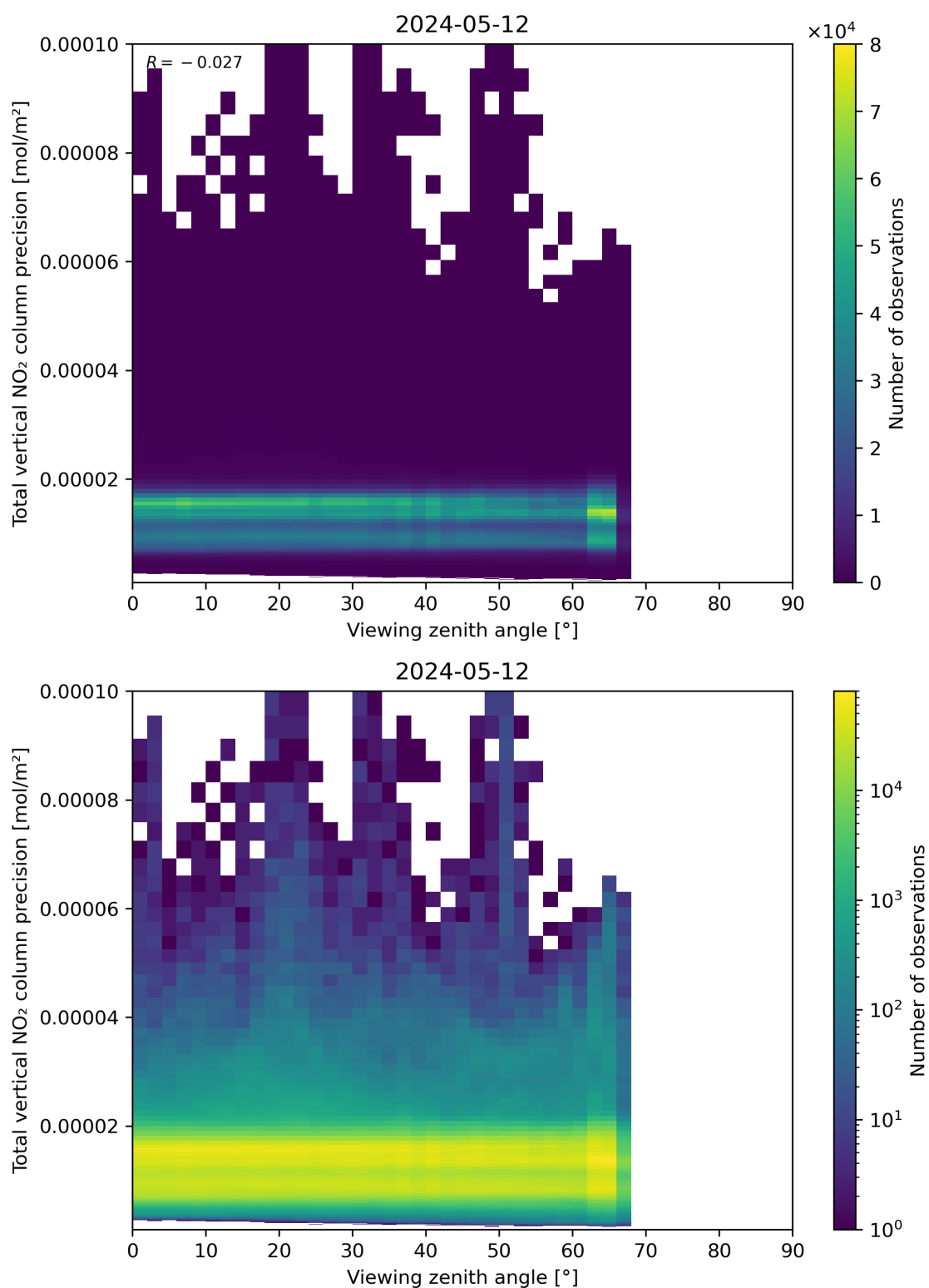
Figure 168: Scatter density plot of “Viewing zenith angle” against “Total vertical NO 2 column precision” for 2024-05-12 to 2024-05-13.
