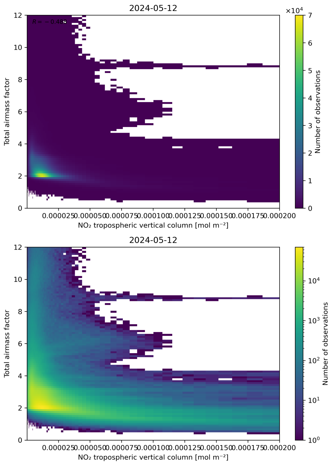
Figure 122: Scatter density plot of “NO 2 tropospheric vertical column” against “Total air mass factor” for 2024-05-12 to 2024-05-13.
