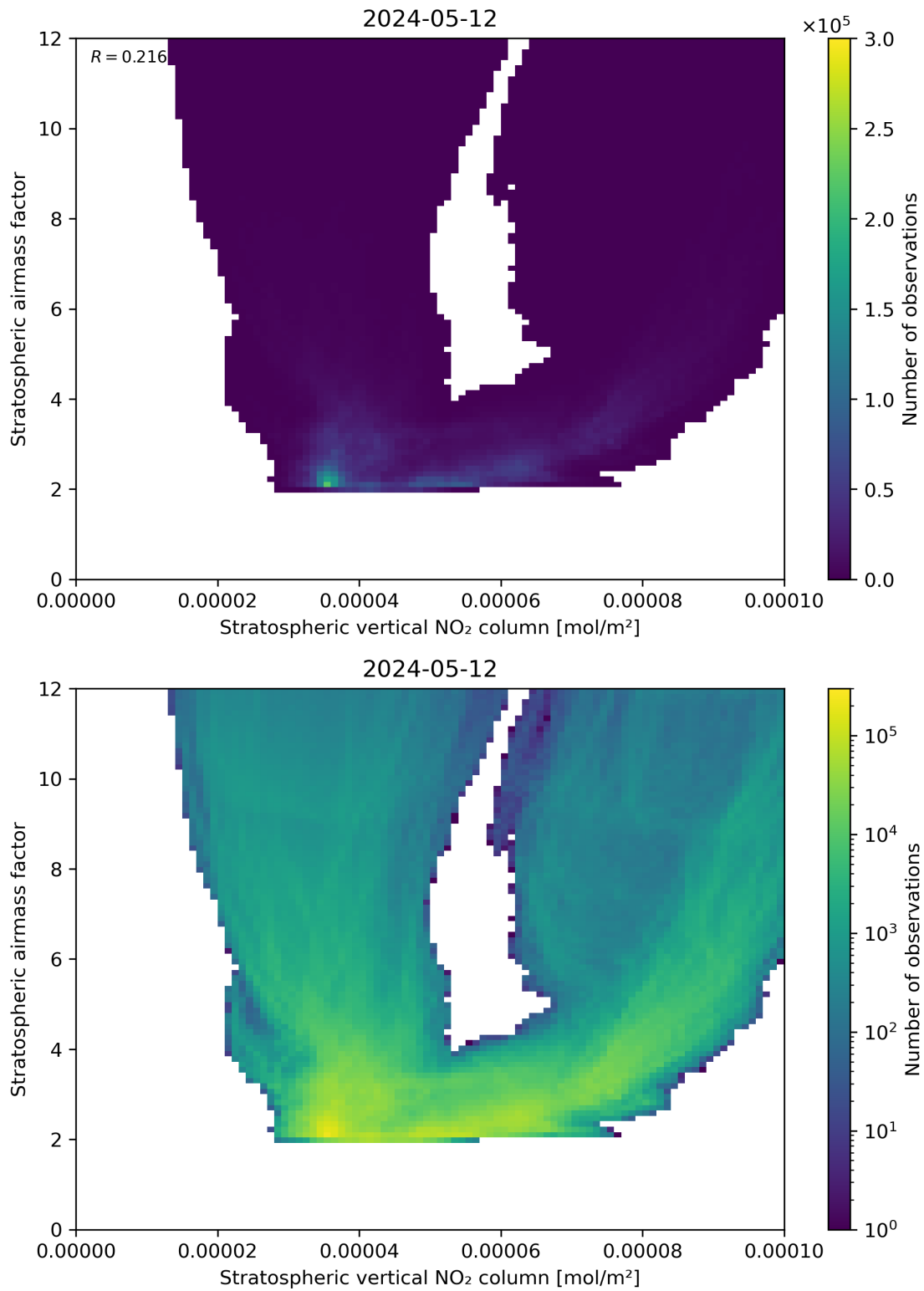
Figure 96: Scatter density plot of “Stratospheric vertical NO 2 column” against “Stratospheric airmass factor” for 2024-05-12 to 2024-05-13.
