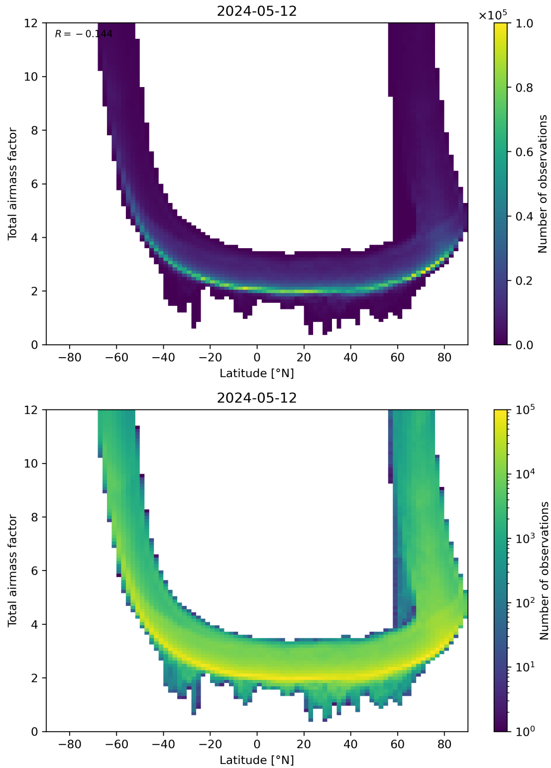
Figure 84: Scatter density plot of “Latitude” against “Total airmass factor” for 2024-05-12 to 2024-05-13.
