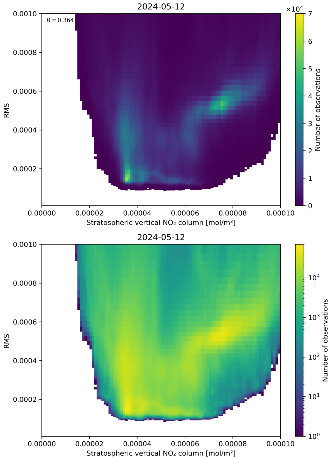
Figure 102: Scatter density plot of “Stratospheric vertical NO 2 column” against “RMS” for 2024-05-12 to 2024-05-13.
