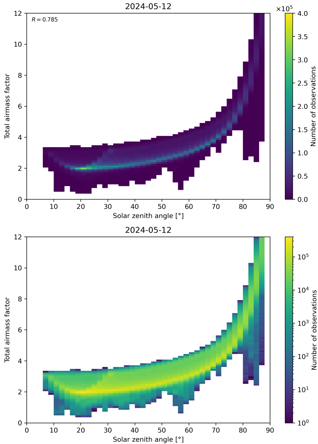
Figure 146: Scatter density plot of “Solar zenith angle” against “Total airmass factor” for 2024-05-12 to 2024-05-13.
