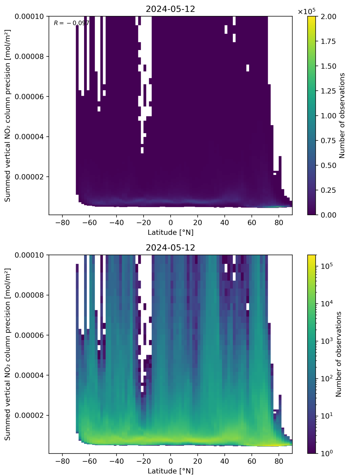
Figure 89: Scatter density plot of “Latitude” against “Summed vertical NO 2 column precision” for 2024-05-12 to 2024-05-13.
