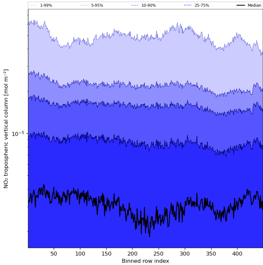
Figure 46: Along track statistics of “NO 2 tropospheric vertical column” for 2024-05-12 to 2024-05-13
