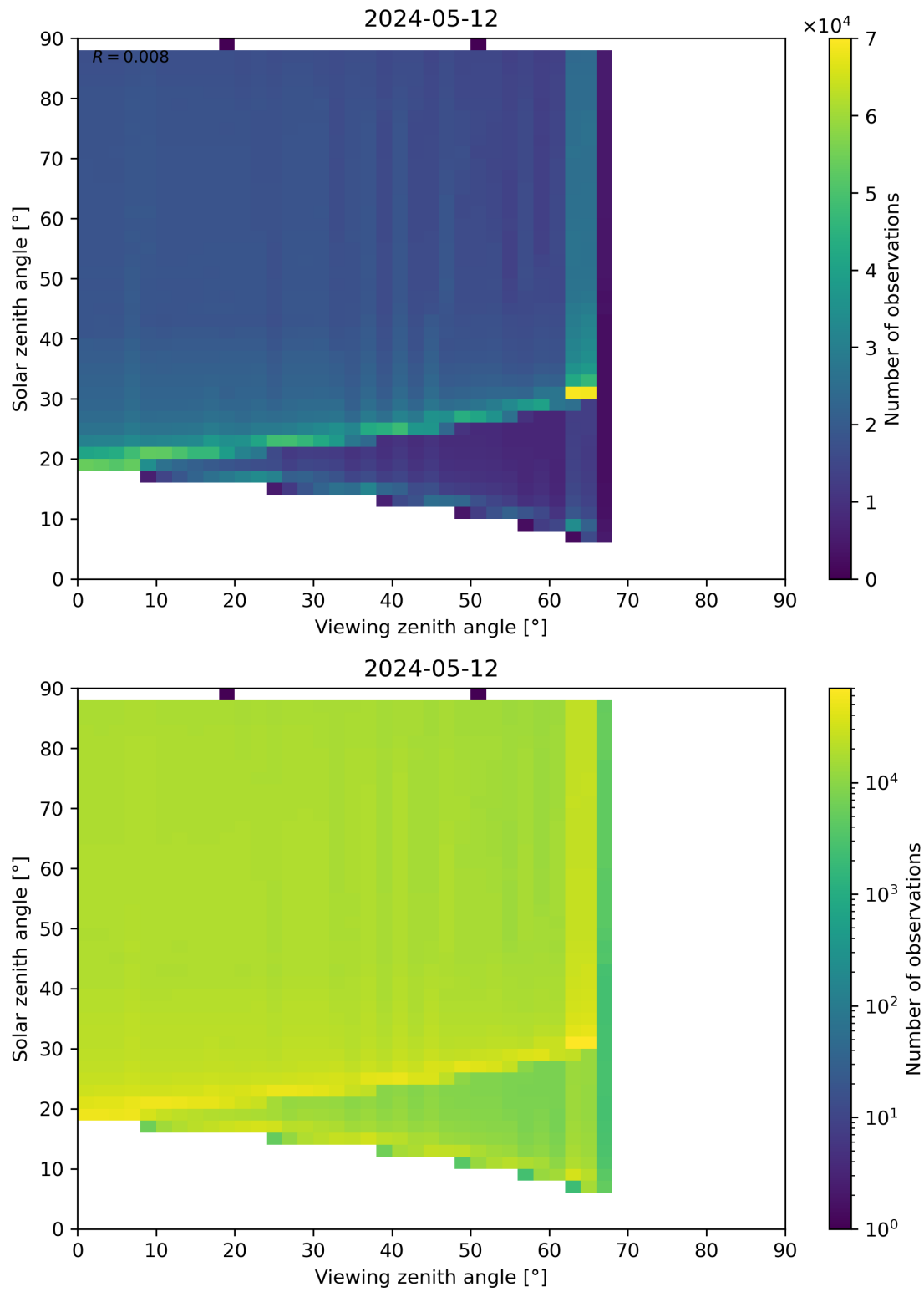
Figure 172: Scatter density plot of “Viewing zenith angle” against “Solar zenith angle” for 2024-05-12 to 2024-05-13.
