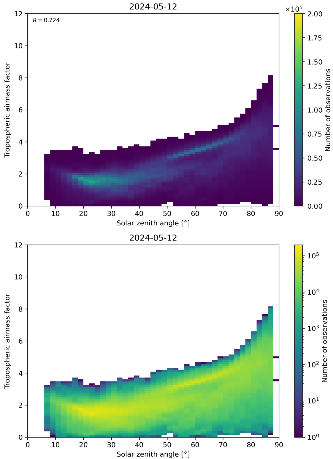
Figure 147: Scatter density plot of “Solar zenith angle” against “Tropospheric airmass factor” for 2024-05-12 to 2024-05-13.
