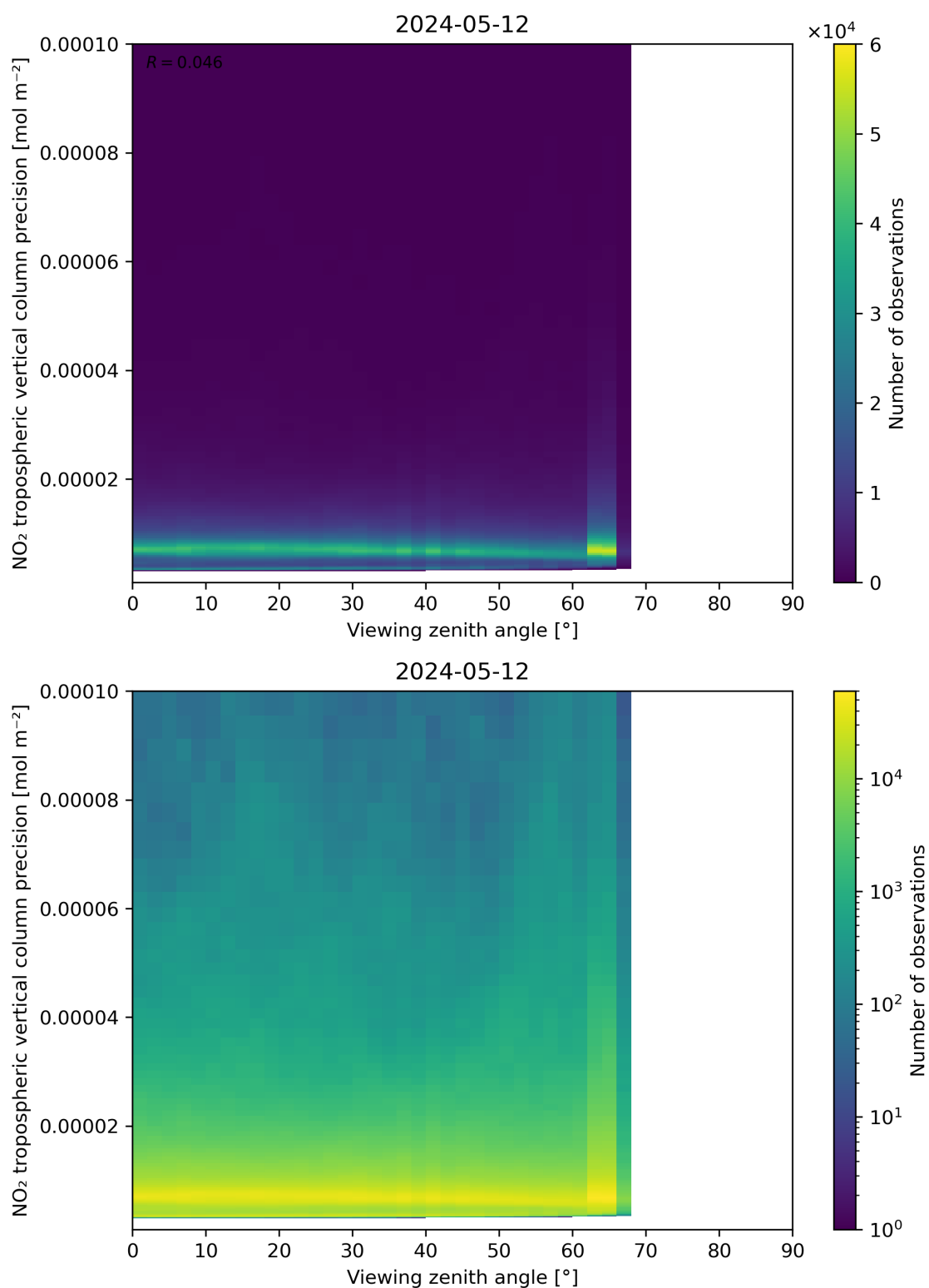
Figure 170: Scatter density plot of “Viewing zenith angle” against “NO 2 tropospheric vertical column precision” for 2024-05-12 to 2024-05-13.
