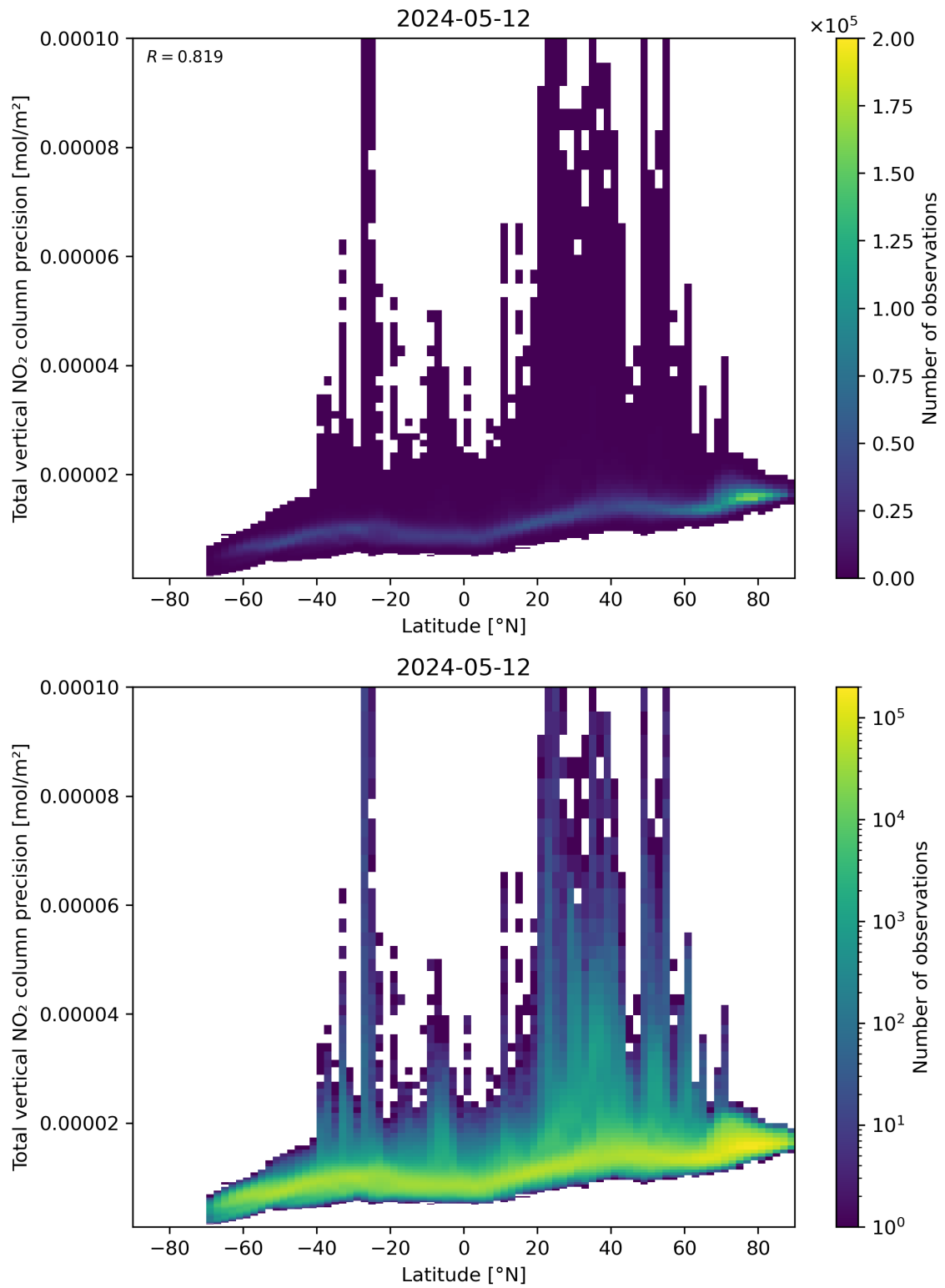
Figure 91: Scatter density plot of “Latitude” against “Total vertical NO 2 column precision” for 2024-05-12 to 2024-05-13.
