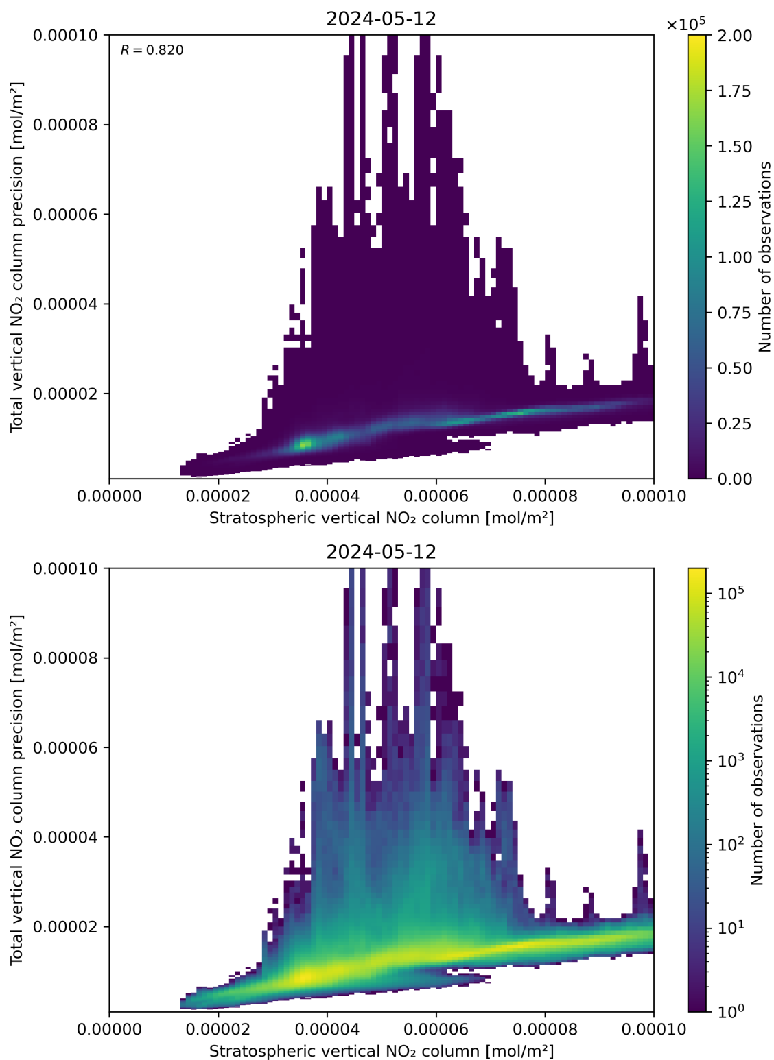
Figure 101: Scatter density plot of “Stratospheric vertical NO 2 column” against “Total vertical NO 2 column precision” for 2024-05-12 to 2024-05-13.
