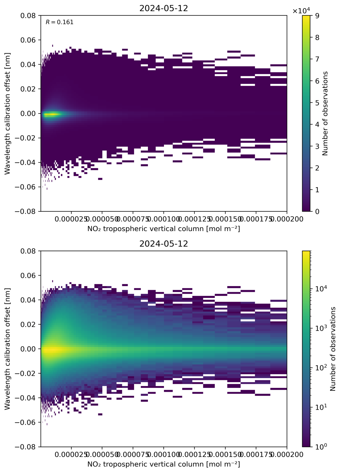
Figure 143: Scatter density plot of “NO 2 tropospheric vertical column” against “Wavelength calibration offset” for 2024-05-12 to 2024-05-13.
