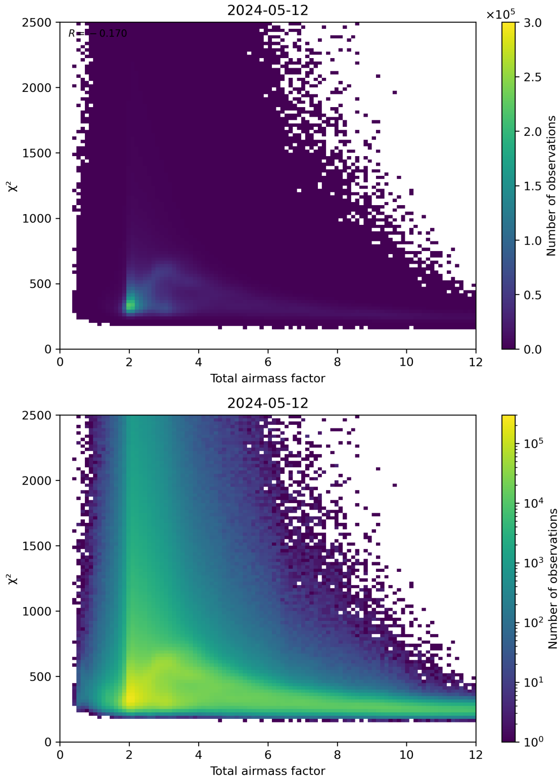
Figure 63: Scatter density plot of “Total airmass factor” against “ \chi^2 ” for 2024-05-12 to 2024-05-13.
