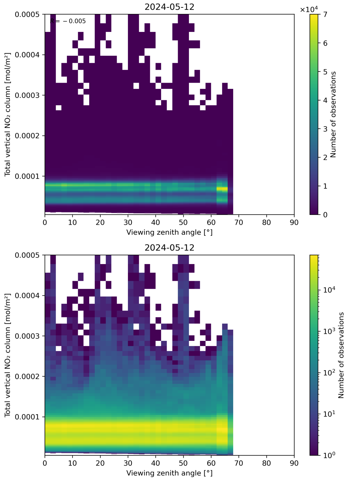
Figure 167: Scatter density plot of “Viewing zenith angle” against “Total vertical NO 2 column” for 2024-05-12 to 2024-05-13.
