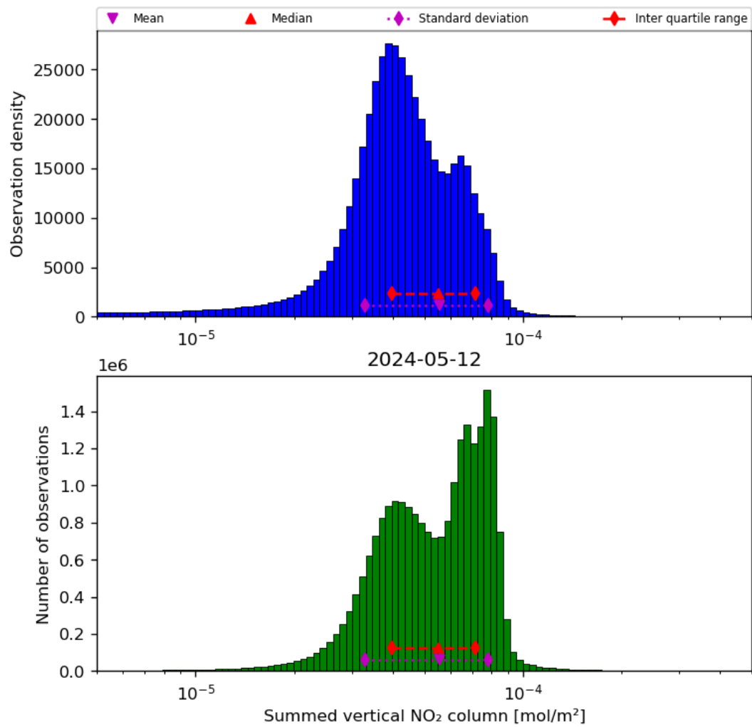
Figure 40: Histogram of “Summed vertical NO 2 column” for 2024-05-12 to 2024-05-13
