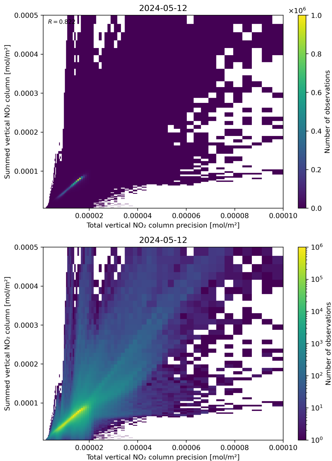
Figure 117: Scatter density plot of “Total vertical NO 2 column precision” against “Summed vertical NO 2 column” for 2024-05-12 to 2024-05-13.
