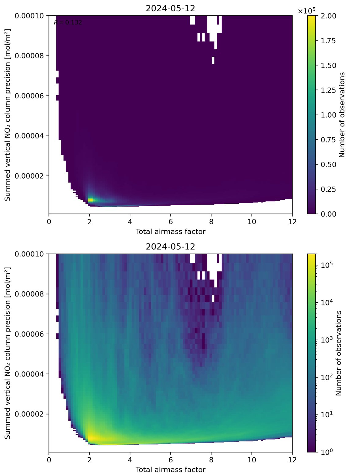
Figure 66: Scatter density plot of “Total airmass factor” against “Summed vertical NO 2 column precision” for 2024-05-12 to 2024-05-13.
