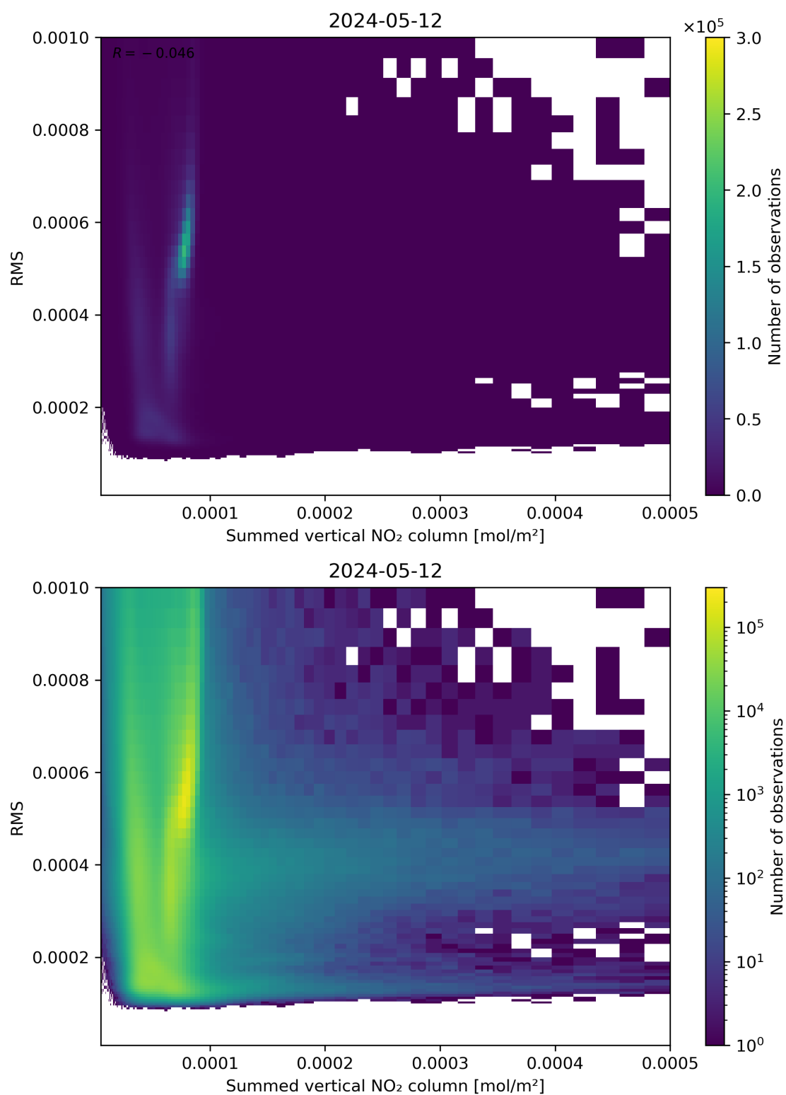
Figure 109: Scatter density plot of “Summed vertical NO 2 column” against “RMS” for 2024-05-12 to 2024-05-13.
