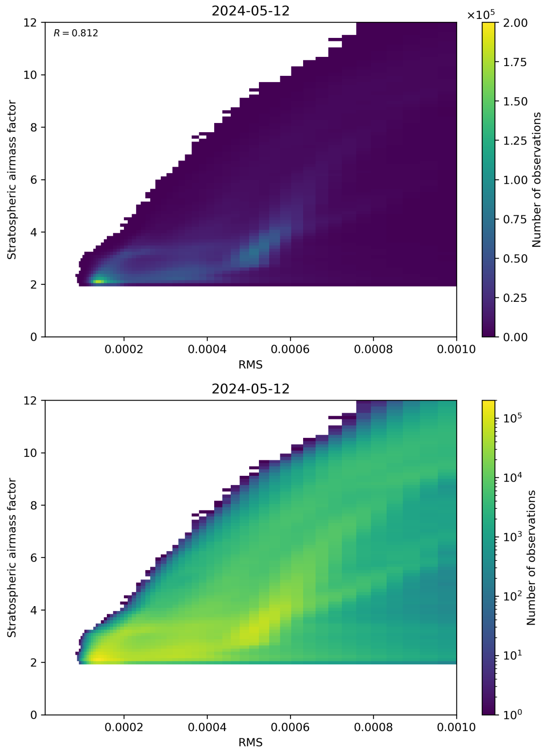
Figure 144: Scatter density plot of “RMS” against “Stratospheric airmass factor” for 2024-05-12 to 2024-05-13.
