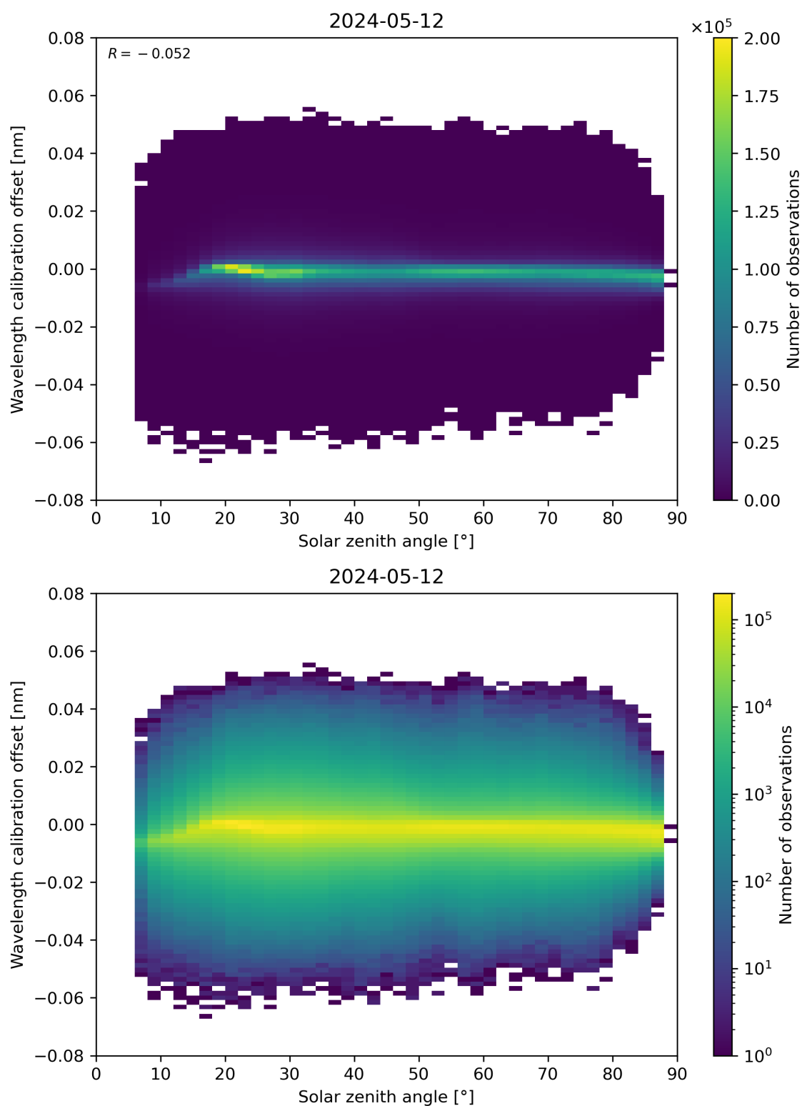
Figure 158: Scatter density plot of “Solar zenith angle” against “Wavelength calibration offset” for 2024-05-12 to 2024-05-13.
