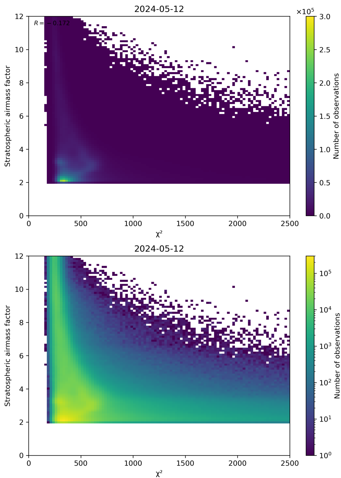
Figure 81: Scatter density plot of “ \chi^2 ” against “Stratospheric airmass factor” for 2024-05-12 to 2024-05-13.
