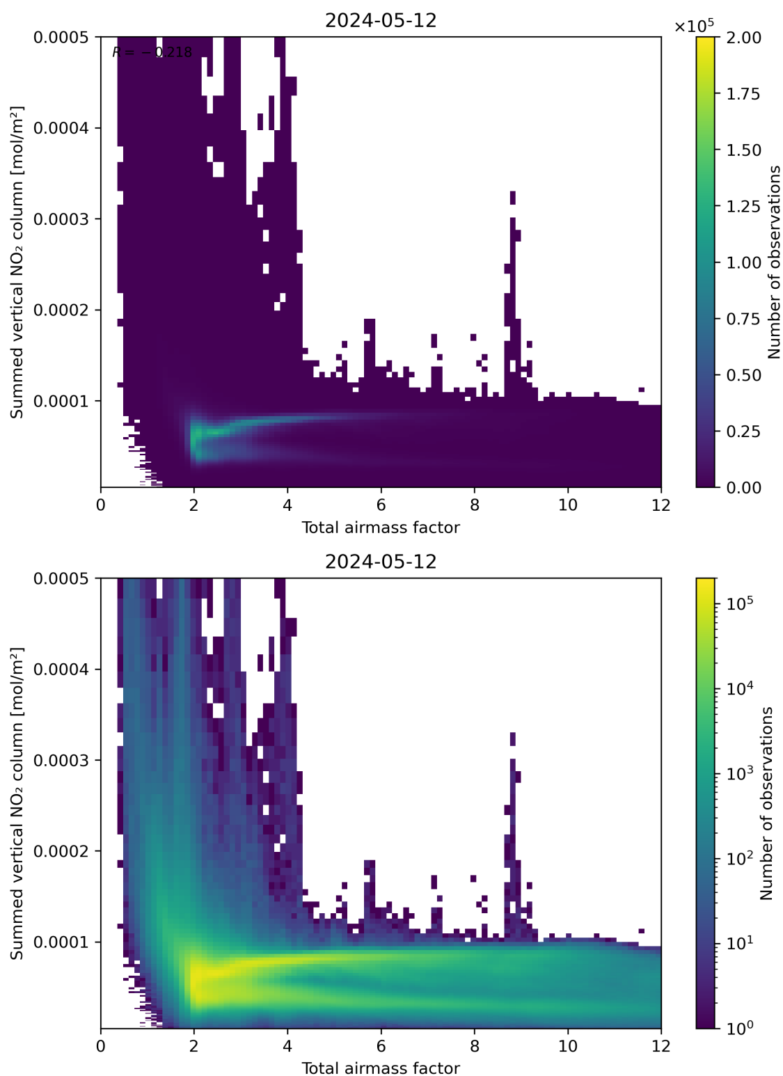
Figure 65: Scatter density plot of “Total airmass factor” against “Summed vertical NO 2 column” for 2024-05-12 to 2024-05-13.
