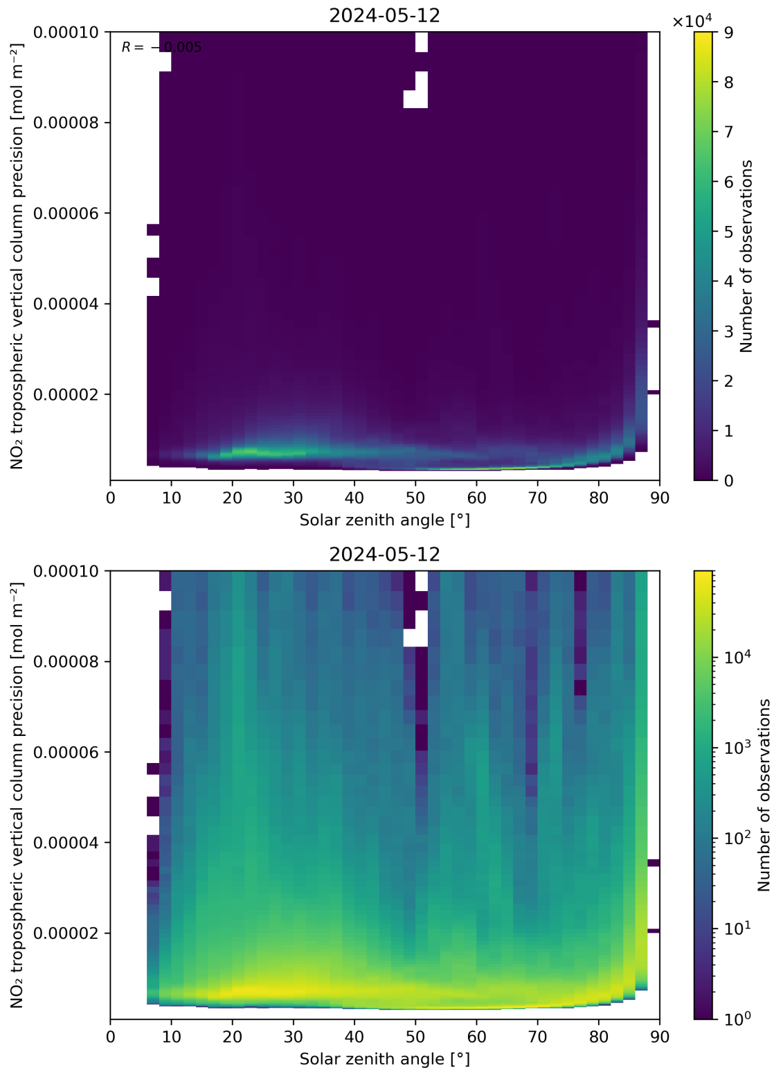
Figure 156: Scatter density plot of “Solar zenith angle” against “NO 2 tropospheric vertical column precision” for 2024-05-12 to 2024-05-13.
