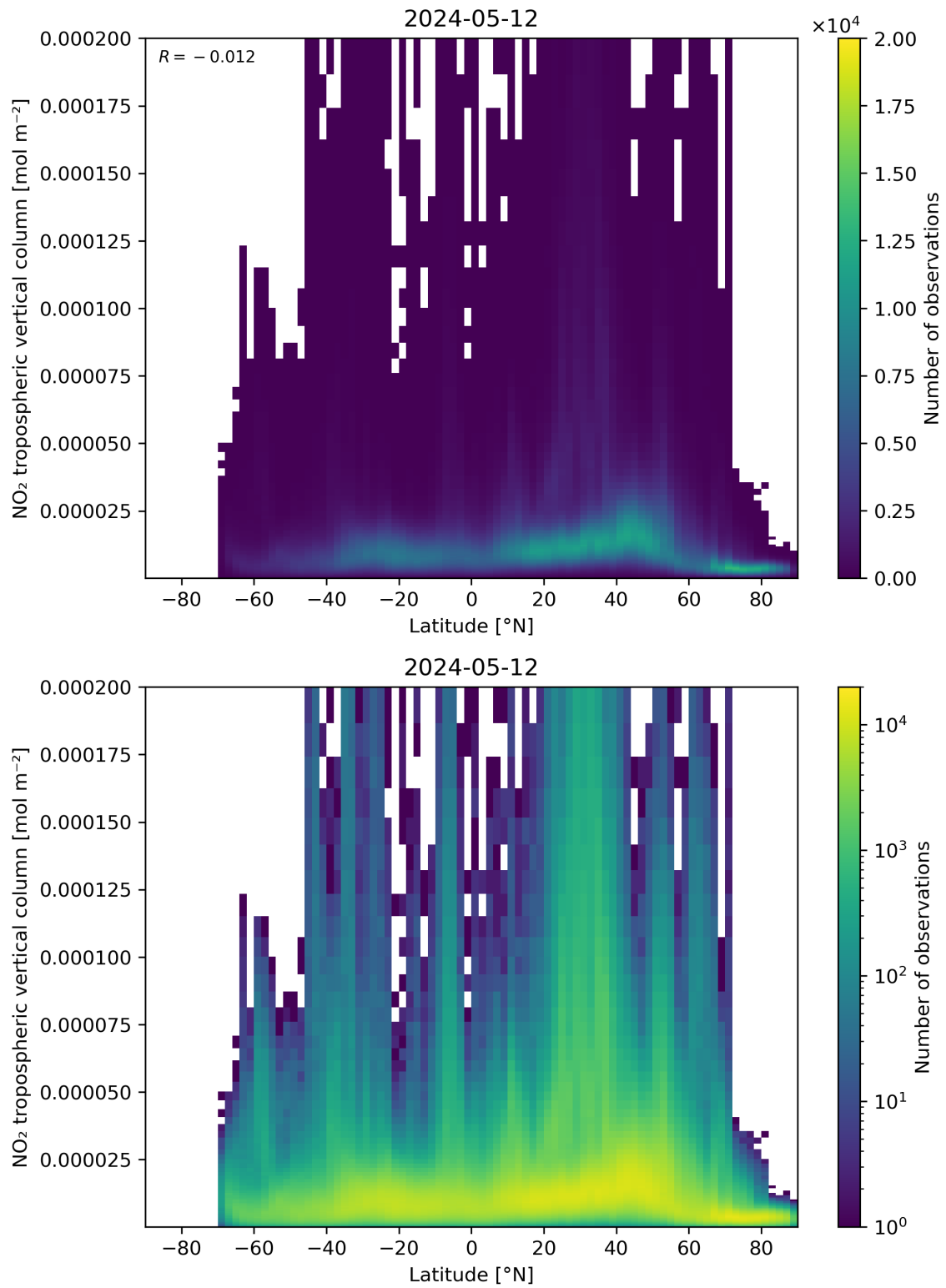
Figure 92: Scatter density plot of “Latitude” against “NO 2 tropospheric vertical column” for 2024-05-12 to 2024-05-13.
