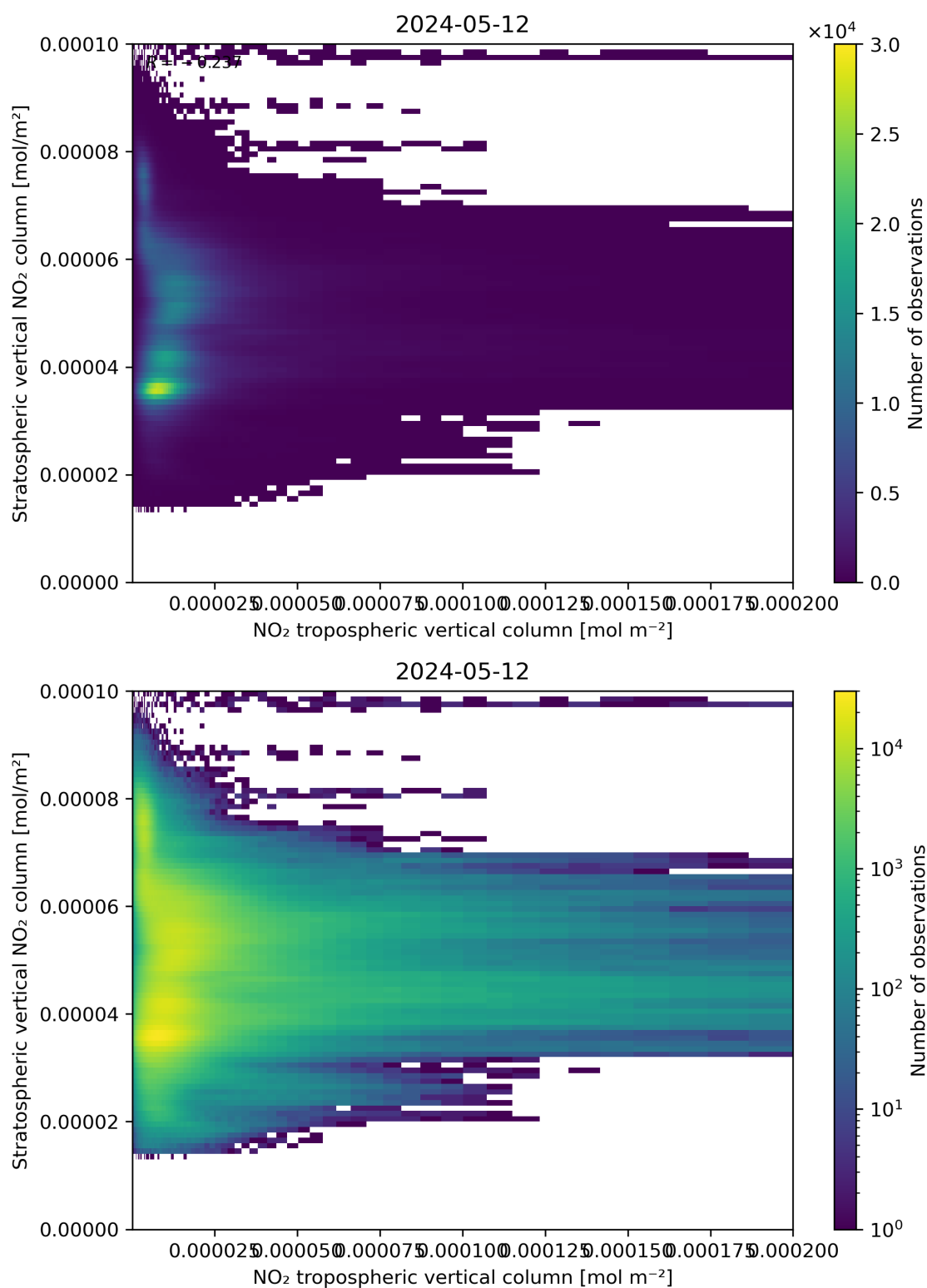
Figure 125: Scatter density plot of “NO 2 tropospheric vertical column” against “Stratospheric vertical NO 2 column” for 2024-05-12 to 2024-05-13.
