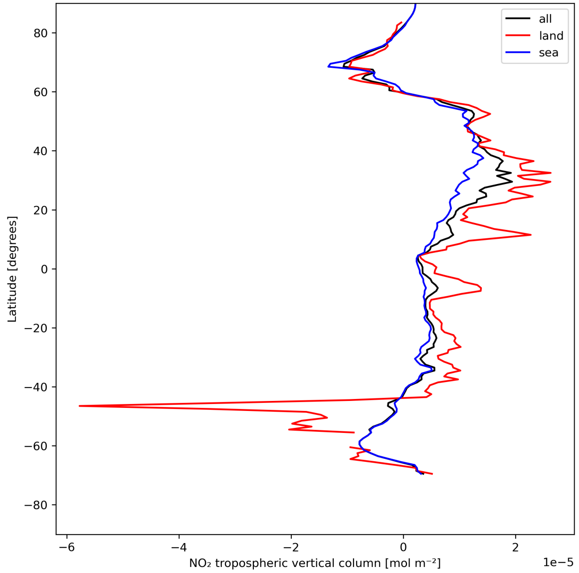
Figure 12: Zonal average of “NO 2 tropospheric vertical column” for 2024-05-12 to 2024-05-13.
