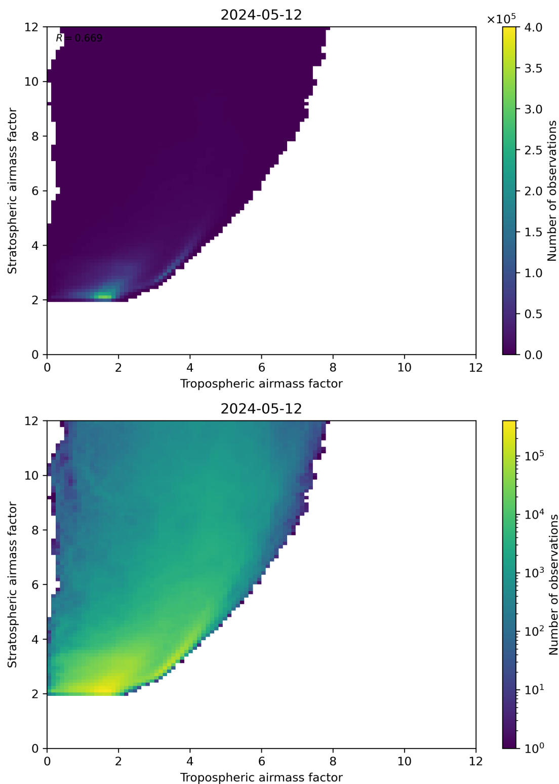
Figure 71: Scatter density plot of “Tropospheric airmass factor” against “Stratospheric airmass factor” for 2024-05-12 to 2024-05-13.
