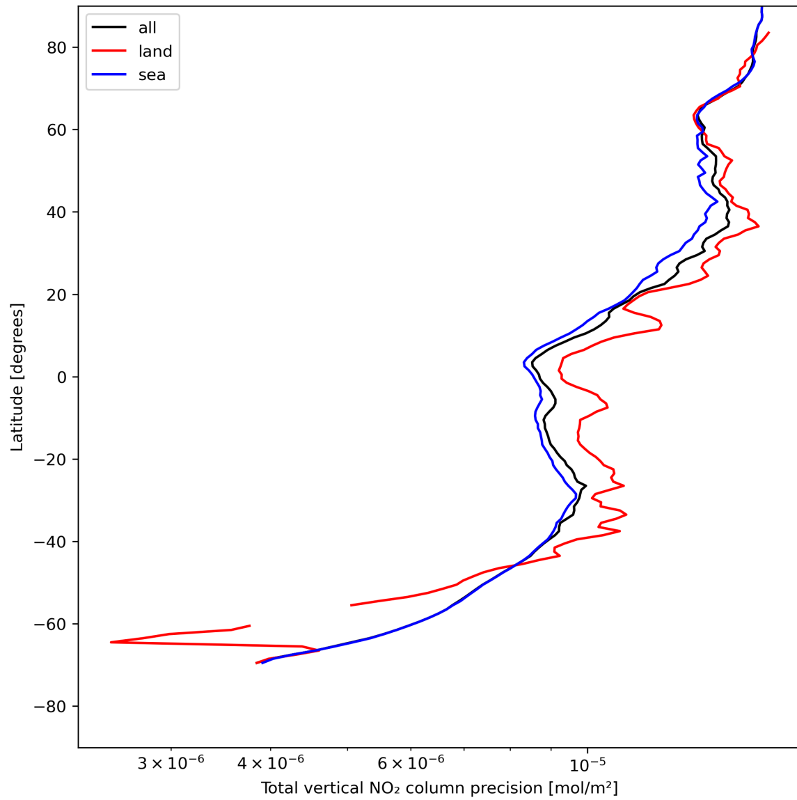
Figure 22: Zonal average of “Total vertical NO 2 column precision” for 2024-05-12 to 2024-05-13.
