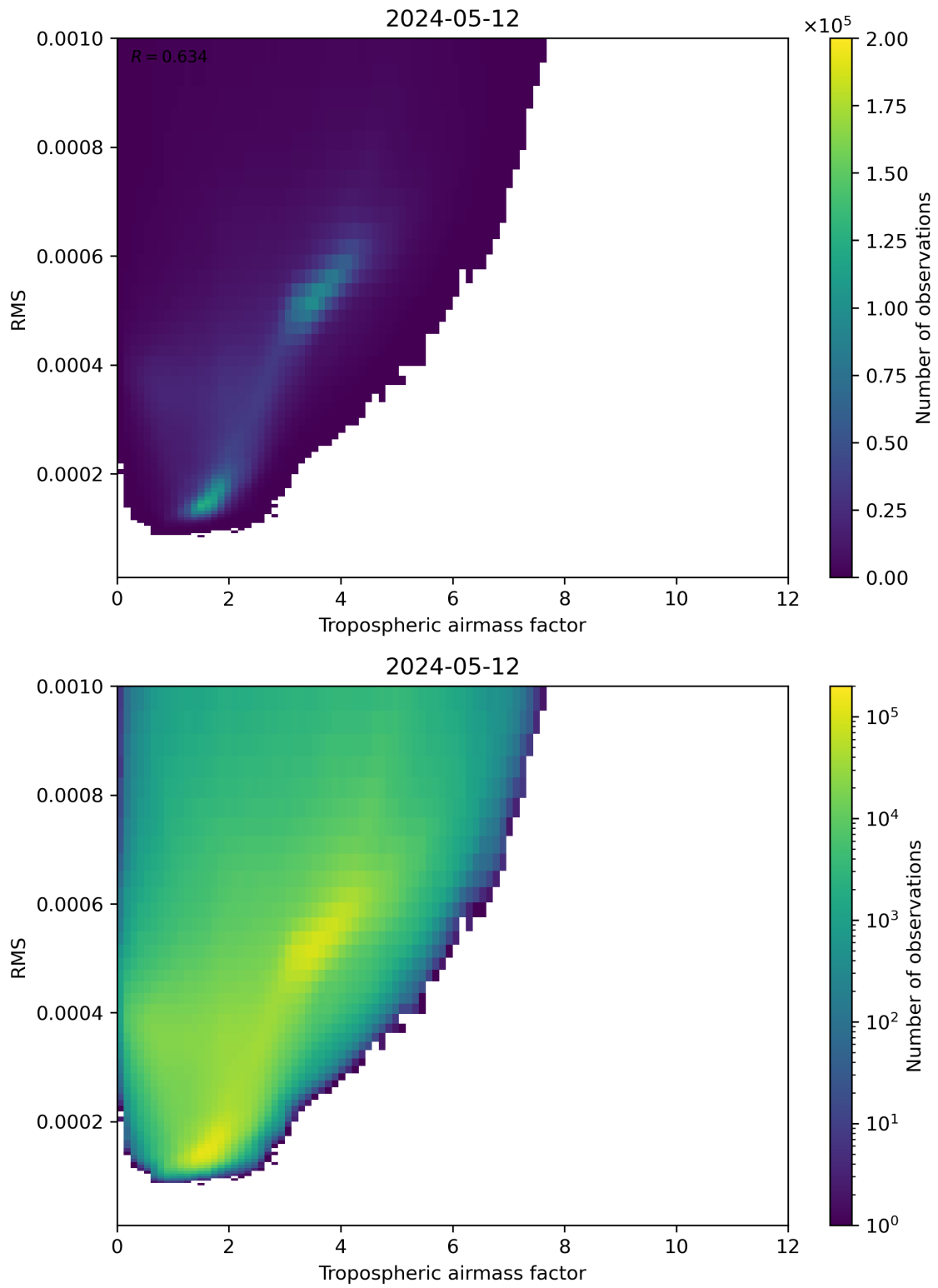
Figure 79: Scatter density plot of “Tropospheric airmass factor” against “RMS” for 2024-05-12 to 2024-05-13.
