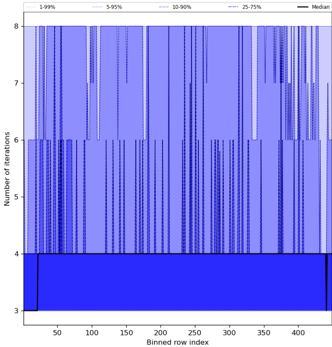
Figure 51: Along track statistics of “Number of iterations” for 2024-05-12 to 2024-05-13
