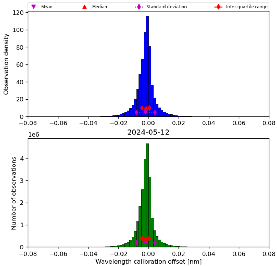
Figure 35: Histogram of “Wavelength calibration offset” for 2024-05-12 to 2024-05-13
