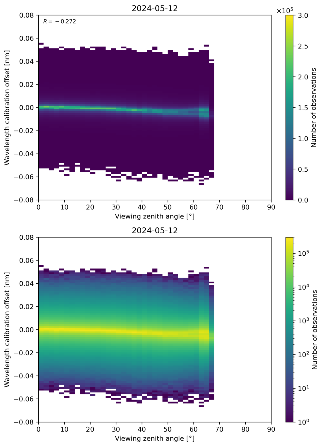
Figure 173: Scatter density plot of “Viewing zenith angle” against “Wavelength calibration offset” for 2024-05-12 to 2024-05-13.
