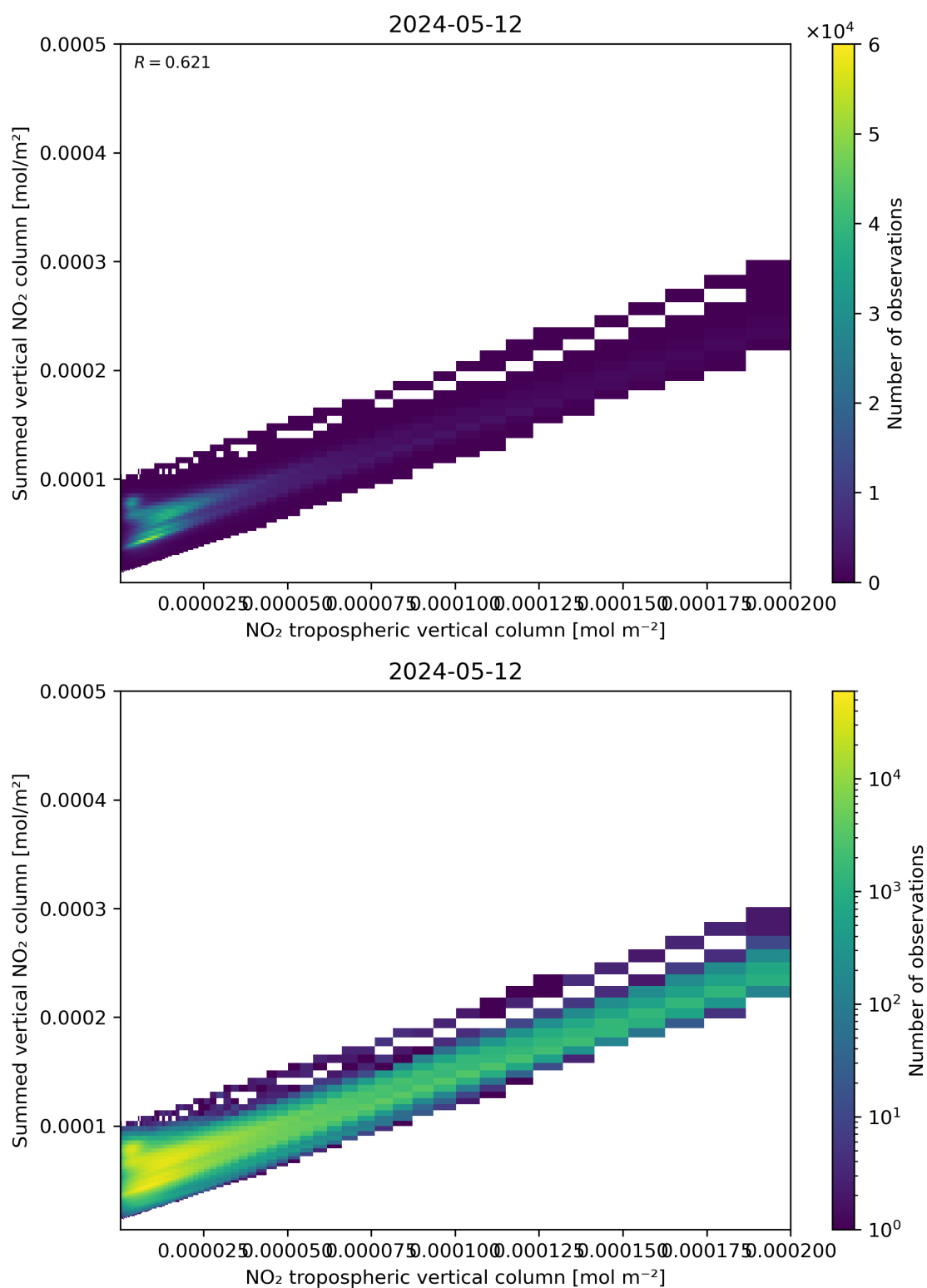
Figure 126: Scatter density plot of “NO 2 tropospheric vertical column” against “Summed vertical NO 2 column” for 2024-05-12 to 2024-05-13.
