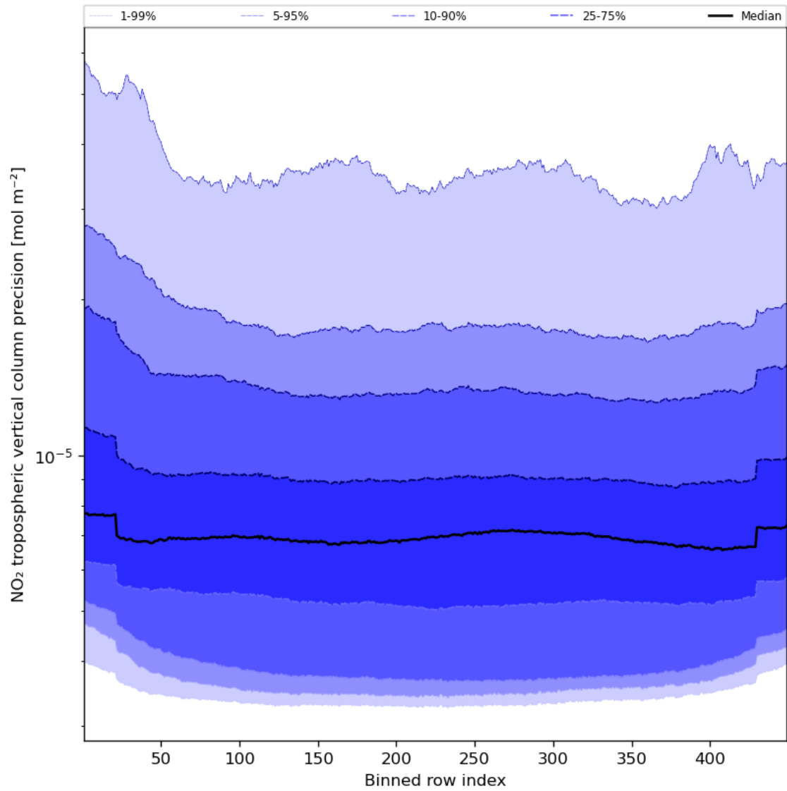
Figure 47: Along track statistics of “NO 2 tropospheric vertical column precision” for 2024-05-12 to 2024-05-13
