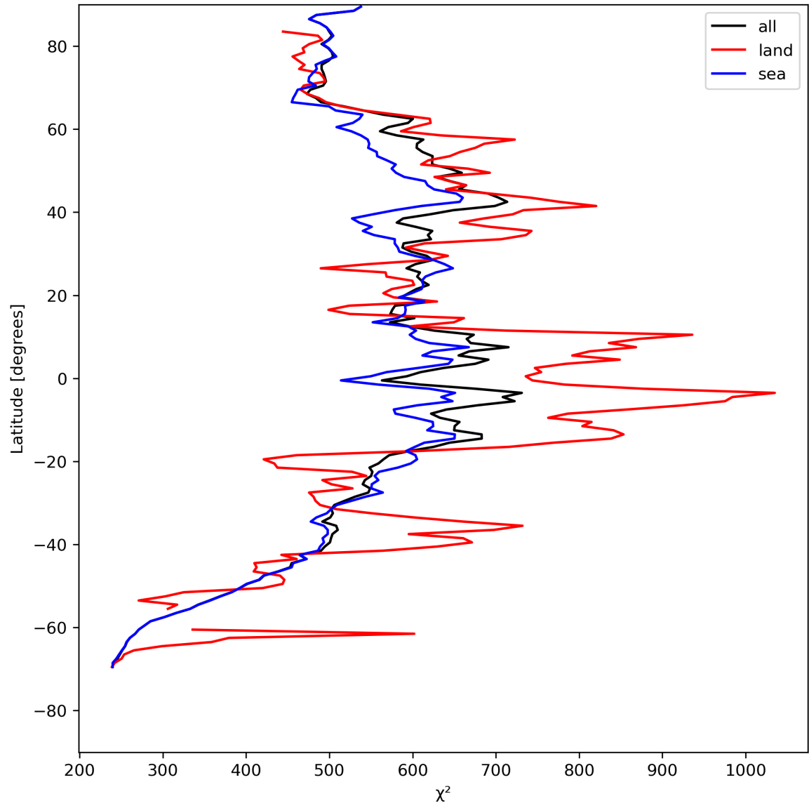
Figure 25: Zonal average of “ \chi^2 ” for 2024-05-12 to 2024-05-13.
