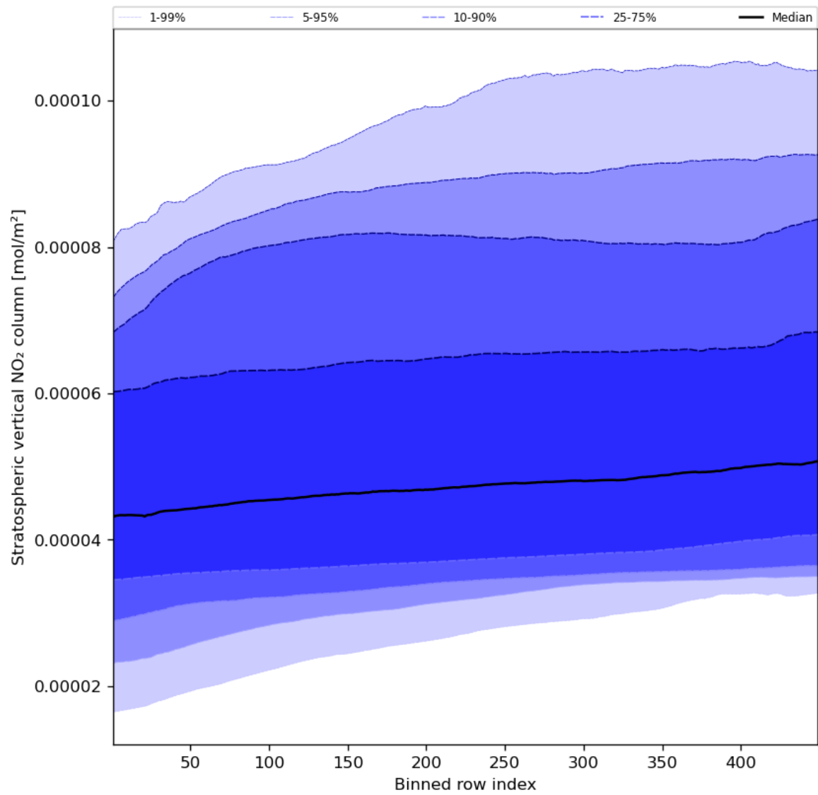
Figure 53: Along track statistics of “Stratospheric vertical NO 2 column” for 2024-05-12 to 2024-05-13
