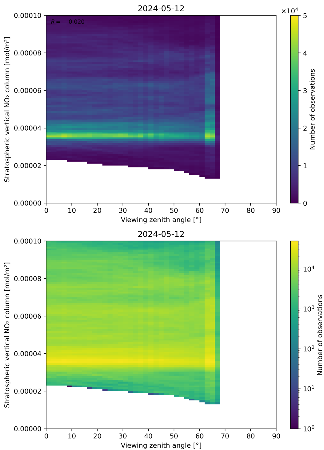
Figure 164: Scatter density plot of “Viewing zenith angle” against “Stratospheric vertical NO 2 column” for 2024-05-12 to 2024-05-13.
