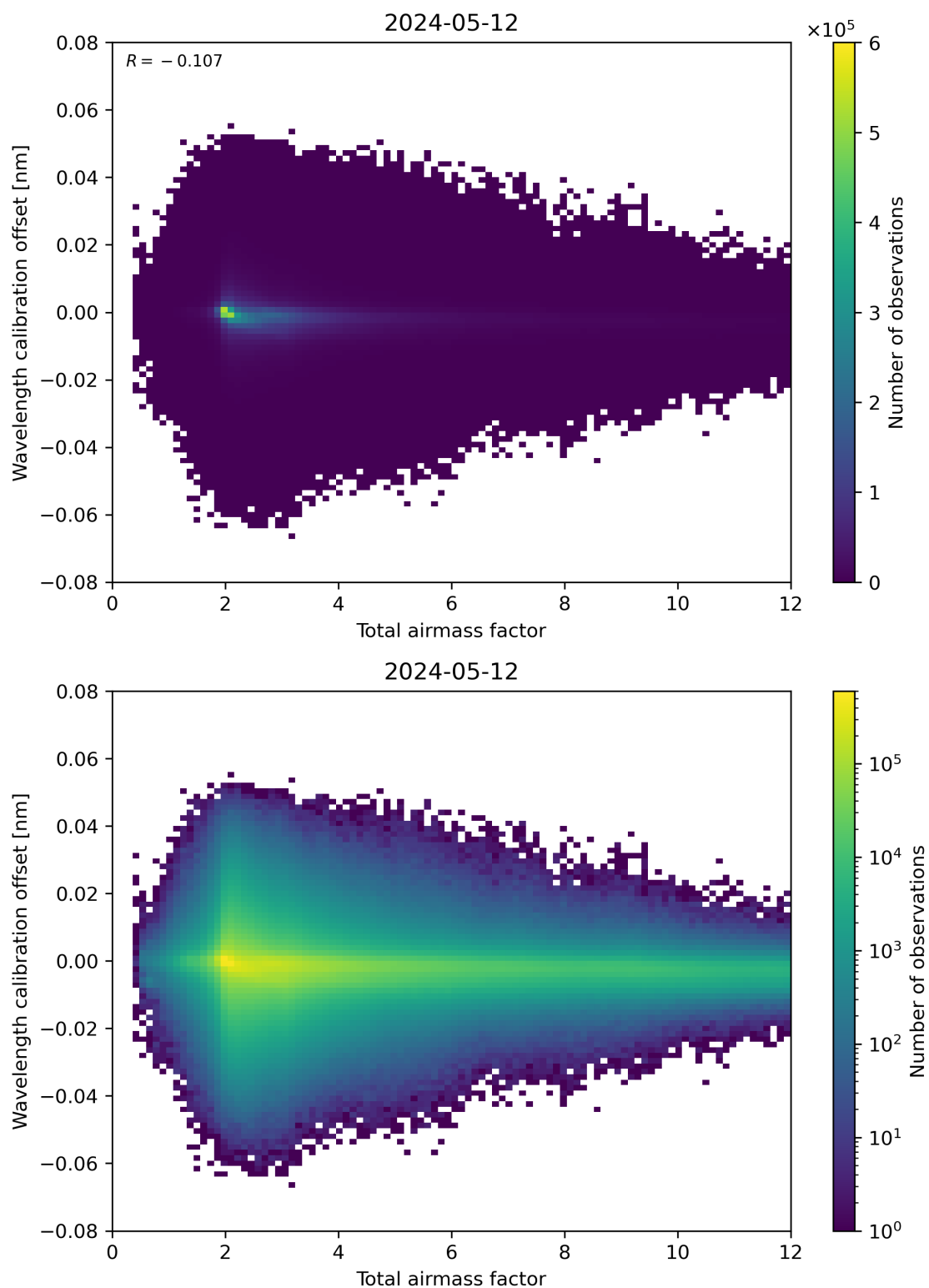
Figure 70: Scatter density plot of “Total airmass factor” against “Wavelength calibration offset” for 2024-05-12 to 2024-05-13.
