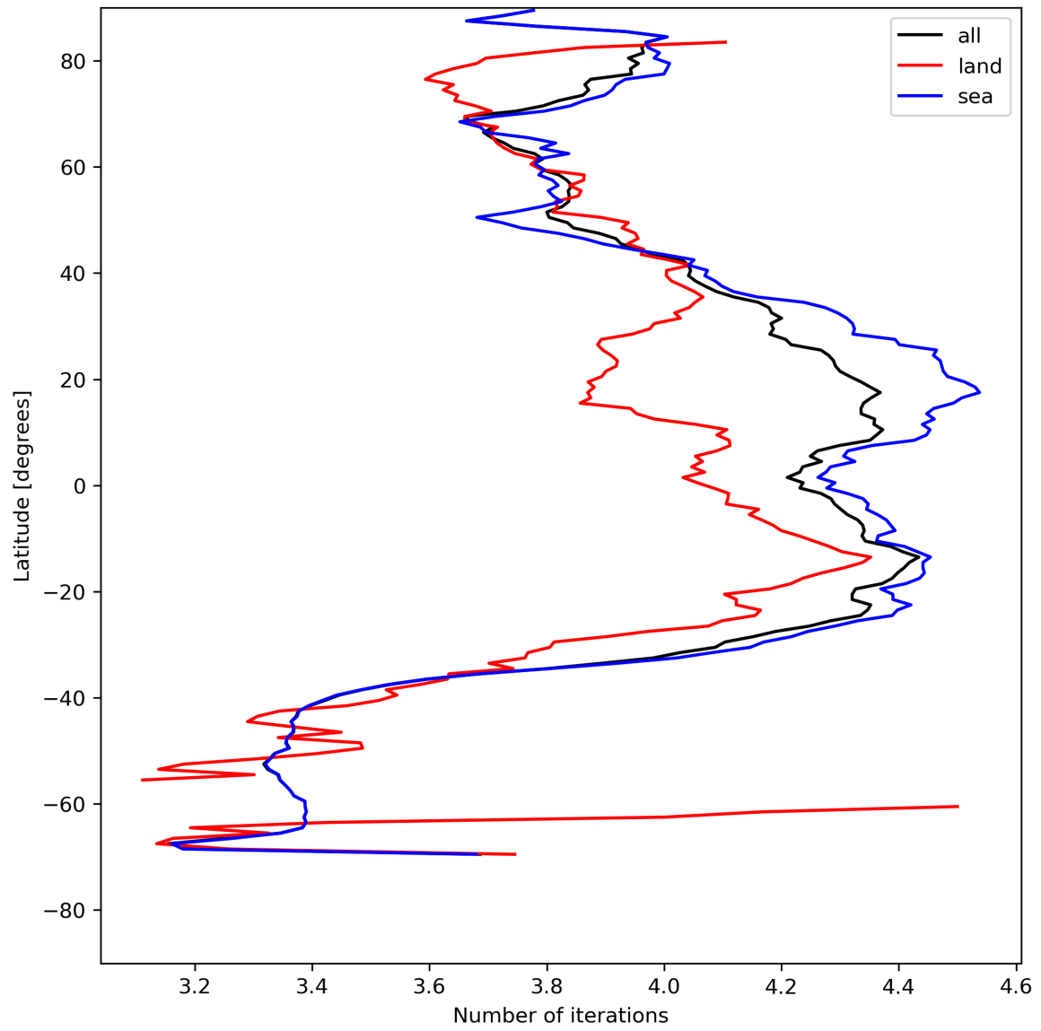
Figure 17: Zonal average of “Number of iterations” for 2024-05-12 to 2024-05-13.
