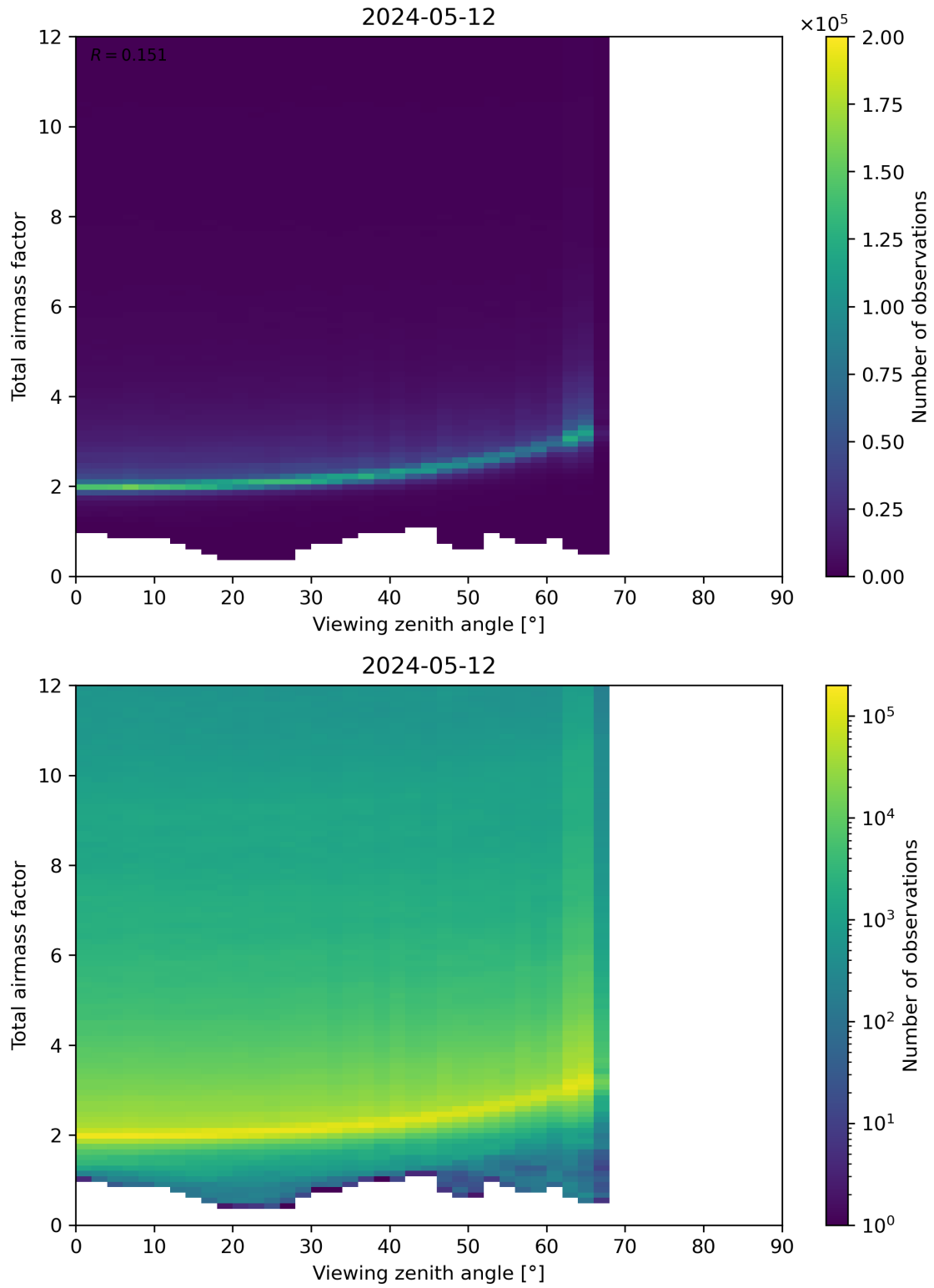
Figure 160: Scatter density plot of “Viewing zenith angle” against “Total airmass factor” for 2024-05-12 to 2024-05-13.
