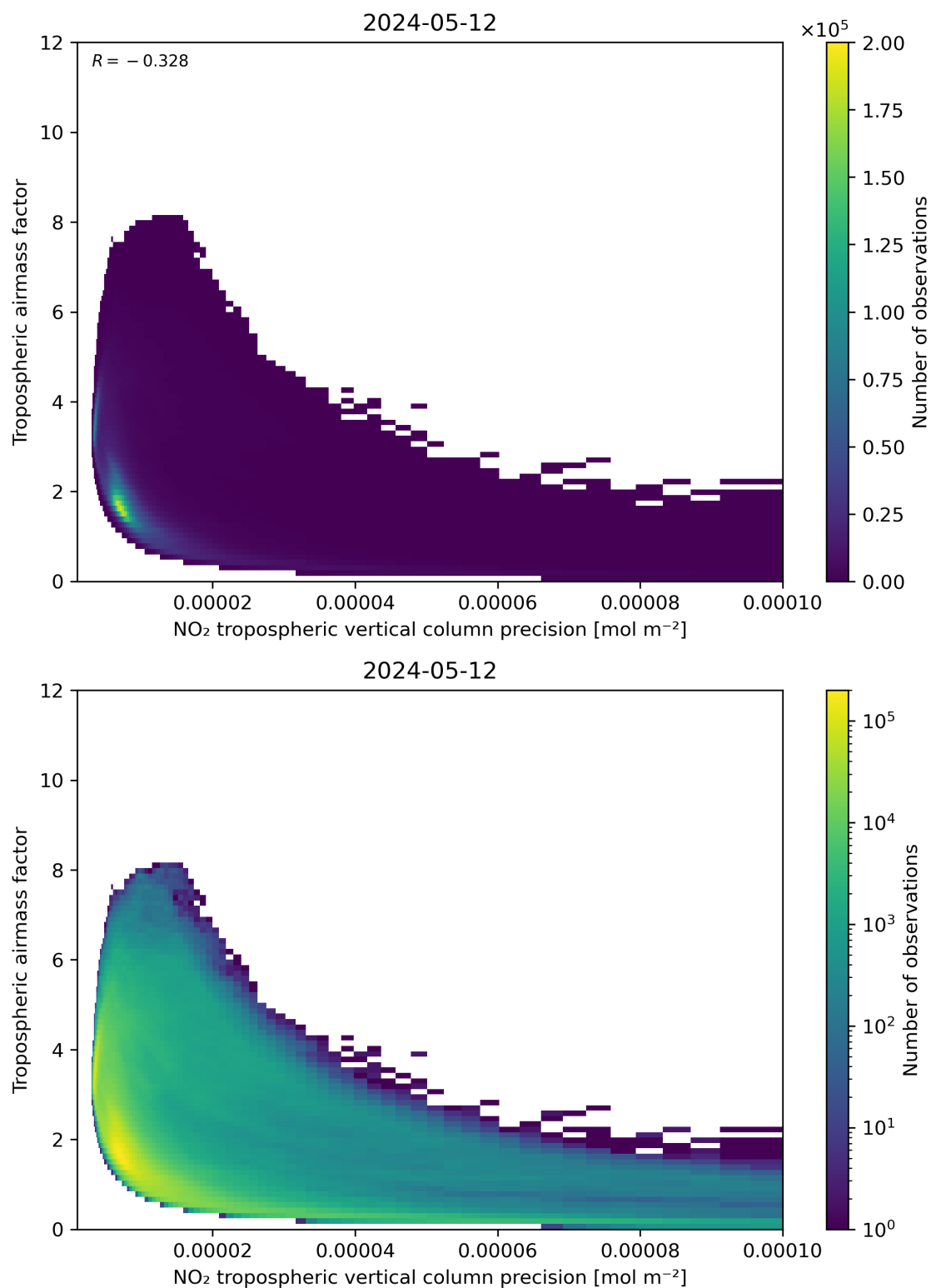
Figure 133: Scatter density plot of “NO 2 tropospheric vertical column precision” against “Tropospheric airmass factor” for 2024-05-12 to 2024-05-13.
