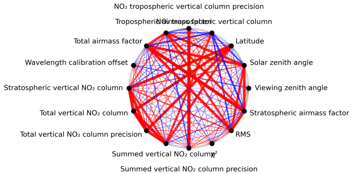
Figure 1: Map of correlation graph for 2024-05-12 to 2024-05-13.
