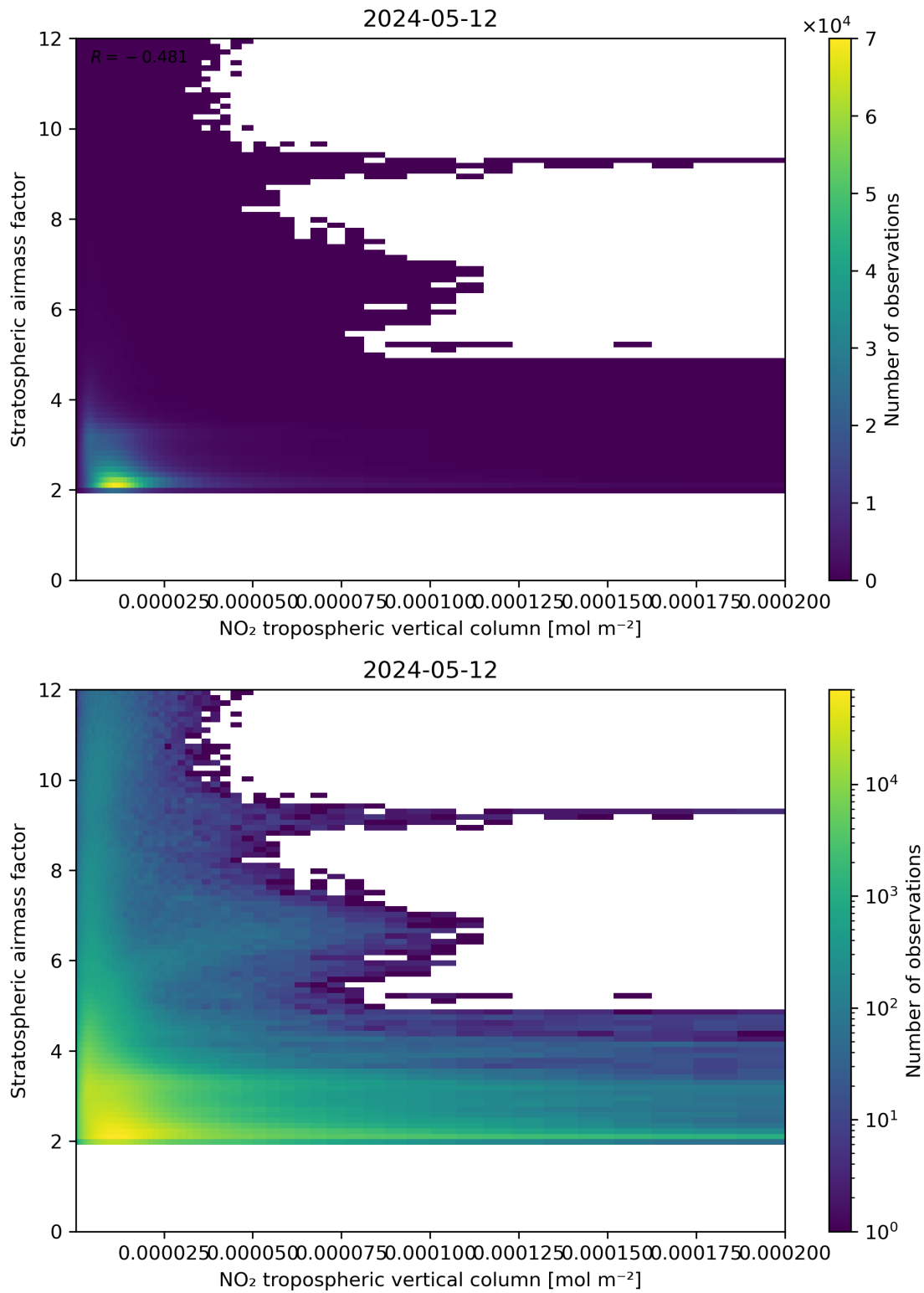
Figure 121: Scatter density plot of “NO 2 tropospheric vertical column” against “Stratospheric air mass factor” for 2024-05-12 to 2024-05-13.
