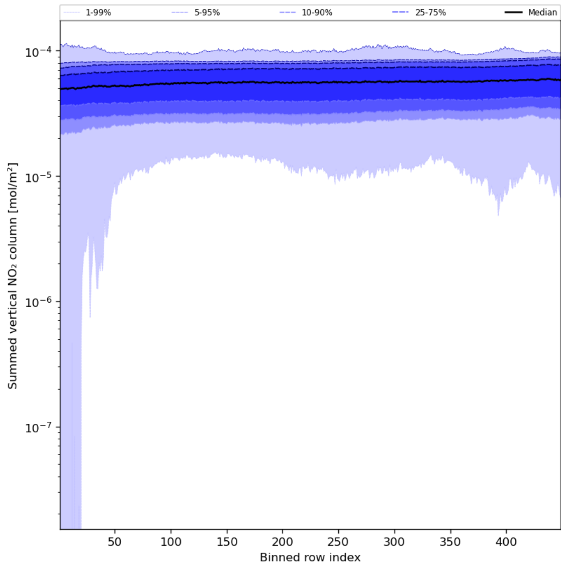
Figure 57: Along track statistics of “Summed vertical NO 2 column” for 2024-05-12 to 2024-05-13
