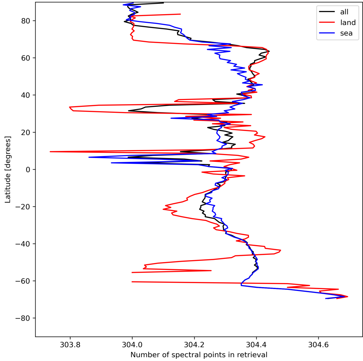
Figure 16: Zonal average of “Number of spectral points in retrieval” for 2024-05-12 to 2024-05-13.
