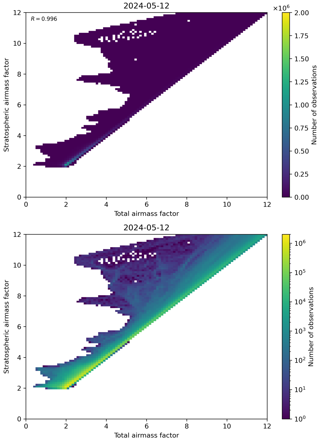
Figure 62: Scatter density plot of “Total airmass factor” against “Stratospheric airmass factor” for 2024-05-12 to 2024-05-13.
