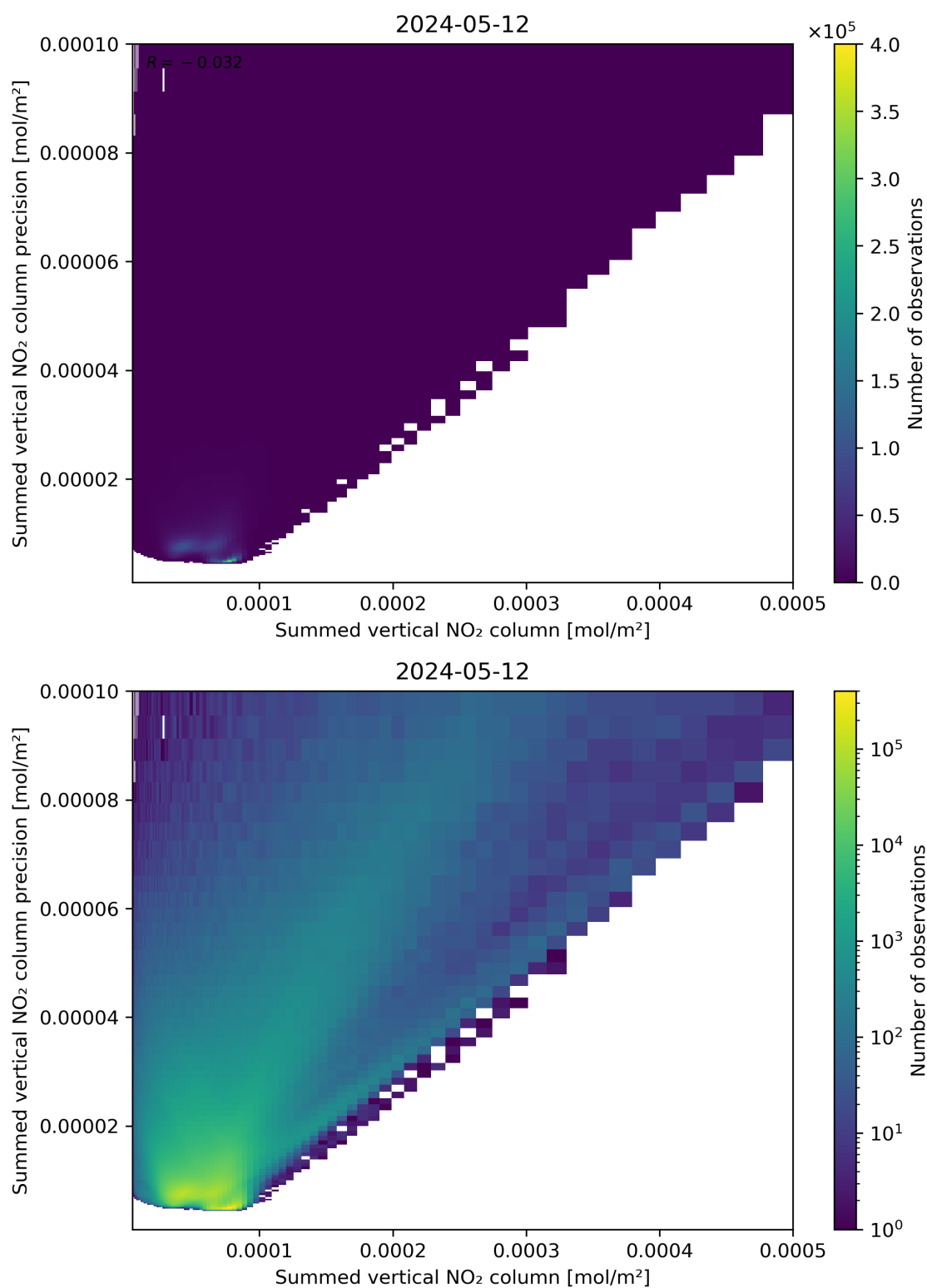
Figure 105: Scatter density plot of “Summed vertical NO 2 column” against “Summed vertical NO 2 column precision” for 2024-05-12 to 2024-05-13.
