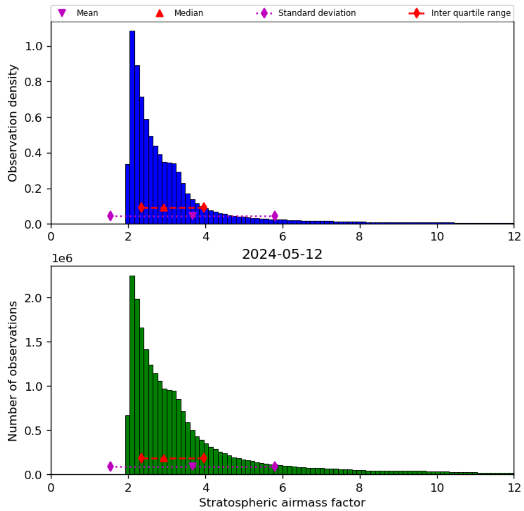
Figure 44: Histogram of “Stratospheric airmass factor” for 2024-05-12 to 2024-05-13
