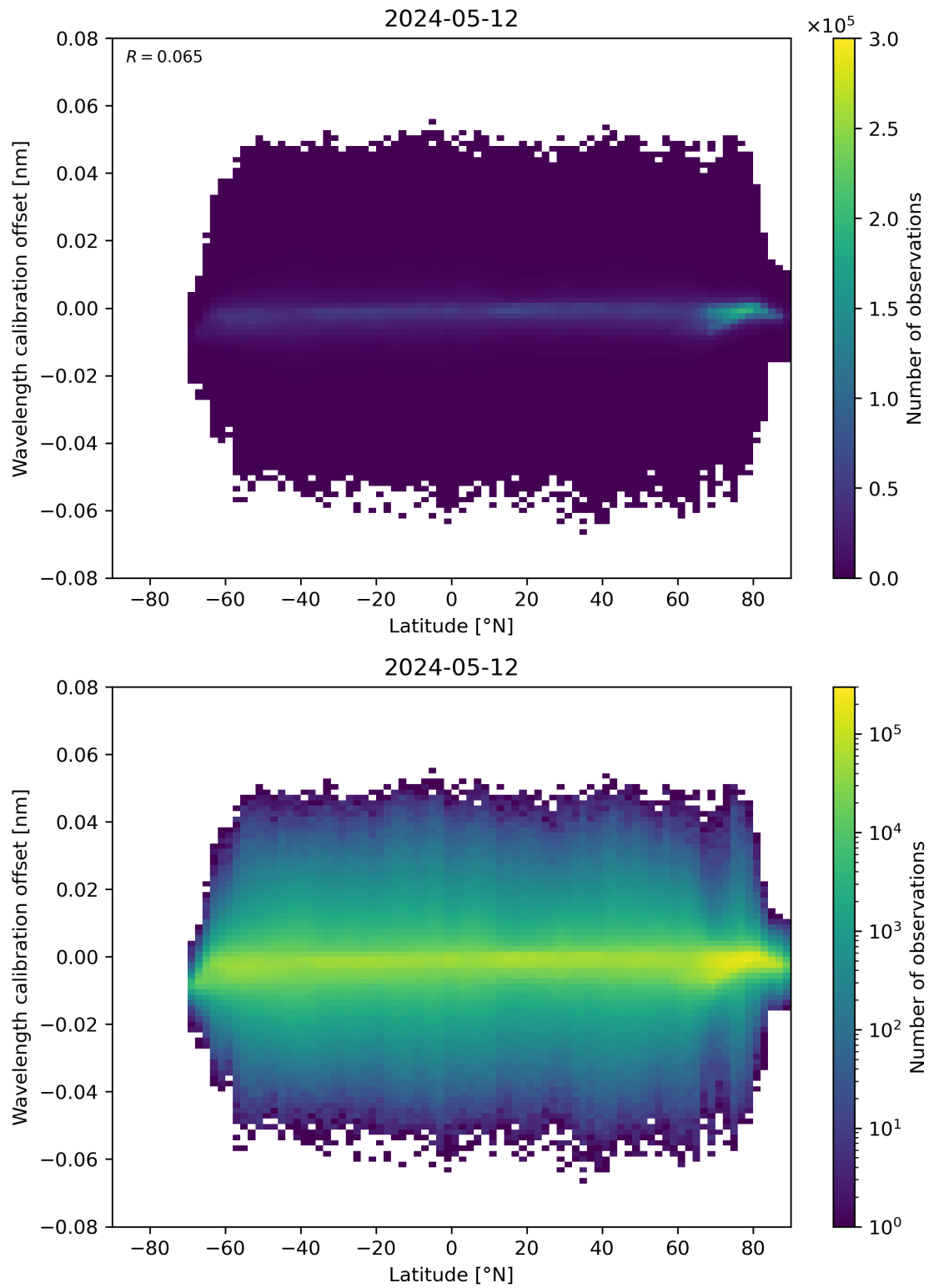
Figure 95: Scatter density plot of “Latitude” against “Wavelength calibration offset” for 2024-05-12 to 2024-05-13.
