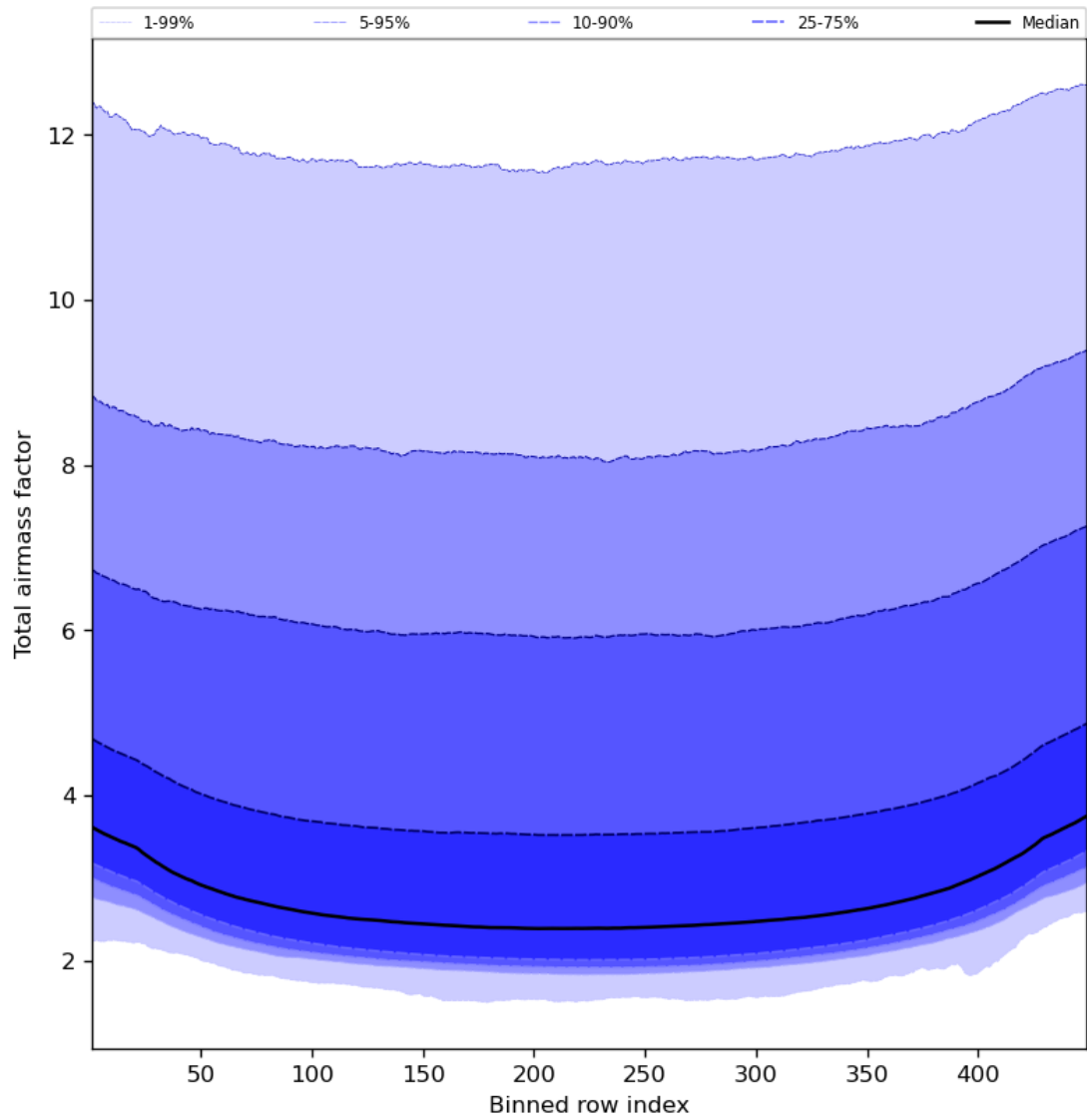
Figure 49: Along track statistics of “Total airmass factor” for 2024-05-12 to 2024-05-13
