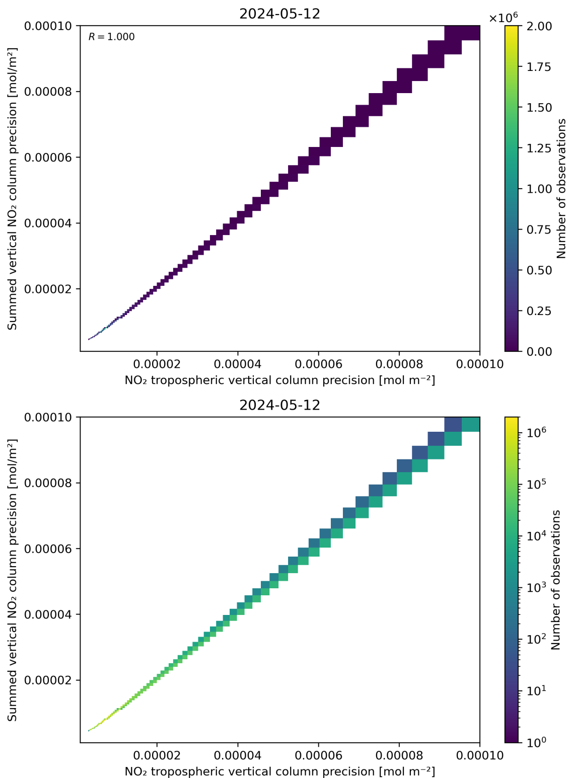
Figure 137: Scatter density plot of “NO 2 tropospheric vertical column precision” against “Summed vertical NO 2 column precision” for 2024-05-12 to 2024-05-13.
