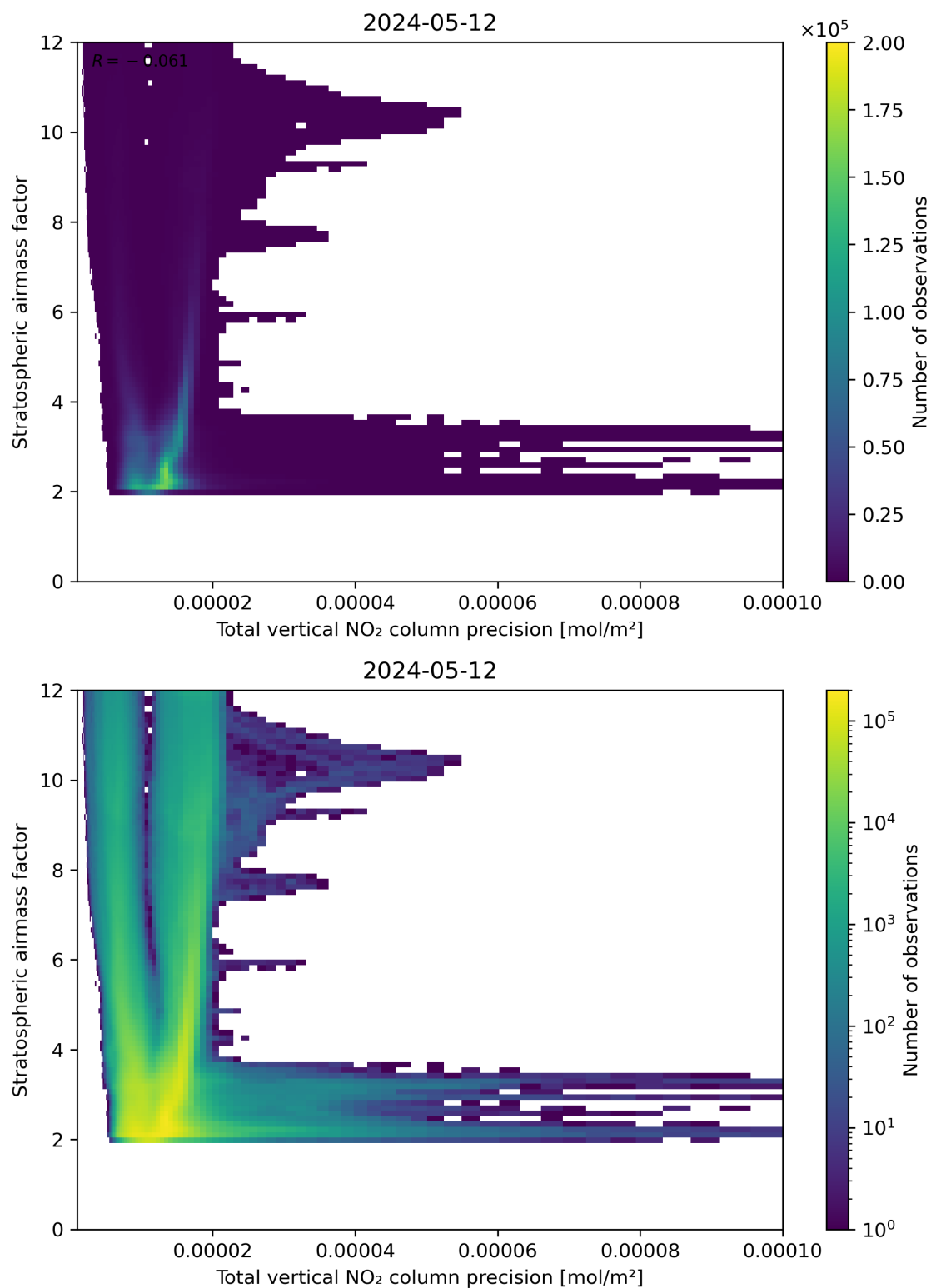
Figure 115: Scatter density plot of “Total vertical NO 2 column precision” against “Stratospheric air mass factor” for 2024-05-12 to 2024-05-13.
