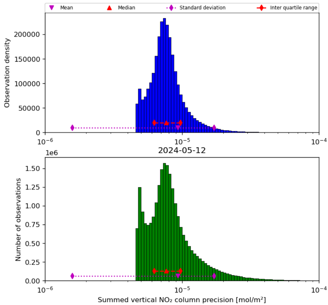
Figure 41: Histogram of “Summed vertical NO 2 column precision” for 2024-05-12 to 2024-05-13
