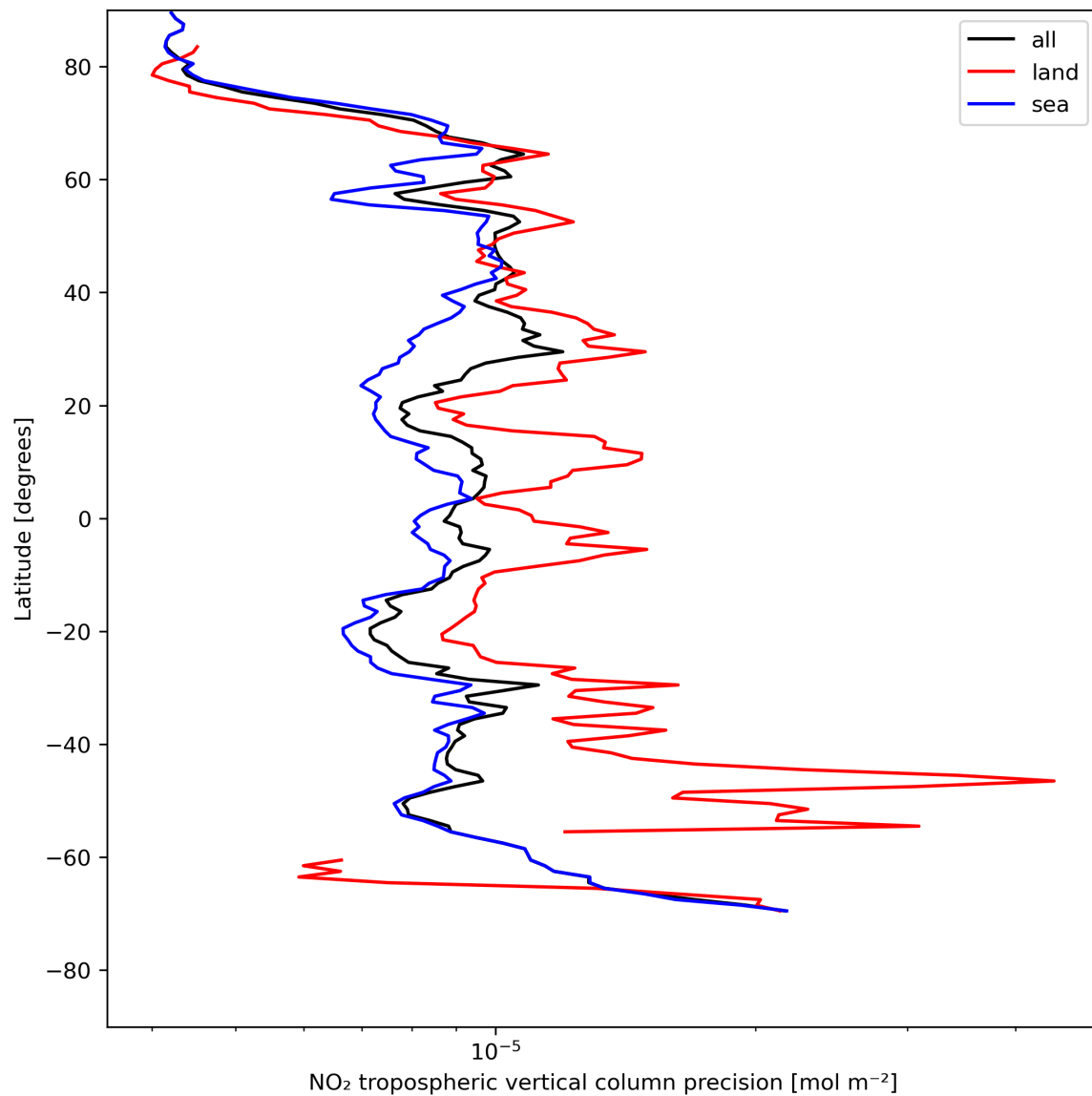
Figure 13: Zonal average of “NO 2 tropospheric vertical column precision” for 2024-05-12 to 2024-05-13.
