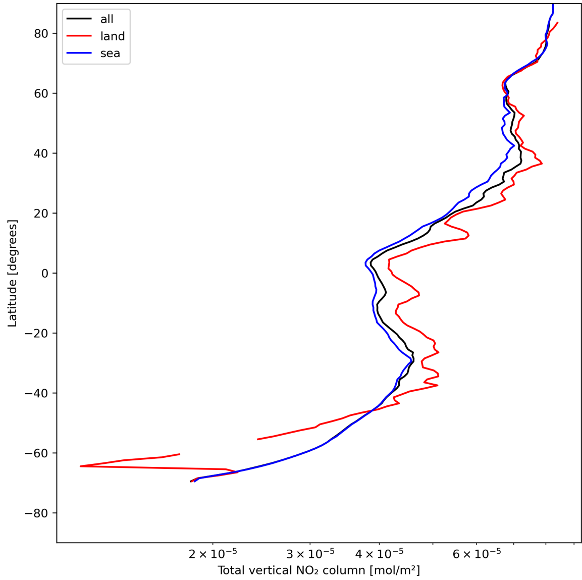
Figure 21: Zonal average of “Total vertical NO 2 column” for 2024-05-12 to 2024-05-13.
