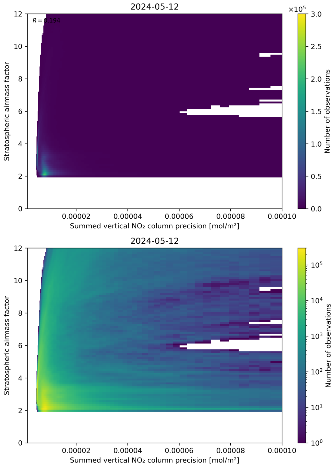
Figure 106: Scatter density plot of “Summed vertical NO 2 column precision” against “Stratospheric airmass factor” for 2024-05-12 to 2024-05-13.
