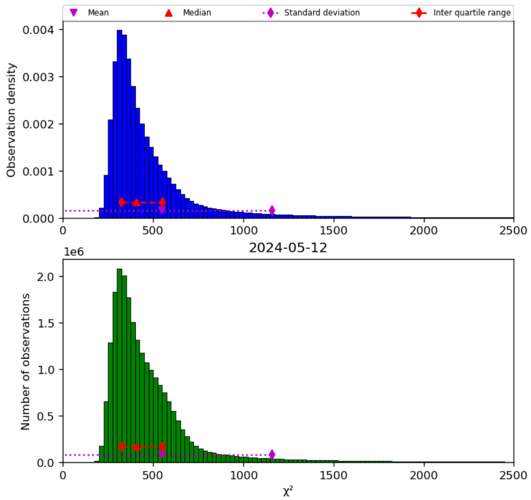
Figure 42: Histogram of “ \chi^2 ” for 2024-05-12 to 2024-05-13
