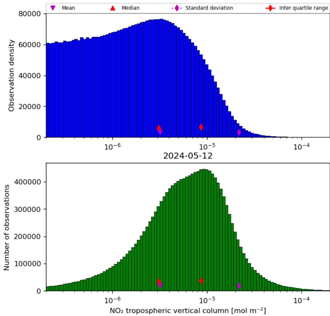
Figure 29: Histogram of “NO 2 tropospheric vertical column” for 2024-05-12 to 2024-05-13
