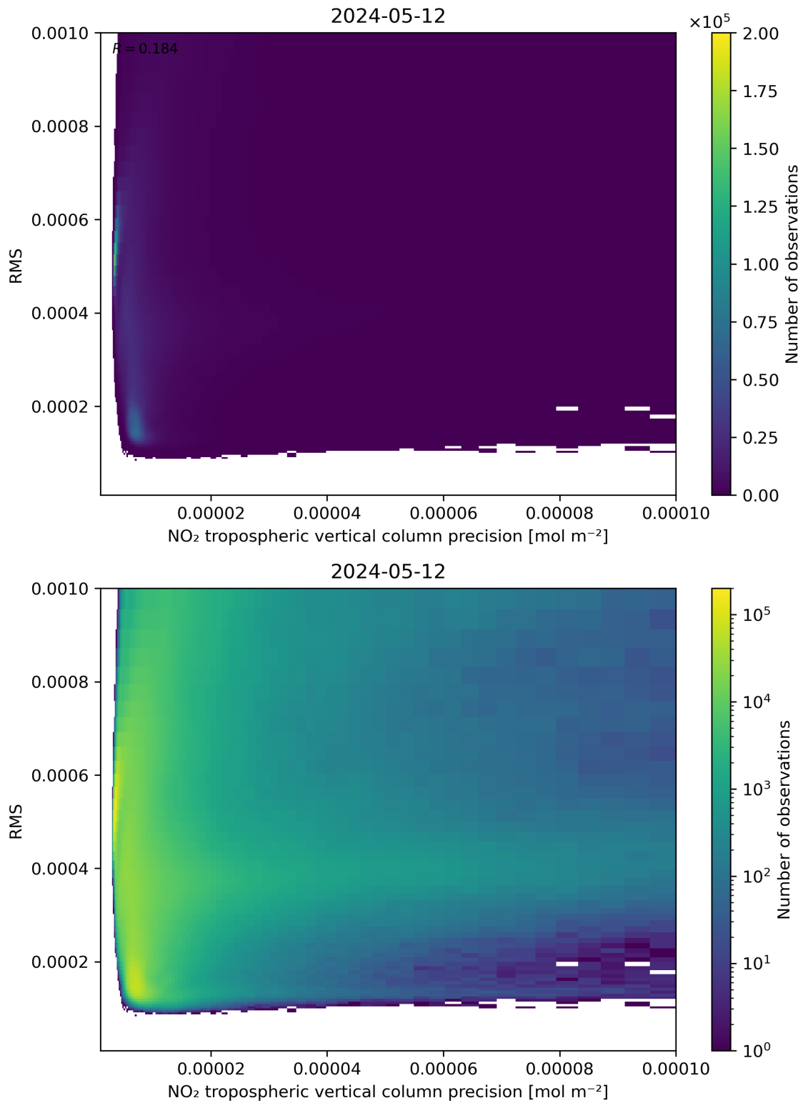
Figure 140: Scatter density plot of “NO 2 tropospheric vertical column precision” against “RMS” for 2024-05-12 to 2024-05-13.
