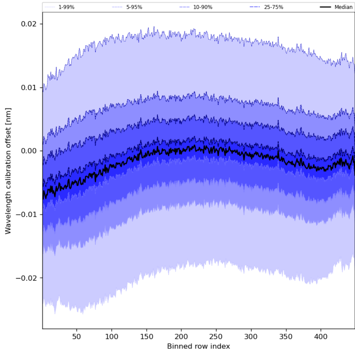
Figure 52: Along track statistics of “Wavelength calibration offset” for 2024-05-12 to 2024-05-13
