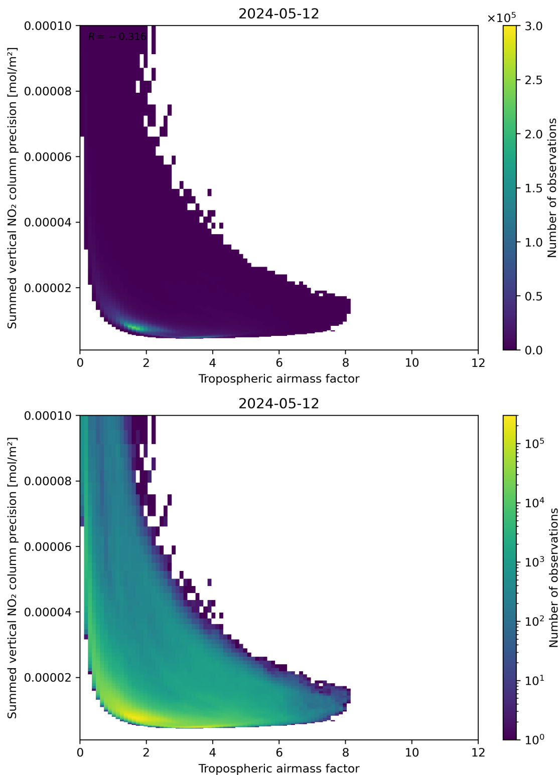
Figure 76: Scatter density plot of “Tropospheric air mass factor” against “Summed vertical NO 2 column precision” for 2024-05-12 to 2024-05-13.
