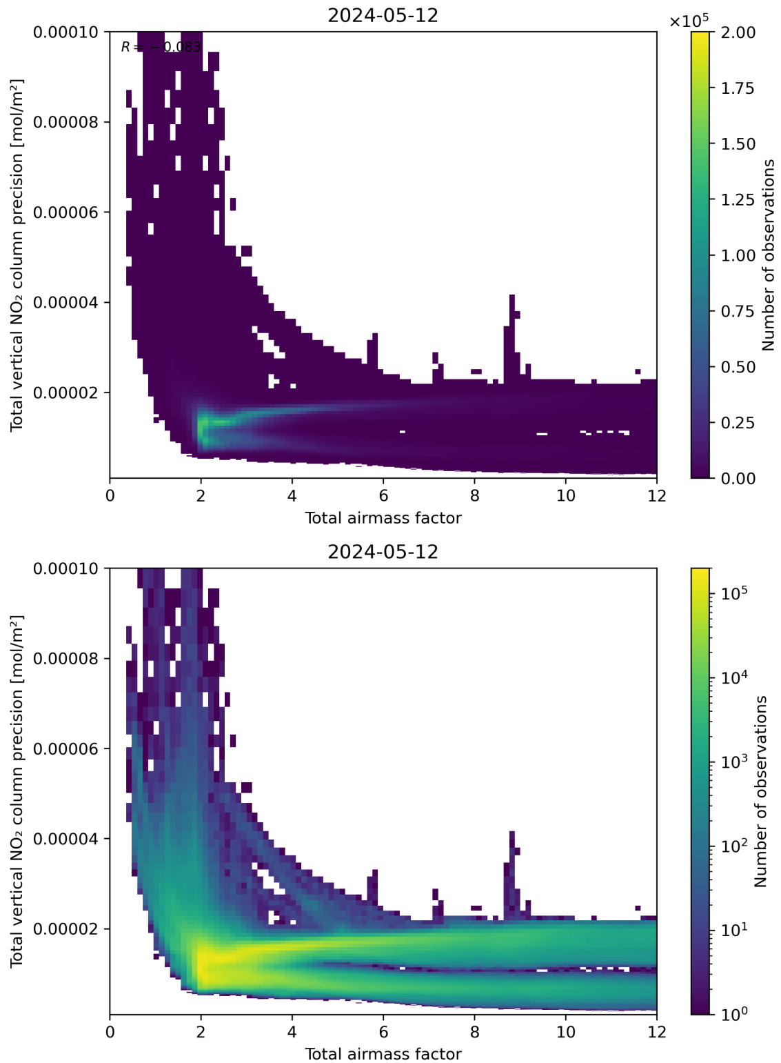
Figure 68: Scatter density plot of “Total airmass factor” against “Total vertical NO 2 column precision” for 2024-05-12 to 2024-05-13.
