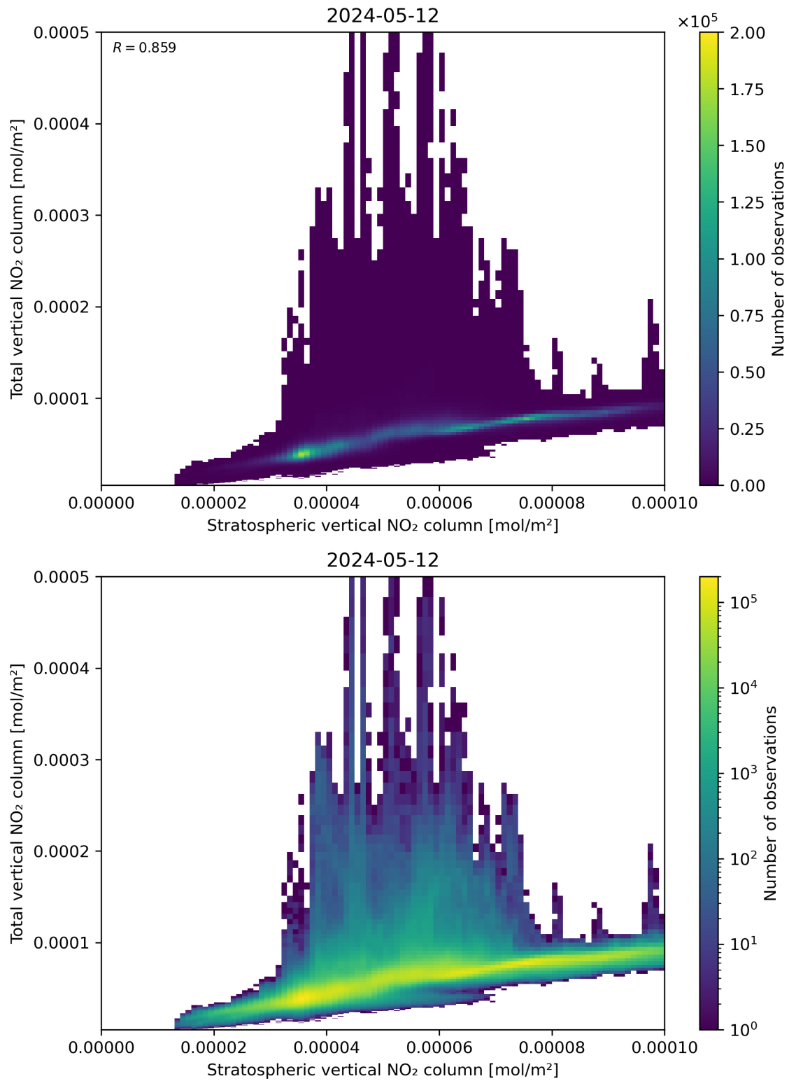
Figure 100: Scatter density plot of “Stratospheric vertical NO 2 column” against “Total vertical NO 2 column” for 2024-05-12 to 2024-05-13.
