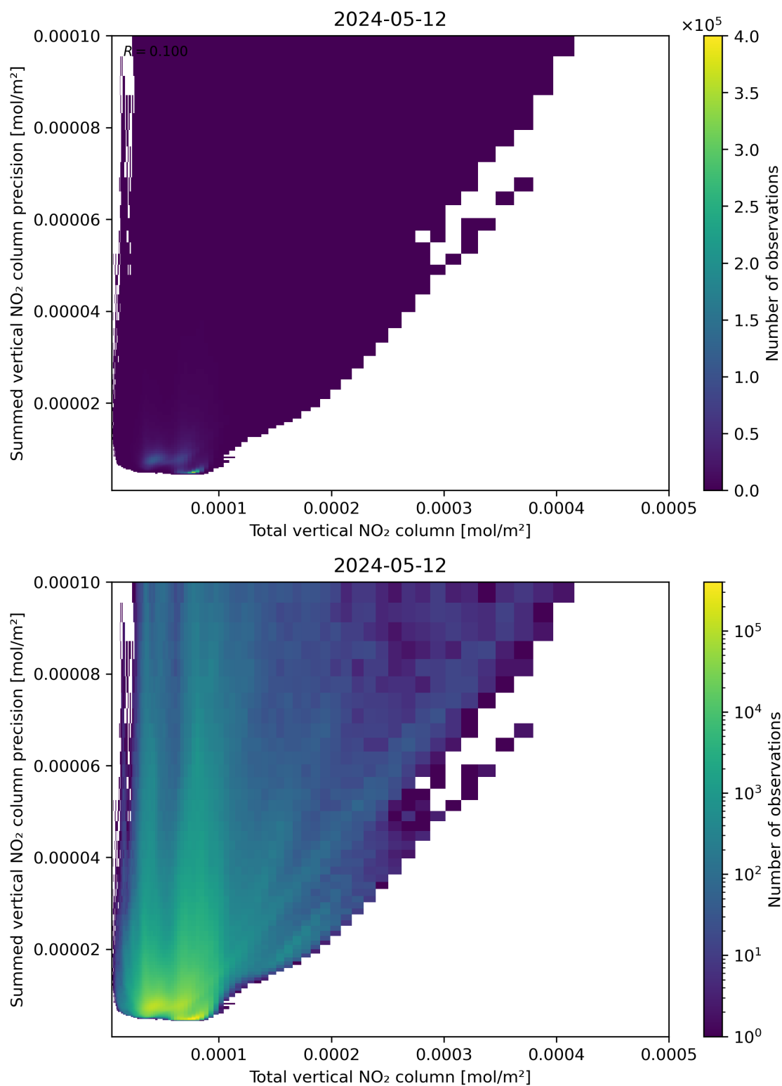
Figure 113: Scatter density plot of “Total vertical NO 2 column” against “Summed vertical NO 2 column precision” for 2024-05-12 to 2024-05-13.
