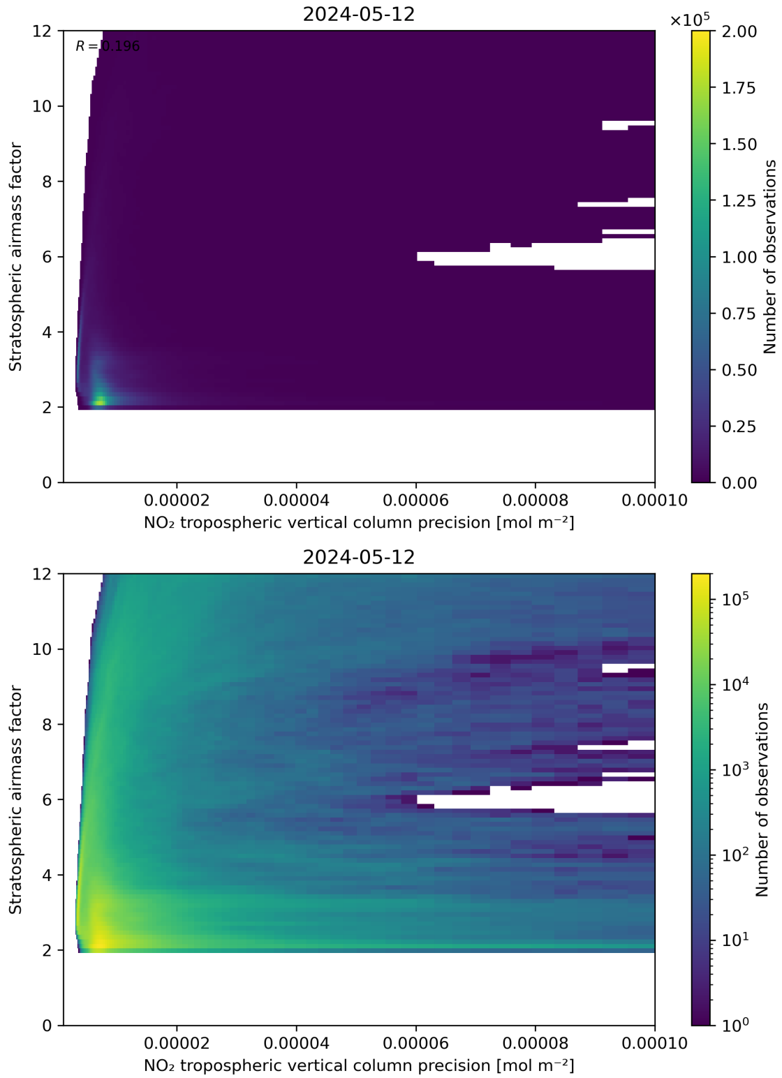
Figure 131: Scatter density plot of “NO 2 tropospheric vertical column precision” against “Stratospheric airmass factor” for 2024-05-12 to 2024-05-13.
