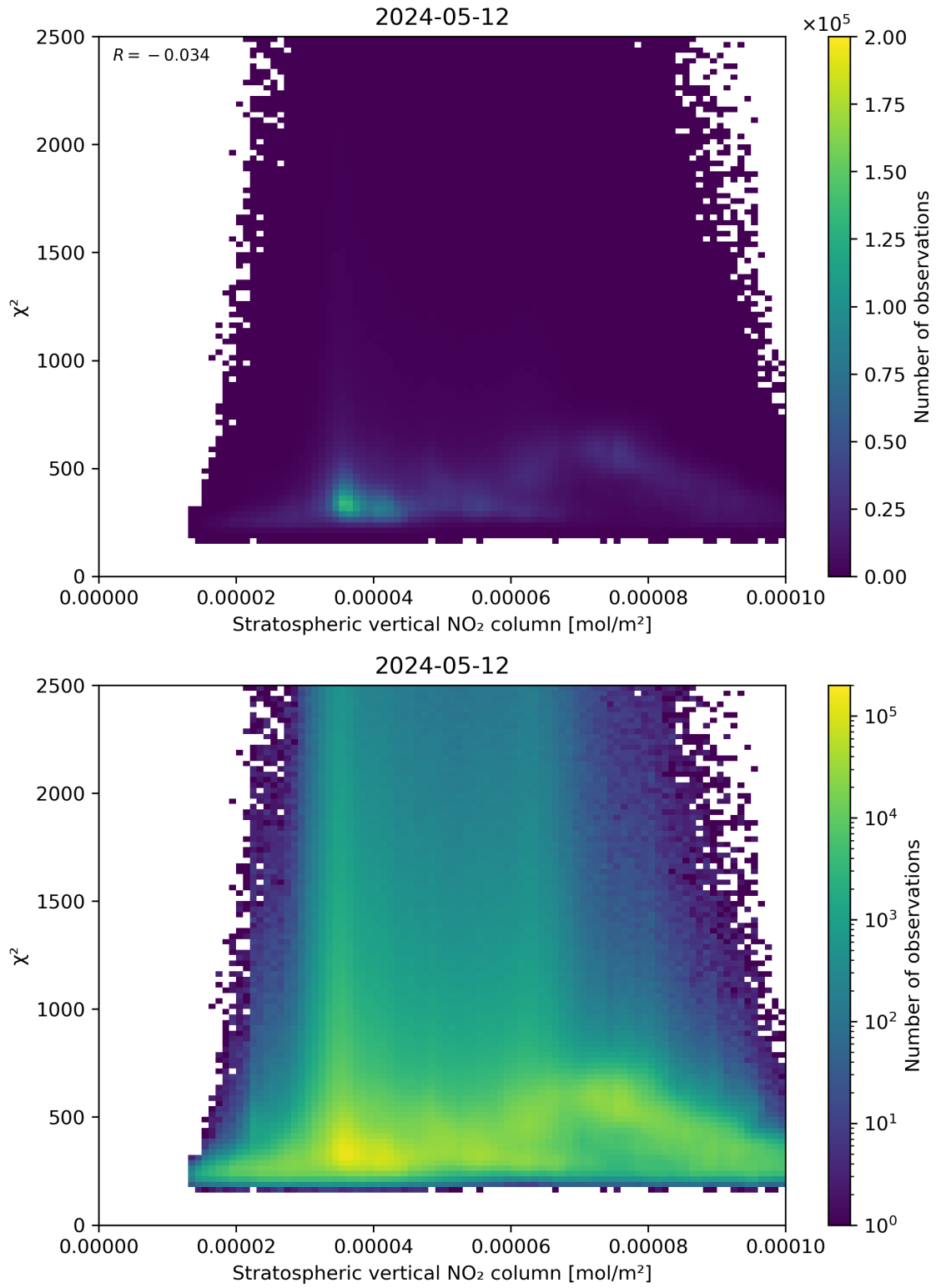
Figure 97: Scatter density plot of “Stratospheric vertical NO 2 column” against “ \chi^2 ” for 2024-05-12 to 2024-05-13.
