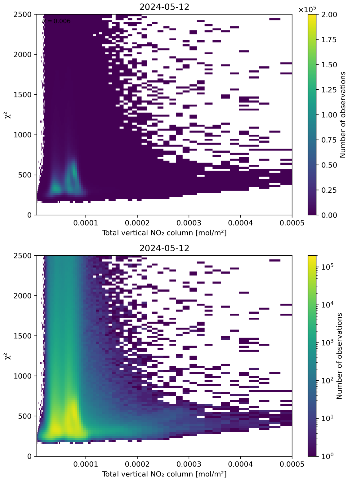
Figure 111: Scatter density plot of “Total vertical NO 2 column” against “ \chi^2 ” for 2024-05-12 to 2024-05-13.
