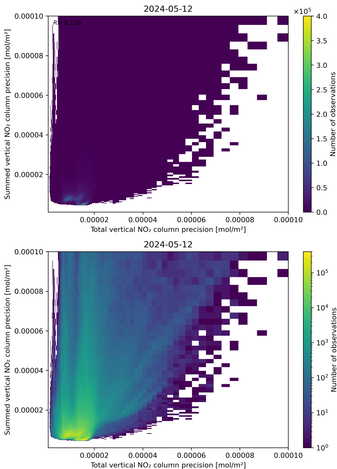
Figure 118: Scatter density plot of “Total vertical NO 2 column precision” against “Summed vertical NO 2 column precision” for 2024-05-12 to 2024-05-13.
