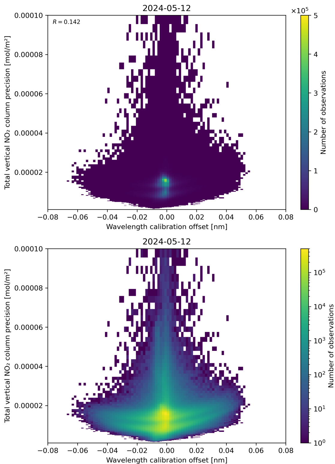
Figure 180: Scatter density plot of “Wavelength calibration offset” against “Total vertical NO 2 column precision” for 2024-05-12 to 2024-05-13.
