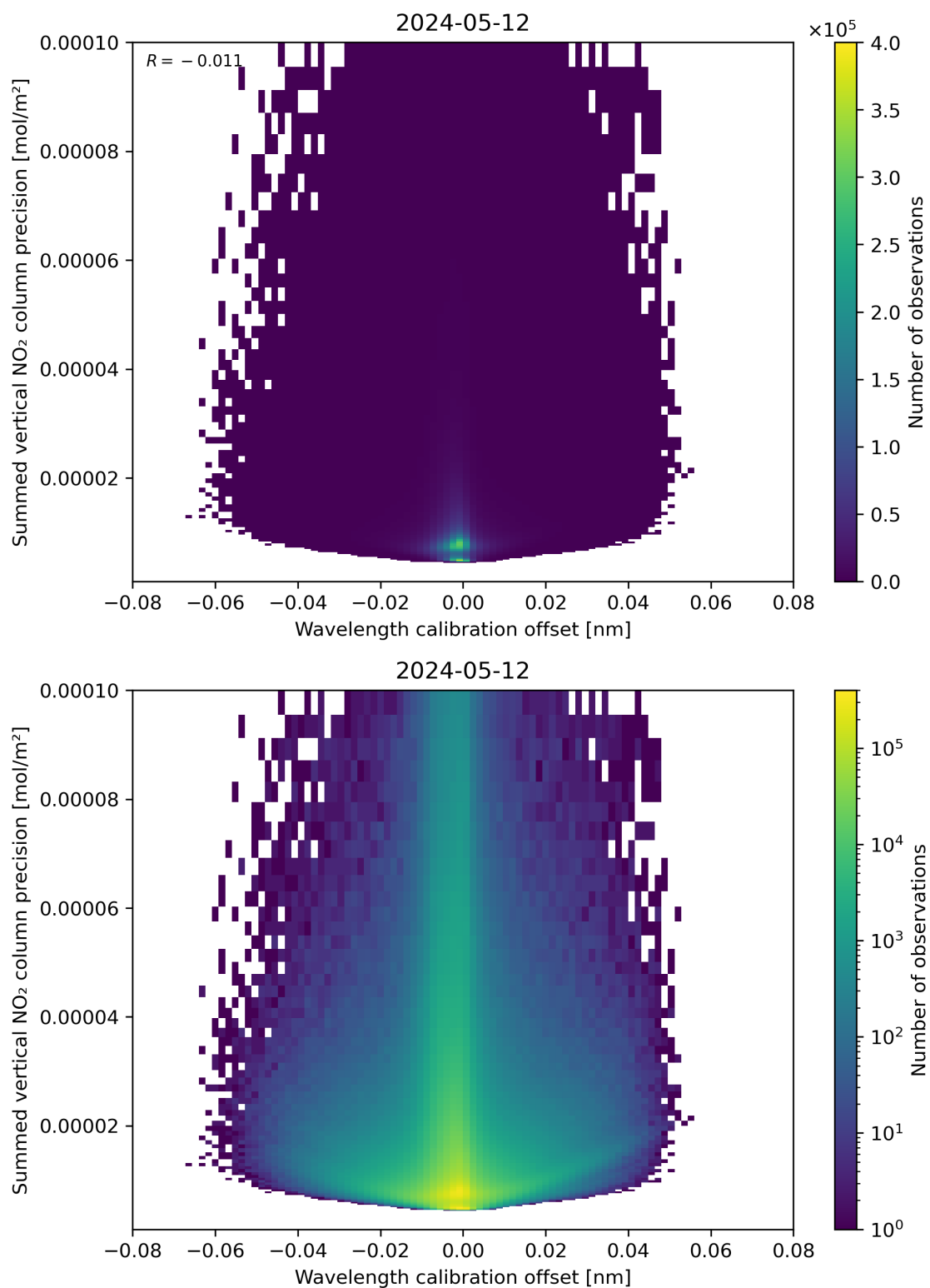
Figure 178: Scatter density plot of “Wavelength calibration offset” against “Summed vertical NO 2 column precision” for 2024-05-12 to 2024-05-13.
