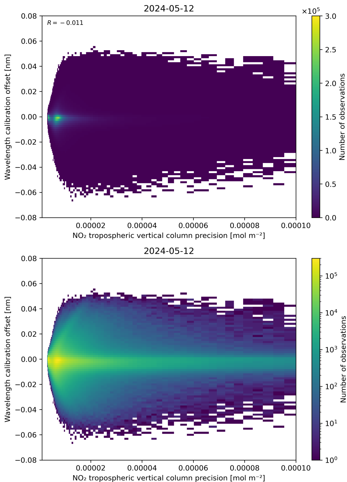
Figure 141: Scatter density plot of “NO 2 tropospheric vertical column precision” against “Wavelength calibration offset” for 2024-05-12 to 2024-05-13.
