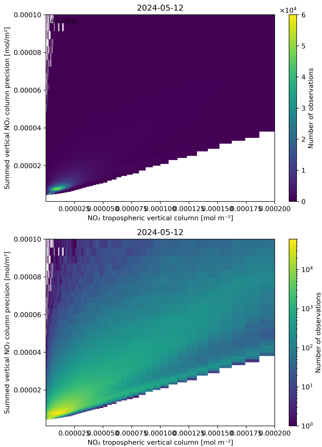
Figure 127: Scatter density plot of “NO 2 tropospheric vertical column” against “Summed vertical NO 2 column precision” for 2024-05-12 to 2024-05-13.
