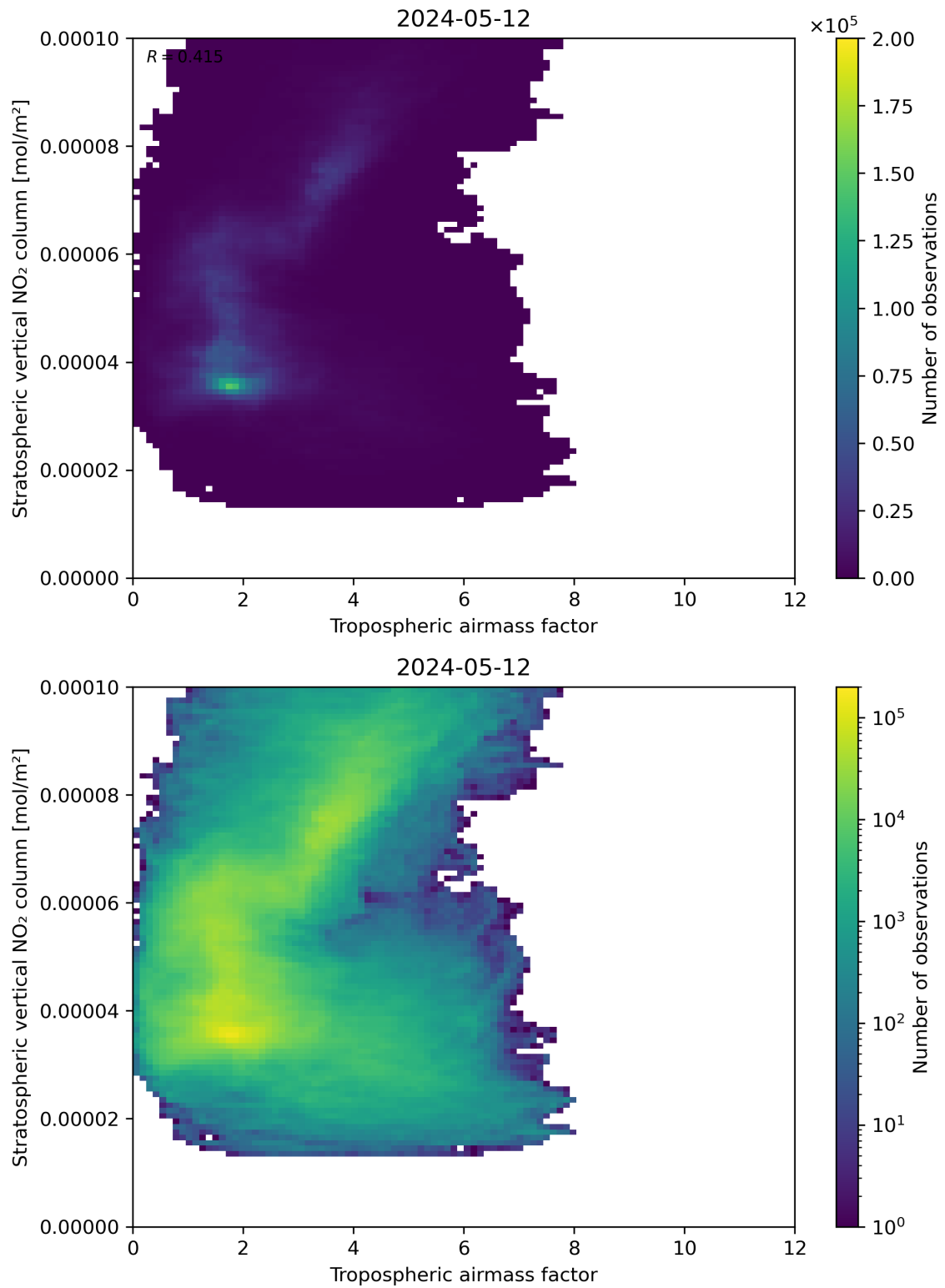
Figure 74: Scatter density plot of “Tropospheric airmass factor” against “Stratospheric vertical NO 2 column” for 2024-05-12 to 2024-05-13.
