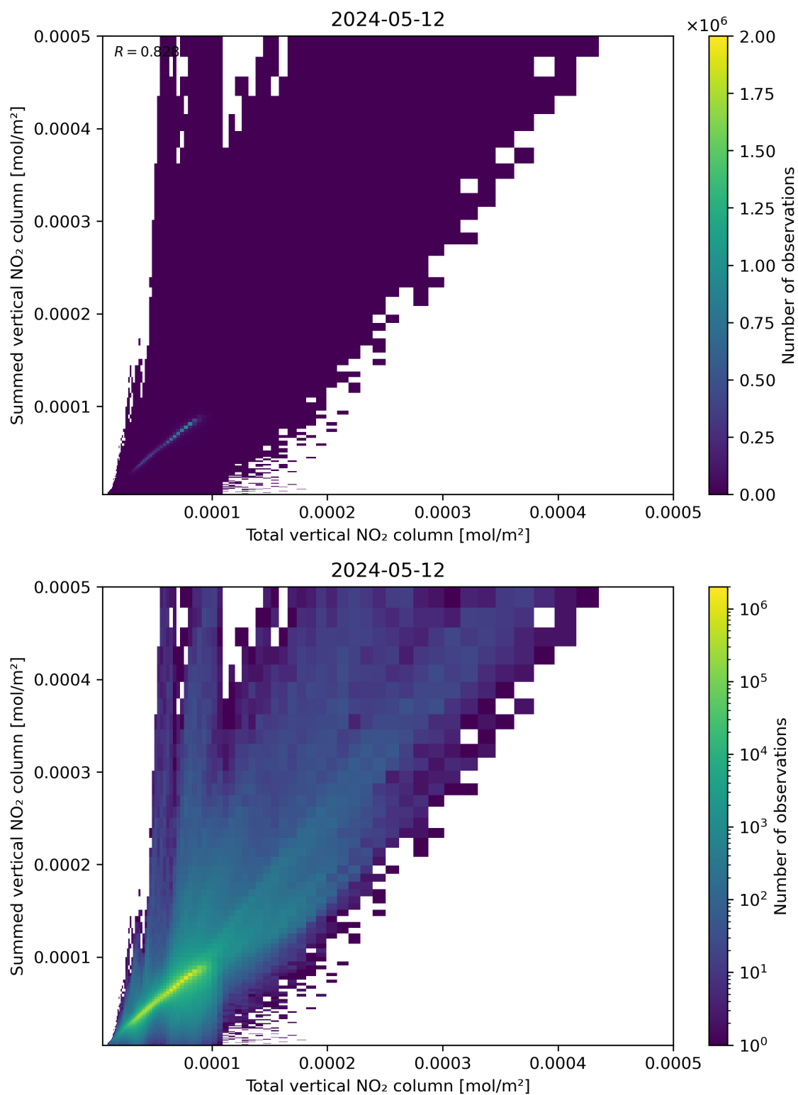
Figure 112: Scatter density plot of “Total vertical NO 2 column” against “Summed vertical NO 2 column” for 2024-05-12 to 2024-05-13.
