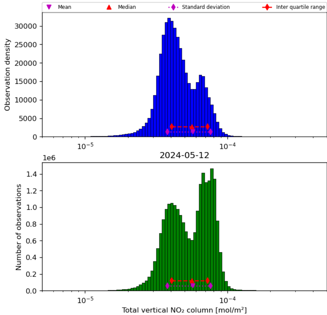
Figure 38: Histogram of “Total vertical NO 2 column” for 2024-05-12 to 2024-05-13
