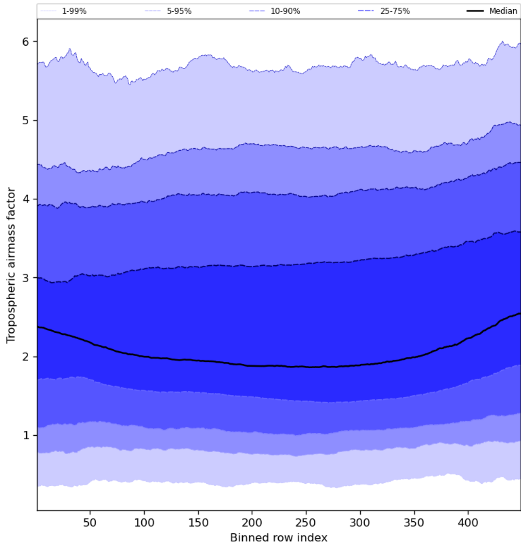
Figure 48: Along track statistics of “Tropospheric air mass factor” for 2024-05-12 to 2024-05-13
