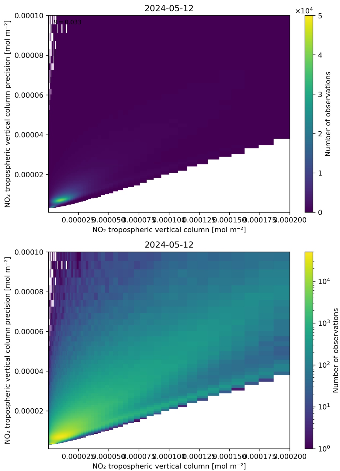
Figure 130: Scatter density plot of “NO 2 tropospheric vertical column” against “NO 2 tropospheric vertical column precision” for 2024-05-12 to 2024-05-13.
