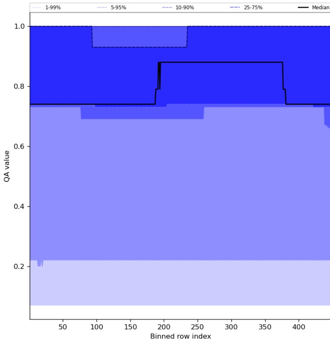
Figure 45: Along track statistics of “QA value” for 2024-05-12 to 2024-05-13
