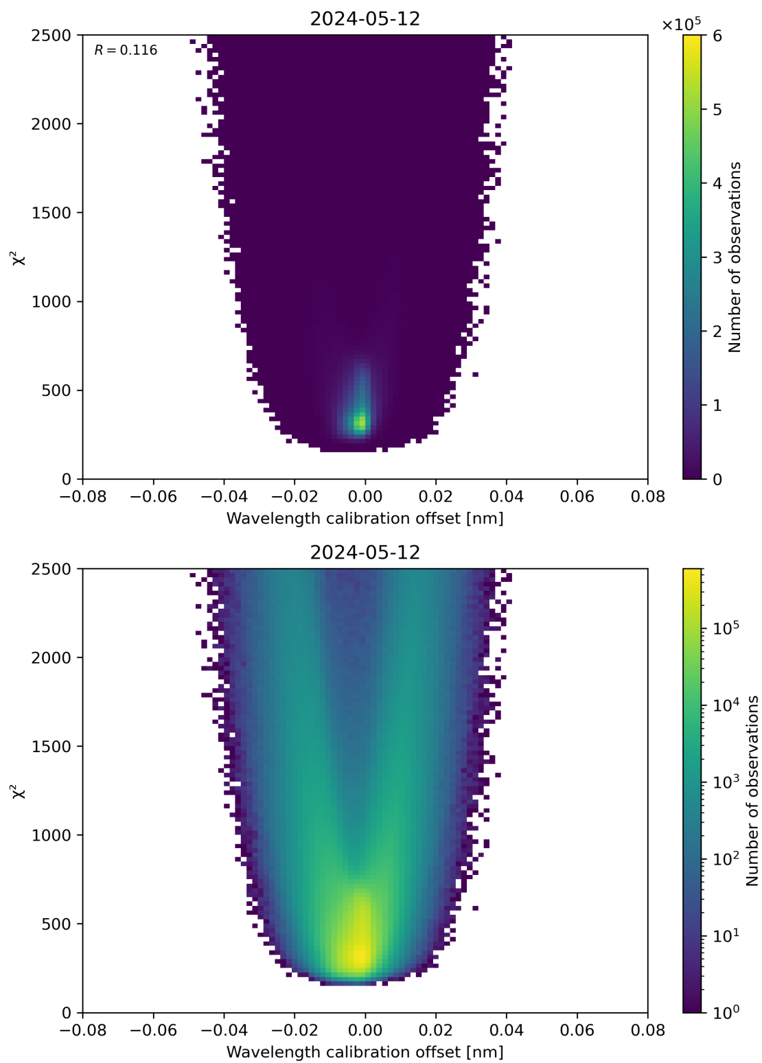
Figure 175: Scatter density plot of “Wavelength calibration offset” against “ \chi^2 ” for 2024-05-12 to 2024-05-13.
