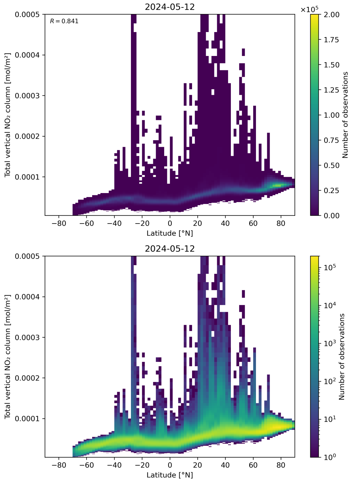
Figure 90: Scatter density plot of “Latitude” against “Total vertical NO 2 column” for 2024-05-12 to 2024-05-13.
