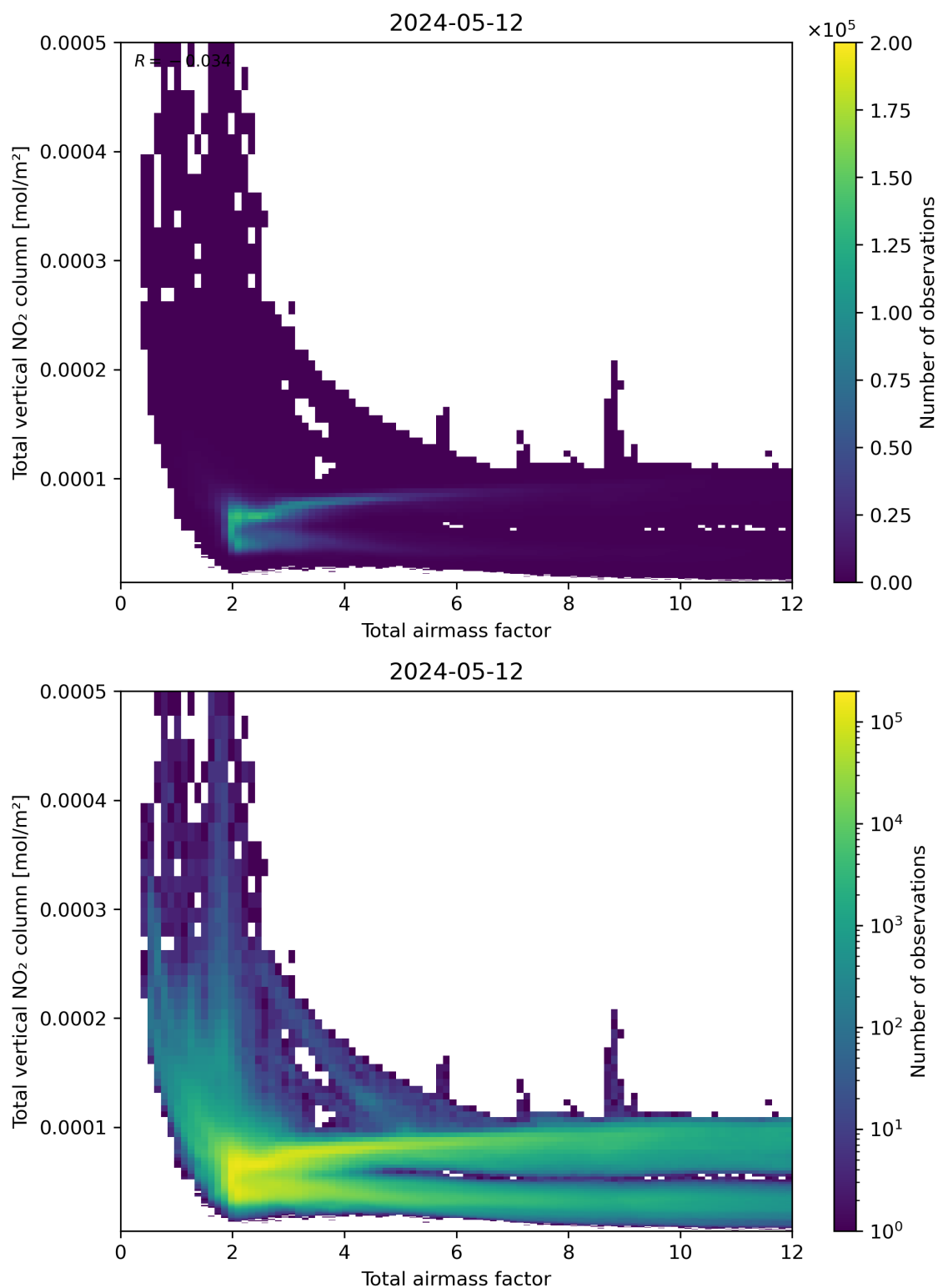
Figure 67: Scatter density plot of “Total airmass factor” against “Total vertical NO 2 column” for 2024-05-12 to 2024-05-13.
