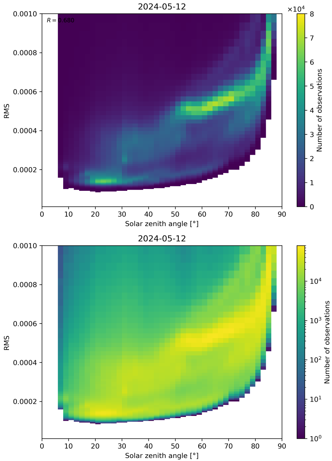
Figure 157: Scatter density plot of “Solar zenith angle” against “RMS” for 2024-05-12 to 2024-05-13.
