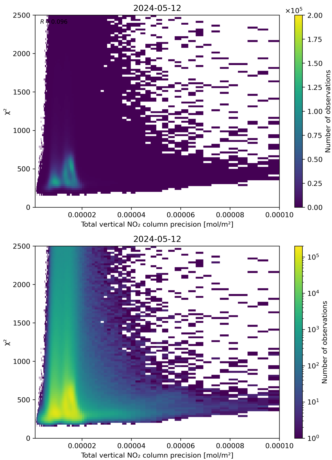
Figure 116: Scatter density plot of “Total vertical NO 2 column precision” against “ \chi^2 ” for 2024-05-12 to 2024-05-13.
