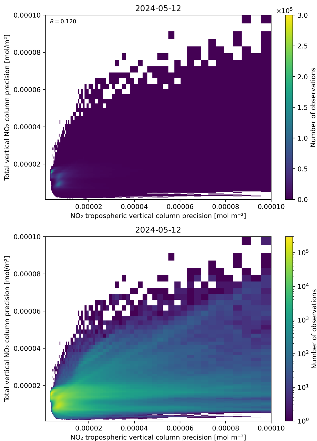
Figure 139: Scatter density plot of “NO 2 tropospheric vertical column precision” against “Total vertical NO 2 column precision” for 2024-05-12 to 2024-05-13.
