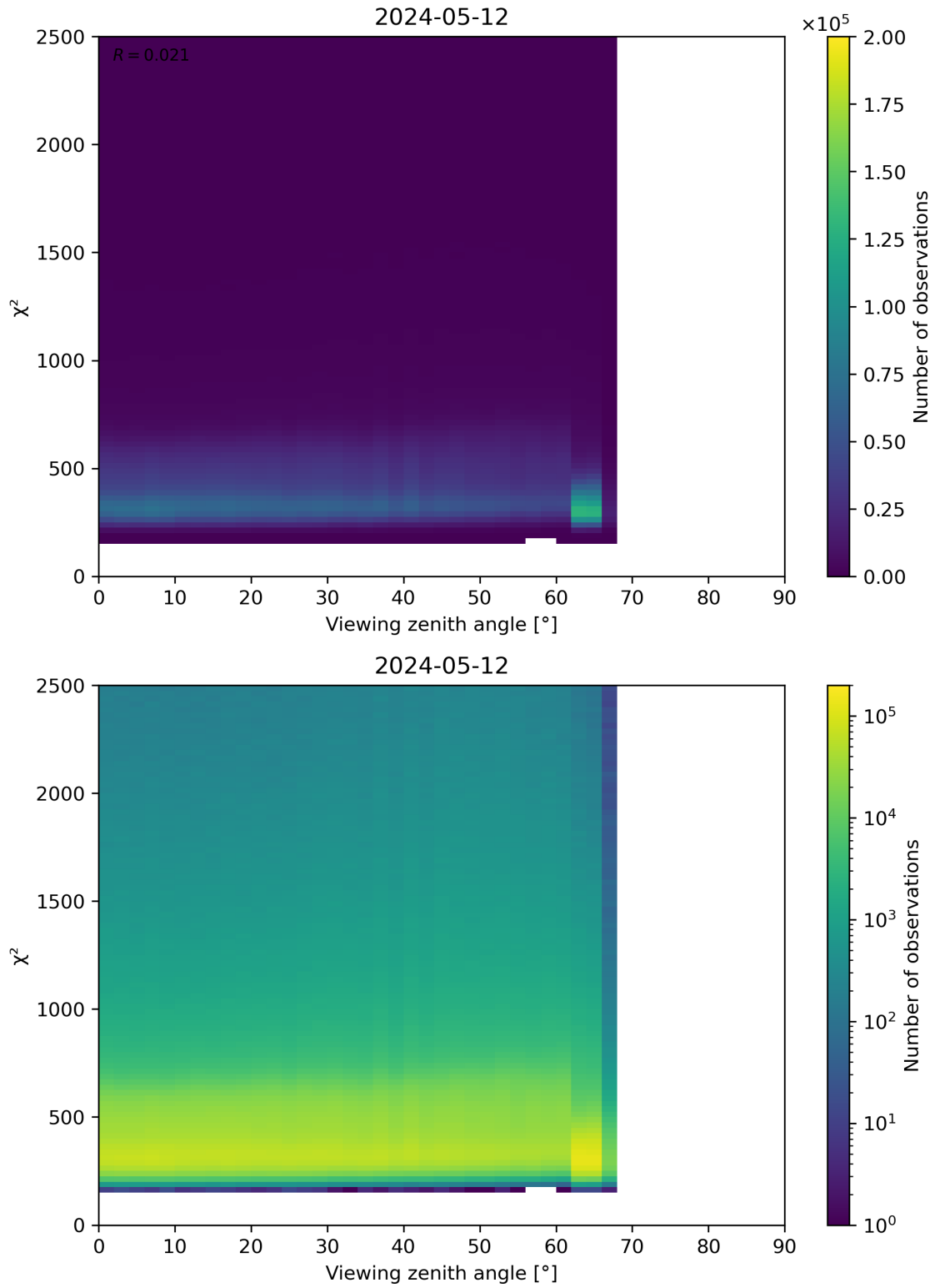
Figure 162: Scatter density plot of “Viewing zenith angle” against “ \chi^2 ” for 2024-05-12 to 2024-05-13.
