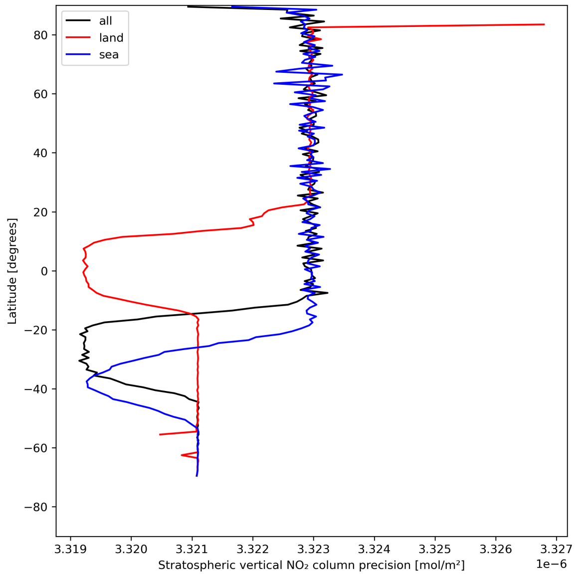
Figure 20: Zonal average of “Stratospheric vertical NO 2 column precision” for 2024-05-12 to 2024-05-13.
