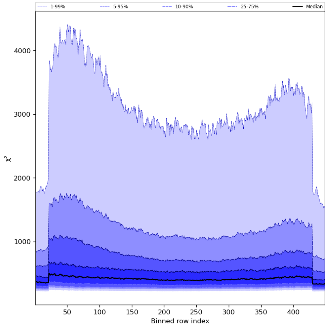
Figure 59: Along track statistics of “ \chi^2 ” for 2024-05-12 to 2024-05-13
