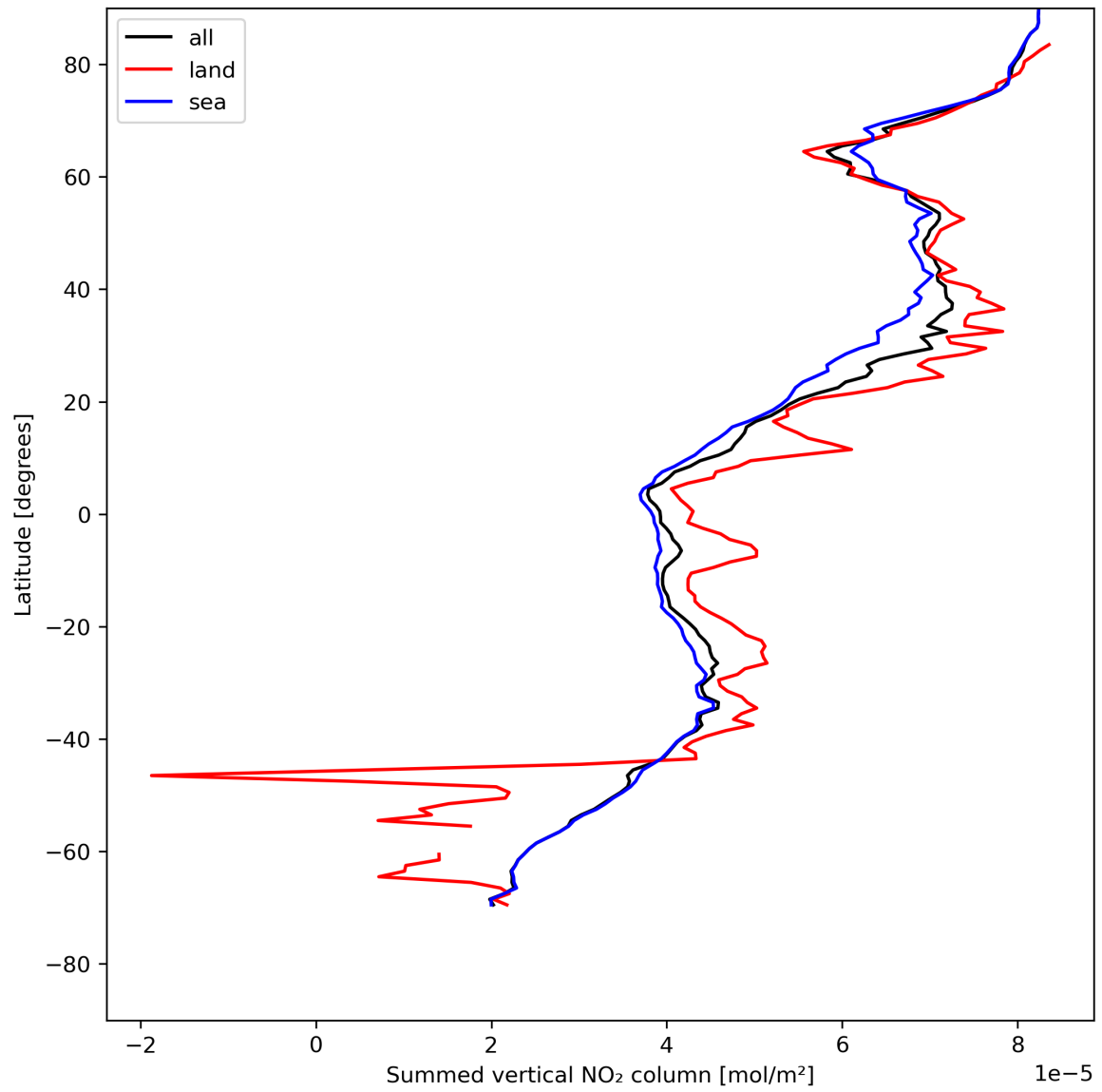
Figure 23: Zonal average of “Summed vertical NO 2 column” for 2024-05-12 to 2024-05-13.
