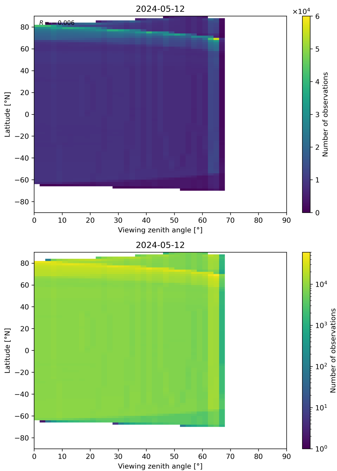
Figure 163: Scatter density plot of “Viewing zenith angle” against “Latitude” for 2024-05-12 to 2024-05-13.
