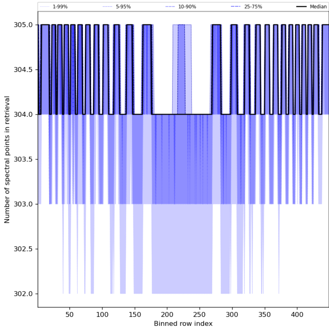
Figure 50: Along track statistics of “Number of spectral points in retrieval” for 2024-05-12 to 2024-05-13
