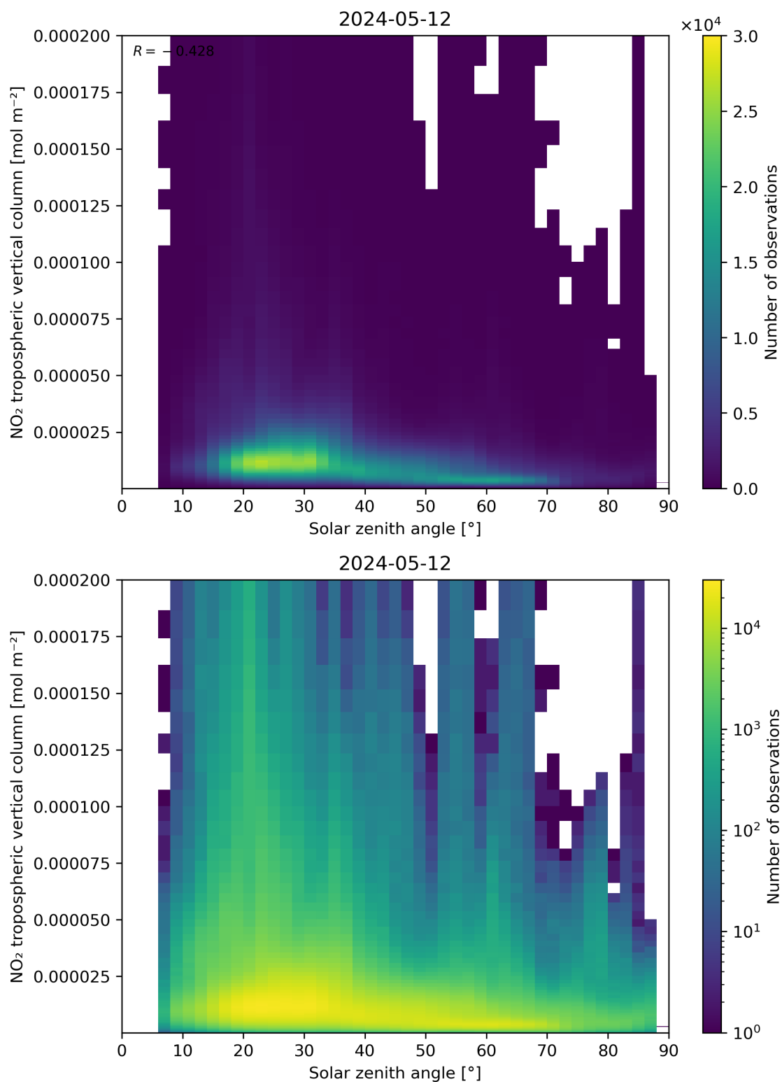
Figure 155: Scatter density plot of “Solar zenith angle” against “NO 2 tropospheric vertical column” for 2024-05-12 to 2024-05-13.
