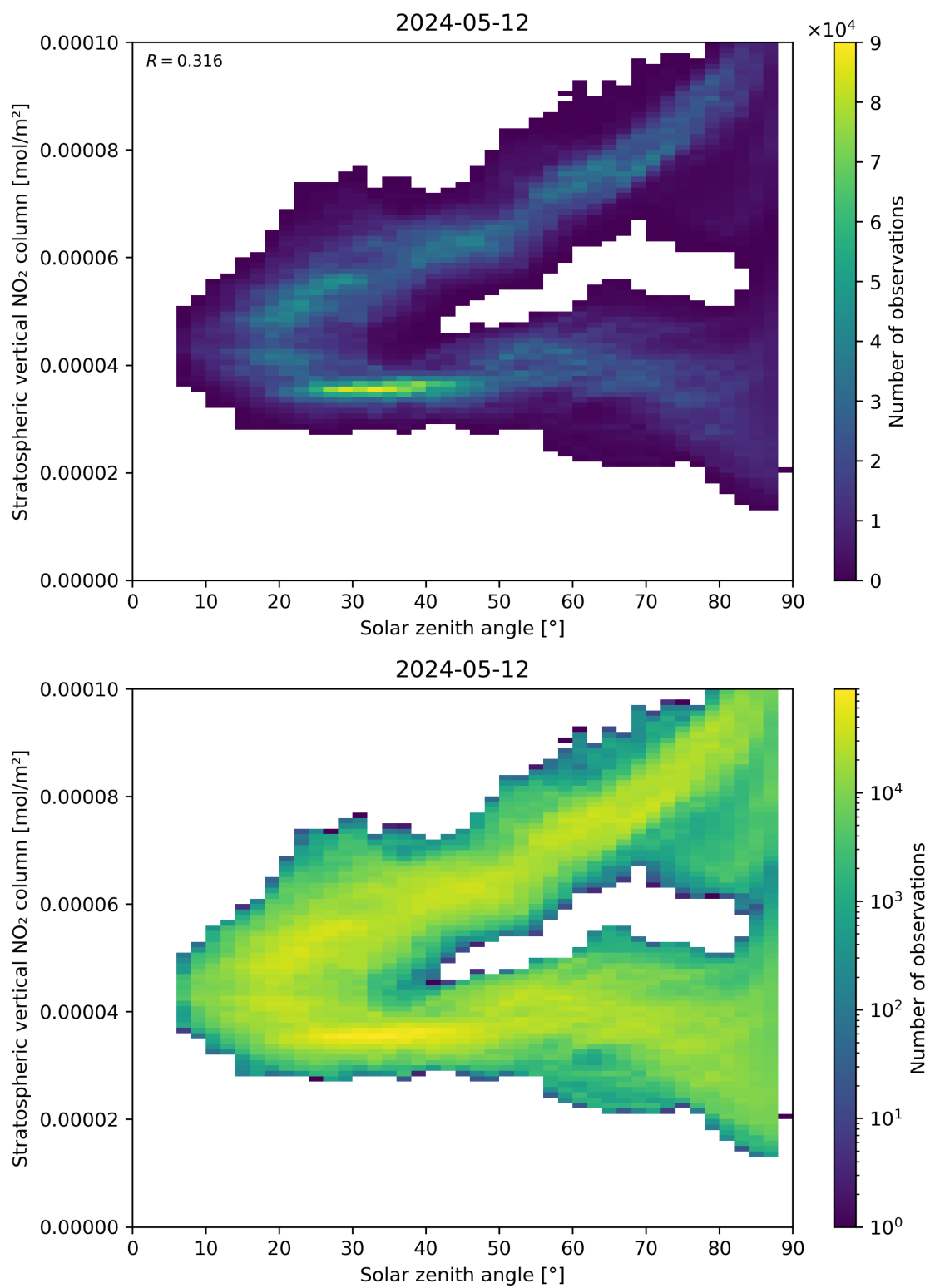
Figure 150: Scatter density plot of “Solar zenith angle” against “Stratospheric vertical NO 2 column” for 2024-05-12 to 2024-05-13.
