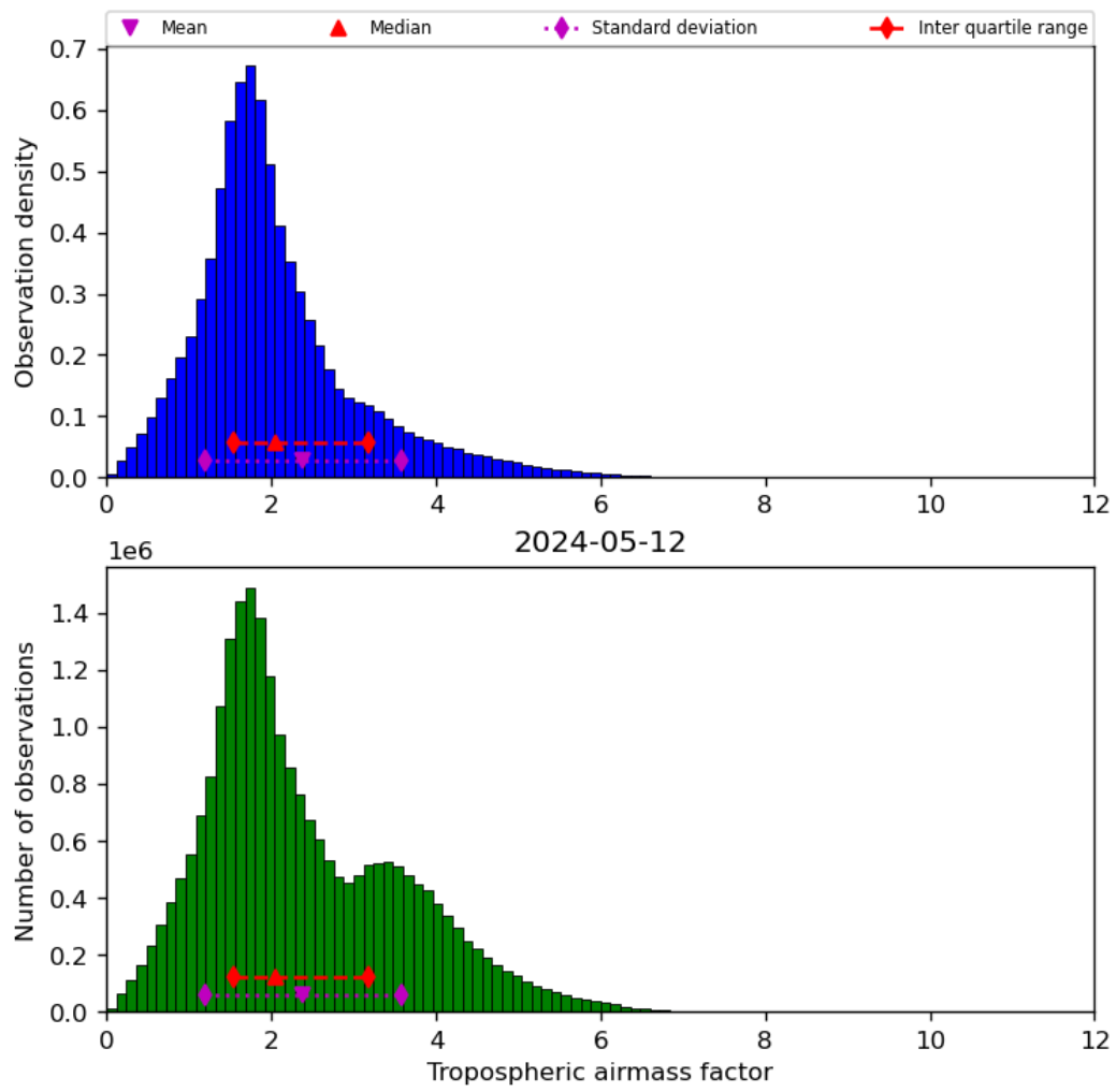
Figure 31: Histogram of “Tropospheric airmass factor” for 2024-05-12 to 2024-05-13
