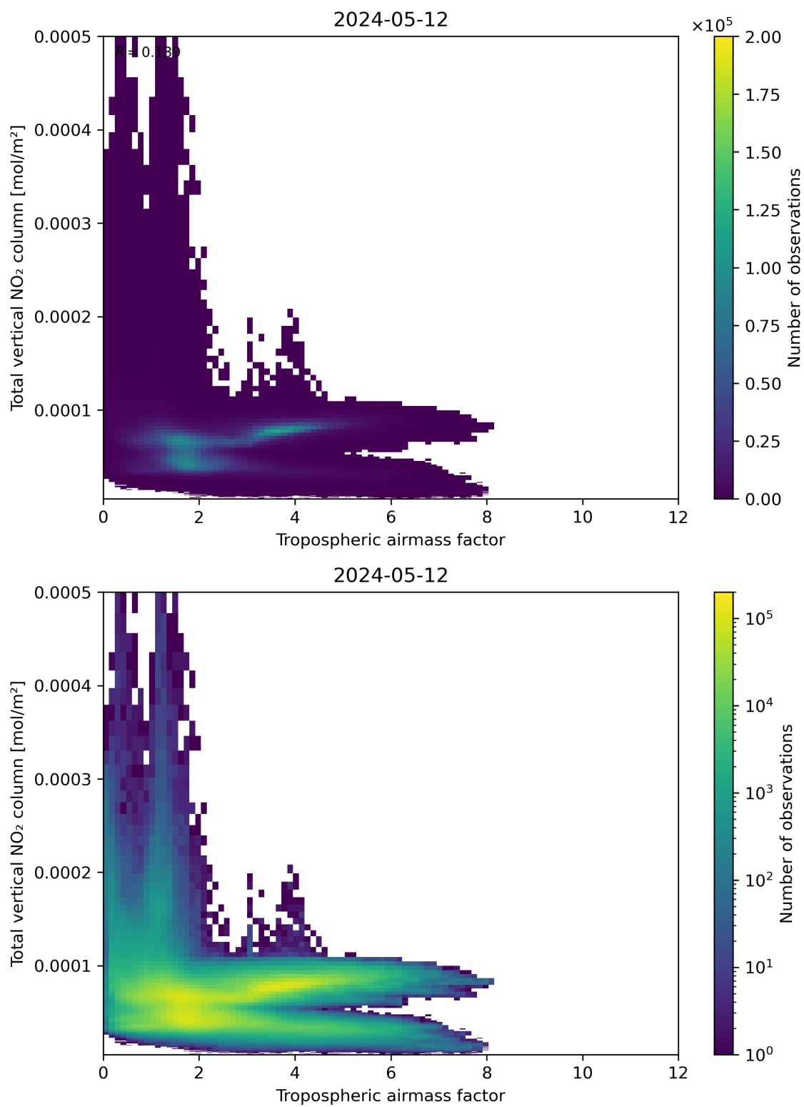
Figure 77: Scatter density plot of “Tropospheric airmass factor” against “Total vertical NO 2 column” for 2024-05-12 to 2024-05-13.
