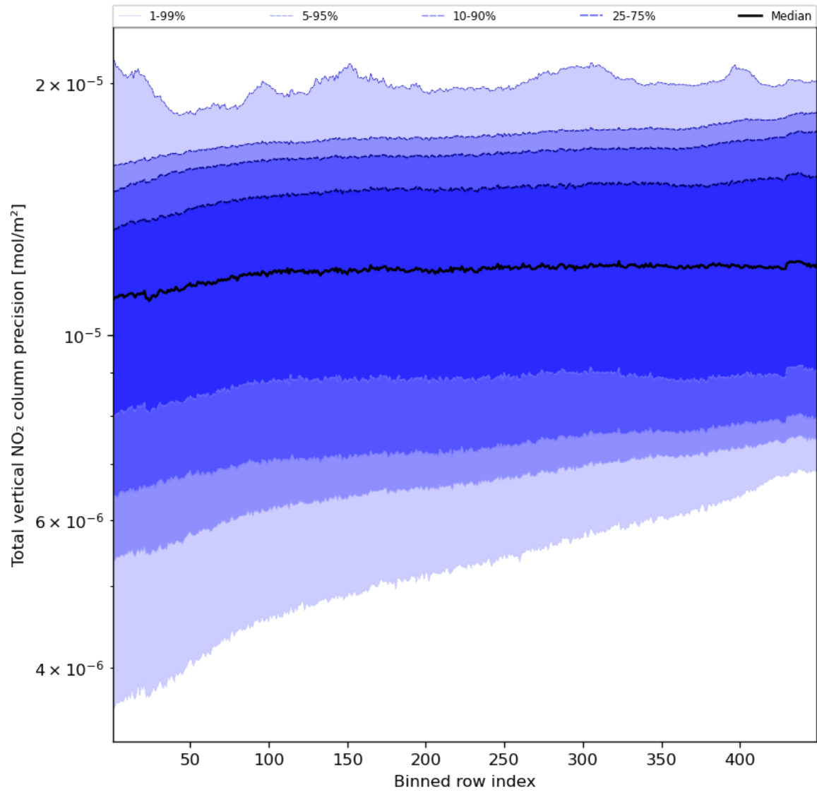
Figure 56: Along track statistics of “Total vertical NO 2 column precision” for 2024-05-12 to 2024-05-13
