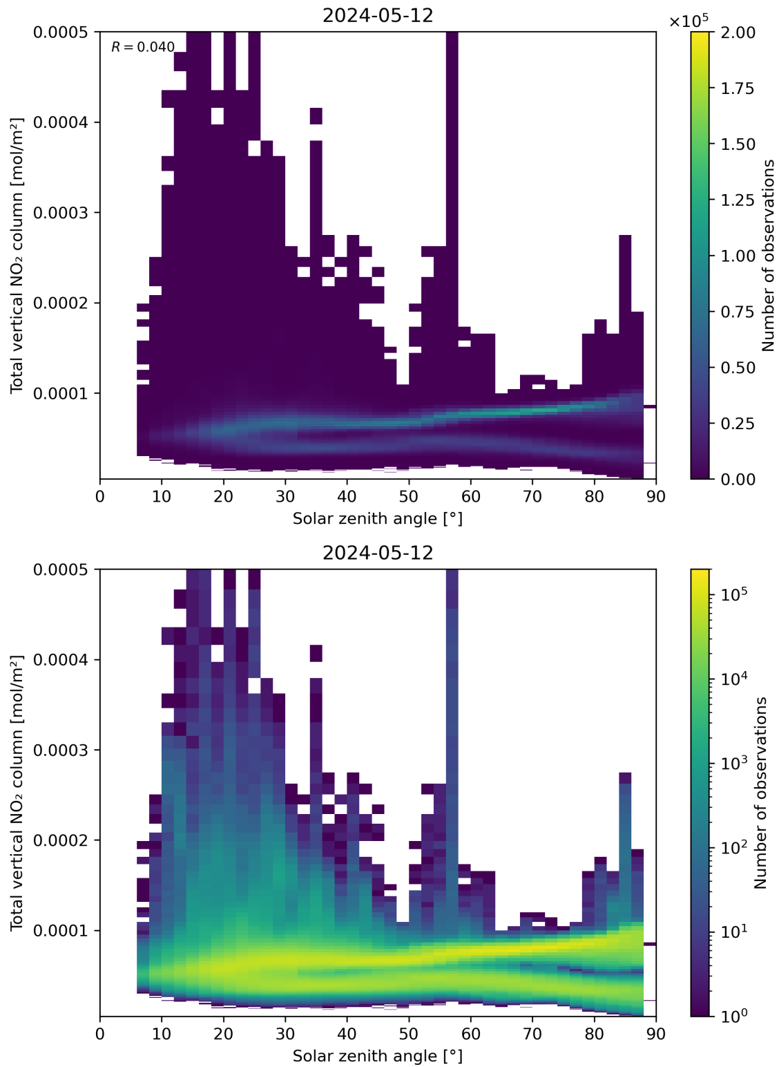
Figure 153: Scatter density plot of “Solar zenith angle” against “Total vertical NO 2 column” for 2024-05-12 to 2024-05-13.
