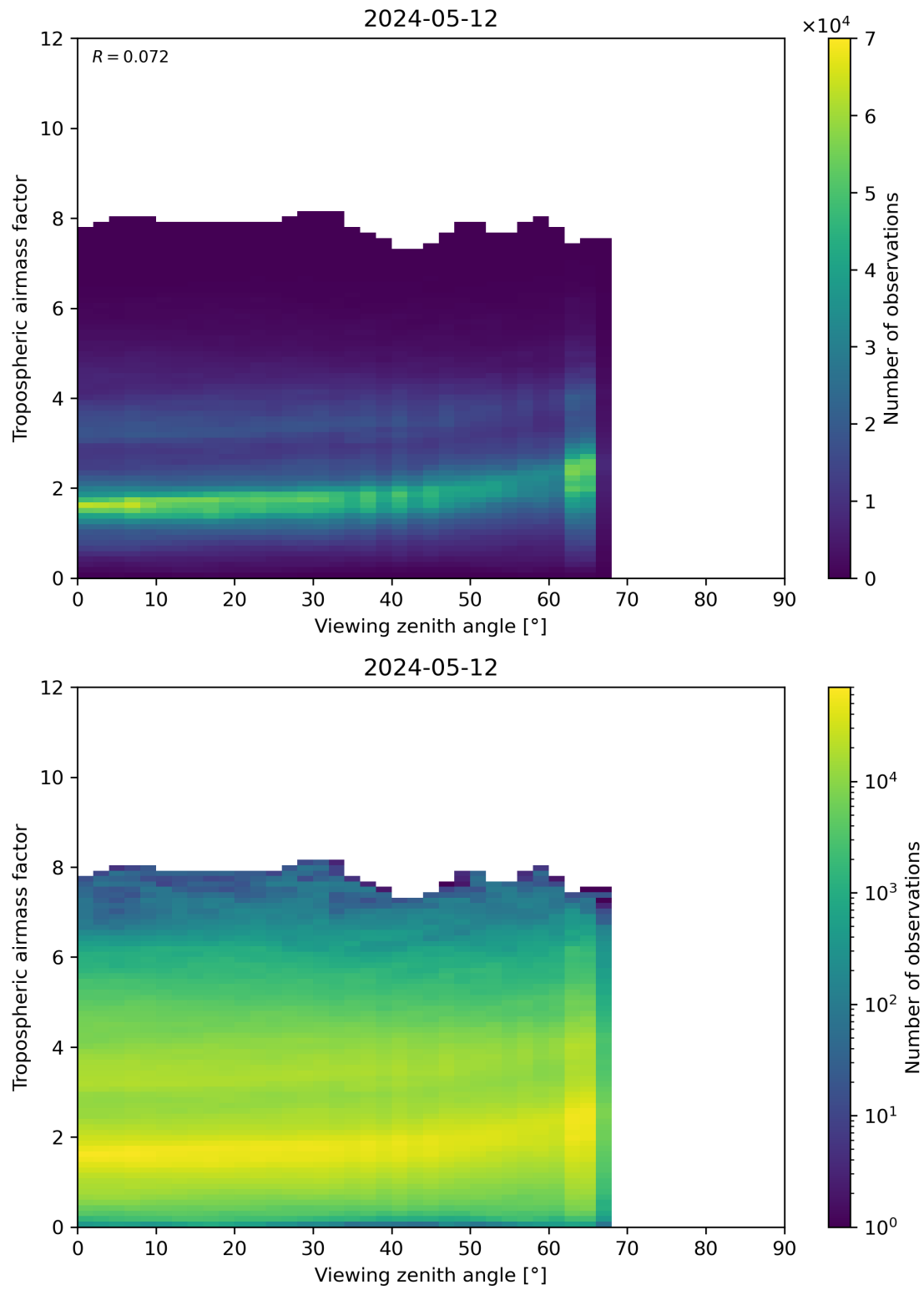
Figure 161: Scatter density plot of “Viewing zenith angle” against “Tropospheric airmass factor” for 2024-05-12 to 2024-05-13.
