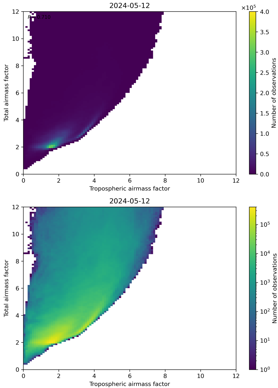
Figure 72: Scatter density plot of “Tropospheric airmass factor” against “Total airmass factor” for 2024-05-12 to 2024-05-13.
