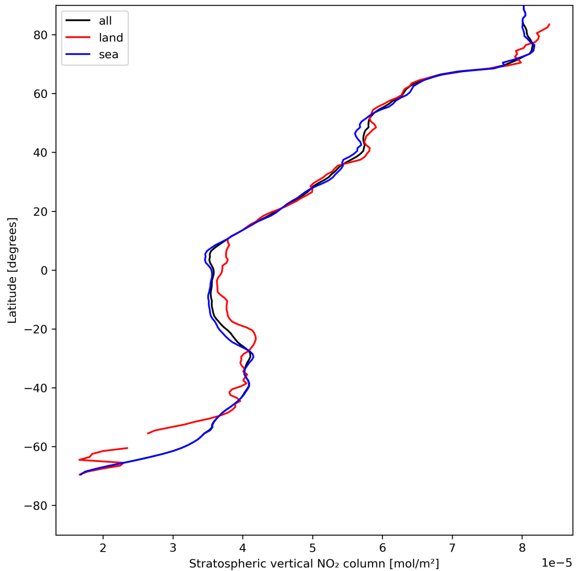
Figure 19: Zonal average of “Stratospheric vertical NO 2 column” for 2024-05-12 to 2024-05-13.
