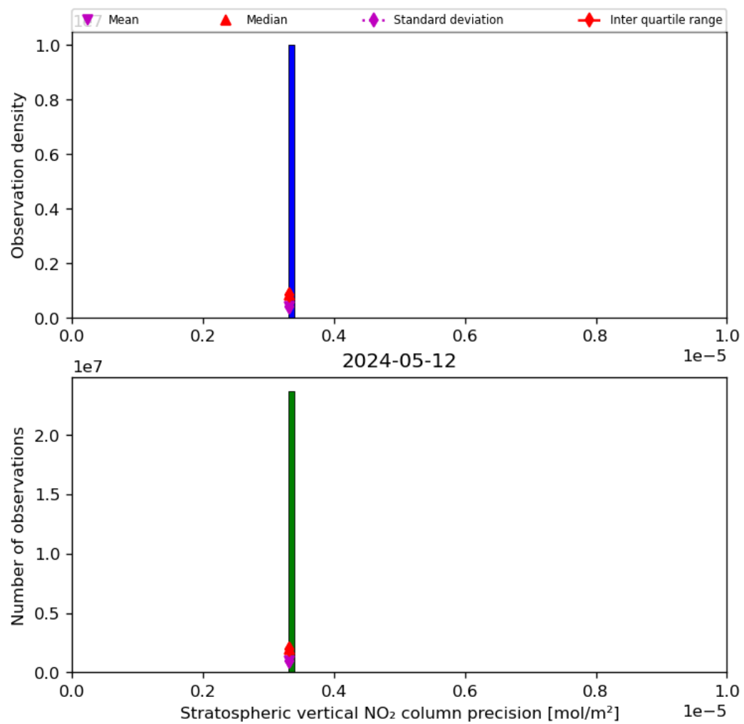
Figure 37: Histogram of “Stratospheric vertical NO 2 column precision” for 2024-05-12 to 2024-05-13
