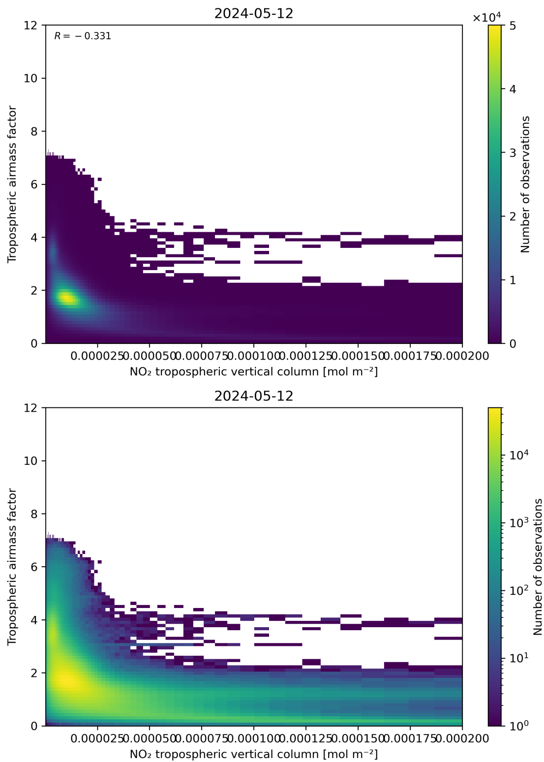
Figure 123: Scatter density plot of “NO 2 tropospheric vertical column” against “Tropospheric air mass factor” for 2024-05-12 to 2024-05-13.
