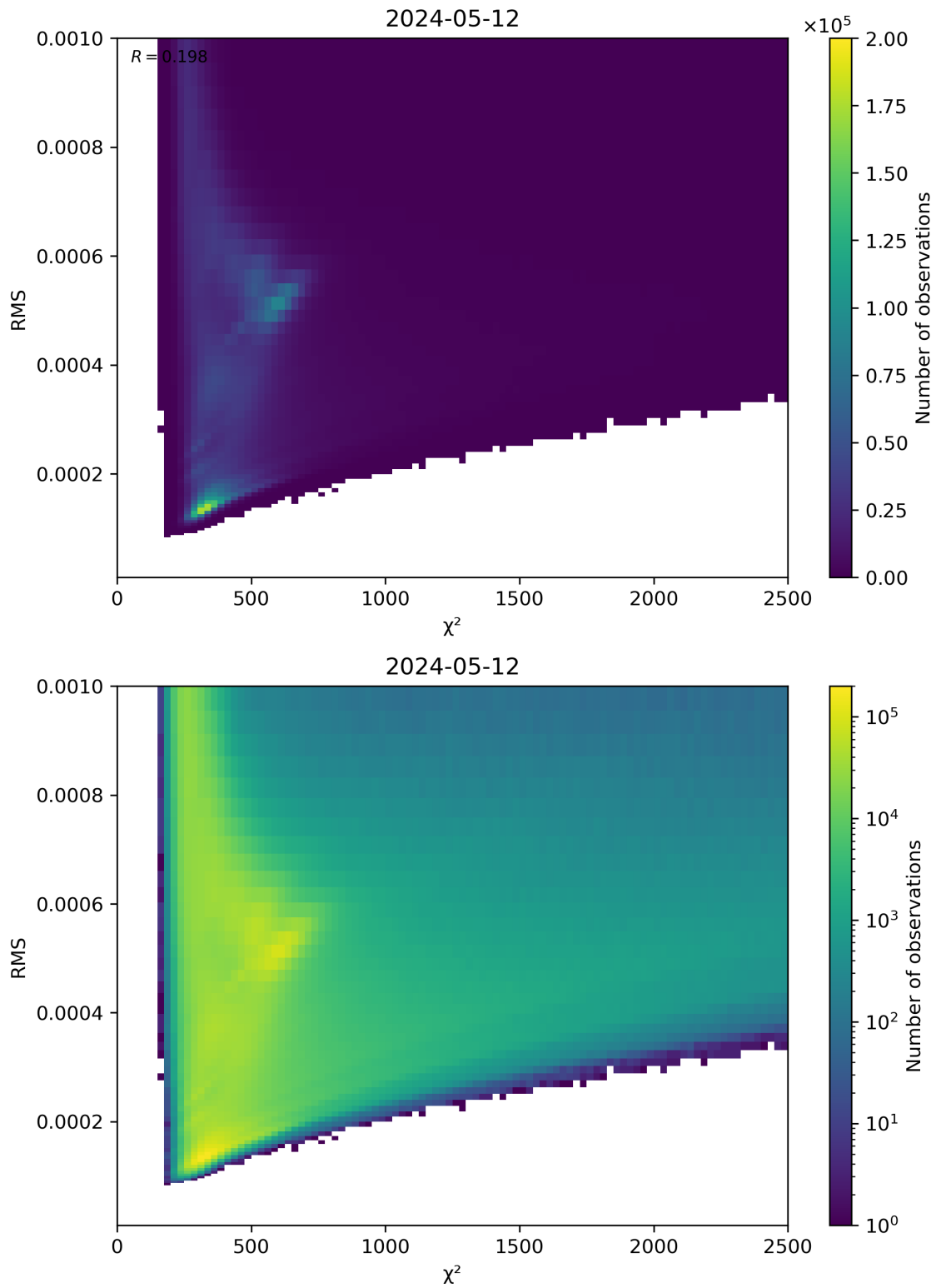
Figure 82: Scatter density plot of “ \chi^2 ” against “RMS” for 2024-05-12 to 2024-05-13.
