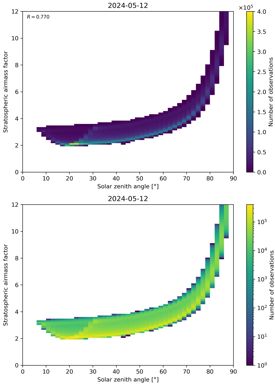
Figure 145: Scatter density plot of “Solar zenith angle” against “Stratospheric airmass factor” for 2024-05-12 to 2024-05-13.
