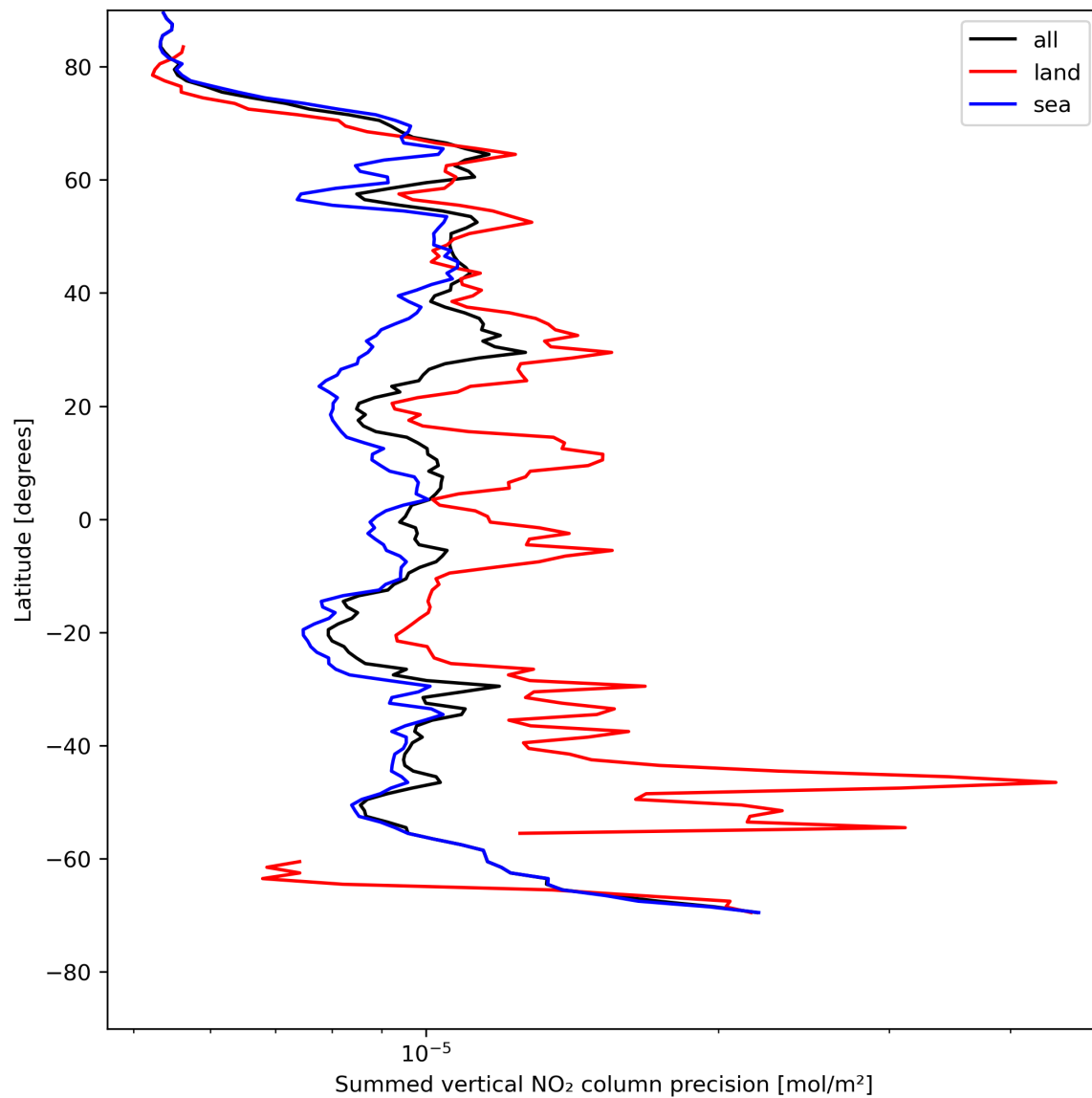
Figure 24: Zonal average of “Summed vertical NO 2 column precision” for 2024-05-12 to 2024-05-13.
