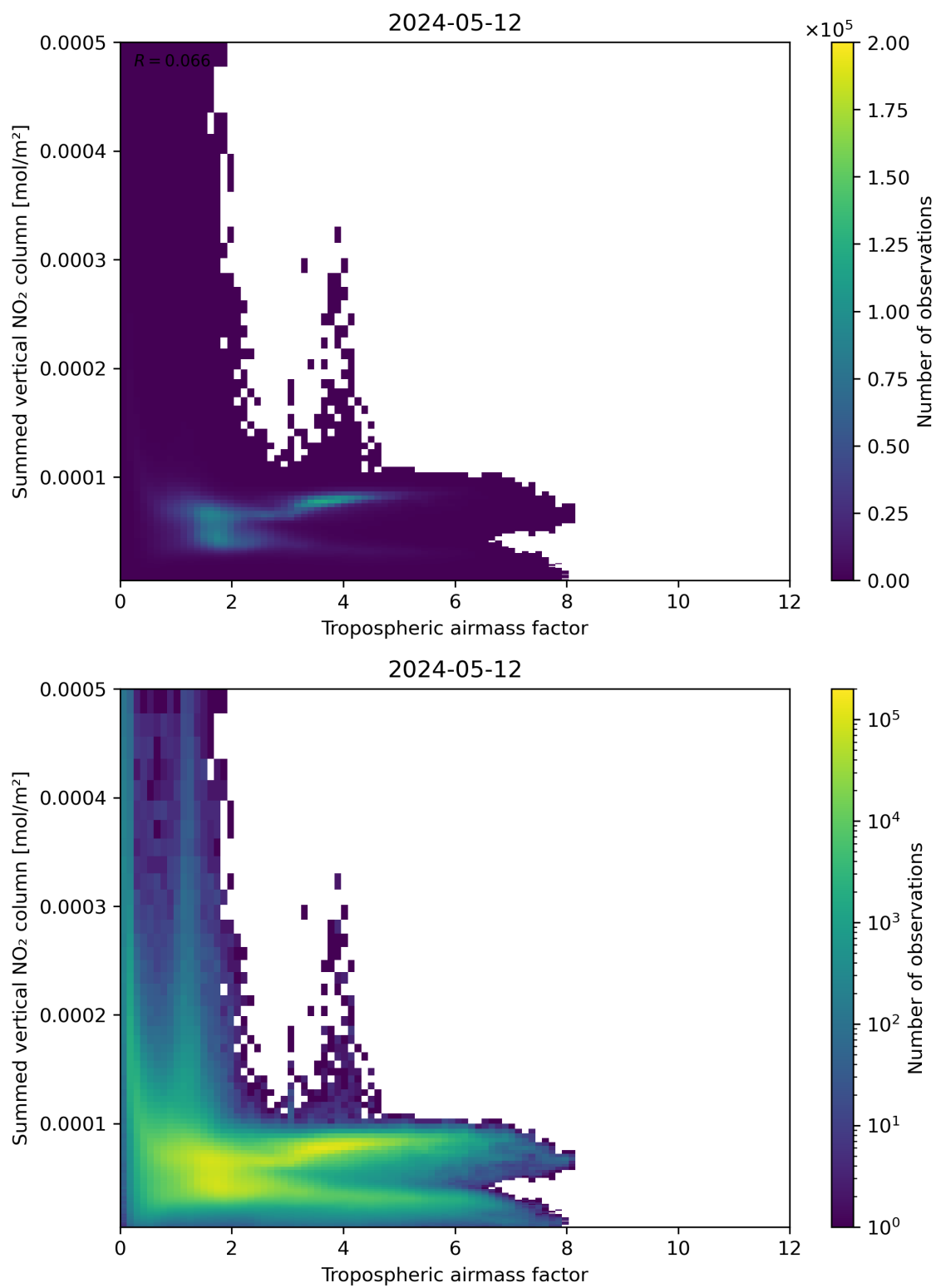
Figure 75: Scatter density plot of “Tropospheric airmass factor” against “Summed vertical NO 2 column” for 2024-05-12 to 2024-05-13.
