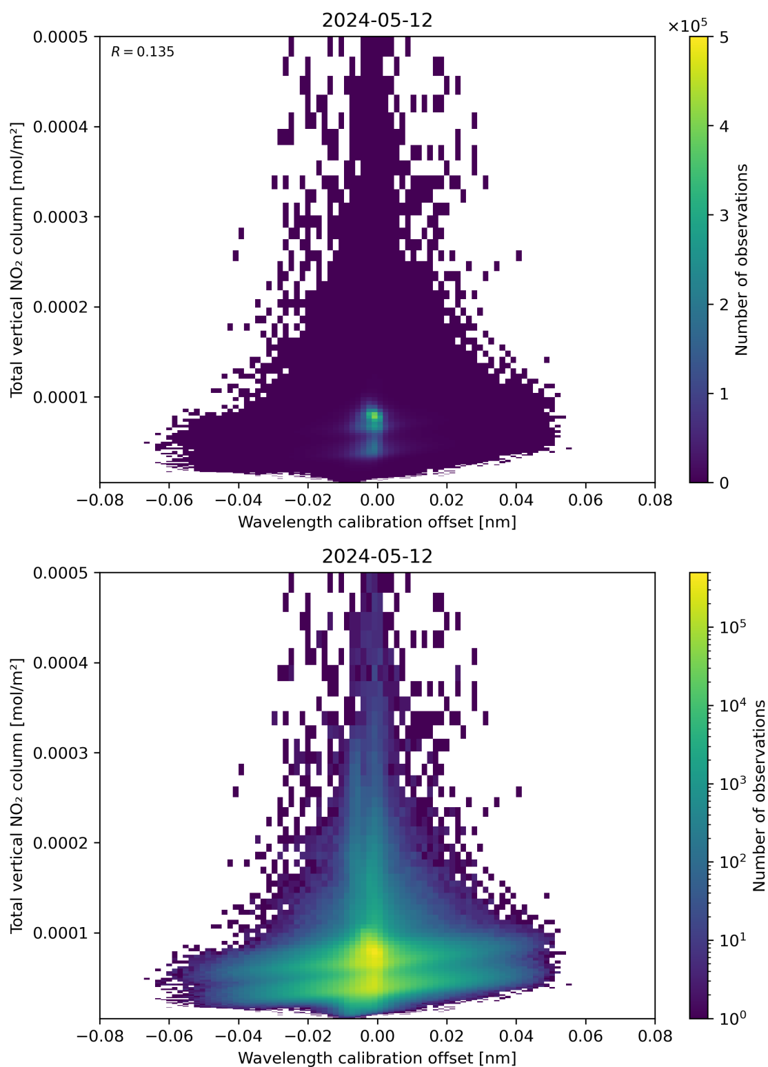
Figure 179: Scatter density plot of “Wavelength calibration offset” against “Total vertical NO 2 column” for 2024-05-12 to 2024-05-13.
