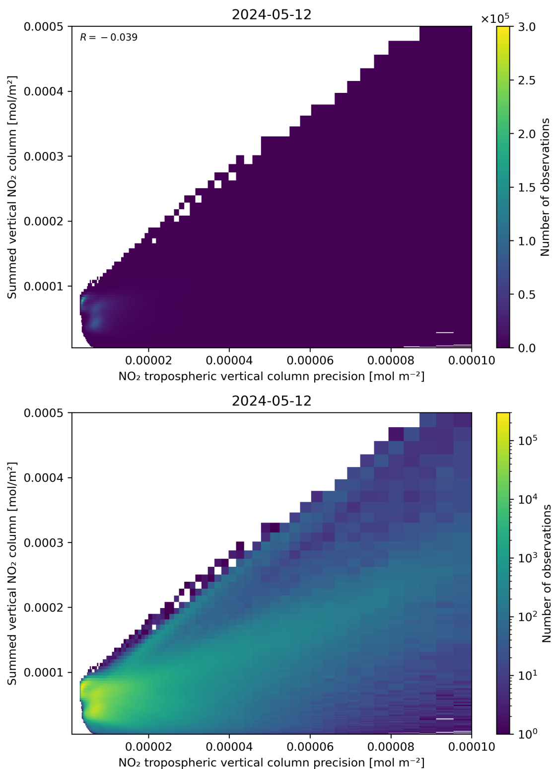
Figure 136: Scatter density plot of “NO 2 tropospheric vertical column precision” against “Summed vertical NO 2 column” for 2024-05-12 to 2024-05-13.
