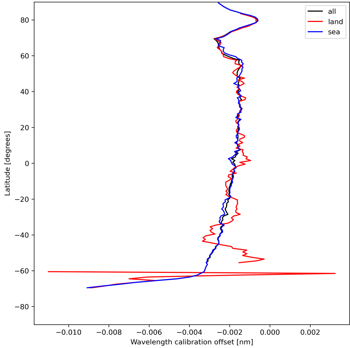
Figure 18: Zonal average of “Wavelength calibration offset” for 2024-05-12 to 2024-05-13.
