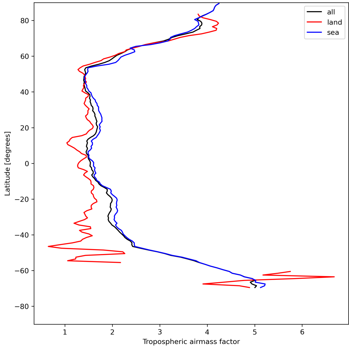
Figure 14: Zonal average of “Tropospheric airmass factor” for 2024-05-12 to 2024-05-13.
