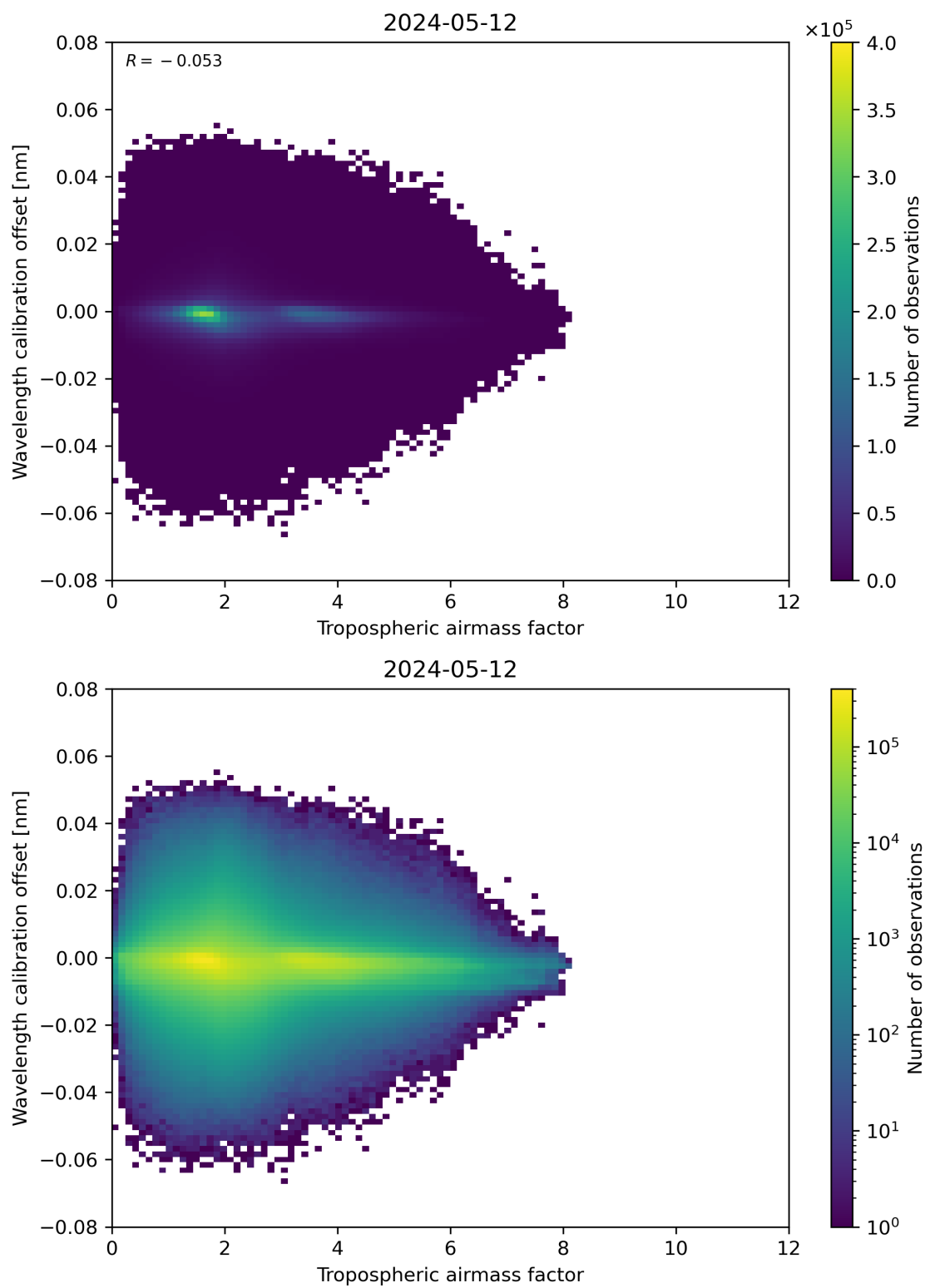
Figure 80: Scatter density plot of “Tropospheric airmass factor” against “Wavelength calibration offset” for 2024-05-12 to 2024-05-13.
