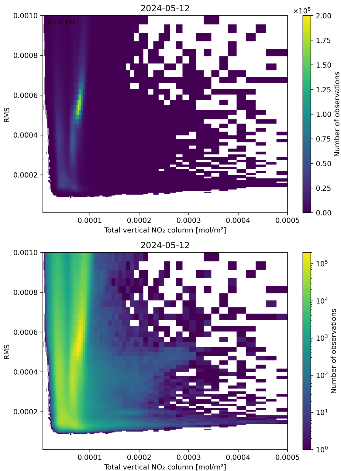
Figure 120: Scatter density plot of “Total vertical NO 2 column” against “RMS” for 2024-05-12 to 2024-05-13.
