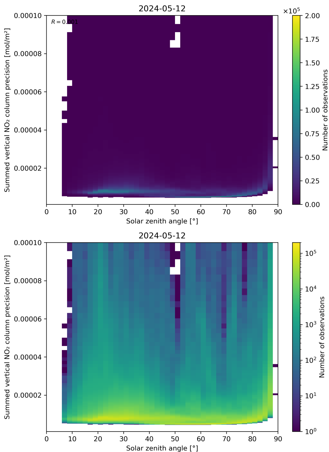
Figure 152: Scatter density plot of “Solar zenith angle” against “Summed vertical NO 2 column precision” for 2024-05-12 to 2024-05-13.
