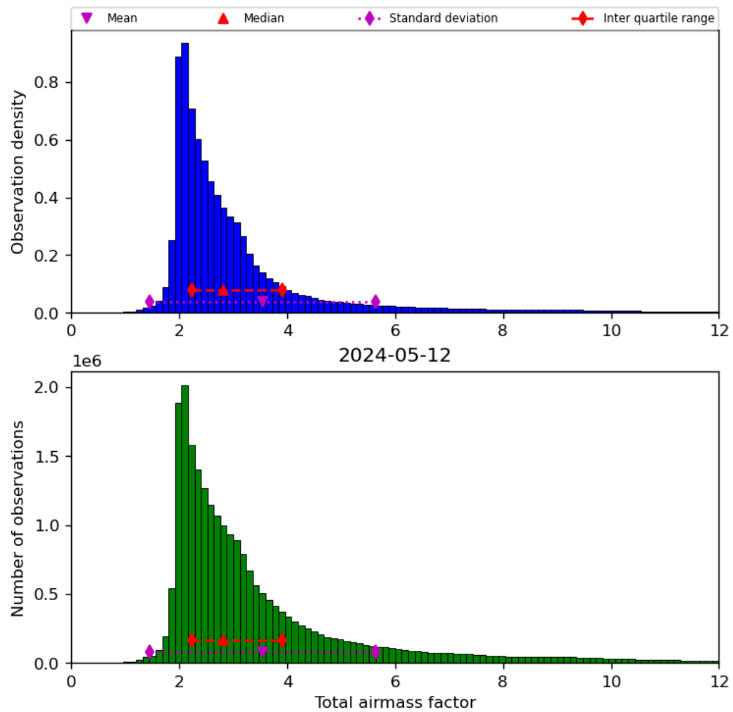
Figure 32: Histogram of “Total airmass factor” for 2024-05-12 to 2024-05-13
