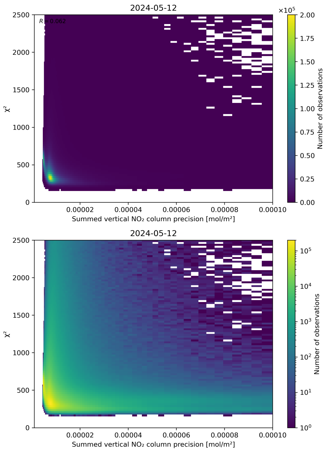
Figure 107: Scatter density plot of “Summed vertical NO 2 column precision” against “ \chi^2 ” for 2024-05-12 to 2024-05-13.
