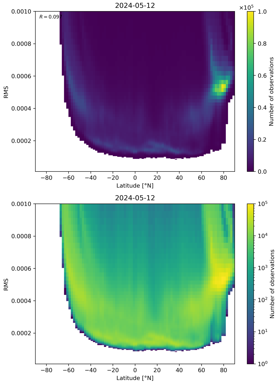
Figure 94: Scatter density plot of “Latitude” against “RMS” for 2024-05-12 to 2024-05-13.
