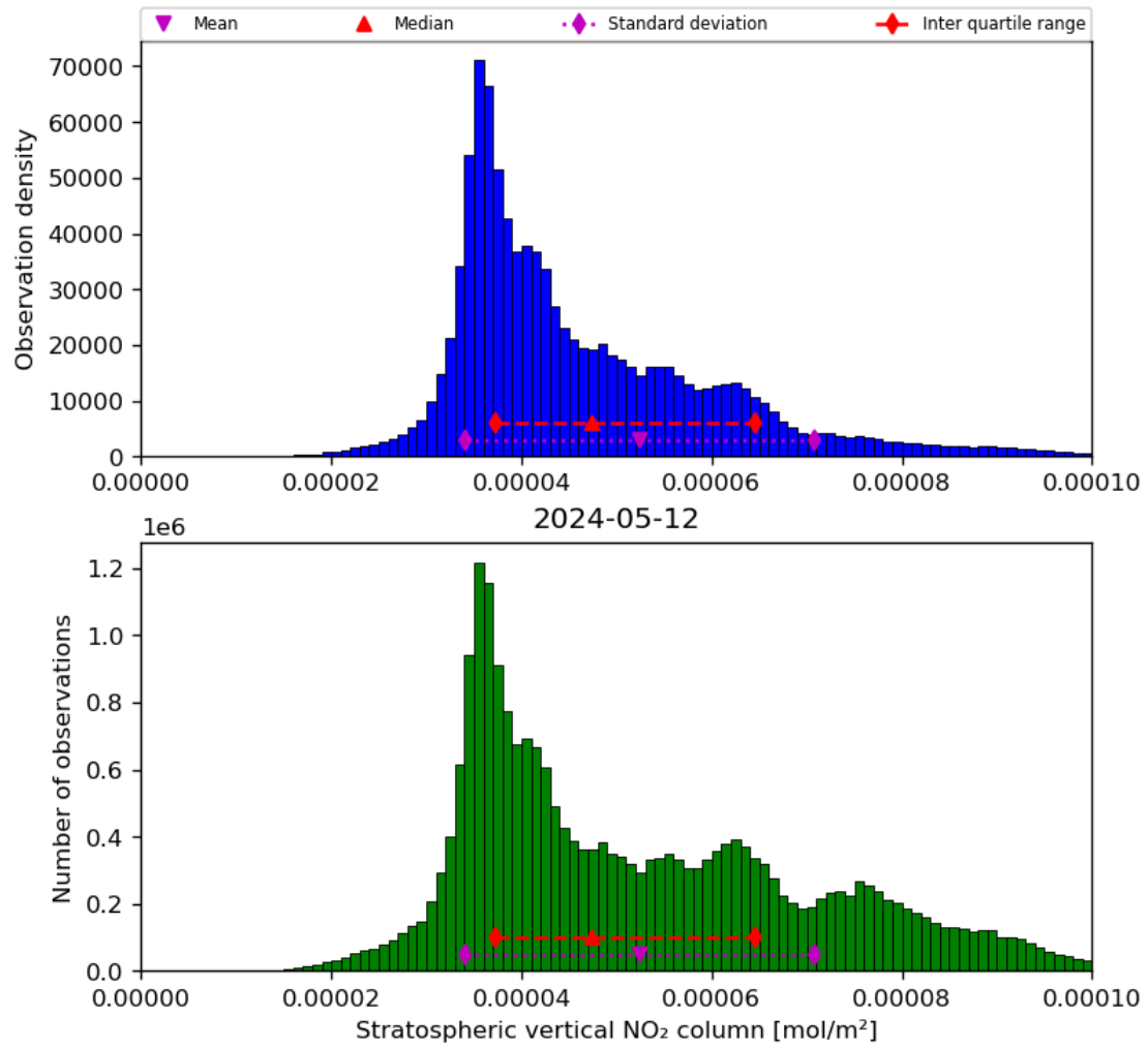
Figure 36: Histogram of “Stratospheric vertical NO 2 column” for 2024-05-12 to 2024-05-13
