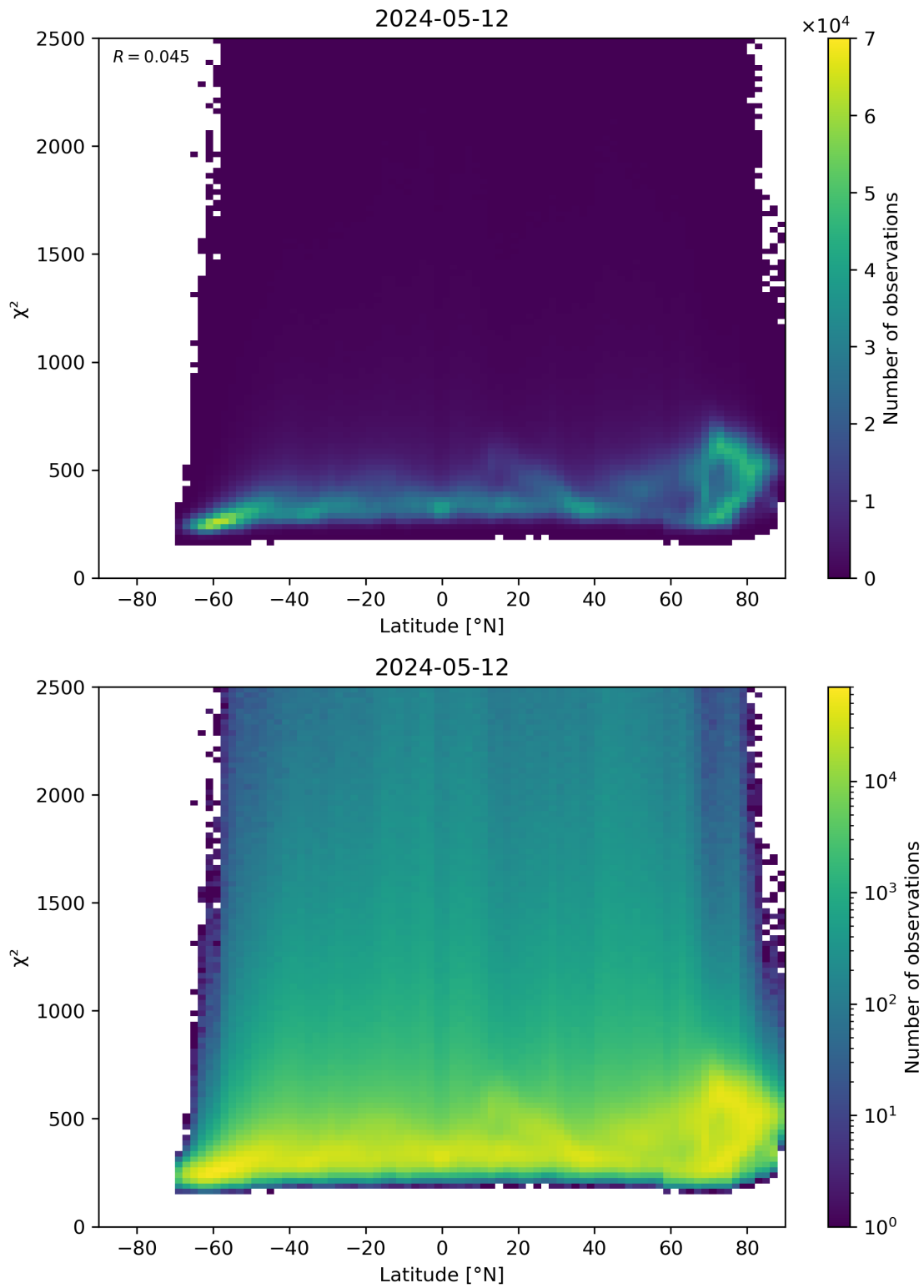
Figure 86: Scatter density plot of “Latitude” against “ \chi^2 ” for 2024-05-12 to 2024-05-13.
