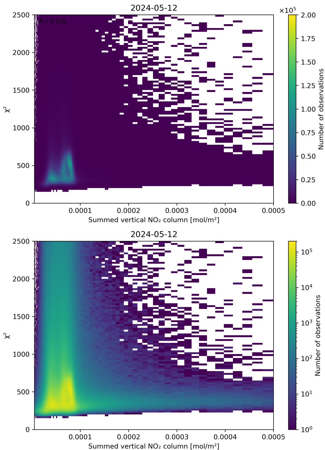
Figure 104: Scatter density plot of “Summed vertical NO 2 column” against “ \chi^2 ” for 2024-05-12 to 2024-05-13.
