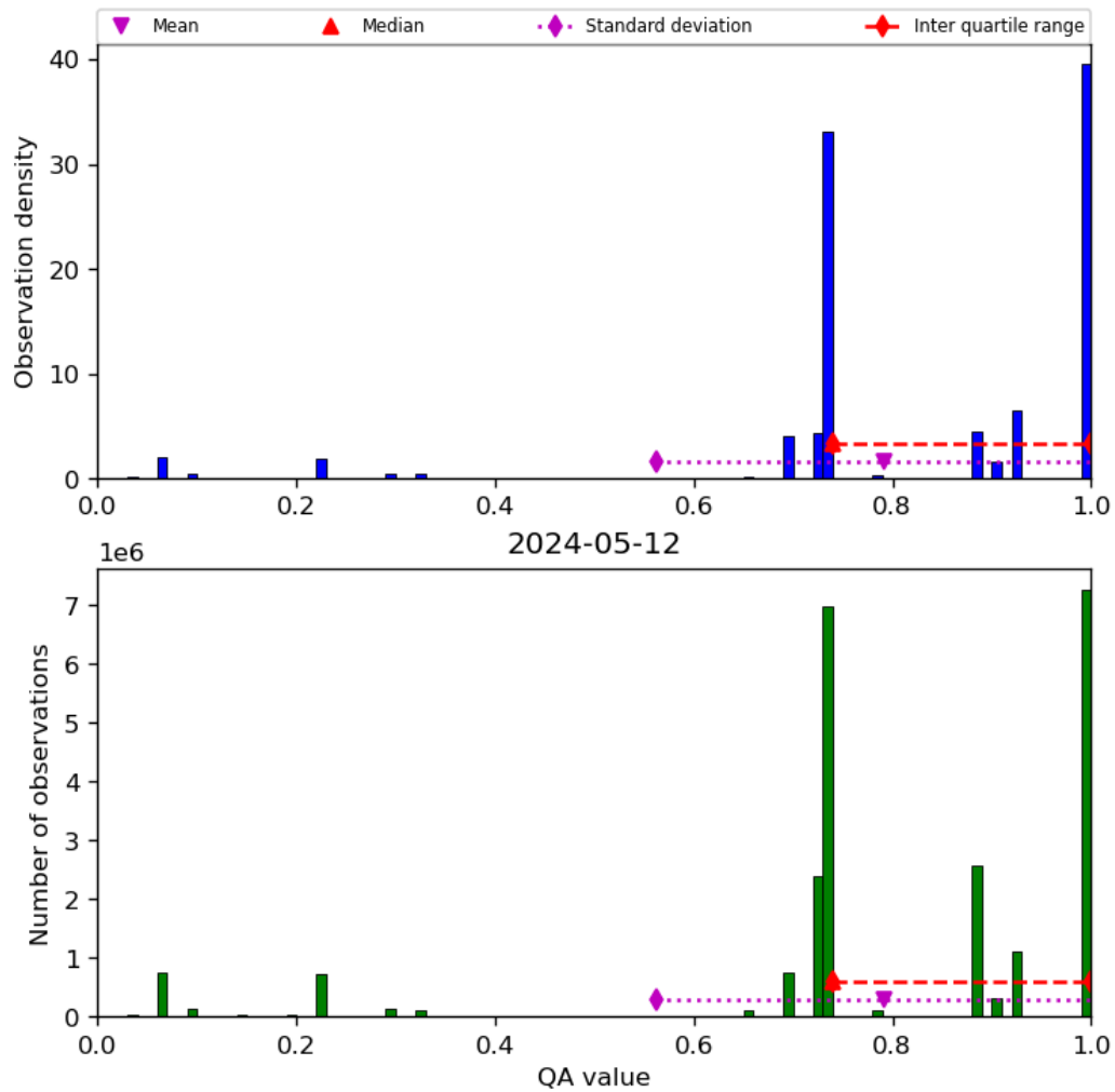
Figure 28: Histogram of “QA value” for 2024-05-12 to 2024-05-13
