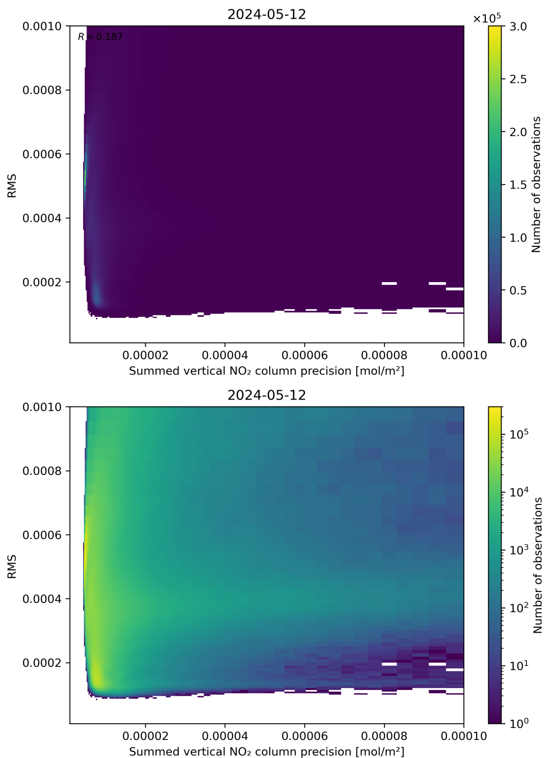
Figure 108: Scatter density plot of “Summed vertical NO 2 column precision” against “RMS” for 2024-05-12 to 2024-05-13.
