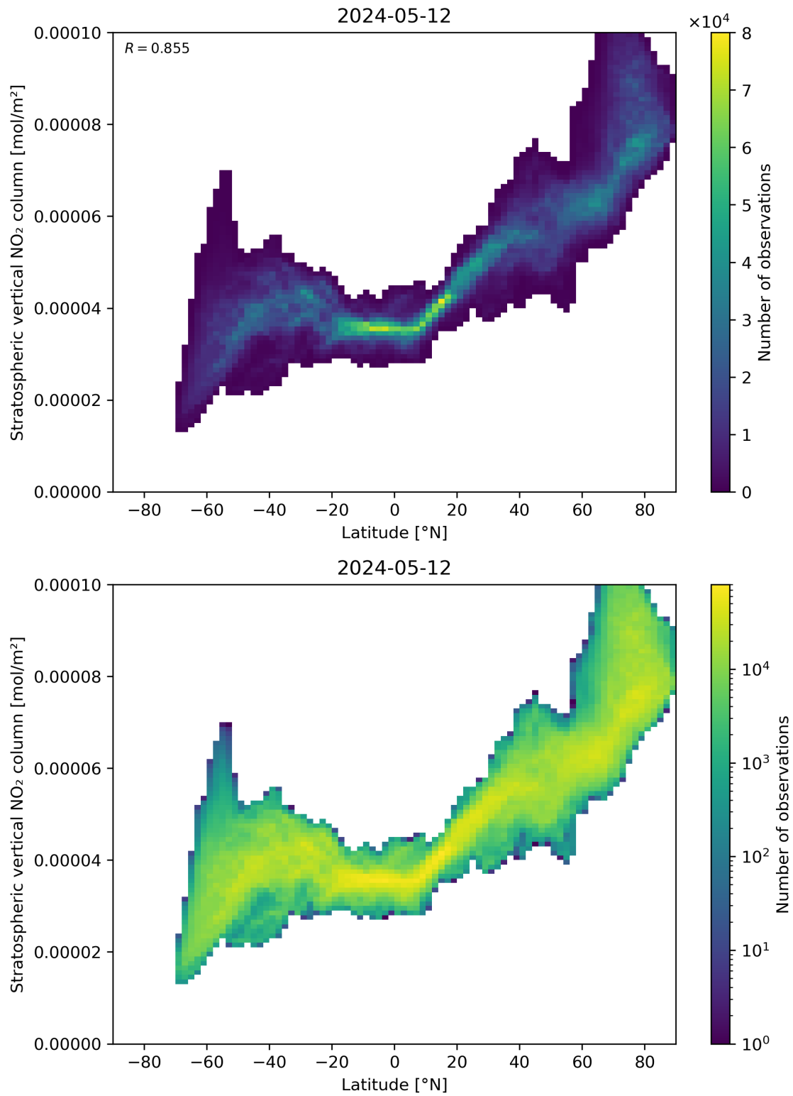
Figure 87: Scatter density plot of “Latitude” against “Stratospheric vertical NO 2 column” for 2024-05-12 to 2024-05-13.
