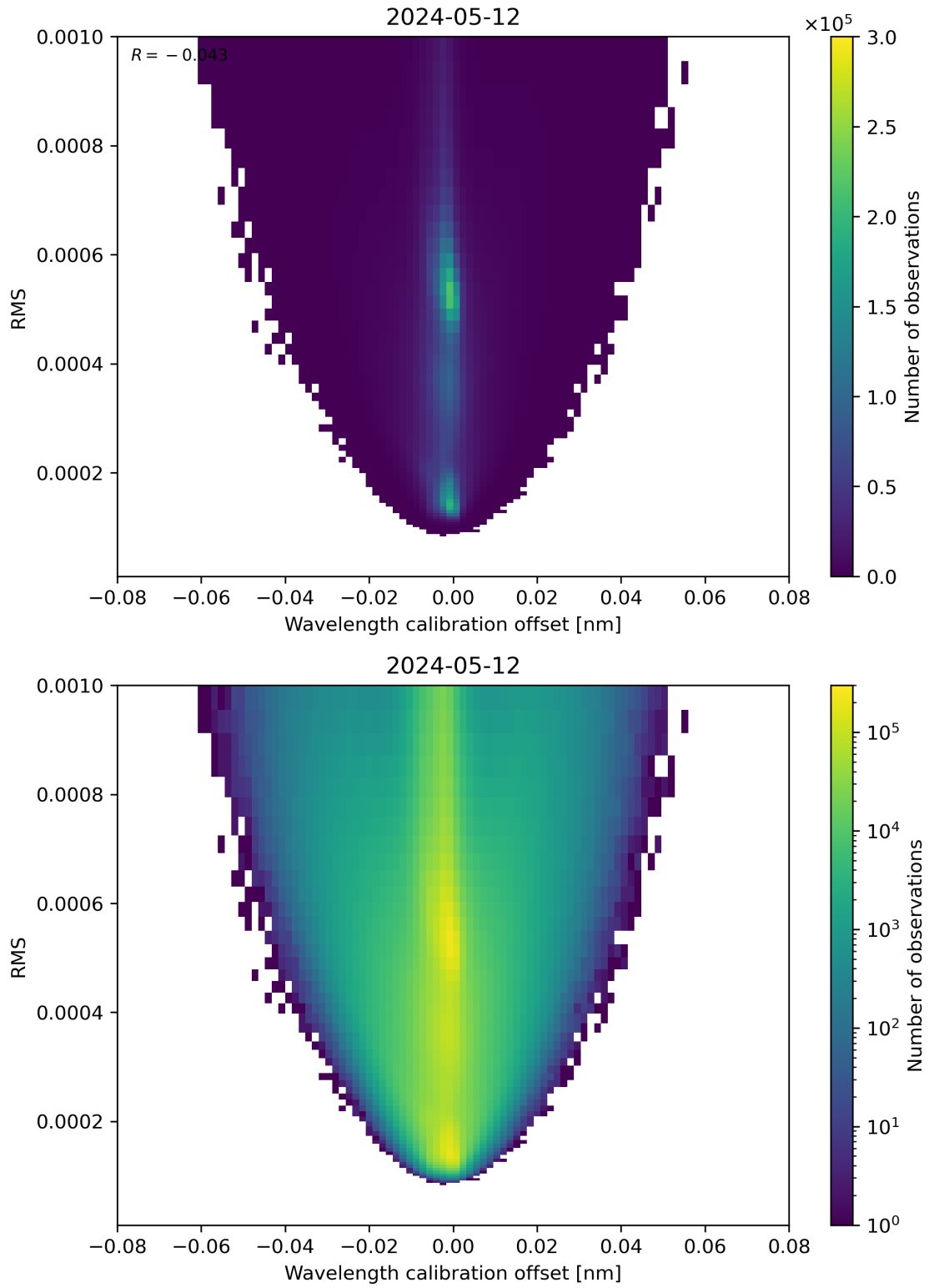
Figure 181: Scatter density plot of “Wavelength calibration offset” against “RMS” for 2024-05-12 to 2024-05-13.
