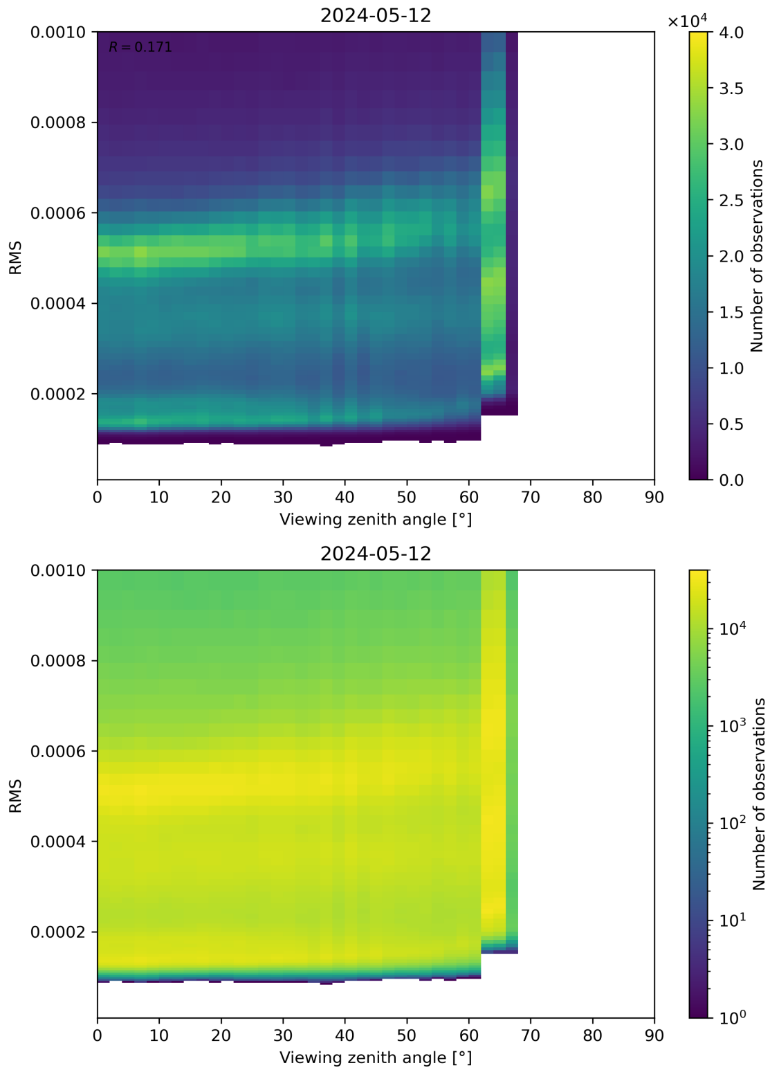
Figure 171: Scatter density plot of “Viewing zenith angle” against “RMS” for 2024-05-12 to 2024-05-13.
