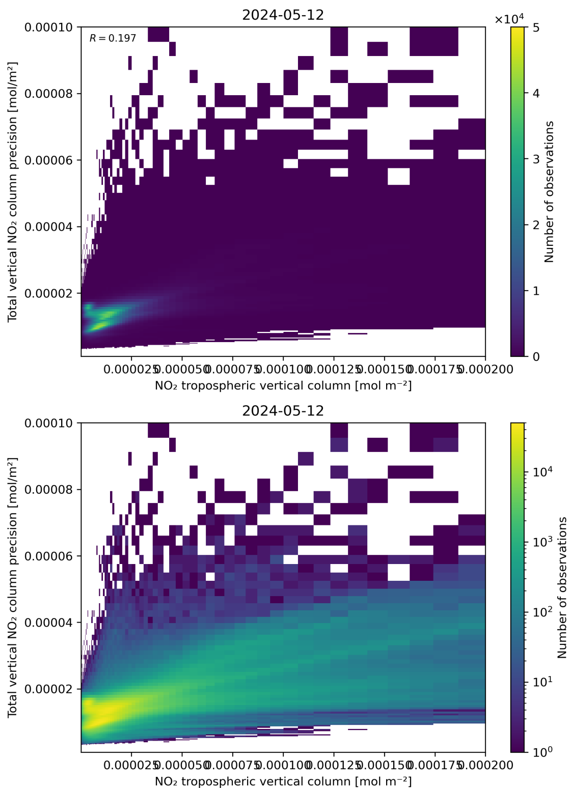
Figure 129: Scatter density plot of “NO 2 tropospheric vertical column” against “Total vertical NO 2 column precision” for 2024-05-12 to 2024-05-13.
