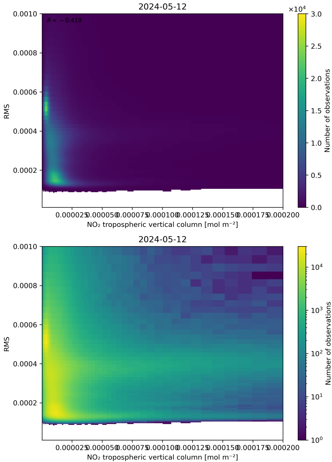
Figure 142: Scatter density plot of “NO 2 tropospheric vertical column” against “RMS” for 2024-05-12 to 2024-05-13.
