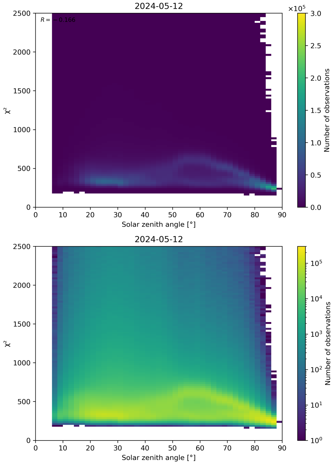
Figure 148: Scatter density plot of “Solar zenith angle” against “ \chi^2 ” for 2024-05-12 to 2024-05-13.
