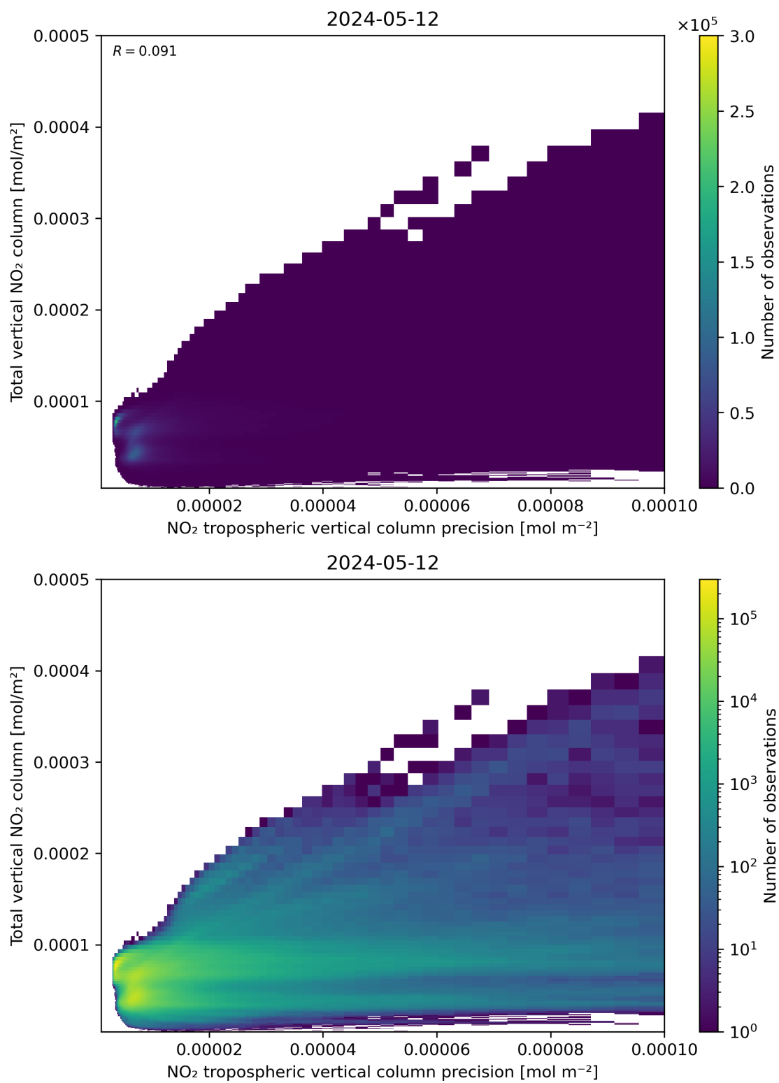
Figure 138: Scatter density plot of “NO 2 tropospheric vertical column precision” against “Total vertical NO 2 column” for 2024-05-12 to 2024-05-13.
