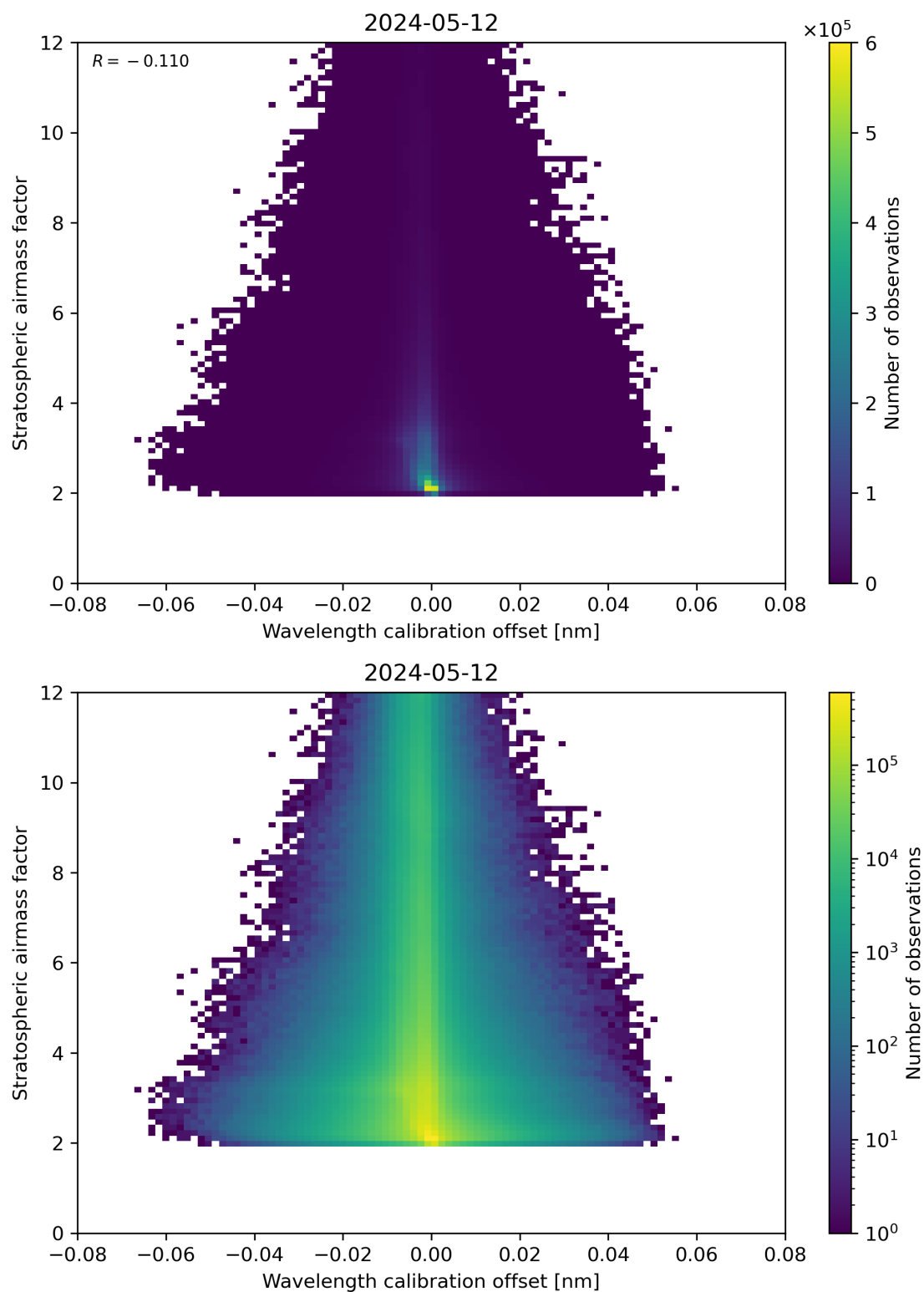
Figure 174: Scatter density plot of “Wavelength calibration offset” against “Stratospheric air mass factor” for 2024-05-12 to 2024-05-13.
