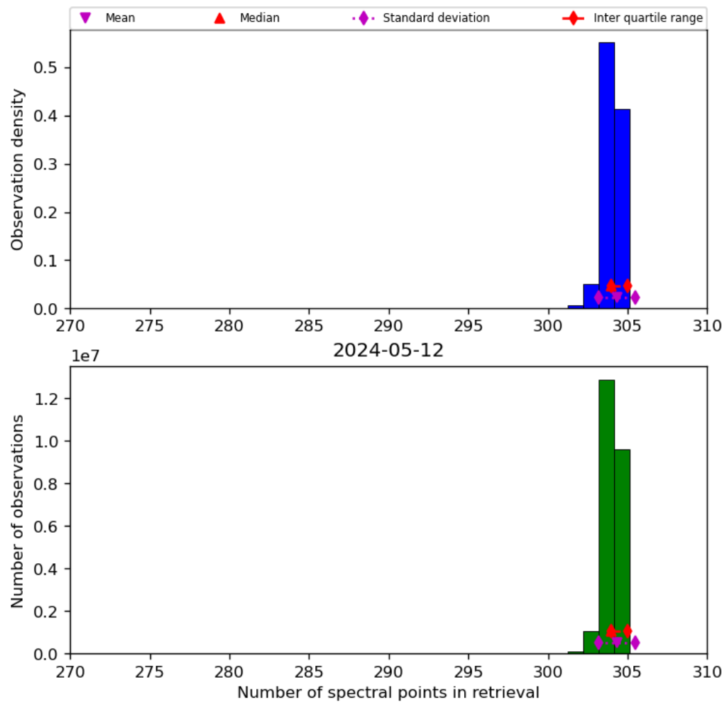
Figure 33: Histogram of “Number of spectral points in retrieval” for 2024-05-12 to 2024-05-13
