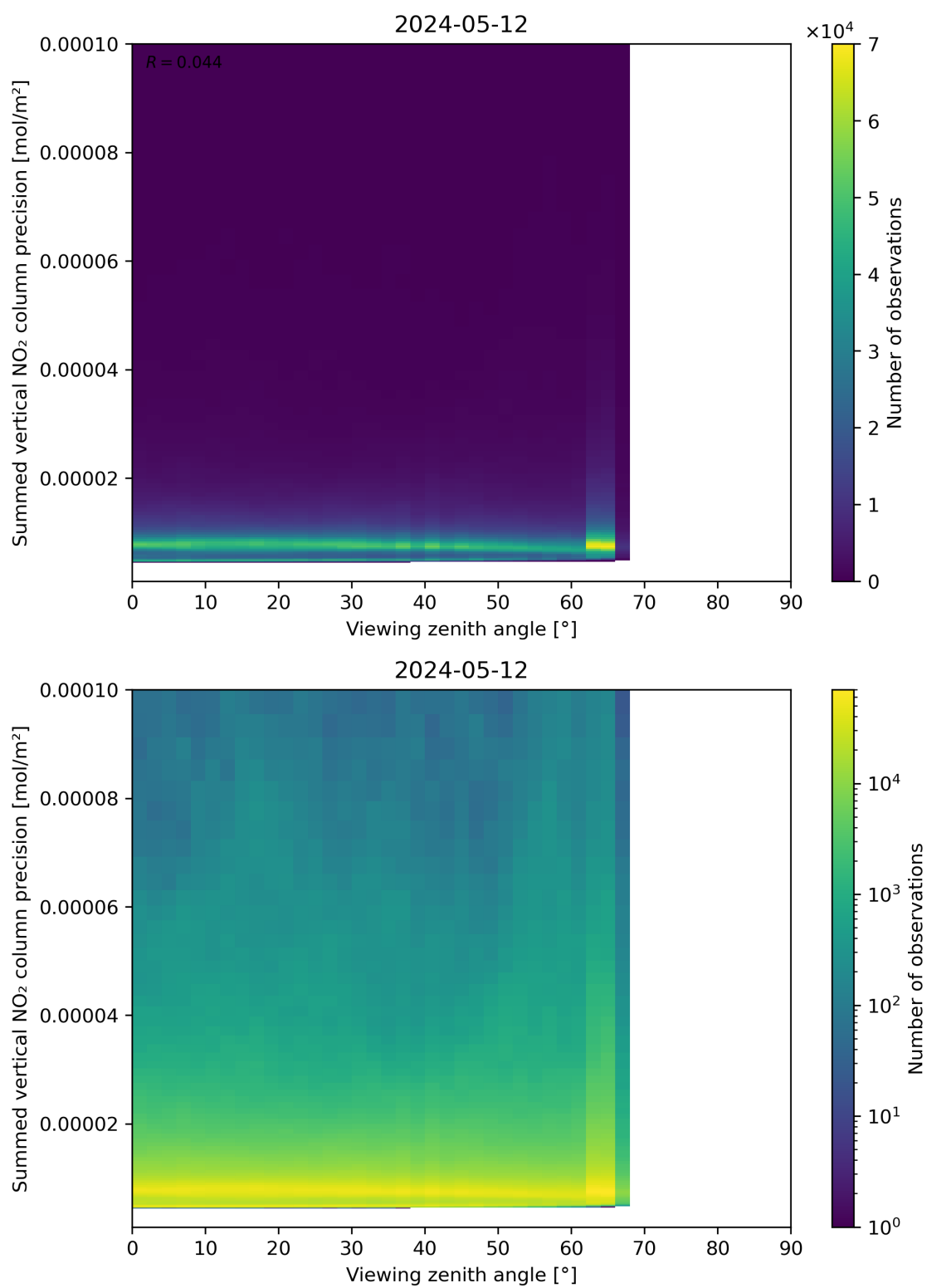
Figure 166: Scatter density plot of “Viewing zenith angle” against “Summed vertical NO 2 column precision” for 2024-05-12 to 2024-05-13.
