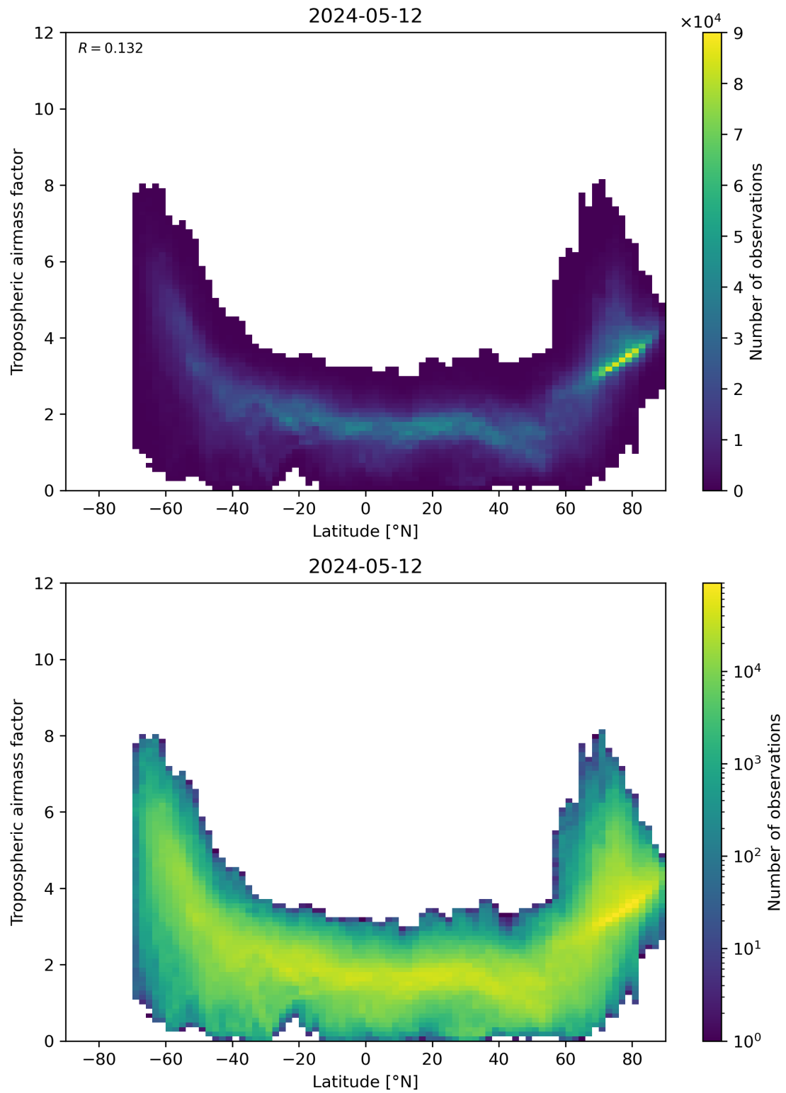
Figure 85: Scatter density plot of “Latitude” against “Tropospheric airmass factor” for 2024-05-12 to 2024-05-13.
