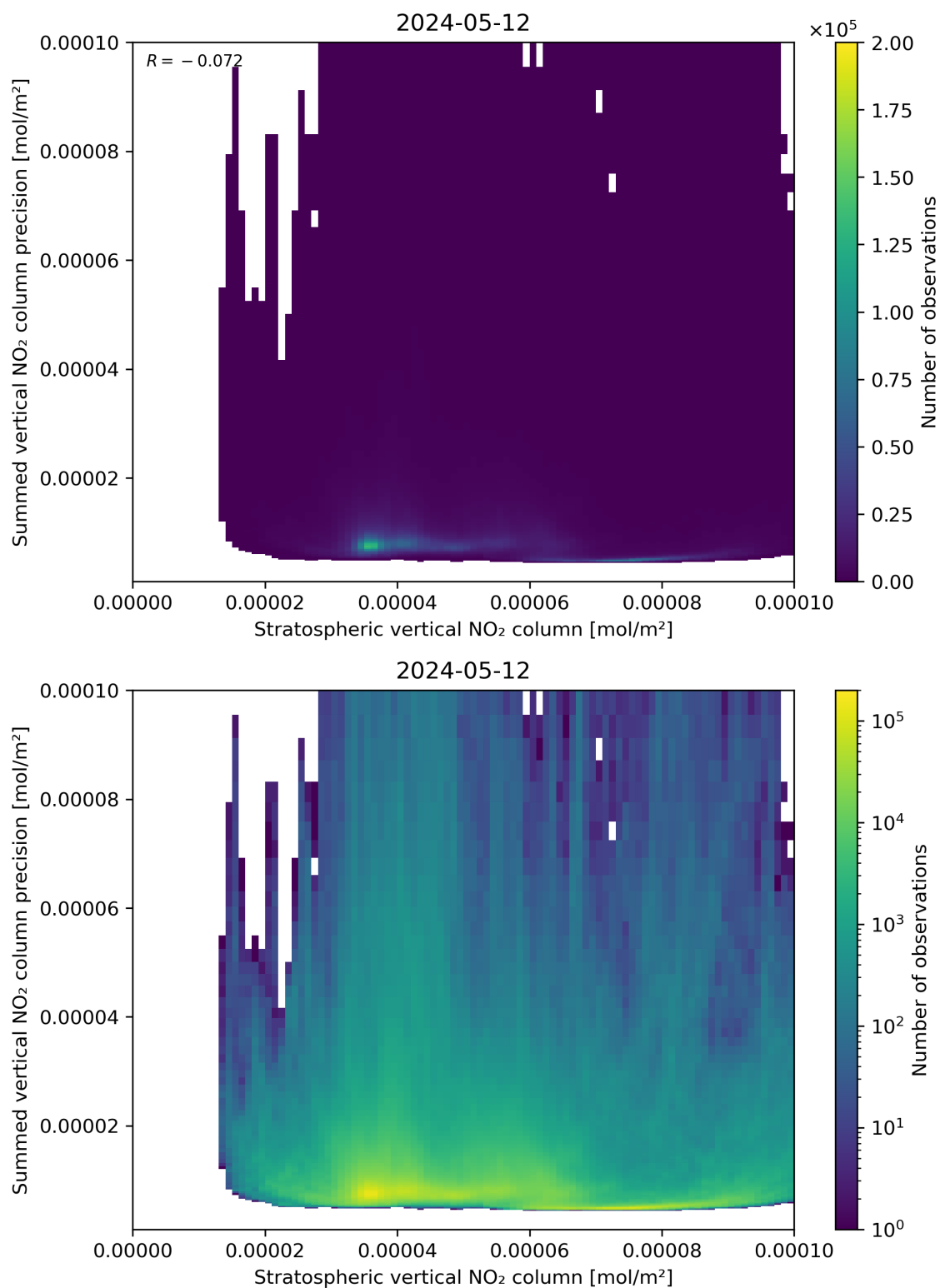
Figure 99: Scatter density plot of “Stratospheric vertical NO 2 column” against “Summed vertical NO 2 column precision” for 2024-05-12 to 2024-05-13.
