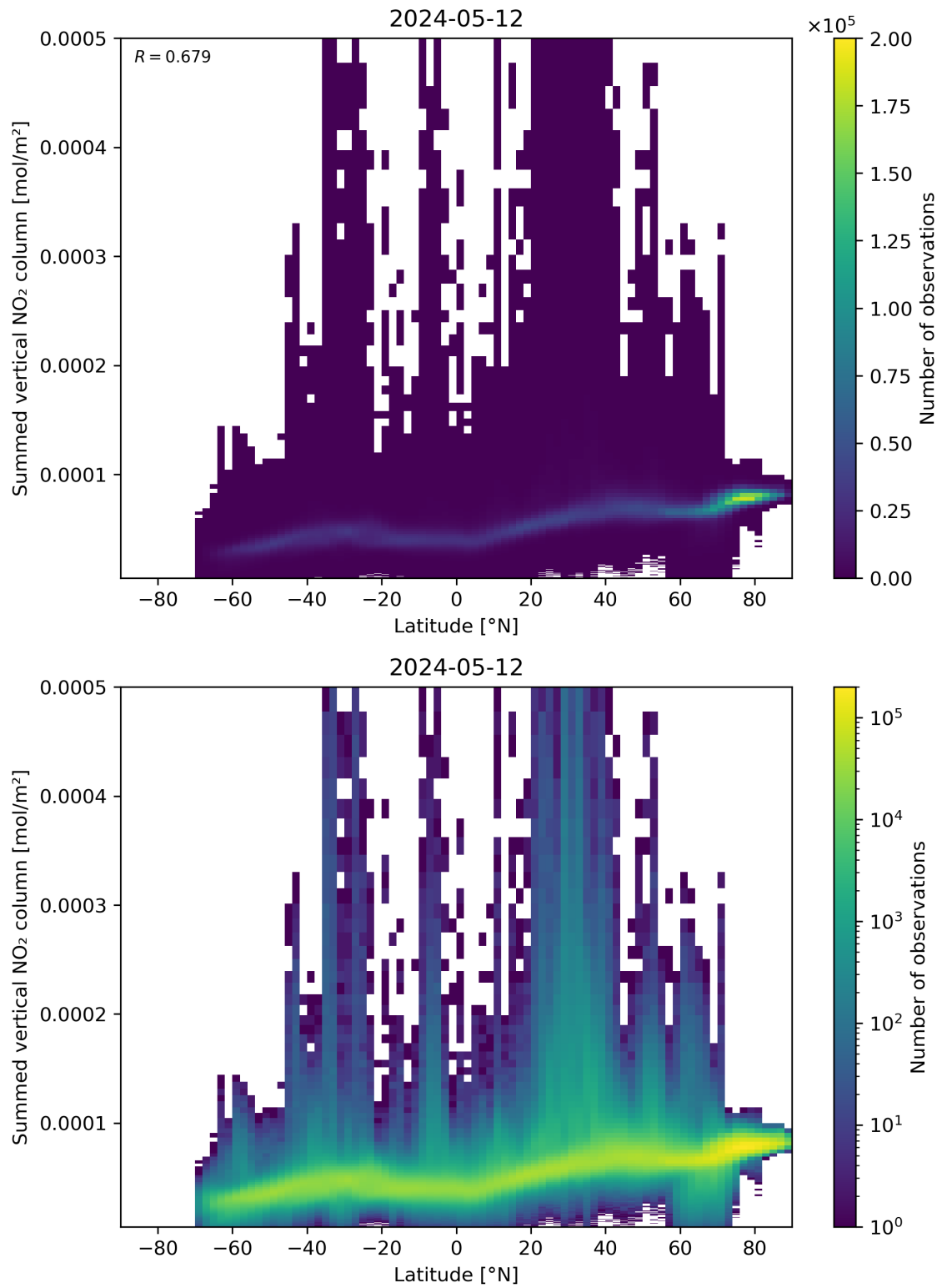
Figure 88: Scatter density plot of “Latitude” against “Summed vertical NO 2 column” for 2024-05-12 to 2024-05-13.
