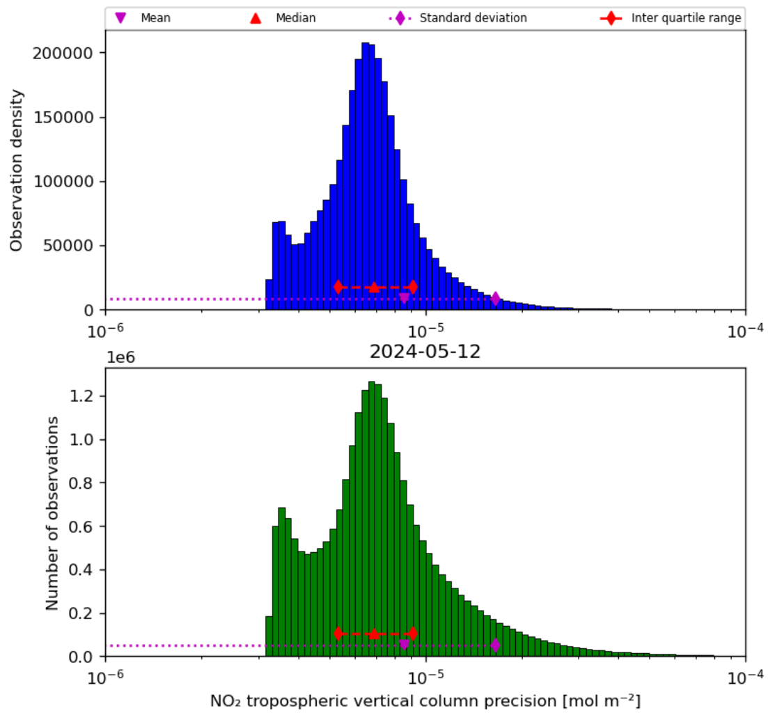
Figure 30: Histogram of “NO 2 tropospheric vertical column precision” for 2024-05-12 to 2024-05-13
