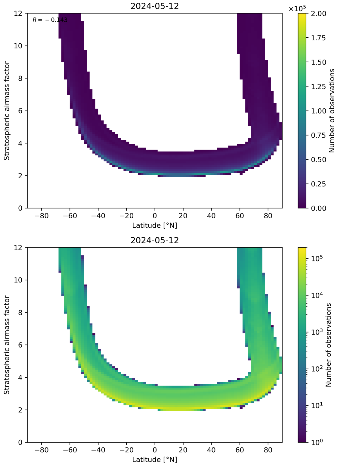
Figure 83: Scatter density plot of “Latitude” against “Stratospheric air mass factor” for 2024-05-12 to 2024-05-13.
