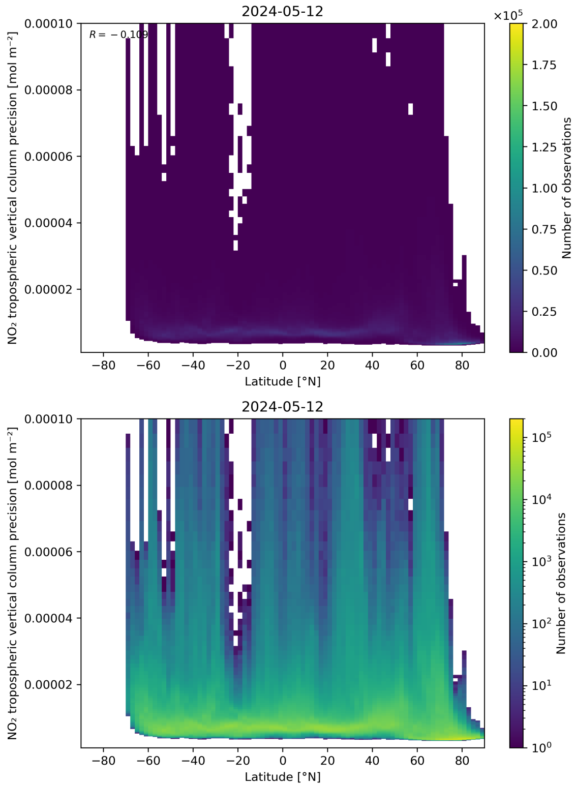
Figure 93: Scatter density plot of “Latitude” against “NO 2 tropospheric vertical column precision” for 2024-05-12 to 2024-05-13.
