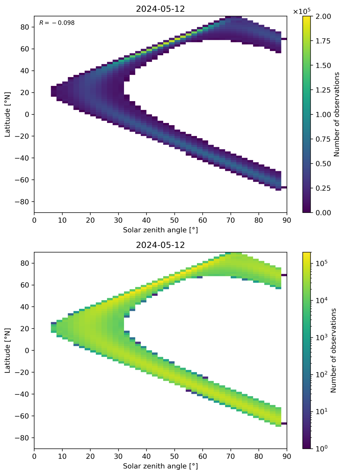
Figure 149: Scatter density plot of “Solar zenith angle” against “Latitude” for 2024-05-12 to 2024-05-13.
