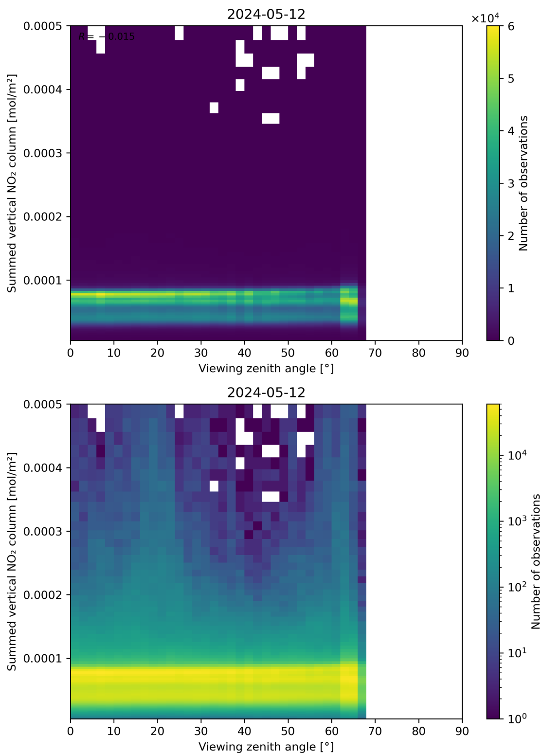
Figure 165: Scatter density plot of “Viewing zenith angle” against “Summed vertical NO 2 column” for 2024-05-12 to 2024-05-13.
