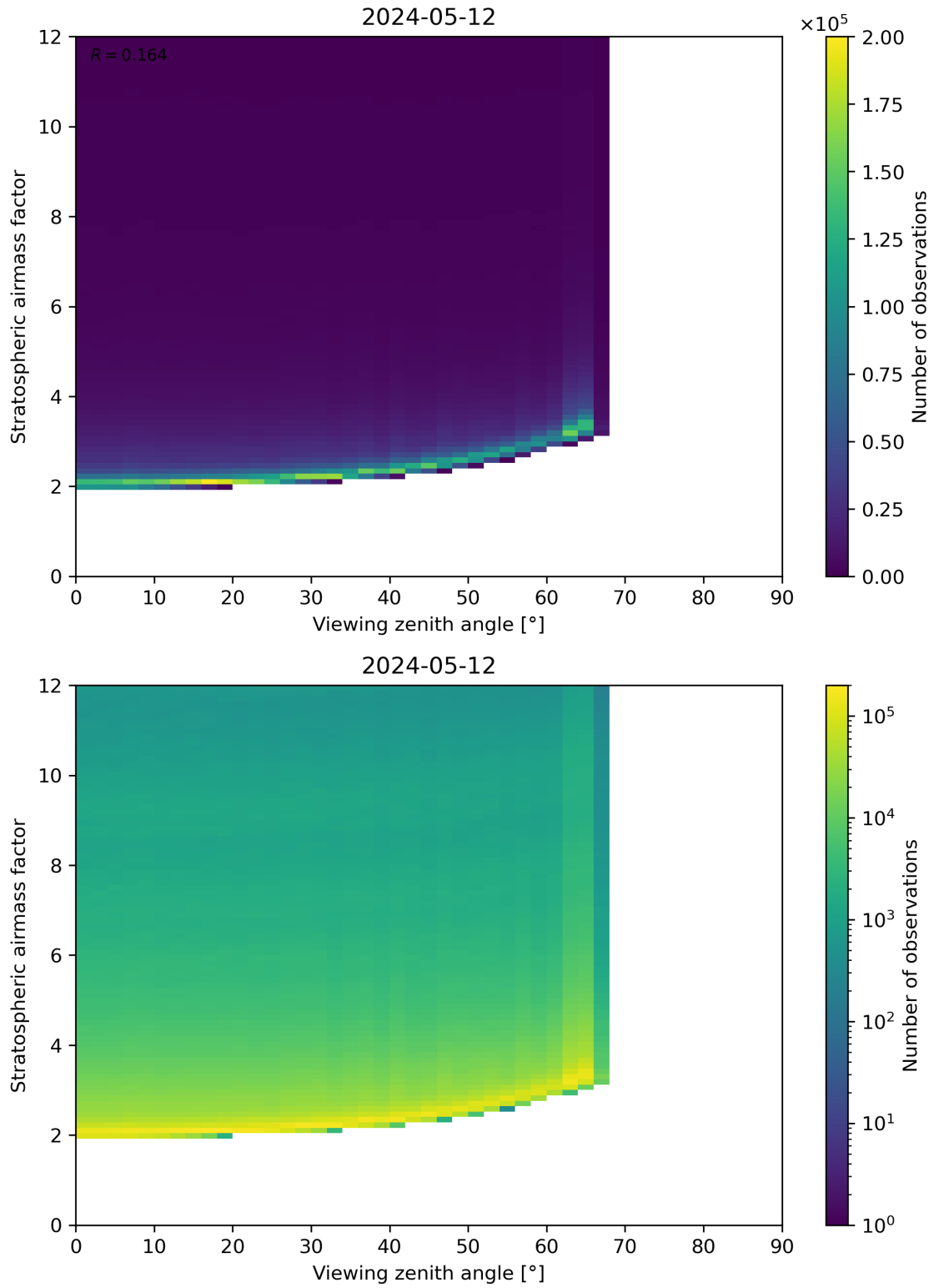
Figure 159: Scatter density plot of “Viewing zenith angle” against “Stratospheric airmass factor” for 2024-05-12 to 2024-05-13.
