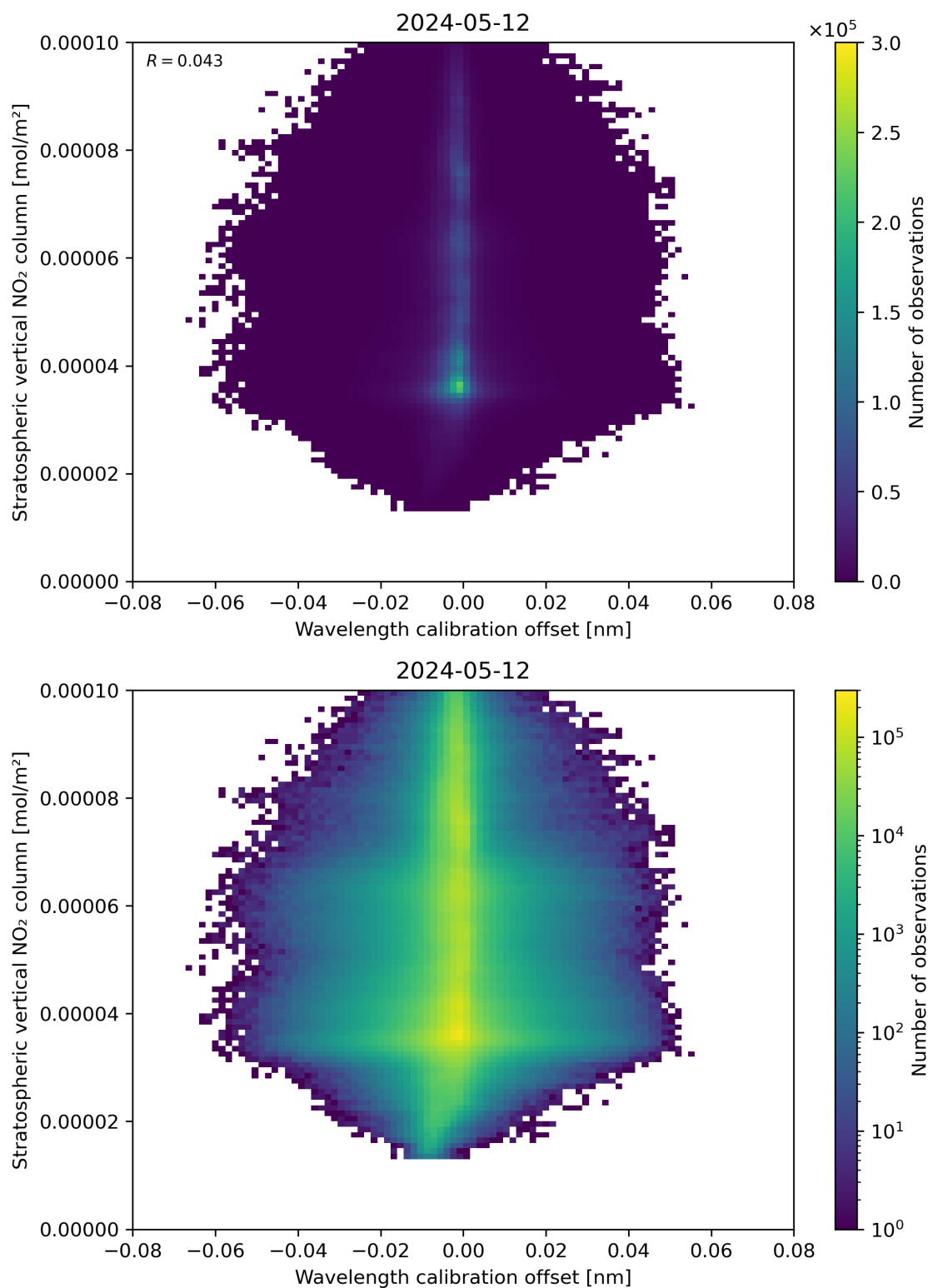
Figure 176: Scatter density plot of “Wavelength calibration offset” against “Stratospheric vertical NO 2 column” for 2024-05-12 to 2024-05-13.
