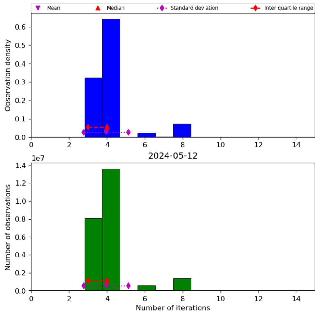
Figure 34: Histogram of “Number of iterations” for 2024-05-12 to 2024-05-13
