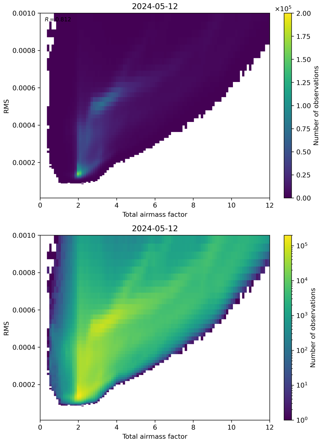
Figure 69: Scatter density plot of “Total airmass factor” against “RMS” for 2024-05-12 to 2024-05-13.
