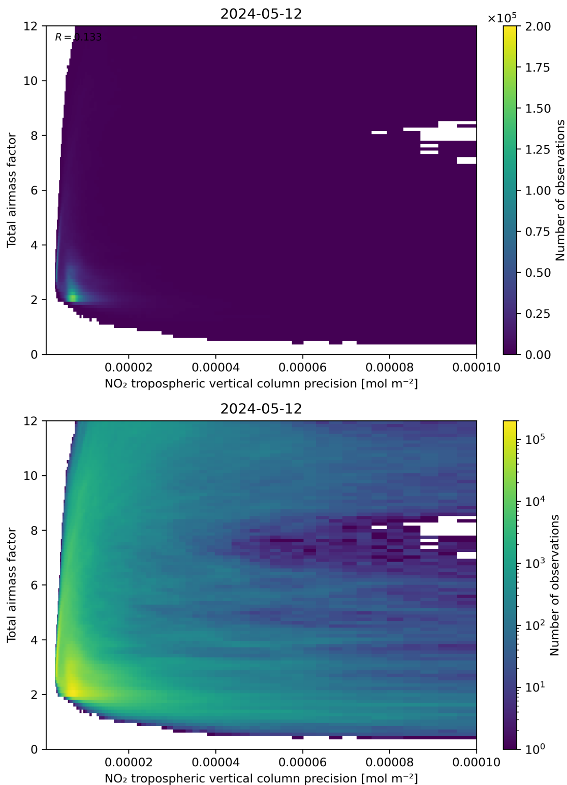
Figure 132: Scatter density plot of “NO 2 tropospheric vertical column precision” against “Total air mass factor” for 2024-05-12 to 2024-05-13.
