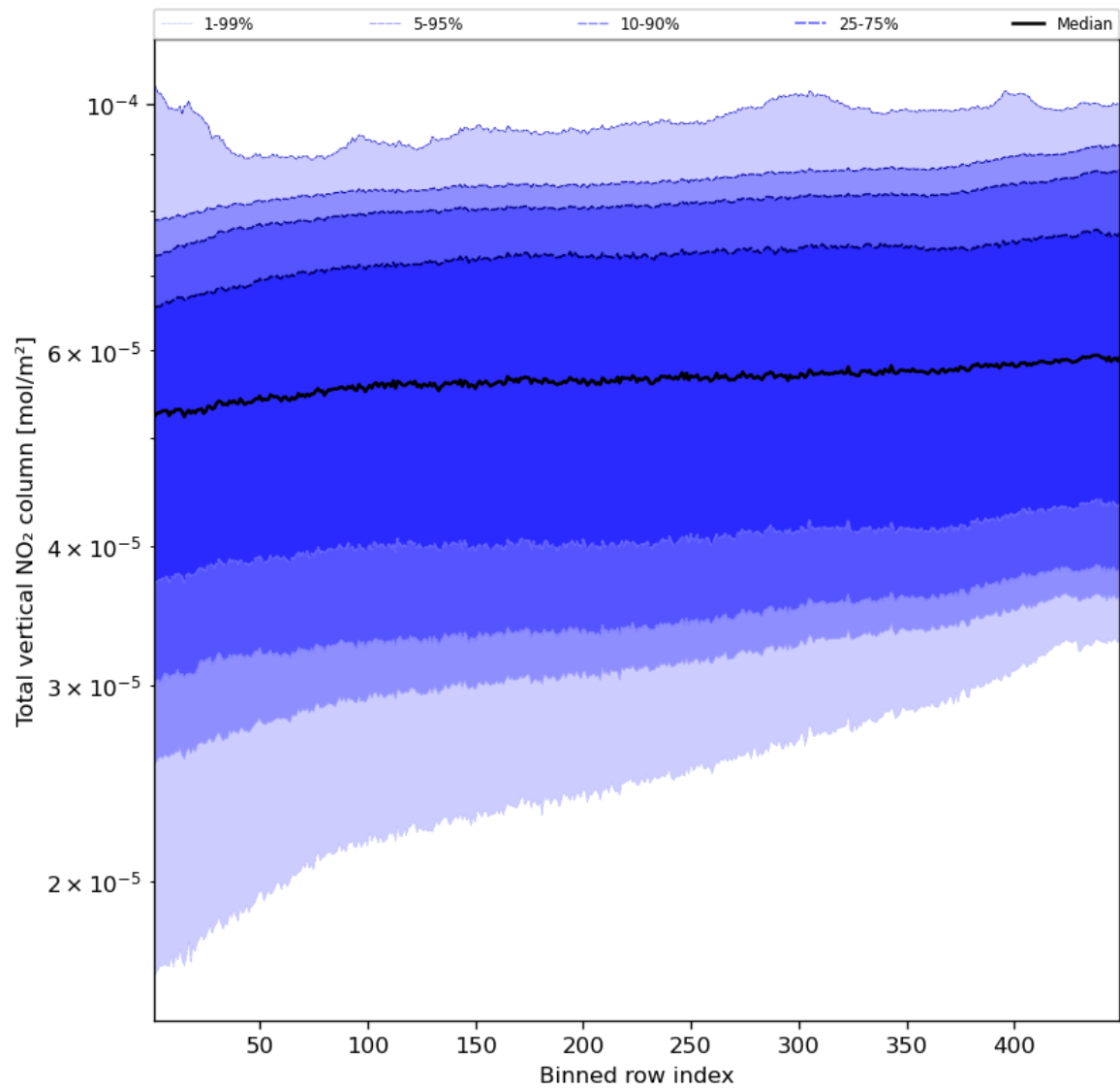
Figure 55: Along track statistics of “Total vertical NO 2 column” for 2024-05-12 to 2024-05-13
