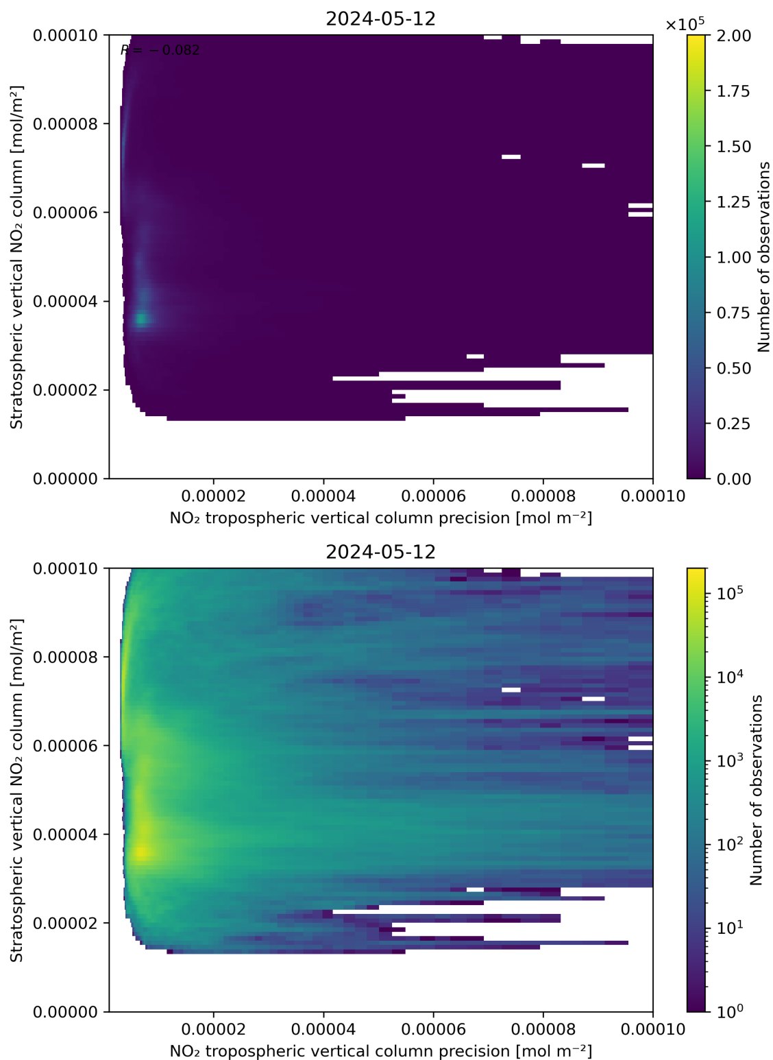
Figure 135: Scatter density plot of “NO 2 tropospheric vertical column precision” against “Stratospheric vertical NO 2 column” for 2024-05-12 to 2024-05-13.
