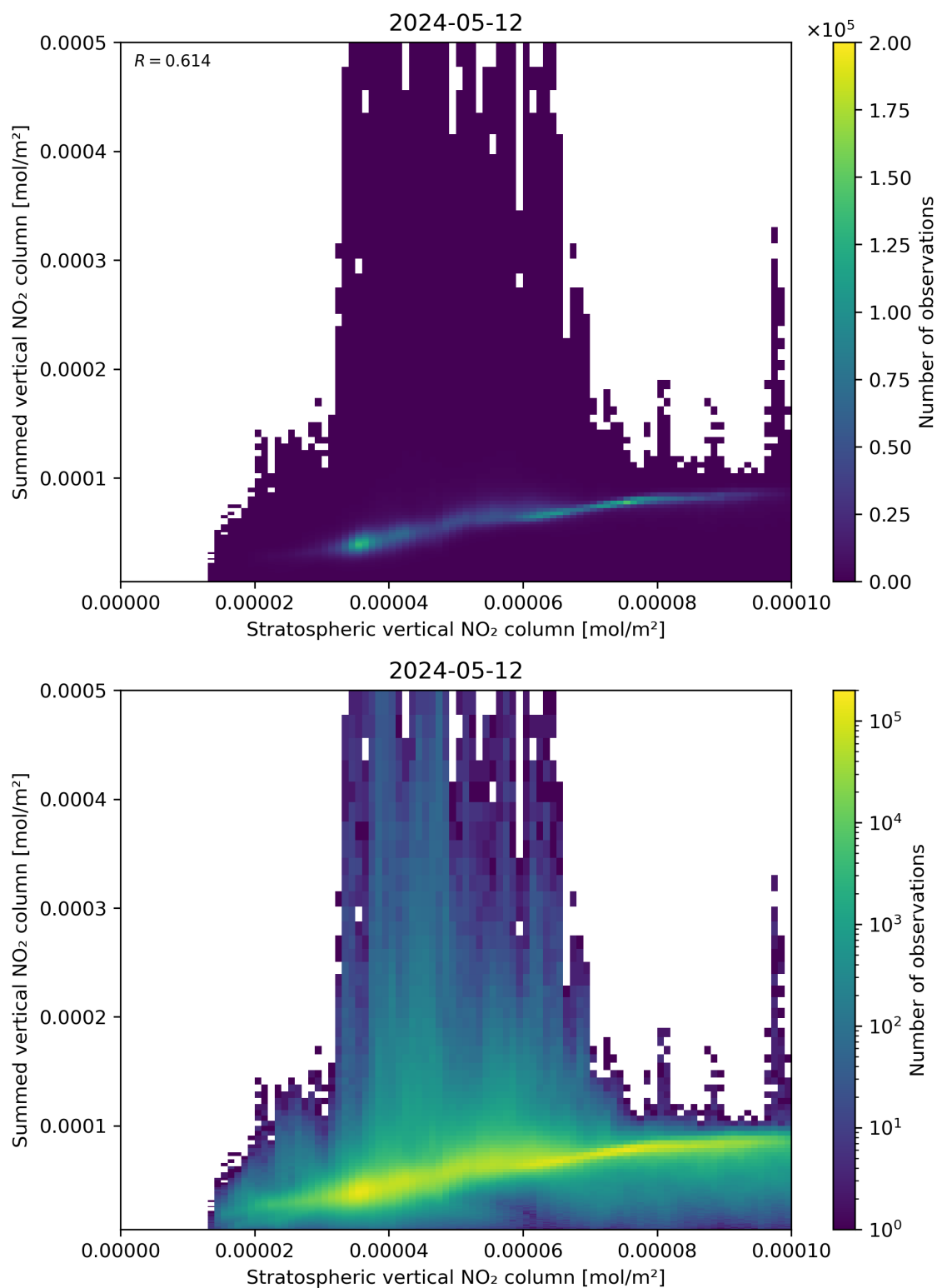
Figure 98: Scatter density plot of “Stratospheric vertical NO 2 column” against “Summed vertical NO 2 column” for 2024-05-12 to 2024-05-13.
