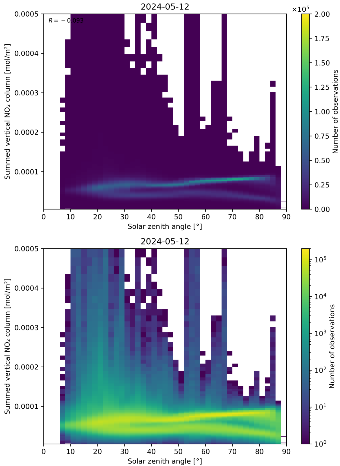
Figure 151: Scatter density plot of “Solar zenith angle” against “Summed vertical NO 2 column” for 2024-05-12 to 2024-05-13.
