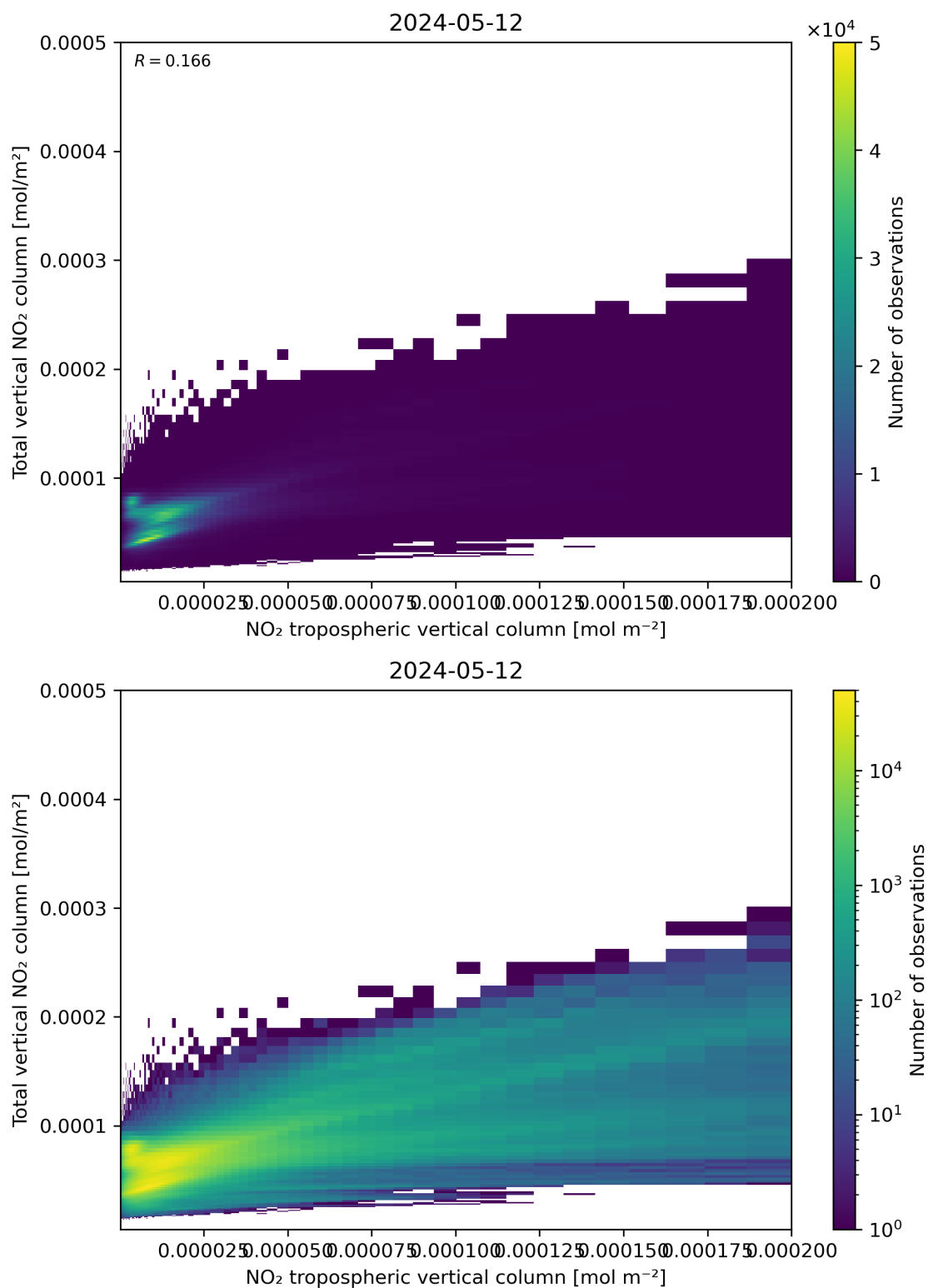
Figure 128: Scatter density plot of “NO 2 tropospheric vertical column” against “Total vertical NO 2 column” for 2024-05-12 to 2024-05-13.
