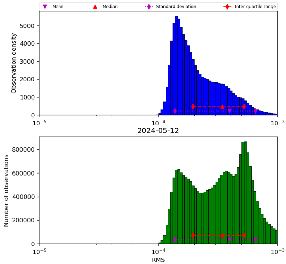
Figure 43: Histogram of “RMS” for 2024-05-12 to 2024-05-13
