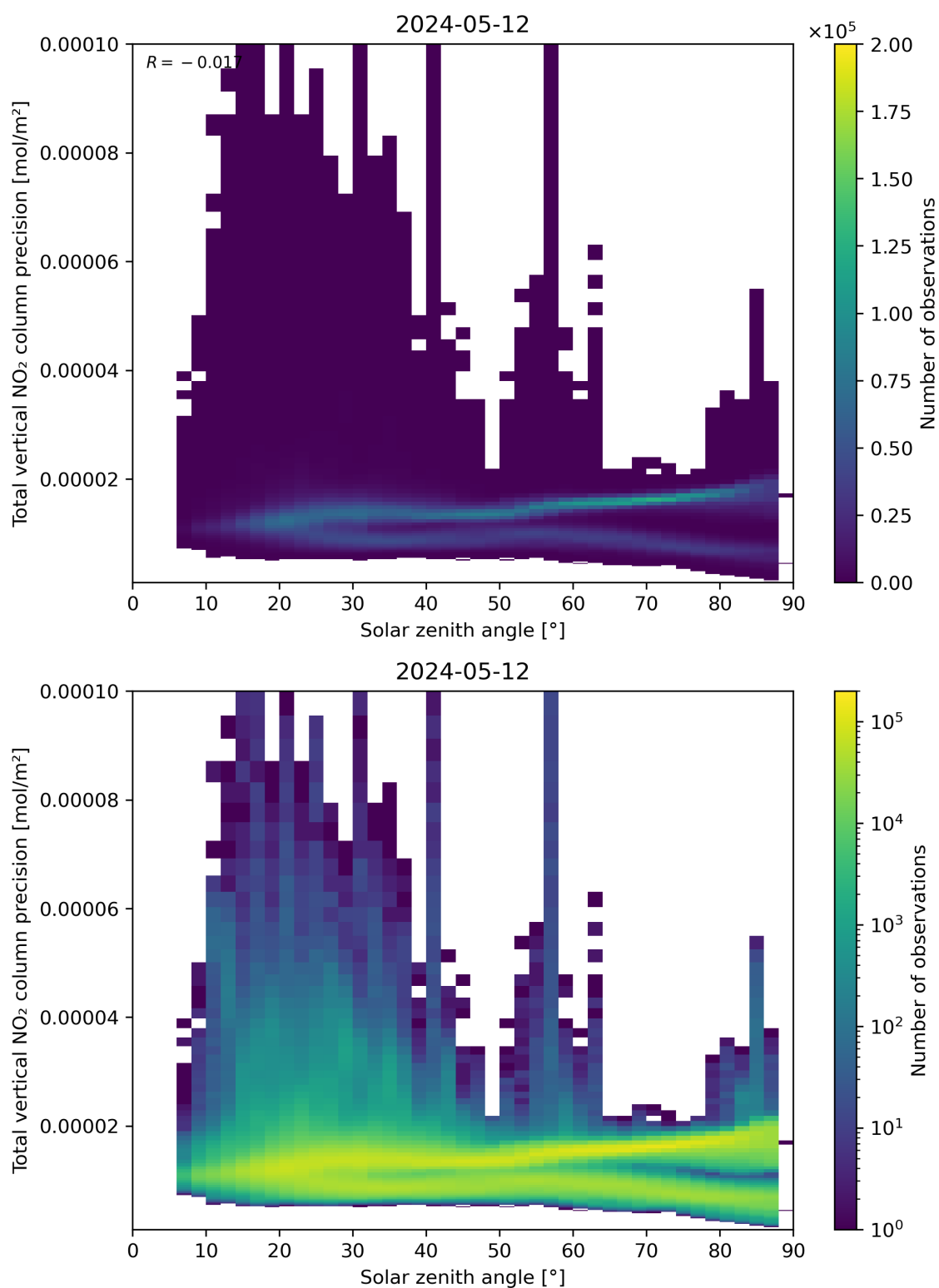
Figure 154: Scatter density plot of “Solar zenith angle” against “Total vertical NO 2 column precision” for 2024-05-12 to 2024-05-13.
