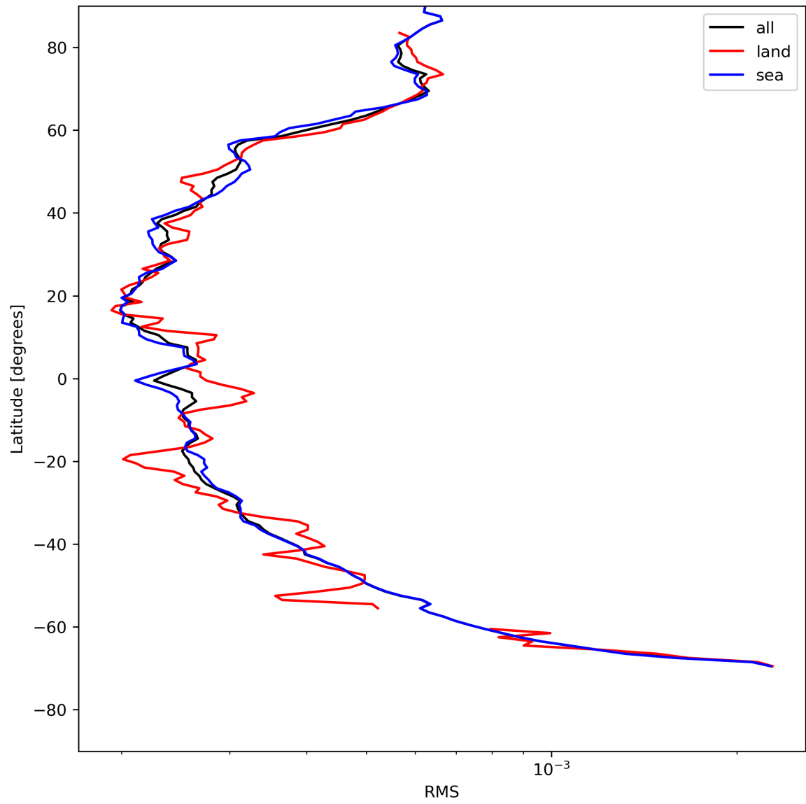
Figure 26: Zonal average of “RMS” for 2024-05-12 to 2024-05-13.
