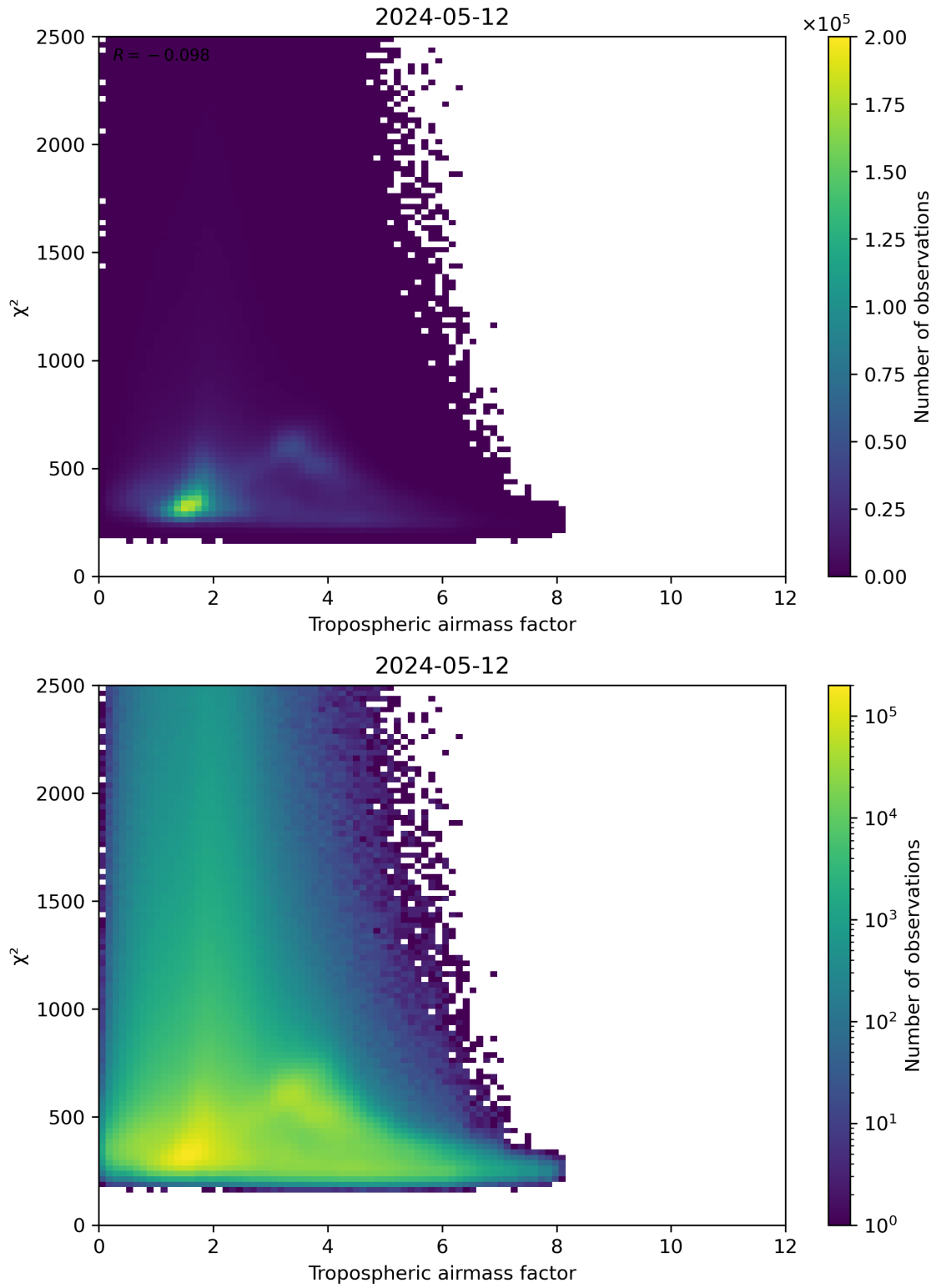
Figure 73: Scatter density plot of “Tropospheric airmass factor” against “ \chi^2 ” for 2024-05-12 to 2024-05-13.
