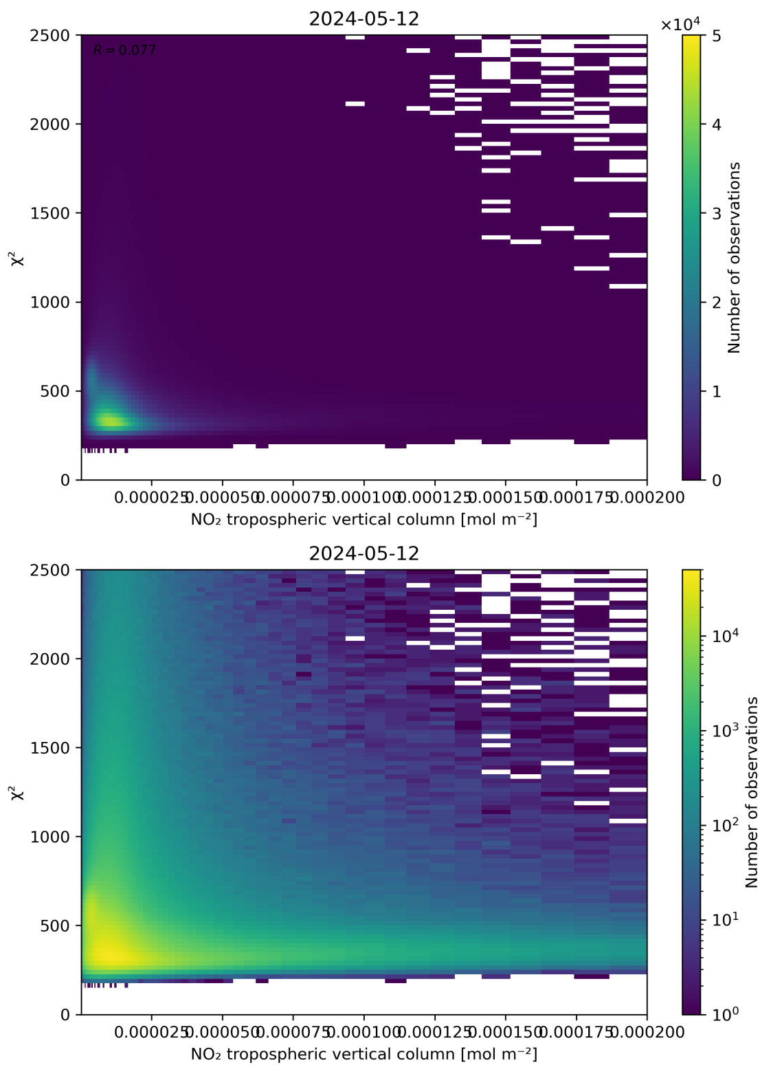
Figure 124: Scatter density plot of “NO 2 tropospheric vertical column” against “ \chi^2 ” for 2024-05-12 to 2024-05-13.
