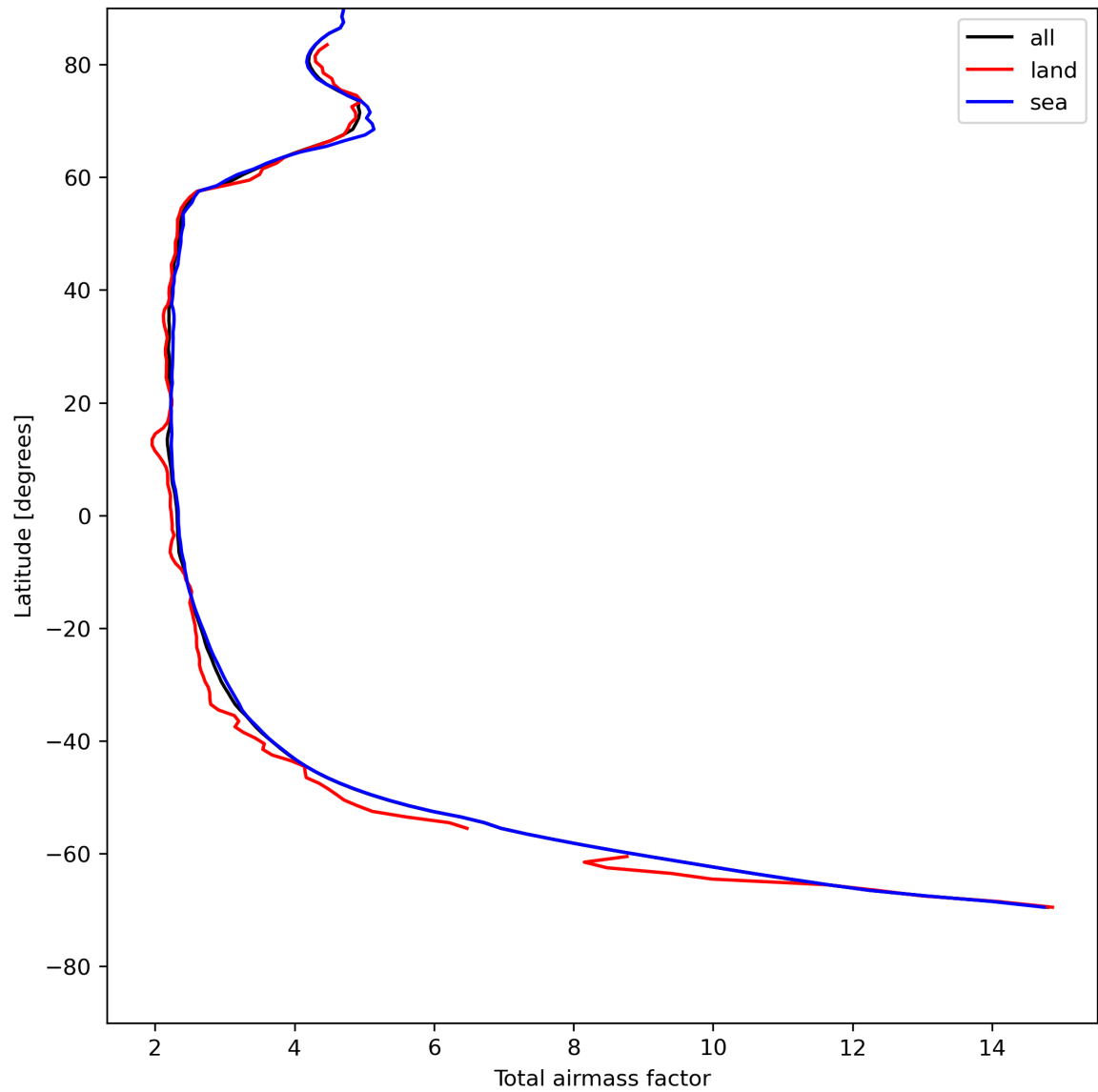
Figure 15: Zonal average of “Total airmass factor” for 2024-05-12 to 2024-05-13.
