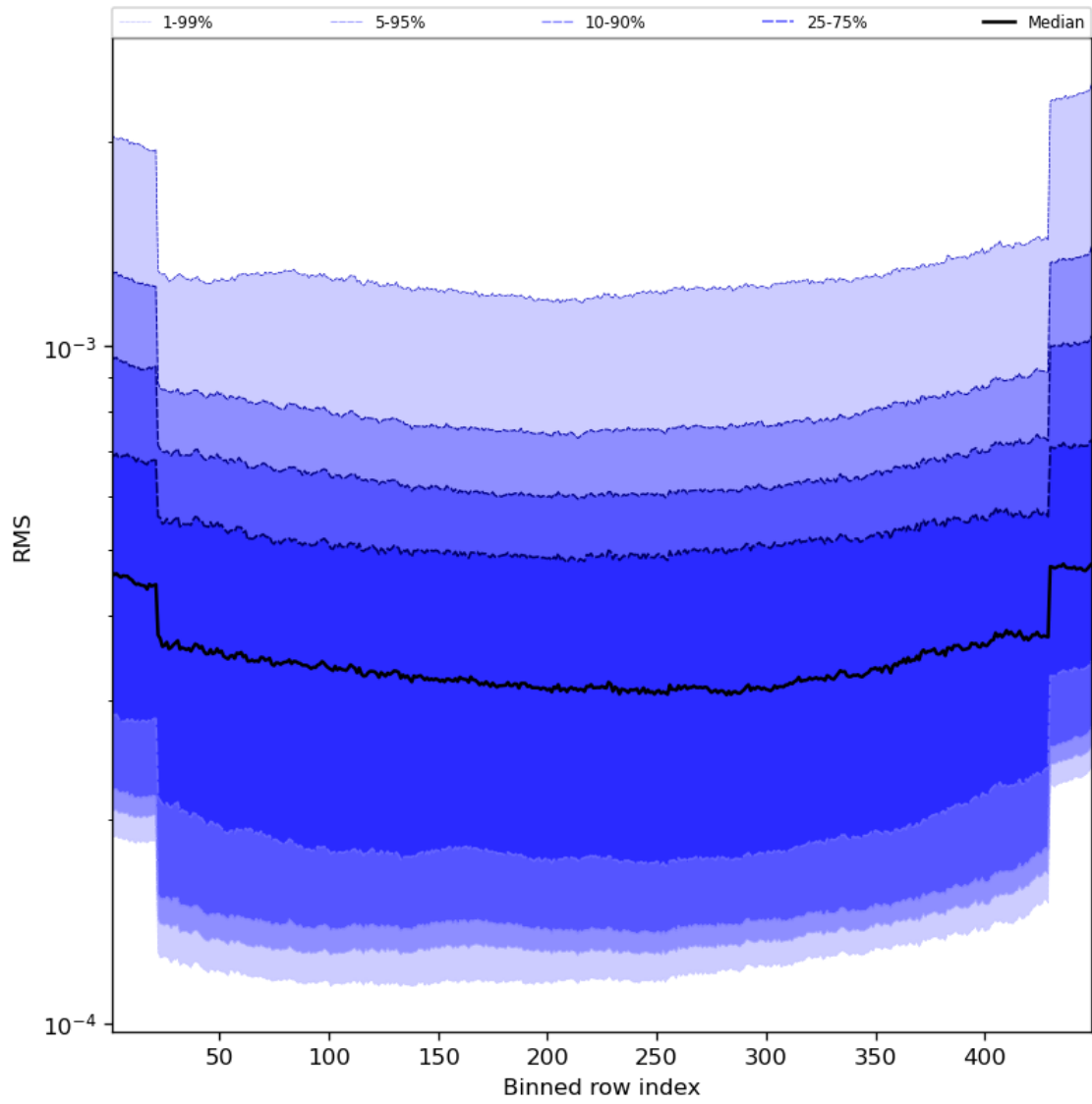
Figure 60: Along track statistics of “RMS” for 2024-05-12 to 2024-05-13
