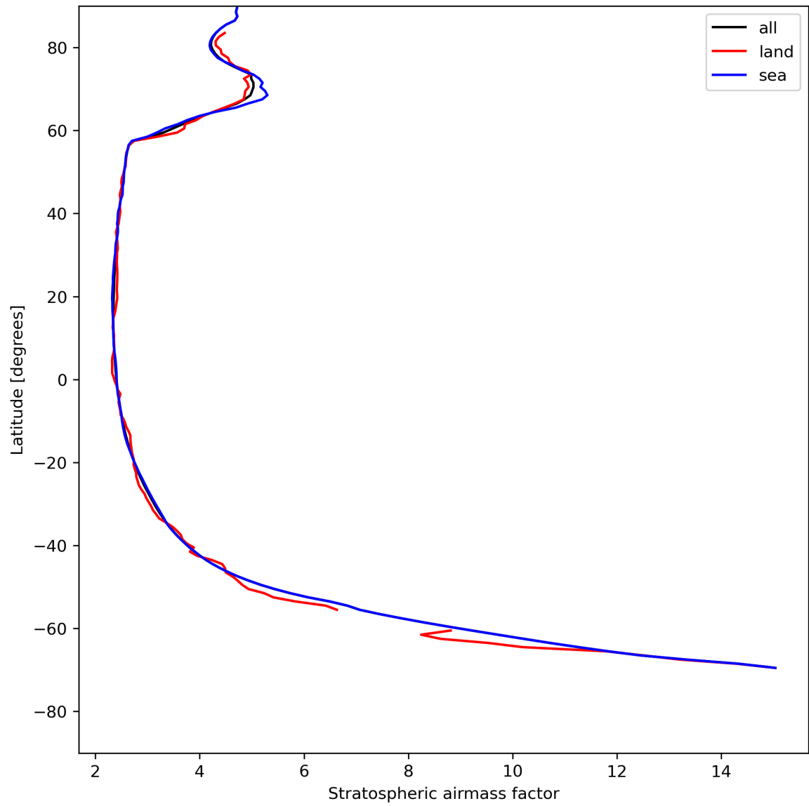
Figure 27: Zonal average of “Stratospheric air mass factor” for 2024-05-12 to 2024-05-13.
