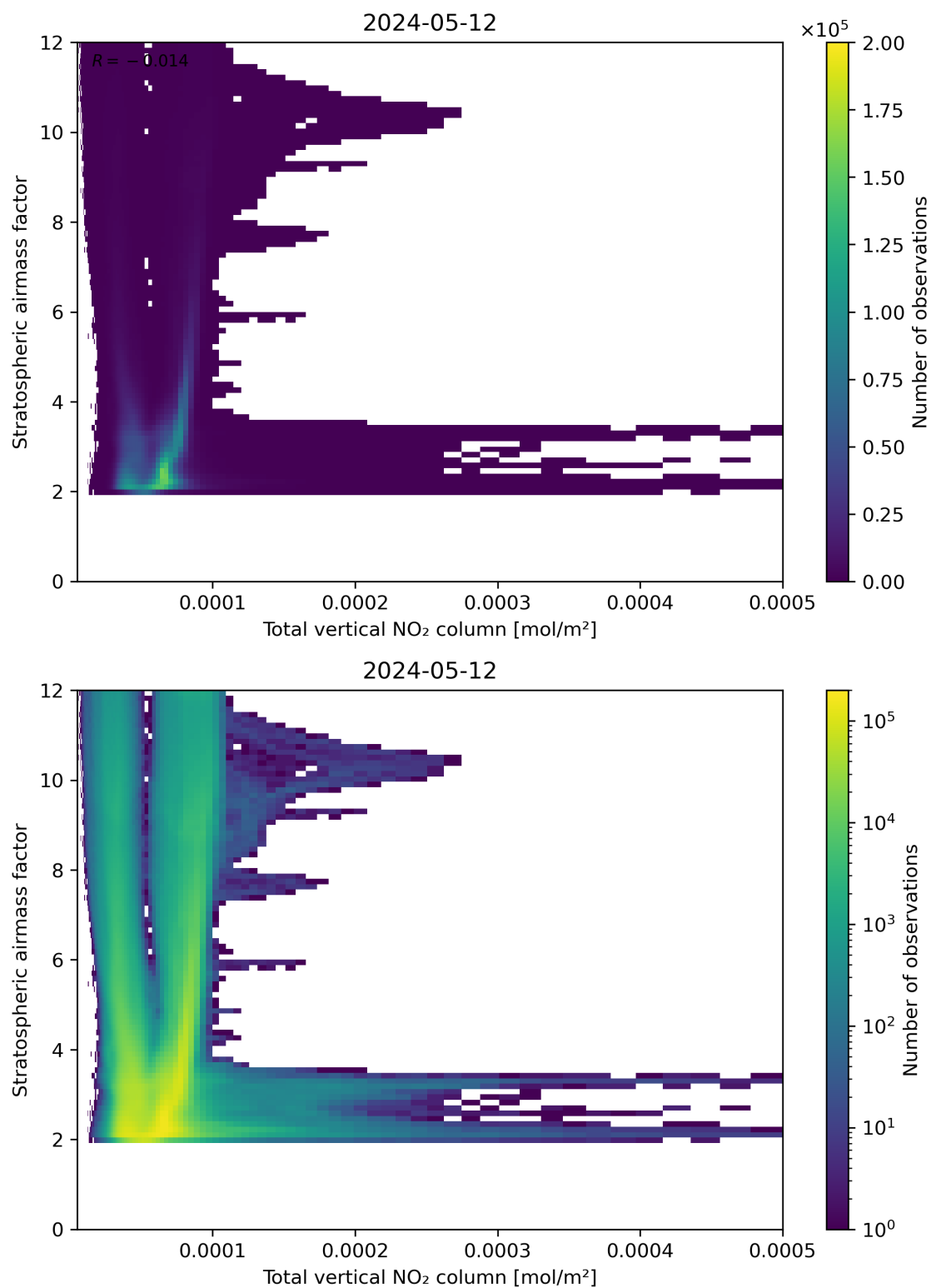
Figure 110: Scatter density plot of “Total vertical NO 2 column” against “Stratospheric airmass factor” for 2024-05-12 to 2024-05-13.
