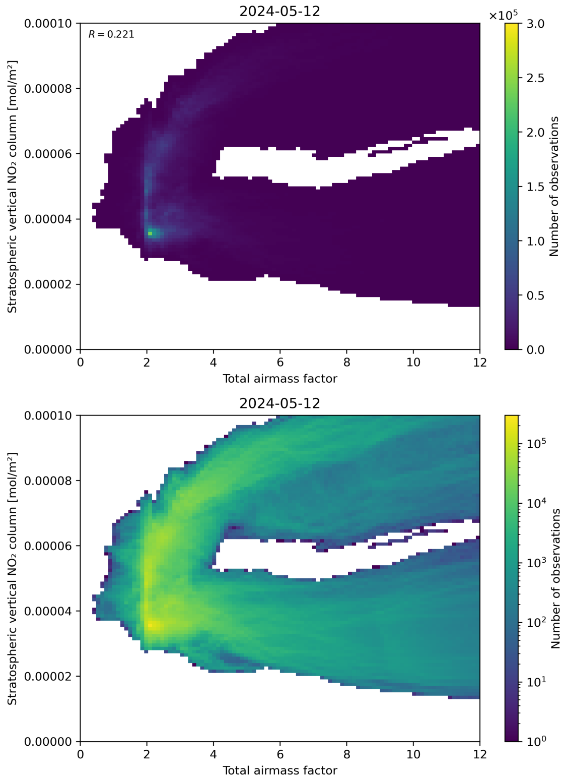
Figure 64: Scatter density plot of “Total airmass factor” against “Stratospheric vertical \text{NO}_2 column” for 2024-05-12 to 2024-05-13.
