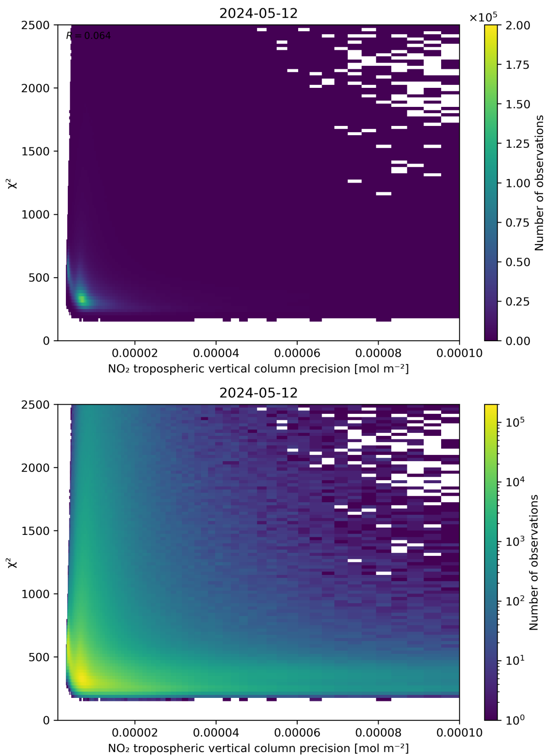
Figure 134: Scatter density plot of “NO 2 tropospheric vertical column precision” against “ \chi^2 ” for 2024-05-12 to 2024-05-13.
