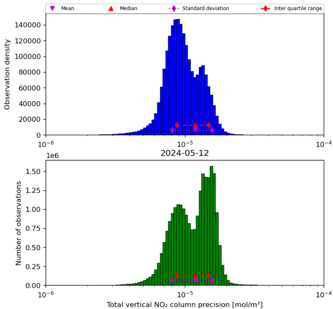
Figure 39: Histogram of “Total vertical NO 2 column precision” for 2024-05-12 to 2024-05-13
