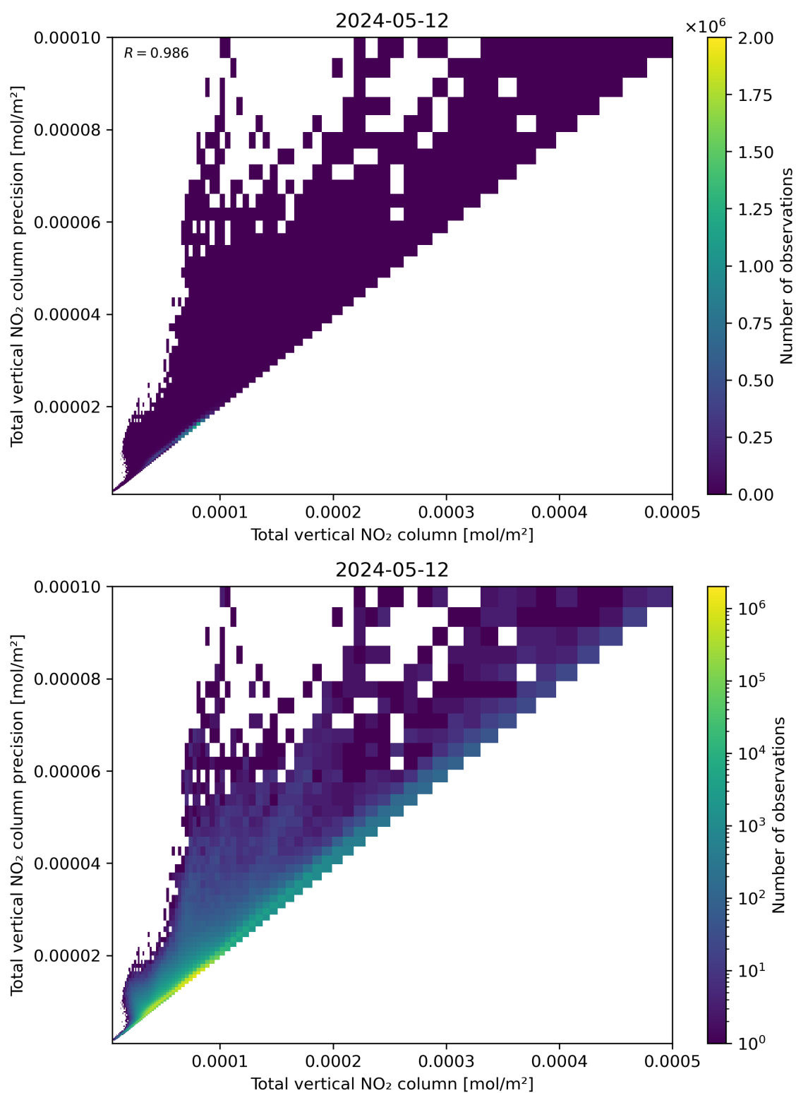
Figure 114: Scatter density plot of “Total vertical NO 2 column” against “Total vertical NO 2 column precision” for 2024-05-12 to 2024-05-13.
