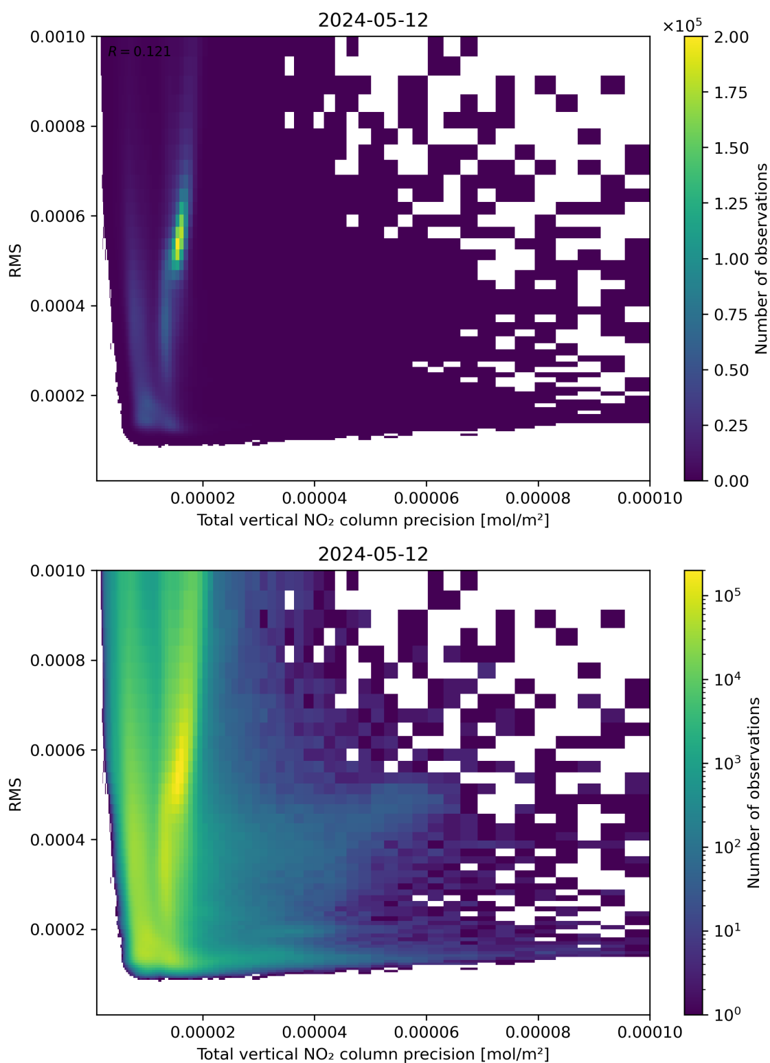
Figure 119: Scatter density plot of “Total vertical NO 2 column precision” against “RMS” for 2024-05-12 to 2024-05-13.
