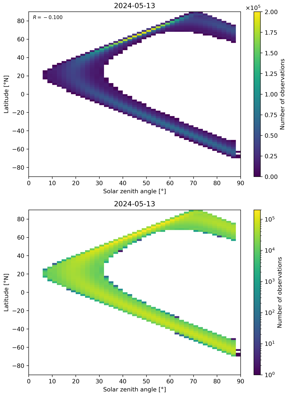
Figure 149: Scatter density plot of “Solar zenith angle” against “Latitude” for 2024-05-12 to 2024-05-14.
