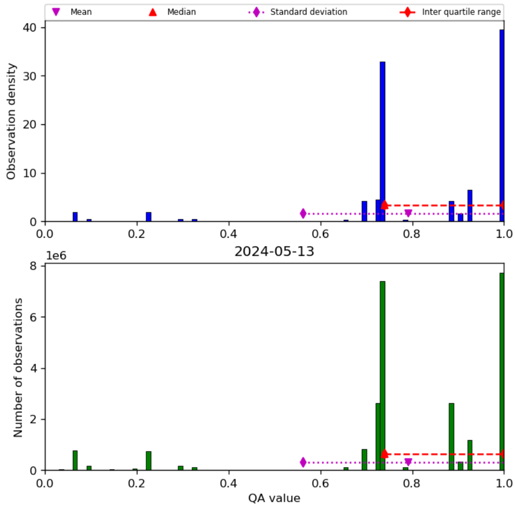
Figure 28: Histogram of “QA value” for 2024-05-12 to 2024-05-14
