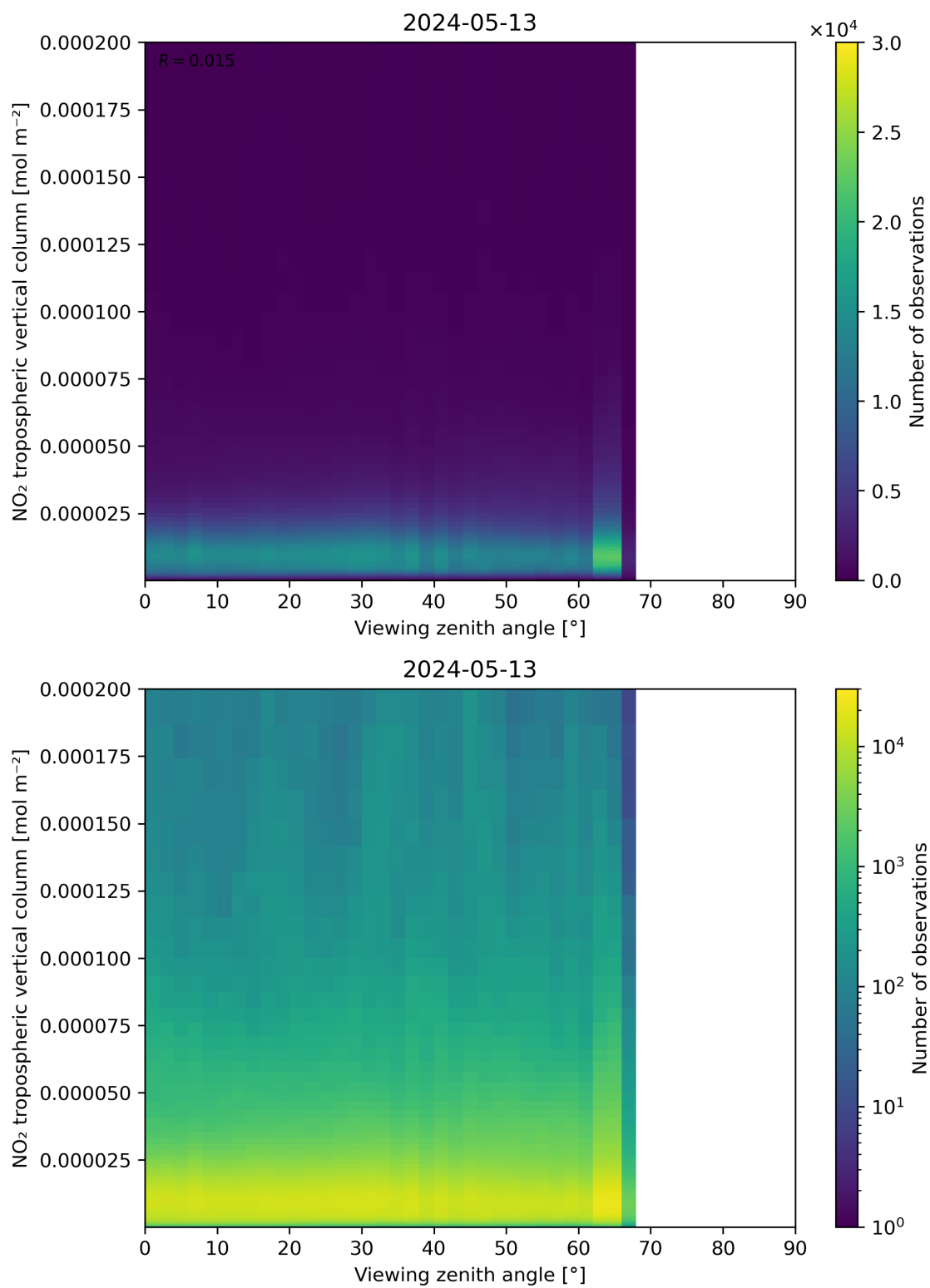
Figure 169: Scatter density plot of “Viewing zenith angle” against “NO 2 tropospheric vertical column” for 2024-05-12 to 2024-05-14.
