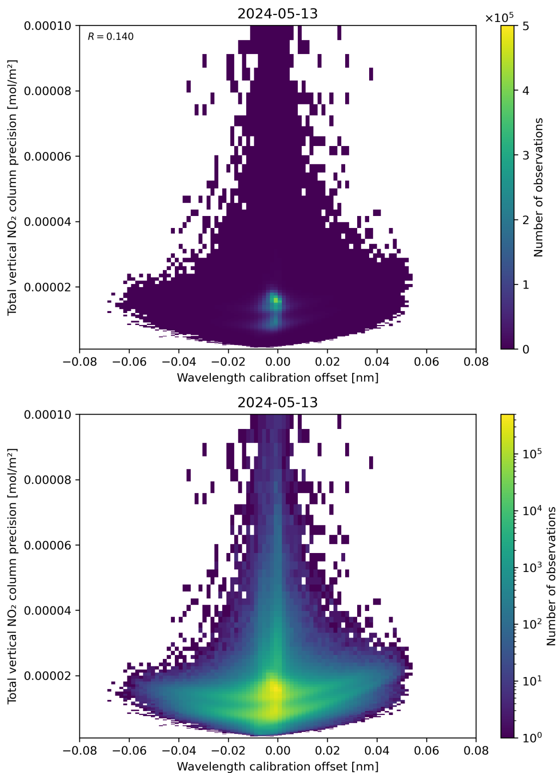
Figure 180: Scatter density plot of “Wavelength calibration offset” against “Total vertical NO 2 column precision” for 2024-05-12 to 2024-05-14.
