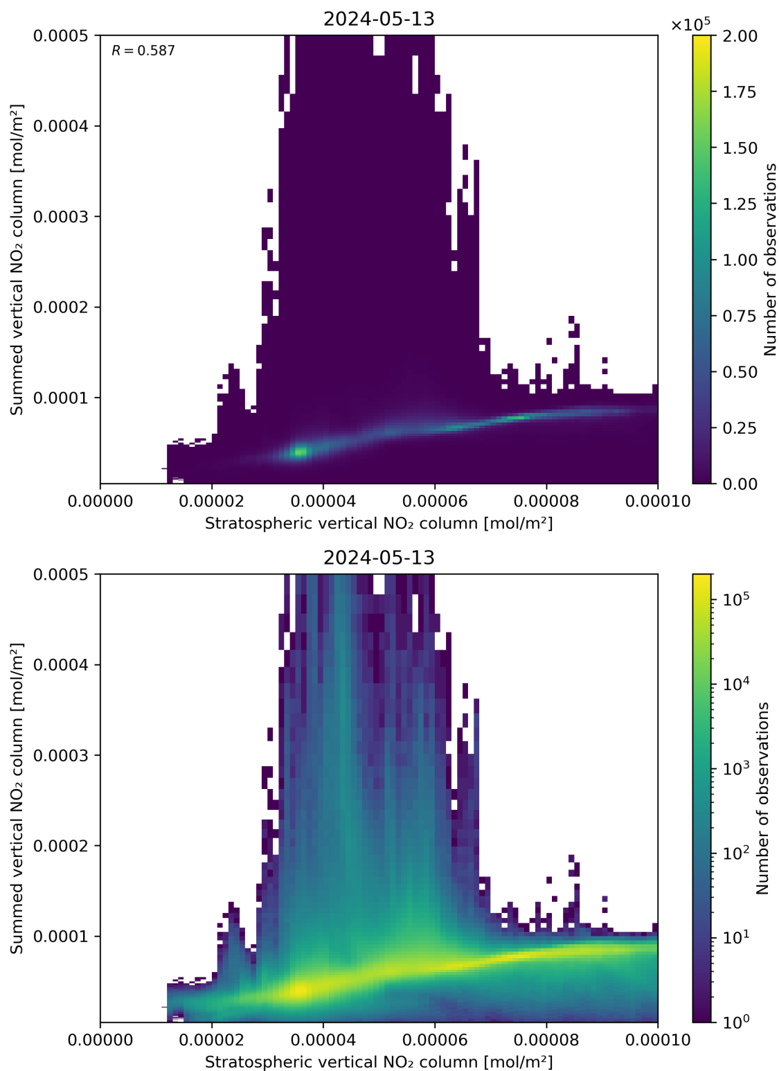
Figure 98: Scatter density plot of “Stratospheric vertical NO 2 column” against “Summed vertical NO 2 column” for 2024-05-12 to 2024-05-14.
