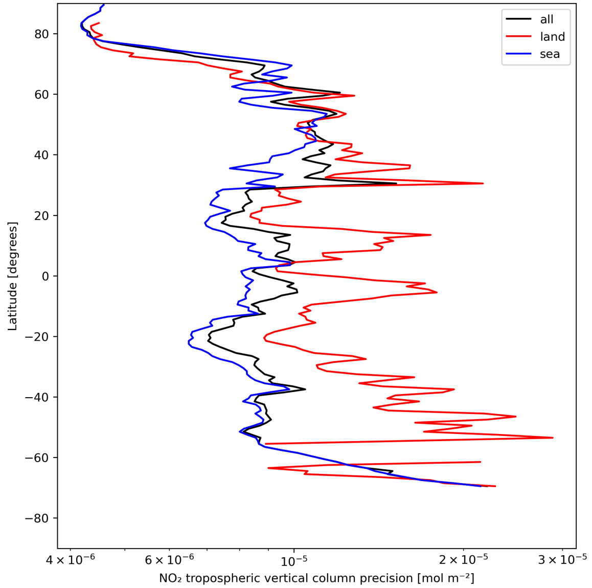
Figure 13: Zonal average of “NO 2 tropospheric vertical column precision” for 2024-05-12 to 2024-05-14.
