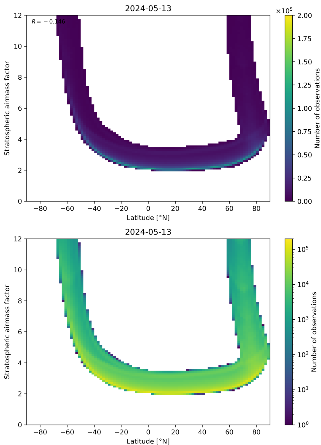
Figure 83: Scatter density plot of “Latitude” against “Stratospheric air mass factor” for 2024-05-12 to 2024-05-14.
