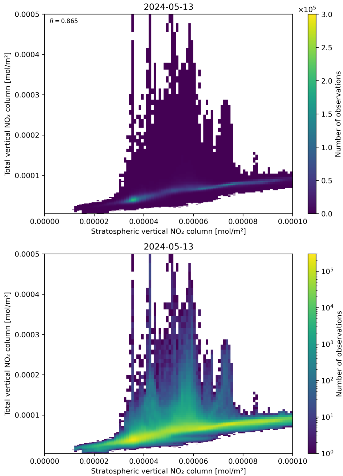
Figure 100: Scatter density plot of “Stratospheric vertical NO 2 column” against “Total vertical NO 2 column” for 2024-05-12 to 2024-05-14.
