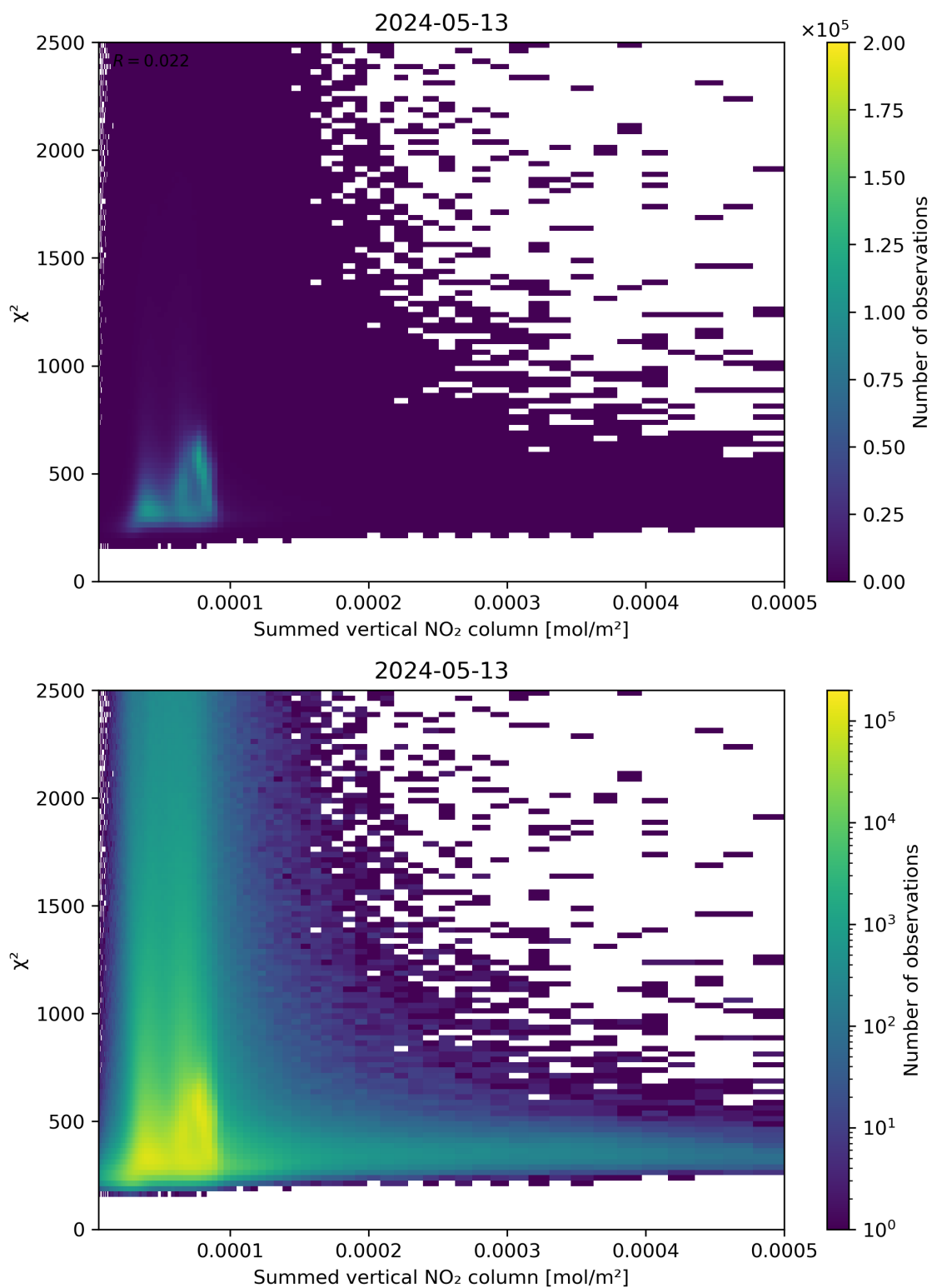
Figure 104: Scatter density plot of “Summed vertical NO 2 column” against “ \chi^2 ” for 2024-05-12 to 2024-05-14.
