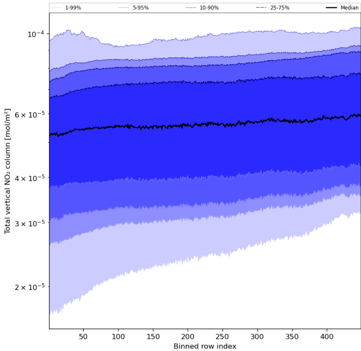
Figure 55: Along track statistics of “Total vertical NO 2 column” for 2024-05-12 to 2024-05-14
