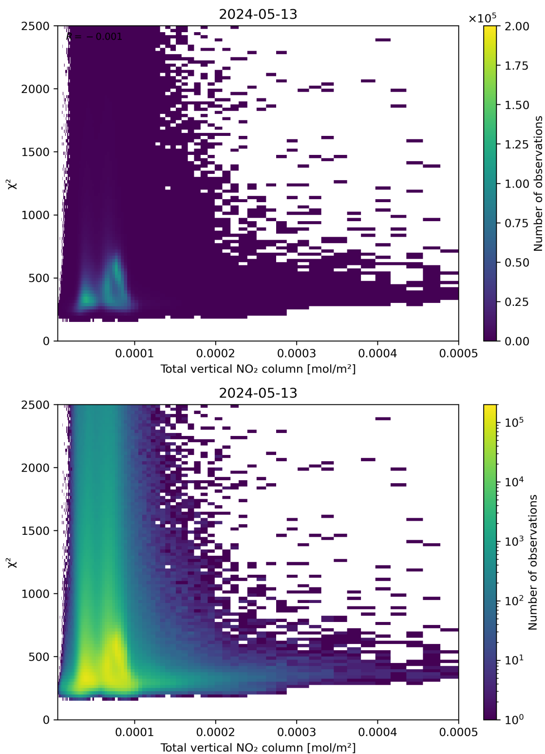
Figure 111: Scatter density plot of “Total vertical NO 2 column” against “ \chi^2 ” for 2024-05-12 to 2024-05-14.
