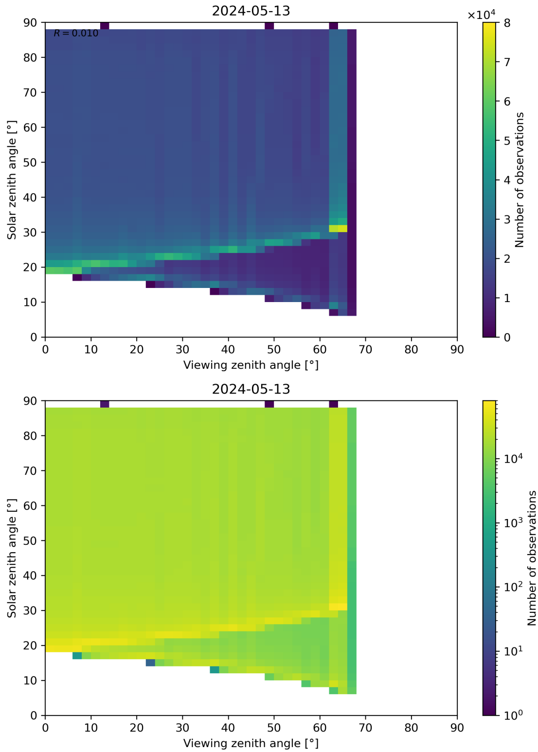
Figure 172: Scatter density plot of “Viewing zenith angle” against “Solar zenith angle” for 2024-05-12 to 2024-05-14.
