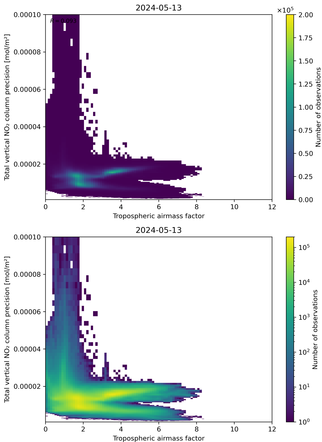
Figure 78: Scatter density plot of “Tropospheric air mass factor” against “Total vertical NO 2 column precision” for 2024-05-12 to 2024-05-14.
