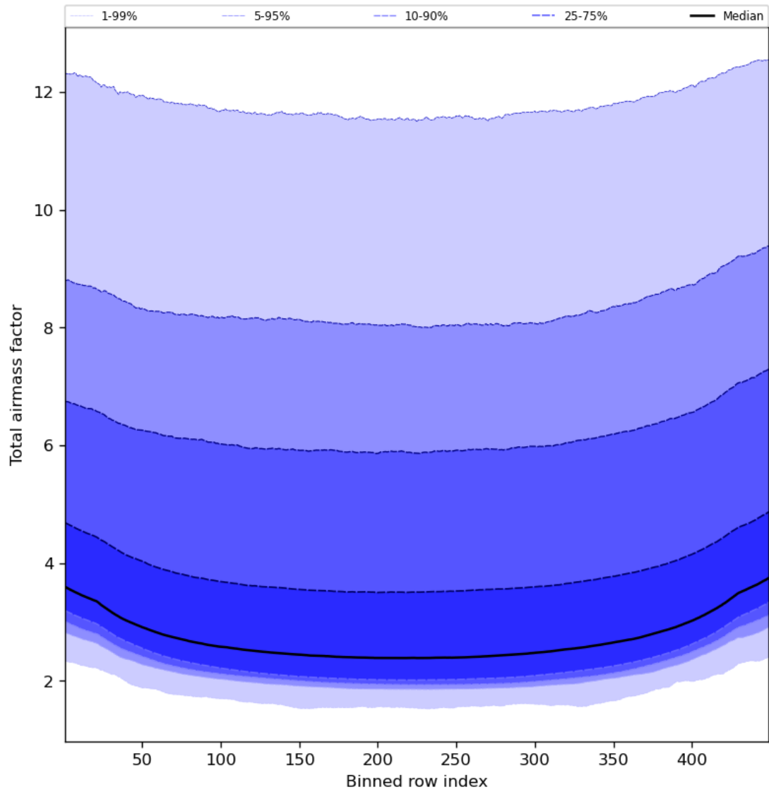
Figure 49: Along track statistics of “Total airmass factor” for 2024-05-12 to 2024-05-14
