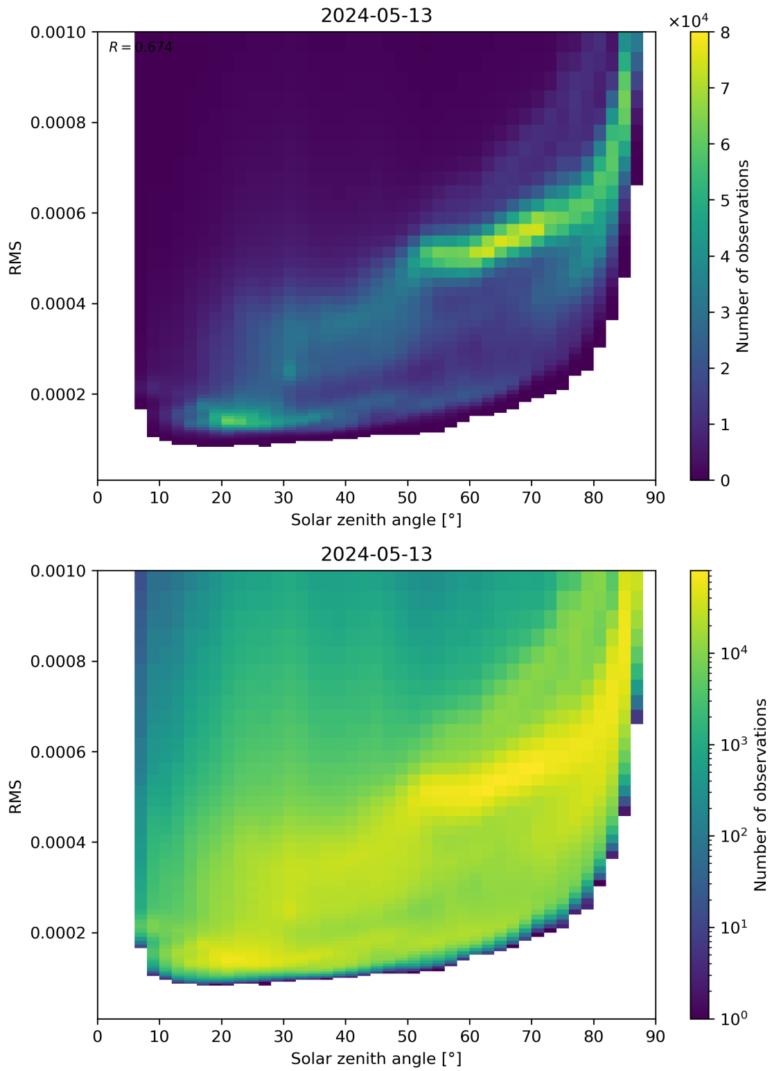
Figure 157: Scatter density plot of “Solar zenith angle” against “RMS” for 2024-05-12 to 2024-05-14.
