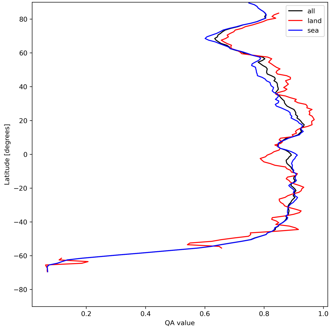
Figure 11: Zonal average of “QA value” for 2024-05-12 to 2024-05-14.
