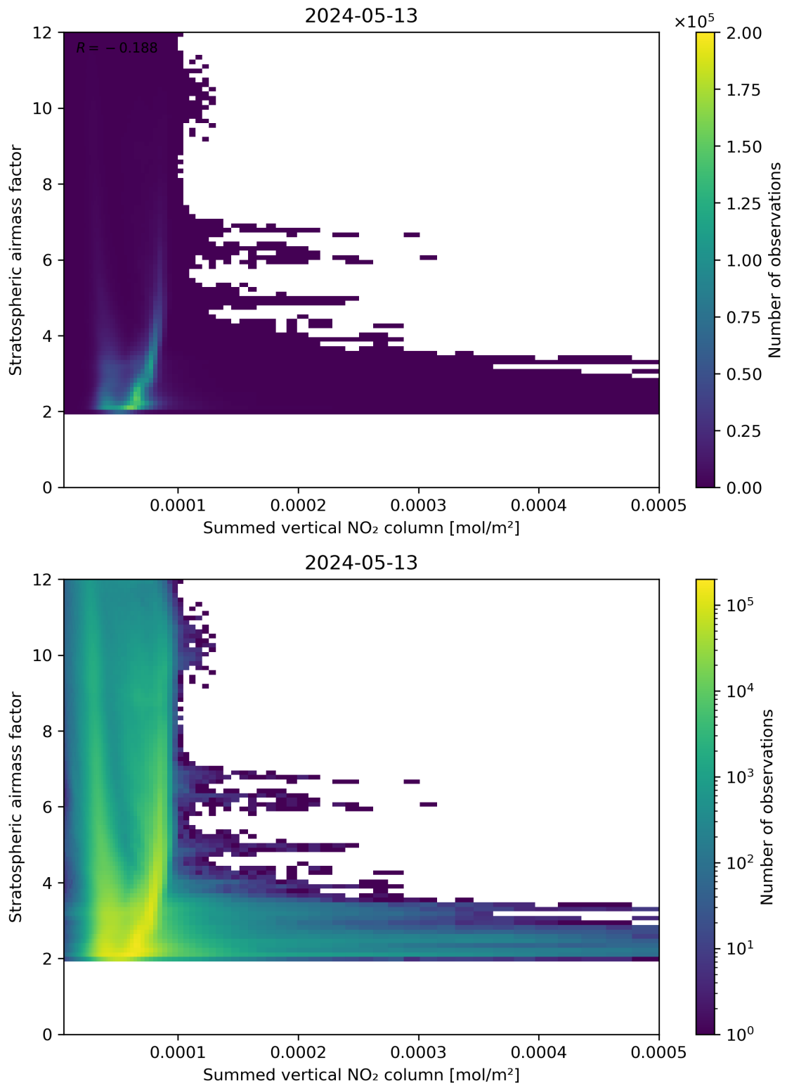
Figure 103: Scatter density plot of “Summed vertical NO 2 column” against “Stratospheric air mass factor” for 2024-05-12 to 2024-05-14.
