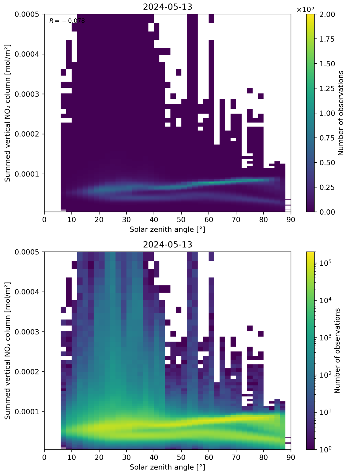
Figure 151: Scatter density plot of “Solar zenith angle” against “Summed vertical NO 2 column” for 2024-05-12 to 2024-05-14.
