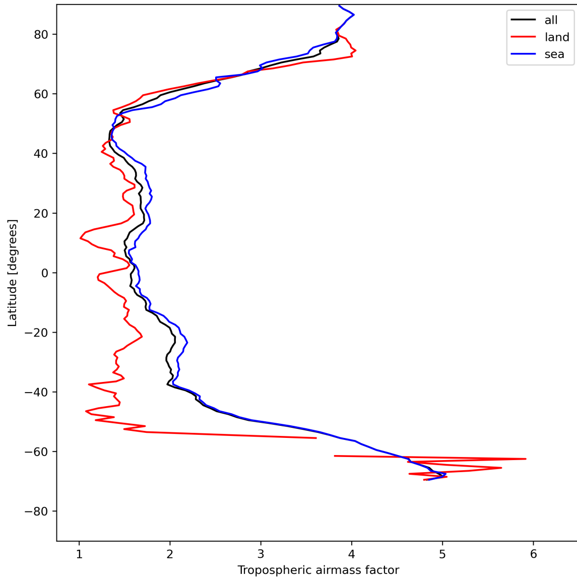
Figure 14: Zonal average of “Tropospheric airmass factor” for 2024-05-12 to 2024-05-14.
