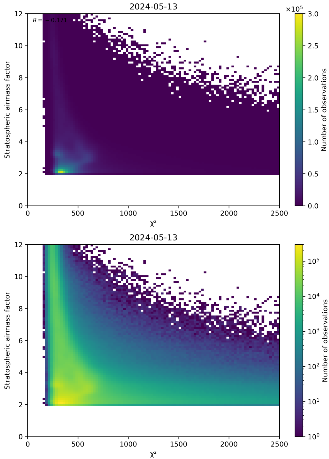
Figure 81: Scatter density plot of “ \chi^2 ” against “Stratospheric airmass factor” for 2024-05-12 to 2024-05-14.
