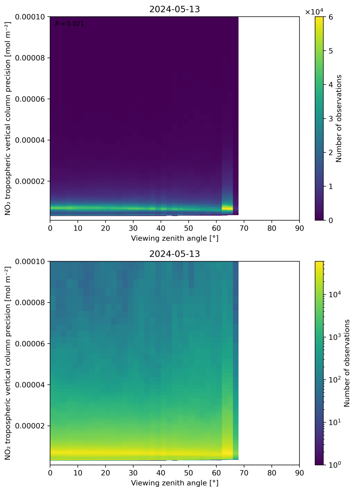
Figure 170: Scatter density plot of “Viewing zenith angle” against “NO 2 tropospheric vertical column precision” for 2024-05-12 to 2024-05-14.
