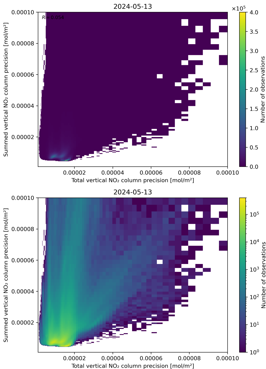
Figure 118: Scatter density plot of “Total vertical NO 2 column precision” against “Summed vertical NO 2 column precision” for 2024-05-12 to 2024-05-14.
