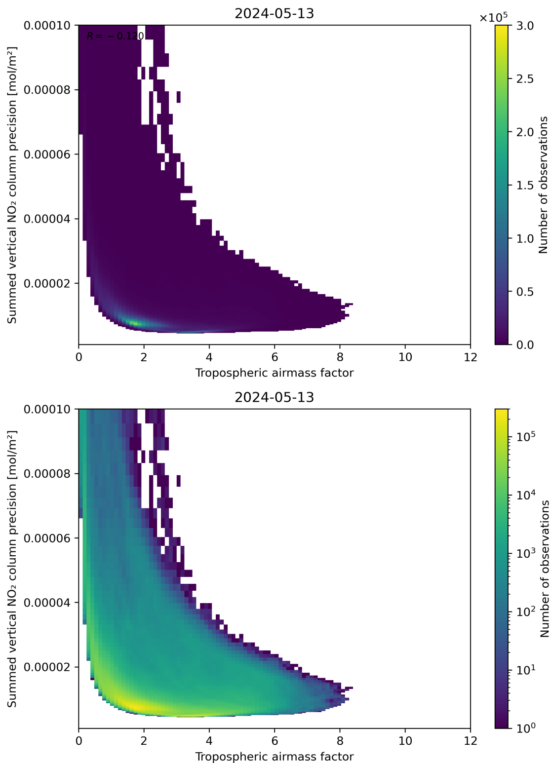
Figure 76: Scatter density plot of “Tropospheric air mass factor” against “Summed vertical NO 2 column precision” for 2024-05-12 to 2024-05-14.
