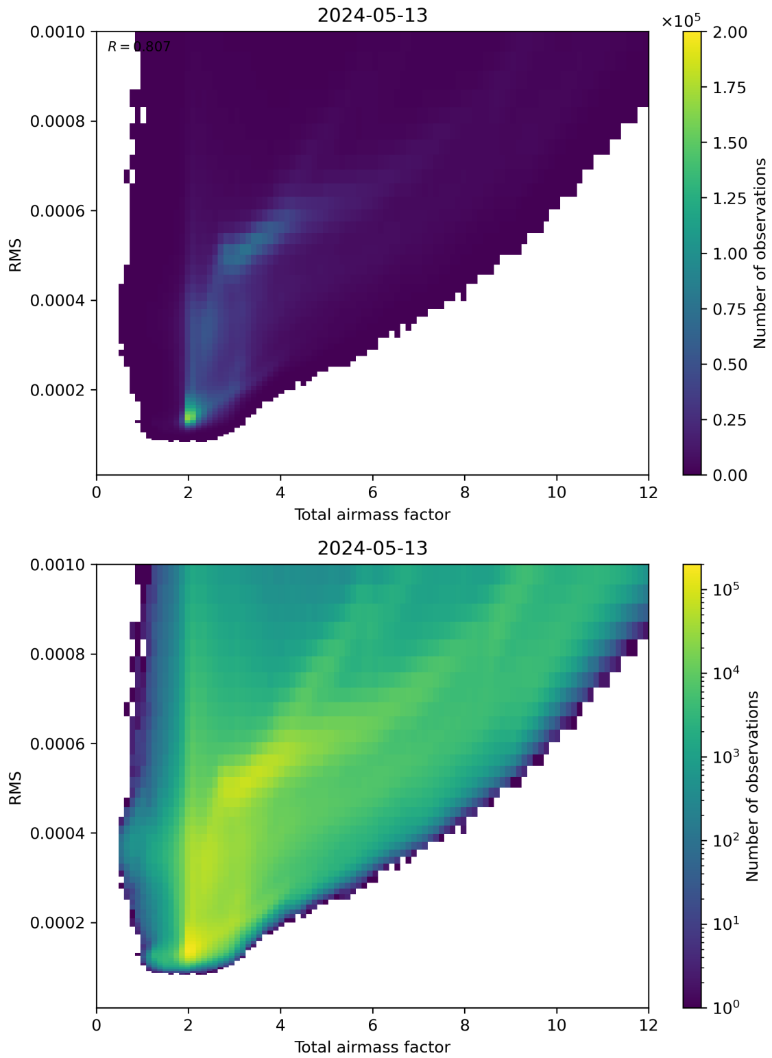
Figure 69: Scatter density plot of “Total airmass factor” against “RMS” for 2024-05-12 to 2024-05-14.
