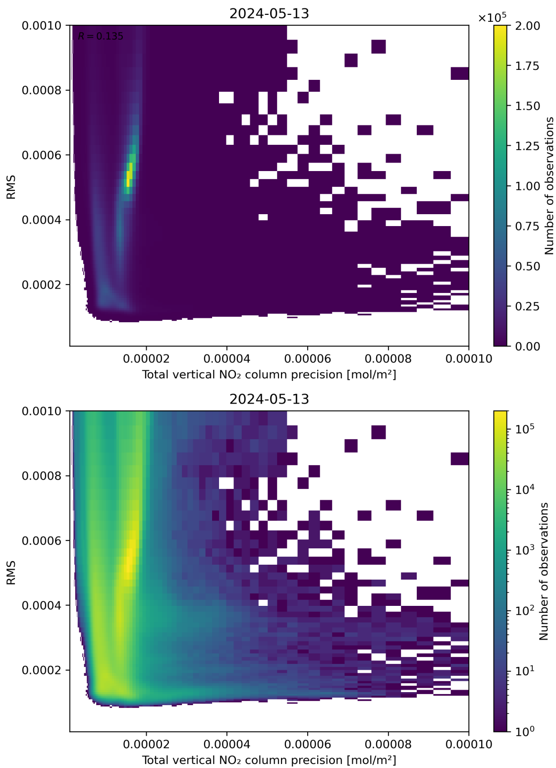
Figure 119: Scatter density plot of “Total vertical NO 2 column precision” against “RMS” for 2024-05-12 to 2024-05-14.
