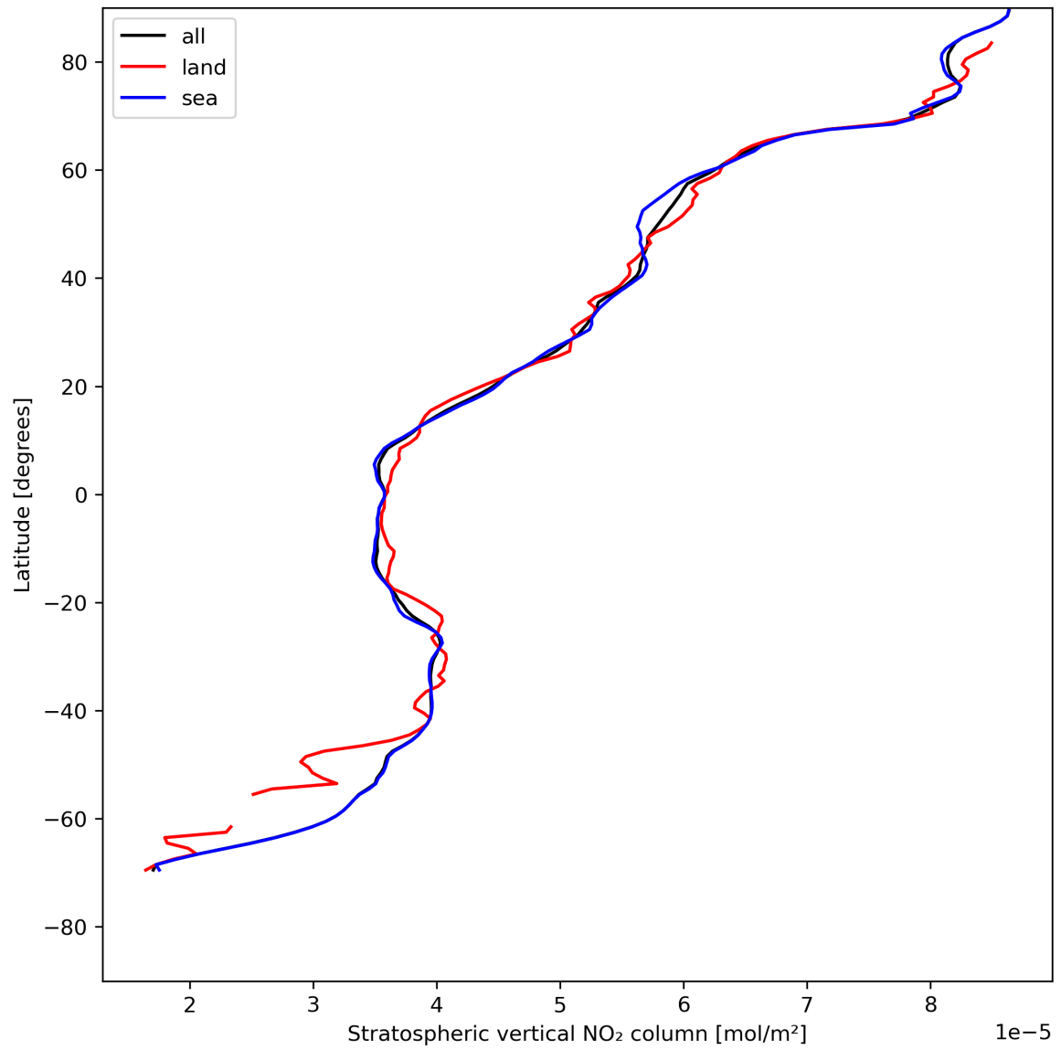
Figure 19: Zonal average of “Stratospheric vertical NO 2 column” for 2024-05-12 to 2024-05-14.
