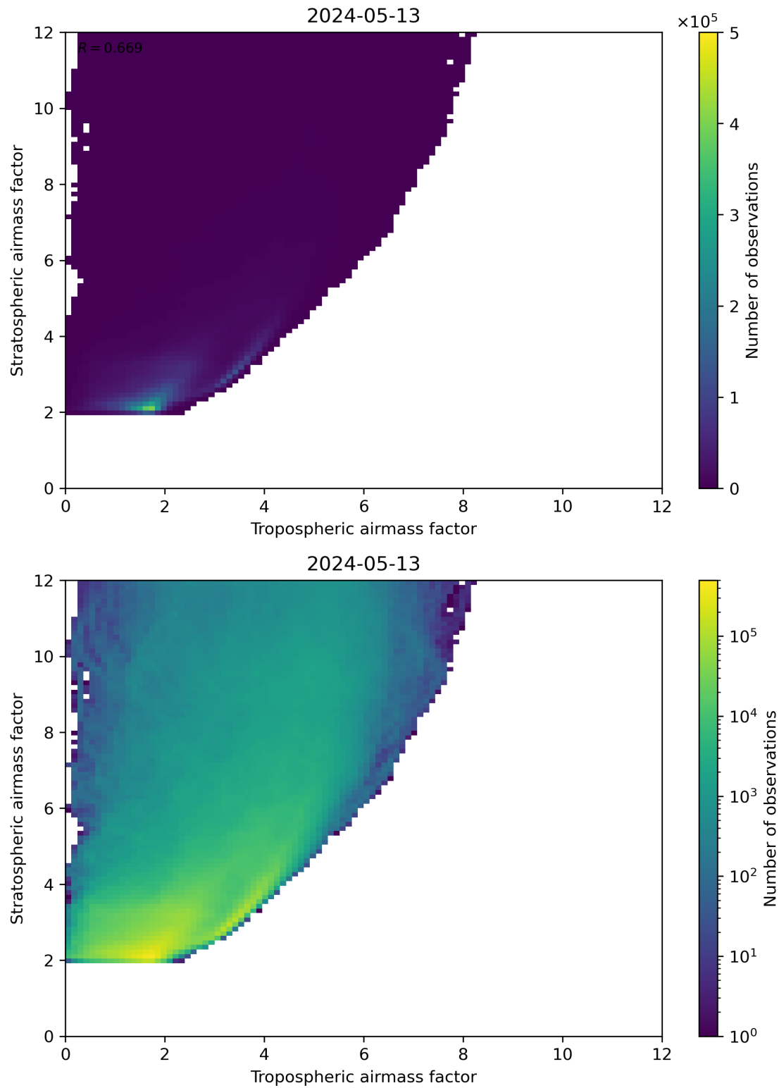
Figure 71: Scatter density plot of “Tropospheric airmass factor” against “Stratospheric airmass factor” for 2024-05-12 to 2024-05-14.
