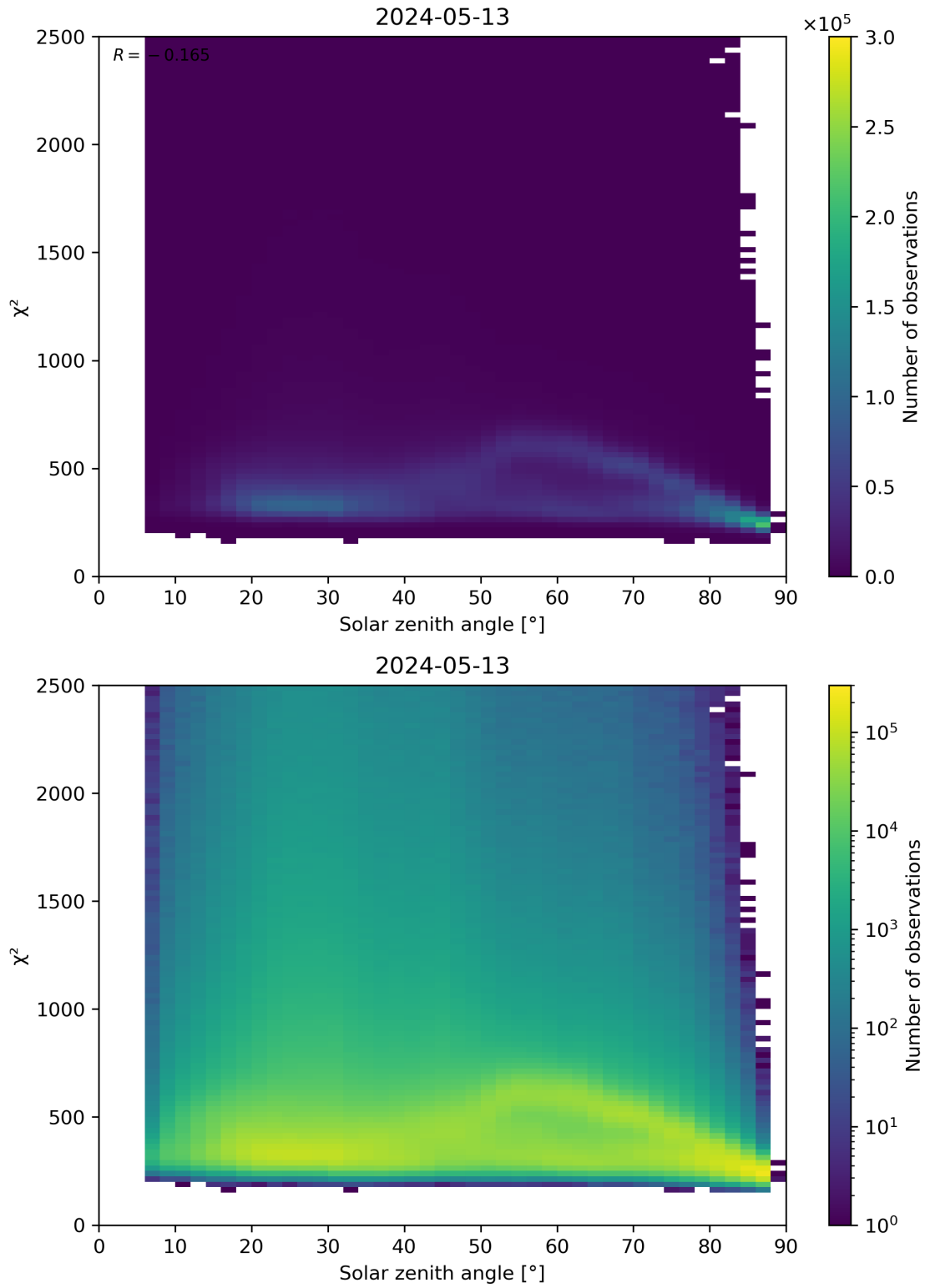
Figure 148: Scatter density plot of “Solar zenith angle” against “ \chi^2 ” for 2024-05-12 to 2024-05-14.
