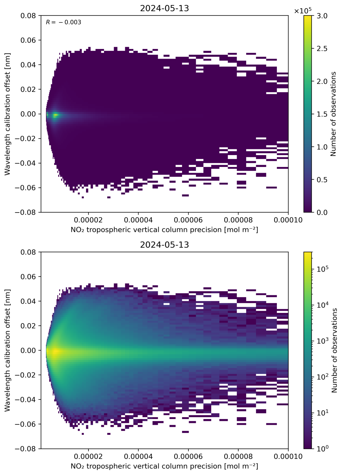
Figure 141: Scatter density plot of “NO 2 tropospheric vertical column precision” against “Wavelength calibration offset” for 2024-05-12 to 2024-05-14.
