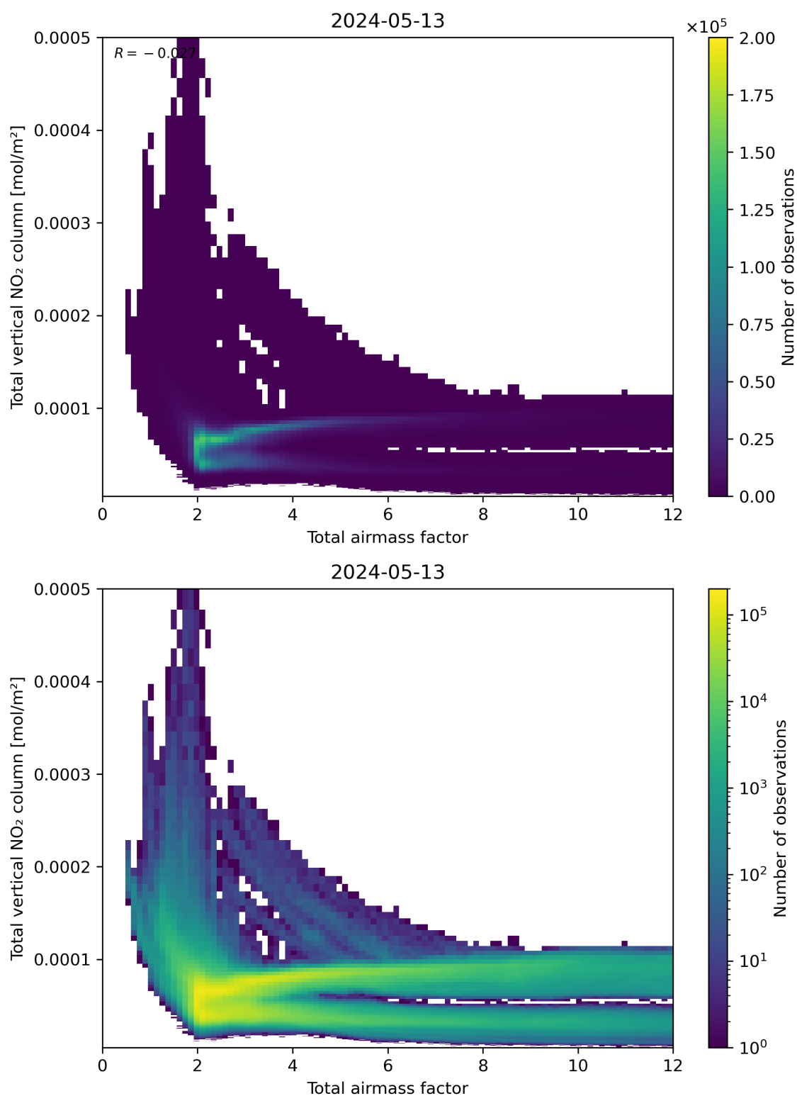
Figure 67: Scatter density plot of “Total airmass factor” against “Total vertical NO 2 column” for 2024-05-12 to 2024-05-14.
