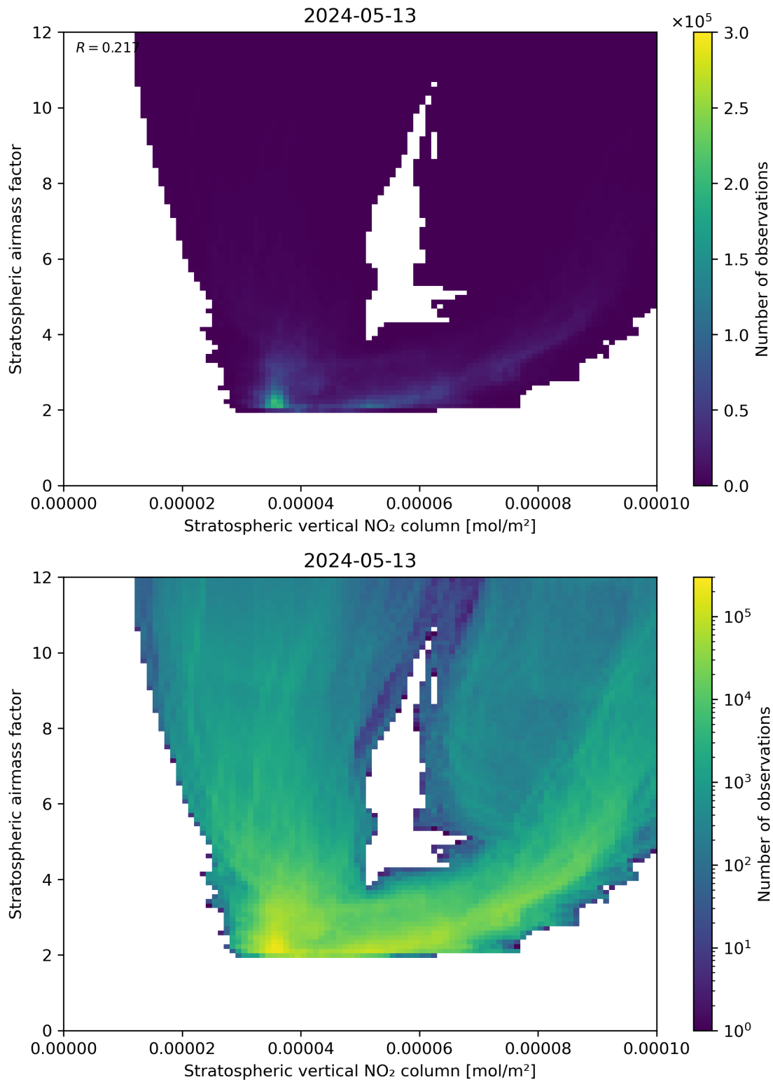
Figure 96: Scatter density plot of “Stratospheric vertical NO 2 column” against “Stratospheric airmass factor” for 2024-05-12 to 2024-05-14.
