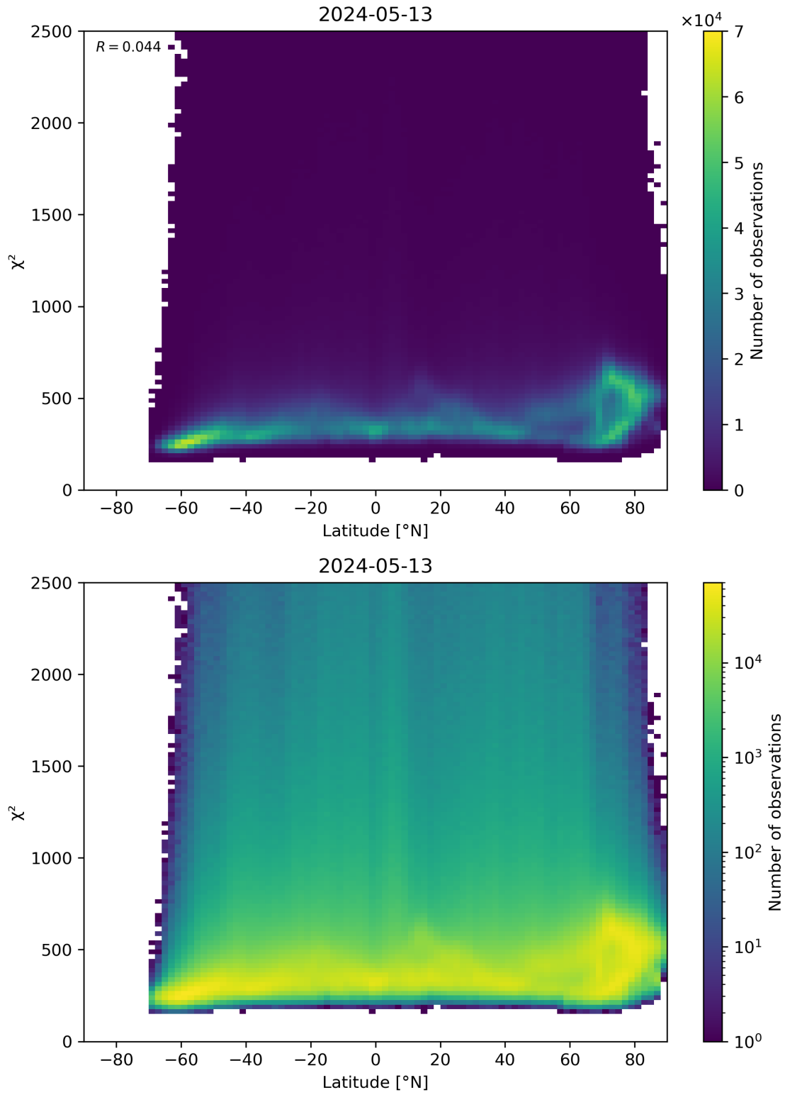
Figure 86: Scatter density plot of “Latitude” against “ \chi^2 ” for 2024-05-12 to 2024-05-14.
