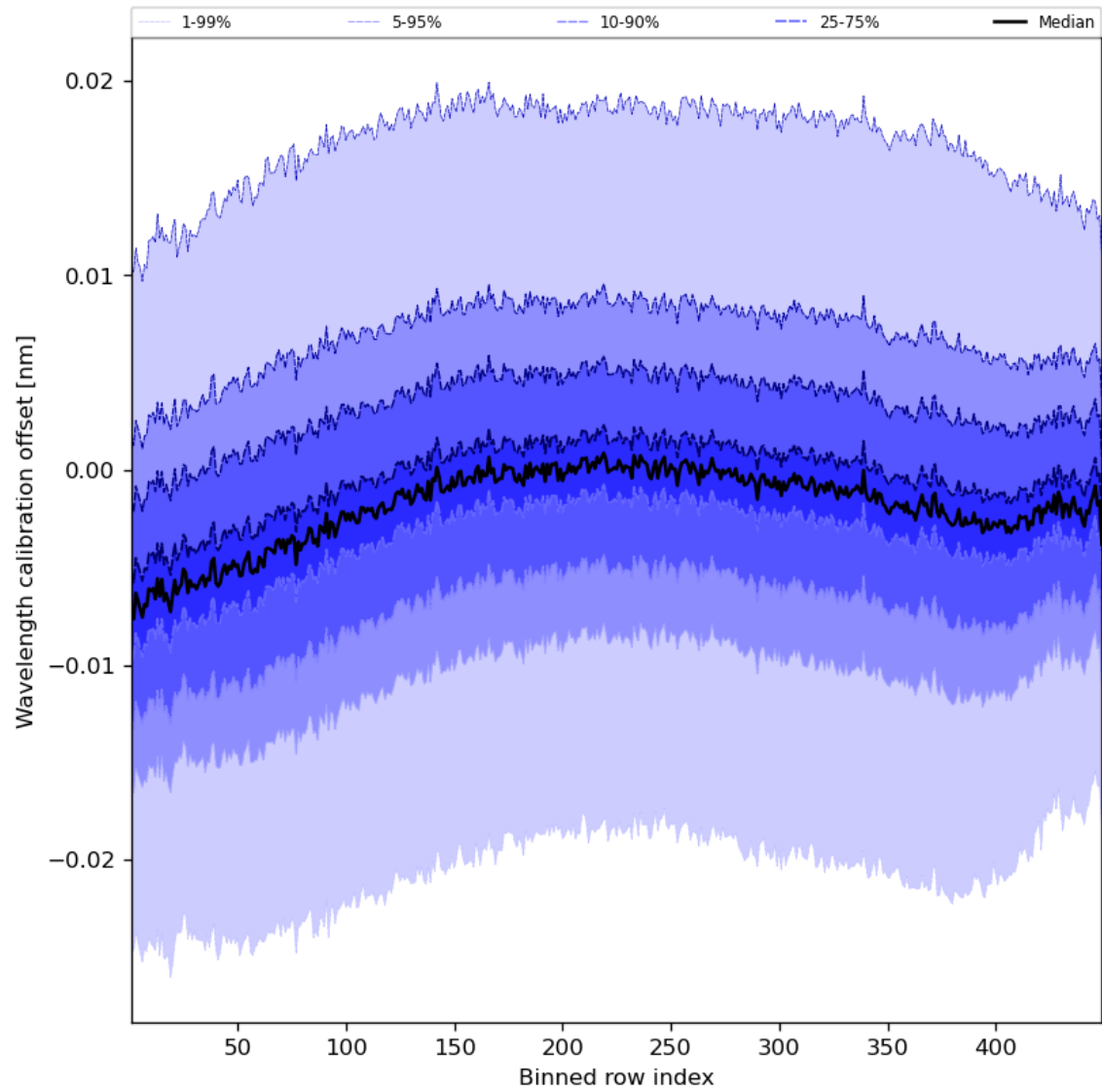
Figure 52: Along track statistics of “Wavelength calibration offset” for 2024-05-12 to 2024-05-14
