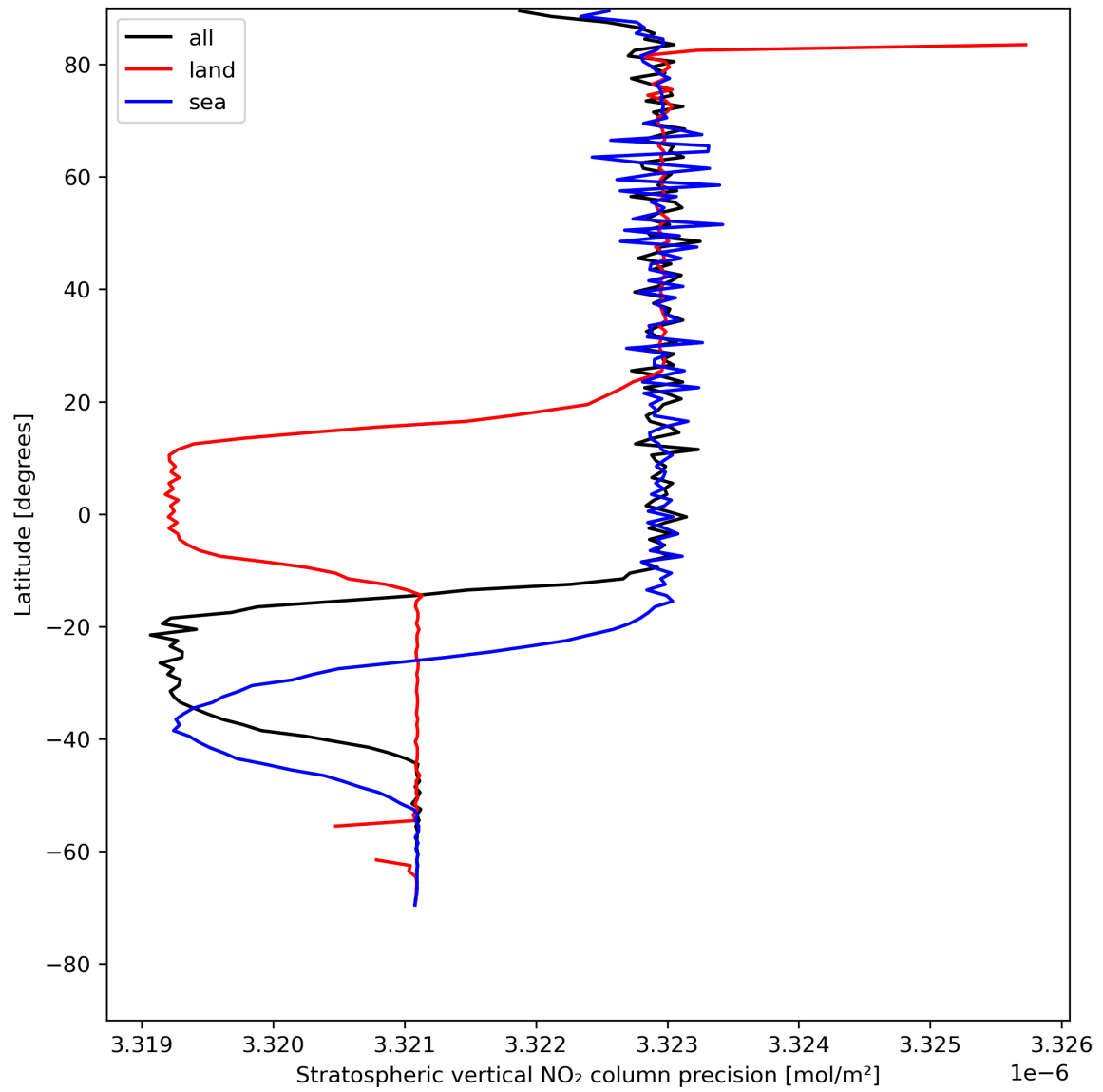
Figure 20: Zonal average of “Stratospheric vertical NO 2 column precision” for 2024-05-12 to 2024-05-14.
