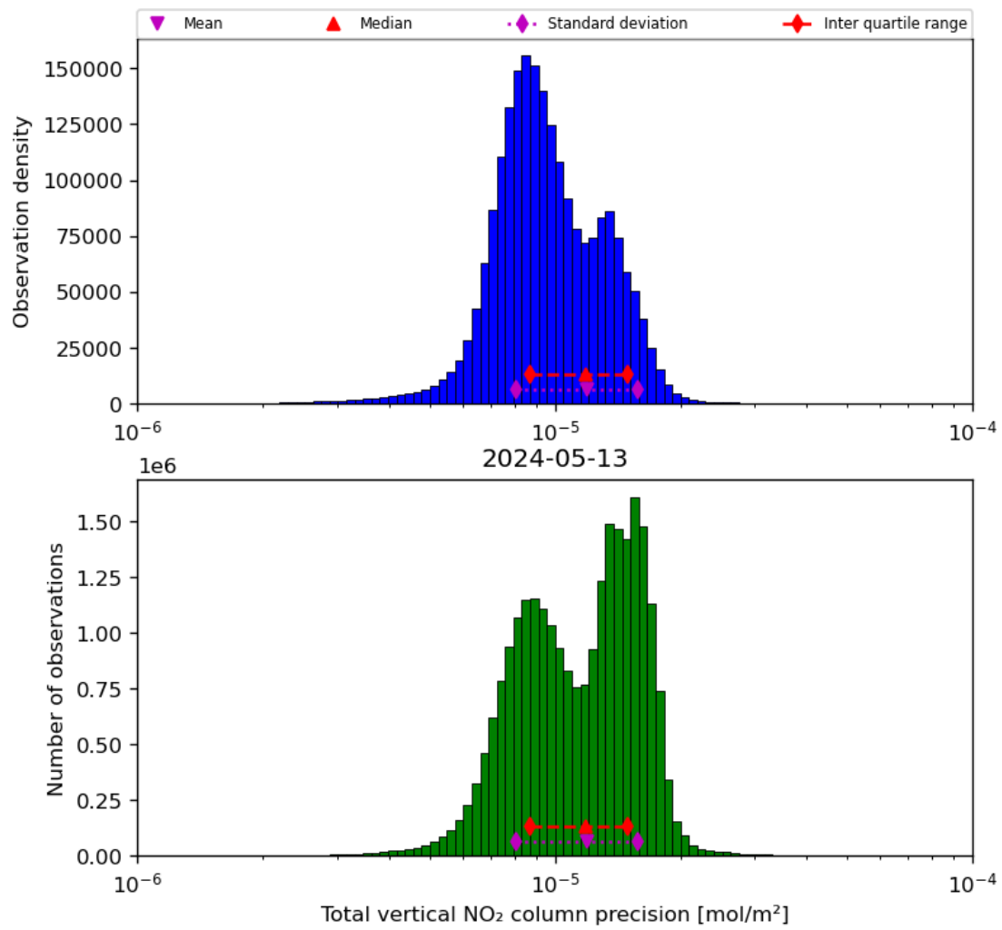
Figure 39: Histogram of “Total vertical NO 2 column precision” for 2024-05-12 to 2024-05-14
