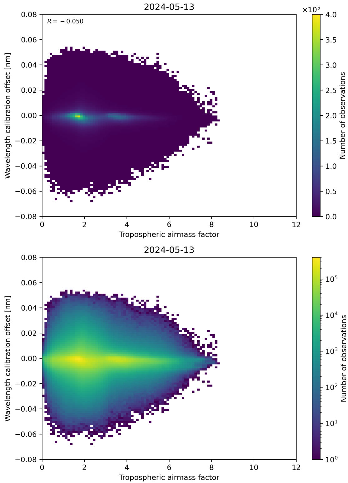
Figure 80: Scatter density plot of “Tropospheric airmass factor” against “Wavelength calibration offset” for 2024-05-12 to 2024-05-14.
