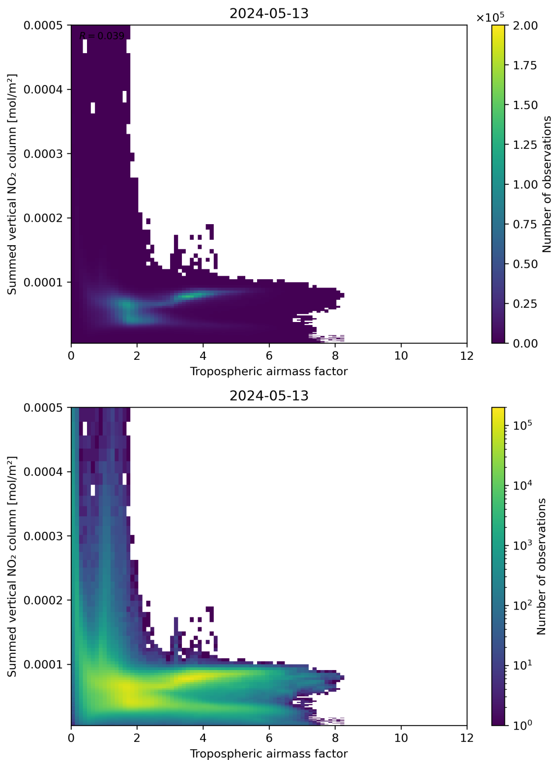
Figure 75: Scatter density plot of “Tropospheric airmass factor” against “Summed vertical NO 2 column” for 2024-05-12 to 2024-05-14.
