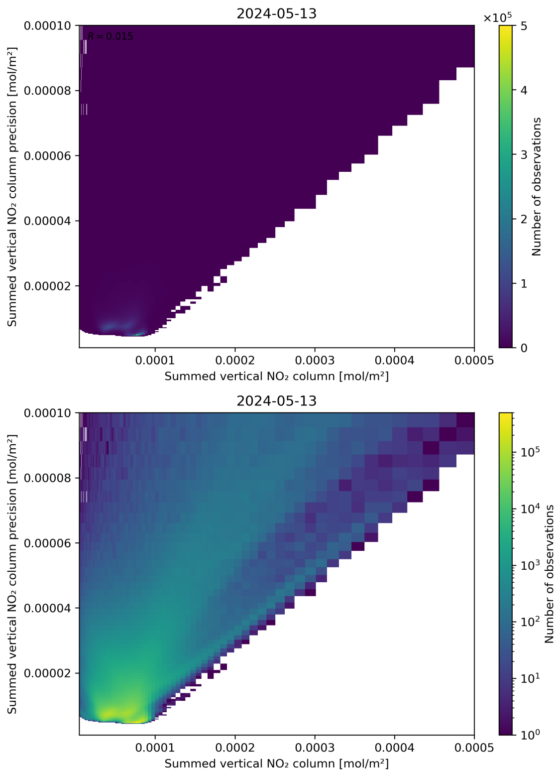
Figure 105: Scatter density plot of “Summed vertical NO 2 column” against “Summed vertical NO 2 column precision” for 2024-05-12 to 2024-05-14.
