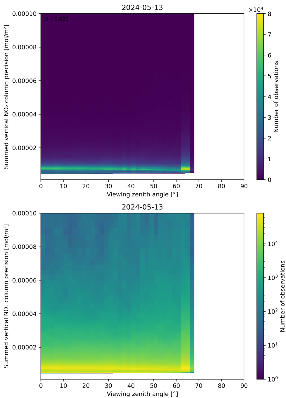
Figure 166: Scatter density plot of “Viewing zenith angle” against “Summed vertical NO 2 column precision” for 2024-05-12 to 2024-05-14.
