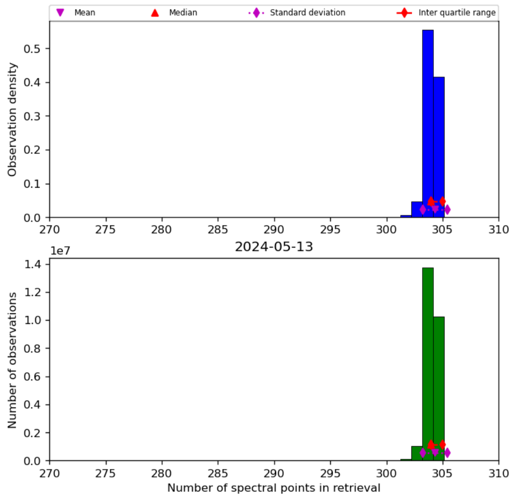
Figure 33: Histogram of “Number of spectral points in retrieval” for 2024-05-12 to 2024-05-14
