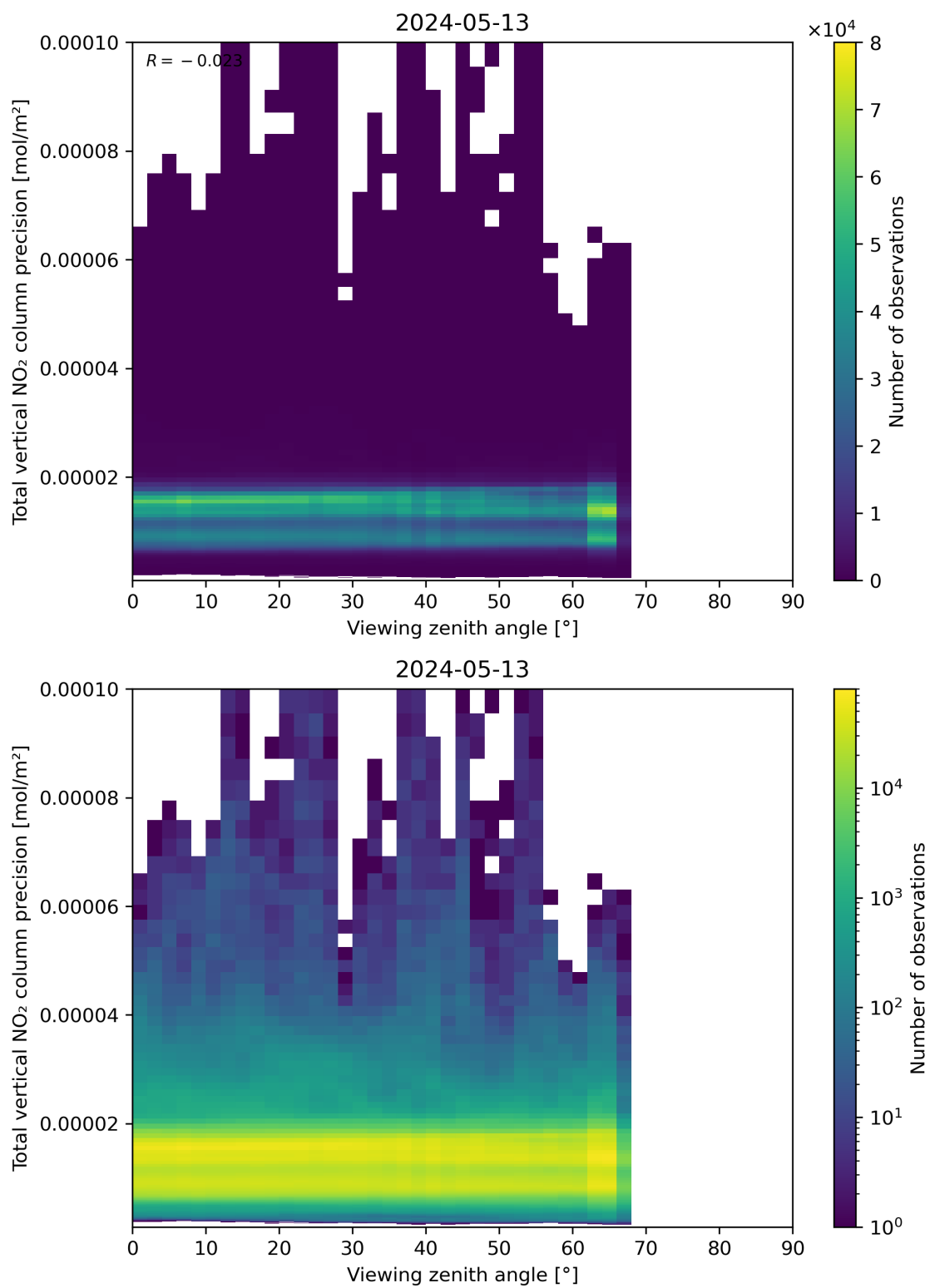
Figure 168: Scatter density plot of “Viewing zenith angle” against “Total vertical NO 2 column precision” for 2024-05-12 to 2024-05-14.
