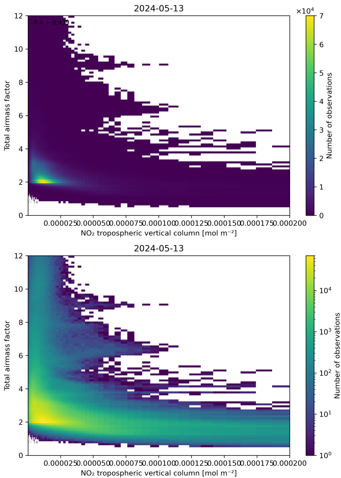
Figure 122: Scatter density plot of “NO 2 tropospheric vertical column” against “Total air mass factor” for 2024-05-12 to 2024-05-14.
