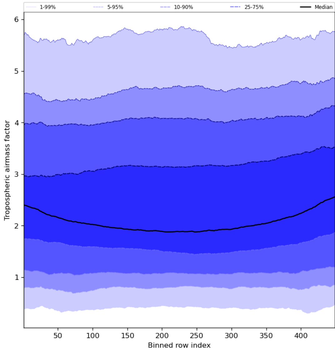
Figure 48: Along track statistics of “Tropospheric airmass factor” for 2024-05-12 to 2024-05-14
