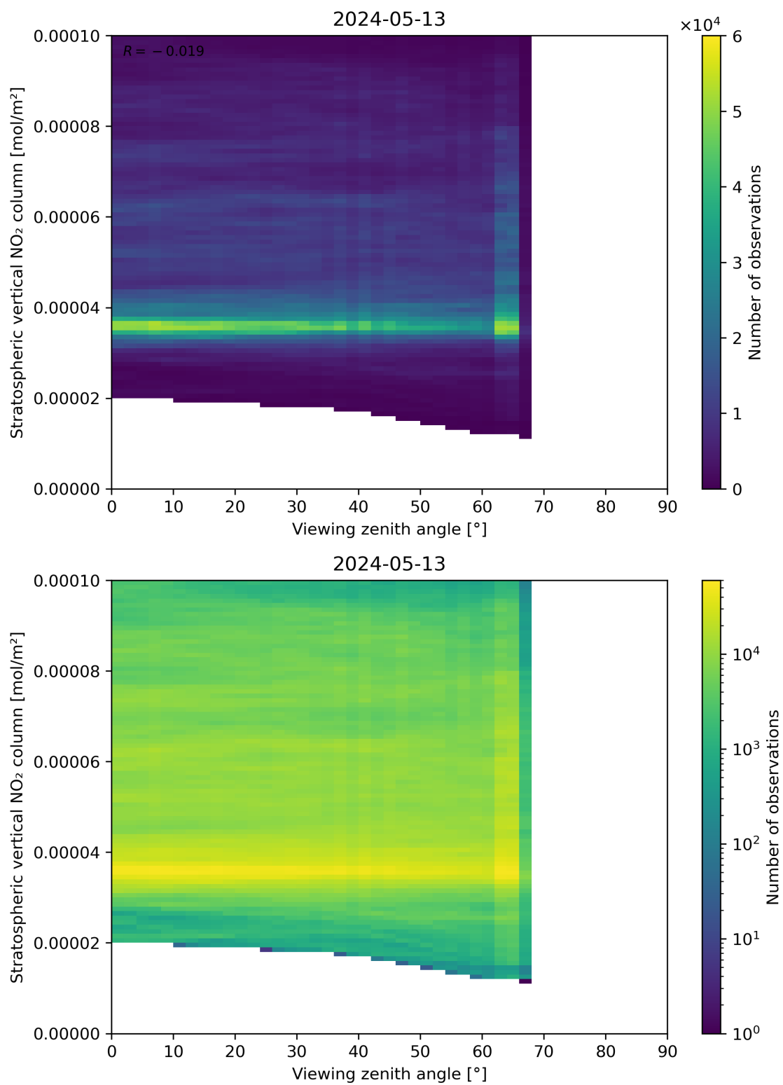
Figure 164: Scatter density plot of “Viewing zenith angle” against “Stratospheric vertical NO 2 column” for 2024-05-12 to 2024-05-14.
