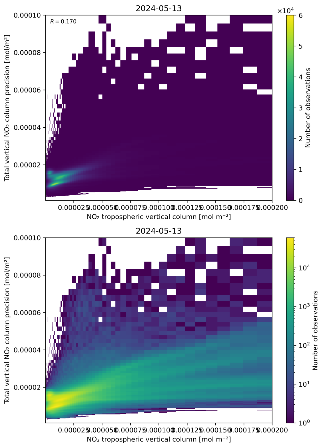
Figure 129: Scatter density plot of “NO 2 tropospheric vertical column” against “Total vertical NO 2 column precision” for 2024-05-12 to 2024-05-14.
