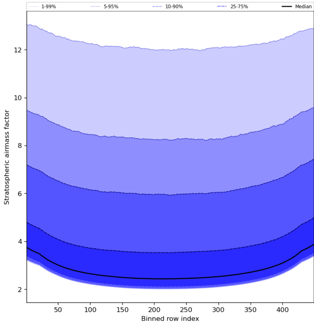
Figure 61: Along track statistics of “Stratospheric airmass factor” for 2024-05-12 to 2024-05-14
