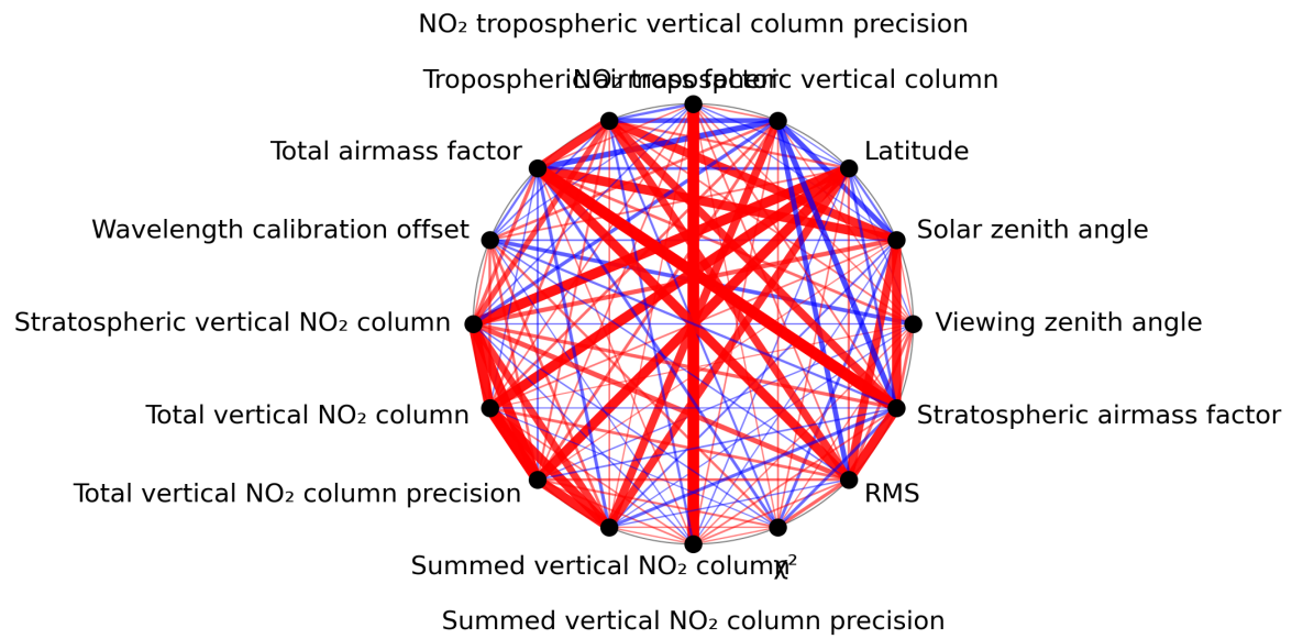
Figure 1: Map of correlation graph for 2024-05-12 to 2024-05-14.
