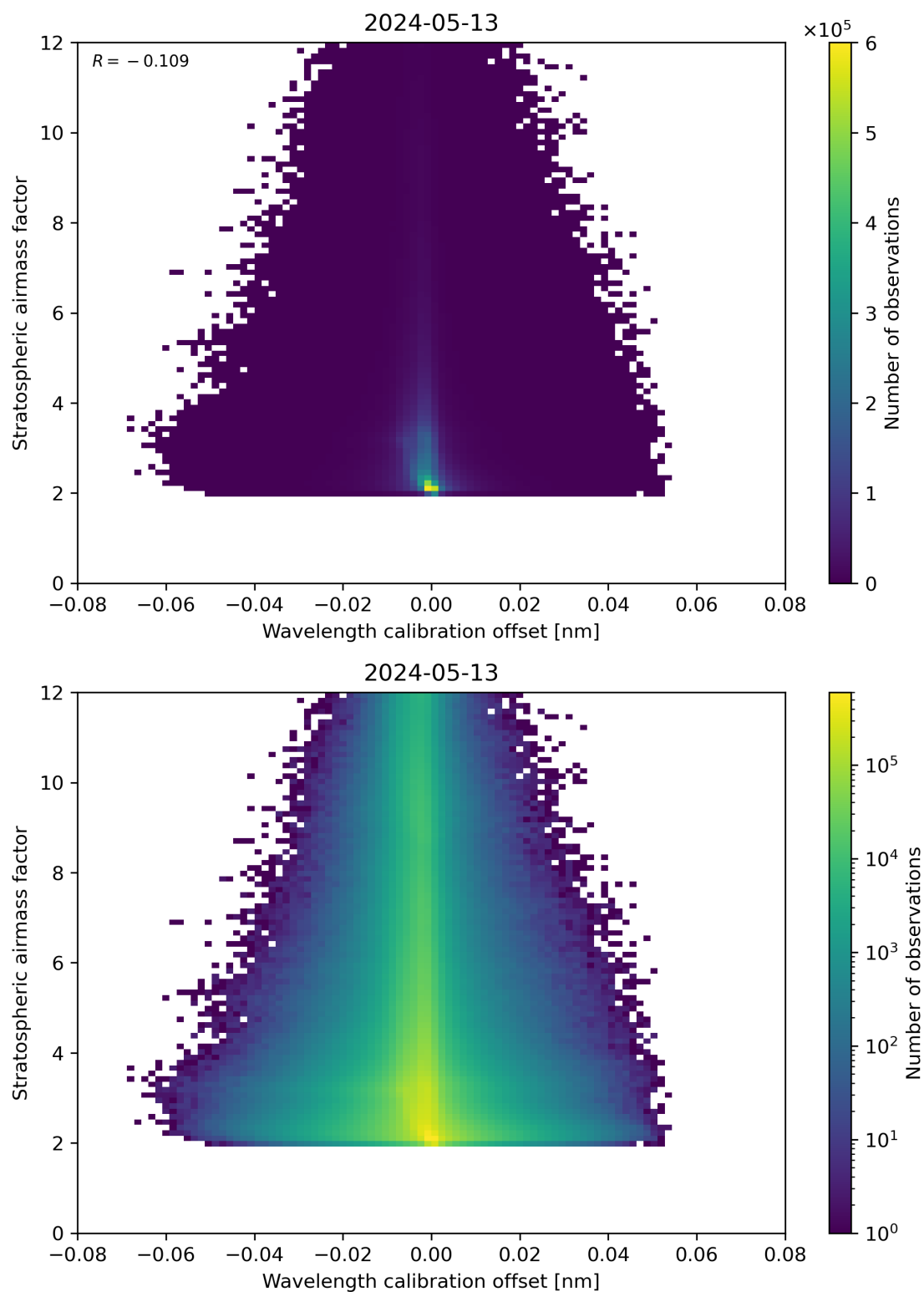
Figure 174: Scatter density plot of “Wavelength calibration offset” against “Stratospheric airmass factor” for 2024-05-12 to 2024-05-14.
