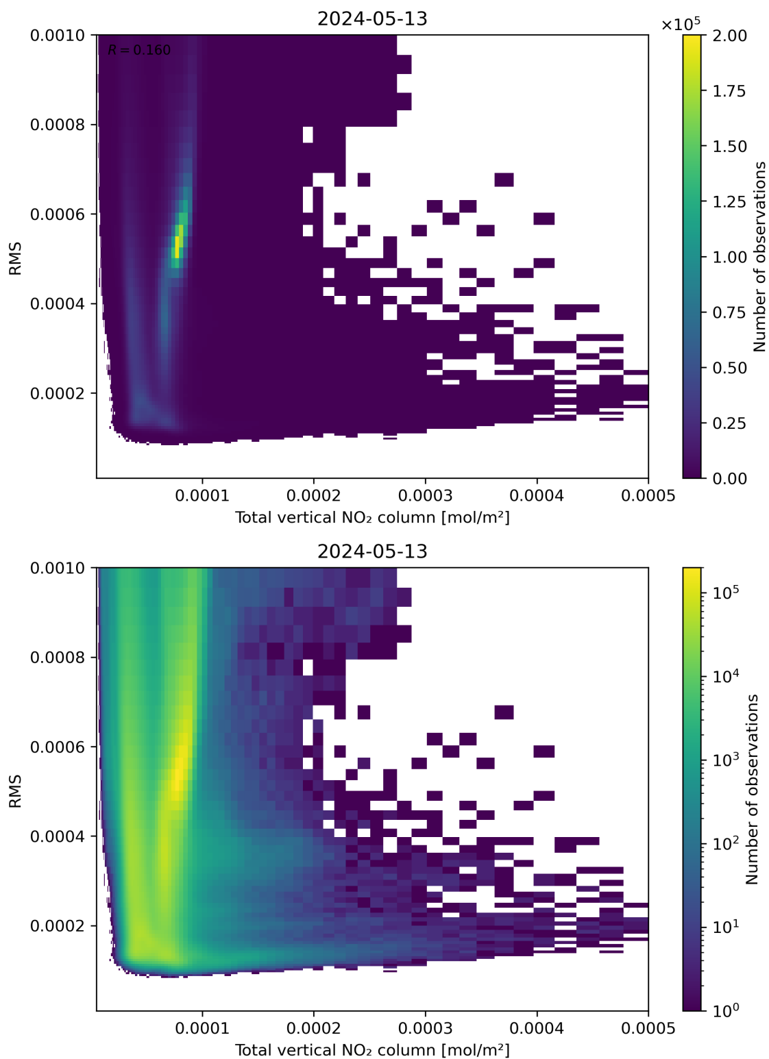
Figure 120: Scatter density plot of “Total vertical NO 2 column” against “RMS” for 2024-05-12 to 2024-05-14.
