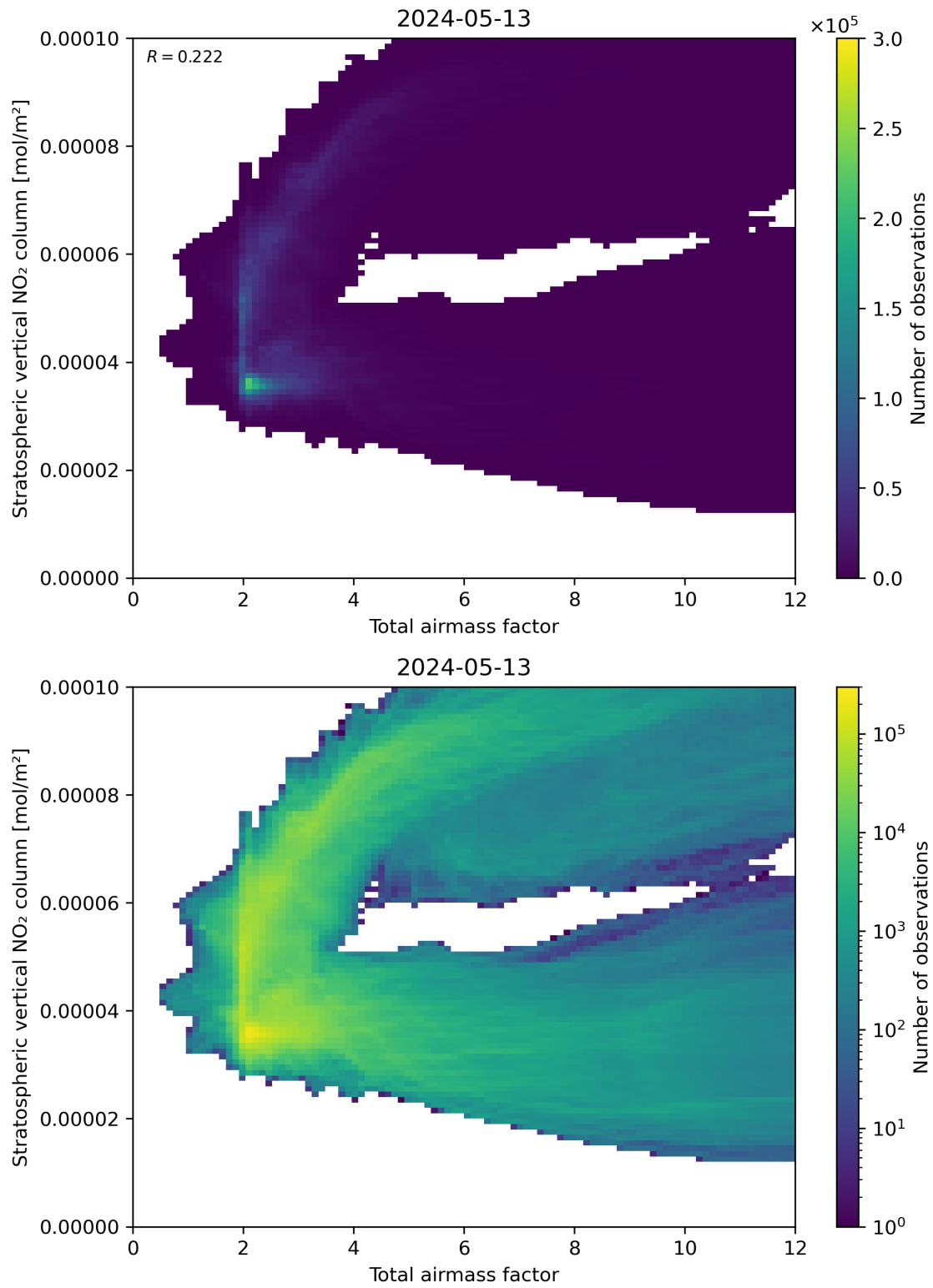
Figure 64: Scatter density plot of “Total airmass factor” against “Stratospheric vertical \text{NO}_2 column” for 2024-05-12 to 2024-05-14.
