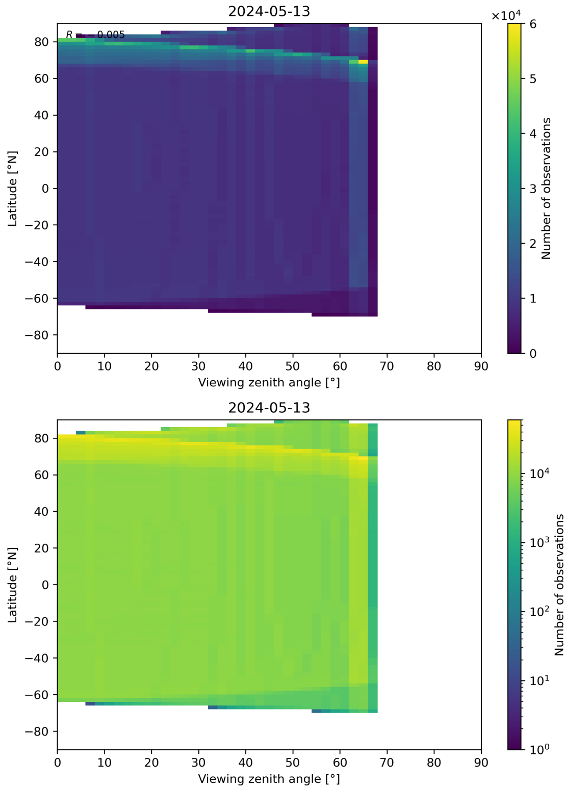
Figure 163: Scatter density plot of “Viewing zenith angle” against “Latitude” for 2024-05-12 to 2024-05-14.
