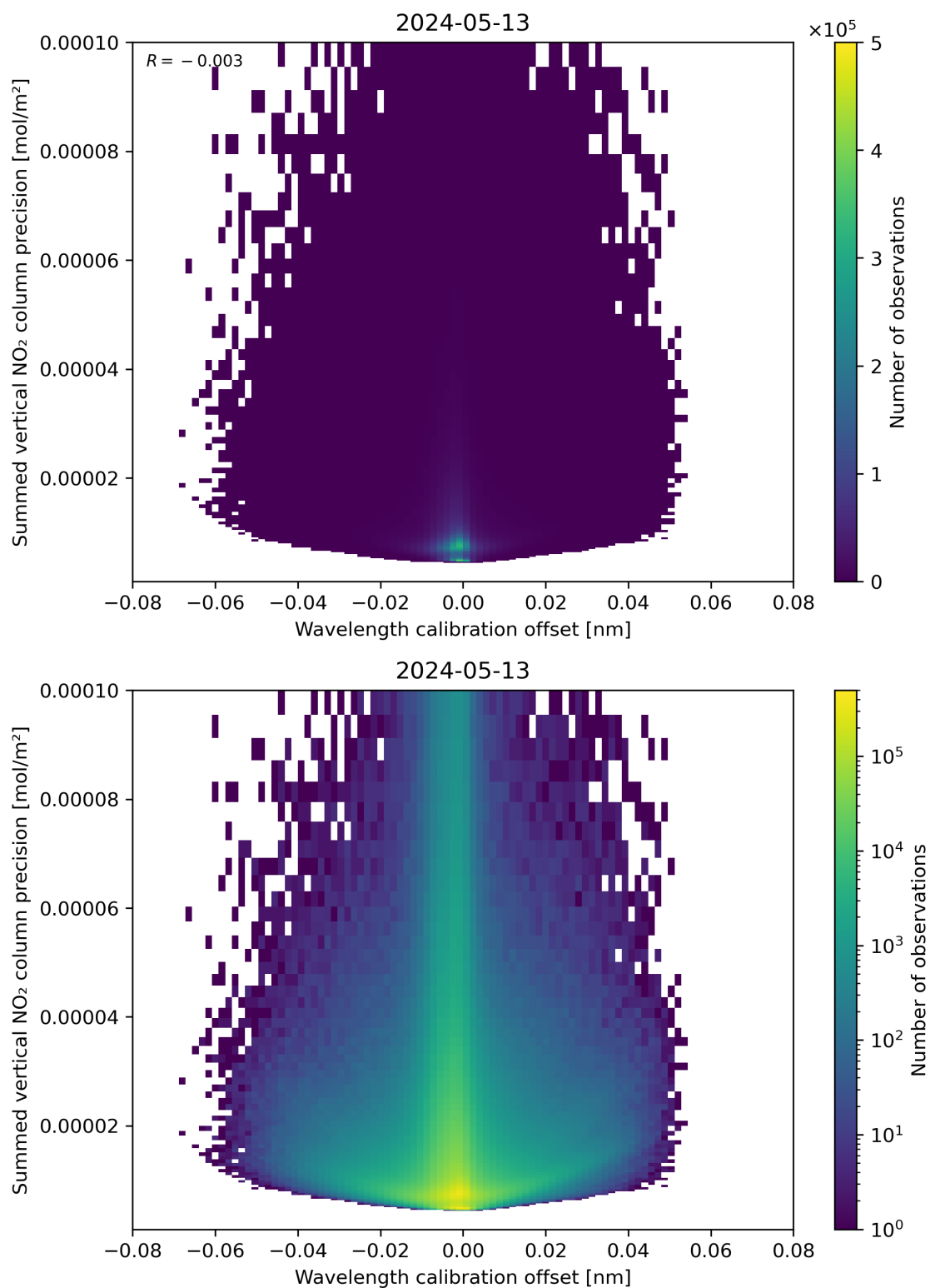
Figure 178: Scatter density plot of “Wavelength calibration offset” against “Summed vertical NO 2 column precision” for 2024-05-12 to 2024-05-14.
