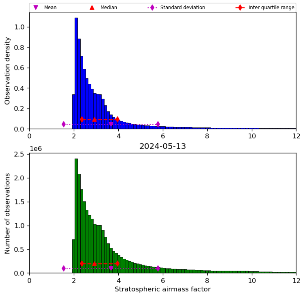
Figure 44: Histogram of “Stratospheric airmass factor” for 2024-05-12 to 2024-05-14
