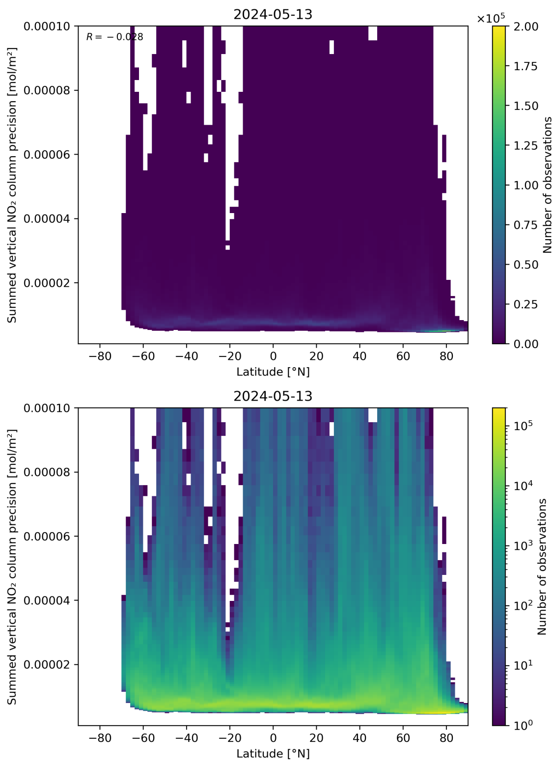
Figure 89: Scatter density plot of “Latitude” against “Summed vertical NO 2 column precision” for 2024-05-12 to 2024-05-14.
