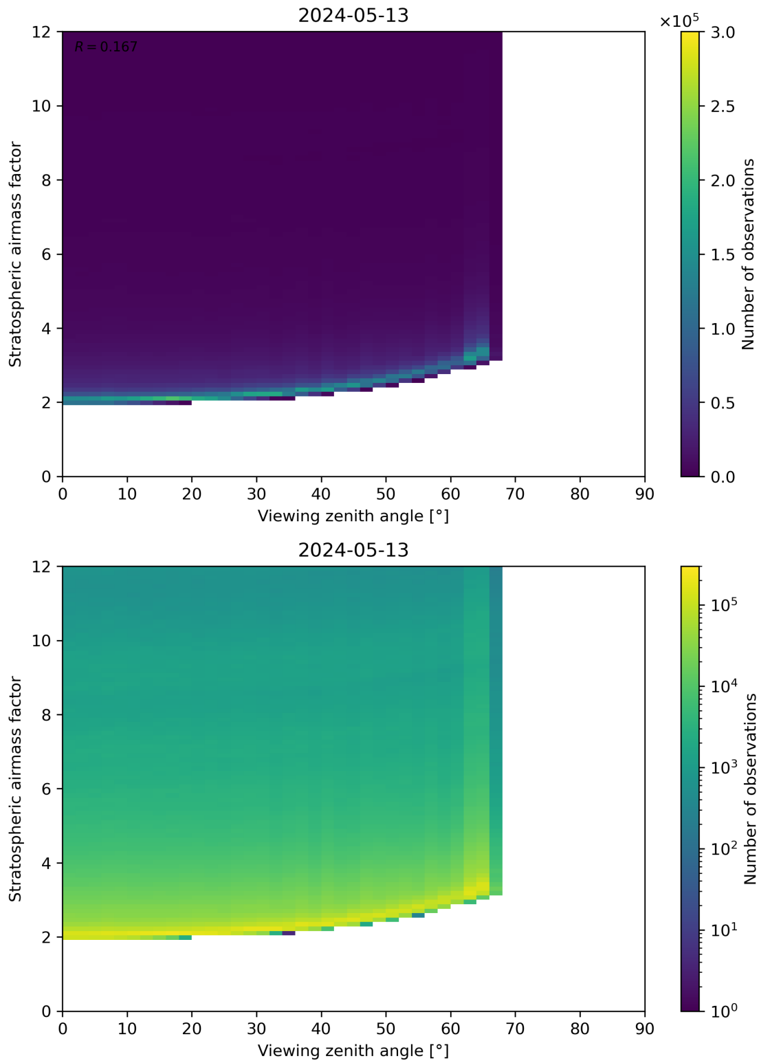
Figure 159: Scatter density plot of “Viewing zenith angle” against “Stratospheric airmass factor” for 2024-05-12 to 2024-05-14.
