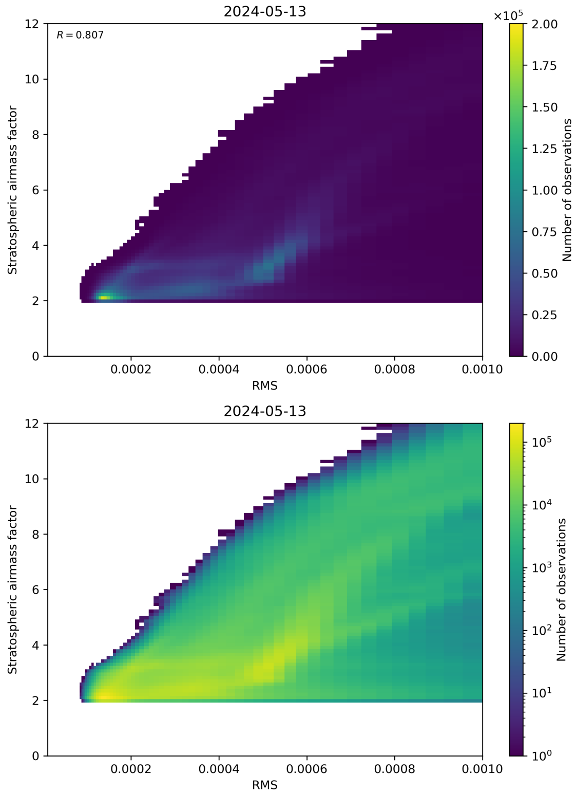
Figure 144: Scatter density plot of “RMS” against “Stratospheric airmass factor” for 2024-05-12 to 2024-05-14.
