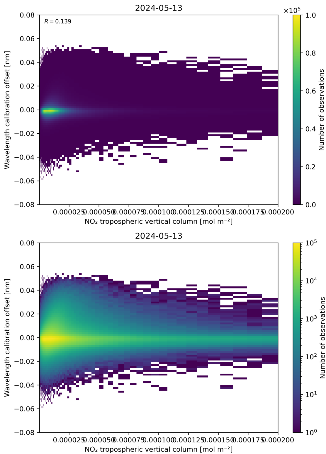
Figure 143: Scatter density plot of “NO 2 tropospheric vertical column” against “Wavelength calibration offset” for 2024-05-12 to 2024-05-14.
