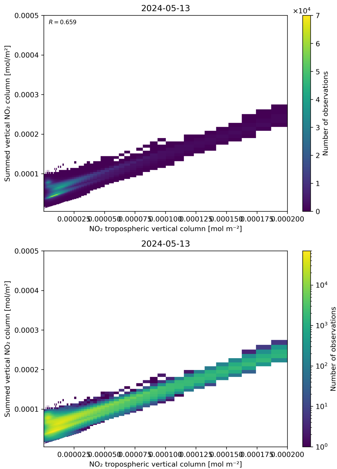
Figure 126: Scatter density plot of “NO 2 tropospheric vertical column” against “Summed vertical NO 2 column” for 2024-05-12 to 2024-05-14.
