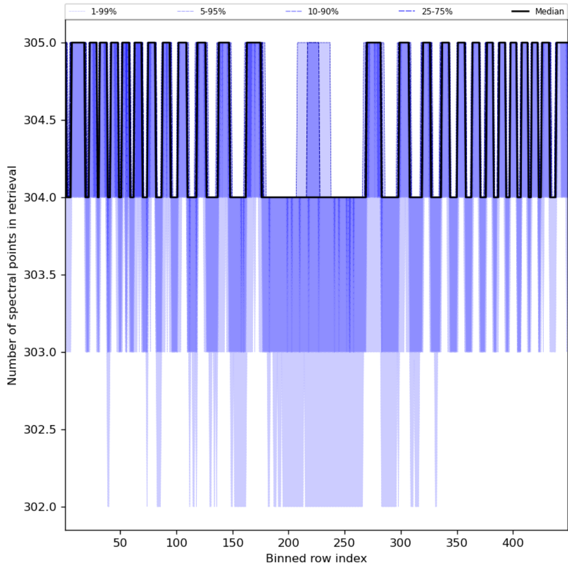
Figure 50: Along track statistics of “Number of spectral points in retrieval” for 2024-05-12 to 2024-05-14
