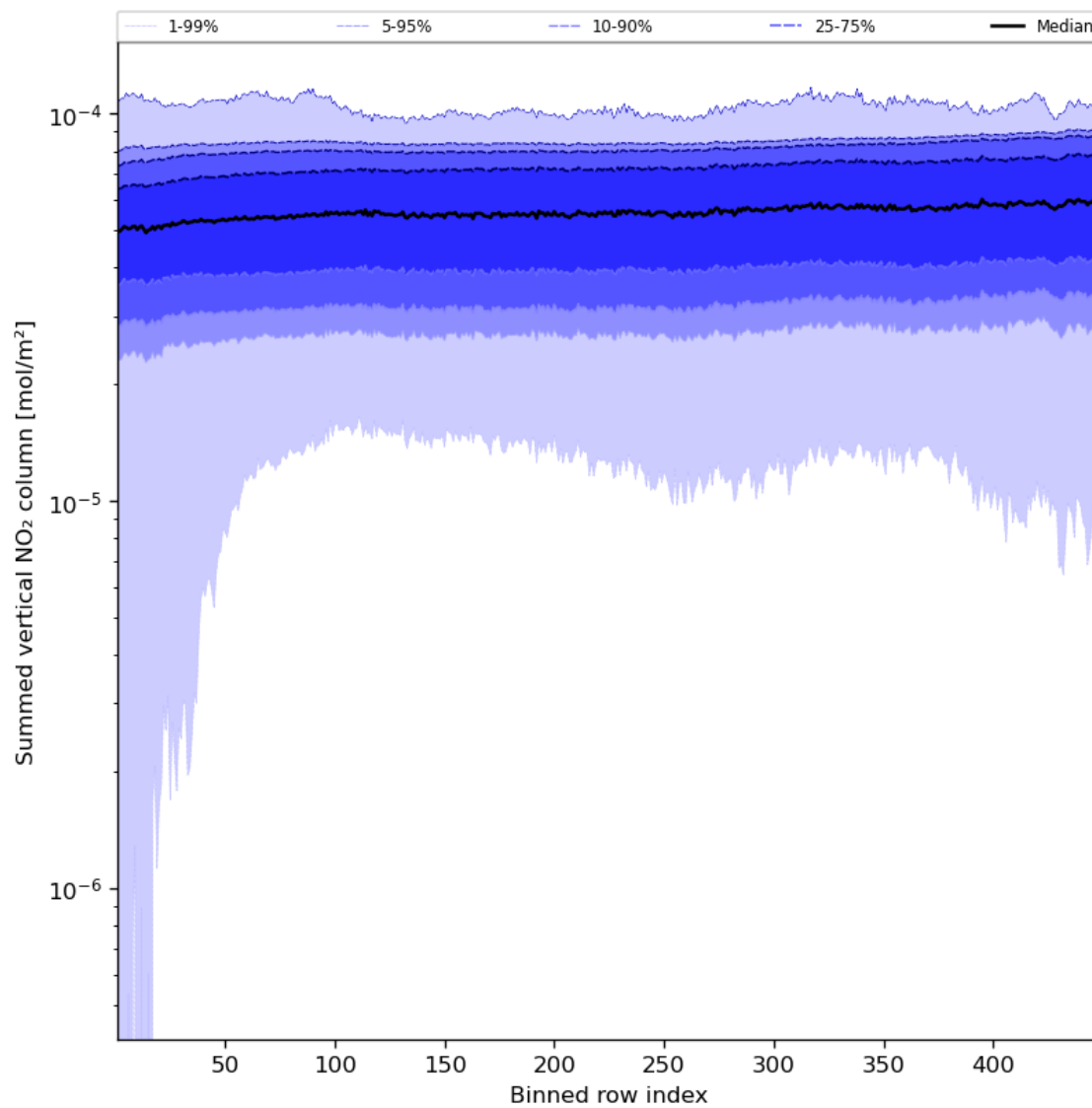
Figure 57: Along track statistics of “Summed vertical NO 2 column” for 2024-05-12 to 2024-05-14
