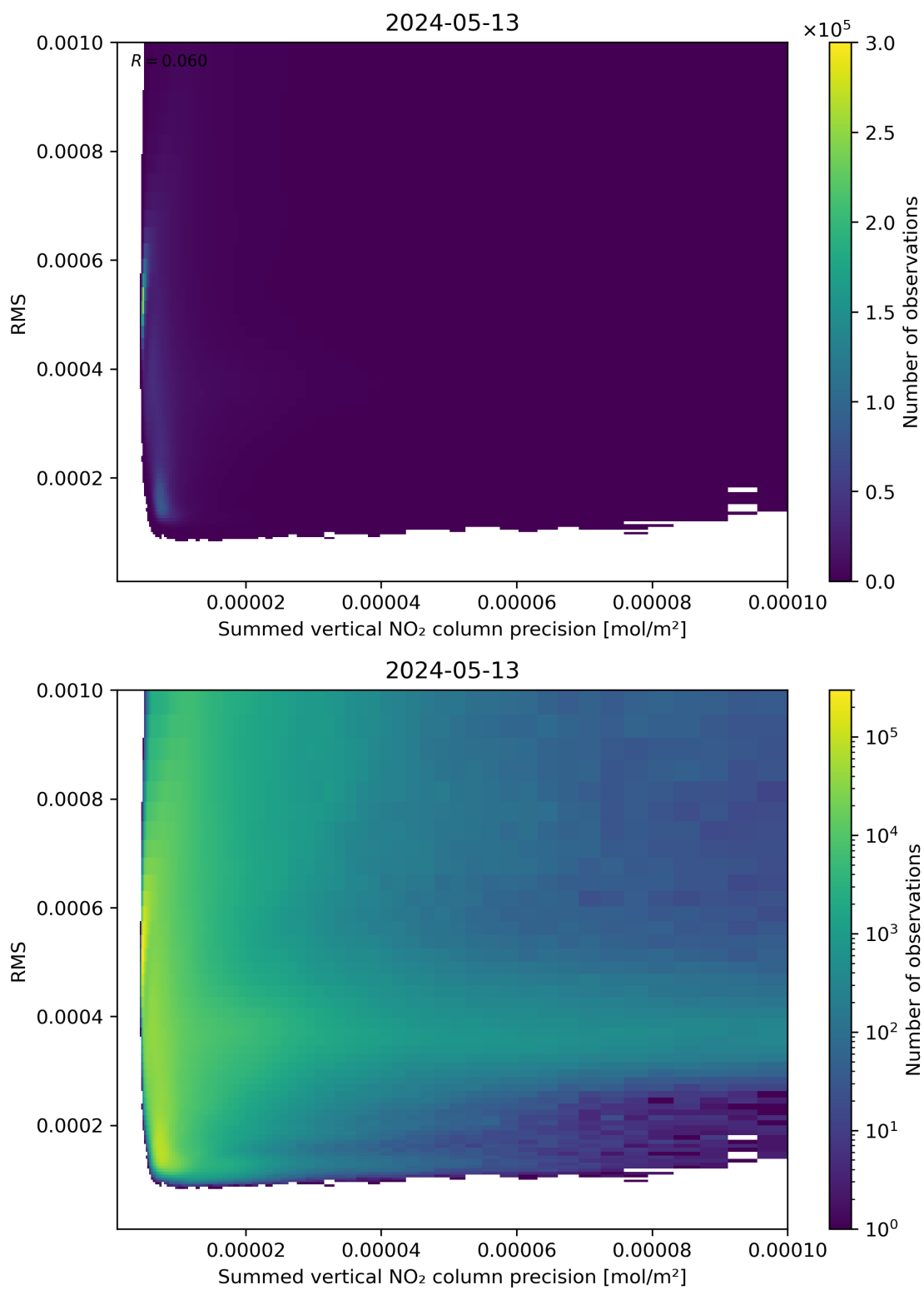
Figure 108: Scatter density plot of “Summed vertical NO 2 column precision” against “RMS” for 2024-05-12 to 2024-05-14.
