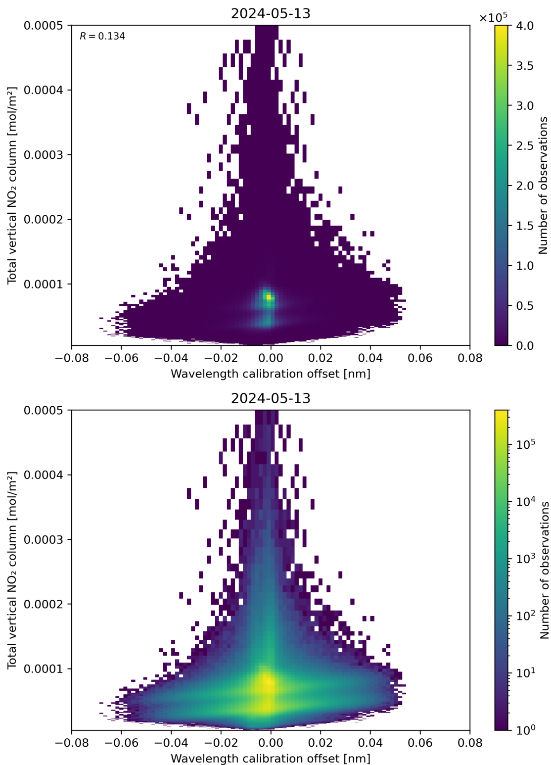
Figure 179: Scatter density plot of “Wavelength calibration offset” against “Total vertical NO 2 column” for 2024-05-12 to 2024-05-14.
