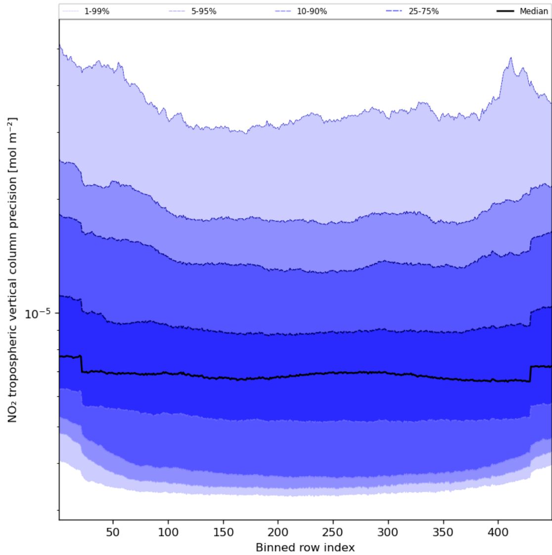
Figure 47: Along track statistics of “NO 2 tropospheric vertical column precision” for 2024-05-12 to 2024-05-14
