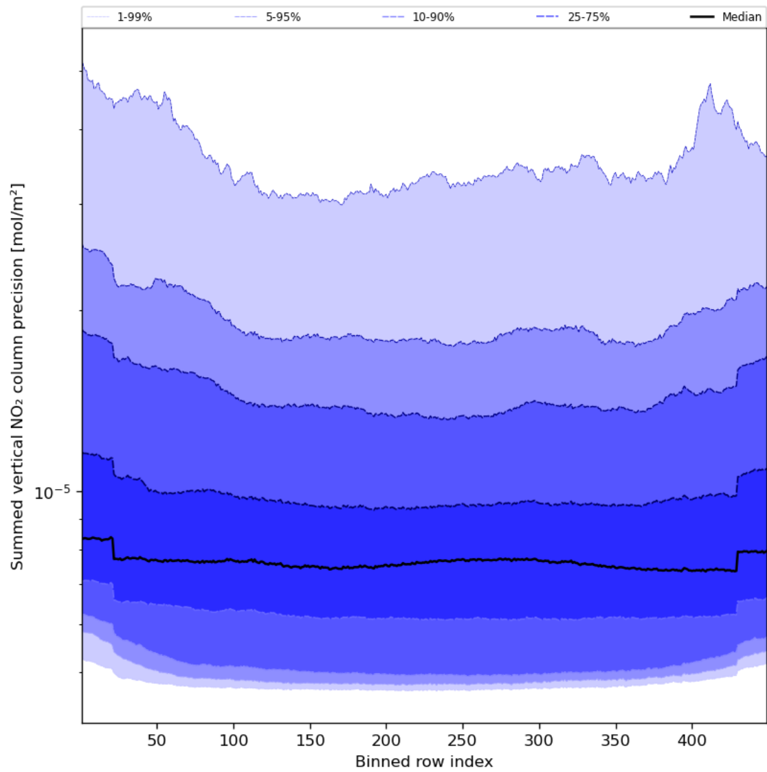
Figure 58: Along track statistics of “Summed vertical NO 2 column precision” for 2024-05-12 to 2024-05-14
