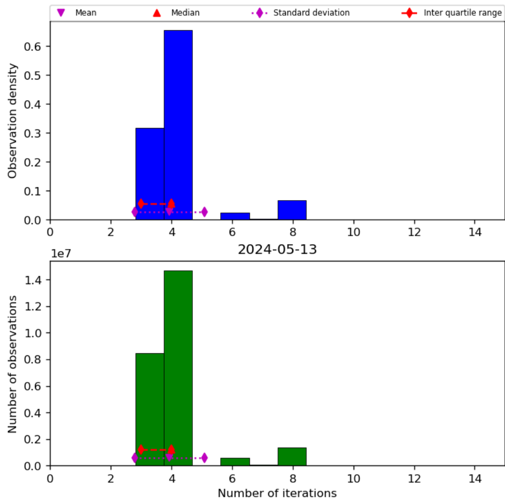
Figure 34: Histogram of “Number of iterations” for 2024-05-12 to 2024-05-14
