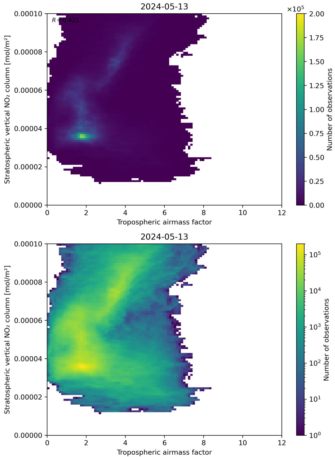
Figure 74: Scatter density plot of “Tropospheric air mass factor” against “Stratospheric vertical NO 2 column” for 2024-05-12 to 2024-05-14.
