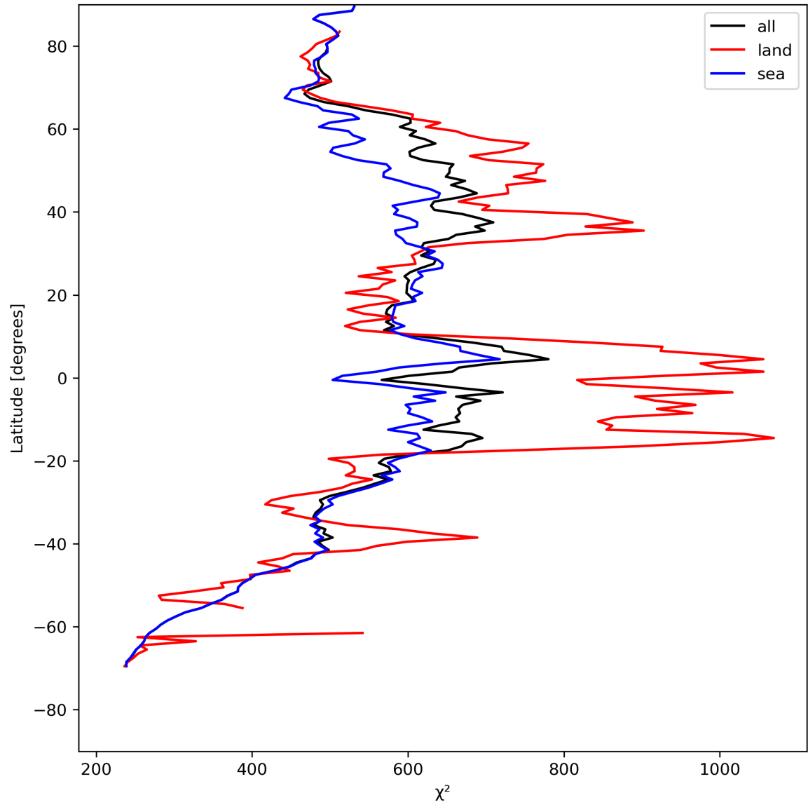
Figure 25: Zonal average of “ \chi^2 ” for 2024-05-12 to 2024-05-14.
