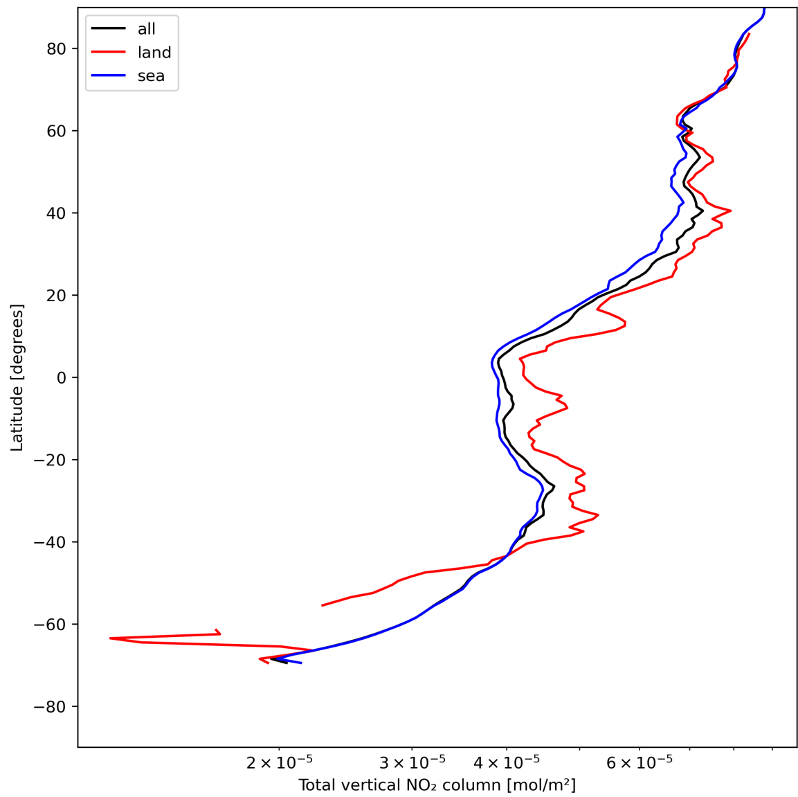
Figure 21: Zonal average of “Total vertical NO 2 column” for 2024-05-12 to 2024-05-14.
