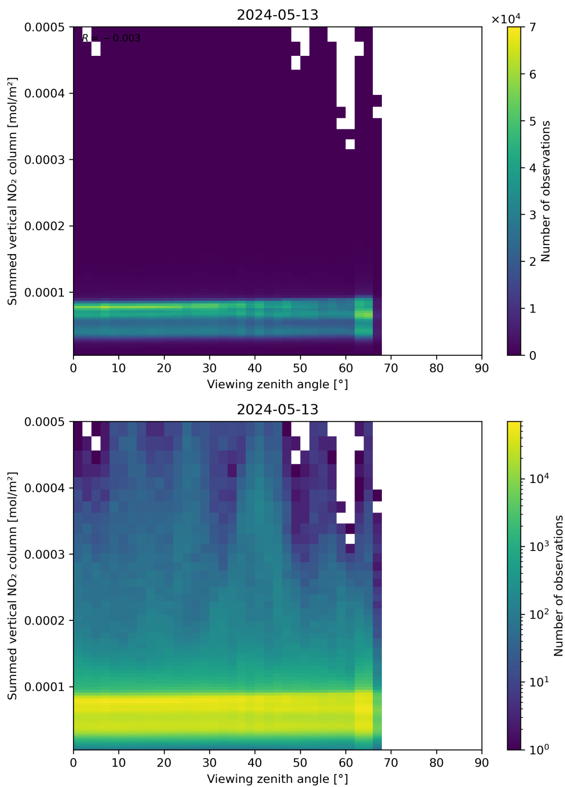
Figure 165: Scatter density plot of “Viewing zenith angle” against “Summed vertical NO 2 column” for 2024-05-12 to 2024-05-14.
