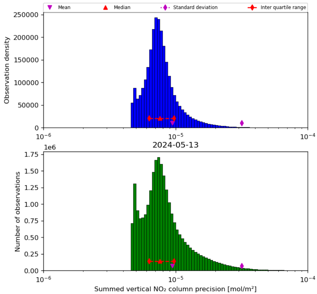
Figure 41: Histogram of "Summed vertical NO 2 column precision" for 2024-05-12 to 2024-05-14
