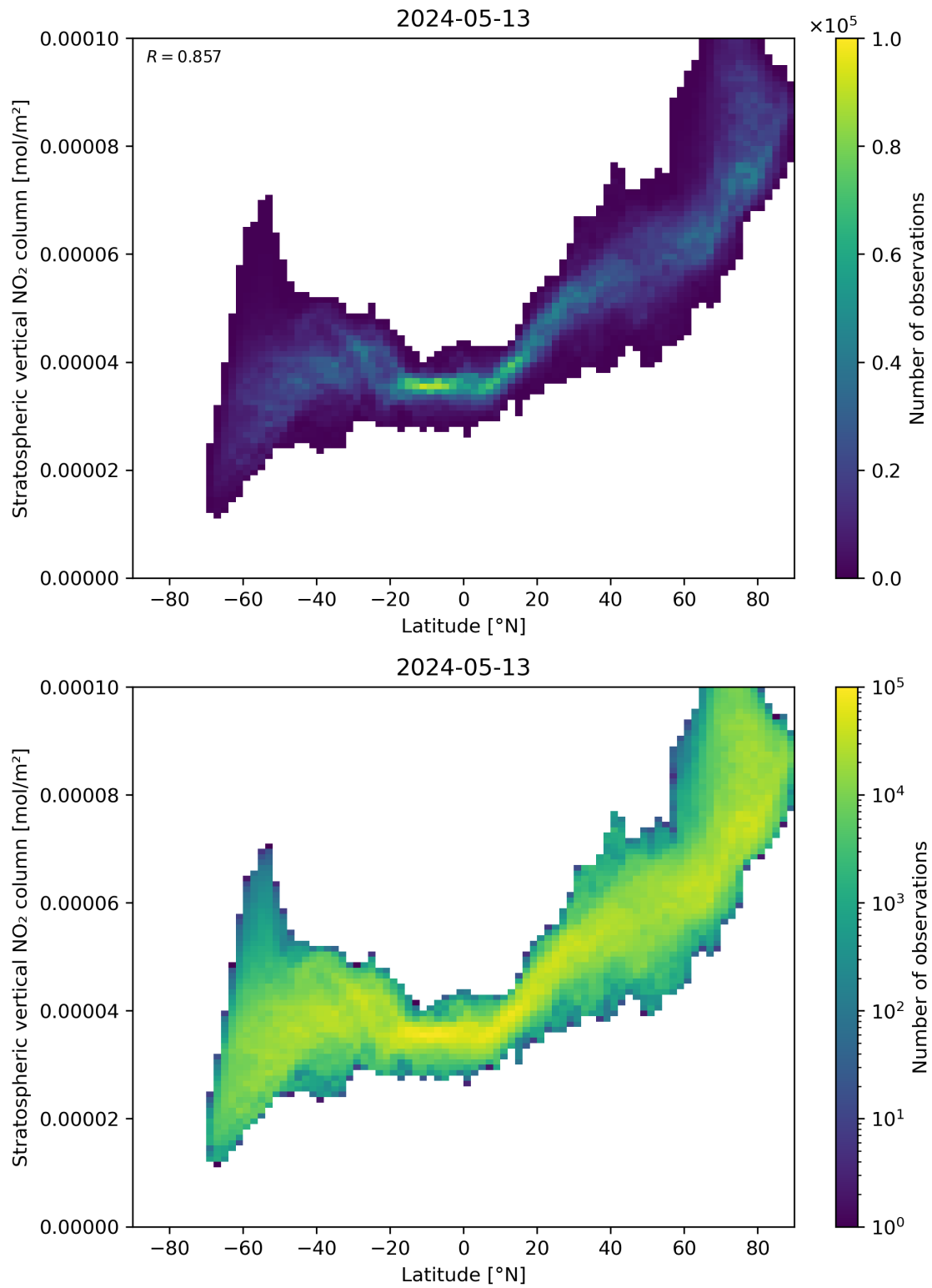
Figure 87: Scatter density plot of “Latitude” against “Stratospheric vertical NO 2 column” for 2024-05-12 to 2024-05-14.
