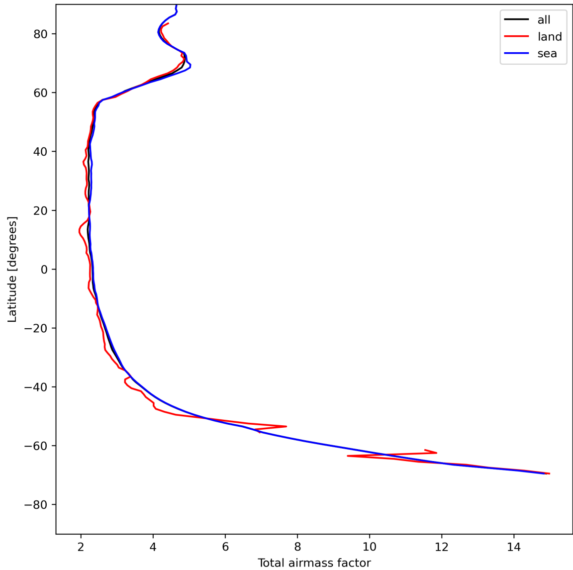
Figure 15: Zonal average of “Total airmass factor” for 2024-05-12 to 2024-05-14.
