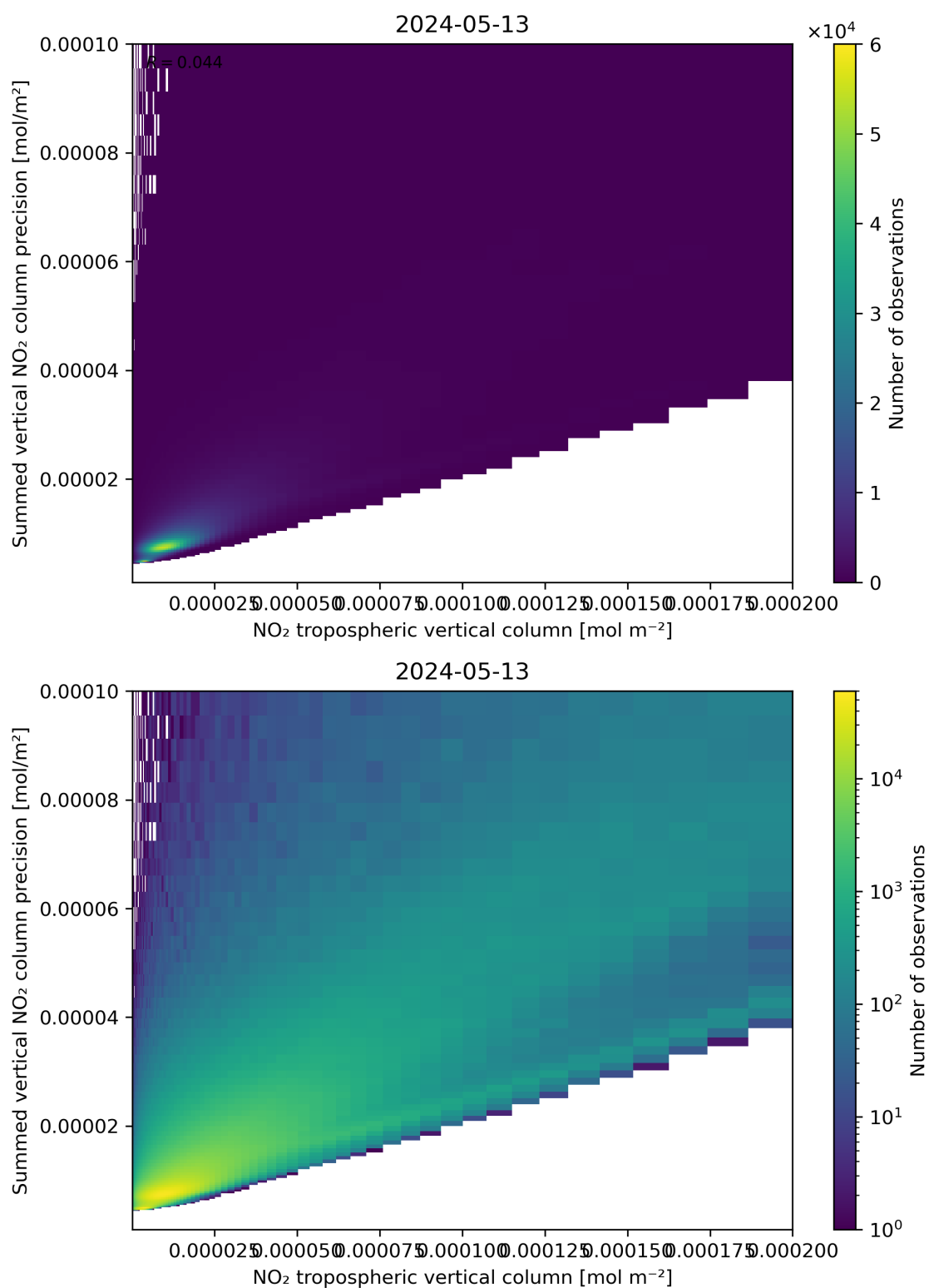
Figure 127: Scatter density plot of “NO 2 tropospheric vertical column” against “Summed vertical NO 2 column precision” for 2024-05-12 to 2024-05-14.
