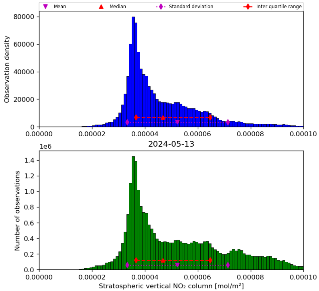
Figure 36: Histogram of “Stratospheric vertical NO 2 column” for 2024-05-12 to 2024-05-14
