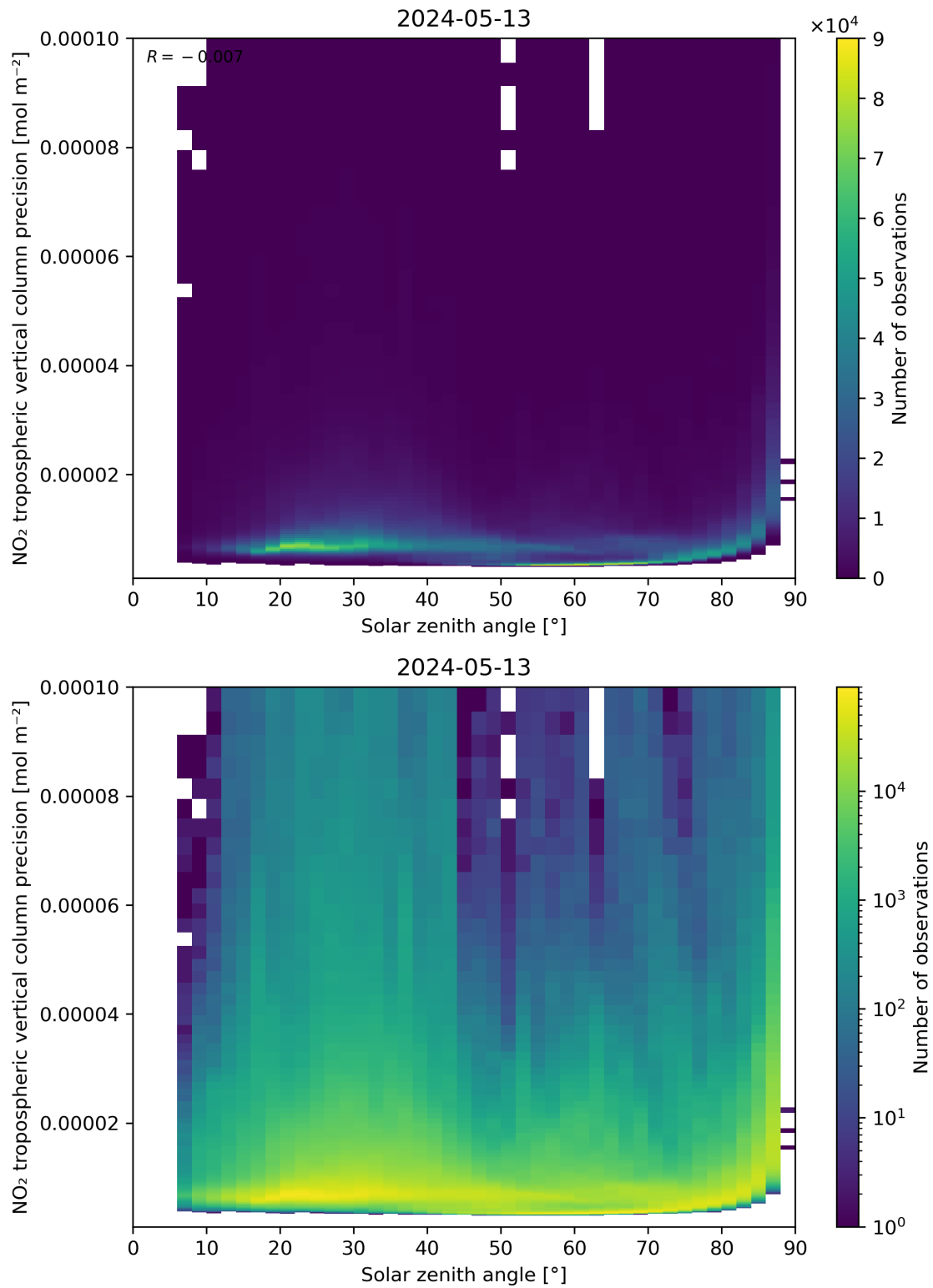
Figure 156: Scatter density plot of “Solar zenith angle” against “NO 2 tropospheric vertical column precision” for 2024-05-12 to 2024-05-14.
