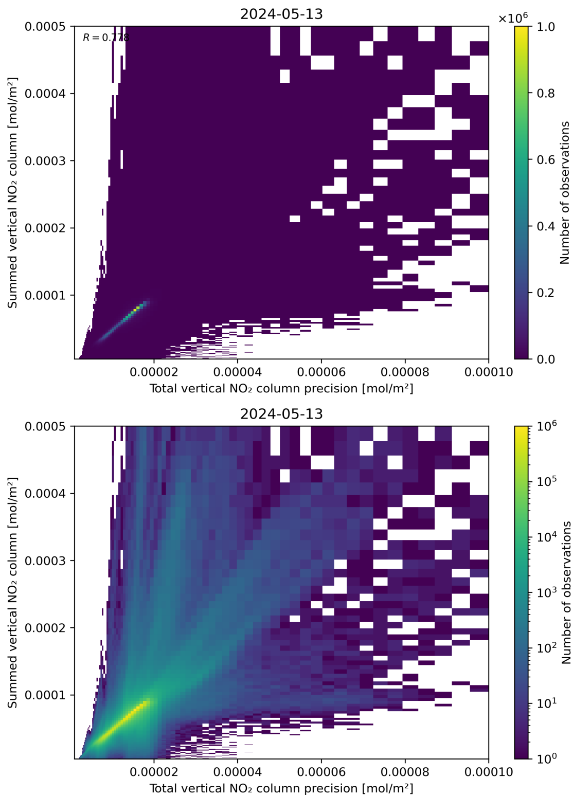
Figure 117: Scatter density plot of “Total vertical NO 2 column precision” against “Summed vertical NO 2 column” for 2024-05-12 to 2024-05-14.
