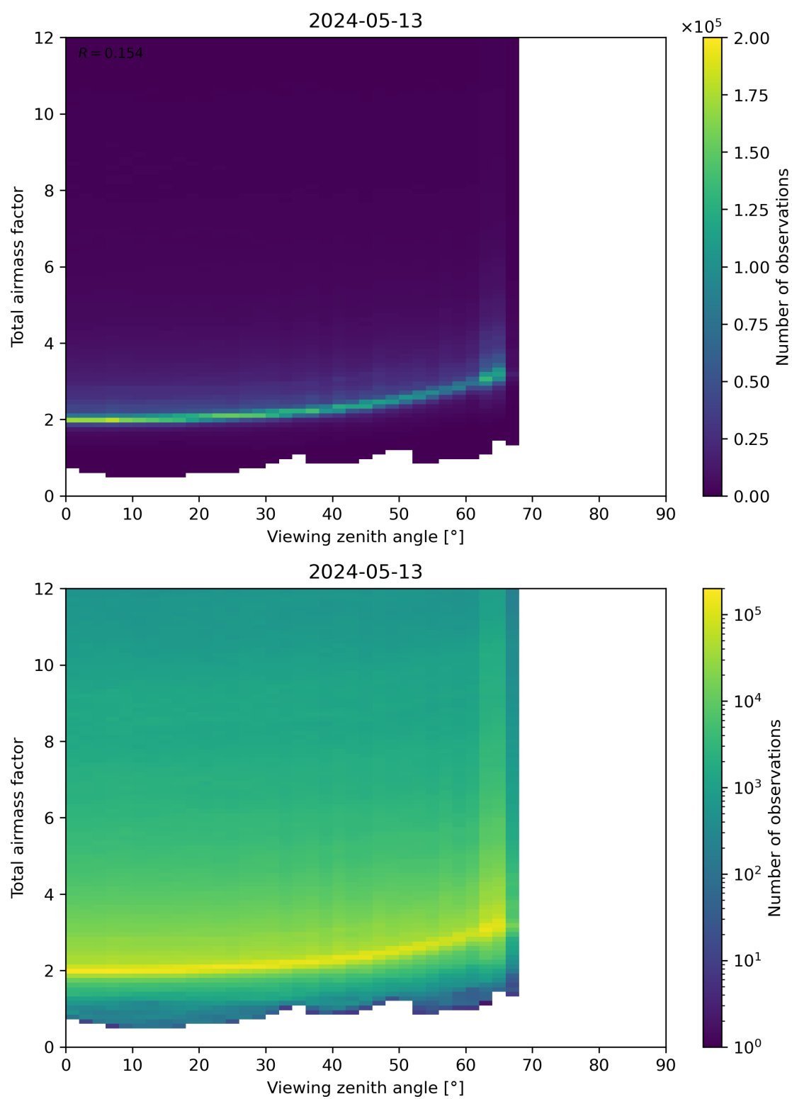
Figure 160: Scatter density plot of “Viewing zenith angle” against “Total airmass factor” for 2024-05-12 to 2024-05-14.
