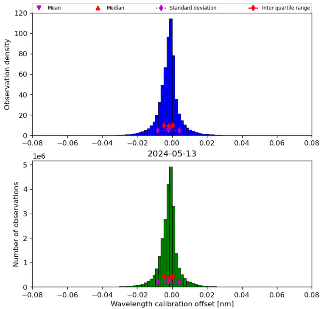
Figure 35: Histogram of “Wavelength calibration offset” for 2024-05-12 to 2024-05-14
