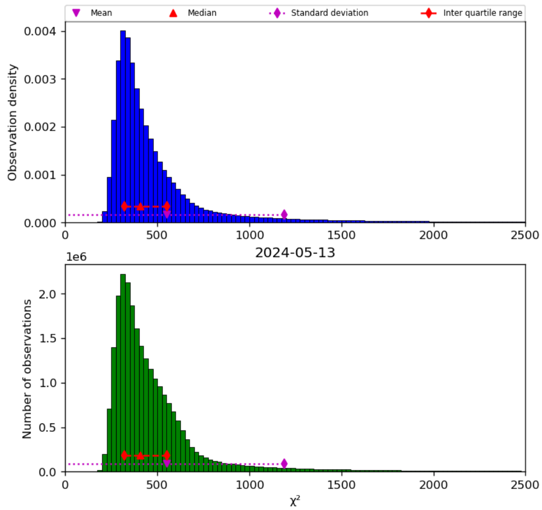
Figure 42: Histogram of “ \chi^2 ” for 2024-05-12 to 2024-05-14
