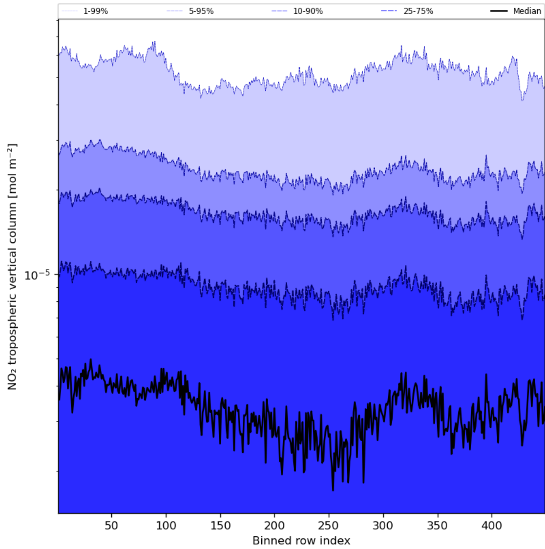
Figure 46: Along track statistics of “NO 2 tropospheric vertical column” for 2024-05-12 to 2024-05-14
