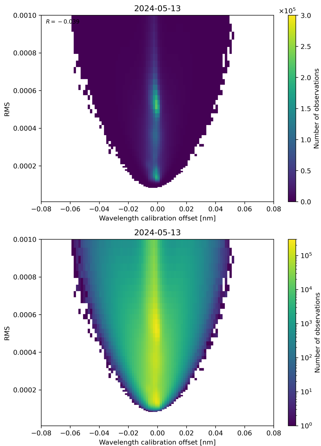
Figure 181: Scatter density plot of “Wavelength calibration offset” against “RMS” for 2024-05-12 to 2024-05-14.
