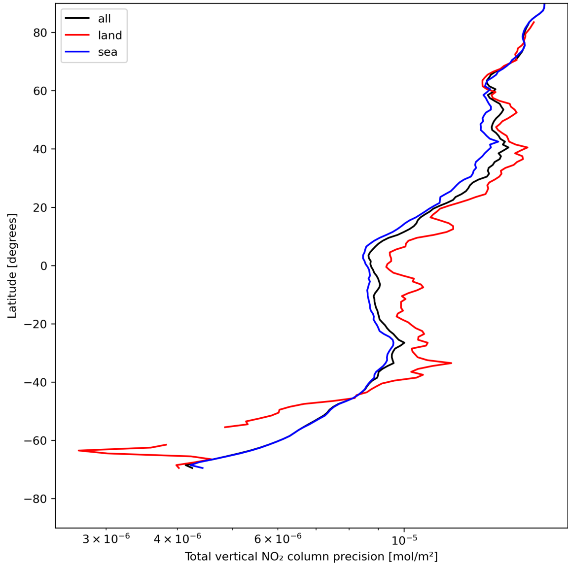
Figure 22: Zonal average of “Total vertical NO 2 column precision” for 2024-05-12 to 2024-05-14.
