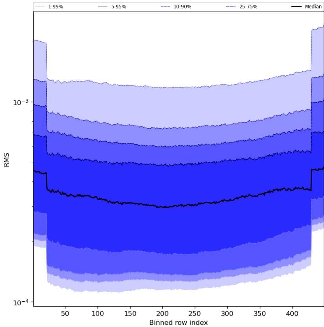
Figure 60: Along track statistics of “RMS” for 2024-05-12 to 2024-05-14
