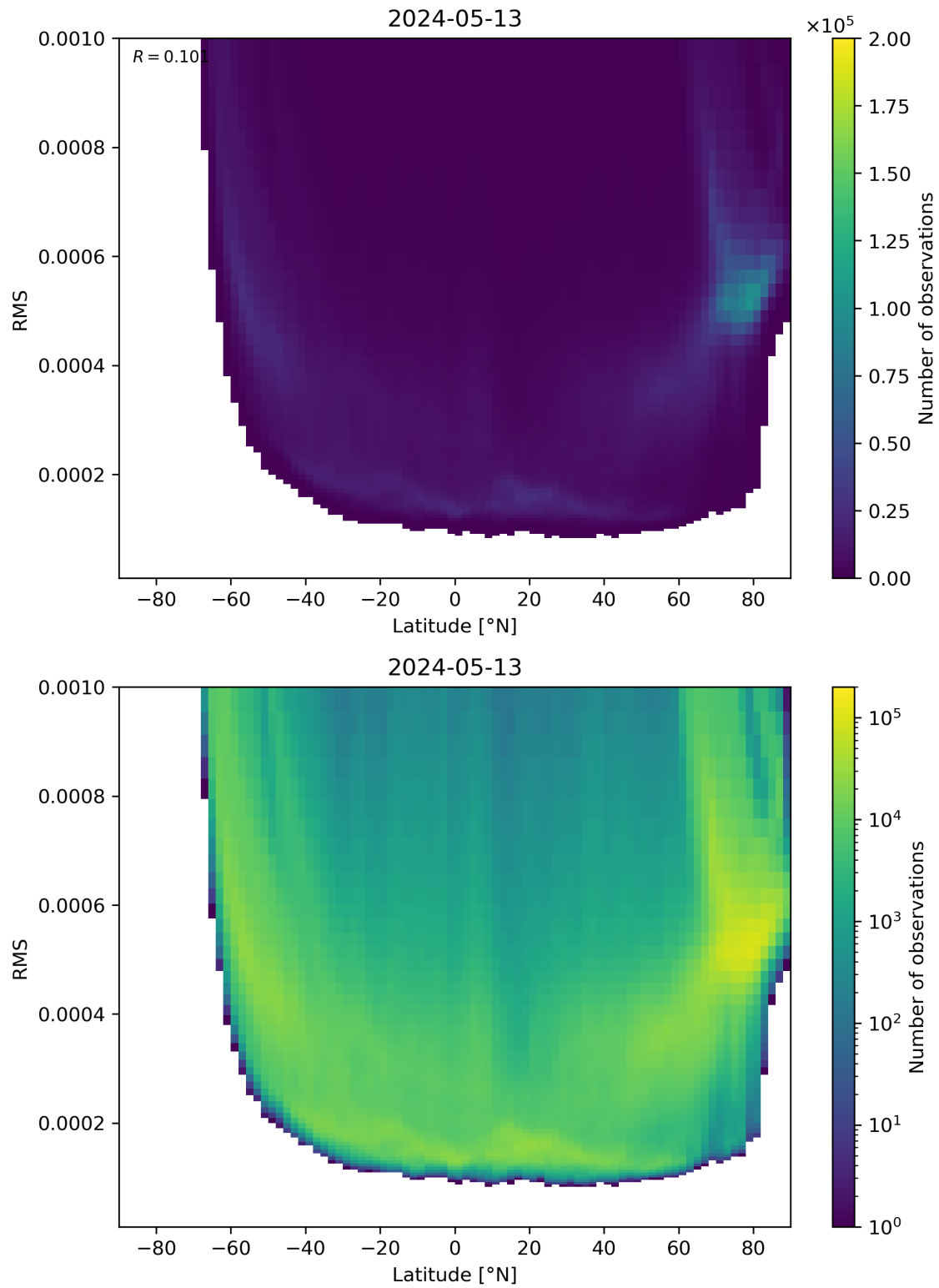
Figure 94: Scatter density plot of “Latitude” against “RMS” for 2024-05-12 to 2024-05-14.
