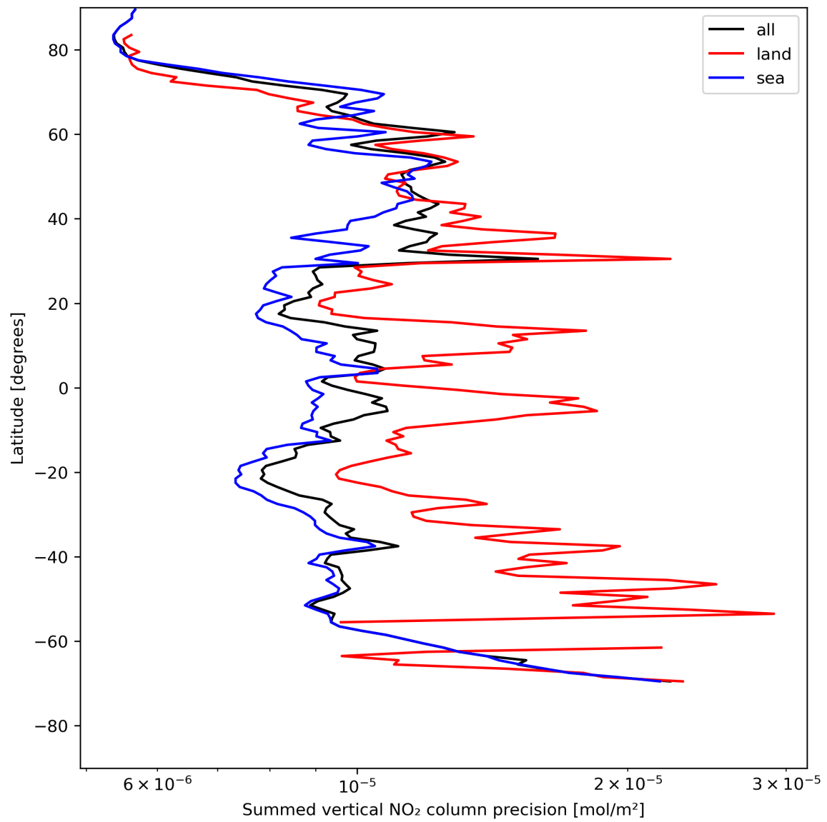
Figure 24: Zonal average of “Summed vertical NO 2 column precision” for 2024-05-12 to 2024-05-14.
