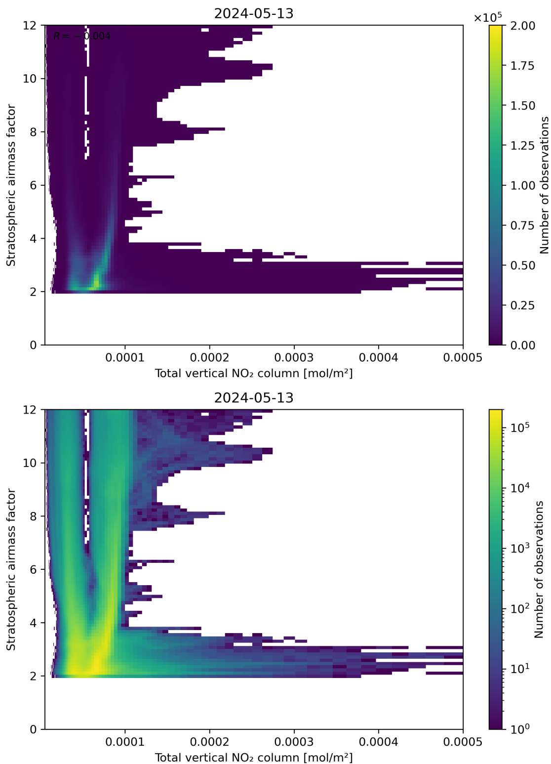
Figure 110: Scatter density plot of “Total vertical NO 2 column” against “Stratospheric air mass factor” for 2024-05-12 to 2024-05-14.
