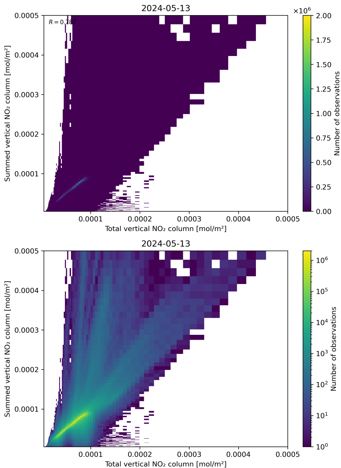
Figure 112: Scatter density plot of “Total vertical NO 2 column” against “Summed vertical NO 2 column” for 2024-05-12 to 2024-05-14.
