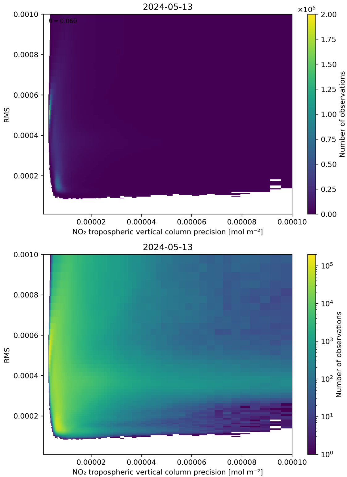
Figure 140: Scatter density plot of “NO 2 tropospheric vertical column precision” against “RMS” for 2024-05-12 to 2024-05-14.
