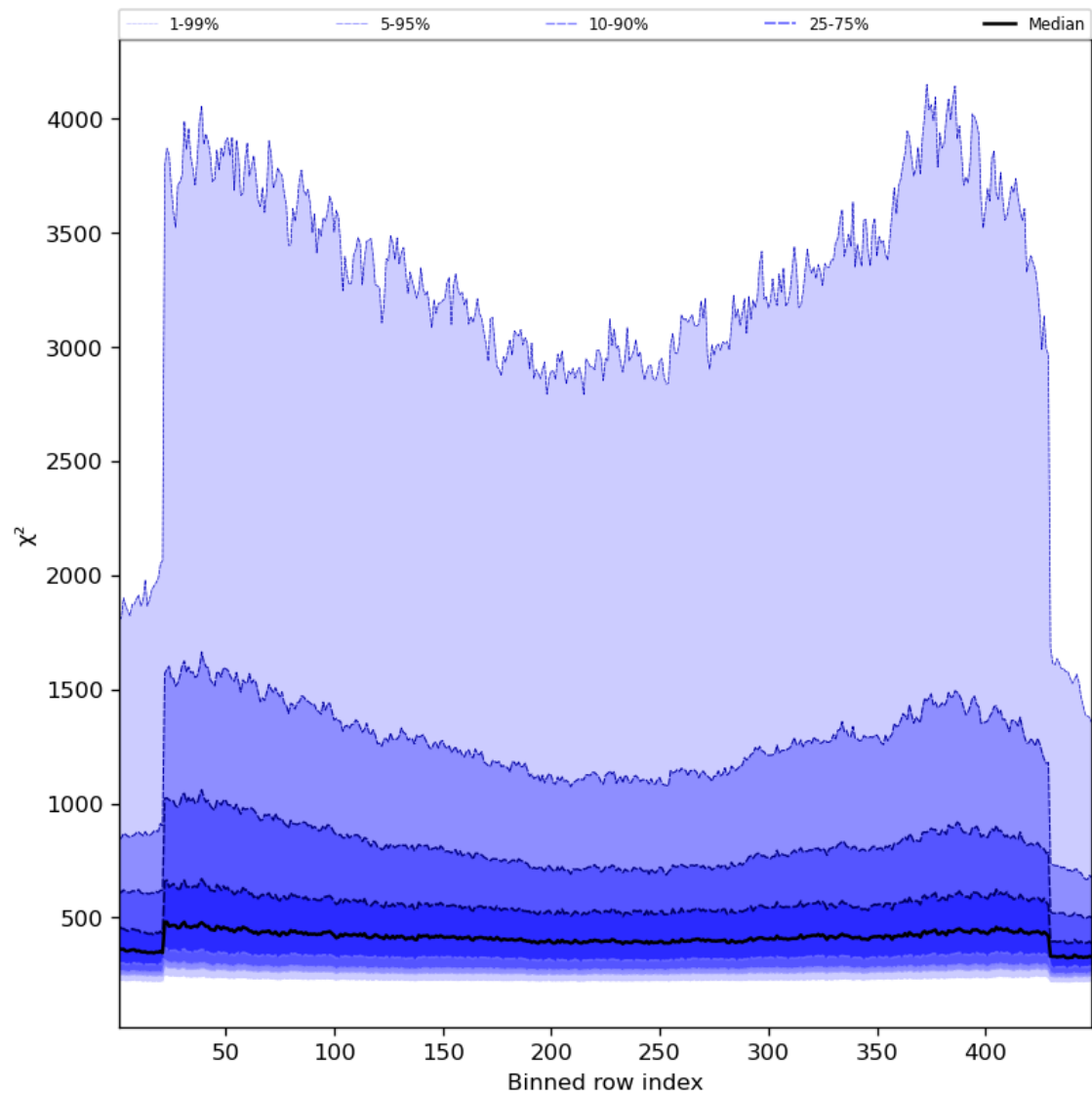
Figure 59: Along track statistics of “ \chi^2 ” for 2024-05-12 to 2024-05-14
