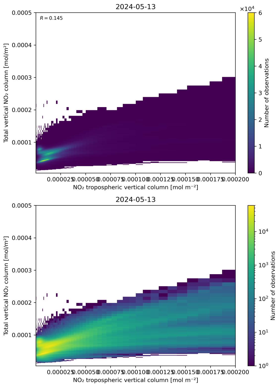
Figure 128: Scatter density plot of “NO 2 tropospheric vertical column” against “Total vertical NO 2 column” for 2024-05-12 to 2024-05-14.
