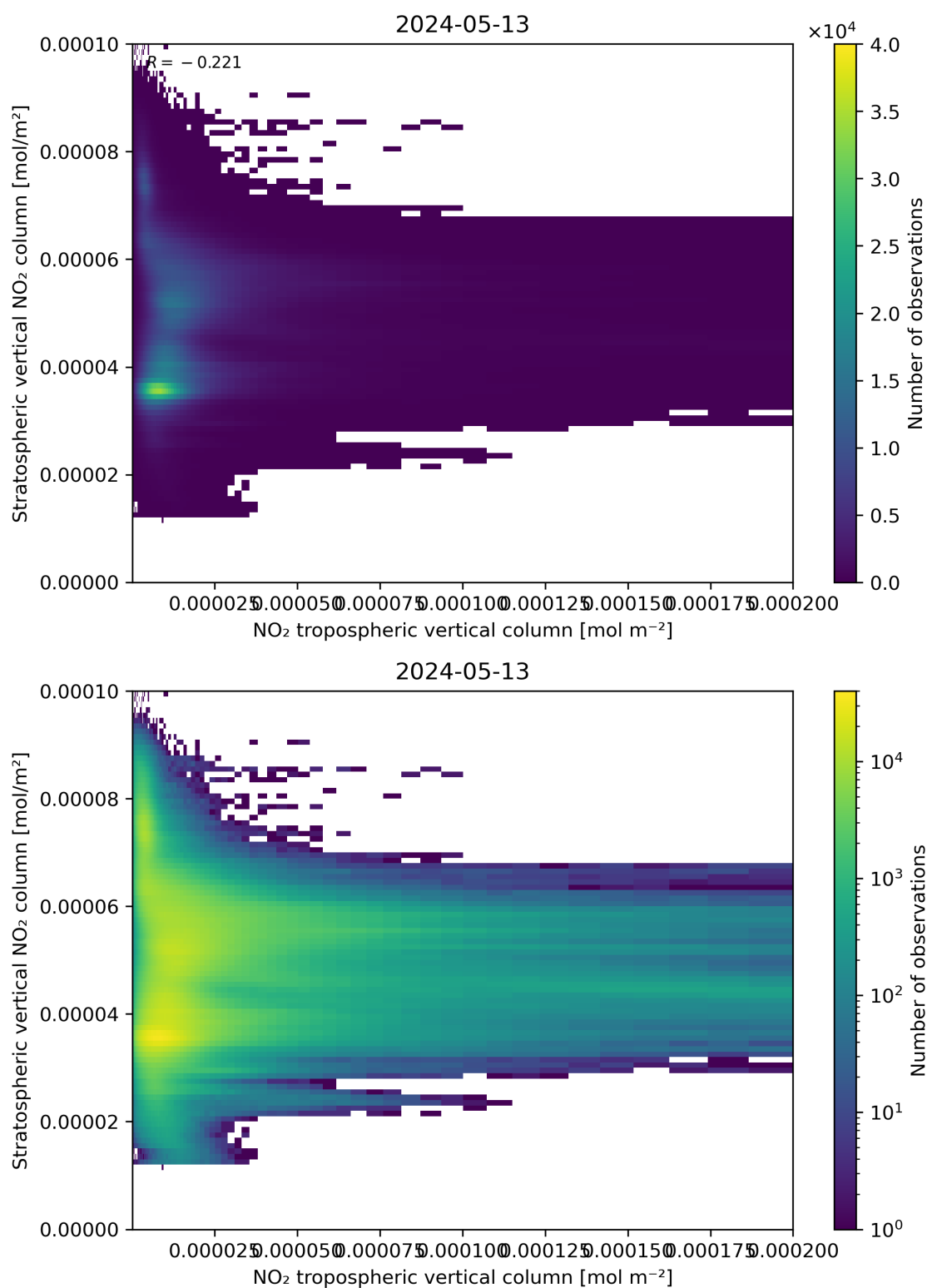
Figure 125: Scatter density plot of “NO 2 tropospheric vertical column” against “Stratospheric vertical NO 2 column” for 2024-05-12 to 2024-05-14.
