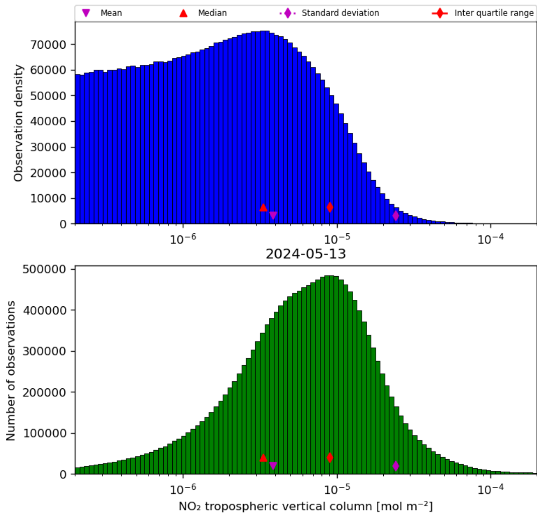
Figure 29: Histogram of “NO 2 tropospheric vertical column” for 2024-05-12 to 2024-05-14
