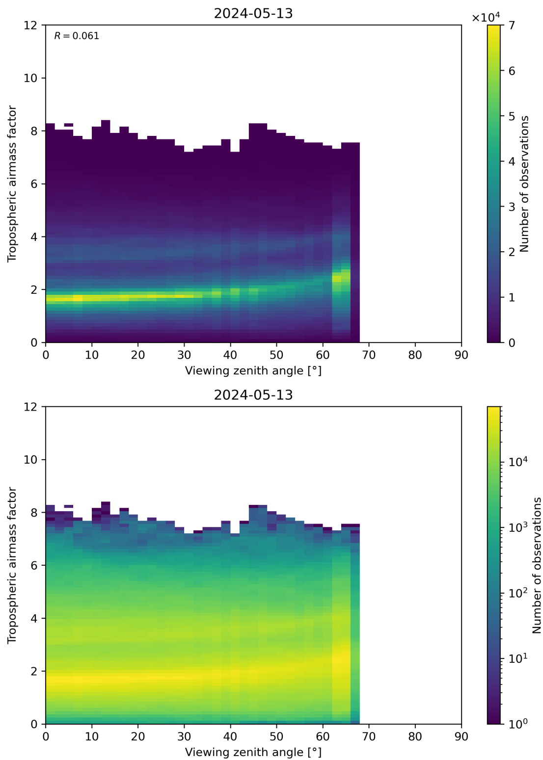
Figure 161: Scatter density plot of “Viewing zenith angle” against “Tropospheric airmass factor” for 2024-05-12 to 2024-05-14.
