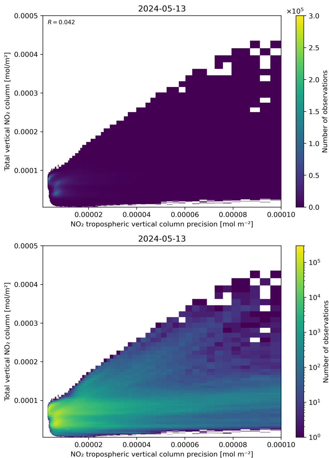
Figure 138: Scatter density plot of “NO 2 tropospheric vertical column precision” against “Total vertical NO 2 column” for 2024-05-12 to 2024-05-14.
