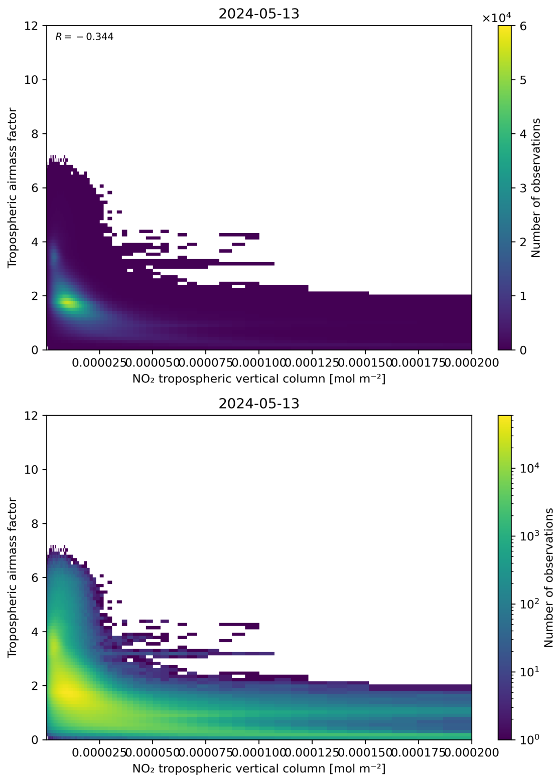
Figure 123: Scatter density plot of “NO 2 tropospheric vertical column” against “Tropospheric airmass factor” for 2024-05-12 to 2024-05-14.
