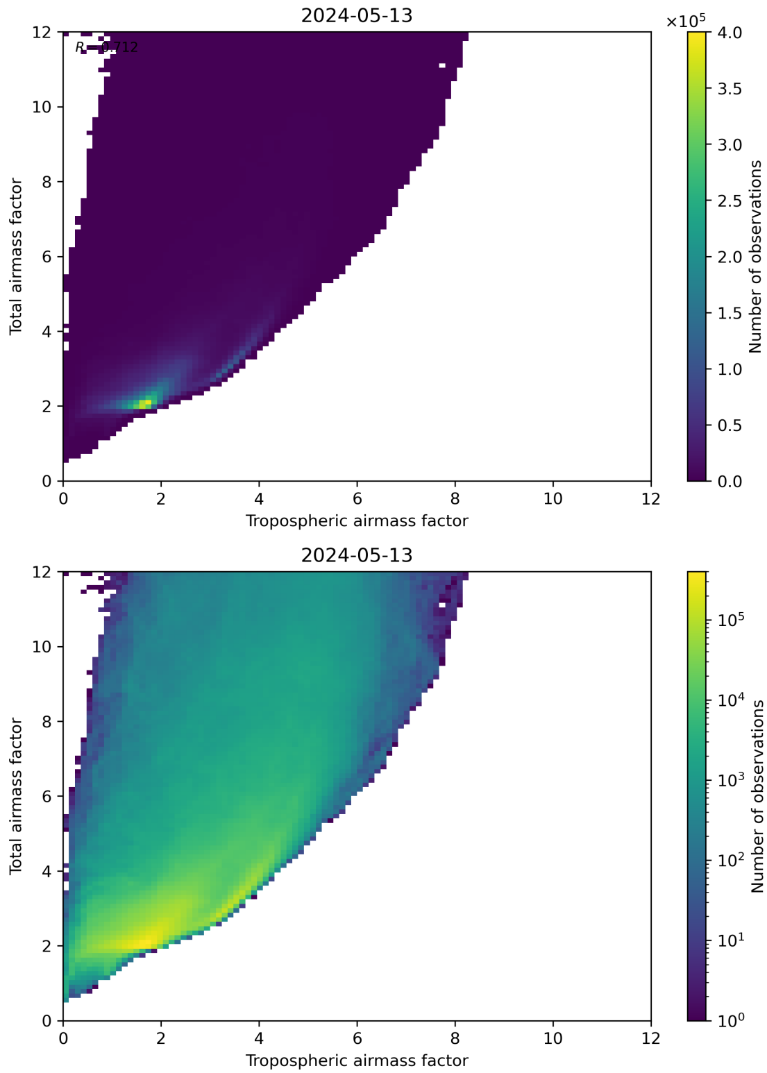
Figure 72: Scatter density plot of “Tropospheric airmass factor” against “Total airmass factor” for 2024-05-12 to 2024-05-14.
