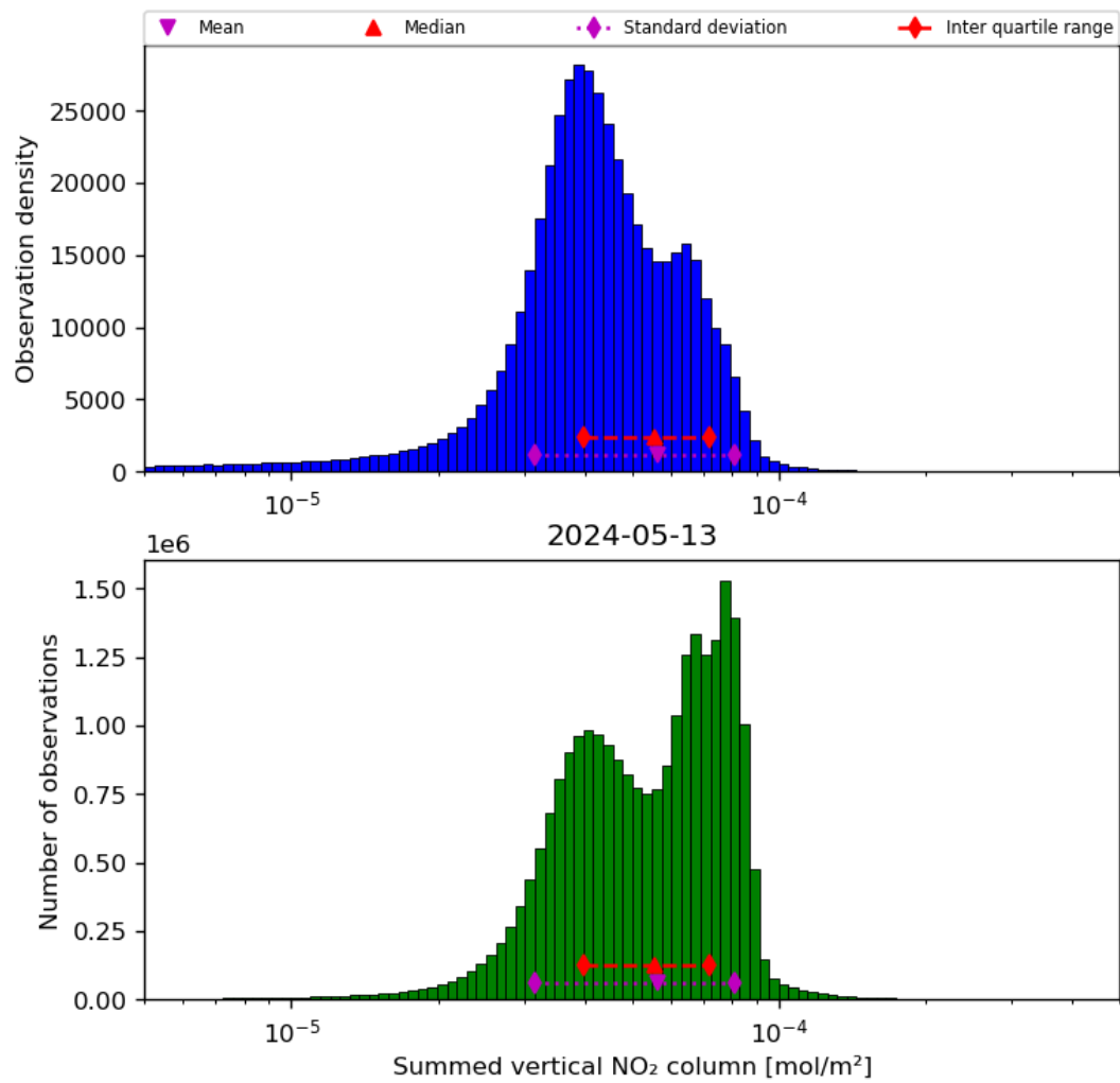
Figure 40: Histogram of “Summed vertical NO 2 column” for 2024-05-12 to 2024-05-14
