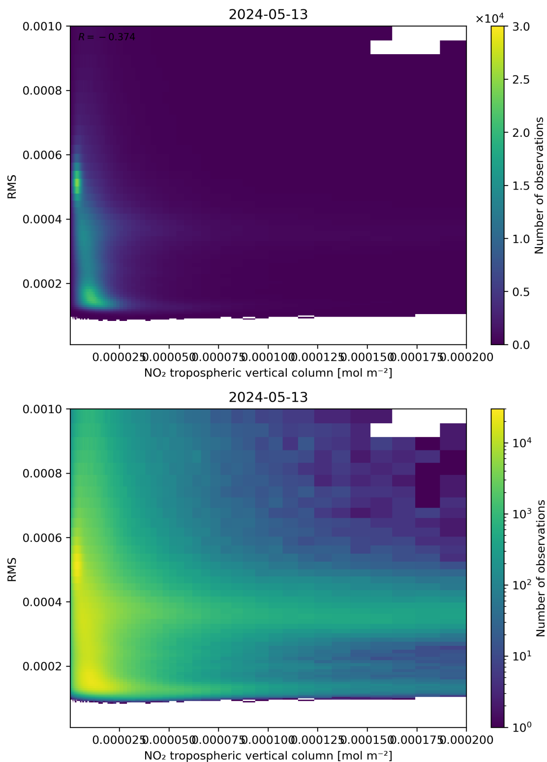
Figure 142: Scatter density plot of “NO 2 tropospheric vertical column” against “RMS” for 2024-05-12 to 2024-05-14.
