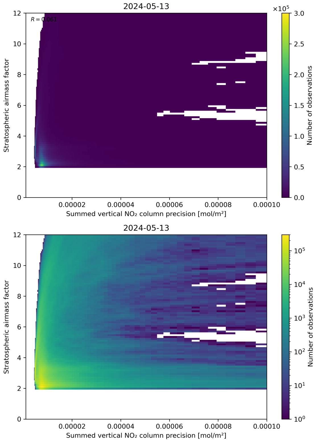
Figure 106: Scatter density plot of “Summed vertical NO 2 column precision” against “Stratospheric airmass factor” for 2024-05-12 to 2024-05-14.
