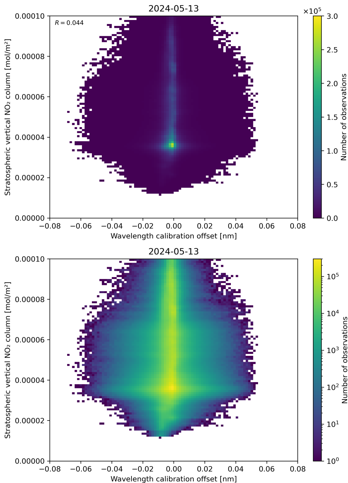
Figure 176: Scatter density plot of “Wavelength calibration offset” against “Stratospheric vertical NO 2 column” for 2024-05-12 to 2024-05-14.
