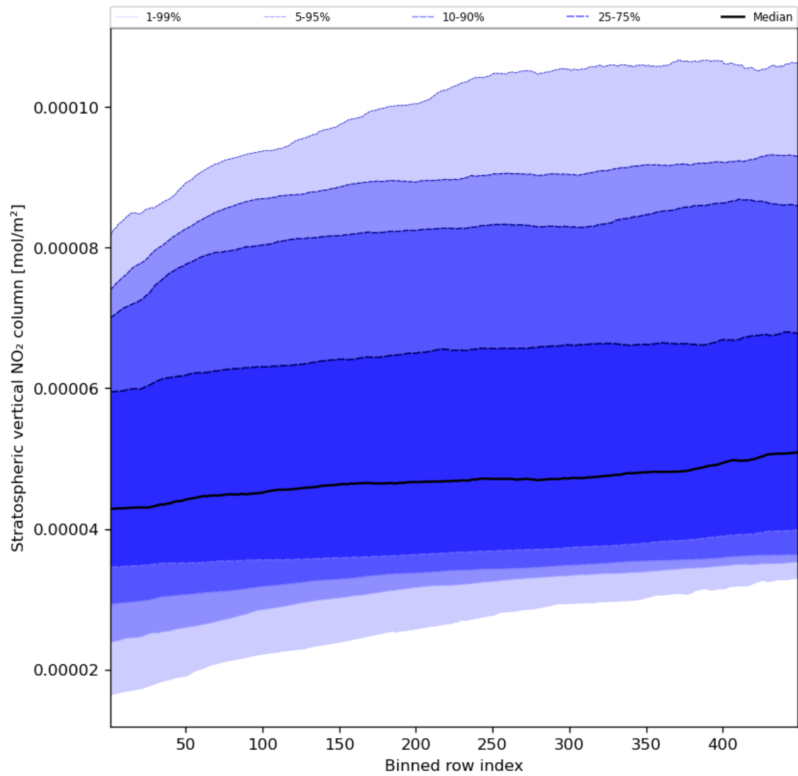
Figure 53: Along track statistics of “Stratospheric vertical NO 2 column” for 2024-05-12 to 2024-05-14
