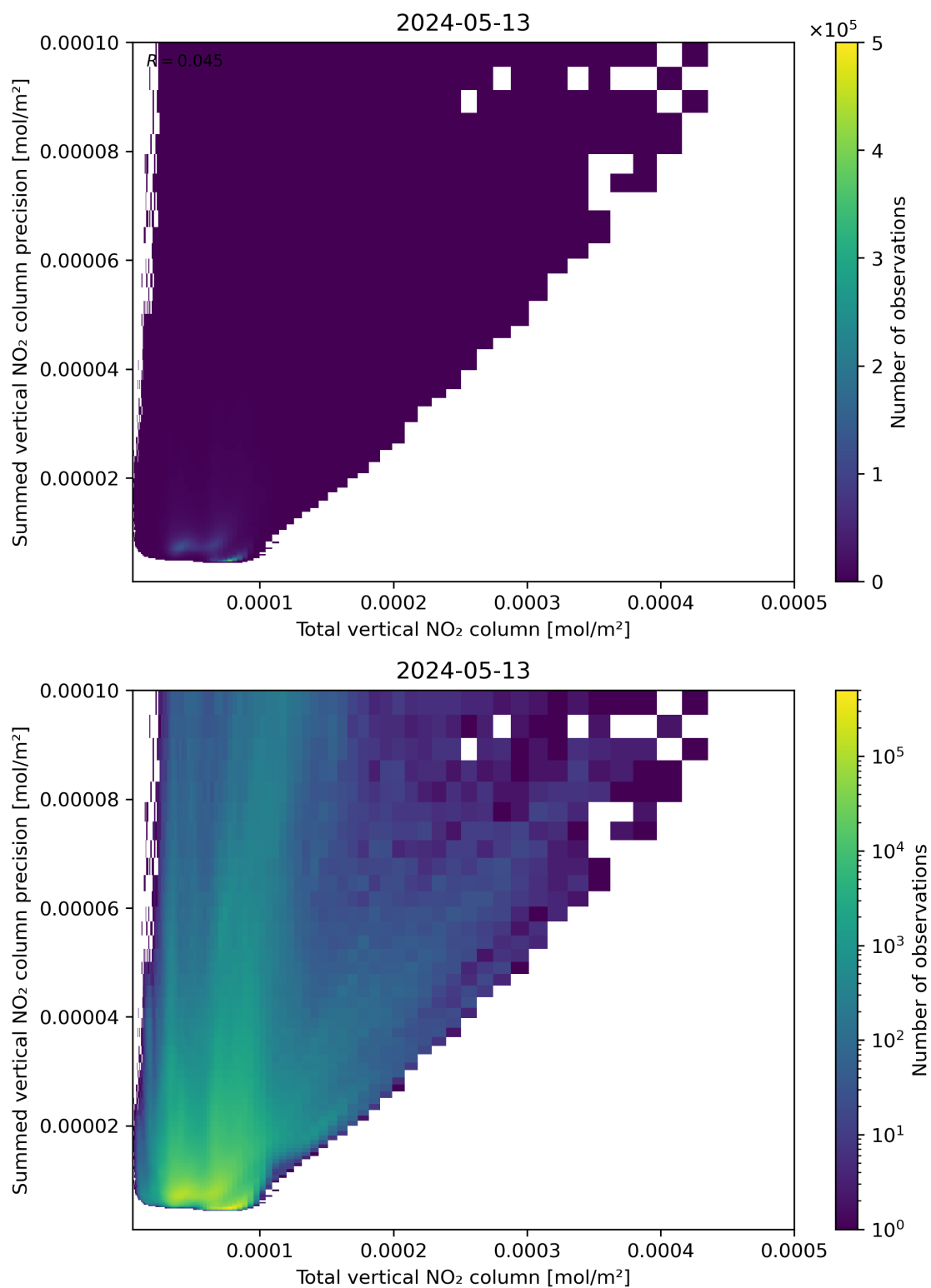
Figure 113: Scatter density plot of “Total vertical NO 2 column” against “Summed vertical NO 2 column precision” for 2024-05-12 to 2024-05-14.
