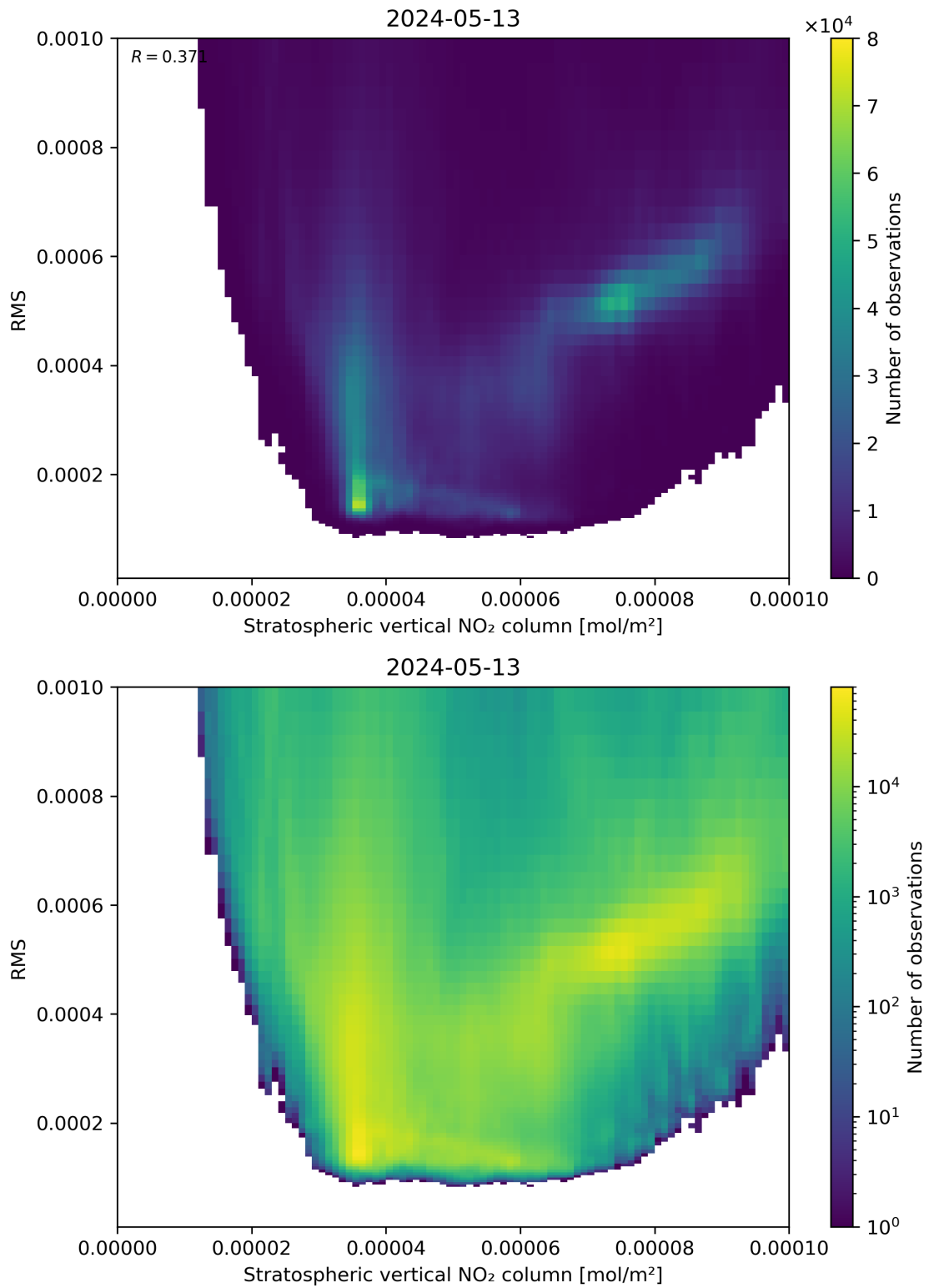
Figure 102: Scatter density plot of “Stratospheric vertical NO 2 column” against “RMS” for 2024-05-12 to 2024-05-14.
