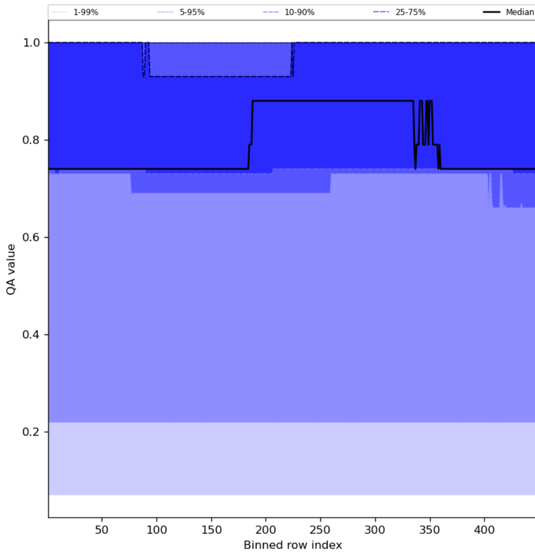
Figure 45: Along track statistics of “QA value” for 2024-05-12 to 2024-05-14
