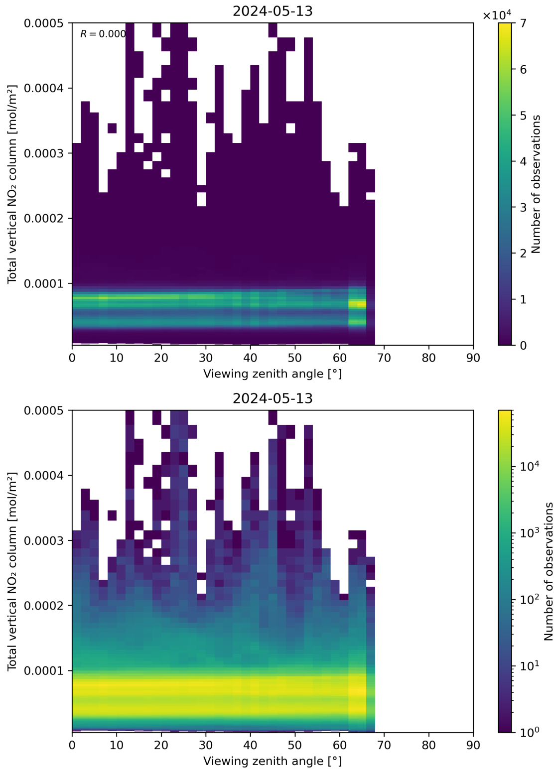
Figure 167: Scatter density plot of “Viewing zenith angle” against “Total vertical NO 2 column” for 2024-05-12 to 2024-05-14.
