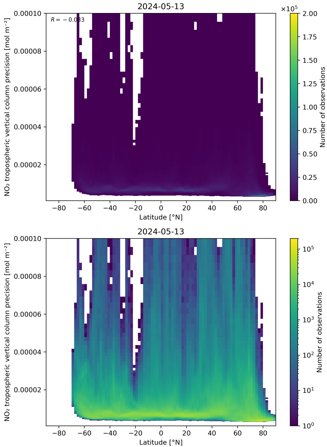
Figure 93: Scatter density plot of “Latitude” against “NO 2 tropospheric vertical column precision” for 2024-05-12 to 2024-05-14.
