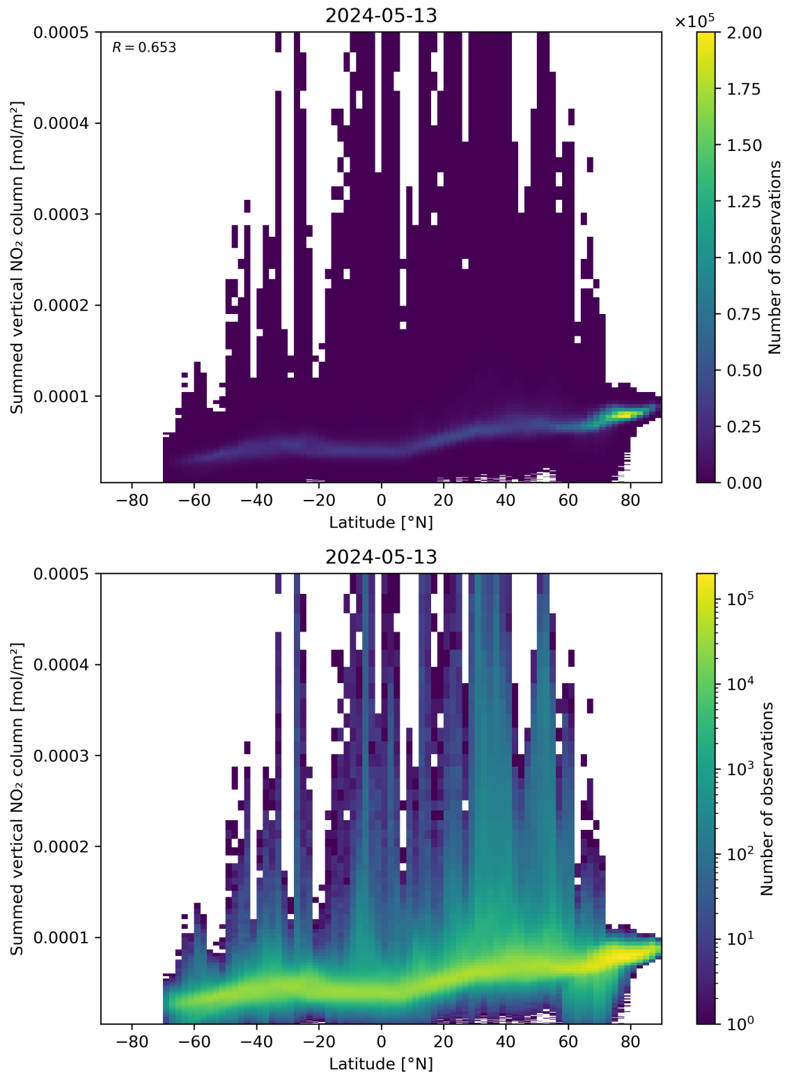
Figure 88: Scatter density plot of “Latitude” against “Summed vertical NO 2 column” for 2024-05-12 to 2024-05-14.
