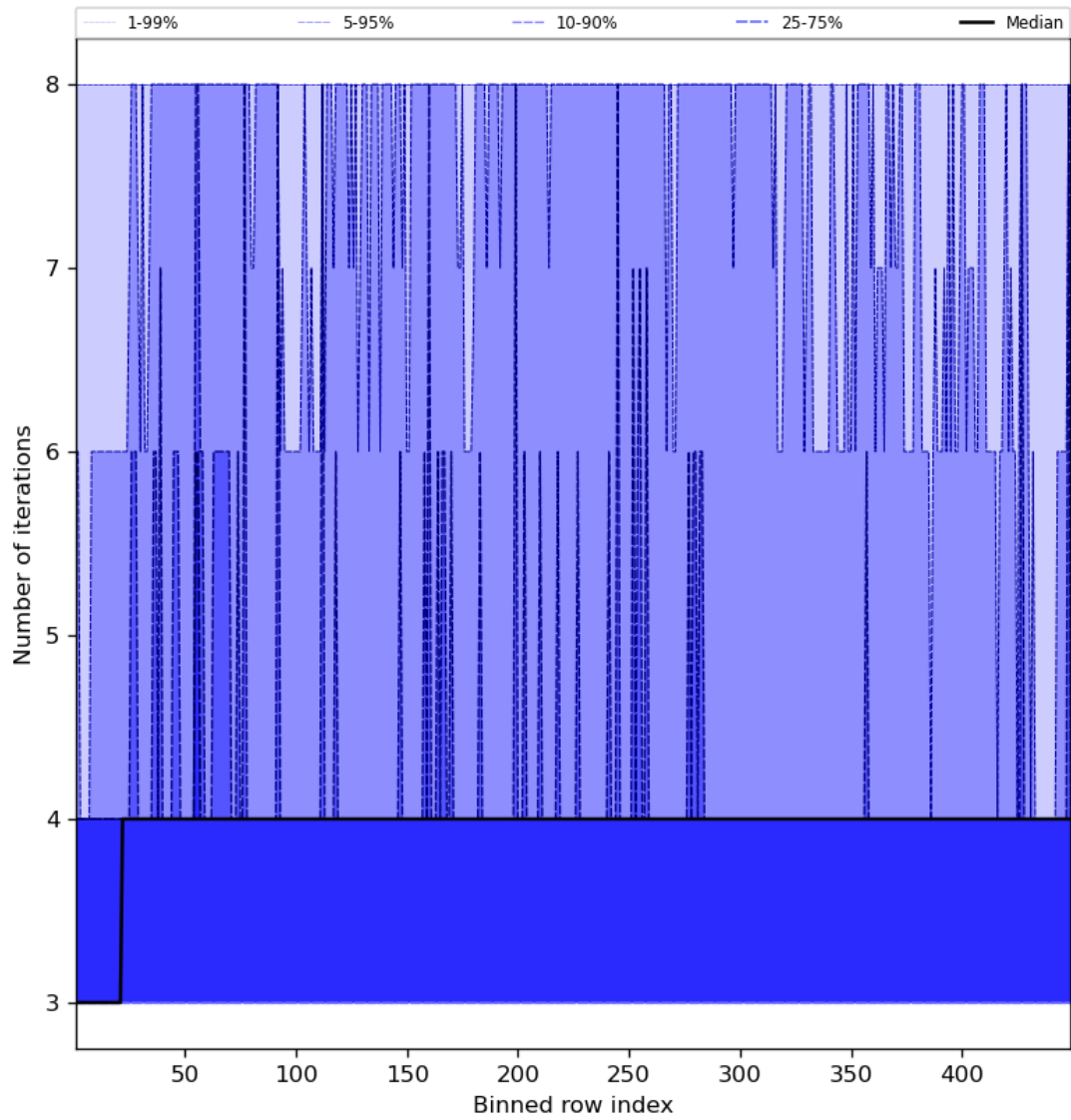
Figure 51: Along track statistics of “Number of iterations” for 2024-05-12 to 2024-05-14
