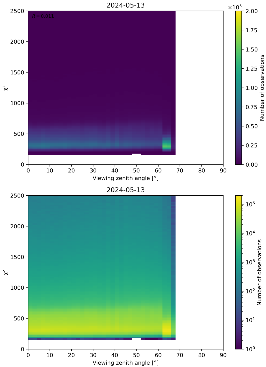
Figure 162: Scatter density plot of “Viewing zenith angle” against “ \chi^2 ” for 2024-05-12 to 2024-05-14.
