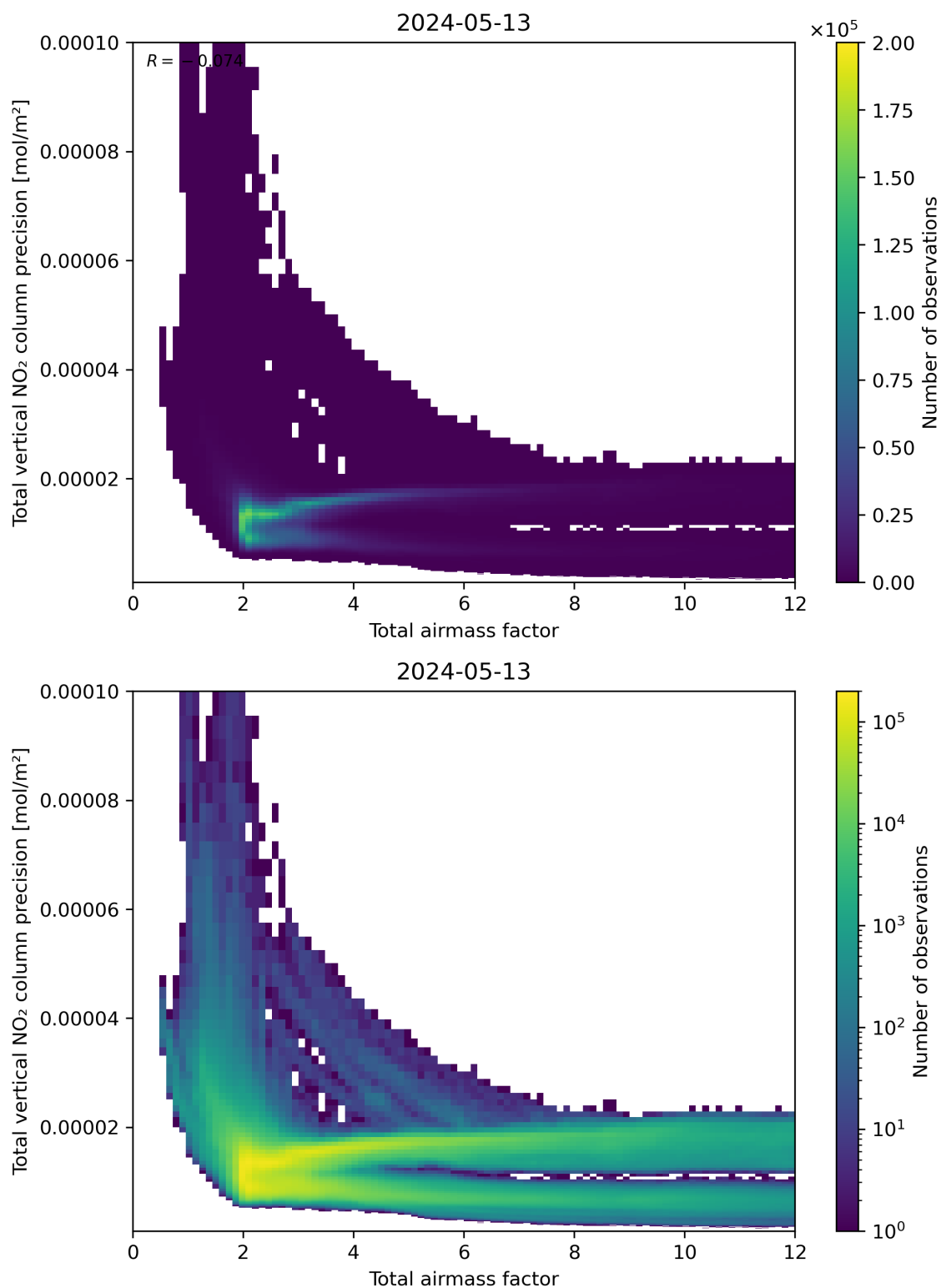
Figure 68: Scatter density plot of “Total airmass factor” against “Total vertical NO 2 column precision” for 2024-05-12 to 2024-05-14.
