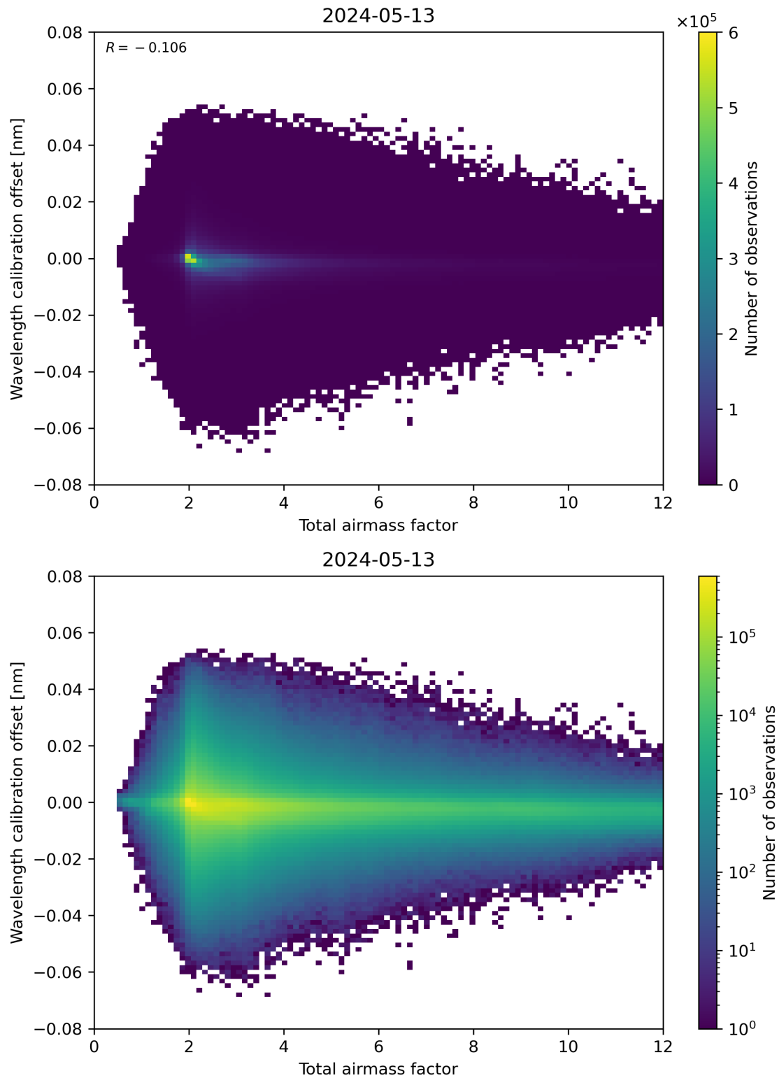
Figure 70: Scatter density plot of “Total airmass factor” against “Wavelength calibration offset” for 2024-05-12 to 2024-05-14.
