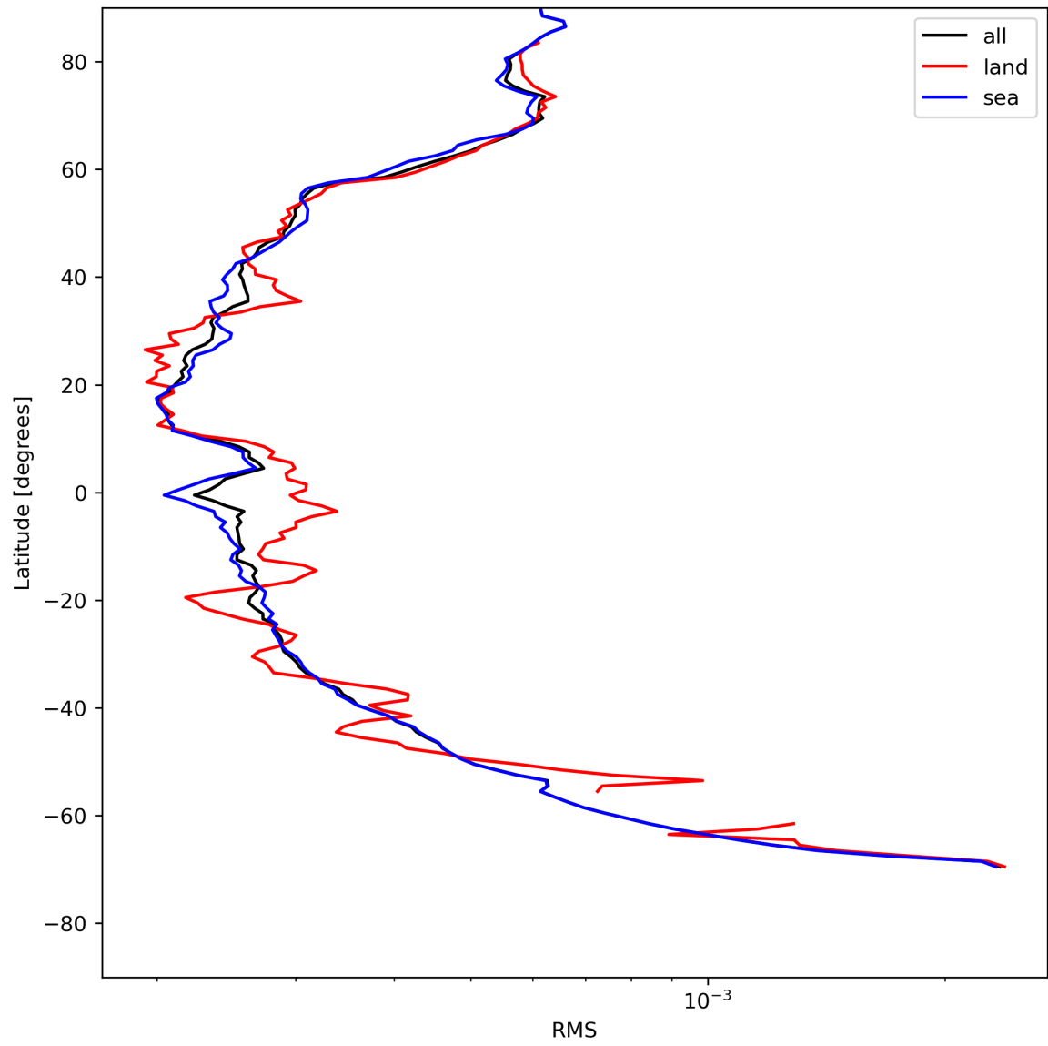
Figure 26: Zonal average of “RMS” for 2024-05-12 to 2024-05-14.
