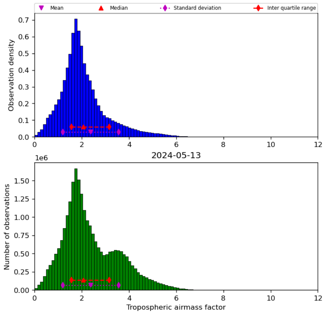
Figure 31: Histogram of “Tropospheric airmass factor” for 2024-05-12 to 2024-05-14
