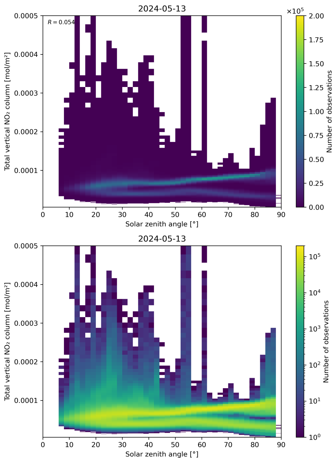
Figure 153: Scatter density plot of “Solar zenith angle” against “Total vertical NO 2 column” for 2024-05-12 to 2024-05-14.
