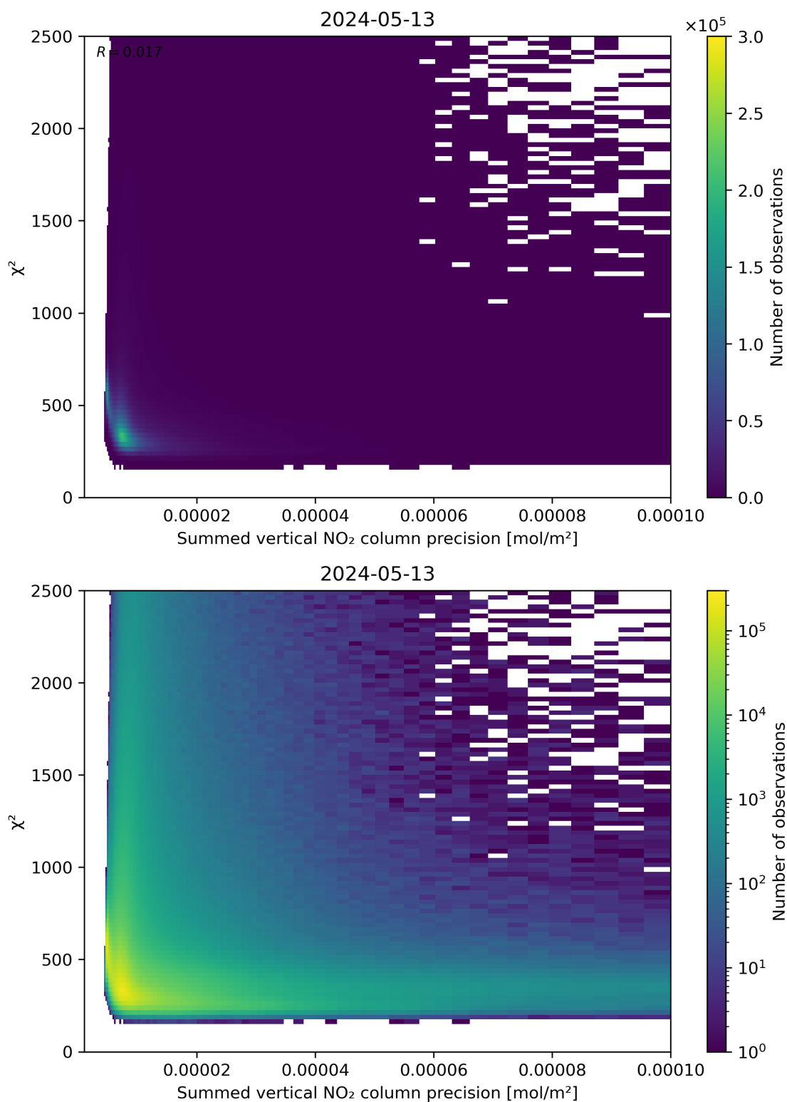
Figure 107: Scatter density plot of “Summed vertical NO 2 column precision” against “ \chi^2 ” for 2024-05-12 to 2024-05-14.
