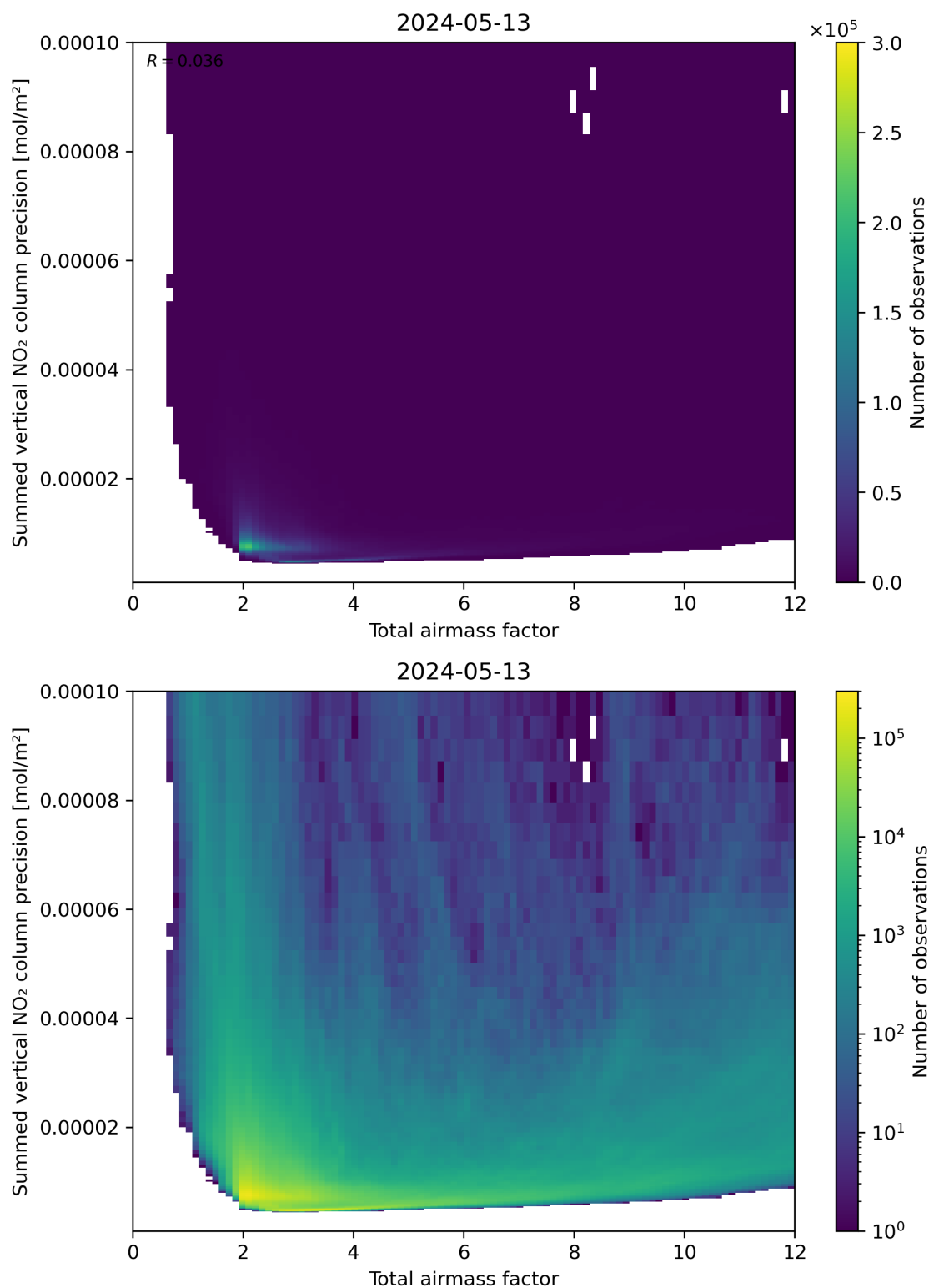
Figure 66: Scatter density plot of “Total airmass factor” against “Summed vertical NO 2 column precision” for 2024-05-12 to 2024-05-14.
