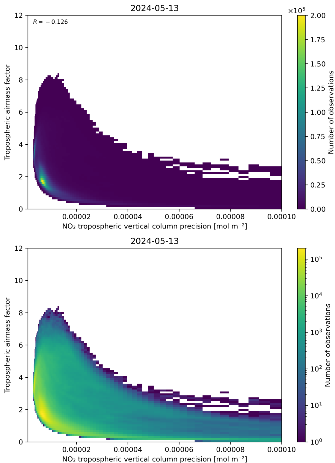
Figure 133: Scatter density plot of “NO 2 tropospheric vertical column precision” against “Tropospheric airmass factor” for 2024-05-12 to 2024-05-14.
