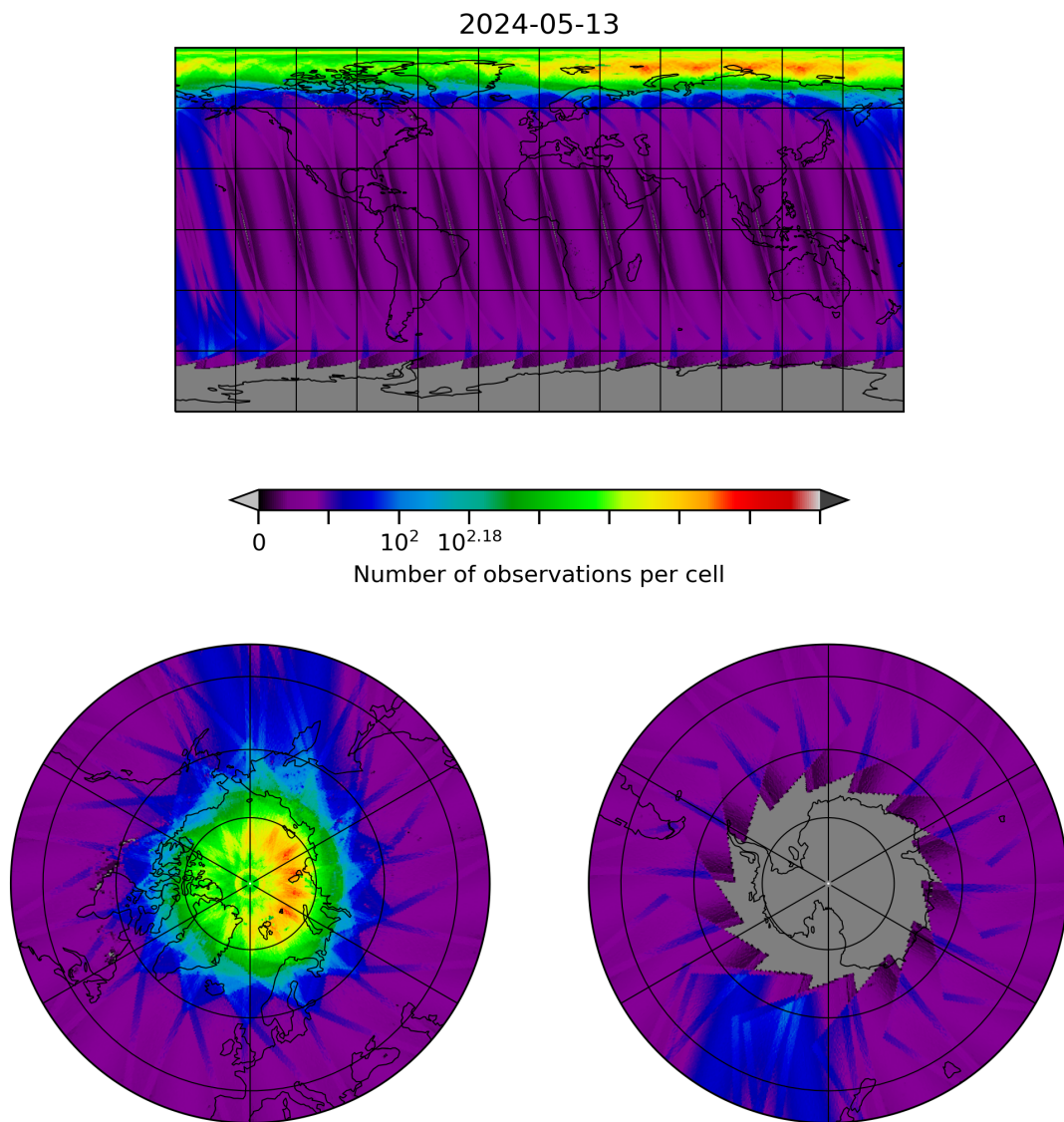
Figure 10: Map of the number of observations for 2024-05-12 to 2024-05-14
