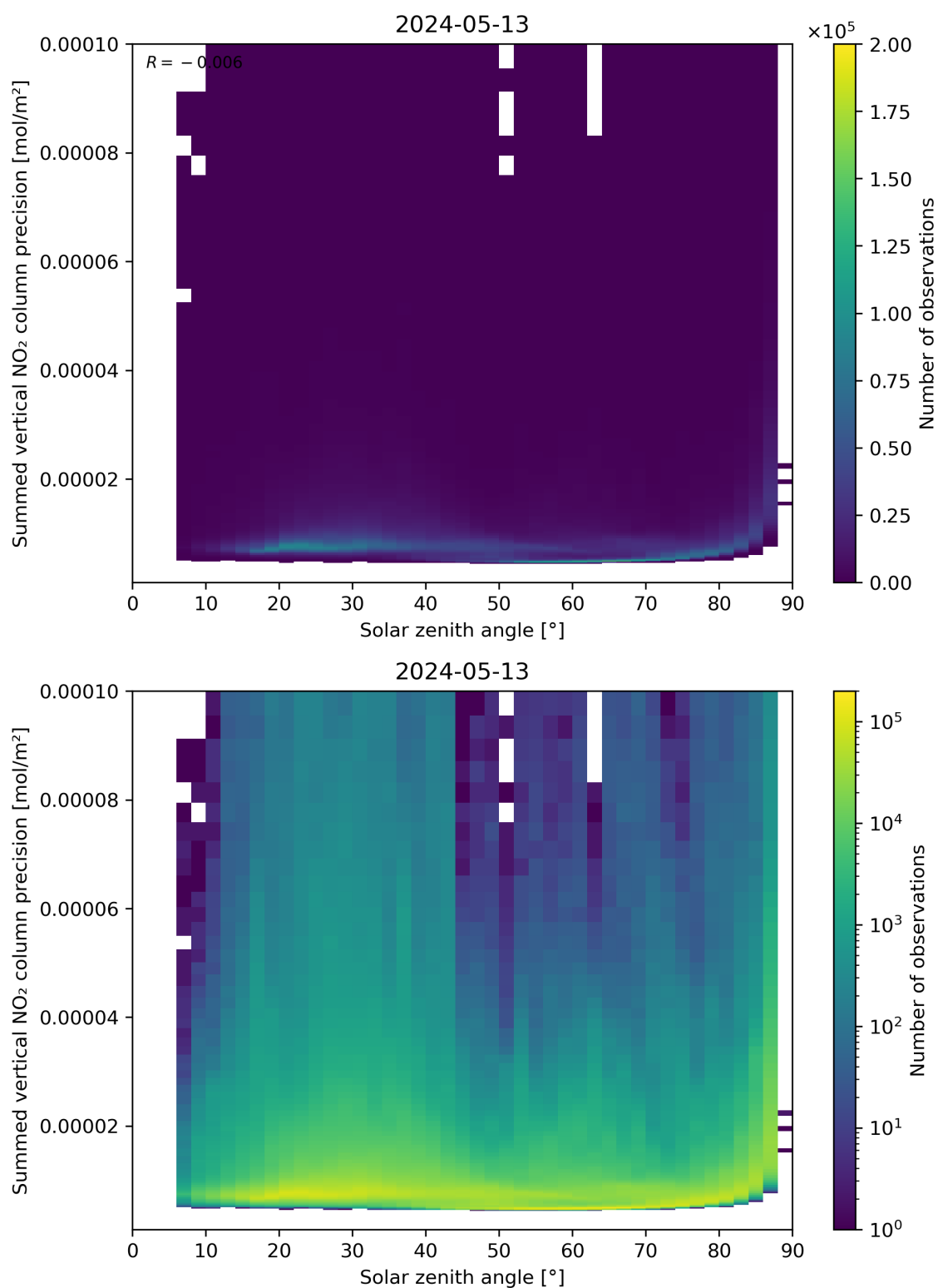
Figure 152: Scatter density plot of “Solar zenith angle” against “Summed vertical NO 2 column precision” for 2024-05-12 to 2024-05-14.
