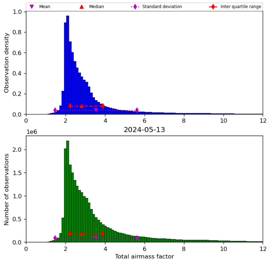
Figure 32: Histogram of “Total airmass factor” for 2024-05-12 to 2024-05-14
