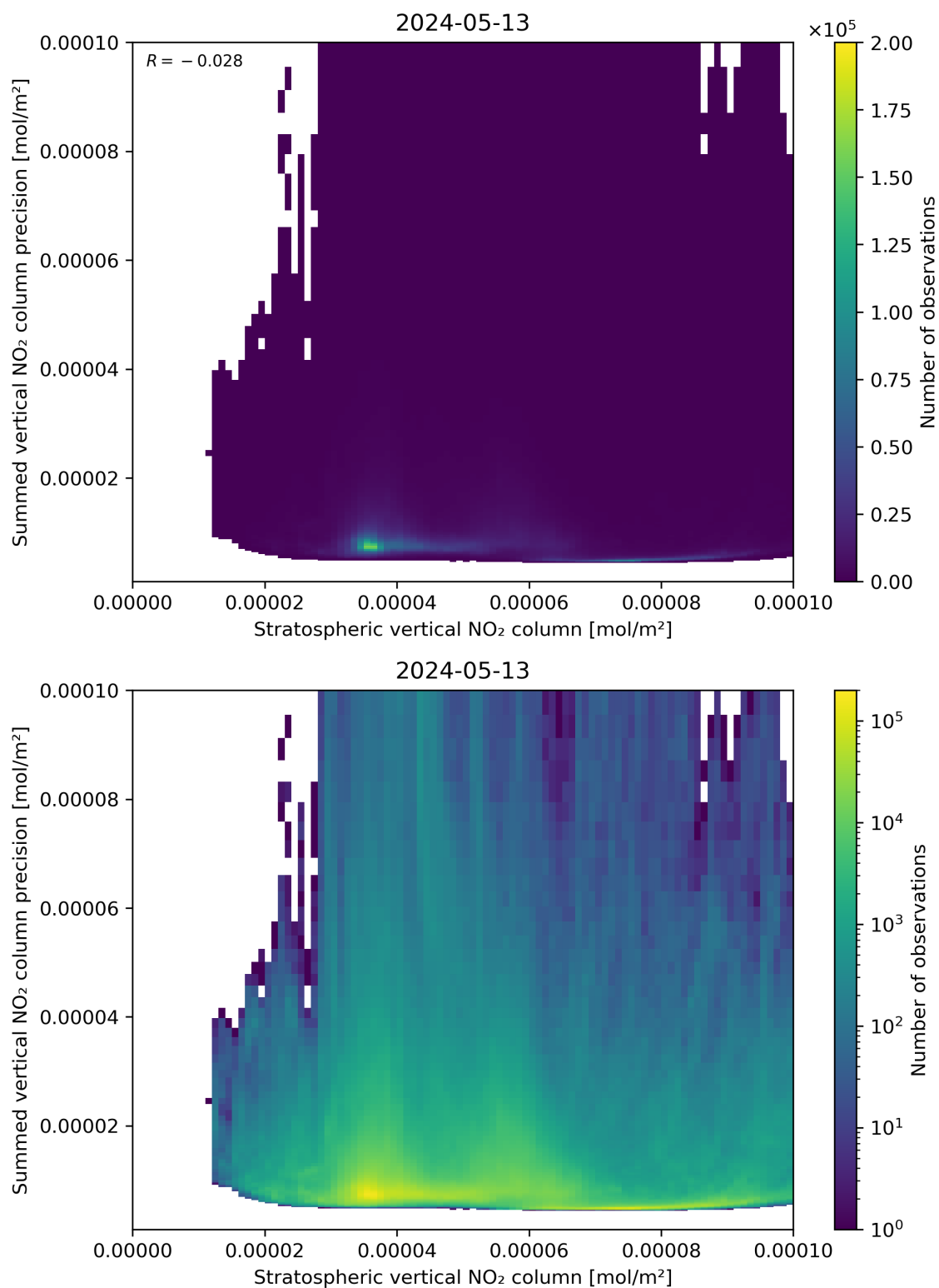
Figure 99: Scatter density plot of “Stratospheric vertical NO 2 column” against “Summed vertical NO 2 column precision” for 2024-05-12 to 2024-05-14.
