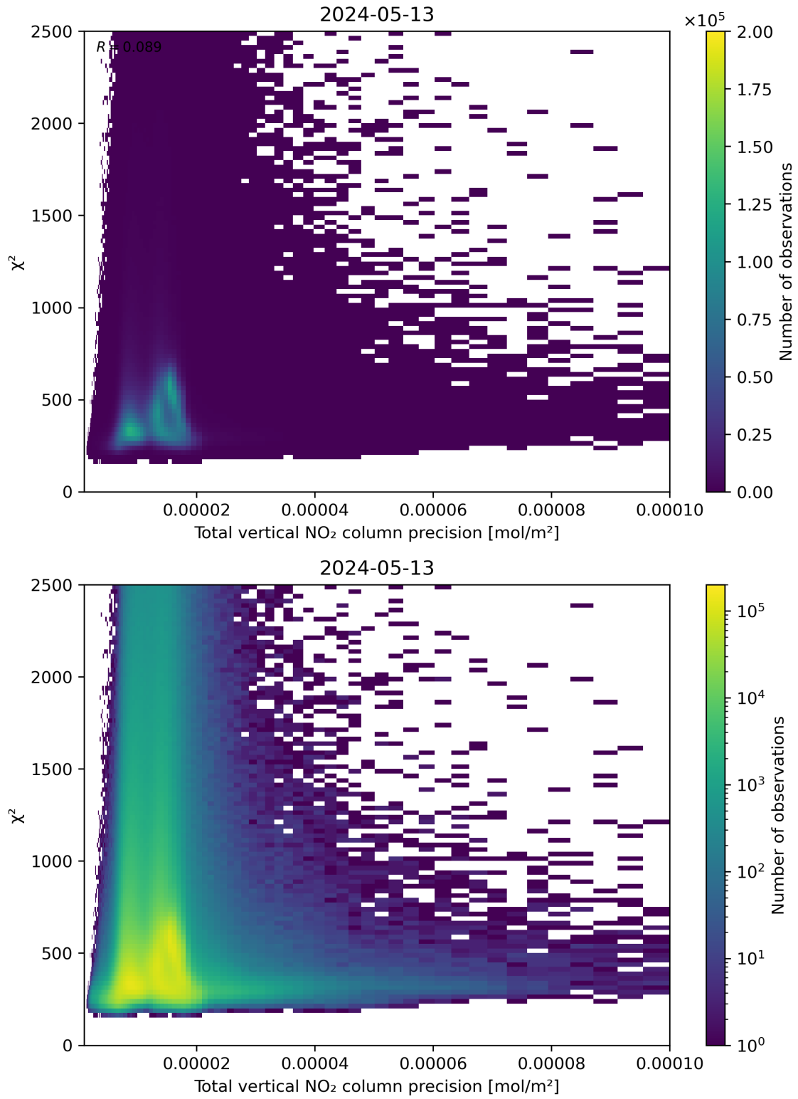
Figure 116: Scatter density plot of “Total vertical NO 2 column precision” against “ \chi^2 ” for 2024-05-12 to 2024-05-14.
