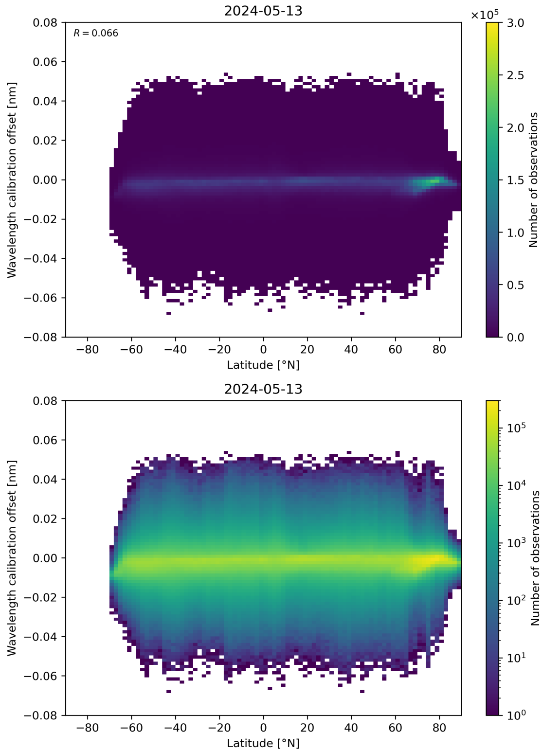
Figure 95: Scatter density plot of “Latitude” against “Wavelength calibration offset” for 2024-05-12 to 2024-05-14.
