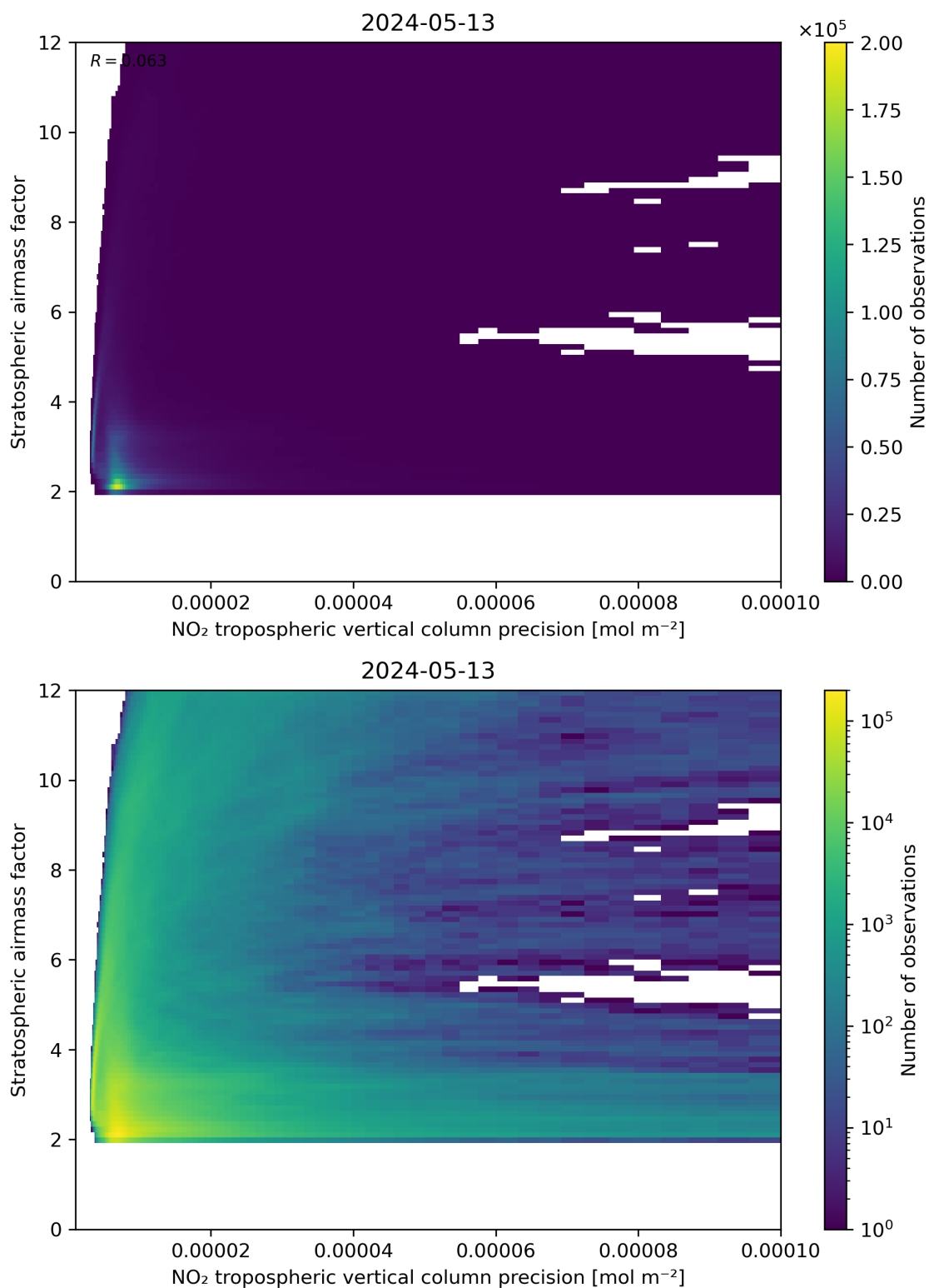
Figure 131: Scatter density plot of “NO 2 tropospheric vertical column precision” against “Stratospheric airmass factor” for 2024-05-12 to 2024-05-14.
