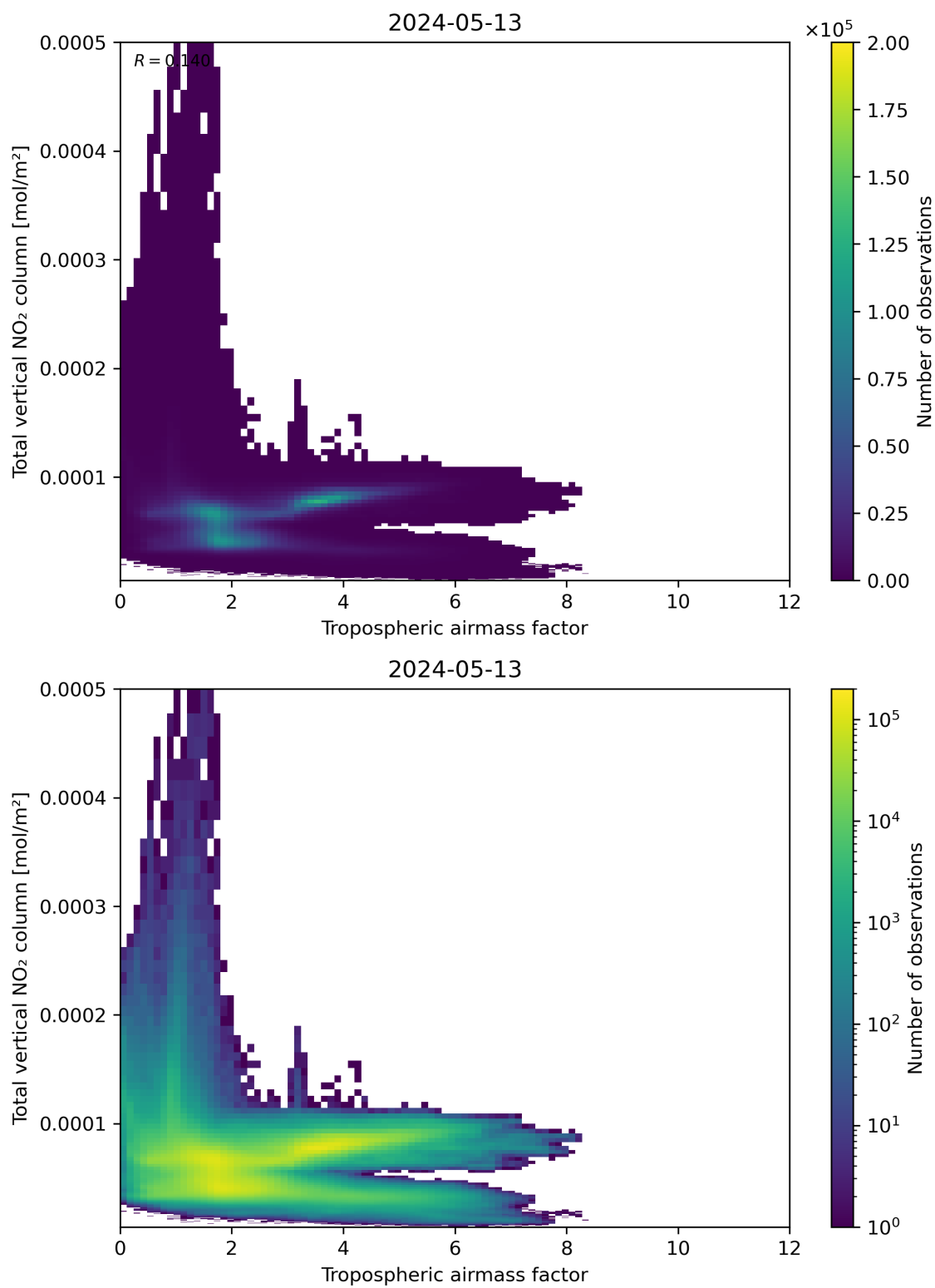
Figure 77: Scatter density plot of “Tropospheric airmass factor” against “Total vertical NO 2 column” for 2024-05-12 to 2024-05-14.
