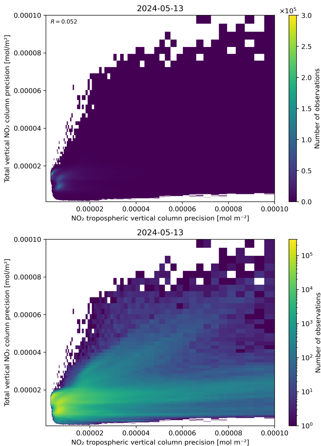
Figure 139: Scatter density plot of “NO 2 tropospheric vertical column precision” against “Total vertical NO 2 column precision” for 2024-05-12 to 2024-05-14.
