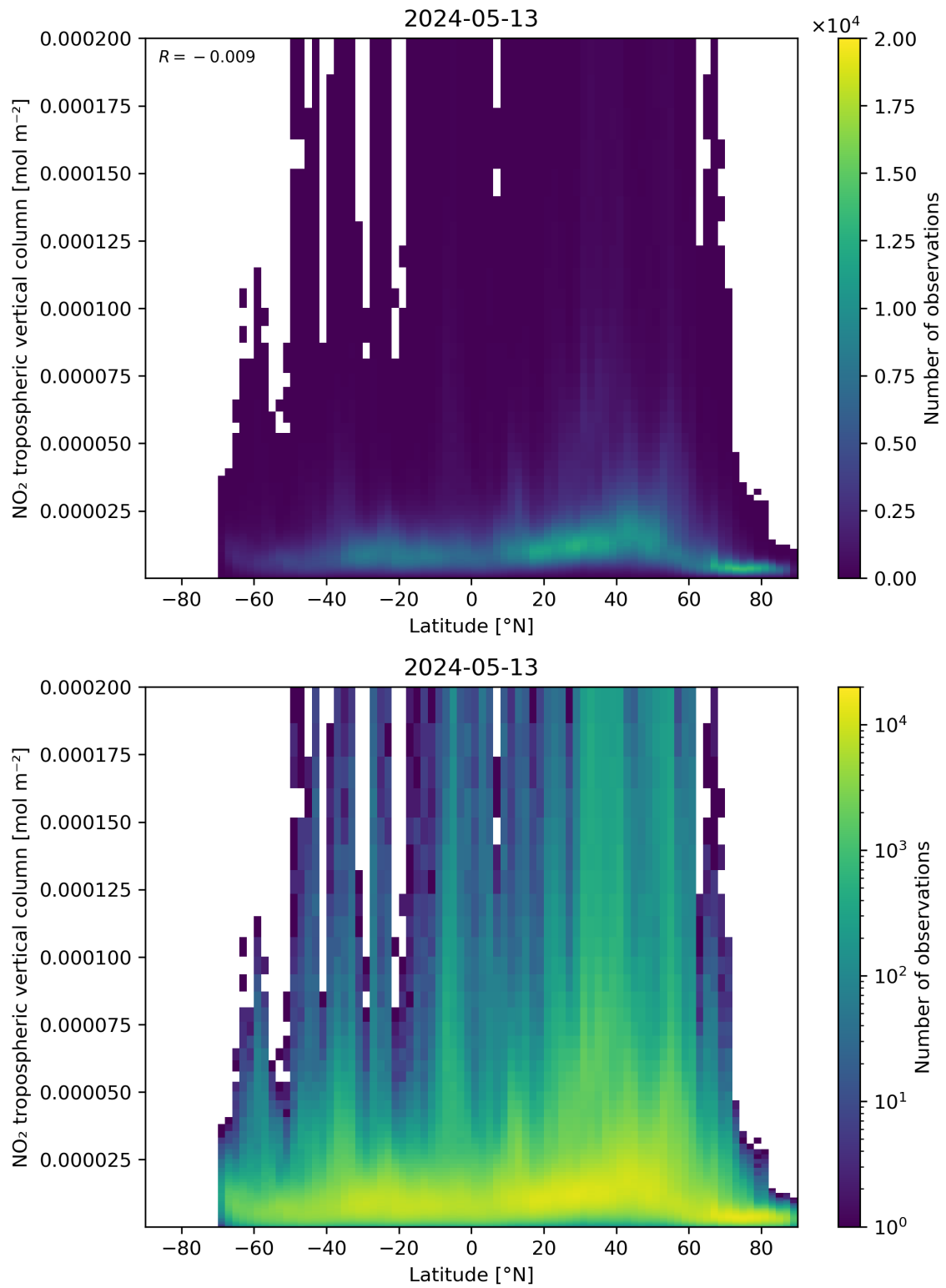
Figure 92: Scatter density plot of “Latitude” against “NO 2 tropospheric vertical column” for 2024-05-12 to 2024-05-14.
