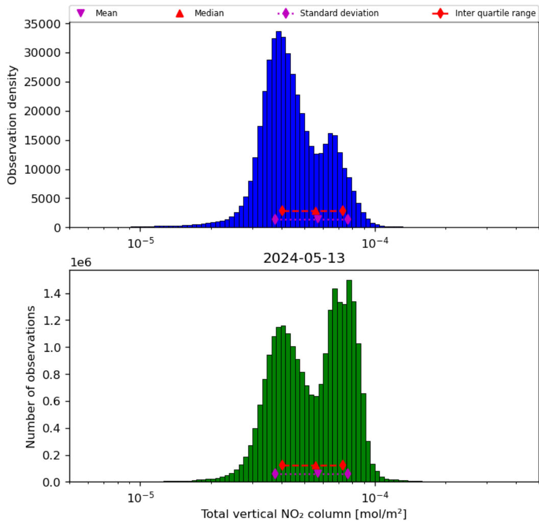
Figure 38: Histogram of “Total vertical NO 2 column” for 2024-05-12 to 2024-05-14
