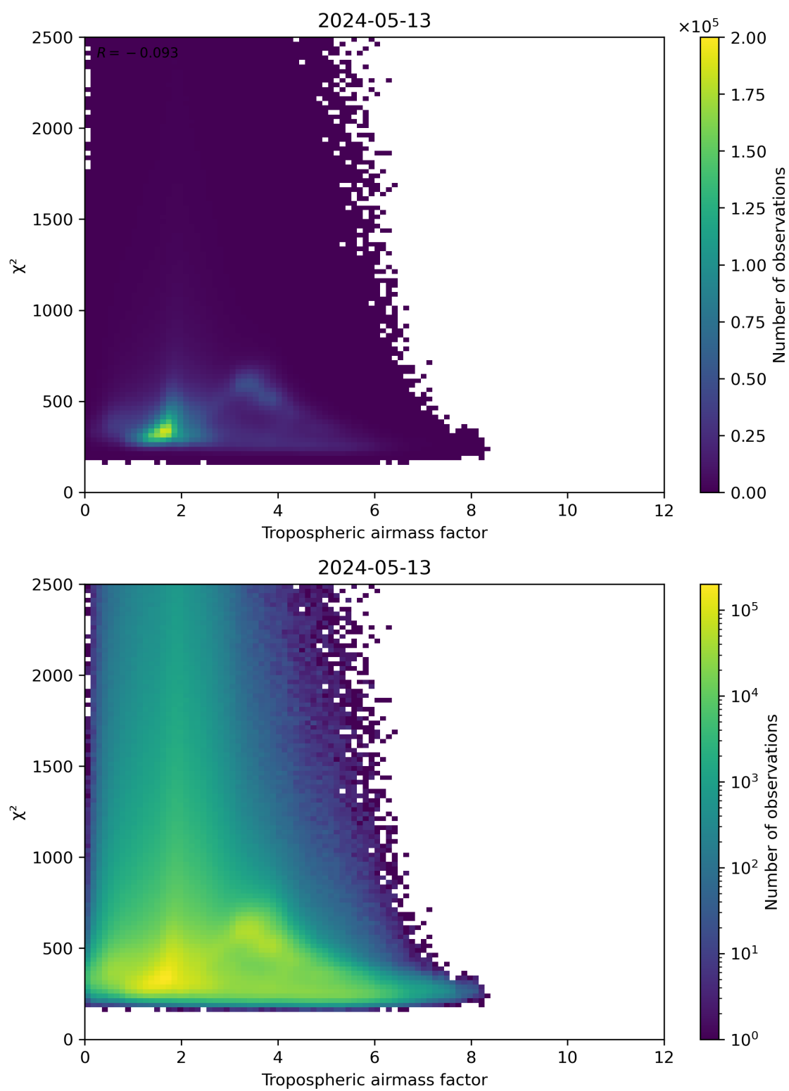
Figure 73: Scatter density plot of “Tropospheric airmass factor” against “ \chi^2 ” for 2024-05-12 to 2024-05-14.
