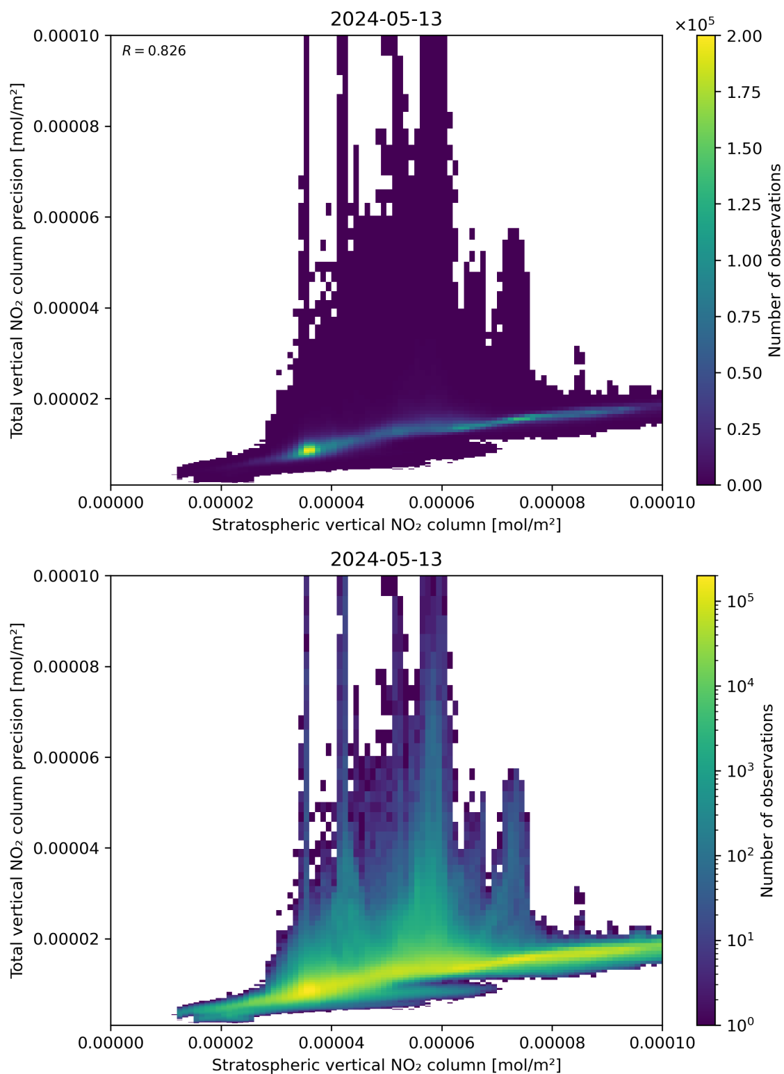
Figure 101: Scatter density plot of “Stratospheric vertical NO 2 column” against “Total vertical NO 2 column precision” for 2024-05-12 to 2024-05-14.
