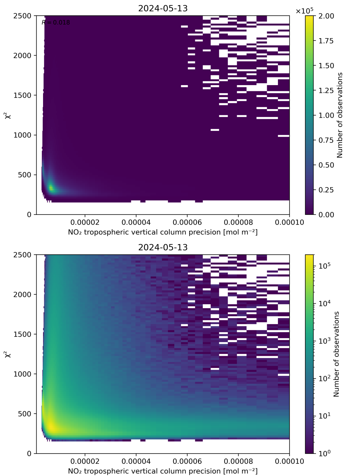
Figure 134: Scatter density plot of “NO 2 tropospheric vertical column precision” against “ \chi^2 ” for 2024-05-12 to 2024-05-14.
