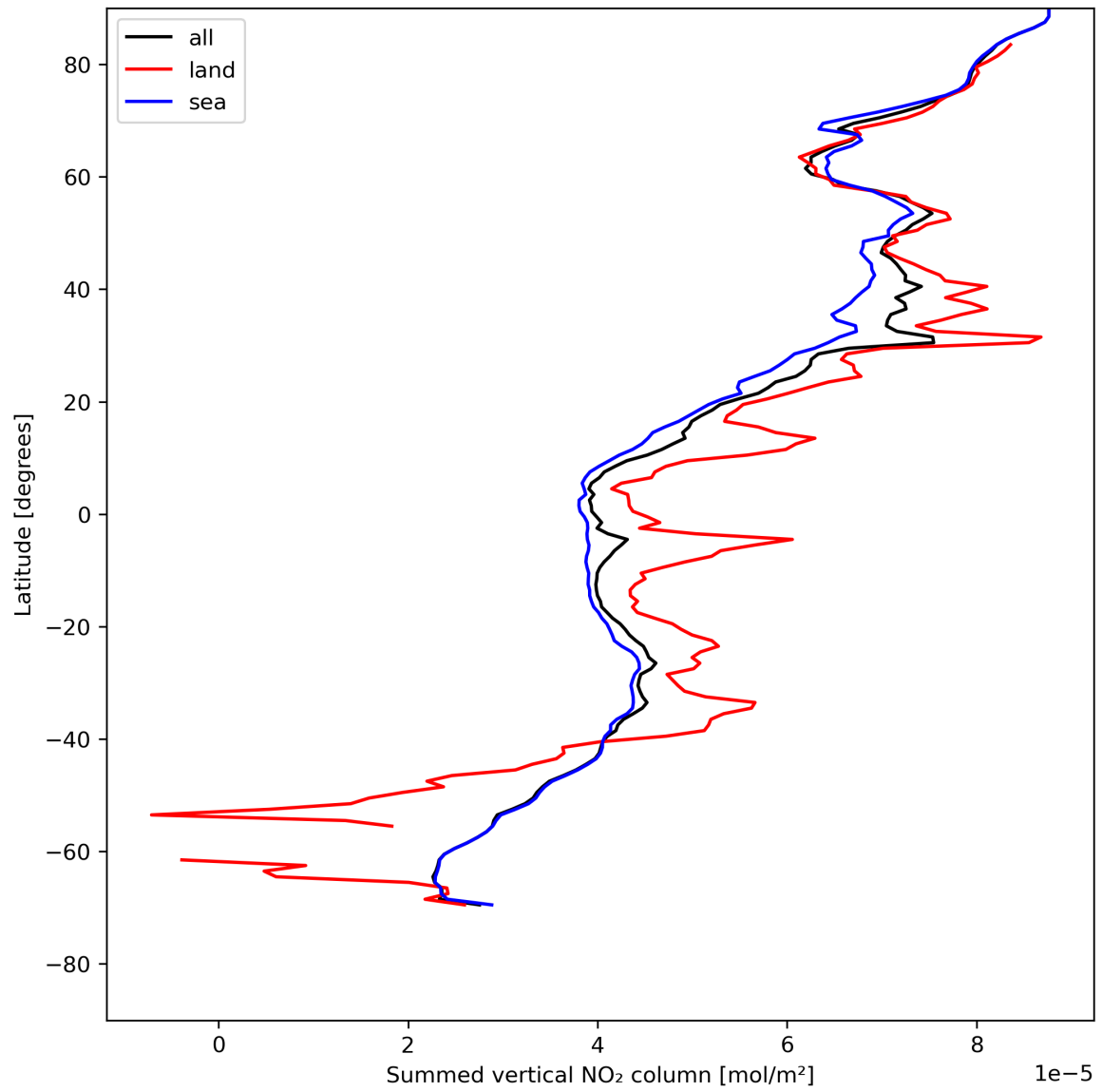
Figure 23: Zonal average of “Summed vertical NO 2 column” for 2024-05-12 to 2024-05-14.
