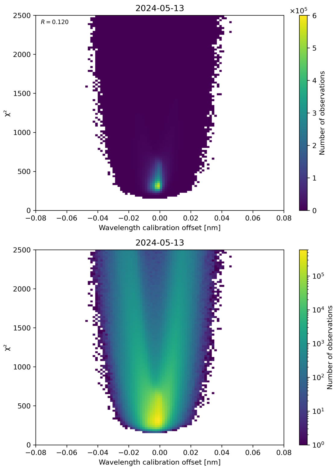
Figure 175: Scatter density plot of “Wavelength calibration offset” against “ \chi^2 ” for 2024-05-12 to 2024-05-14.
