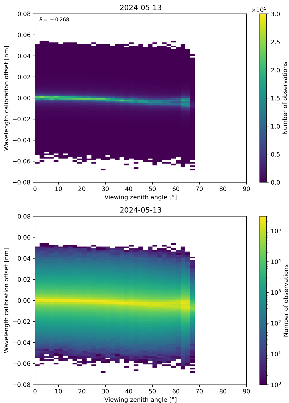
Figure 173: Scatter density plot of “Viewing zenith angle” against “Wavelength calibration offset” for 2024-05-12 to 2024-05-14.
