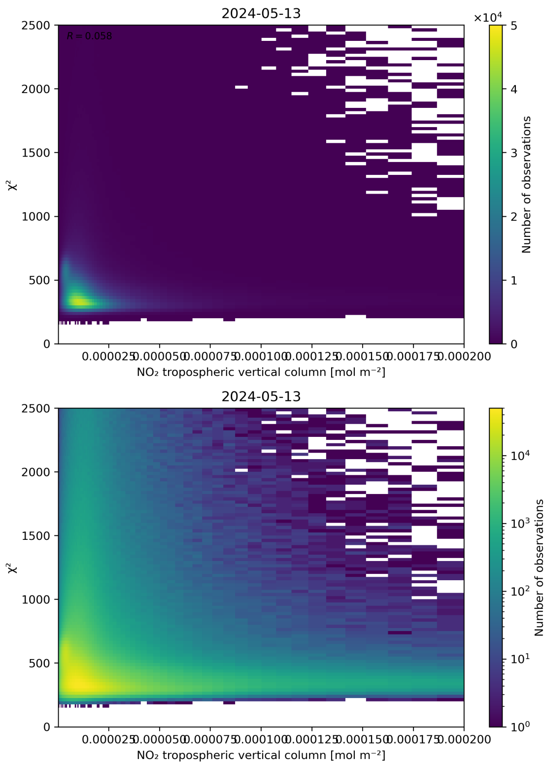
Figure 124: Scatter density plot of “NO 2 tropospheric vertical column” against “ \chi^2 ” for 2024-05-12 to 2024-05-14.
