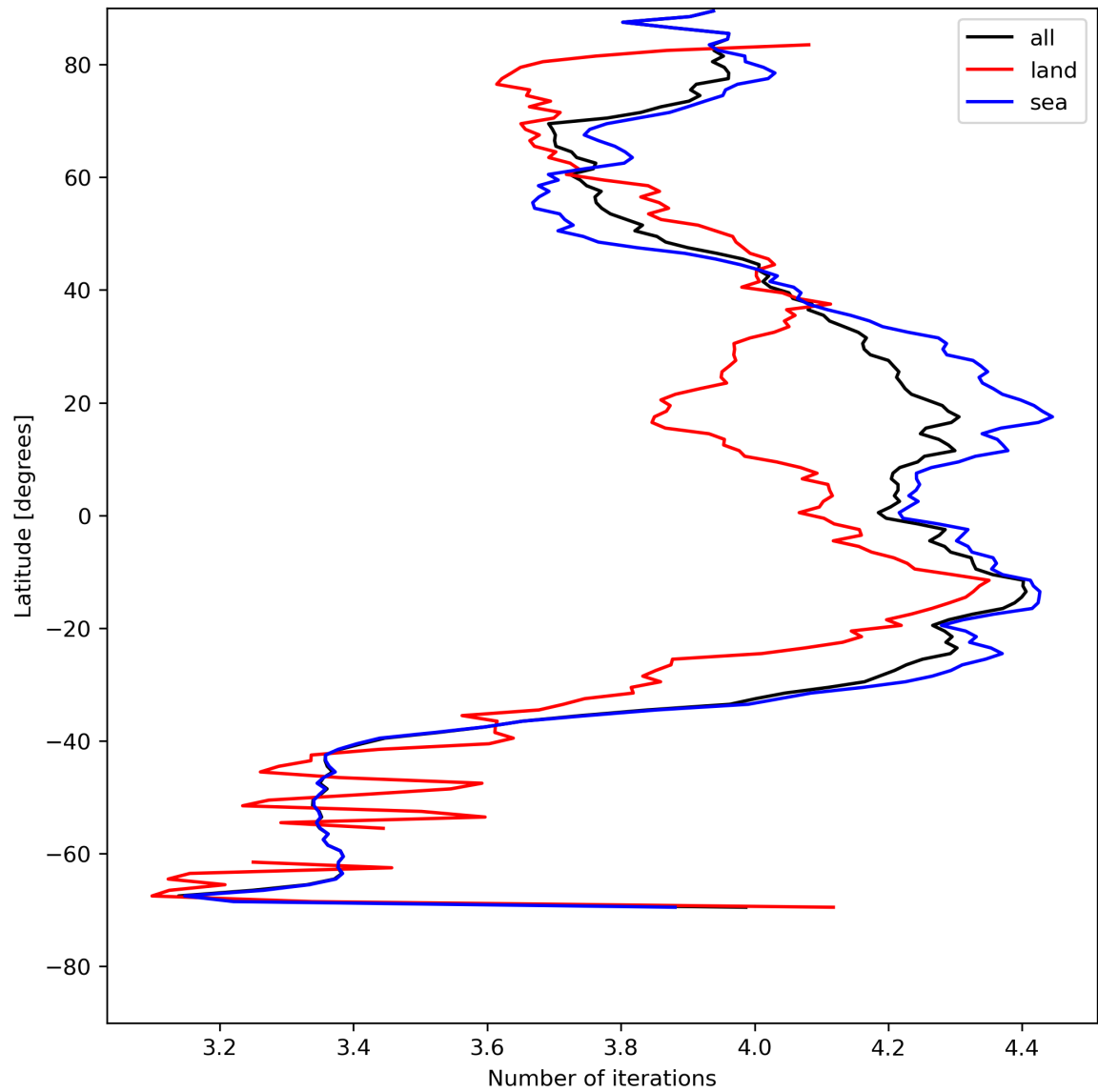
Figure 17: Zonal average of “Number of iterations” for 2024-05-12 to 2024-05-14.
