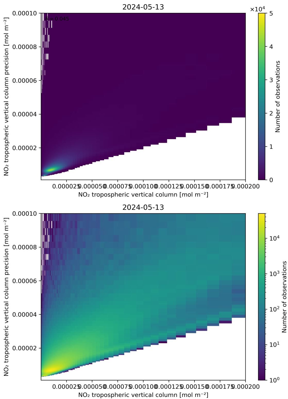
Figure 130: Scatter density plot of “NO 2 tropospheric vertical column” against “NO 2 tropospheric vertical column precision” for 2024-05-12 to 2024-05-14.
