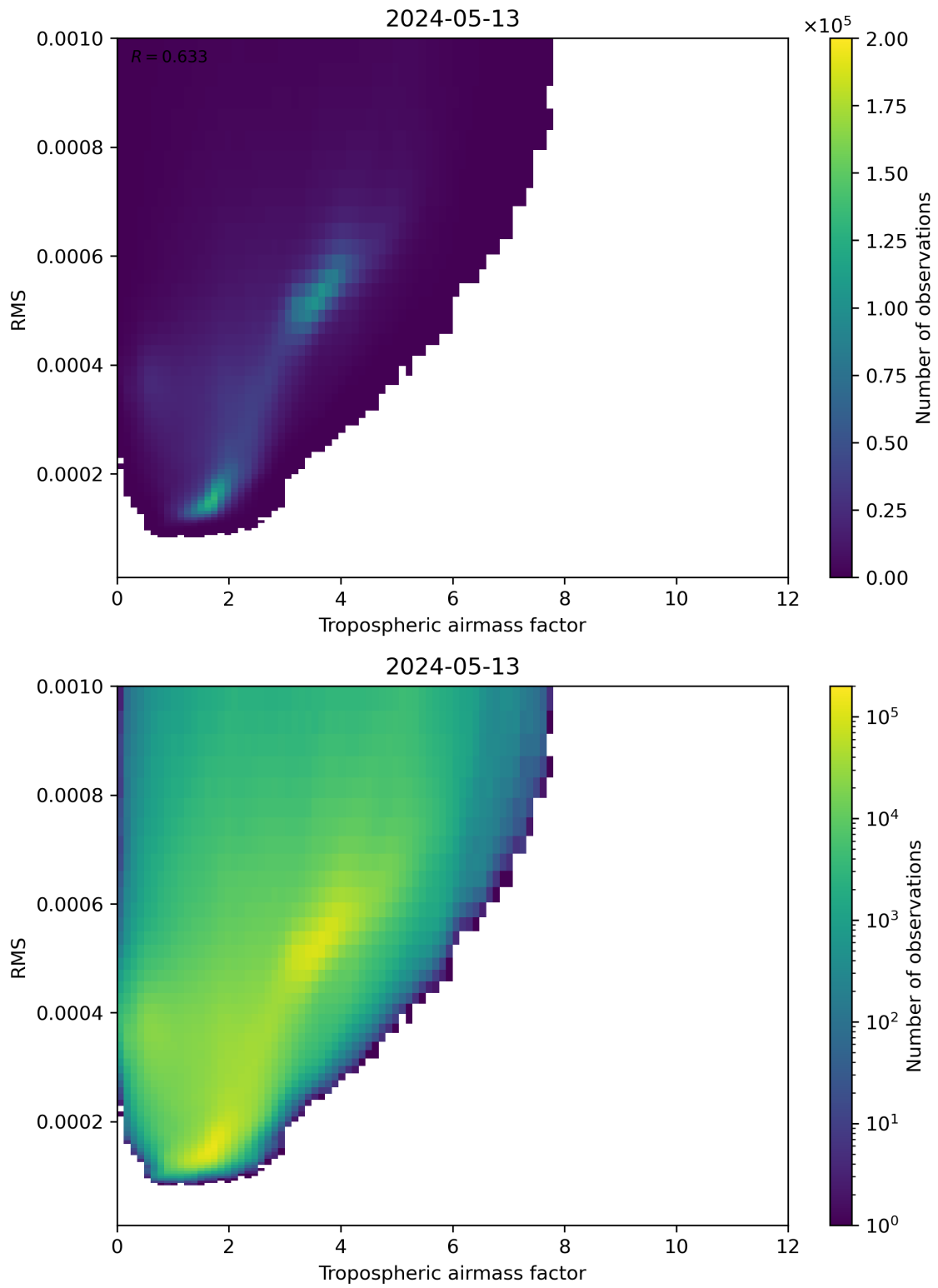
Figure 79: Scatter density plot of “Tropospheric airmass factor” against “RMS” for 2024-05-12 to 2024-05-14.
