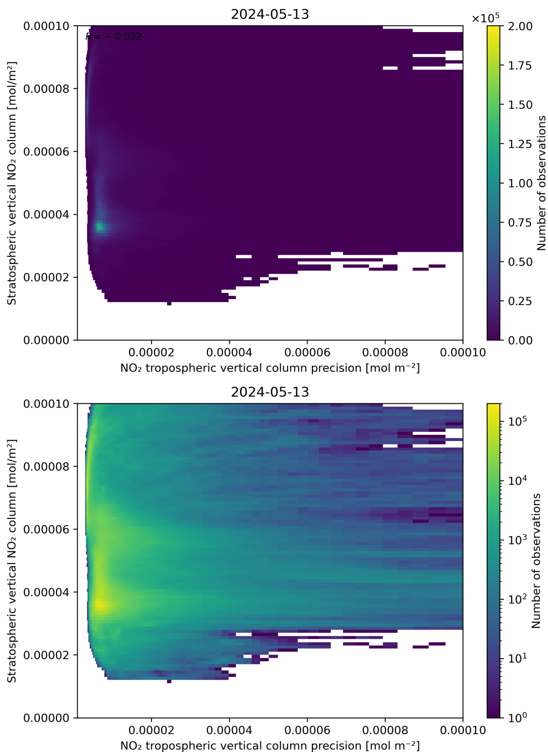
Figure 135: Scatter density plot of “NO 2 tropospheric vertical column precision” against “Stratospheric vertical NO 2 column” for 2024-05-12 to 2024-05-14.
