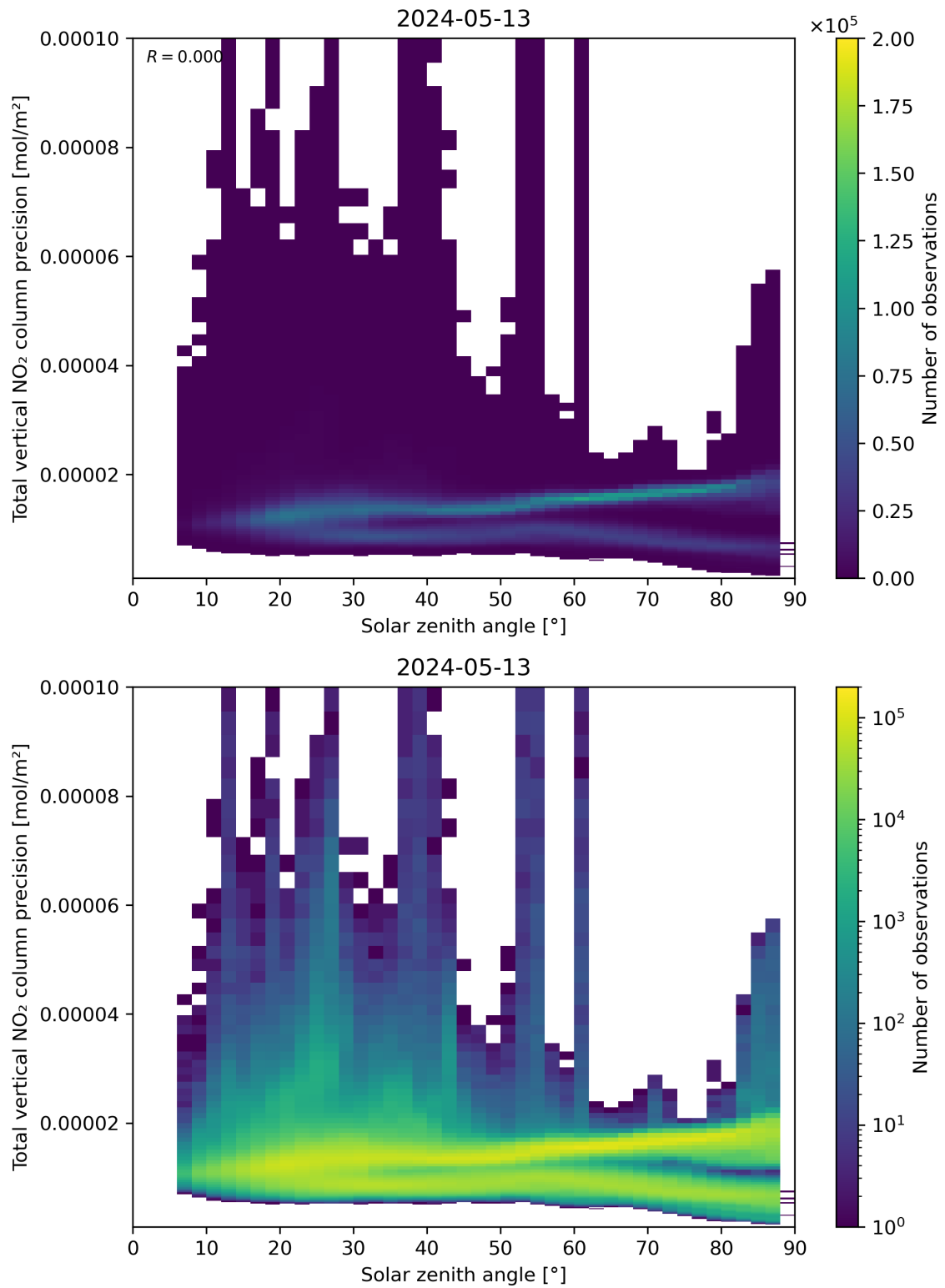
Figure 154: Scatter density plot of “Solar zenith angle” against “Total vertical NO 2 column precision” for 2024-05-12 to 2024-05-14.
