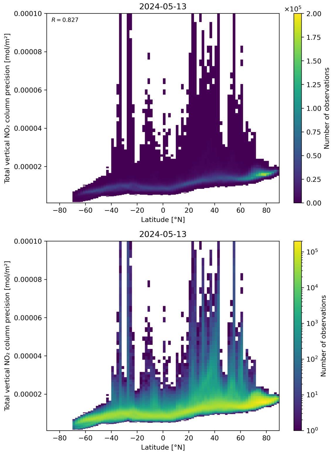
Figure 91: Scatter density plot of “Latitude” against “Total vertical NO 2 column precision” for 2024-05-12 to 2024-05-14.
