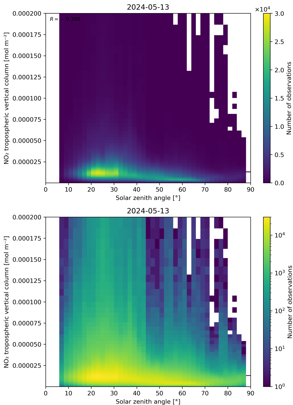
Figure 155: Scatter density plot of “Solar zenith angle” against “NO 2 tropospheric vertical column” for 2024-05-12 to 2024-05-14.
