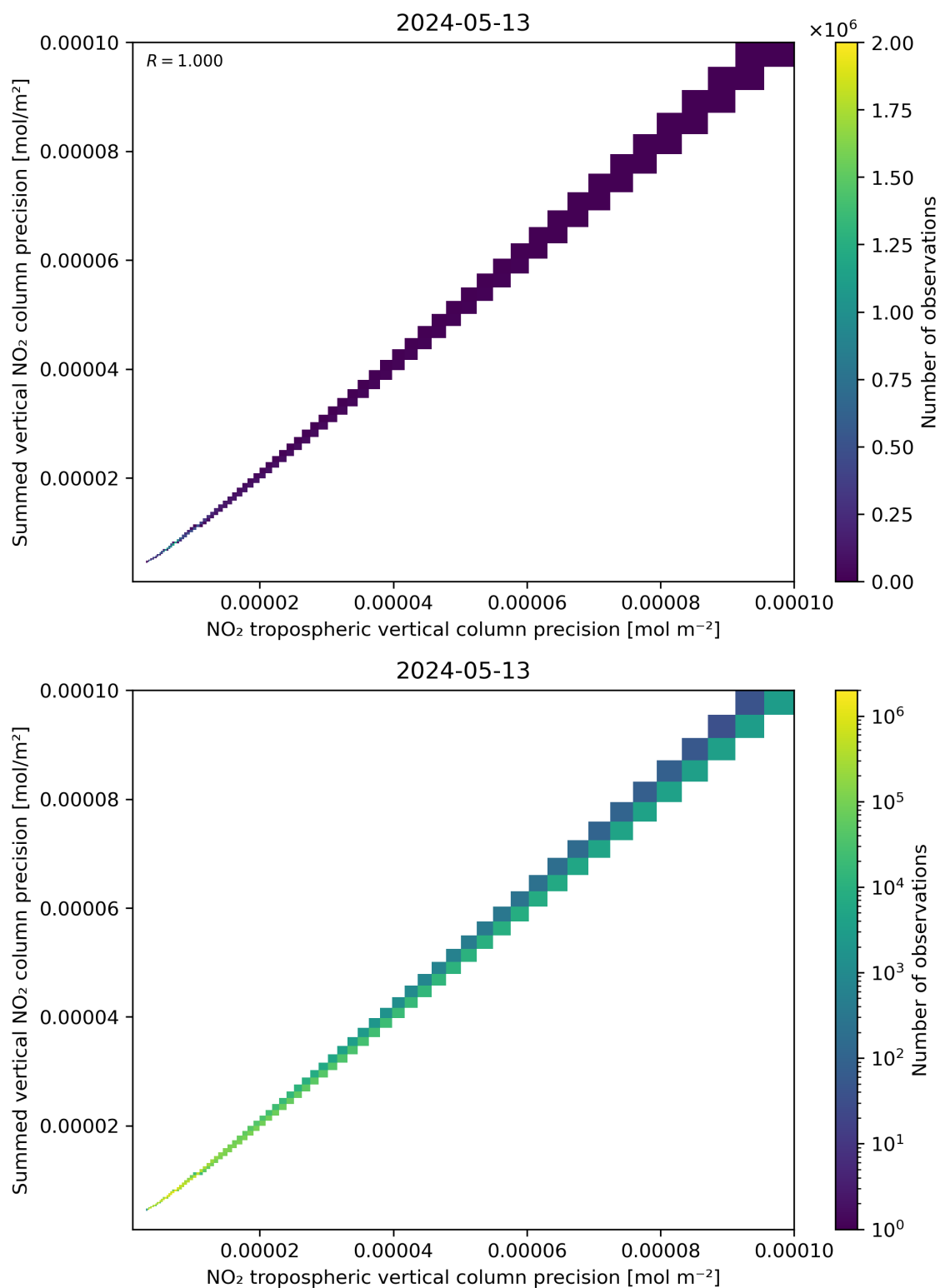
Figure 137: Scatter density plot of “NO 2 tropospheric vertical column precision” against “Summed vertical NO 2 column precision” for 2024-05-12 to 2024-05-14.
