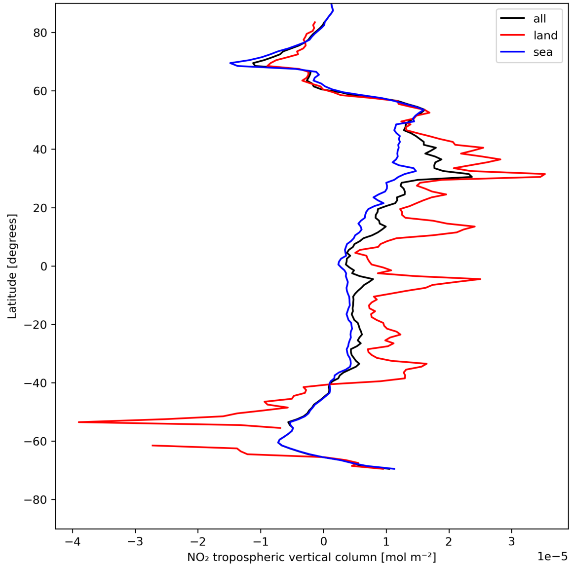
Figure 12: Zonal average of “NO 2 tropospheric vertical column” for 2024-05-12 to 2024-05-14.
