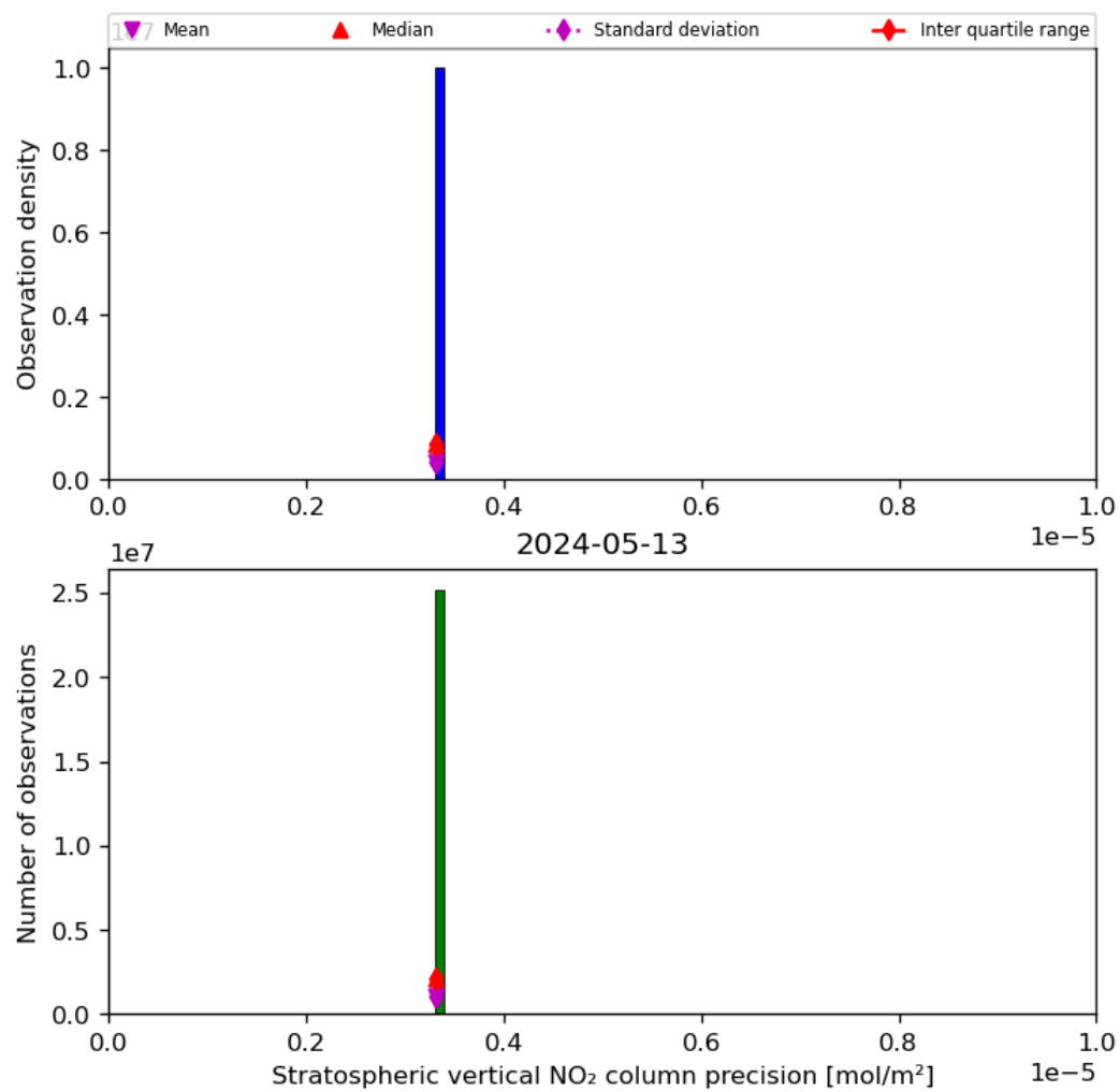
Figure 37: Histogram of “Stratospheric vertical NO 2 column precision” for 2024-05-12 to 2024-05-14
