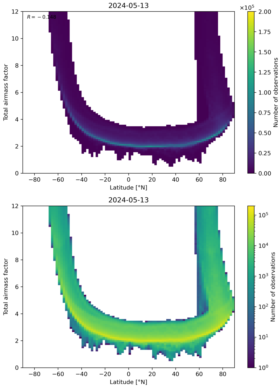
Figure 84: Scatter density plot of “Latitude” against “Total airmass factor” for 2024-05-12 to 2024-05-14.
