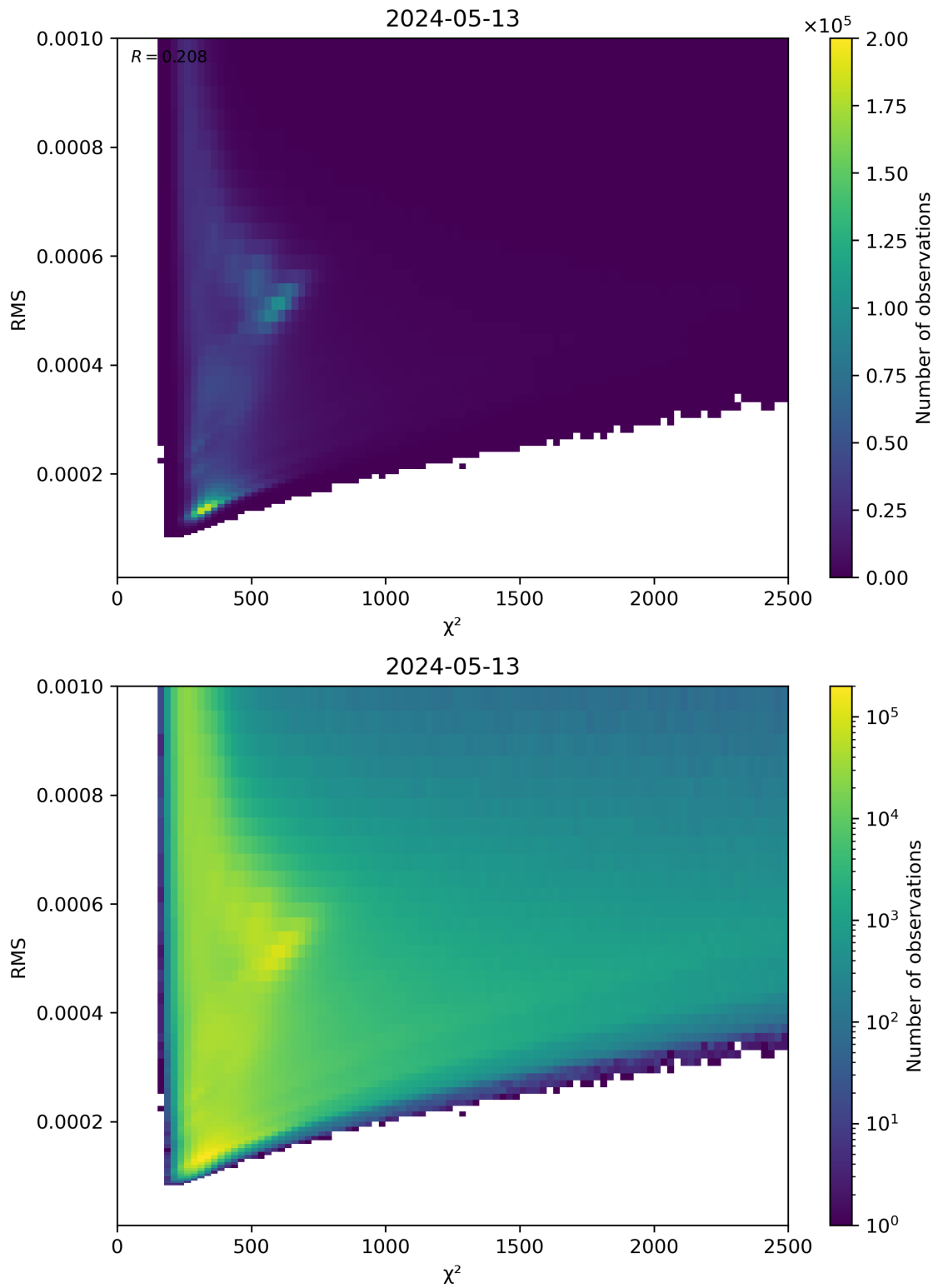
Figure 82: Scatter density plot of “ \chi^2 ” against “RMS” for 2024-05-12 to 2024-05-14.
