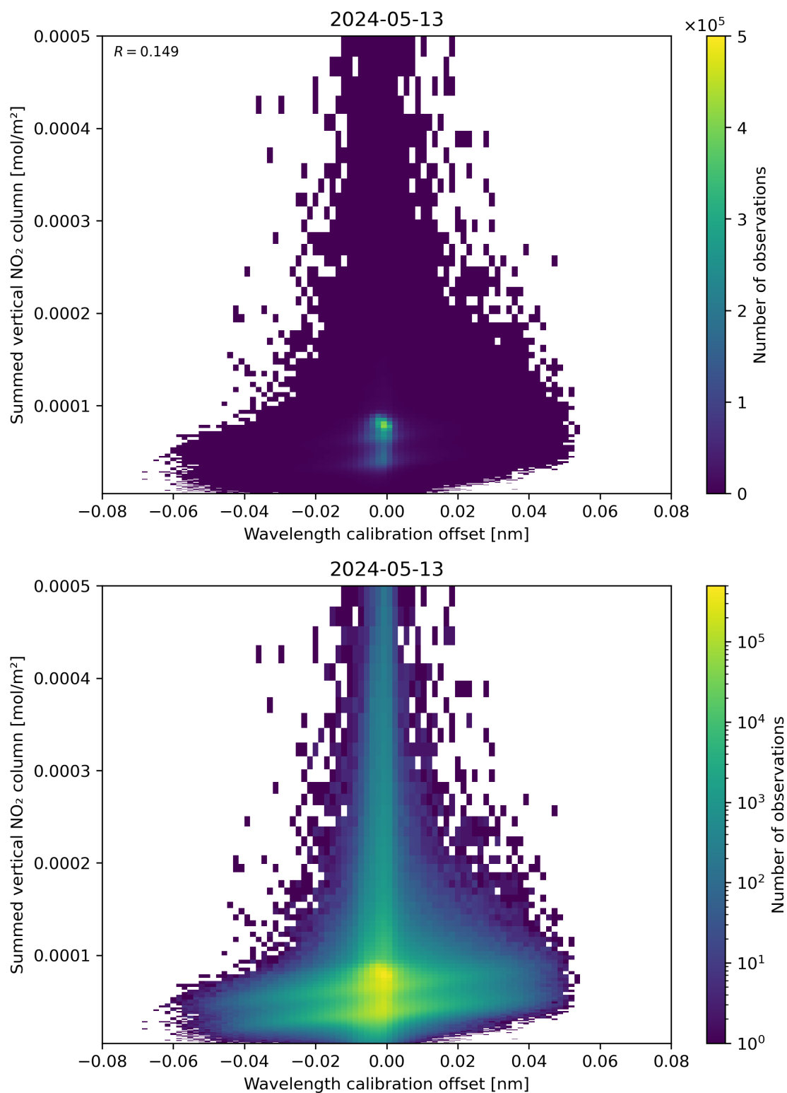
Figure 177: Scatter density plot of “Wavelength calibration offset” against “Summed vertical NO 2 column” for 2024-05-12 to 2024-05-14.
