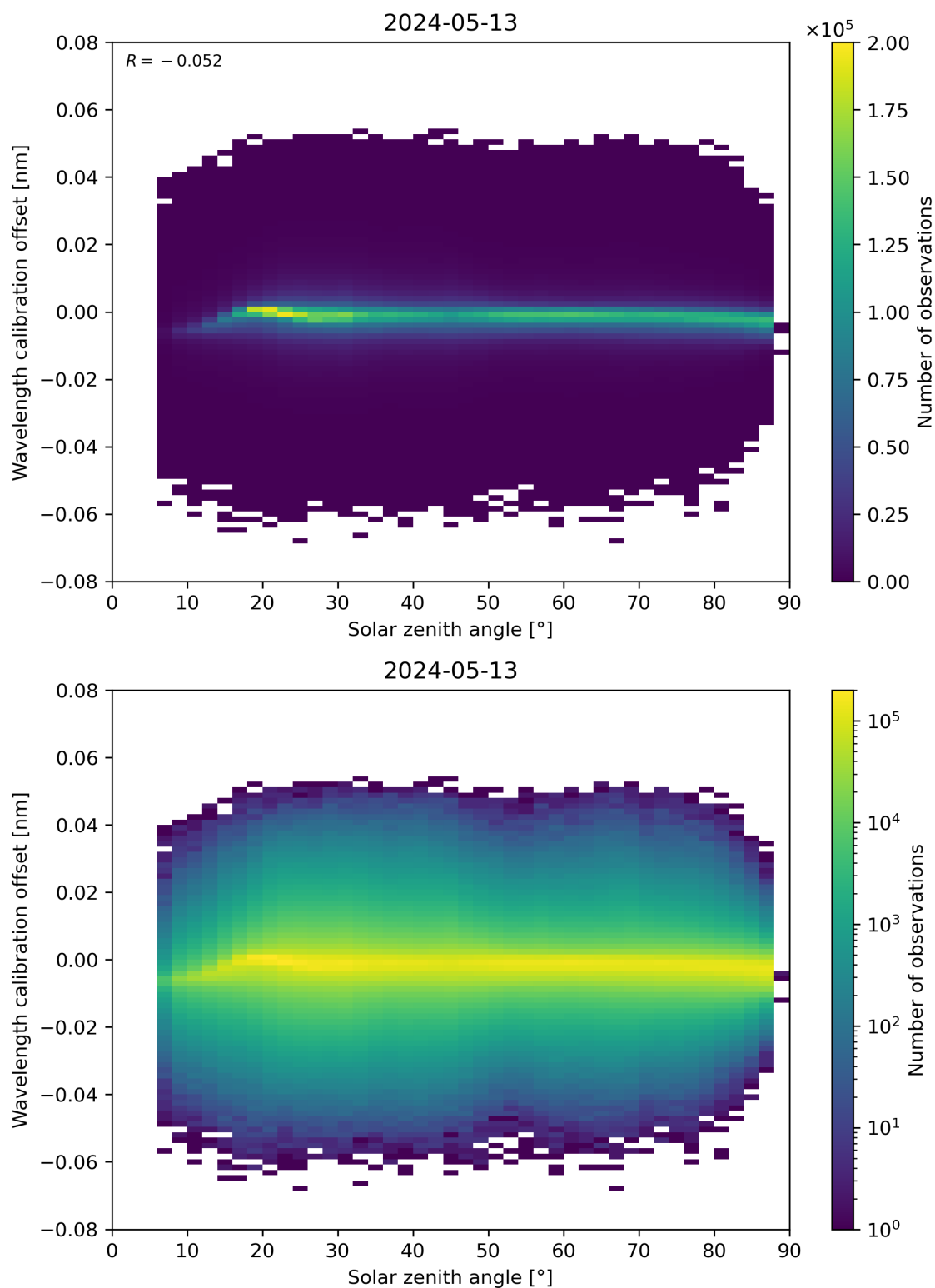
Figure 158: Scatter density plot of “Solar zenith angle” against “Wavelength calibration offset” for 2024-05-12 to 2024-05-14.
