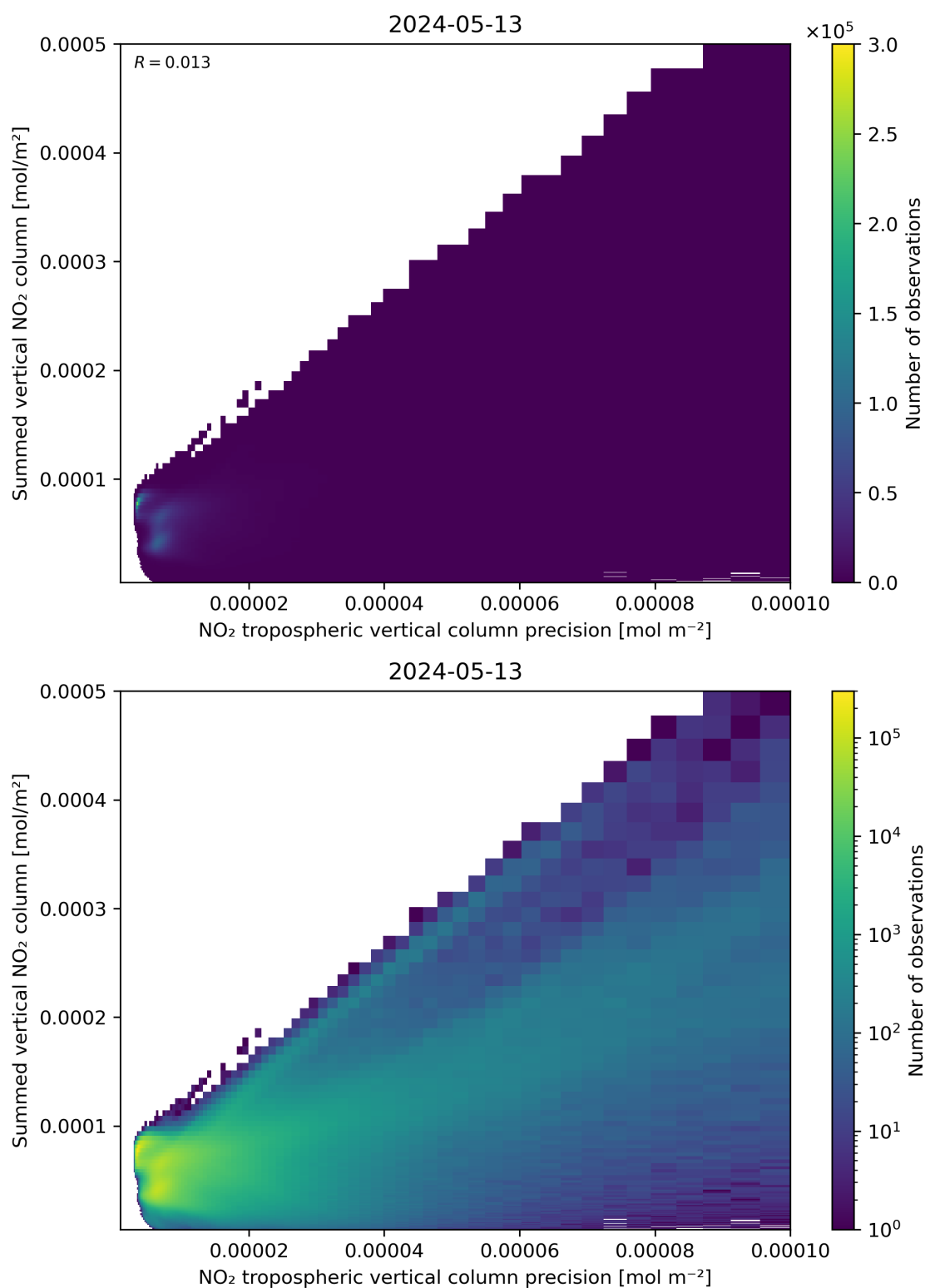
Figure 136: Scatter density plot of “NO 2 tropospheric vertical column precision” against “Summed vertical NO 2 column” for 2024-05-12 to 2024-05-14.
