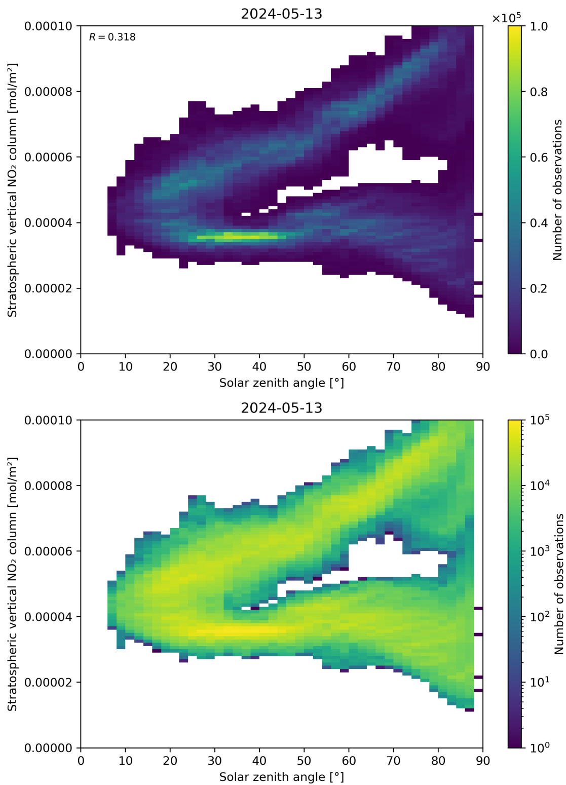
Figure 150: Scatter density plot of “Solar zenith angle” against “Stratospheric vertical NO 2 column” for 2024-05-12 to 2024-05-14.
