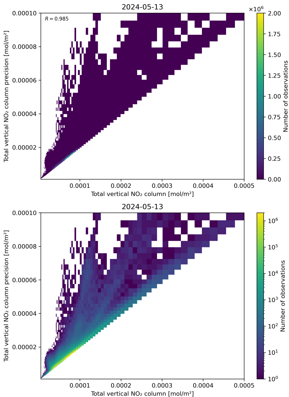
Figure 114: Scatter density plot of “Total vertical NO 2 column” against “Total vertical NO 2 column precision” for 2024-05-12 to 2024-05-14.
