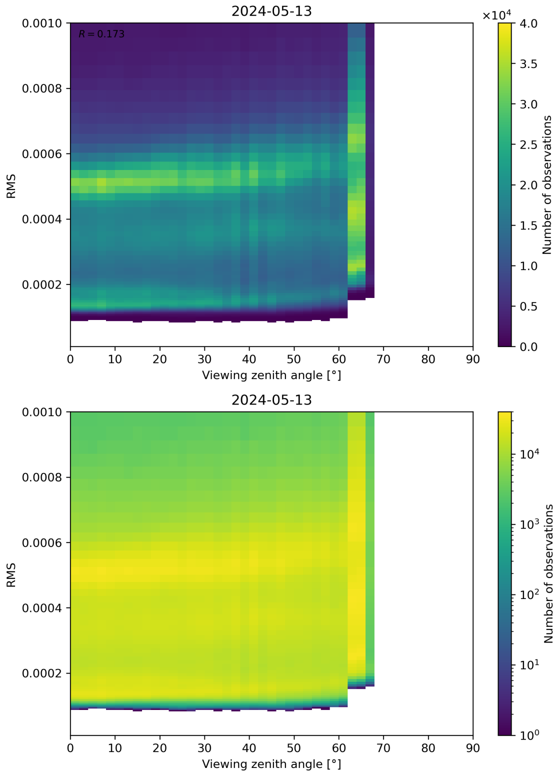
Figure 171: Scatter density plot of “Viewing zenith angle” against “RMS” for 2024-05-12 to 2024-05-14.
