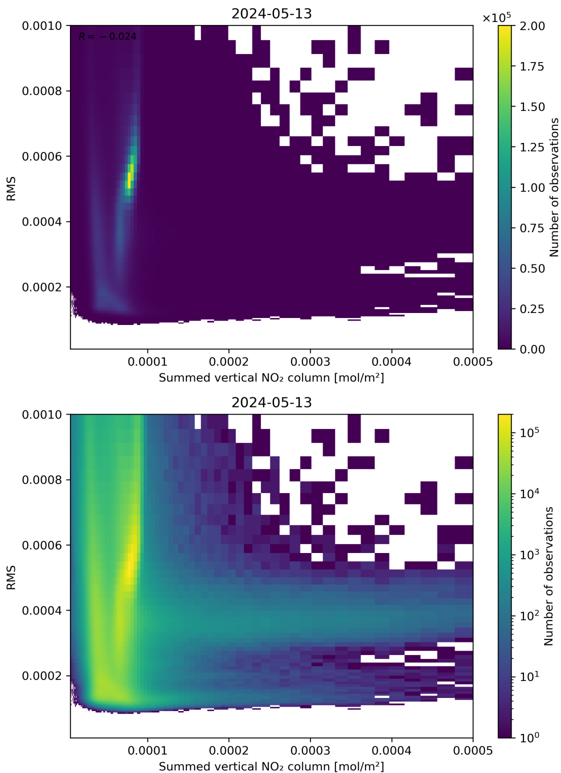
Figure 109: Scatter density plot of “Summed vertical NO 2 column” against “RMS” for 2024-05-12 to 2024-05-14.
