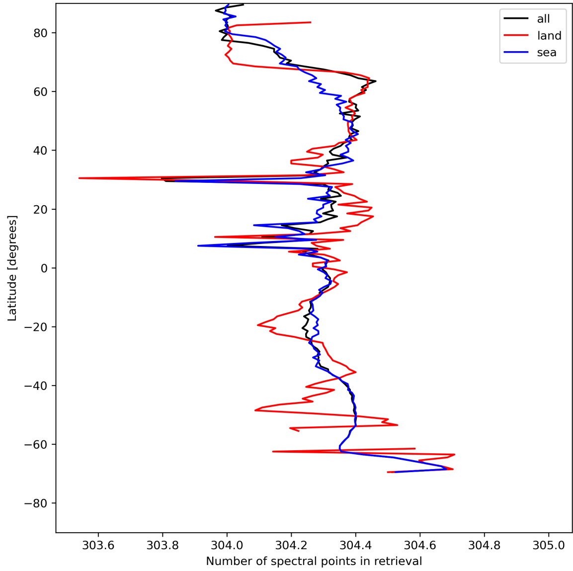
Figure 16: Zonal average of “Number of spectral points in retrieval” for 2024-05-12 to 2024-05-14.
