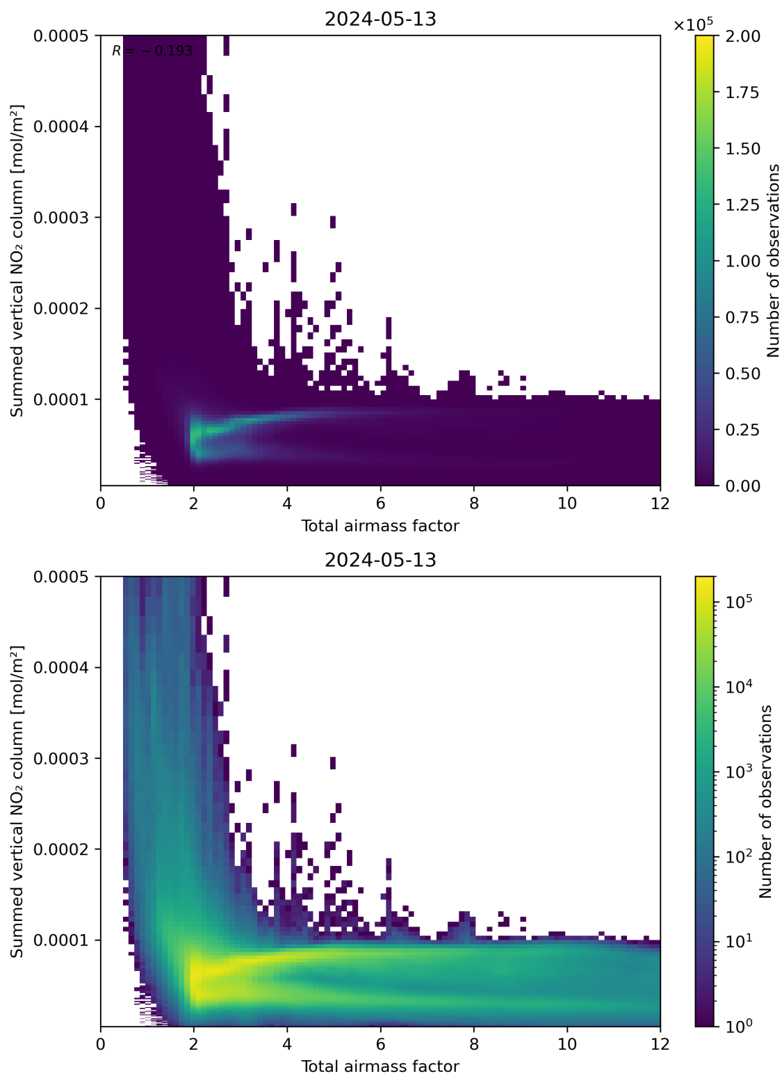
Figure 65: Scatter density plot of “Total airmass factor” against “Summed vertical NO 2 column” for 2024-05-12 to 2024-05-14.
