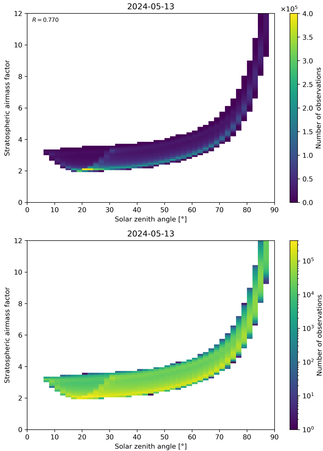
Figure 145: Scatter density plot of “Solar zenith angle” against “Stratospheric airmass factor” for 2024-05-12 to 2024-05-14.
