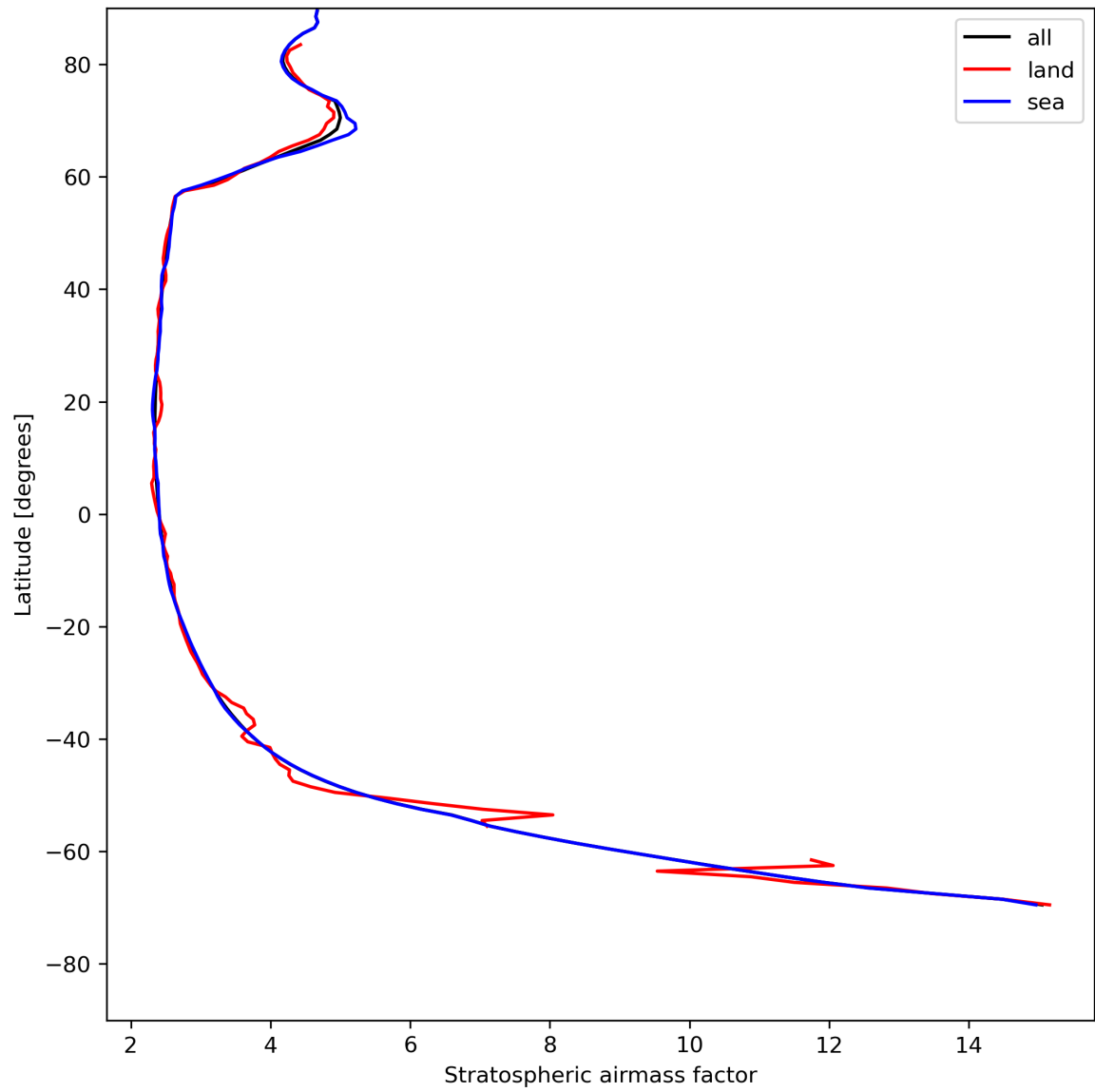
Figure 27: Zonal average of “Stratospheric airmass factor” for 2024-05-12 to 2024-05-14.
