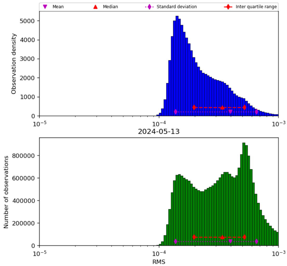
Figure 43: Histogram of “RMS” for 2024-05-12 to 2024-05-14
