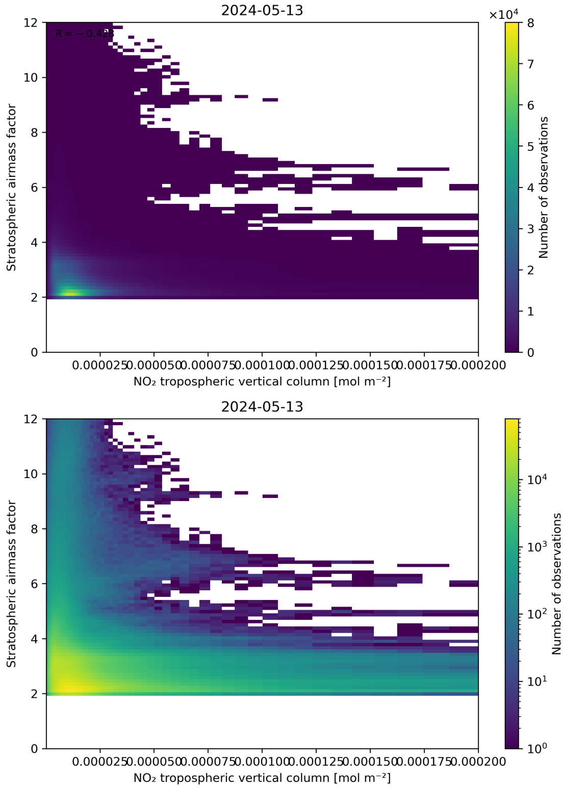
Figure 121: Scatter density plot of “NO 2 tropospheric vertical column” against “Stratospheric air mass factor” for 2024-05-12 to 2024-05-14.
