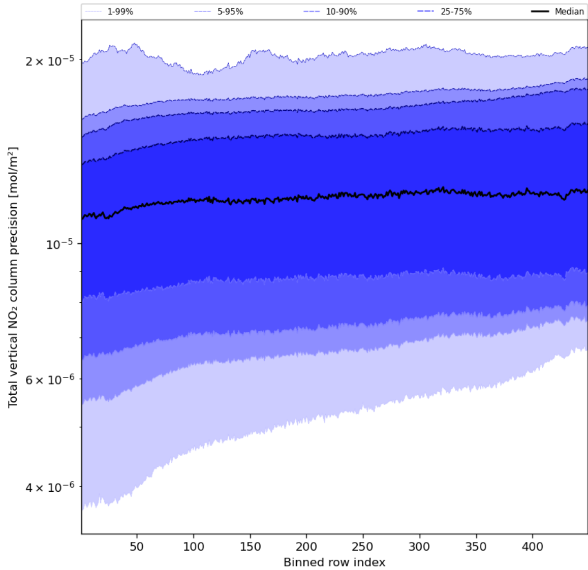
Figure 56: Along track statistics of “Total vertical NO 2 column precision” for 2024-05-12 to 2024-05-14
