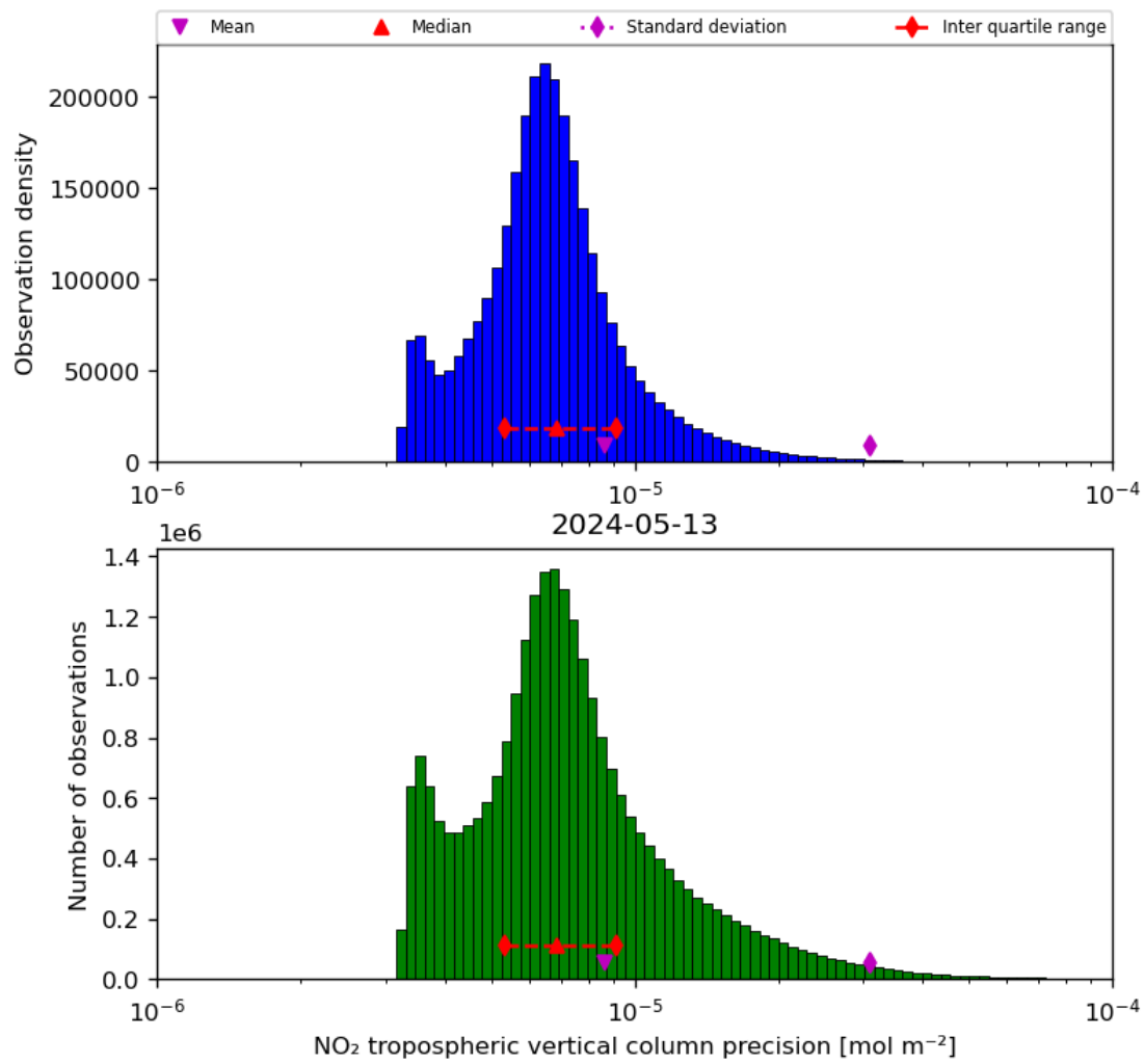
Figure 30: Histogram of “NO 2 tropospheric vertical column precision” for 2024-05-12 to 2024-05-14
