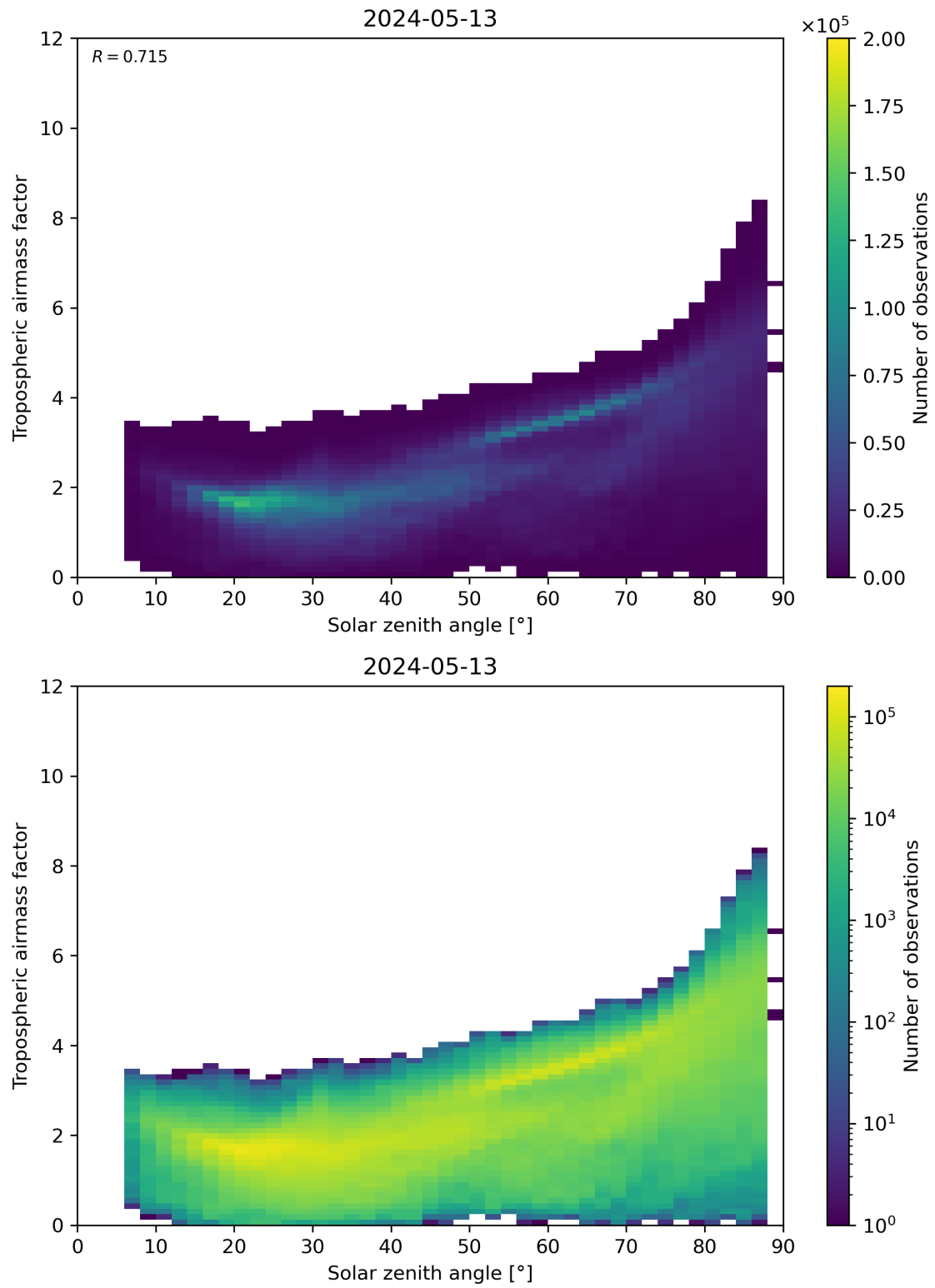
Figure 147: Scatter density plot of “Solar zenith angle” against “Tropospheric airmass factor” for 2024-05-12 to 2024-05-14.
