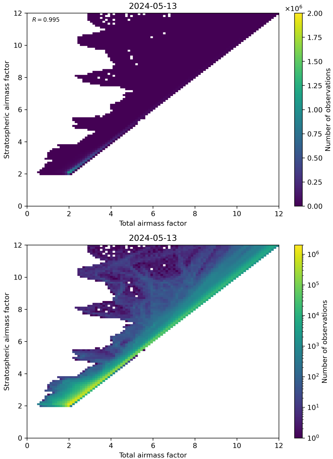
Figure 62: Scatter density plot of “Total airmass factor” against “Stratospheric airmass factor” for 2024-05-12 to 2024-05-14.
