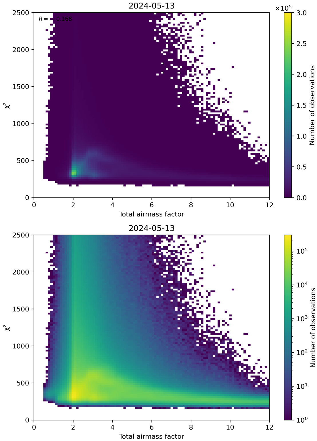
Figure 63: Scatter density plot of “Total airmass factor” against “ \chi^2 ” for 2024-05-12 to 2024-05-14.
