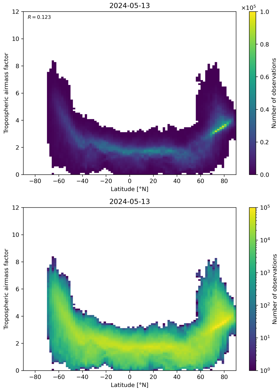
Figure 85: Scatter density plot of “Latitude” against “Tropospheric airmass factor” for 2024-05-12 to 2024-05-14.
