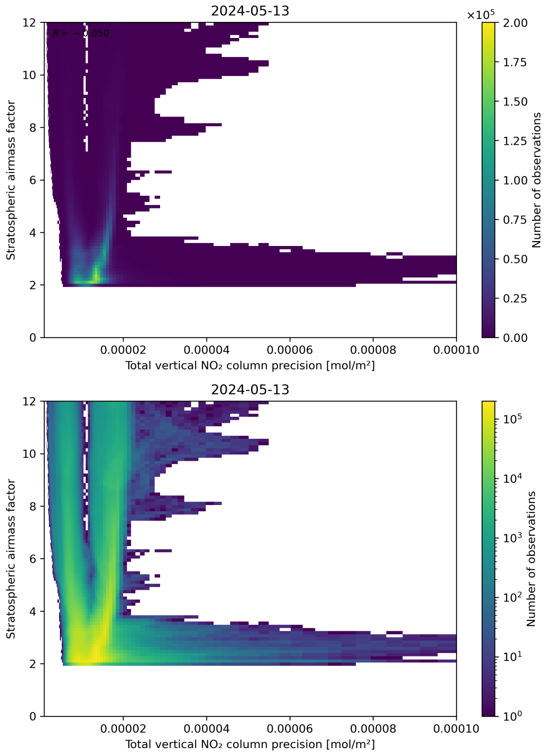
Figure 115: Scatter density plot of “Total vertical NO 2 column precision” against “Stratospheric air mass factor” for 2024-05-12 to 2024-05-14.
