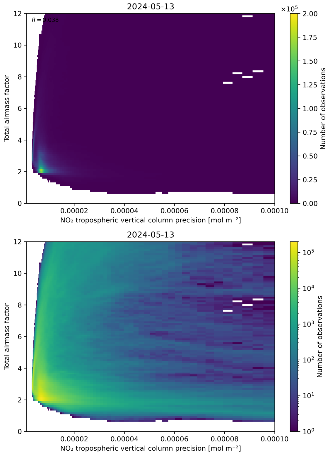
Figure 132: Scatter density plot of “NO 2 tropospheric vertical column precision” against “Total air mass factor” for 2024-05-12 to 2024-05-14.
