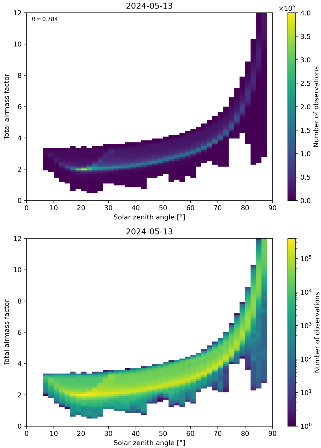
Figure 146: Scatter density plot of “Solar zenith angle” against “Total air mass factor” for 2024-05-12 to 2024-05-14.
