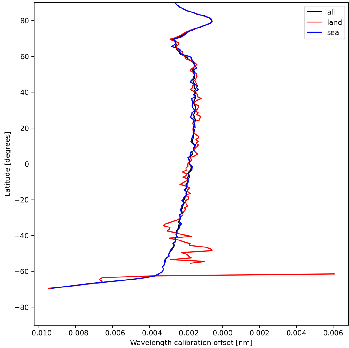
Figure 18: Zonal average of “Wavelength calibration offset” for 2024-05-12 to 2024-05-14.
