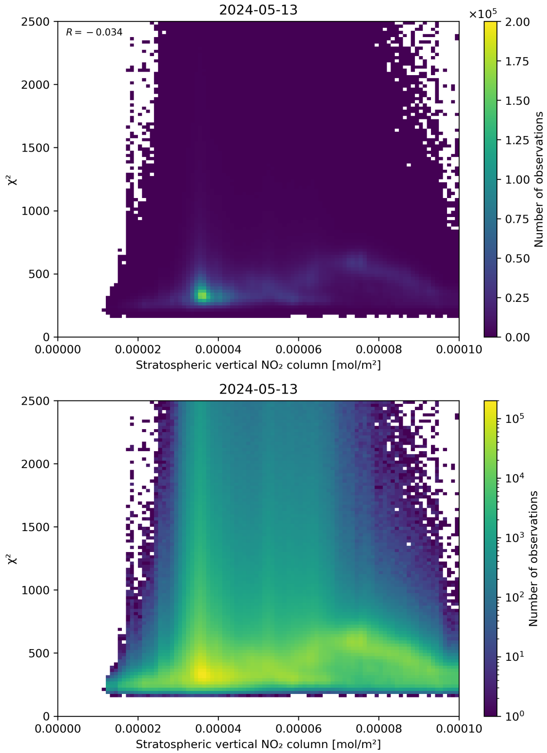
Figure 97: Scatter density plot of “Stratospheric vertical NO 2 column” against “ \chi^2 ” for 2024-05-12 to 2024-05-14.
