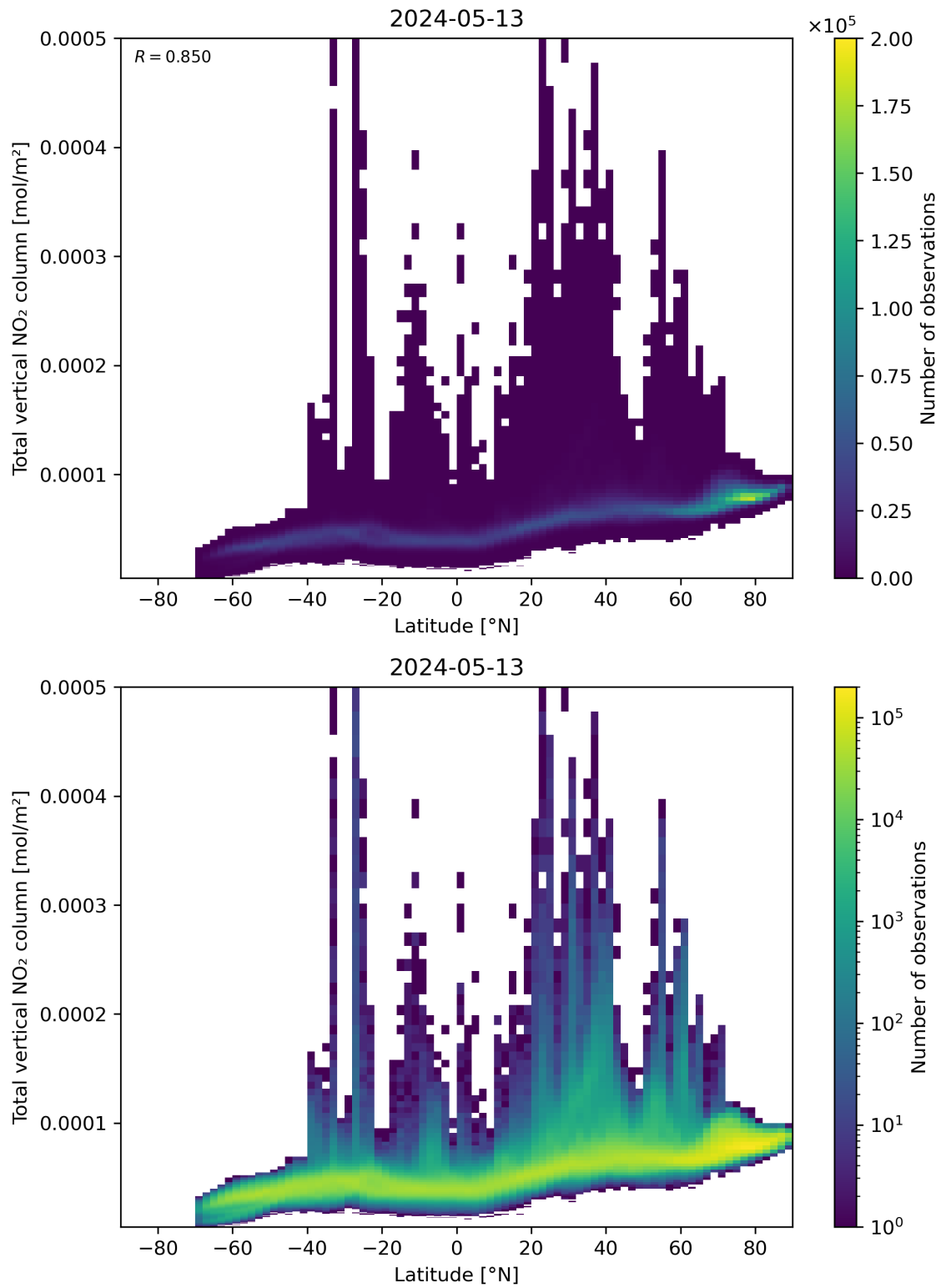
Figure 90: Scatter density plot of “Latitude” against “Total vertical NO 2 column” for 2024-05-12 to 2024-05-14.
