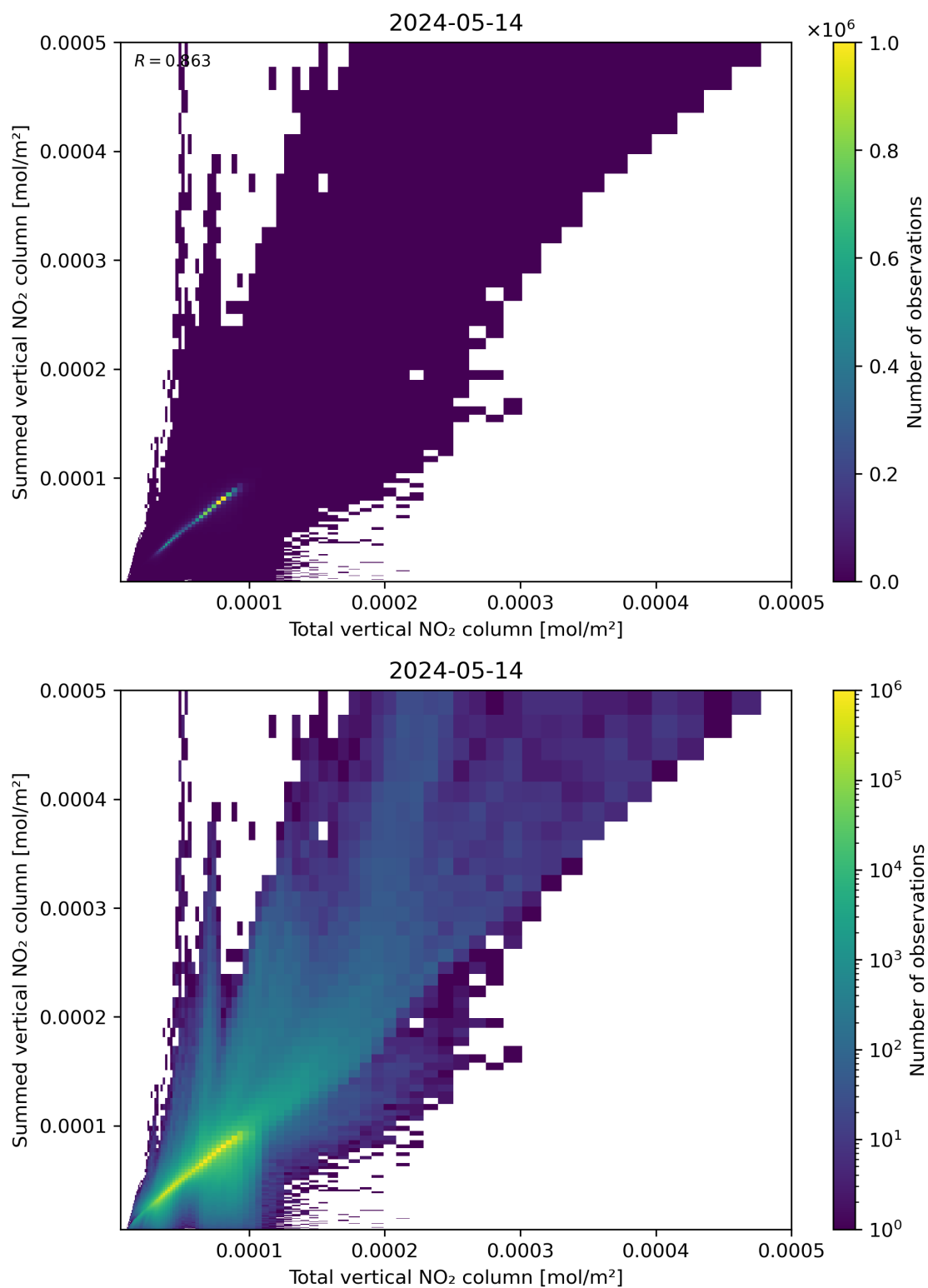
Figure 112: Scatter density plot of “Total vertical NO 2 column” against “Summed vertical NO 2 column” for 2024-05-13 to 2024-05-15.
