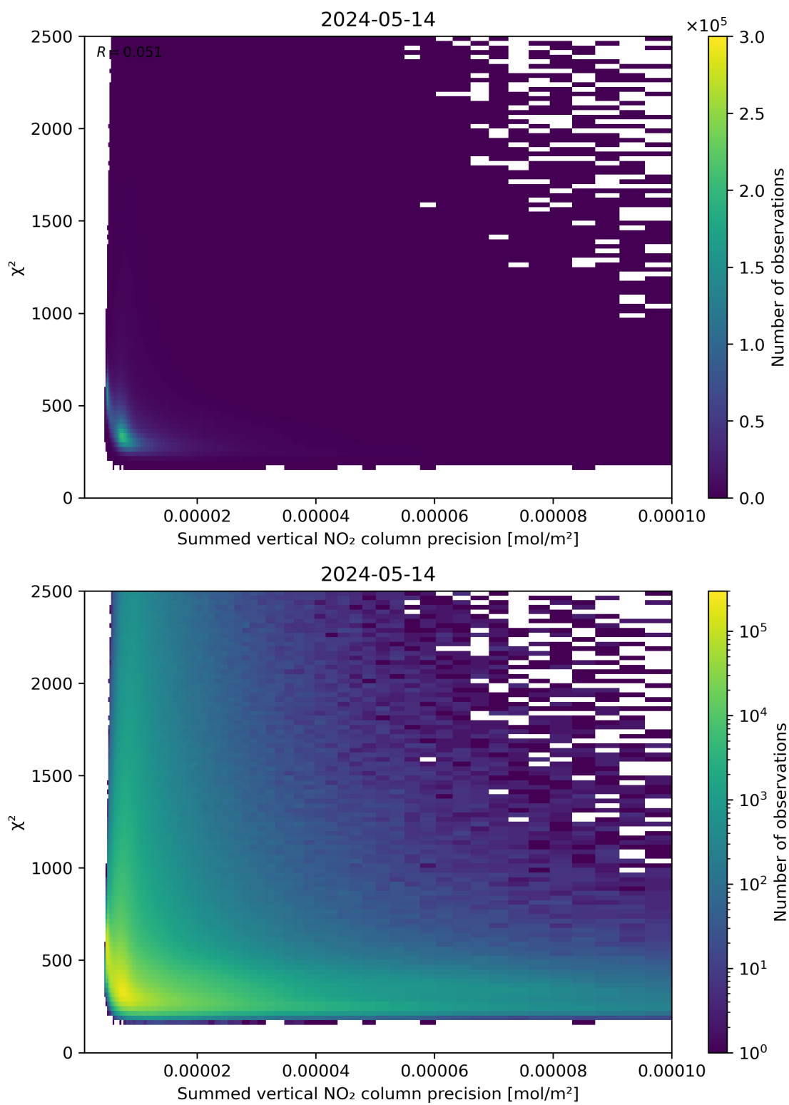
Figure 107: Scatter density plot of “Summed vertical NO 2 column precision” against “ \chi^2 ” for 2024-05-13 to 2024-05-15.
