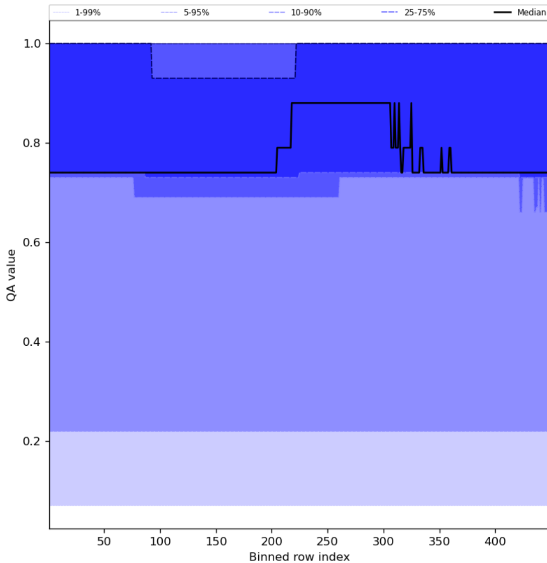
Figure 45: Along track statistics of “QA value” for 2024-05-13 to 2024-05-15
