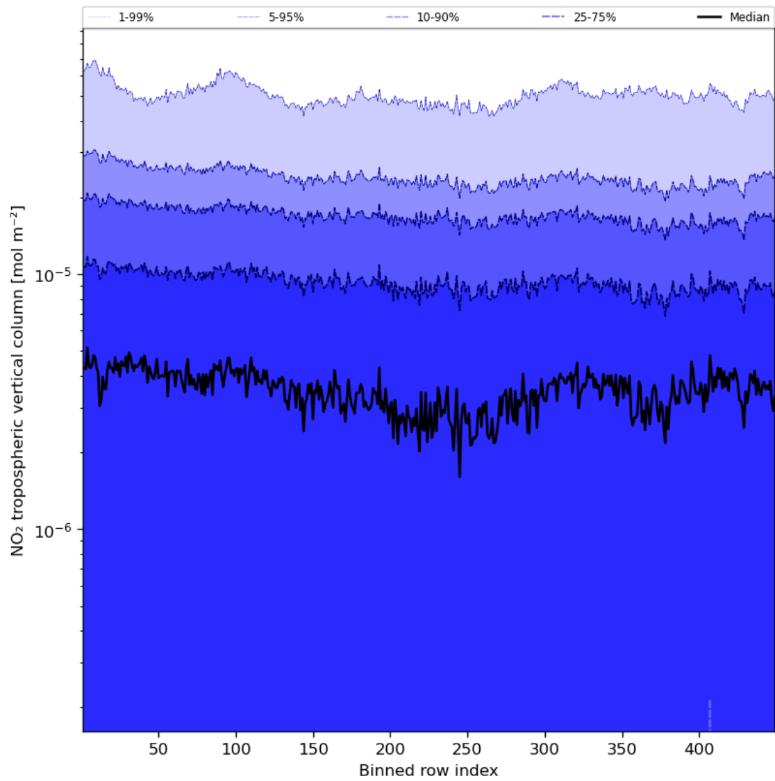
Figure 46: Along track statistics of “NO 2 tropospheric vertical column” for 2024-05-13 to 2024-05-15
