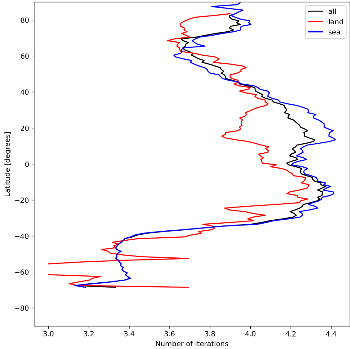
Figure 17: Zonal average of “Number of iterations” for 2024-05-13 to 2024-05-15.
