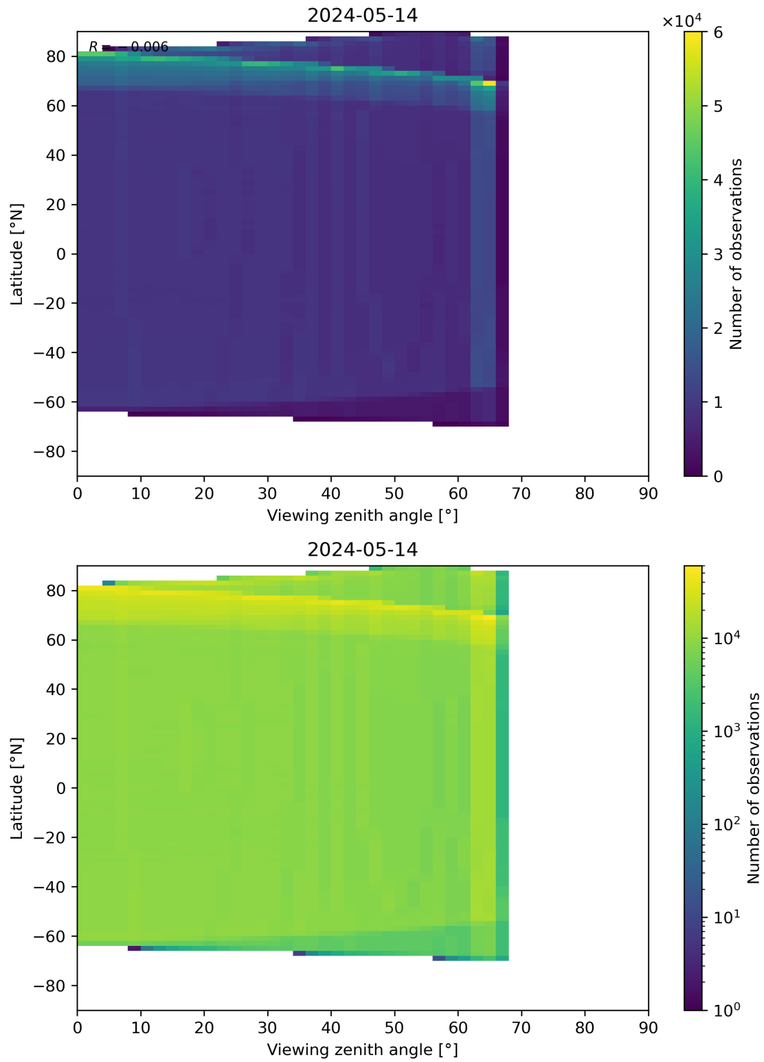
Figure 163: Scatter density plot of “Viewing zenith angle” against “Latitude” for 2024-05-13 to 2024-05-15.
