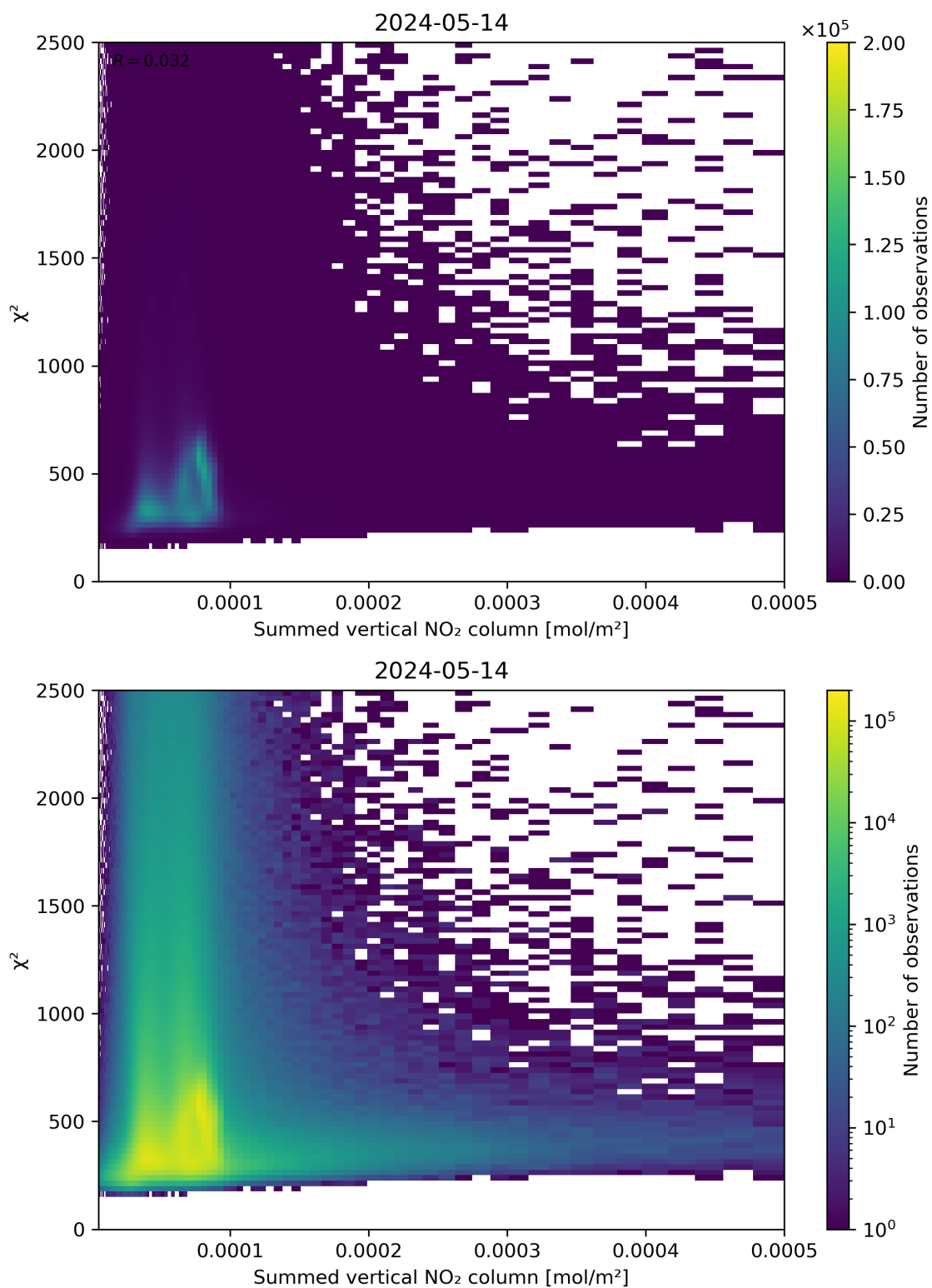
Figure 104: Scatter density plot of “Summed vertical NO 2 column” against “ \chi^2 ” for 2024-05-13 to 2024-05-15.
