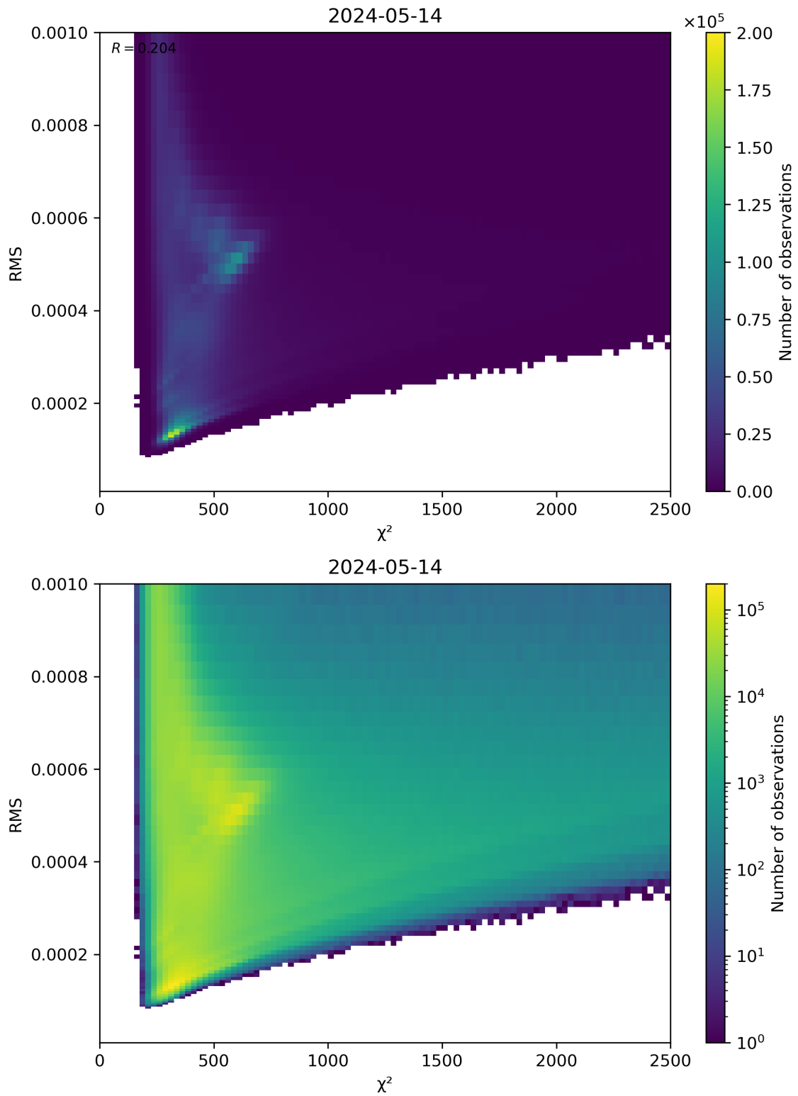
Figure 82: Scatter density plot of “ \chi^2 ” against “RMS” for 2024-05-13 to 2024-05-15.
