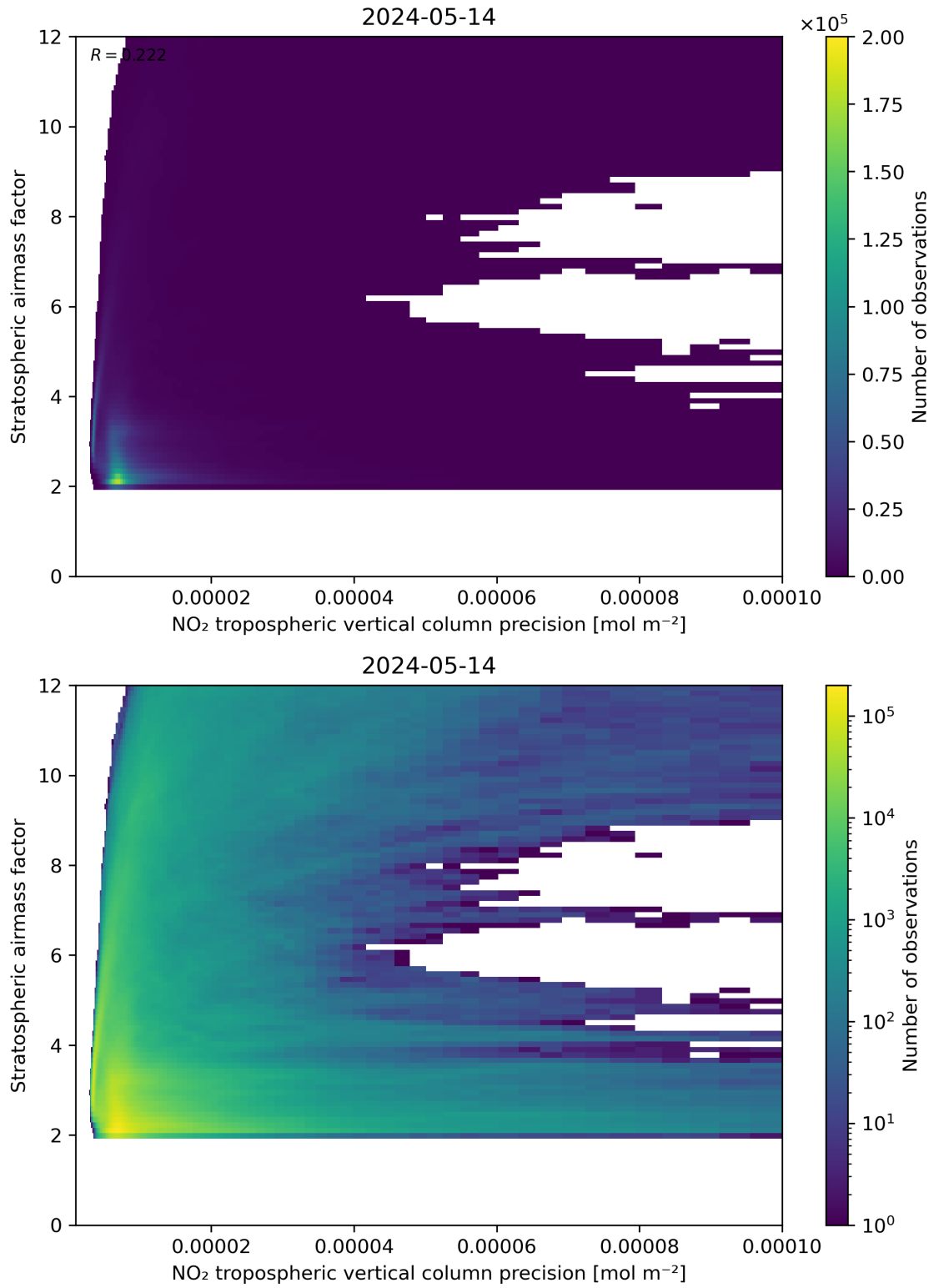
Figure 131: Scatter density plot of “NO 2 tropospheric vertical column precision” against “Stratospheric airmass factor” for 2024-05-13 to 2024-05-15.
