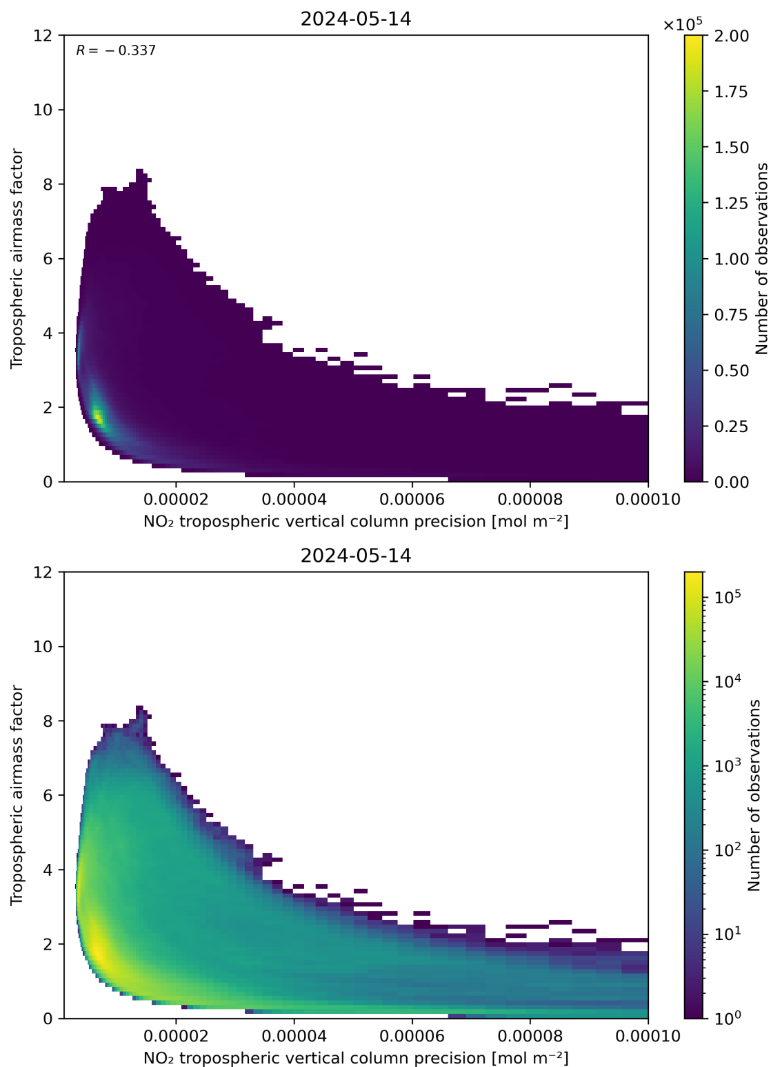
Figure 133: Scatter density plot of “NO 2 tropospheric vertical column precision” against “Tropospheric airmass factor” for 2024-05-13 to 2024-05-15.
