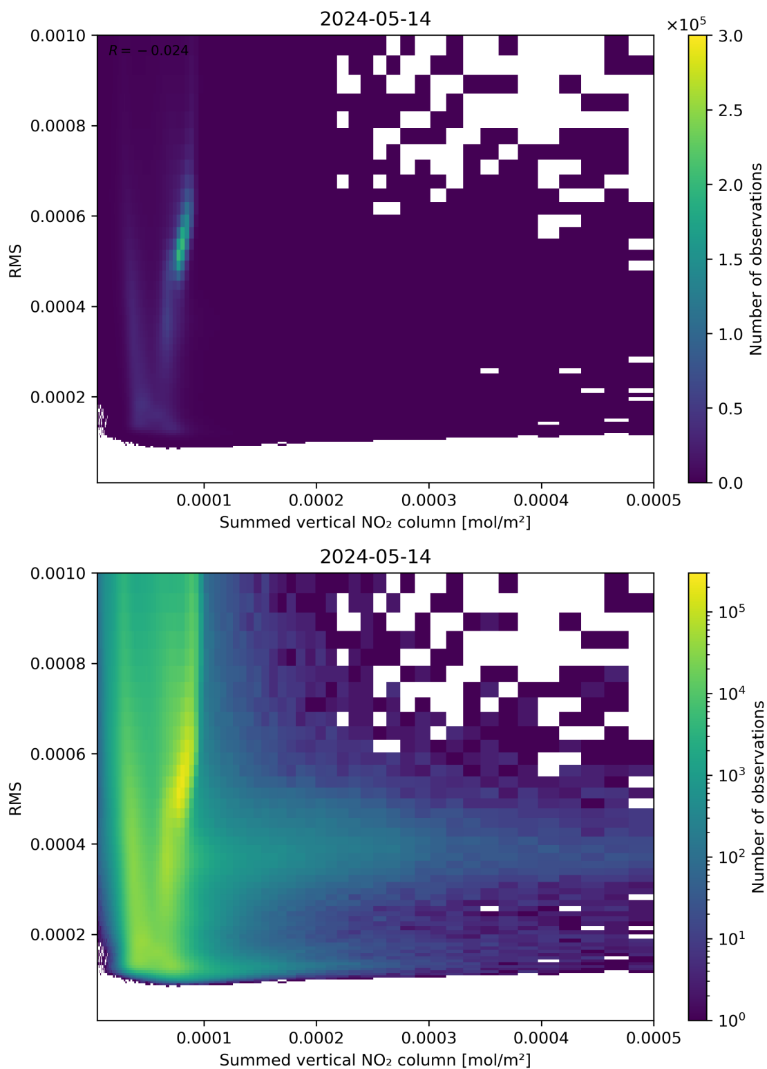
Figure 109: Scatter density plot of “Summed vertical NO 2 column” against “RMS” for 2024-05-13 to 2024-05-15.
