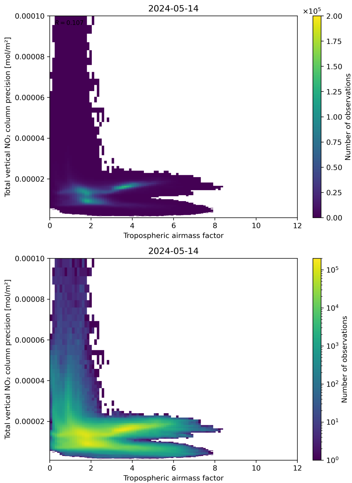
Figure 78: Scatter density plot of “Tropospheric air mass factor” against “Total vertical NO 2 column precision” for 2024-05-13 to 2024-05-15.
