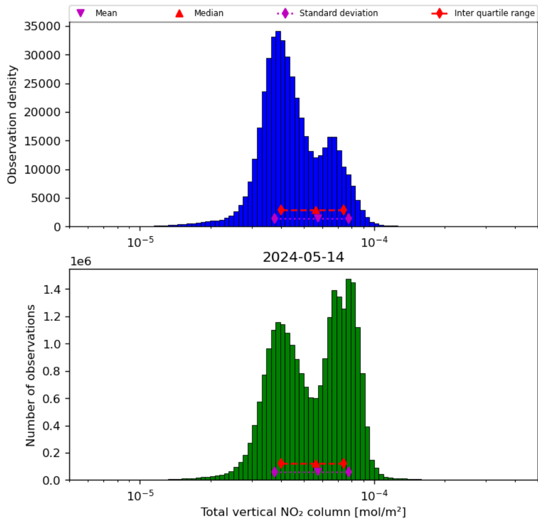
Figure 38: Histogram of “Total vertical NO 2 column” for 2024-05-13 to 2024-05-15
