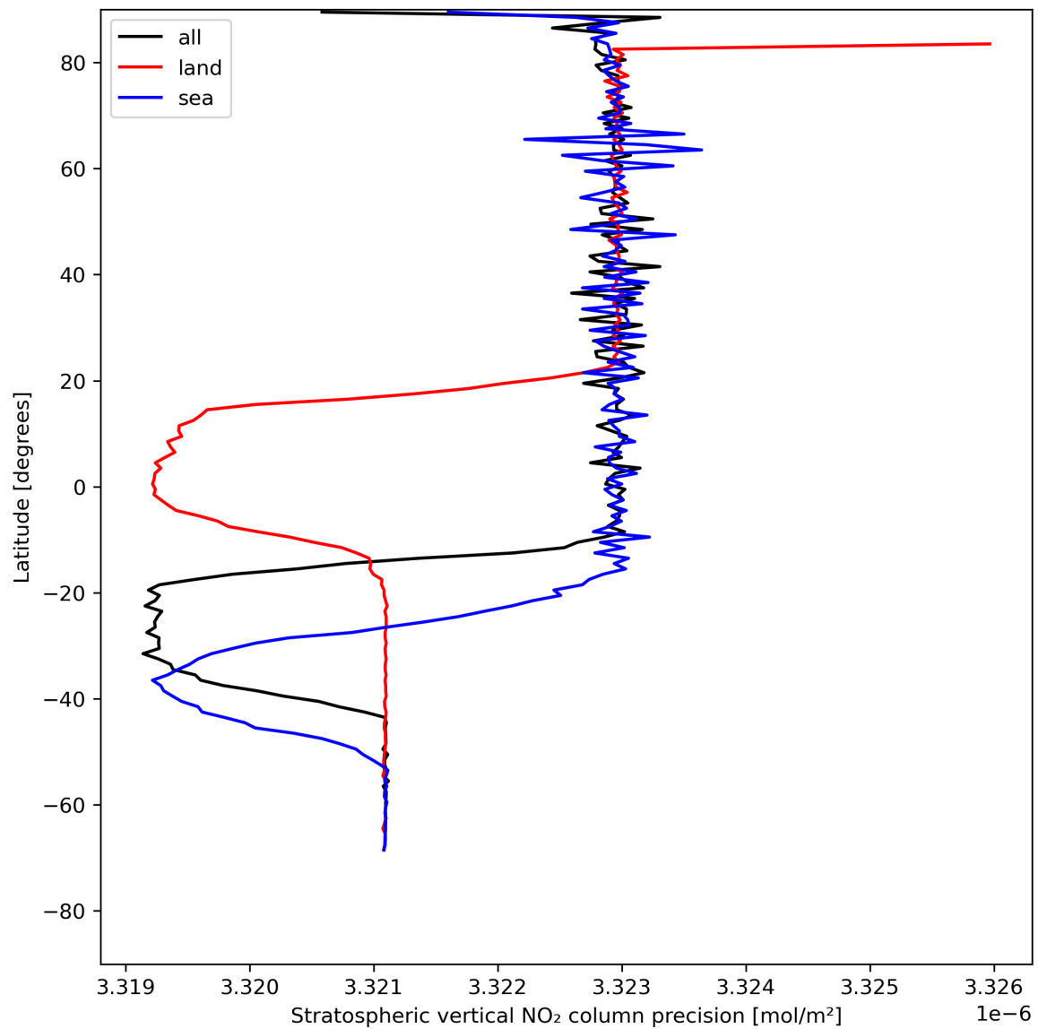
Figure 20: Zonal average of “Stratospheric vertical NO 2 column precision” for 2024-05-13 to 2024-05-15.
