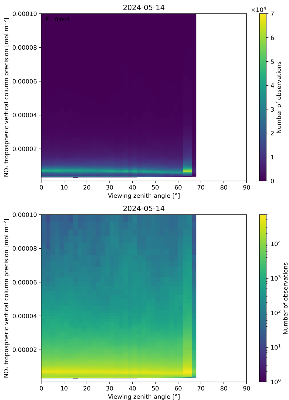
Figure 170: Scatter density plot of “Viewing zenith angle” against “NO 2 tropospheric vertical column precision” for 2024-05-13 to 2024-05-15.
