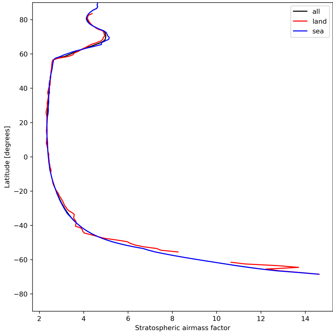
Figure 27: Zonal average of “Stratospheric air mass factor” for 2024-05-13 to 2024-05-15.
