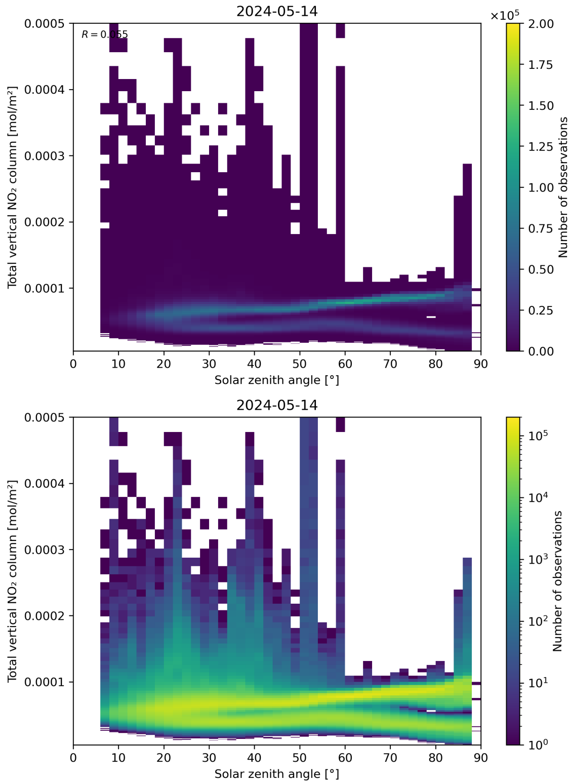
Figure 153: Scatter density plot of “Solar zenith angle” against “Total vertical NO 2 column” for 2024-05-13 to 2024-05-15.
