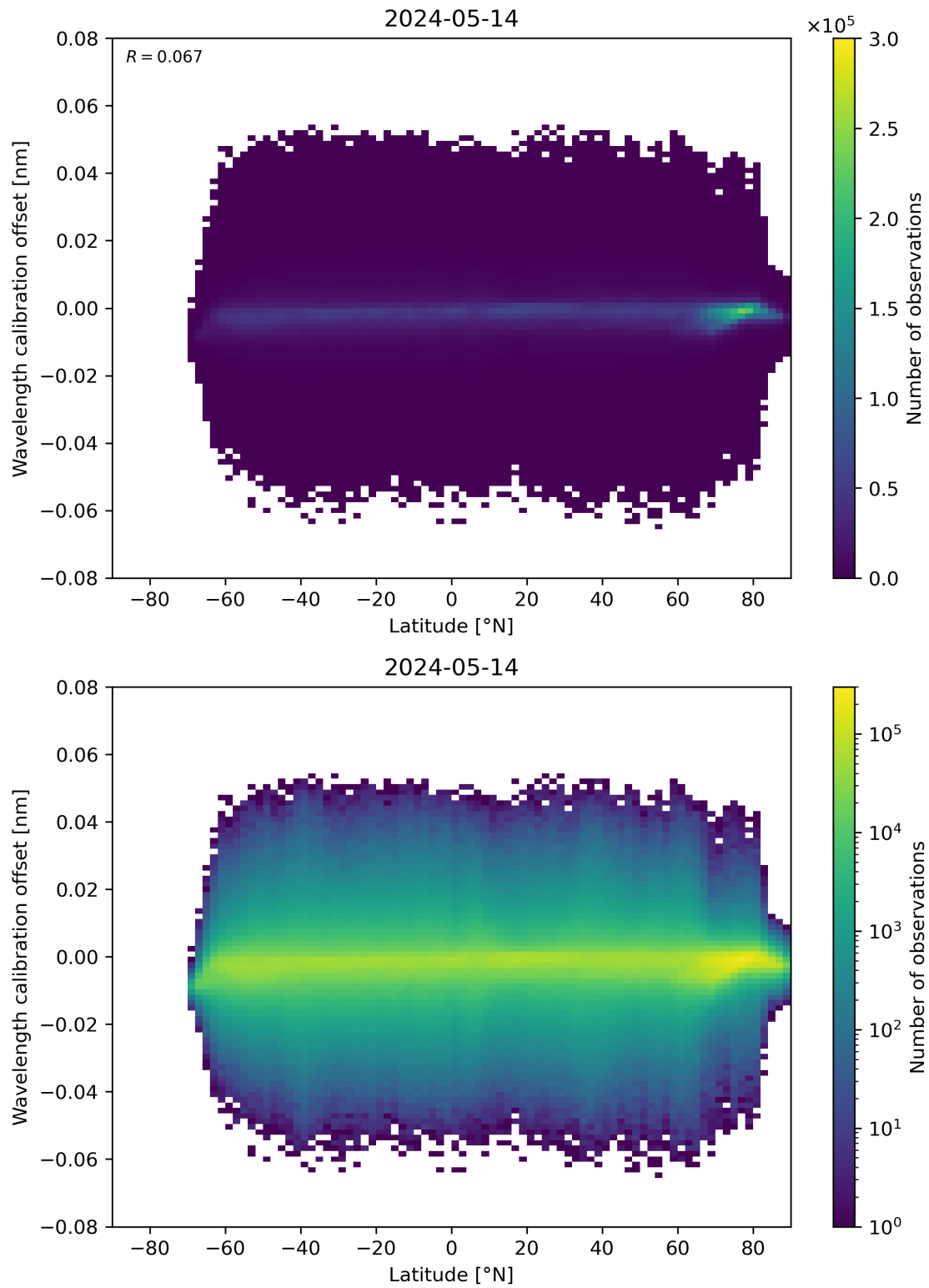
Figure 95: Scatter density plot of “Latitude” against “Wavelength calibration offset” for 2024-05-13 to 2024-05-15.
