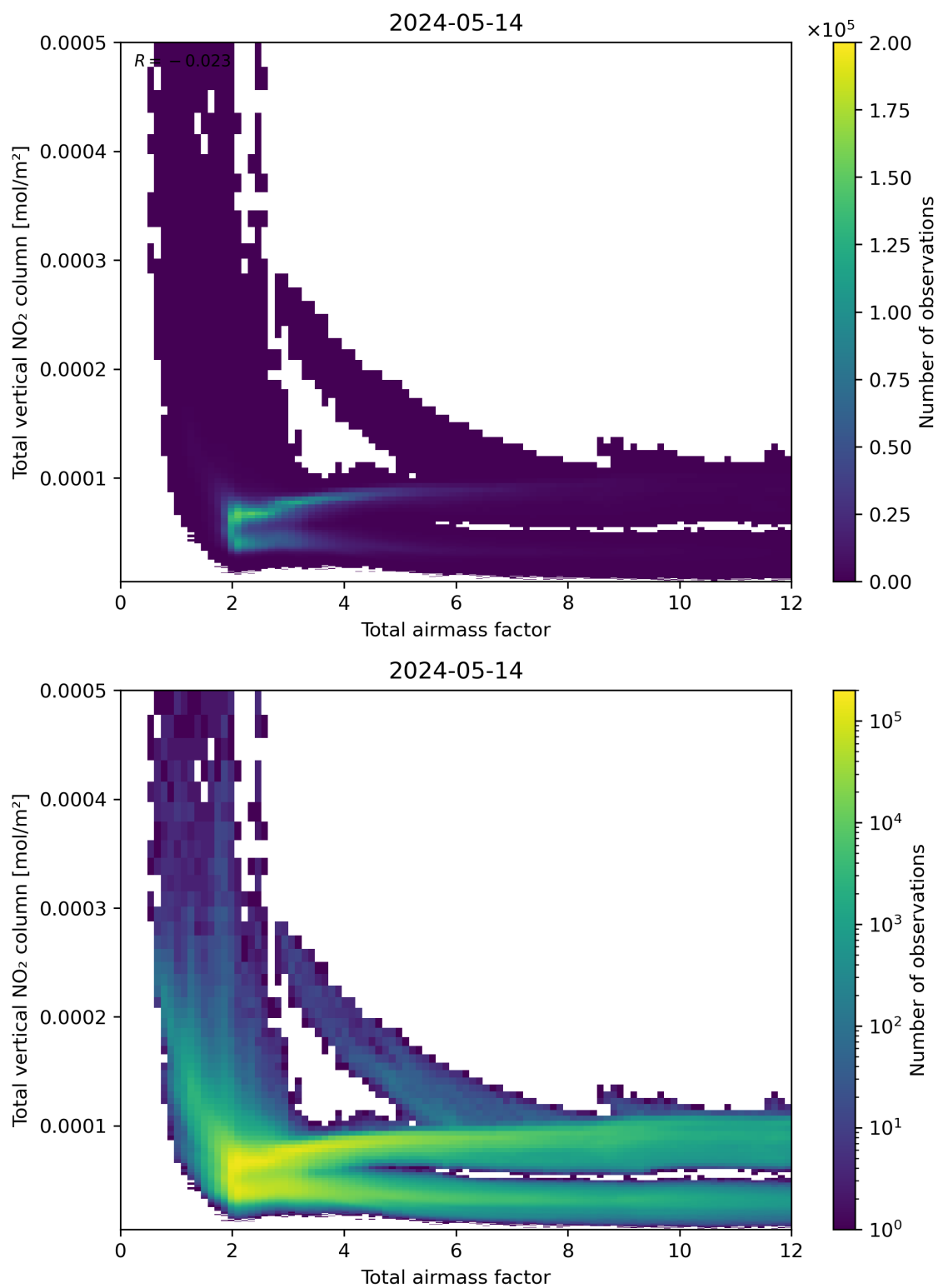
Figure 67: Scatter density plot of “Total airmass factor” against “Total vertical NO 2 column” for 2024-05-13 to 2024-05-15.
