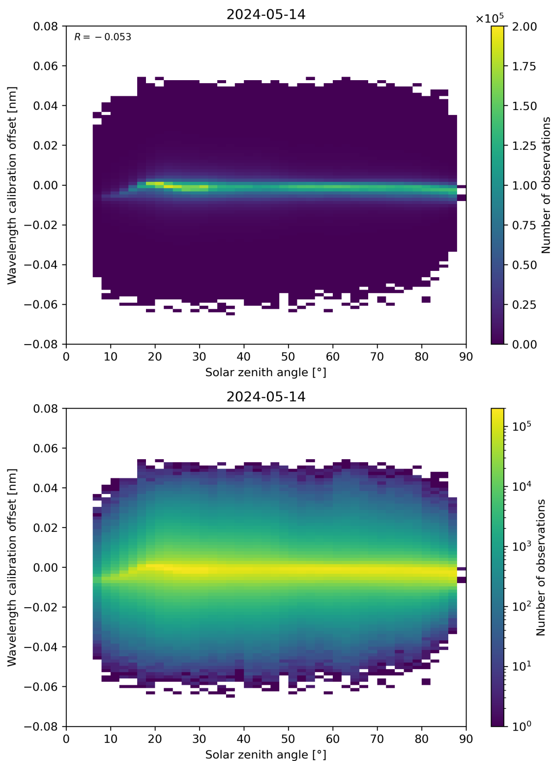
Figure 158: Scatter density plot of “Solar zenith angle” against “Wavelength calibration offset” for 2024-05-13 to 2024-05-15.
