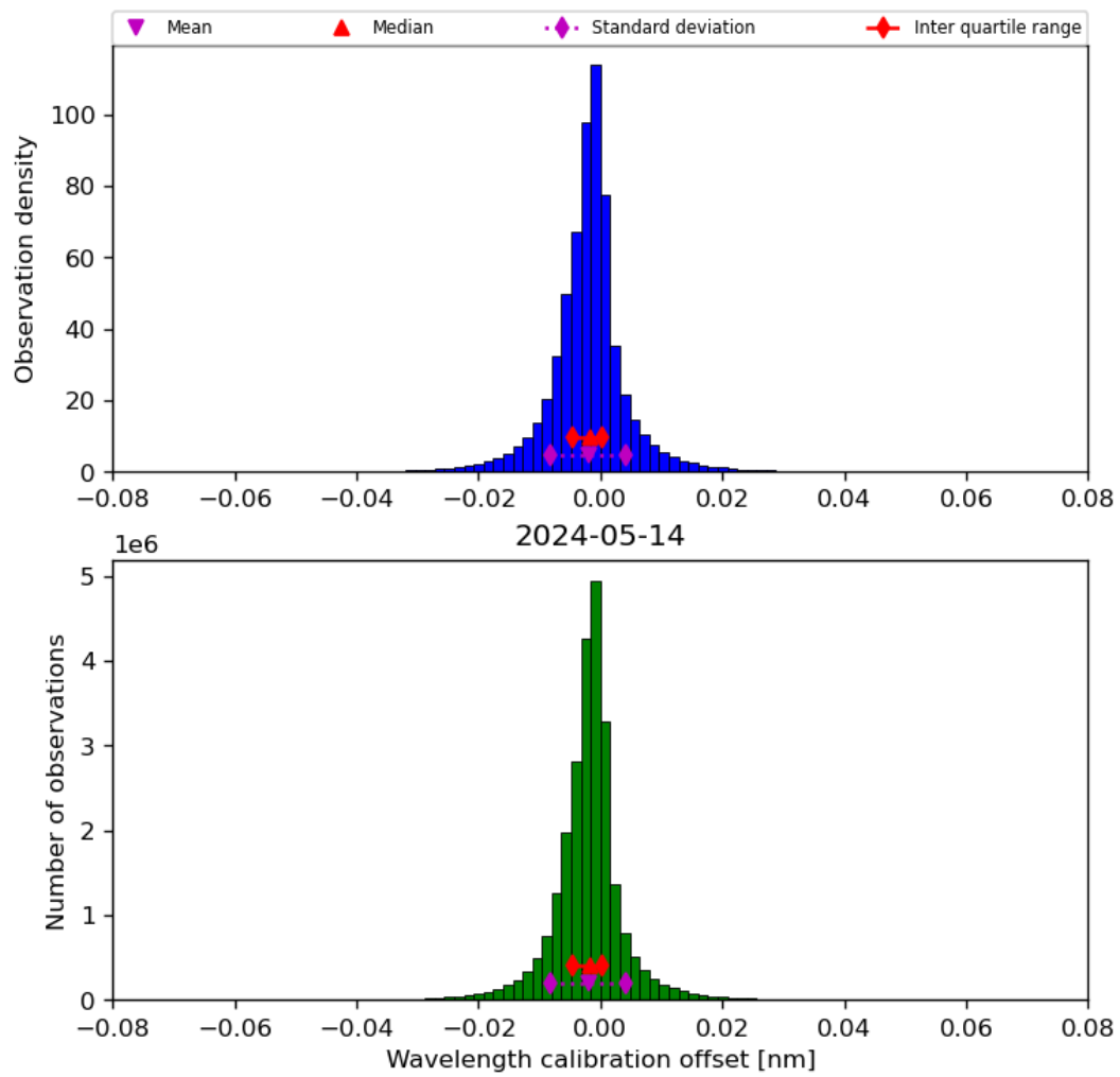
Figure 35: Histogram of “Wavelength calibration offset” for 2024-05-13 to 2024-05-15
