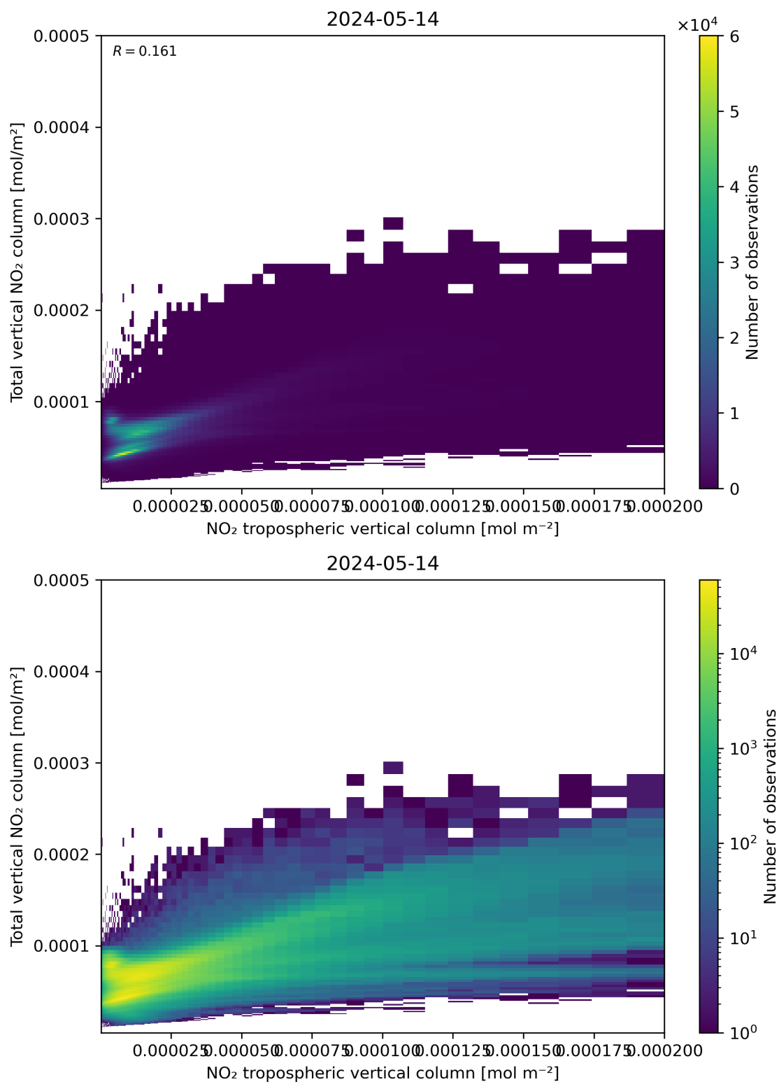
Figure 128: Scatter density plot of “NO 2 tropospheric vertical column” against “Total vertical NO 2 column” for 2024-05-13 to 2024-05-15.
