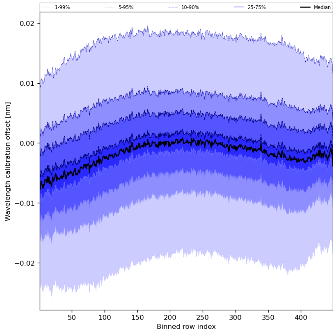
Figure 52: Along track statistics of “Wavelength calibration offset” for 2024-05-13 to 2024-05-15
