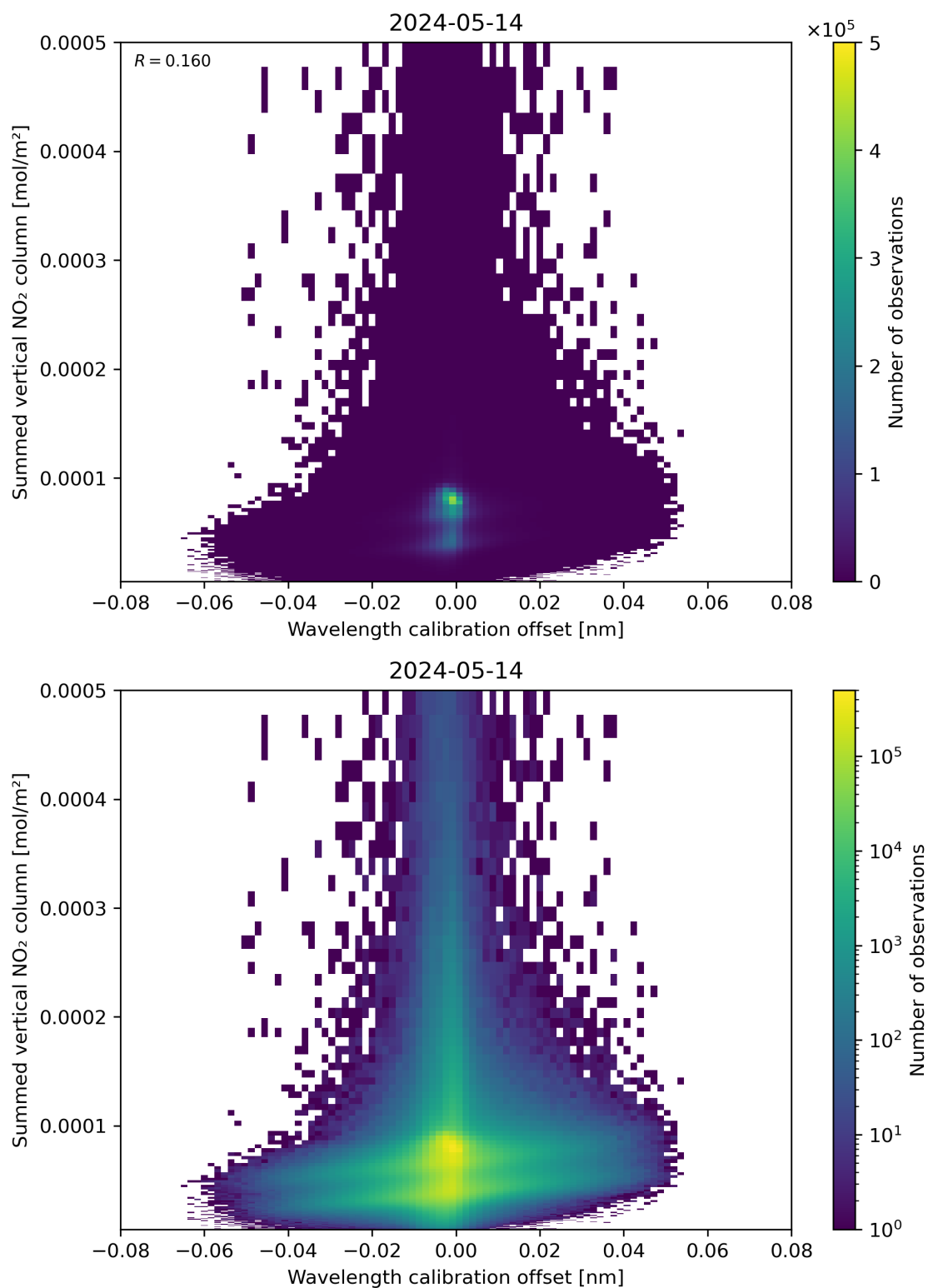
Figure 177: Scatter density plot of “Wavelength calibration offset” against “Summed vertical NO 2 column” for 2024-05-13 to 2024-05-15.
