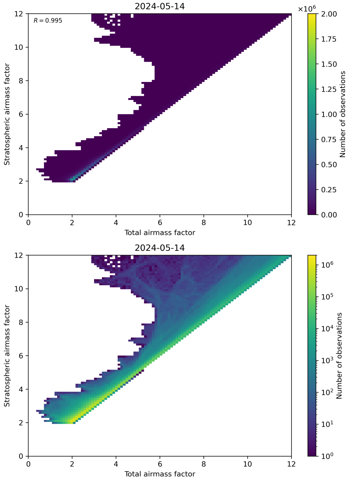
Figure 62: Scatter density plot of “Total airmass factor” against “Stratospheric airmass factor” for 2024-05-13 to 2024-05-15.
