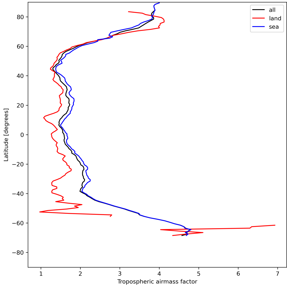
Figure 14: Zonal average of “Tropospheric airmass factor” for 2024-05-13 to 2024-05-15.
