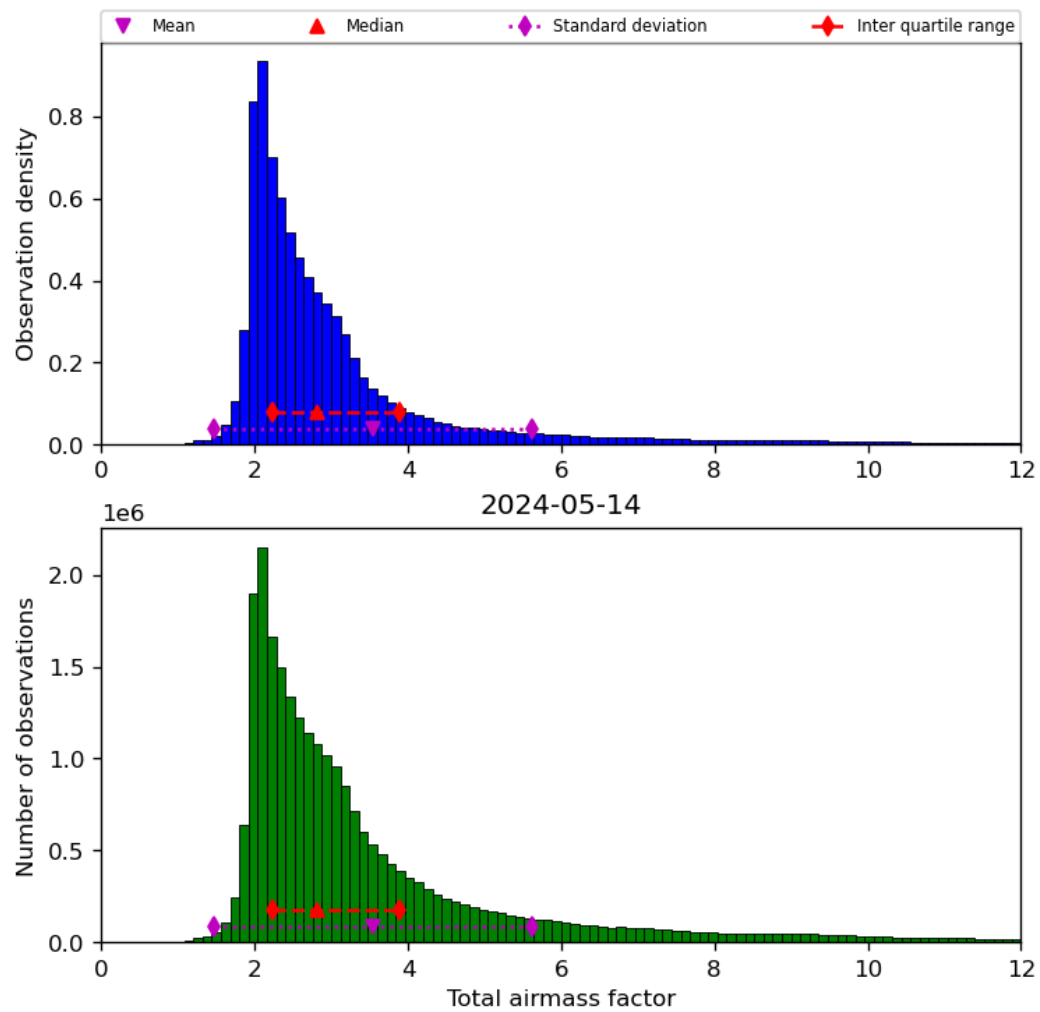
Figure 32: Histogram of “Total airmass factor” for 2024-05-13 to 2024-05-15
