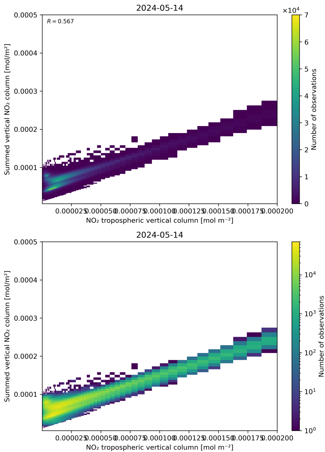
Figure 126: Scatter density plot of “NO 2 tropospheric vertical column” against “Summed vertical NO 2 column” for 2024-05-13 to 2024-05-15.
