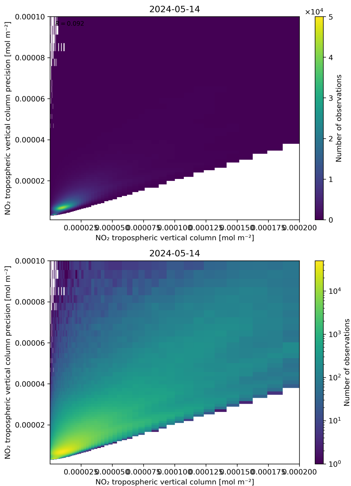
Figure 130: Scatter density plot of “NO 2 tropospheric vertical column” against “NO 2 tropospheric vertical column precision” for 2024-05-13 to 2024-05-15.
