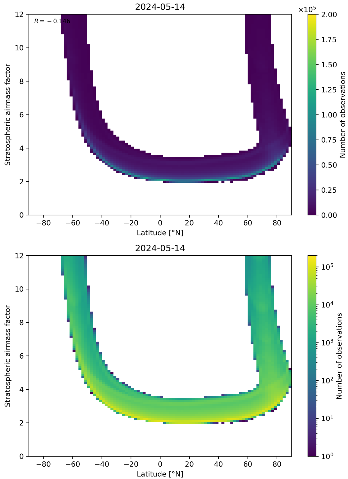
Figure 83: Scatter density plot of “Latitude” against “Stratospheric air mass factor” for 2024-05-13 to 2024-05-15.
