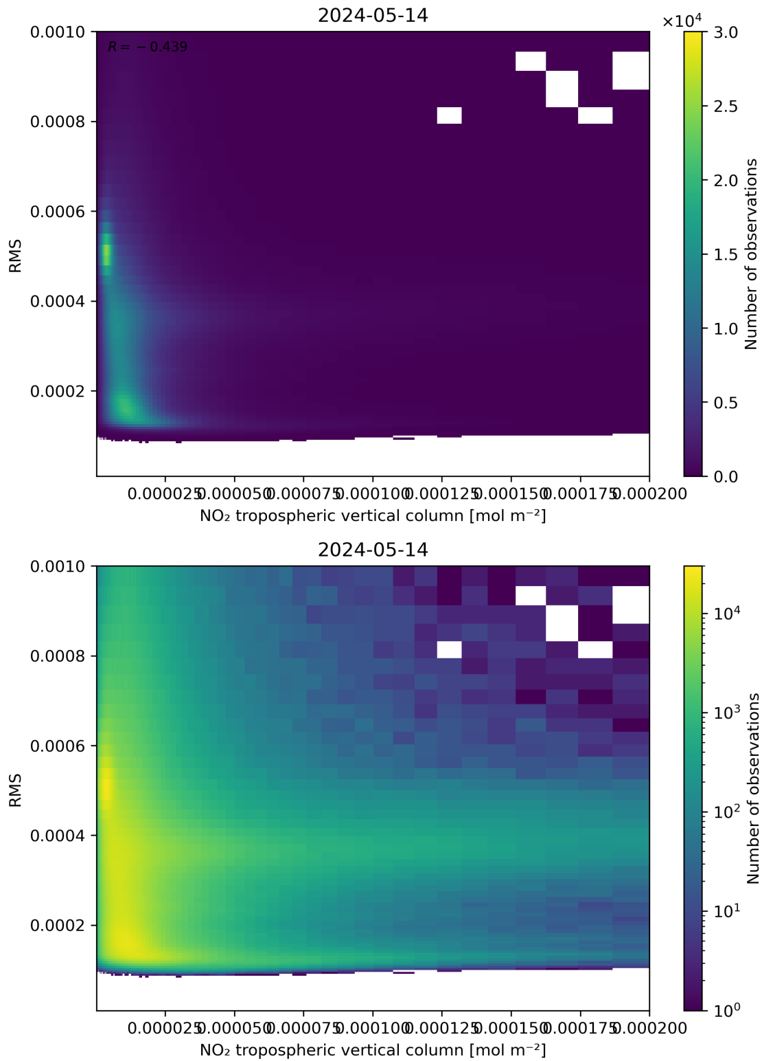
Figure 142: Scatter density plot of “NO 2 tropospheric vertical column” against “RMS” for 2024-05-13 to 2024-05-15.
