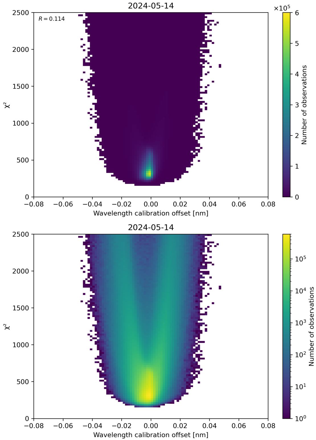
Figure 175: Scatter density plot of “Wavelength calibration offset” against “ \chi^2 ” for 2024-05-13 to 2024-05-15.
