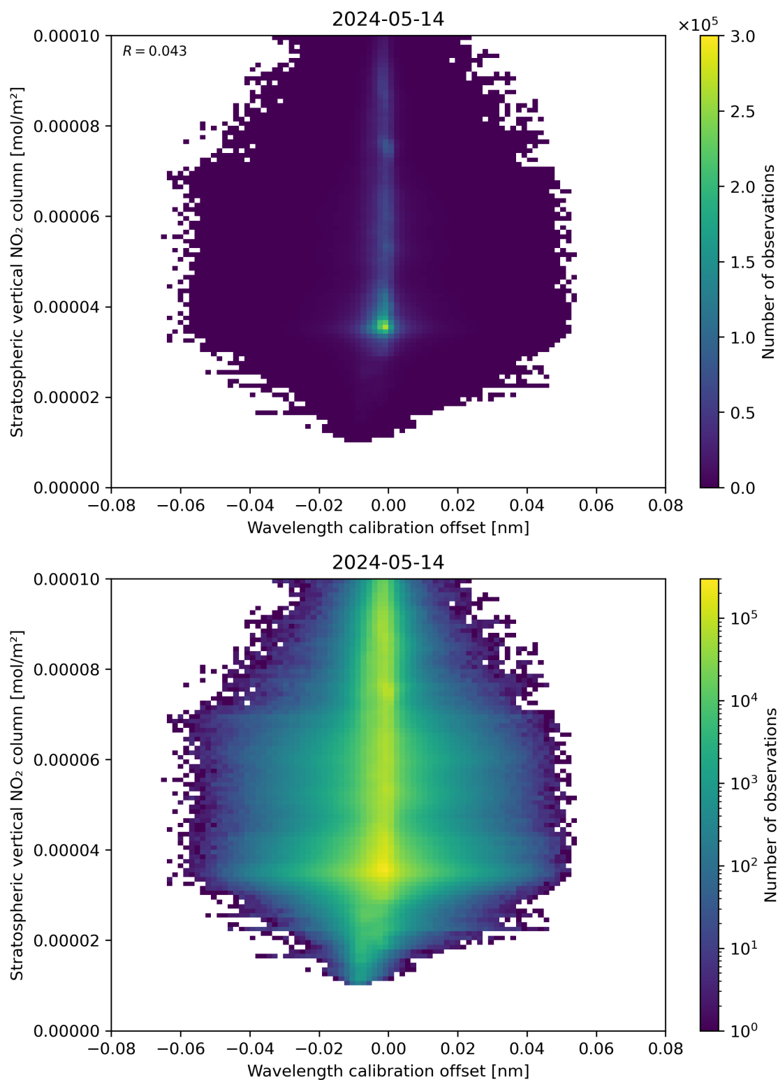
Figure 176: Scatter density plot of “Wavelength calibration offset” against “Stratospheric vertical NO 2 column” for 2024-05-13 to 2024-05-15.
