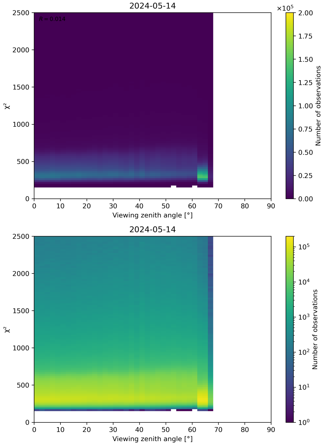
Figure 162: Scatter density plot of “Viewing zenith angle” against “ \chi^2 ” for 2024-05-13 to 2024-05-15.
