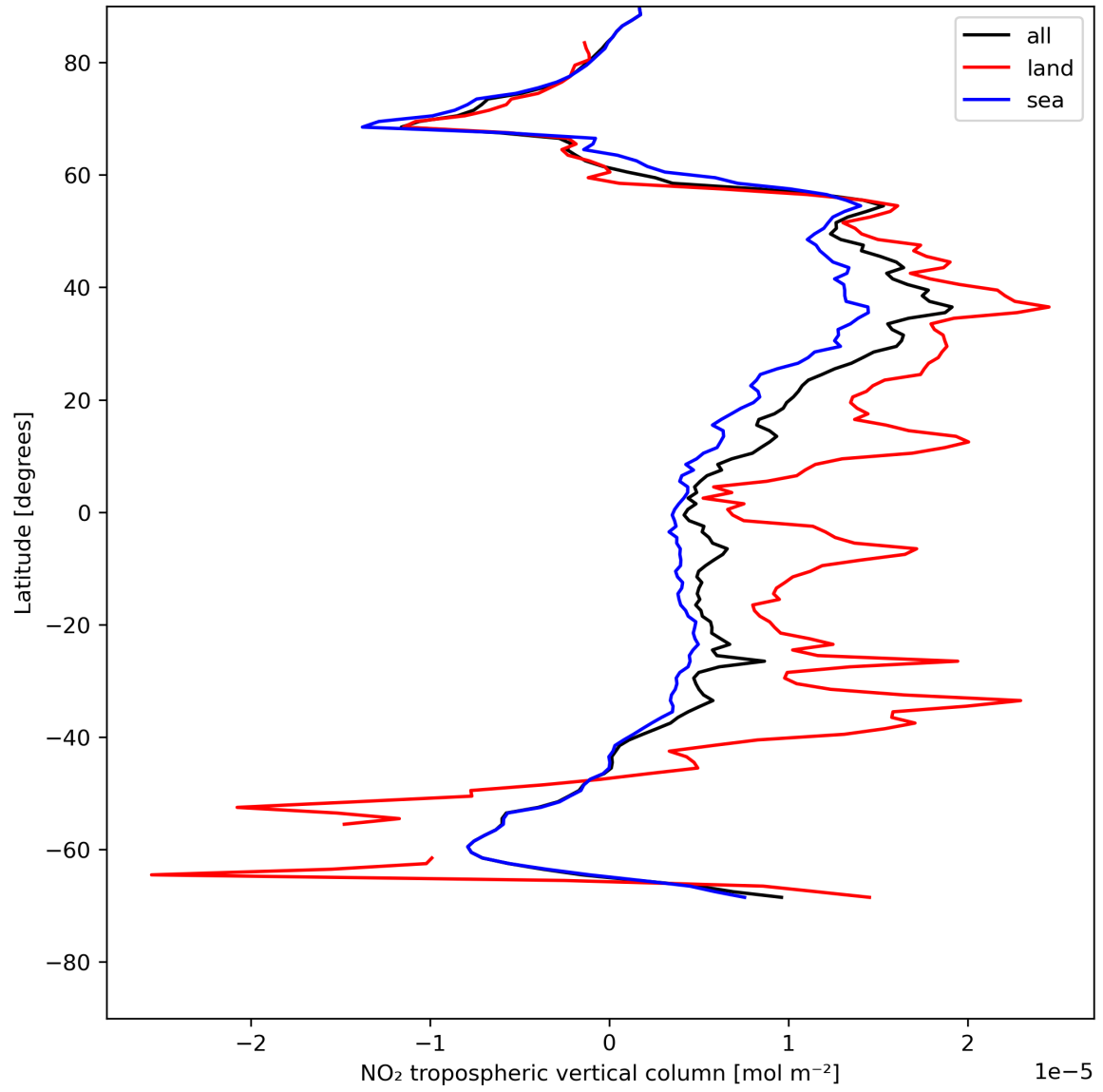
Figure 12: Zonal average of “NO 2 tropospheric vertical column” for 2024-05-13 to 2024-05-15.
