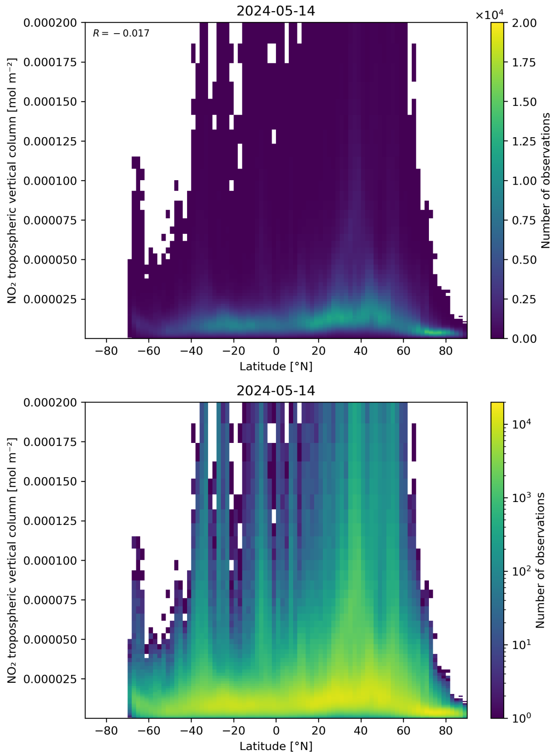
Figure 92: Scatter density plot of “Latitude” against “NO 2 tropospheric vertical column” for 2024-05-13 to 2024-05-15.
