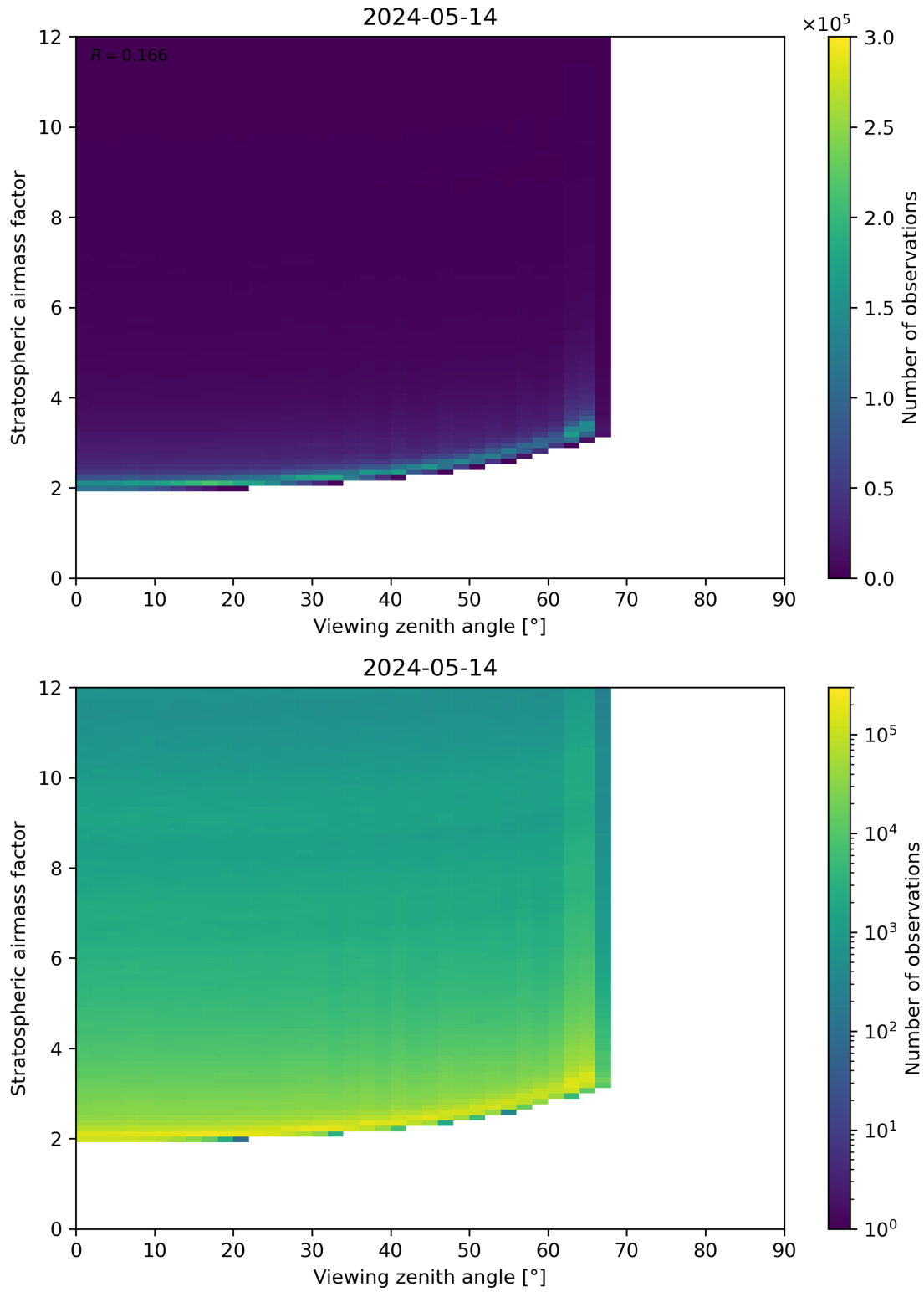
Figure 159: Scatter density plot of “Viewing zenith angle” against “Stratospheric airmass factor” for 2024-05-13 to 2024-05-15.
