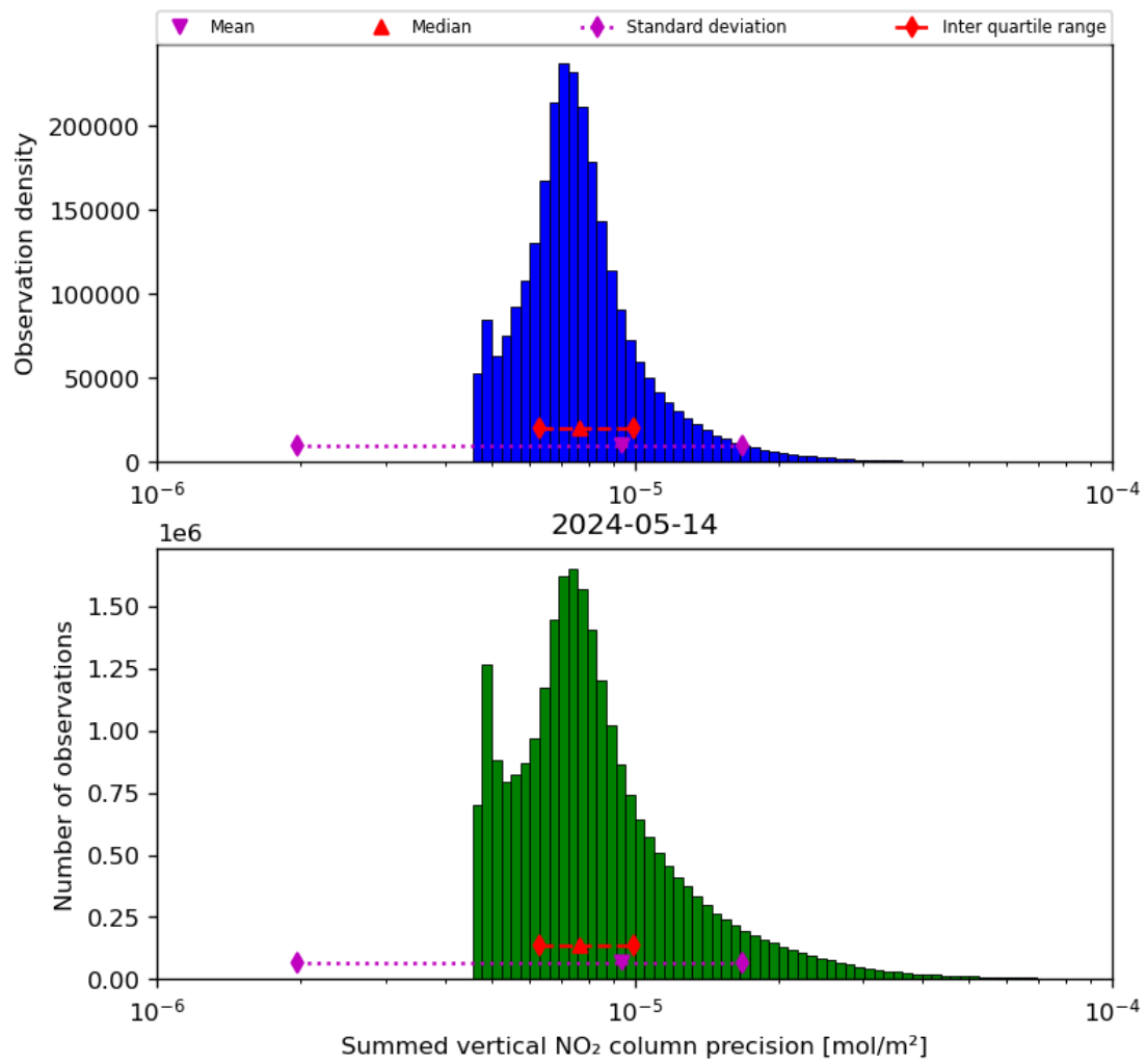
Figure 41: Histogram of "Summed vertical NO 2 column precision" for 2024-05-13 to 2024-05-15
