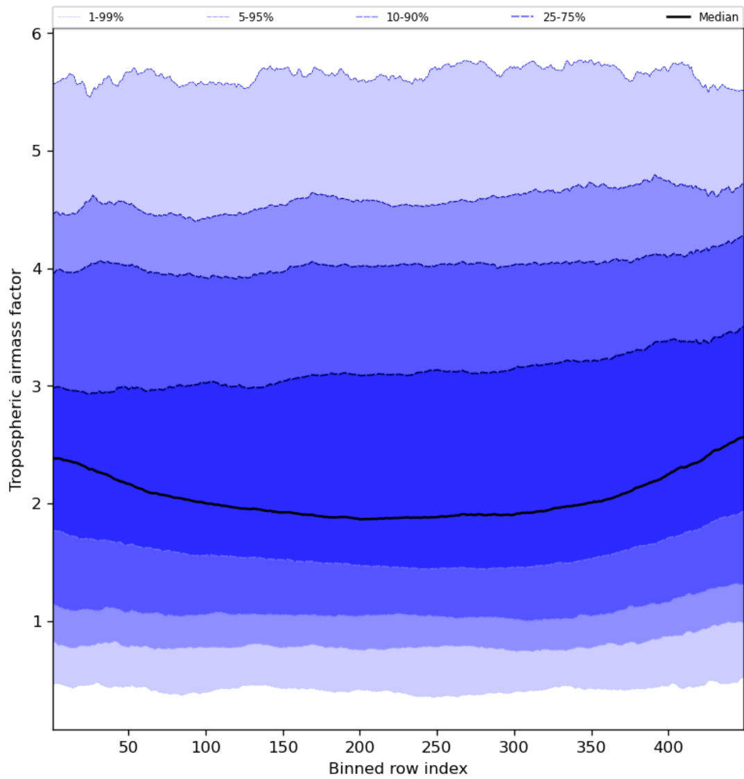
Figure 48: Along track statistics of “Tropospheric airmass factor” for 2024-05-13 to 2024-05-15
