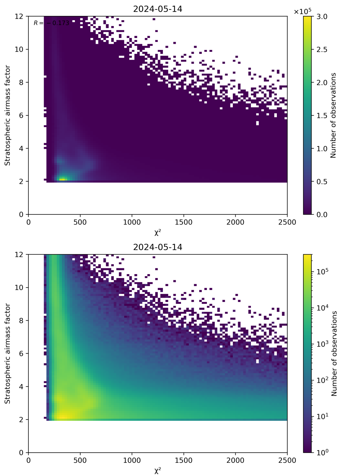
Figure 81: Scatter density plot of “ \chi^2 ” against “Stratospheric airmass factor” for 2024-05-13 to 2024-05-15.
