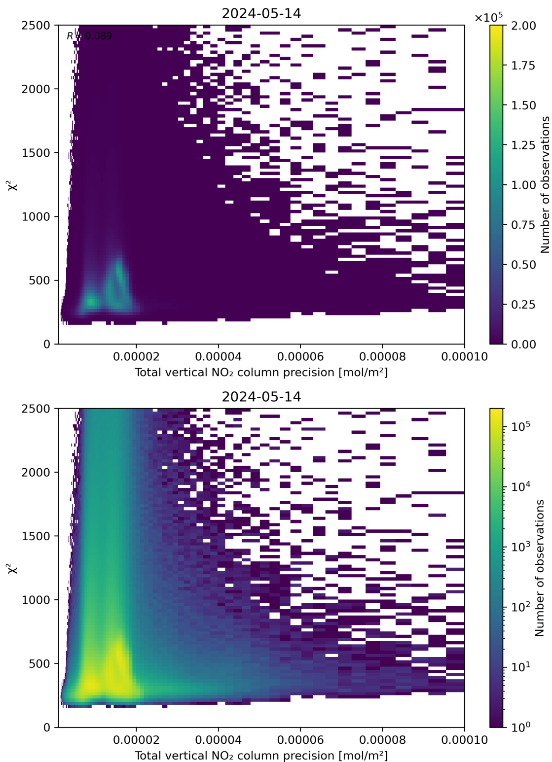
Figure 116: Scatter density plot of “Total vertical NO 2 column precision” against “ \chi^2 ” for 2024-05-13 to 2024-05-15.
