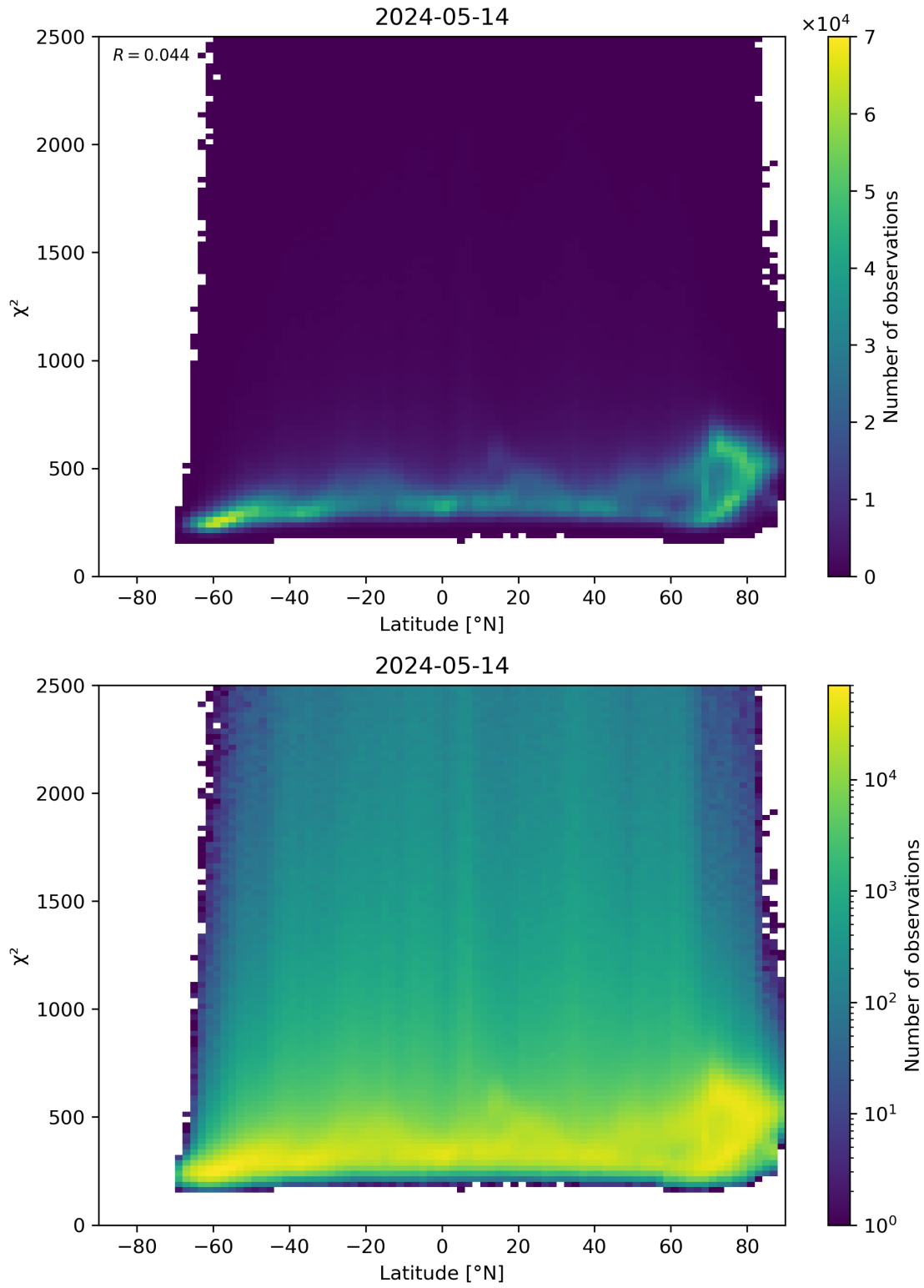
Figure 86: Scatter density plot of “Latitude” against “ \chi^2 ” for 2024-05-13 to 2024-05-15.
