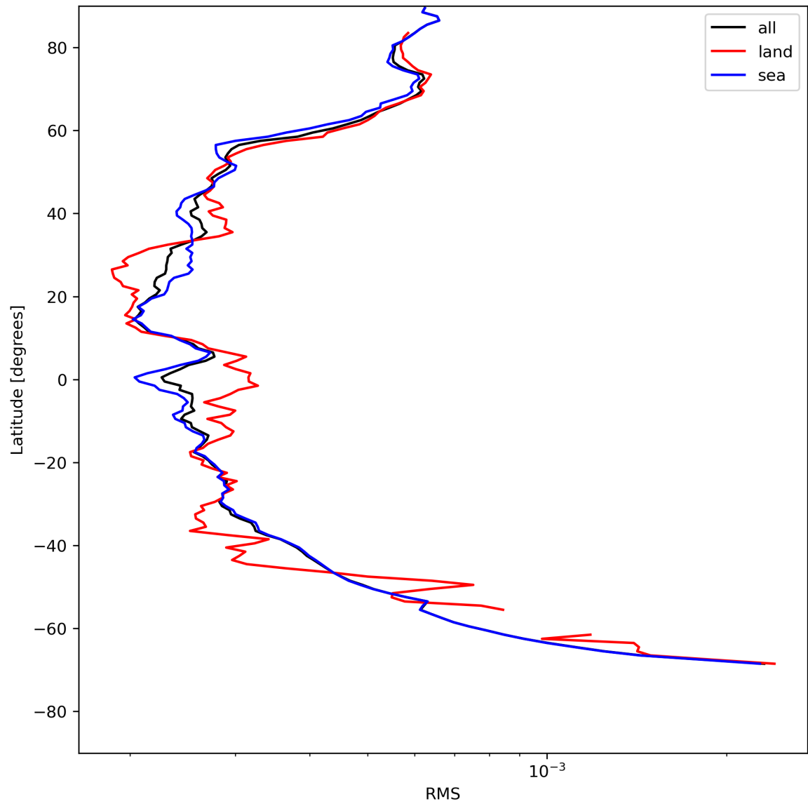
Figure 26: Zonal average of “RMS” for 2024-05-13 to 2024-05-15.
