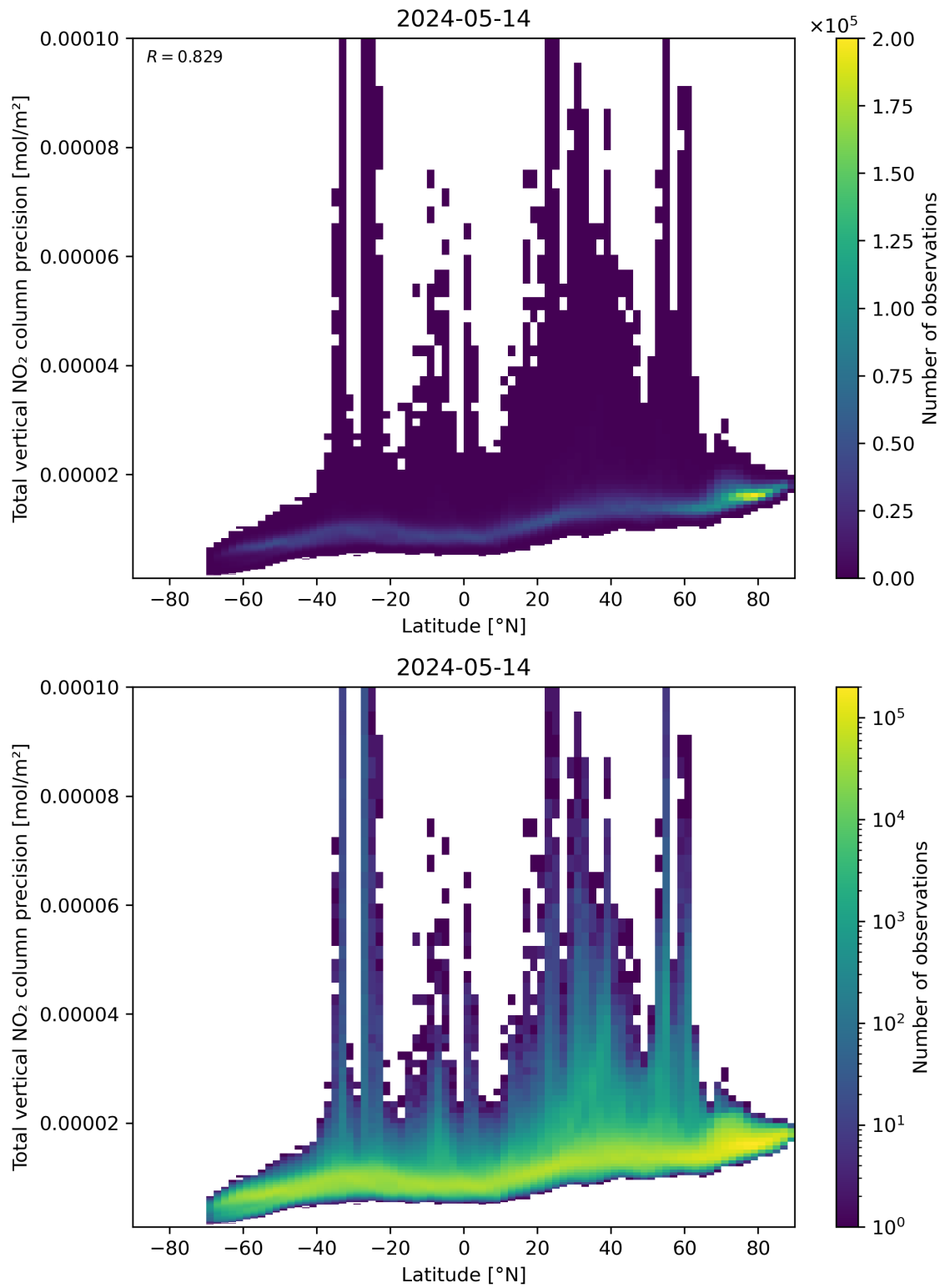
Figure 91: Scatter density plot of “Latitude” against “Total vertical NO 2 column precision” for 2024-05-13 to 2024-05-15.
