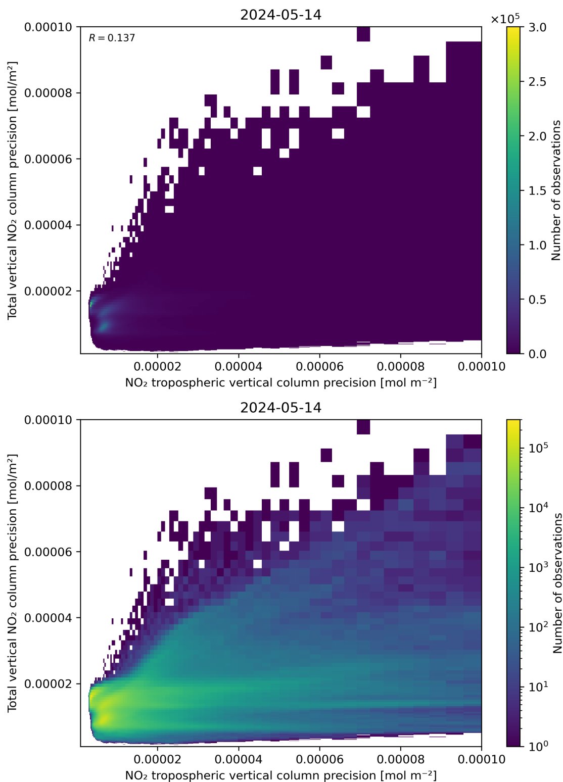
Figure 139: Scatter density plot of “NO 2 tropospheric vertical column precision” against “Total vertical NO 2 column precision” for 2024-05-13 to 2024-05-15.
