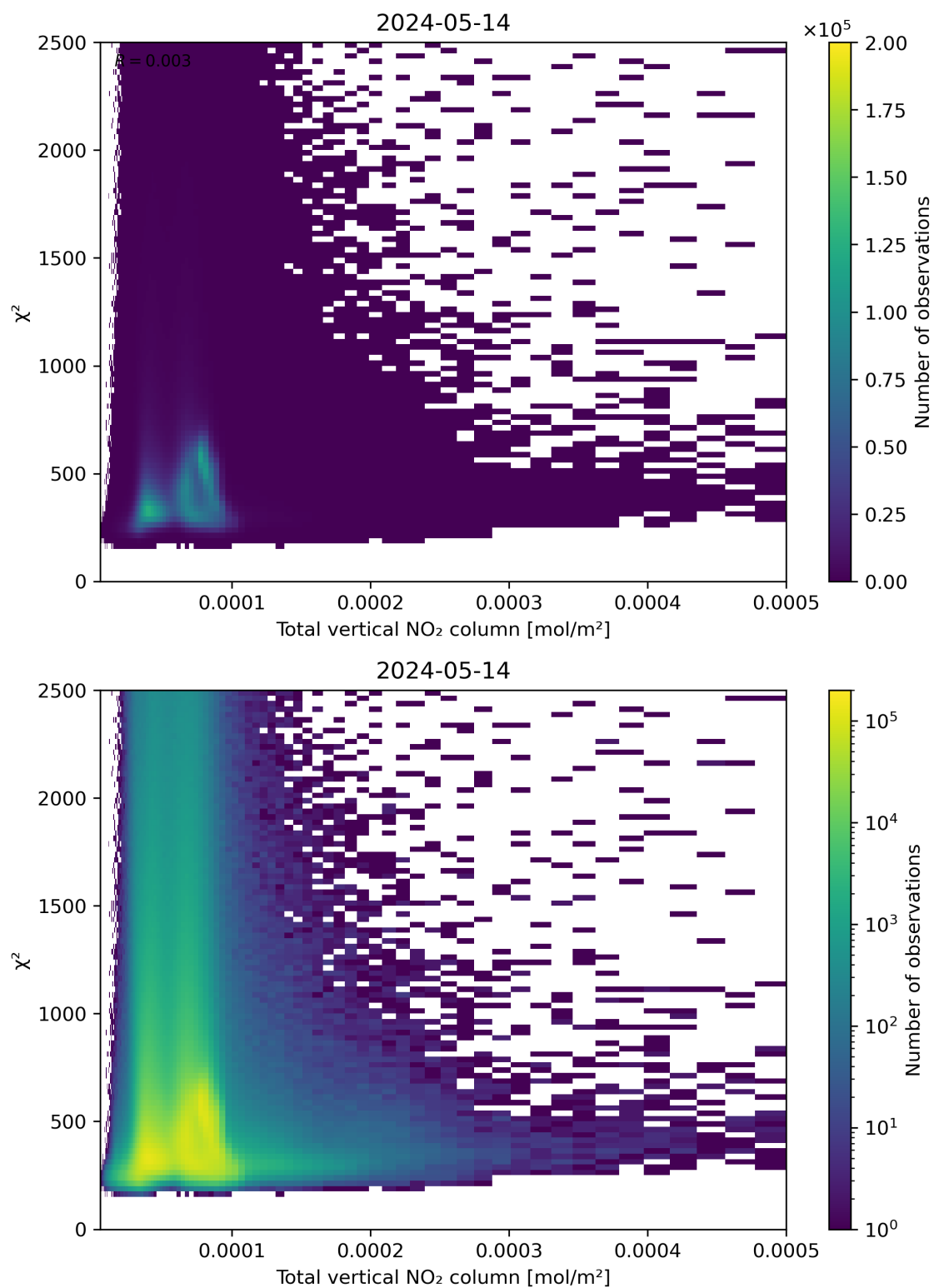
Figure 111: Scatter density plot of “Total vertical NO 2 column” against “ \chi^2 ” for 2024-05-13 to 2024-05-15.
