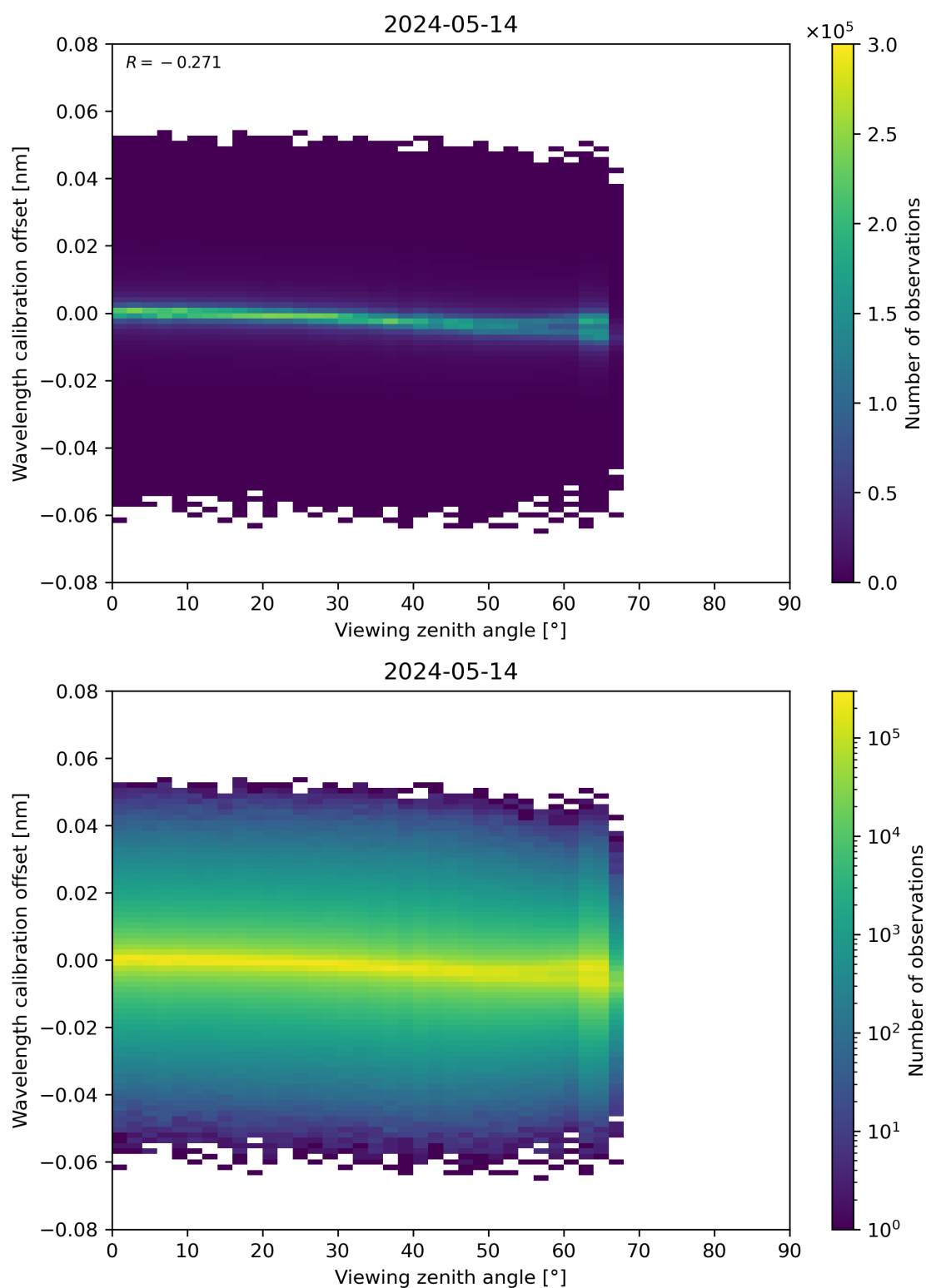
Figure 173: Scatter density plot of “Viewing zenith angle” against “Wavelength calibration offset” for 2024-05-13 to 2024-05-15.
