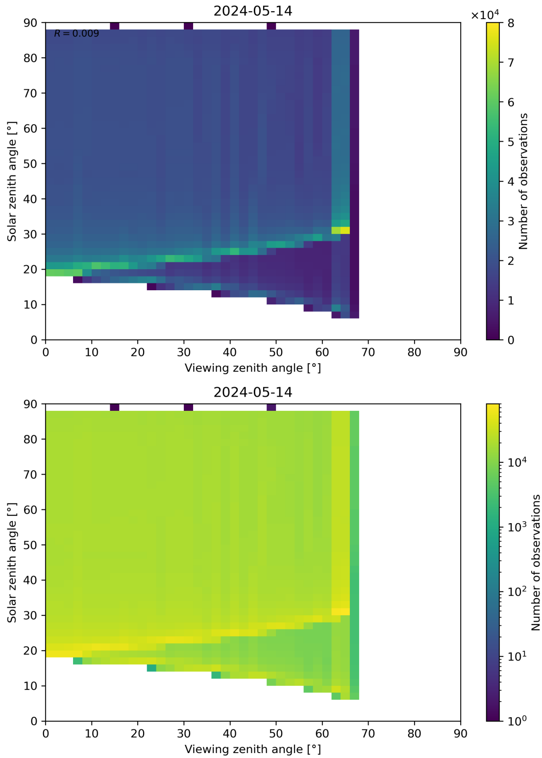
Figure 172: Scatter density plot of “Viewing zenith angle” against “Solar zenith angle” for 2024-05-13 to 2024-05-15.
