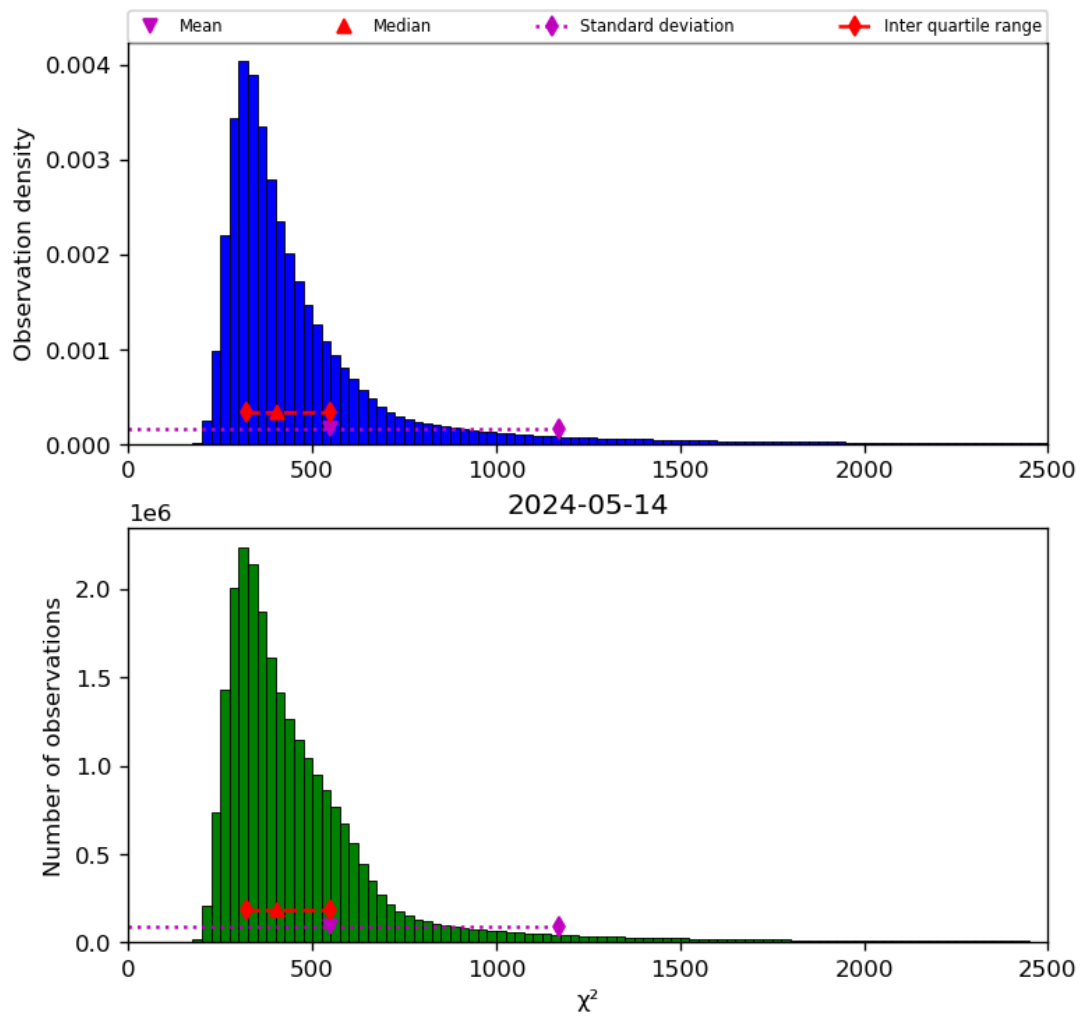
Figure 42: Histogram of “ \chi^2 ” for 2024-05-13 to 2024-05-15
