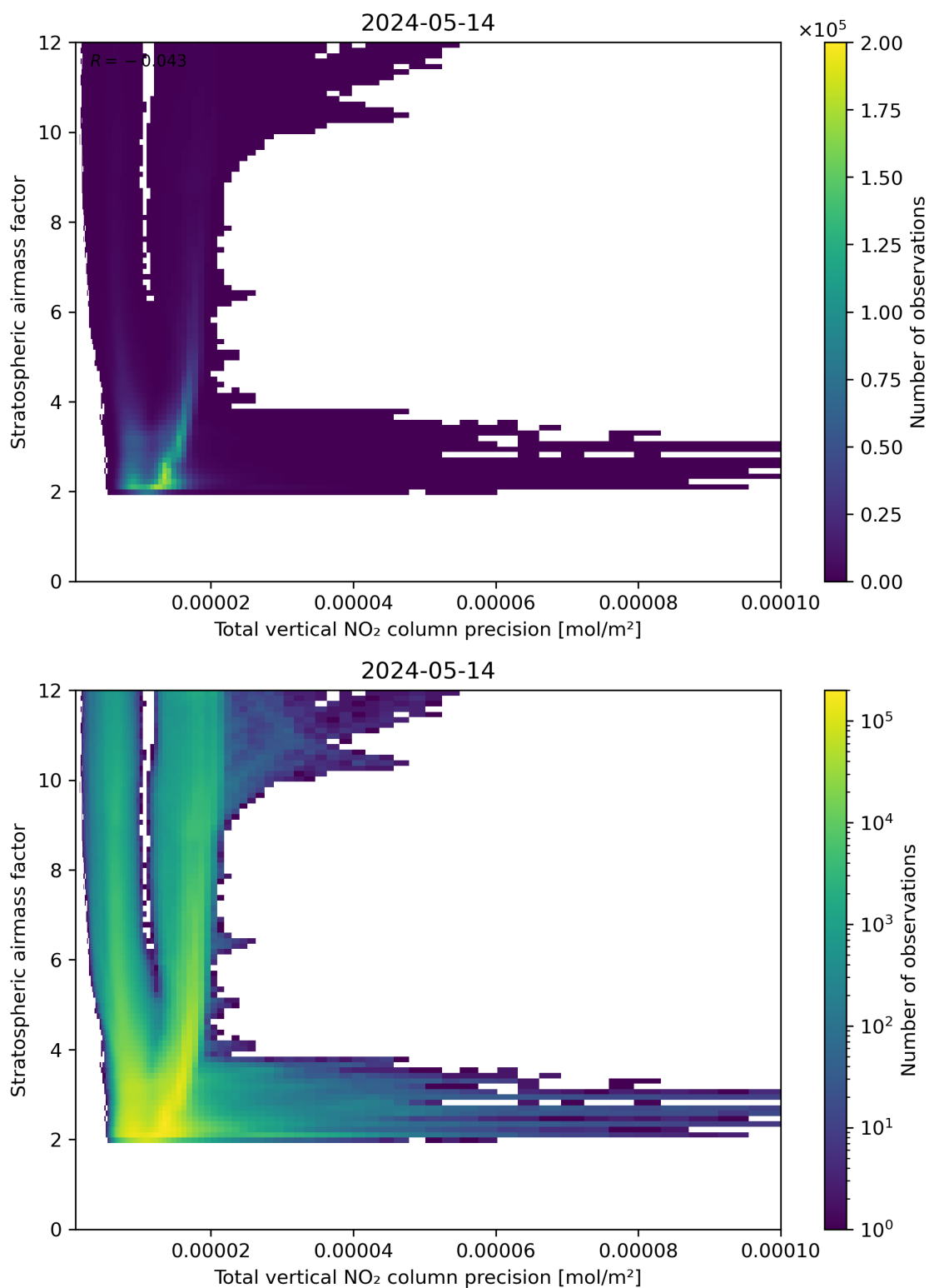
Figure 115: Scatter density plot of “Total vertical NO 2 column precision” against “Stratospheric air mass factor” for 2024-05-13 to 2024-05-15.
