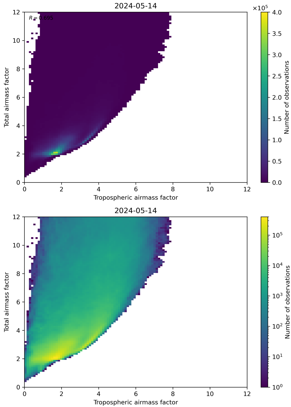
Figure 72: Scatter density plot of “Tropospheric airmass factor” against “Total airmass factor” for 2024-05-13 to 2024-05-15.
