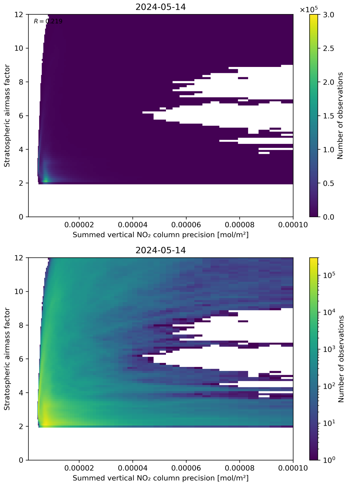
Figure 106: Scatter density plot of “Summed vertical NO 2 column precision” against “Stratospheric airmass factor” for 2024-05-13 to 2024-05-15.
