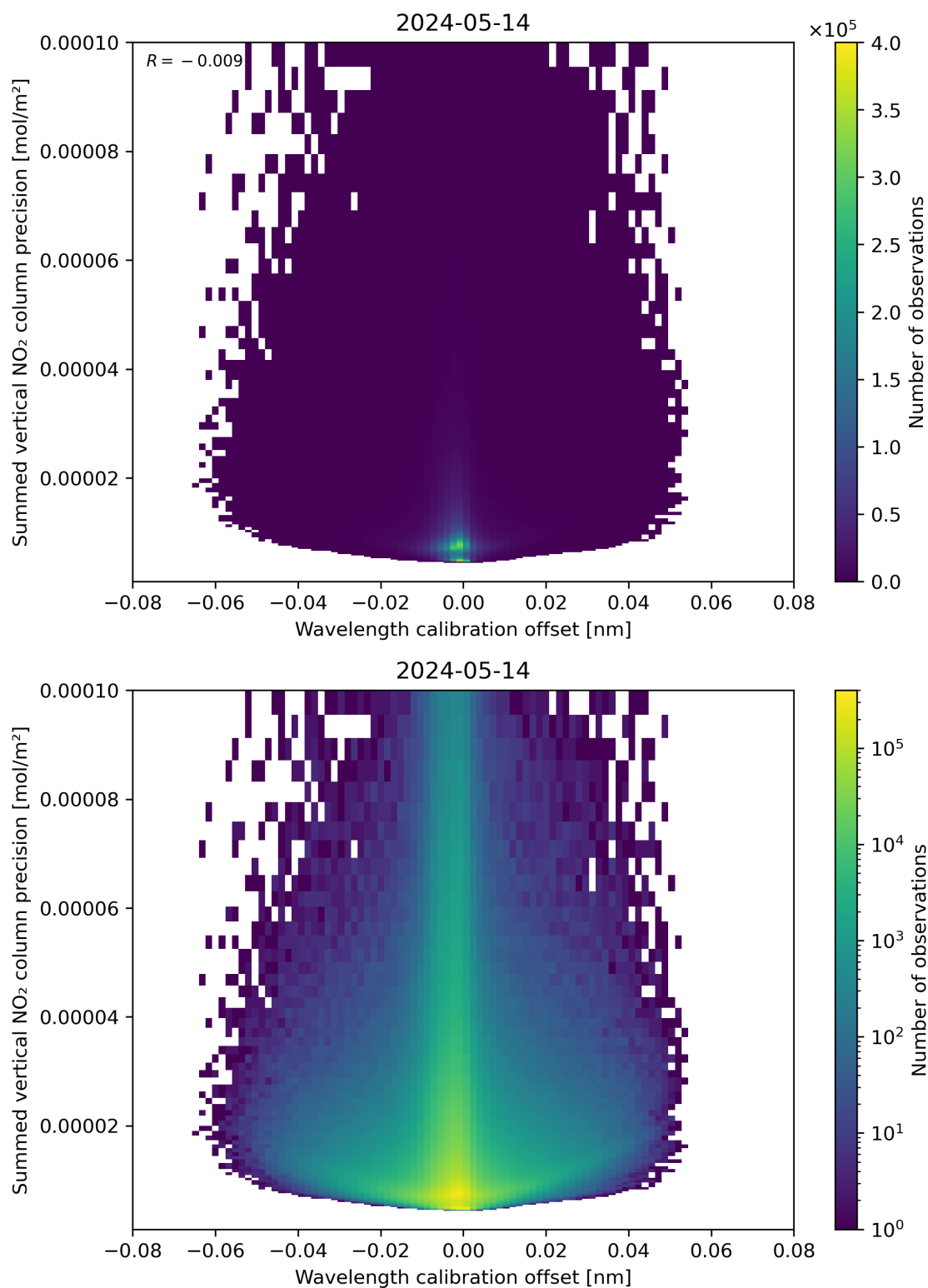
Figure 178: Scatter density plot of “Wavelength calibration offset” against “Summed vertical NO 2 column precision” for 2024-05-13 to 2024-05-15.
