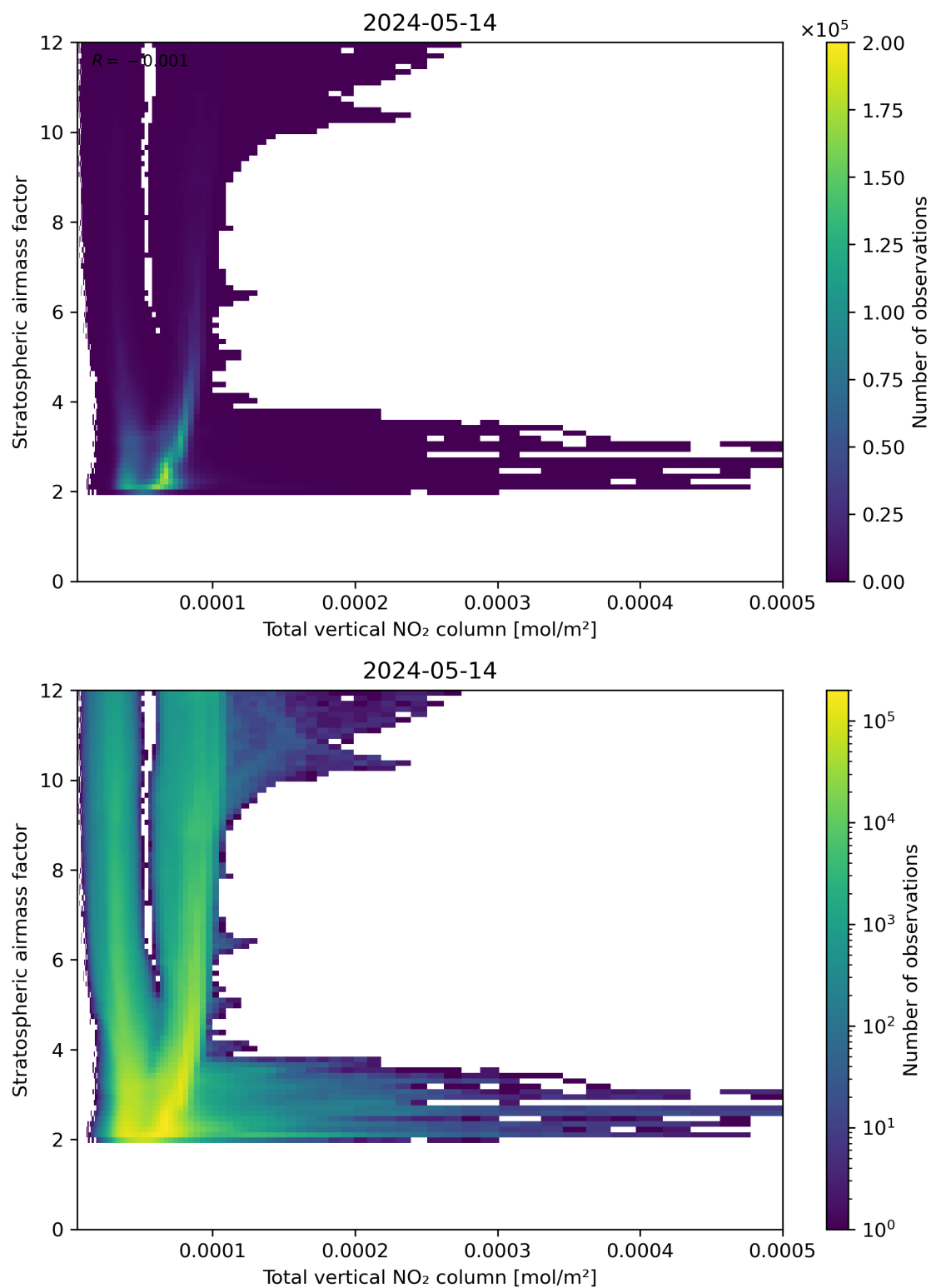
Figure 110: Scatter density plot of “Total vertical NO 2 column” against “Stratospheric airmass factor” for 2024-05-13 to 2024-05-15.
