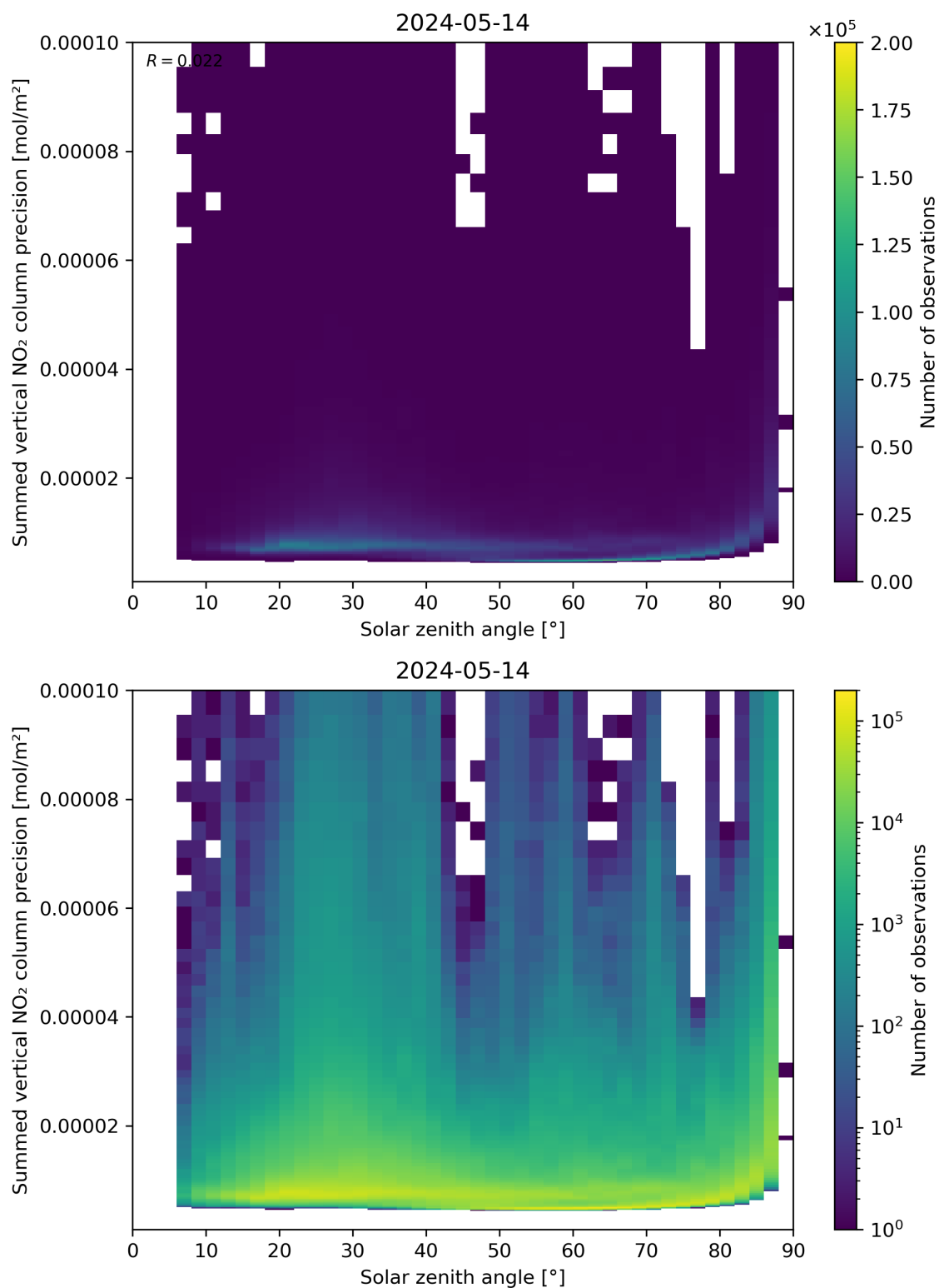
Figure 152: Scatter density plot of “Solar zenith angle” against “Summed vertical NO 2 column precision” for 2024-05-13 to 2024-05-15.
