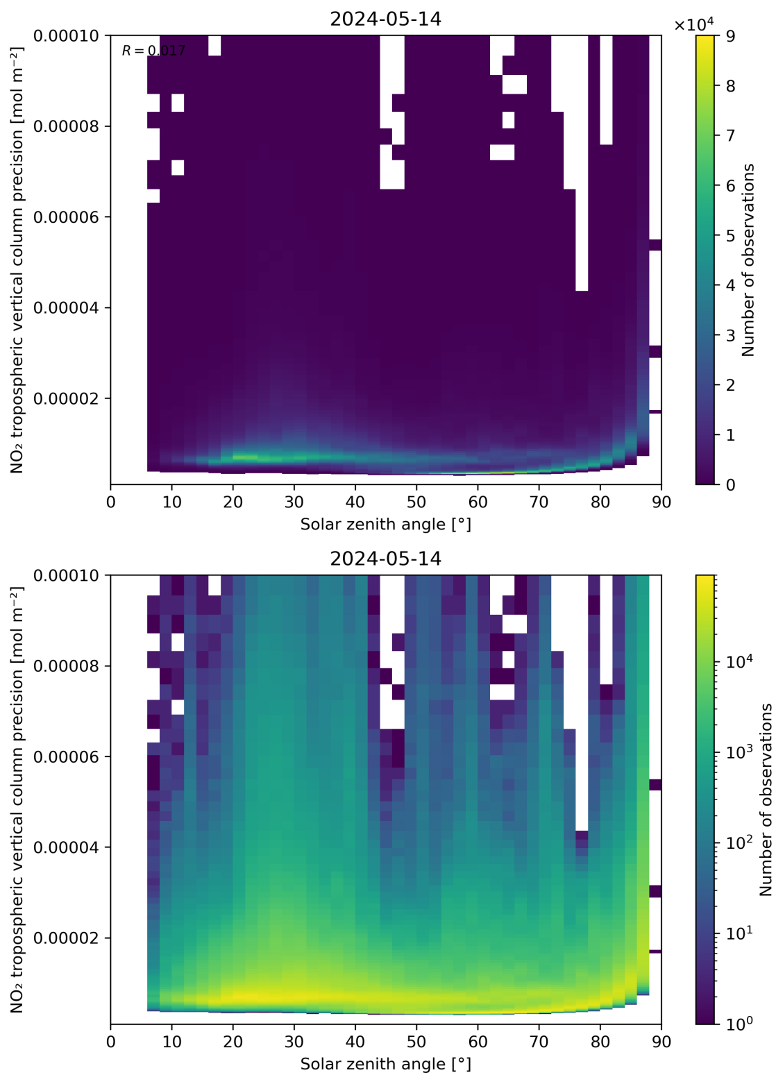
Figure 156: Scatter density plot of “Solar zenith angle” against “NO 2 tropospheric vertical column precision” for 2024-05-13 to 2024-05-15.
