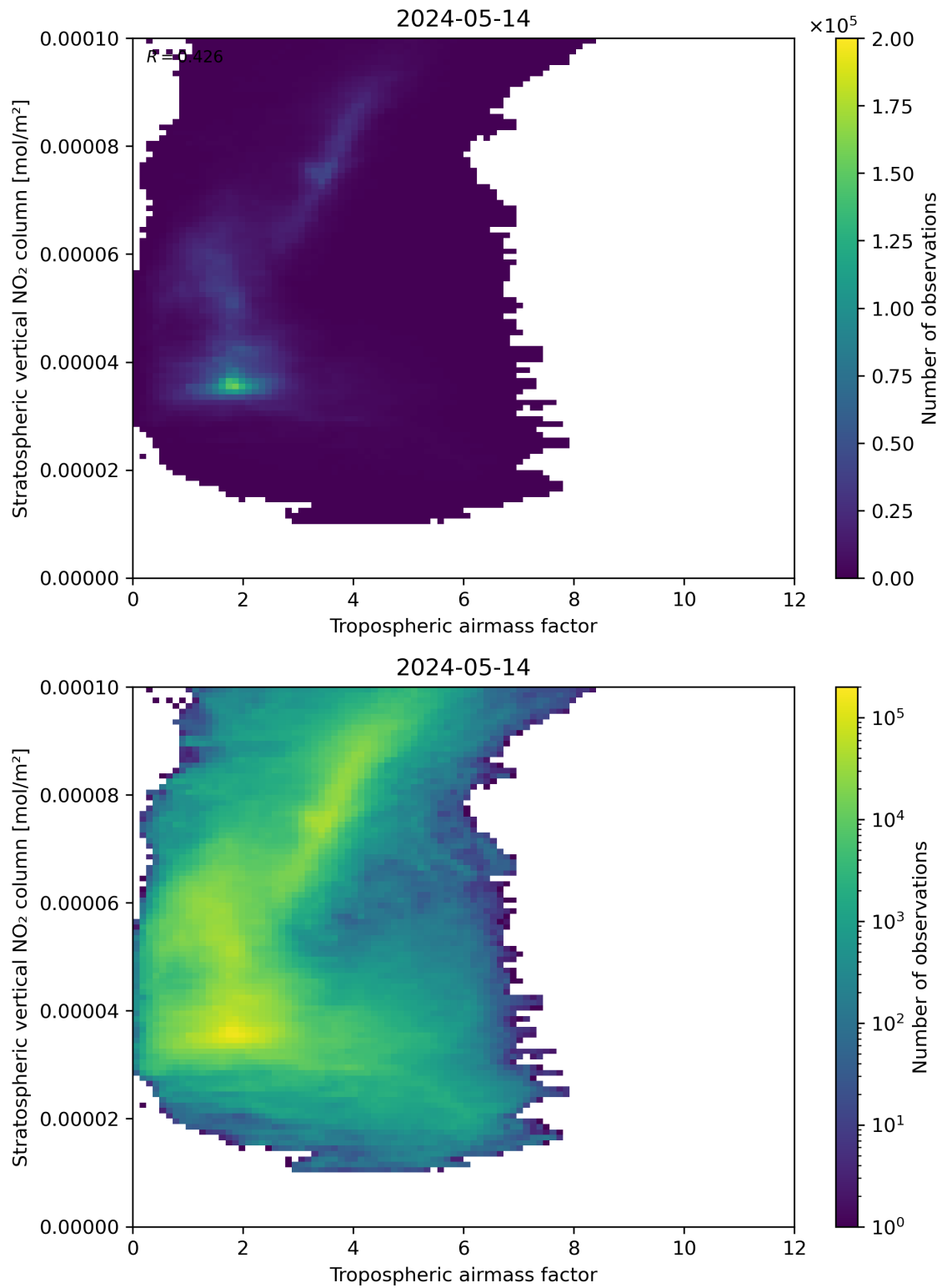
Figure 74: Scatter density plot of “Tropospheric air mass factor” against “Stratospheric vertical NO 2 column” for 2024-05-13 to 2024-05-15.
