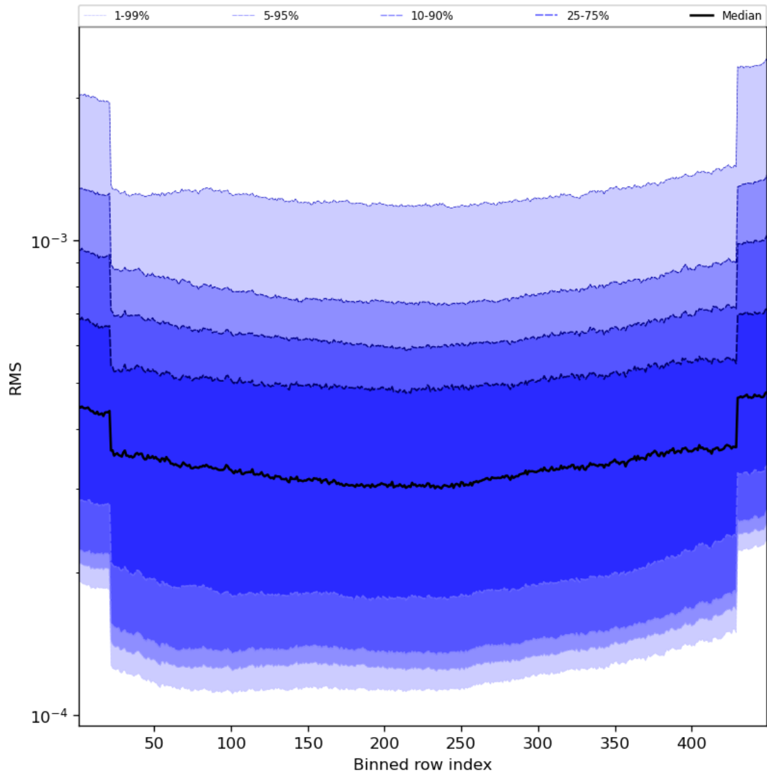
Figure 60: Along track statistics of “RMS” for 2024-05-13 to 2024-05-15
