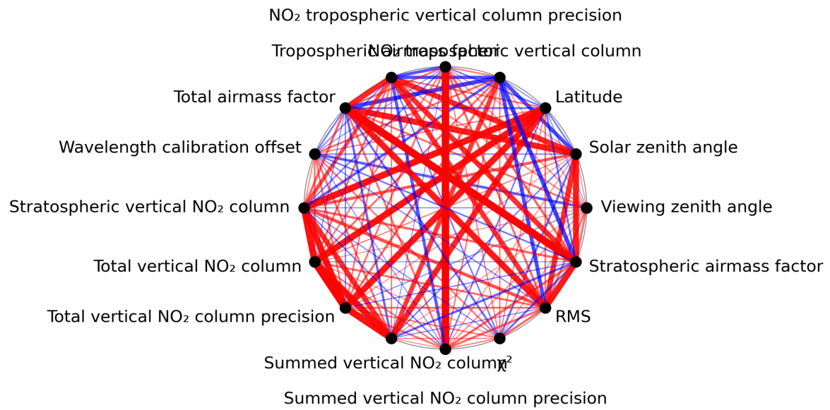
Figure 1: Map of correlation graph for 2024-05-13 to 2024-05-15.
