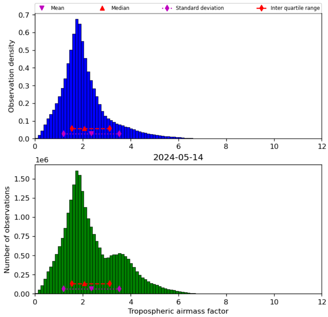
Figure 31: Histogram of “Tropospheric airmass factor” for 2024-05-13 to 2024-05-15
