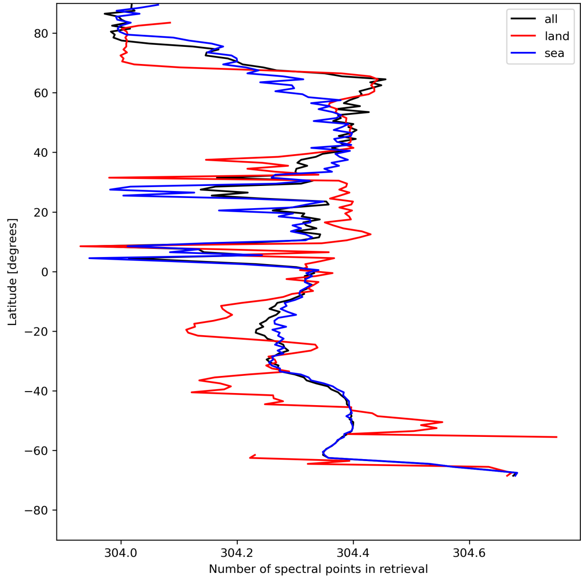
Figure 16: Zonal average of “Number of spectral points in retrieval” for 2024-05-13 to 2024-05-15.
