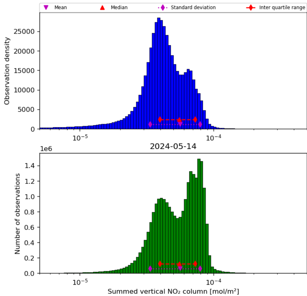
Figure 40: Histogram of “Summed vertical NO 2 column” for 2024-05-13 to 2024-05-15
