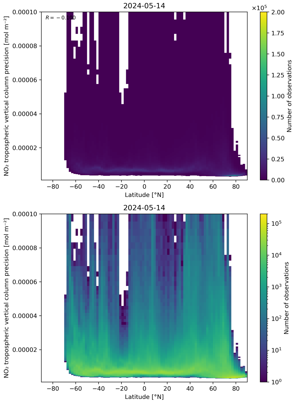
Figure 93: Scatter density plot of “Latitude” against “NO 2 tropospheric vertical column precision” for 2024-05-13 to 2024-05-15.
