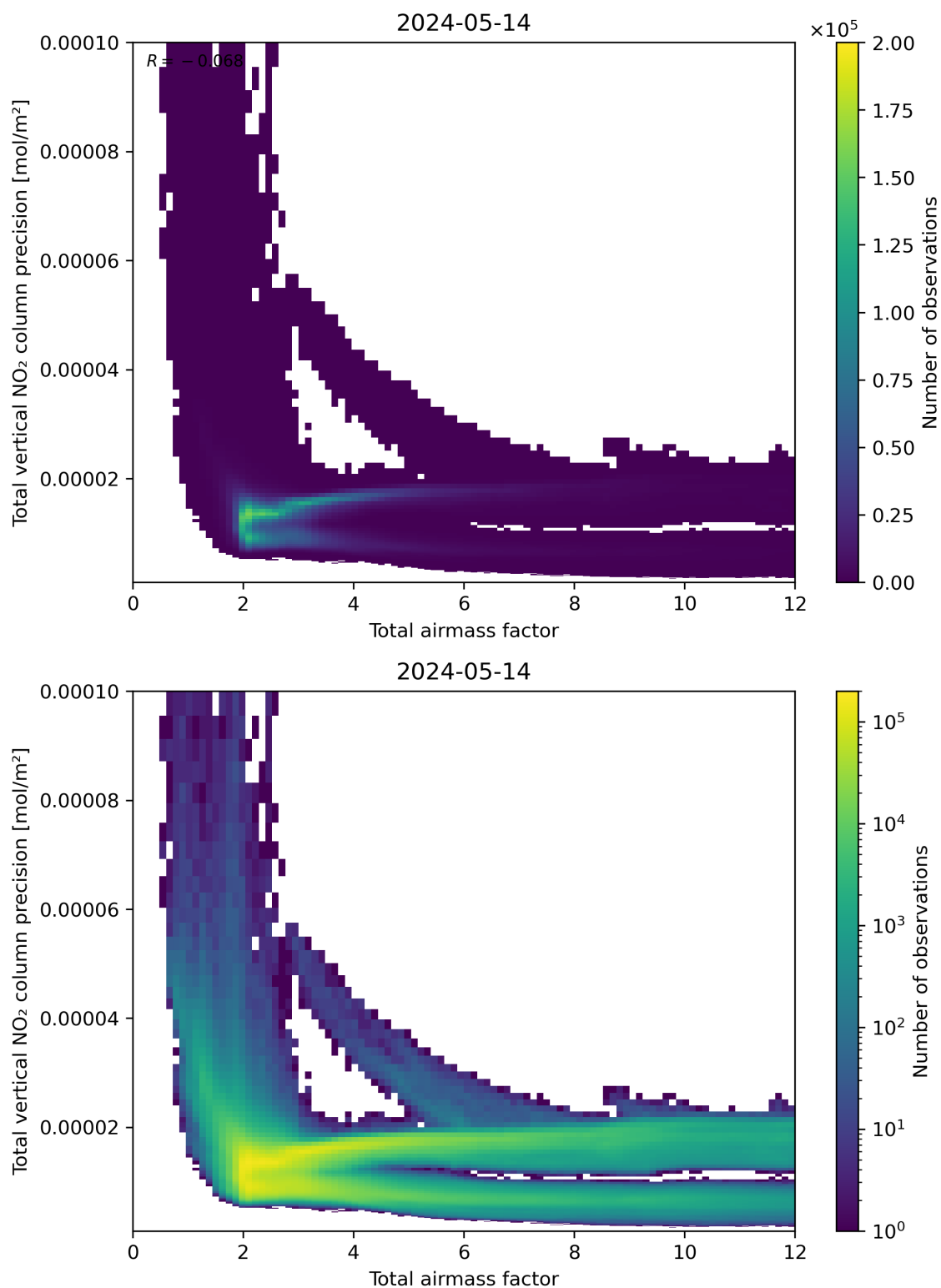
Figure 68: Scatter density plot of “Total airmass factor” against “Total vertical NO 2 column precision” for 2024-05-13 to 2024-05-15.
