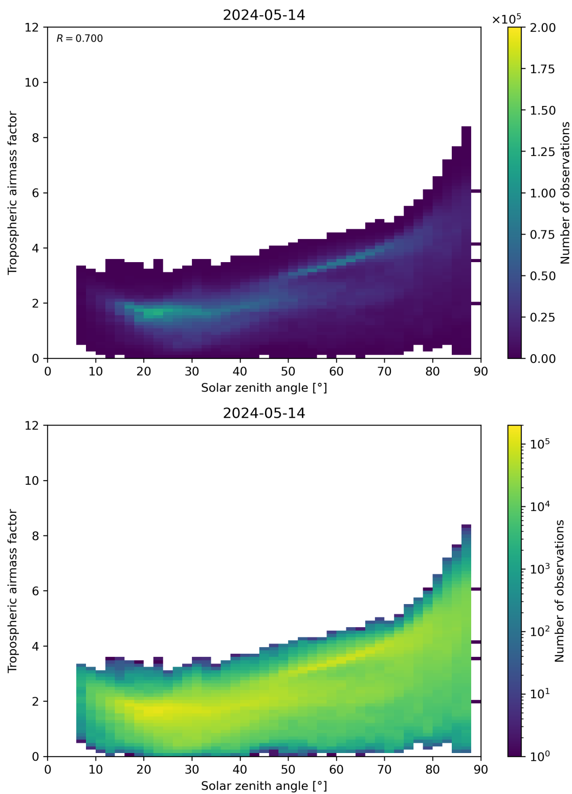
Figure 147: Scatter density plot of “Solar zenith angle” against “Tropospheric airmass factor” for 2024-05-13 to 2024-05-15.
