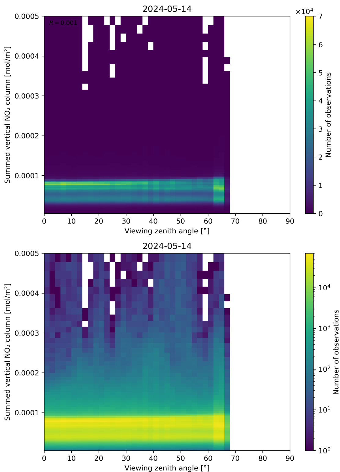
Figure 165: Scatter density plot of “Viewing zenith angle” against “Summed vertical NO 2 column” for 2024-05-13 to 2024-05-15.
