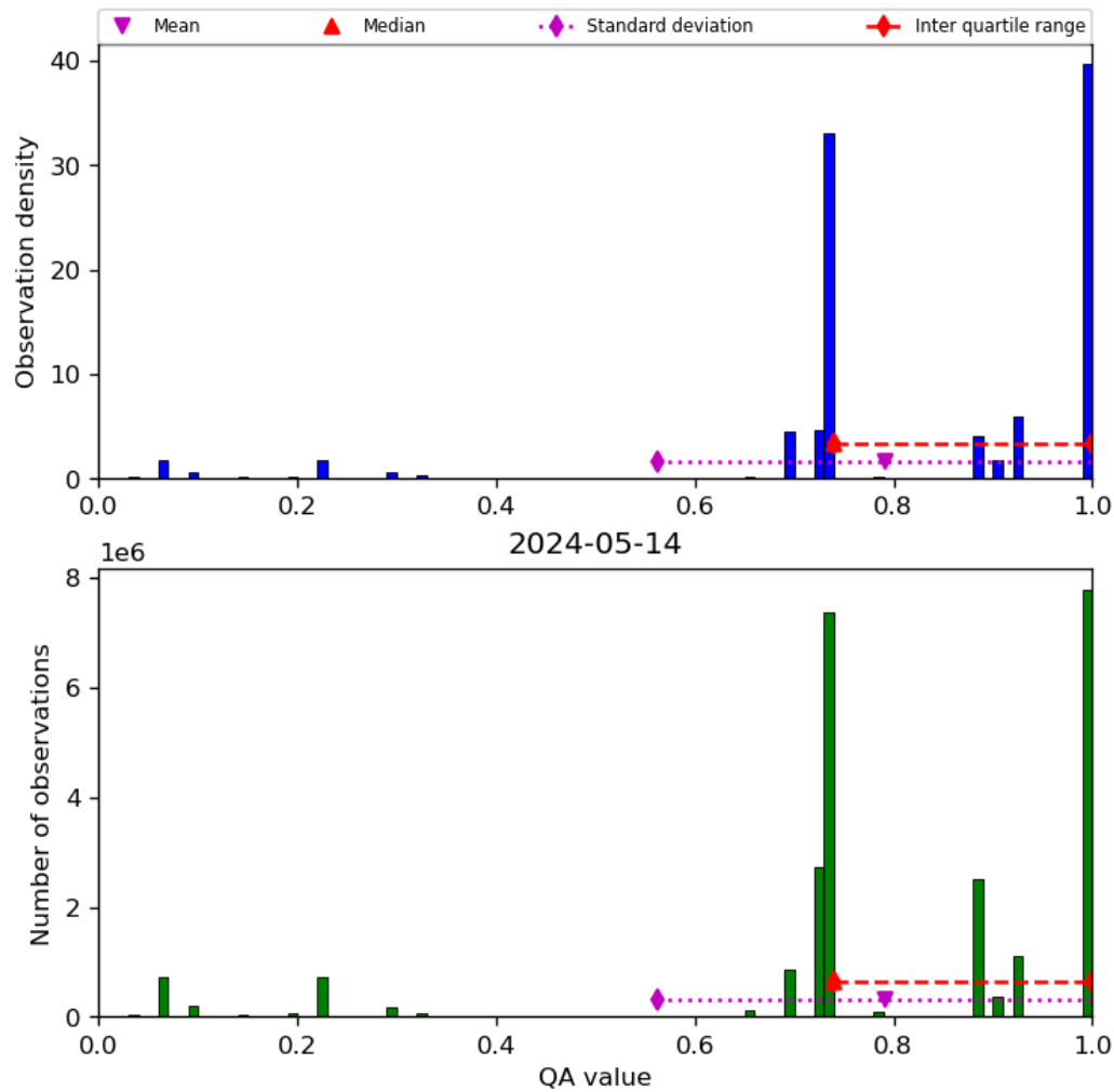
Figure 28: Histogram of “QA value” for 2024-05-13 to 2024-05-15
