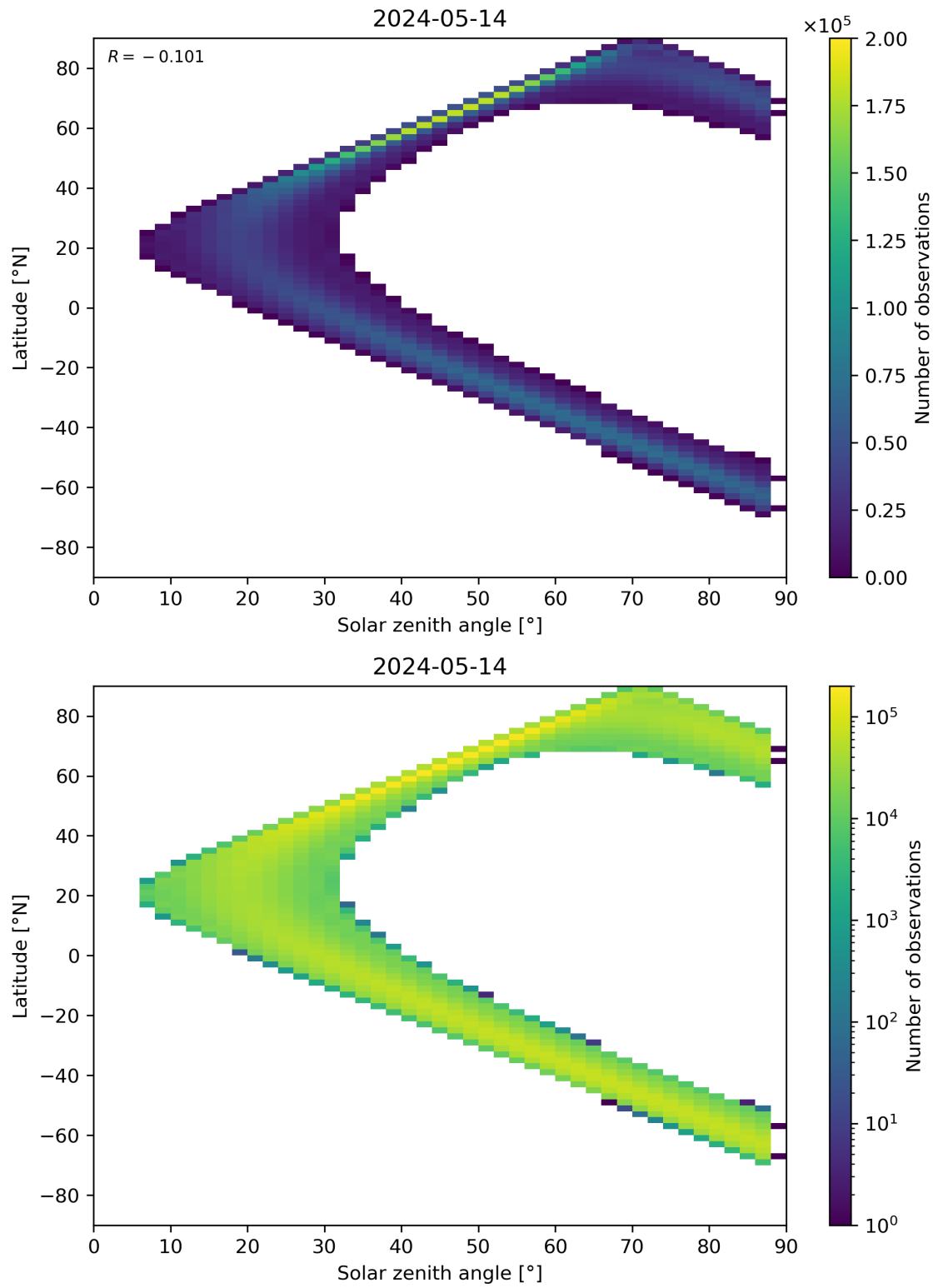
Figure 149: Scatter density plot of “Solar zenith angle” against “Latitude” for 2024-05-13 to 2024-05-15.
