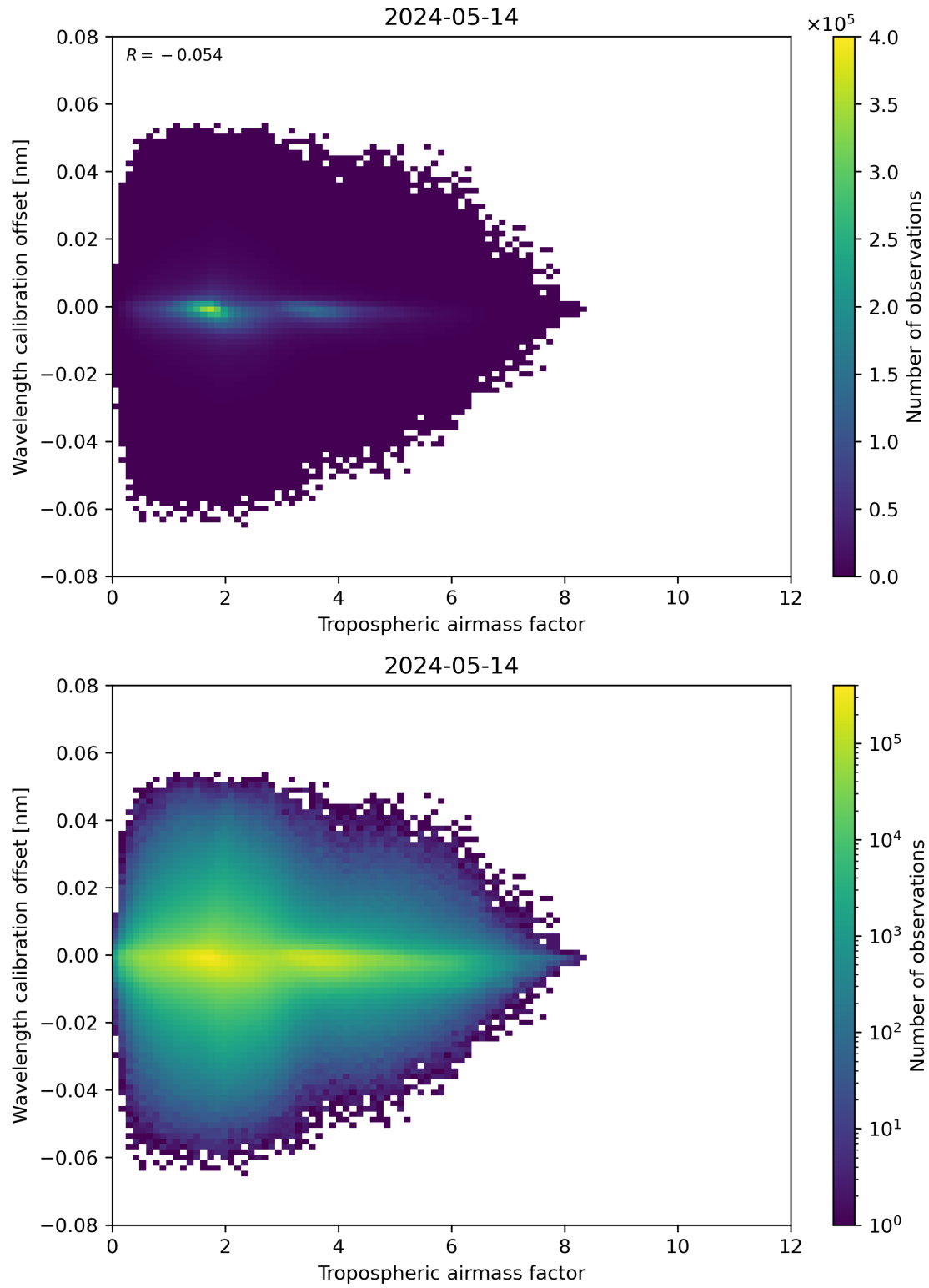
Figure 80: Scatter density plot of “Tropospheric airmass factor” against “Wavelength calibration offset” for 2024-05-13 to 2024-05-15.
