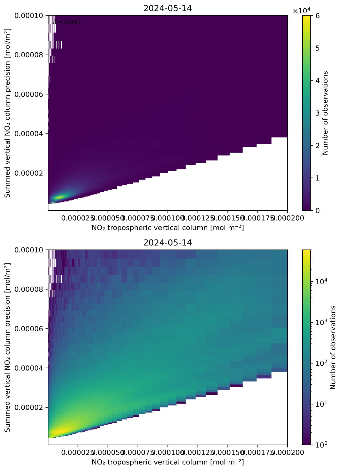
Figure 127: Scatter density plot of “NO 2 tropospheric vertical column” against “Summed vertical NO 2 column precision” for 2024-05-13 to 2024-05-15.
