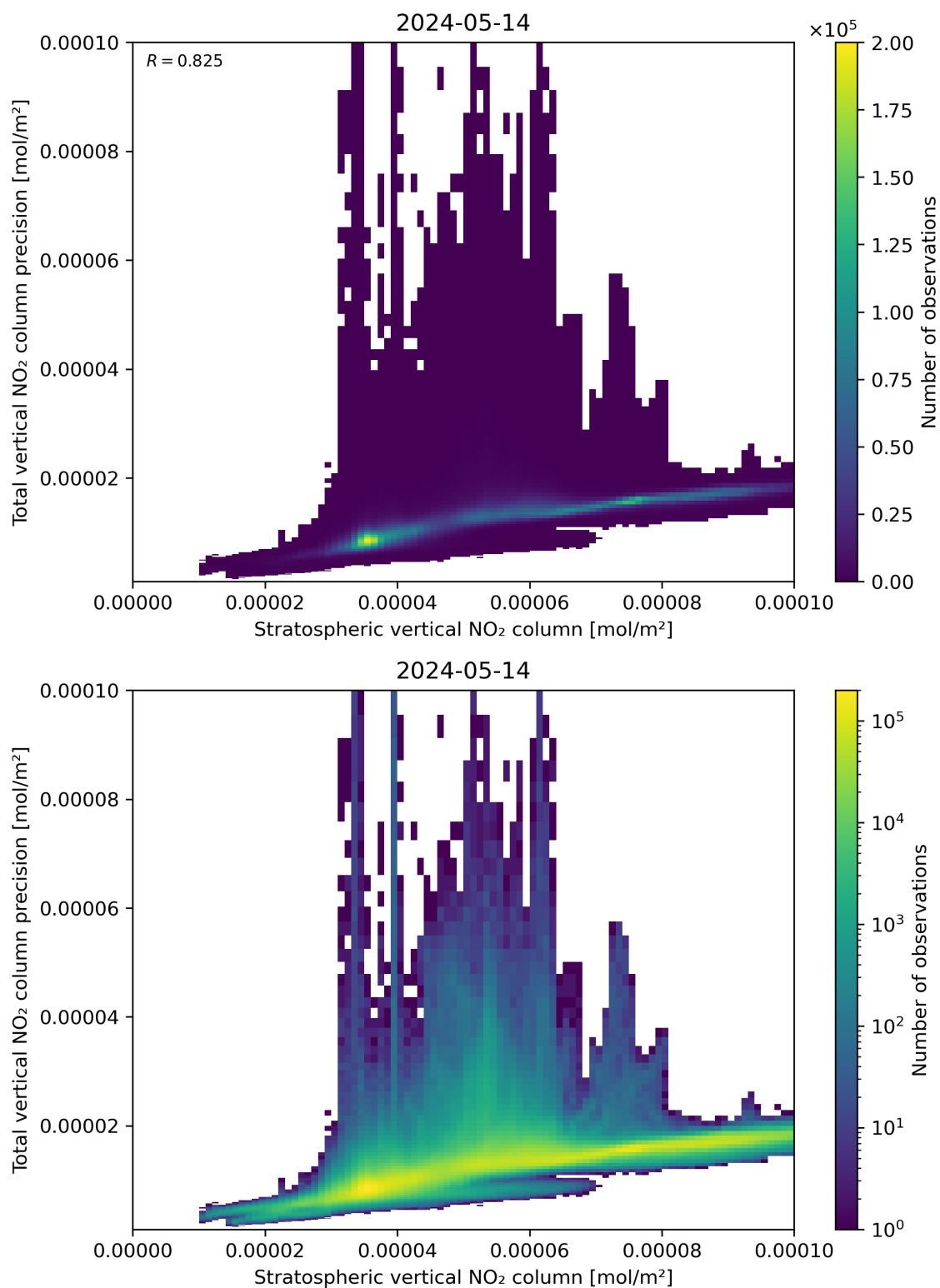
Figure 101: Scatter density plot of “Stratospheric vertical NO 2 column” against “Total vertical NO 2 column precision” for 2024-05-13 to 2024-05-15.
