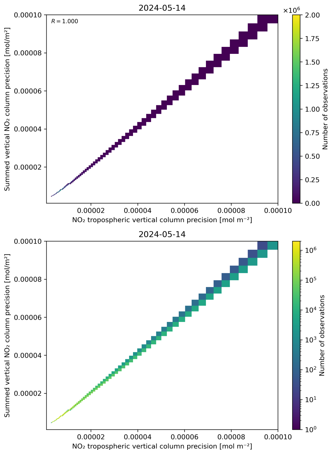
Figure 137: Scatter density plot of “NO 2 tropospheric vertical column precision” against “Summed vertical NO 2 column precision” for 2024-05-13 to 2024-05-15.
