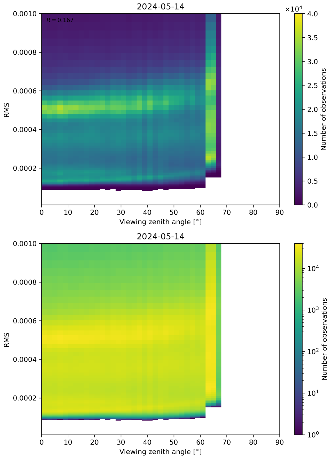
Figure 171: Scatter density plot of “Viewing zenith angle” against “RMS” for 2024-05-13 to 2024-05-15.
