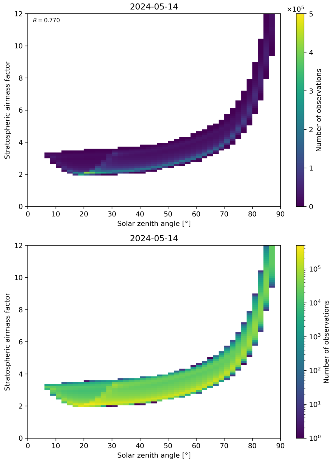
Figure 145: Scatter density plot of “Solar zenith angle” against “Stratospheric airmass factor” for 2024-05-13 to 2024-05-15.
