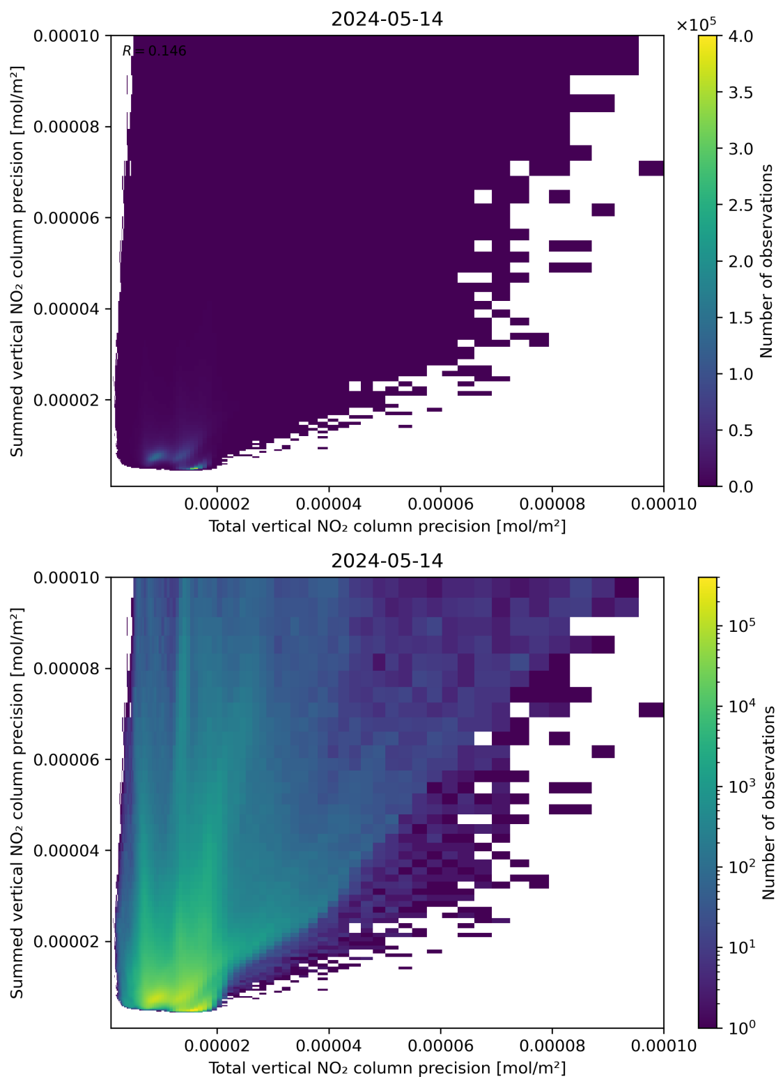
Figure 118: Scatter density plot of “Total vertical NO 2 column precision” against “Summed vertical NO 2 column precision” for 2024-05-13 to 2024-05-15.
