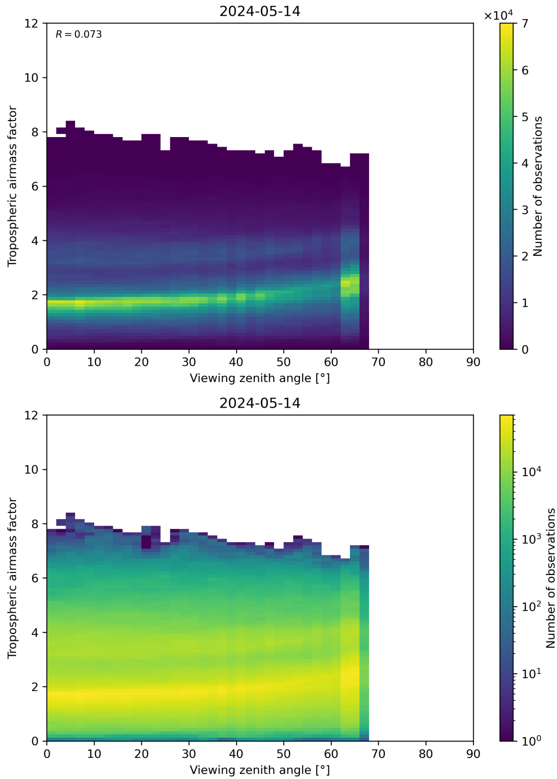
Figure 161: Scatter density plot of “Viewing zenith angle” against “Tropospheric airmass factor” for 2024-05-13 to 2024-05-15.
