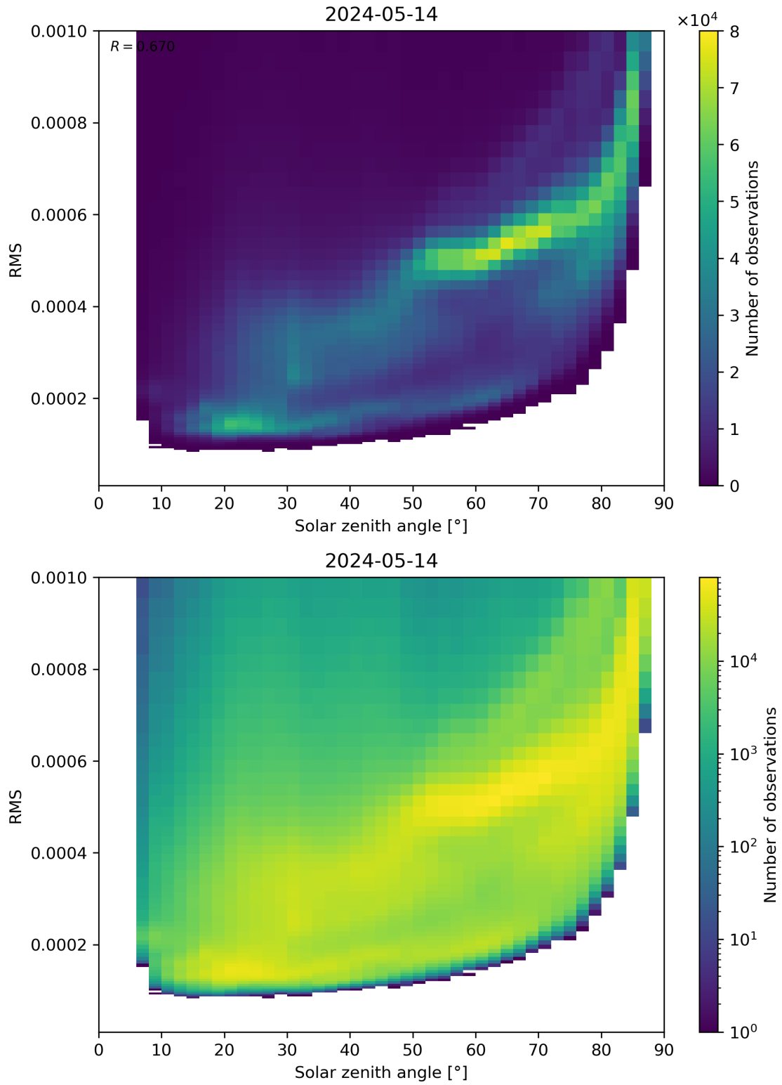
Figure 157: Scatter density plot of “Solar zenith angle” against “RMS” for 2024-05-13 to 2024-05-15.
