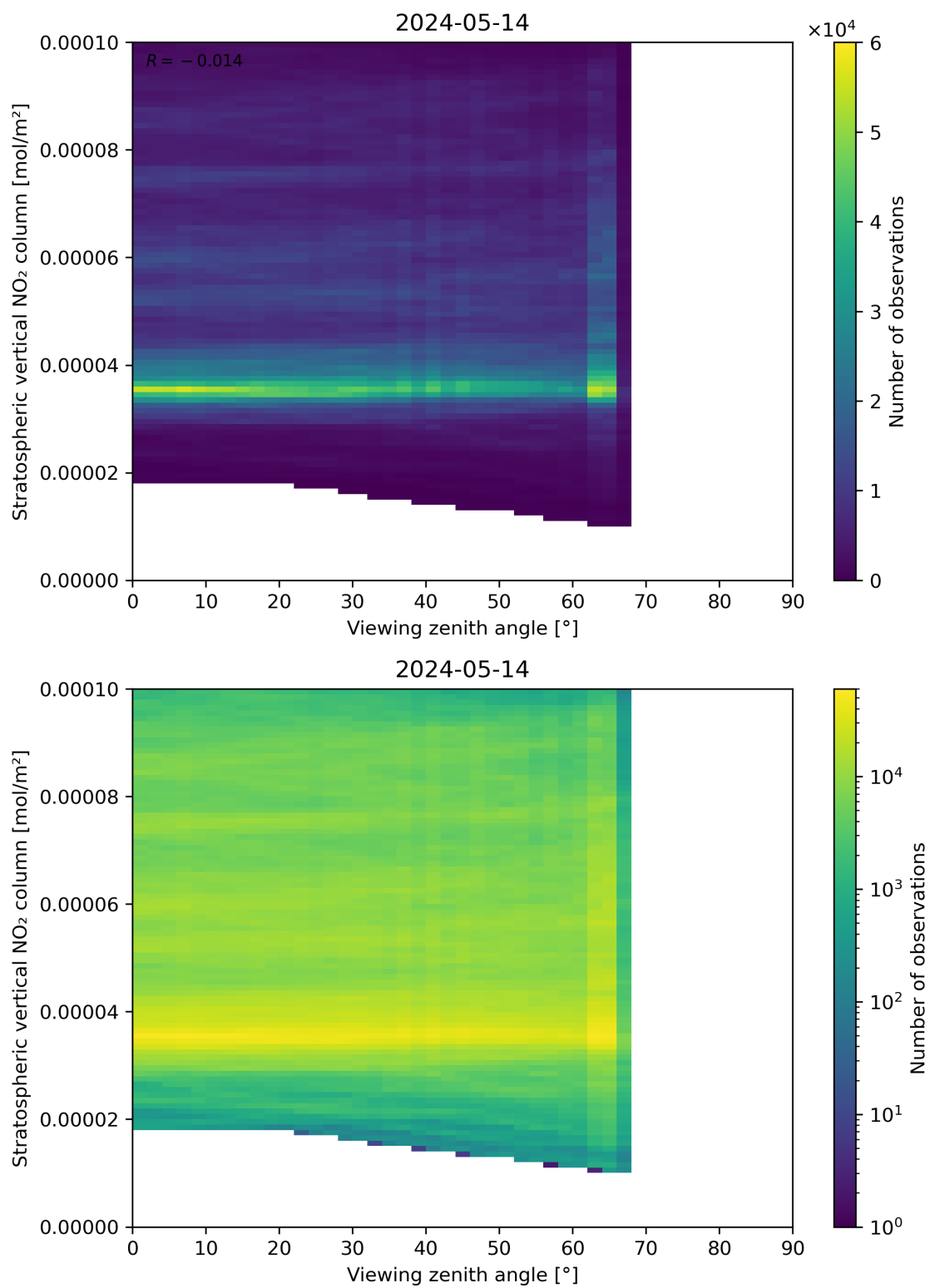
Figure 164: Scatter density plot of “Viewing zenith angle” against “Stratospheric vertical NO 2 column” for 2024-05-13 to 2024-05-15.
