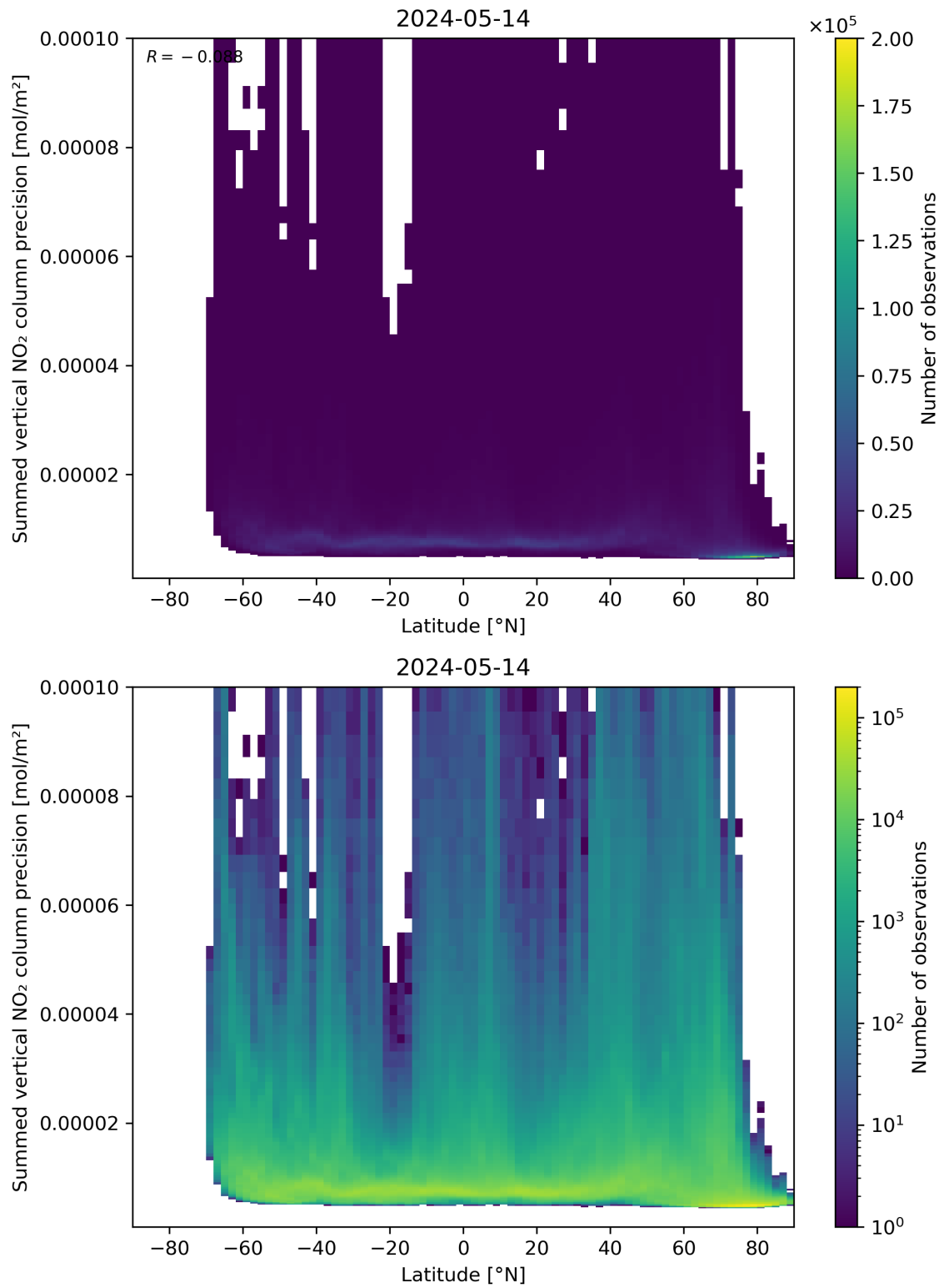
Figure 89: Scatter density plot of “Latitude” against “Summed vertical NO 2 column precision” for 2024-05-13 to 2024-05-15.
