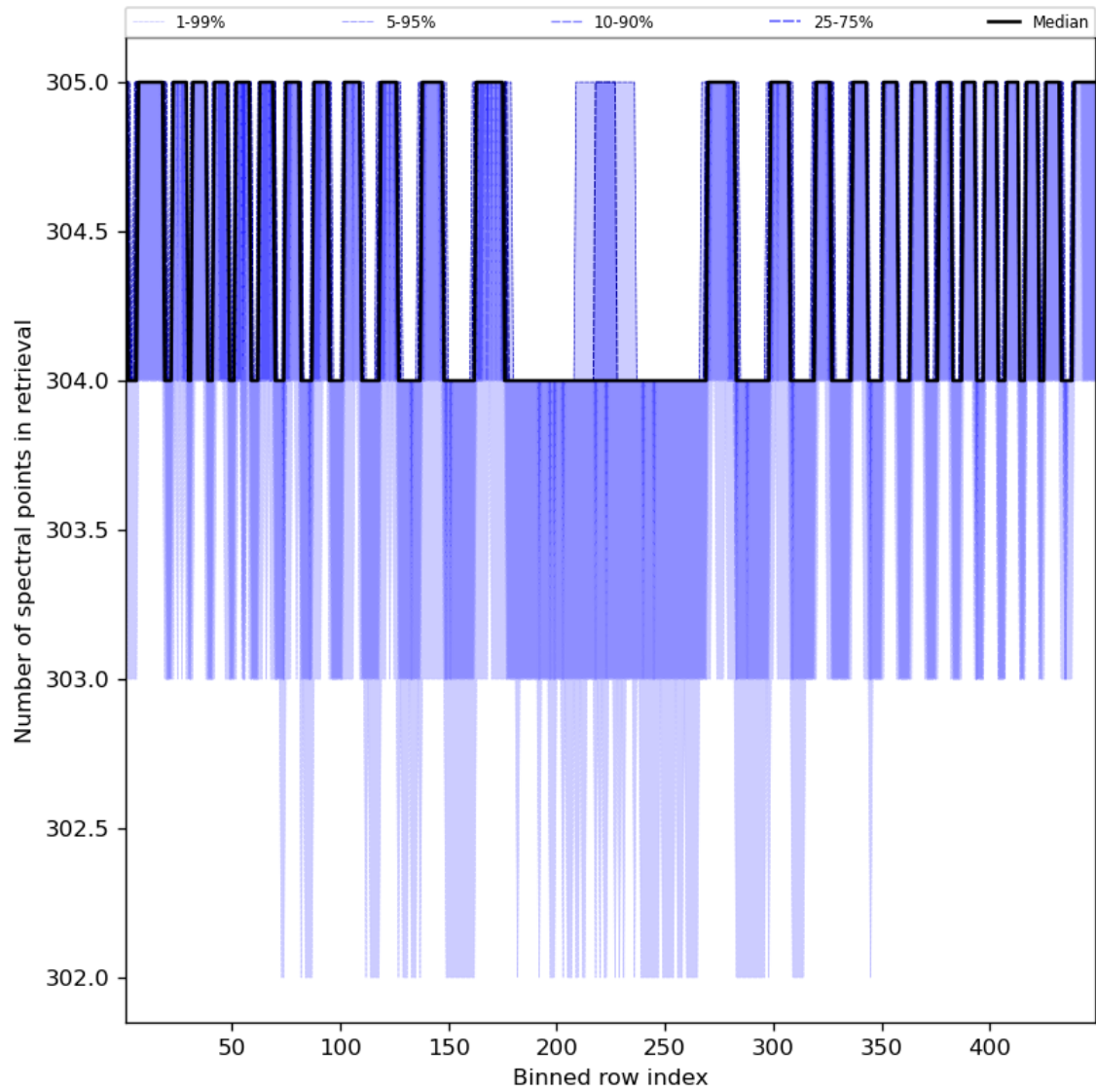
Figure 50: Along track statistics of “Number of spectral points in retrieval” for 2024-05-13 to 2024-05-15
