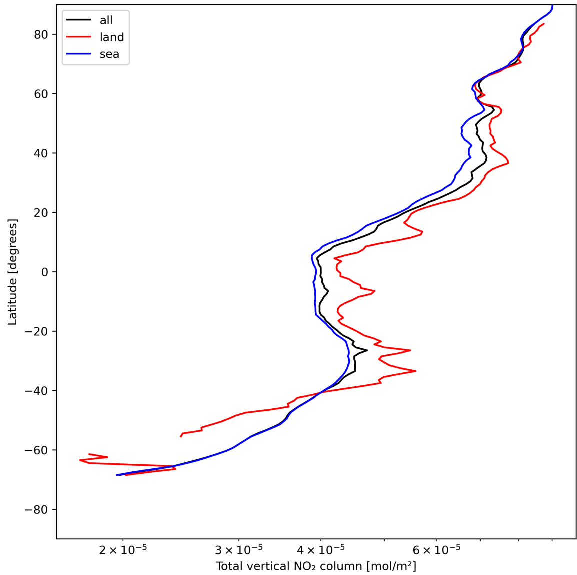
Figure 21: Zonal average of “Total vertical NO 2 column” for 2024-05-13 to 2024-05-15.
