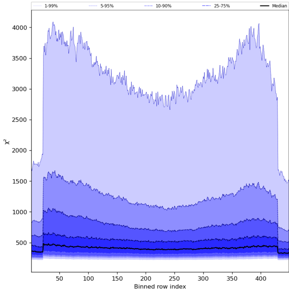
Figure 59: Along track statistics of “ \chi^2 ” for 2024-05-13 to 2024-05-15
