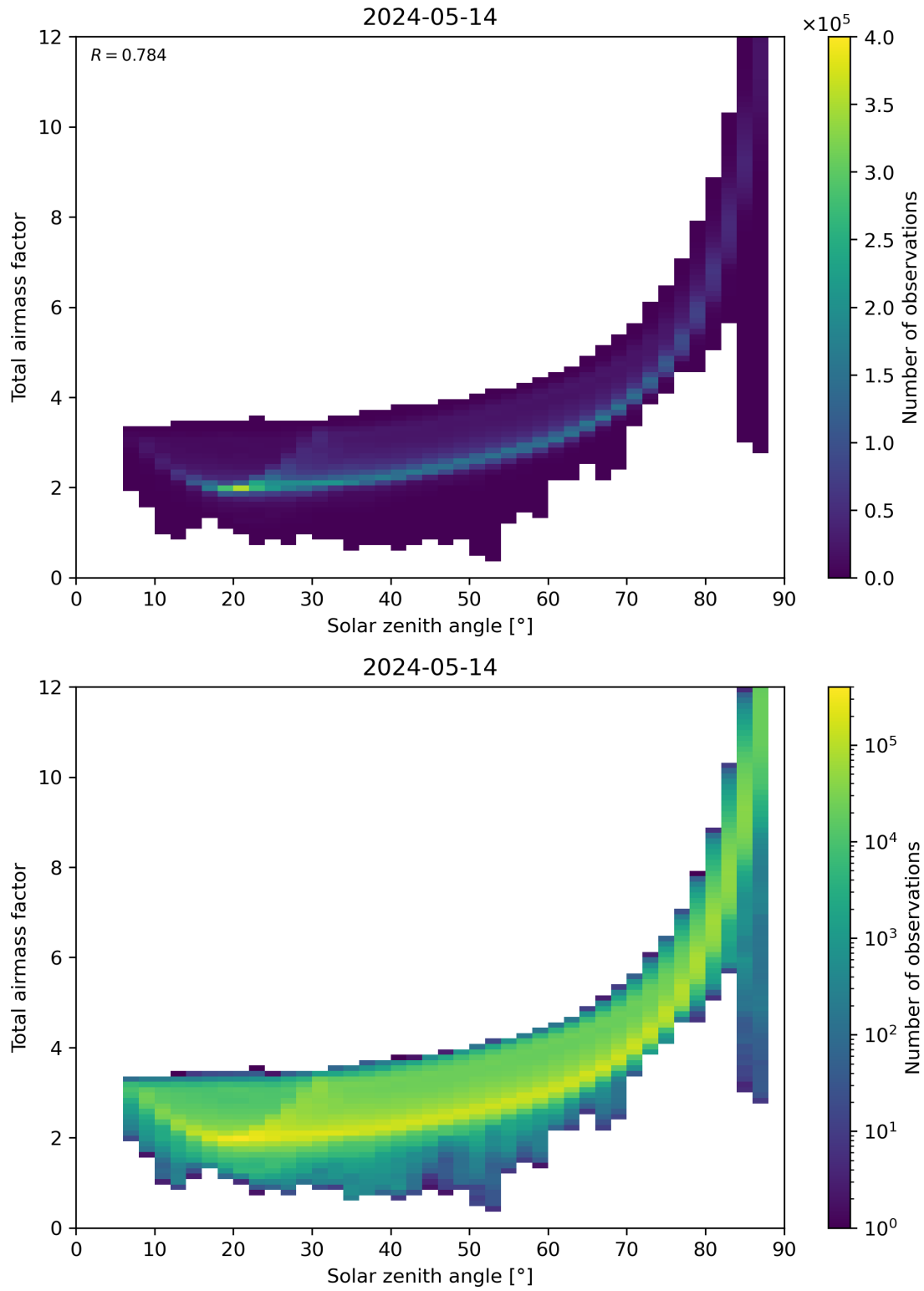
Figure 146: Scatter density plot of “Solar zenith angle” against “Total air mass factor” for 2024-05-13 to 2024-05-15.
