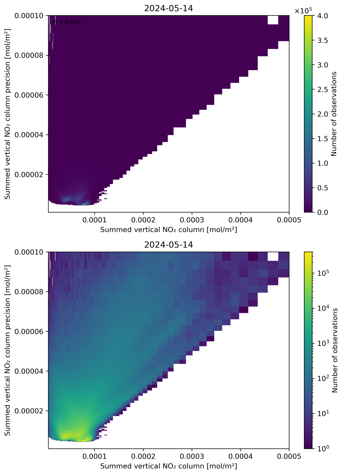
Figure 105: Scatter density plot of “Summed vertical NO 2 column” against “Summed vertical NO 2 column precision” for 2024-05-13 to 2024-05-15.
