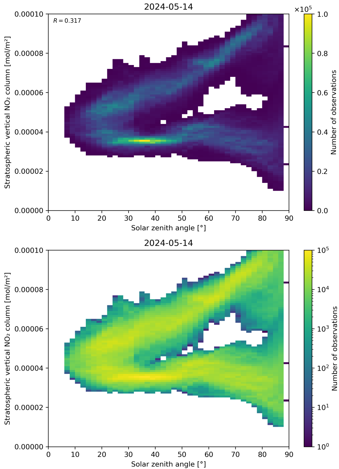
Figure 150: Scatter density plot of “Solar zenith angle” against “Stratospheric vertical NO 2 column” for 2024-05-13 to 2024-05-15.
