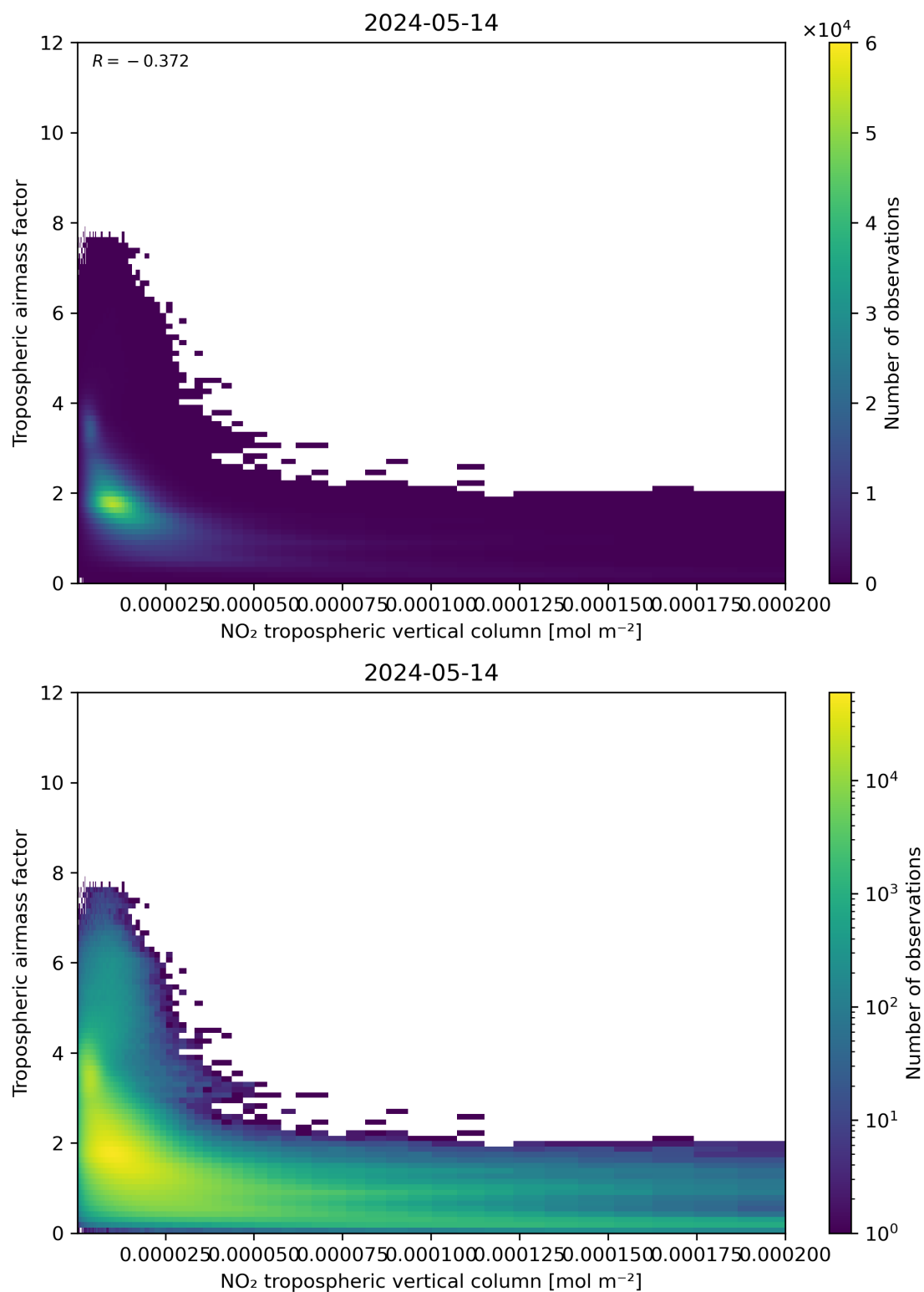
Figure 123: Scatter density plot of “NO 2 tropospheric vertical column” against “Tropospheric airmass factor” for 2024-05-13 to 2024-05-15.
