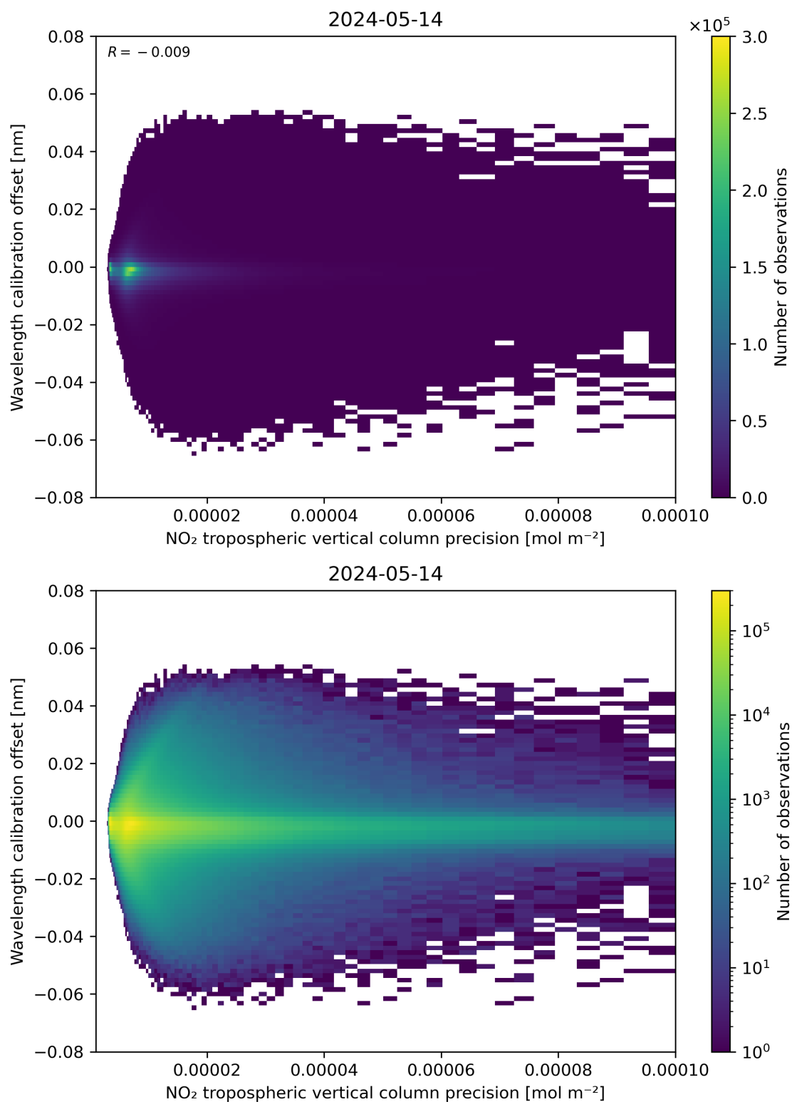
Figure 141: Scatter density plot of “NO 2 tropospheric vertical column precision” against “Wavelength calibration offset” for 2024-05-13 to 2024-05-15.
