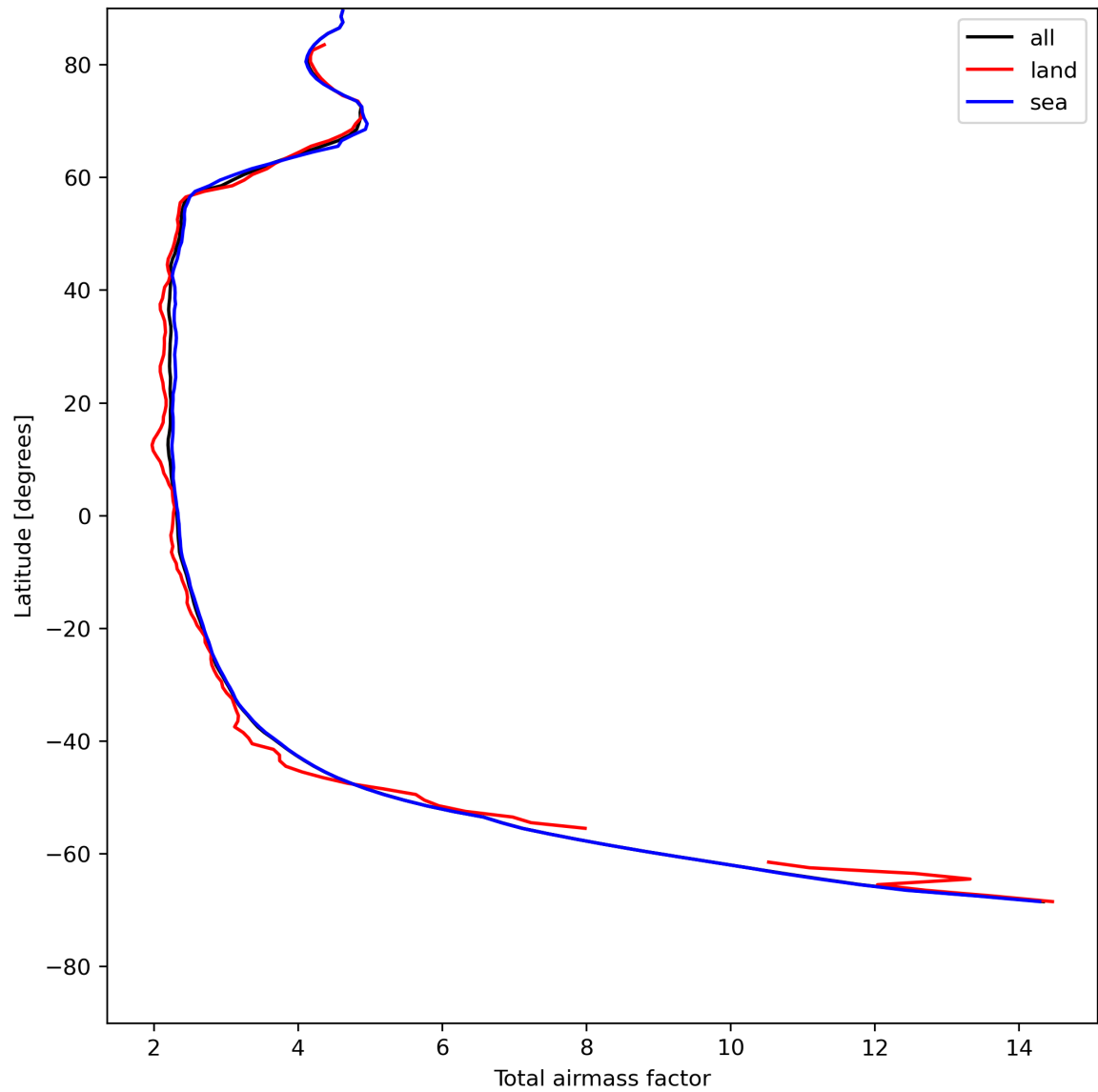
Figure 15: Zonal average of “Total airmass factor” for 2024-05-13 to 2024-05-15.
