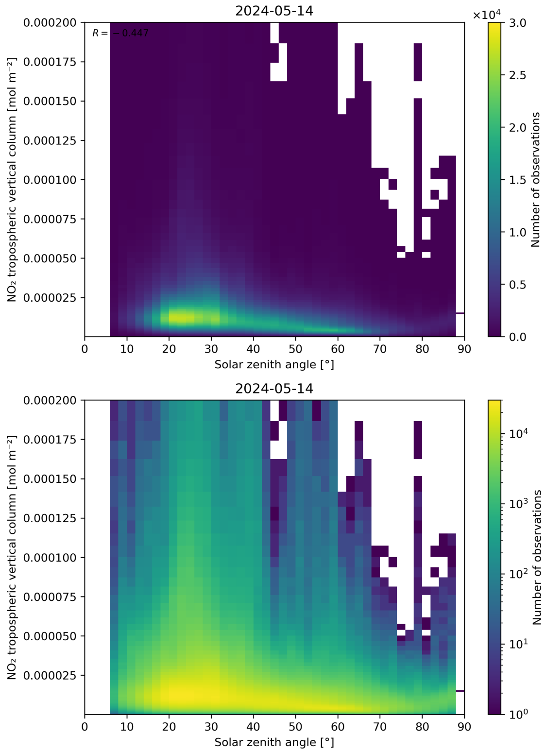
Figure 155: Scatter density plot of “Solar zenith angle” against “NO 2 tropospheric vertical column” for 2024-05-13 to 2024-05-15.
