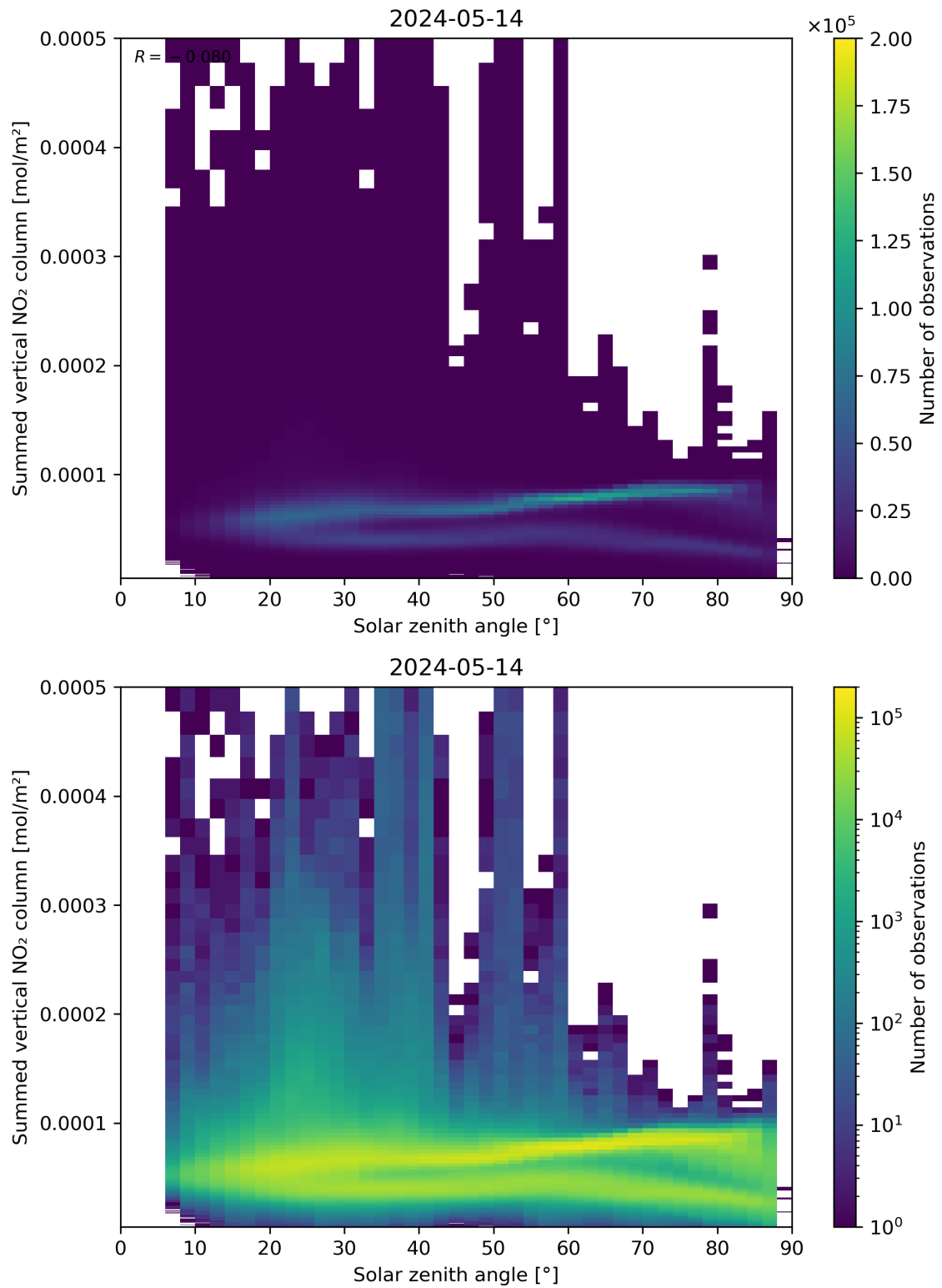
Figure 151: Scatter density plot of “Solar zenith angle” against “Summed vertical NO 2 column” for 2024-05-13 to 2024-05-15.
