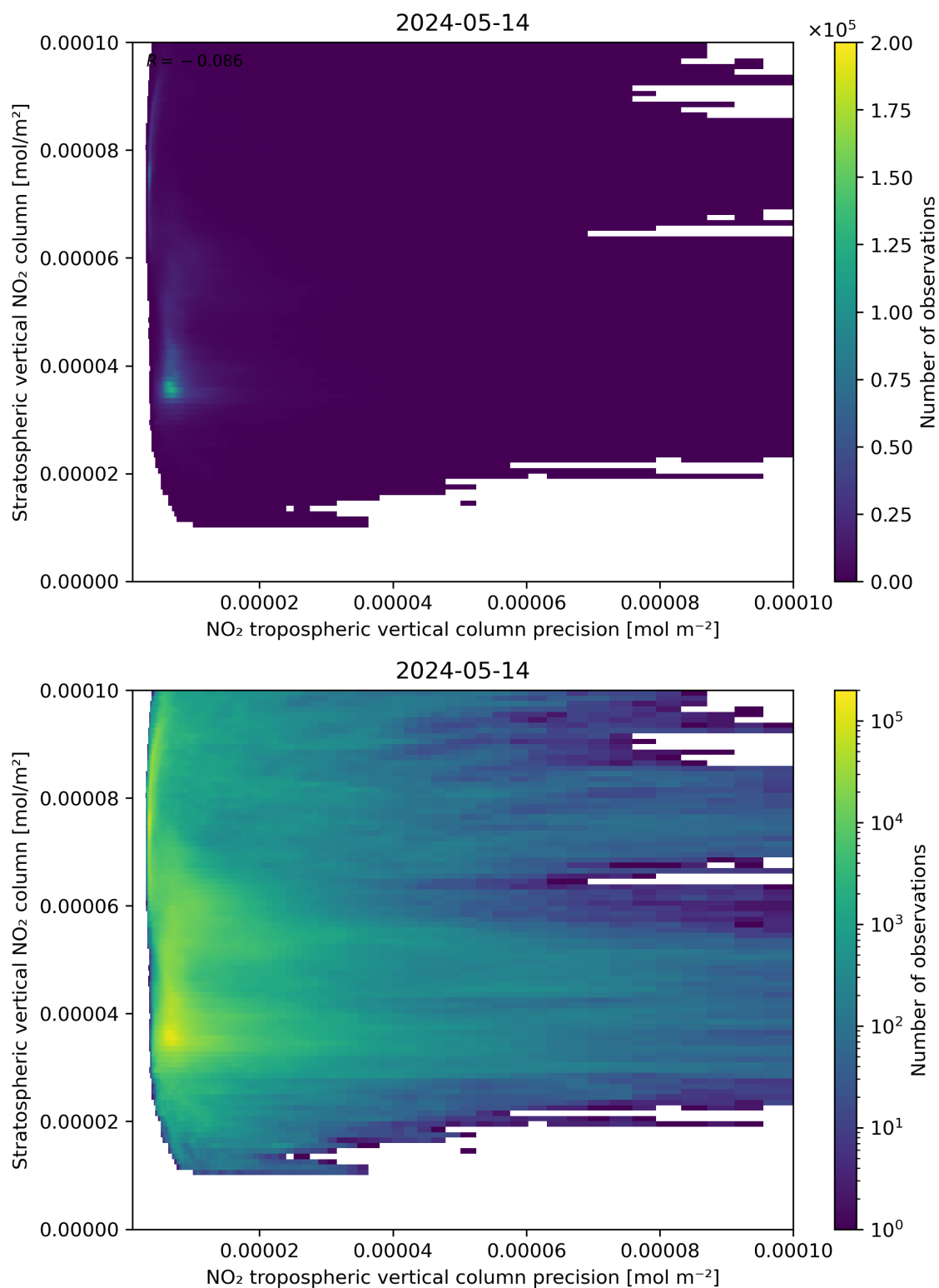
Figure 135: Scatter density plot of “NO 2 tropospheric vertical column precision” against “Stratospheric vertical NO 2 column” for 2024-05-13 to 2024-05-15.
