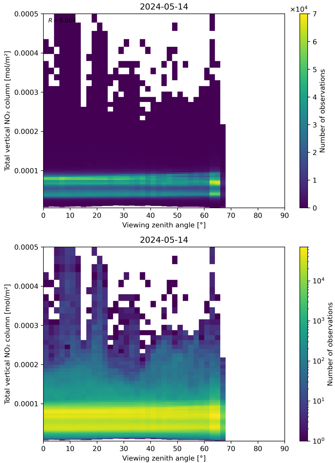
Figure 167: Scatter density plot of “Viewing zenith angle” against “Total vertical NO 2 column” for 2024-05-13 to 2024-05-15.
