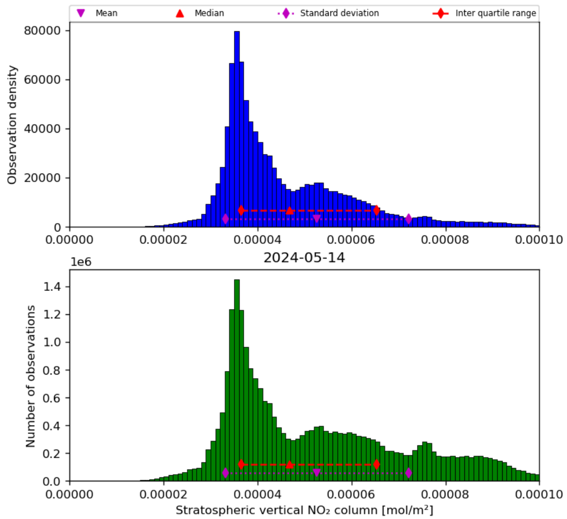
Figure 36: Histogram of “Stratospheric vertical NO 2 column” for 2024-05-13 to 2024-05-15
