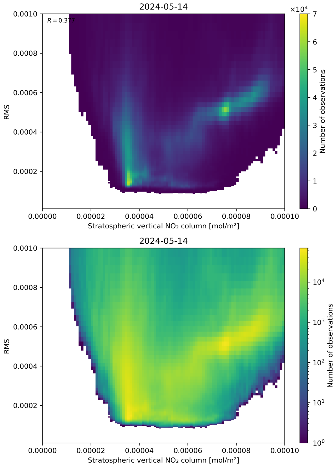
Figure 102: Scatter density plot of “Stratospheric vertical NO 2 column” against “RMS” for 2024-05-13 to 2024-05-15.
