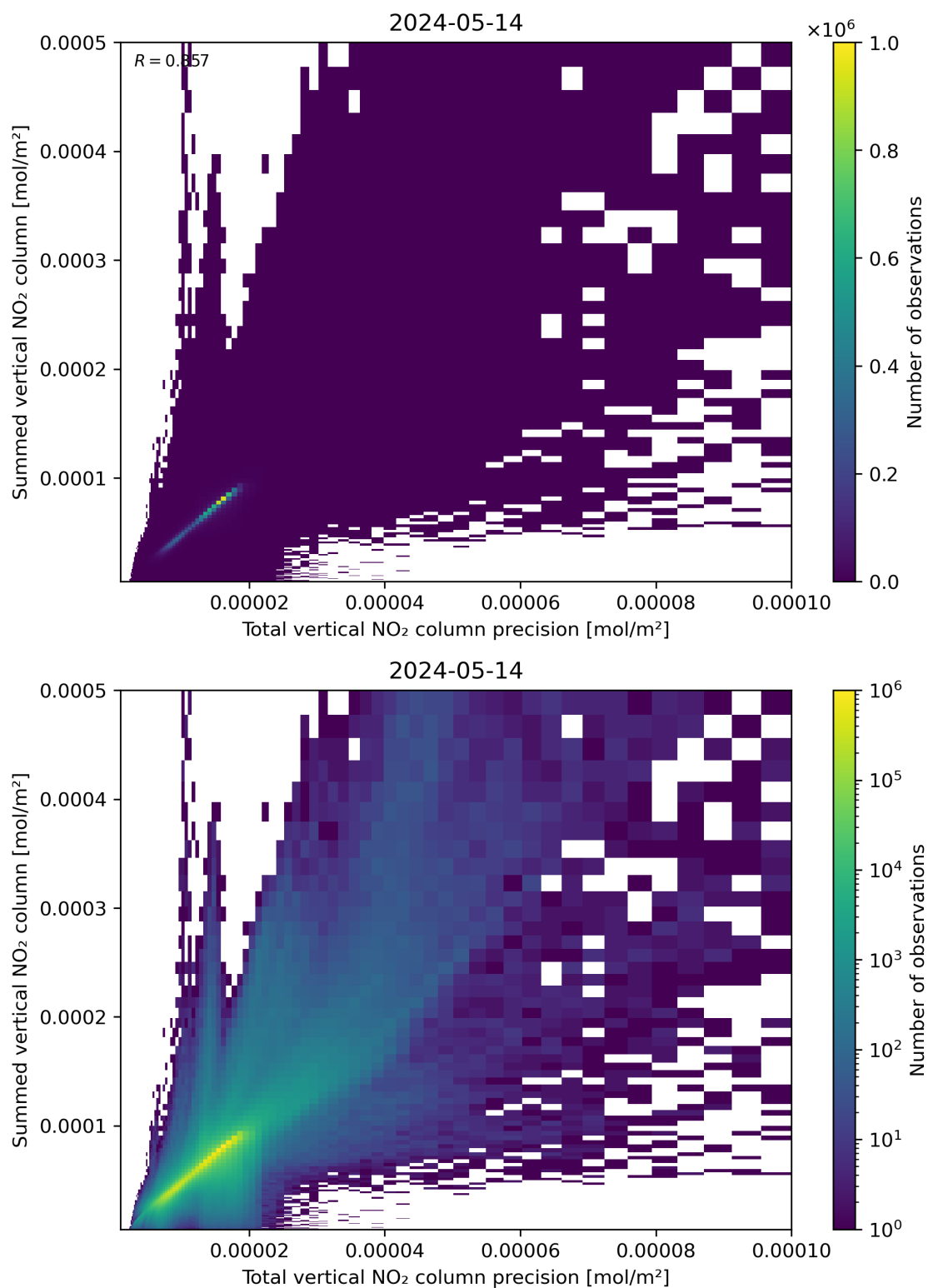
Figure 117: Scatter density plot of “Total vertical NO 2 column precision” against “Summed vertical NO 2 column” for 2024-05-13 to 2024-05-15.
