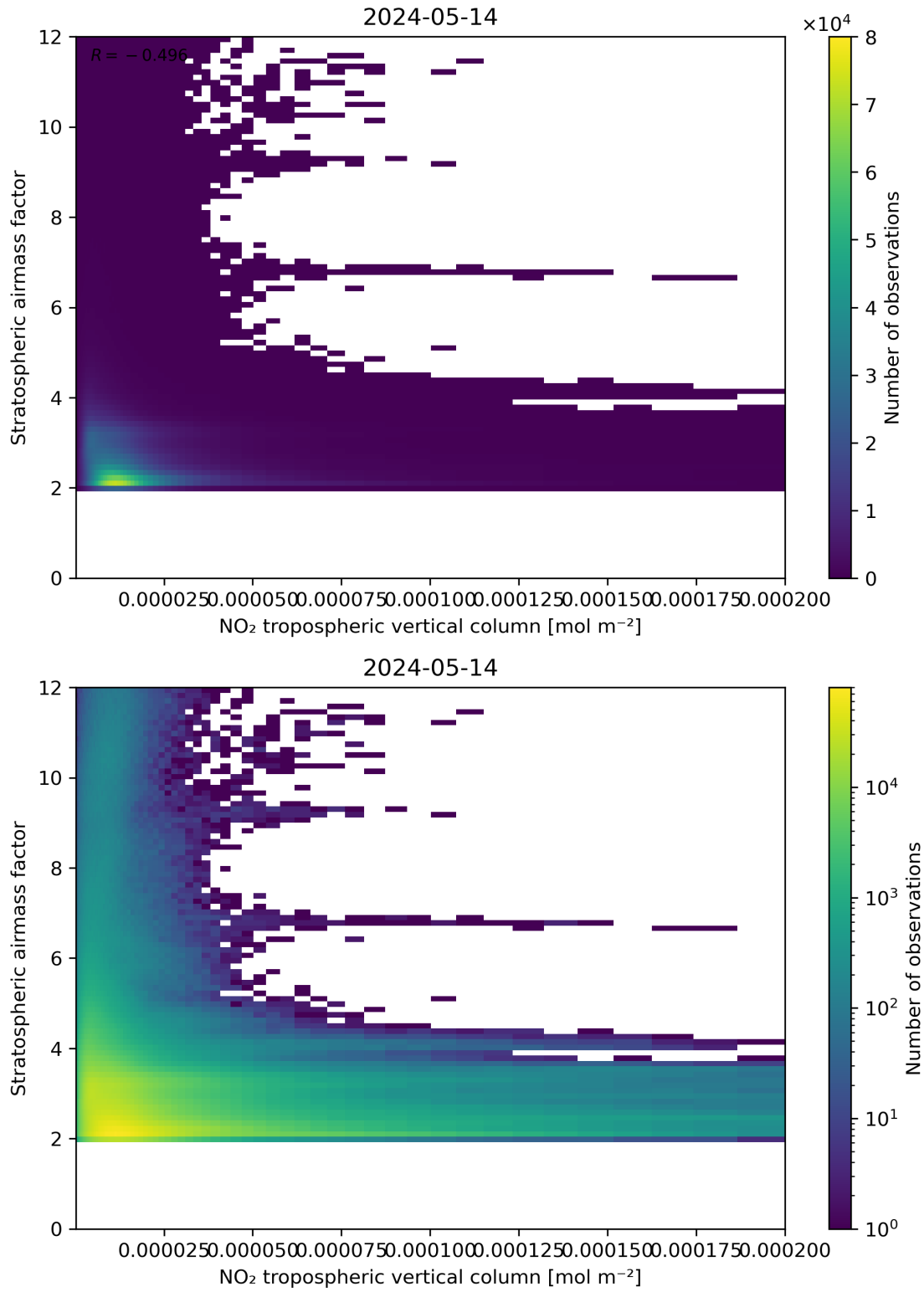
Figure 121: Scatter density plot of “NO 2 tropospheric vertical column” against “Stratospheric air mass factor” for 2024-05-13 to 2024-05-15.
