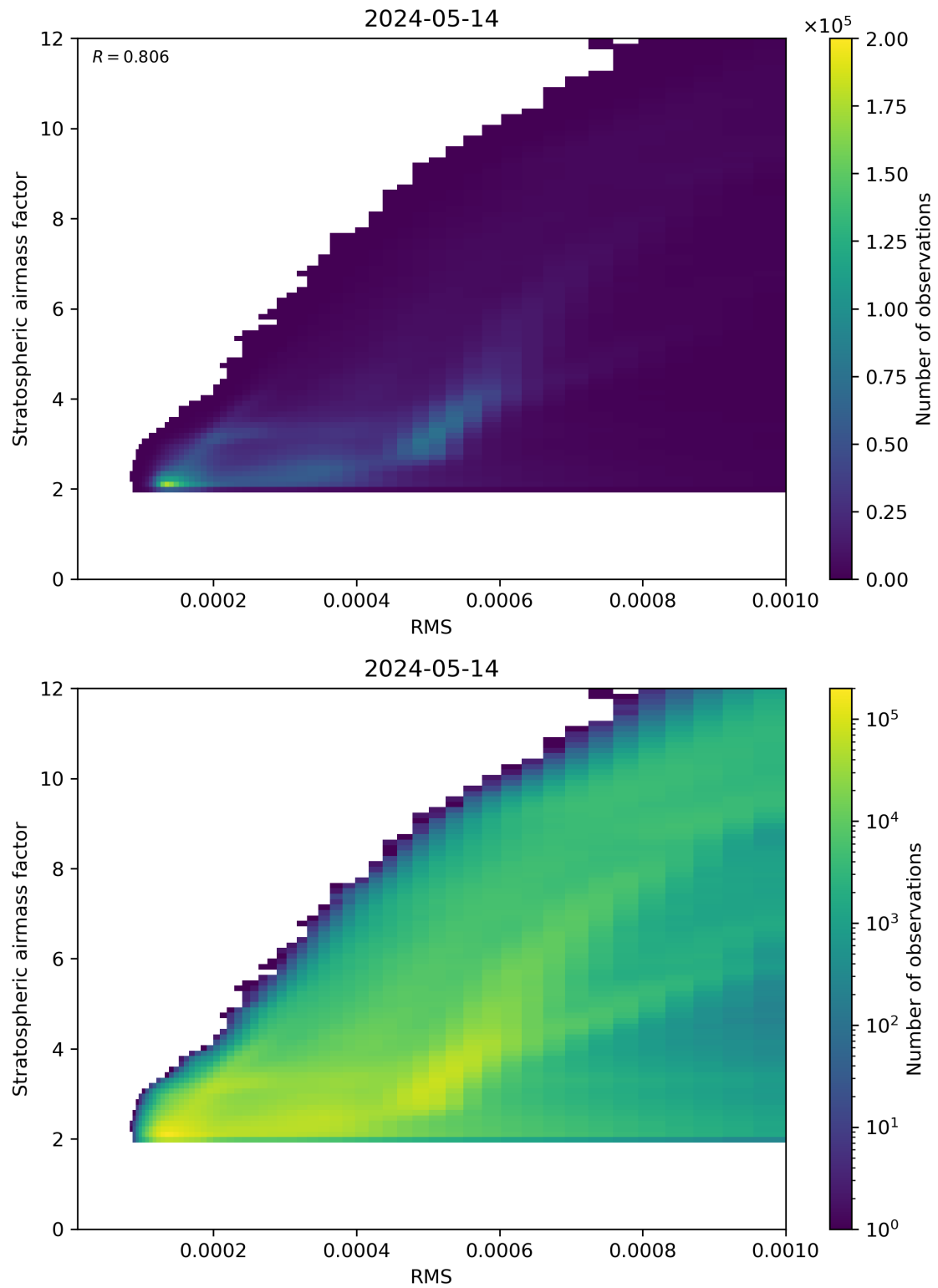
Figure 144: Scatter density plot of “RMS” against “Stratospheric airmass factor” for 2024-05-13 to 2024-05-15.
