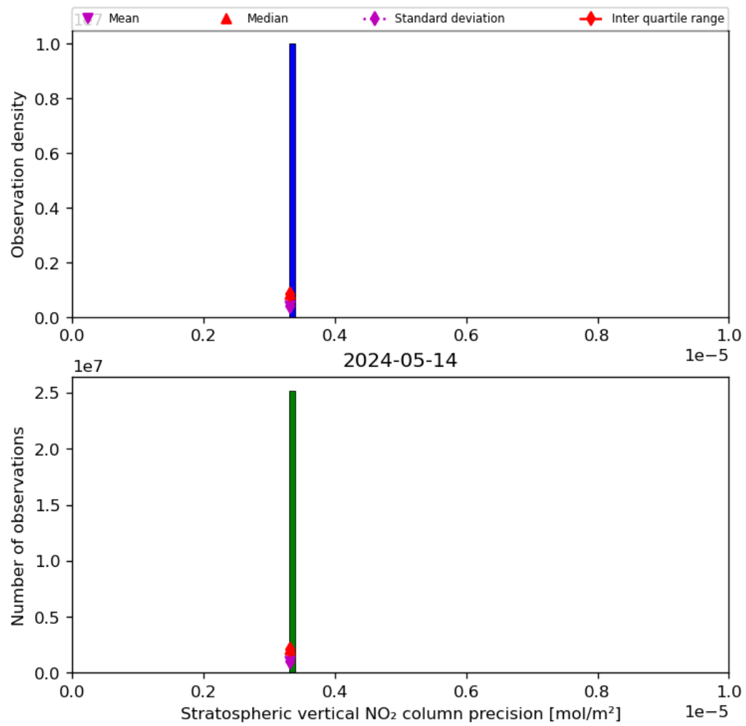
Figure 37: Histogram of “Stratospheric vertical NO 2 column precision” for 2024-05-13 to 2024-05-15
