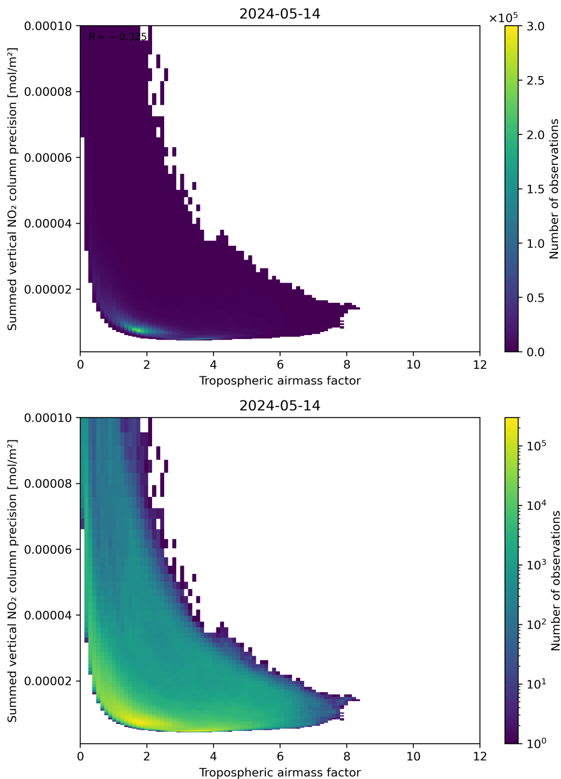
Figure 76: Scatter density plot of “Tropospheric air mass factor” against “Summed vertical NO 2 column precision” for 2024-05-13 to 2024-05-15.
