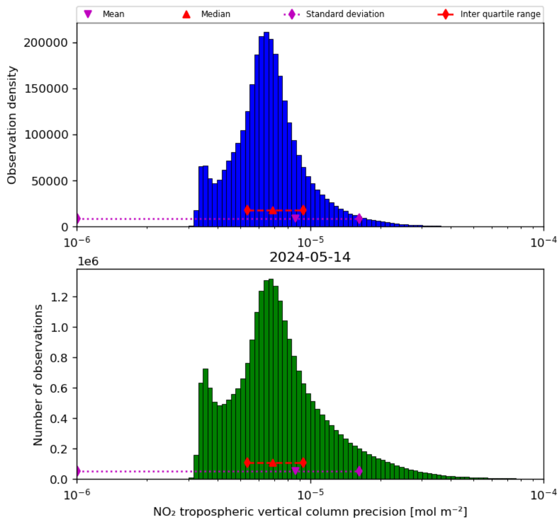
Figure 30: Histogram of “NO 2 tropospheric vertical column precision” for 2024-05-13 to 2024-05-15
