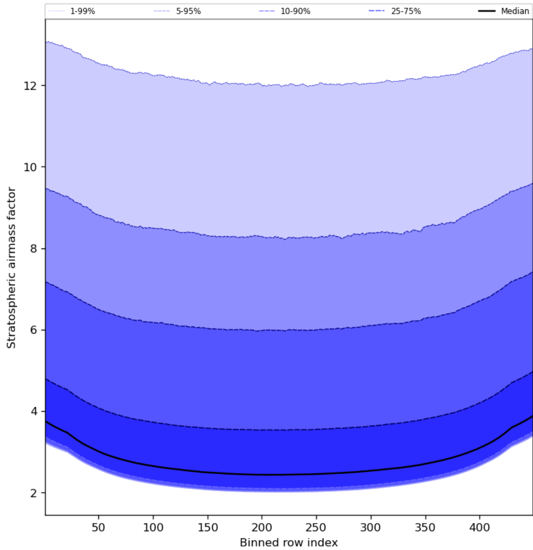
Figure 61: Along track statistics of “Stratospheric airmass factor” for 2024-05-13 to 2024-05-15
