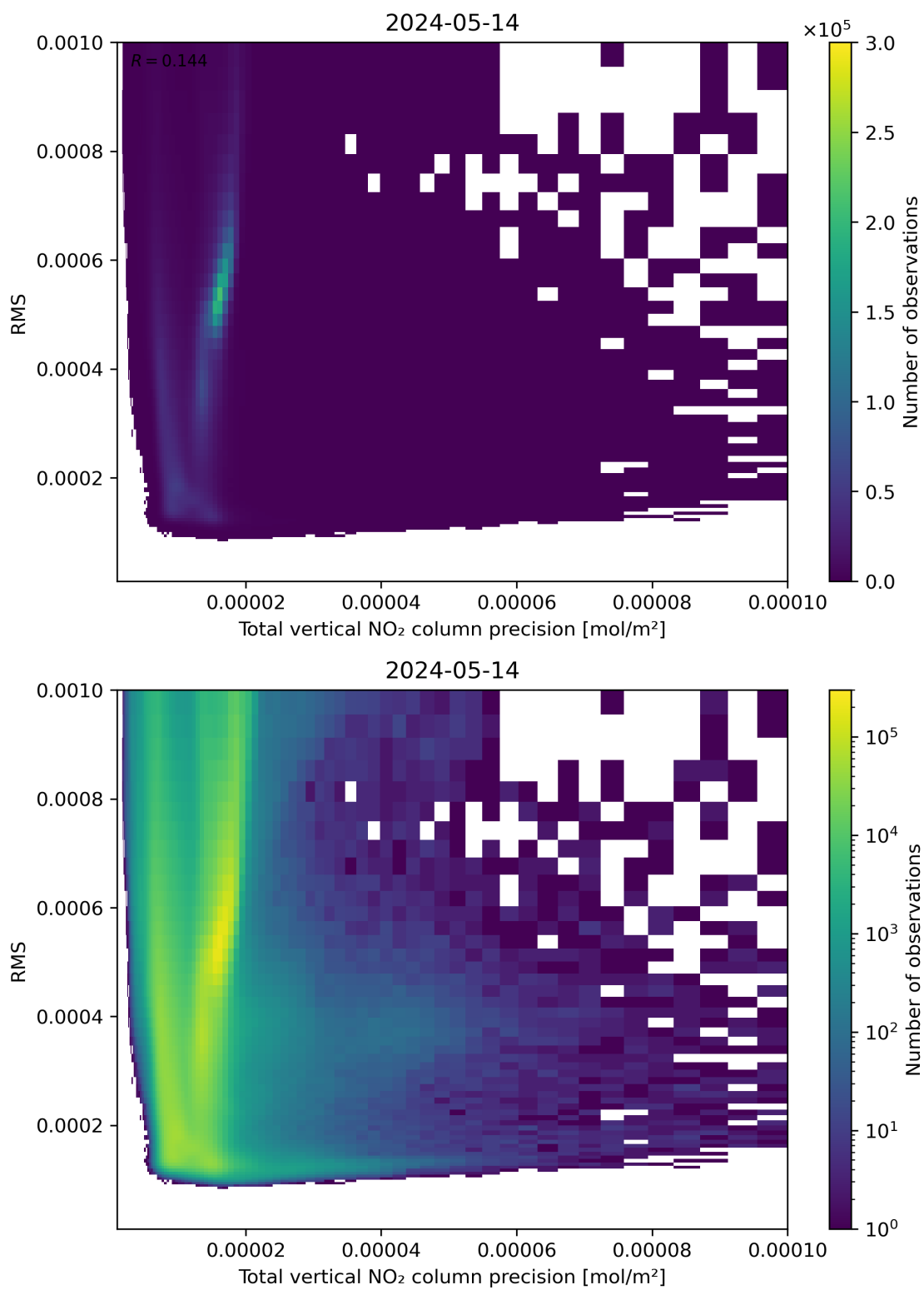
Figure 119: Scatter density plot of “Total vertical NO 2 column precision” against “RMS” for 2024-05-13 to 2024-05-15.
