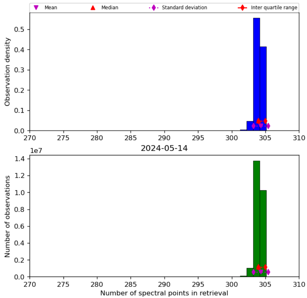
Figure 33: Histogram of “Number of spectral points in retrieval” for 2024-05-13 to 2024-05-15
