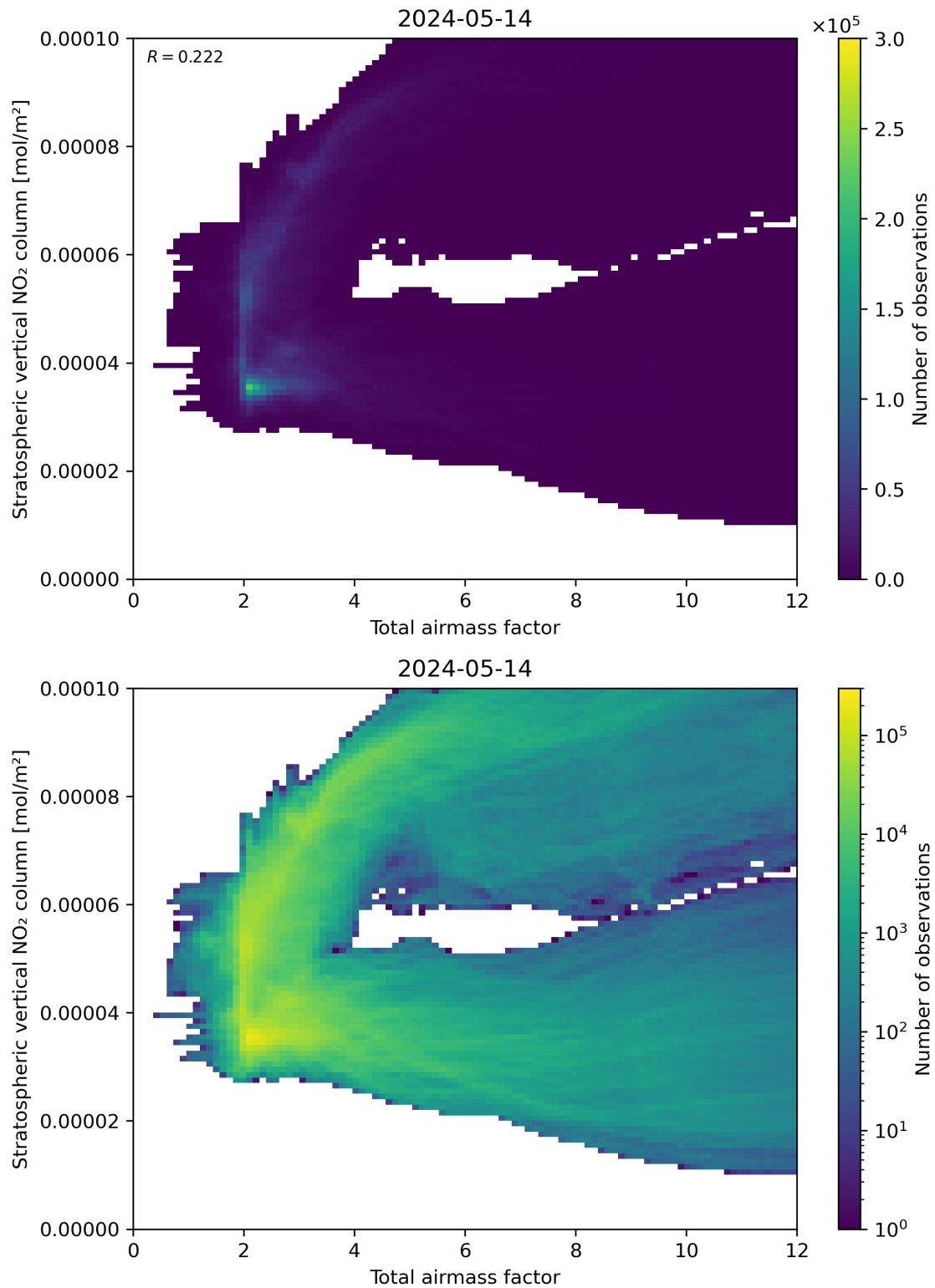
Figure 64: Scatter density plot of “Total airmass factor” against “Stratospheric vertical \text{NO}_2 column” for 2024-05-13 to 2024-05-15.
