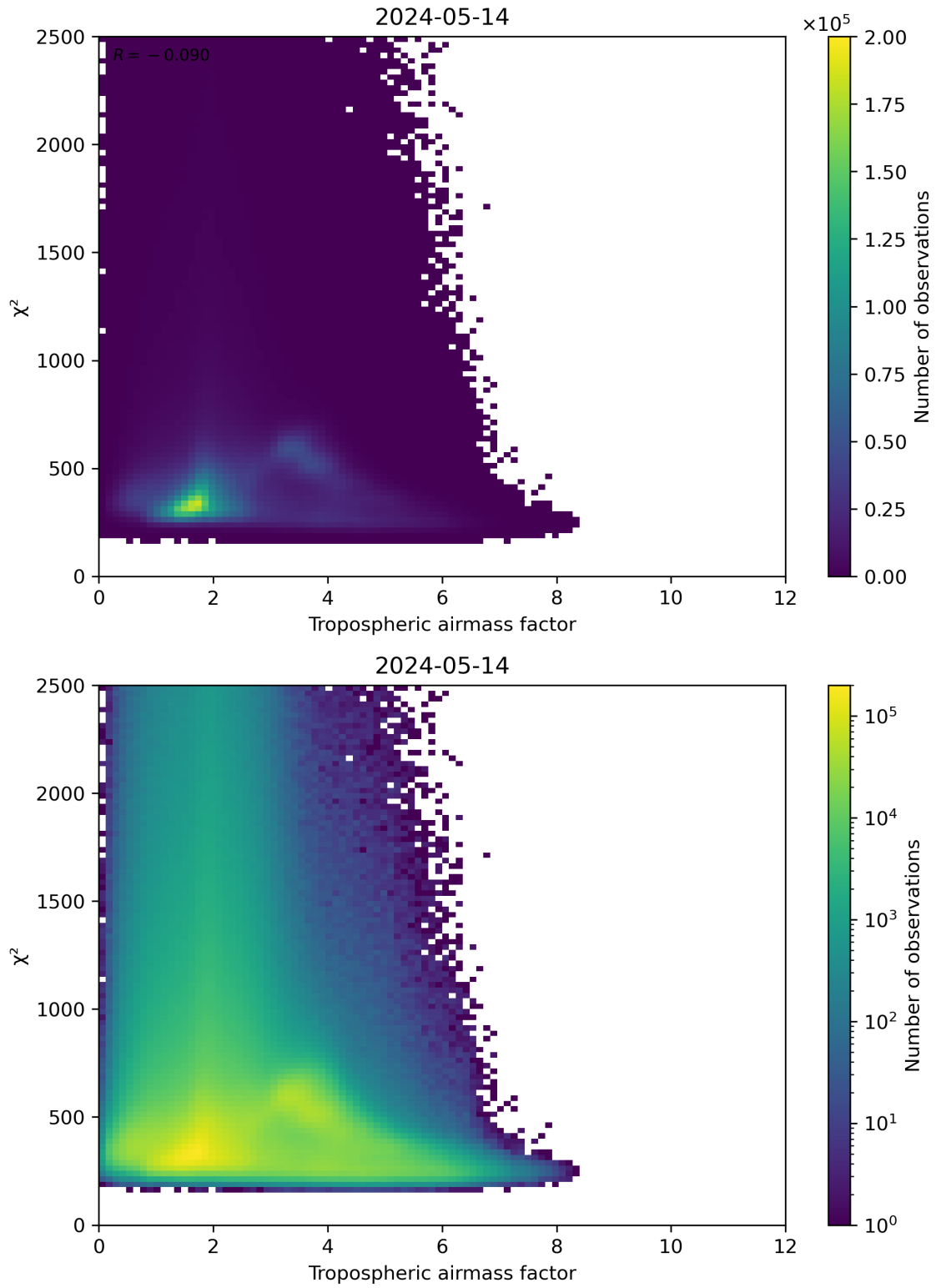
Figure 73: Scatter density plot of “Tropospheric airmass factor” against “ \chi^2 ” for 2024-05-13 to 2024-05-15.
