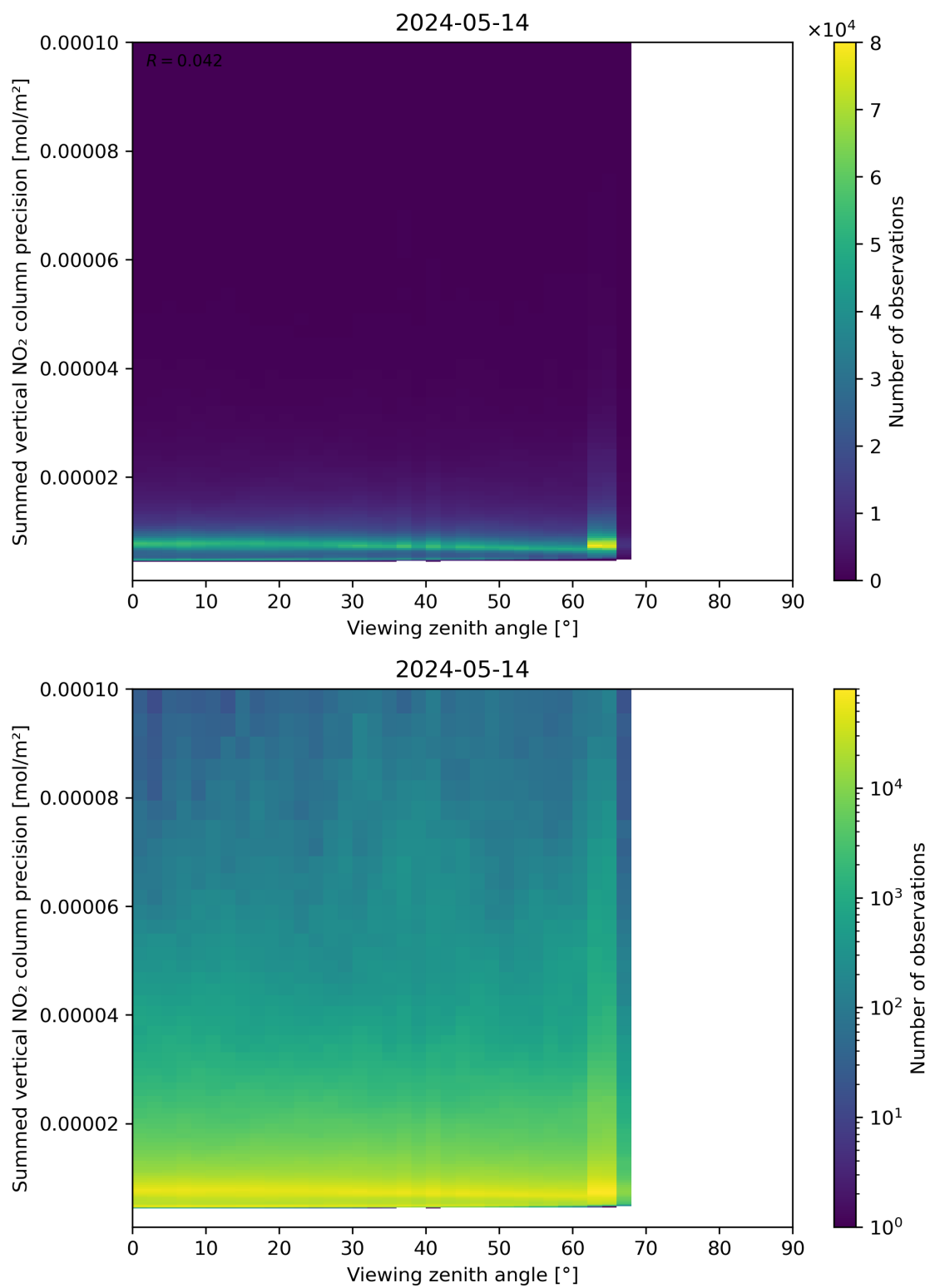
Figure 166: Scatter density plot of “Viewing zenith angle” against “Summed vertical NO 2 column precision” for 2024-05-13 to 2024-05-15.
