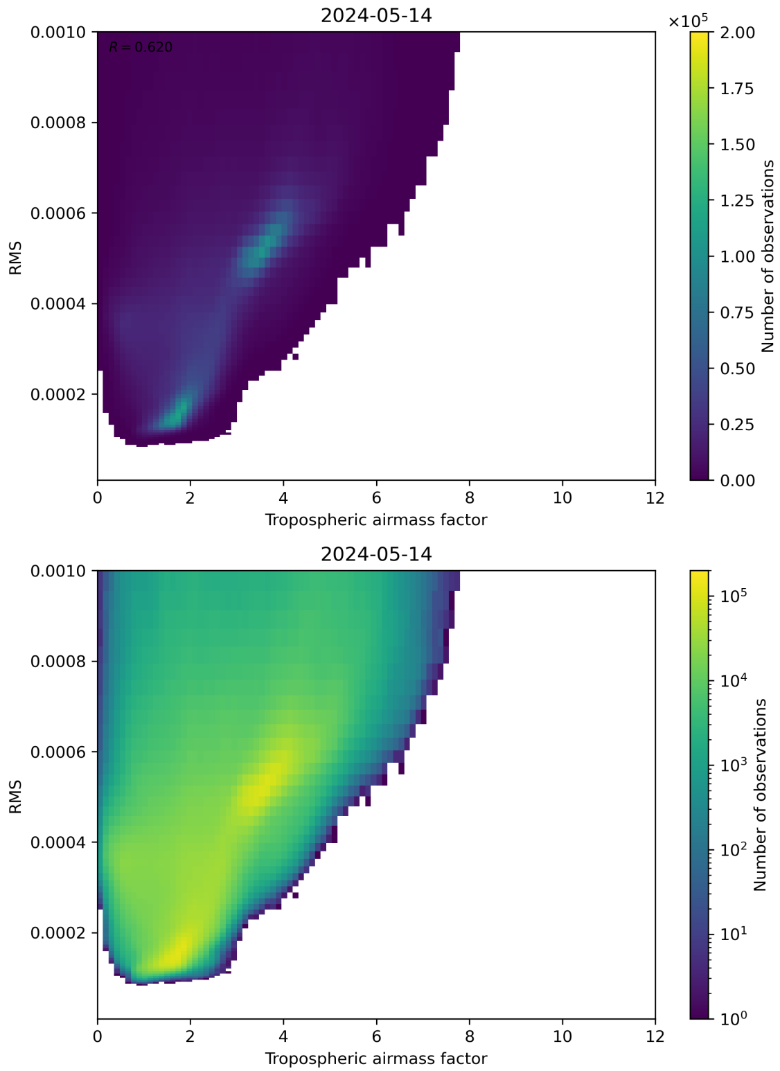
Figure 79: Scatter density plot of “Tropospheric airmass factor” against “RMS” for 2024-05-13 to 2024-05-15.
