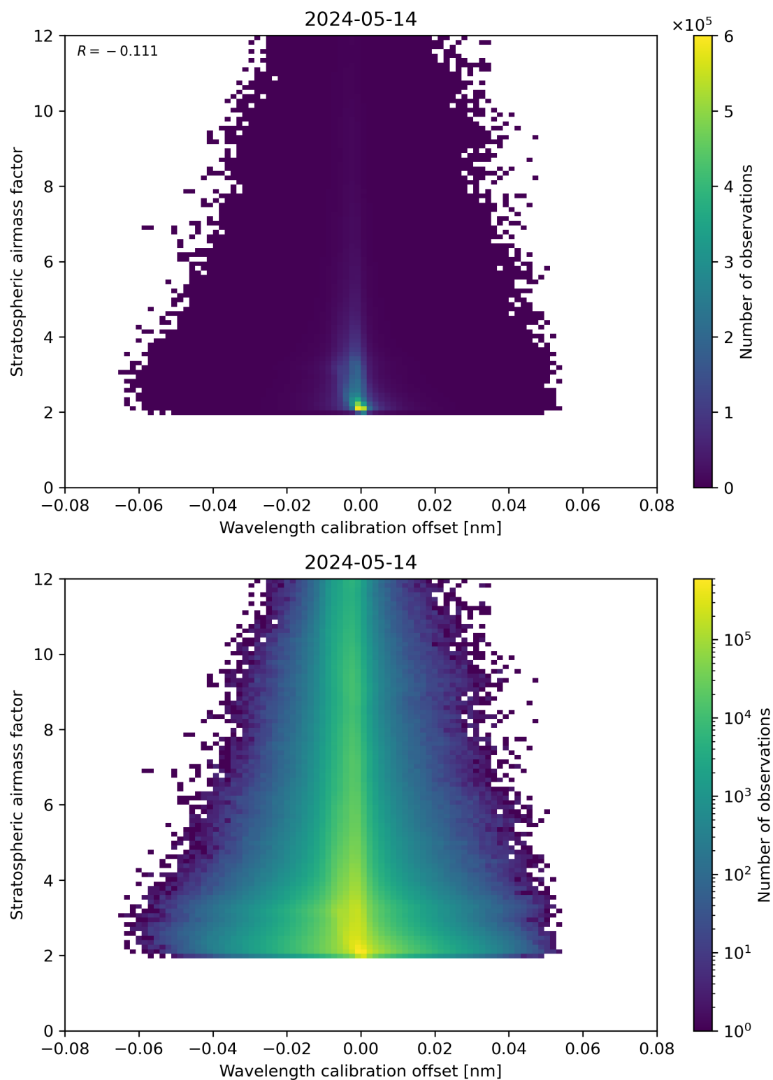
Figure 174: Scatter density plot of “Wavelength calibration offset” against “Stratospheric airmass factor” for 2024-05-13 to 2024-05-15.
