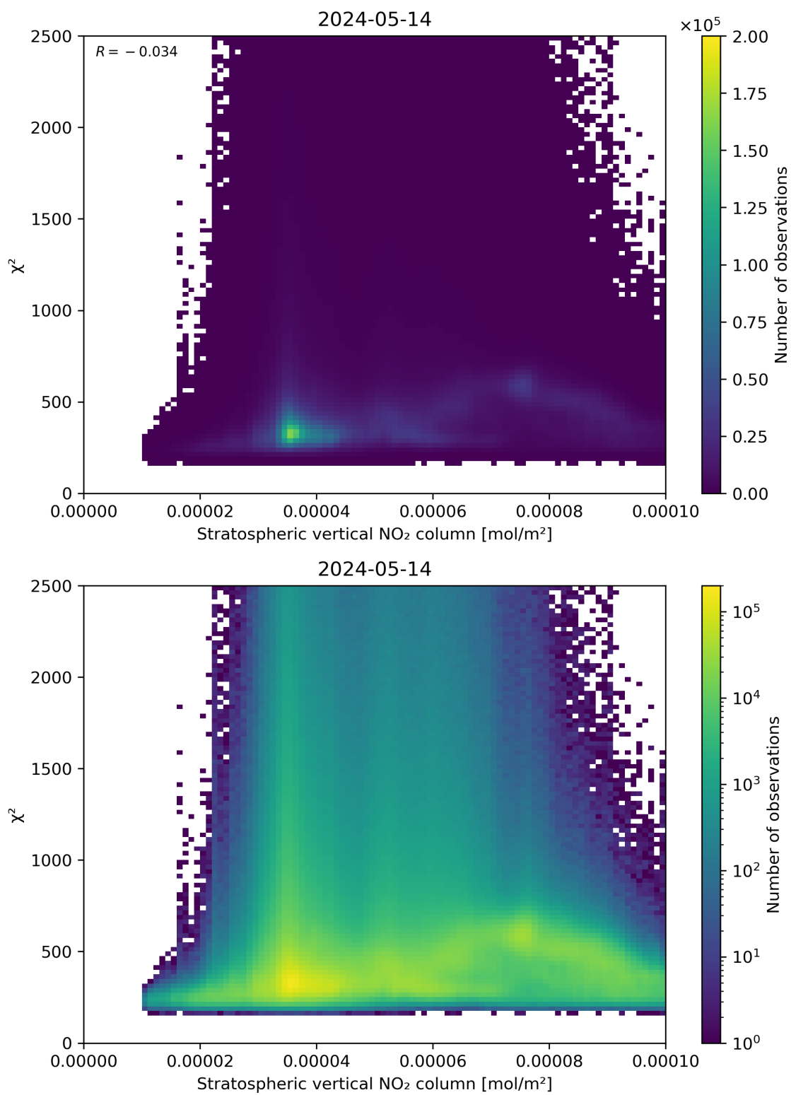
Figure 97: Scatter density plot of “Stratospheric vertical NO 2 column” against “ \chi^2 ” for 2024-05-13 to 2024-05-15.
