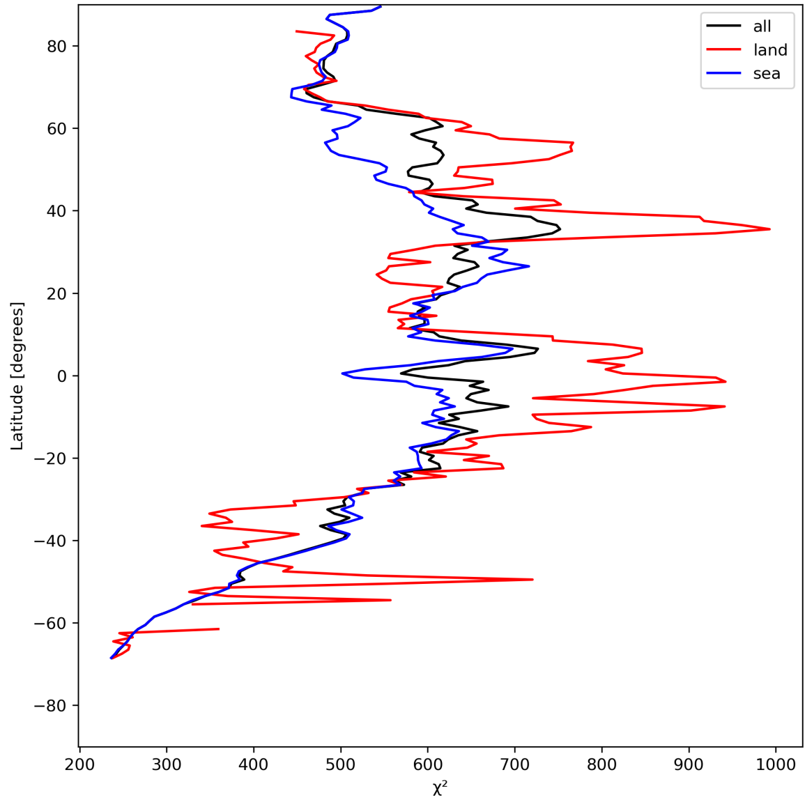
Figure 25: Zonal average of “ \chi^2 ” for 2024-05-13 to 2024-05-15.
