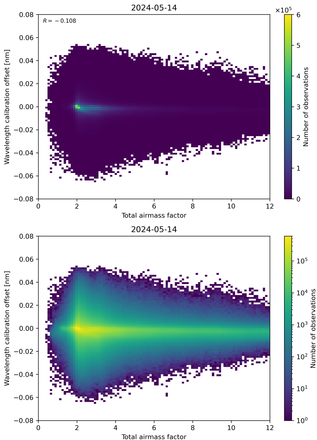
Figure 70: Scatter density plot of “Total airmass factor” against “Wavelength calibration offset” for 2024-05-13 to 2024-05-15.
