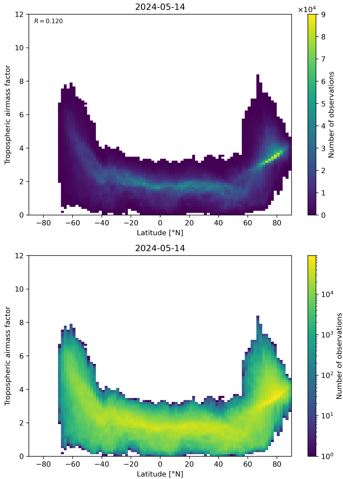
Figure 85: Scatter density plot of “Latitude” against “Tropospheric airmass factor” for 2024-05-13 to 2024-05-15.
