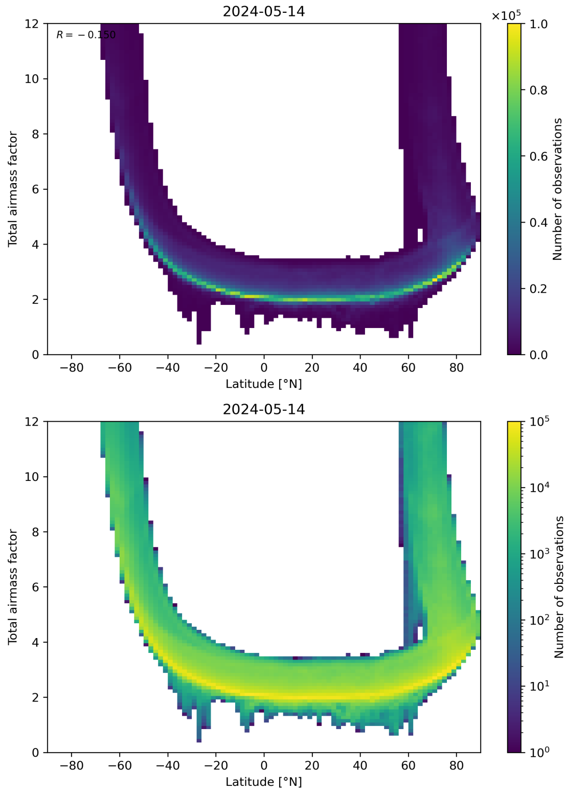
Figure 84: Scatter density plot of “Latitude” against “Total airmass factor” for 2024-05-13 to 2024-05-15.
