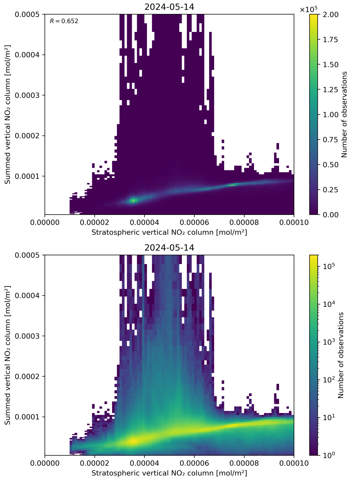
Figure 98: Scatter density plot of “Stratospheric vertical NO 2 column” against “Summed vertical NO 2 column” for 2024-05-13 to 2024-05-15.
