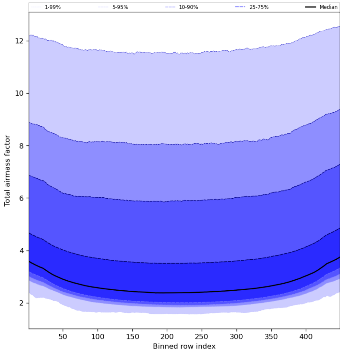
Figure 49: Along track statistics of “Total airmass factor” for 2024-05-13 to 2024-05-15
