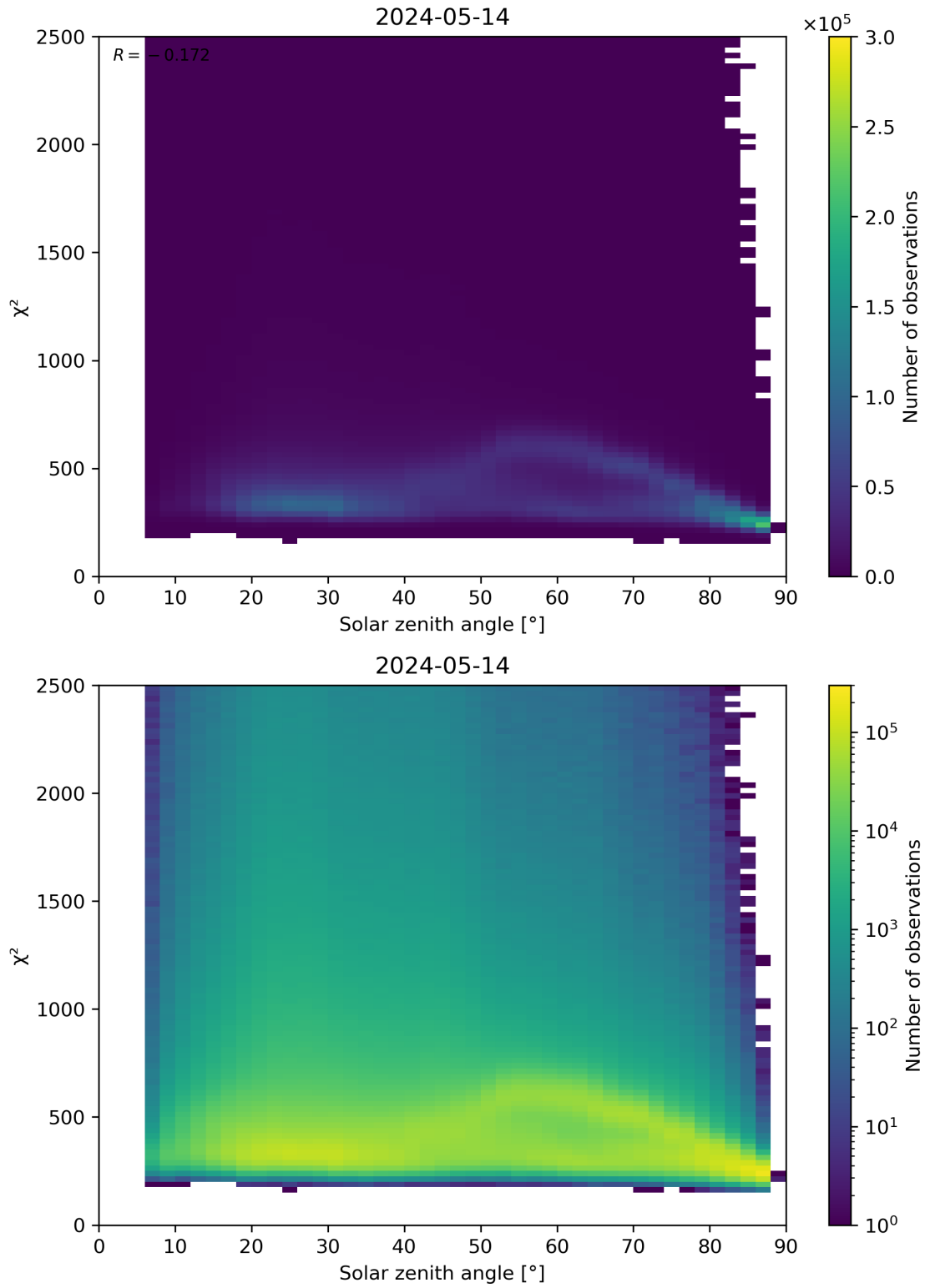
Figure 148: Scatter density plot of “Solar zenith angle” against “ \chi^2 ” for 2024-05-13 to 2024-05-15.
