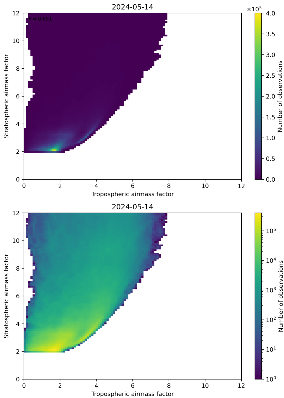
Figure 71: Scatter density plot of “Tropospheric airmass factor” against “Stratospheric airmass factor” for 2024-05-13 to 2024-05-15.
