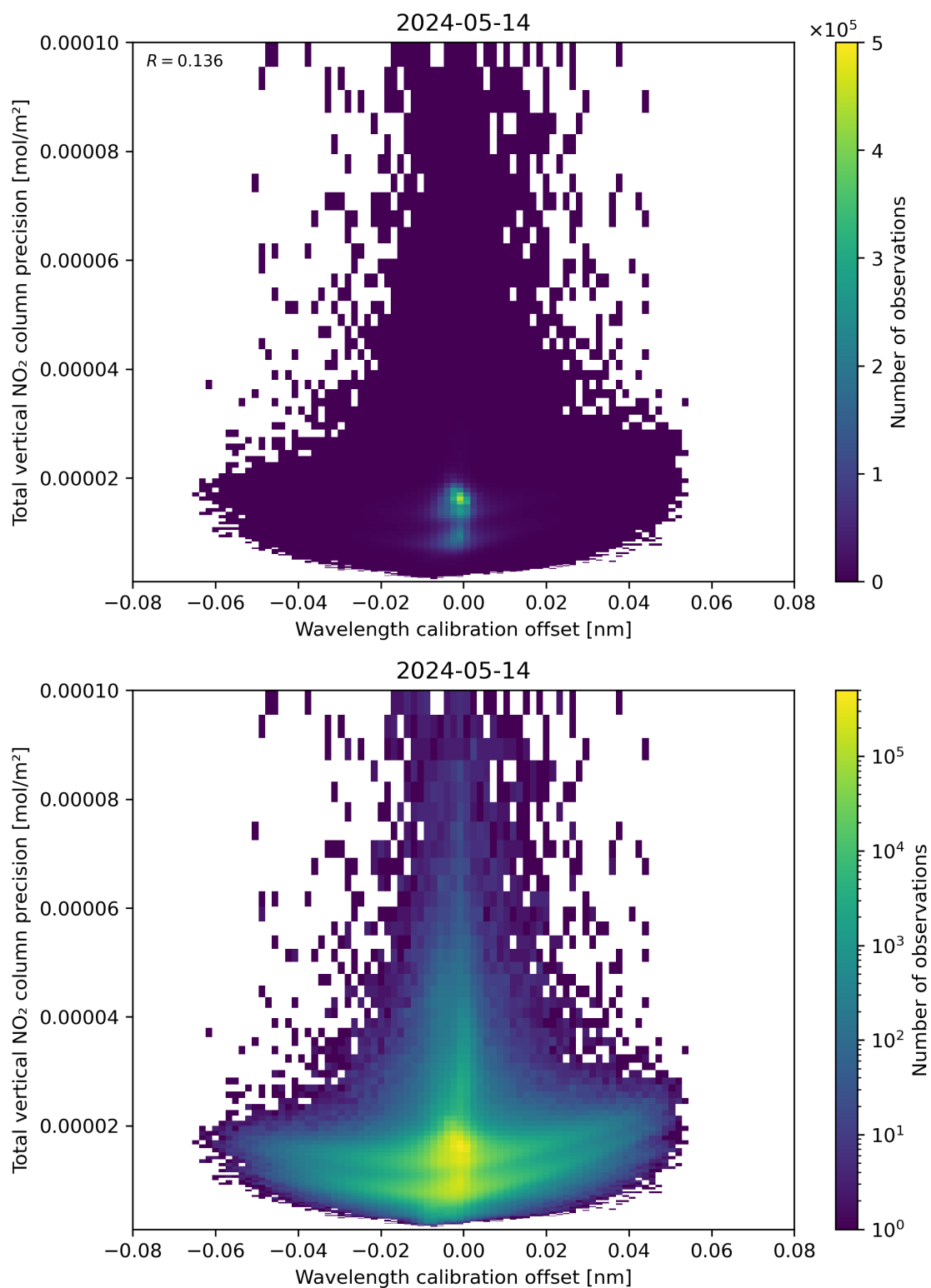
Figure 180: Scatter density plot of “Wavelength calibration offset” against “Total vertical NO 2 column precision” for 2024-05-13 to 2024-05-15.
