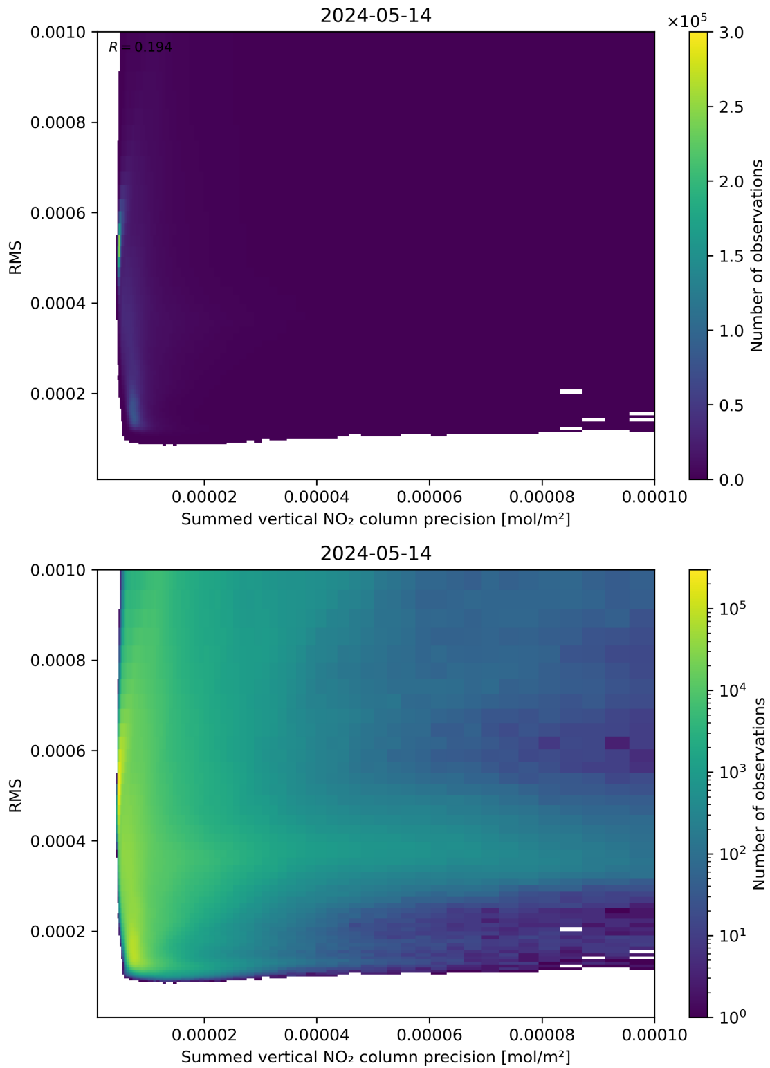
Figure 108: Scatter density plot of “Summed vertical NO 2 column precision” against “RMS” for 2024-05-13 to 2024-05-15.
