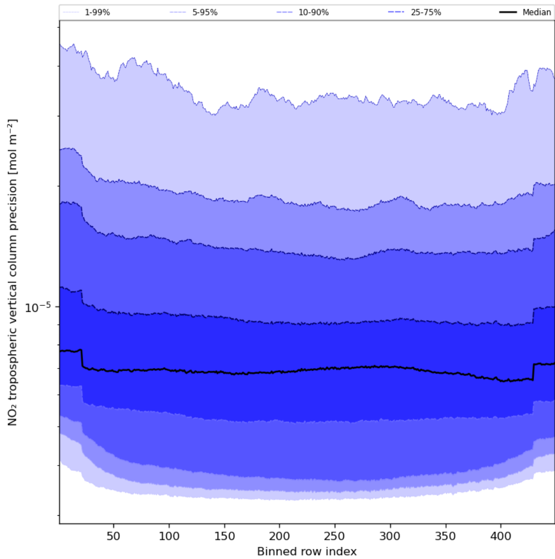
Figure 47: Along track statistics of “NO 2 tropospheric vertical column precision” for 2024-05-13 to 2024-05-15
