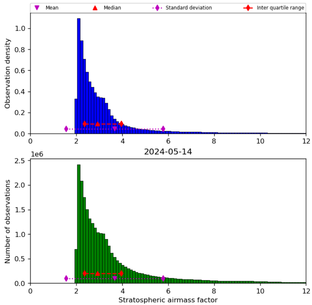
Figure 44: Histogram of “Stratospheric airmass factor” for 2024-05-13 to 2024-05-15
