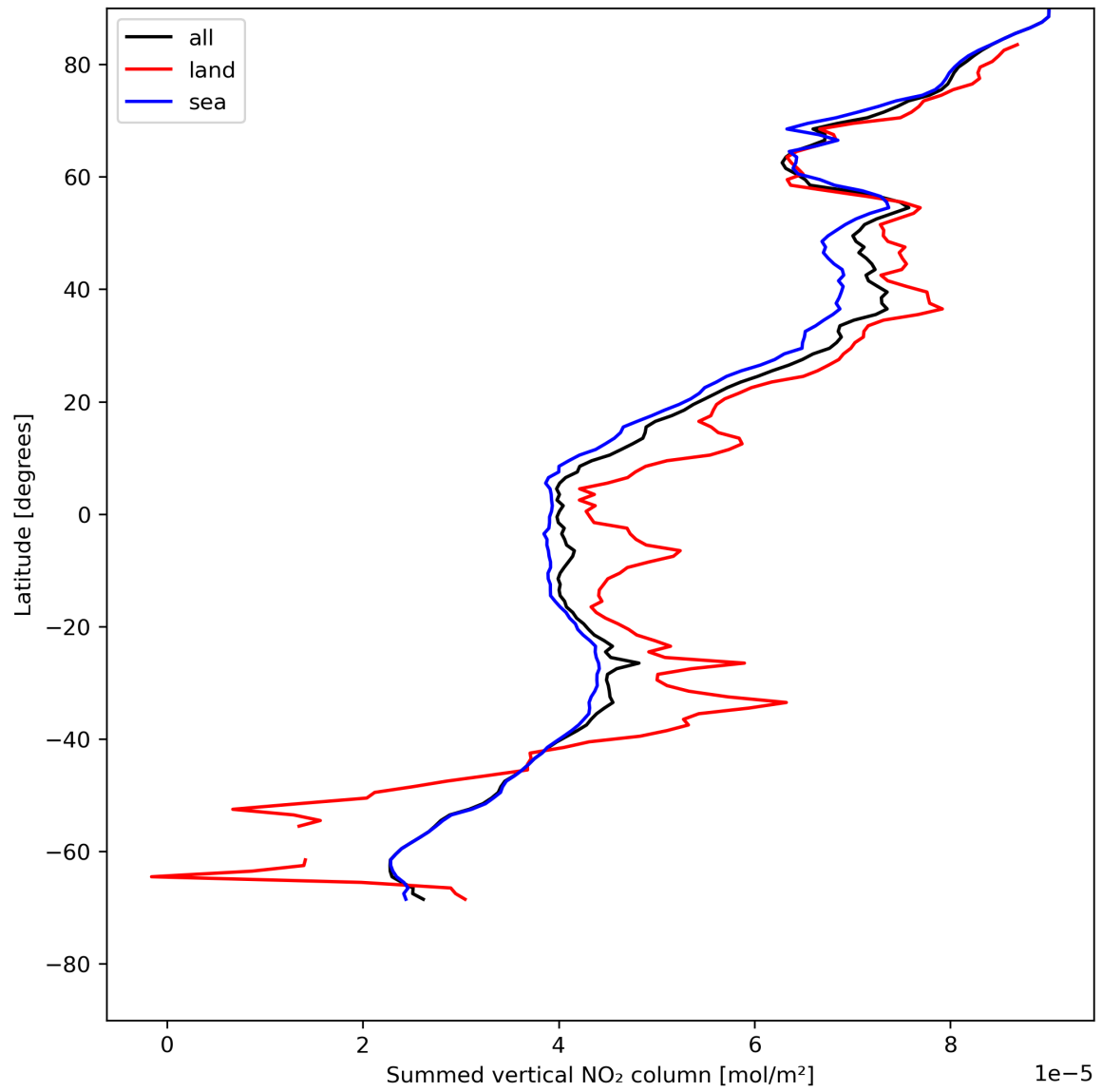
Figure 23: Zonal average of “Summed vertical NO 2 column” for 2024-05-13 to 2024-05-15.
