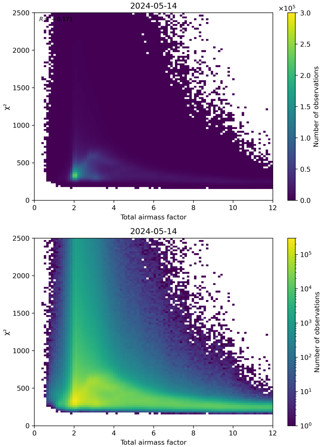
Figure 63: Scatter density plot of “Total airmass factor” against “ \chi^2 ” for 2024-05-13 to 2024-05-15.
