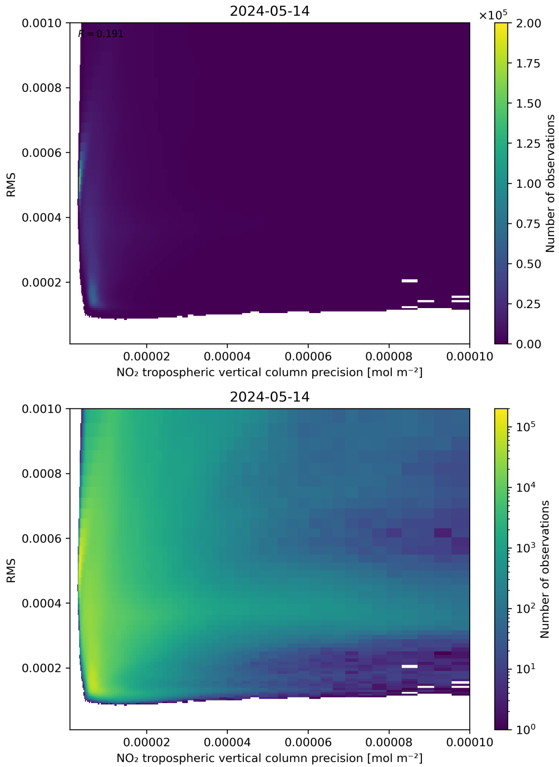
Figure 140: Scatter density plot of “NO 2 tropospheric vertical column precision” against “RMS” for 2024-05-13 to 2024-05-15.
