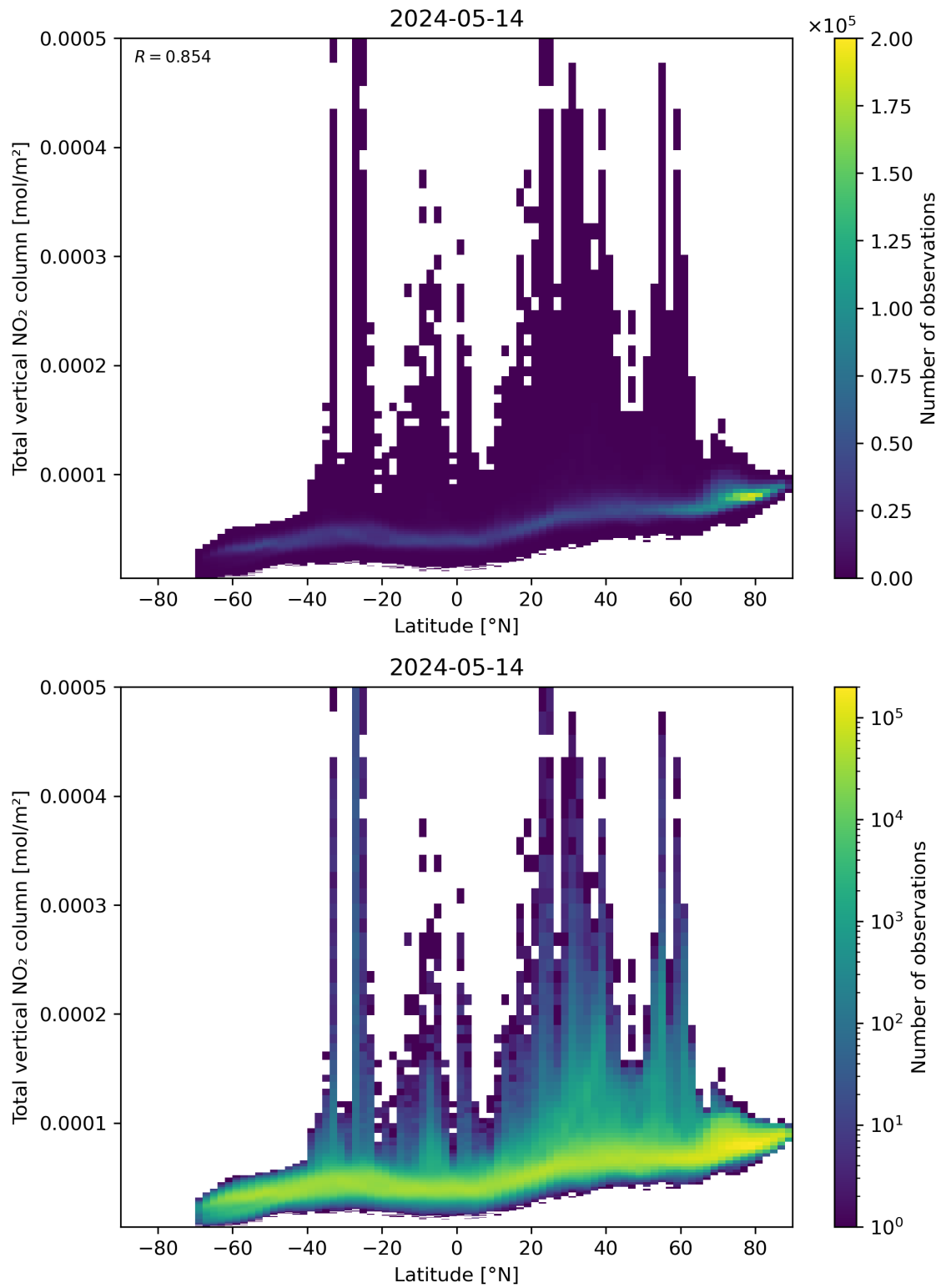
Figure 90: Scatter density plot of “Latitude” against “Total vertical NO 2 column” for 2024-05-13 to 2024-05-15.
