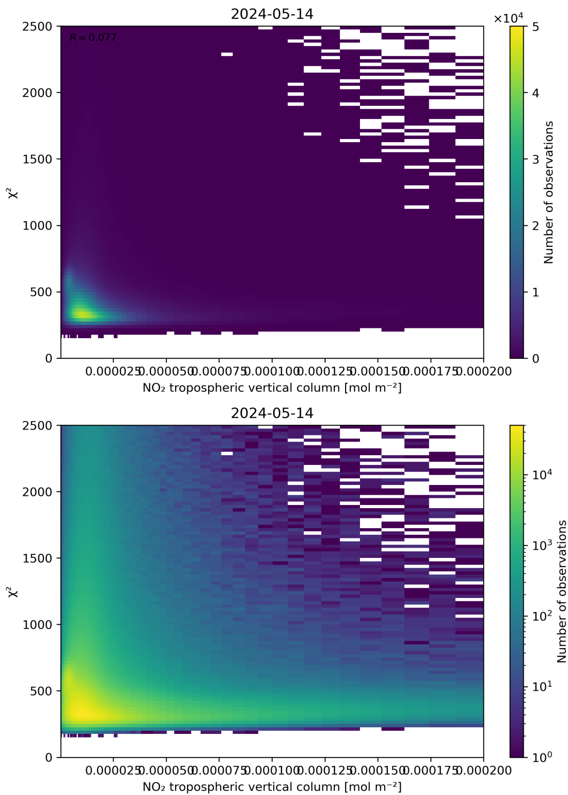
Figure 124: Scatter density plot of “NO 2 tropospheric vertical column” against “ \chi^2 ” for 2024-05-13 to 2024-05-15.
