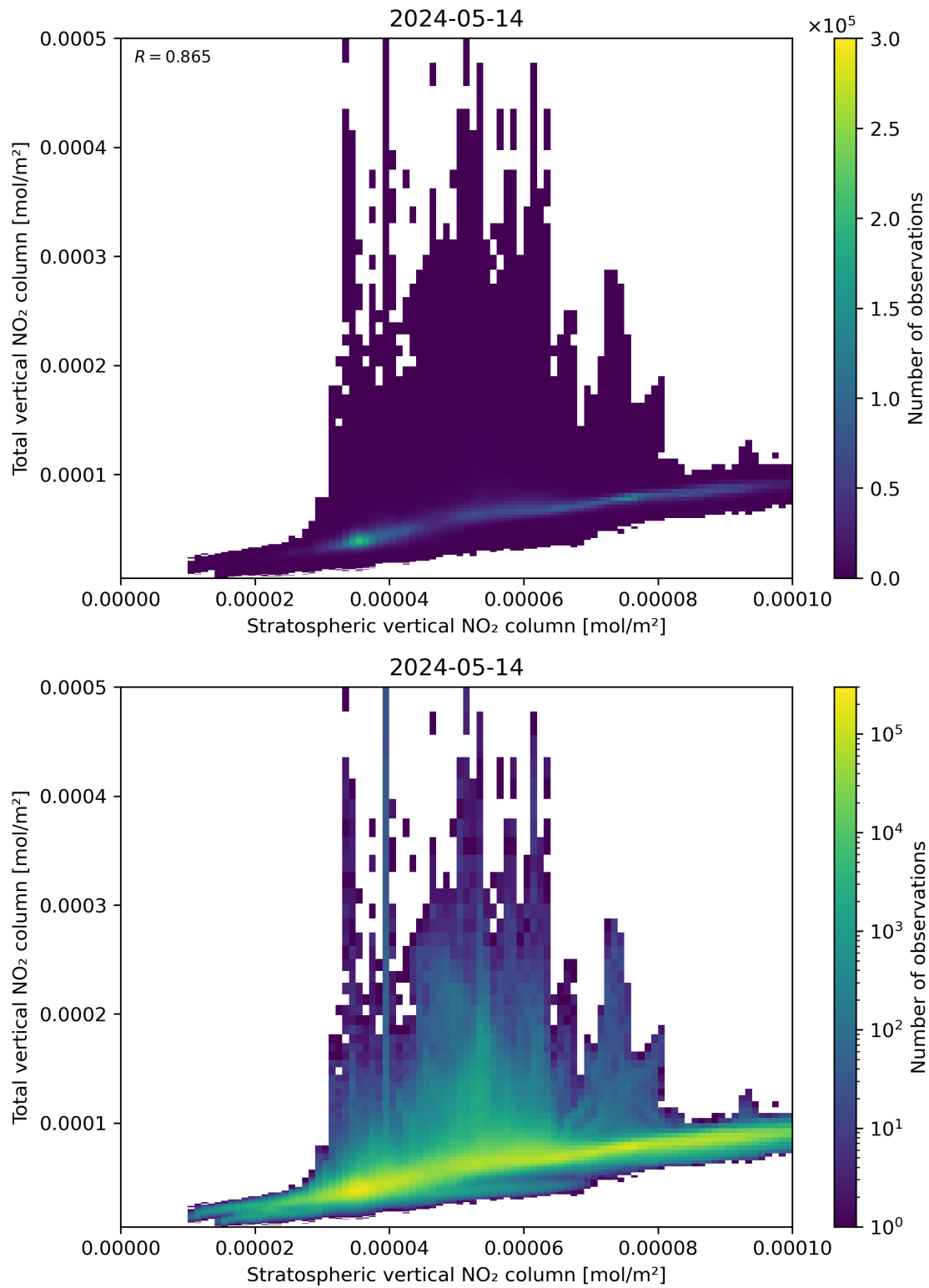
Figure 100: Scatter density plot of “Stratospheric vertical NO 2 column” against “Total vertical NO 2 column” for 2024-05-13 to 2024-05-15.
