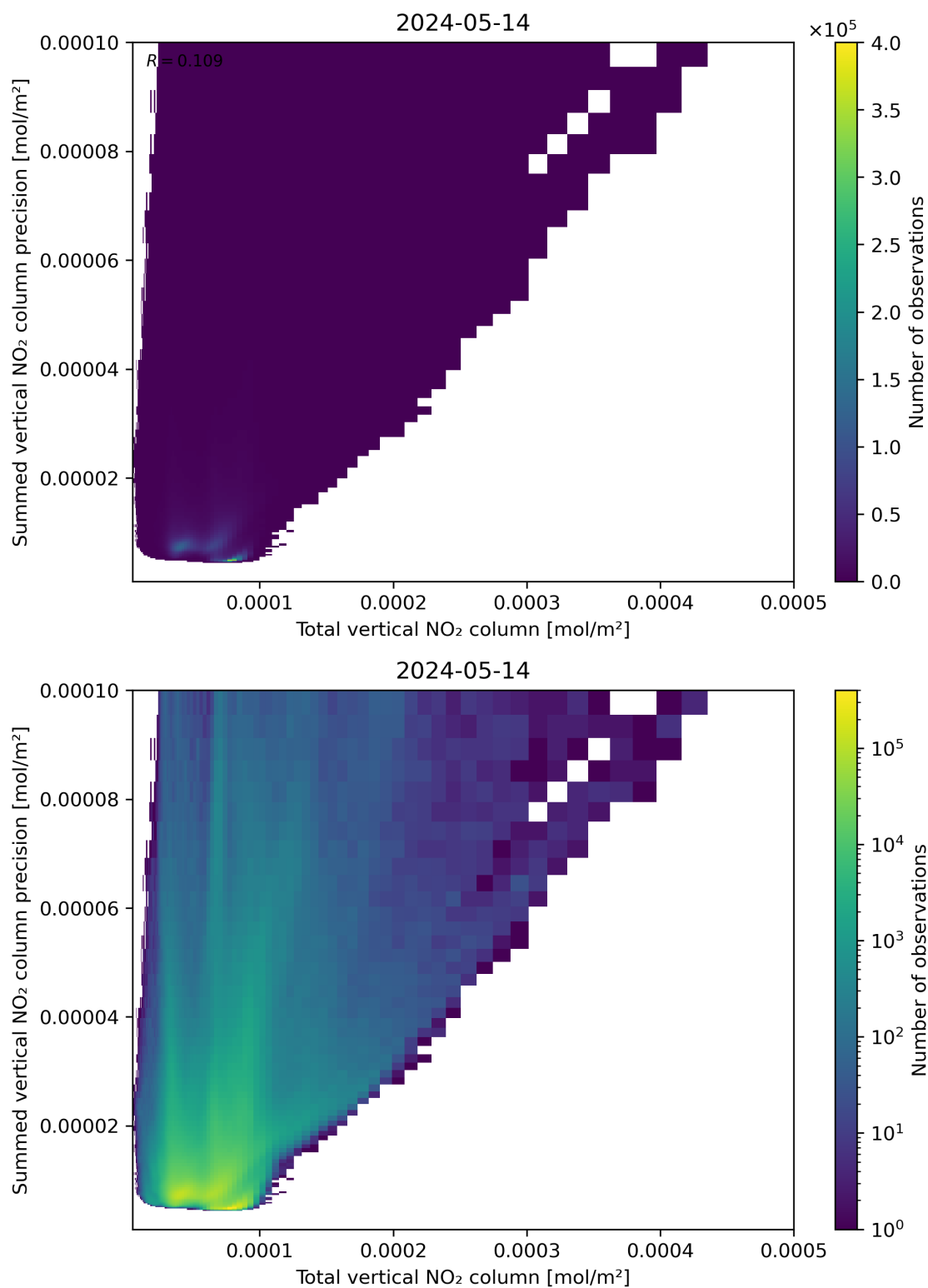
Figure 113: Scatter density plot of “Total vertical NO 2 column” against “Summed vertical NO 2 column precision” for 2024-05-13 to 2024-05-15.
