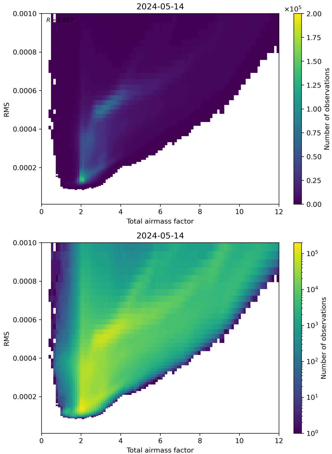
Figure 69: Scatter density plot of “Total airmass factor” against “RMS” for 2024-05-13 to 2024-05-15.
