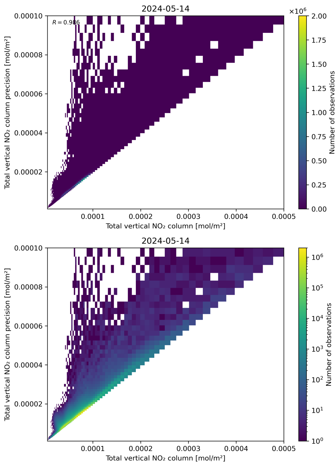
Figure 114: Scatter density plot of “Total vertical NO 2 column” against “Total vertical NO 2 column precision” for 2024-05-13 to 2024-05-15.
