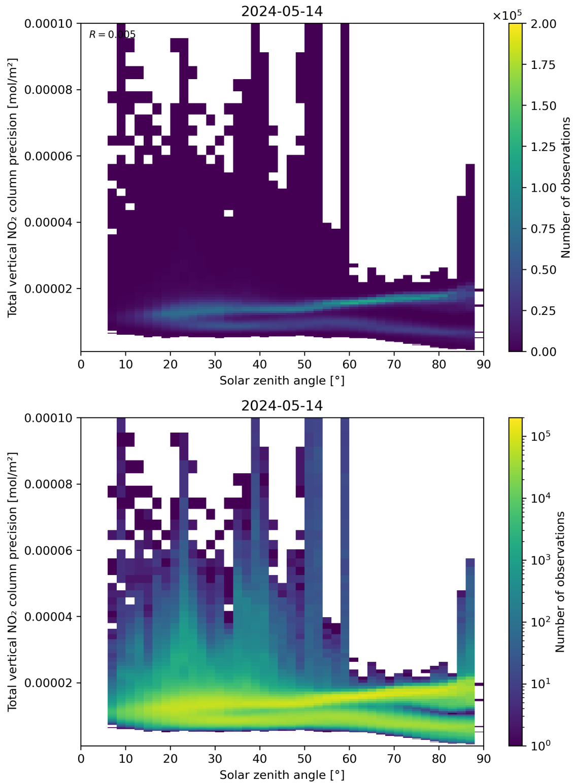
Figure 154: Scatter density plot of “Solar zenith angle” against “Total vertical NO 2 column precision” for 2024-05-13 to 2024-05-15.
