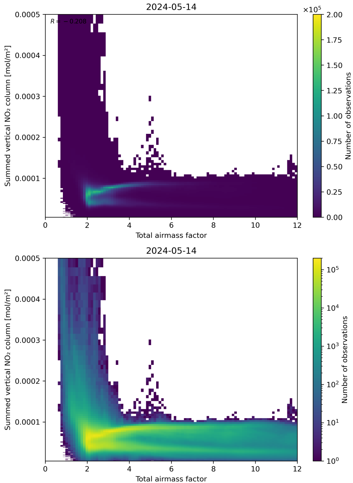
Figure 65: Scatter density plot of “Total airmass factor” against “Summed vertical NO 2 column” for 2024-05-13 to 2024-05-15.
