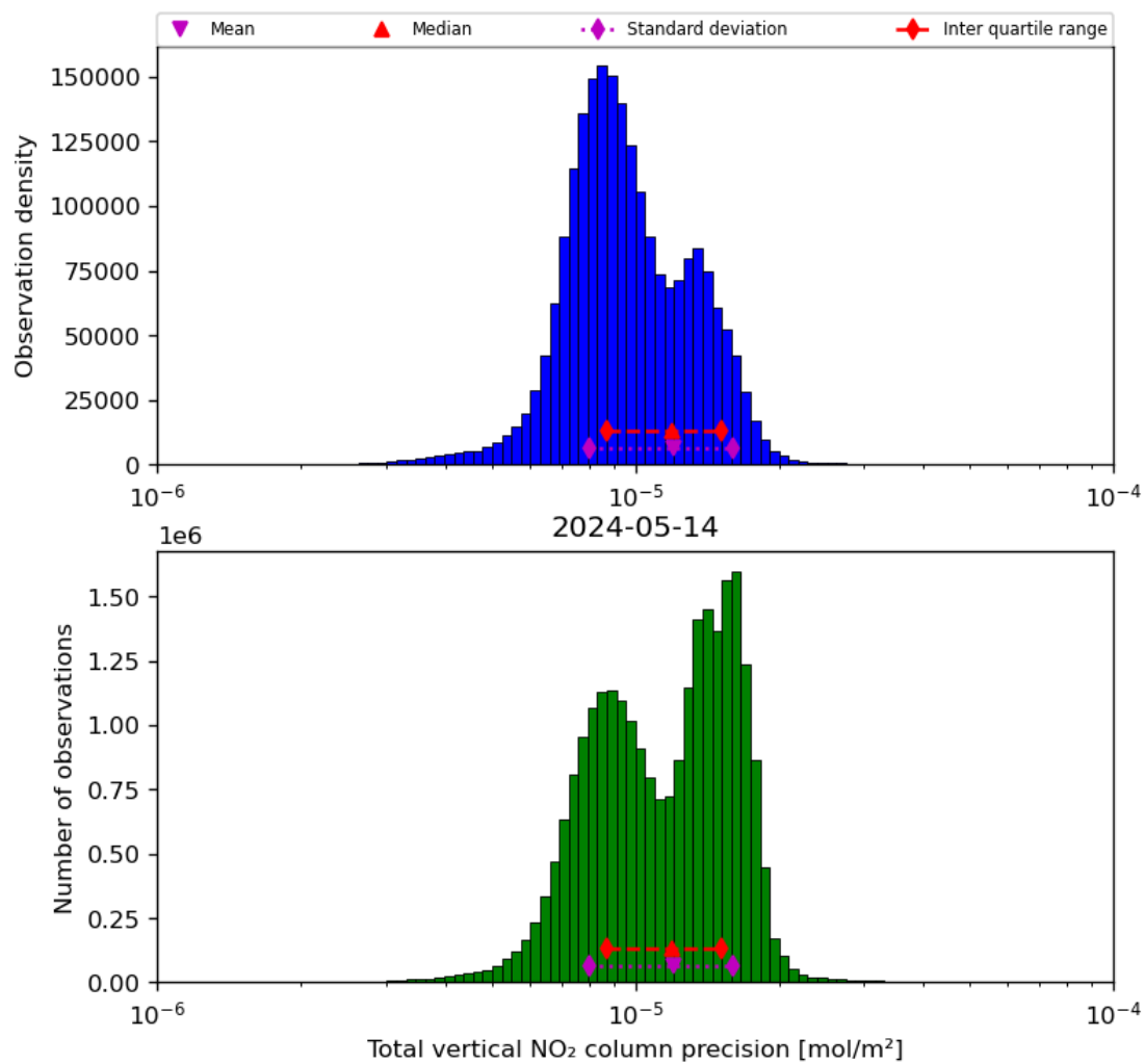
Figure 39: Histogram of “Total vertical NO 2 column precision” for 2024-05-13 to 2024-05-15
