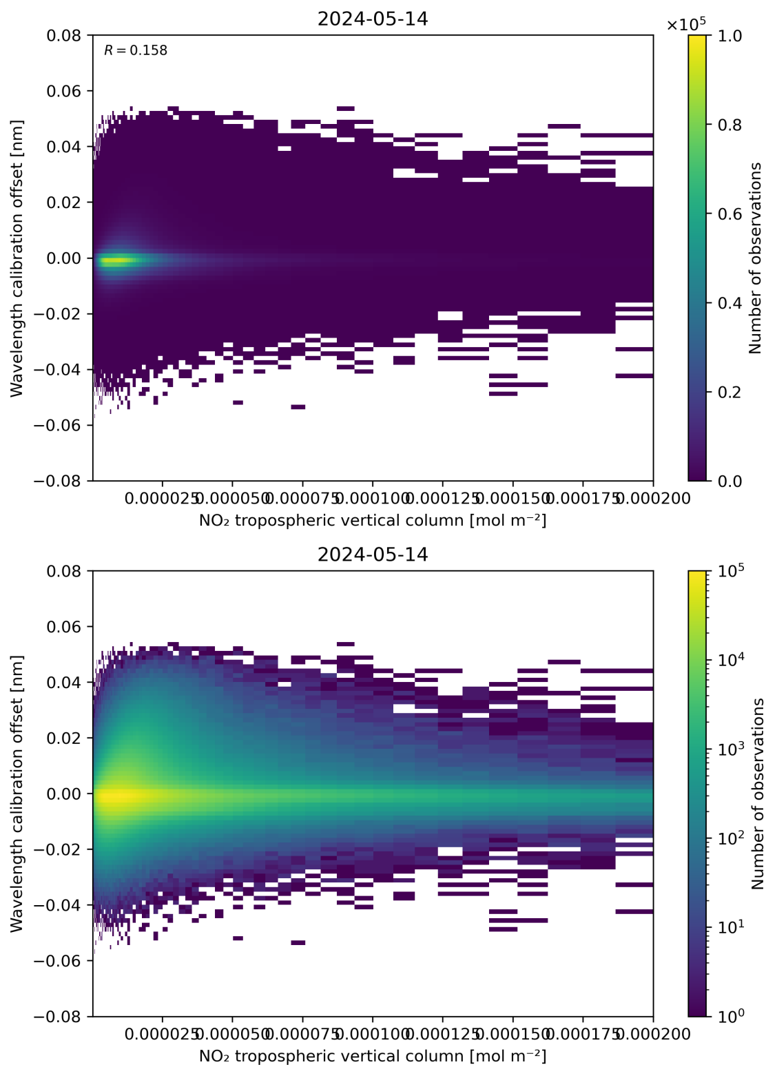
Figure 143: Scatter density plot of “NO 2 tropospheric vertical column” against “Wavelength calibration offset” for 2024-05-13 to 2024-05-15.
