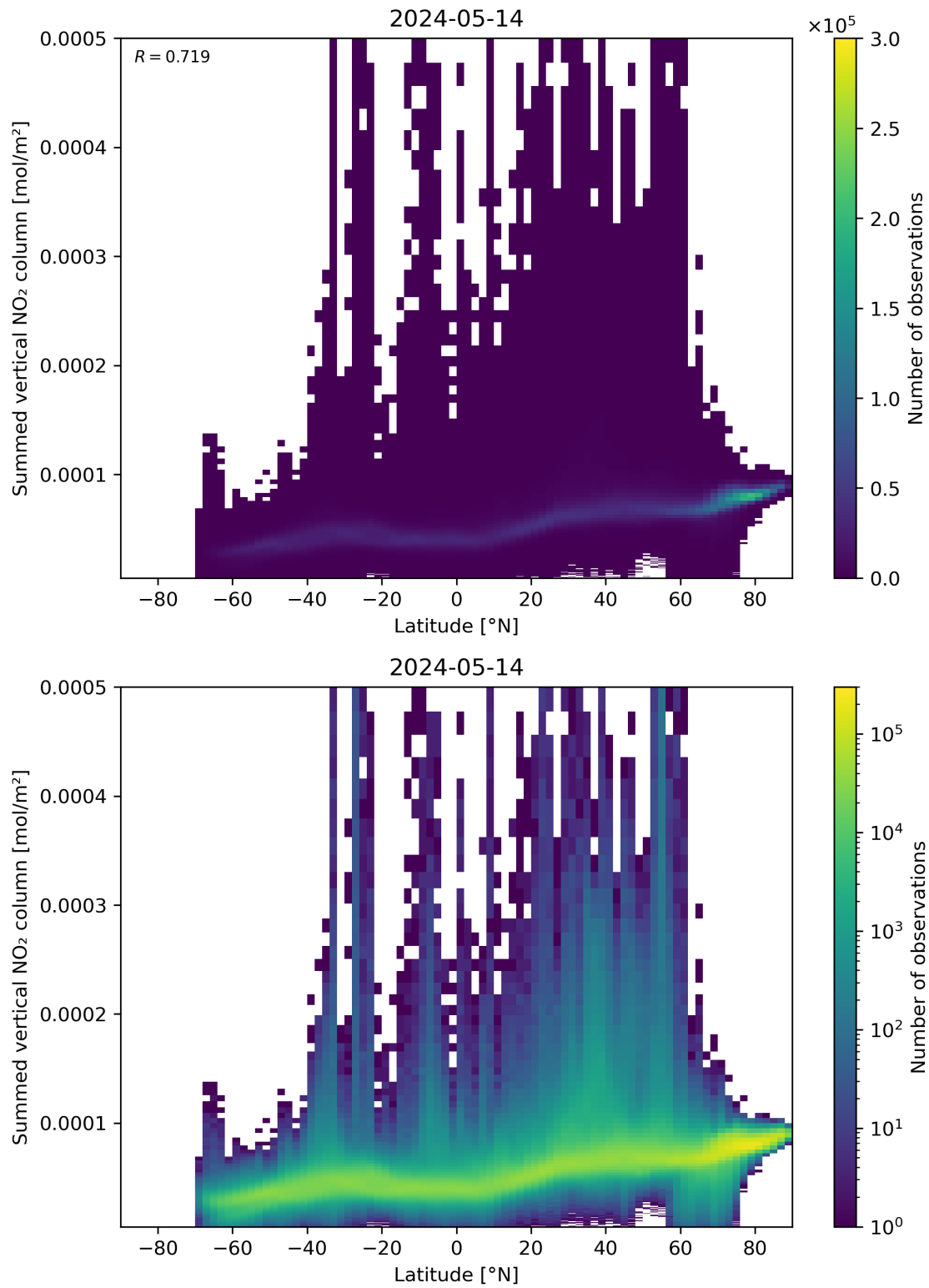
Figure 88: Scatter density plot of “Latitude” against “Summed vertical NO 2 column” for 2024-05-13 to 2024-05-15.
