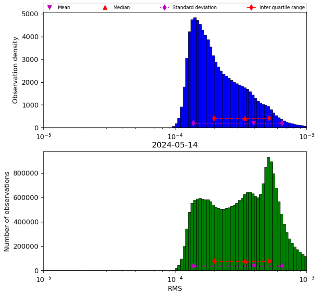
Figure 43: Histogram of “RMS” for 2024-05-13 to 2024-05-15
