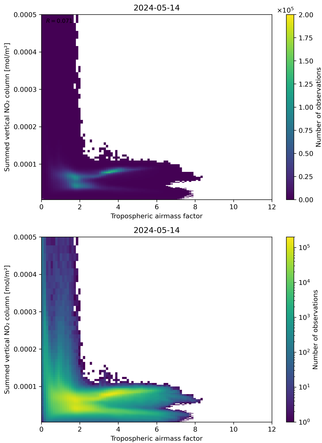
Figure 75: Scatter density plot of “Tropospheric airmass factor” against “Summed vertical NO 2 column” for 2024-05-13 to 2024-05-15.
