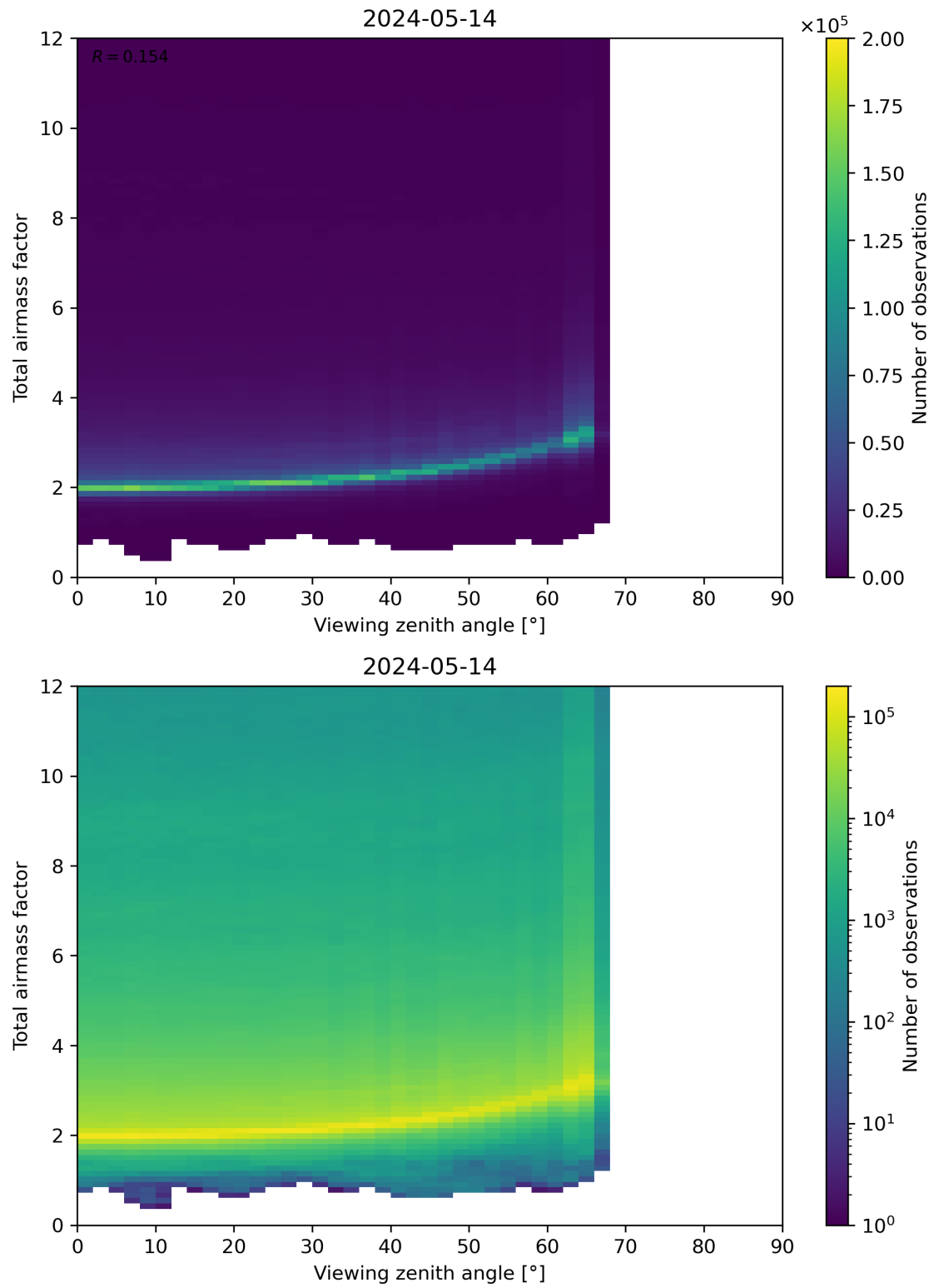
Figure 160: Scatter density plot of “Viewing zenith angle” against “Total airmass factor” for 2024-05-13 to 2024-05-15.
