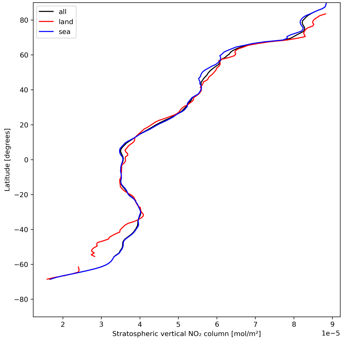
Figure 19: Zonal average of “Stratospheric vertical NO 2 column” for 2024-05-13 to 2024-05-15.
