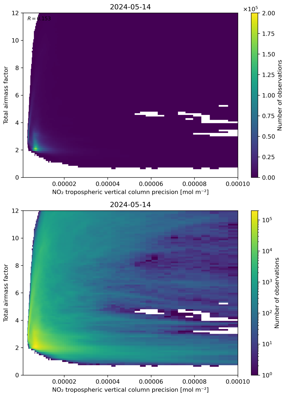
Figure 132: Scatter density plot of “NO 2 tropospheric vertical column precision” against “Total air mass factor” for 2024-05-13 to 2024-05-15.
