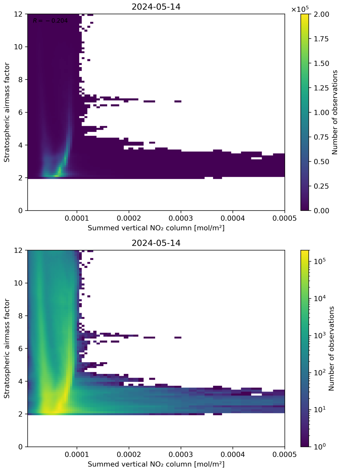
Figure 103: Scatter density plot of “Summed vertical NO 2 column” against “Stratospheric airmass factor” for 2024-05-13 to 2024-05-15.
