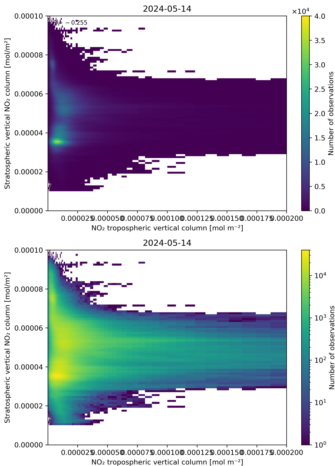
Figure 125: Scatter density plot of “NO 2 tropospheric vertical column” against “Stratospheric vertical NO 2 column” for 2024-05-13 to 2024-05-15.
