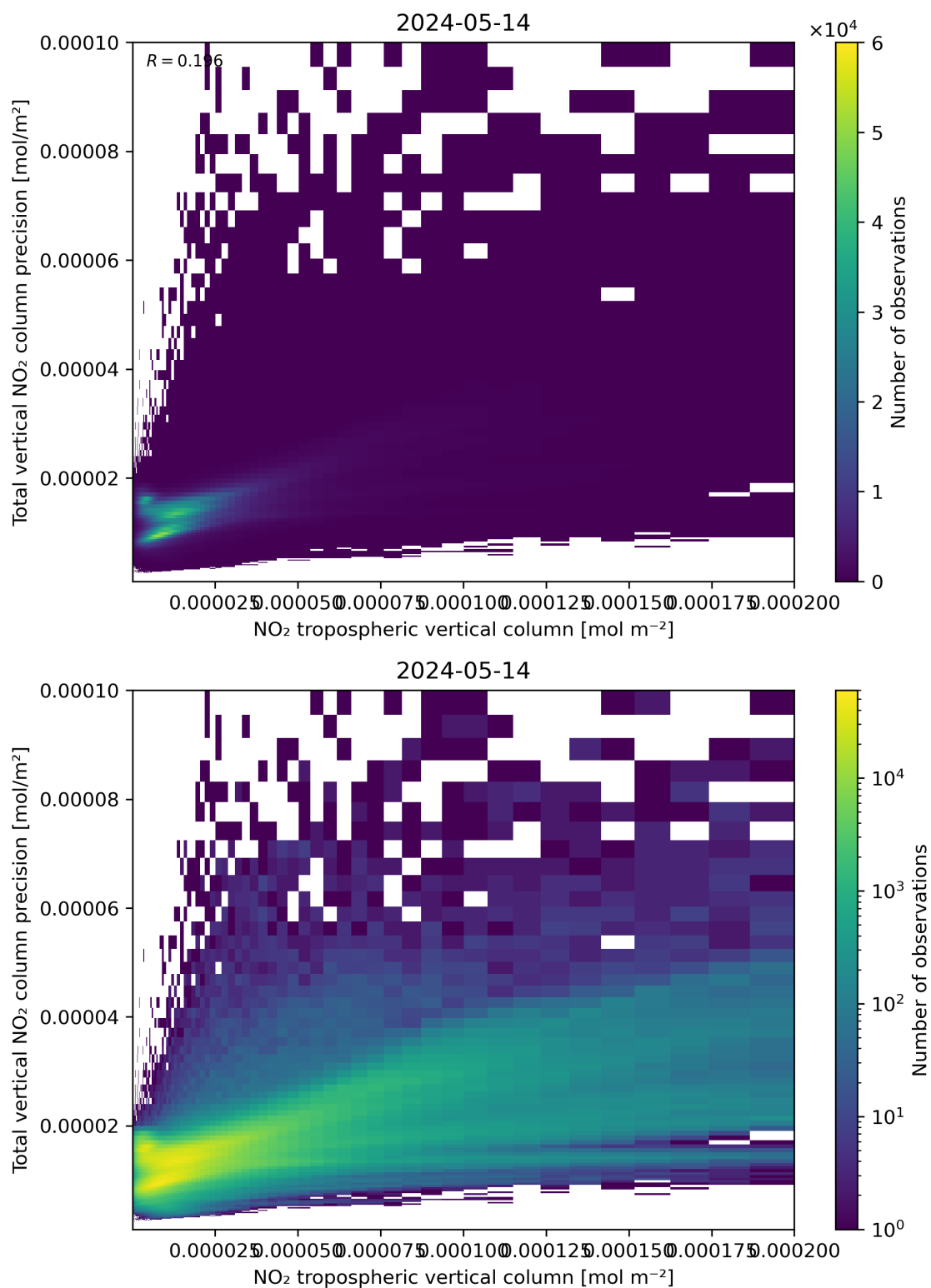
Figure 129: Scatter density plot of “NO 2 tropospheric vertical column” against “Total vertical NO 2 column precision” for 2024-05-13 to 2024-05-15.
