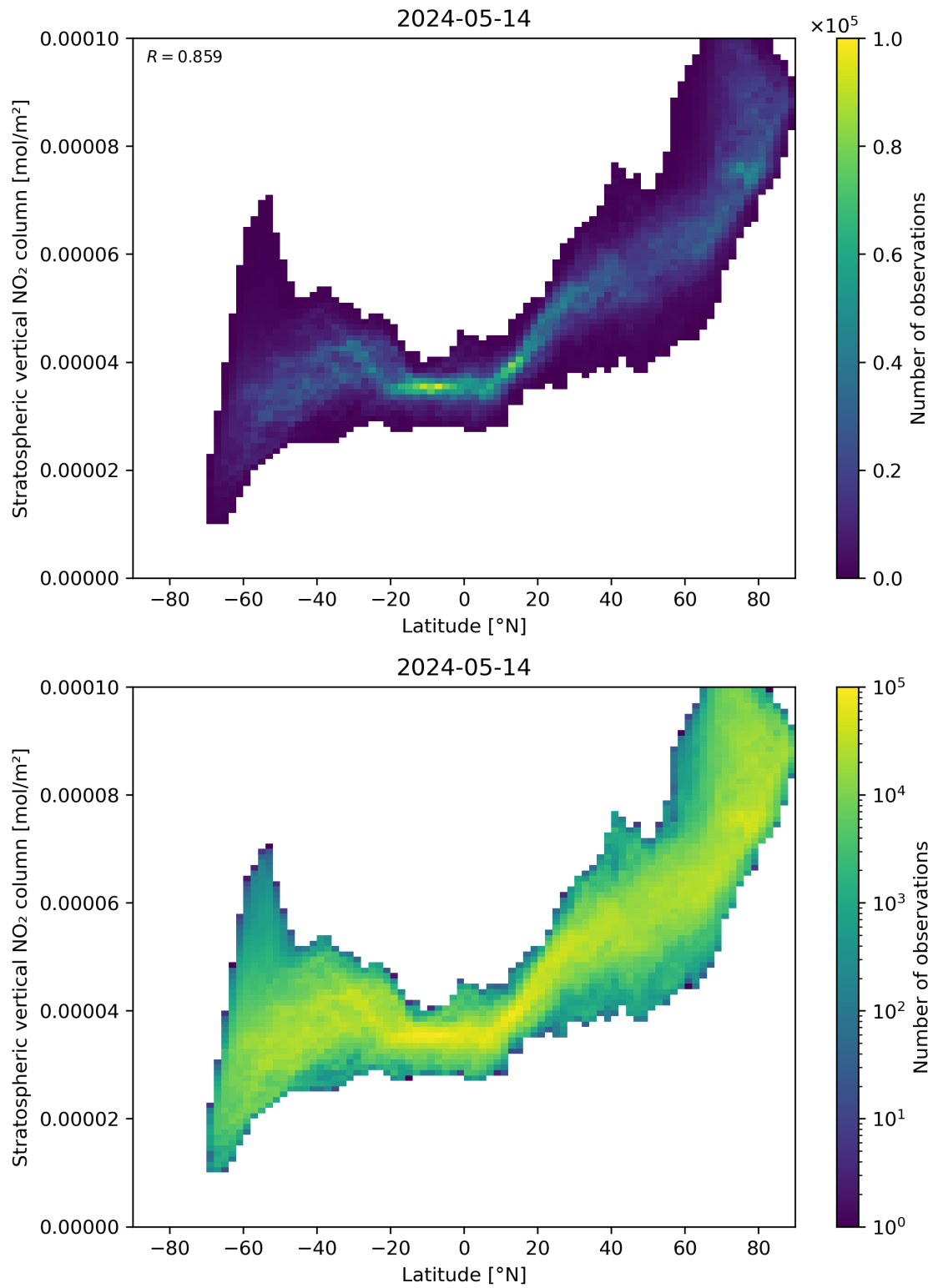
Figure 87: Scatter density plot of “Latitude” against “Stratospheric vertical NO 2 column” for 2024-05-13 to 2024-05-15.
