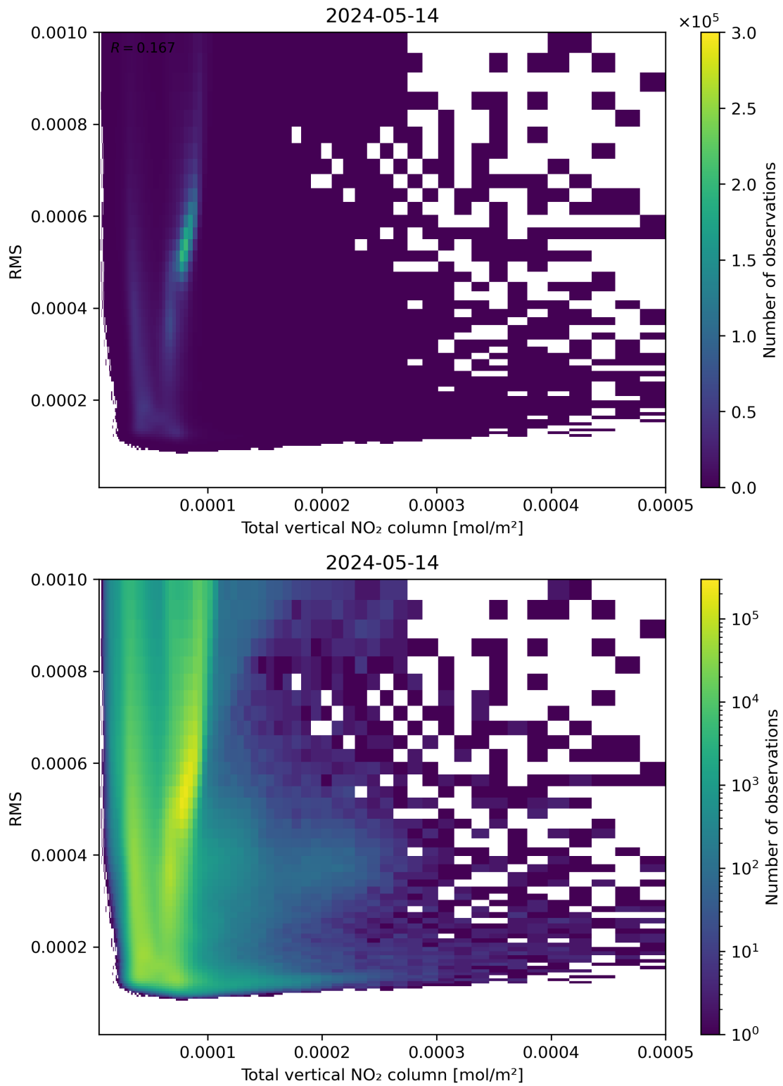
Figure 120: Scatter density plot of “Total vertical NO 2 column” against “RMS” for 2024-05-13 to 2024-05-15.
