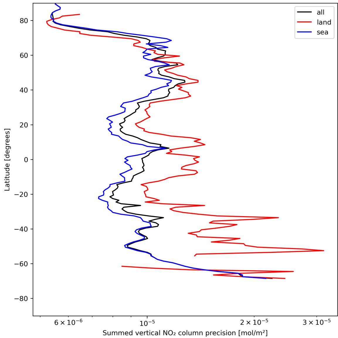
Figure 24: Zonal average of “Summed vertical NO 2 column precision” for 2024-05-13 to 2024-05-15.
