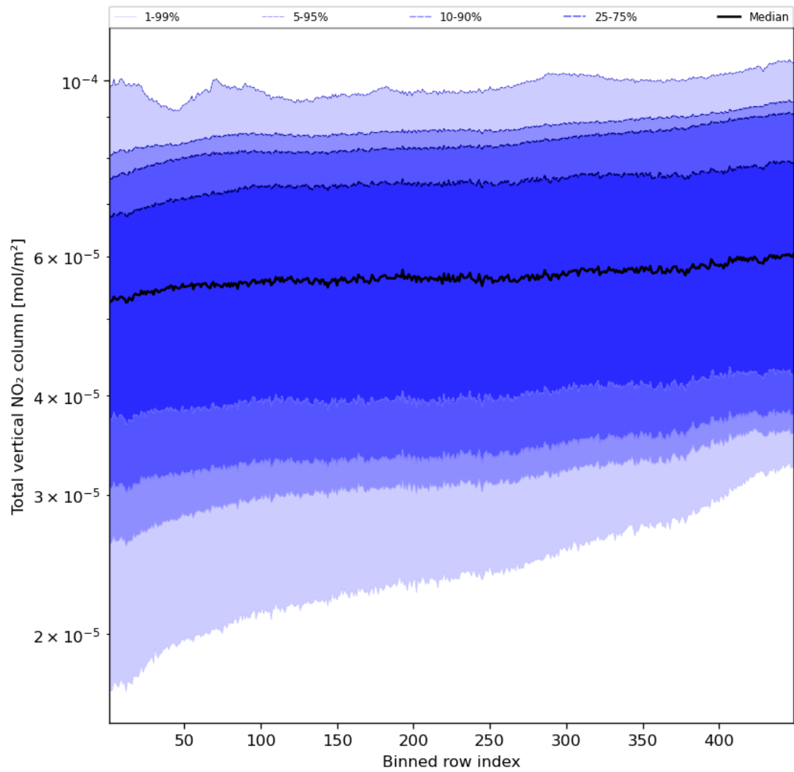
Figure 55: Along track statistics of “Total vertical NO 2 column” for 2024-05-13 to 2024-05-15
