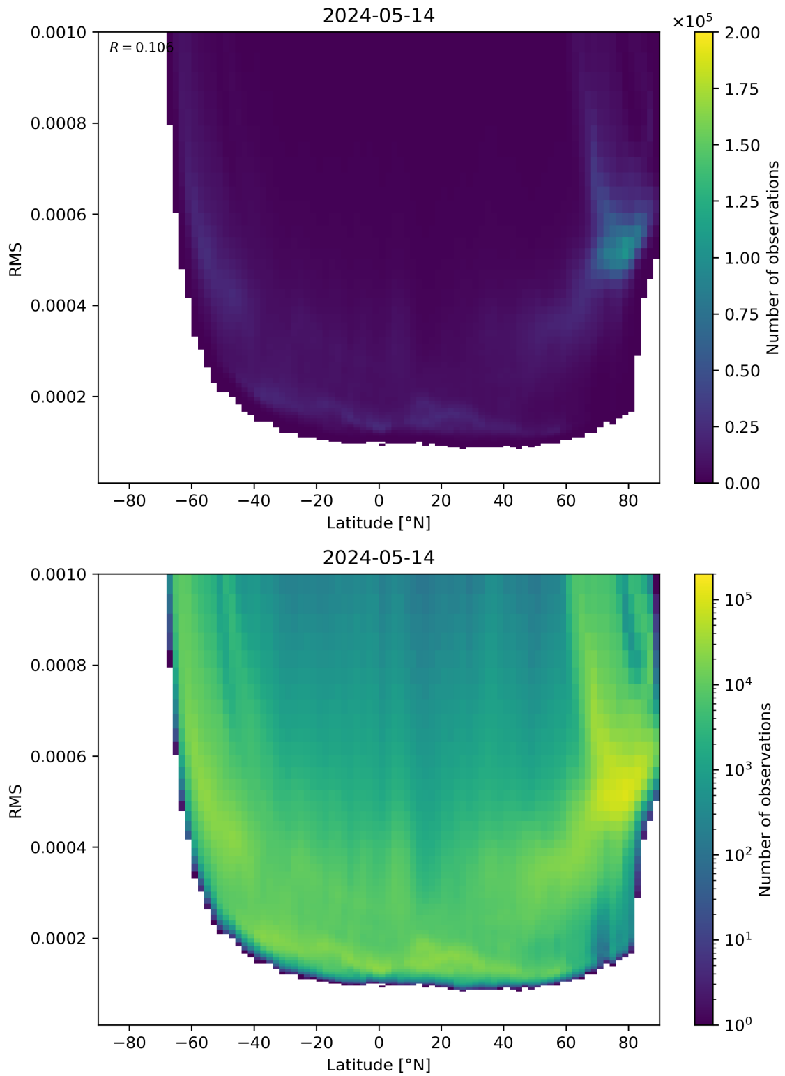
Figure 94: Scatter density plot of “Latitude” against “RMS” for 2024-05-13 to 2024-05-15.
