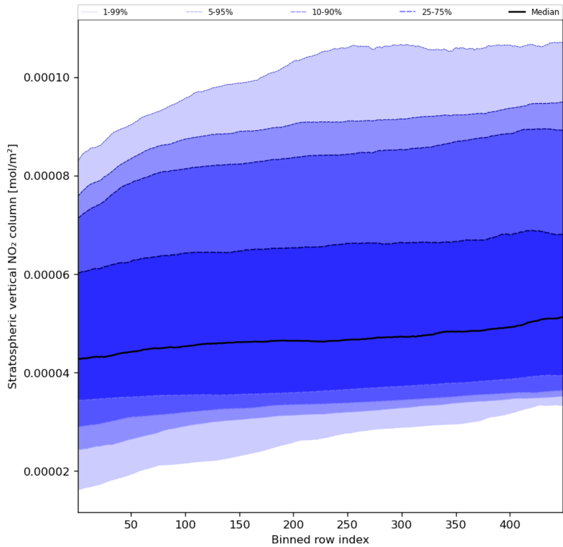
Figure 53: Along track statistics of “Stratospheric vertical NO 2 column” for 2024-05-13 to 2024-05-15
