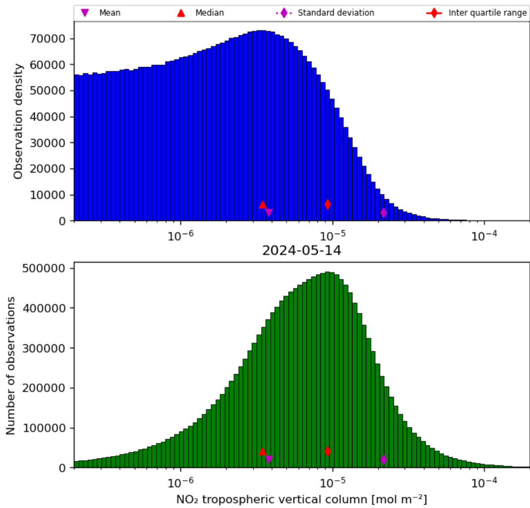
Figure 29: Histogram of “NO 2 tropospheric vertical column” for 2024-05-13 to 2024-05-15
