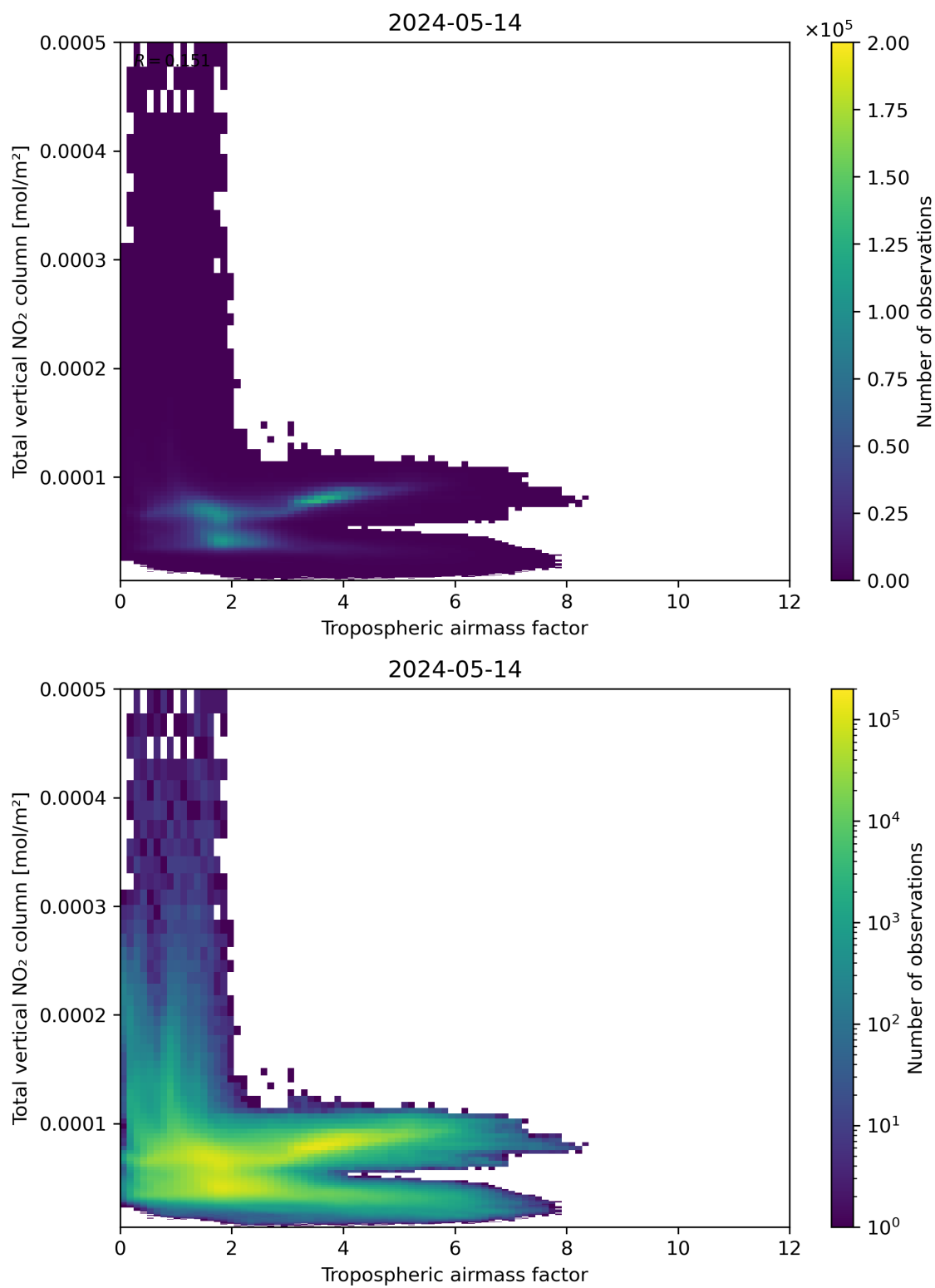
Figure 77: Scatter density plot of “Tropospheric airmass factor” against “Total vertical NO 2 column” for 2024-05-13 to 2024-05-15.
