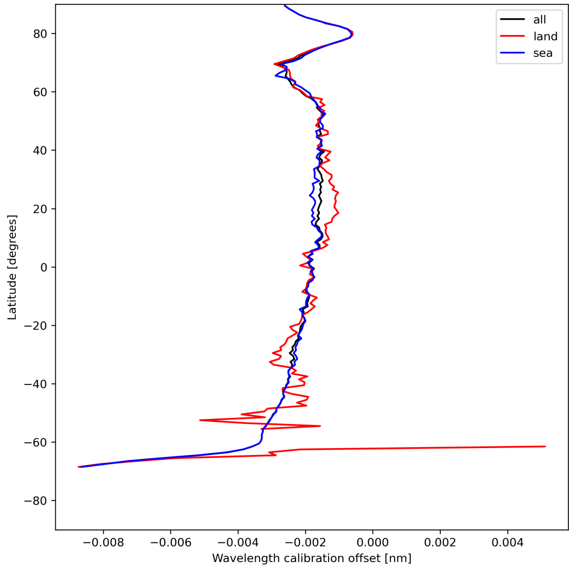
Figure 18: Zonal average of “Wavelength calibration offset” for 2024-05-13 to 2024-05-15.
