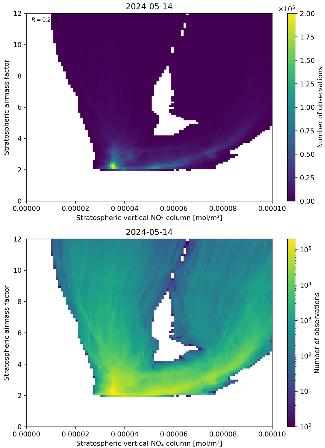
Figure 96: Scatter density plot of “Stratospheric vertical NO 2 column” against “Stratospheric airmass factor” for 2024-05-13 to 2024-05-15.
