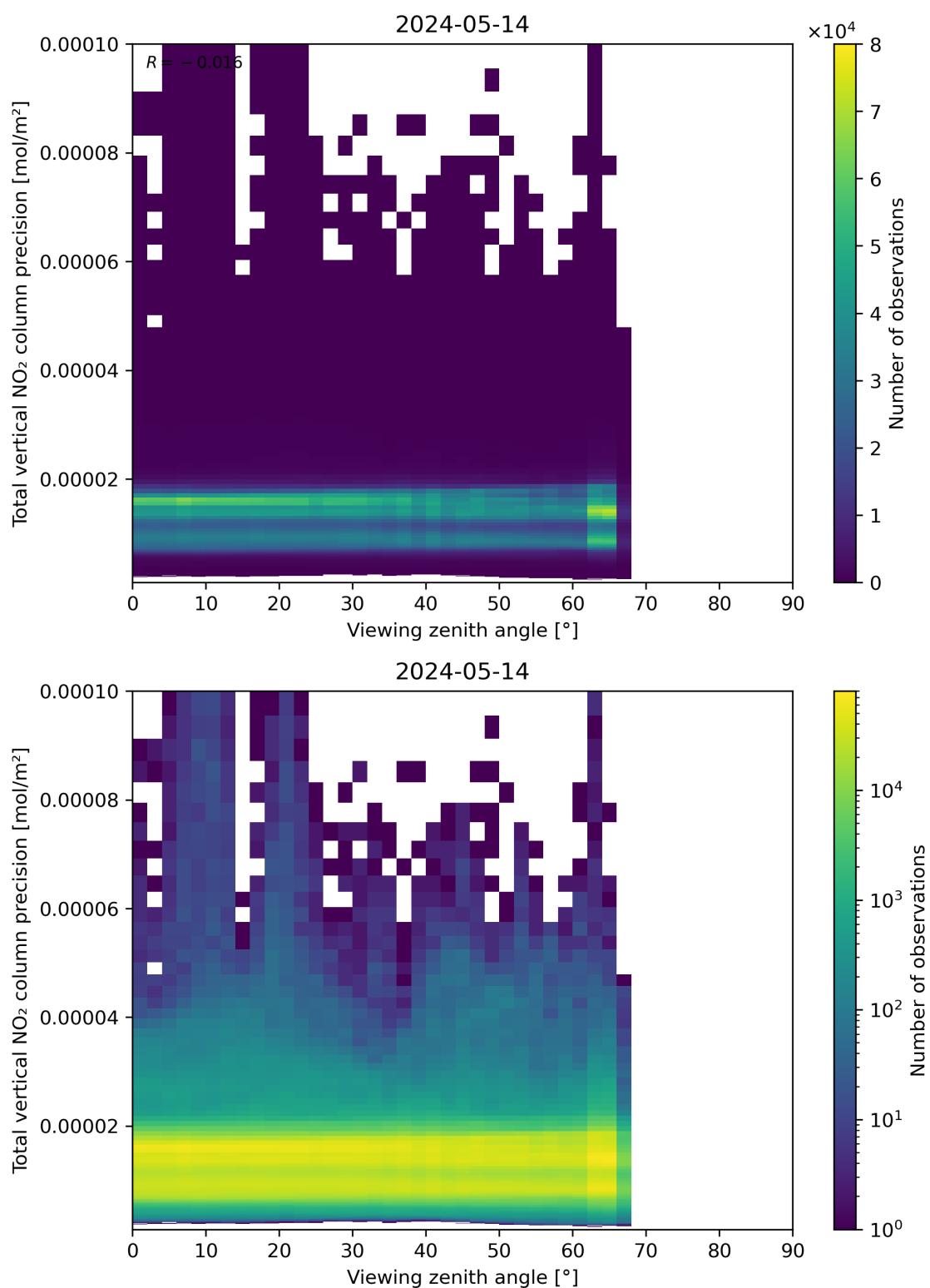
Figure 168: Scatter density plot of “Viewing zenith angle” against “Total vertical NO 2 column precision” for 2024-05-13 to 2024-05-15.
