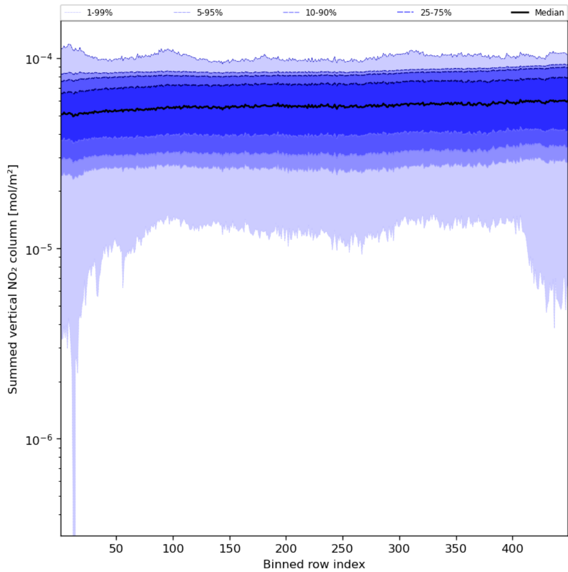
Figure 57: Along track statistics of “Summed vertical NO 2 column” for 2024-05-13 to 2024-05-15
