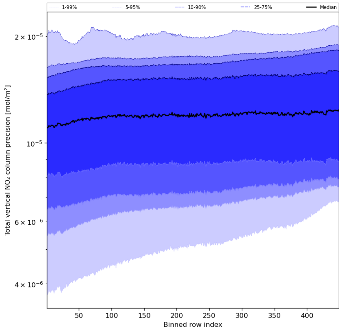
Figure 56: Along track statistics of “Total vertical NO 2 column precision” for 2024-05-13 to 2024-05-15
