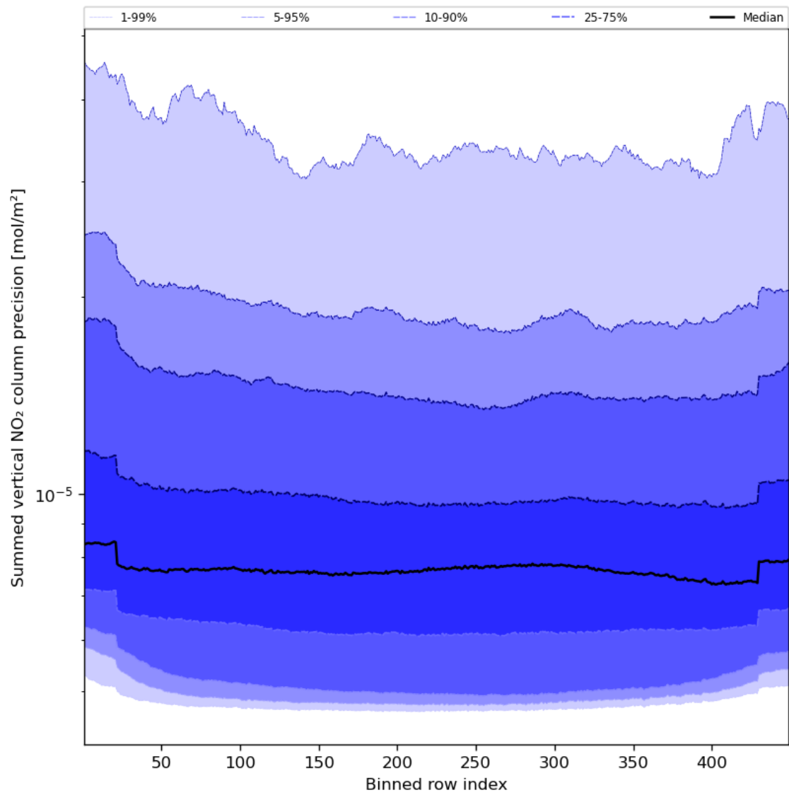
Figure 58: Along track statistics of “Summed vertical NO 2 column precision” for 2024-05-13 to 2024-05-15
