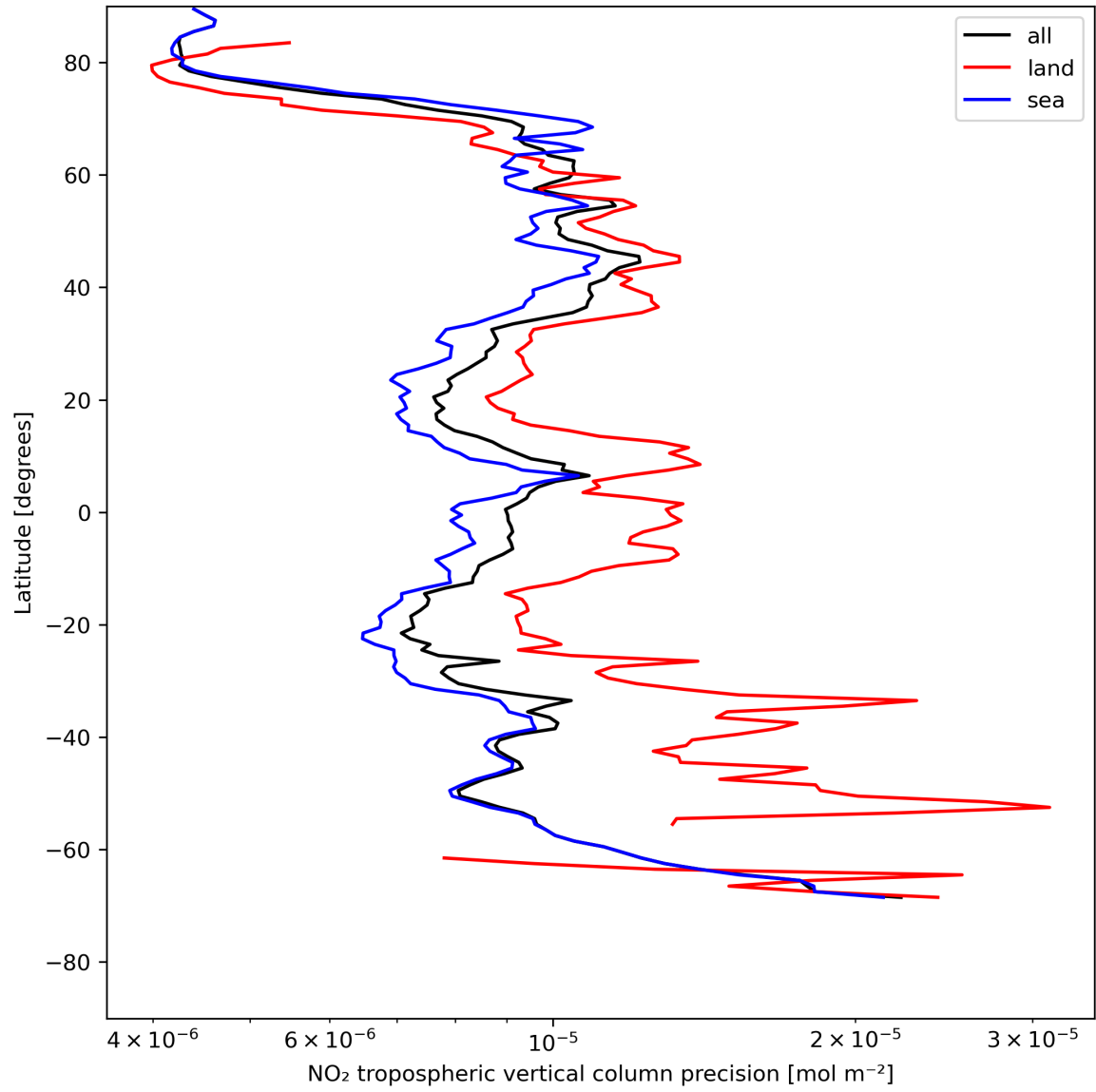
Figure 13: Zonal average of “NO 2 tropospheric vertical column precision” for 2024-05-13 to 2024-05-15.
