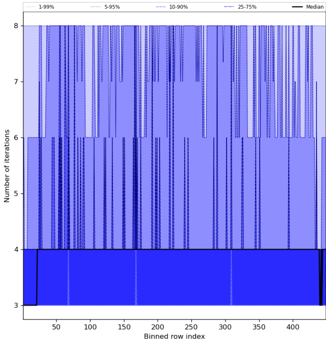
Figure 51: Along track statistics of “Number of iterations” for 2024-05-13 to 2024-05-15
