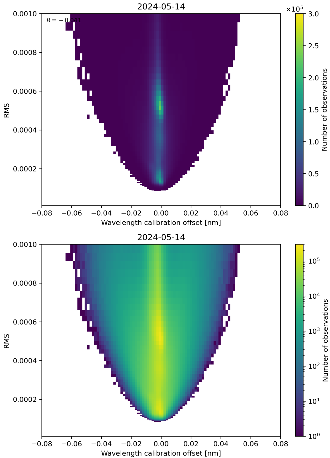
Figure 181: Scatter density plot of “Wavelength calibration offset” against “RMS” for 2024-05-13 to 2024-05-15.
