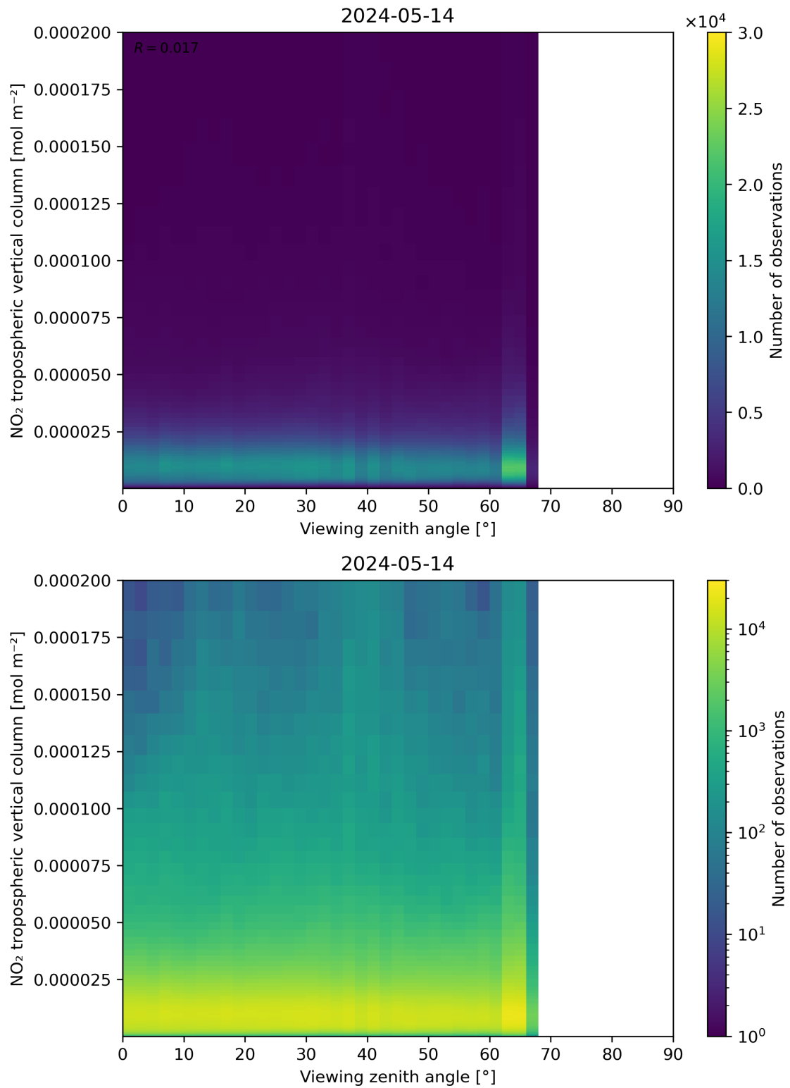
Figure 169: Scatter density plot of “Viewing zenith angle” against “NO 2 tropospheric vertical column” for 2024-05-13 to 2024-05-15.
