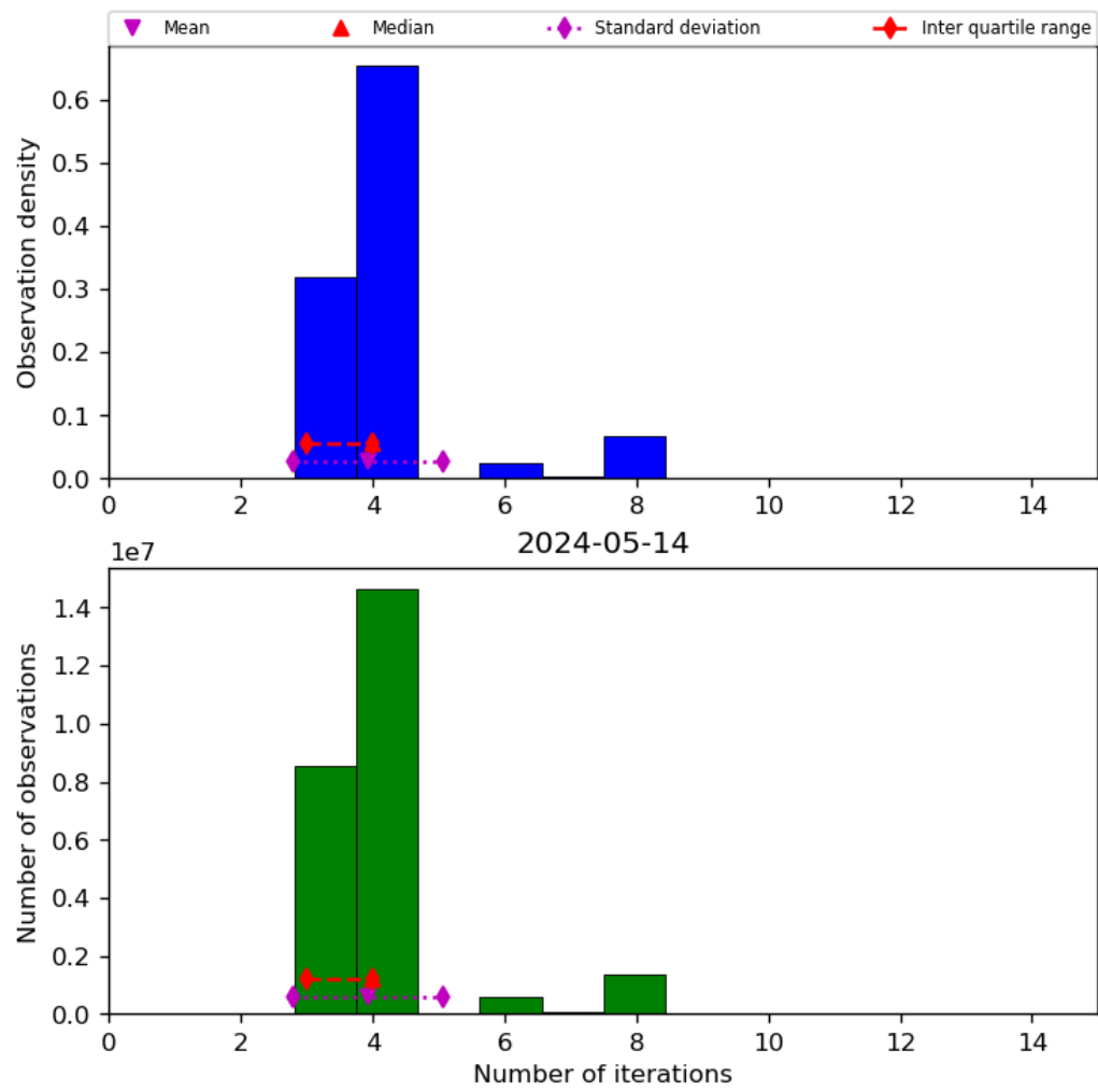
Figure 34: Histogram of “Number of iterations” for 2024-05-13 to 2024-05-15
