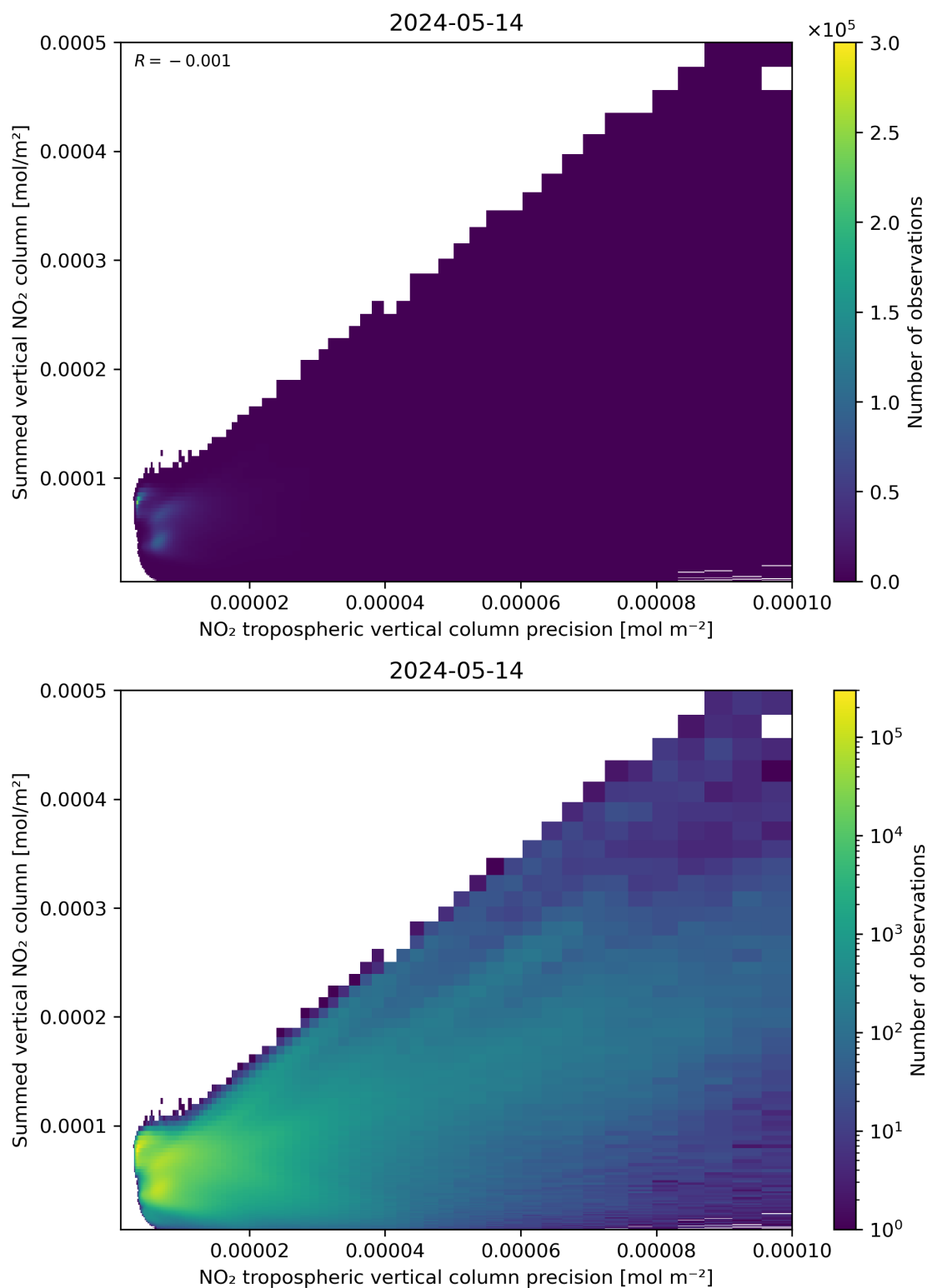
Figure 136: Scatter density plot of “NO 2 tropospheric vertical column precision” against “Summed vertical NO 2 column” for 2024-05-13 to 2024-05-15.
