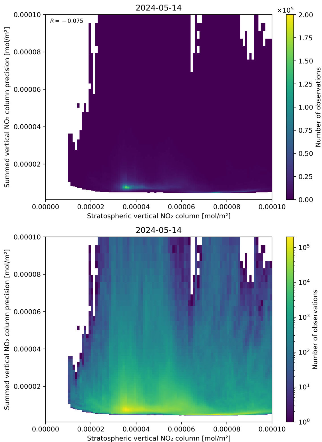
Figure 99: Scatter density plot of “Stratospheric vertical NO 2 column” against “Summed vertical NO 2 column precision” for 2024-05-13 to 2024-05-15.
