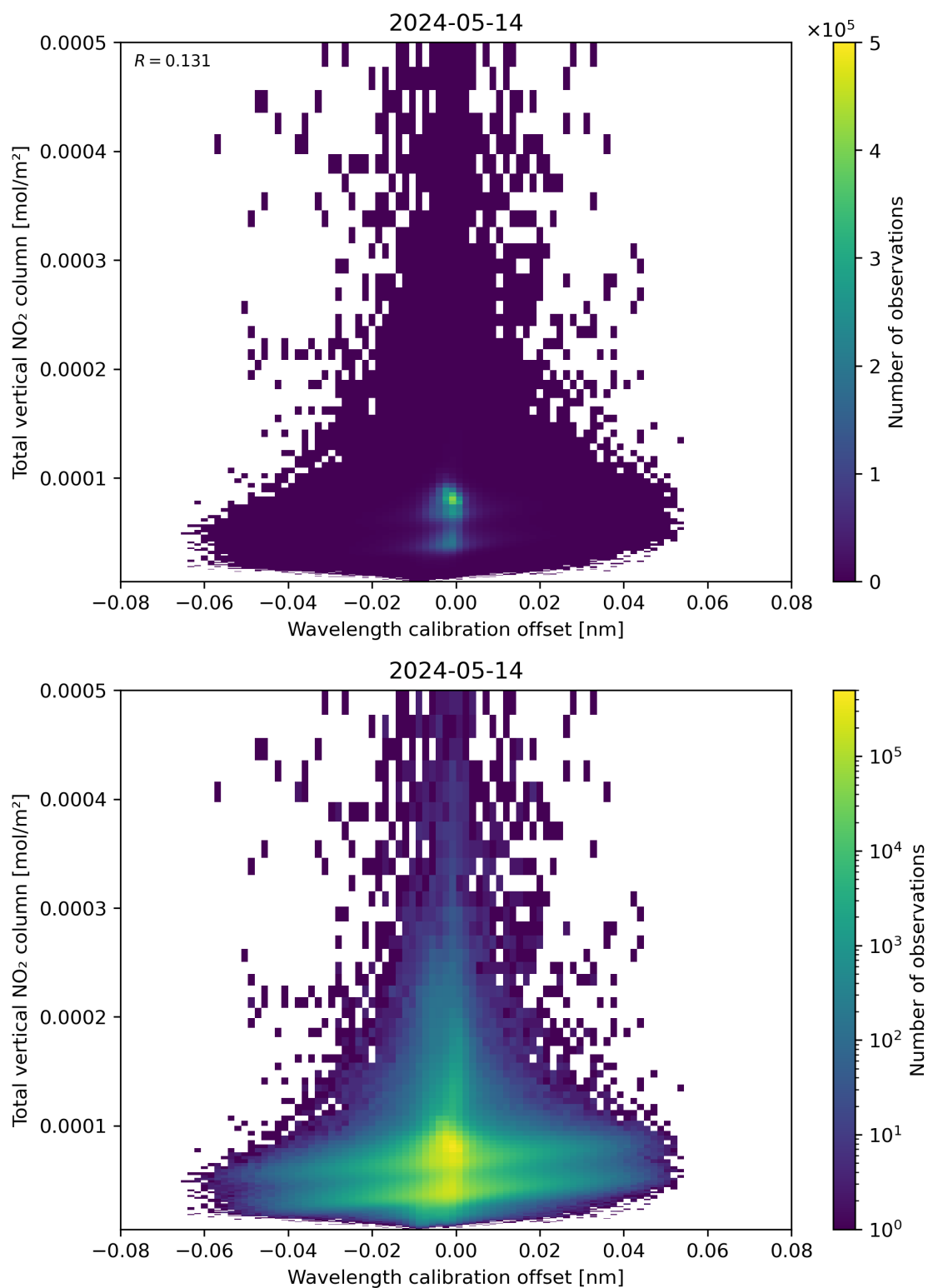
Figure 179: Scatter density plot of “Wavelength calibration offset” against “Total vertical NO 2 column” for 2024-05-13 to 2024-05-15.
