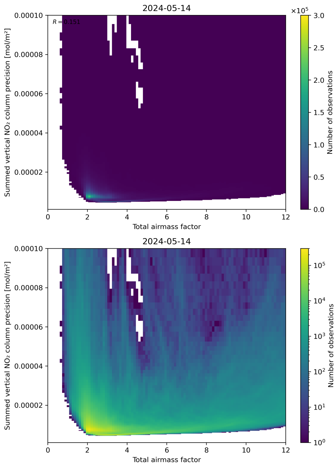
Figure 66: Scatter density plot of “Total airmass factor” against “Summed vertical NO 2 column precision” for 2024-05-13 to 2024-05-15.
