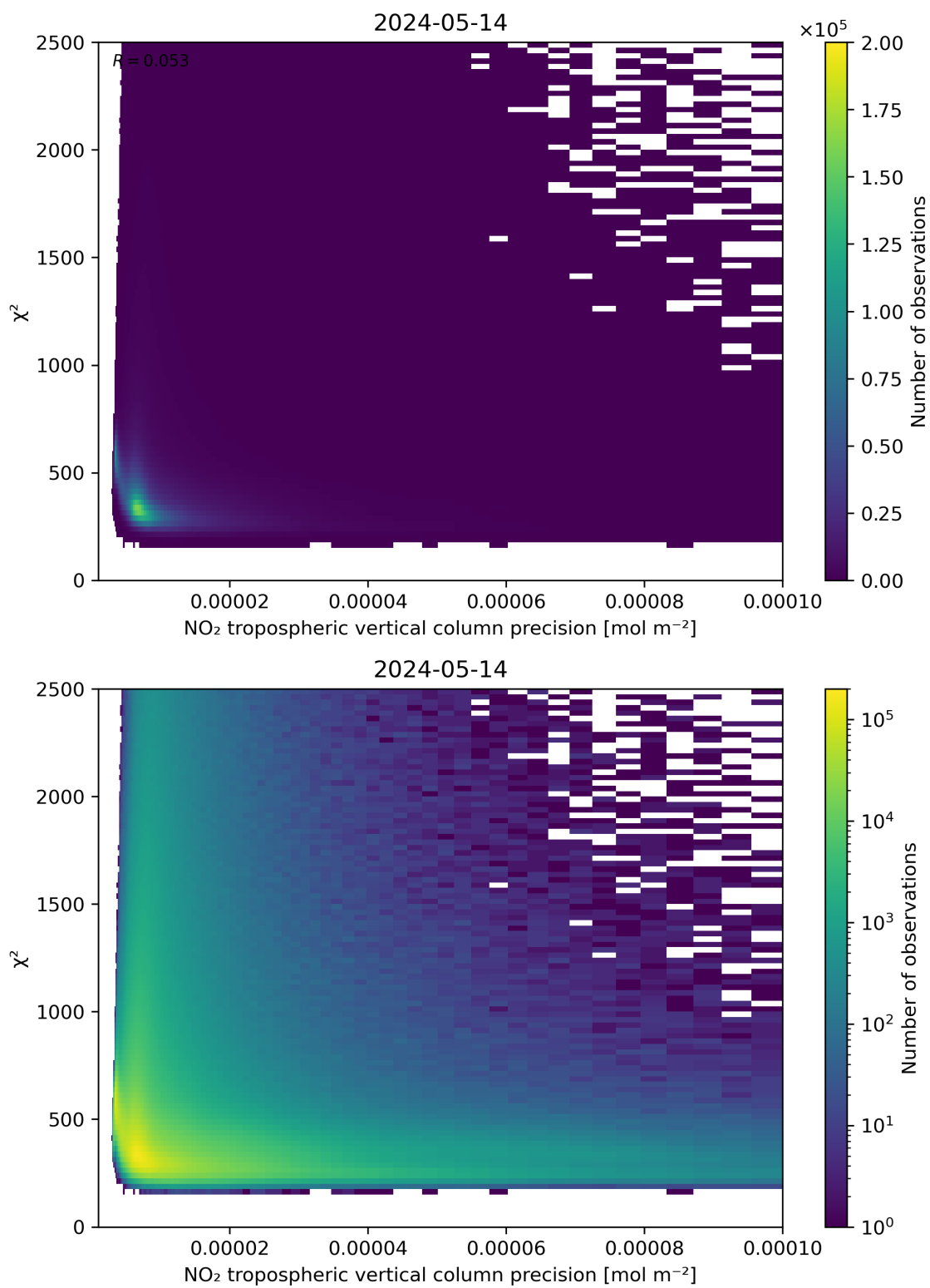
Figure 134: Scatter density plot of “NO 2 tropospheric vertical column precision” against “ \chi^2 ” for 2024-05-13 to 2024-05-15.
