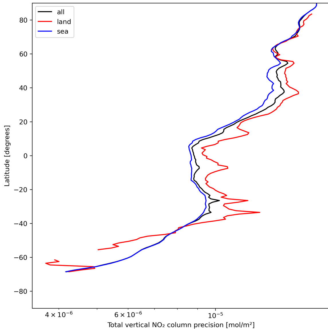
Figure 22: Zonal average of “Total vertical NO 2 column precision” for 2024-05-13 to 2024-05-15.
