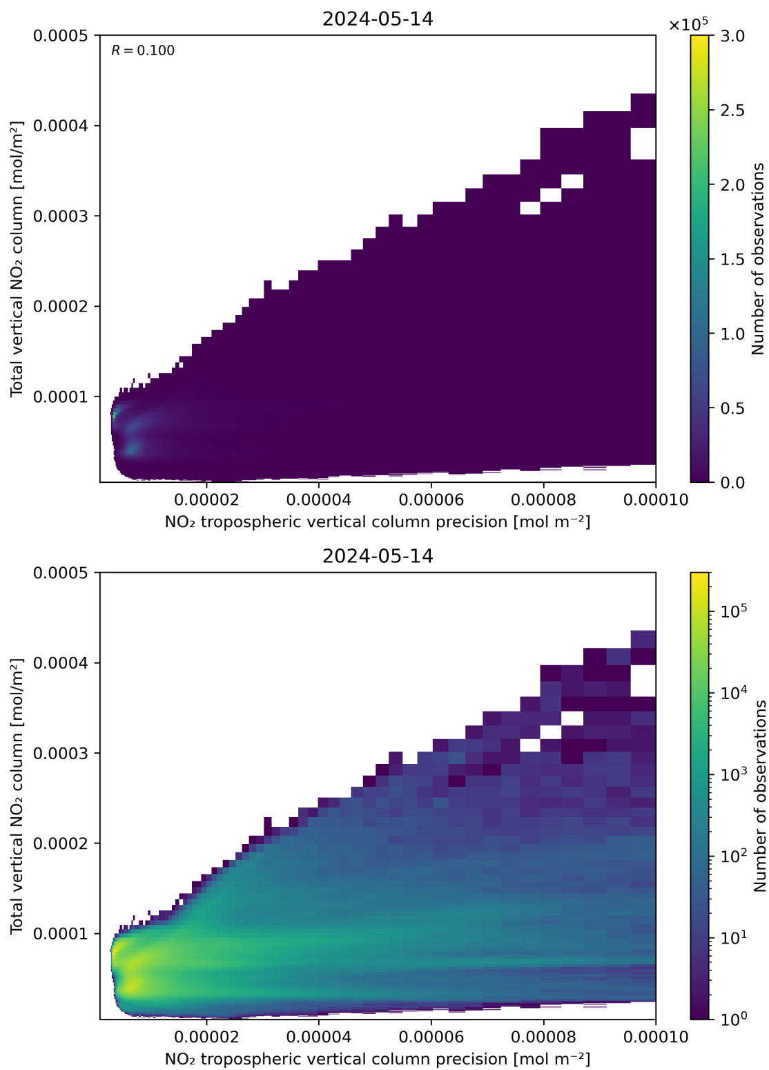
Figure 138: Scatter density plot of “NO 2 tropospheric vertical column precision” against “Total vertical NO 2 column” for 2024-05-13 to 2024-05-15.
