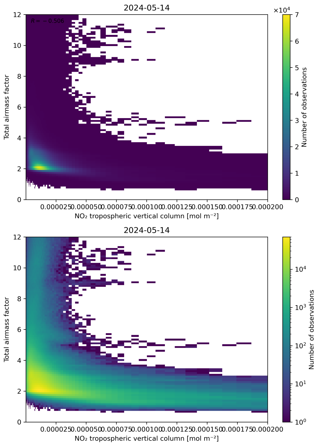
Figure 122: Scatter density plot of “NO 2 tropospheric vertical column” against “Total air mass factor” for 2024-05-13 to 2024-05-15.
