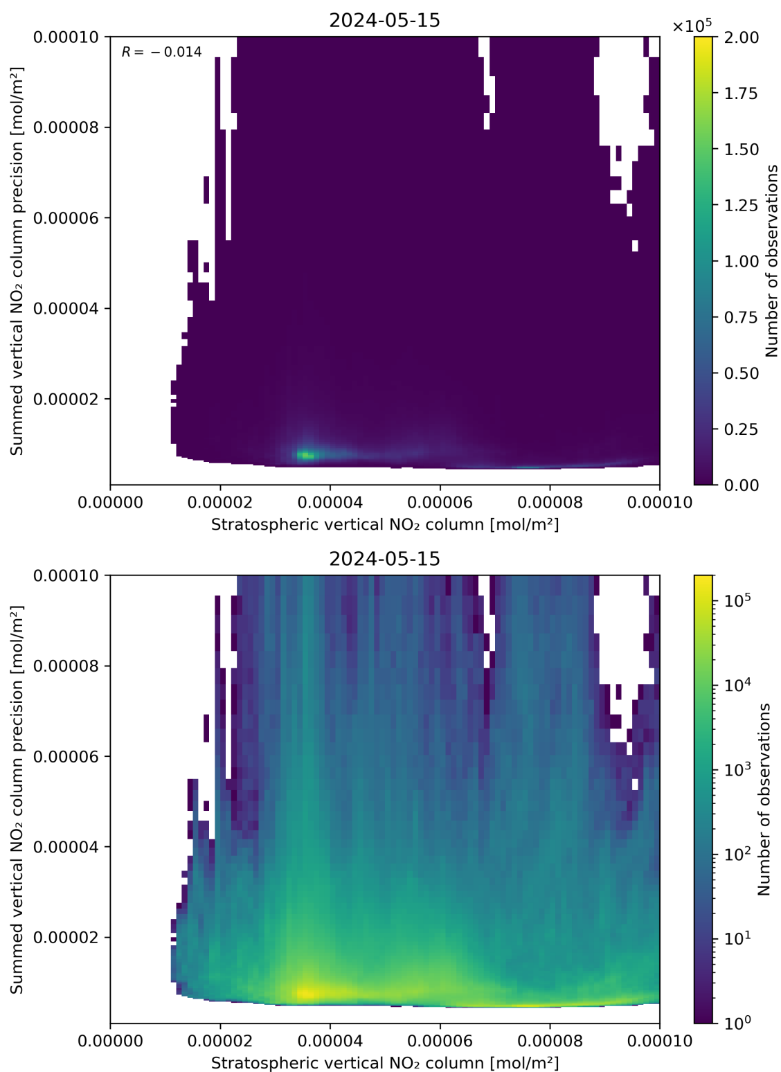
Figure 99: Scatter density plot of “Stratospheric vertical NO 2 column” against “Summed vertical NO 2 column precision” for 2024-05-14 to 2024-05-16.
