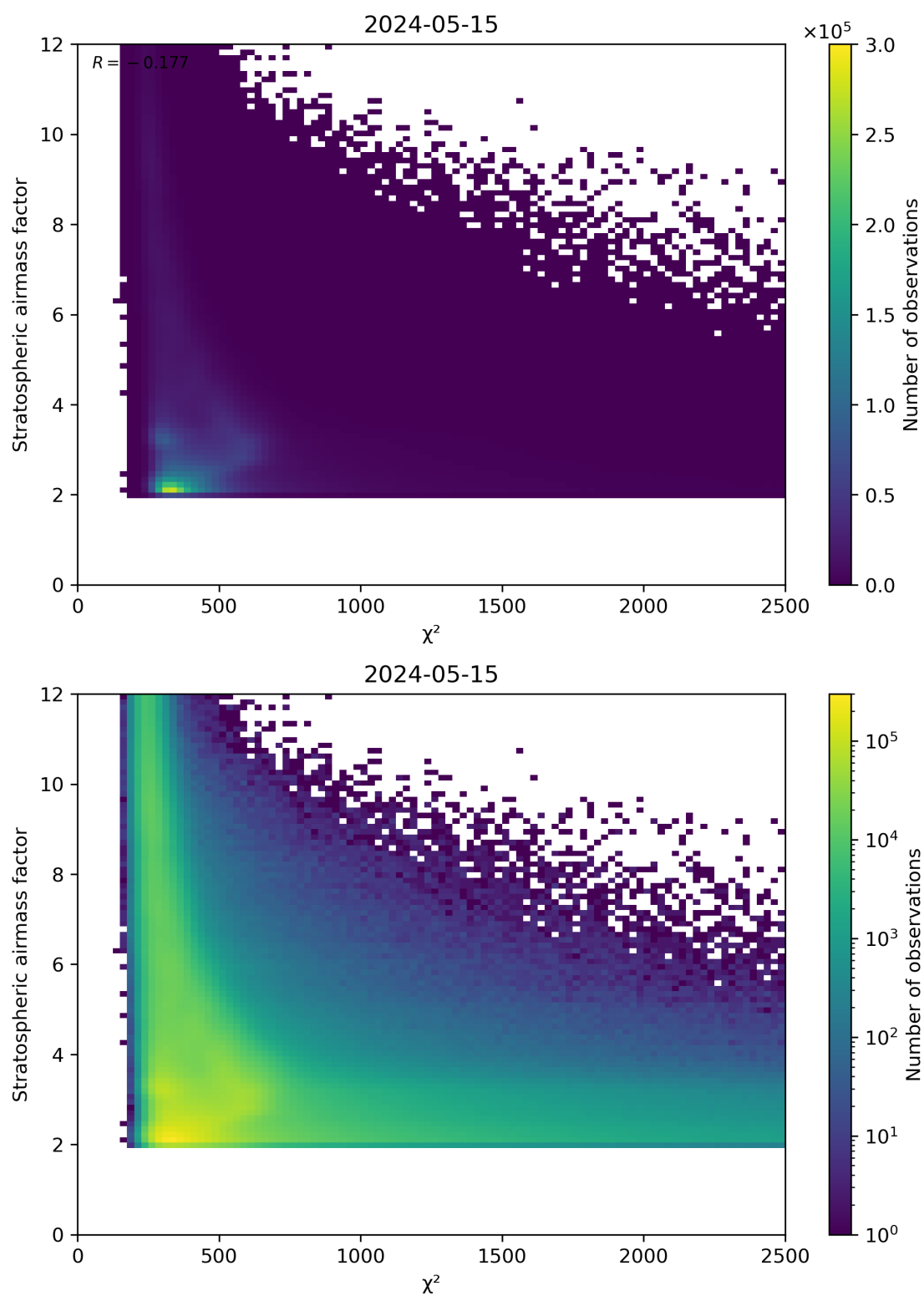
Figure 81: Scatter density plot of “ \chi^2 ” against “Stratospheric airmass factor” for 2024-05-14 to 2024-05-16.
