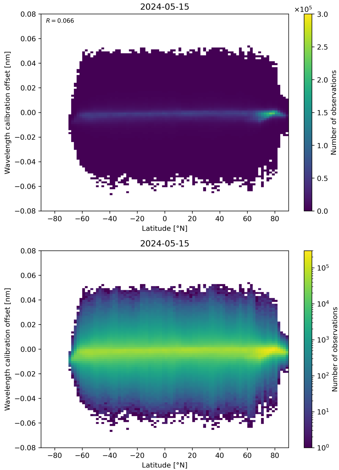
Figure 95: Scatter density plot of “Latitude” against “Wavelength calibration offset” for 2024-05-14 to 2024-05-16.
