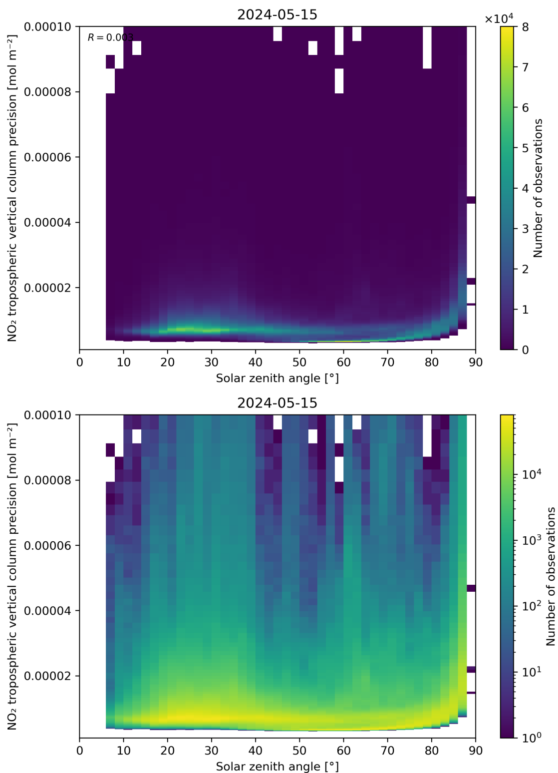
Figure 156: Scatter density plot of “Solar zenith angle” against “NO 2 tropospheric vertical column precision” for 2024-05-14 to 2024-05-16.
