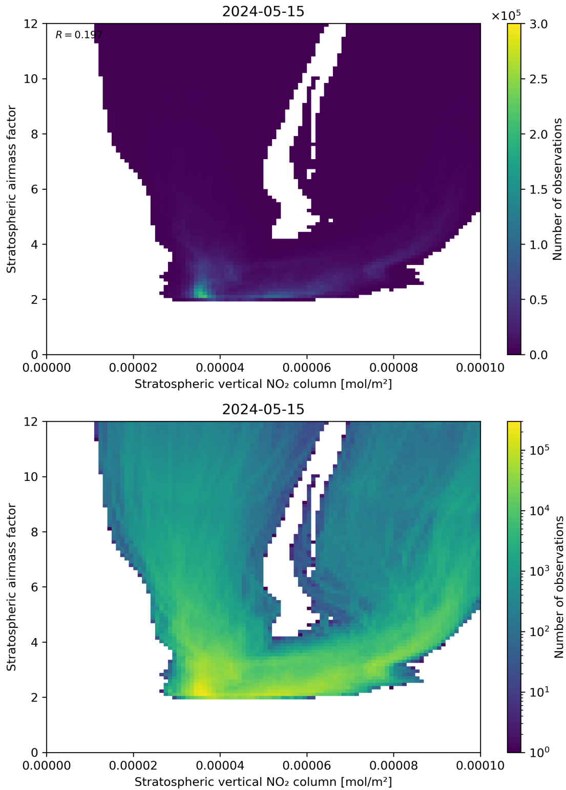
Figure 96: Scatter density plot of “Stratospheric vertical NO 2 column” against “Stratospheric airmass factor” for 2024-05-14 to 2024-05-16.
