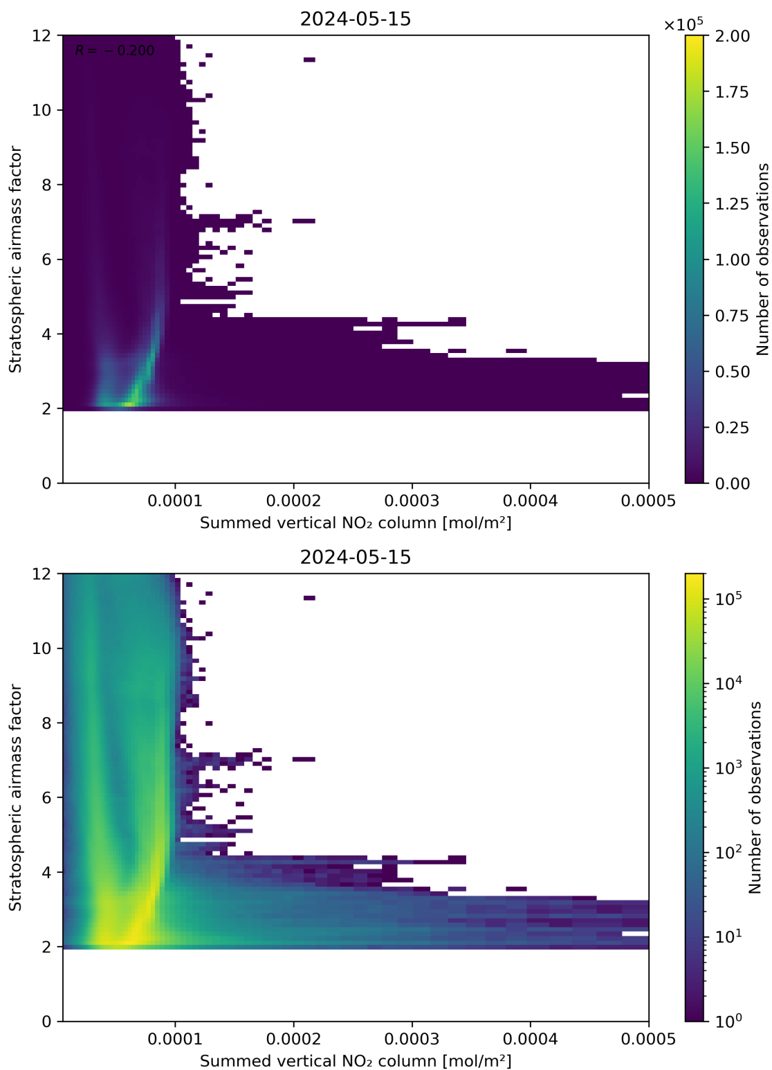
Figure 103: Scatter density plot of “Summed vertical NO 2 column” against “Stratospheric airmass factor” for 2024-05-14 to 2024-05-16.
