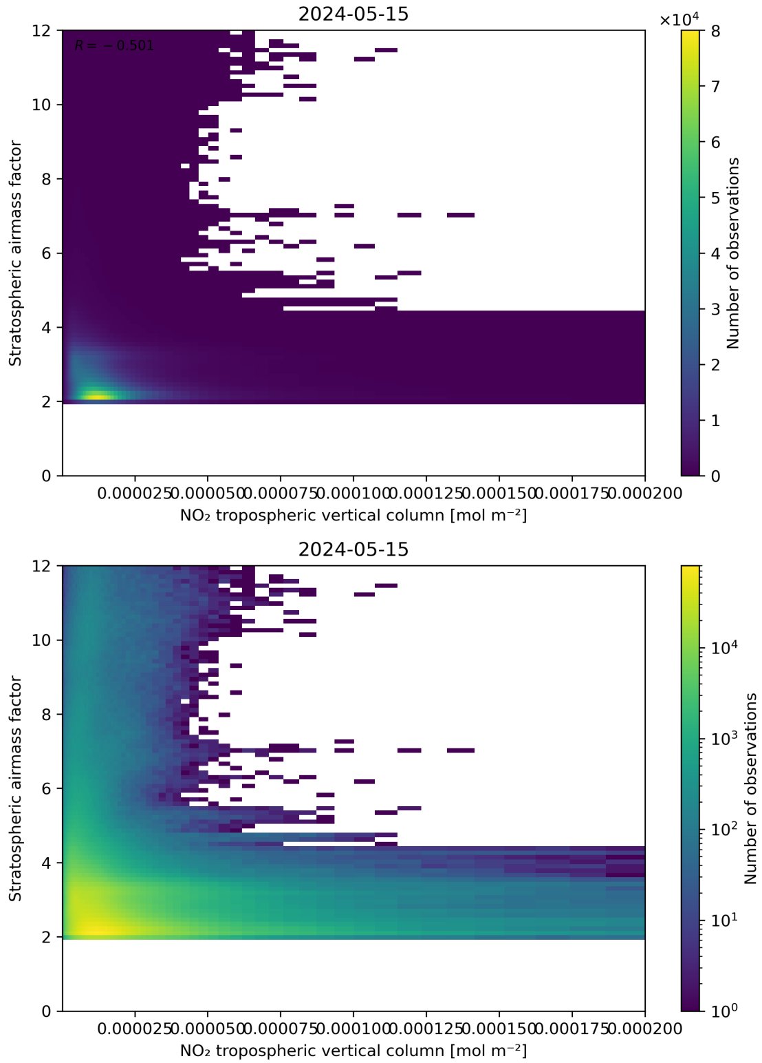
Figure 121: Scatter density plot of “NO 2 tropospheric vertical column” against “Stratospheric air mass factor” for 2024-05-14 to 2024-05-16.
