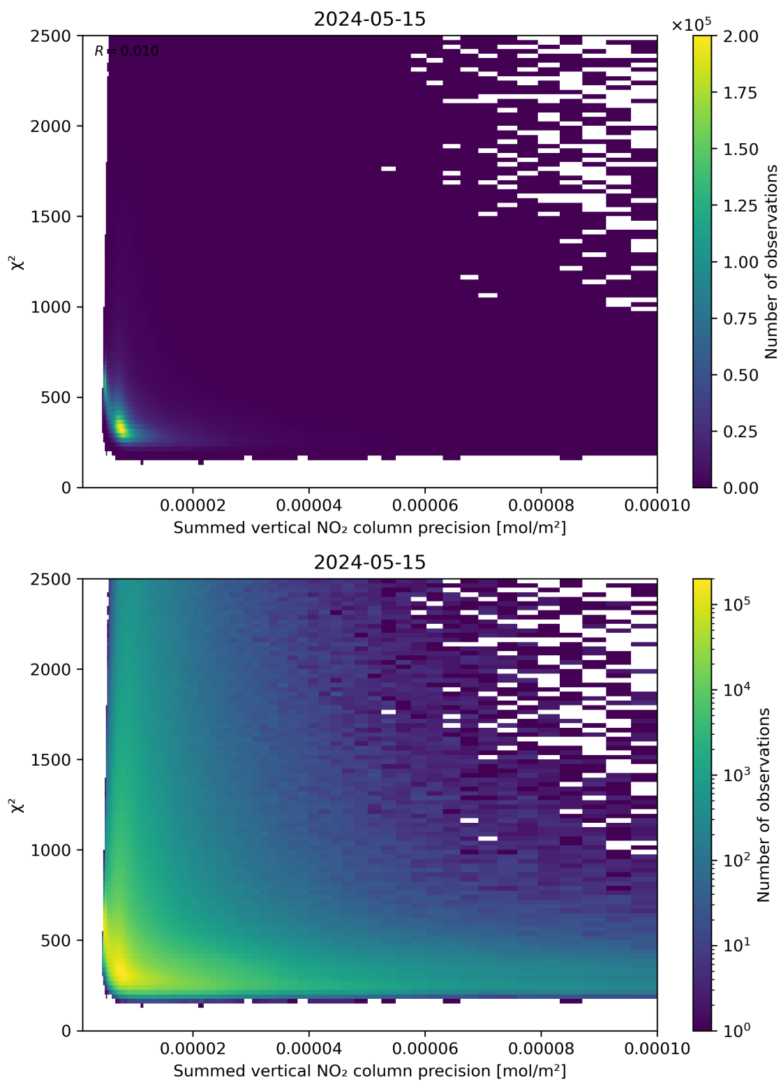
Figure 107: Scatter density plot of “Summed vertical NO 2 column precision” against “ \chi^2 ” for 2024-05-14 to 2024-05-16.
