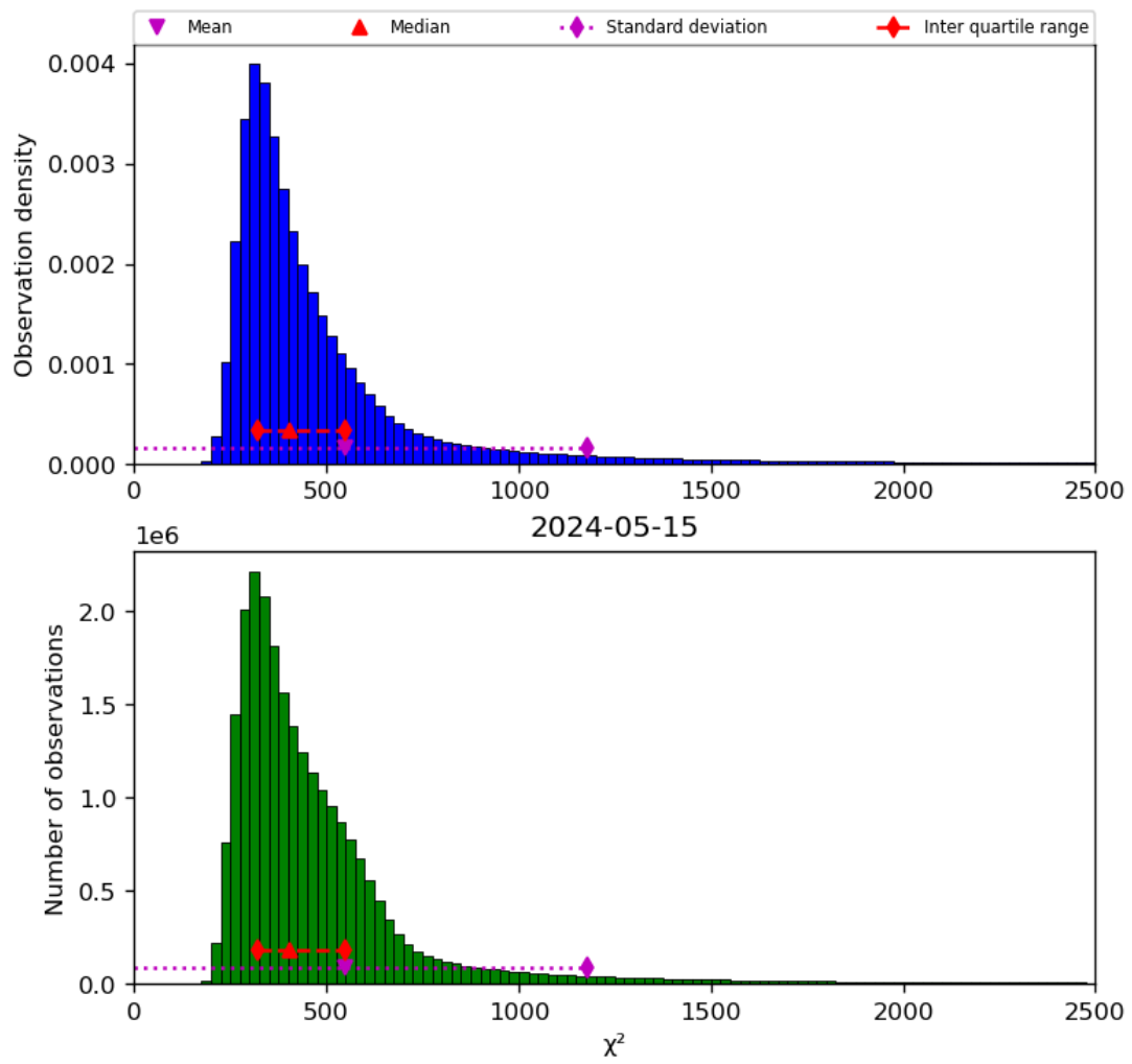
Figure 42: Histogram of “ \chi^2 ” for 2024-05-14 to 2024-05-16
