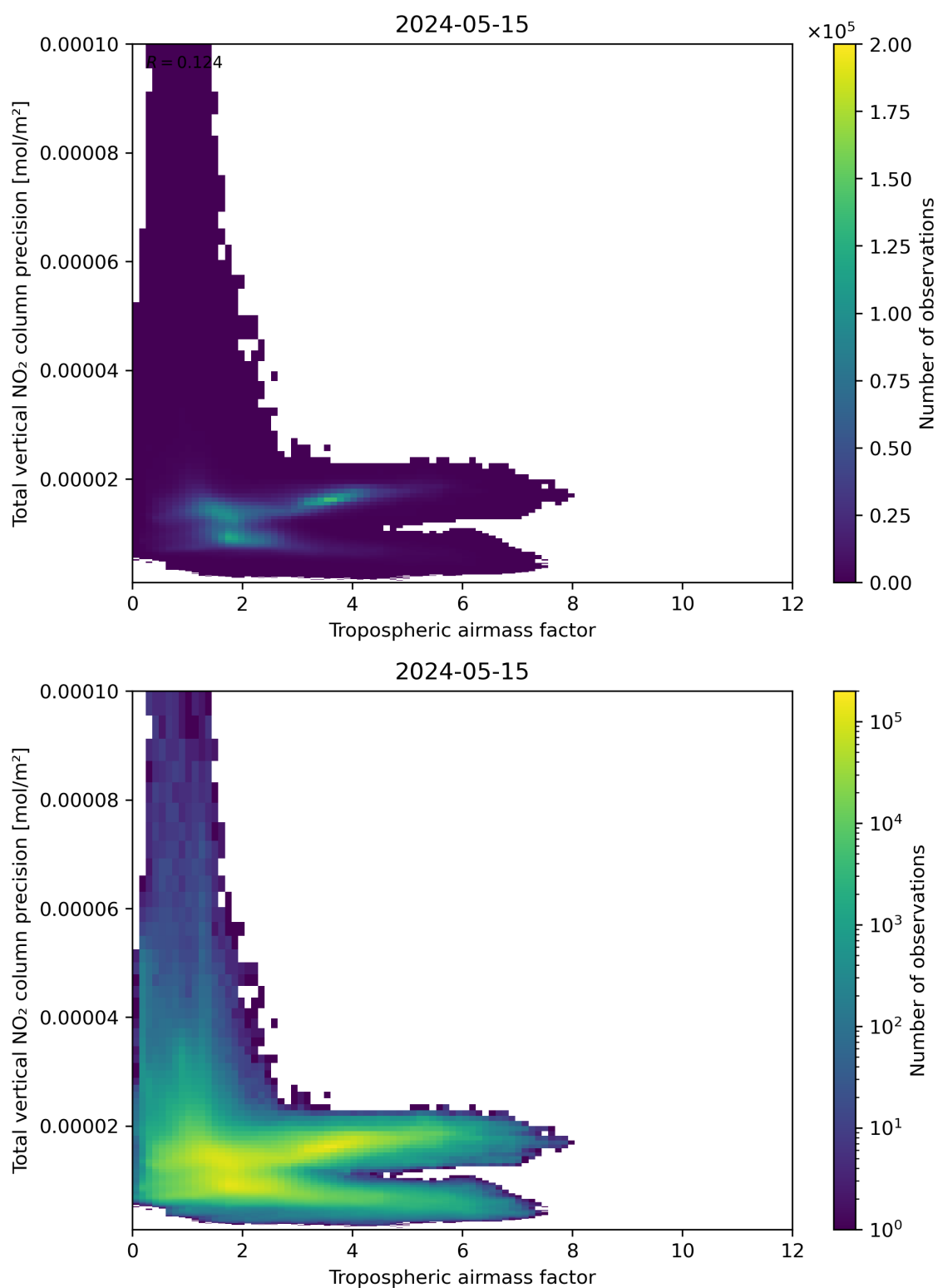
Figure 78: Scatter density plot of “Tropospheric air mass factor” against “Total vertical NO 2 column precision” for 2024-05-14 to 2024-05-16.
