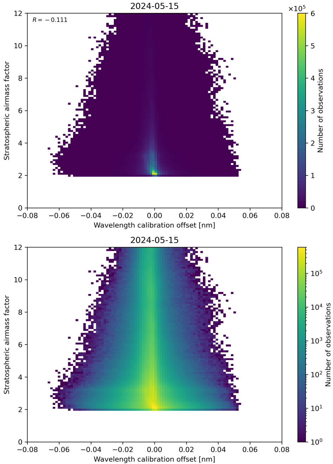
Figure 174: Scatter density plot of “Wavelength calibration offset” against “Stratospheric airmass factor” for 2024-05-14 to 2024-05-16.
