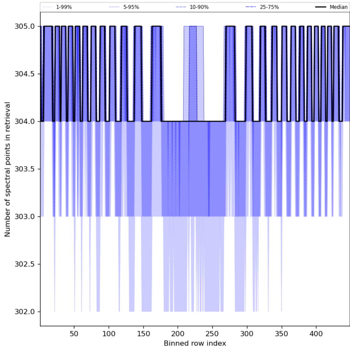
Figure 50: Along track statistics of “Number of spectral points in retrieval” for 2024-05-14 to 2024-05-16
