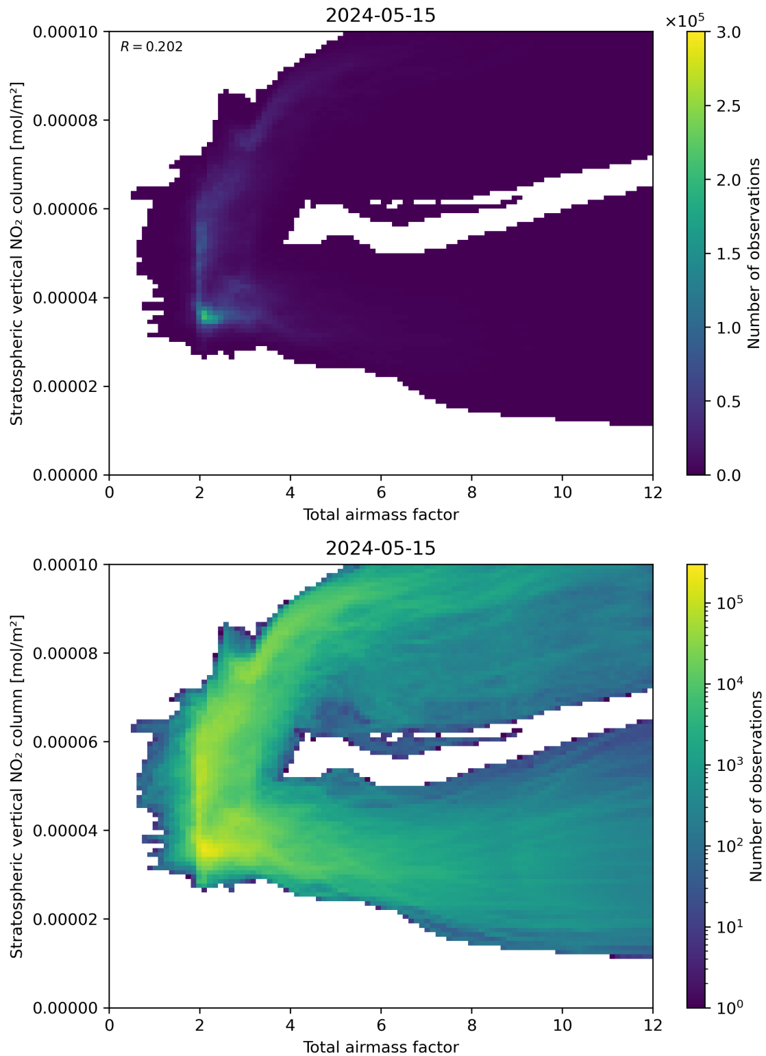
Figure 64: Scatter density plot of “Total airmass factor” against “Stratospheric vertical \text{NO}_2 column” for 2024-05-14 to 2024-05-16.
