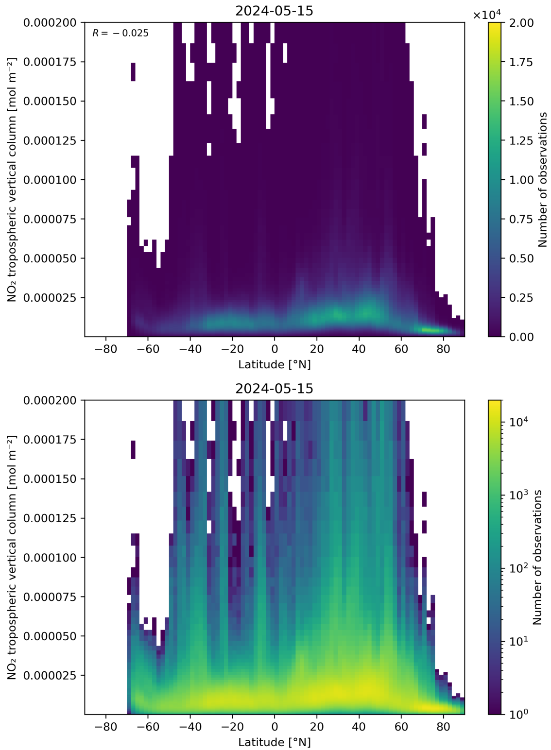
Figure 92: Scatter density plot of “Latitude” against “NO 2 tropospheric vertical column” for 2024-05-14 to 2024-05-16.
