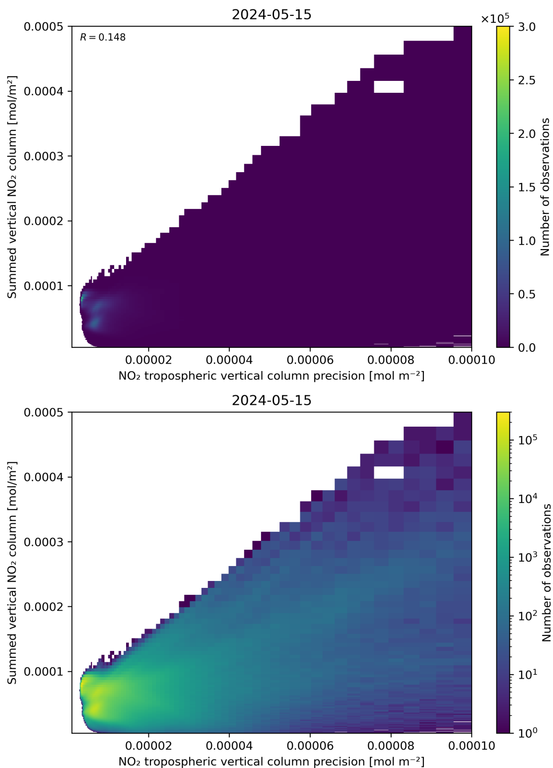
Figure 136: Scatter density plot of “NO 2 tropospheric vertical column precision” against “Summed vertical NO 2 column” for 2024-05-14 to 2024-05-16.
