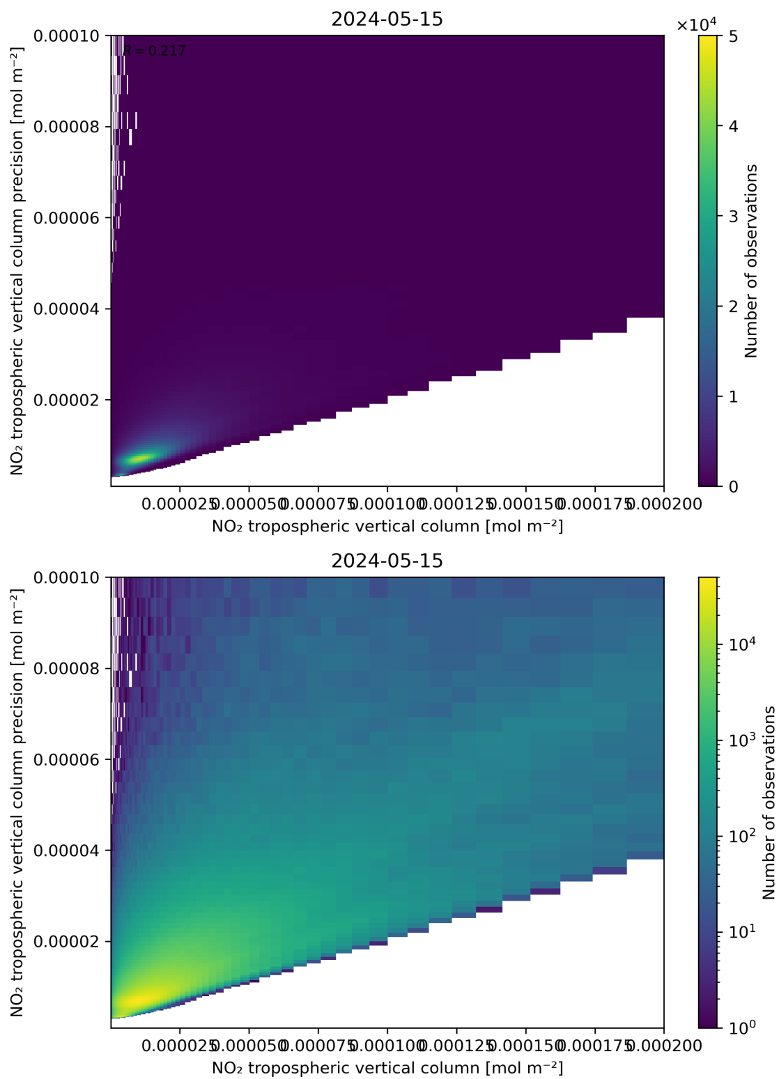
Figure 130: Scatter density plot of “NO 2 tropospheric vertical column” against “NO 2 tropospheric vertical column precision” for 2024-05-14 to 2024-05-16.
