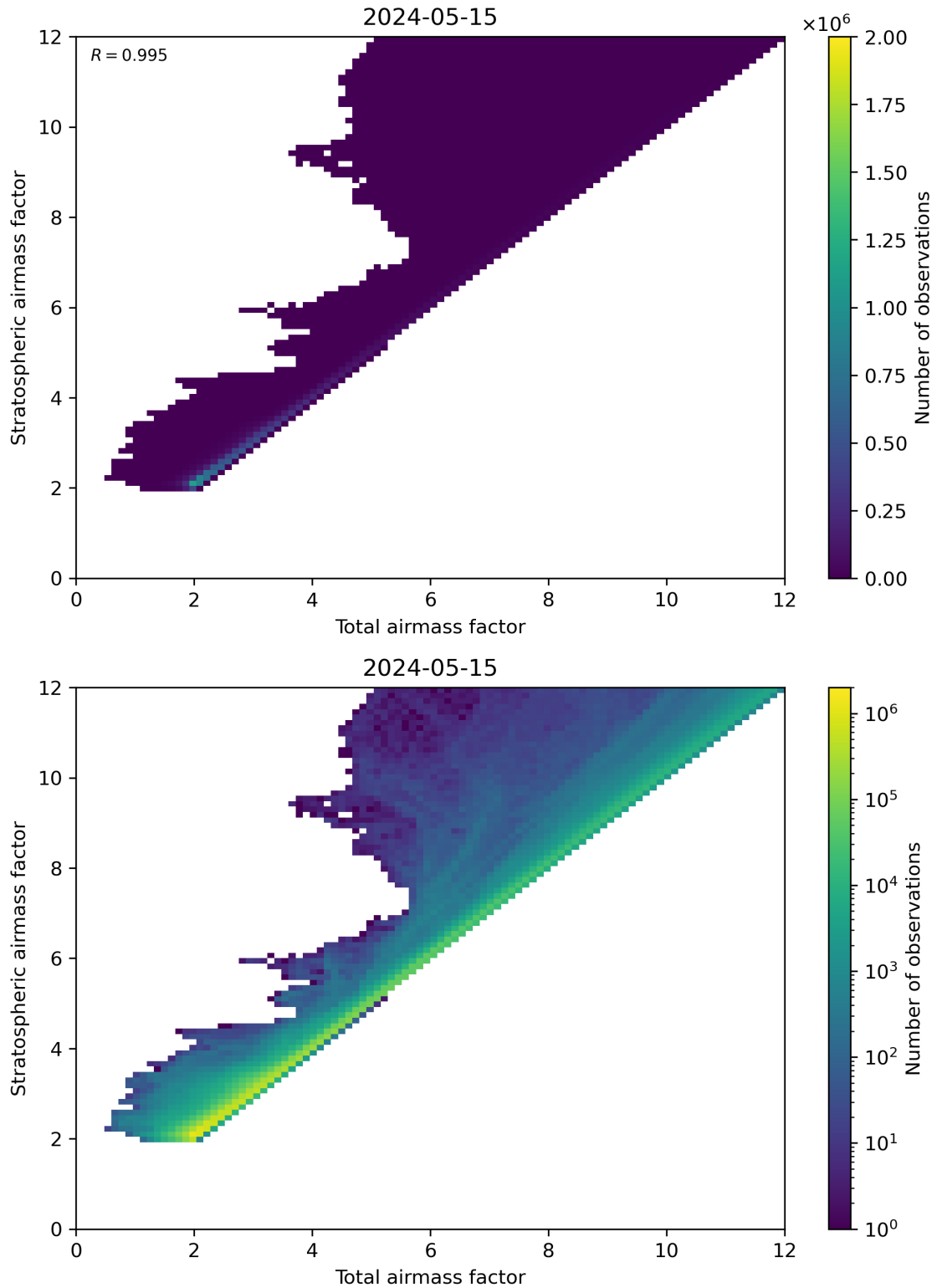
Figure 62: Scatter density plot of “Total airmass factor” against “Stratospheric airmass factor” for 2024-05-14 to 2024-05-16.
