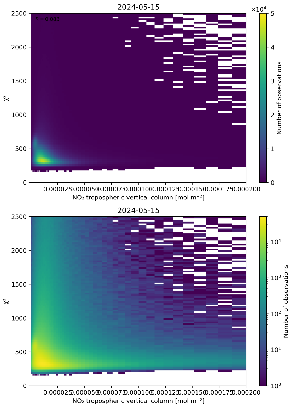
Figure 124: Scatter density plot of “NO 2 tropospheric vertical column” against “ \chi^2 ” for 2024-05-14 to 2024-05-16.
