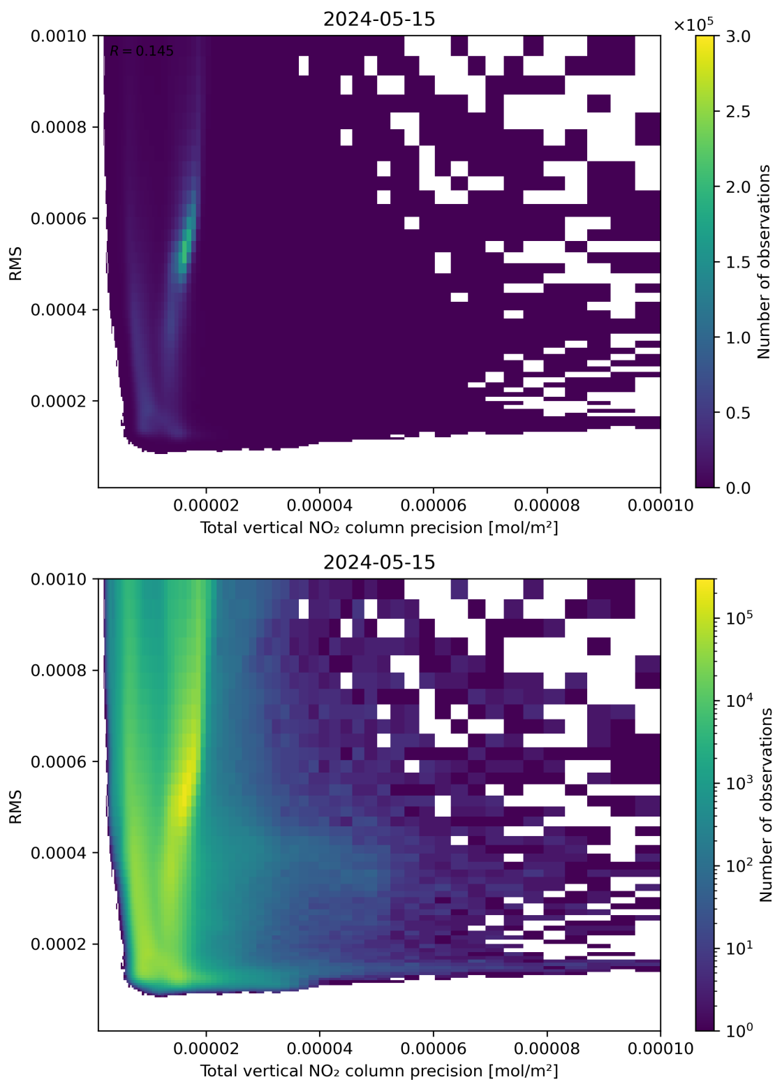
Figure 119: Scatter density plot of “Total vertical NO 2 column precision” against “RMS” for 2024-05-14 to 2024-05-16.
