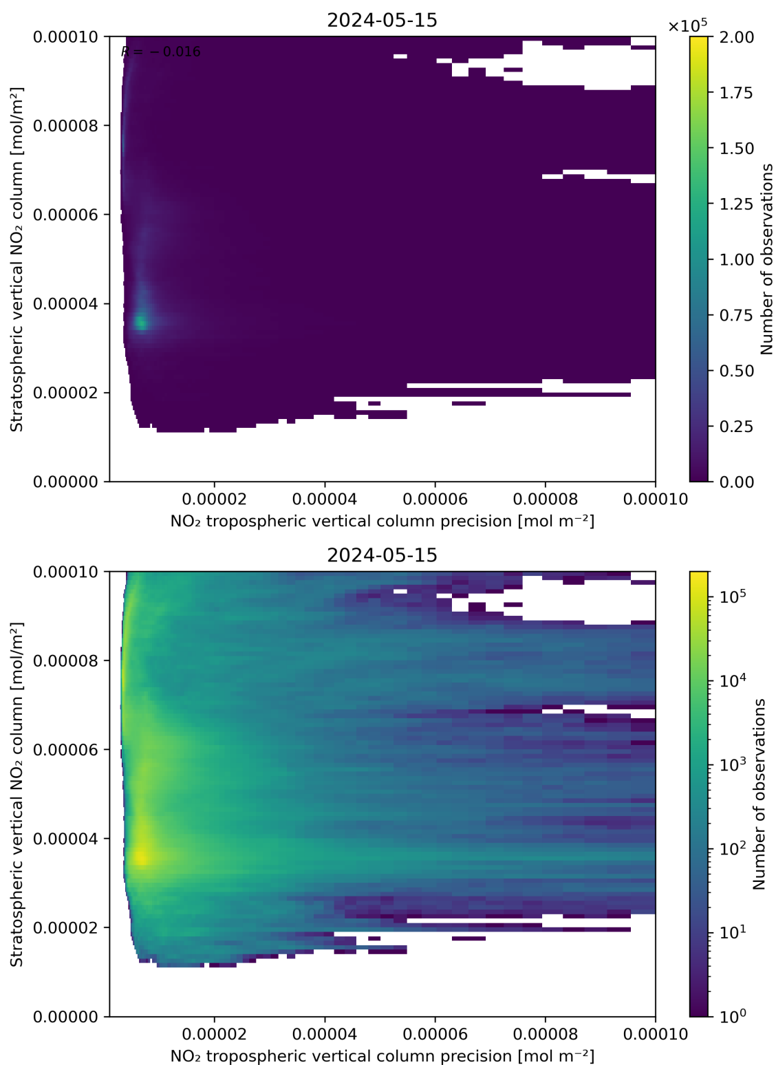
Figure 135: Scatter density plot of “NO 2 tropospheric vertical column precision” against “Stratospheric vertical NO 2 column” for 2024-05-14 to 2024-05-16.
