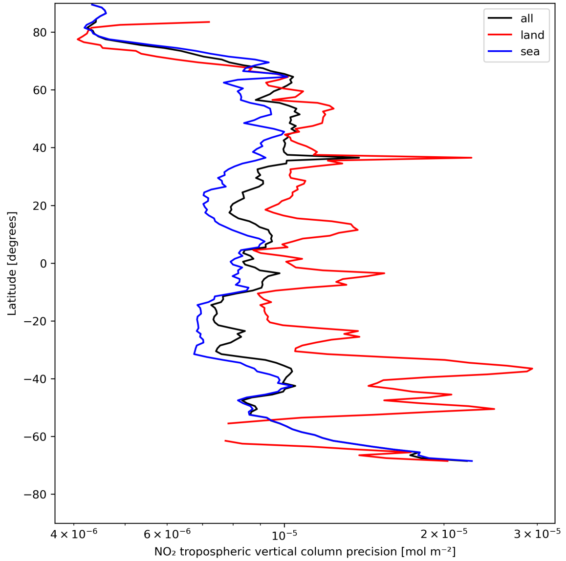
Figure 13: Zonal average of “NO 2 tropospheric vertical column precision” for 2024-05-14 to 2024-05-16.
