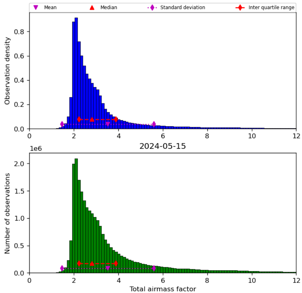
Figure 32: Histogram of “Total airmass factor” for 2024-05-14 to 2024-05-16
