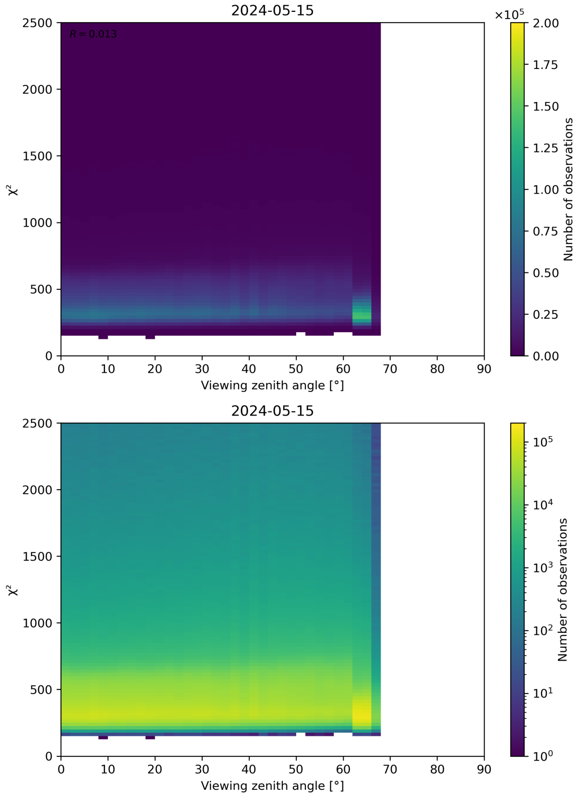
Figure 162: Scatter density plot of “Viewing zenith angle” against “ \chi^2 ” for 2024-05-14 to 2024-05-16.
