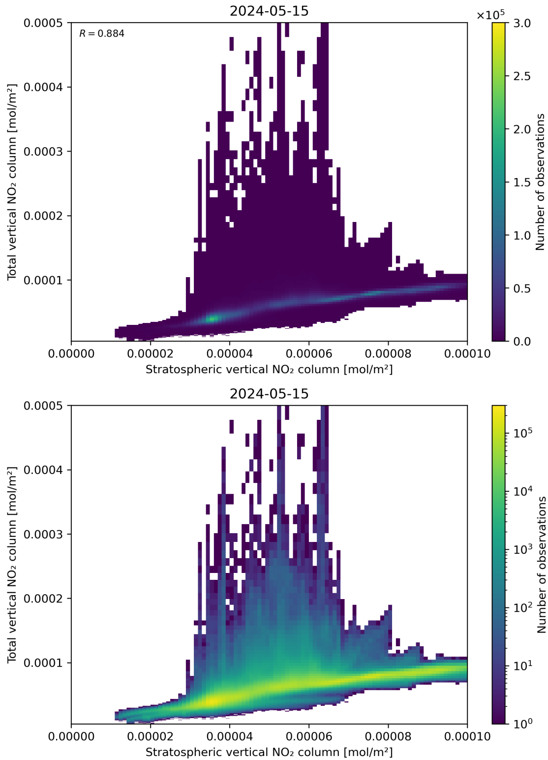
Figure 100: Scatter density plot of “Stratospheric vertical NO 2 column” against “Total vertical NO 2 column” for 2024-05-14 to 2024-05-16.
