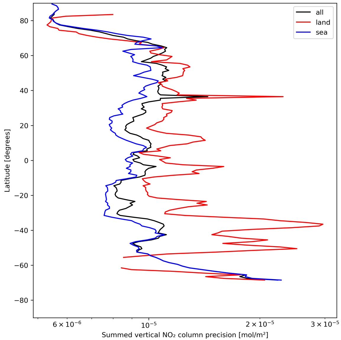
Figure 24: Zonal average of “Summed vertical NO 2 column precision” for 2024-05-14 to 2024-05-16.
