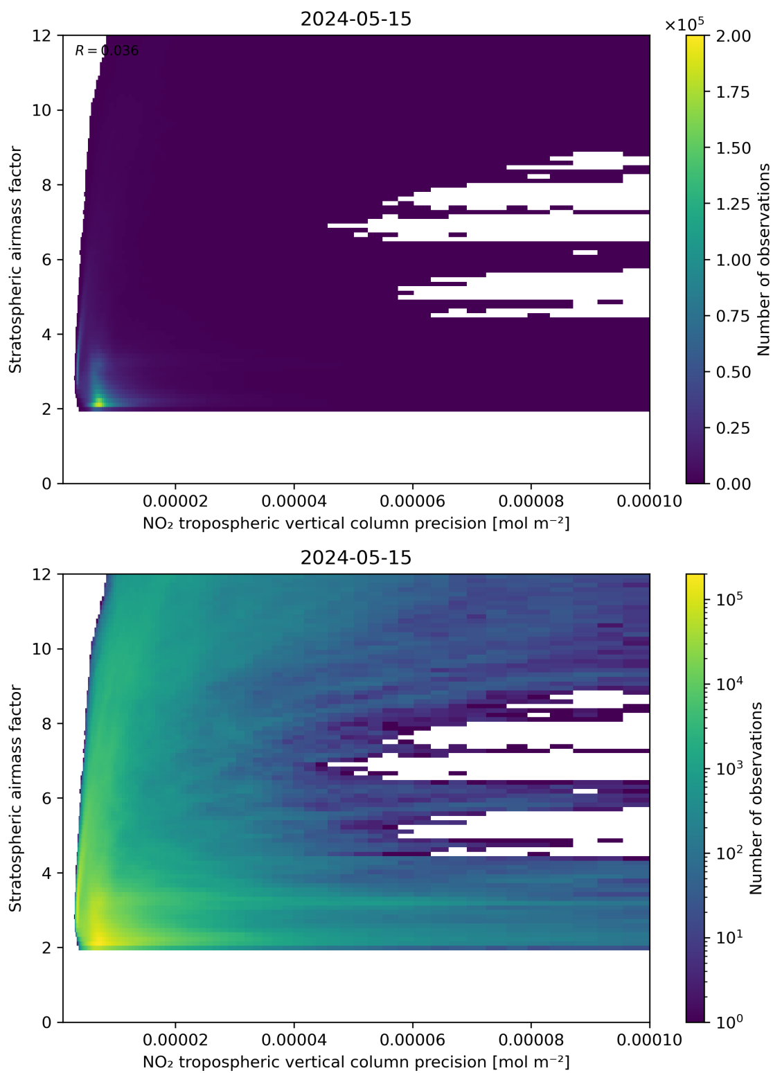
Figure 131: Scatter density plot of “NO 2 tropospheric vertical column precision” against “Stratospheric airmass factor” for 2024-05-14 to 2024-05-16.
