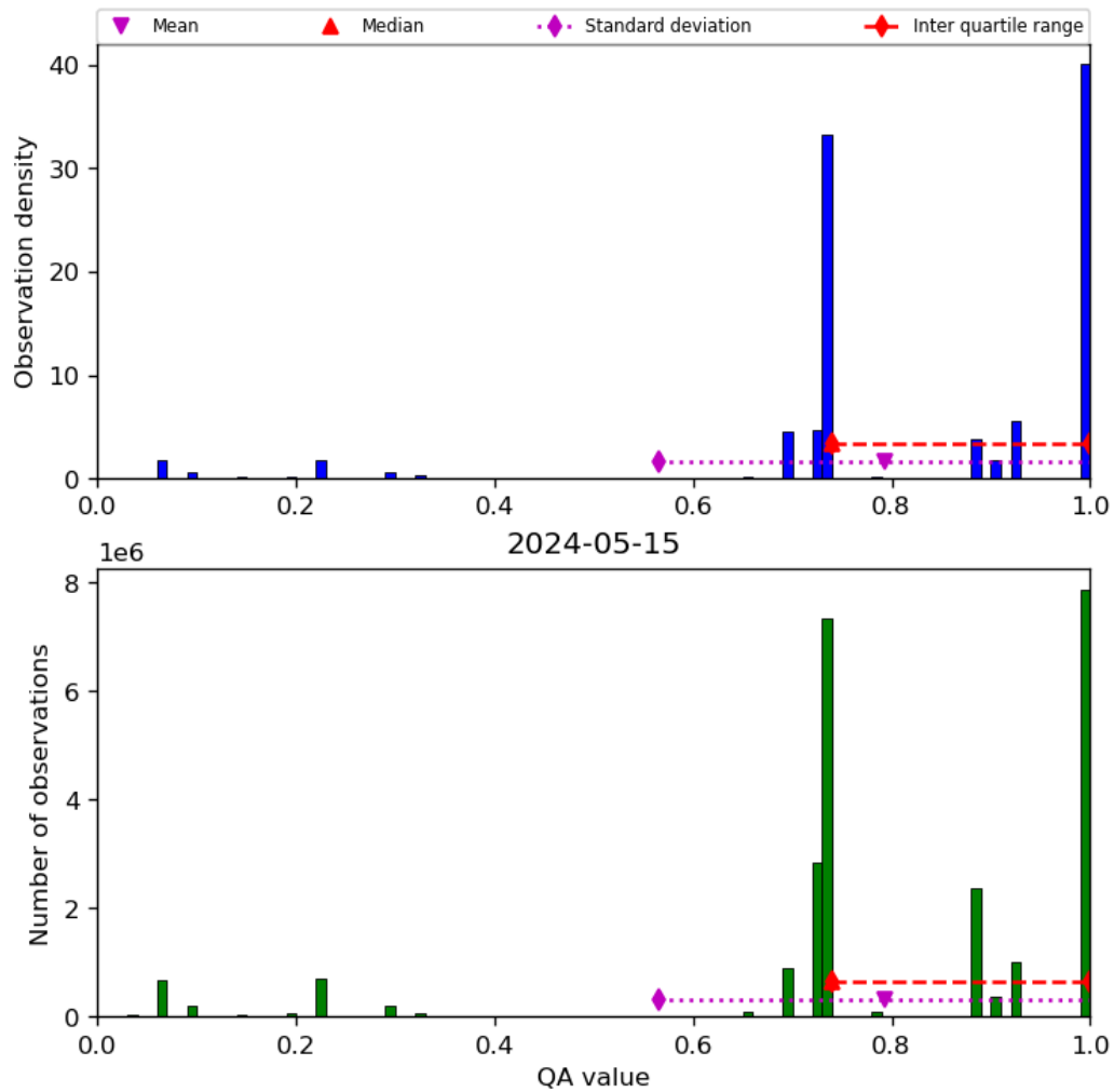
Figure 28: Histogram of “QA value” for 2024-05-14 to 2024-05-16
