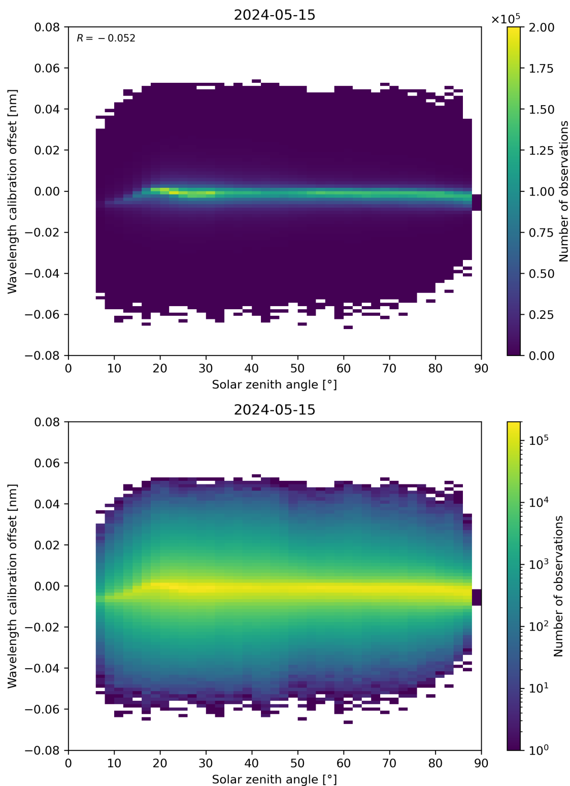
Figure 158: Scatter density plot of “Solar zenith angle” against “Wavelength calibration offset” for 2024-05-14 to 2024-05-16.
