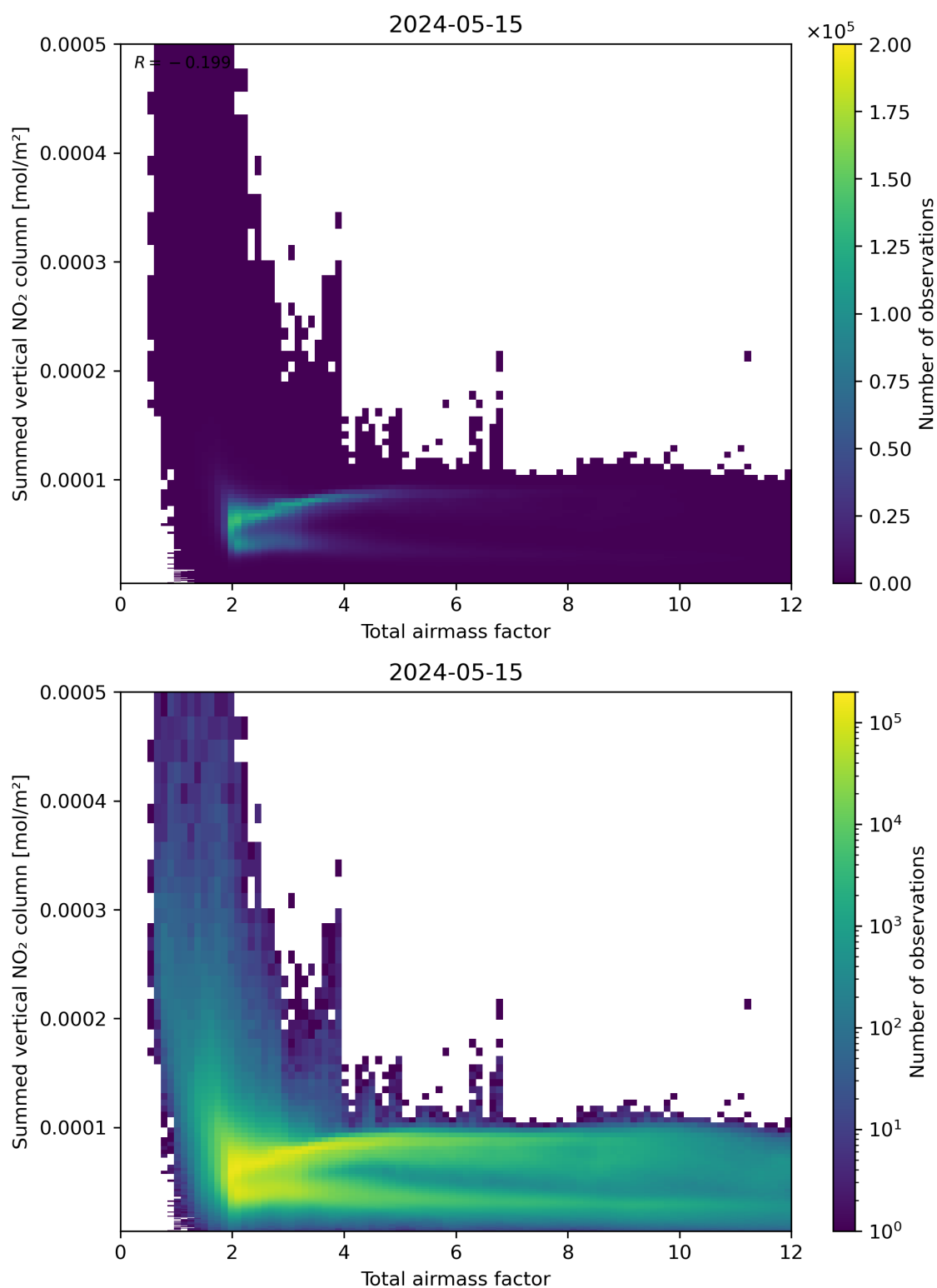
Figure 65: Scatter density plot of “Total airmass factor” against “Summed vertical NO 2 column” for 2024-05-14 to 2024-05-16.
