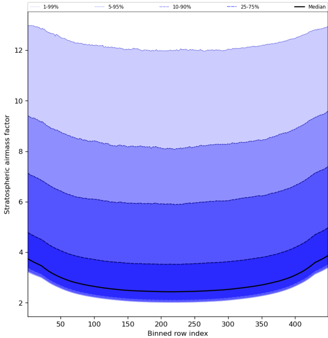
Figure 61: Along track statistics of “Stratospheric airmass factor” for 2024-05-14 to 2024-05-16
