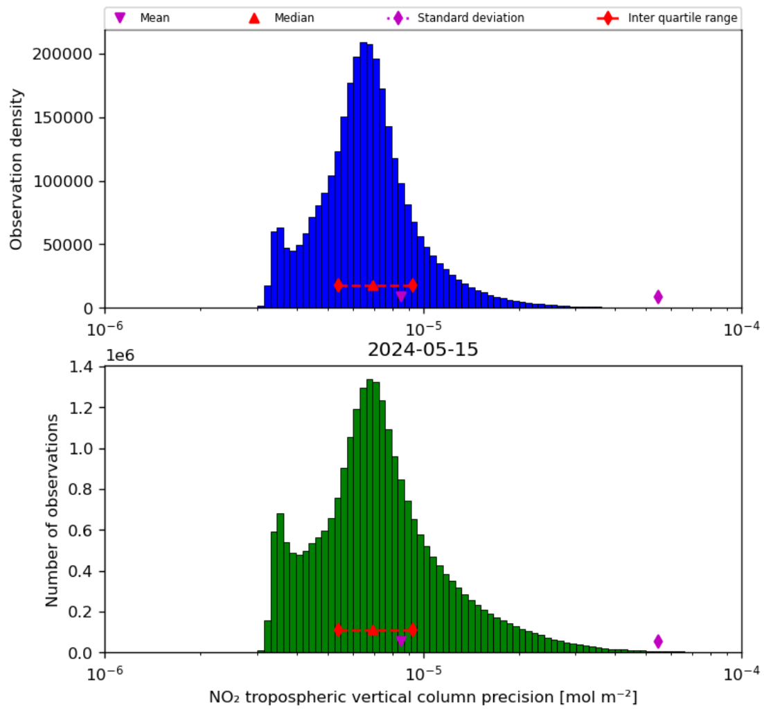
Figure 30: Histogram of “NO 2 tropospheric vertical column precision” for 2024-05-14 to 2024-05-16
