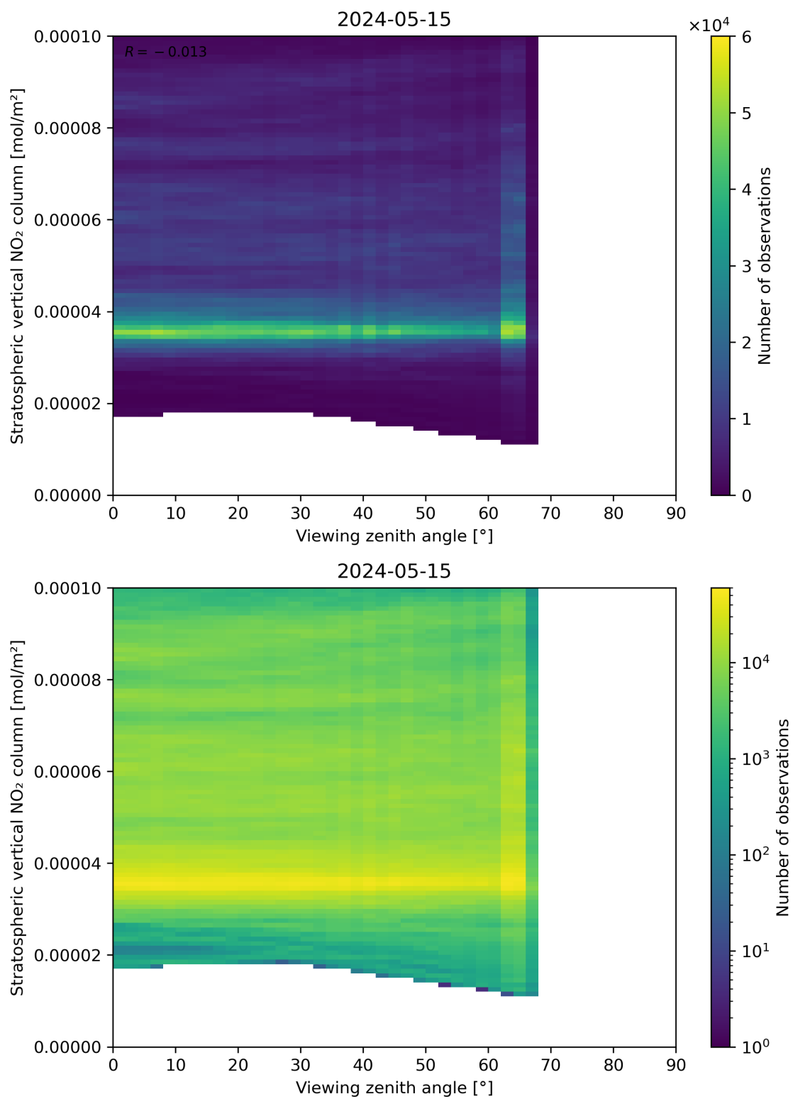
Figure 164: Scatter density plot of “Viewing zenith angle” against “Stratospheric vertical NO 2 column” for 2024-05-14 to 2024-05-16.
