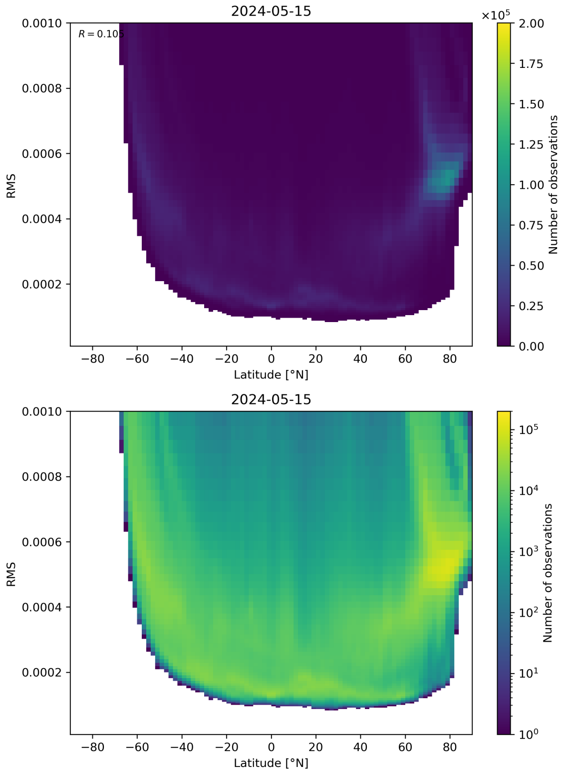
Figure 94: Scatter density plot of “Latitude” against “RMS” for 2024-05-14 to 2024-05-16.
