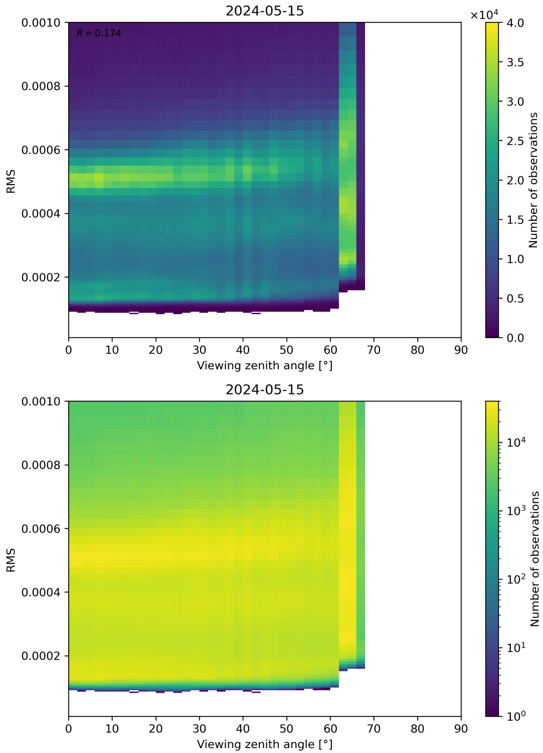
Figure 171: Scatter density plot of “Viewing zenith angle” against “RMS” for 2024-05-14 to 2024-05-16.
