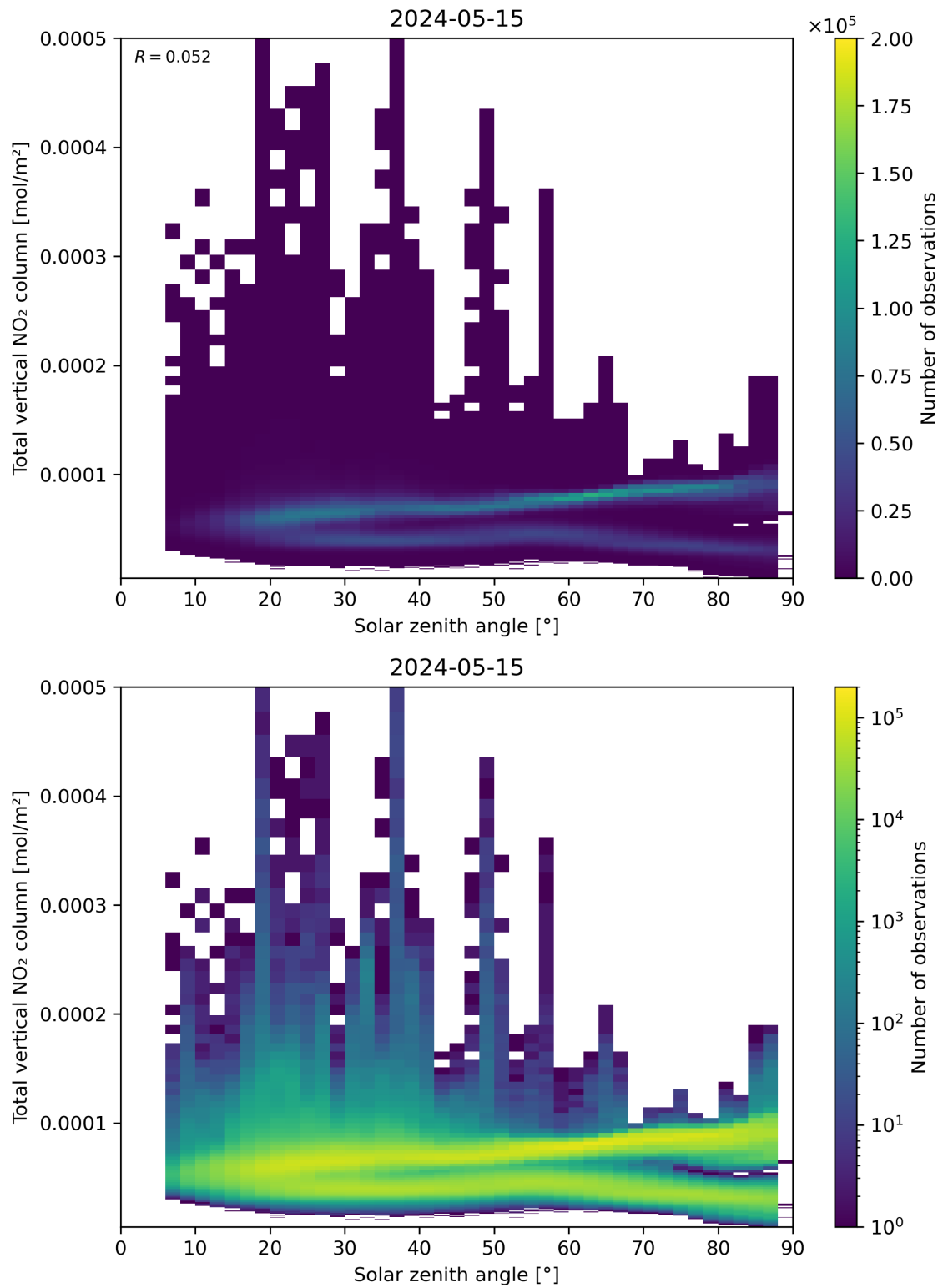
Figure 153: Scatter density plot of “Solar zenith angle” against “Total vertical \text{NO}_2 column” for 2024-05-14 to 2024-05-16.
