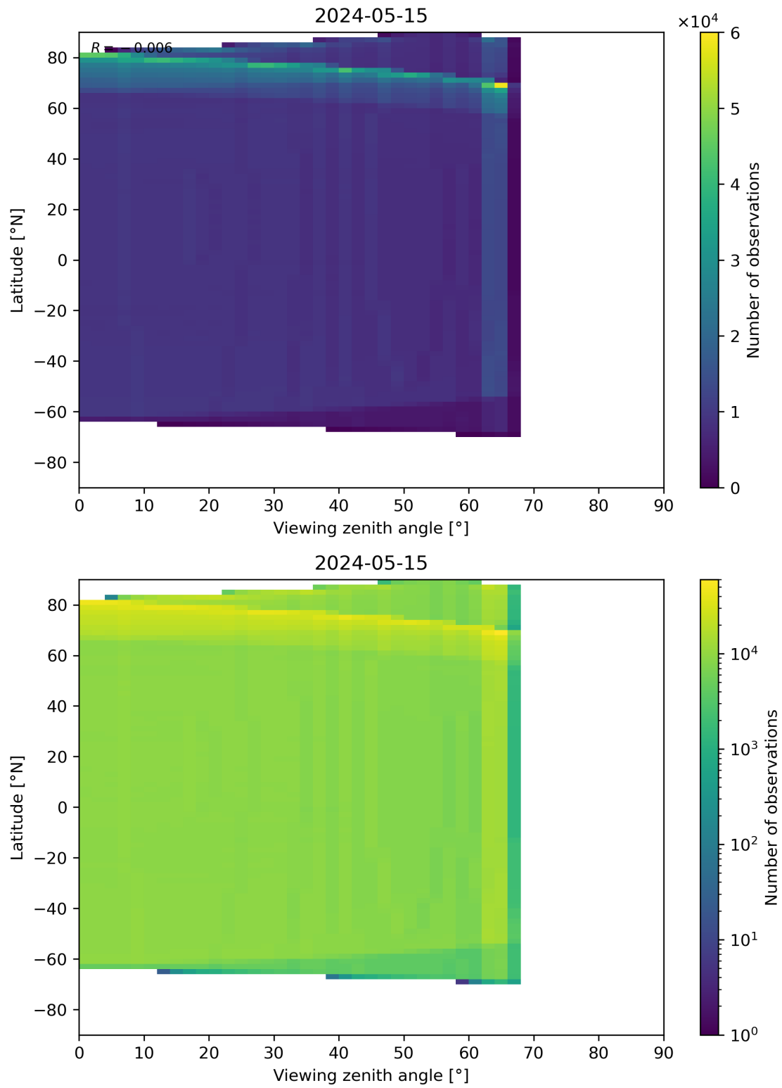
Figure 163: Scatter density plot of “Viewing zenith angle” against “Latitude” for 2024-05-14 to 2024-05-16.
