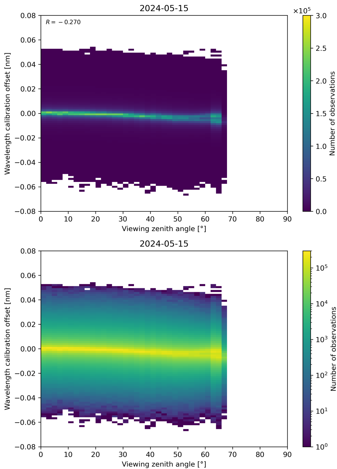
Figure 173: Scatter density plot of “Viewing zenith angle” against “Wavelength calibration offset” for 2024-05-14 to 2024-05-16.
