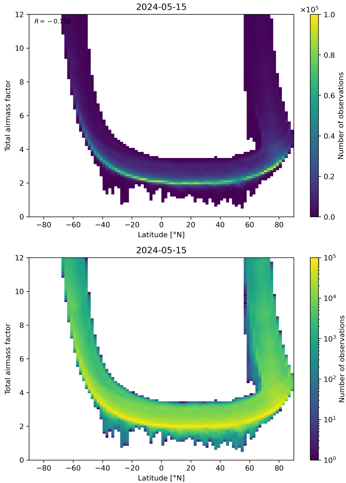
Figure 84: Scatter density plot of “Latitude” against “Total airmass factor” for 2024-05-14 to 2024-05-16.
