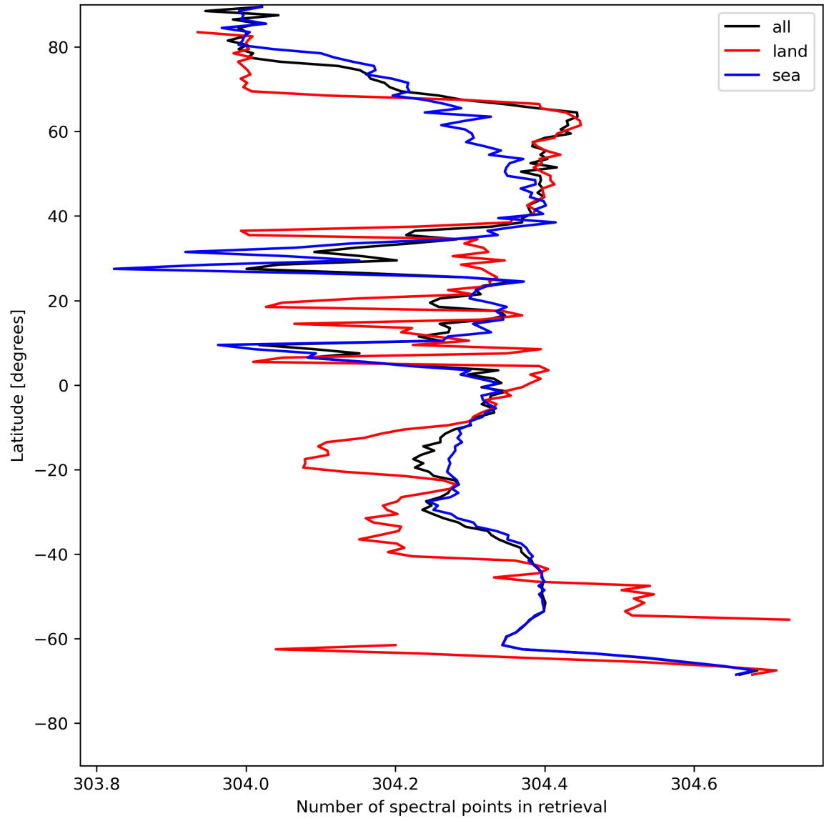
Figure 16: Zonal average of “Number of spectral points in retrieval” for 2024-05-14 to 2024-05-16.
