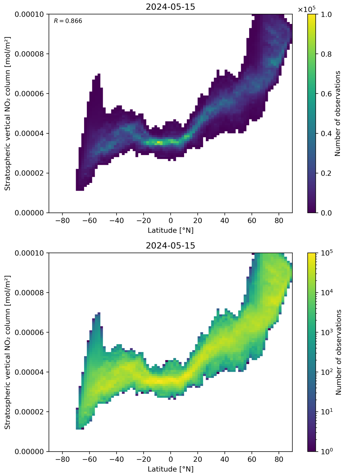
Figure 87: Scatter density plot of “Latitude” against “Stratospheric vertical NO 2 column” for 2024-05-14 to 2024-05-16.
