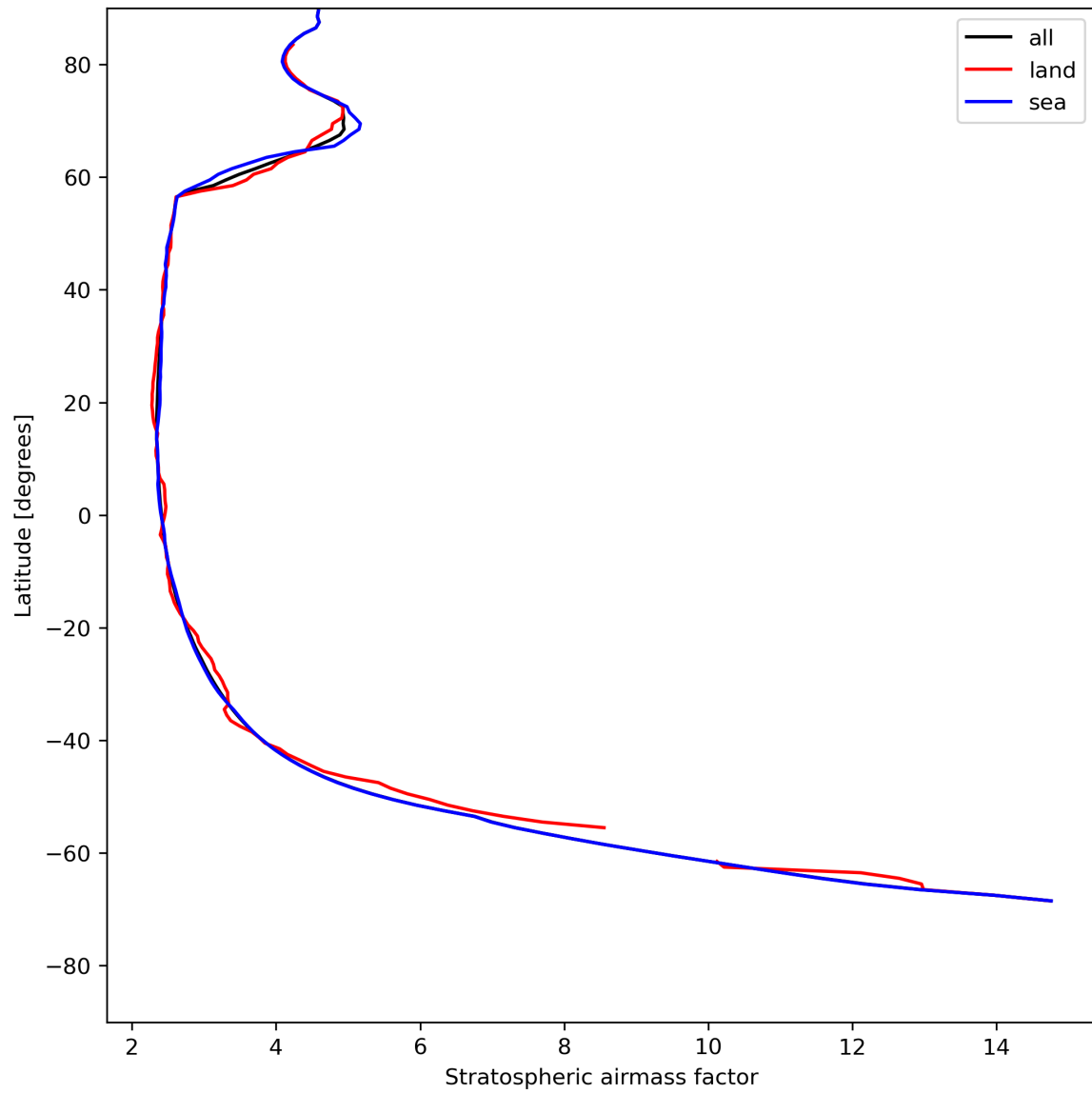
Figure 27: Zonal average of “Stratospheric airmass factor” for 2024-05-14 to 2024-05-16.
