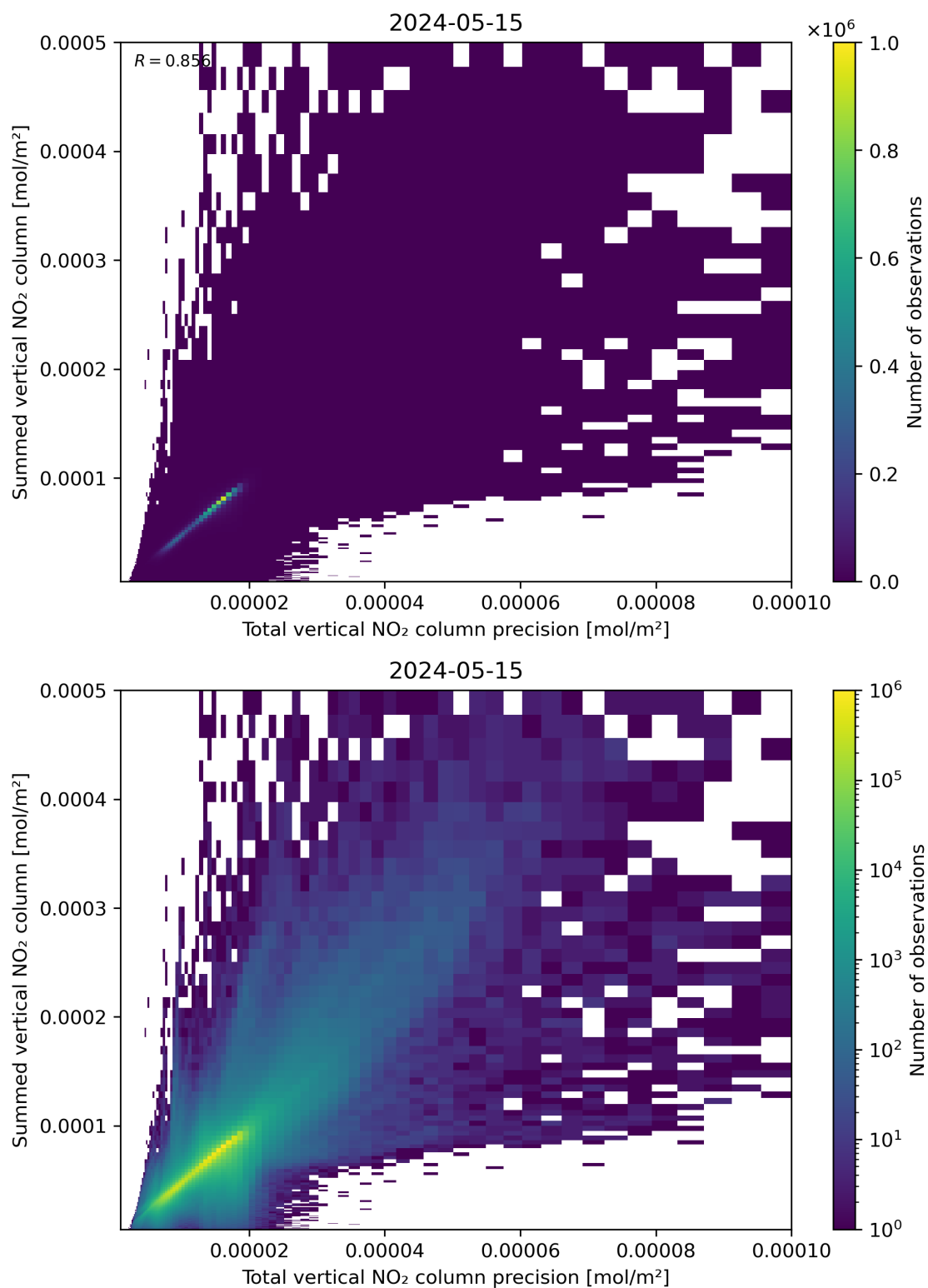
Figure 117: Scatter density plot of “Total vertical NO 2 column precision” against “Summed vertical NO 2 column” for 2024-05-14 to 2024-05-16.
