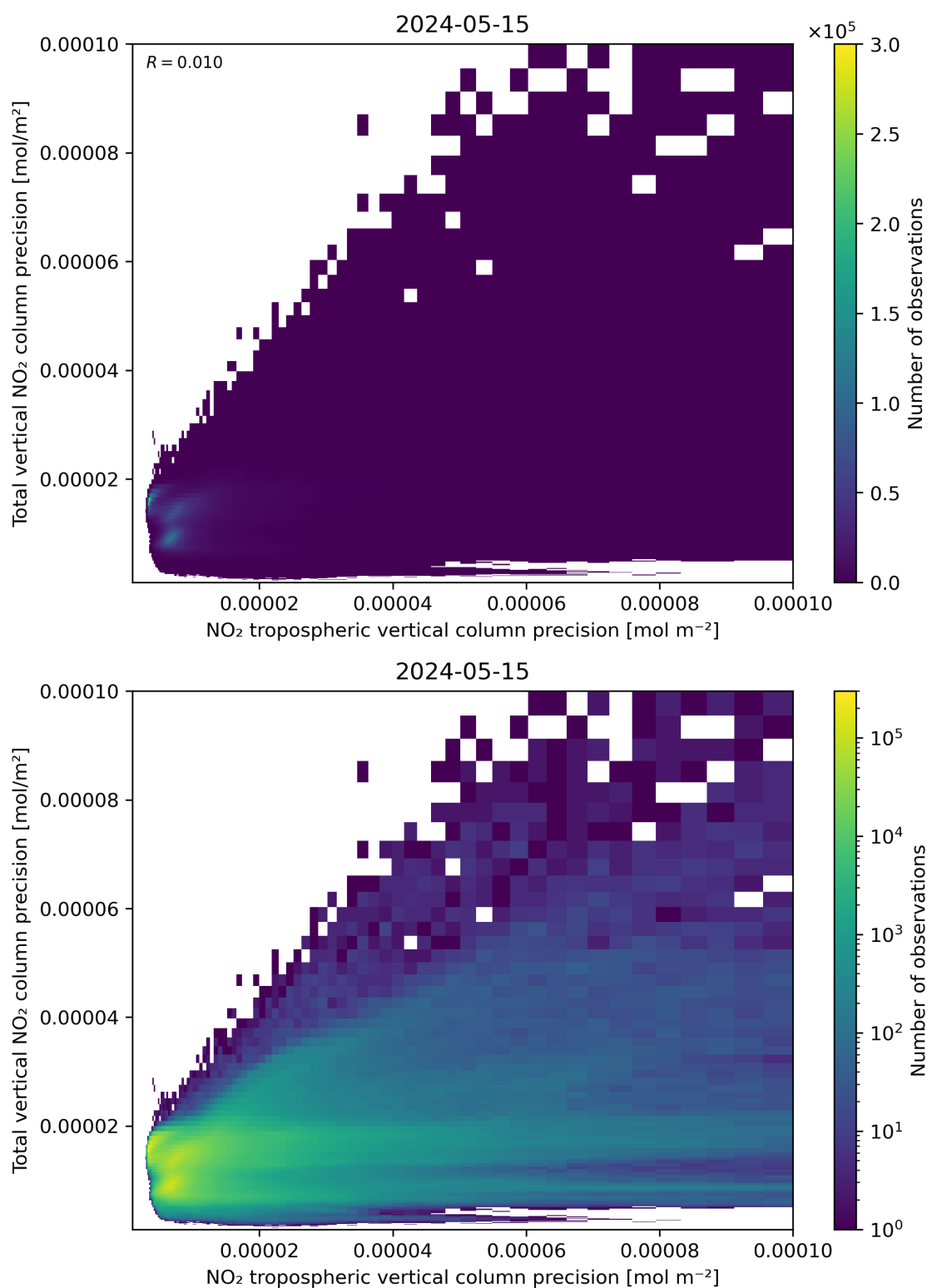
Figure 139: Scatter density plot of “NO 2 tropospheric vertical column precision” against “Total vertical NO 2 column precision” for 2024-05-14 to 2024-05-16.
