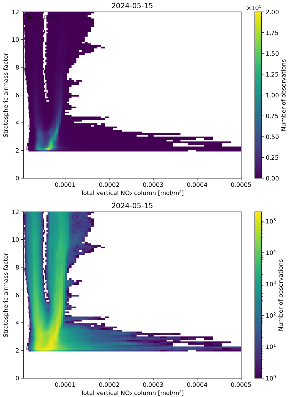
Figure 110: Scatter density plot of “Total vertical NO 2 column” against “Stratospheric airmass factor” for 2024-05-14 to 2024-05-16.
