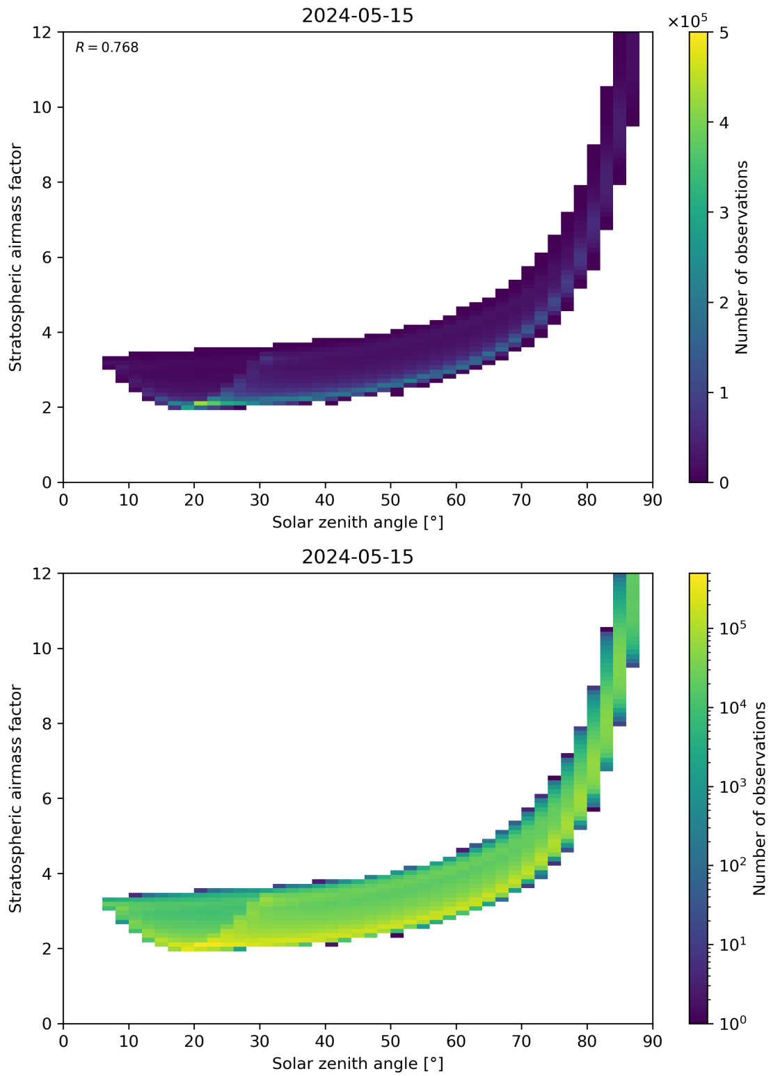
Figure 145: Scatter density plot of “Solar zenith angle” against “Stratospheric airmass factor” for 2024-05-14 to 2024-05-16.
