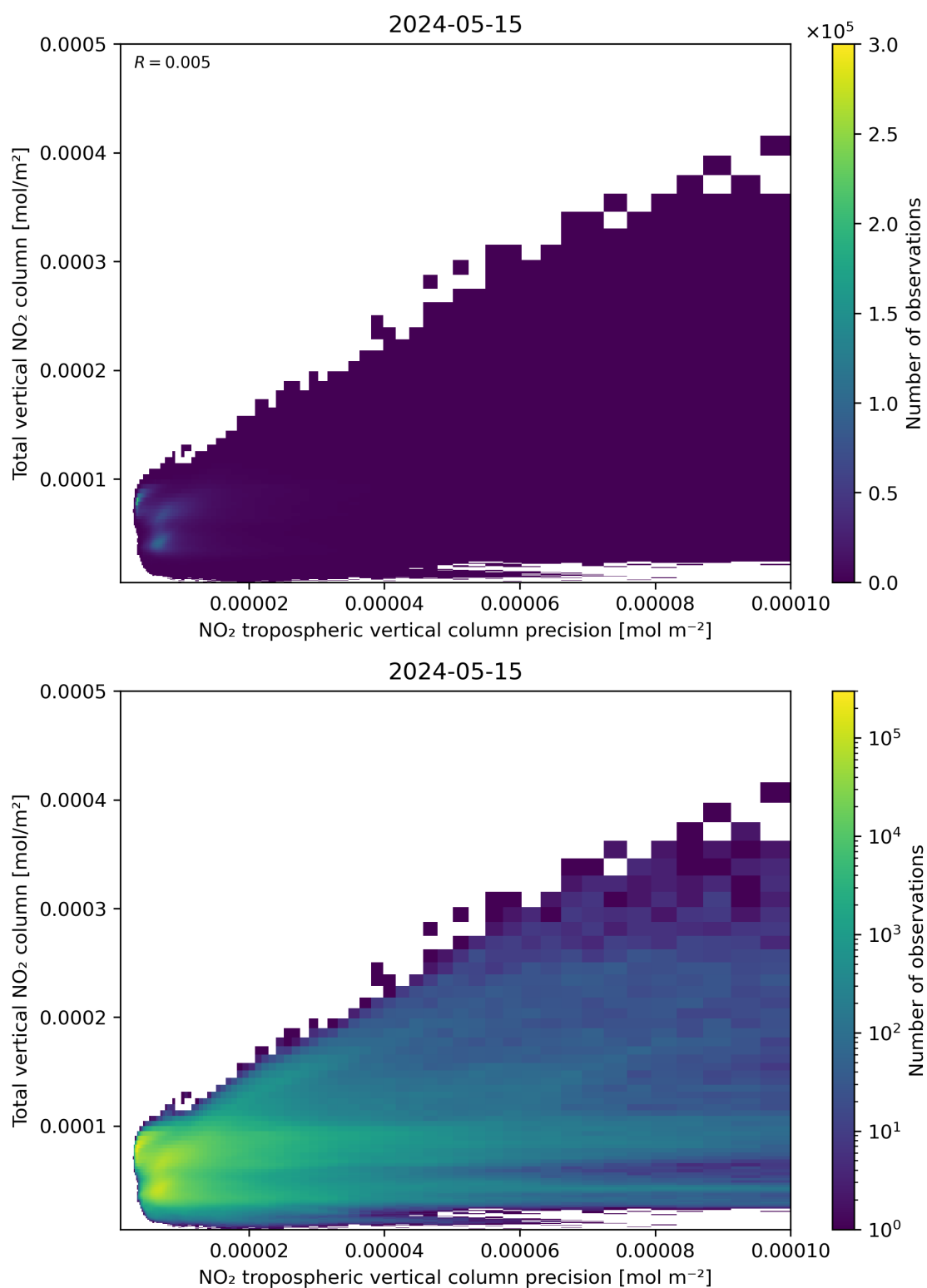
Figure 138: Scatter density plot of “NO 2 tropospheric vertical column precision” against “Total vertical NO 2 column” for 2024-05-14 to 2024-05-16.
