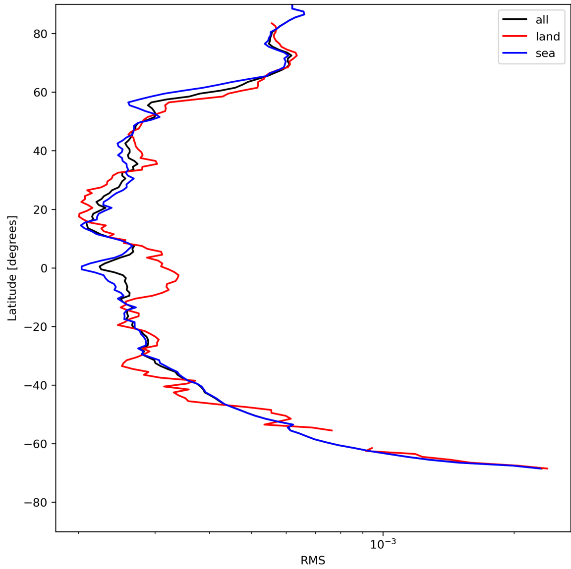
Figure 26: Zonal average of “RMS” for 2024-05-14 to 2024-05-16.
