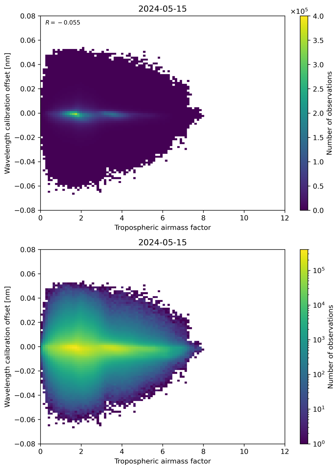
Figure 80: Scatter density plot of “Tropospheric airmass factor” against “Wavelength calibration offset” for 2024-05-14 to 2024-05-16.
