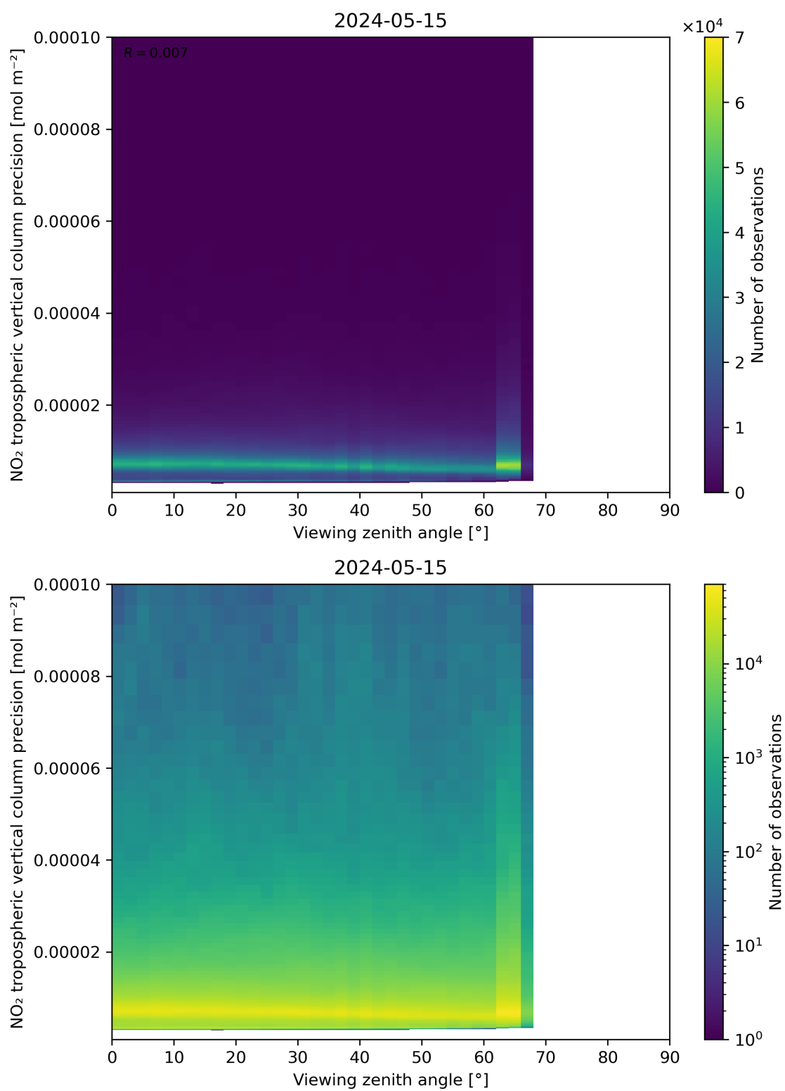
Figure 170: Scatter density plot of “Viewing zenith angle” against “NO 2 tropospheric vertical column precision” for 2024-05-14 to 2024-05-16.
