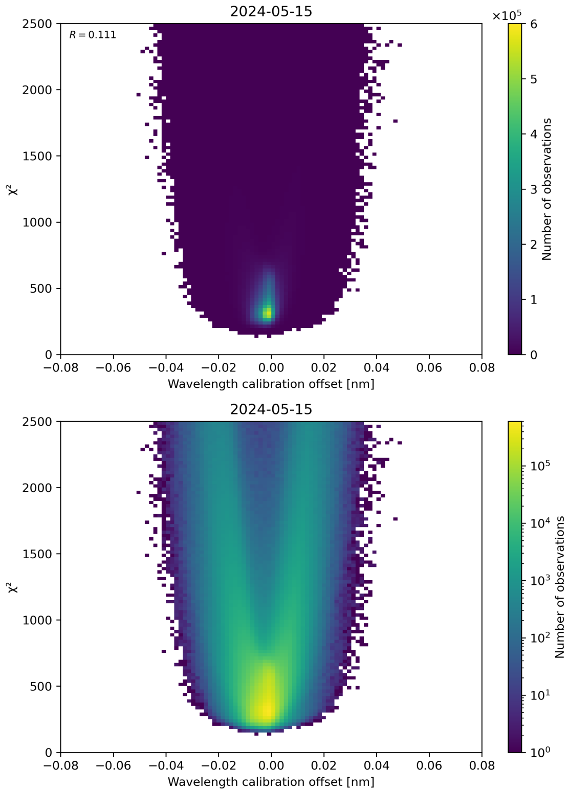
Figure 175: Scatter density plot of “Wavelength calibration offset” against “ \chi^2 ” for 2024-05-14 to 2024-05-16.
