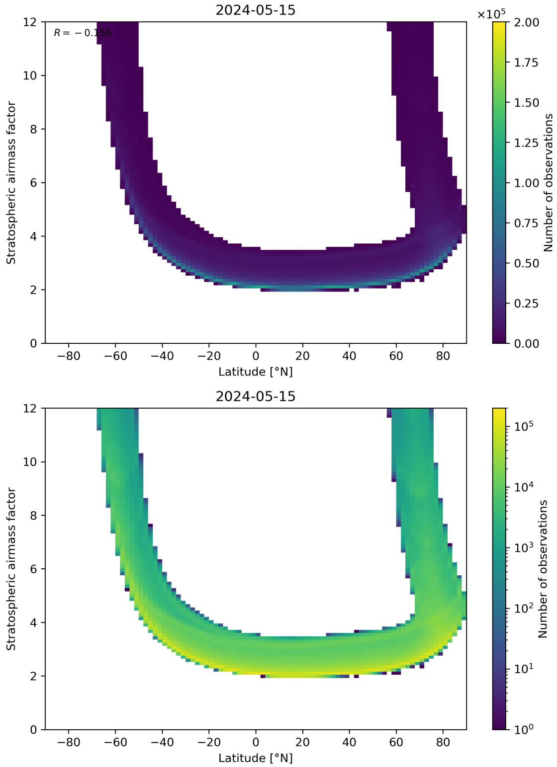
Figure 83: Scatter density plot of “Latitude” against “Stratospheric air mass factor” for 2024-05-14 to 2024-05-16.
