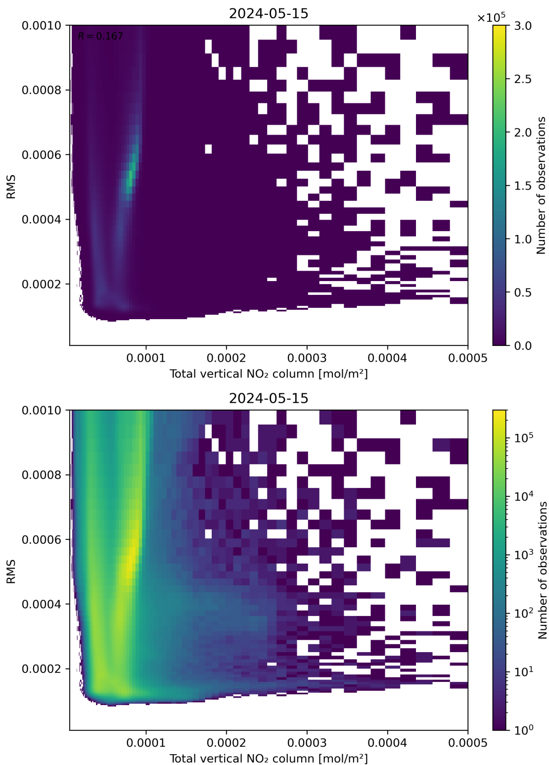
Figure 120: Scatter density plot of “Total vertical NO 2 column” against “RMS” for 2024-05-14 to 2024-05-16.
