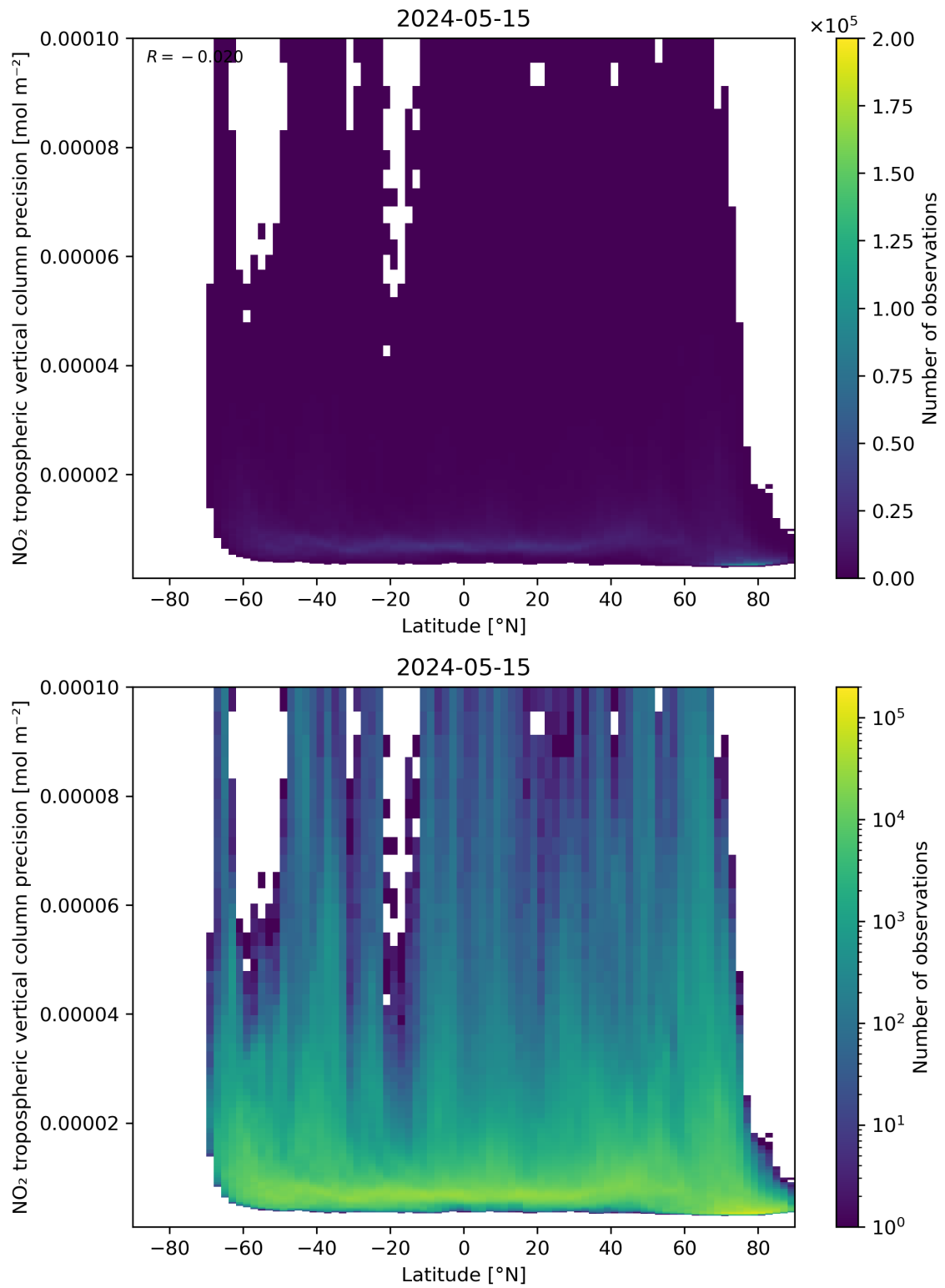
Figure 93: Scatter density plot of “Latitude” against “NO 2 tropospheric vertical column precision” for 2024-05-14 to 2024-05-16.
