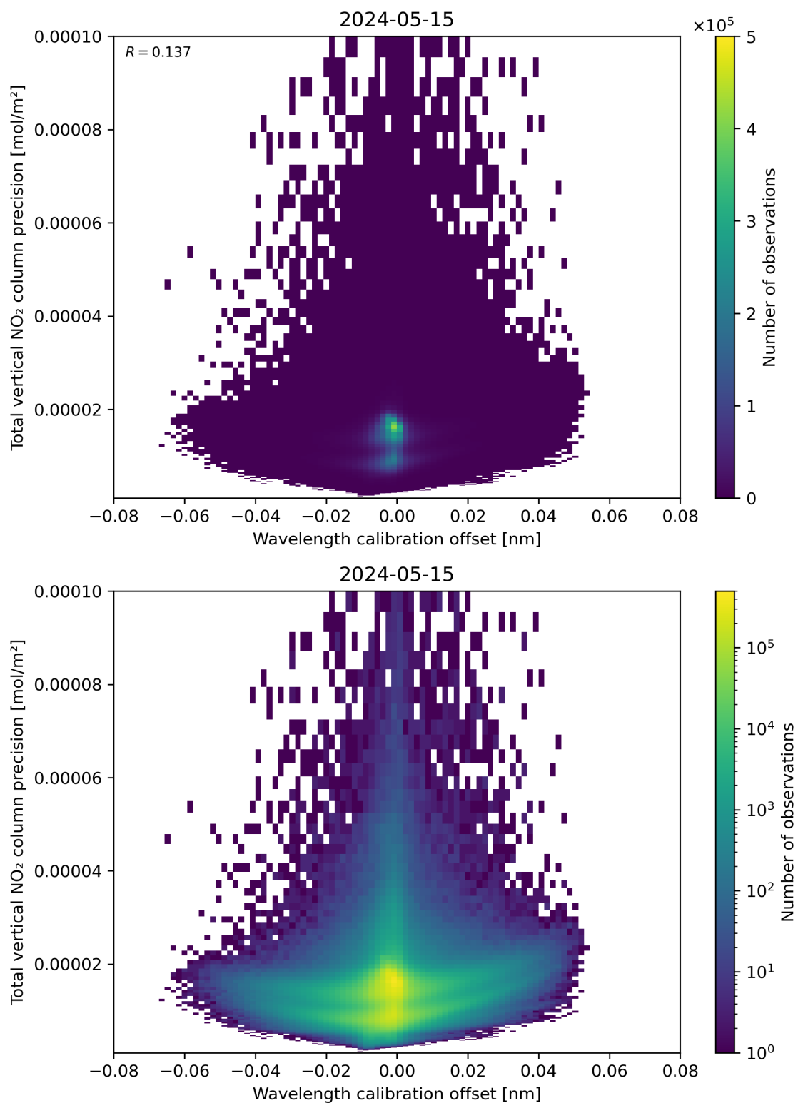
Figure 180: Scatter density plot of “Wavelength calibration offset” against “Total vertical NO 2 column precision” for 2024-05-14 to 2024-05-16.
