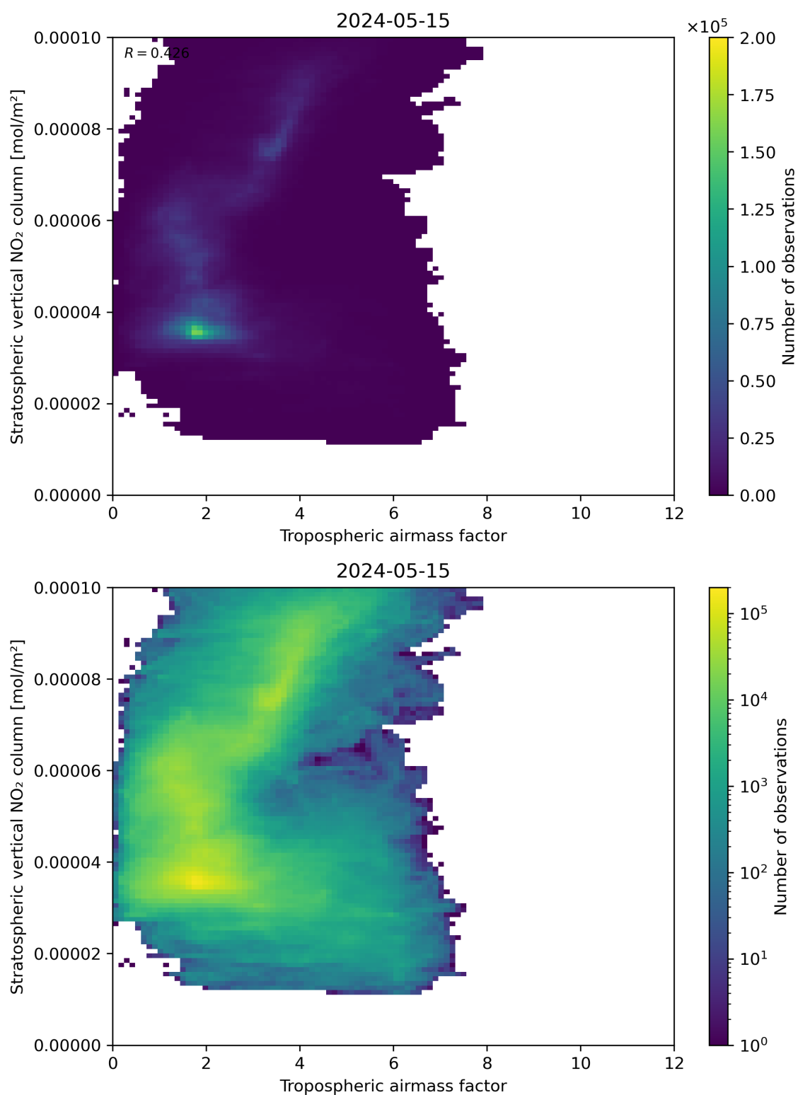
Figure 74: Scatter density plot of “Tropospheric air mass factor” against “Stratospheric vertical NO 2 column” for 2024-05-14 to 2024-05-16.
