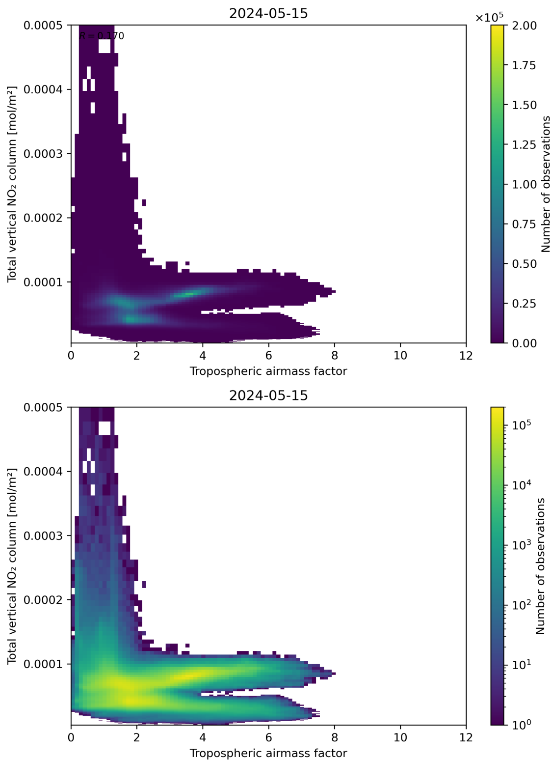
Figure 77: Scatter density plot of “Tropospheric airmass factor” against “Total vertical NO 2 column” for 2024-05-14 to 2024-05-16.
