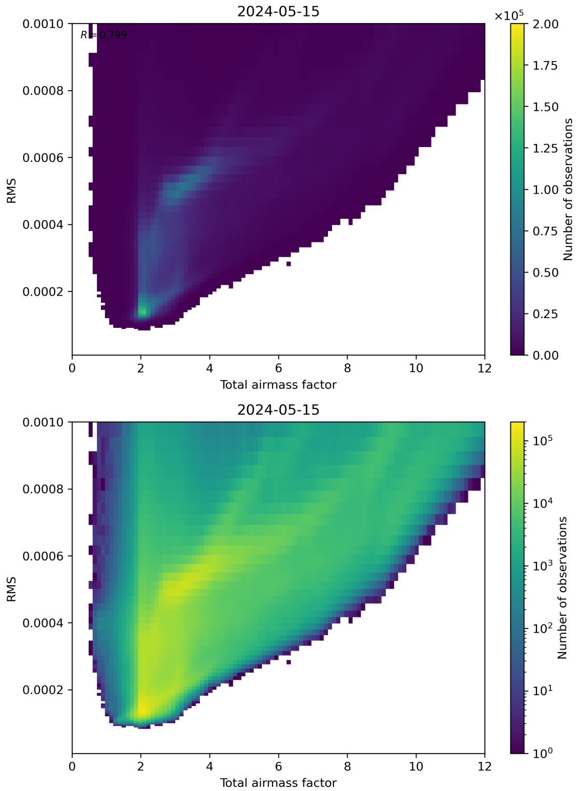
Figure 69: Scatter density plot of “Total airmass factor” against “RMS” for 2024-05-14 to 2024-05-16.
