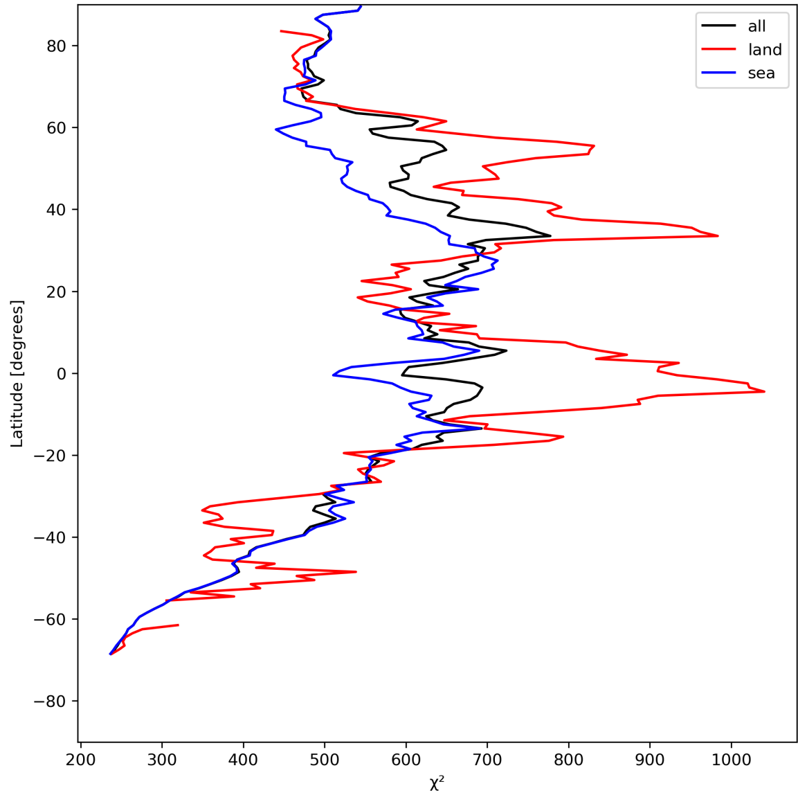
Figure 25: Zonal average of “ \chi^2 ” for 2024-05-14 to 2024-05-16.
