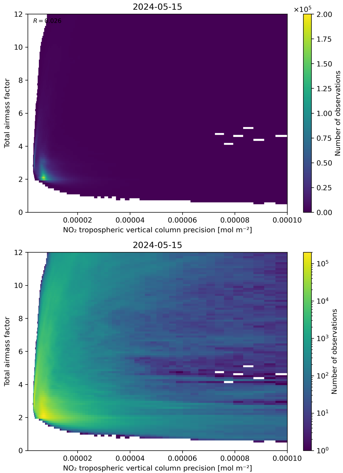
Figure 132: Scatter density plot of “NO 2 tropospheric vertical column precision” against “Total air mass factor” for 2024-05-14 to 2024-05-16.
