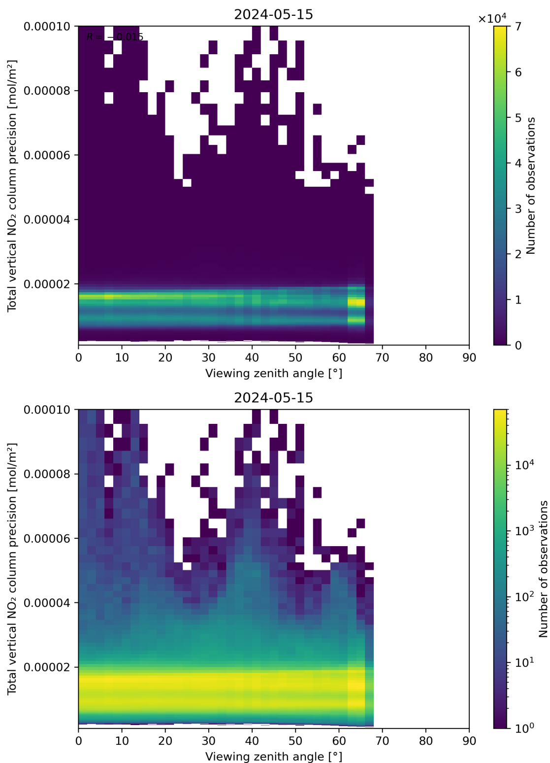
Figure 168: Scatter density plot of “Viewing zenith angle” against “Total vertical NO 2 column precision” for 2024-05-14 to 2024-05-16.
