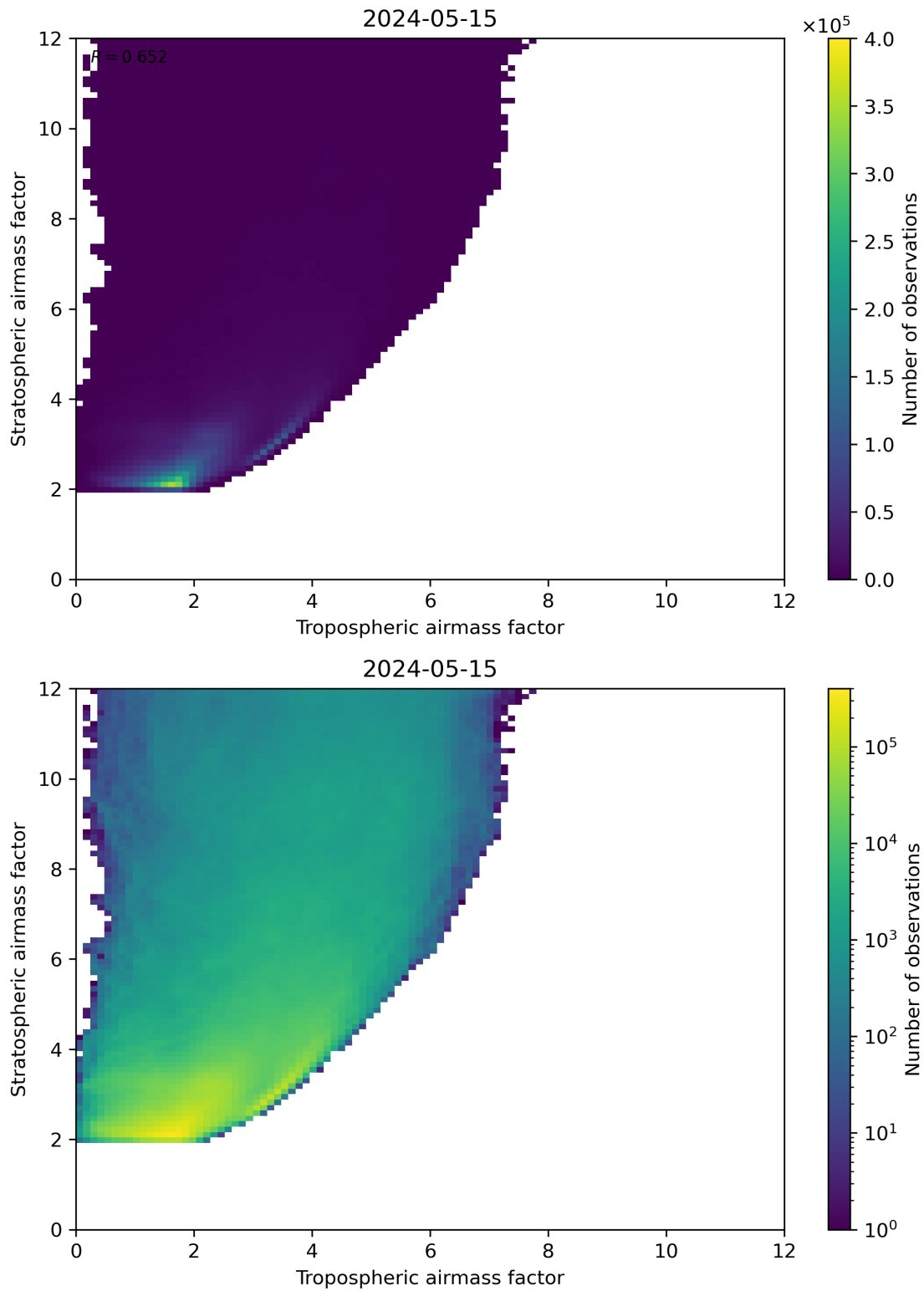
Figure 71: Scatter density plot of “Tropospheric airmass factor” against “Stratospheric airmass factor” for 2024-05-14 to 2024-05-16.
