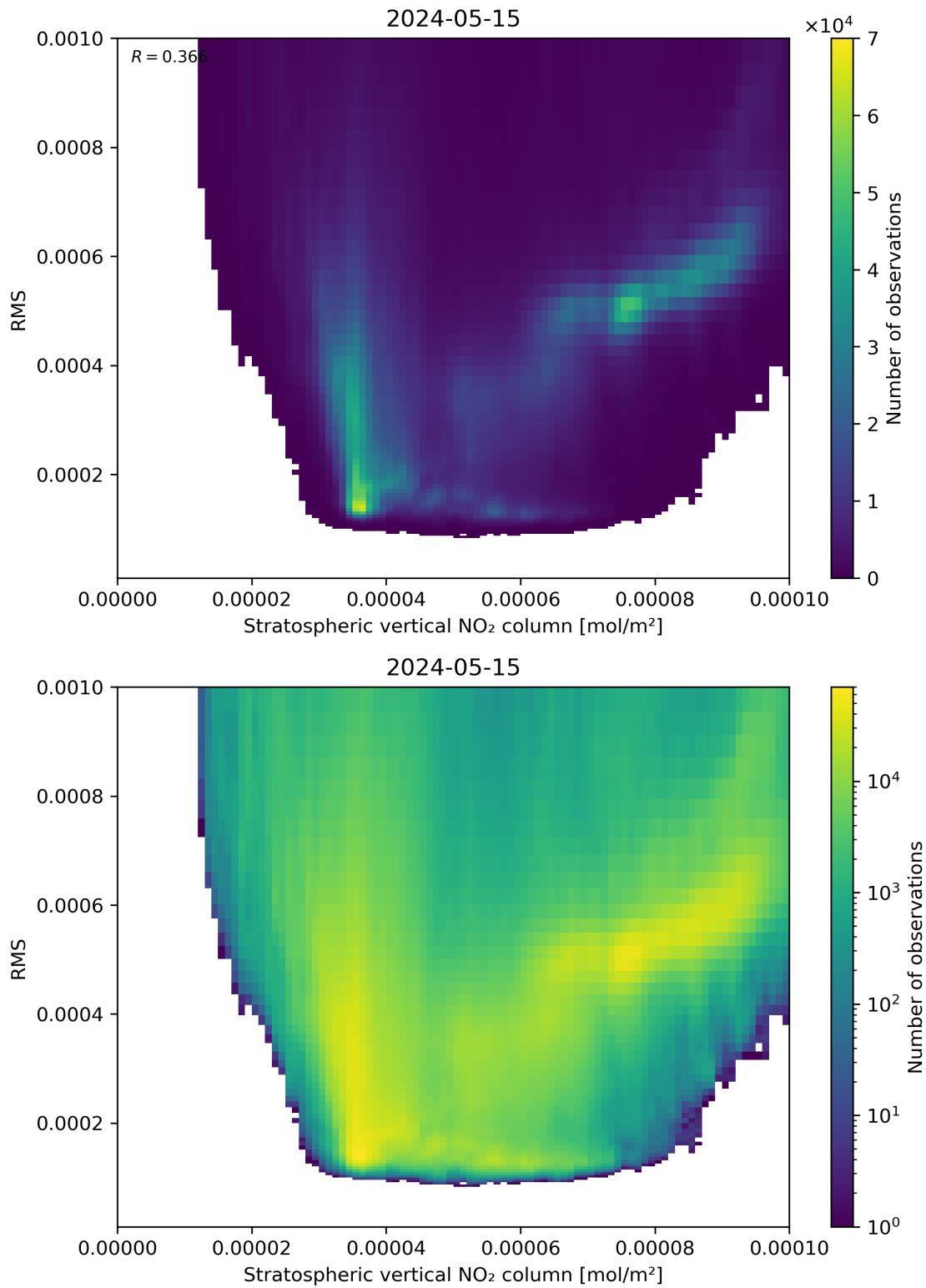
Figure 102: Scatter density plot of “Stratospheric vertical NO 2 column” against “RMS” for 2024-05-14 to 2024-05-16.
