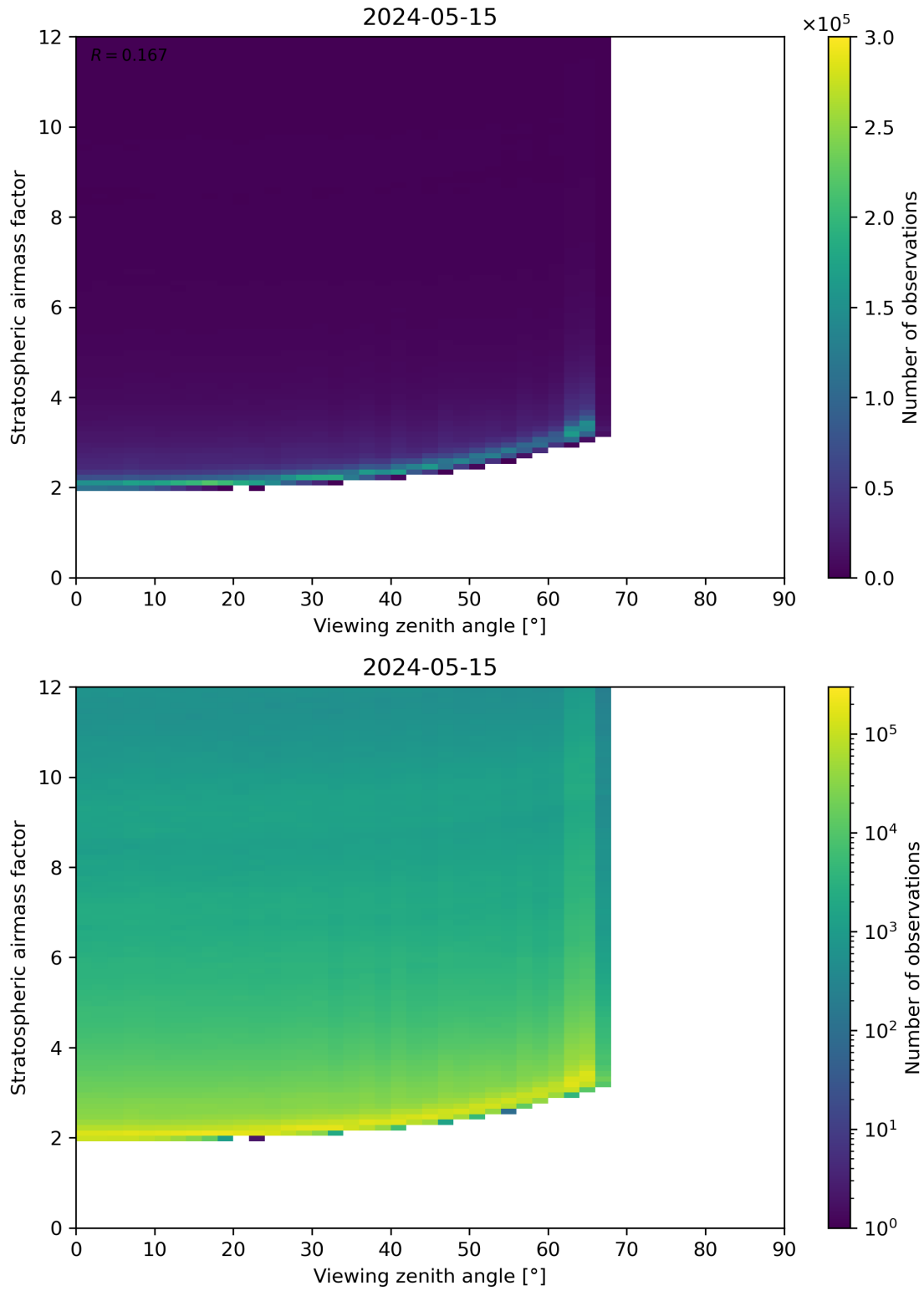
Figure 159: Scatter density plot of “Viewing zenith angle” against “Stratospheric airmass factor” for 2024-05-14 to 2024-05-16.
