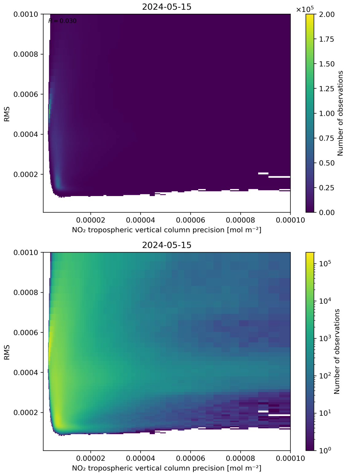
Figure 140: Scatter density plot of “NO 2 tropospheric vertical column precision” against “RMS” for 2024-05-14 to 2024-05-16.
