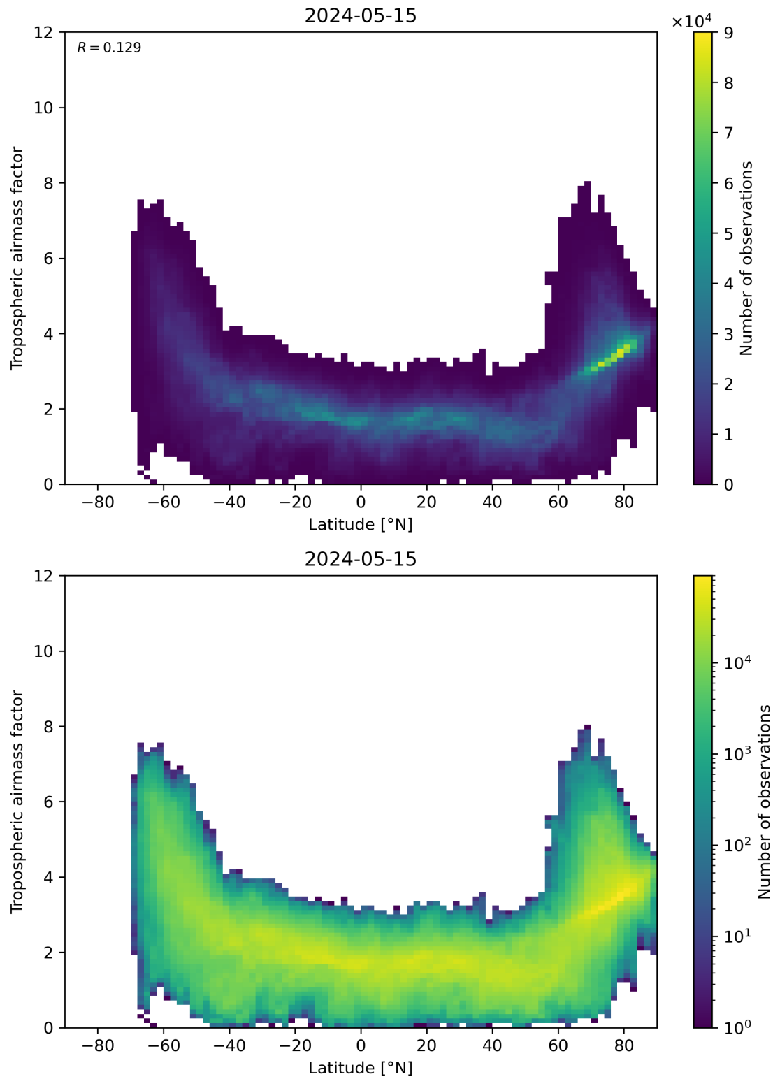
Figure 85: Scatter density plot of “Latitude” against “Tropospheric airmass factor” for 2024-05-14 to 2024-05-16.
