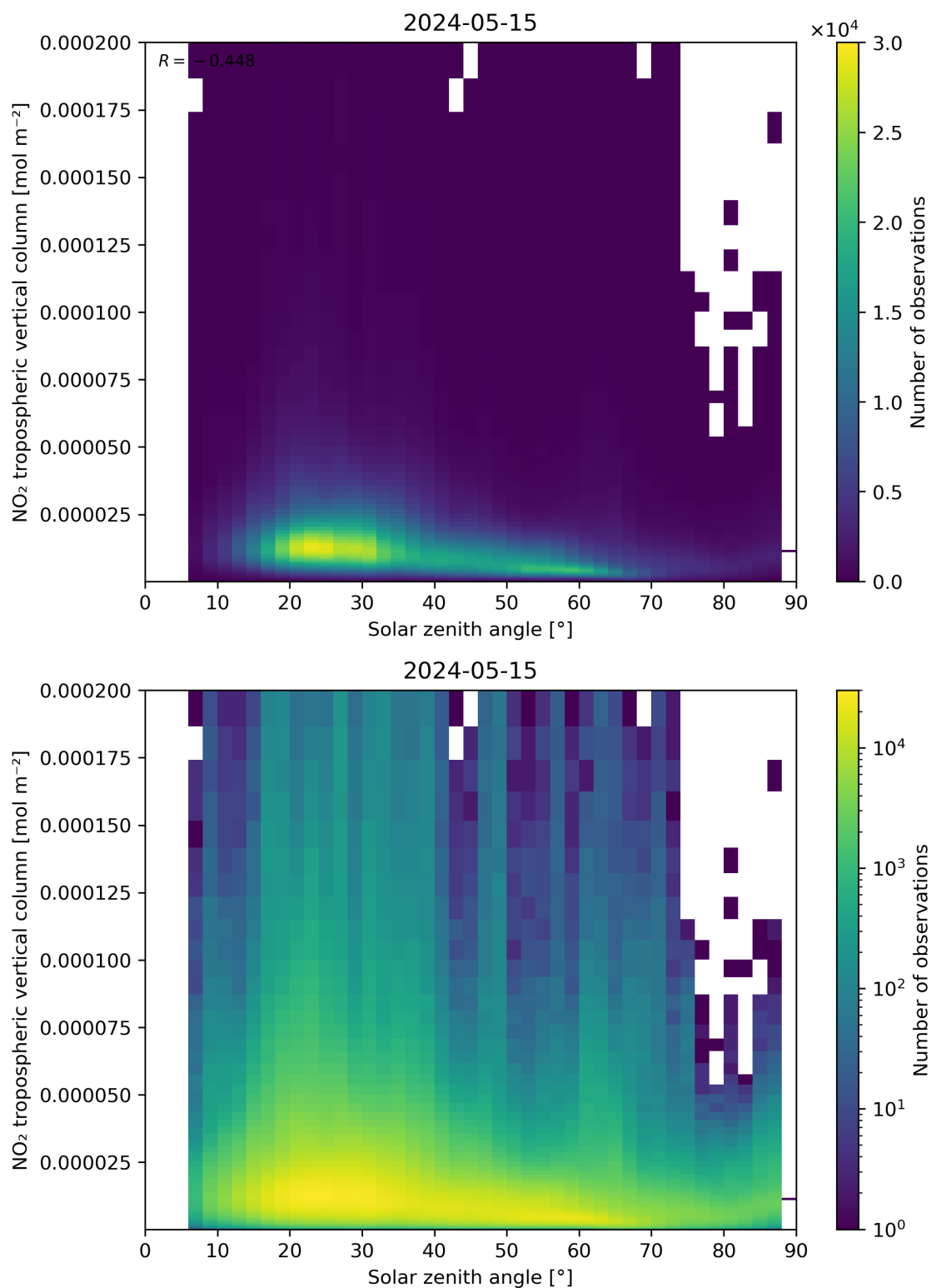
Figure 155: Scatter density plot of “Solar zenith angle” against “NO 2 tropospheric vertical column” for 2024-05-14 to 2024-05-16.
