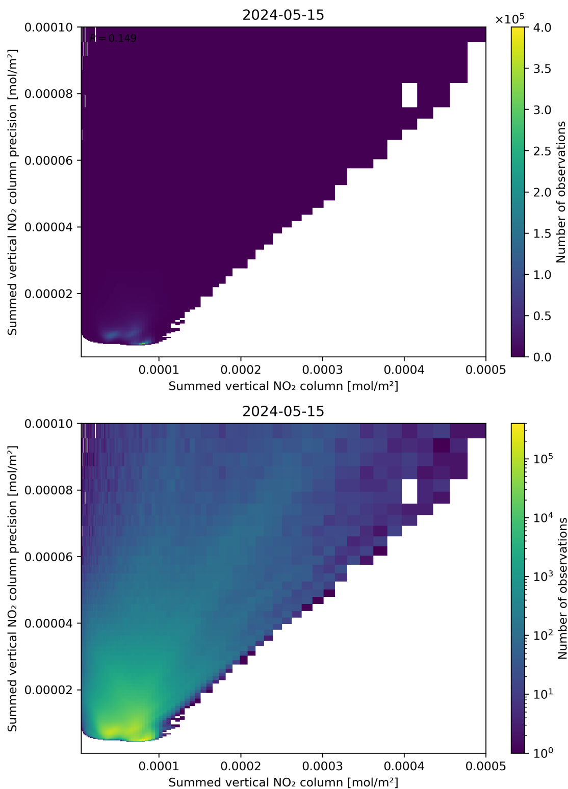
Figure 105: Scatter density plot of “Summed vertical NO 2 column” against “Summed vertical NO 2 column precision” for 2024-05-14 to 2024-05-16.
