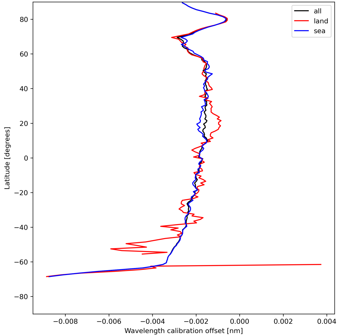
Figure 18: Zonal average of “Wavelength calibration offset” for 2024-05-14 to 2024-05-16.
