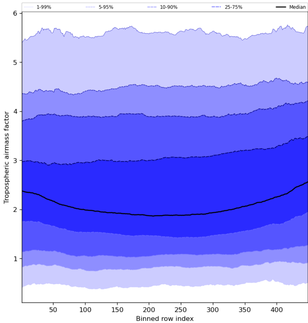
Figure 48: Along track statistics of “Tropospheric airmass factor” for 2024-05-14 to 2024-05-16
