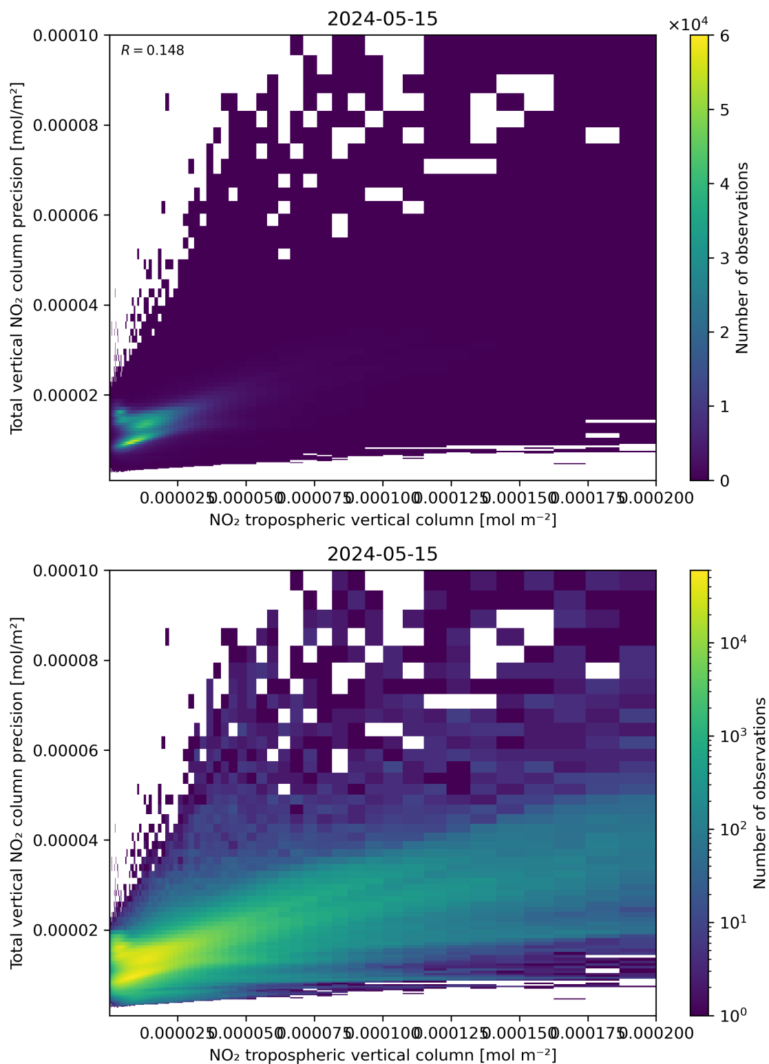
Figure 129: Scatter density plot of “NO 2 tropospheric vertical column” against “Total vertical NO 2 column precision” for 2024-05-14 to 2024-05-16.
