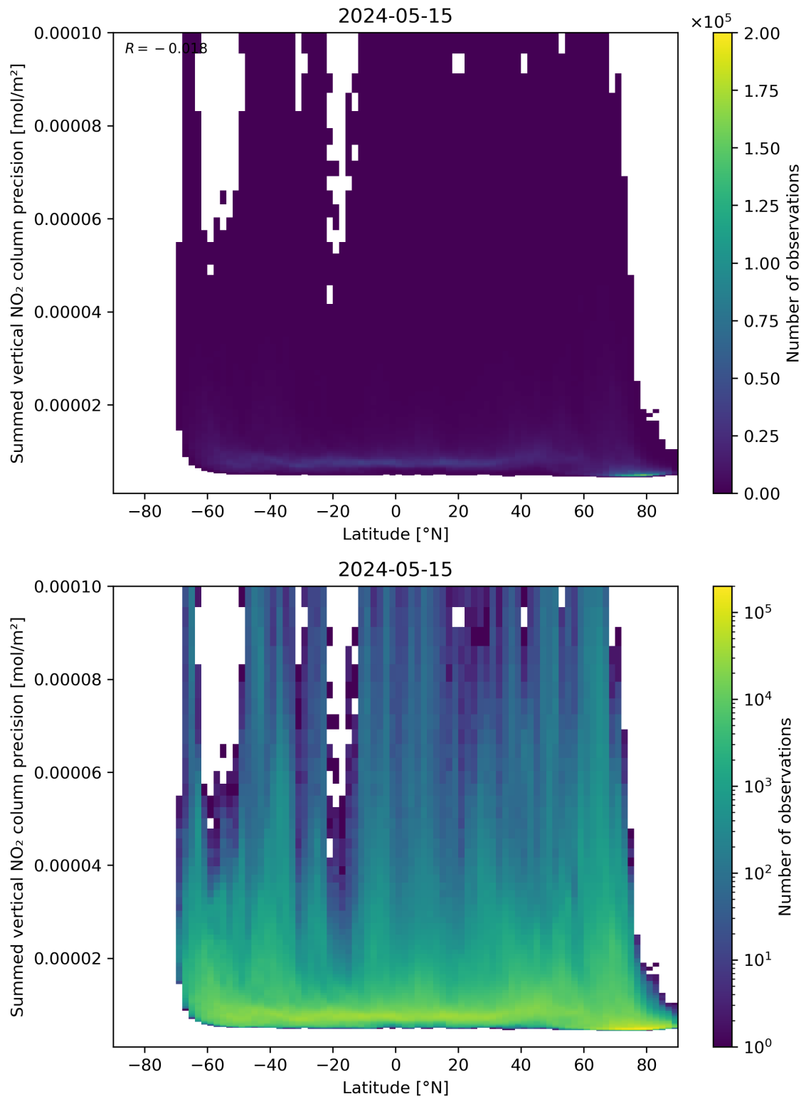
Figure 89: Scatter density plot of “Latitude” against “Summed vertical NO 2 column precision” for 2024-05-14 to 2024-05-16.
