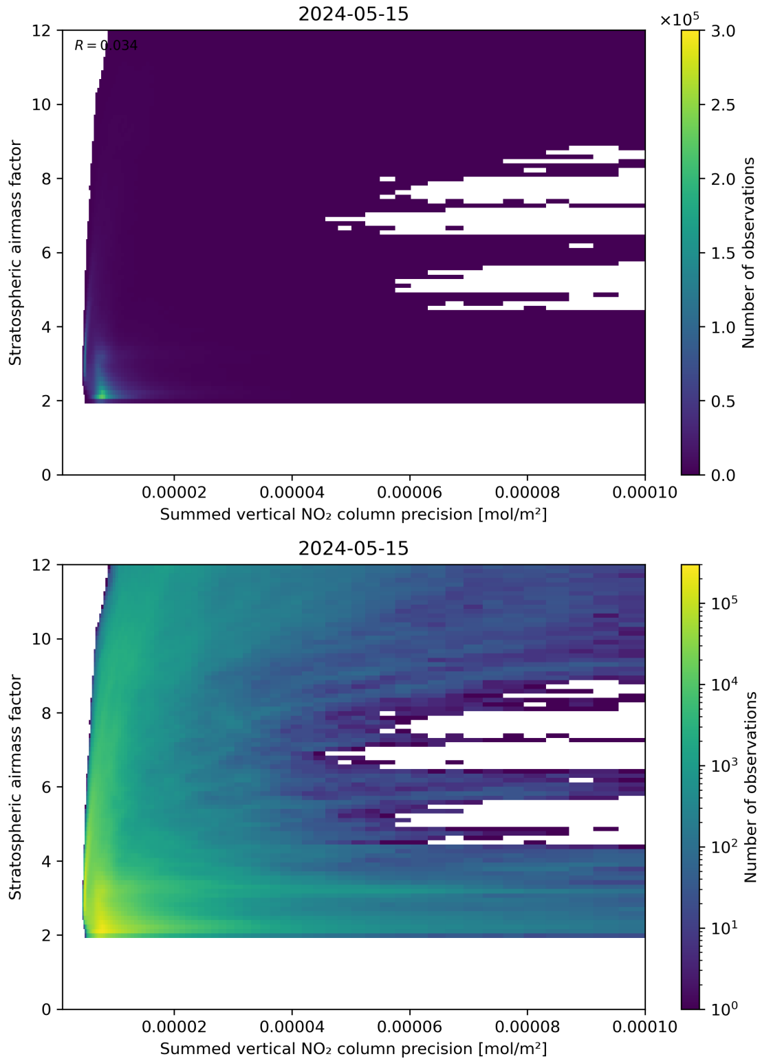
Figure 106: Scatter density plot of “Summed vertical NO 2 column precision” against “Stratospheric airmass factor” for 2024-05-14 to 2024-05-16.
