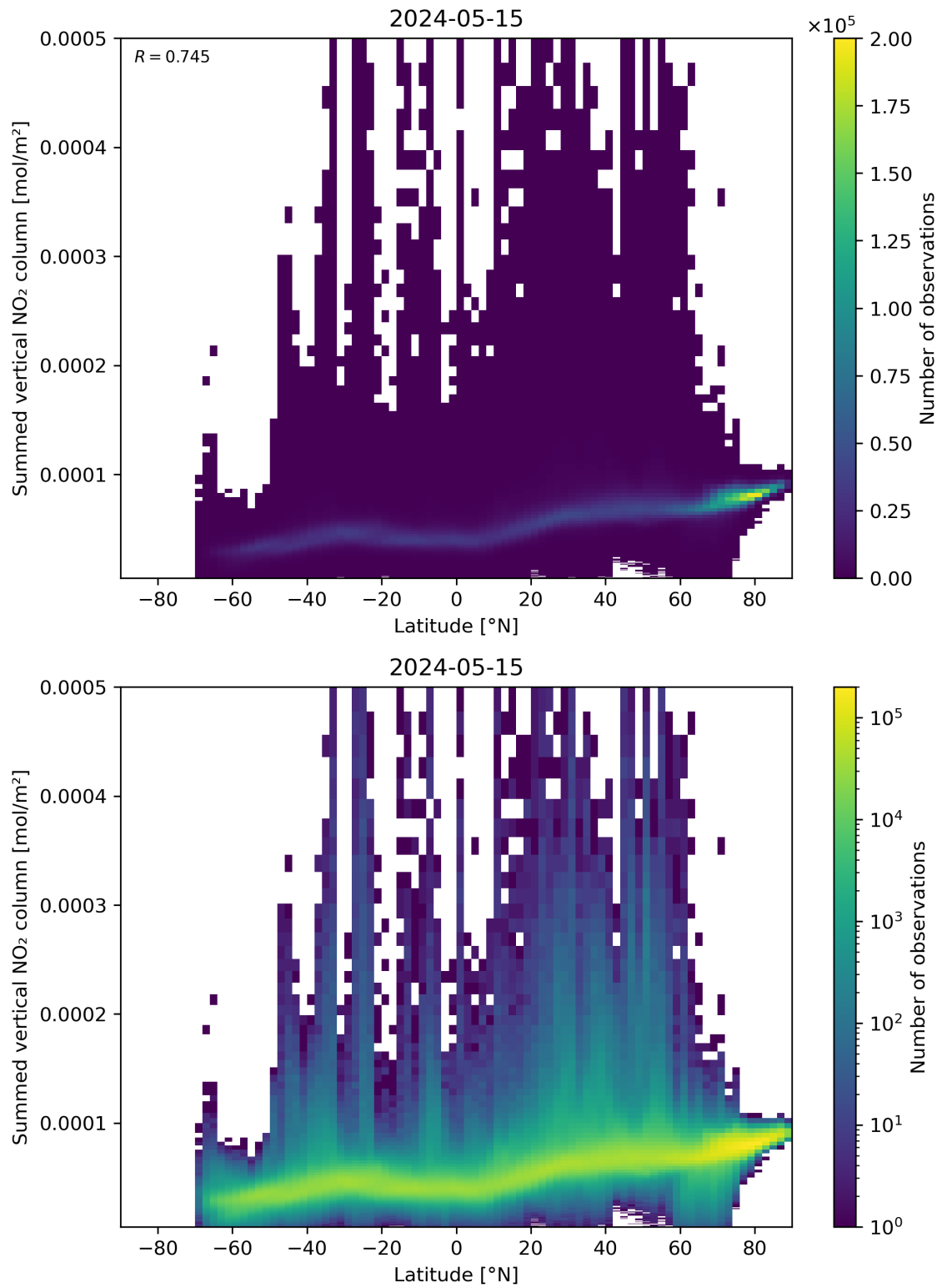
Figure 88: Scatter density plot of “Latitude” against “Summed vertical NO 2 column” for 2024-05-14 to 2024-05-16.
