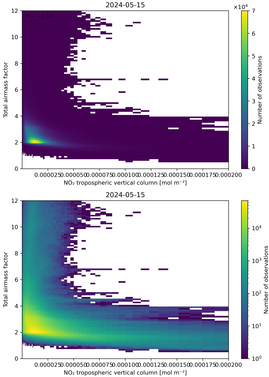
Figure 122: Scatter density plot of “NO 2 tropospheric vertical column” against “Total air mass factor” for 2024-05-14 to 2024-05-16.
