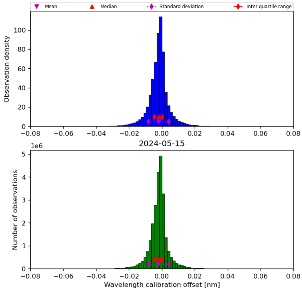
Figure 35: Histogram of “Wavelength calibration offset” for 2024-05-14 to 2024-05-16
