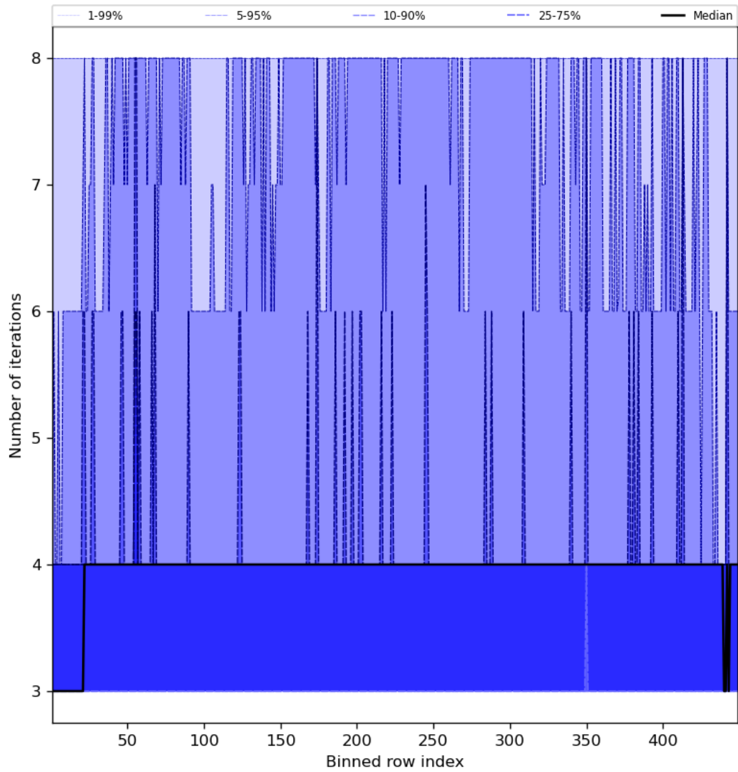
Figure 51: Along track statistics of “Number of iterations” for 2024-05-14 to 2024-05-16
