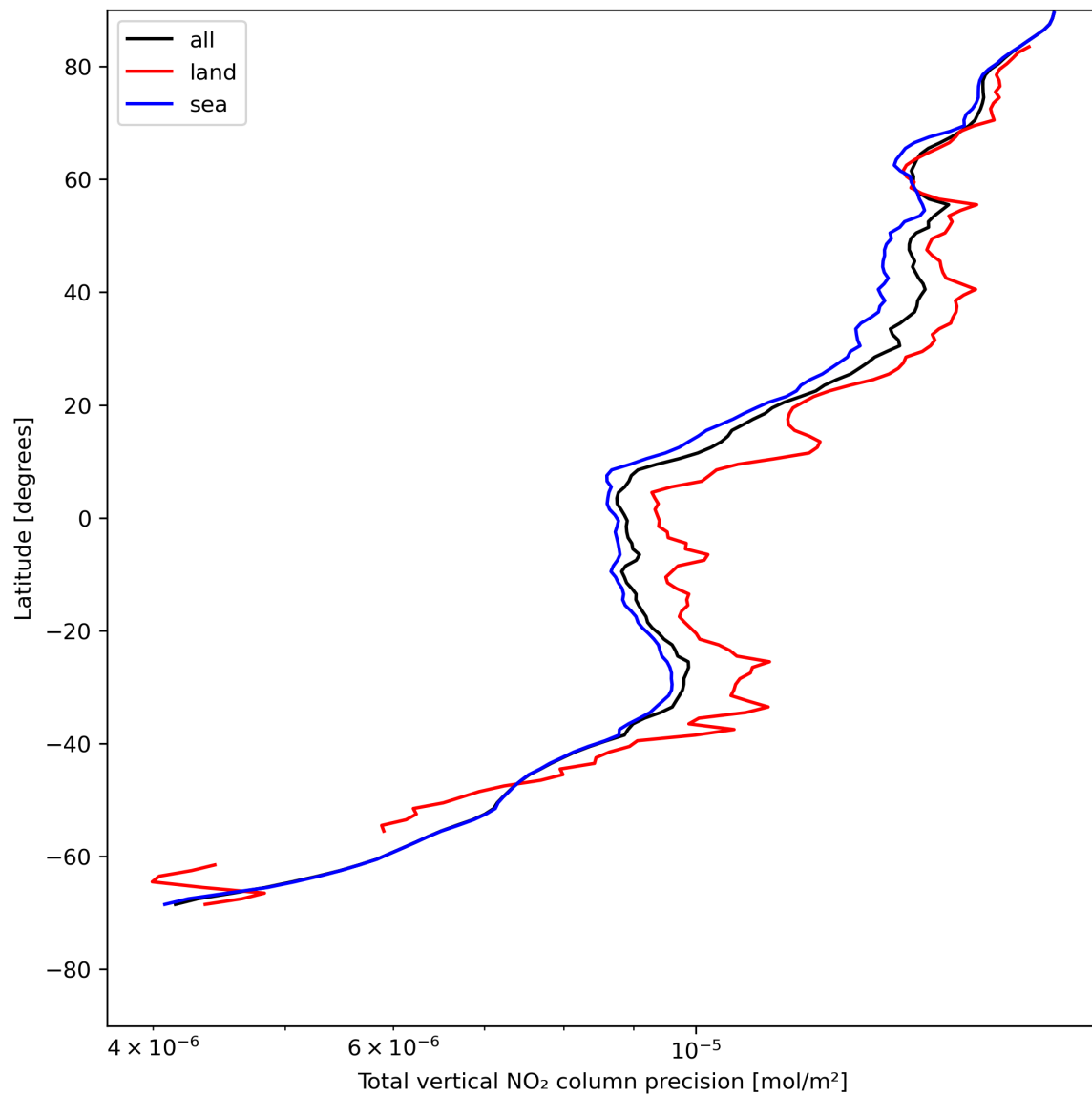
Figure 22: Zonal average of “Total vertical NO 2 column precision” for 2024-05-14 to 2024-05-16.
