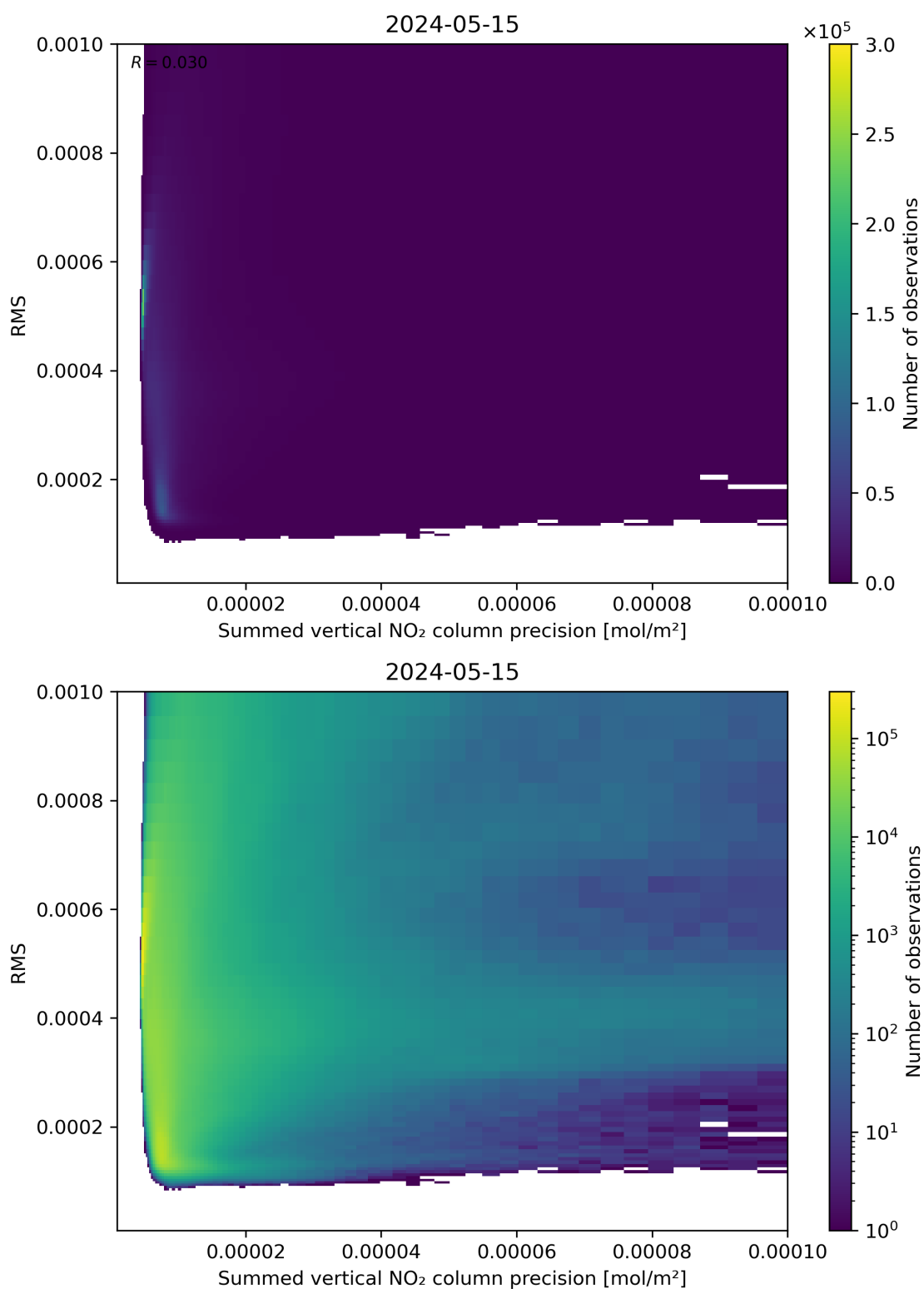
Figure 108: Scatter density plot of “Summed vertical NO 2 column precision” against “RMS” for 2024-05-14 to 2024-05-16.
