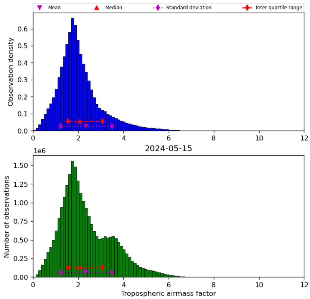
Figure 31: Histogram of “Tropospheric airmass factor” for 2024-05-14 to 2024-05-16
