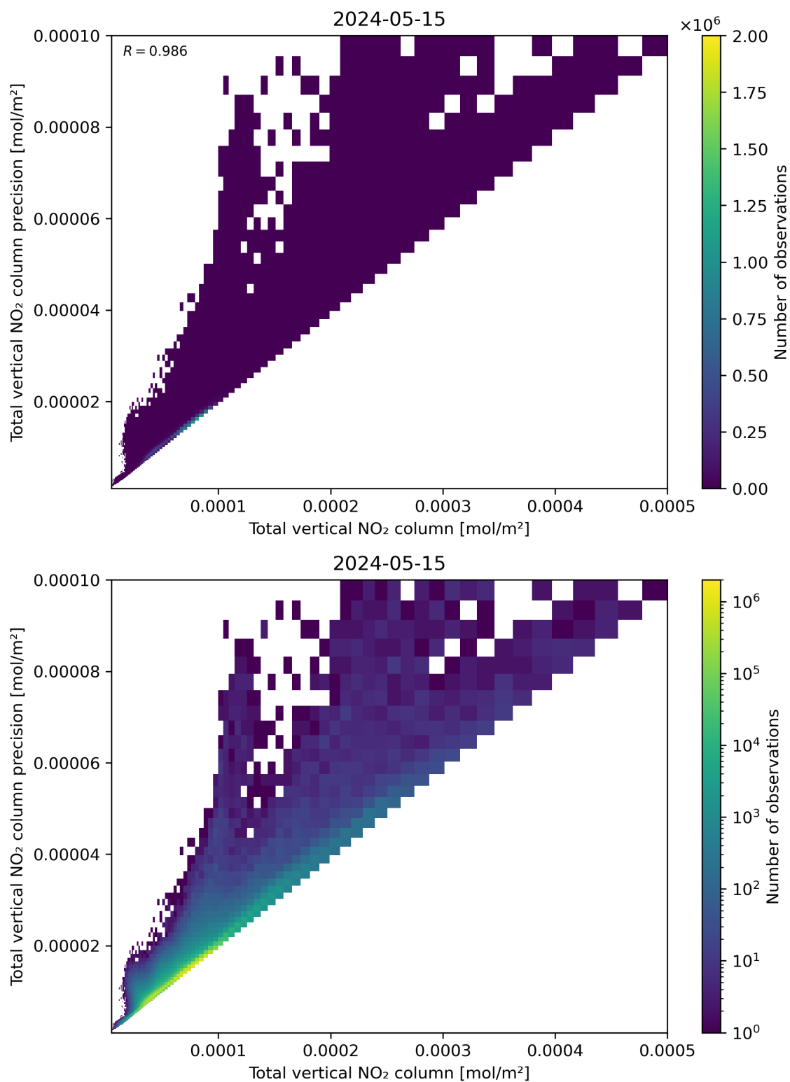
Figure 114: Scatter density plot of “Total vertical NO 2 column” against “Total vertical NO 2 column precision” for 2024-05-14 to 2024-05-16.
