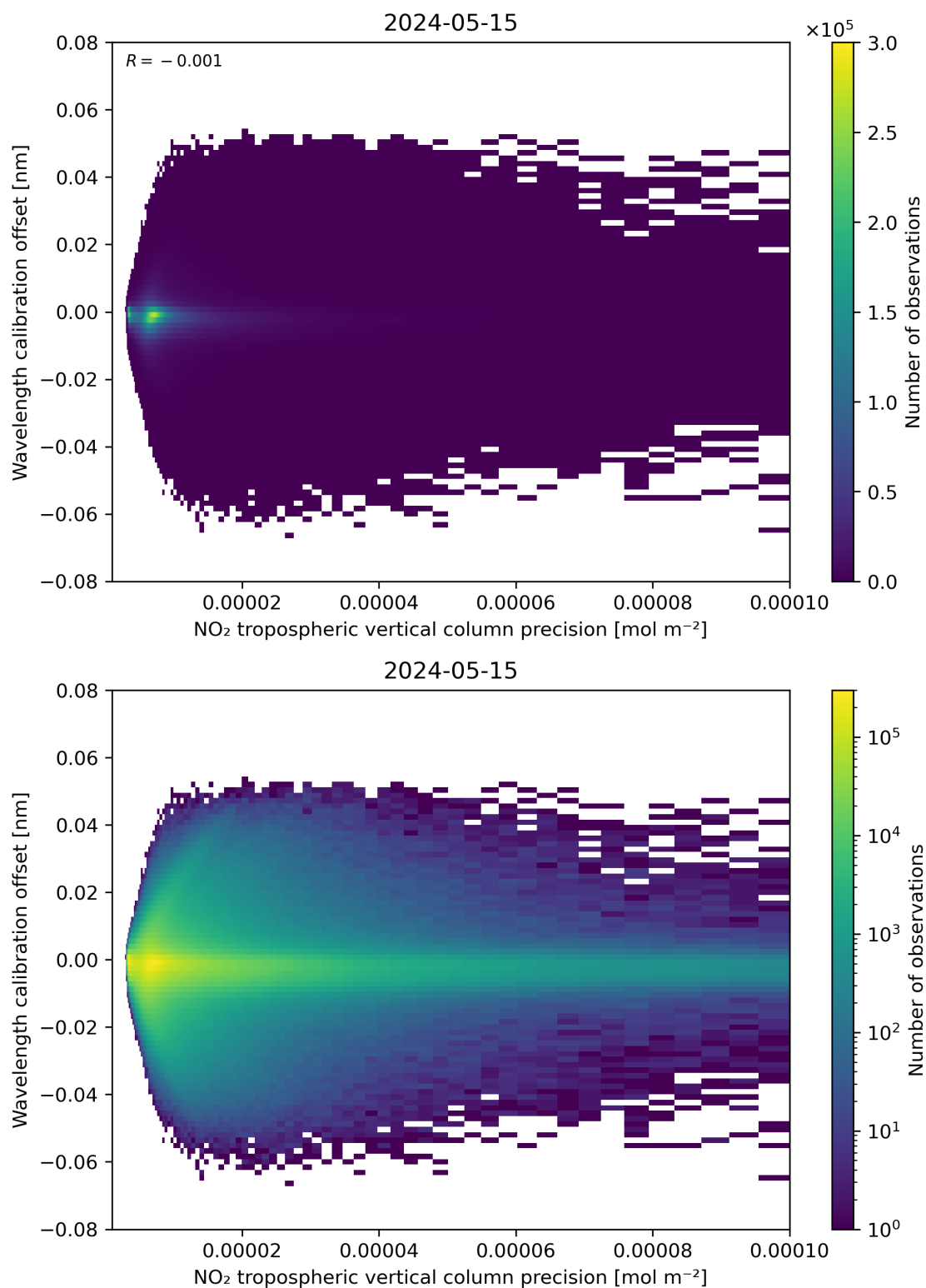
Figure 141: Scatter density plot of “NO 2 tropospheric vertical column precision” against “Wavelength calibration offset” for 2024-05-14 to 2024-05-16.
