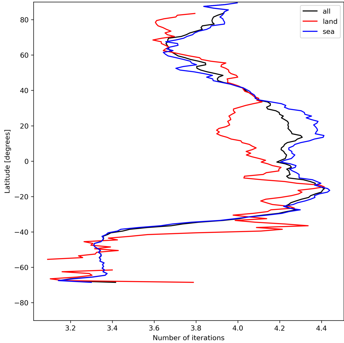
Figure 17: Zonal average of “Number of iterations” for 2024-05-14 to 2024-05-16.
