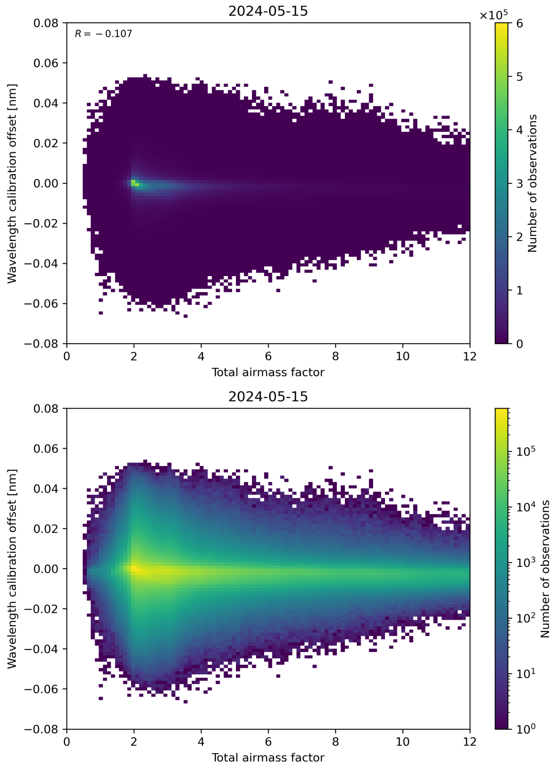
Figure 70: Scatter density plot of “Total airmass factor” against “Wavelength calibration offset” for 2024-05-14 to 2024-05-16.
