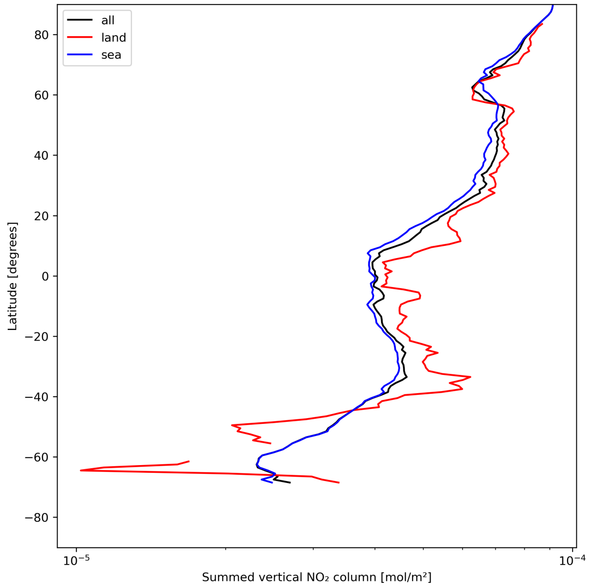
Figure 23: Zonal average of “Summed vertical NO 2 column” for 2024-05-14 to 2024-05-16.
