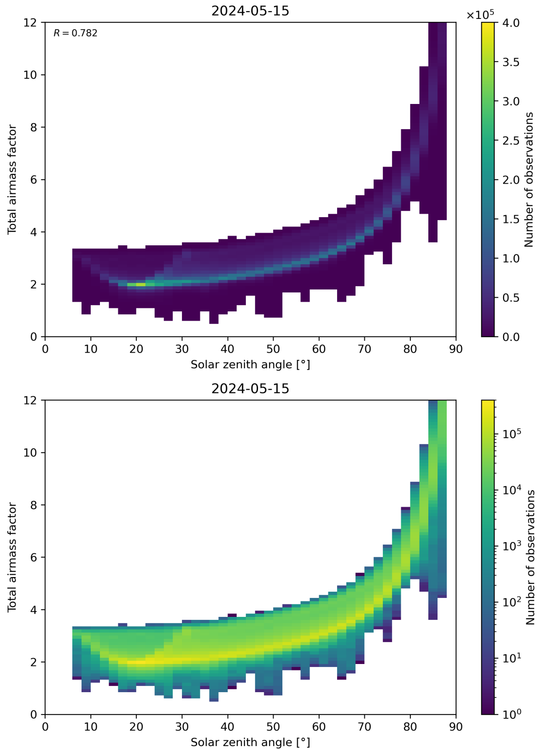
Figure 146: Scatter density plot of “Solar zenith angle” against “Total air mass factor” for 2024-05-14 to 2024-05-16.
