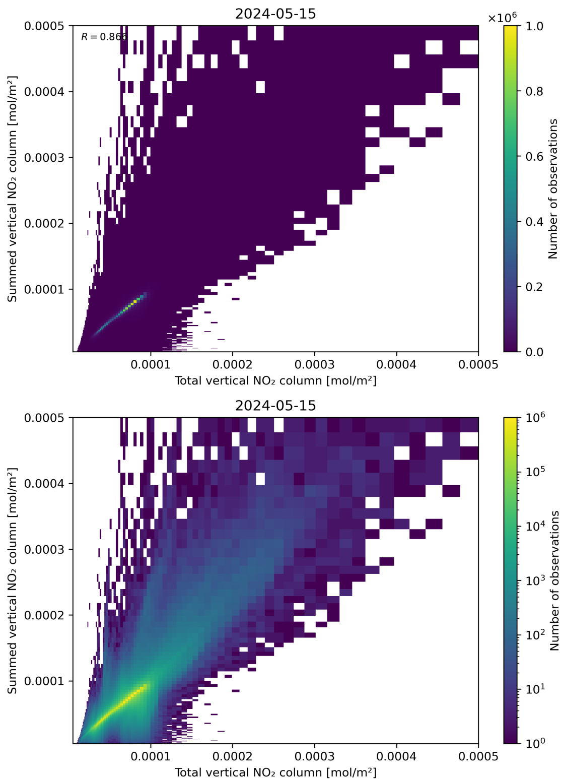
Figure 112: Scatter density plot of “Total vertical NO 2 column” against “Summed vertical NO 2 column” for 2024-05-14 to 2024-05-16.
