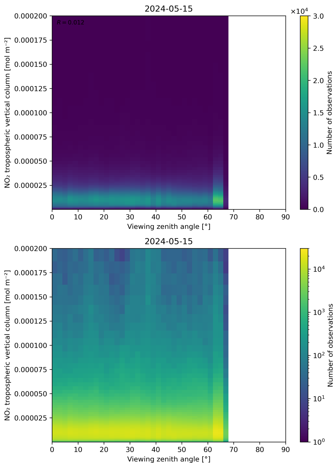
Figure 169: Scatter density plot of “Viewing zenith angle” against “NO 2 tropospheric vertical column” for 2024-05-14 to 2024-05-16.
