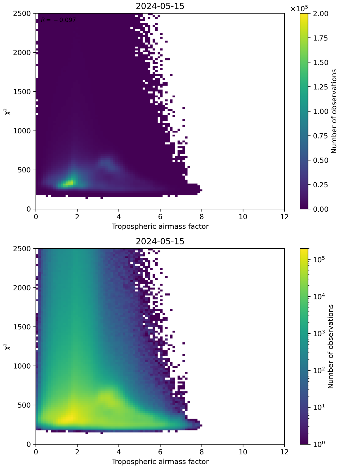
Figure 73: Scatter density plot of “Tropospheric airmass factor” against “ \chi^2 ” for 2024-05-14 to 2024-05-16.
