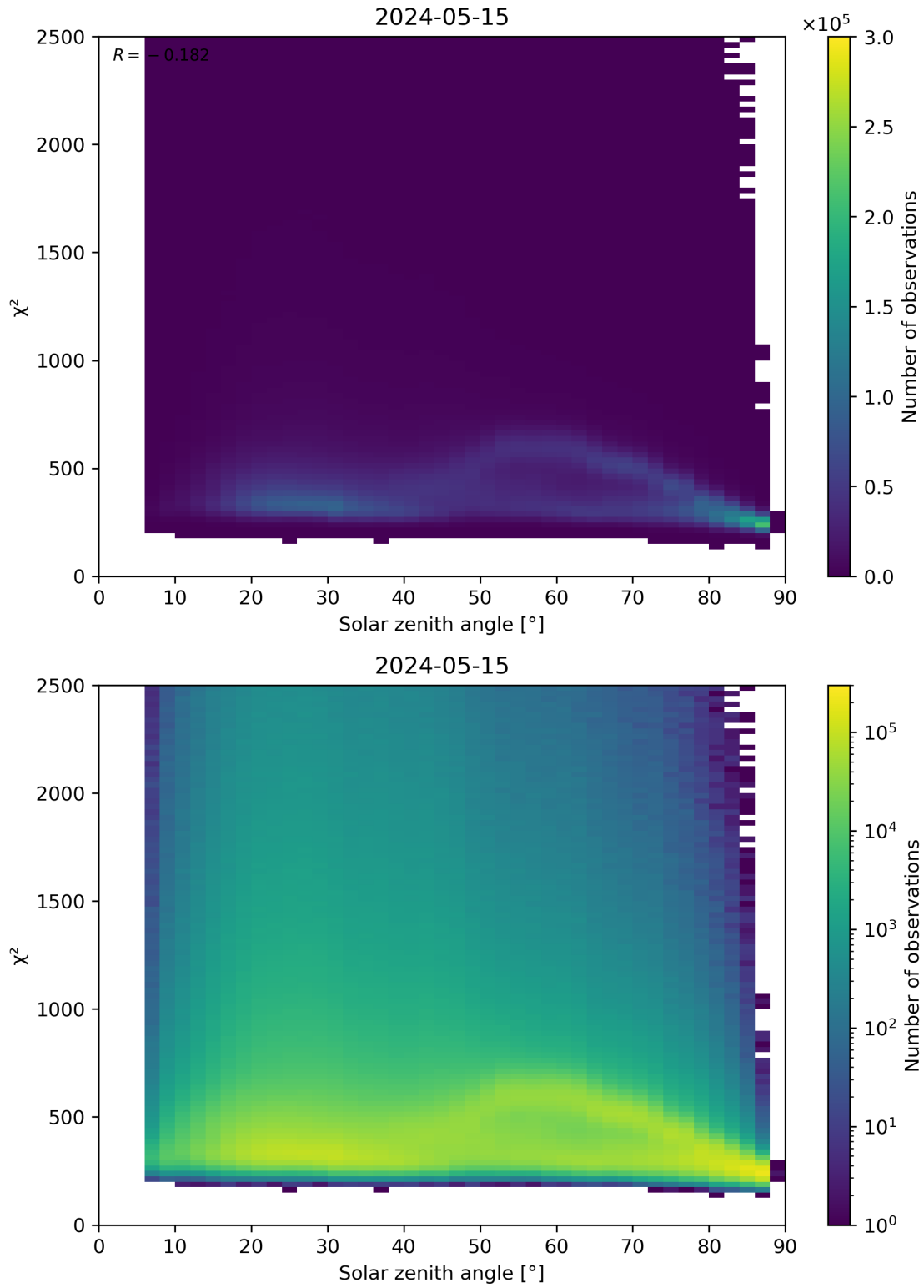
Figure 148: Scatter density plot of “Solar zenith angle” against “ \chi^2 ” for 2024-05-14 to 2024-05-16.
