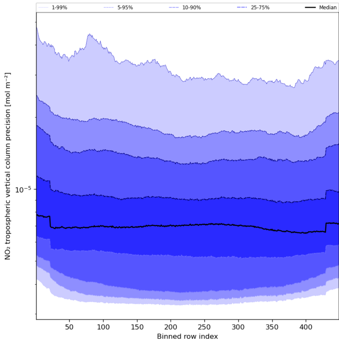
Figure 47: Along track statistics of “NO 2 tropospheric vertical column precision” for 2024-05-14 to 2024-05-16
