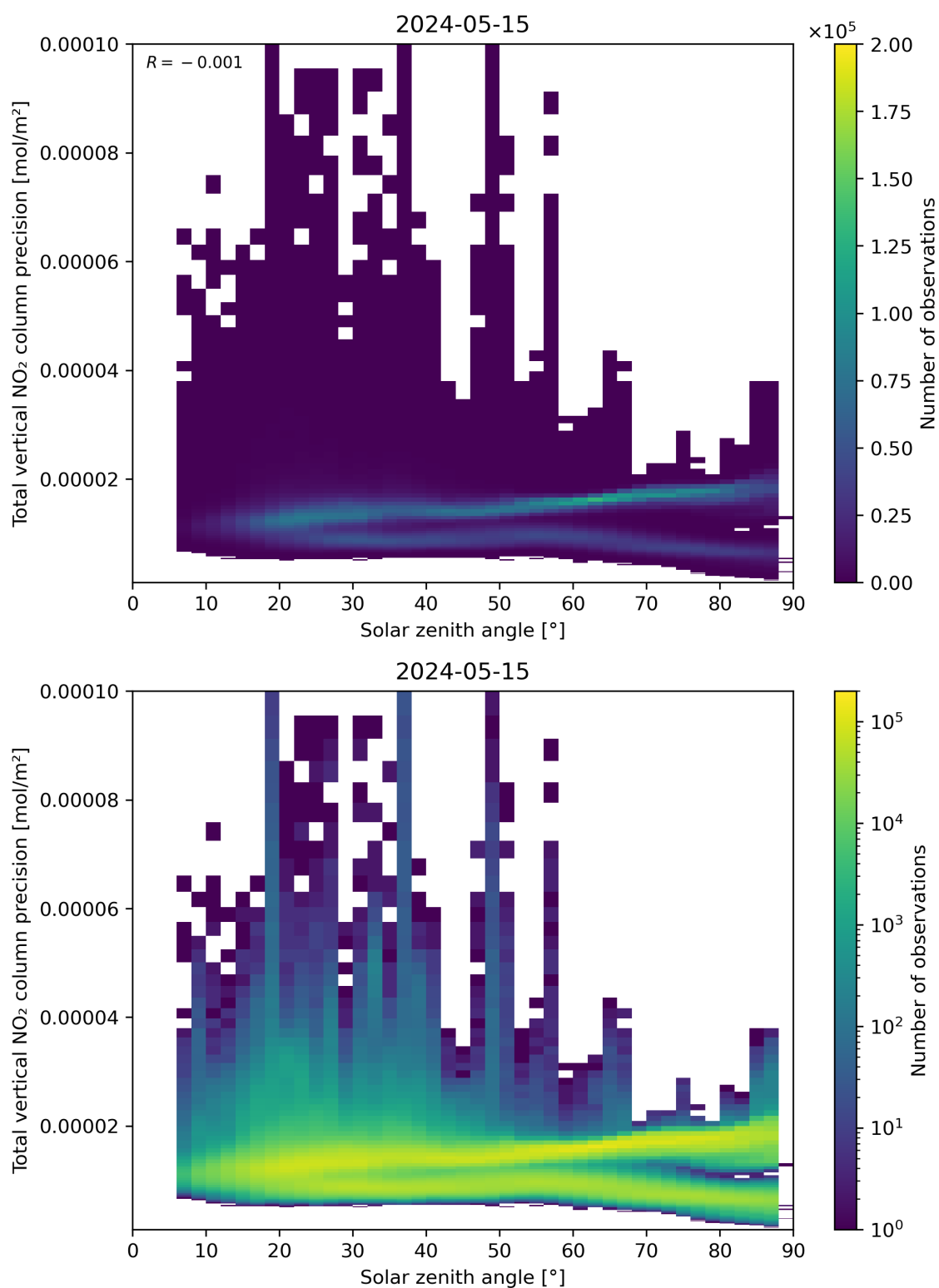
Figure 154: Scatter density plot of “Solar zenith angle” against “Total vertical NO 2 column precision” for 2024-05-14 to 2024-05-16.
