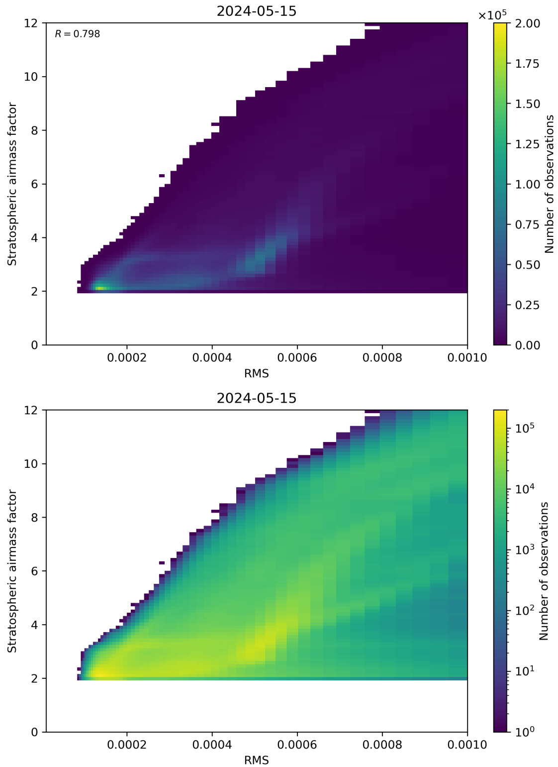
Figure 144: Scatter density plot of “RMS” against “Stratospheric airmass factor” for 2024-05-14 to 2024-05-16.
