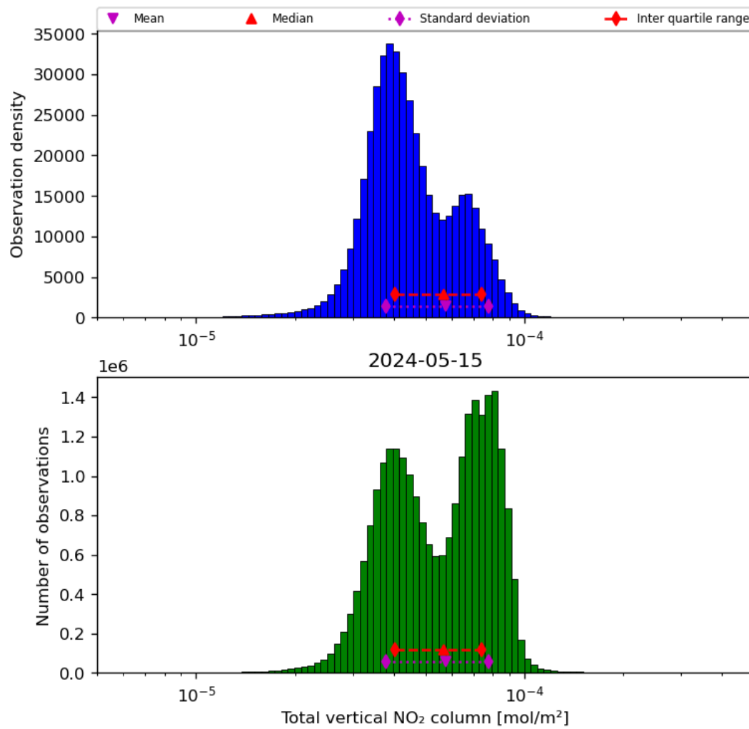
Figure 38: Histogram of “Total vertical NO 2 column” for 2024-05-14 to 2024-05-16
