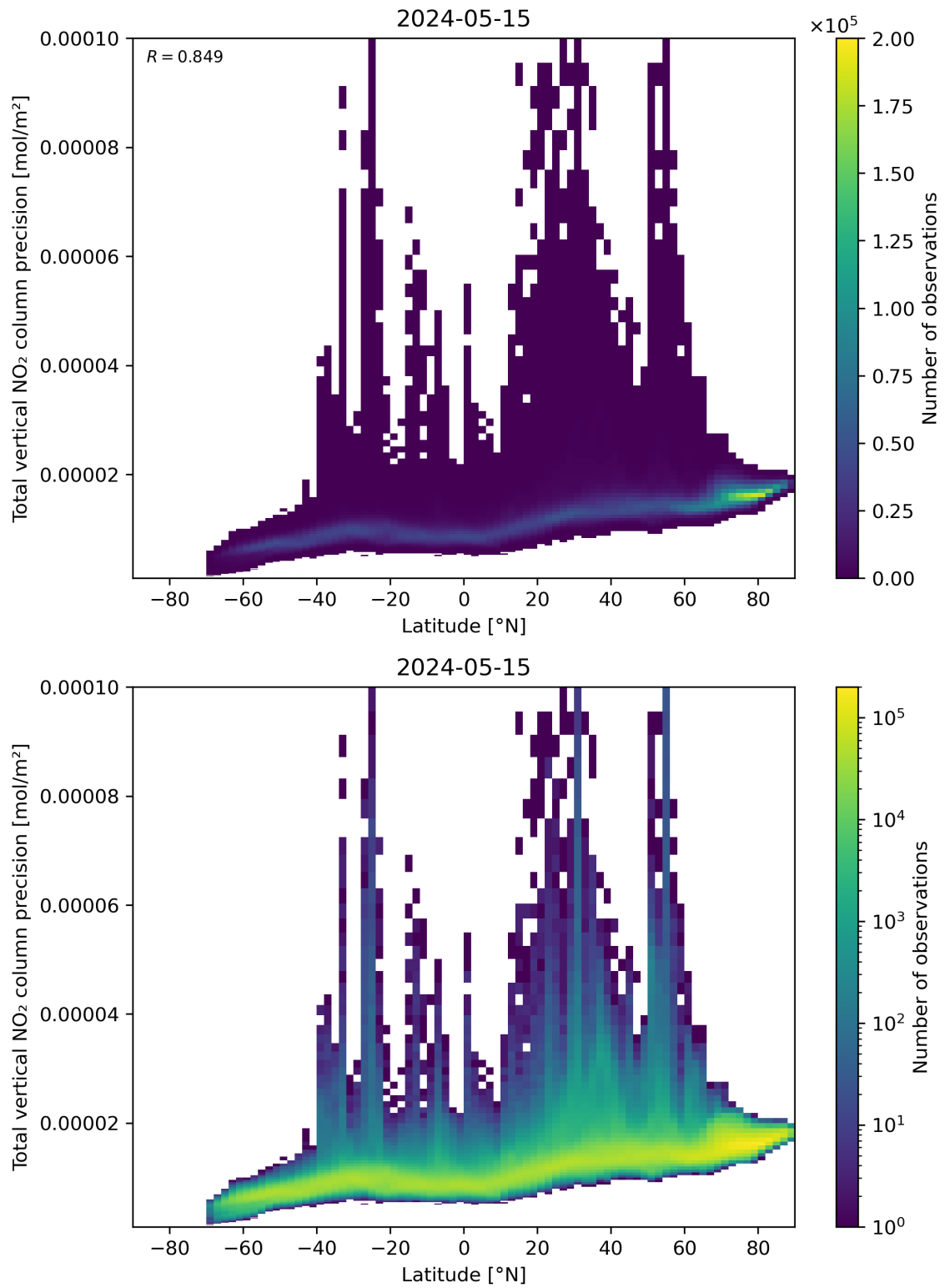
Figure 91: Scatter density plot of “Latitude” against “Total vertical NO 2 column precision” for 2024-05-14 to 2024-05-16.
