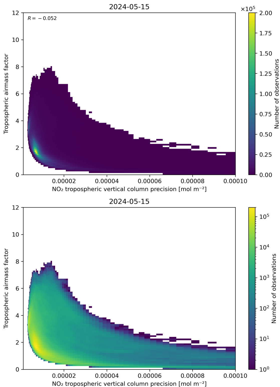
Figure 133: Scatter density plot of “NO 2 tropospheric vertical column precision” against “Tropospheric airmass factor” for 2024-05-14 to 2024-05-16.
