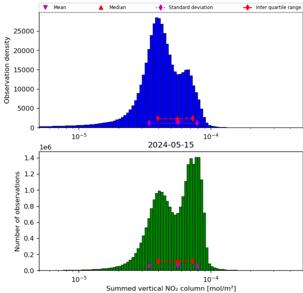
Figure 40: Histogram of “Summed vertical NO 2 column” for 2024-05-14 to 2024-05-16
