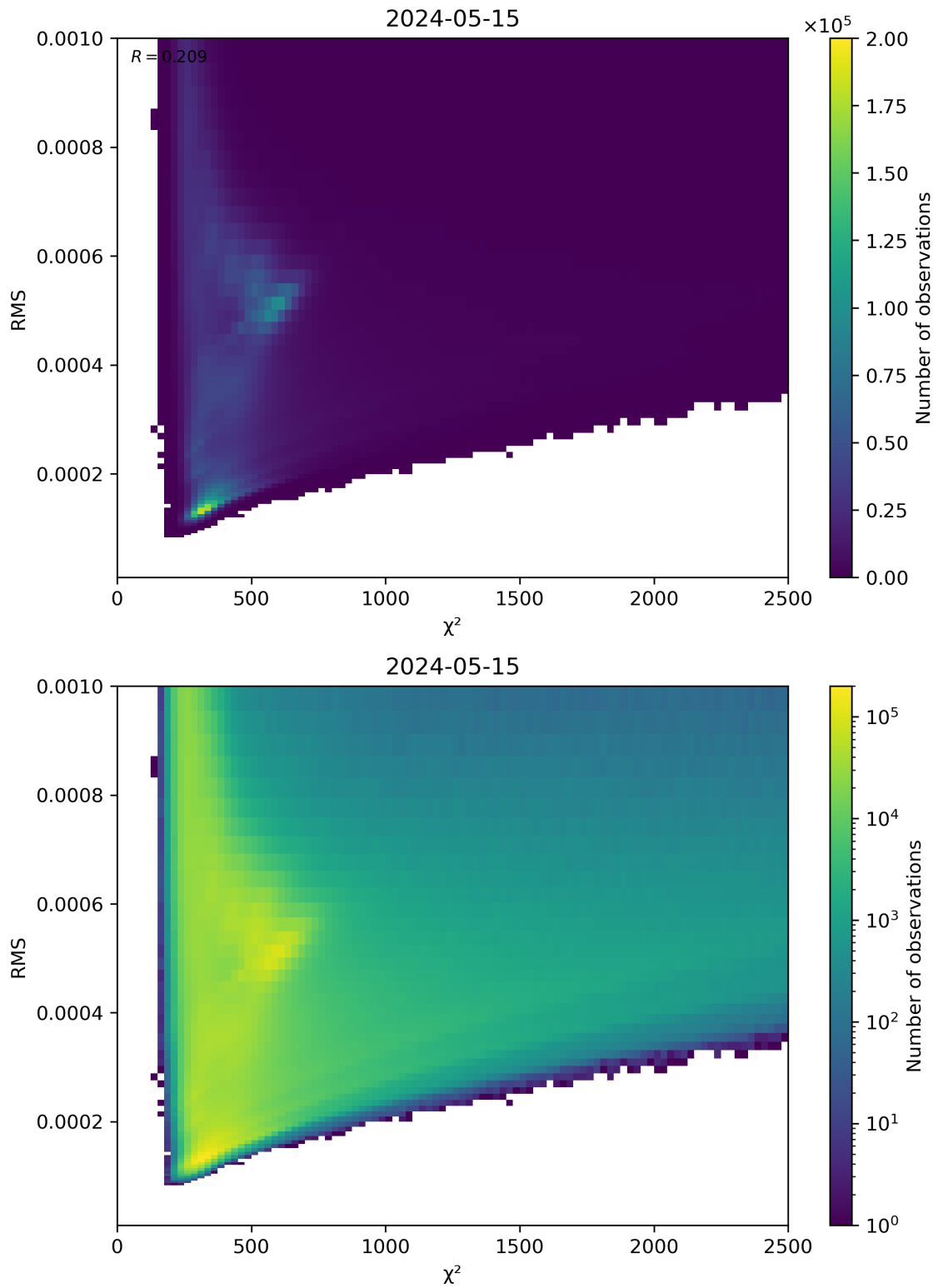
Figure 82: Scatter density plot of “ \chi^2 ” against “RMS” for 2024-05-14 to 2024-05-16.
