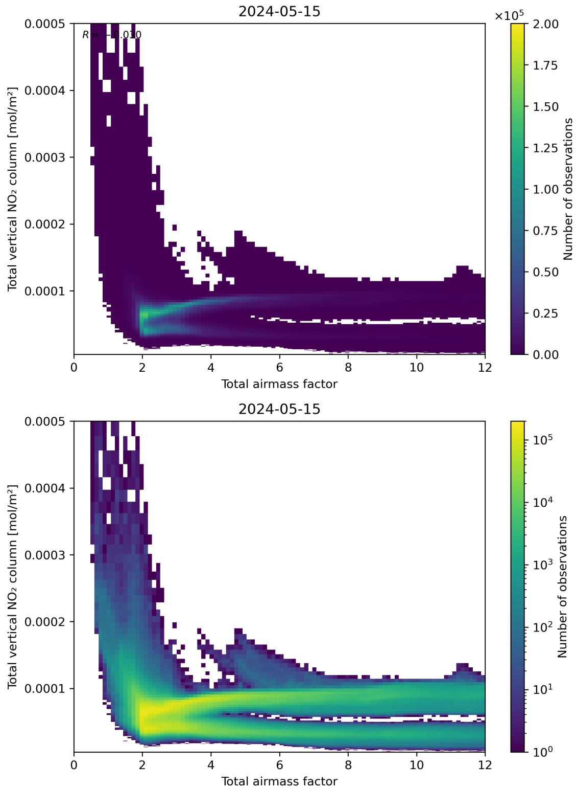
Figure 67: Scatter density plot of “Total air mass factor” against “Total vertical NO 2 column” for 2024-05-14 to 2024-05-16.
