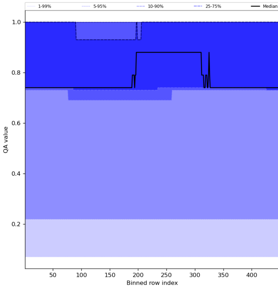
Figure 45: Along track statistics of “QA value” for 2024-05-14 to 2024-05-16
