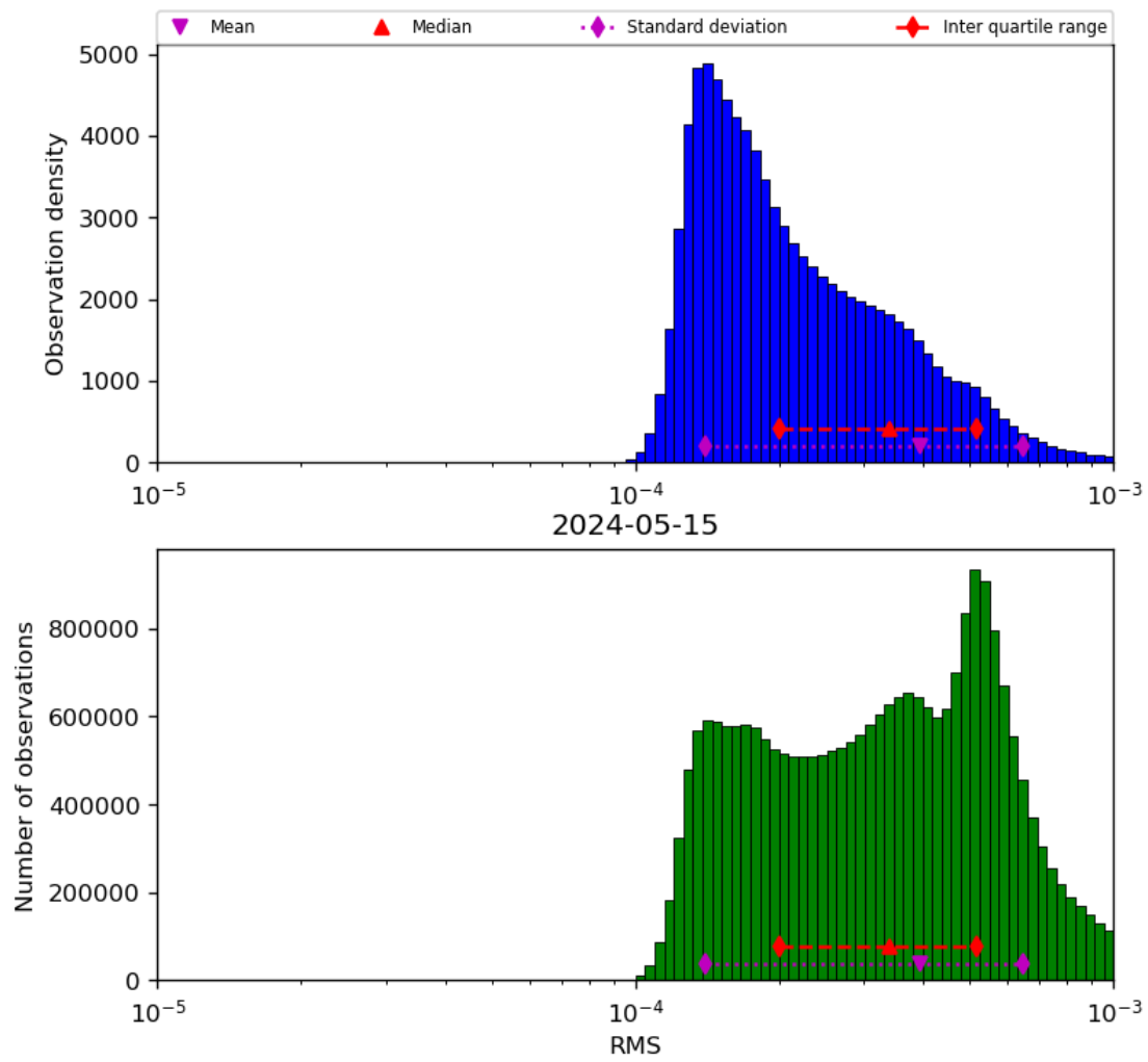
Figure 43: Histogram of “RMS” for 2024-05-14 to 2024-05-16
