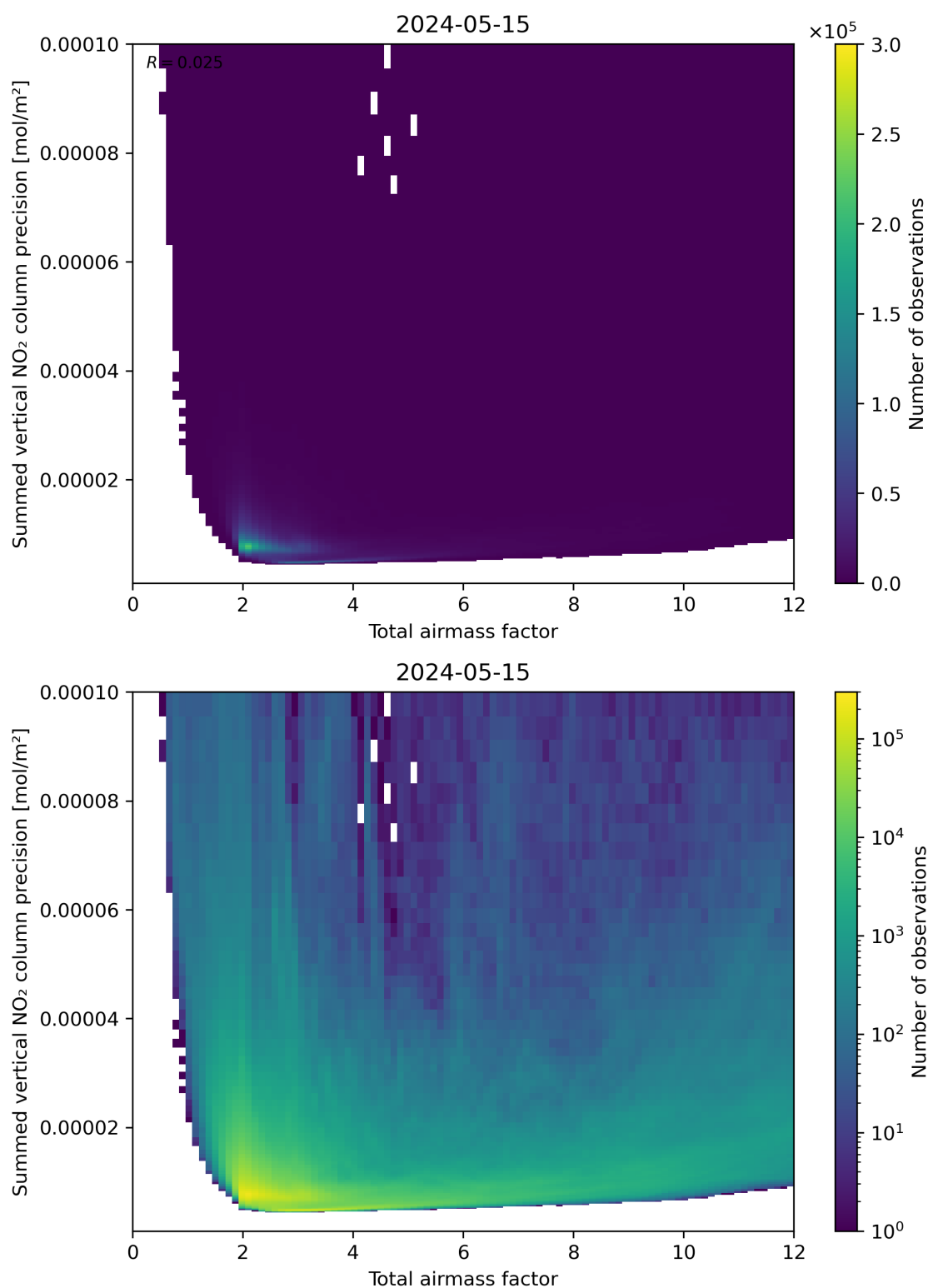
Figure 66: Scatter density plot of “Total airmass factor” against “Summed vertical NO 2 column precision” for 2024-05-14 to 2024-05-16.
