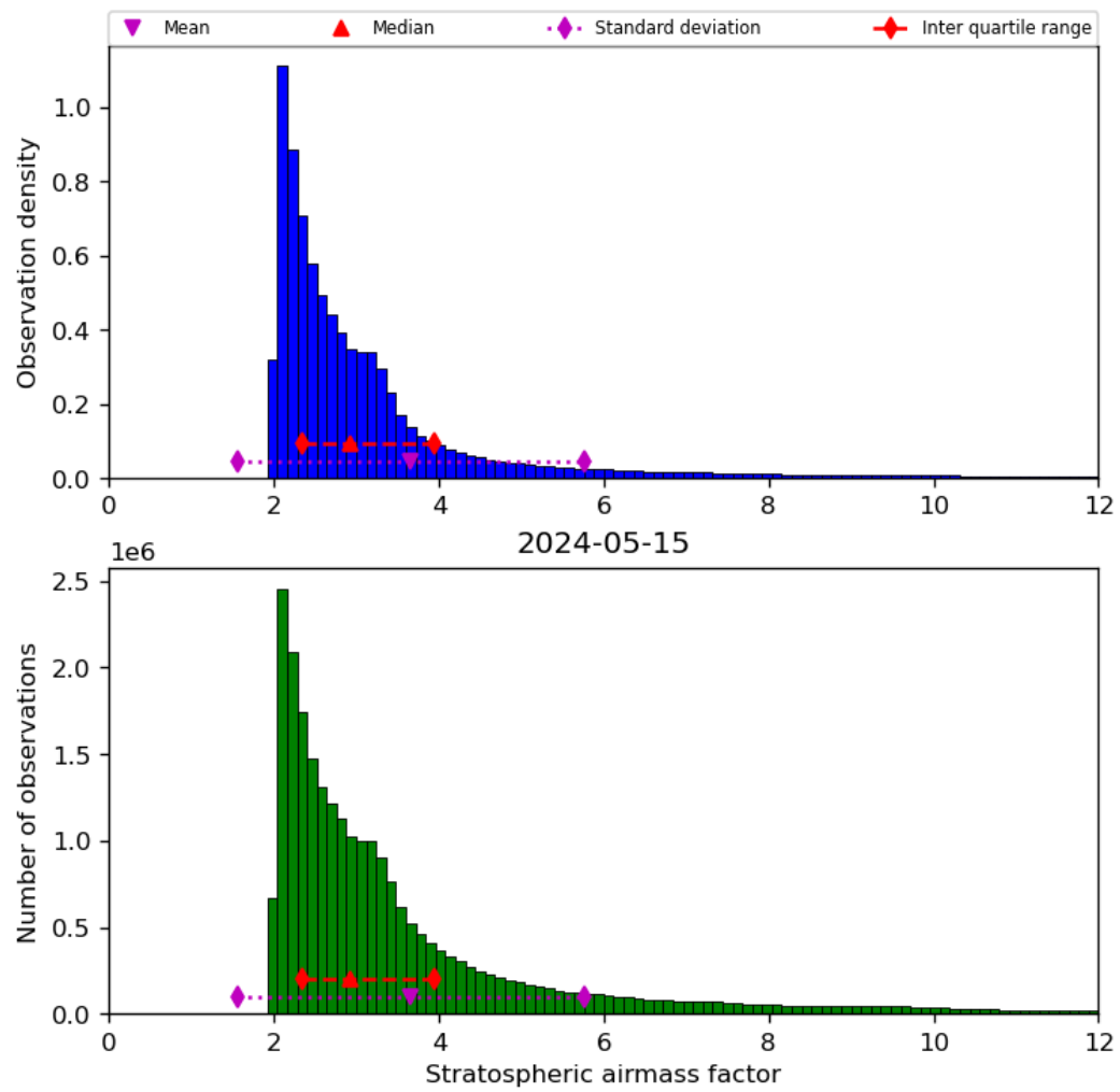
Figure 44: Histogram of “Stratospheric airmass factor” for 2024-05-14 to 2024-05-16
