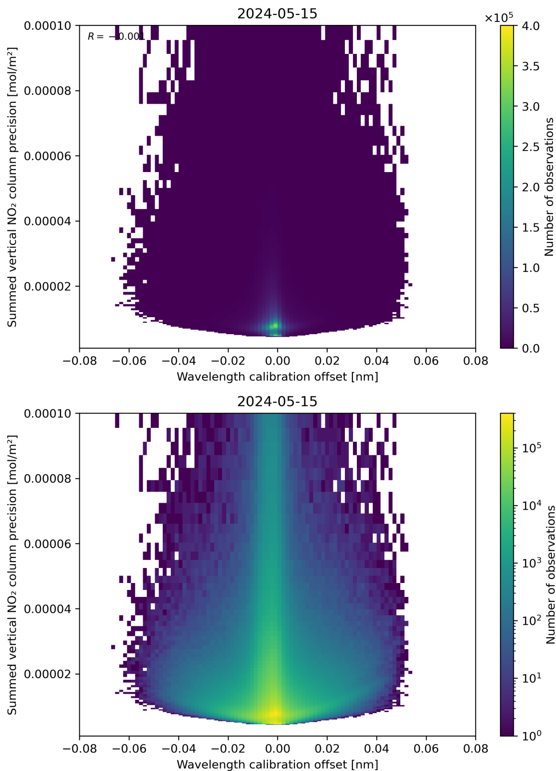
Figure 178: Scatter density plot of “Wavelength calibration offset” against “Summed vertical NO 2 column precision” for 2024-05-14 to 2024-05-16.
