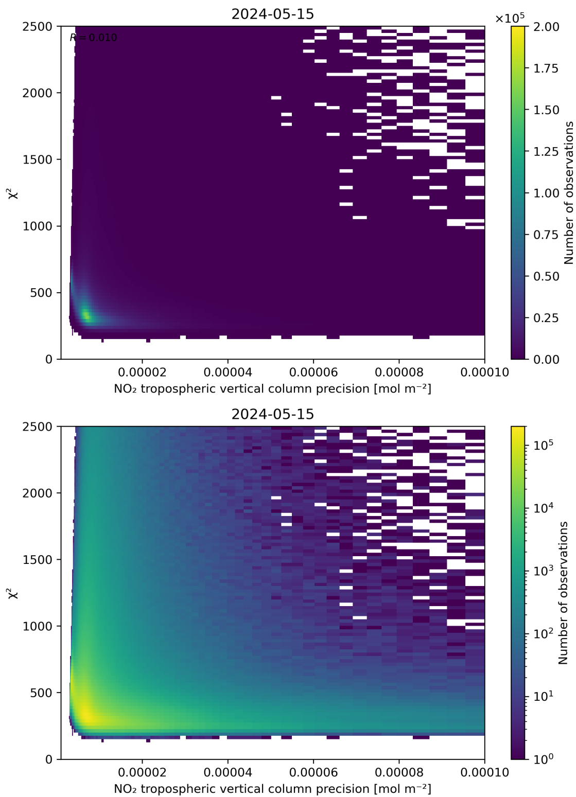
Figure 134: Scatter density plot of “NO 2 tropospheric vertical column precision” against “ \chi^2 ” for 2024-05-14 to 2024-05-16.
