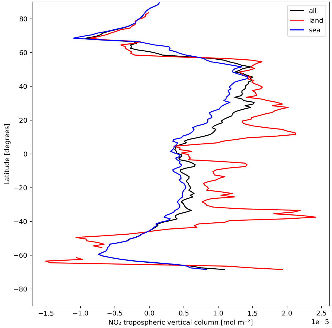
Figure 12: Zonal average of “NO 2 tropospheric vertical column” for 2024-05-14 to 2024-05-16.
