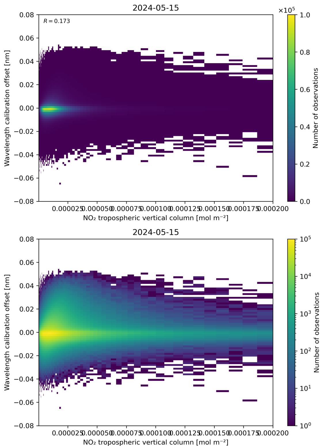
Figure 143: Scatter density plot of “NO 2 tropospheric vertical column” against “Wavelength calibration offset” for 2024-05-14 to 2024-05-16.
