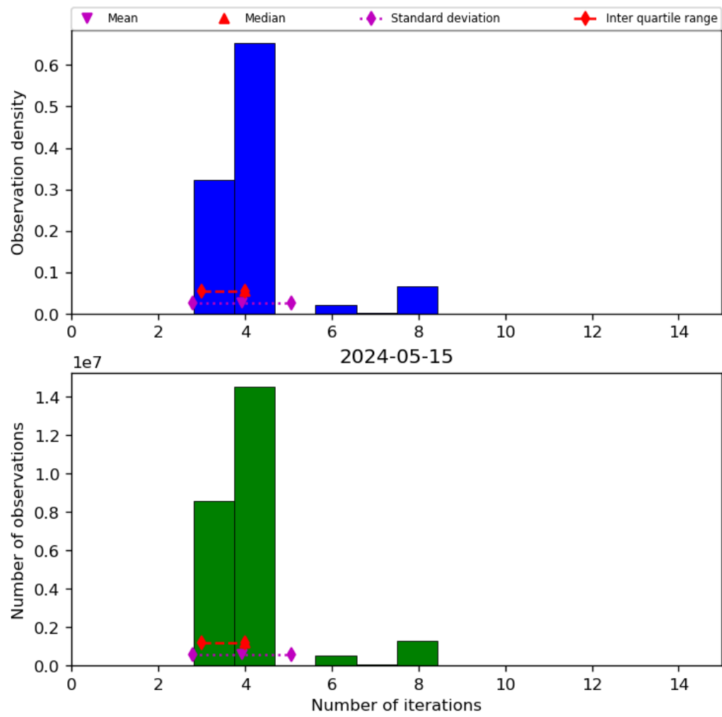
Figure 34: Histogram of “Number of iterations” for 2024-05-14 to 2024-05-16
