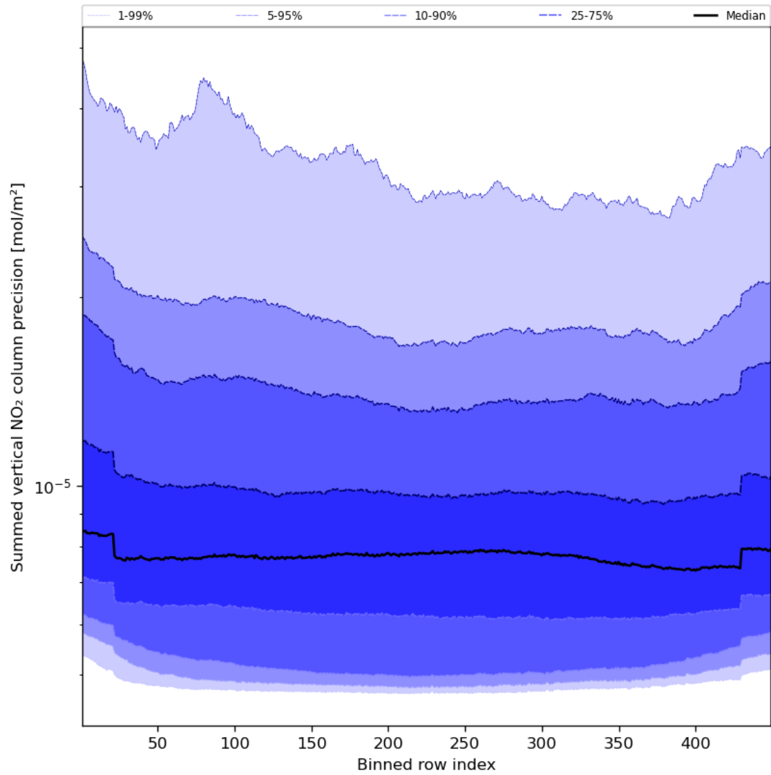
Figure 58: Along track statistics of “Summed vertical NO 2 column precision” for 2024-05-14 to 2024-05-16
