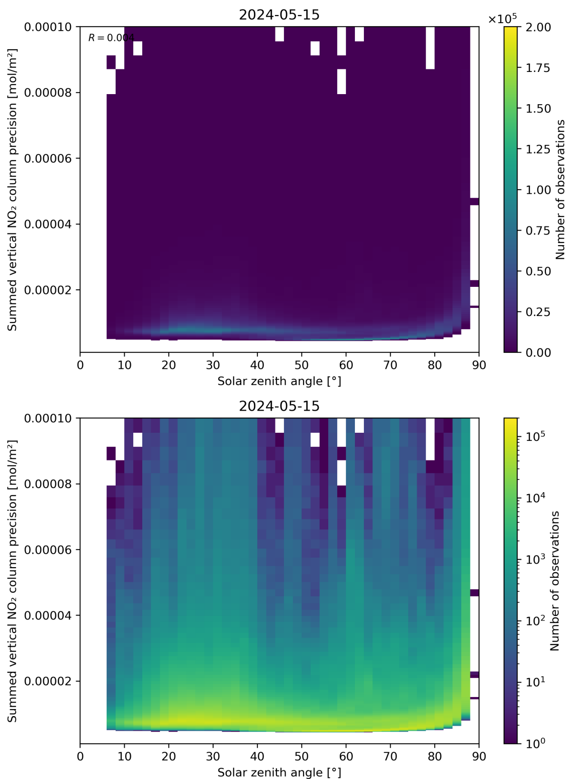
Figure 152: Scatter density plot of “Solar zenith angle” against “Summed vertical NO 2 column precision” for 2024-05-14 to 2024-05-16.
