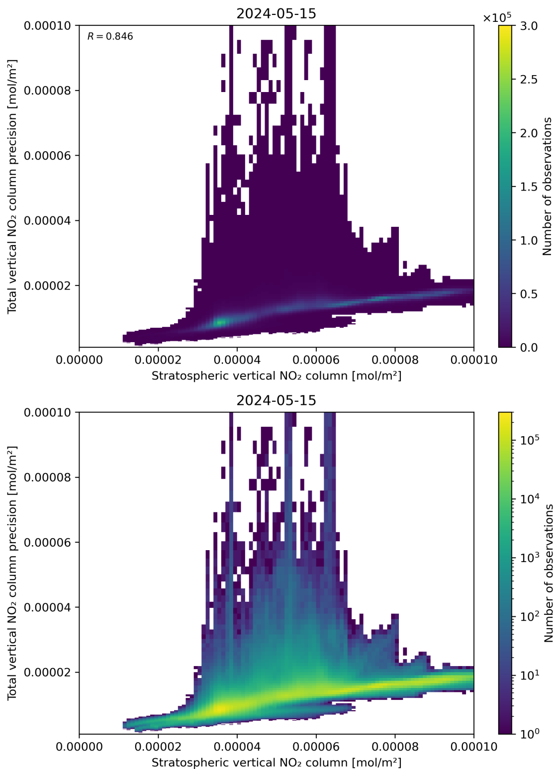
Figure 101: Scatter density plot of “Stratospheric vertical NO 2 column” against “Total vertical NO 2 column precision” for 2024-05-14 to 2024-05-16.
