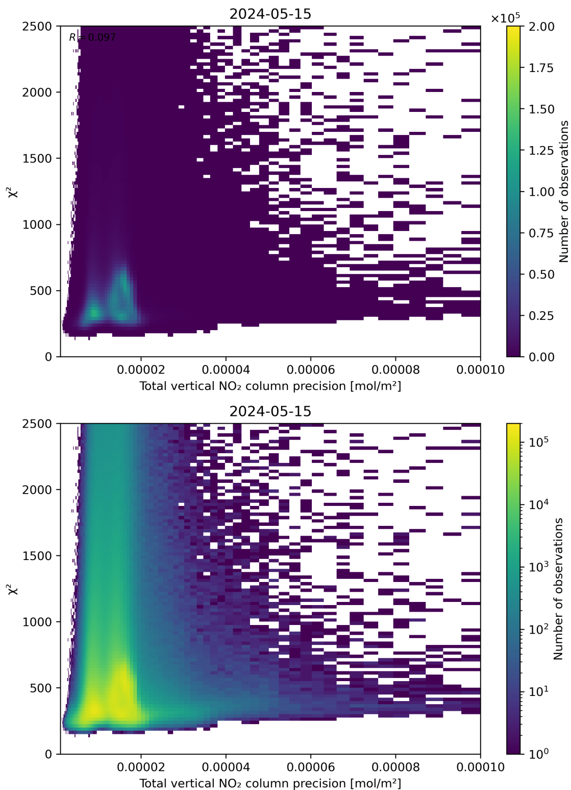
Figure 116: Scatter density plot of “Total vertical NO 2 column precision” against “ \chi^2 ” for 2024-05-14 to 2024-05-16.
