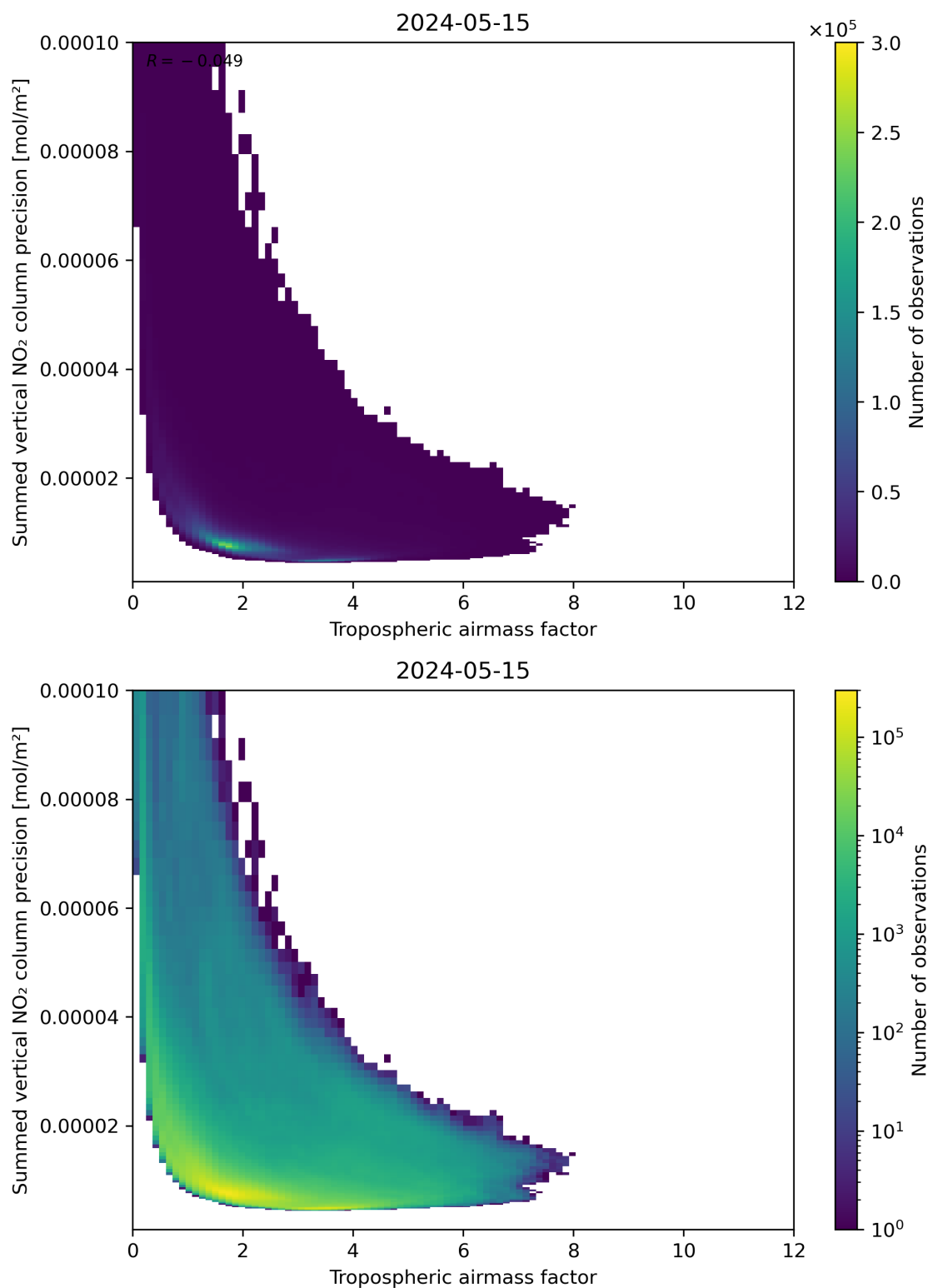
Figure 76: Scatter density plot of “Tropospheric air mass factor” against “Summed vertical NO 2 column precision” for 2024-05-14 to 2024-05-16.
