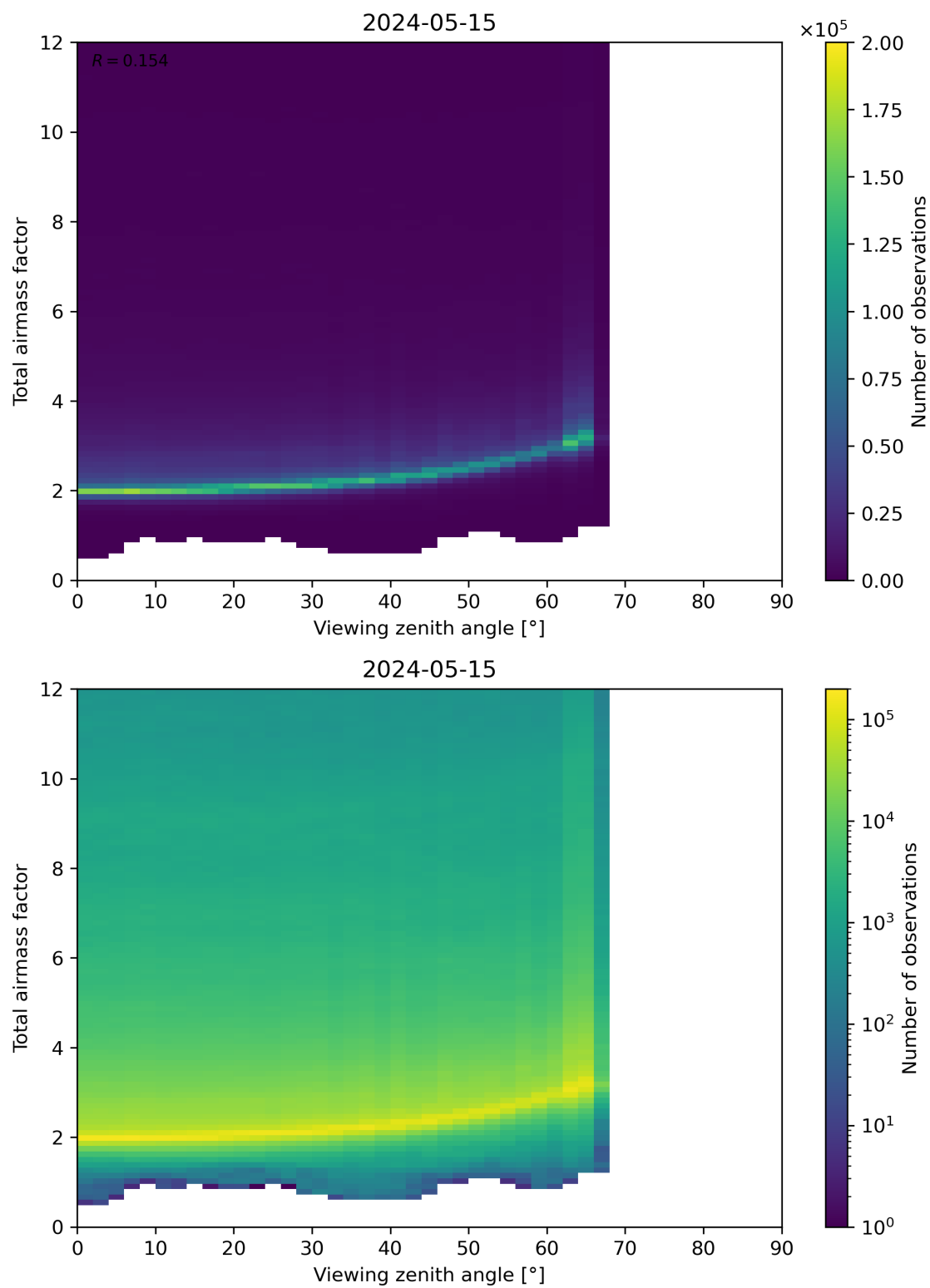
Figure 160: Scatter density plot of “Viewing zenith angle” against “Total airmass factor” for 2024-05-14 to 2024-05-16.
