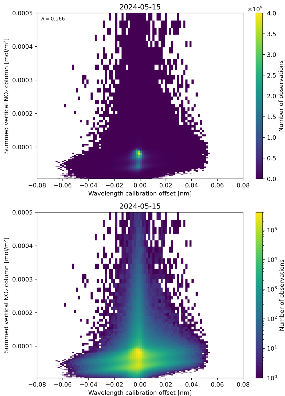
Figure 177: Scatter density plot of “Wavelength calibration offset” against “Summed vertical NO 2 column” for 2024-05-14 to 2024-05-16.
