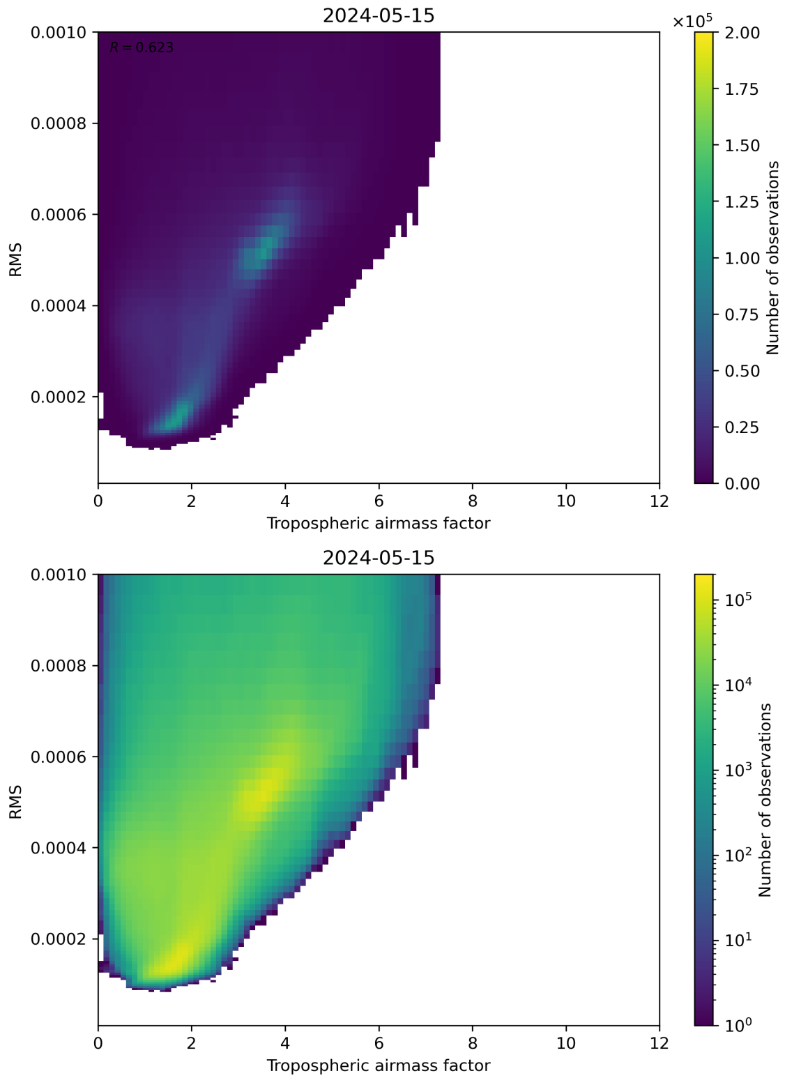
Figure 79: Scatter density plot of “Tropospheric airmass factor” against “RMS” for 2024-05-14 to 2024-05-16.
