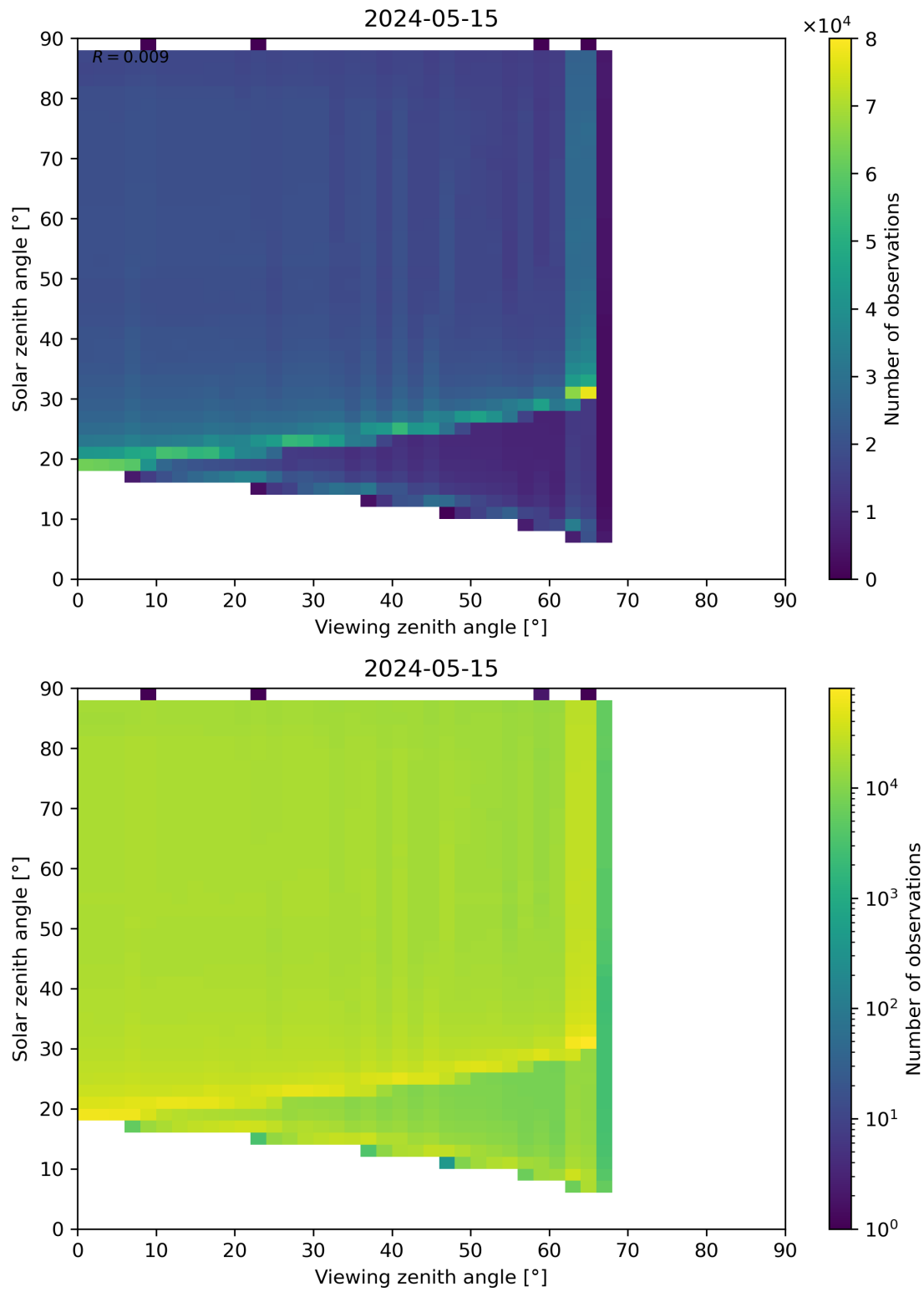
Figure 172: Scatter density plot of “Viewing zenith angle” against “Solar zenith angle” for 2024-05-14 to 2024-05-16.
