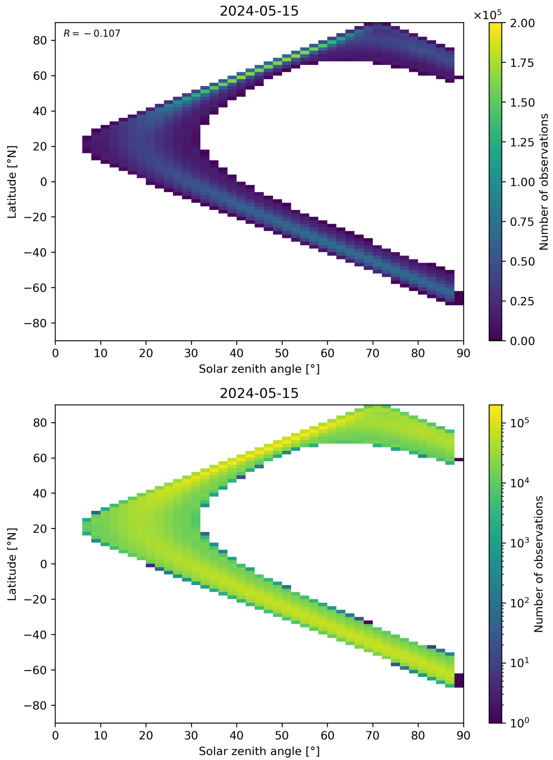
Figure 149: Scatter density plot of “Solar zenith angle” against “Latitude” for 2024-05-14 to 2024-05-16.
