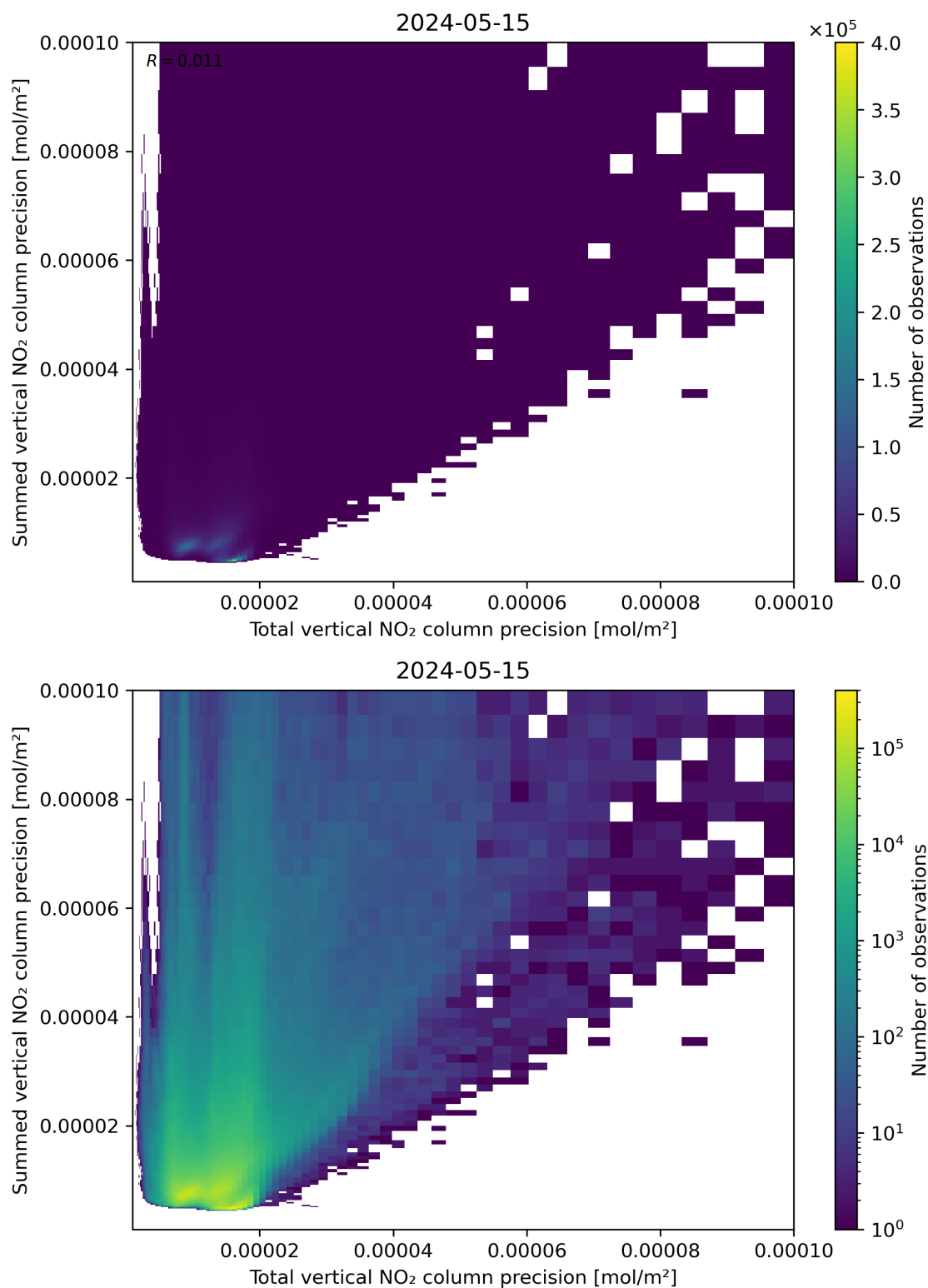
Figure 118: Scatter density plot of “Total vertical NO 2 column precision” against “Summed vertical NO 2 column precision” for 2024-05-14 to 2024-05-16.
