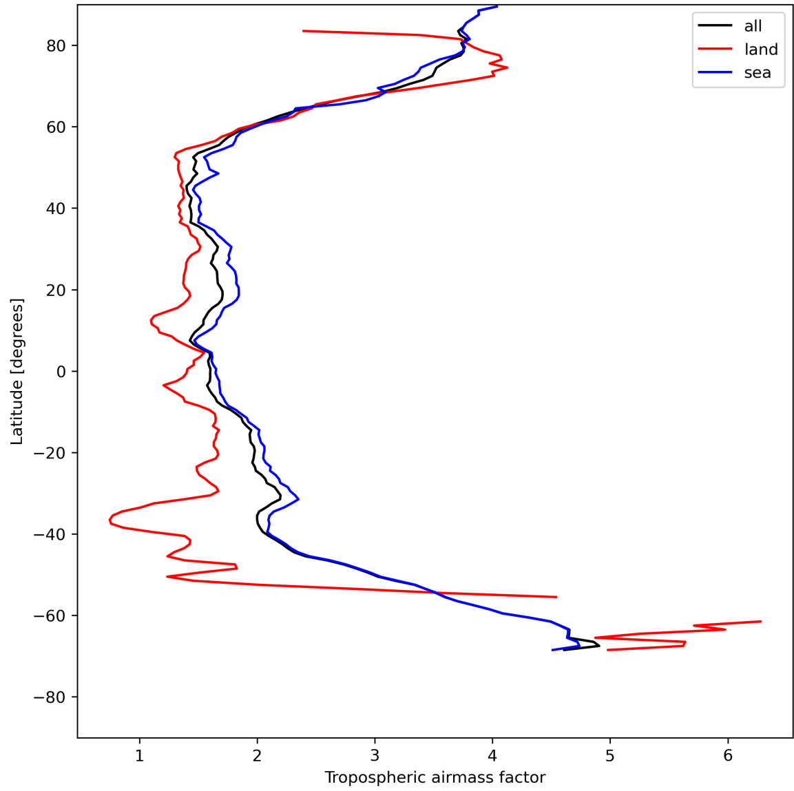
Figure 14: Zonal average of “Tropospheric airmass factor” for 2024-05-14 to 2024-05-16.
