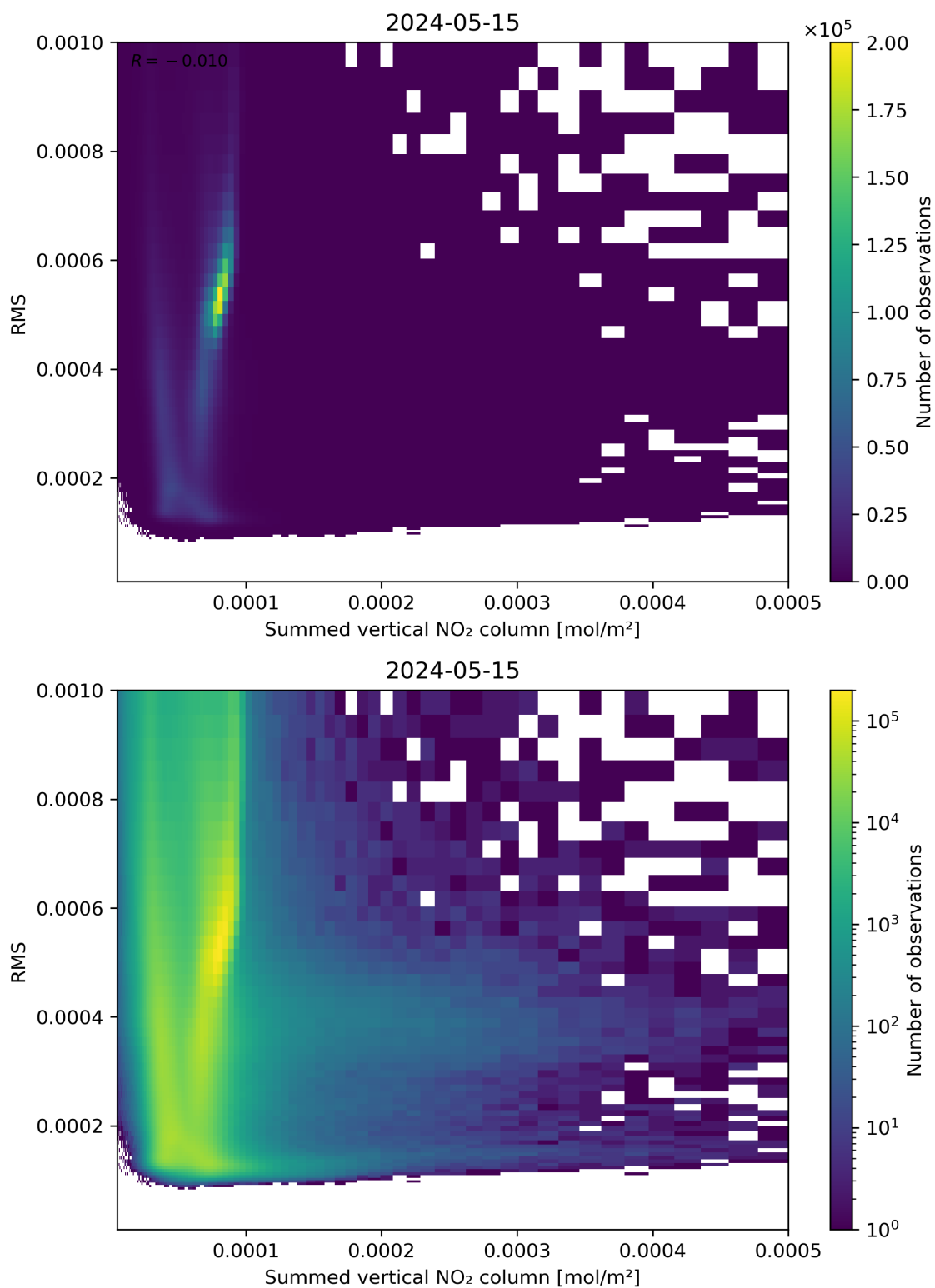
Figure 109: Scatter density plot of “Summed vertical NO 2 column” against “RMS” for 2024-05-14 to 2024-05-16.
