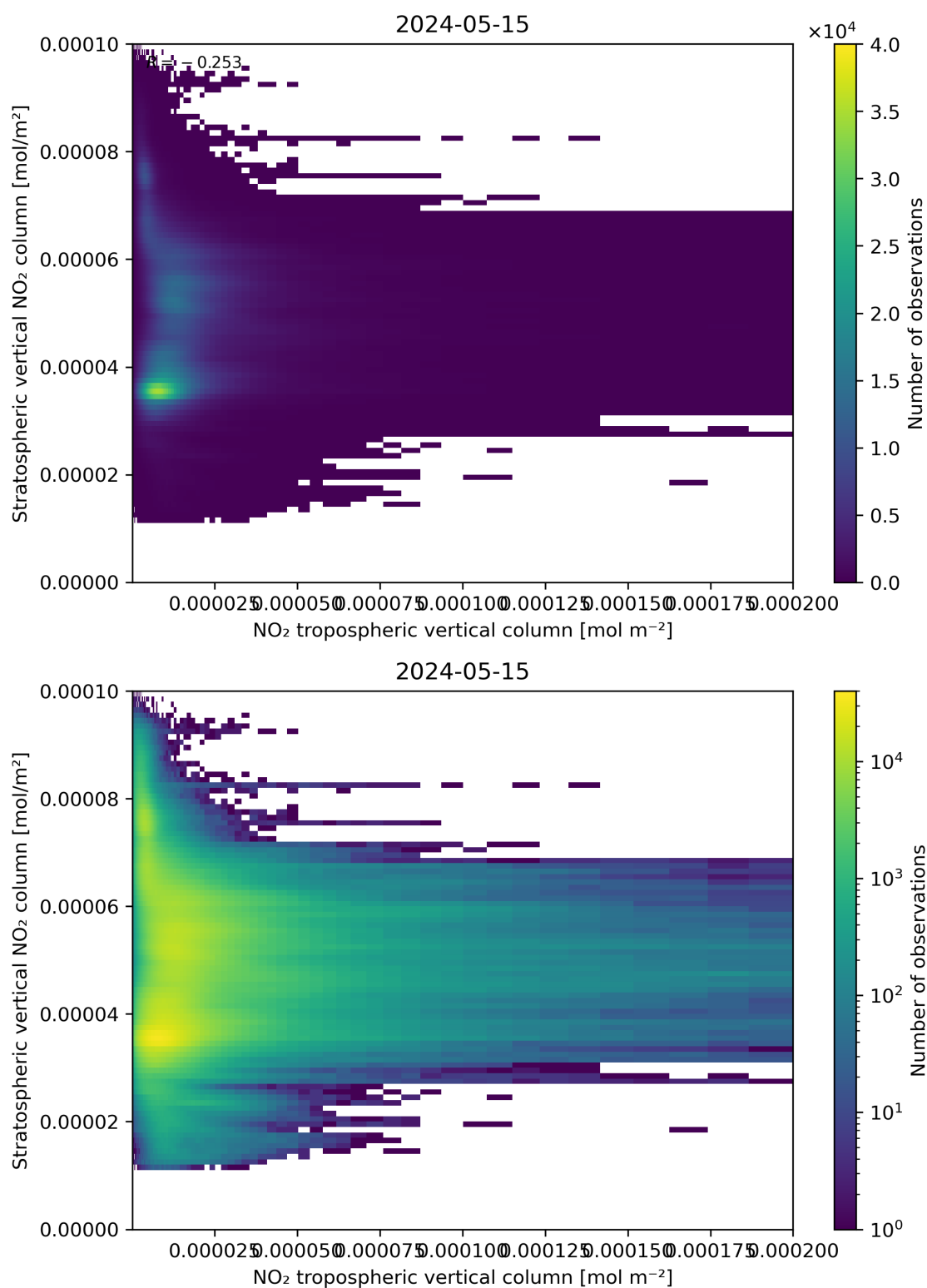
Figure 125: Scatter density plot of “NO 2 tropospheric vertical column” against “Stratospheric vertical NO 2 column” for 2024-05-14 to 2024-05-16.
