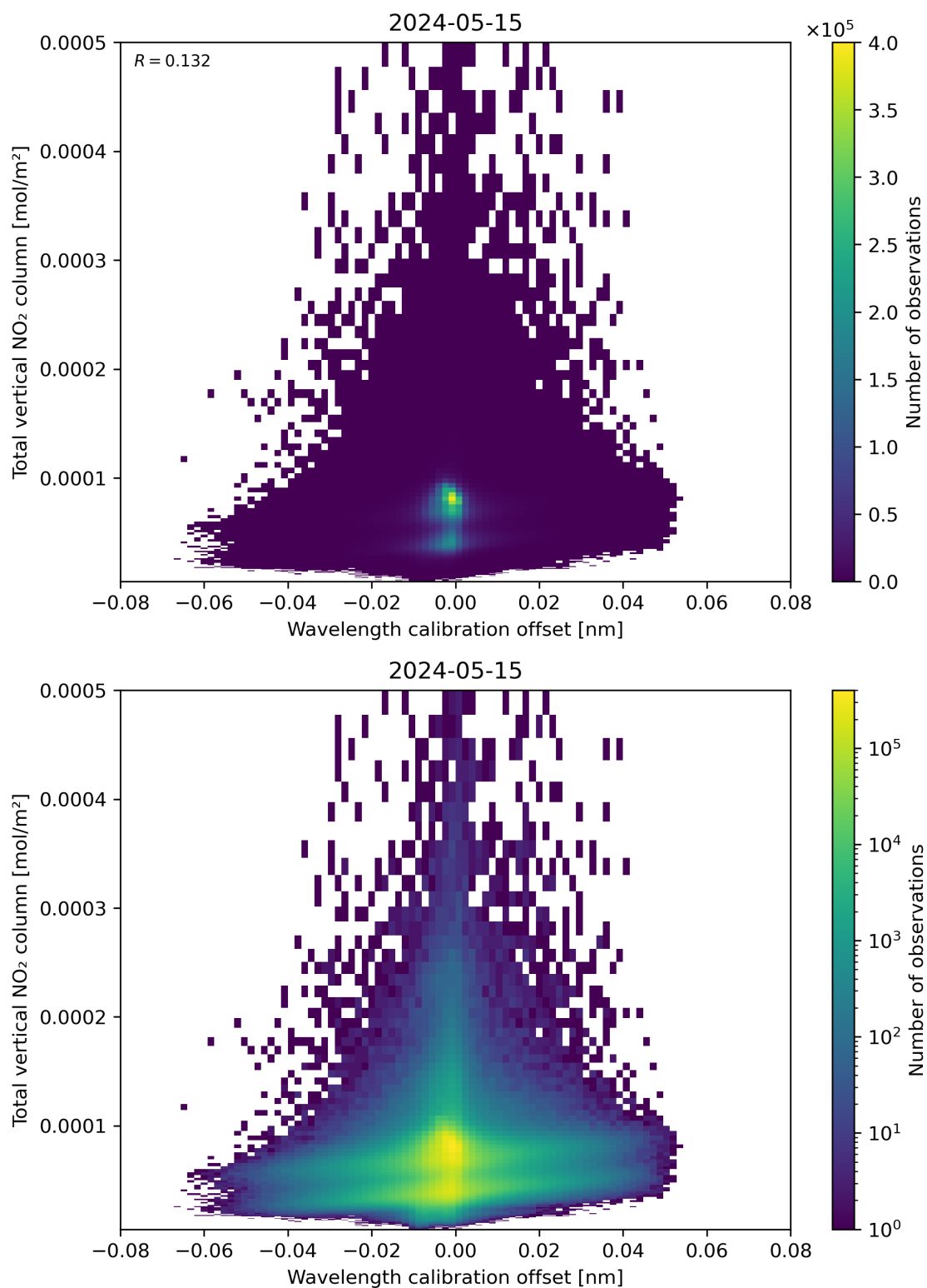
Figure 179: Scatter density plot of “Wavelength calibration offset” against “Total vertical NO 2 column” for 2024-05-14 to 2024-05-16.
