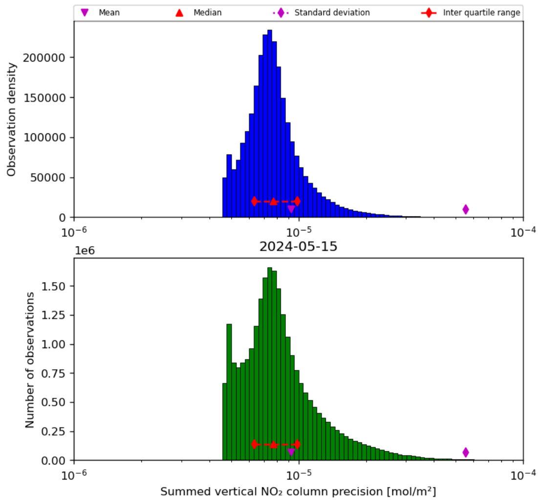
Figure 41: Histogram of “Summed vertical NO 2 column precision” for 2024-05-14 to 2024-05-16
