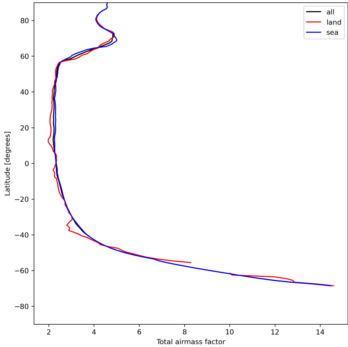
Figure 15: Zonal average of “Total airmass factor” for 2024-05-14 to 2024-05-16.
