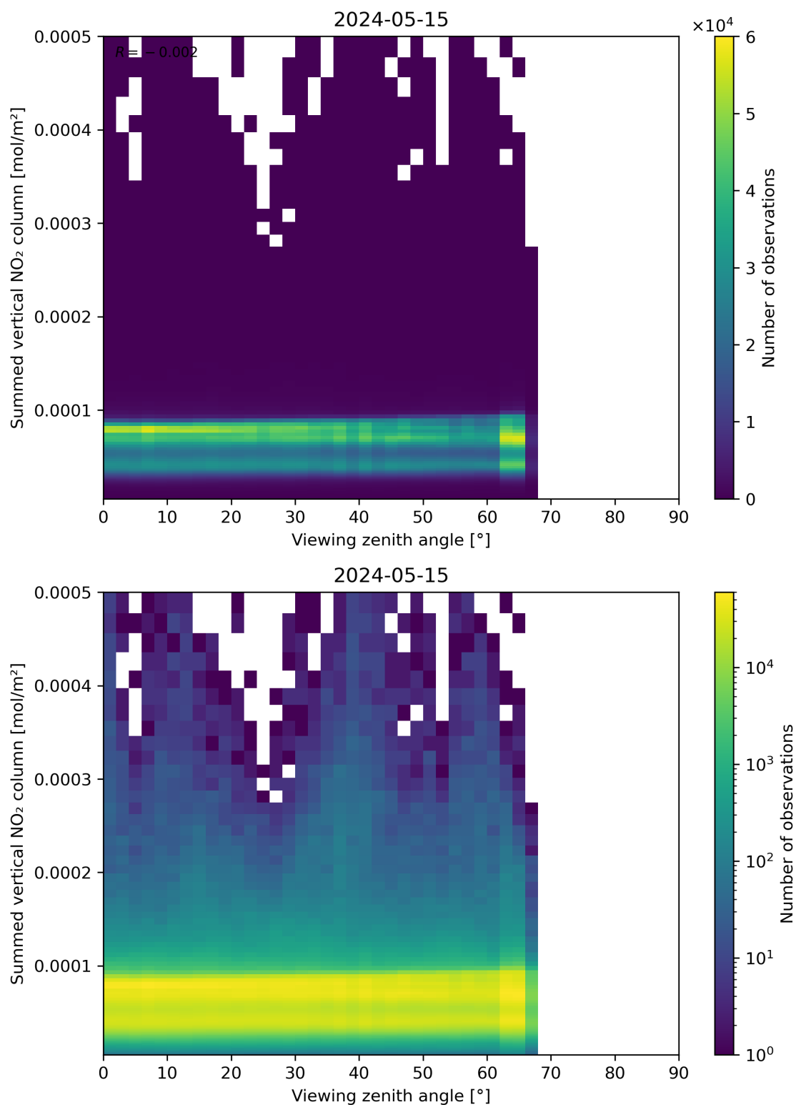
Figure 165: Scatter density plot of “Viewing zenith angle” against “Summed vertical NO 2 column” for 2024-05-14 to 2024-05-16.
