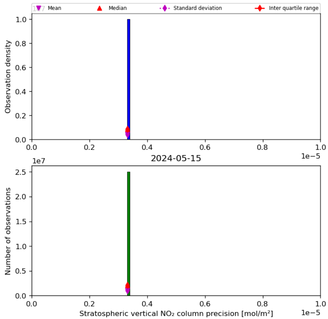
Figure 37: Histogram of “Stratospheric vertical NO 2 column precision” for 2024-05-14 to 2024-05-16
