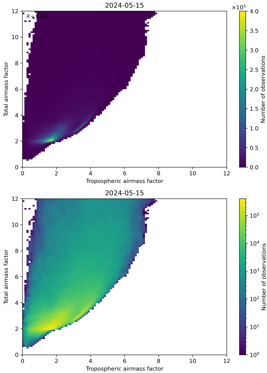
Figure 72: Scatter density plot of “Tropospheric airmass factor” against “Total airmass factor” for 2024-05-14 to 2024-05-16.
