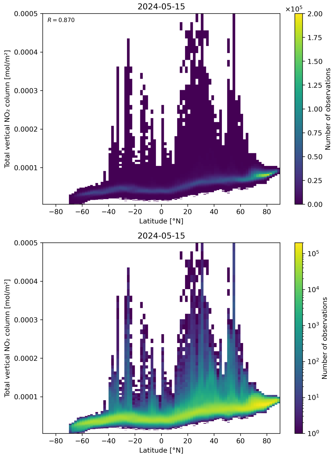
Figure 90: Scatter density plot of “Latitude” against “Total vertical NO 2 column” for 2024-05-14 to 2024-05-16.
