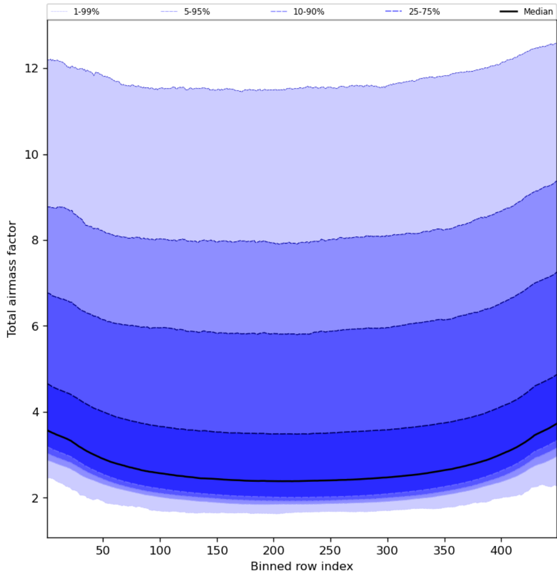
Figure 49: Along track statistics of “Total airmass factor” for 2024-05-14 to 2024-05-16
