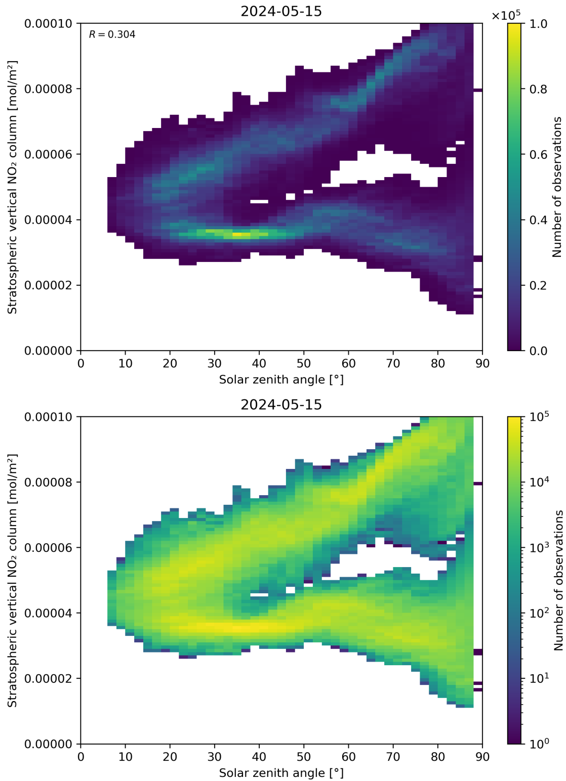
Figure 150: Scatter density plot of “Solar zenith angle” against “Stratospheric vertical NO 2 column” for 2024-05-14 to 2024-05-16.
