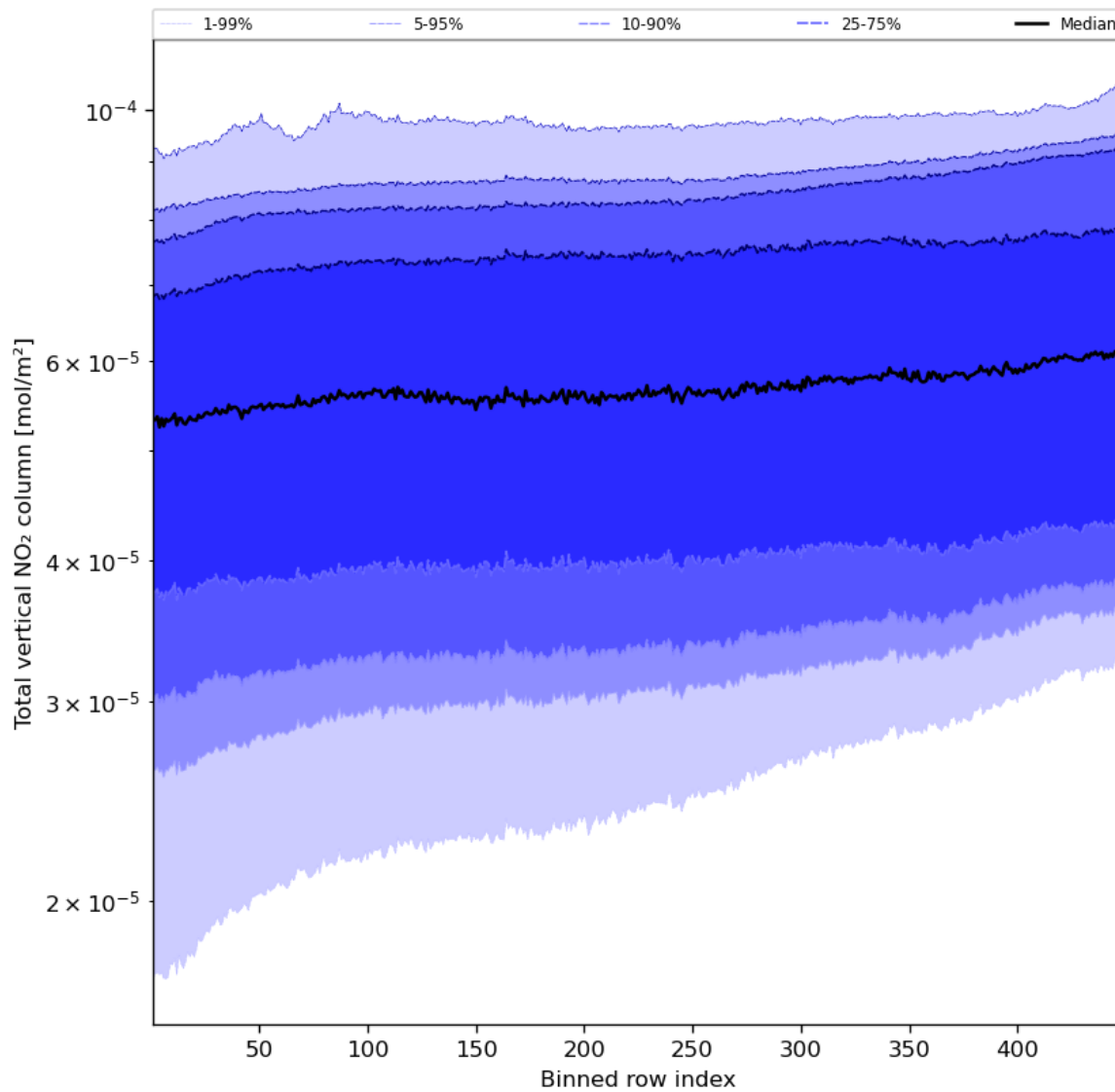
Figure 55: Along track statistics of “Total vertical NO 2 column” for 2024-05-14 to 2024-05-16
