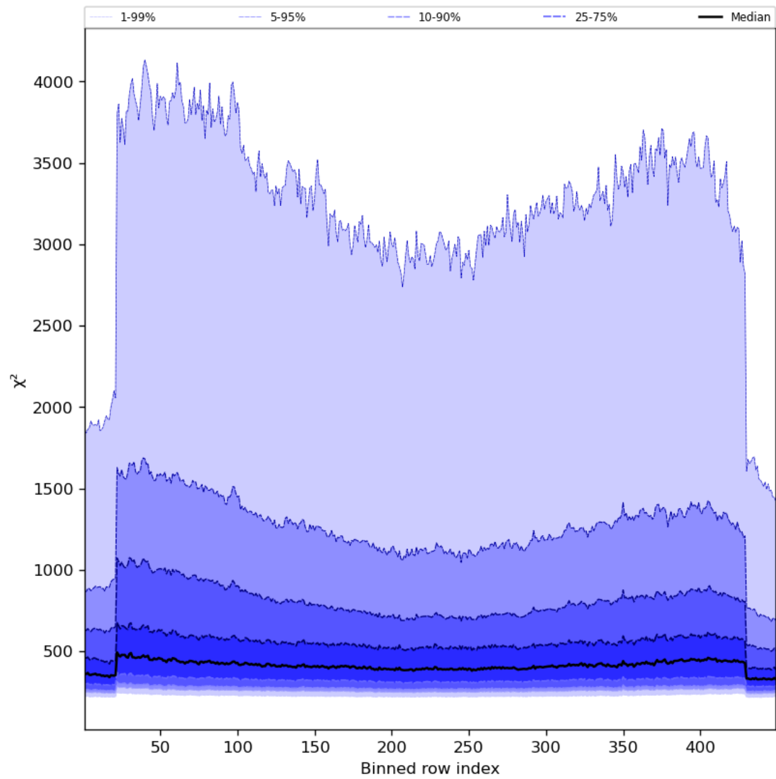
Figure 59: Along track statistics of “ \chi^2 ” for 2024-05-14 to 2024-05-16
