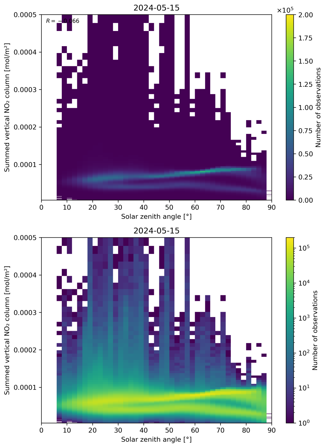
Figure 151: Scatter density plot of “Solar zenith angle” against “Summed vertical NO 2 column” for 2024-05-14 to 2024-05-16.
