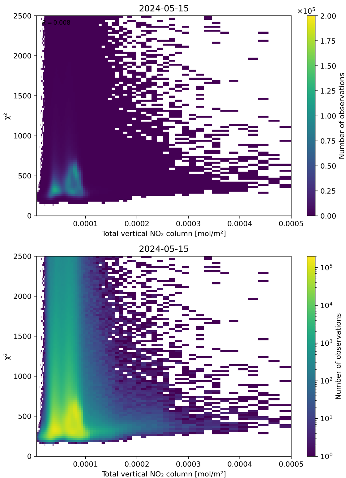
Figure 111: Scatter density plot of “Total vertical NO 2 column” against “ \chi^2 ” for 2024-05-14 to 2024-05-16.
