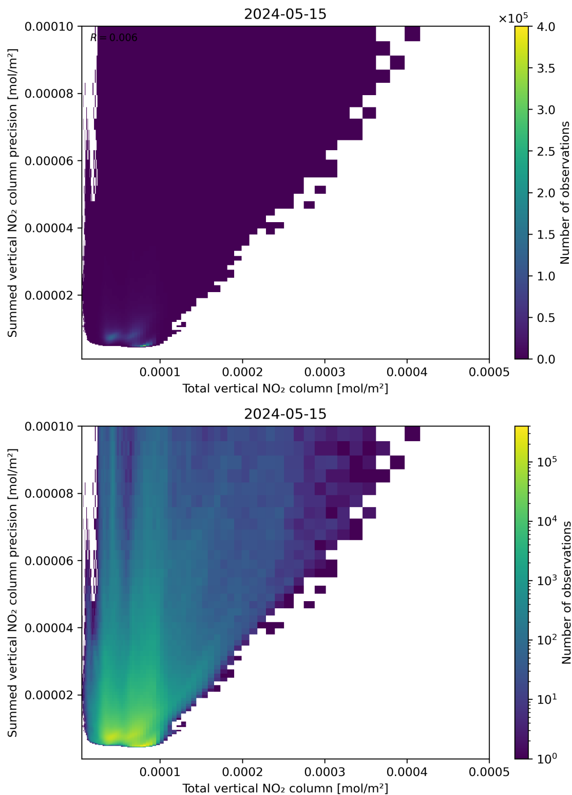
Figure 113: Scatter density plot of “Total vertical NO 2 column” against “Summed vertical NO 2 column precision” for 2024-05-14 to 2024-05-16.
