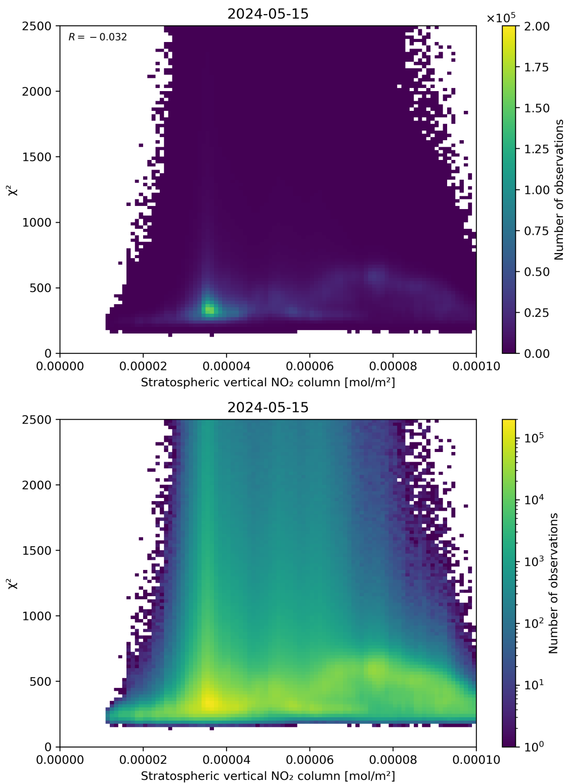
Figure 97: Scatter density plot of “Stratospheric vertical NO 2 column” against “ \chi^2 ” for 2024-05-14 to 2024-05-16.
