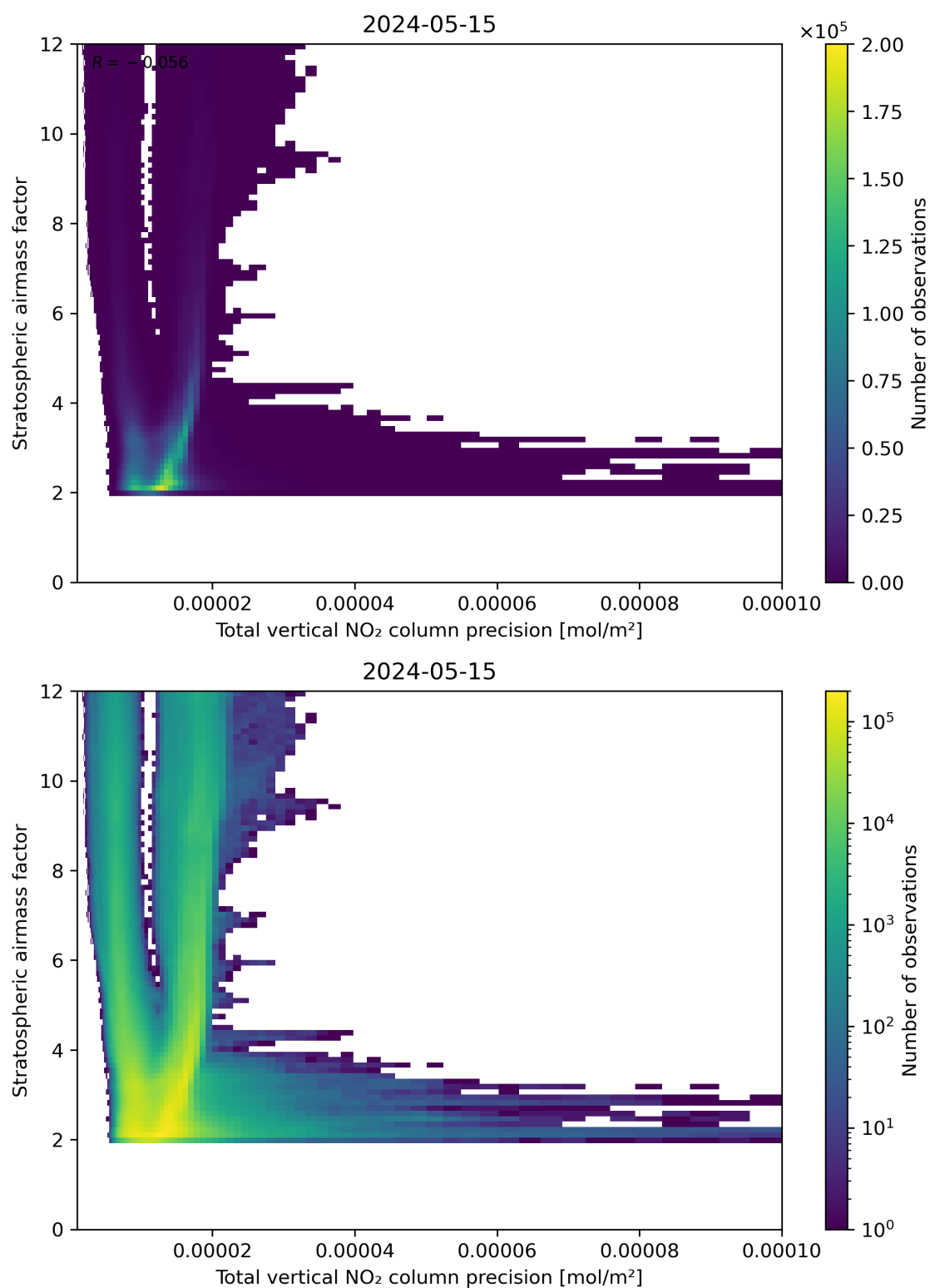
Figure 115: Scatter density plot of “Total vertical NO 2 column precision” against “Stratospheric air mass factor” for 2024-05-14 to 2024-05-16.
