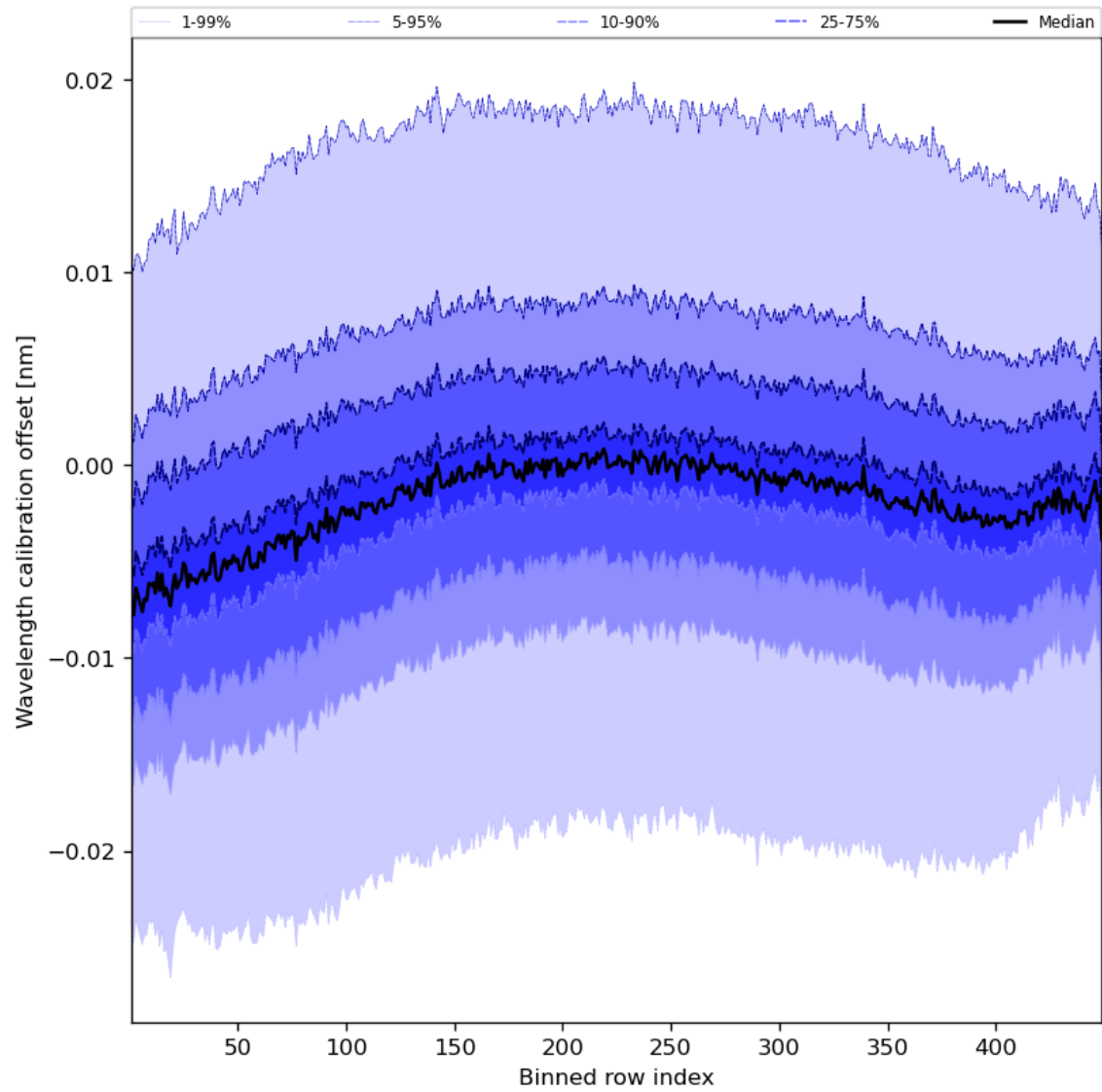
Figure 52: Along track statistics of “Wavelength calibration offset” for 2024-05-14 to 2024-05-16
