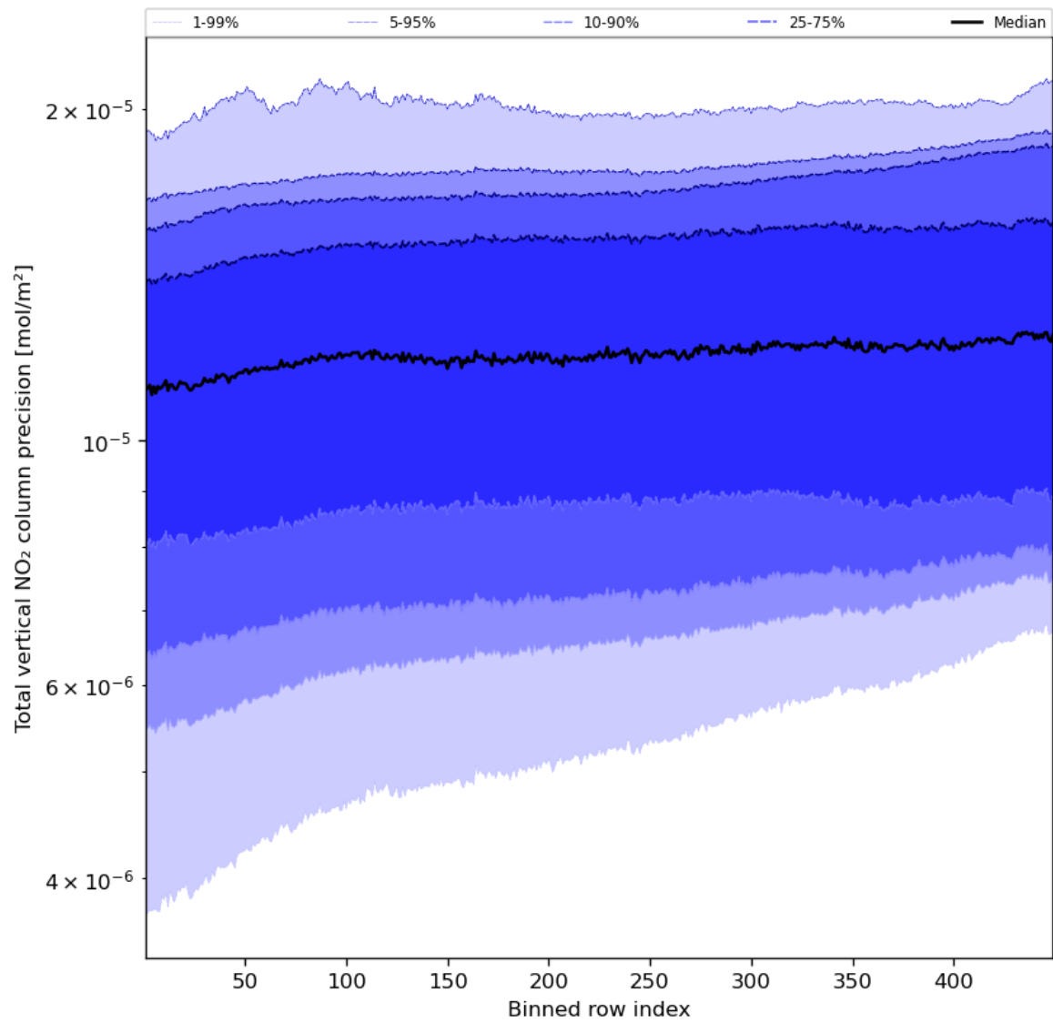
Figure 56: Along track statistics of “Total vertical NO 2 column precision” for 2024-05-14 to 2024-05-16
