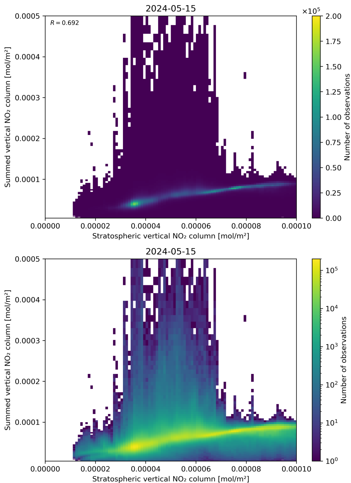
Figure 98: Scatter density plot of “Stratospheric vertical NO 2 column” against “Summed vertical NO 2 column” for 2024-05-14 to 2024-05-16.
