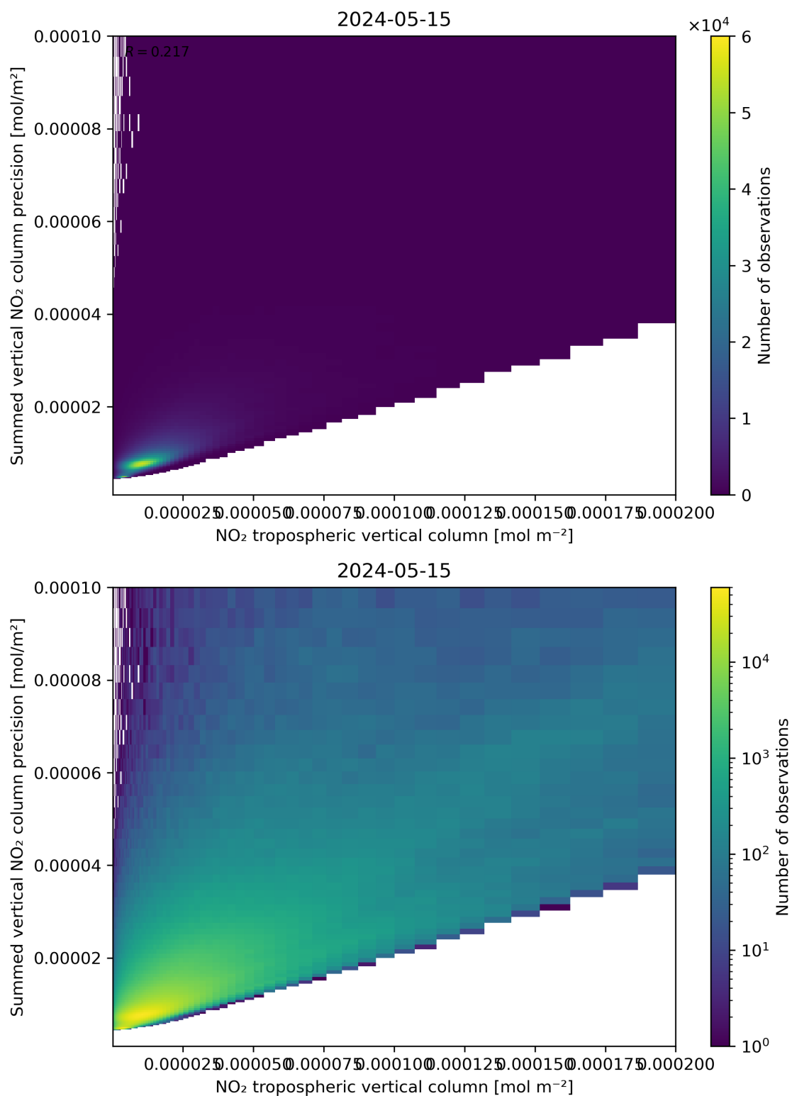
Figure 127: Scatter density plot of “NO 2 tropospheric vertical column” against “Summed vertical NO 2 column precision” for 2024-05-14 to 2024-05-16.
