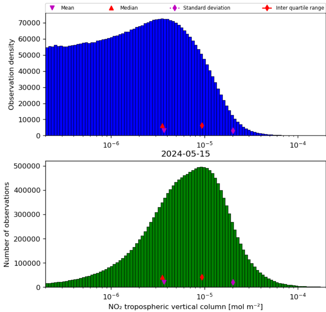
Figure 29: Histogram of “NO 2 tropospheric vertical column” for 2024-05-14 to 2024-05-16
