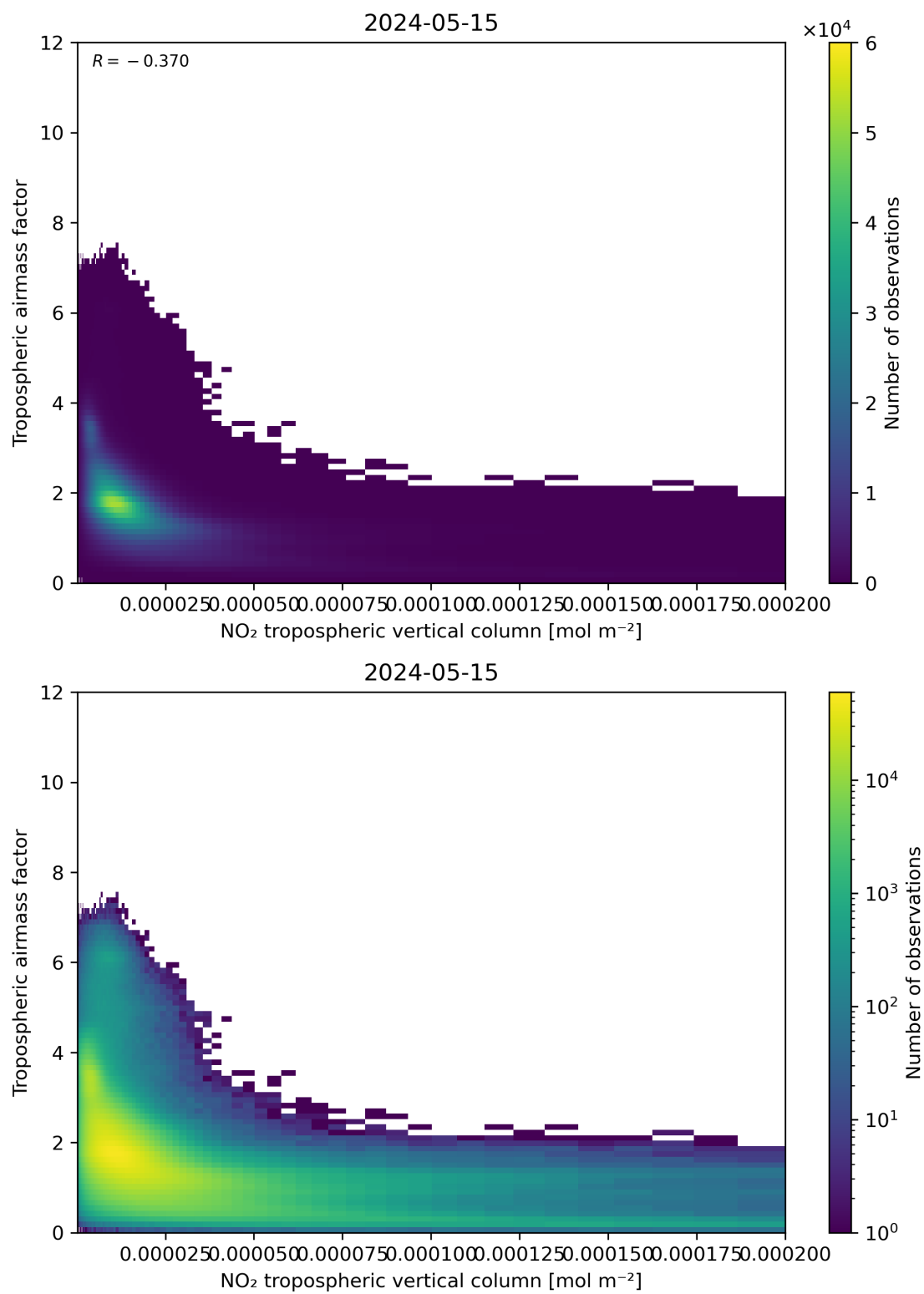
Figure 123: Scatter density plot of “NO 2 tropospheric vertical column” against “Tropospheric airmass factor” for 2024-05-14 to 2024-05-16.
