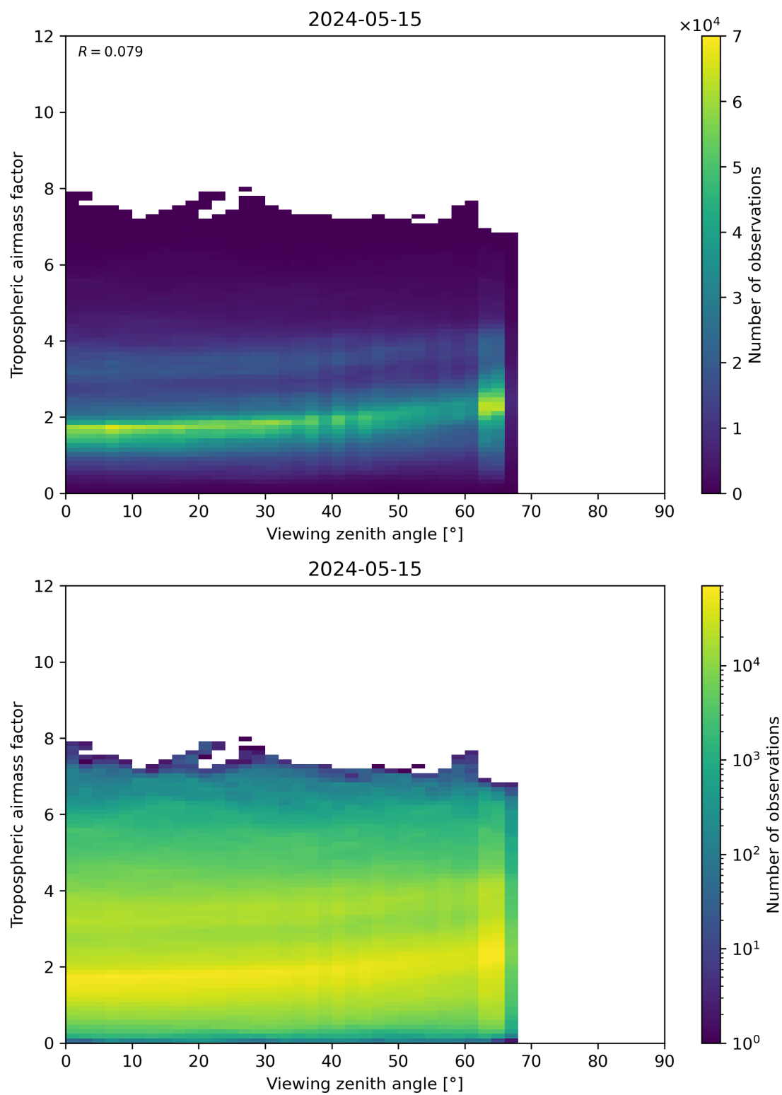
Figure 161: Scatter density plot of “Viewing zenith angle” against “Tropospheric airmass factor” for 2024-05-14 to 2024-05-16.
