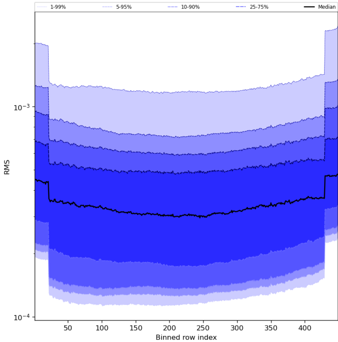
Figure 60: Along track statistics of “RMS” for 2024-05-14 to 2024-05-16
