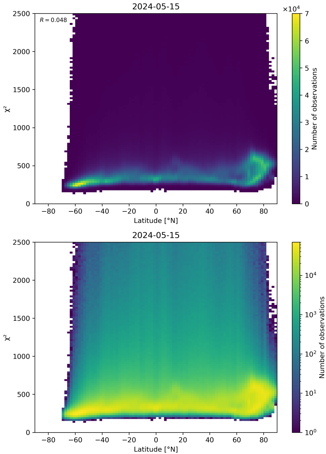
Figure 86: Scatter density plot of “Latitude” against “ \chi^2 ” for 2024-05-14 to 2024-05-16.
