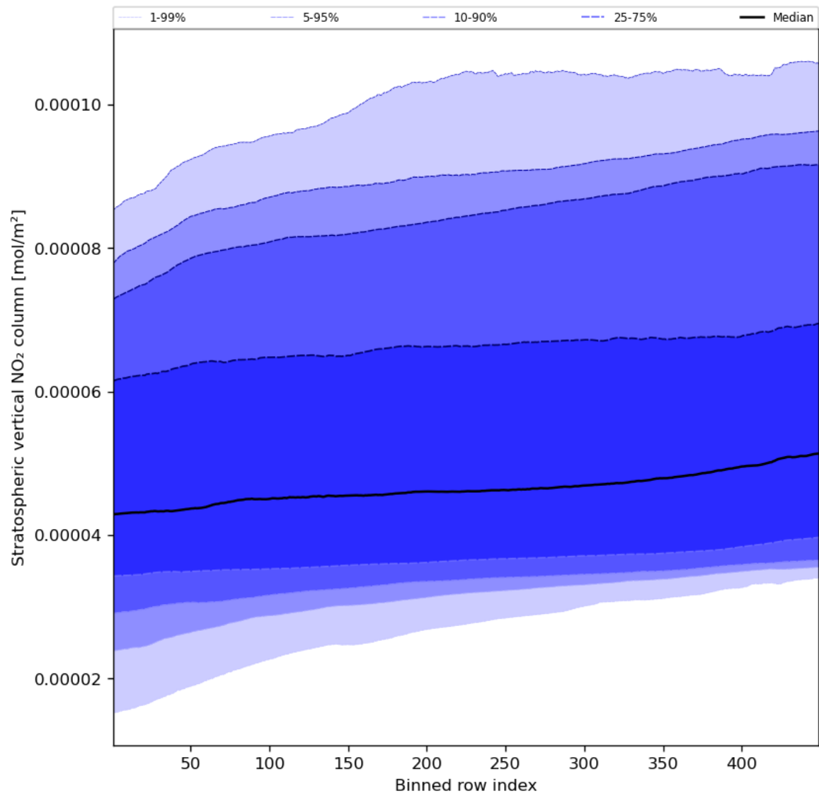
Figure 53: Along track statistics of “Stratospheric vertical NO 2 column” for 2024-05-14 to 2024-05-16
