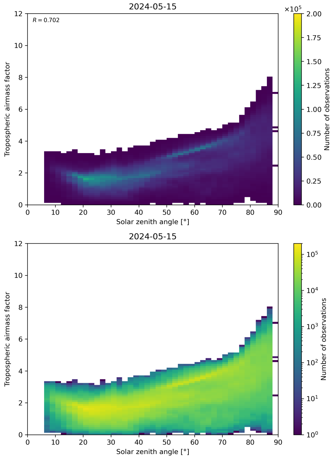
Figure 147: Scatter density plot of “Solar zenith angle” against “Tropospheric airmass factor” for 2024-05-14 to 2024-05-16.
