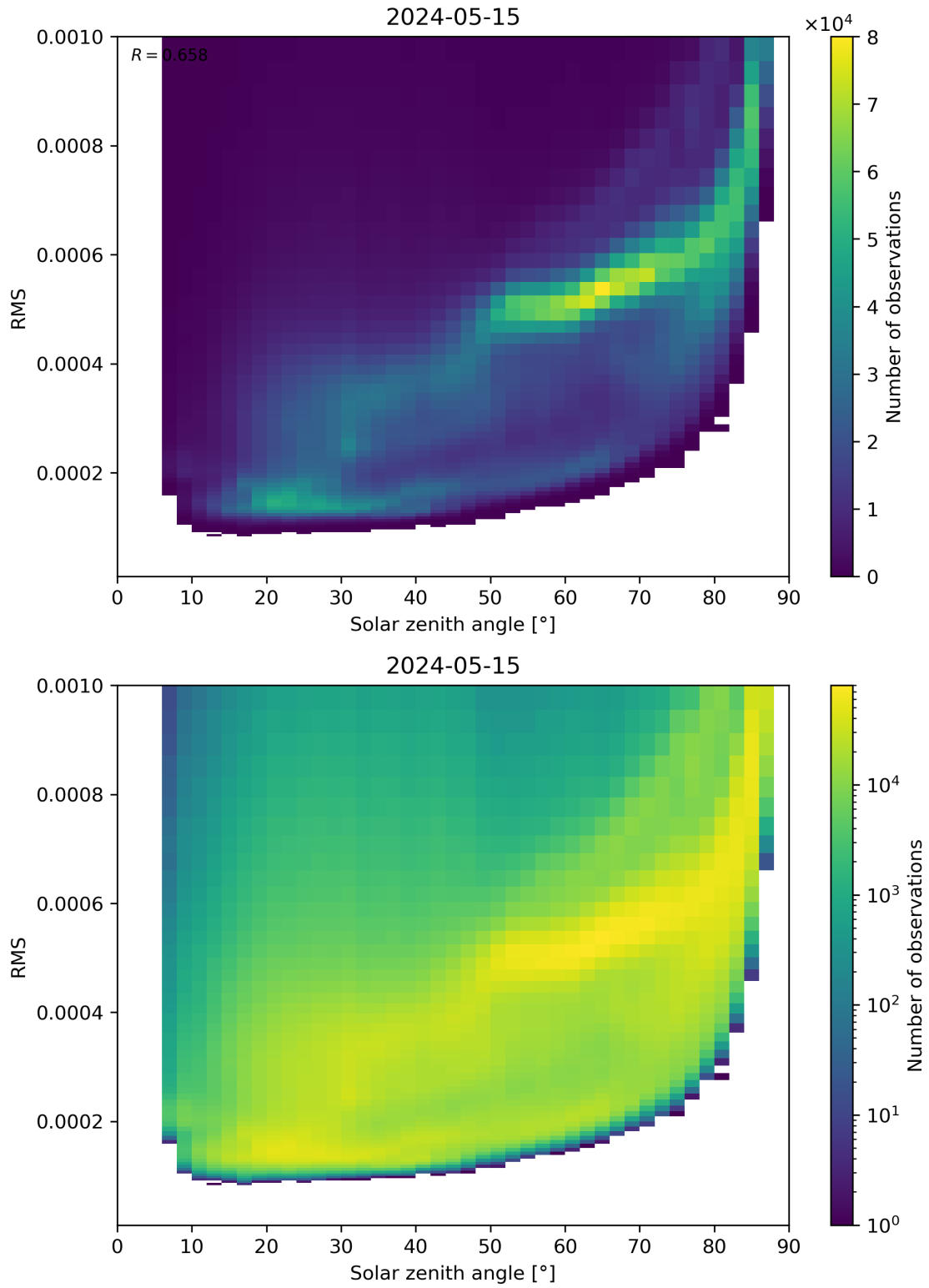
Figure 157: Scatter density plot of “Solar zenith angle” against “RMS” for 2024-05-14 to 2024-05-16.
