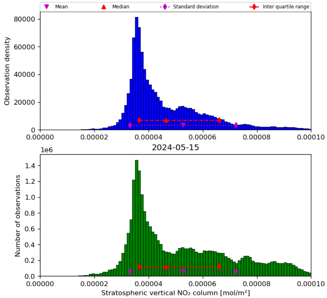
Figure 36: Histogram of “Stratospheric vertical NO 2 column” for 2024-05-14 to 2024-05-16
