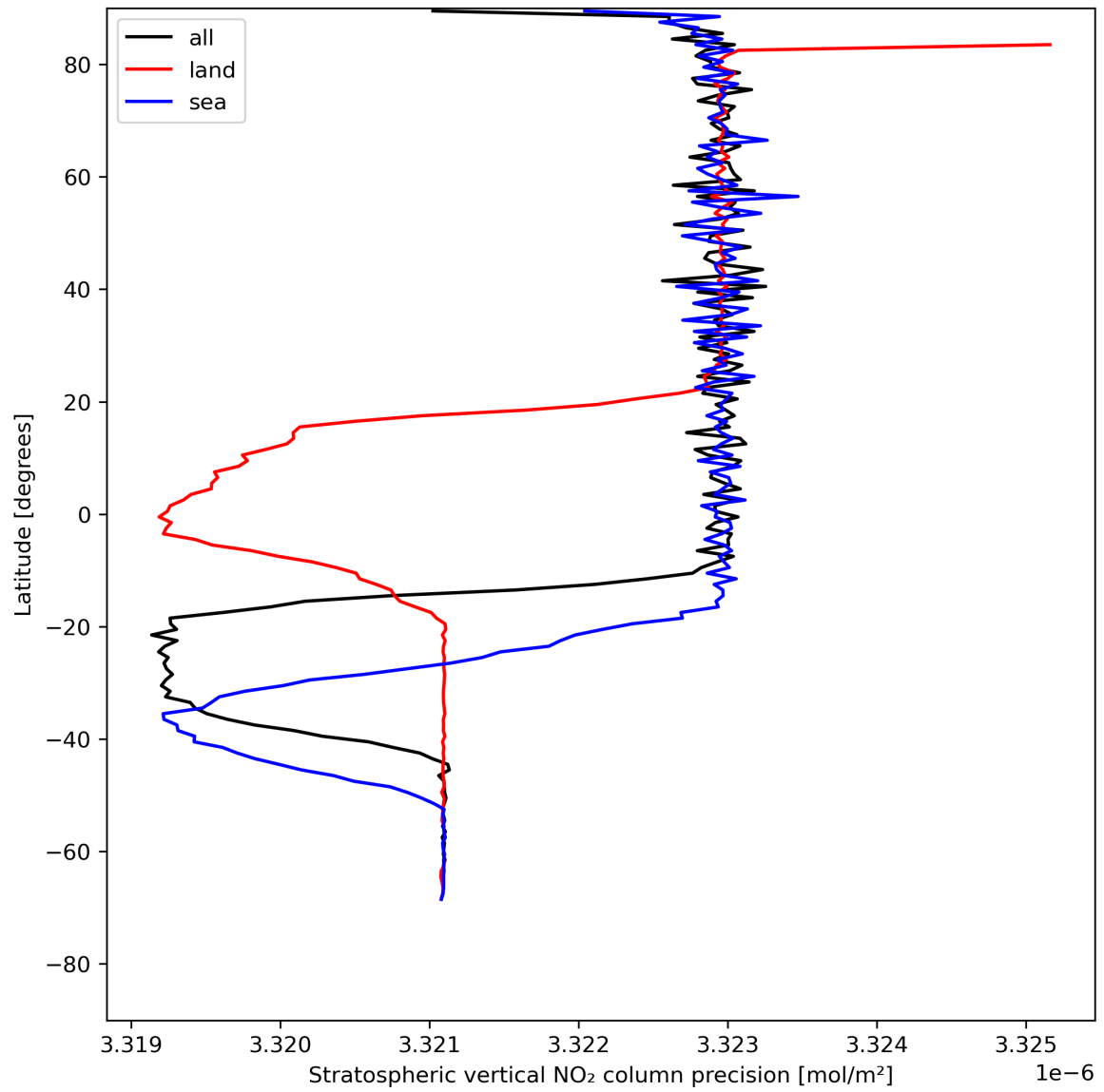
Figure 20: Zonal average of “Stratospheric vertical NO 2 column precision” for 2024-05-14 to 2024-05-16.
