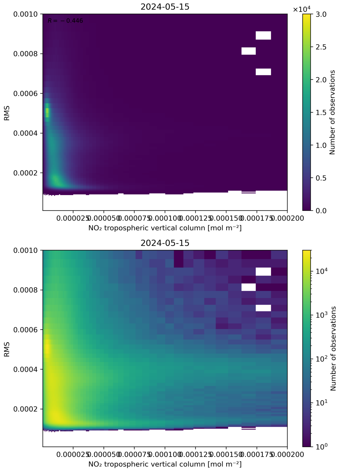
Figure 142: Scatter density plot of “NO 2 tropospheric vertical column” against “RMS” for 2024-05-14 to 2024-05-16.
