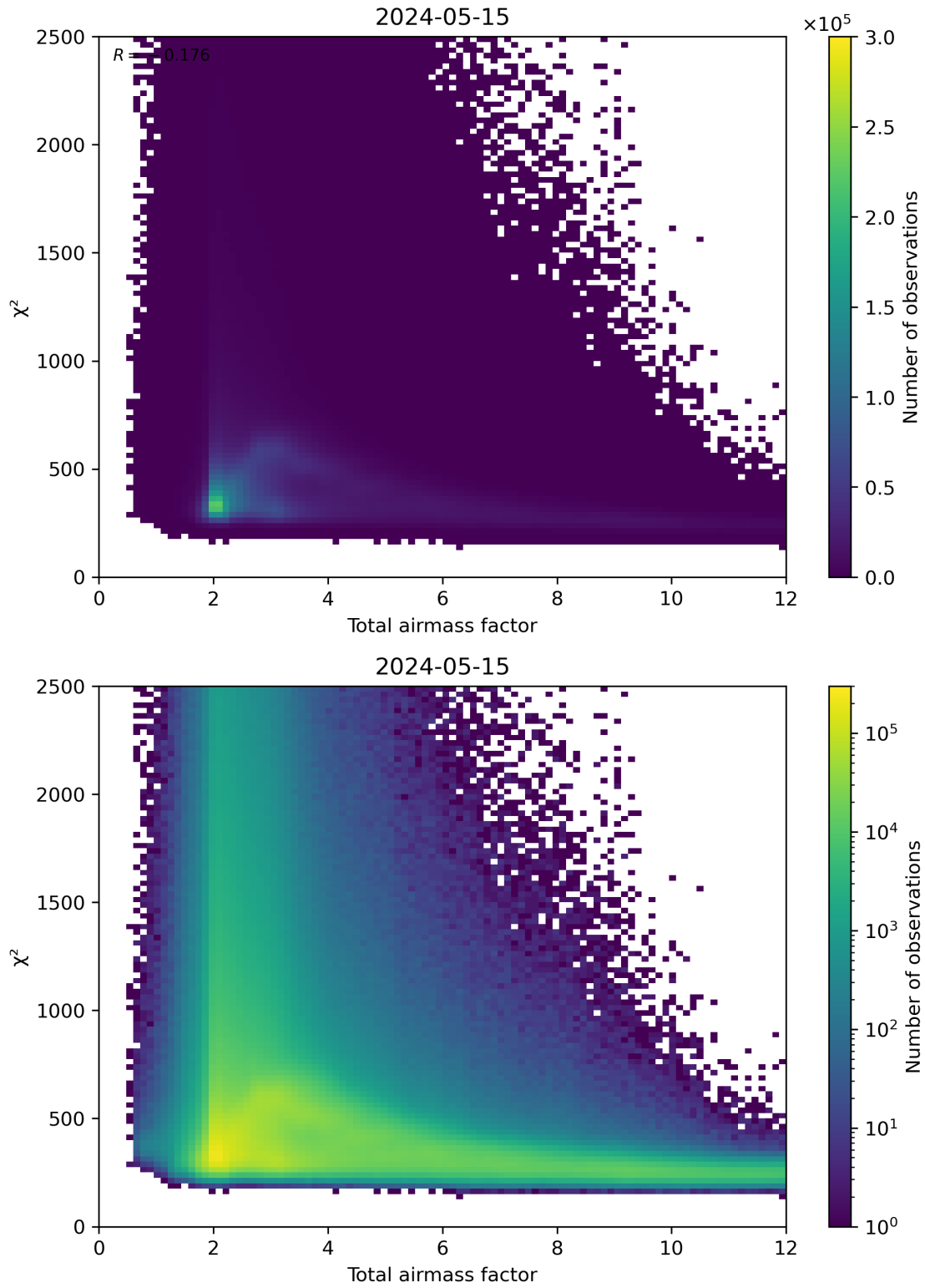
Figure 63: Scatter density plot of “Total airmass factor” against “ \chi^2 ” for 2024-05-14 to 2024-05-16.
