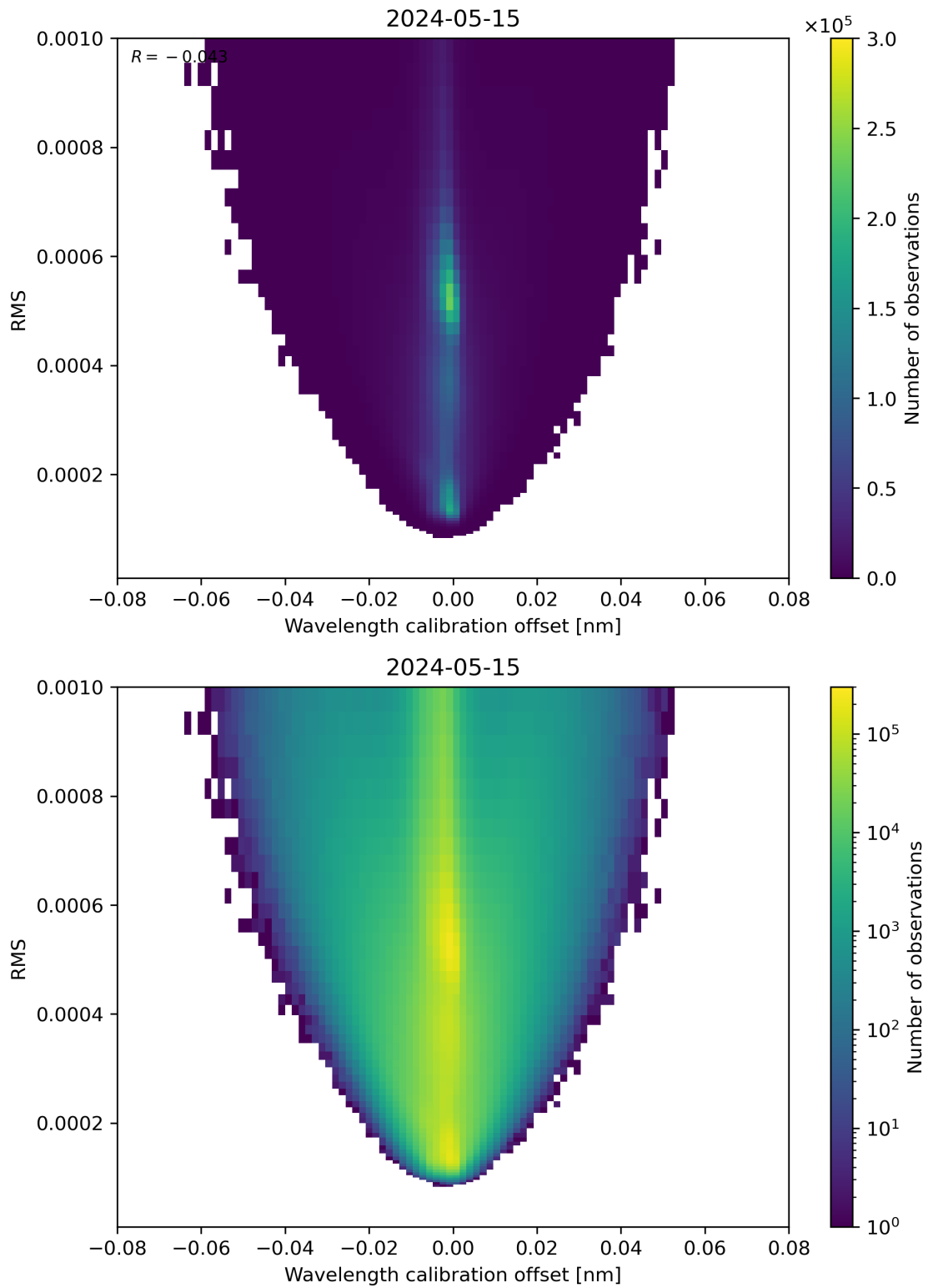
Figure 181: Scatter density plot of “Wavelength calibration offset” against “RMS” for 2024-05-14 to 2024-05-16.
