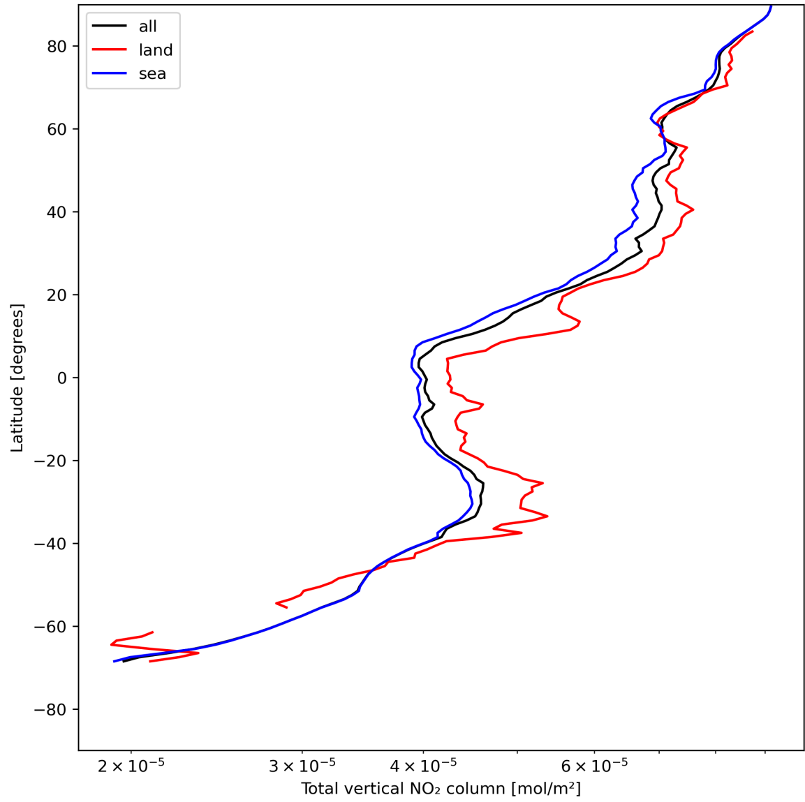
Figure 21: Zonal average of “Total vertical NO 2 column” for 2024-05-14 to 2024-05-16.
