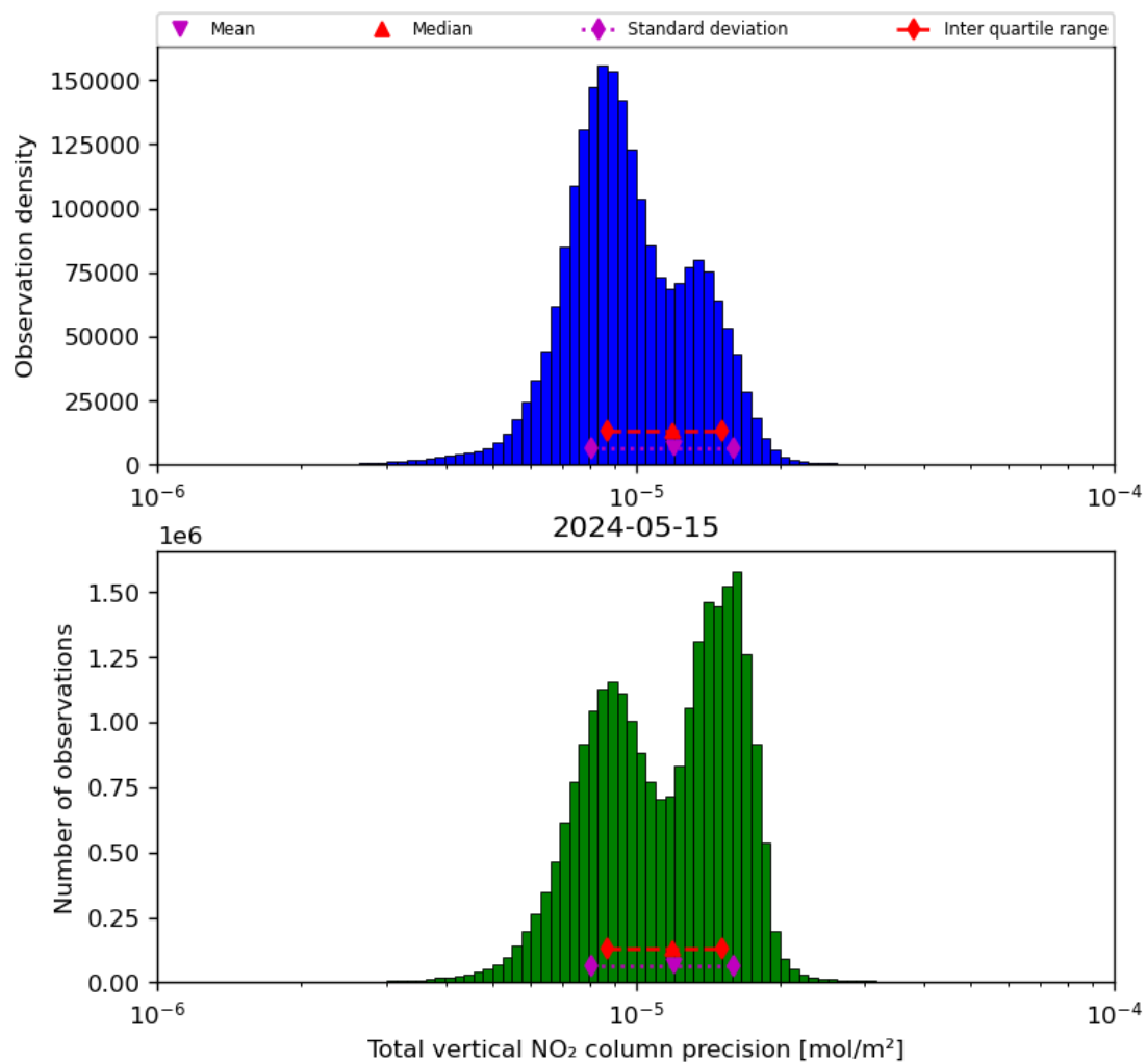
Figure 39: Histogram of “Total vertical NO 2 column precision” for 2024-05-14 to 2024-05-16
