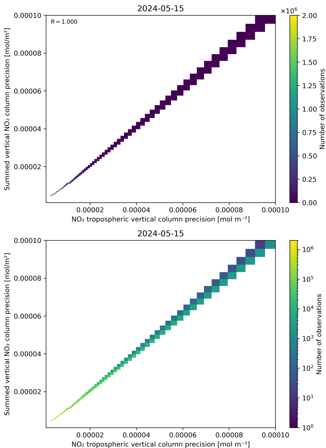
Figure 137: Scatter density plot of “NO 2 tropospheric vertical column precision” against “Summed vertical NO 2 column precision” for 2024-05-14 to 2024-05-16.
