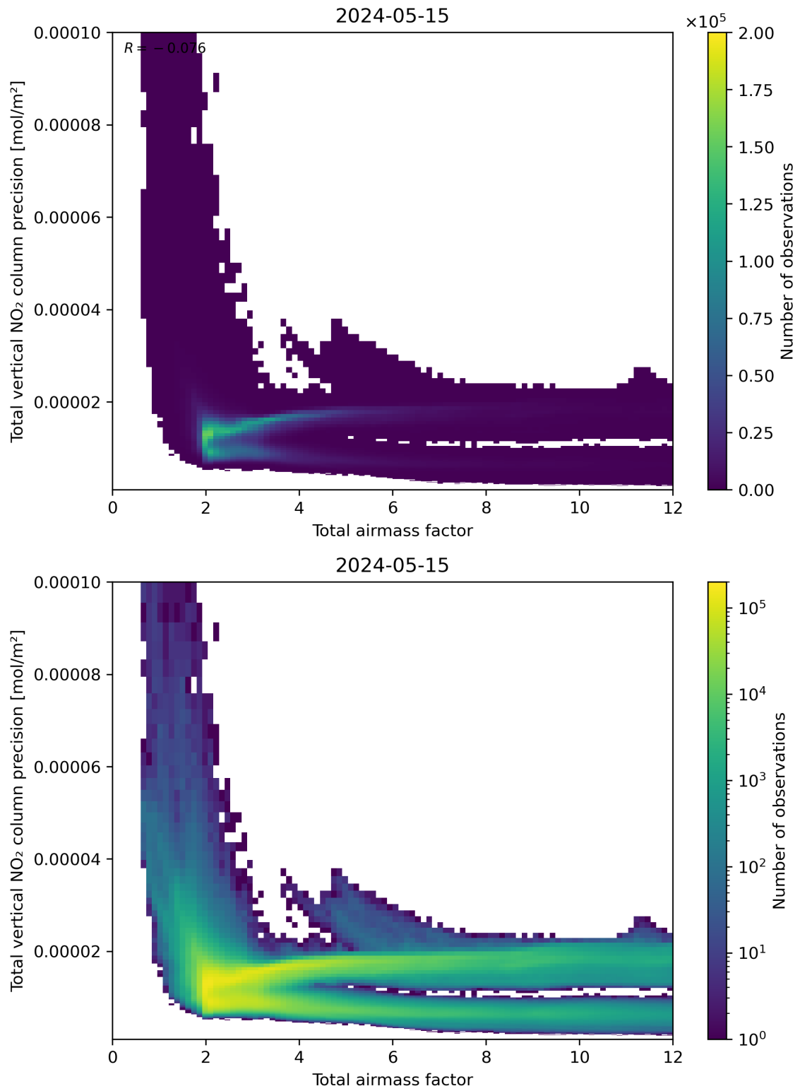
Figure 68: Scatter density plot of “Total airmass factor” against “Total vertical NO 2 column precision” for 2024-05-14 to 2024-05-16.
