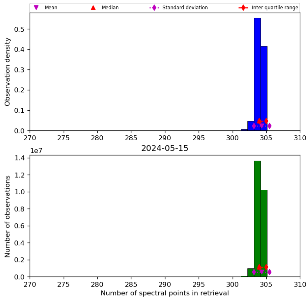
Figure 33: Histogram of “Number of spectral points in retrieval” for 2024-05-14 to 2024-05-16
