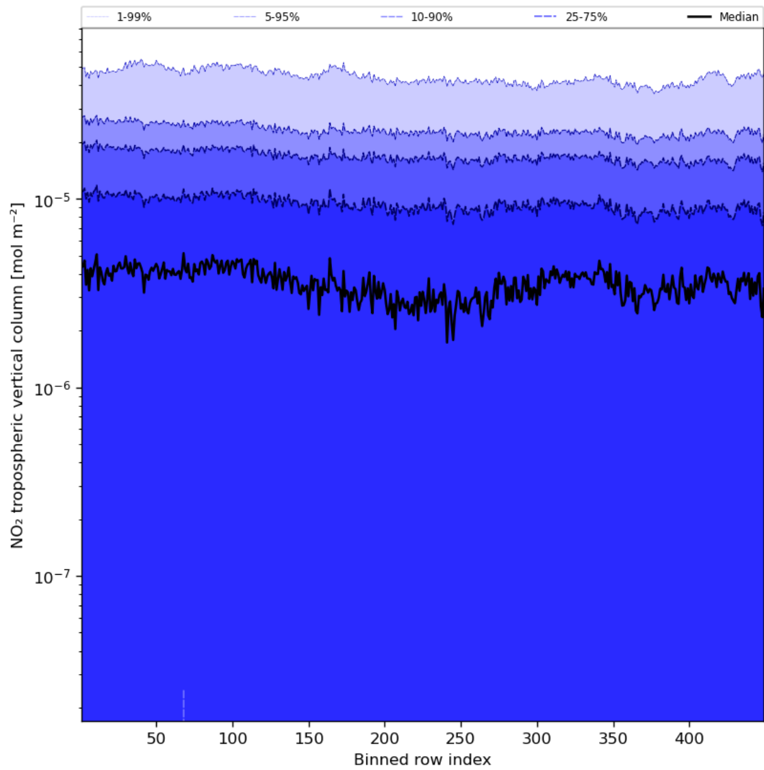
Figure 46: Along track statistics of “NO 2 tropospheric vertical column” for 2024-05-14 to 2024-05-16
