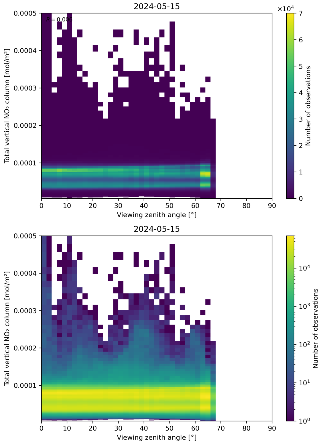
Figure 167: Scatter density plot of “Viewing zenith angle” against “Total vertical NO 2 column” for 2024-05-14 to 2024-05-16.
