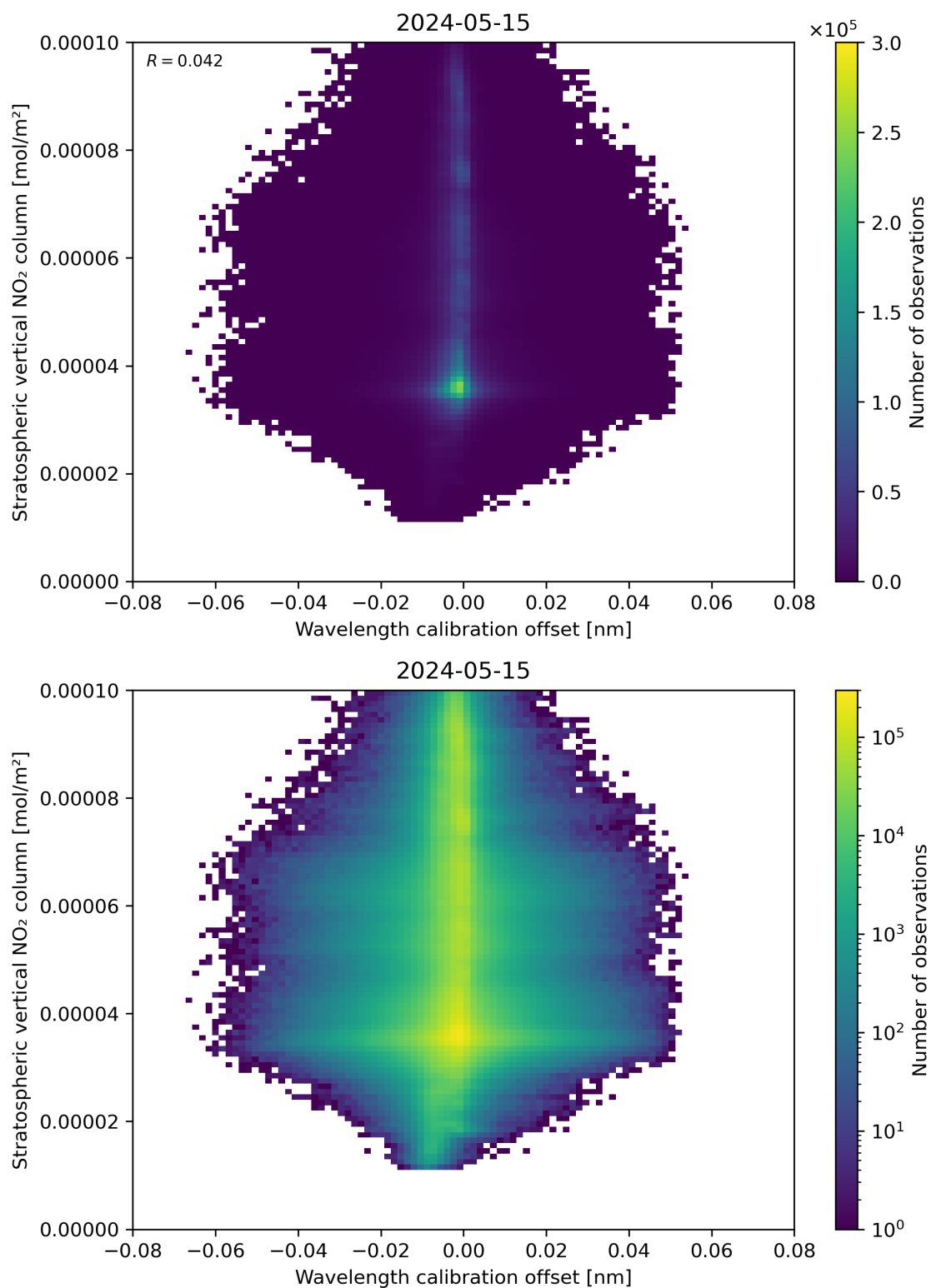
Figure 176: Scatter density plot of “Wavelength calibration offset” against “Stratospheric vertical NO 2 column” for 2024-05-14 to 2024-05-16.
