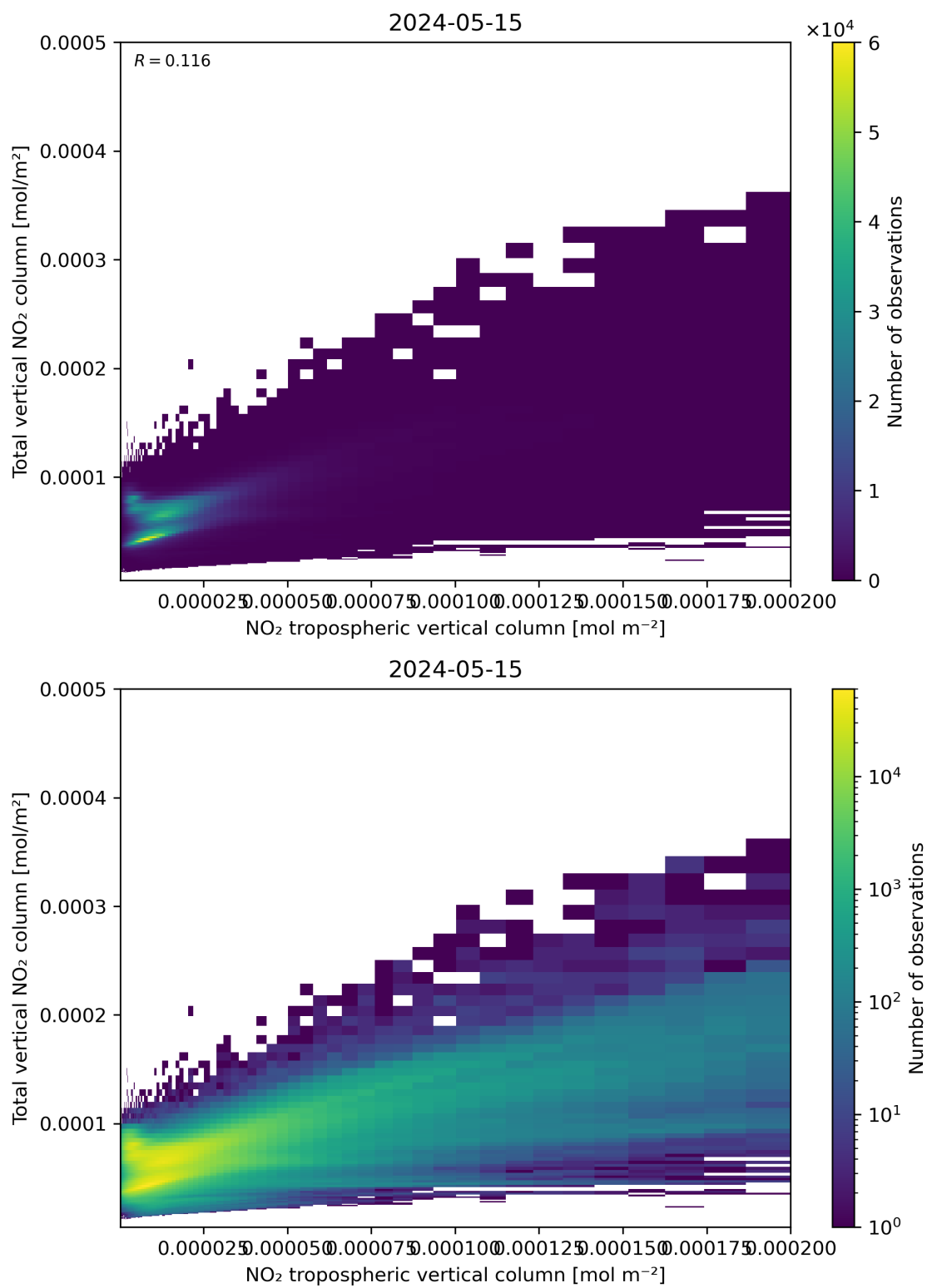
Figure 128: Scatter density plot of “NO 2 tropospheric vertical column” against “Total vertical NO 2 column” for 2024-05-14 to 2024-05-16.
