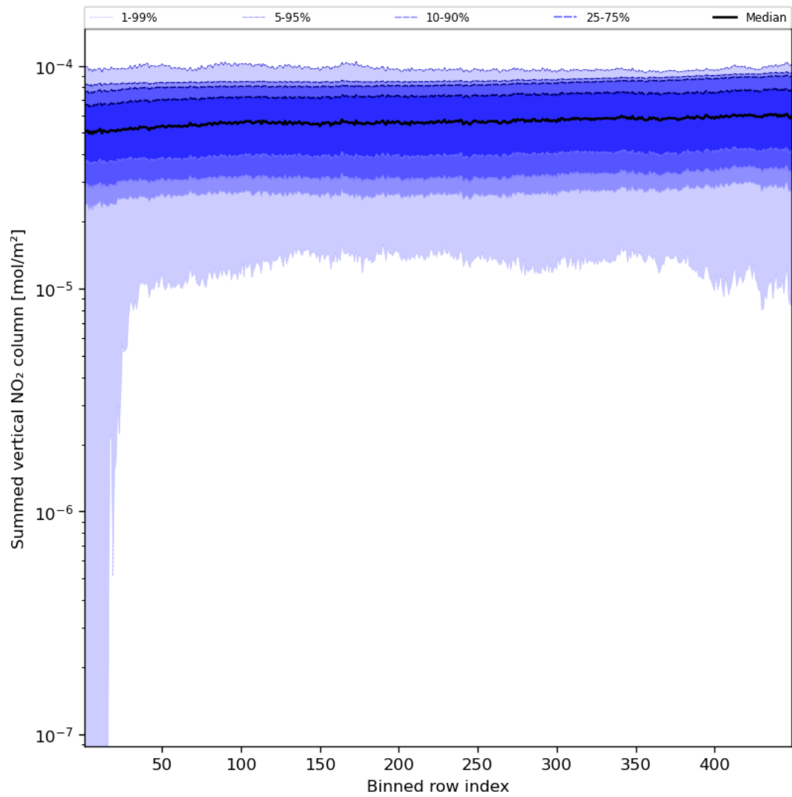
Figure 57: Along track statistics of “Summed vertical NO 2 column” for 2024-05-14 to 2024-05-16
