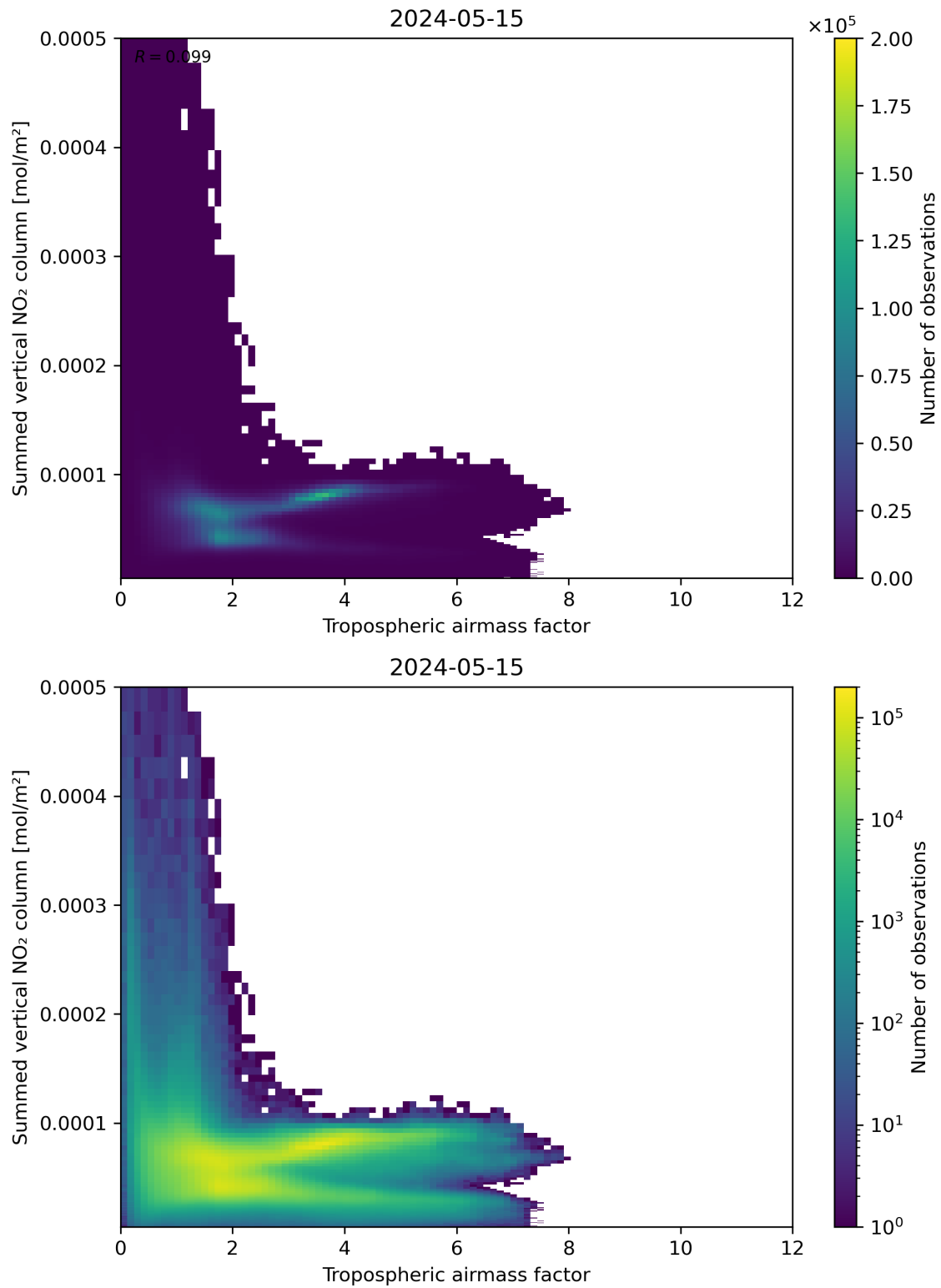
Figure 75: Scatter density plot of “Tropospheric airmass factor” against “Summed vertical NO 2 column” for 2024-05-14 to 2024-05-16.
