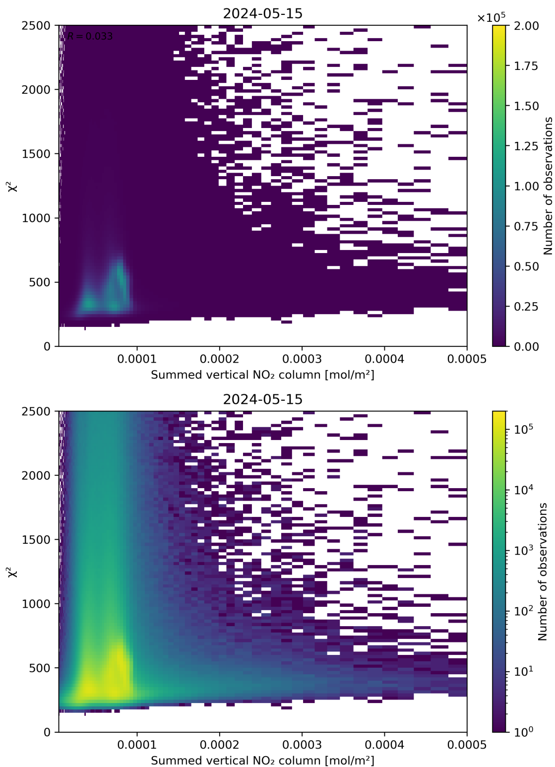
Figure 104: Scatter density plot of “Summed vertical NO 2 column” against “ \chi^2 ” for 2024-05-14 to 2024-05-16.
