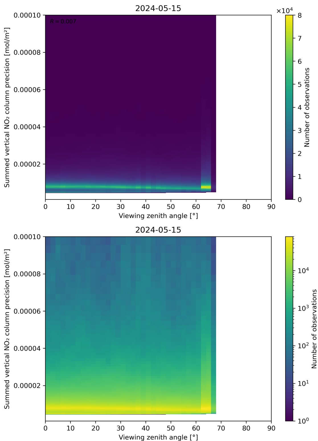
Figure 166: Scatter density plot of “Viewing zenith angle” against “Summed vertical NO 2 column precision” for 2024-05-14 to 2024-05-16.
