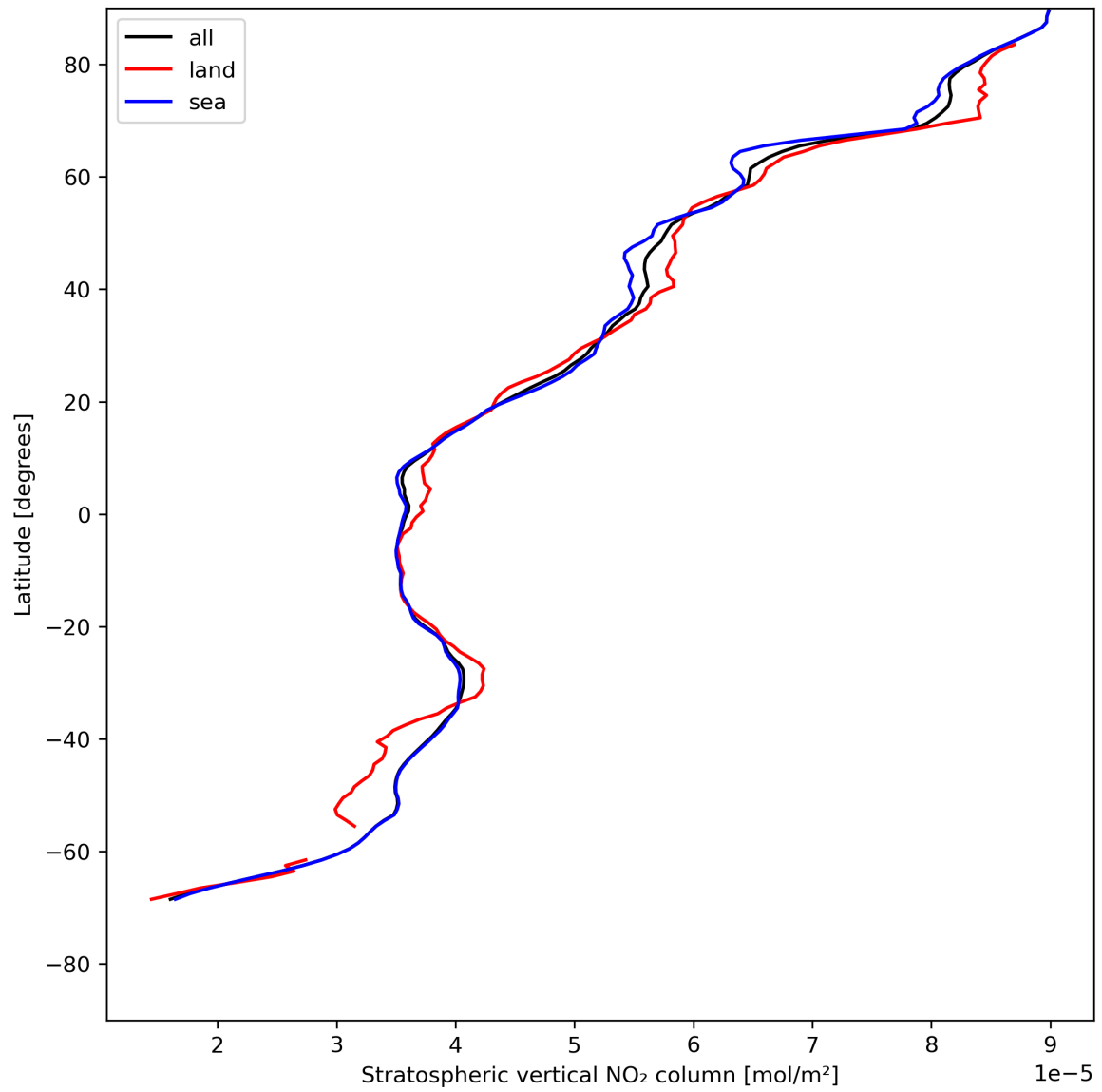
Figure 19: Zonal average of “Stratospheric vertical NO 2 column” for 2024-05-14 to 2024-05-16.
