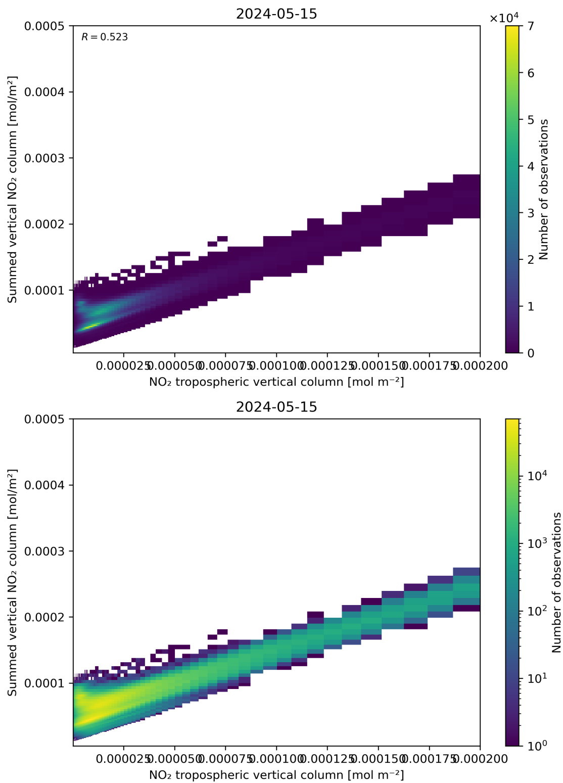
Figure 126: Scatter density plot of “NO 2 tropospheric vertical column” against “Summed vertical NO 2 column” for 2024-05-14 to 2024-05-16.
