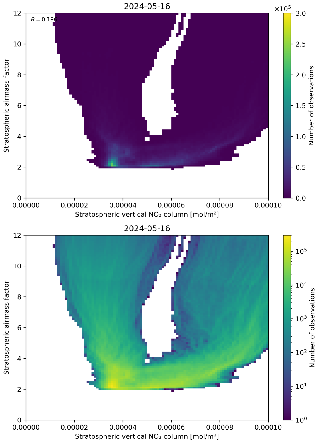
Figure 96: Scatter density plot of “Stratospheric vertical NO 2 column” against “Stratospheric airmass factor” for 2024-05-15 to 2024-05-17.
