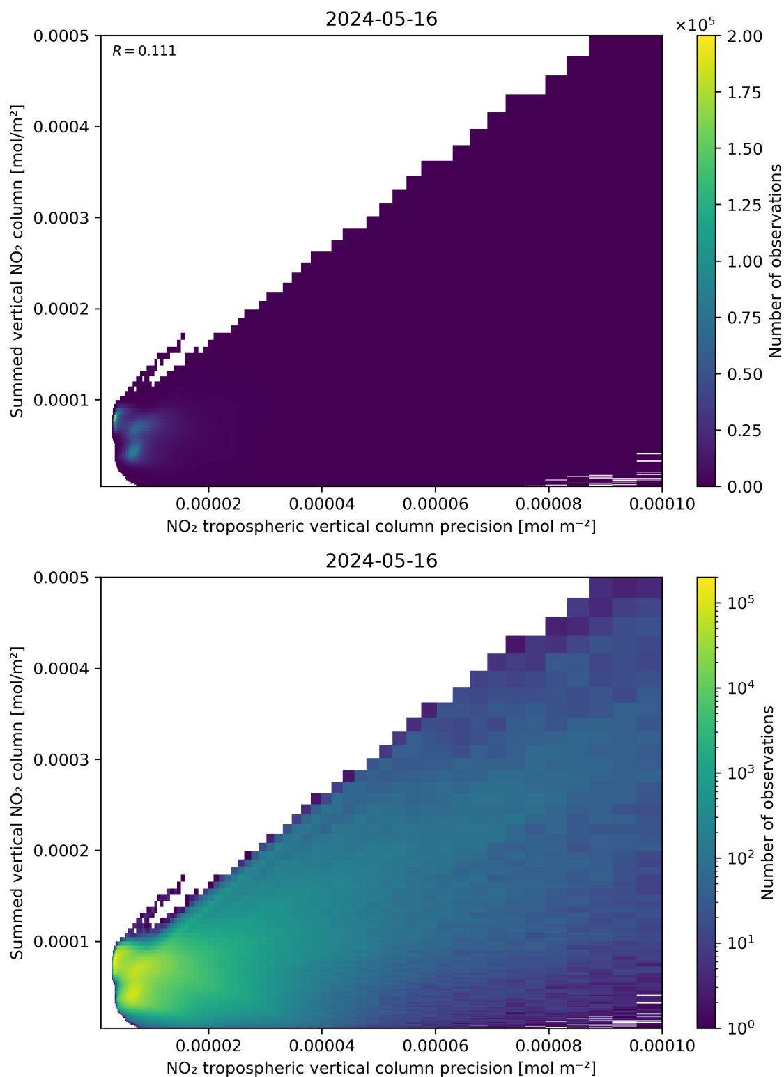
Figure 136: Scatter density plot of “NO 2 tropospheric vertical column precision” against “Summed vertical NO 2 column” for 2024-05-15 to 2024-05-17.
