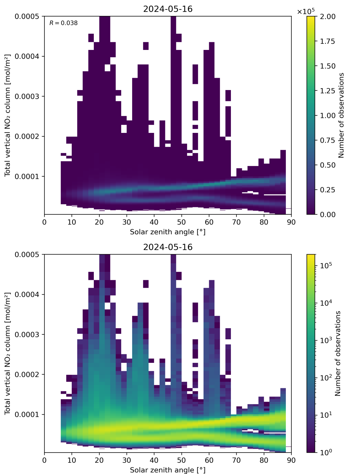
Figure 153: Scatter density plot of “Solar zenith angle” against “Total vertical NO 2 column” for 2024-05-15 to 2024-05-17.
