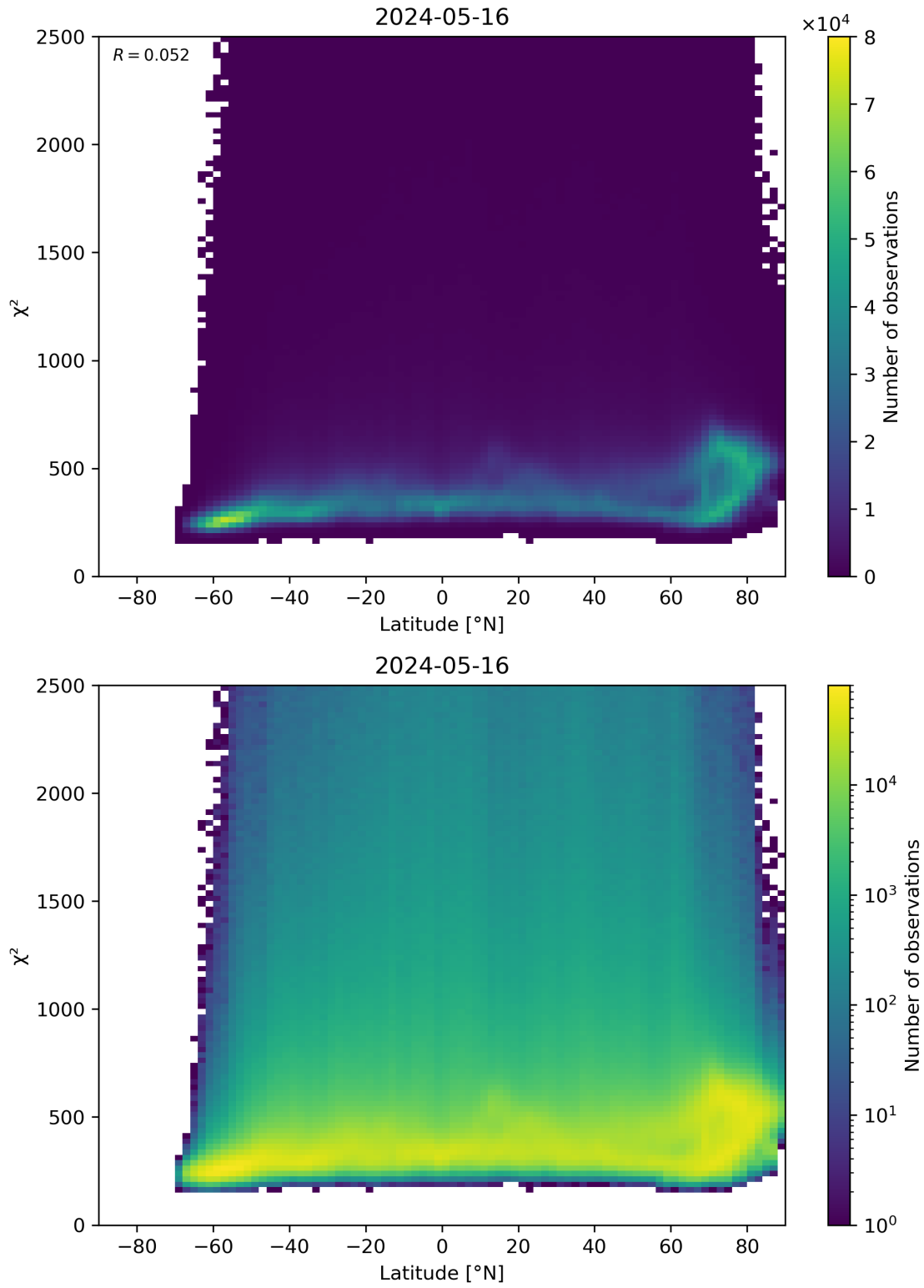
Figure 86: Scatter density plot of “Latitude” against “ \chi^2 ” for 2024-05-15 to 2024-05-17.
