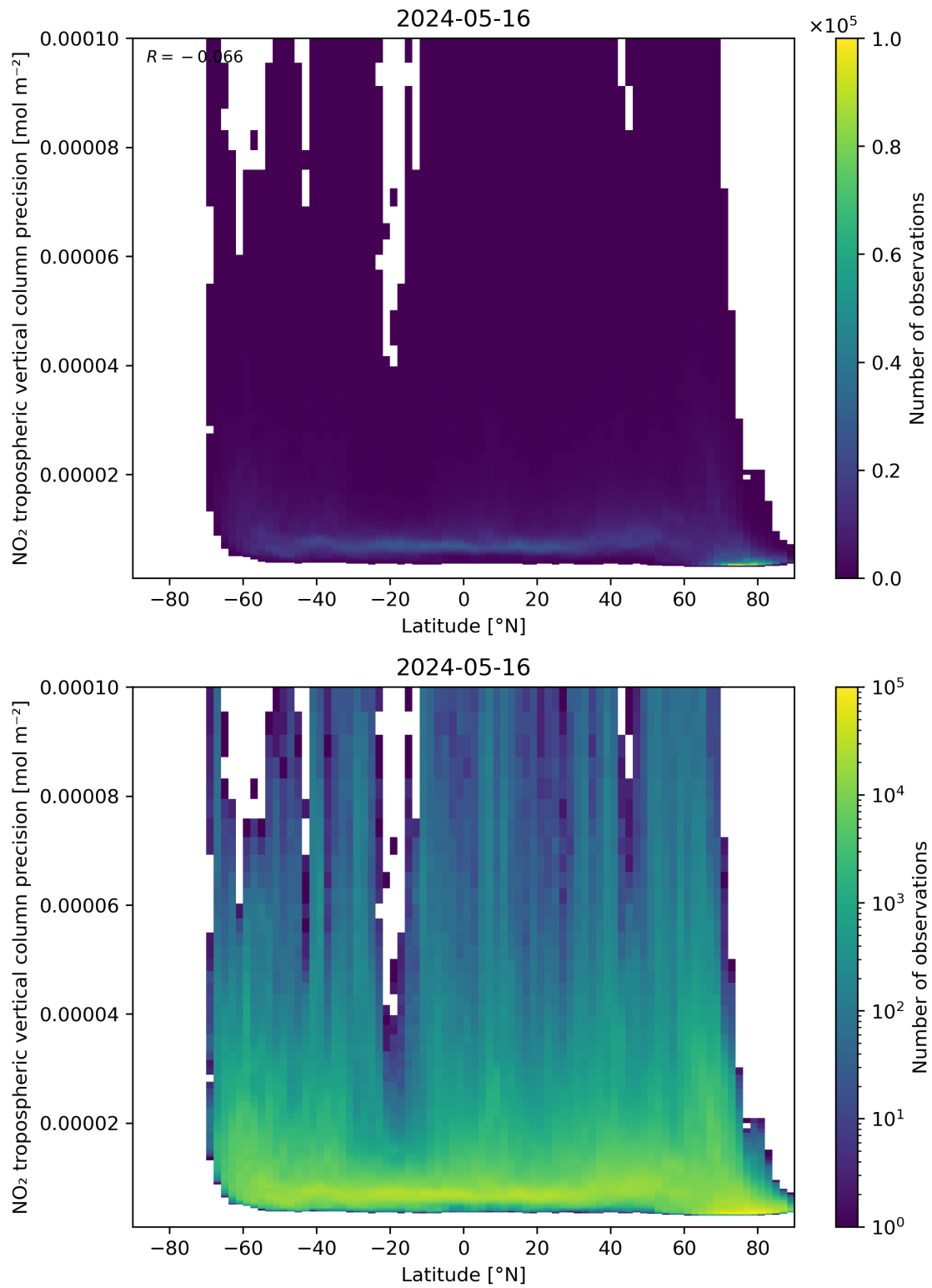
Figure 93: Scatter density plot of “Latitude” against “NO 2 tropospheric vertical column precision” for 2024-05-15 to 2024-05-17.
