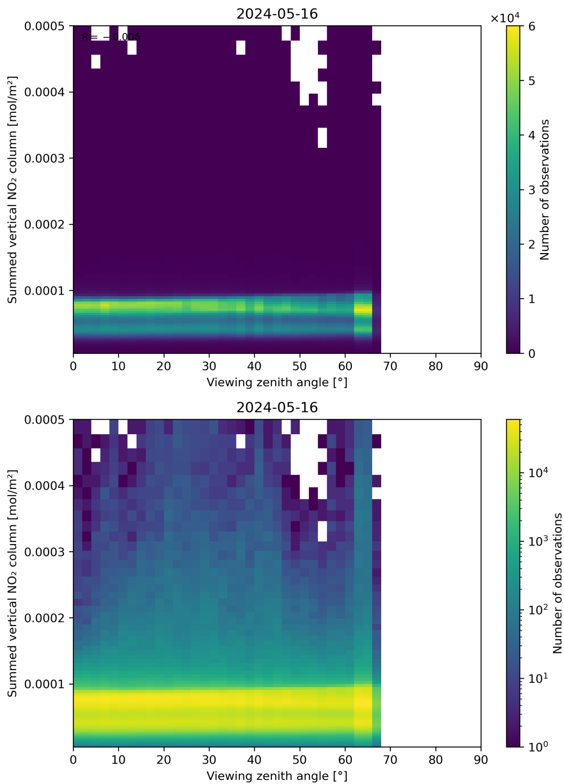
Figure 165: Scatter density plot of “Viewing zenith angle” against “Summed vertical NO 2 column” for 2024-05-15 to 2024-05-17.
