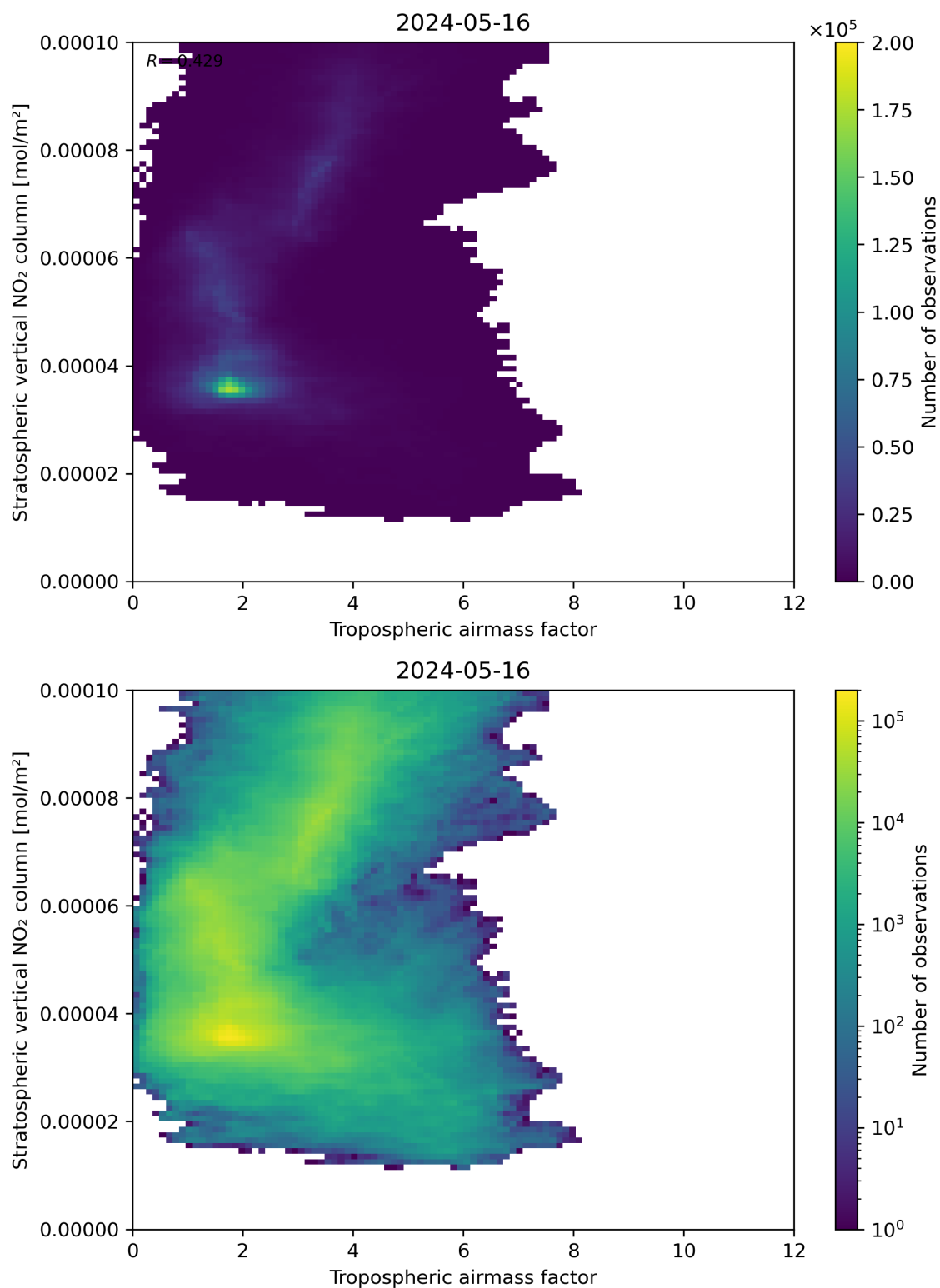
Figure 74: Scatter density plot of “Tropospheric air mass factor” against “Stratospheric vertical NO 2 column” for 2024-05-15 to 2024-05-17.
