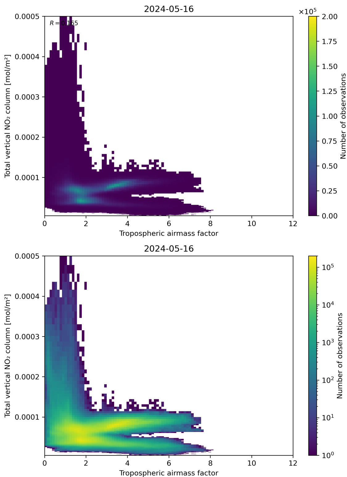
Figure 77: Scatter density plot of “Tropospheric airmass factor” against “Total vertical NO 2 column” for 2024-05-15 to 2024-05-17.
