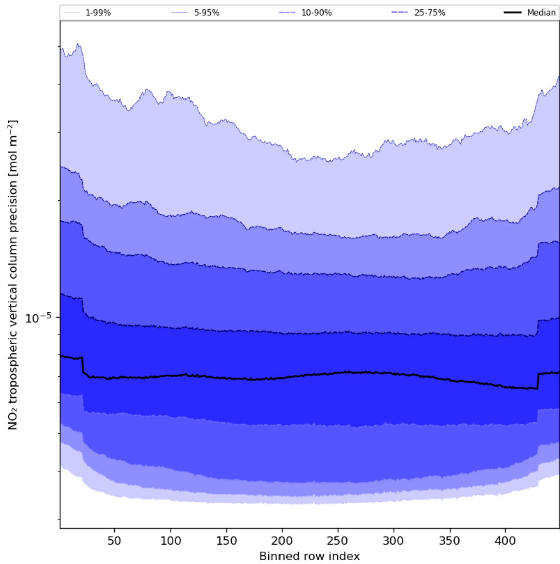
Figure 47: Along track statistics of “NO 2 tropospheric vertical column precision” for 2024-05-15 to 2024-05-17
