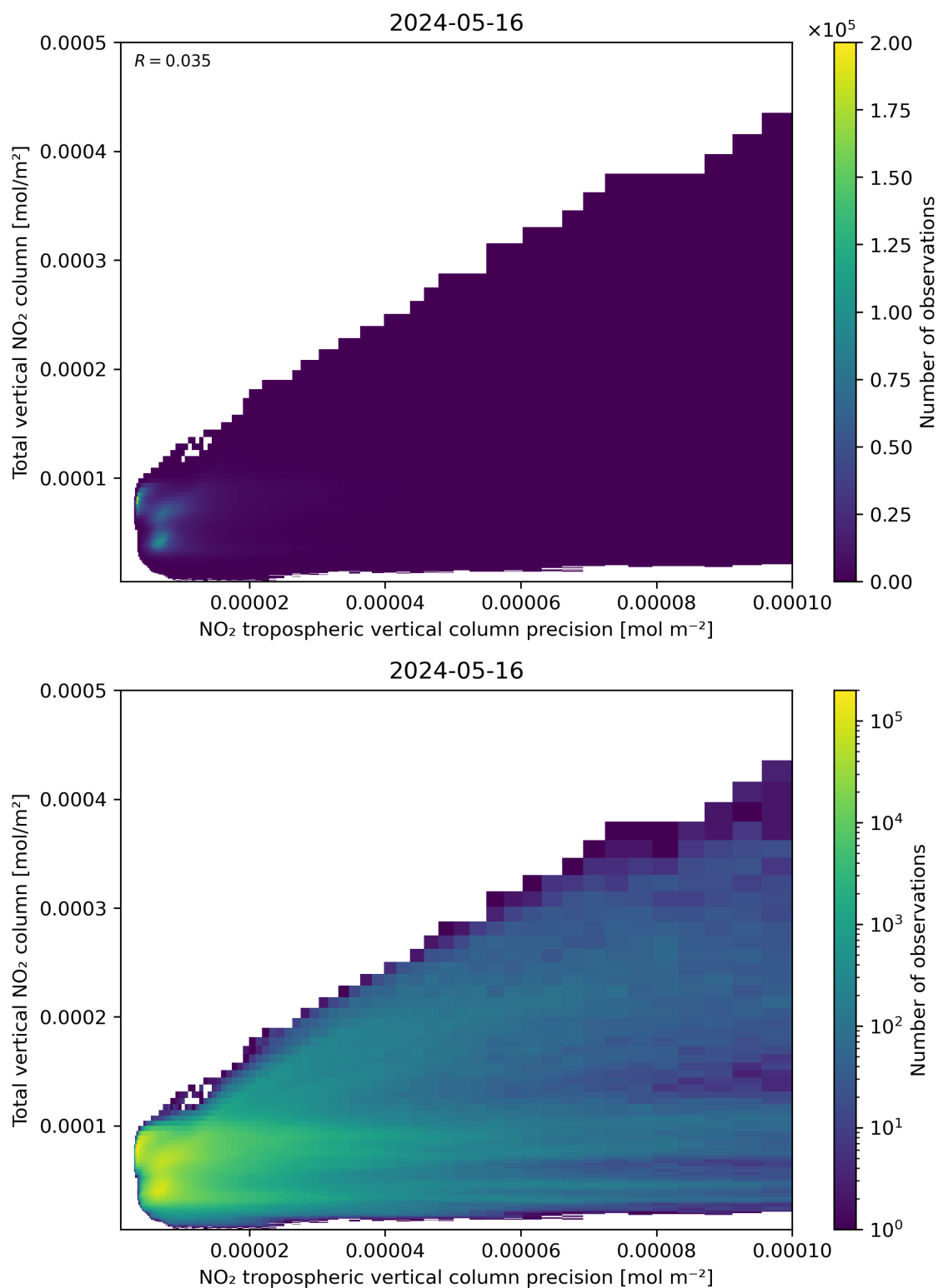
Figure 138: Scatter density plot of “NO 2 tropospheric vertical column precision” against “Total vertical NO 2 column” for 2024-05-15 to 2024-05-17.
