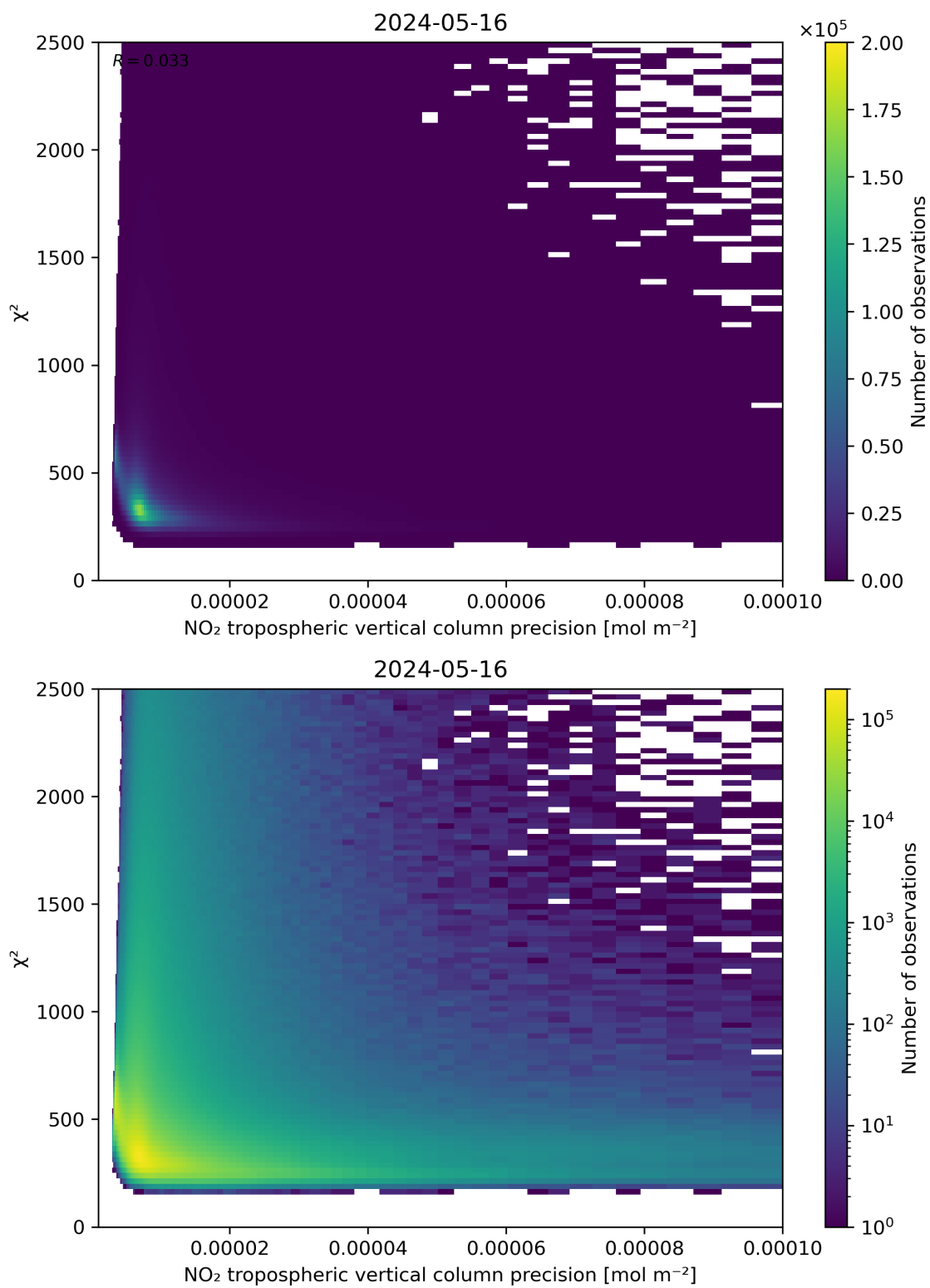
Figure 134: Scatter density plot of “NO 2 tropospheric vertical column precision” against “ \chi^2 ” for 2024-05-15 to 2024-05-17.
