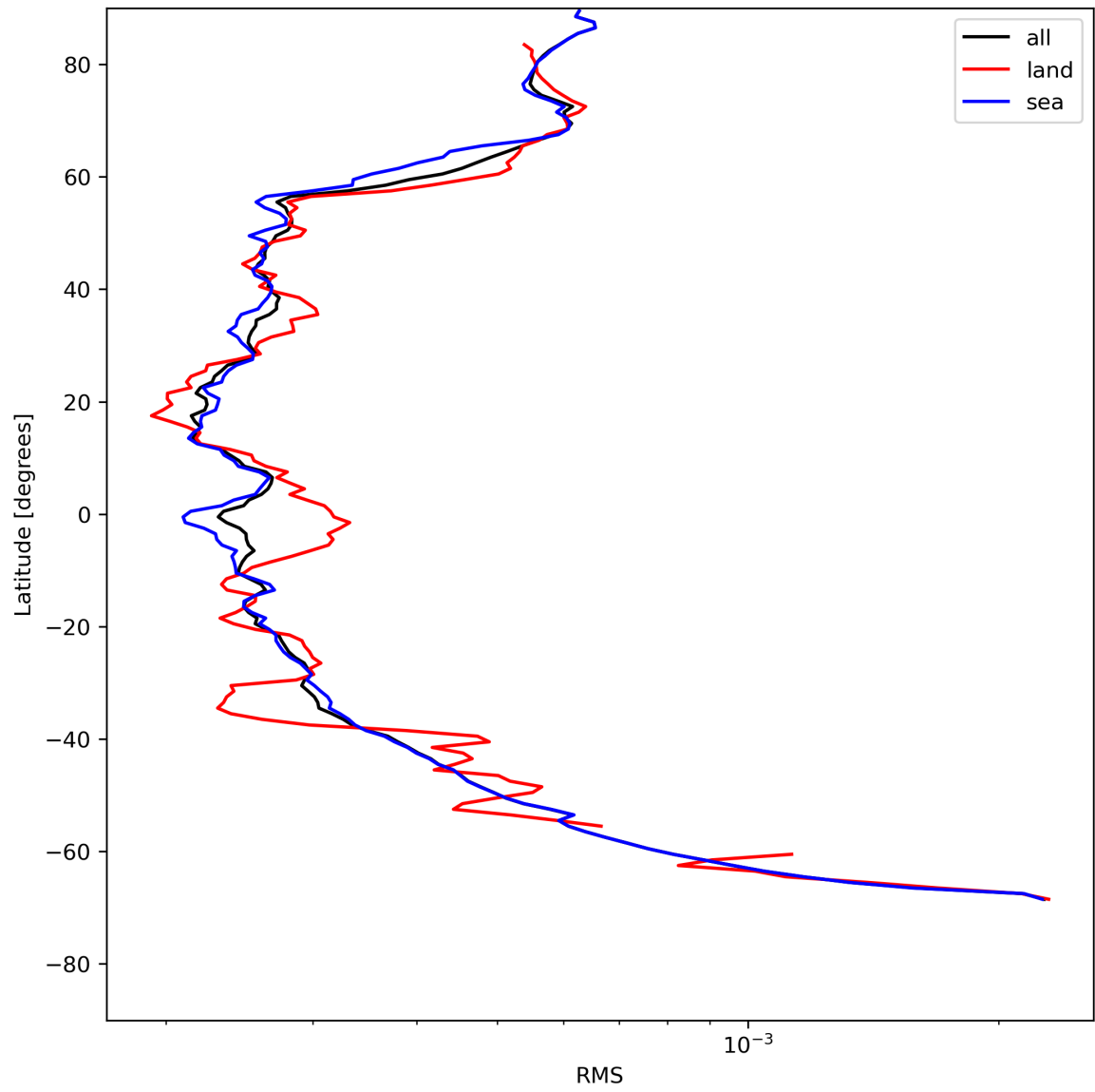
Figure 26: Zonal average of “RMS” for 2024-05-15 to 2024-05-17.
