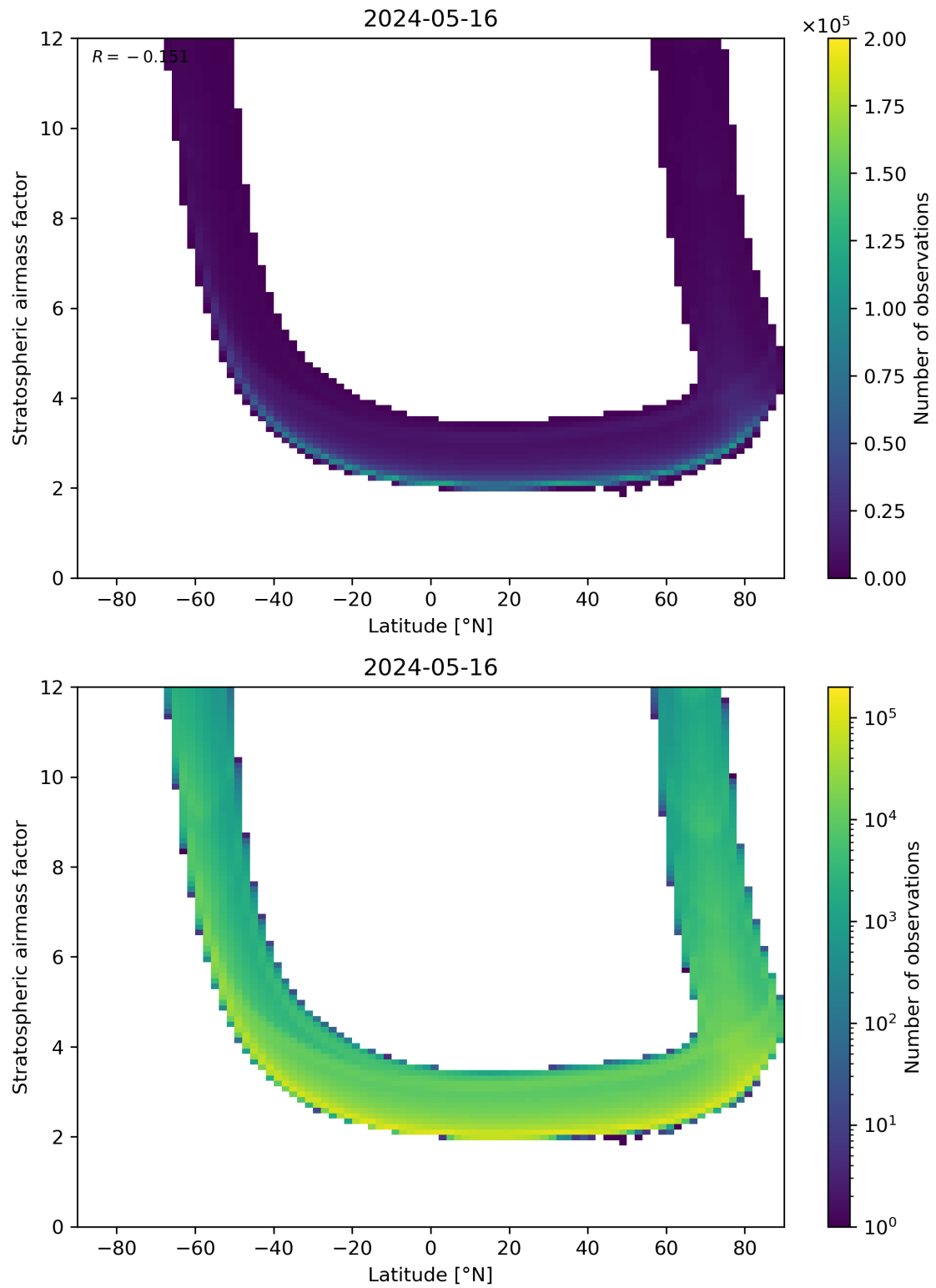
Figure 83: Scatter density plot of “Latitude” against “Stratospheric air mass factor” for 2024-05-15 to 2024-05-17.
