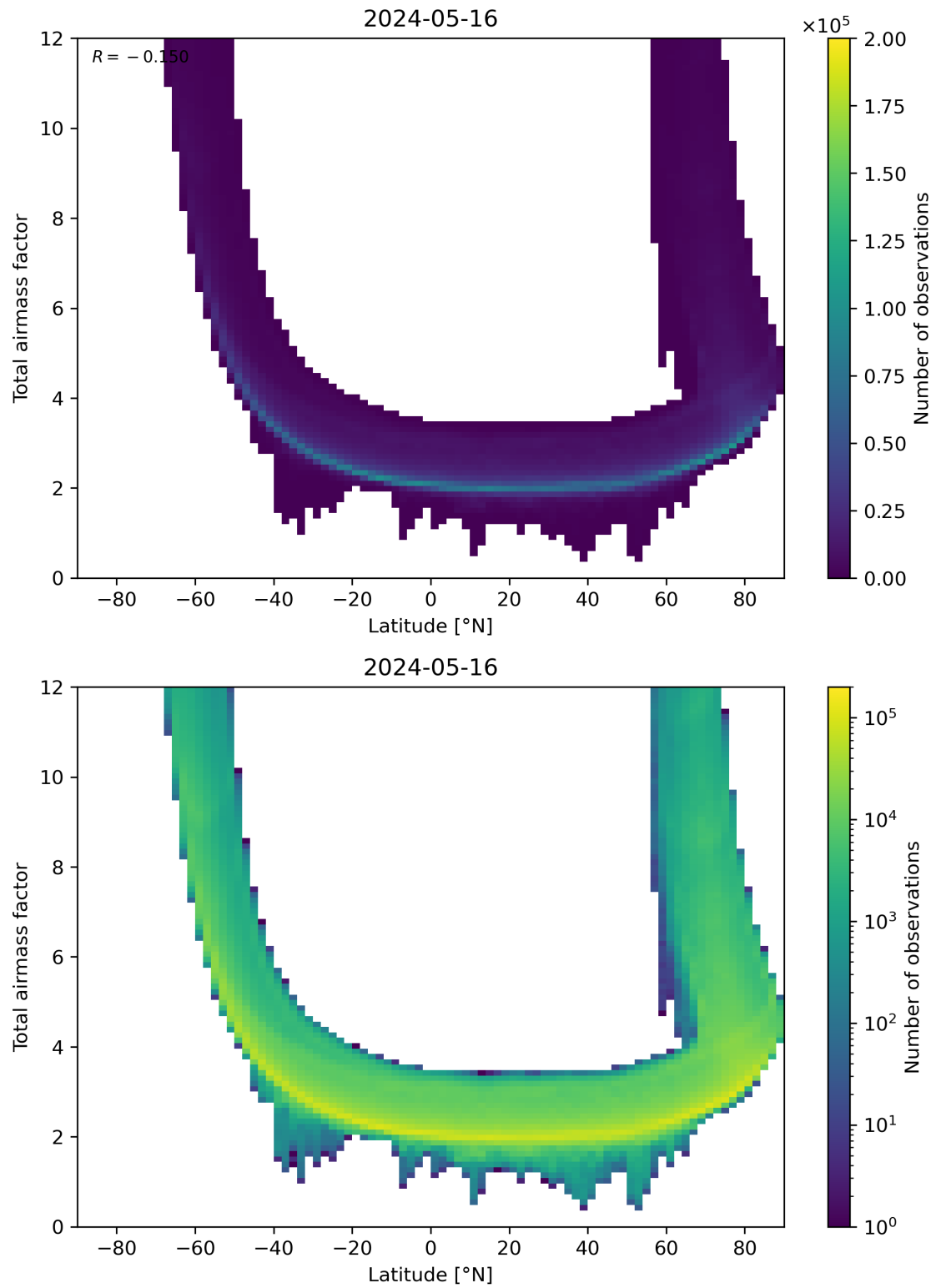
Figure 84: Scatter density plot of “Latitude” against “Total airmass factor” for 2024-05-15 to 2024-05-17.
