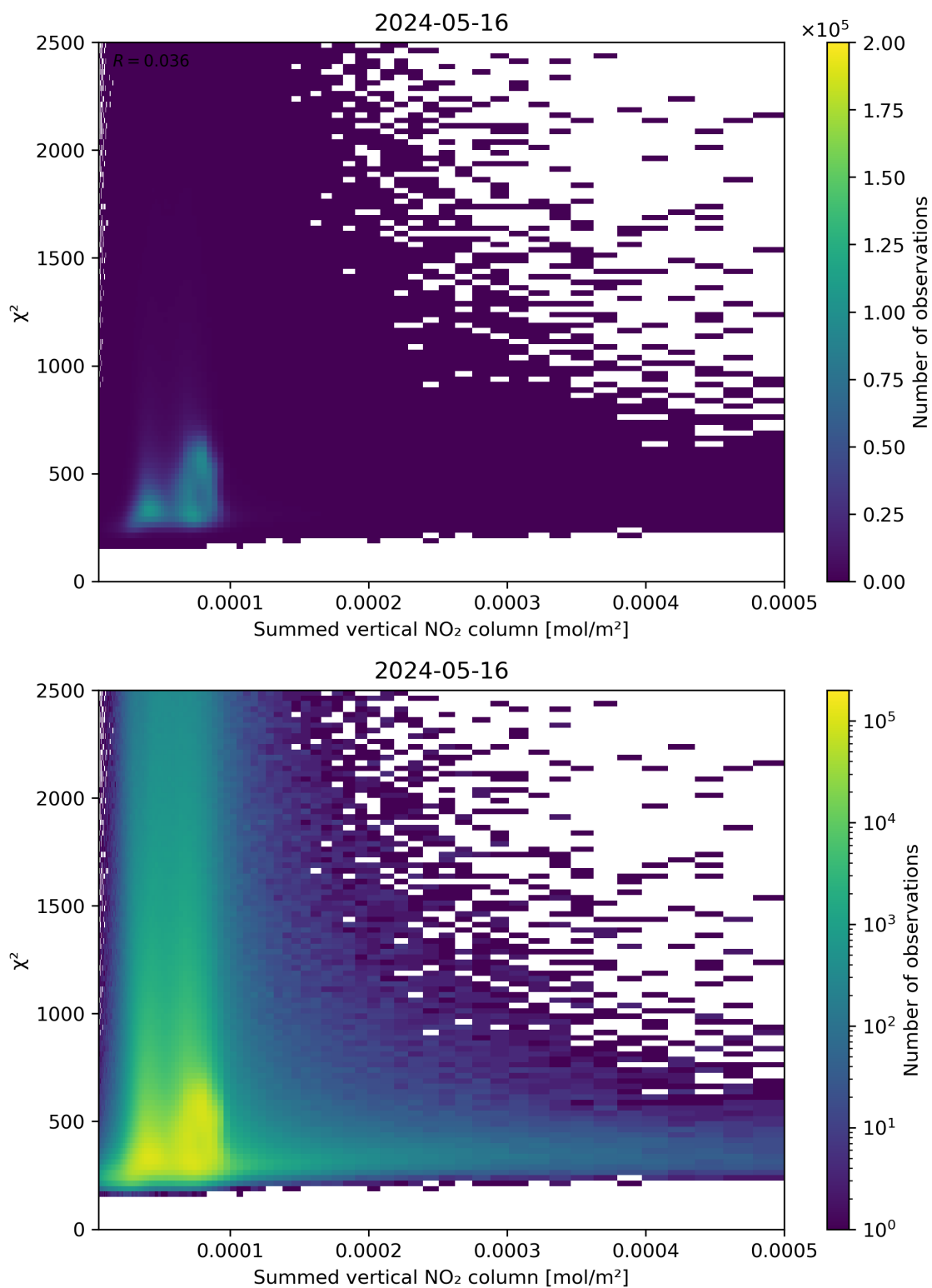
Figure 104: Scatter density plot of “Summed vertical NO 2 column” against “ \chi^2 ” for 2024-05-15 to 2024-05-17.
