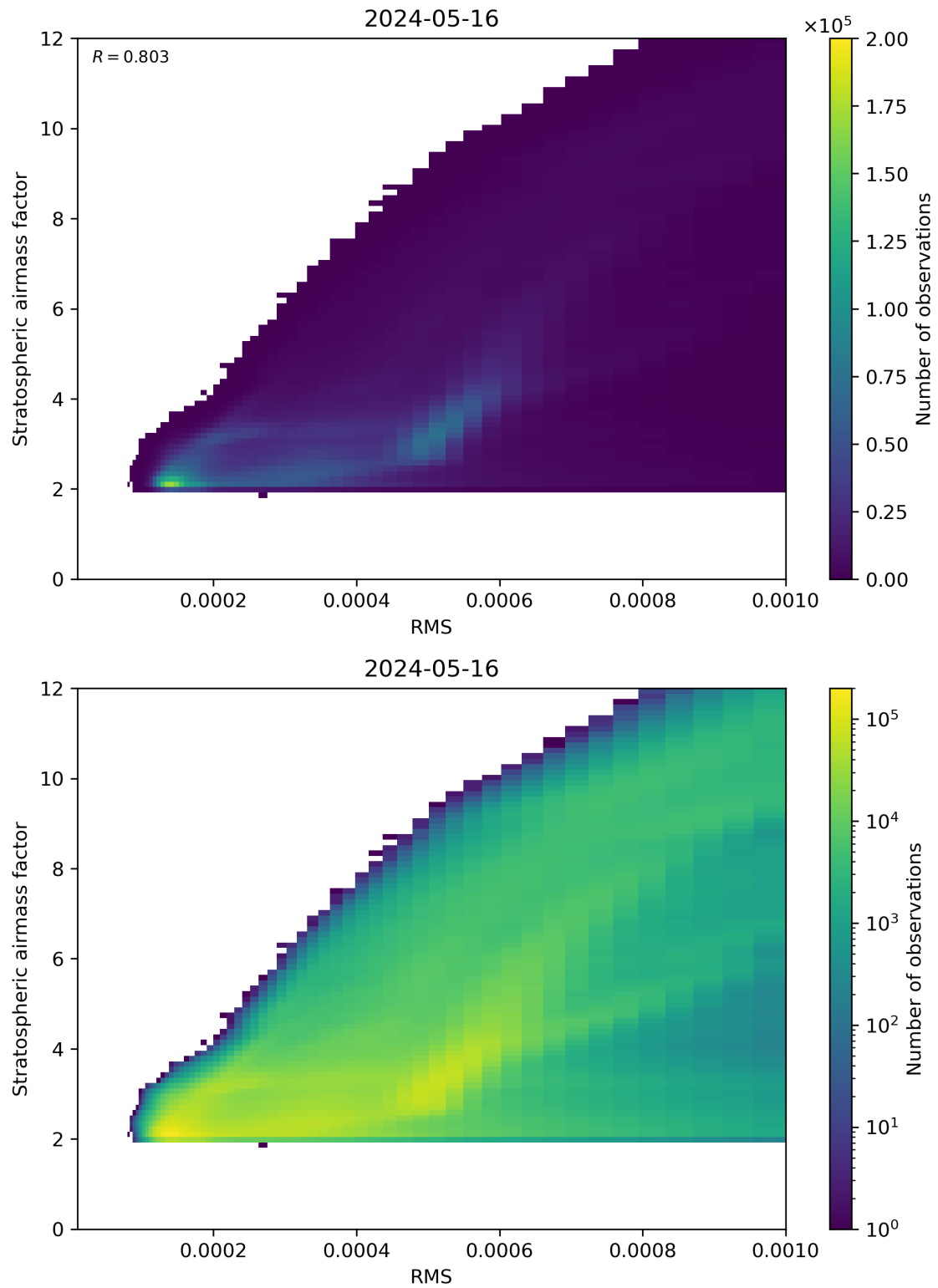
Figure 144: Scatter density plot of “RMS” against “Stratospheric airmass factor” for 2024-05-15 to 2024-05-17.
