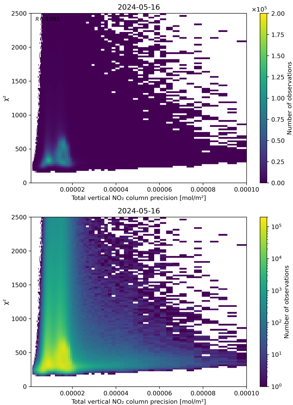
Figure 116: Scatter density plot of “Total vertical NO 2 column precision” against “ \chi^2 ” for 2024-05-15 to 2024-05-17.
