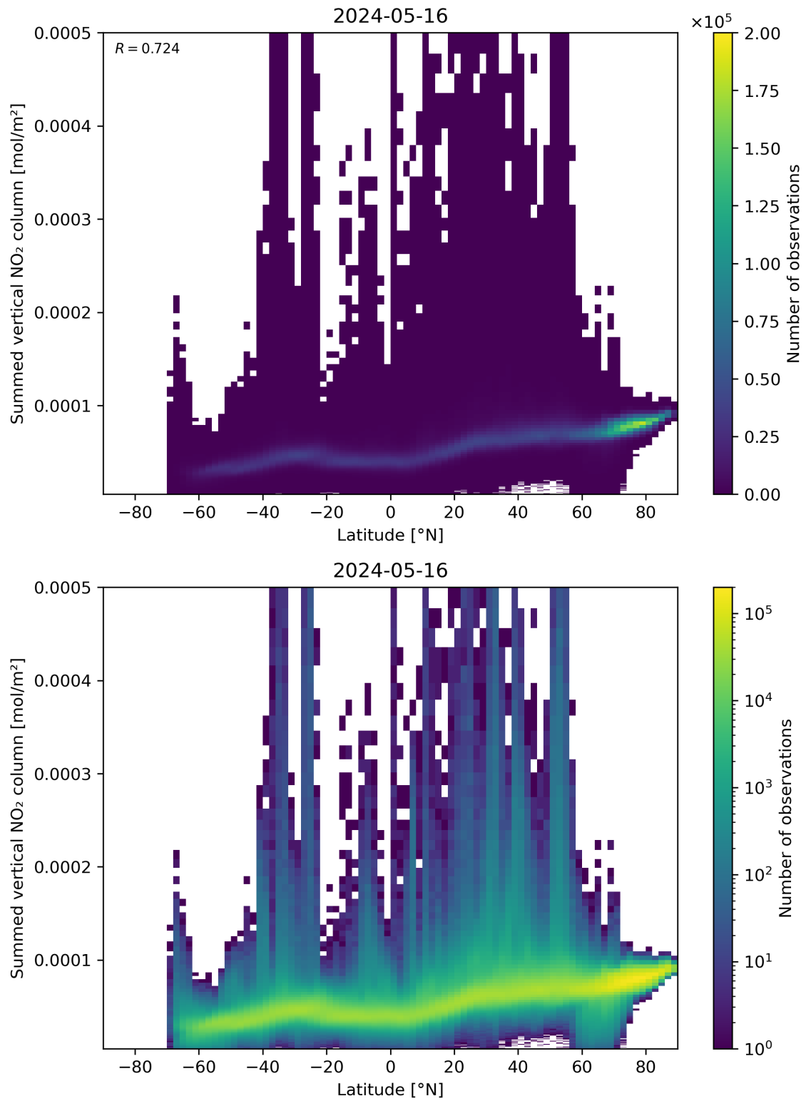
Figure 88: Scatter density plot of “Latitude” against “Summed vertical NO 2 column” for 2024-05-15 to 2024-05-17.
