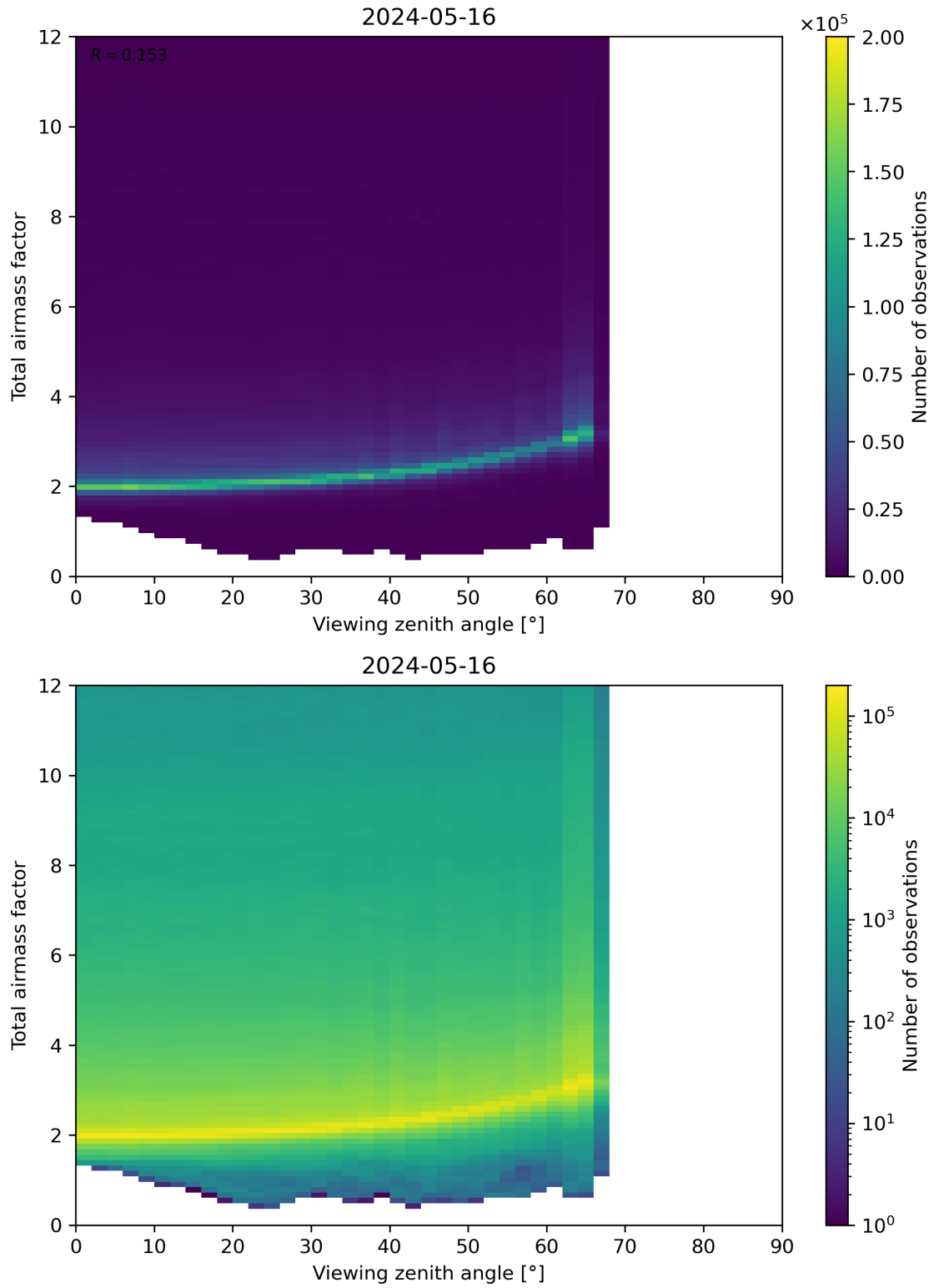
Figure 160: Scatter density plot of “Viewing zenith angle” against “Total airmass factor” for 2024-05-15 to 2024-05-17.
