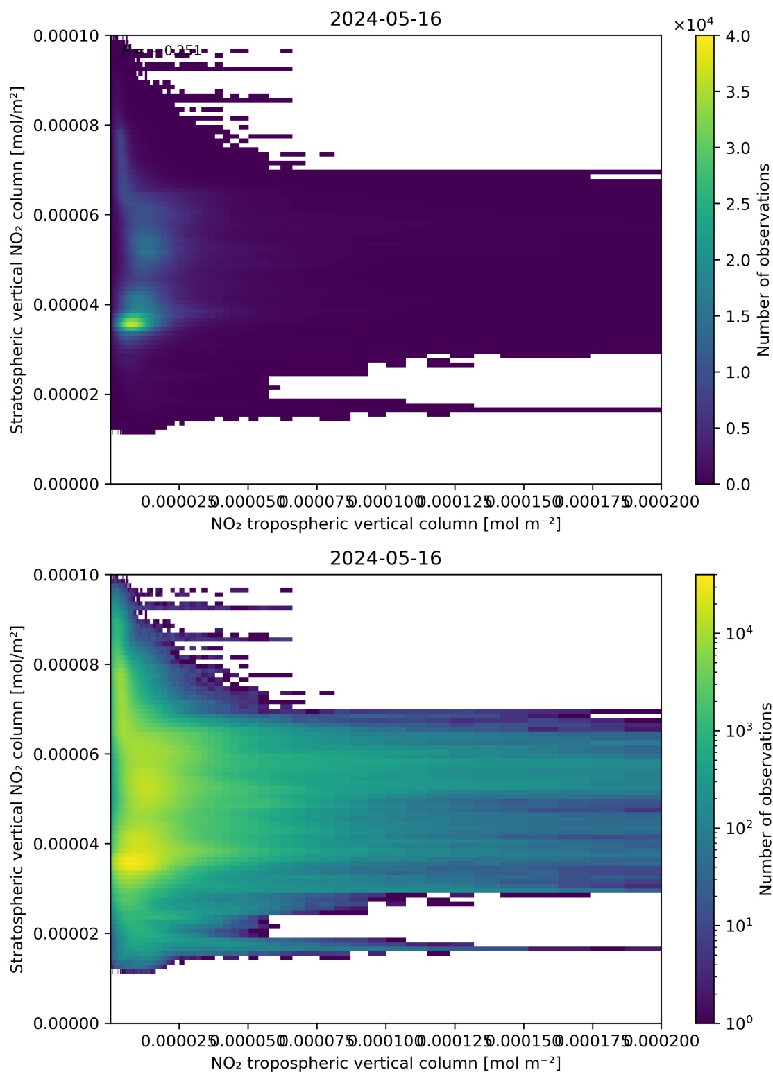
Figure 125: Scatter density plot of “NO 2 tropospheric vertical column” against “Stratospheric vertical NO 2 column” for 2024-05-15 to 2024-05-17.
