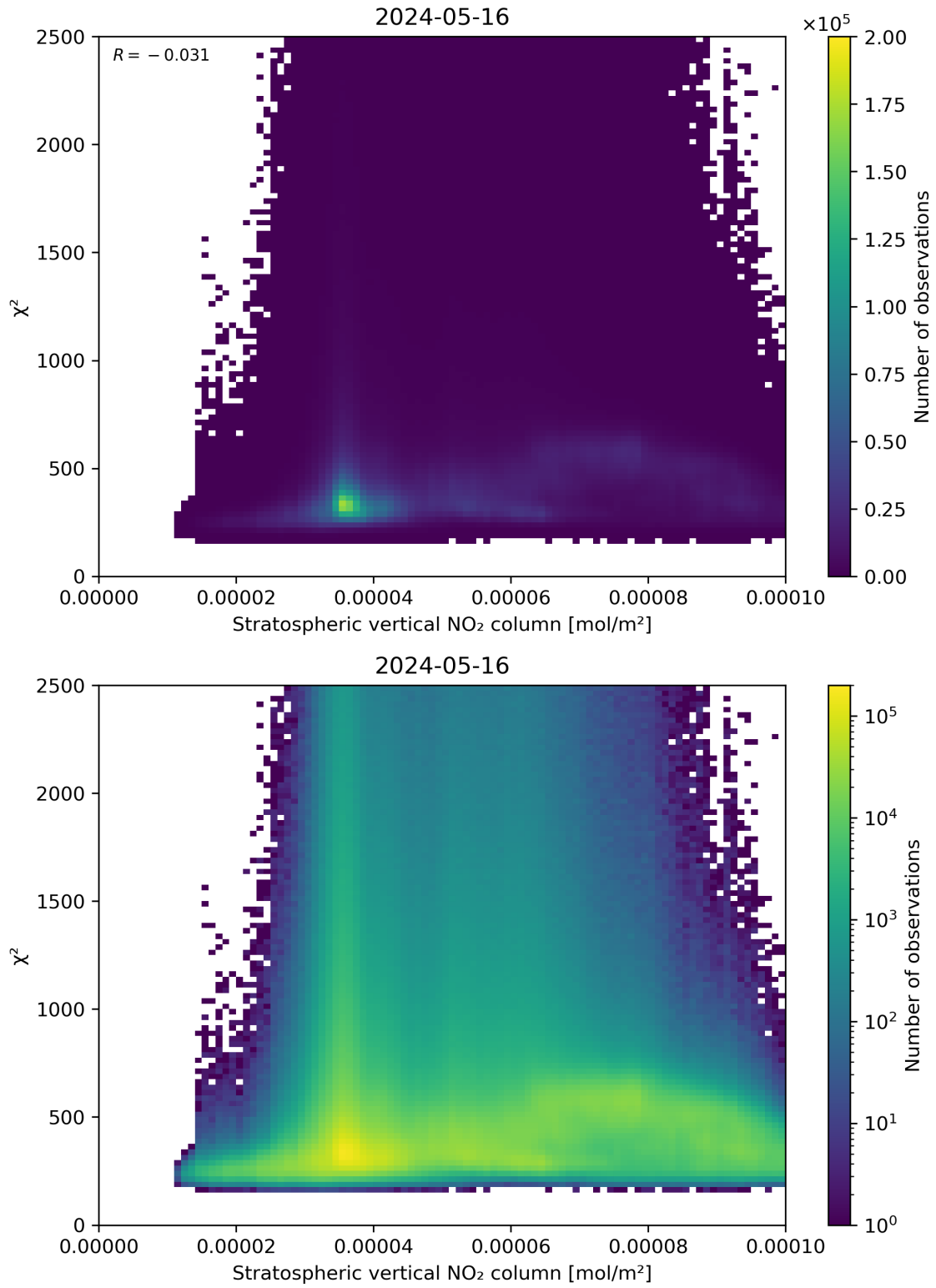
Figure 97: Scatter density plot of “Stratospheric vertical NO 2 column” against “ \chi^2 ” for 2024-05-15 to 2024-05-17.
