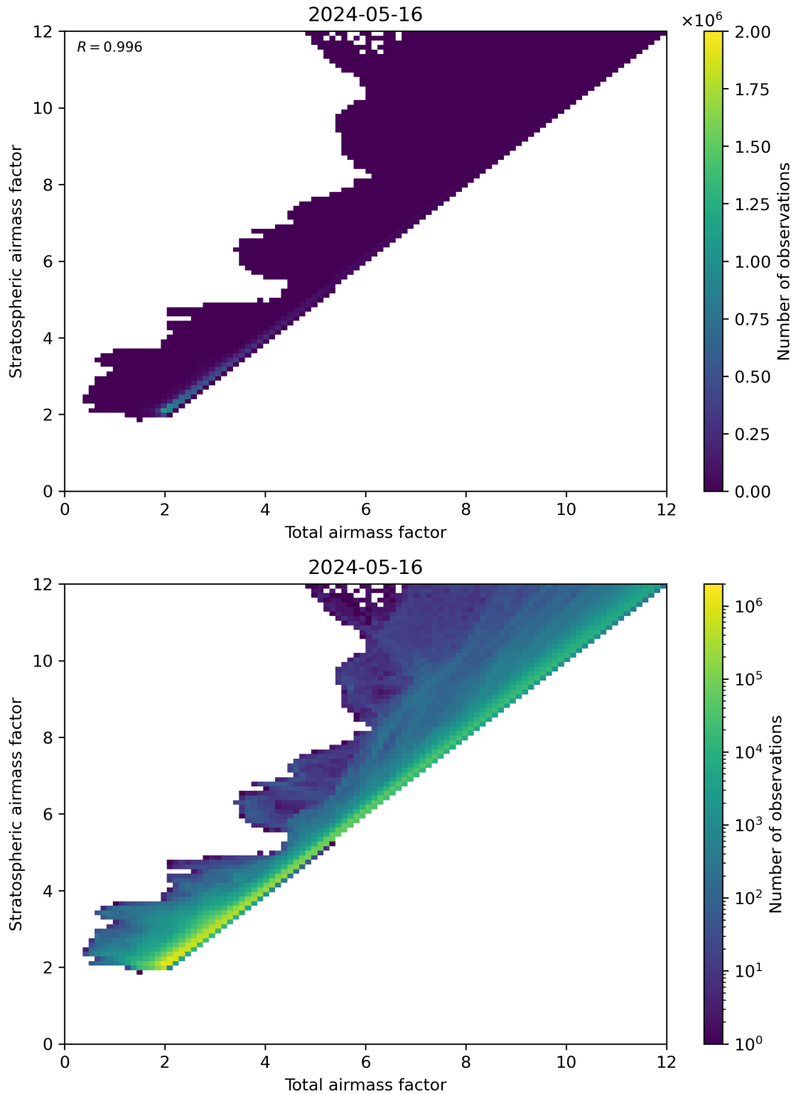
Figure 62: Scatter density plot of “Total airmass factor” against “Stratospheric airmass factor” for 2024-05-15 to 2024-05-17.
