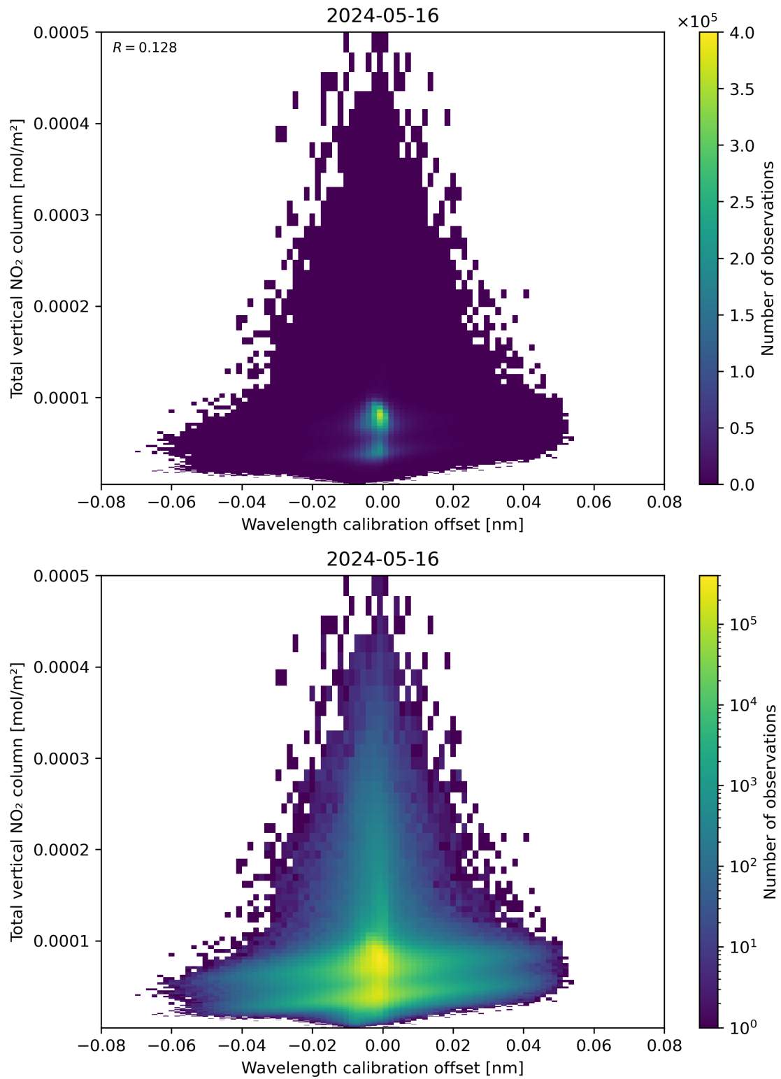
Figure 179: Scatter density plot of “Wavelength calibration offset” against “Total vertical NO 2 column” for 2024-05-15 to 2024-05-17.
