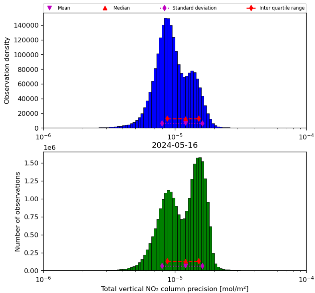
Figure 39: Histogram of “Total vertical NO 2 column precision” for 2024-05-15 to 2024-05-17
