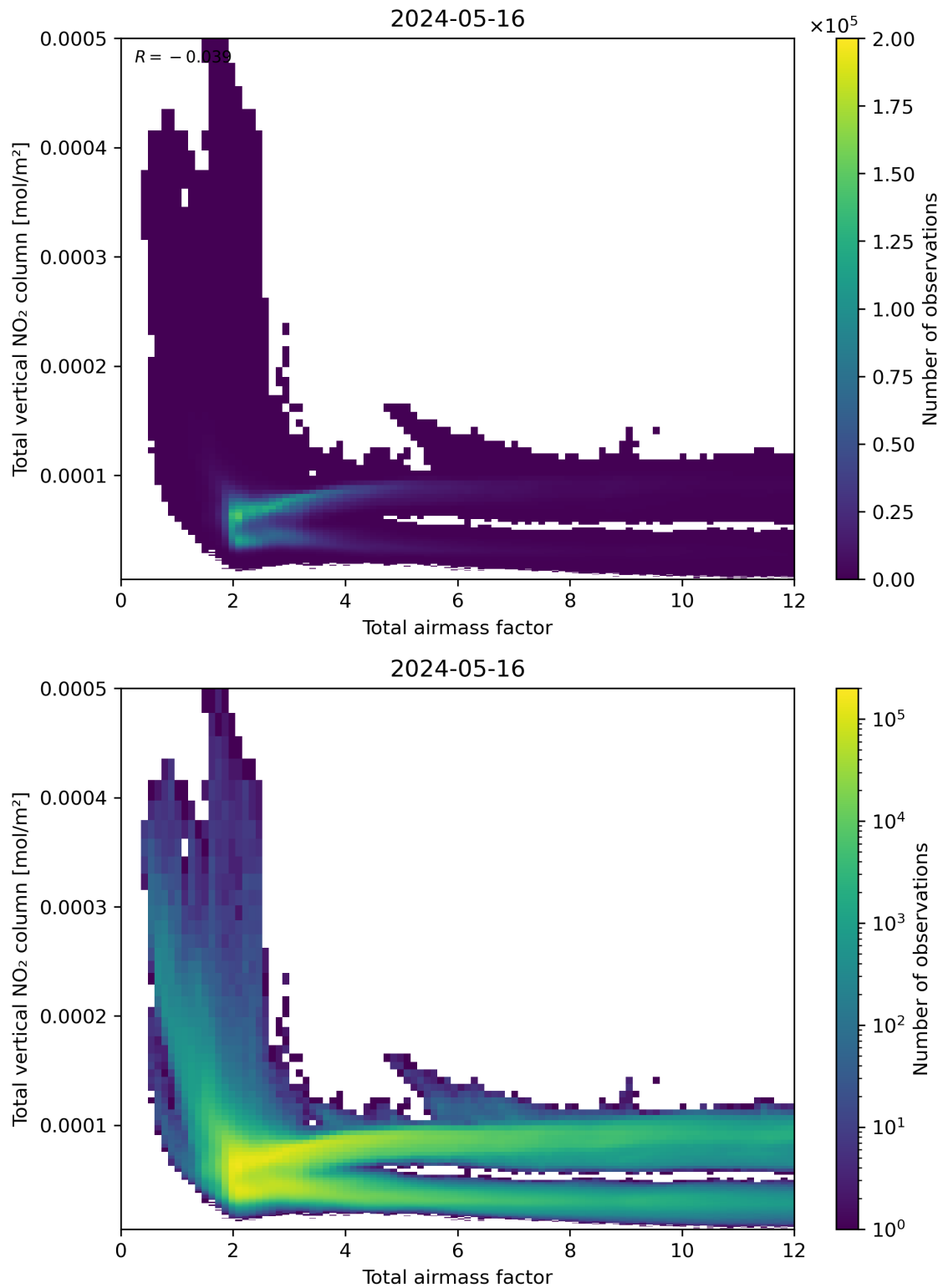
Figure 67: Scatter density plot of “Total air mass factor” against “Total vertical NO 2 column” for 2024-05-15 to 2024-05-17.
