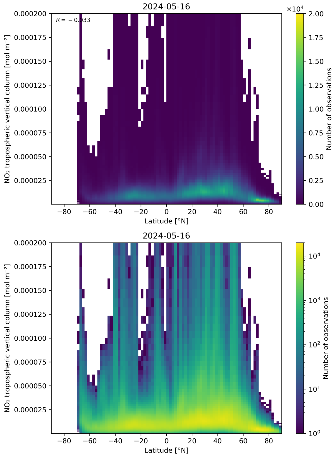
Figure 92: Scatter density plot of “Latitude” against “NO 2 tropospheric vertical column” for 2024-05-15 to 2024-05-17.
