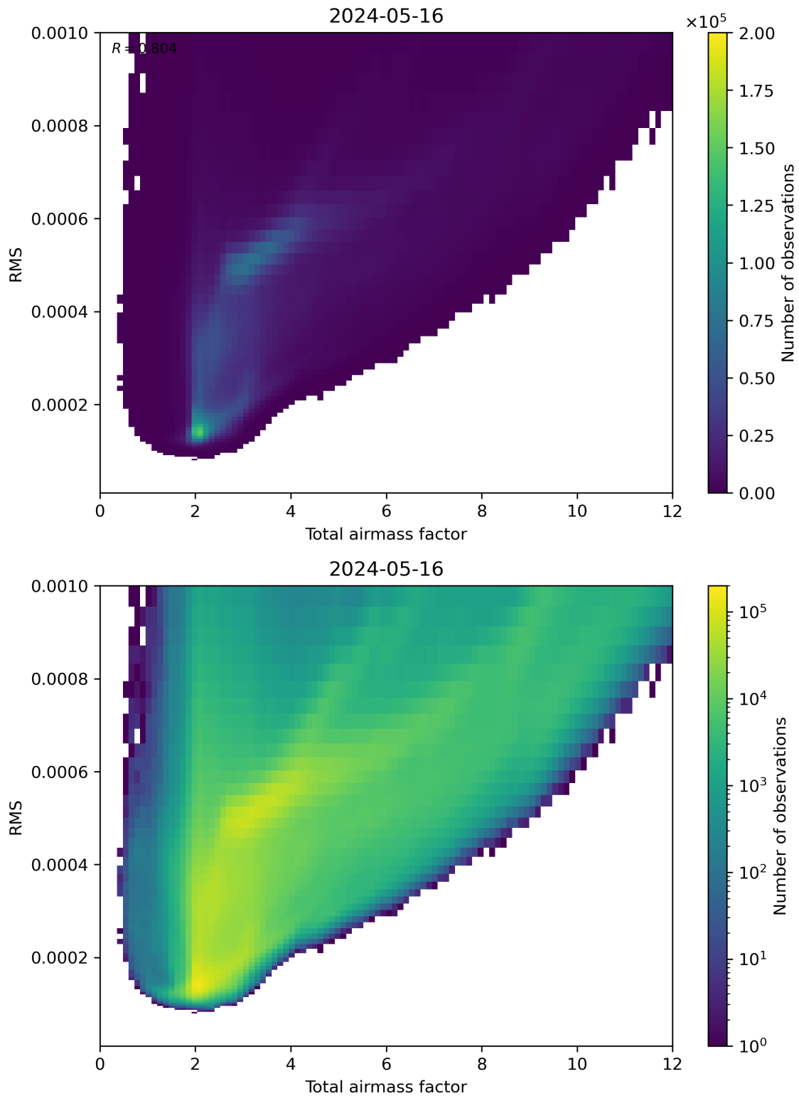
Figure 69: Scatter density plot of “Total airmass factor” against “RMS” for 2024-05-15 to 2024-05-17.
