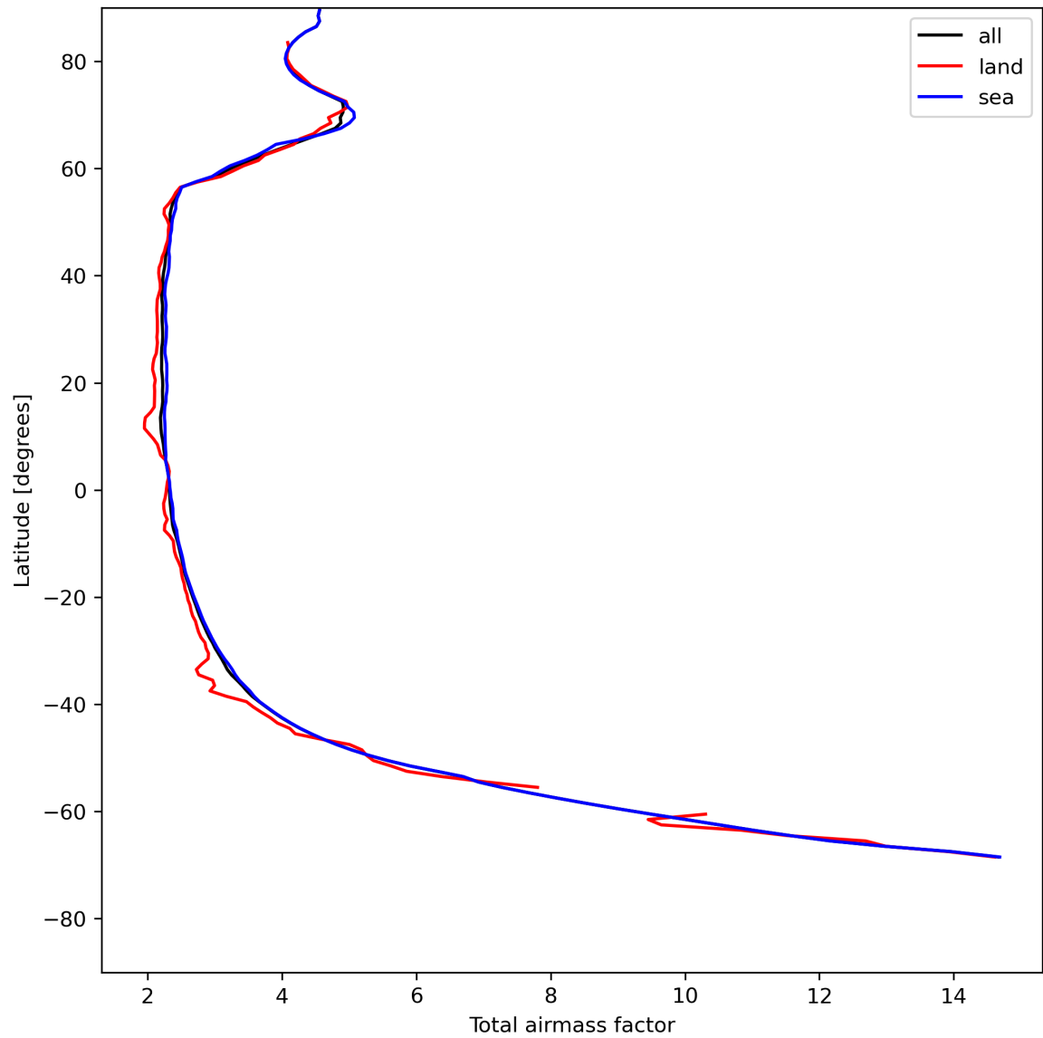
Figure 15: Zonal average of “Total airmass factor” for 2024-05-15 to 2024-05-17.
