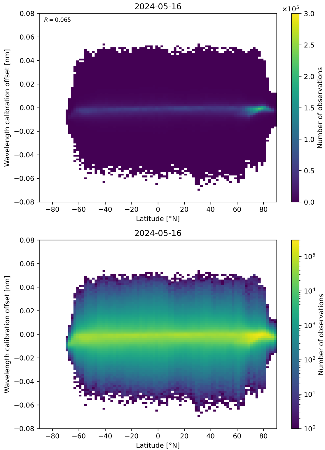
Figure 95: Scatter density plot of “Latitude” against “Wavelength calibration offset” for 2024-05-15 to 2024-05-17.
