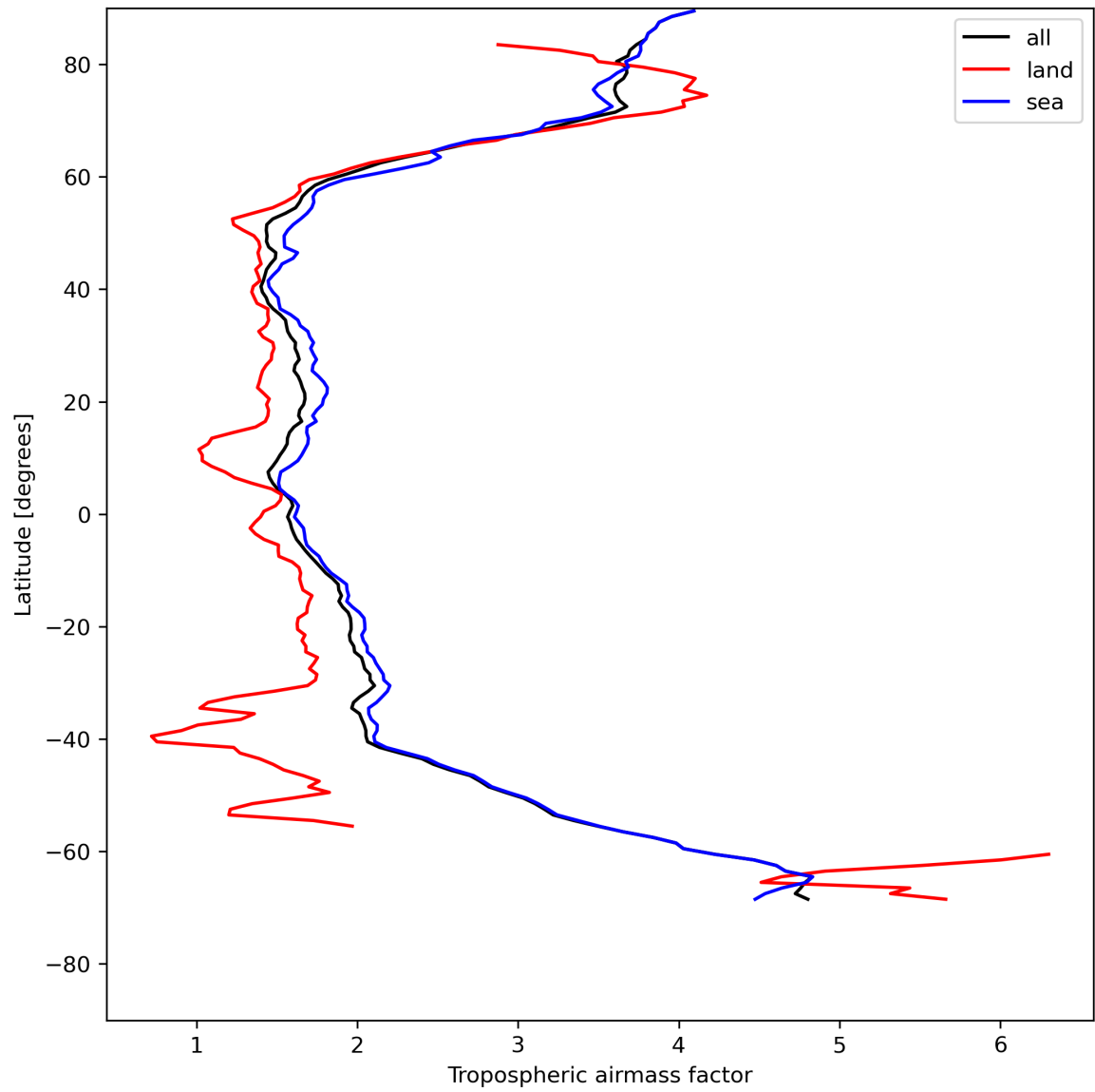
Figure 14: Zonal average of “Tropospheric airmass factor” for 2024-05-15 to 2024-05-17.
