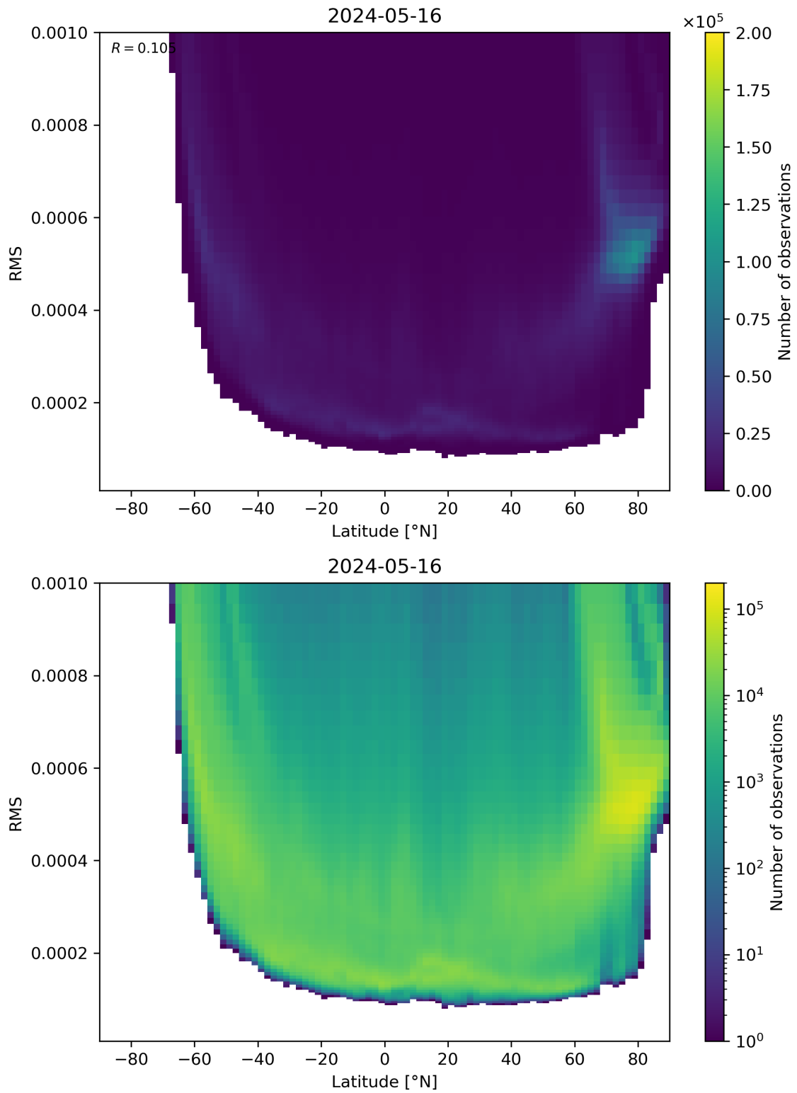
Figure 94: Scatter density plot of “Latitude” against “RMS” for 2024-05-15 to 2024-05-17.
