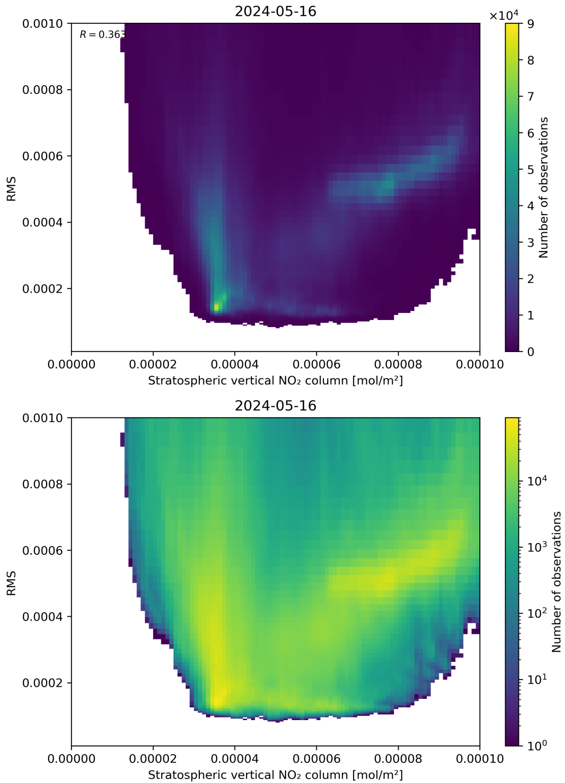
Figure 102: Scatter density plot of “Stratospheric vertical NO 2 column” against “RMS” for 2024-05-15 to 2024-05-17.
