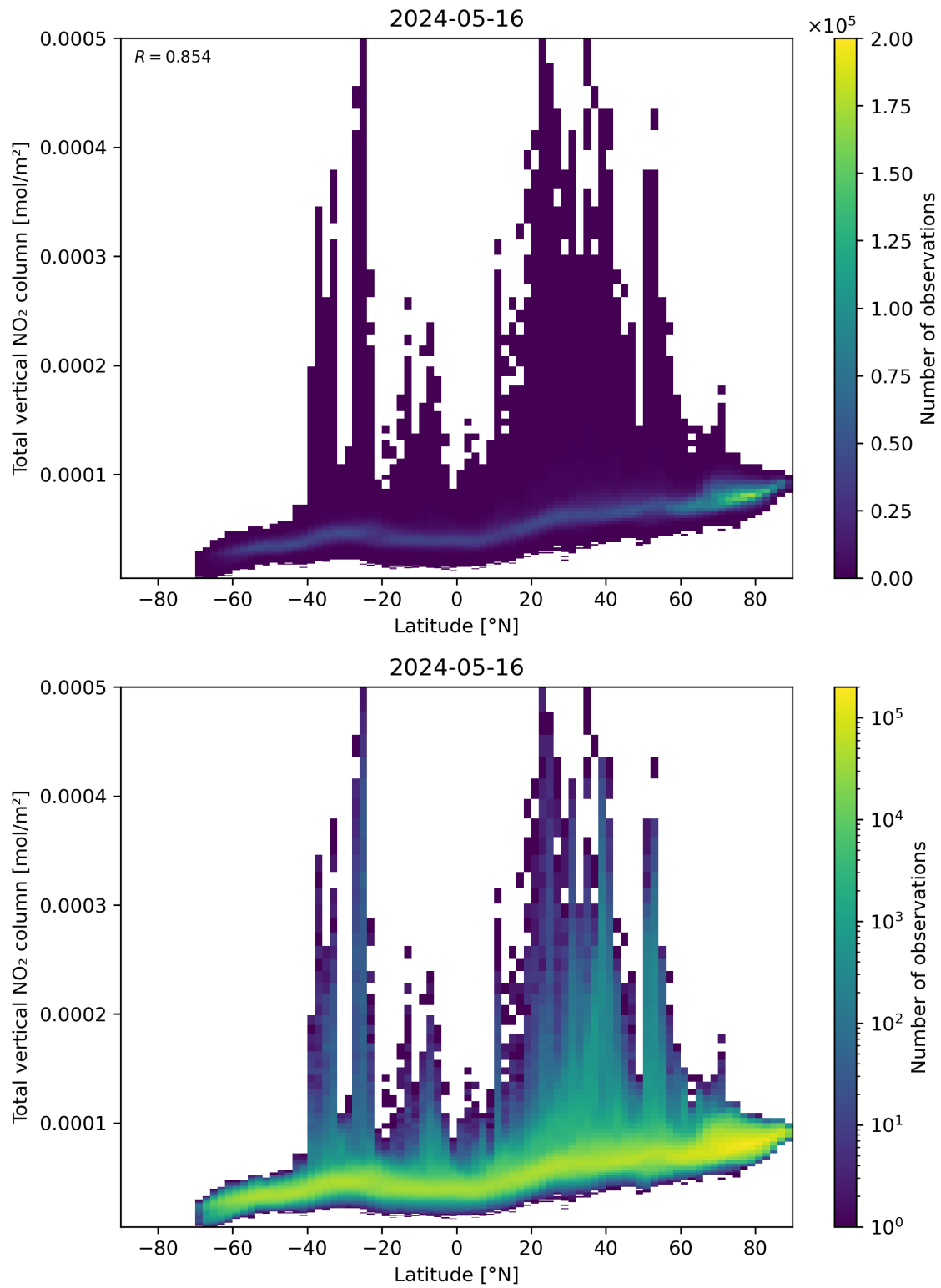
Figure 90: Scatter density plot of “Latitude” against “Total vertical NO 2 column” for 2024-05-15 to 2024-05-17.
