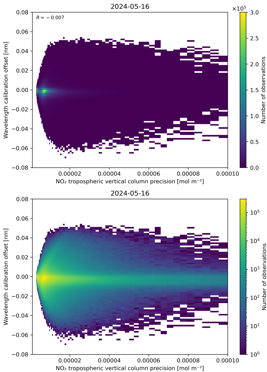
Figure 141: Scatter density plot of “NO 2 tropospheric vertical column precision” against “Wavelength calibration offset” for 2024-05-15 to 2024-05-17.
