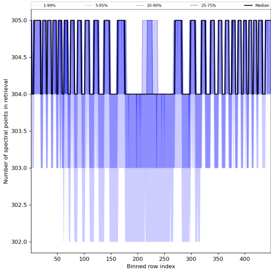
Figure 50: Along track statistics of “Number of spectral points in retrieval” for 2024-05-15 to 2024-05-17
