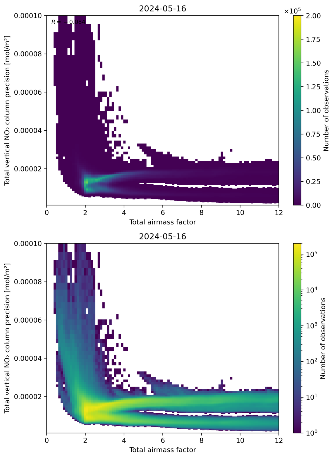
Figure 68: Scatter density plot of “Total airmass factor” against “Total vertical NO 2 column precision” for 2024-05-15 to 2024-05-17.
