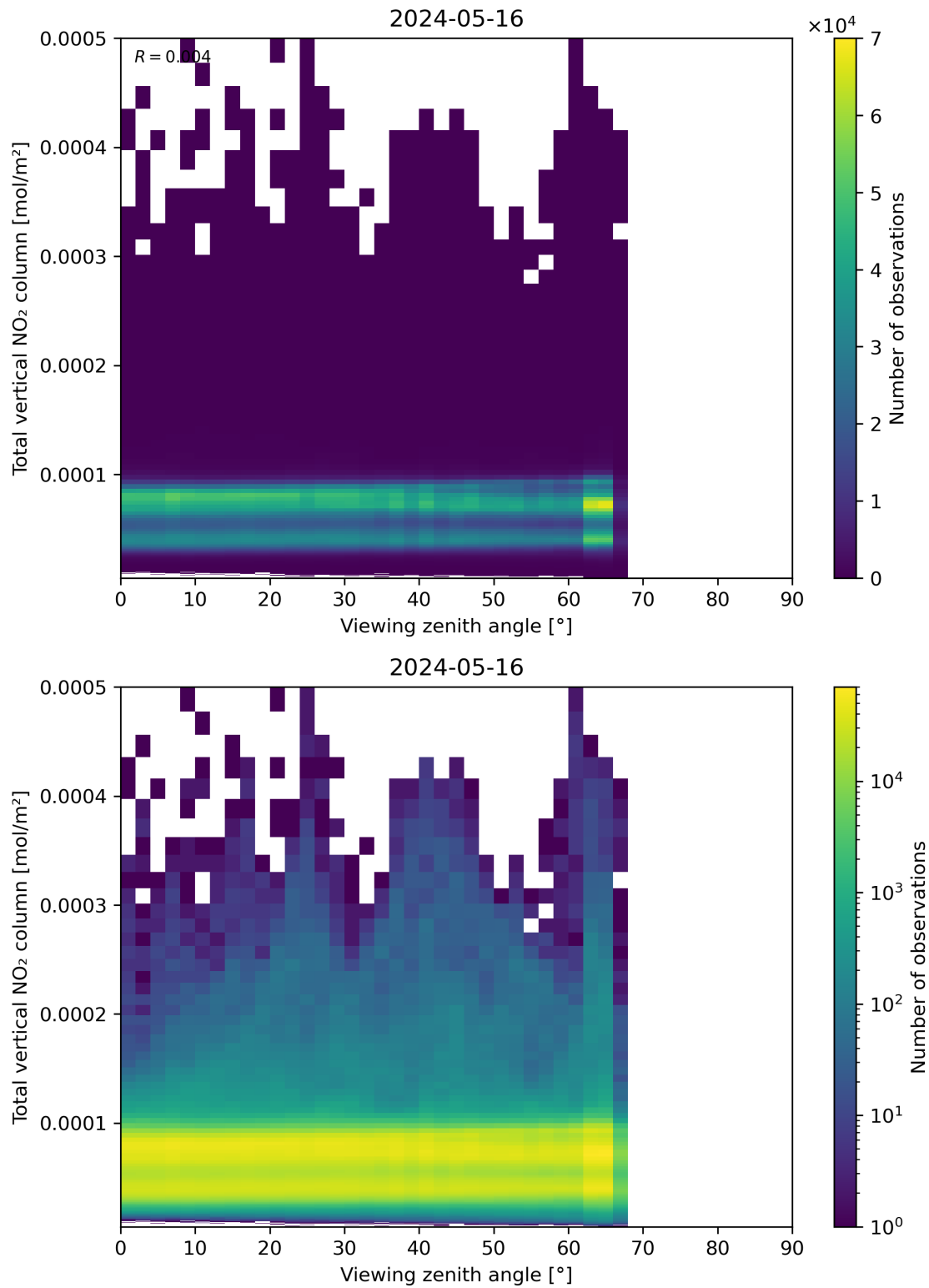
Figure 167: Scatter density plot of “Viewing zenith angle” against “Total vertical NO 2 column” for 2024-05-15 to 2024-05-17.
