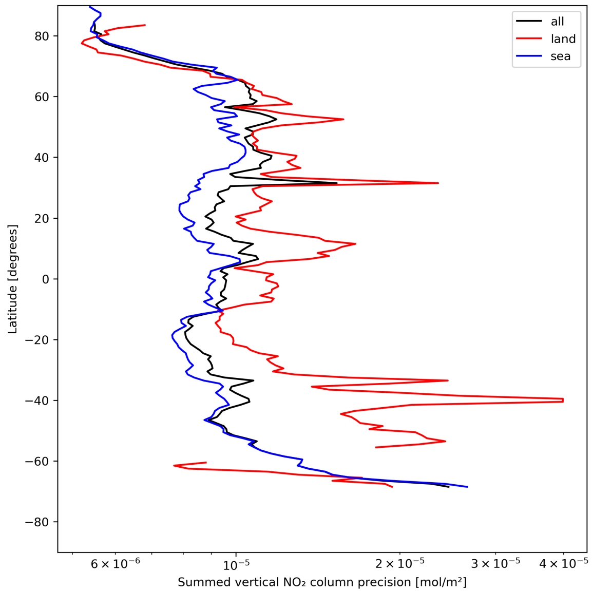
Figure 24: Zonal average of “Summed vertical NO 2 column precision” for 2024-05-15 to 2024-05-17.
