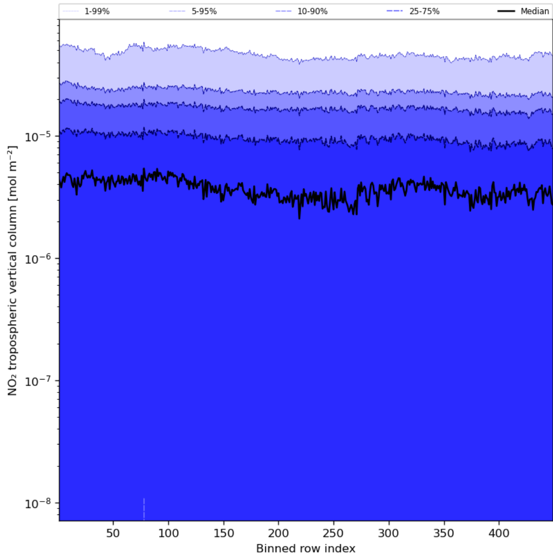
Figure 46: Along track statistics of “NO 2 tropospheric vertical column” for 2024-05-15 to 2024-05-17
