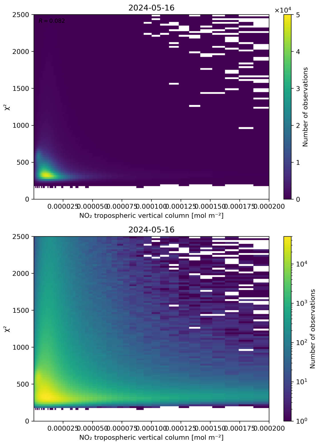
Figure 124: Scatter density plot of “NO 2 tropospheric vertical column” against “ \chi^2 ” for 2024-05-15 to 2024-05-17.
