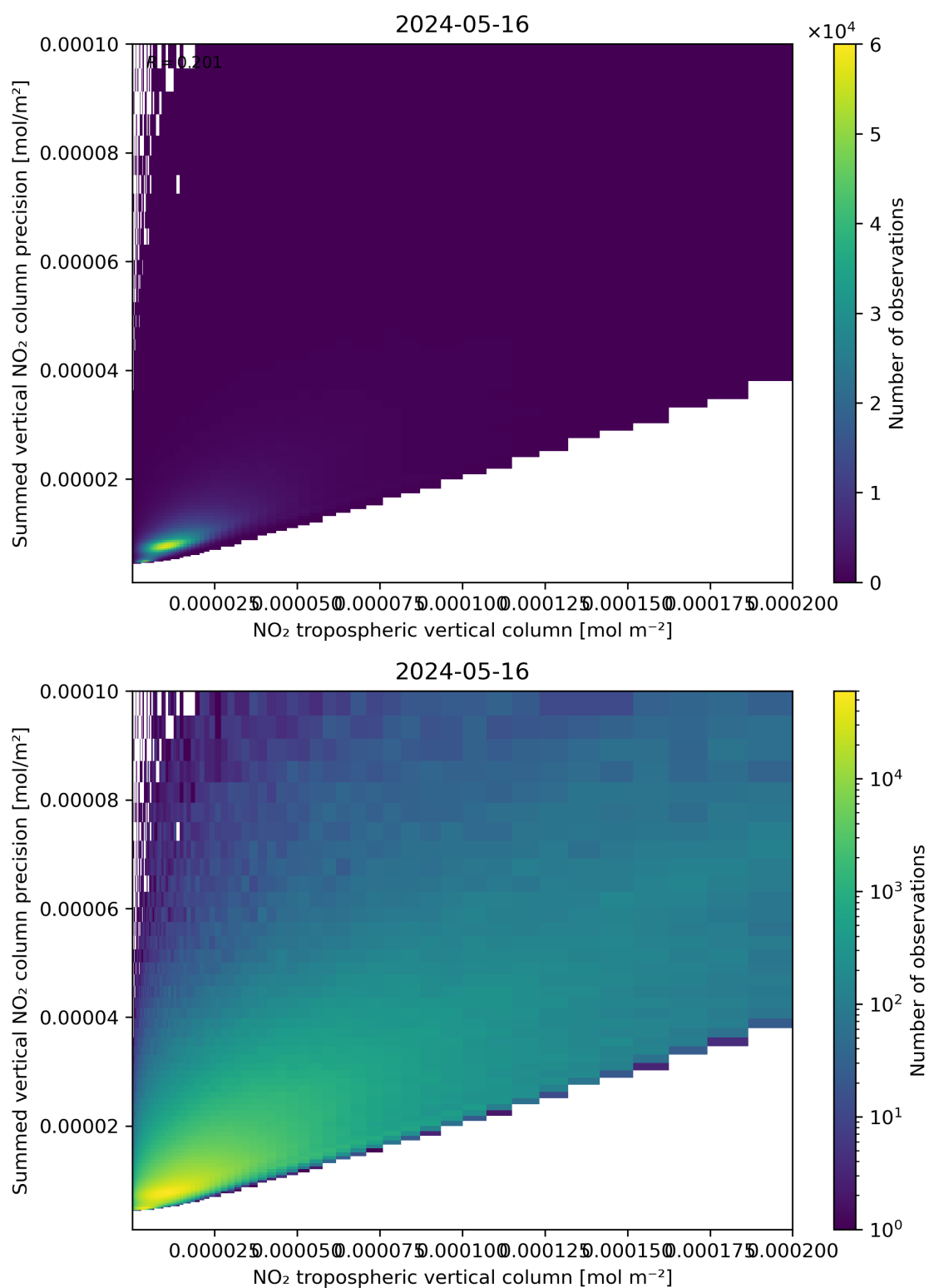
Figure 127: Scatter density plot of “NO 2 tropospheric vertical column” against “Summed vertical NO 2 column precision” for 2024-05-15 to 2024-05-17.
