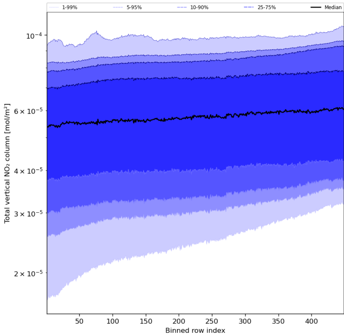
Figure 55: Along track statistics of “Total vertical NO 2 column” for 2024-05-15 to 2024-05-17
