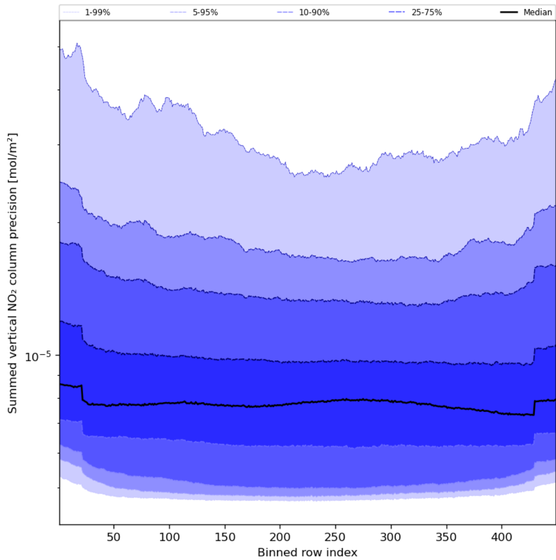
Figure 58: Along track statistics of “Summed vertical NO 2 column precision” for 2024-05-15 to 2024-05-17
