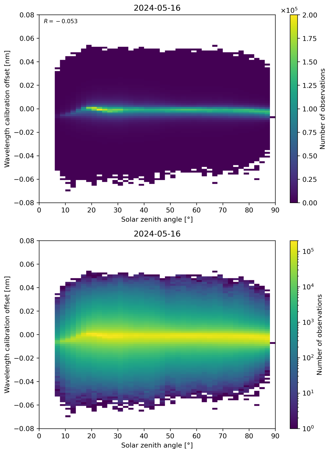
Figure 158: Scatter density plot of “Solar zenith angle” against “Wavelength calibration offset” for 2024-05-15 to 2024-05-17.
