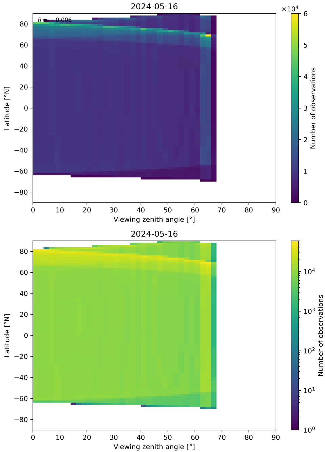
Figure 163: Scatter density plot of “Viewing zenith angle” against “Latitude” for 2024-05-15 to 2024-05-17.
