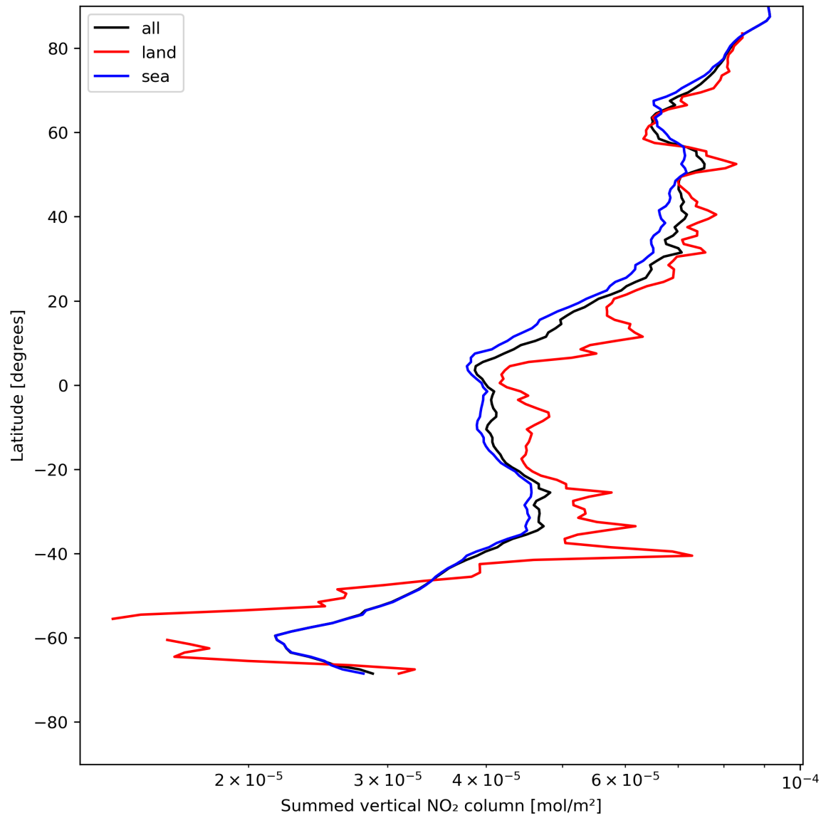
Figure 23: Zonal average of “Summed vertical NO 2 column” for 2024-05-15 to 2024-05-17.
