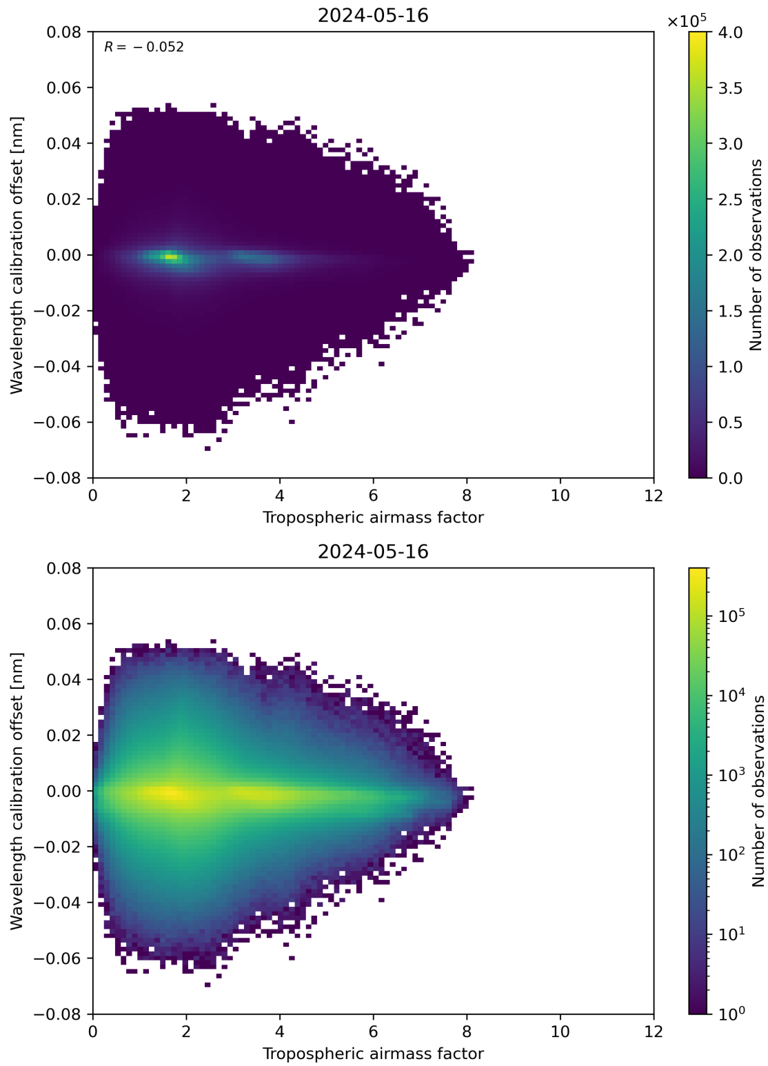
Figure 80: Scatter density plot of “Tropospheric airmass factor” against “Wavelength calibration offset” for 2024-05-15 to 2024-05-17.
