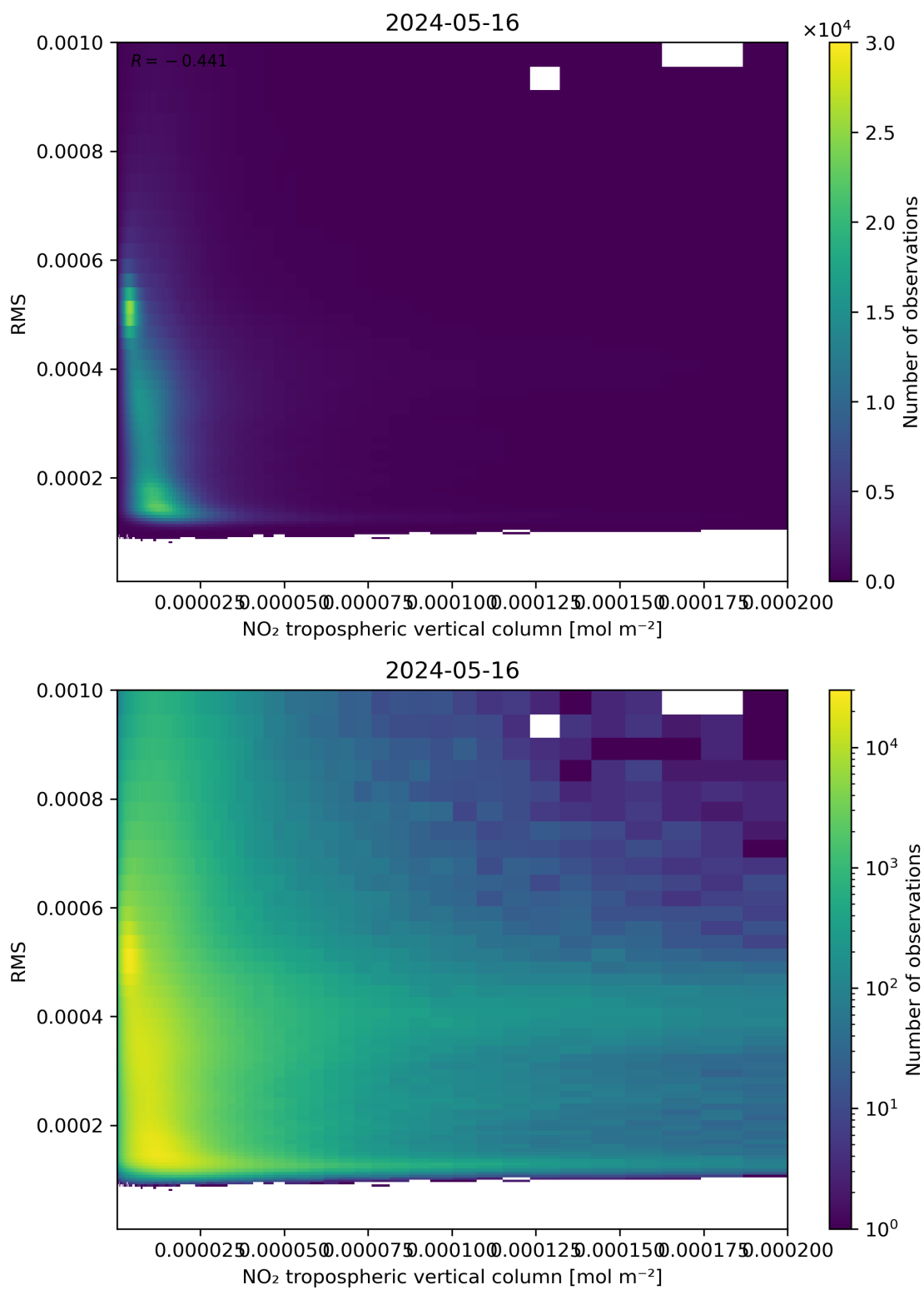
Figure 142: Scatter density plot of “NO 2 tropospheric vertical column” against “RMS” for 2024-05-15 to 2024-05-17.
