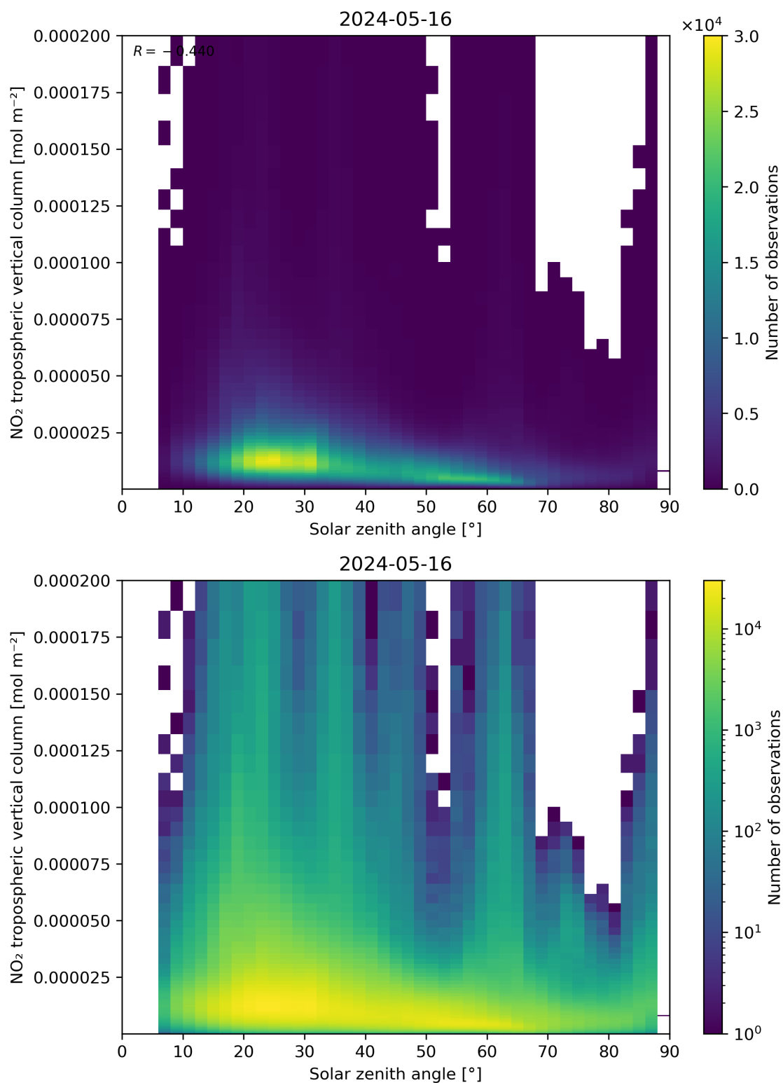
Figure 155: Scatter density plot of “Solar zenith angle” against “NO 2 tropospheric vertical column” for 2024-05-15 to 2024-05-17.
