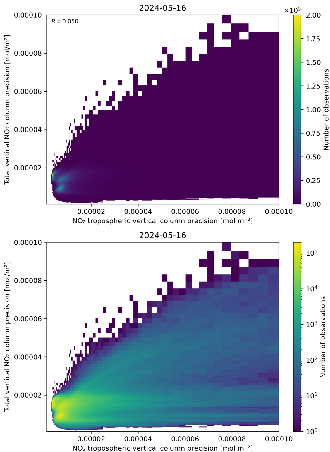
Figure 139: Scatter density plot of “NO 2 tropospheric vertical column precision” against “Total vertical NO 2 column precision” for 2024-05-15 to 2024-05-17.
