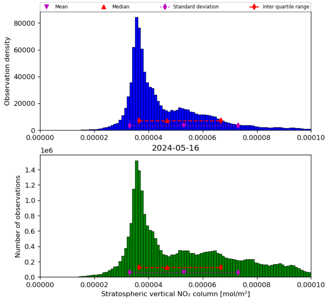
Figure 36: Histogram of “Stratospheric vertical NO 2 column” for 2024-05-15 to 2024-05-17
