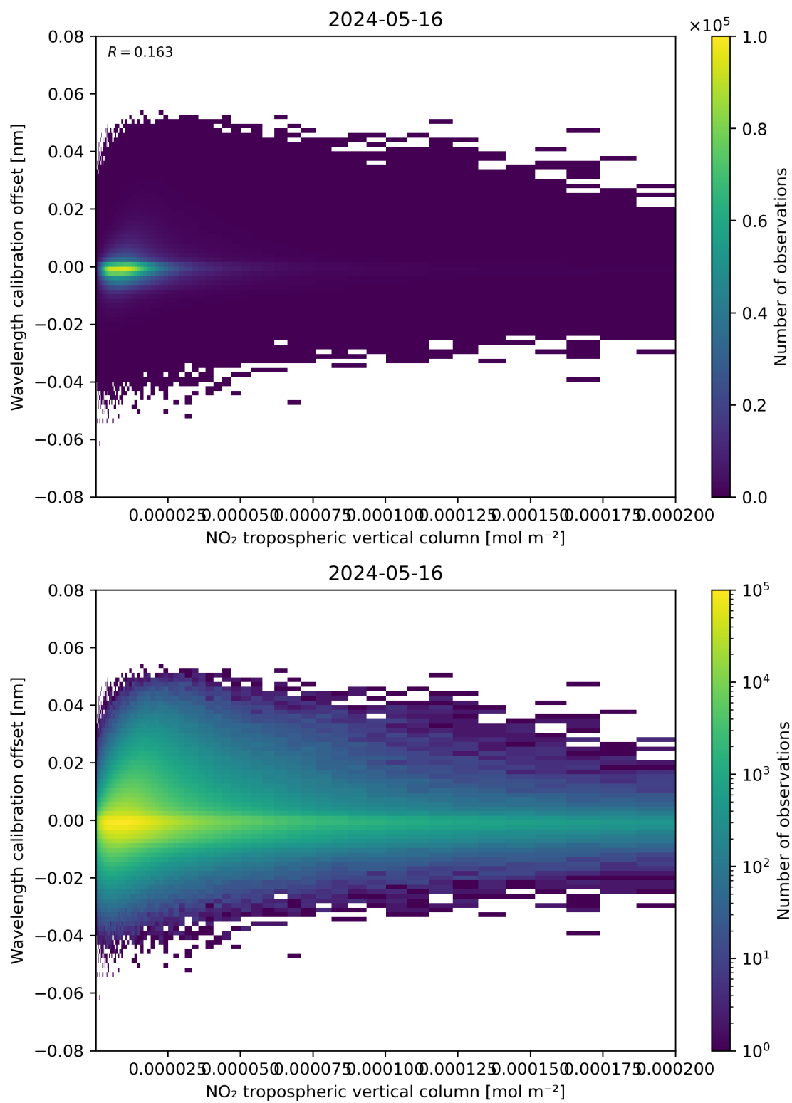
Figure 143: Scatter density plot of “NO 2 tropospheric vertical column” against “Wavelength calibration offset” for 2024-05-15 to 2024-05-17.
