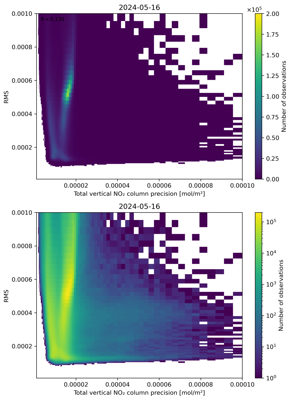
Figure 119: Scatter density plot of “Total vertical NO 2 column precision” against “RMS” for 2024-05-15 to 2024-05-17.
