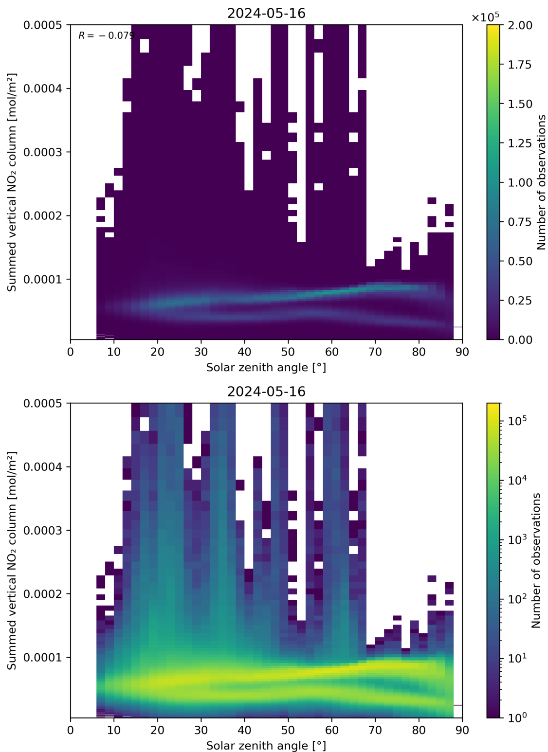
Figure 151: Scatter density plot of “Solar zenith angle” against “Summed vertical NO 2 column” for 2024-05-15 to 2024-05-17.
