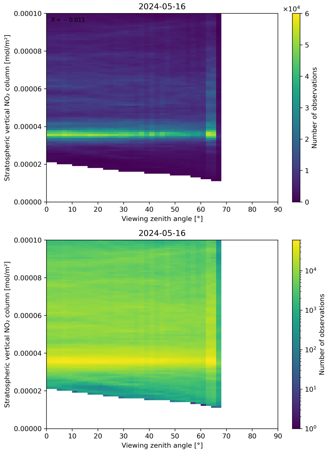
Figure 164: Scatter density plot of “Viewing zenith angle” against “Stratospheric vertical NO 2 column” for 2024-05-15 to 2024-05-17.
