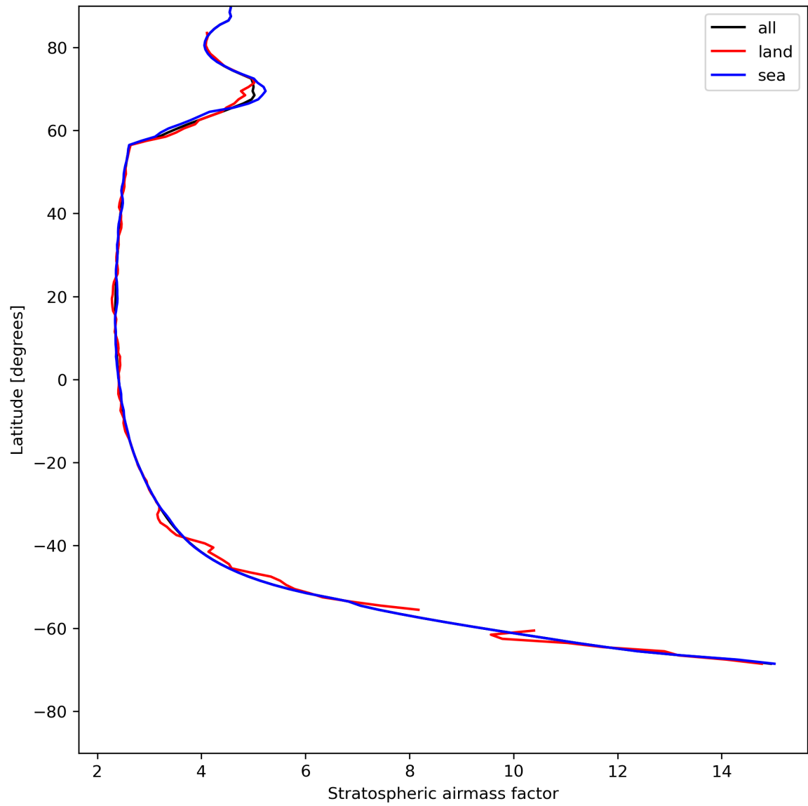
Figure 27: Zonal average of “Stratospheric airmass factor” for 2024-05-15 to 2024-05-17.
