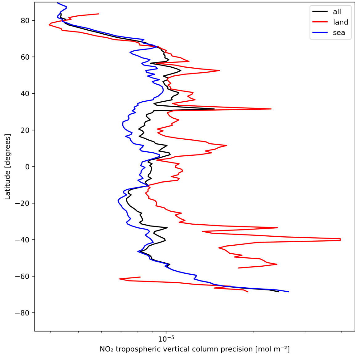
Figure 13: Zonal average of “NO 2 tropospheric vertical column precision” for 2024-05-15 to 2024-05-17.
