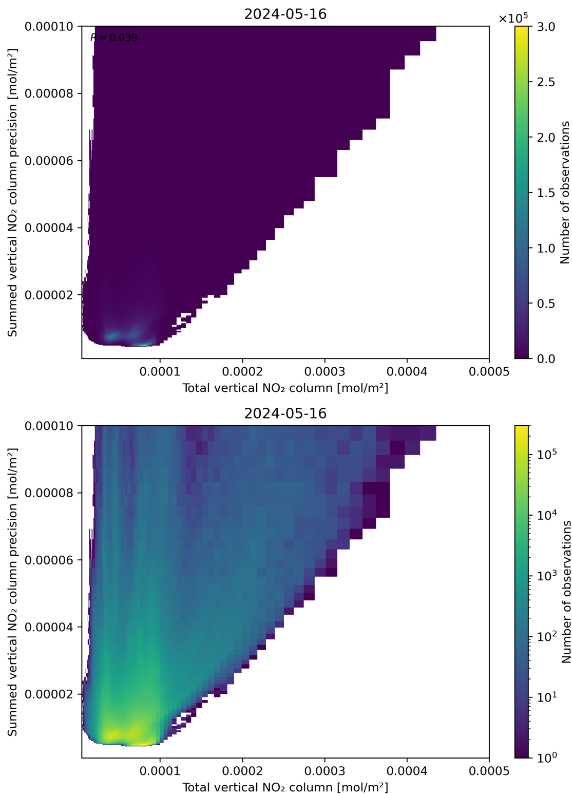
Figure 113: Scatter density plot of “Total vertical NO 2 column” against “Summed vertical NO 2 column precision” for 2024-05-15 to 2024-05-17.
