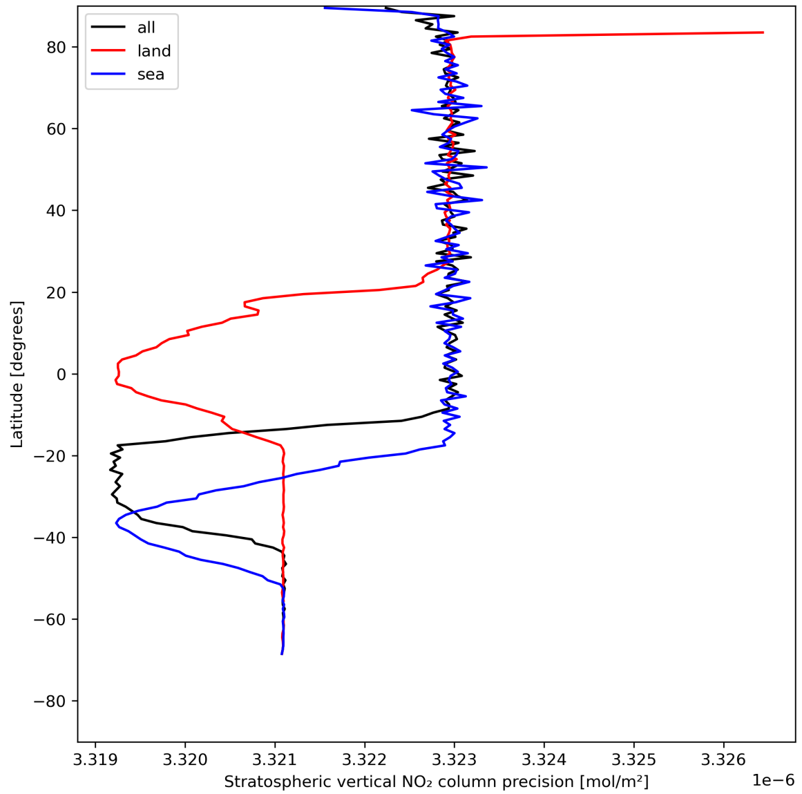
Figure 20: Zonal average of “Stratospheric vertical NO 2 column precision” for 2024-05-15 to 2024-05-17.
