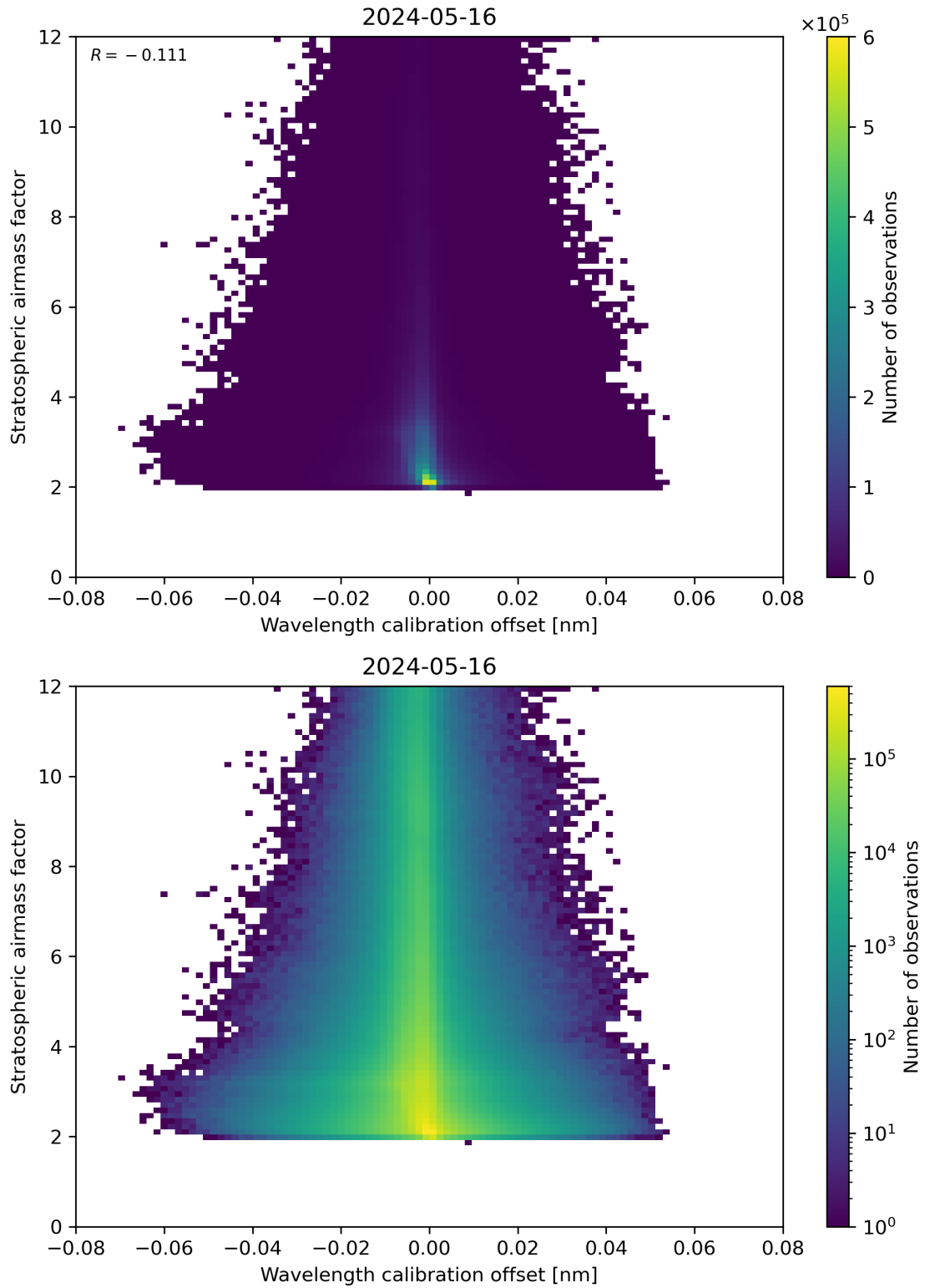
Figure 174: Scatter density plot of “Wavelength calibration offset” against “Stratospheric airmass factor” for 2024-05-15 to 2024-05-17.
