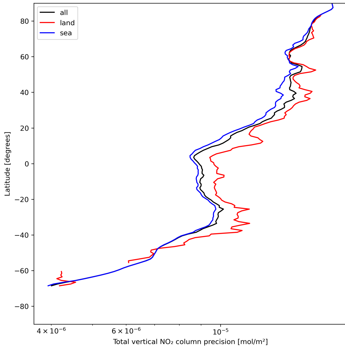
Figure 22: Zonal average of “Total vertical NO 2 column precision” for 2024-05-15 to 2024-05-17.
