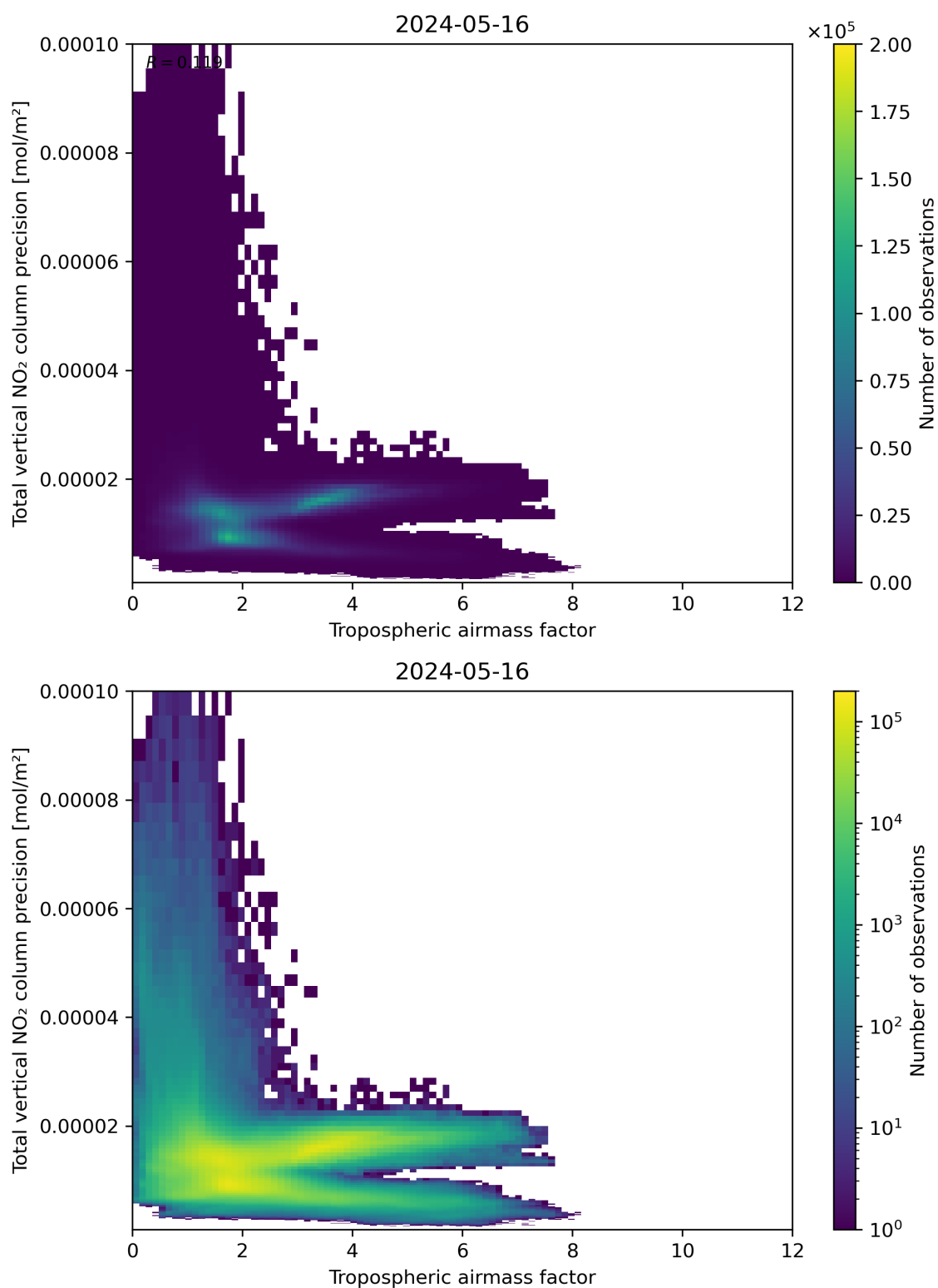
Figure 78: Scatter density plot of “Tropospheric air mass factor” against “Total vertical NO 2 column precision” for 2024-05-15 to 2024-05-17.
