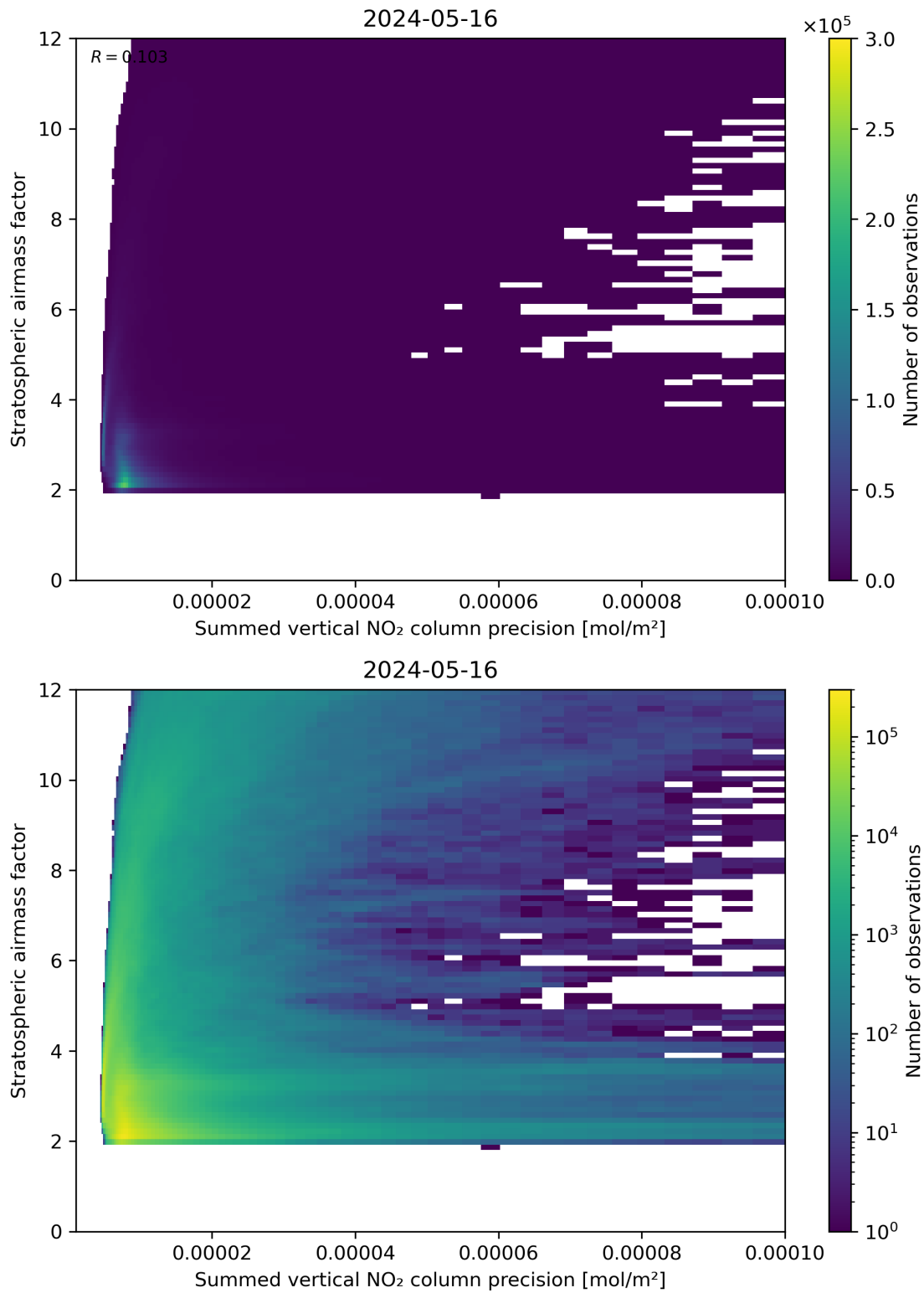
Figure 106: Scatter density plot of “Summed vertical NO 2 column precision” against “Stratospheric airmass factor” for 2024-05-15 to 2024-05-17.
