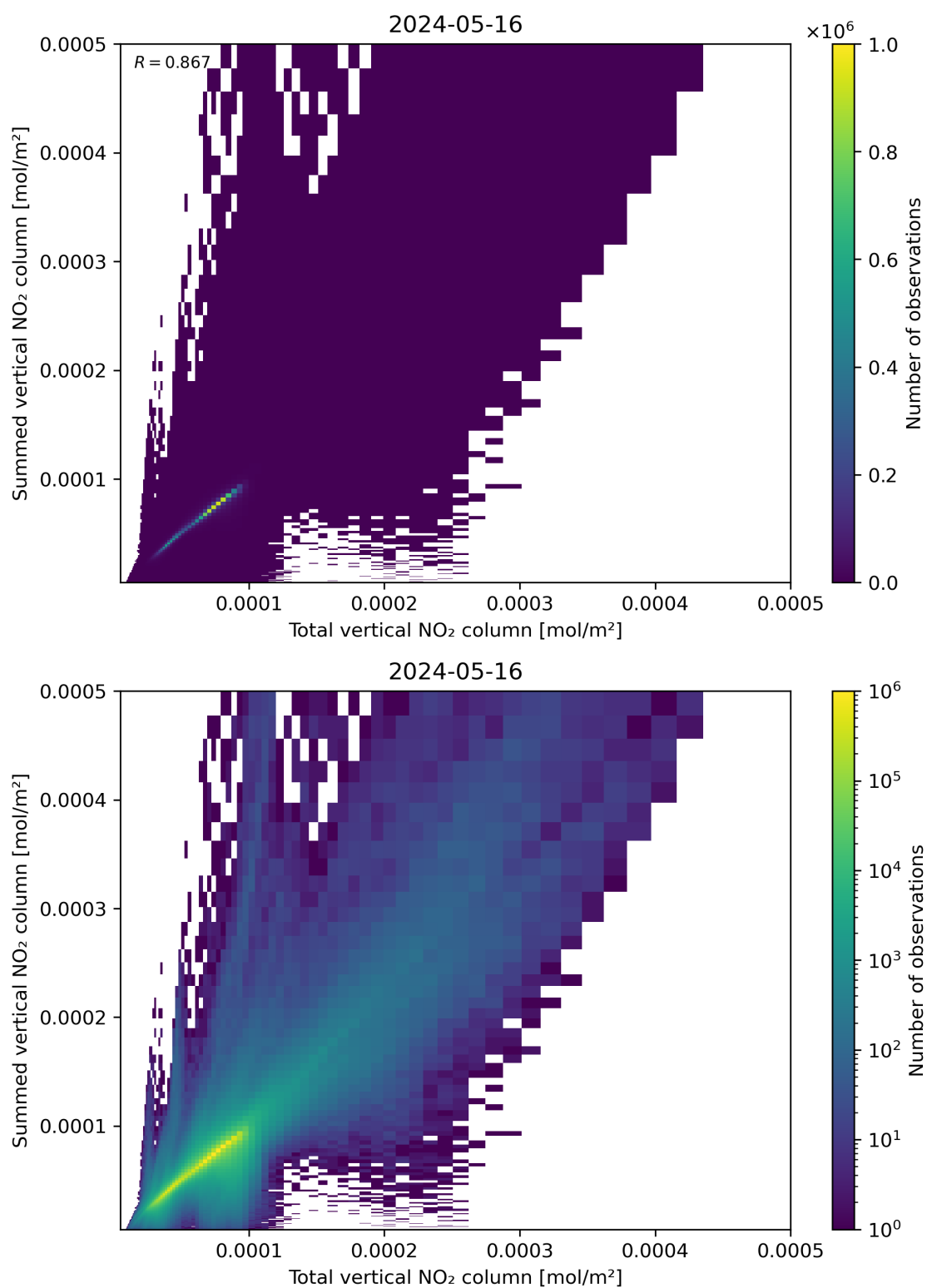
Figure 112: Scatter density plot of “Total vertical NO 2 column” against “Summed vertical NO 2 column” for 2024-05-15 to 2024-05-17.
