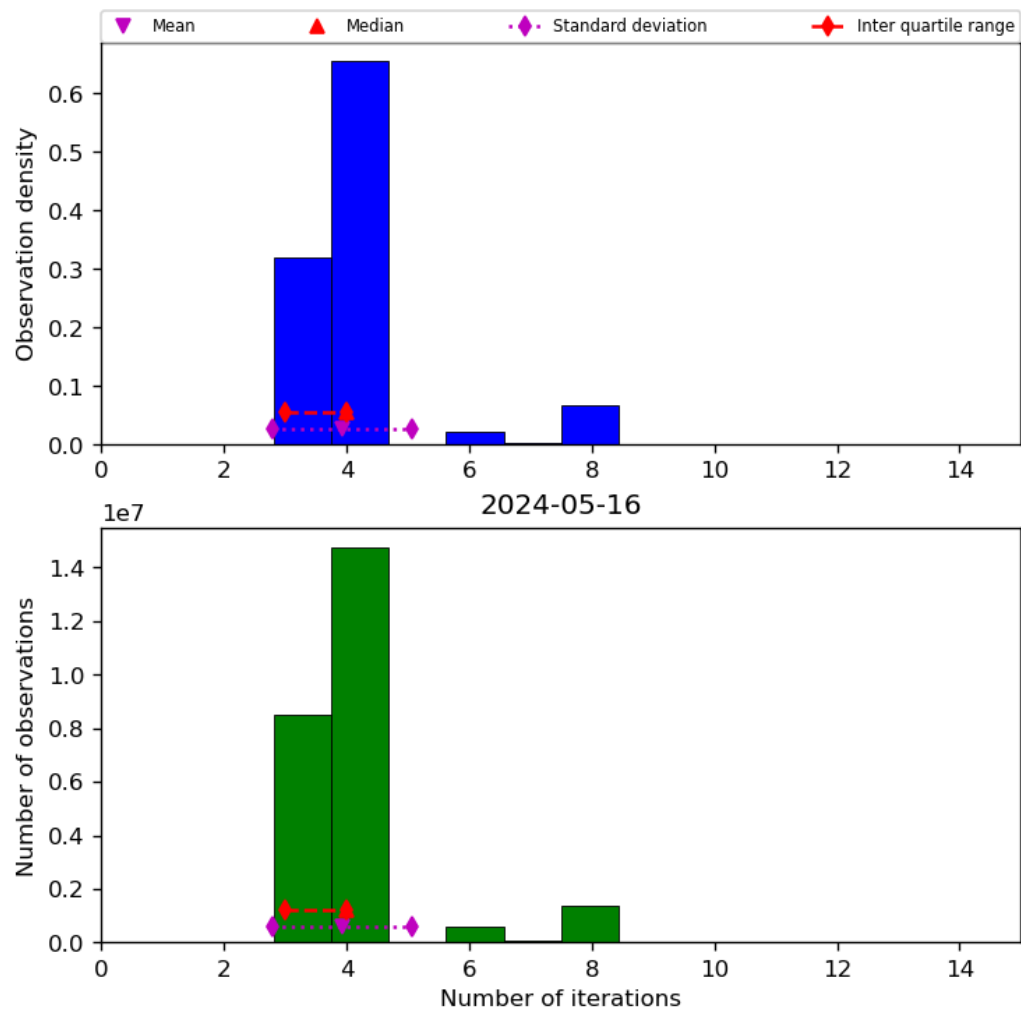
Figure 34: Histogram of "Number of iterations" for 2024-05-15 to 2024-05-17
