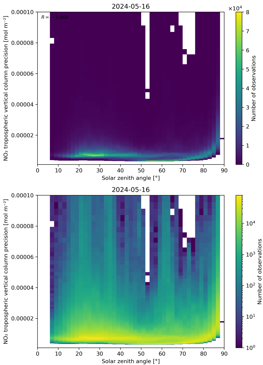
Figure 156: Scatter density plot of “Solar zenith angle” against “NO 2 tropospheric vertical column precision” for 2024-05-15 to 2024-05-17.
