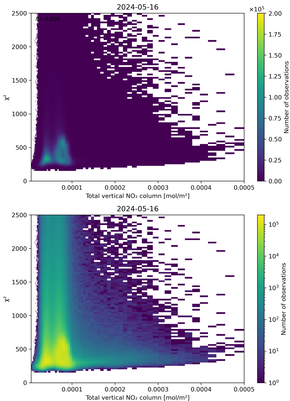
Figure 111: Scatter density plot of “Total vertical NO 2 column” against “ \chi^2 ” for 2024-05-15 to 2024-05-17.
