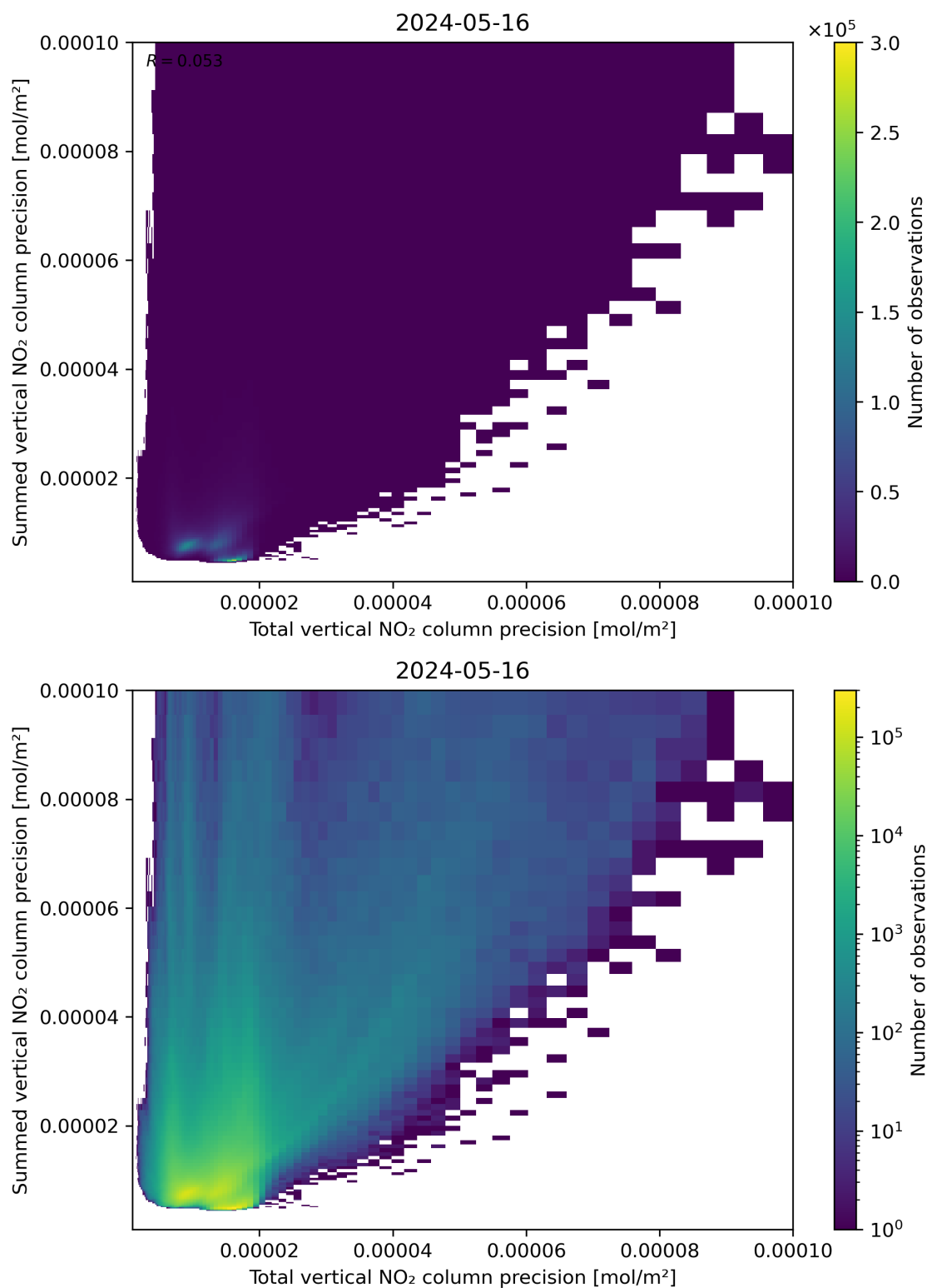
Figure 118: Scatter density plot of “Total vertical NO 2 column precision” against “Summed vertical NO 2 column precision” for 2024-05-15 to 2024-05-17.
