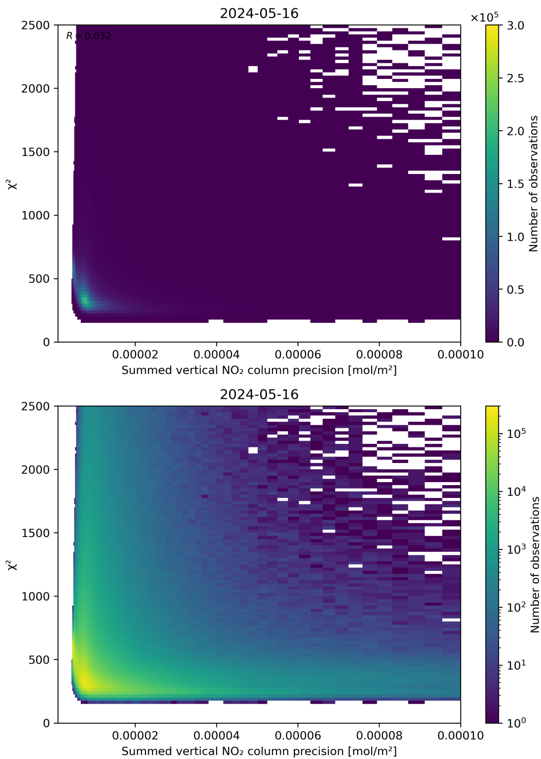
Figure 107: Scatter density plot of “Summed vertical NO 2 column precision” against “ \chi^2 ” for 2024-05-15 to 2024-05-17.
