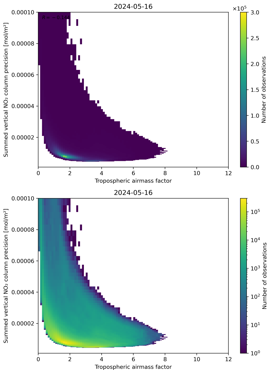
Figure 76: Scatter density plot of “Tropospheric air mass factor” against “Summed vertical NO 2 column precision” for 2024-05-15 to 2024-05-17.
