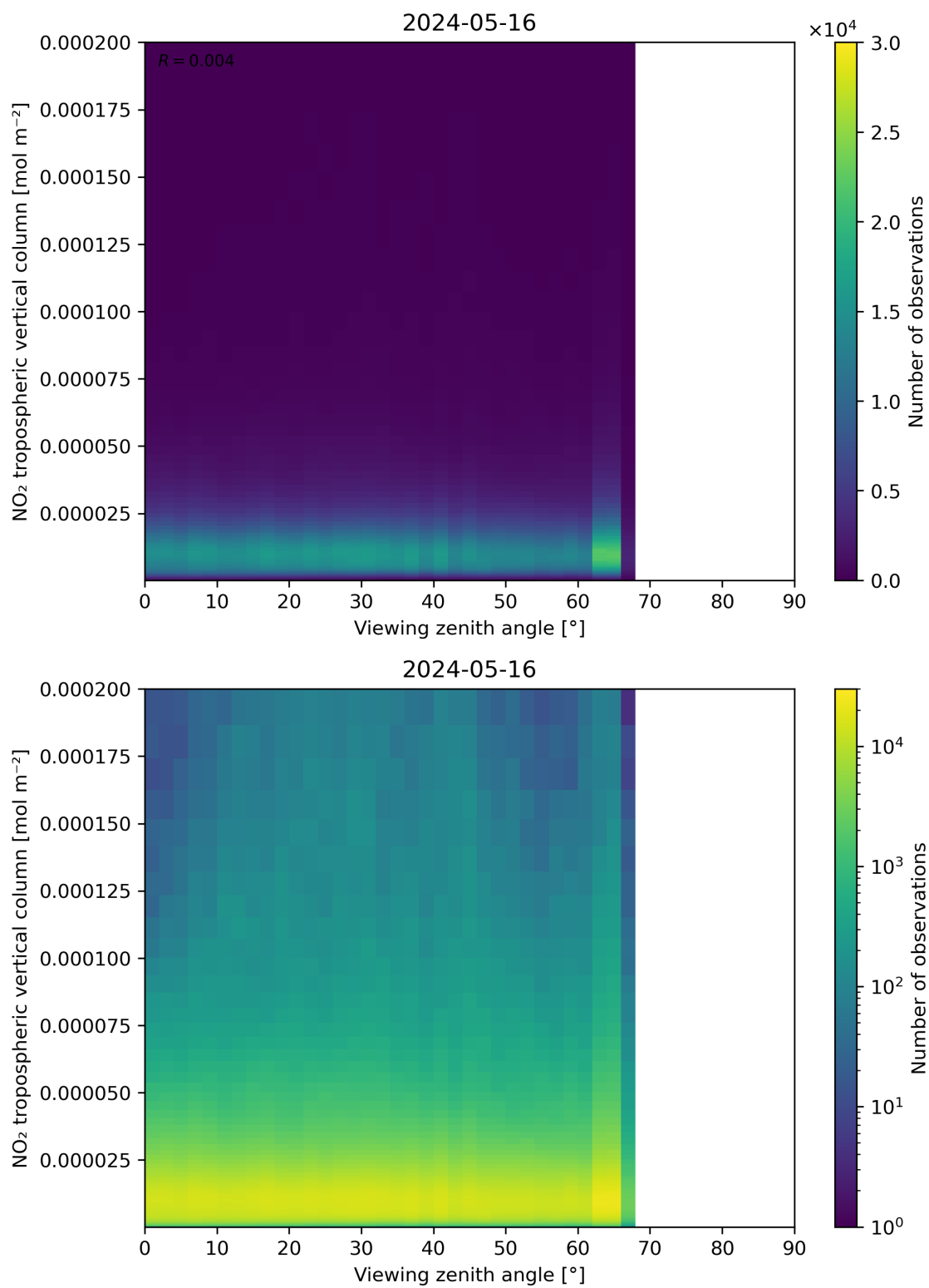
Figure 169: Scatter density plot of “Viewing zenith angle” against “NO 2 tropospheric vertical column” for 2024-05-15 to 2024-05-17.
