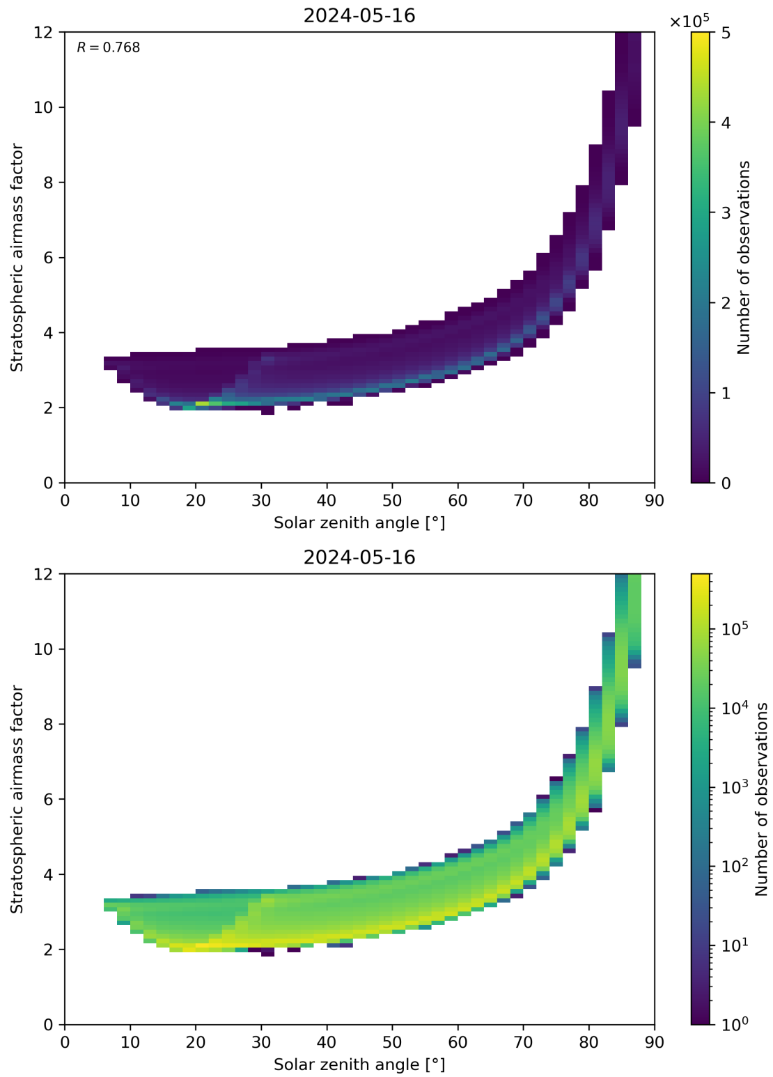
Figure 145: Scatter density plot of “Solar zenith angle” against “Stratospheric airmass factor” for 2024-05-15 to 2024-05-17.
