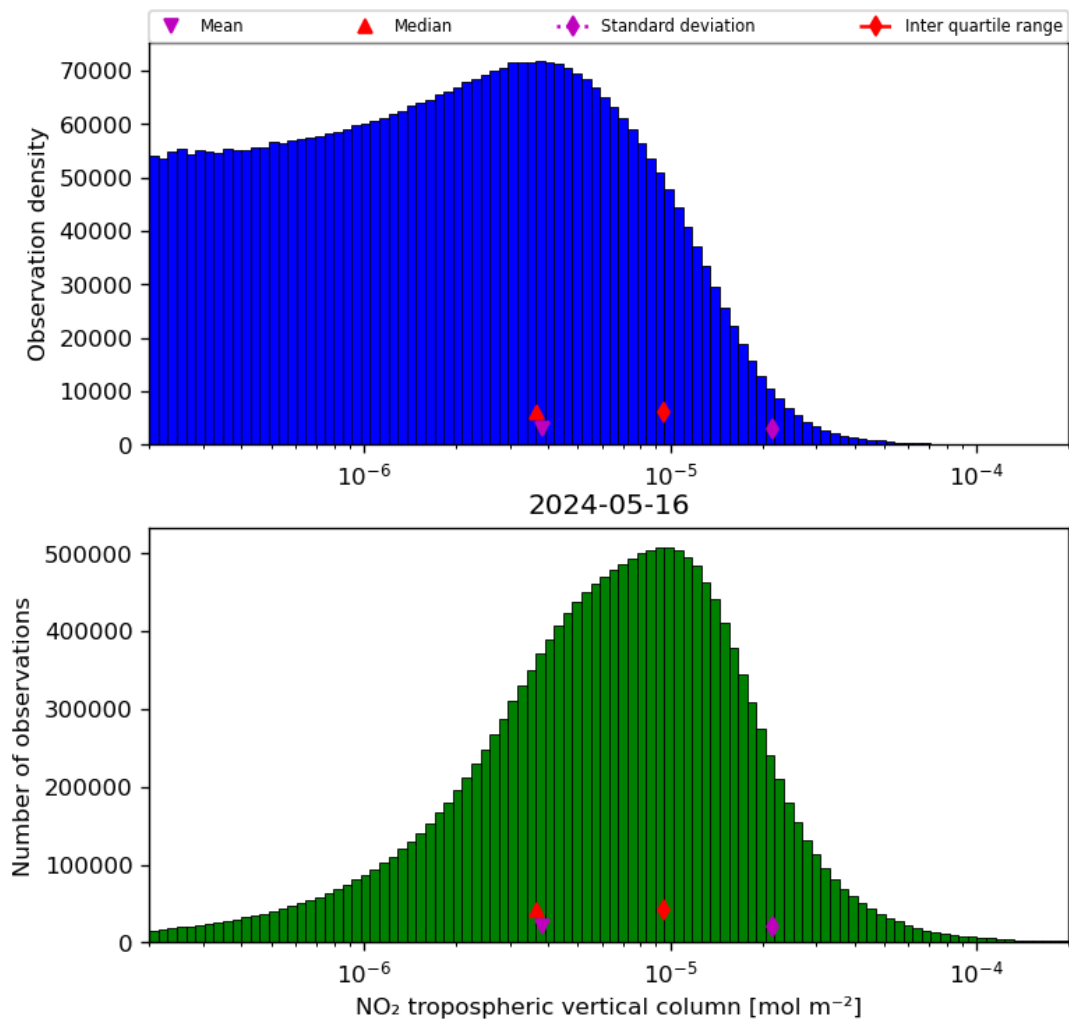
Figure 29: Histogram of “NO 2 tropospheric vertical column” for 2024-05-15 to 2024-05-17
