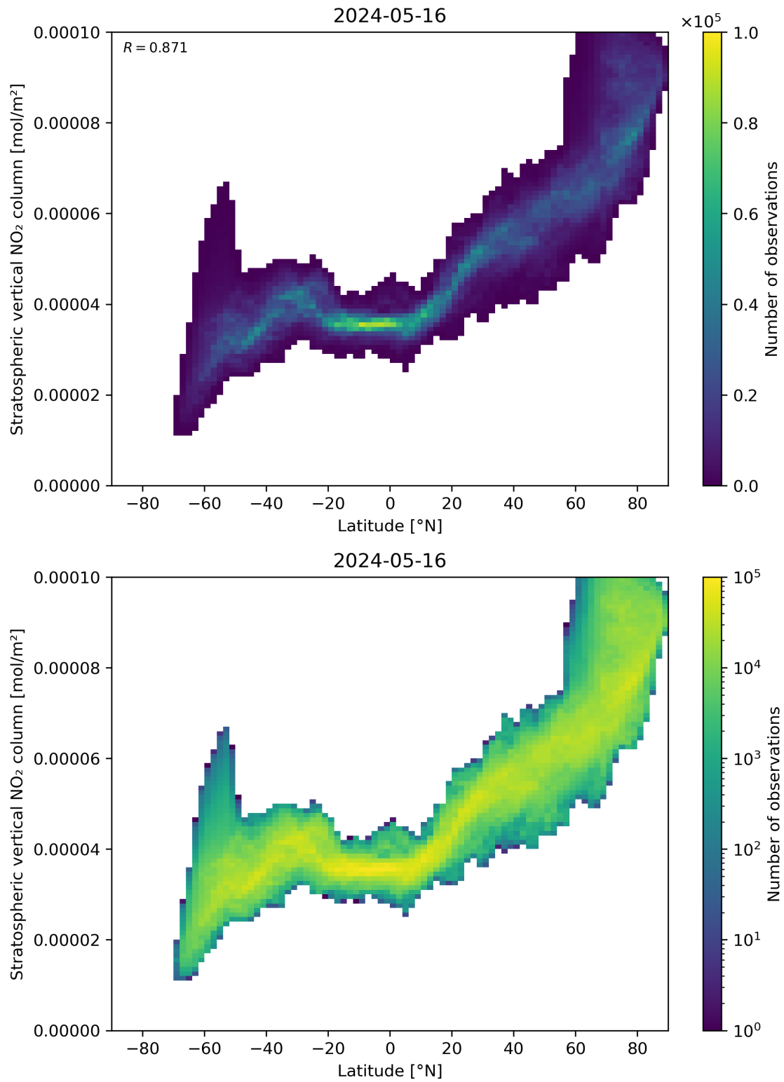
Figure 87: Scatter density plot of “Latitude” against “Stratospheric vertical \text{NO}_2 column” for 2024-05-15 to 2024-05-17.
