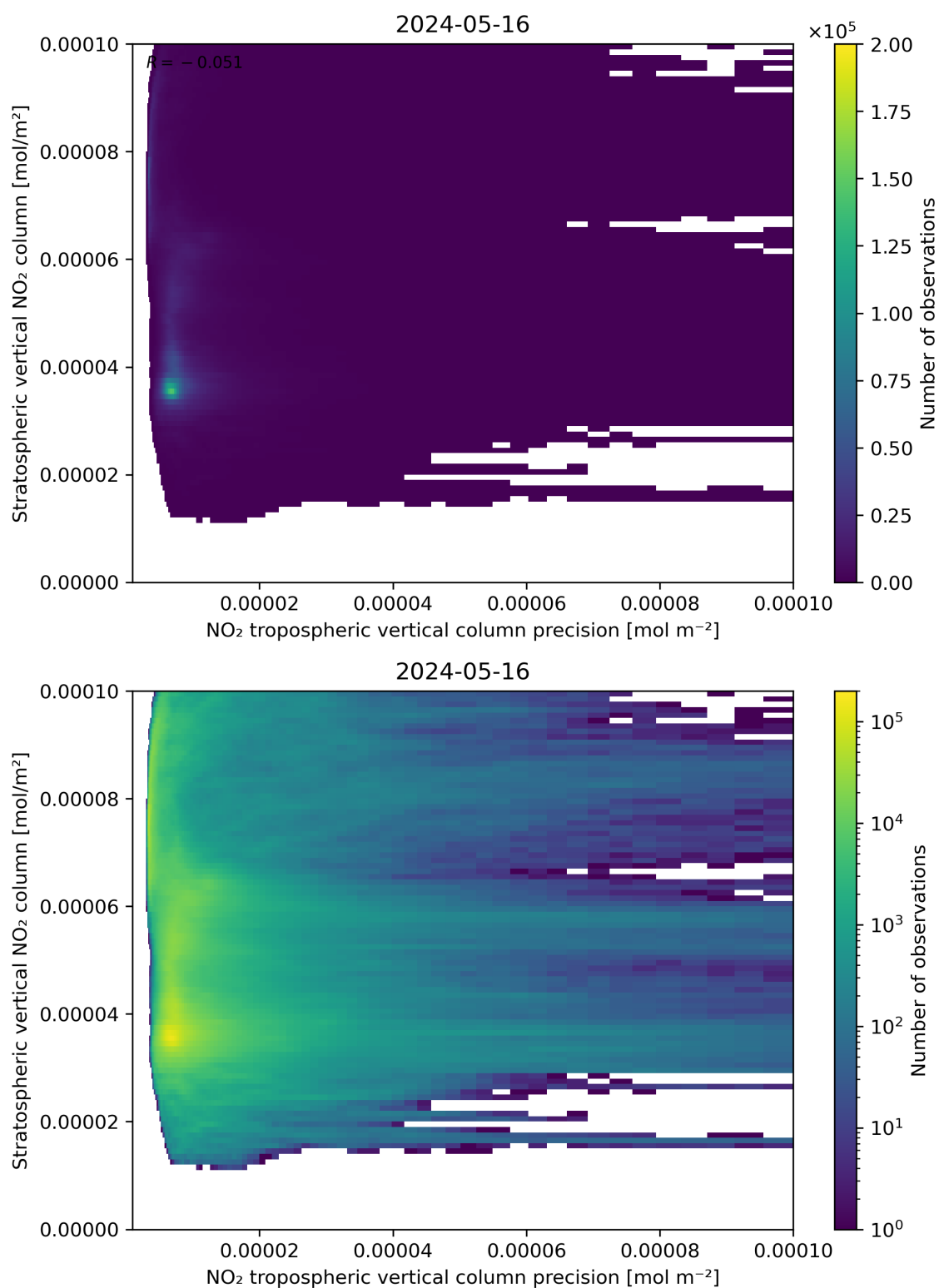
Figure 135: Scatter density plot of “NO 2 tropospheric vertical column precision” against “Stratospheric vertical NO 2 column” for 2024-05-15 to 2024-05-17.
