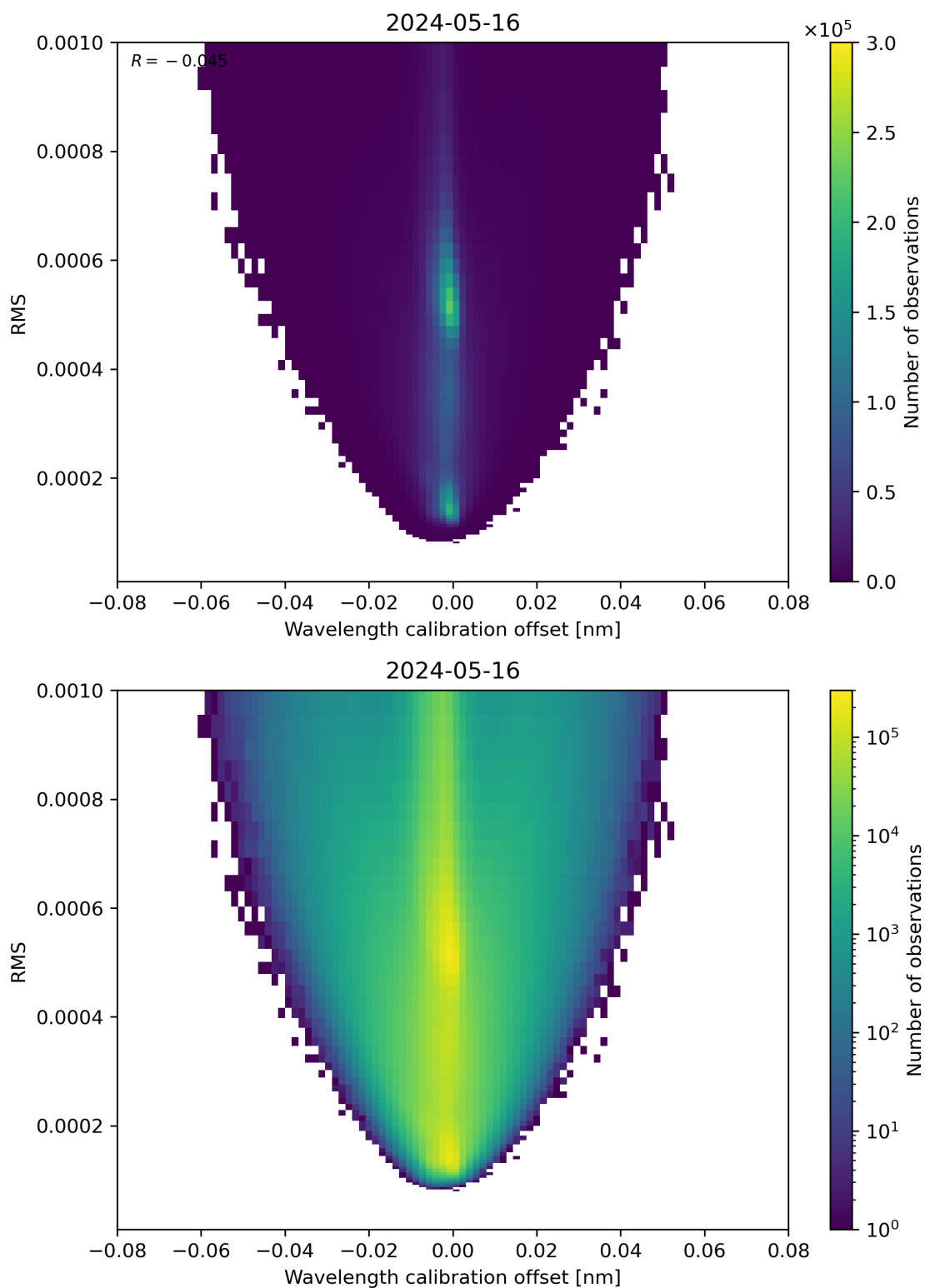
Figure 181: Scatter density plot of “Wavelength calibration offset” against “RMS” for 2024-05-15 to 2024-05-17.
