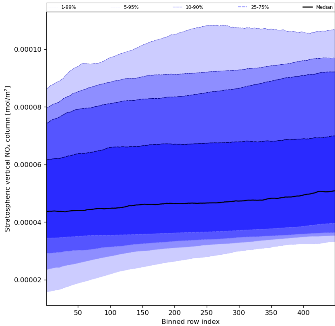
Figure 53: Along track statistics of “Stratospheric vertical NO 2 column” for 2024-05-15 to 2024-05-17
