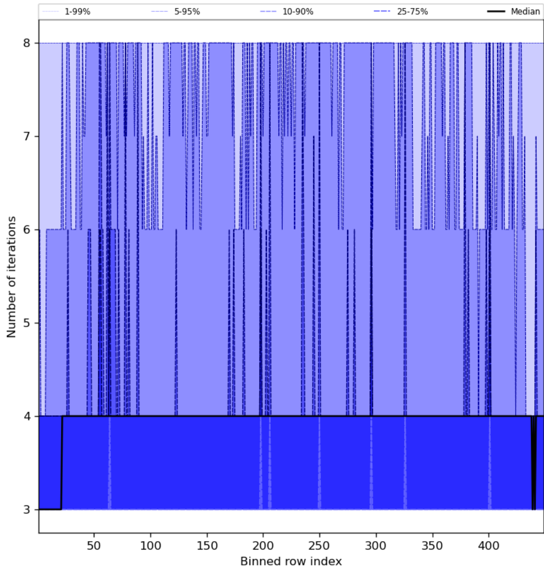
Figure 51: Along track statistics of “Number of iterations” for 2024-05-15 to 2024-05-17
