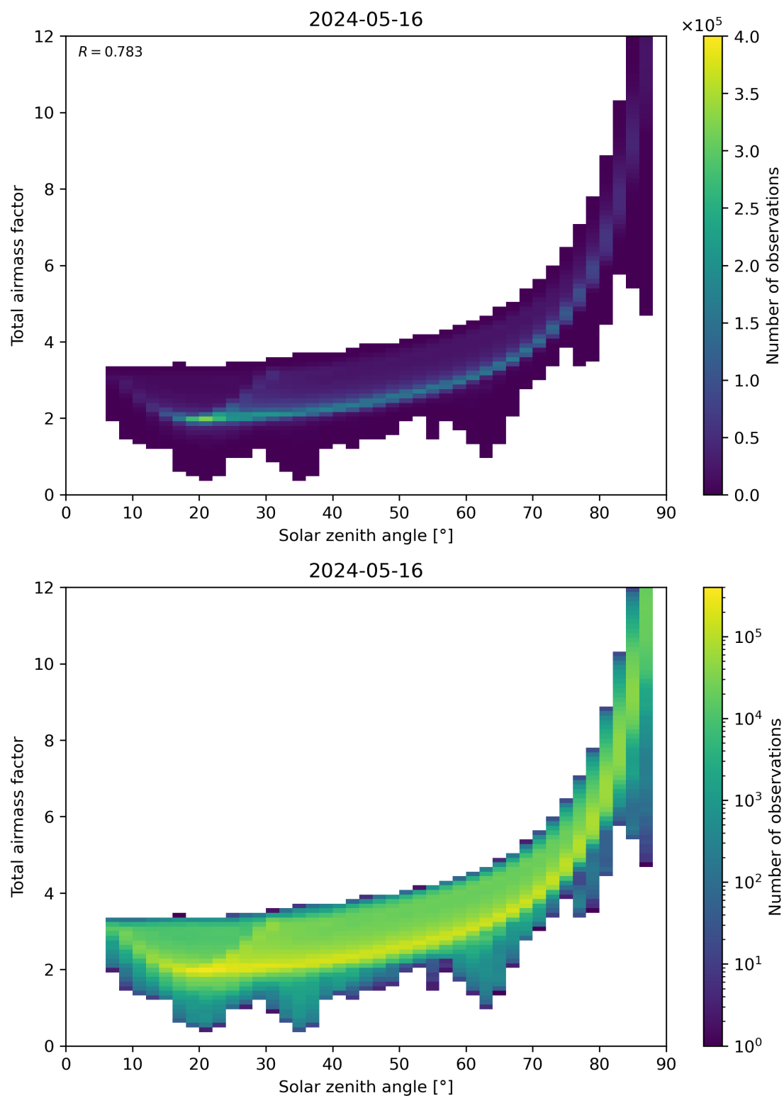
Figure 146: Scatter density plot of “Solar zenith angle” against “Total air mass factor” for 2024-05-15 to 2024-05-17.
