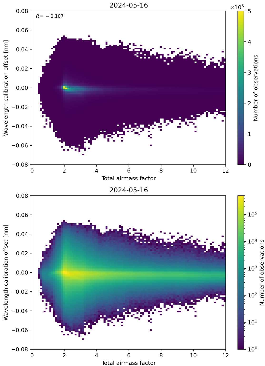
Figure 70: Scatter density plot of “Total airmass factor” against “Wavelength calibration offset” for 2024-05-15 to 2024-05-17.
