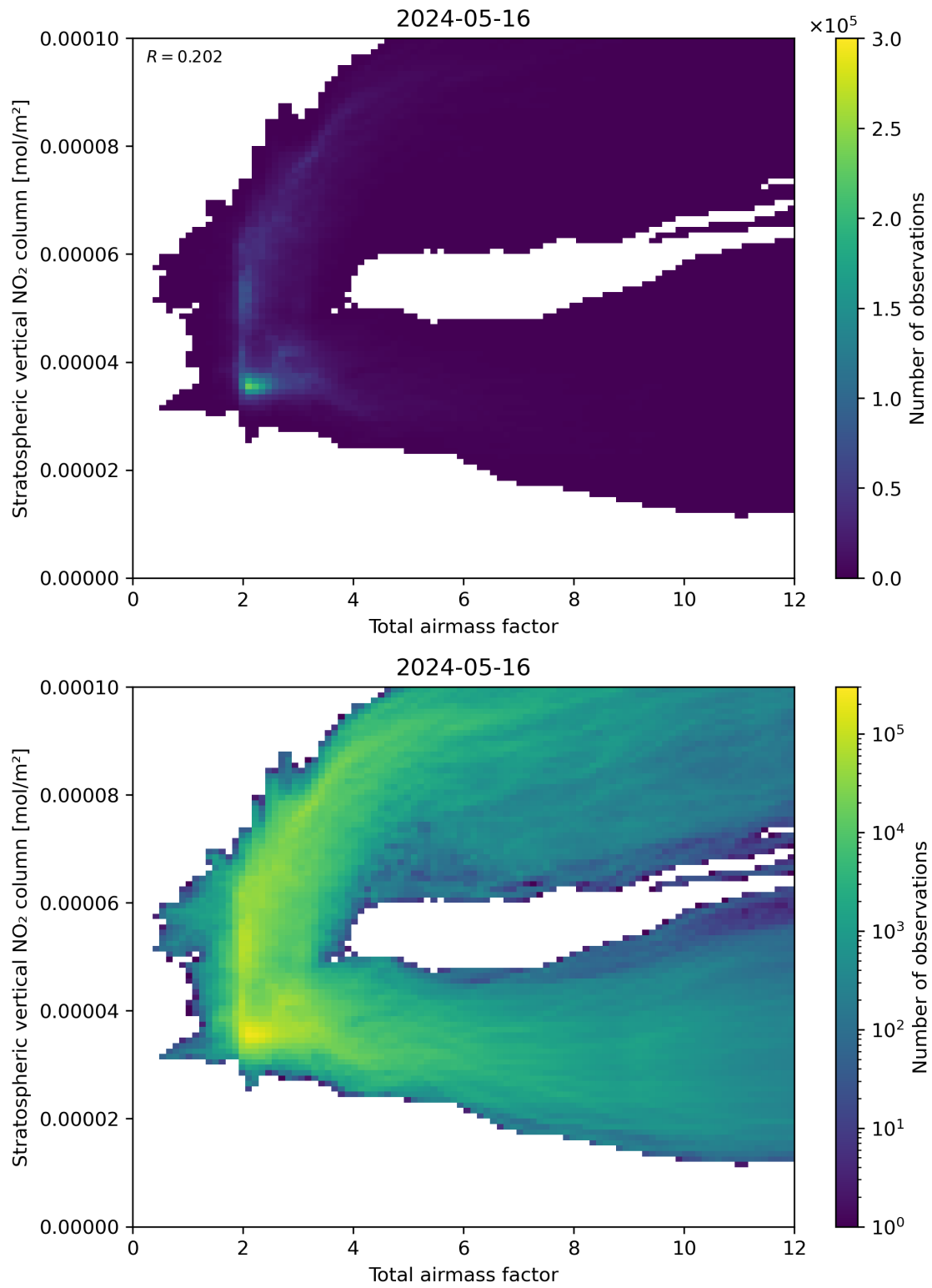
Figure 64: Scatter density plot of “Total airmass factor” against “Stratospheric vertical \text{NO}_2 column” for 2024-05-15 to 2024-05-17.
