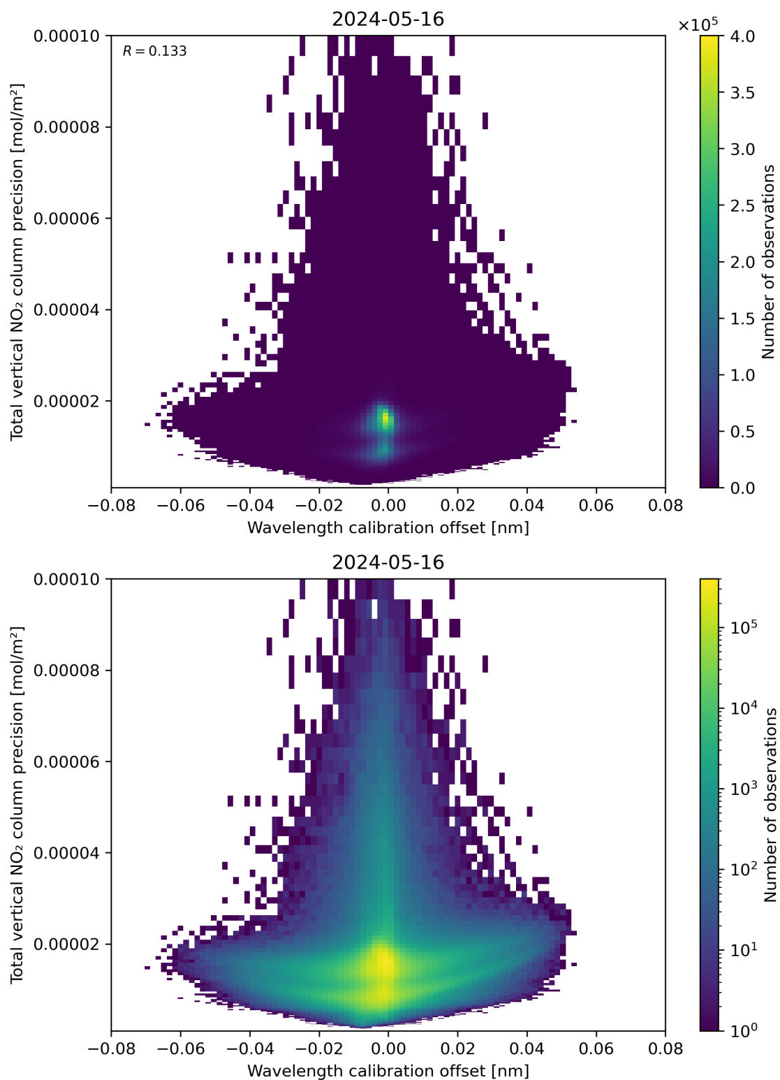
Figure 180: Scatter density plot of “Wavelength calibration offset” against “Total vertical NO 2 column precision” for 2024-05-15 to 2024-05-17.
