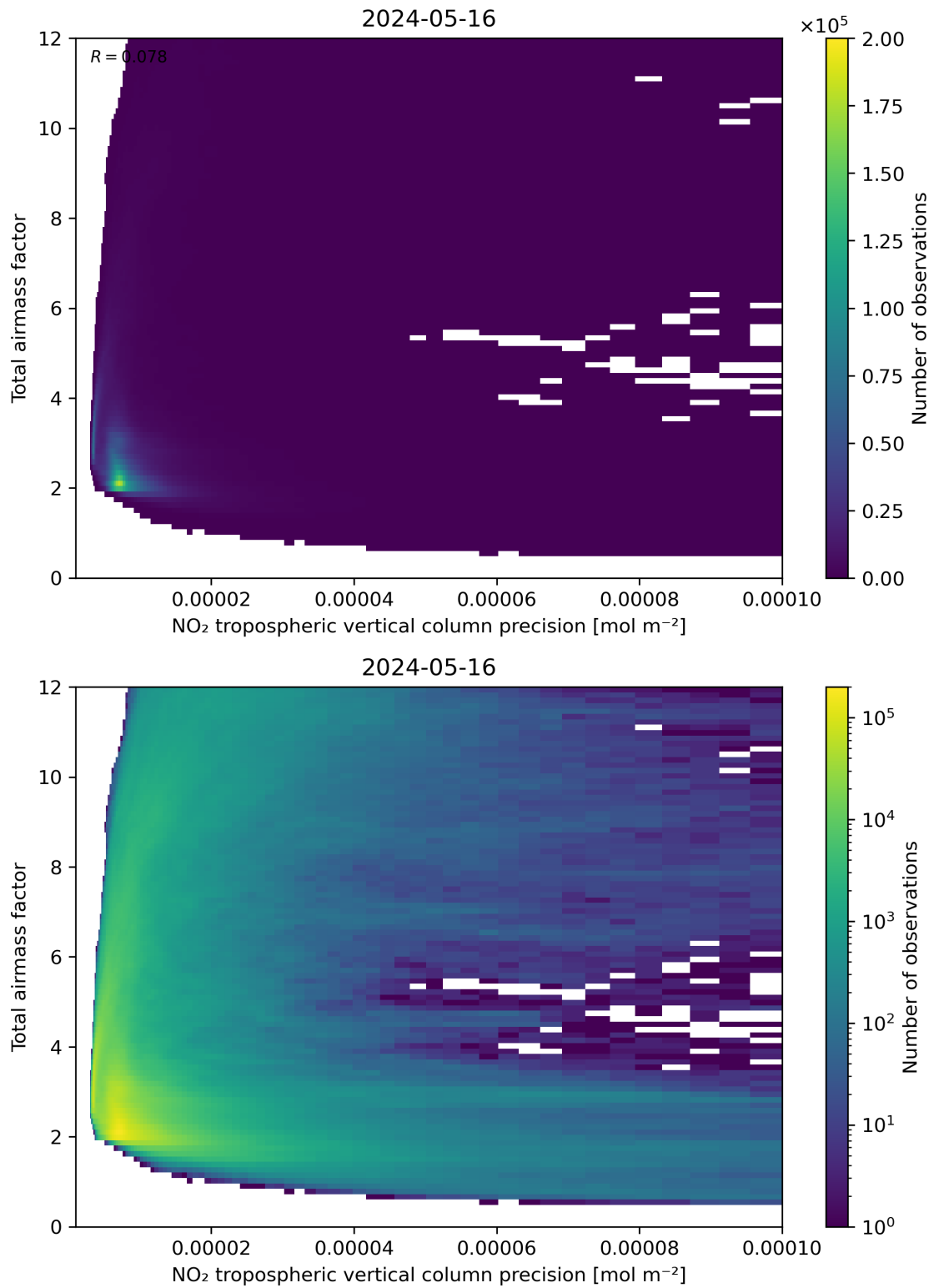
Figure 132: Scatter density plot of “NO 2 tropospheric vertical column precision” against “Total air mass factor” for 2024-05-15 to 2024-05-17.
