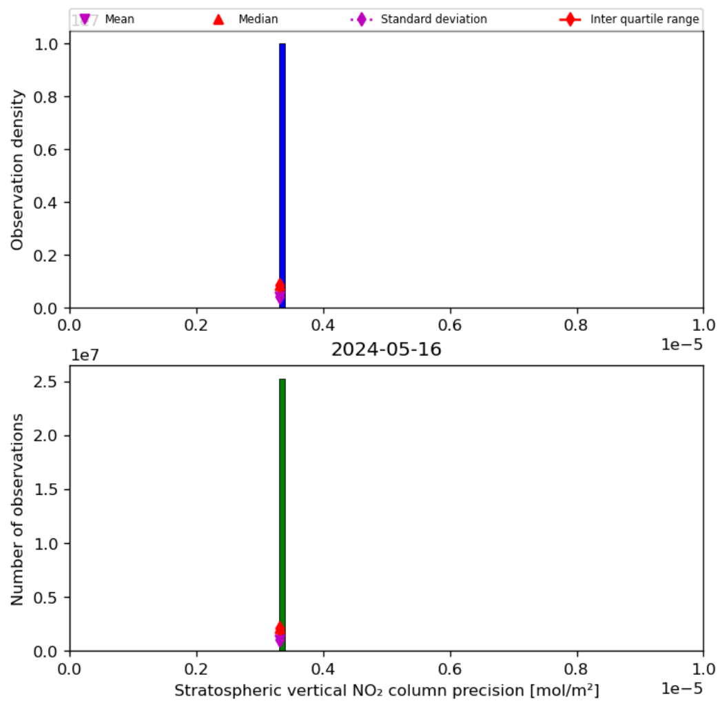
Figure 37: Histogram of “Stratospheric vertical NO 2 column precision” for 2024-05-15 to 2024-05-17
