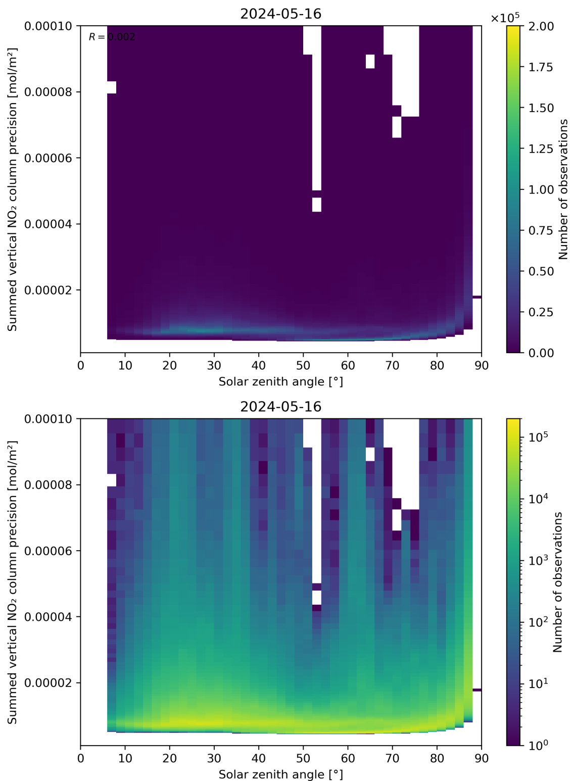
Figure 152: Scatter density plot of “Solar zenith angle” against “Summed vertical NO 2 column precision” for 2024-05-15 to 2024-05-17.
