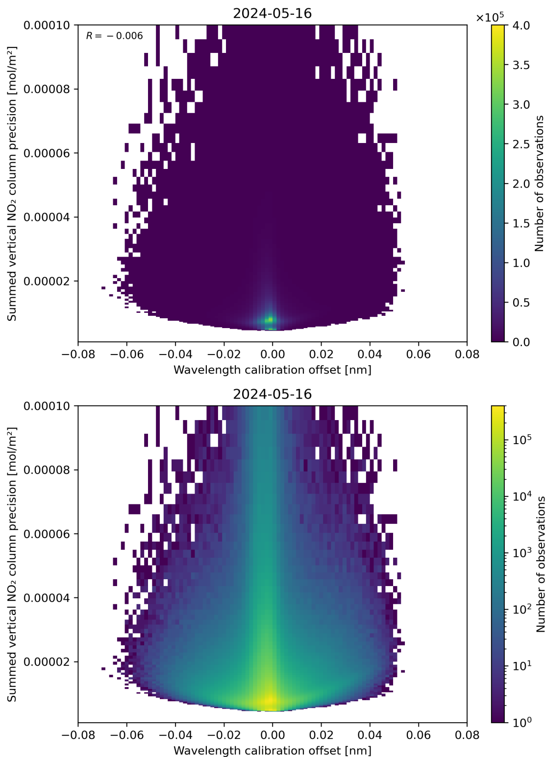
Figure 178: Scatter density plot of “Wavelength calibration offset” against “Summed vertical NO 2 column precision” for 2024-05-15 to 2024-05-17.
