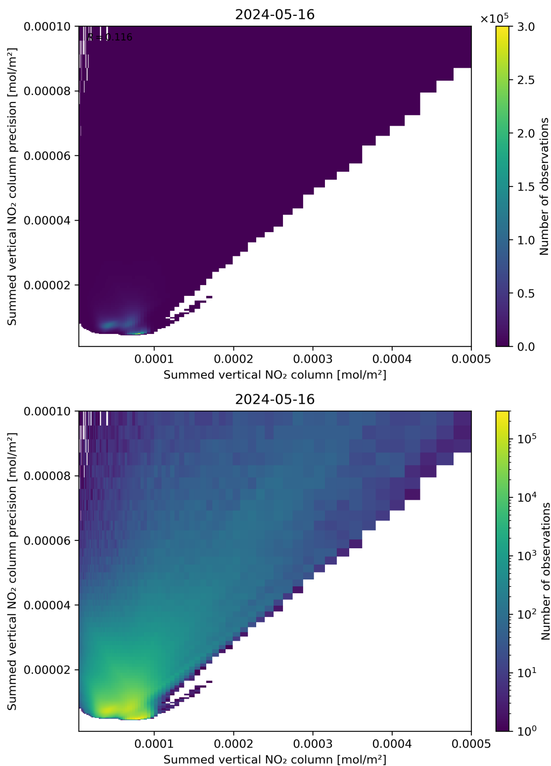
Figure 105: Scatter density plot of “Summed vertical NO 2 column” against “Summed vertical NO 2 column precision” for 2024-05-15 to 2024-05-17.
