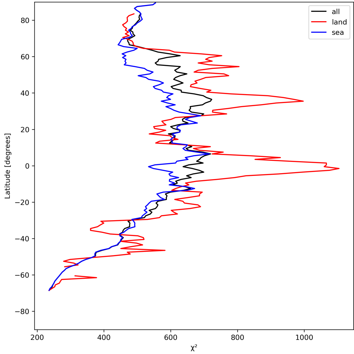
Figure 25: Zonal average of “ \chi^2 ” for 2024-05-15 to 2024-05-17.
