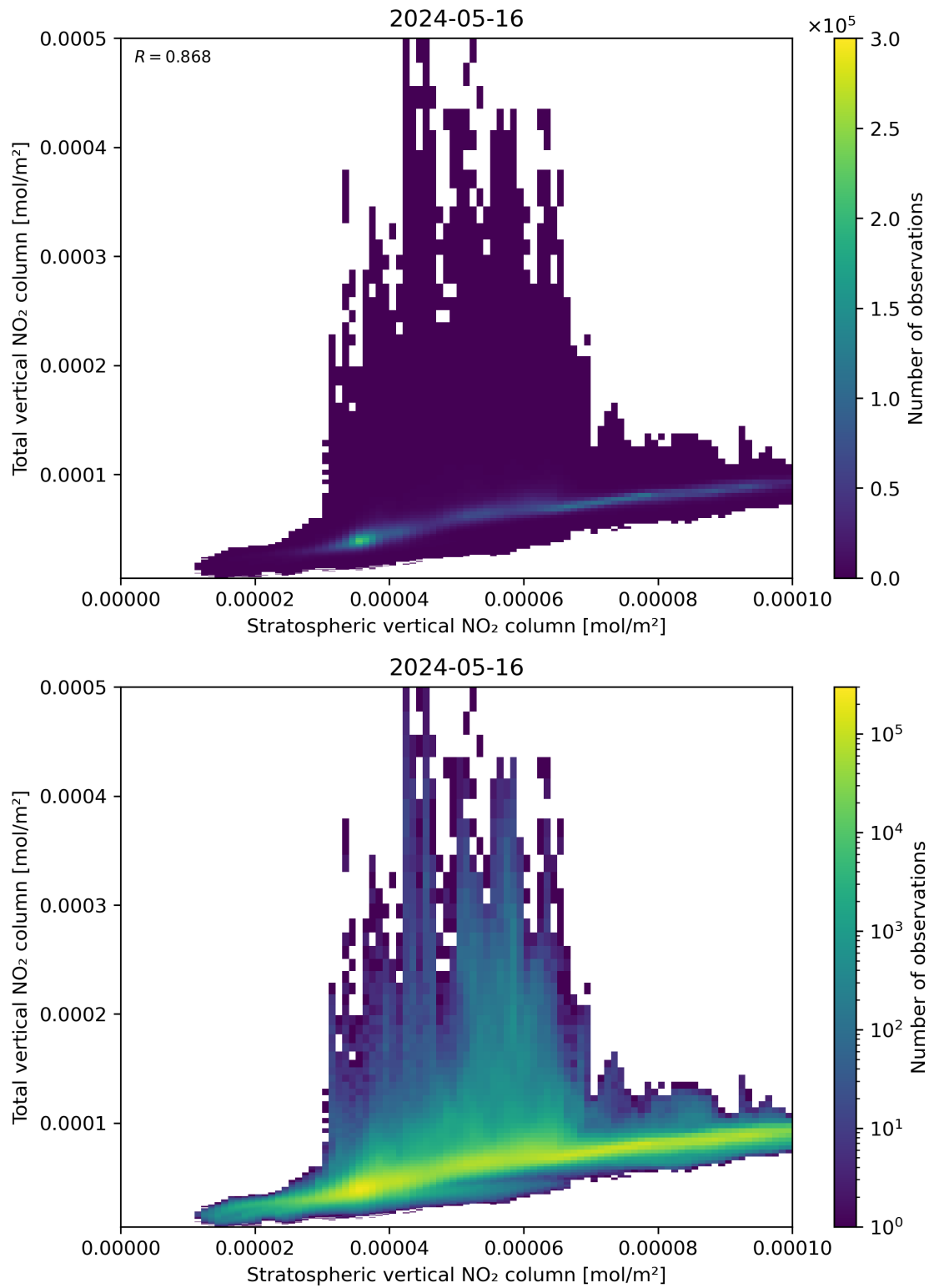
Figure 100: Scatter density plot of “Stratospheric vertical NO 2 column” against “Total vertical NO 2 column” for 2024-05-15 to 2024-05-17.
