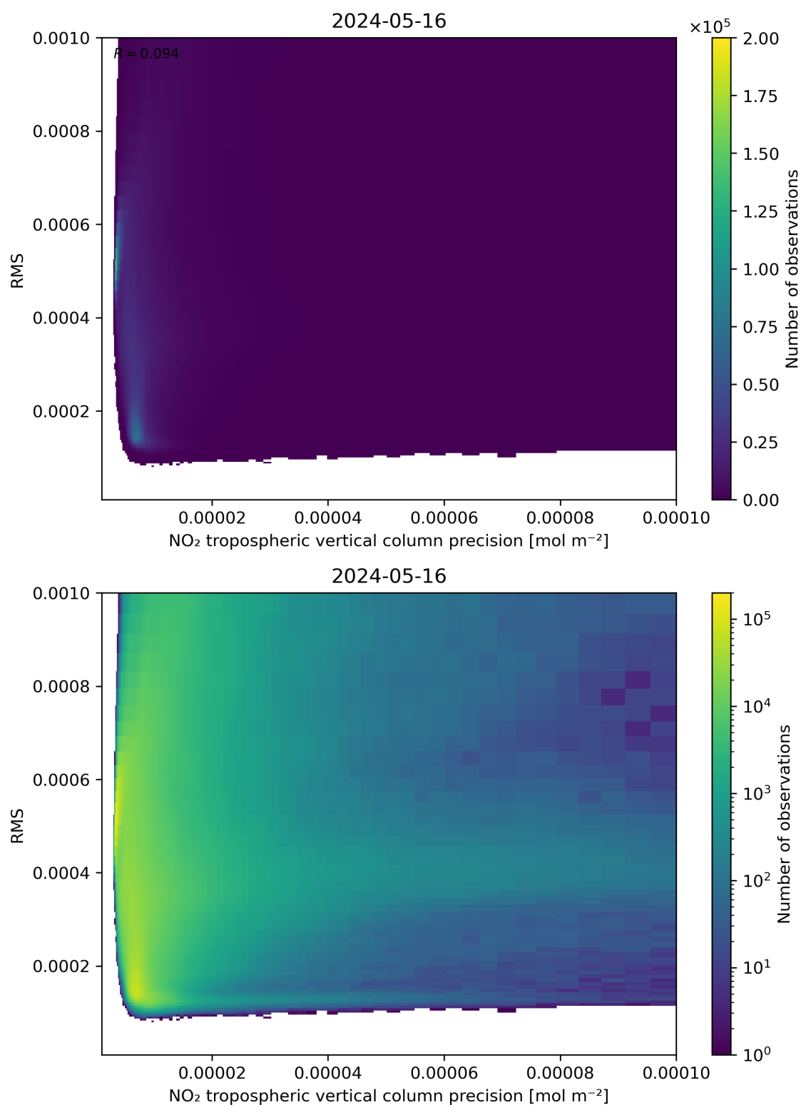
Figure 140: Scatter density plot of “NO 2 tropospheric vertical column precision” against “RMS” for 2024-05-15 to 2024-05-17.
