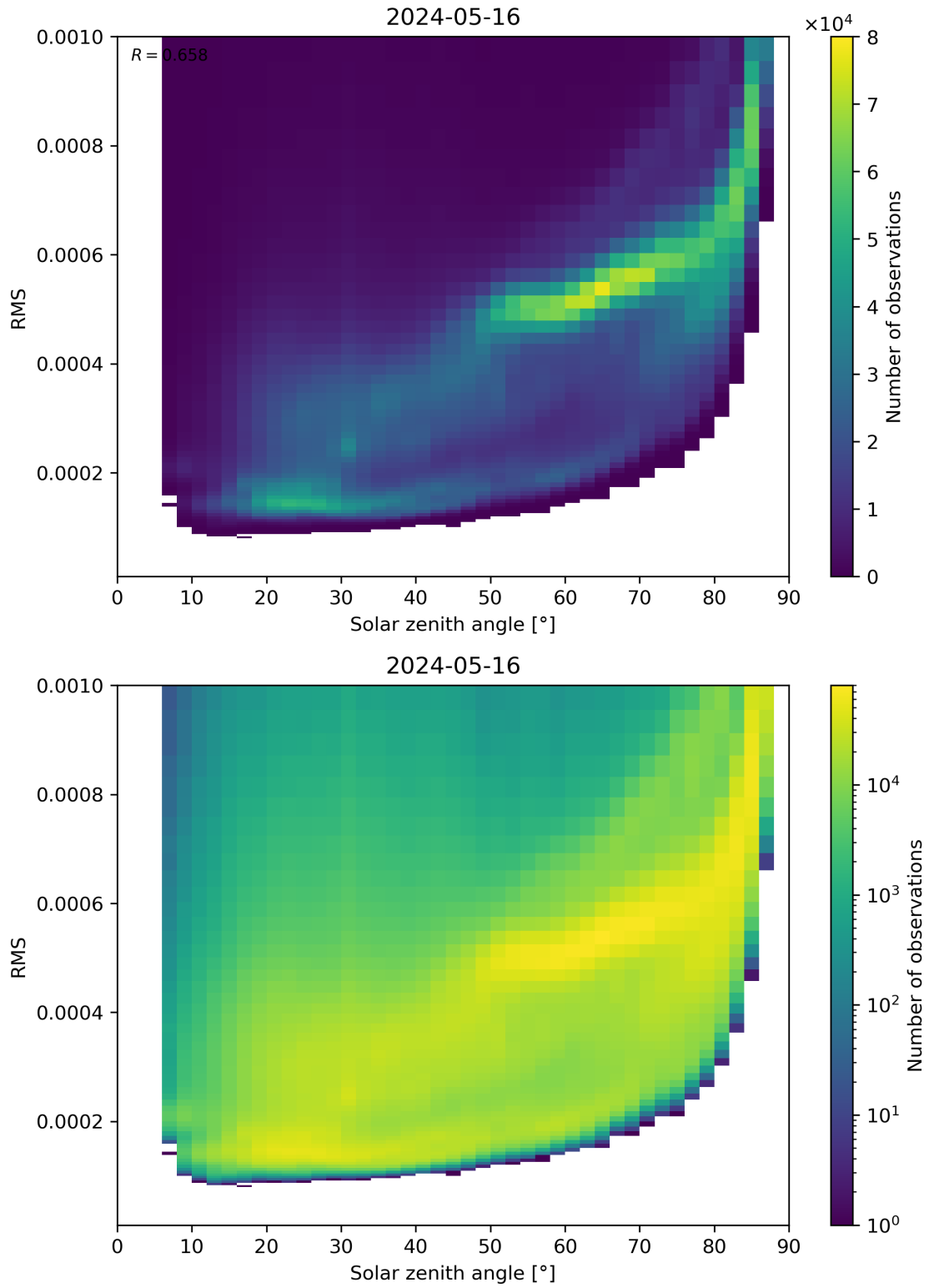
Figure 157: Scatter density plot of “Solar zenith angle” against “RMS” for 2024-05-15 to 2024-05-17.
