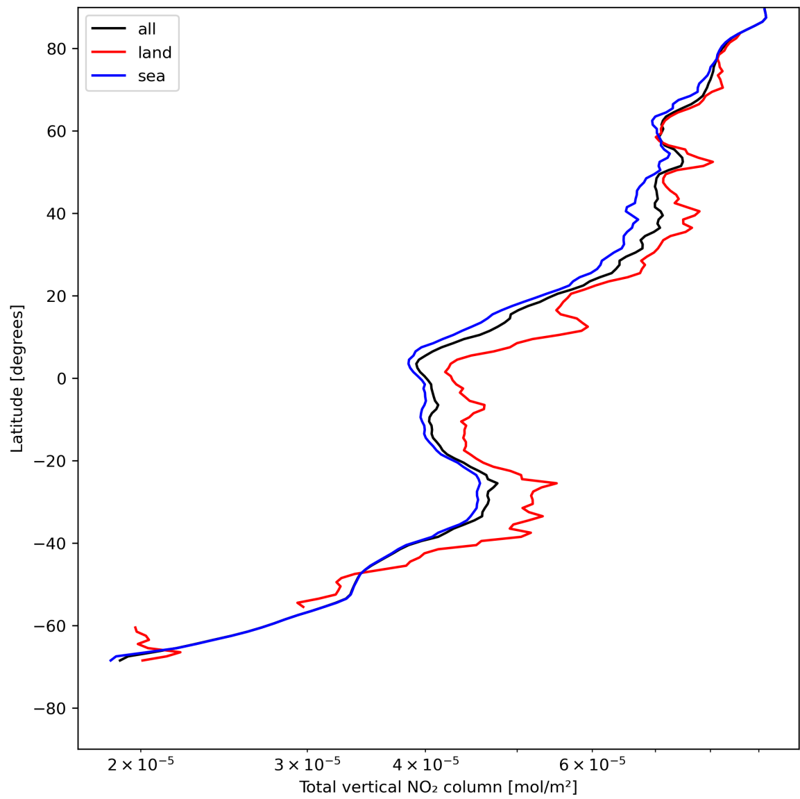
Figure 21: Zonal average of “Total vertical NO 2 column” for 2024-05-15 to 2024-05-17.
