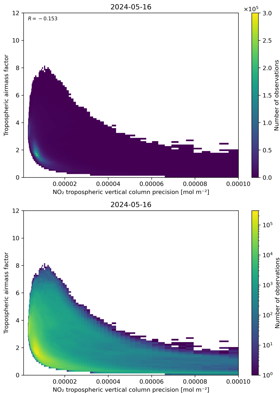
Figure 133: Scatter density plot of “NO 2 tropospheric vertical column precision” against “Tropospheric air mass factor” for 2024-05-15 to 2024-05-17.
