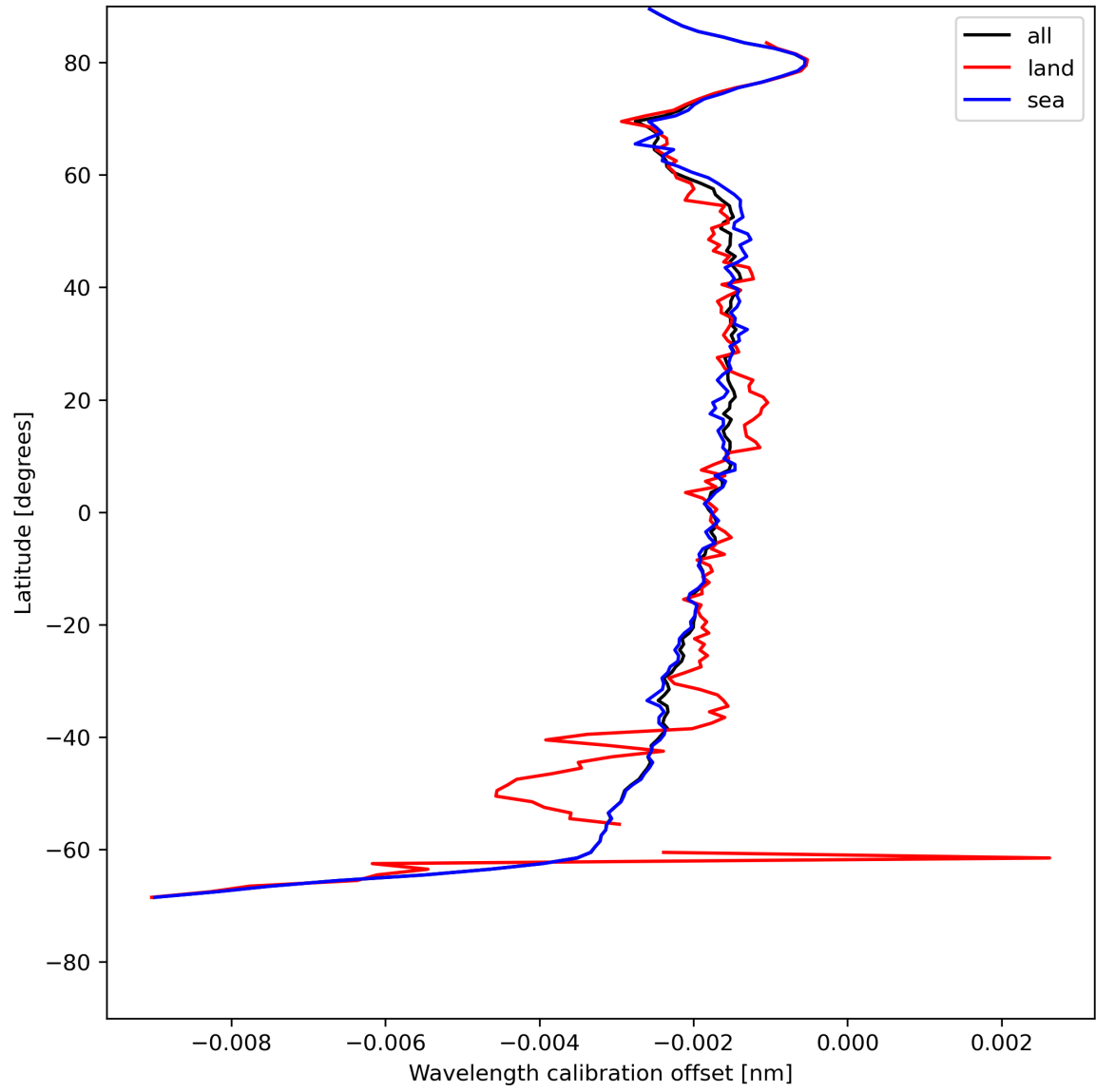
Figure 18: Zonal average of “Wavelength calibration offset” for 2024-05-15 to 2024-05-17.
