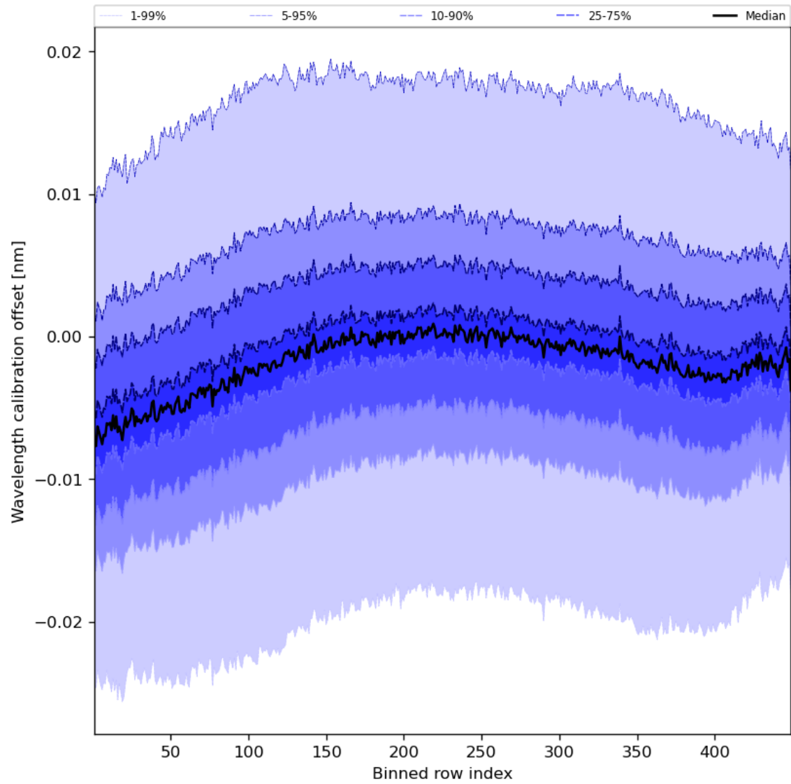
Figure 52: Along track statistics of “Wavelength calibration offset” for 2024-05-15 to 2024-05-17
