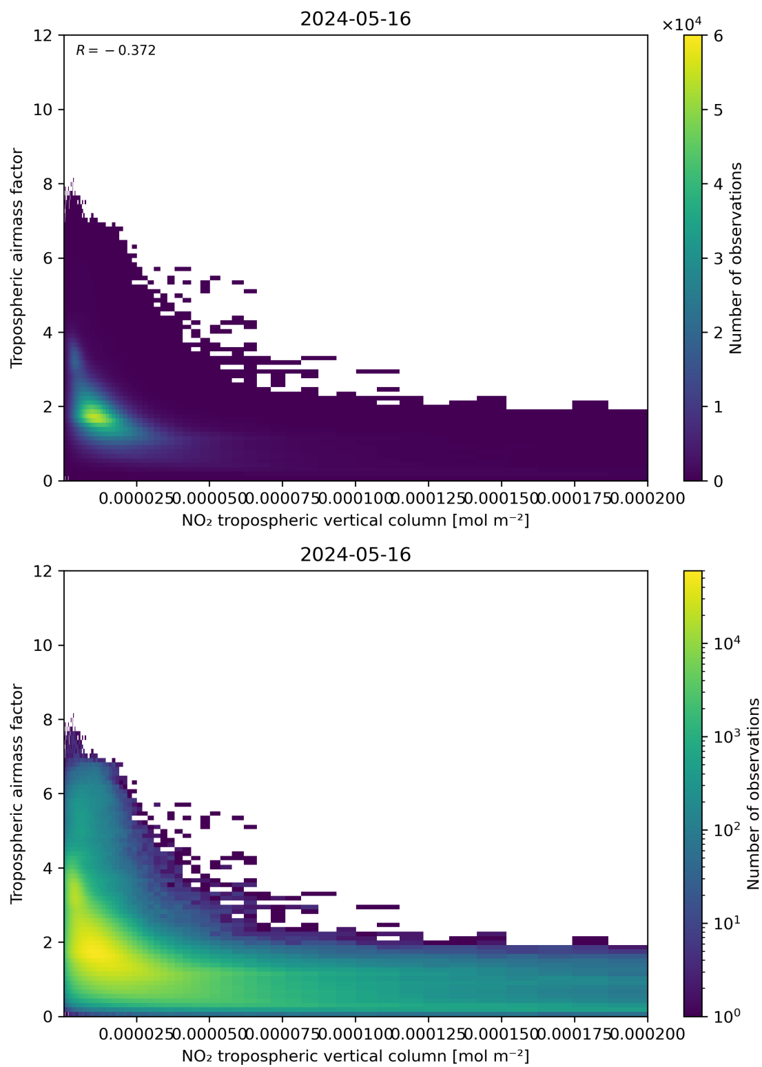
Figure 123: Scatter density plot of “NO 2 tropospheric vertical column” against “Tropospheric air mass factor” for 2024-05-15 to 2024-05-17.
