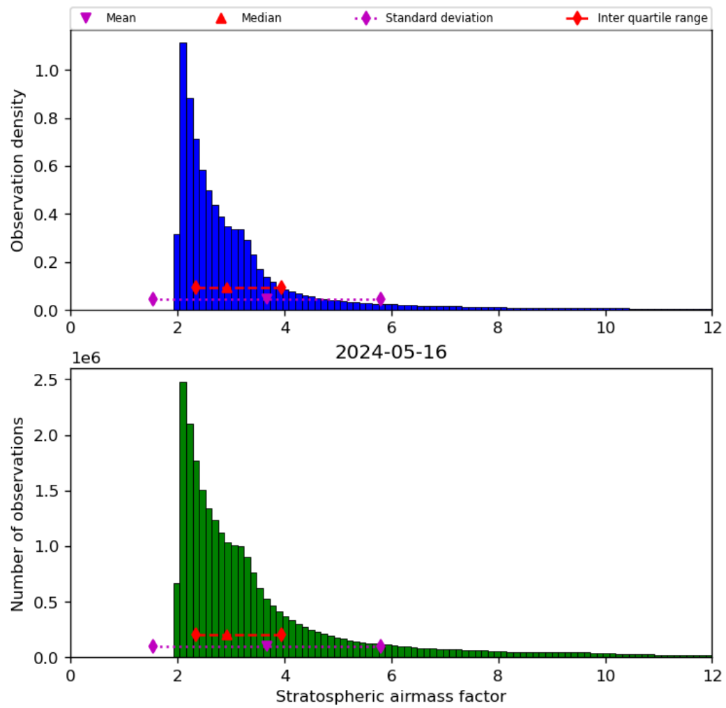
Figure 44: Histogram of “Stratospheric airmass factor” for 2024-05-15 to 2024-05-17
