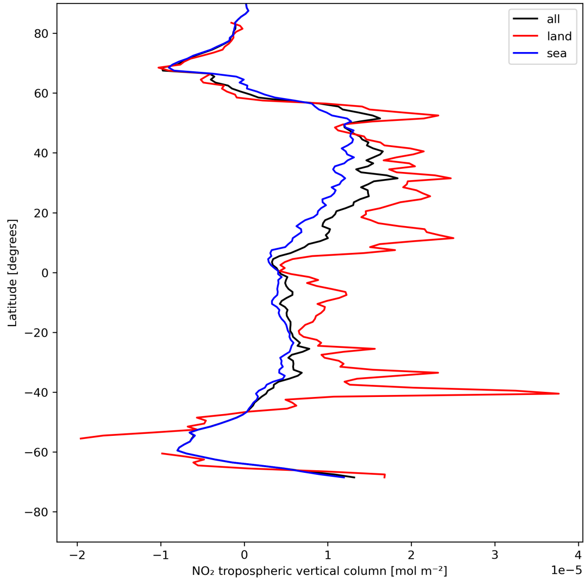
Figure 12: Zonal average of “NO 2 tropospheric vertical column” for 2024-05-15 to 2024-05-17.
