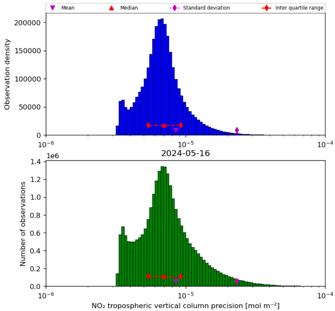
Figure 30: Histogram of “NO 2 tropospheric vertical column precision” for 2024-05-15 to 2024-05-17
