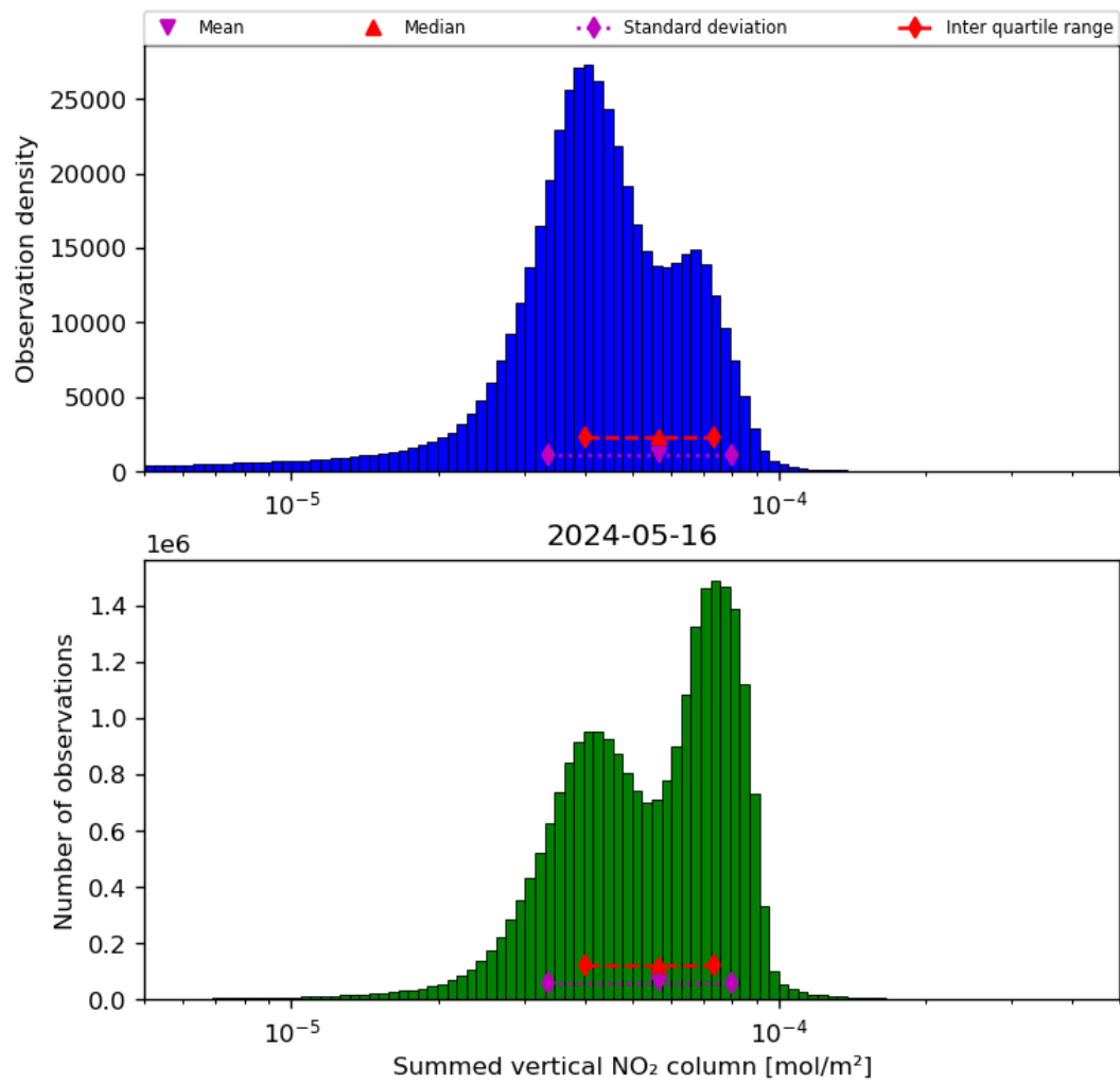
Figure 40: Histogram of “Summed vertical NO 2 column” for 2024-05-15 to 2024-05-17
