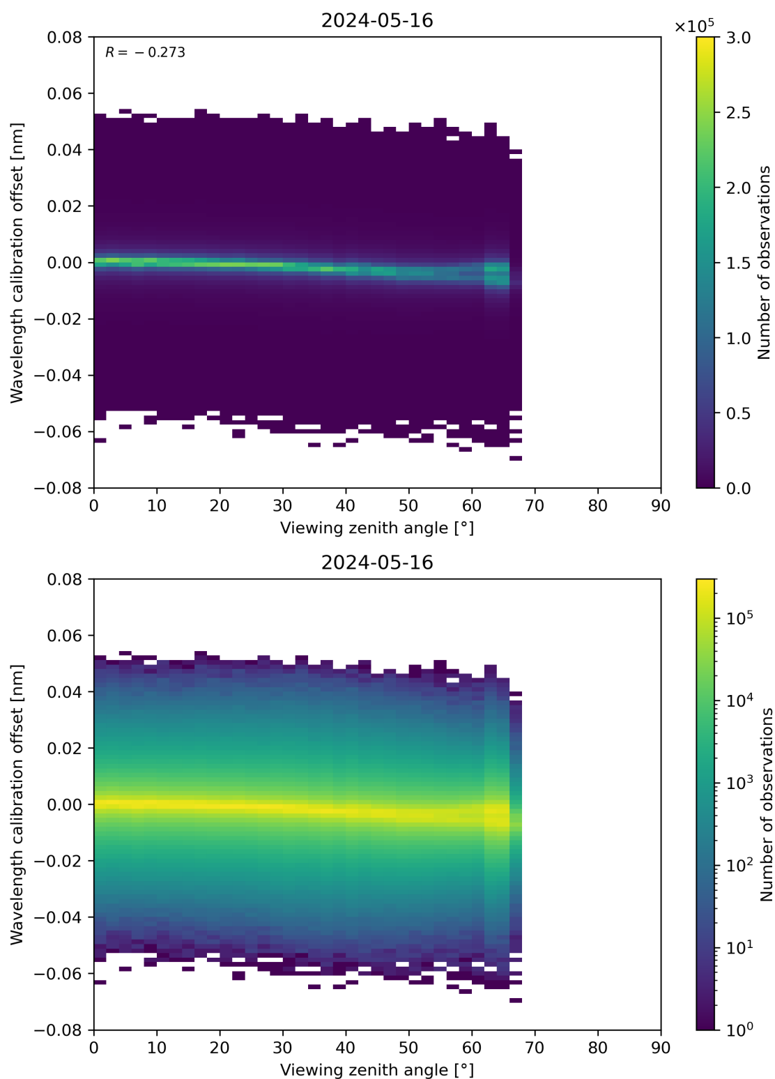
Figure 173: Scatter density plot of “Viewing zenith angle” against “Wavelength calibration offset” for 2024-05-15 to 2024-05-17.
