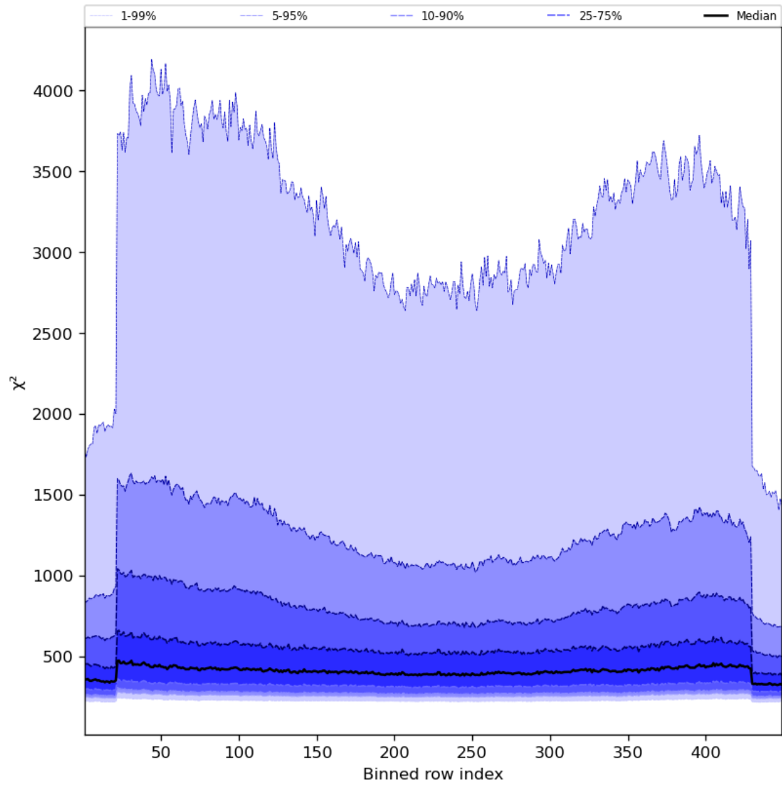
Figure 59: Along track statistics of “ \chi^2 ” for 2024-05-15 to 2024-05-17
