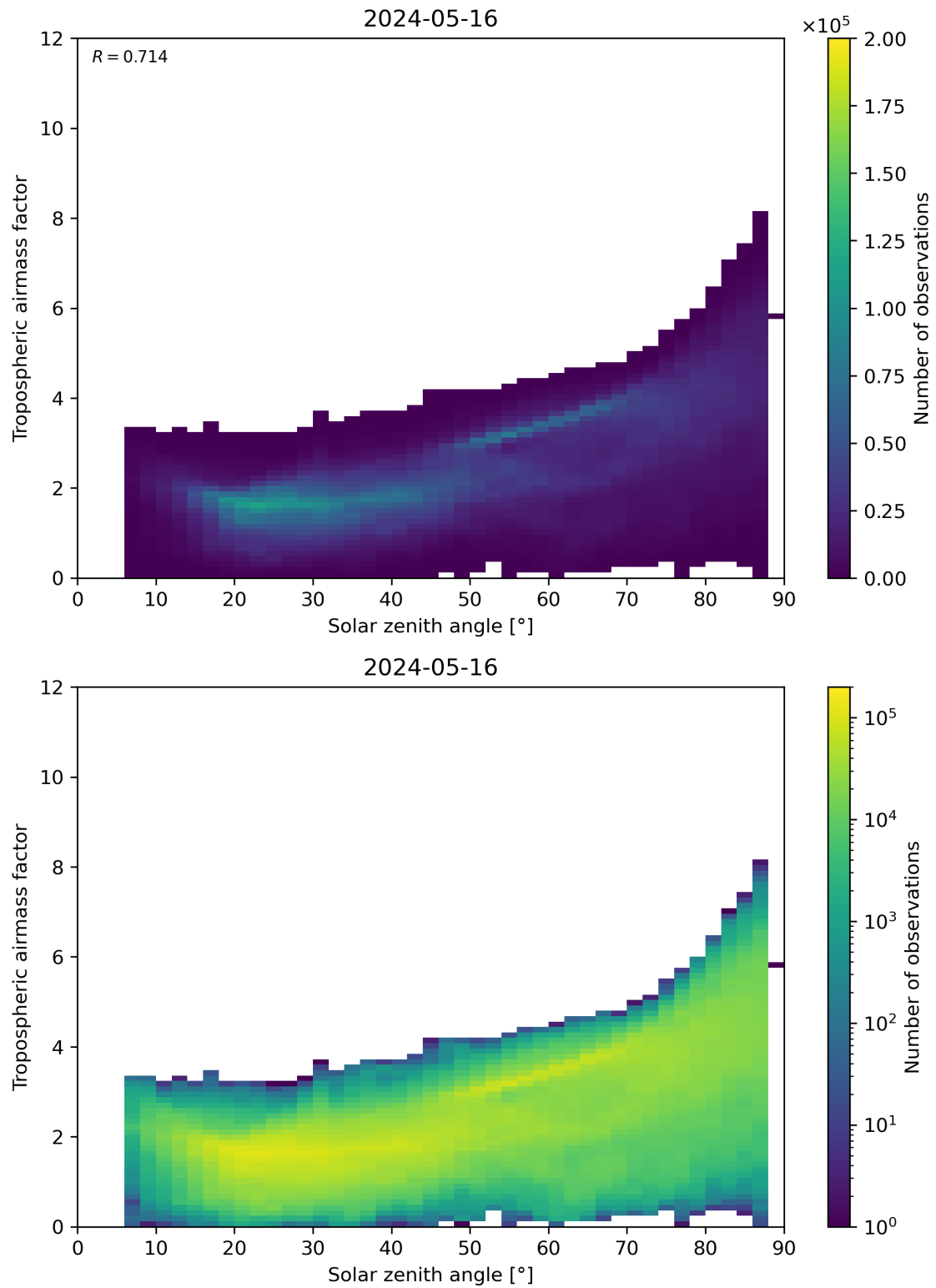
Figure 147: Scatter density plot of “Solar zenith angle” against “Tropospheric airmass factor” for 2024-05-15 to 2024-05-17.
