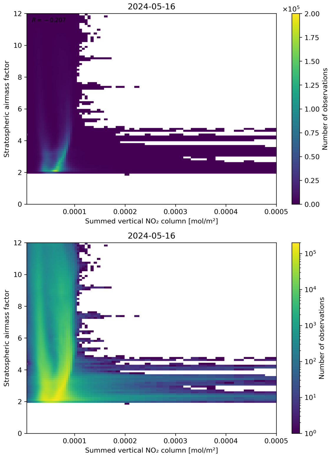
Figure 103: Scatter density plot of “Summed vertical NO 2 column” against “Stratospheric airmass factor” for 2024-05-15 to 2024-05-17.
