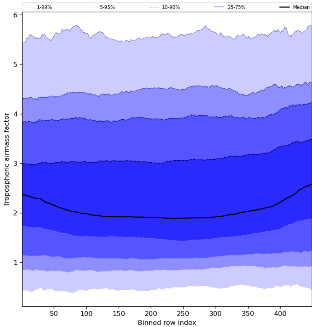
Figure 48: Along track statistics of “Tropospheric airmass factor” for 2024-05-15 to 2024-05-17
