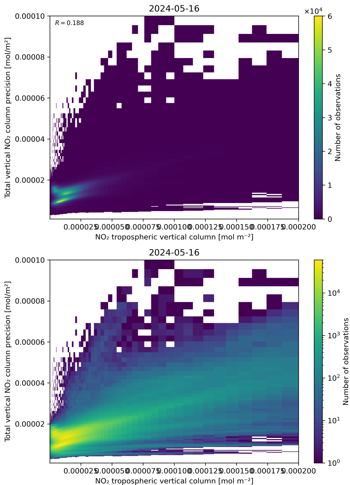
Figure 129: Scatter density plot of “NO 2 tropospheric vertical column” against “Total vertical NO 2 column precision” for 2024-05-15 to 2024-05-17.
