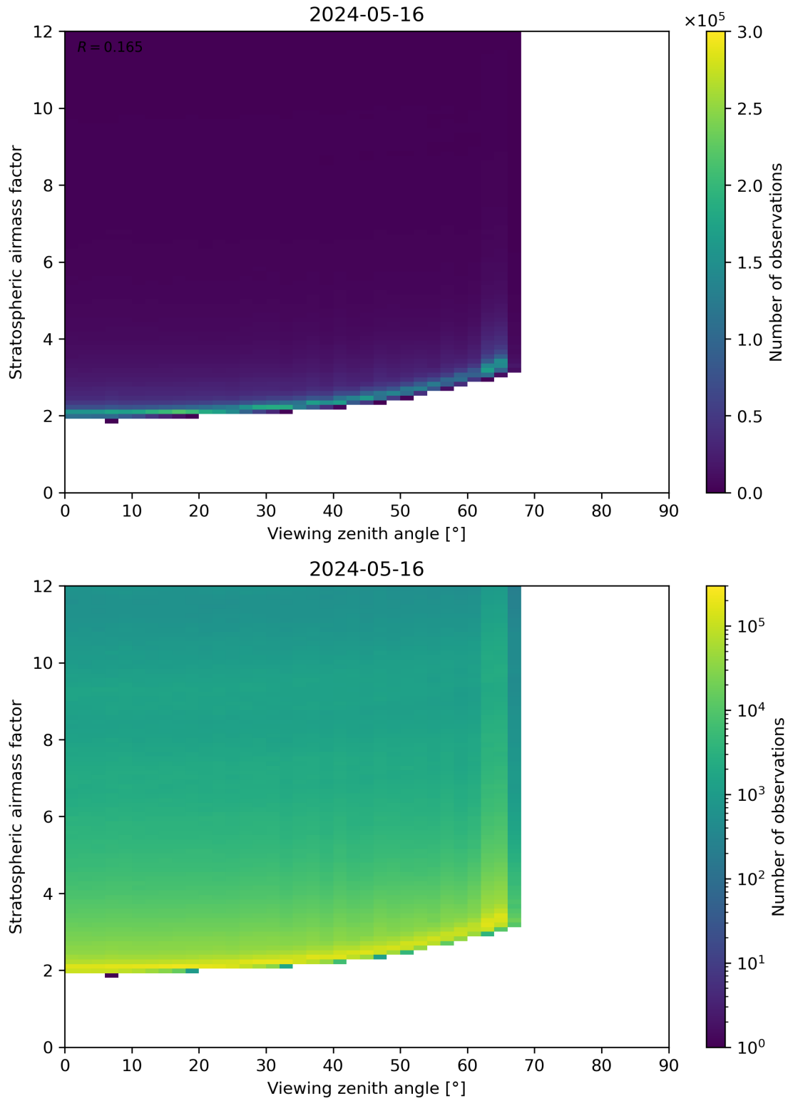
Figure 159: Scatter density plot of “Viewing zenith angle” against “Stratospheric airmass factor” for 2024-05-15 to 2024-05-17.
