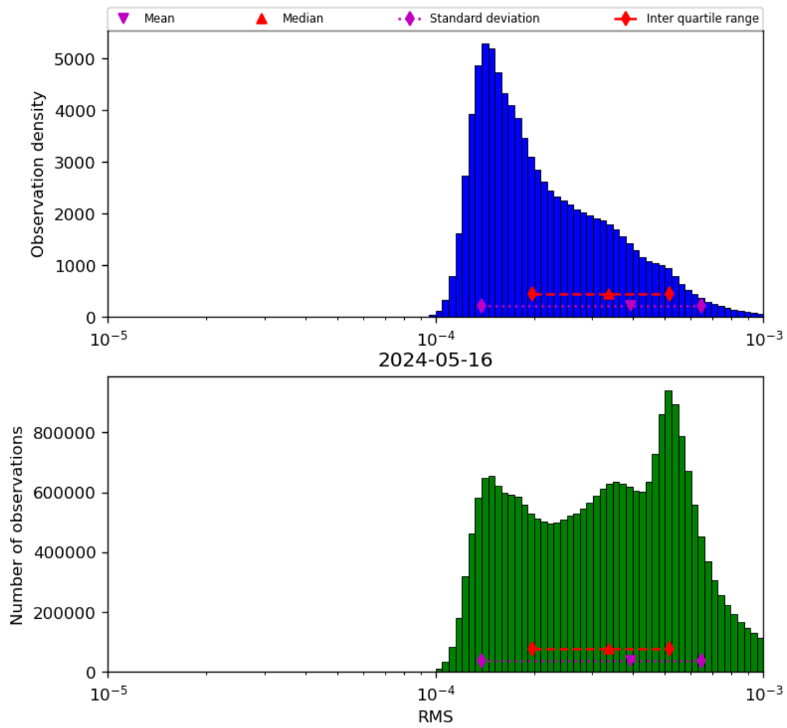
Figure 43: Histogram of “RMS” for 2024-05-15 to 2024-05-17
