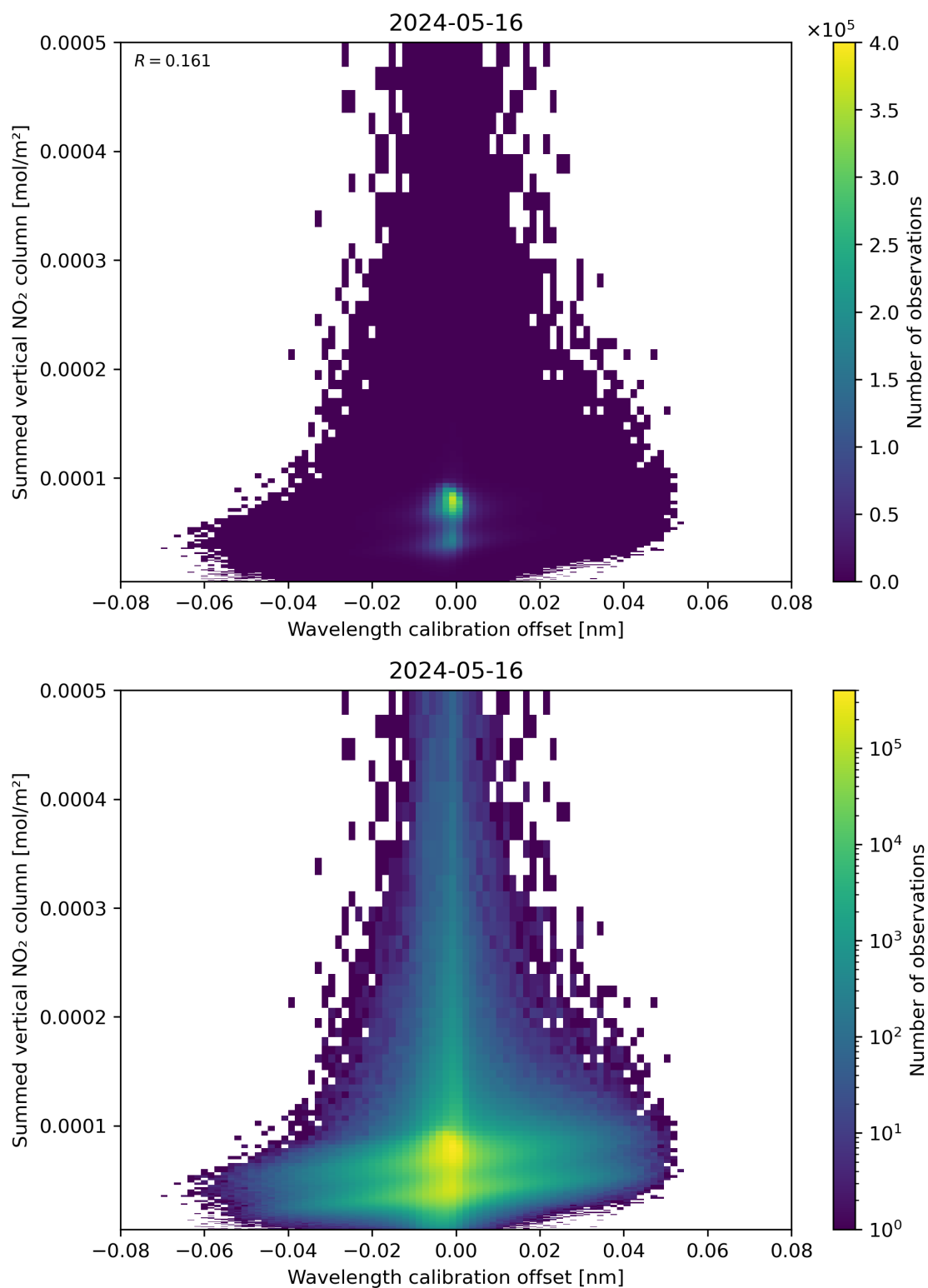
Figure 177: Scatter density plot of “Wavelength calibration offset” against “Summed vertical NO 2 column” for 2024-05-15 to 2024-05-17.
