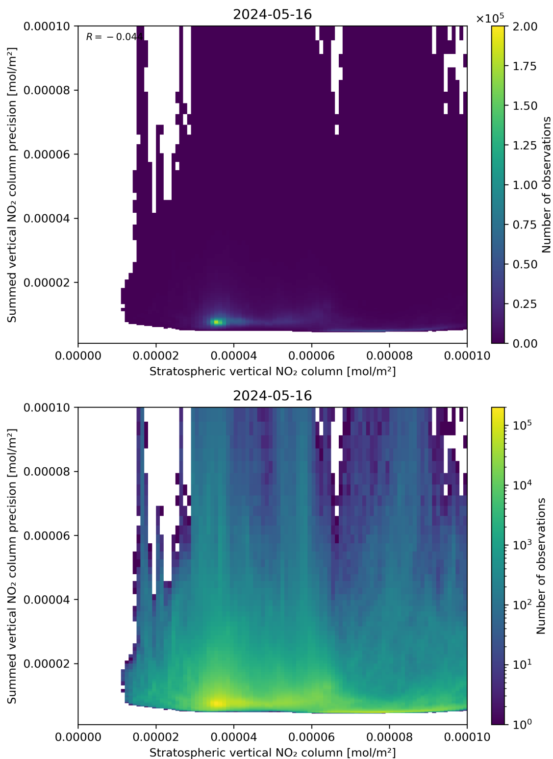
Figure 99: Scatter density plot of “Stratospheric vertical NO 2 column” against “Summed vertical NO 2 column precision” for 2024-05-15 to 2024-05-17.
