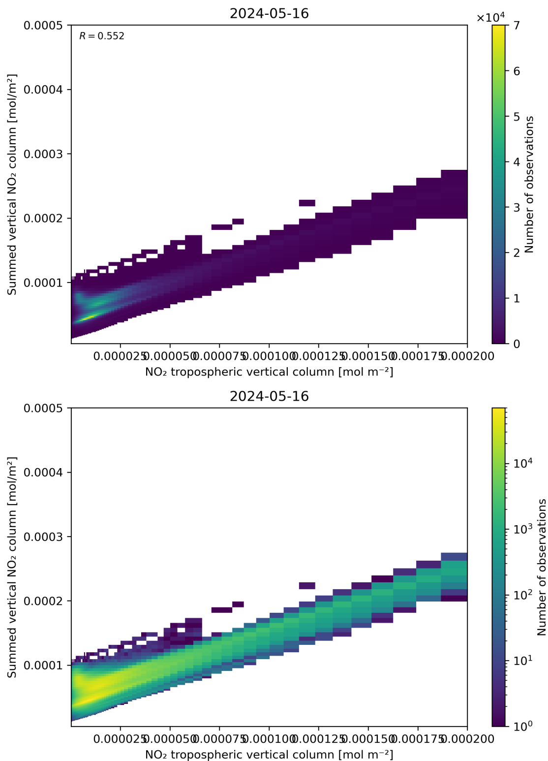
Figure 126: Scatter density plot of “NO 2 tropospheric vertical column” against “Summed vertical NO 2 column” for 2024-05-15 to 2024-05-17.
