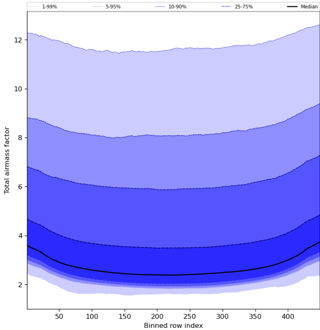
Figure 49: Along track statistics of “Total airmass factor” for 2024-05-15 to 2024-05-17
