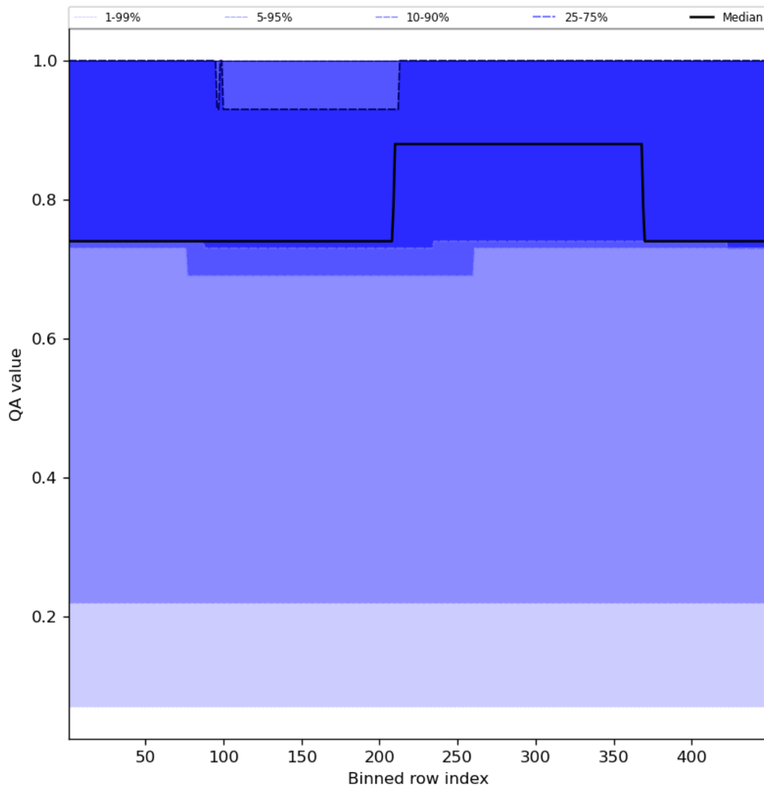
Figure 45: Along track statistics of “QA value” for 2024-05-15 to 2024-05-17
