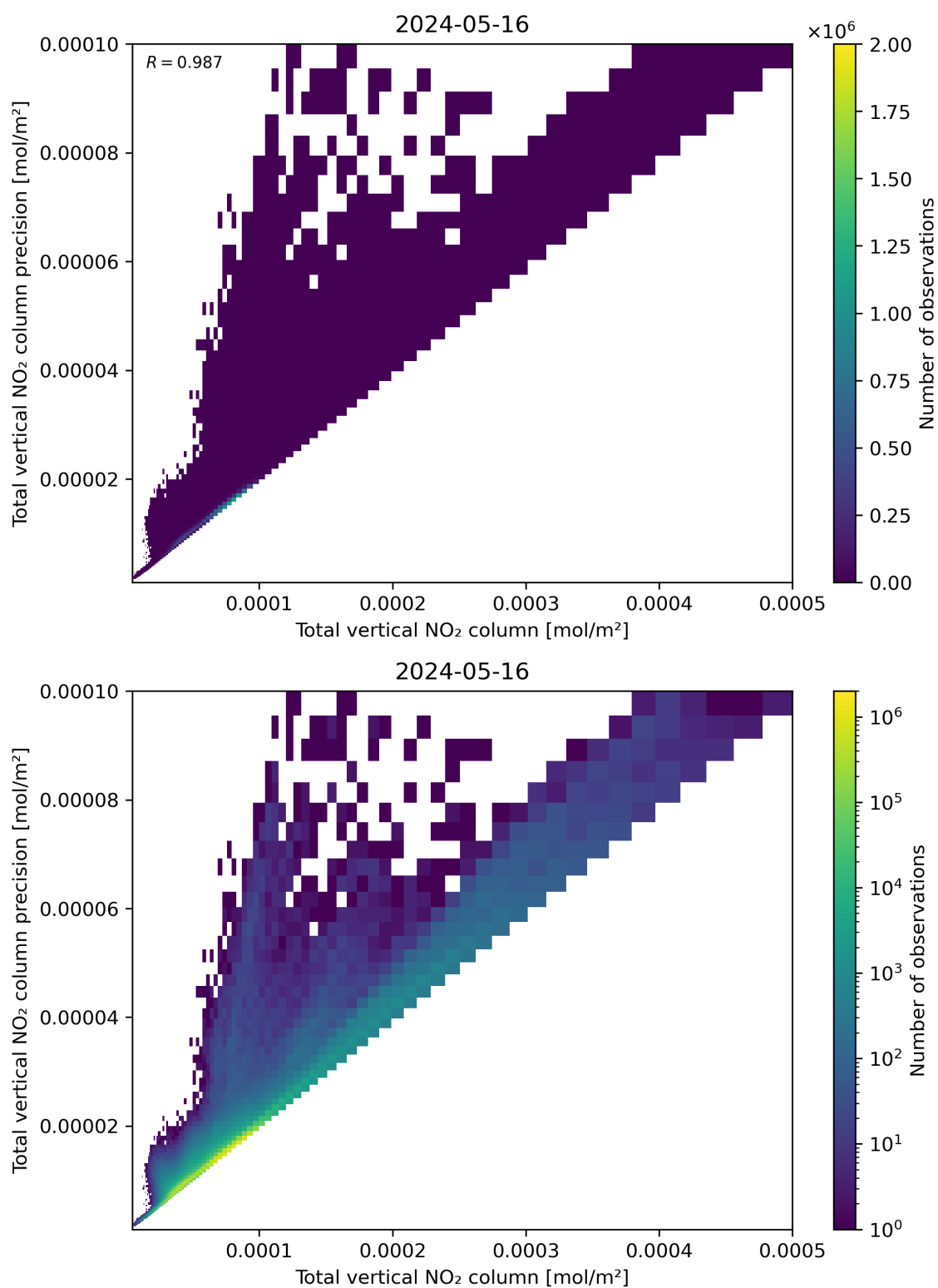
Figure 114: Scatter density plot of “Total vertical NO 2 column” against “Total vertical NO 2 column precision” for 2024-05-15 to 2024-05-17.
