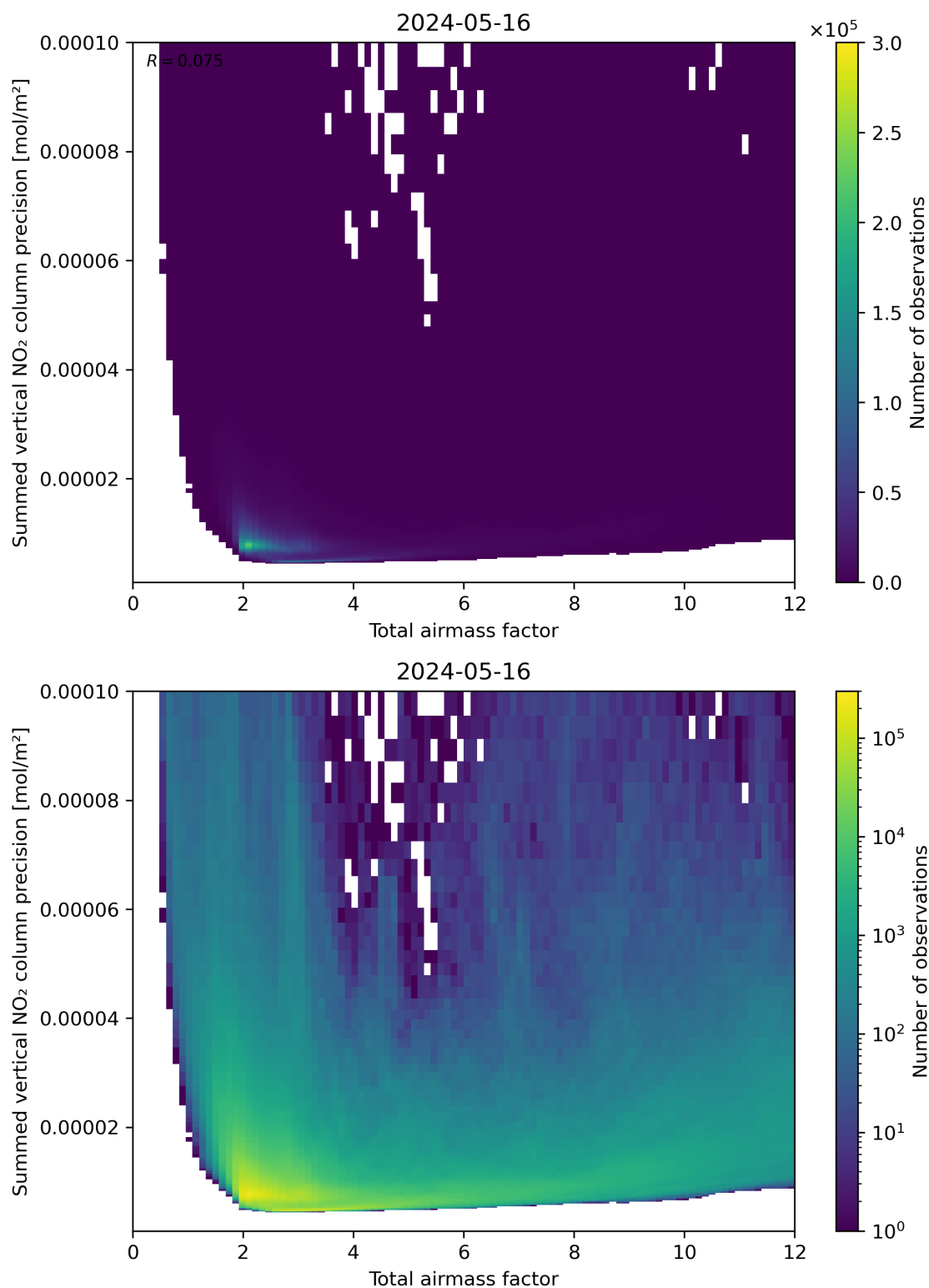
Figure 66: Scatter density plot of “Total airmass factor” against “Summed vertical NO 2 column precision” for 2024-05-15 to 2024-05-17.
