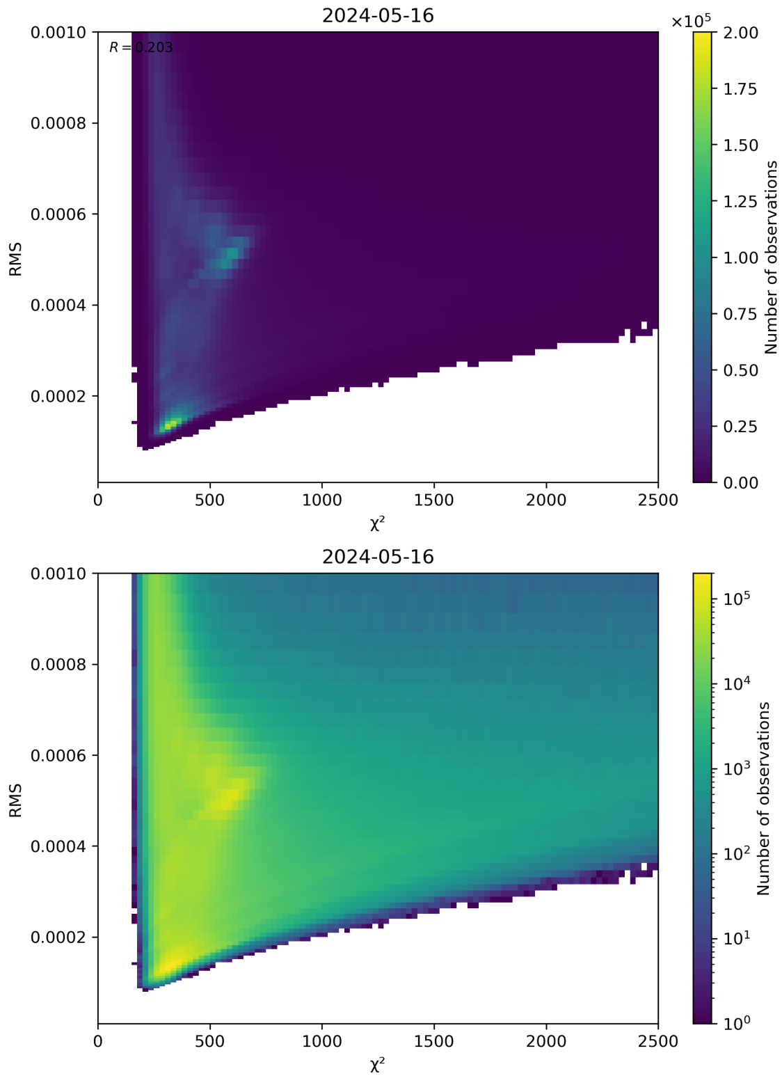
Figure 82: Scatter density plot of “ \chi^2 ” against “RMS” for 2024-05-15 to 2024-05-17.
