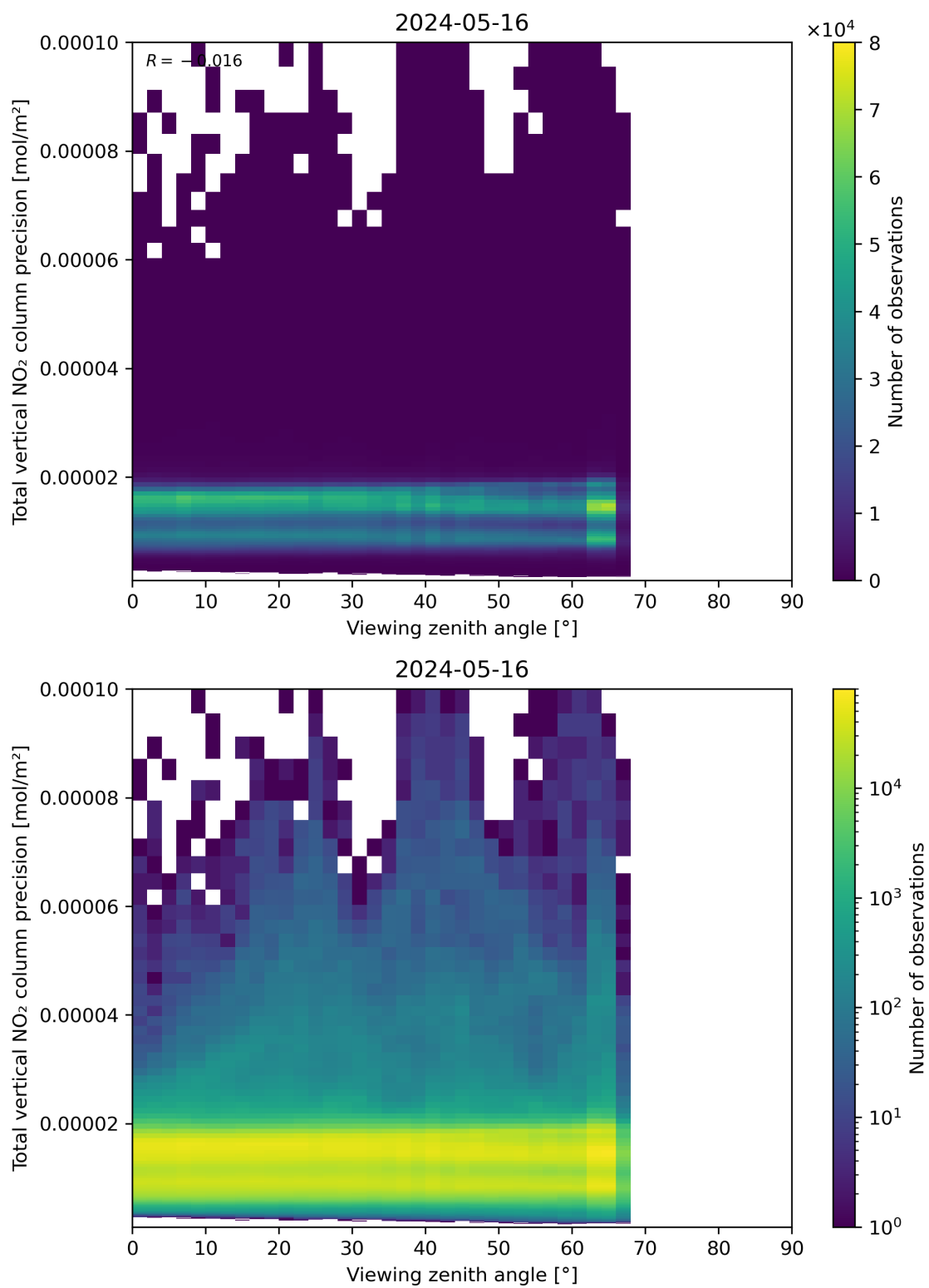
Figure 168: Scatter density plot of “Viewing zenith angle” against “Total vertical NO 2 column precision” for 2024-05-15 to 2024-05-17.
