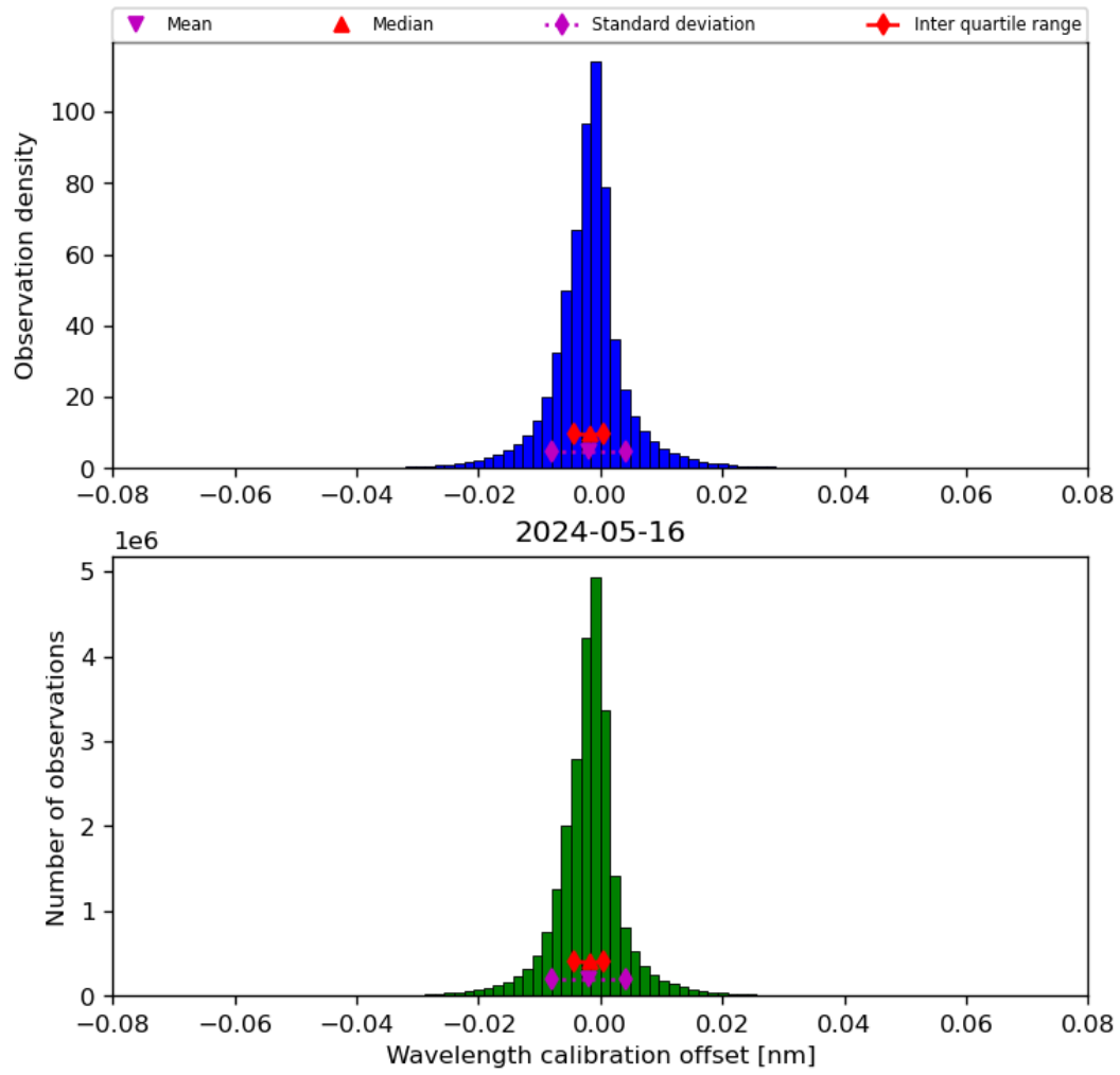
Figure 35: Histogram of “Wavelength calibration offset” for 2024-05-15 to 2024-05-17
