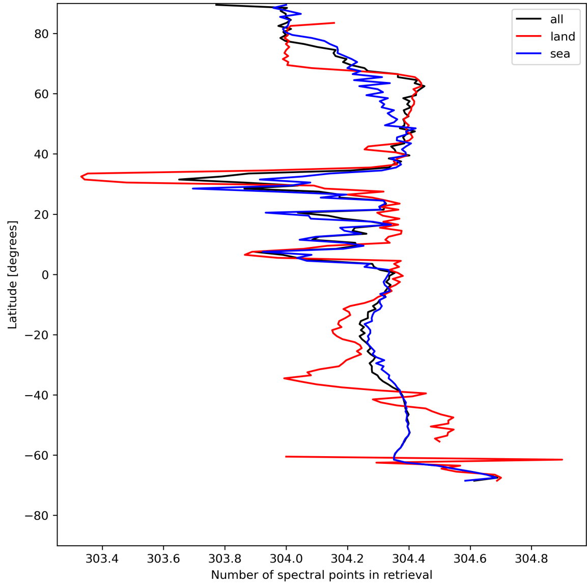
Figure 16: Zonal average of “Number of spectral points in retrieval” for 2024-05-15 to 2024-05-17.
