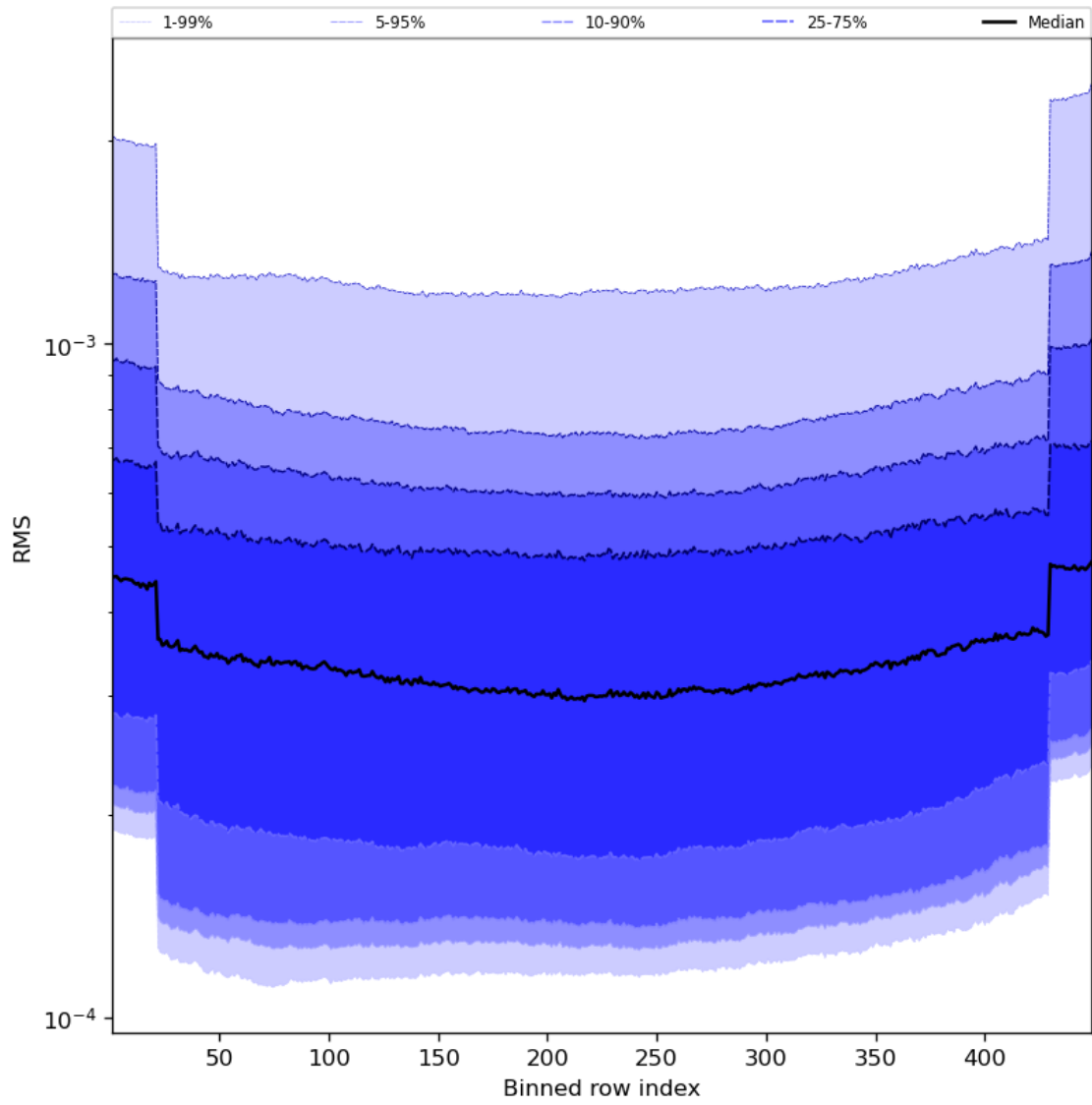
Figure 60: Along track statistics of “RMS” for 2024-05-15 to 2024-05-17
