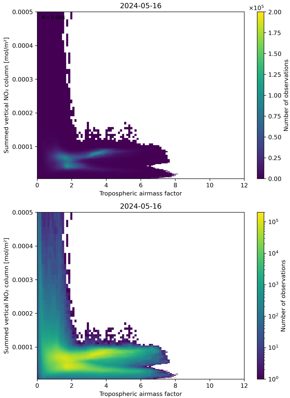
Figure 75: Scatter density plot of “Tropospheric airmass factor” against “Summed vertical NO 2 column” for 2024-05-15 to 2024-05-17.
