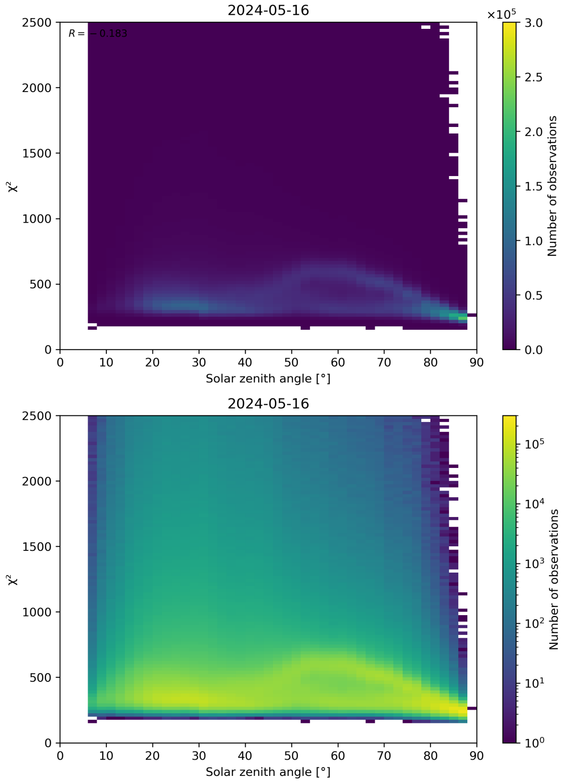
Figure 148: Scatter density plot of “Solar zenith angle” against “ \chi^2 ” for 2024-05-15 to 2024-05-17.
