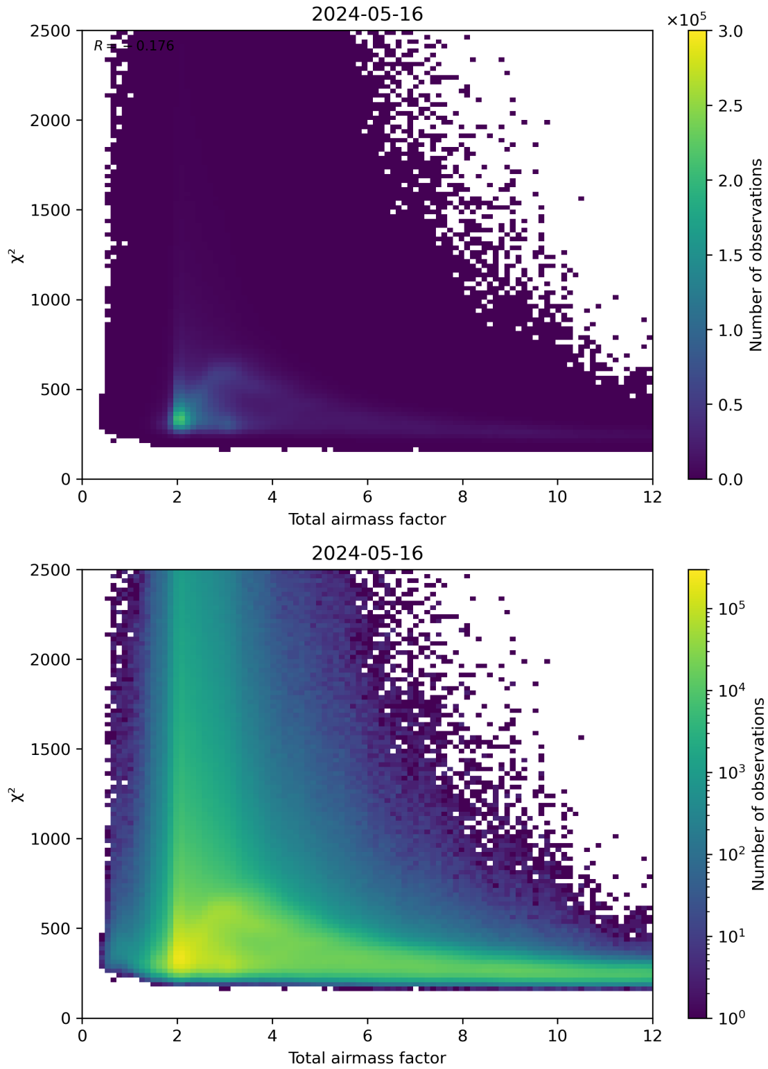
Figure 63: Scatter density plot of “Total airmass factor” against “ \chi^2 ” for 2024-05-15 to 2024-05-17.
