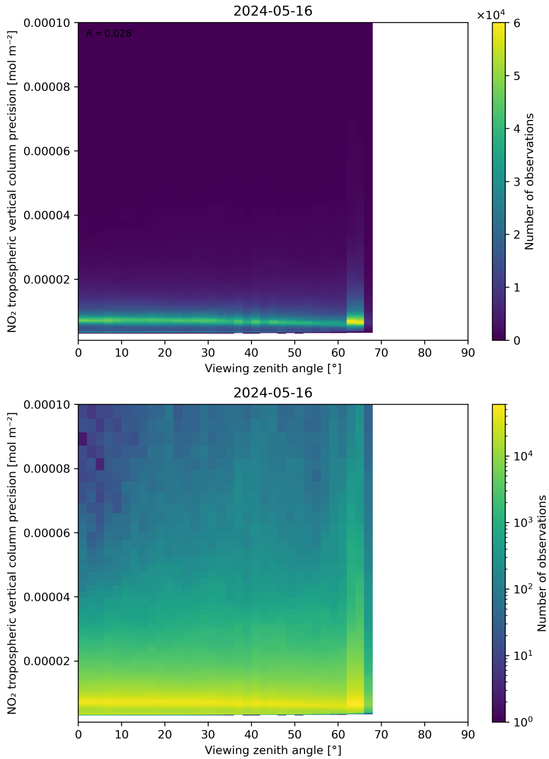
Figure 170: Scatter density plot of “Viewing zenith angle” against “NO 2 tropospheric vertical column precision” for 2024-05-15 to 2024-05-17.
