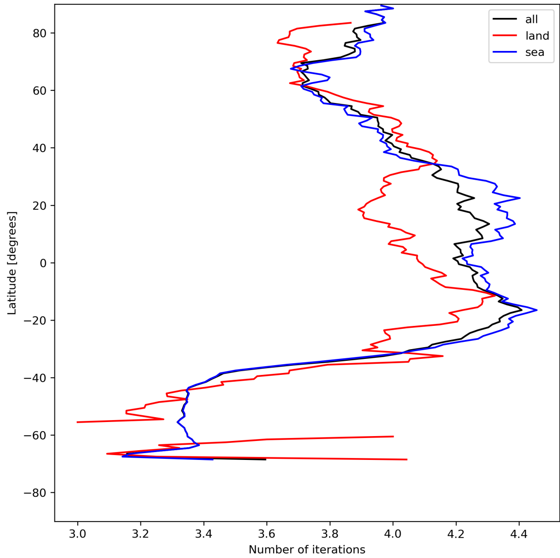
Figure 17: Zonal average of “Number of iterations” for 2024-05-15 to 2024-05-17.
