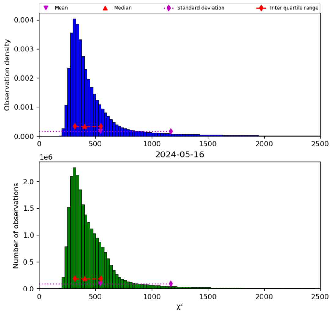
Figure 42: Histogram of “ \chi^2 ” for 2024-05-15 to 2024-05-17
