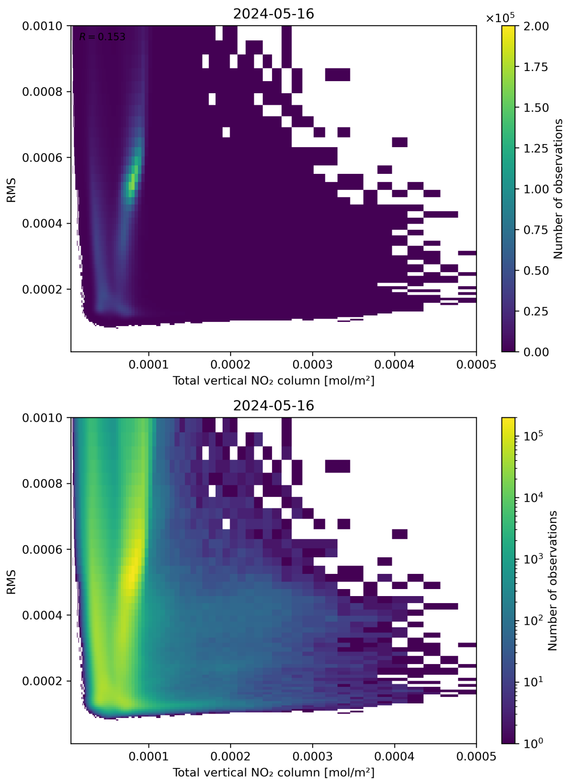
Figure 120: Scatter density plot of “Total vertical NO 2 column” against “RMS” for 2024-05-15 to 2024-05-17.
