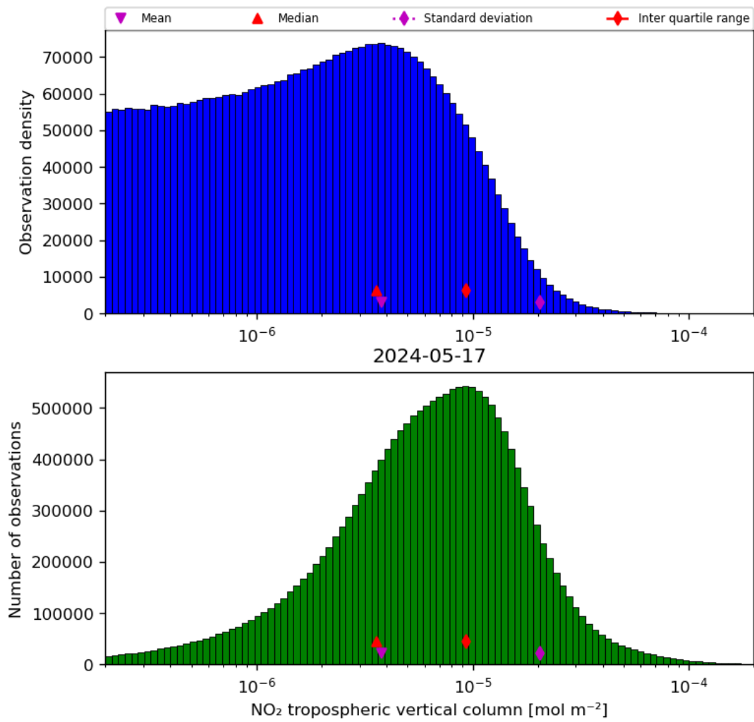
Figure 29: Histogram of “NO 2 tropospheric vertical column” for 2024-05-16 to 2024-05-18
