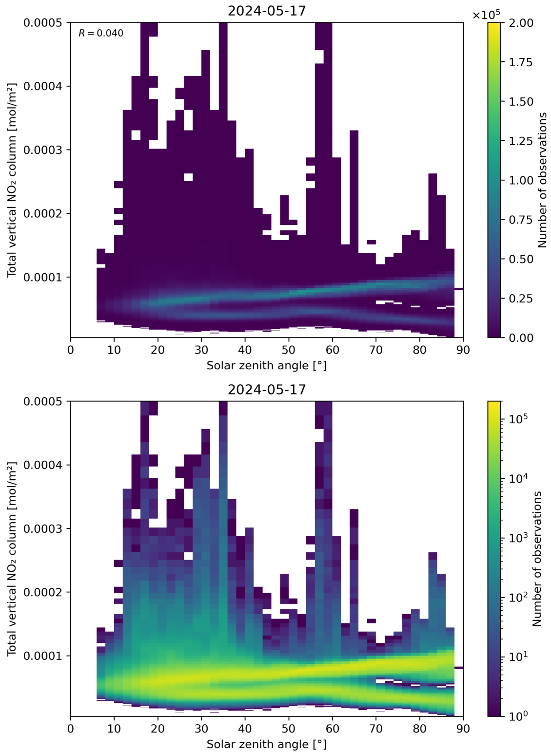
Figure 153: Scatter density plot of “Solar zenith angle” against “Total vertical NO 2 column” for 2024-05-16 to 2024-05-18.
