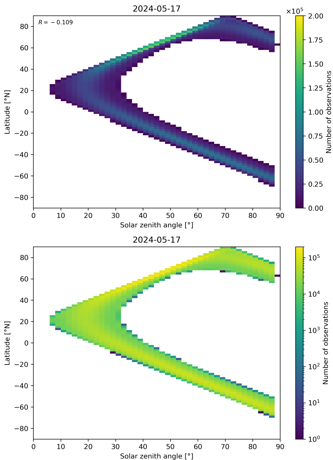
Figure 149: Scatter density plot of “Solar zenith angle” against “Latitude” for 2024-05-16 to 2024-05-18.
