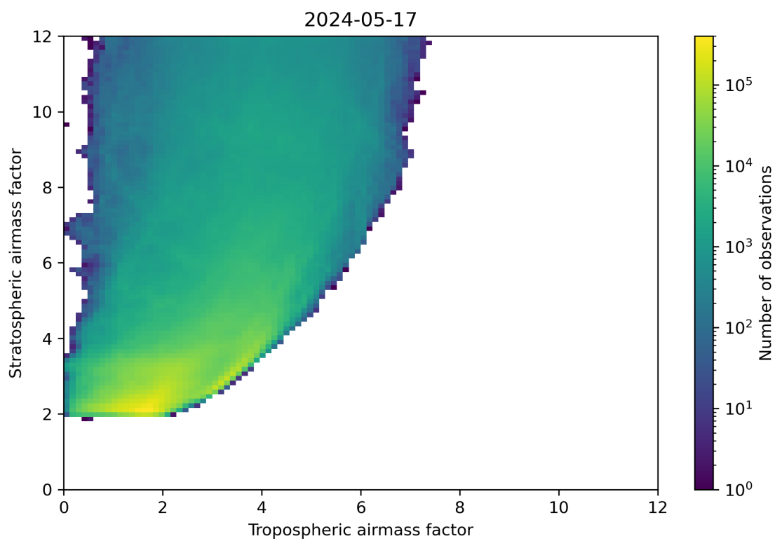
Figure 71: Scatter density plot of “Tropospheric airmass factor” against “Stratospheric airmass factor” for 2024-05-16 to 2024-05-18.
