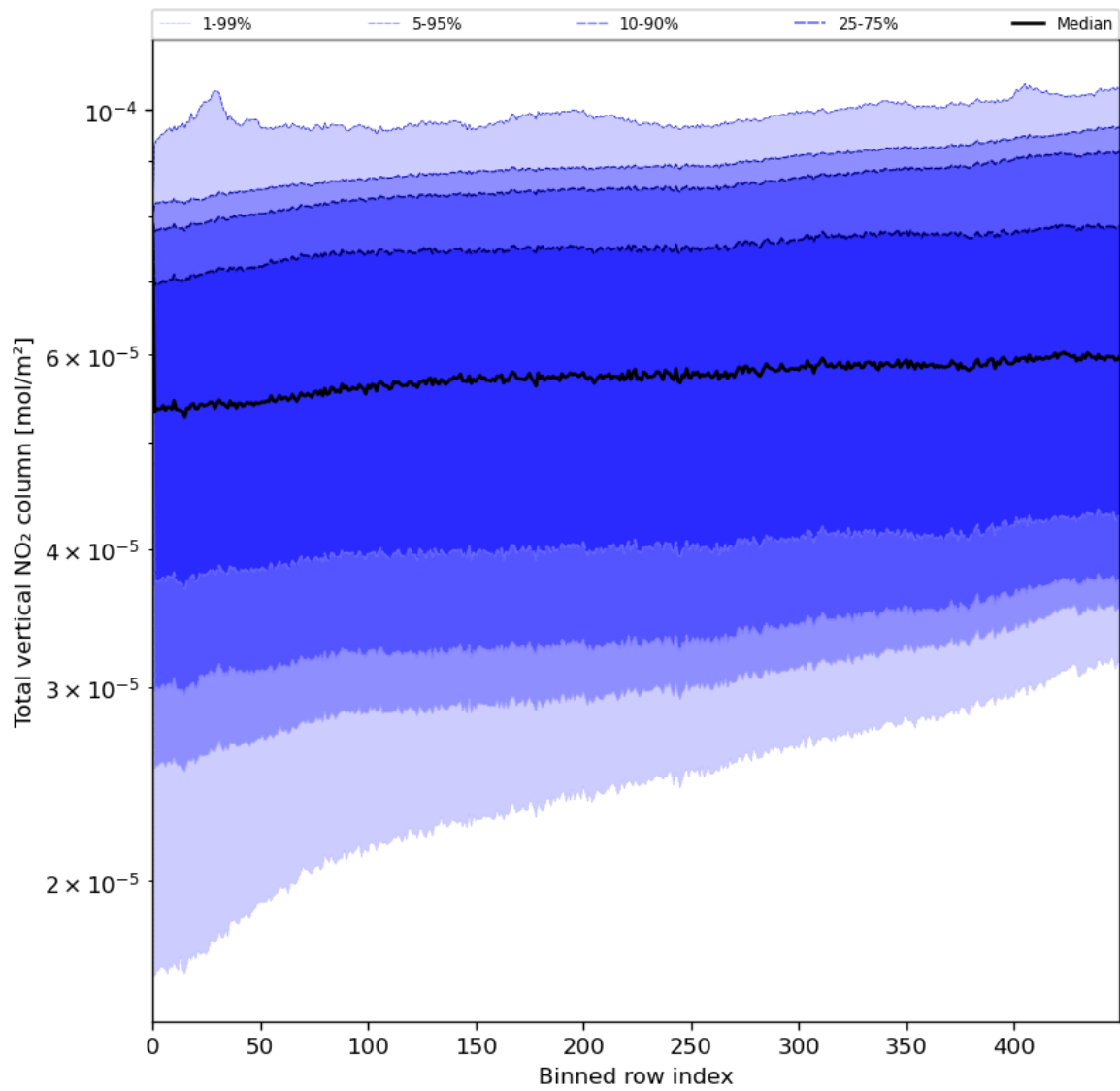
Figure 55: Along track statistics of “Total vertical NO 2 column” for 2024-05-16 to 2024-05-18
