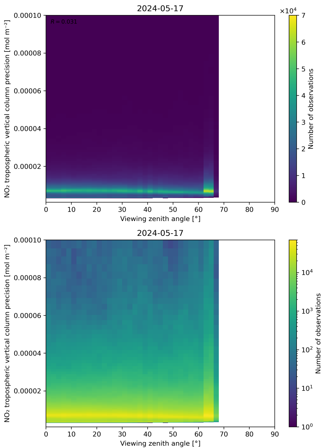
Figure 170: Scatter density plot of “Viewing zenith angle” against “NO 2 tropospheric vertical column precision” for 2024-05-16 to 2024-05-18.
