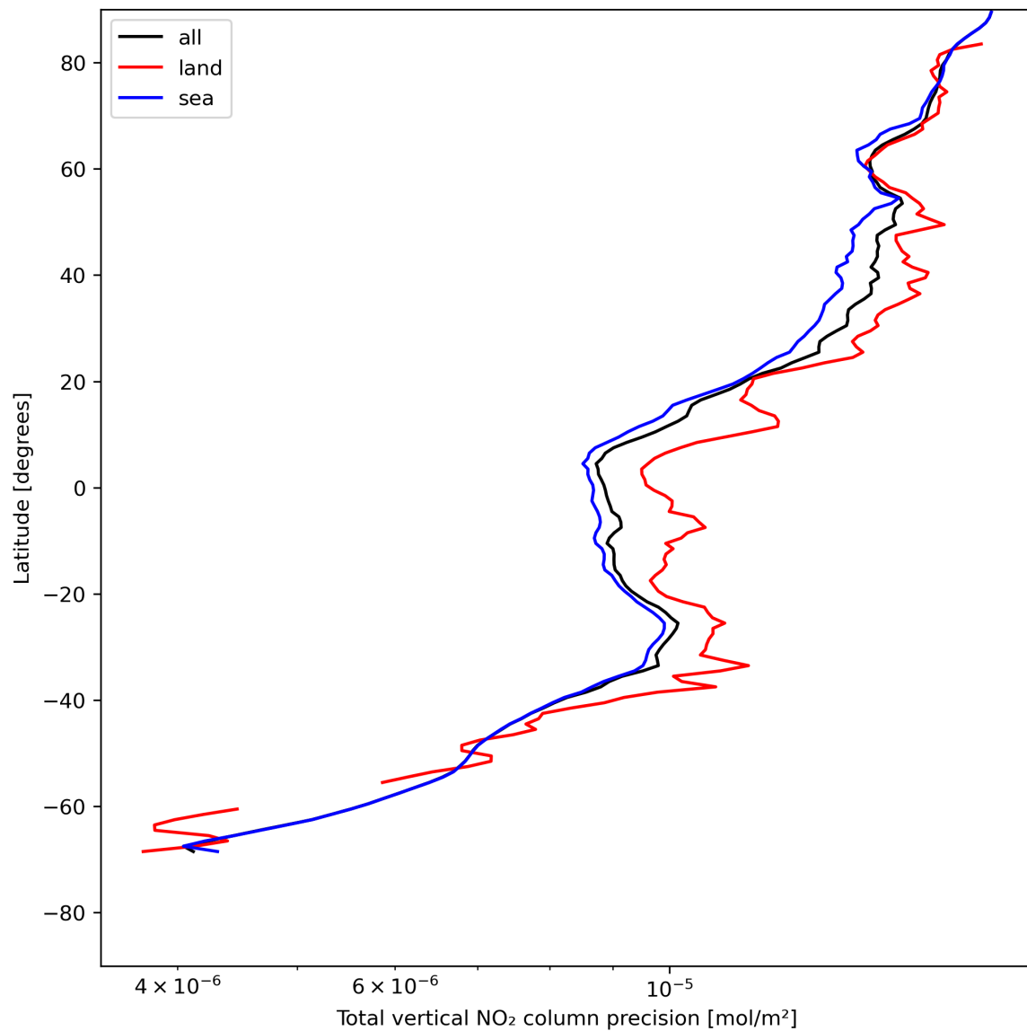
Figure 22: Zonal average of “Total vertical NO 2 column precision” for 2024-05-16 to 2024-05-18.
