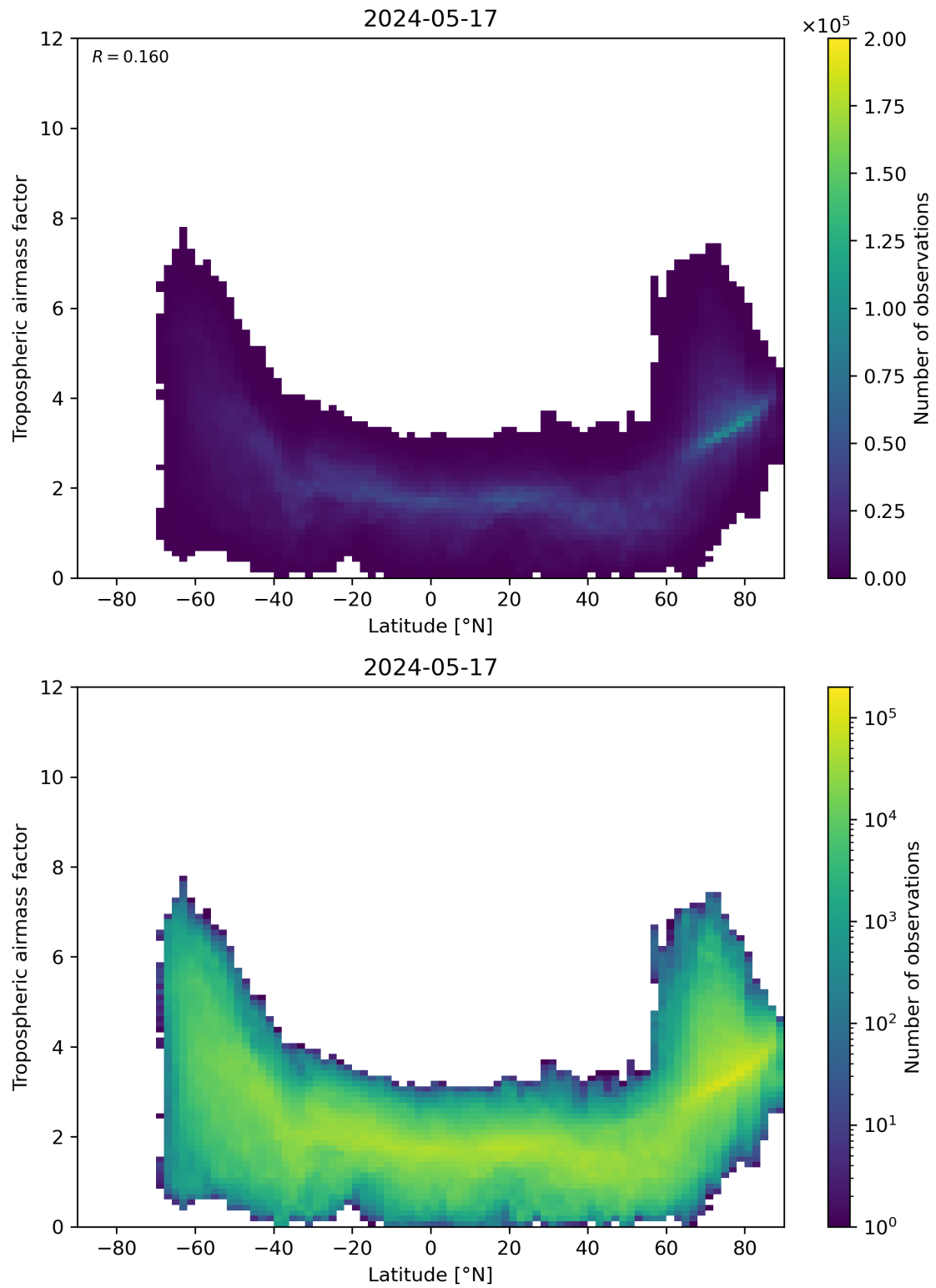
Figure 85: Scatter density plot of “Latitude” against “Tropospheric airmass factor” for 2024-05-16 to 2024-05-18.
