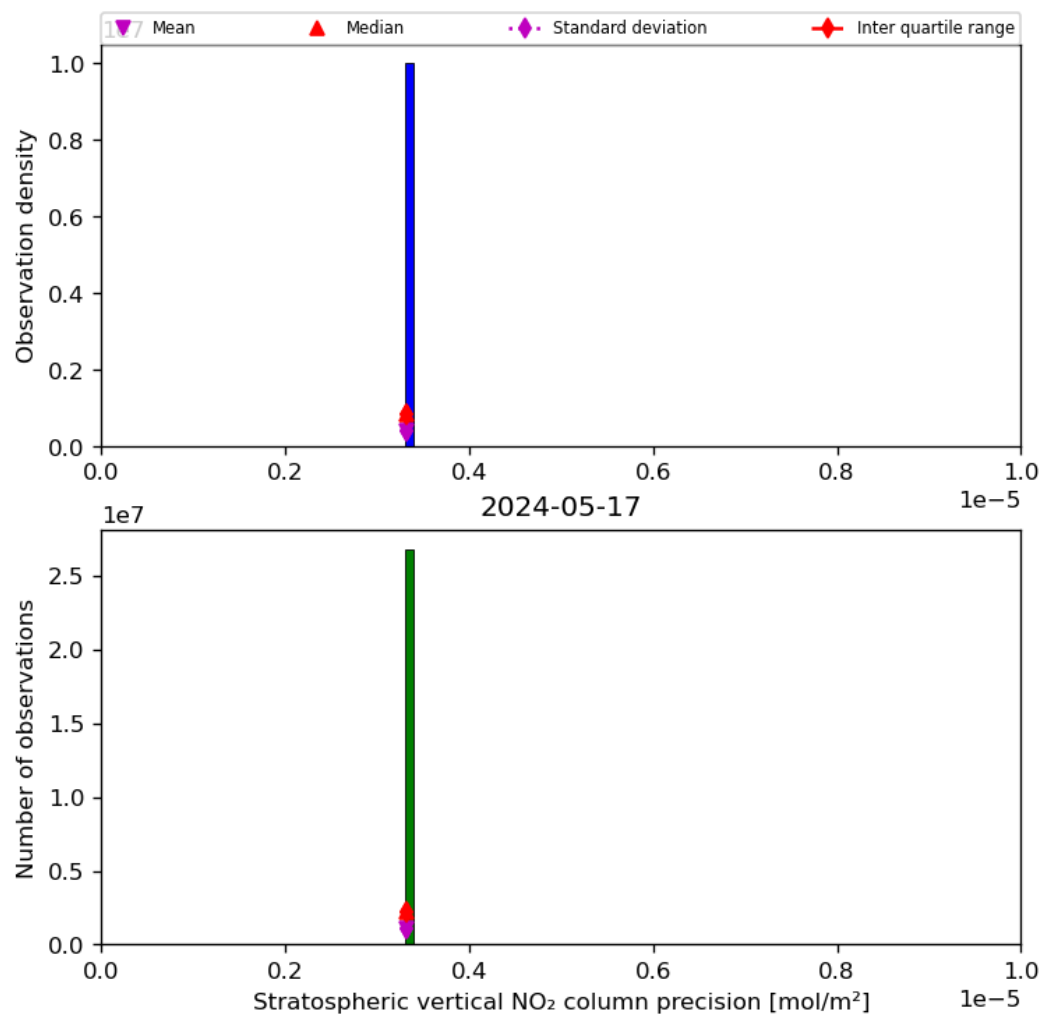
Figure 37: Histogram of “Stratospheric vertical NO 2 column precision” for 2024-05-16 to 2024-05-18
