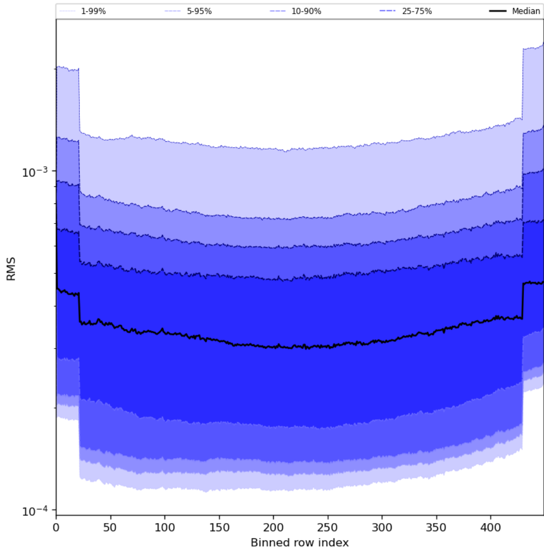
Figure 60: Along track statistics of “RMS” for 2024-05-16 to 2024-05-18
