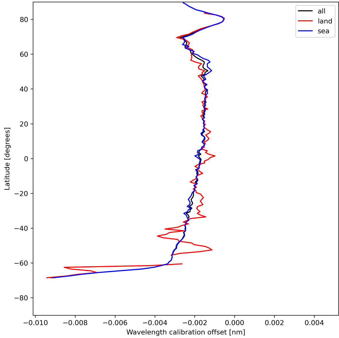
Figure 18: Zonal average of “Wavelength calibration offset” for 2024-05-16 to 2024-05-18.
