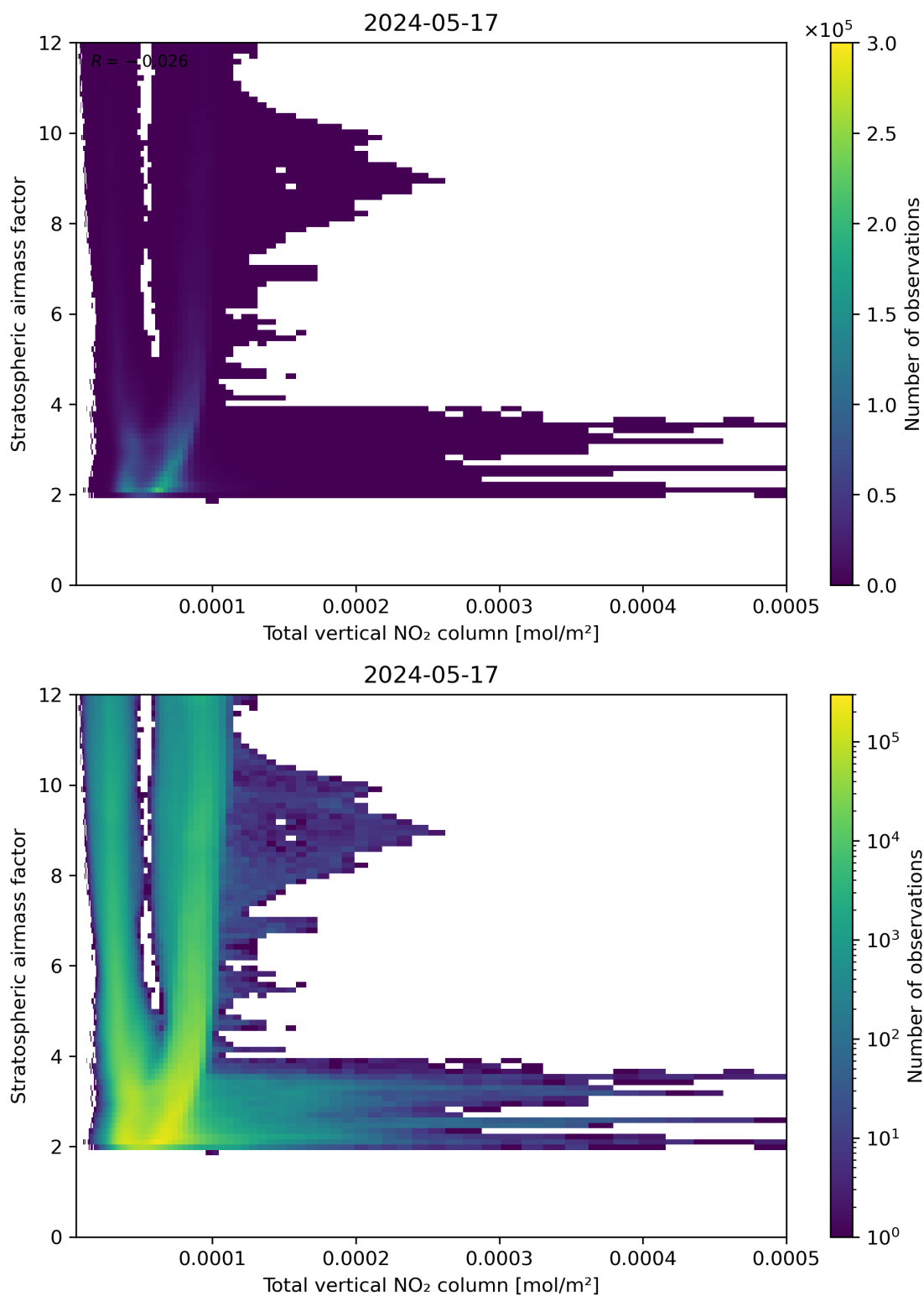
Figure 110: Scatter density plot of “Total vertical NO 2 column” against “Stratospheric airmass factor” for 2024-05-16 to 2024-05-18.
