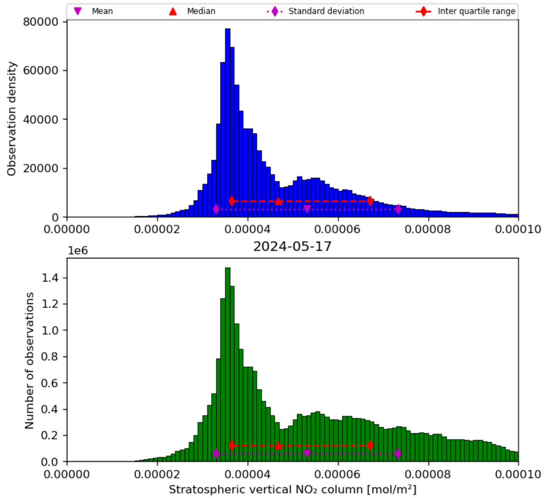
Figure 36: Histogram of “Stratospheric vertical NO 2 column” for 2024-05-16 to 2024-05-18
