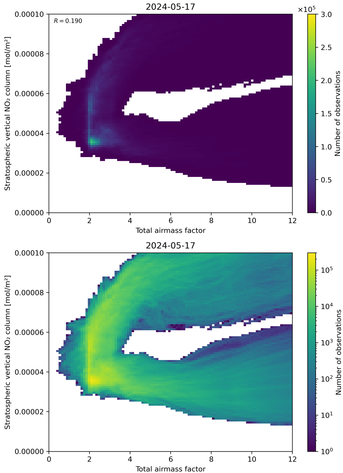
Figure 64: Scatter density plot of “Total airmass factor” against “Stratospheric vertical \text{NO}_2 column” for 2024-05-16 to 2024-05-18.
