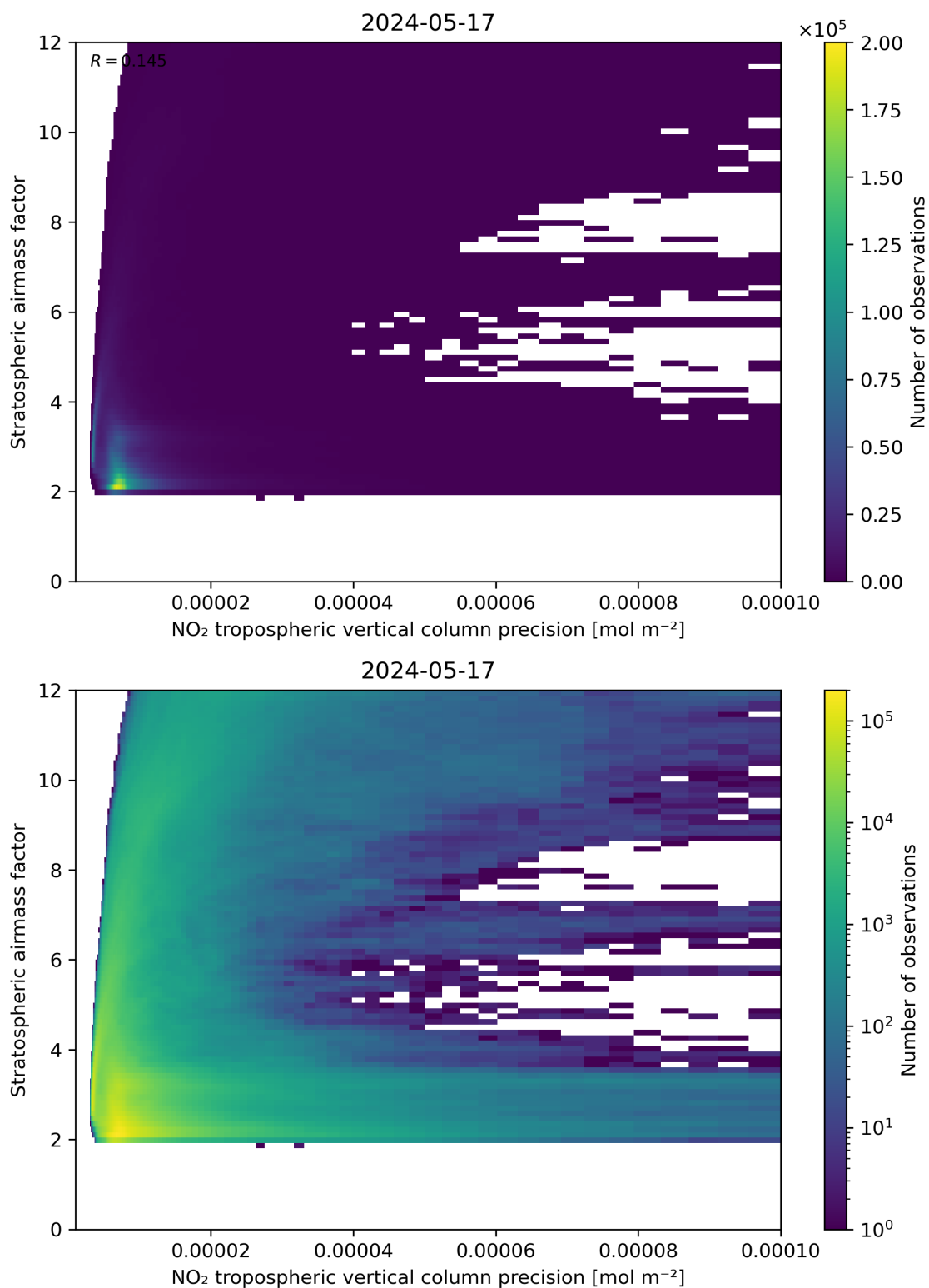
Figure 131: Scatter density plot of “NO 2 tropospheric vertical column precision” against “Stratospheric airmass factor” for 2024-05-16 to 2024-05-18.
