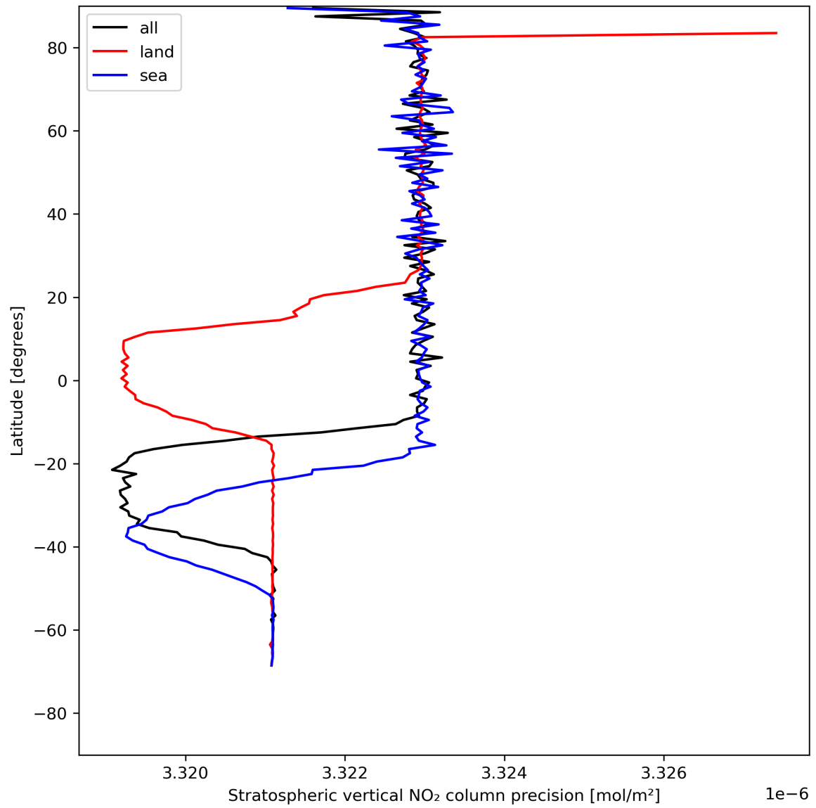
Figure 20: Zonal average of “Stratospheric vertical NO 2 column precision” for 2024-05-16 to 2024-05-18.
