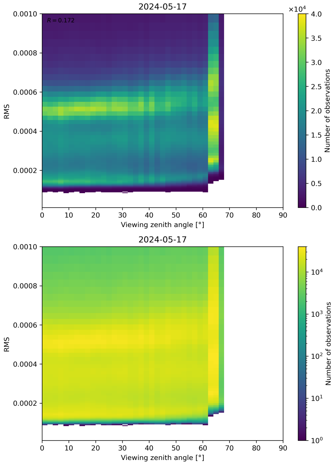
Figure 171: Scatter density plot of “Viewing zenith angle” against “RMS” for 2024-05-16 to 2024-05-18.
