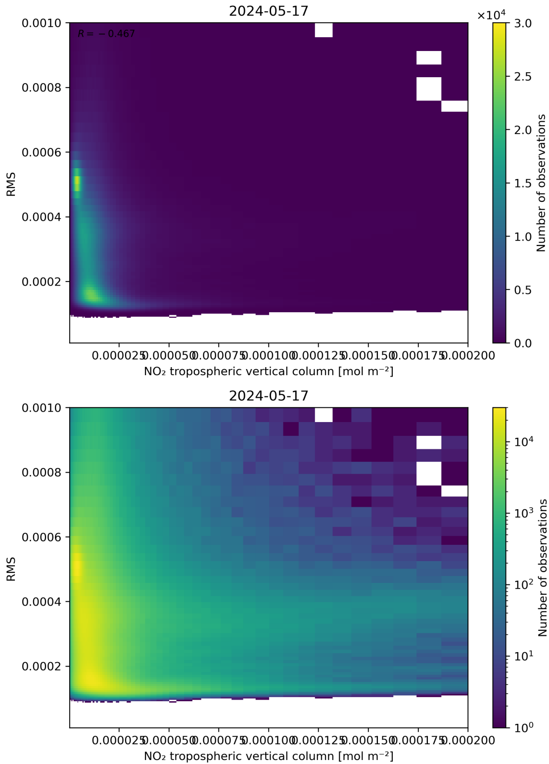
Figure 142: Scatter density plot of “NO 2 tropospheric vertical column” against “RMS” for 2024-05-16 to 2024-05-18.
