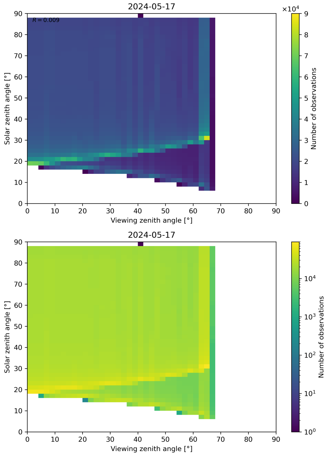
Figure 172: Scatter density plot of “Viewing zenith angle” against “Solar zenith angle” for 2024-05-16 to 2024-05-18.
