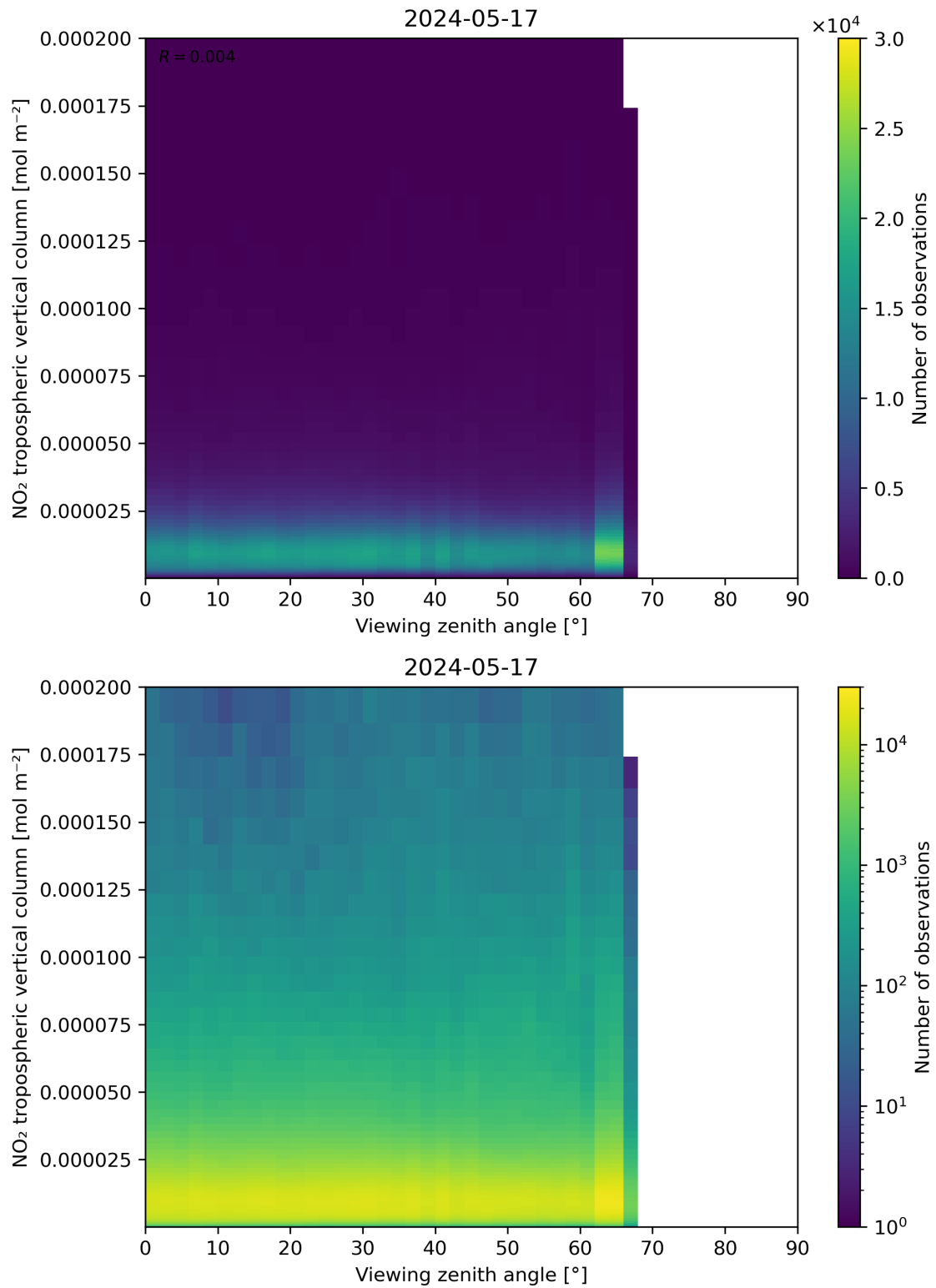
Figure 169: Scatter density plot of “Viewing zenith angle” against “NO 2 tropospheric vertical column” for 2024-05-16 to 2024-05-18.
