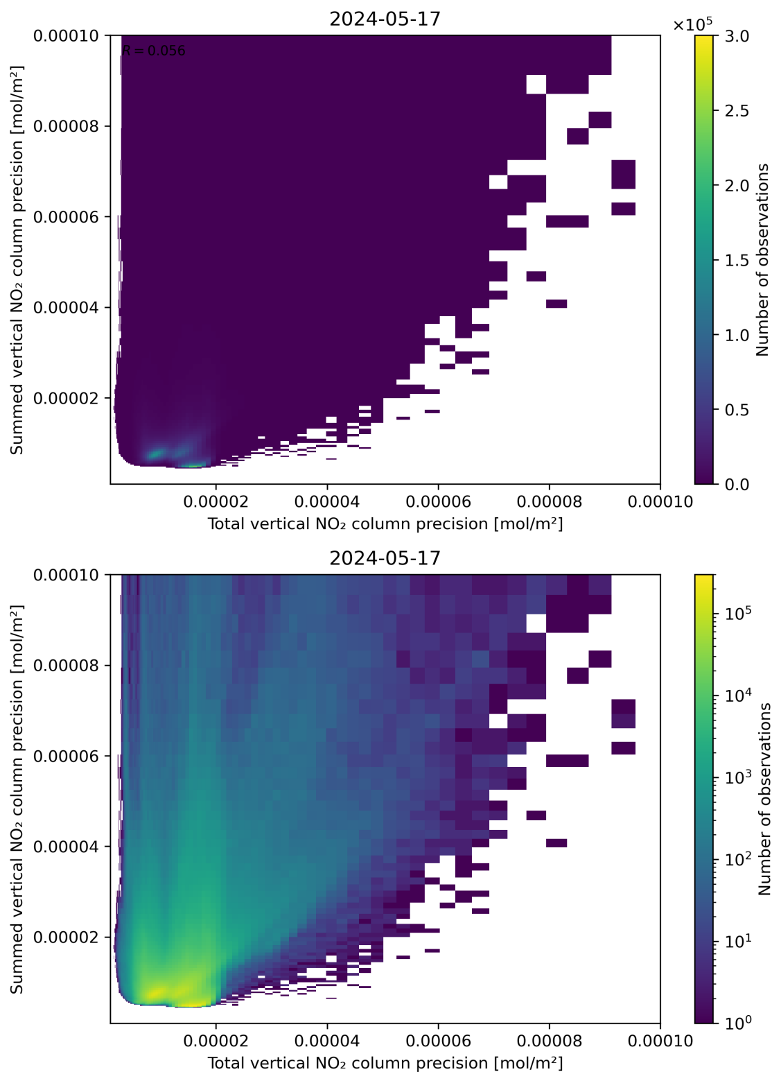
Figure 118: Scatter density plot of “Total vertical NO 2 column precision” against “Summed vertical NO 2 column precision” for 2024-05-16 to 2024-05-18.
