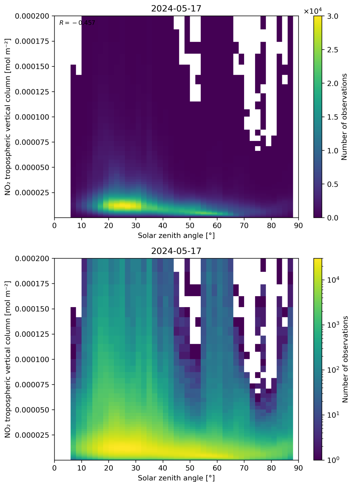
Figure 155: Scatter density plot of “Solar zenith angle” against “NO 2 tropospheric vertical column” for 2024-05-16 to 2024-05-18.
