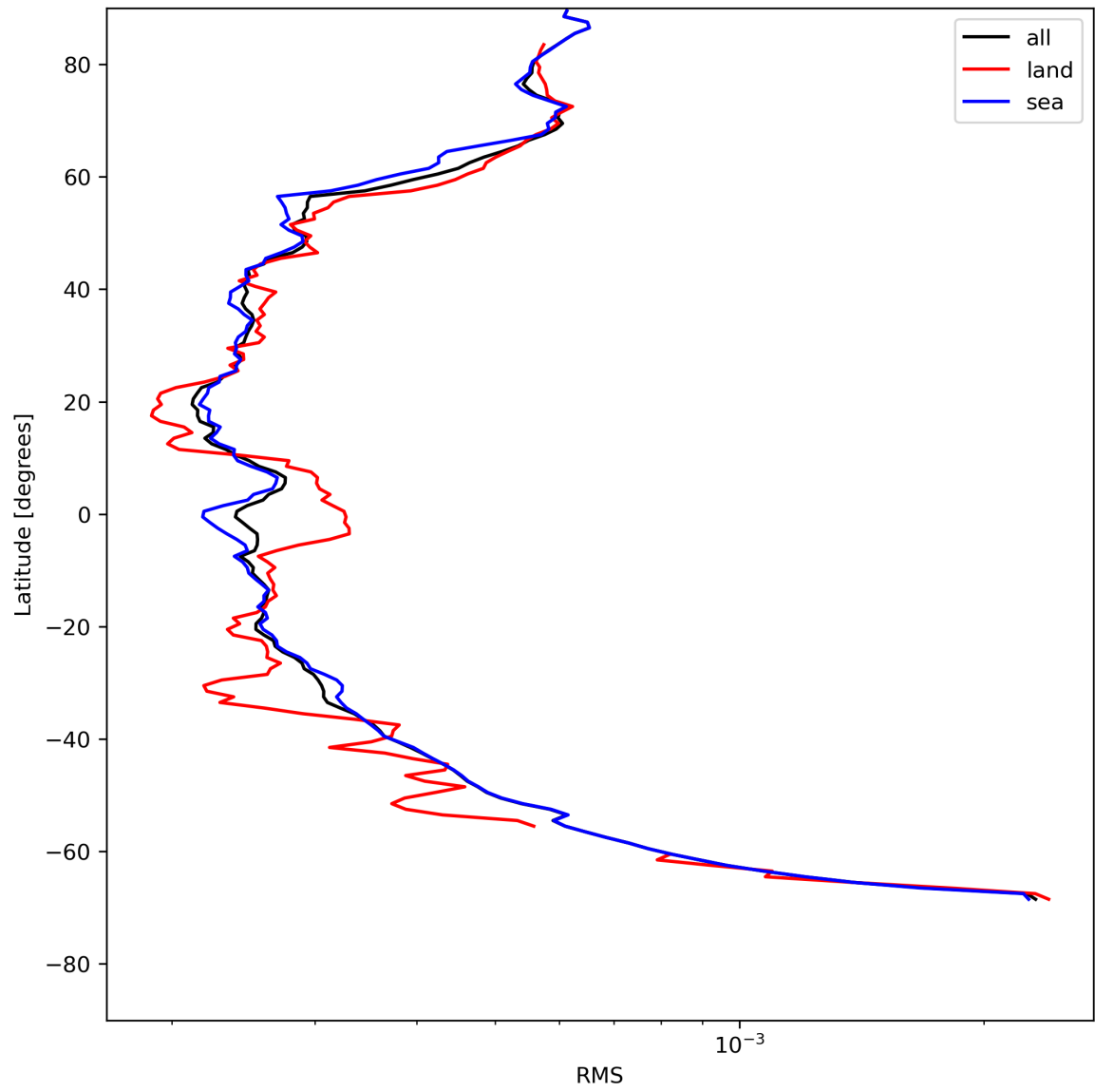
Figure 26: Zonal average of “RMS” for 2024-05-16 to 2024-05-18.
