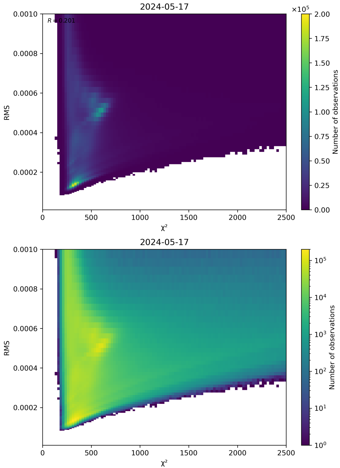
Figure 82: Scatter density plot of “ \chi^2 ” against “RMS” for 2024-05-16 to 2024-05-18.
