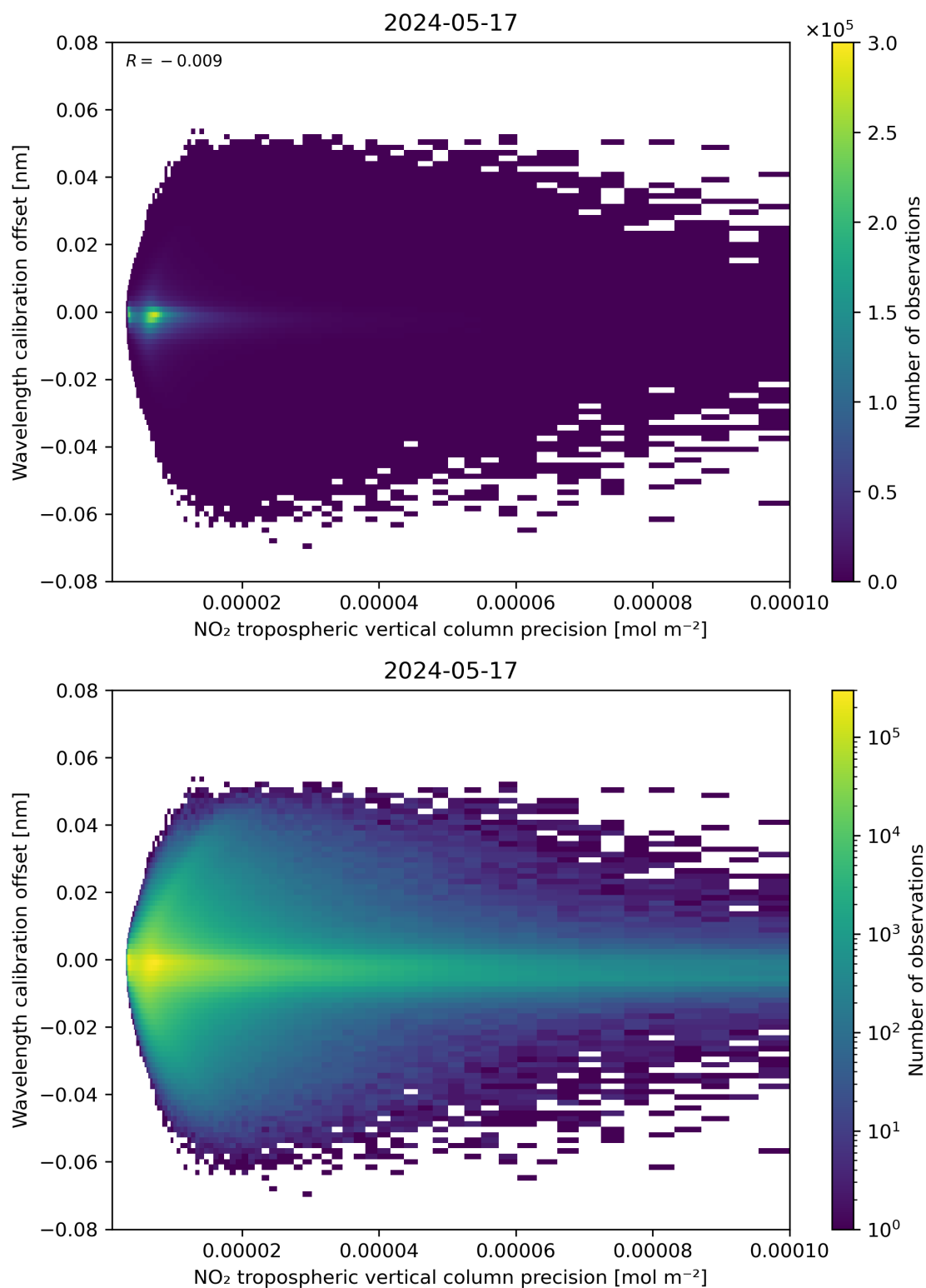
Figure 141: Scatter density plot of “NO 2 tropospheric vertical column precision” against “Wavelength calibration offset” for 2024-05-16 to 2024-05-18.
