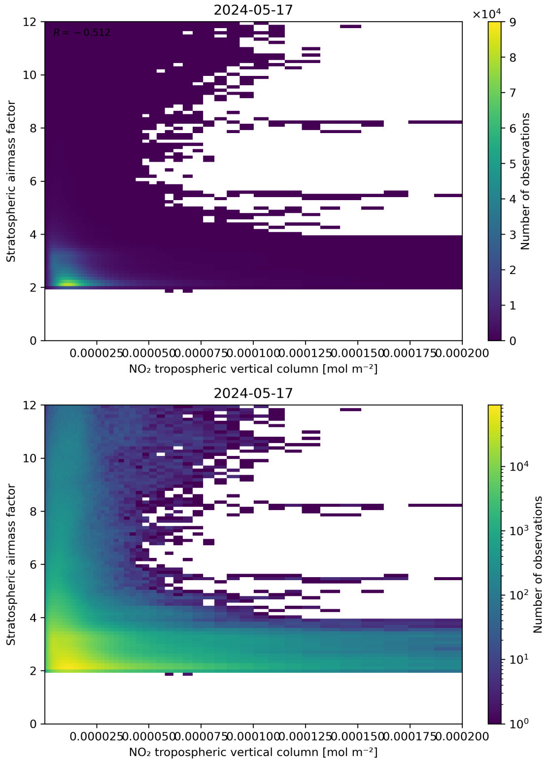
Figure 121: Scatter density plot of “NO 2 tropospheric vertical column” against “Stratospheric air mass factor” for 2024-05-16 to 2024-05-18.
