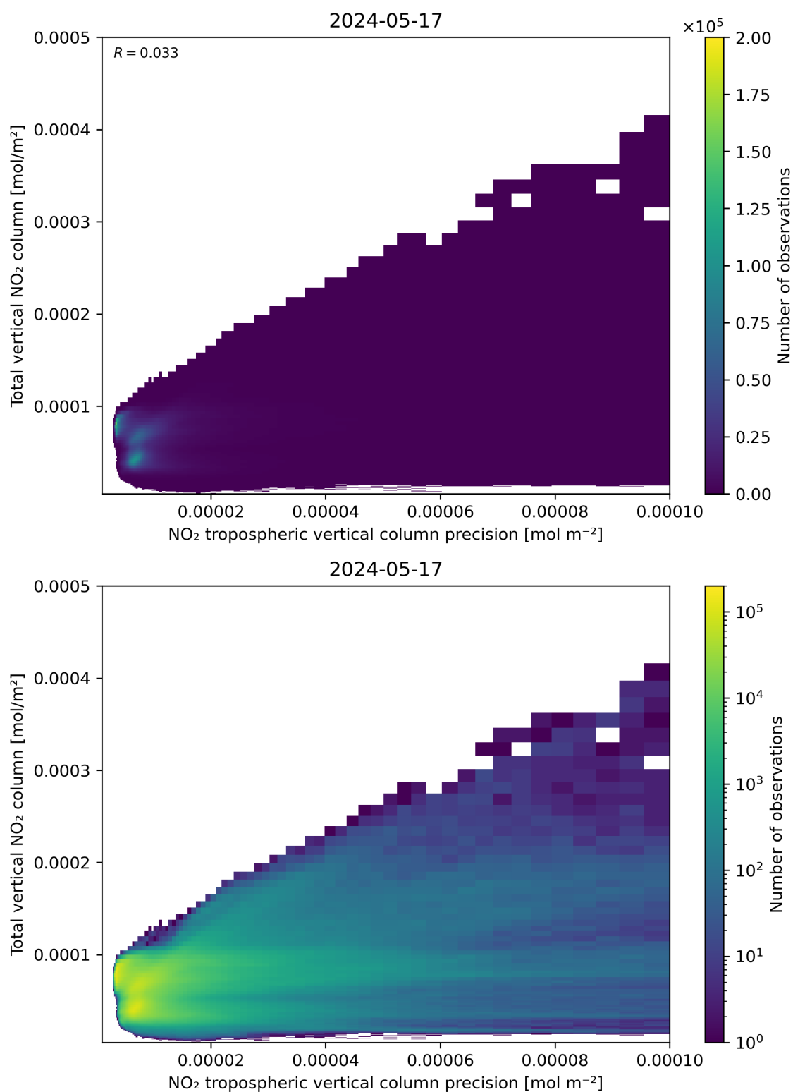
Figure 138: Scatter density plot of “NO 2 tropospheric vertical column precision” against “Total vertical NO 2 column” for 2024-05-16 to 2024-05-18.
