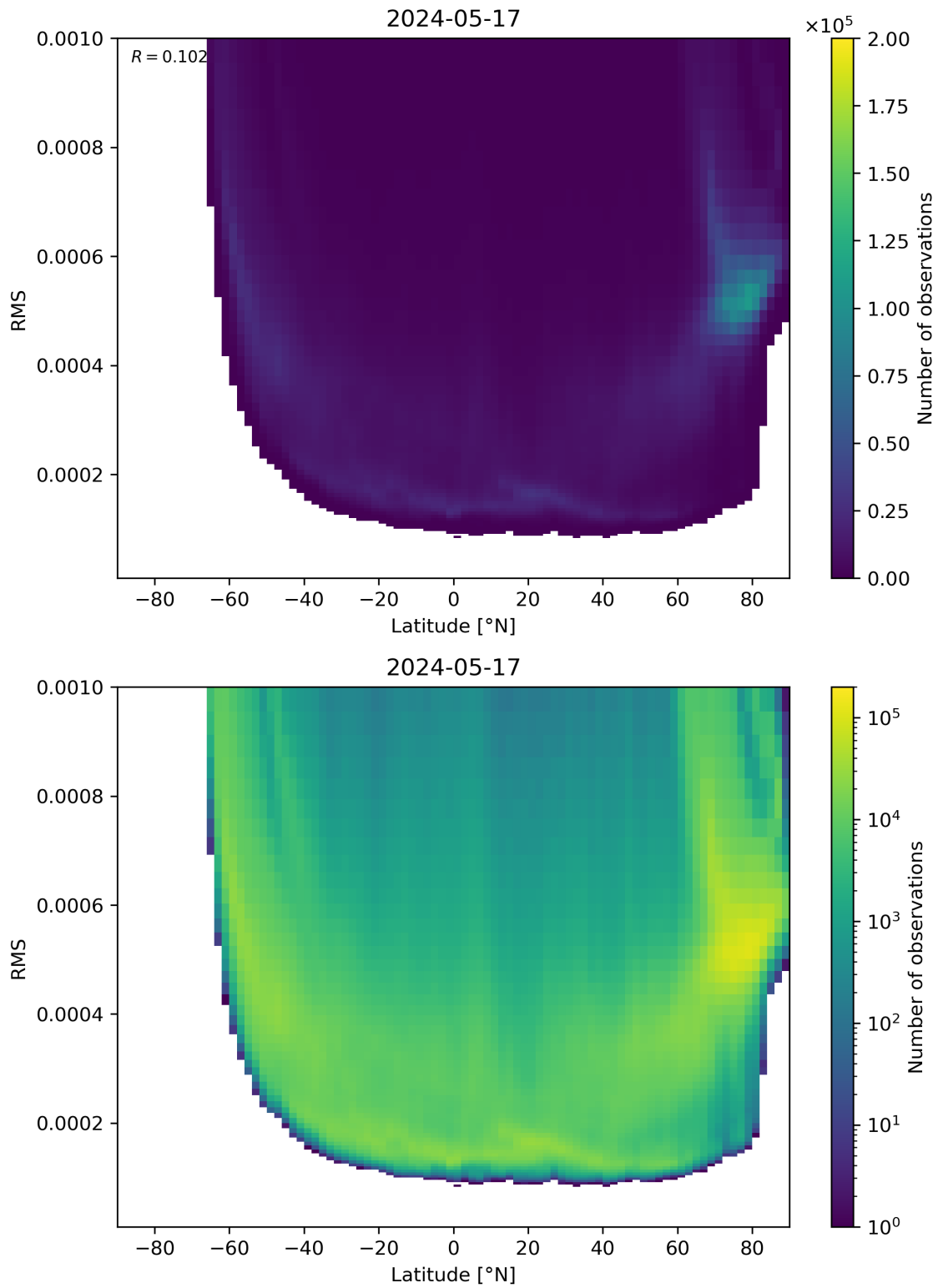
Figure 94: Scatter density plot of “Latitude” against “RMS” for 2024-05-16 to 2024-05-18.
