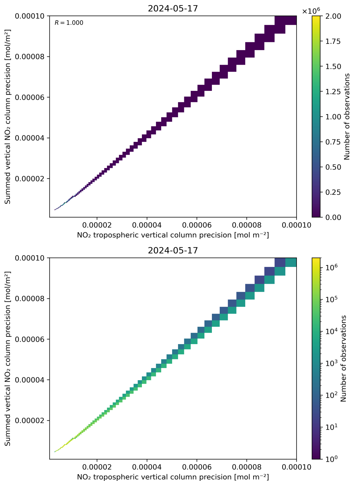
Figure 137: Scatter density plot of “NO 2 tropospheric vertical column precision” against “Summed vertical NO 2 column precision” for 2024-05-16 to 2024-05-18.
