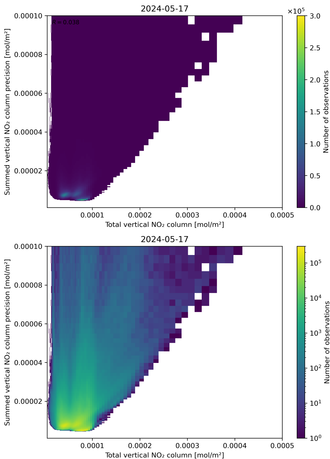
Figure 113: Scatter density plot of “Total vertical NO 2 column” against “Summed vertical NO 2 column precision” for 2024-05-16 to 2024-05-18.
