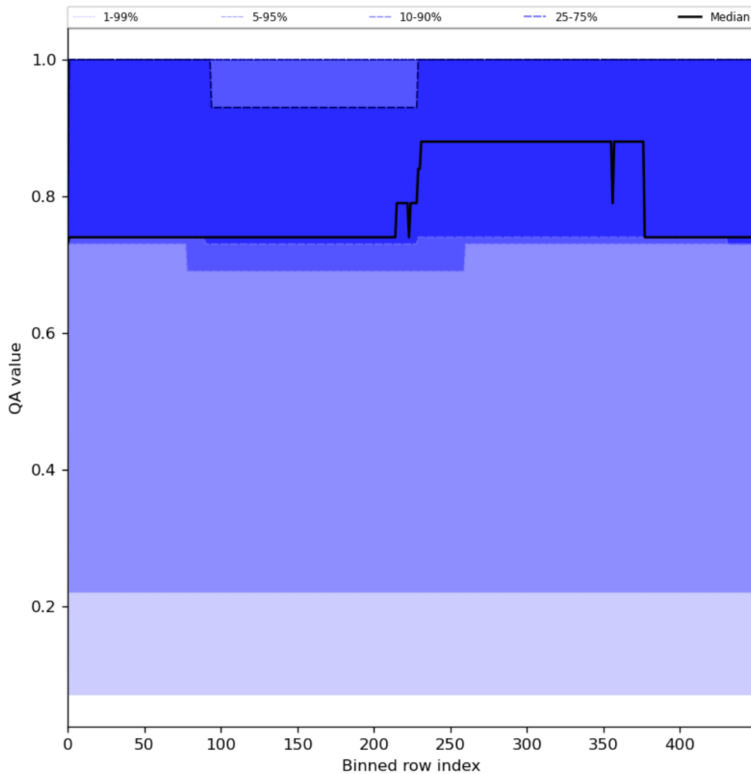
Figure 45: Along track statistics of “QA value” for 2024-05-16 to 2024-05-18
