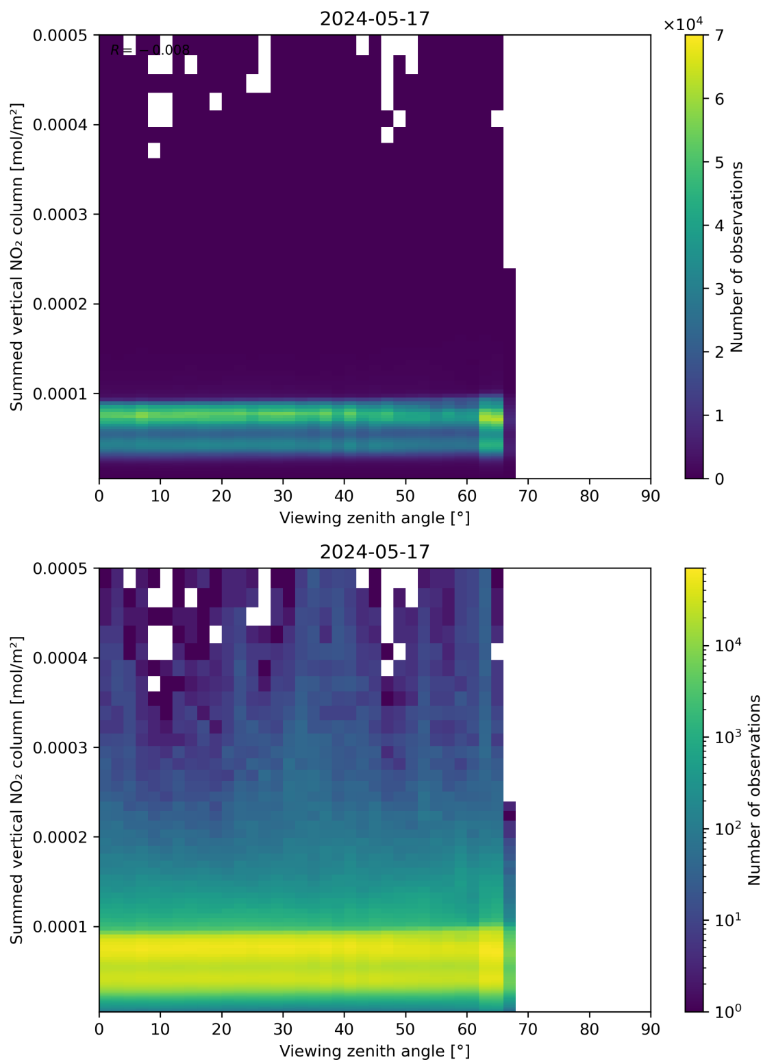
Figure 165: Scatter density plot of “Viewing zenith angle” against “Summed vertical NO 2 column” for 2024-05-16 to 2024-05-18.
