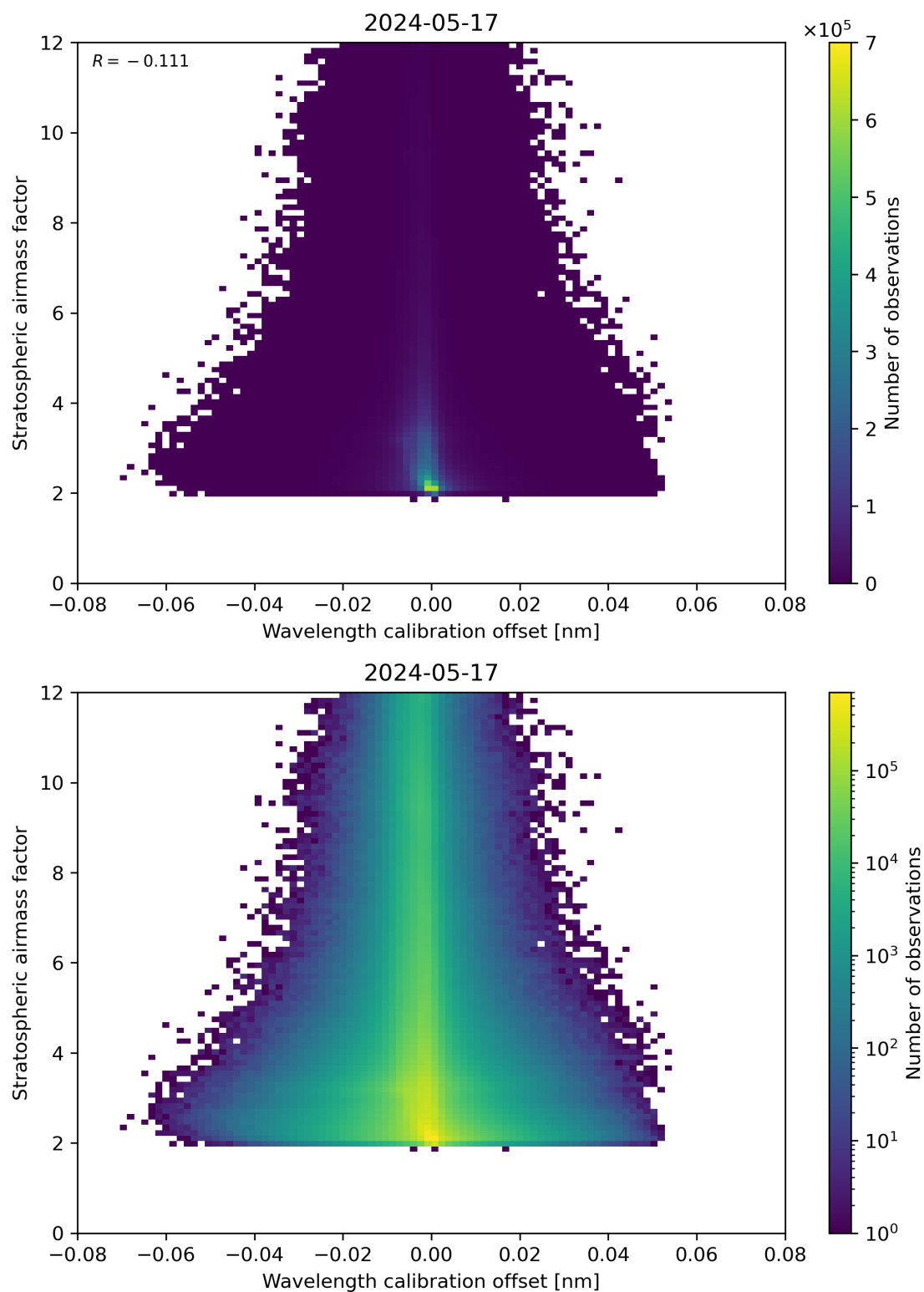
Figure 174: Scatter density plot of “Wavelength calibration offset” against “Stratospheric airmass factor” for 2024-05-16 to 2024-05-18.
