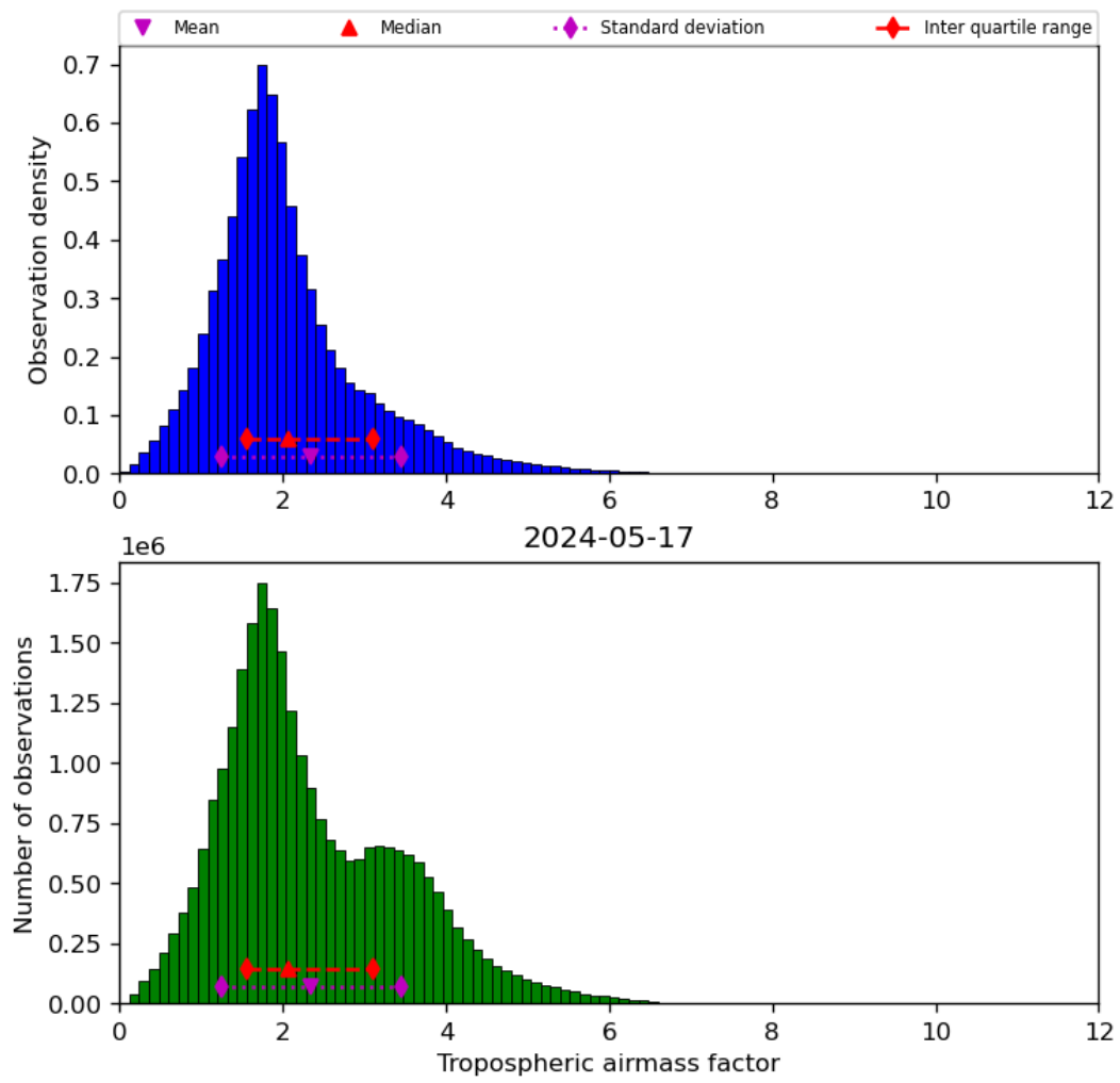
Figure 31: Histogram of “Tropospheric airmass factor” for 2024-05-16 to 2024-05-18
