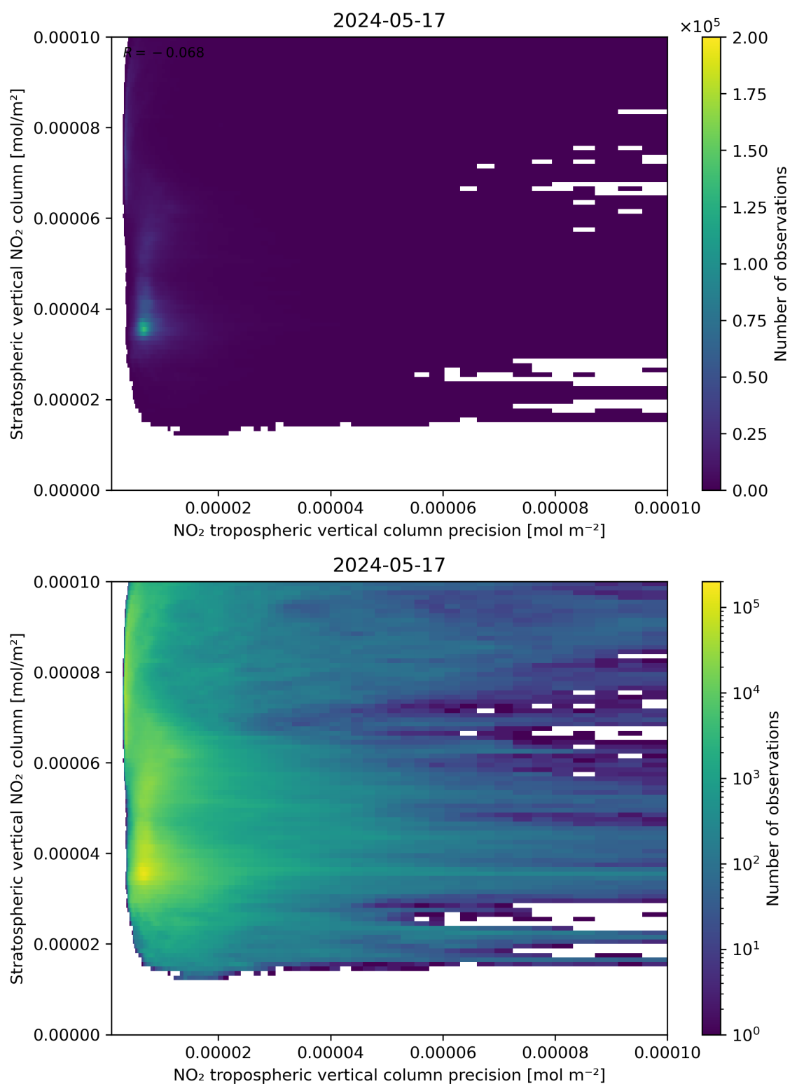
Figure 135: Scatter density plot of “NO 2 tropospheric vertical column precision” against “Stratospheric vertical NO 2 column” for 2024-05-16 to 2024-05-18.
