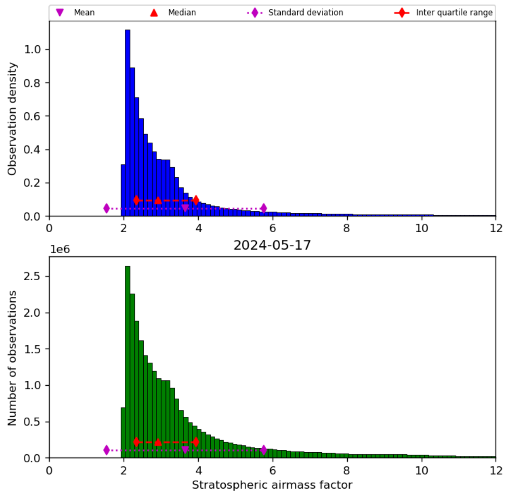
Figure 44: Histogram of “Stratospheric airmass factor” for 2024-05-16 to 2024-05-18
