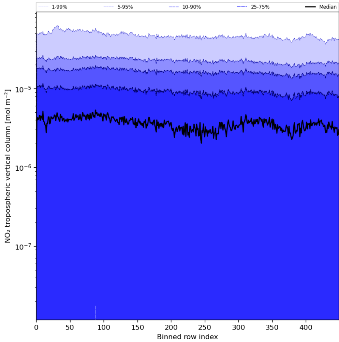
Figure 46: Along track statistics of “NO 2 tropospheric vertical column” for 2024-05-16 to 2024-05-18
