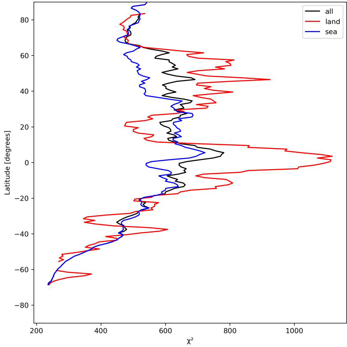
Figure 25: Zonal average of “ \chi^2 ” for 2024-05-16 to 2024-05-18.
