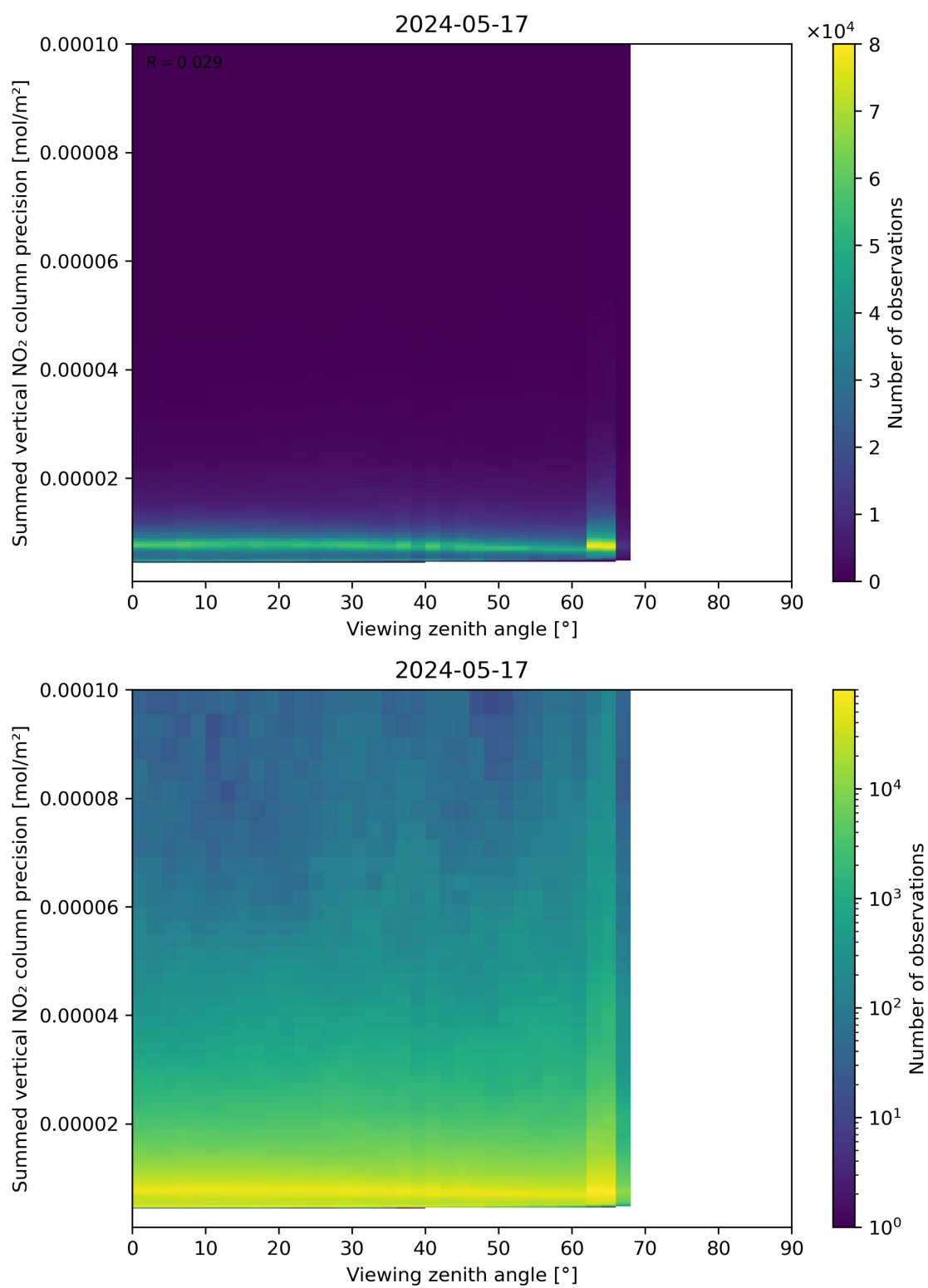
Figure 166: Scatter density plot of “Viewing zenith angle” against “Summed vertical NO 2 column precision” for 2024-05-16 to 2024-05-18.
