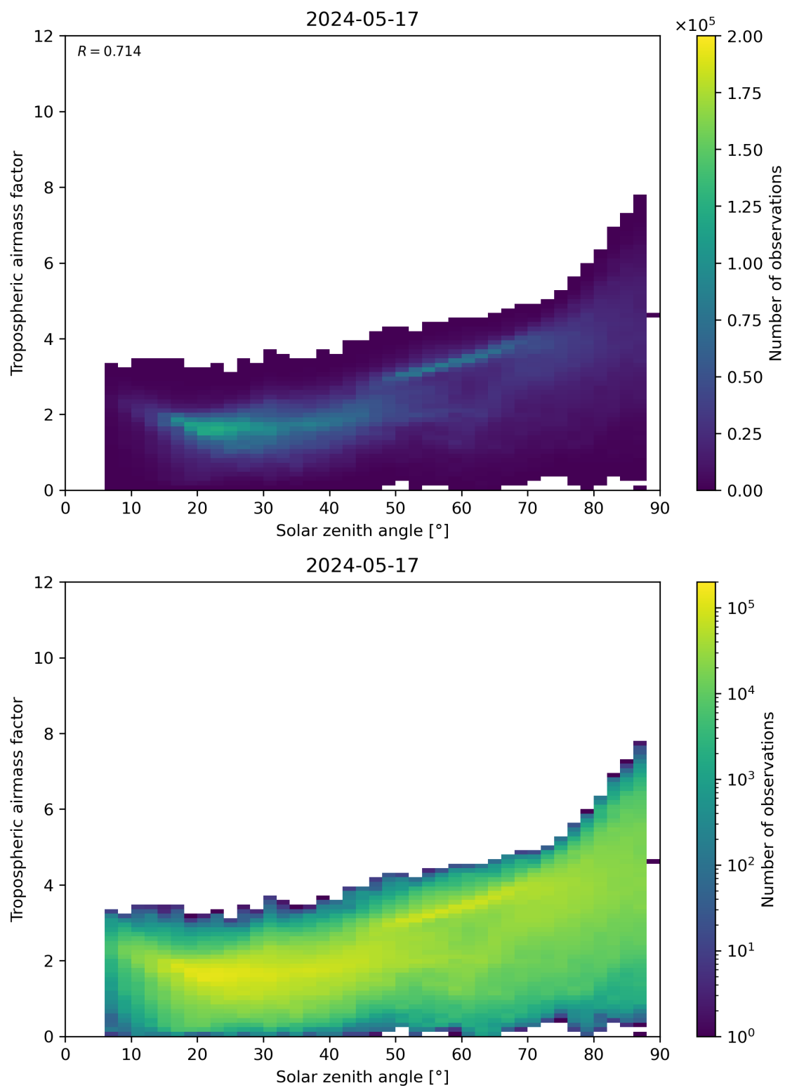
Figure 147: Scatter density plot of “Solar zenith angle” against “Tropospheric airmass factor” for 2024-05-16 to 2024-05-18.
