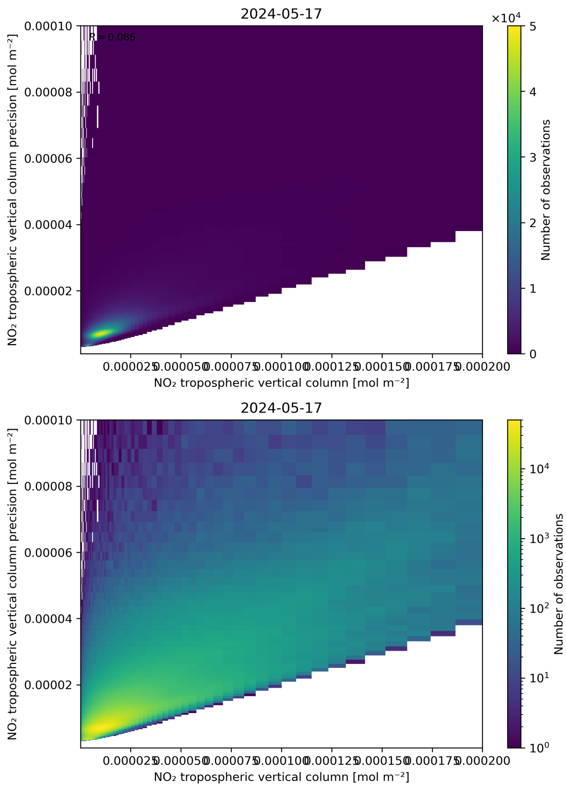
Figure 130: Scatter density plot of “NO 2 tropospheric vertical column” against “NO 2 tropospheric vertical column precision” for 2024-05-16 to 2024-05-18.
