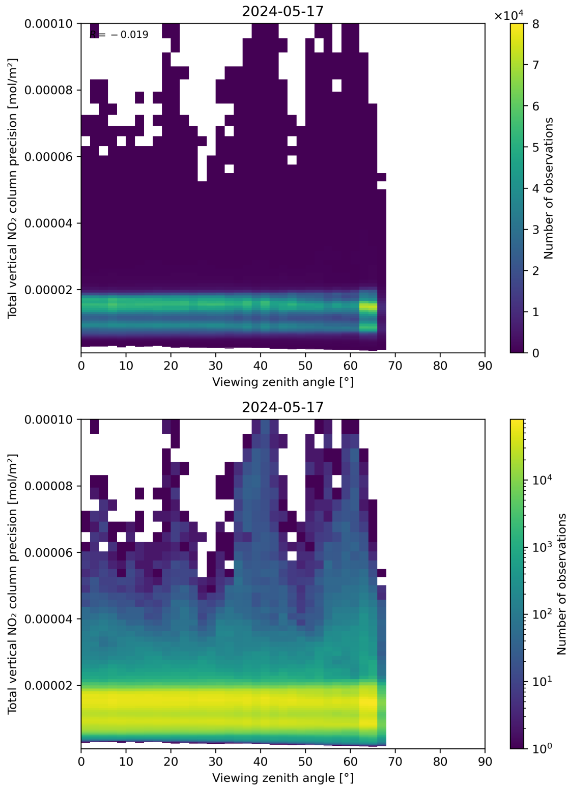
Figure 168: Scatter density plot of “Viewing zenith angle” against “Total vertical NO 2 column precision” for 2024-05-16 to 2024-05-18.
