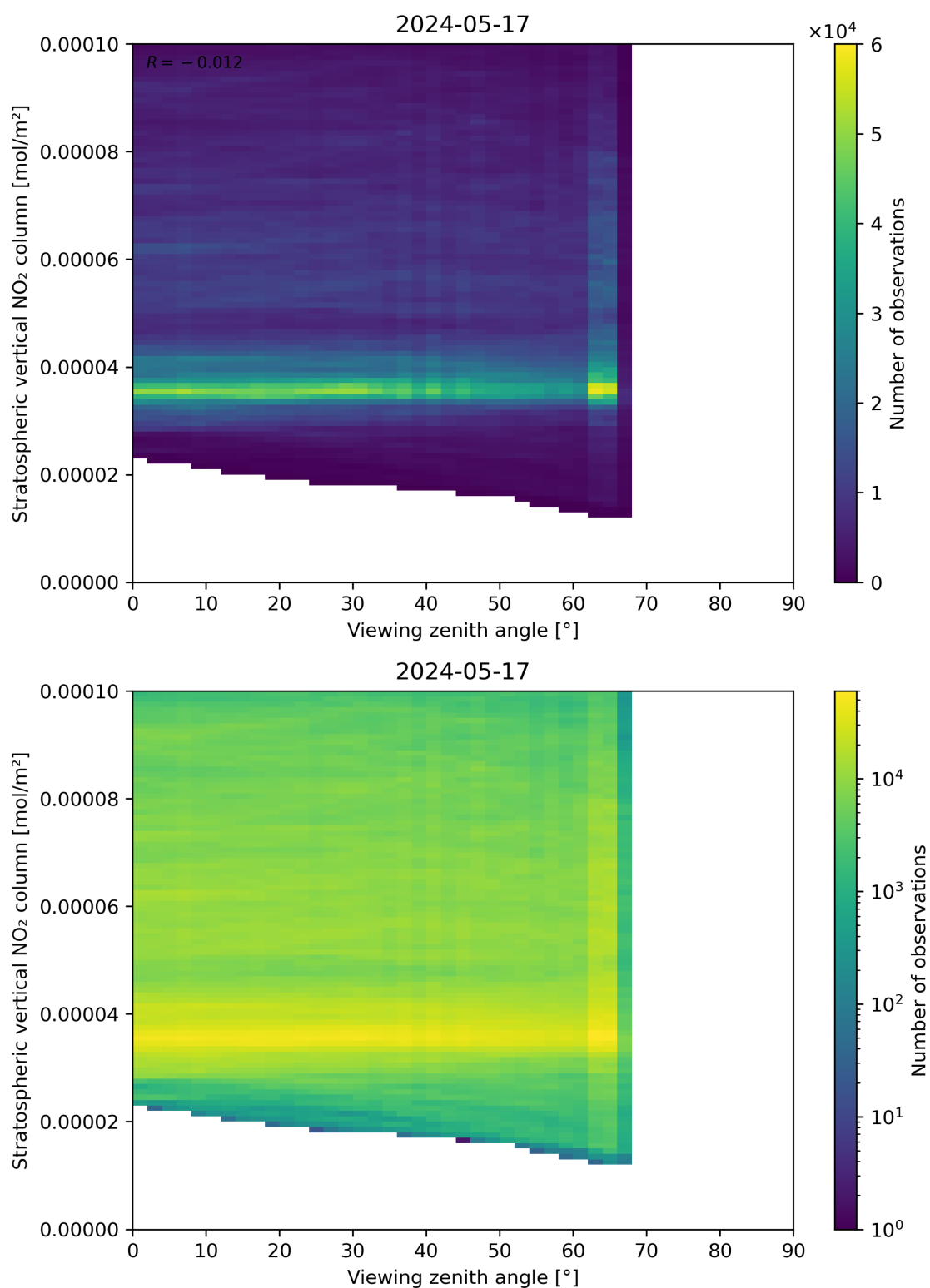
Figure 164: Scatter density plot of “Viewing zenith angle” against “Stratospheric vertical NO 2 column” for 2024-05-16 to 2024-05-18.
