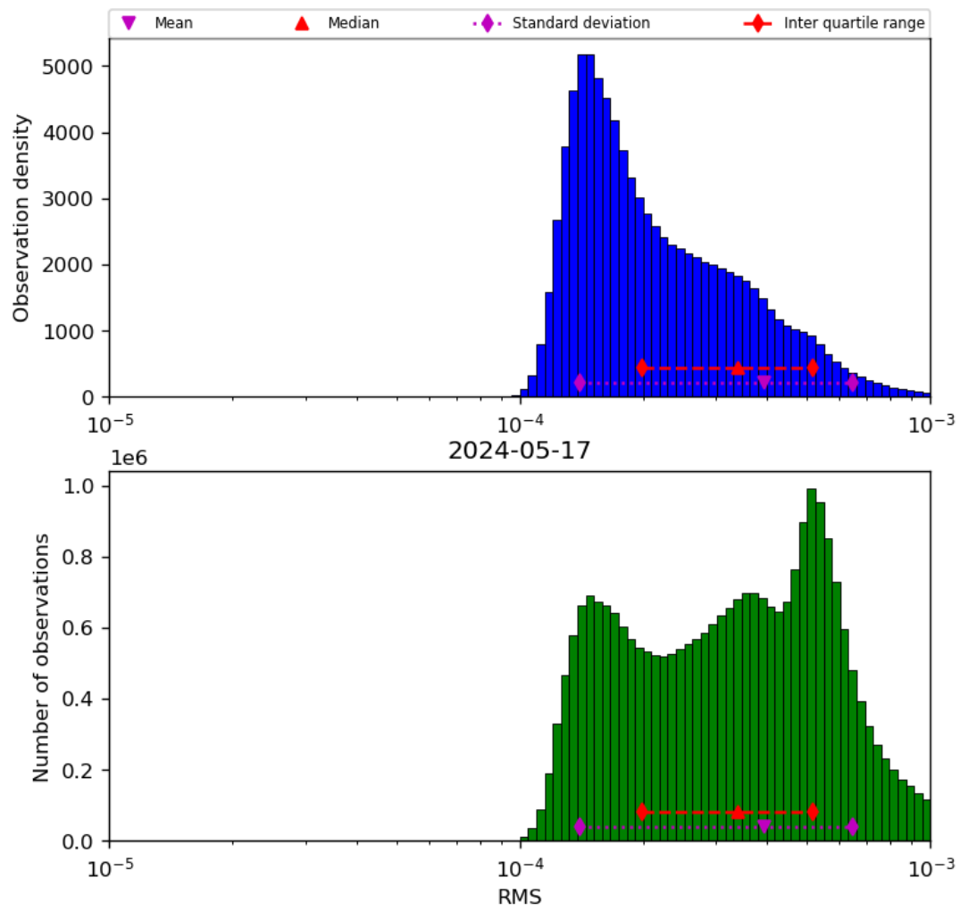
Figure 43: Histogram of “RMS” for 2024-05-16 to 2024-05-18
