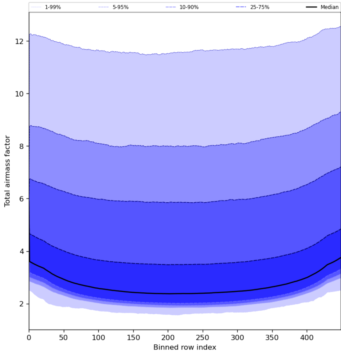
Figure 49: Along track statistics of “Total airmass factor” for 2024-05-16 to 2024-05-18
