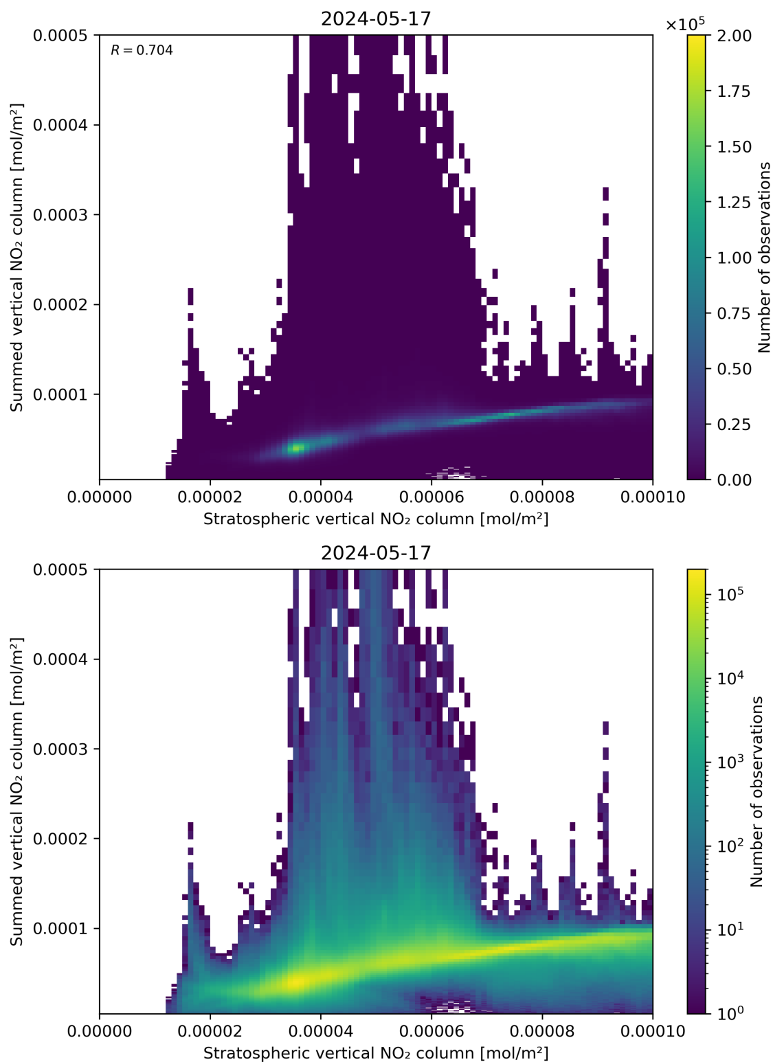
Figure 98: Scatter density plot of “Stratospheric vertical NO 2 column” against “Summed vertical NO 2 column” for 2024-05-16 to 2024-05-18.
