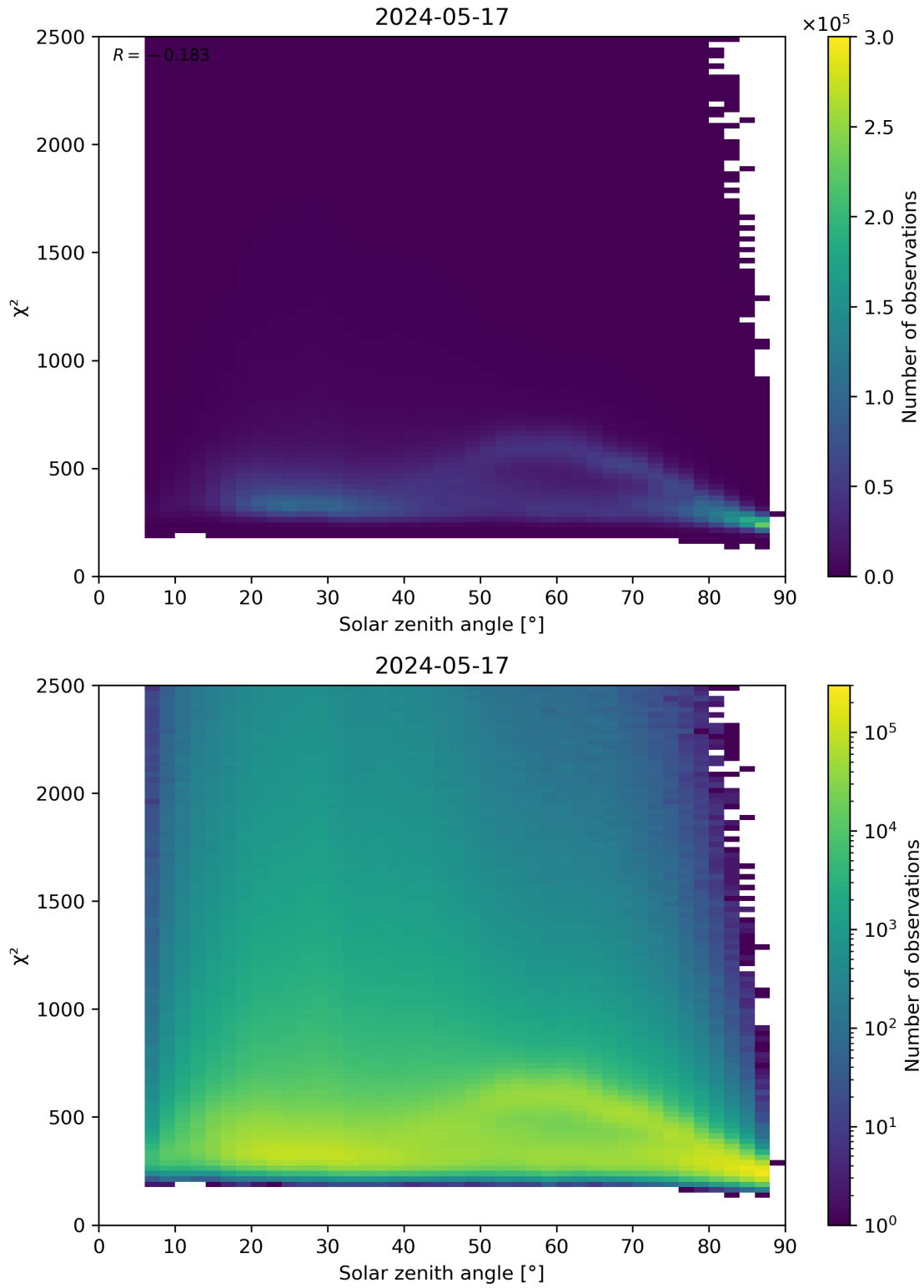
Figure 148: Scatter density plot of “Solar zenith angle” against “ \chi^2 ” for 2024-05-16 to 2024-05-18.
