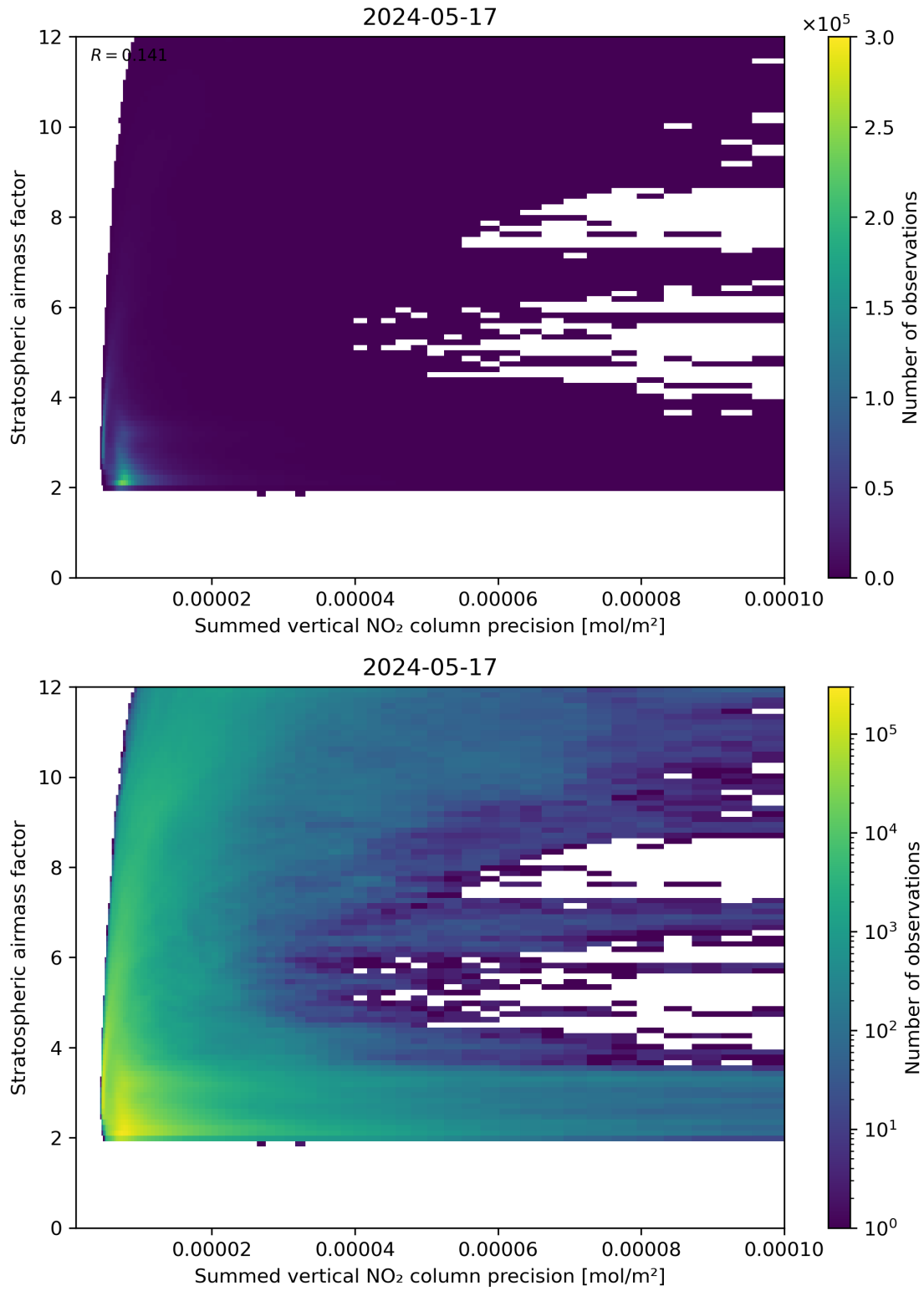
Figure 106: Scatter density plot of “Summed vertical NO 2 column precision” against “Stratospheric airmass factor” for 2024-05-16 to 2024-05-18.
