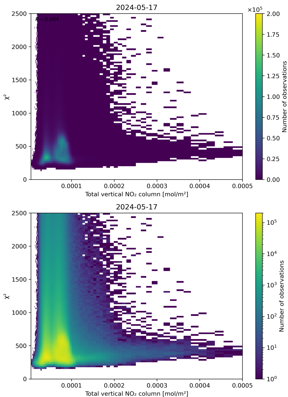
Figure 111: Scatter density plot of “Total vertical NO 2 column” against “ \chi^2 ” for 2024-05-16 to 2024-05-18.
