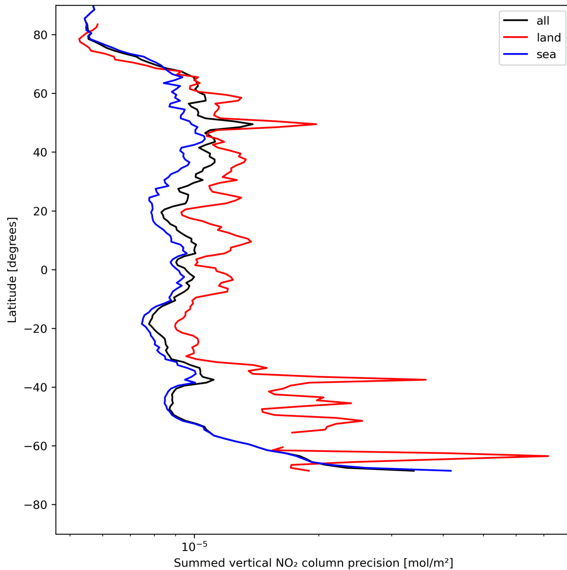
Figure 24: Zonal average of “Summed vertical NO 2 column precision” for 2024-05-16 to 2024-05-18.
