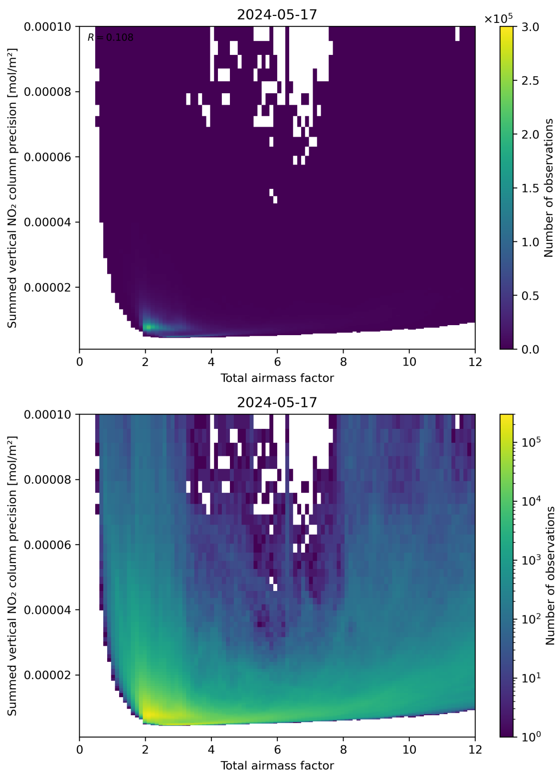
Figure 66: Scatter density plot of “Total airmass factor” against “Summed vertical NO 2 column precision” for 2024-05-16 to 2024-05-18.
