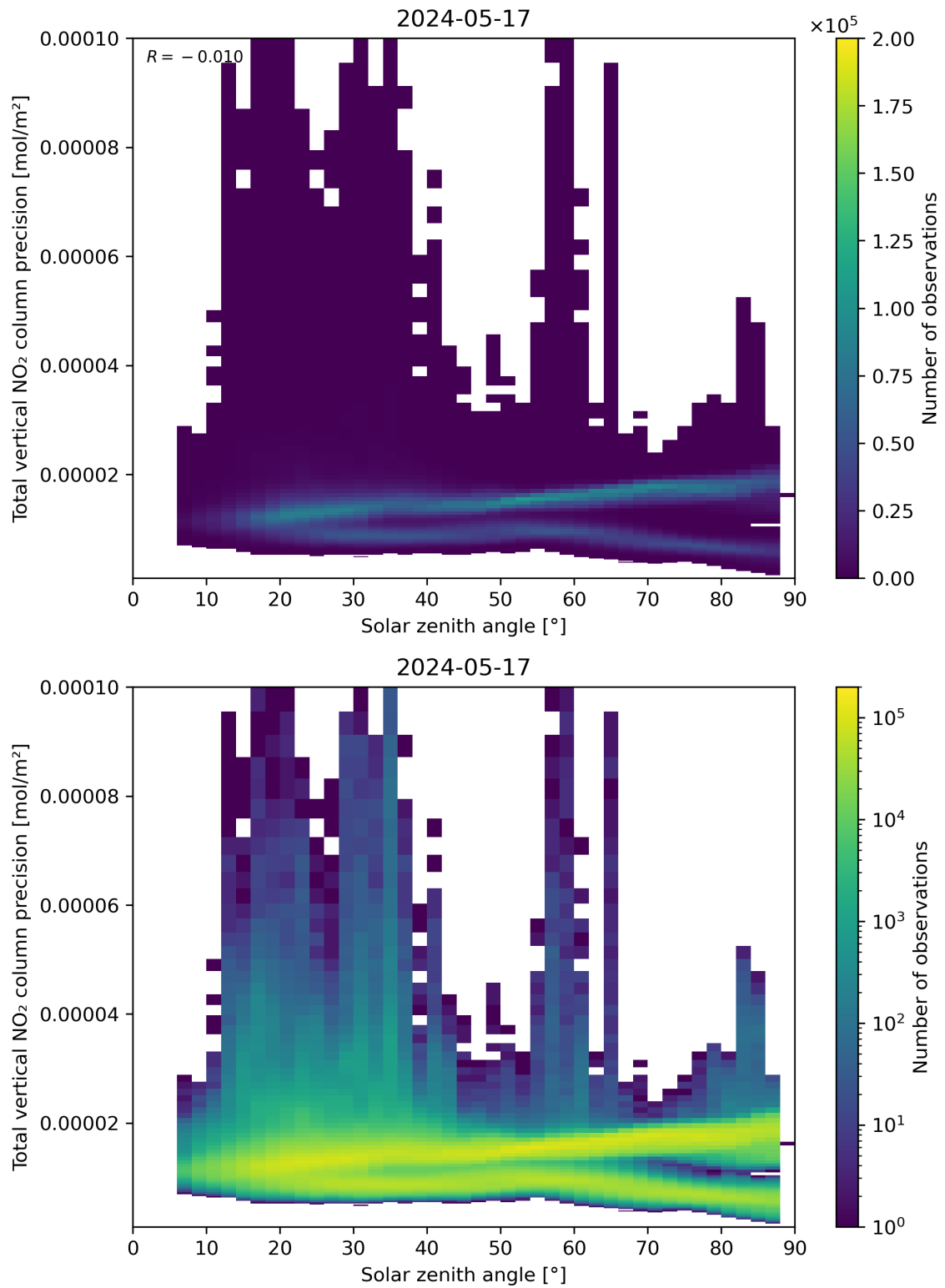
Figure 154: Scatter density plot of “Solar zenith angle” against “Total vertical NO 2 column precision” for 2024-05-16 to 2024-05-18.
