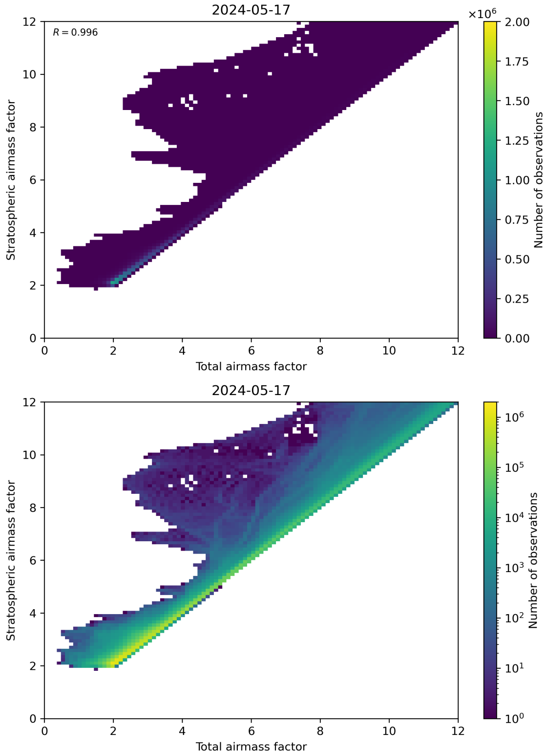
Figure 62: Scatter density plot of “Total airmass factor” against “Stratospheric airmass factor” for 2024-05-16 to 2024-05-18.
