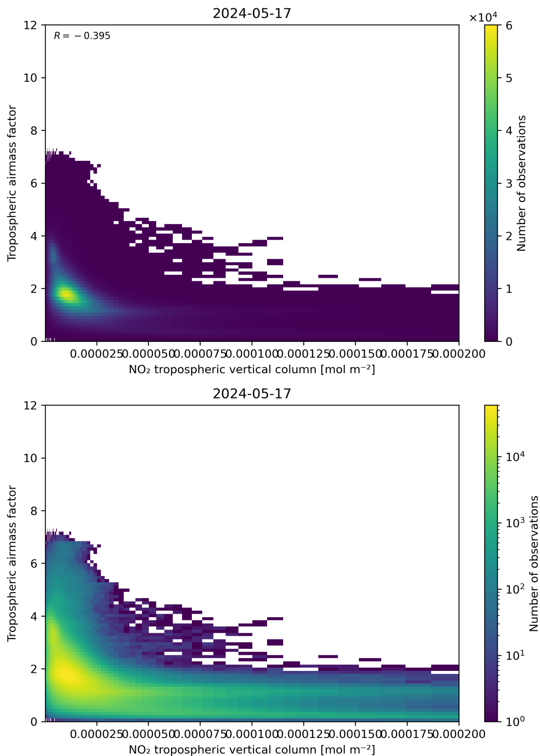
Figure 123: Scatter density plot of “NO 2 tropospheric vertical column” against “Tropospheric air mass factor” for 2024-05-16 to 2024-05-18.
