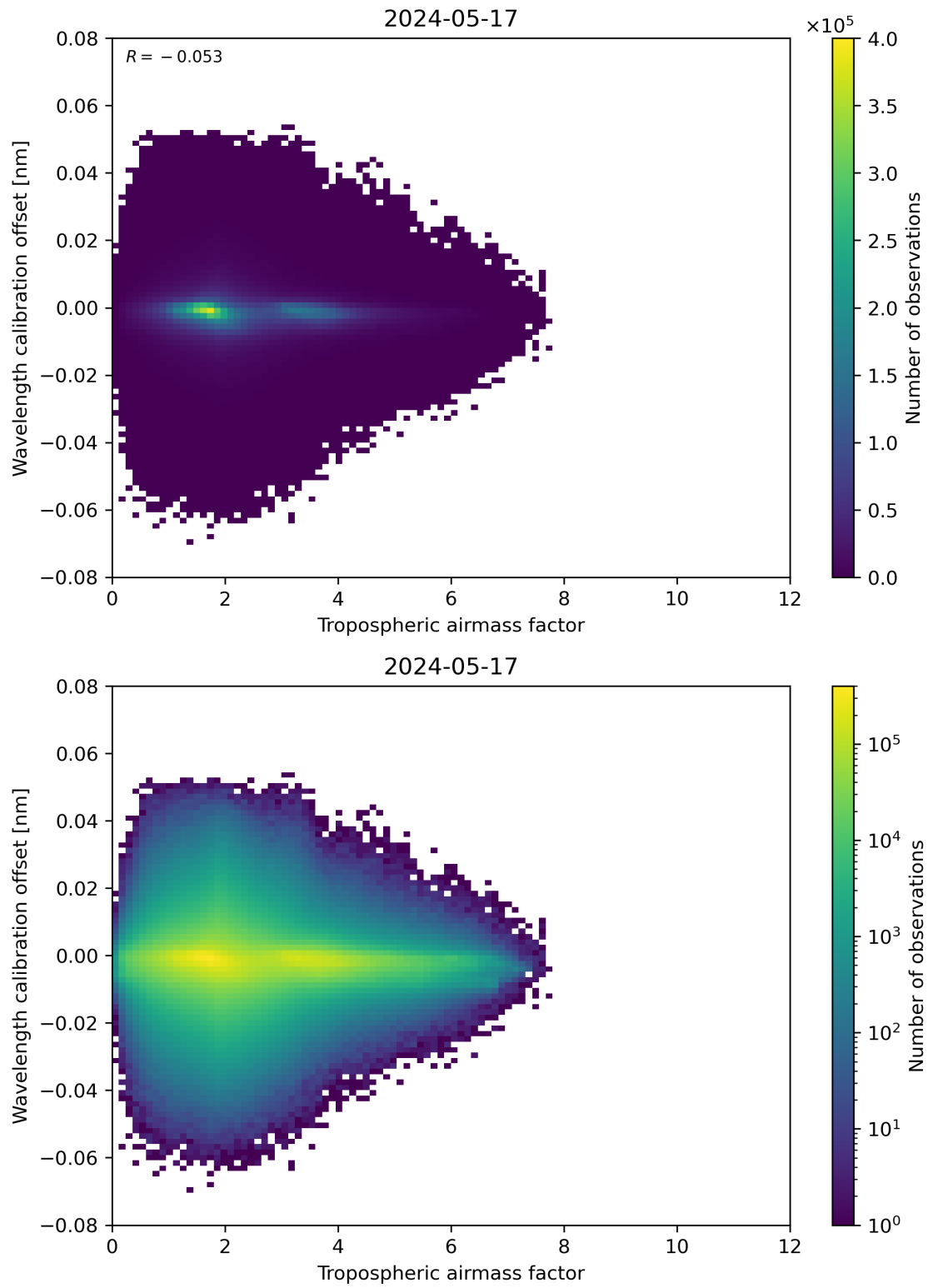
Figure 80: Scatter density plot of “Tropospheric airmass factor” against “Wavelength calibration offset” for 2024-05-16 to 2024-05-18.
