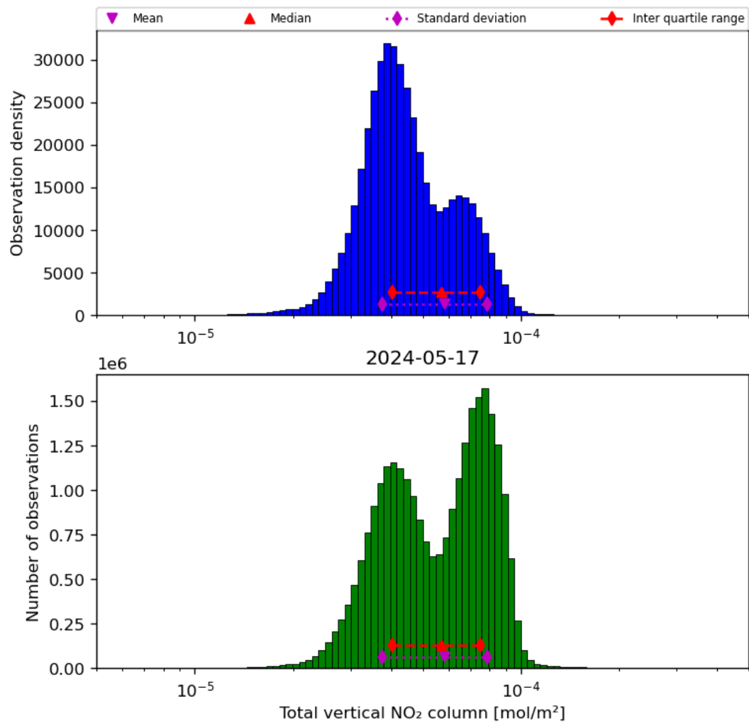
Figure 38: Histogram of “Total vertical NO 2 column” for 2024-05-16 to 2024-05-18
