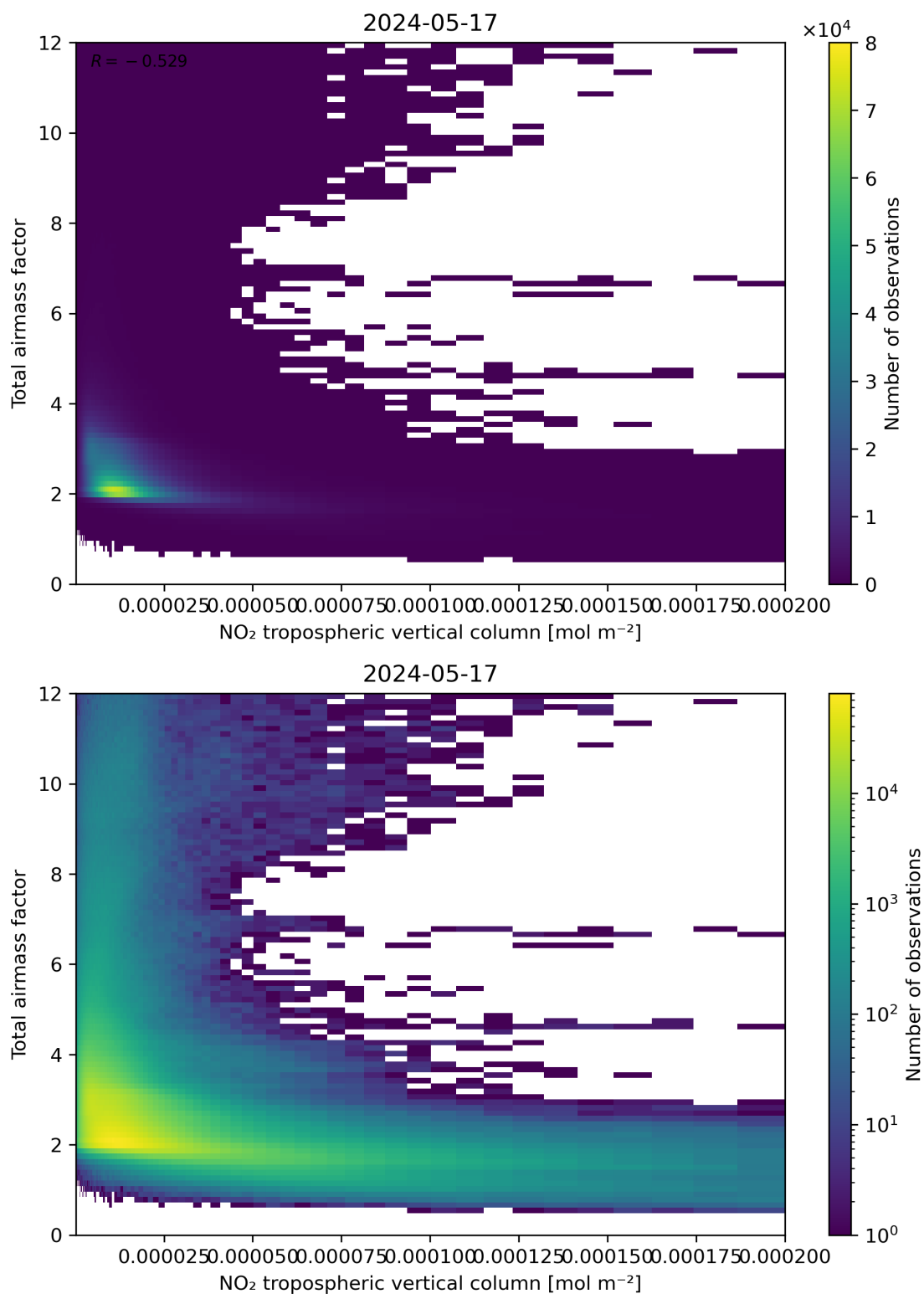
Figure 122: Scatter density plot of “NO 2 tropospheric vertical column” against “Total air mass factor” for 2024-05-16 to 2024-05-18.
