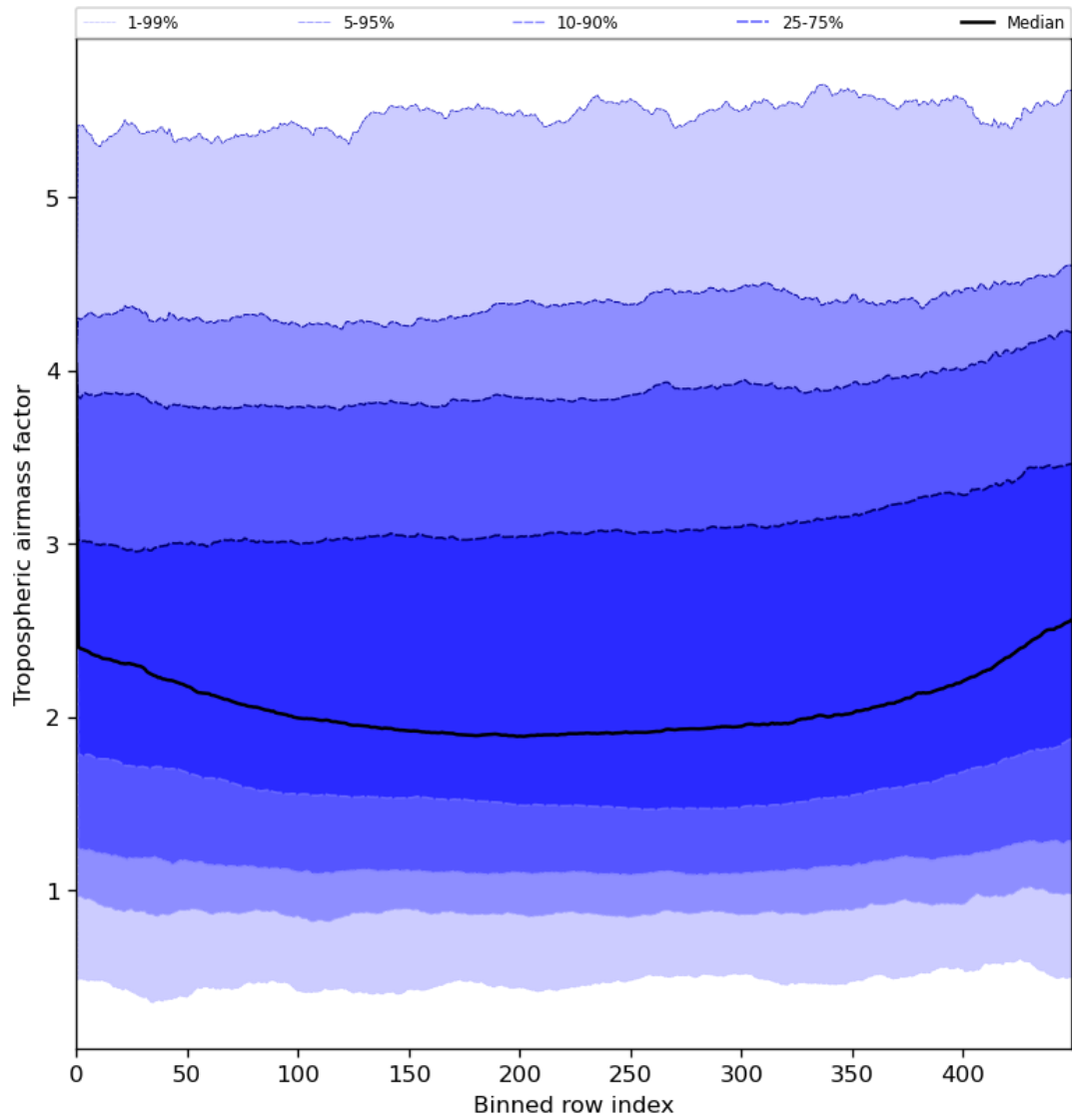
Figure 48: Along track statistics of “Tropospheric airmass factor” for 2024-05-16 to 2024-05-18
