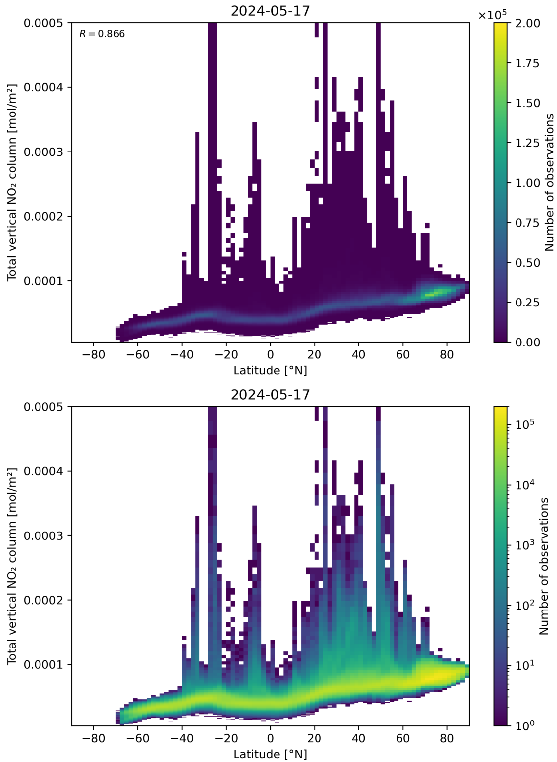
Figure 90: Scatter density plot of “Latitude” against “Total vertical NO 2 column” for 2024-05-16 to 2024-05-18.
