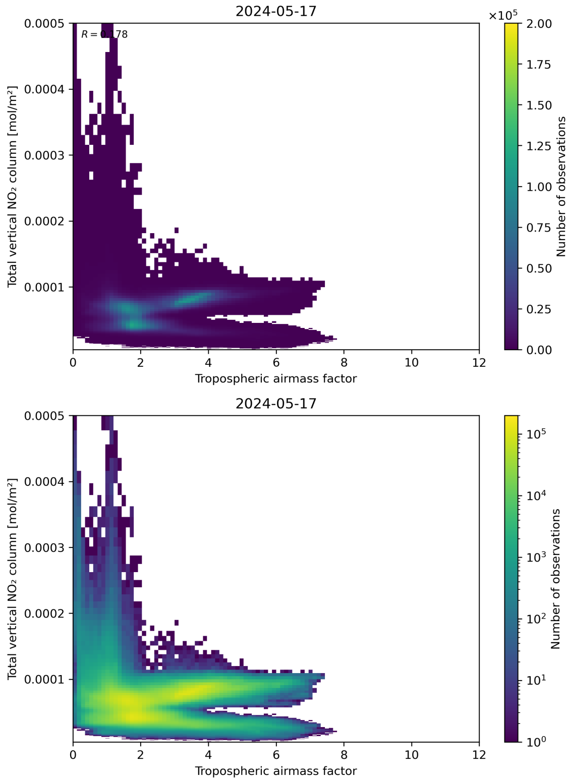
Figure 77: Scatter density plot of “Tropospheric airmass factor” against “Total vertical NO 2 column” for 2024-05-16 to 2024-05-18.
