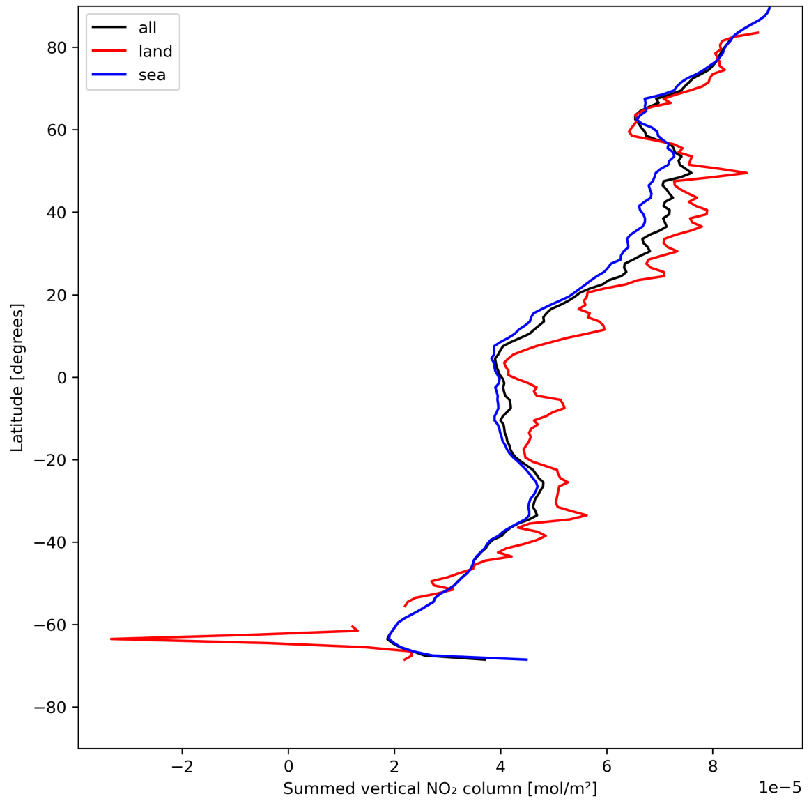
Figure 23: Zonal average of “Summed vertical NO 2 column” for 2024-05-16 to 2024-05-18.
