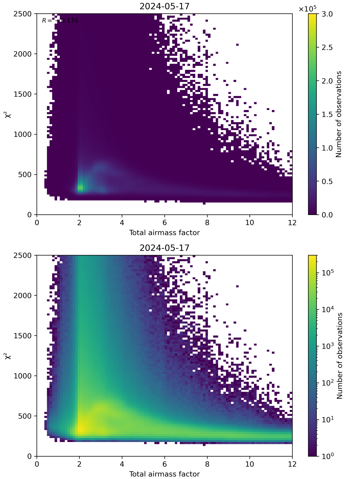
Figure 63: Scatter density plot of “Total airmass factor” against “ \chi^2 ” for 2024-05-16 to 2024-05-18.
