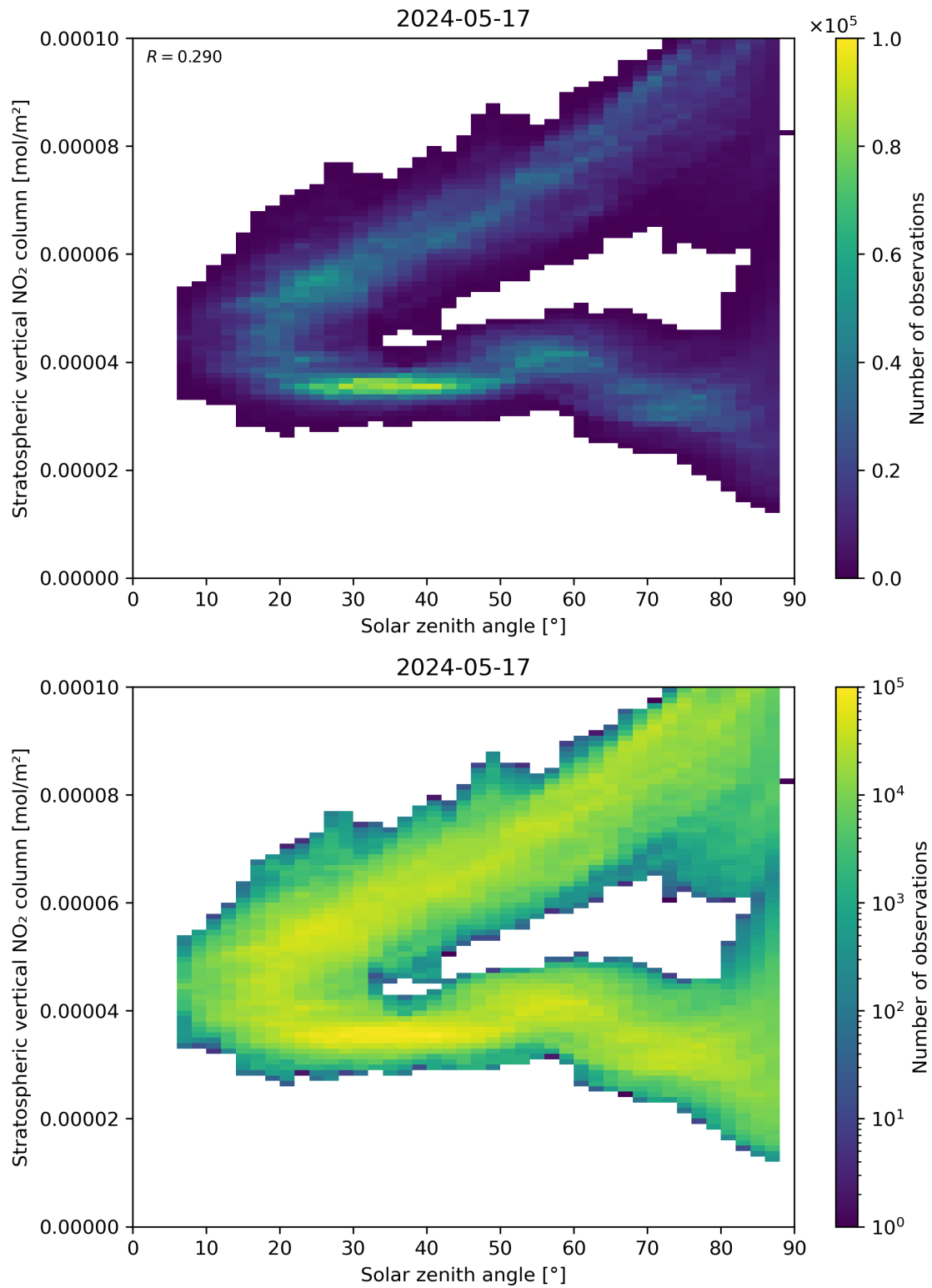
Figure 150: Scatter density plot of “Solar zenith angle” against “Stratospheric vertical \text{NO}_2 column” for 2024-05-16 to 2024-05-18.
