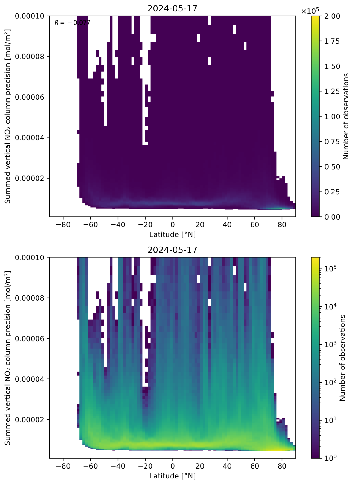
Figure 89: Scatter density plot of “Latitude” against “Summed vertical NO 2 column precision” for 2024-05-16 to 2024-05-18.
