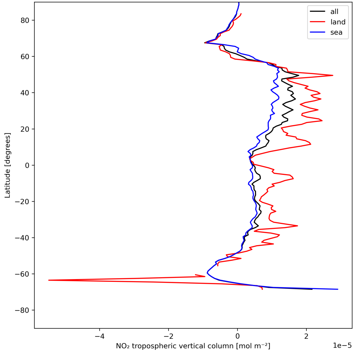
Figure 12: Zonal average of “NO 2 tropospheric vertical column” for 2024-05-16 to 2024-05-18.
