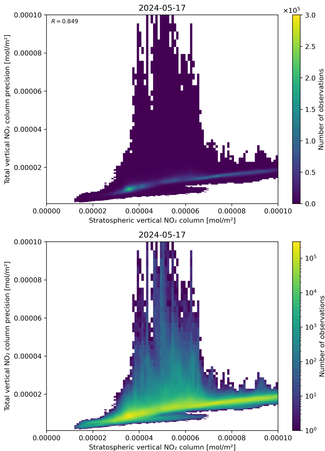
Figure 101: Scatter density plot of “Stratospheric vertical NO 2 column” against “Total vertical NO 2 column precision” for 2024-05-16 to 2024-05-18.
