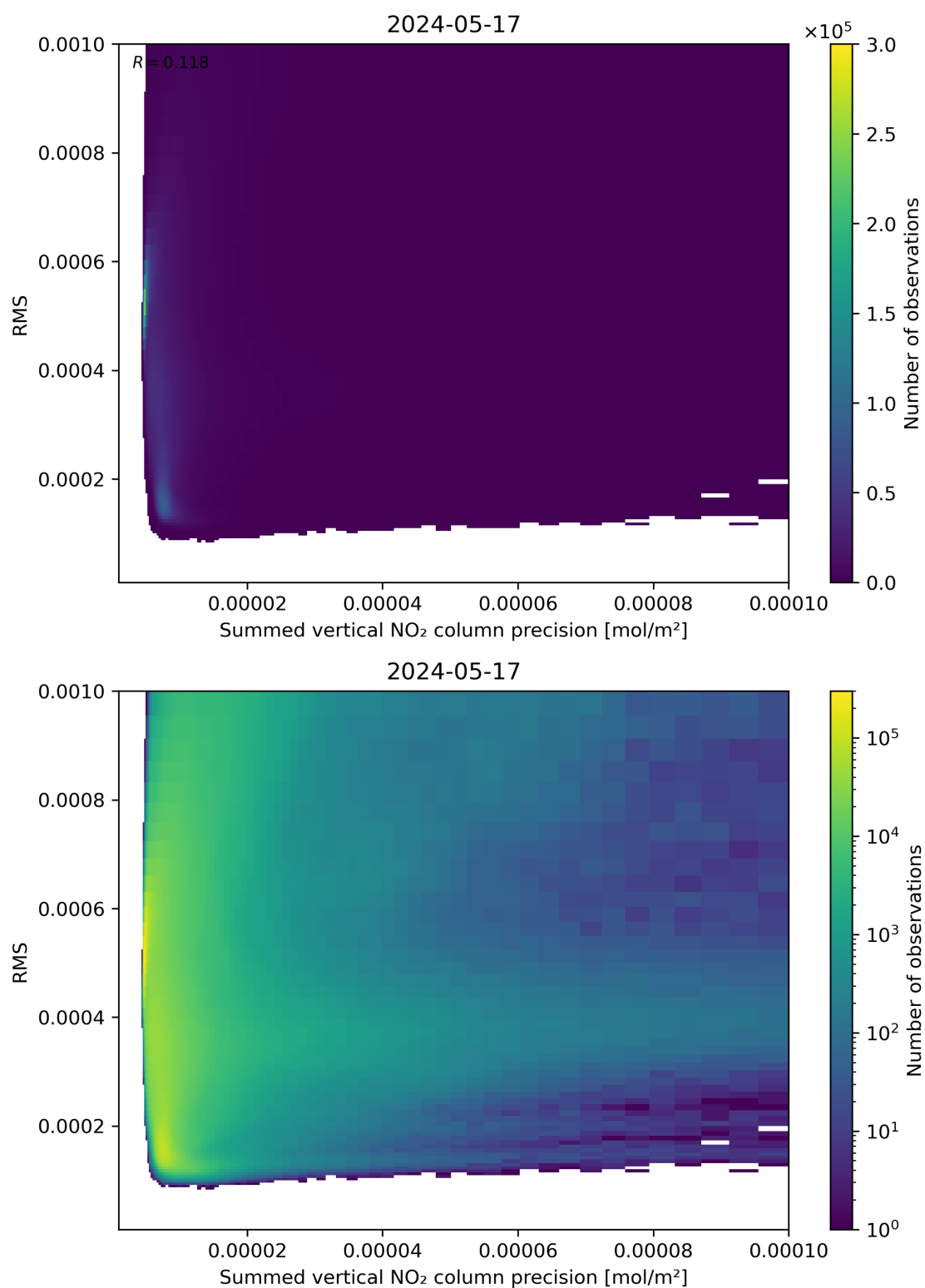
Figure 108: Scatter density plot of “Summed vertical NO 2 column precision” against “RMS” for 2024-05-16 to 2024-05-18.
