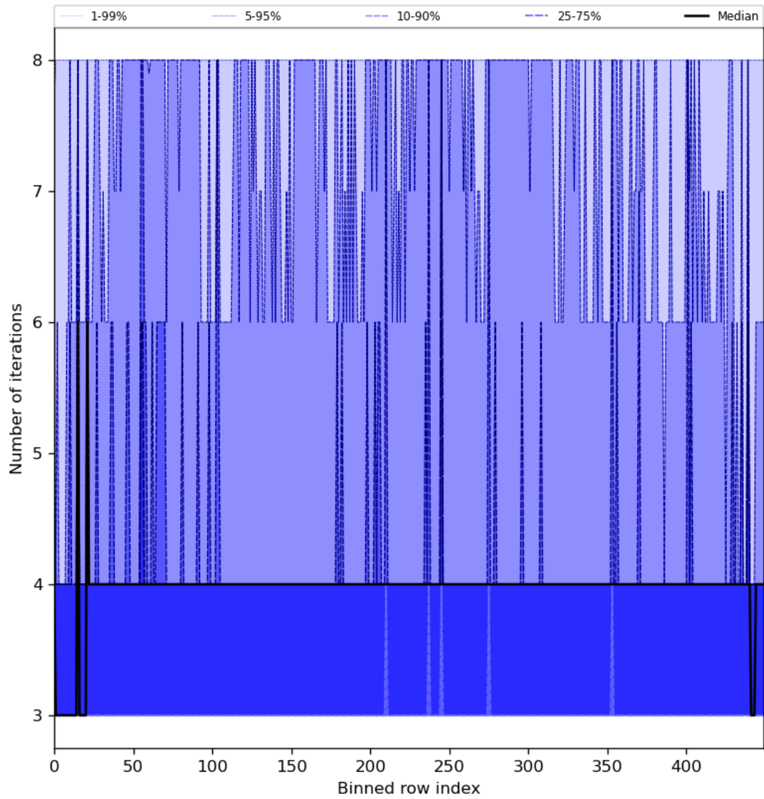
Figure 51: Along track statistics of “Number of iterations” for 2024-05-16 to 2024-05-18
