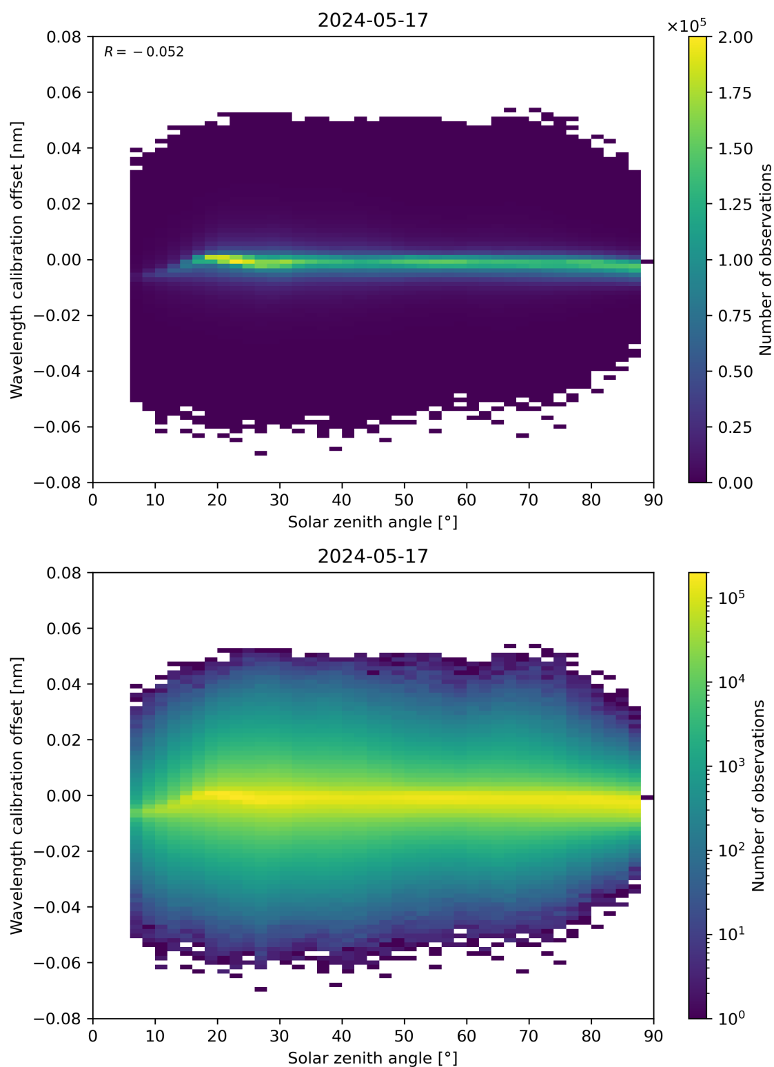
Figure 158: Scatter density plot of “Solar zenith angle” against “Wavelength calibration offset” for 2024-05-16 to 2024-05-18.
