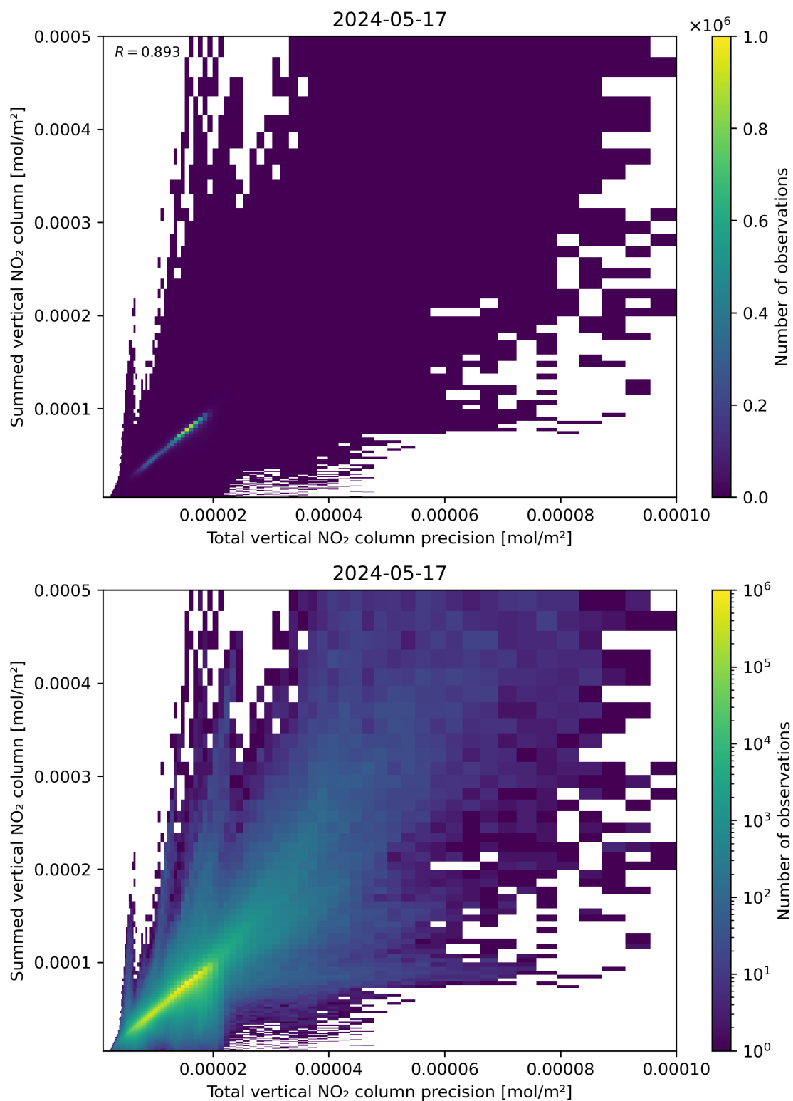
Figure 117: Scatter density plot of “Total vertical NO 2 column precision” against “Summed vertical NO 2 column” for 2024-05-16 to 2024-05-18.
