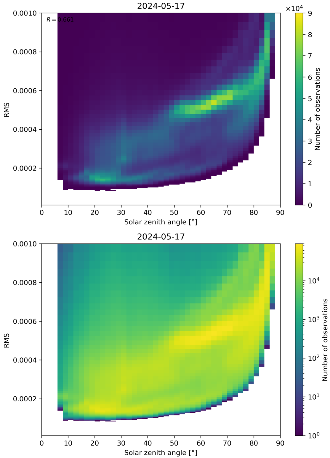
Figure 157: Scatter density plot of “Solar zenith angle” against “RMS” for 2024-05-16 to 2024-05-18.
