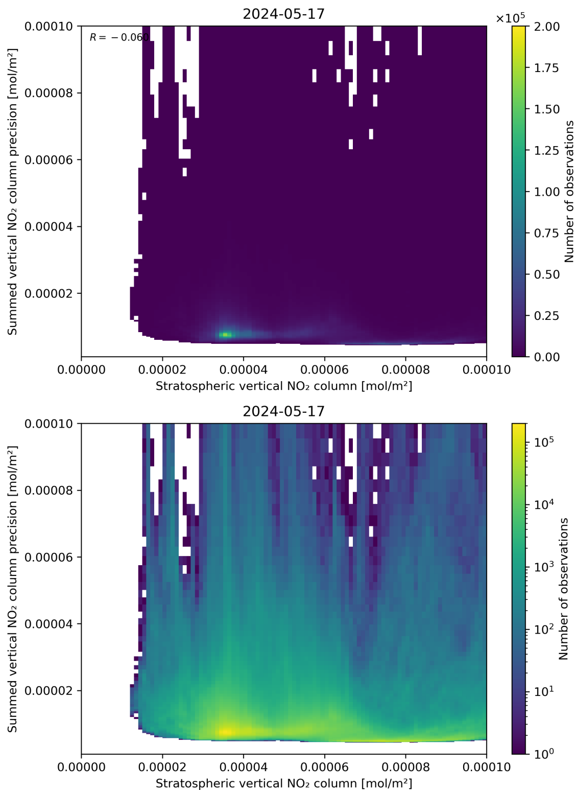
Figure 99: Scatter density plot of “Stratospheric vertical NO 2 column” against “Summed vertical NO 2 column precision” for 2024-05-16 to 2024-05-18.
