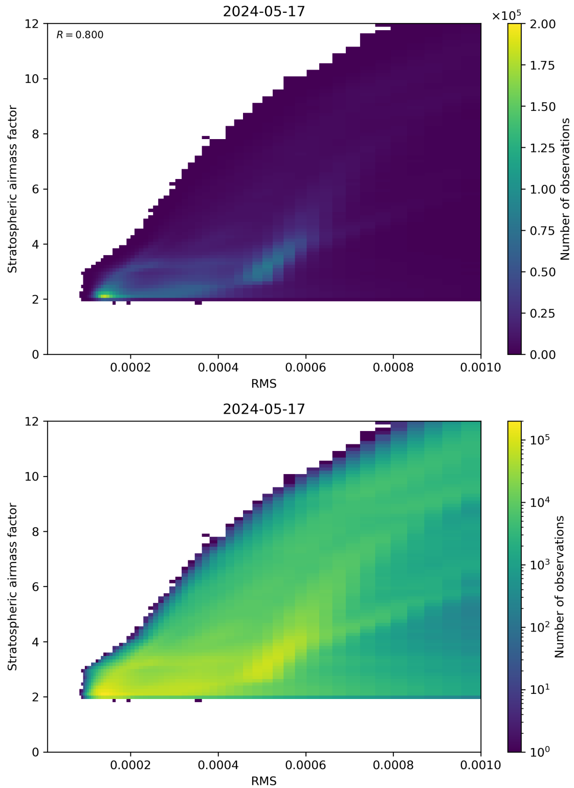
Figure 144: Scatter density plot of “RMS” against “Stratospheric airmass factor” for 2024-05-16 to 2024-05-18.
