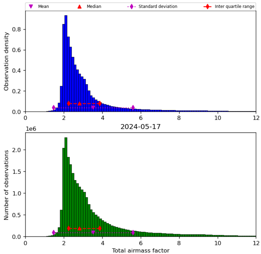
Figure 32: Histogram of “Total airmass factor” for 2024-05-16 to 2024-05-18
