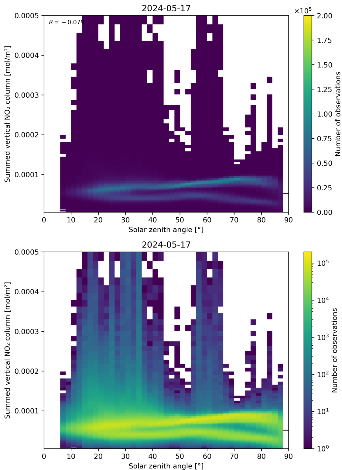
Figure 151: Scatter density plot of “Solar zenith angle” against “Summed vertical NO 2 column” for 2024-05-16 to 2024-05-18.
