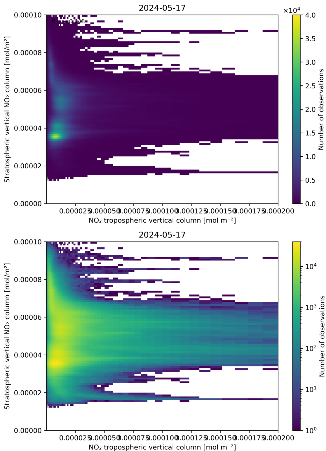
Figure 125: Scatter density plot of “NO 2 tropospheric vertical column” against “Stratospheric vertical NO 2 column” for 2024-05-16 to 2024-05-18.
