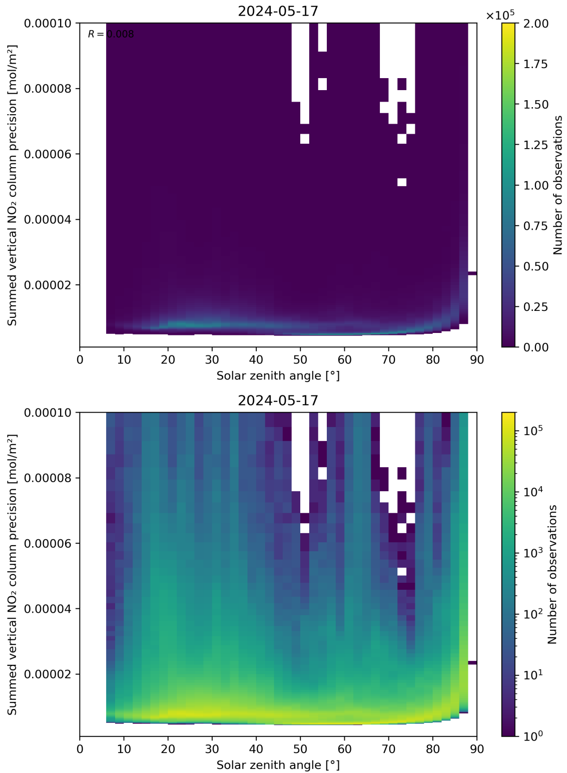
Figure 152: Scatter density plot of “Solar zenith angle” against “Summed vertical NO 2 column precision” for 2024-05-16 to 2024-05-18.
