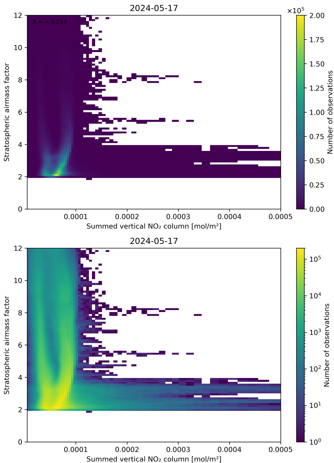
Figure 103: Scatter density plot of “Summed vertical NO 2 column” against “Stratospheric air mass factor” for 2024-05-16 to 2024-05-18.
