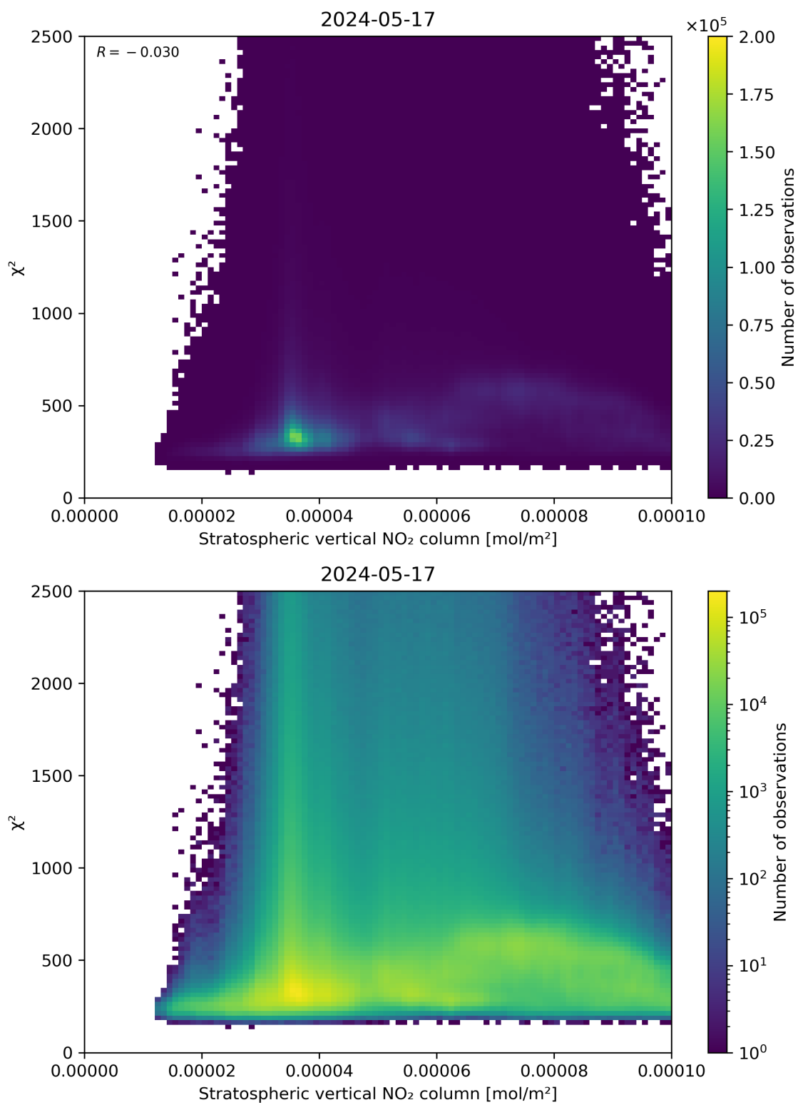
Figure 97: Scatter density plot of “Stratospheric vertical NO 2 column” against “ \chi^2 ” for 2024-05-16 to 2024-05-18.
