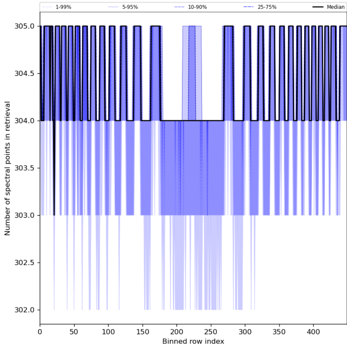
Figure 50: Along track statistics of “Number of spectral points in retrieval” for 2024-05-16 to 2024-05-18
