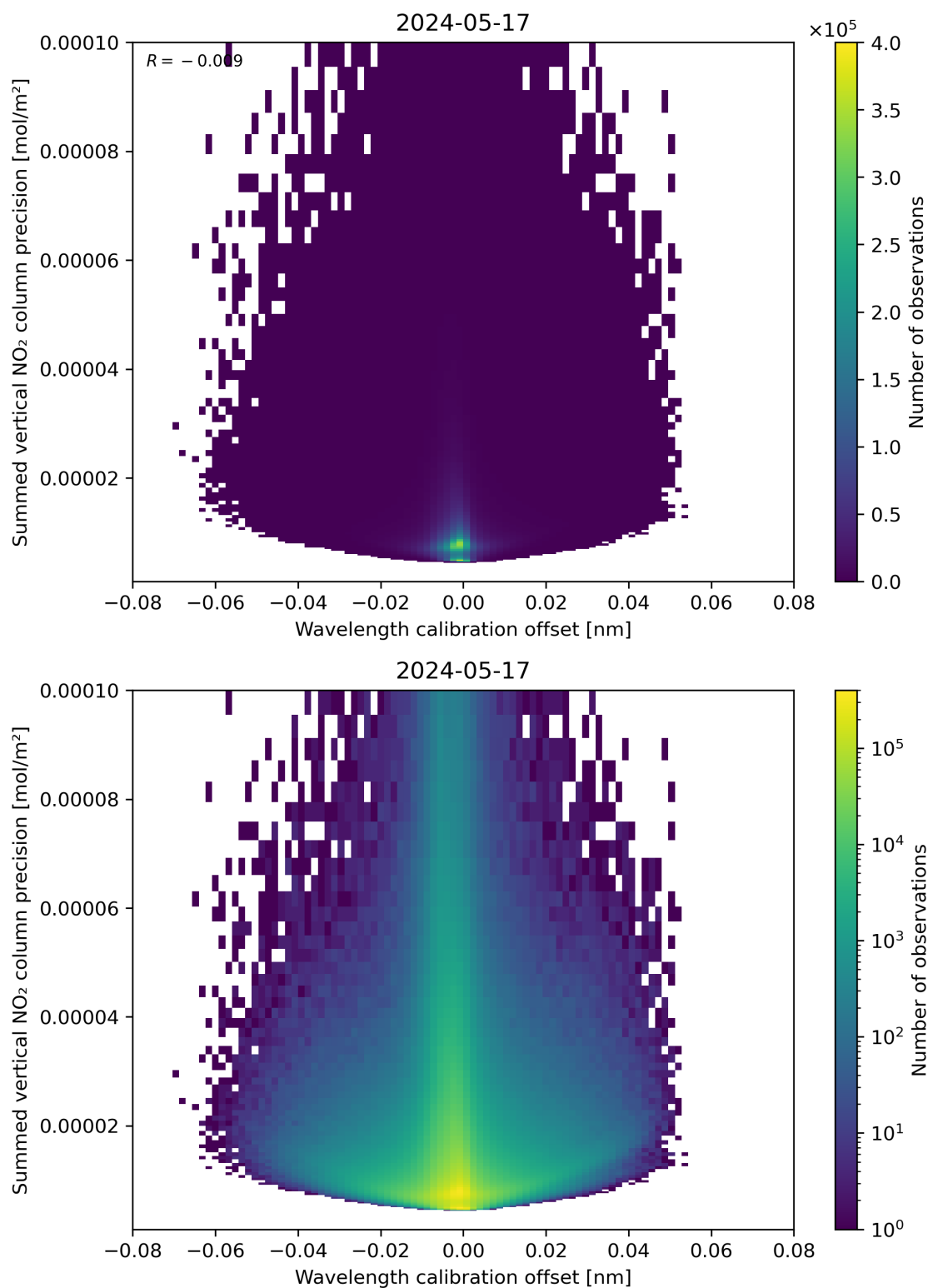
Figure 178: Scatter density plot of “Wavelength calibration offset” against “Summed vertical NO 2 column precision” for 2024-05-16 to 2024-05-18.
