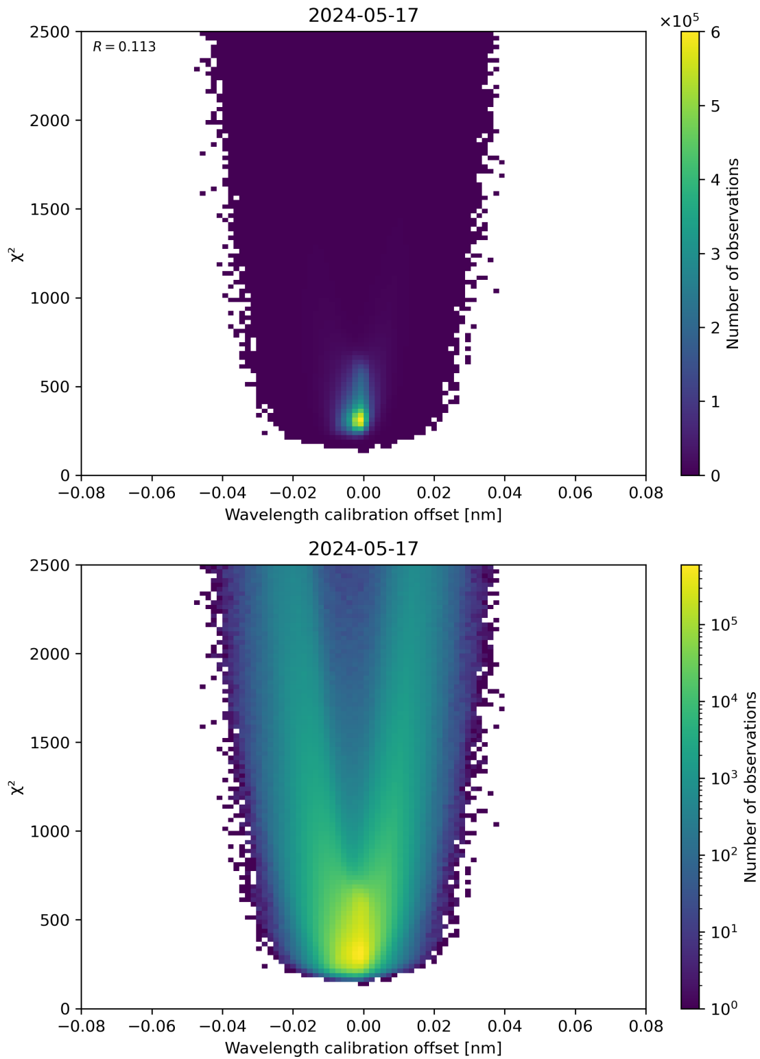
Figure 175: Scatter density plot of “Wavelength calibration offset” against “ \chi^2 ” for 2024-05-16 to 2024-05-18.
