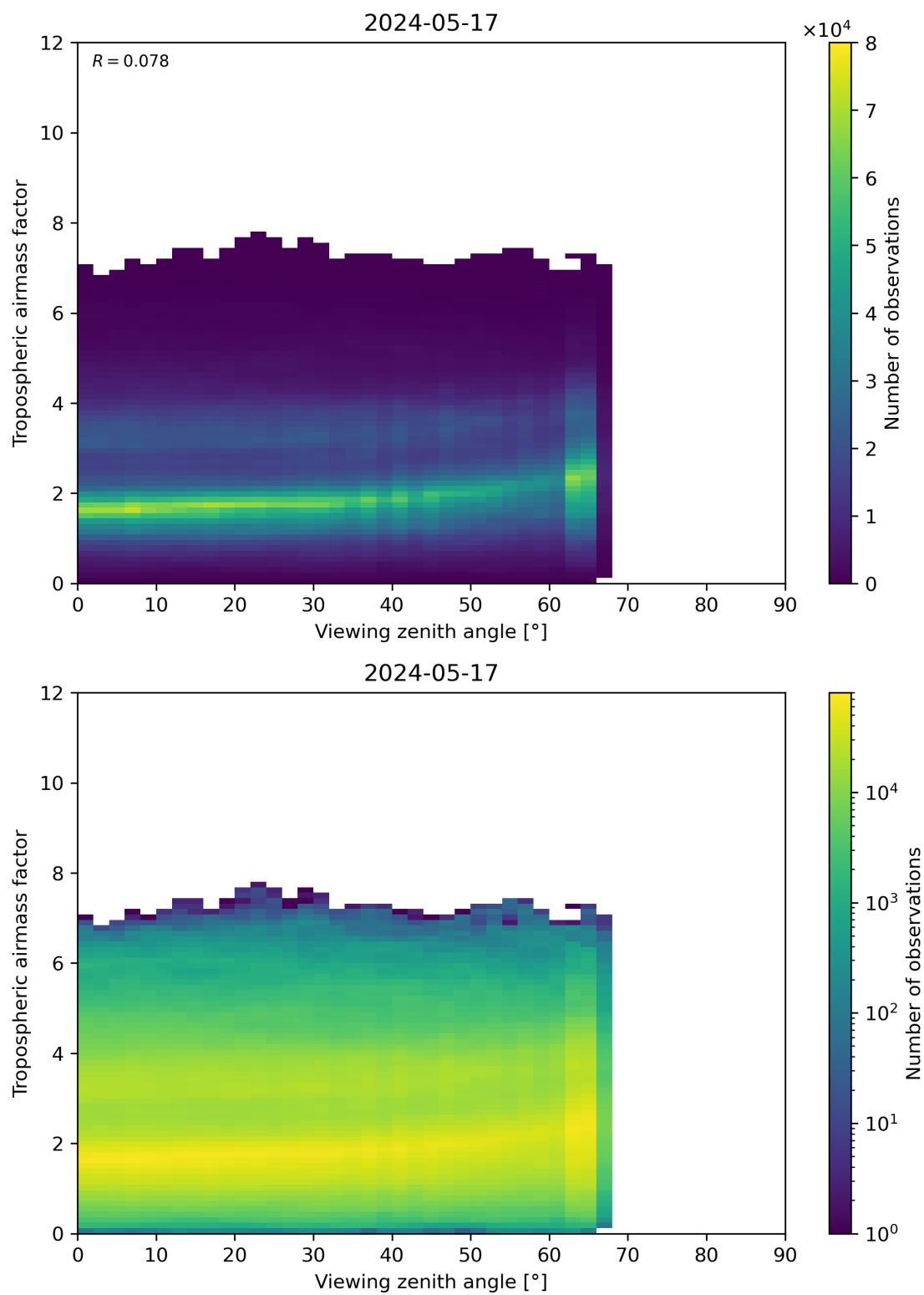
Figure 161: Scatter density plot of “Viewing zenith angle” against “Tropospheric airmass factor” for 2024-05-16 to 2024-05-18.
