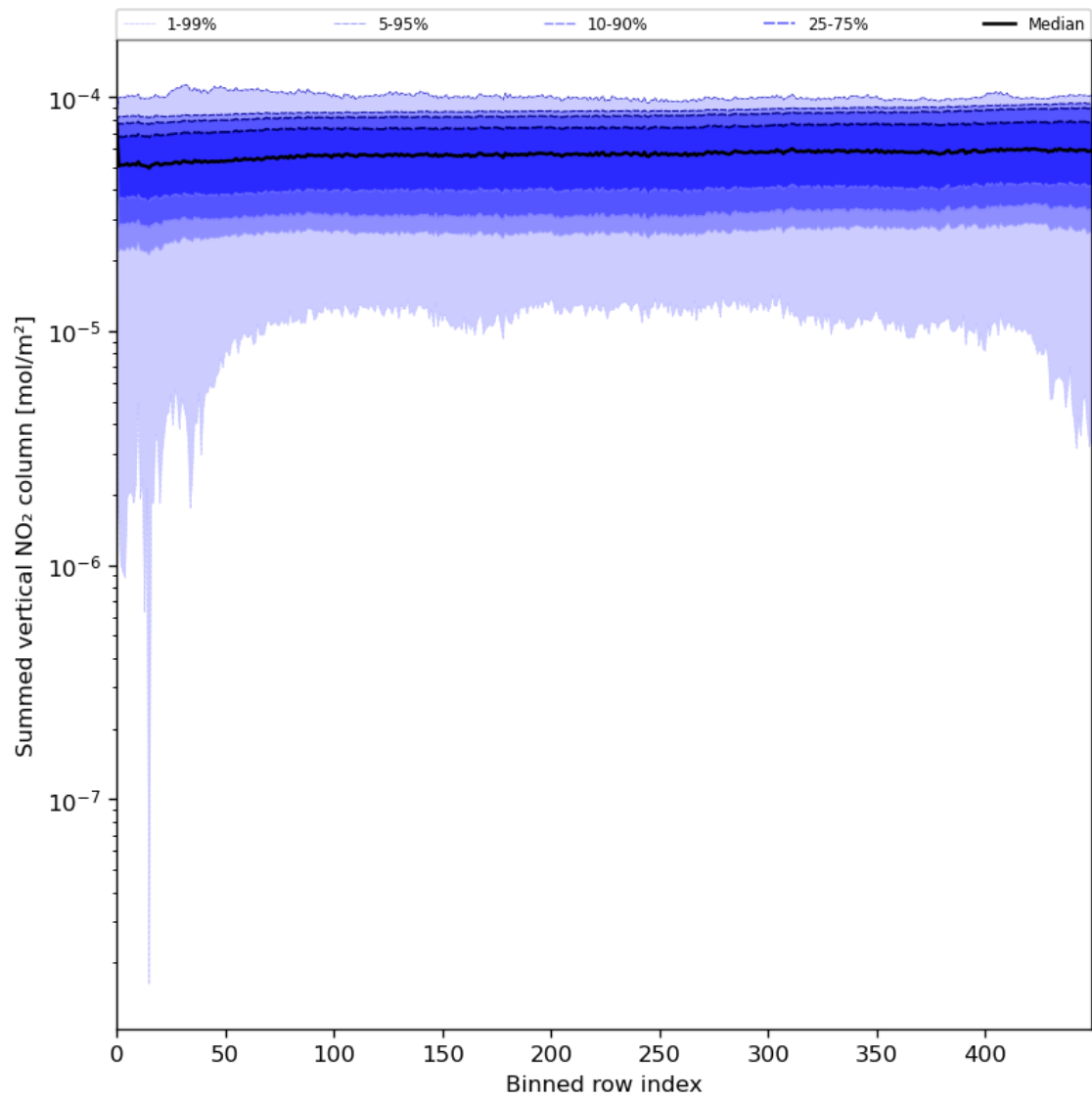
Figure 57: Along track statistics of “Summed vertical NO 2 column” for 2024-05-16 to 2024-05-18
