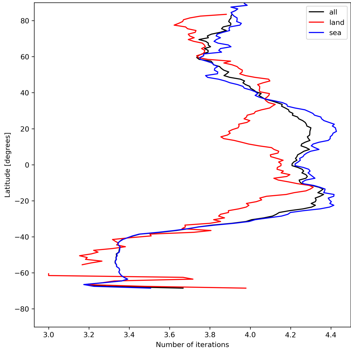
Figure 17: Zonal average of “Number of iterations” for 2024-05-16 to 2024-05-18.
