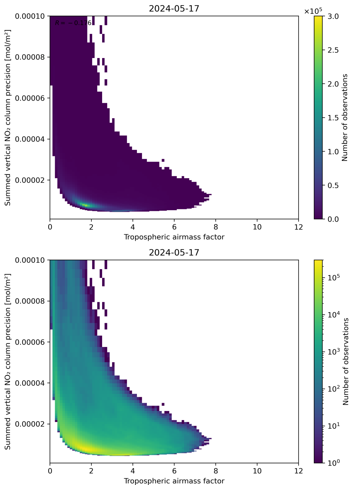
Figure 76: Scatter density plot of “Tropospheric air mass factor” against “Summed vertical NO 2 column precision” for 2024-05-16 to 2024-05-18.
