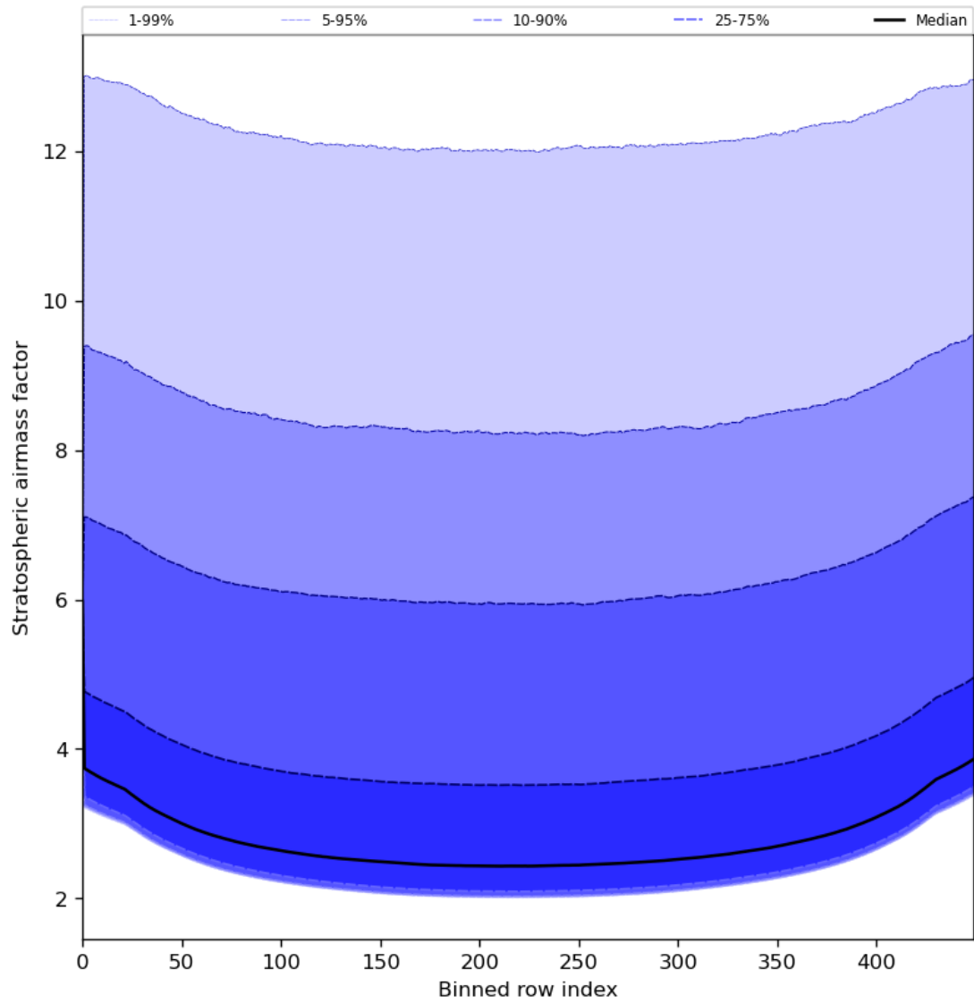
Figure 61: Along track statistics of “Stratospheric airmass factor” for 2024-05-16 to 2024-05-18
