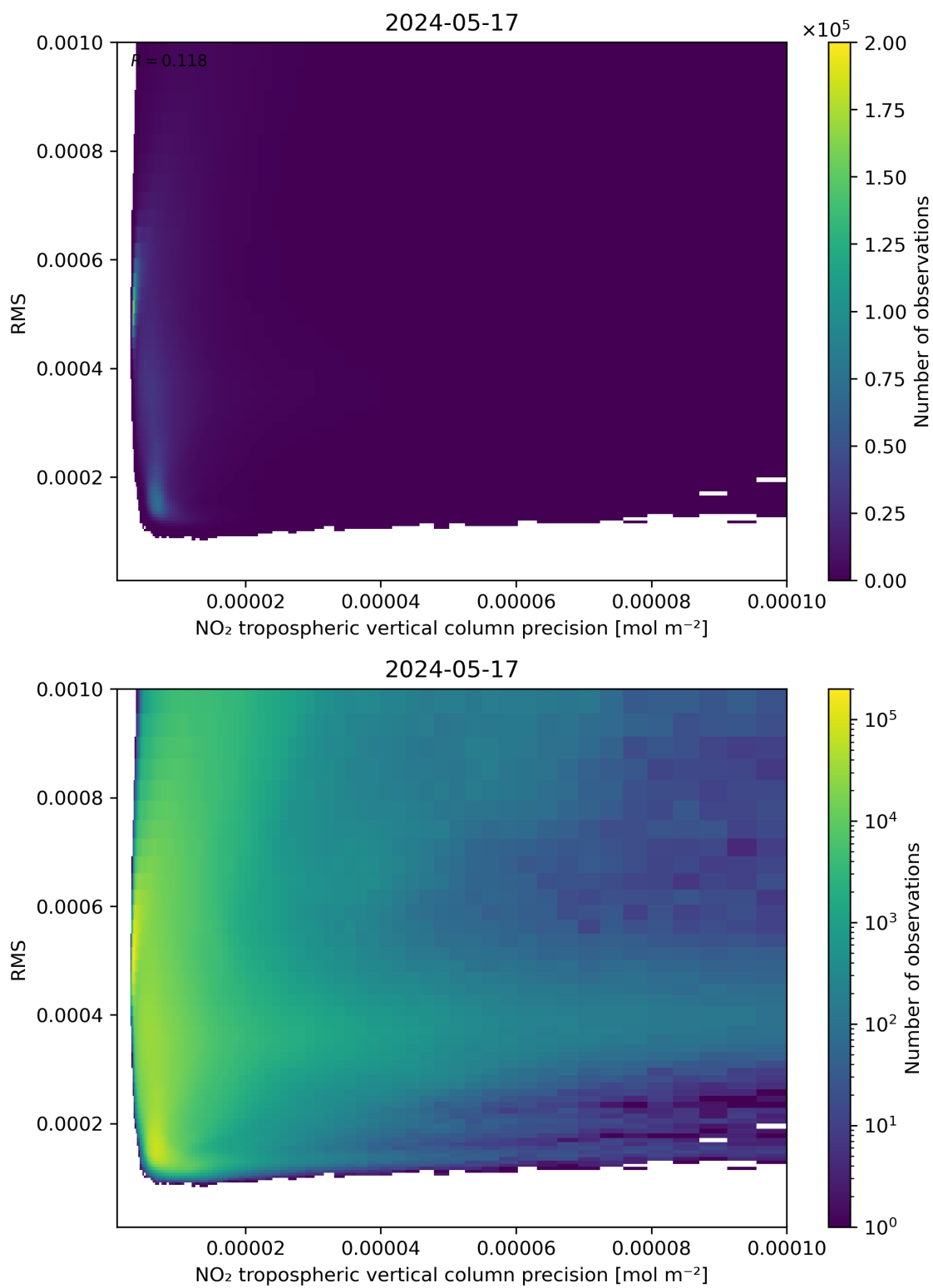
Figure 140: Scatter density plot of “NO 2 tropospheric vertical column precision” against “RMS” for 2024-05-16 to 2024-05-18.
