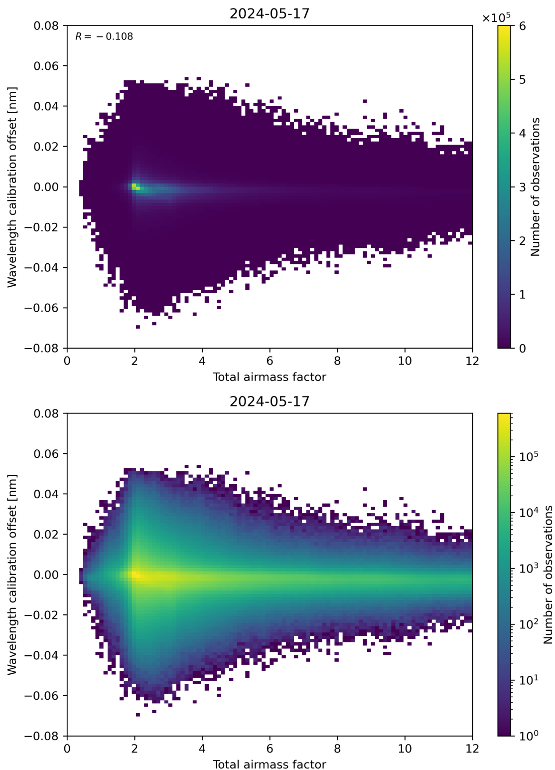
Figure 70: Scatter density plot of “Total airmass factor” against “Wavelength calibration offset” for 2024-05-16 to 2024-05-18.
