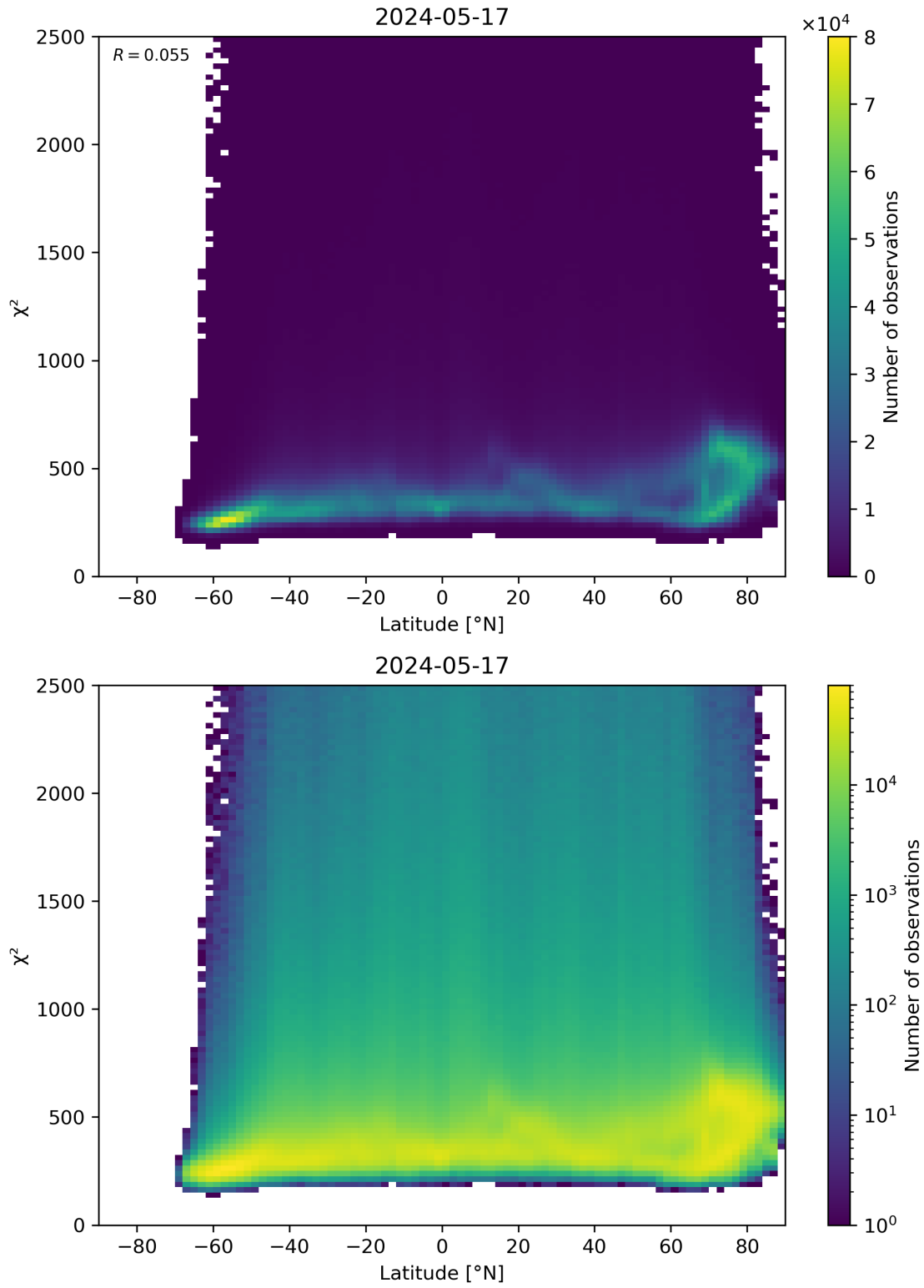
Figure 86: Scatter density plot of “Latitude” against “ \chi^2 ” for 2024-05-16 to 2024-05-18.
