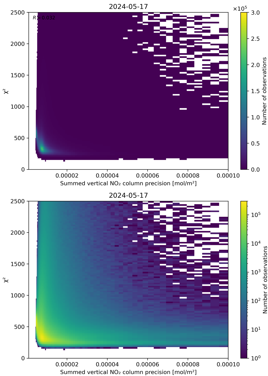
Figure 107: Scatter density plot of “Summed vertical NO 2 column precision” against “ \chi^2 ” for 2024-05-16 to 2024-05-18.
