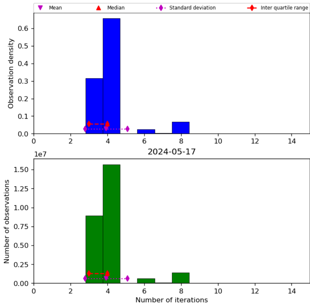
Figure 34: Histogram of “Number of iterations” for 2024-05-16 to 2024-05-18
