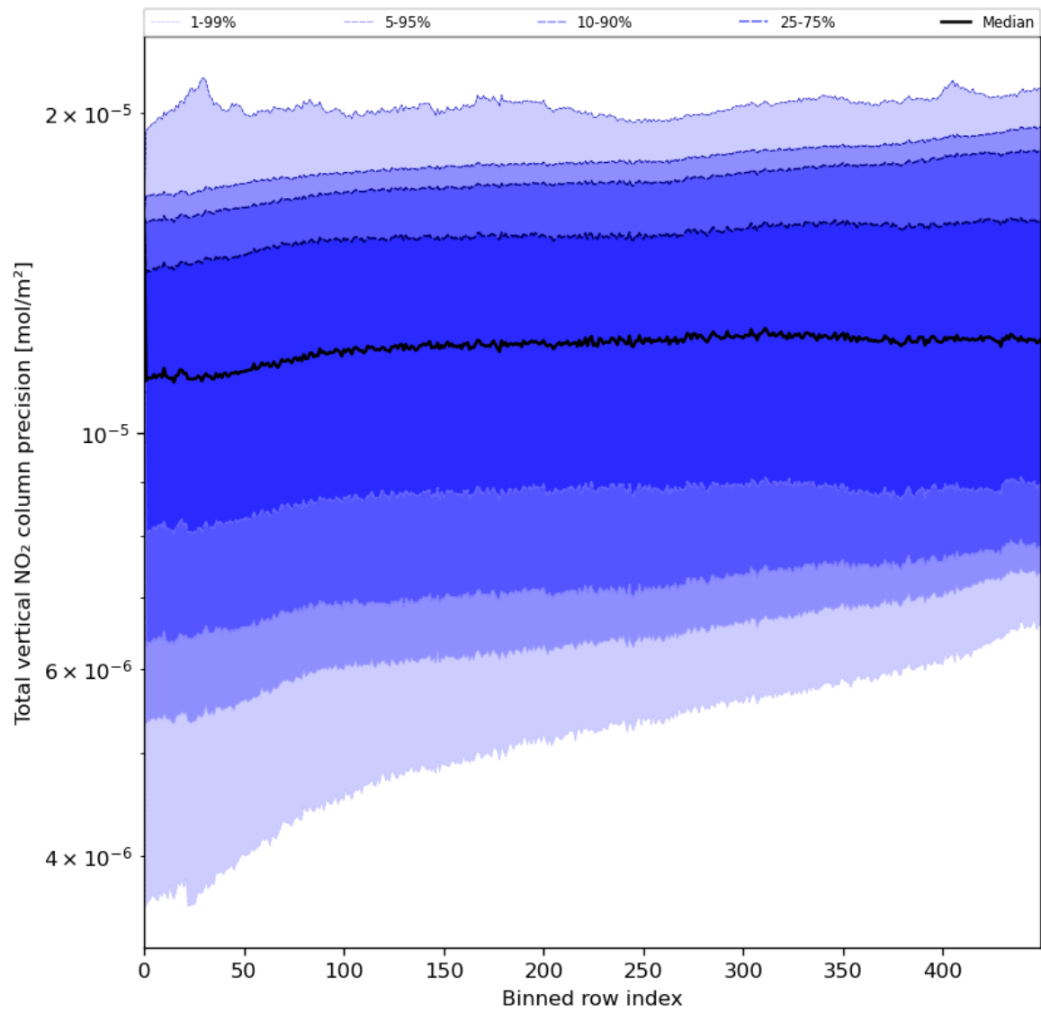
Figure 56: Along track statistics of “Total vertical NO 2 column precision” for 2024-05-16 to 2024-05-18
