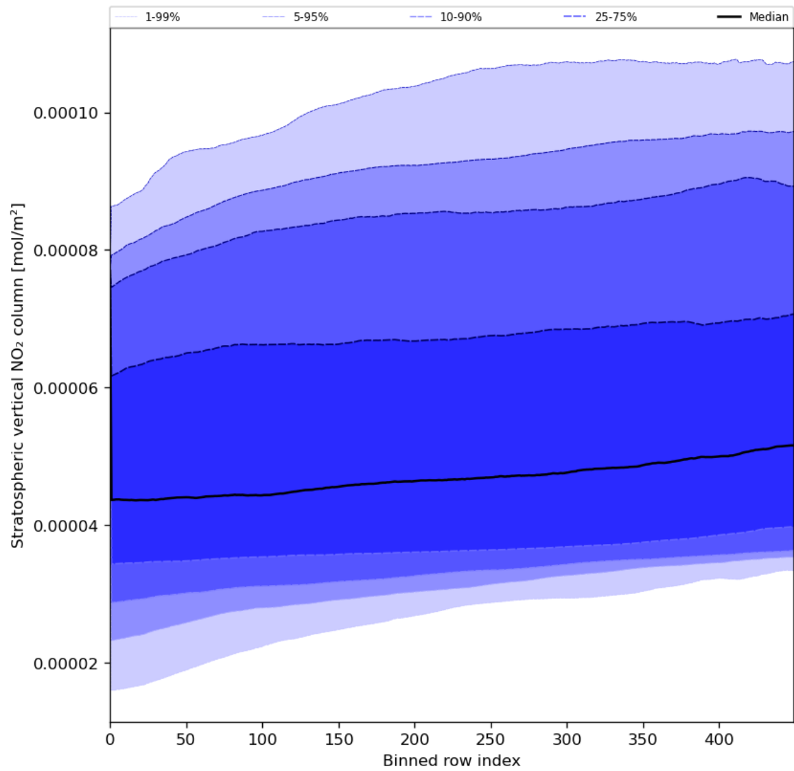
Figure 53: Along track statistics of “Stratospheric vertical NO 2 column” for 2024-05-16 to 2024-05-18
