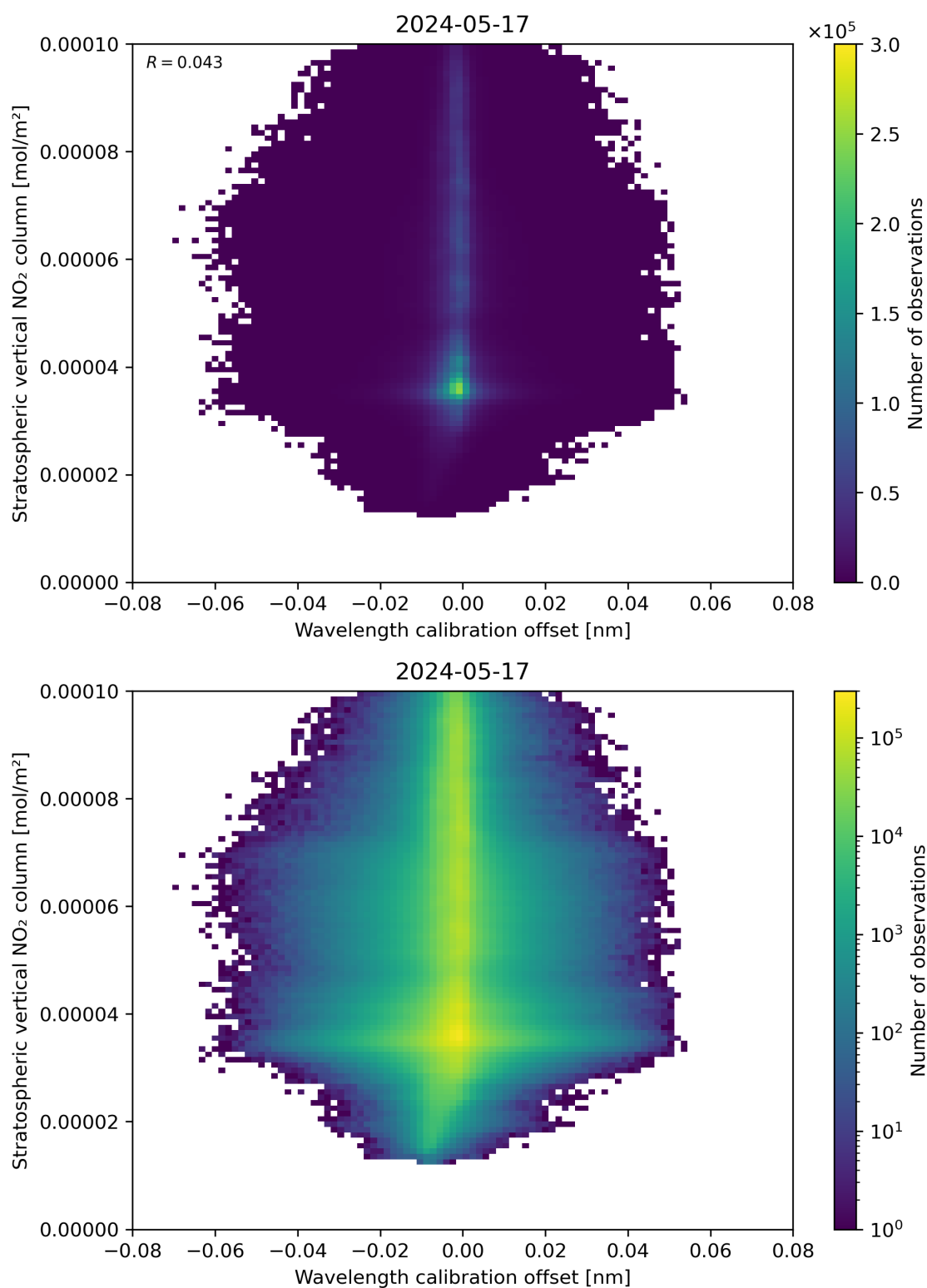
Figure 176: Scatter density plot of “Wavelength calibration offset” against “Stratospheric vertical NO 2 column” for 2024-05-16 to 2024-05-18.
