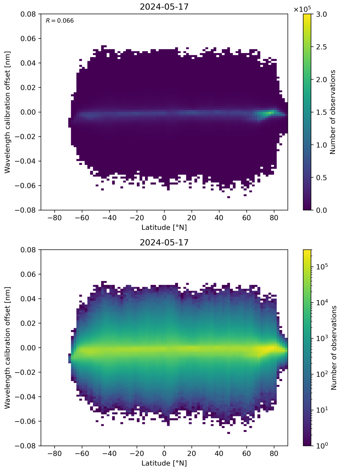
Figure 95: Scatter density plot of “Latitude” against “Wavelength calibration offset” for 2024-05-16 to 2024-05-18.
