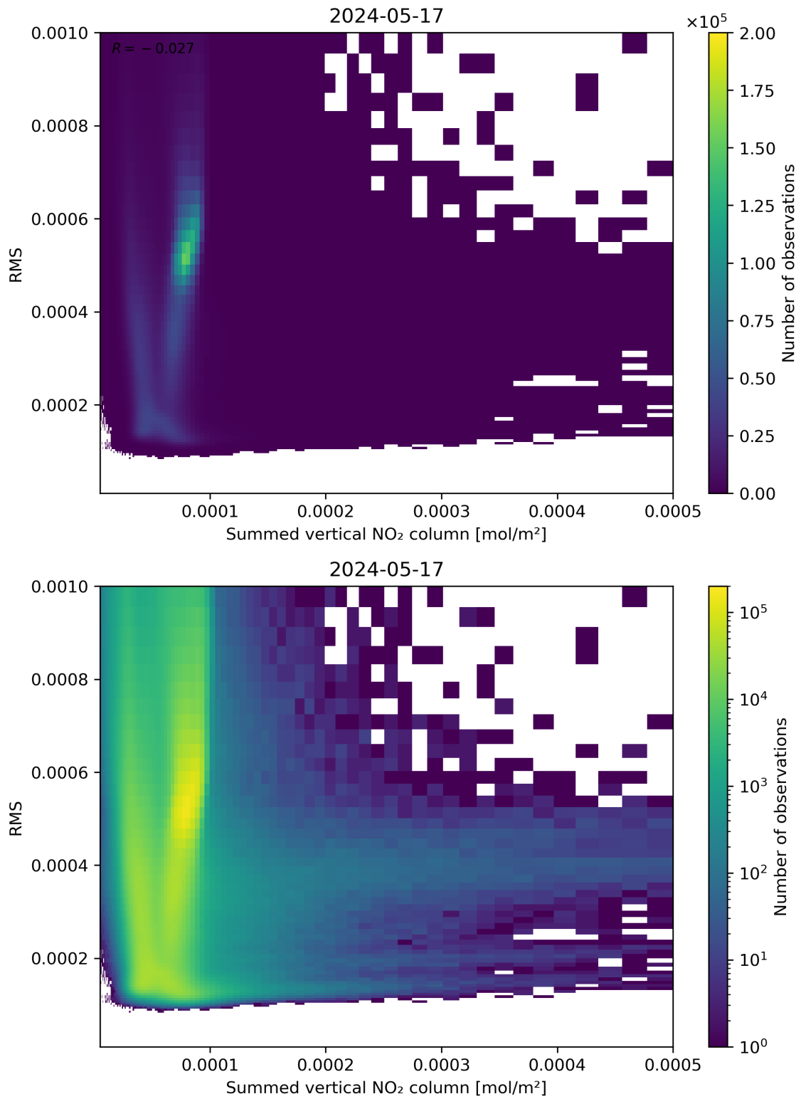
Figure 109: Scatter density plot of “Summed vertical NO 2 column” against “RMS” for 2024-05-16 to 2024-05-18.
