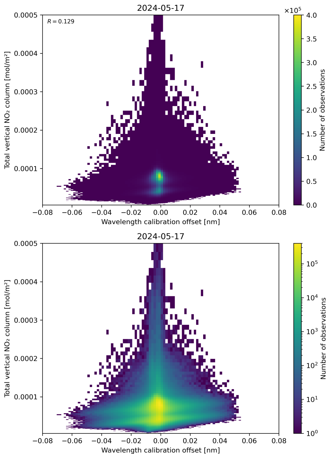
Figure 179: Scatter density plot of “Wavelength calibration offset” against “Total vertical NO 2 column” for 2024-05-16 to 2024-05-18.
