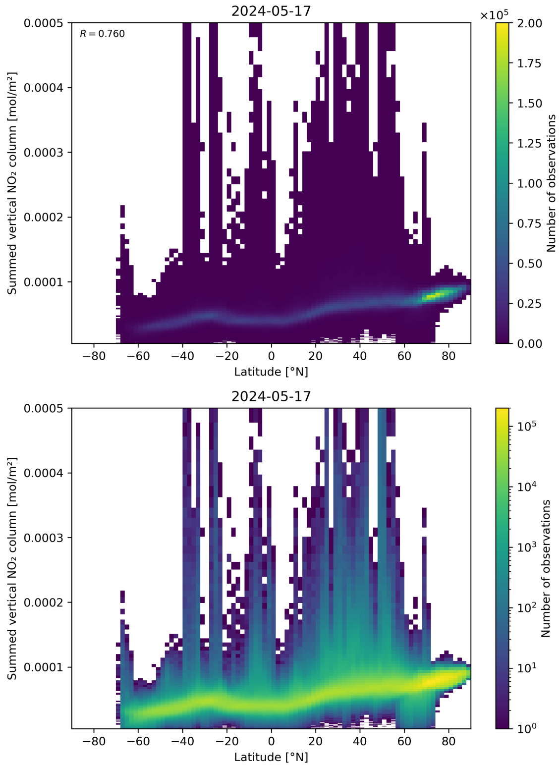
Figure 88: Scatter density plot of “Latitude” against “Summed vertical NO 2 column” for 2024-05-16 to 2024-05-18.
