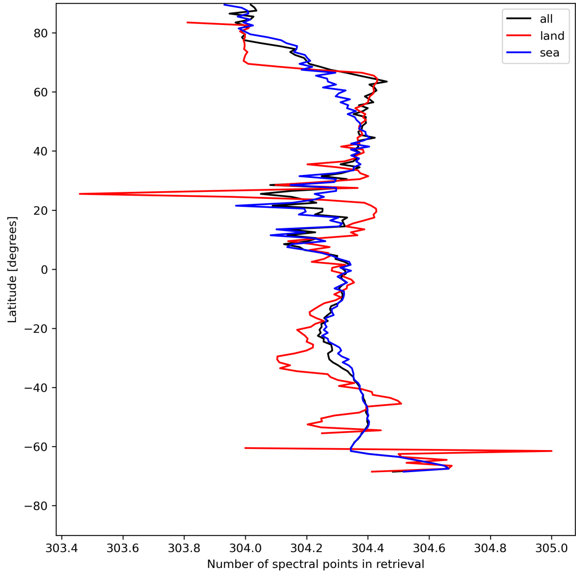
Figure 16: Zonal average of “Number of spectral points in retrieval” for 2024-05-16 to 2024-05-18.
