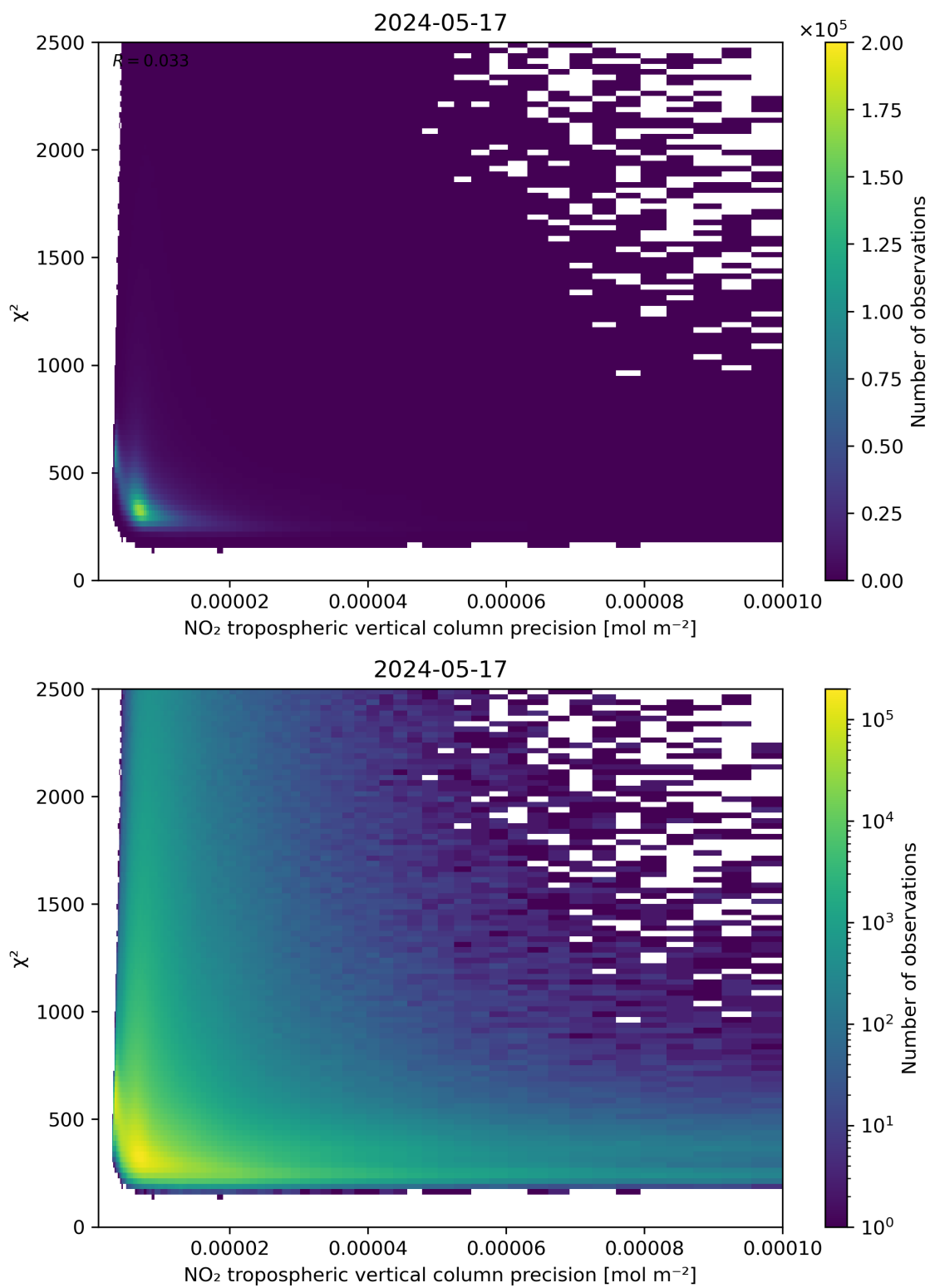
Figure 134: Scatter density plot of “NO 2 tropospheric vertical column precision” against “ \chi^2 ” for 2024-05-16 to 2024-05-18.
