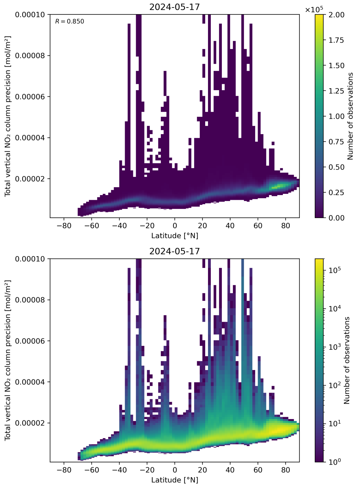
Figure 91: Scatter density plot of “Latitude” against “Total vertical NO 2 column precision” for 2024-05-16 to 2024-05-18.
