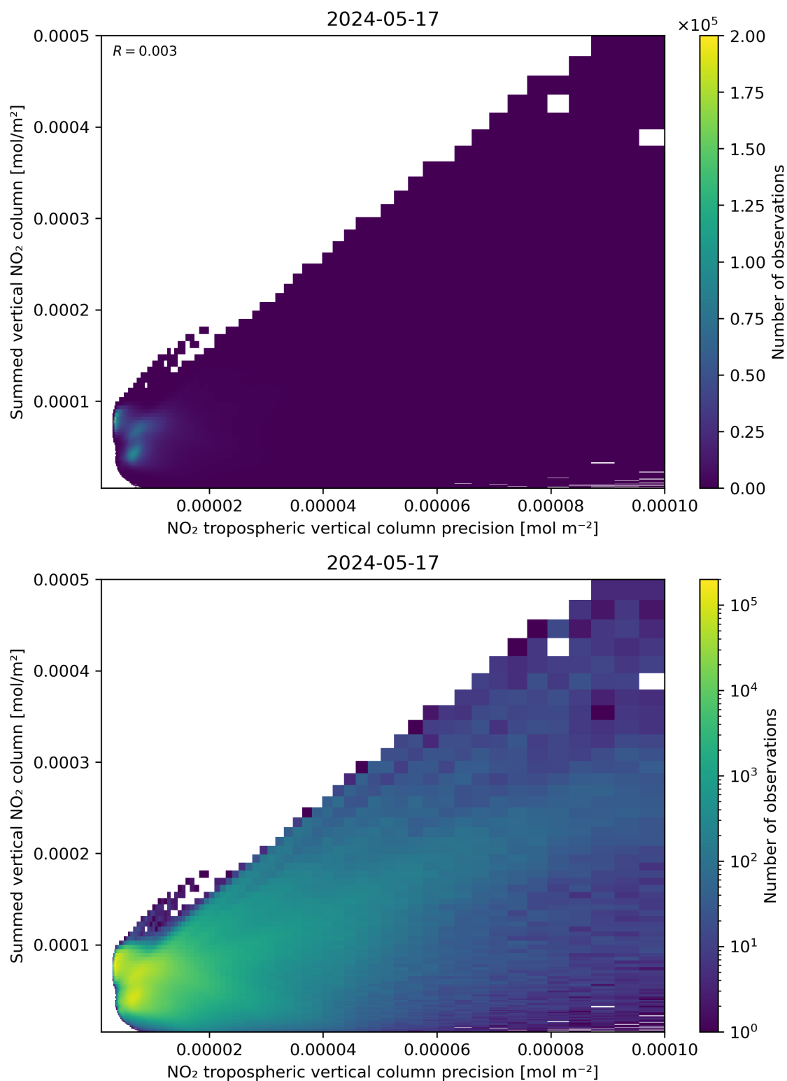
Figure 136: Scatter density plot of “NO 2 tropospheric vertical column precision” against “Summed vertical NO 2 column” for 2024-05-16 to 2024-05-18.
