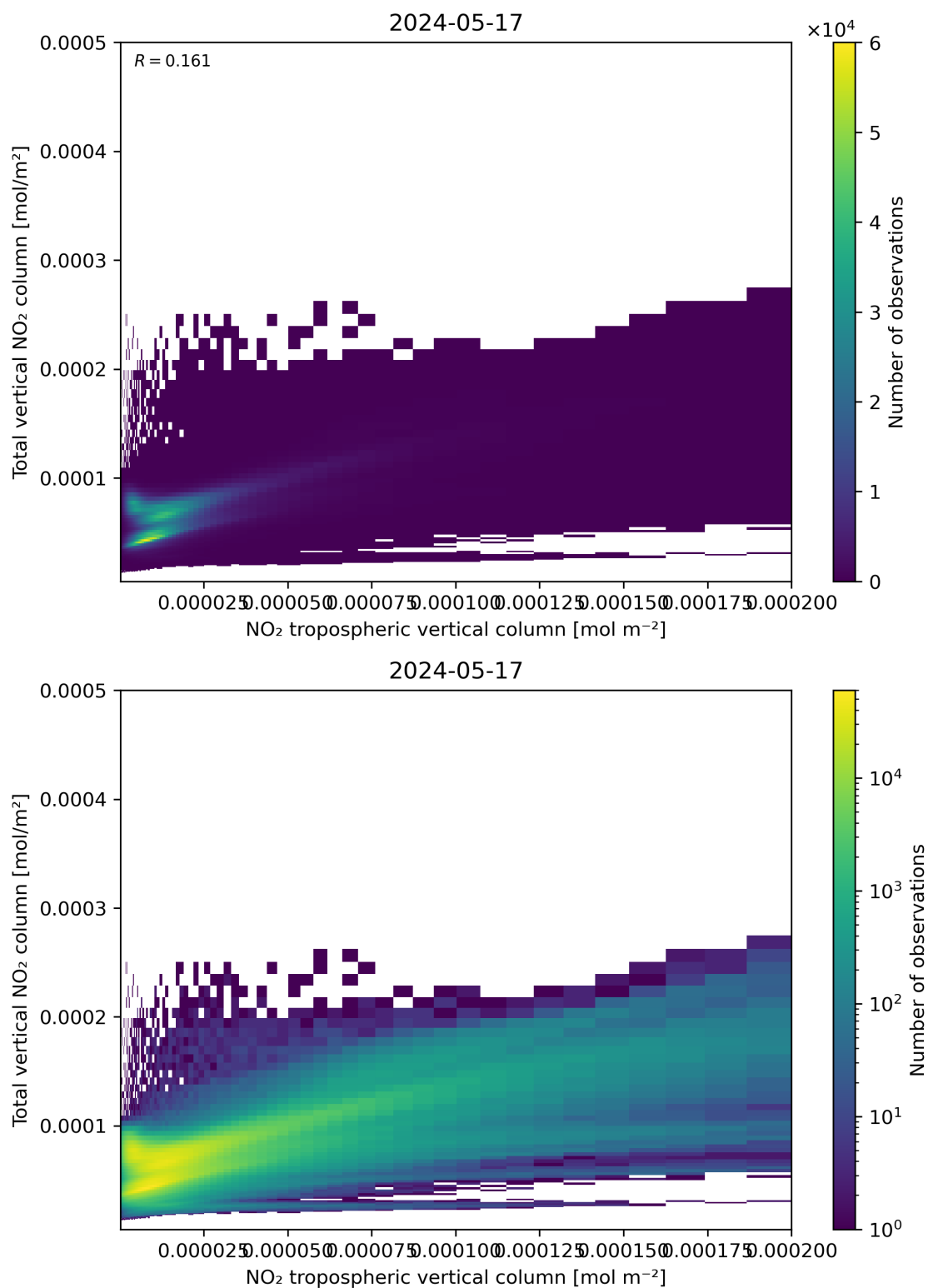
Figure 128: Scatter density plot of “NO 2 tropospheric vertical column” against “Total vertical NO 2 column” for 2024-05-16 to 2024-05-18.
