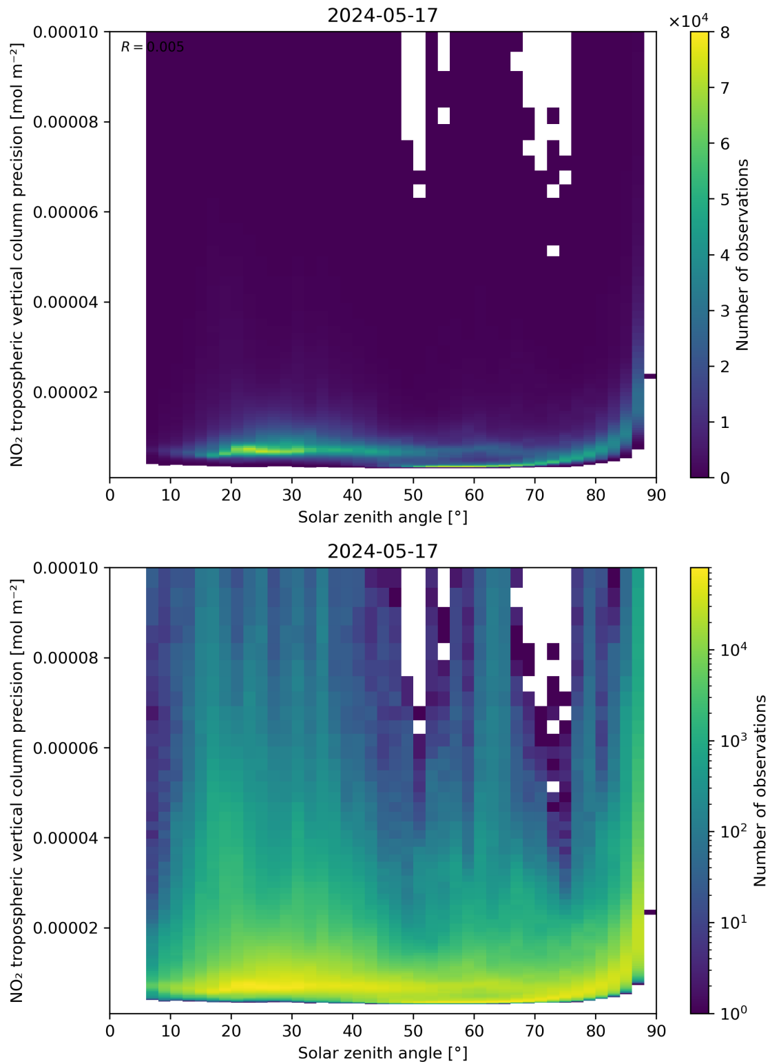
Figure 156: Scatter density plot of “Solar zenith angle” against “NO 2 tropospheric vertical column precision” for 2024-05-16 to 2024-05-18.
