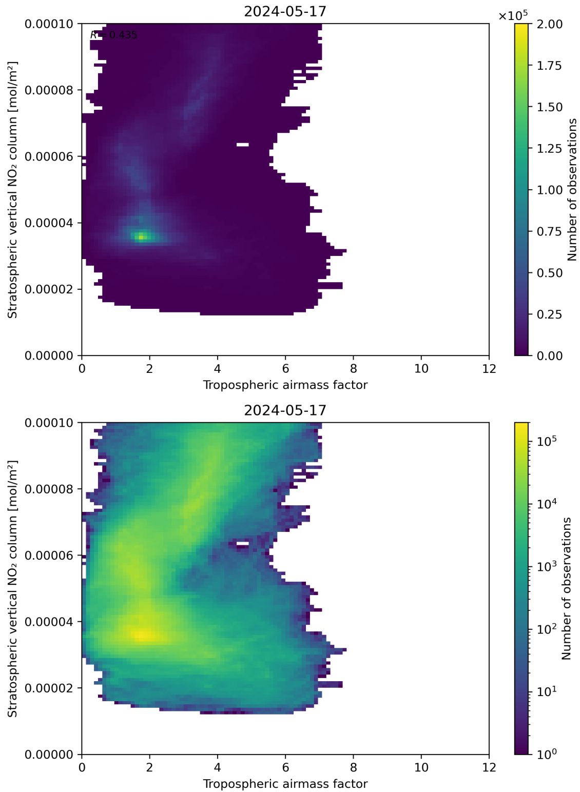
Figure 74: Scatter density plot of “Tropospheric air mass factor” against “Stratospheric vertical NO 2 column” for 2024-05-16 to 2024-05-18.
