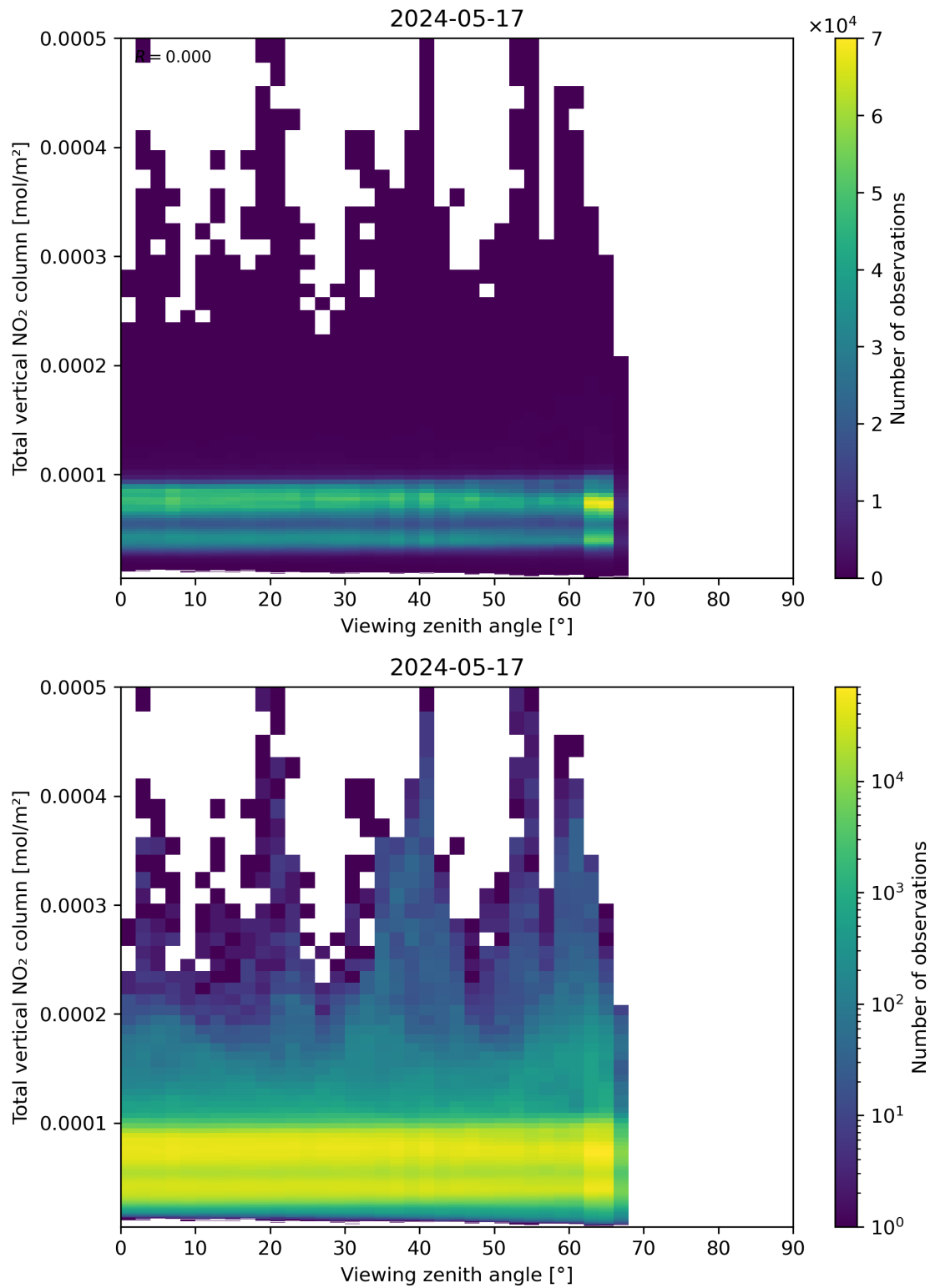
Figure 167: Scatter density plot of “Viewing zenith angle” against “Total vertical NO 2 column” for 2024-05-16 to 2024-05-18.
