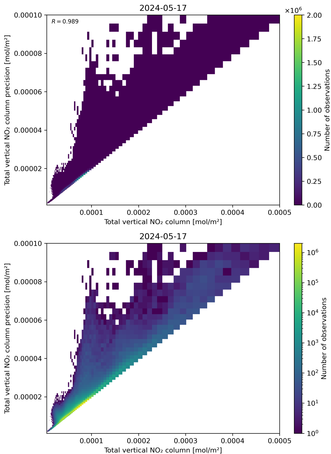
Figure 114: Scatter density plot of “Total vertical NO 2 column” against “Total vertical NO 2 column precision” for 2024-05-16 to 2024-05-18.
