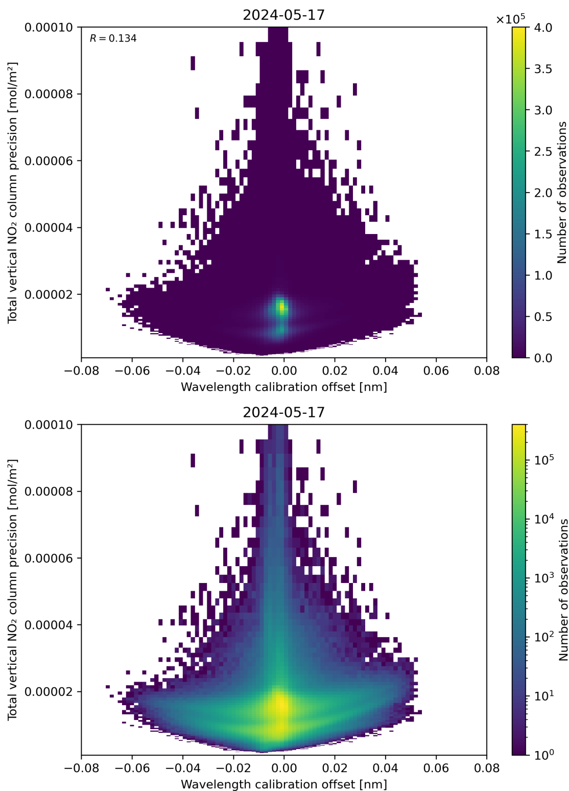
Figure 180: Scatter density plot of “Wavelength calibration offset” against “Total vertical NO 2 column precision” for 2024-05-16 to 2024-05-18.
