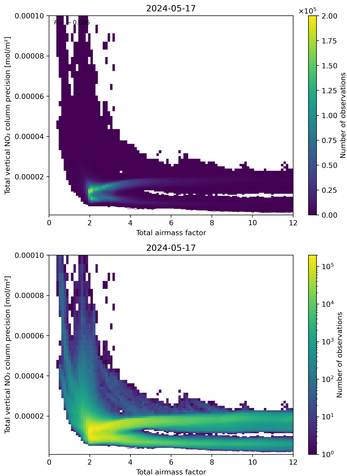
Figure 68: Scatter density plot of “Total airmass factor” against “Total vertical NO 2 column precision” for 2024-05-16 to 2024-05-18.
