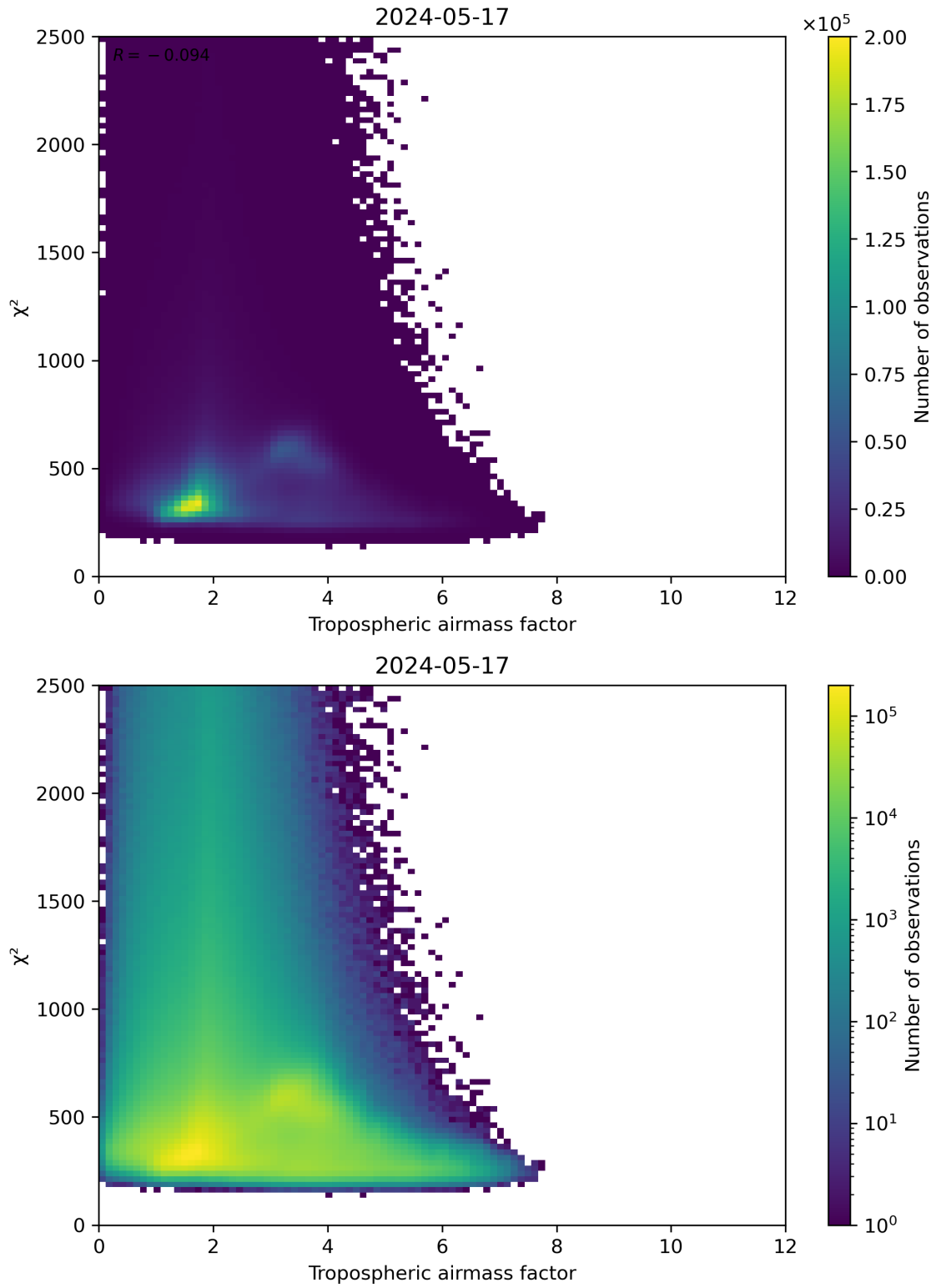
Figure 73: Scatter density plot of “Tropospheric airmass factor” against “ \chi^2 ” for 2024-05-16 to 2024-05-18.
