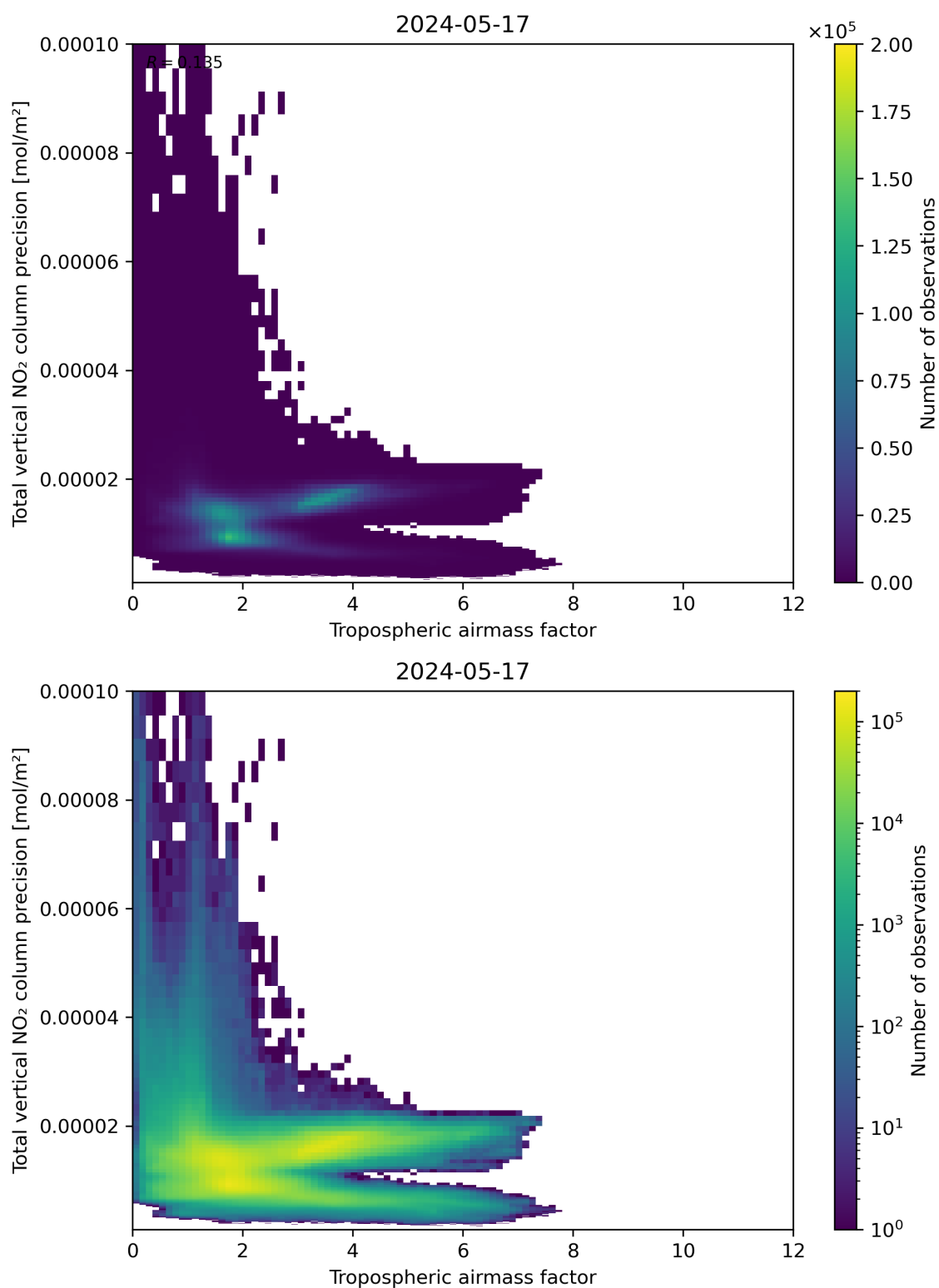
Figure 78: Scatter density plot of “Tropospheric air mass factor” against “Total vertical NO 2 column precision” for 2024-05-16 to 2024-05-18.
