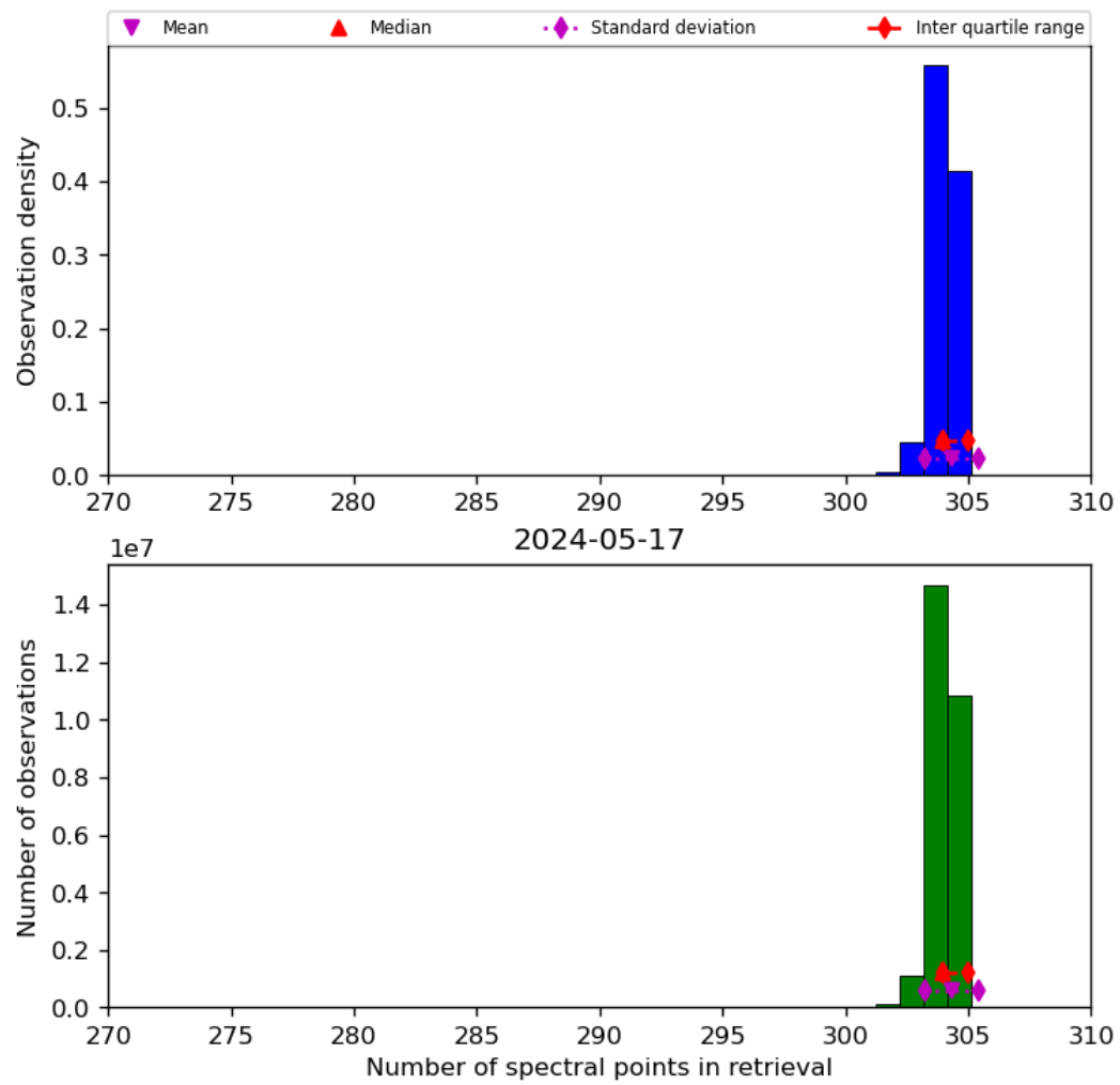
Figure 33: Histogram of "Number of spectral points in retrieval" for 2024-05-16 to 2024-05-18
