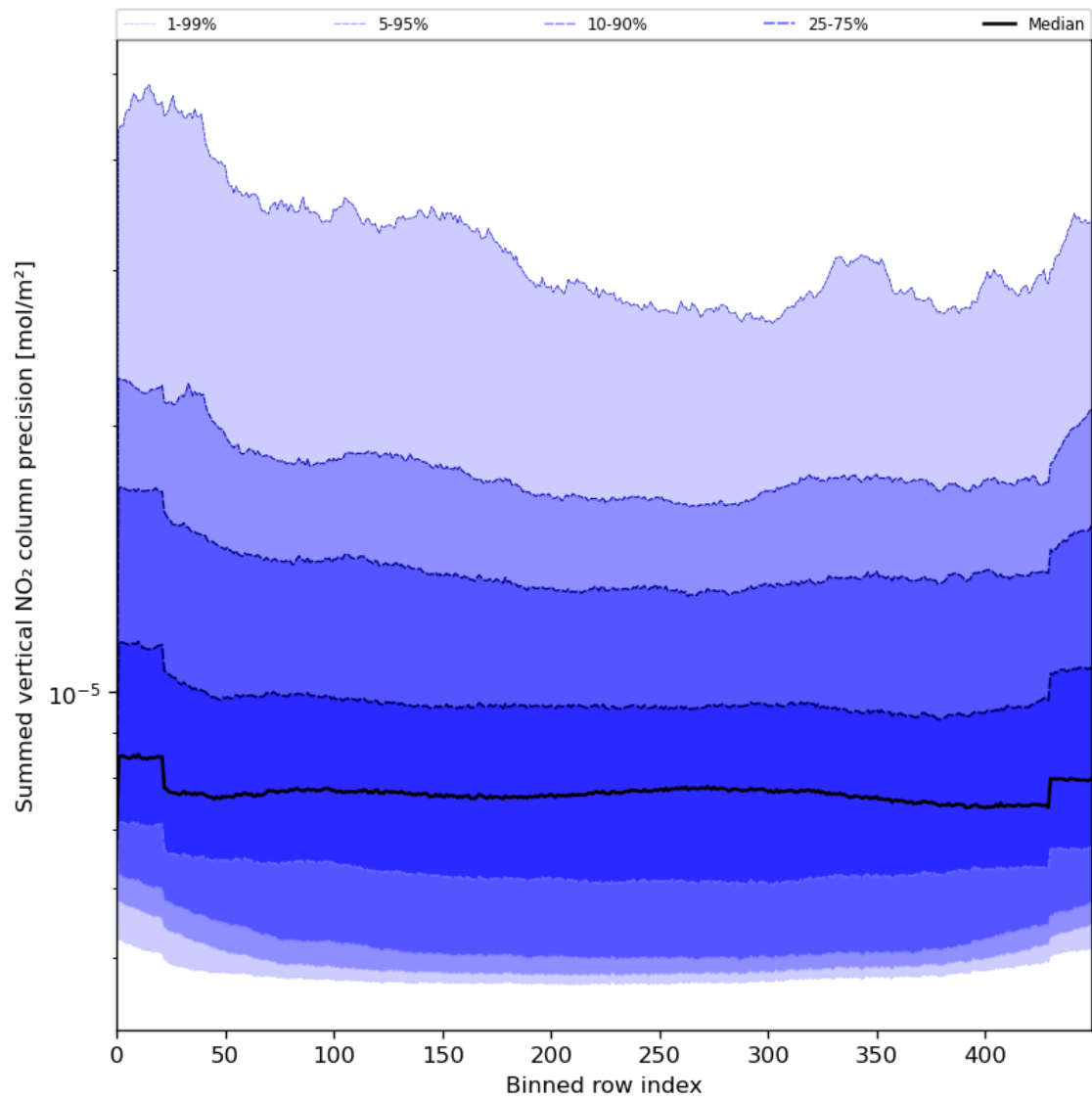
Figure 58: Along track statistics of “Summed vertical NO 2 column precision” for 2024-05-16 to 2024-05-18
