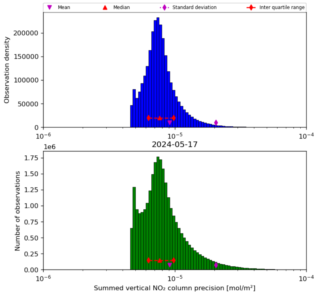
Figure 41: Histogram of “Summed vertical NO 2 column precision” for 2024-05-16 to 2024-05-18
