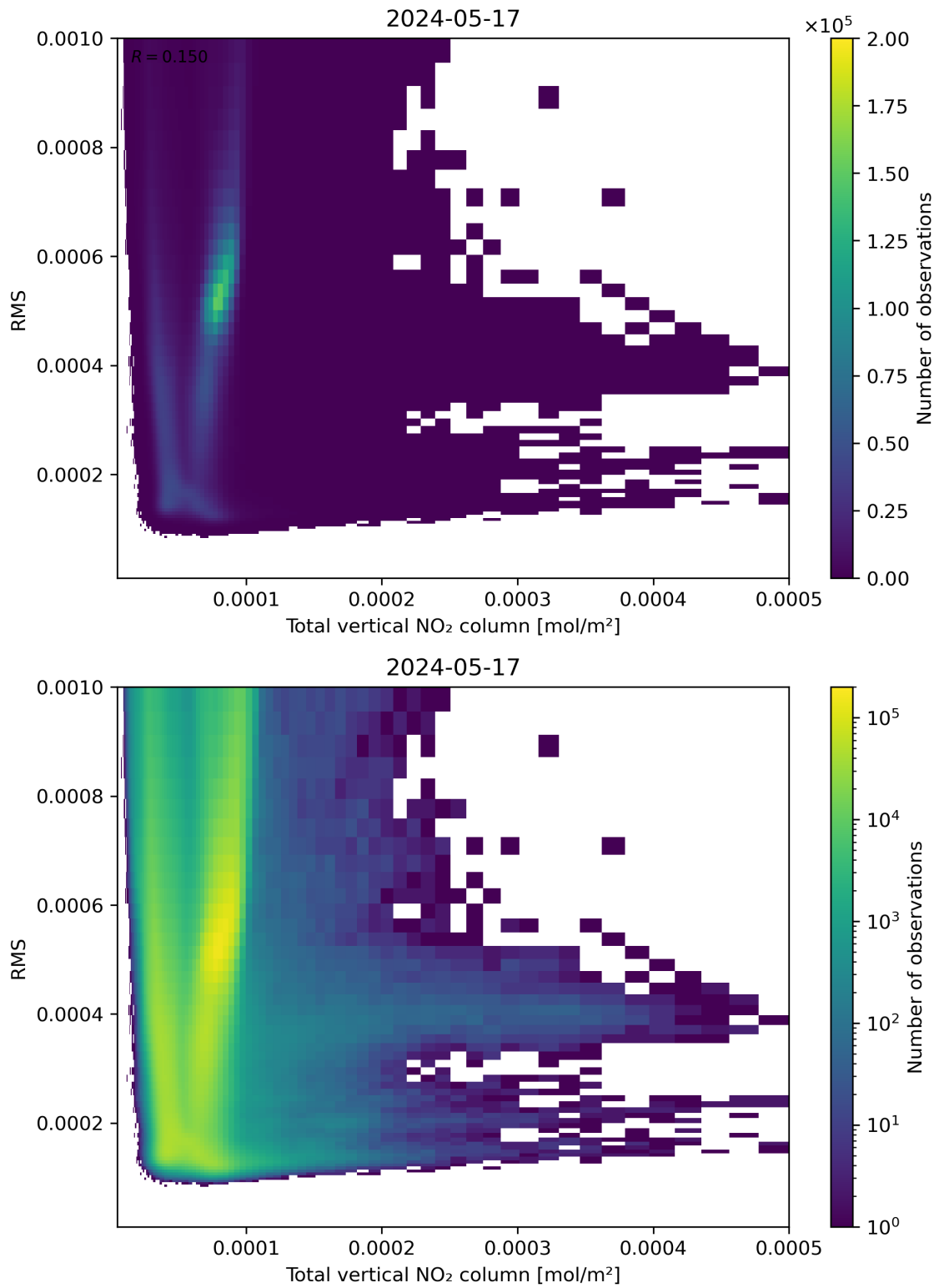
Figure 120: Scatter density plot of “Total vertical NO 2 column” against “RMS” for 2024-05-16 to 2024-05-18.
