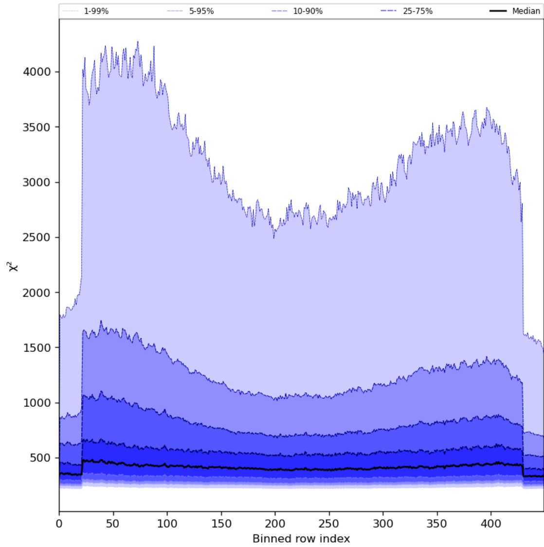
Figure 59: Along track statistics of “ \chi^2 ” for 2024-05-16 to 2024-05-18
