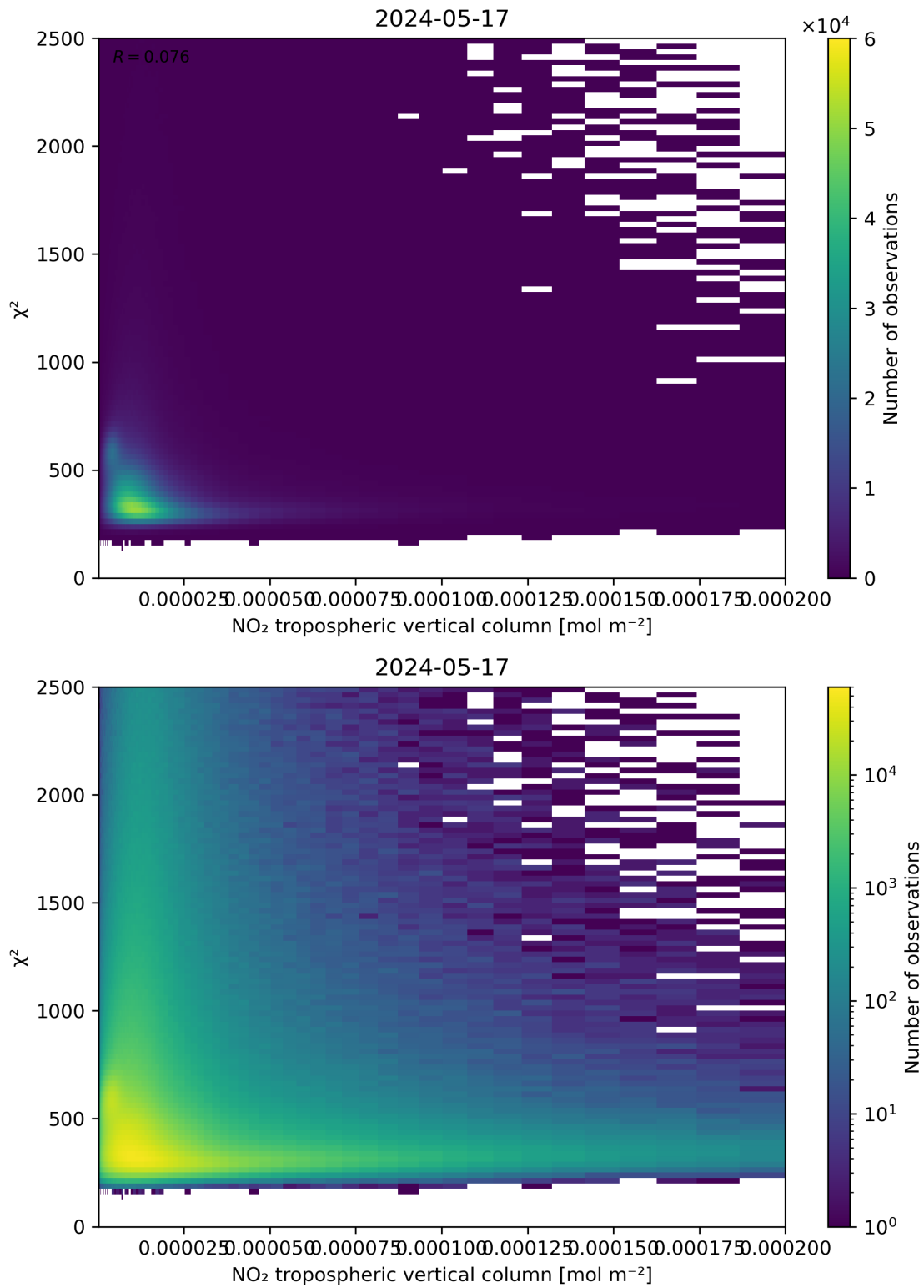
Figure 124: Scatter density plot of “NO 2 tropospheric vertical column” against “ \chi^2 ” for 2024-05-16 to 2024-05-18.
