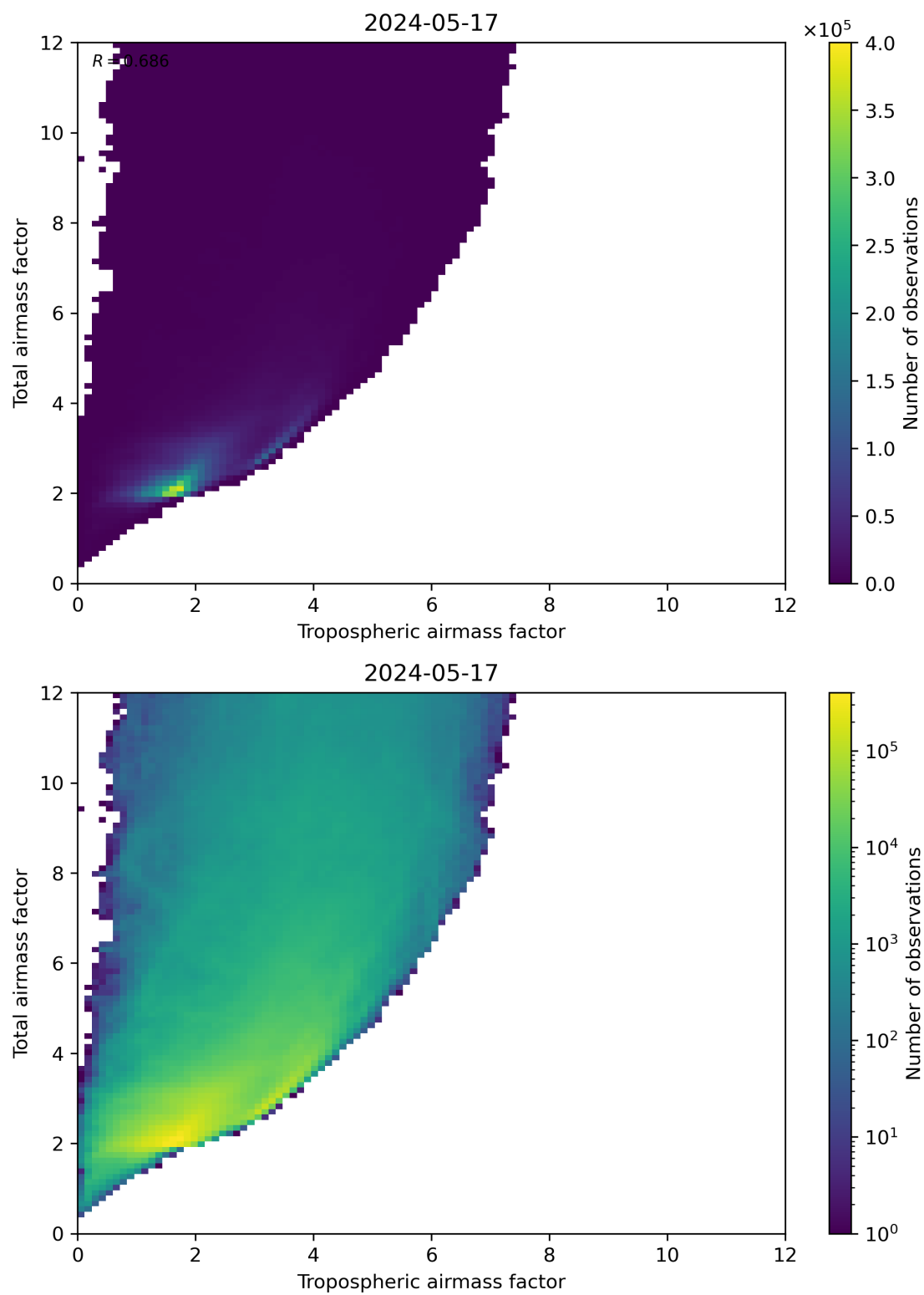
Figure 72: Scatter density plot of “Tropospheric airmass factor” against “Total airmass factor” for 2024-05-16 to 2024-05-18.
