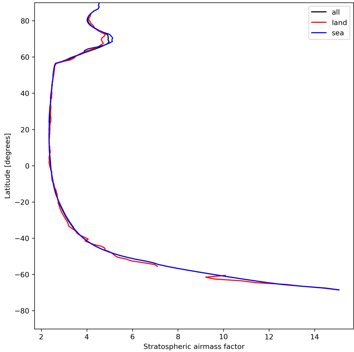
Figure 27: Zonal average of “Stratospheric air mass factor” for 2024-05-16 to 2024-05-18.
