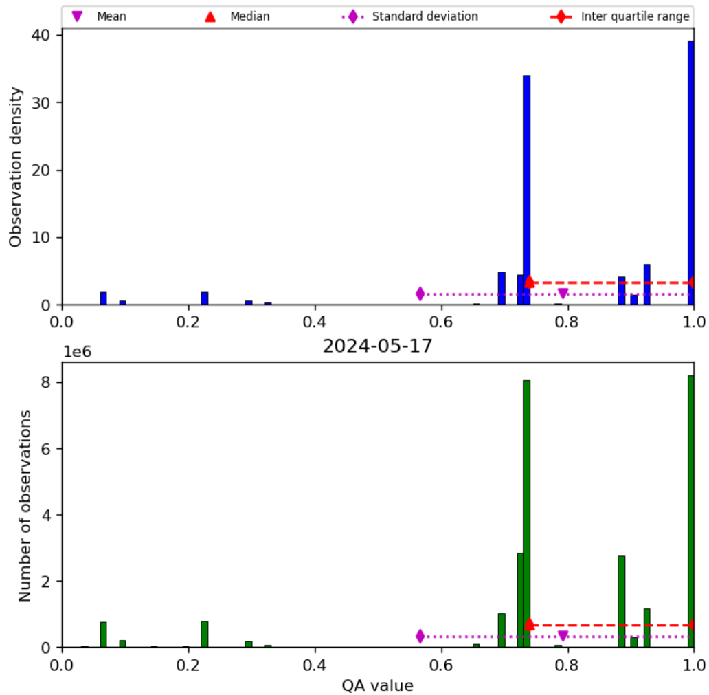
Figure 28: Histogram of “QA value” for 2024-05-16 to 2024-05-18
