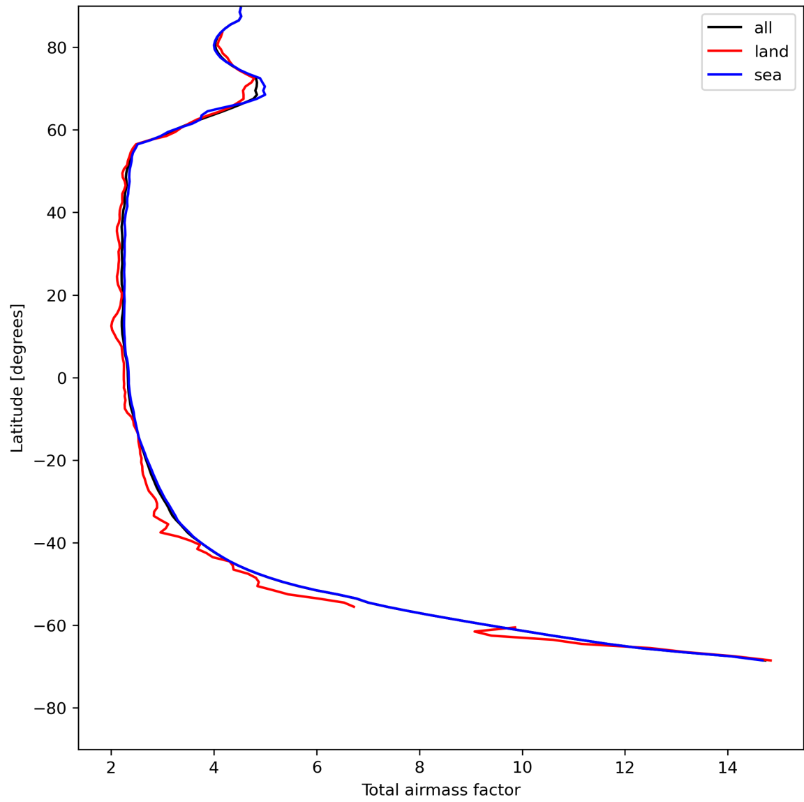
Figure 15: Zonal average of “Total airmass factor” for 2024-05-16 to 2024-05-18.
