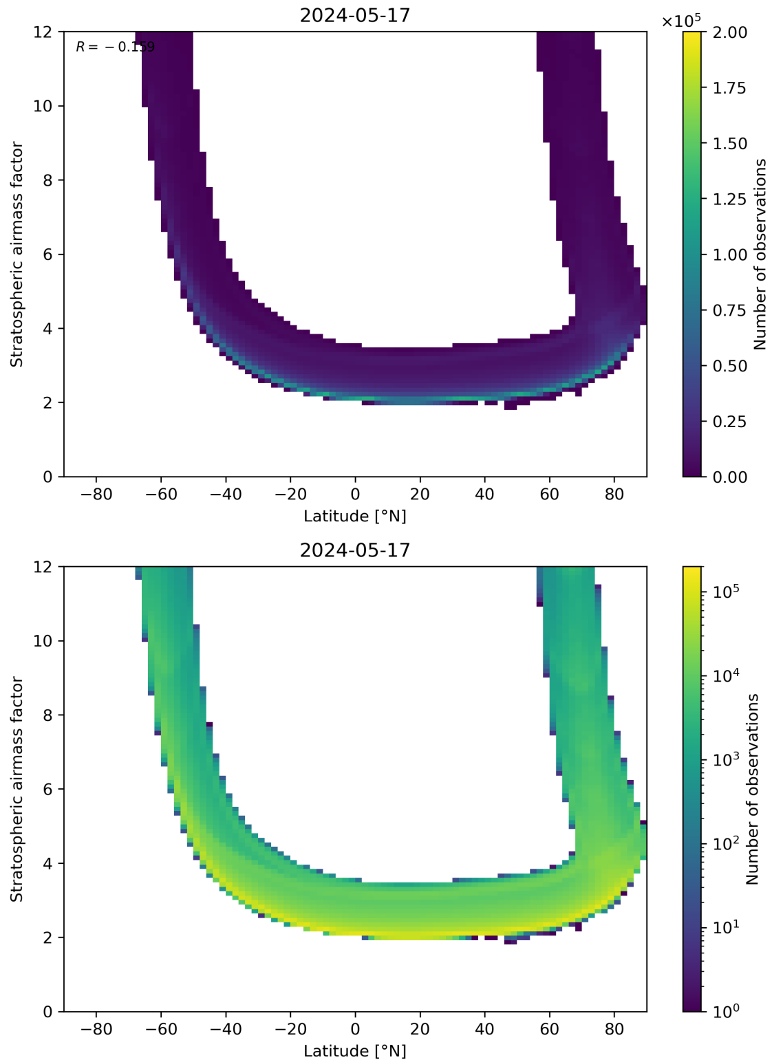
Figure 83: Scatter density plot of “Latitude” against “Stratospheric air mass factor” for 2024-05-16 to 2024-05-18.
