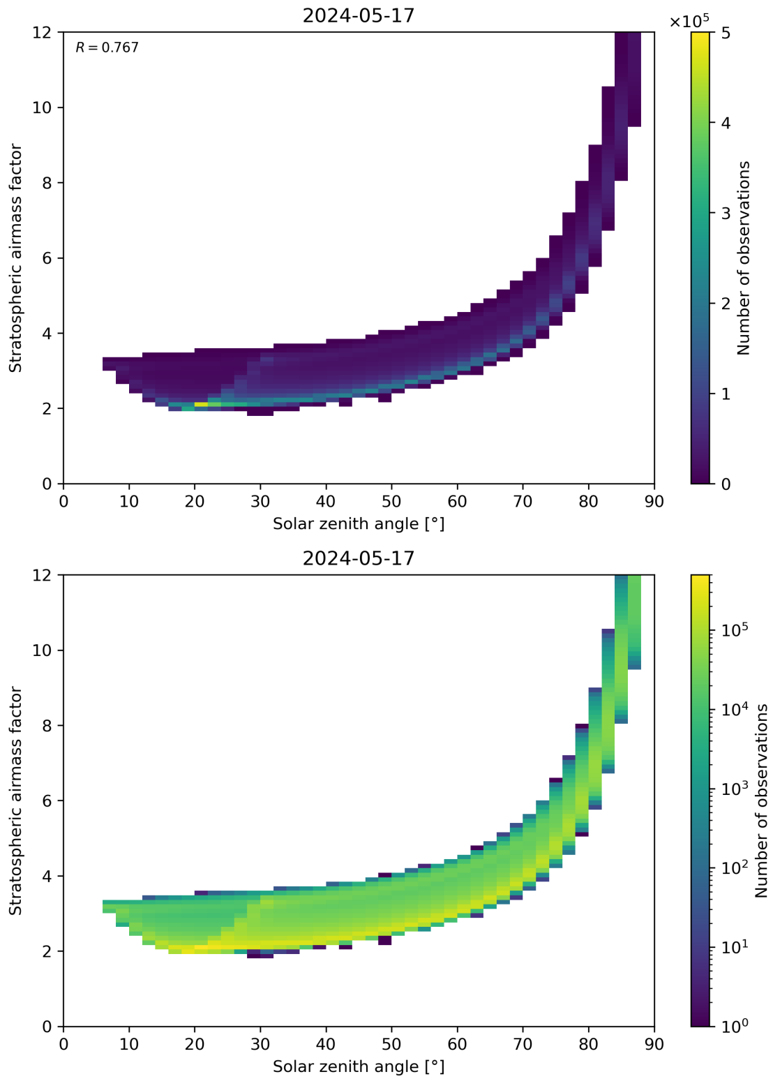
Figure 145: Scatter density plot of “Solar zenith angle” against “Stratospheric airmass factor” for 2024-05-16 to 2024-05-18.
