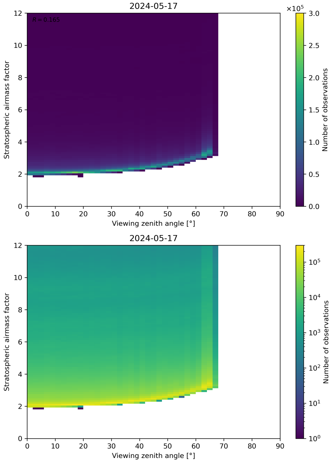
Figure 159: Scatter density plot of “Viewing zenith angle” against “Stratospheric airmass factor” for 2024-05-16 to 2024-05-18.
