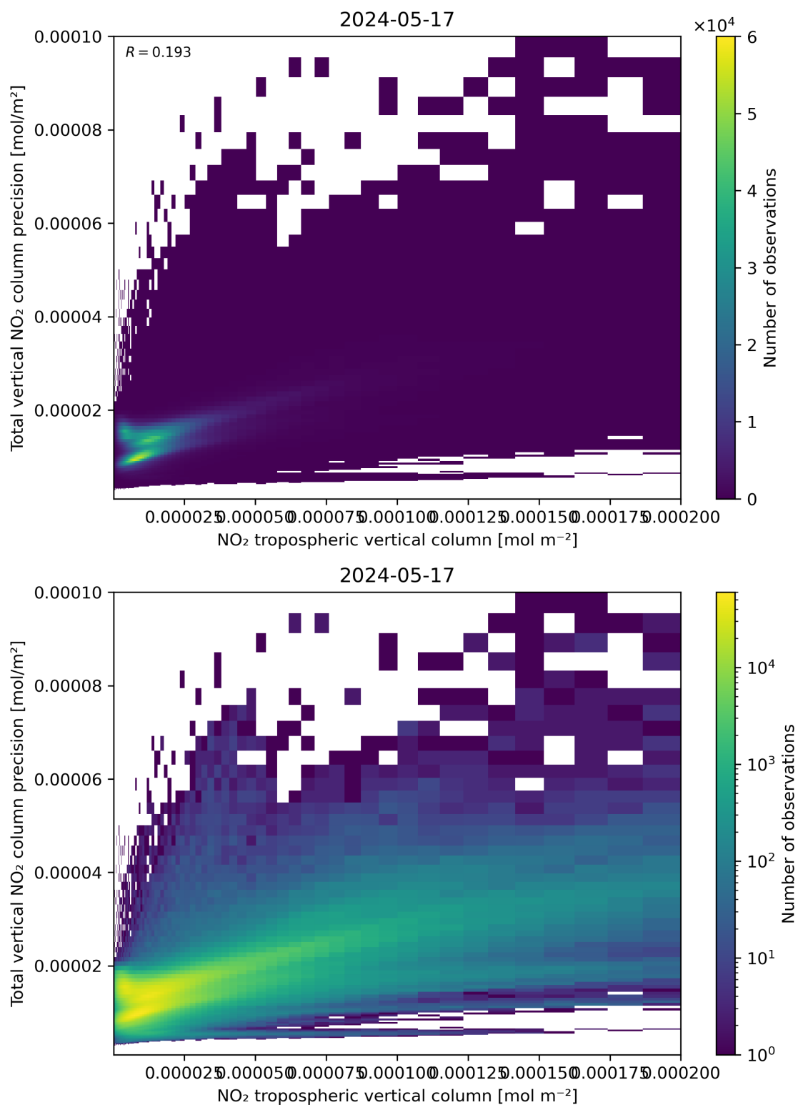
Figure 129: Scatter density plot of “NO 2 tropospheric vertical column” against “Total vertical NO 2 column precision” for 2024-05-16 to 2024-05-18.
