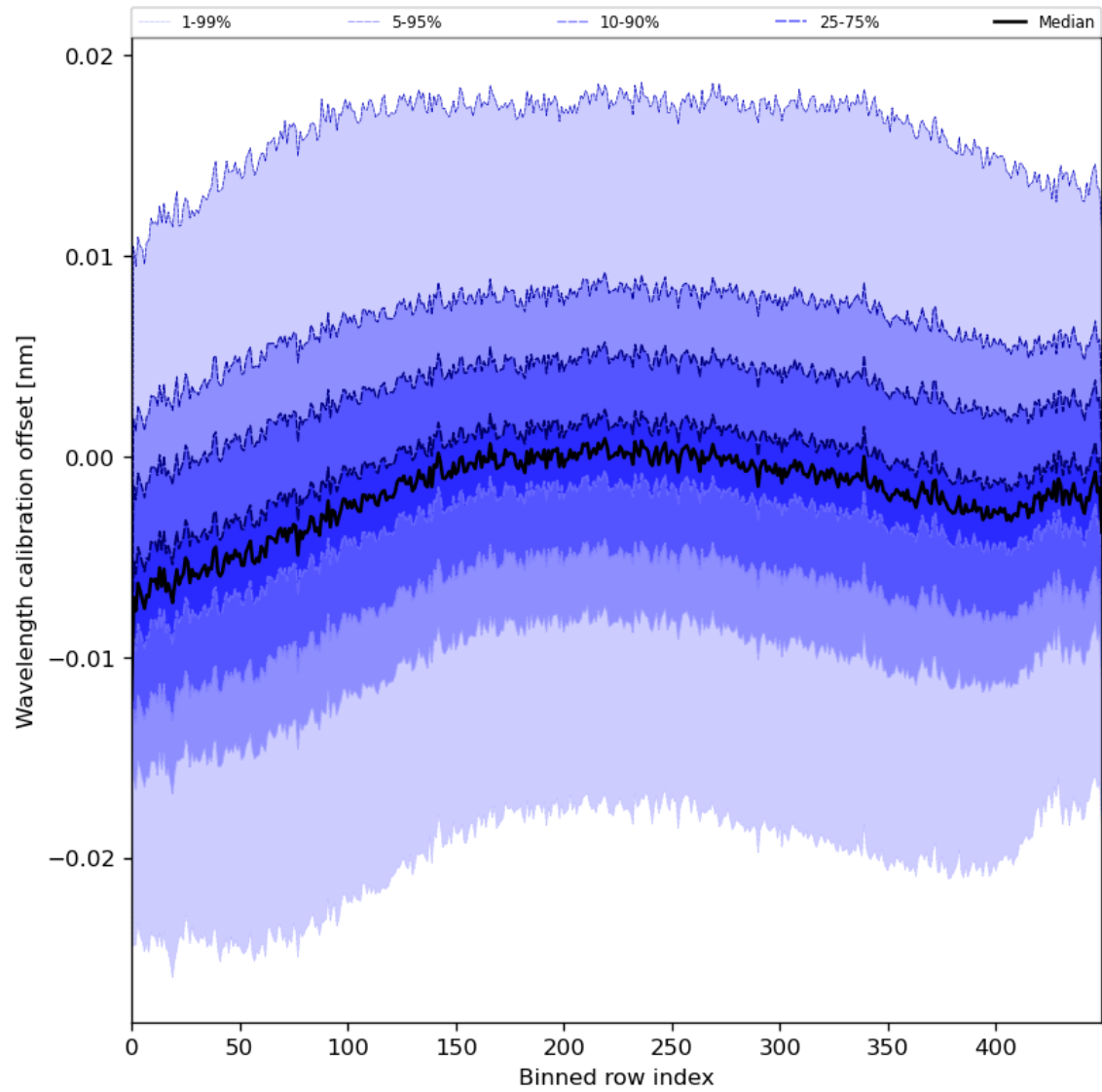
Figure 52: Along track statistics of “Wavelength calibration offset” for 2024-05-16 to 2024-05-18
