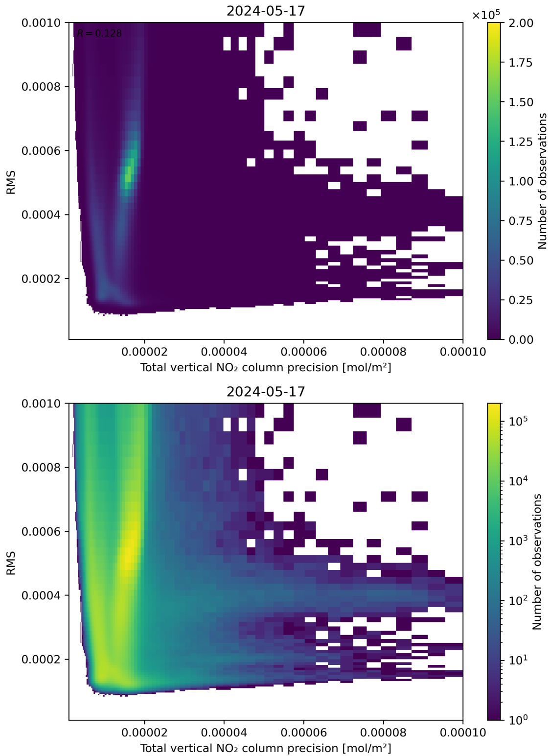
Figure 119: Scatter density plot of “Total vertical NO 2 column precision” against “RMS” for 2024-05-16 to 2024-05-18.
