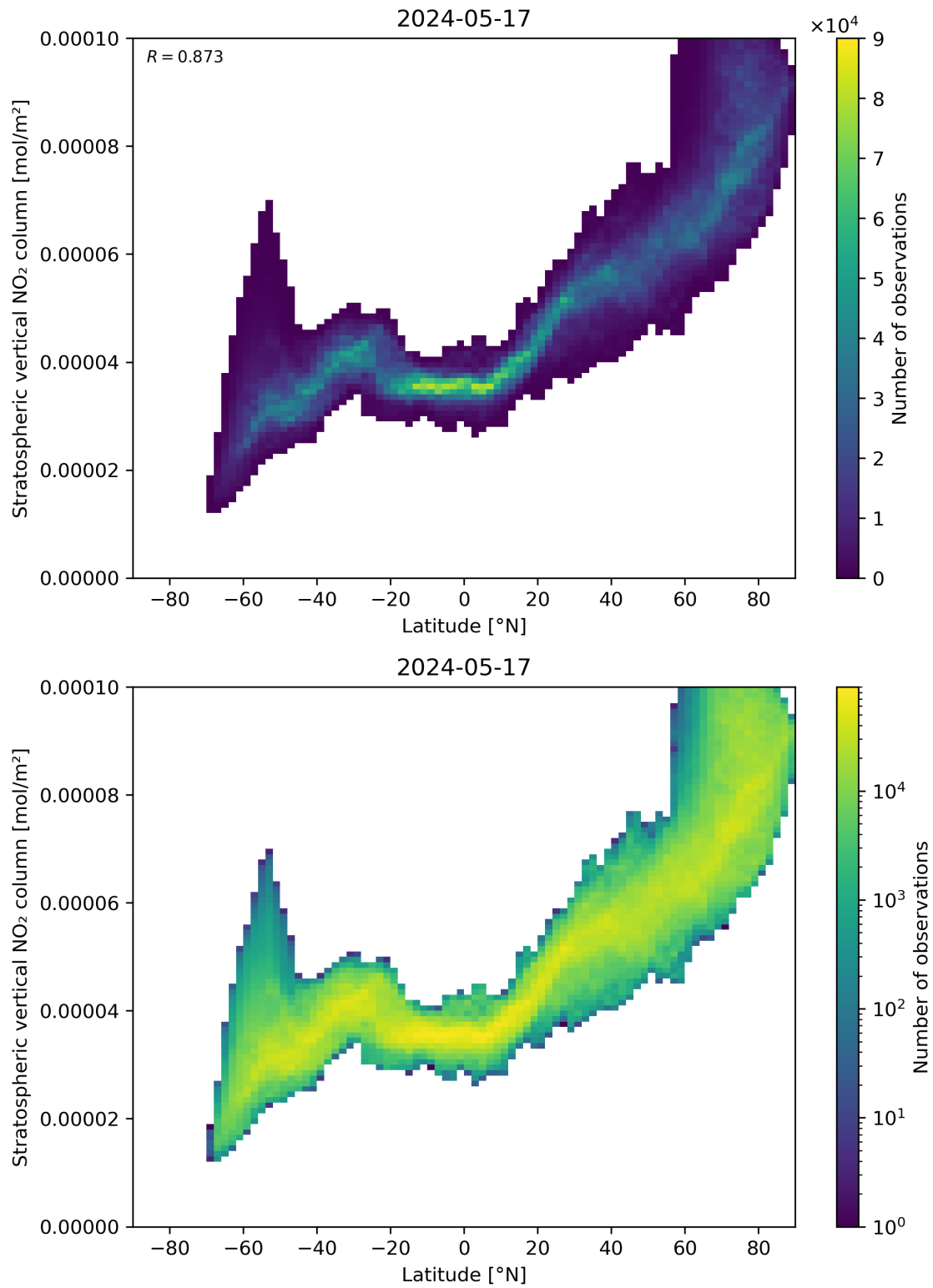
Figure 87: Scatter density plot of “Latitude” against “Stratospheric vertical NO 2 column” for 2024-05-16 to 2024-05-18.
