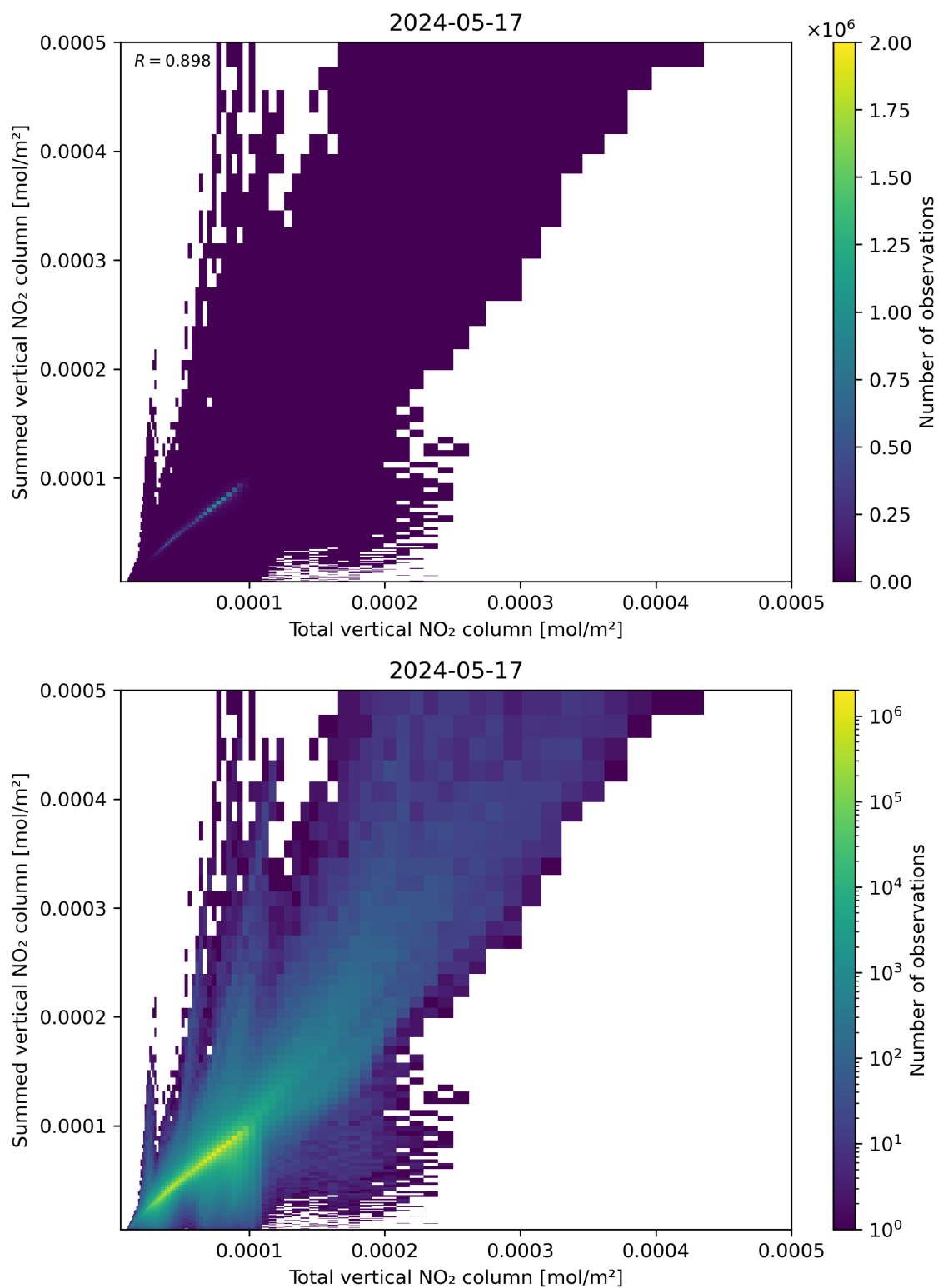
Figure 112: Scatter density plot of “Total vertical NO 2 column” against “Summed vertical NO 2 column” for 2024-05-16 to 2024-05-18.
