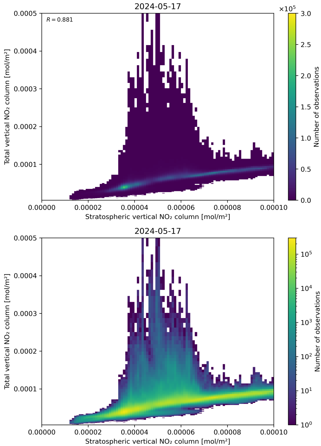
Figure 100: Scatter density plot of “Stratospheric vertical NO 2 column” against “Total vertical NO 2 column” for 2024-05-16 to 2024-05-18.
