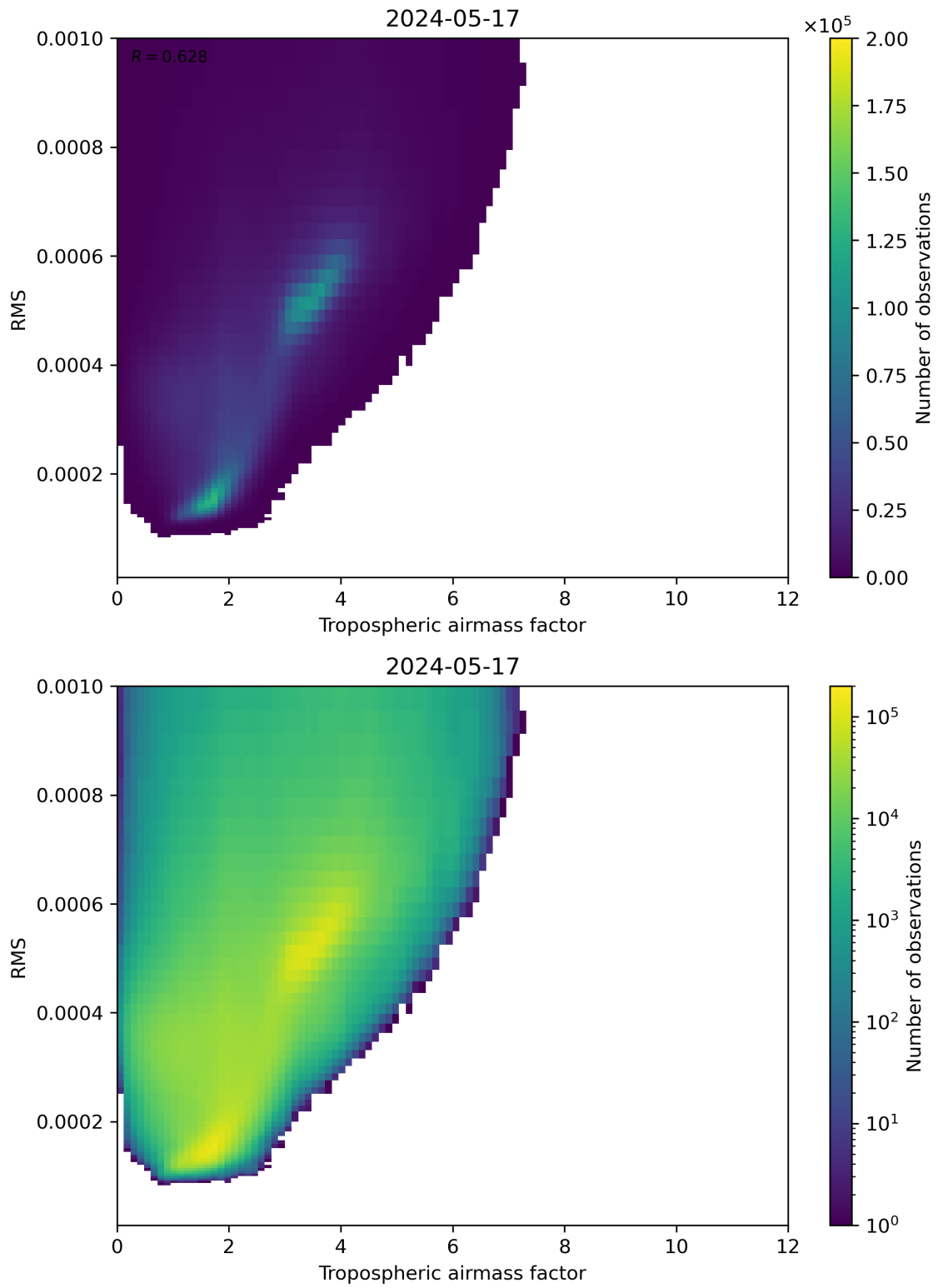
Figure 79: Scatter density plot of “Tropospheric airmass factor” against “RMS” for 2024-05-16 to 2024-05-18.
