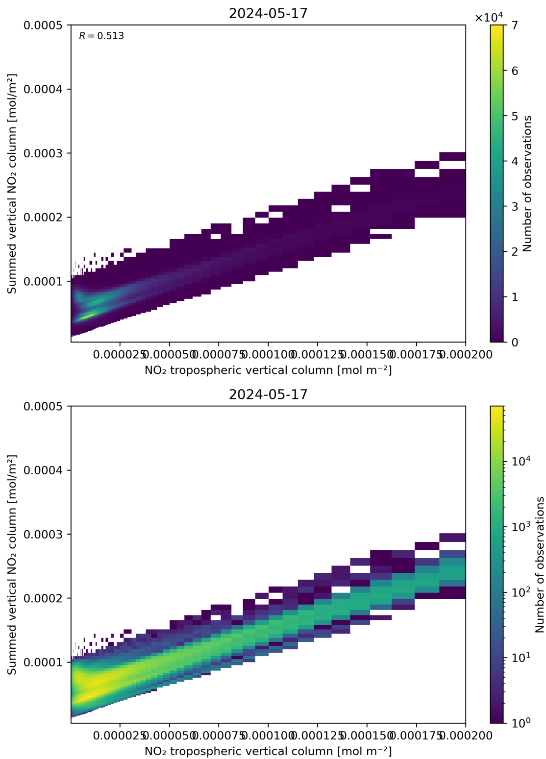
Figure 126: Scatter density plot of “NO 2 tropospheric vertical column” against “Summed vertical NO 2 column” for 2024-05-16 to 2024-05-18.
