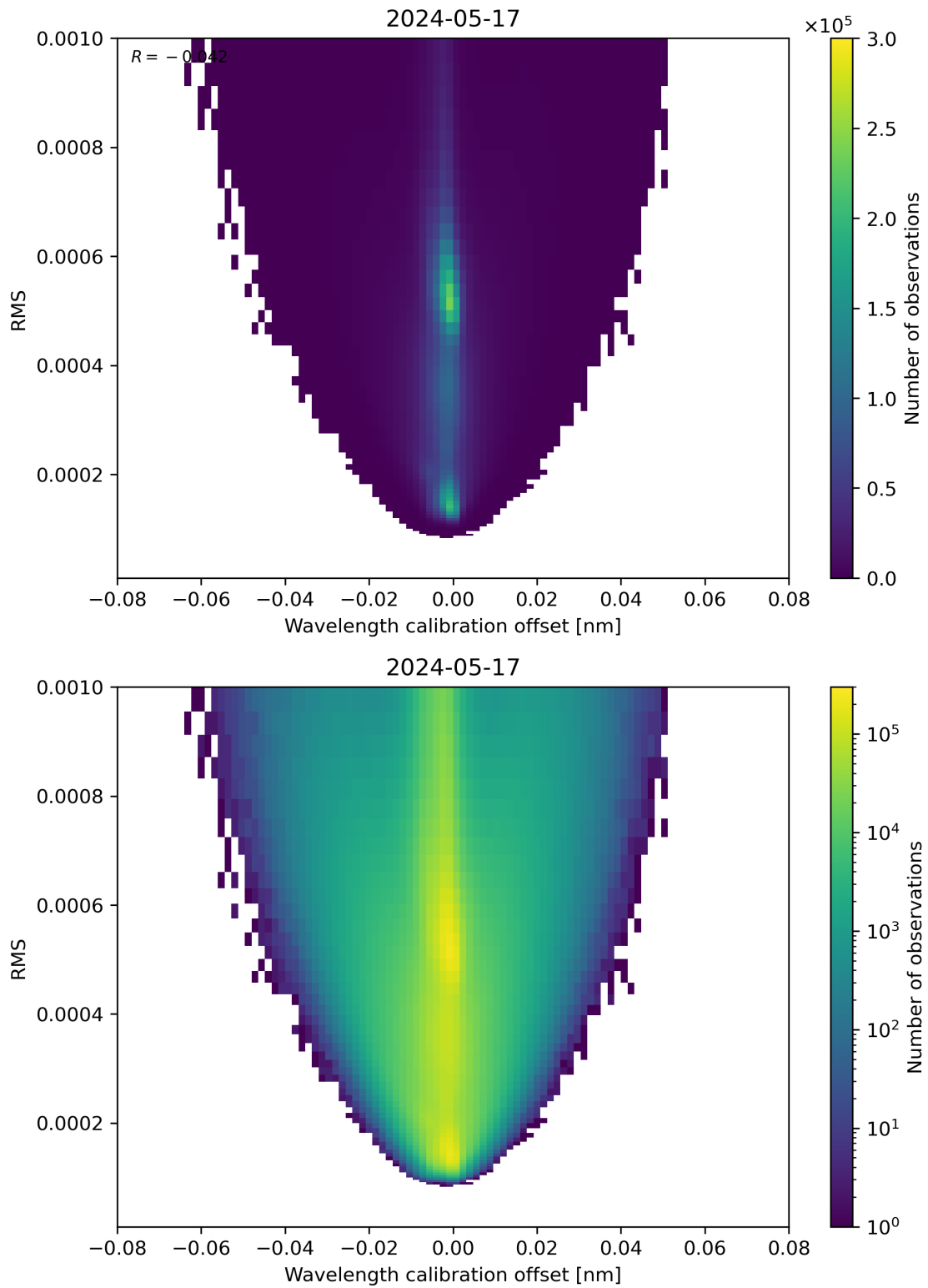
Figure 181: Scatter density plot of “Wavelength calibration offset” against “RMS” for 2024-05-16 to 2024-05-18.
