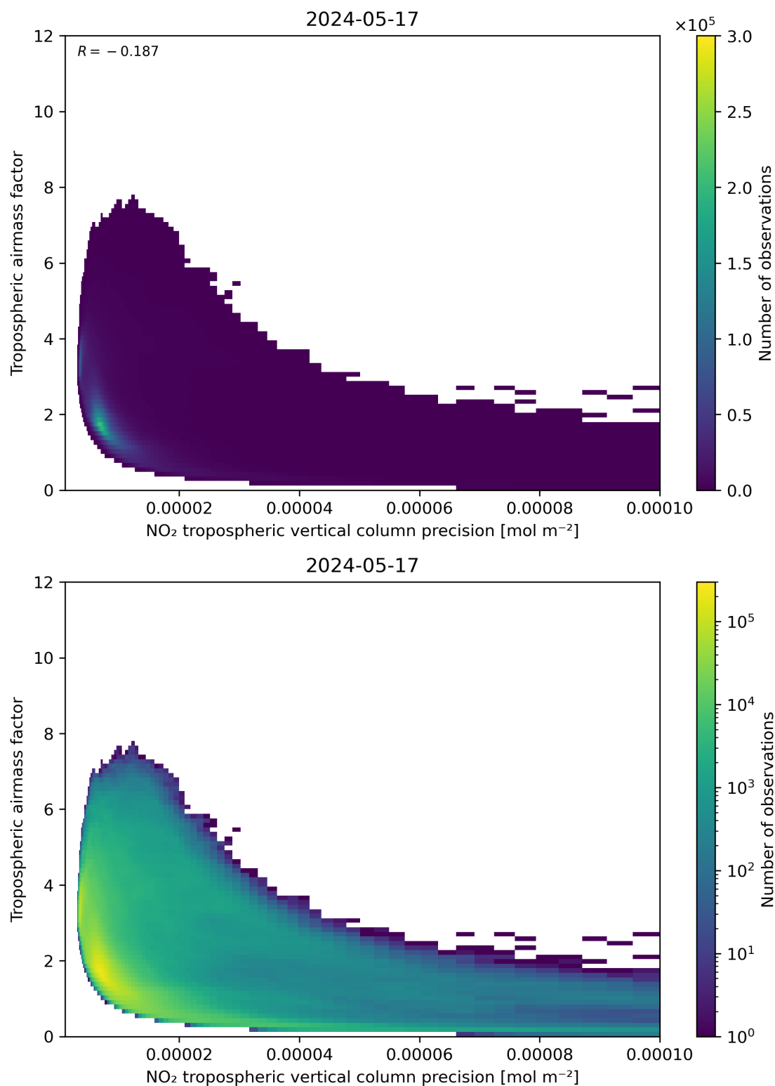
Figure 133: Scatter density plot of “NO 2 tropospheric vertical column precision” against “Tropospheric airmass factor” for 2024-05-16 to 2024-05-18.
