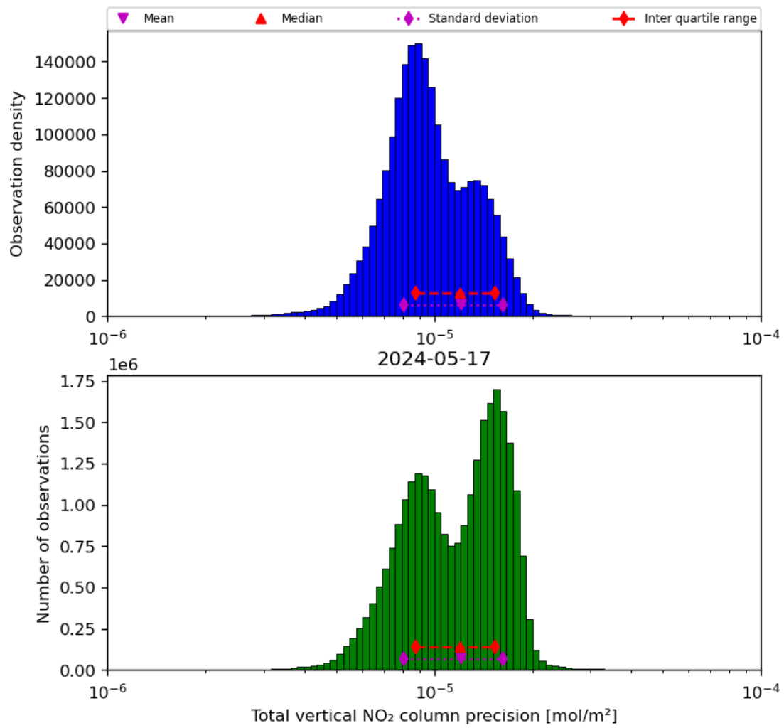
Figure 39: Histogram of “Total vertical NO 2 column precision” for 2024-05-16 to 2024-05-18
