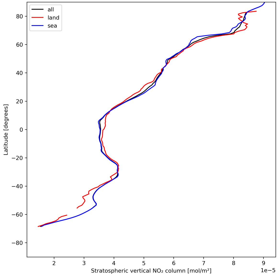
Figure 19: Zonal average of “Stratospheric vertical NO 2 column” for 2024-05-16 to 2024-05-18.
