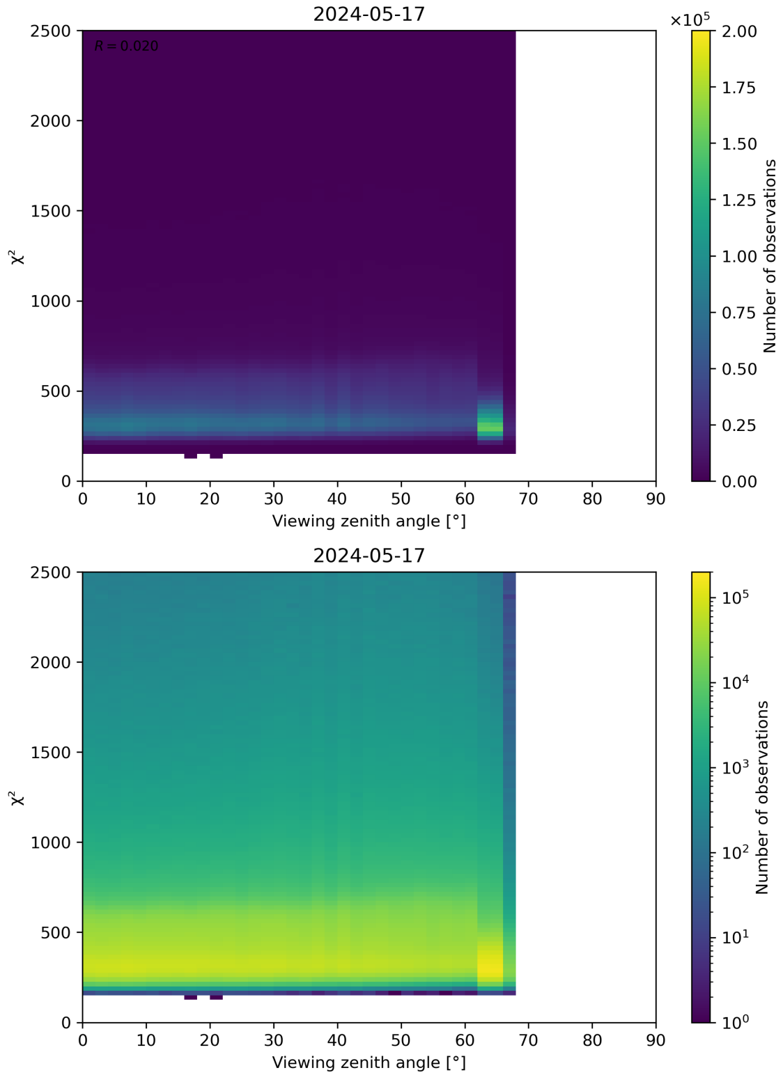
Figure 162: Scatter density plot of “Viewing zenith angle” against “ \chi^2 ” for 2024-05-16 to 2024-05-18.
