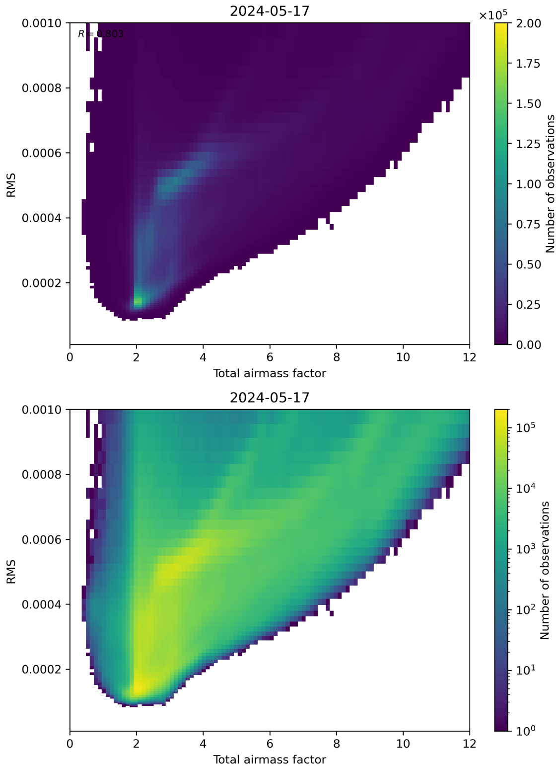
Figure 69: Scatter density plot of “Total airmass factor” against “RMS” for 2024-05-16 to 2024-05-18.
