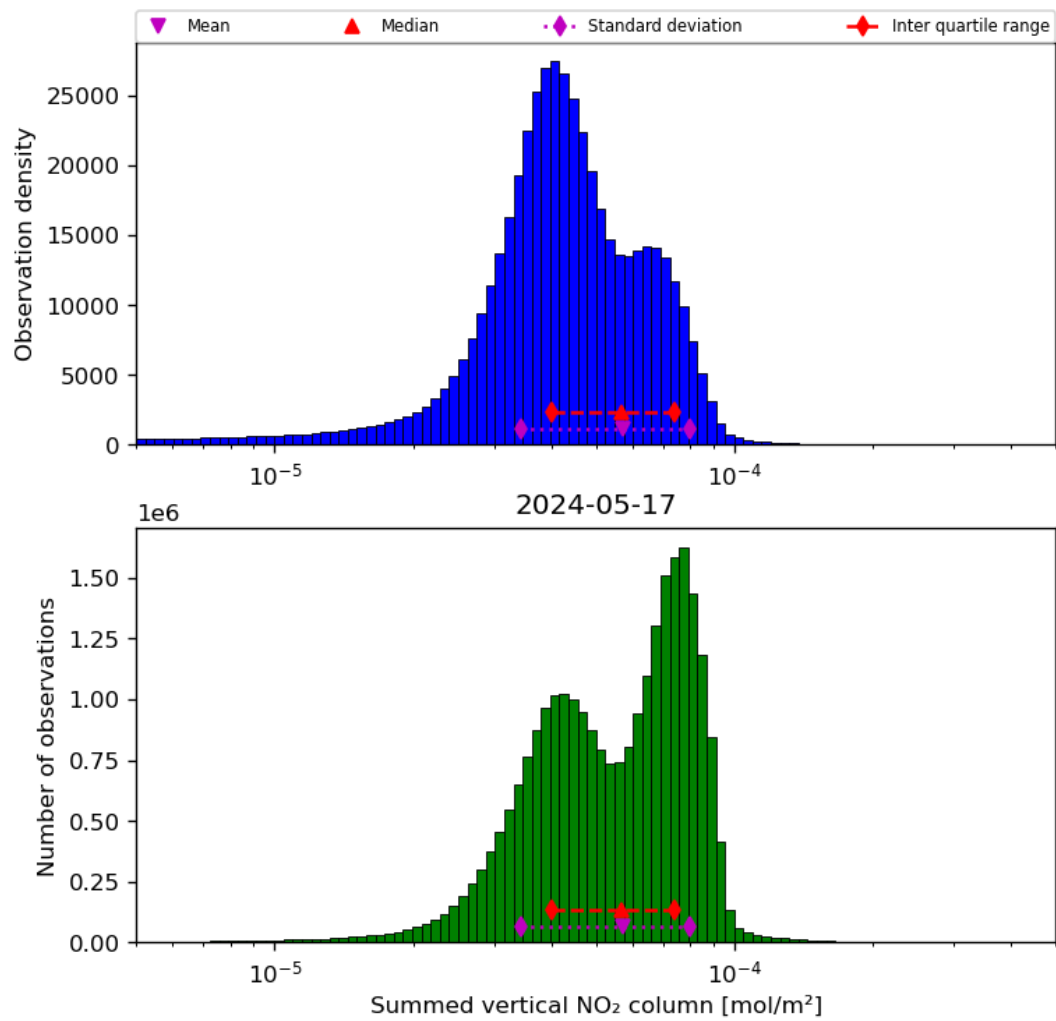
Figure 40: Histogram of “Summed vertical NO 2 column” for 2024-05-16 to 2024-05-18
