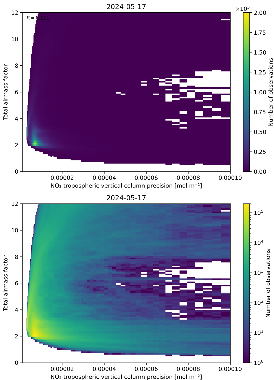
Figure 132: Scatter density plot of “NO 2 tropospheric vertical column precision” against “Total air mass factor” for 2024-05-16 to 2024-05-18.
