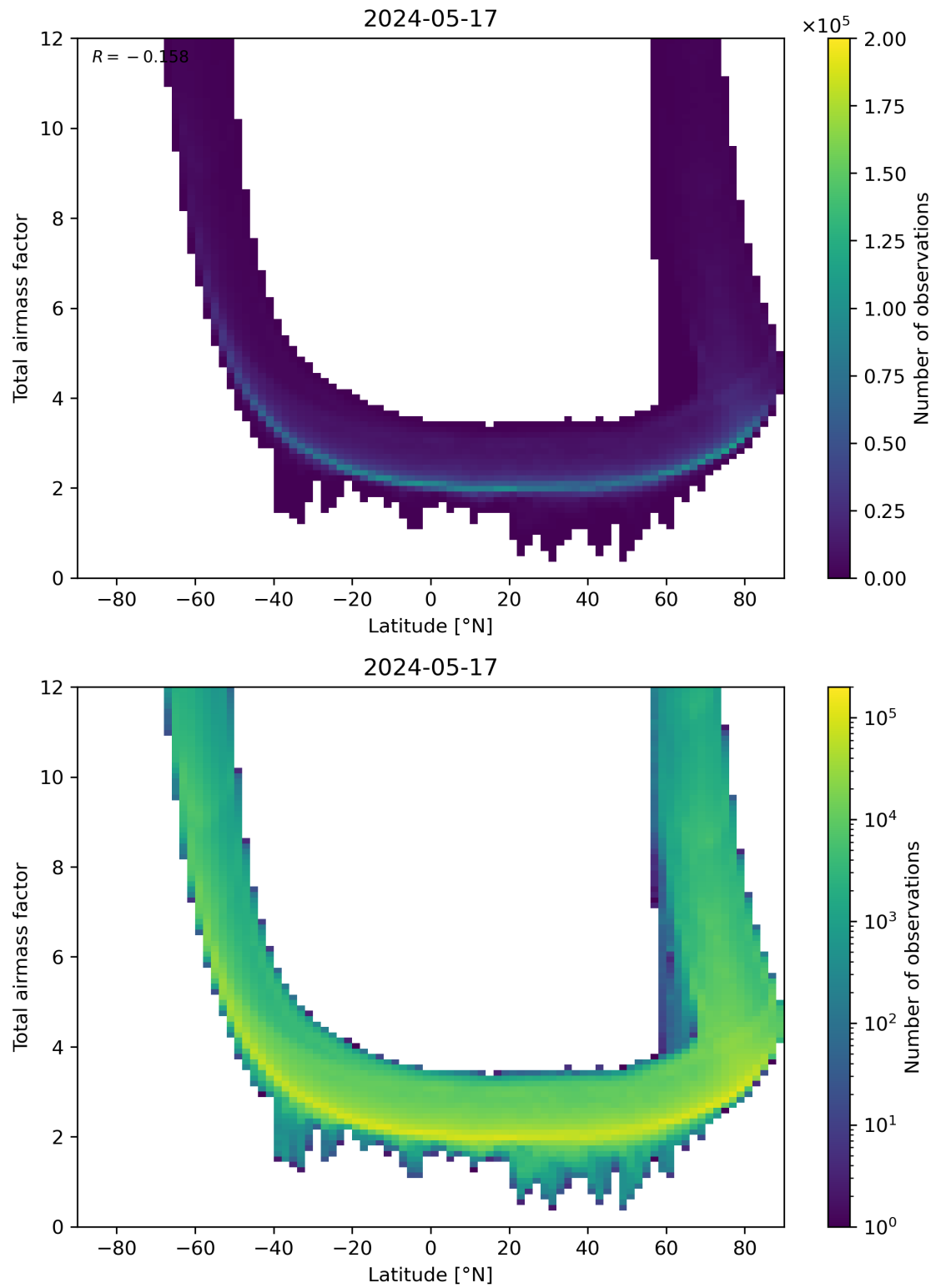
Figure 84: Scatter density plot of “Latitude” against “Total airmass factor” for 2024-05-16 to 2024-05-18.
