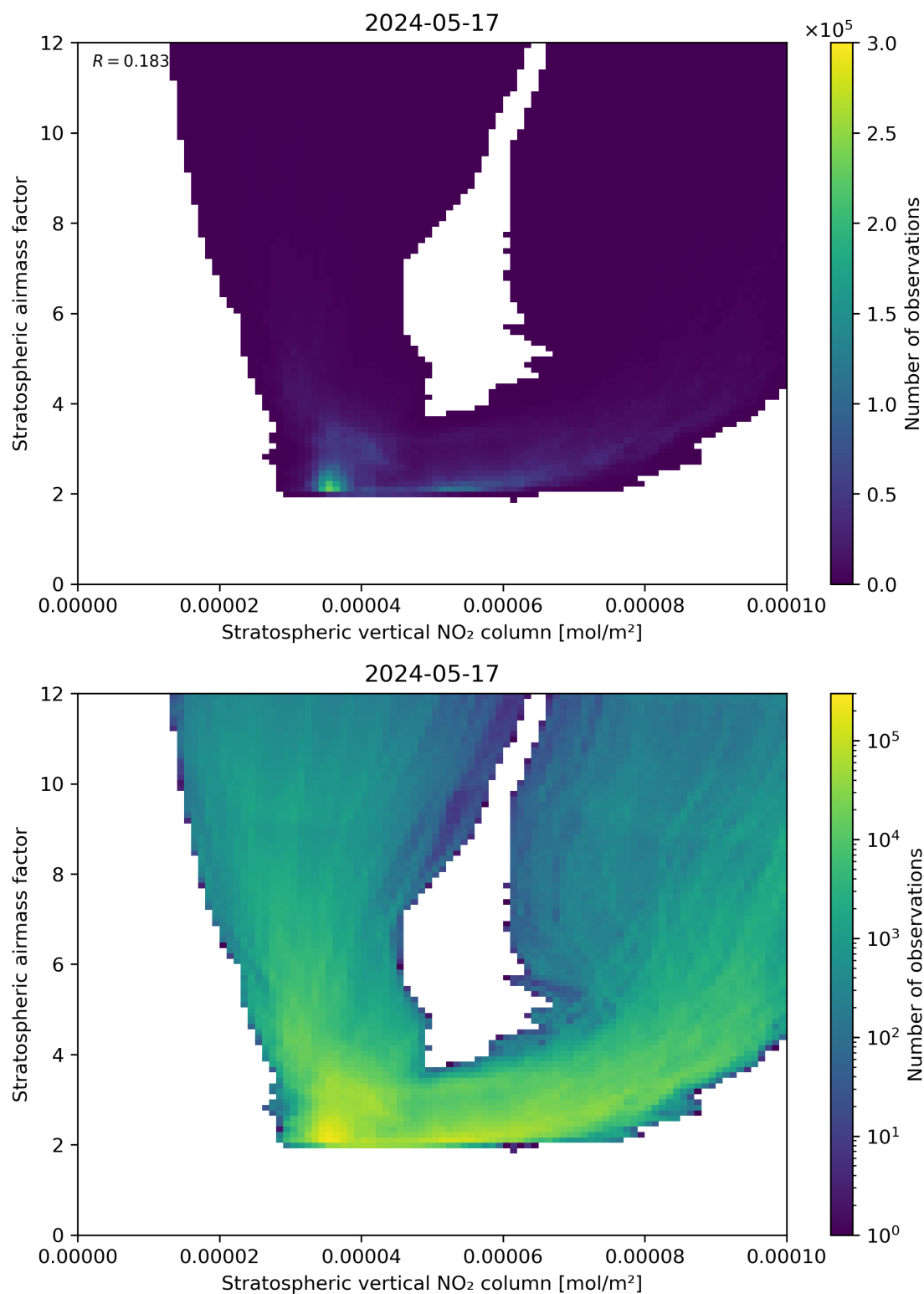
Figure 96: Scatter density plot of “Stratospheric vertical NO 2 column” against “Stratospheric airmass factor” for 2024-05-16 to 2024-05-18.
