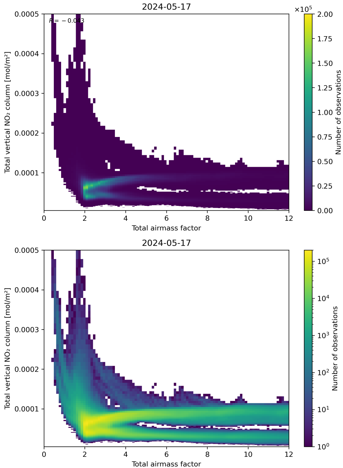
Figure 67: Scatter density plot of “Total airmass factor” against “Total vertical NO 2 column” for 2024-05-16 to 2024-05-18.
