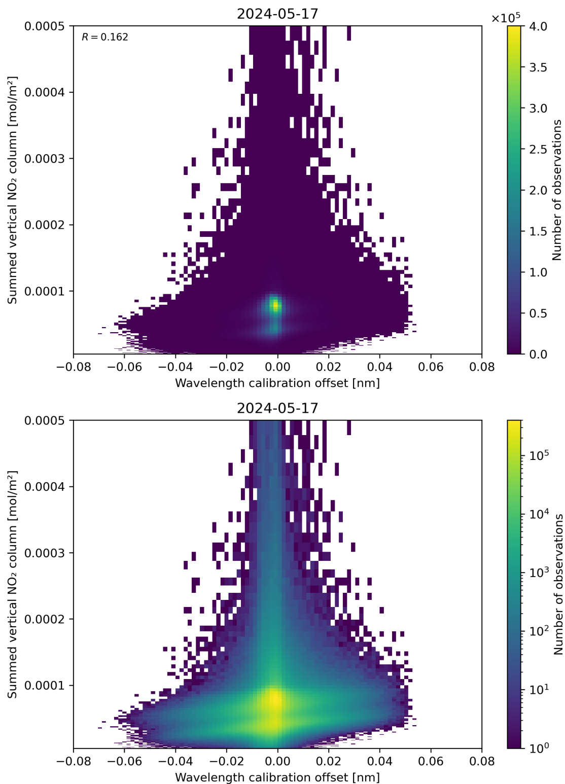
Figure 177: Scatter density plot of “Wavelength calibration offset” against “Summed vertical NO 2 column” for 2024-05-16 to 2024-05-18.
