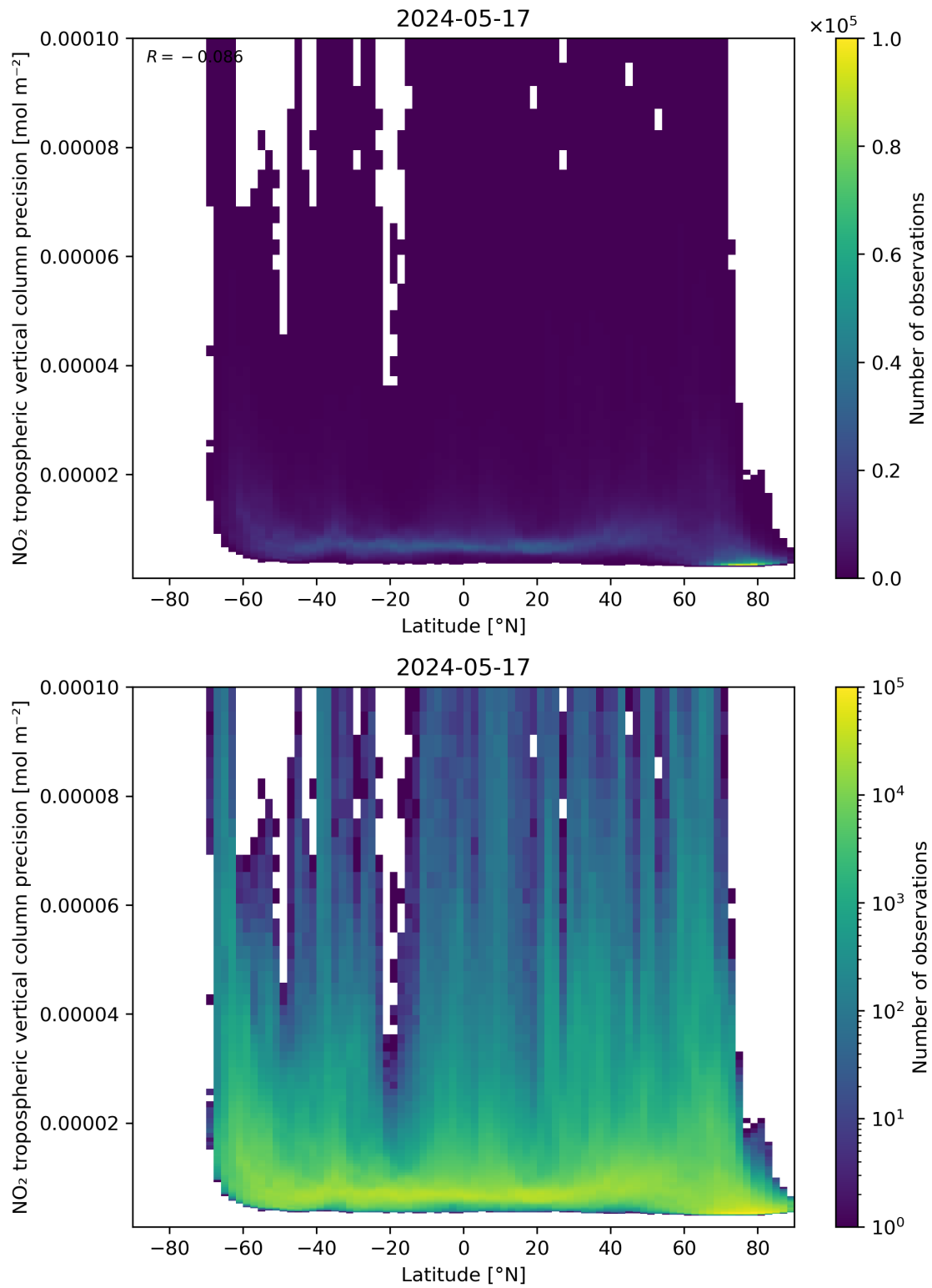
Figure 93: Scatter density plot of “Latitude” against “NO 2 tropospheric vertical column precision” for 2024-05-16 to 2024-05-18.
