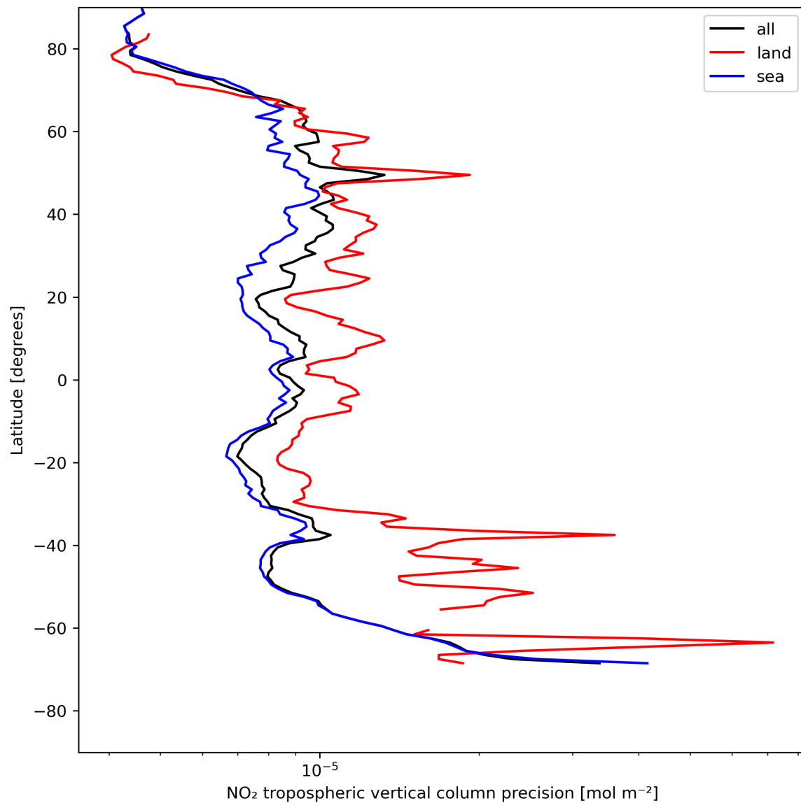
Figure 13: Zonal average of “NO 2 tropospheric vertical column precision” for 2024-05-16 to 2024-05-18.
