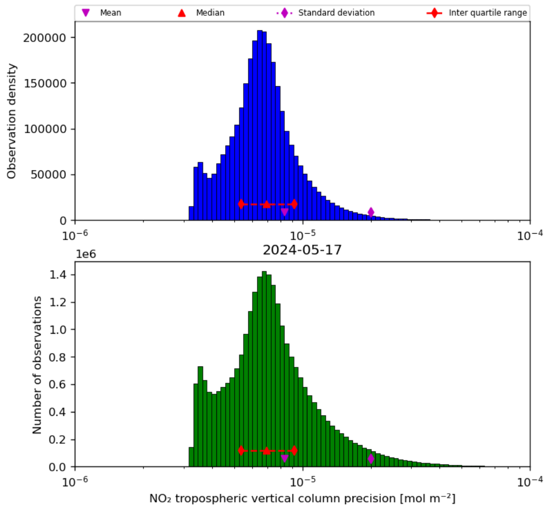
Figure 30: Histogram of “NO 2 tropospheric vertical column precision” for 2024-05-16 to 2024-05-18
