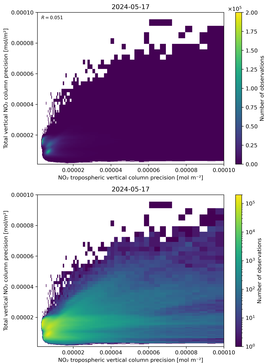
Figure 139: Scatter density plot of “NO 2 tropospheric vertical column precision” against “Total vertical NO 2 column precision” for 2024-05-16 to 2024-05-18.
