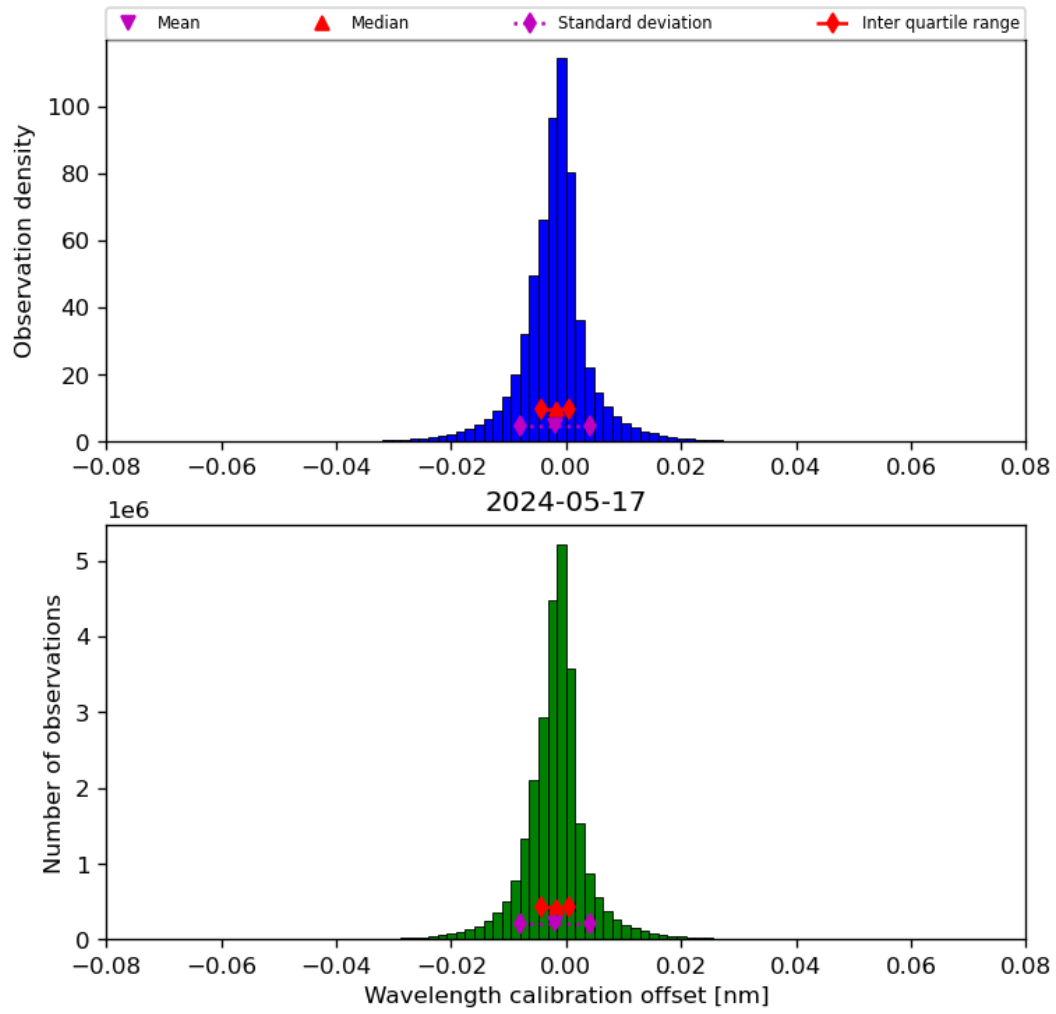
Figure 35: Histogram of “Wavelength calibration offset” for 2024-05-16 to 2024-05-18
