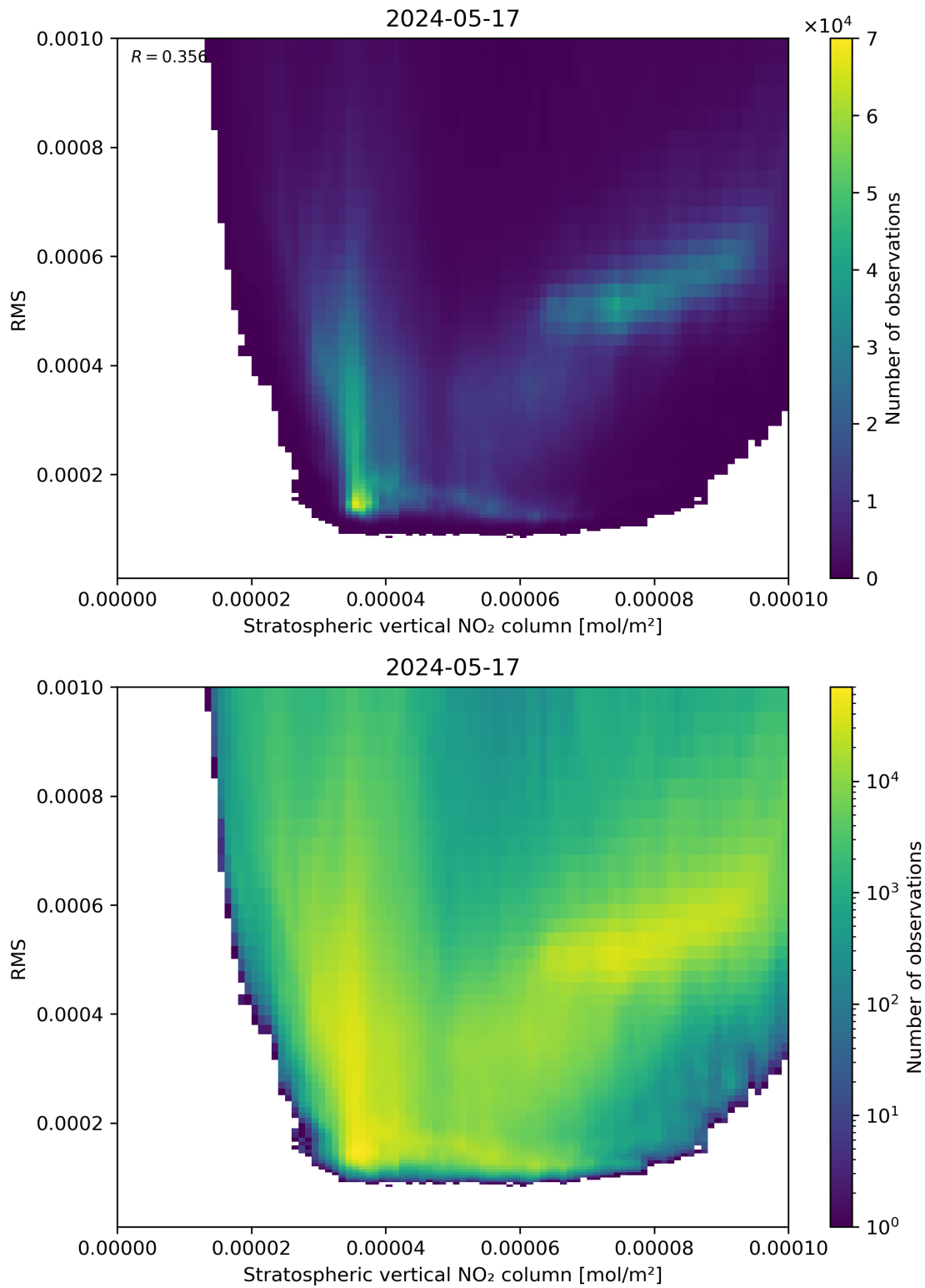
Figure 102: Scatter density plot of “Stratospheric vertical NO 2 column” against “RMS” for 2024-05-16 to 2024-05-18.
