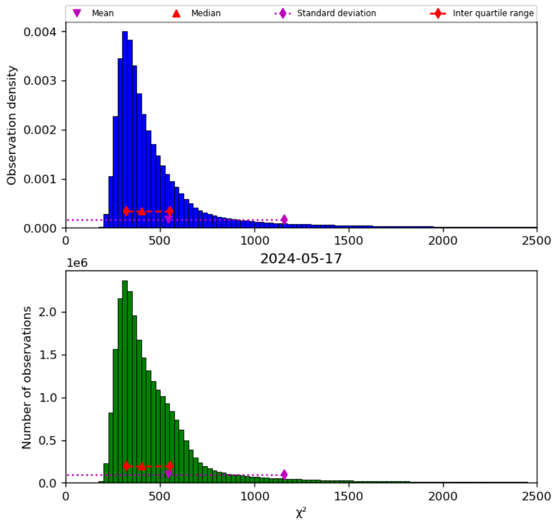
Figure 42: Histogram of “ \chi^2 ” for 2024-05-16 to 2024-05-18
