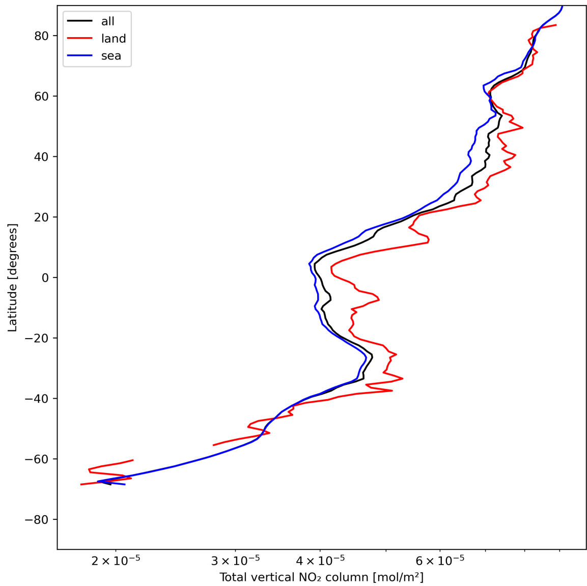
Figure 21: Zonal average of “Total vertical NO 2 column” for 2024-05-16 to 2024-05-18.
