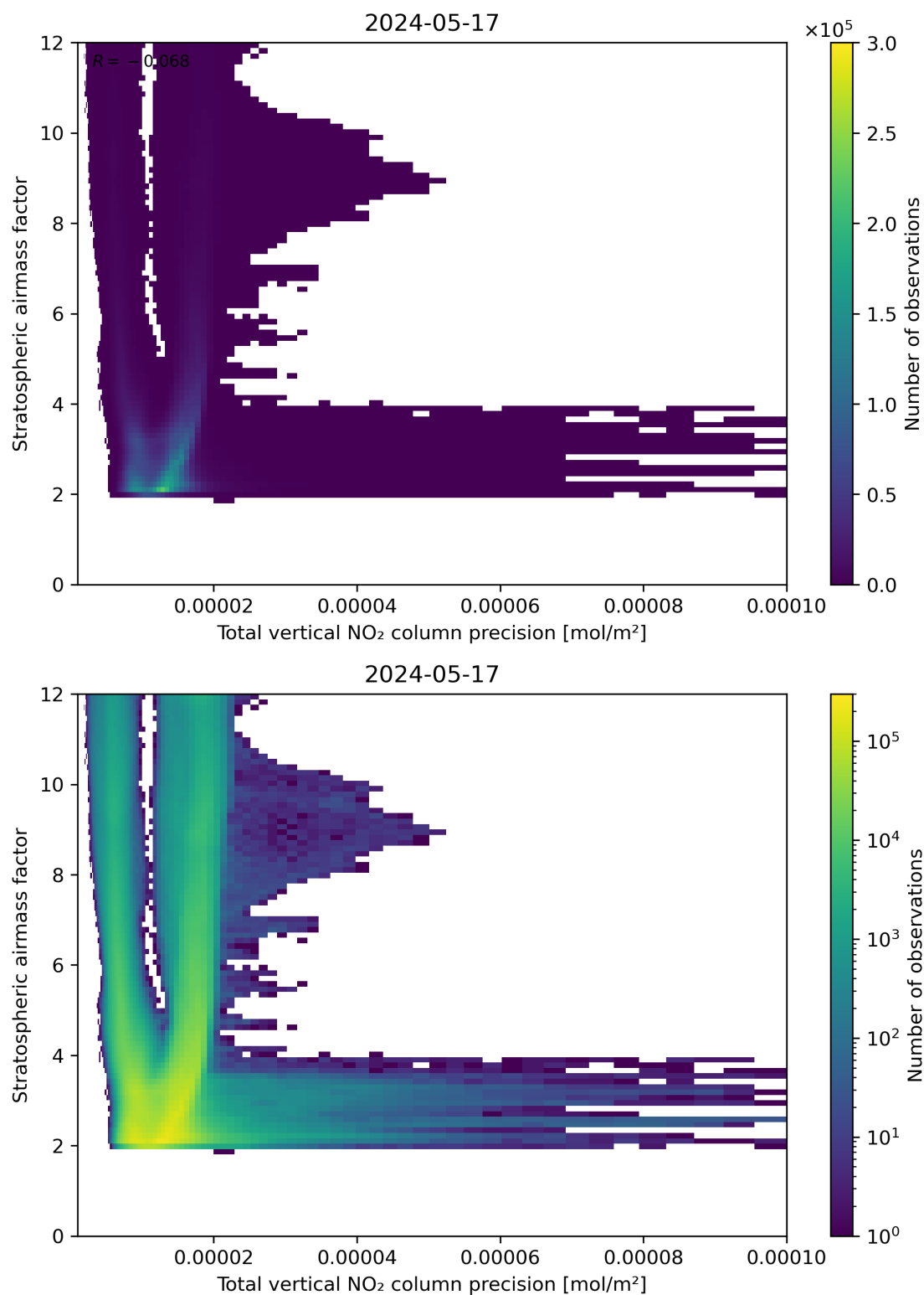
Figure 115: Scatter density plot of “Total vertical NO 2 column precision” against “Stratospheric air mass factor” for 2024-05-16 to 2024-05-18.
