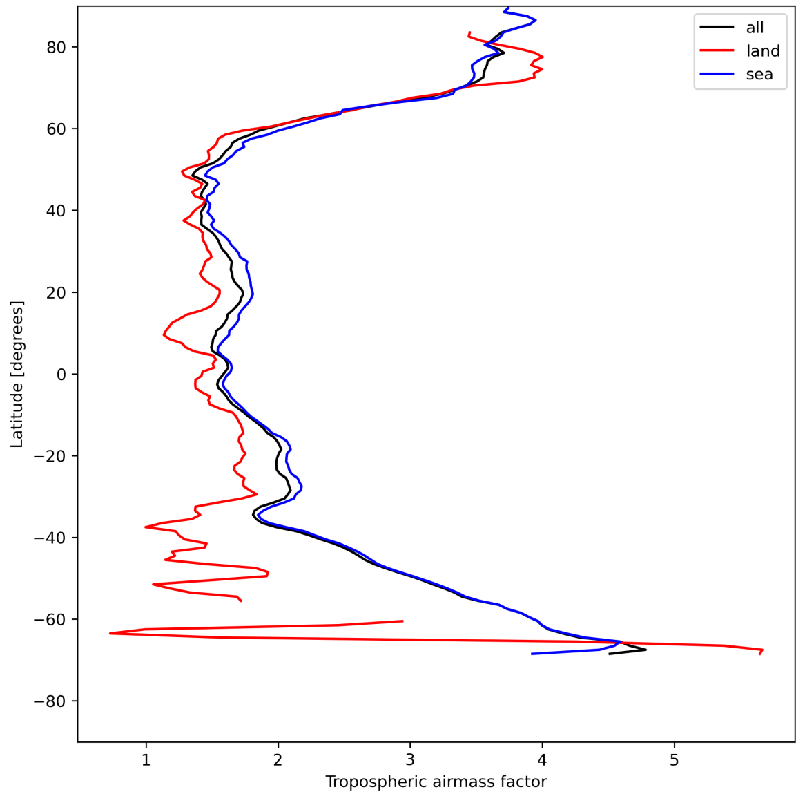
Figure 14: Zonal average of “Tropospheric airmass factor” for 2024-05-16 to 2024-05-18.
