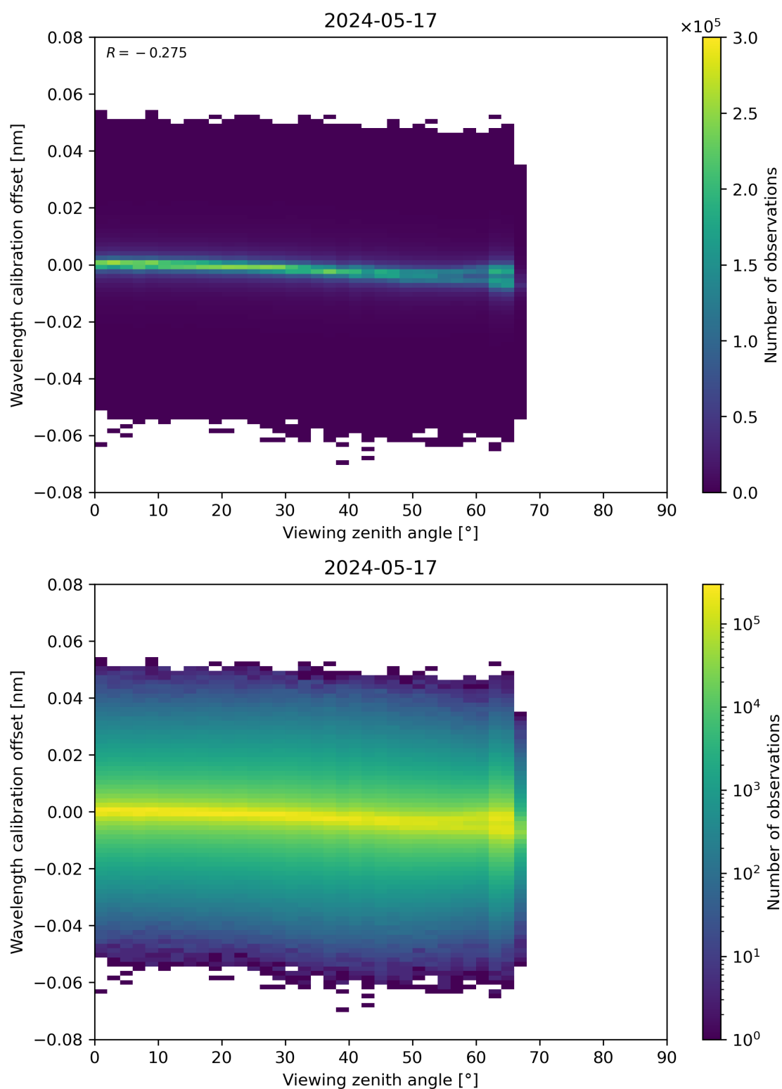
Figure 173: Scatter density plot of “Viewing zenith angle” against “Wavelength calibration offset” for 2024-05-16 to 2024-05-18.
