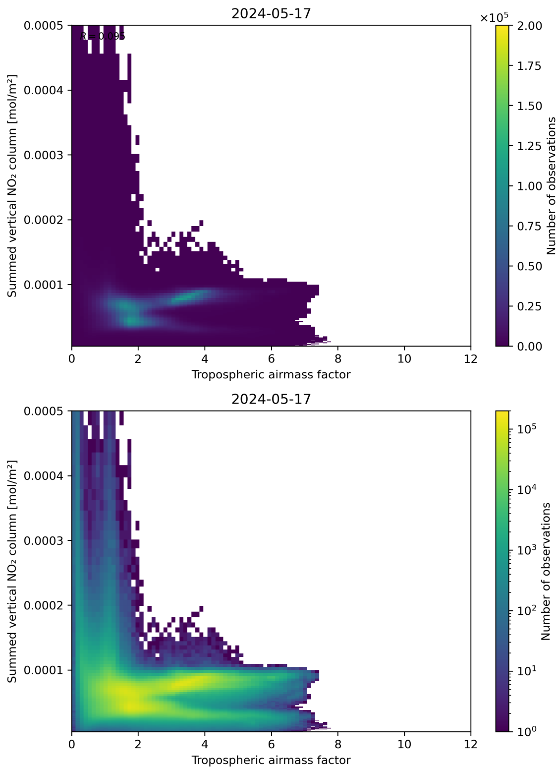
Figure 75: Scatter density plot of “Tropospheric airmass factor” against “Summed vertical NO 2 column” for 2024-05-16 to 2024-05-18.
