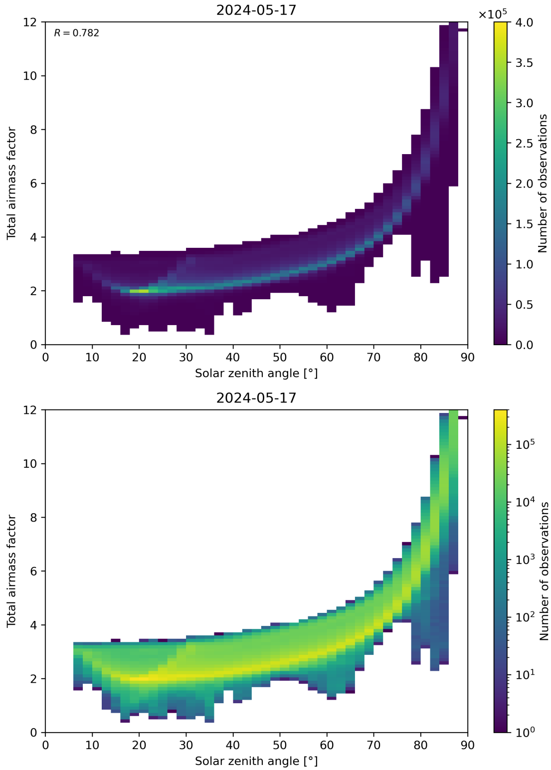
Figure 146: Scatter density plot of “Solar zenith angle” against “Total air mass factor” for 2024-05-16 to 2024-05-18.
