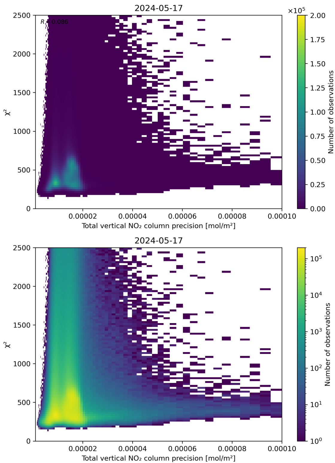
Figure 116: Scatter density plot of “Total vertical NO 2 column precision” against “ \chi^2 ” for 2024-05-16 to 2024-05-18.
