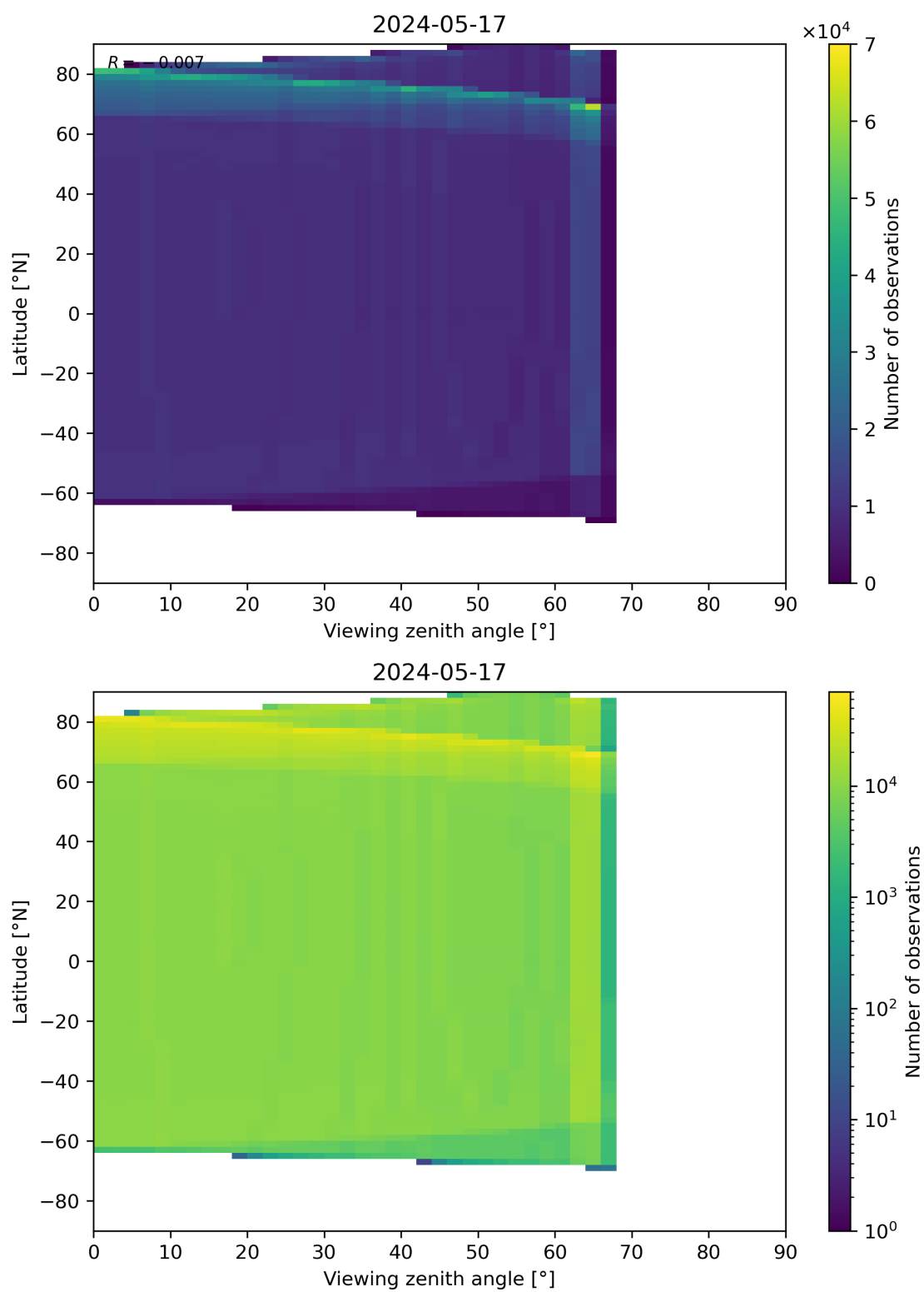
Figure 163: Scatter density plot of “Viewing zenith angle” against “Latitude” for 2024-05-16 to 2024-05-18.
