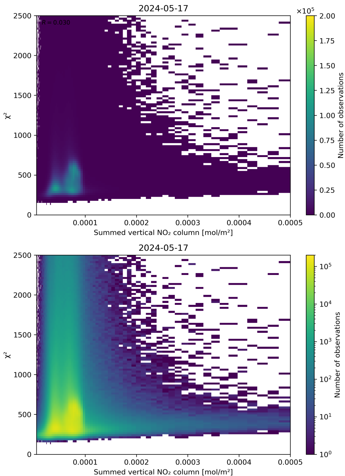
Figure 104: Scatter density plot of “Summed vertical NO 2 column” against “ \chi^2 ” for 2024-05-16 to 2024-05-18.
