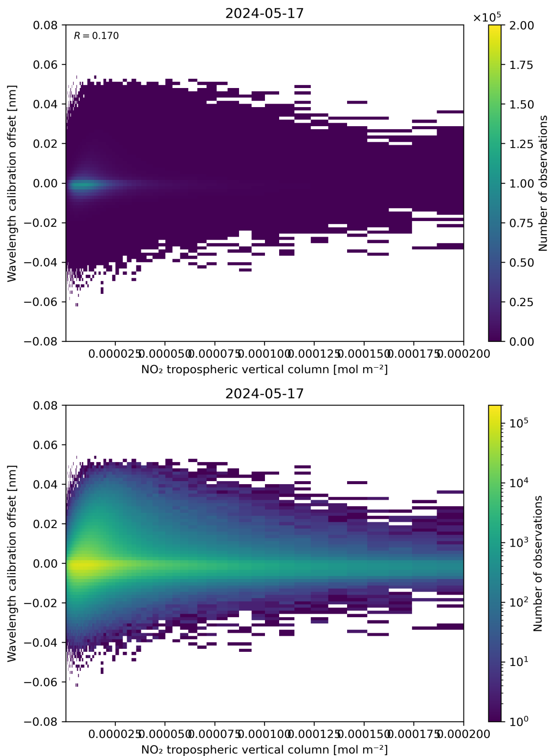
Figure 143: Scatter density plot of “NO 2 tropospheric vertical column” against “Wavelength calibration offset” for 2024-05-16 to 2024-05-18.
