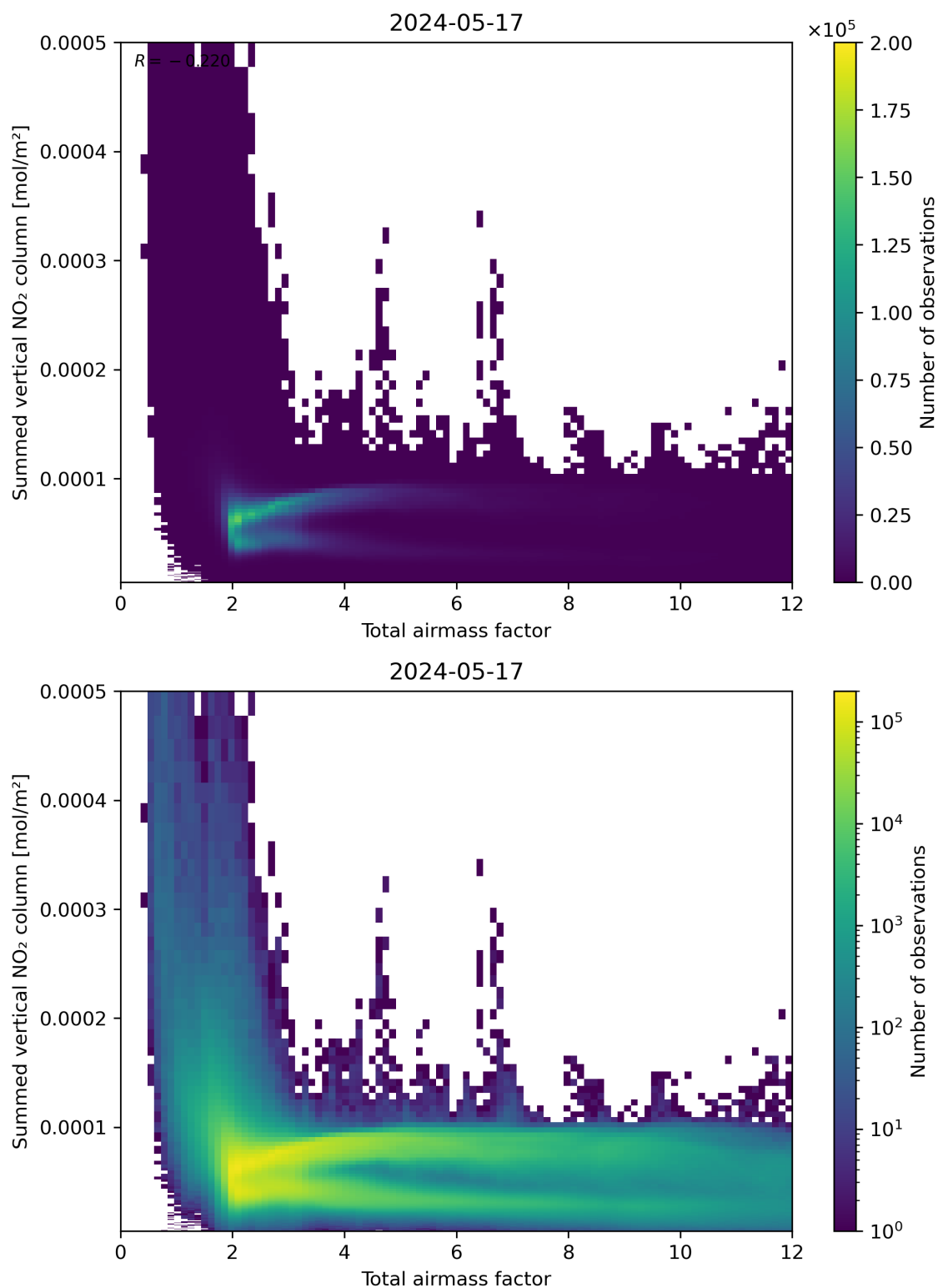
Figure 65: Scatter density plot of “Total airmass factor” against “Summed vertical NO 2 column” for 2024-05-16 to 2024-05-18.
