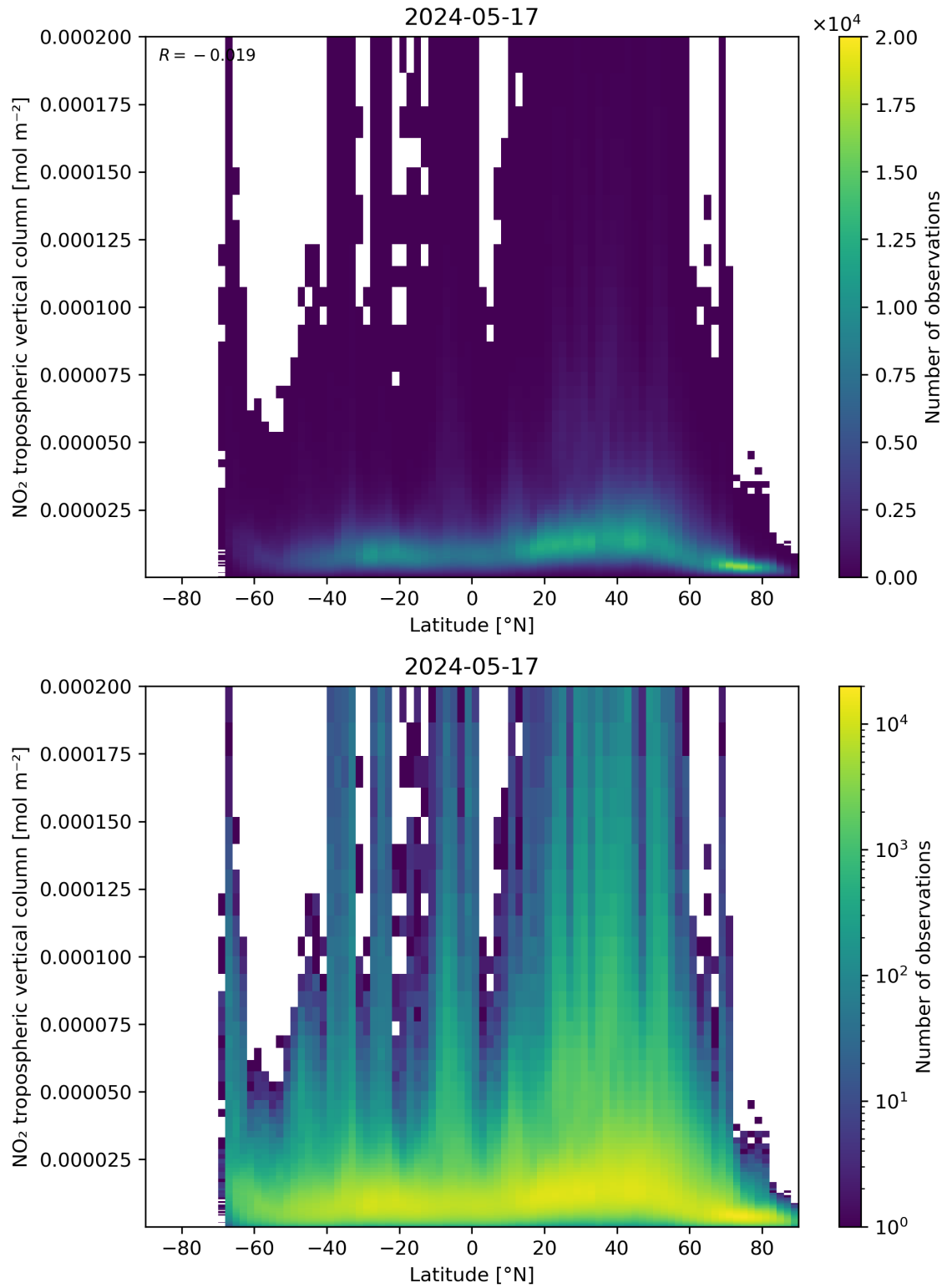
Figure 92: Scatter density plot of “Latitude” against “NO 2 tropospheric vertical column” for 2024-05-16 to 2024-05-18.
