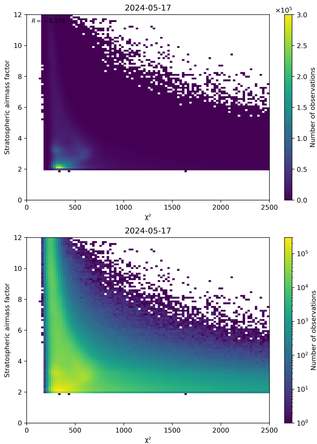
Figure 81: Scatter density plot of “ \chi^2 ” against “Stratospheric airmass factor” for 2024-05-16 to 2024-05-18.
