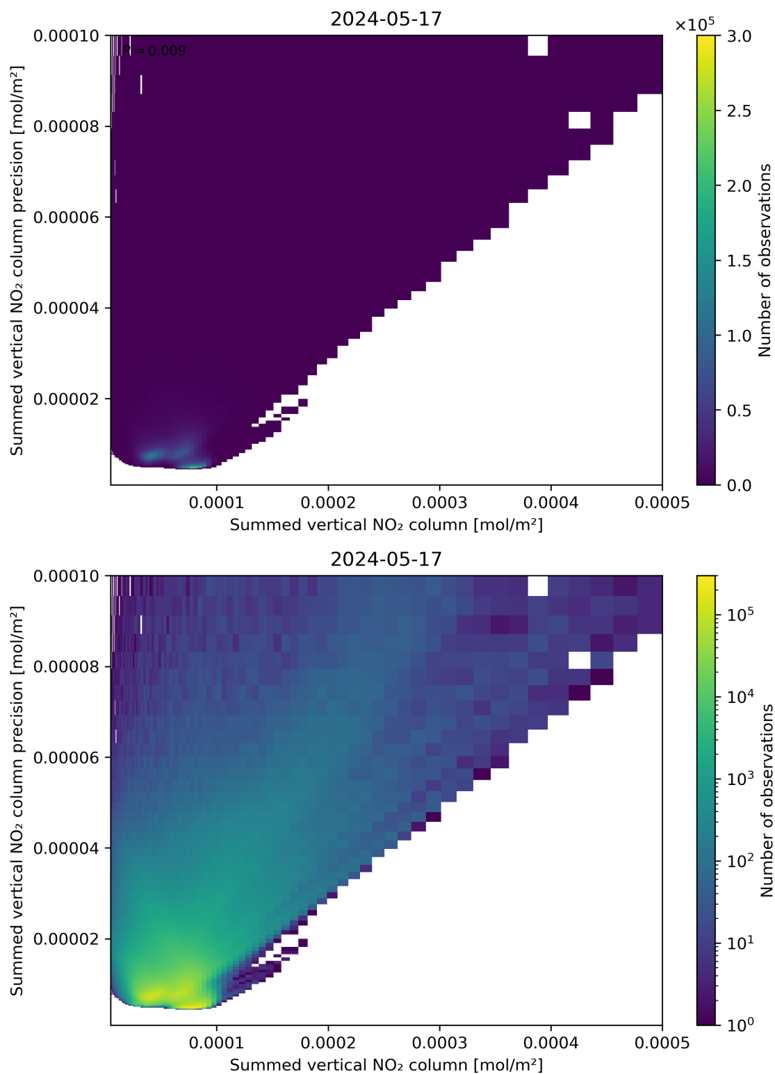
Figure 105: Scatter density plot of “Summed vertical NO 2 column” against “Summed vertical NO 2 column precision” for 2024-05-16 to 2024-05-18.
