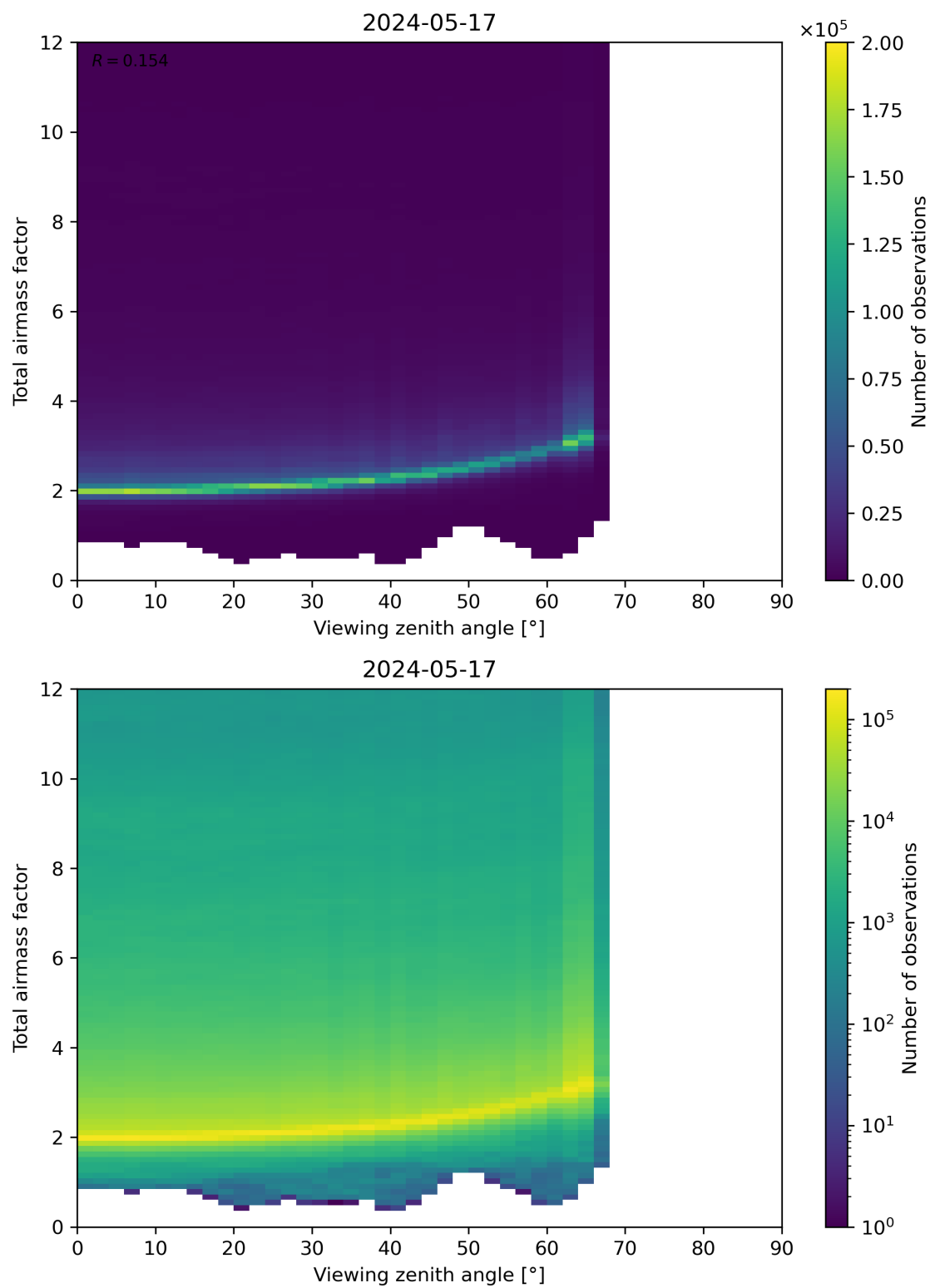
Figure 160: Scatter density plot of “Viewing zenith angle” against “Total airmass factor” for 2024-05-16 to 2024-05-18.
