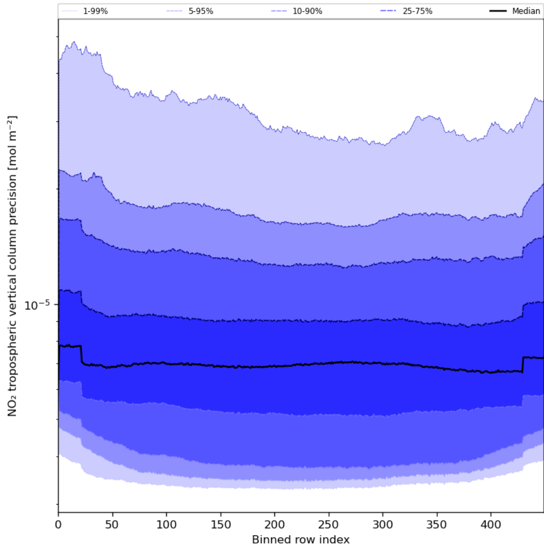
Figure 47: Along track statistics of “NO 2 tropospheric vertical column precision” for 2024-05-16 to 2024-05-18
