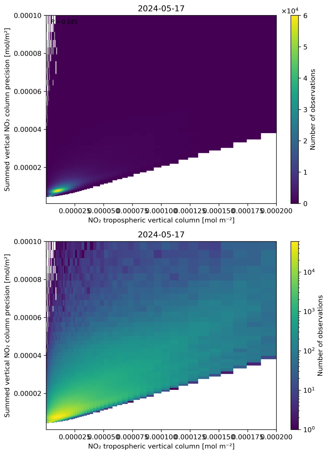
Figure 127: Scatter density plot of “NO 2 tropospheric vertical column” against “Summed vertical NO 2 column precision” for 2024-05-16 to 2024-05-18.
