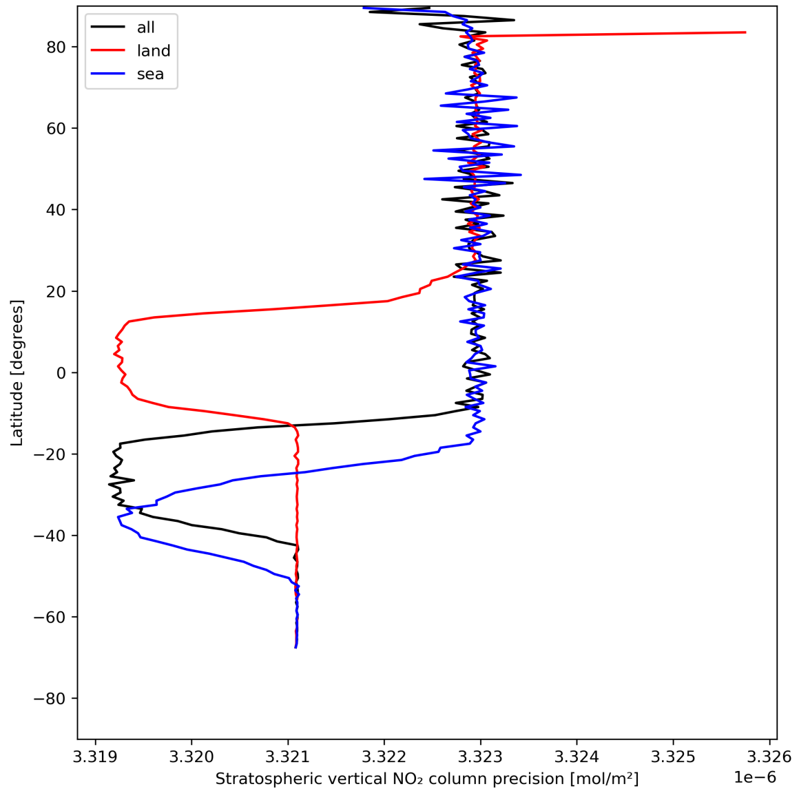
Figure 20: Zonal average of “Stratospheric vertical NO 2 column precision” for 2024-05-18 to 2024-05-19.
