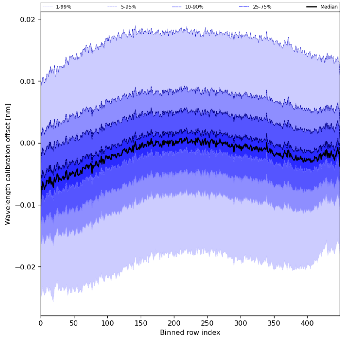
Figure 52: Along track statistics of “Wavelength calibration offset” for 2024-05-18 to 2024-05-19
