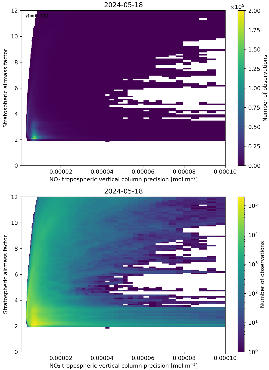
Figure 131: Scatter density plot of “NO 2 tropospheric vertical column precision” against “Stratospheric airmass factor” for 2024-05-18 to 2024-05-19.
