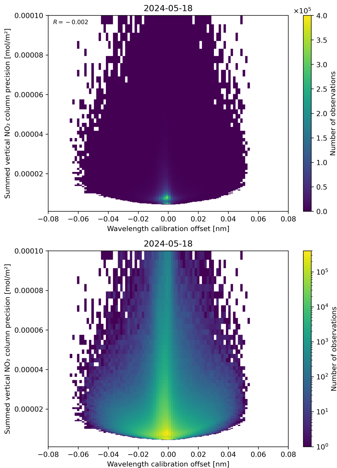
Figure 178: Scatter density plot of “Wavelength calibration offset” against “Summed vertical NO 2 column precision” for 2024-05-18 to 2024-05-19.
