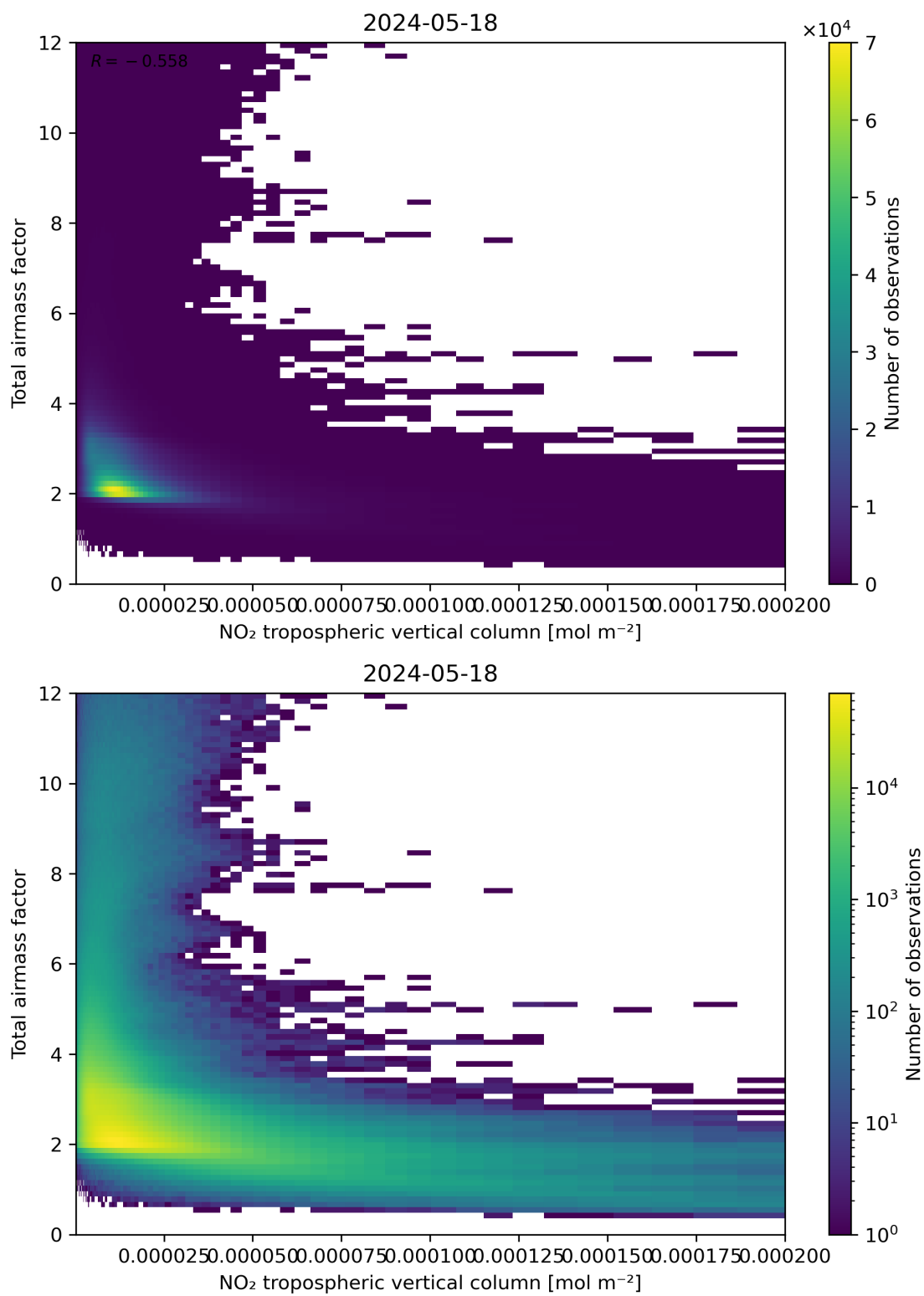
Figure 122: Scatter density plot of “NO 2 tropospheric vertical column” against “Total air mass factor” for 2024-05-18 to 2024-05-19.
