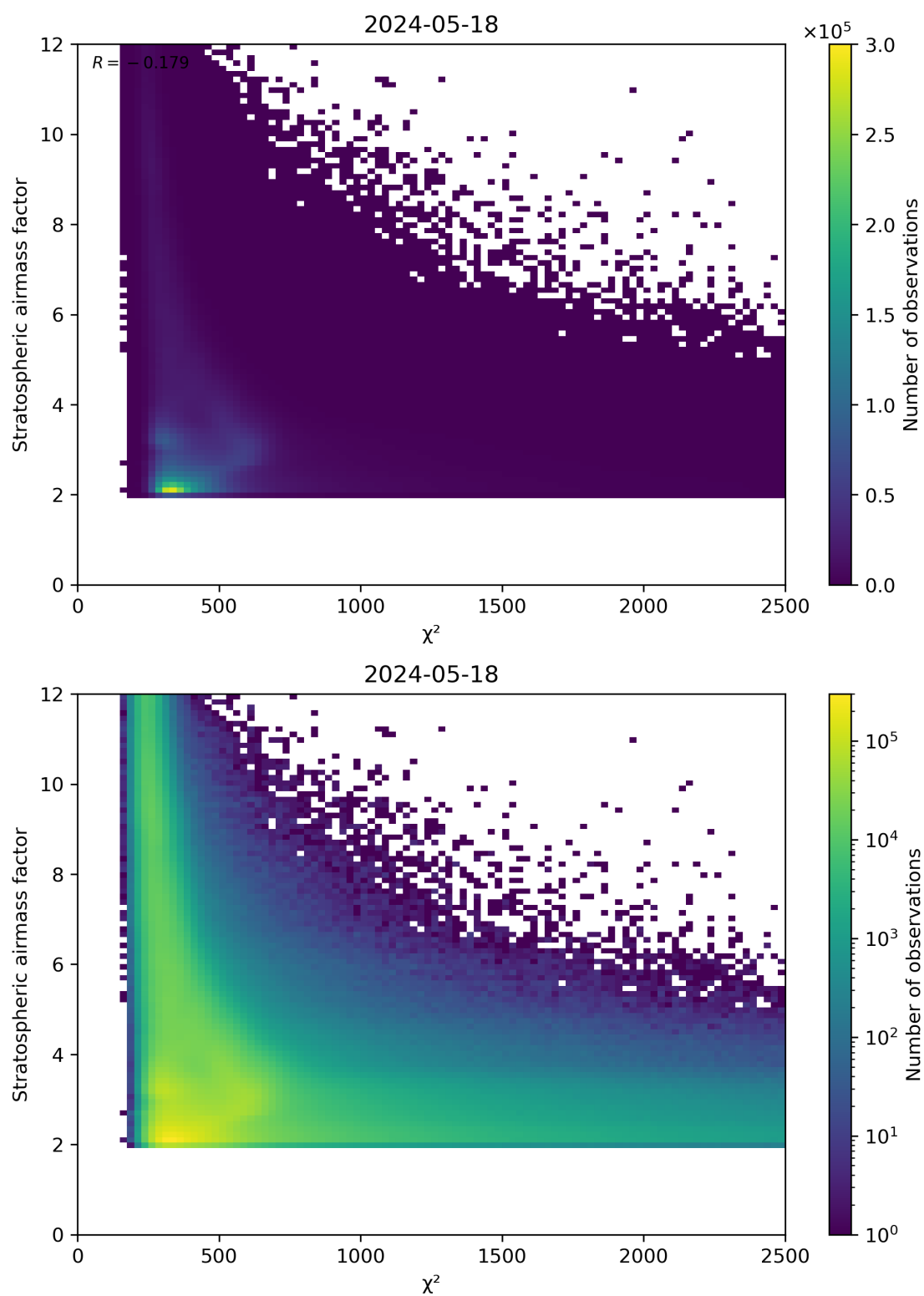
Figure 81: Scatter density plot of “ \chi^2 ” against “Stratospheric air mass factor” for 2024-05-18 to 2024-05-19.
