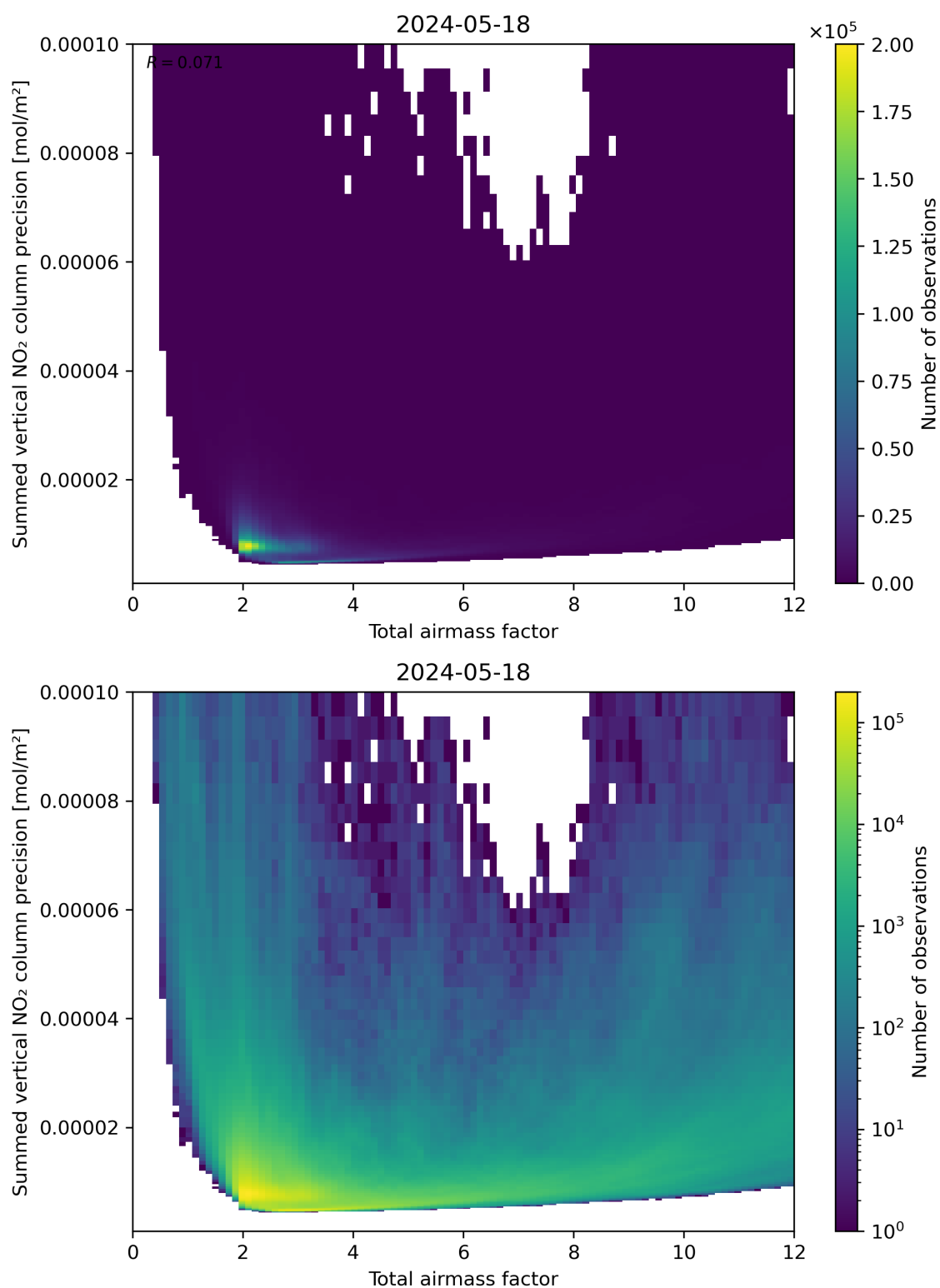
Figure 66: Scatter density plot of “Total airmass factor” against “Summed vertical NO 2 column precision” for 2024-05-18 to 2024-05-19.
