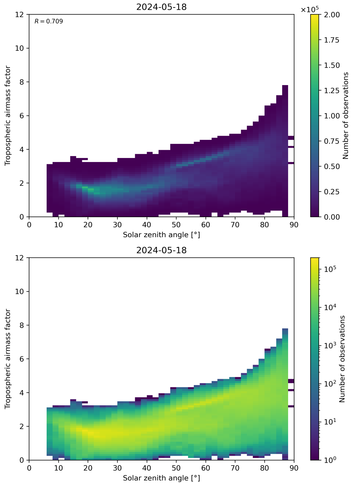
Figure 147: Scatter density plot of “Solar zenith angle” against “Tropospheric airmass factor” for 2024-05-18 to 2024-05-19.
