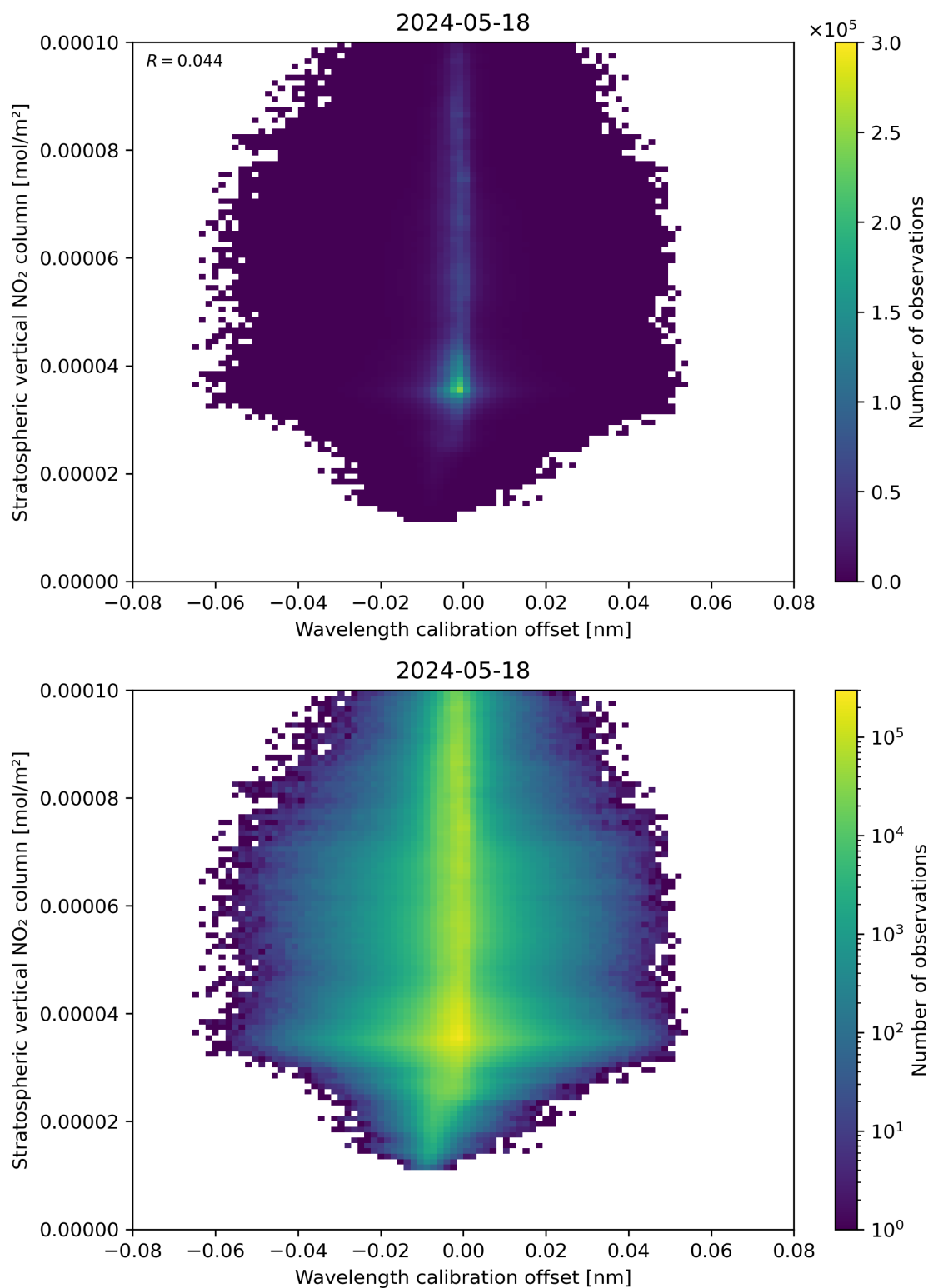
Figure 176: Scatter density plot of “Wavelength calibration offset” against “Stratospheric vertical NO 2 column” for 2024-05-18 to 2024-05-19.
