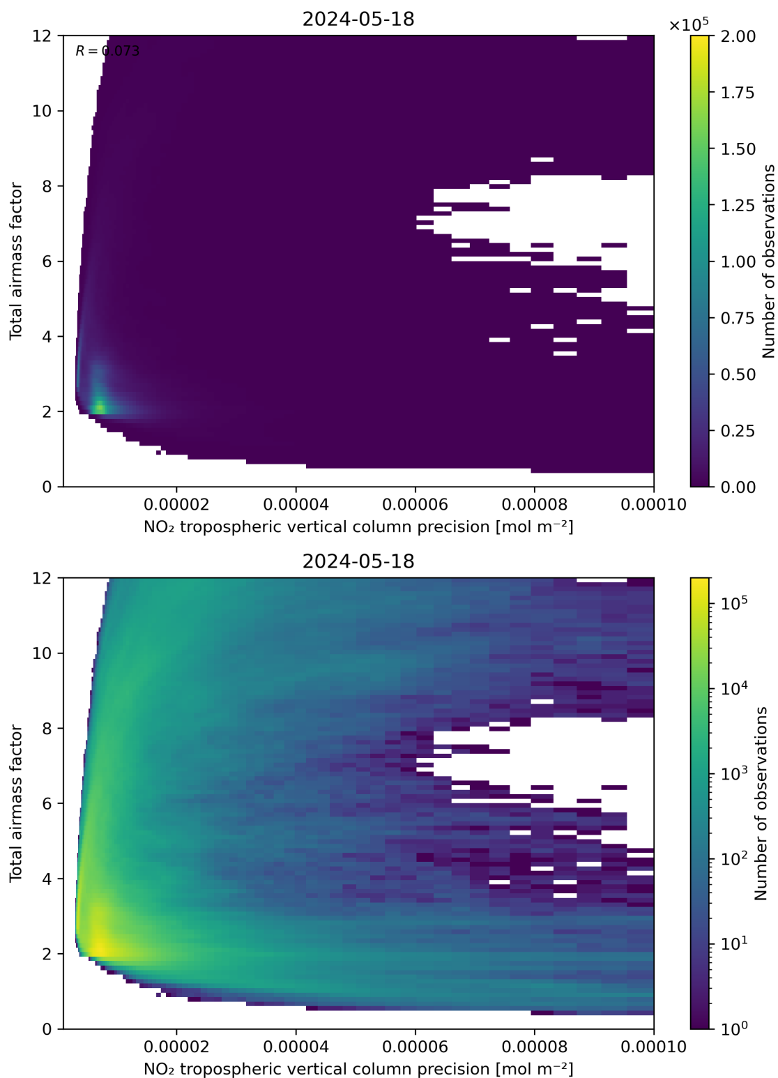
Figure 132: Scatter density plot of “NO 2 tropospheric vertical column precision” against “Total air mass factor” for 2024-05-18 to 2024-05-19.
