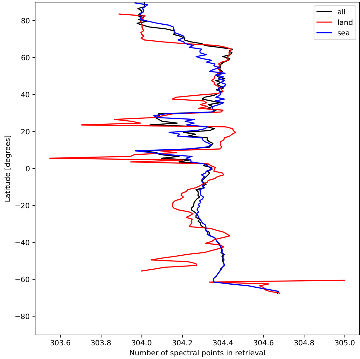
Figure 16: Zonal average of “Number of spectral points in retrieval” for 2024-05-18 to 2024-05-19.
