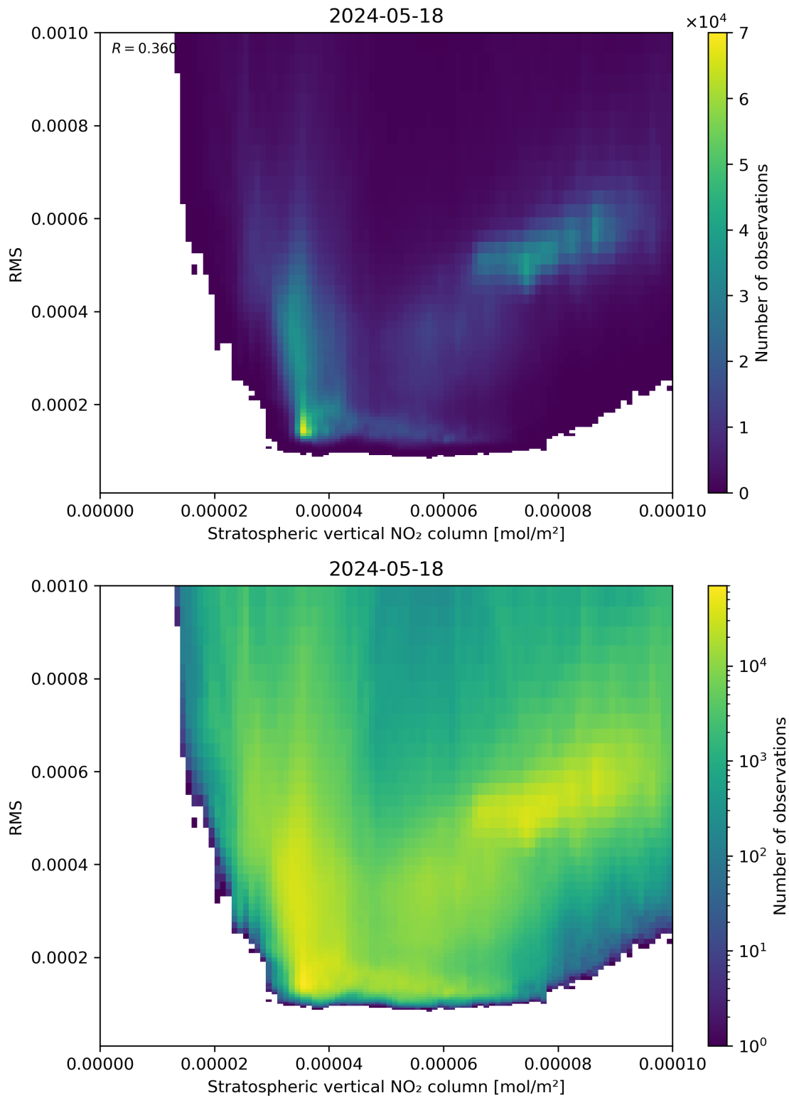
Figure 102: Scatter density plot of “Stratospheric vertical NO 2 column” against “RMS” for 2024-05-18 to 2024-05-19.
