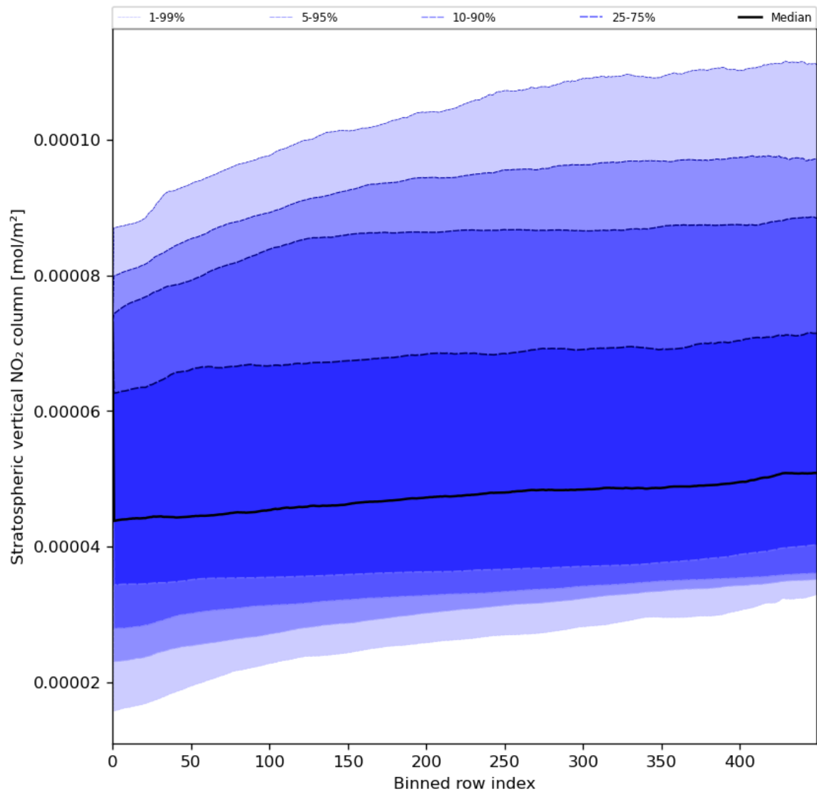
Figure 53: Along track statistics of “Stratospheric vertical NO 2 column” for 2024-05-18 to 2024-05-19
