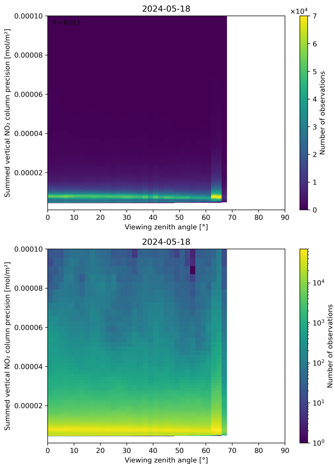
Figure 166: Scatter density plot of “Viewing zenith angle” against “Summed vertical NO 2 column precision” for 2024-05-18 to 2024-05-19.
