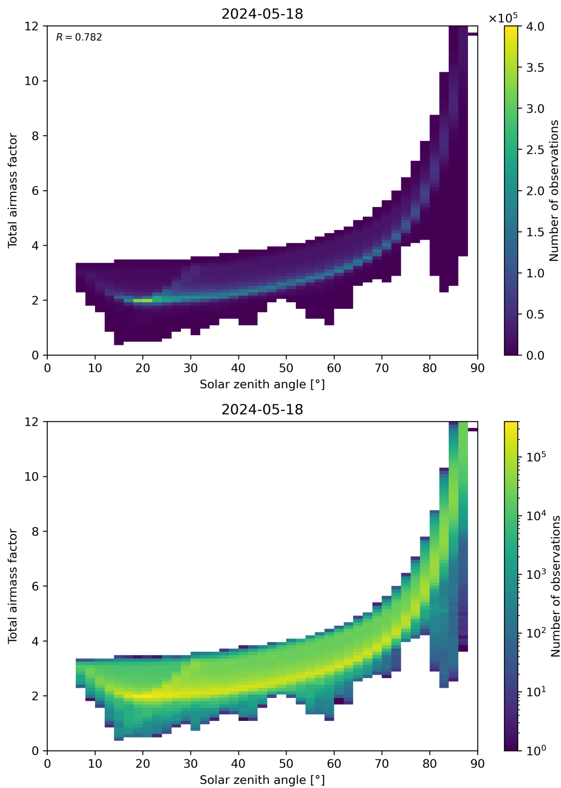
Figure 146: Scatter density plot of “Solar zenith angle” against “Total air mass factor” for 2024-05-18 to 2024-05-19.
