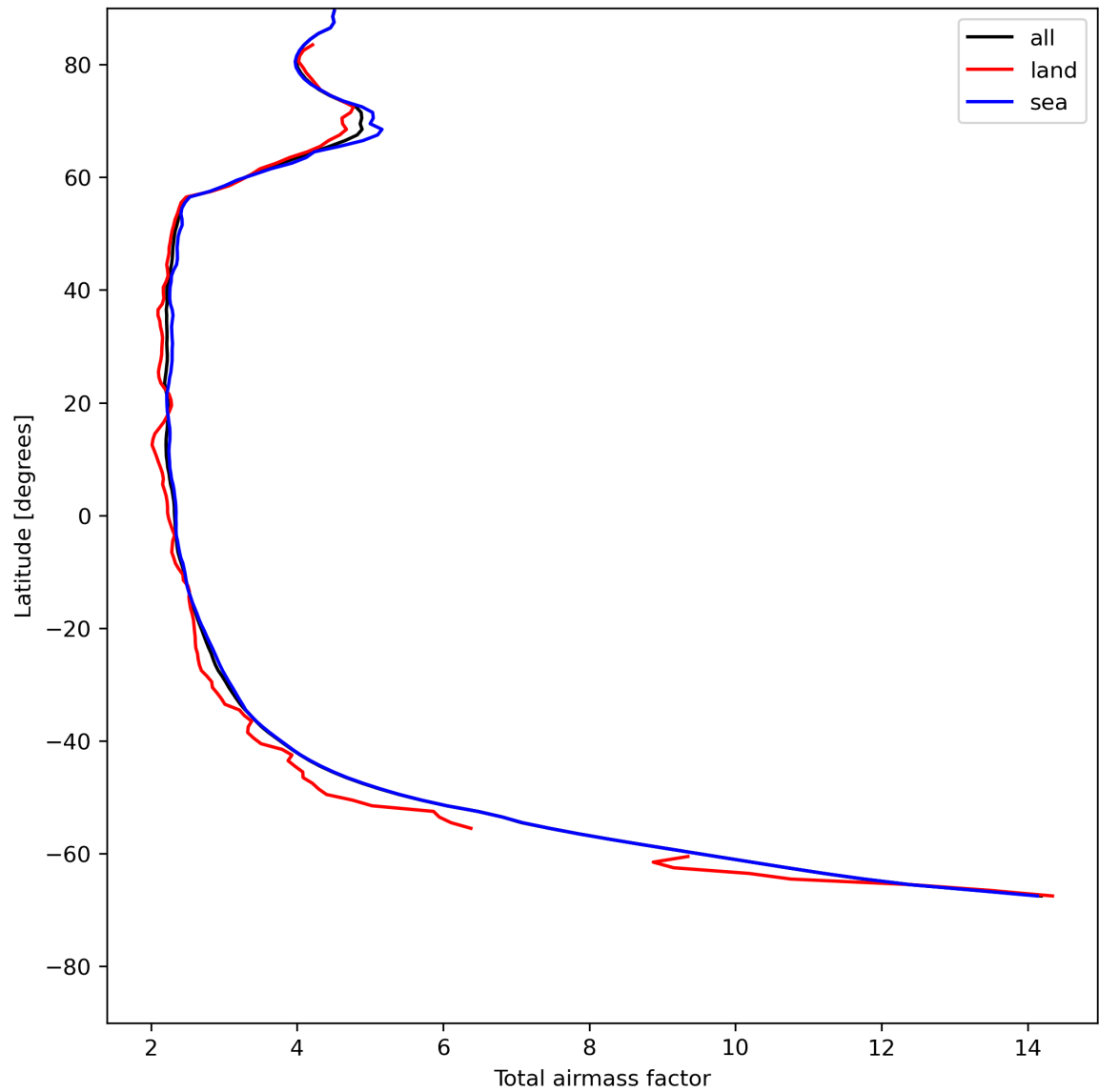
Figure 15: Zonal average of “Total airmass factor” for 2024-05-18 to 2024-05-19.
