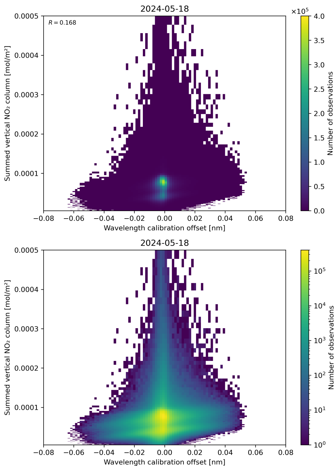
Figure 177: Scatter density plot of “Wavelength calibration offset” against “Summed vertical NO 2 column” for 2024-05-18 to 2024-05-19.
