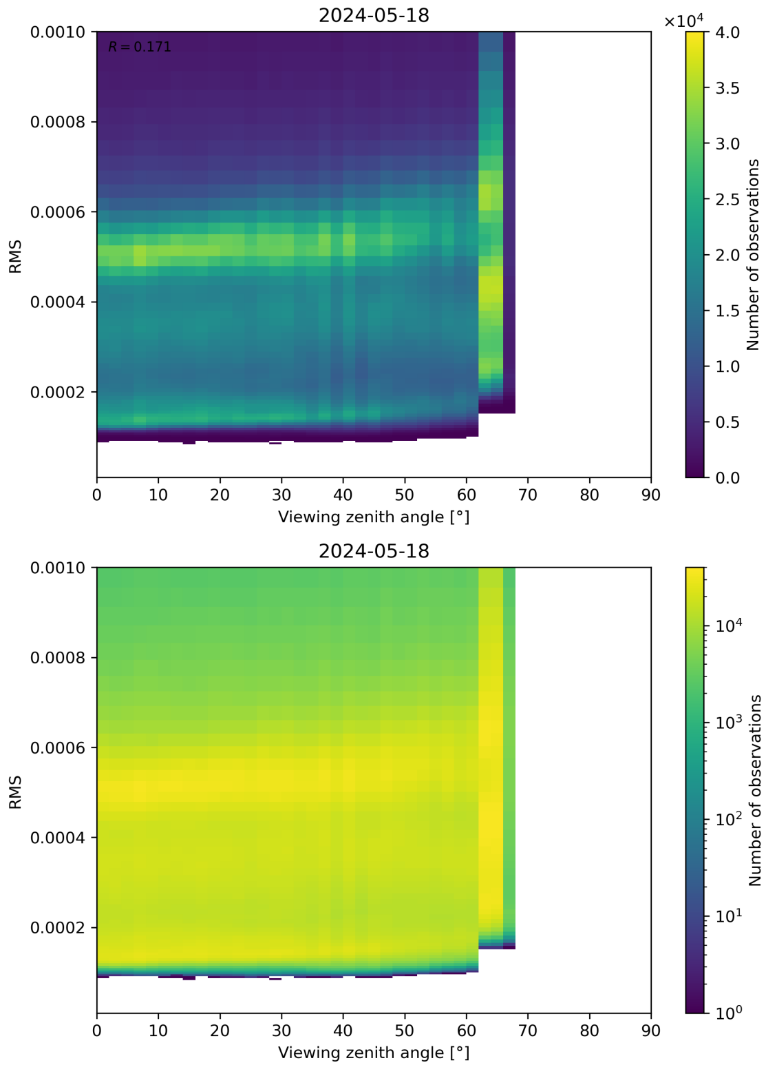
Figure 171: Scatter density plot of “Viewing zenith angle” against “RMS” for 2024-05-18 to 2024-05-19.
