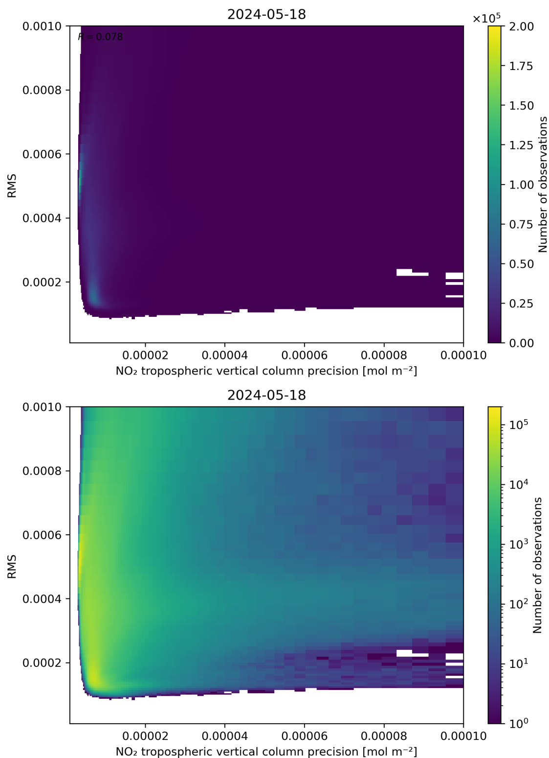
Figure 140: Scatter density plot of “NO 2 tropospheric vertical column precision” against “RMS” for 2024-05-18 to 2024-05-19.
