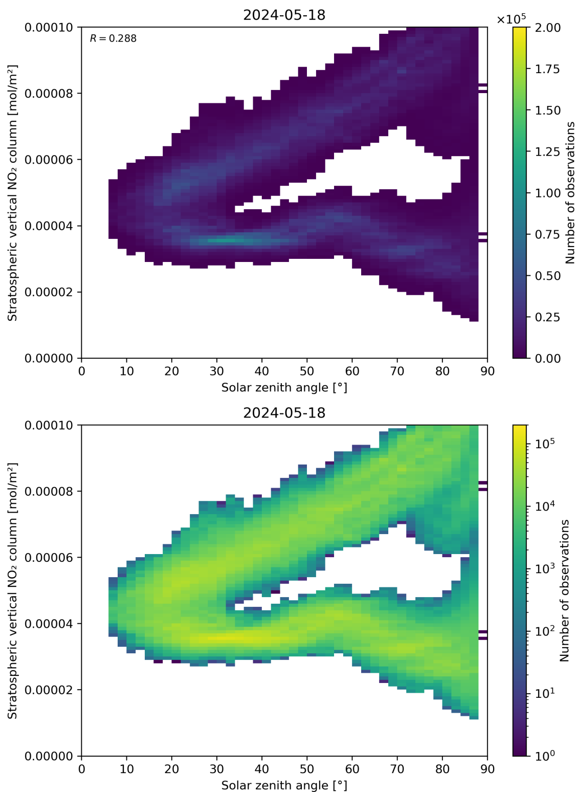
Figure 150: Scatter density plot of “Solar zenith angle” against “Stratospheric vertical NO 2 column” for 2024-05-18 to 2024-05-19.
