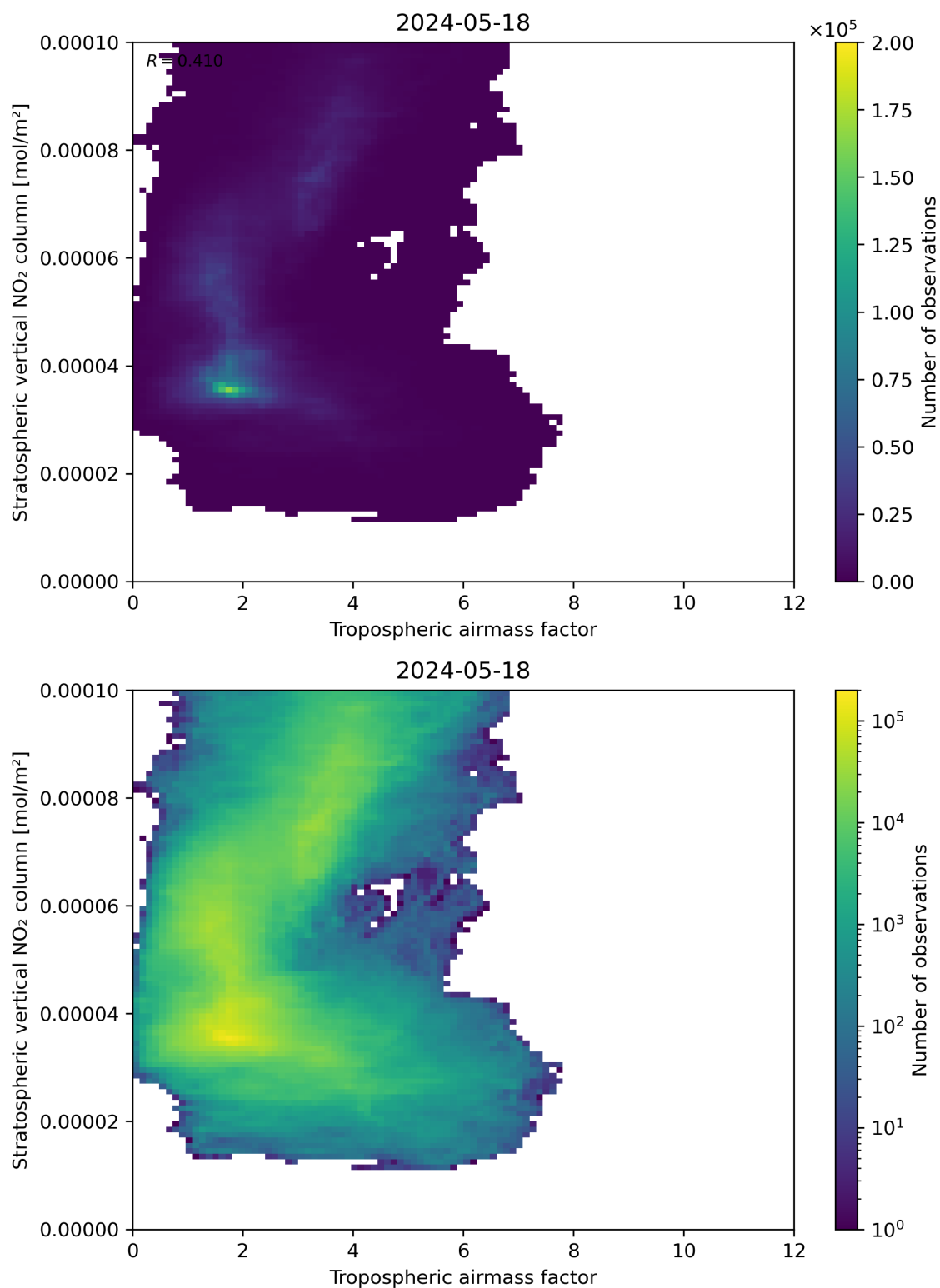
Figure 74: Scatter density plot of “Tropospheric air mass factor” against “Stratospheric vertical NO 2 column” for 2024-05-18 to 2024-05-19.
