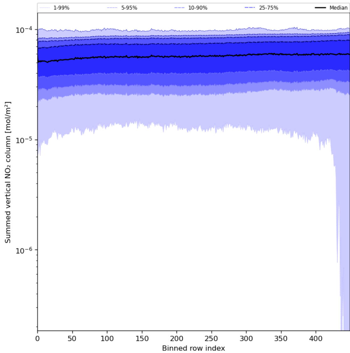
Figure 57: Along track statistics of “Summed vertical NO 2 column” for 2024-05-18 to 2024-05-19
