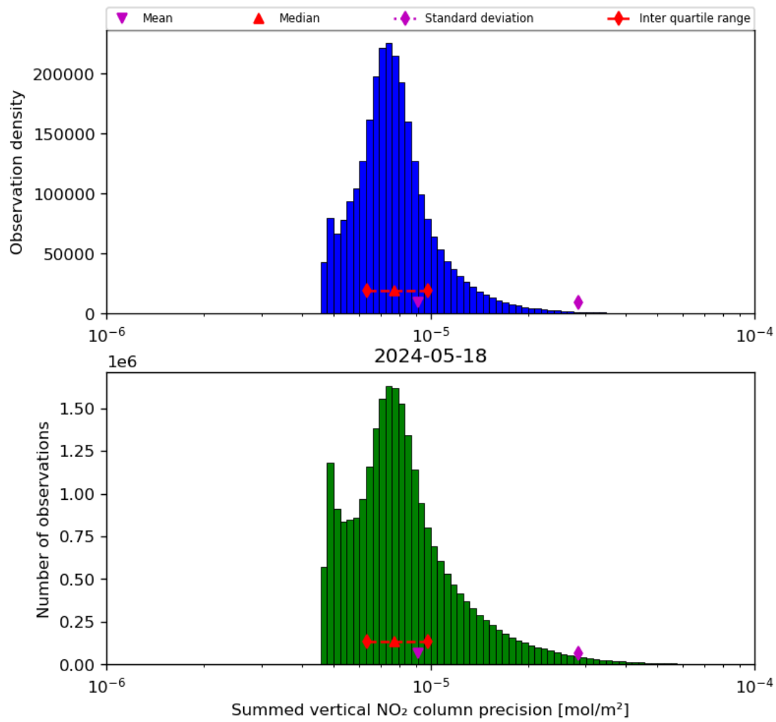
Figure 41: Histogram of “Summed vertical NO 2 column precision” for 2024-05-18 to 2024-05-19
