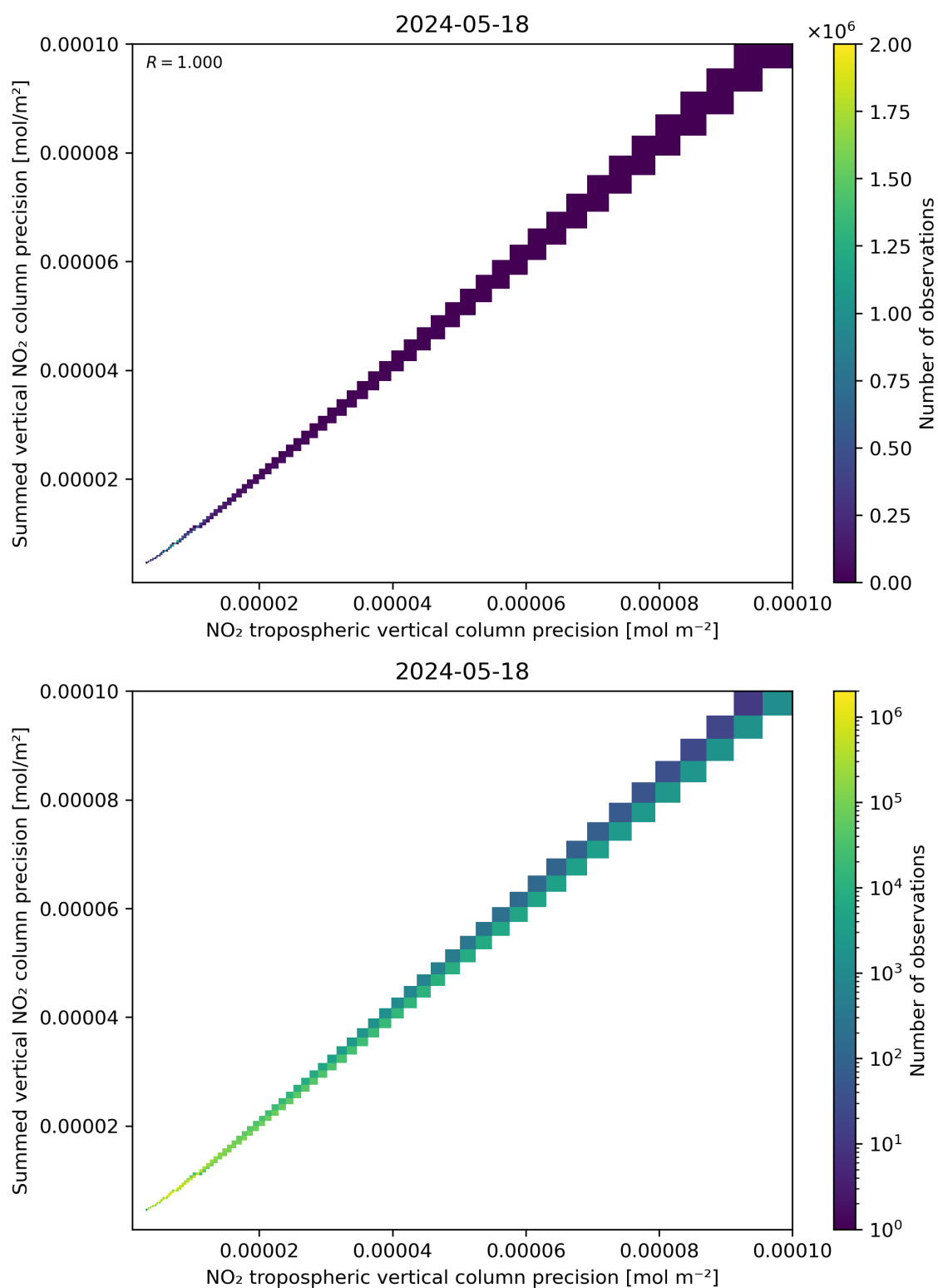
Figure 137: Scatter density plot of “NO 2 tropospheric vertical column precision” against “Summed vertical NO 2 column precision” for 2024-05-18 to 2024-05-19.
