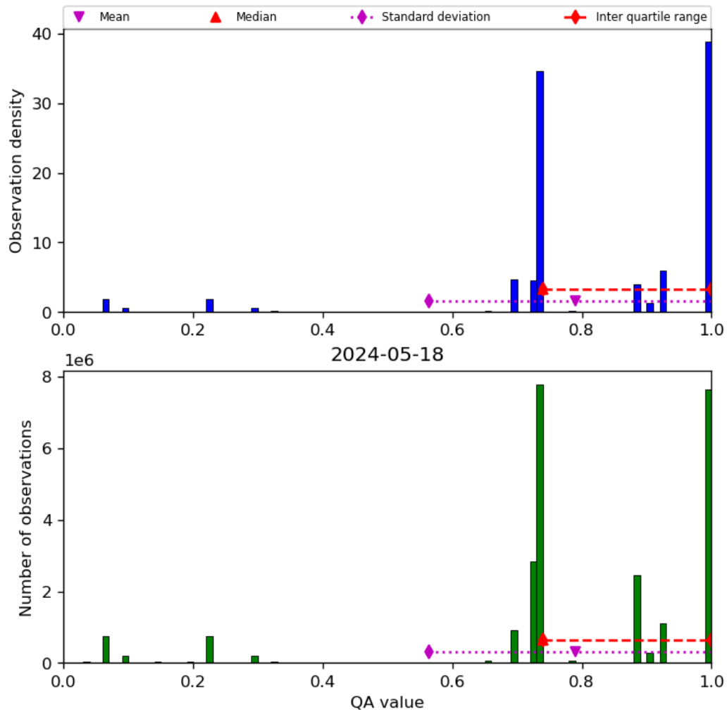
Figure 28: Histogram of “QA value” for 2024-05-18 to 2024-05-19
