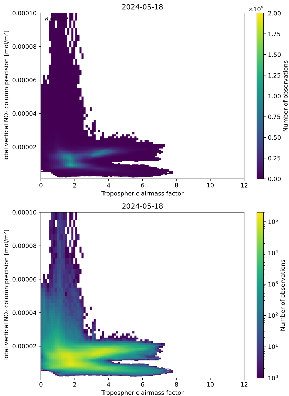
Figure 78: Scatter density plot of “Tropospheric air mass factor” against “Total vertical NO 2 column precision” for 2024-05-18 to 2024-05-19.
