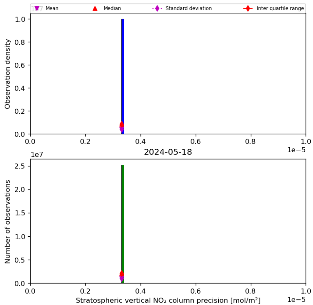
Figure 37: Histogram of “Stratospheric vertical NO 2 column precision” for 2024-05-18 to 2024-05-19
