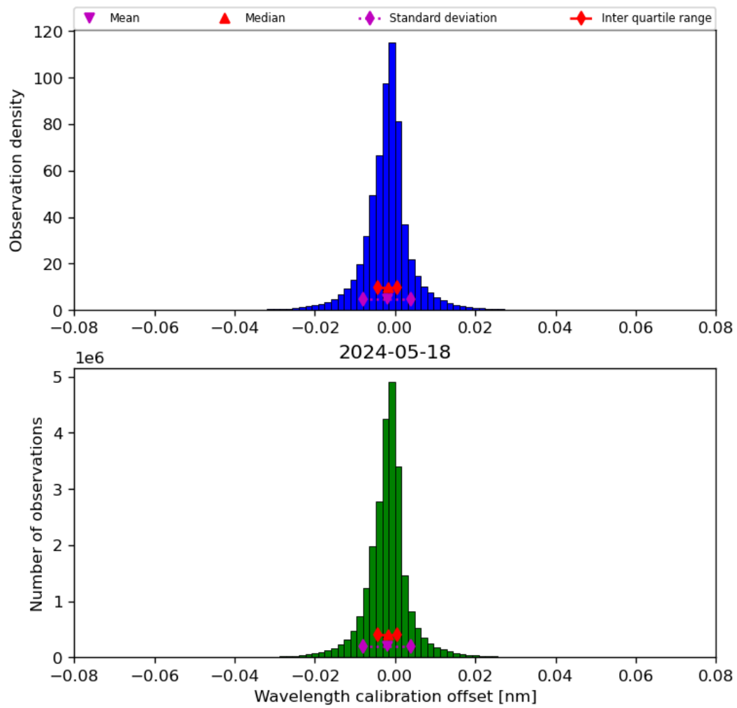
Figure 35: Histogram of “Wavelength calibration offset” for 2024-05-18 to 2024-05-19
