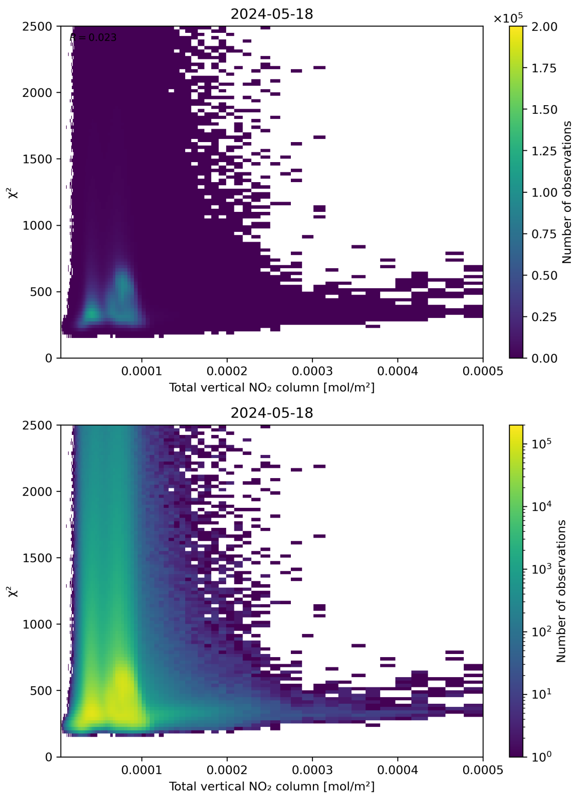
Figure 111: Scatter density plot of “Total vertical NO 2 column” against “ \chi^2 ” for 2024-05-18 to 2024-05-19.
