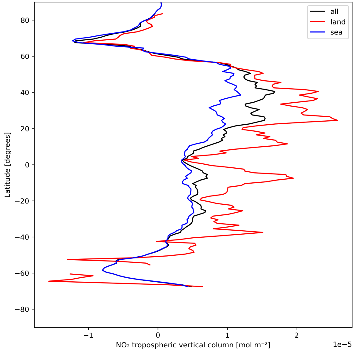
Figure 12: Zonal average of “NO 2 tropospheric vertical column” for 2024-05-18 to 2024-05-19.
