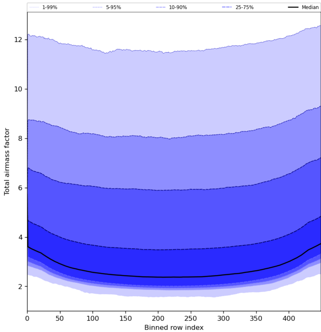
Figure 49: Along track statistics of “Total airmass factor” for 2024-05-18 to 2024-05-19
