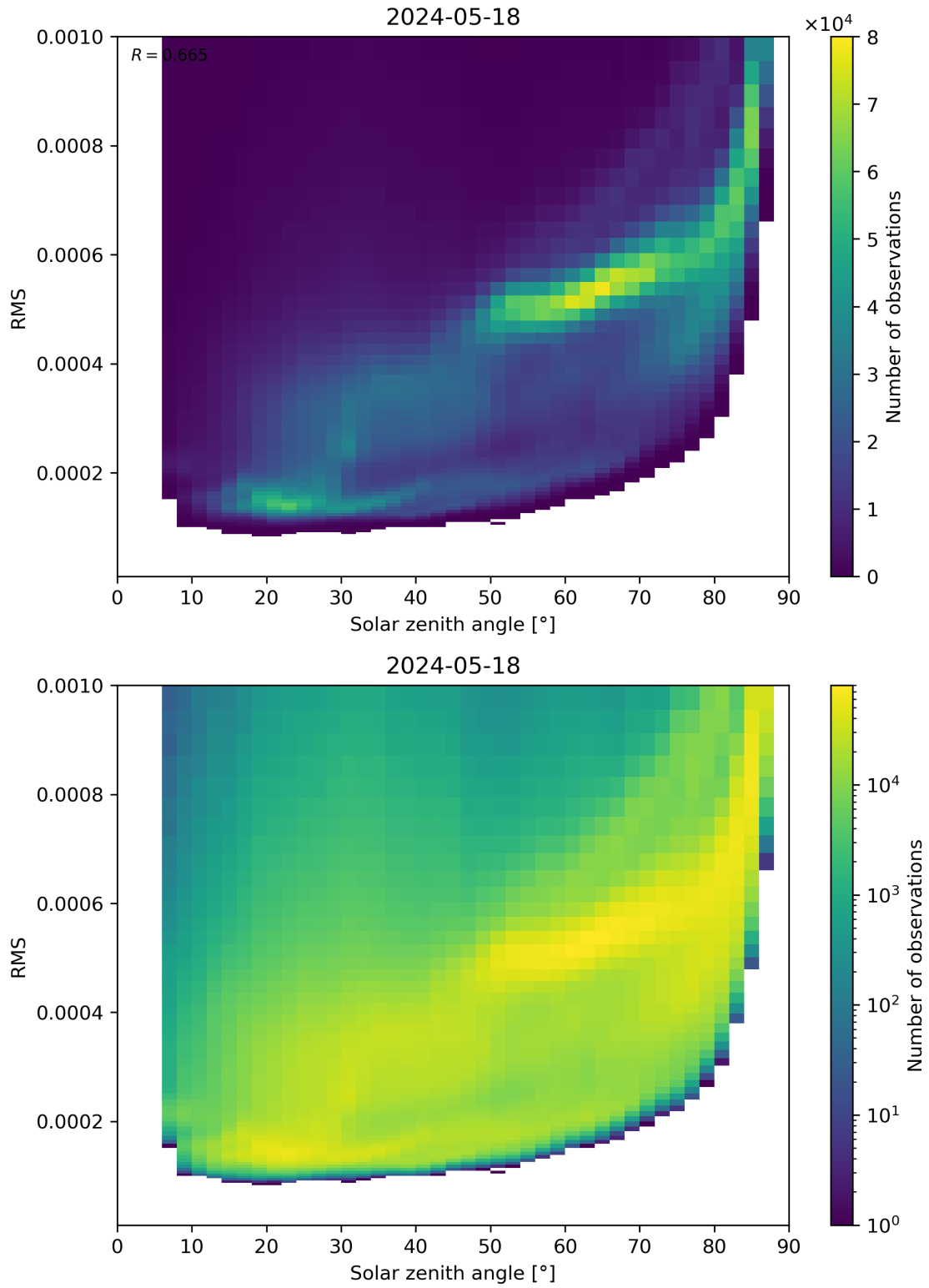
Figure 157: Scatter density plot of “Solar zenith angle” against “RMS” for 2024-05-18 to 2024-05-19.
