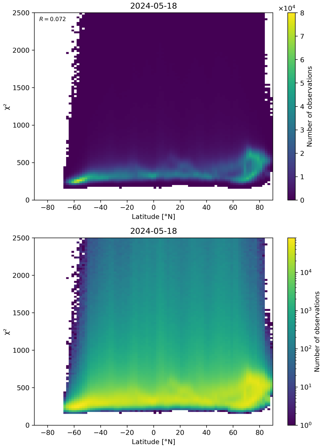
Figure 86: Scatter density plot of “Latitude” against “ \chi^2 ” for 2024-05-18 to 2024-05-19.
