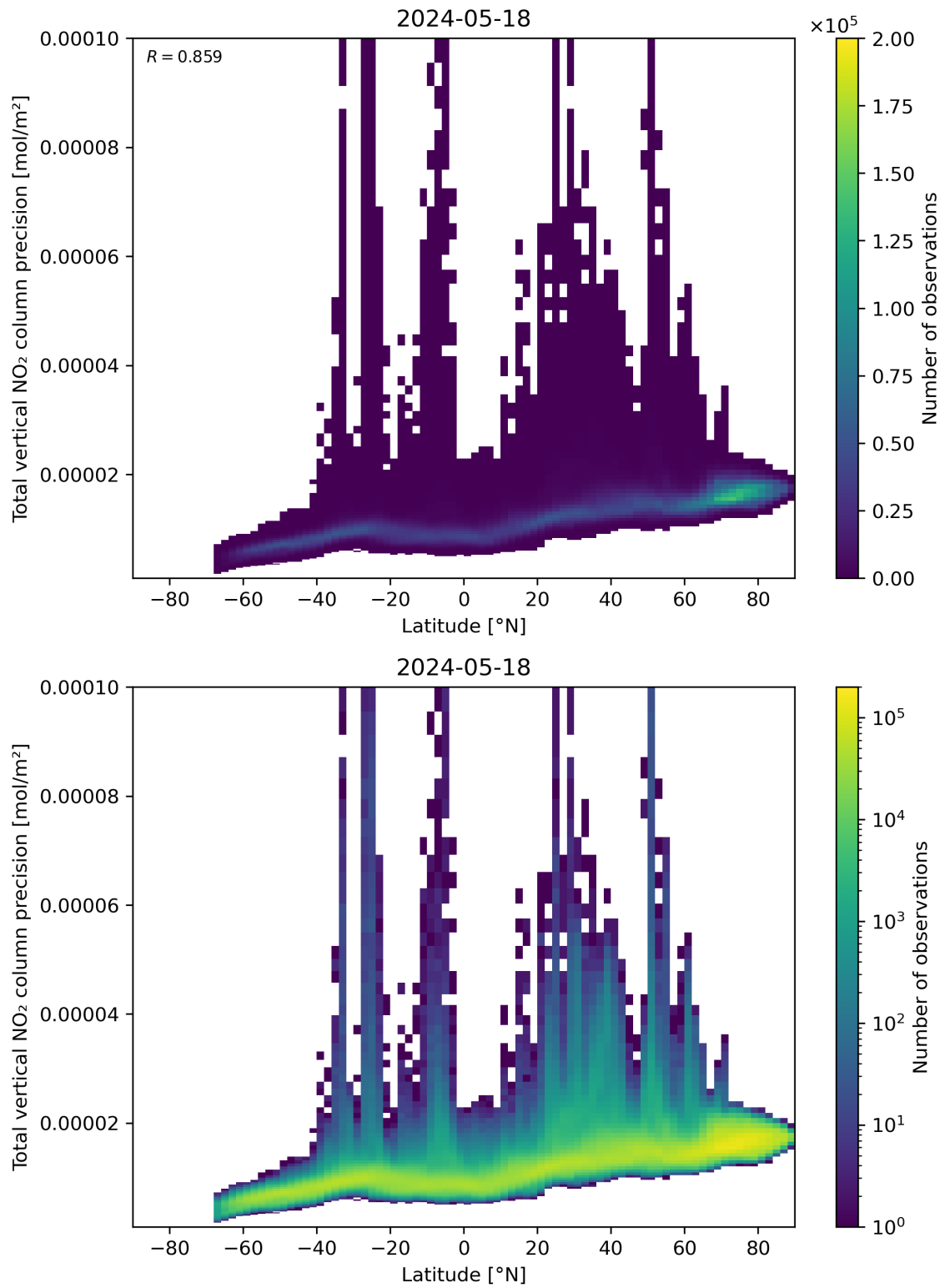
Figure 91: Scatter density plot of “Latitude” against “Total vertical NO 2 column precision” for 2024-05-18 to 2024-05-19.
