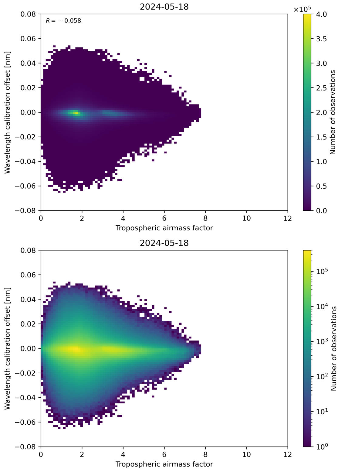
Figure 80: Scatter density plot of “Tropospheric airmass factor” against “Wavelength calibration offset” for 2024-05-18 to 2024-05-19.
