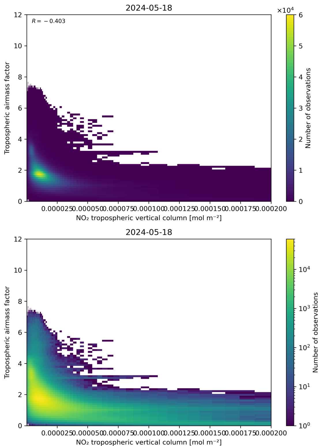
Figure 123: Scatter density plot of “NO 2 tropospheric vertical column” against “Tropospheric airmass factor” for 2024-05-18 to 2024-05-19.
