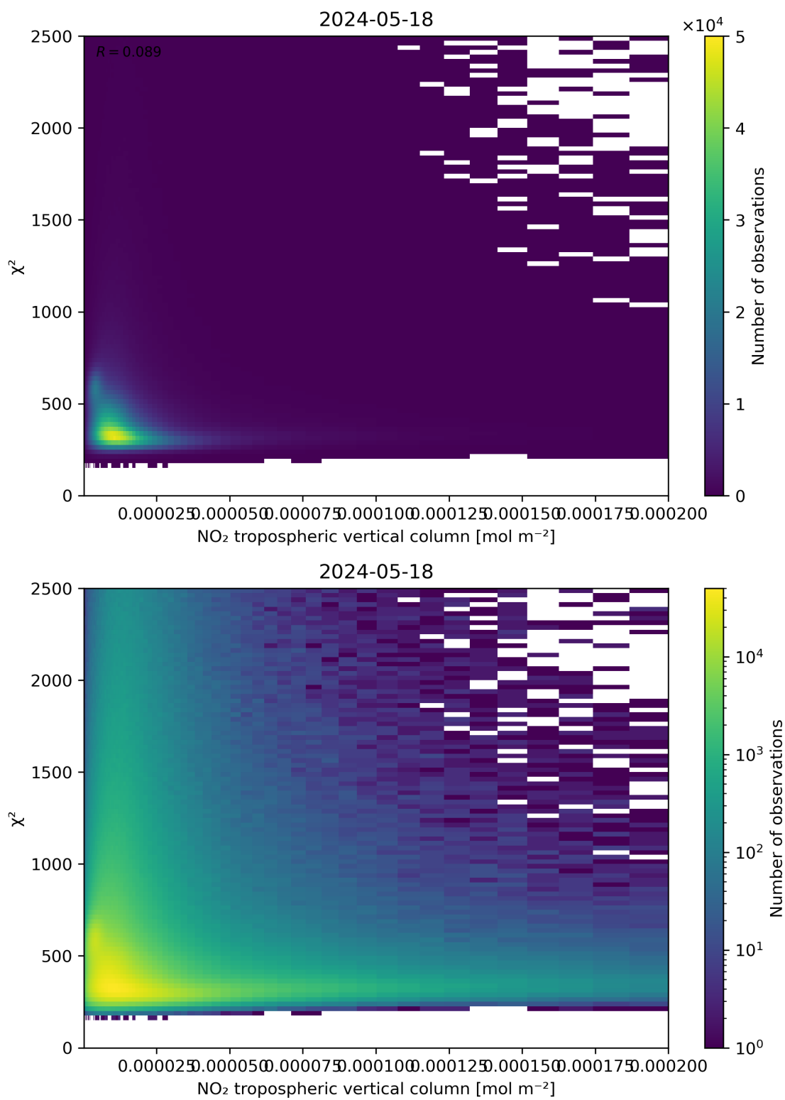
Figure 124: Scatter density plot of “NO 2 tropospheric vertical column” against “ \chi^2 ” for 2024-05-18 to 2024-05-19.
