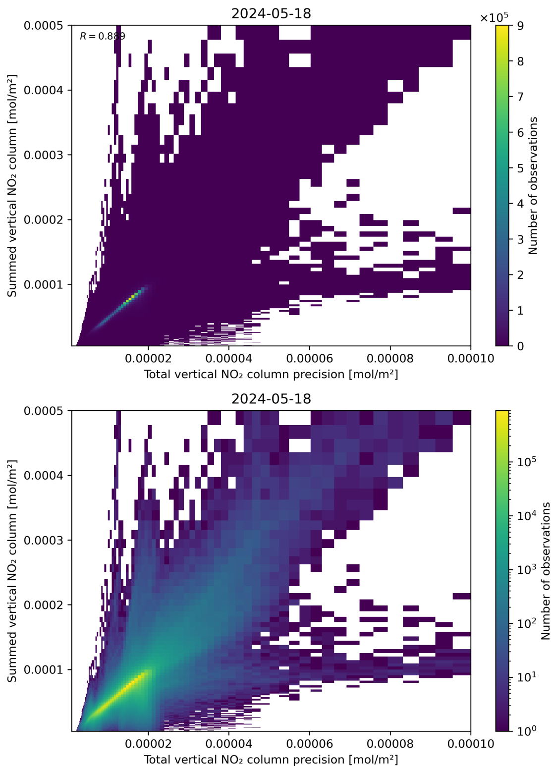
Figure 117: Scatter density plot of “Total vertical NO 2 column precision” against “Summed vertical NO 2 column” for 2024-05-18 to 2024-05-19.
