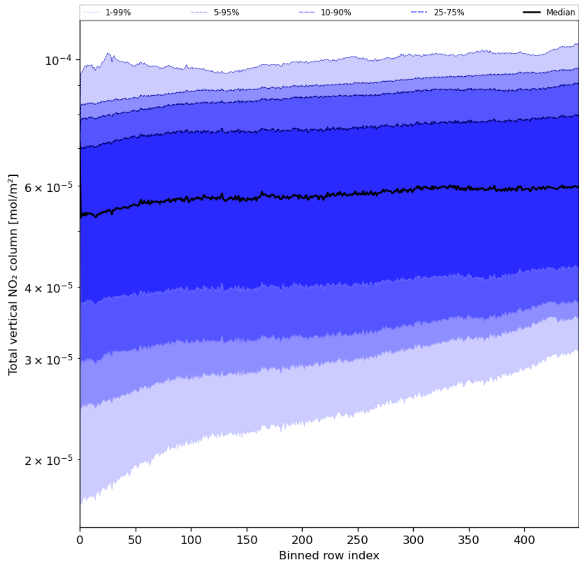
Figure 55: Along track statistics of “Total vertical NO 2 column” for 2024-05-18 to 2024-05-19
