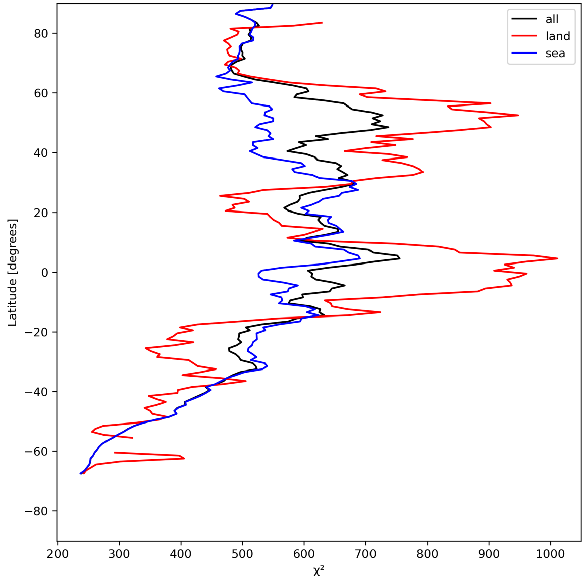
Figure 25: Zonal average of “ \chi^2 ” for 2024-05-18 to 2024-05-19.
