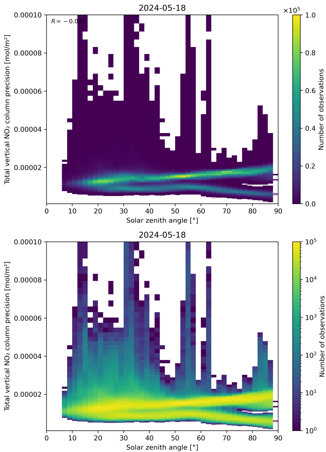
Figure 154: Scatter density plot of “Solar zenith angle” against “Total vertical NO 2 column precision” for 2024-05-18 to 2024-05-19.
