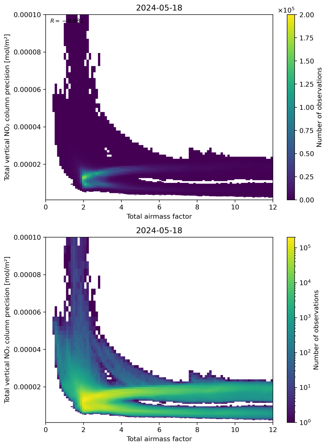
Figure 68: Scatter density plot of “Total airmass factor” against “Total vertical NO 2 column precision” for 2024-05-18 to 2024-05-19.
