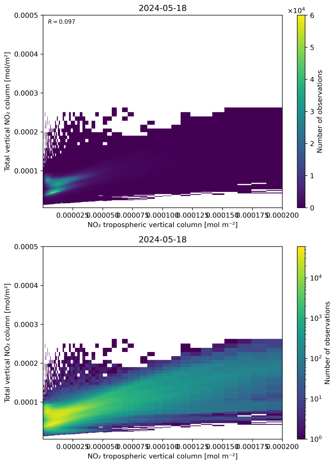
Figure 128: Scatter density plot of “NO 2 tropospheric vertical column” against “Total vertical NO 2 column” for 2024-05-18 to 2024-05-19.
