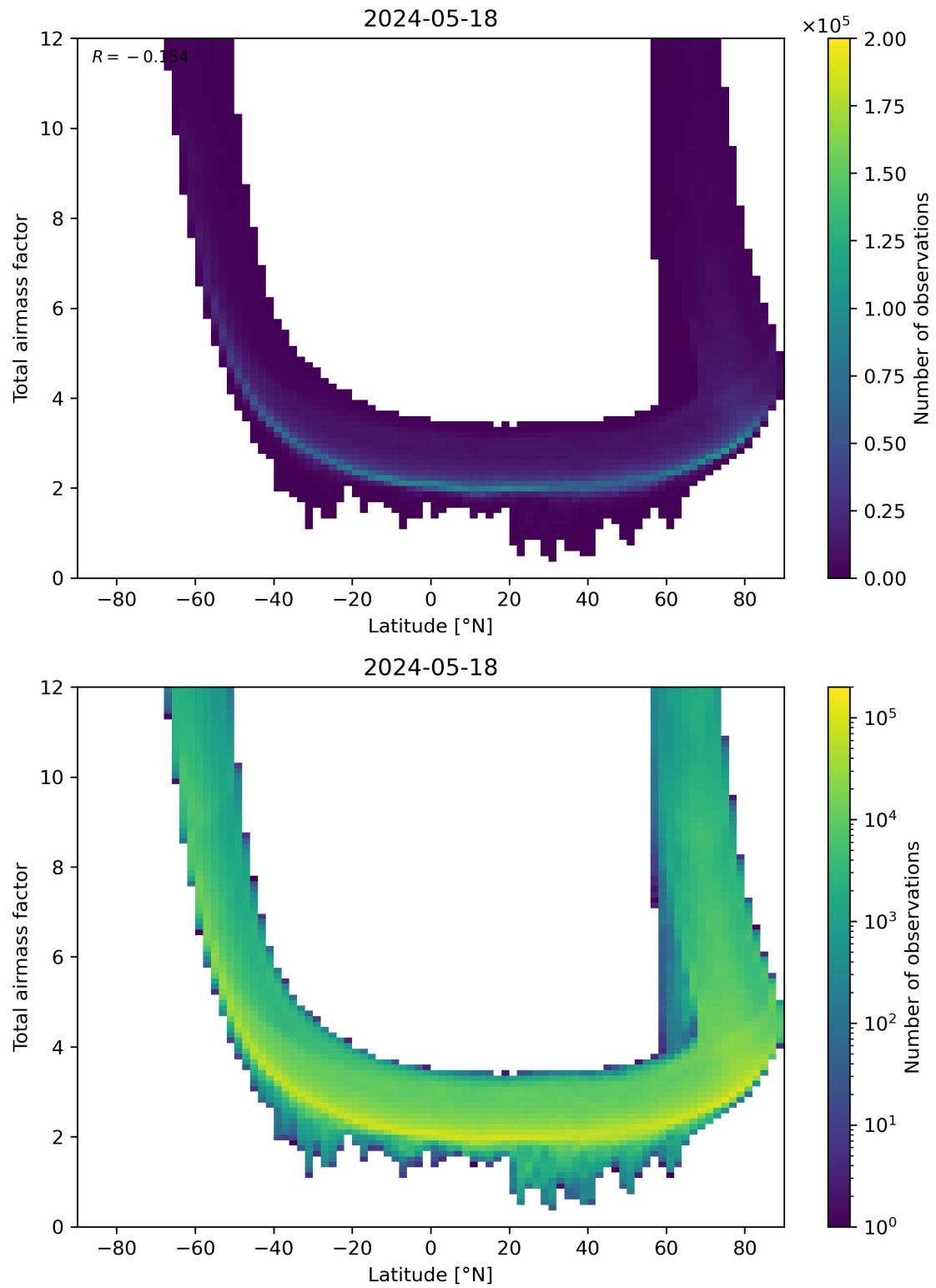
Figure 84: Scatter density plot of “Latitude” against “Total airmass factor” for 2024-05-18 to 2024-05-19.
