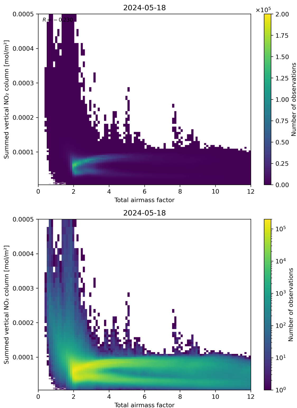
Figure 65: Scatter density plot of “Total airmass factor” against “Summed vertical NO 2 column” for 2024-05-18 to 2024-05-19.
