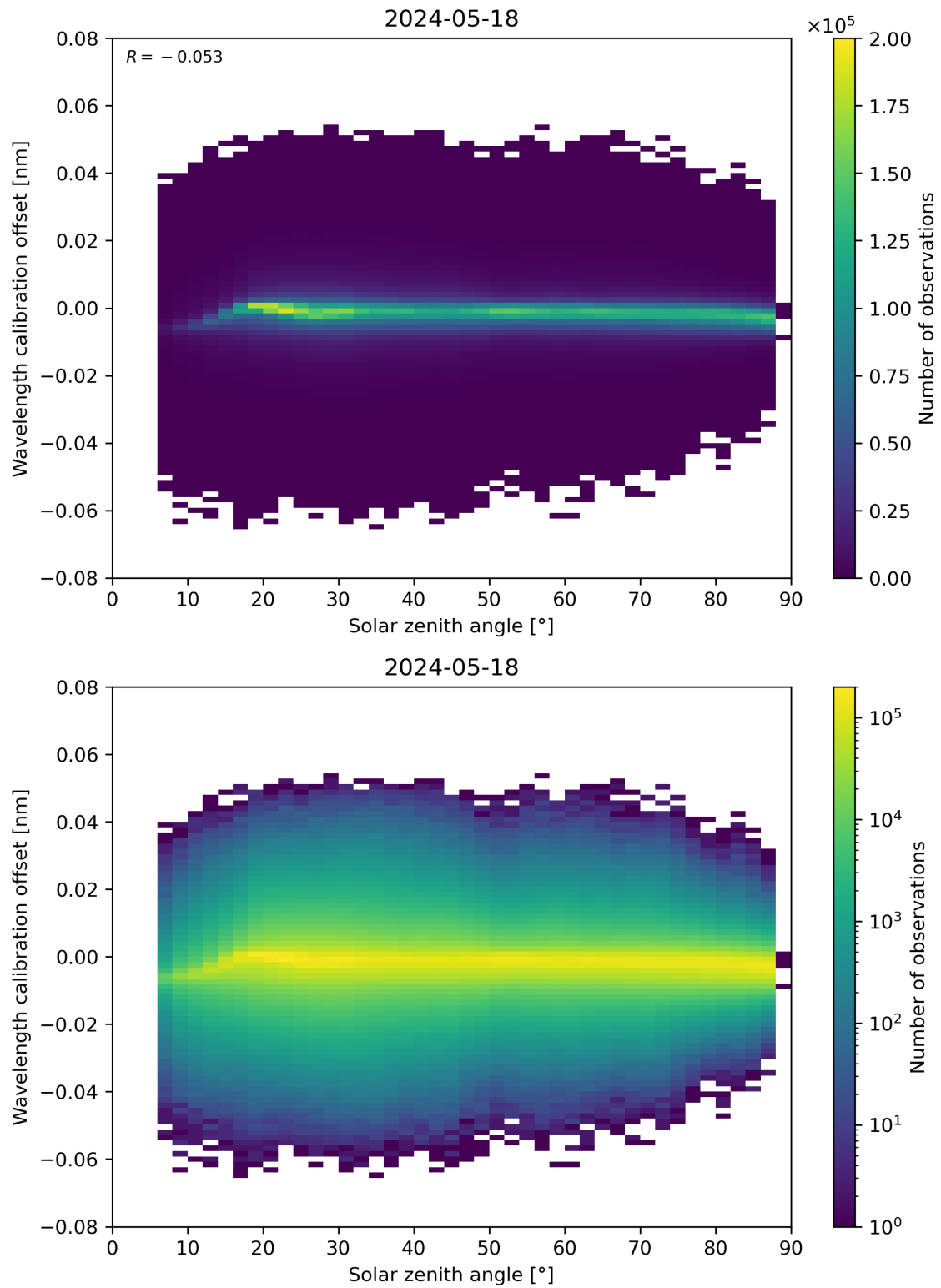
Figure 158: Scatter density plot of “Solar zenith angle” against “Wavelength calibration offset” for 2024-05-18 to 2024-05-19.
