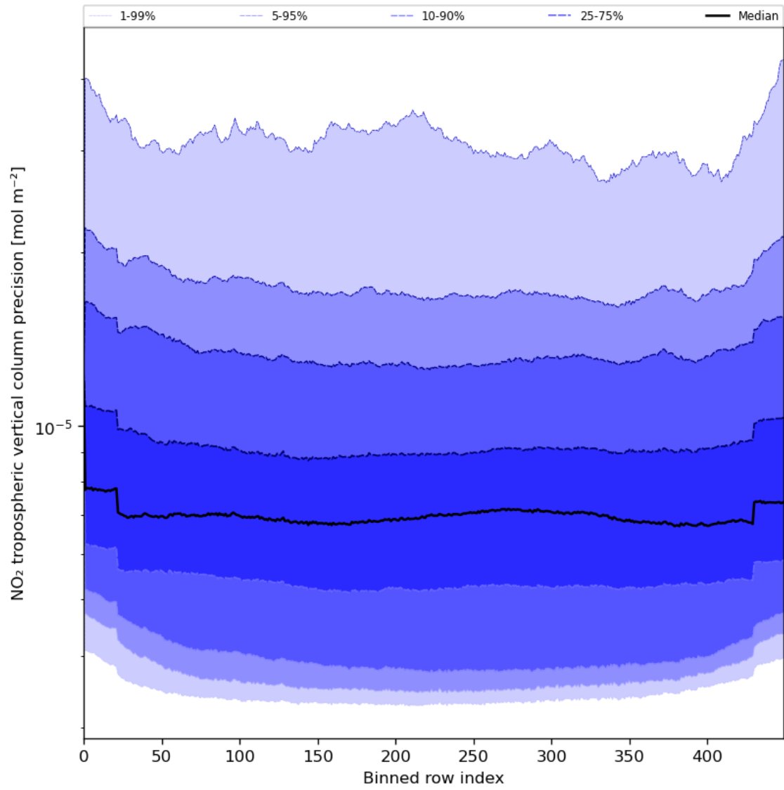
Figure 47: Along track statistics of “NO 2 tropospheric vertical column precision” for 2024-05-18 to 2024-05-19
