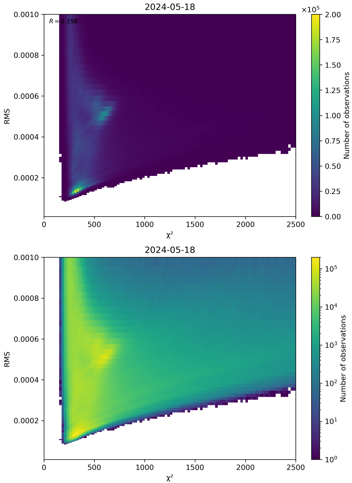
Figure 82: Scatter density plot of “ \chi^2 ” against “RMS” for 2024-05-18 to 2024-05-19.
