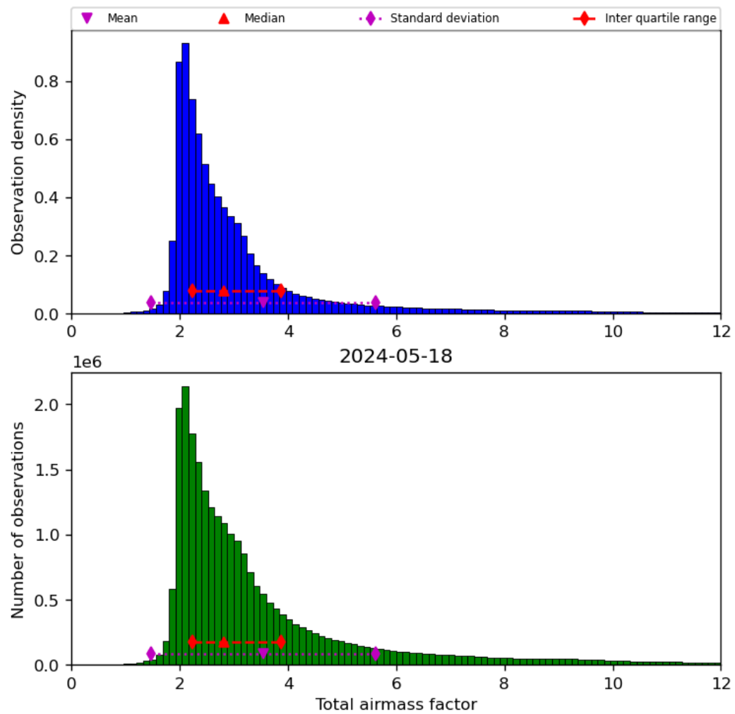
Figure 32: Histogram of “Total airmass factor” for 2024-05-18 to 2024-05-19
