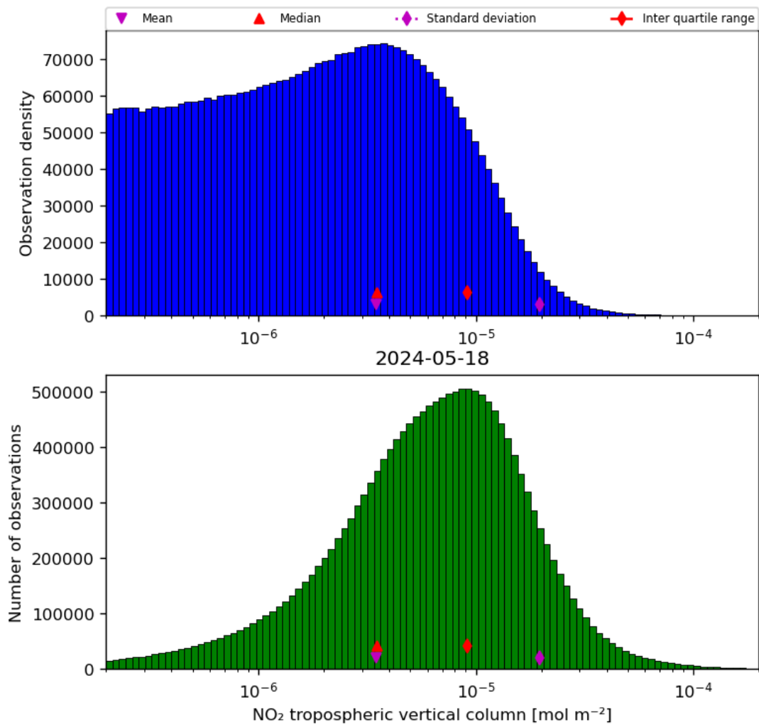
Figure 29: Histogram of “NO 2 tropospheric vertical column” for 2024-05-18 to 2024-05-19
