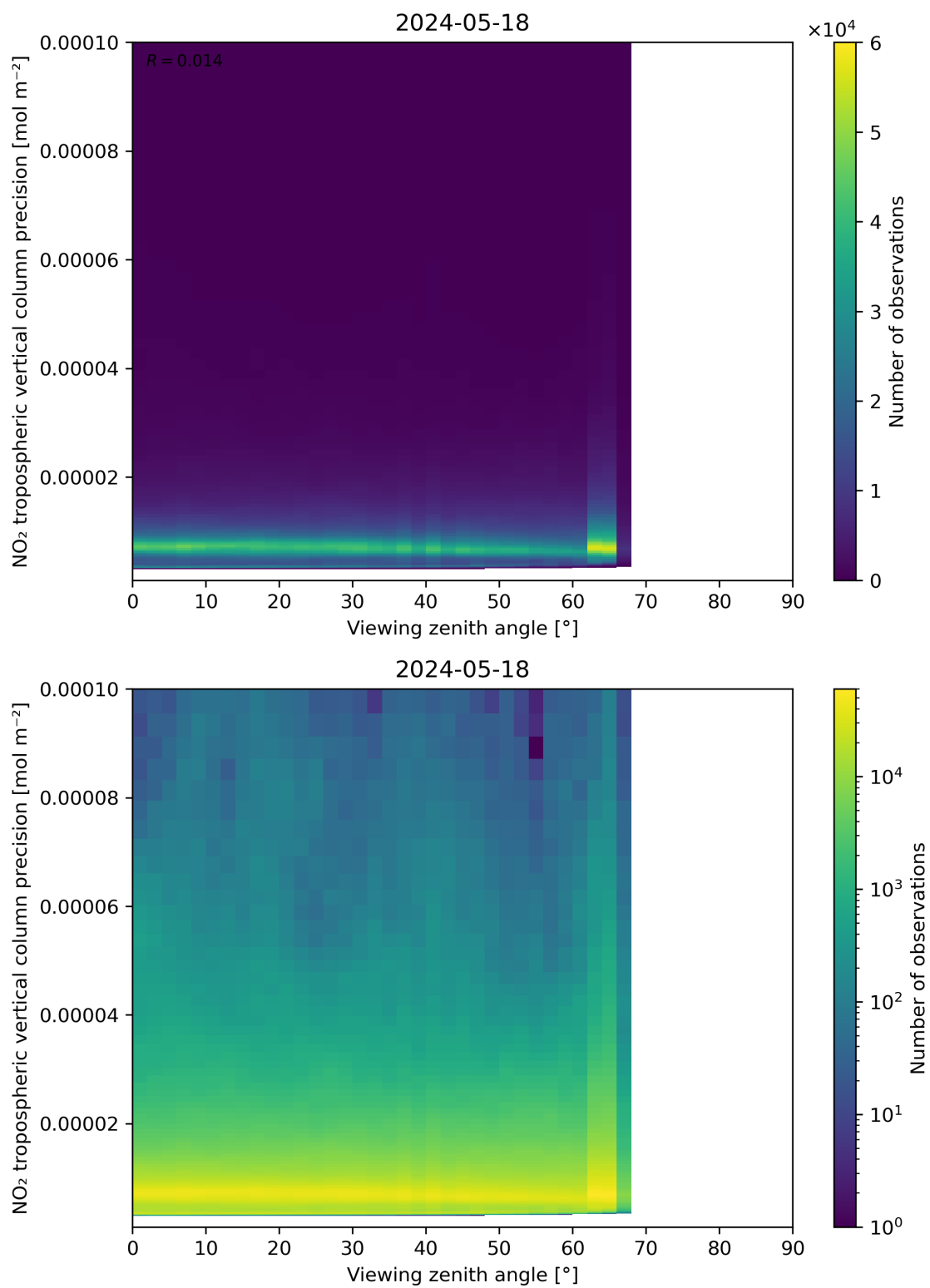
Figure 170: Scatter density plot of “Viewing zenith angle” against “NO 2 tropospheric vertical column precision” for 2024-05-18 to 2024-05-19.
