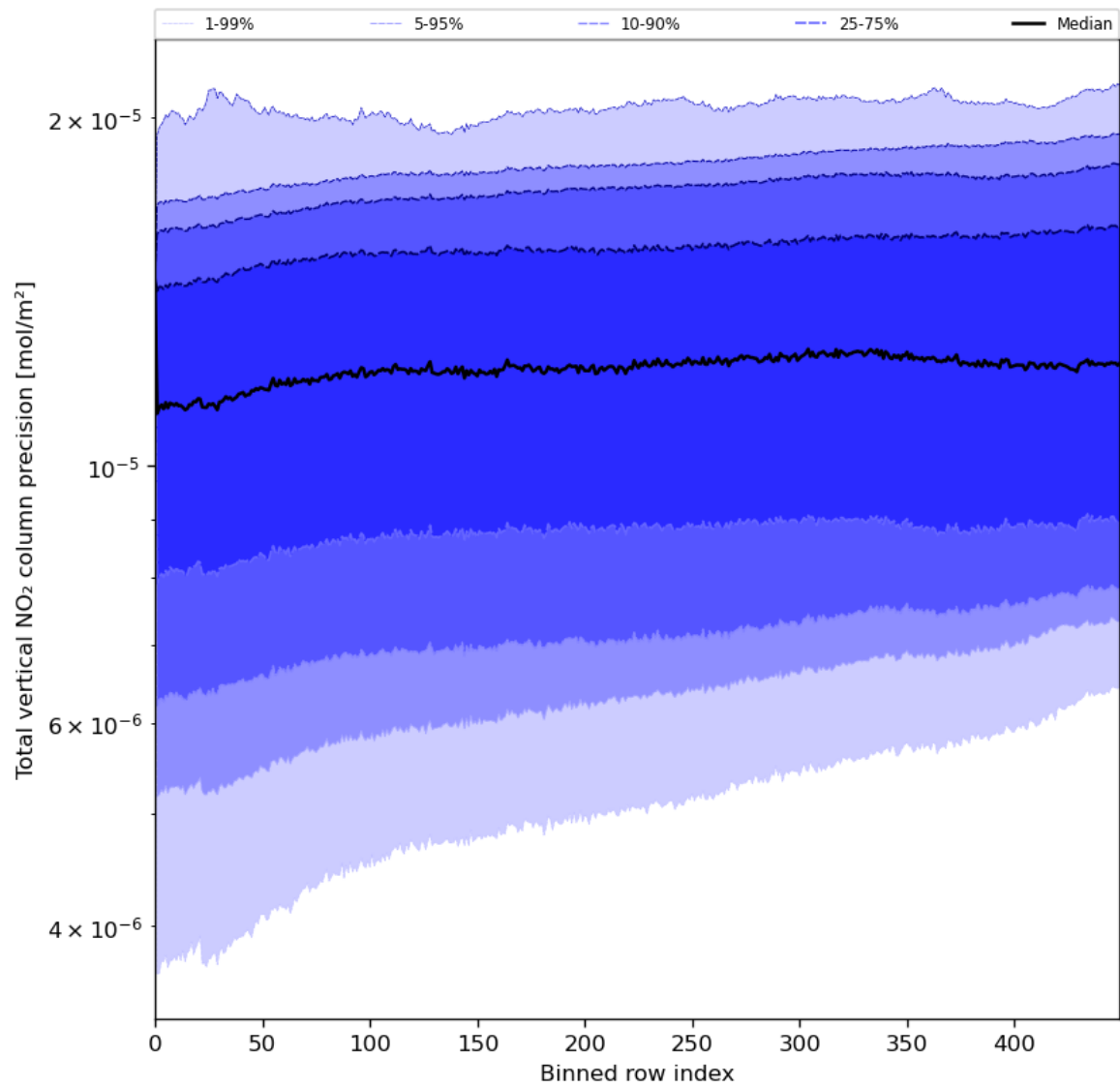
Figure 56: Along track statistics of “Total vertical NO 2 column precision” for 2024-05-18 to 2024-05-19
