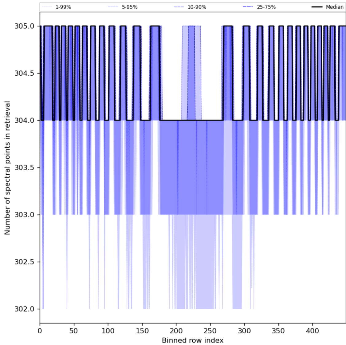
Figure 50: Along track statistics of “Number of spectral points in retrieval” for 2024-05-18 to 2024-05-19
