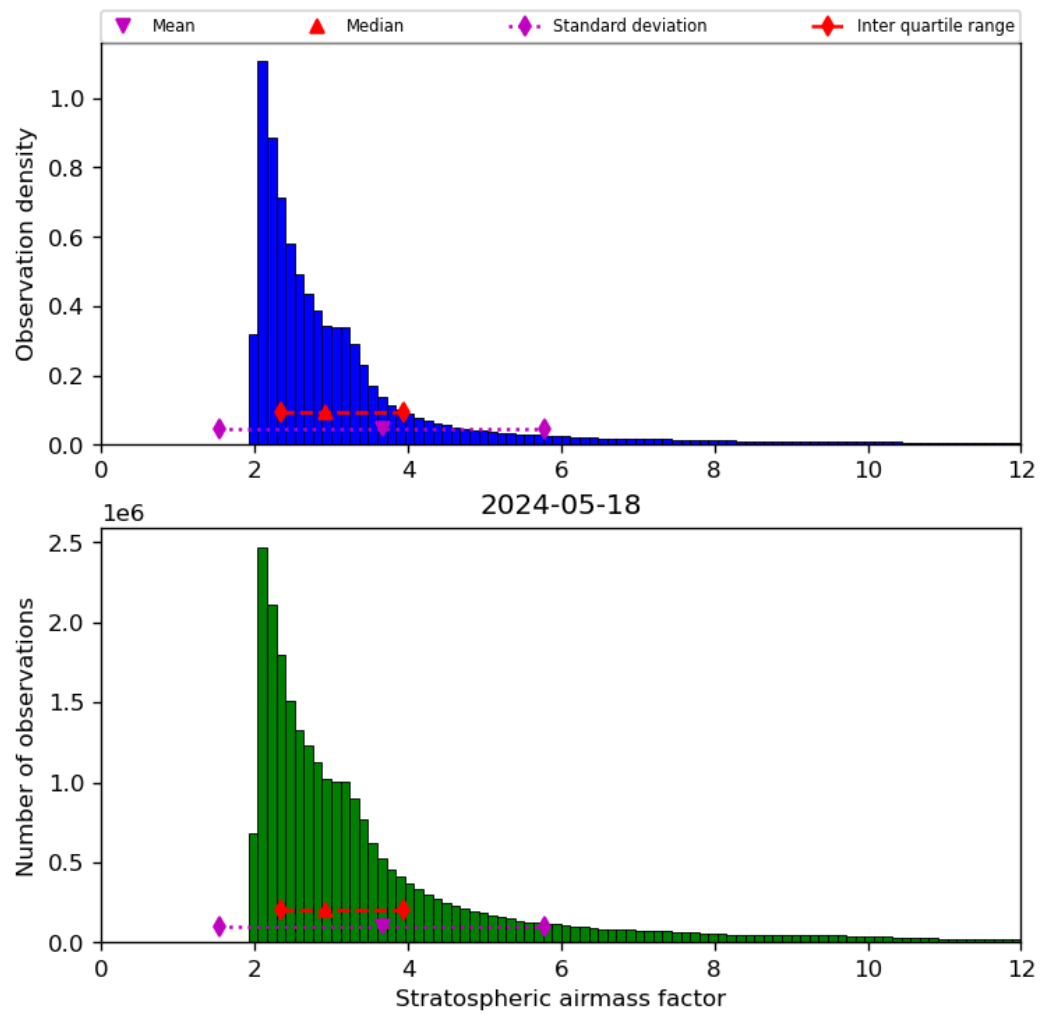
Figure 44: Histogram of “Stratospheric airmass factor” for 2024-05-18 to 2024-05-19
