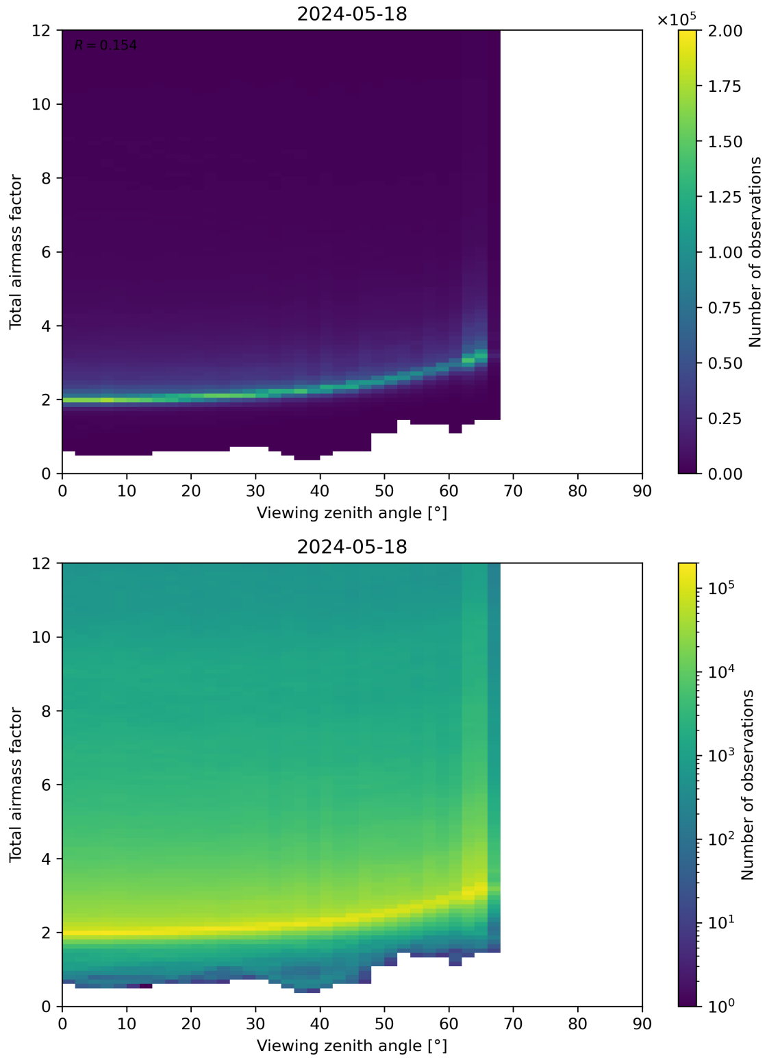
Figure 160: Scatter density plot of “Viewing zenith angle” against “Total airmass factor” for 2024-05-18 to 2024-05-19.
