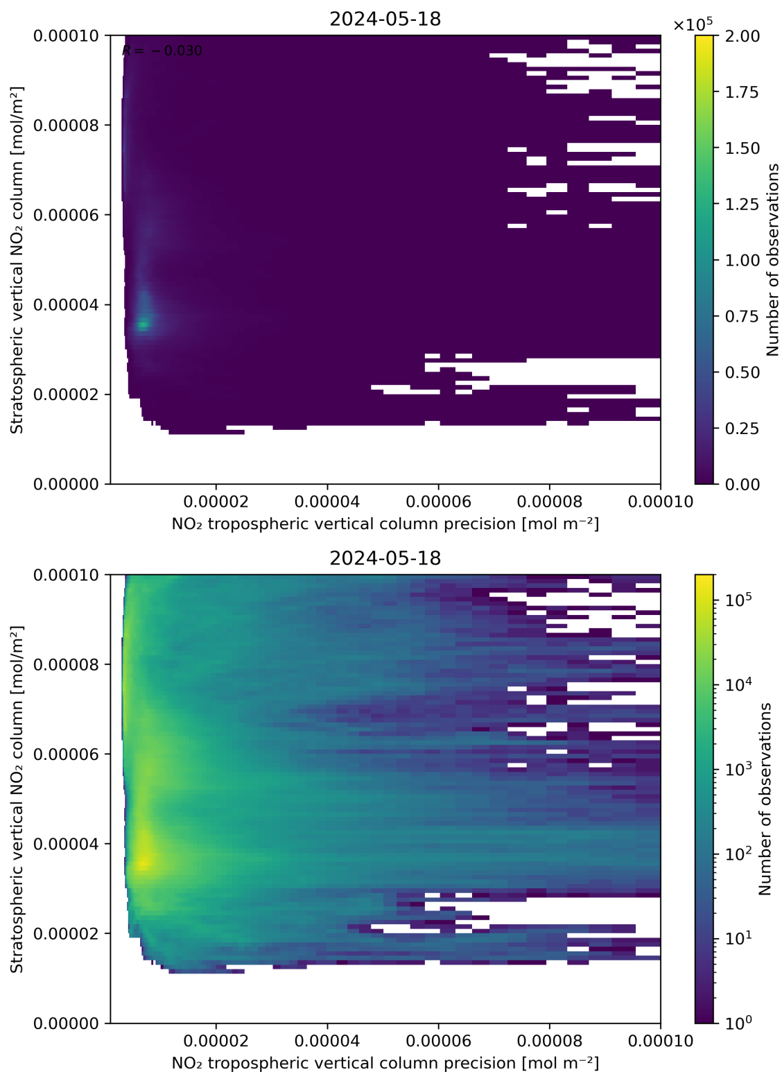
Figure 135: Scatter density plot of “NO 2 tropospheric vertical column precision” against “Stratospheric vertical NO 2 column” for 2024-05-18 to 2024-05-19.
