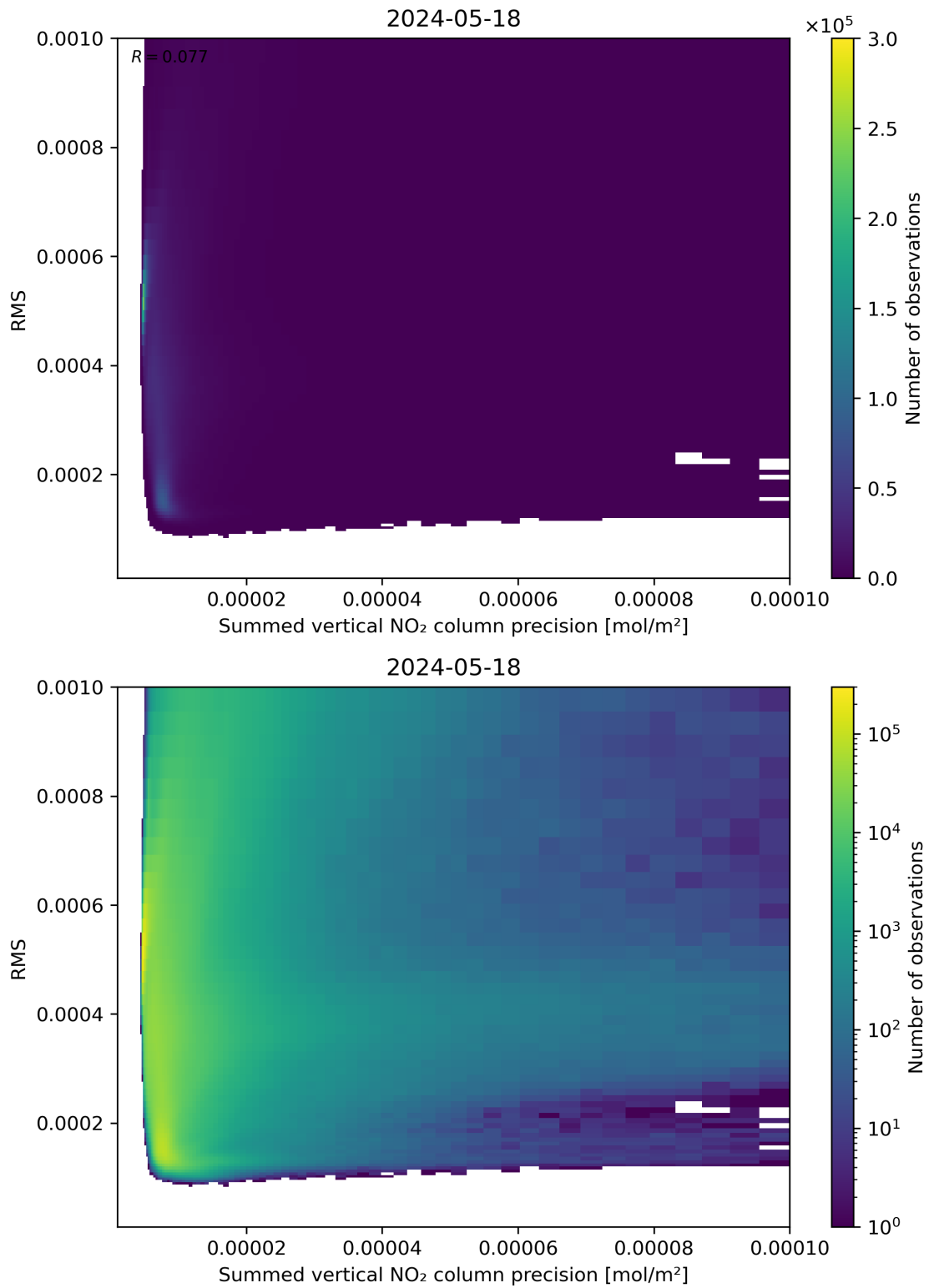
Figure 108: Scatter density plot of “Summed vertical NO 2 column precision” against “RMS” for 2024-05-18 to 2024-05-19.
