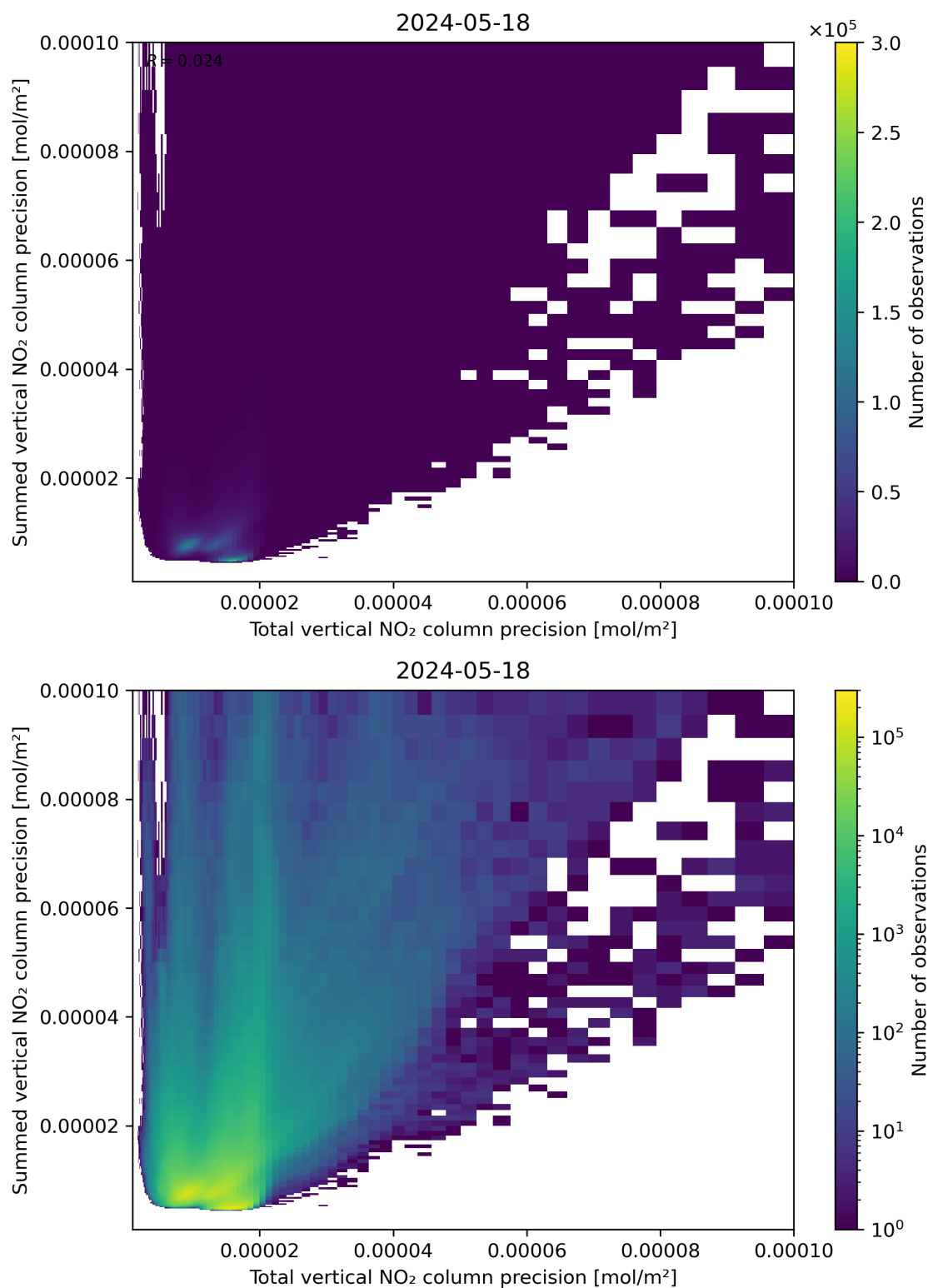
Figure 118: Scatter density plot of “Total vertical NO 2 column precision” against “Summed vertical NO 2 column precision” for 2024-05-18 to 2024-05-19.
