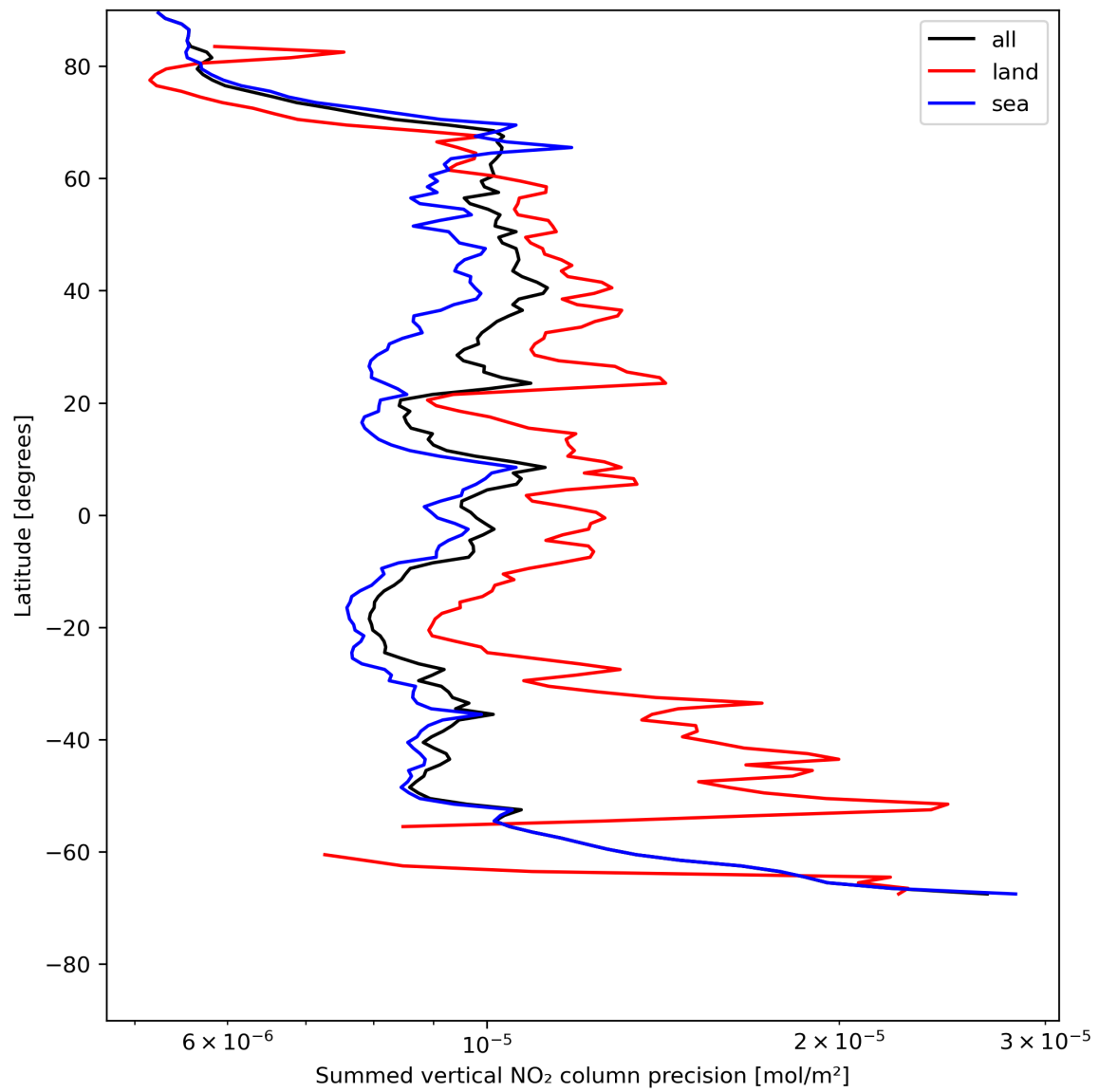
Figure 24: Zonal average of “Summed vertical NO 2 column precision” for 2024-05-18 to 2024-05-19.
