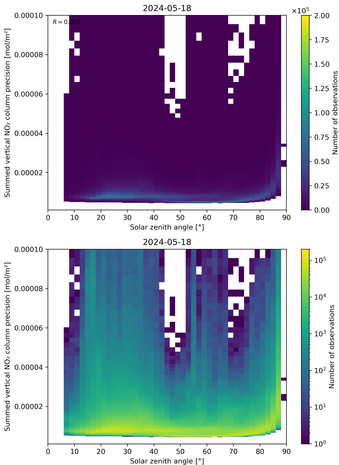
Figure 152: Scatter density plot of “Solar zenith angle” against “Summed vertical NO 2 column precision” for 2024-05-18 to 2024-05-19.
