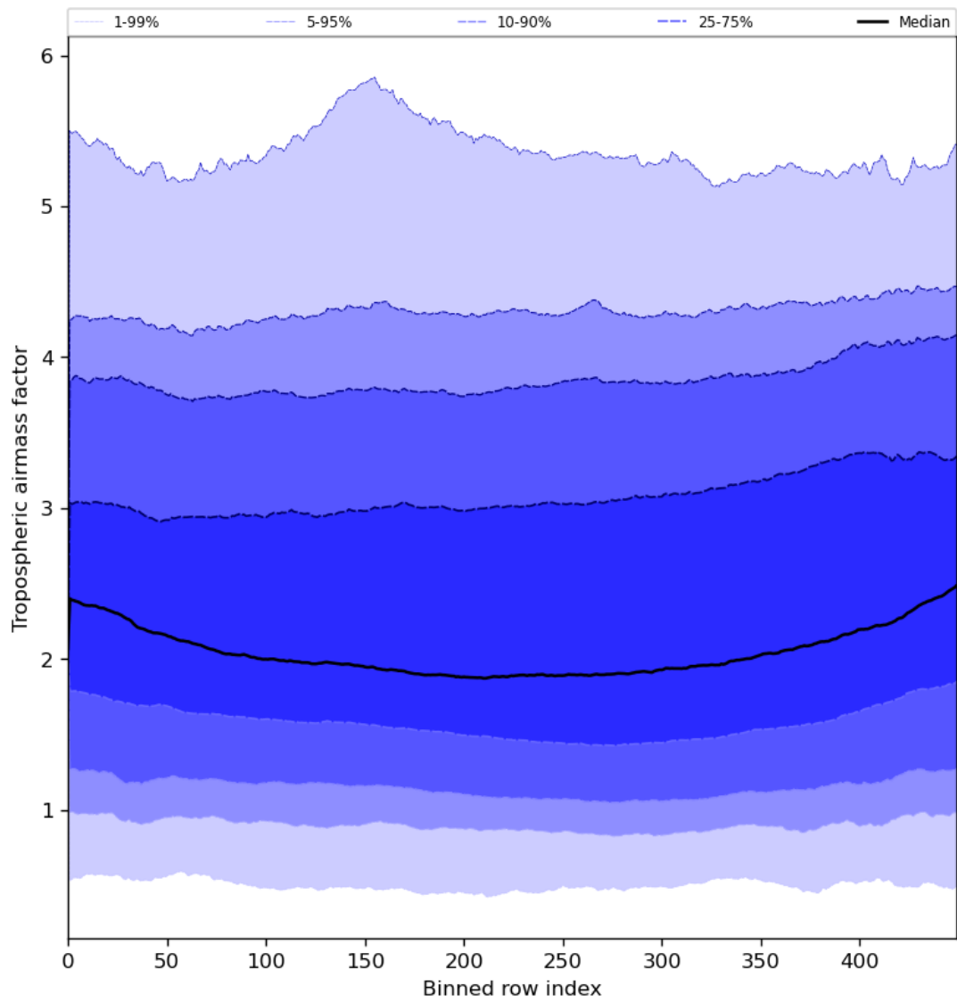
Figure 48: Along track statistics of “Tropospheric airmass factor” for 2024-05-18 to 2024-05-19
