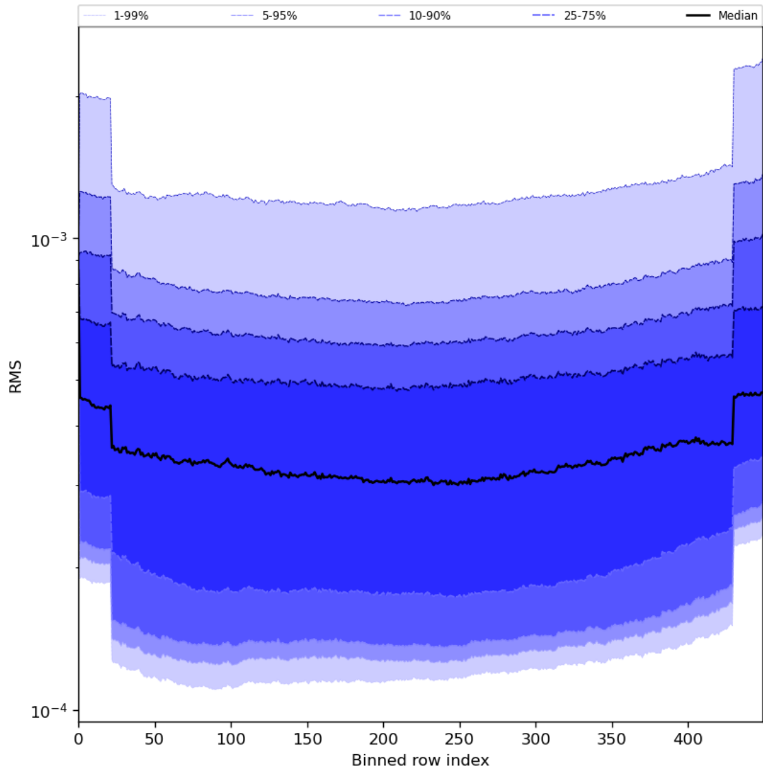
Figure 60: Along track statistics of “RMS” for 2024-05-18 to 2024-05-19
