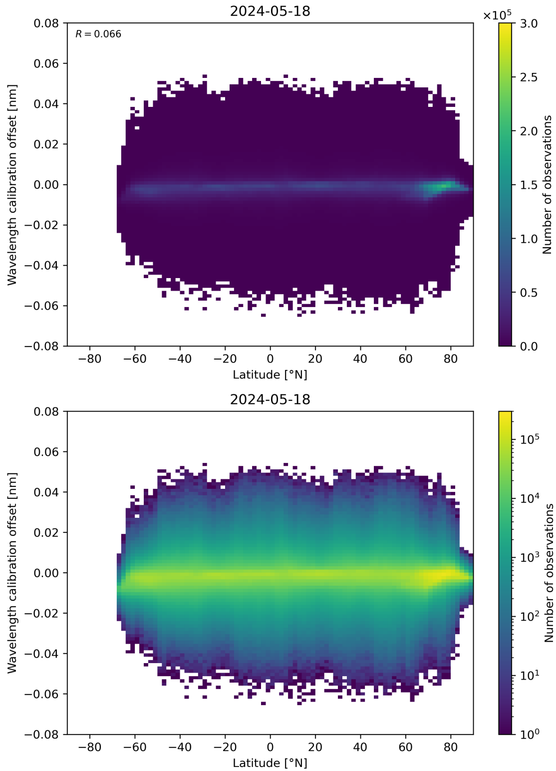
Figure 95: Scatter density plot of “Latitude” against “Wavelength calibration offset” for 2024-05-18 to 2024-05-19.
