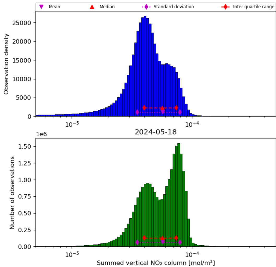
Figure 40: Histogram of “Summed vertical NO 2 column” for 2024-05-18 to 2024-05-19
