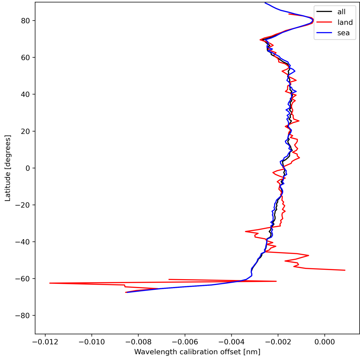
Figure 18: Zonal average of “Wavelength calibration offset” for 2024-05-18 to 2024-05-19.
