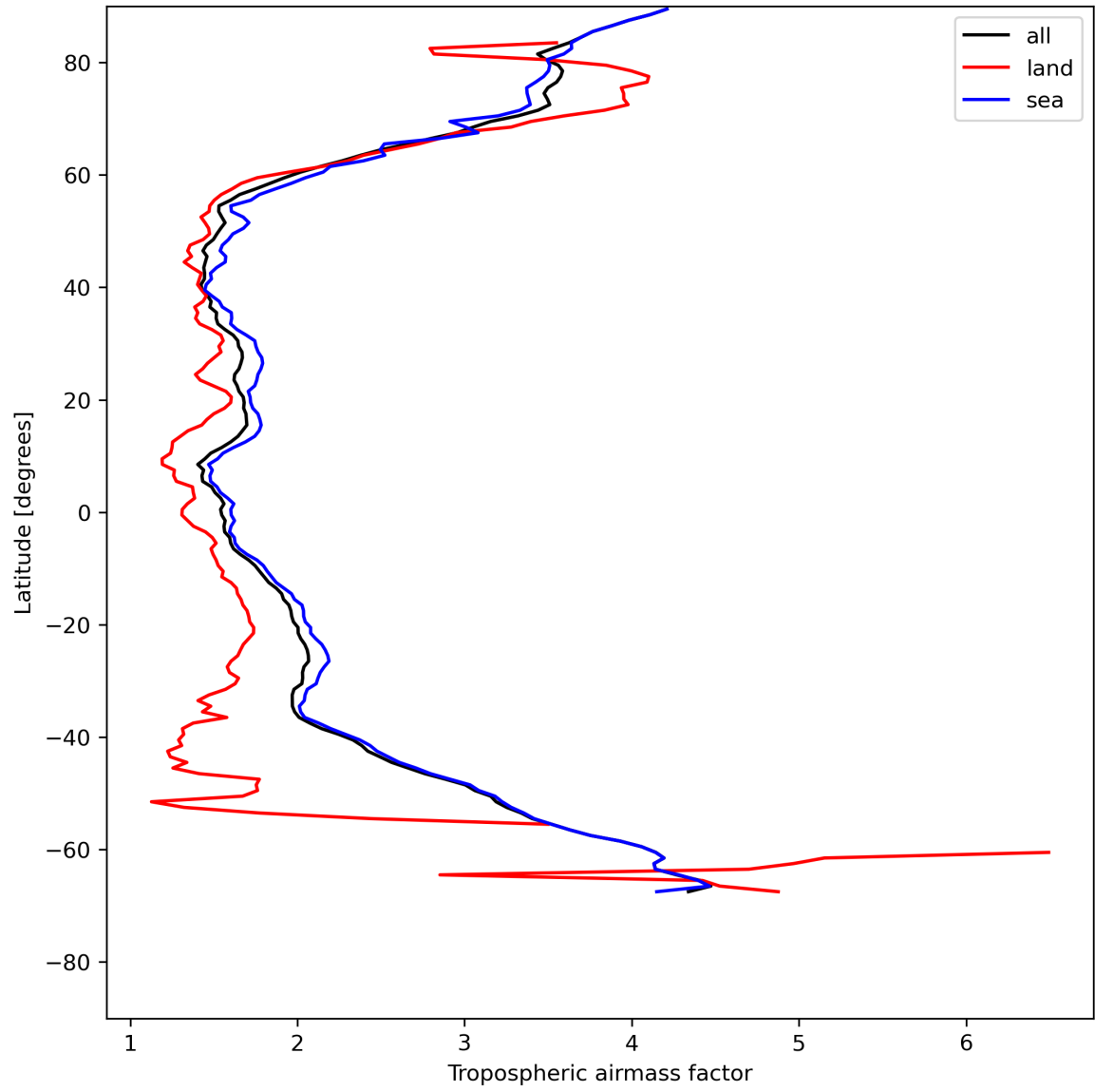
Figure 14: Zonal average of “Tropospheric air mass factor” for 2024-05-18 to 2024-05-19.
