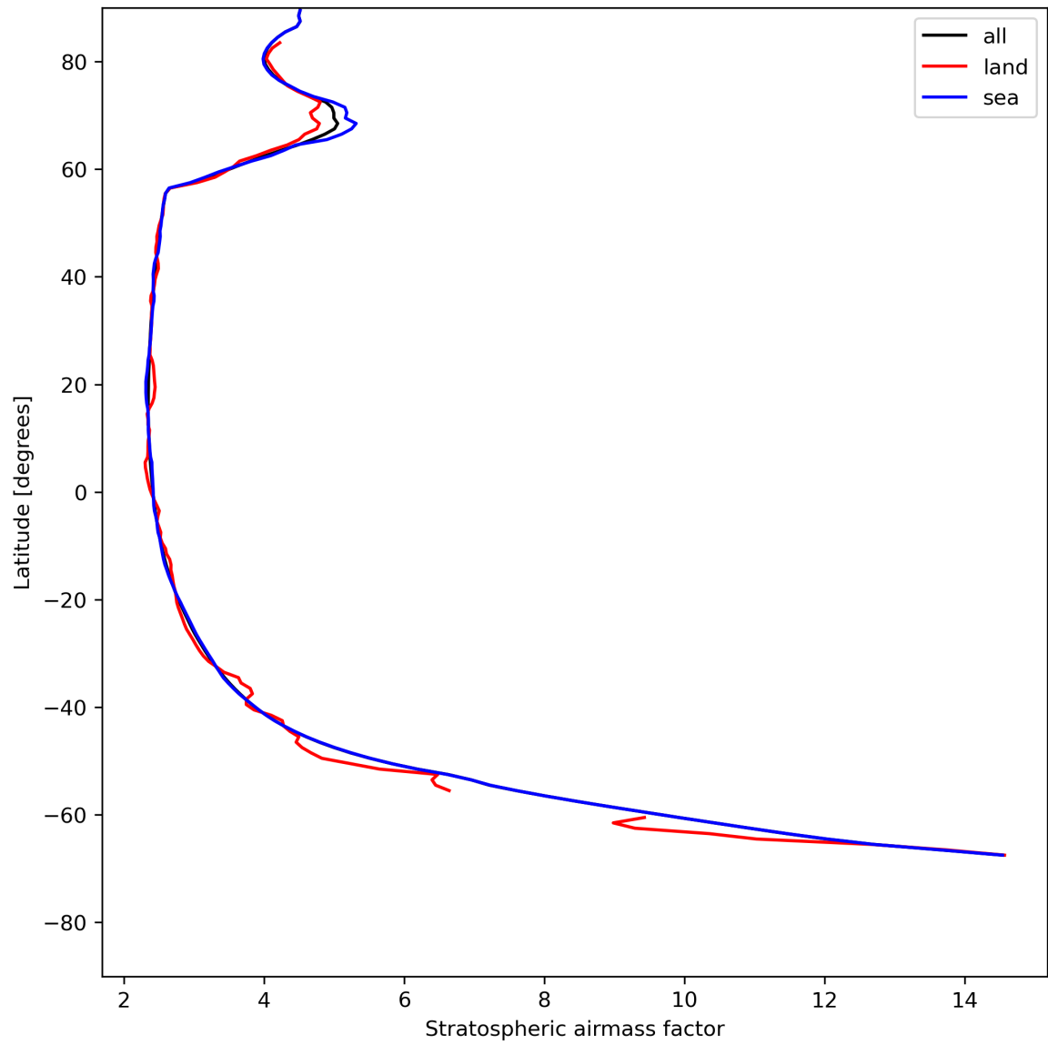
Figure 27: Zonal average of “Stratospheric airmass factor” for 2024-05-18 to 2024-05-19.
