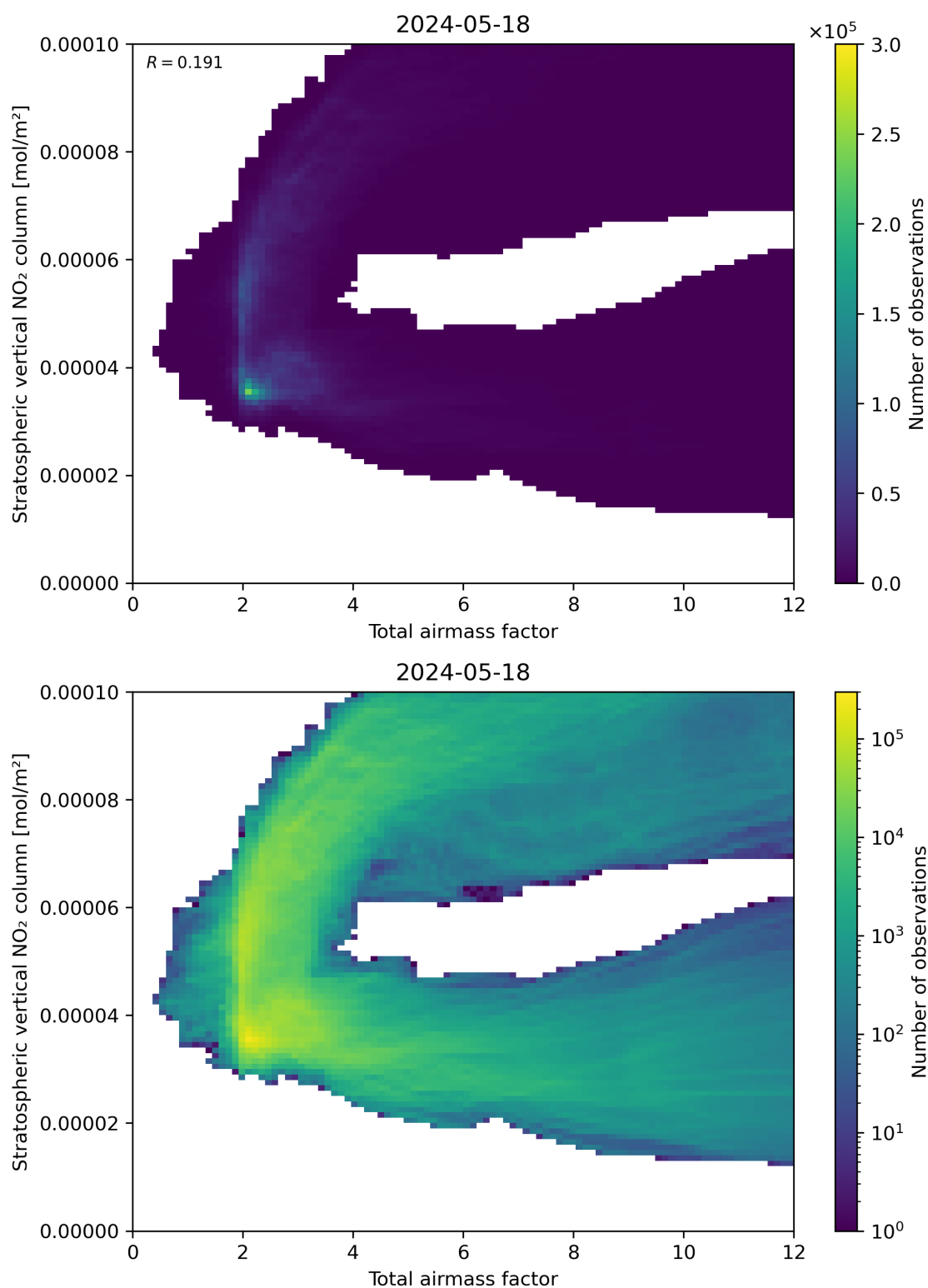
Figure 64: Scatter density plot of “Total airmass factor” against “Stratospheric vertical \text{NO}_2 column” for 2024-05-18 to 2024-05-19.
