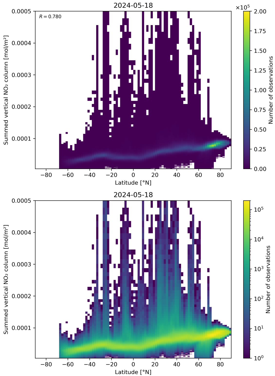
Figure 88: Scatter density plot of “Latitude” against “Summed vertical NO 2 column” for 2024-05-18 to 2024-05-19.
