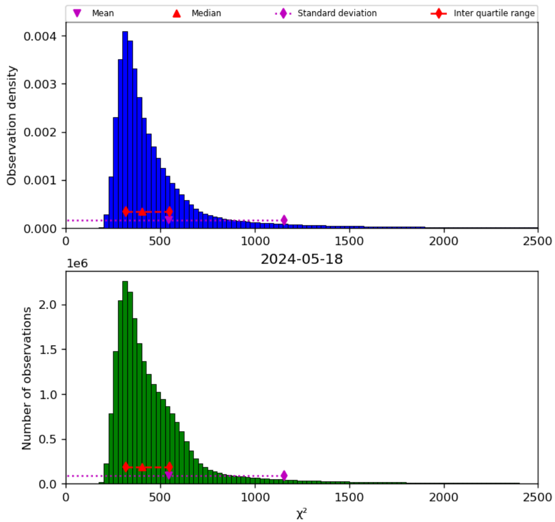
Figure 42: Histogram of “ \chi^2 ” for 2024-05-18 to 2024-05-19
