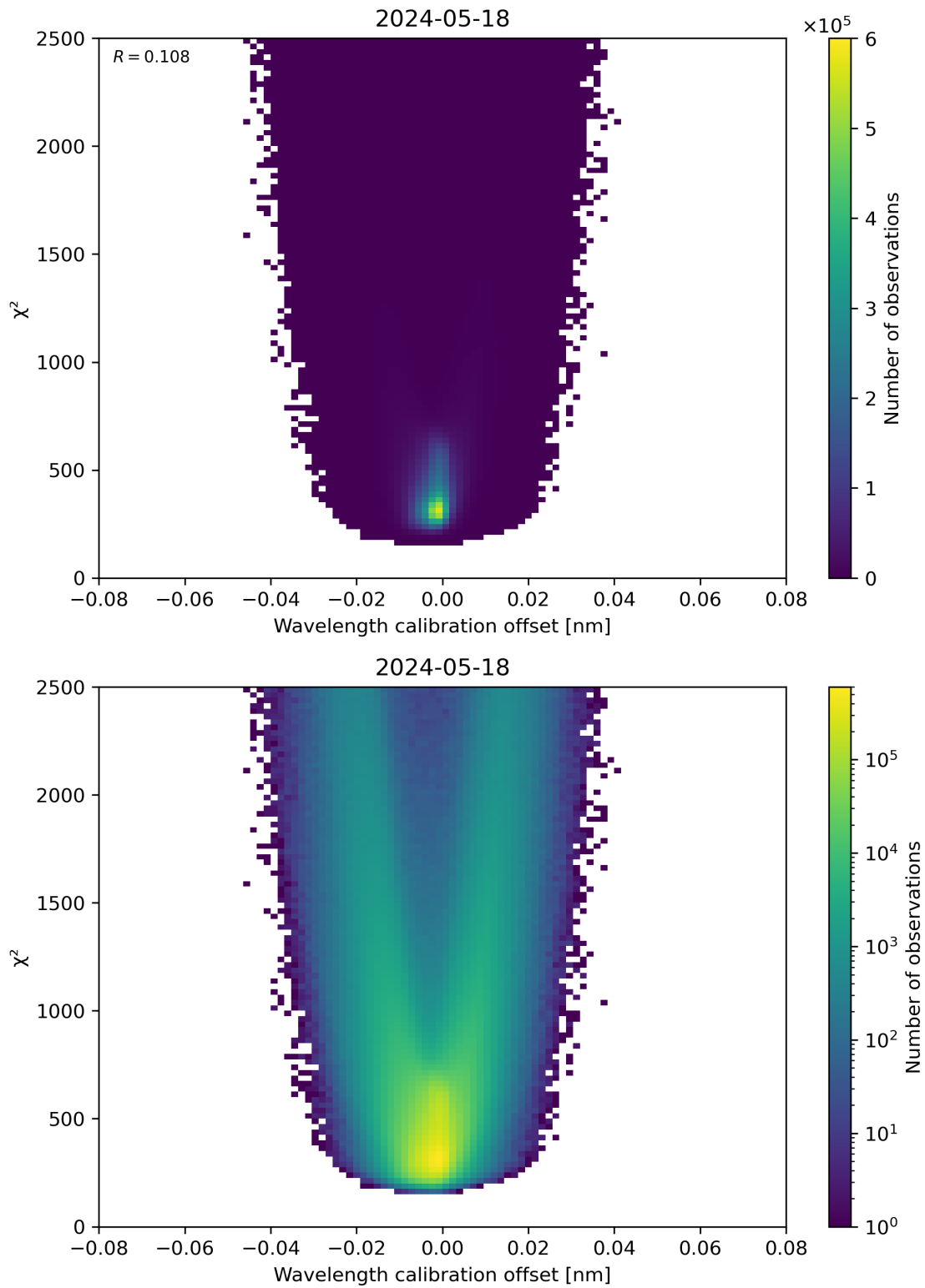
Figure 175: Scatter density plot of “Wavelength calibration offset” against “ \chi^2 ” for 2024-05-18 to 2024-05-19.
