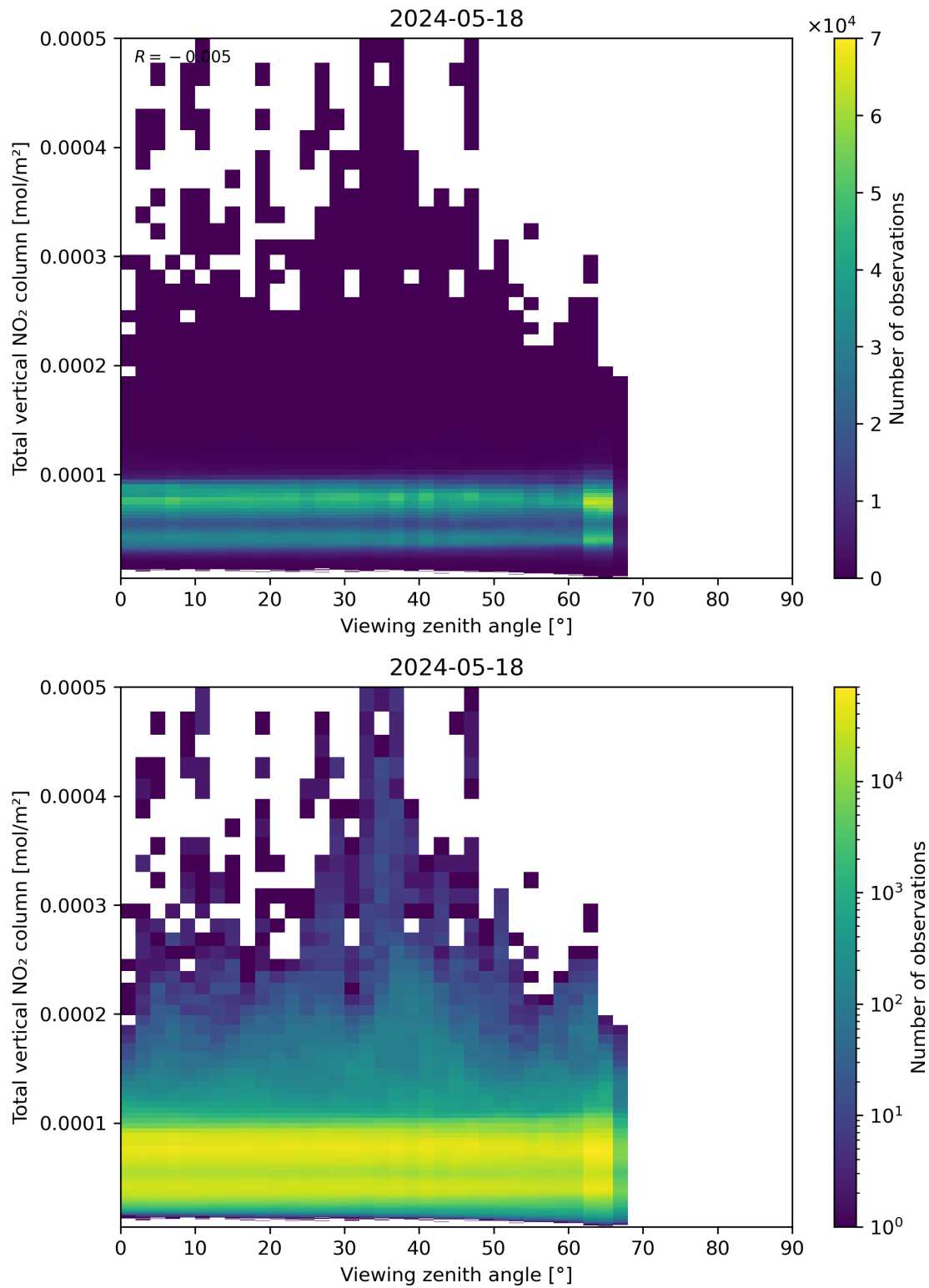
Figure 167: Scatter density plot of “Viewing zenith angle” against “Total vertical NO 2 column” for 2024-05-18 to 2024-05-19.
