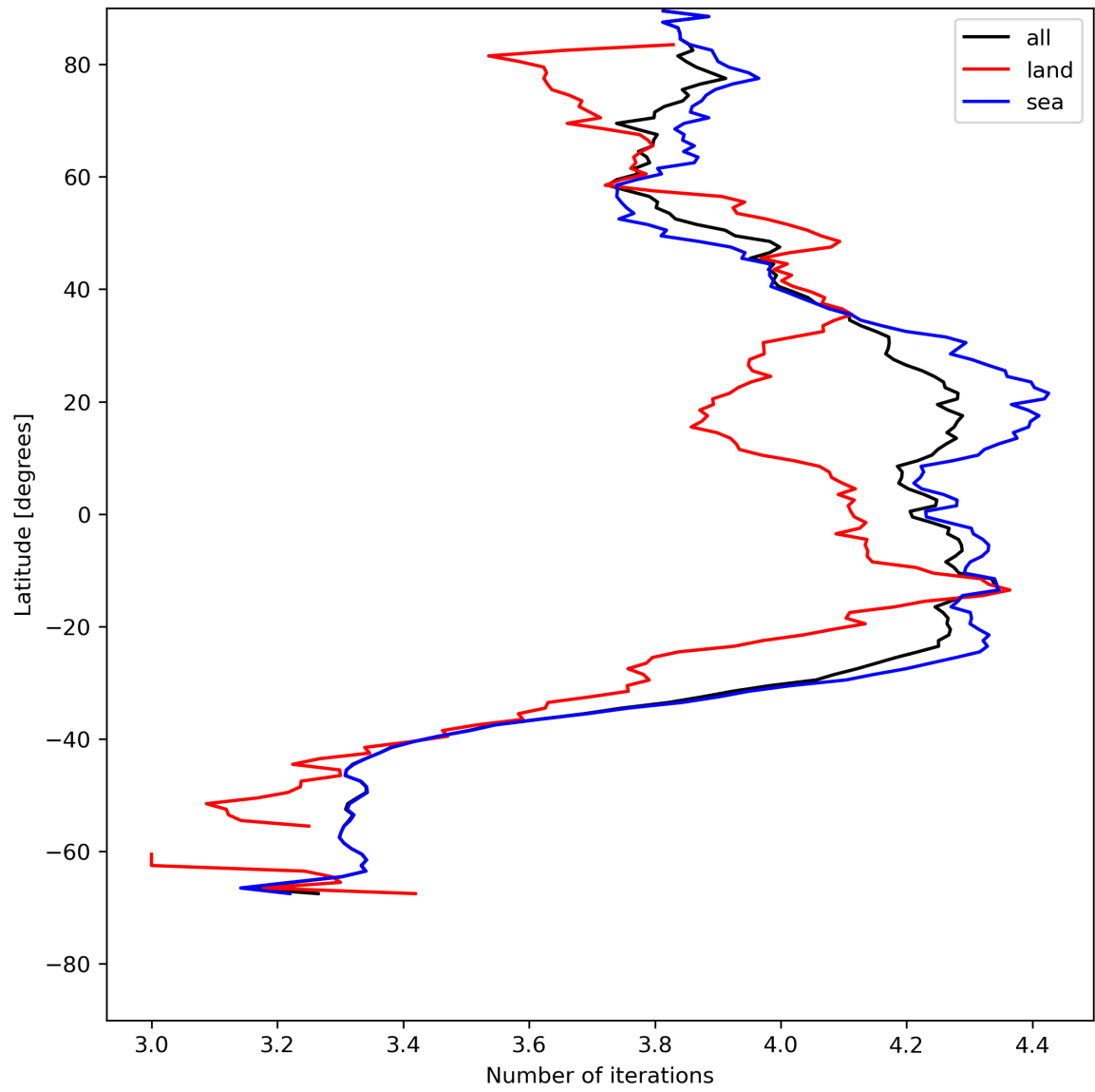
Figure 17: Zonal average of “Number of iterations” for 2024-05-18 to 2024-05-19.
