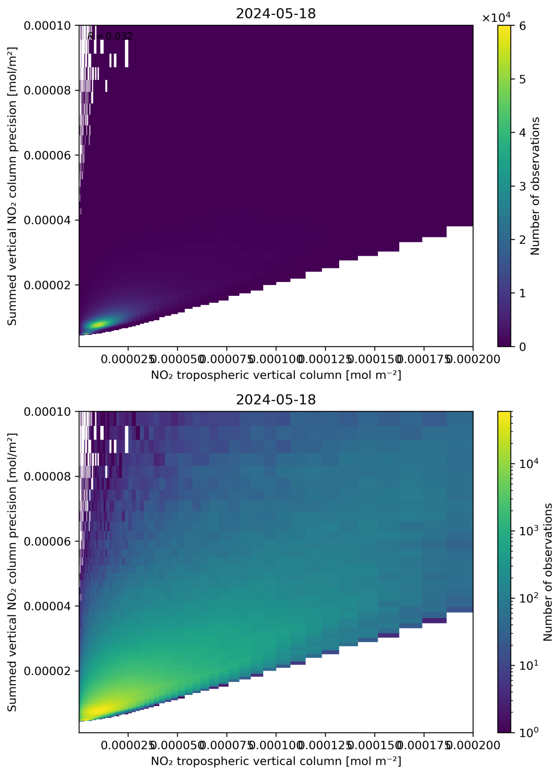
Figure 127: Scatter density plot of “NO 2 tropospheric vertical column” against “Summed vertical NO 2 column precision” for 2024-05-18 to 2024-05-19.
