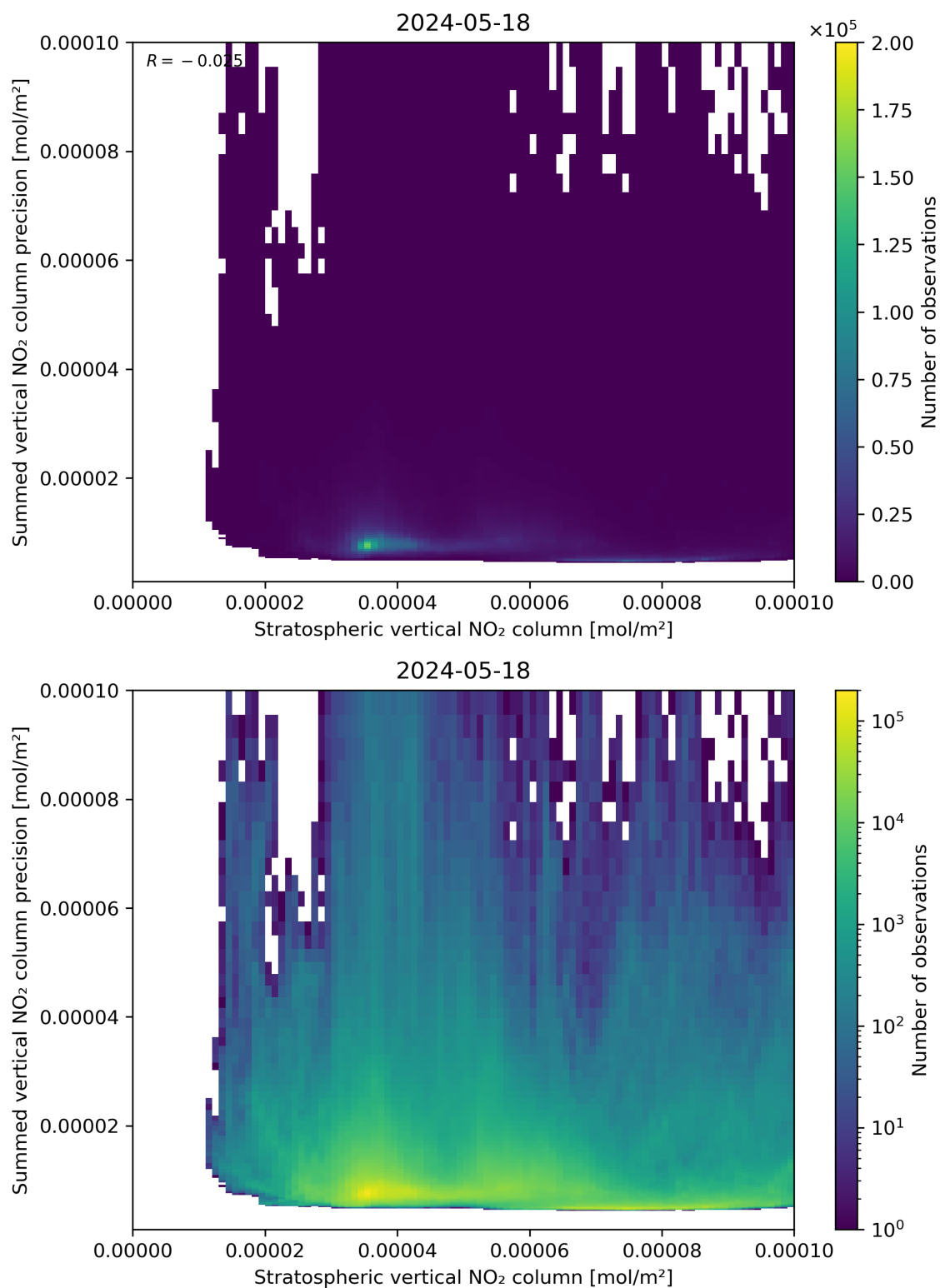
Figure 99: Scatter density plot of “Stratospheric vertical NO 2 column” against “Summed vertical NO 2 column precision” for 2024-05-18 to 2024-05-19.
