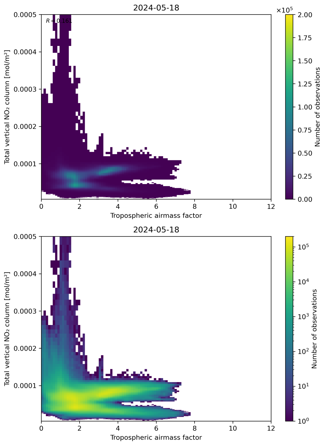
Figure 77: Scatter density plot of “Tropospheric airmass factor” against “Total vertical NO 2 column” for 2024-05-18 to 2024-05-19.
