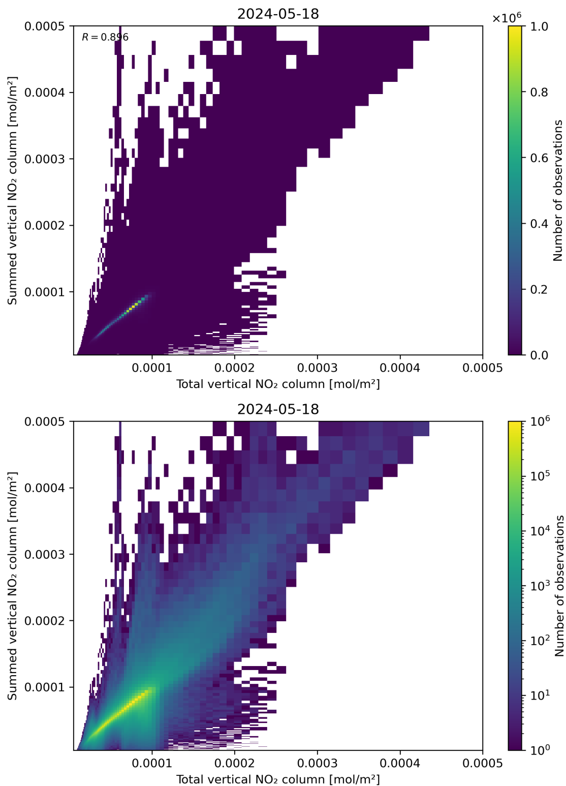
Figure 112: Scatter density plot of “Total vertical NO 2 column” against “Summed vertical NO 2 column” for 2024-05-18 to 2024-05-19.
