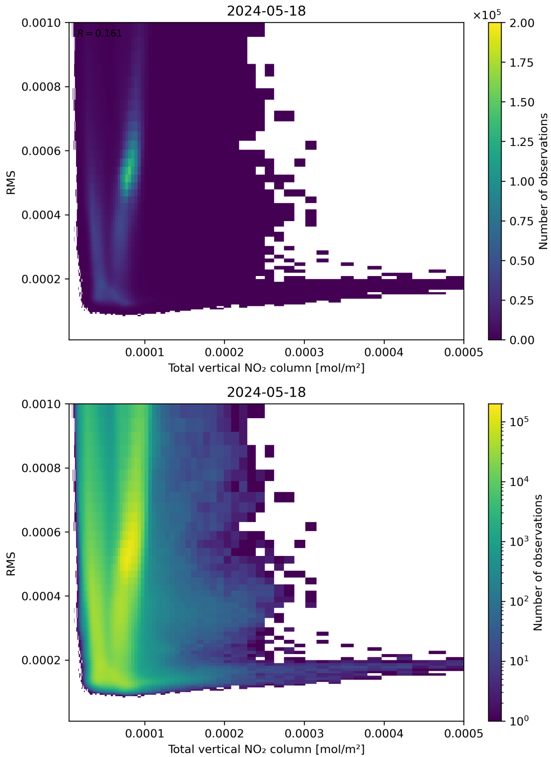
Figure 120: Scatter density plot of “Total vertical NO 2 column” against “RMS” for 2024-05-18 to 2024-05-19.
