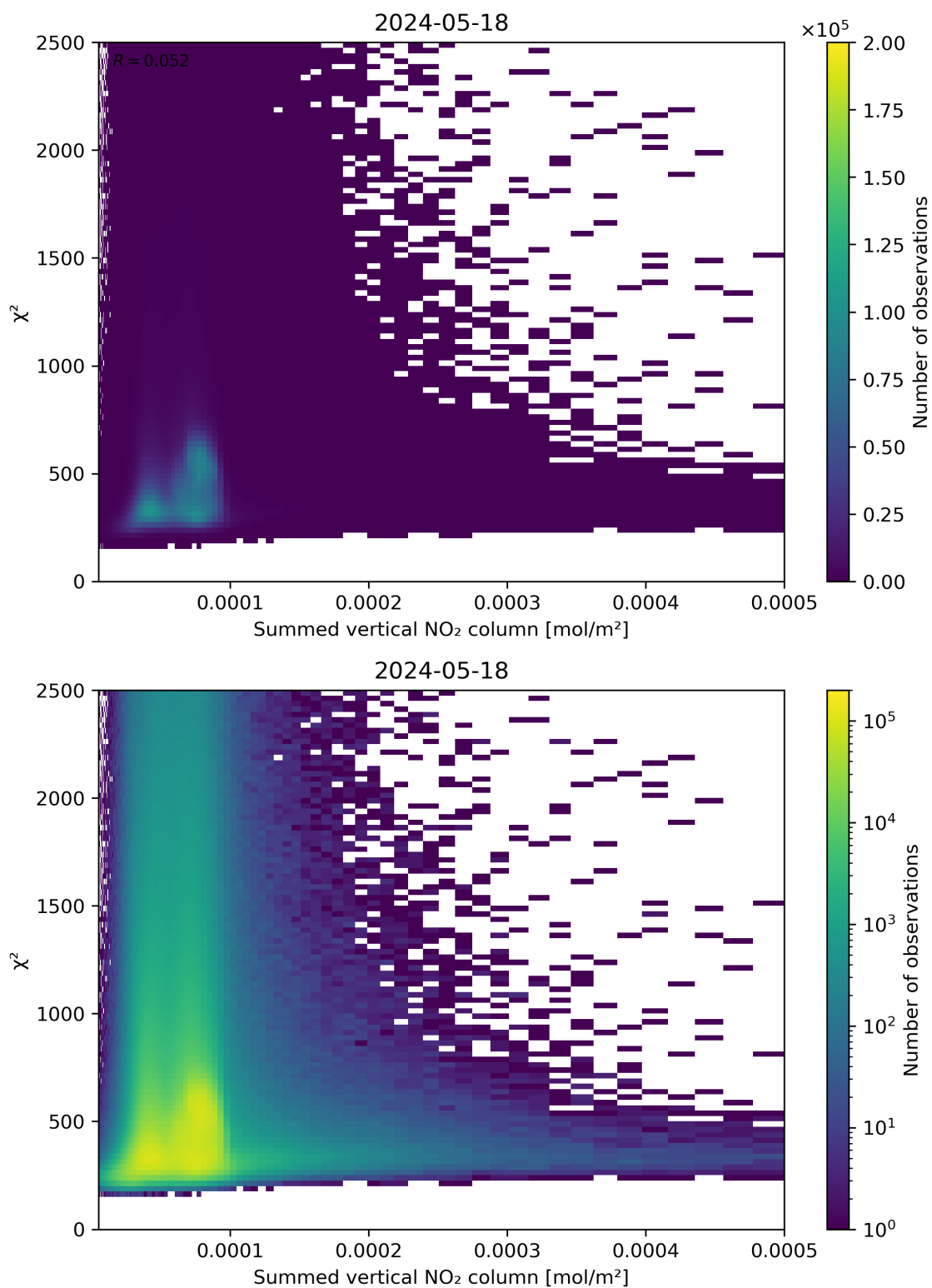
Figure 104: Scatter density plot of “Summed vertical NO 2 column” against “ \chi^2 ” for 2024-05-18 to 2024-05-19.
