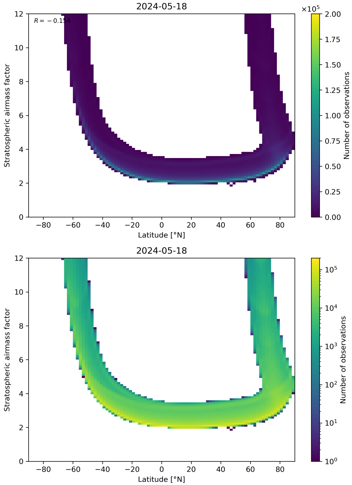
Figure 83: Scatter density plot of “Latitude” against “Stratospheric air mass factor” for 2024-05-18 to 2024-05-19.
