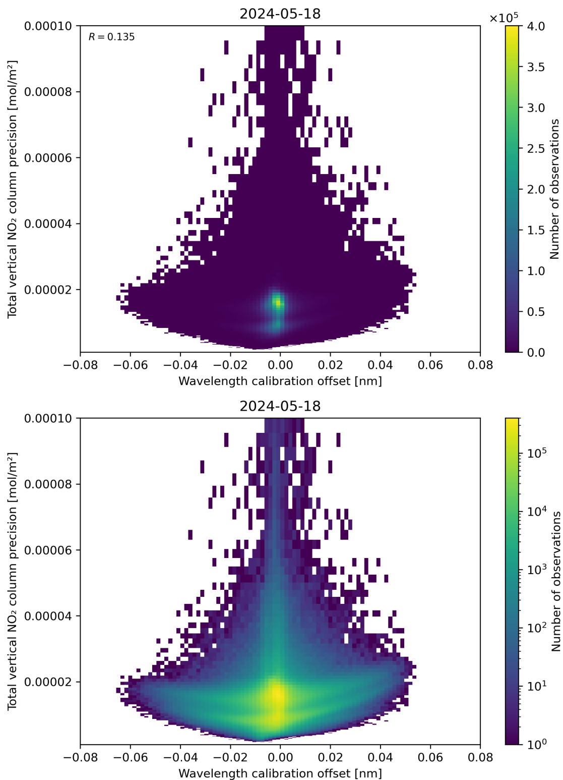
Figure 180: Scatter density plot of “Wavelength calibration offset” against “Total vertical NO 2 column precision” for 2024-05-18 to 2024-05-19.
