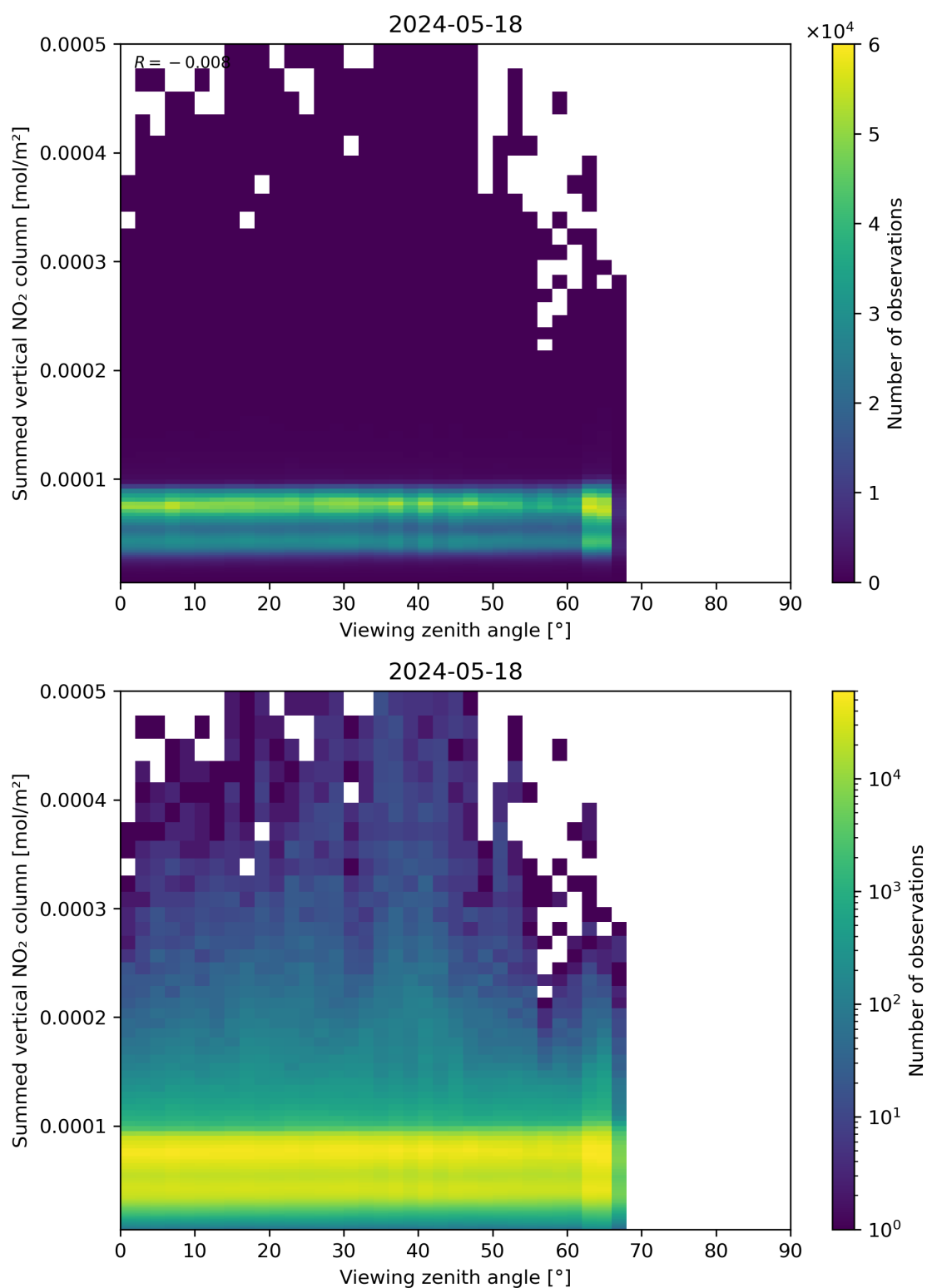
Figure 165: Scatter density plot of “Viewing zenith angle” against “Summed vertical NO 2 column” for 2024-05-18 to 2024-05-19.
