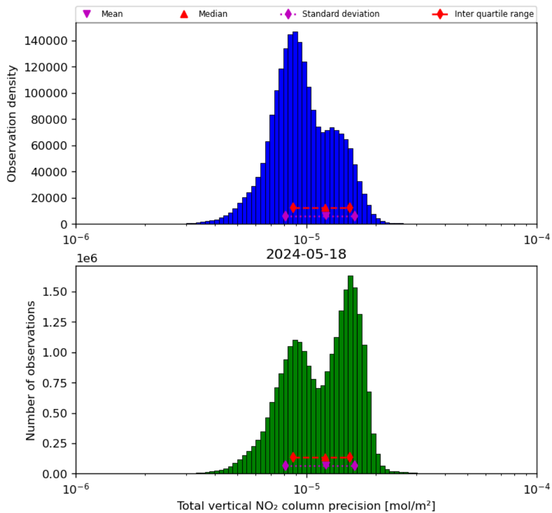
Figure 39: Histogram of “Total vertical NO 2 column precision” for 2024-05-18 to 2024-05-19
