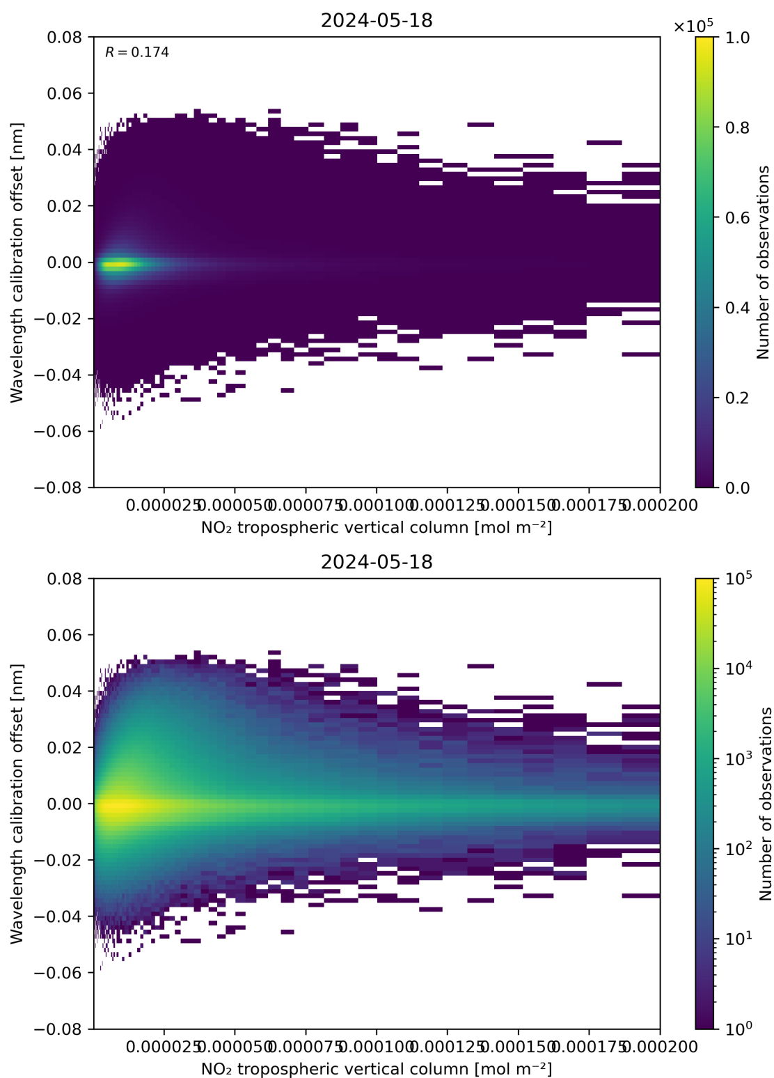
Figure 143: Scatter density plot of “NO 2 tropospheric vertical column” against “Wavelength calibration offset” for 2024-05-18 to 2024-05-19.
