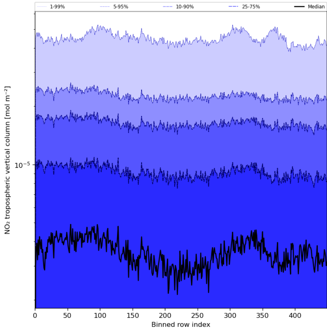
Figure 46: Along track statistics of “NO 2 tropospheric vertical column” for 2024-05-18 to 2024-05-19
