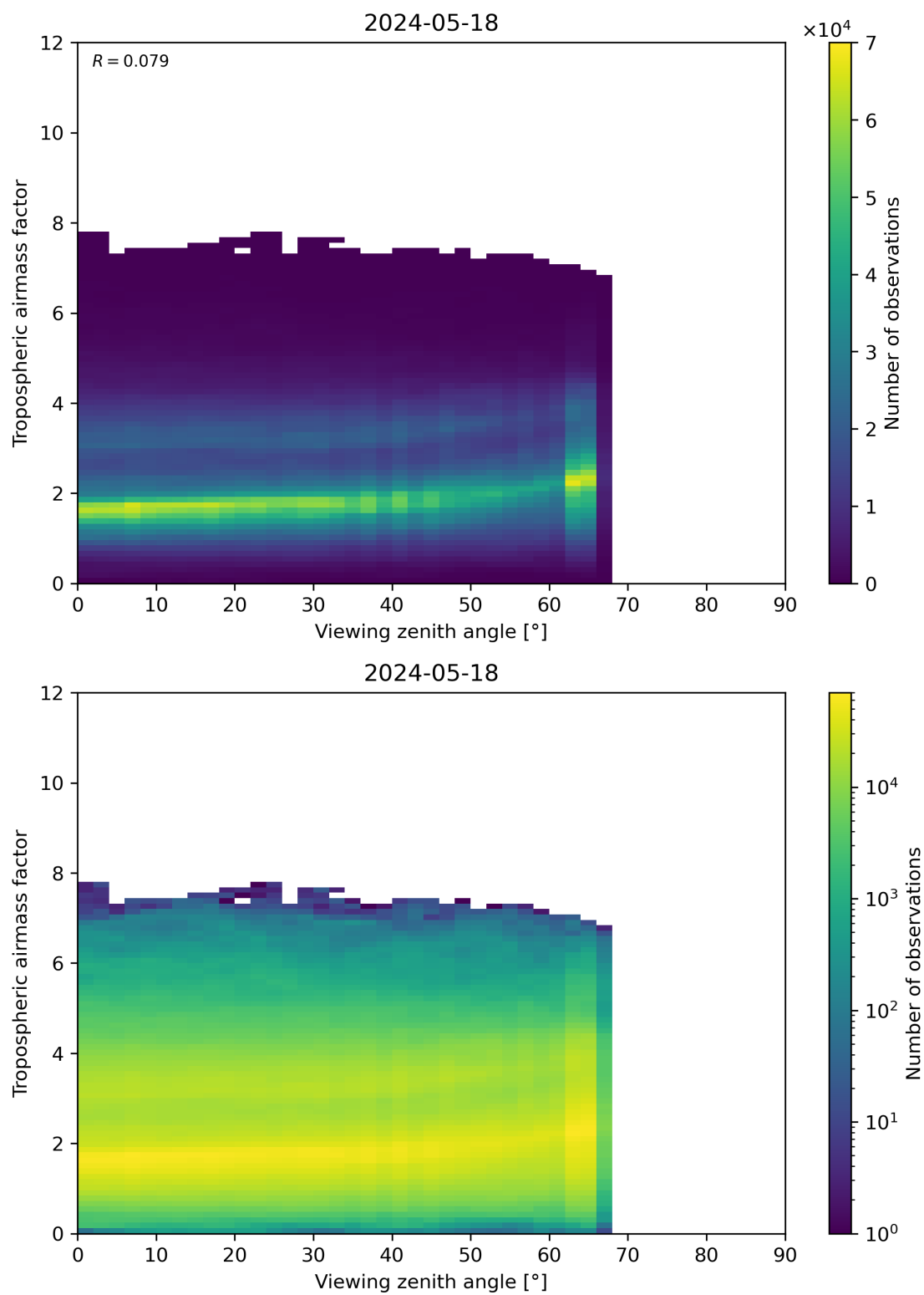
Figure 161: Scatter density plot of “Viewing zenith angle” against “Tropospheric airmass factor” for 2024-05-18 to 2024-05-19.
