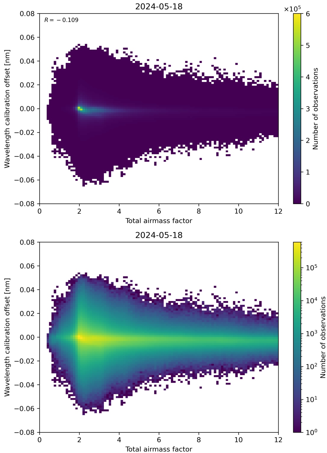
Figure 70: Scatter density plot of “Total airmass factor” against “Wavelength calibration offset” for 2024-05-18 to 2024-05-19.
