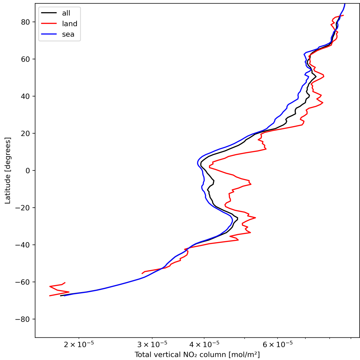
Figure 21: Zonal average of “Total vertical NO 2 column” for 2024-05-18 to 2024-05-19.
