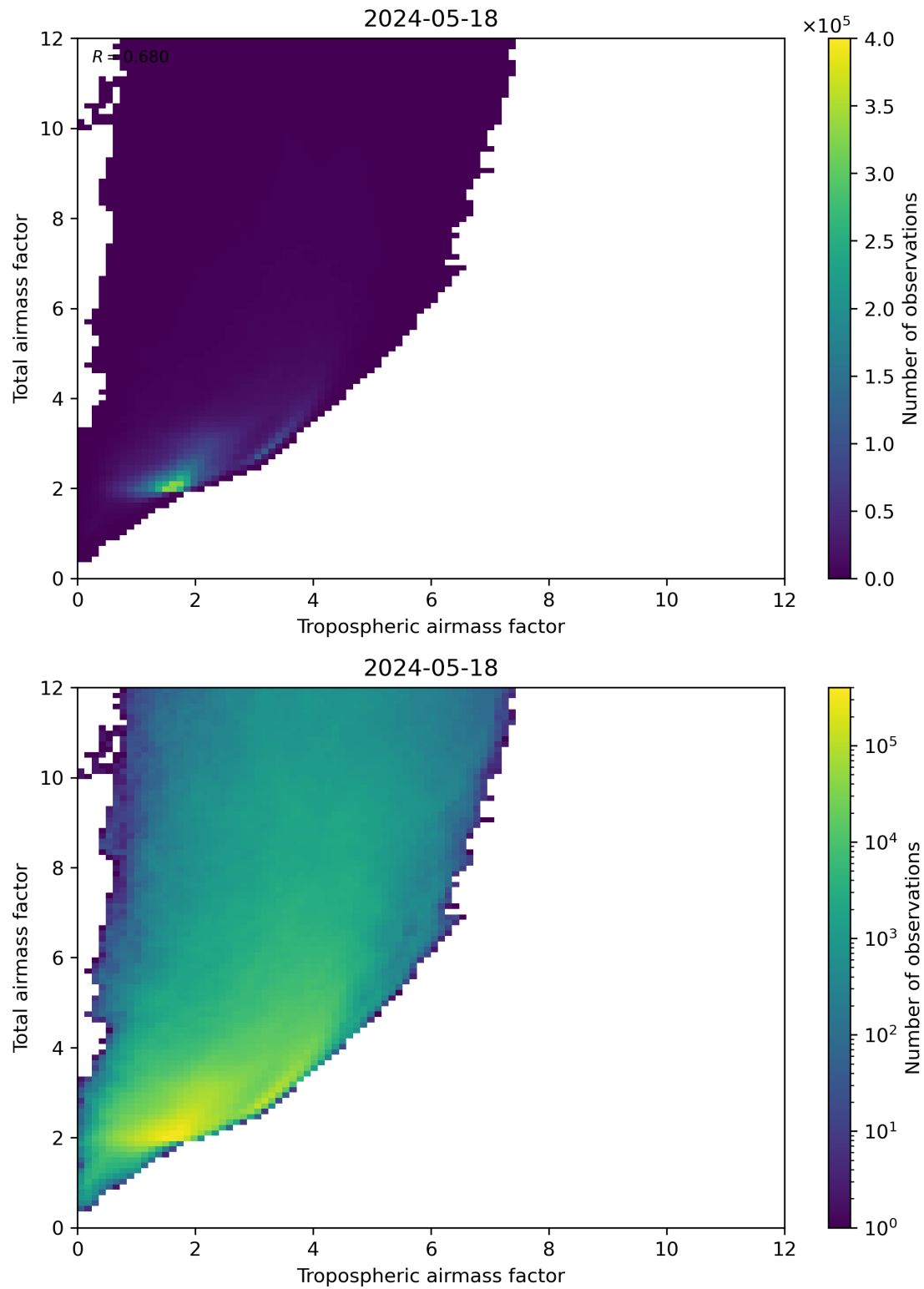
Figure 72: Scatter density plot of “Tropospheric airmass factor” against “Total airmass factor” for 2024-05-18 to 2024-05-19.
