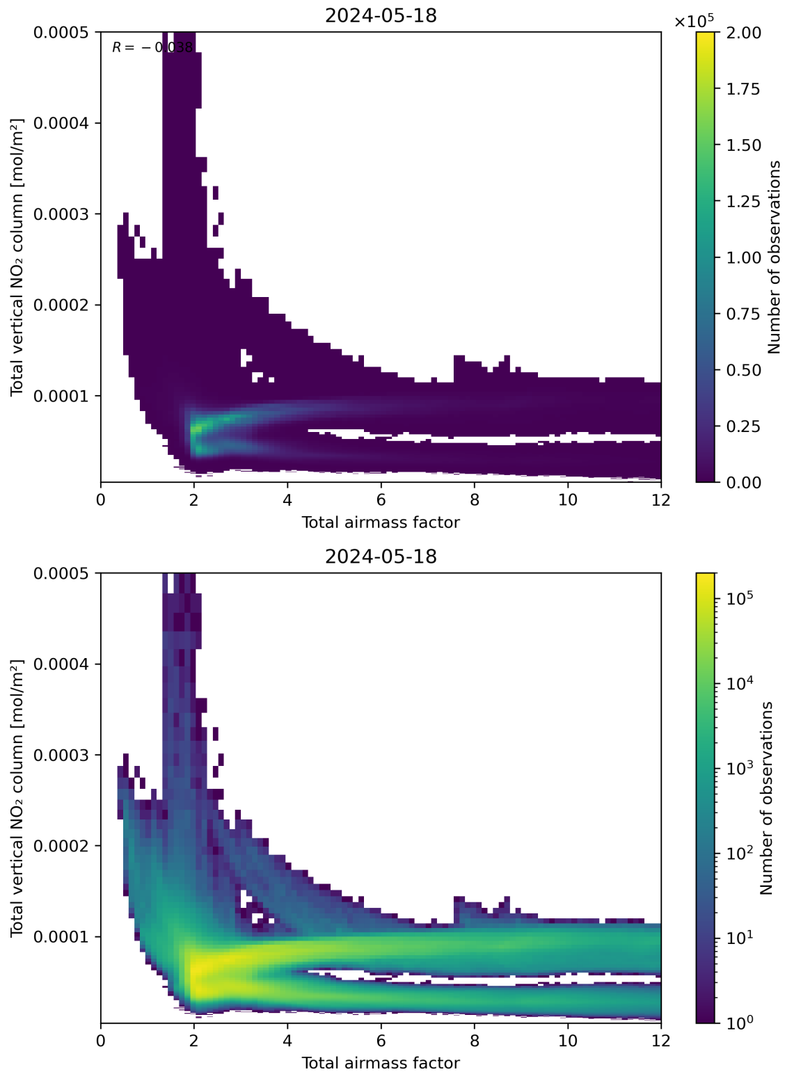
Figure 67: Scatter density plot of “Total airmass factor” against “Total vertical NO 2 column” for 2024-05-18 to 2024-05-19.
