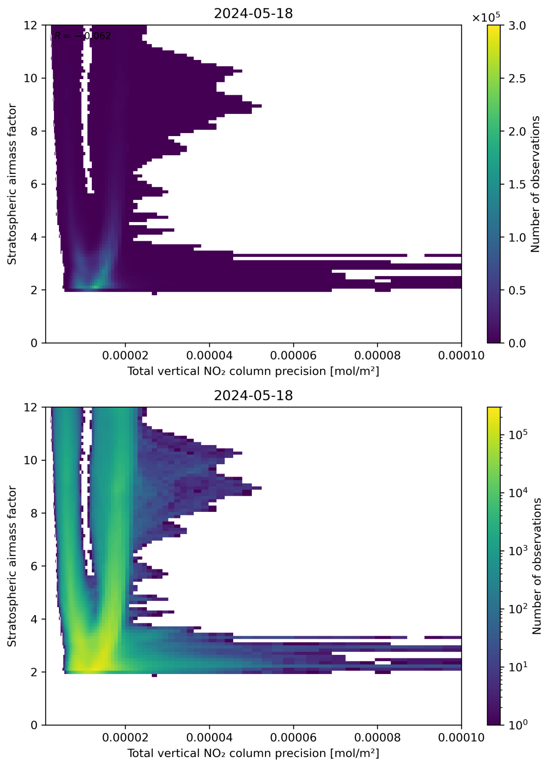
Figure 115: Scatter density plot of “Total vertical NO 2 column precision” against “Stratospheric air mass factor” for 2024-05-18 to 2024-05-19.
