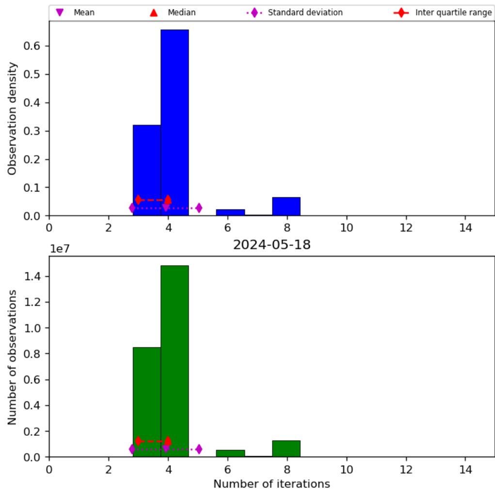
Figure 34: Histogram of “Number of iterations” for 2024-05-18 to 2024-05-19
