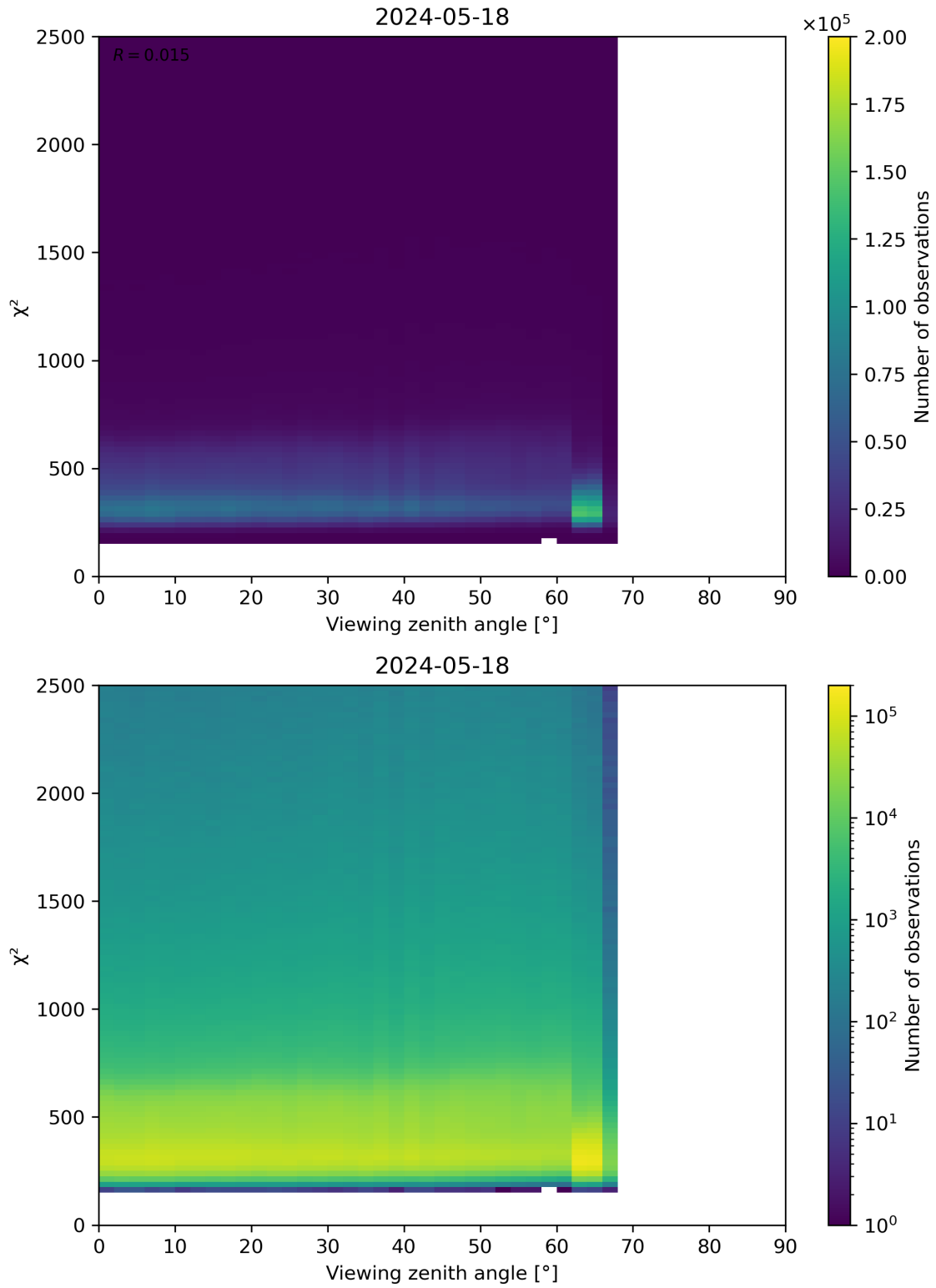
Figure 162: Scatter density plot of “Viewing zenith angle” against “ \chi^2 ” for 2024-05-18 to 2024-05-19.
