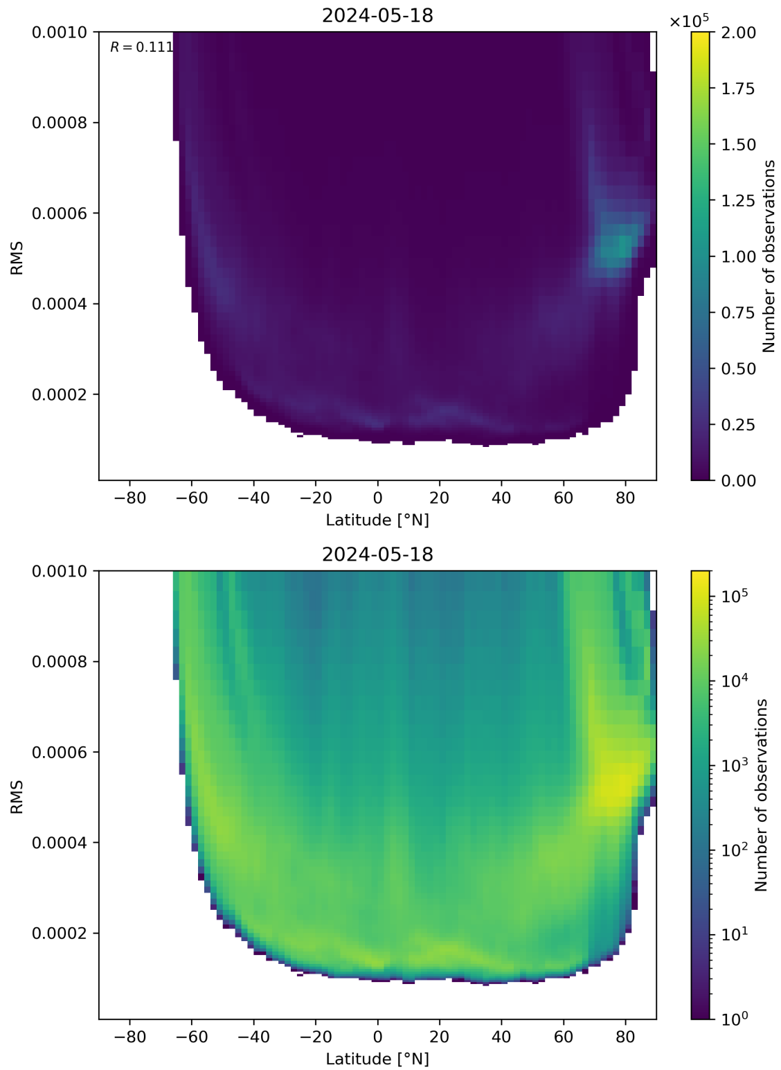
Figure 94: Scatter density plot of “Latitude” against “RMS” for 2024-05-18 to 2024-05-19.
