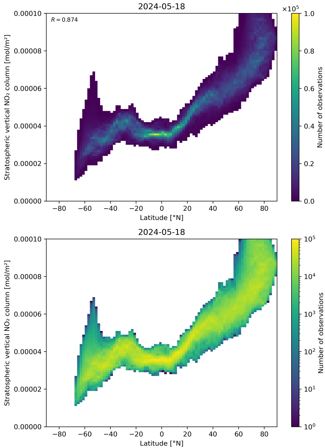
Figure 87: Scatter density plot of “Latitude” against “Stratospheric vertical NO 2 column” for 2024-05-18 to 2024-05-19.
