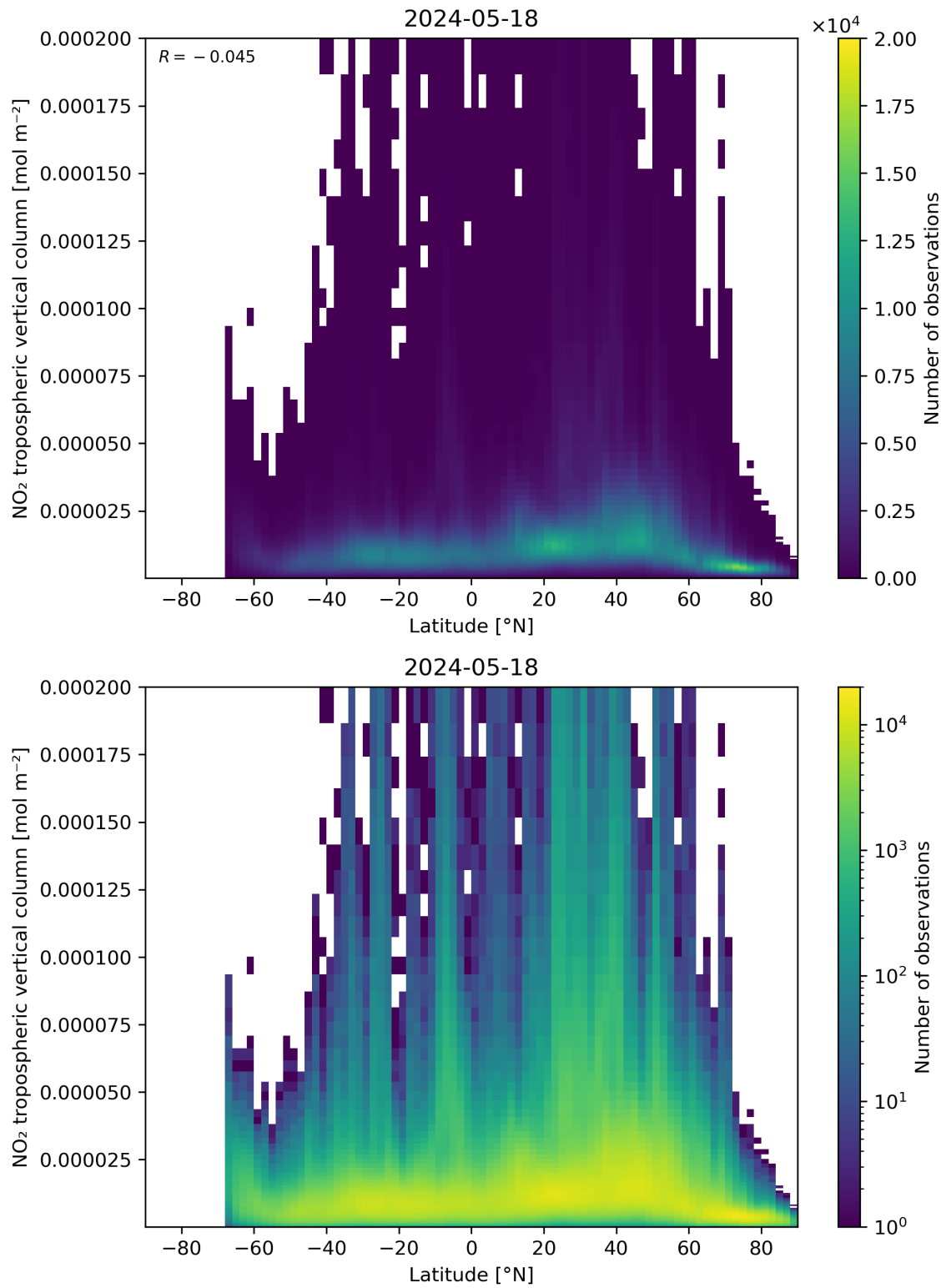
Figure 92: Scatter density plot of “Latitude” against “NO 2 tropospheric vertical column” for 2024-05-18 to 2024-05-19.
