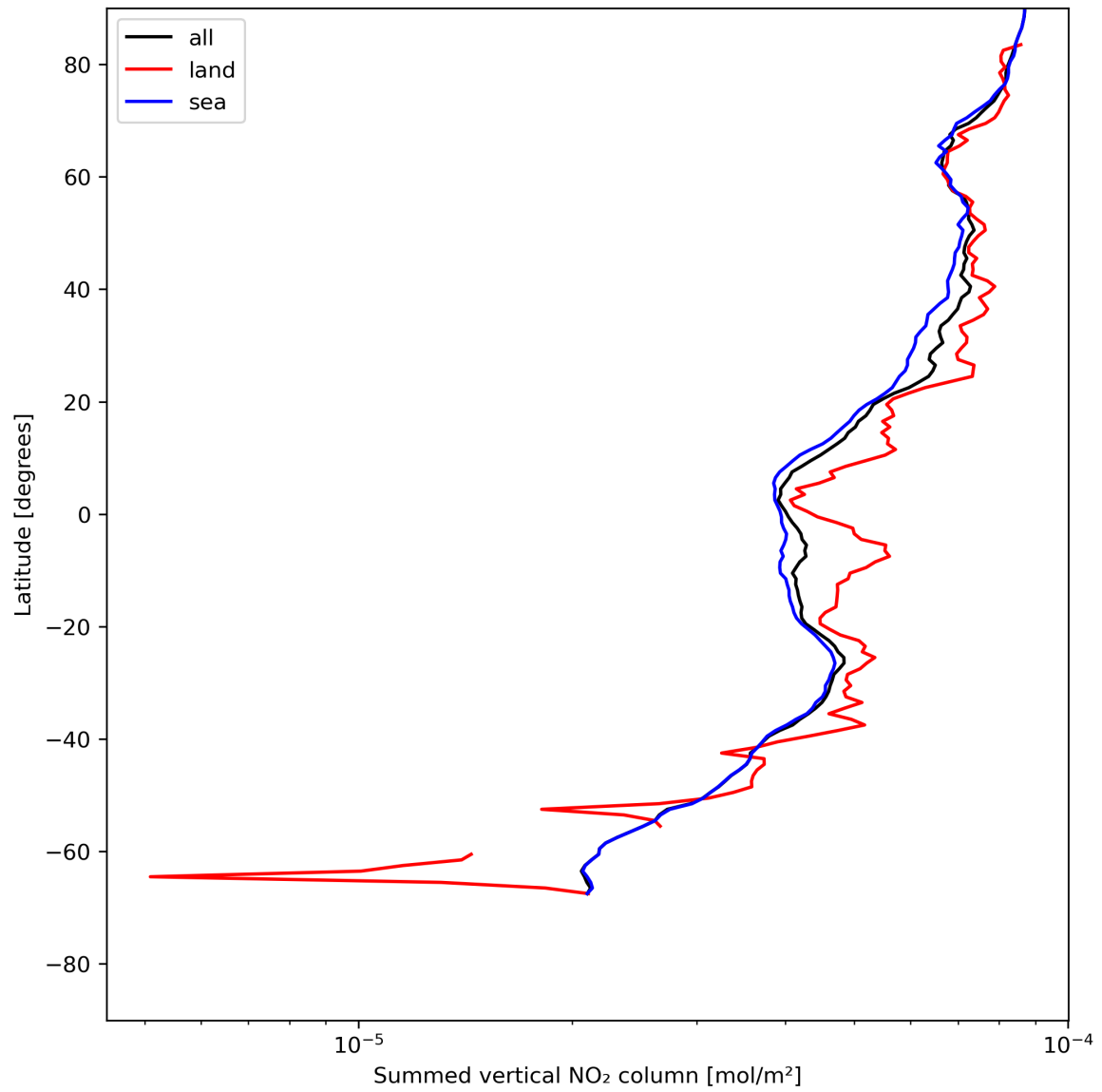
Figure 23: Zonal average of “Summed vertical NO 2 column” for 2024-05-18 to 2024-05-19.
