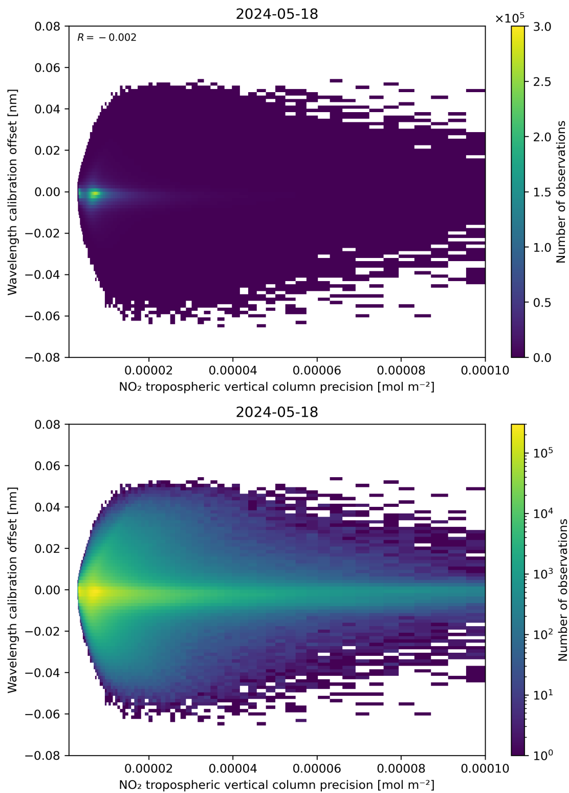
Figure 141: Scatter density plot of “NO 2 tropospheric vertical column precision” against “Wavelength calibration offset” for 2024-05-18 to 2024-05-19.
