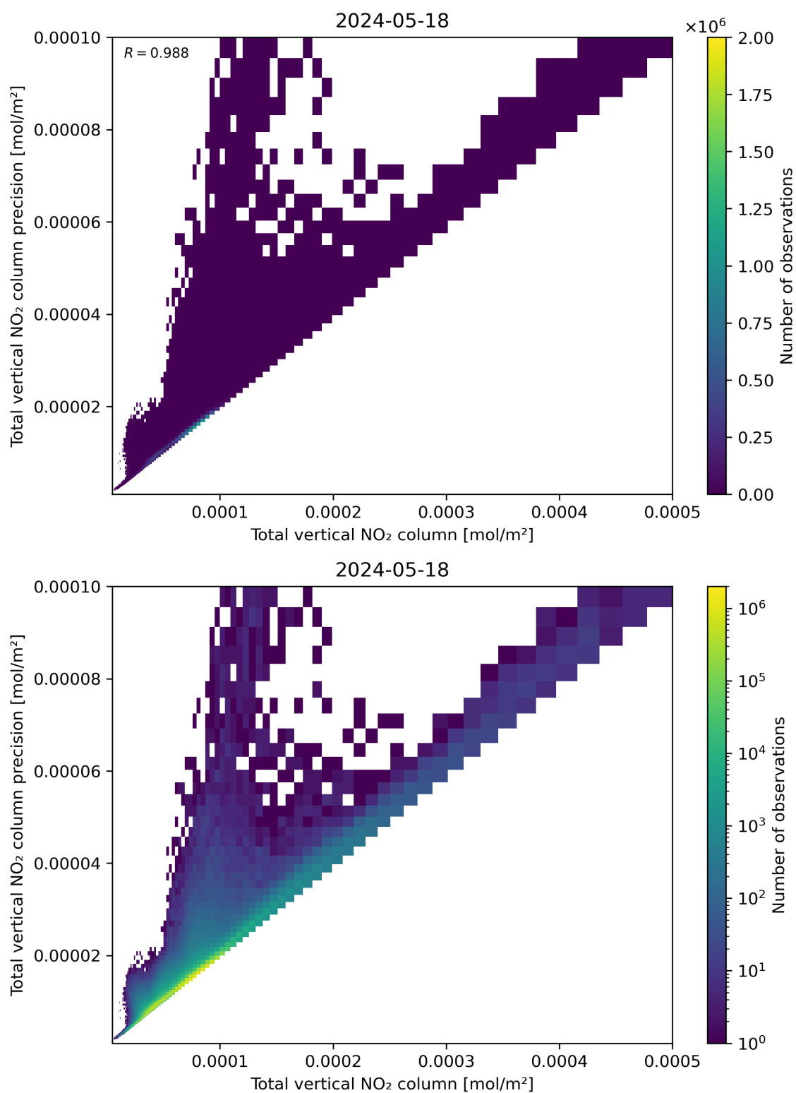
Figure 114: Scatter density plot of “Total vertical NO 2 column” against “Total vertical NO 2 column precision” for 2024-05-18 to 2024-05-19.
