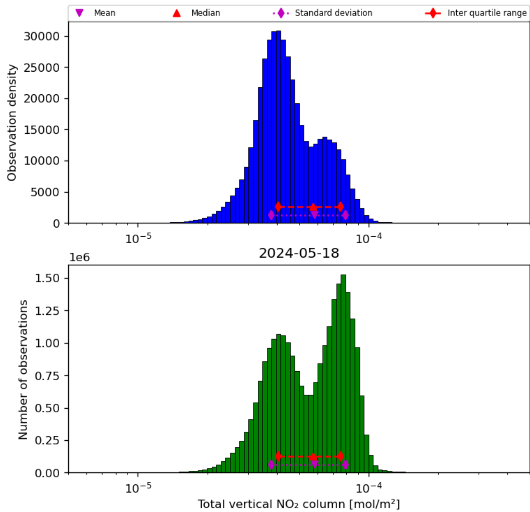
Figure 38: Histogram of "Total vertical NO 2 column" for 2024-05-18 to 2024-05-19
