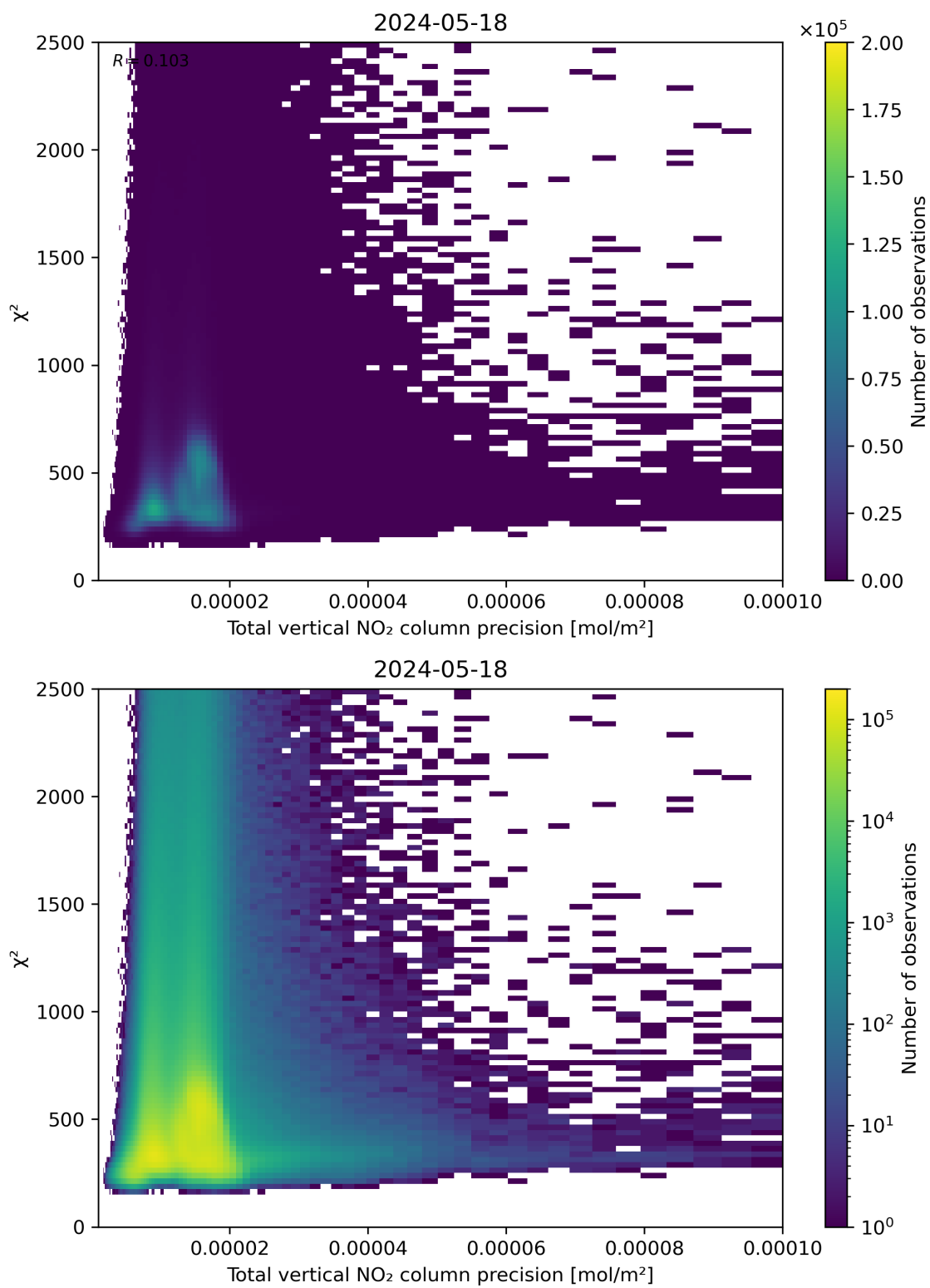
Figure 116: Scatter density plot of “Total vertical NO 2 column precision” against “ \chi^2 ” for 2024-05-18 to 2024-05-19.
