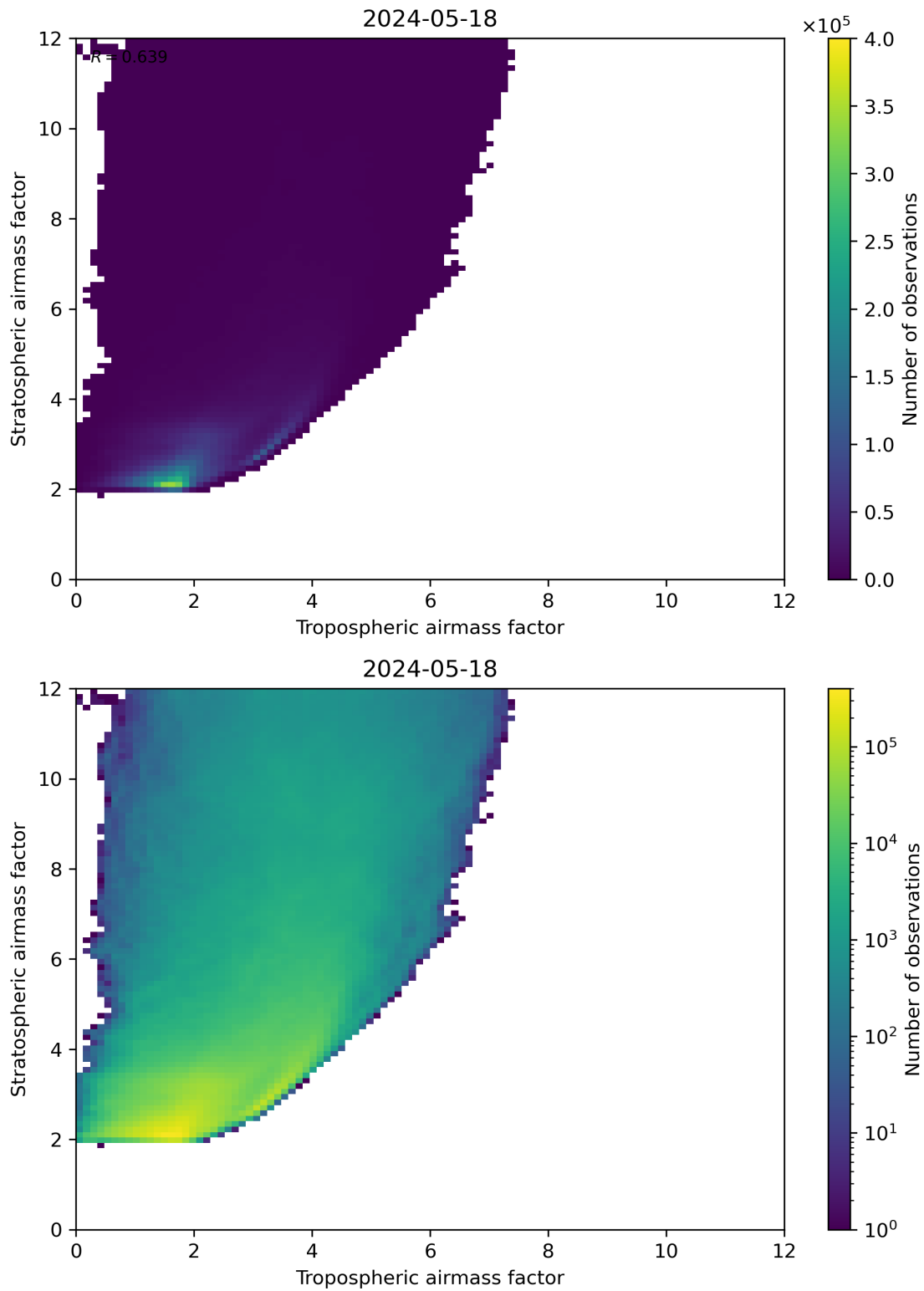
Figure 71: Scatter density plot of “Tropospheric airmass factor” against “Stratospheric airmass factor” for 2024-05-18 to 2024-05-19.
