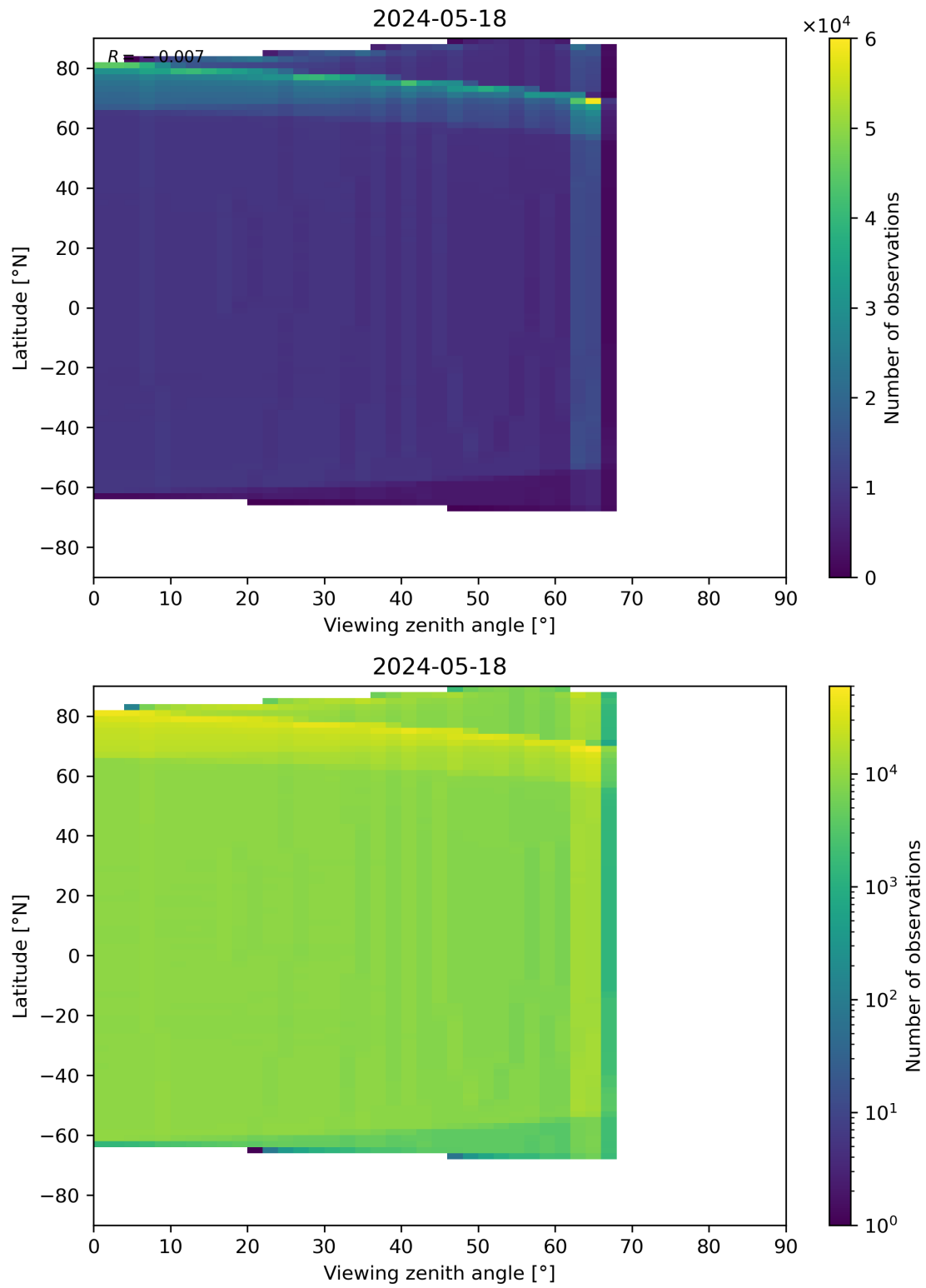
Figure 163: Scatter density plot of “Viewing zenith angle” against “Latitude” for 2024-05-18 to 2024-05-19.
