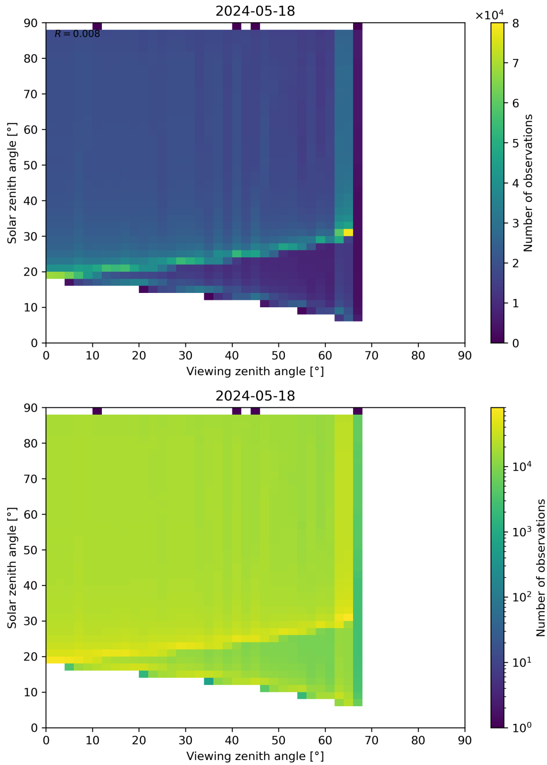
Figure 172: Scatter density plot of “Viewing zenith angle” against “Solar zenith angle” for 2024-05-18 to 2024-05-19.
