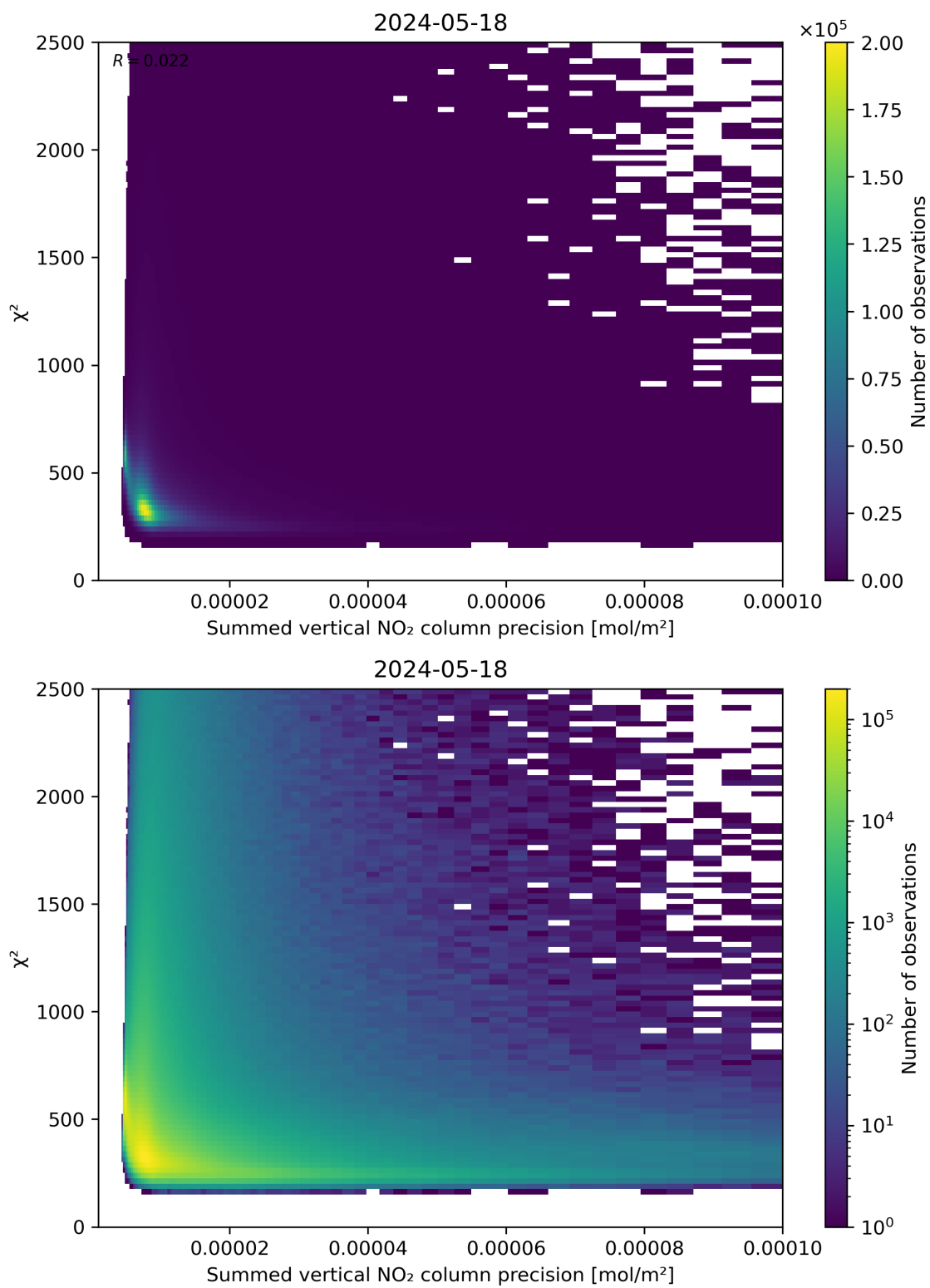
Figure 107: Scatter density plot of “Summed vertical NO 2 column precision” against “ \chi^2 ” for 2024-05-18 to 2024-05-19.
