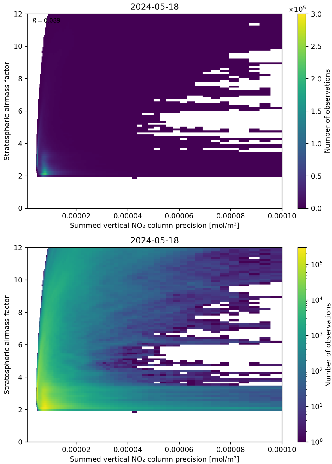
Figure 106: Scatter density plot of “Summed vertical NO 2 column precision” against “Stratospheric airmass factor” for 2024-05-18 to 2024-05-19.
