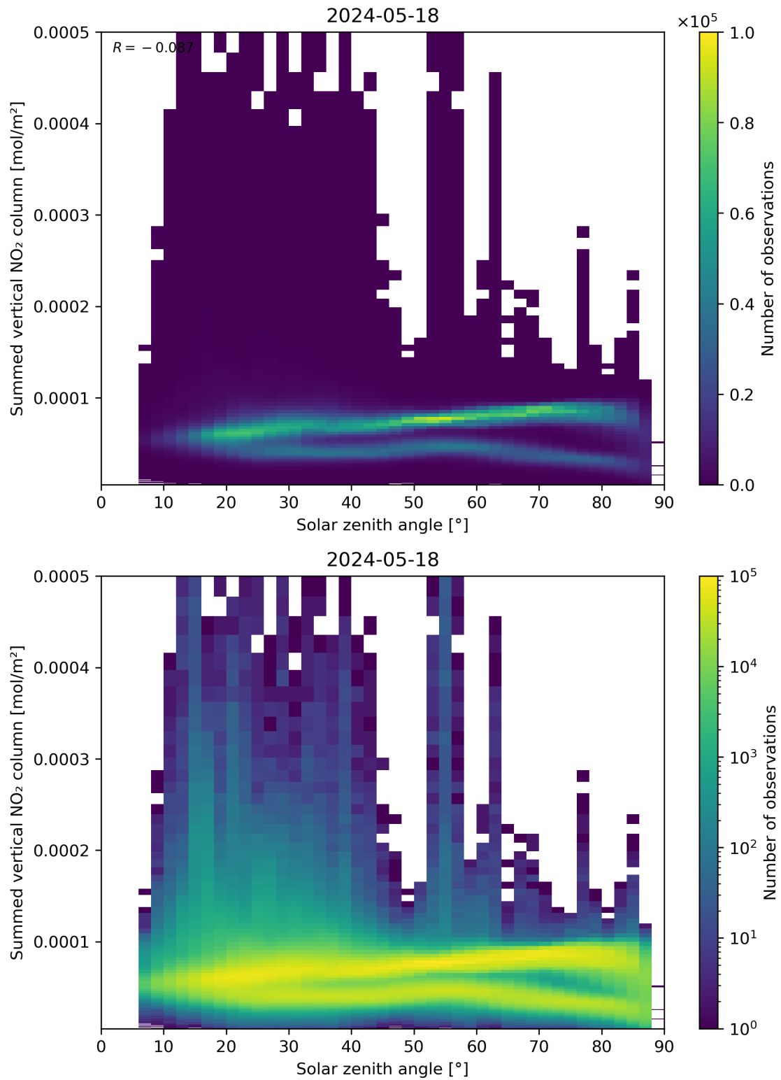
Figure 151: Scatter density plot of “Solar zenith angle” against “Summed vertical NO 2 column” for 2024-05-18 to 2024-05-19.
