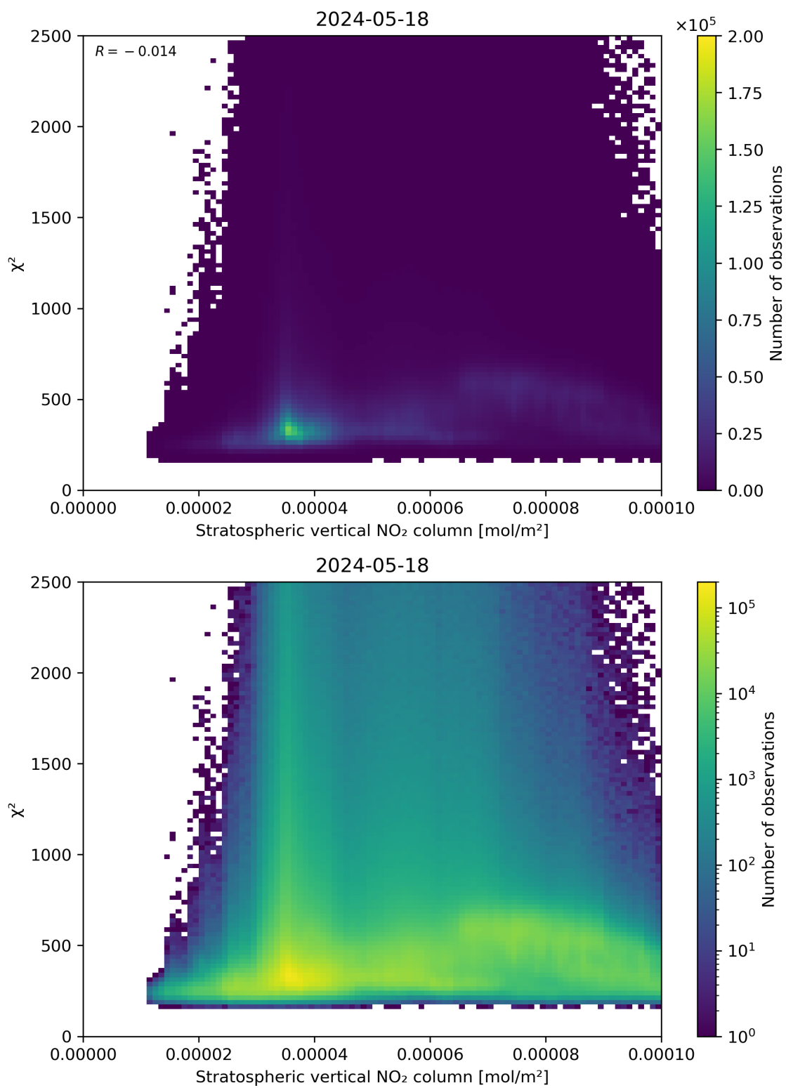
Figure 97: Scatter density plot of “Stratospheric vertical NO 2 column” against “ \chi^2 ” for 2024-05-18 to 2024-05-19.
