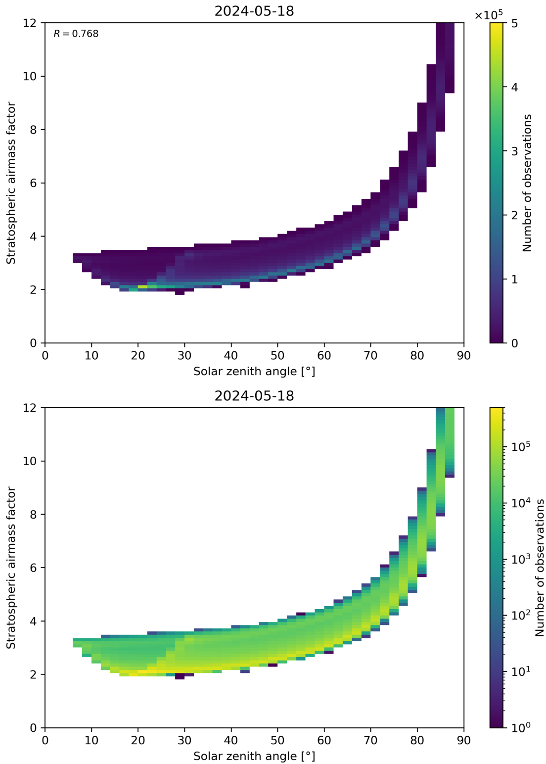
Figure 145: Scatter density plot of “Solar zenith angle” against “Stratospheric airmass factor” for 2024-05-18 to 2024-05-19.
