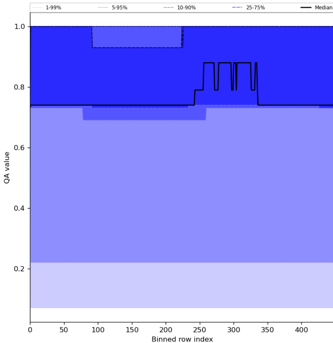
Figure 45: Along track statistics of “QA value” for 2024-05-18 to 2024-05-19
