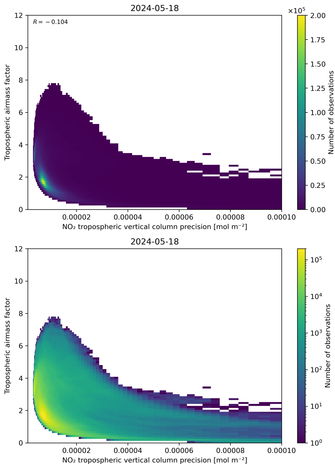
Figure 133: Scatter density plot of “NO 2 tropospheric vertical column precision” against “Tropospheric airmass factor” for 2024-05-18 to 2024-05-19.
