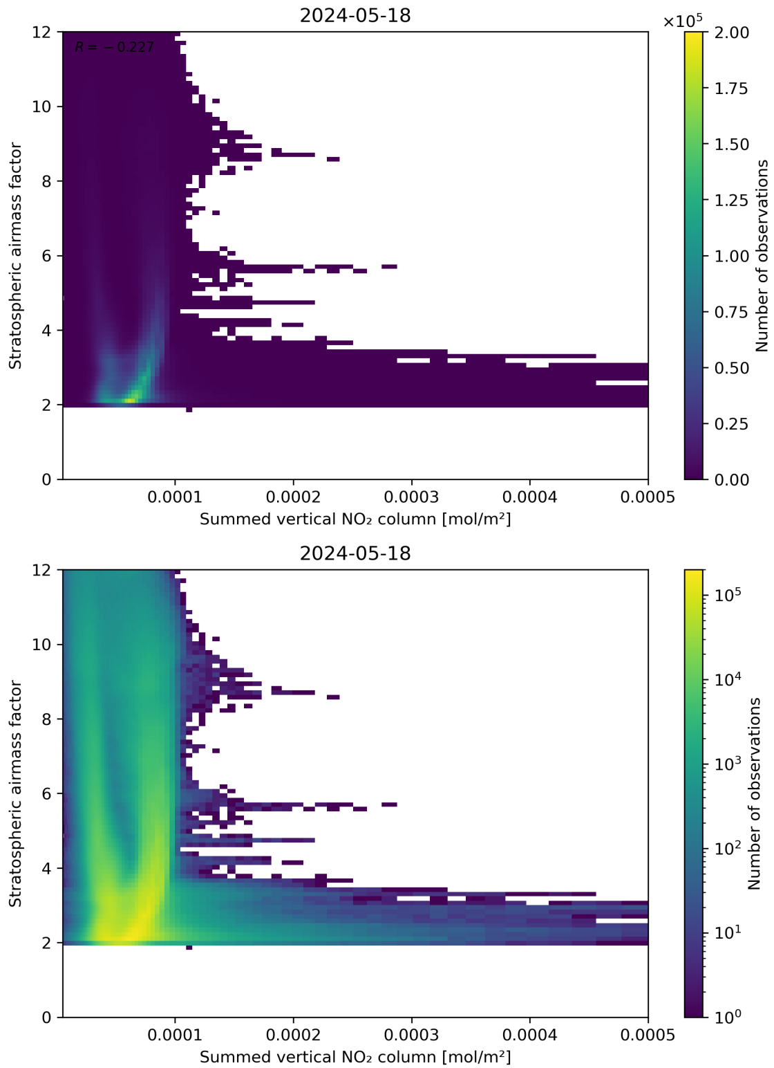
Figure 103: Scatter density plot of “Summed vertical NO 2 column” against “Stratospheric airmass factor” for 2024-05-18 to 2024-05-19.
