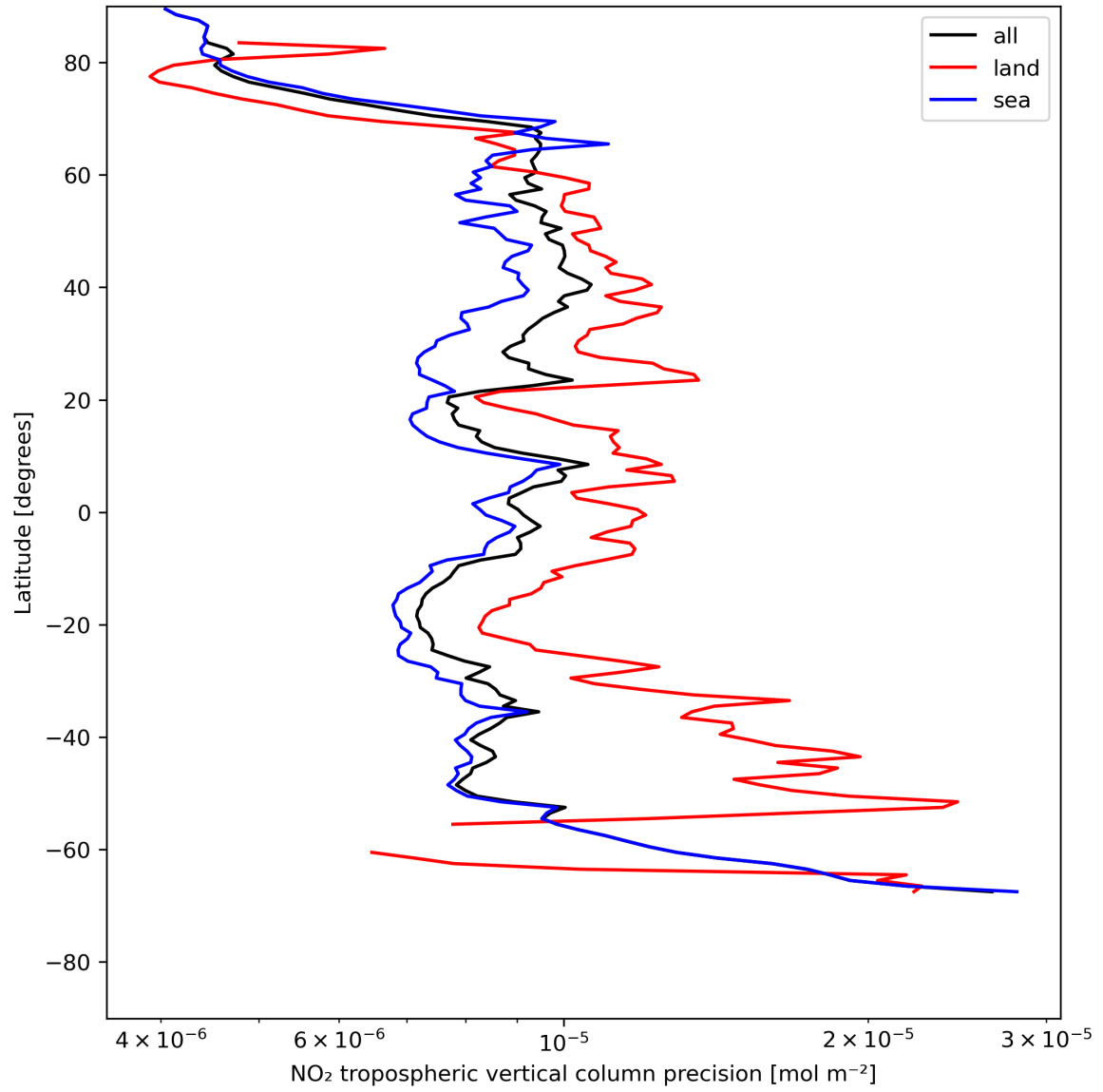
Figure 13: Zonal average of “NO 2 tropospheric vertical column precision” for 2024-05-18 to 2024-05-19.
