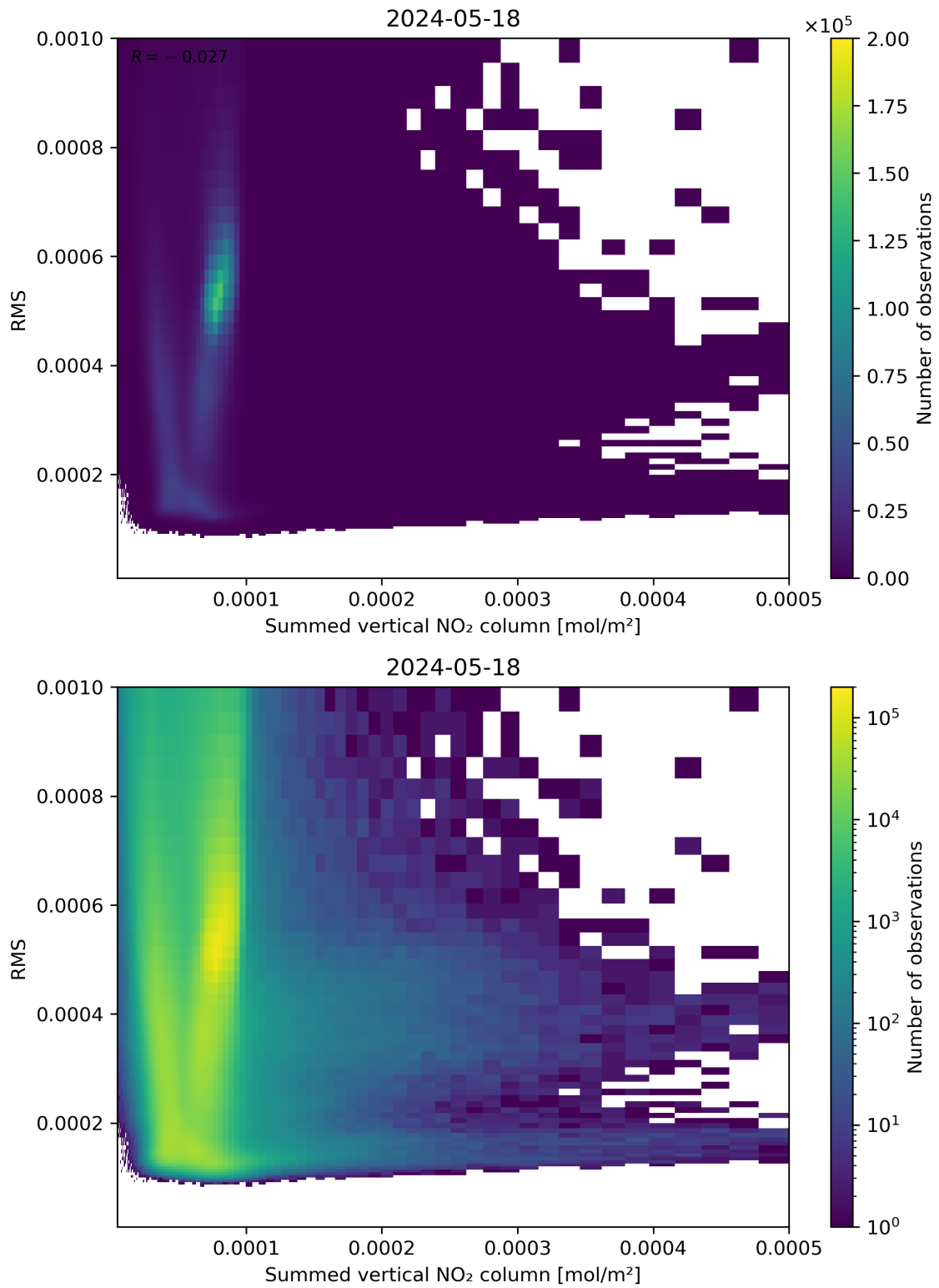
Figure 109: Scatter density plot of “Summed vertical NO 2 column” against “RMS” for 2024-05-18 to 2024-05-19.
