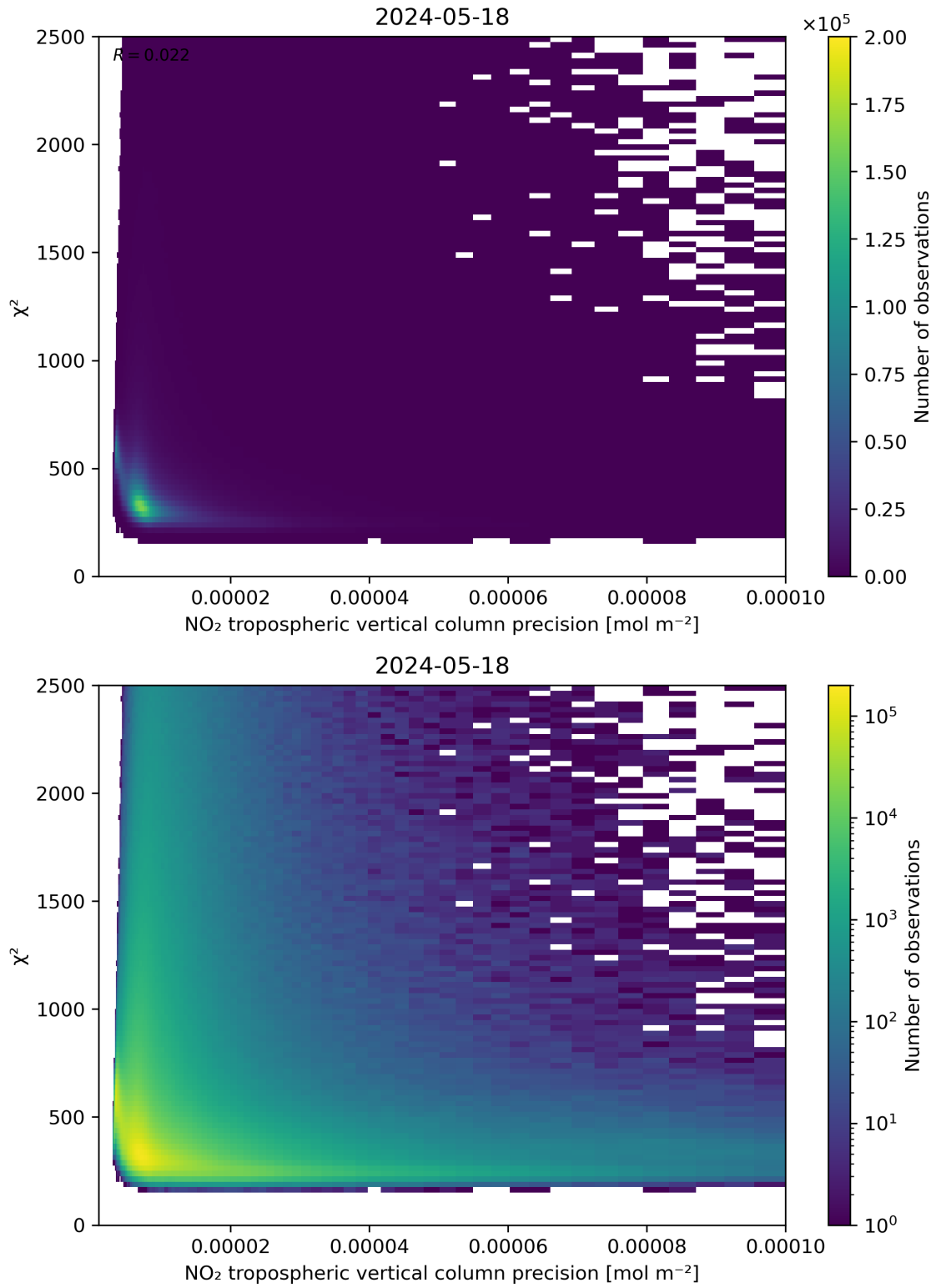
Figure 134: Scatter density plot of “NO 2 tropospheric vertical column precision” against “ \chi^2 ” for 2024-05-18 to 2024-05-19.
