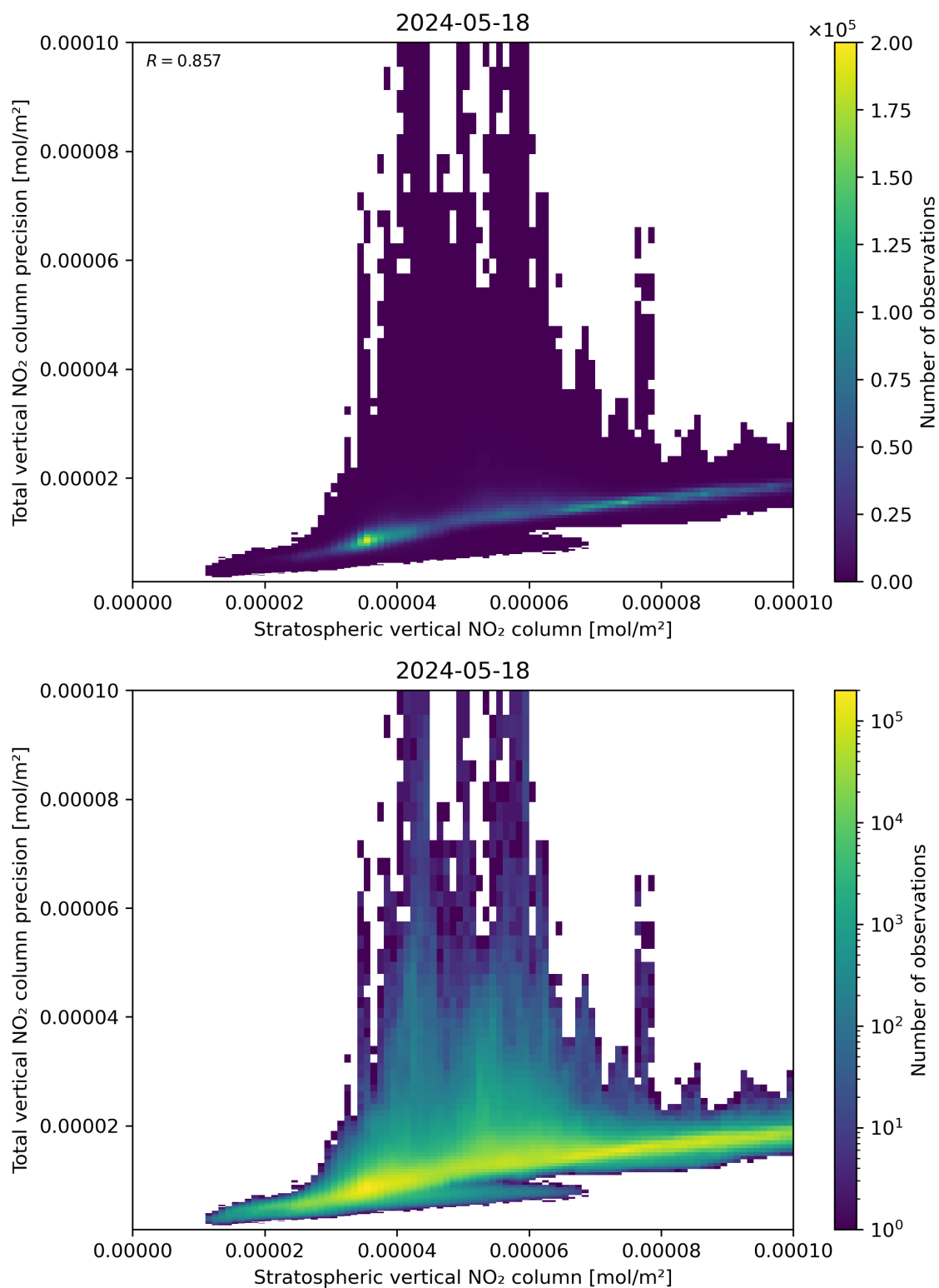
Figure 101: Scatter density plot of “Stratospheric vertical NO 2 column” against “Total vertical NO 2 column precision” for 2024-05-18 to 2024-05-19.
