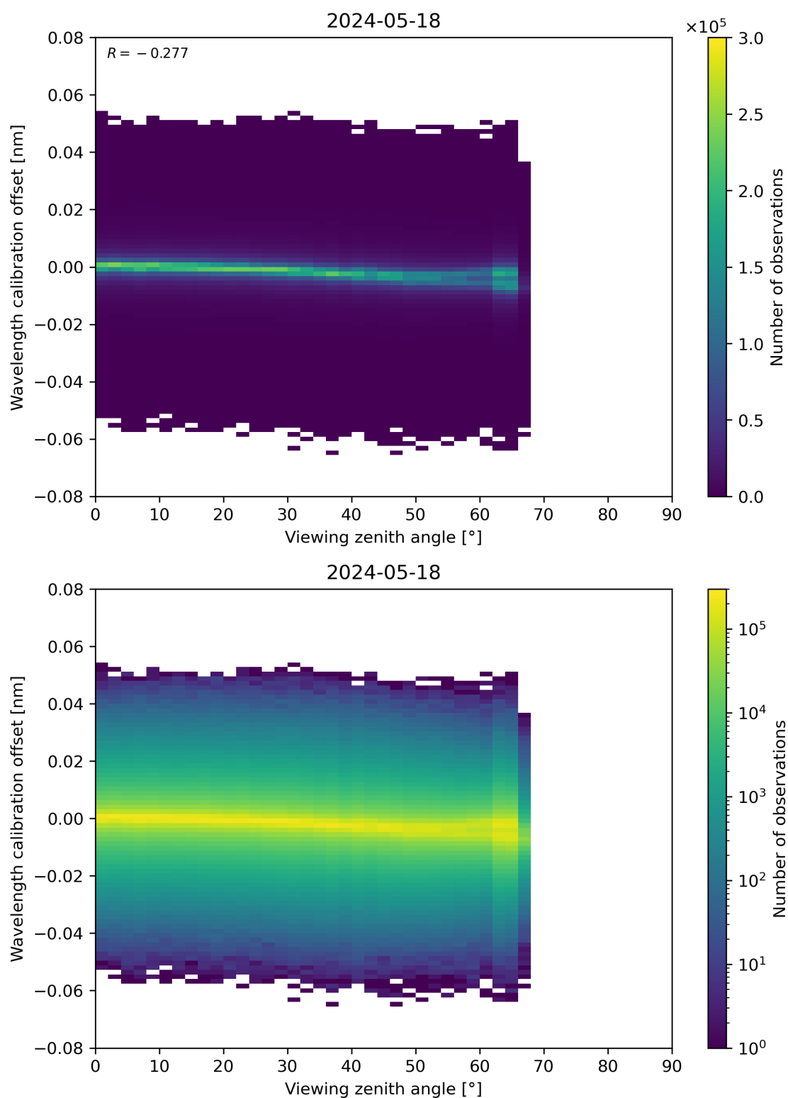
Figure 173: Scatter density plot of “Viewing zenith angle” against “Wavelength calibration offset” for 2024-05-18 to 2024-05-19.
