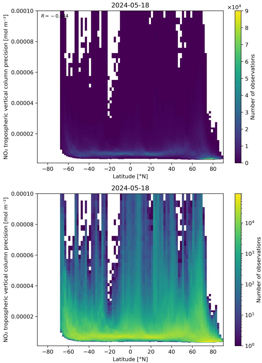
Figure 93: Scatter density plot of “Latitude” against “NO 2 tropospheric vertical column precision” for 2024-05-18 to 2024-05-19.
