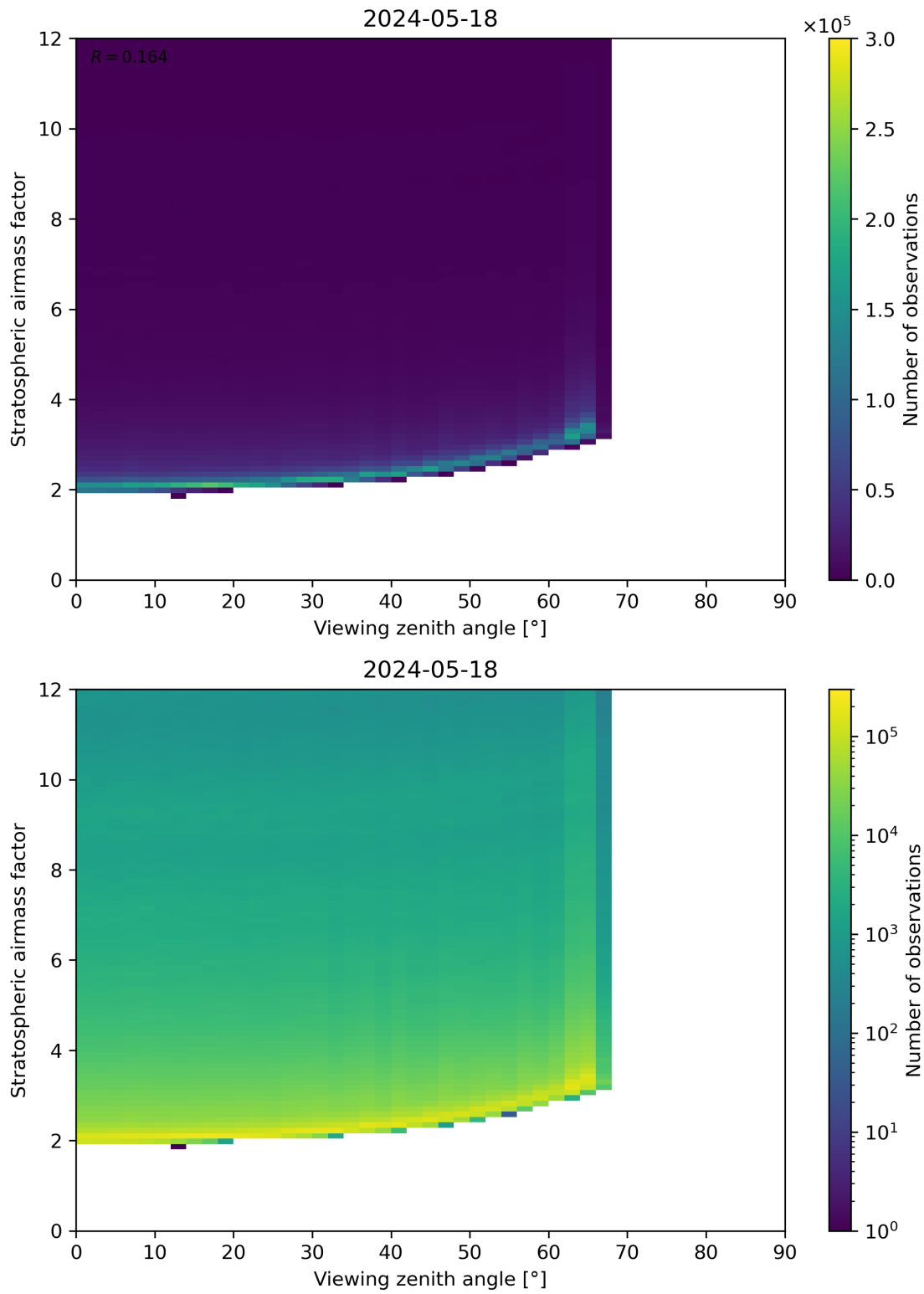
Figure 159: Scatter density plot of “Viewing zenith angle” against “Stratospheric airmass factor” for 2024-05-18 to 2024-05-19.
