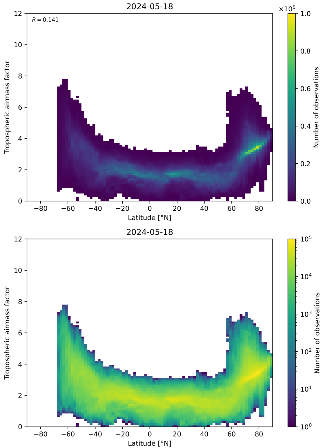
Figure 85: Scatter density plot of “Latitude” against “Tropospheric airmass factor” for 2024-05-18 to 2024-05-19.
