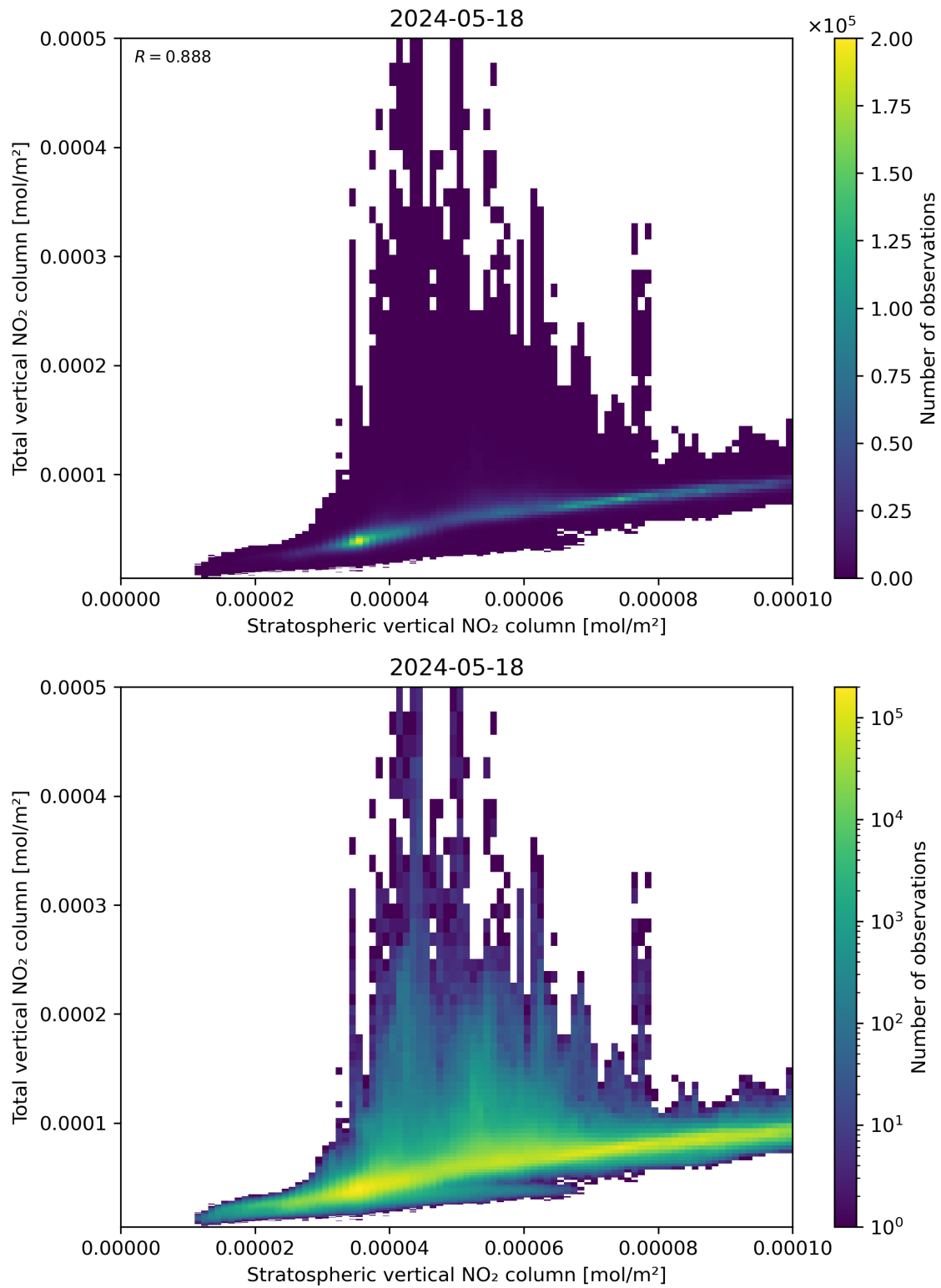
Figure 100: Scatter density plot of “Stratospheric vertical NO 2 column” against “Total vertical NO 2 column” for 2024-05-18 to 2024-05-19.
