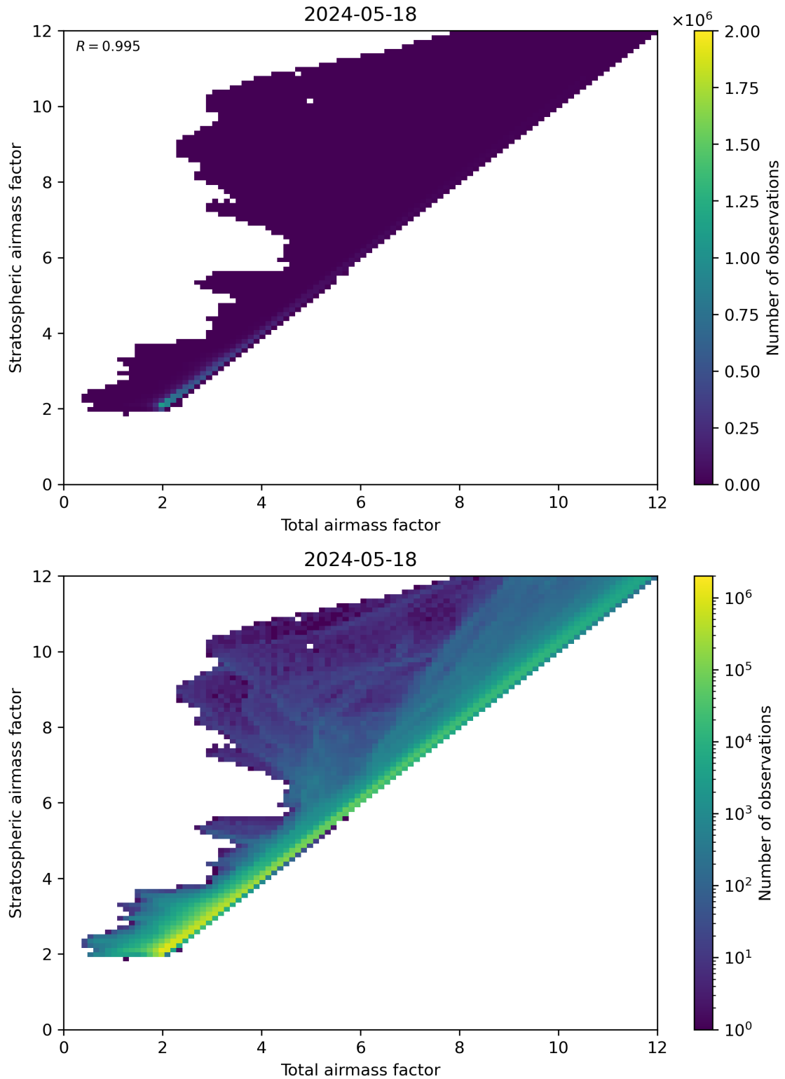
Figure 62: Scatter density plot of “Total airmass factor” against “Stratospheric airmass factor” for 2024-05-18 to 2024-05-19.
