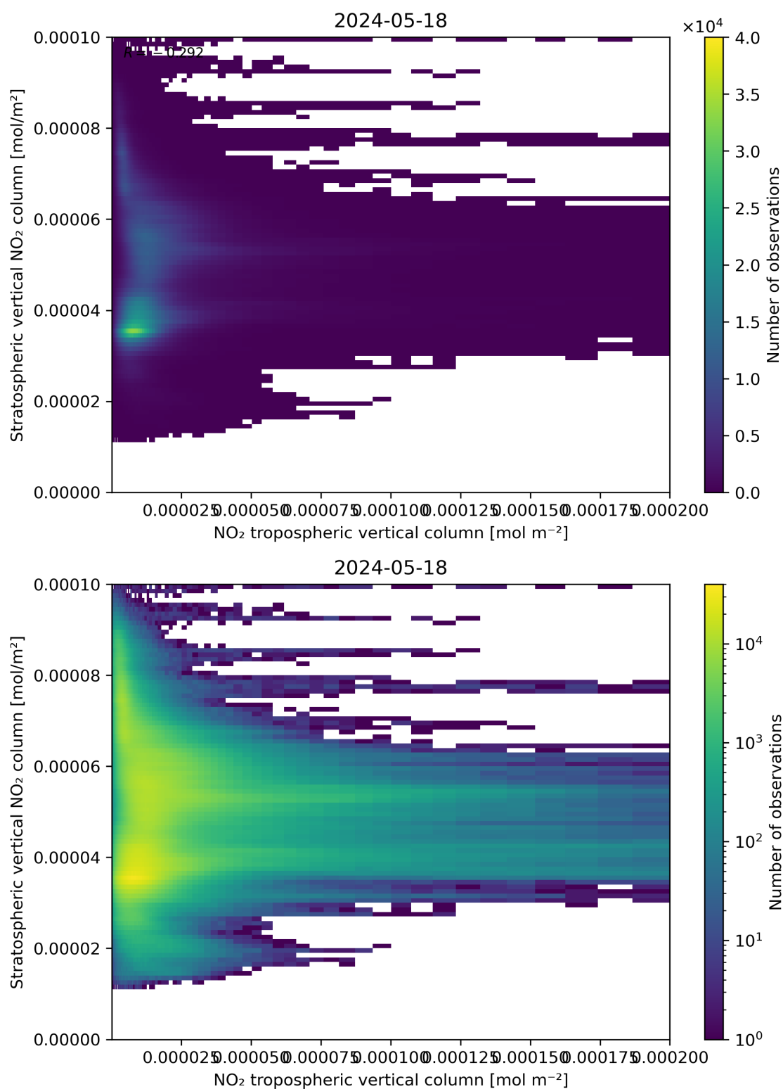
Figure 125: Scatter density plot of “NO 2 tropospheric vertical column” against “Stratospheric vertical NO 2 column” for 2024-05-18 to 2024-05-19.
