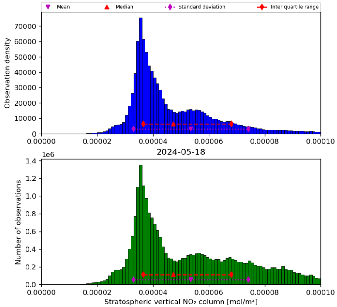
Figure 36: Histogram of “Stratospheric vertical NO 2 column” for 2024-05-18 to 2024-05-19
