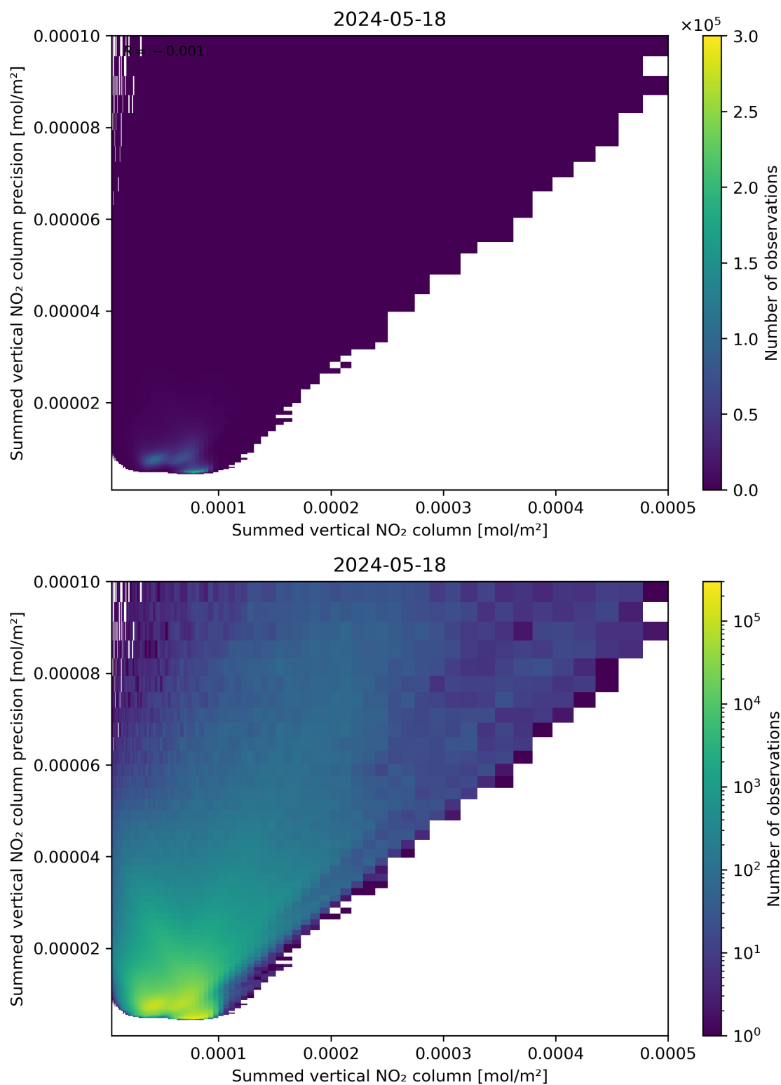
Figure 105: Scatter density plot of “Summed vertical NO 2 column” against “Summed vertical NO 2 column precision” for 2024-05-18 to 2024-05-19.
