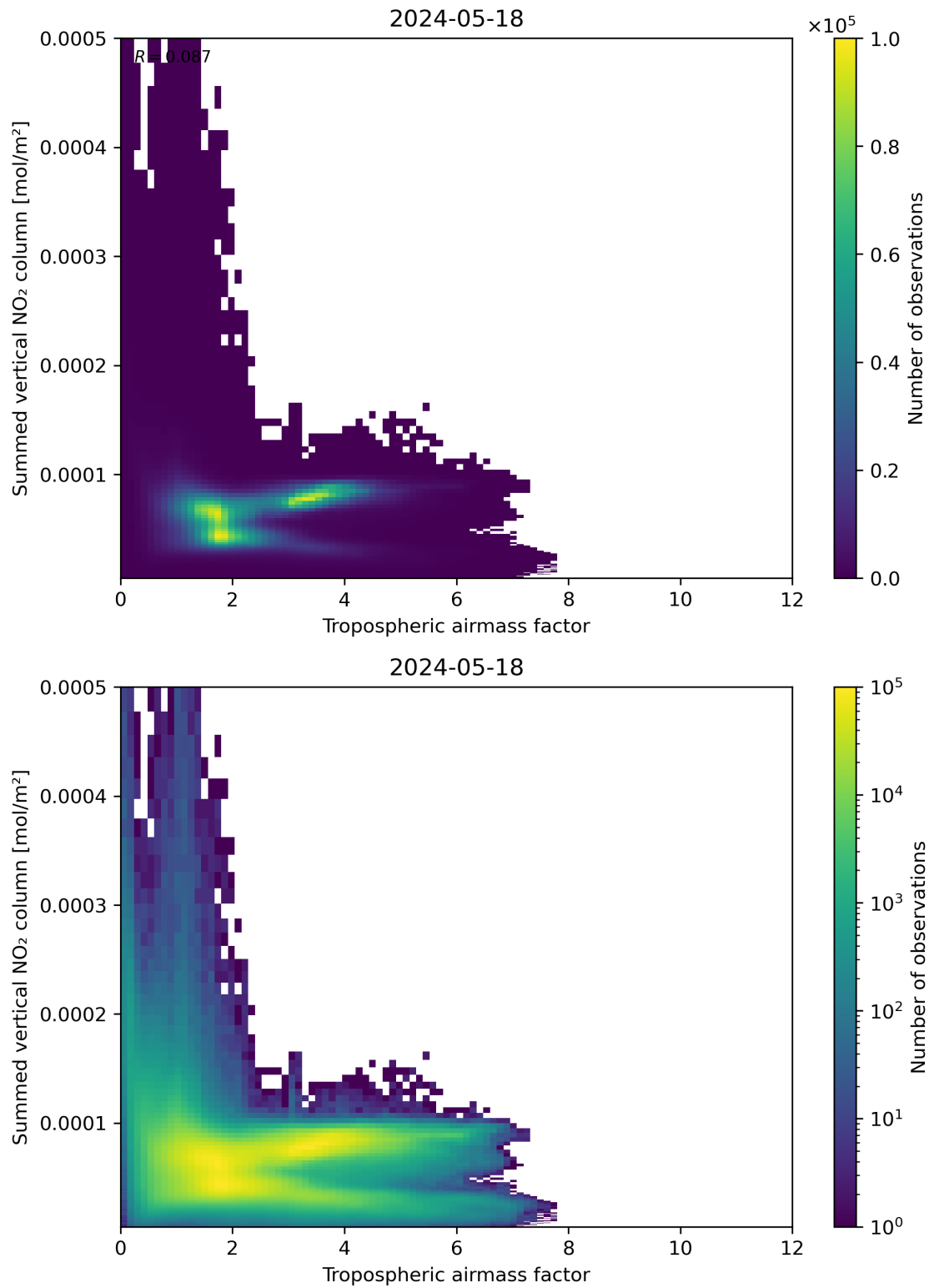
Figure 75: Scatter density plot of “Tropospheric air mass factor” against “Summed vertical NO 2 column” for 2024-05-18 to 2024-05-19.
