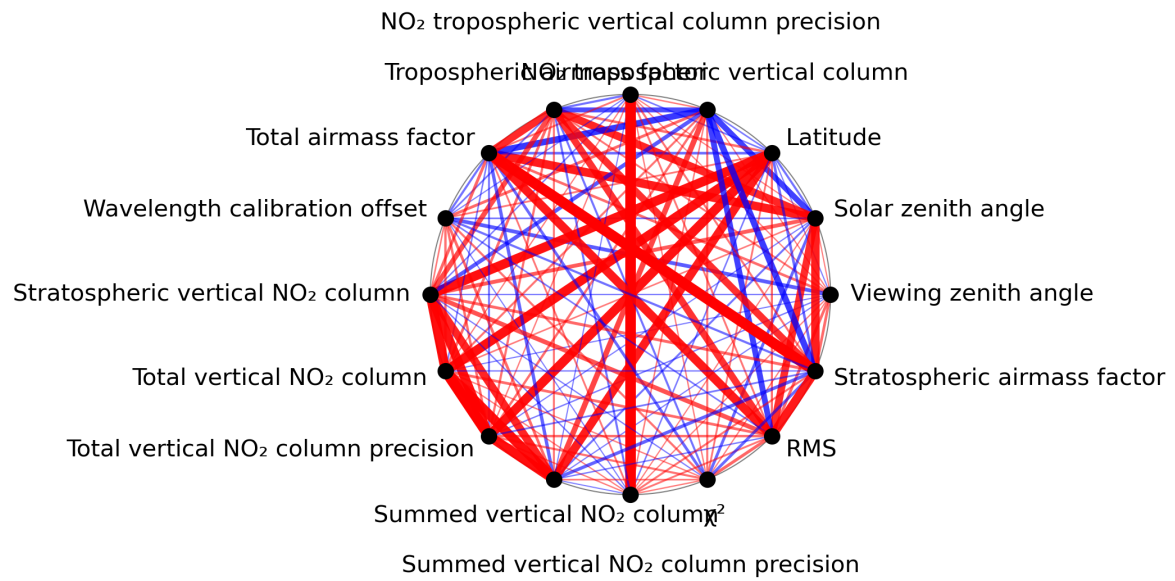
Figure 1: Map of correlation graph for 2024-05-18 to 2024-05-19.
