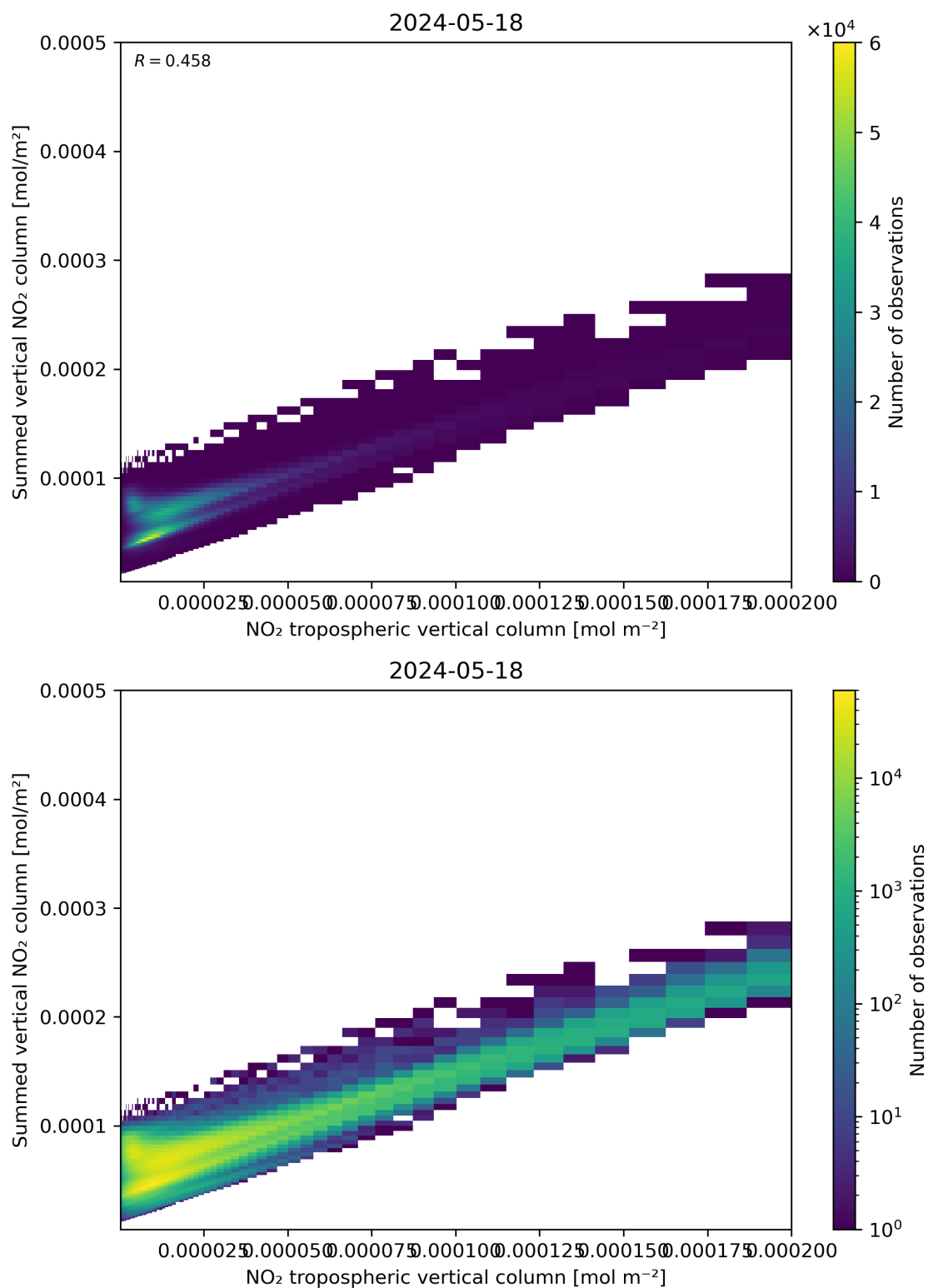
Figure 126: Scatter density plot of “NO 2 tropospheric vertical column” against “Summed vertical NO 2 column” for 2024-05-18 to 2024-05-19.
