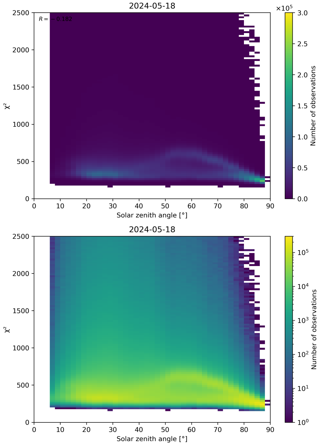
Figure 148: Scatter density plot of “Solar zenith angle” against “ \chi^2 ” for 2024-05-18 to 2024-05-19.
