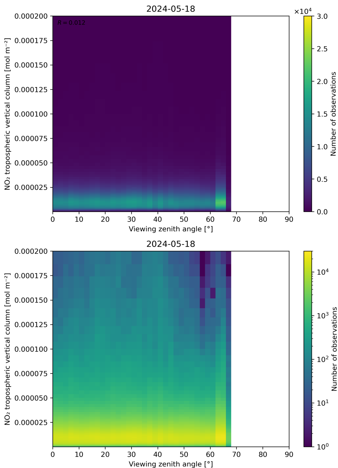
Figure 169: Scatter density plot of “Viewing zenith angle” against “NO 2 tropospheric vertical column” for 2024-05-18 to 2024-05-19.
