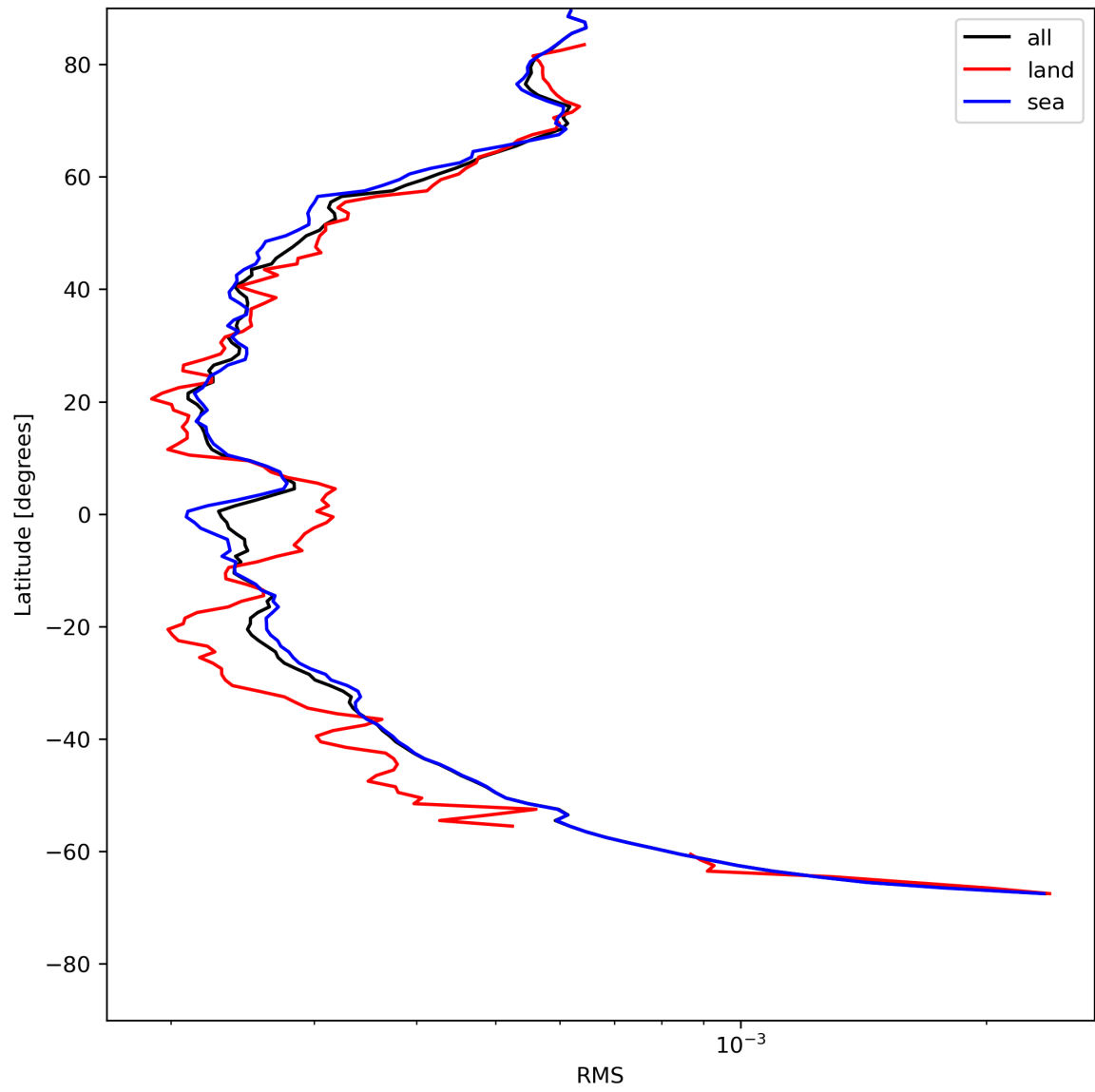
Figure 26: Zonal average of “RMS” for 2024-05-18 to 2024-05-19.
