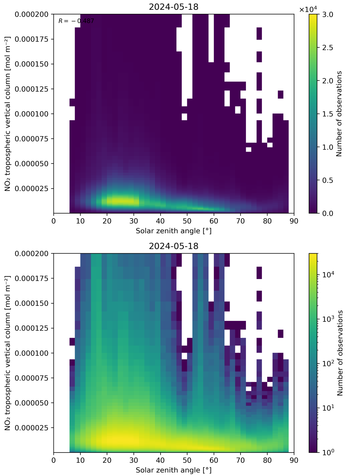
Figure 155: Scatter density plot of “Solar zenith angle” against “NO 2 tropospheric vertical column” for 2024-05-18 to 2024-05-19.
