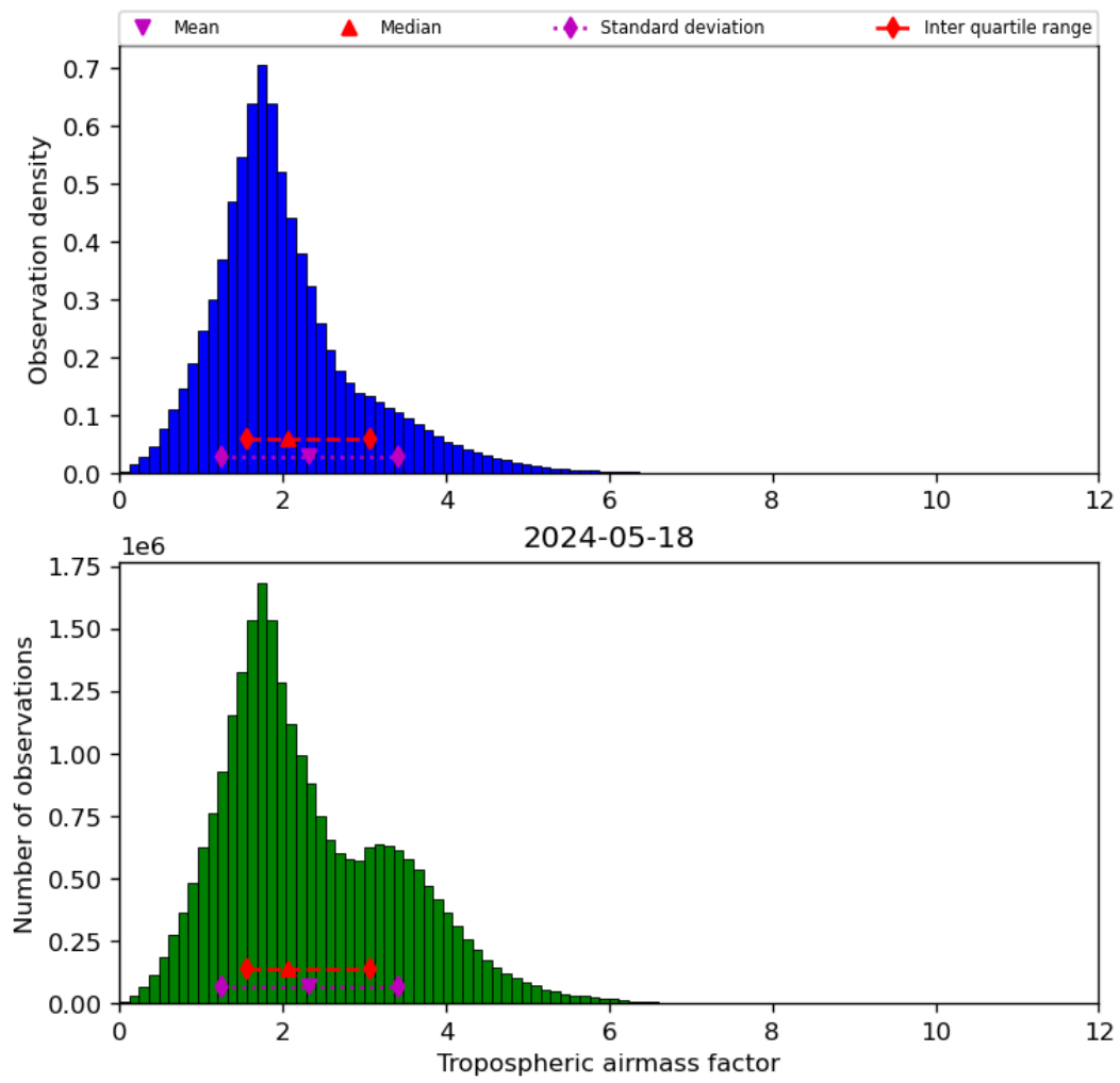
Figure 31: Histogram of “Tropospheric airmass factor” for 2024-05-18 to 2024-05-19
