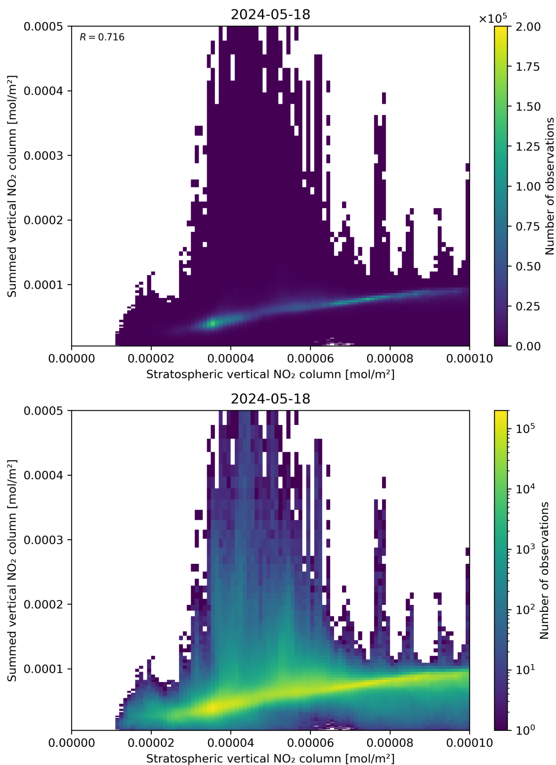
Figure 98: Scatter density plot of “Stratospheric vertical NO 2 column” against “Summed vertical NO 2 column” for 2024-05-18 to 2024-05-19.
