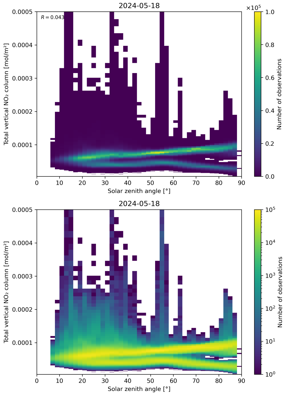
Figure 153: Scatter density plot of “Solar zenith angle” against “Total vertical NO 2 column” for 2024-05-18 to 2024-05-19.
