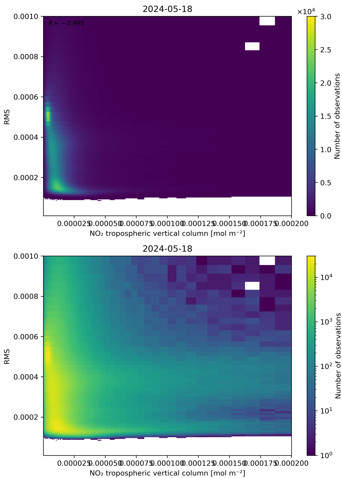
Figure 142: Scatter density plot of “NO 2 tropospheric vertical column” against “RMS” for 2024-05-18 to 2024-05-19.
