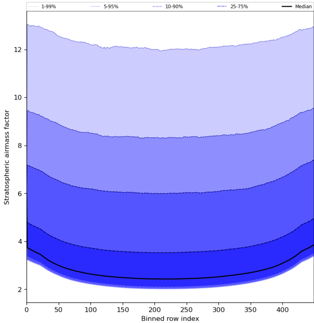
Figure 61: Along track statistics of “Stratospheric airmass factor” for 2024-05-18 to 2024-05-19
