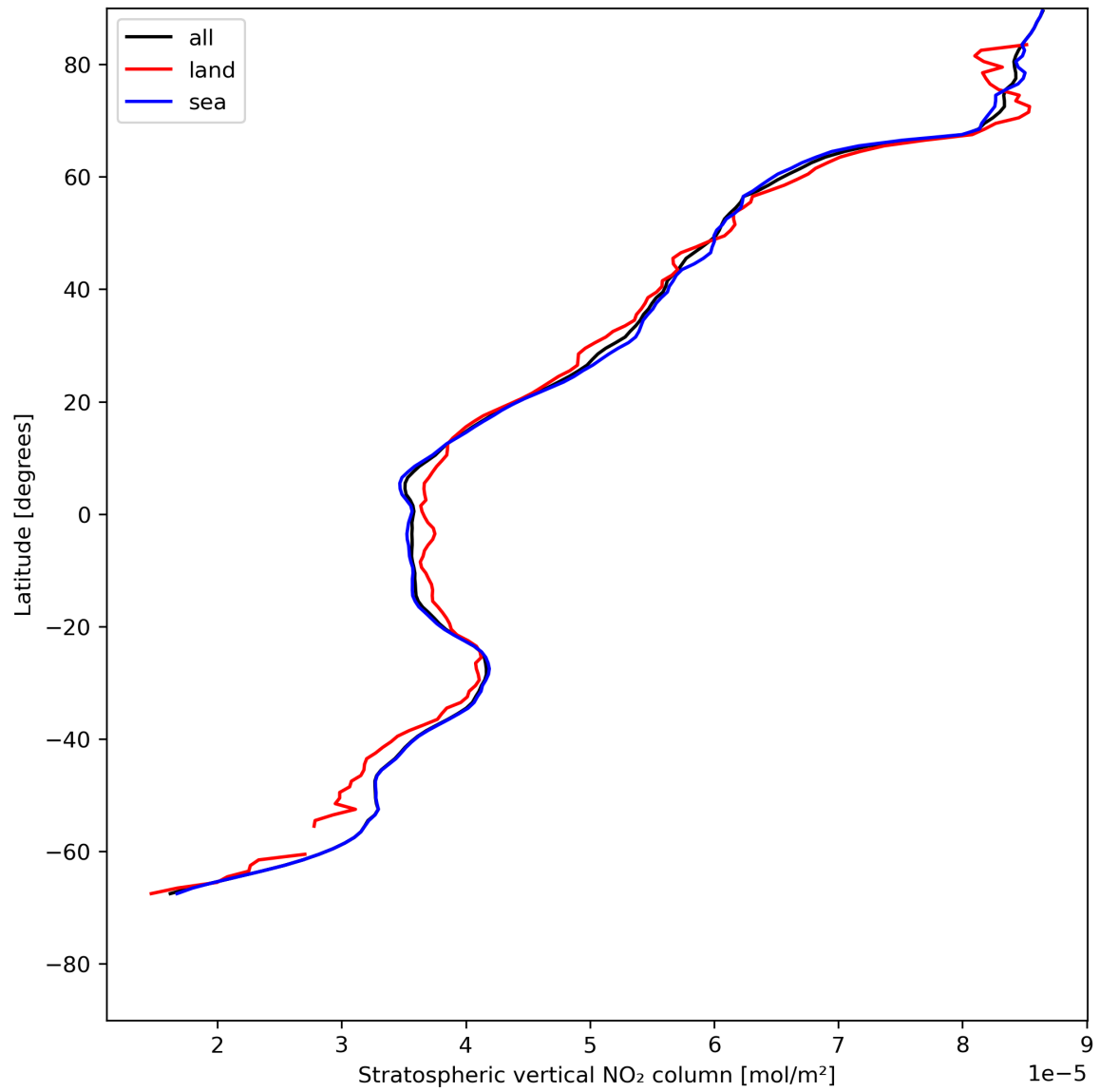
Figure 19: Zonal average of “Stratospheric vertical NO 2 column” for 2024-05-18 to 2024-05-19.
