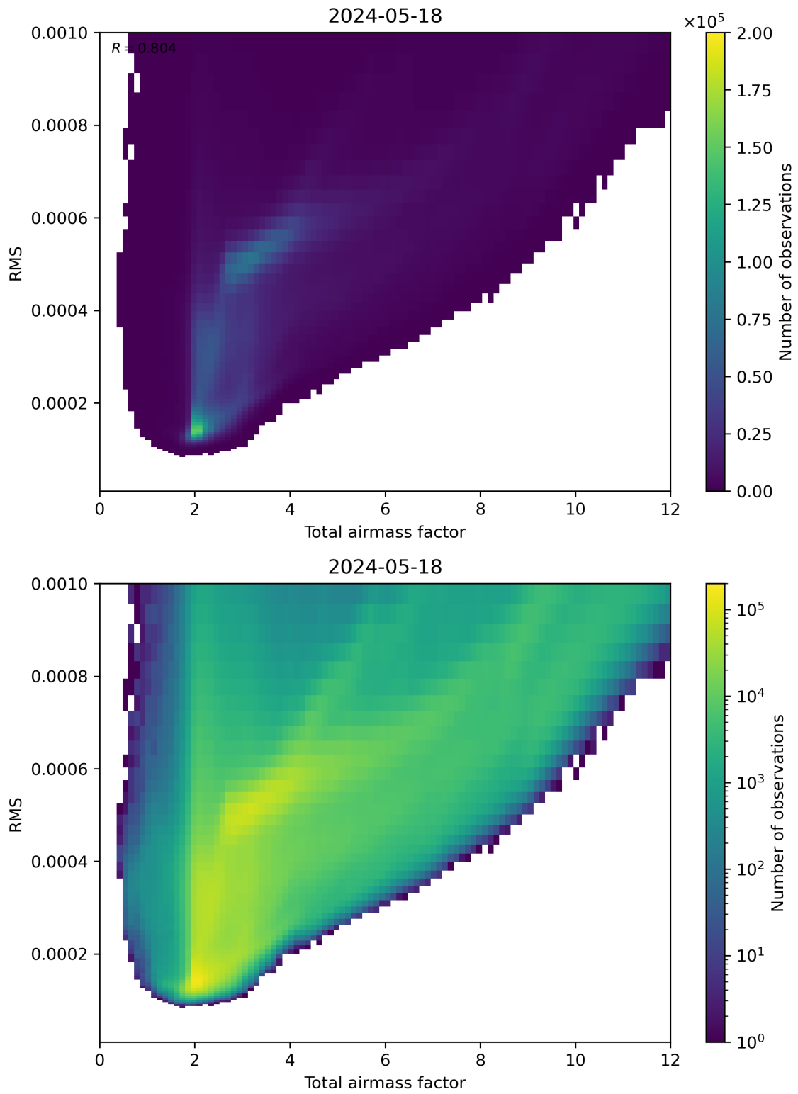
Figure 69: Scatter density plot of “Total airmass factor” against “RMS” for 2024-05-18 to 2024-05-19.
