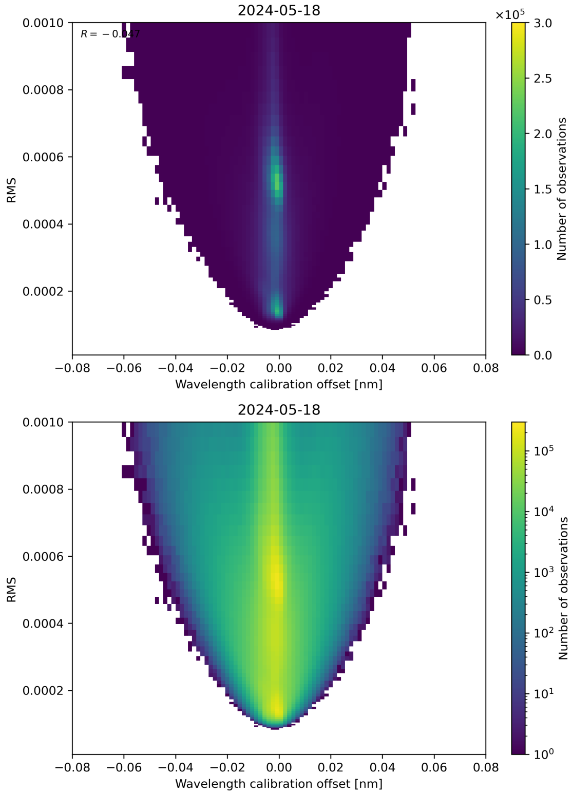
Figure 181: Scatter density plot of “Wavelength calibration offset” against “RMS” for 2024-05-18 to 2024-05-19.
