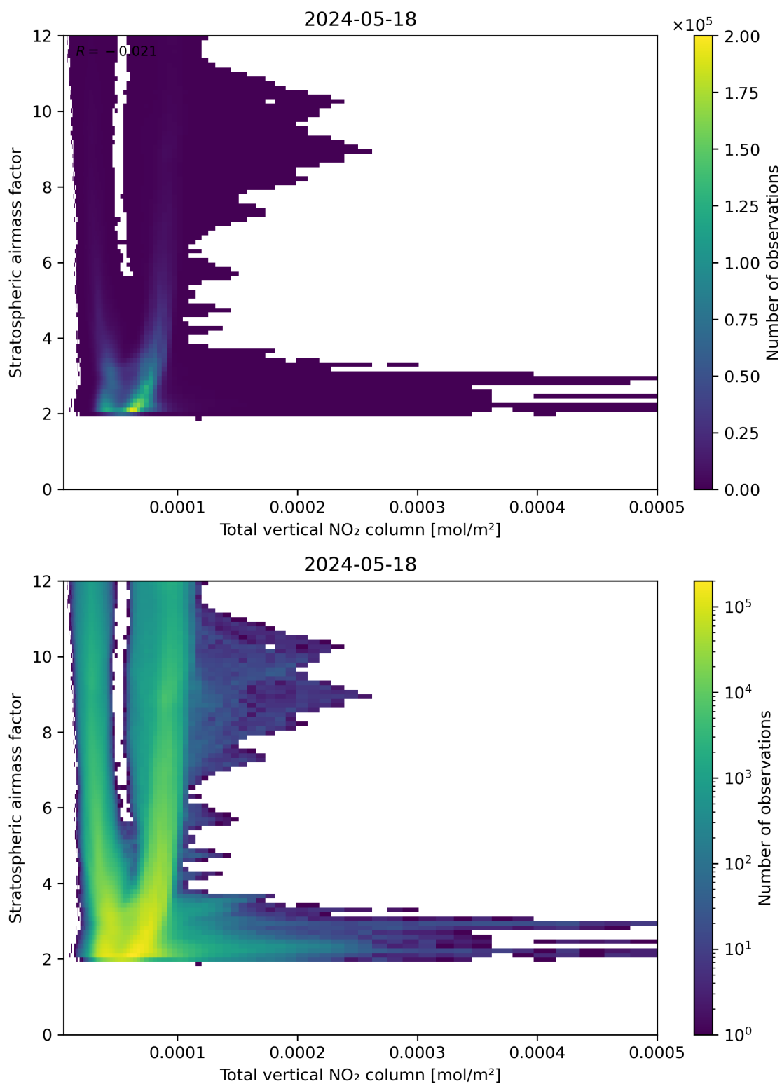
Figure 110: Scatter density plot of “Total vertical NO 2 column” against “Stratospheric airmass factor” for 2024-05-18 to 2024-05-19.
