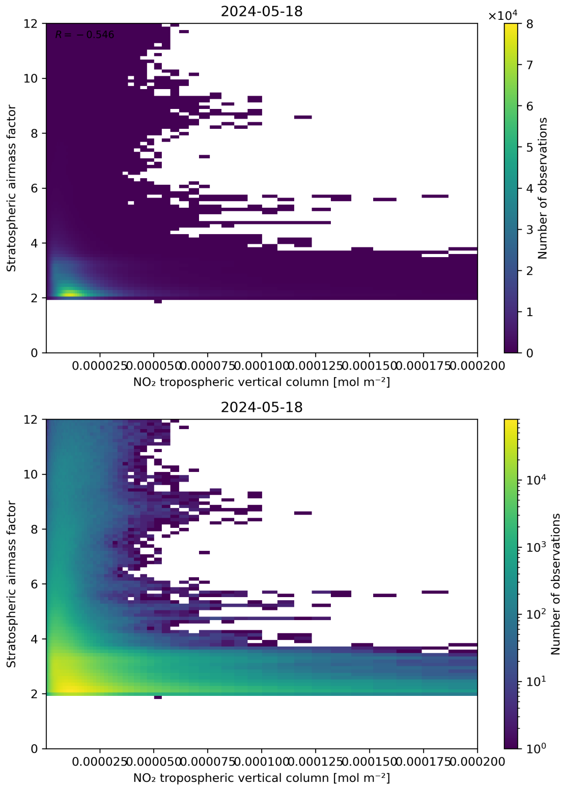
Figure 121: Scatter density plot of “NO 2 tropospheric vertical column” against “Stratospheric air mass factor” for 2024-05-18 to 2024-05-19.
