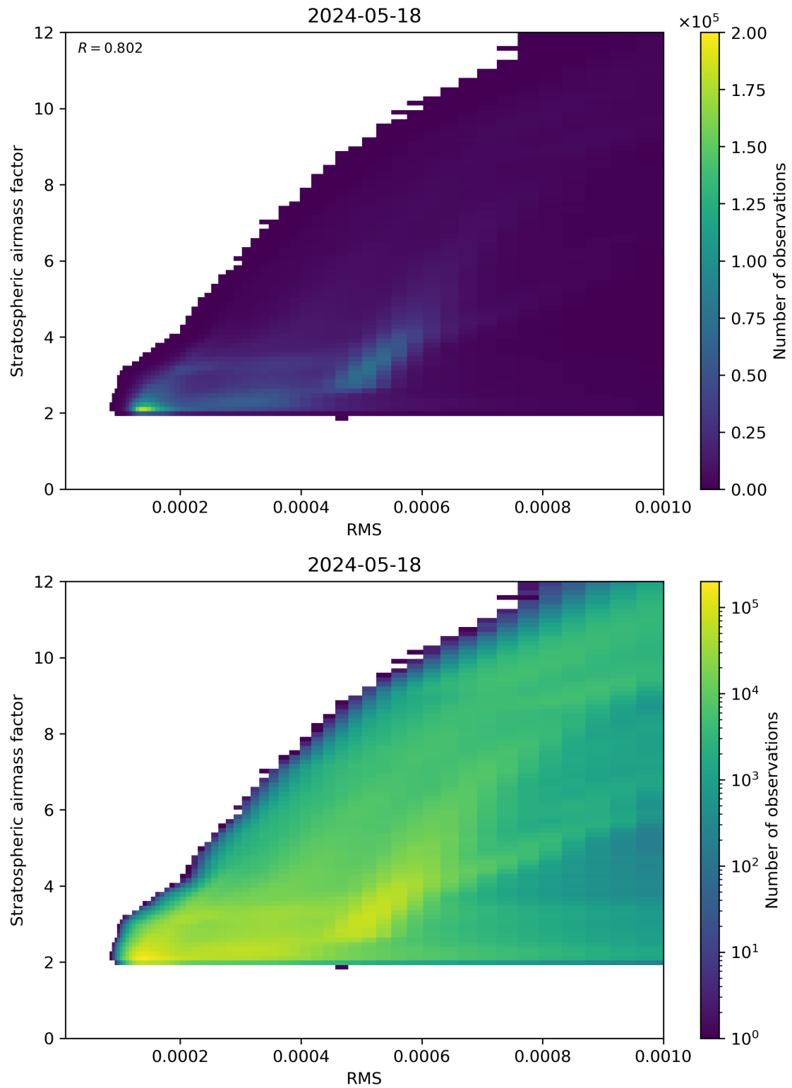
Figure 144: Scatter density plot of “RMS” against “Stratospheric airmass factor” for 2024-05-18 to 2024-05-19.
