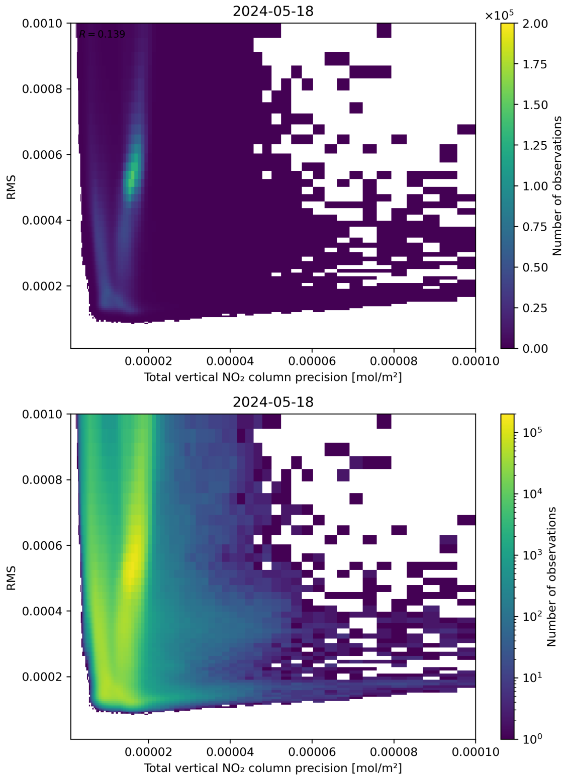
Figure 119: Scatter density plot of “Total vertical NO 2 column precision” against “RMS” for 2024-05-18 to 2024-05-19.
