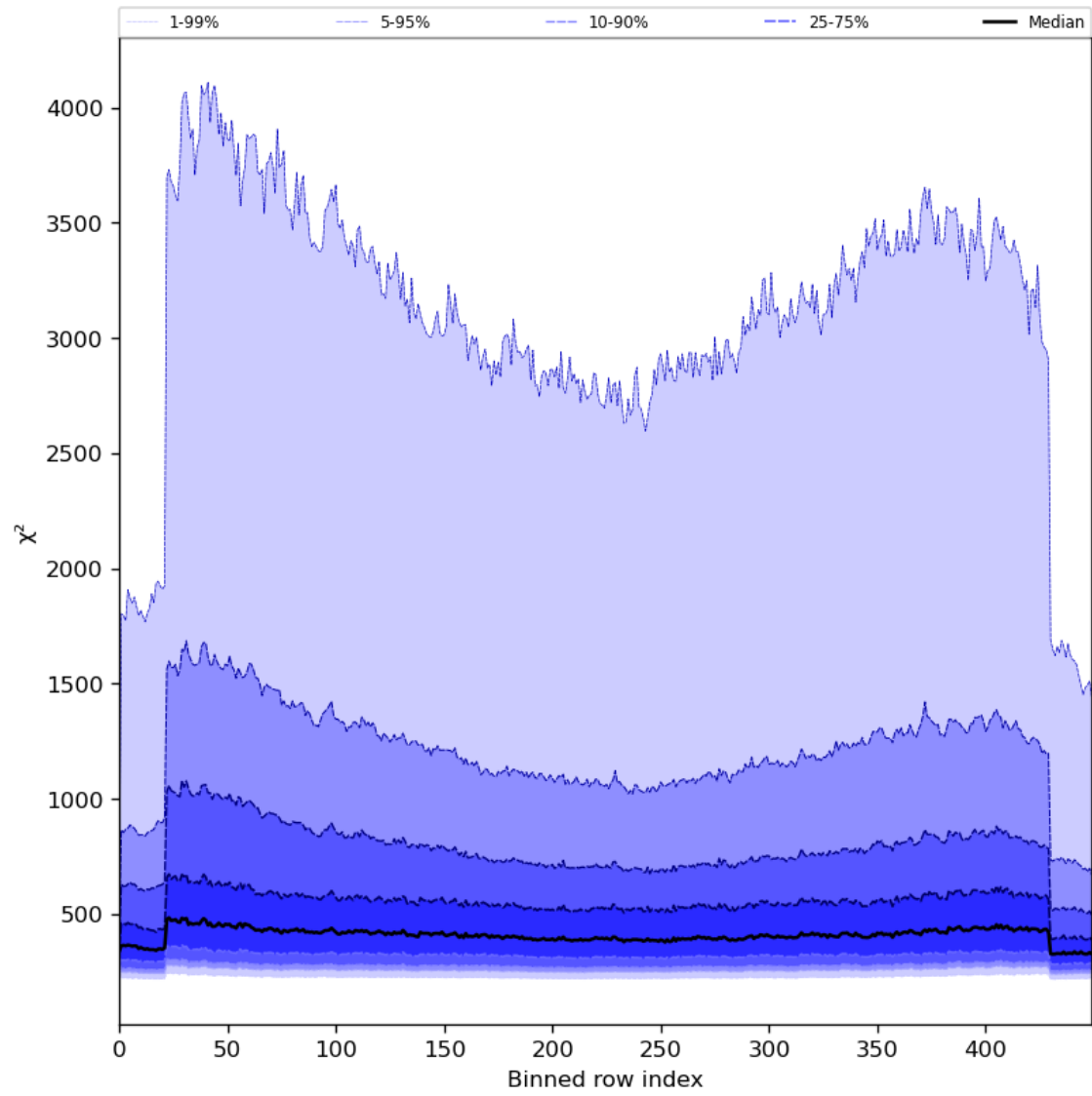
Figure 59: Along track statistics of “ \chi^2 ” for 2024-05-18 to 2024-05-19
