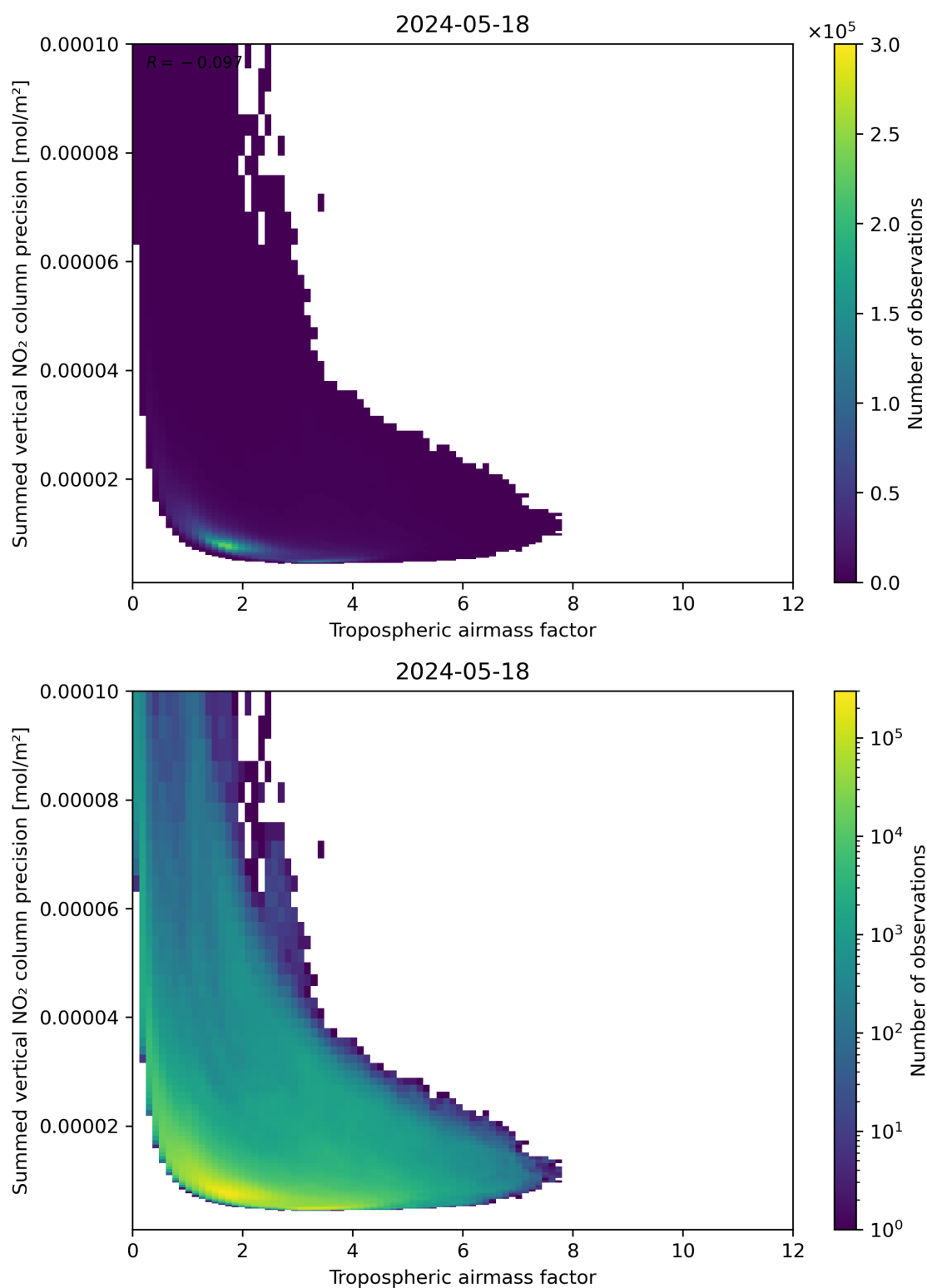
Figure 76: Scatter density plot of “Tropospheric air mass factor” against “Summed vertical NO 2 column precision” for 2024-05-18 to 2024-05-19.
