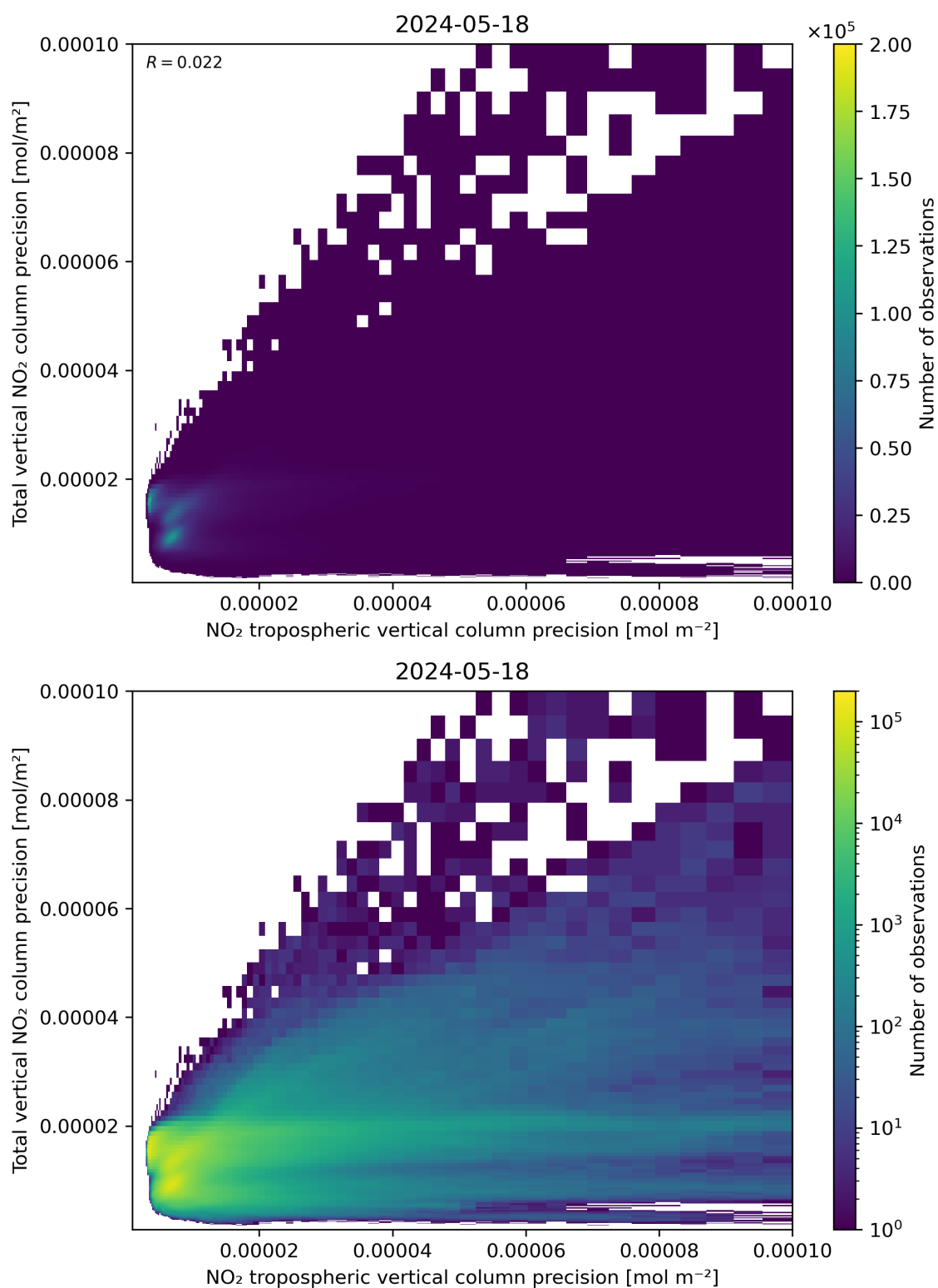
Figure 139: Scatter density plot of “NO 2 tropospheric vertical column precision” against “Total vertical NO 2 column precision” for 2024-05-18 to 2024-05-19.
