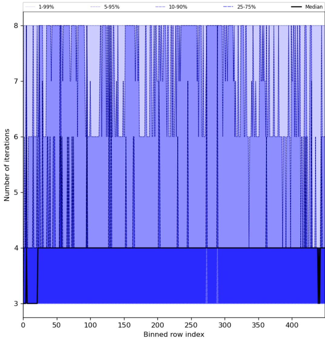
Figure 51: Along track statistics of “Number of iterations” for 2024-05-18 to 2024-05-19
