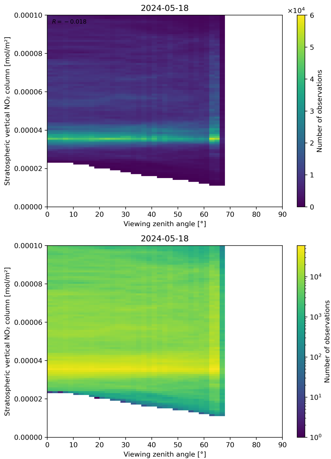
Figure 164: Scatter density plot of “Viewing zenith angle” against “Stratospheric vertical NO 2 column” for 2024-05-18 to 2024-05-19.
