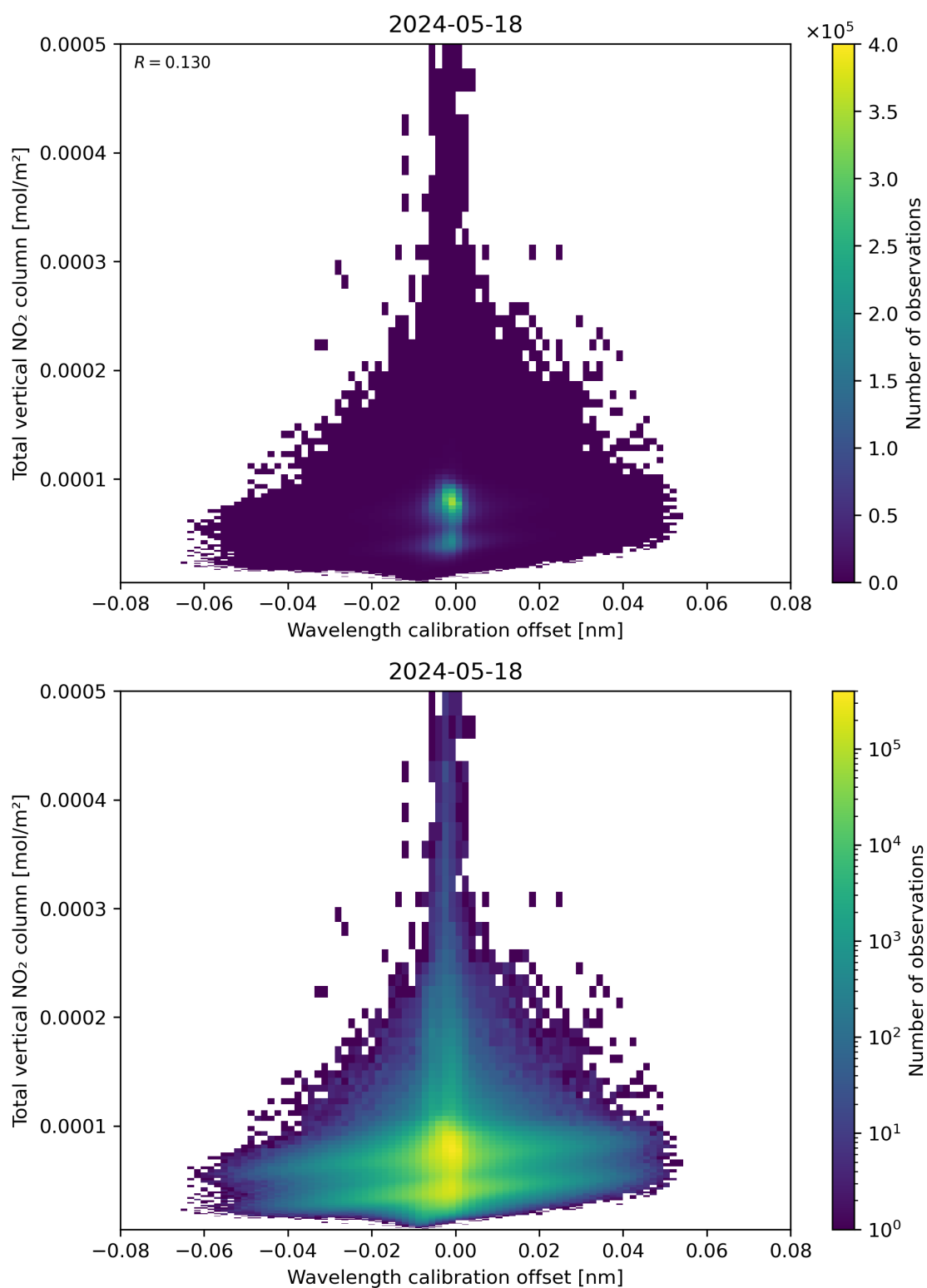
Figure 179: Scatter density plot of “Wavelength calibration offset” against “Total vertical NO 2 column” for 2024-05-18 to 2024-05-19.
