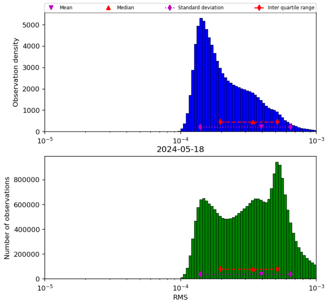
Figure 43: Histogram of “RMS” for 2024-05-18 to 2024-05-19
