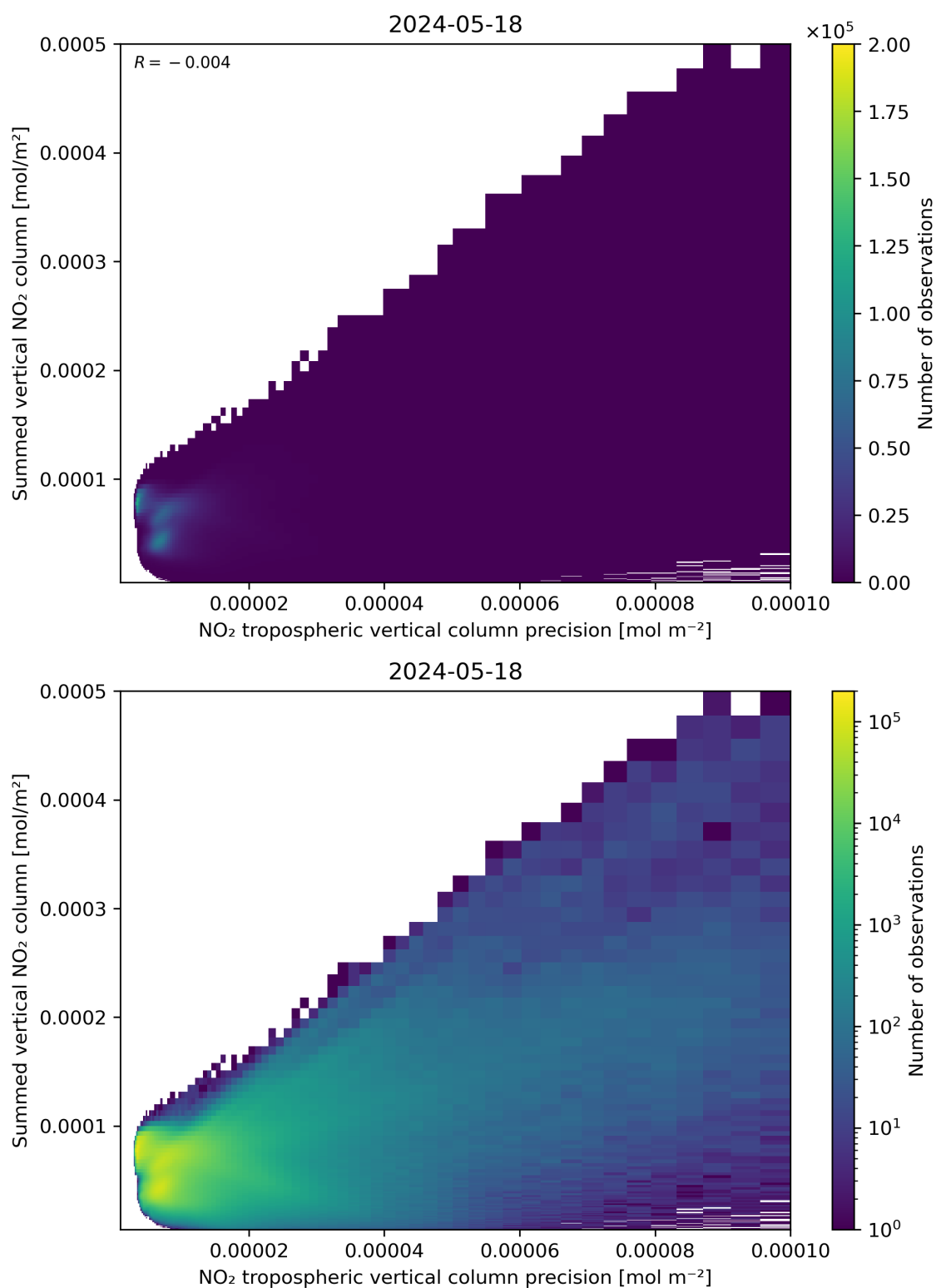
Figure 136: Scatter density plot of “NO 2 tropospheric vertical column precision” against “Summed vertical NO 2 column” for 2024-05-18 to 2024-05-19.
