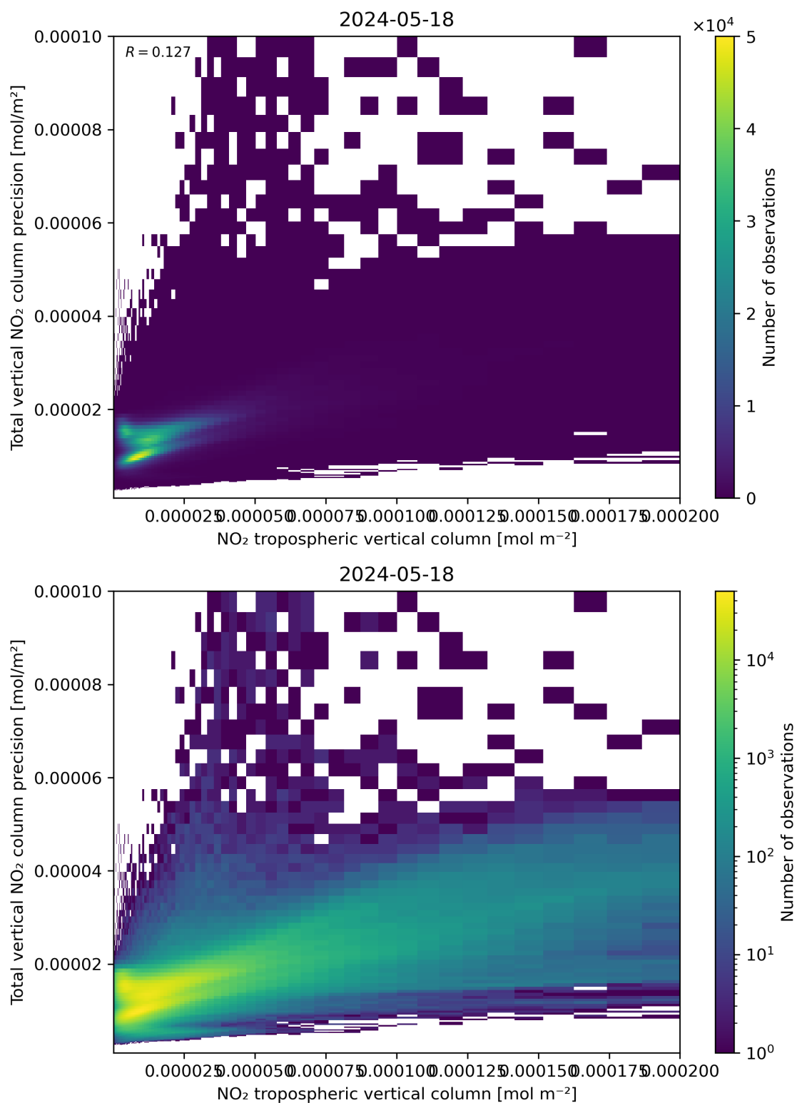
Figure 129: Scatter density plot of “NO 2 tropospheric vertical column” against “Total vertical NO 2 column precision” for 2024-05-18 to 2024-05-19.
