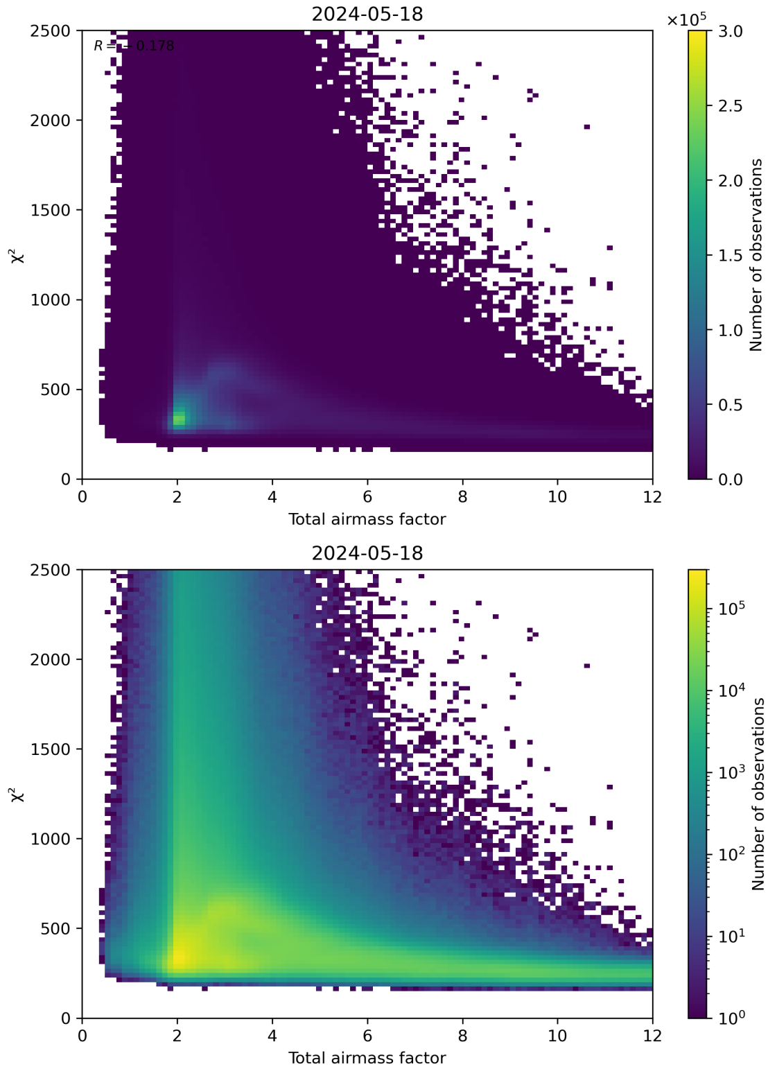
Figure 63: Scatter density plot of “Total airmass factor” against “ \chi^2 ” for 2024-05-18 to 2024-05-19.
