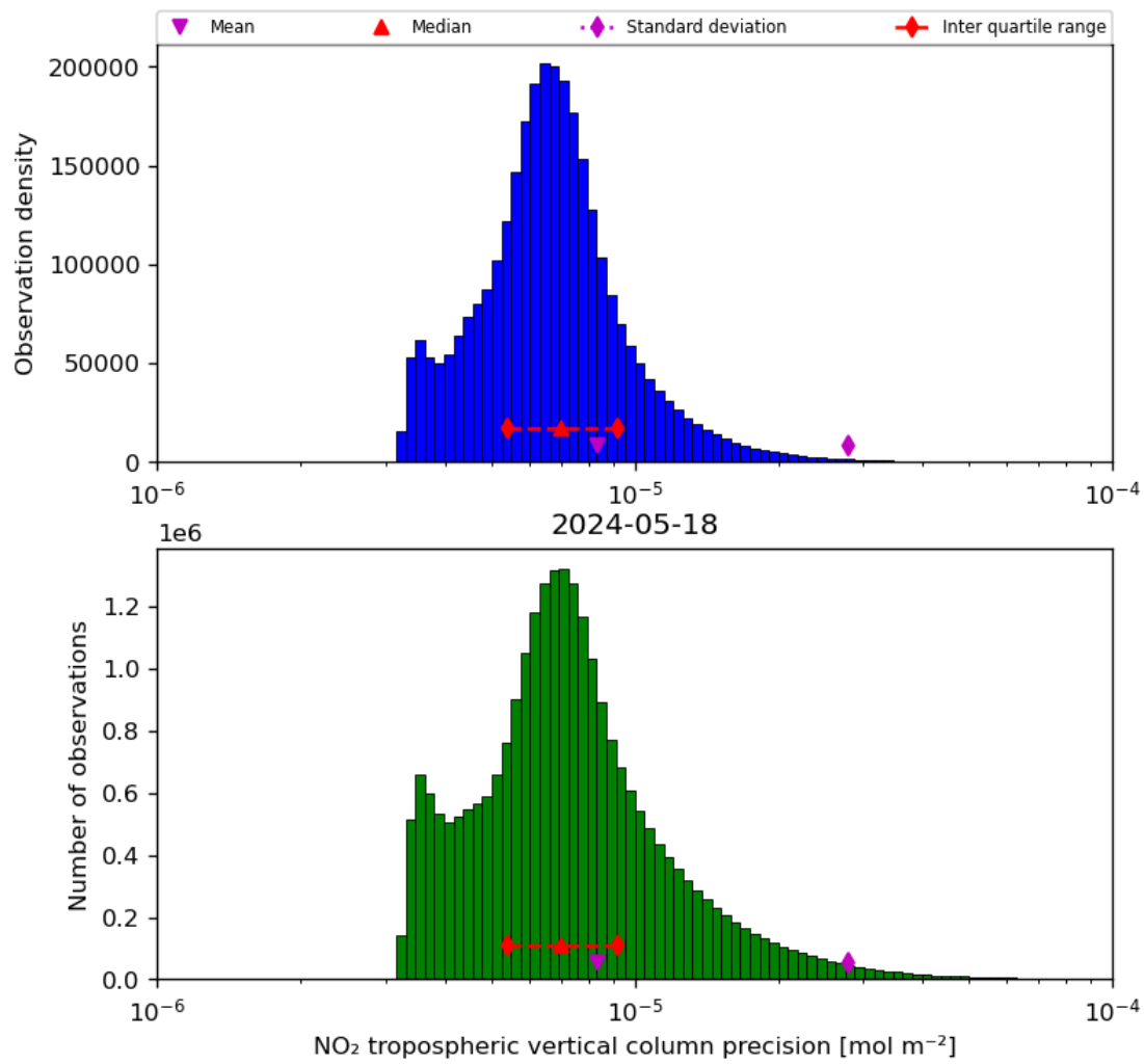
Figure 30: Histogram of “NO 2 tropospheric vertical column precision” for 2024-05-18 to 2024-05-19
