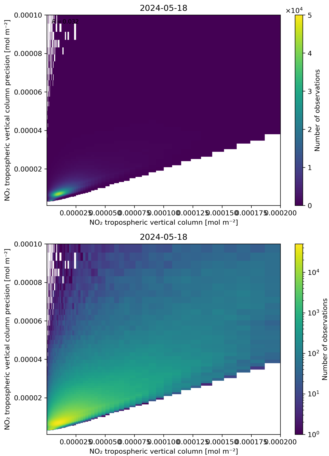
Figure 130: Scatter density plot of “NO 2 tropospheric vertical column” against “NO 2 tropospheric vertical column precision” for 2024-05-18 to 2024-05-19.
