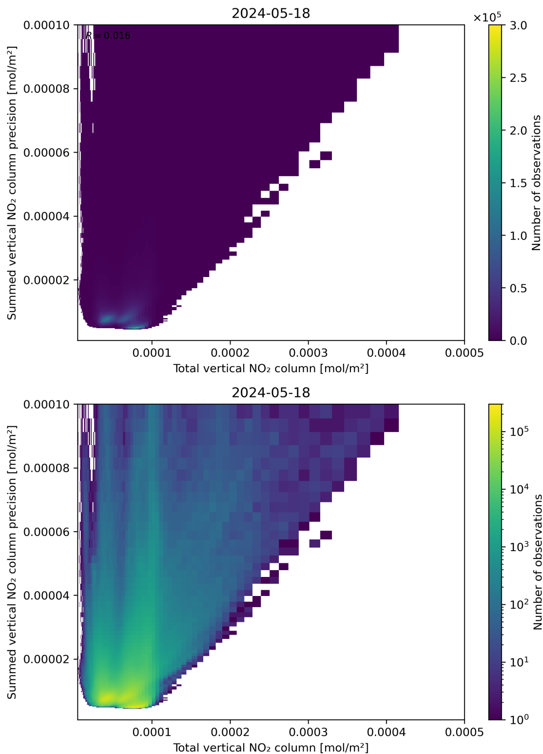
Figure 113: Scatter density plot of “Total vertical NO 2 column” against “Summed vertical NO 2 column precision” for 2024-05-18 to 2024-05-19.
