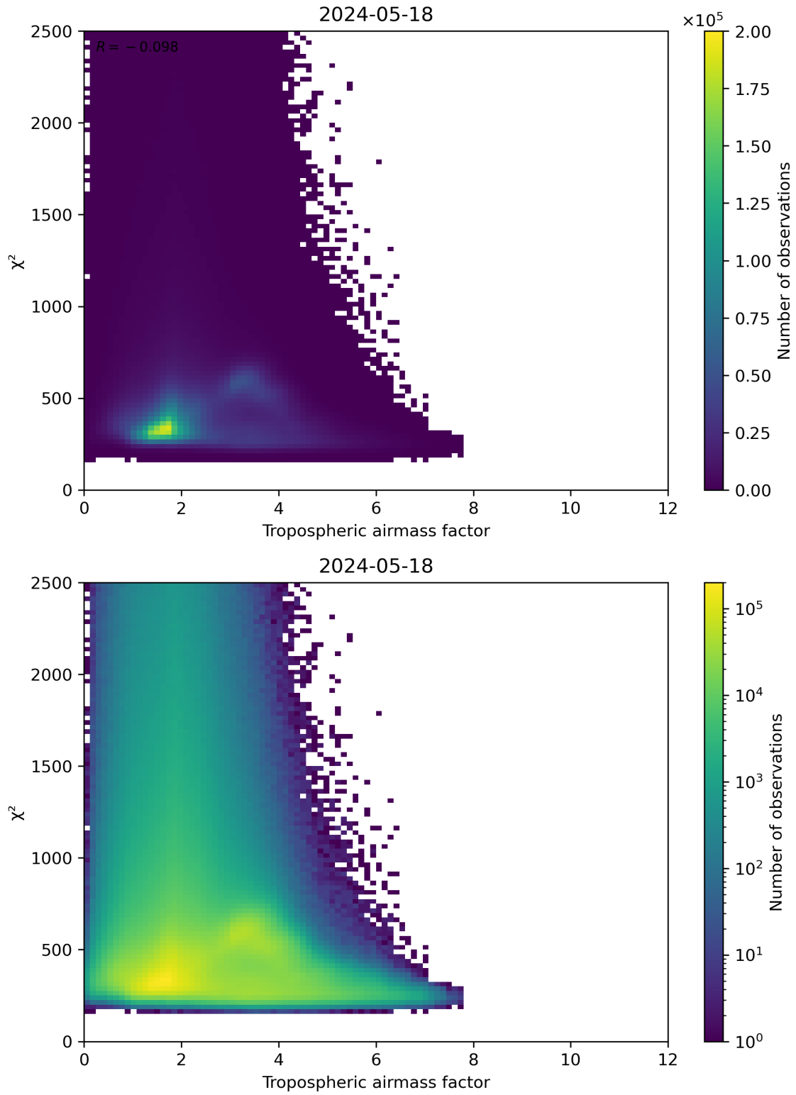
Figure 73: Scatter density plot of “Tropospheric airmass factor” against “ \chi^2 ” for 2024-05-18 to 2024-05-19.
