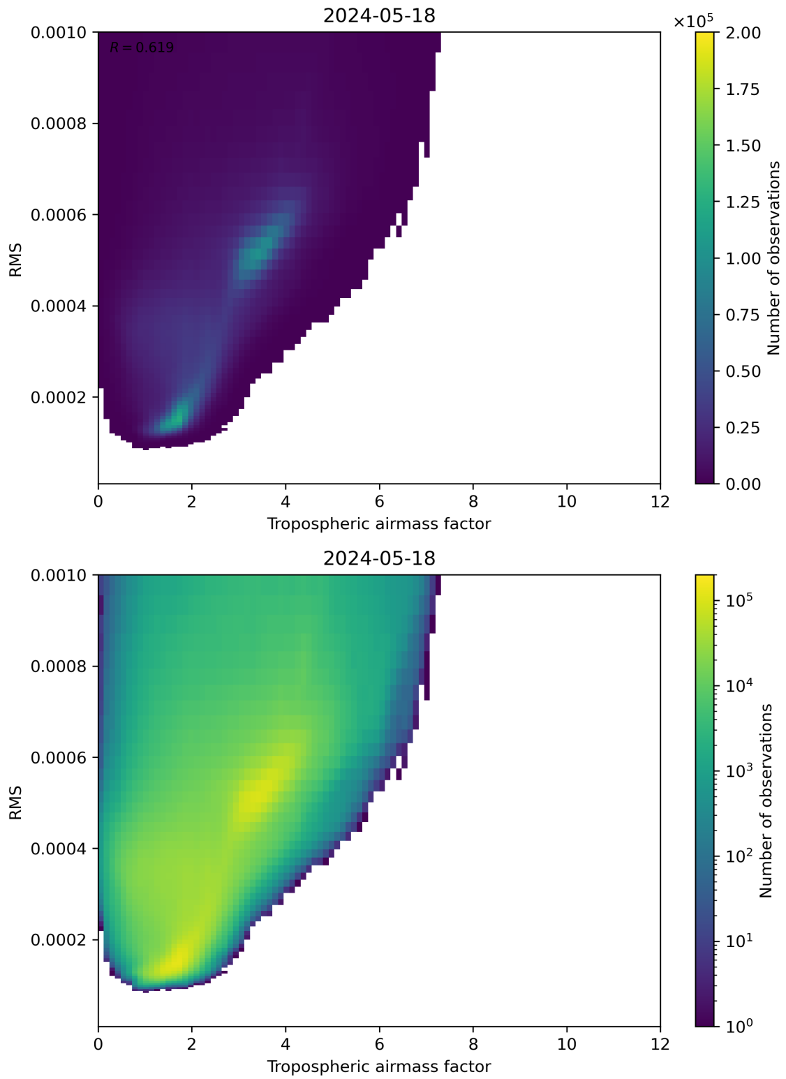
Figure 79: Scatter density plot of “Tropospheric airmass factor” against “RMS” for 2024-05-18 to 2024-05-19.
