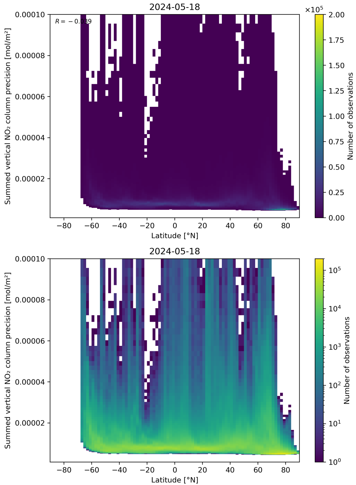
Figure 89: Scatter density plot of “Latitude” against “Summed vertical NO 2 column precision” for 2024-05-18 to 2024-05-19.
