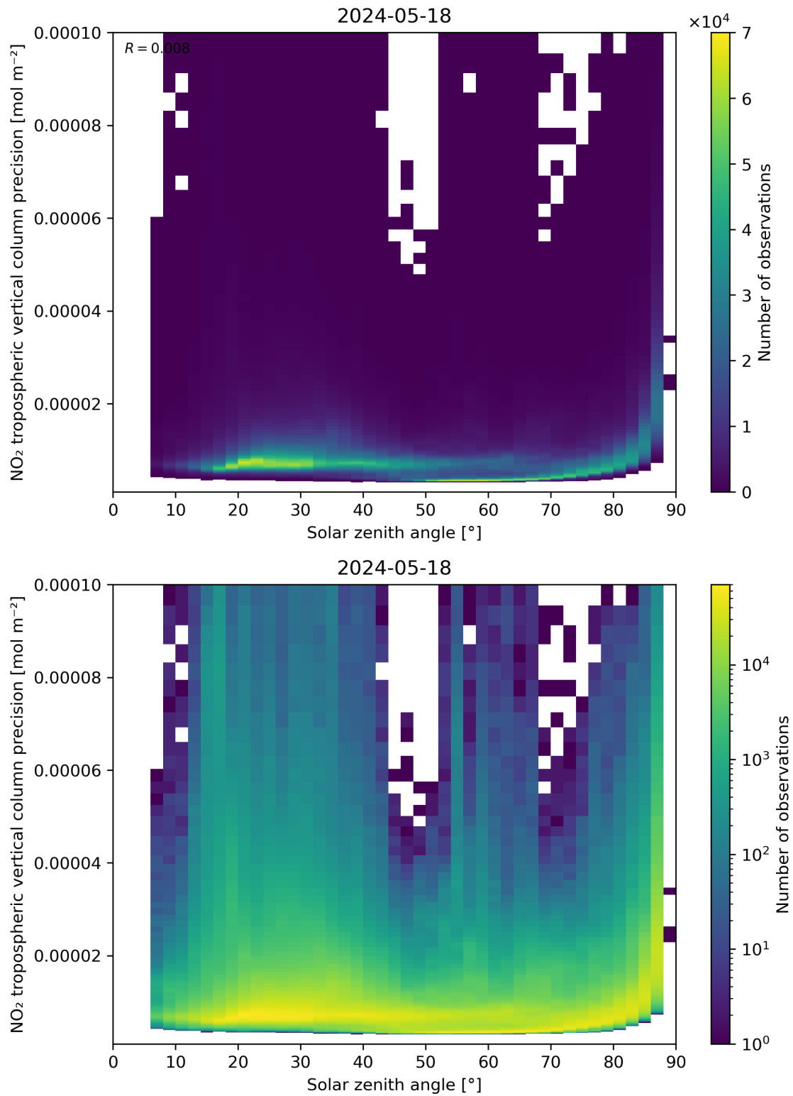
Figure 156: Scatter density plot of “Solar zenith angle” against “NO 2 tropospheric vertical column precision” for 2024-05-18 to 2024-05-19.
