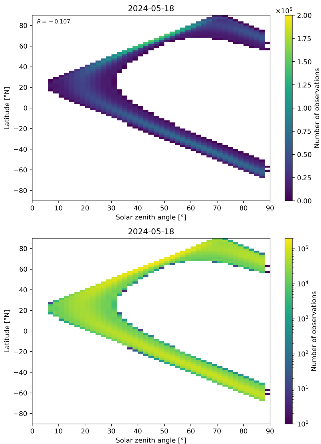
Figure 149: Scatter density plot of “Solar zenith angle” against “Latitude” for 2024-05-18 to 2024-05-19.
