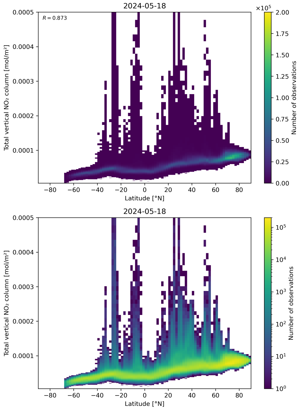
Figure 90: Scatter density plot of “Latitude” against “Total vertical NO 2 column” for 2024-05-18 to 2024-05-19.
