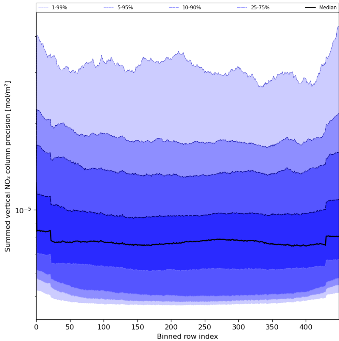
Figure 58: Along track statistics of “Summed vertical NO 2 column precision” for 2024-05-18 to 2024-05-19
