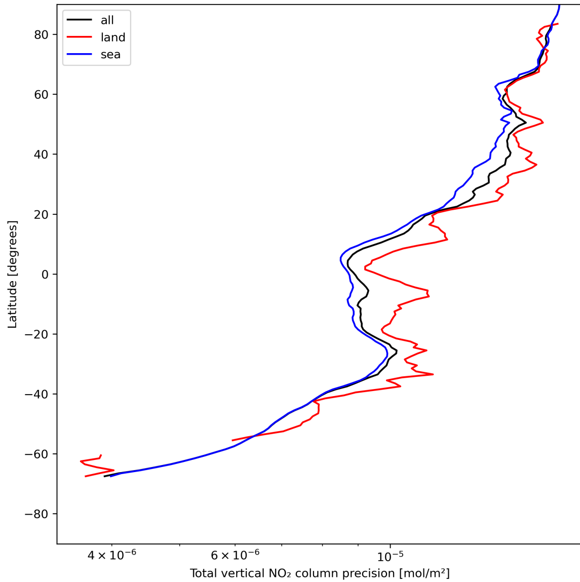
Figure 22: Zonal average of “Total vertical NO 2 column precision” for 2024-05-18 to 2024-05-19.
