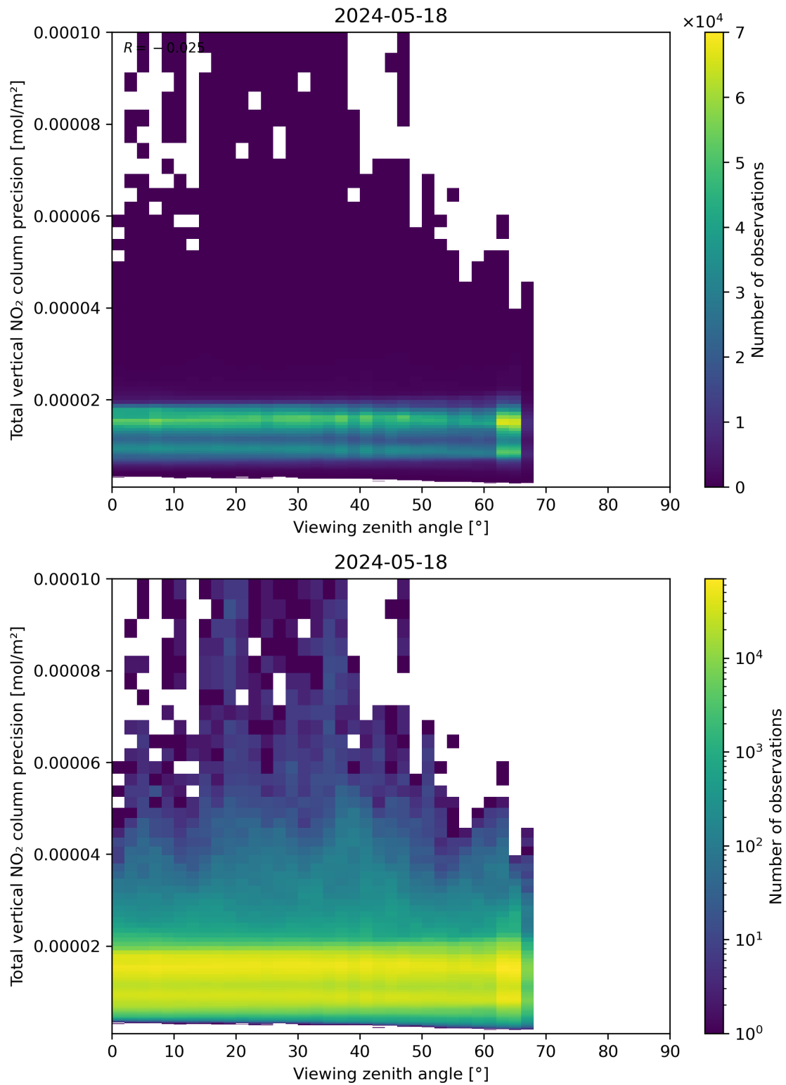
Figure 168: Scatter density plot of “Viewing zenith angle” against “Total vertical NO 2 column precision” for 2024-05-18 to 2024-05-19.
