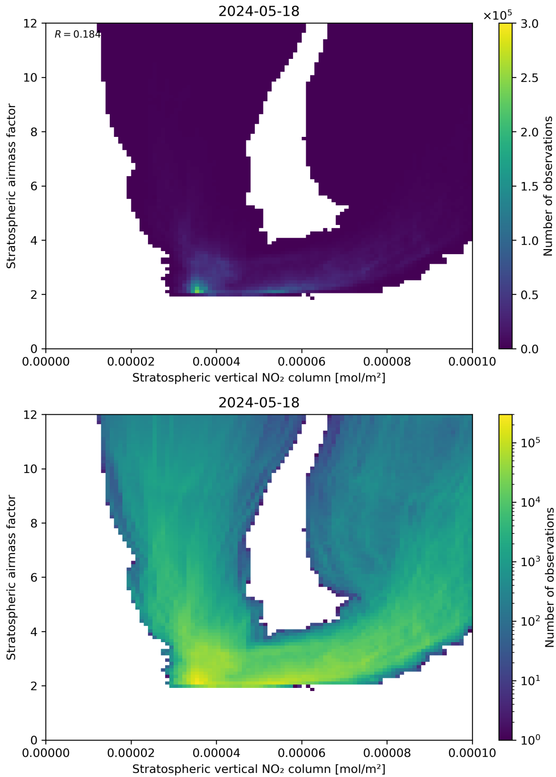
Figure 96: Scatter density plot of “Stratospheric vertical NO 2 column” against “Stratospheric airmass factor” for 2024-05-18 to 2024-05-19.
