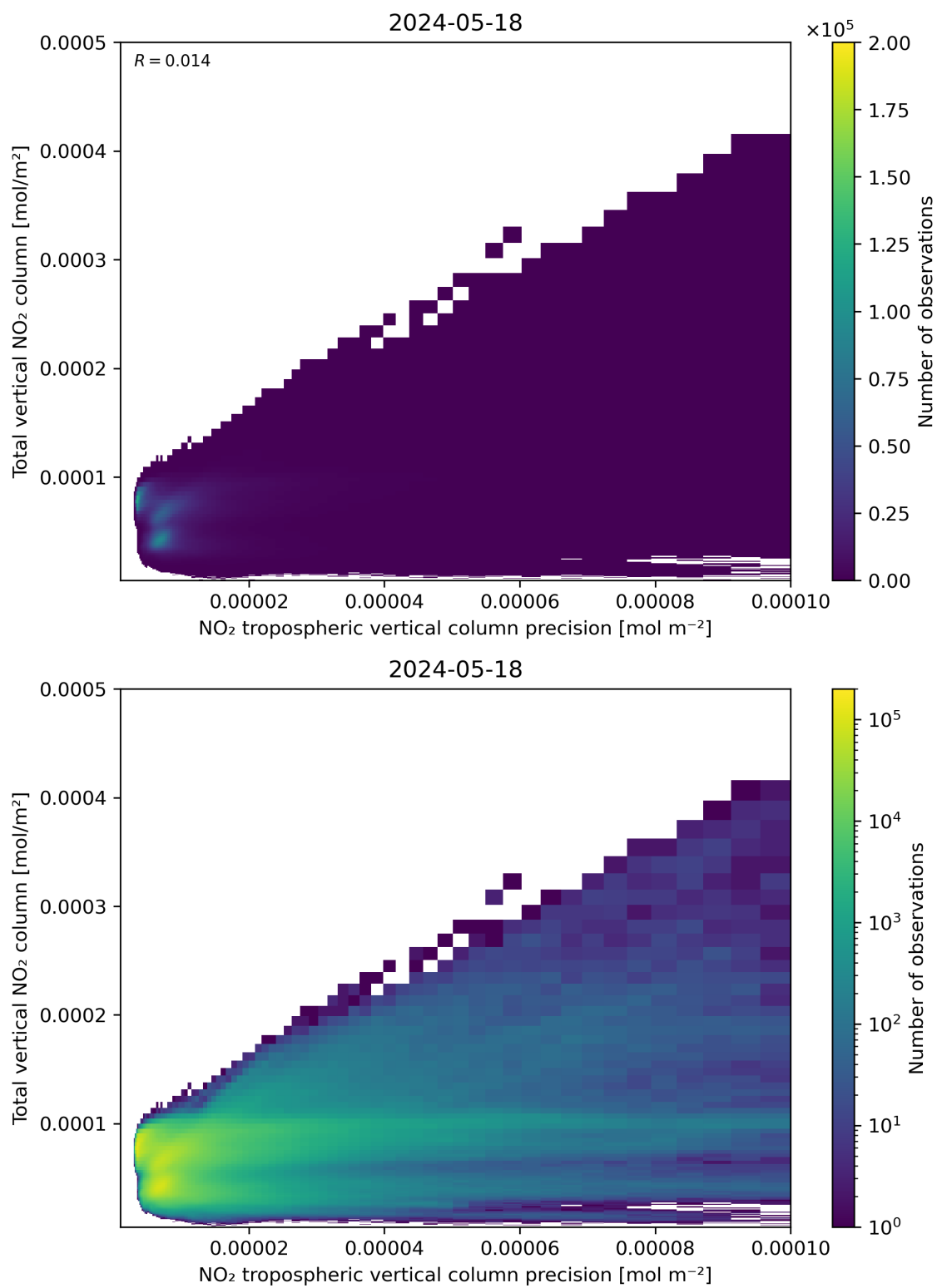
Figure 138: Scatter density plot of “NO 2 tropospheric vertical column precision” against “Total vertical NO 2 column” for 2024-05-18 to 2024-05-19.
