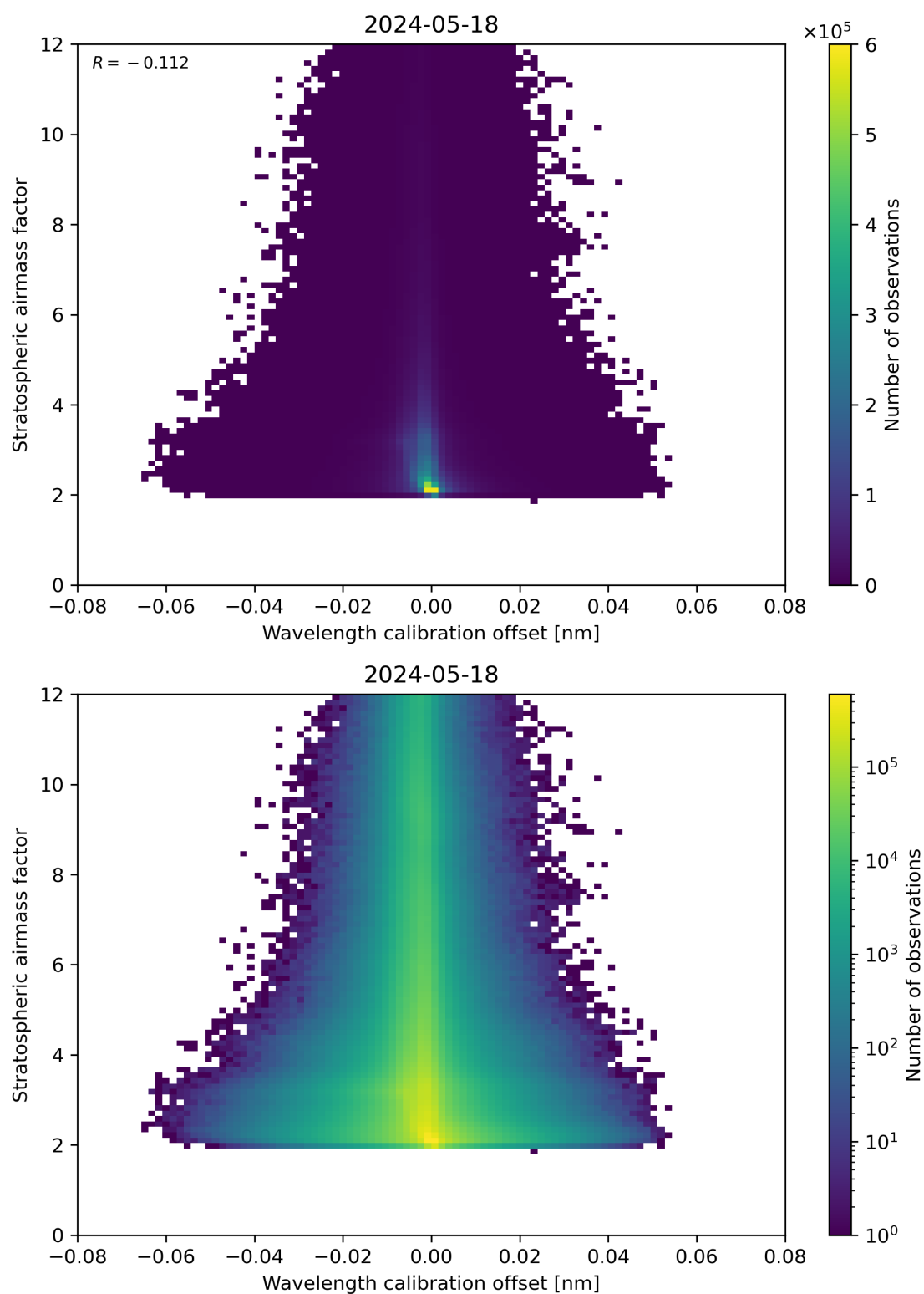
Figure 174: Scatter density plot of “Wavelength calibration offset” against “Stratospheric airmass factor” for 2024-05-18 to 2024-05-19.
