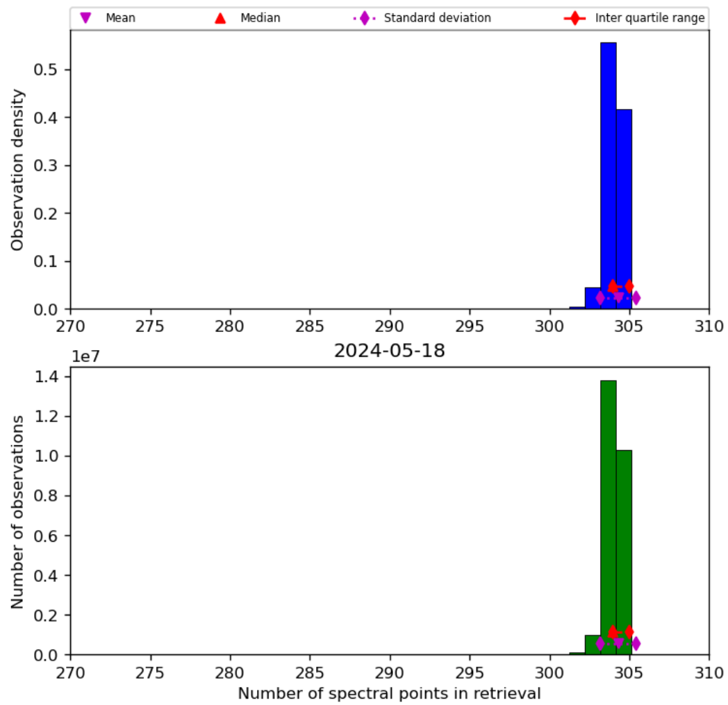
Figure 33: Histogram of “Number of spectral points in retrieval” for 2024-05-18 to 2024-05-19
