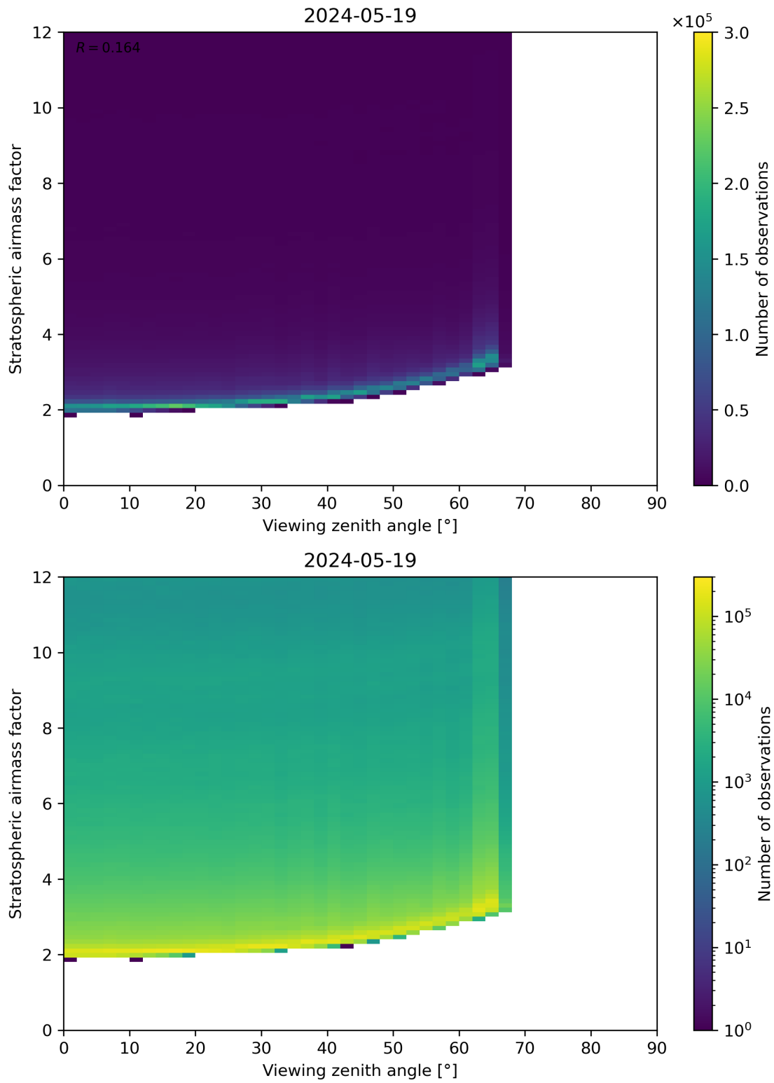
Figure 159: Scatter density plot of “Viewing zenith angle” against “Stratospheric airmass factor” for 2024-05-18 to 2024-05-20.
