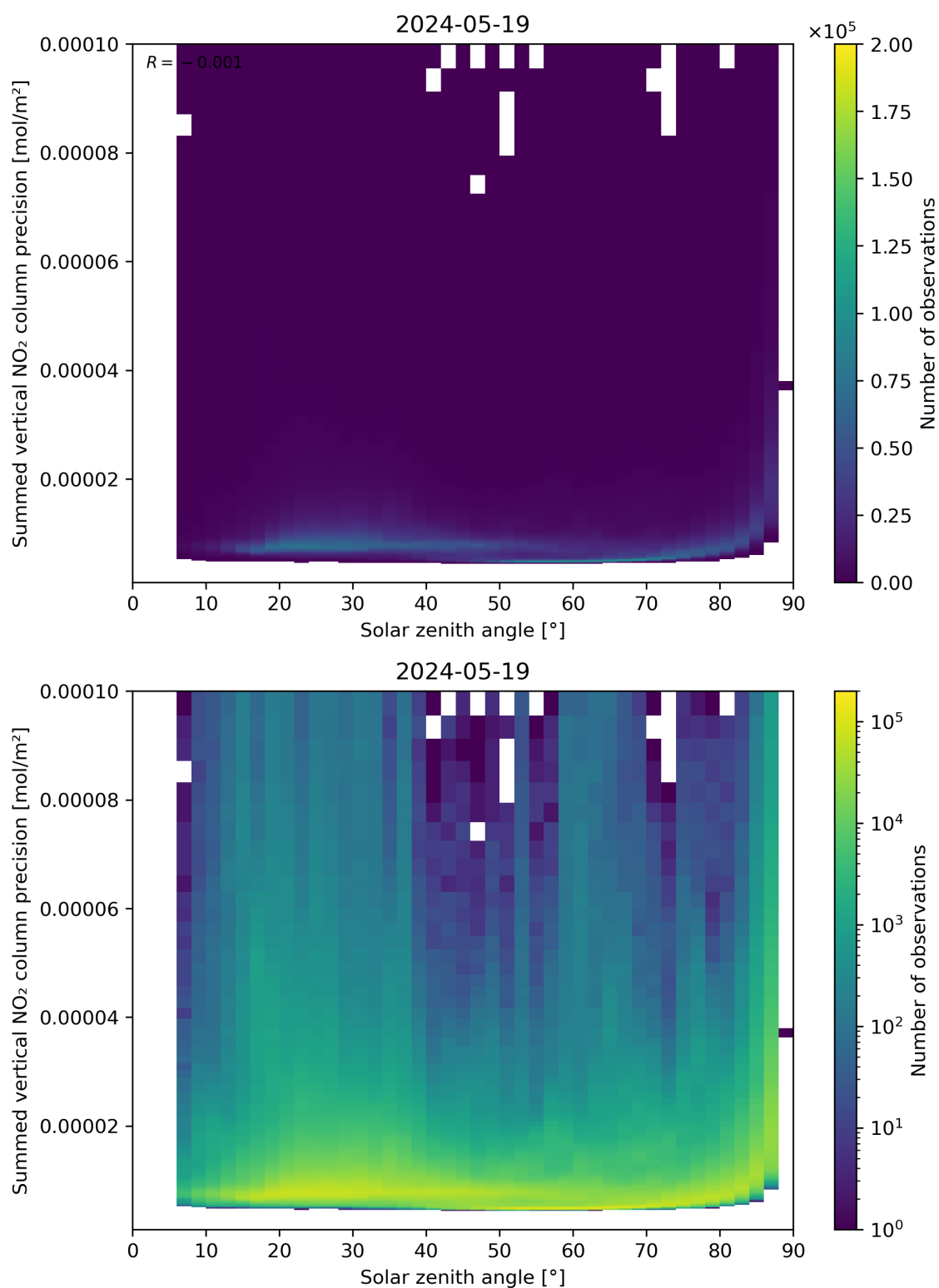
Figure 152: Scatter density plot of “Solar zenith angle” against “Summed vertical NO 2 column precision” for 2024-05-18 to 2024-05-20.
