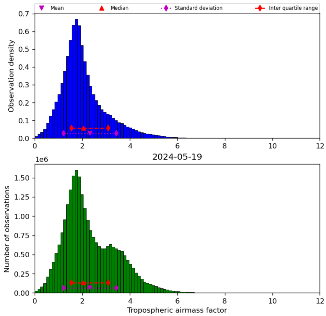
Figure 31: Histogram of “Tropospheric airmass factor” for 2024-05-18 to 2024-05-20
