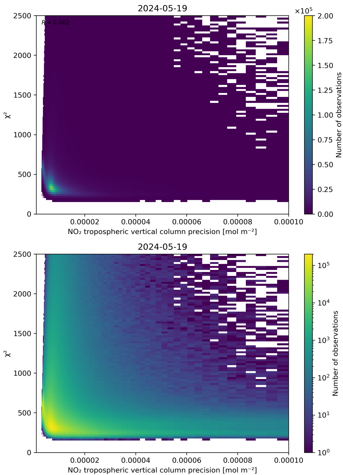
Figure 134: Scatter density plot of “NO 2 tropospheric vertical column precision” against “ \chi^2 ” for 2024-05-18 to 2024-05-20.
