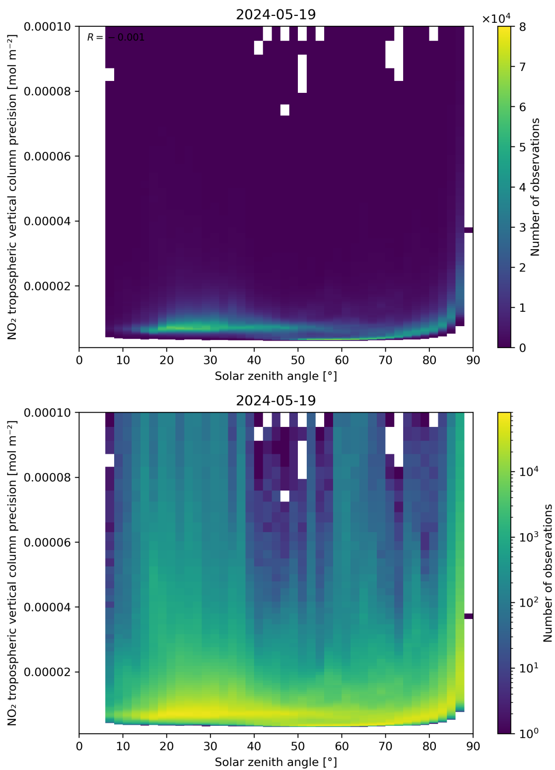
Figure 156: Scatter density plot of “Solar zenith angle” against “NO 2 tropospheric vertical column precision” for 2024-05-18 to 2024-05-20.
