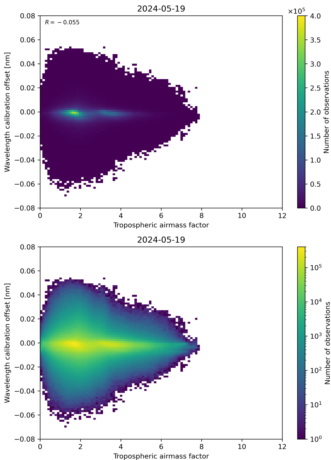
Figure 80: Scatter density plot of “Tropospheric airmass factor” against “Wavelength calibration offset” for 2024-05-18 to 2024-05-20.
