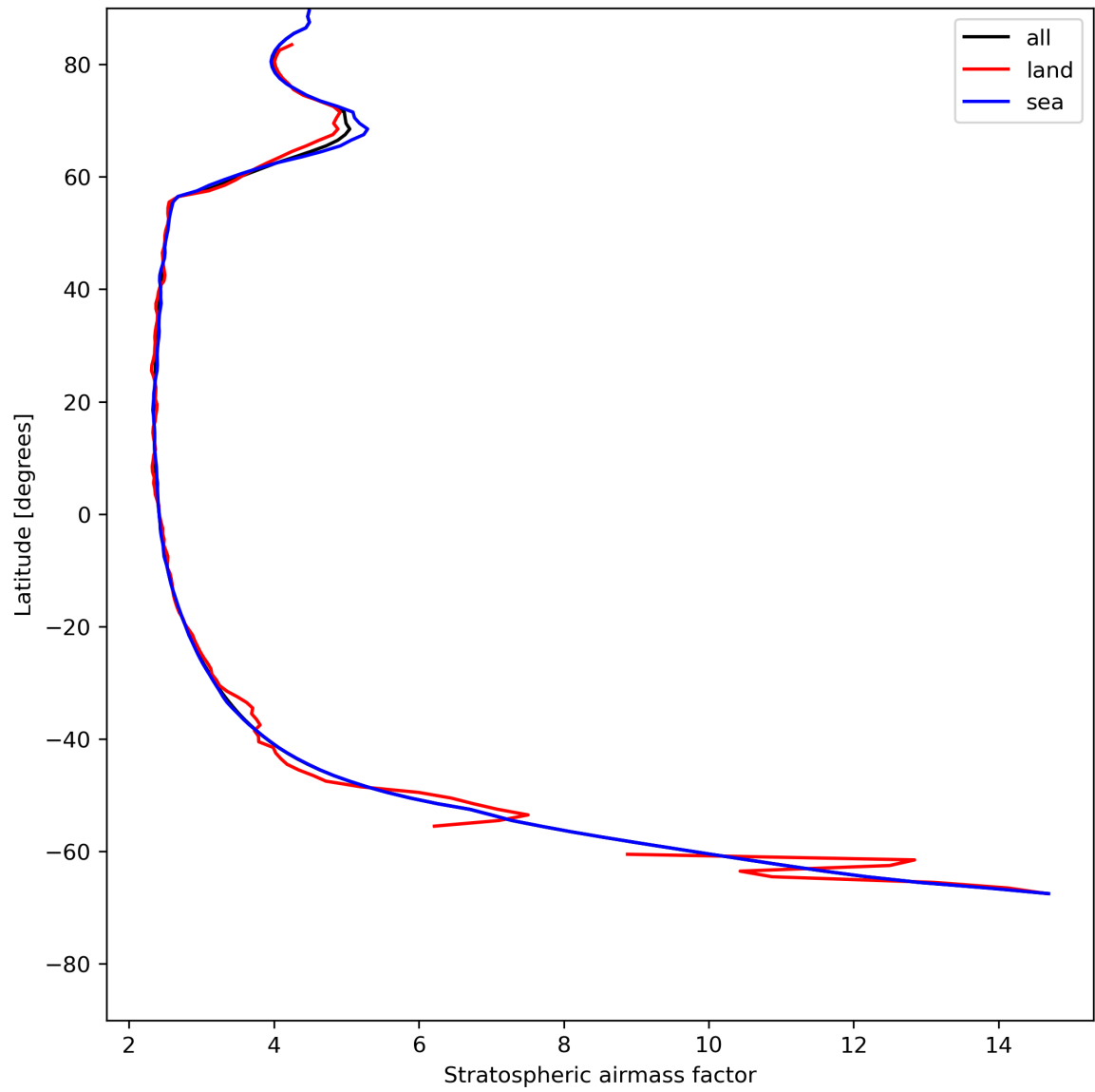
Figure 27: Zonal average of “Stratospheric air mass factor” for 2024-05-18 to 2024-05-20.
