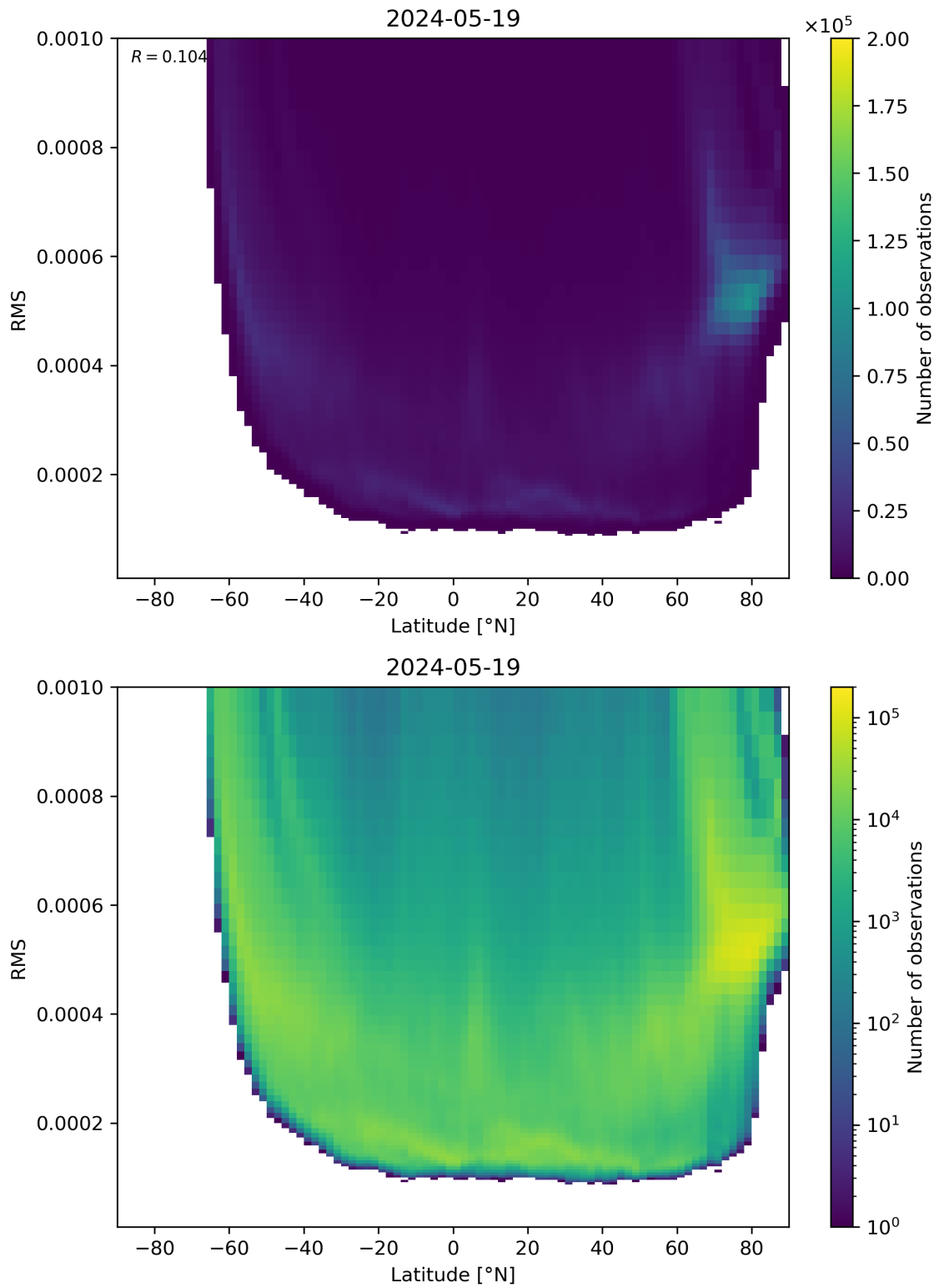
Figure 94: Scatter density plot of “Latitude” against “RMS” for 2024-05-18 to 2024-05-20.
