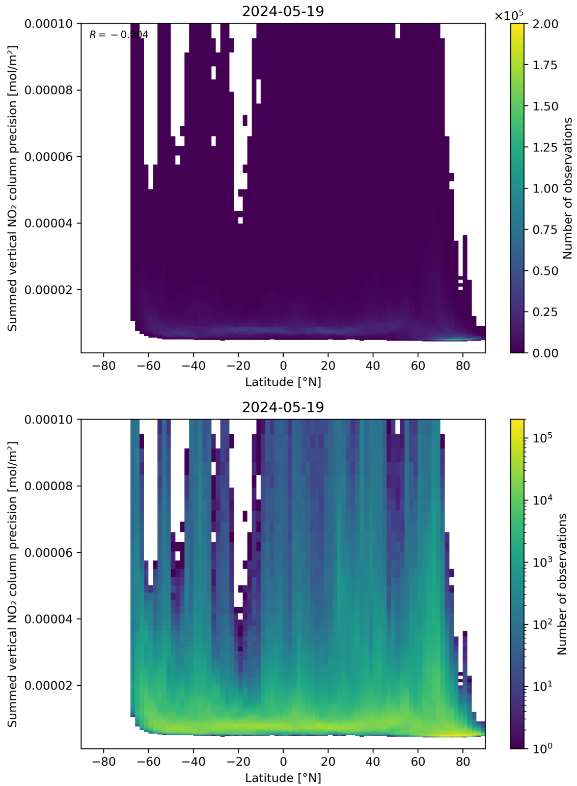
Figure 89: Scatter density plot of “Latitude” against “Summed vertical NO 2 column precision” for 2024-05-18 to 2024-05-20.
