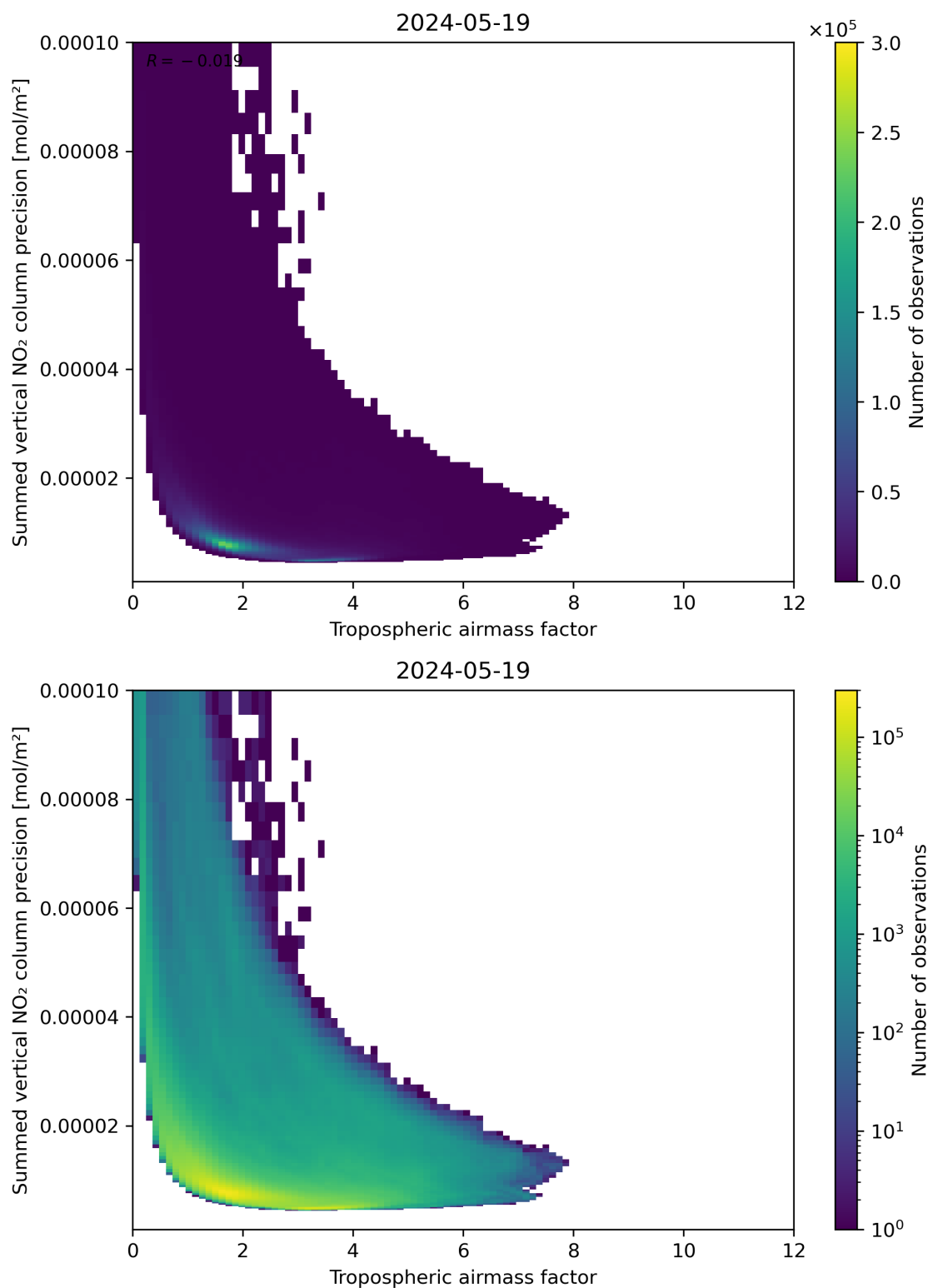
Figure 76: Scatter density plot of “Tropospheric air mass factor” against “Summed vertical NO 2 column precision” for 2024-05-18 to 2024-05-20.
