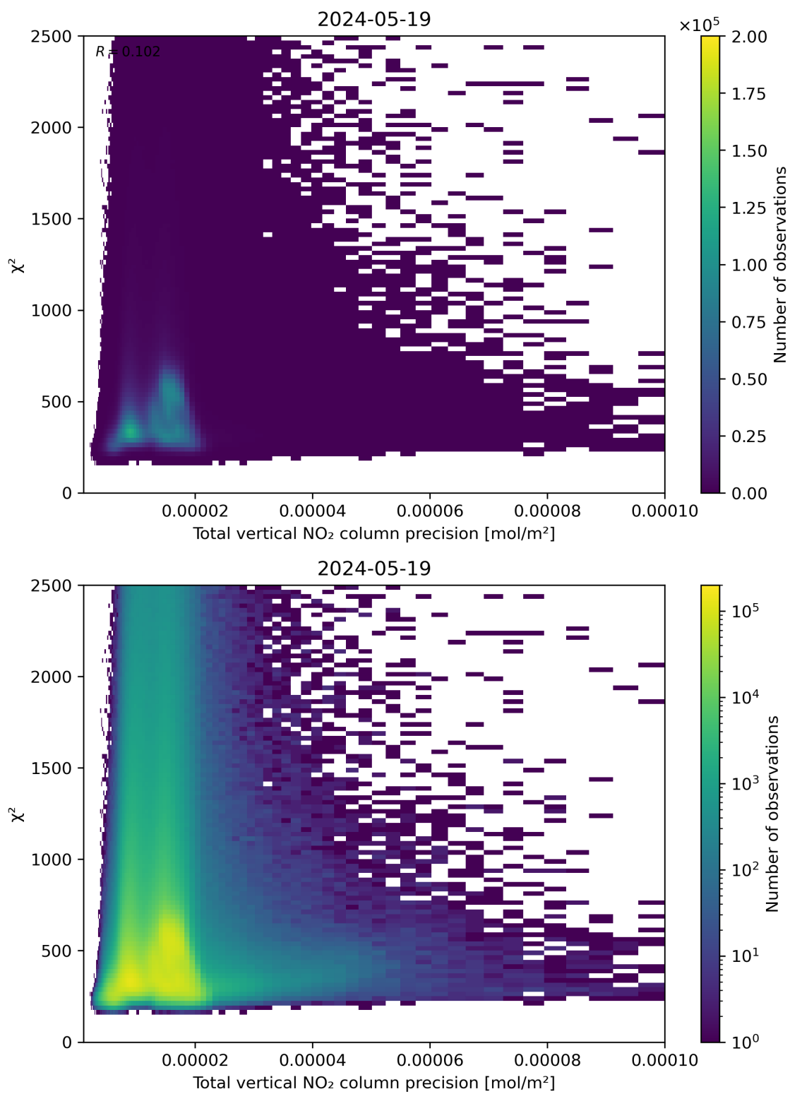
Figure 116: Scatter density plot of “Total vertical NO 2 column precision” against “ \chi^2 ” for 2024-05-18 to 2024-05-20.
