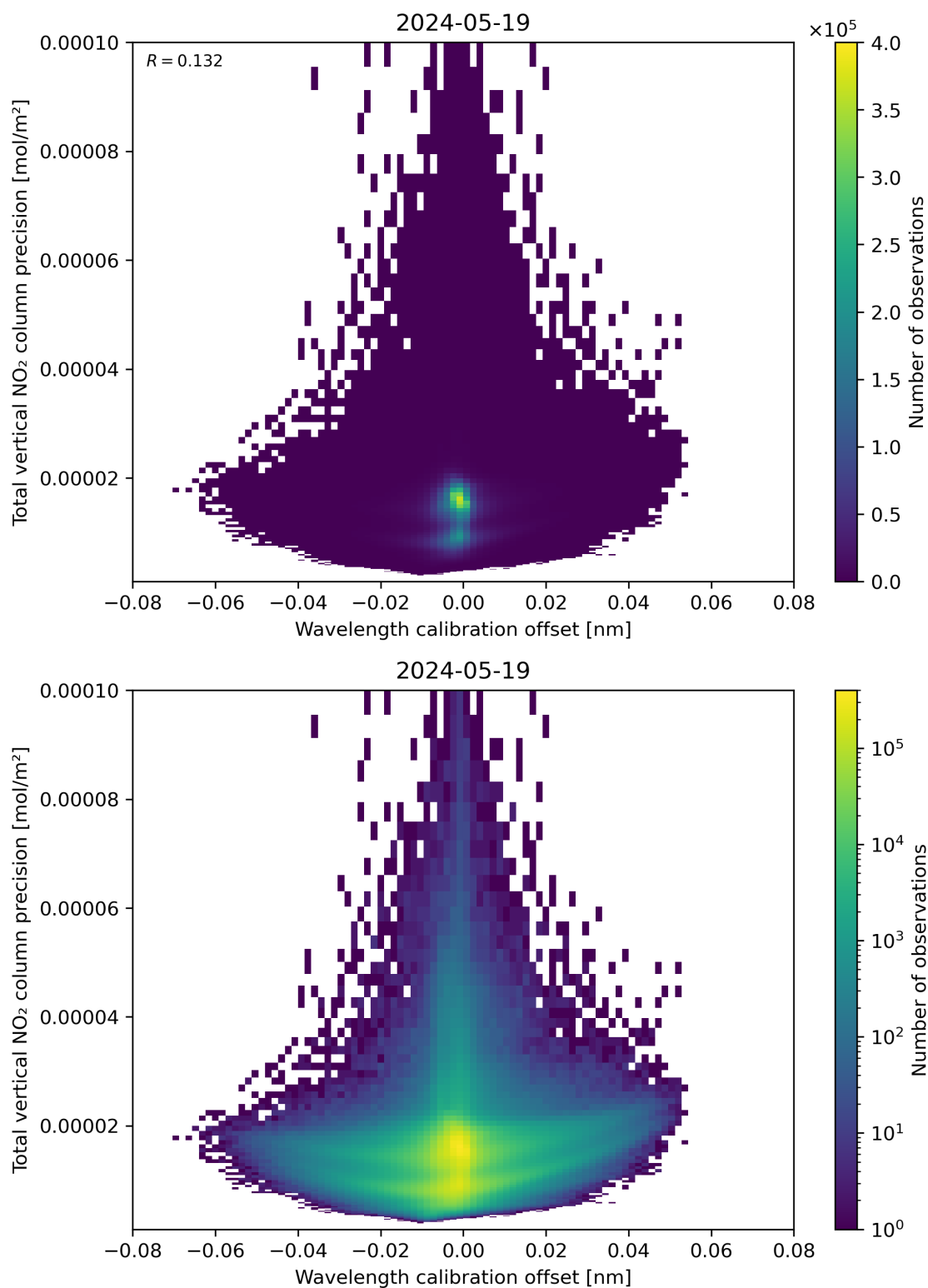
Figure 180: Scatter density plot of “Wavelength calibration offset” against “Total vertical NO 2 column precision” for 2024-05-18 to 2024-05-20.
