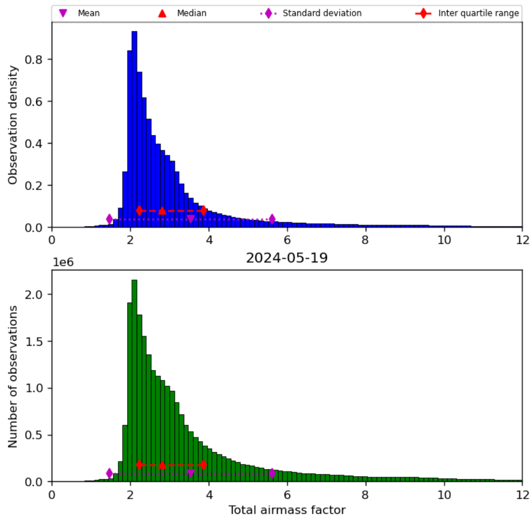
Figure 32: Histogram of “Total airmass factor” for 2024-05-18 to 2024-05-20
