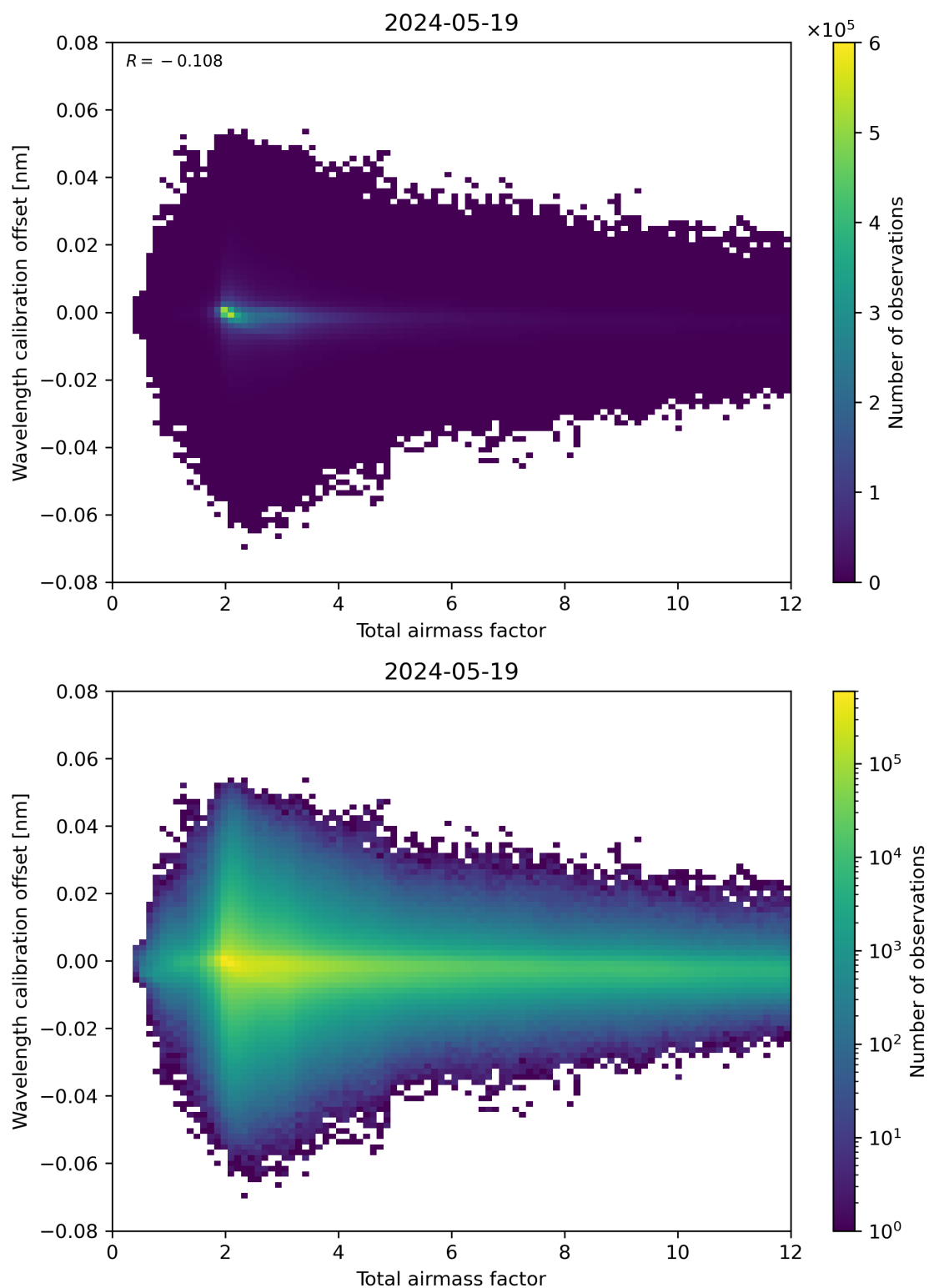
Figure 70: Scatter density plot of “Total airmass factor” against “Wavelength calibration offset” for 2024-05-18 to 2024-05-20.
