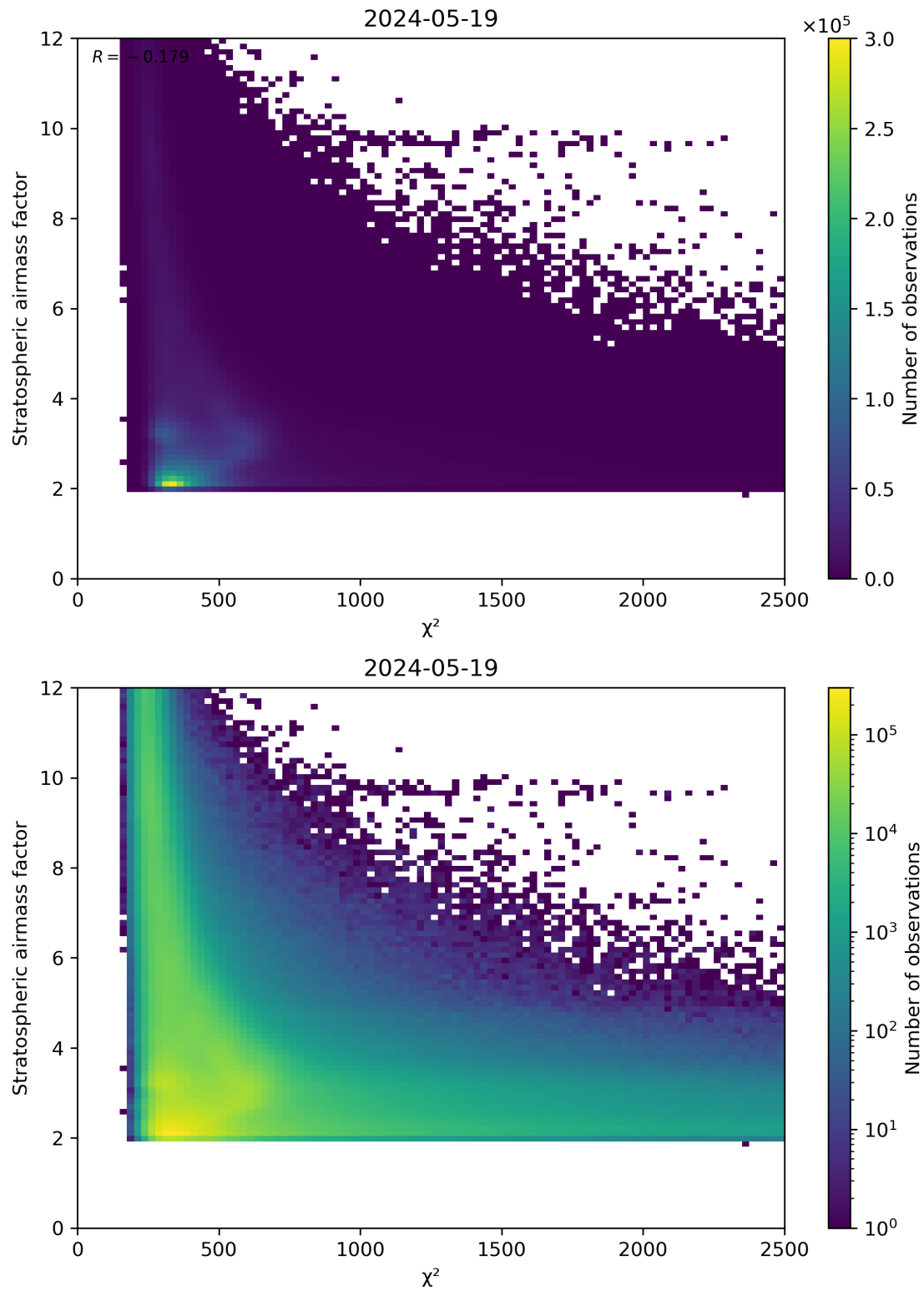
Figure 81: Scatter density plot of “ \chi^2 ” against “Stratospheric airmass factor” for 2024-05-18 to 2024-05-20.
