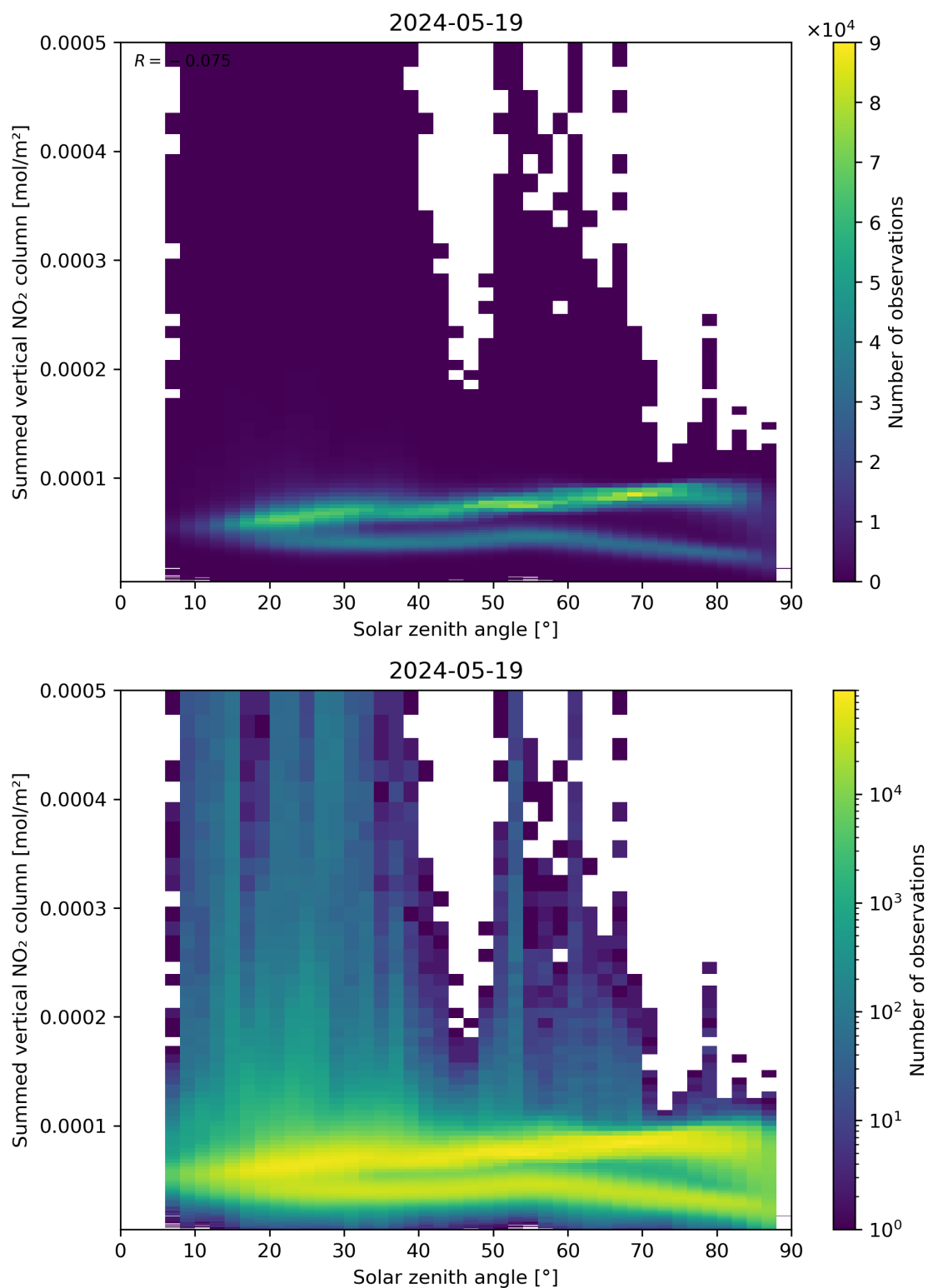
Figure 151: Scatter density plot of “Solar zenith angle” against “Summed vertical NO 2 column” for 2024-05-18 to 2024-05-20.
