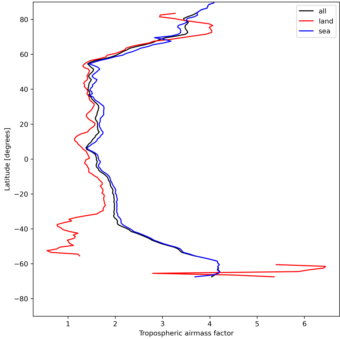
Figure 14: Zonal average of “Tropospheric airmass factor” for 2024-05-18 to 2024-05-20.
