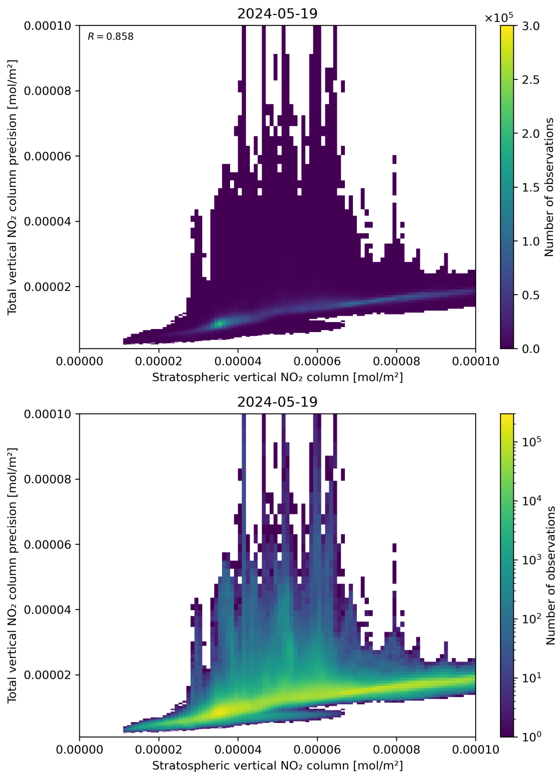
Figure 101: Scatter density plot of “Stratospheric vertical NO 2 column” against “Total vertical NO 2 column precision” for 2024-05-18 to 2024-05-20.
