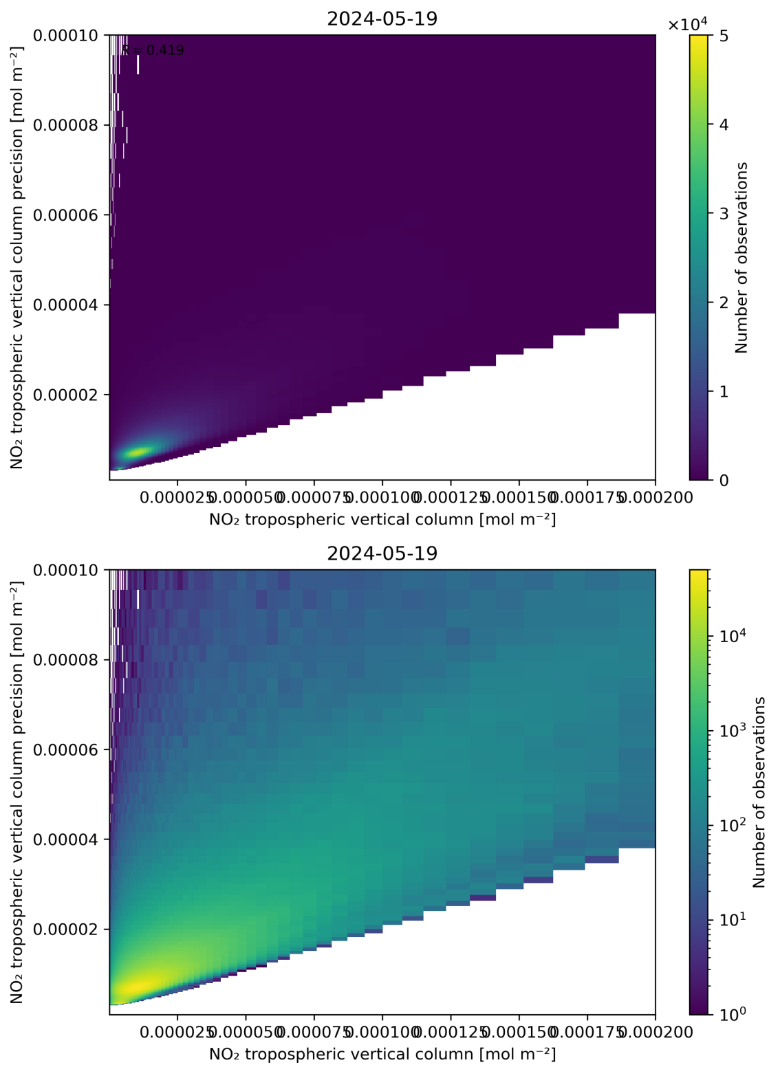
Figure 130: Scatter density plot of “NO 2 tropospheric vertical column” against “NO 2 tropospheric vertical column precision” for 2024-05-18 to 2024-05-20.
