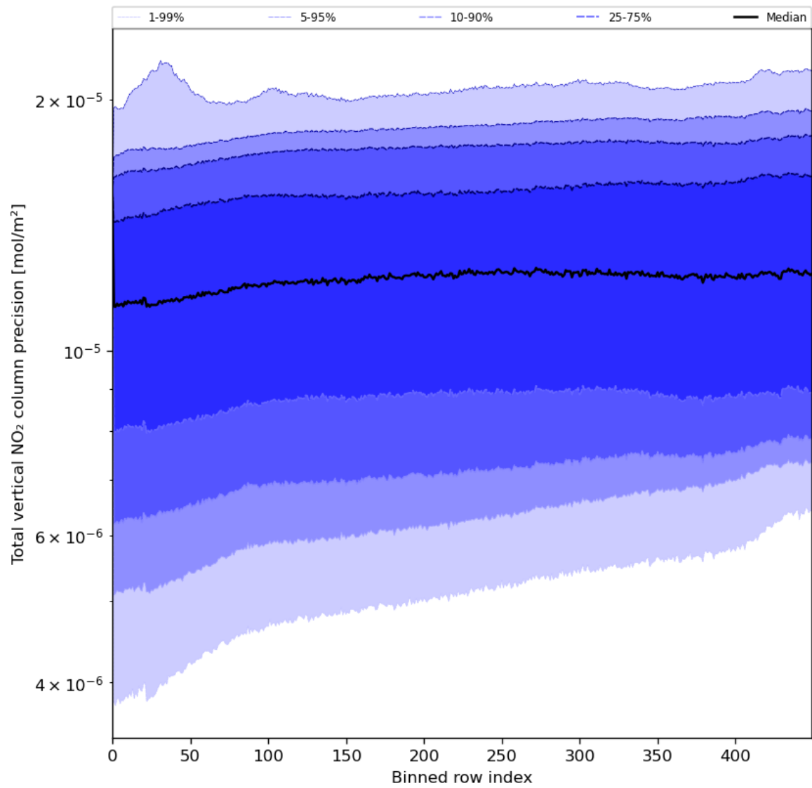
Figure 56: Along track statistics of "Total vertical NO 2 column precision" for 2024-05-18 to 2024-05-20
