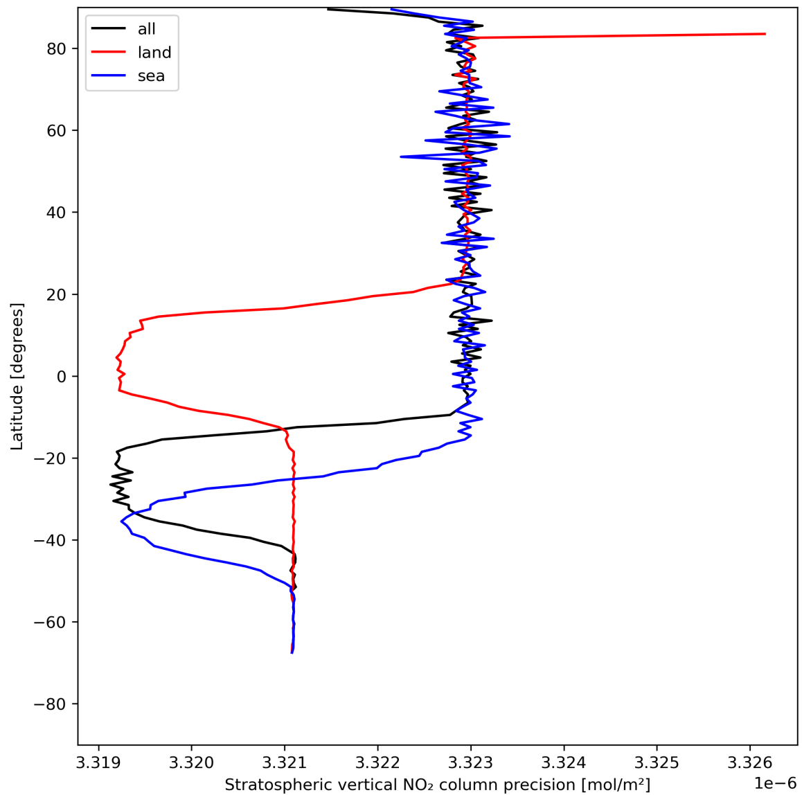
Figure 20: Zonal average of “Stratospheric vertical NO 2 column precision” for 2024-05-18 to 2024-05-20.
