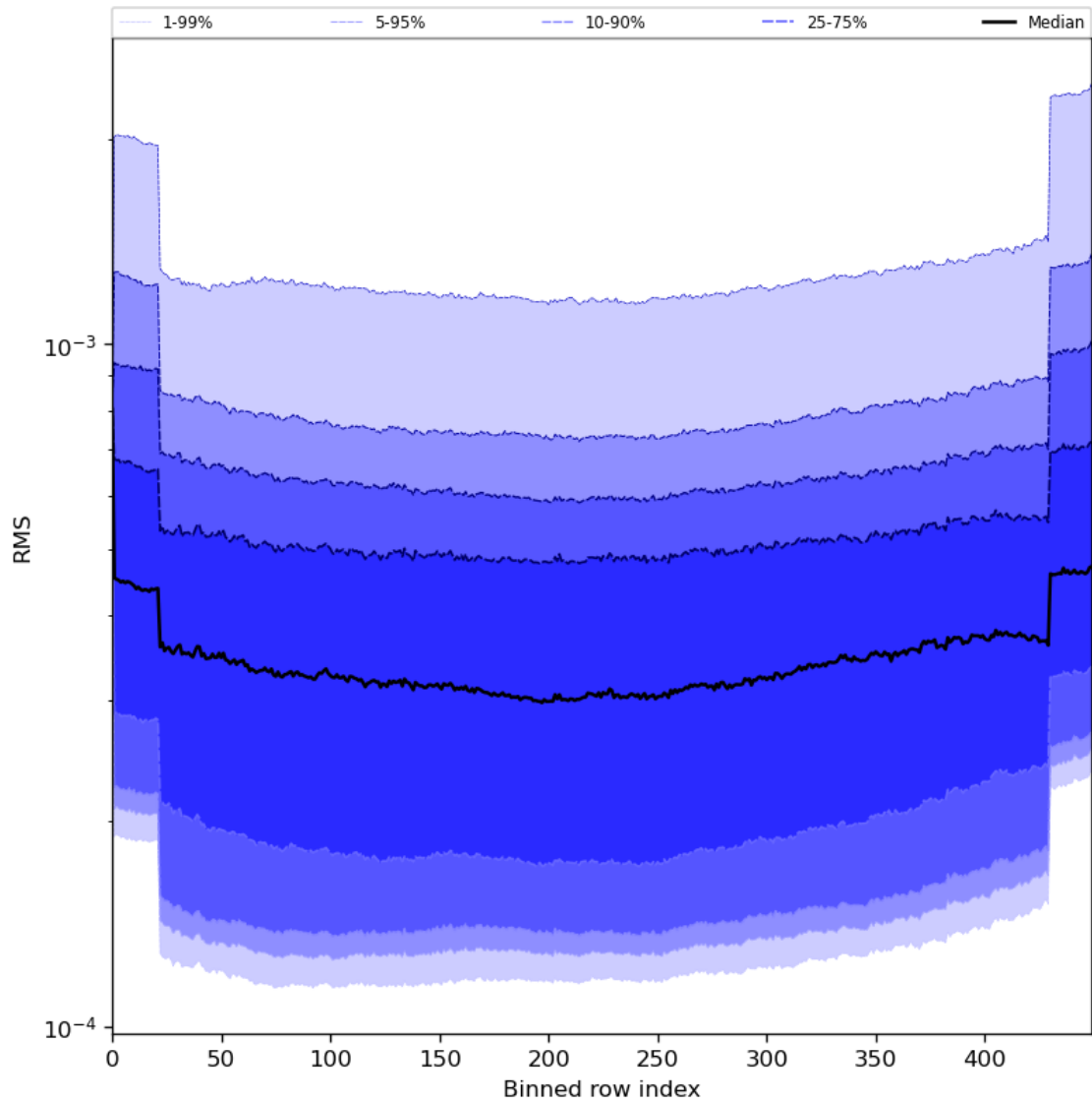
Figure 60: Along track statistics of “RMS” for 2024-05-18 to 2024-05-20
