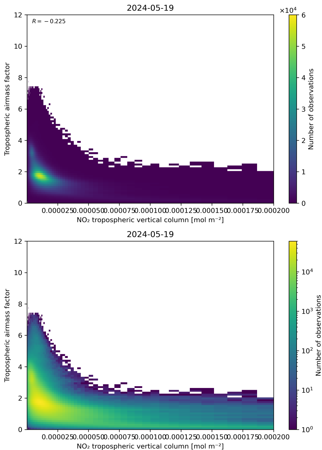
Figure 123: Scatter density plot of “NO 2 tropospheric vertical column” against “Tropospheric airmass factor” for 2024-05-18 to 2024-05-20.
