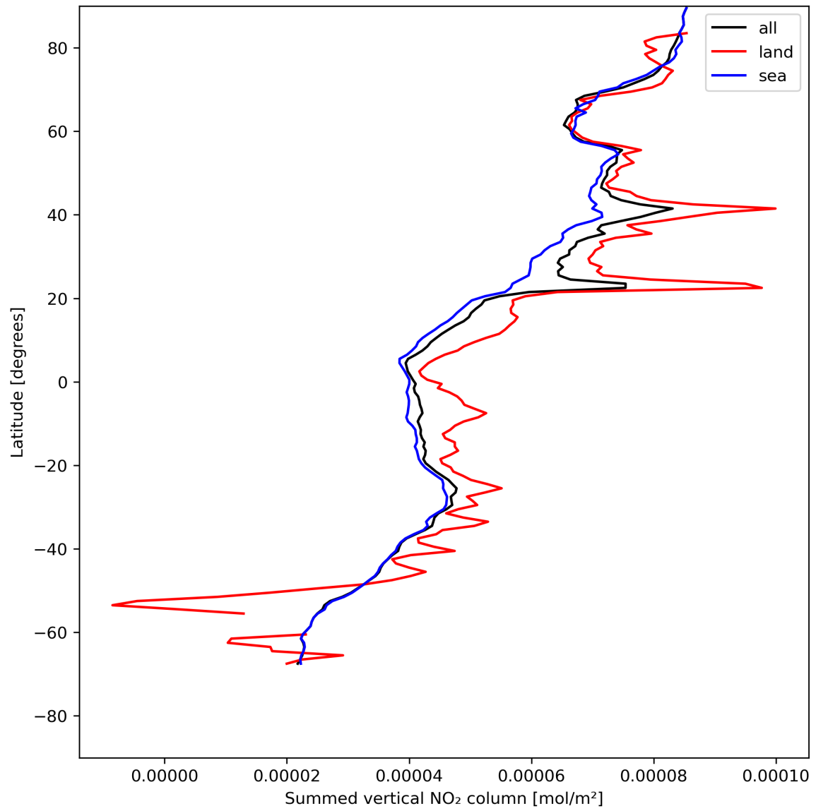
Figure 23: Zonal average of “Summed vertical NO 2 column” for 2024-05-18 to 2024-05-20.
