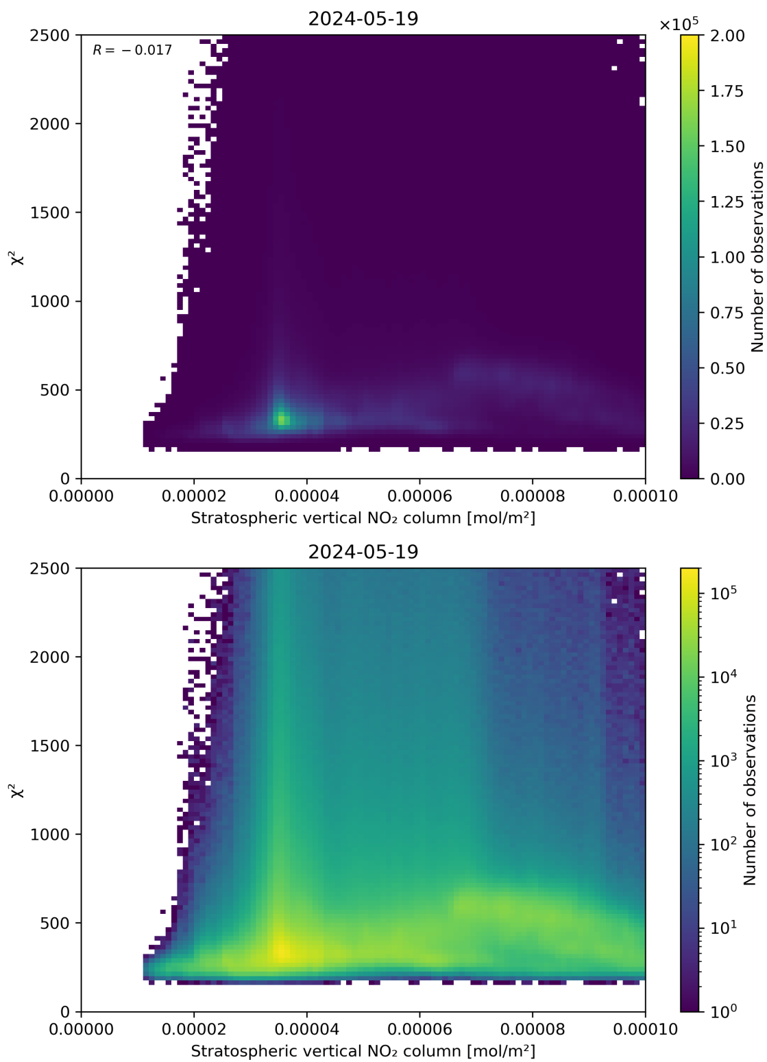
Figure 97: Scatter density plot of “Stratospheric vertical NO 2 column” against “ \chi^2 ” for 2024-05-18 to 2024-05-20.
