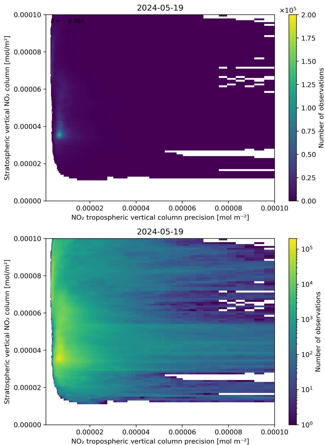
Figure 135: Scatter density plot of “NO 2 tropospheric vertical column precision” against “Stratospheric vertical NO 2 column” for 2024-05-18 to 2024-05-20.
