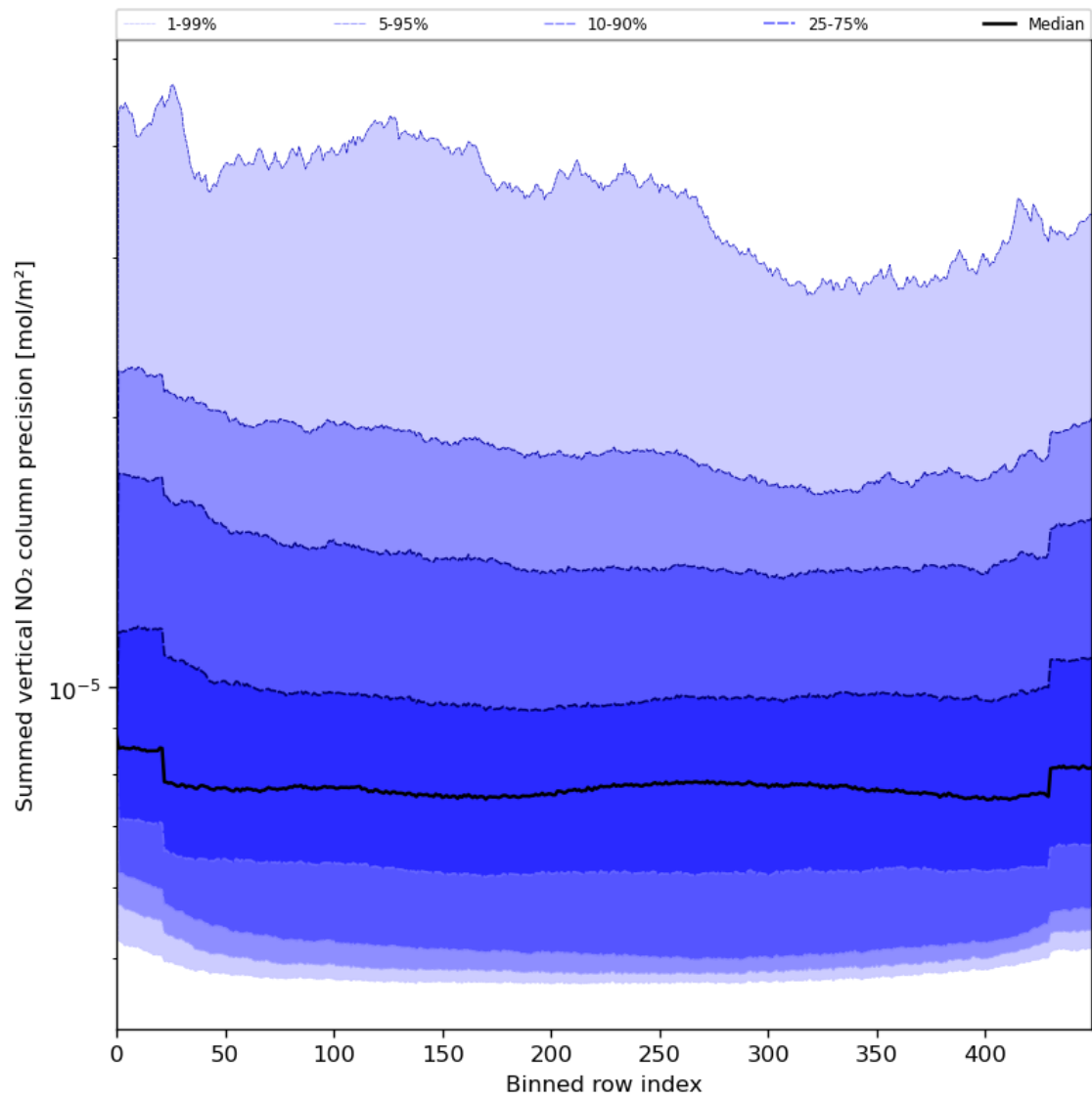
Figure 58: Along track statistics of “Summed vertical NO 2 column precision” for 2024-05-18 to 2024-05-20
