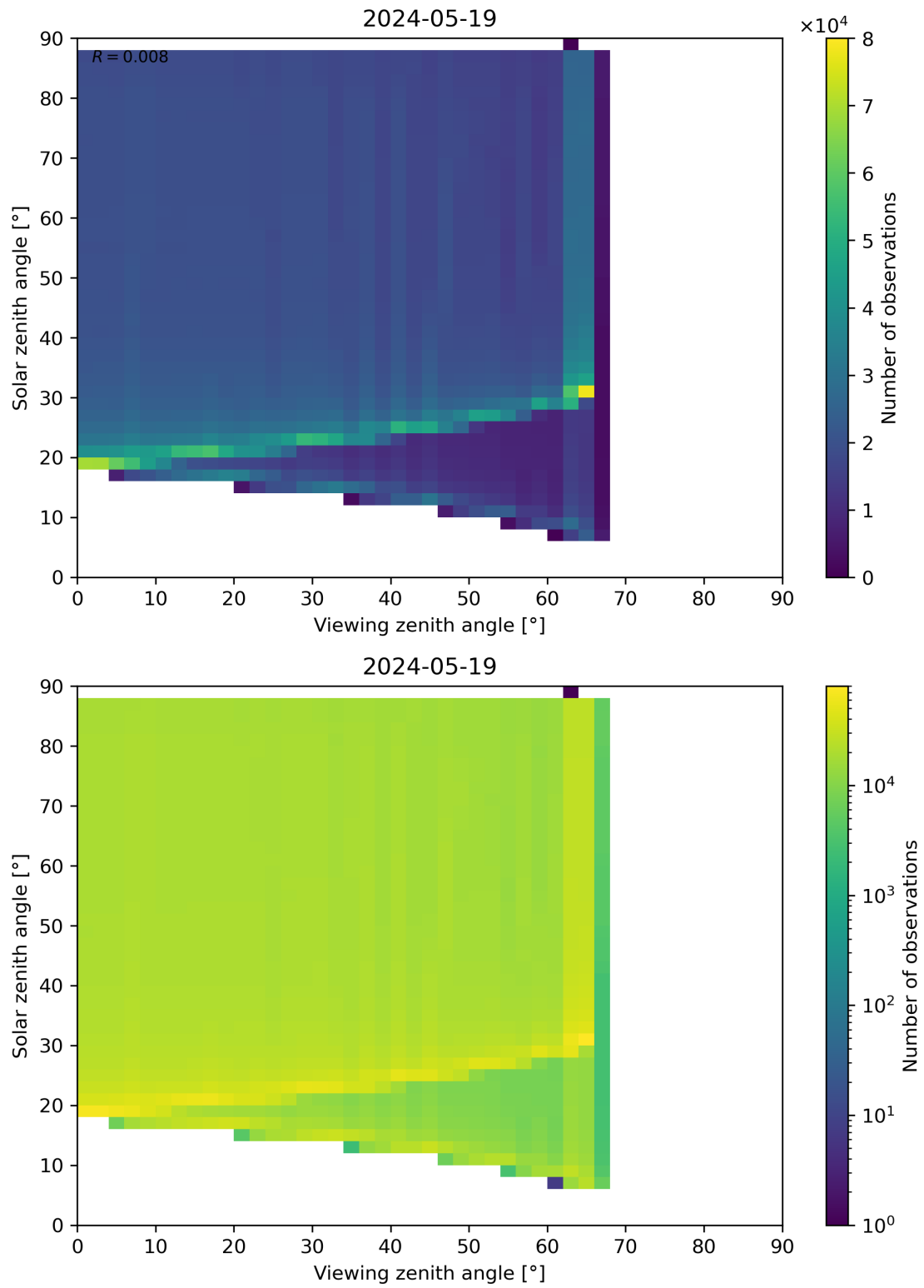
Figure 172: Scatter density plot of “Viewing zenith angle” against “Solar zenith angle” for 2024-05-18 to 2024-05-20.
