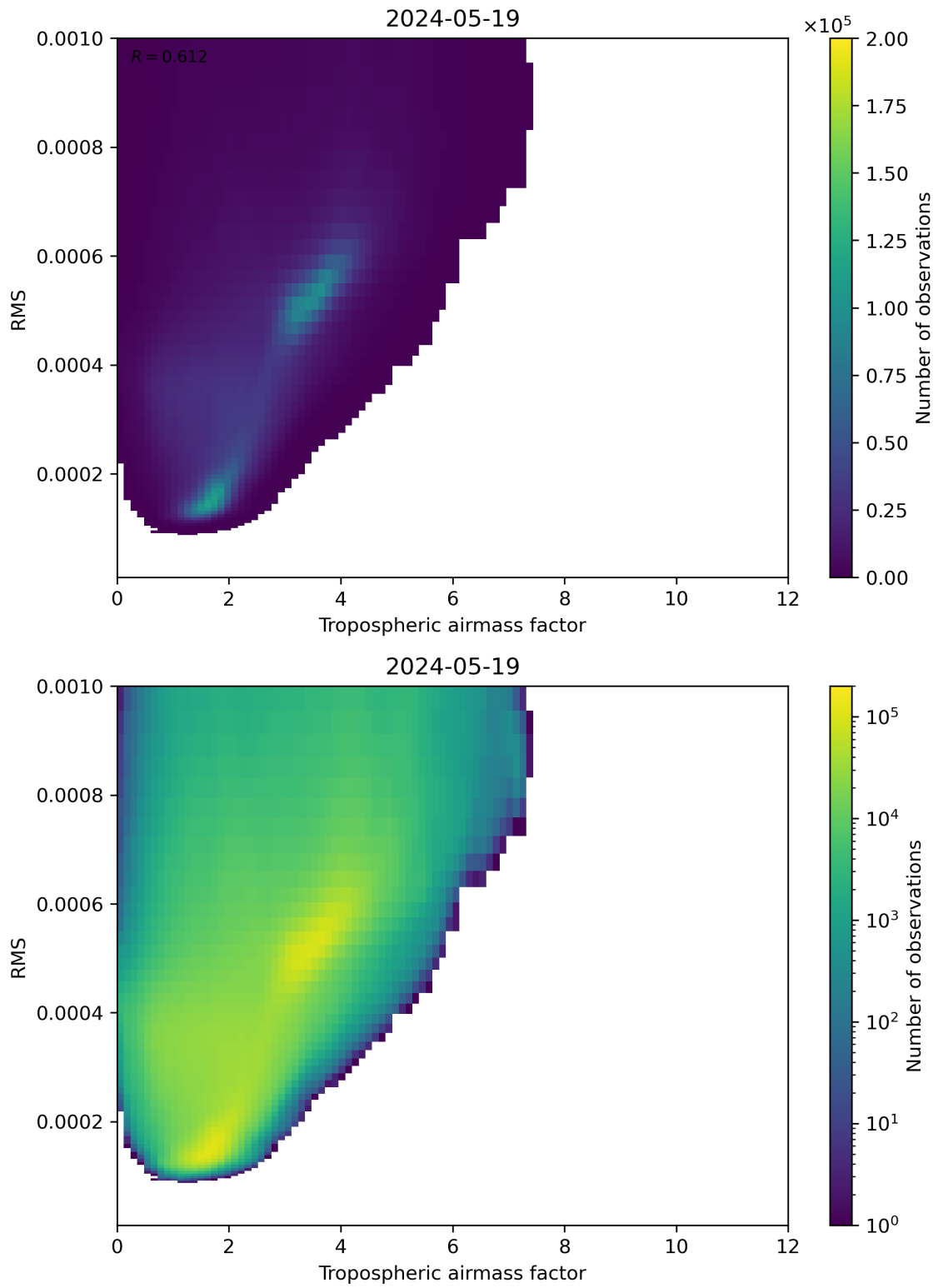
Figure 79: Scatter density plot of “Tropospheric airmass factor” against “RMS” for 2024-05-18 to 2024-05-20.
