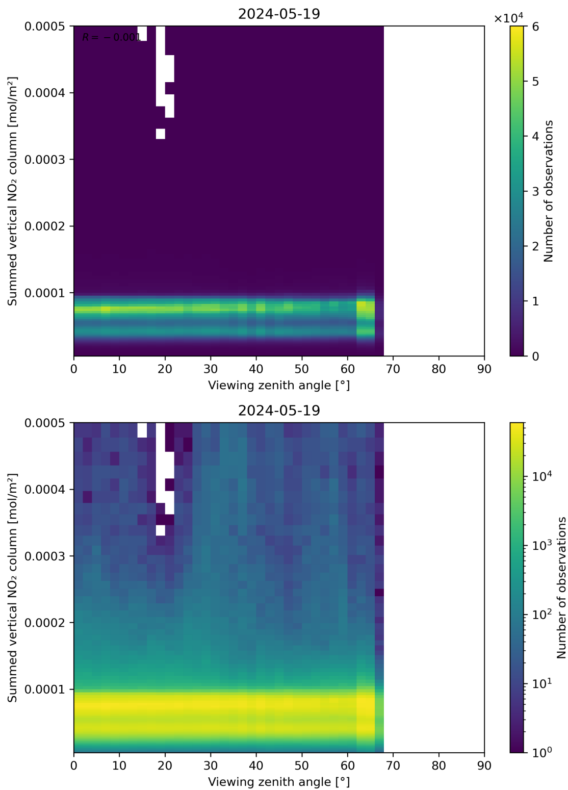
Figure 165: Scatter density plot of “Viewing zenith angle” against “Summed vertical NO 2 column” for 2024-05-18 to 2024-05-20.
