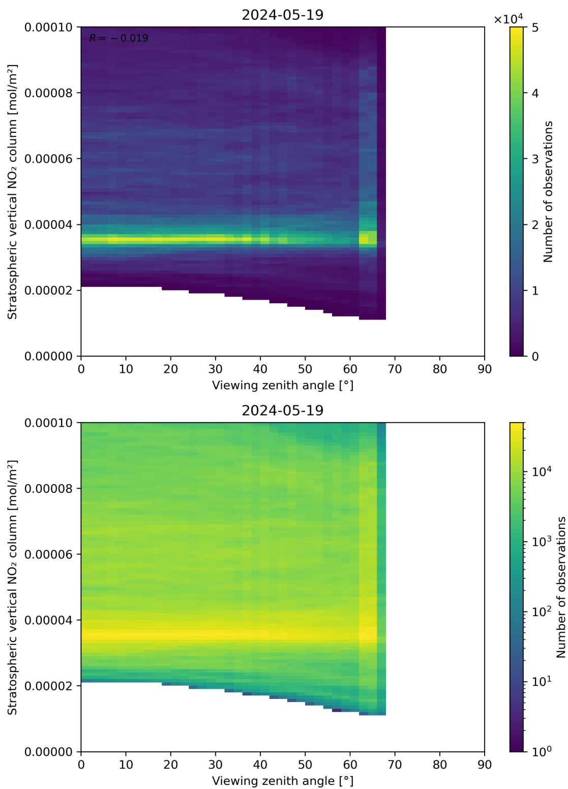
Figure 164: Scatter density plot of “Viewing zenith angle” against “Stratospheric vertical NO 2 column” for 2024-05-18 to 2024-05-20.
