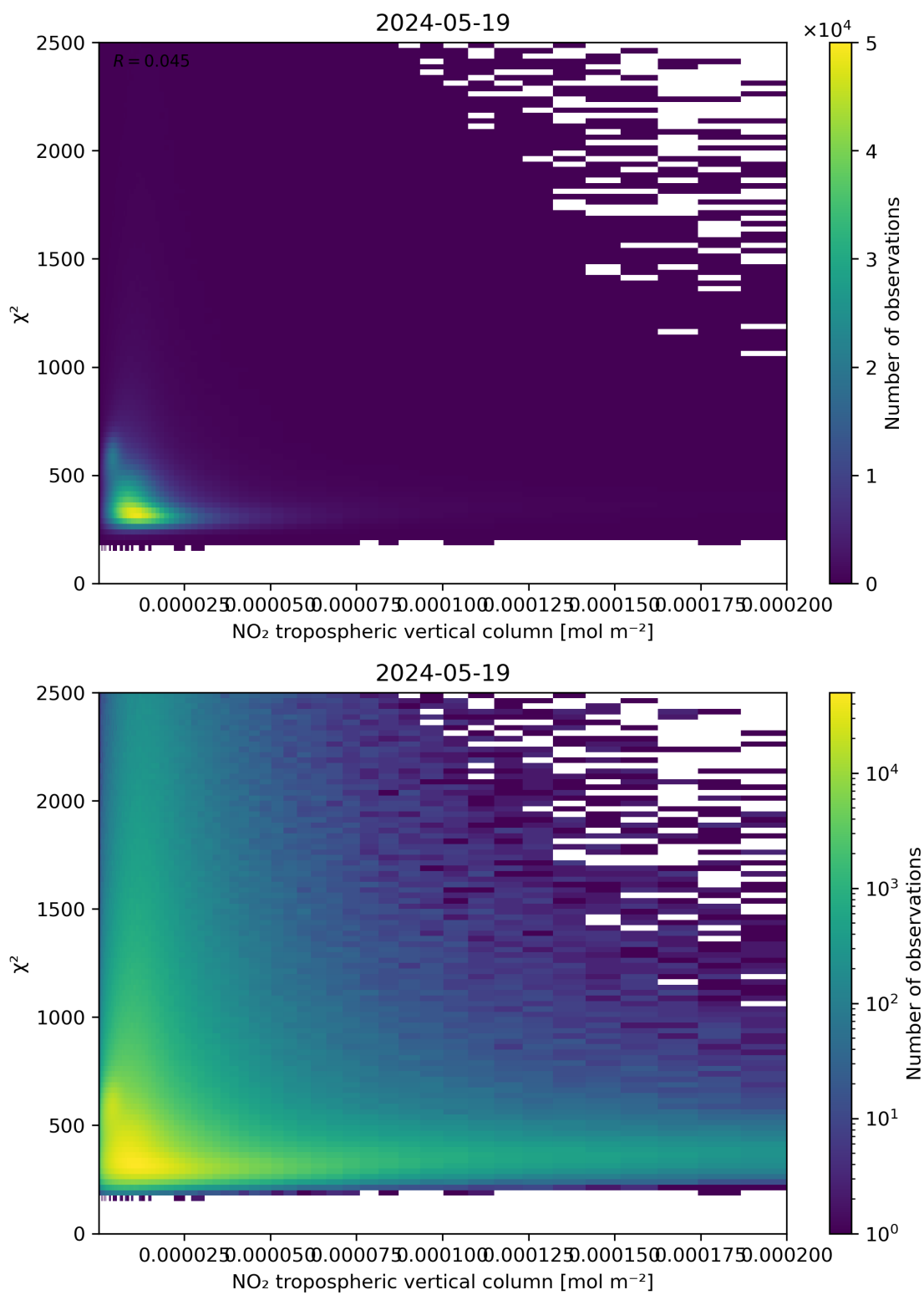
Figure 124: Scatter density plot of “NO 2 tropospheric vertical column” against “ \chi^2 ” for 2024-05-18 to 2024-05-20.
