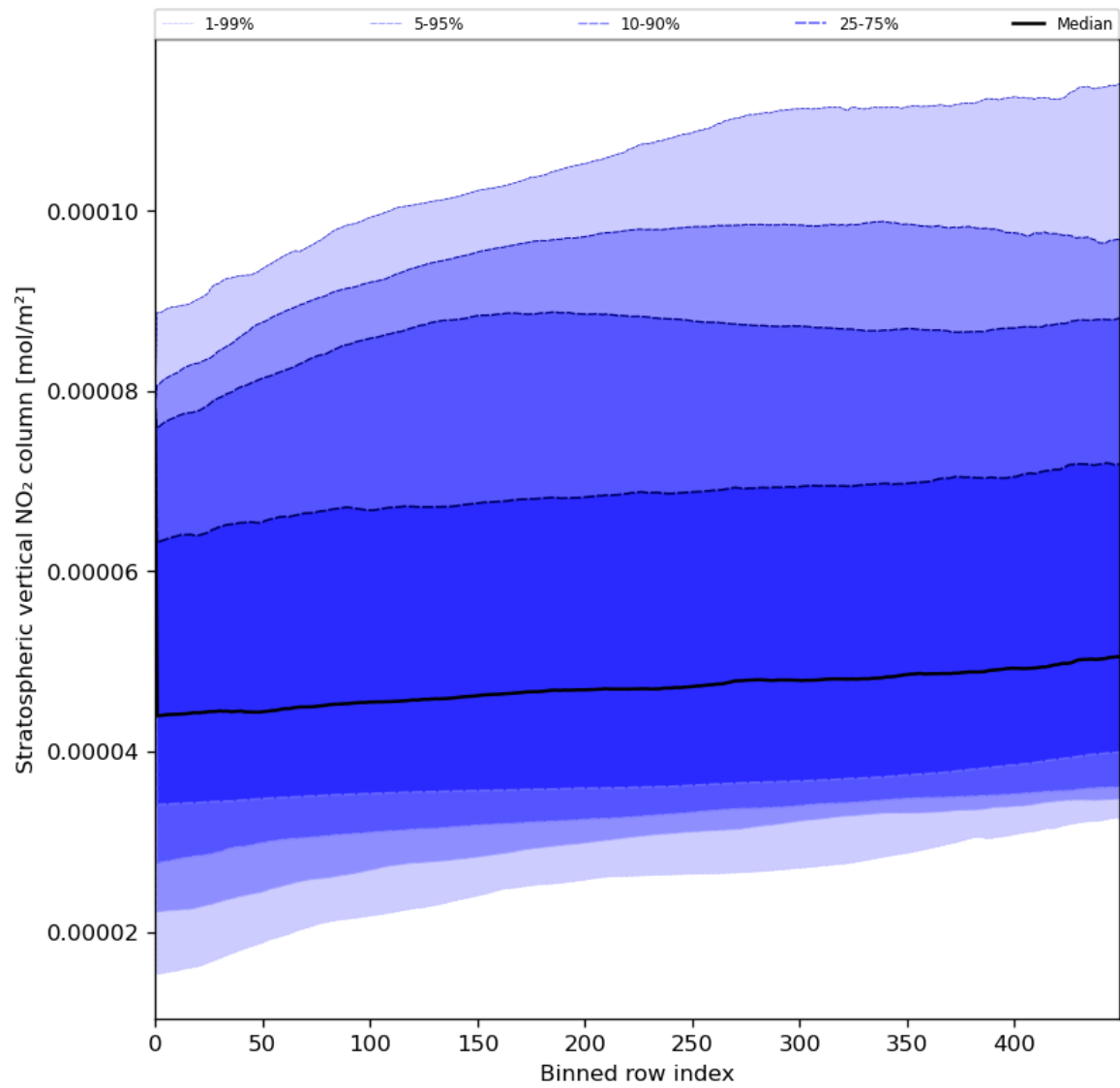
Figure 53: Along track statistics of “Stratospheric vertical NO 2 column” for 2024-05-18 to 2024-05-20
