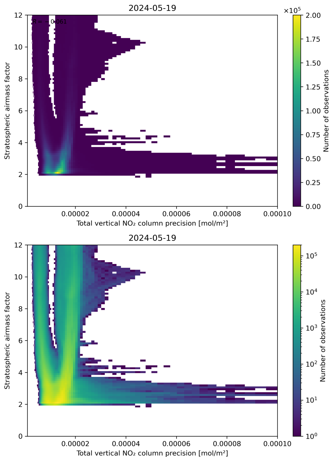
Figure 115: Scatter density plot of “Total vertical NO 2 column precision” against “Stratospheric air mass factor” for 2024-05-18 to 2024-05-20.
