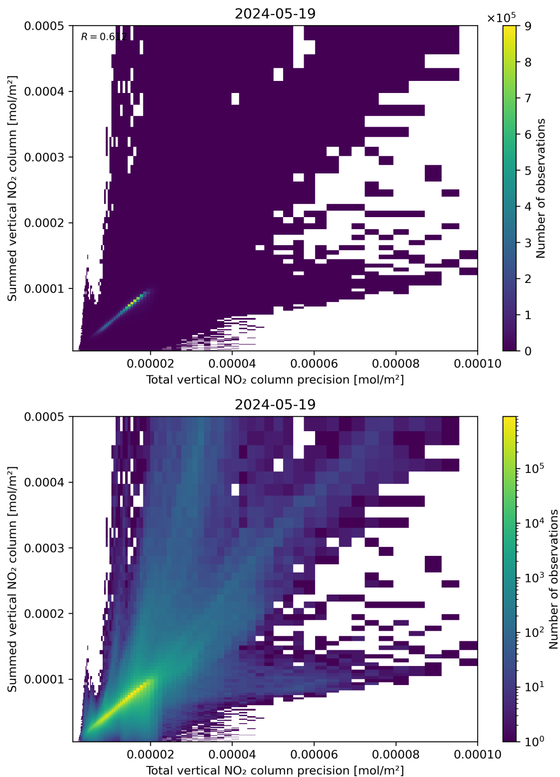
Figure 117: Scatter density plot of “Total vertical NO 2 column precision” against “Summed vertical NO 2 column” for 2024-05-18 to 2024-05-20.
