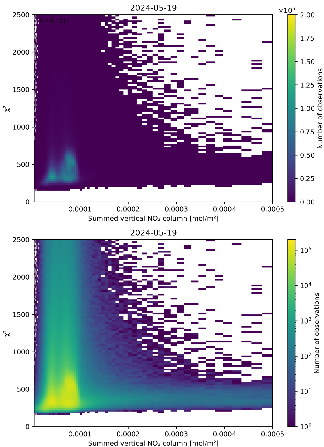
Figure 104: Scatter density plot of “Summed vertical NO 2 column” against “ \chi^2 ” for 2024-05-18 to 2024-05-20.
