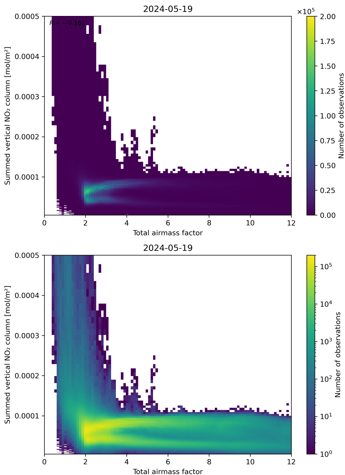
Figure 65: Scatter density plot of “Total airmass factor” against “Summed vertical NO 2 column” for 2024-05-18 to 2024-05-20.
