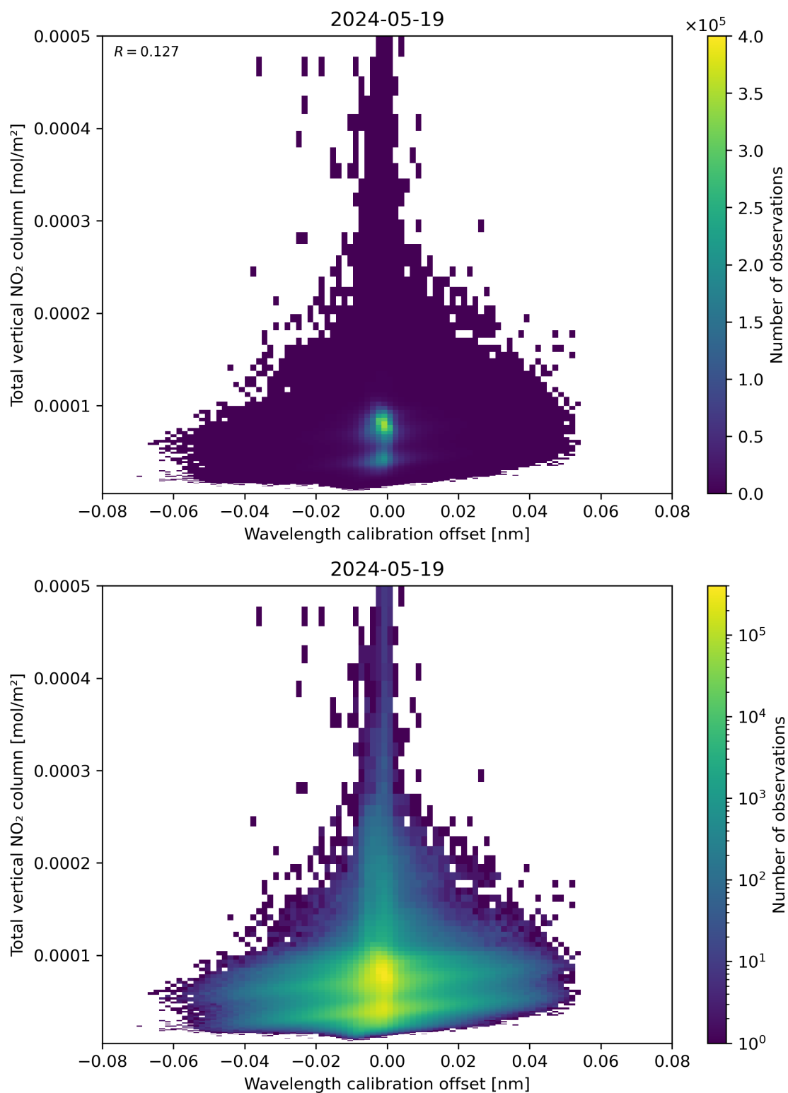
Figure 179: Scatter density plot of “Wavelength calibration offset” against “Total vertical NO 2 column” for 2024-05-18 to 2024-05-20.
