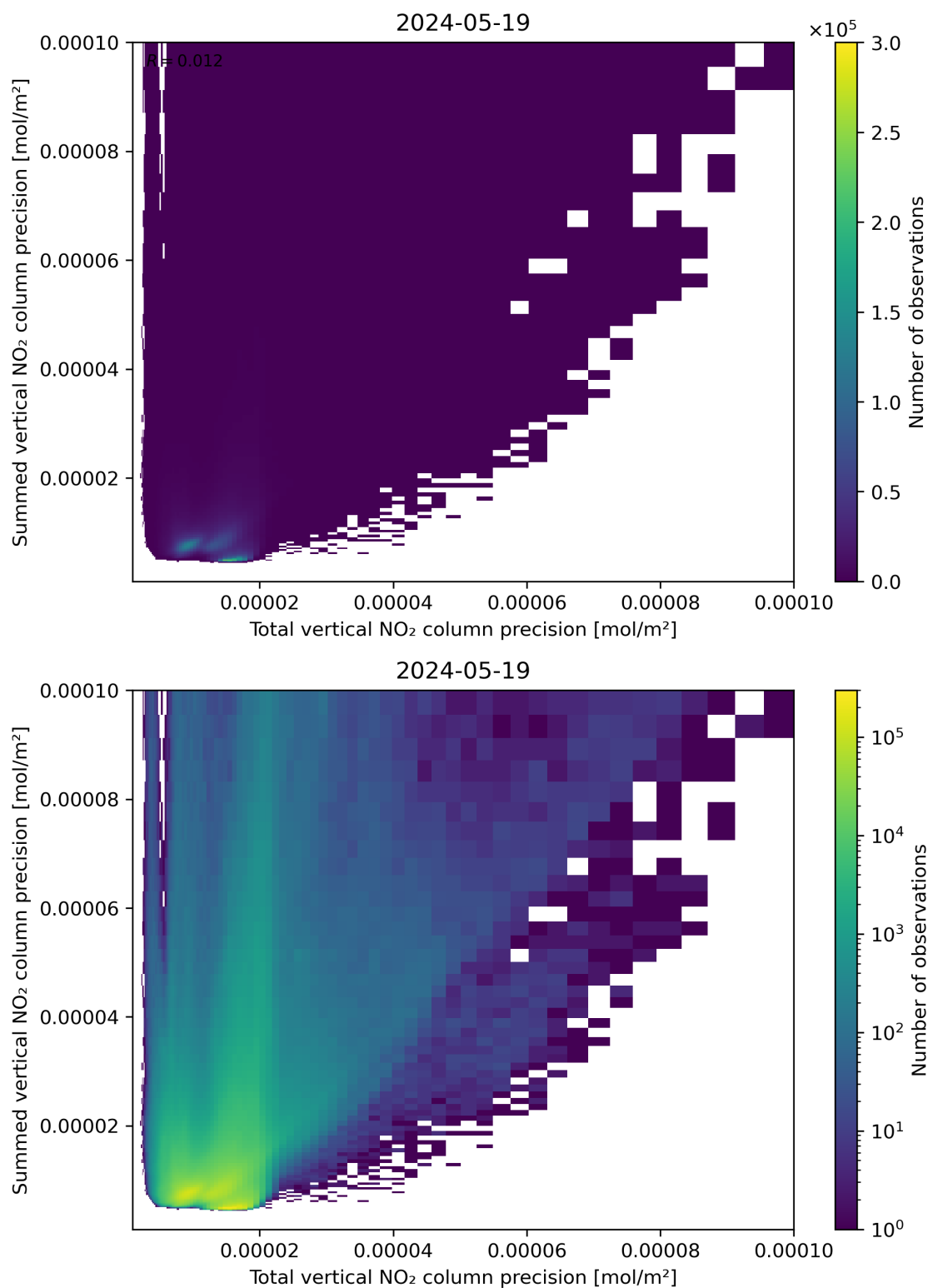
Figure 118: Scatter density plot of “Total vertical NO 2 column precision” against “Summed vertical NO 2 column precision” for 2024-05-18 to 2024-05-20.
