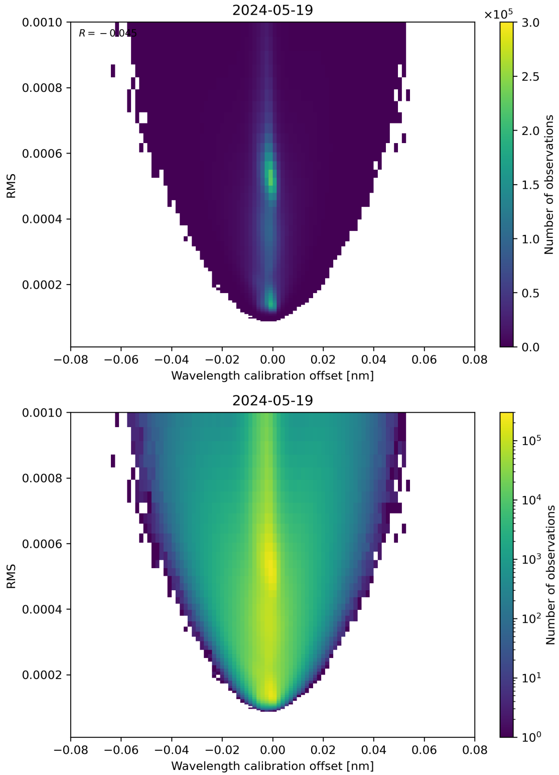
Figure 181: Scatter density plot of “Wavelength calibration offset” against “RMS” for 2024-05-18 to 2024-05-20.
