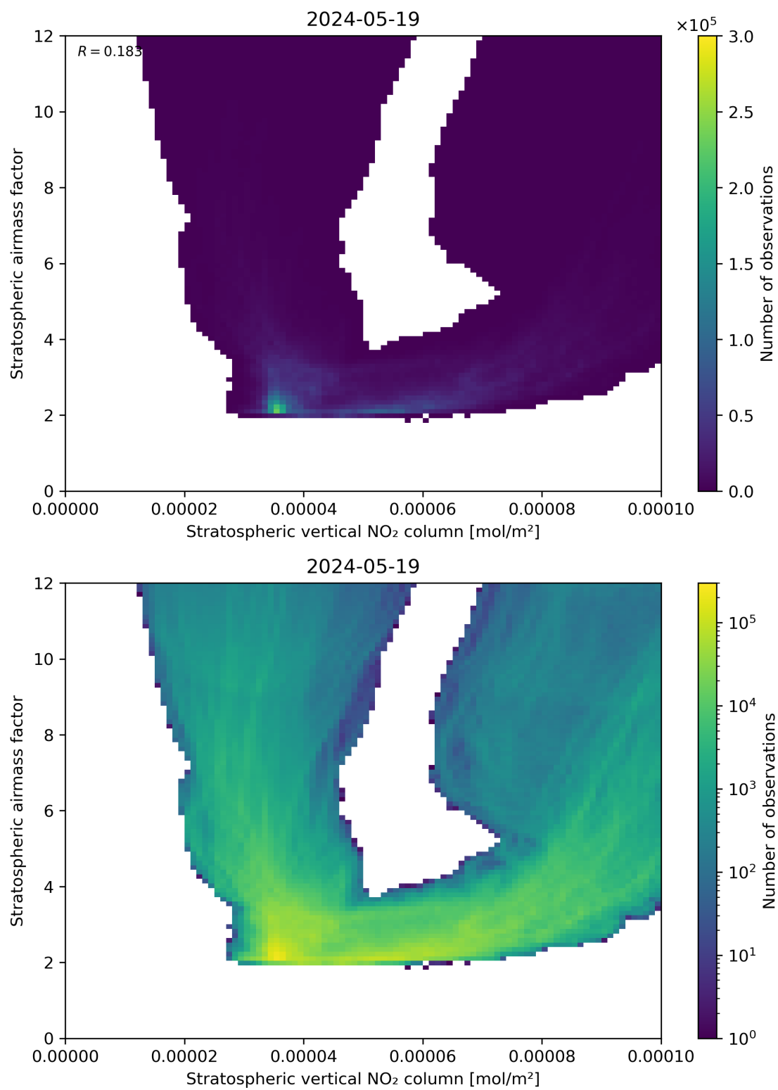
Figure 96: Scatter density plot of “Stratospheric vertical NO 2 column” against “Stratospheric airmass factor” for 2024-05-18 to 2024-05-20.
