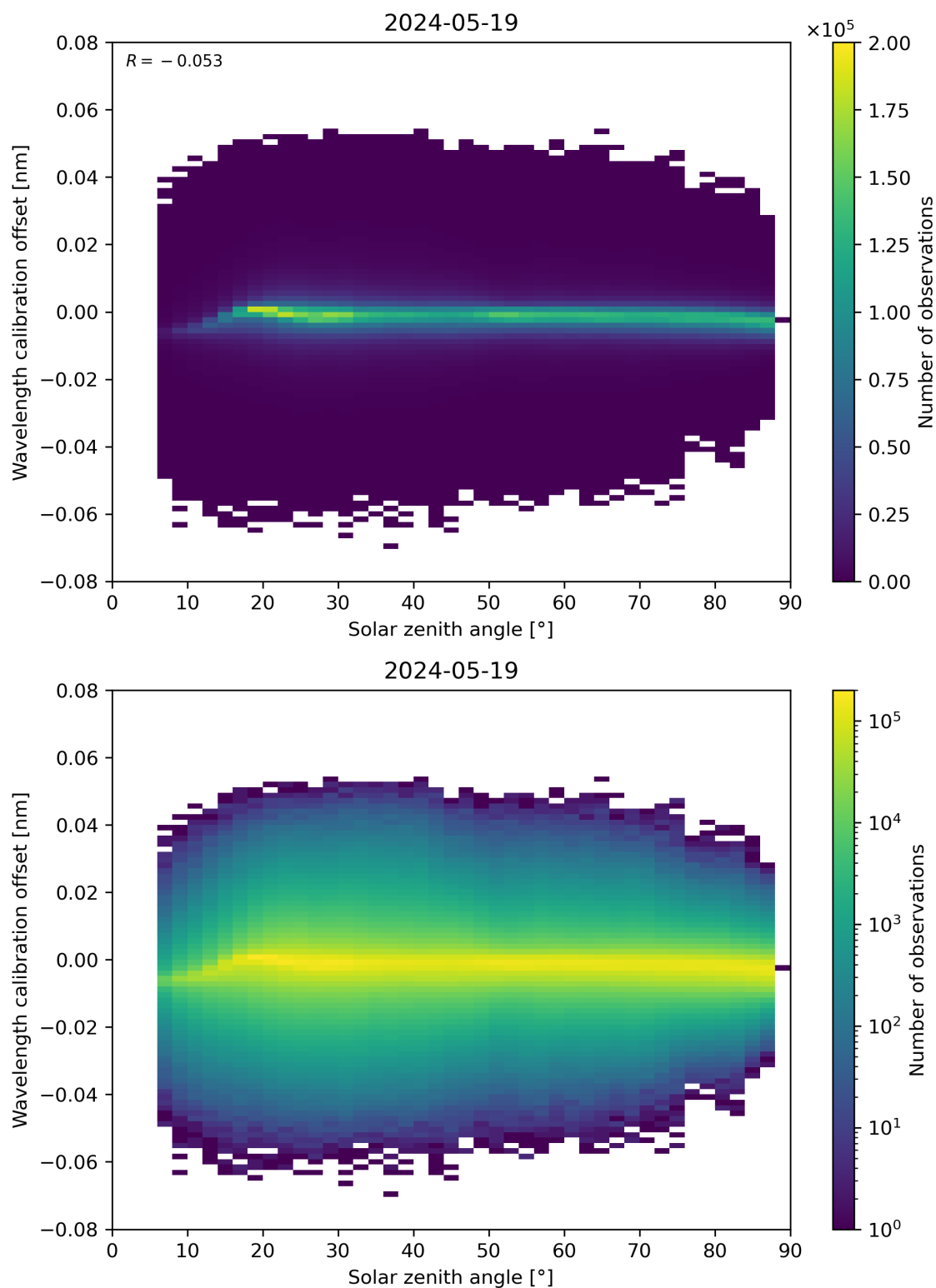
Figure 158: Scatter density plot of “Solar zenith angle” against “Wavelength calibration offset” for 2024-05-18 to 2024-05-20.
