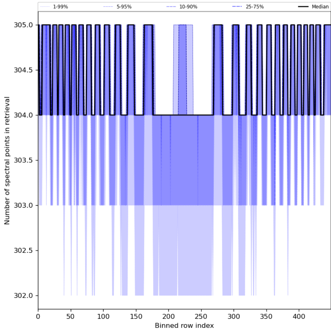
Figure 50: Along track statistics of “Number of spectral points in retrieval” for 2024-05-18 to 2024-05-20
