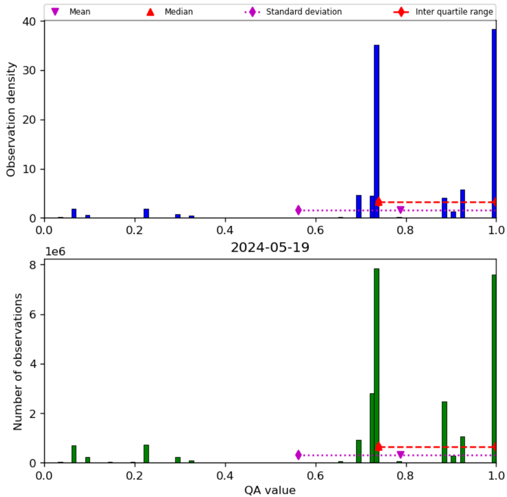
Figure 28: Histogram of “QA value” for 2024-05-18 to 2024-05-20
