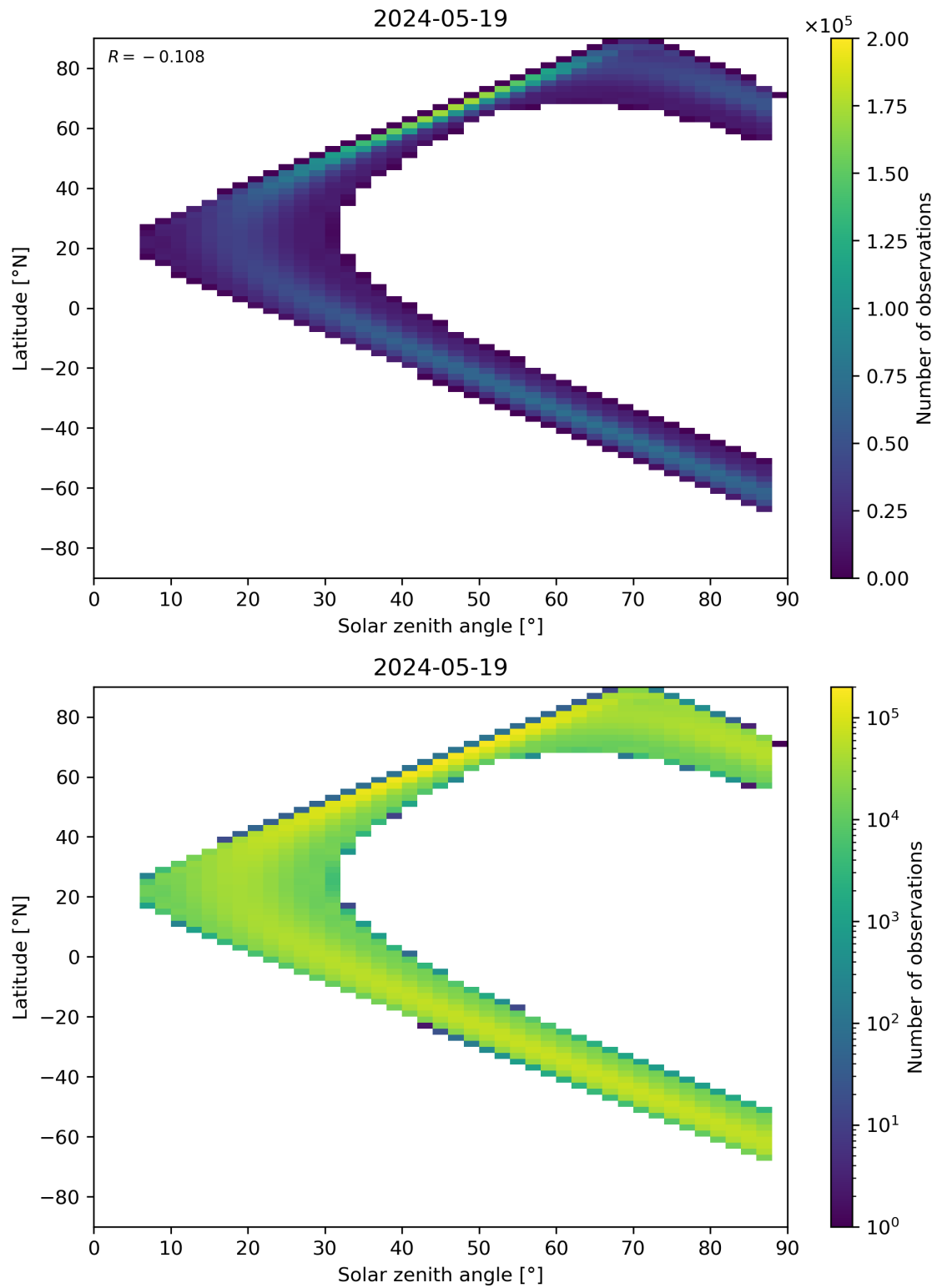
Figure 149: Scatter density plot of “Solar zenith angle” against “Latitude” for 2024-05-18 to 2024-05-20.
