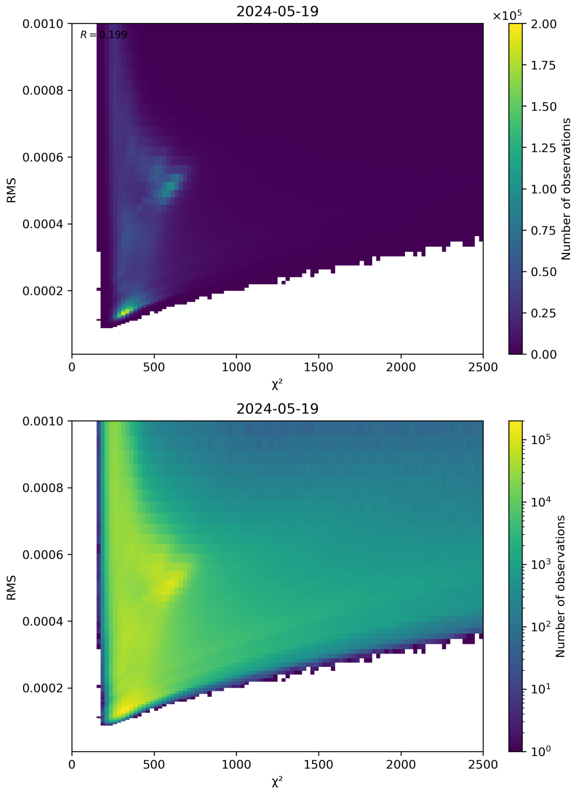
Figure 82: Scatter density plot of “ \chi^2 ” against “RMS” for 2024-05-18 to 2024-05-20.
