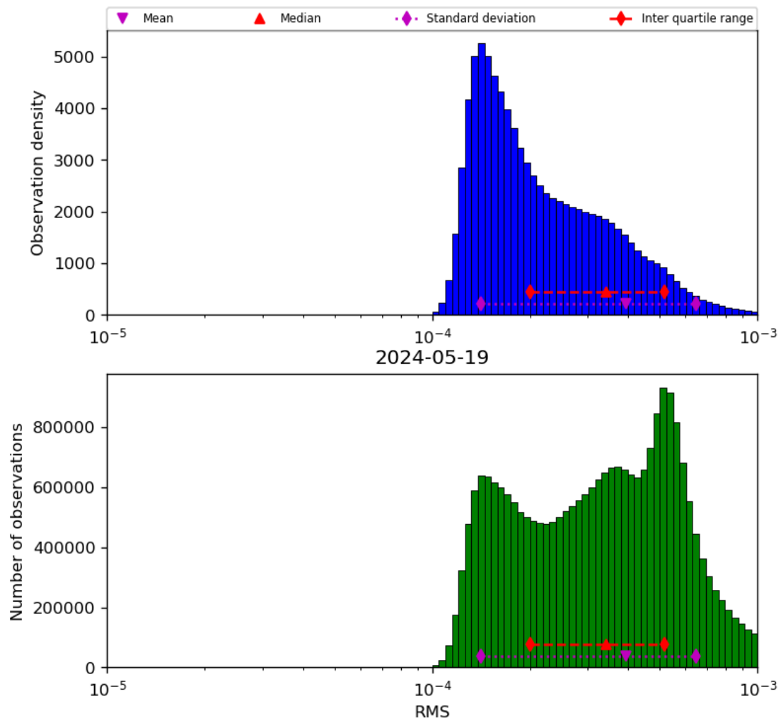
Figure 43: Histogram of “RMS” for 2024-05-18 to 2024-05-20
