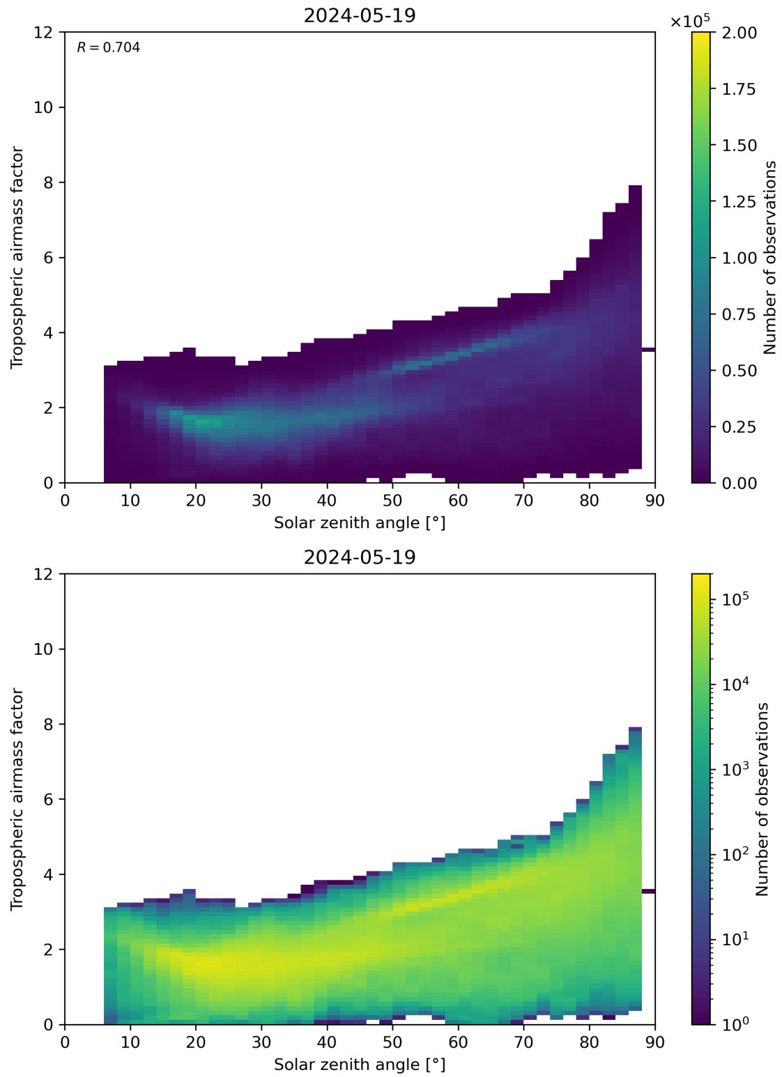
Figure 147: Scatter density plot of “Solar zenith angle” against “Tropospheric airmass factor” for 2024-05-18 to 2024-05-20.
