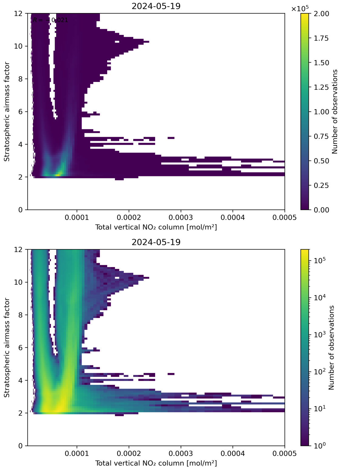
Figure 110: Scatter density plot of “Total vertical NO 2 column” against “Stratospheric airmass factor” for 2024-05-18 to 2024-05-20.
