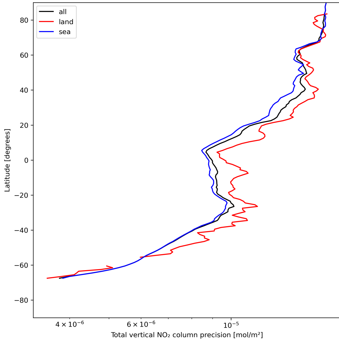
Figure 22: Zonal average of “Total vertical NO 2 column precision” for 2024-05-18 to 2024-05-20.
