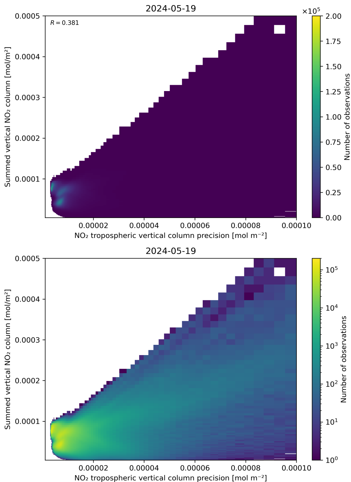
Figure 136: Scatter density plot of “NO 2 tropospheric vertical column precision” against “Summed vertical NO 2 column” for 2024-05-18 to 2024-05-20.
