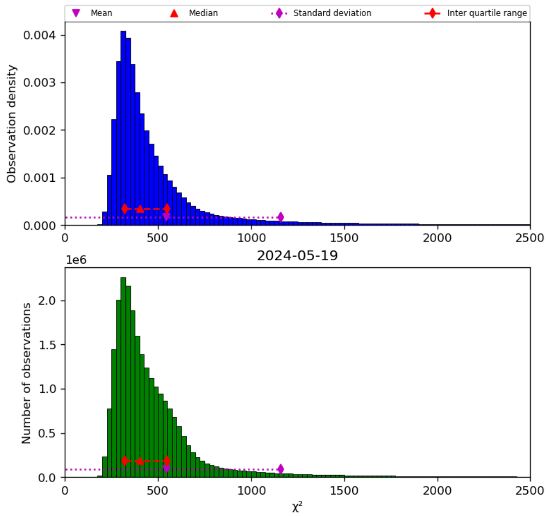
Figure 42: Histogram of “ \chi^2 ” for 2024-05-18 to 2024-05-20
