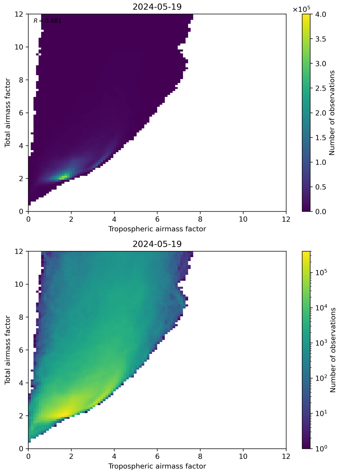
Figure 72: Scatter density plot of “Tropospheric airmass factor” against “Total airmass factor” for 2024-05-18 to 2024-05-20.
