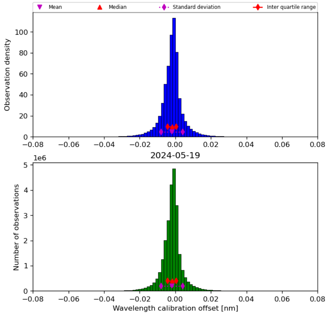
Figure 35: Histogram of “Wavelength calibration offset” for 2024-05-18 to 2024-05-20
