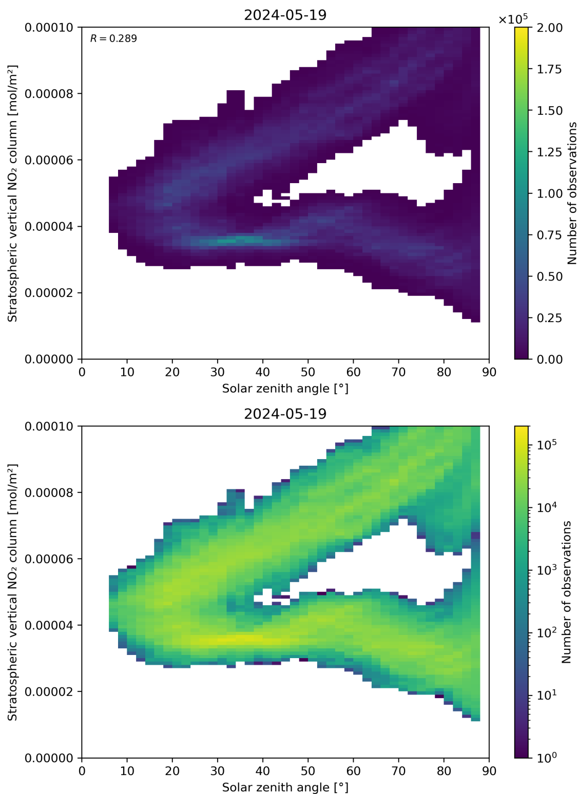
Figure 150: Scatter density plot of “Solar zenith angle” against “Stratospheric vertical NO 2 column” for 2024-05-18 to 2024-05-20.
