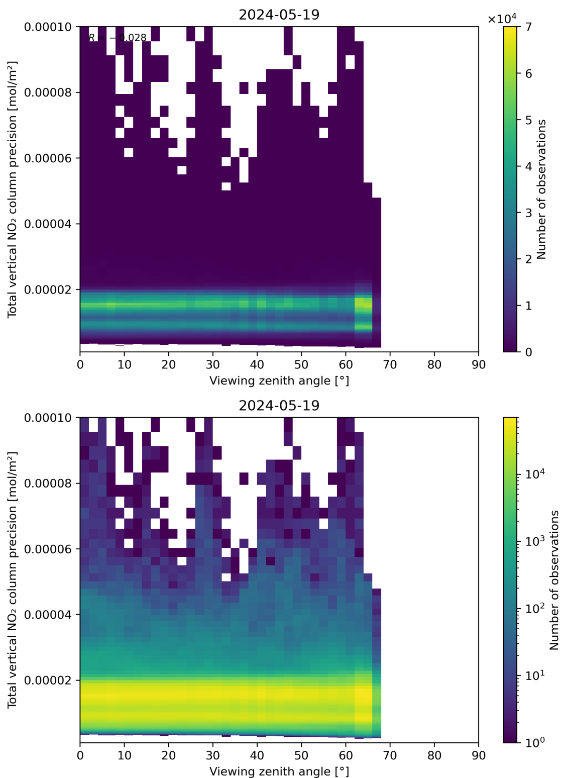
Figure 168: Scatter density plot of “Viewing zenith angle” against “Total vertical NO 2 column precision” for 2024-05-18 to 2024-05-20.
