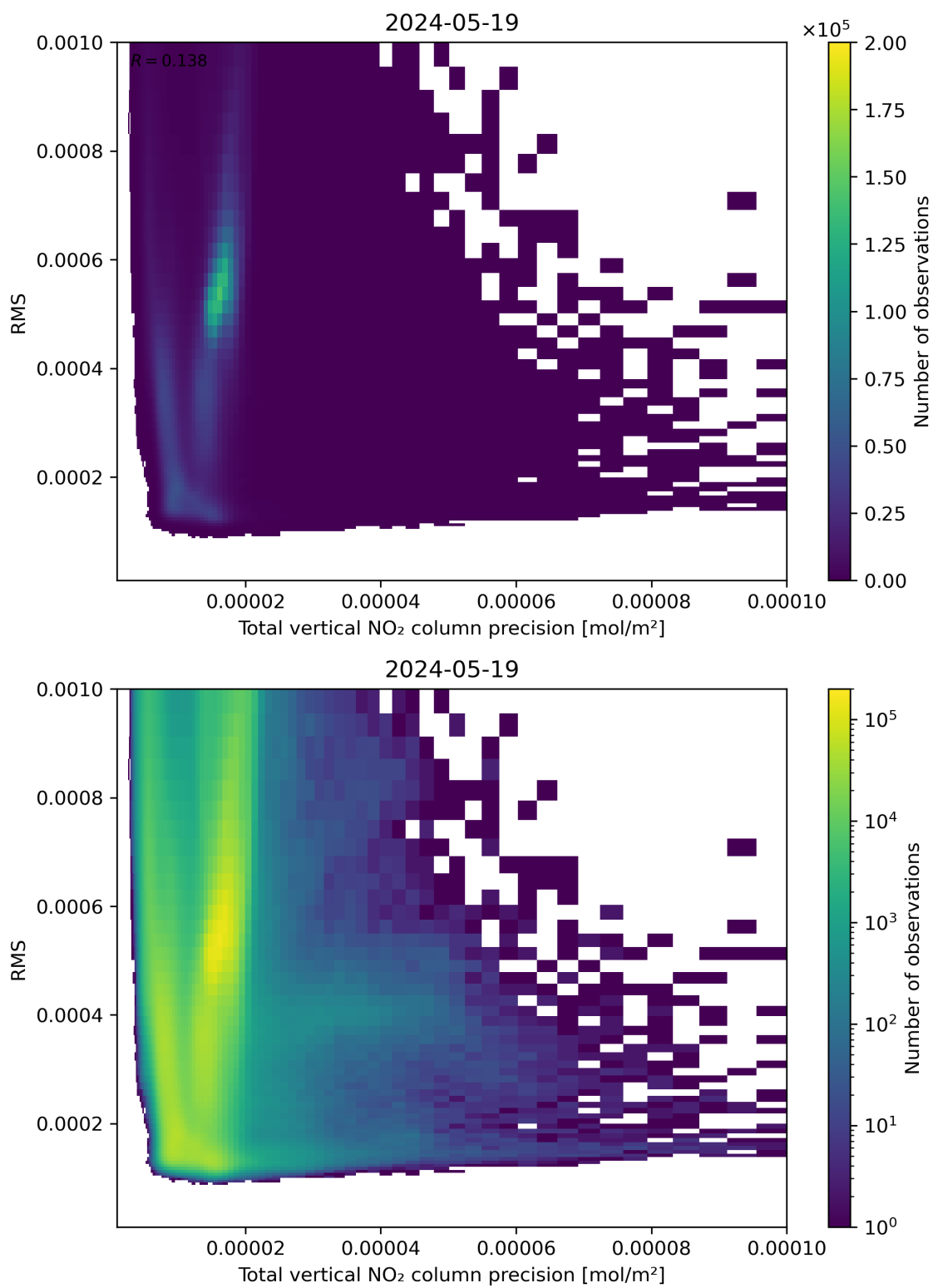
Figure 119: Scatter density plot of “Total vertical NO 2 column precision” against “RMS” for 2024-05-18 to 2024-05-20.
