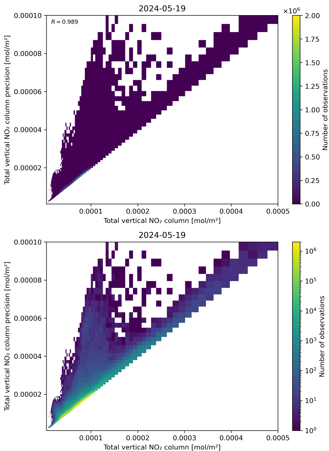
Figure 114: Scatter density plot of “Total vertical NO 2 column” against “Total vertical NO 2 column precision” for 2024-05-18 to 2024-05-20.
