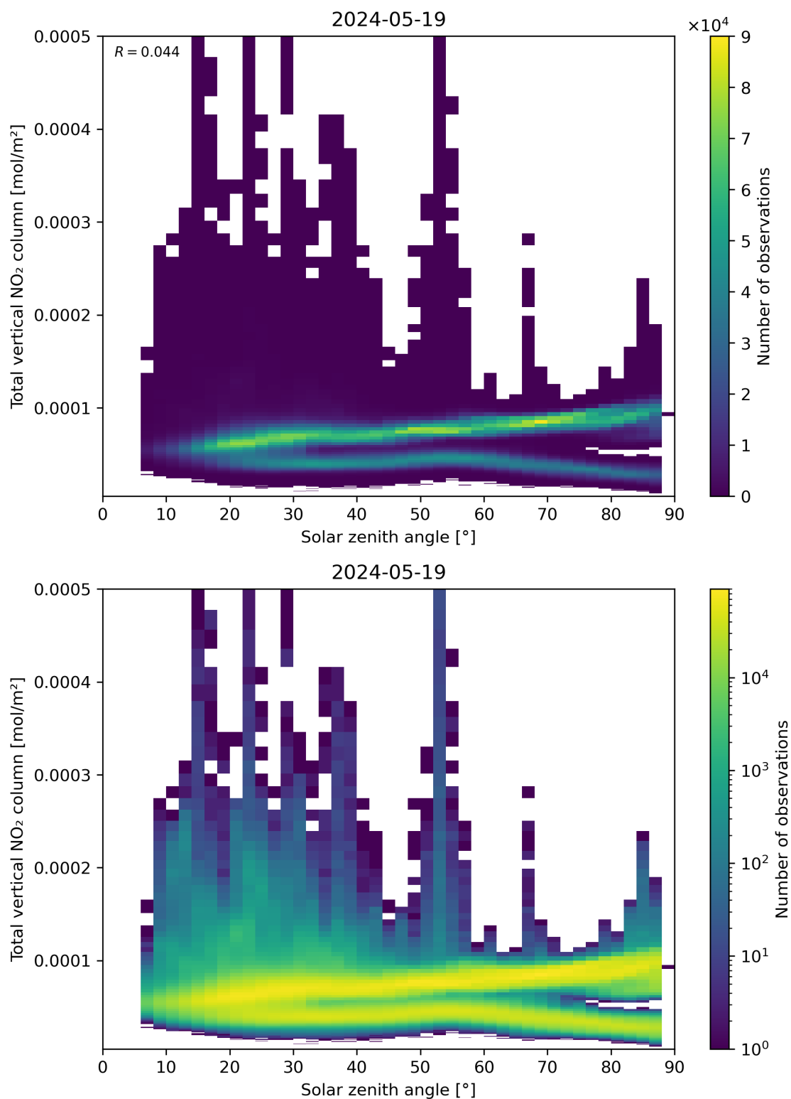
Figure 153: Scatter density plot of “Solar zenith angle” against “Total vertical NO 2 column” for 2024-05-18 to 2024-05-20.
