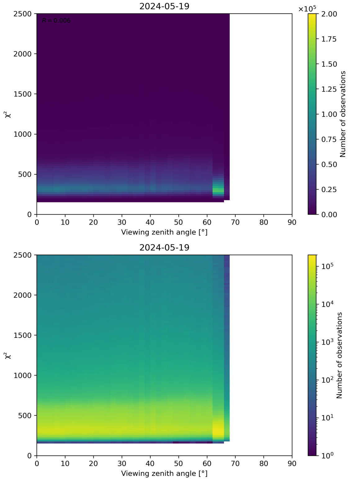
Figure 162: Scatter density plot of “Viewing zenith angle” against “ \chi^2 ” for 2024-05-18 to 2024-05-20.
