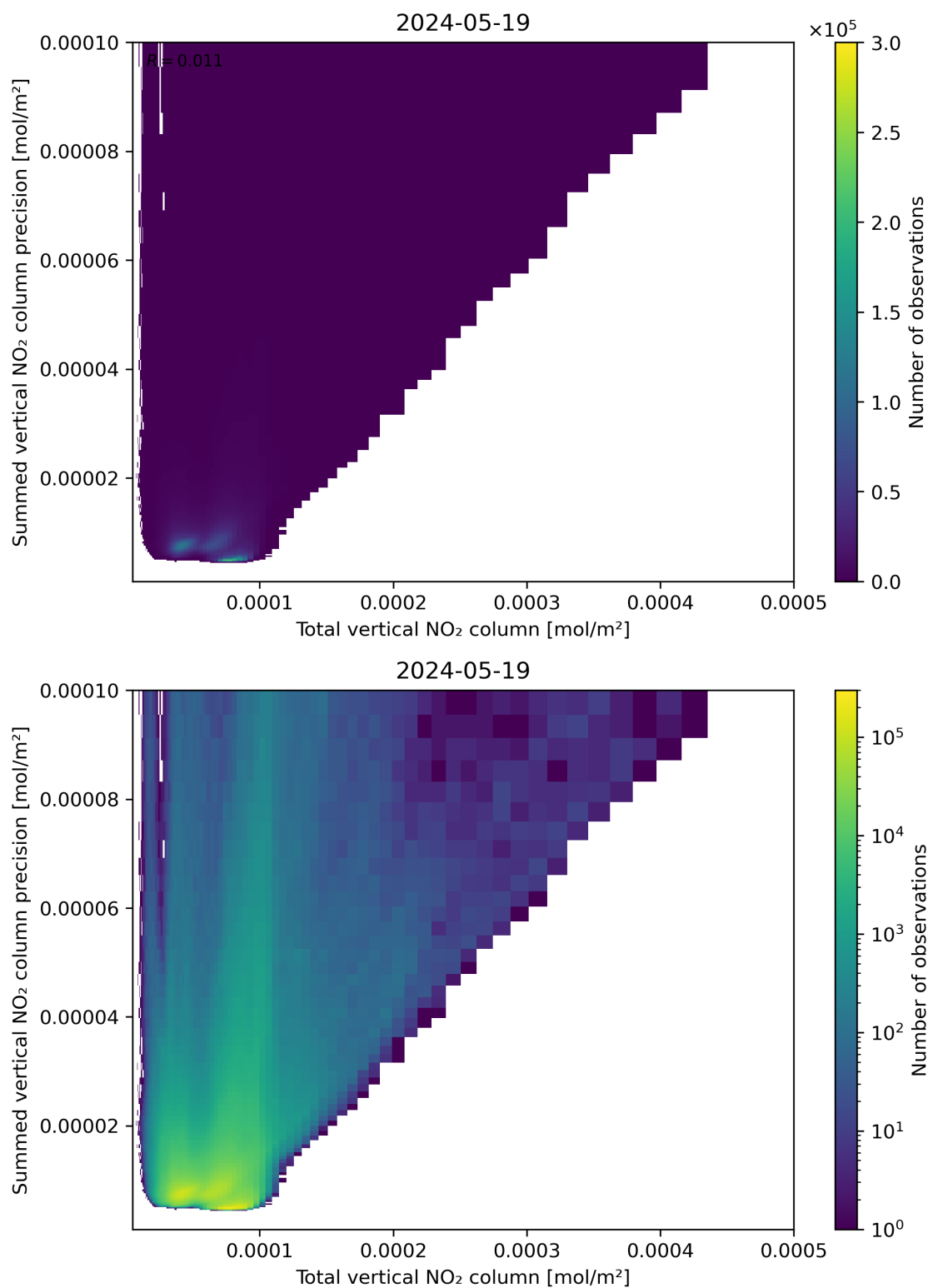
Figure 113: Scatter density plot of “Total vertical NO 2 column” against “Summed vertical NO 2 column precision” for 2024-05-18 to 2024-05-20.
