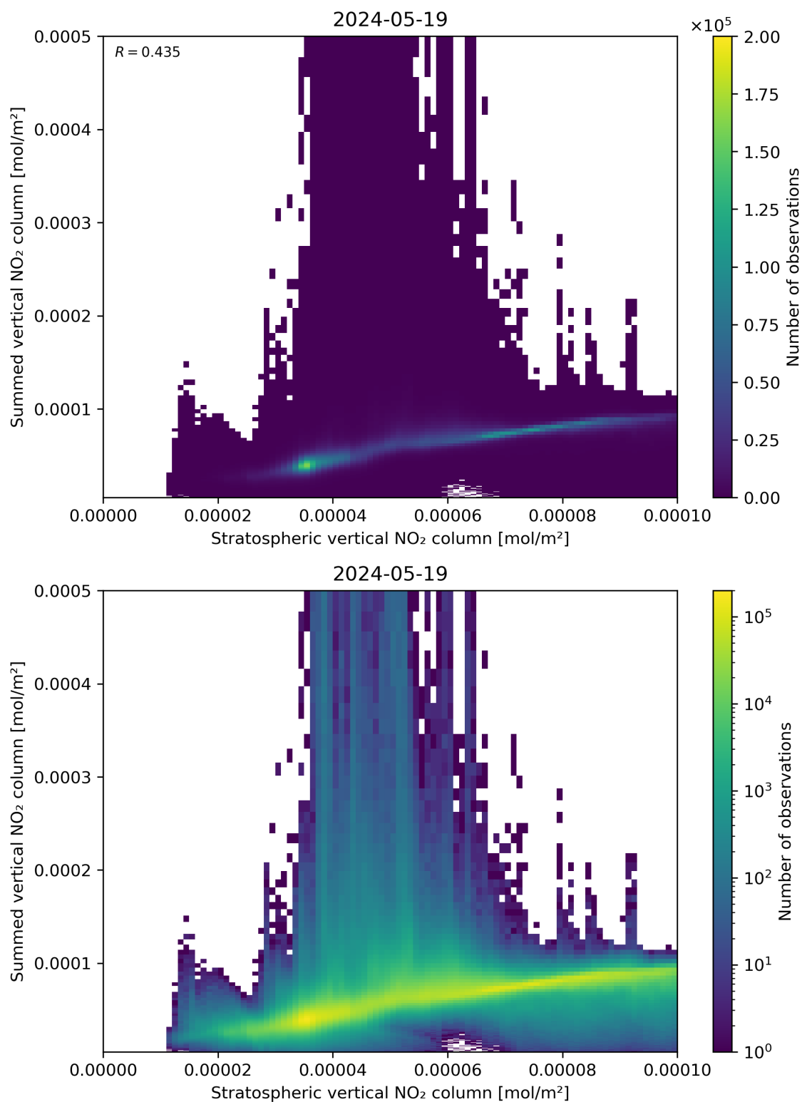
Figure 98: Scatter density plot of “Stratospheric vertical NO 2 column” against “Summed vertical NO 2 column” for 2024-05-18 to 2024-05-20.
