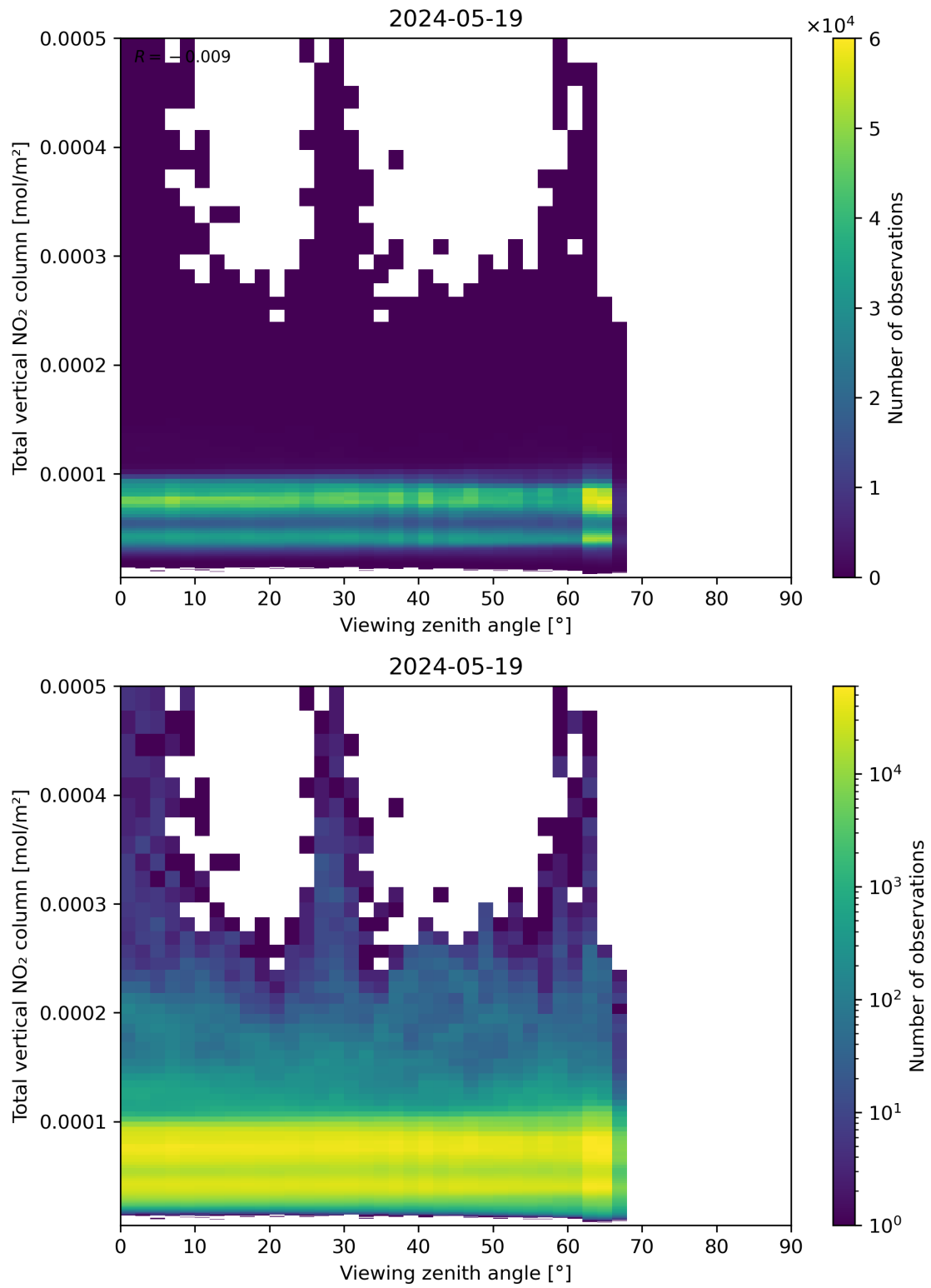
Figure 167: Scatter density plot of “Viewing zenith angle” against “Total vertical NO 2 column” for 2024-05-18 to 2024-05-20.
