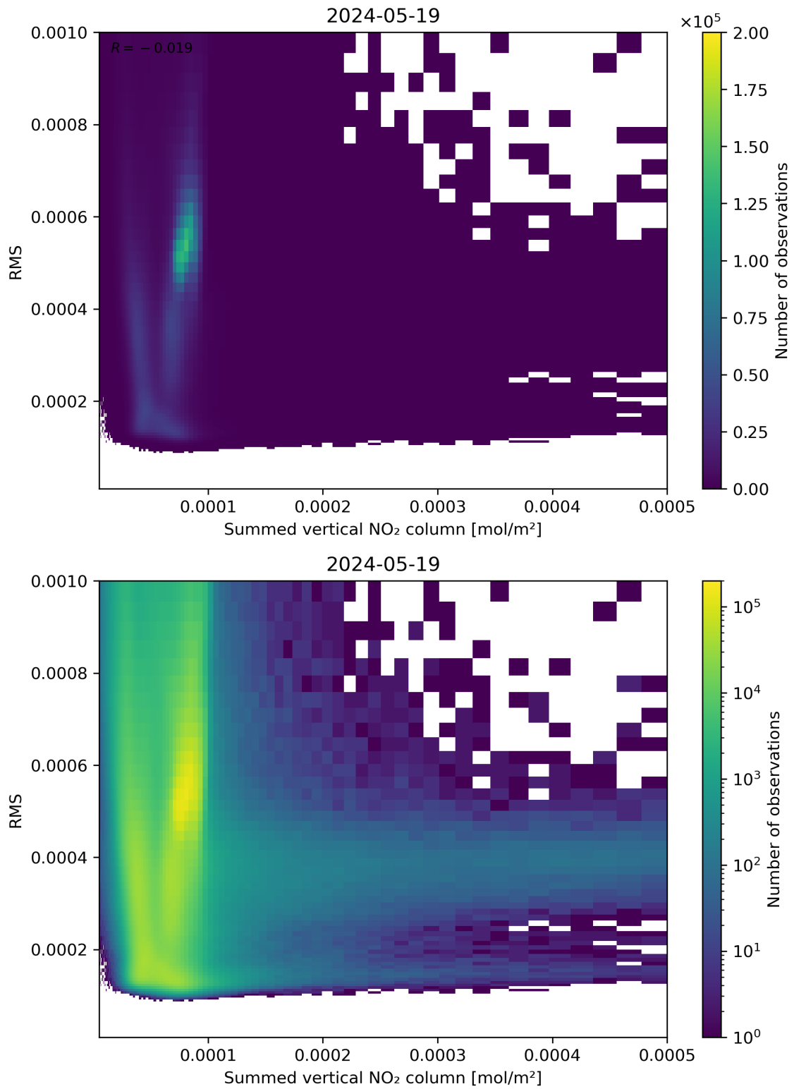
Figure 109: Scatter density plot of “Summed vertical NO 2 column” against “RMS” for 2024-05-18 to 2024-05-20.
