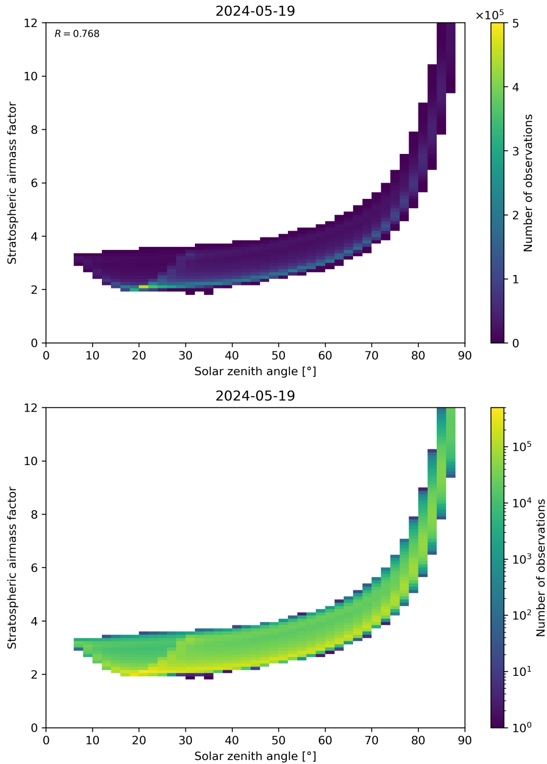
Figure 145: Scatter density plot of “Solar zenith angle” against “Stratospheric airmass factor” for 2024-05-18 to 2024-05-20.
