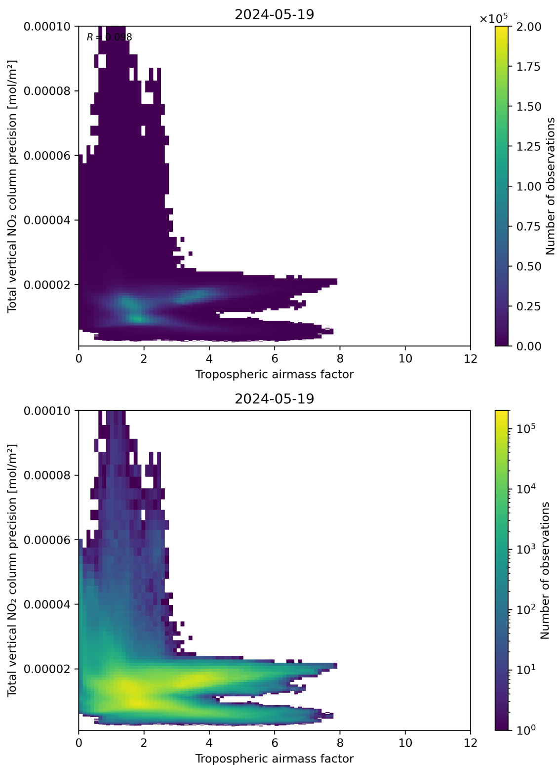
Figure 78: Scatter density plot of “Tropospheric air mass factor” against “Total vertical NO 2 column precision” for 2024-05-18 to 2024-05-20.
