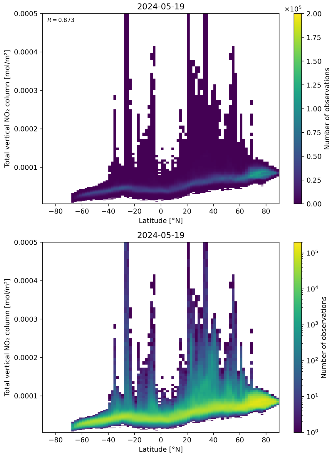
Figure 90: Scatter density plot of “Latitude” against “Total vertical NO 2 column” for 2024-05-18 to 2024-05-20.
