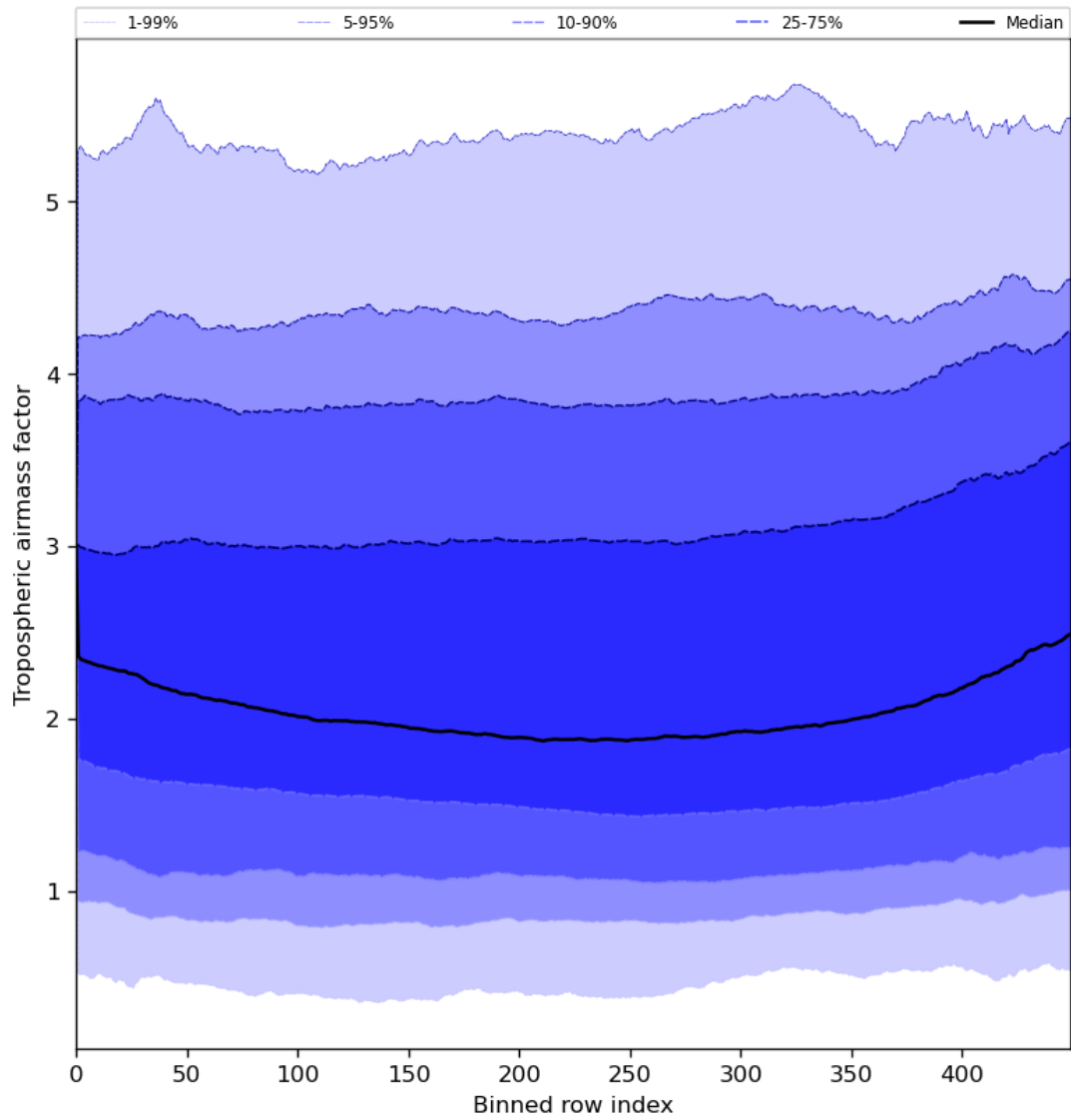
Figure 48: Along track statistics of “Tropospheric airmass factor” for 2024-05-18 to 2024-05-20
