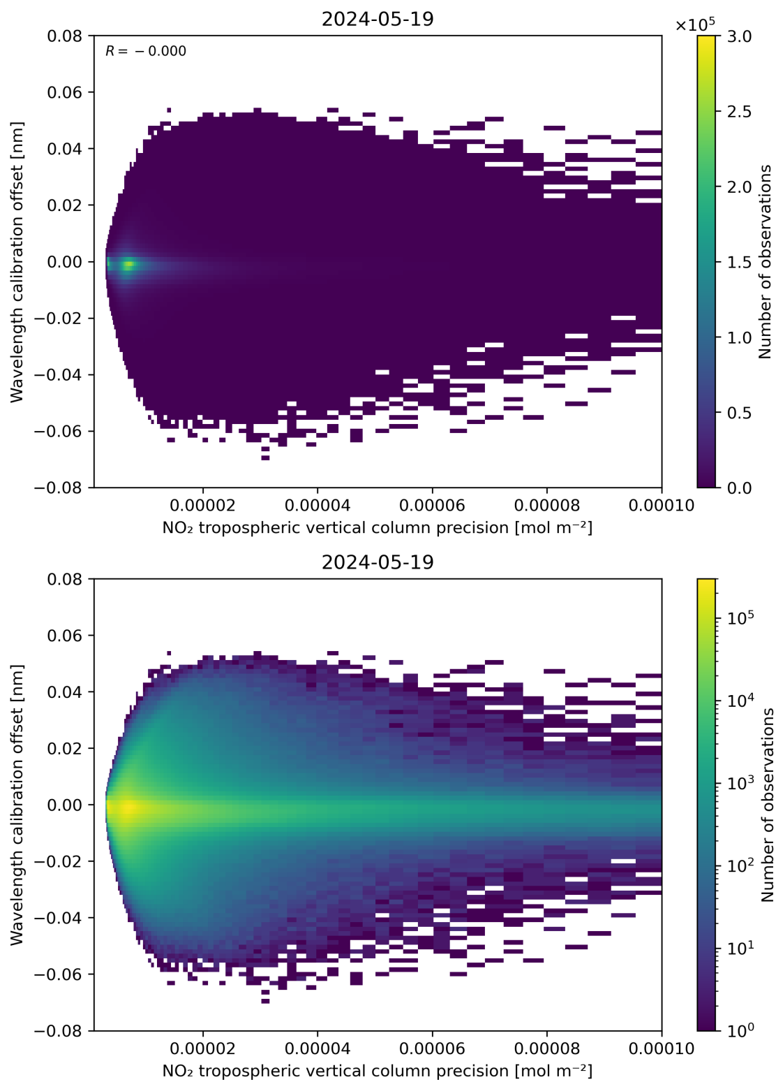
Figure 141: Scatter density plot of “NO 2 tropospheric vertical column precision” against “Wavelength calibration offset” for 2024-05-18 to 2024-05-20.
