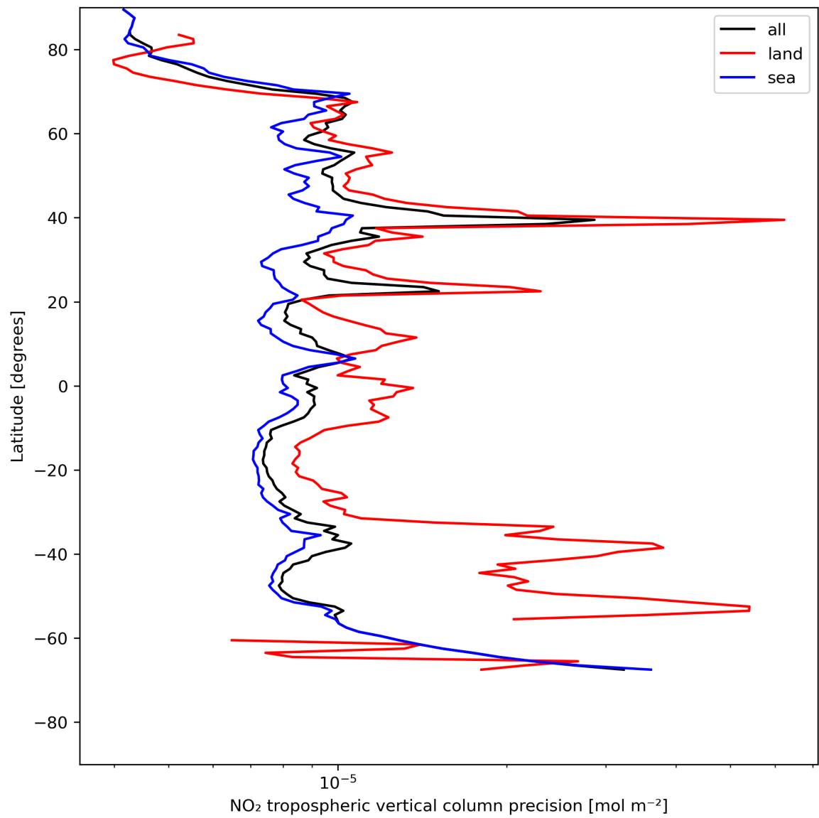
Figure 13: Zonal average of “NO 2 tropospheric vertical column precision” for 2024-05-18 to 2024-05-20.
