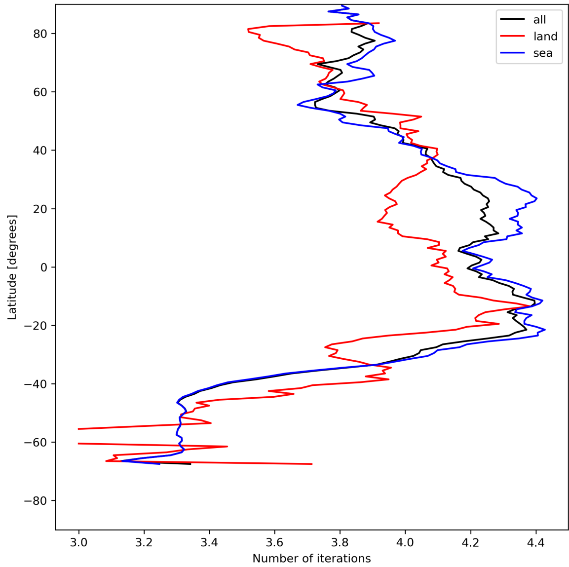
Figure 17: Zonal average of “Number of iterations” for 2024-05-18 to 2024-05-20.
