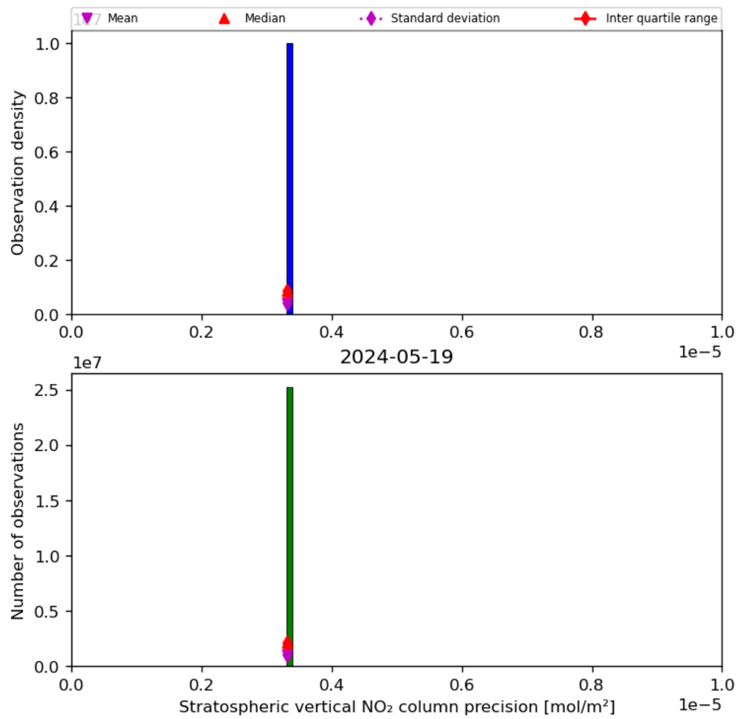
Figure 37: Histogram of “Stratospheric vertical NO 2 column precision” for 2024-05-18 to 2024-05-20
