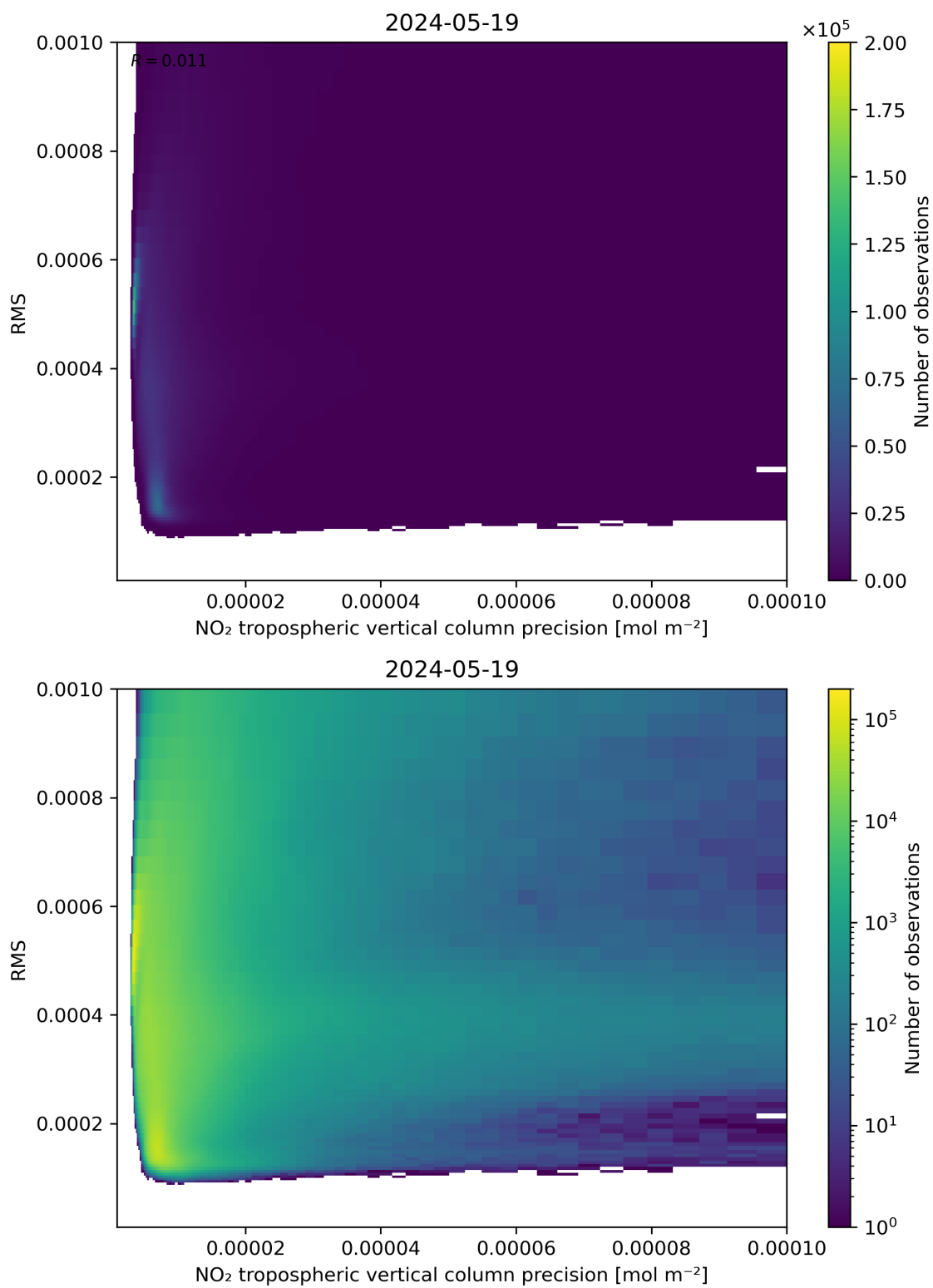
Figure 140: Scatter density plot of “NO 2 tropospheric vertical column precision” against “RMS” for 2024-05-18 to 2024-05-20.
