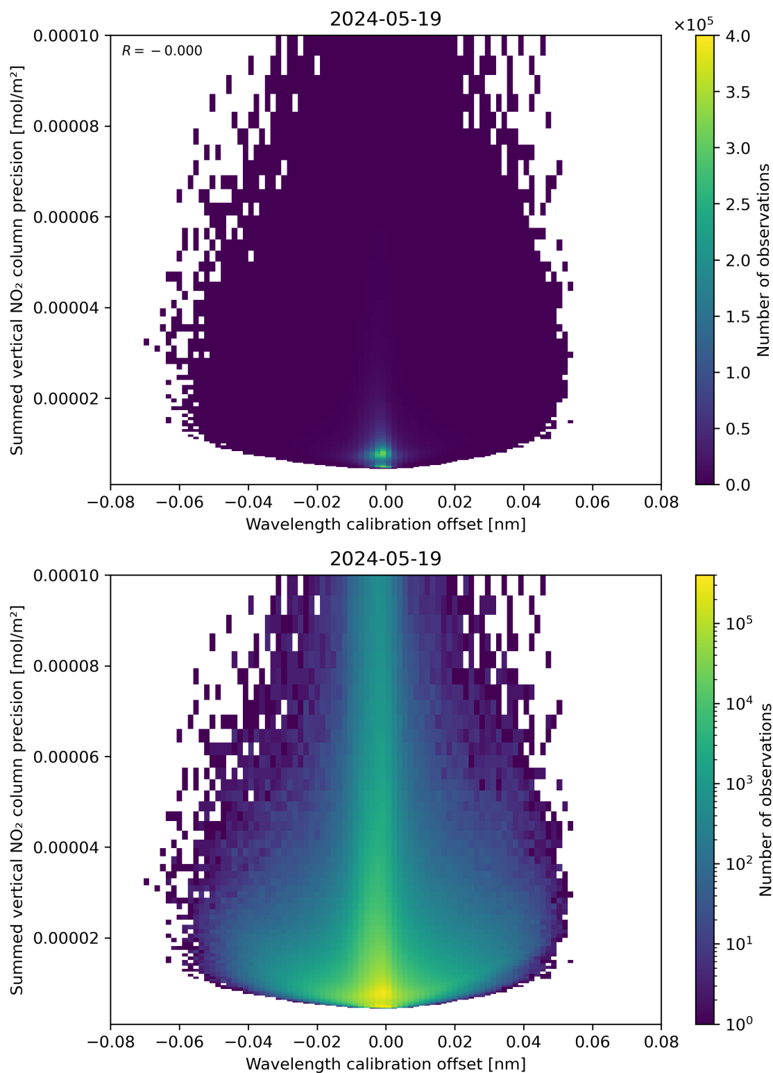
Figure 178: Scatter density plot of “Wavelength calibration offset” against “Summed vertical NO 2 column precision” for 2024-05-18 to 2024-05-20.
