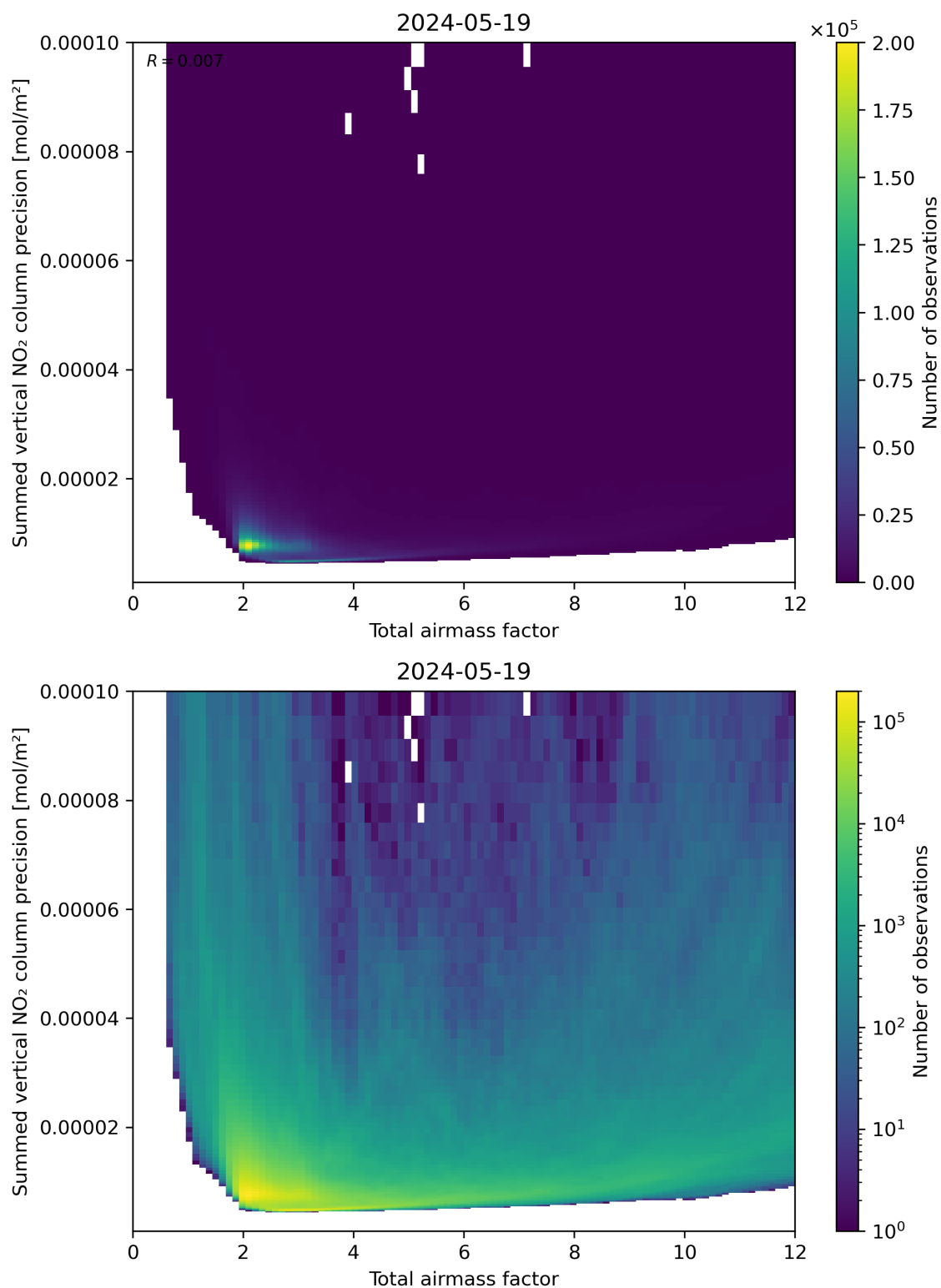
Figure 66: Scatter density plot of “Total airmass factor” against “Summed vertical NO 2 column precision” for 2024-05-18 to 2024-05-20.
