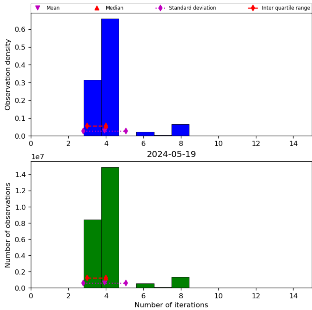
Figure 34: Histogram of “Number of iterations” for 2024-05-18 to 2024-05-20
