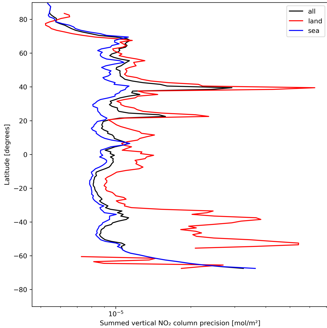
Figure 24: Zonal average of “Summed vertical NO 2 column precision” for 2024-05-18 to 2024-05-20.
