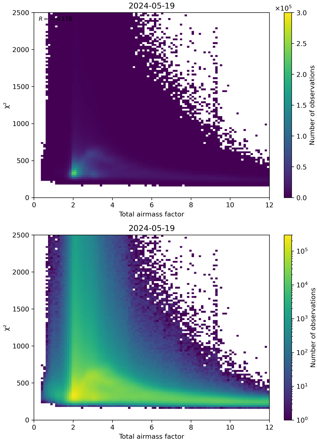
Figure 63: Scatter density plot of “Total airmass factor” against “ \chi^2 ” for 2024-05-18 to 2024-05-20.
