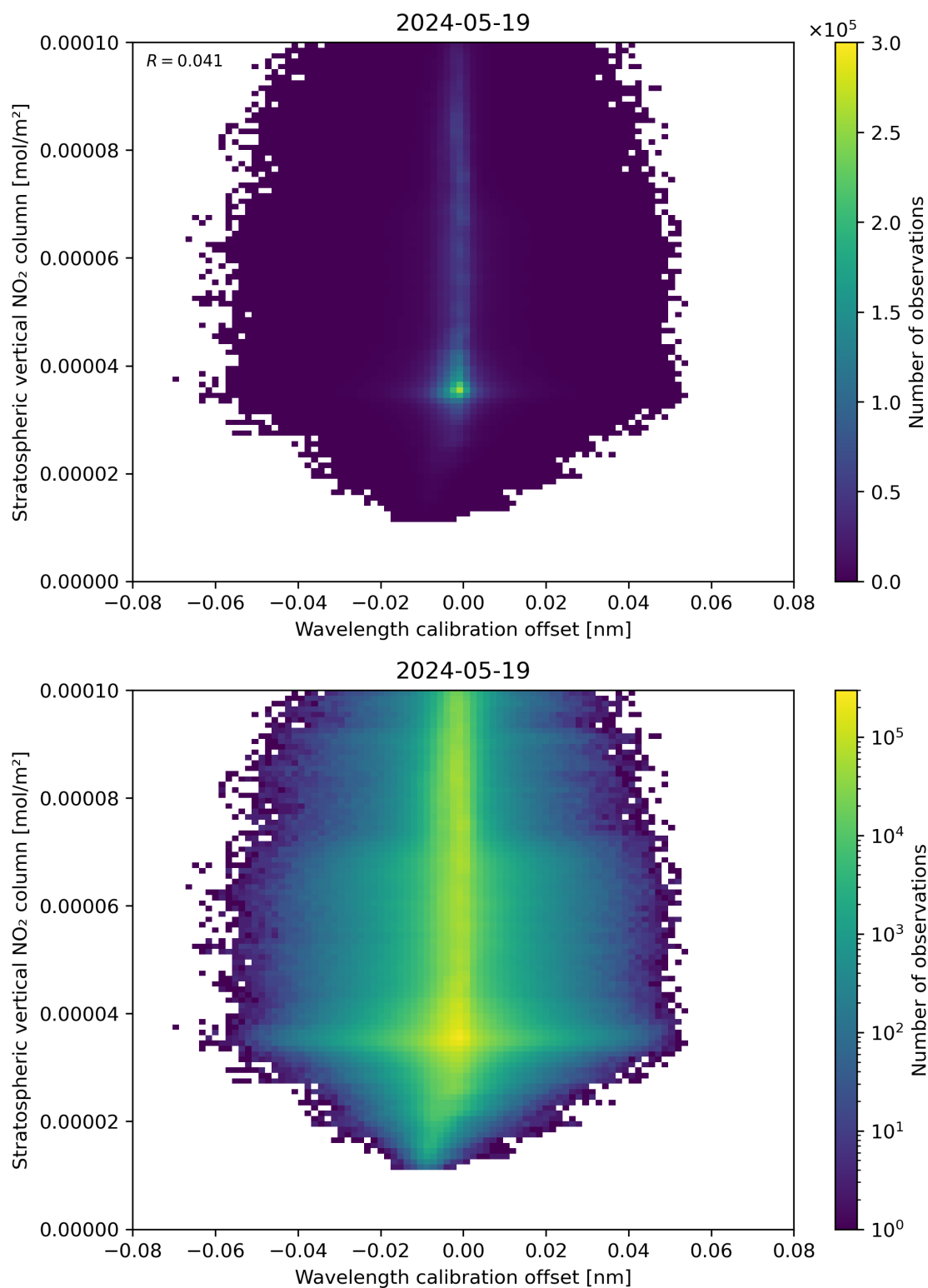
Figure 176: Scatter density plot of “Wavelength calibration offset” against “Stratospheric vertical NO 2 column” for 2024-05-18 to 2024-05-20.
