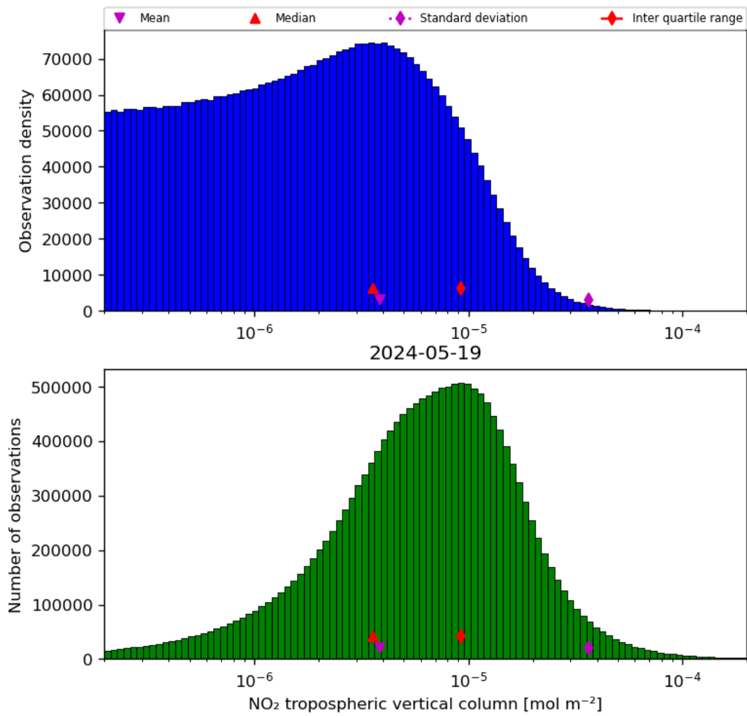
Figure 29: Histogram of “NO 2 tropospheric vertical column” for 2024-05-18 to 2024-05-20
