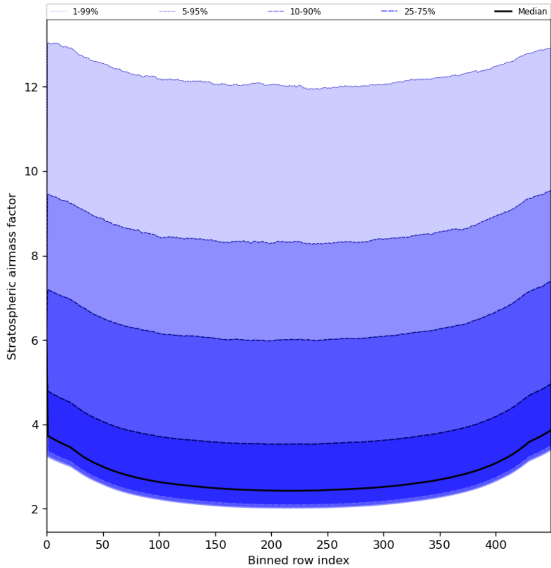
Figure 61: Along track statistics of “Stratospheric airmass factor” for 2024-05-18 to 2024-05-20
