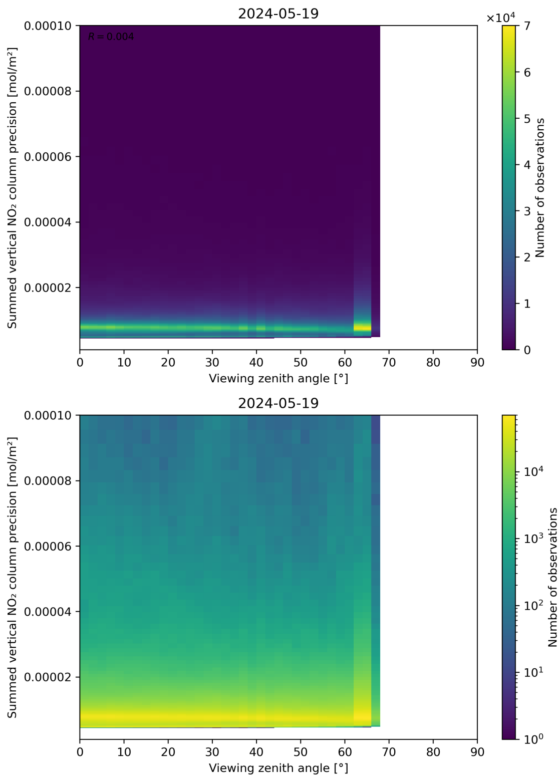
Figure 166: Scatter density plot of “Viewing zenith angle” against “Summed vertical NO 2 column precision” for 2024-05-18 to 2024-05-20.
