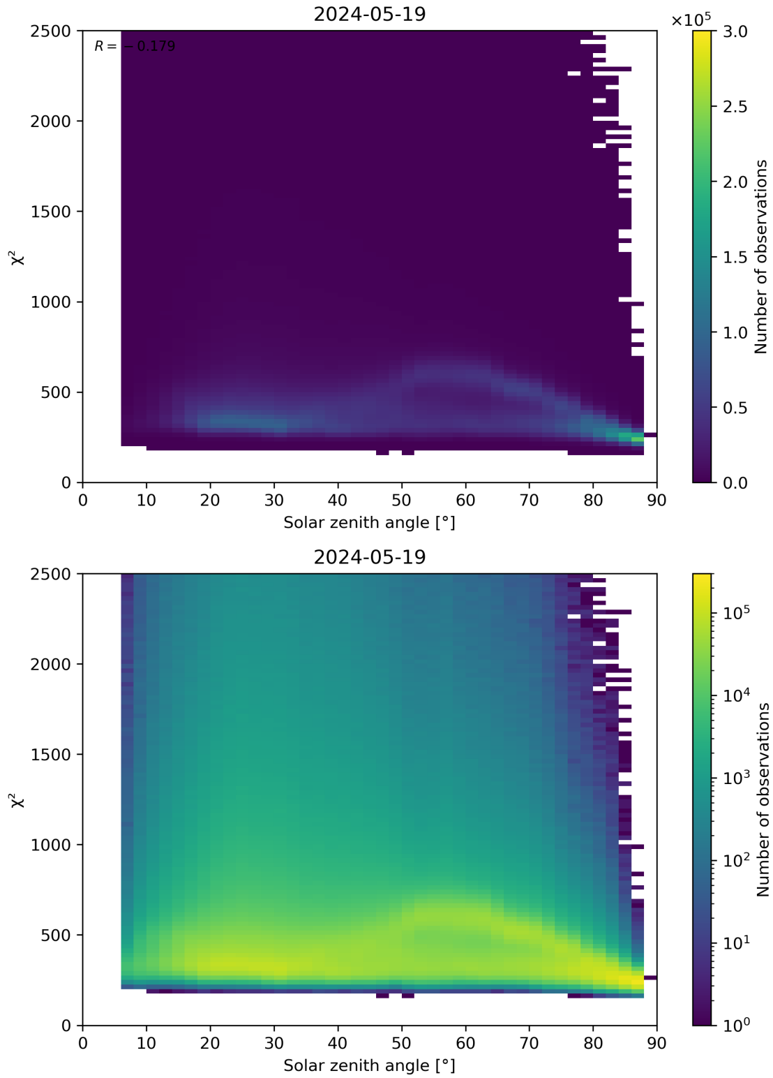
Figure 148: Scatter density plot of “Solar zenith angle” against “ \chi^2 ” for 2024-05-18 to 2024-05-20.
