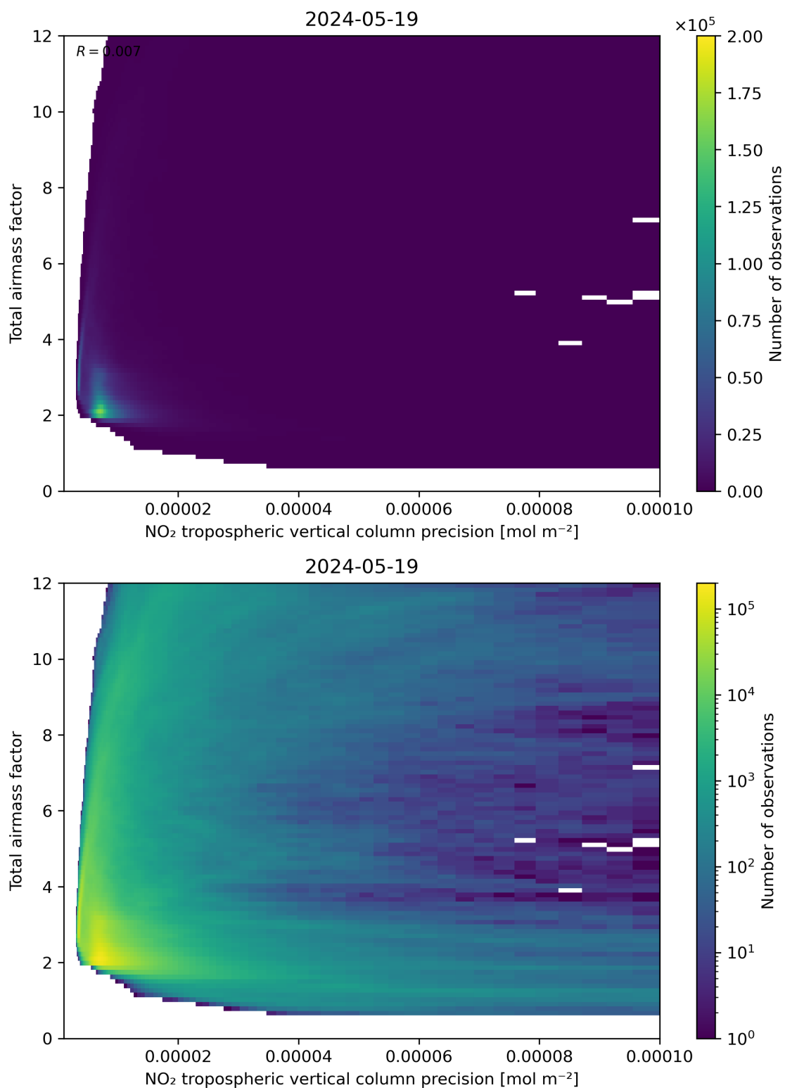
Figure 132: Scatter density plot of “NO 2 tropospheric vertical column precision” against “Total air mass factor” for 2024-05-18 to 2024-05-20.
