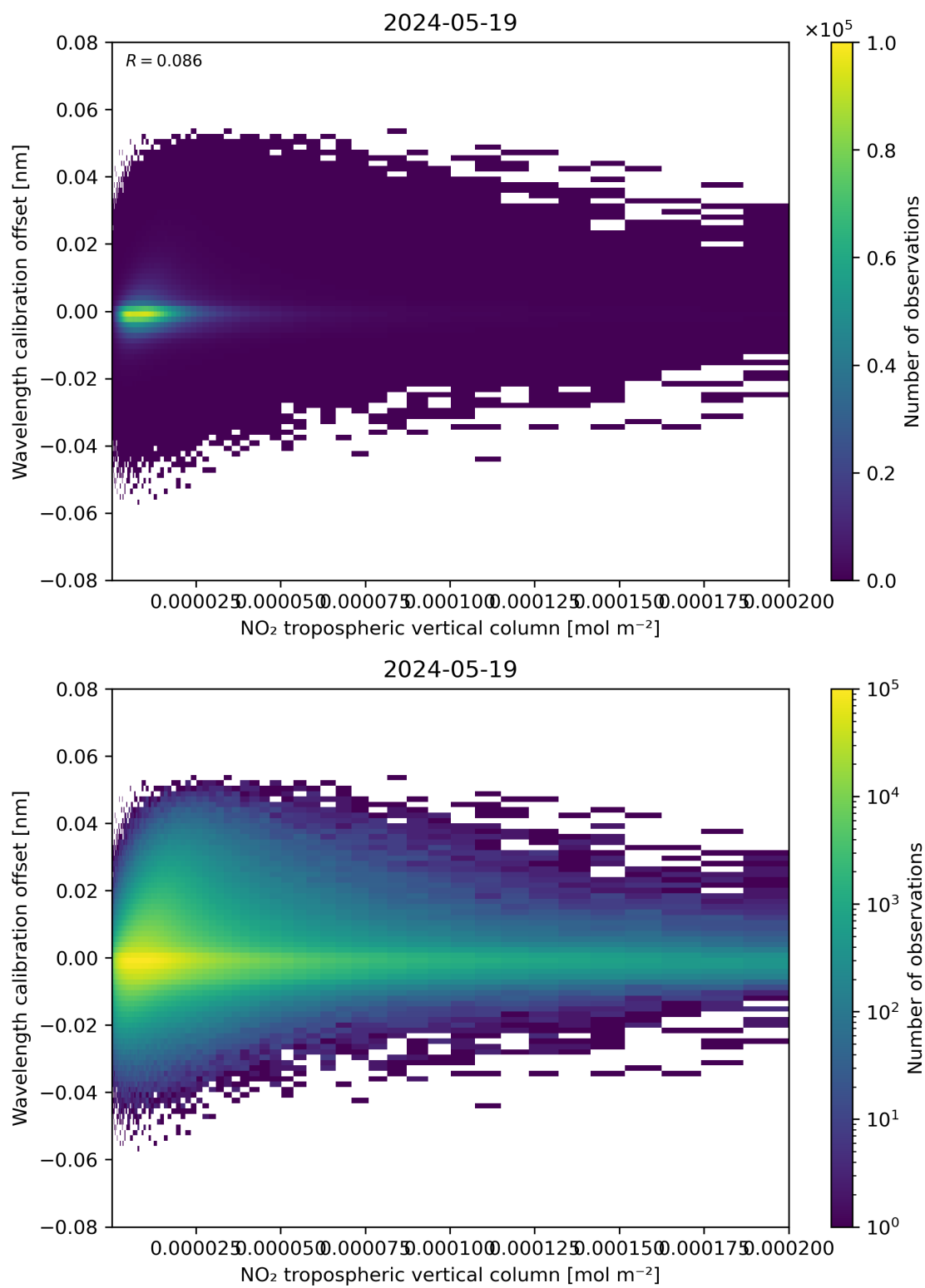
Figure 143: Scatter density plot of “NO 2 tropospheric vertical column” against “Wavelength calibration offset” for 2024-05-18 to 2024-05-20.
