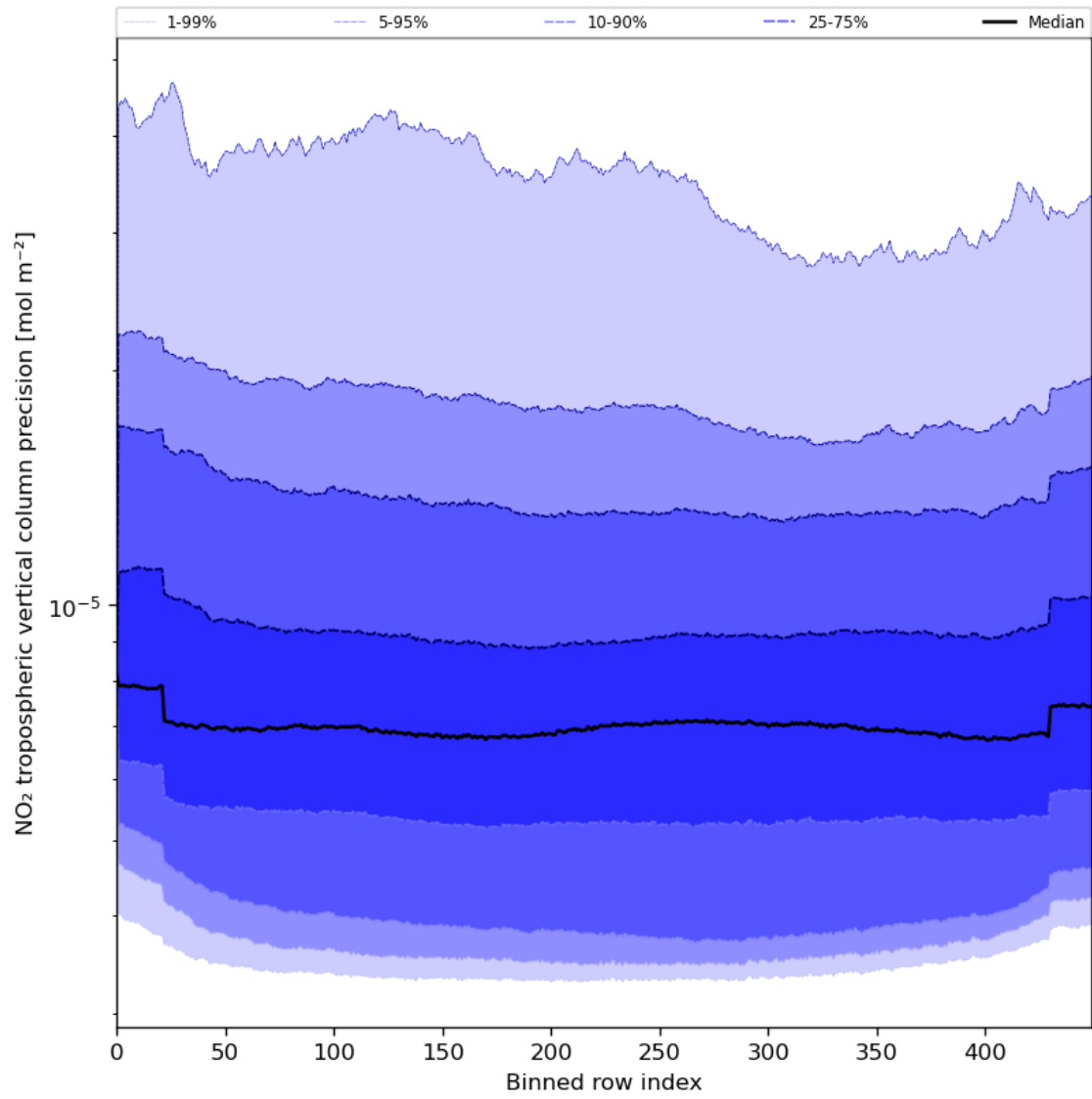
Figure 47: Along track statistics of “NO 2 tropospheric vertical column precision” for 2024-05-18 to 2024-05-20
