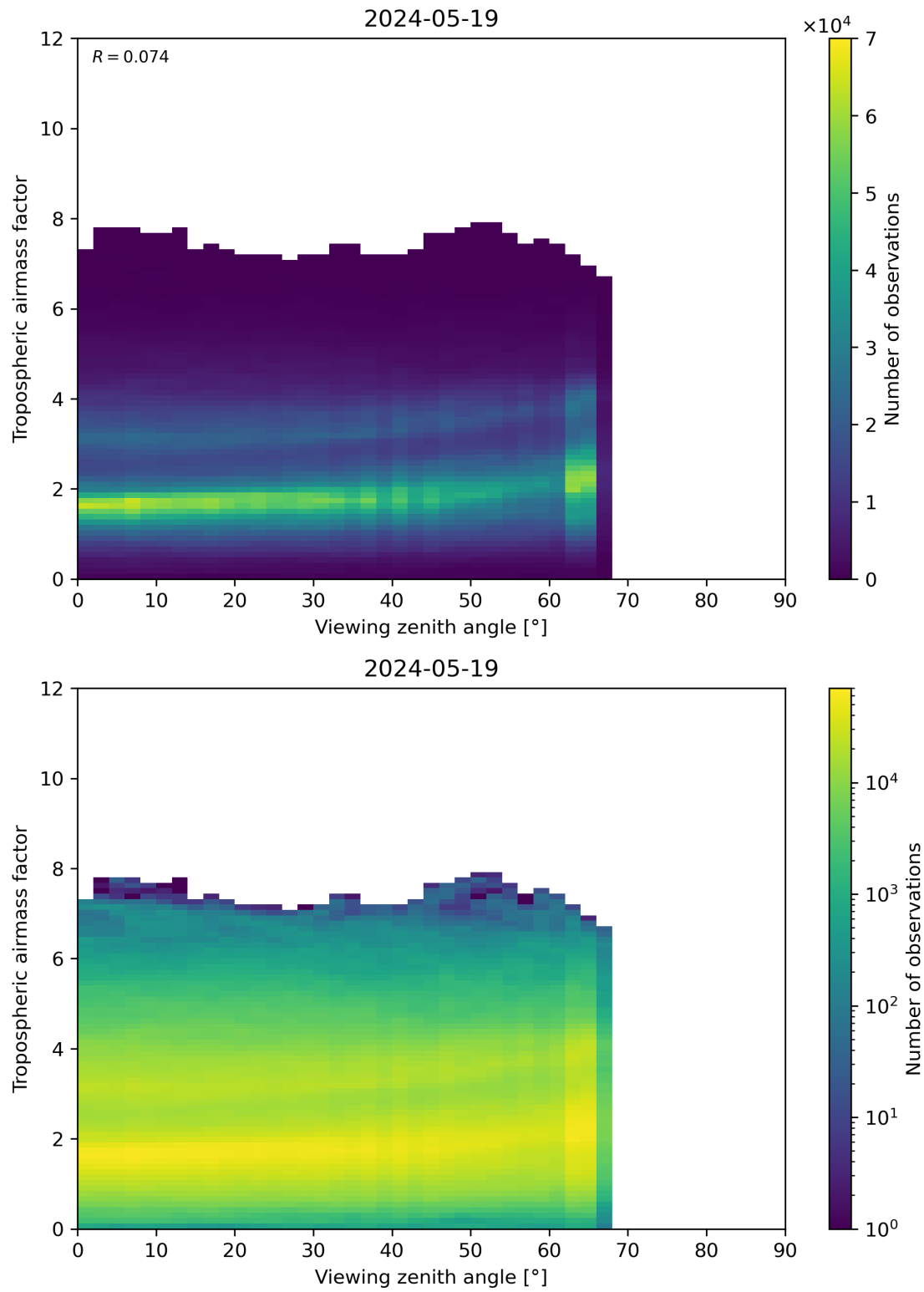
Figure 161: Scatter density plot of “Viewing zenith angle” against “Tropospheric airmass factor” for 2024-05-18 to 2024-05-20.
