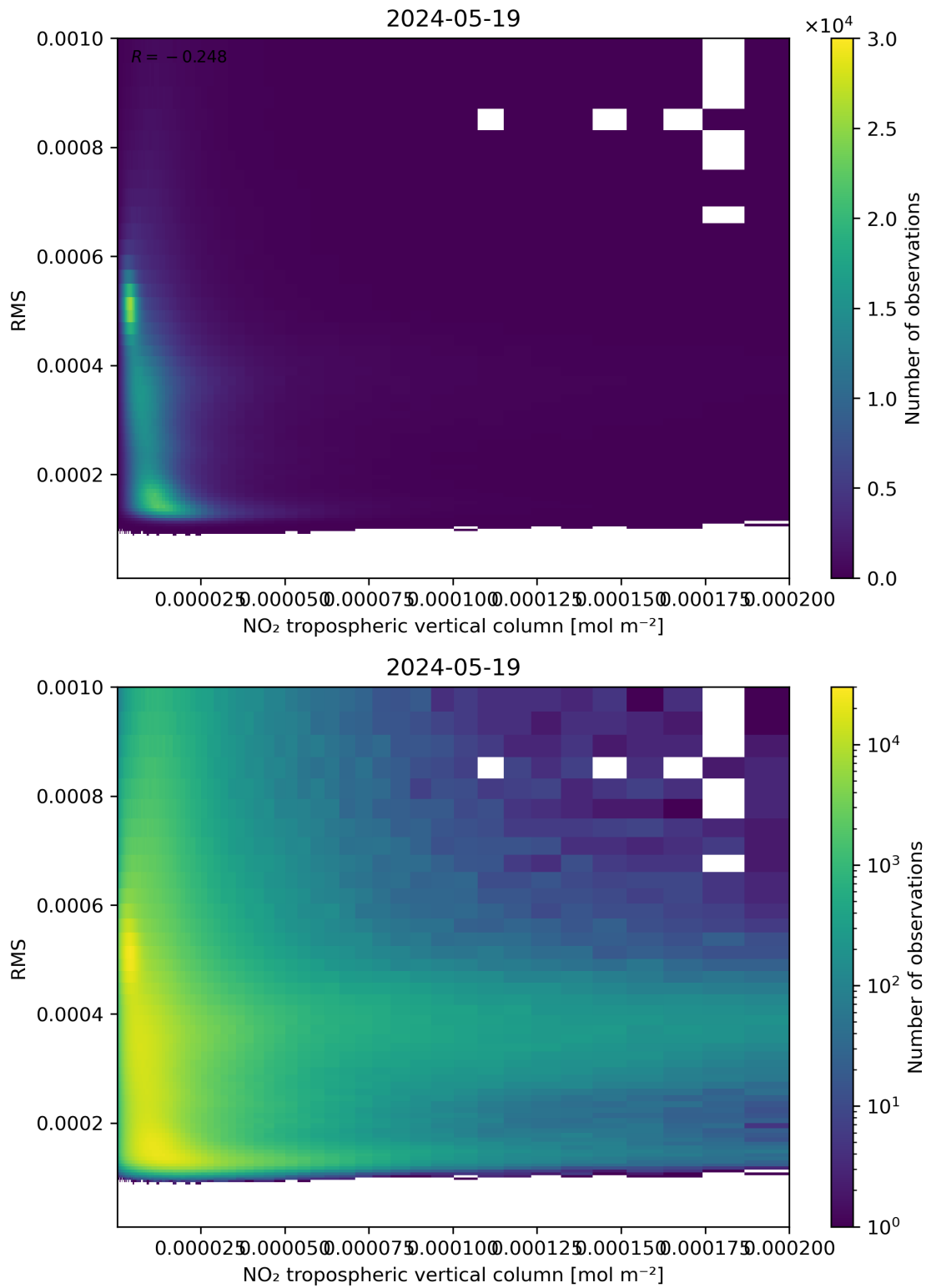
Figure 142: Scatter density plot of “NO 2 tropospheric vertical column” against “RMS” for 2024-05-18 to 2024-05-20.
