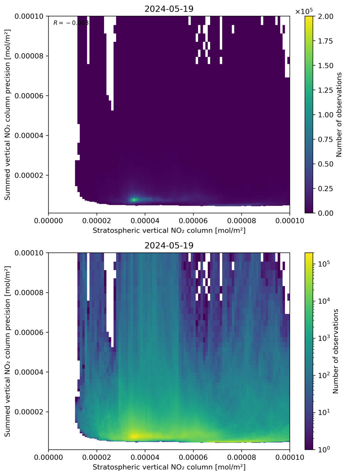
Figure 99: Scatter density plot of “Stratospheric vertical NO 2 column” against “Summed vertical NO 2 column precision” for 2024-05-18 to 2024-05-20.
