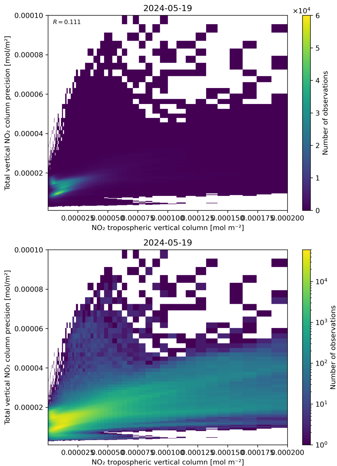
Figure 129: Scatter density plot of “NO 2 tropospheric vertical column” against “Total vertical NO 2 column precision” for 2024-05-18 to 2024-05-20.
