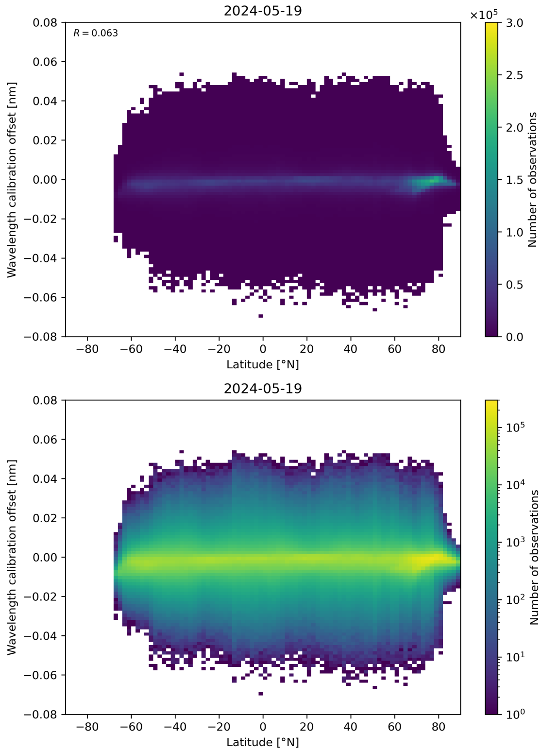
Figure 95: Scatter density plot of “Latitude” against “Wavelength calibration offset” for 2024-05-18 to 2024-05-20.
