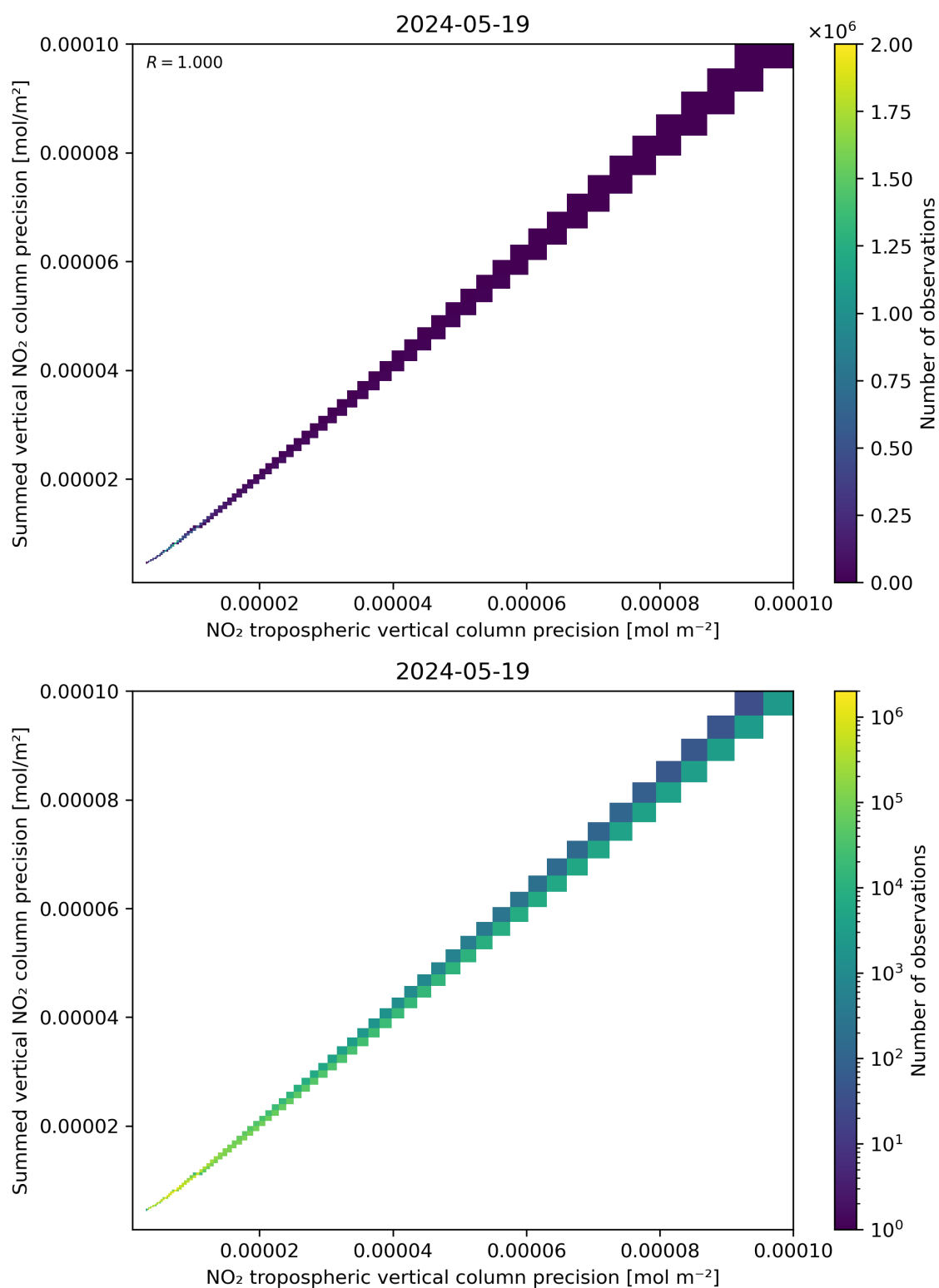
Figure 137: Scatter density plot of “NO 2 tropospheric vertical column precision” against “Summed vertical NO 2 column precision” for 2024-05-18 to 2024-05-20.
