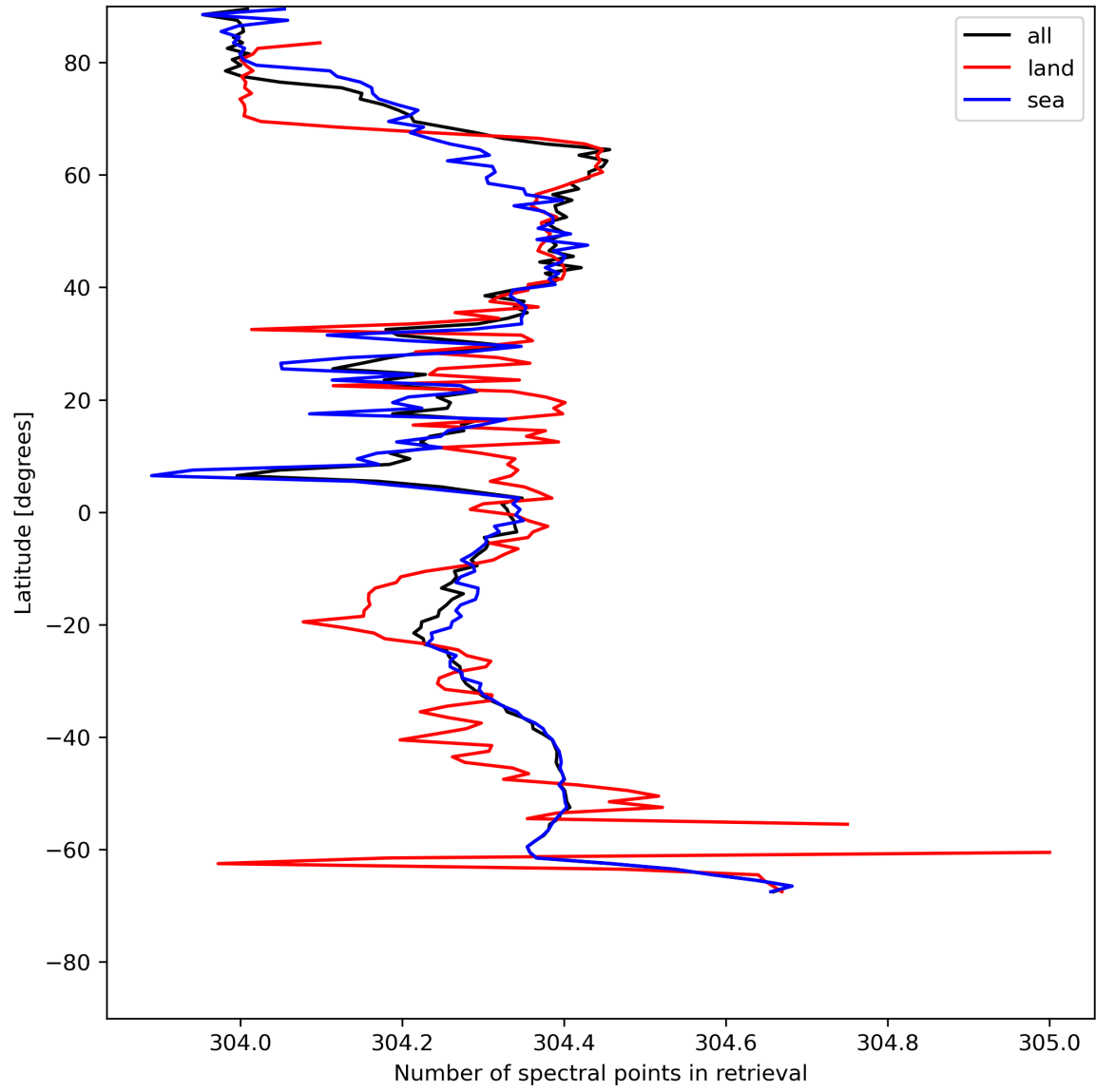
Figure 16: Zonal average of “Number of spectral points in retrieval” for 2024-05-18 to 2024-05-20.
