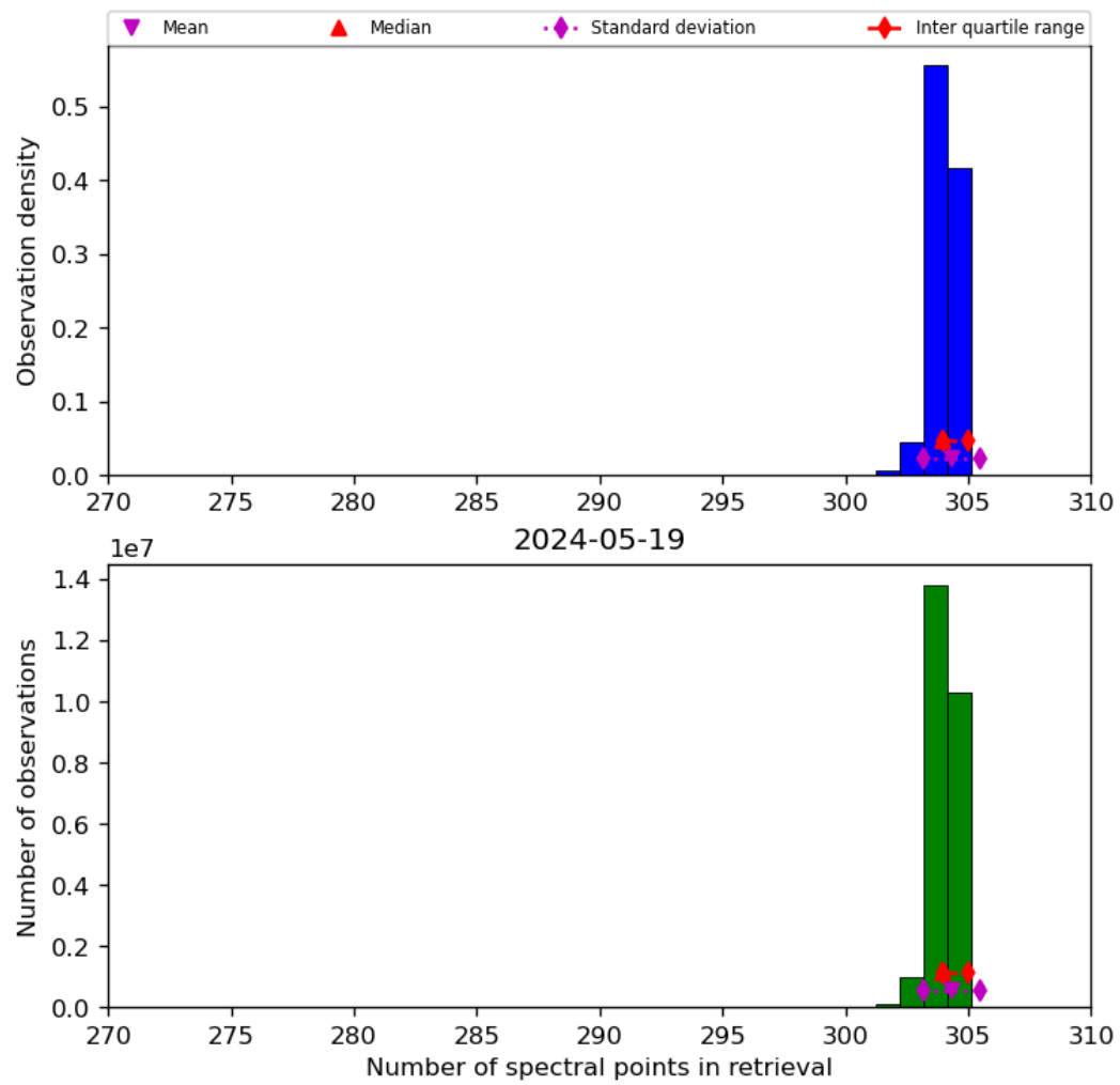
Figure 33: Histogram of “Number of spectral points in retrieval” for 2024-05-18 to 2024-05-20
