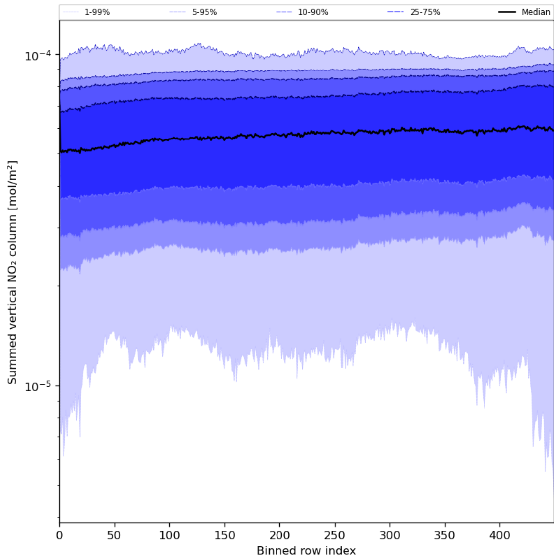
Figure 57: Along track statistics of “Summed vertical NO 2 column” for 2024-05-18 to 2024-05-20
