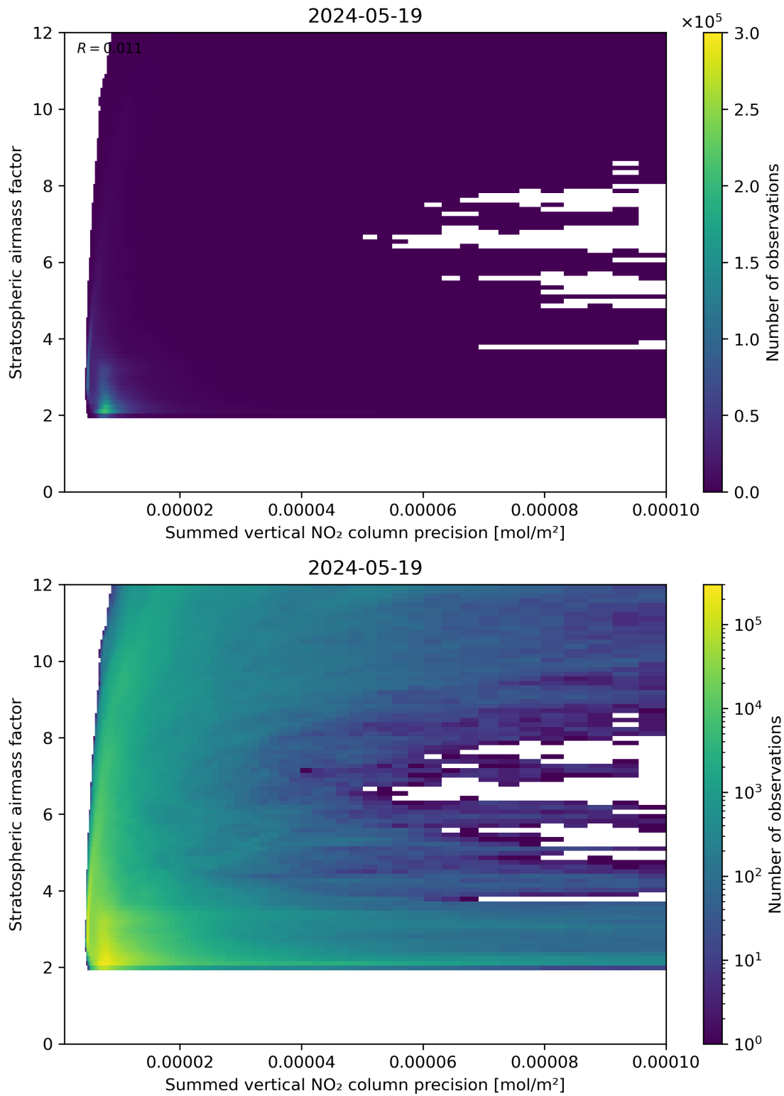
Figure 106: Scatter density plot of “Summed vertical NO 2 column precision” against “Stratospheric airmass factor” for 2024-05-18 to 2024-05-20.
