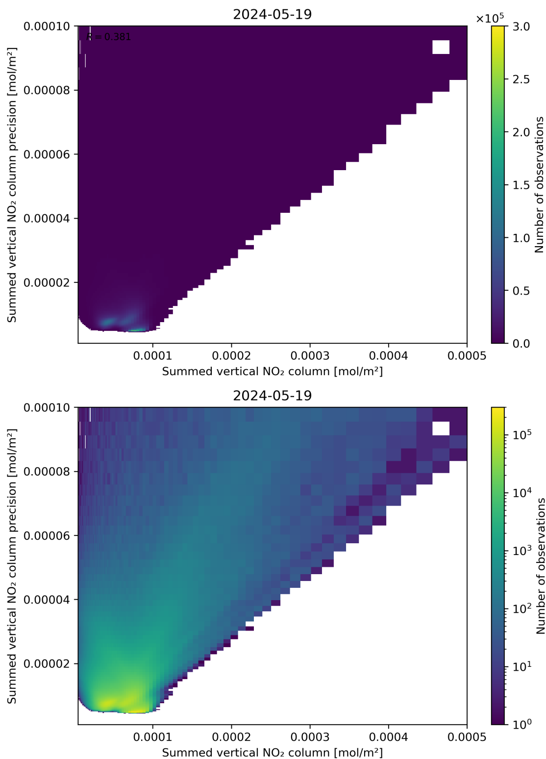
Figure 105: Scatter density plot of “Summed vertical NO 2 column” against “Summed vertical NO 2 column precision” for 2024-05-18 to 2024-05-20.
