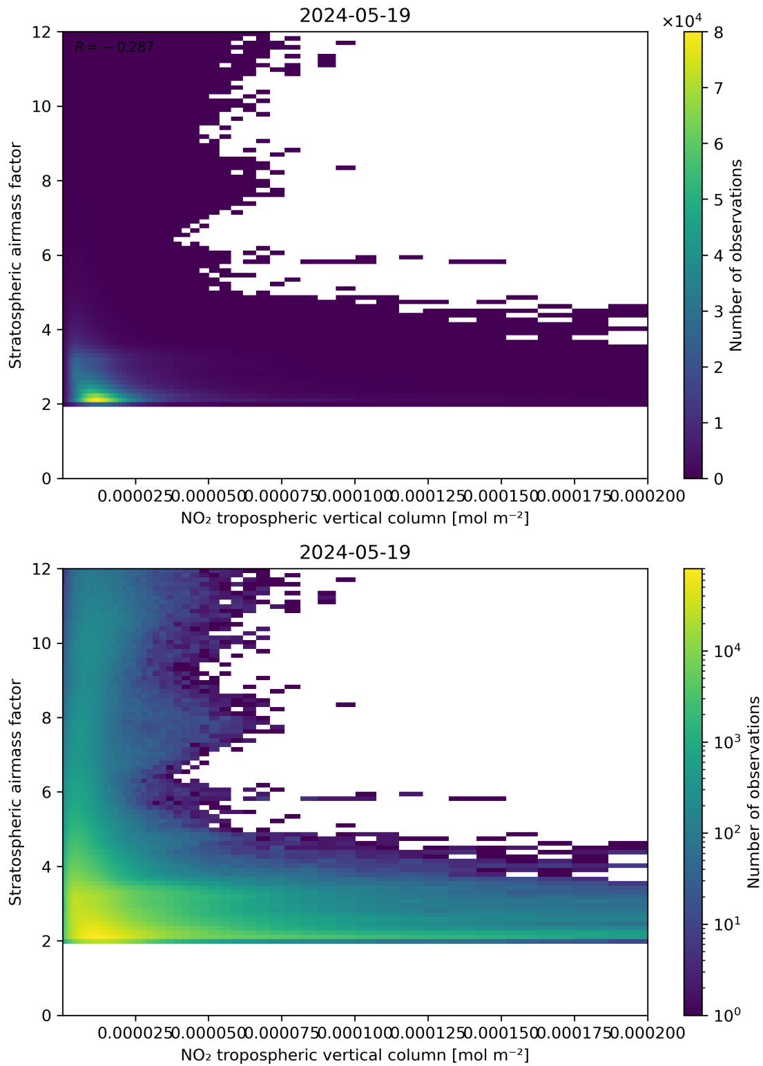
Figure 121: Scatter density plot of “NO 2 tropospheric vertical column” against “Stratospheric air mass factor” for 2024-05-18 to 2024-05-20.
