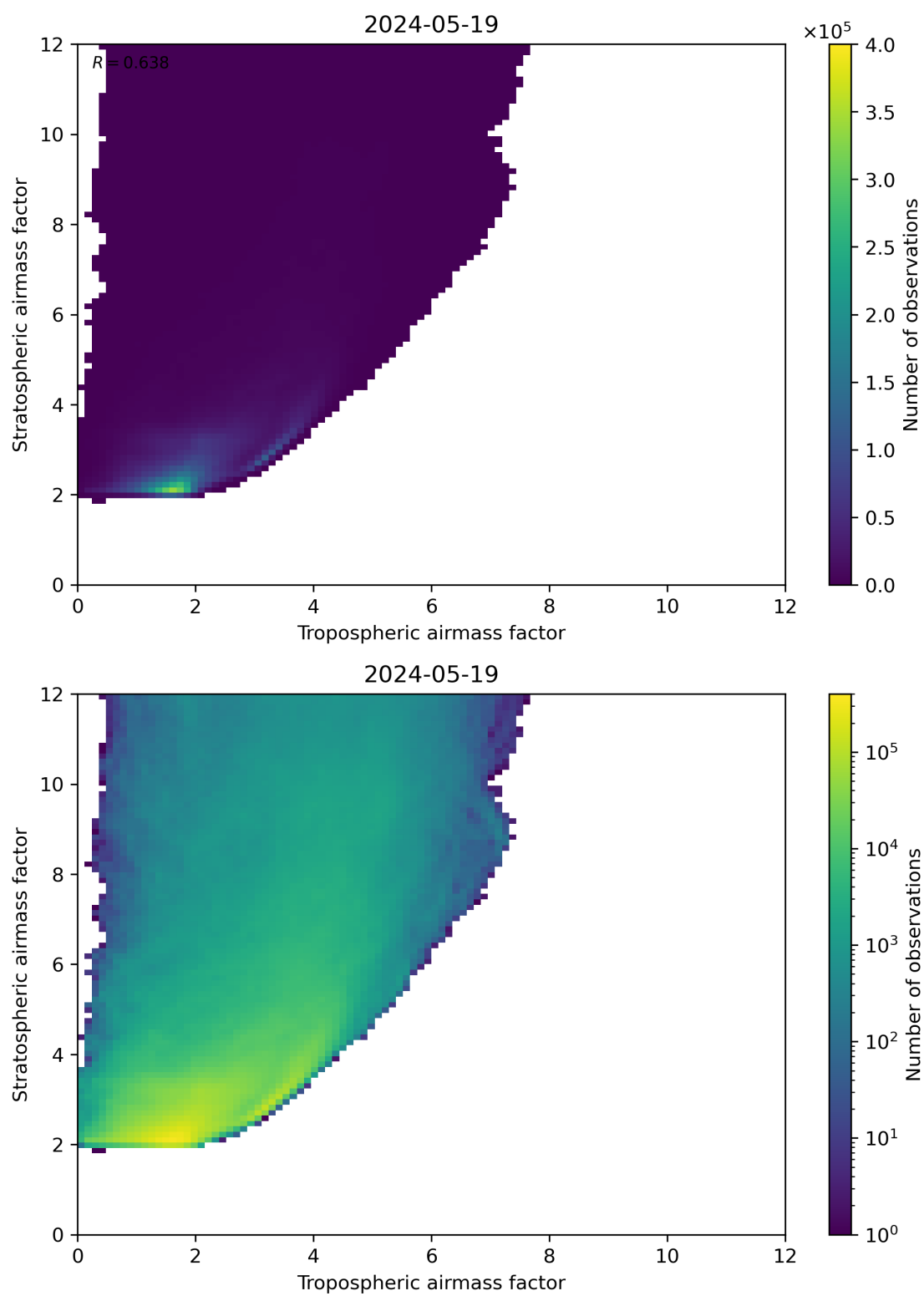
Figure 71: Scatter density plot of “Tropospheric airmass factor” against “Stratospheric airmass factor” for 2024-05-18 to 2024-05-20.
