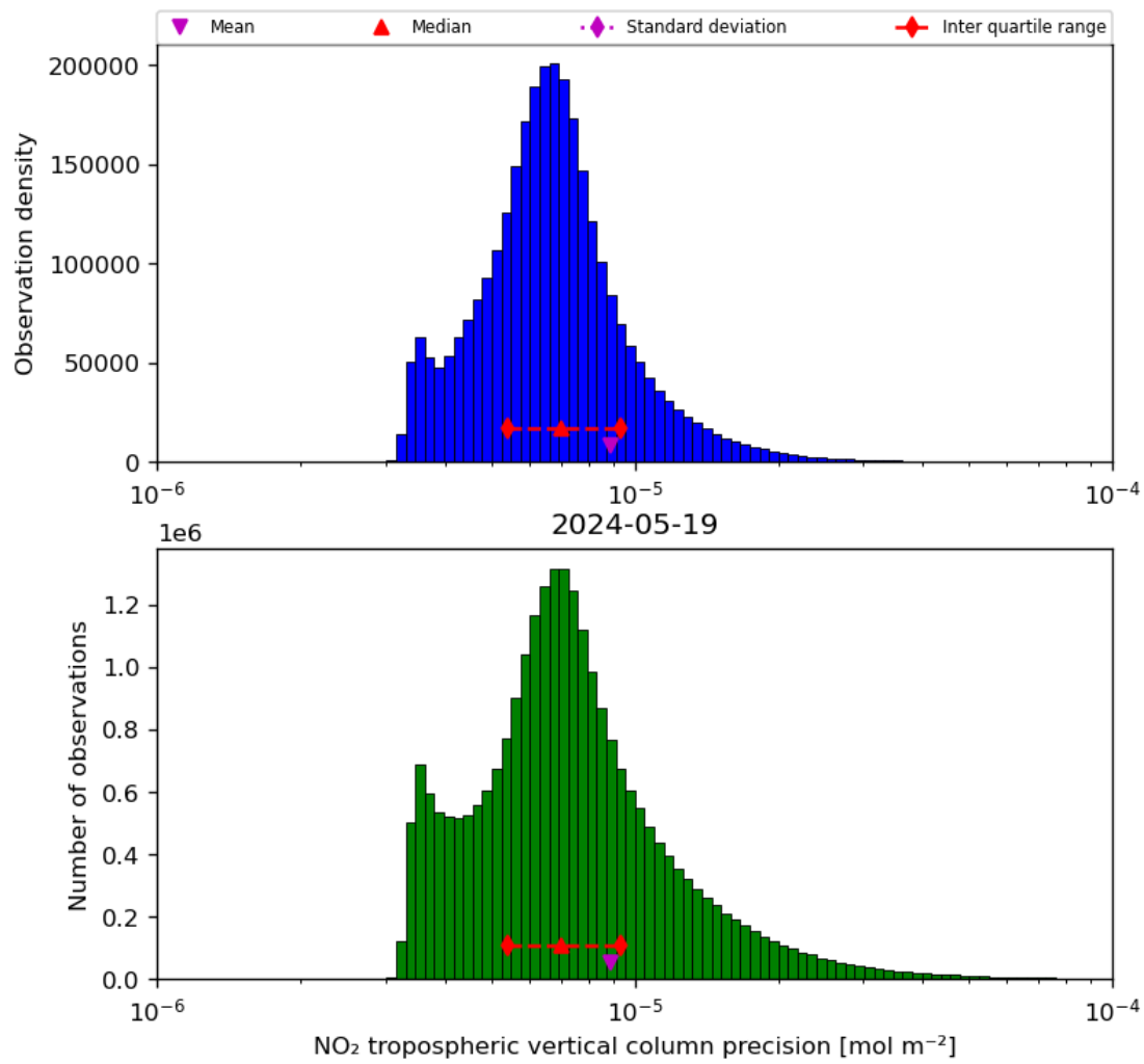
Figure 30: Histogram of “NO 2 tropospheric vertical column precision” for 2024-05-18 to 2024-05-20
