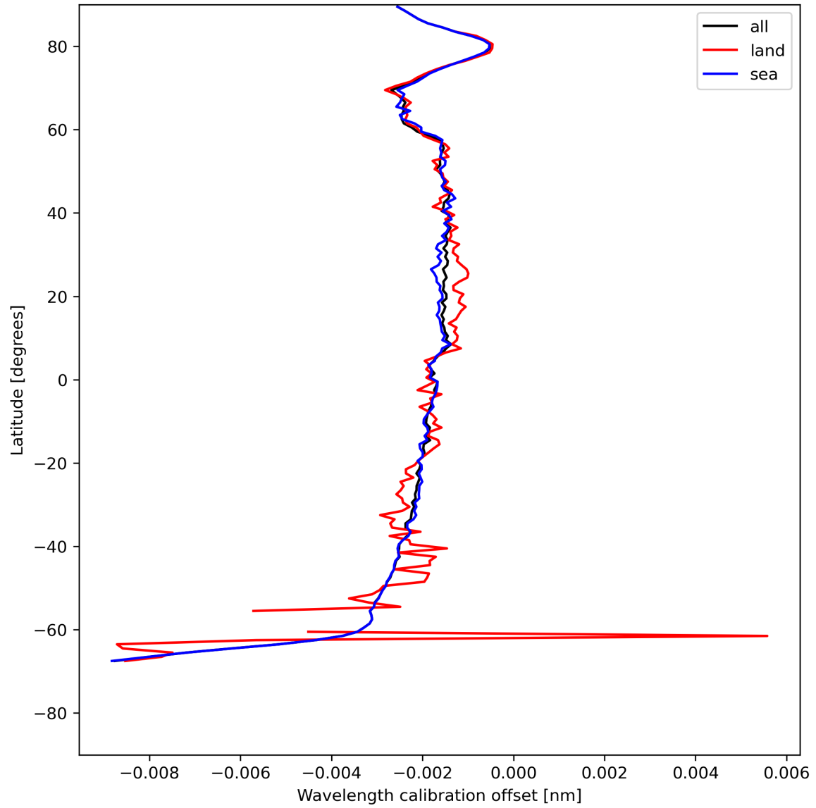
Figure 18: Zonal average of “Wavelength calibration offset” for 2024-05-18 to 2024-05-20.
