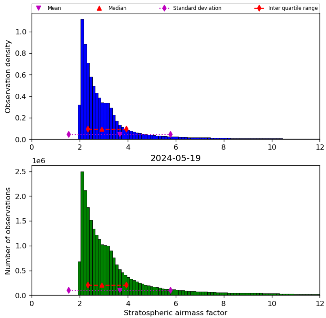
Figure 44: Histogram of “Stratospheric airmass factor” for 2024-05-18 to 2024-05-20
