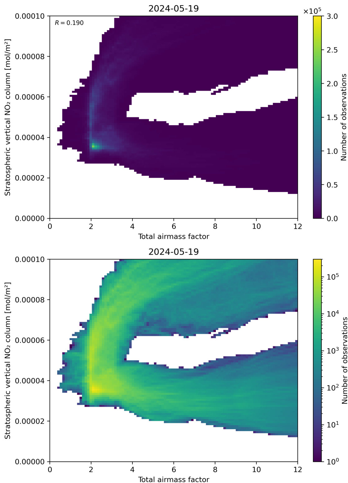
Figure 64: Scatter density plot of “Total airmass factor” against “Stratospheric vertical \text{NO}_2 column” for 2024-05-18 to 2024-05-20.
