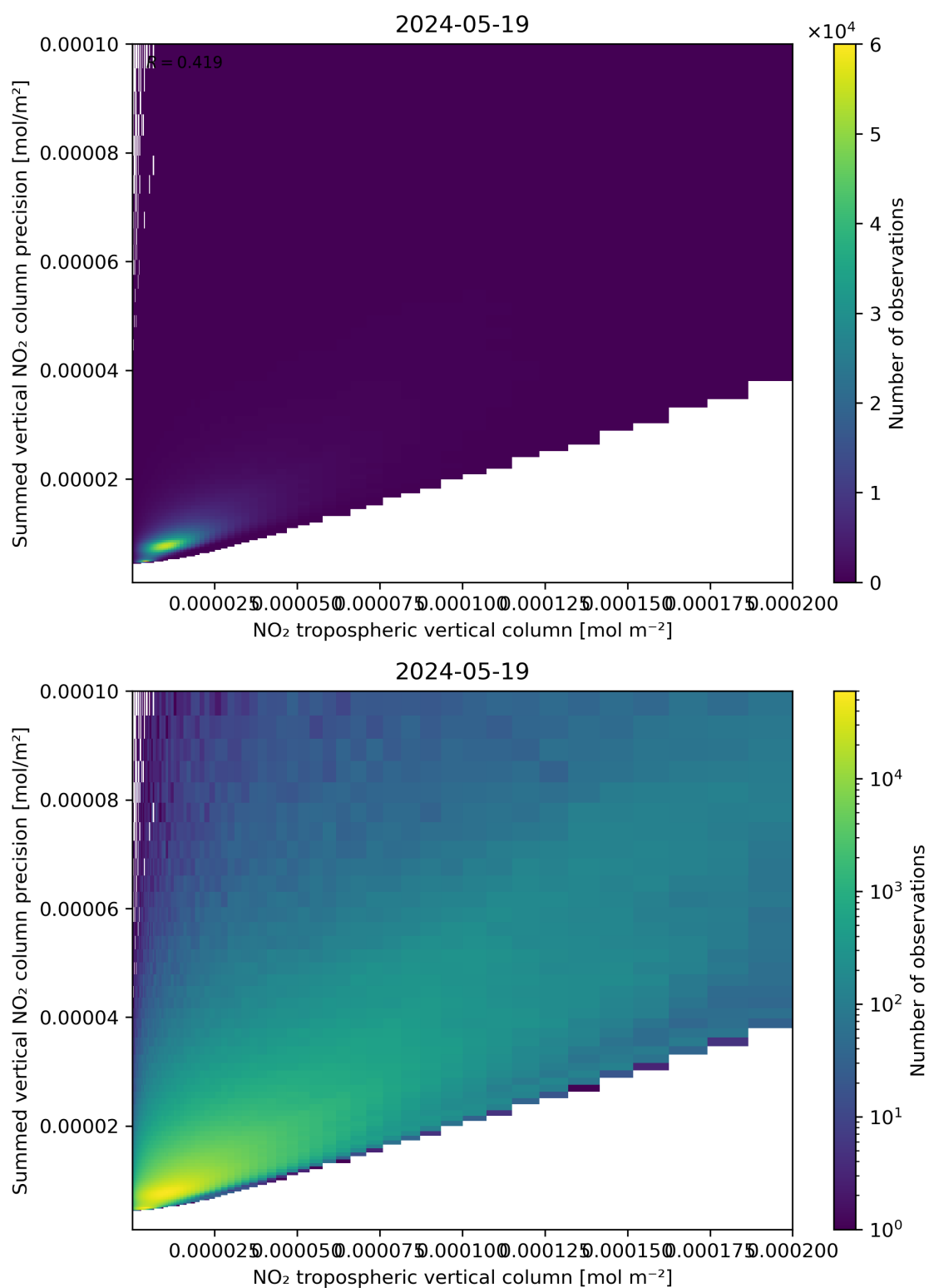
Figure 127: Scatter density plot of “NO 2 tropospheric vertical column” against “Summed vertical NO 2 column precision” for 2024-05-18 to 2024-05-20.
