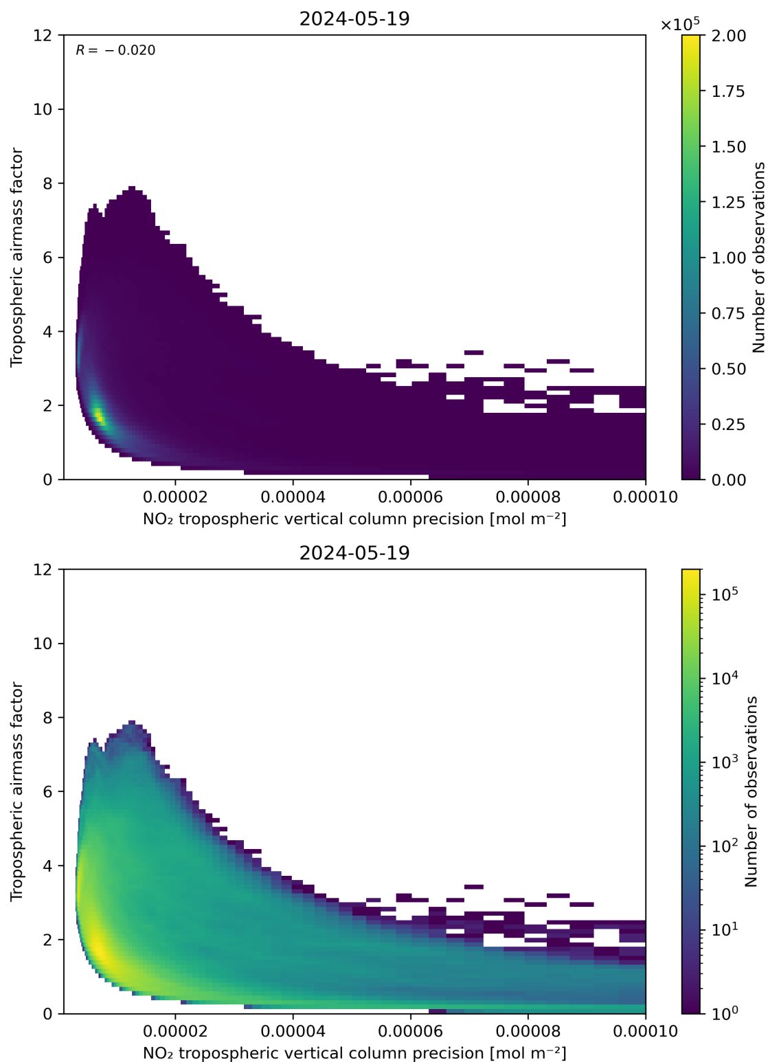
Figure 133: Scatter density plot of “NO 2 tropospheric vertical column precision” against “Tropospheric airmass factor” for 2024-05-18 to 2024-05-20.
