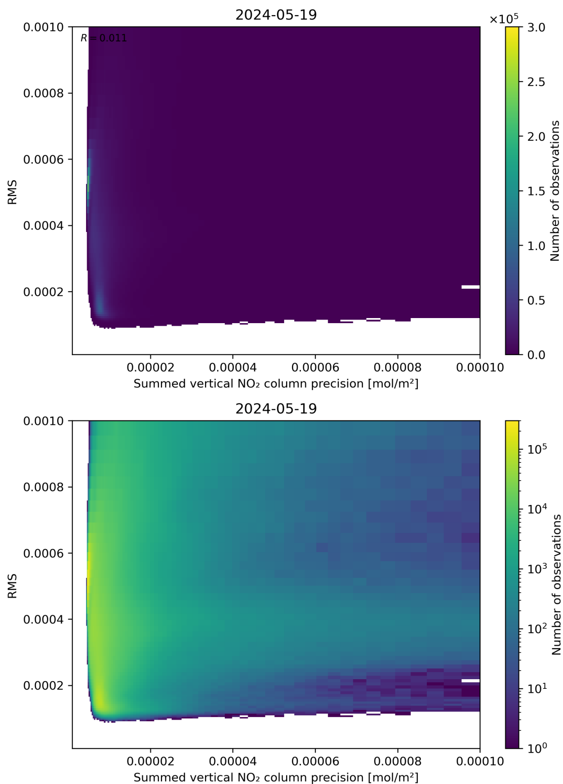
Figure 108: Scatter density plot of “Summed vertical NO 2 column precision” against “RMS” for 2024-05-18 to 2024-05-20.
