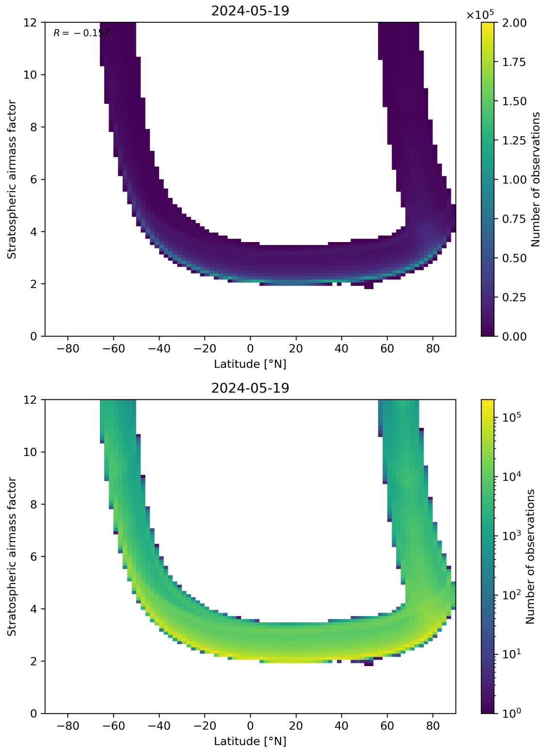
Figure 83: Scatter density plot of “Latitude” against “Stratospheric air mass factor” for 2024-05-18 to 2024-05-20.
