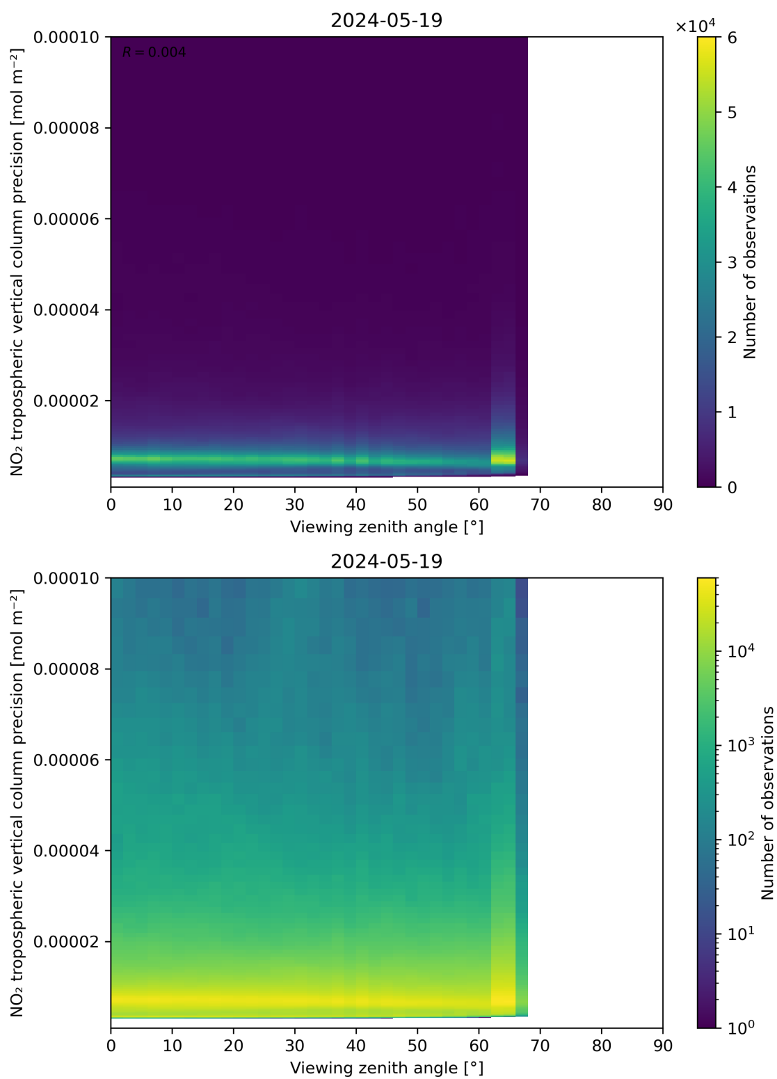
Figure 170: Scatter density plot of “Viewing zenith angle” against “NO 2 tropospheric vertical column precision” for 2024-05-18 to 2024-05-20.
