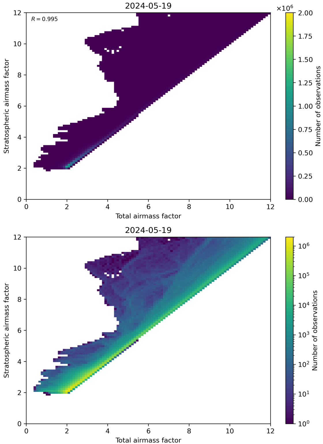
Figure 62: Scatter density plot of “Total airmass factor” against “Stratospheric airmass factor” for 2024-05-18 to 2024-05-20.
