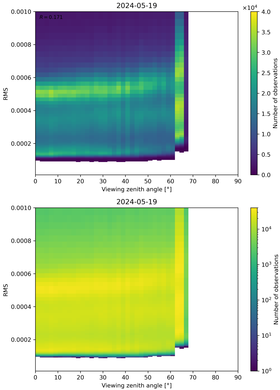
Figure 171: Scatter density plot of “Viewing zenith angle” against “RMS” for 2024-05-18 to 2024-05-20.
