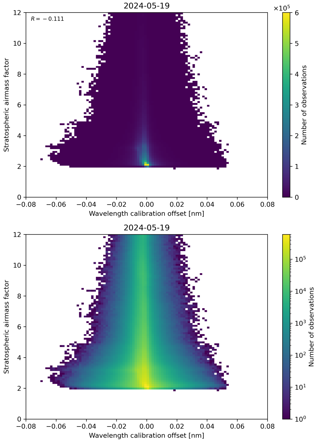
Figure 174: Scatter density plot of “Wavelength calibration offset” against “Stratospheric airmass factor” for 2024-05-18 to 2024-05-20.
