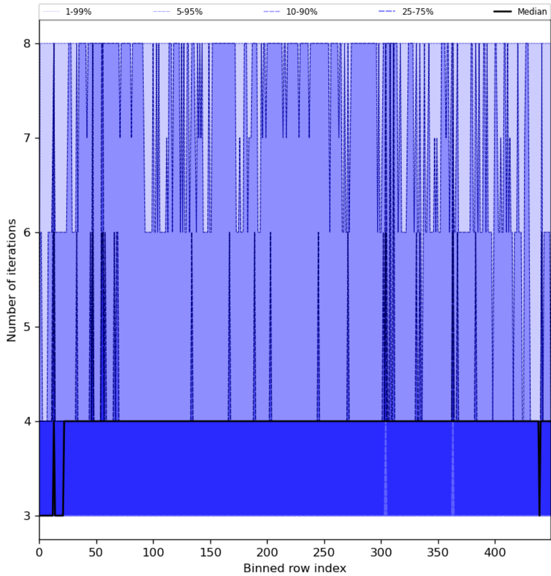
Figure 51: Along track statistics of “Number of iterations” for 2024-05-18 to 2024-05-20
