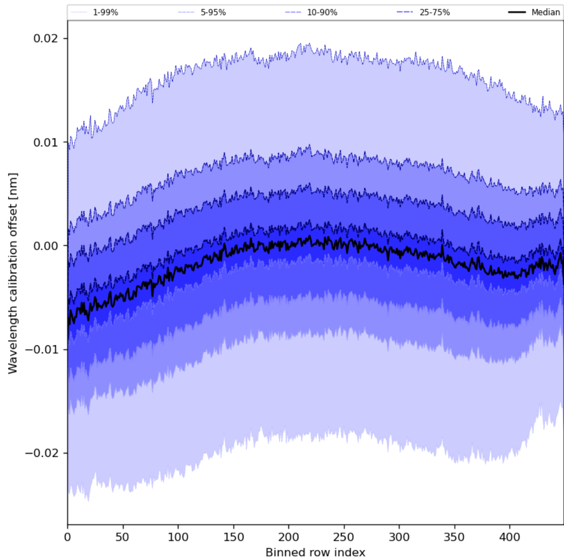
Figure 52: Along track statistics of “Wavelength calibration offset” for 2024-05-18 to 2024-05-20
