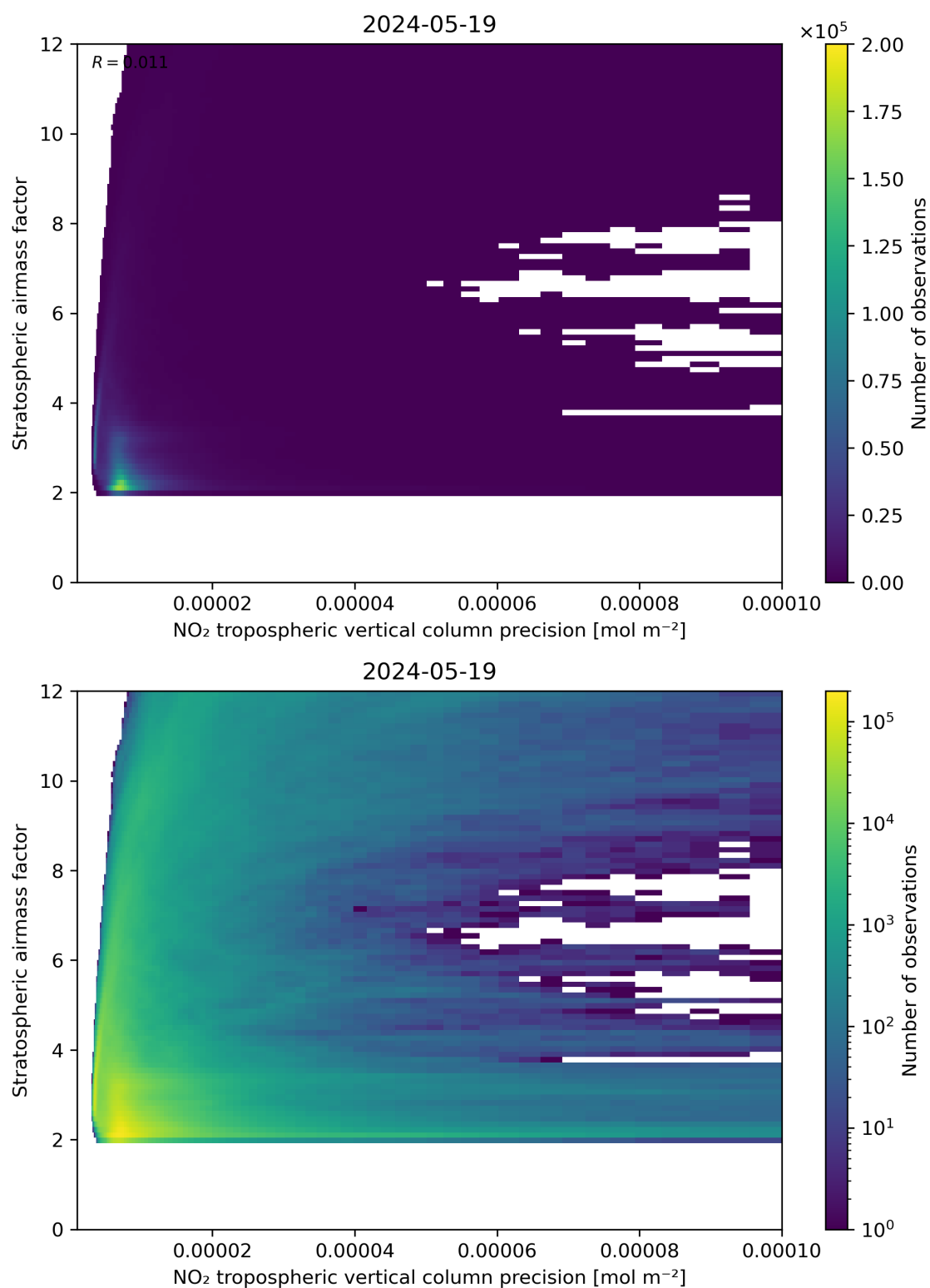
Figure 131: Scatter density plot of “NO 2 tropospheric vertical column precision” against “Stratospheric airmass factor” for 2024-05-18 to 2024-05-20.
