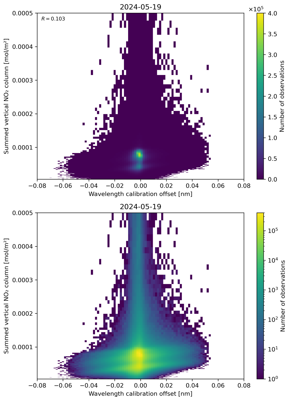
Figure 177: Scatter density plot of “Wavelength calibration offset” against “Summed vertical NO 2 column” for 2024-05-18 to 2024-05-20.
