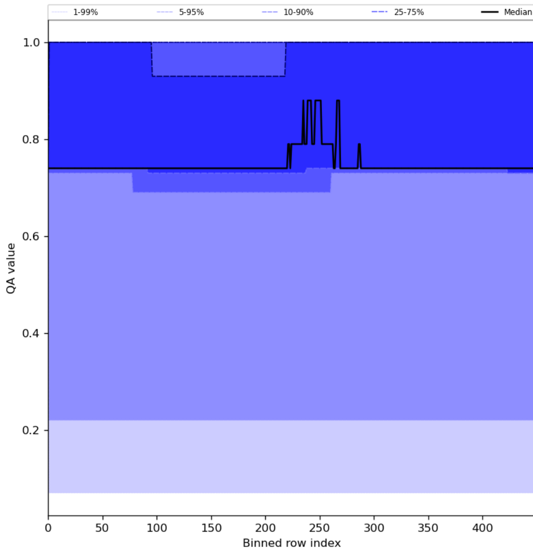
Figure 45: Along track statistics of “QA value” for 2024-05-18 to 2024-05-20
