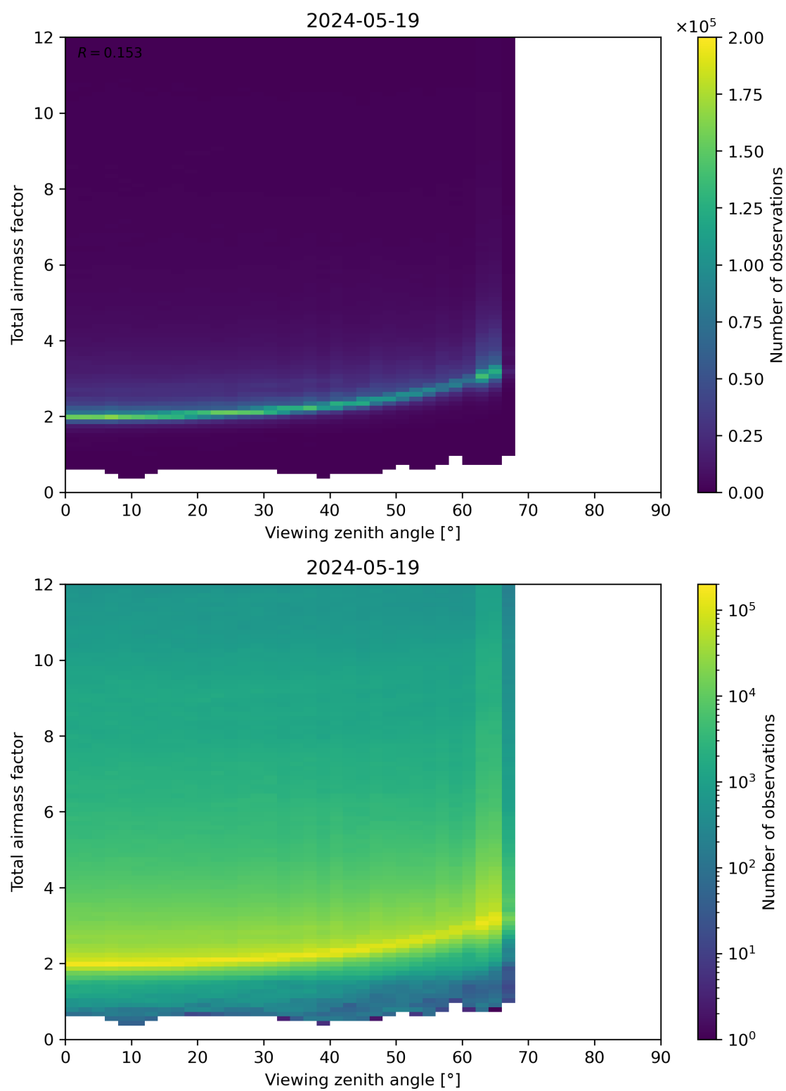
Figure 160: Scatter density plot of “Viewing zenith angle” against “Total airmass factor” for 2024-05-18 to 2024-05-20.
