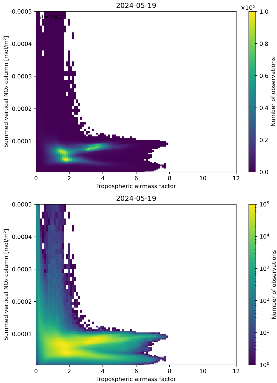
Figure 75: Scatter density plot of “Tropospheric air mass factor” against “Summed vertical NO 2 column” for 2024-05-18 to 2024-05-20.
