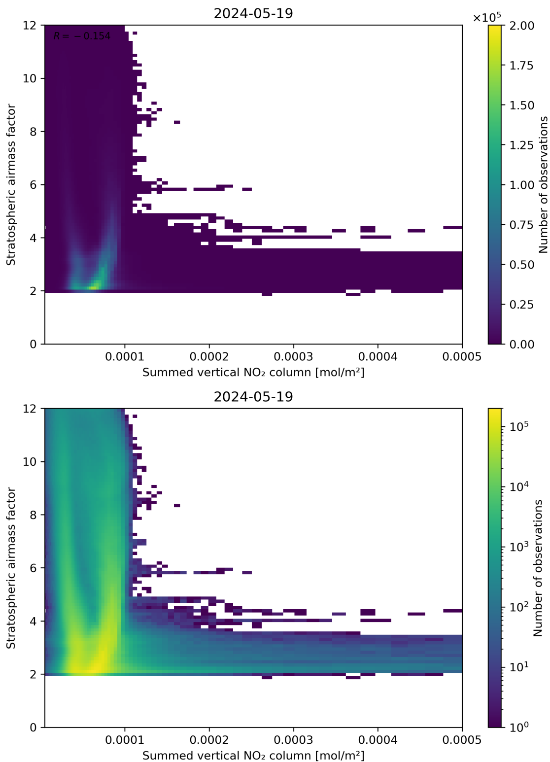
Figure 103: Scatter density plot of “Summed vertical NO 2 column” against “Stratospheric air mass factor” for 2024-05-18 to 2024-05-20.
