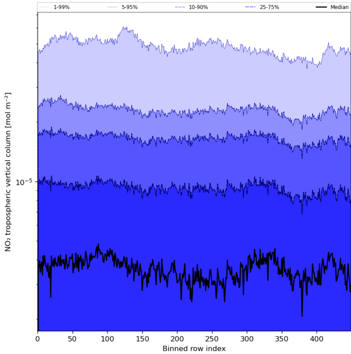
Figure 46: Along track statistics of “NO 2 tropospheric vertical column” for 2024-05-18 to 2024-05-20
