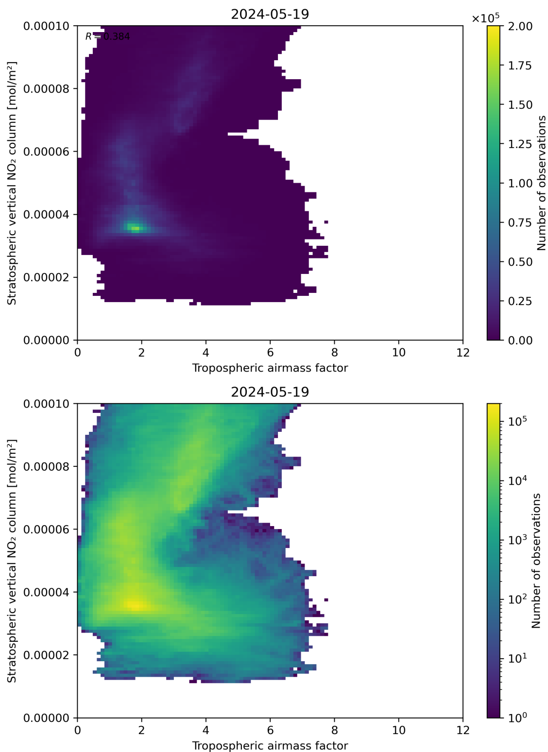
Figure 74: Scatter density plot of “Tropospheric air mass factor” against “Stratospheric vertical NO 2 column” for 2024-05-18 to 2024-05-20.
