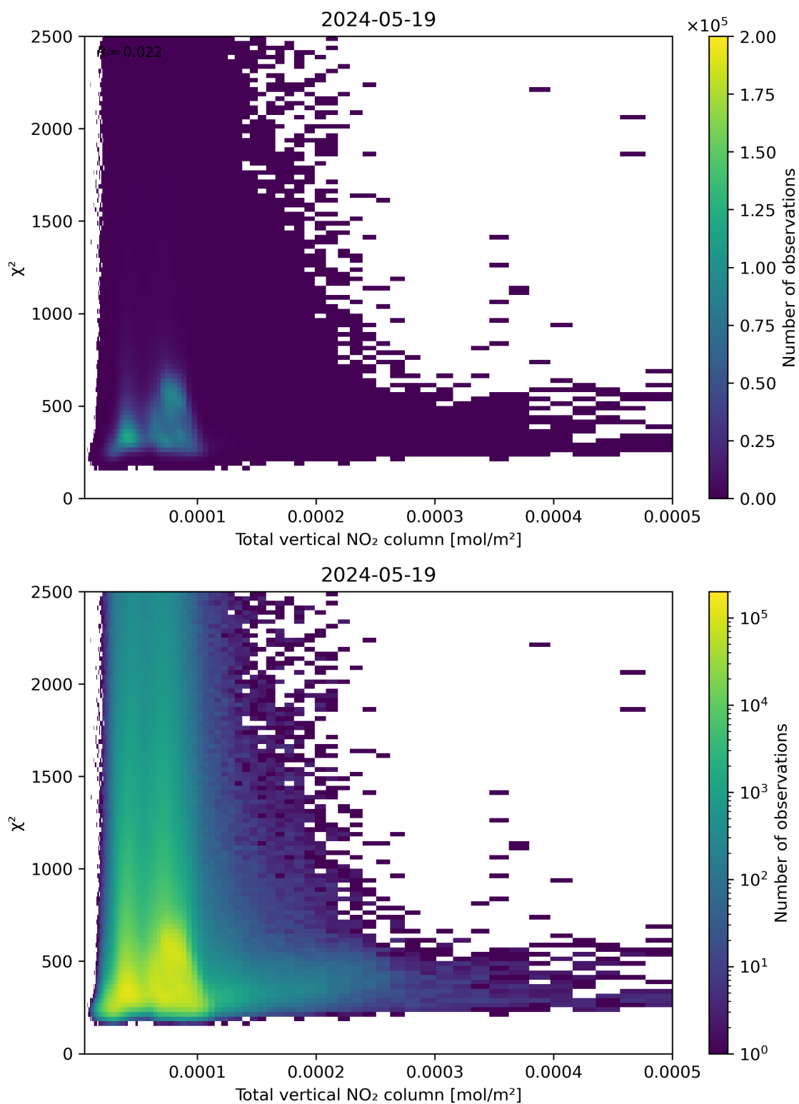
Figure 111: Scatter density plot of “Total vertical NO 2 column” against “ \chi^2 ” for 2024-05-18 to 2024-05-20.
