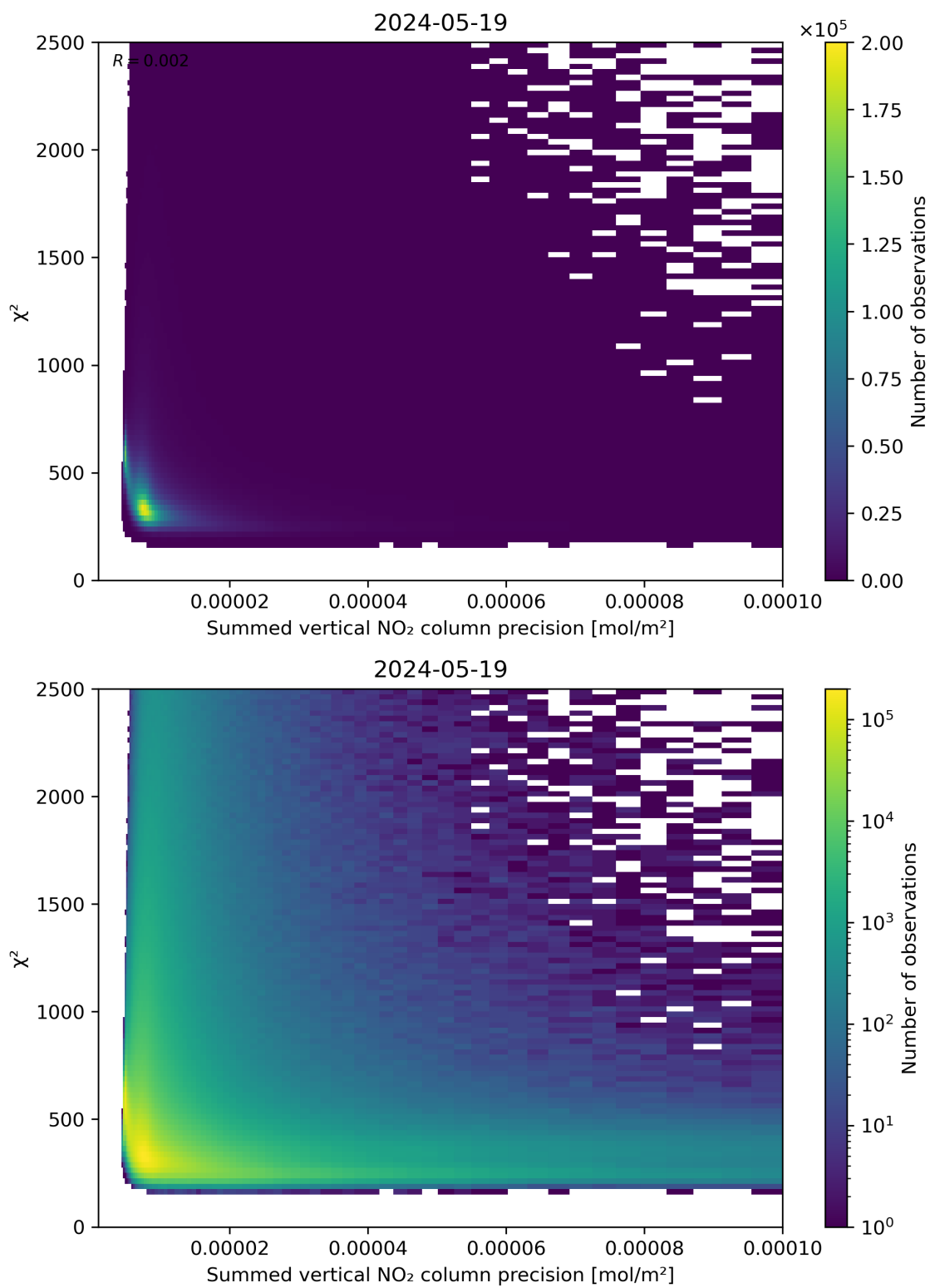
Figure 107: Scatter density plot of “Summed vertical NO 2 column precision” against “ \chi^2 ” for 2024-05-18 to 2024-05-20.
