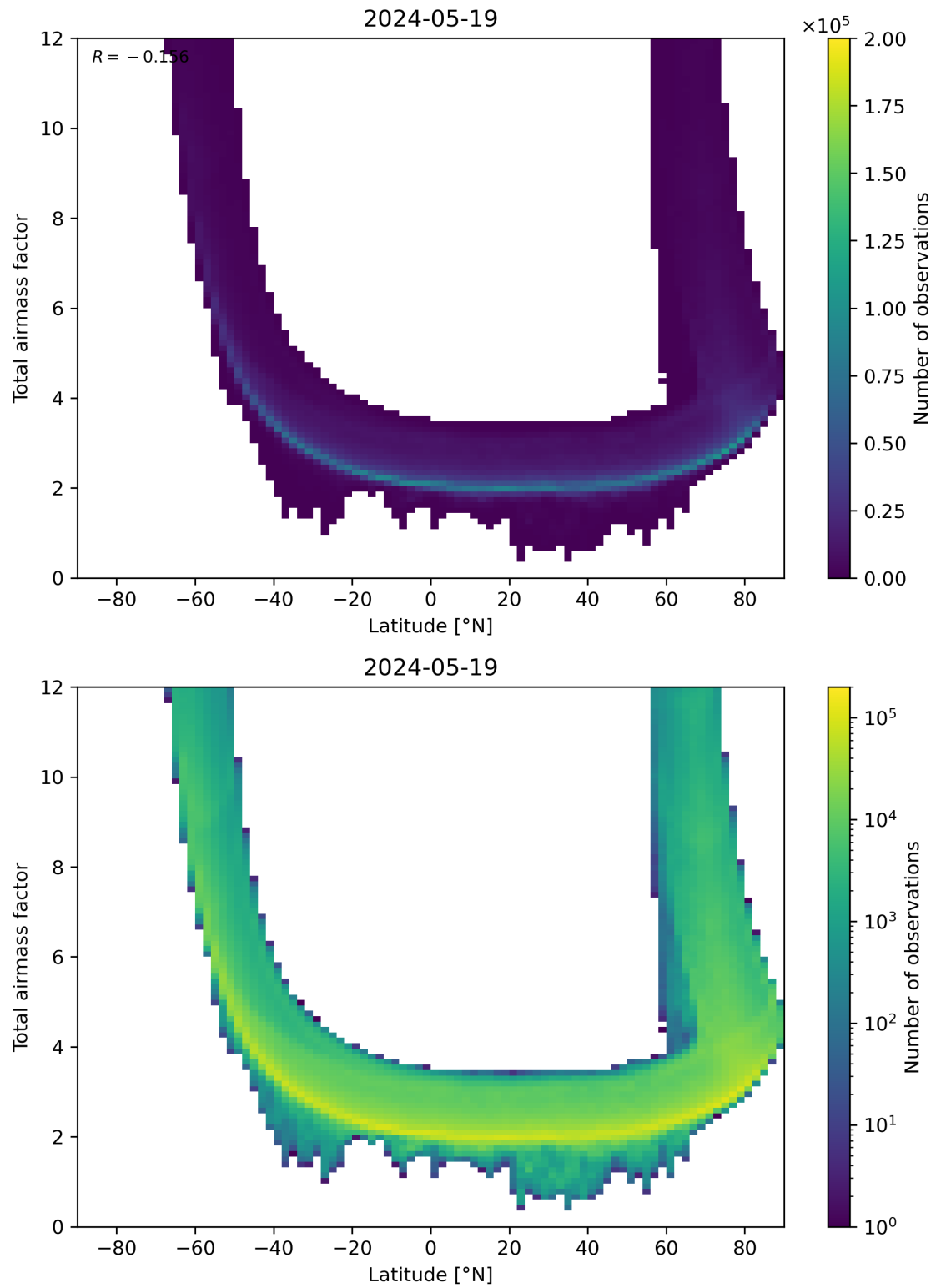
Figure 84: Scatter density plot of “Latitude” against “Total airmass factor” for 2024-05-18 to 2024-05-20.
