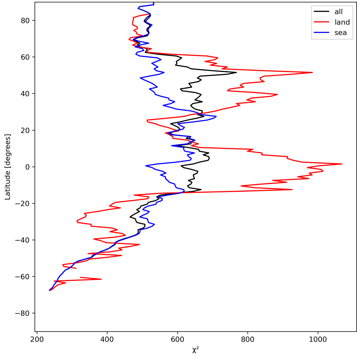
Figure 25: Zonal average of “ \chi^2 ” for 2024-05-18 to 2024-05-20.
