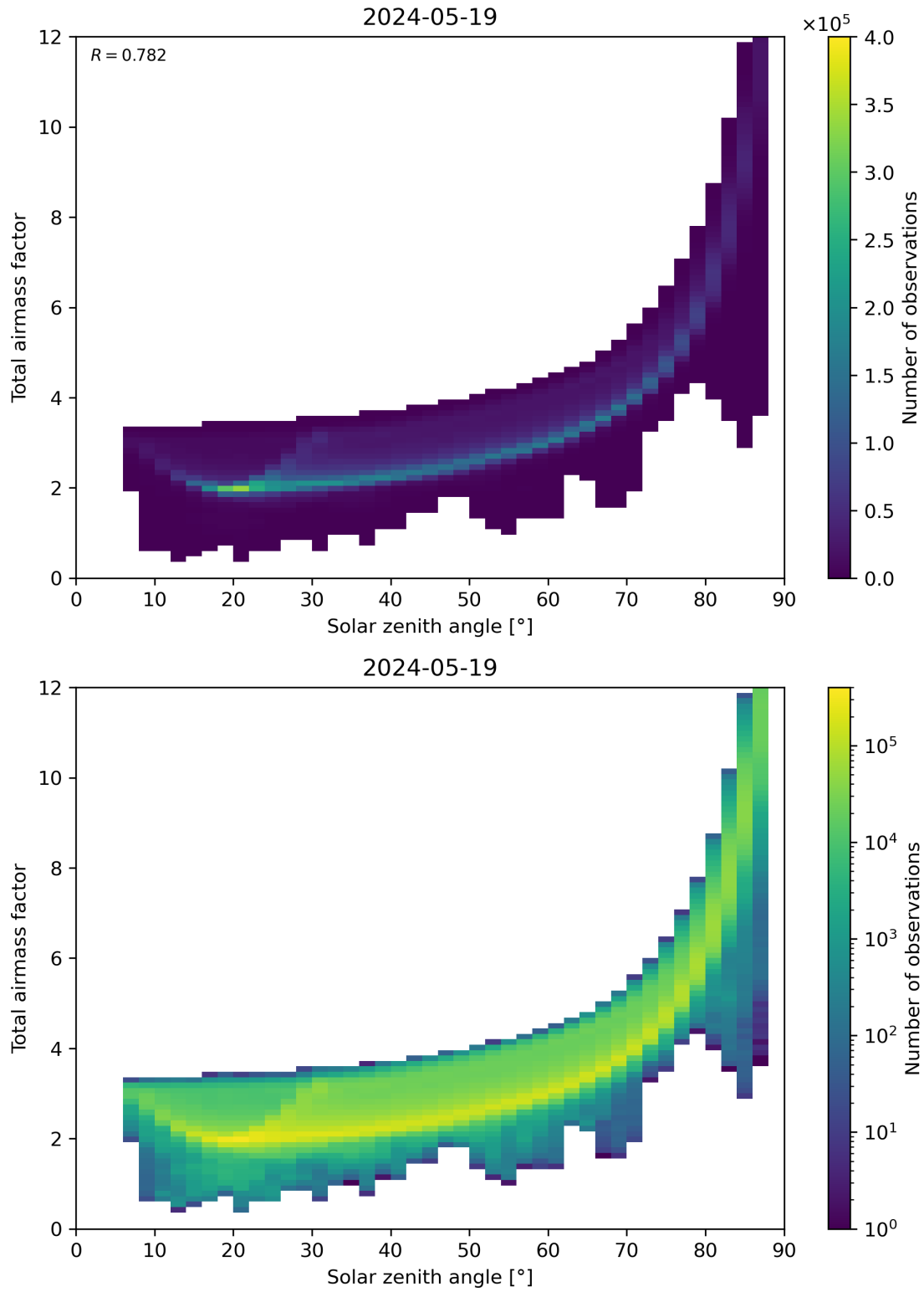
Figure 146: Scatter density plot of “Solar zenith angle” against “Total air mass factor” for 2024-05-18 to 2024-05-20.
