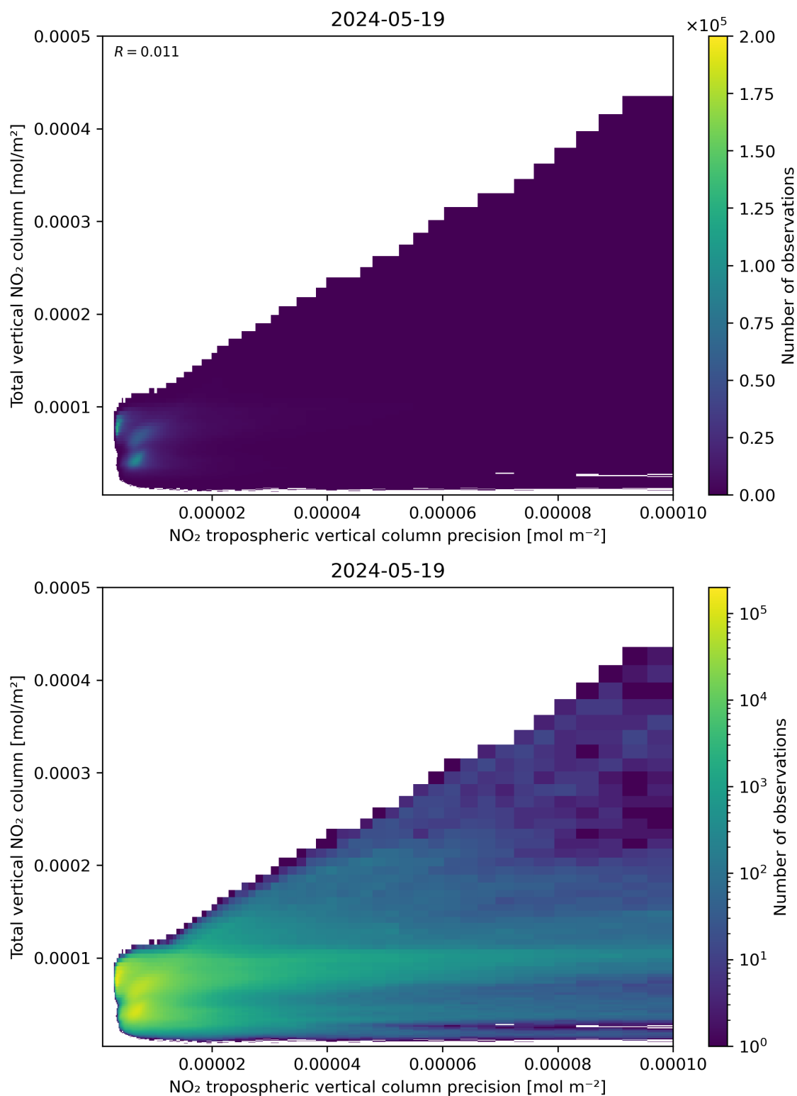
Figure 138: Scatter density plot of “NO 2 tropospheric vertical column precision” against “Total vertical NO 2 column” for 2024-05-18 to 2024-05-20.
