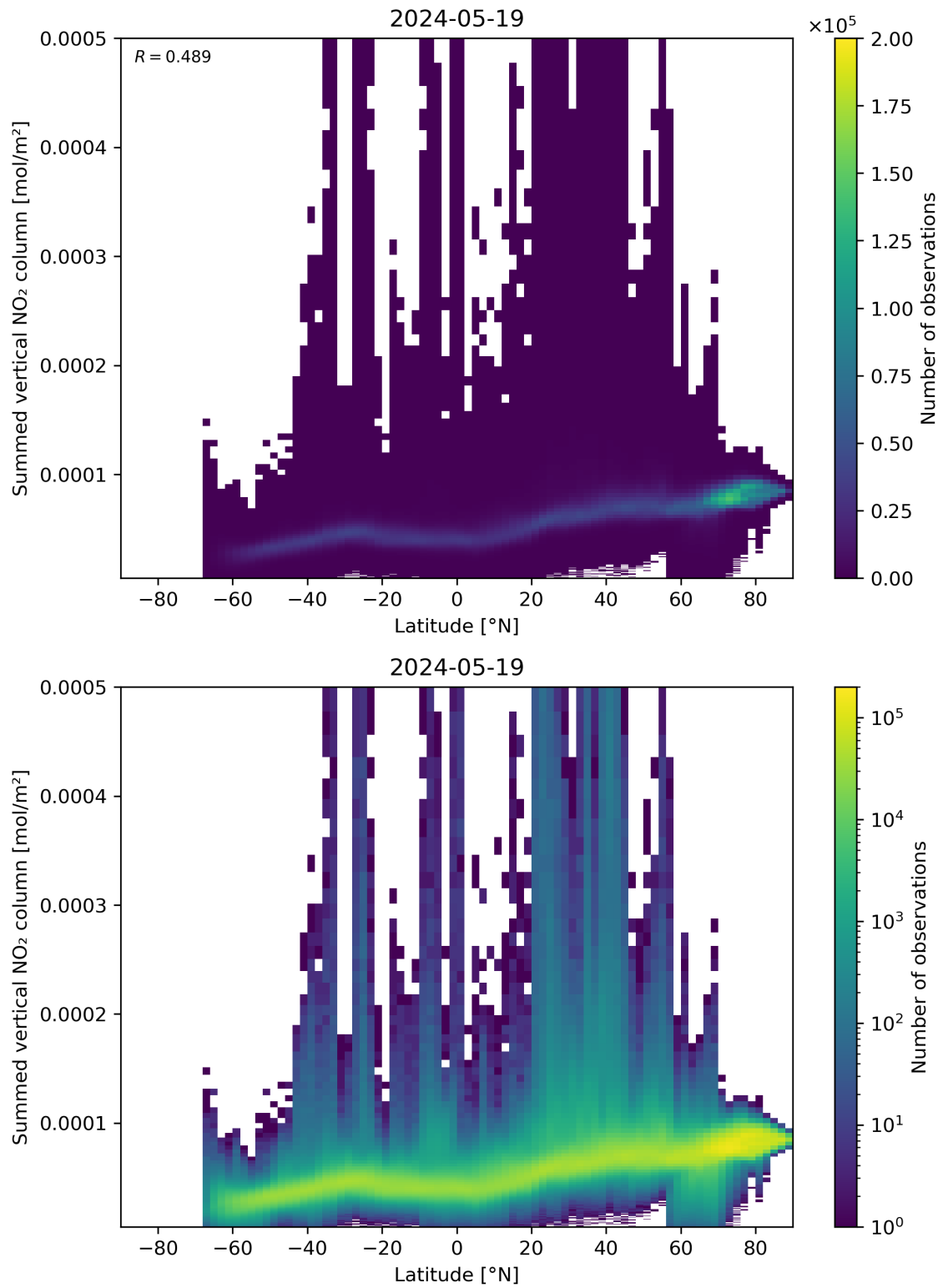
Figure 88: Scatter density plot of “Latitude” against “Summed vertical NO 2 column” for 2024-05-18 to 2024-05-20.
