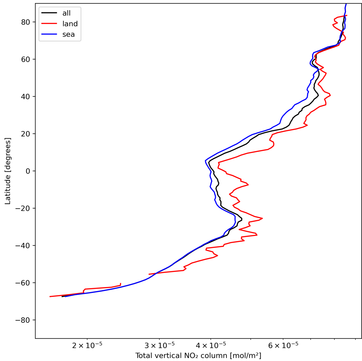
Figure 21: Zonal average of “Total vertical NO 2 column” for 2024-05-18 to 2024-05-20.
