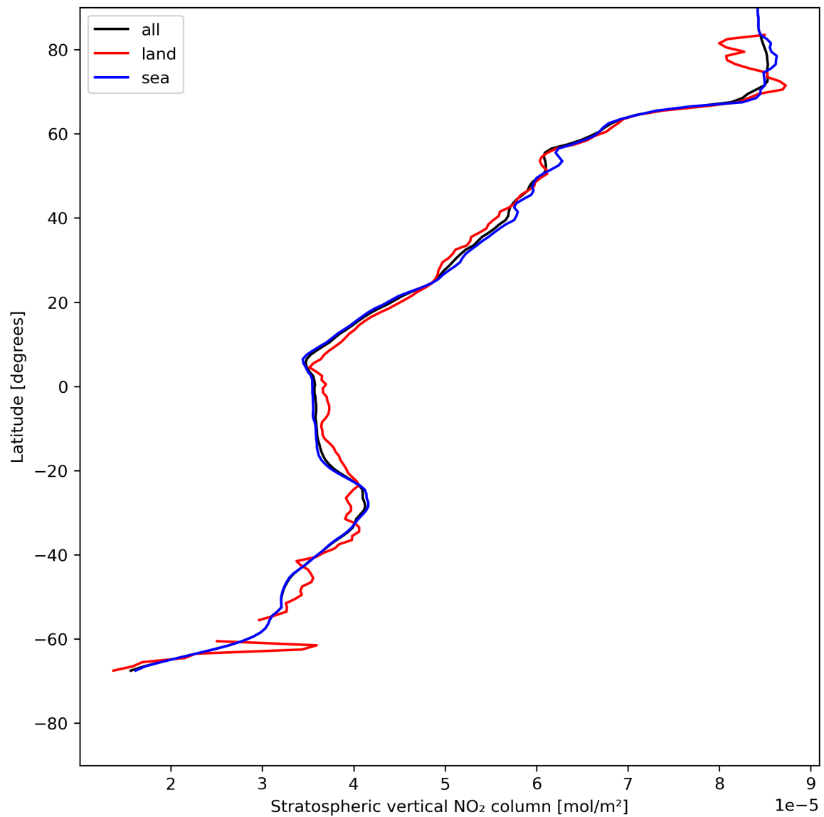
Figure 19: Zonal average of “Stratospheric vertical NO 2 column” for 2024-05-18 to 2024-05-20.
