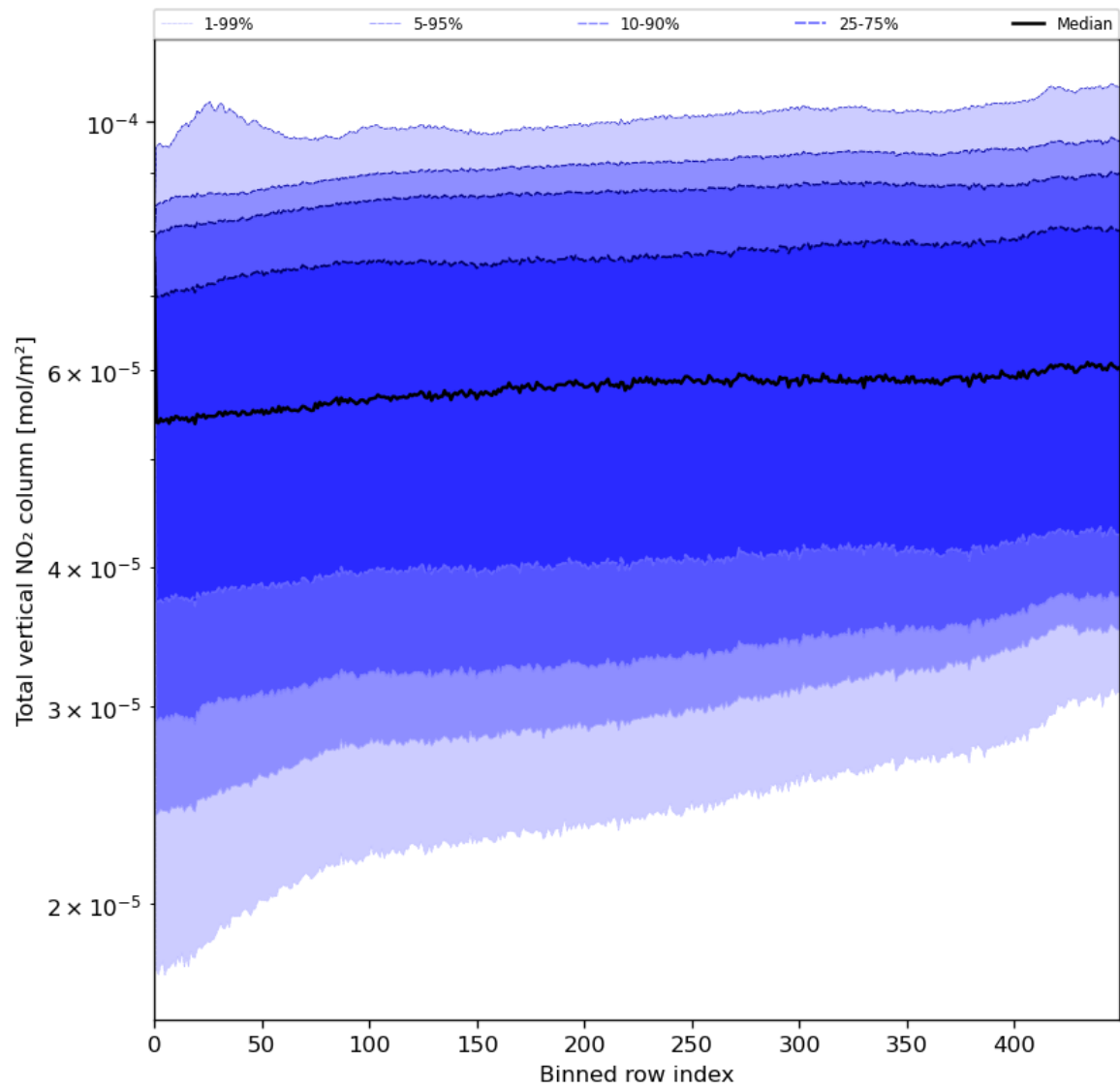
Figure 55: Along track statistics of “Total vertical NO 2 column” for 2024-05-18 to 2024-05-20
