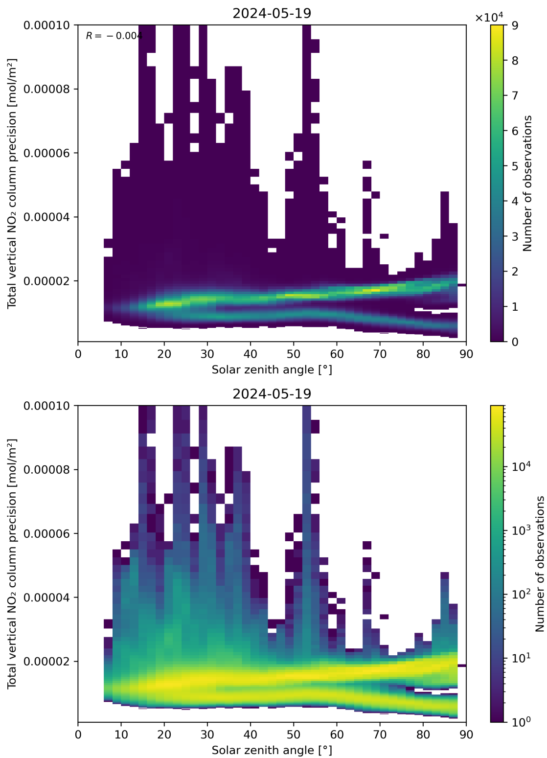
Figure 154: Scatter density plot of “Solar zenith angle” against “Total vertical NO 2 column precision” for 2024-05-18 to 2024-05-20.
