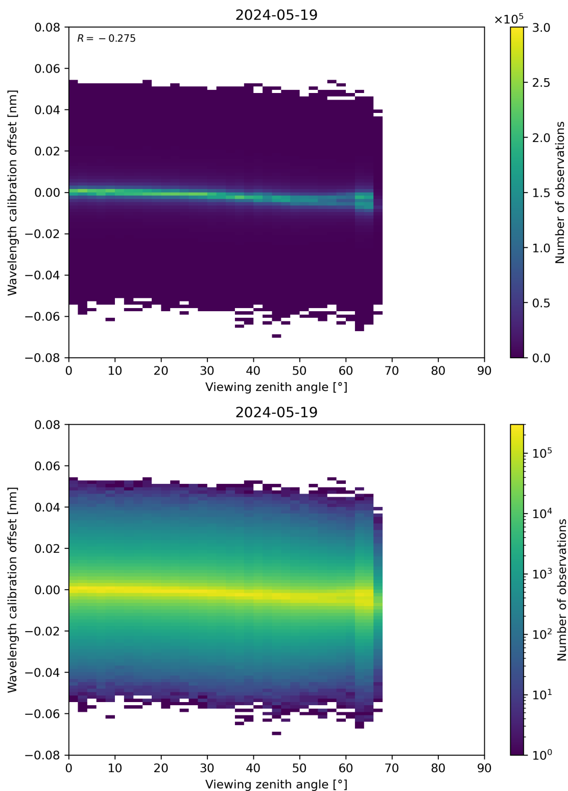
Figure 173: Scatter density plot of “Viewing zenith angle” against “Wavelength calibration offset” for 2024-05-18 to 2024-05-20.
