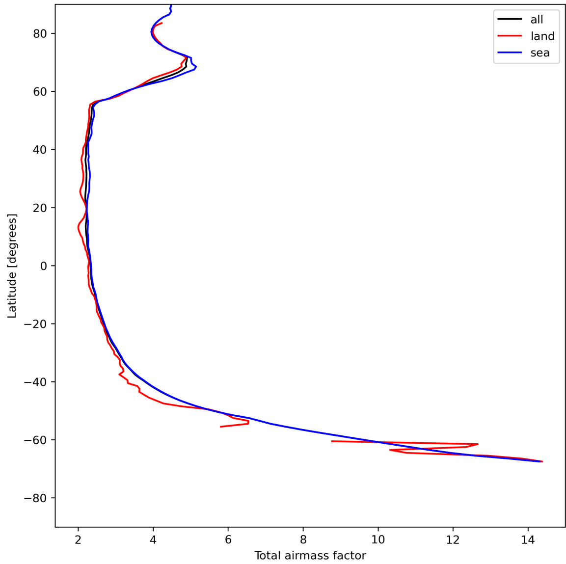
Figure 15: Zonal average of “Total airmass factor” for 2024-05-18 to 2024-05-20.
