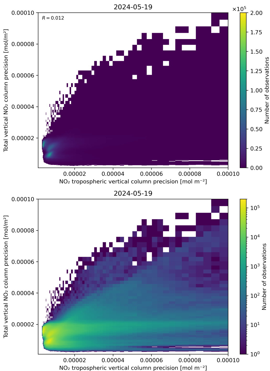
Figure 139: Scatter density plot of “NO 2 tropospheric vertical column precision” against “Total vertical NO 2 column precision” for 2024-05-18 to 2024-05-20.
