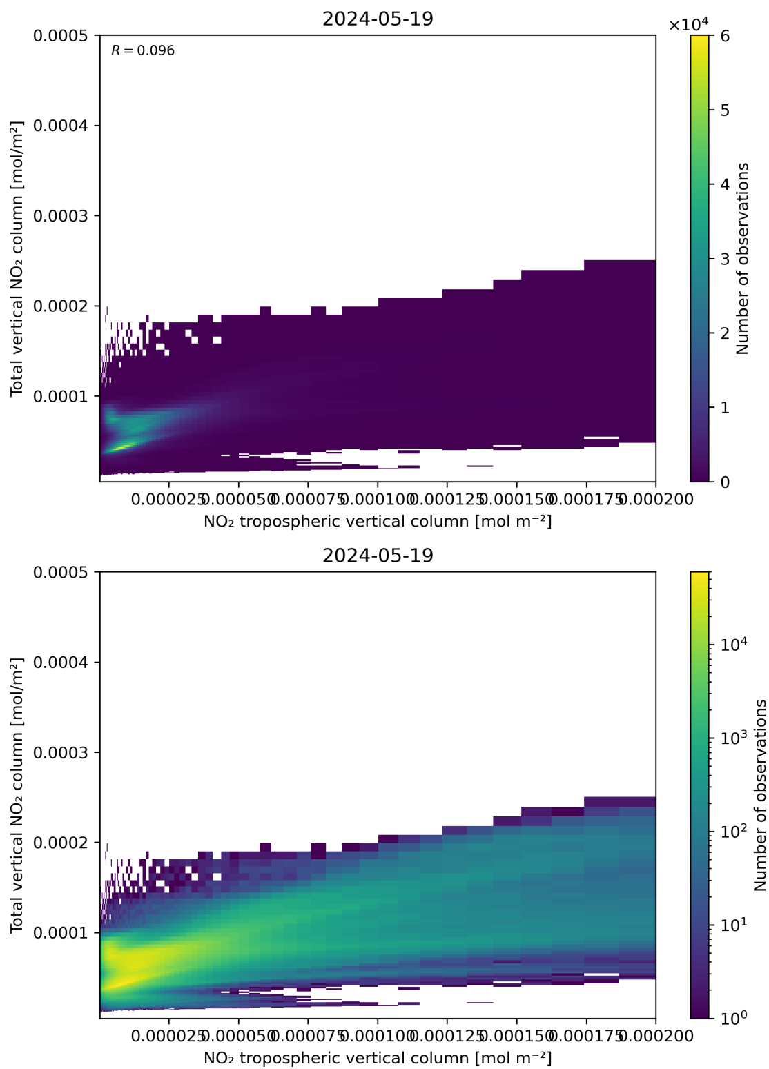
Figure 128: Scatter density plot of “NO 2 tropospheric vertical column” against “Total vertical NO 2 column” for 2024-05-18 to 2024-05-20.
