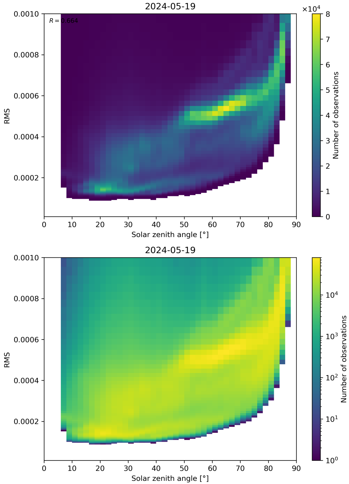
Figure 157: Scatter density plot of “Solar zenith angle” against “RMS” for 2024-05-18 to 2024-05-20.
