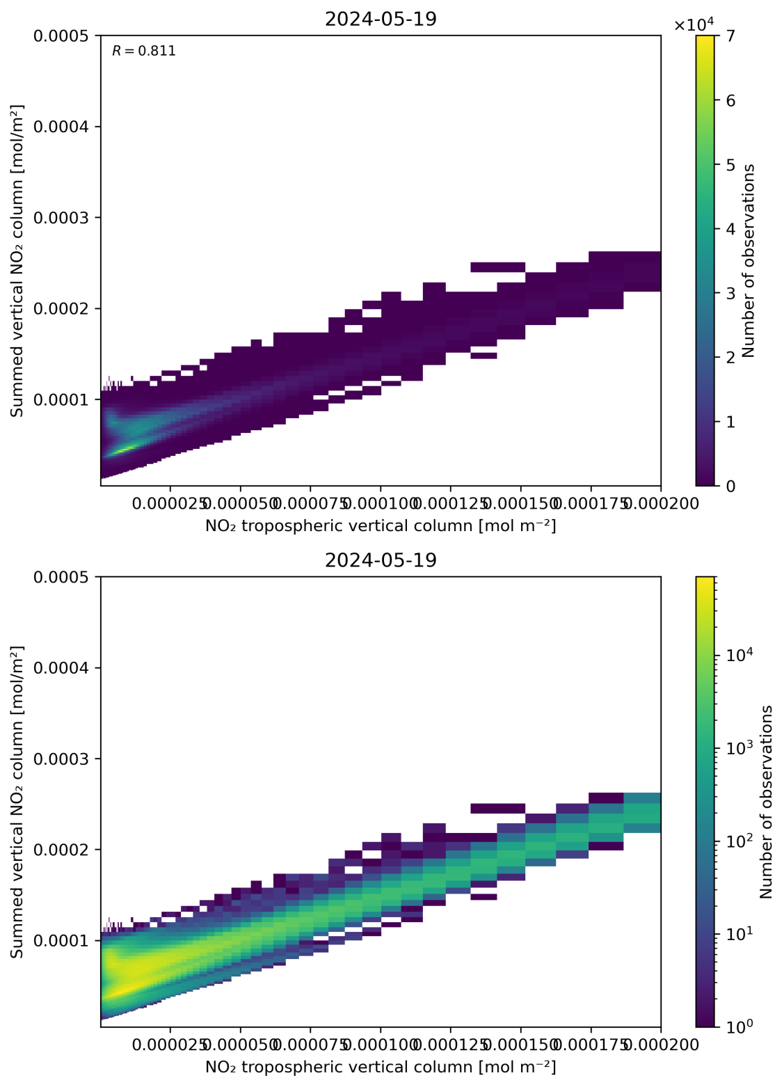
Figure 126: Scatter density plot of “NO 2 tropospheric vertical column” against “Summed vertical NO 2 column” for 2024-05-18 to 2024-05-20.
