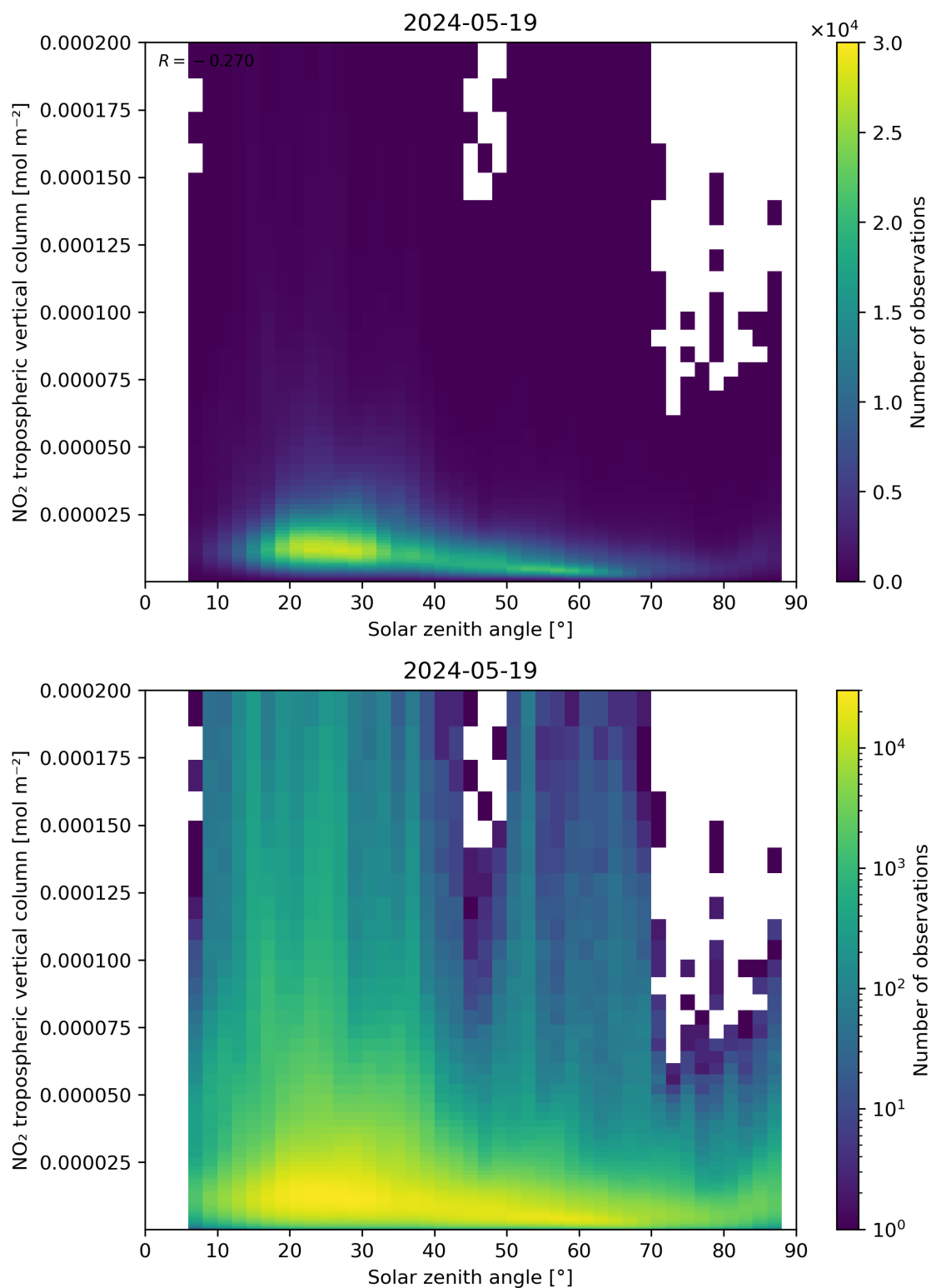
Figure 155: Scatter density plot of “Solar zenith angle” against “NO 2 tropospheric vertical column” for 2024-05-18 to 2024-05-20.
