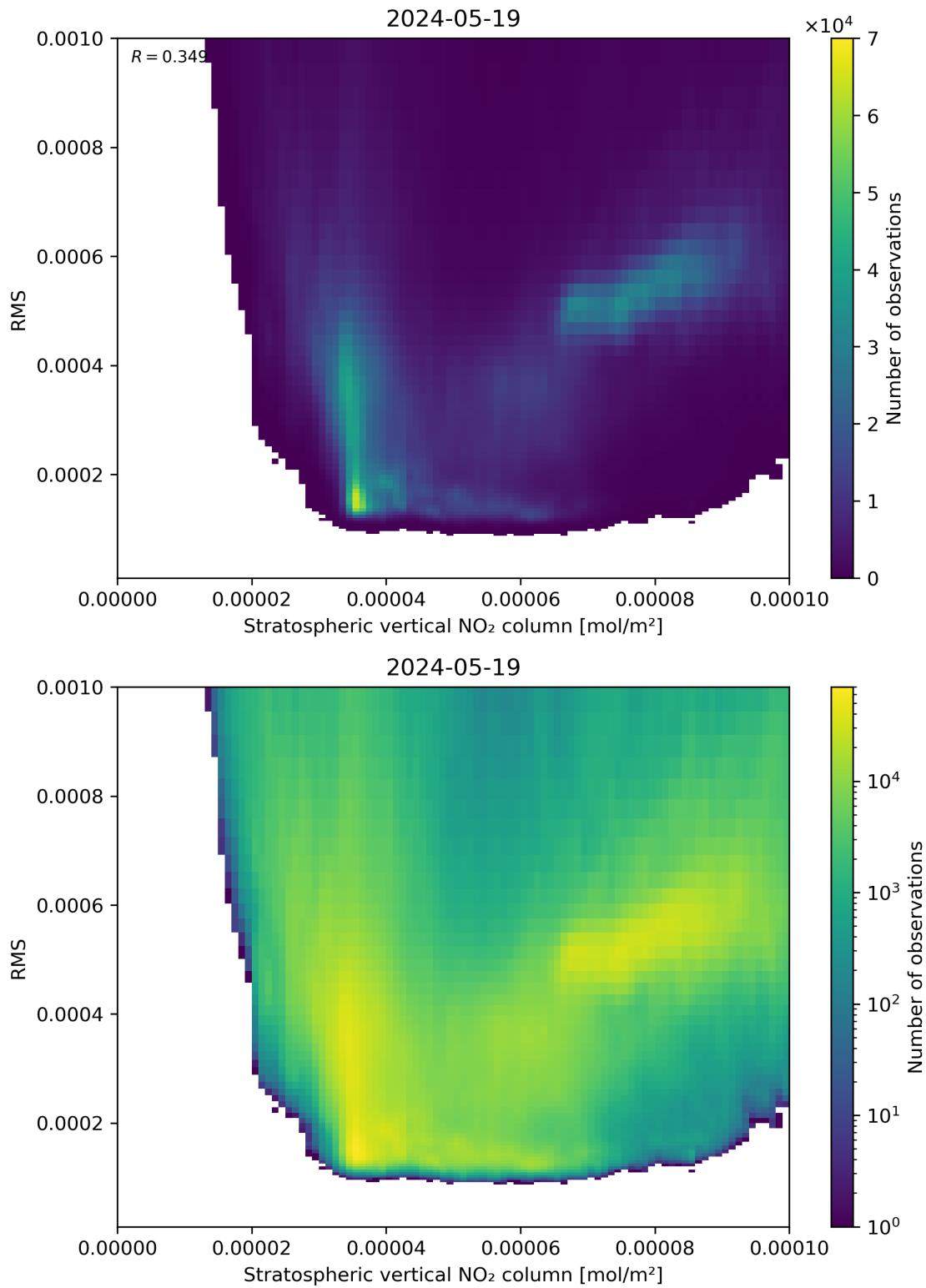
Figure 102: Scatter density plot of “Stratospheric vertical NO 2 column” against “RMS” for 2024-05-18 to 2024-05-20.
