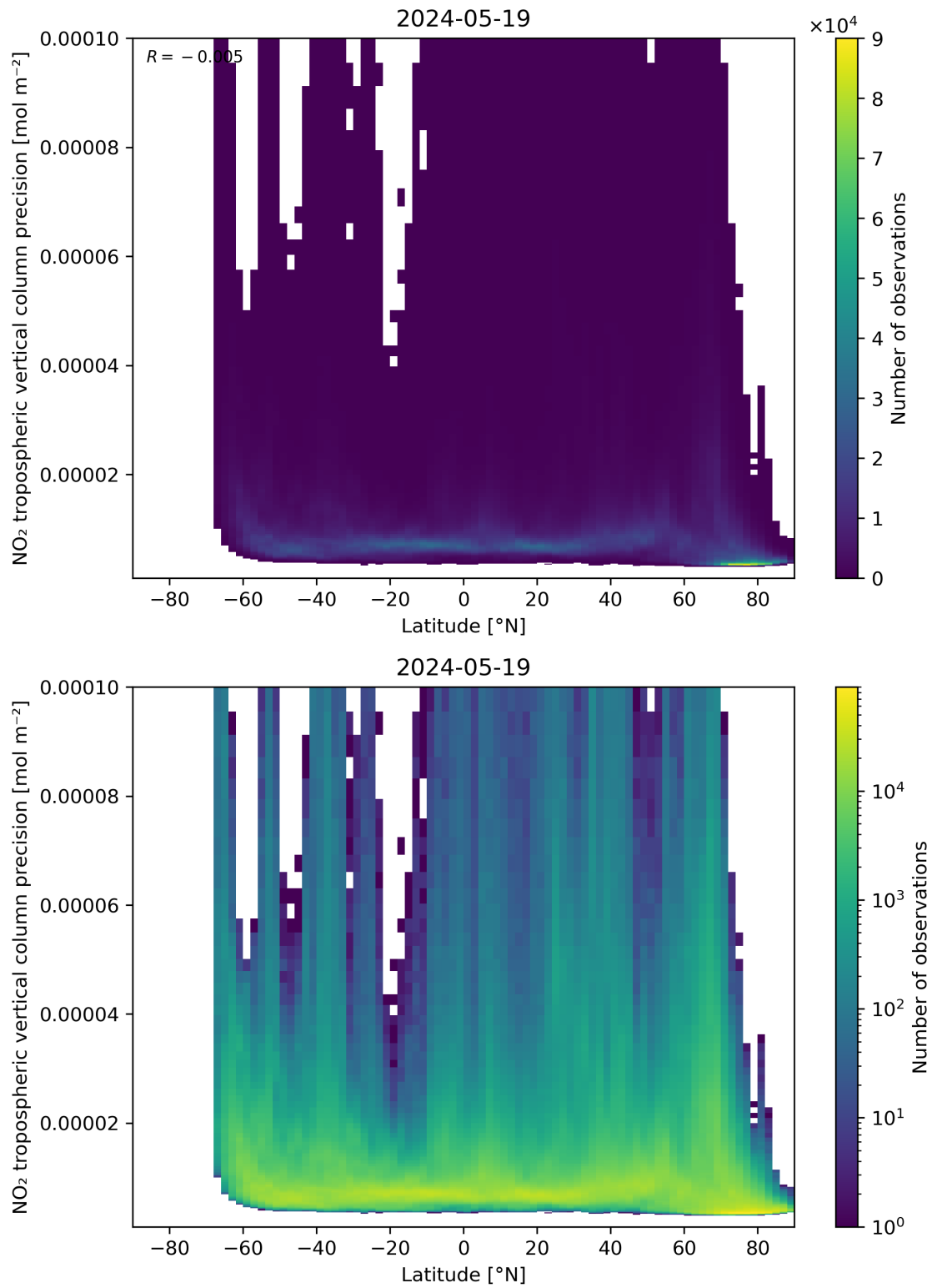
Figure 93: Scatter density plot of “Latitude” against “NO 2 tropospheric vertical column precision” for 2024-05-18 to 2024-05-20.
