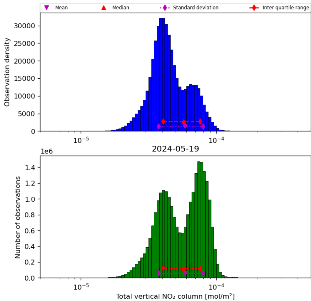
Figure 38: Histogram of “Total vertical NO 2 column” for 2024-05-18 to 2024-05-20
