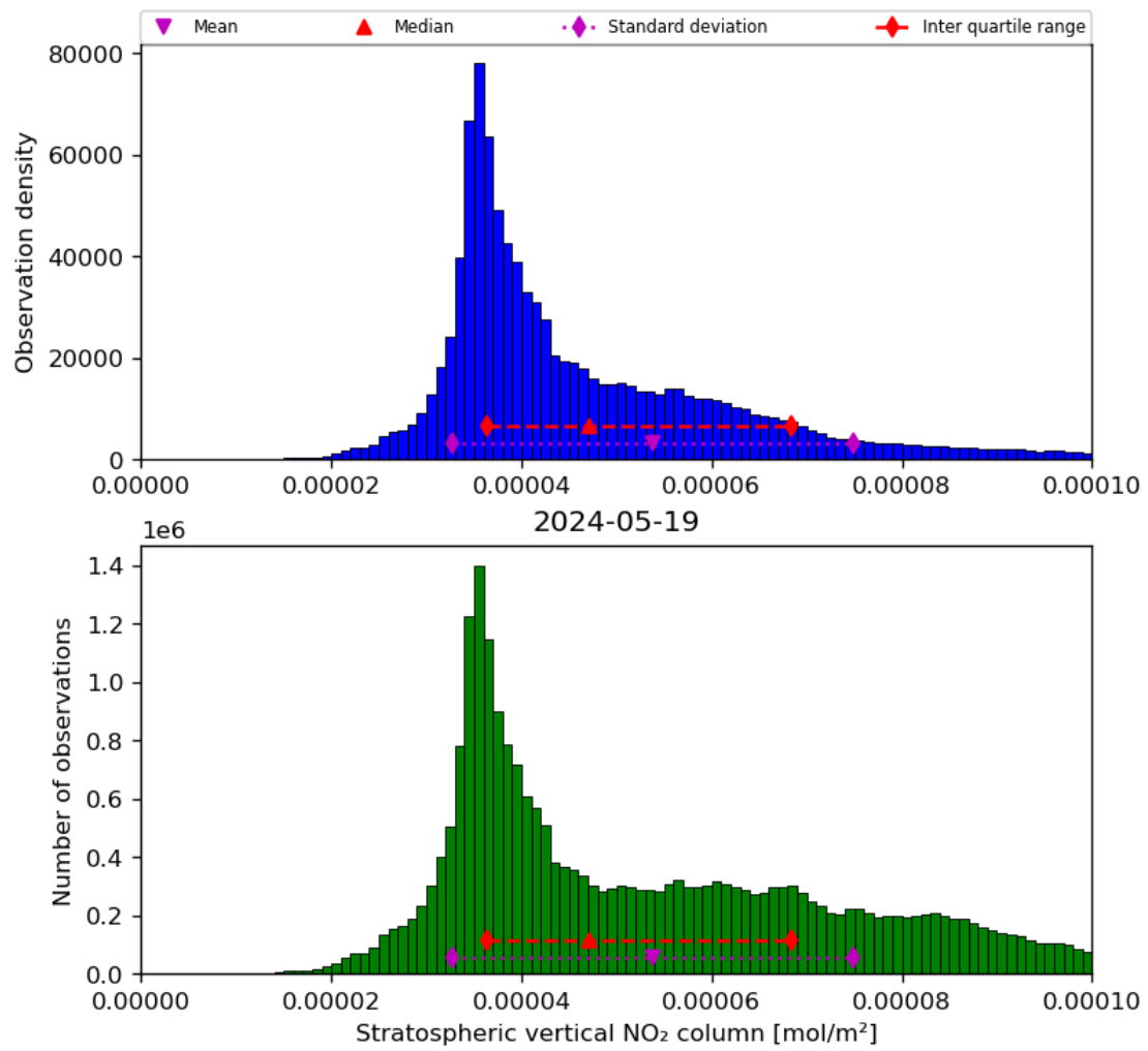
Figure 36: Histogram of “Stratospheric vertical NO 2 column” for 2024-05-18 to 2024-05-20
