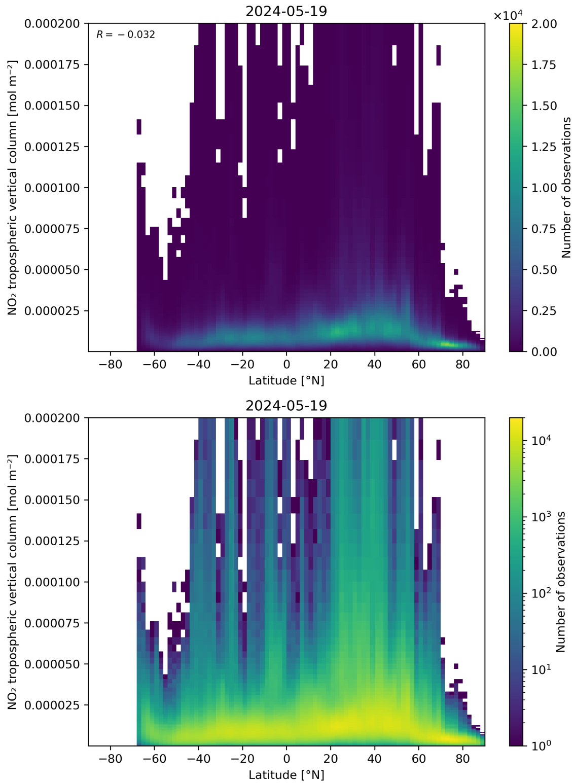
Figure 92: Scatter density plot of “Latitude” against “NO 2 tropospheric vertical column” for 2024-05-18 to 2024-05-20.
