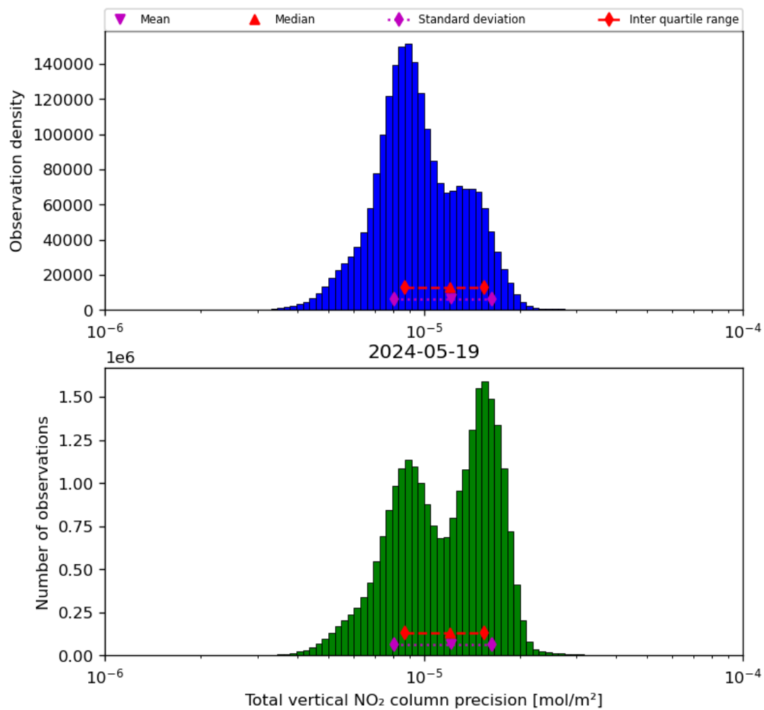
Figure 39: Histogram of “Total vertical NO 2 column precision” for 2024-05-18 to 2024-05-20
