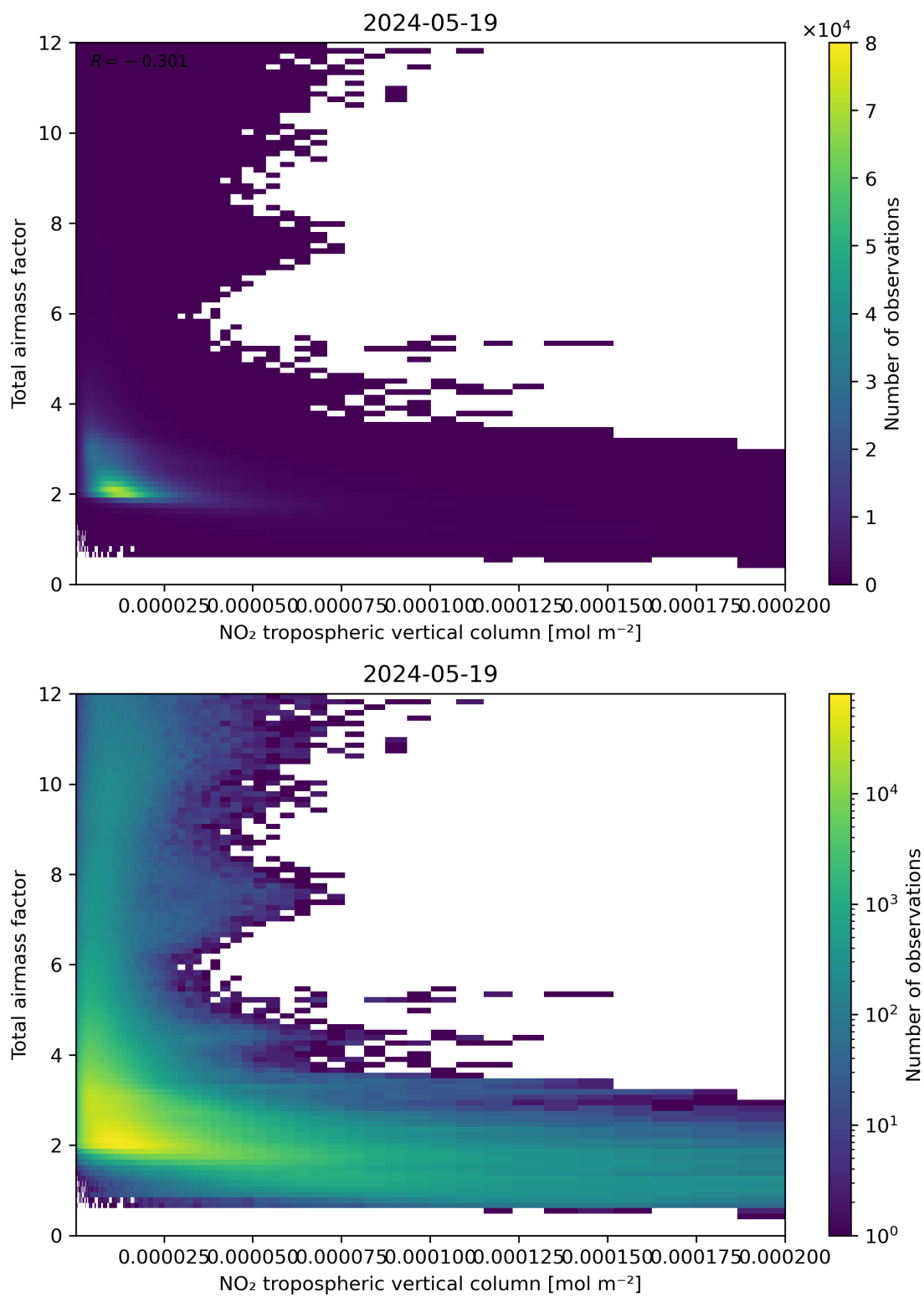
Figure 122: Scatter density plot of “NO 2 tropospheric vertical column” against “Total air mass factor” for 2024-05-18 to 2024-05-20.
