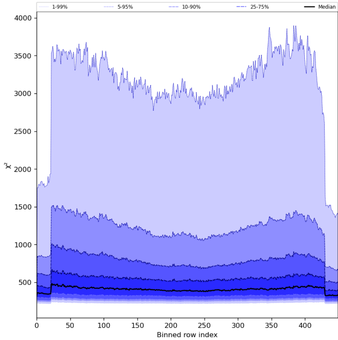
Figure 59: Along track statistics of “ \chi^2 ” for 2024-05-18 to 2024-05-20
