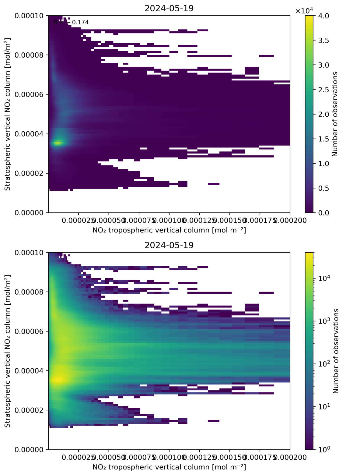
Figure 125: Scatter density plot of “NO 2 tropospheric vertical column” against “Stratospheric vertical NO 2 column” for 2024-05-18 to 2024-05-20.
