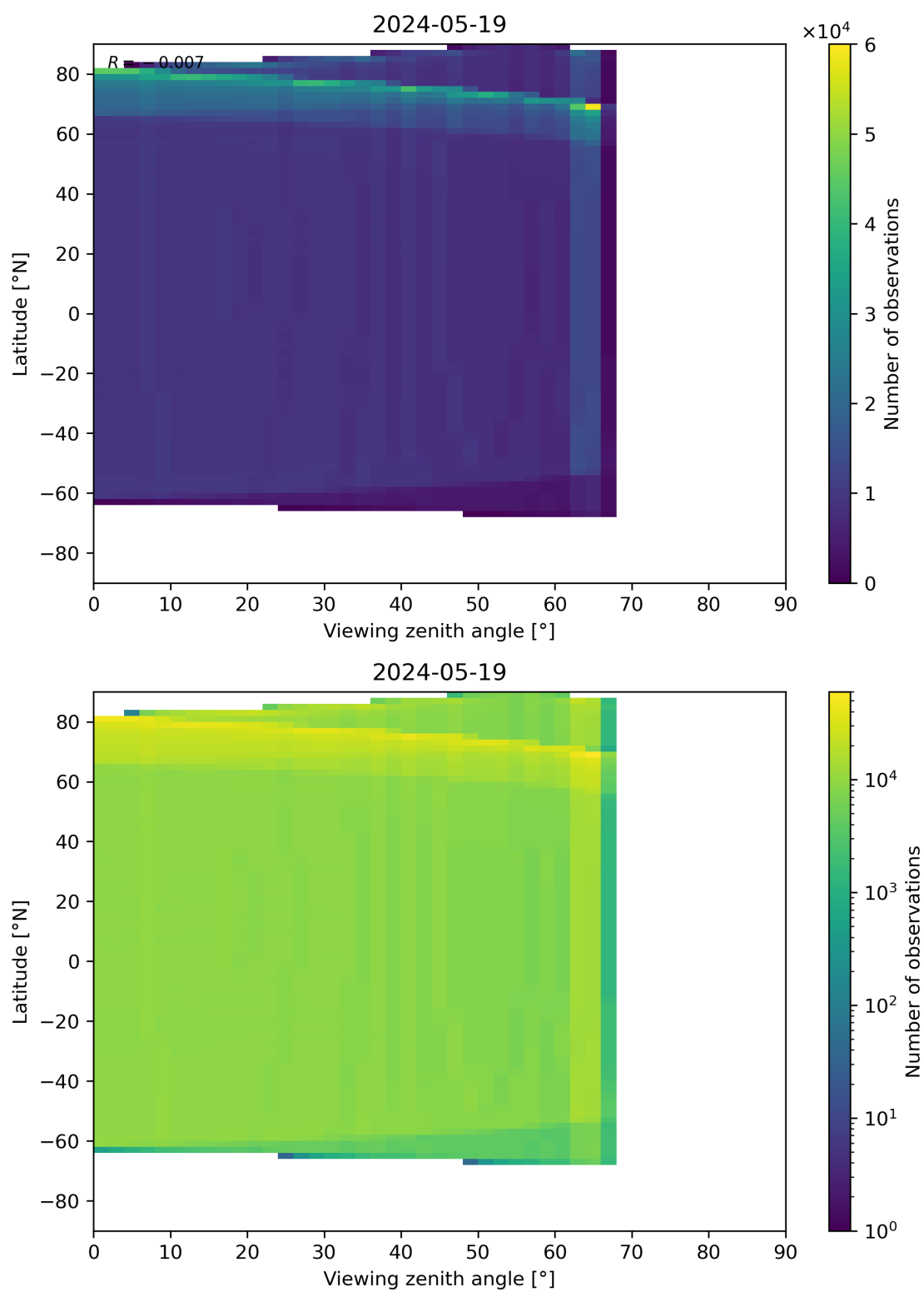
Figure 163: Scatter density plot of “Viewing zenith angle” against “Latitude” for 2024-05-18 to 2024-05-20.
