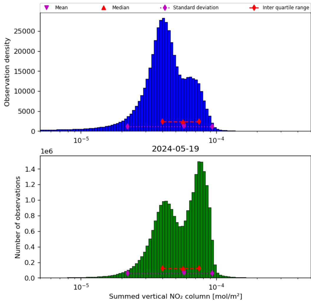
Figure 40: Histogram of “Summed vertical NO 2 column” for 2024-05-18 to 2024-05-20
