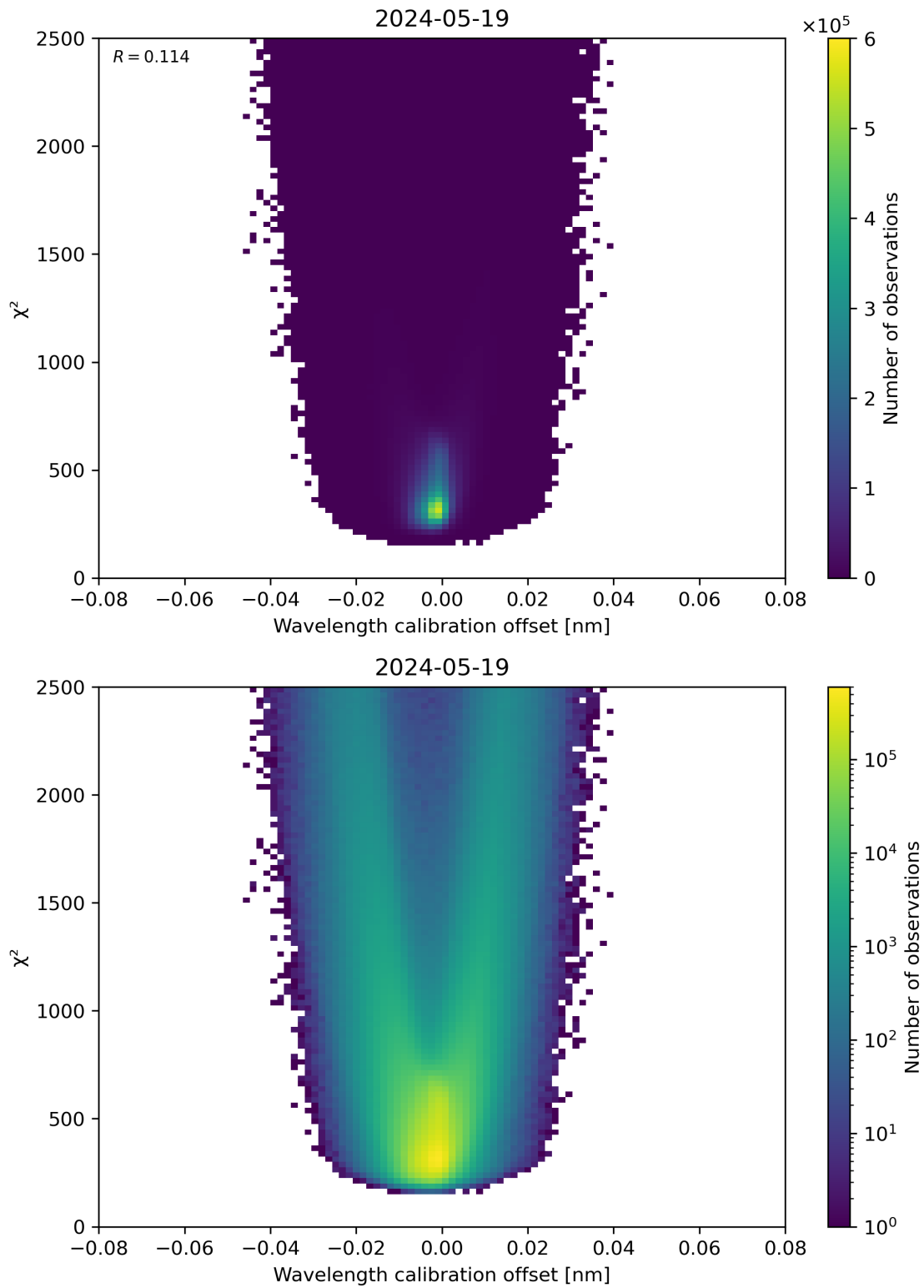
Figure 175: Scatter density plot of “Wavelength calibration offset” against “ \chi^2 ” for 2024-05-18 to 2024-05-20.
