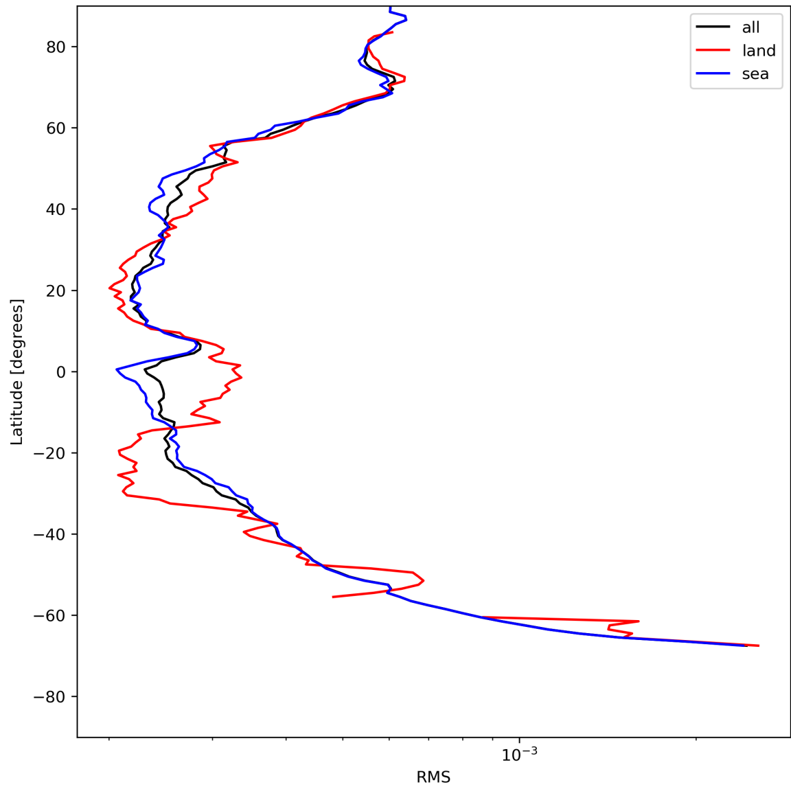
Figure 26: Zonal average of “RMS” for 2024-05-18 to 2024-05-20.
