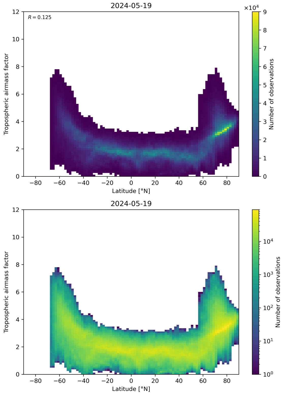
Figure 85: Scatter density plot of “Latitude” against “Tropospheric airmass factor” for 2024-05-18 to 2024-05-20.
