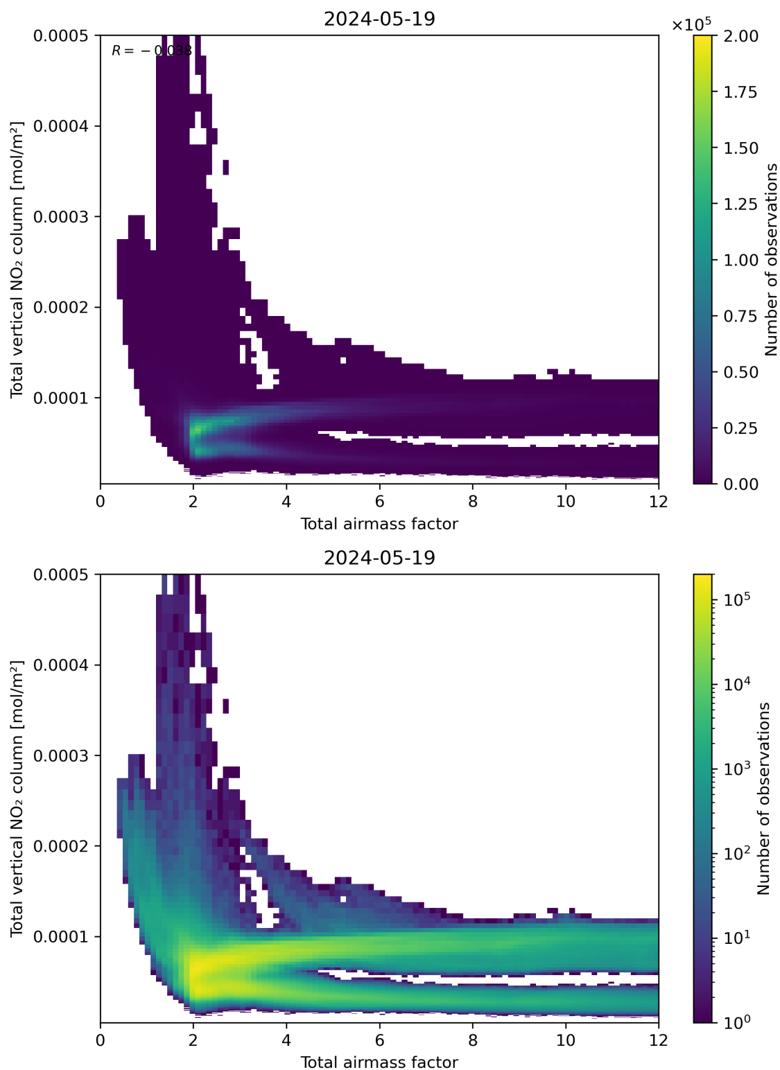
Figure 67: Scatter density plot of “Total airmass factor” against “Total vertical NO 2 column” for 2024-05-18 to 2024-05-20.
