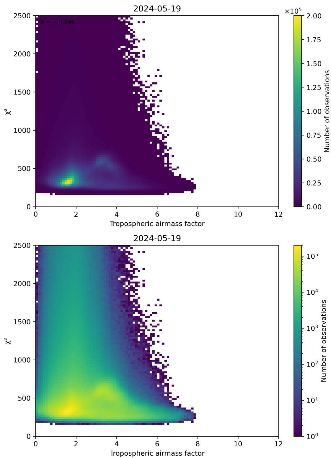
Figure 73: Scatter density plot of “Tropospheric airmass factor” against “ \chi^2 ” for 2024-05-18 to 2024-05-20.
