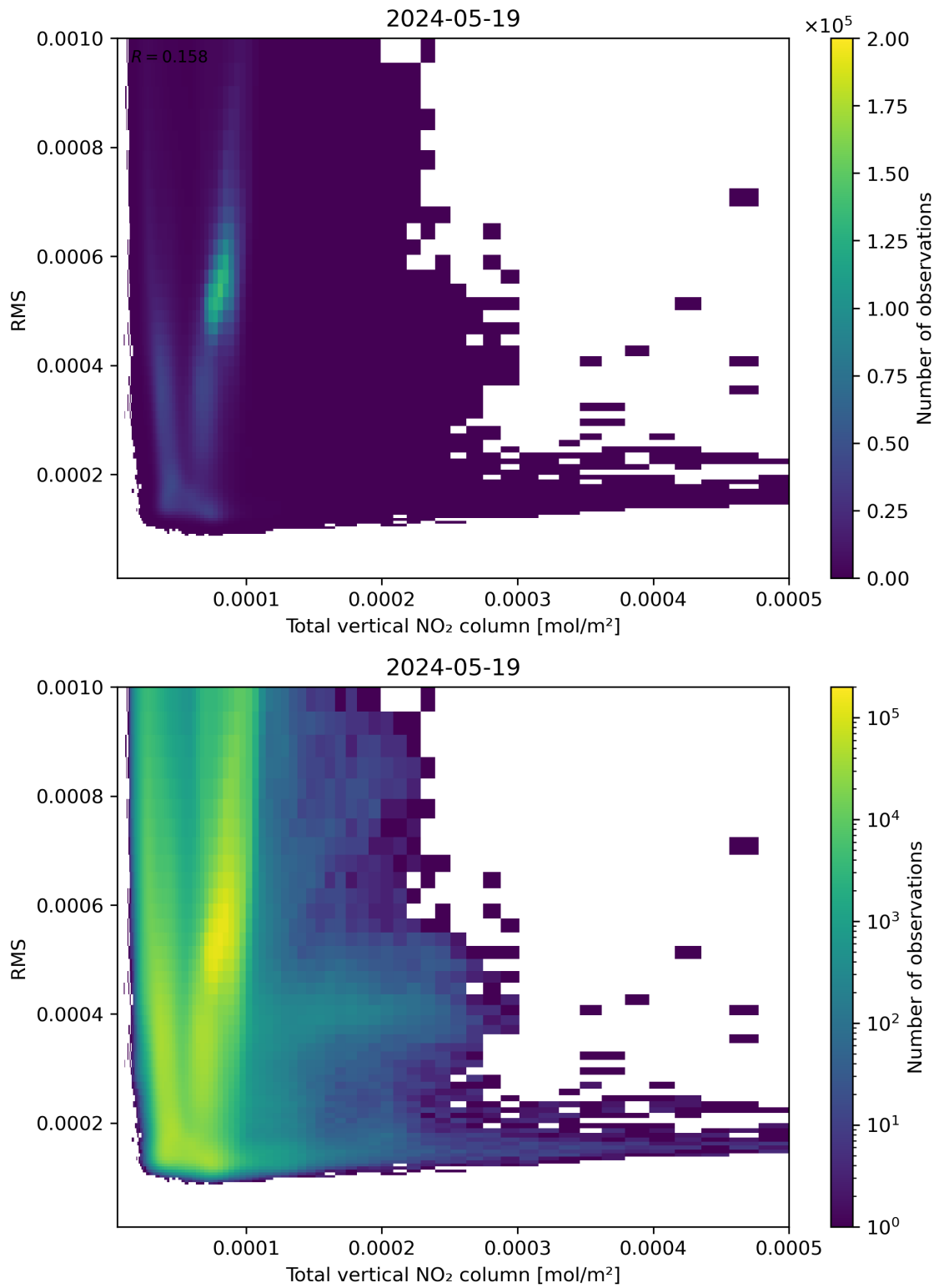
Figure 120: Scatter density plot of “Total vertical NO 2 column” against “RMS” for 2024-05-18 to 2024-05-20.
