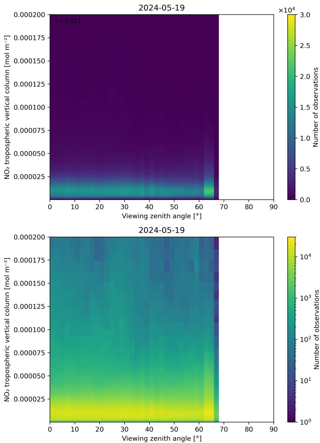
Figure 169: Scatter density plot of “Viewing zenith angle” against “NO 2 tropospheric vertical column” for 2024-05-18 to 2024-05-20.
