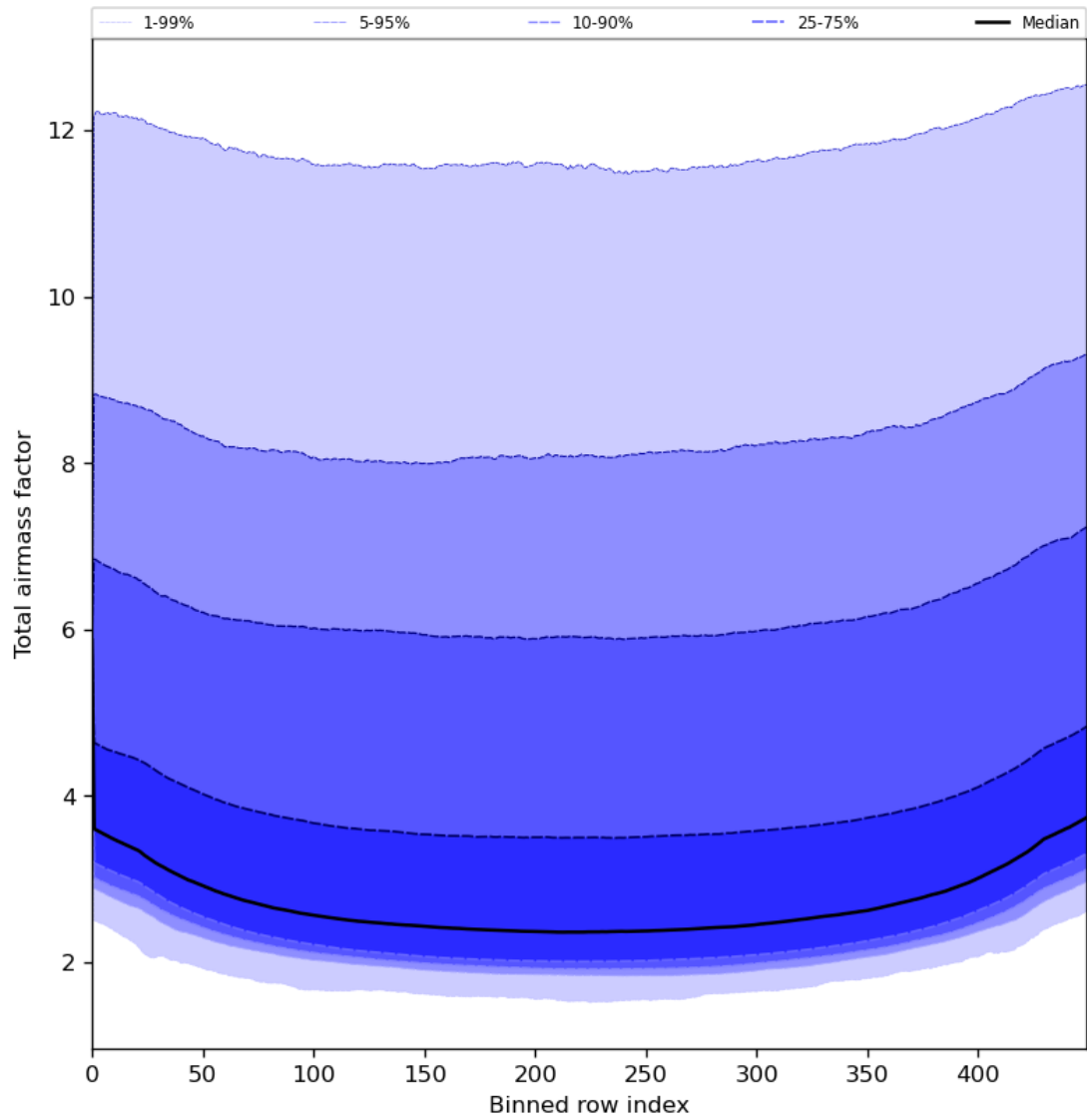
Figure 49: Along track statistics of “Total airmass factor” for 2024-05-18 to 2024-05-20
