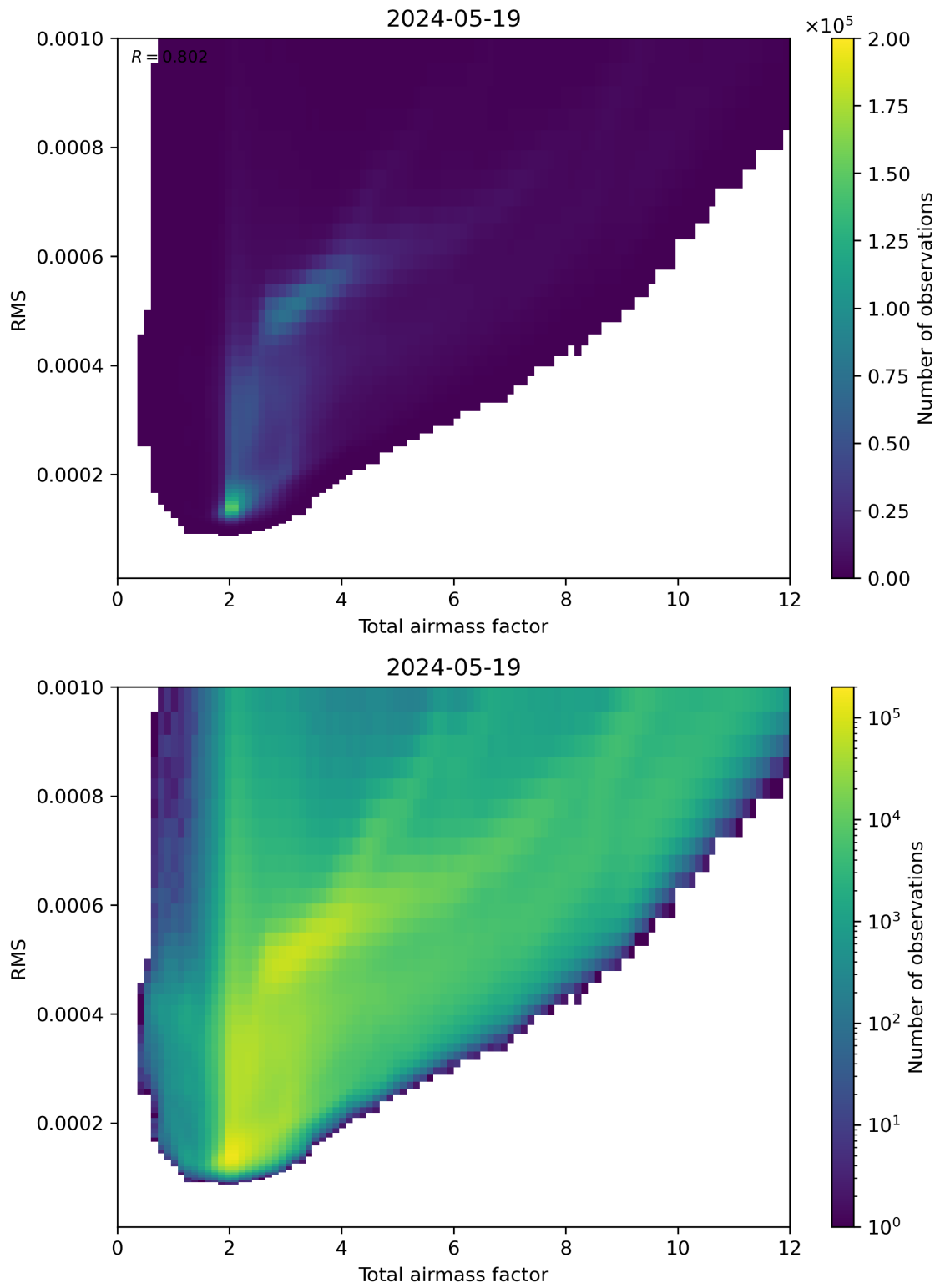
Figure 69: Scatter density plot of “Total airmass factor” against “RMS” for 2024-05-18 to 2024-05-20.
