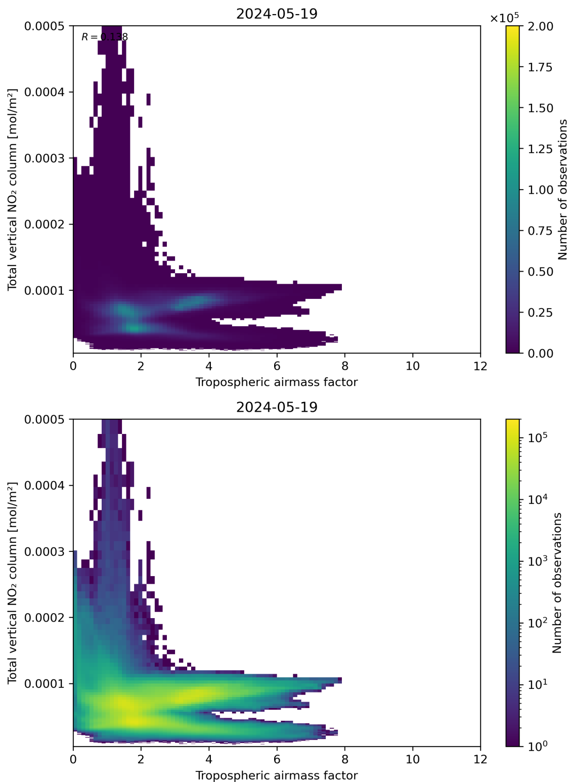
Figure 77: Scatter density plot of “Tropospheric airmass factor” against “Total vertical NO 2 column” for 2024-05-18 to 2024-05-20.
