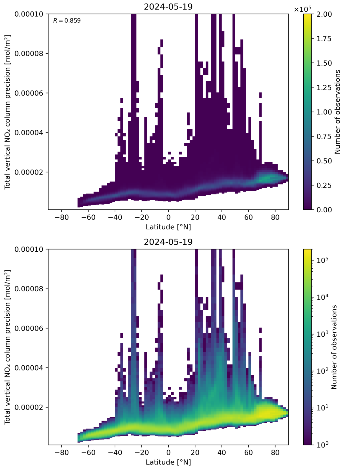
Figure 91: Scatter density plot of “Latitude” against “Total vertical NO 2 column precision” for 2024-05-18 to 2024-05-20.
