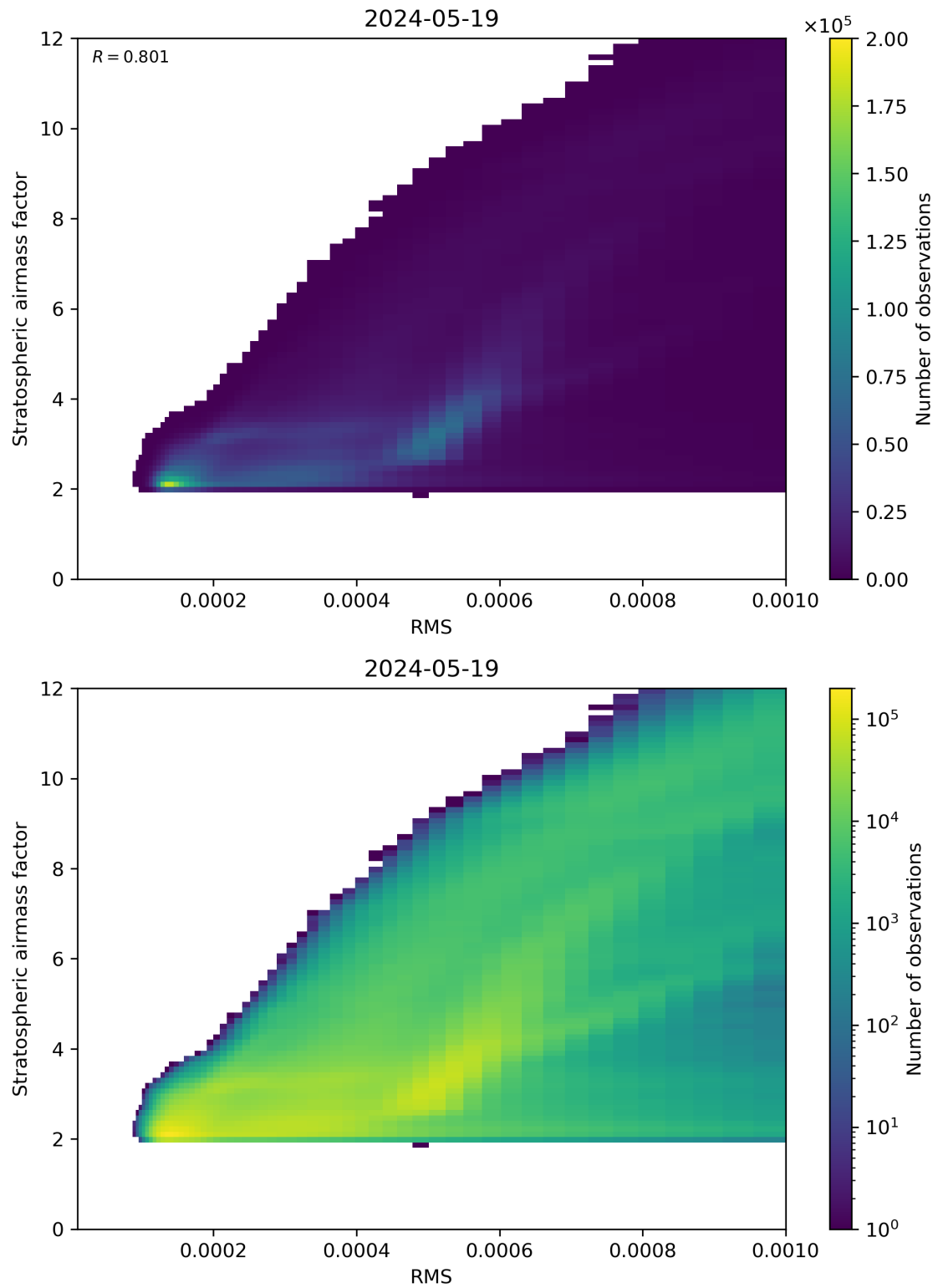
Figure 144: Scatter density plot of “RMS” against “Stratospheric airmass factor” for 2024-05-18 to 2024-05-20.
