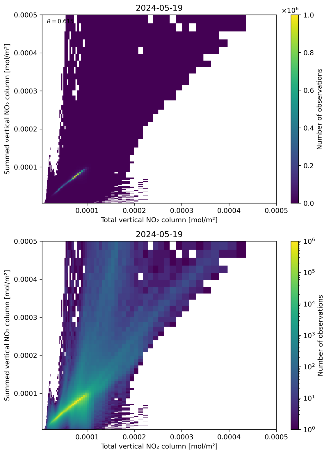
Figure 112: Scatter density plot of “Total vertical NO 2 column” against “Summed vertical NO 2 column” for 2024-05-18 to 2024-05-20.
