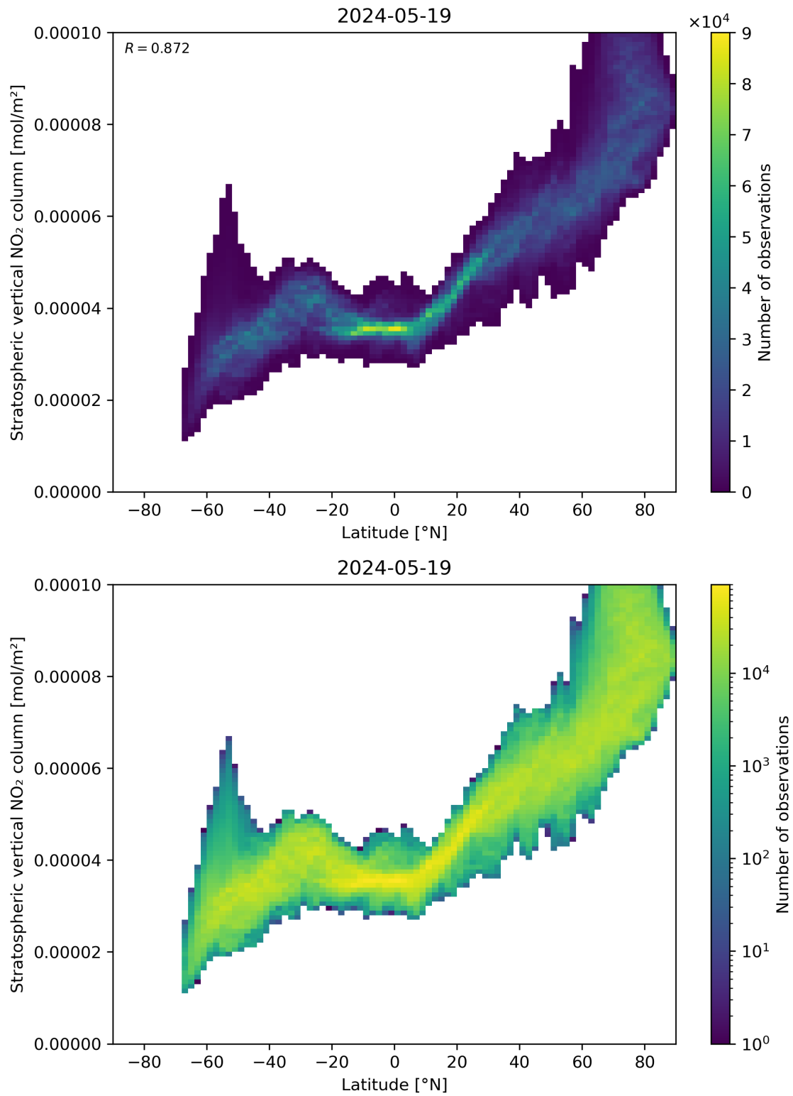
Figure 87: Scatter density plot of “Latitude” against “Stratospheric vertical NO 2 column” for 2024-05-18 to 2024-05-20.
