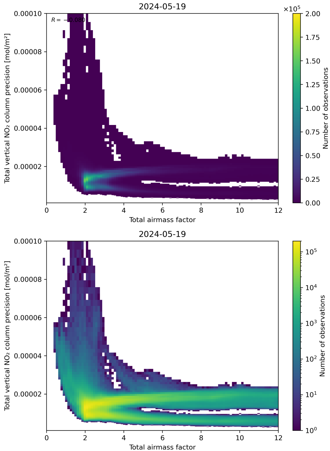
Figure 68: Scatter density plot of “Total airmass factor” against “Total vertical NO 2 column precision” for 2024-05-18 to 2024-05-20.
