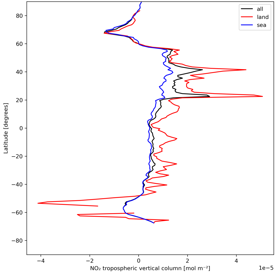
Figure 12: Zonal average of “NO 2 tropospheric vertical column” for 2024-05-18 to 2024-05-20.
