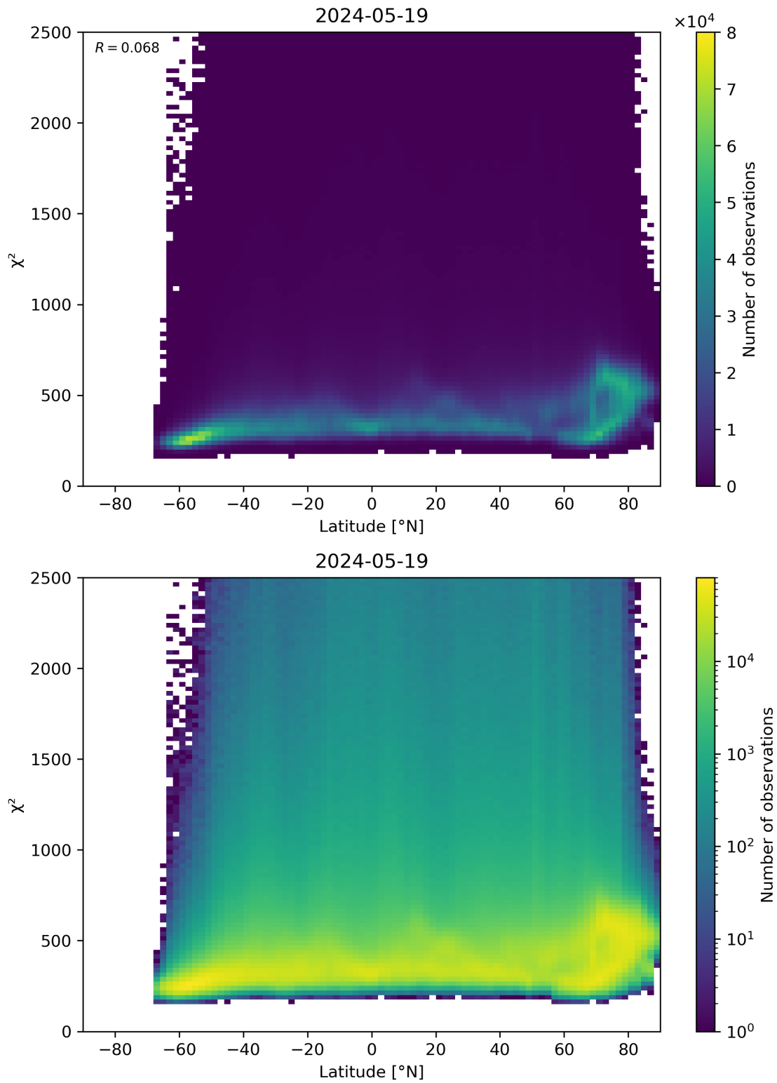
Figure 86: Scatter density plot of “Latitude” against “ \chi^2 ” for 2024-05-18 to 2024-05-20.
