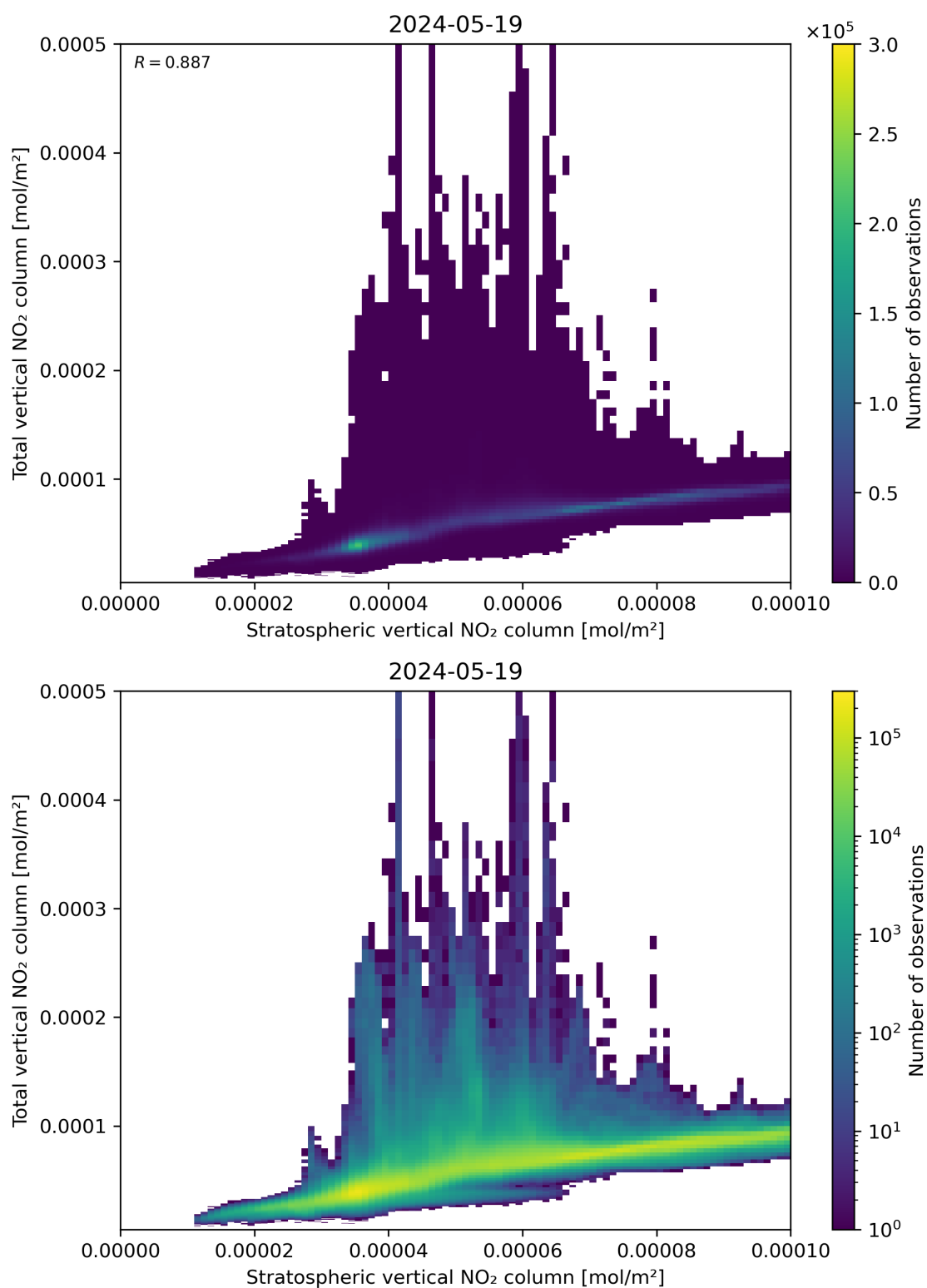
Figure 100: Scatter density plot of “Stratospheric vertical NO 2 column” against “Total vertical NO 2 column” for 2024-05-18 to 2024-05-20.
