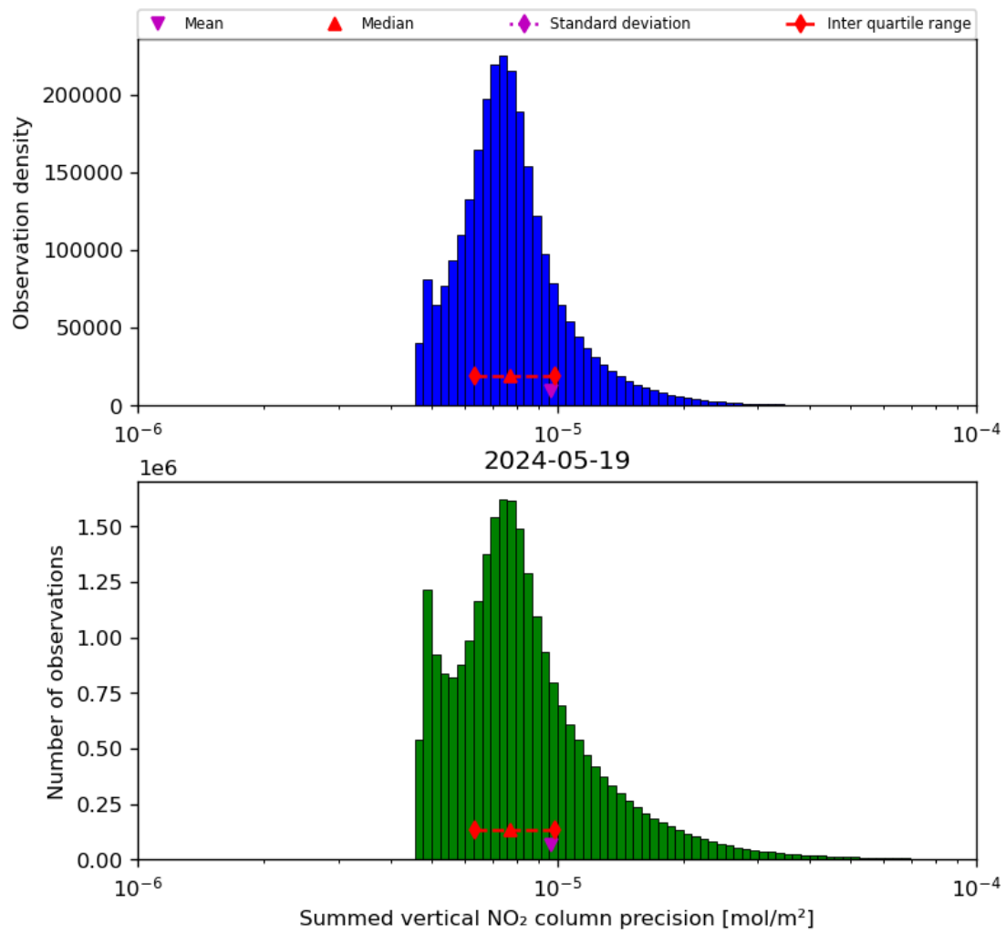
Figure 41: Histogram of “Summed vertical NO 2 column precision” for 2024-05-18 to 2024-05-20
