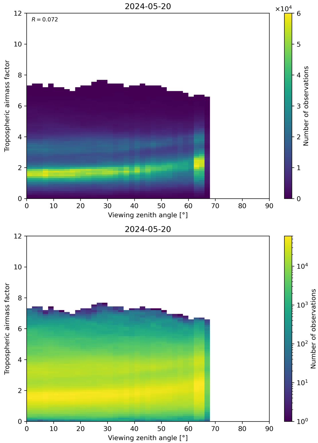
Figure 161: Scatter density plot of “Viewing zenith angle” against “Tropospheric airmass factor” for 2024-05-19 to 2024-05-21.
