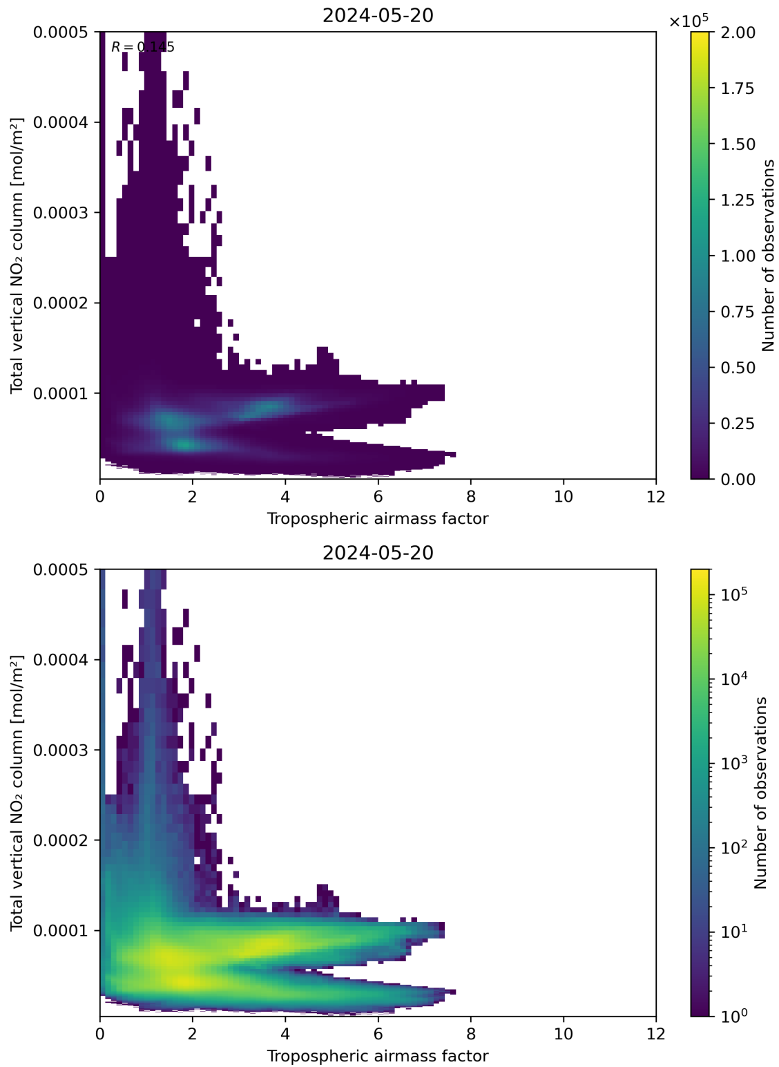
Figure 77: Scatter density plot of “Tropospheric airmass factor” against “Total vertical NO 2 column” for 2024-05-19 to 2024-05-21.
