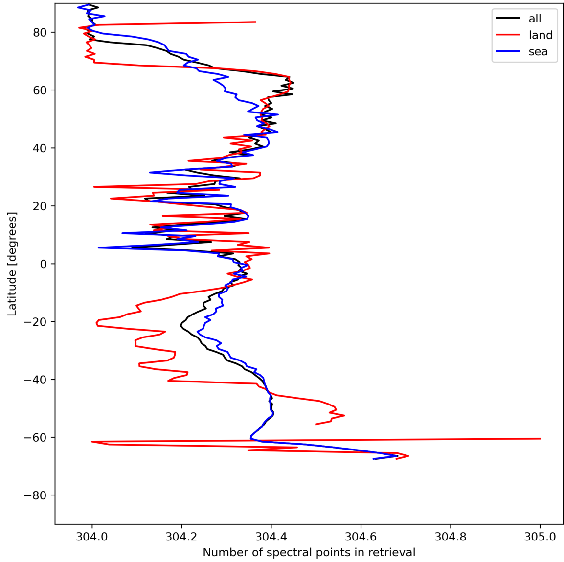
Figure 16: Zonal average of “Number of spectral points in retrieval” for 2024-05-19 to 2024-05-21.
