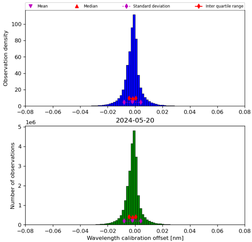
Figure 35: Histogram of “Wavelength calibration offset” for 2024-05-19 to 2024-05-21
