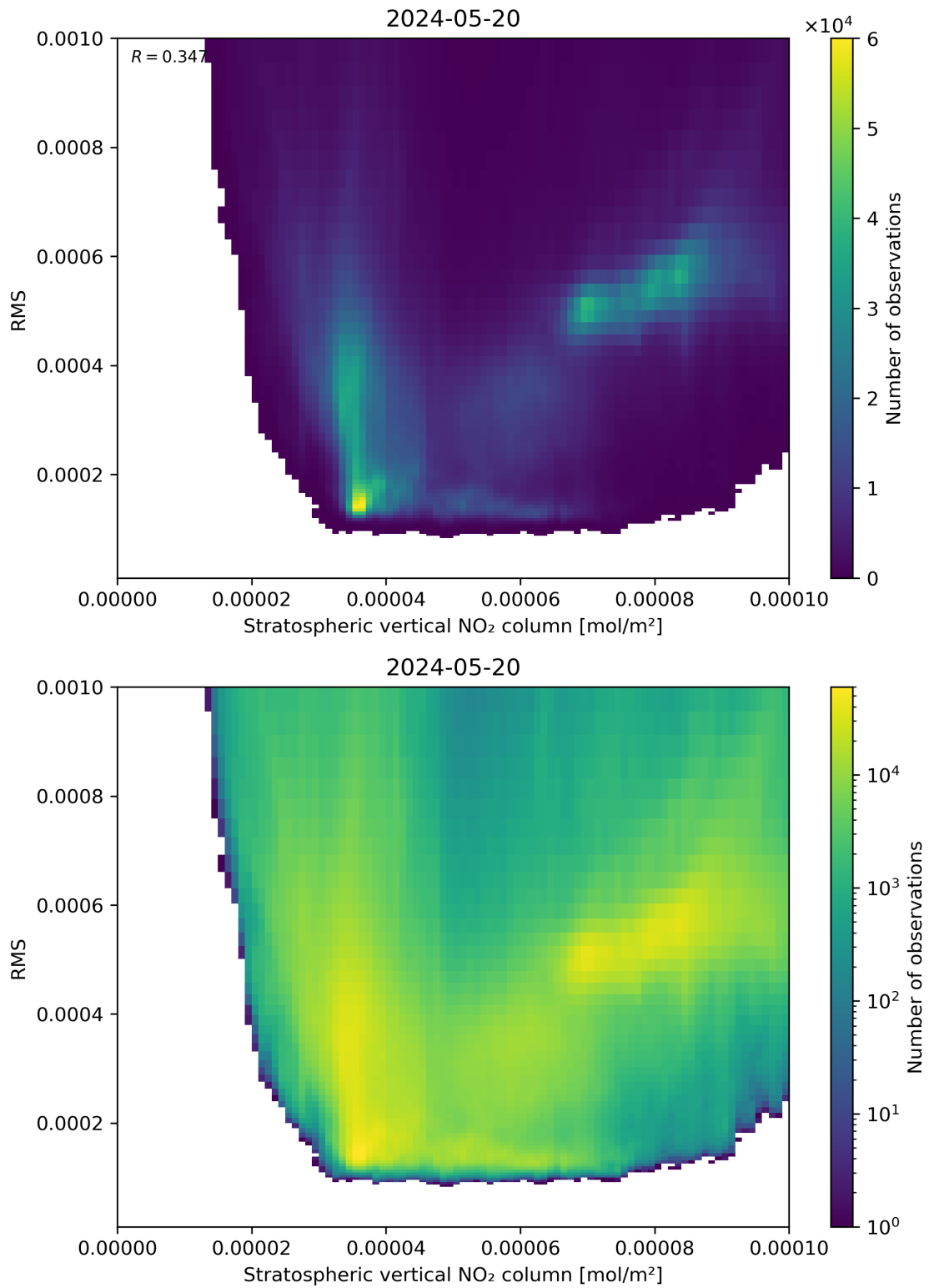
Figure 102: Scatter density plot of “Stratospheric vertical NO 2 column” against “RMS” for 2024-05-19 to 2024-05-21.
