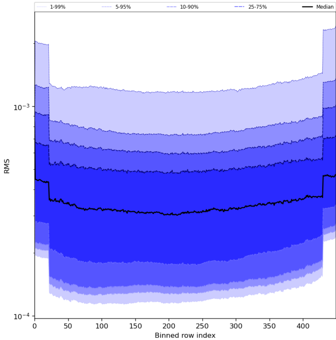
Figure 60: Along track statistics of “RMS” for 2024-05-19 to 2024-05-21
