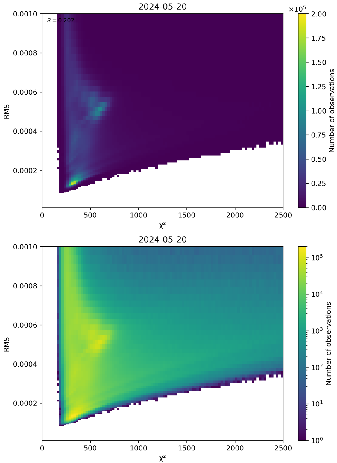
Figure 82: Scatter density plot of “ \chi^2 ” against “RMS” for 2024-05-19 to 2024-05-21.
