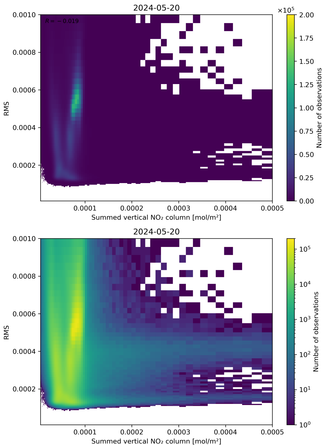
Figure 109: Scatter density plot of “Summed vertical NO 2 column” against “RMS” for 2024-05-19 to 2024-05-21.
