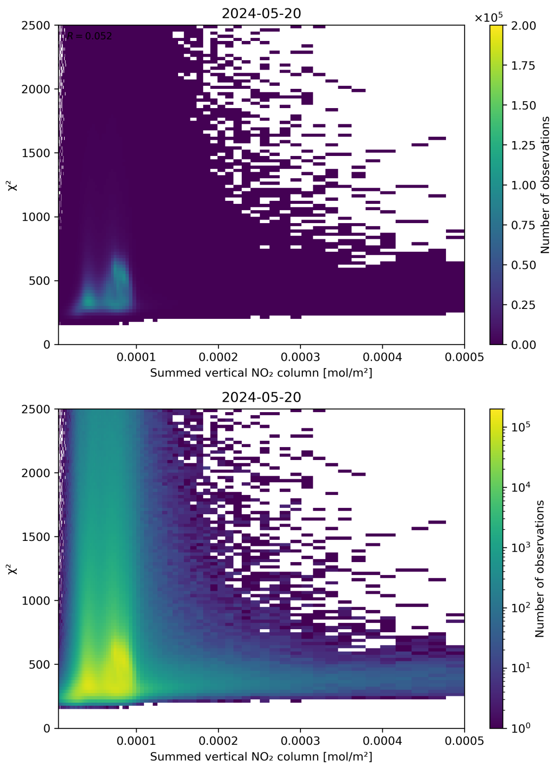
Figure 104: Scatter density plot of “Summed vertical NO 2 column” against “ \chi^2 ” for 2024-05-19 to 2024-05-21.
