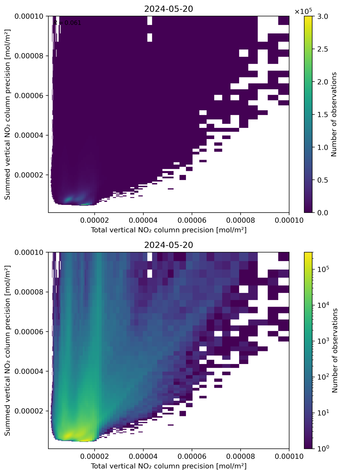
Figure 118: Scatter density plot of “Total vertical NO 2 column precision” against “Summed vertical NO 2 column precision” for 2024-05-19 to 2024-05-21.
