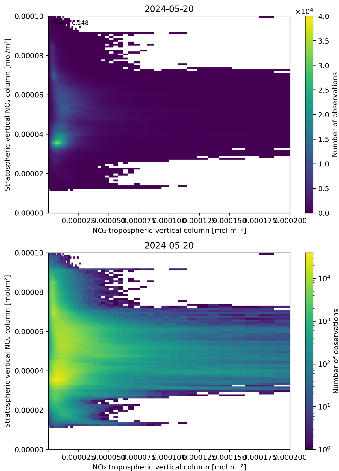
Figure 125: Scatter density plot of “NO 2 tropospheric vertical column” against “Stratospheric vertical NO 2 column” for 2024-05-19 to 2024-05-21.
