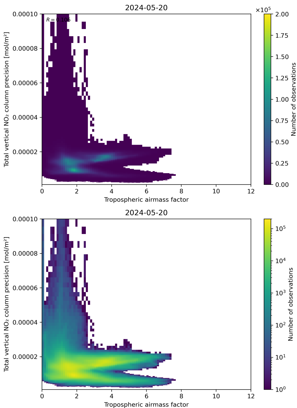
Figure 78: Scatter density plot of “Tropospheric air mass factor” against “Total vertical NO 2 column precision” for 2024-05-19 to 2024-05-21.
