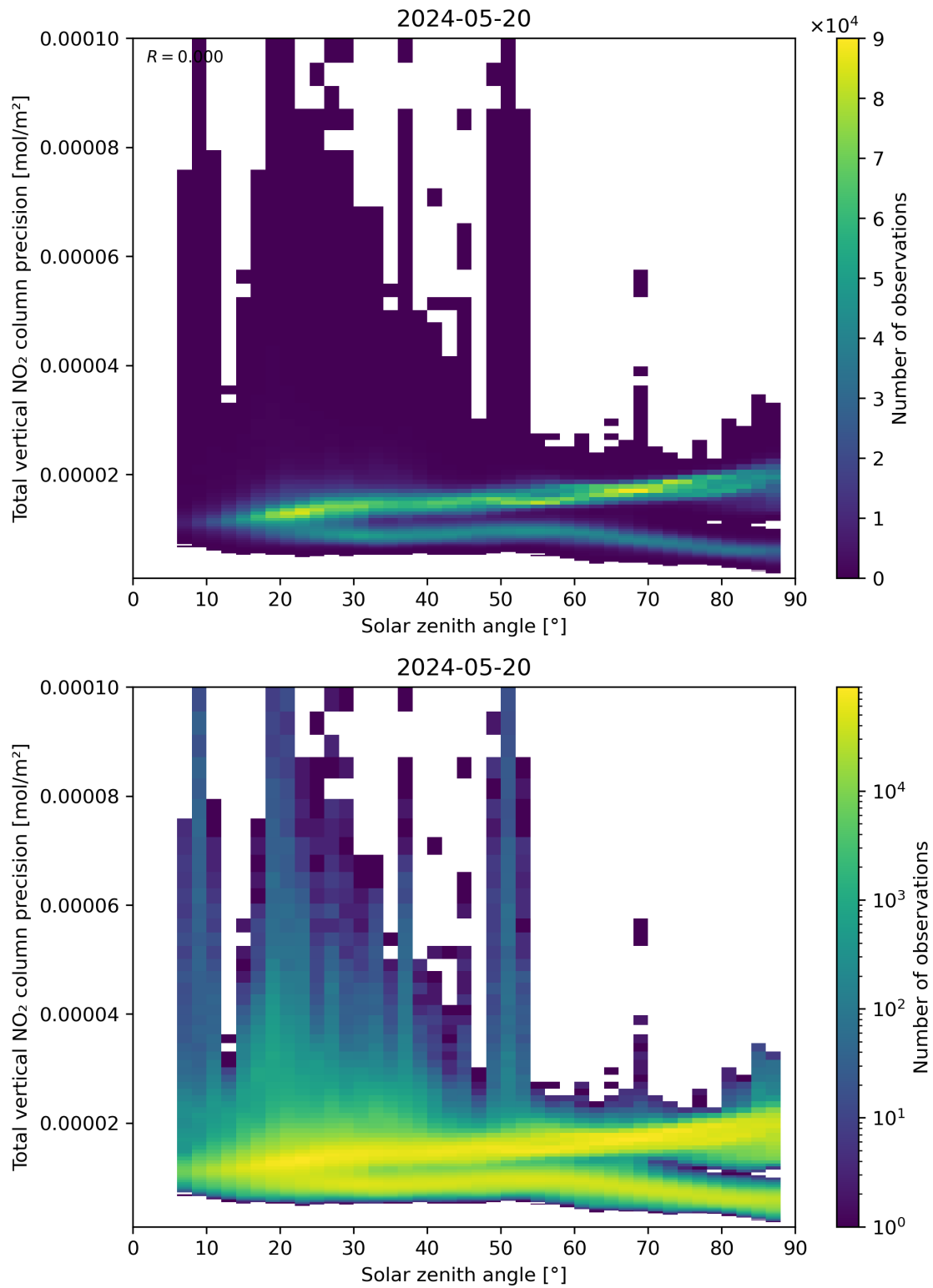
Figure 154: Scatter density plot of “Solar zenith angle” against “Total vertical NO 2 column precision” for 2024-05-19 to 2024-05-21.
