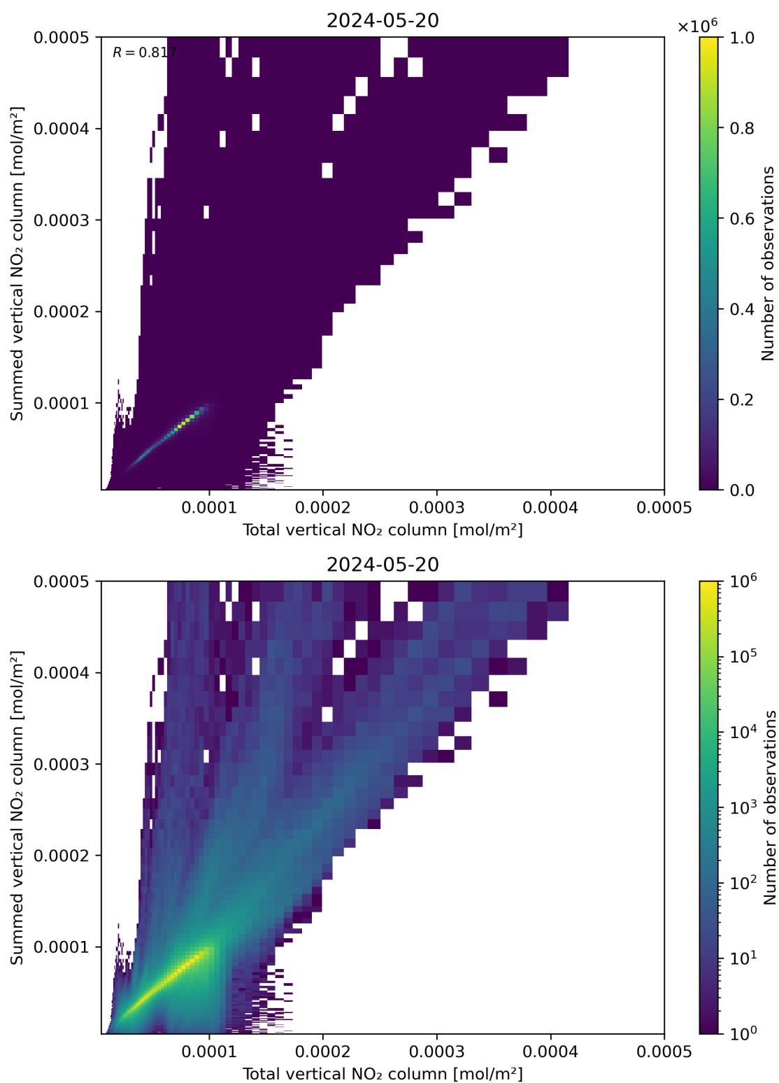
Figure 112: Scatter density plot of “Total vertical NO 2 column” against “Summed vertical NO 2 column” for 2024-05-19 to 2024-05-21.
