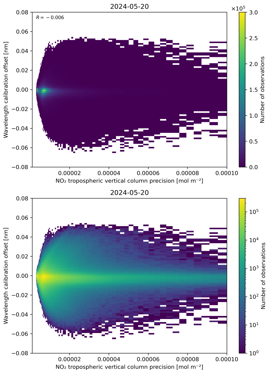
Figure 141: Scatter density plot of “NO 2 tropospheric vertical column precision” against “Wavelength calibration offset” for 2024-05-19 to 2024-05-21.
