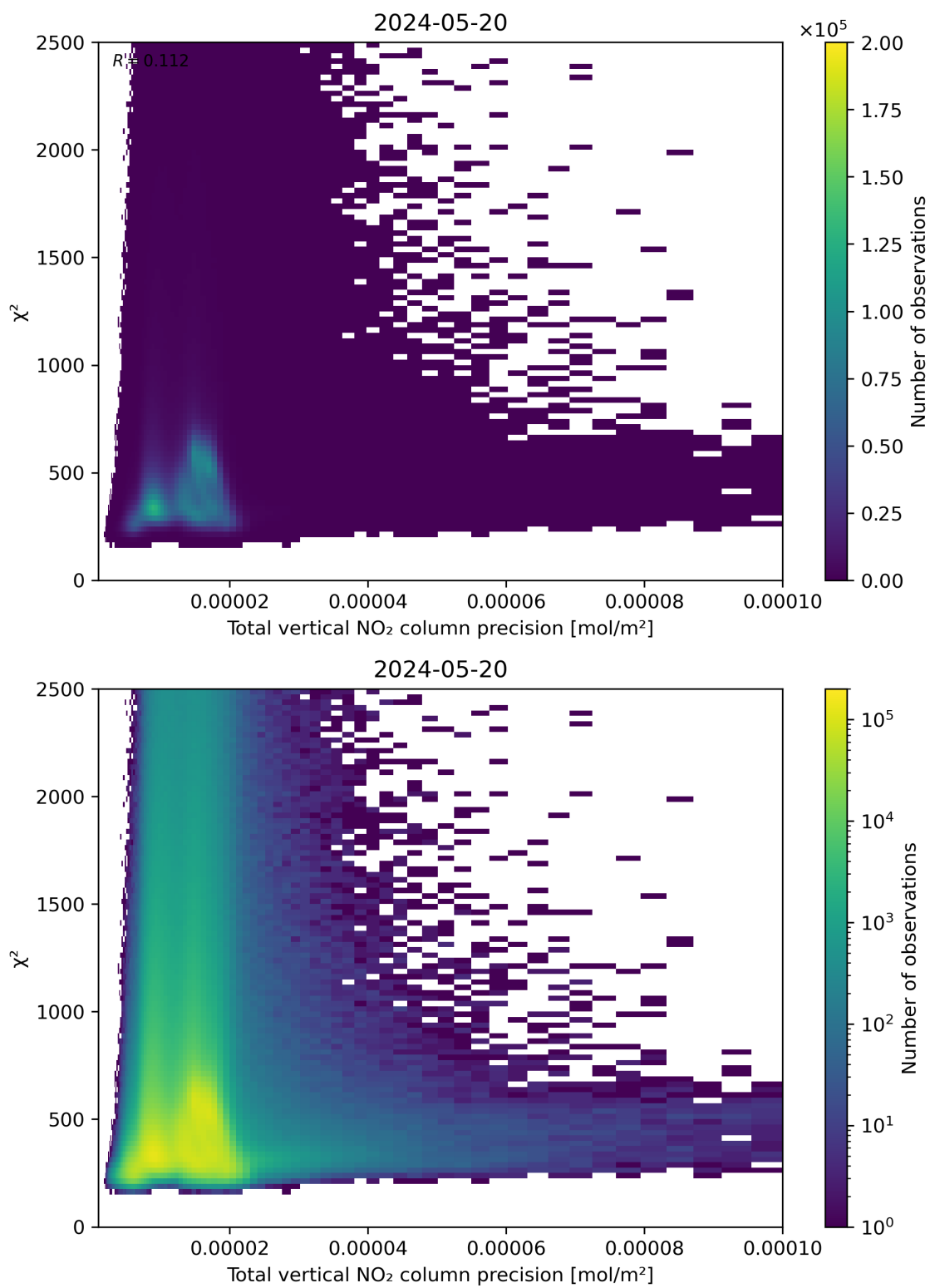
Figure 116: Scatter density plot of “Total vertical NO 2 column precision” against “ \chi^2 ” for 2024-05-19 to 2024-05-21.
