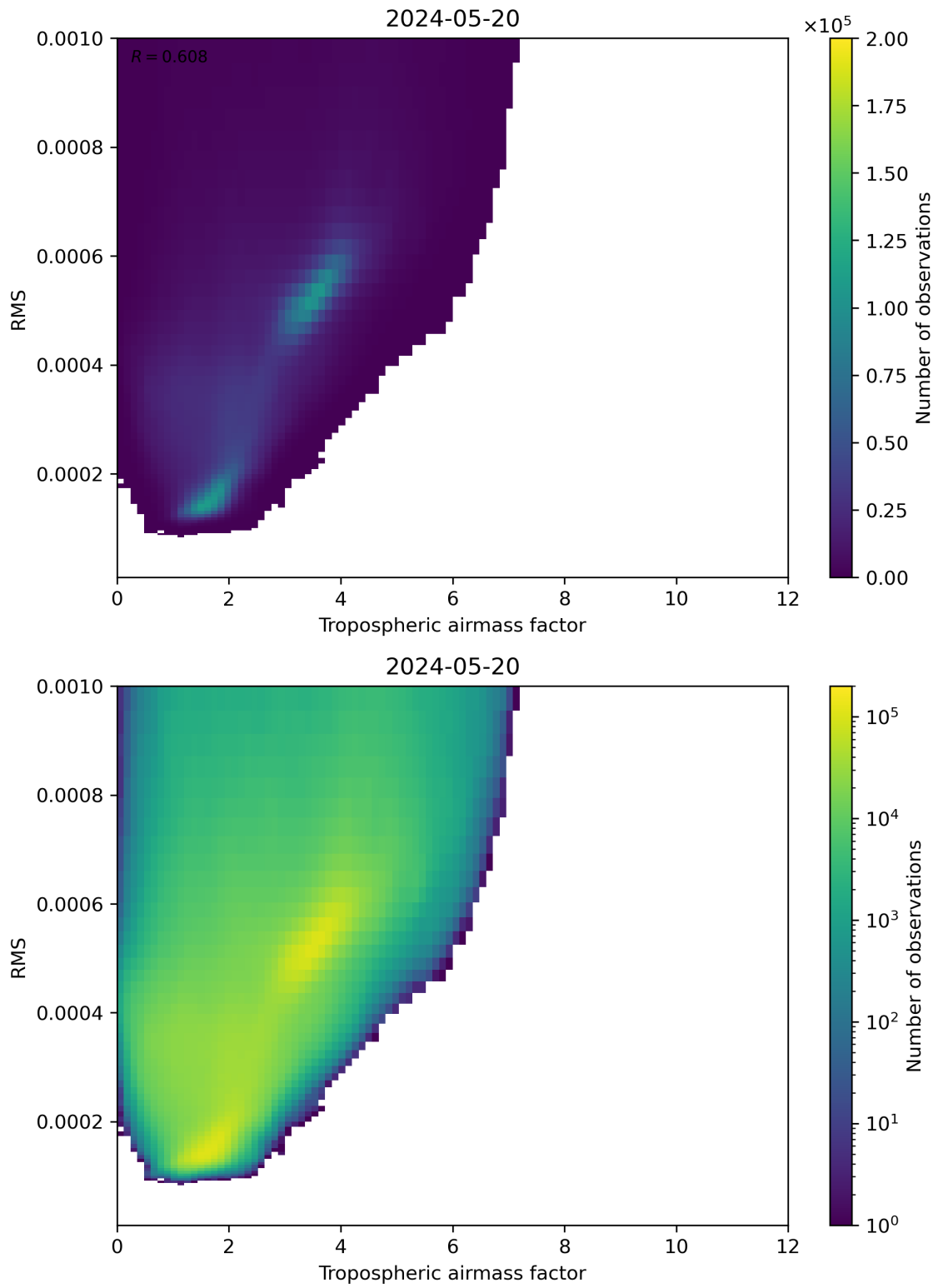
Figure 79: Scatter density plot of “Tropospheric airmass factor” against “RMS” for 2024-05-19 to 2024-05-21.
