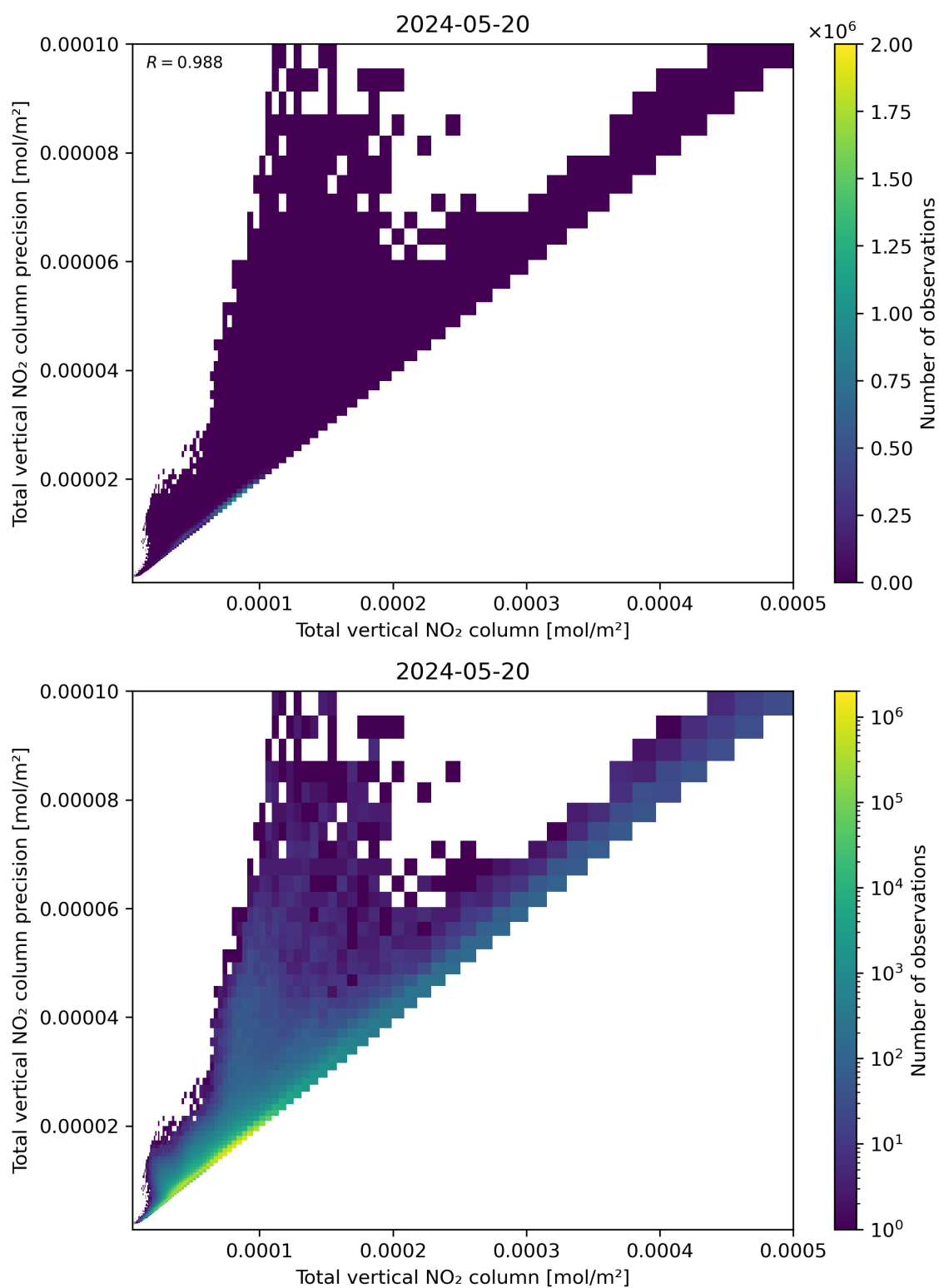
Figure 114: Scatter density plot of “Total vertical NO 2 column” against “Total vertical NO 2 column precision” for 2024-05-19 to 2024-05-21.
