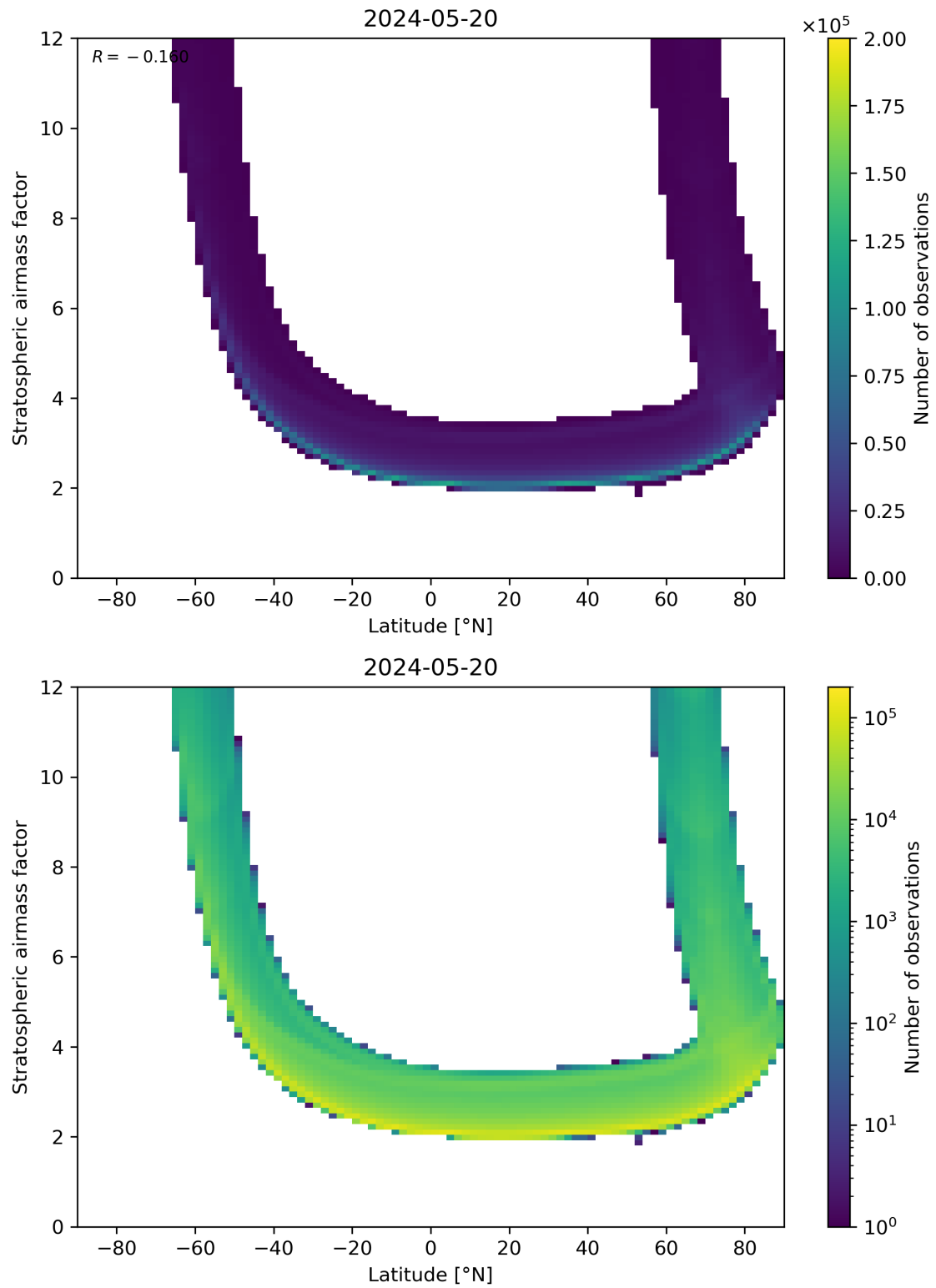
Figure 83: Scatter density plot of “Latitude” against “Stratospheric air mass factor” for 2024-05-19 to 2024-05-21.
