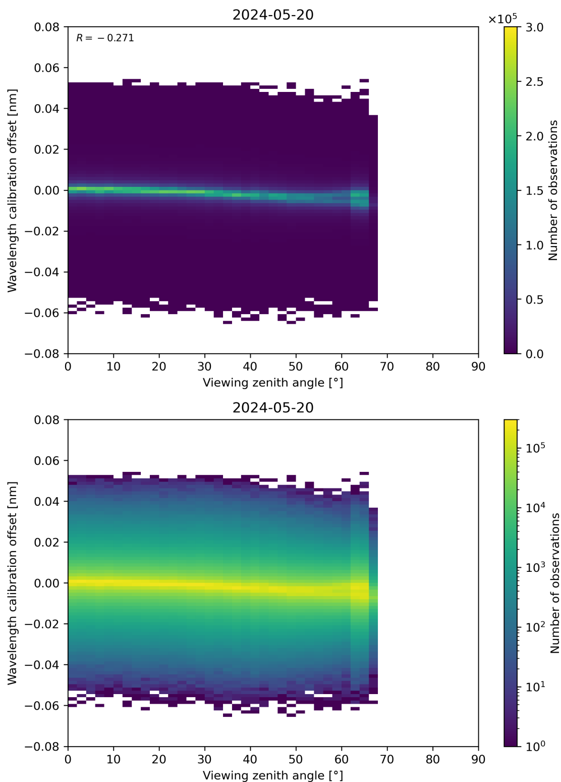
Figure 173: Scatter density plot of “Viewing zenith angle” against “Wavelength calibration offset” for 2024-05-19 to 2024-05-21.
