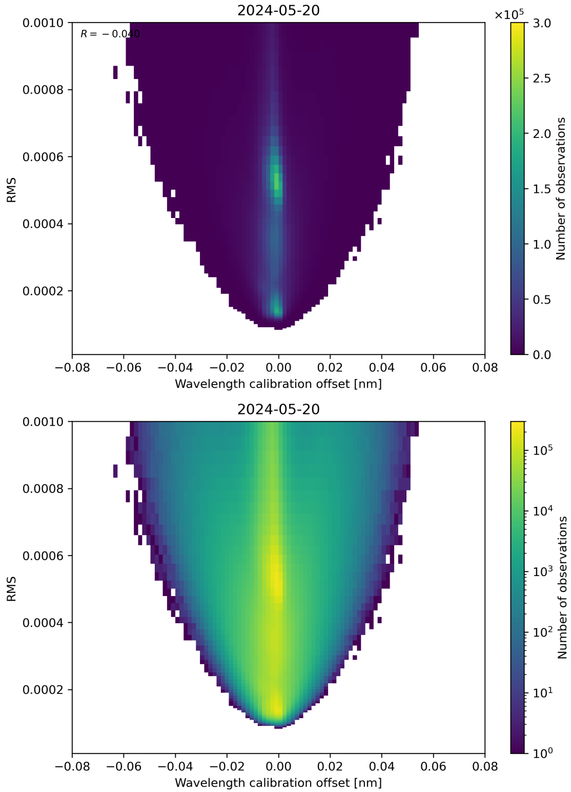
Figure 181: Scatter density plot of “Wavelength calibration offset” against “RMS” for 2024-05-19 to 2024-05-21.
