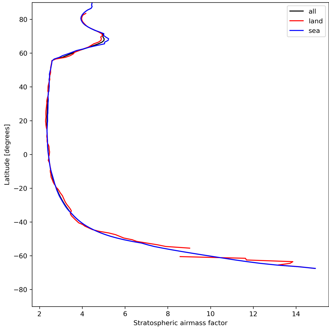
Figure 27: Zonal average of “Stratospheric air mass factor” for 2024-05-19 to 2024-05-21.
