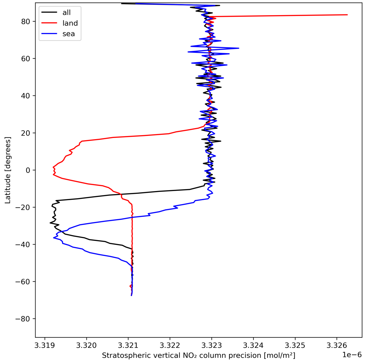
Figure 20: Zonal average of “Stratospheric vertical NO 2 column precision” for 2024-05-19 to 2024-05-21.
