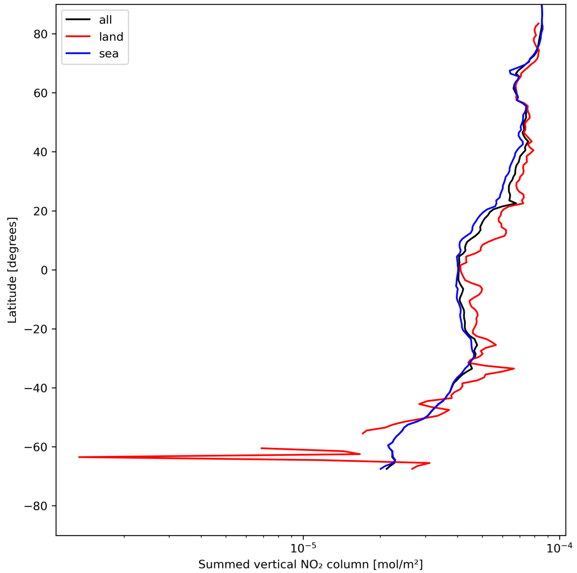
Figure 23: Zonal average of “Summed vertical NO 2 column” for 2024-05-19 to 2024-05-21.
