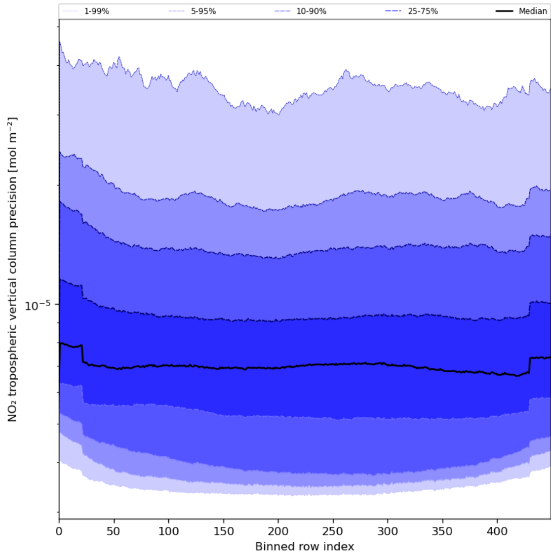
Figure 47: Along track statistics of “NO 2 tropospheric vertical column precision” for 2024-05-19 to 2024-05-21
