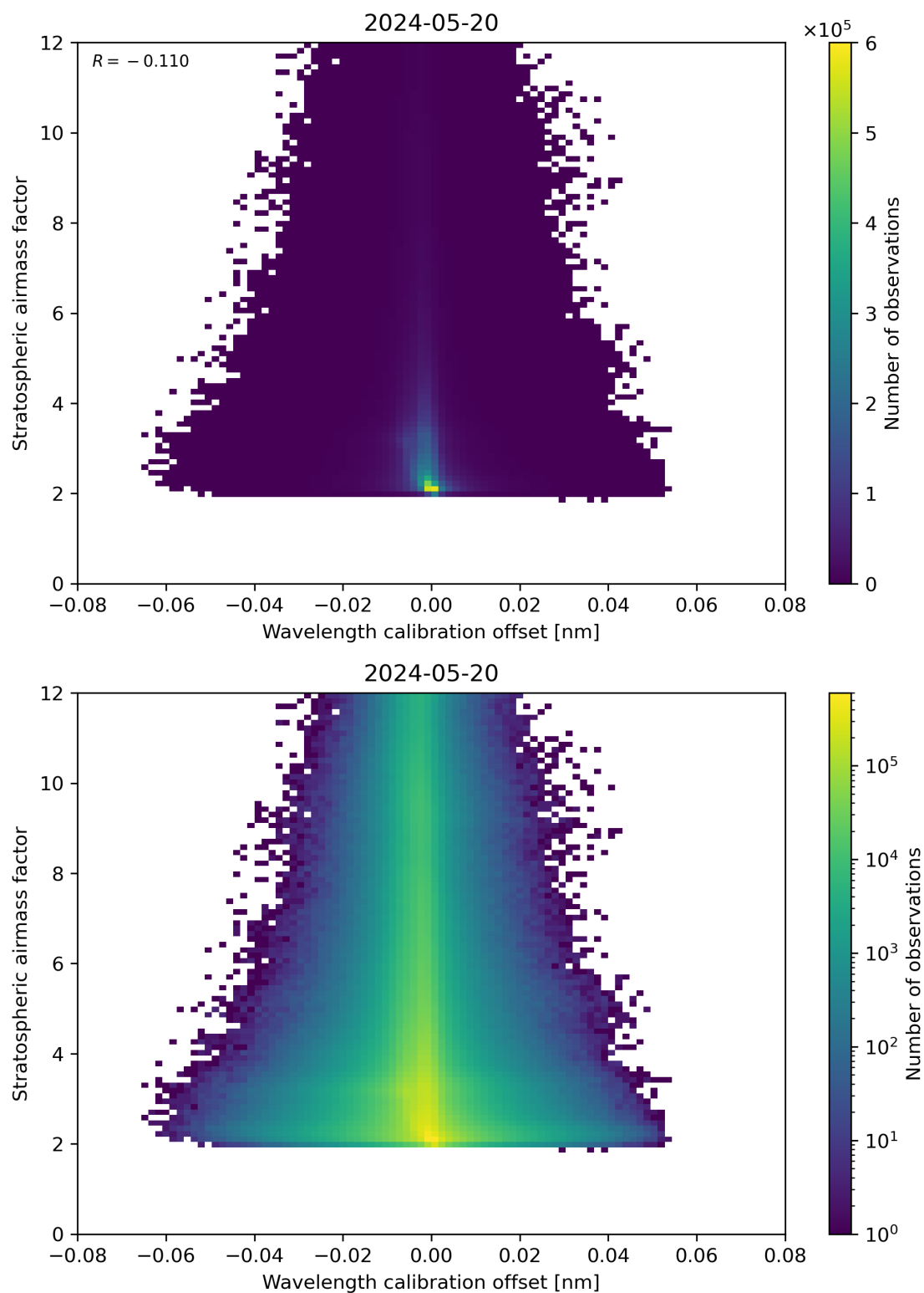
Figure 174: Scatter density plot of “Wavelength calibration offset” against “Stratospheric airmass factor” for 2024-05-19 to 2024-05-21.
