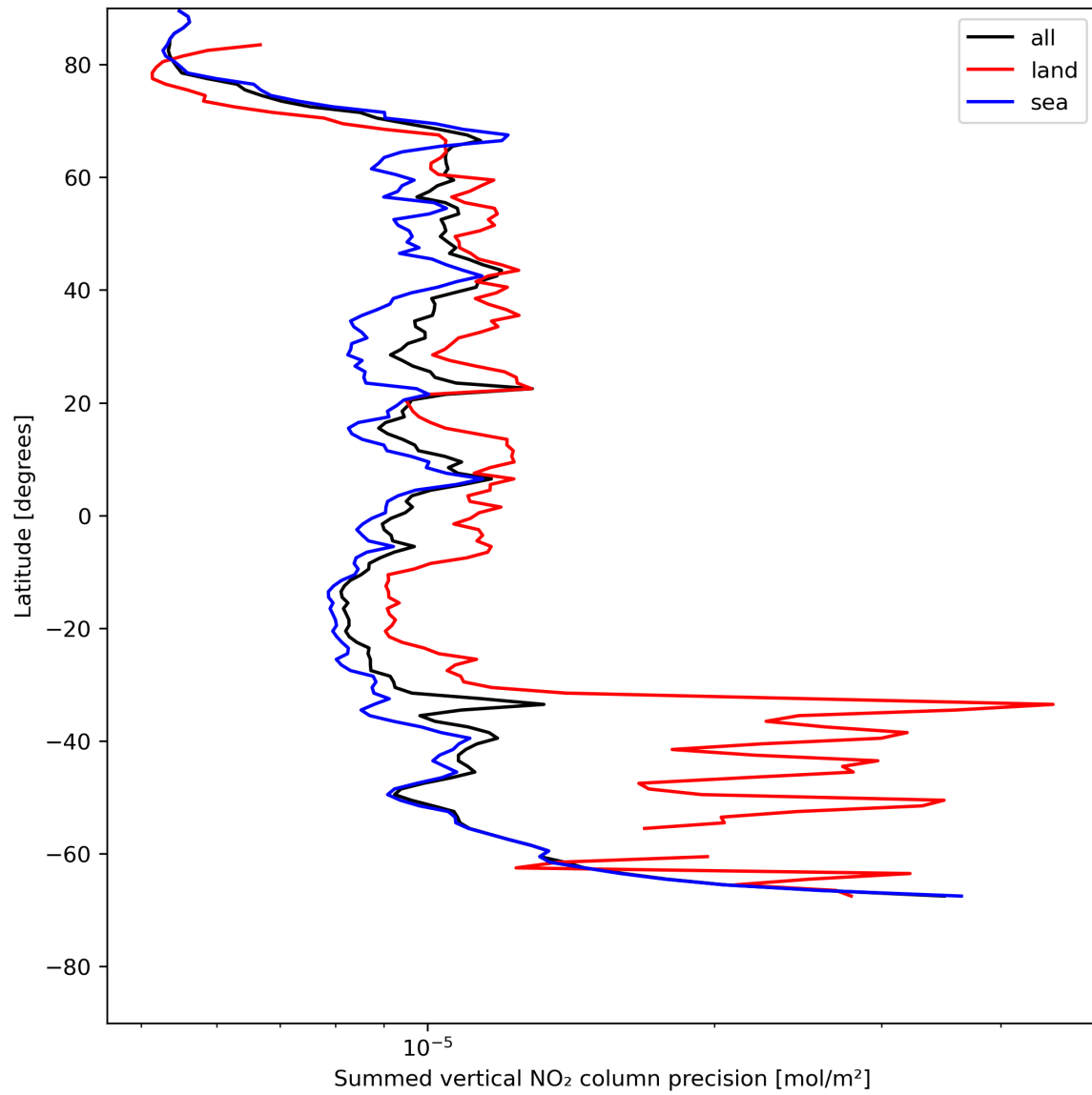
Figure 24: Zonal average of “Summed vertical NO 2 column precision” for 2024-05-19 to 2024-05-21.
