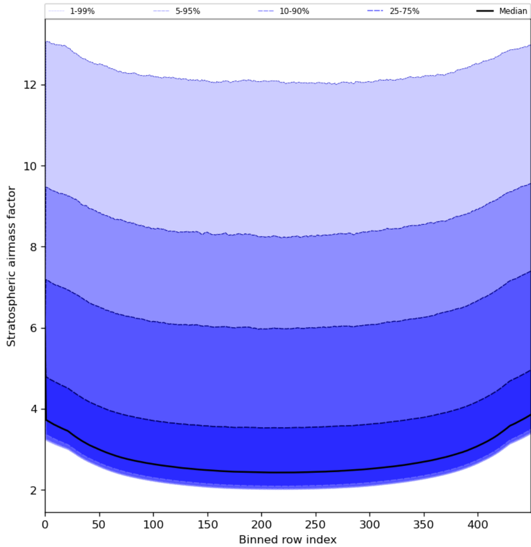
Figure 61: Along track statistics of “Stratospheric air mass factor” for 2024-05-19 to 2024-05-21
