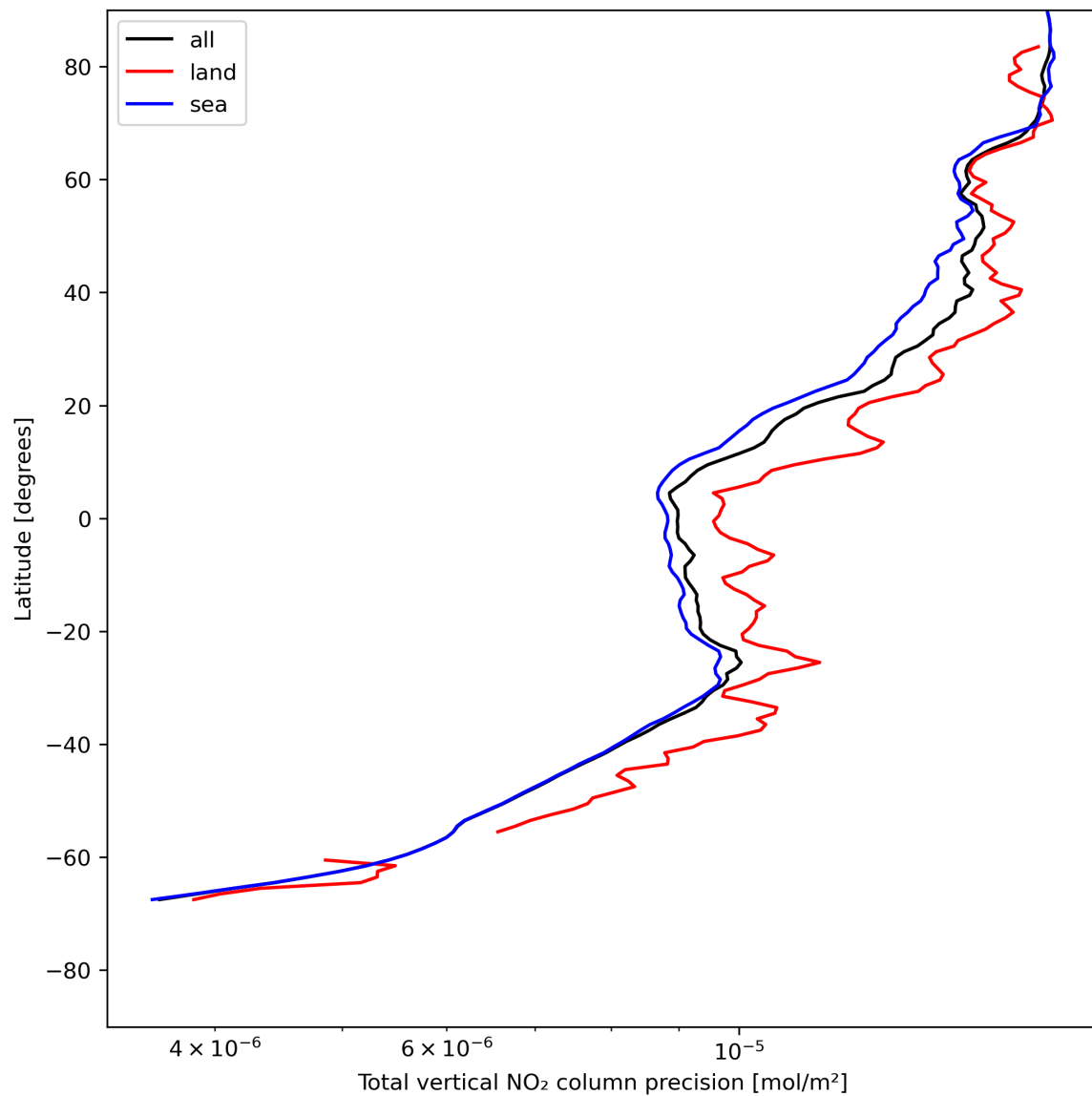
Figure 22: Zonal average of “Total vertical NO 2 column precision” for 2024-05-19 to 2024-05-21.
