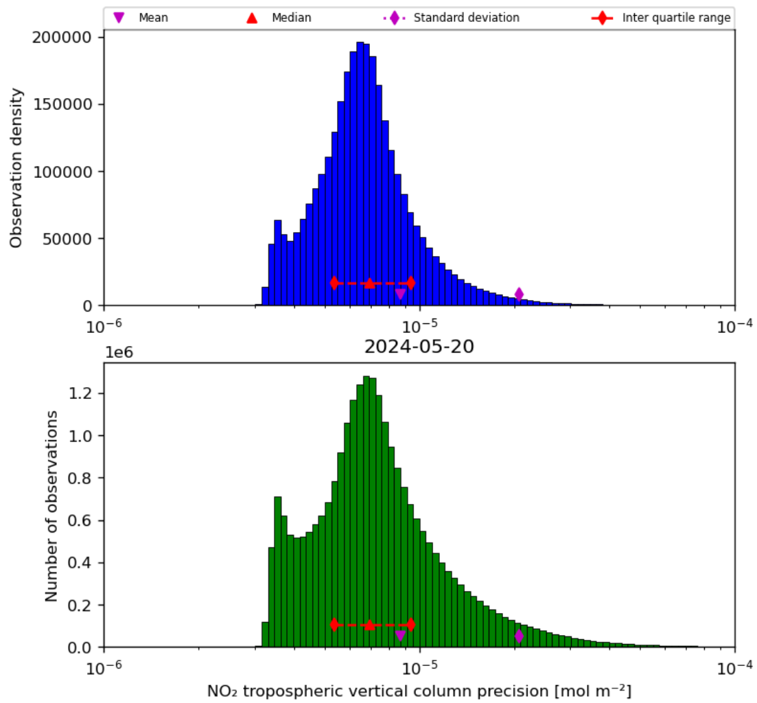
Figure 30: Histogram of “NO 2 tropospheric vertical column precision” for 2024-05-19 to 2024-05-21
