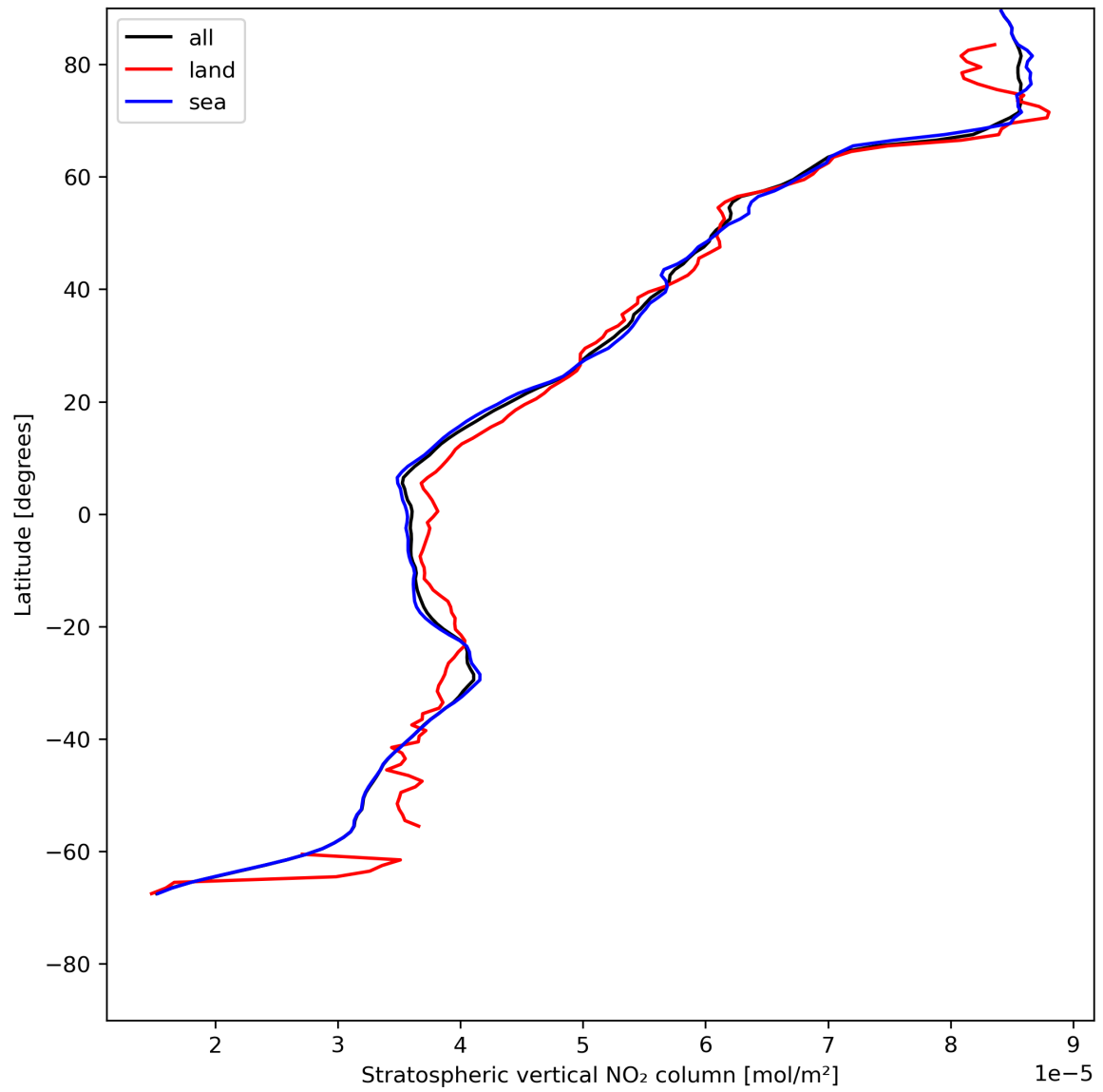
Figure 19: Zonal average of “Stratospheric vertical NO 2 column” for 2024-05-19 to 2024-05-21.
