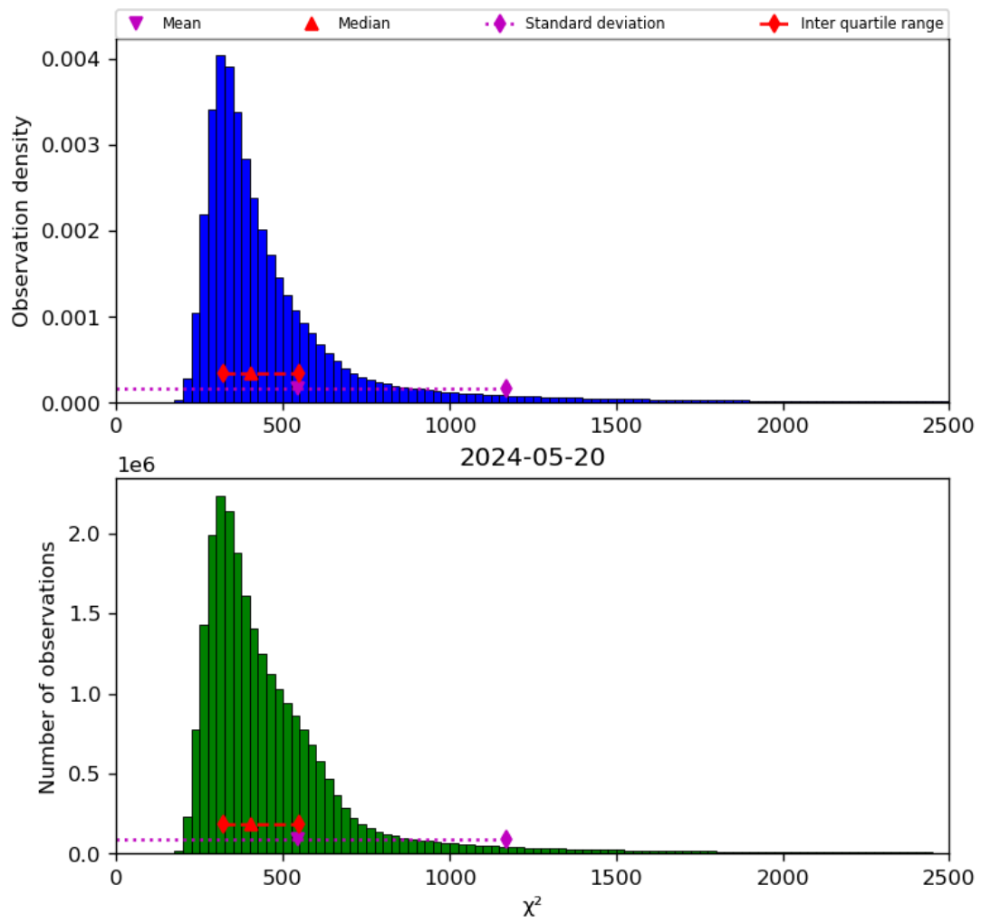
Figure 42: Histogram of “ \chi^2 ” for 2024-05-19 to 2024-05-21
