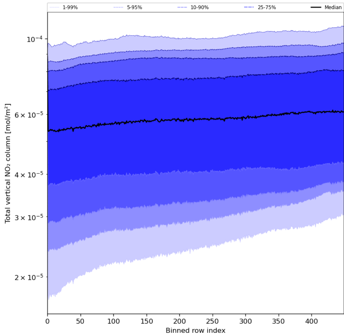
Figure 55: Along track statistics of “Total vertical NO 2 column” for 2024-05-19 to 2024-05-21
