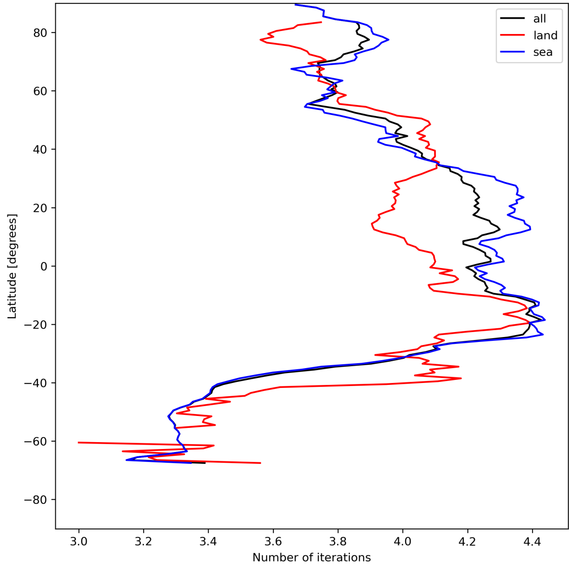
Figure 17: Zonal average of “Number of iterations” for 2024-05-19 to 2024-05-21.
