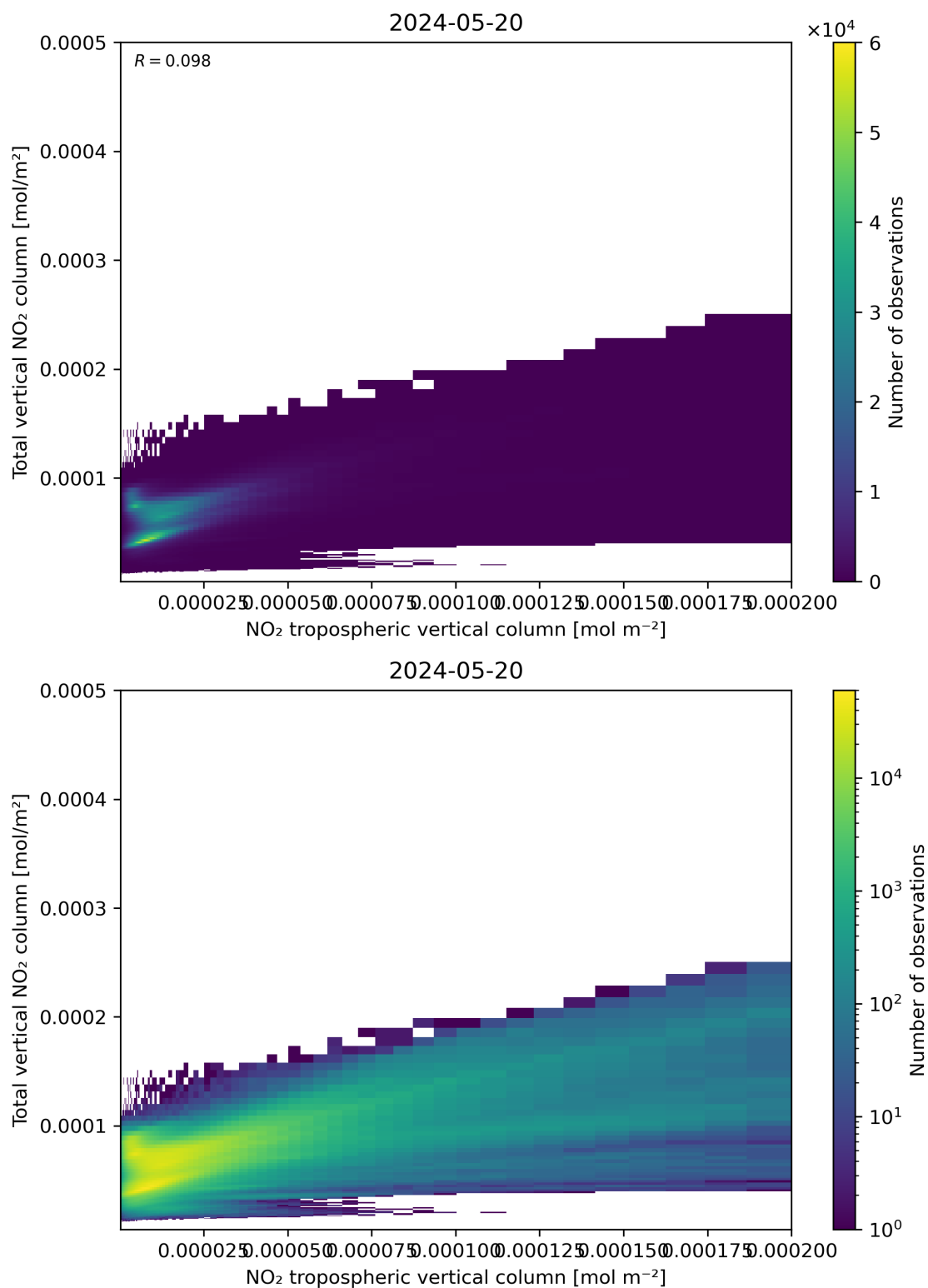
Figure 128: Scatter density plot of “NO 2 tropospheric vertical column” against “Total vertical NO 2 column” for 2024-05-19 to 2024-05-21.
