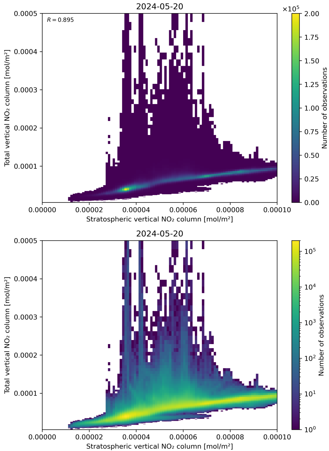
Figure 100: Scatter density plot of “Stratospheric vertical NO 2 column” against “Total vertical NO 2 column” for 2024-05-19 to 2024-05-21.
