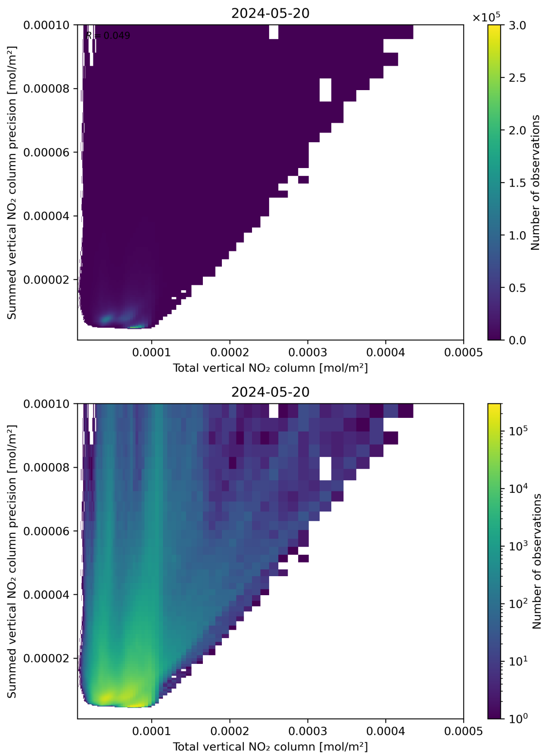
Figure 113: Scatter density plot of “Total vertical NO 2 column” against “Summed vertical NO 2 column precision” for 2024-05-19 to 2024-05-21.
