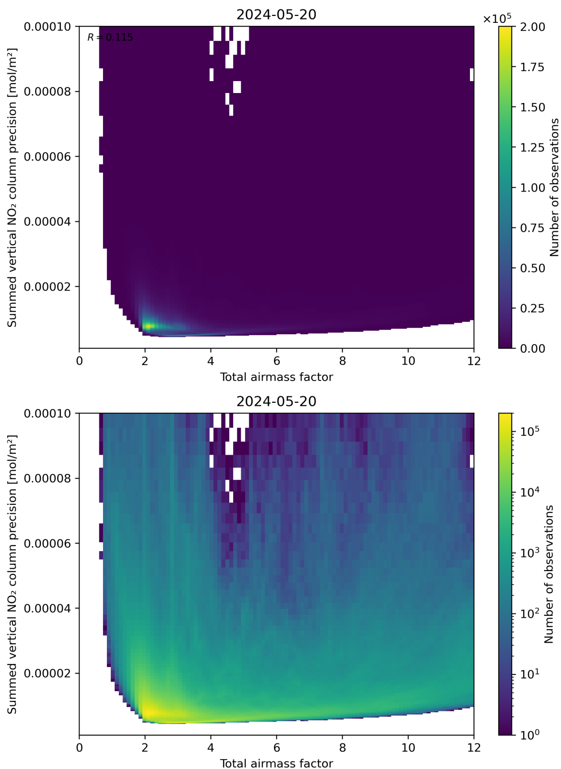
Figure 66: Scatter density plot of “Total airmass factor” against “Summed vertical NO 2 column precision” for 2024-05-19 to 2024-05-21.
