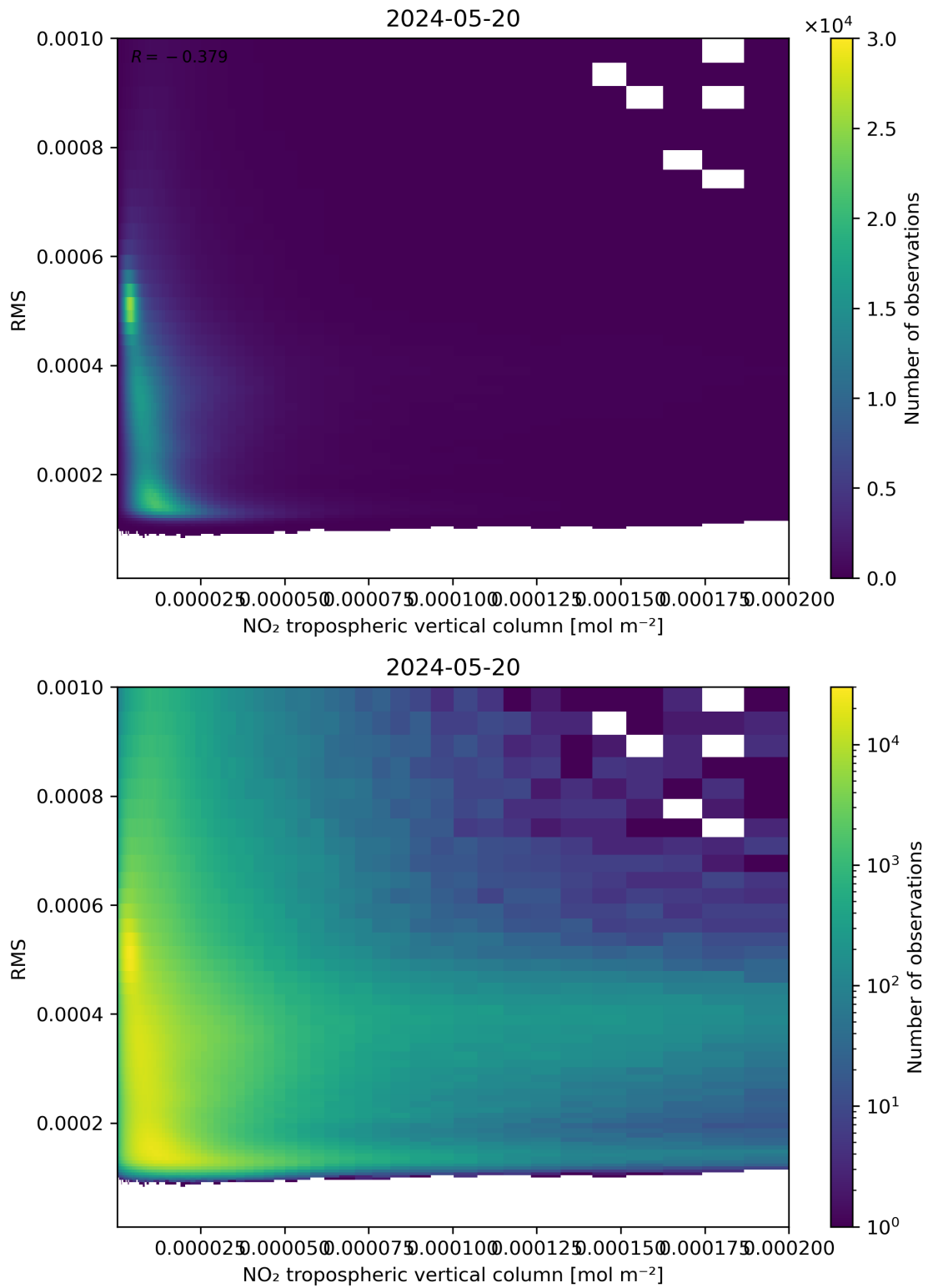
Figure 142: Scatter density plot of “NO 2 tropospheric vertical column” against “RMS” for 2024-05-19 to 2024-05-21.
