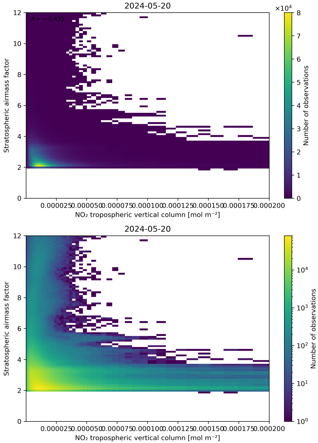
Figure 121: Scatter density plot of “NO 2 tropospheric vertical column” against “Stratospheric air mass factor” for 2024-05-19 to 2024-05-21.
