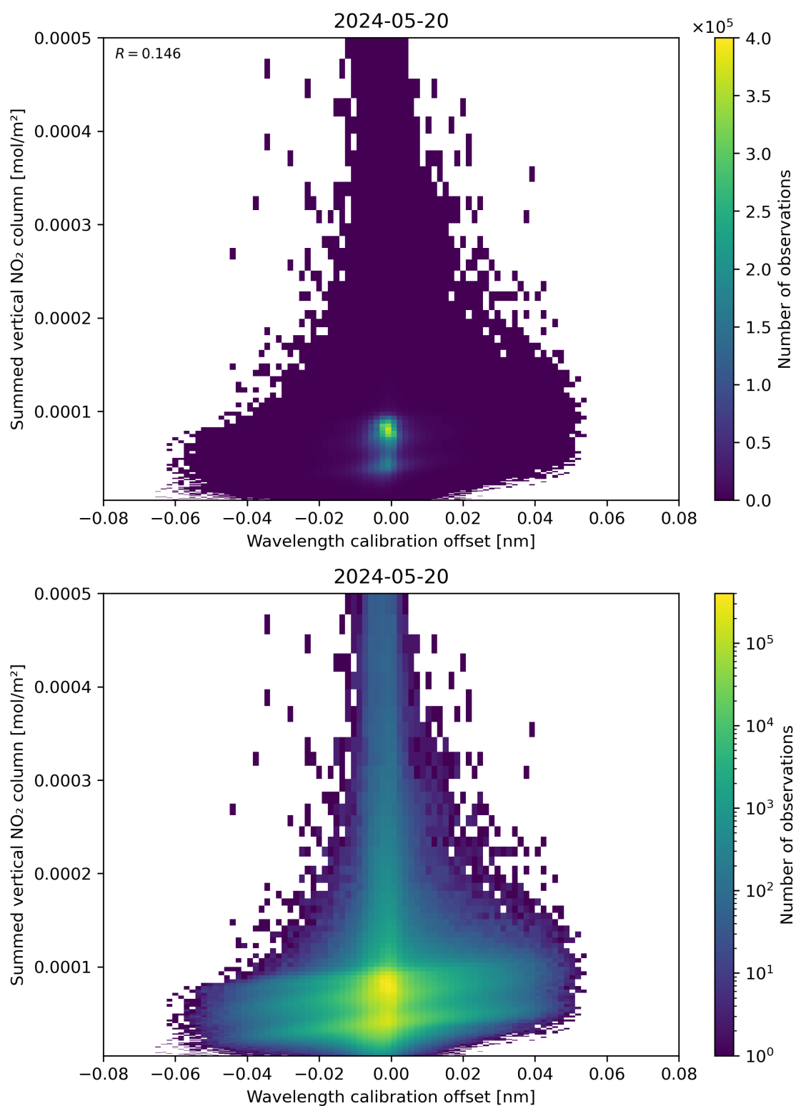
Figure 177: Scatter density plot of “Wavelength calibration offset” against “Summed vertical NO 2 column” for 2024-05-19 to 2024-05-21.
