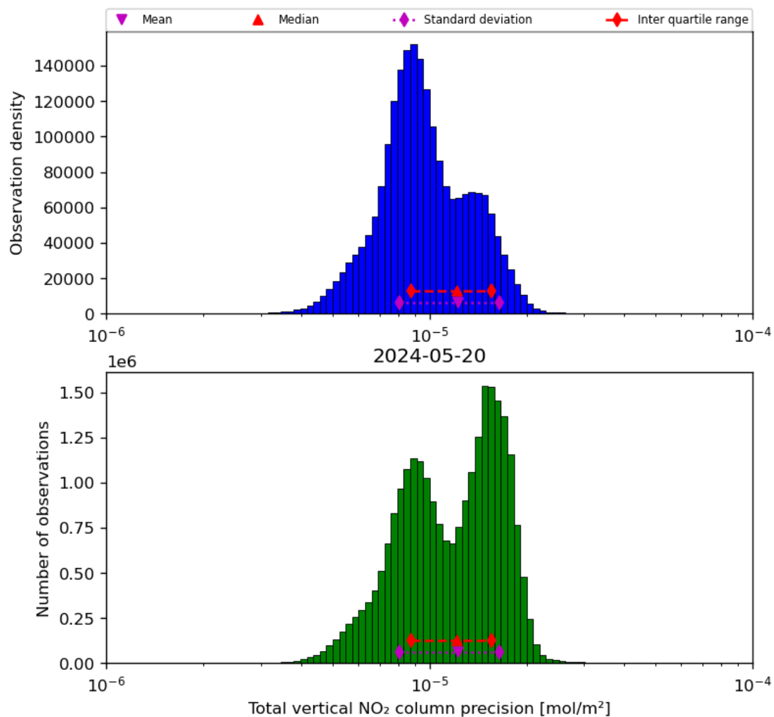
Figure 39: Histogram of “Total vertical NO 2 column precision” for 2024-05-19 to 2024-05-21
