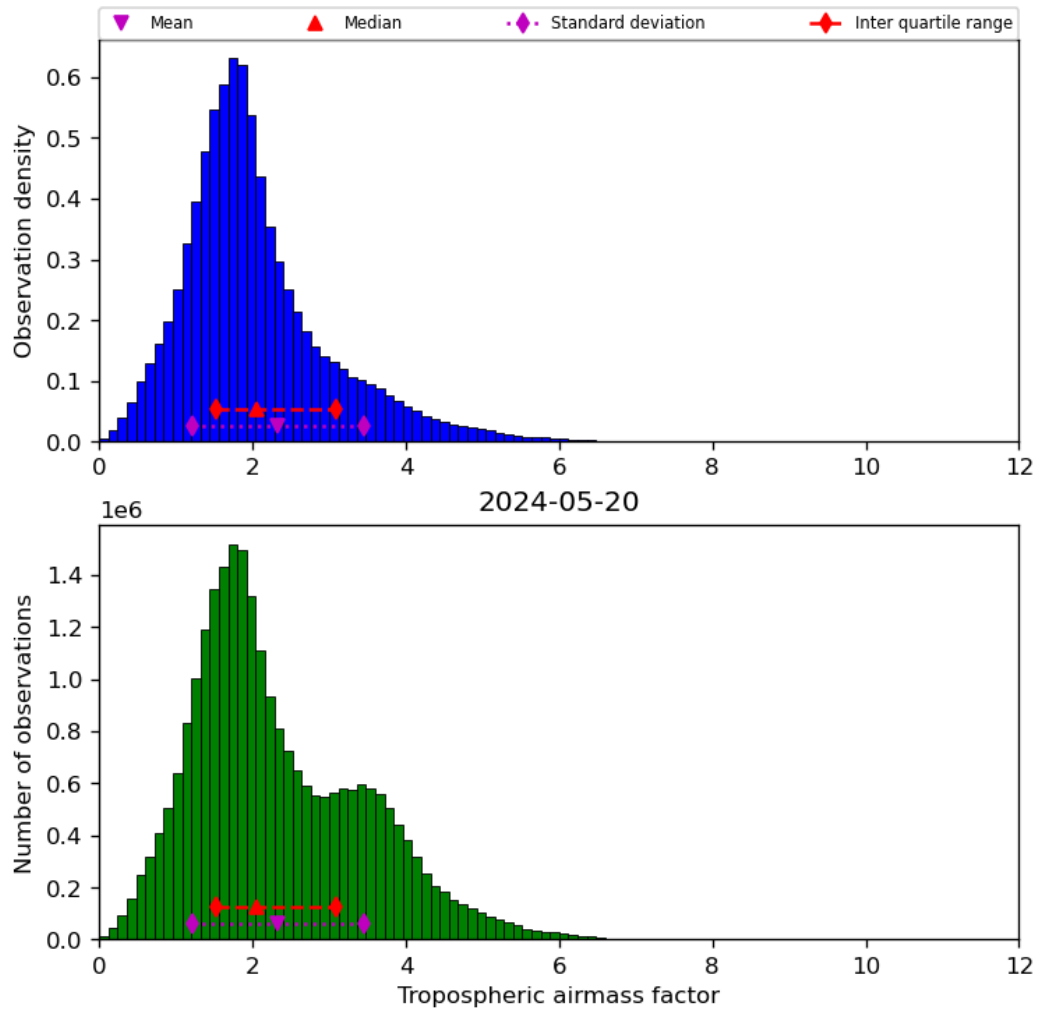
Figure 31: Histogram of “Tropospheric airmass factor” for 2024-05-19 to 2024-05-21
