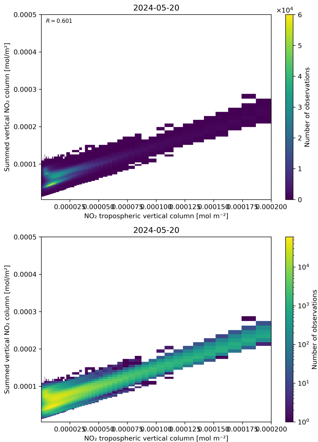
Figure 126: Scatter density plot of “NO 2 tropospheric vertical column” against “Summed vertical NO 2 column” for 2024-05-19 to 2024-05-21.
