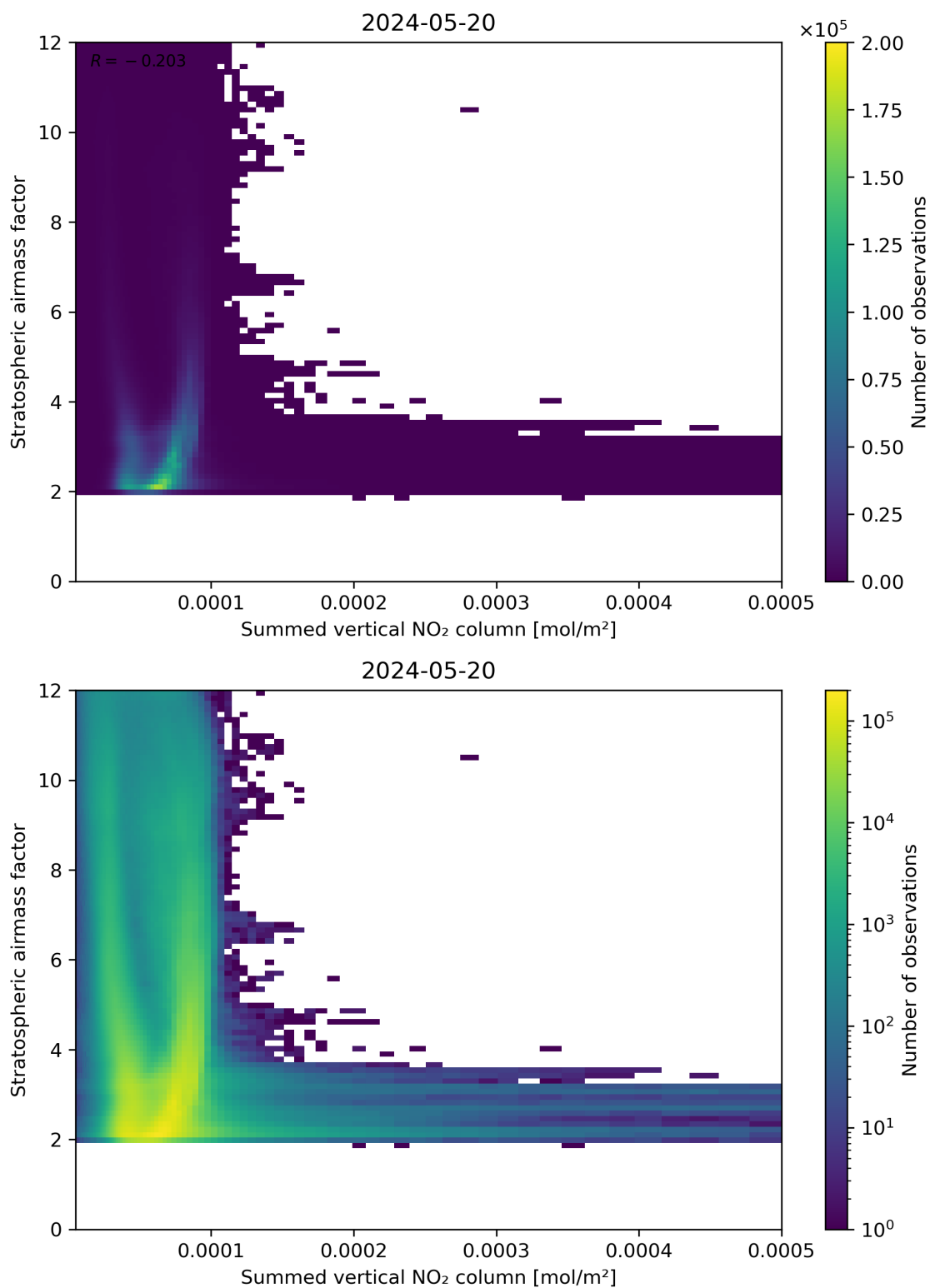
Figure 103: Scatter density plot of “Summed vertical NO 2 column” against “Stratospheric air mass factor” for 2024-05-19 to 2024-05-21.
