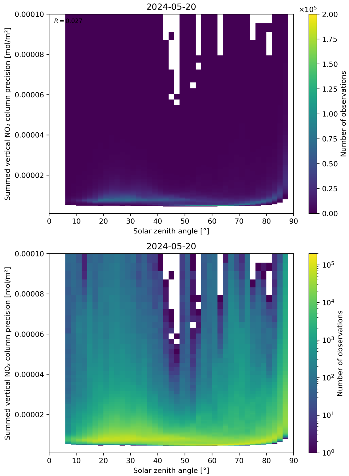
Figure 152: Scatter density plot of “Solar zenith angle” against “Summed vertical NO 2 column precision” for 2024-05-19 to 2024-05-21.
