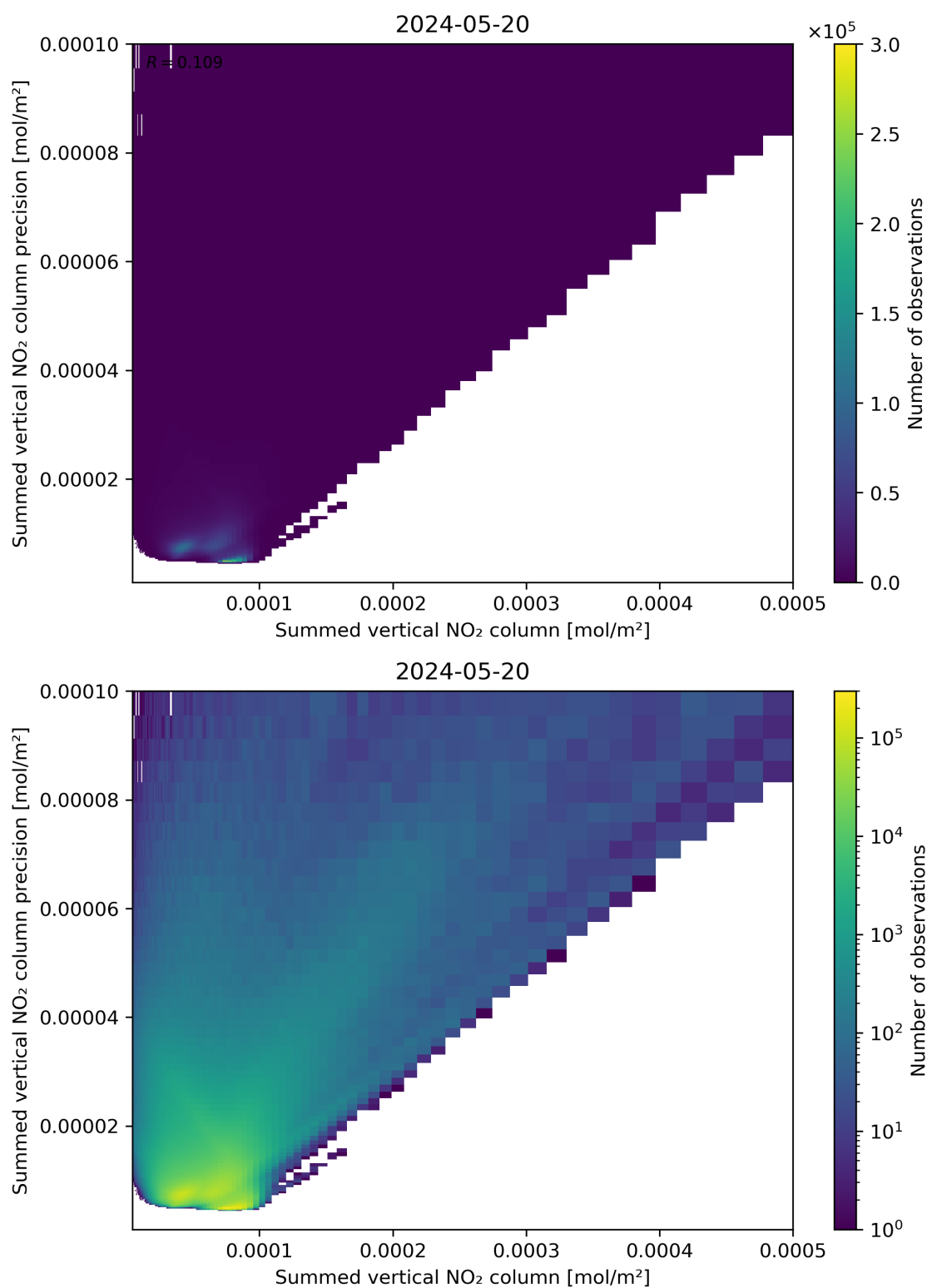
Figure 105: Scatter density plot of “Summed vertical NO 2 column” against “Summed vertical NO 2 column precision” for 2024-05-19 to 2024-05-21.
