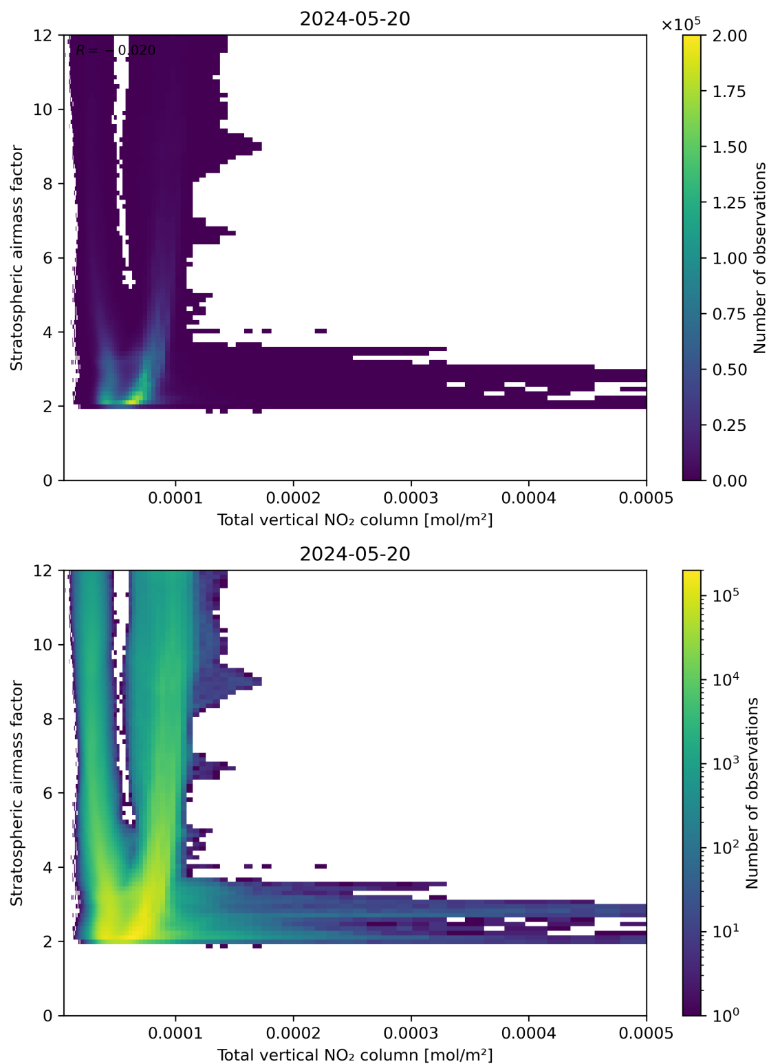
Figure 110: Scatter density plot of “Total vertical NO 2 column” against “Stratospheric airmass factor” for 2024-05-19 to 2024-05-21.
