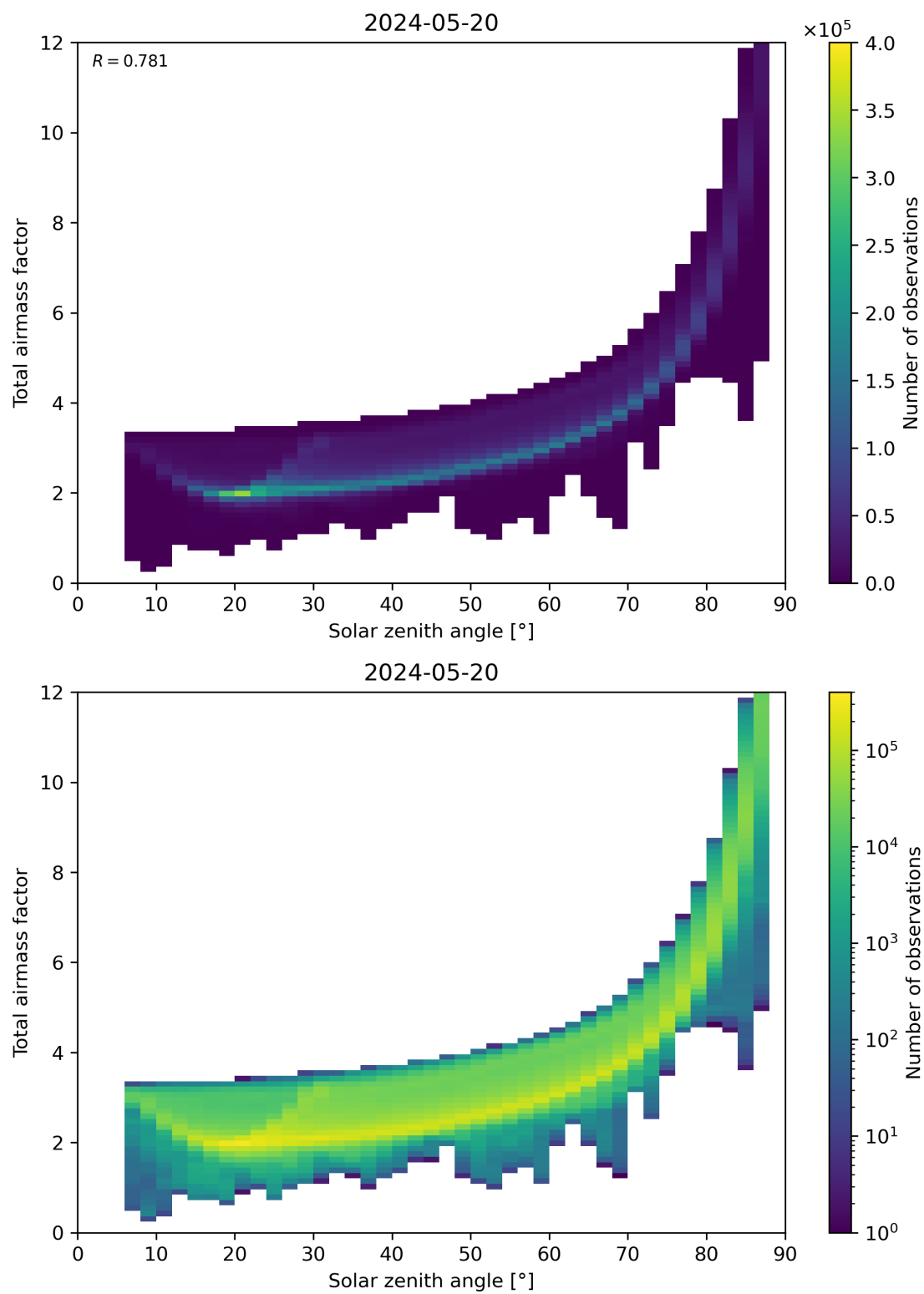
Figure 146: Scatter density plot of “Solar zenith angle” against “Total air mass factor” for 2024-05-19 to 2024-05-21.
