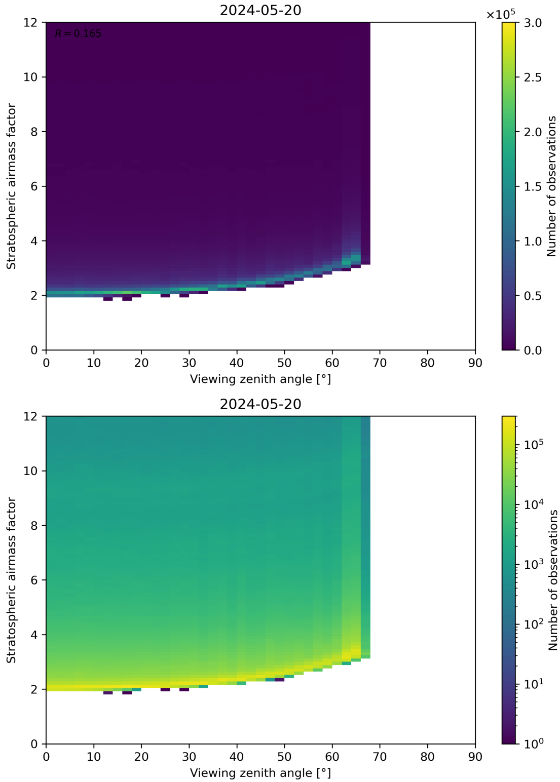
Figure 159: Scatter density plot of “Viewing zenith angle” against “Stratospheric airmass factor” for 2024-05-19 to 2024-05-21.
