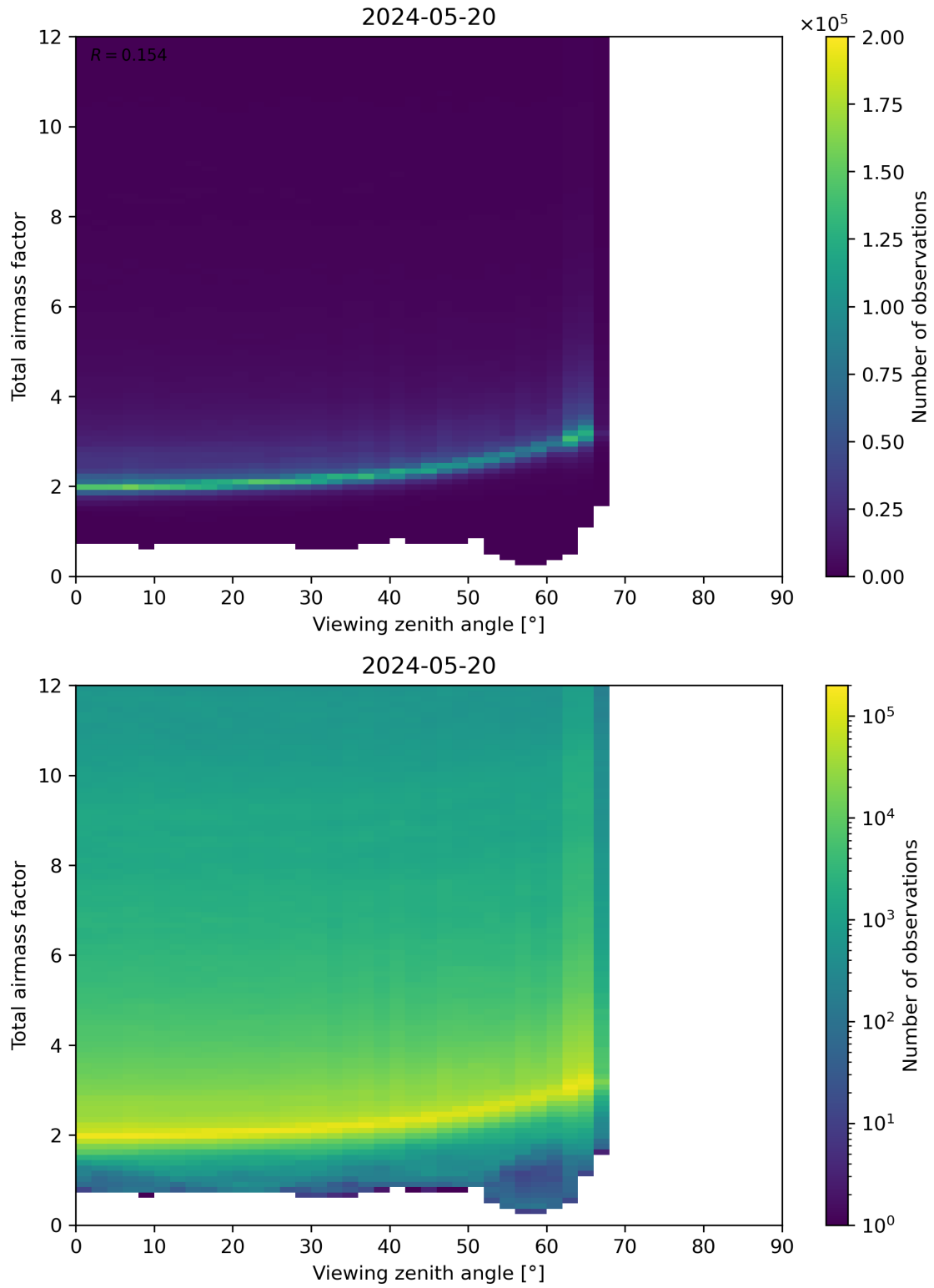
Figure 160: Scatter density plot of “Viewing zenith angle” against “Total airmass factor” for 2024-05-19 to 2024-05-21.
