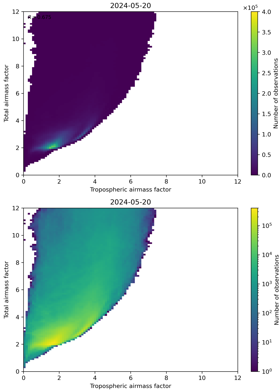
Figure 72: Scatter density plot of “Tropospheric airmass factor” against “Total airmass factor” for 2024-05-19 to 2024-05-21.
