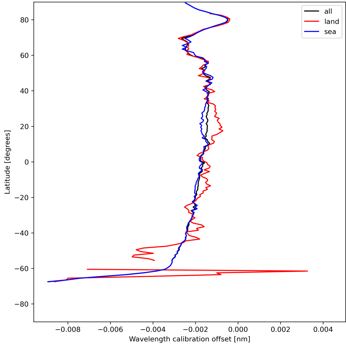
Figure 18: Zonal average of “Wavelength calibration offset” for 2024-05-19 to 2024-05-21.
