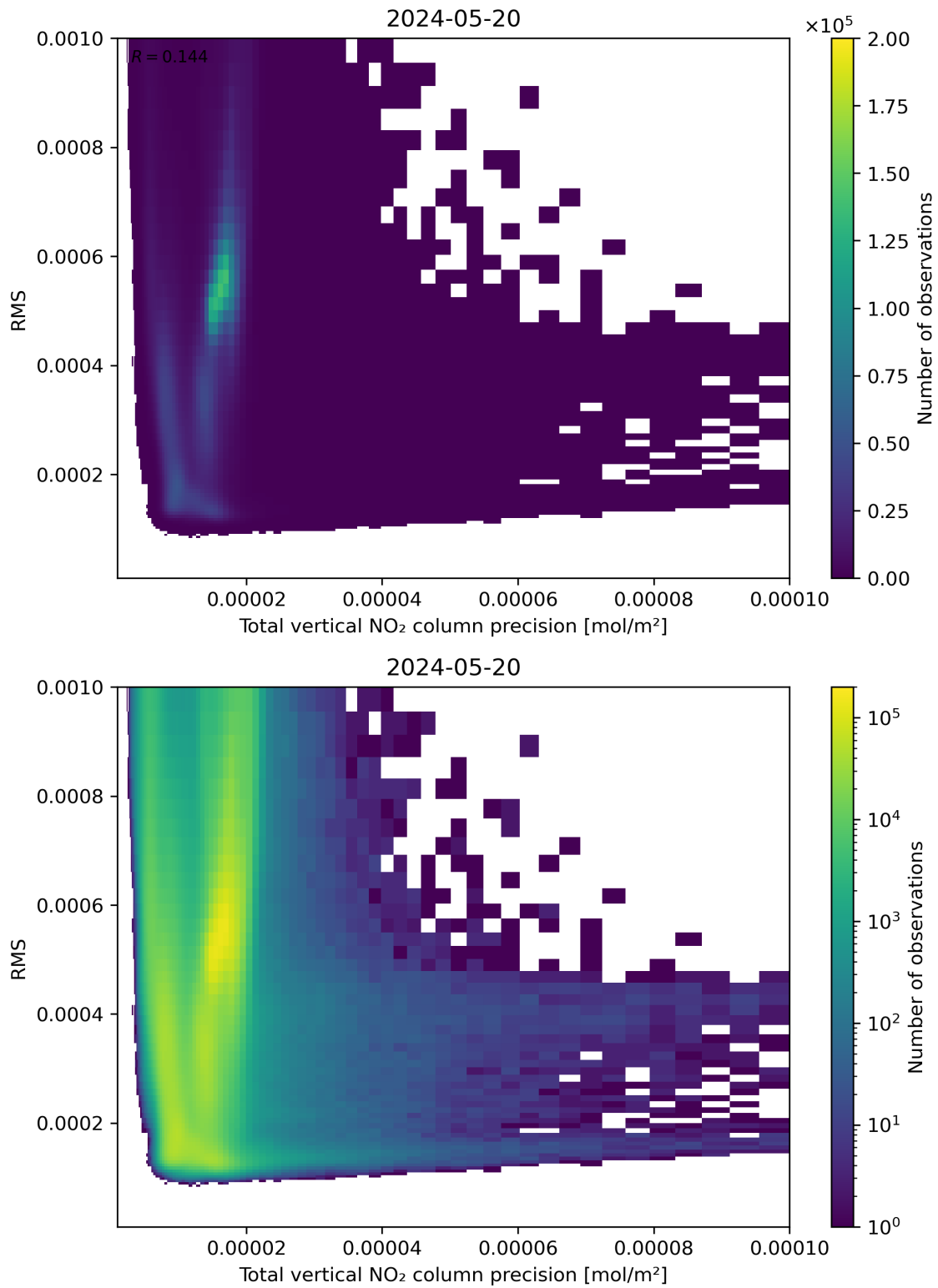
Figure 119: Scatter density plot of “Total vertical NO 2 column precision” against “RMS” for 2024-05-19 to 2024-05-21.
