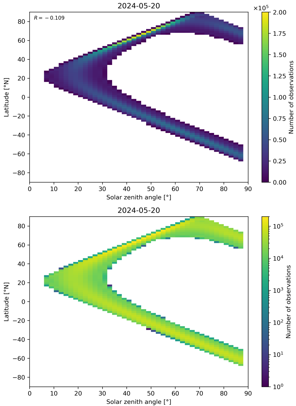
Figure 149: Scatter density plot of “Solar zenith angle” against “Latitude” for 2024-05-19 to 2024-05-21.
