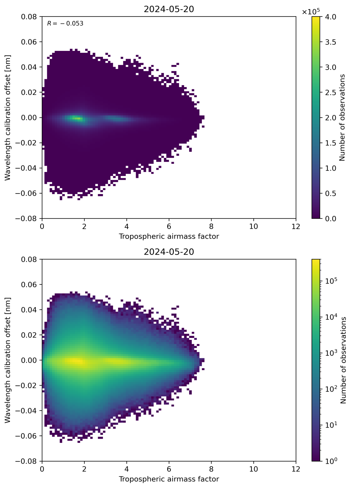
Figure 80: Scatter density plot of “Tropospheric airmass factor” against “Wavelength calibration offset” for 2024-05-19 to 2024-05-21.
