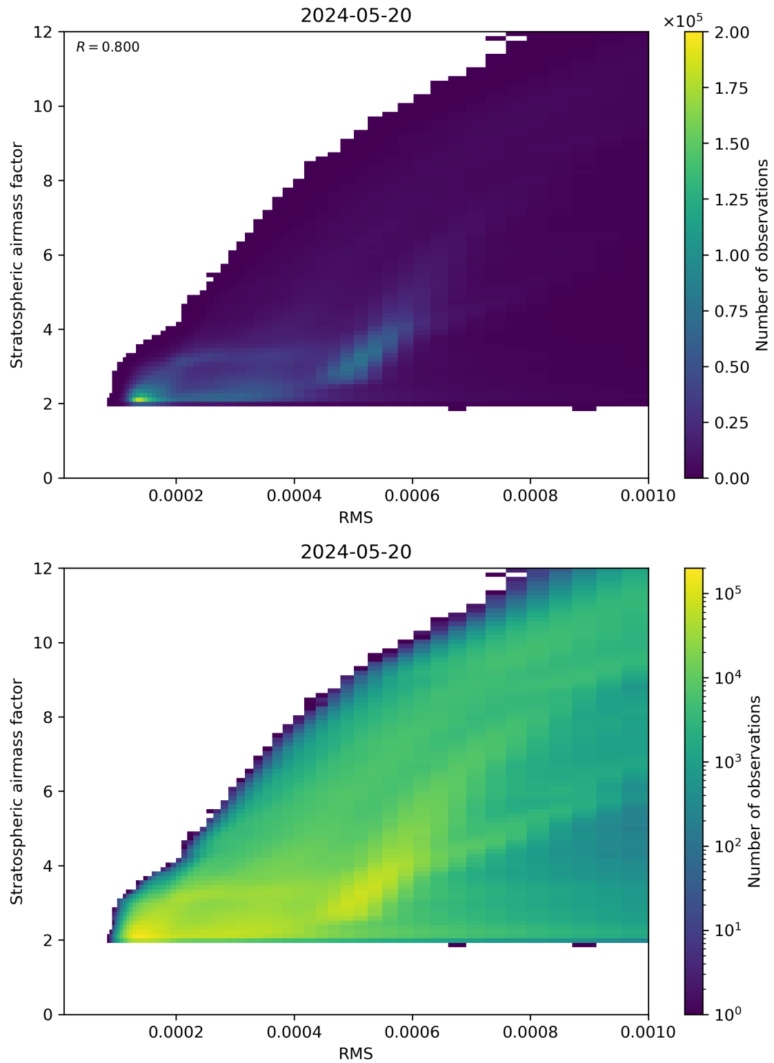
Figure 144: Scatter density plot of “RMS” against “Stratospheric airmass factor” for 2024-05-19 to 2024-05-21.
