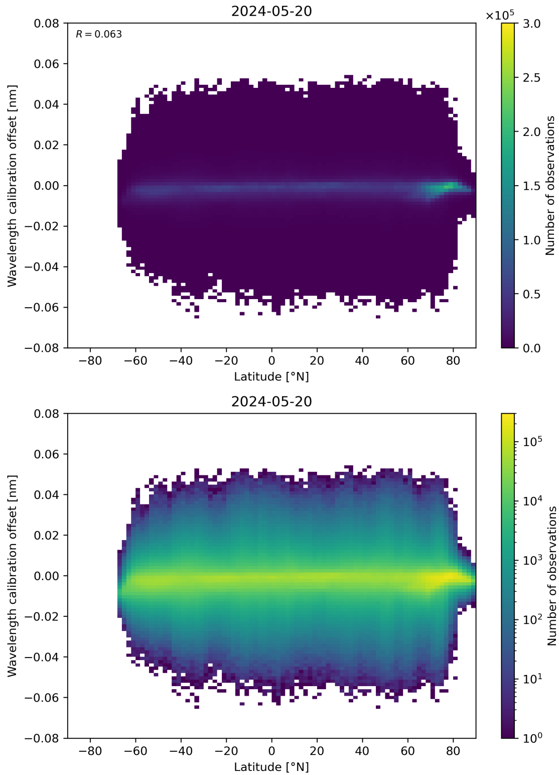
Figure 95: Scatter density plot of “Latitude” against “Wavelength calibration offset” for 2024-05-19 to 2024-05-21.
