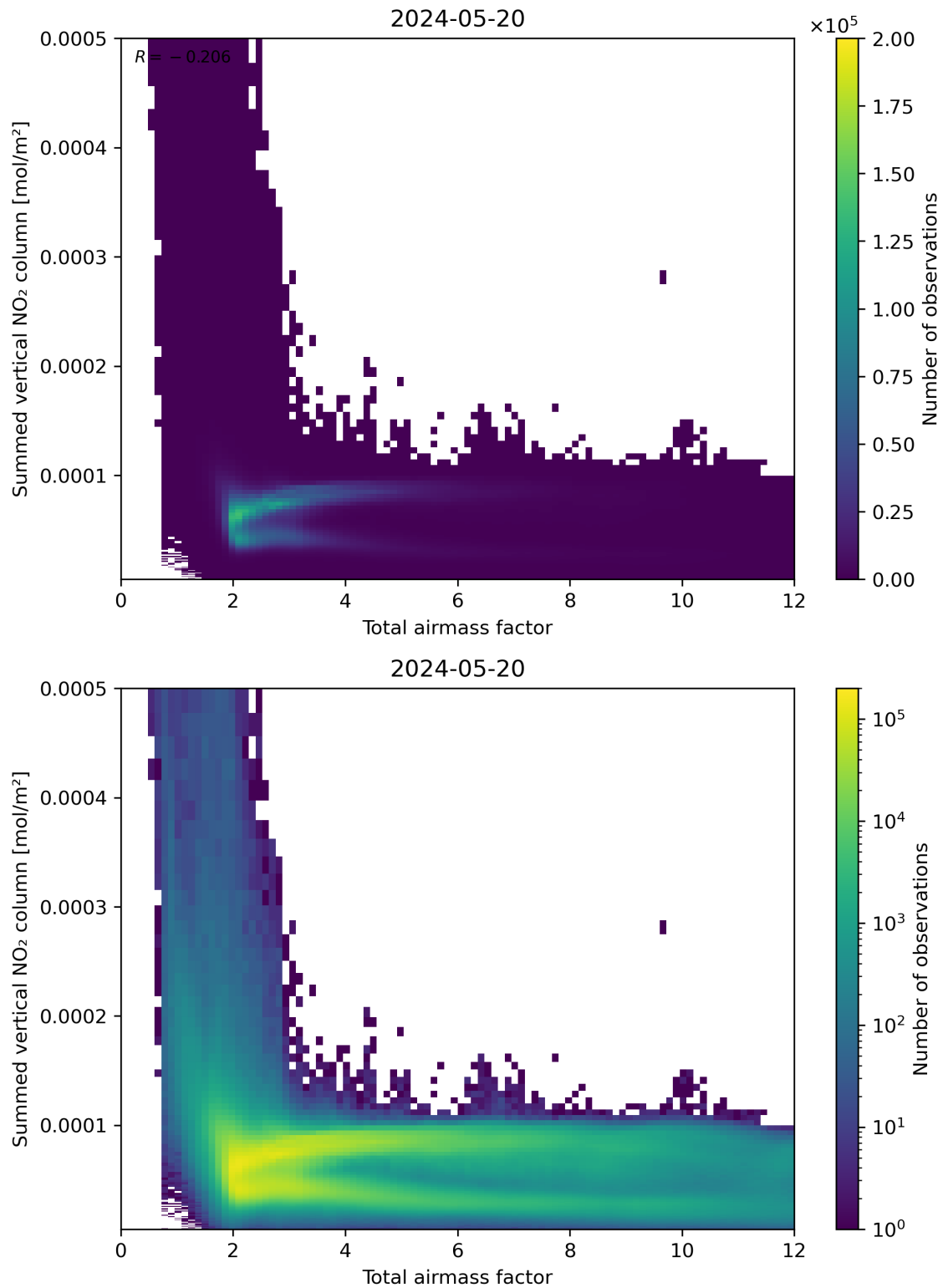
Figure 65: Scatter density plot of “Total airmass factor” against “Summed vertical NO 2 column” for 2024-05-19 to 2024-05-21.
