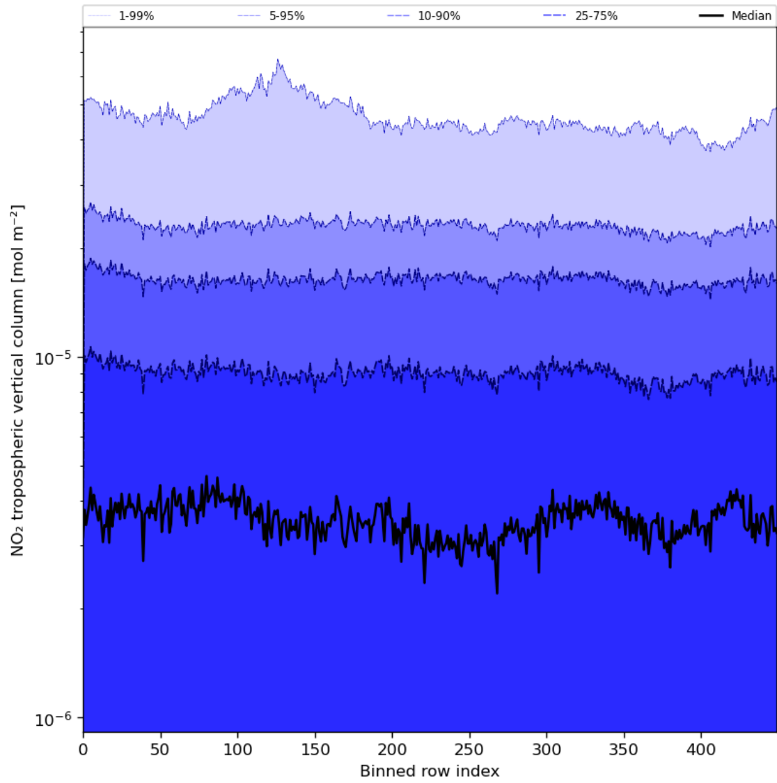
Figure 46: Along track statistics of “NO 2 tropospheric vertical column” for 2024-05-19 to 2024-05-21
