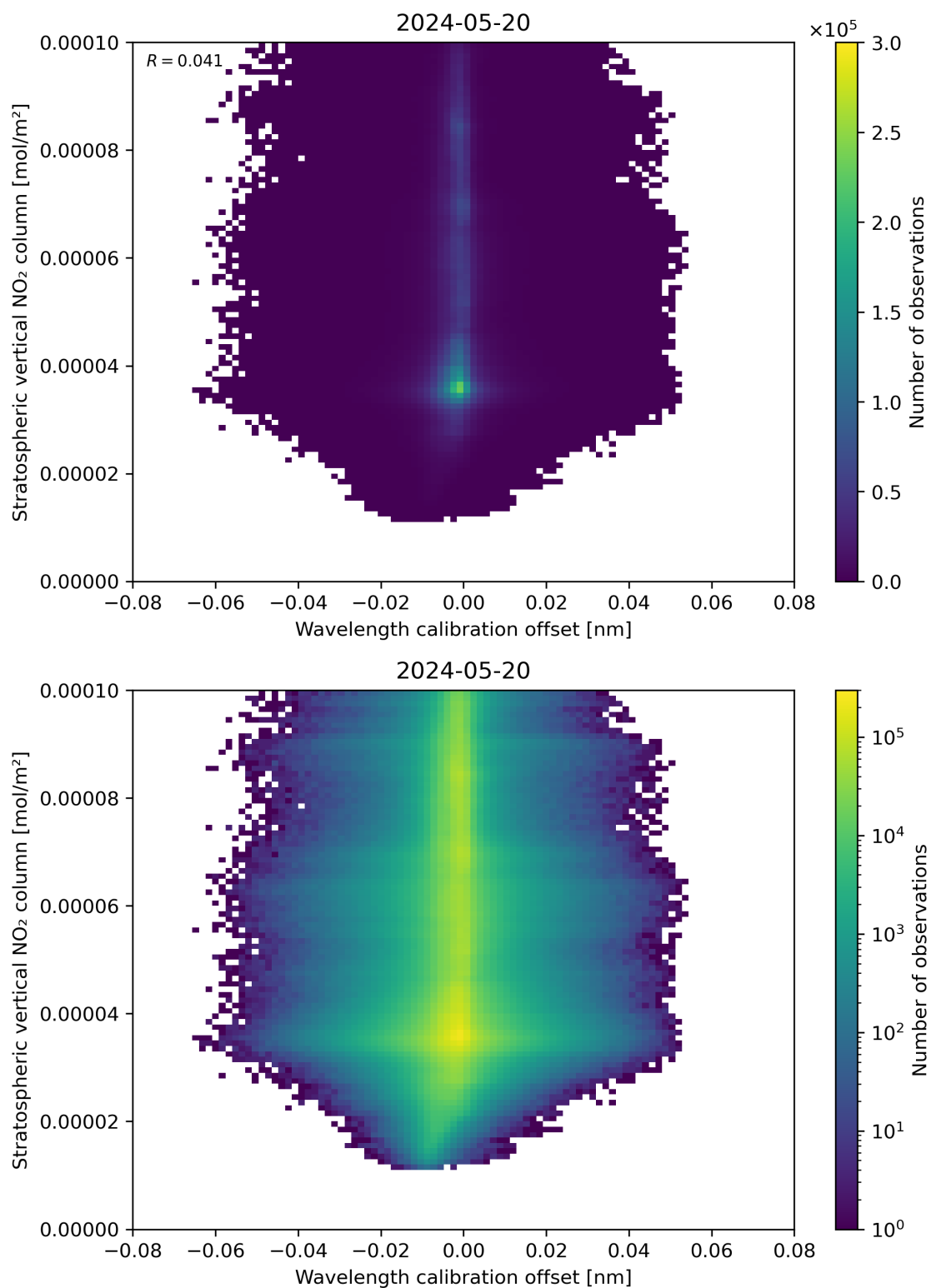
Figure 176: Scatter density plot of “Wavelength calibration offset” against “Stratospheric vertical NO 2 column” for 2024-05-19 to 2024-05-21.
