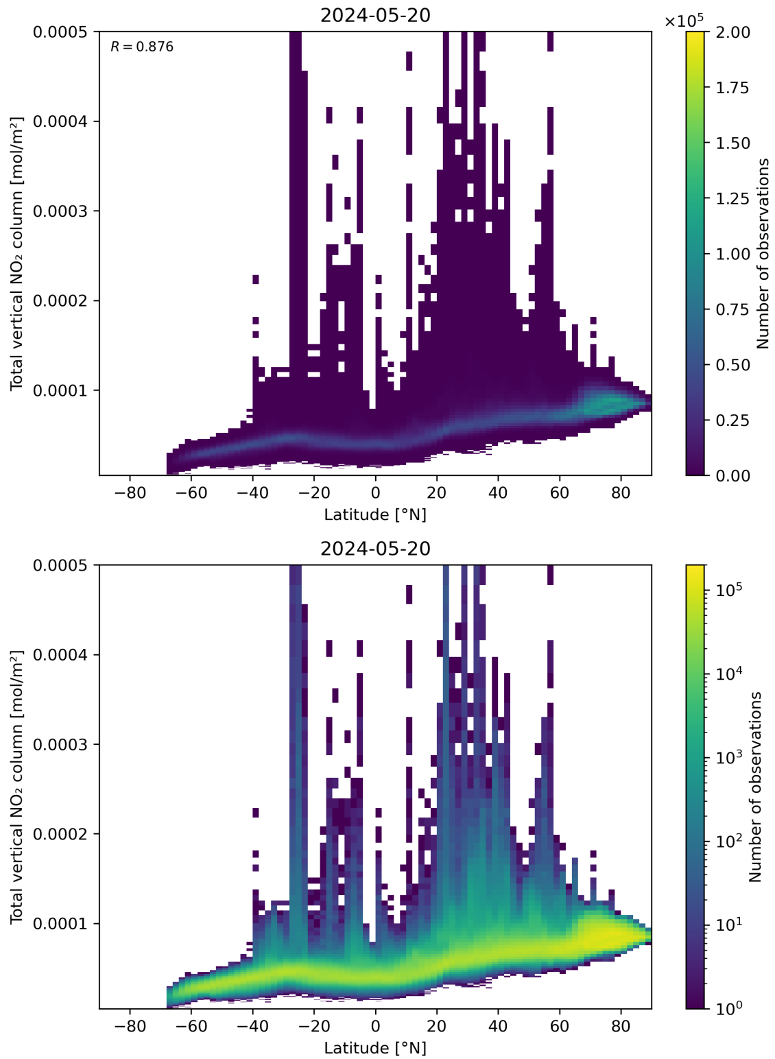
Figure 90: Scatter density plot of “Latitude” against “Total vertical NO 2 column” for 2024-05-19 to 2024-05-21.
