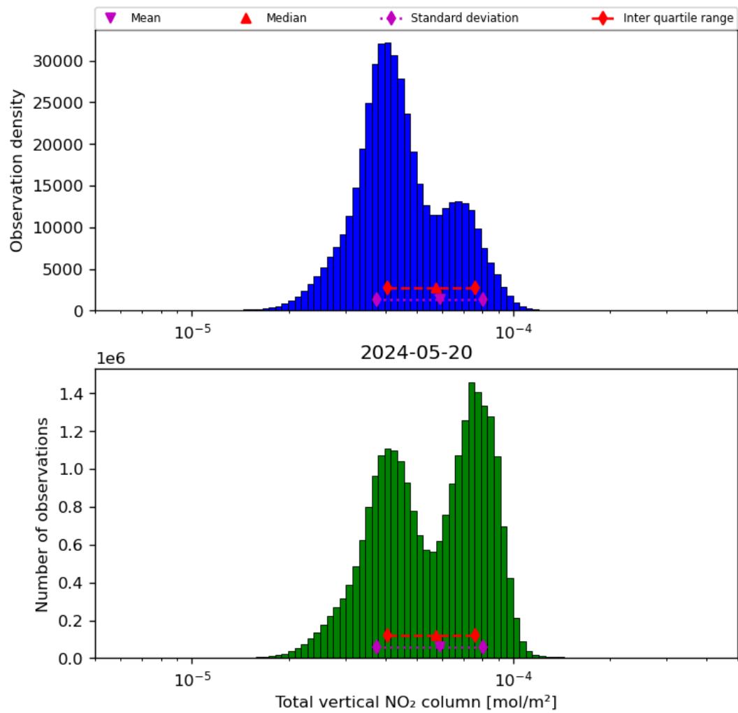
Figure 38: Histogram of “Total vertical NO 2 column” for 2024-05-19 to 2024-05-21
