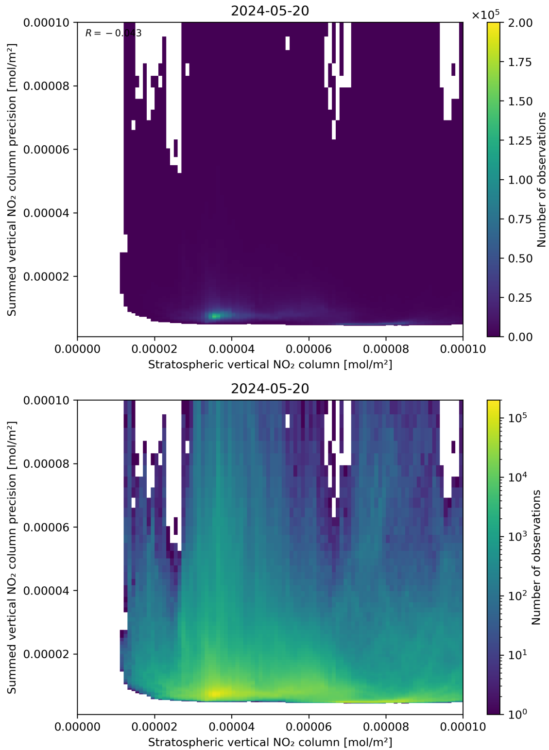
Figure 99: Scatter density plot of “Stratospheric vertical NO 2 column” against “Summed vertical NO 2 column precision” for 2024-05-19 to 2024-05-21.
