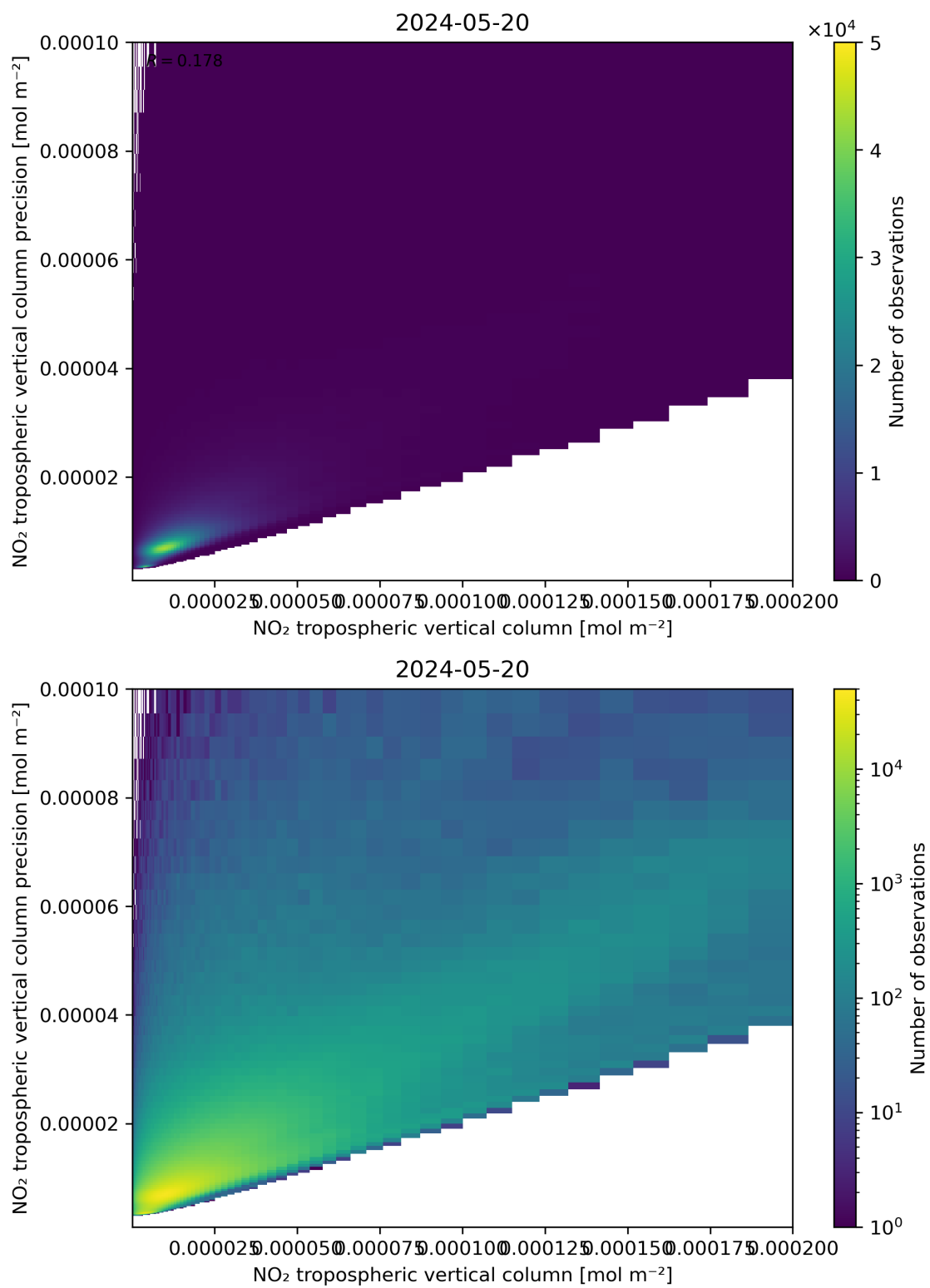
Figure 130: Scatter density plot of “NO 2 tropospheric vertical column” against “NO 2 tropospheric vertical column precision” for 2024-05-19 to 2024-05-21.
