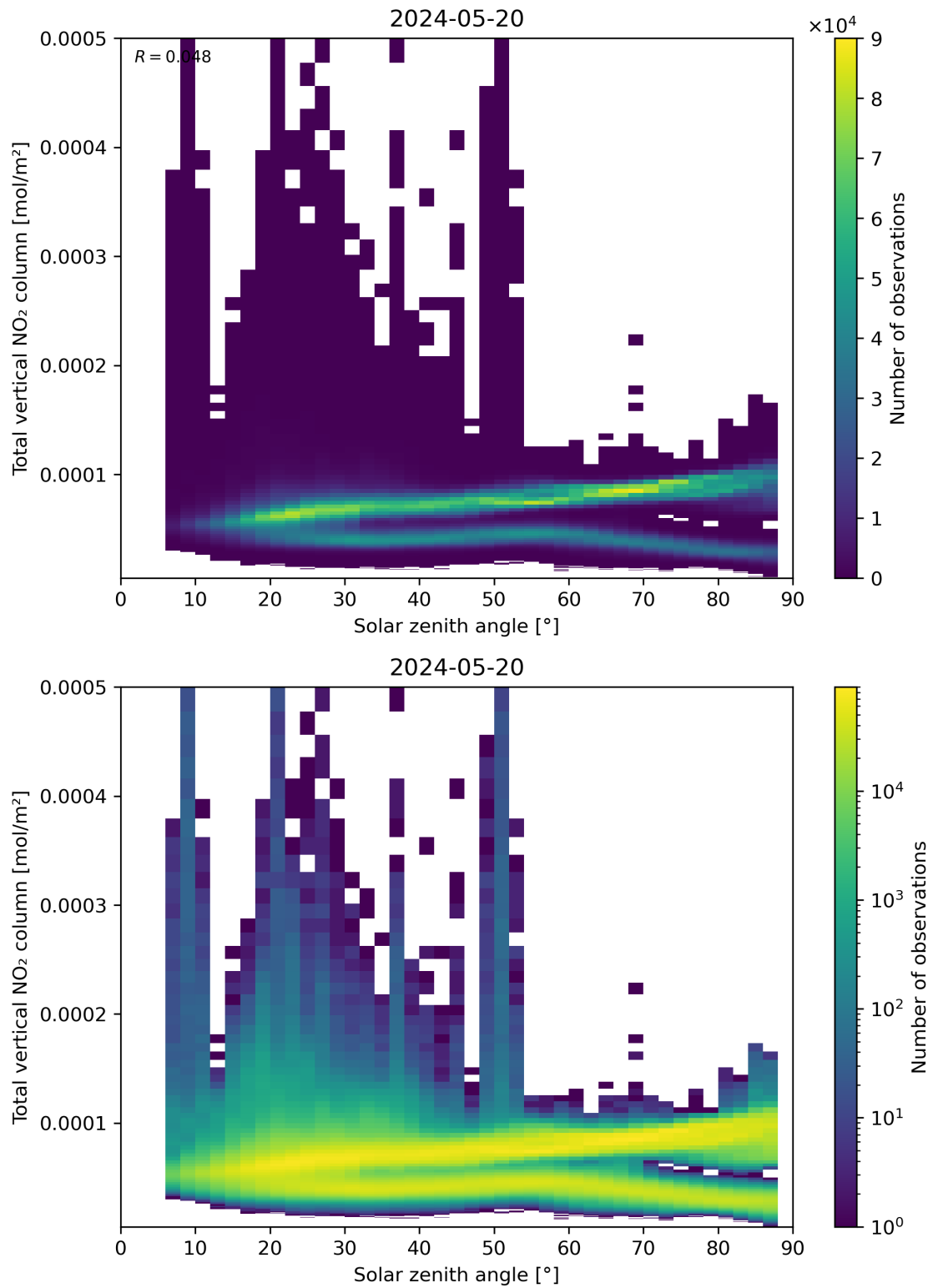
Figure 153: Scatter density plot of “Solar zenith angle” against “Total vertical NO 2 column” for 2024-05-19 to 2024-05-21.
