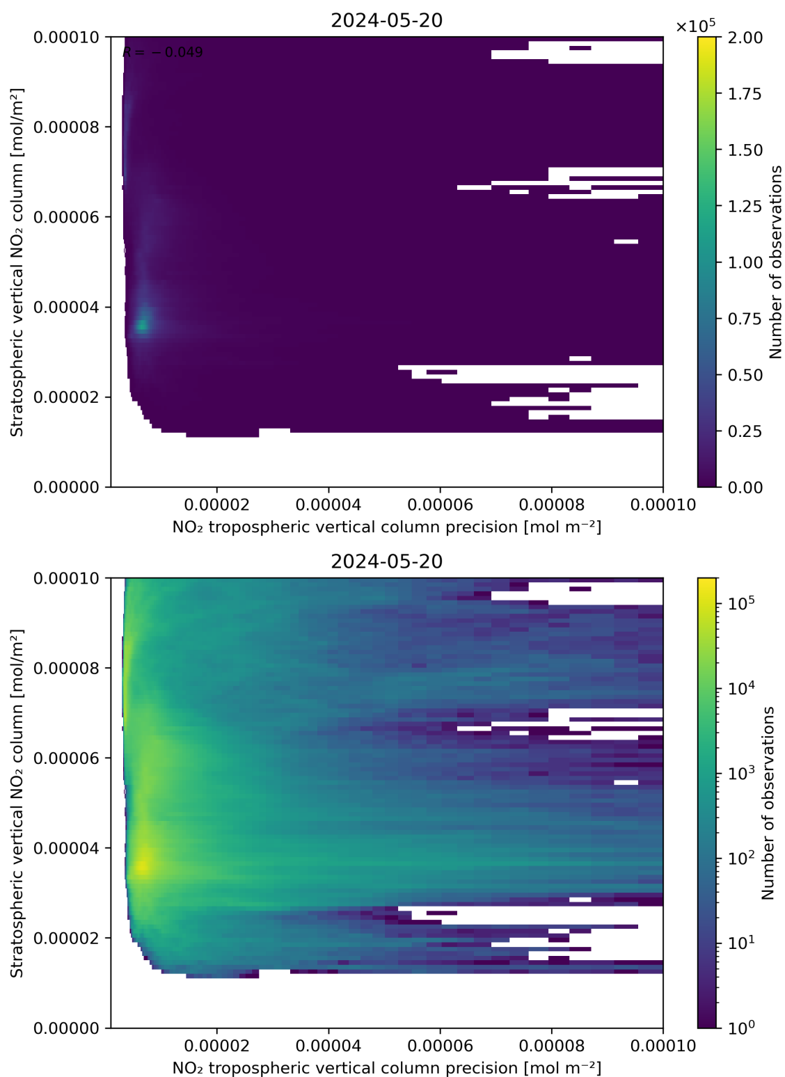
Figure 135: Scatter density plot of “NO 2 tropospheric vertical column precision” against “Stratospheric vertical NO 2 column” for 2024-05-19 to 2024-05-21.
