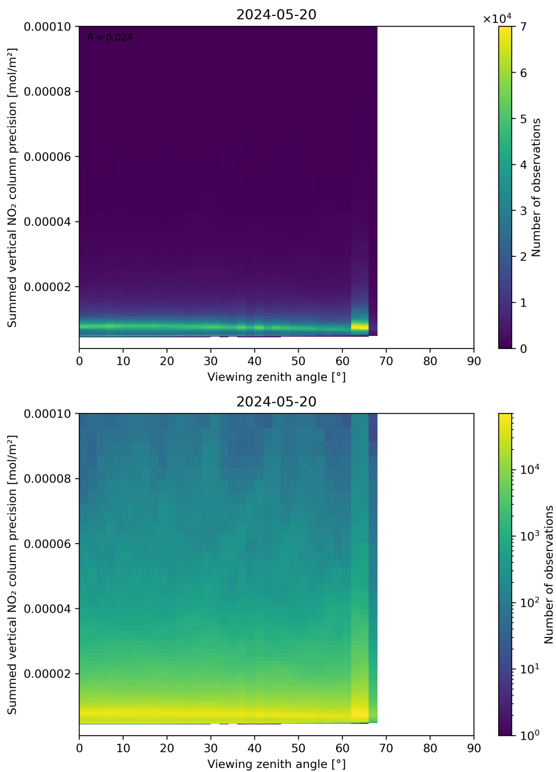
Figure 166: Scatter density plot of “Viewing zenith angle” against “Summed vertical NO 2 column precision” for 2024-05-19 to 2024-05-21.
