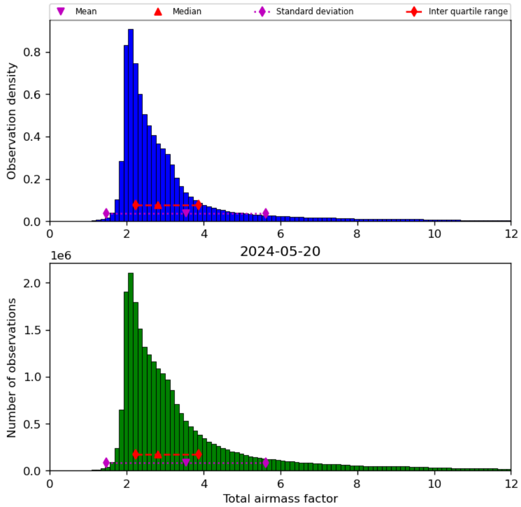
Figure 32: Histogram of “Total airmass factor” for 2024-05-19 to 2024-05-21
