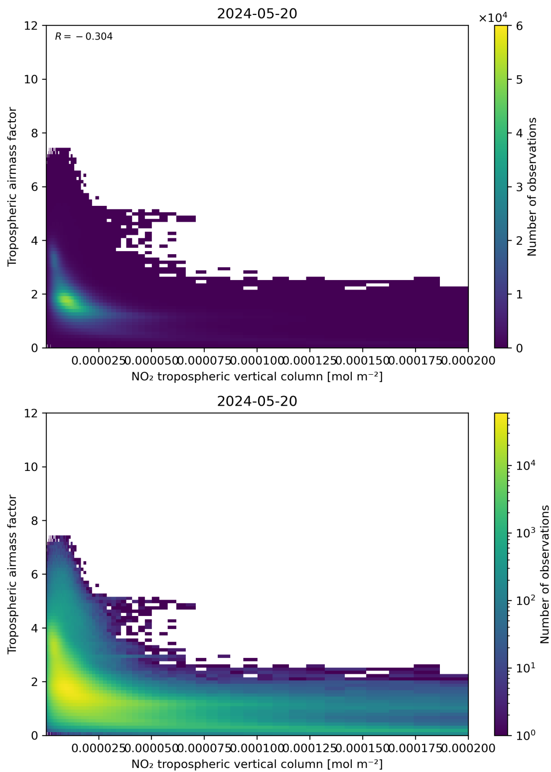
Figure 123: Scatter density plot of “NO 2 tropospheric vertical column” against “Tropospheric airmass factor” for 2024-05-19 to 2024-05-21.
