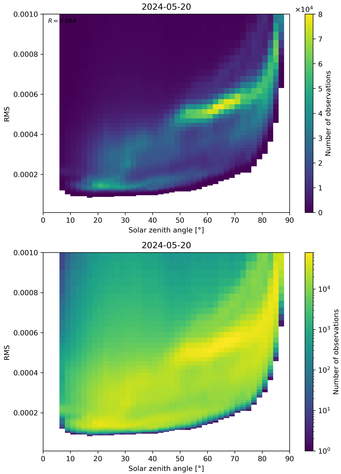
Figure 157: Scatter density plot of “Solar zenith angle” against “RMS” for 2024-05-19 to 2024-05-21.
