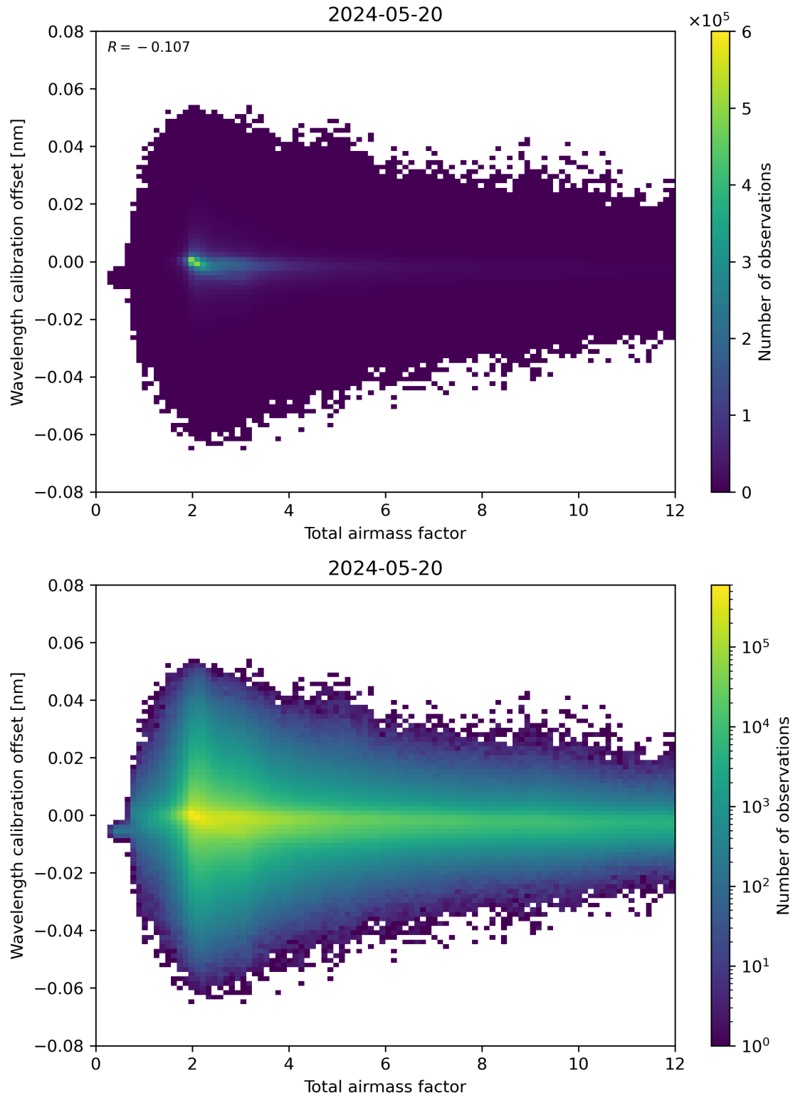
Figure 70: Scatter density plot of “Total airmass factor” against “Wavelength calibration offset” for 2024-05-19 to 2024-05-21.
