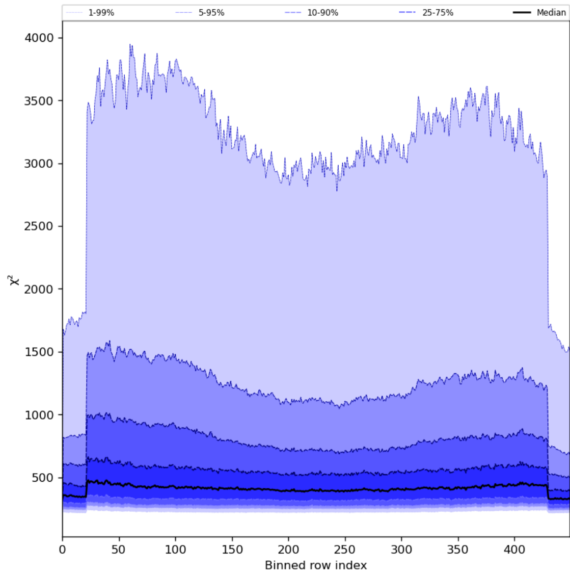
Figure 59: Along track statistics of “ \chi^2 ” for 2024-05-19 to 2024-05-21
