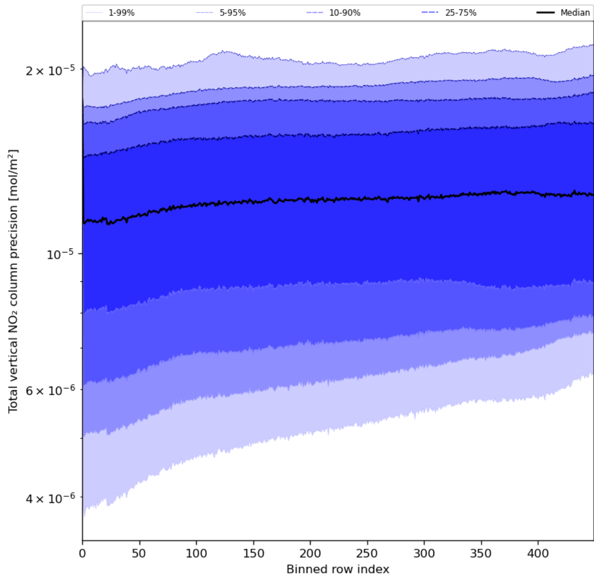
Figure 56: Along track statistics of “Total vertical NO 2 column precision” for 2024-05-19 to 2024-05-21
