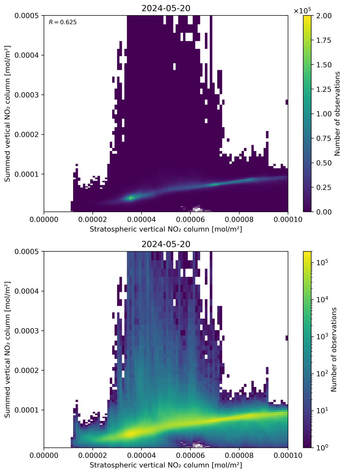
Figure 98: Scatter density plot of “Stratospheric vertical NO 2 column” against “Summed vertical NO 2 column” for 2024-05-19 to 2024-05-21.
