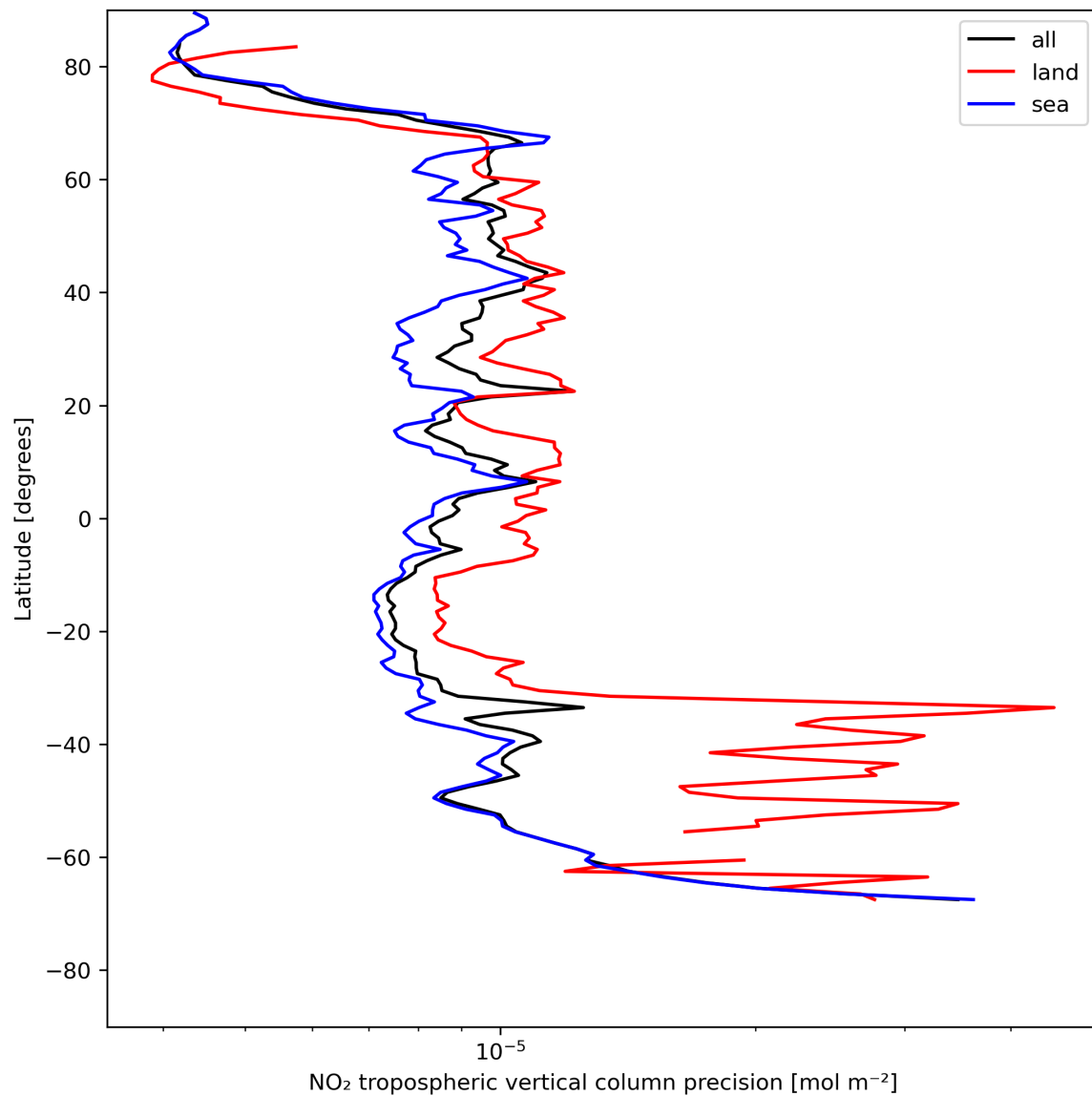
Figure 13: Zonal average of “NO 2 tropospheric vertical column precision” for 2024-05-19 to 2024-05-21.
