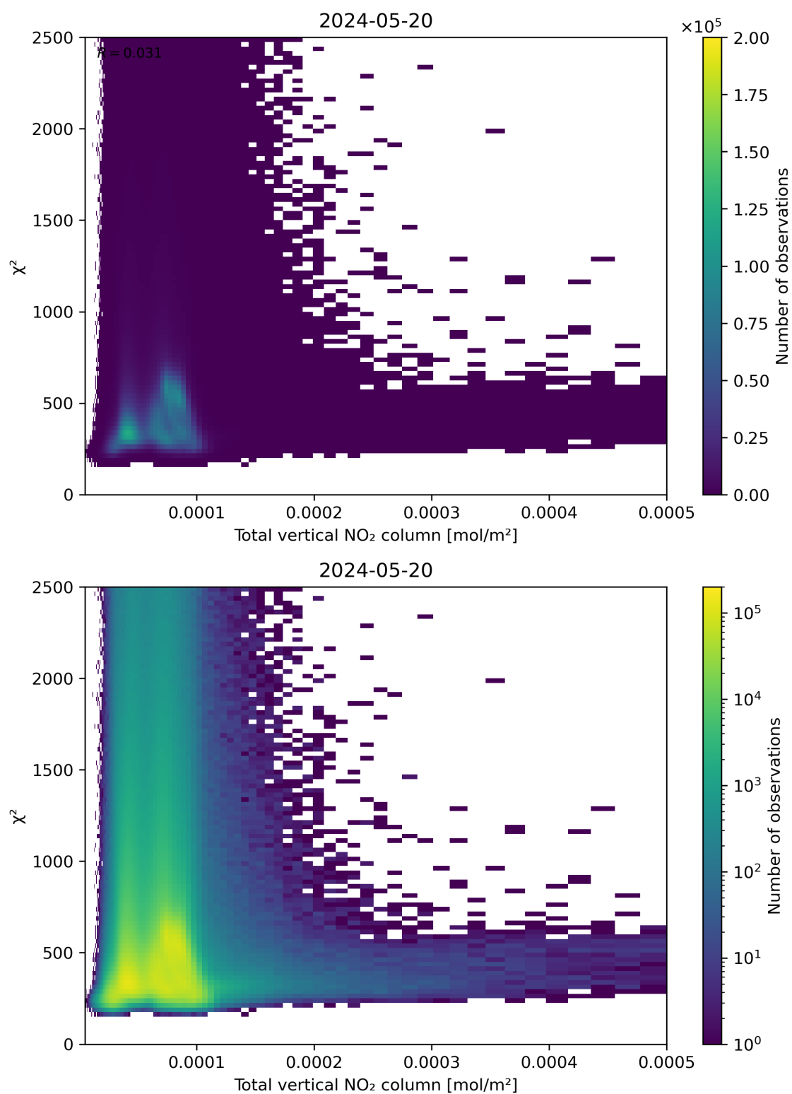
Figure 111: Scatter density plot of “Total vertical NO 2 column” against “ \chi^2 ” for 2024-05-19 to 2024-05-21.
