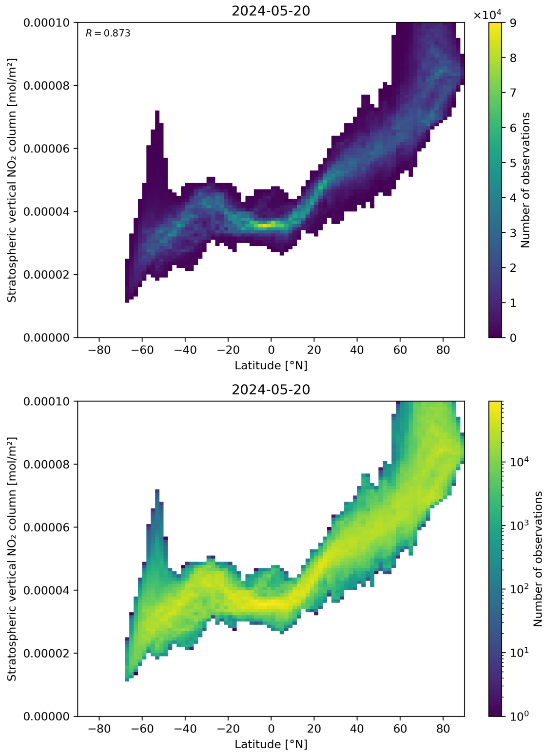
Figure 87: Scatter density plot of “Latitude” against “Stratospheric vertical NO 2 column” for 2024-05-19 to 2024-05-21.
