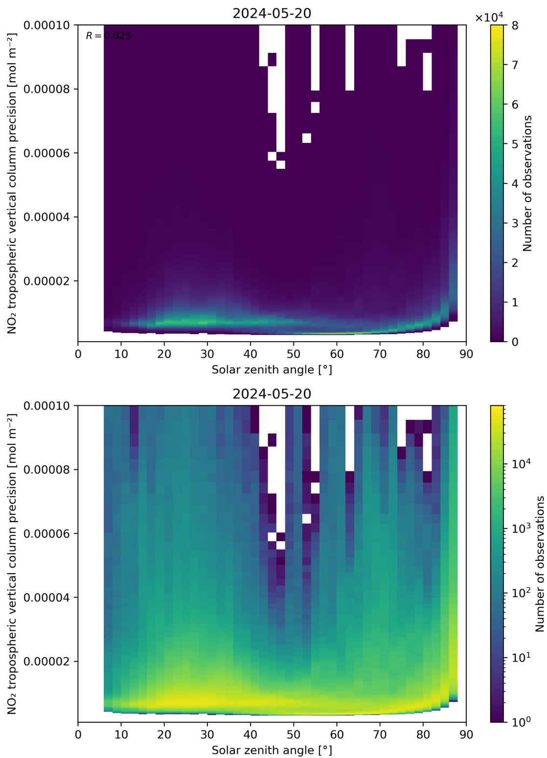
Figure 156: Scatter density plot of “Solar zenith angle” against “NO 2 tropospheric vertical column precision” for 2024-05-19 to 2024-05-21.
