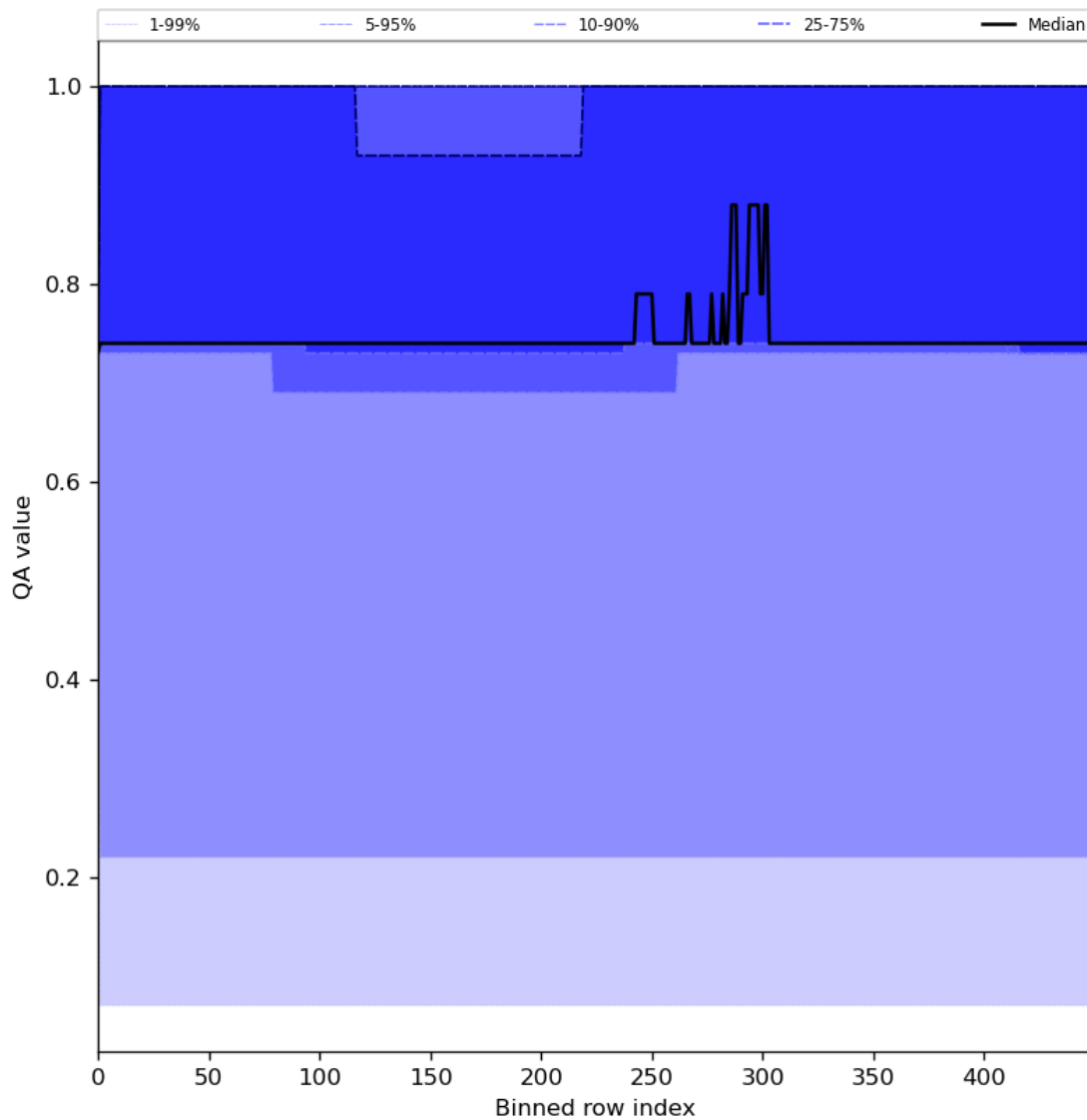
Figure 45: Along track statistics of “QA value” for 2024-05-19 to 2024-05-21
