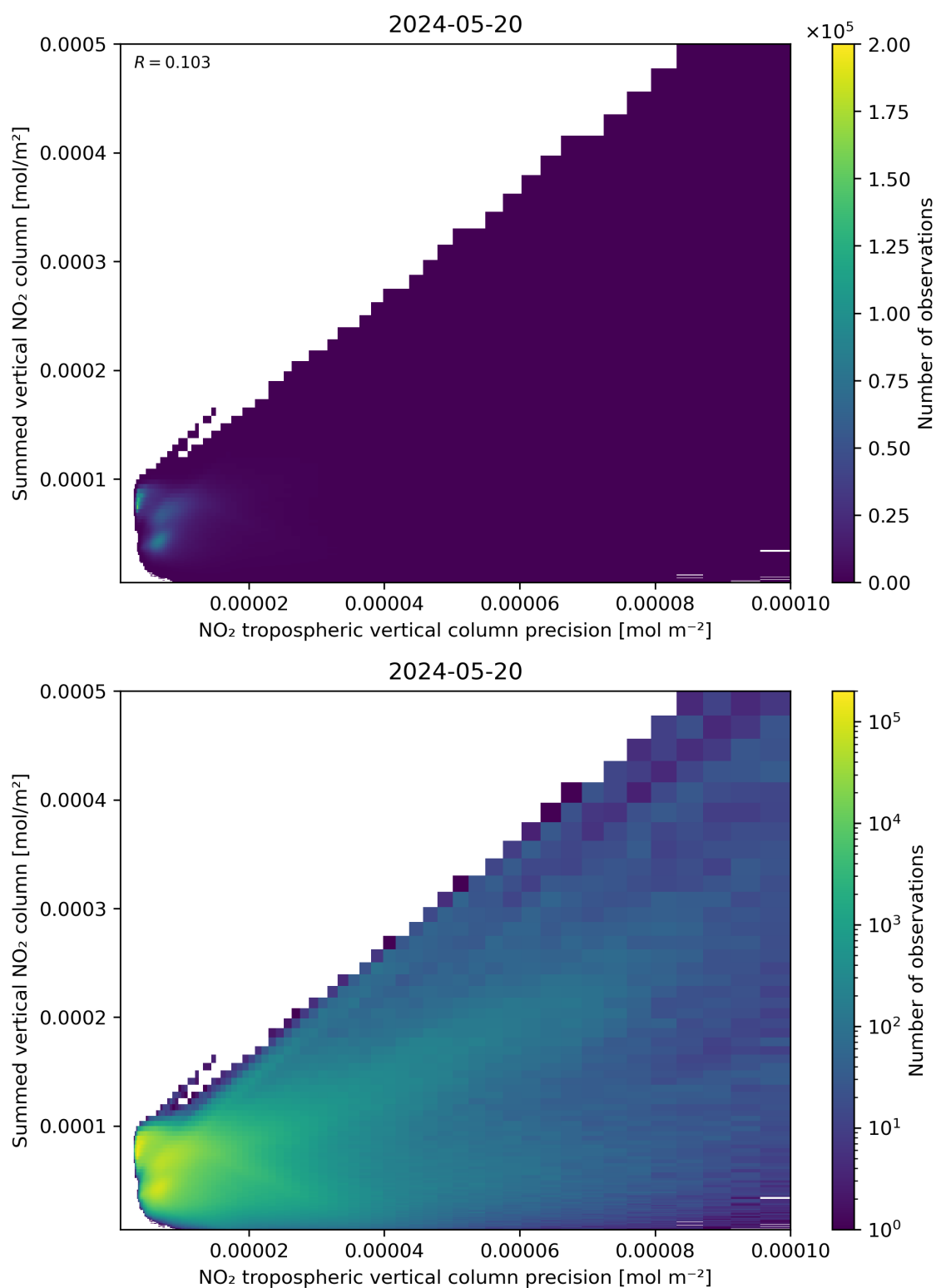
Figure 136: Scatter density plot of “NO 2 tropospheric vertical column precision” against “Summed vertical NO 2 column” for 2024-05-19 to 2024-05-21.
