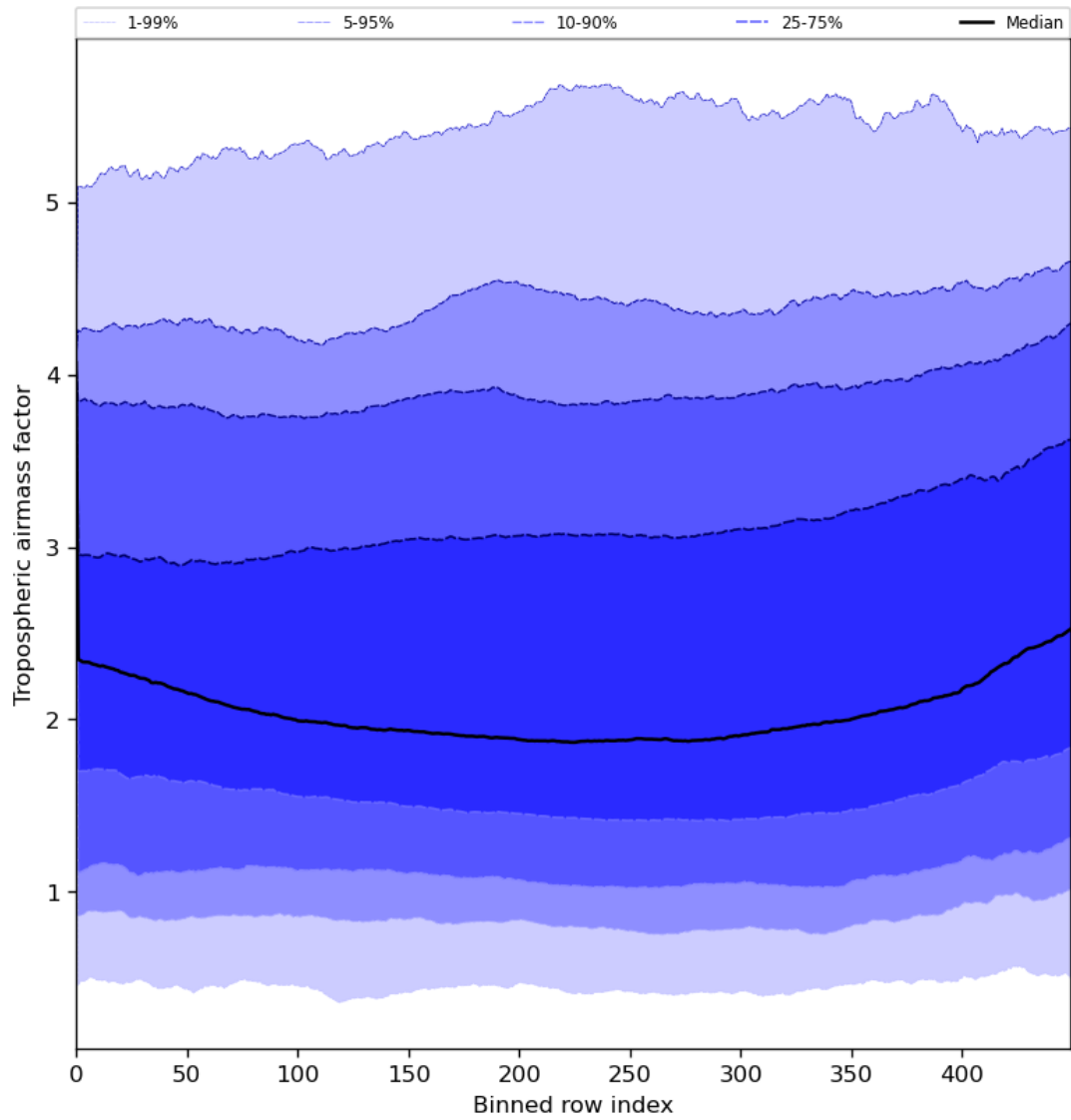
Figure 48: Along track statistics of “Tropospheric airmass factor” for 2024-05-19 to 2024-05-21
