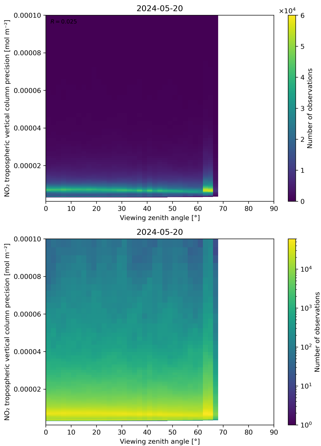
Figure 170: Scatter density plot of “Viewing zenith angle” against “NO 2 tropospheric vertical column precision” for 2024-05-19 to 2024-05-21.
