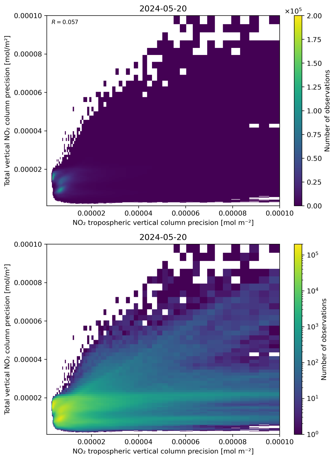
Figure 139: Scatter density plot of “NO 2 tropospheric vertical column precision” against “Total vertical NO 2 column precision” for 2024-05-19 to 2024-05-21.
