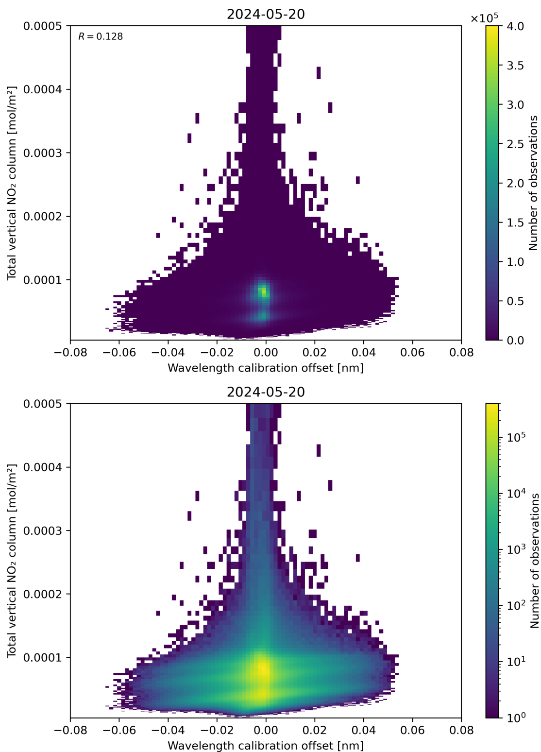
Figure 179: Scatter density plot of “Wavelength calibration offset” against “Total vertical NO 2 column” for 2024-05-19 to 2024-05-21.
