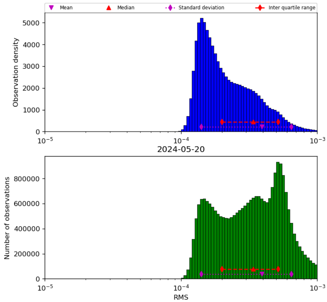
Figure 43: Histogram of “RMS” for 2024-05-19 to 2024-05-21
