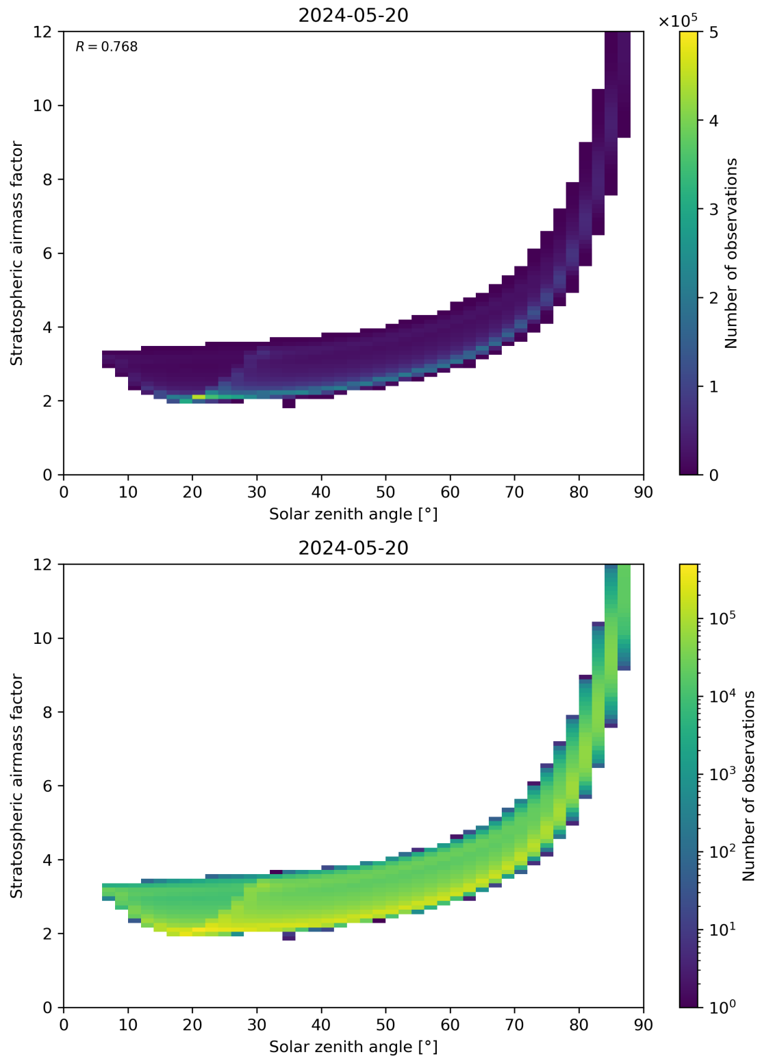
Figure 145: Scatter density plot of “Solar zenith angle” against “Stratospheric airmass factor” for 2024-05-19 to 2024-05-21.
