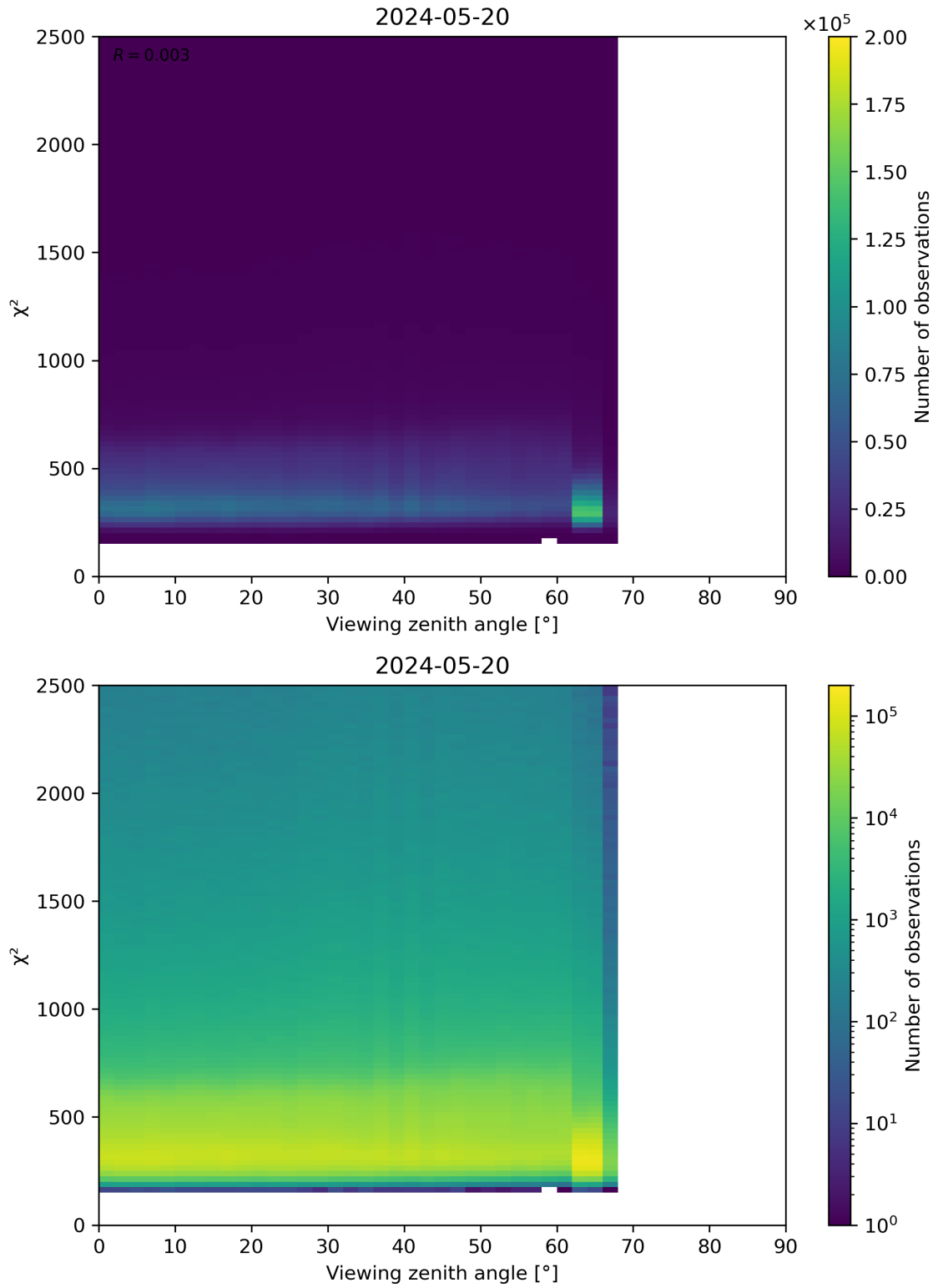
Figure 162: Scatter density plot of “Viewing zenith angle” against “ \chi^2 ” for 2024-05-19 to 2024-05-21.
