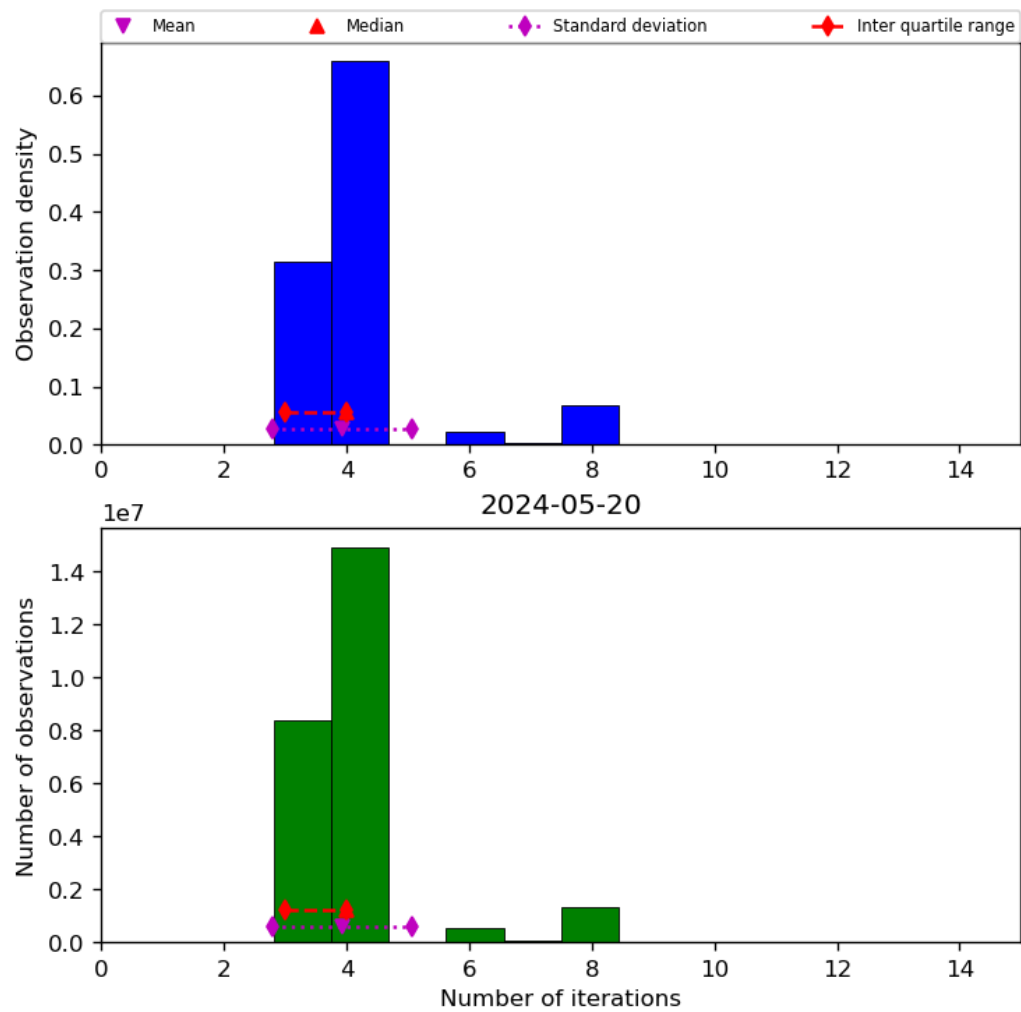
Figure 34: Histogram of “Number of iterations” for 2024-05-19 to 2024-05-21
