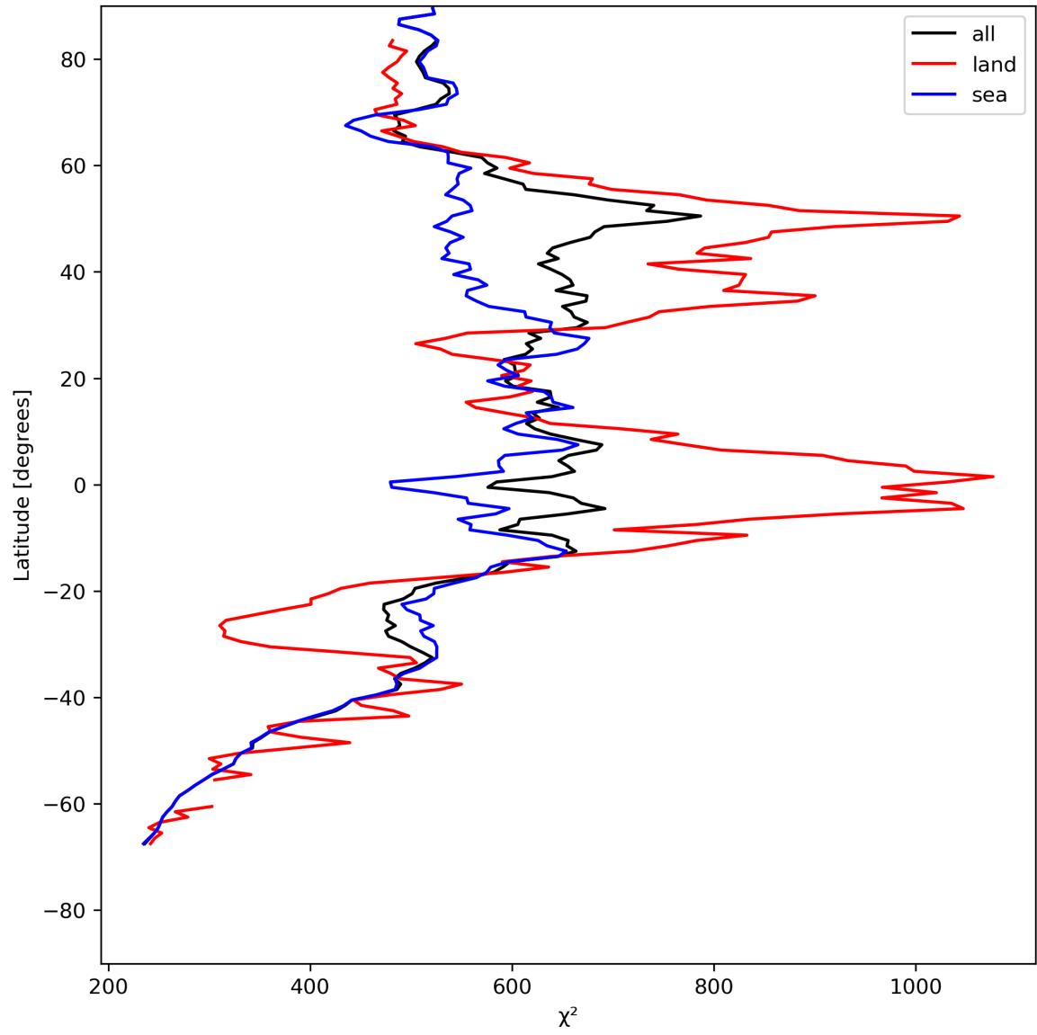
Figure 25: Zonal average of “ \chi^2 ” for 2024-05-19 to 2024-05-21.
