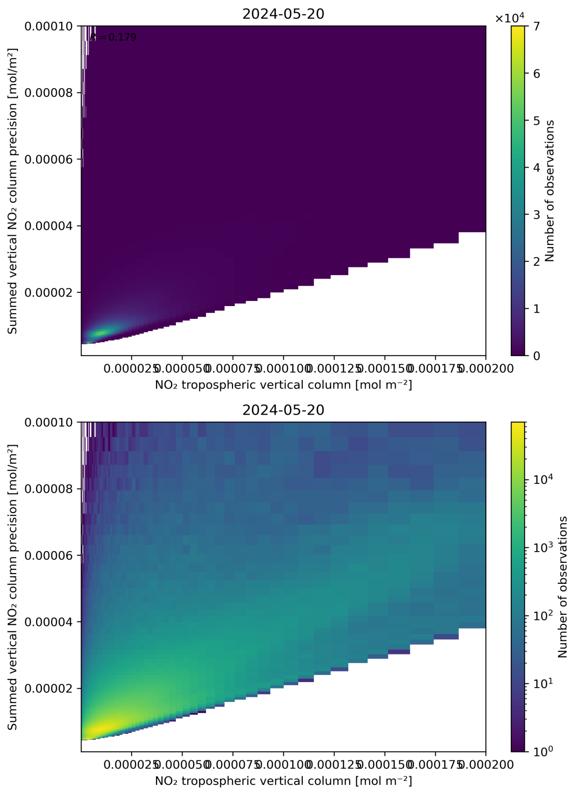
Figure 127: Scatter density plot of “NO 2 tropospheric vertical column” against “Summed vertical NO 2 column precision” for 2024-05-19 to 2024-05-21.
