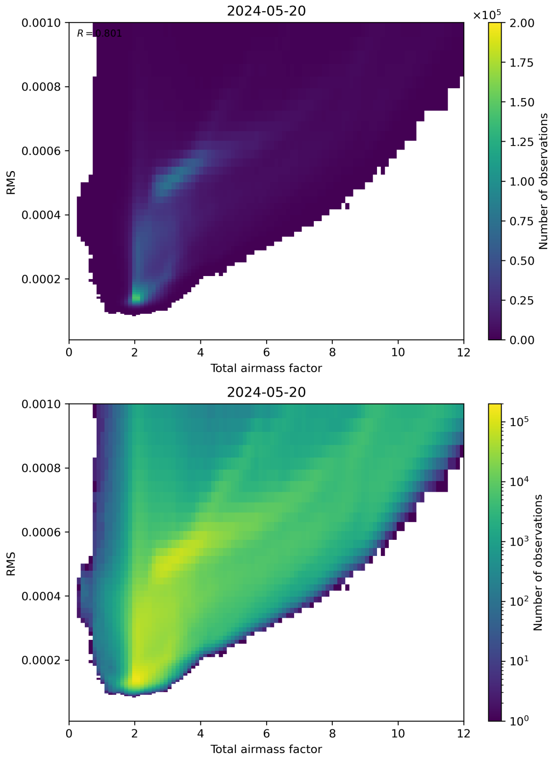
Figure 69: Scatter density plot of “Total airmass factor” against “RMS” for 2024-05-19 to 2024-05-21.
