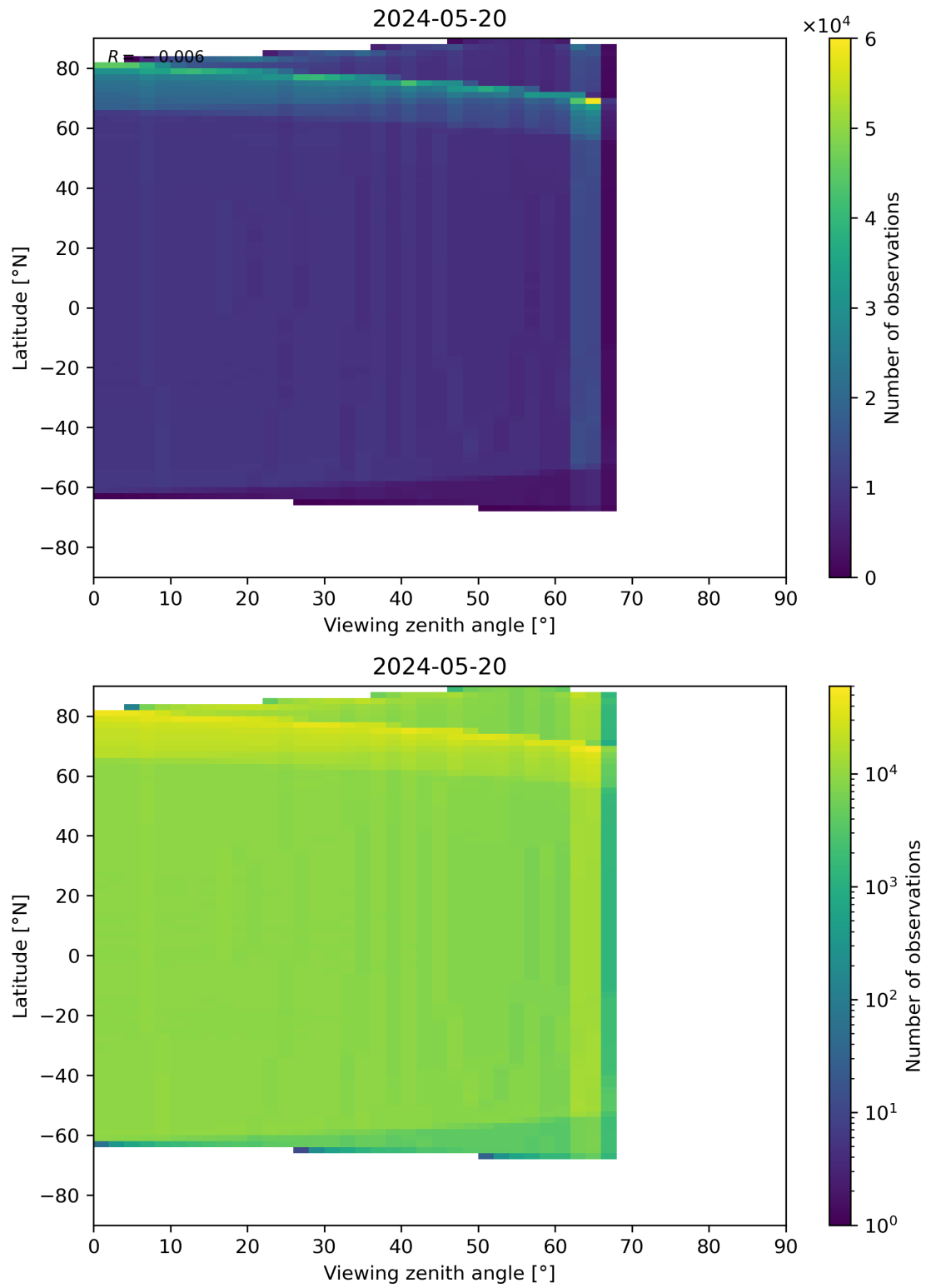
Figure 163: Scatter density plot of “Viewing zenith angle” against “Latitude” for 2024-05-19 to 2024-05-21.
