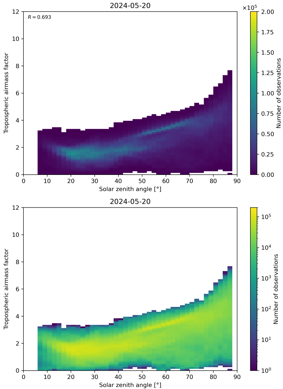
Figure 147: Scatter density plot of “Solar zenith angle” against “Tropospheric airmass factor” for 2024-05-19 to 2024-05-21.
