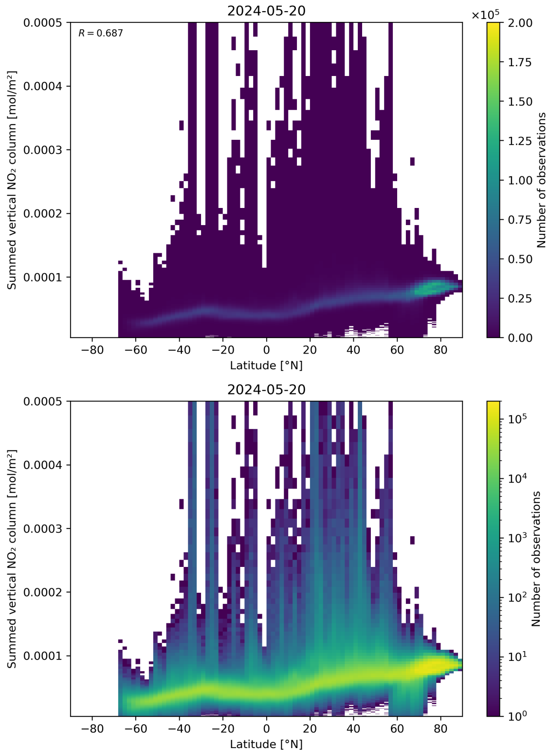
Figure 88: Scatter density plot of “Latitude” against “Summed vertical NO 2 column” for 2024-05-19 to 2024-05-21.
