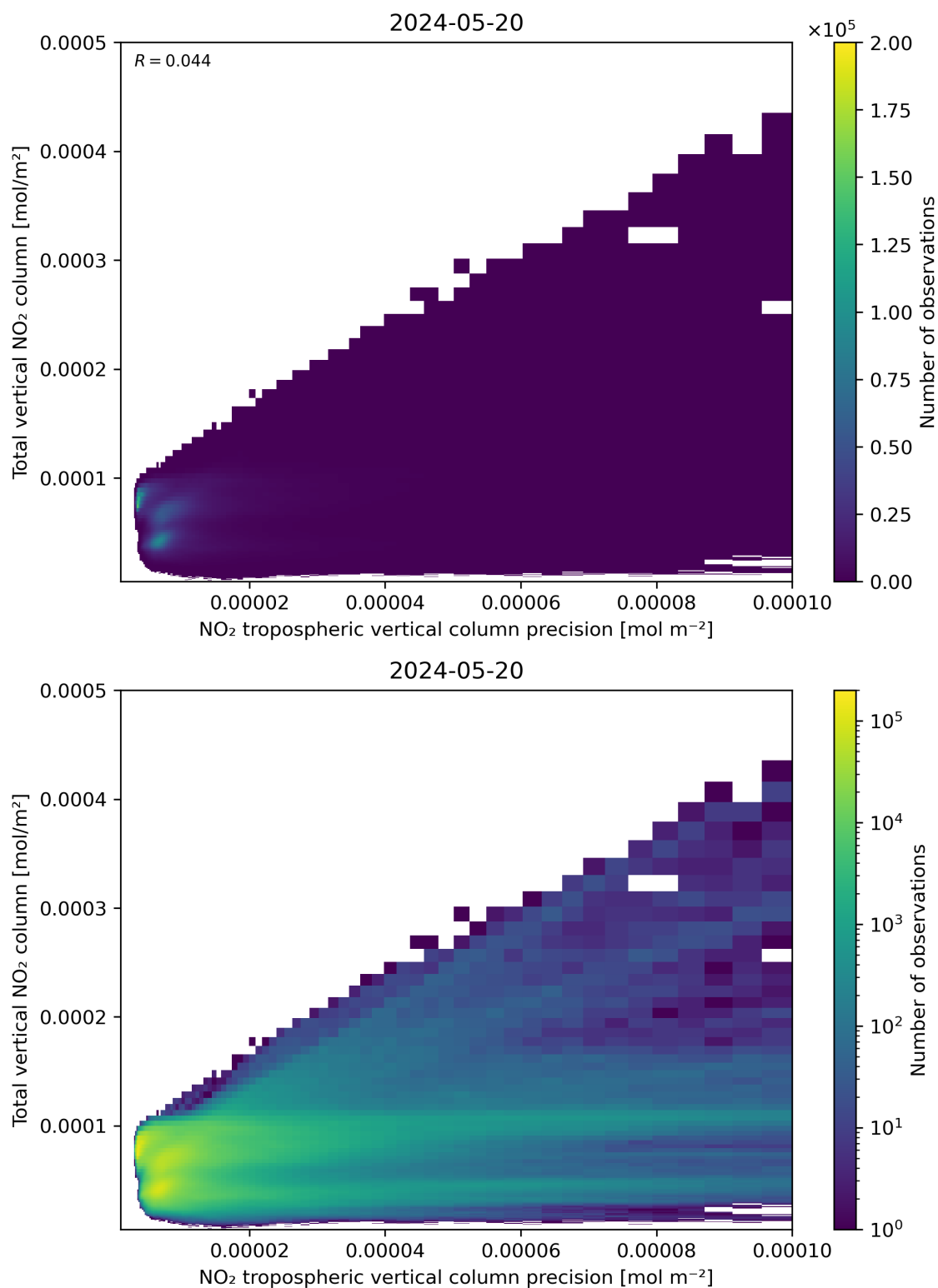
Figure 138: Scatter density plot of “NO 2 tropospheric vertical column precision” against “Total vertical NO 2 column” for 2024-05-19 to 2024-05-21.
