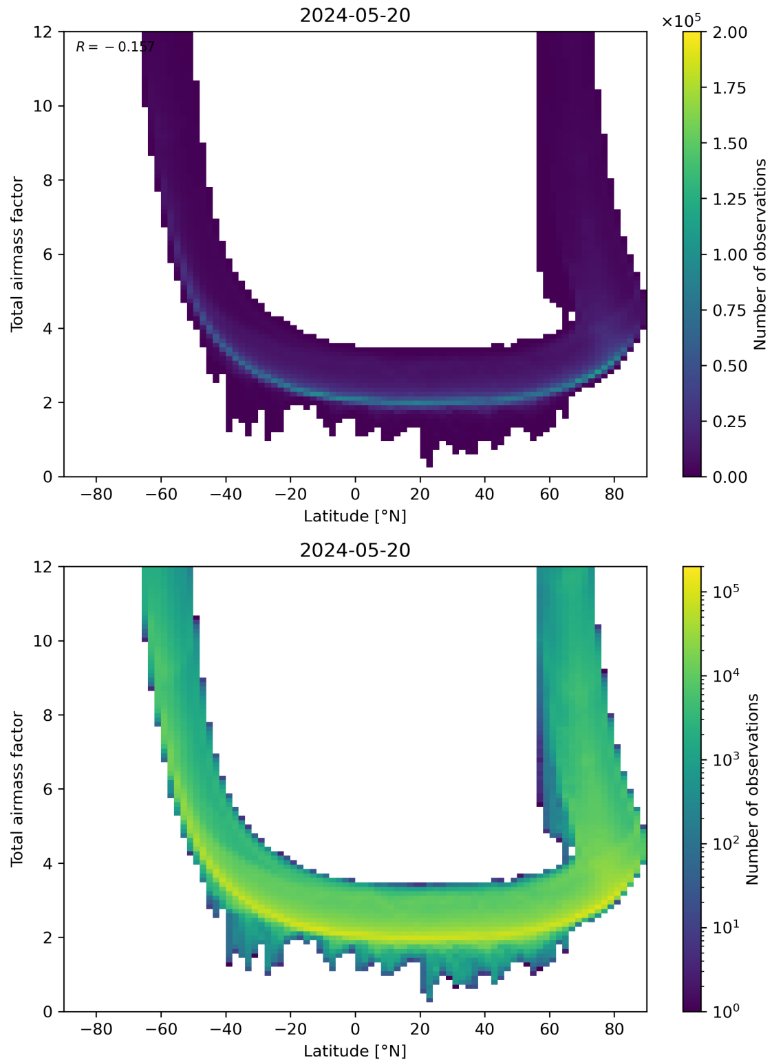
Figure 84: Scatter density plot of “Latitude” against “Total airmass factor” for 2024-05-19 to 2024-05-21.
