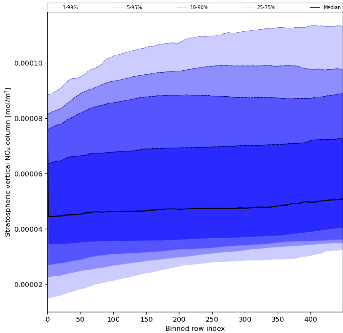
Figure 53: Along track statistics of “Stratospheric vertical NO 2 column” for 2024-05-19 to 2024-05-21
