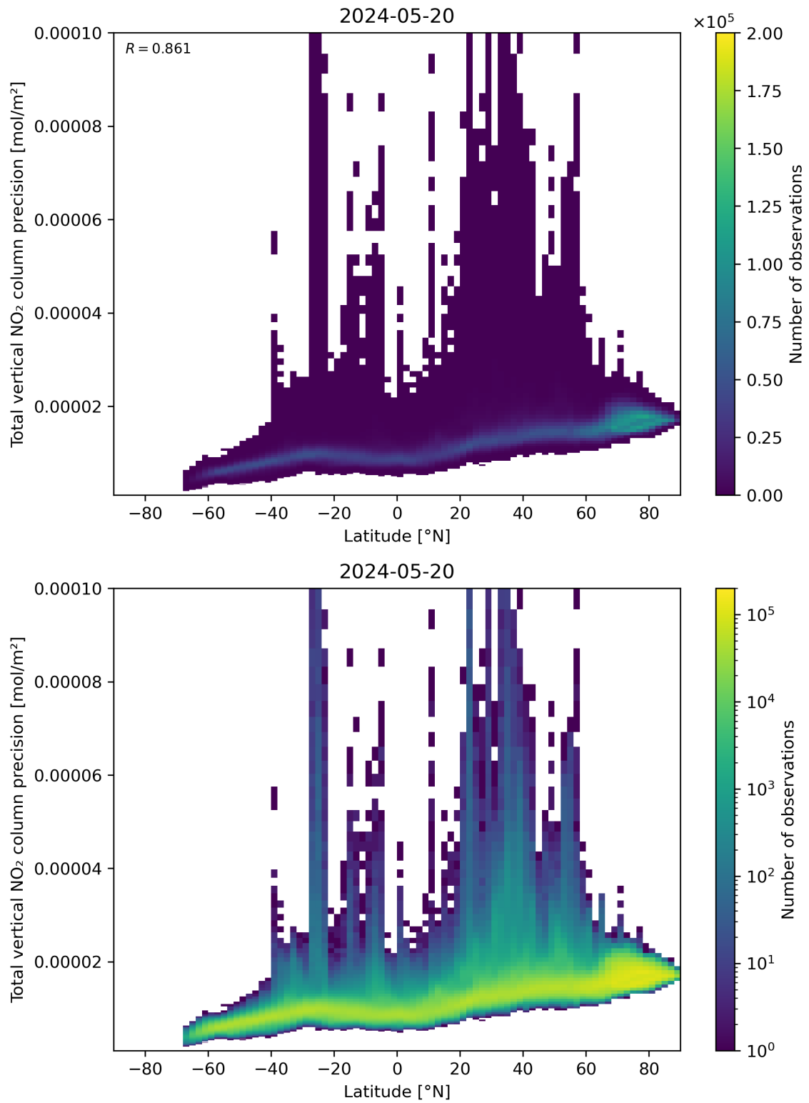
Figure 91: Scatter density plot of “Latitude” against “Total vertical NO 2 column precision” for 2024-05-19 to 2024-05-21.
