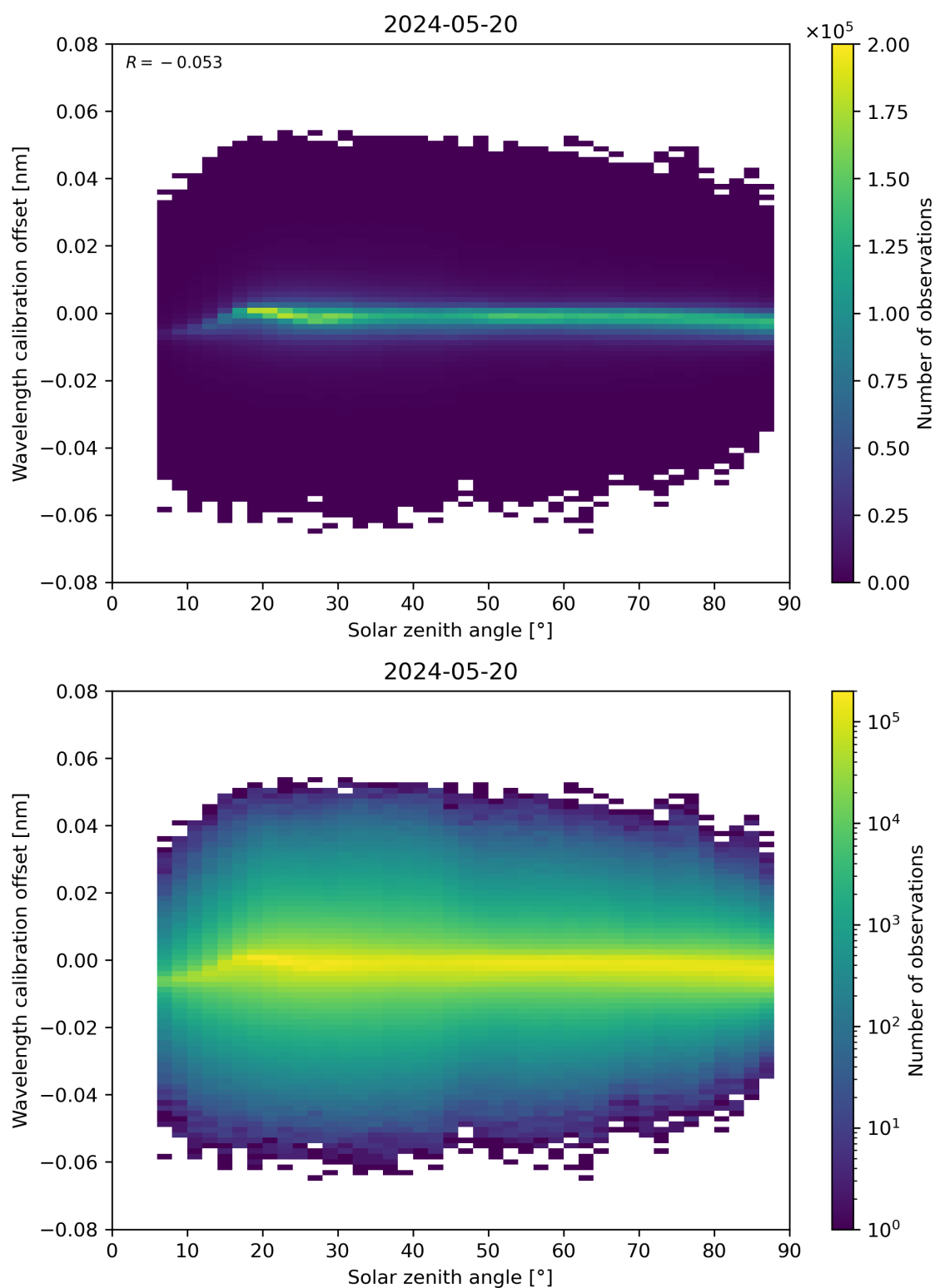
Figure 158: Scatter density plot of “Solar zenith angle” against “Wavelength calibration offset” for 2024-05-19 to 2024-05-21.
