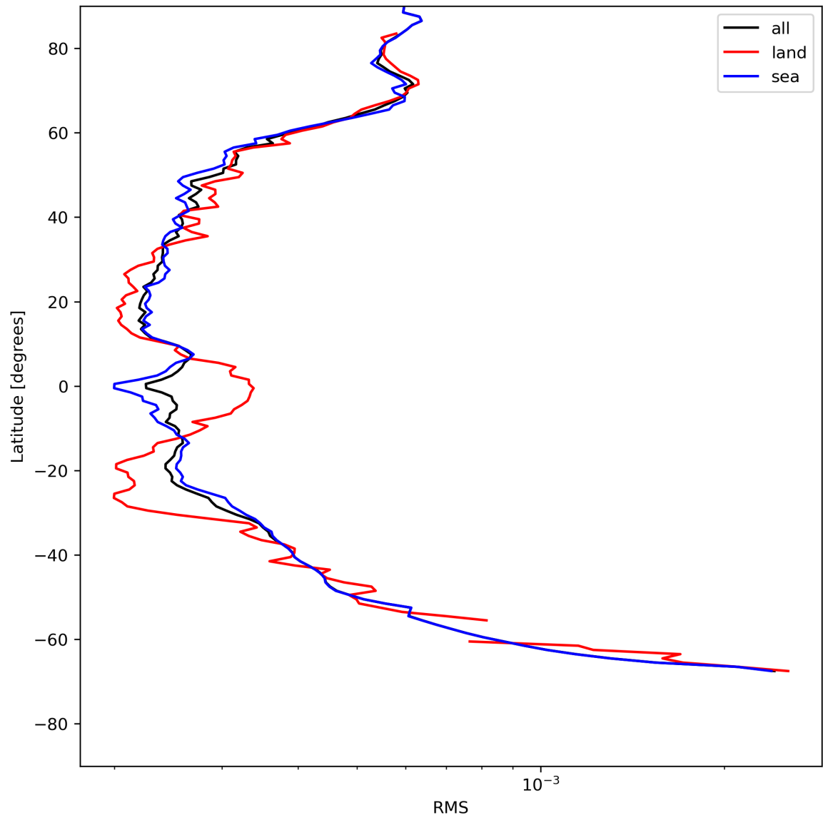
Figure 26: Zonal average of “RMS” for 2024-05-19 to 2024-05-21.
