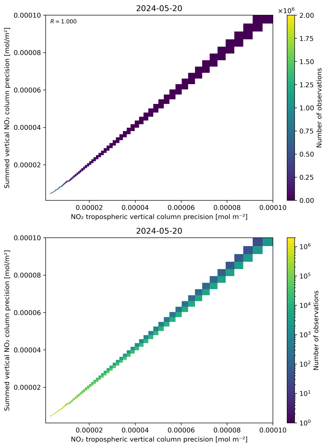
Figure 137: Scatter density plot of “NO 2 tropospheric vertical column precision” against “Summed vertical NO 2 column precision” for 2024-05-19 to 2024-05-21.
