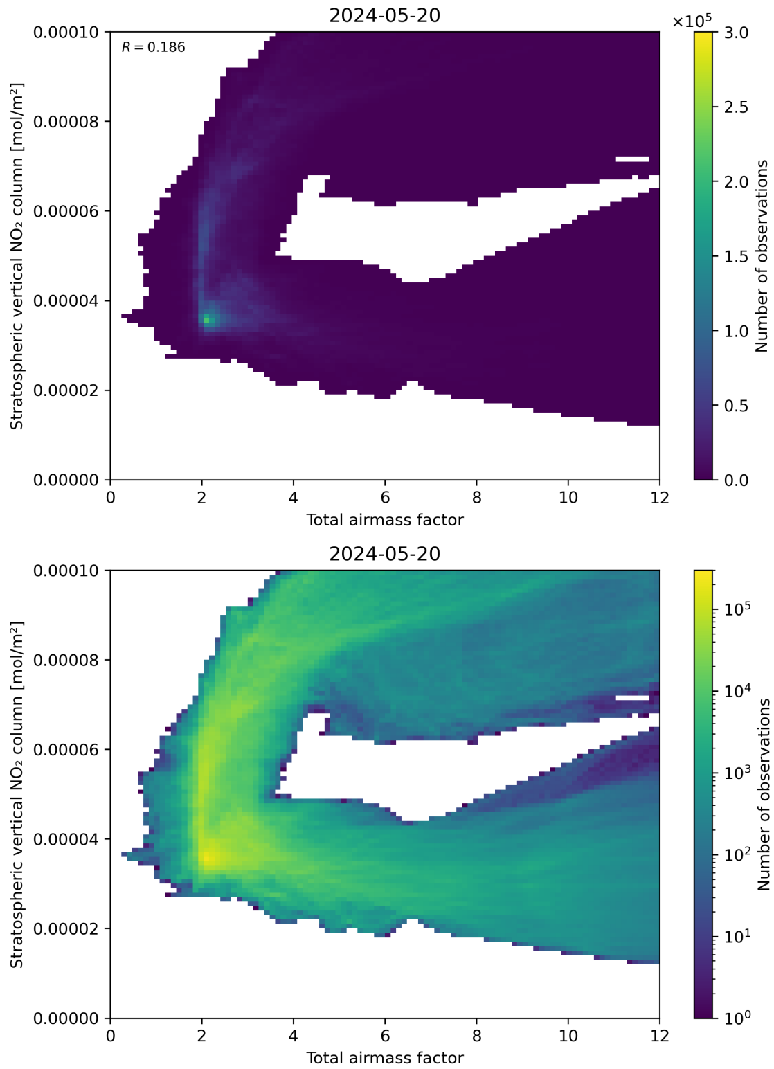
Figure 64: Scatter density plot of “Total airmass factor” against “Stratospheric vertical NO 2 column” for 2024-05-19 to 2024-05-21.
