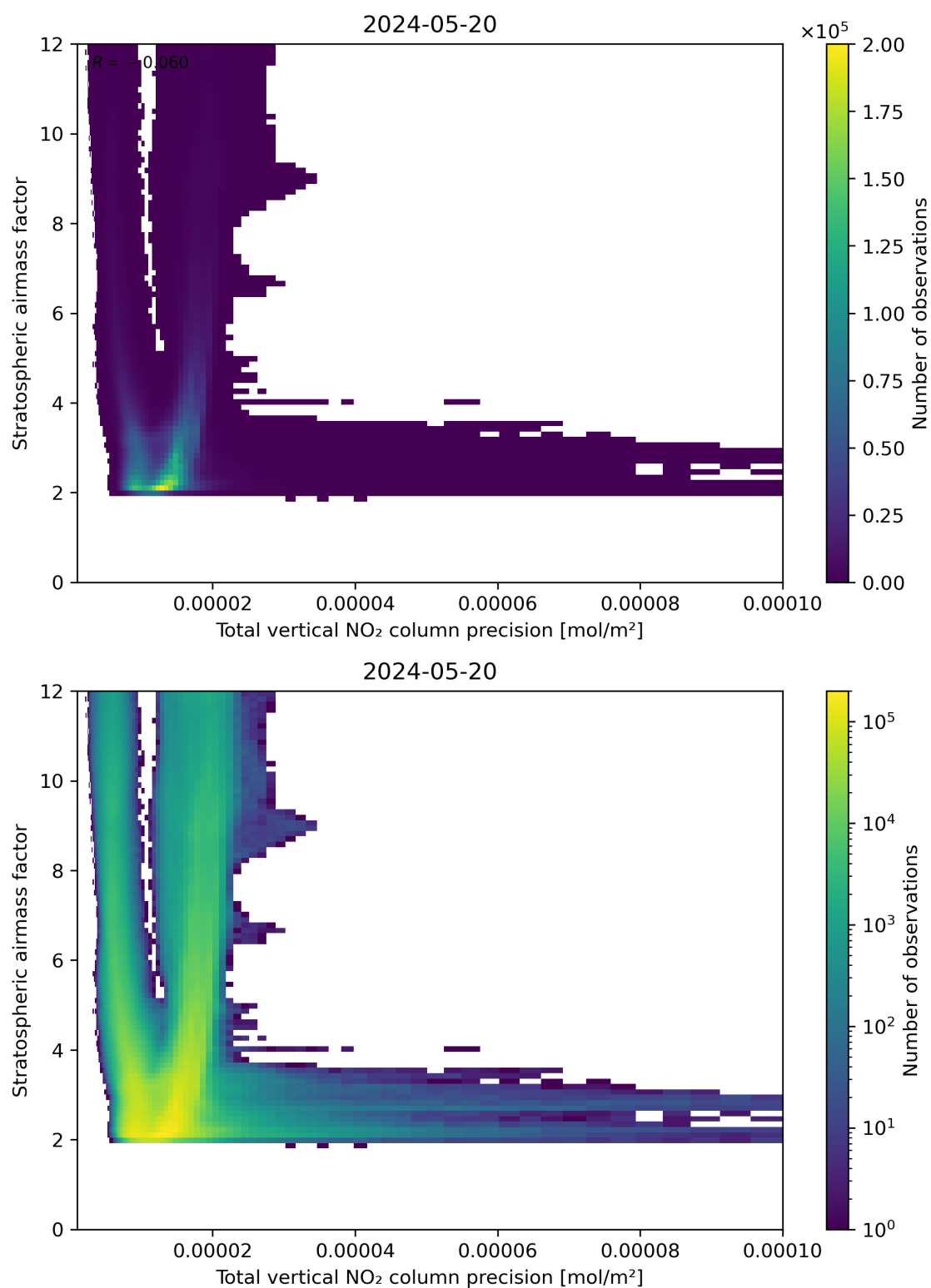
Figure 115: Scatter density plot of “Total vertical NO 2 column precision” against “Stratospheric air mass factor” for 2024-05-19 to 2024-05-21.
