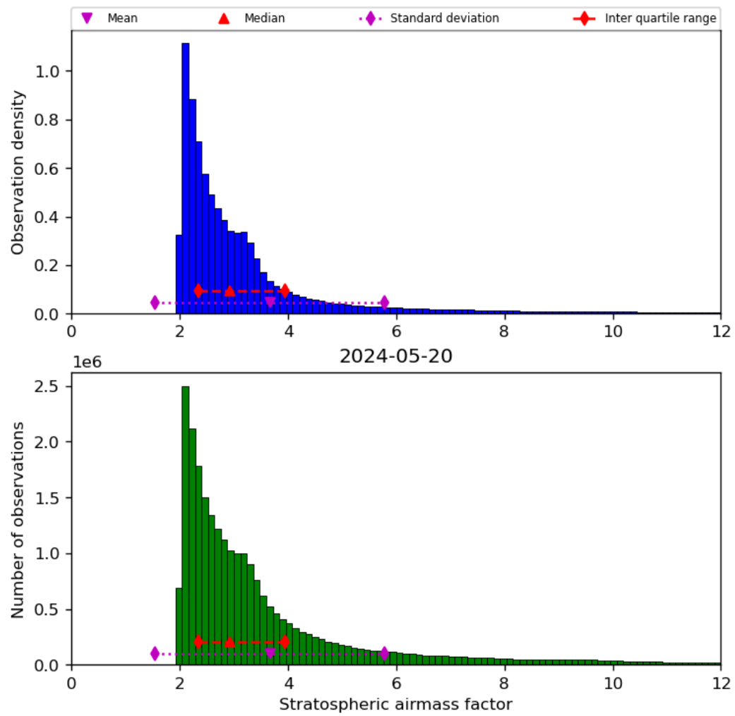
Figure 44: Histogram of “Stratospheric airmass factor” for 2024-05-19 to 2024-05-21
