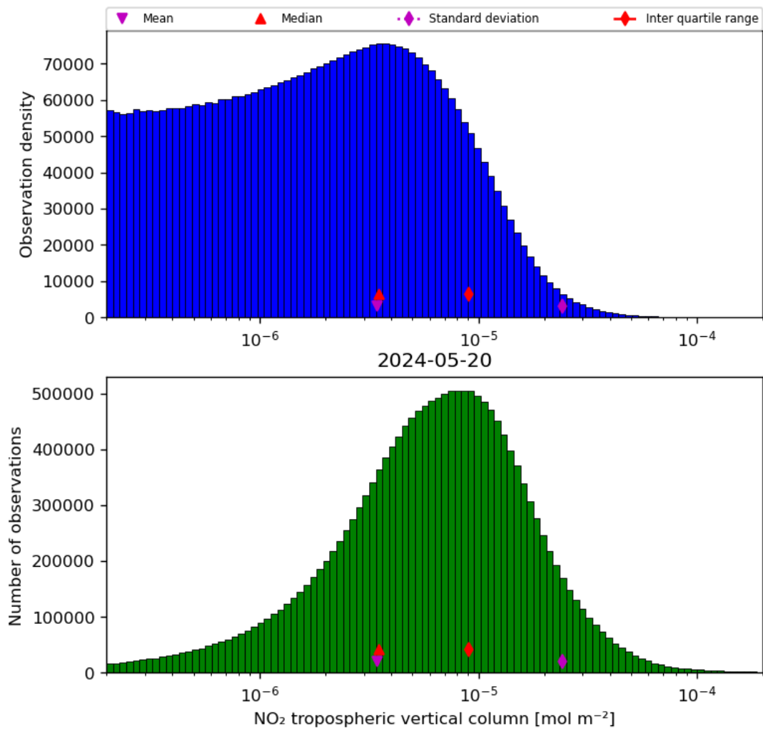
Figure 29: Histogram of “NO 2 tropospheric vertical column” for 2024-05-19 to 2024-05-21
