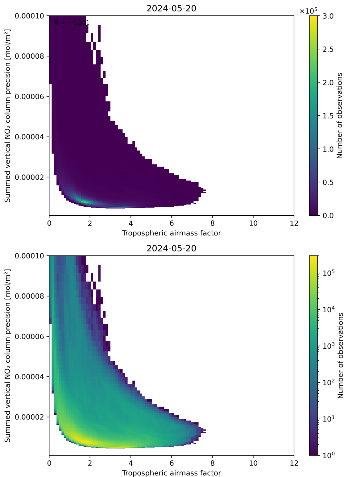
Figure 76: Scatter density plot of “Tropospheric air mass factor” against “Summed vertical NO 2 column precision” for 2024-05-19 to 2024-05-21.
