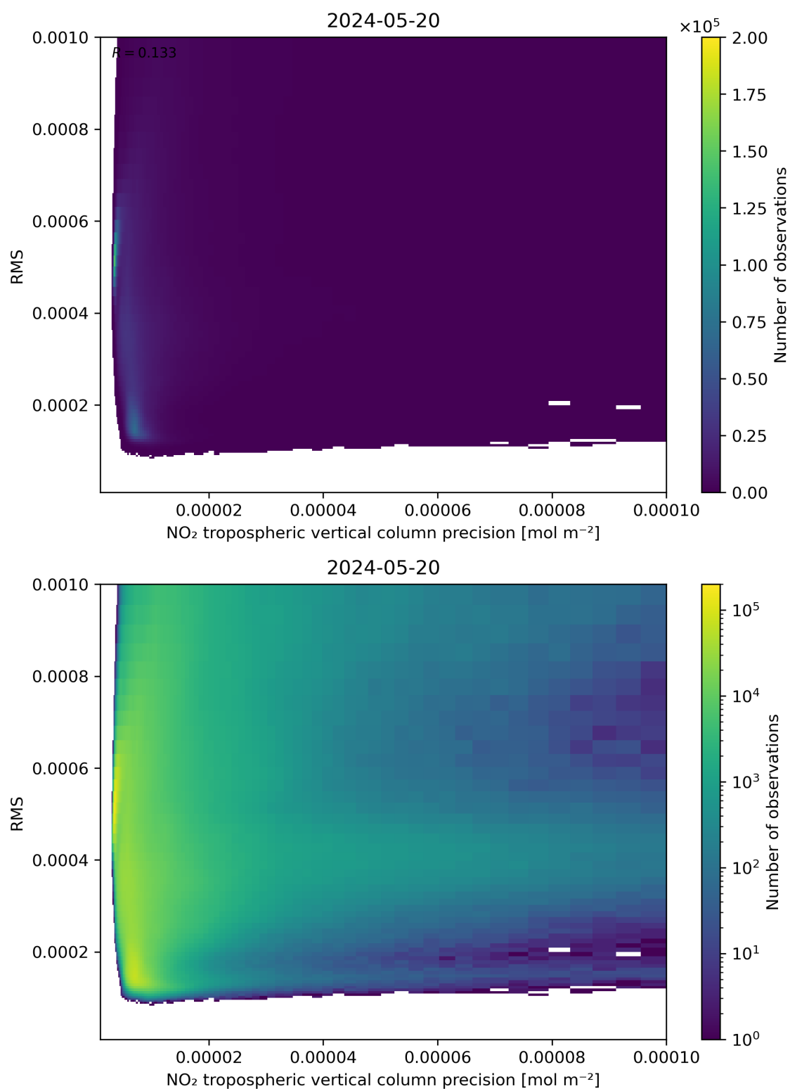
Figure 140: Scatter density plot of “NO 2 tropospheric vertical column precision” against “RMS” for 2024-05-19 to 2024-05-21.
