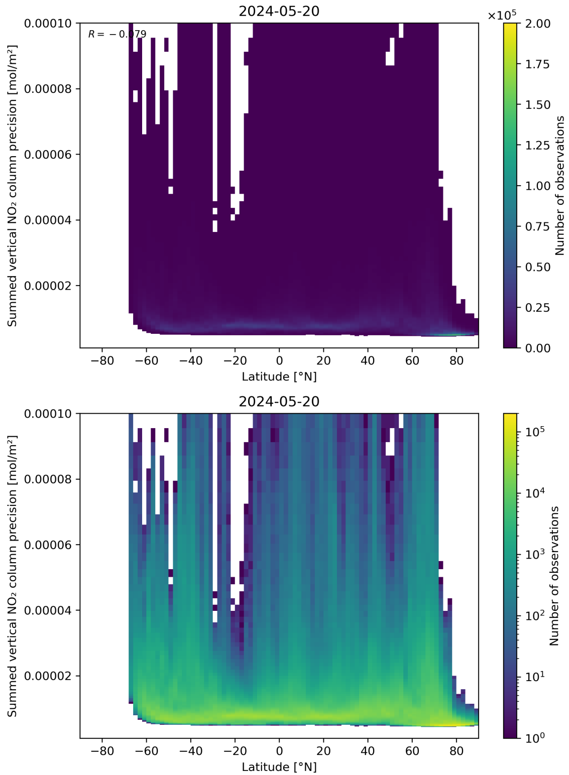
Figure 89: Scatter density plot of “Latitude” against “Summed vertical NO 2 column precision” for 2024-05-19 to 2024-05-21.
