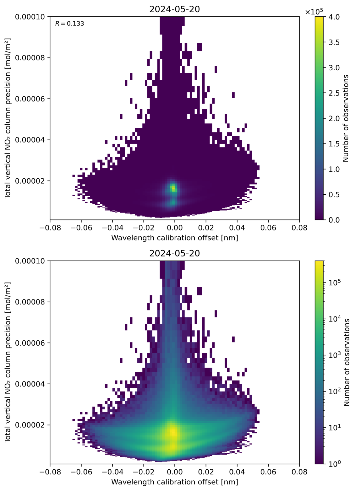
Figure 180: Scatter density plot of “Wavelength calibration offset” against “Total vertical NO 2 column precision” for 2024-05-19 to 2024-05-21.
