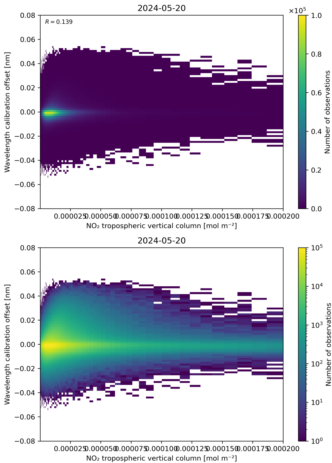
Figure 143: Scatter density plot of “NO 2 tropospheric vertical column” against “Wavelength calibration offset” for 2024-05-19 to 2024-05-21.
