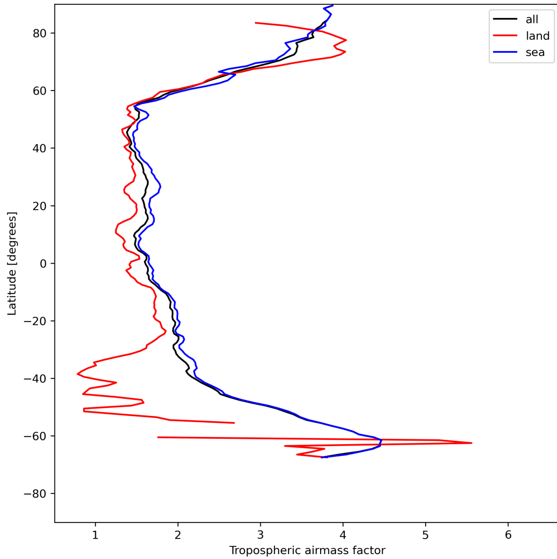
Figure 14: Zonal average of “Tropospheric airmass factor” for 2024-05-19 to 2024-05-21.
