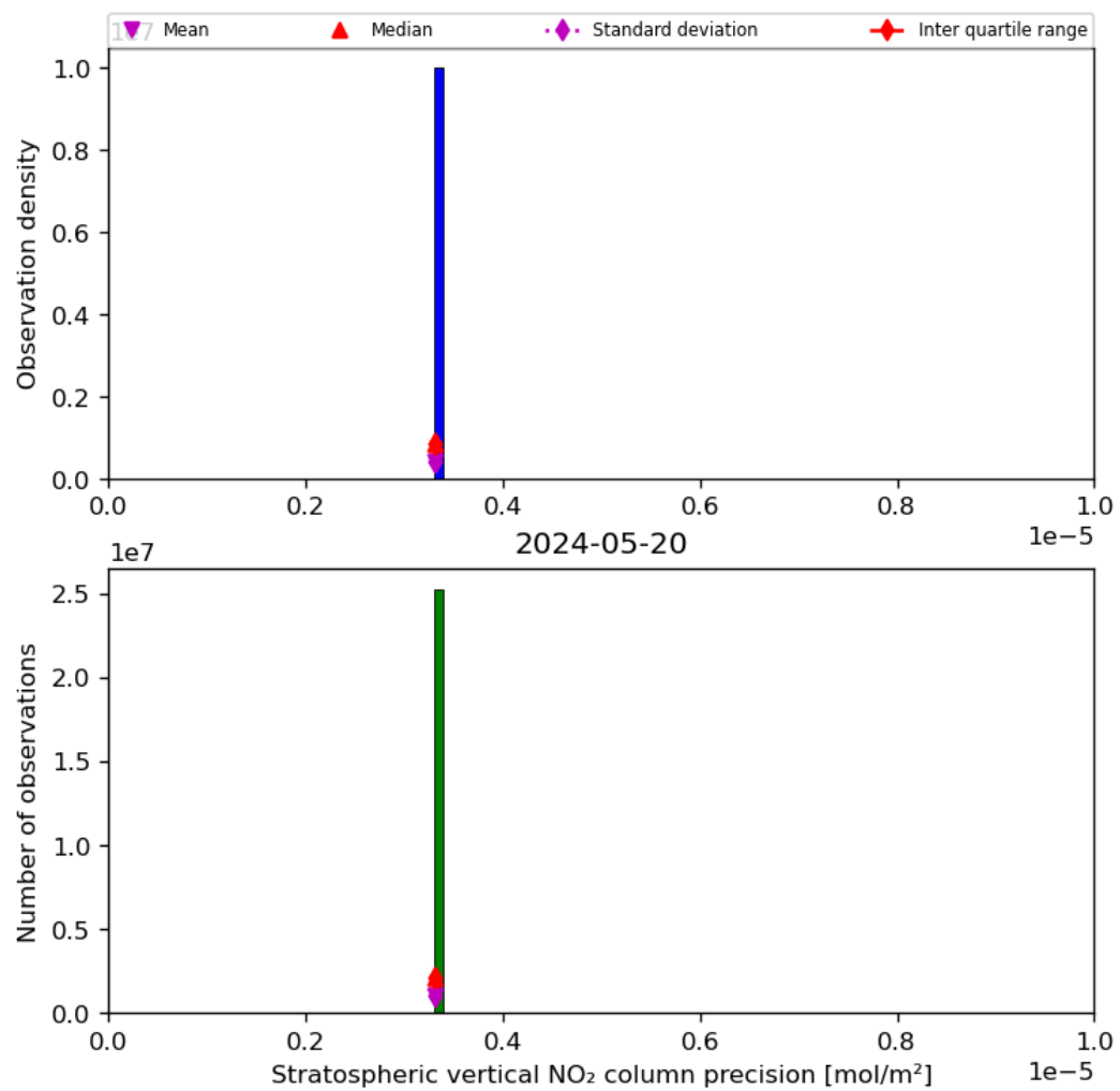
Figure 37: Histogram of “Stratospheric vertical NO 2 column precision” for 2024-05-19 to 2024-05-21
