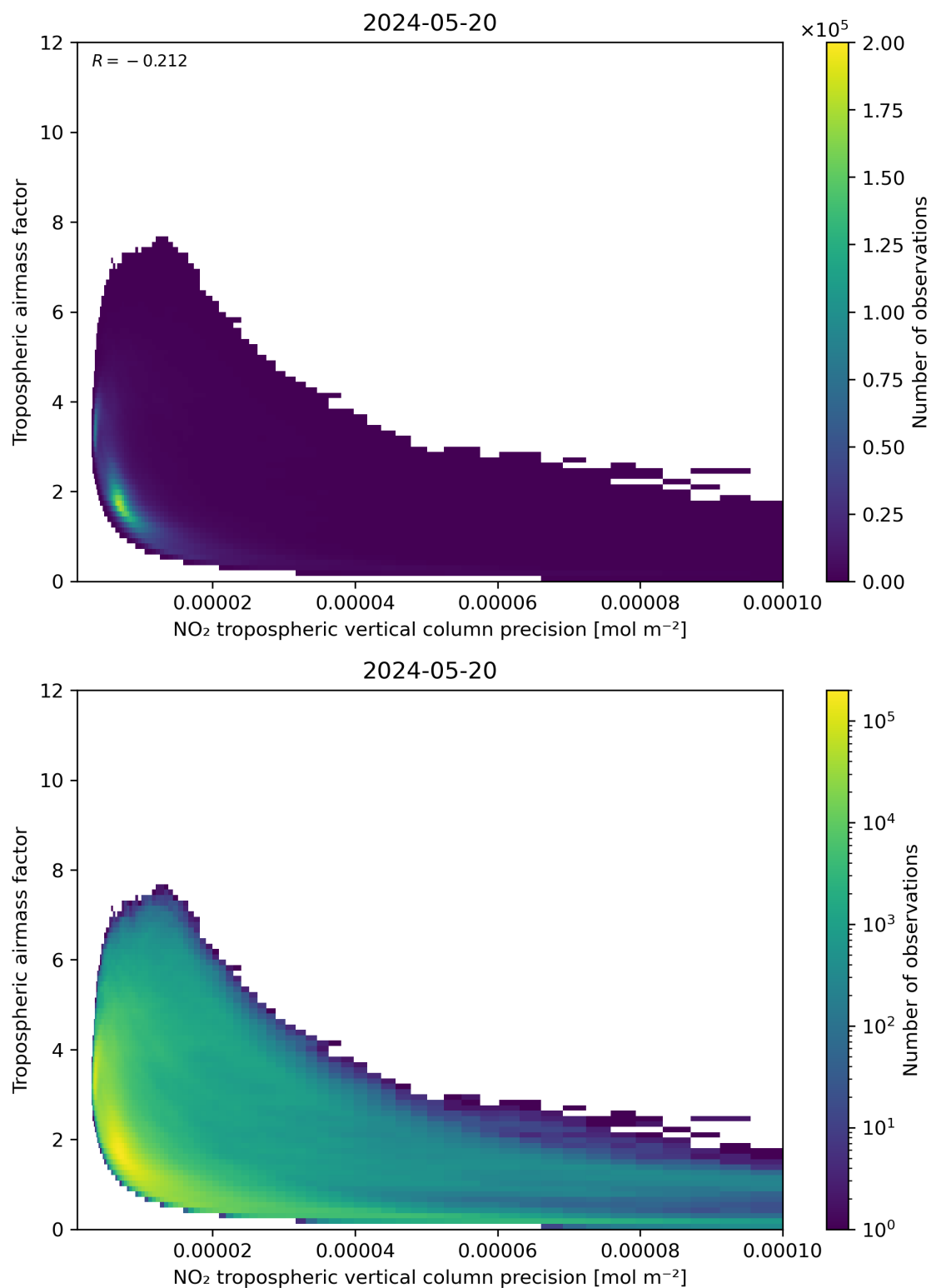
Figure 133: Scatter density plot of “NO 2 tropospheric vertical column precision” against “Tropospheric air mass factor” for 2024-05-19 to 2024-05-21.
