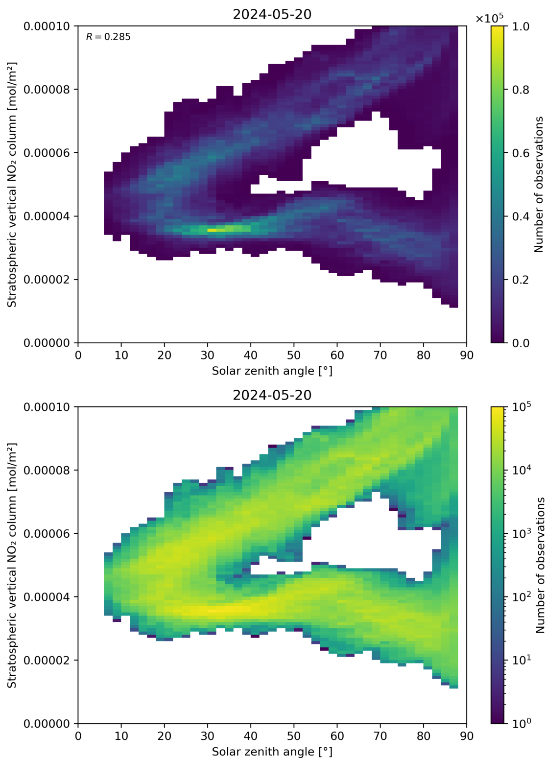
Figure 150: Scatter density plot of “Solar zenith angle” against “Stratospheric vertical NO 2 column” for 2024-05-19 to 2024-05-21.
