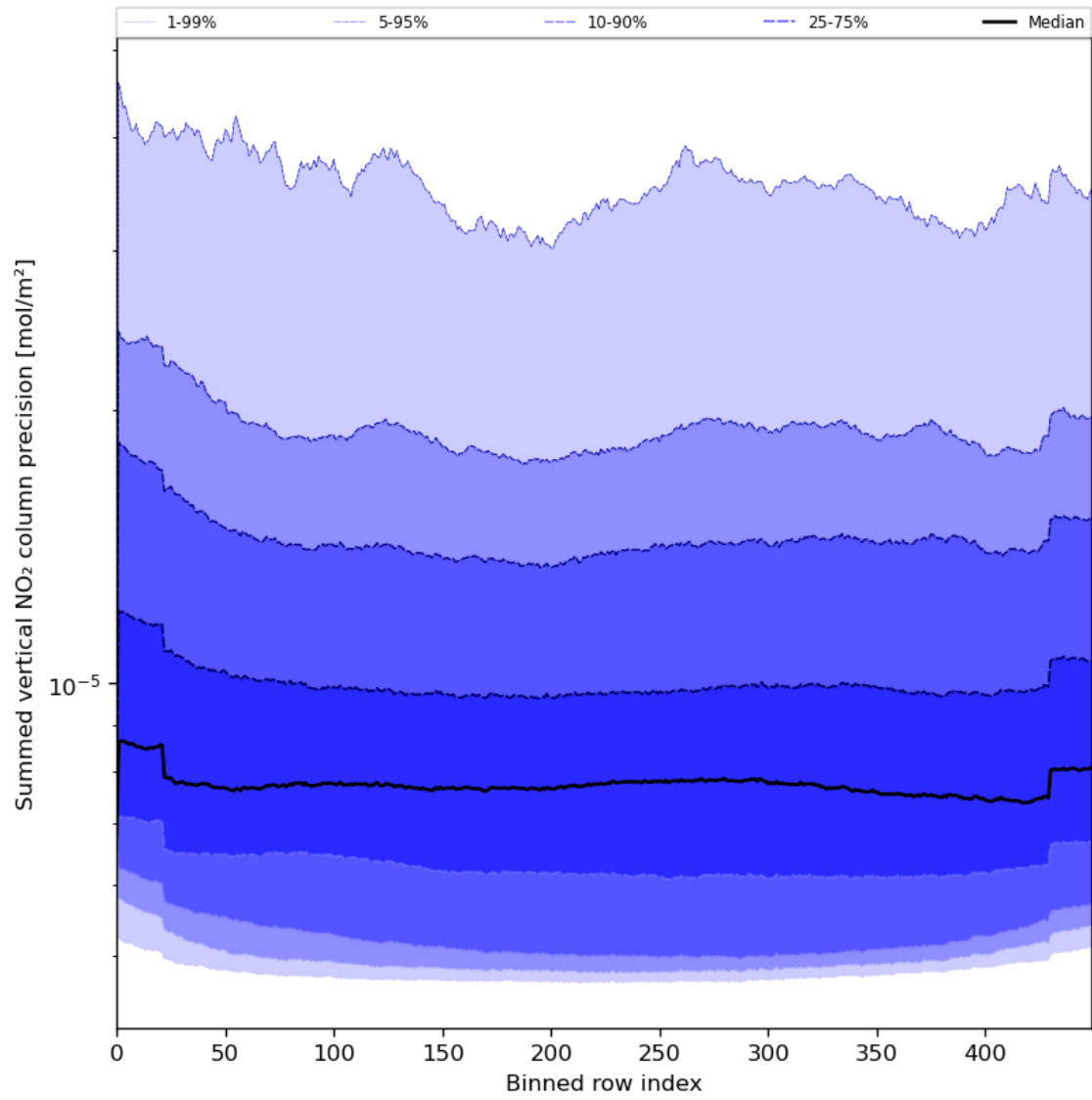
Figure 58: Along track statistics of “Summed vertical NO 2 column precision” for 2024-05-19 to 2024-05-21
