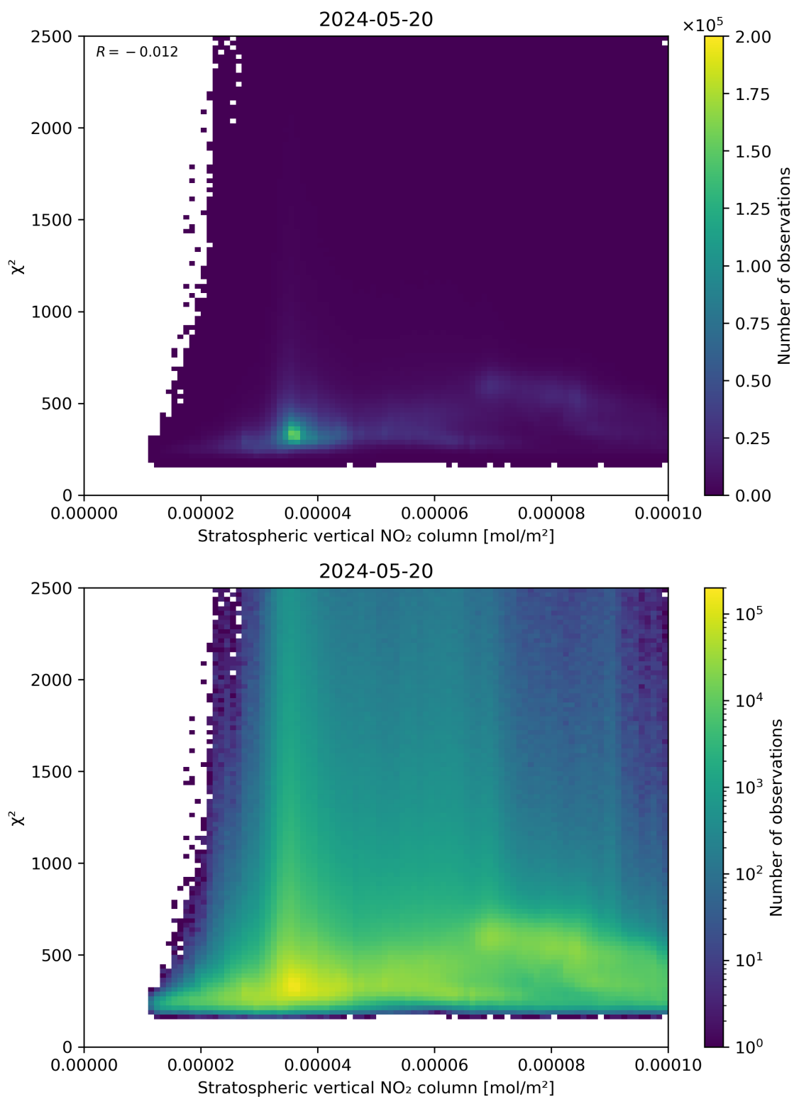
Figure 97: Scatter density plot of “Stratospheric vertical NO 2 column” against “ \chi^2 ” for 2024-05-19 to 2024-05-21.
