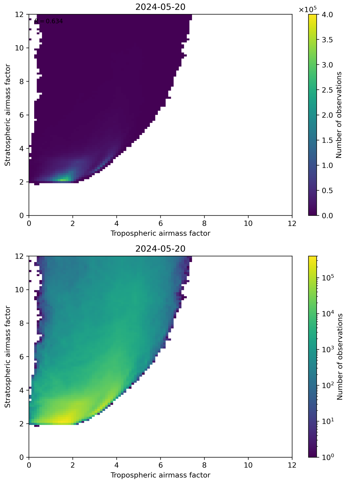
Figure 71: Scatter density plot of “Tropospheric airmass factor” against “Stratospheric airmass factor” for 2024-05-19 to 2024-05-21.
