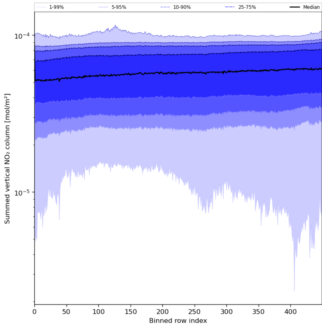
Figure 57: Along track statistics of “Summed vertical NO 2 column” for 2024-05-19 to 2024-05-21
