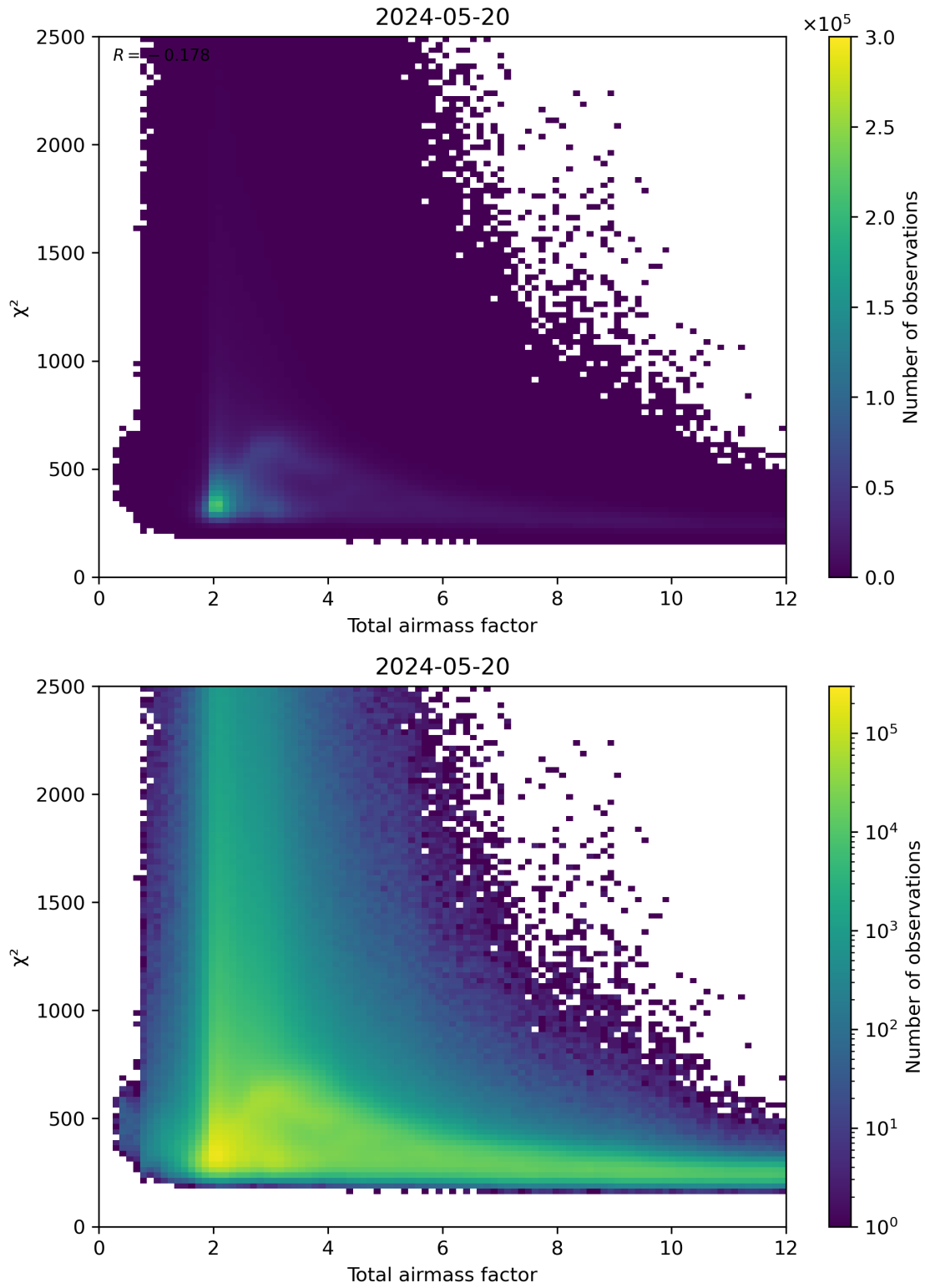
Figure 63: Scatter density plot of “Total airmass factor” against “ \chi^2 ” for 2024-05-19 to 2024-05-21.
