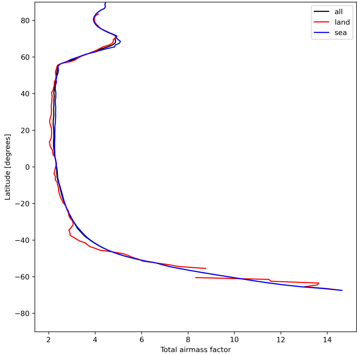
Figure 15: Zonal average of “Total airmass factor” for 2024-05-19 to 2024-05-21.
