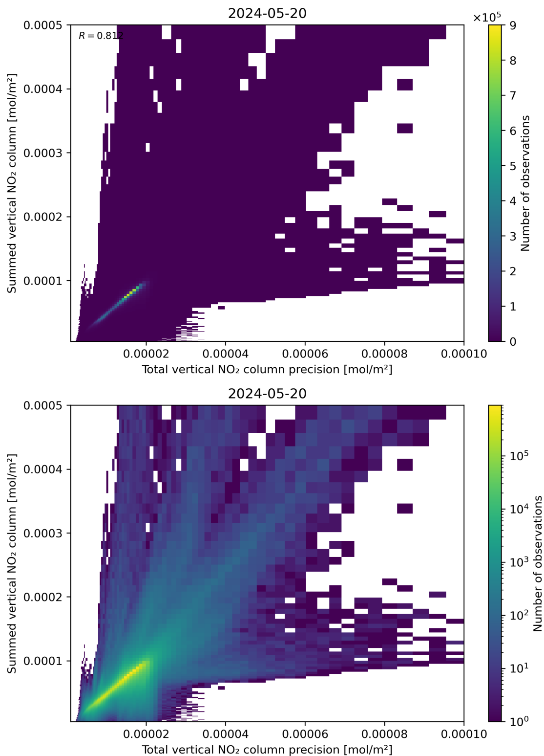
Figure 117: Scatter density plot of “Total vertical NO 2 column precision” against “Summed vertical NO 2 column” for 2024-05-19 to 2024-05-21.
