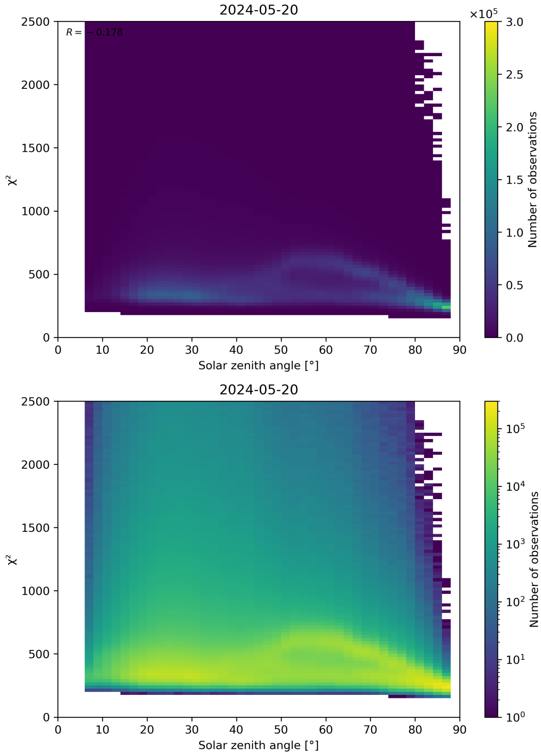
Figure 148: Scatter density plot of “Solar zenith angle” against “ \chi^2 ” for 2024-05-19 to 2024-05-21.
