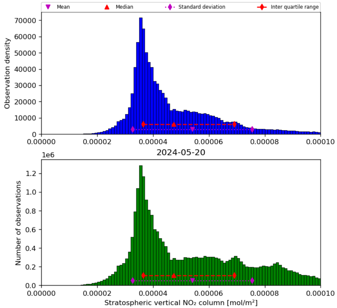
Figure 36: Histogram of “Stratospheric vertical NO 2 column” for 2024-05-19 to 2024-05-21
