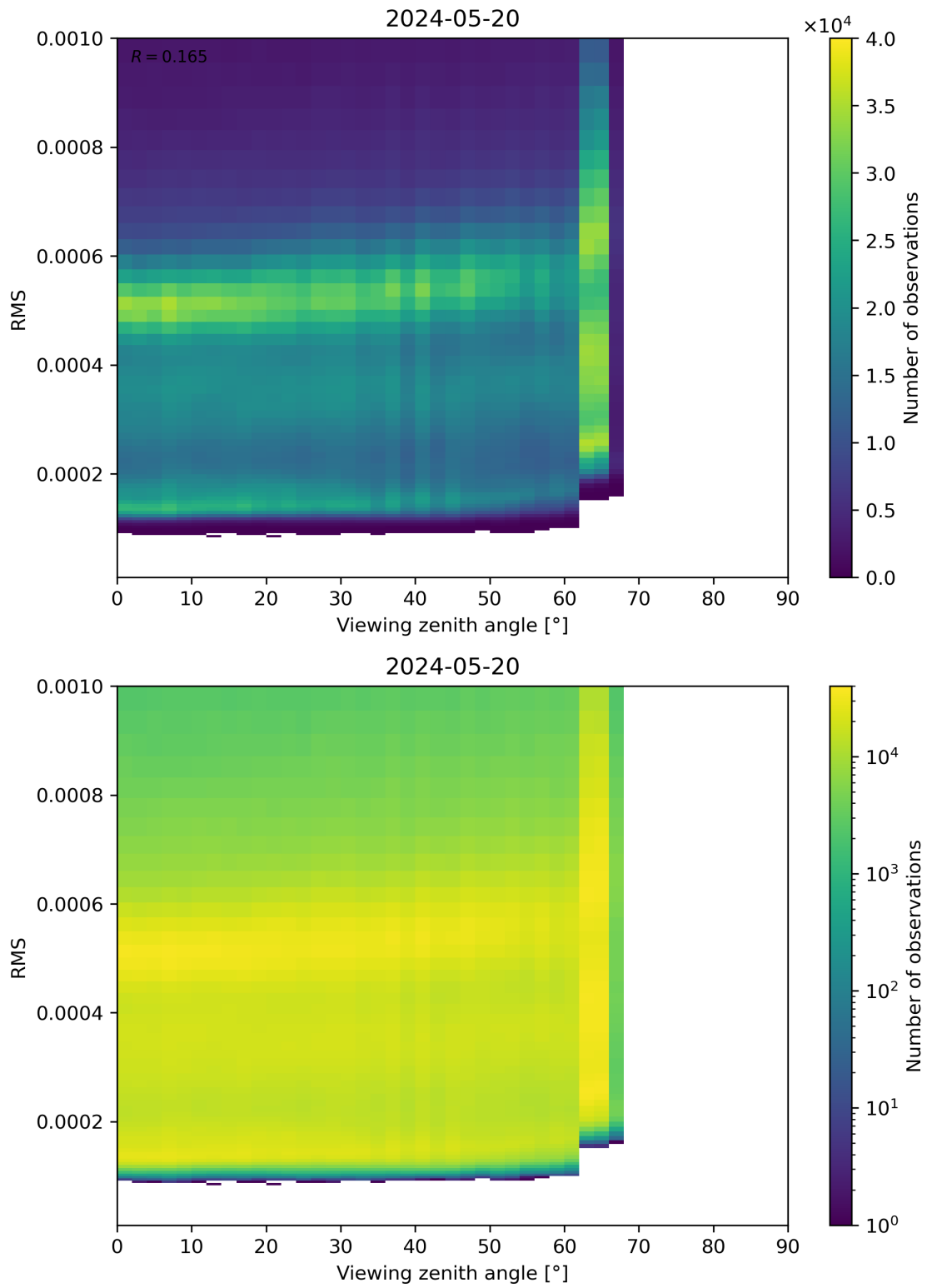
Figure 171: Scatter density plot of “Viewing zenith angle” against “RMS” for 2024-05-19 to 2024-05-21.
