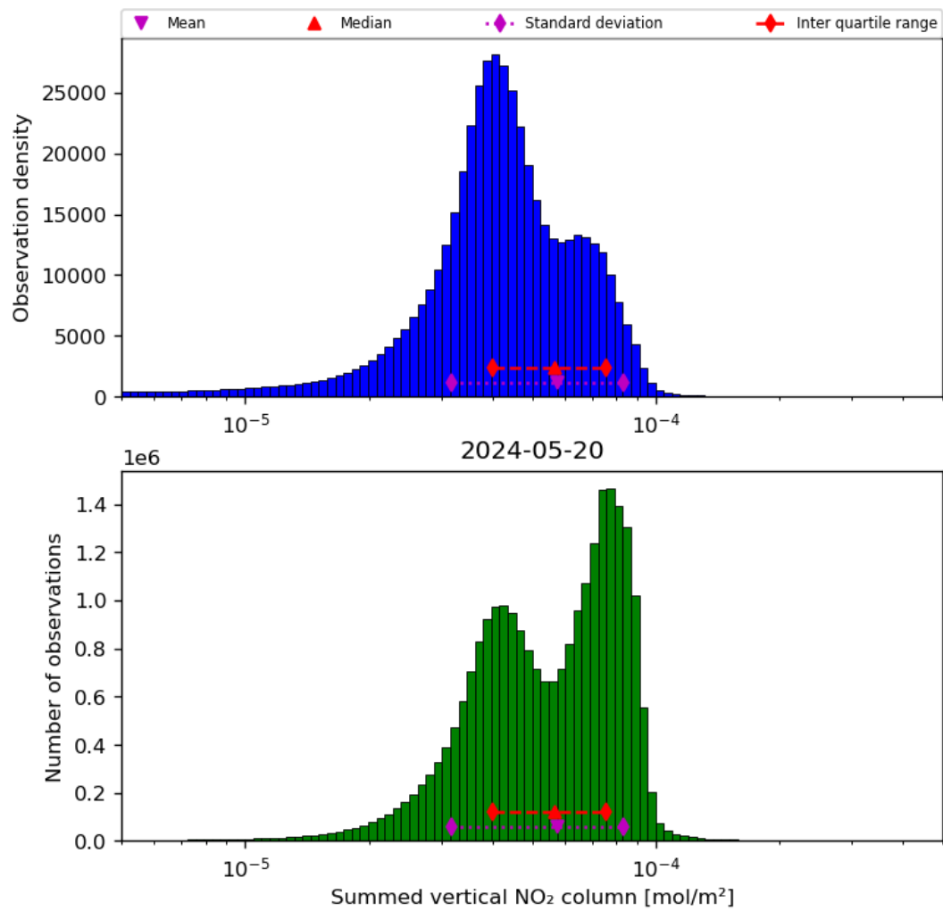
Figure 40: Histogram of “Summed vertical NO 2 column” for 2024-05-19 to 2024-05-21
