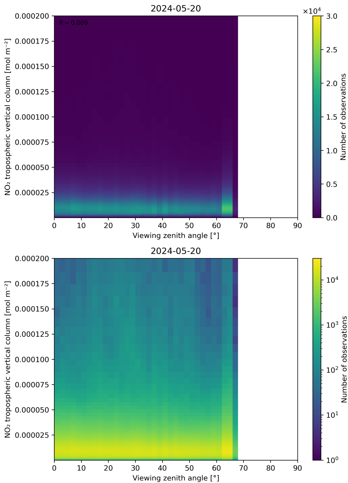
Figure 169: Scatter density plot of “Viewing zenith angle” against “NO 2 tropospheric vertical column” for 2024-05-19 to 2024-05-21.
