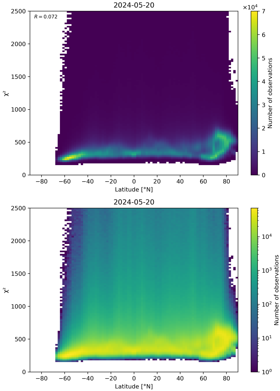
Figure 86: Scatter density plot of “Latitude” against “ \chi^2 ” for 2024-05-19 to 2024-05-21.
