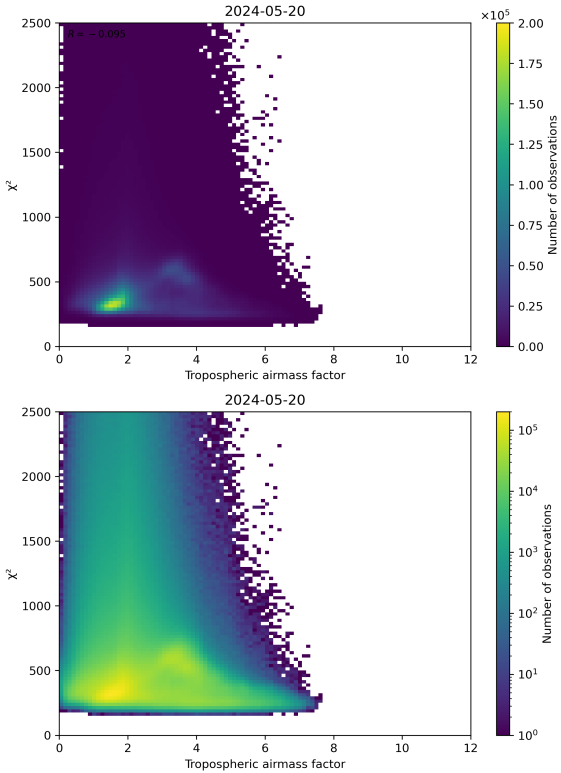
Figure 73: Scatter density plot of “Tropospheric airmass factor” against “ \chi^2 ” for 2024-05-19 to 2024-05-21.
