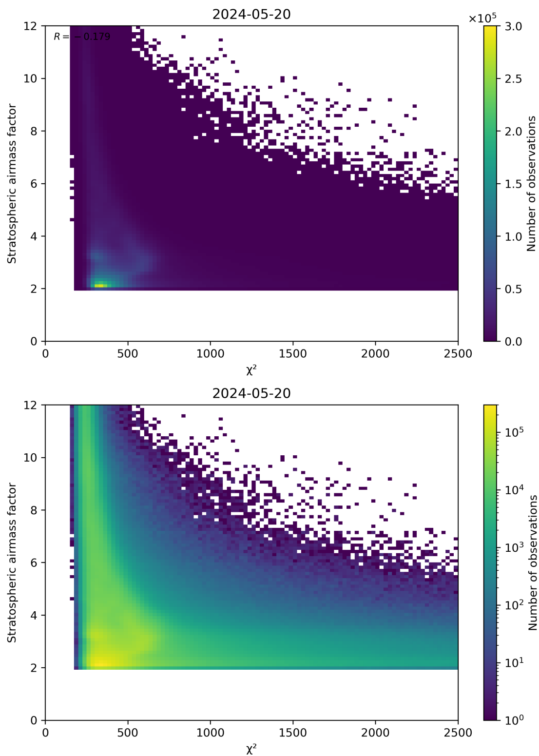
Figure 81: Scatter density plot of “ \chi^2 ” against “Stratospheric airmass factor” for 2024-05-19 to 2024-05-21.
