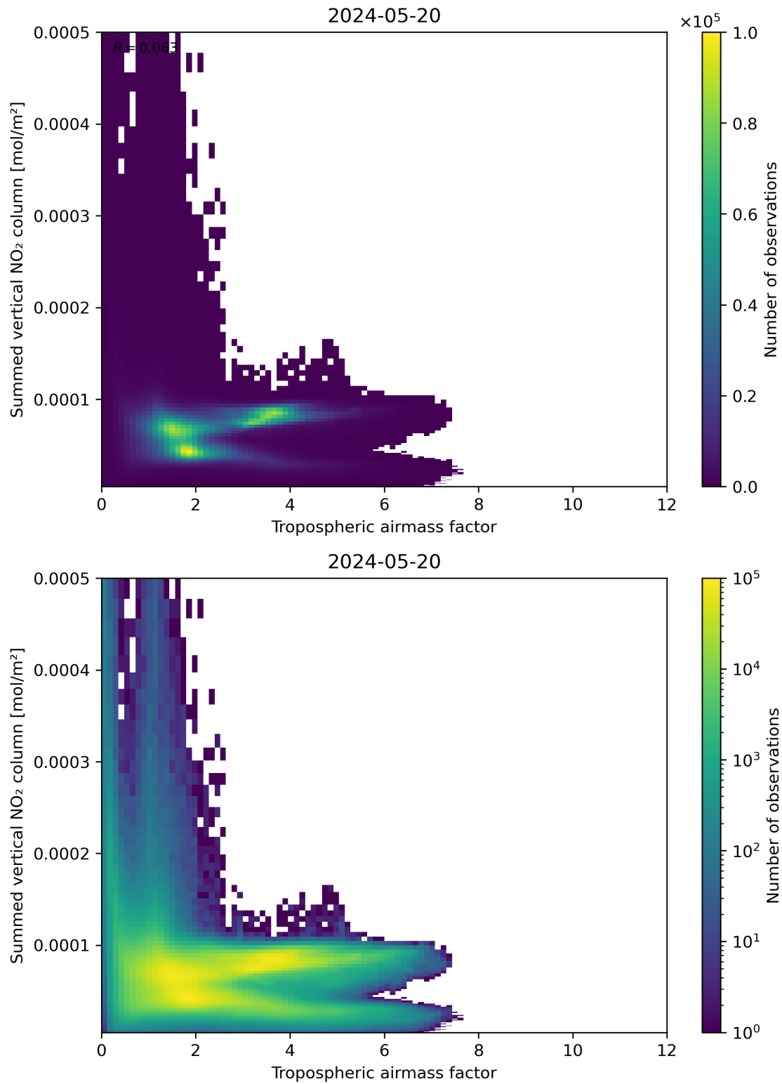
Figure 75: Scatter density plot of “Tropospheric airmass factor” against “Summed vertical NO 2 column” for 2024-05-19 to 2024-05-21.
