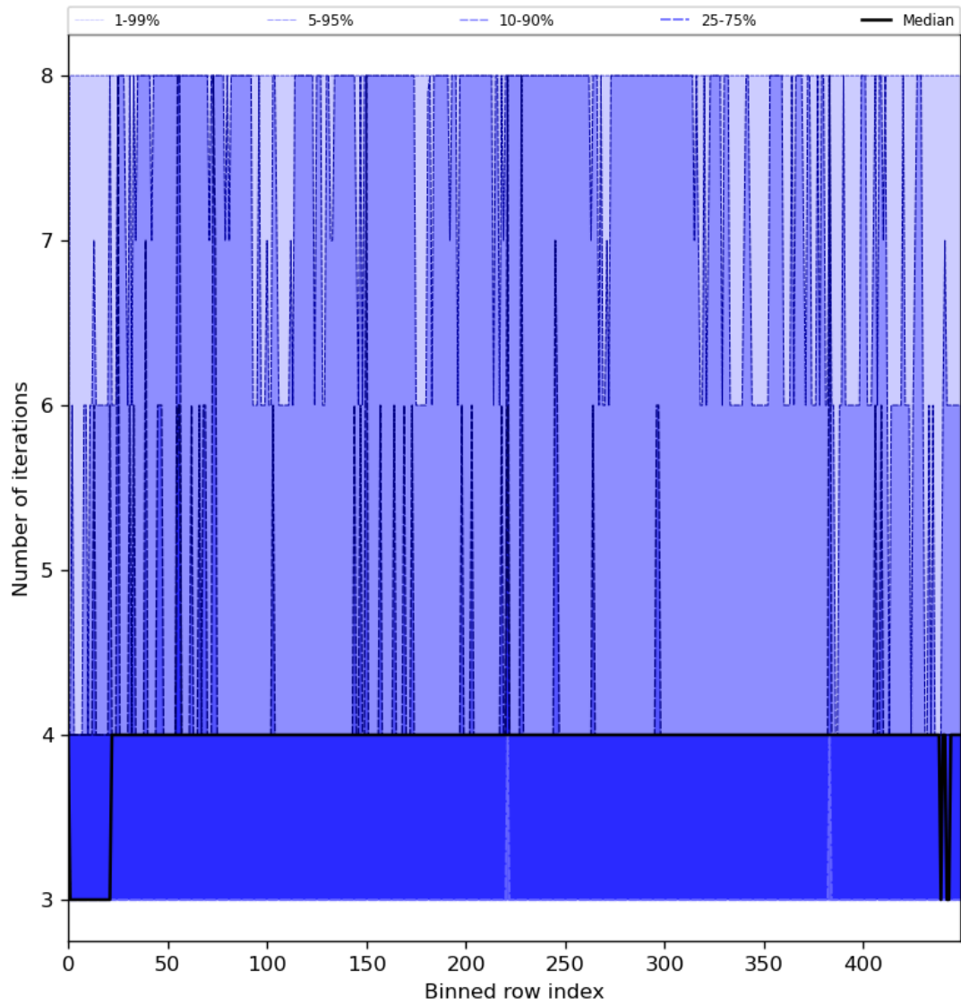
Figure 51: Along track statistics of “Number of iterations” for 2024-05-19 to 2024-05-21
