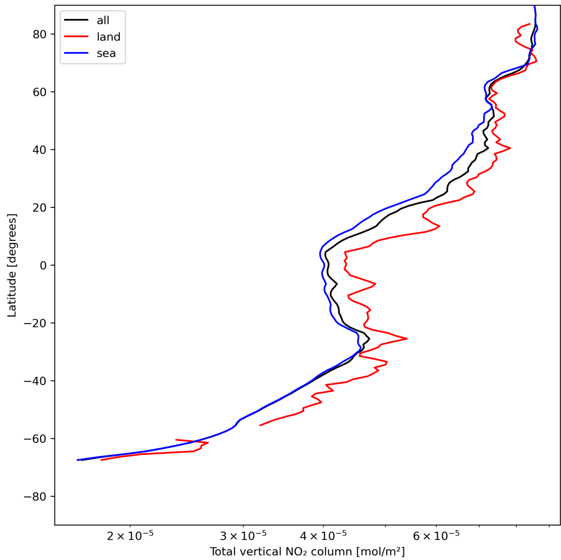
Figure 21: Zonal average of “Total vertical NO 2 column” for 2024-05-19 to 2024-05-21.
