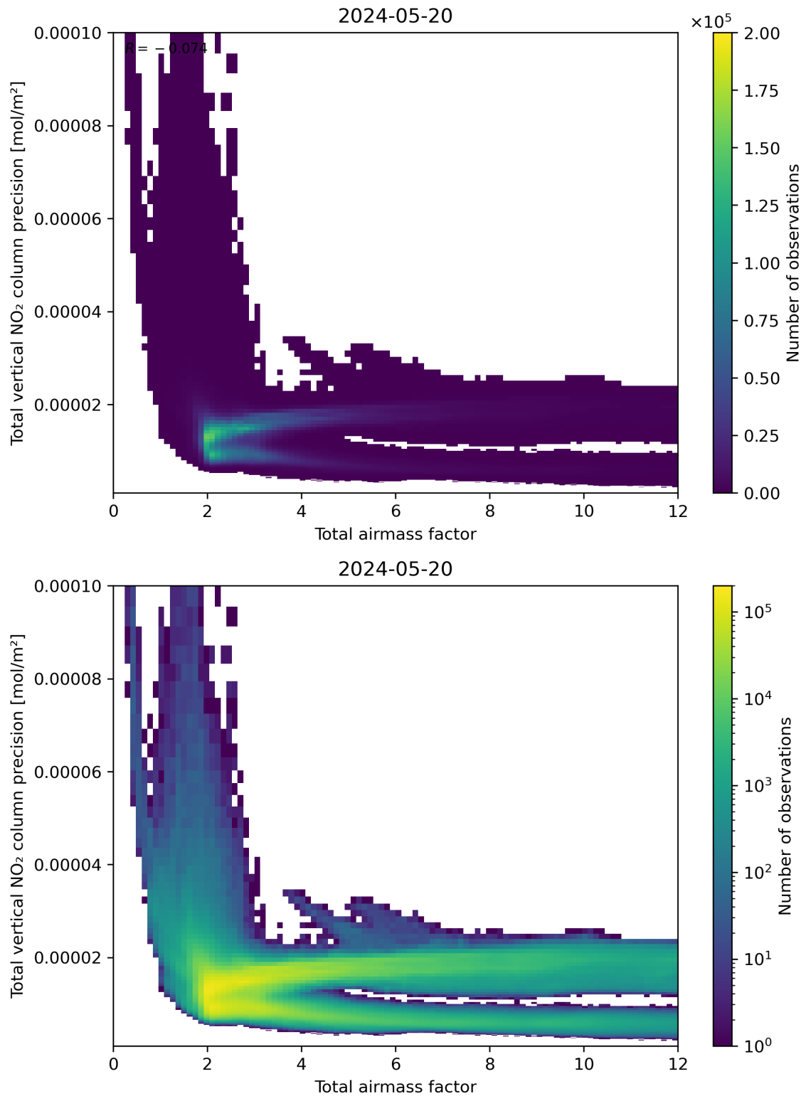
Figure 68: Scatter density plot of “Total airmass factor” against “Total vertical NO 2 column precision” for 2024-05-19 to 2024-05-21.
