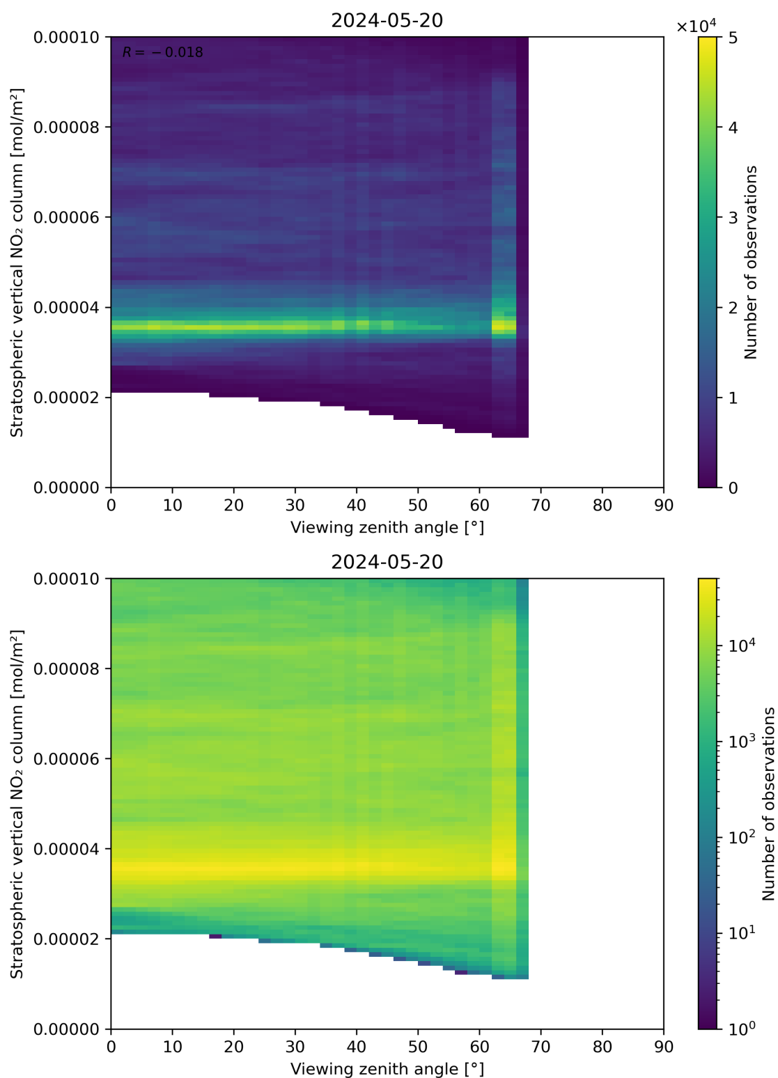
Figure 164: Scatter density plot of “Viewing zenith angle” against “Stratospheric vertical NO 2 column” for 2024-05-19 to 2024-05-21.
