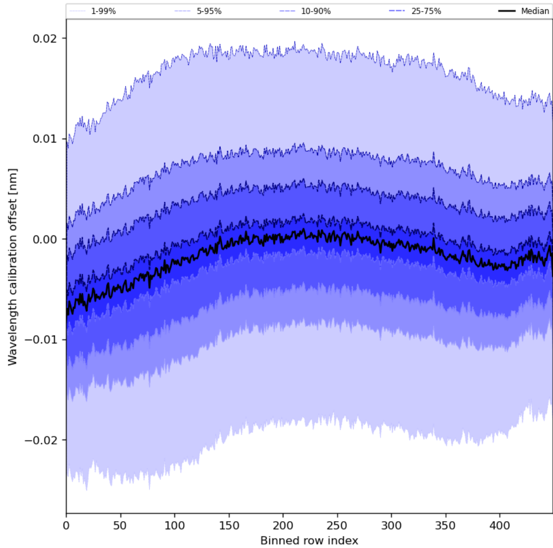
Figure 52: Along track statistics of “Wavelength calibration offset” for 2024-05-19 to 2024-05-21
