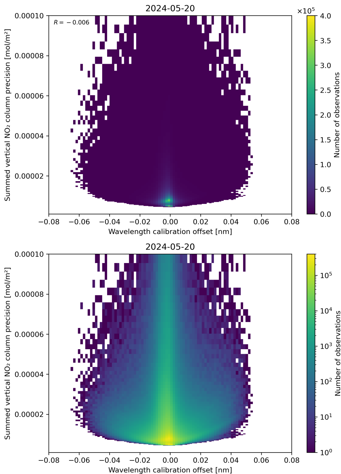
Figure 178: Scatter density plot of “Wavelength calibration offset” against “Summed vertical NO 2 column precision” for 2024-05-19 to 2024-05-21.
