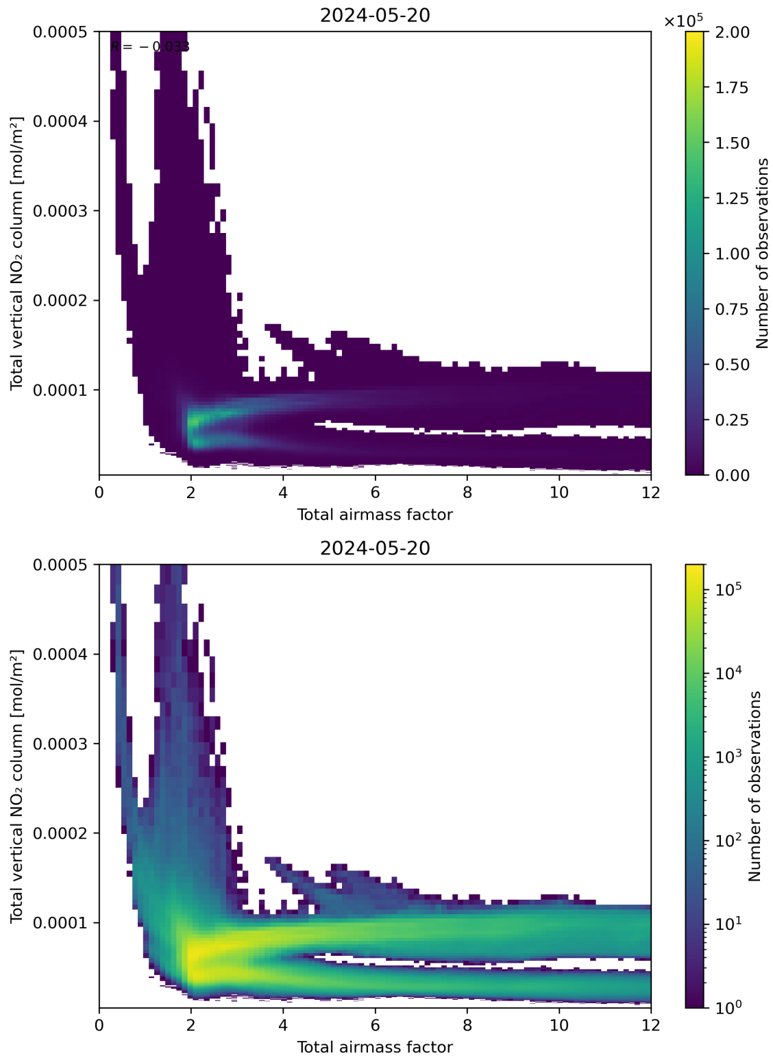
Figure 67: Scatter density plot of “Total airmass factor” against “Total vertical NO 2 column” for 2024-05-19 to 2024-05-21.
