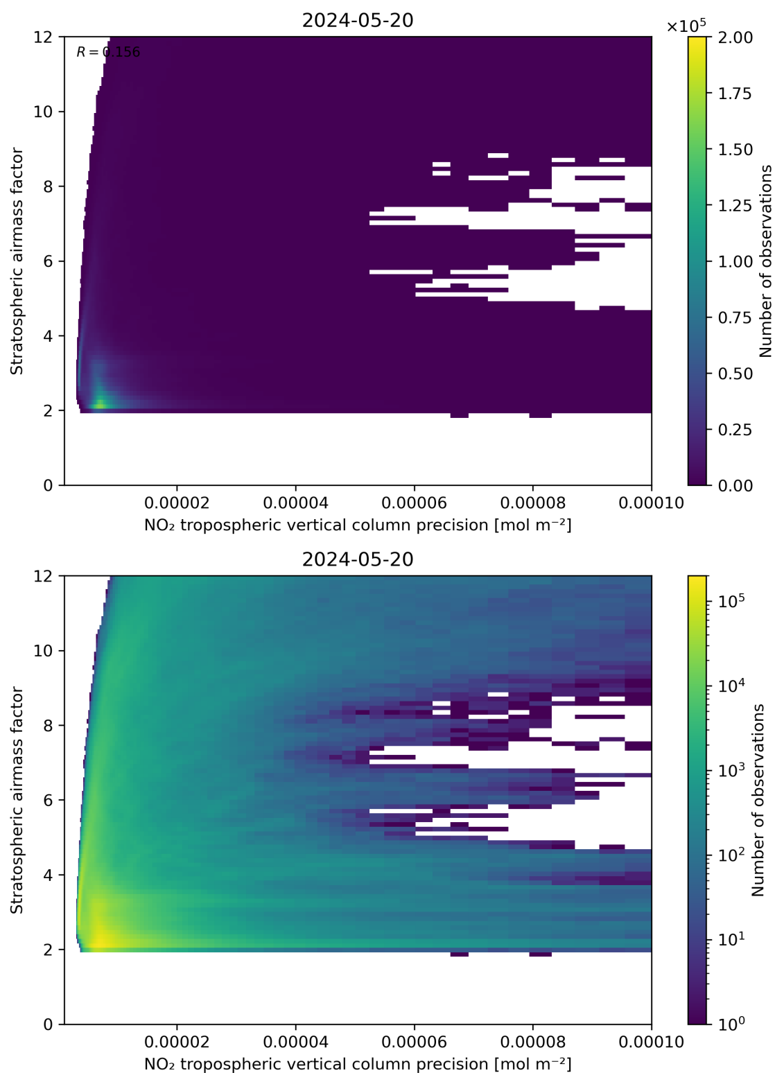
Figure 131: Scatter density plot of “NO 2 tropospheric vertical column precision” against “Stratospheric airmass factor” for 2024-05-19 to 2024-05-21.
