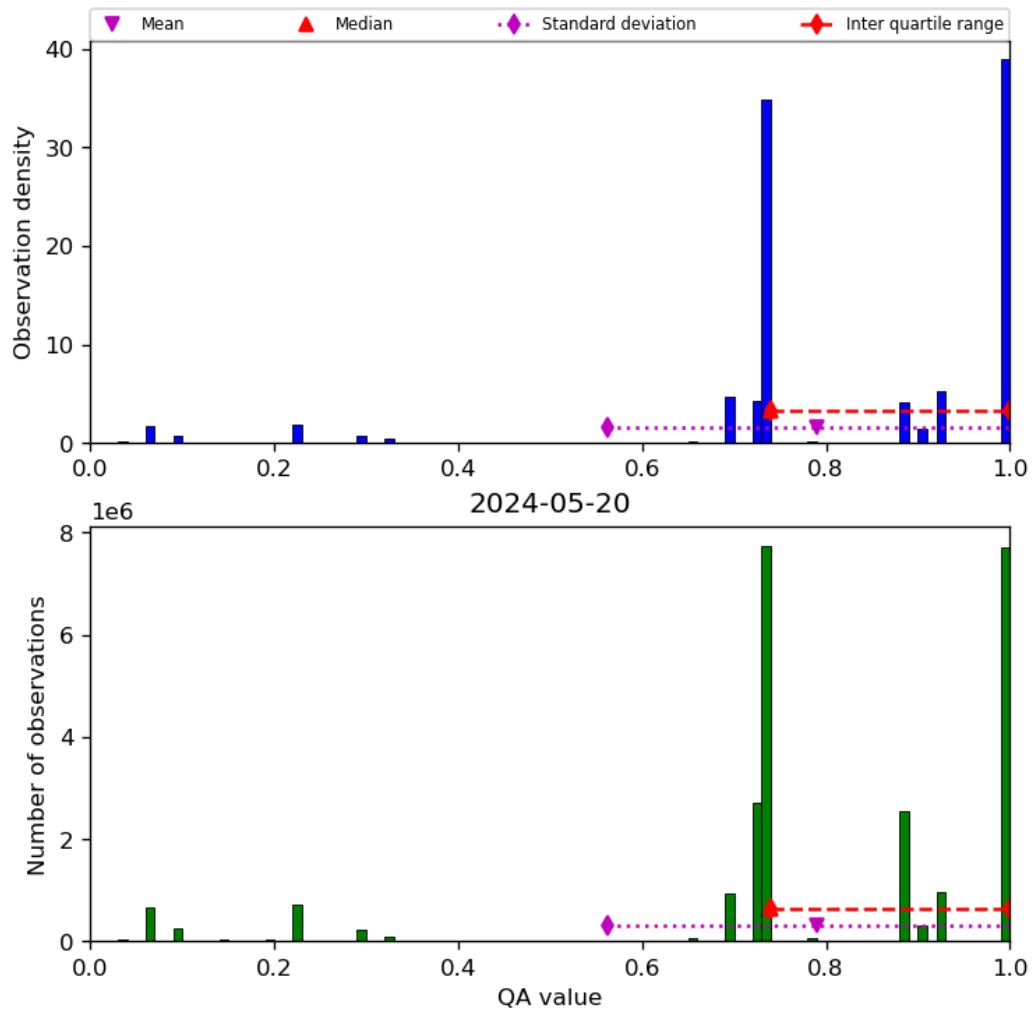
Figure 28: Histogram of “QA value” for 2024-05-19 to 2024-05-21
