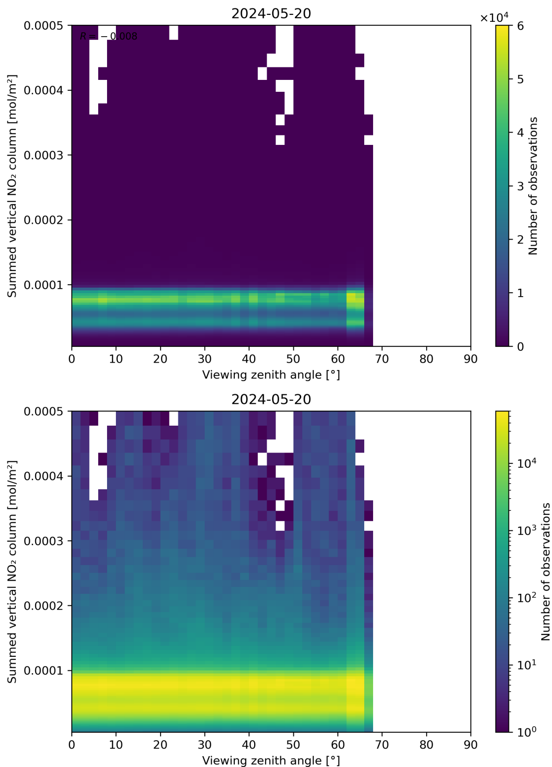
Figure 165: Scatter density plot of “Viewing zenith angle” against “Summed vertical NO 2 column” for 2024-05-19 to 2024-05-21.
