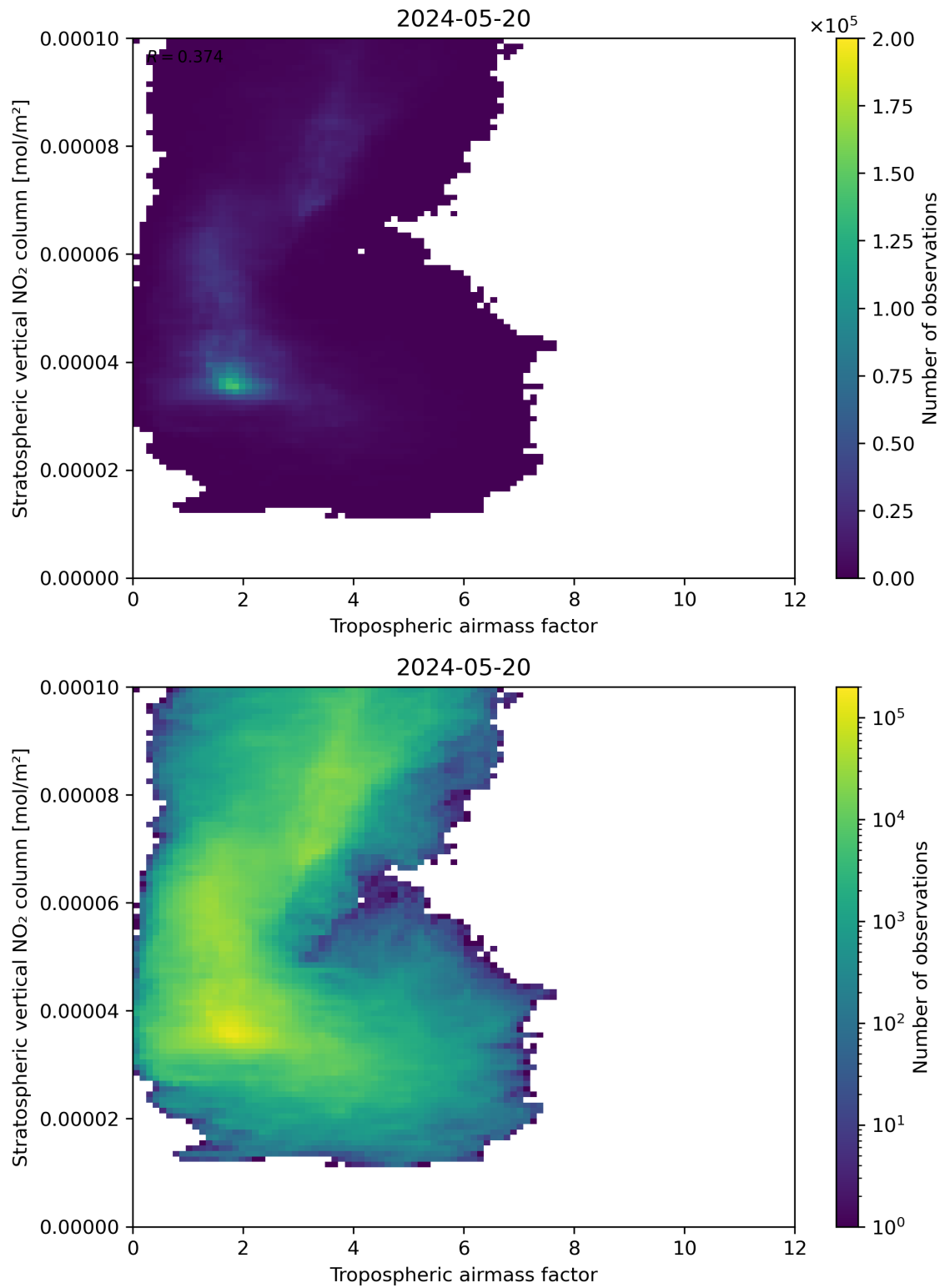
Figure 74: Scatter density plot of “Tropospheric air mass factor” against “Stratospheric vertical NO 2 column” for 2024-05-19 to 2024-05-21.
