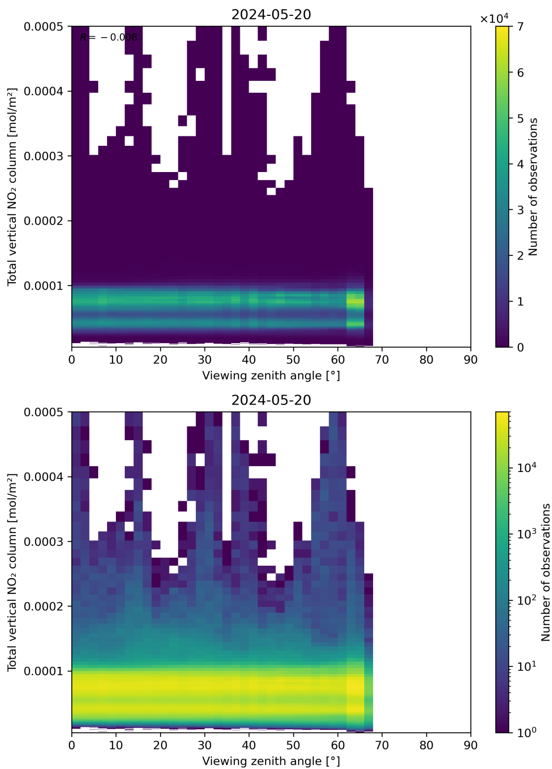
Figure 167: Scatter density plot of “Viewing zenith angle” against “Total vertical NO 2 column” for 2024-05-19 to 2024-05-21.
