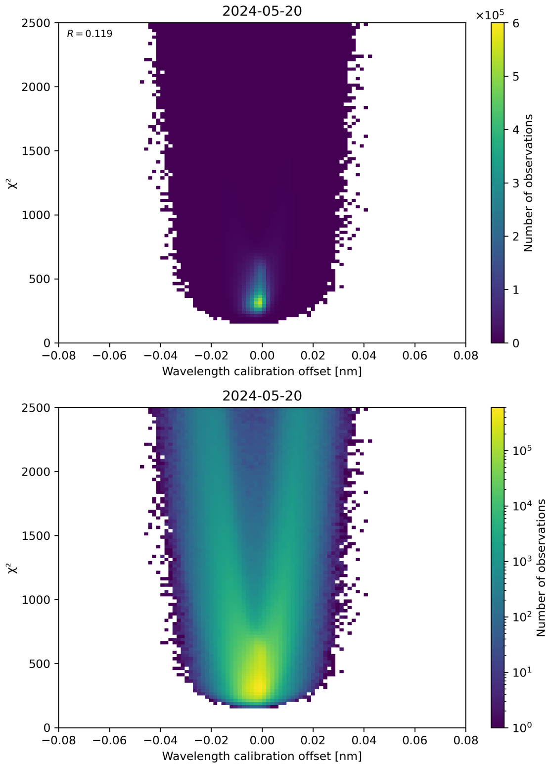
Figure 175: Scatter density plot of “Wavelength calibration offset” against “ \chi^2 ” for 2024-05-19 to 2024-05-21.
