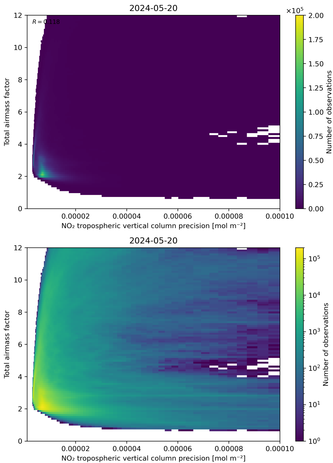
Figure 132: Scatter density plot of “NO 2 tropospheric vertical column precision” against “Total air mass factor” for 2024-05-19 to 2024-05-21.
