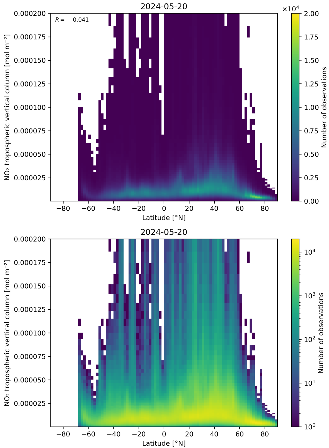
Figure 92: Scatter density plot of “Latitude” against “NO 2 tropospheric vertical column” for 2024-05-19 to 2024-05-21.
