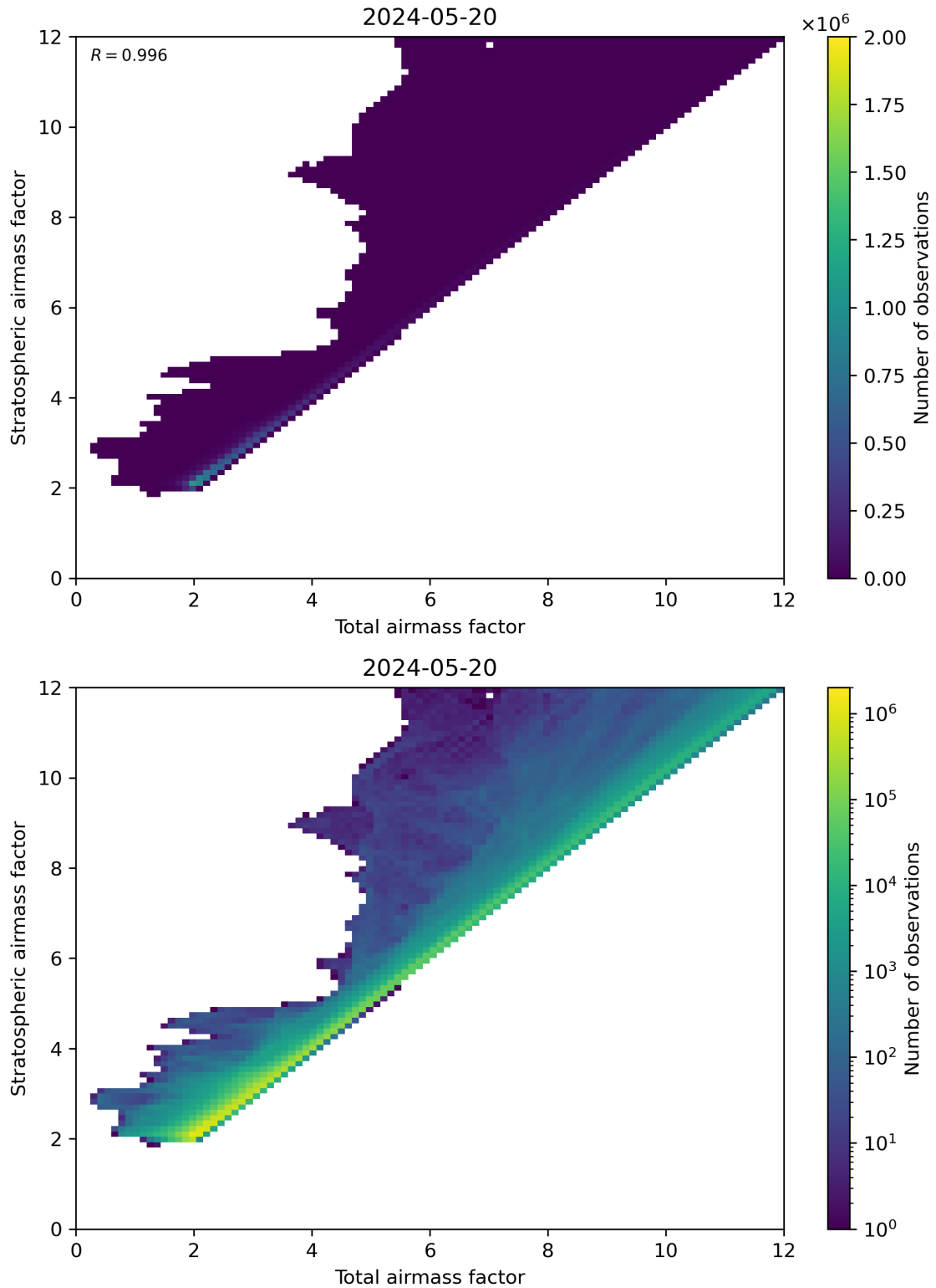
Figure 62: Scatter density plot of “Total airmass factor” against “Stratospheric airmass factor” for 2024-05-19 to 2024-05-21.
