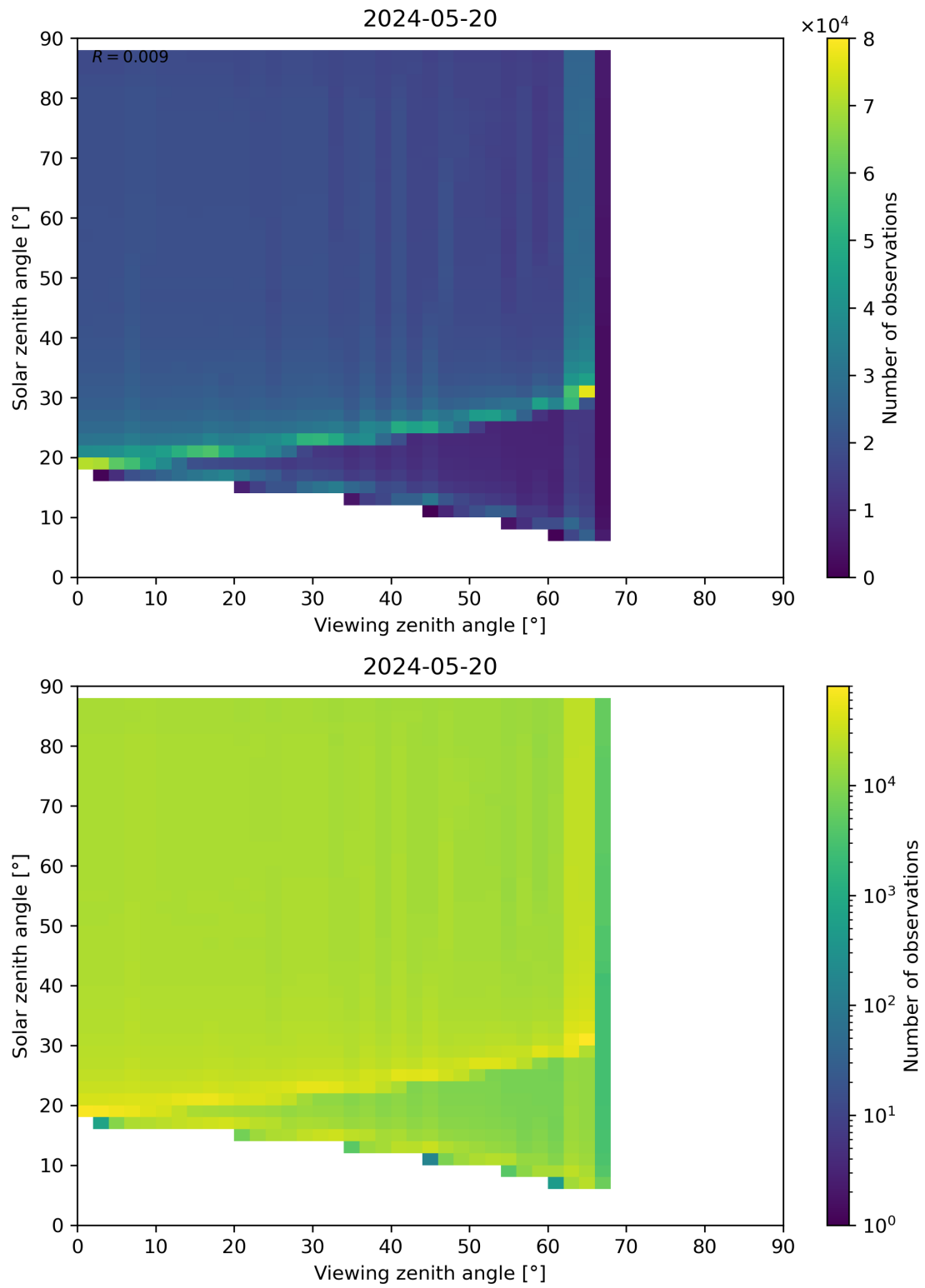
Figure 172: Scatter density plot of “Viewing zenith angle” against “Solar zenith angle” for 2024-05-19 to 2024-05-21.
