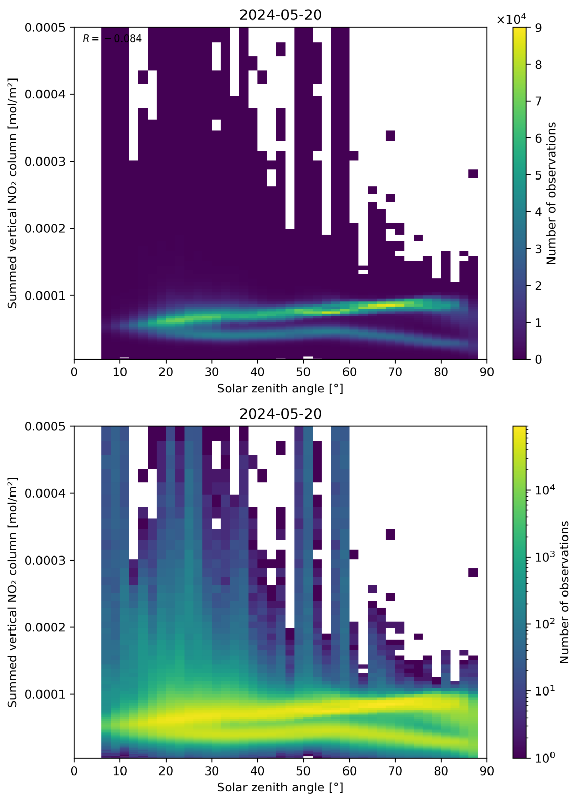
Figure 151: Scatter density plot of “Solar zenith angle” against “Summed vertical NO 2 column” for 2024-05-19 to 2024-05-21.
