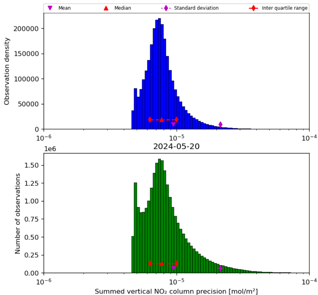
Figure 41: Histogram of “Summed vertical NO 2 column precision” for 2024-05-19 to 2024-05-21
