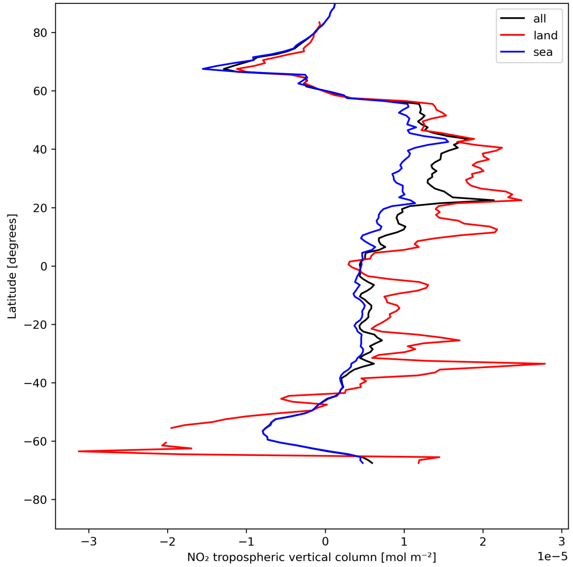
Figure 12: Zonal average of “NO 2 tropospheric vertical column” for 2024-05-19 to 2024-05-21.
