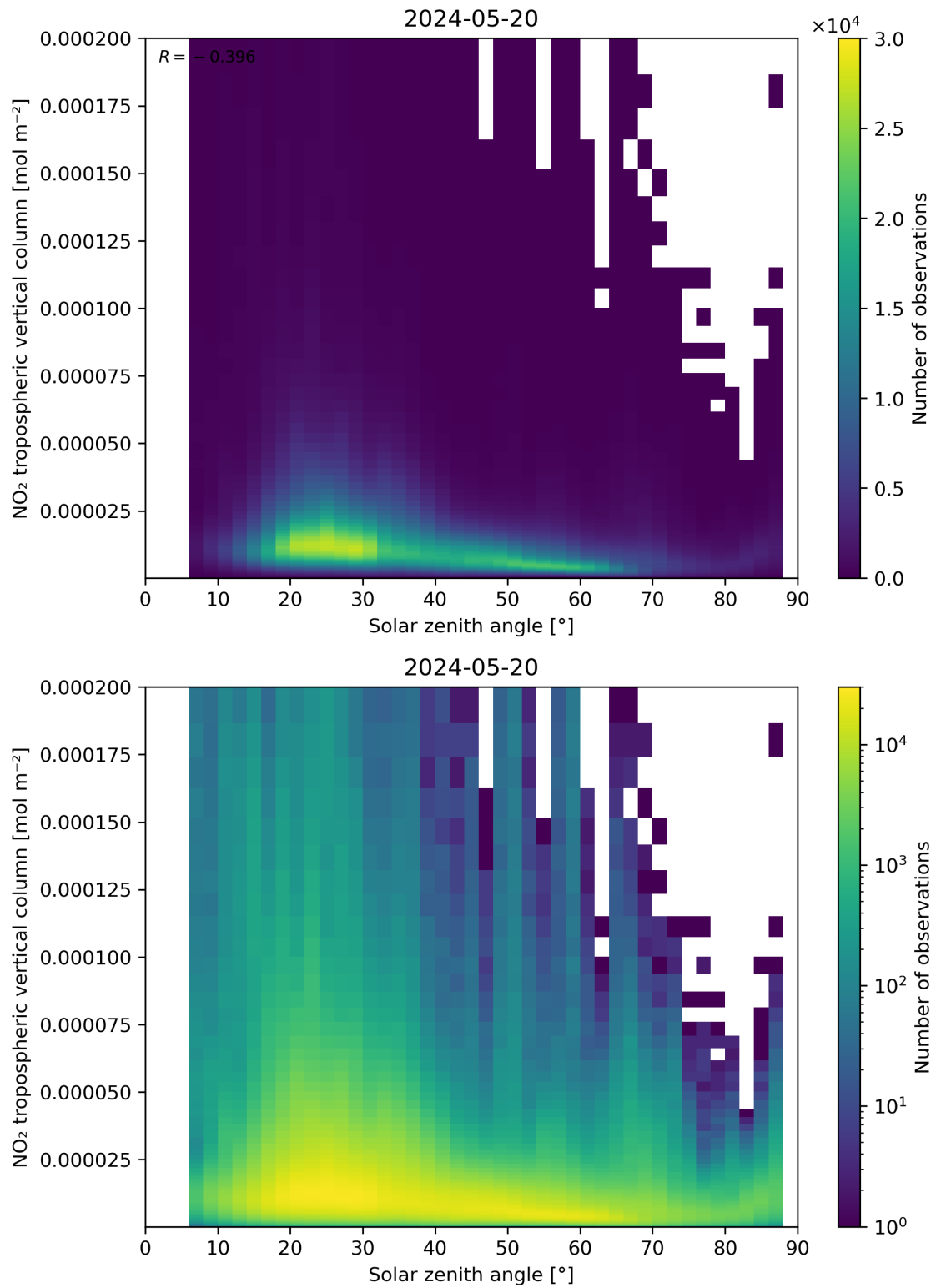
Figure 155: Scatter density plot of “Solar zenith angle” against “NO 2 tropospheric vertical column” for 2024-05-19 to 2024-05-21.
