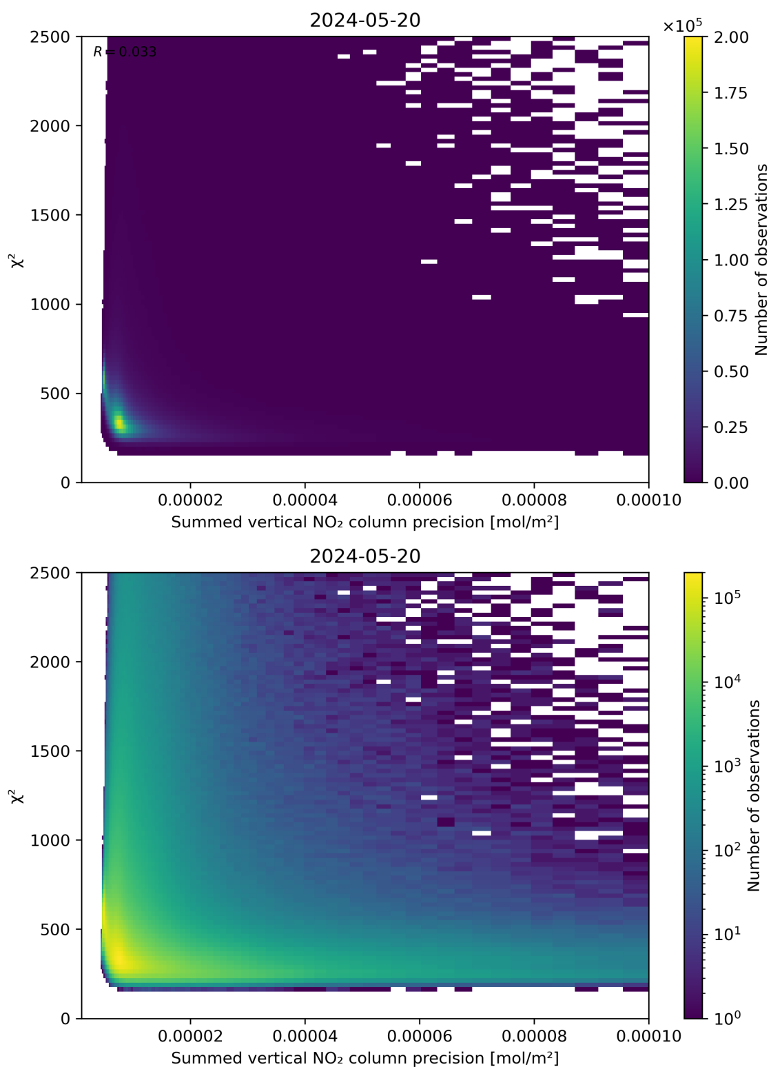
Figure 107: Scatter density plot of “Summed vertical NO 2 column precision” against “ \chi^2 ” for 2024-05-19 to 2024-05-21.
