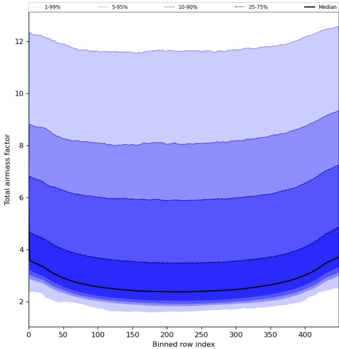
Figure 49: Along track statistics of “Total airmass factor” for 2024-05-19 to 2024-05-21
