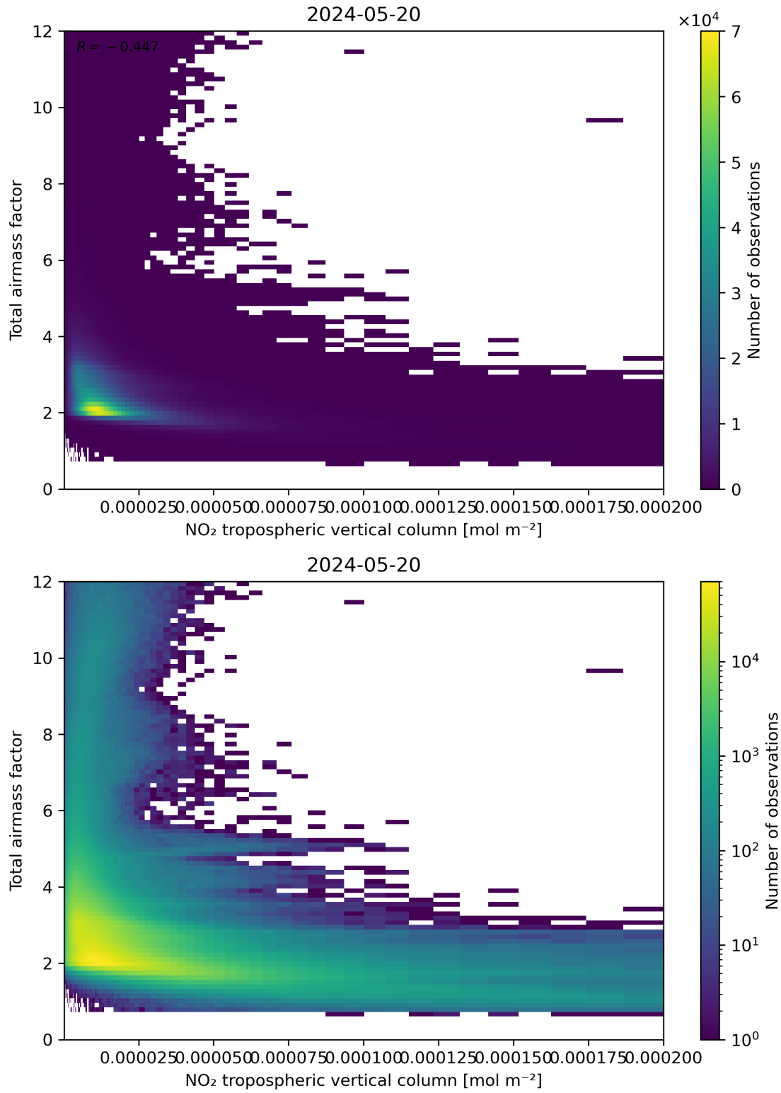
Figure 122: Scatter density plot of “NO 2 tropospheric vertical column” against “Total airmass factor” for 2024-05-19 to 2024-05-21.
