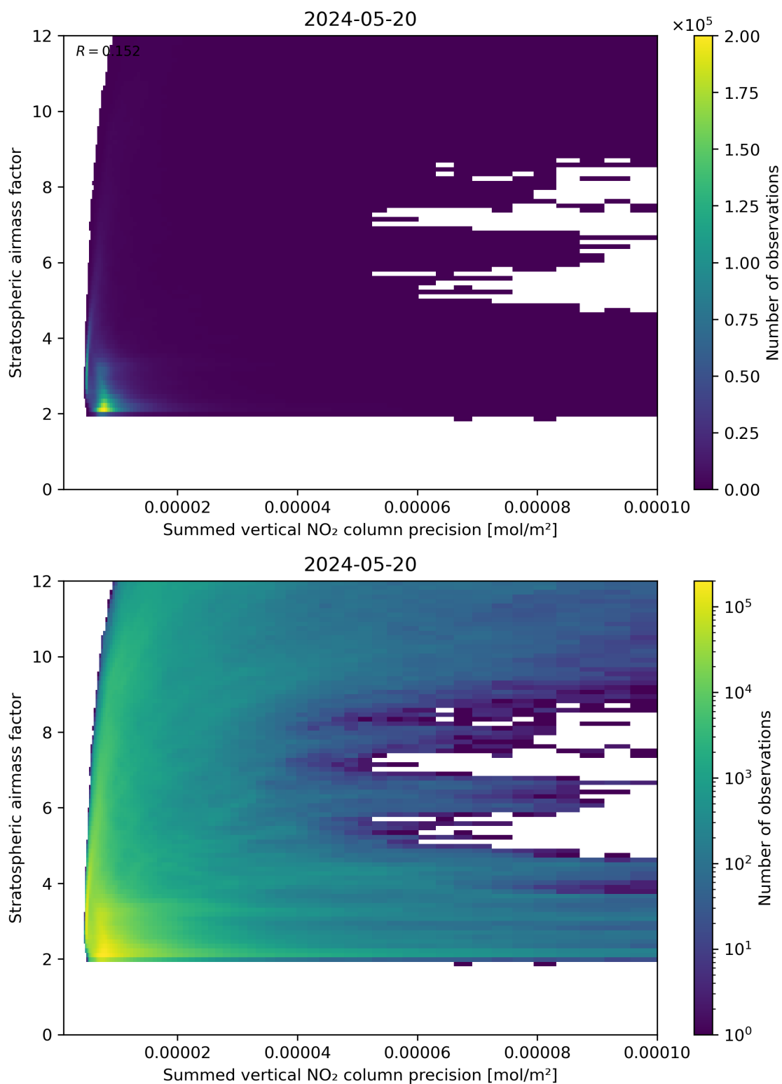
Figure 106: Scatter density plot of “Summed vertical NO 2 column precision” against “Stratospheric airmass factor” for 2024-05-19 to 2024-05-21.
