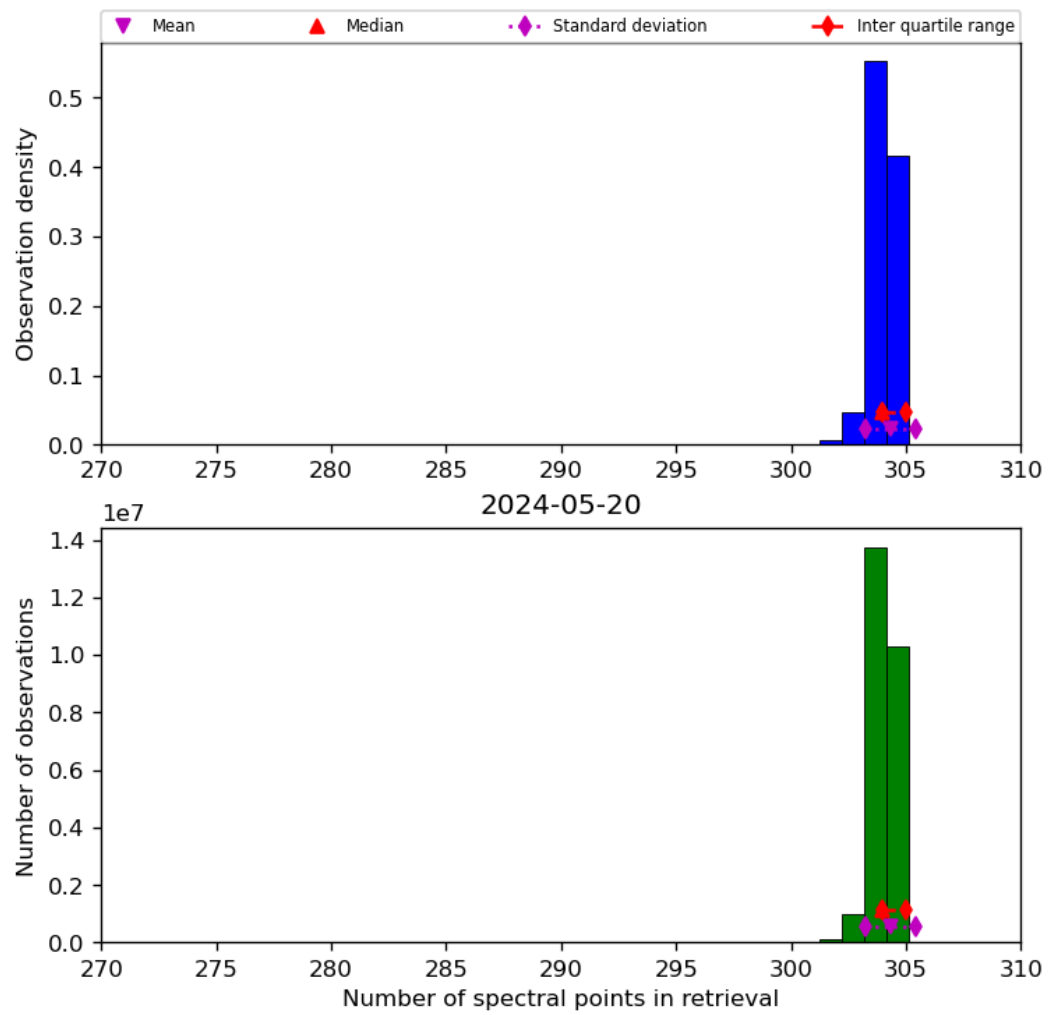
Figure 33: Histogram of “Number of spectral points in retrieval” for 2024-05-19 to 2024-05-21
