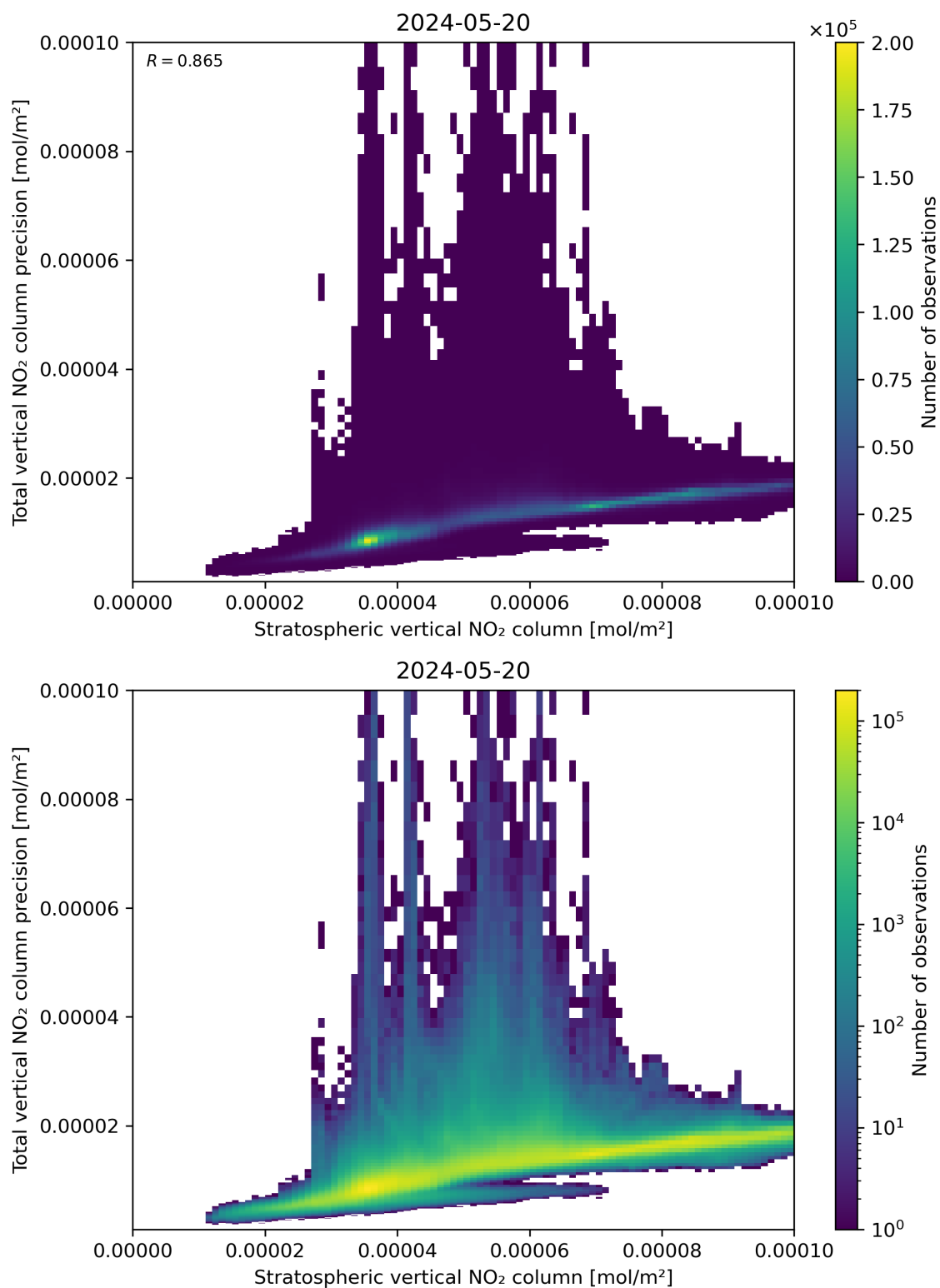
Figure 101: Scatter density plot of “Stratospheric vertical NO 2 column” against “Total vertical NO 2 column precision” for 2024-05-19 to 2024-05-21.
