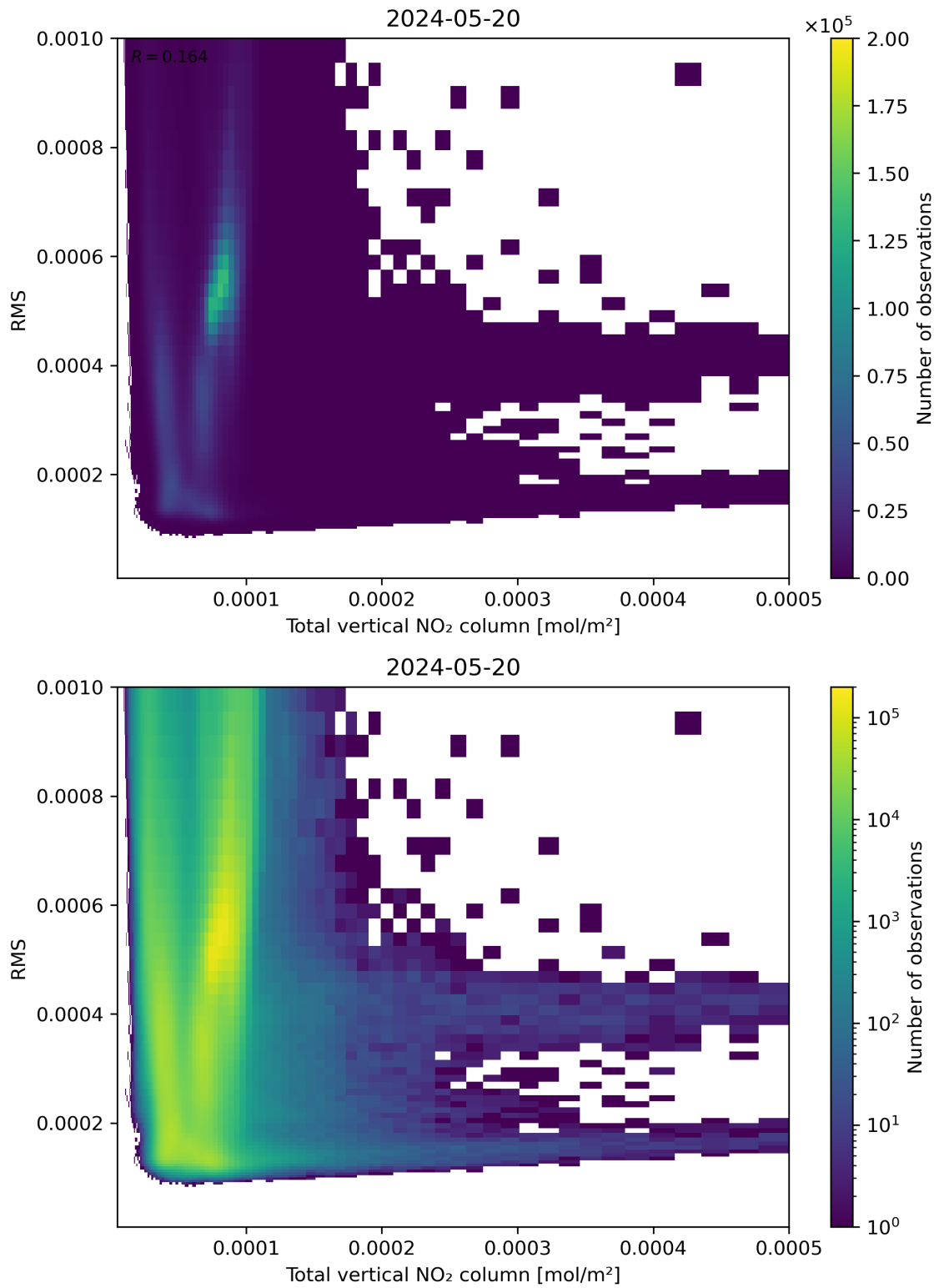
Figure 120: Scatter density plot of “Total vertical NO 2 column” against “RMS” for 2024-05-19 to 2024-05-21.
