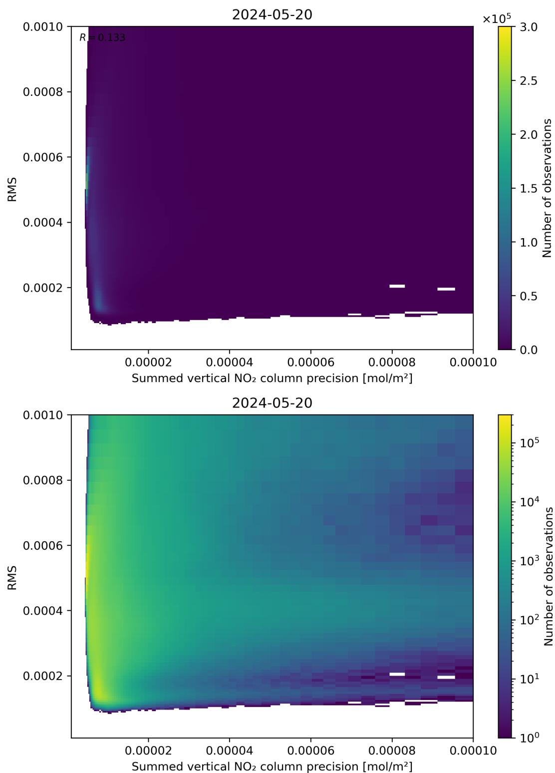
Figure 108: Scatter density plot of “Summed vertical NO 2 column precision” against “RMS” for 2024-05-19 to 2024-05-21.
