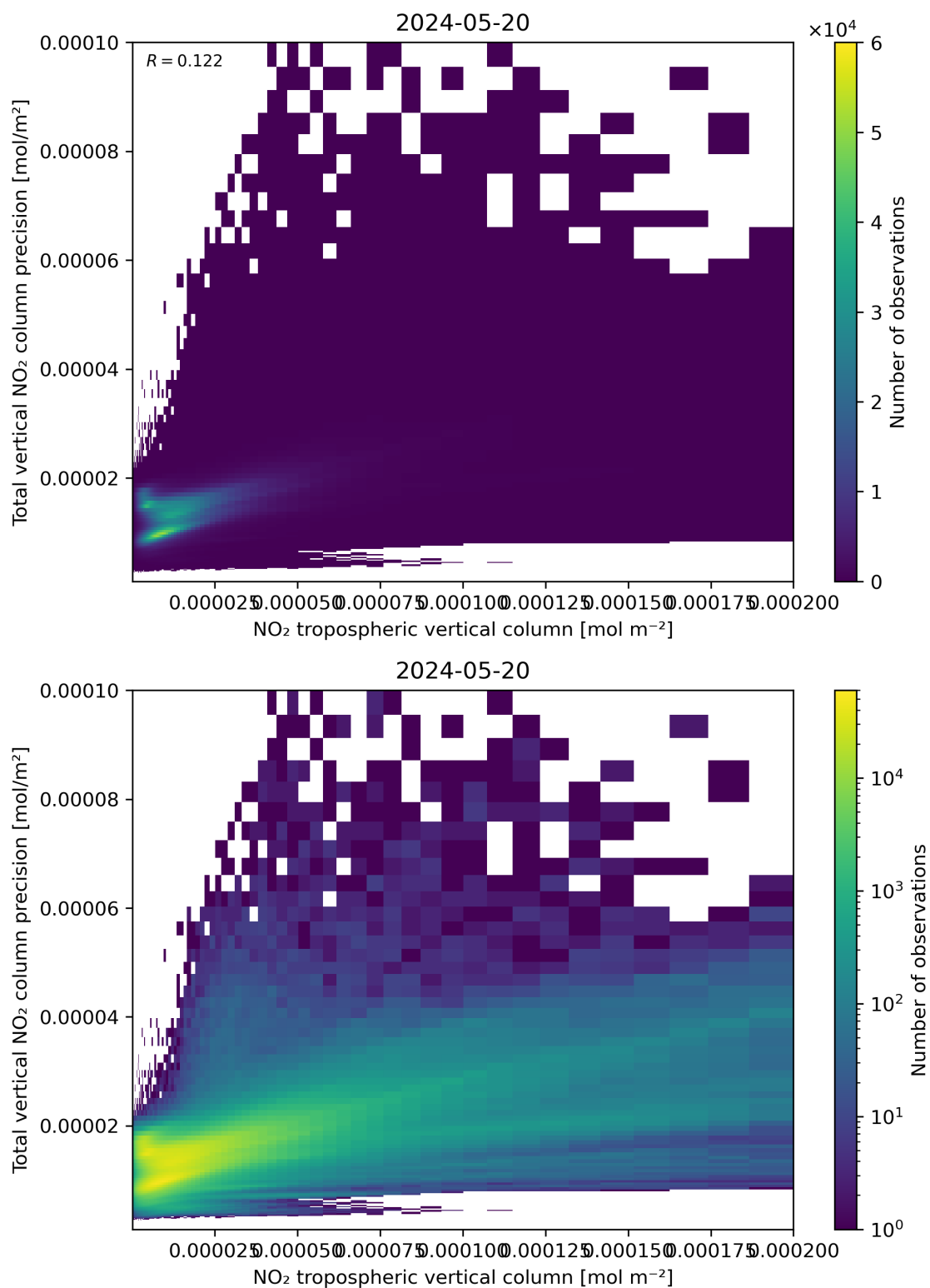
Figure 129: Scatter density plot of “NO 2 tropospheric vertical column” against “Total vertical NO 2 column precision” for 2024-05-19 to 2024-05-21.
