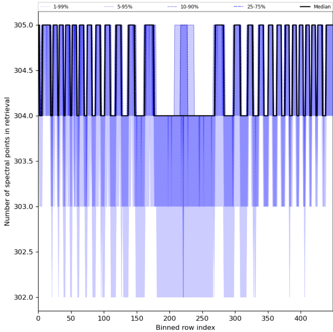
Figure 50: Along track statistics of “Number of spectral points in retrieval” for 2024-05-19 to 2024-05-21
