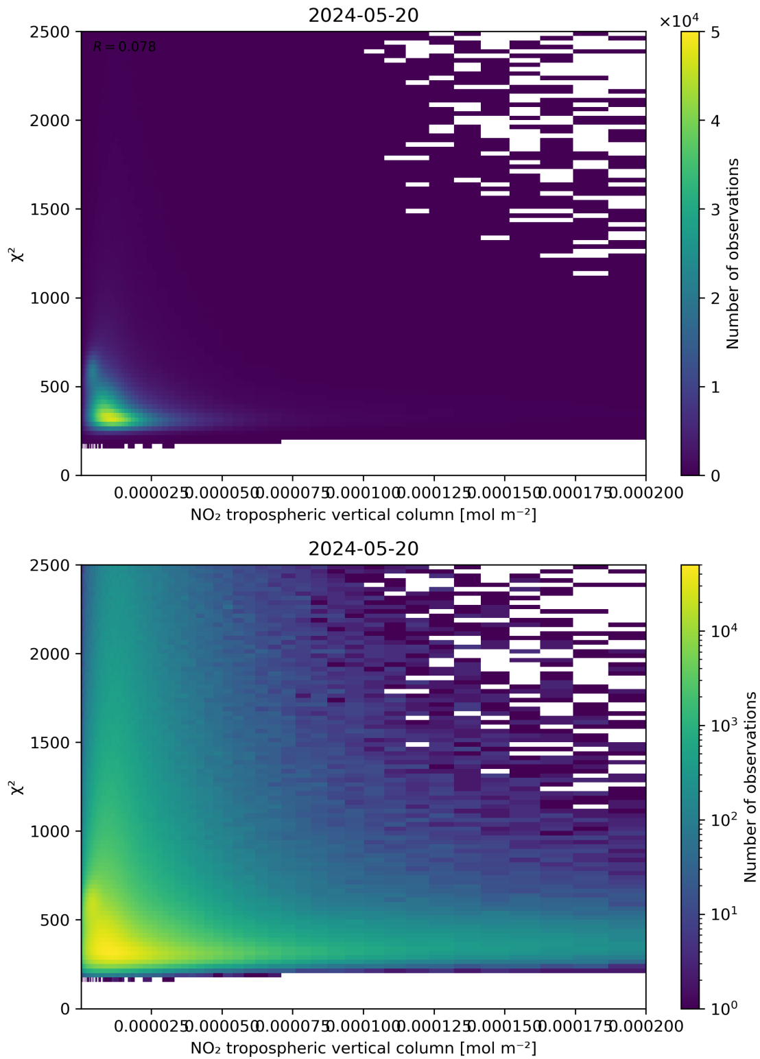
Figure 124: Scatter density plot of “NO 2 tropospheric vertical column” against “ \chi^2 ” for 2024-05-19 to 2024-05-21.
