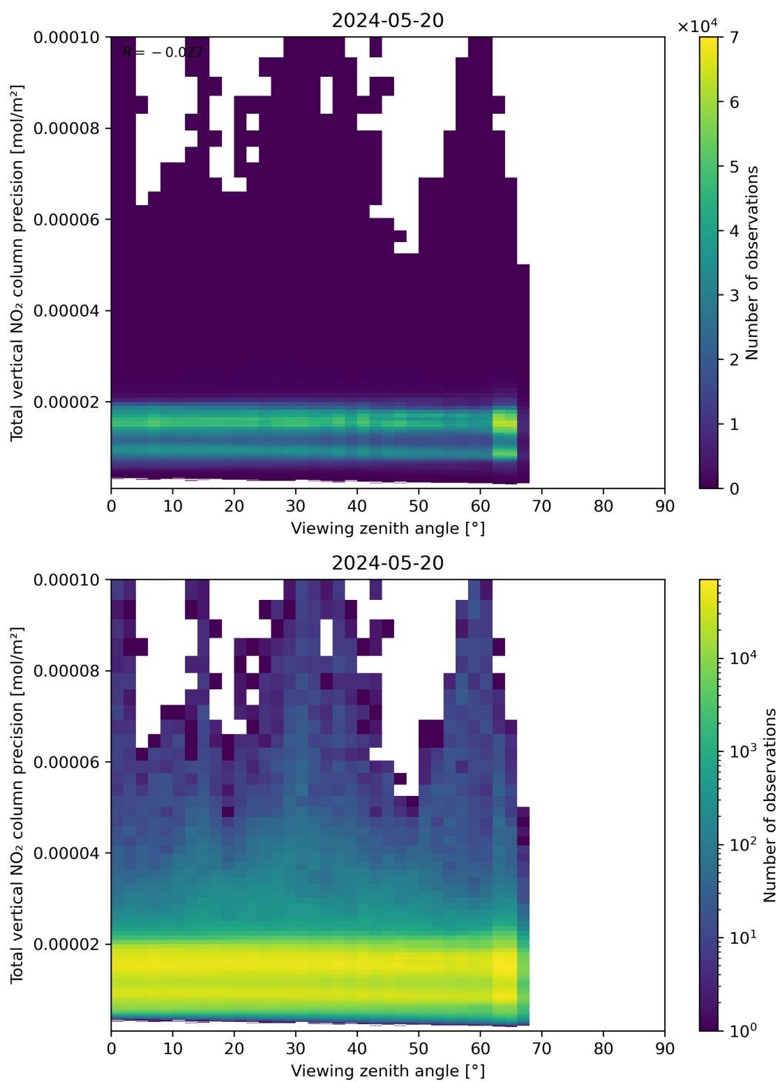
Figure 168: Scatter density plot of “Viewing zenith angle” against “Total vertical NO 2 column precision” for 2024-05-19 to 2024-05-21.
