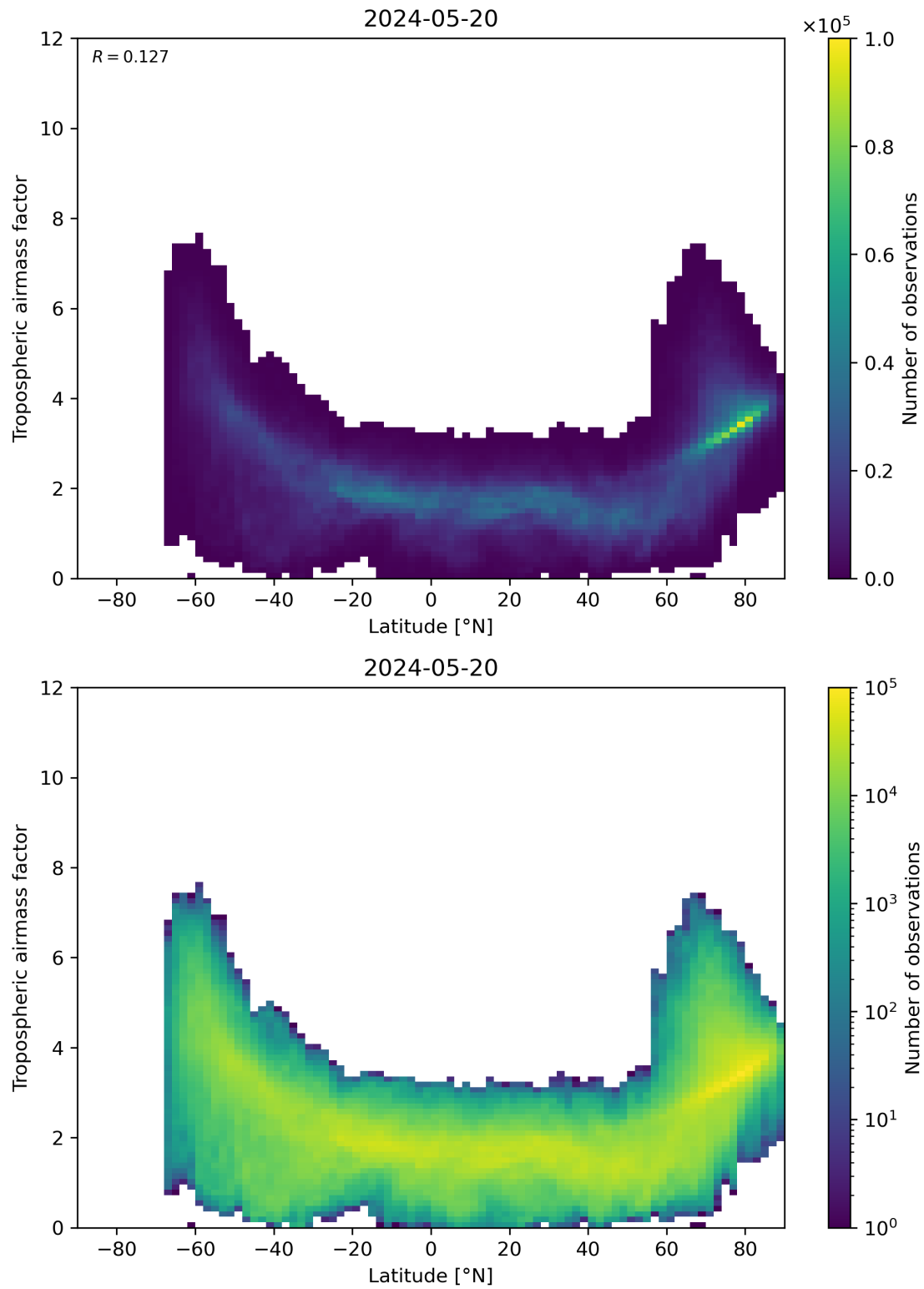
Figure 85: Scatter density plot of “Latitude” against “Tropospheric air mass factor” for 2024-05-19 to 2024-05-21.
