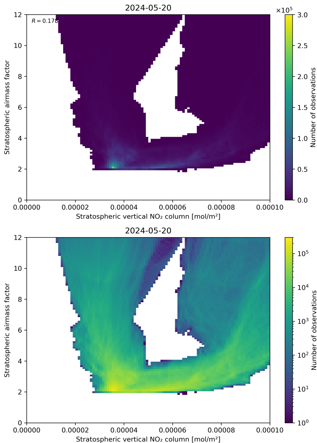
Figure 96: Scatter density plot of “Stratospheric vertical NO 2 column” against “Stratospheric airmass factor” for 2024-05-19 to 2024-05-21.
