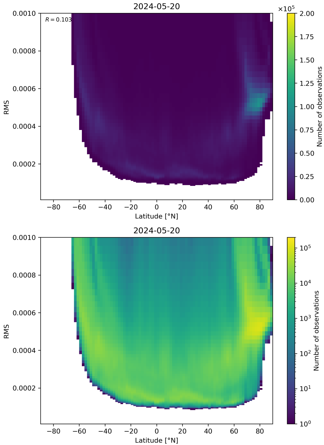
Figure 94: Scatter density plot of “Latitude” against “RMS” for 2024-05-19 to 2024-05-21.
