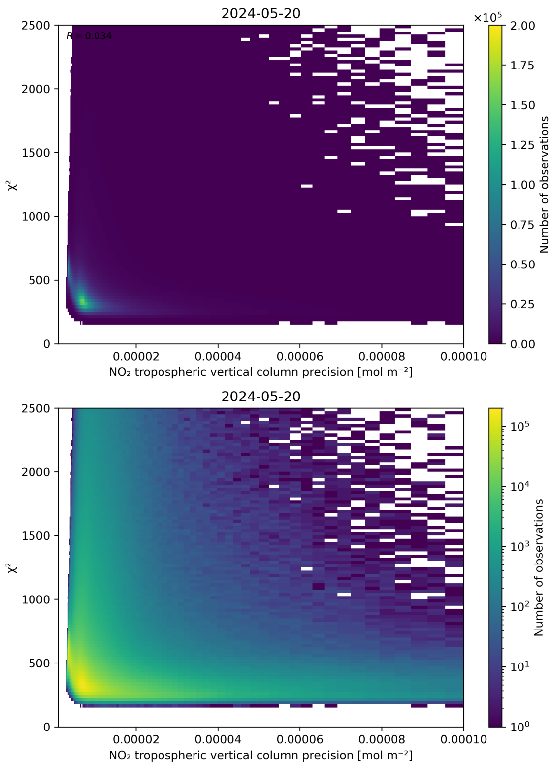
Figure 134: Scatter density plot of “NO 2 tropospheric vertical column precision” against “ \chi^2 ” for 2024-05-19 to 2024-05-21.
