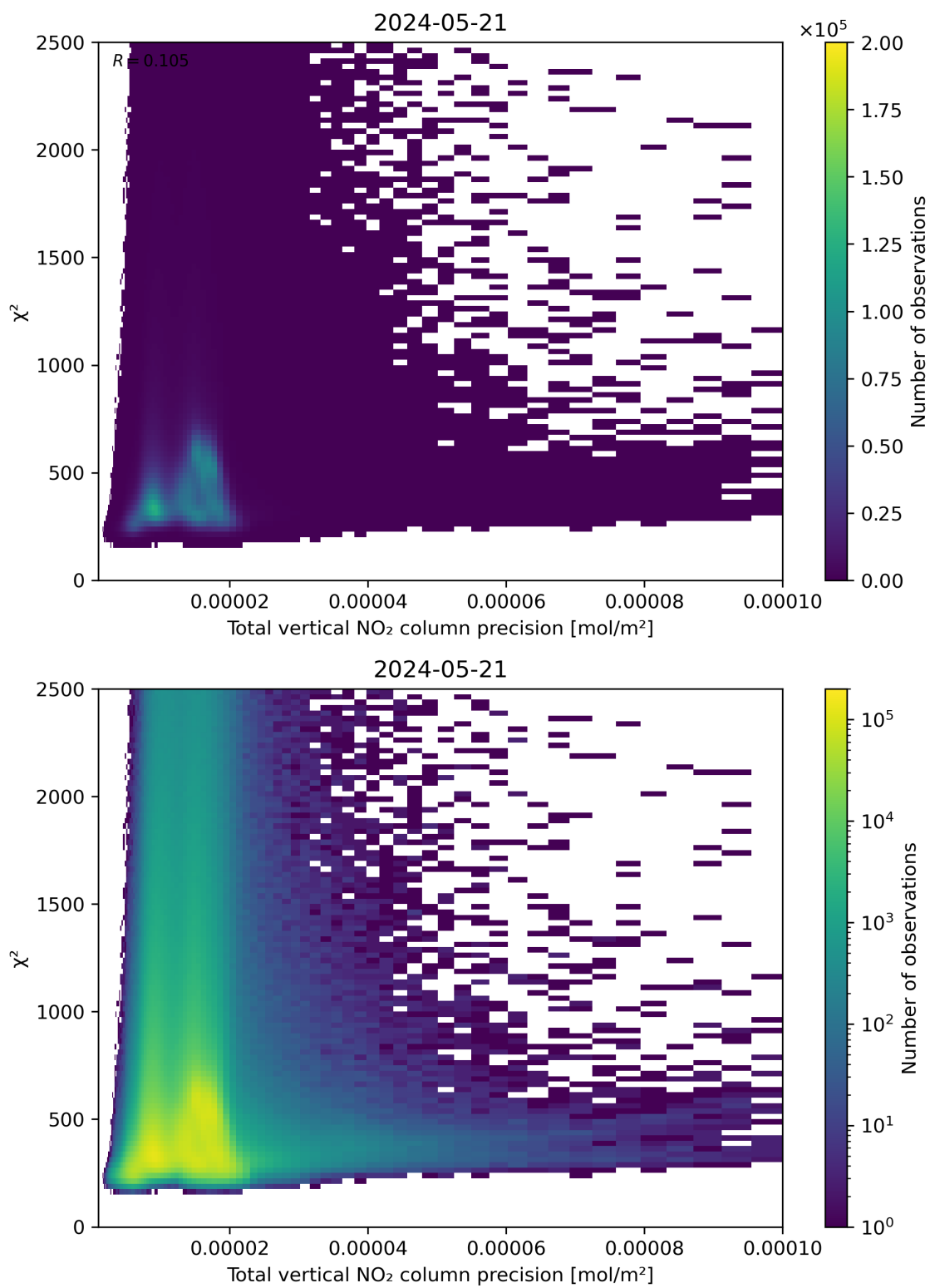
Figure 116: Scatter density plot of “Total vertical NO 2 column precision” against “ \chi^2 ” for 2024-05-20 to 2024-05-22.
