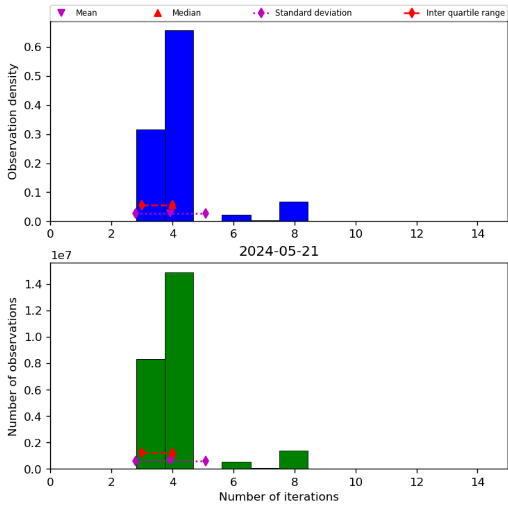
Figure 34: Histogram of “Number of iterations” for 2024-05-20 to 2024-05-22
