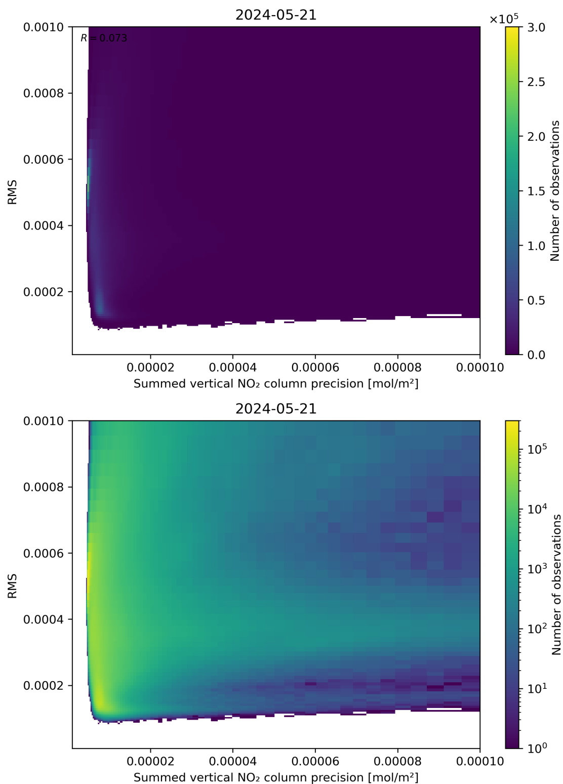
Figure 108: Scatter density plot of “Summed vertical NO 2 column precision” against “RMS” for 2024-05-20 to 2024-05-22.
