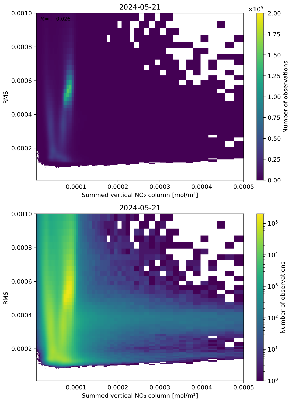
Figure 109: Scatter density plot of “Summed vertical NO 2 column” against “RMS” for 2024-05-20 to 2024-05-22.
