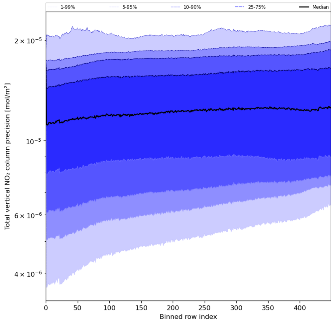
Figure 56: Along track statistics of “Total vertical NO 2 column precision” for 2024-05-20 to 2024-05-22
