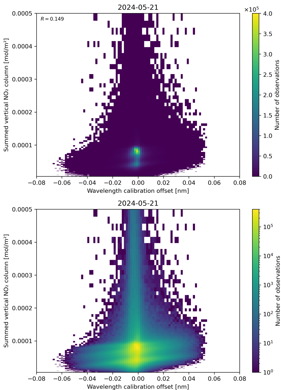
Figure 177: Scatter density plot of “Wavelength calibration offset” against “Summed vertical NO 2 column” for 2024-05-20 to 2024-05-22.
