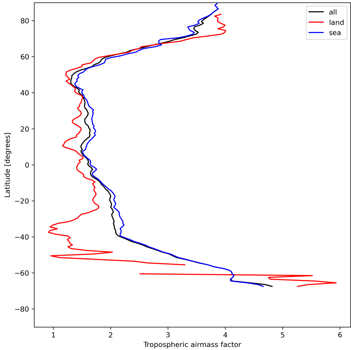
Figure 14: Zonal average of “Tropospheric airmass factor” for 2024-05-20 to 2024-05-22.
