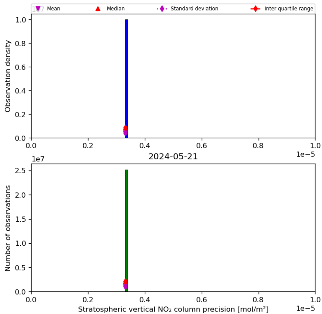
Figure 37: Histogram of “Stratospheric vertical NO 2 column precision” for 2024-05-20 to 2024-05-22
