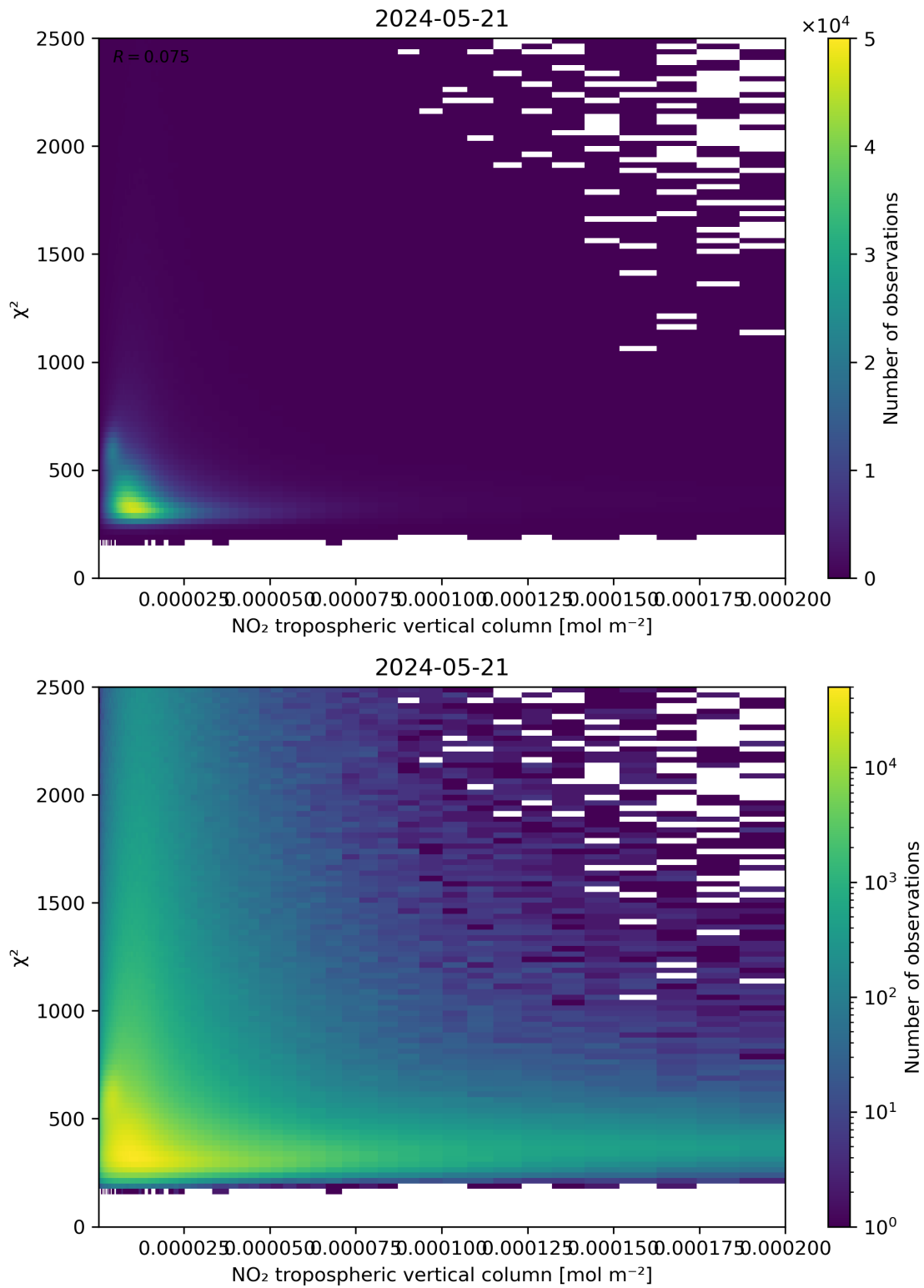
Figure 124: Scatter density plot of “NO 2 tropospheric vertical column” against “ \chi^2 ” for 2024-05-20 to 2024-05-22.
