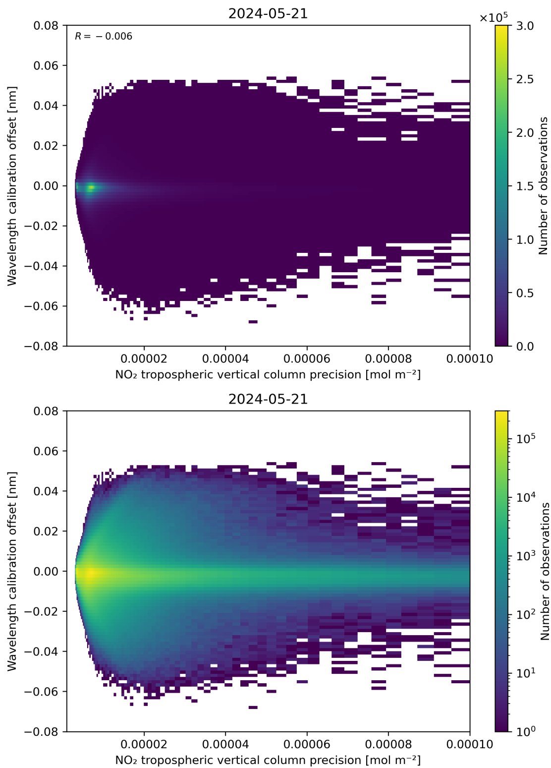
Figure 141: Scatter density plot of “NO 2 tropospheric vertical column precision” against “Wavelength calibration offset” for 2024-05-20 to 2024-05-22.
