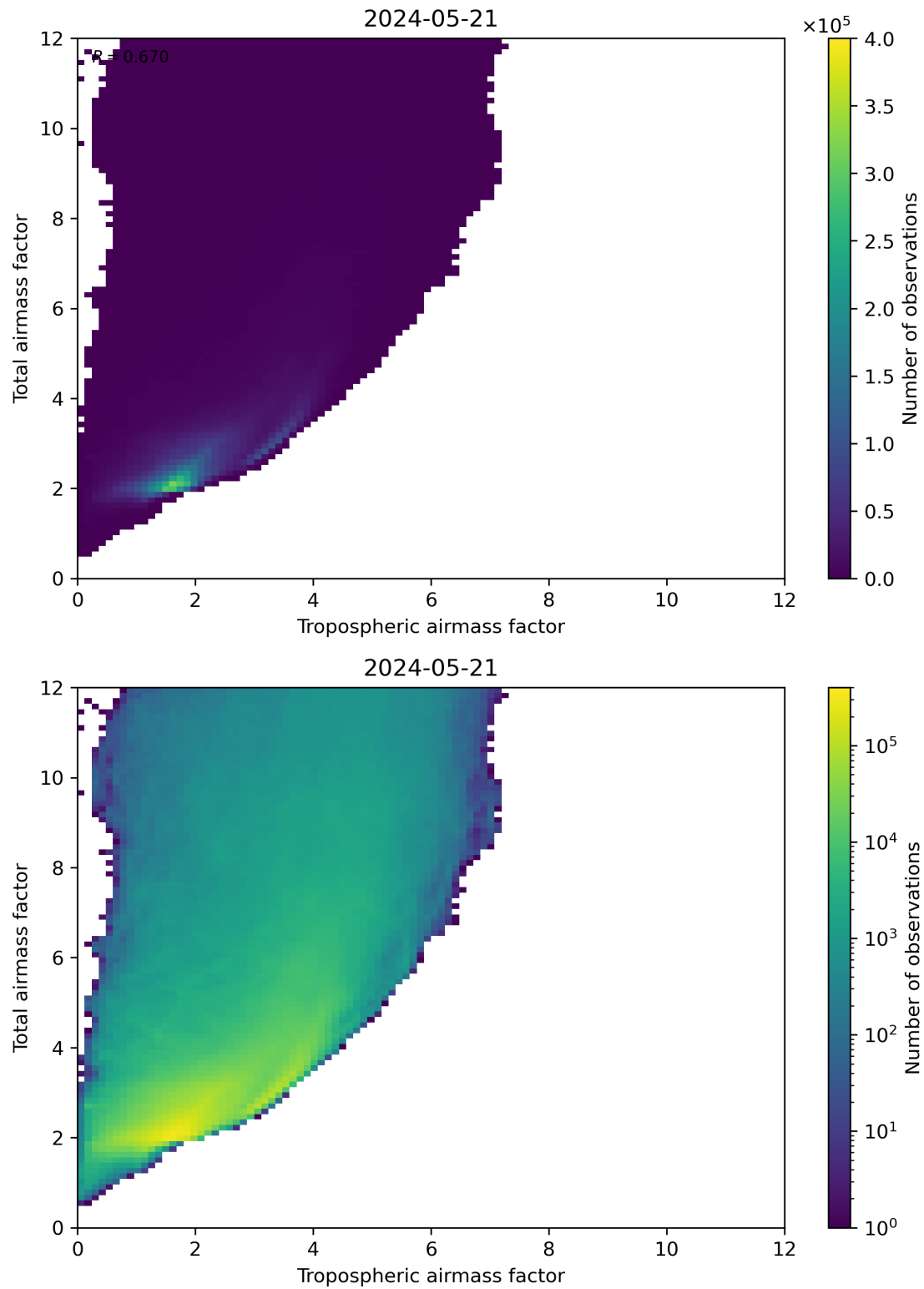
Figure 72: Scatter density plot of “Tropospheric airmass factor” against “Total airmass factor” for 2024-05-20 to 2024-05-22.
