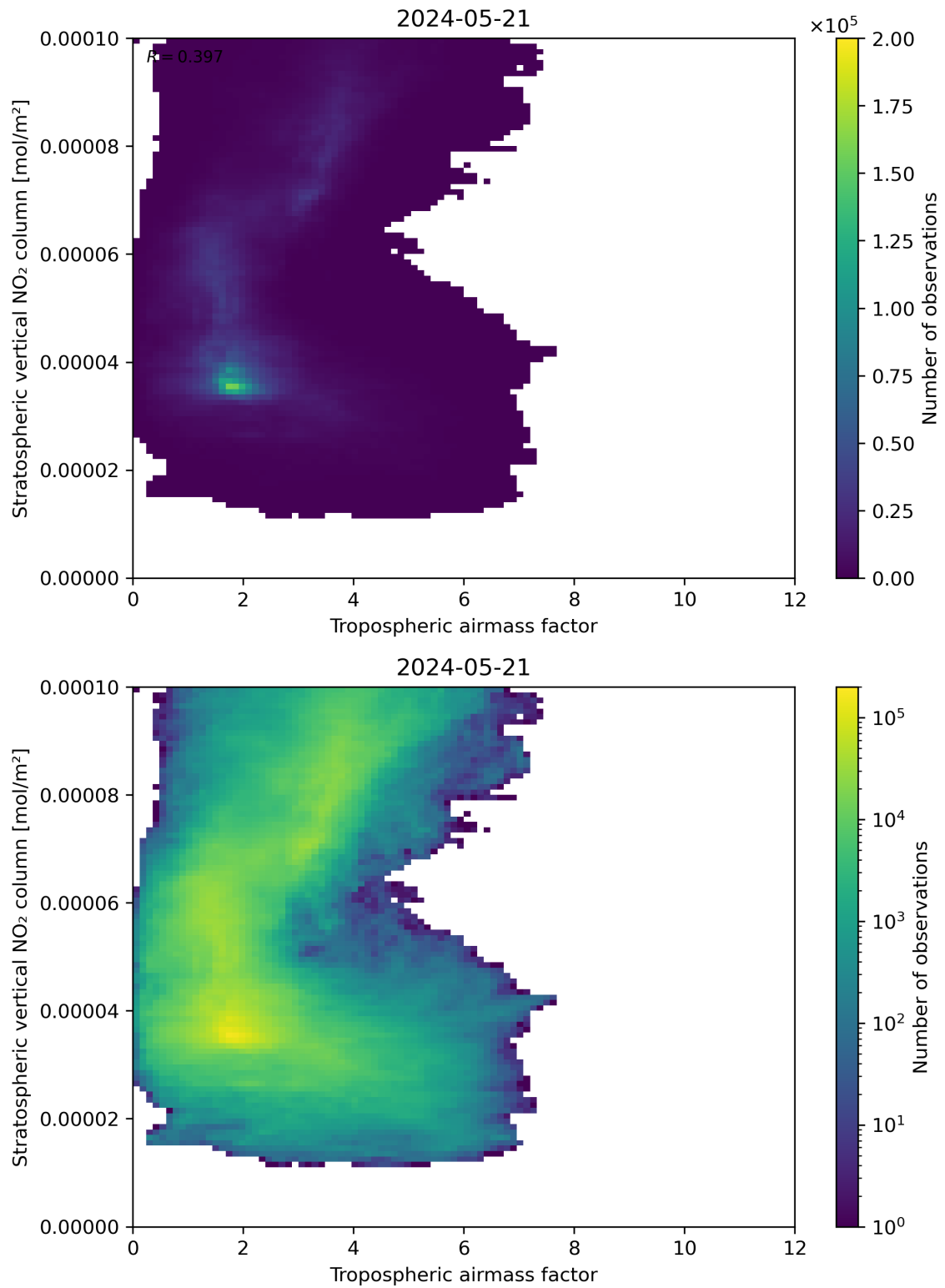
Figure 74: Scatter density plot of “Tropospheric air mass factor” against “Stratospheric vertical NO 2 column” for 2024-05-20 to 2024-05-22.
