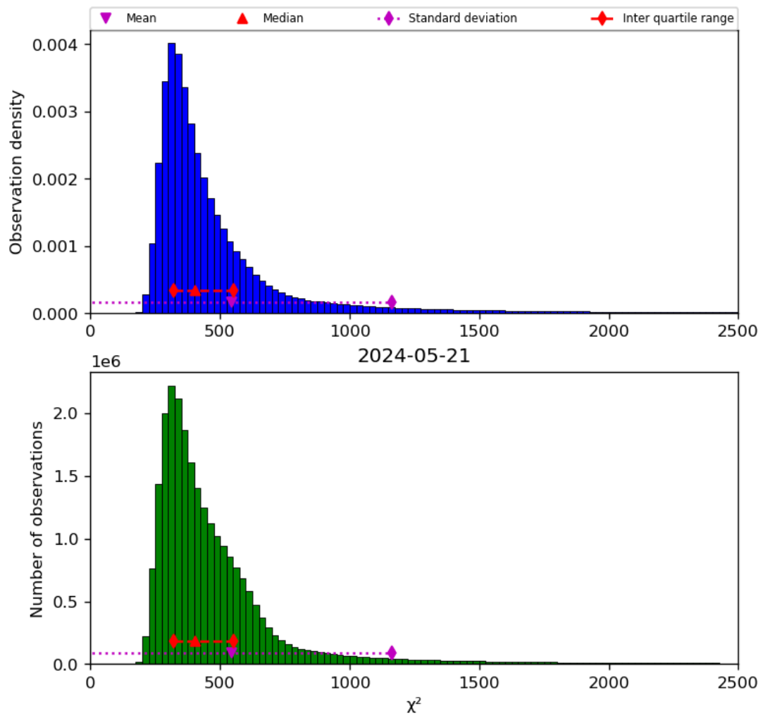
Figure 42: Histogram of “ \chi^2 ” for 2024-05-20 to 2024-05-22
