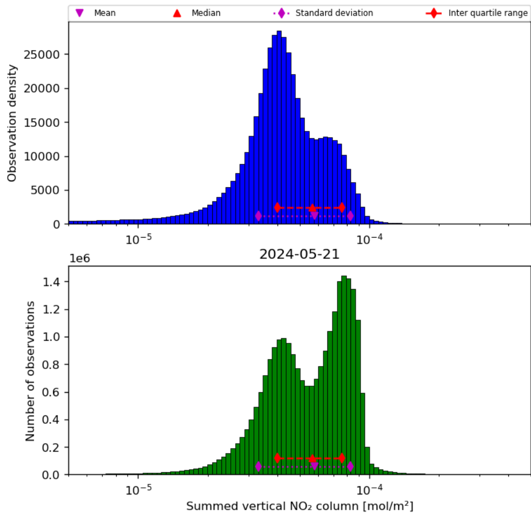
Figure 40: Histogram of “Summed vertical NO 2 column” for 2024-05-20 to 2024-05-22
