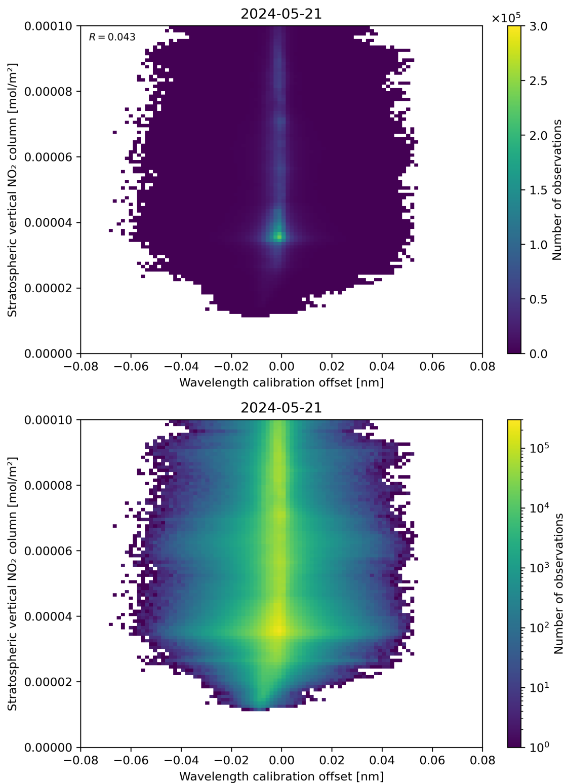
Figure 176: Scatter density plot of “Wavelength calibration offset” against “Stratospheric vertical NO 2 column” for 2024-05-20 to 2024-05-22.
