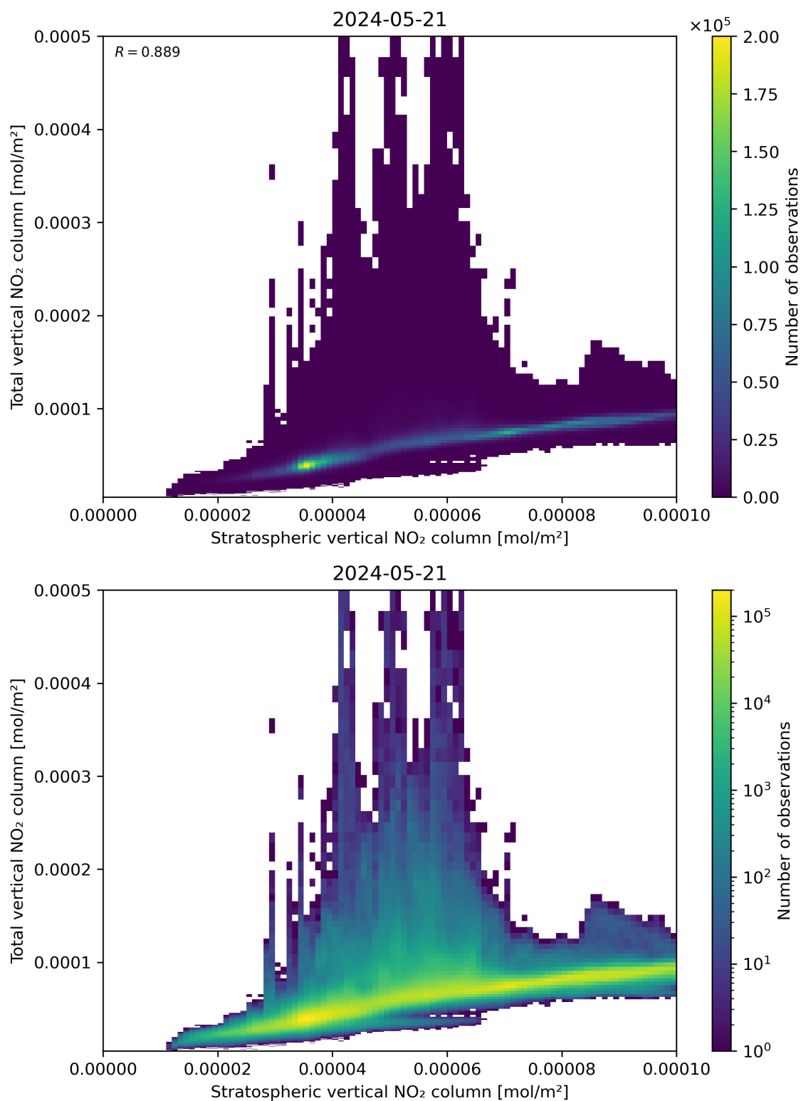
Figure 100: Scatter density plot of “Stratospheric vertical NO 2 column” against “Total vertical NO 2 column” for 2024-05-20 to 2024-05-22.
