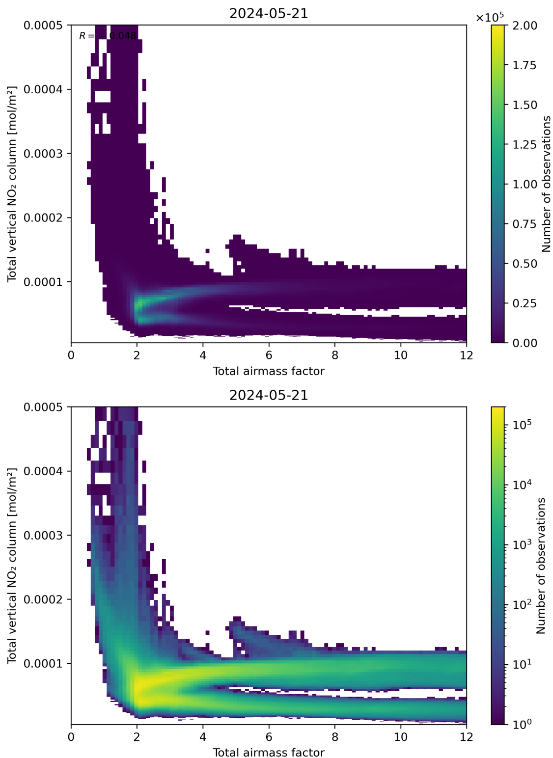
Figure 67: Scatter density plot of “Total airmass factor” against “Total vertical NO 2 column” for 2024-05-20 to 2024-05-22.
