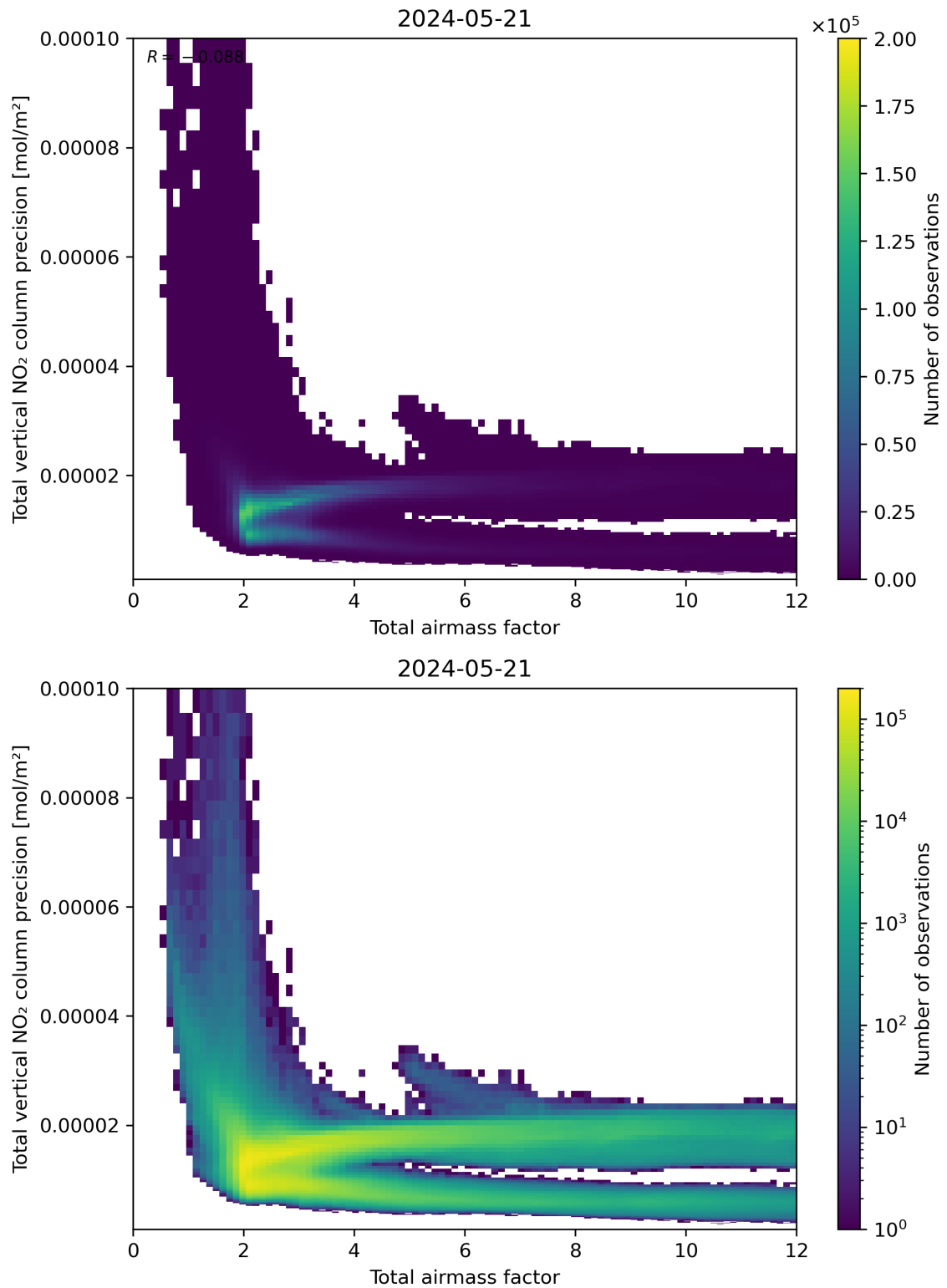
Figure 68: Scatter density plot of “Total airmass factor” against “Total vertical NO 2 column precision” for 2024-05-20 to 2024-05-22.
