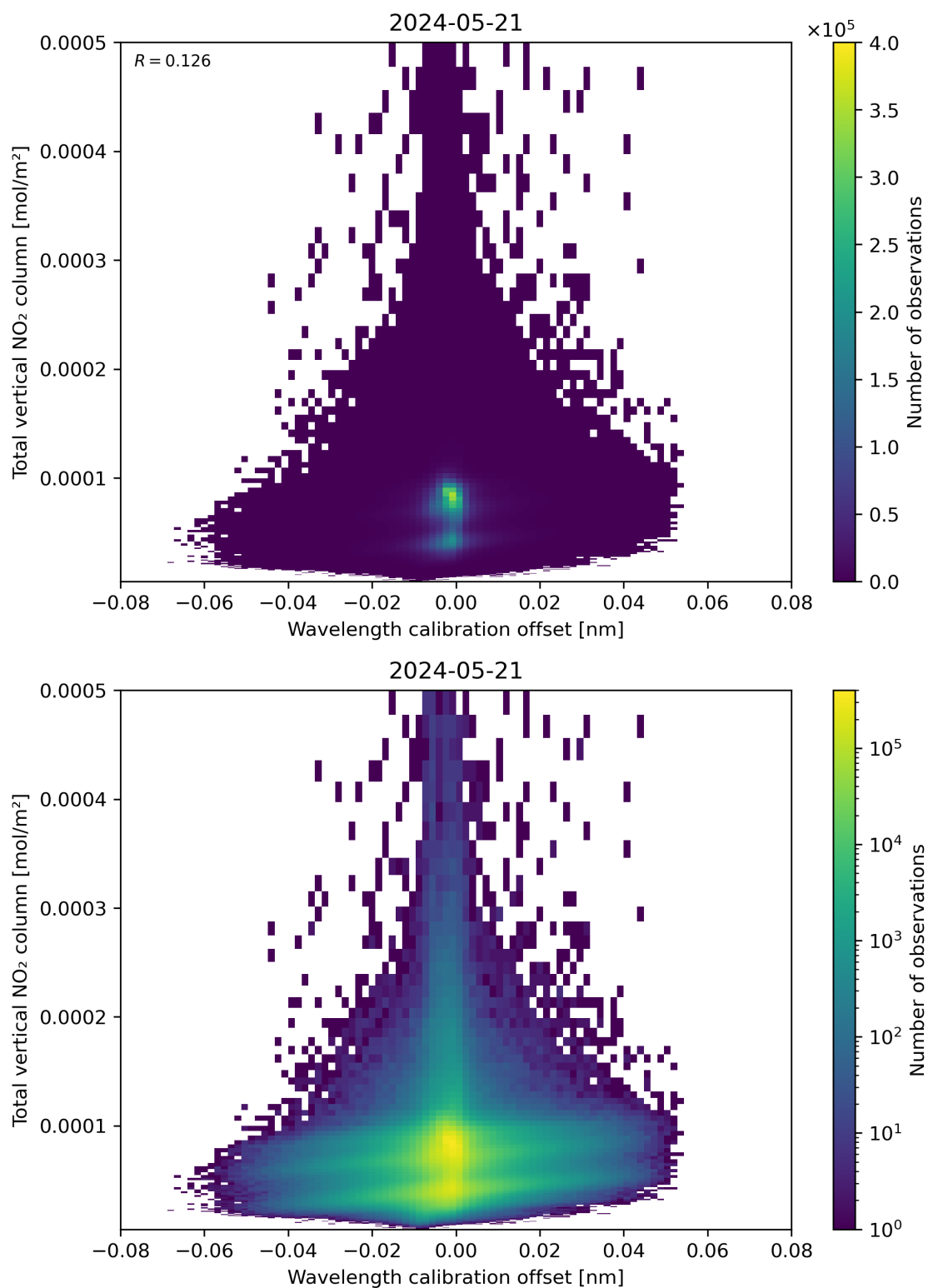
Figure 179: Scatter density plot of “Wavelength calibration offset” against “Total vertical NO 2 column” for 2024-05-20 to 2024-05-22.
