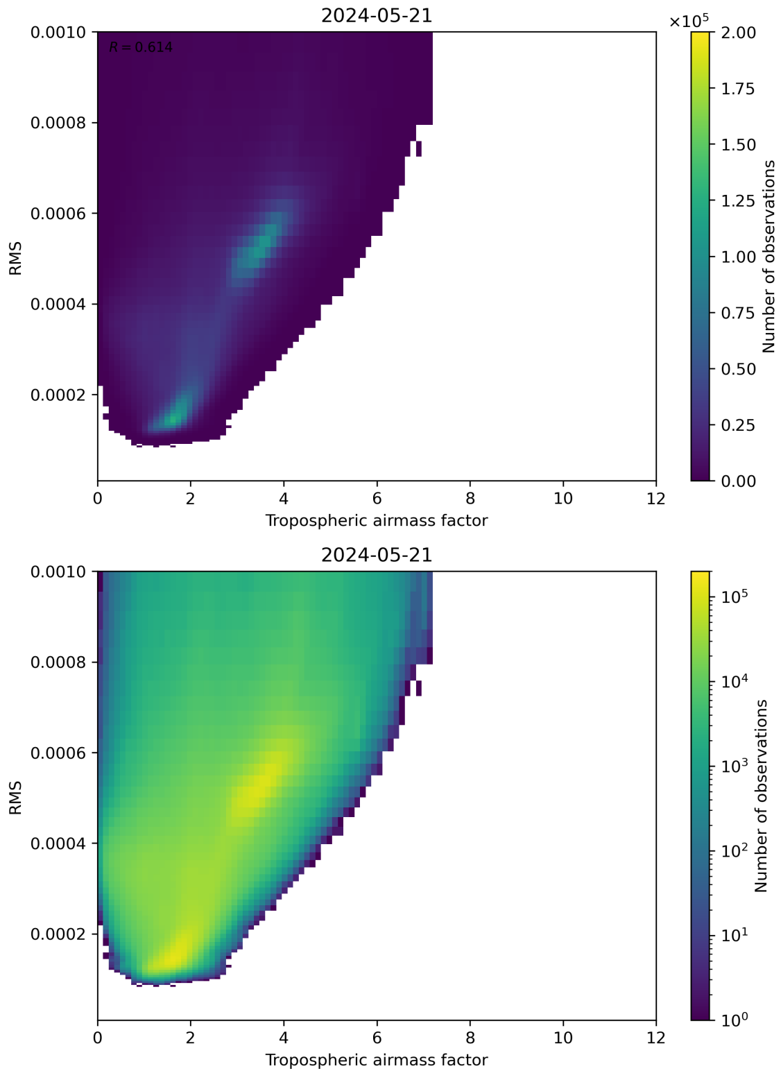
Figure 79: Scatter density plot of “Tropospheric airmass factor” against “RMS” for 2024-05-20 to 2024-05-22.
