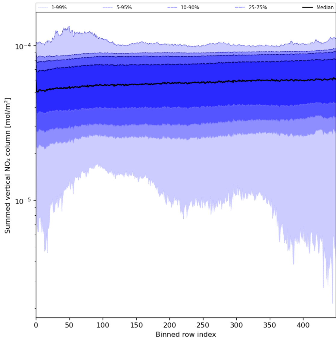
Figure 57: Along track statistics of “Summed vertical NO 2 column” for 2024-05-20 to 2024-05-22
