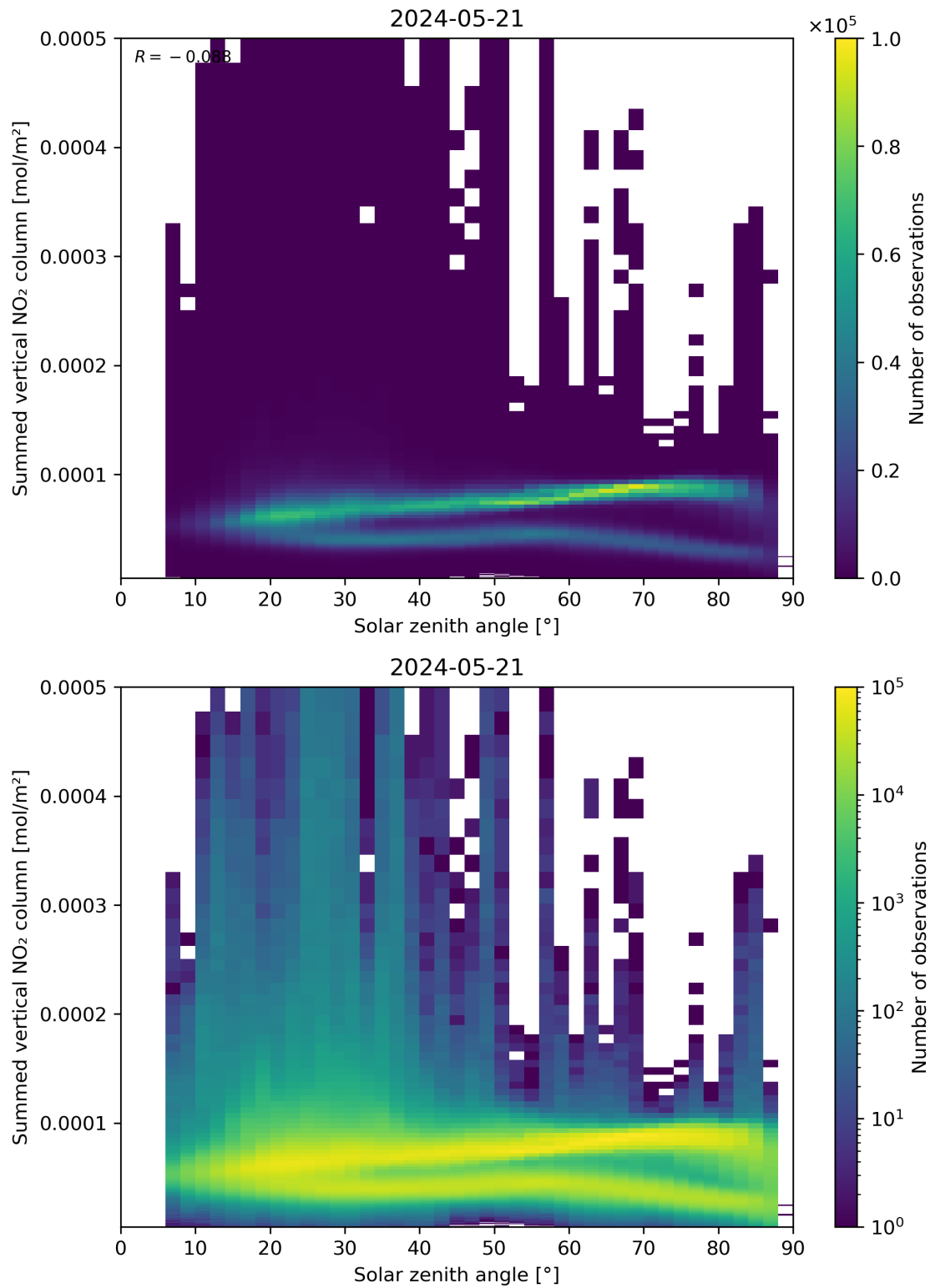
Figure 151: Scatter density plot of “Solar zenith angle” against “Summed vertical NO 2 column” for 2024-05-20 to 2024-05-22.
