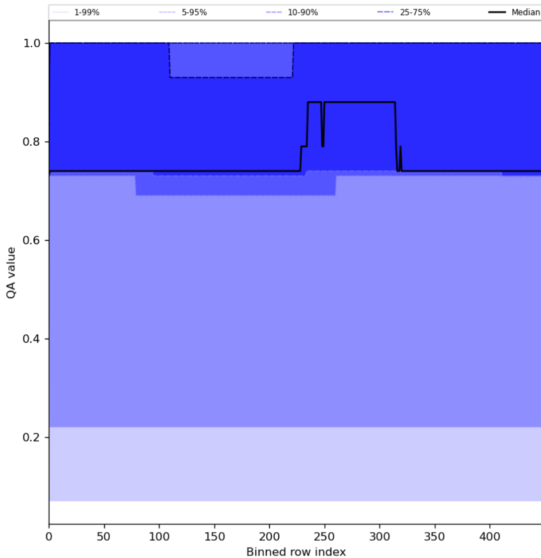
Figure 45: Along track statistics of “QA value” for 2024-05-20 to 2024-05-22
