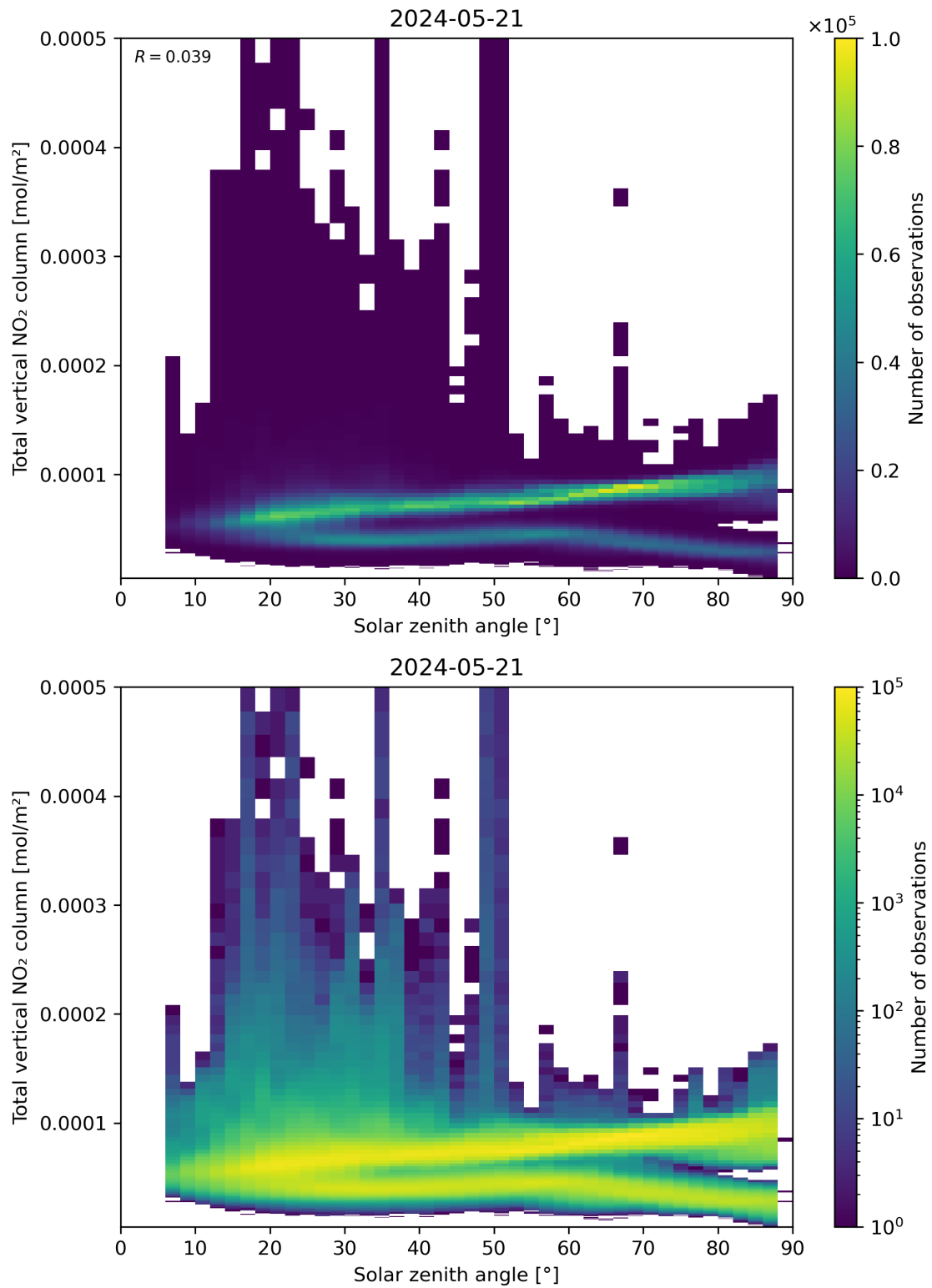
Figure 153: Scatter density plot of “Solar zenith angle” against “Total vertical NO 2 column” for 2024-05-20 to 2024-05-22.
