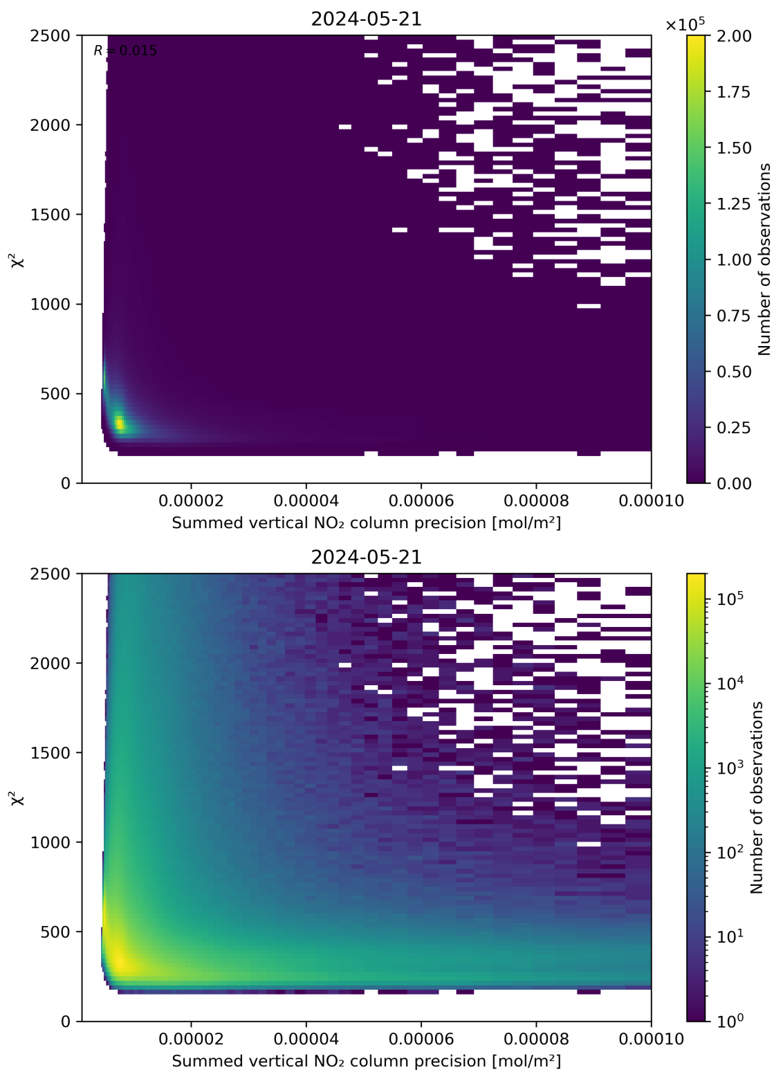
Figure 107: Scatter density plot of “Summed vertical NO 2 column precision” against “ \chi^2 ” for 2024-05-20 to 2024-05-22.
