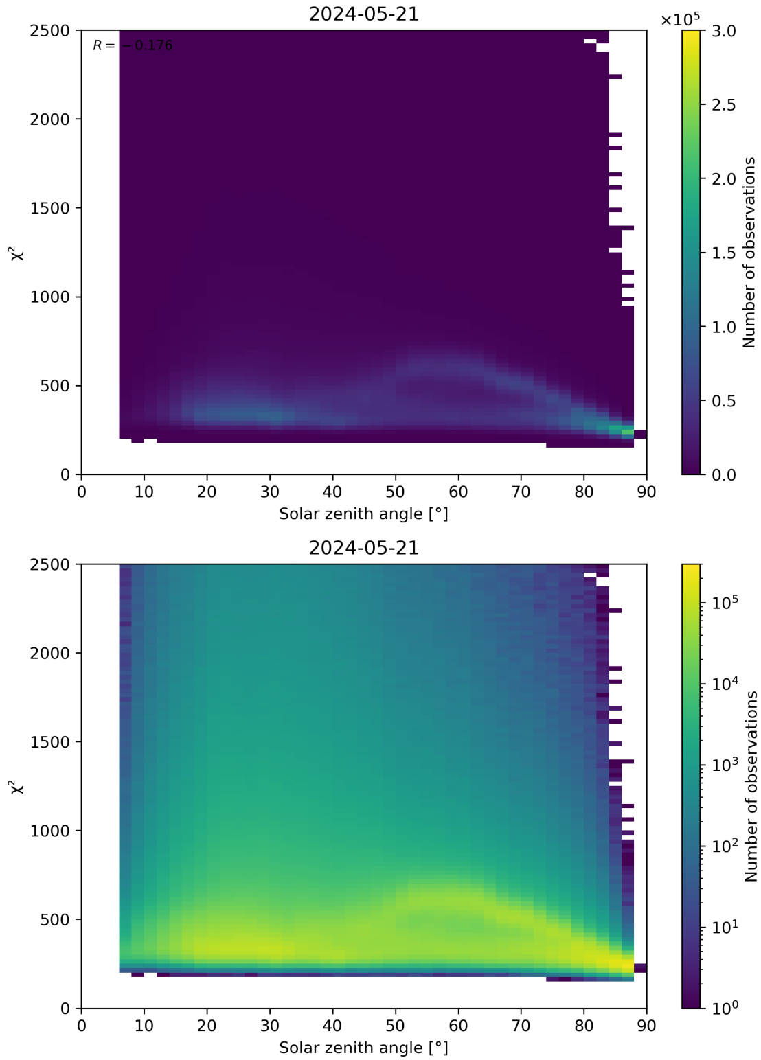
Figure 148: Scatter density plot of “Solar zenith angle” against “ \chi^2 ” for 2024-05-20 to 2024-05-22.
