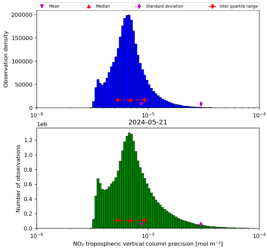
Figure 30: Histogram of “NO 2 tropospheric vertical column precision” for 2024-05-20 to 2024-05-22
