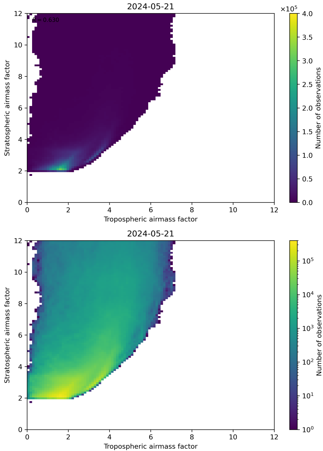
Figure 71: Scatter density plot of “Tropospheric airmass factor” against “Stratospheric airmass factor” for 2024-05-20 to 2024-05-22.
