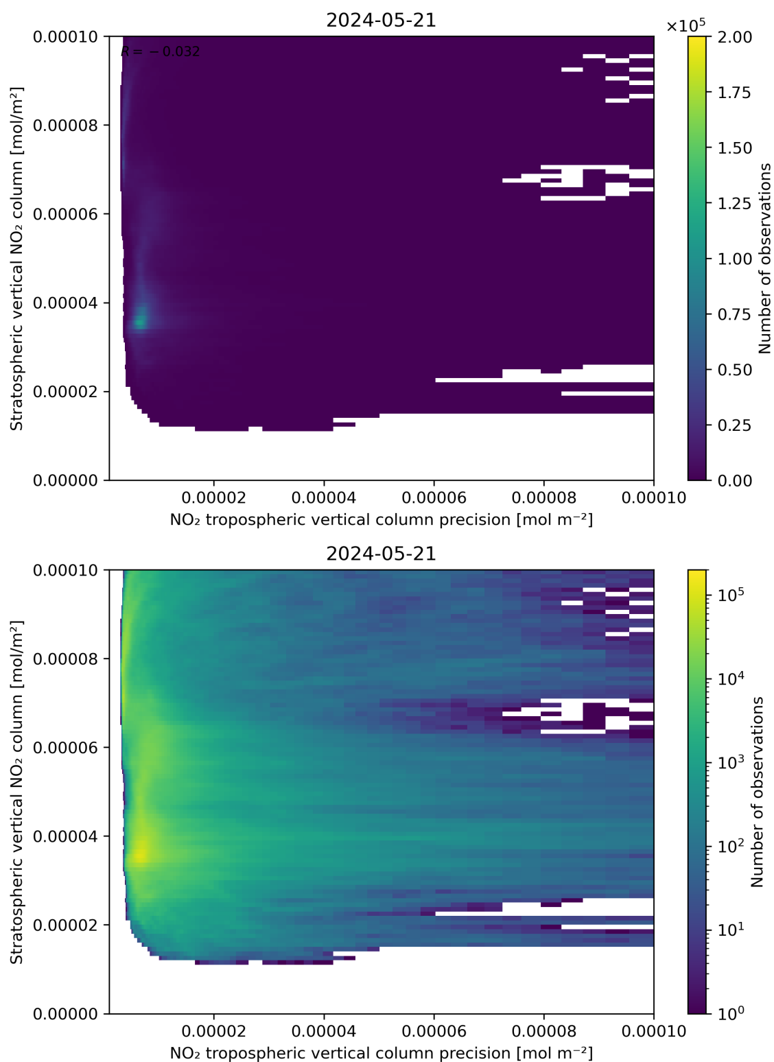
Figure 135: Scatter density plot of “NO 2 tropospheric vertical column precision” against “Stratospheric vertical NO 2 column” for 2024-05-20 to 2024-05-22.
