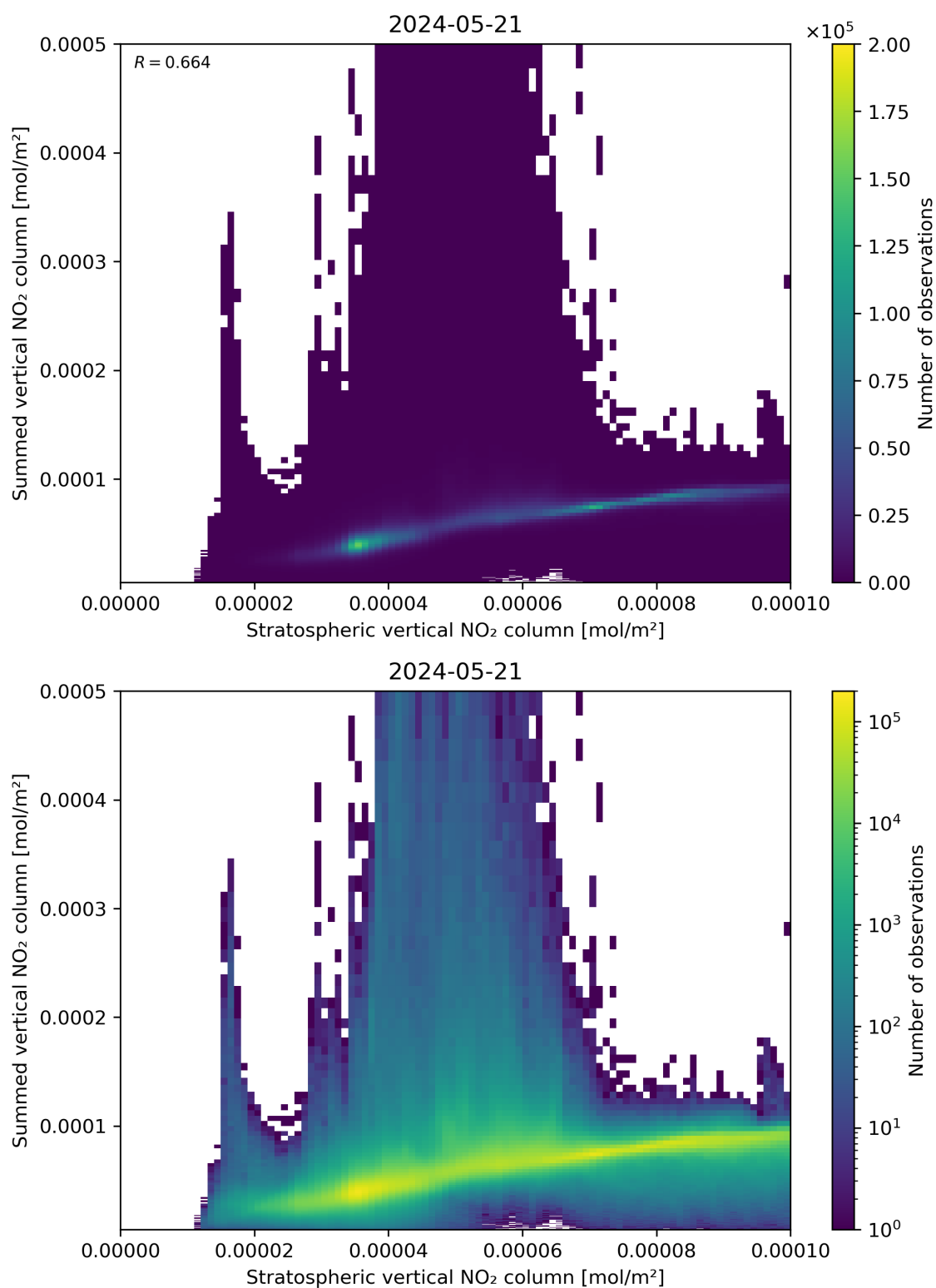
Figure 98: Scatter density plot of “Stratospheric vertical NO 2 column” against “Summed vertical NO 2 column” for 2024-05-20 to 2024-05-22.
