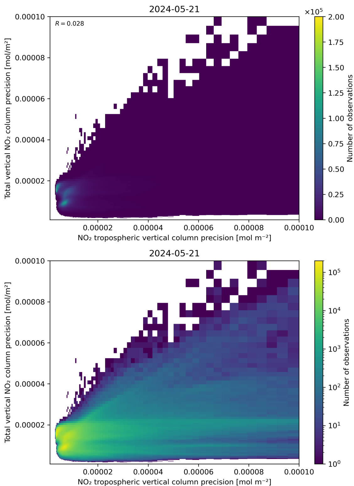
Figure 139: Scatter density plot of “NO 2 tropospheric vertical column precision” against “Total vertical NO 2 column precision” for 2024-05-20 to 2024-05-22.
