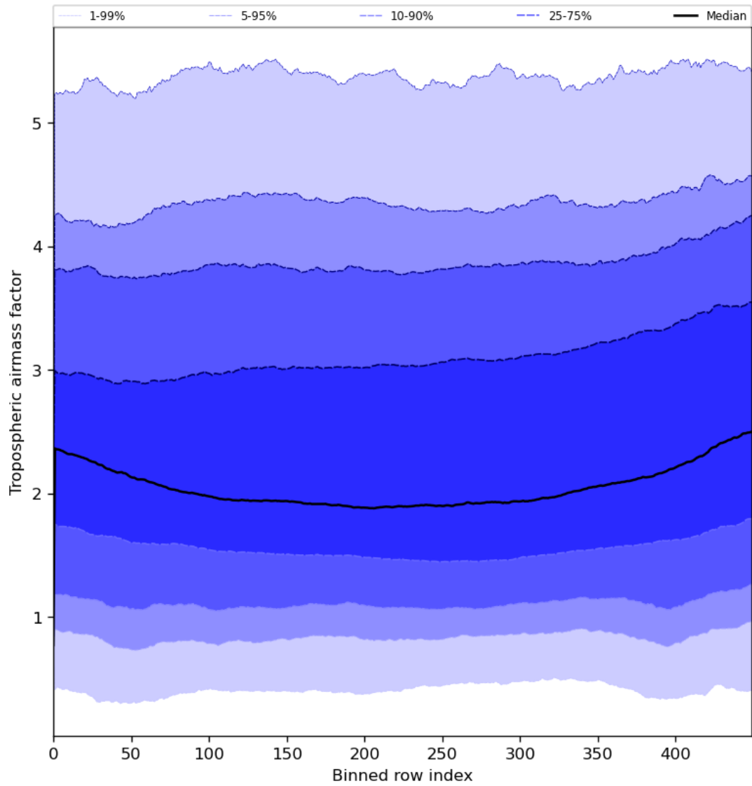
Figure 48: Along track statistics of “Tropospheric airmass factor” for 2024-05-20 to 2024-05-22
