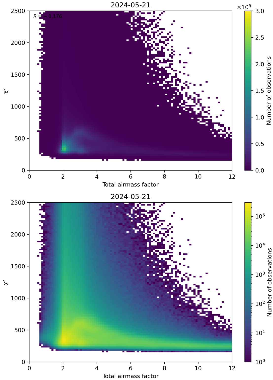
Figure 63: Scatter density plot of “Total airmass factor” against “ \chi^2 ” for 2024-05-20 to 2024-05-22.
