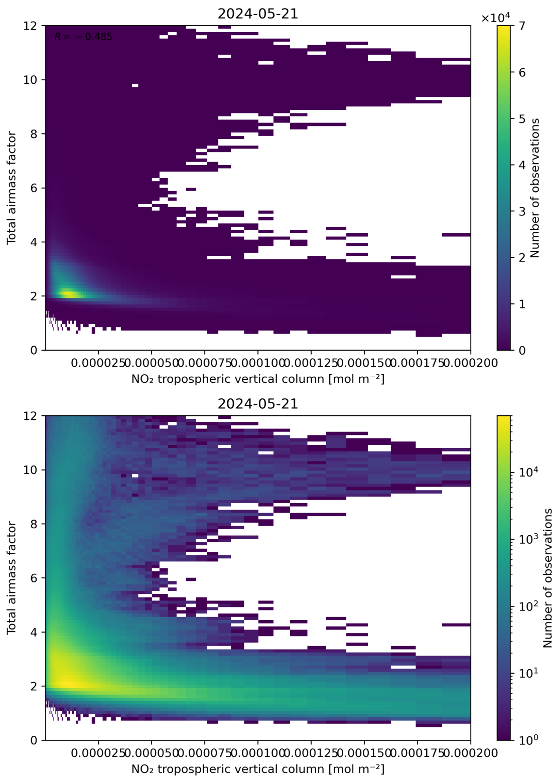
Figure 122: Scatter density plot of “NO 2 tropospheric vertical column” against “Total airmass factor” for 2024-05-20 to 2024-05-22.
