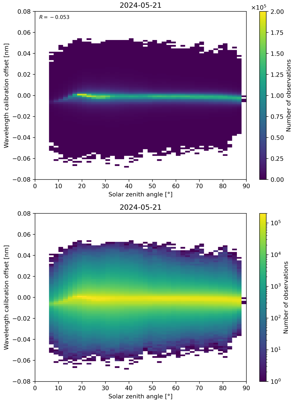
Figure 158: Scatter density plot of “Solar zenith angle” against “Wavelength calibration offset” for 2024-05-20 to 2024-05-22.
