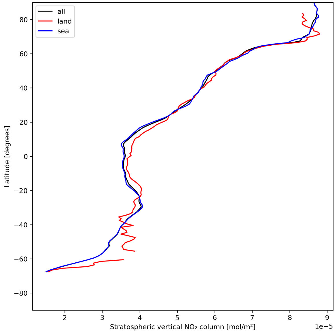
Figure 19: Zonal average of “Stratospheric vertical NO 2 column” for 2024-05-20 to 2024-05-22.
