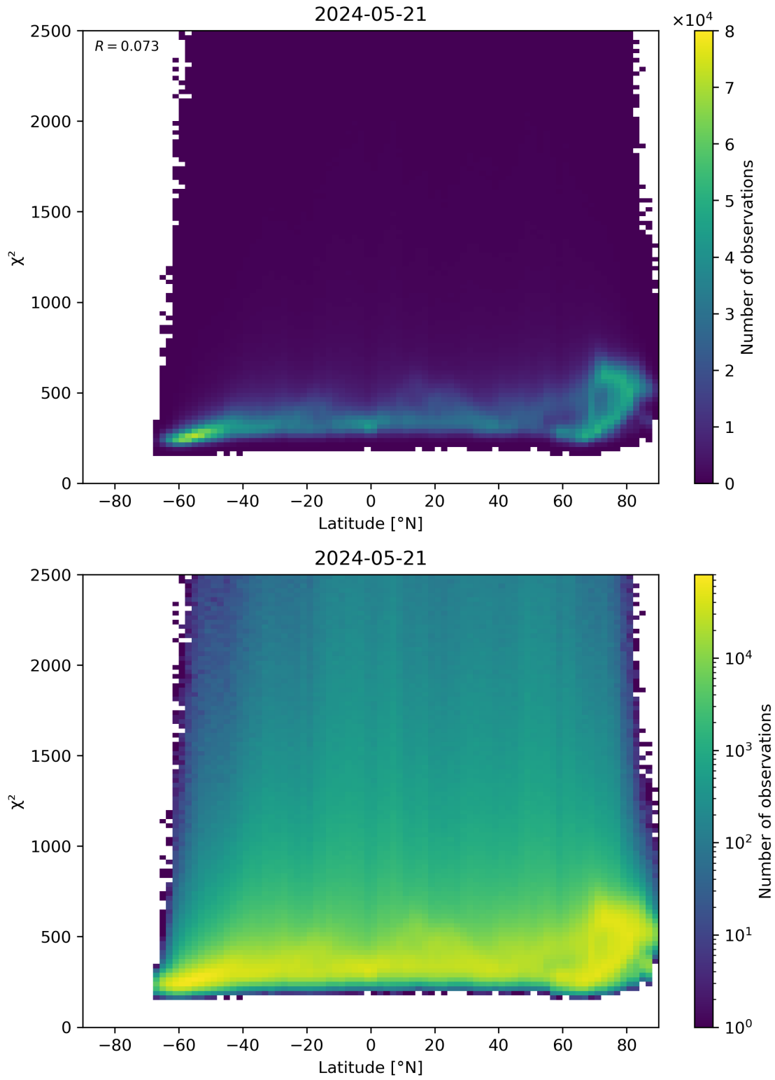
Figure 86: Scatter density plot of “Latitude” against “ \chi^2 ” for 2024-05-20 to 2024-05-22.
