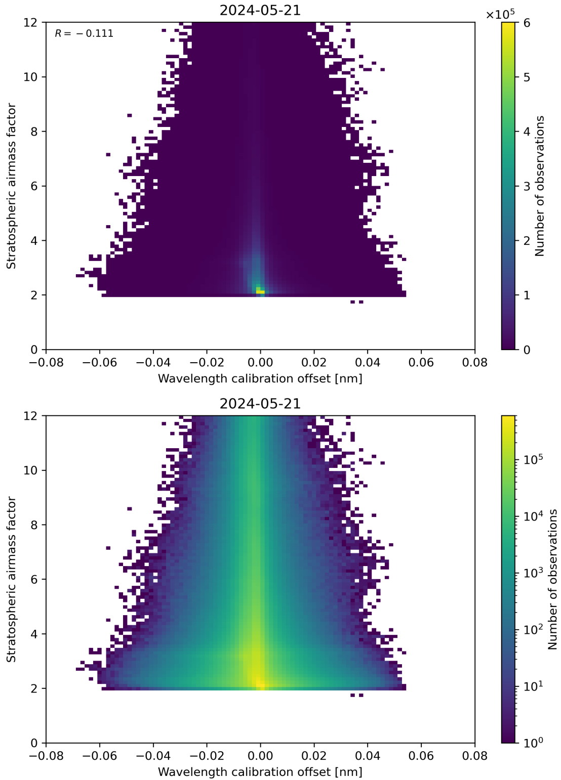
Figure 174: Scatter density plot of “Wavelength calibration offset” against “Stratospheric airmass factor” for 2024-05-20 to 2024-05-22.
