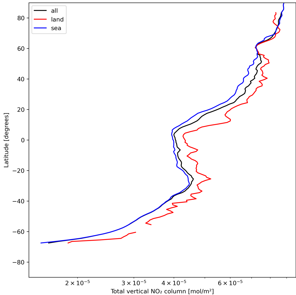
Figure 21: Zonal average of “Total vertical NO 2 column” for 2024-05-20 to 2024-05-22.
