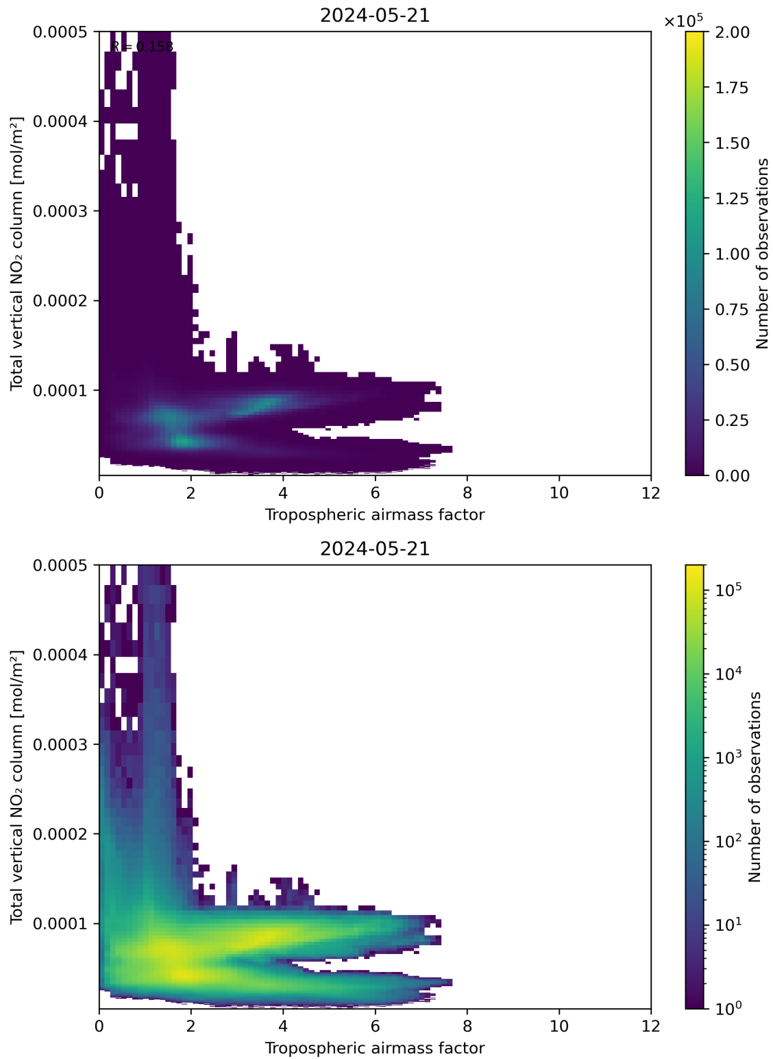
Figure 77: Scatter density plot of “Tropospheric airmass factor” against “Total vertical NO 2 column” for 2024-05-20 to 2024-05-22.
