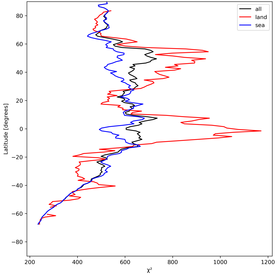
Figure 25: Zonal average of “ \chi^2 ” for 2024-05-20 to 2024-05-22.
