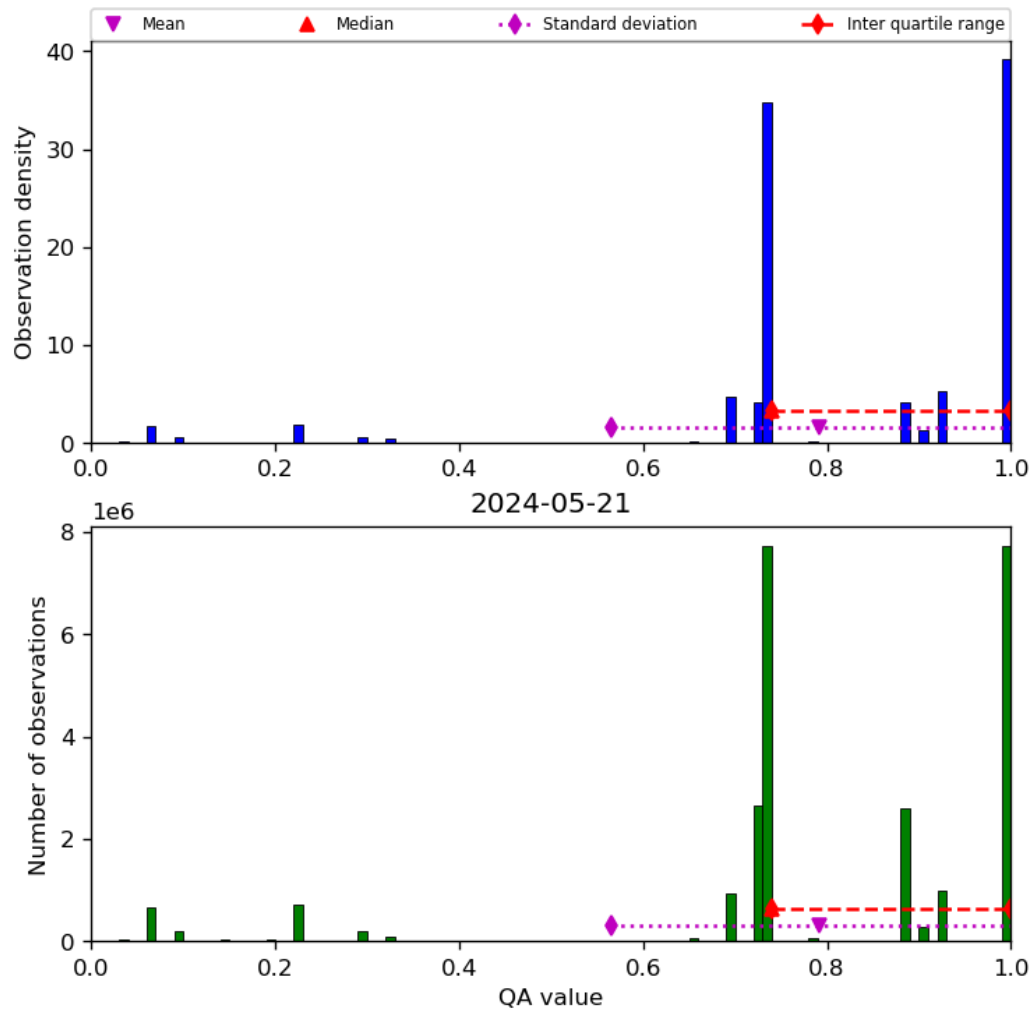
Figure 28: Histogram of “QA value” for 2024-05-20 to 2024-05-22
