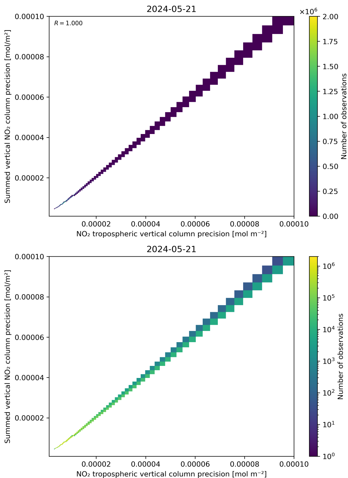
Figure 137: Scatter density plot of “NO 2 tropospheric vertical column precision” against “Summed vertical NO 2 column precision” for 2024-05-20 to 2024-05-22.
