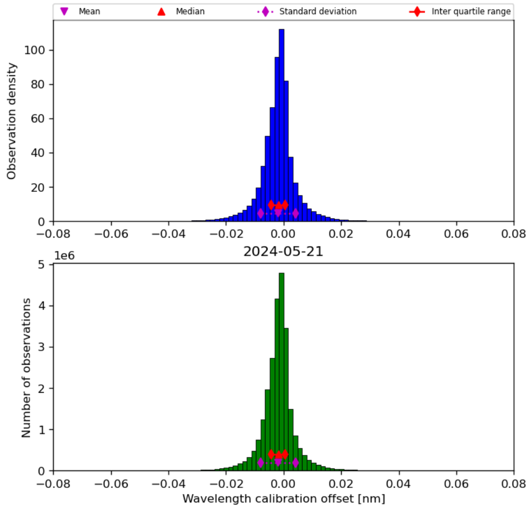
Figure 35: Histogram of “Wavelength calibration offset” for 2024-05-20 to 2024-05-22
