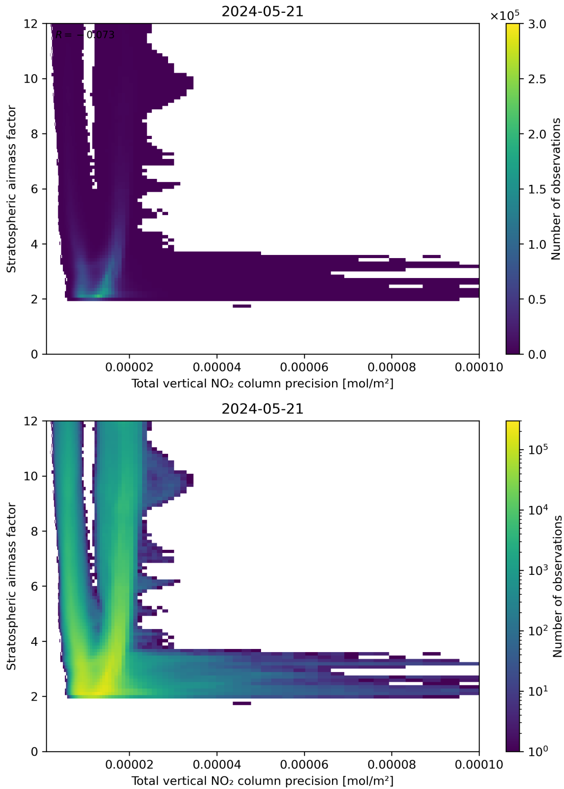
Figure 115: Scatter density plot of “Total vertical NO 2 column precision” against “Stratospheric airmass factor” for 2024-05-20 to 2024-05-22.
