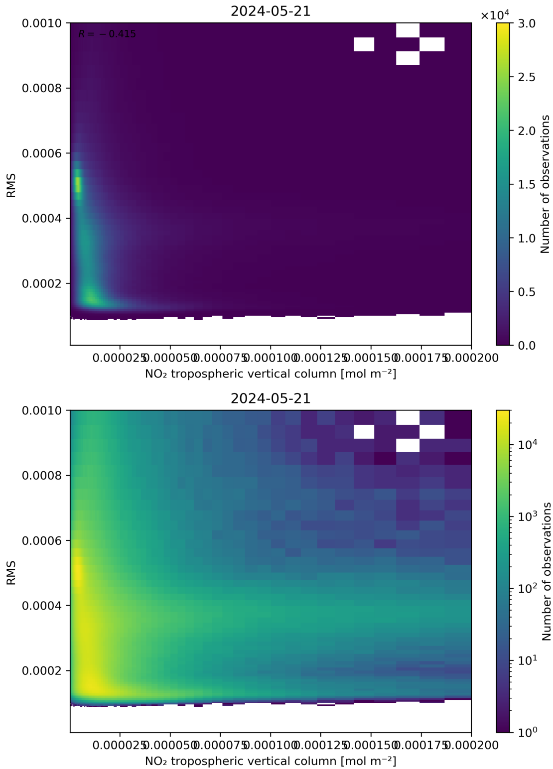
Figure 142: Scatter density plot of “NO 2 tropospheric vertical column” against “RMS” for 2024-05-20 to 2024-05-22.
