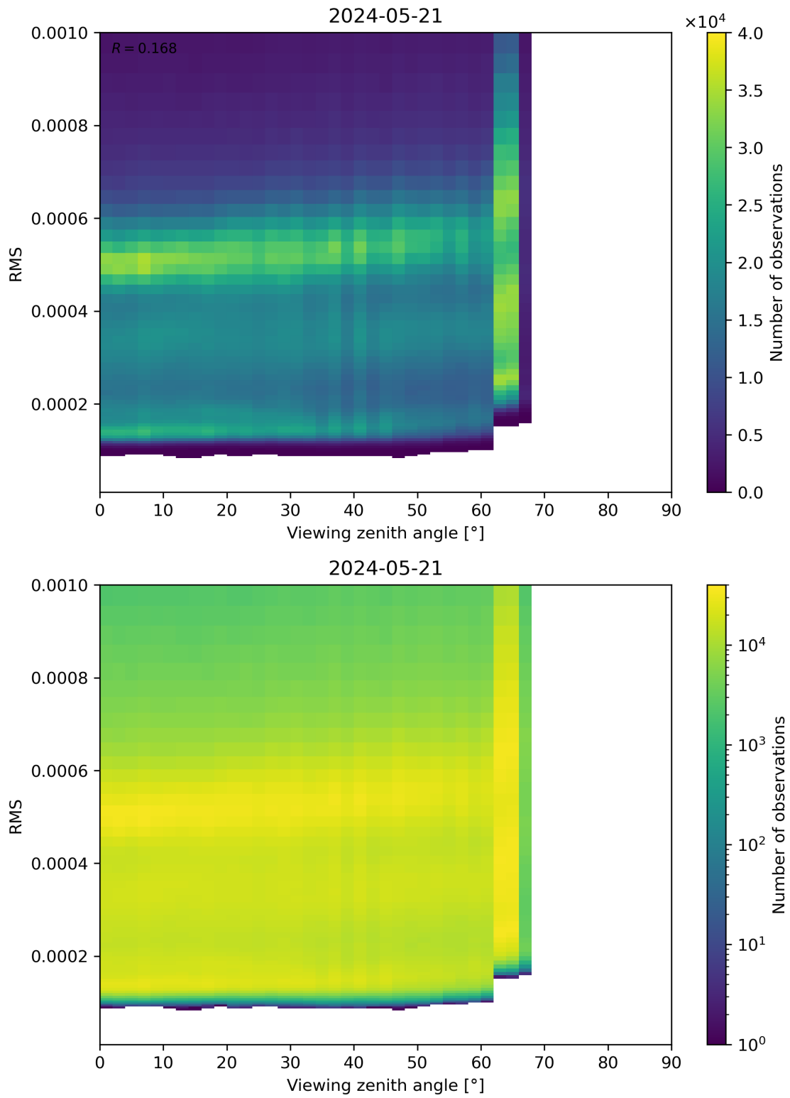
Figure 171: Scatter density plot of “Viewing zenith angle” against “RMS” for 2024-05-20 to 2024-05-22.
