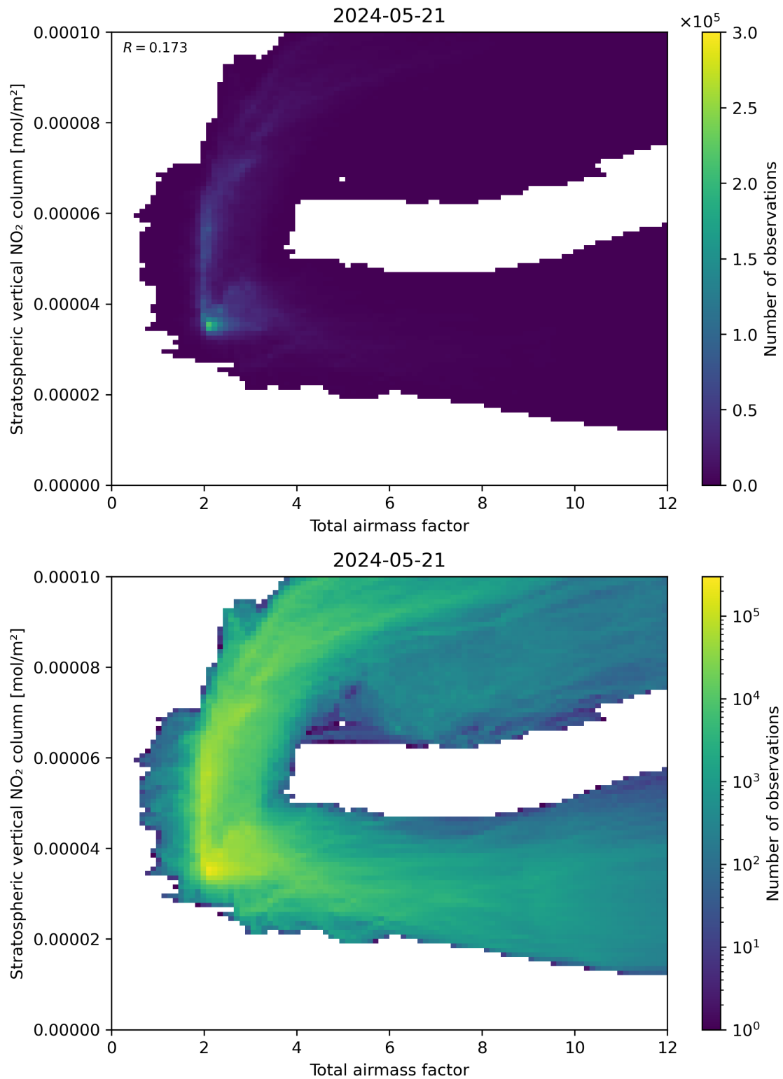
Figure 64: Scatter density plot of “Total airmass factor” against “Stratospheric vertical \text{NO}_2 column” for 2024-05-20 to 2024-05-22.
