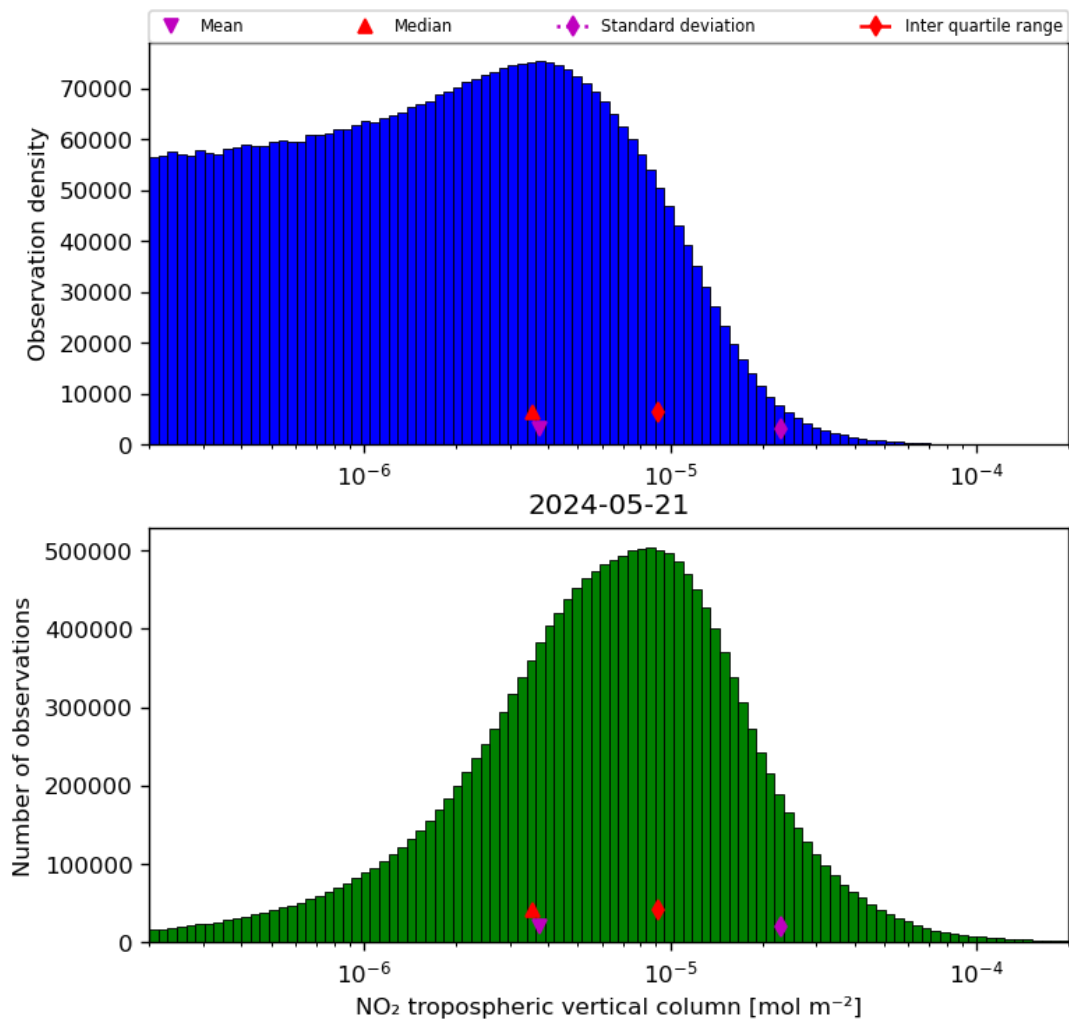
Figure 29: Histogram of “ \text{NO}_2 tropospheric vertical column” for 2024-05-20 to 2024-05-22
