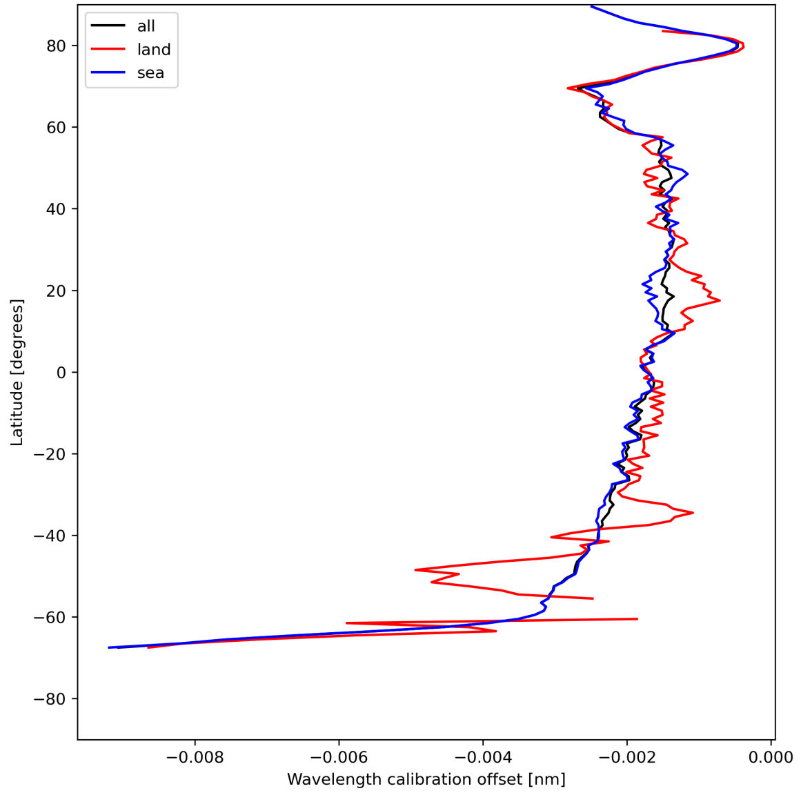
Figure 18: Zonal average of “Wavelength calibration offset” for 2024-05-20 to 2024-05-22.
