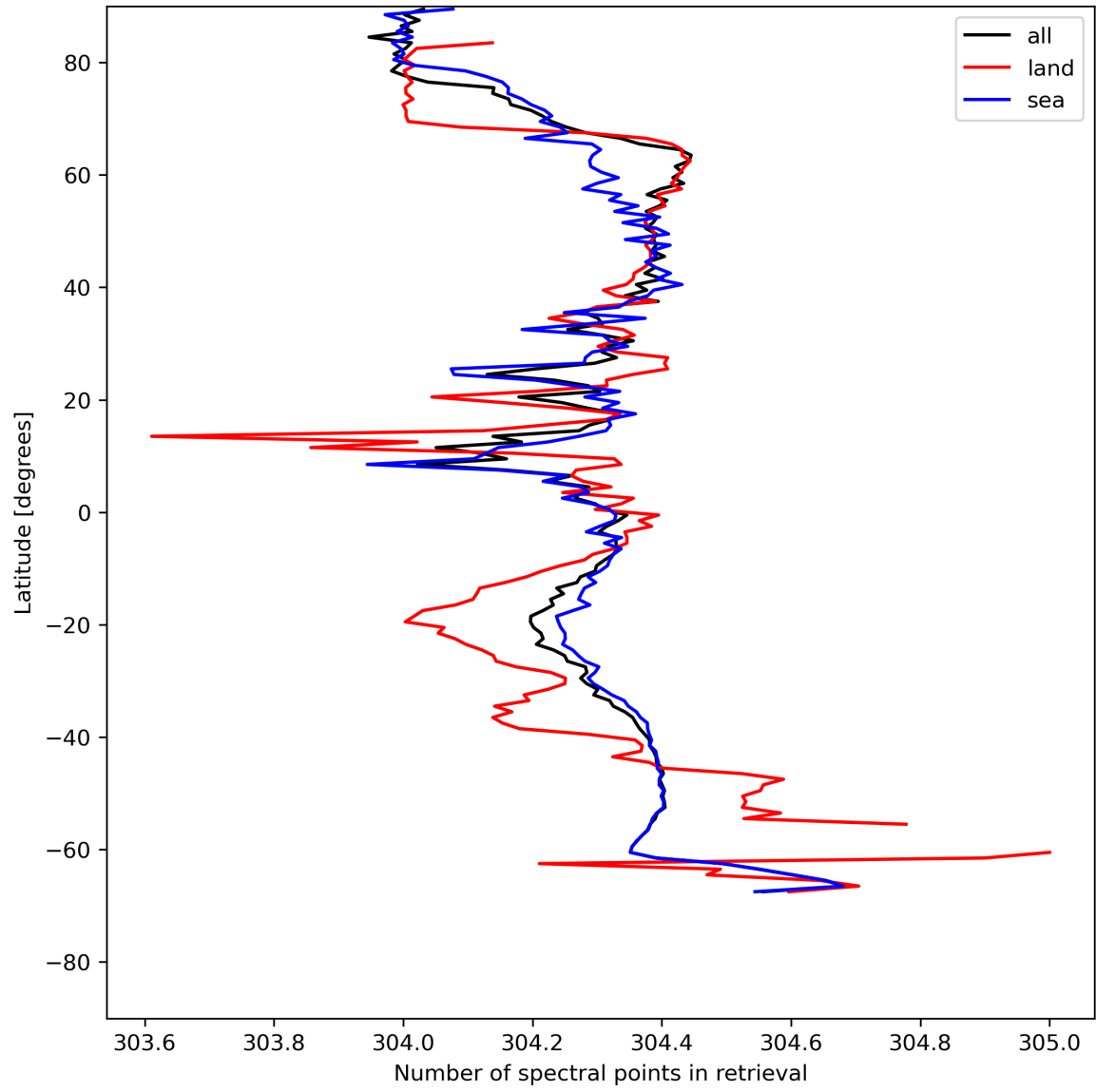
Figure 16: Zonal average of “Number of spectral points in retrieval” for 2024-05-20 to 2024-05-22.
