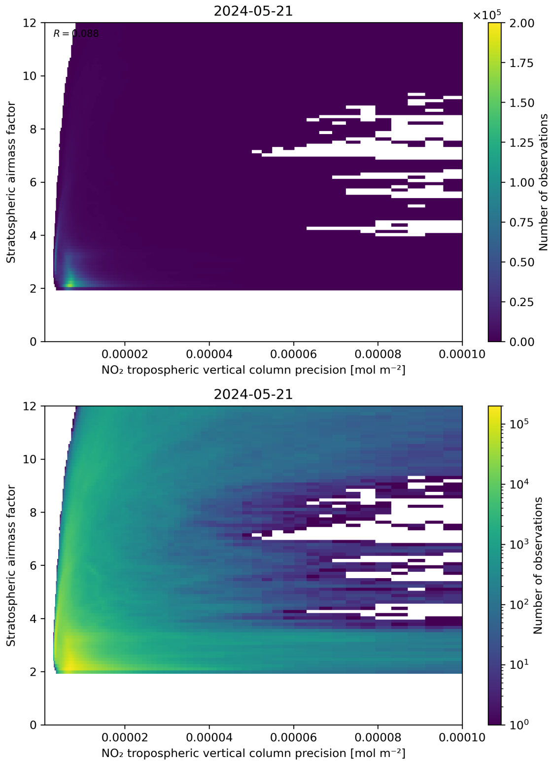
Figure 131: Scatter density plot of “NO 2 tropospheric vertical column precision” against “Stratospheric airmass factor” for 2024-05-20 to 2024-05-22.
