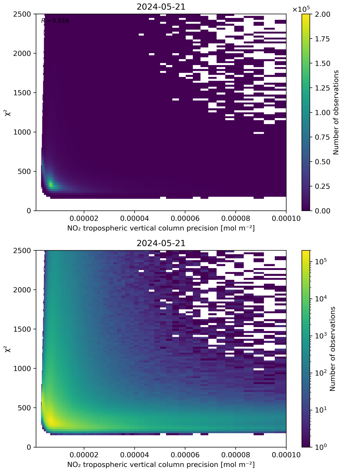
Figure 134: Scatter density plot of “NO 2 tropospheric vertical column precision” against “ \chi^2 ” for 2024-05-20 to 2024-05-22.
