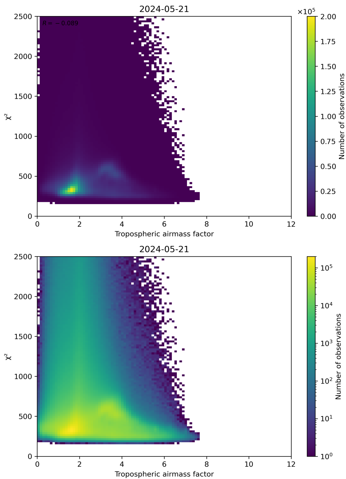
Figure 73: Scatter density plot of “Tropospheric airmass factor” against “ \chi^2 ” for 2024-05-20 to 2024-05-22.
