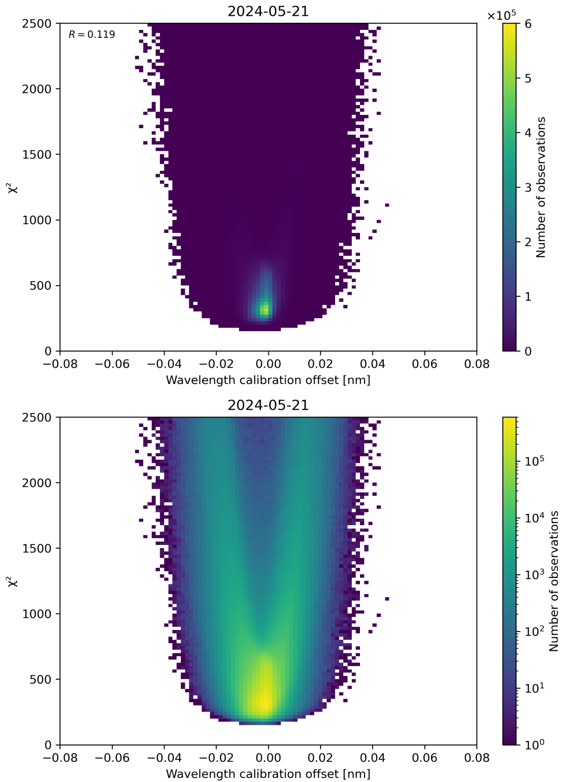
Figure 175: Scatter density plot of “Wavelength calibration offset” against “ \chi^2 ” for 2024-05-20 to 2024-05-22.
