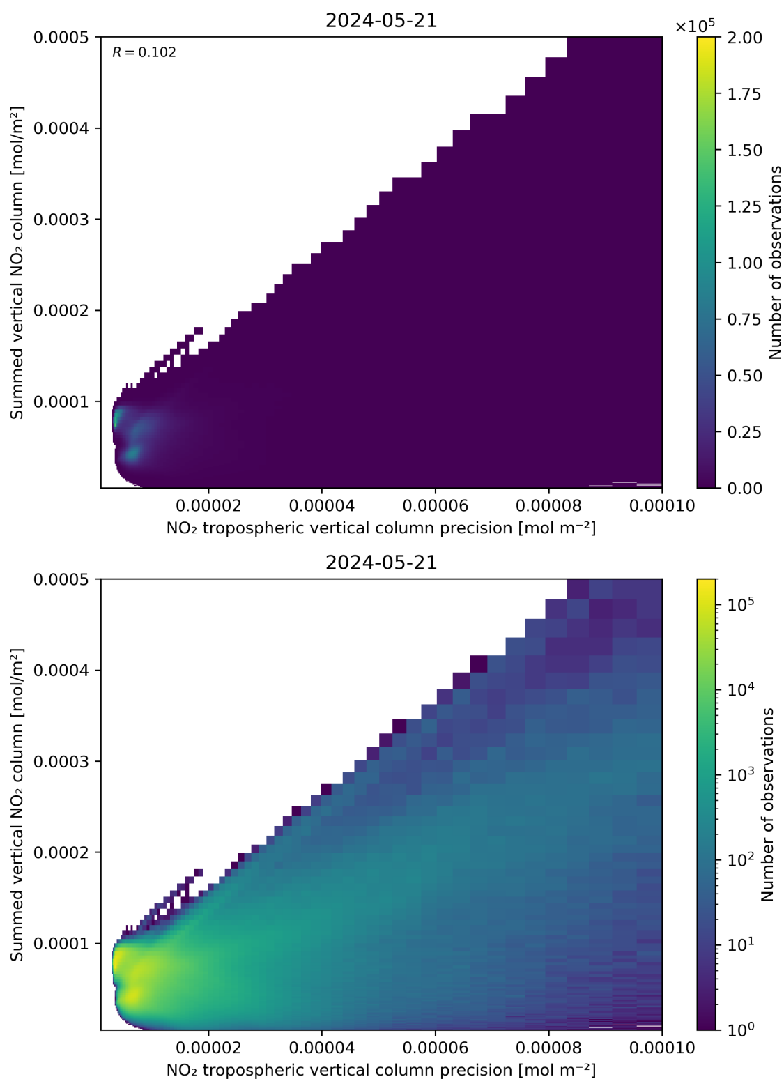
Figure 136: Scatter density plot of “NO 2 tropospheric vertical column precision” against “Summed vertical NO 2 column” for 2024-05-20 to 2024-05-22.
