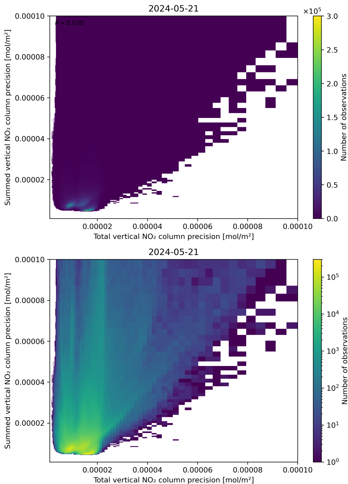
Figure 118: Scatter density plot of “Total vertical NO 2 column precision” against “Summed vertical NO 2 column precision” for 2024-05-20 to 2024-05-22.
