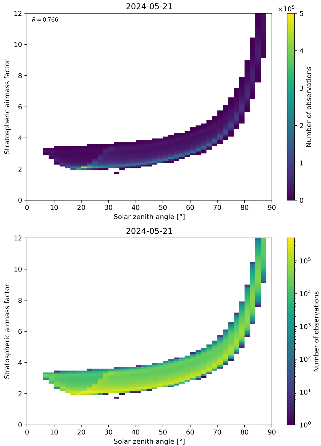
Figure 145: Scatter density plot of “Solar zenith angle” against “Stratospheric airmass factor” for 2024-05-20 to 2024-05-22.
