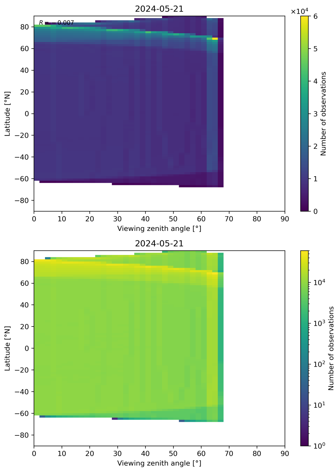
Figure 163: Scatter density plot of “Viewing zenith angle” against “Latitude” for 2024-05-20 to 2024-05-22.
