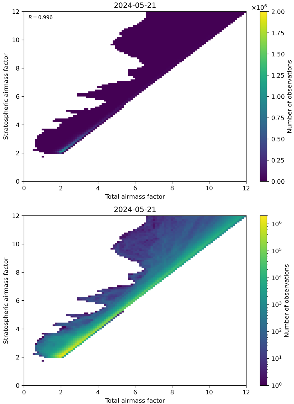
Figure 62: Scatter density plot of “Total airmass factor” against “Stratospheric airmass factor” for 2024-05-20 to 2024-05-22.
