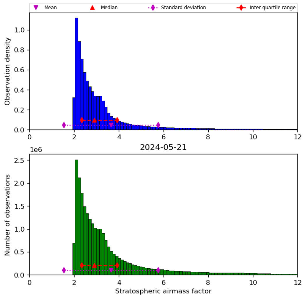
Figure 44: Histogram of “Stratospheric airmass factor” for 2024-05-20 to 2024-05-22
