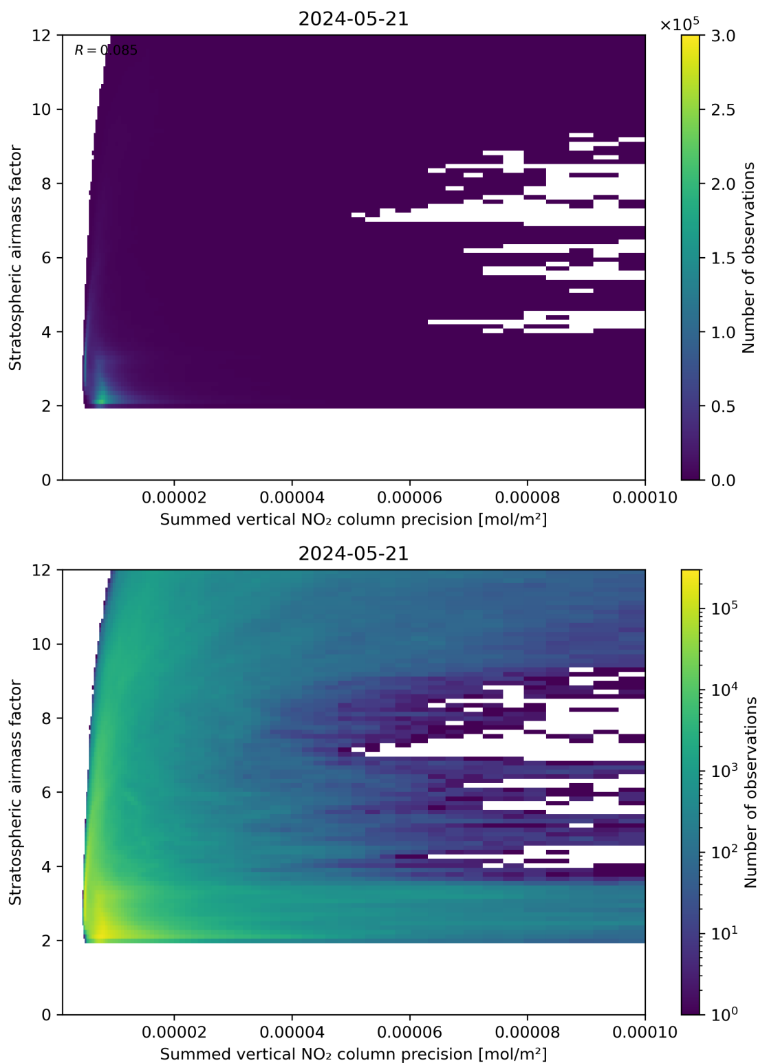
Figure 106: Scatter density plot of “Summed vertical NO 2 column precision” against “Stratospheric airmass factor” for 2024-05-20 to 2024-05-22.
