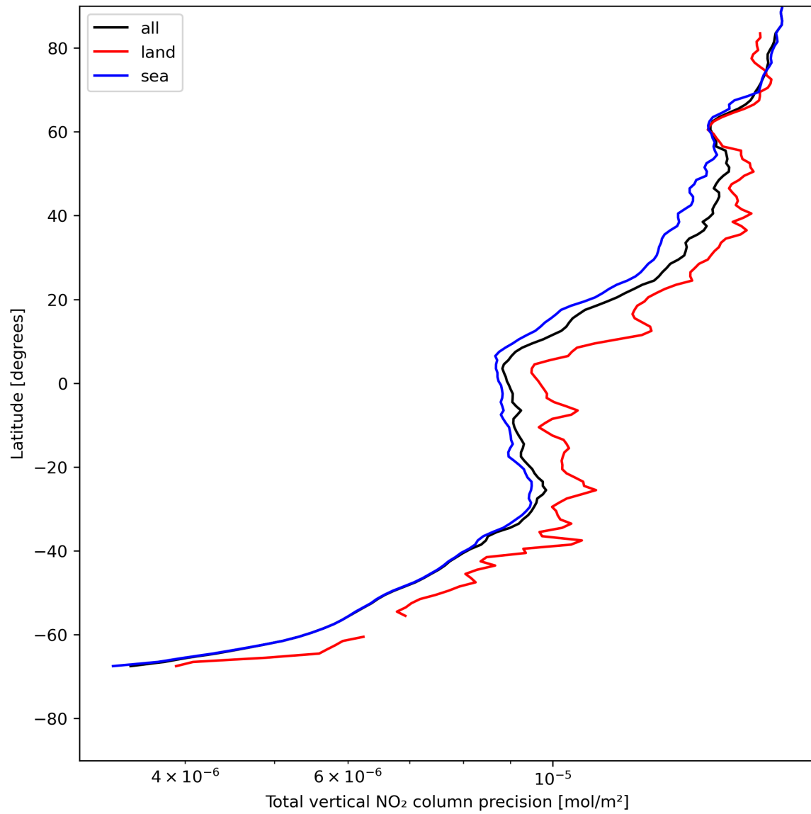
Figure 22: Zonal average of “Total vertical NO 2 column precision” for 2024-05-20 to 2024-05-22.
