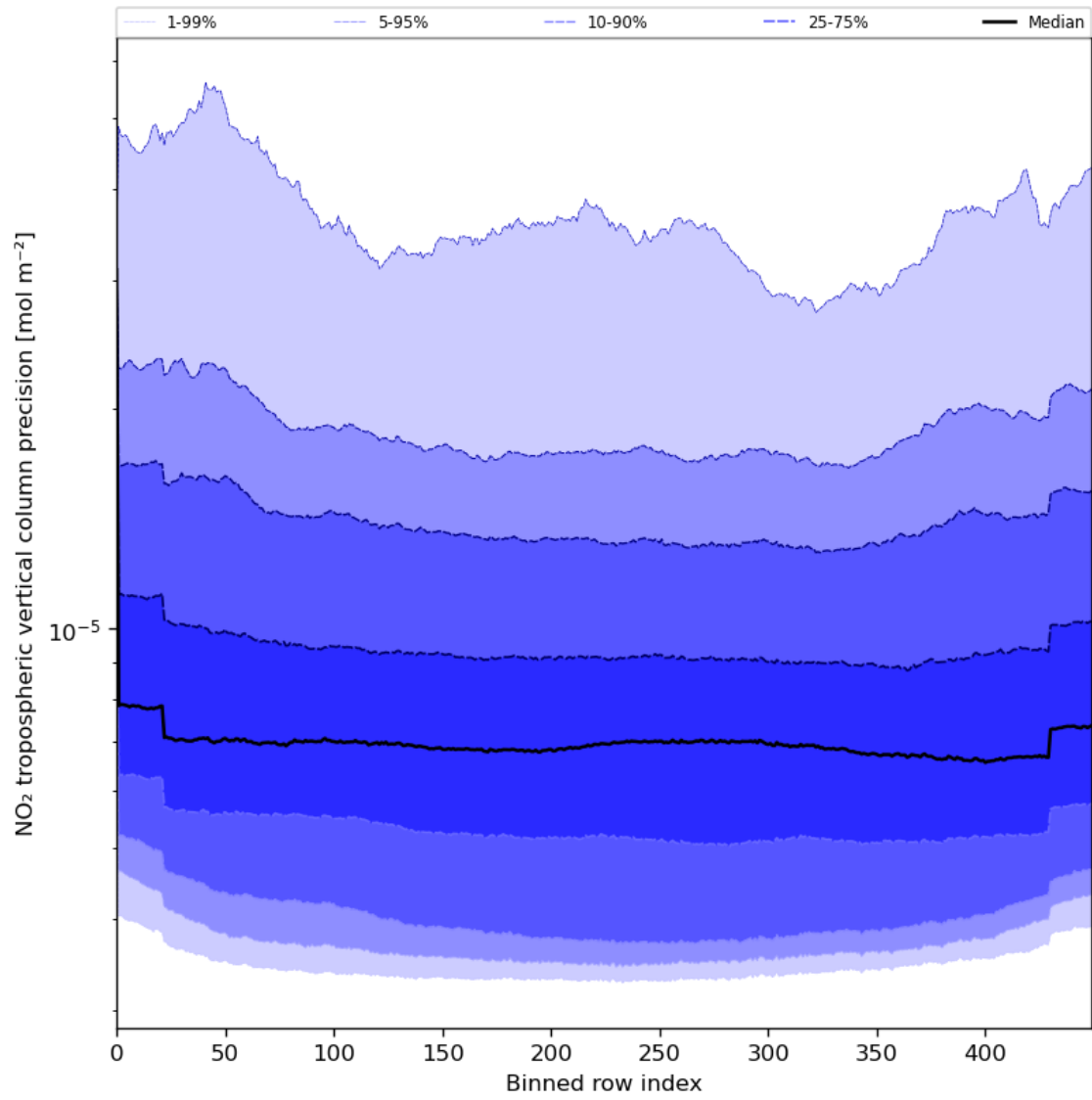
Figure 47: Along track statistics of “NO 2 tropospheric vertical column precision” for 2024-05-20 to 2024-05-22
