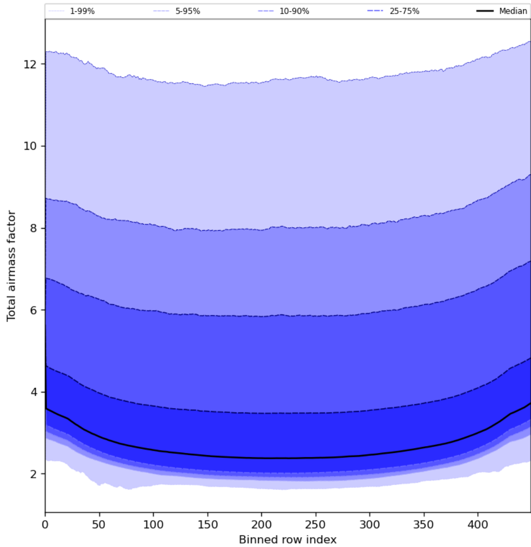
Figure 49: Along track statistics of “Total airmass factor” for 2024-05-20 to 2024-05-22
