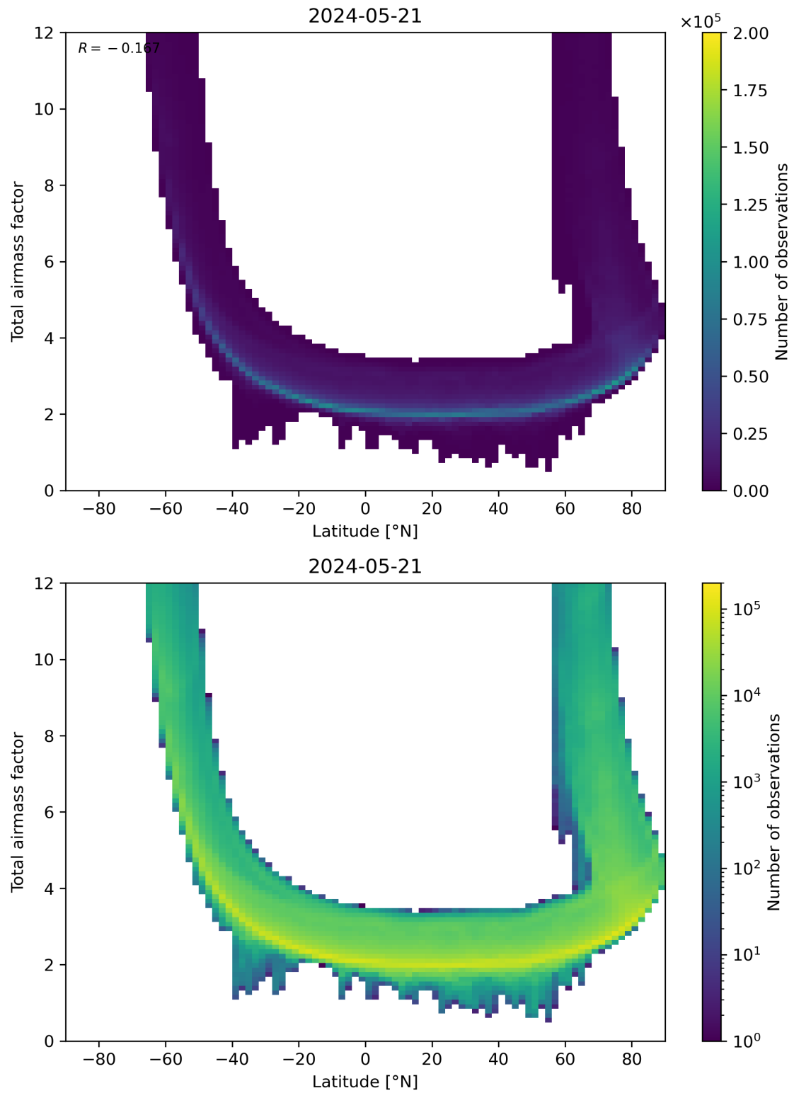
Figure 84: Scatter density plot of “Latitude” against “Total airmass factor” for 2024-05-20 to 2024-05-22.
