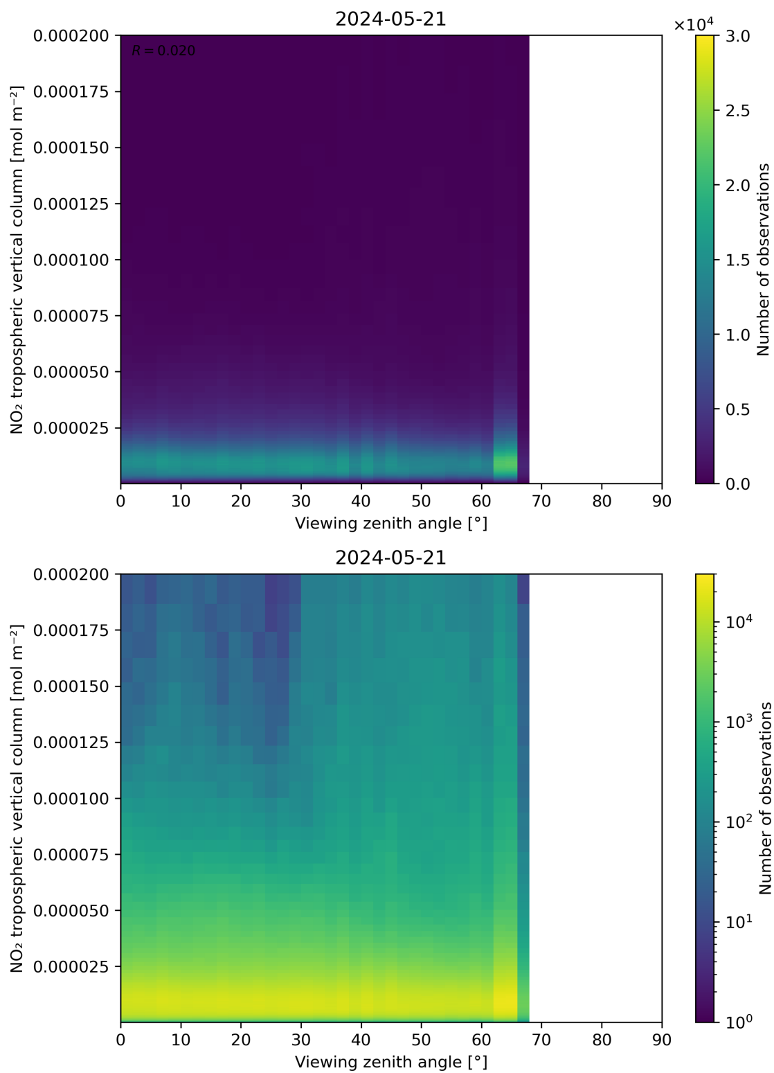
Figure 169: Scatter density plot of “Viewing zenith angle” against “NO 2 tropospheric vertical column” for 2024-05-20 to 2024-05-22.
