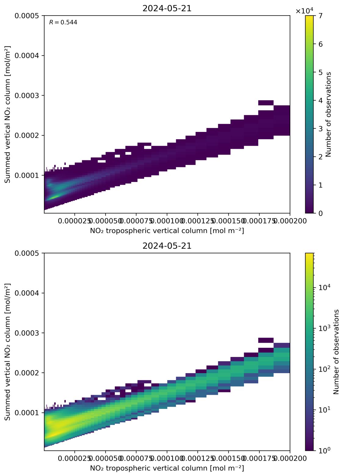
Figure 126: Scatter density plot of “NO 2 tropospheric vertical column” against “Summed vertical NO 2 column” for 2024-05-20 to 2024-05-22.
