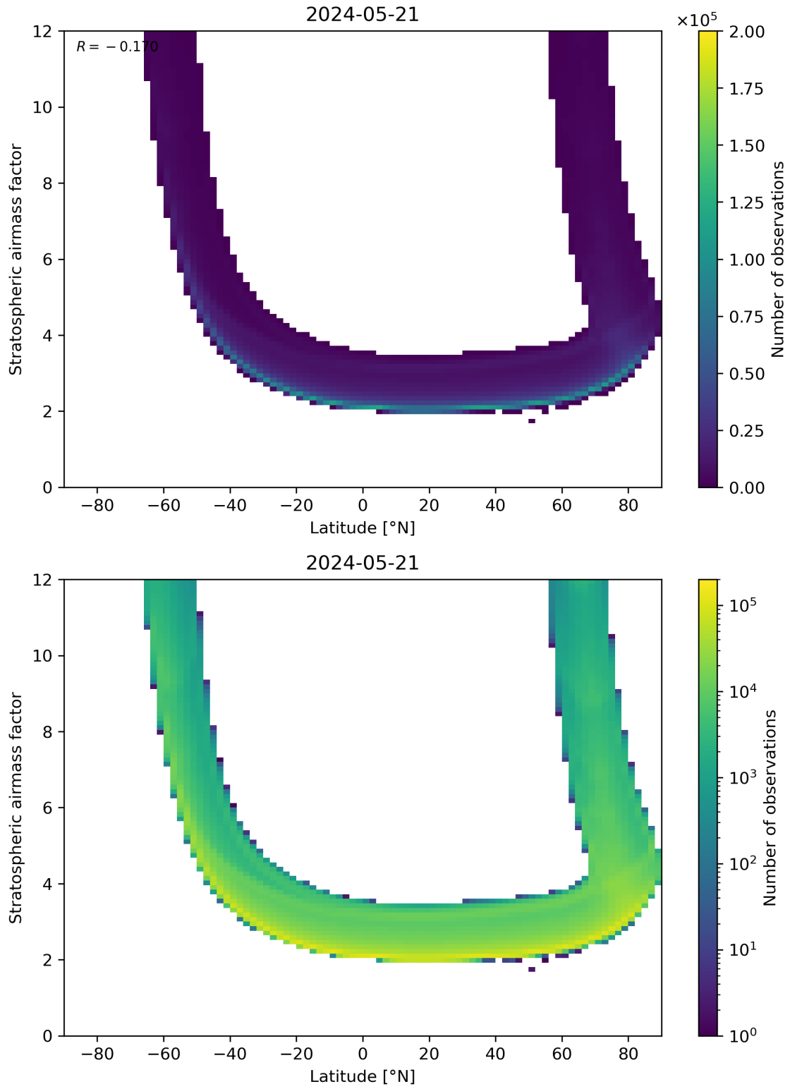
Figure 83: Scatter density plot of “Latitude” against “Stratospheric air mass factor” for 2024-05-20 to 2024-05-22.
