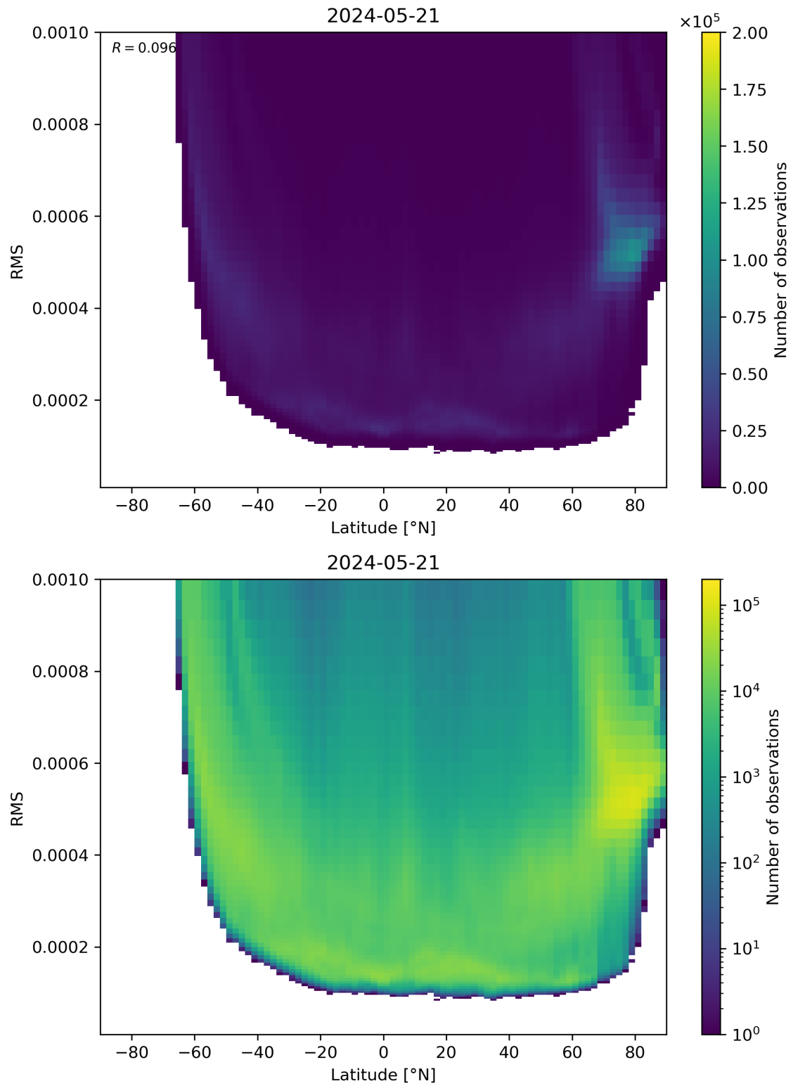
Figure 94: Scatter density plot of “Latitude” against “RMS” for 2024-05-20 to 2024-05-22.
