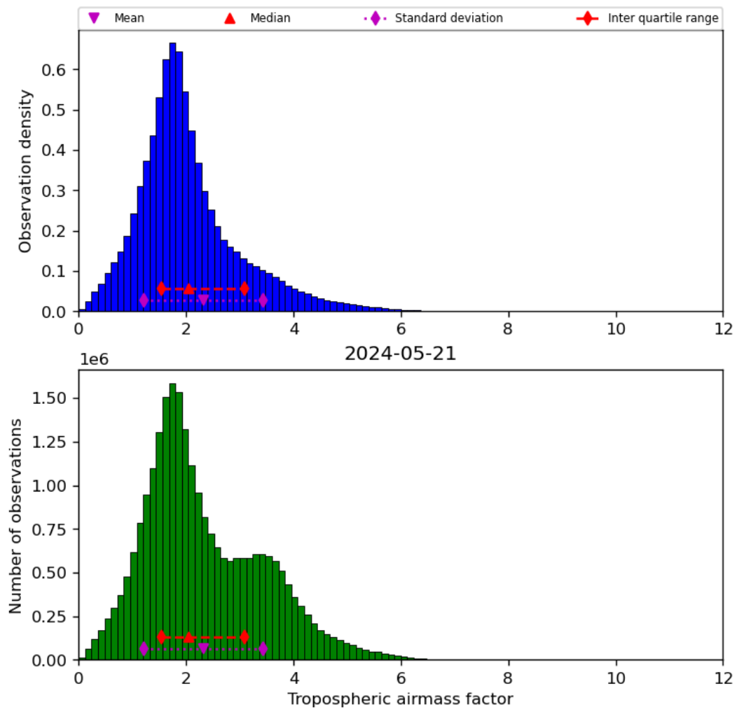
Figure 31: Histogram of “Tropospheric airmass factor” for 2024-05-20 to 2024-05-22
