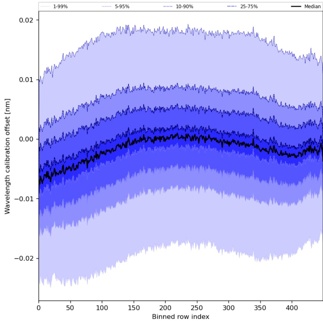
Figure 52: Along track statistics of “Wavelength calibration offset” for 2024-05-20 to 2024-05-22
