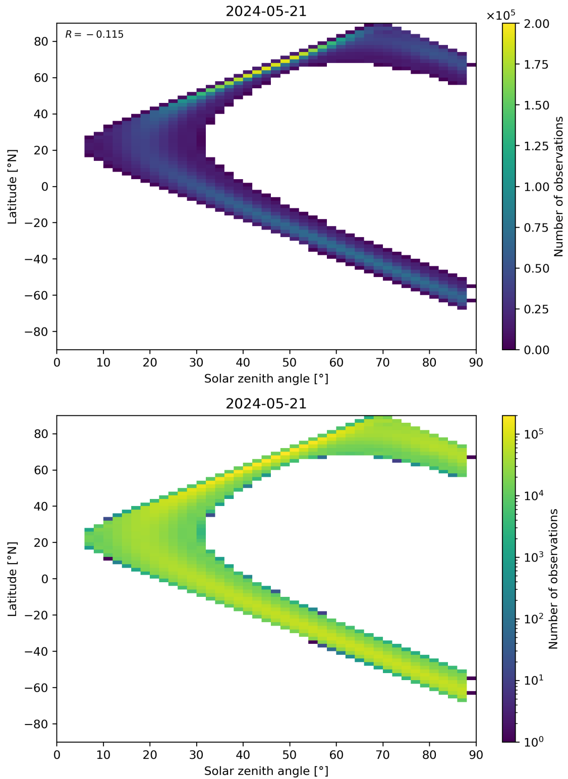
Figure 149: Scatter density plot of “Solar zenith angle” against “Latitude” for 2024-05-20 to 2024-05-22.
