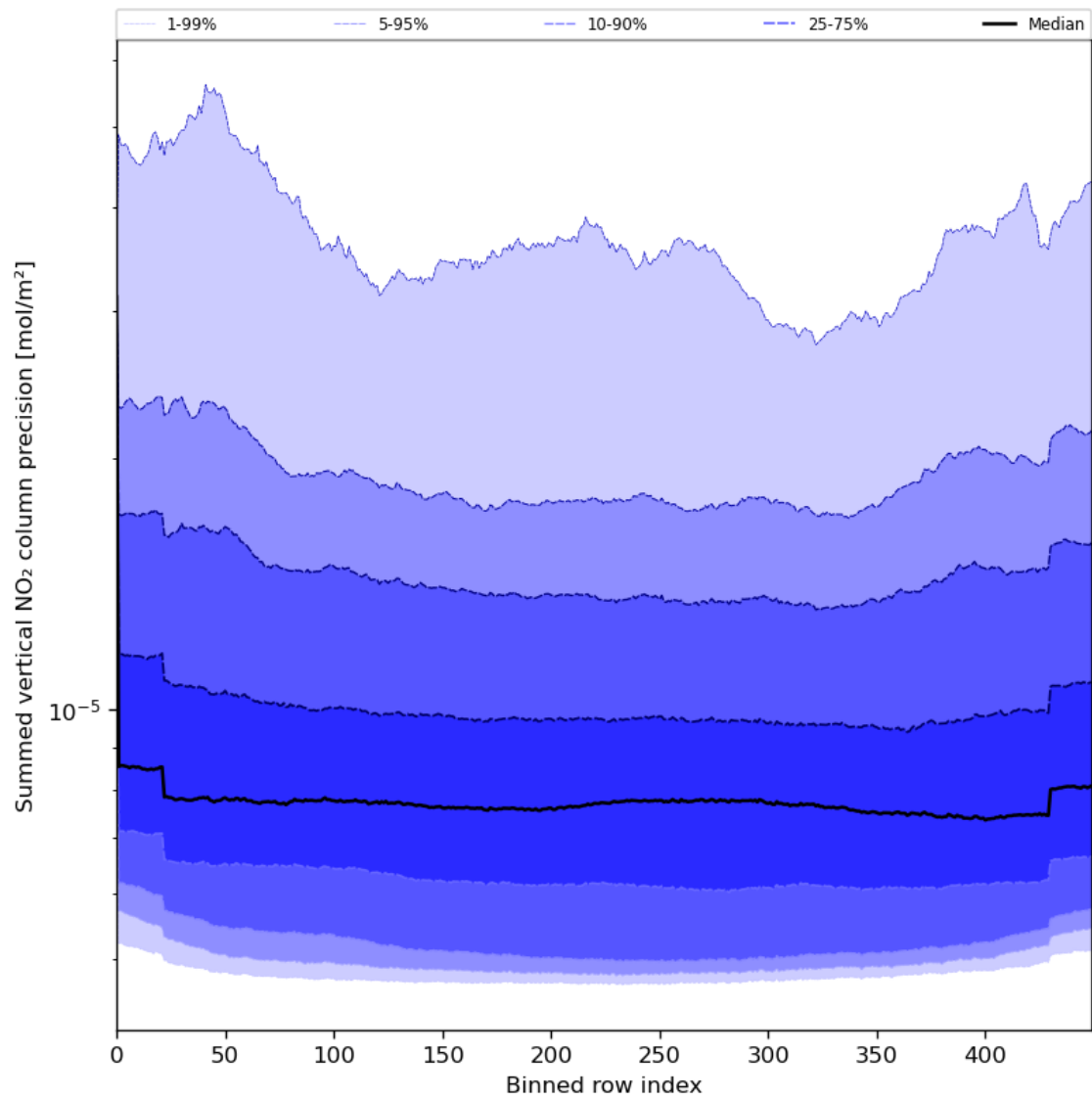
Figure 58: Along track statistics of “Summed vertical NO 2 column precision” for 2024-05-20 to 2024-05-22
