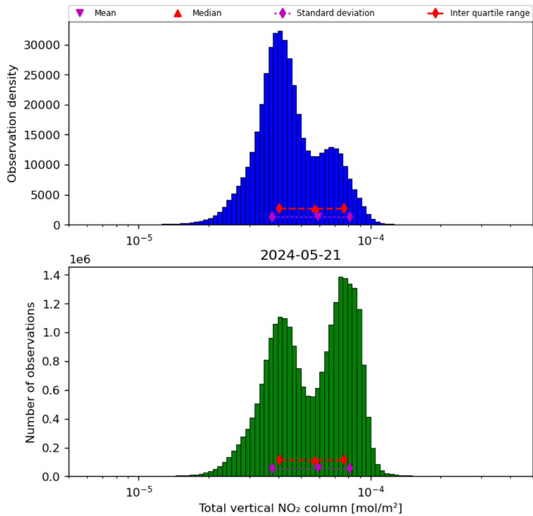
Figure 38: Histogram of “Total vertical NO 2 column” for 2024-05-20 to 2024-05-22
