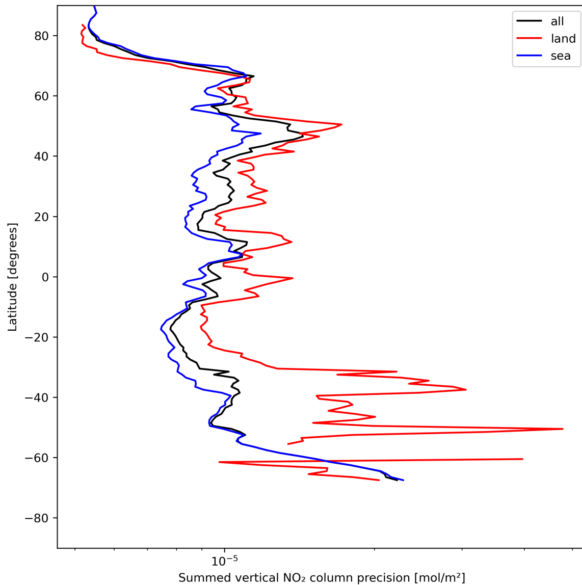
Figure 24: Zonal average of “Summed vertical NO 2 column precision” for 2024-05-20 to 2024-05-22.
