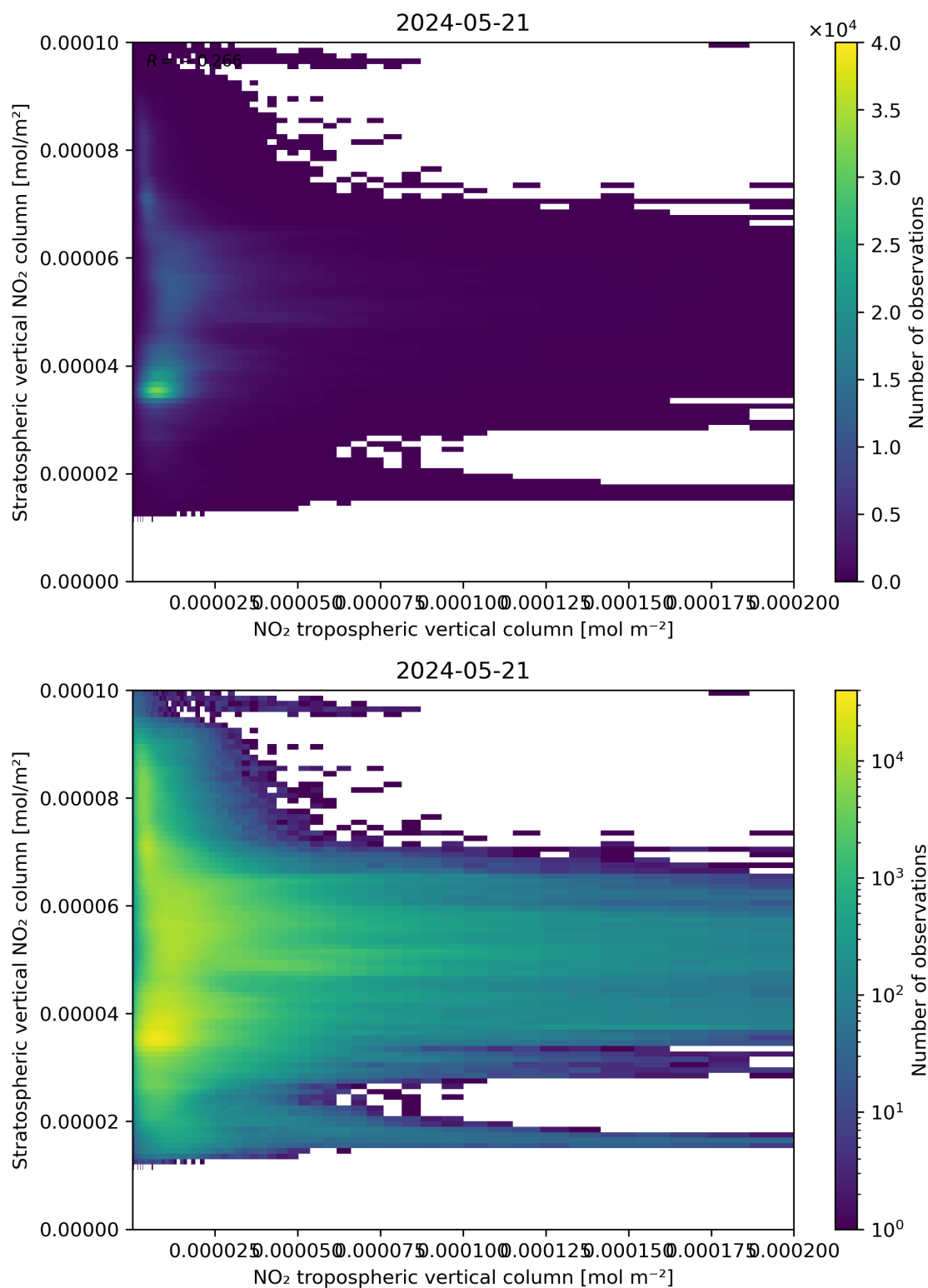
Figure 125: Scatter density plot of “NO 2 tropospheric vertical column” against “Stratospheric vertical NO 2 column” for 2024-05-20 to 2024-05-22.
