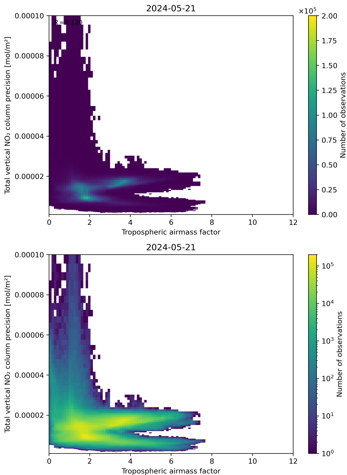
Figure 78: Scatter density plot of “Tropospheric air mass factor” against “Total vertical NO 2 column precision” for 2024-05-20 to 2024-05-22.
