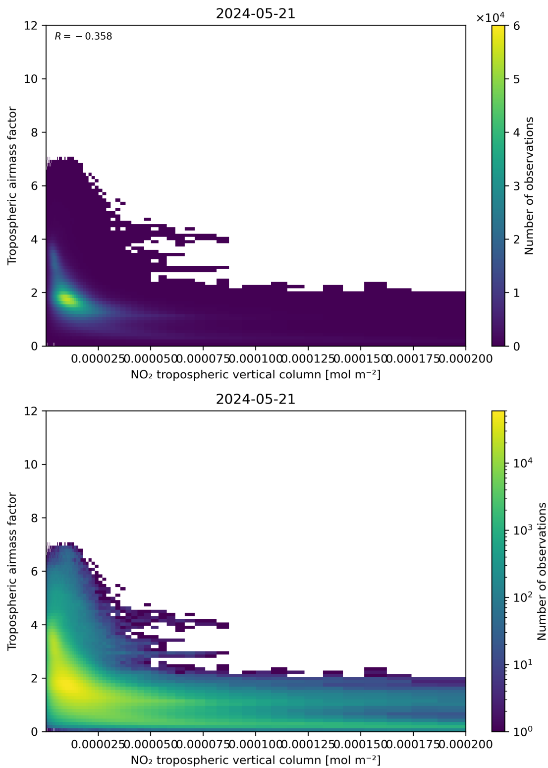
Figure 123: Scatter density plot of “NO 2 tropospheric vertical column” against “Tropospheric airmass factor” for 2024-05-20 to 2024-05-22.
