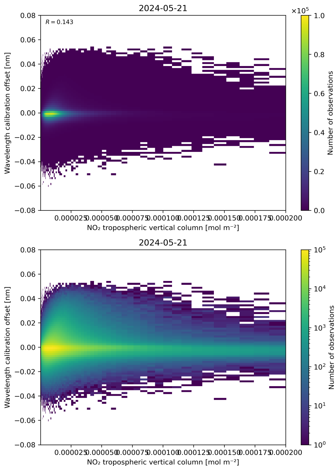
Figure 143: Scatter density plot of “NO 2 tropospheric vertical column” against “Wavelength calibration offset” for 2024-05-20 to 2024-05-22.
