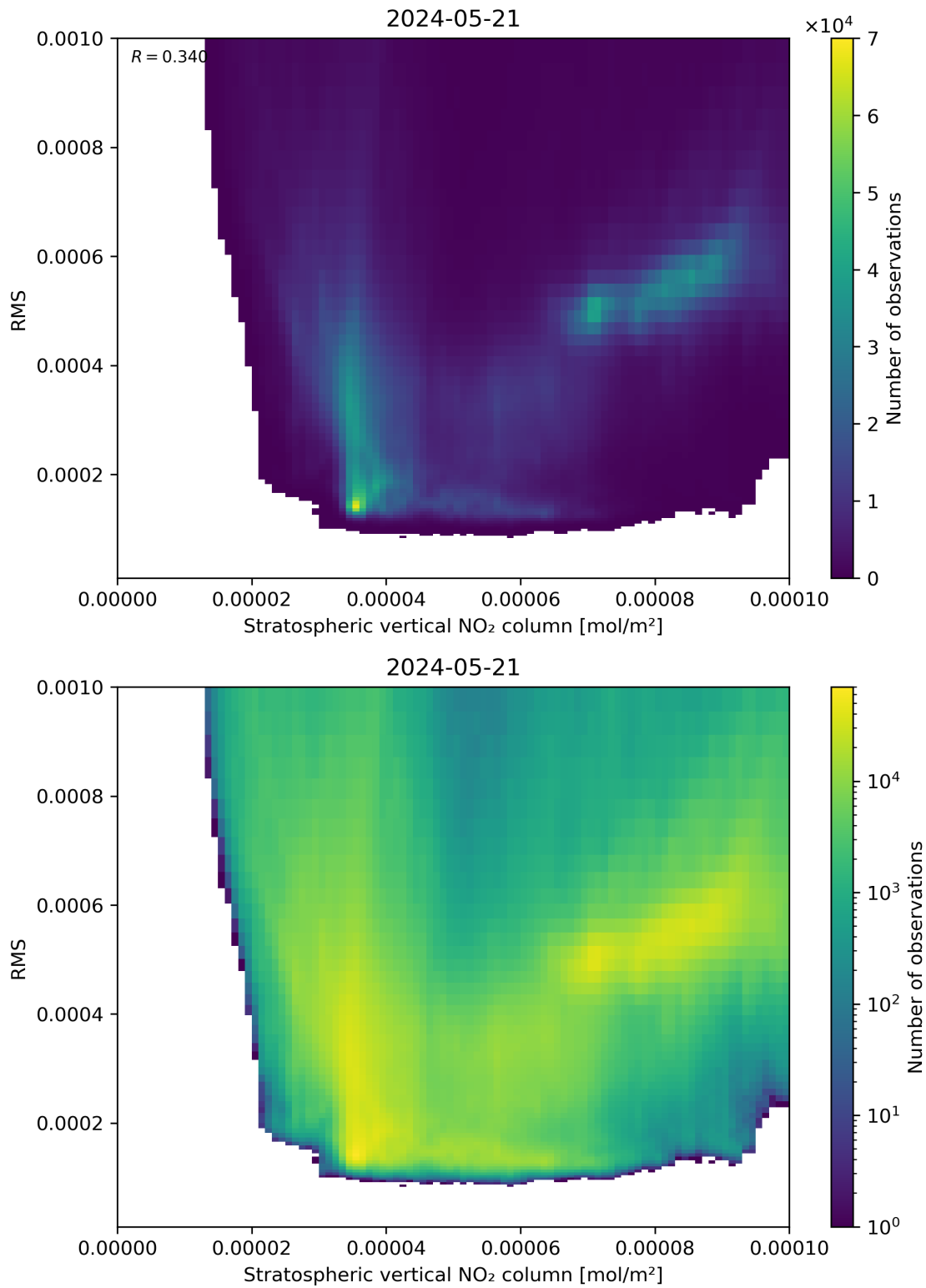
Figure 102: Scatter density plot of “Stratospheric vertical NO 2 column” against “RMS” for 2024-05-20 to 2024-05-22.
