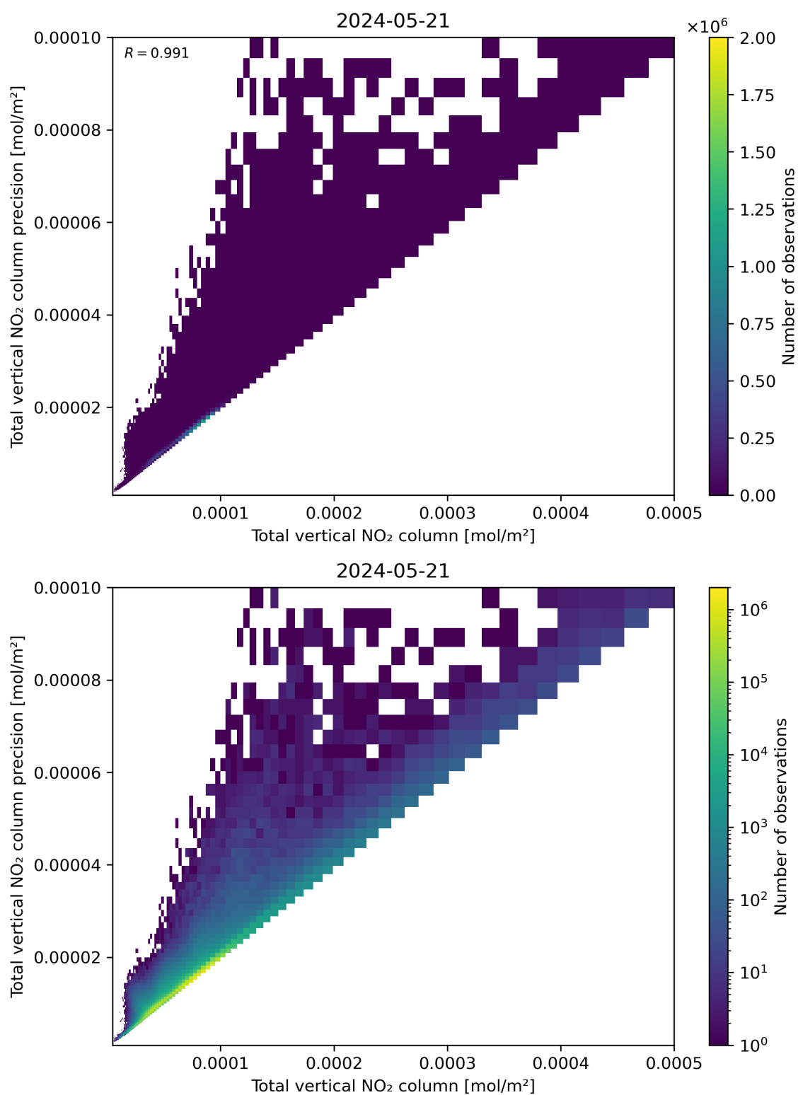
Figure 114: Scatter density plot of “Total vertical NO 2 column” against “Total vertical NO 2 column precision” for 2024-05-20 to 2024-05-22.
