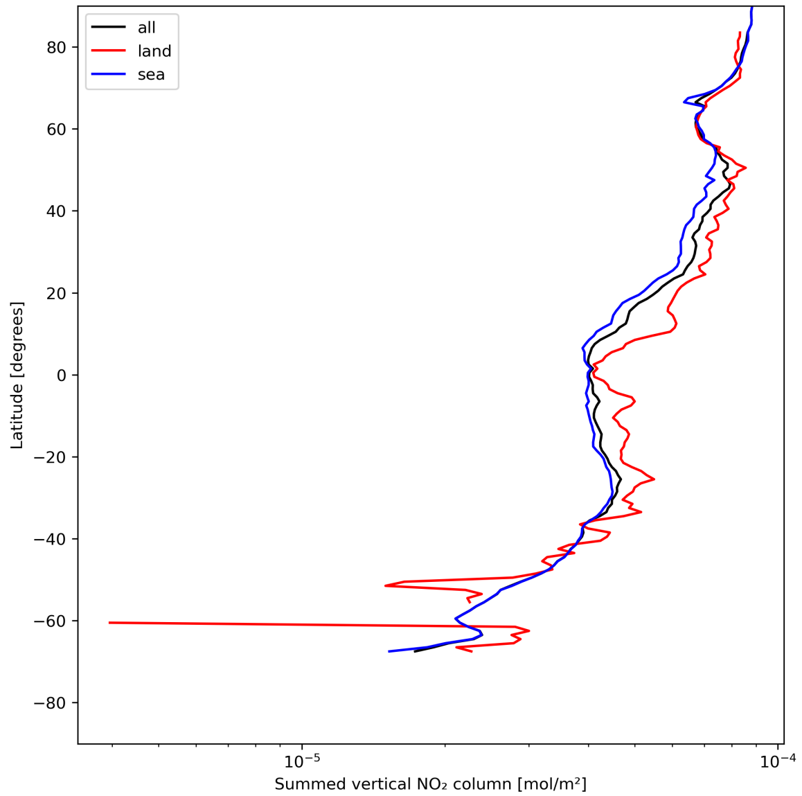
Figure 23: Zonal average of “Summed vertical NO 2 column” for 2024-05-20 to 2024-05-22.
