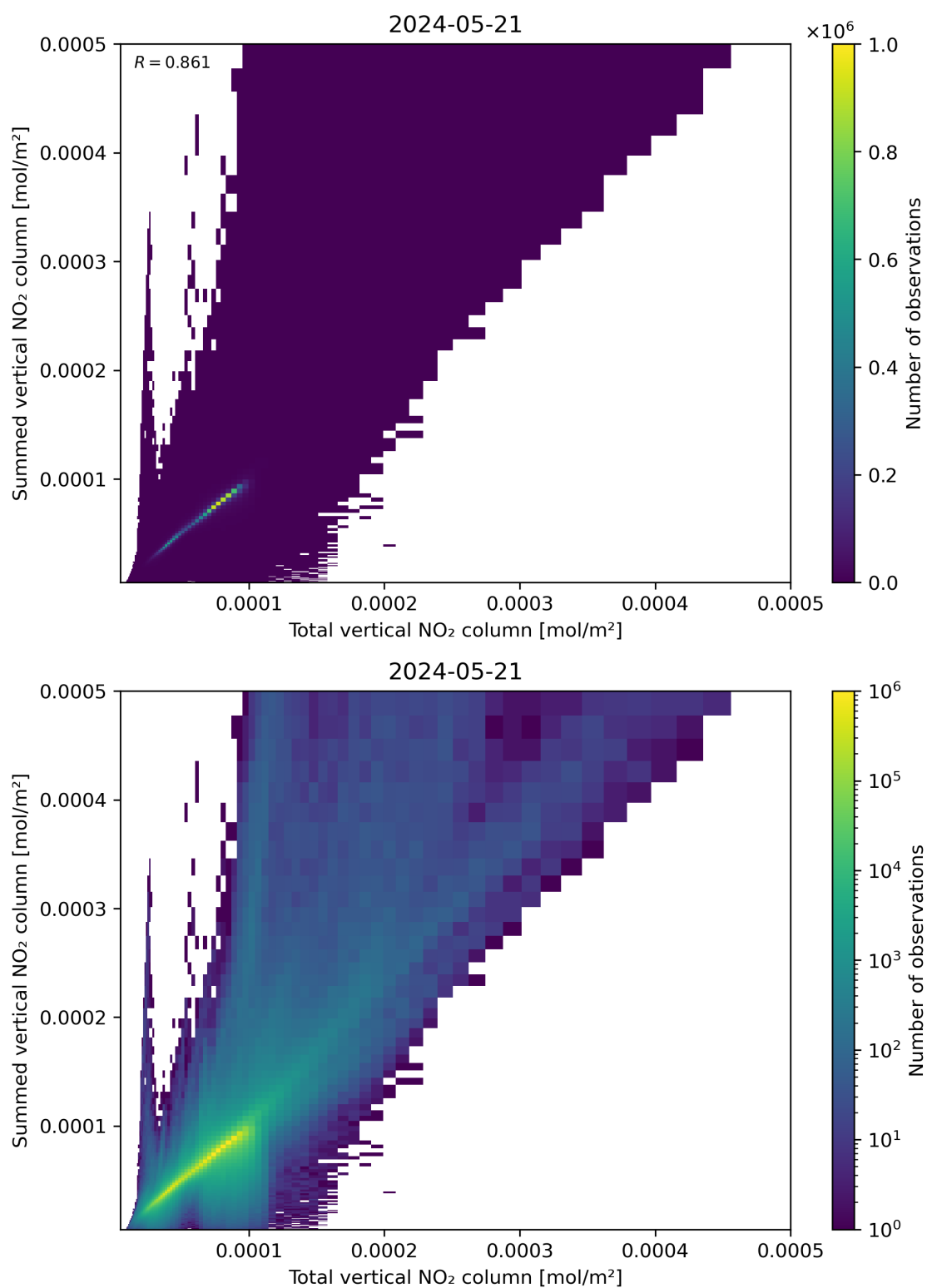
Figure 112: Scatter density plot of “Total vertical NO 2 column” against “Summed vertical NO 2 column” for 2024-05-20 to 2024-05-22.
