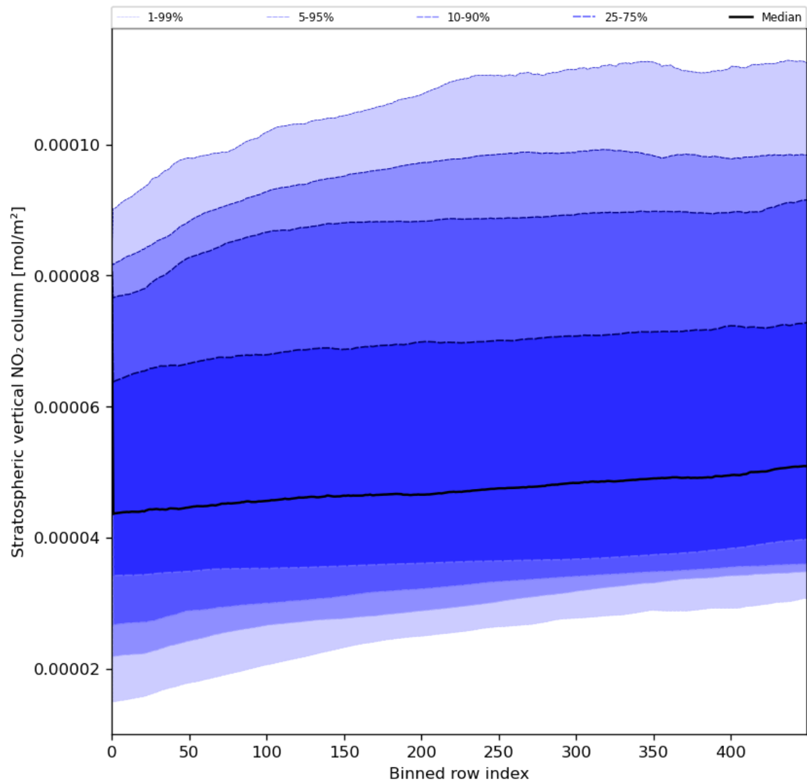
Figure 53: Along track statistics of “Stratospheric vertical NO 2 column” for 2024-05-20 to 2024-05-22
