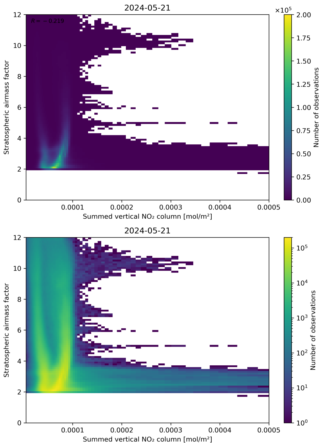
Figure 103: Scatter density plot of “Summed vertical NO 2 column” against “Stratospheric airmass factor” for 2024-05-20 to 2024-05-22.
