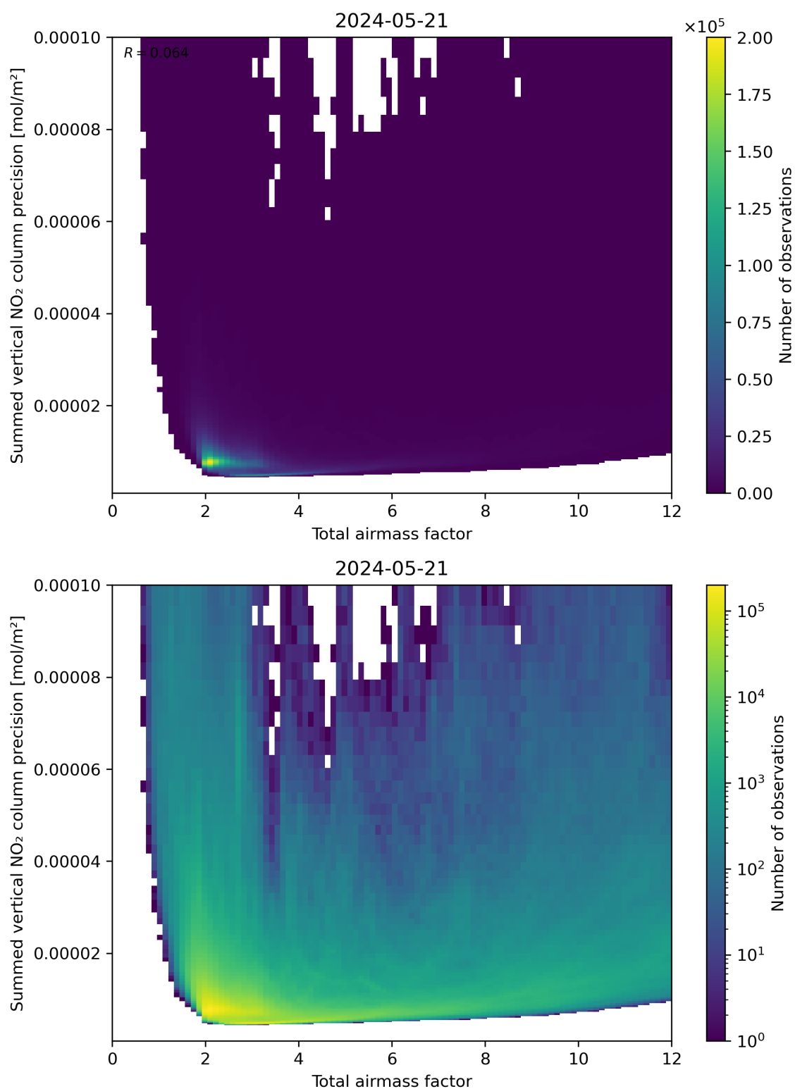
Figure 66: Scatter density plot of “Total airmass factor” against “Summed vertical NO 2 column precision” for 2024-05-20 to 2024-05-22.
