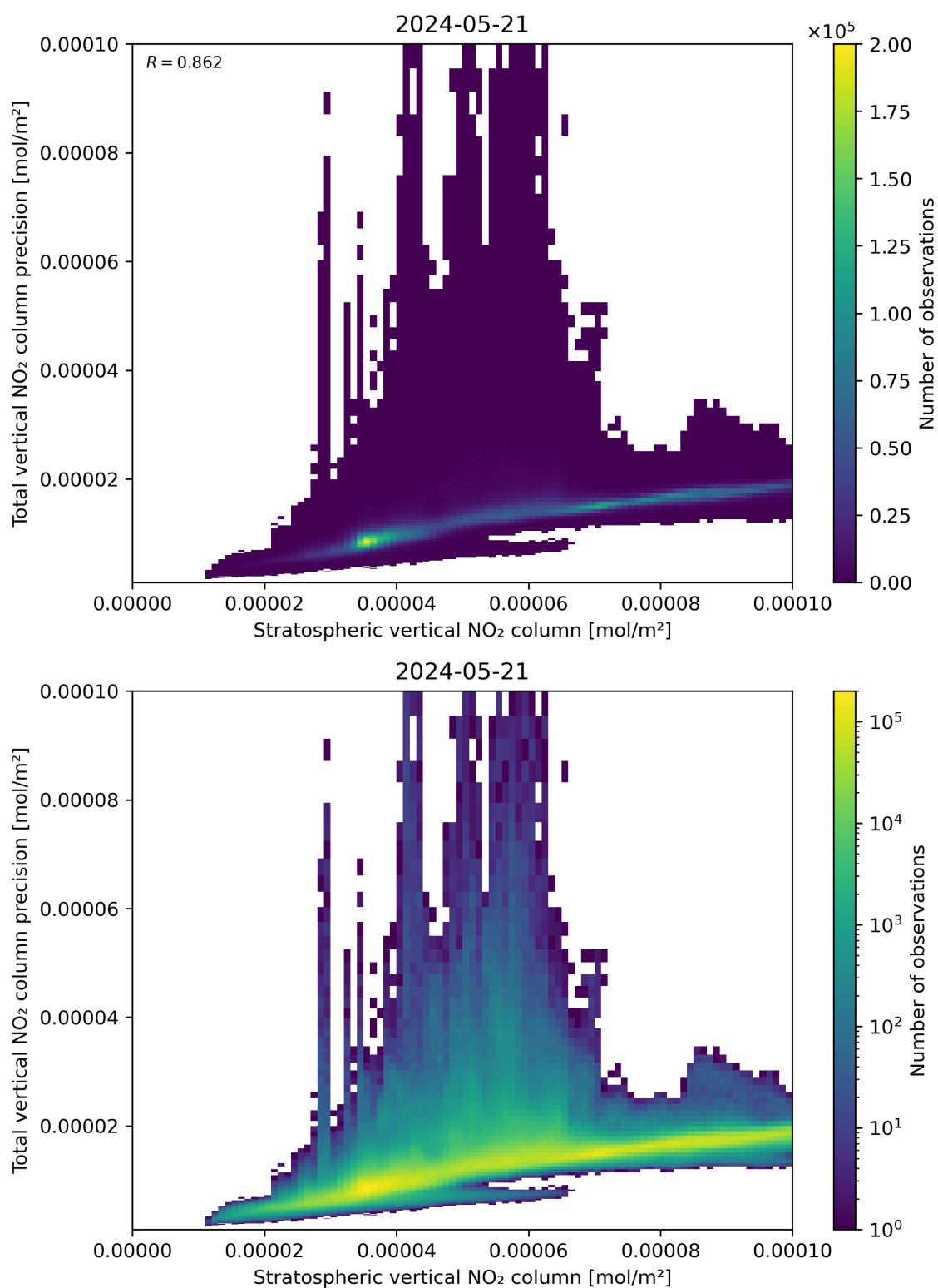
Figure 101: Scatter density plot of “Stratospheric vertical NO 2 column” against “Total vertical NO 2 column precision” for 2024-05-20 to 2024-05-22.
