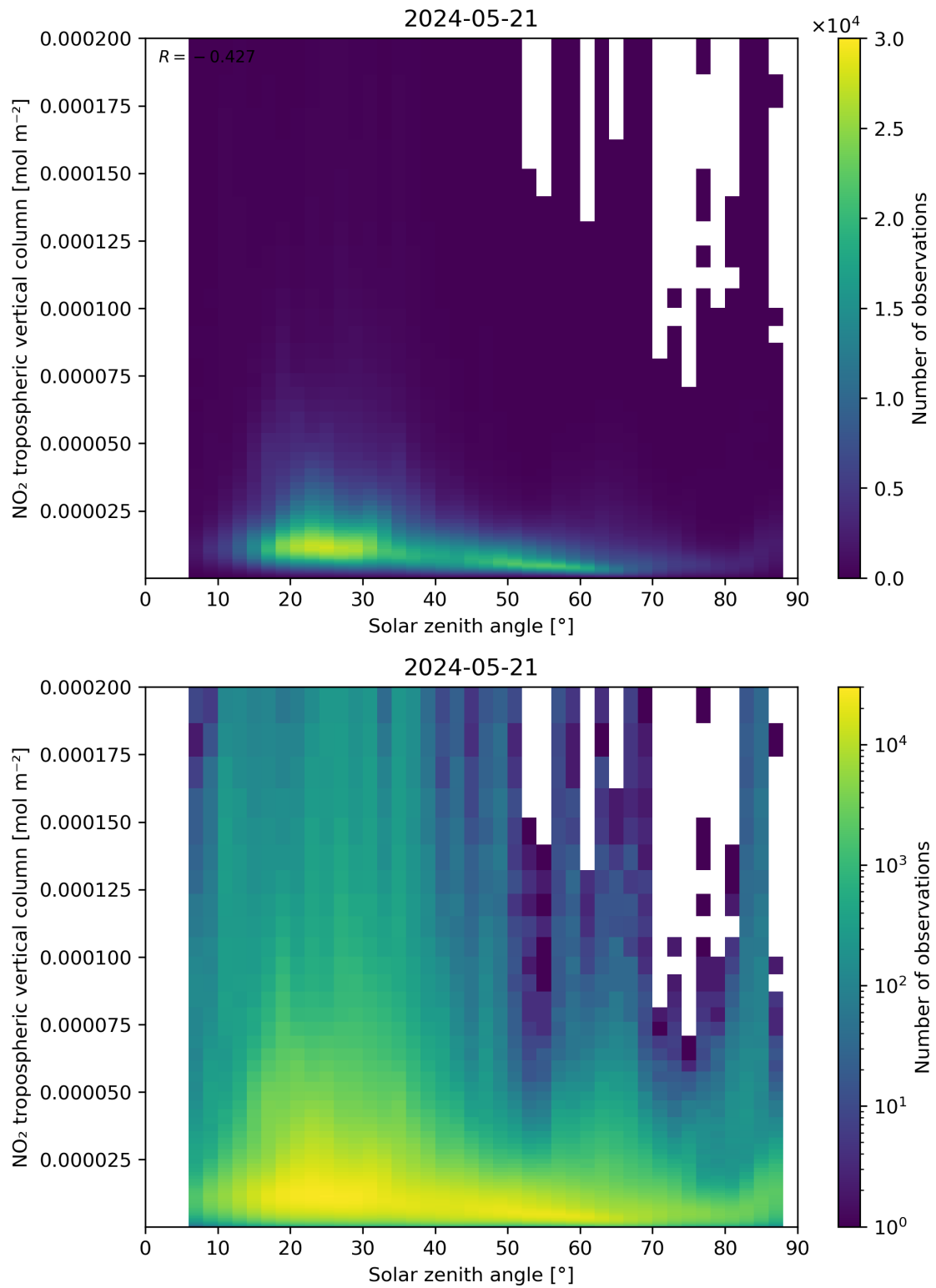
Figure 155: Scatter density plot of “Solar zenith angle” against “NO 2 tropospheric vertical column” for 2024-05-20 to 2024-05-22.
