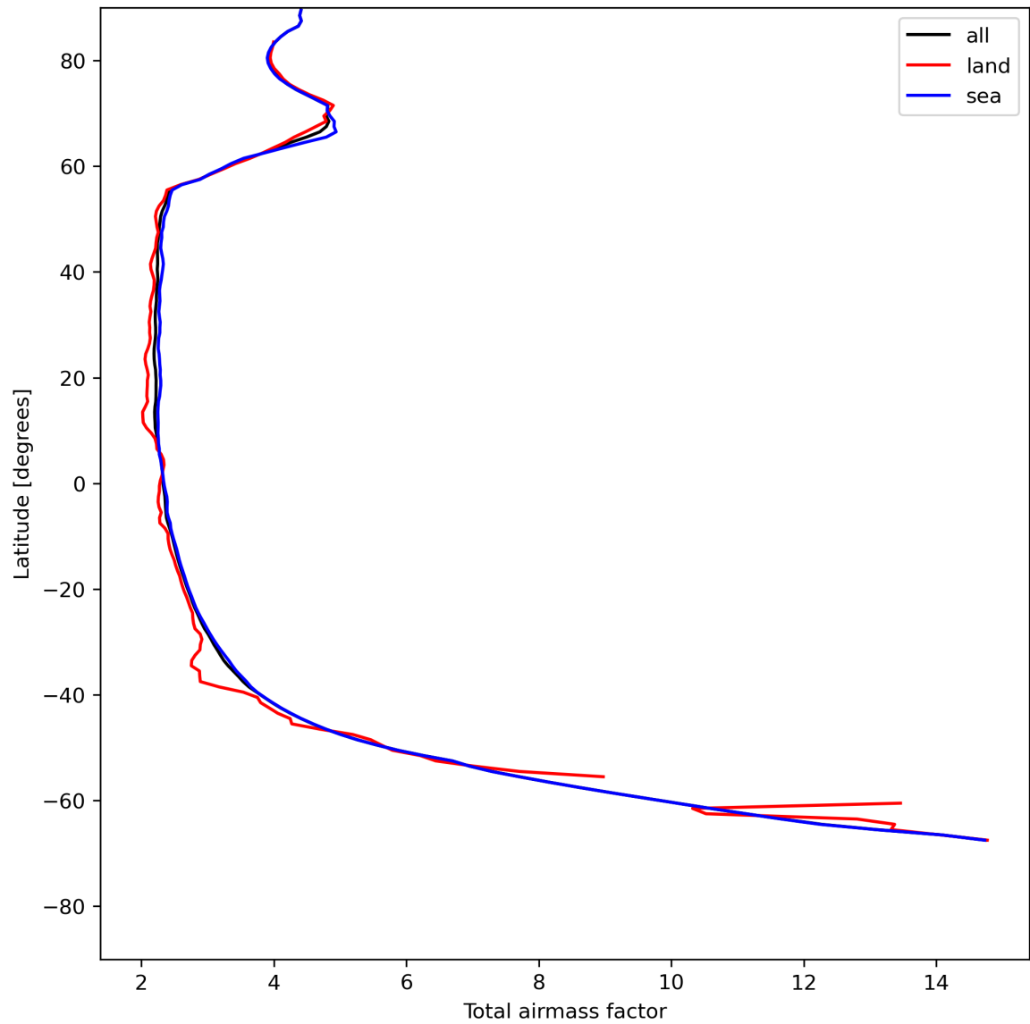
Figure 15: Zonal average of “Total airmass factor” for 2024-05-20 to 2024-05-22.
