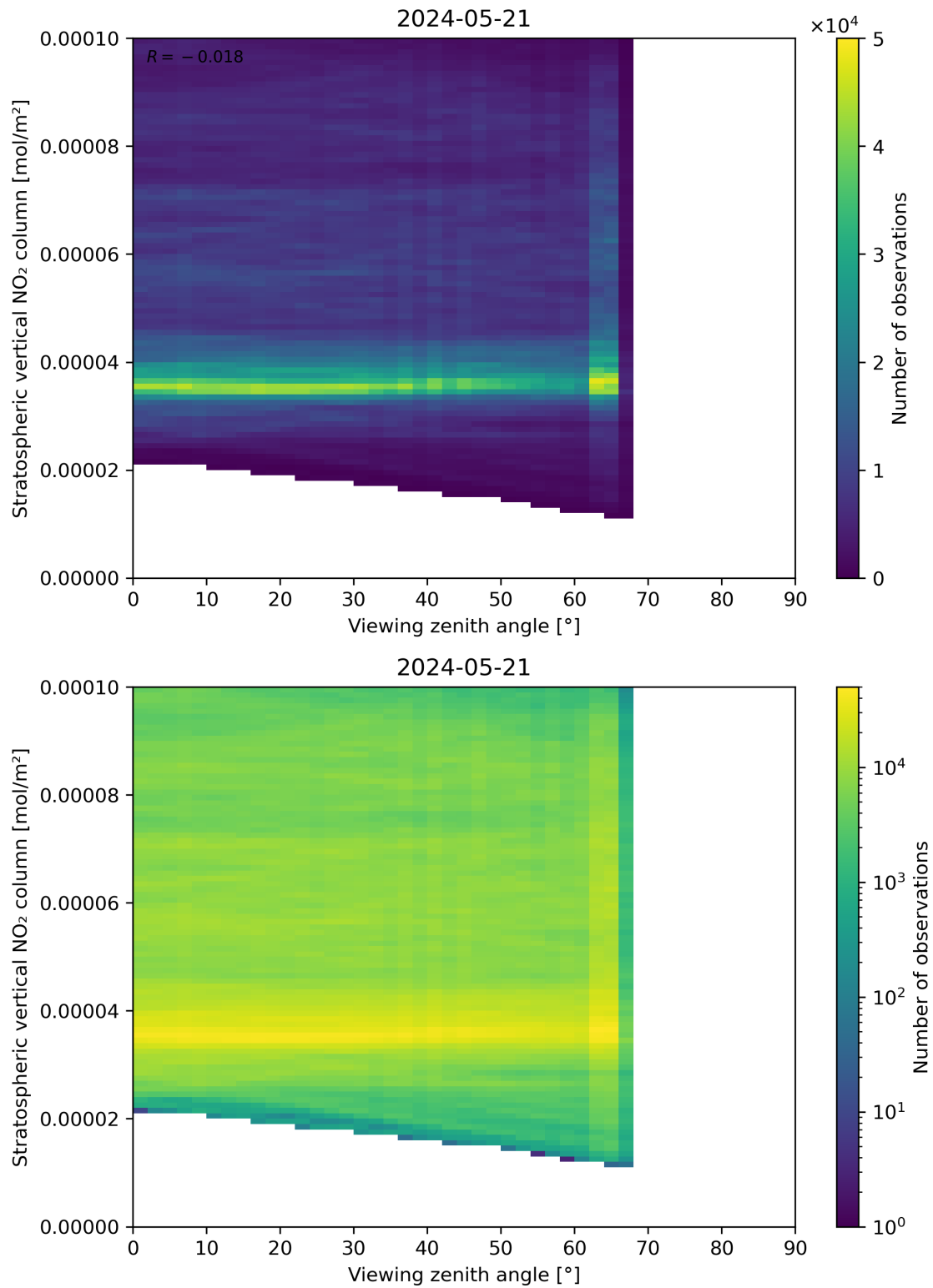
Figure 164: Scatter density plot of “Viewing zenith angle” against “Stratospheric vertical NO 2 column” for 2024-05-20 to 2024-05-22.
