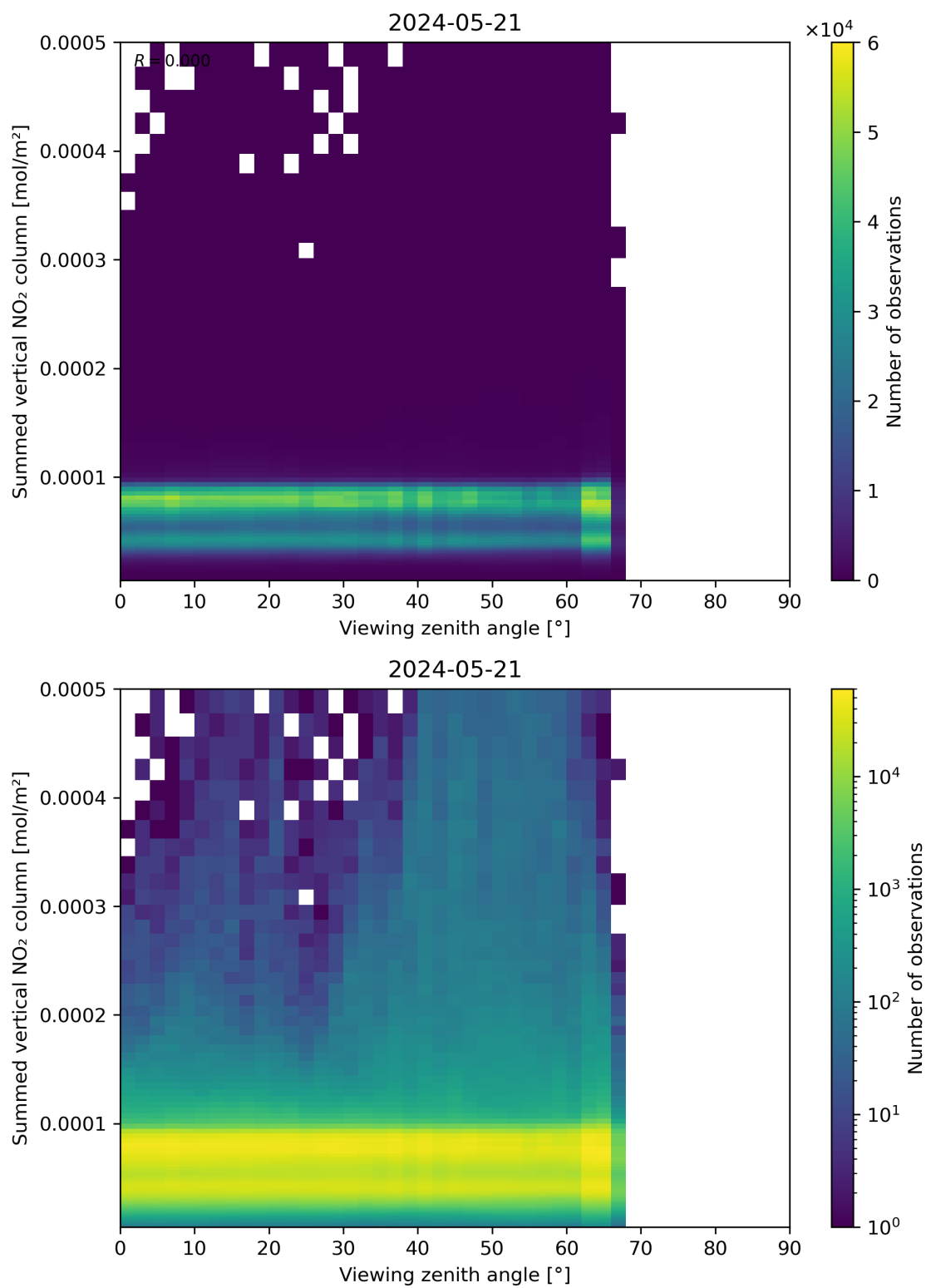
Figure 165: Scatter density plot of “Viewing zenith angle” against “Summed vertical NO 2 column” for 2024-05-20 to 2024-05-22.
