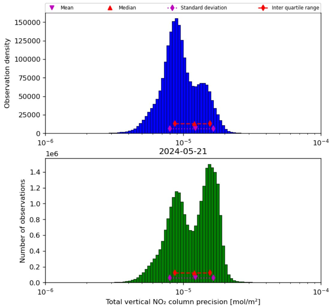
Figure 39: Histogram of “Total vertical NO 2 column precision” for 2024-05-20 to 2024-05-22
