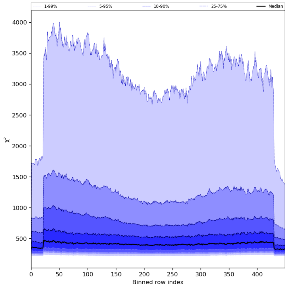
Figure 59: Along track statistics of “ \chi^2 ” for 2024-05-20 to 2024-05-22
