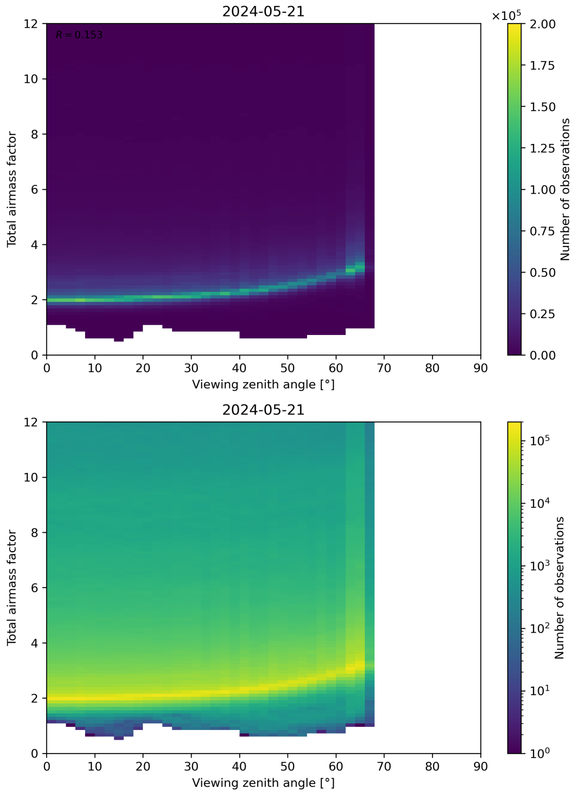
Figure 160: Scatter density plot of “Viewing zenith angle” against “Total airmass factor” for 2024-05-20 to 2024-05-22.
