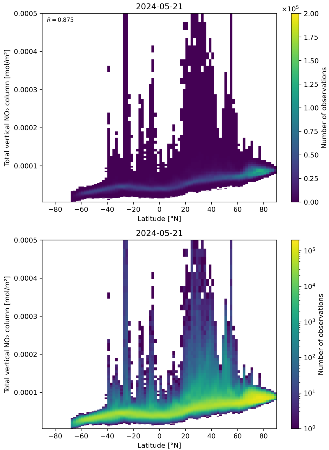
Figure 90: Scatter density plot of “Latitude” against “Total vertical NO 2 column” for 2024-05-20 to 2024-05-22.
