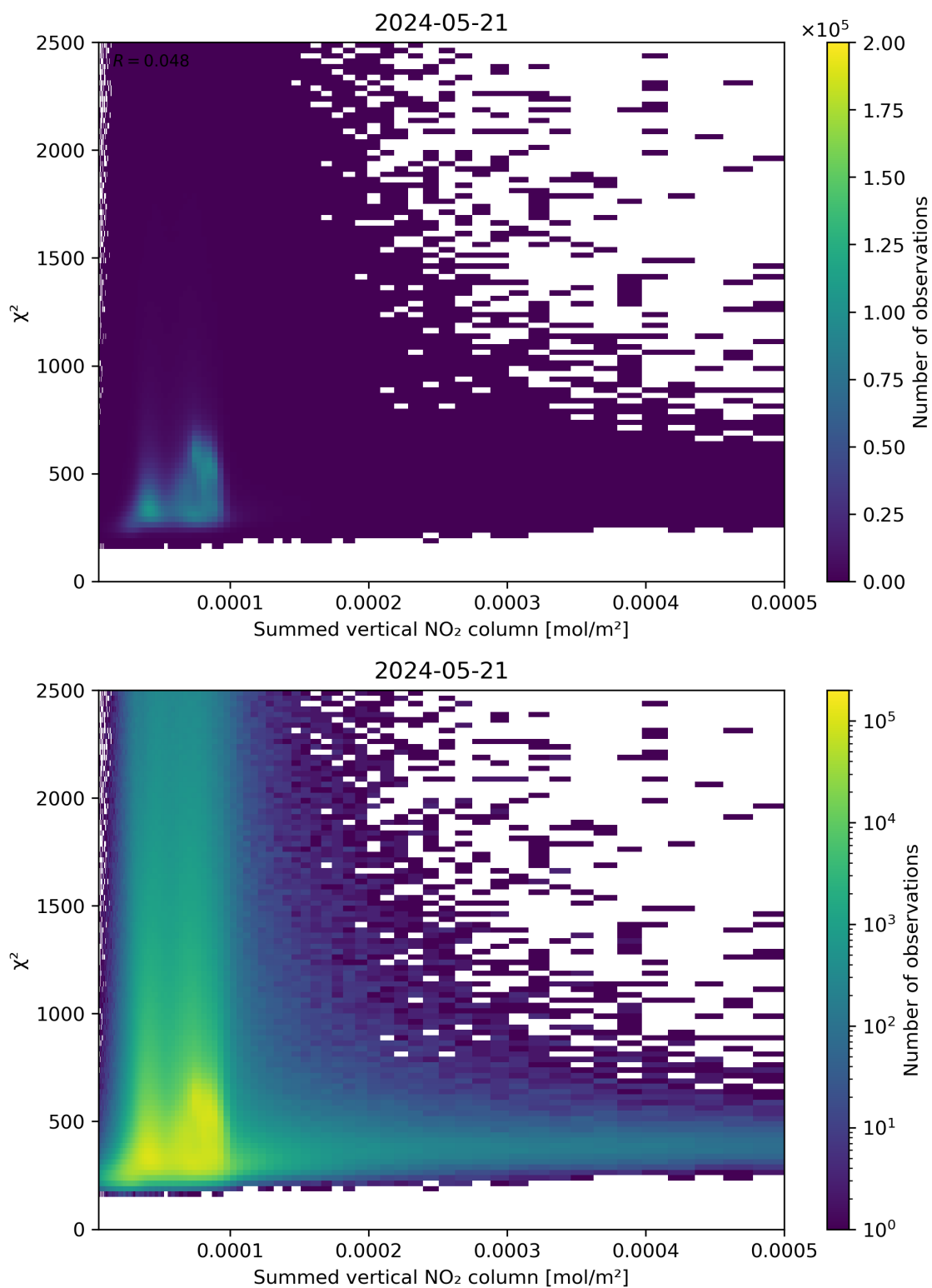
Figure 104: Scatter density plot of “Summed vertical NO 2 column” against “ \chi^2 ” for 2024-05-20 to 2024-05-22.
