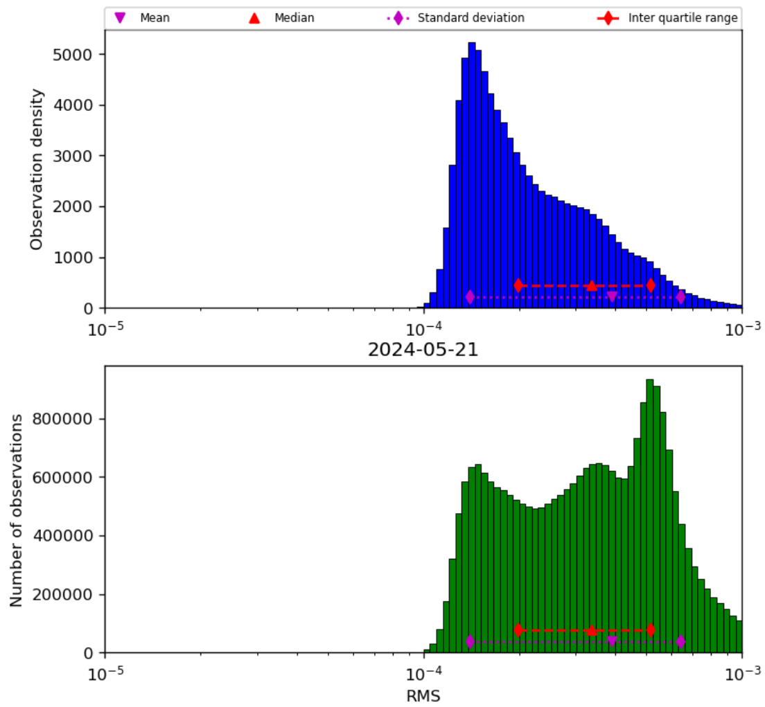
Figure 43: Histogram of “RMS” for 2024-05-20 to 2024-05-22
