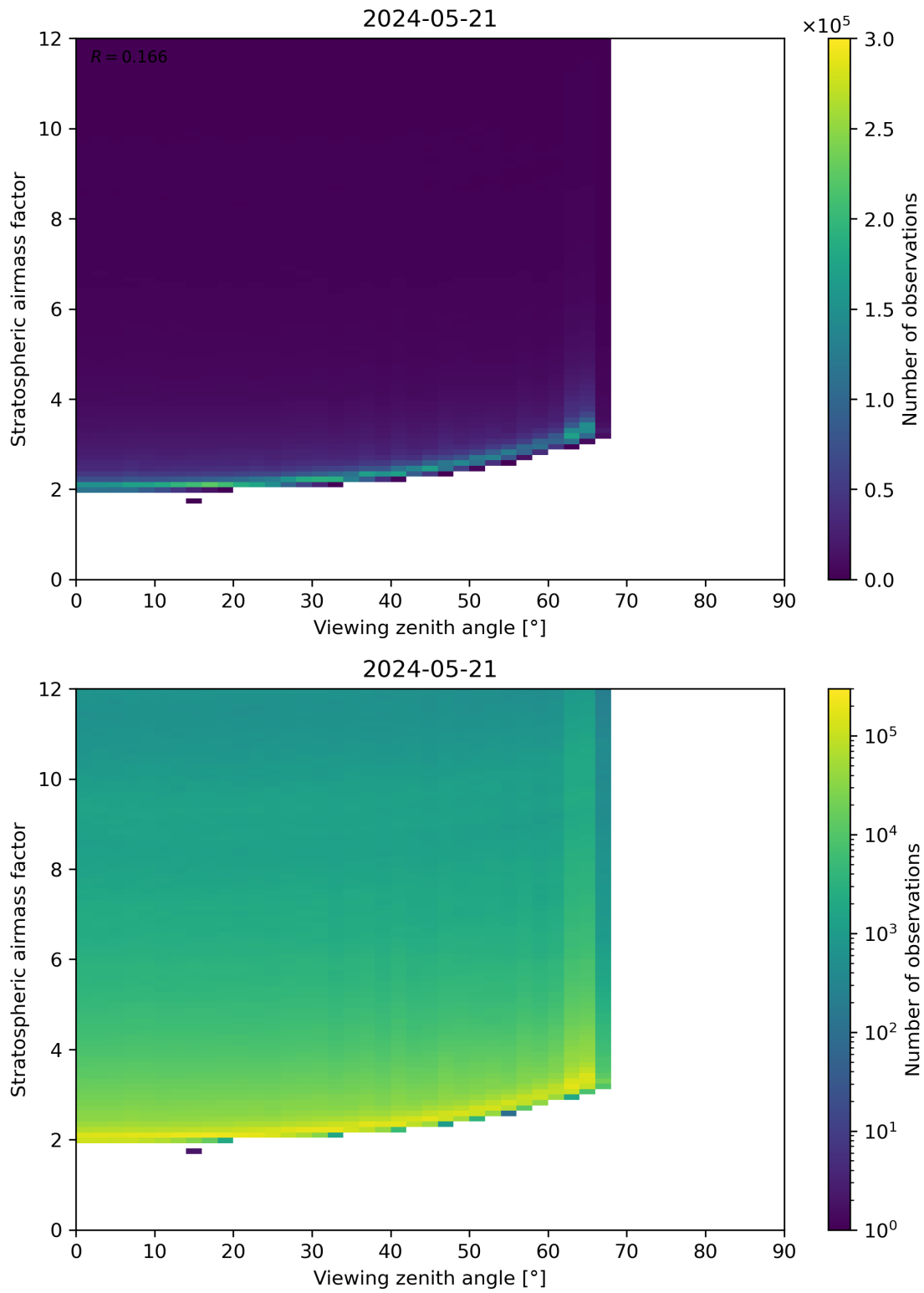
Figure 159: Scatter density plot of “Viewing zenith angle” against “Stratospheric airmass factor” for 2024-05-20 to 2024-05-22.
