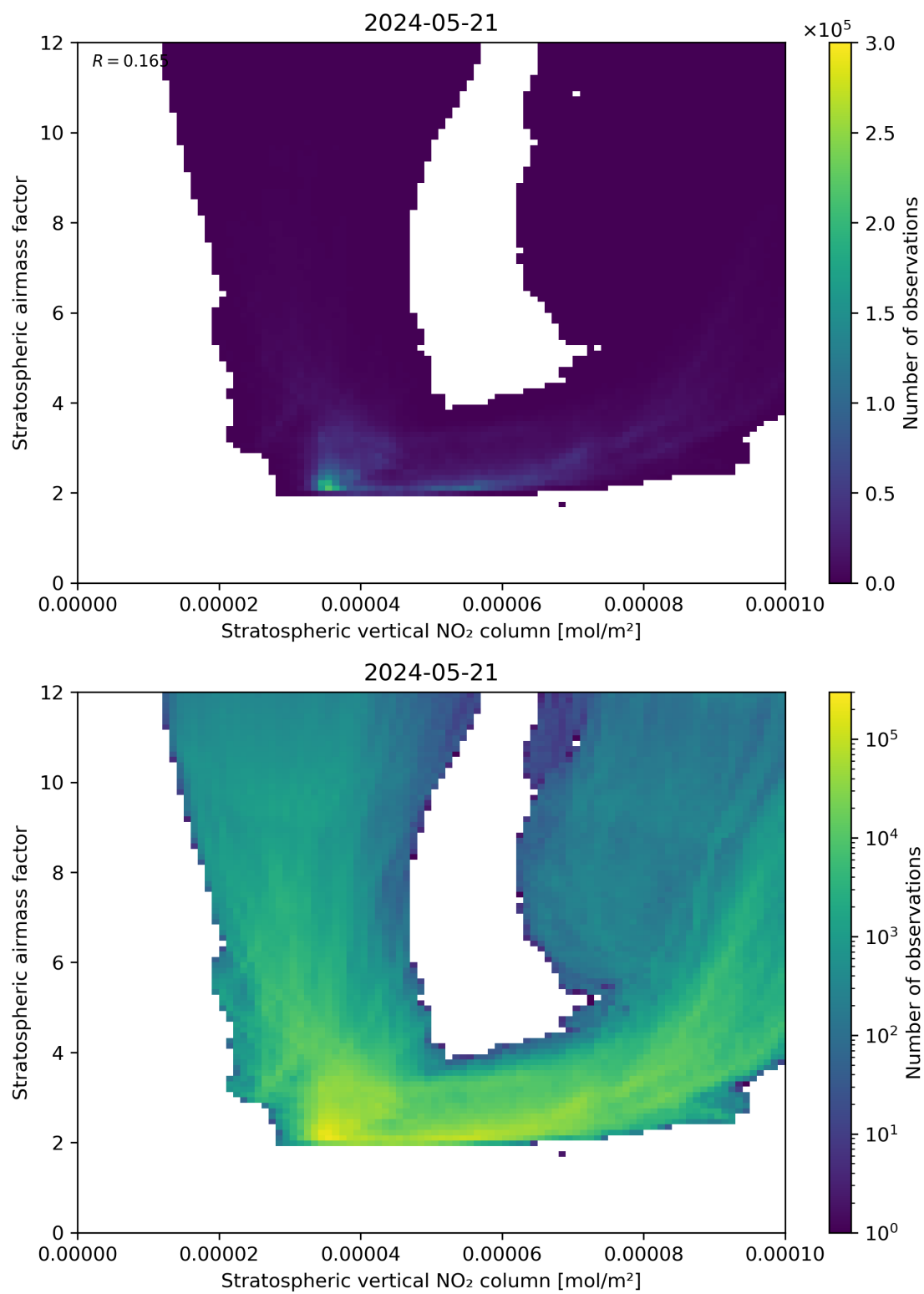
Figure 96: Scatter density plot of “Stratospheric vertical NO 2 column” against “Stratospheric airmass factor” for 2024-05-20 to 2024-05-22.
