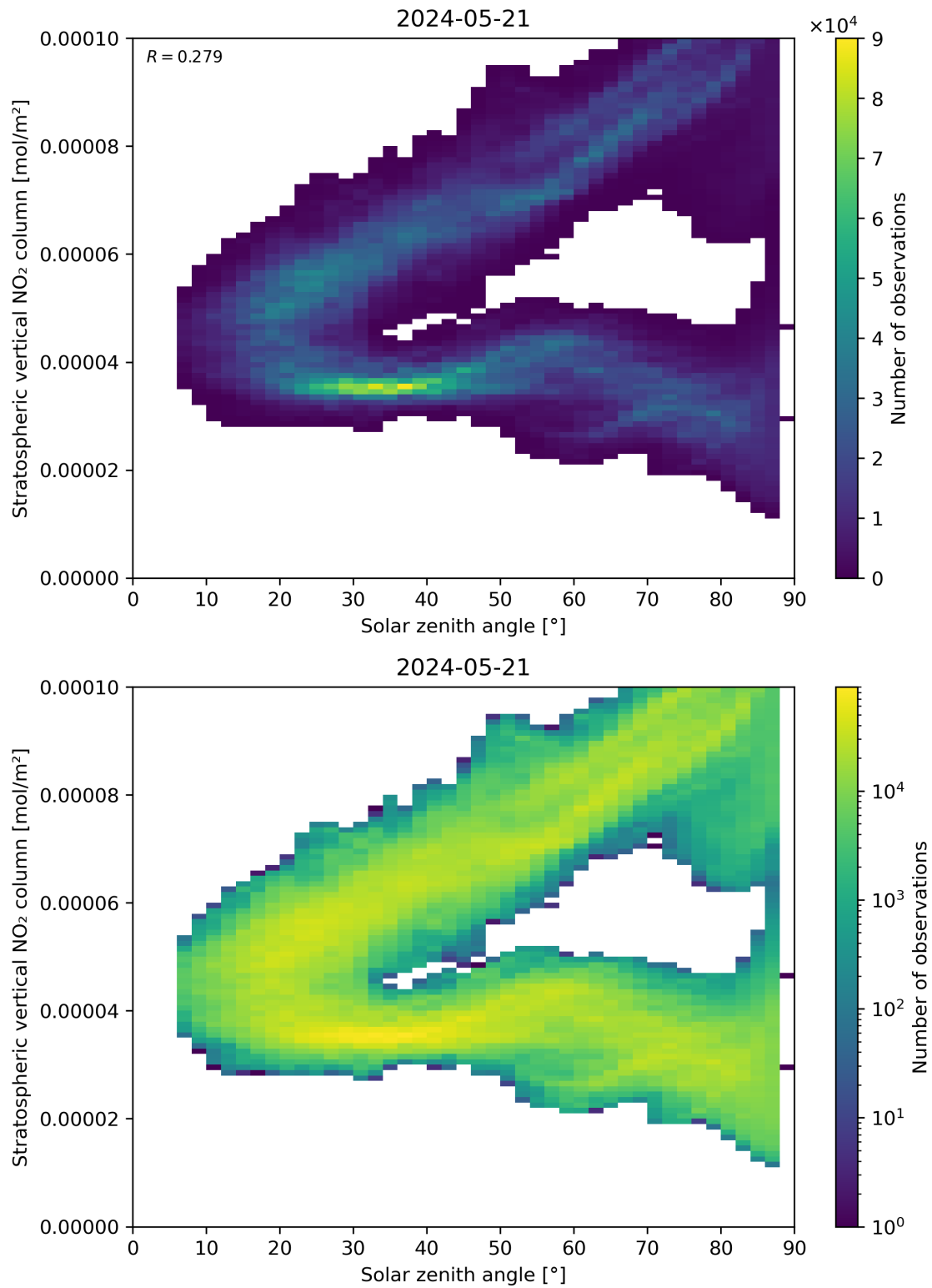
Figure 150: Scatter density plot of “Solar zenith angle” against “Stratospheric vertical NO 2 column” for 2024-05-20 to 2024-05-22.
