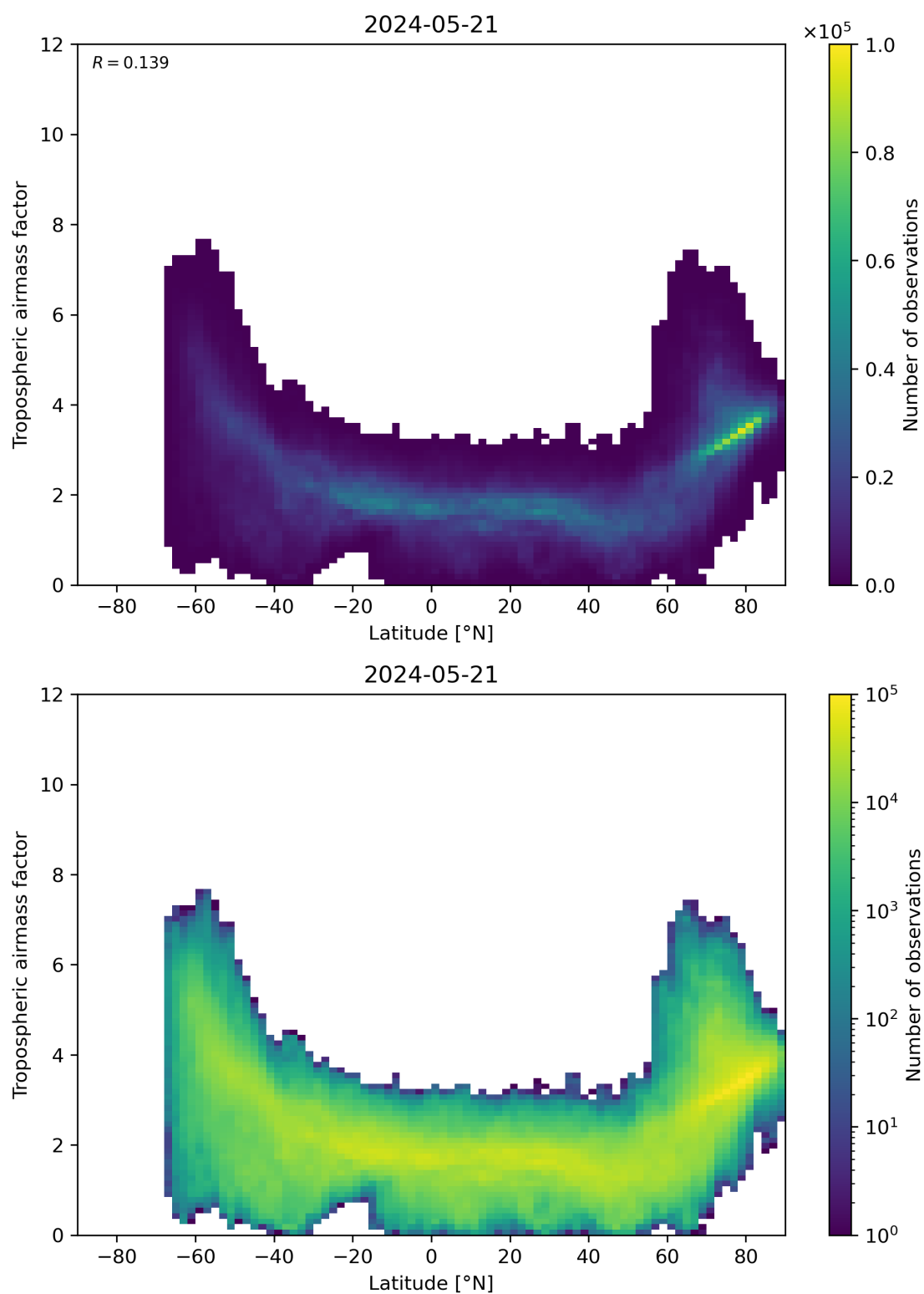
Figure 85: Scatter density plot of “Latitude” against “Tropospheric airmass factor” for 2024-05-20 to 2024-05-22.
