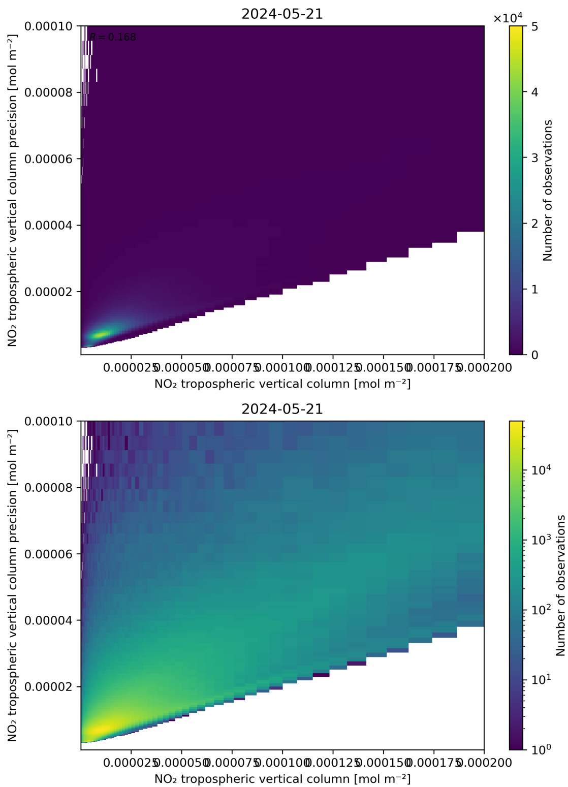
Figure 130: Scatter density plot of “NO 2 tropospheric vertical column” against “NO 2 tropospheric vertical column precision” for 2024-05-20 to 2024-05-22.
