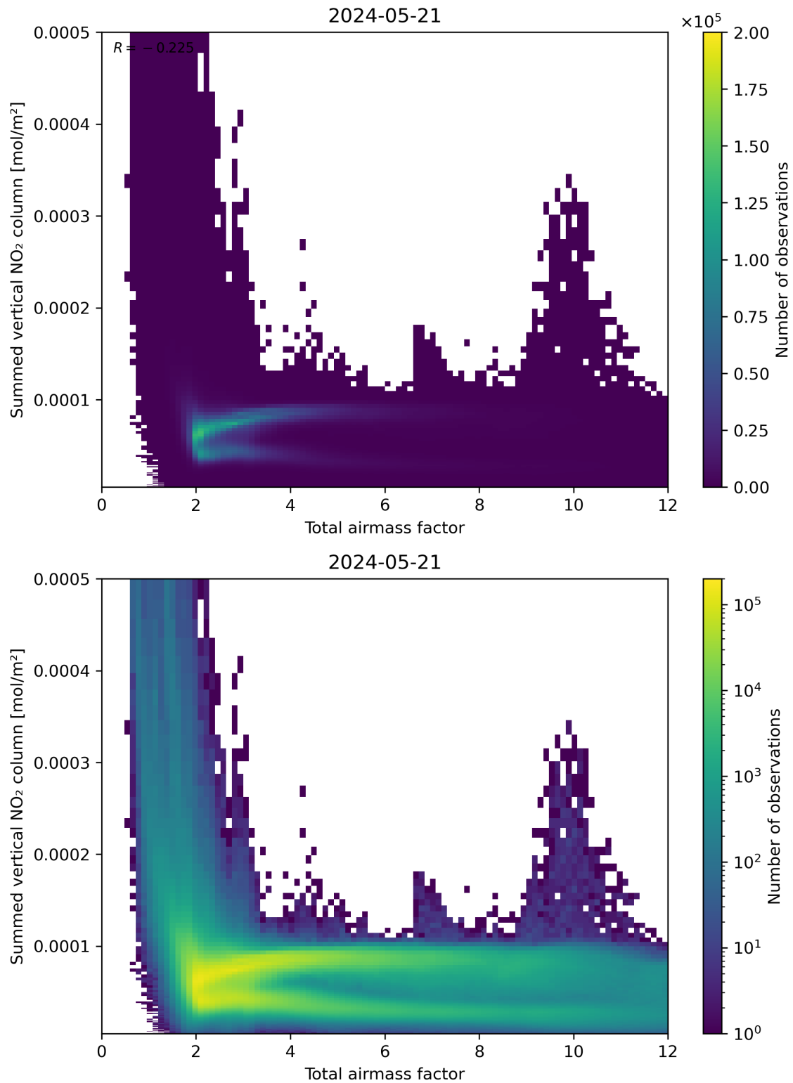
Figure 65: Scatter density plot of “Total airmass factor” against “Summed vertical NO 2 column” for 2024-05-20 to 2024-05-22.
