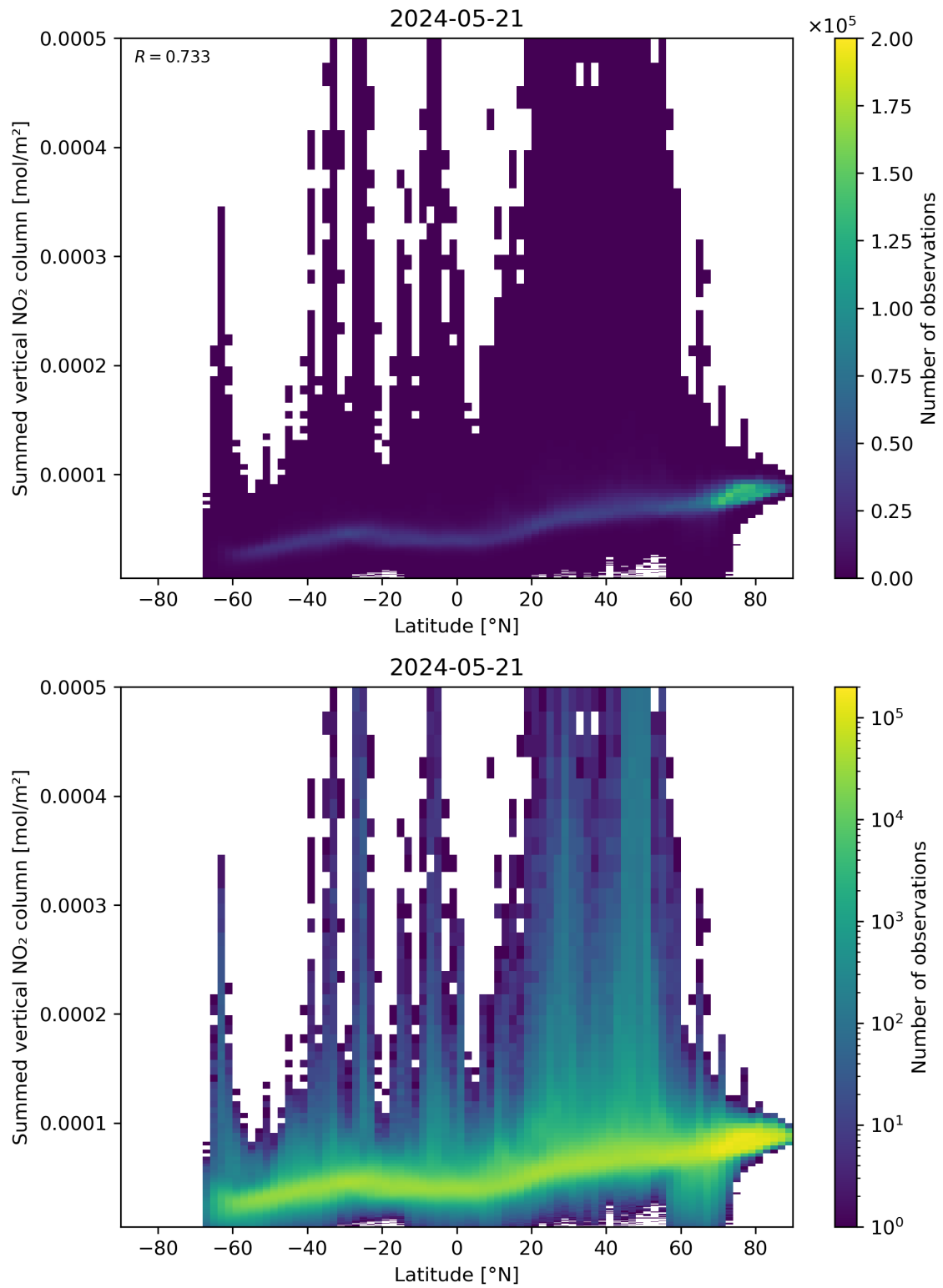
Figure 88: Scatter density plot of “Latitude” against “Summed vertical NO 2 column” for 2024-05-20 to 2024-05-22.
