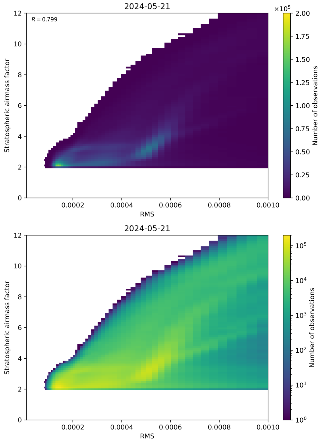
Figure 144: Scatter density plot of “RMS” against “Stratospheric airmass factor” for 2024-05-20 to 2024-05-22.
