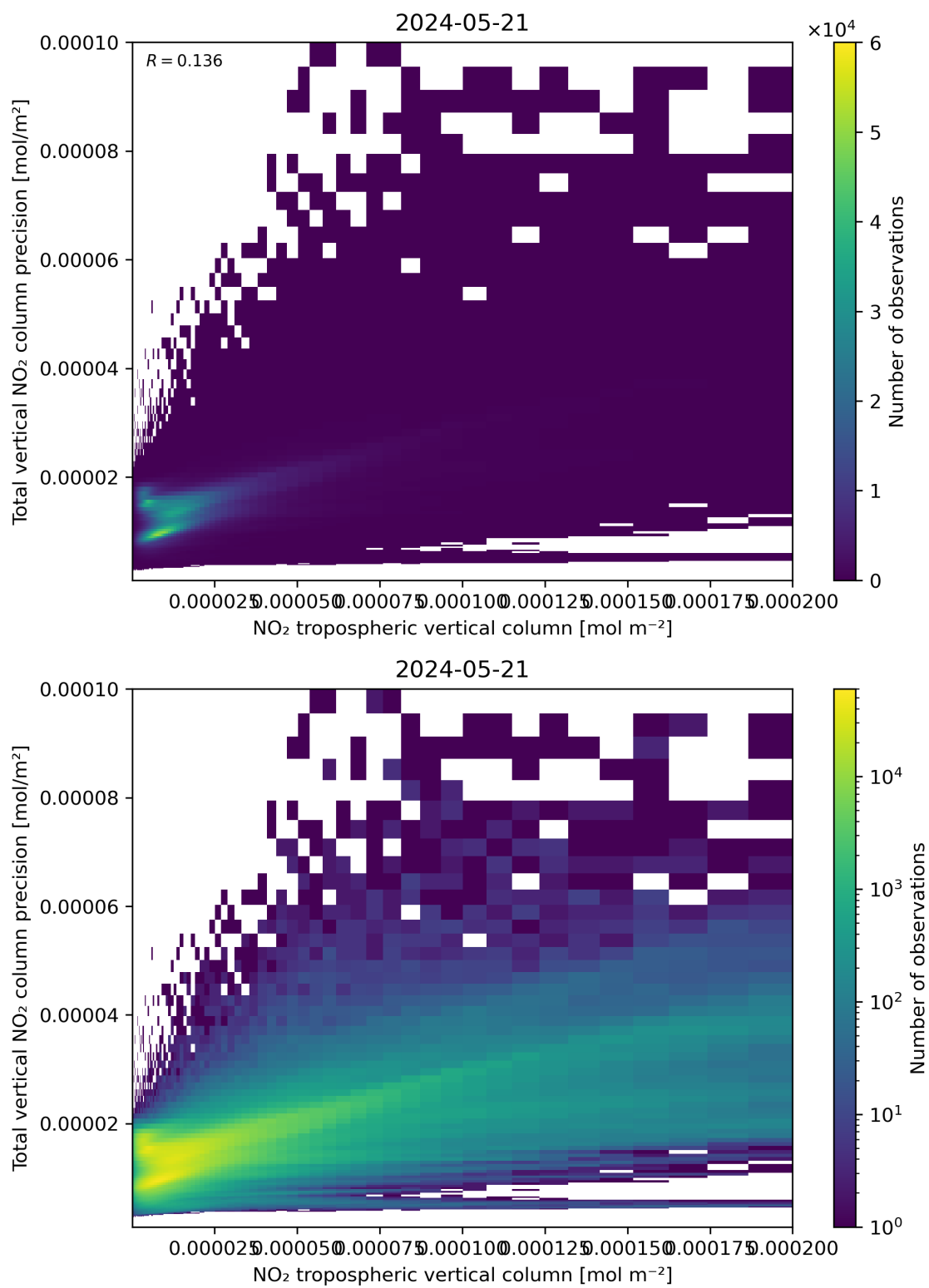
Figure 129: Scatter density plot of “NO 2 tropospheric vertical column” against “Total vertical NO 2 column precision” for 2024-05-20 to 2024-05-22.
