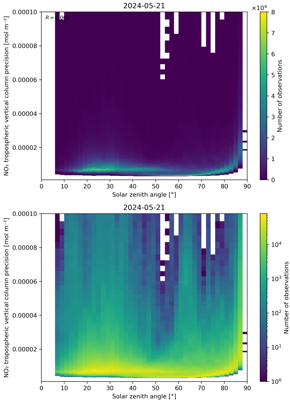
Figure 156: Scatter density plot of “Solar zenith angle” against “NO 2 tropospheric vertical column precision” for 2024-05-20 to 2024-05-22.
