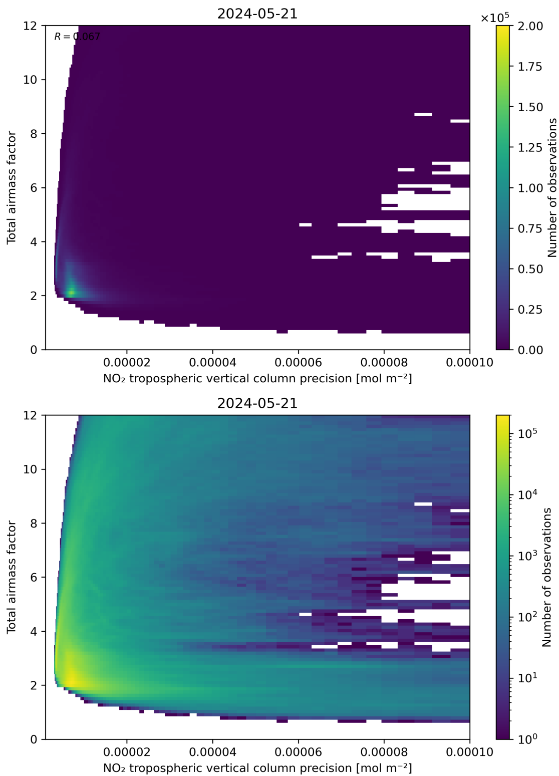
Figure 132: Scatter density plot of “NO 2 tropospheric vertical column precision” against “Total airmass factor” for 2024-05-20 to 2024-05-22.
