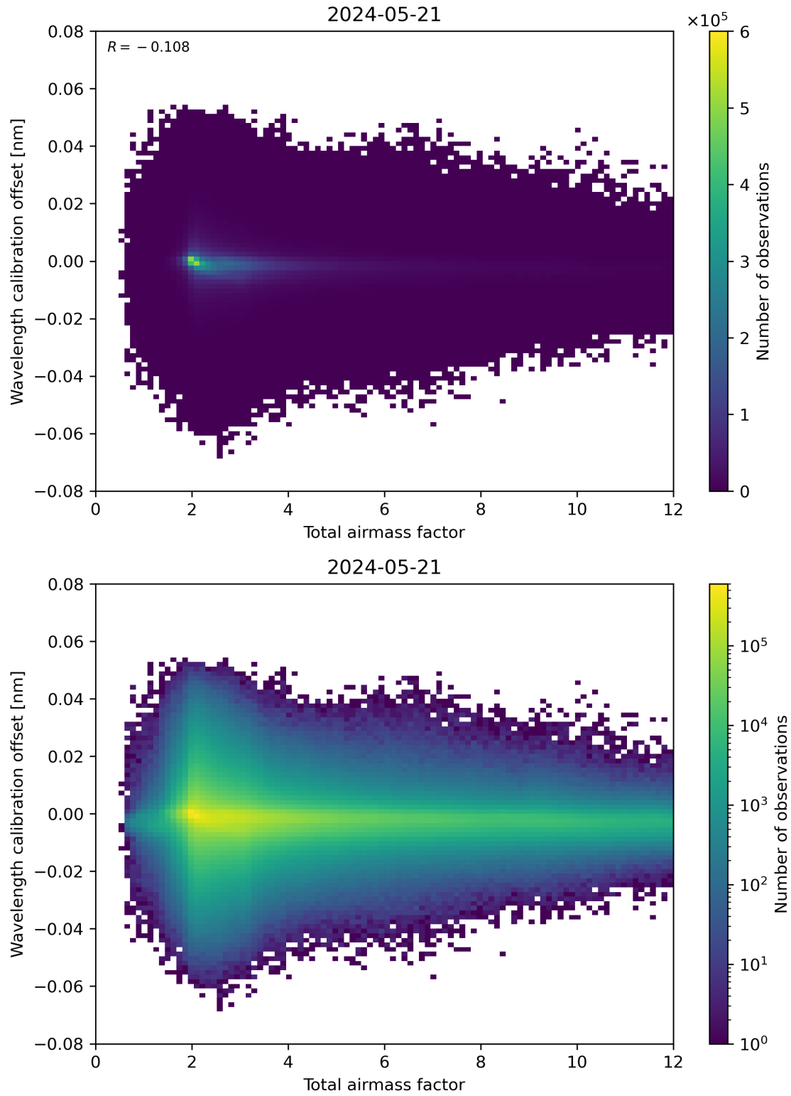
Figure 70: Scatter density plot of “Total airmass factor” against “Wavelength calibration offset” for 2024-05-20 to 2024-05-22.
