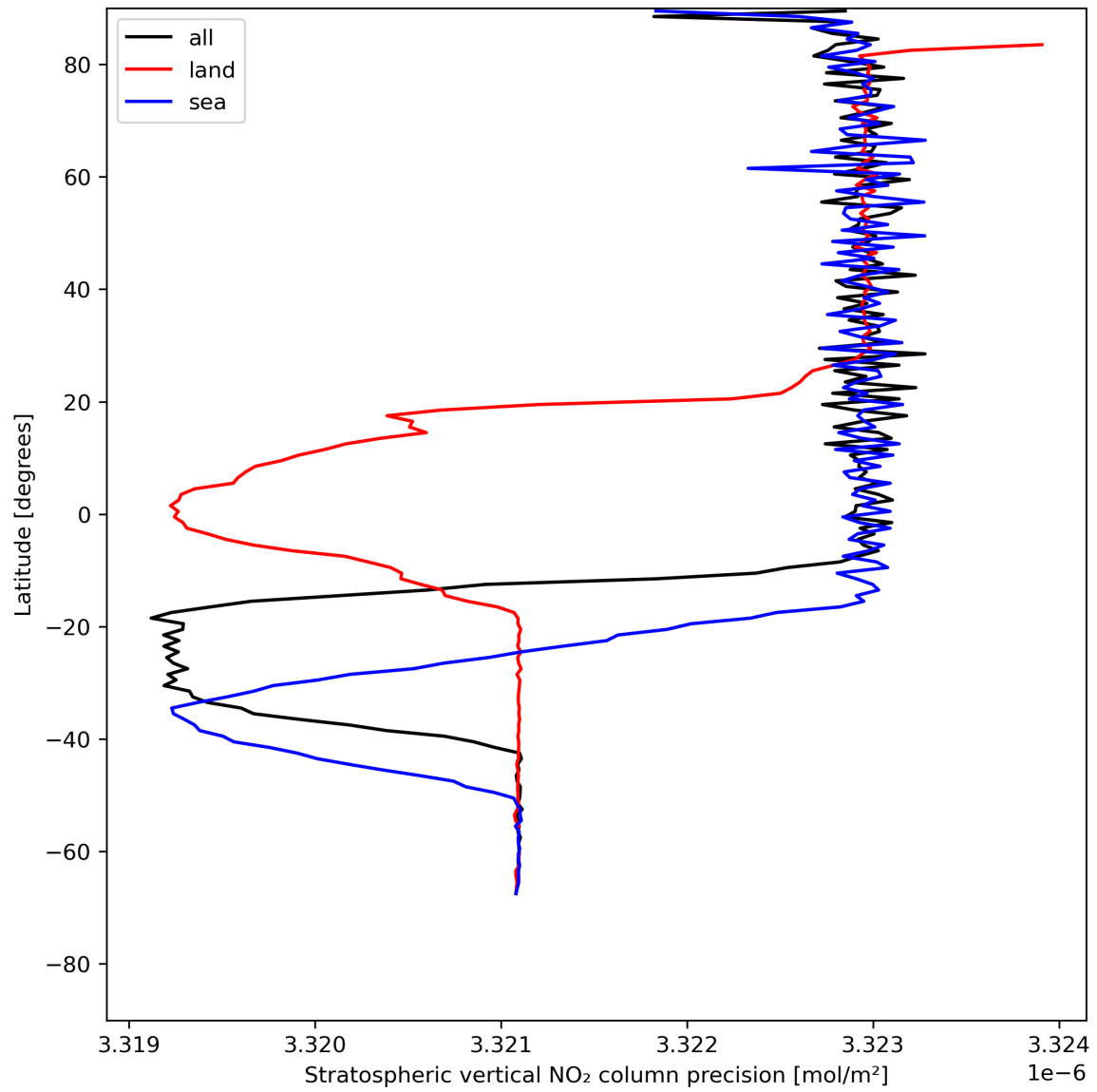
Figure 20: Zonal average of “Stratospheric vertical NO 2 column precision” for 2024-05-20 to 2024-05-22.
