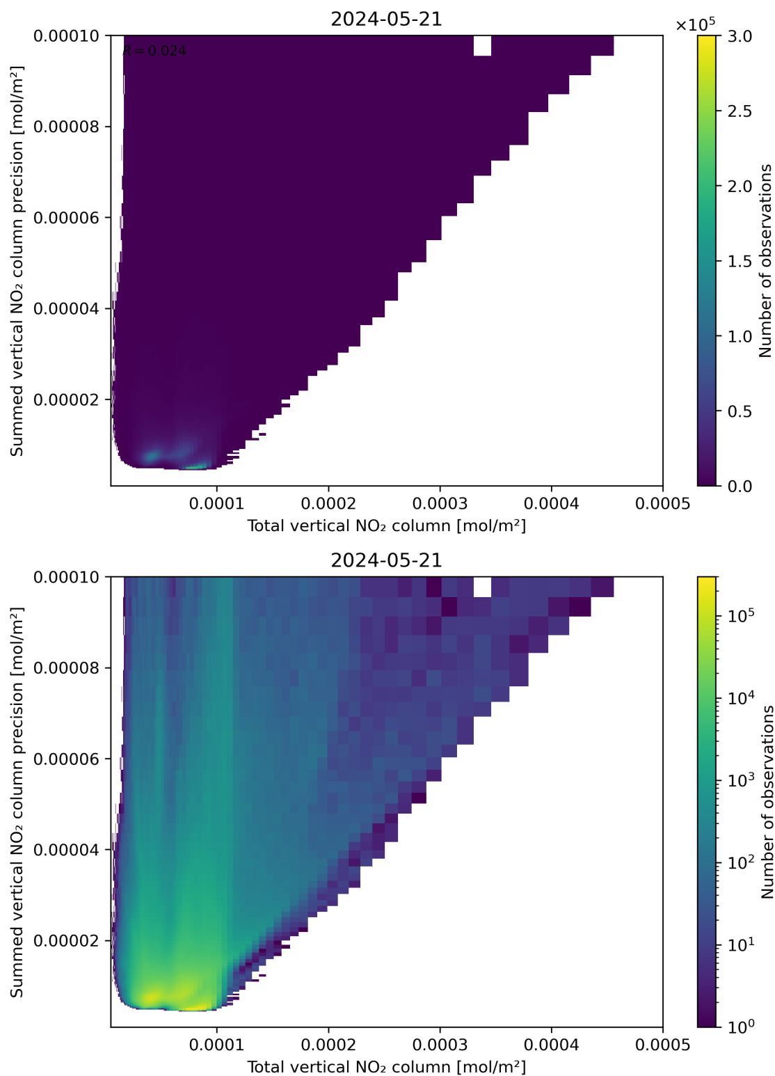
Figure 113: Scatter density plot of “Total vertical NO 2 column” against “Summed vertical NO 2 column precision” for 2024-05-20 to 2024-05-22.
