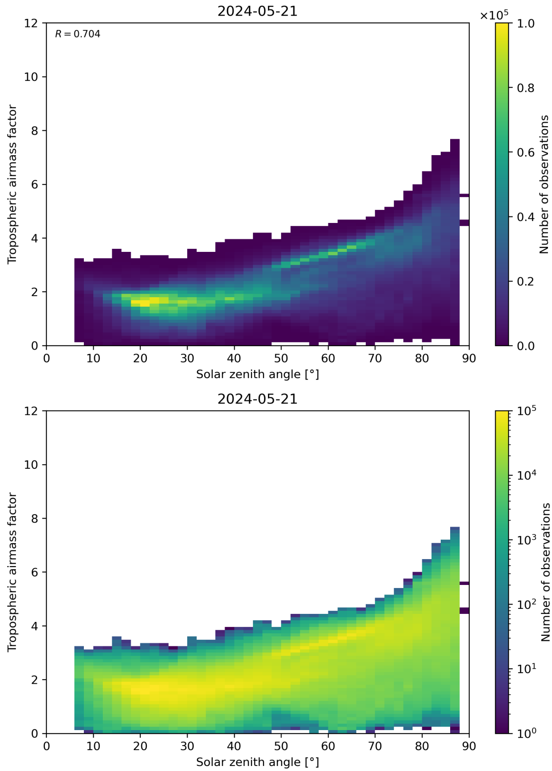
Figure 147: Scatter density plot of “Solar zenith angle” against “Tropospheric airmass factor” for 2024-05-20 to 2024-05-22.
