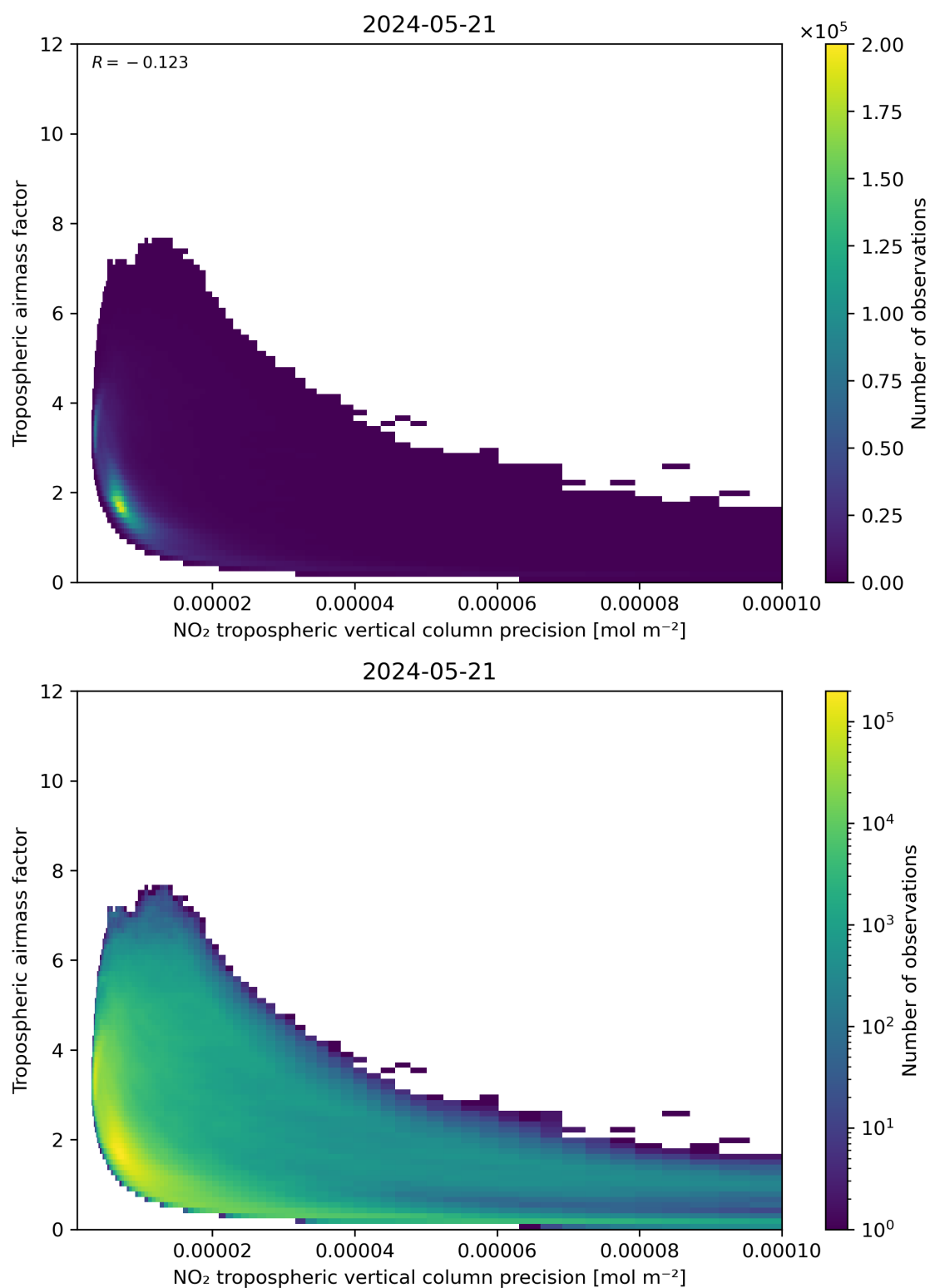
Figure 133: Scatter density plot of “NO 2 tropospheric vertical column precision” against “Tropospheric air mass factor” for 2024-05-20 to 2024-05-22.
