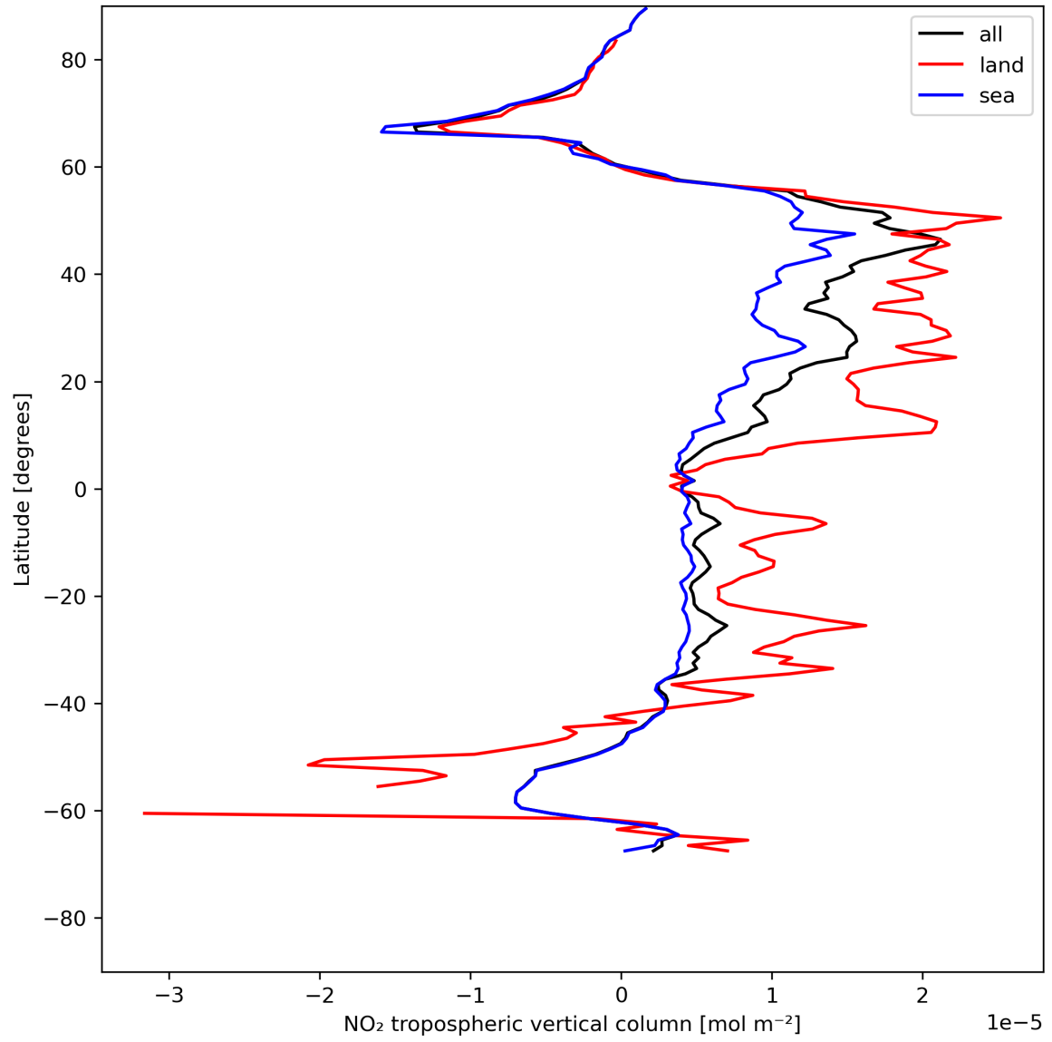
Figure 12: Zonal average of “NO 2 tropospheric vertical column” for 2024-05-20 to 2024-05-22.
