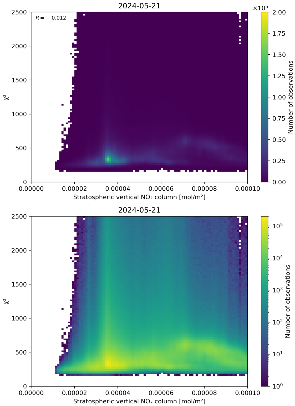
Figure 97: Scatter density plot of “Stratospheric vertical NO 2 column” against “ \chi^2 ” for 2024-05-20 to 2024-05-22.
