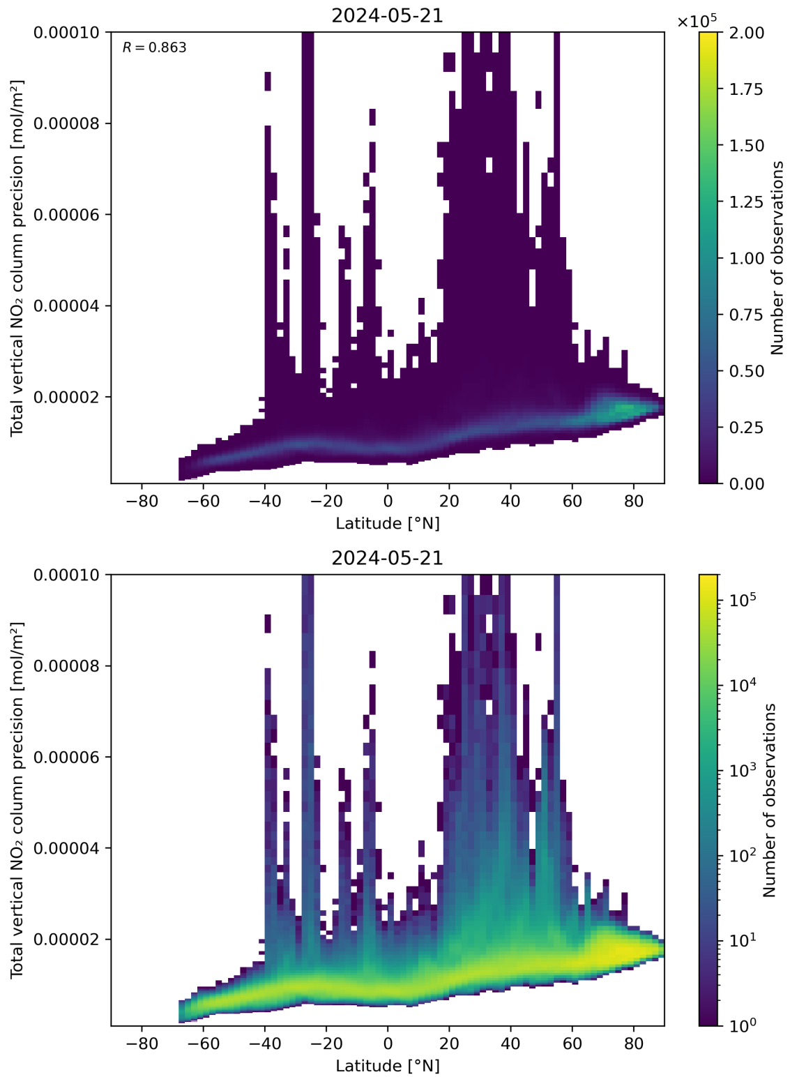
Figure 91: Scatter density plot of “Latitude” against “Total vertical NO 2 column precision” for 2024-05-20 to 2024-05-22.
