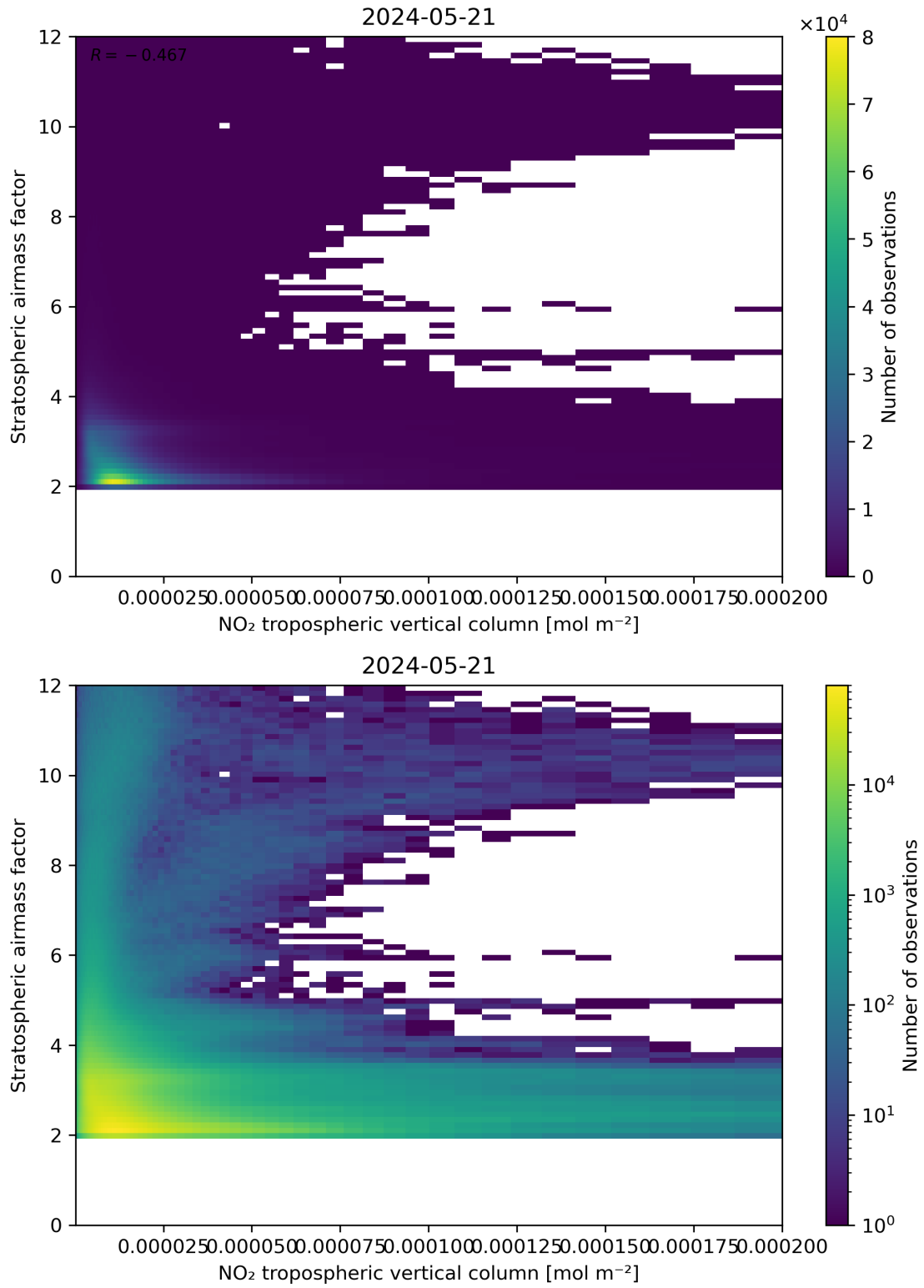
Figure 121: Scatter density plot of “NO 2 tropospheric vertical column” against “Stratospheric air mass factor” for 2024-05-20 to 2024-05-22.
