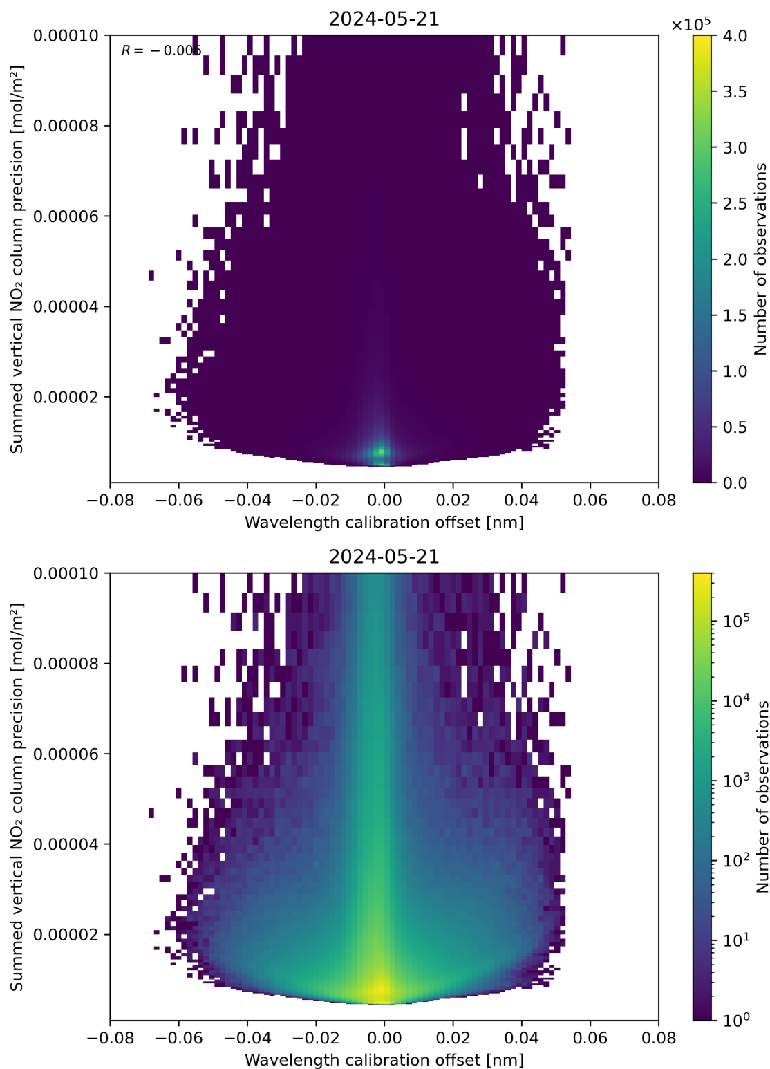
Figure 178: Scatter density plot of “Wavelength calibration offset” against “Summed vertical NO 2 column precision” for 2024-05-20 to 2024-05-22.
