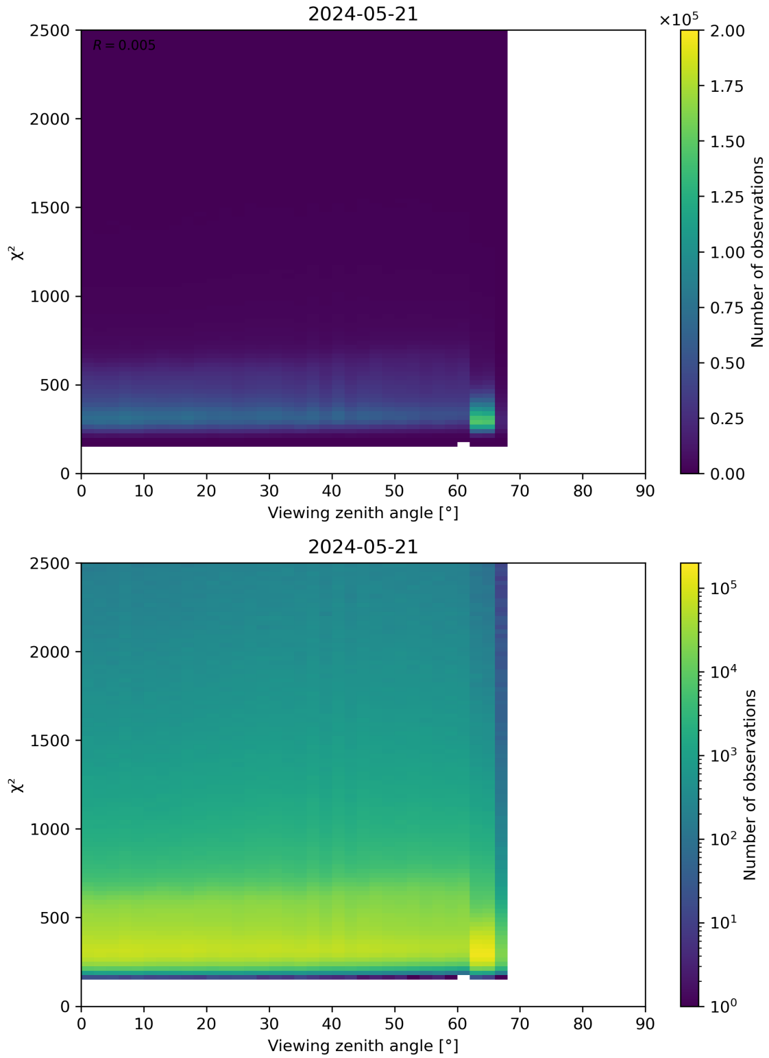
Figure 162: Scatter density plot of “Viewing zenith angle” against “ \chi^2 ” for 2024-05-20 to 2024-05-22.
