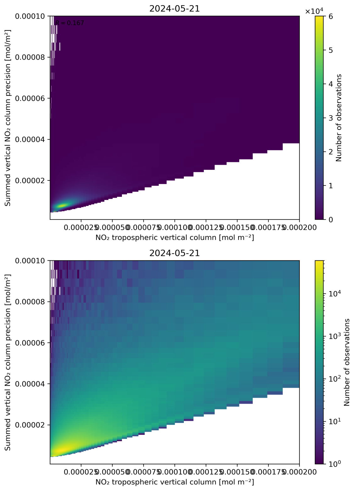
Figure 127: Scatter density plot of “NO 2 tropospheric vertical column” against “Summed vertical NO 2 column precision” for 2024-05-20 to 2024-05-22.
