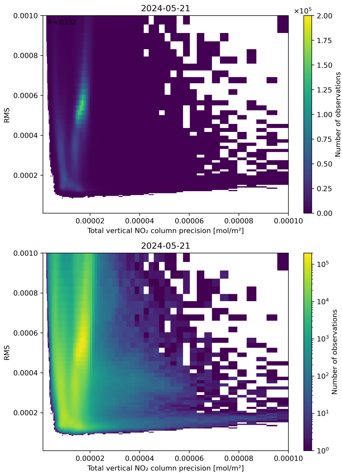
Figure 119: Scatter density plot of “Total vertical NO 2 column precision” against “RMS” for 2024-05-20 to 2024-05-22.
