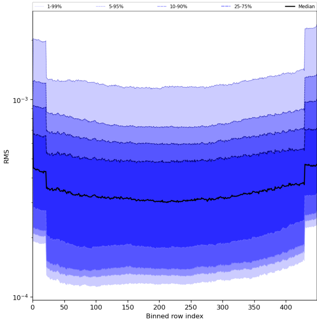
Figure 60: Along track statistics of “RMS” for 2024-05-20 to 2024-05-22
