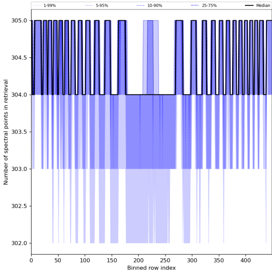
Figure 50: Along track statistics of “Number of spectral points in retrieval” for 2024-05-20 to 2024-05-22
