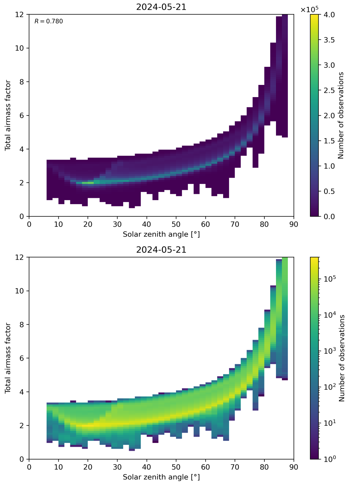
Figure 146: Scatter density plot of “Solar zenith angle” against “Total air mass factor” for 2024-05-20 to 2024-05-22.
