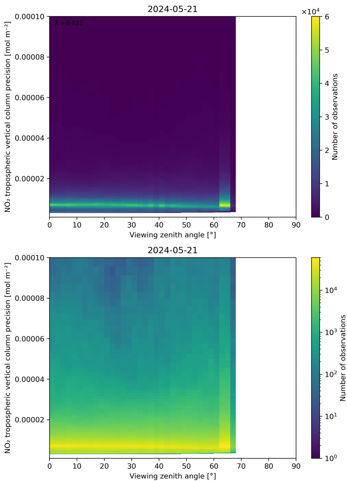
Figure 170: Scatter density plot of “Viewing zenith angle” against “NO 2 tropospheric vertical column precision” for 2024-05-20 to 2024-05-22.
