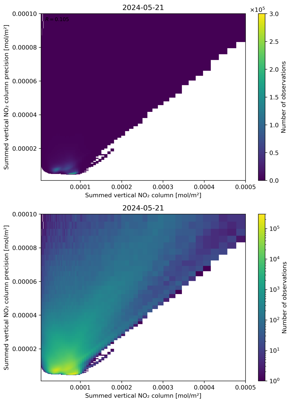
Figure 105: Scatter density plot of “Summed vertical NO 2 column” against “Summed vertical NO 2 column precision” for 2024-05-20 to 2024-05-22.
