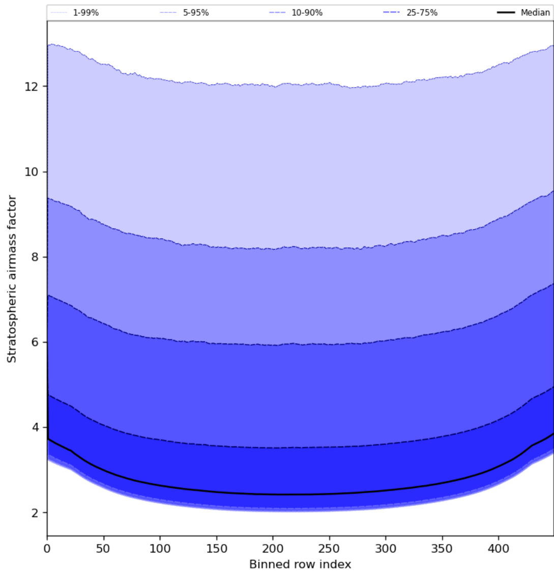
Figure 61: Along track statistics of “Stratospheric airmass factor” for 2024-05-20 to 2024-05-22
