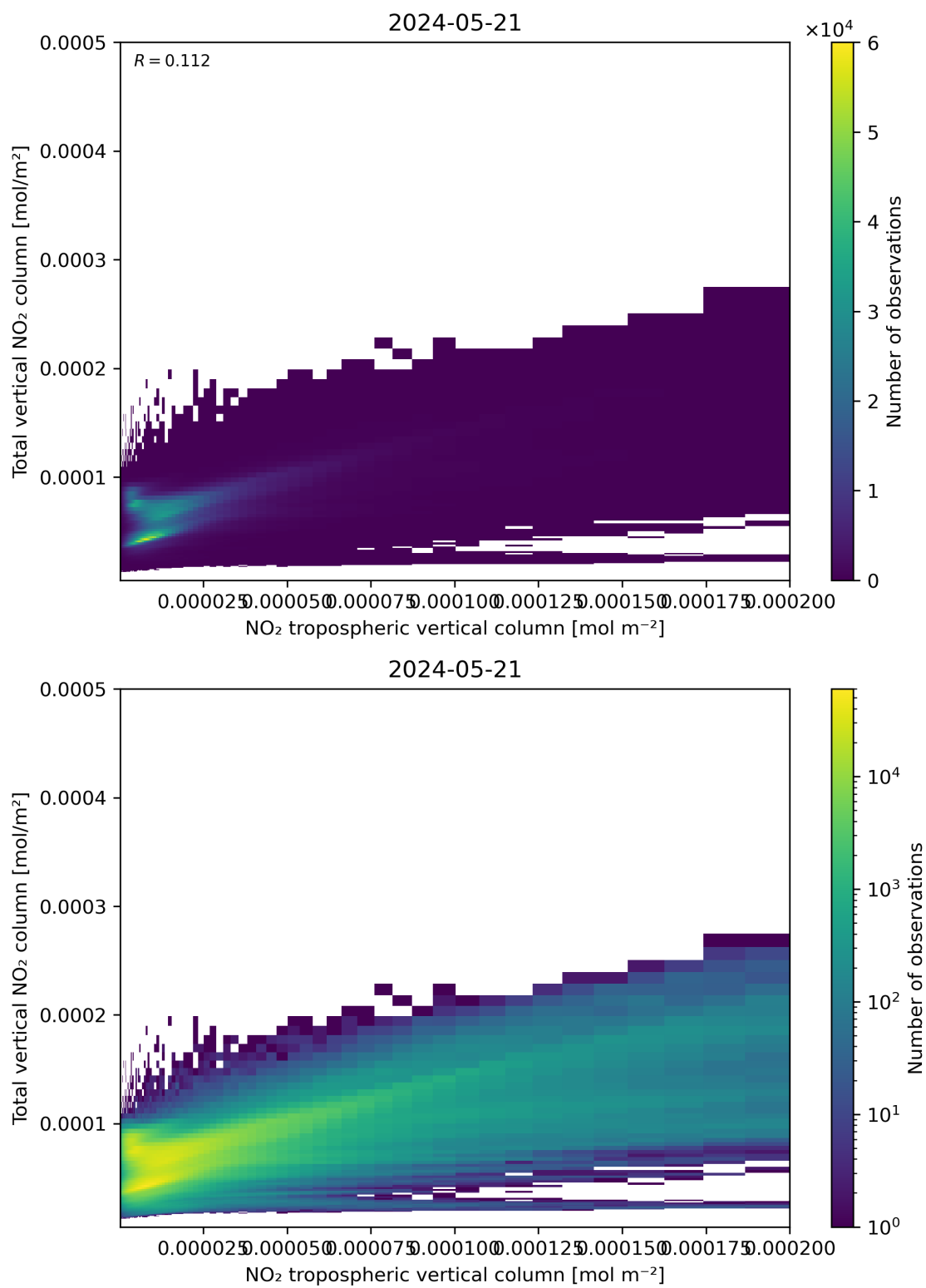
Figure 128: Scatter density plot of “NO 2 tropospheric vertical column” against “Total vertical NO 2 column” for 2024-05-20 to 2024-05-22.
