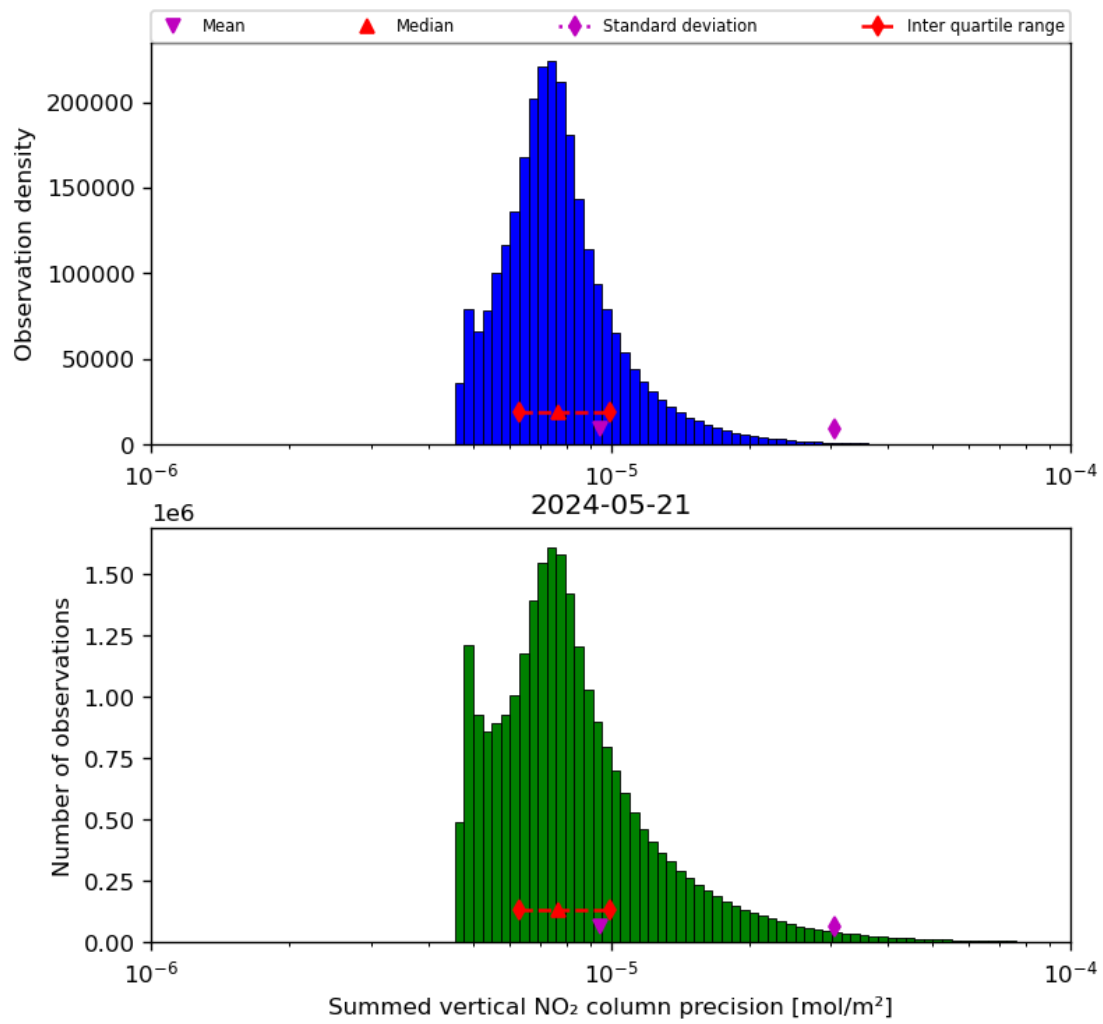
Figure 41: Histogram of "Summed vertical NO 2 column precision" for 2024-05-20 to 2024-05-22
