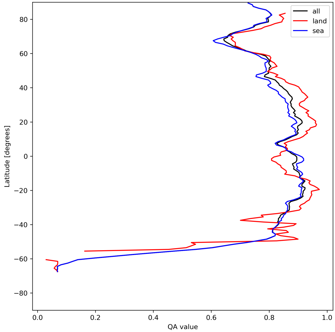
Figure 11: Zonal average of “QA value” for 2024-05-20 to 2024-05-22.
