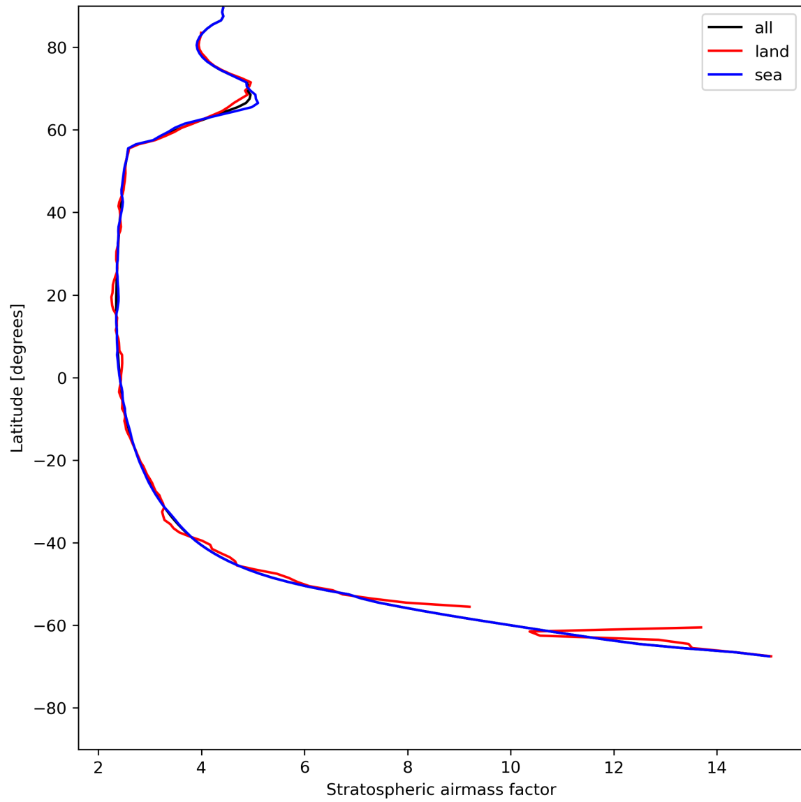
Figure 27: Zonal average of “Stratospheric airmass factor” for 2024-05-20 to 2024-05-22.
