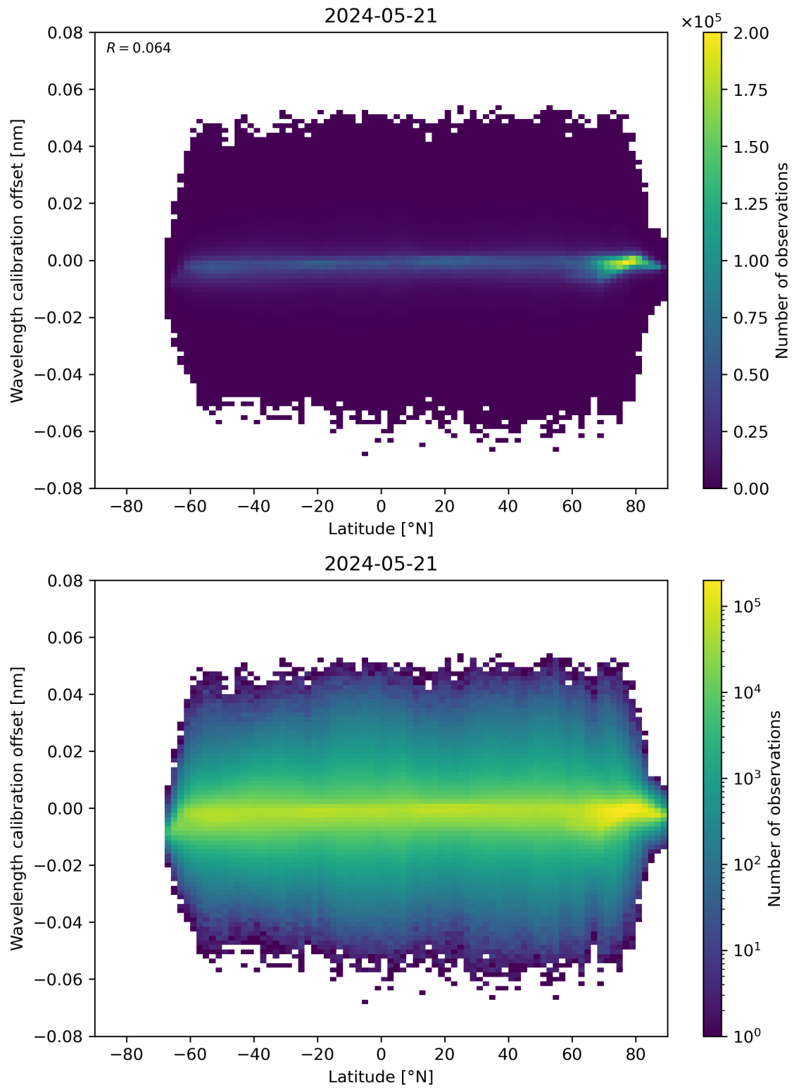
Figure 95: Scatter density plot of “Latitude” against “Wavelength calibration offset” for 2024-05-20 to 2024-05-22.
