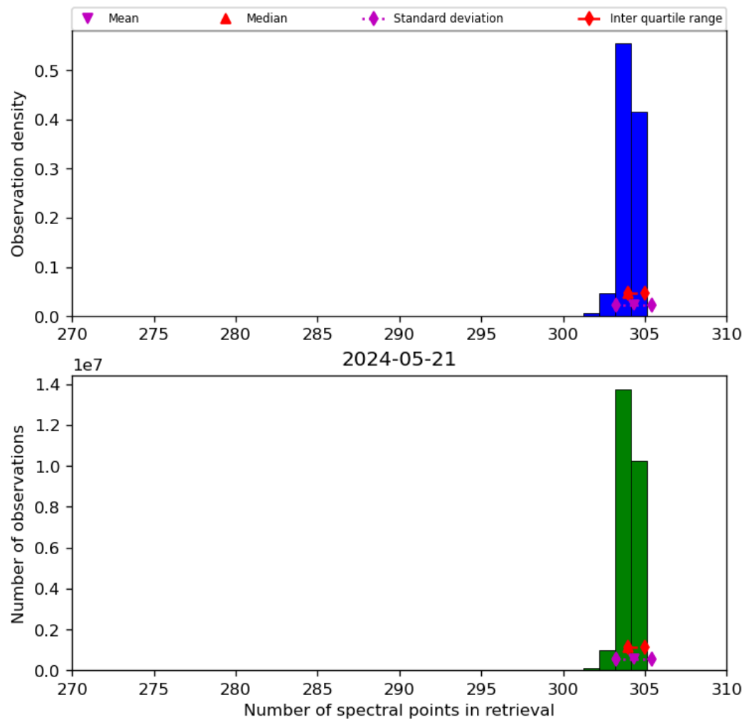
Figure 33: Histogram of “Number of spectral points in retrieval” for 2024-05-20 to 2024-05-22
