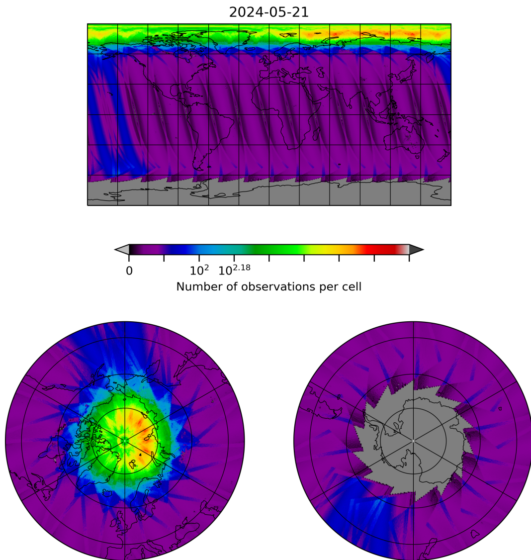
Figure 10: Map of the number of observations for 2024-05-20 to 2024-05-22
