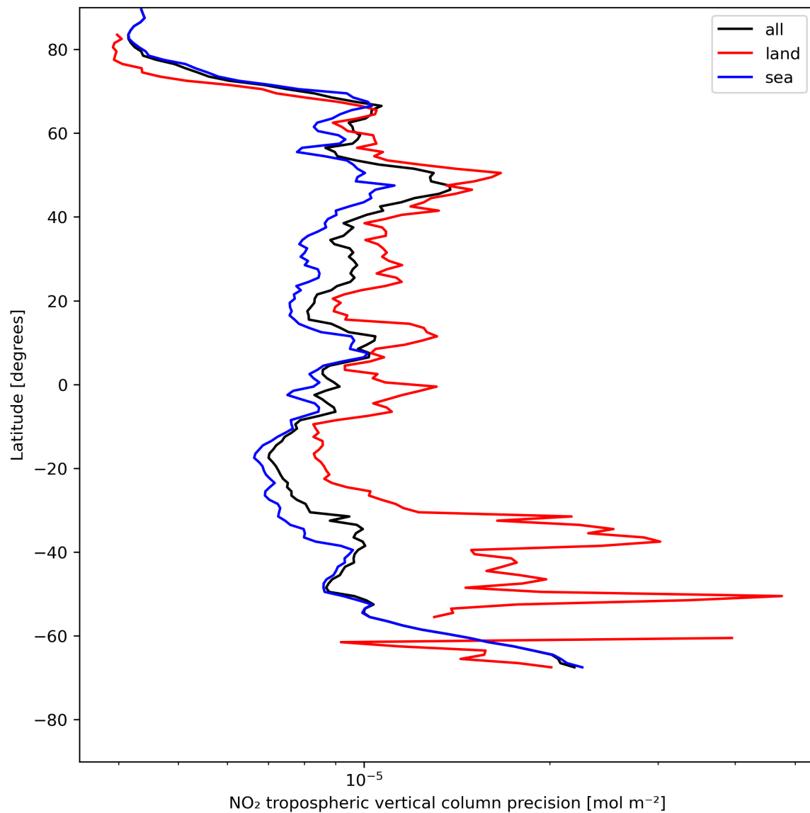
Figure 13: Zonal average of “NO 2 tropospheric vertical column precision” for 2024-05-20 to 2024-05-22.
