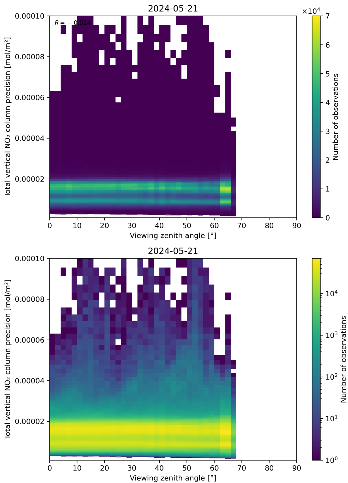
Figure 168: Scatter density plot of “Viewing zenith angle” against “Total vertical NO 2 column precision” for 2024-05-20 to 2024-05-22.
