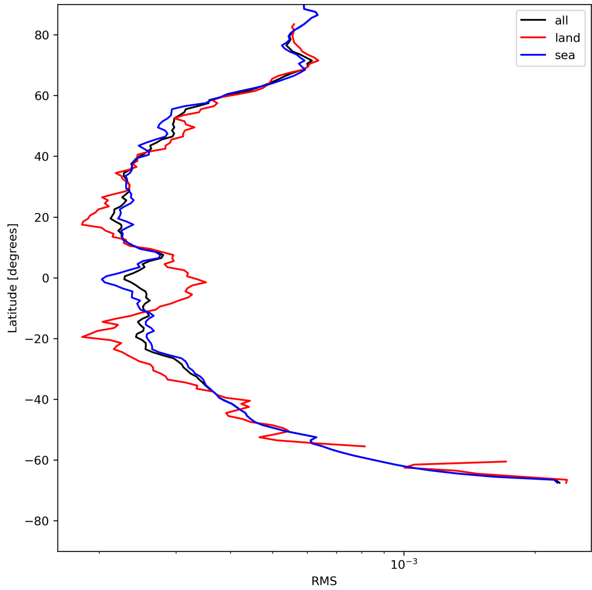
Figure 26: Zonal average of “RMS” for 2024-05-20 to 2024-05-22.
