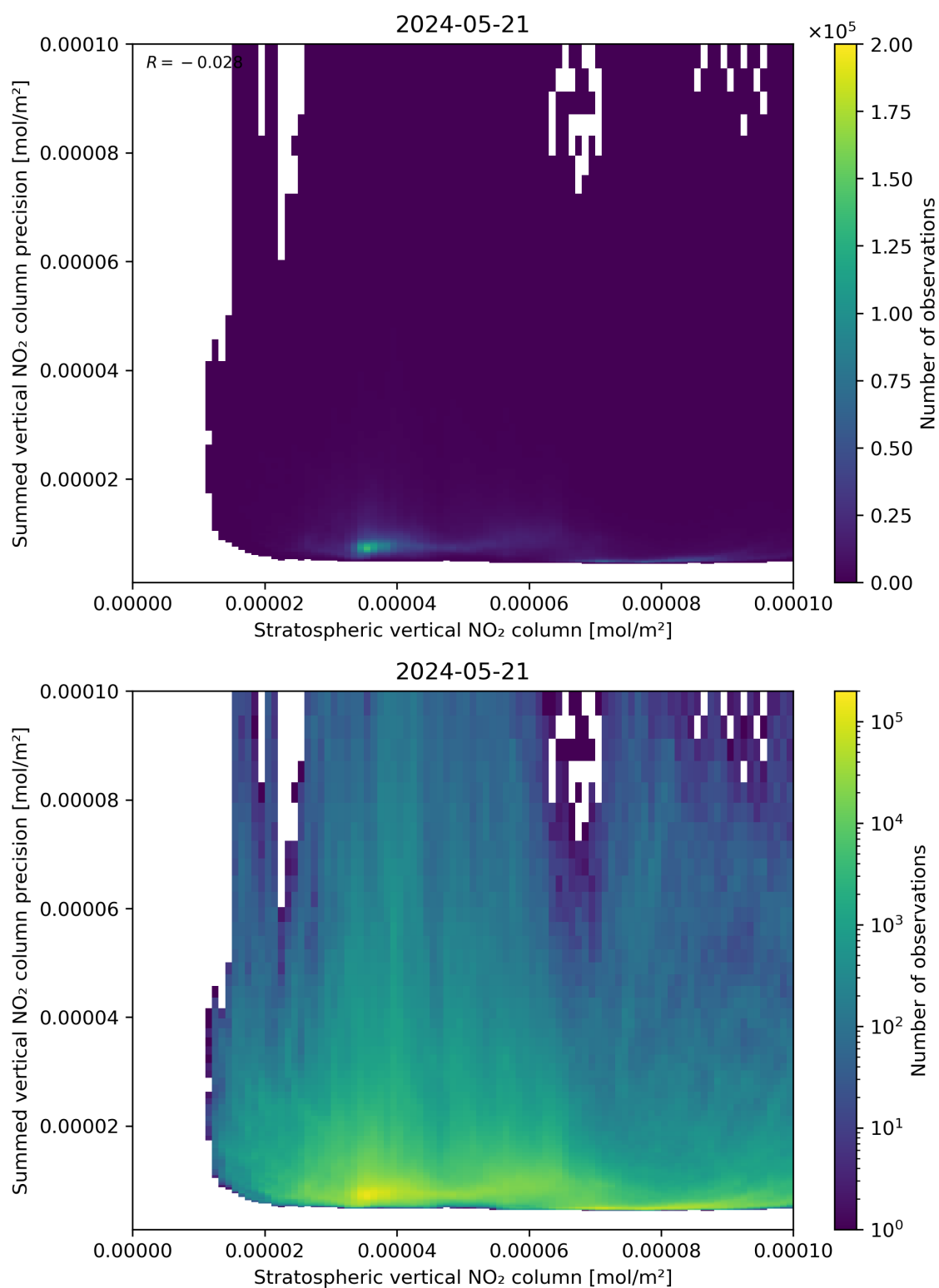
Figure 99: Scatter density plot of “Stratospheric vertical NO 2 column” against “Summed vertical NO 2 column precision” for 2024-05-20 to 2024-05-22.
