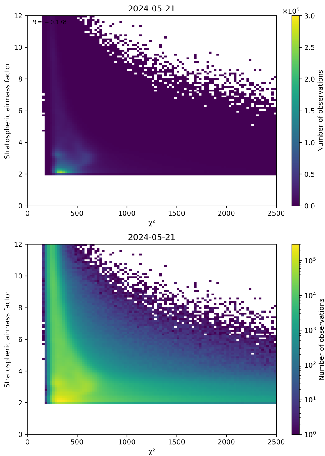
Figure 81: Scatter density plot of “ \chi^2 ” against “Stratospheric airmass factor” for 2024-05-20 to 2024-05-22.
