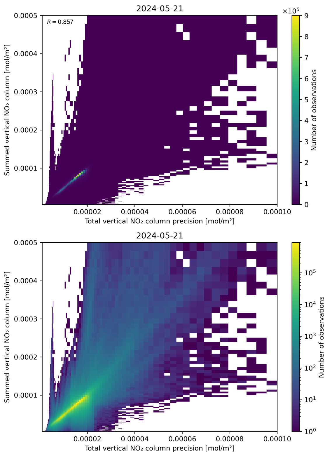
Figure 117: Scatter density plot of “Total vertical NO 2 column precision” against “Summed vertical NO 2 column” for 2024-05-20 to 2024-05-22.
