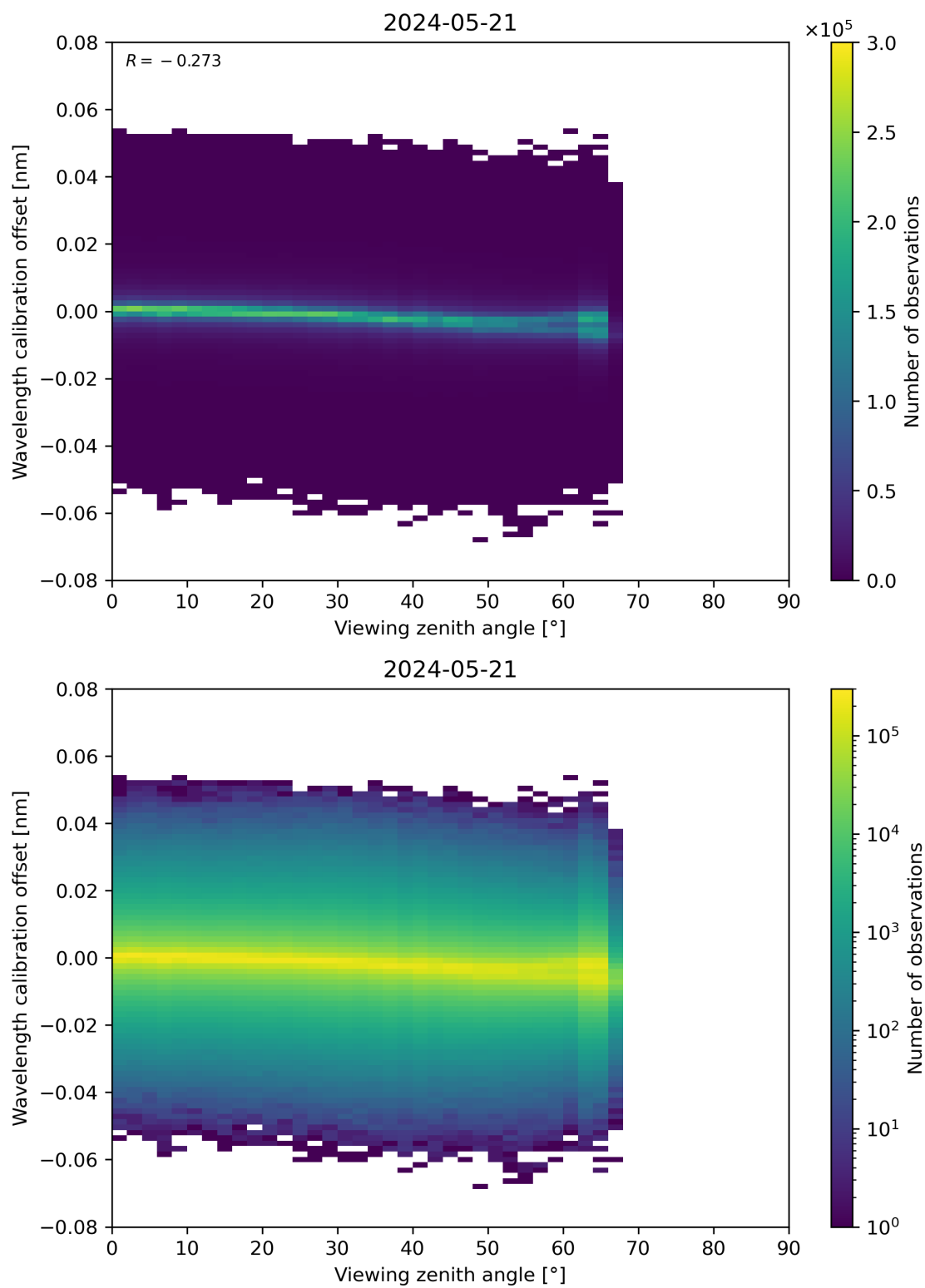
Figure 173: Scatter density plot of “Viewing zenith angle” against “Wavelength calibration offset” for 2024-05-20 to 2024-05-22.
