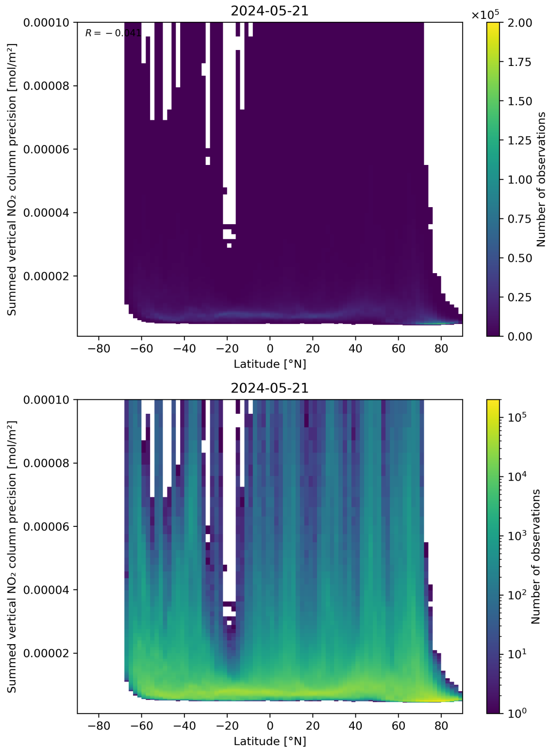
Figure 89: Scatter density plot of “Latitude” against “Summed vertical NO 2 column precision” for 2024-05-20 to 2024-05-22.
