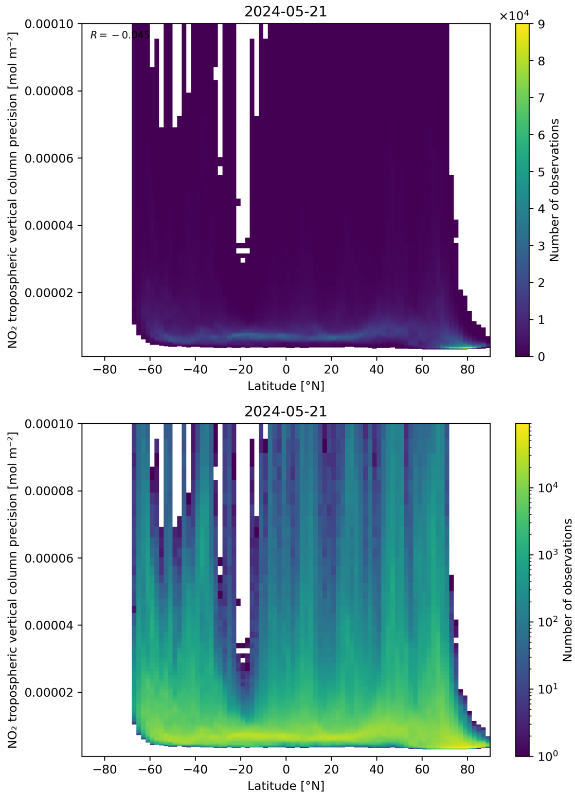
Figure 93: Scatter density plot of “Latitude” against “NO 2 tropospheric vertical column precision” for 2024-05-20 to 2024-05-22.
