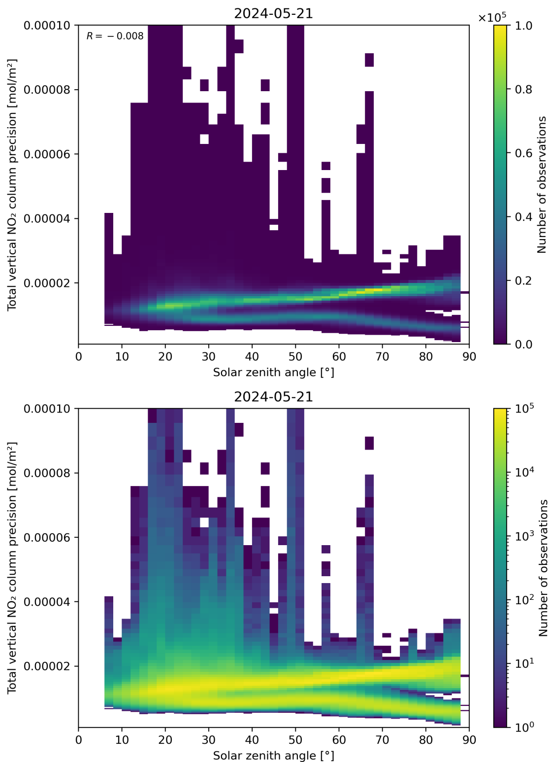
Figure 154: Scatter density plot of “Solar zenith angle” against “Total vertical NO 2 column precision” for 2024-05-20 to 2024-05-22.
