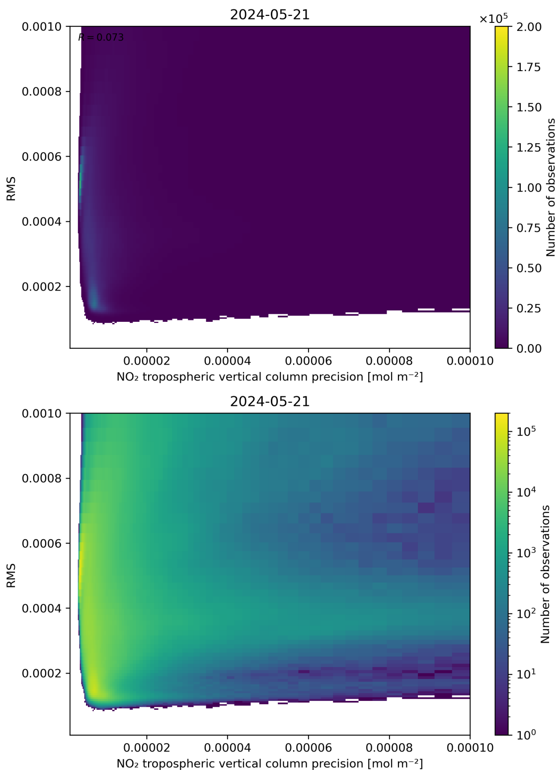
Figure 140: Scatter density plot of “NO 2 tropospheric vertical column precision” against “RMS” for 2024-05-20 to 2024-05-22.
