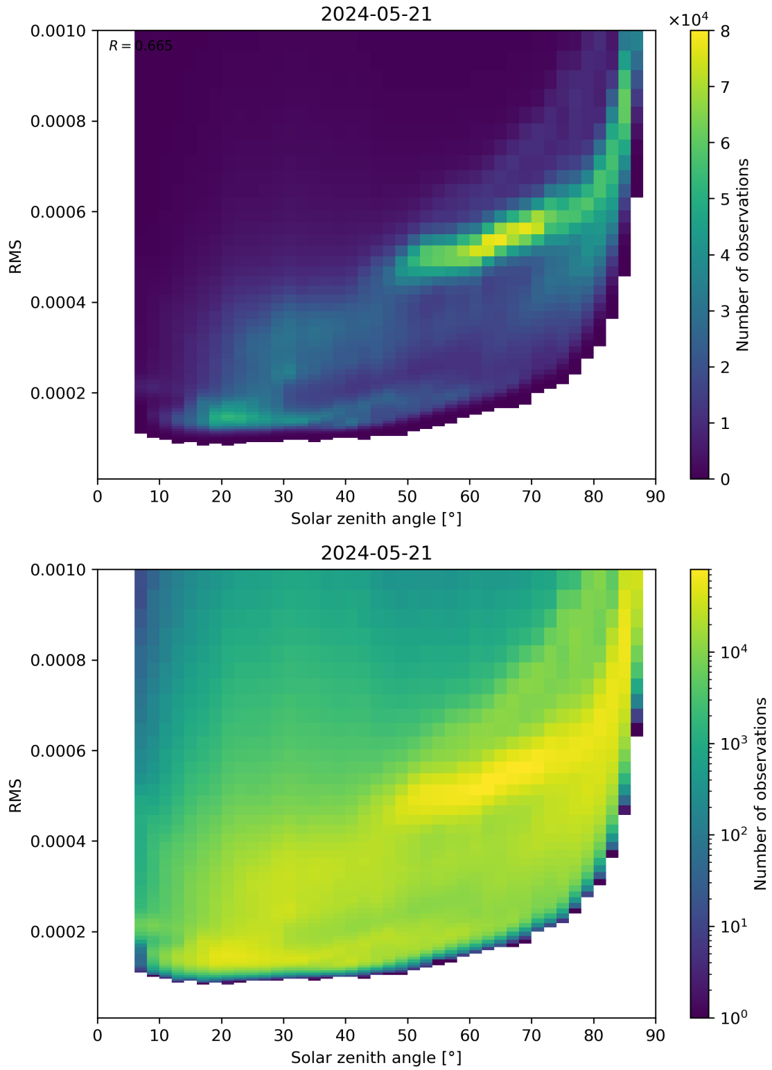
Figure 157: Scatter density plot of “Solar zenith angle” against “RMS” for 2024-05-20 to 2024-05-22.
