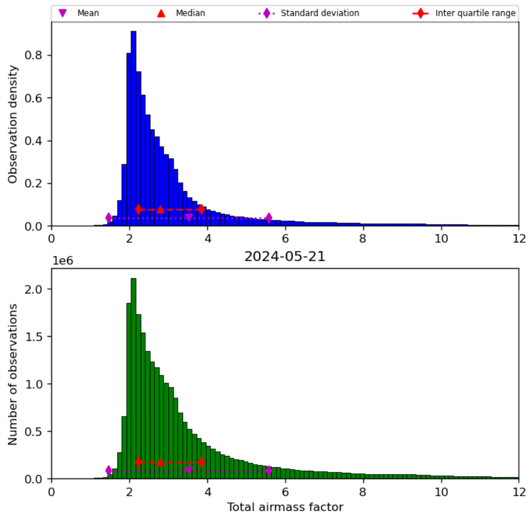
Figure 32: Histogram of “Total airmass factor” for 2024-05-20 to 2024-05-22
