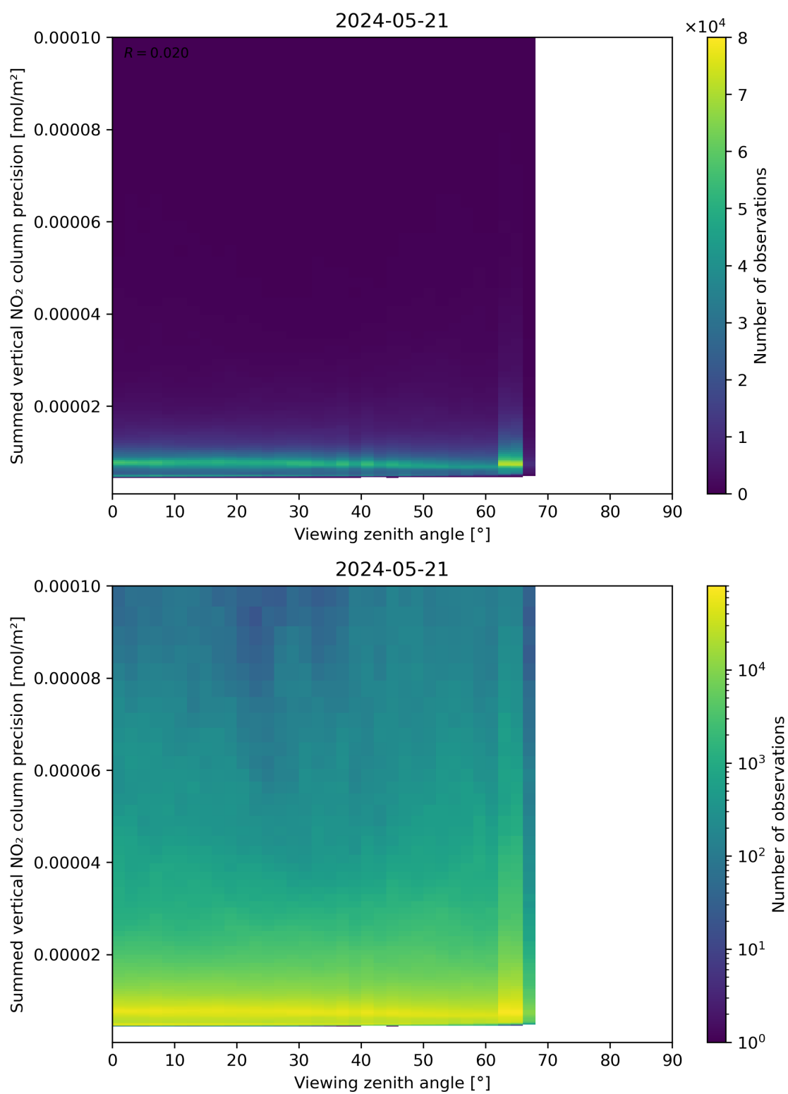
Figure 166: Scatter density plot of “Viewing zenith angle” against “Summed vertical NO 2 column precision” for 2024-05-20 to 2024-05-22.
