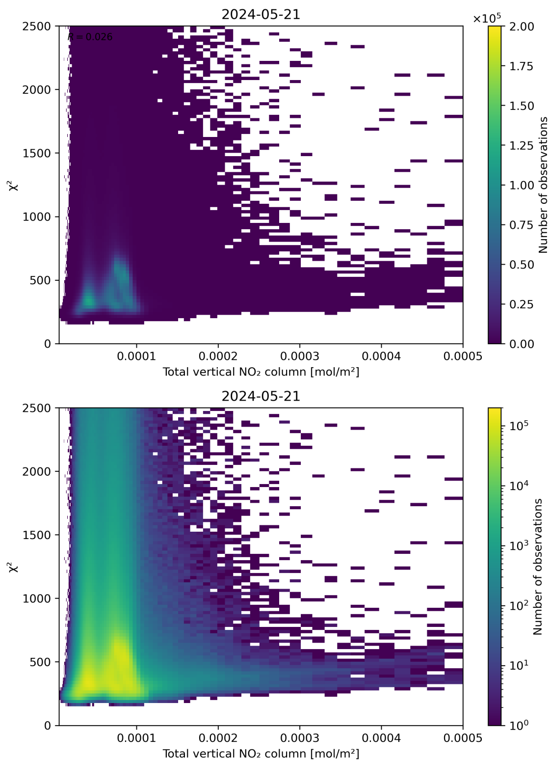
Figure 111: Scatter density plot of “Total vertical NO 2 column” against “ \chi^2 ” for 2024-05-20 to 2024-05-22.
