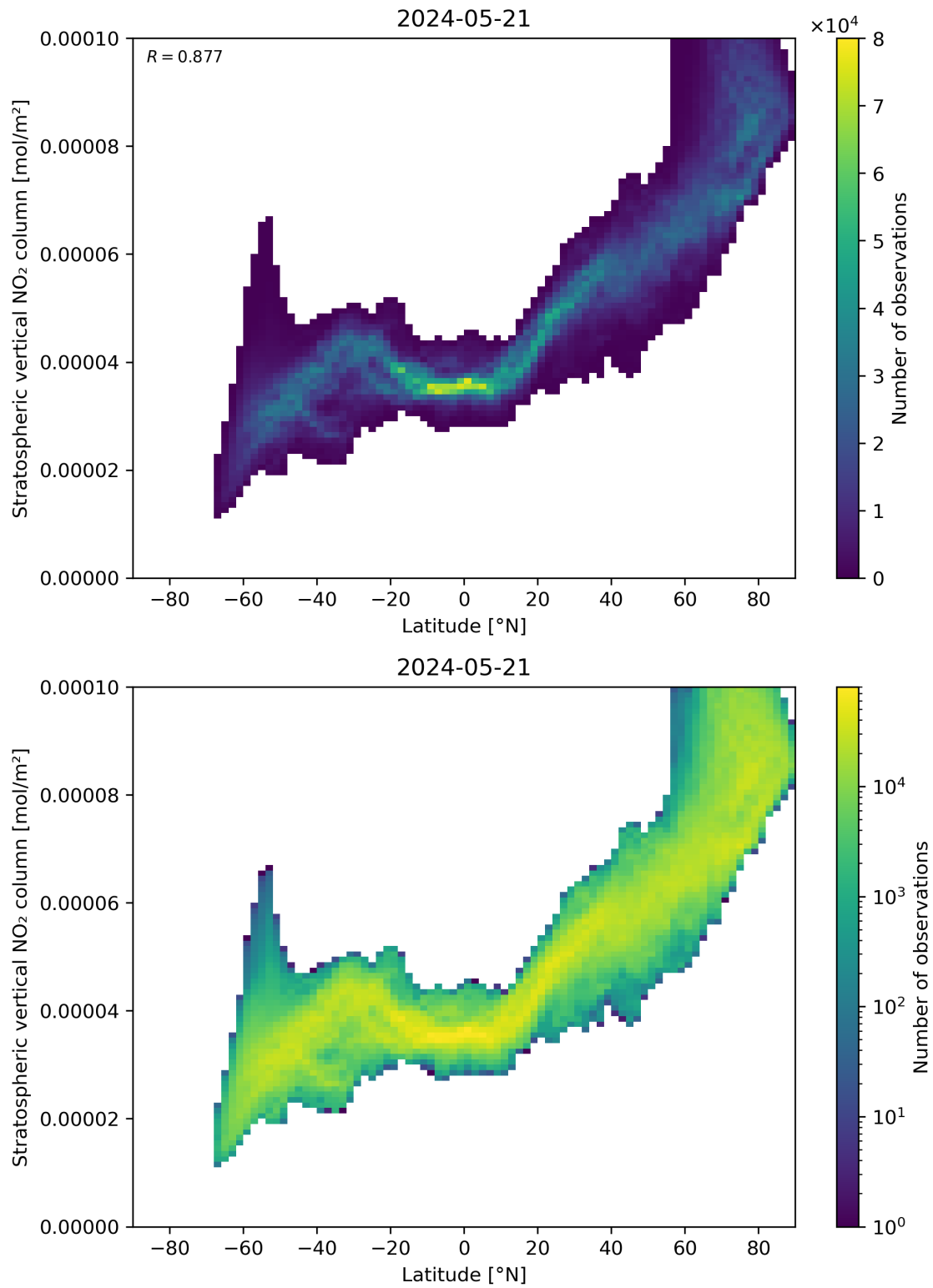
Figure 87: Scatter density plot of “Latitude” against “Stratospheric vertical NO 2 column” for 2024-05-20 to 2024-05-22.
