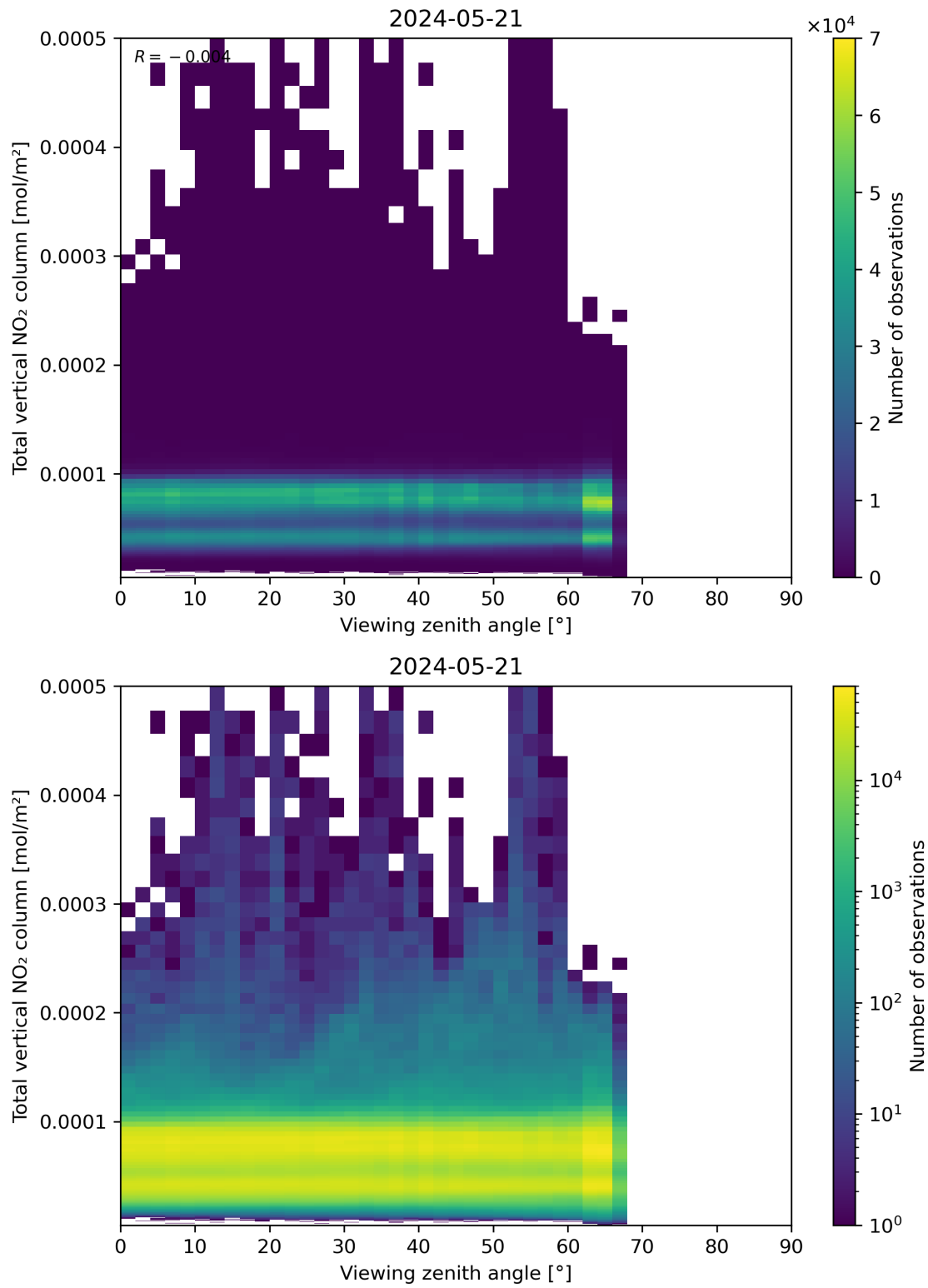
Figure 167: Scatter density plot of “Viewing zenith angle” against “Total vertical NO 2 column” for 2024-05-20 to 2024-05-22.
