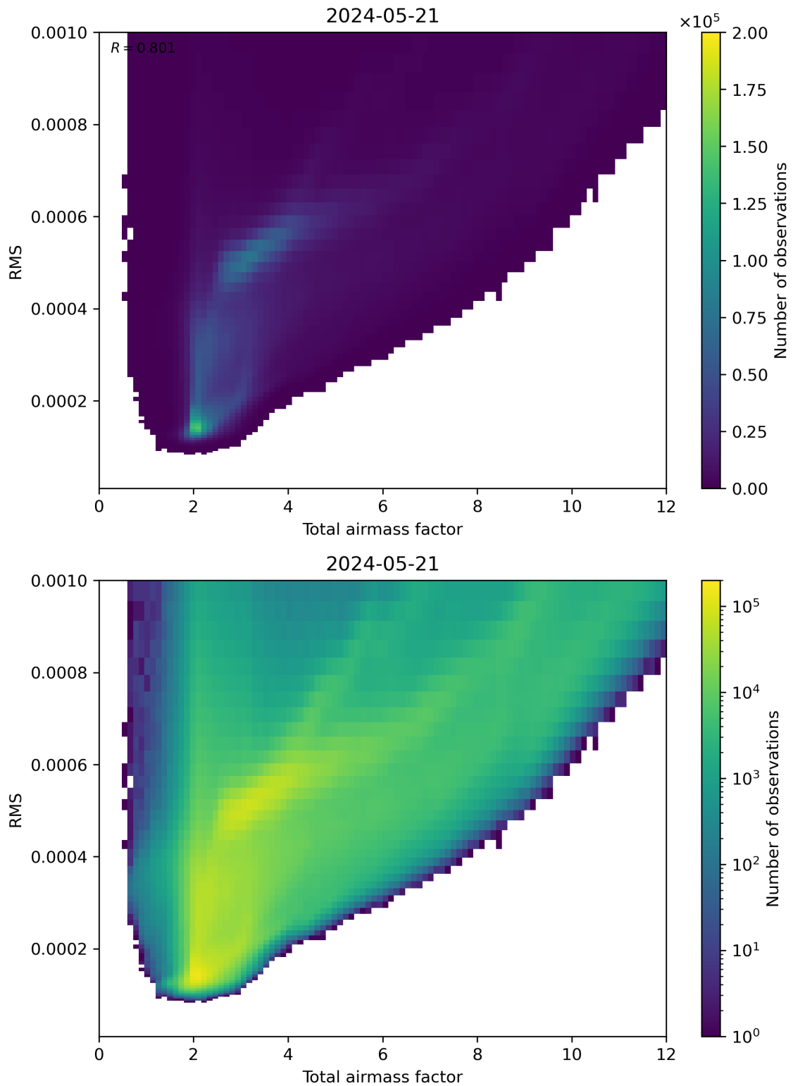
Figure 69: Scatter density plot of “Total airmass factor” against “RMS” for 2024-05-20 to 2024-05-22.
