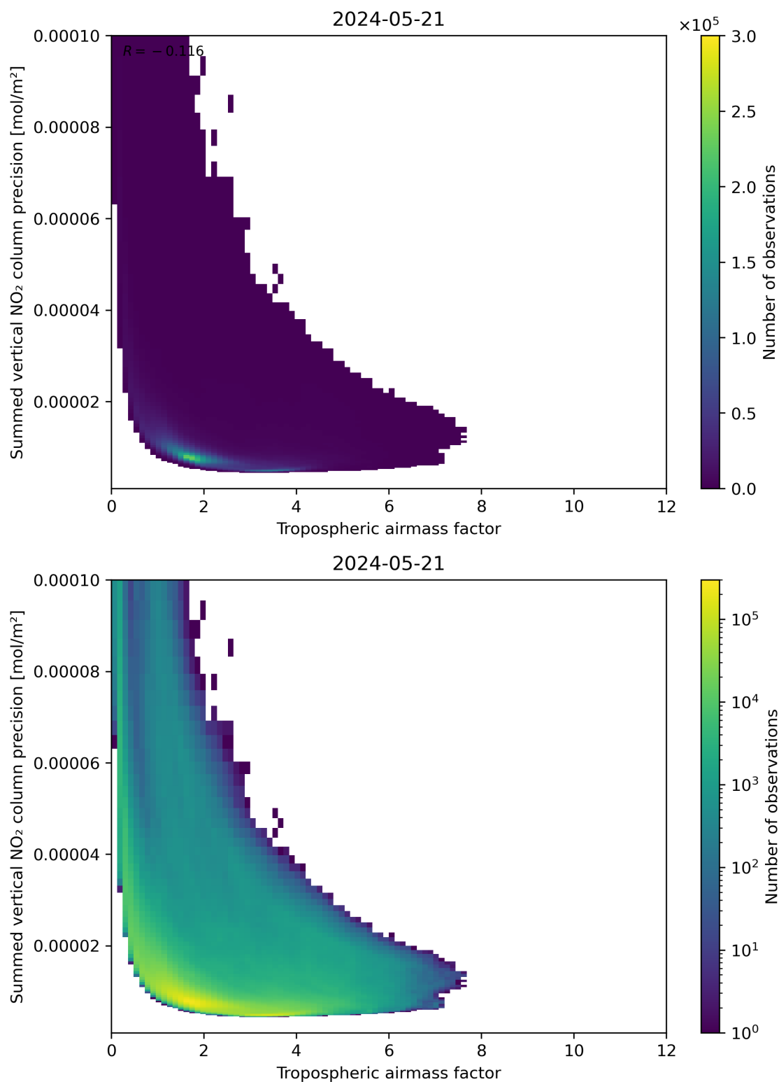
Figure 76: Scatter density plot of “Tropospheric air mass factor” against “Summed vertical NO 2 column precision” for 2024-05-20 to 2024-05-22.
