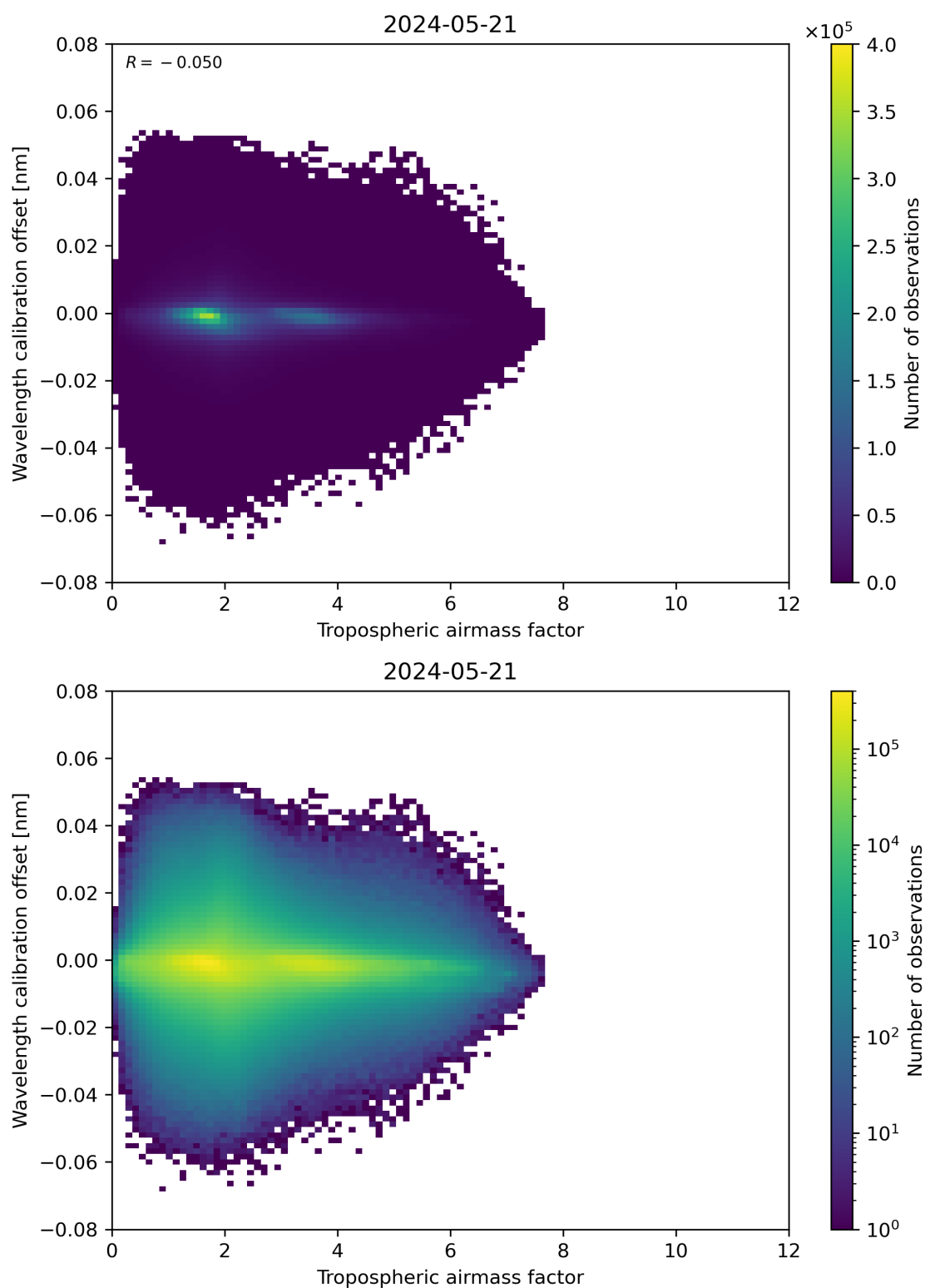
Figure 80: Scatter density plot of “Tropospheric airmass factor” against “Wavelength calibration offset” for 2024-05-20 to 2024-05-22.
