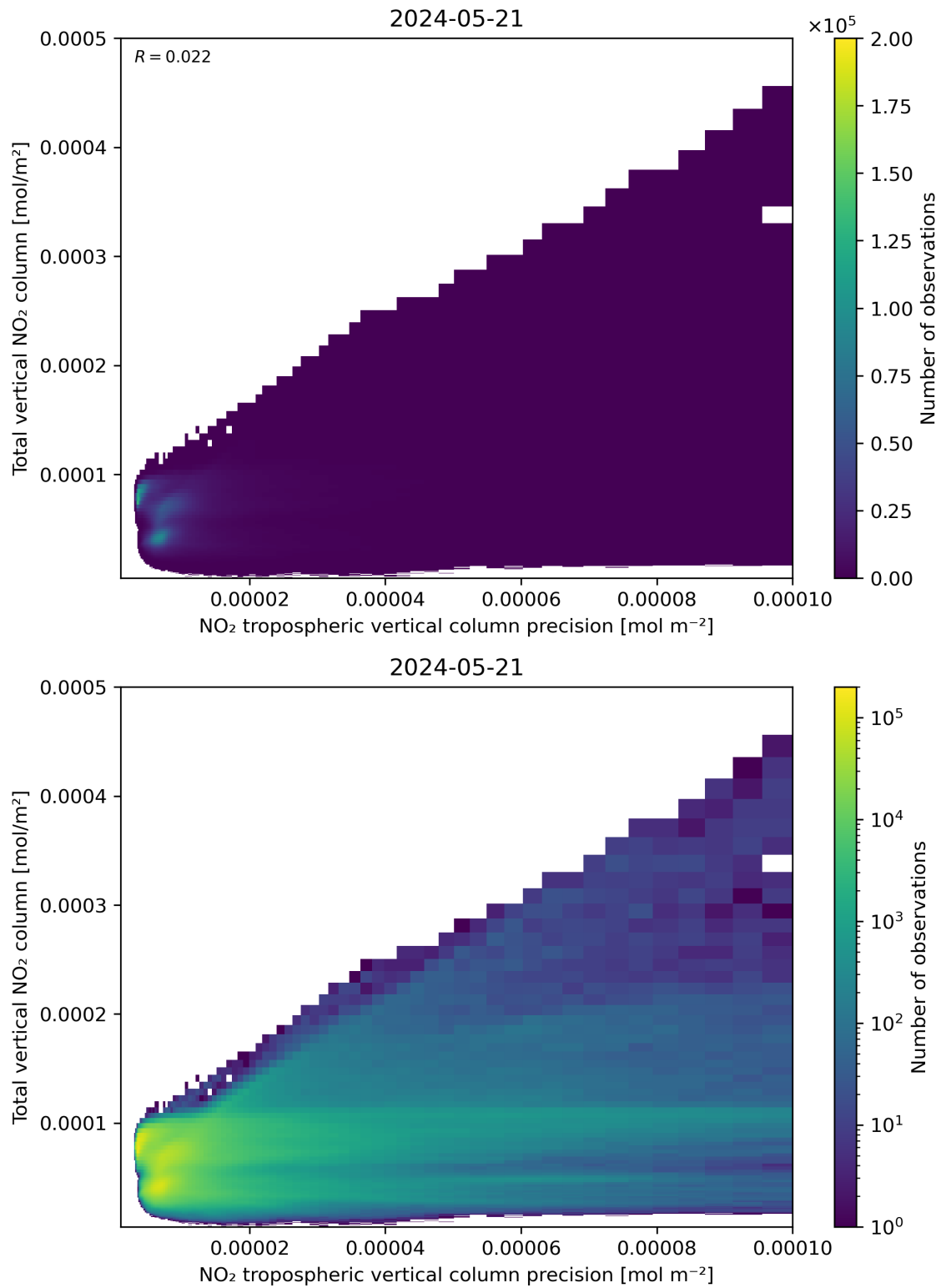
Figure 138: Scatter density plot of “NO 2 tropospheric vertical column precision” against “Total vertical NO 2 column” for 2024-05-20 to 2024-05-22.
