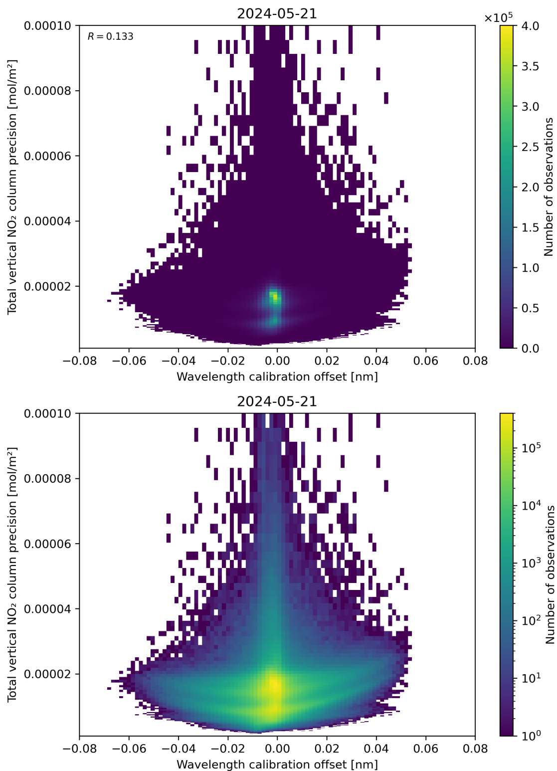
Figure 180: Scatter density plot of “Wavelength calibration offset” against “Total vertical NO 2 column precision” for 2024-05-20 to 2024-05-22.
