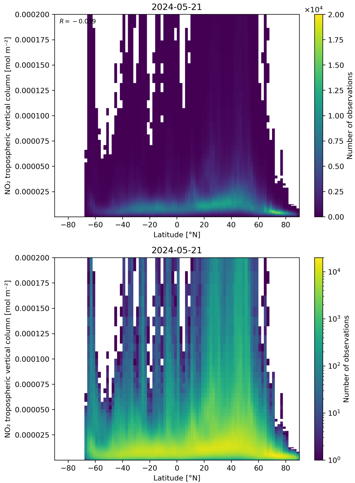
Figure 92: Scatter density plot of “Latitude” against “NO 2 tropospheric vertical column” for 2024-05-20 to 2024-05-22.
