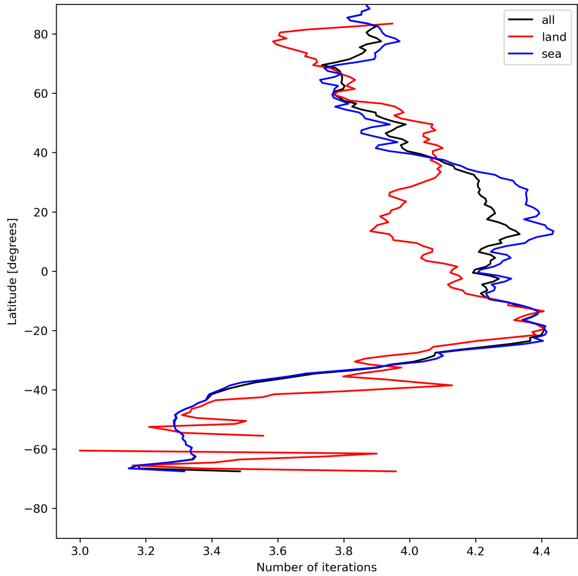
Figure 17: Zonal average of “Number of iterations” for 2024-05-20 to 2024-05-22.
