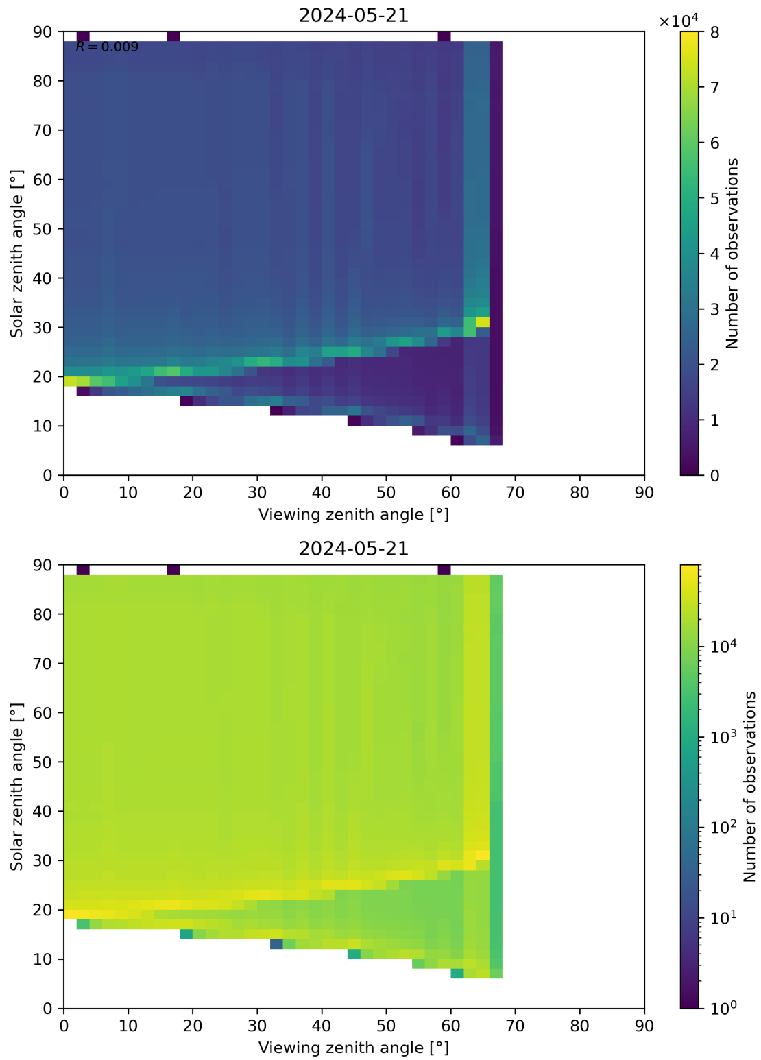
Figure 172: Scatter density plot of “Viewing zenith angle” against “Solar zenith angle” for 2024-05-20 to 2024-05-22.
