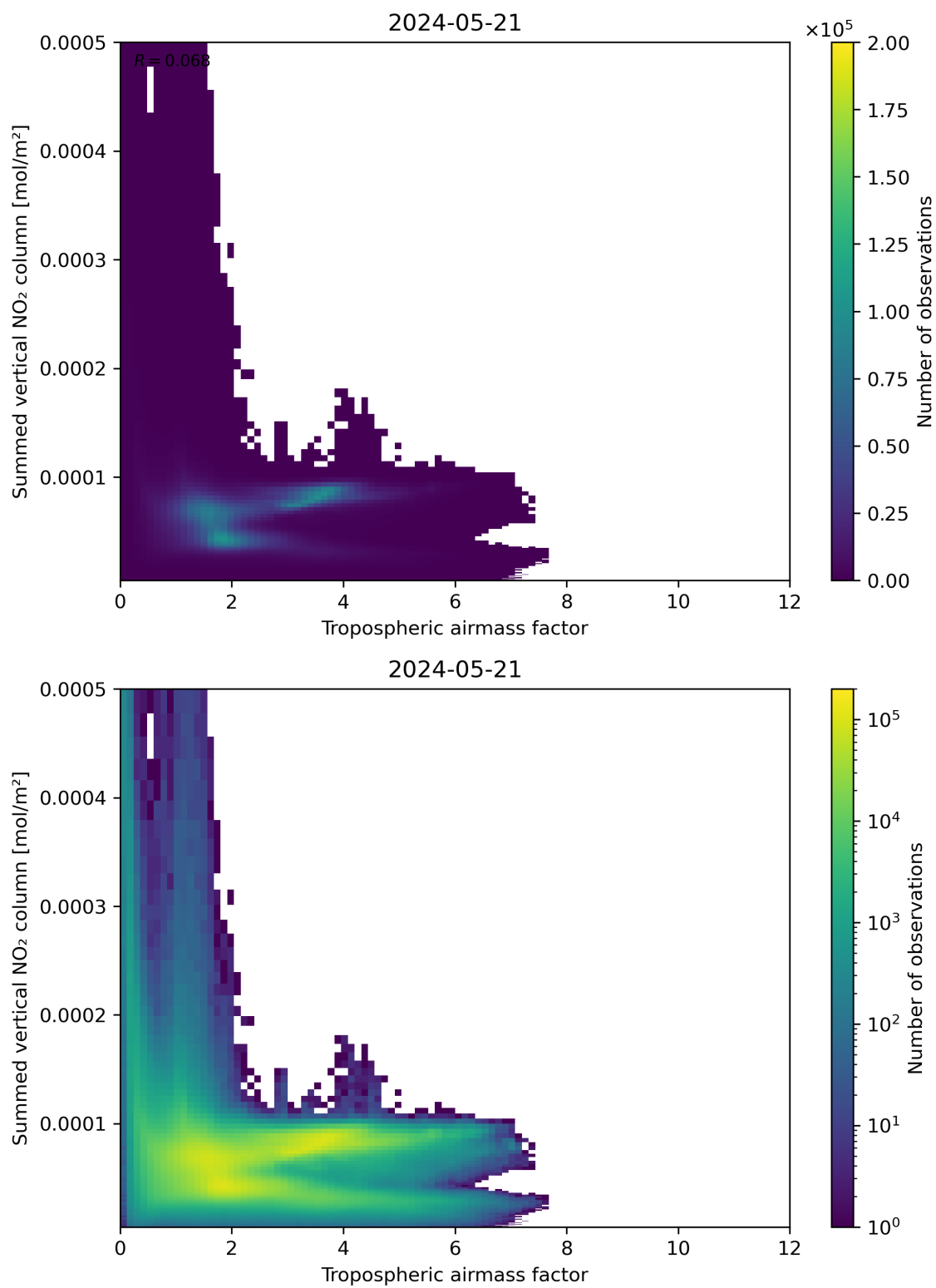
Figure 75: Scatter density plot of “Tropospheric airmass factor” against “Summed vertical NO 2 column” for 2024-05-20 to 2024-05-22.
