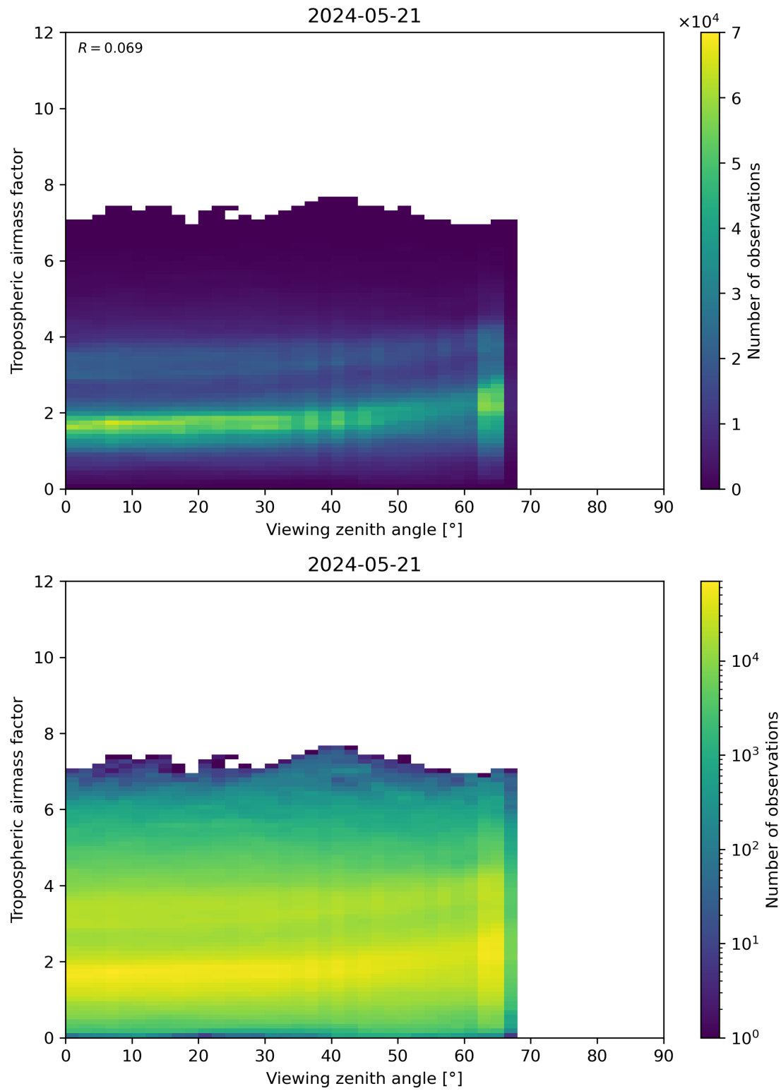
Figure 161: Scatter density plot of “Viewing zenith angle” against “Tropospheric airmass factor” for 2024-05-20 to 2024-05-22.
