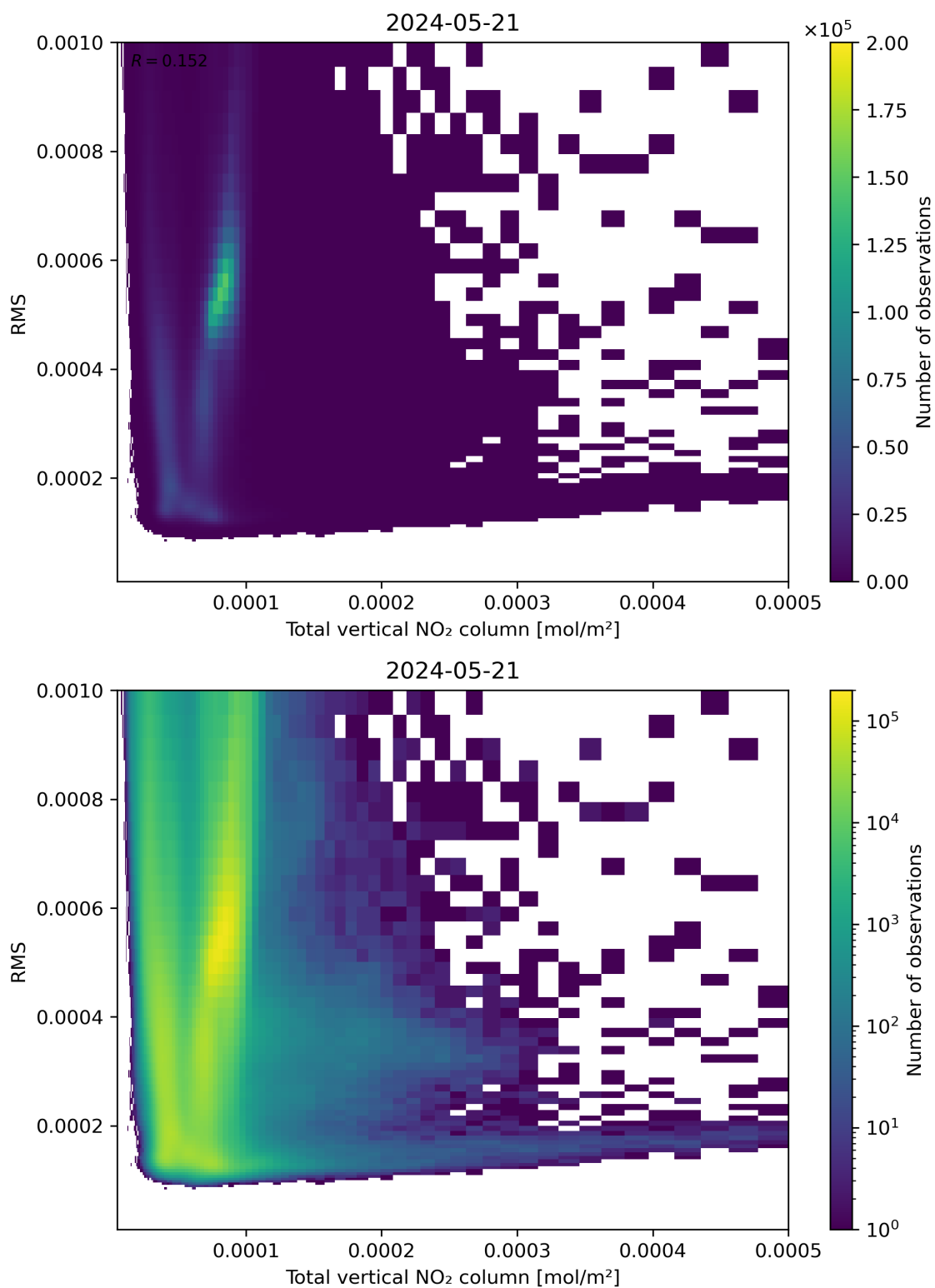
Figure 120: Scatter density plot of “Total vertical NO 2 column” against “RMS” for 2024-05-20 to 2024-05-22.
