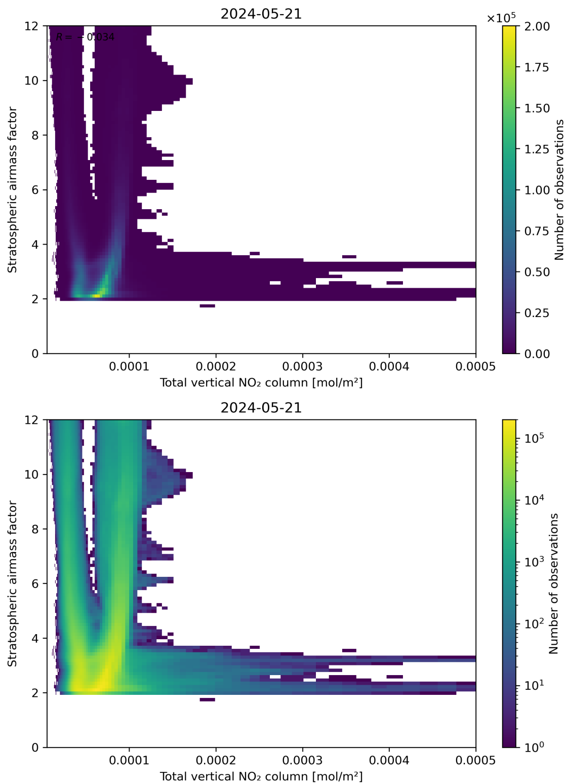
Figure 110: Scatter density plot of “Total vertical NO 2 column” against “Stratospheric airmass factor” for 2024-05-20 to 2024-05-22.
