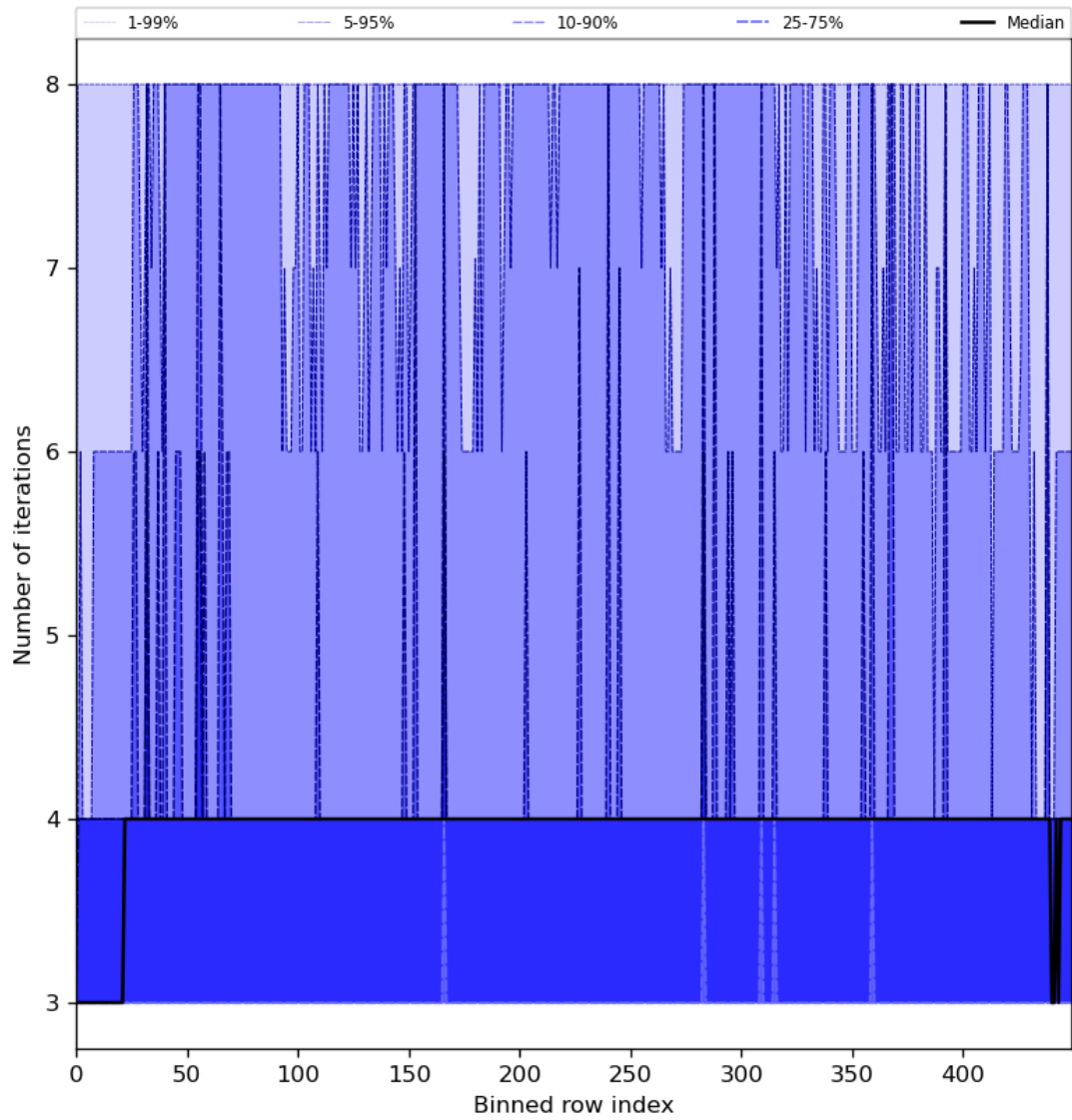
Figure 51: Along track statistics of “Number of iterations” for 2024-05-20 to 2024-05-22
