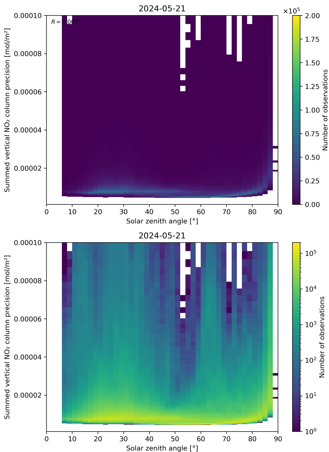
Figure 152: Scatter density plot of “Solar zenith angle” against “Summed vertical NO 2 column precision” for 2024-05-20 to 2024-05-22.
