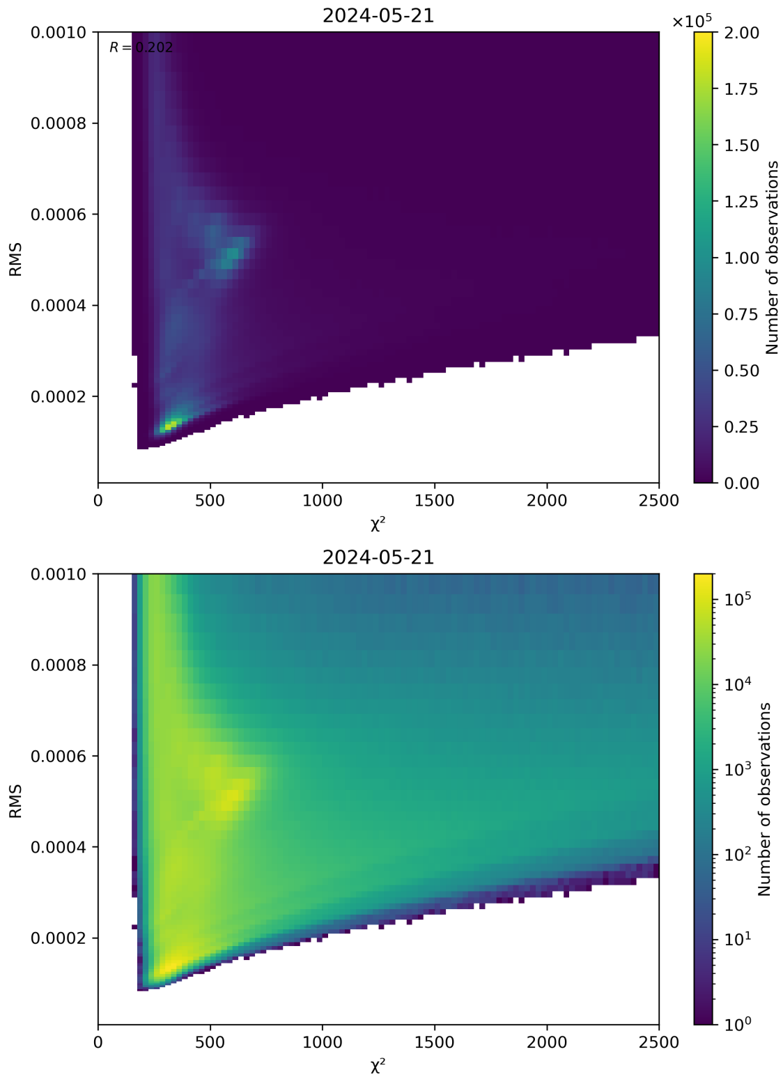
Figure 82: Scatter density plot of “ \chi^2 ” against “RMS” for 2024-05-20 to 2024-05-22.
