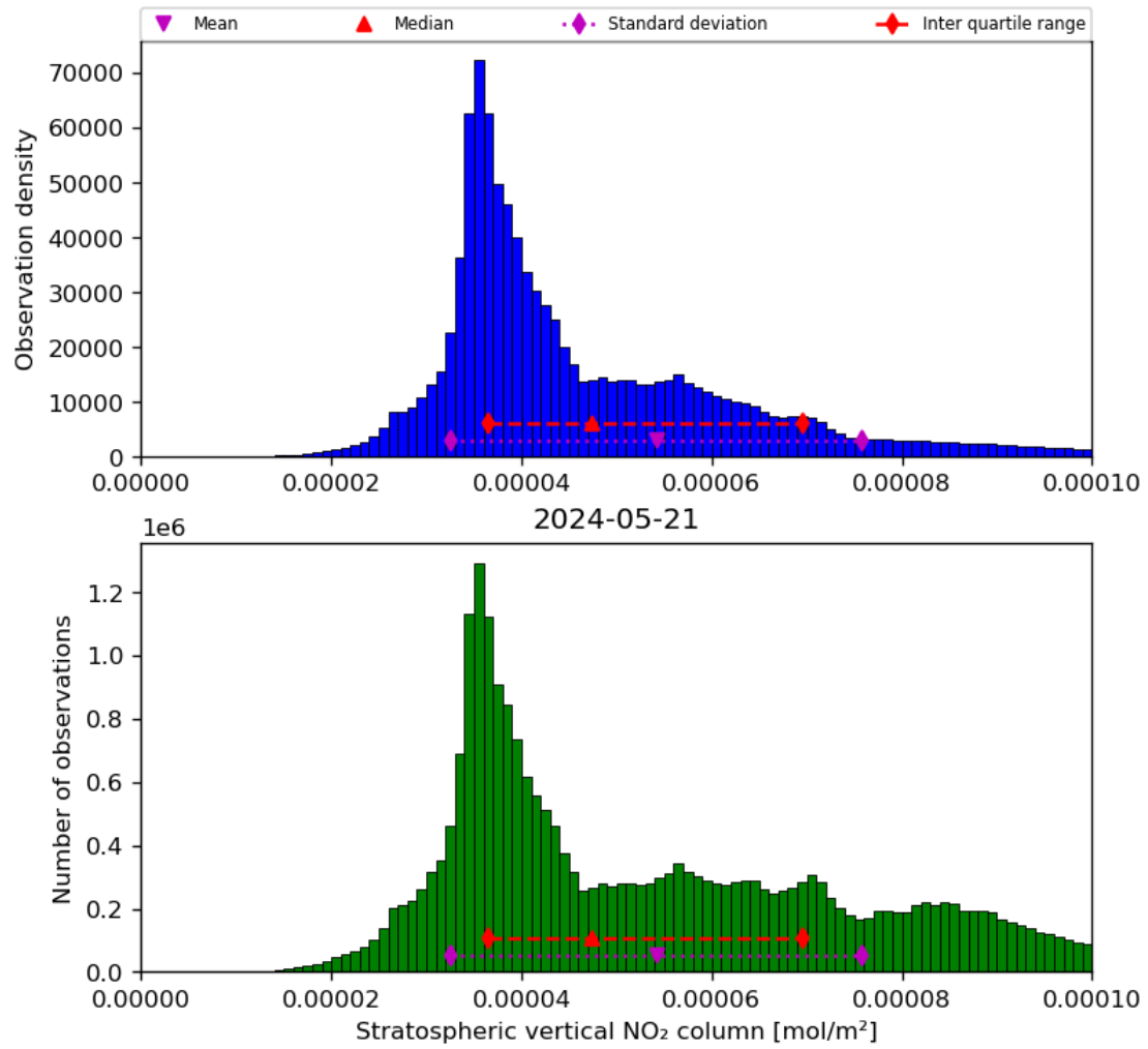
Figure 36: Histogram of “Stratospheric vertical NO 2 column” for 2024-05-20 to 2024-05-22
