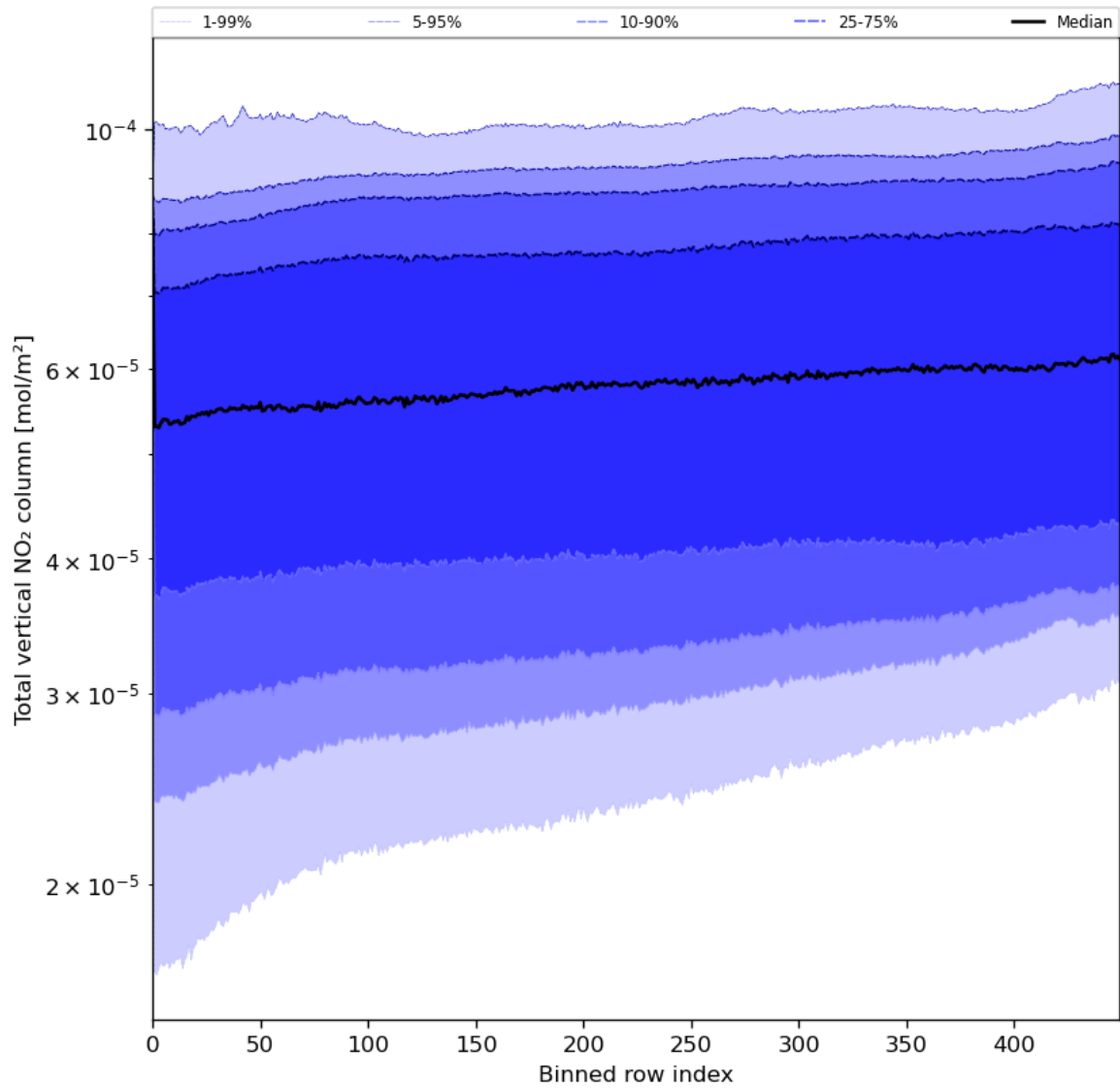
Figure 55: Along track statistics of “Total vertical NO 2 column” for 2024-05-20 to 2024-05-22
