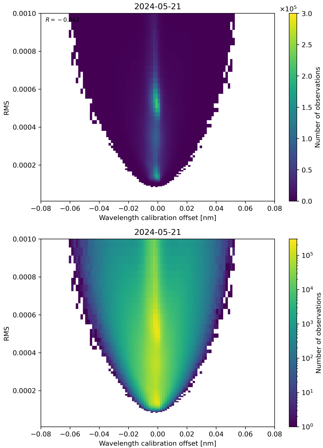
Figure 181: Scatter density plot of “Wavelength calibration offset” against “RMS” for 2024-05-20 to 2024-05-22.
