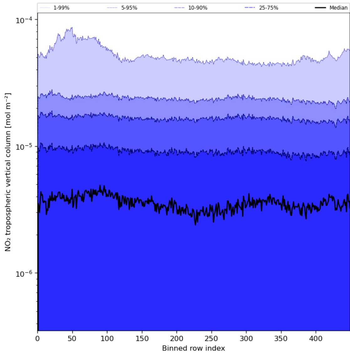
Figure 46: Along track statistics of “NO 2 tropospheric vertical column” for 2024-05-20 to 2024-05-22
