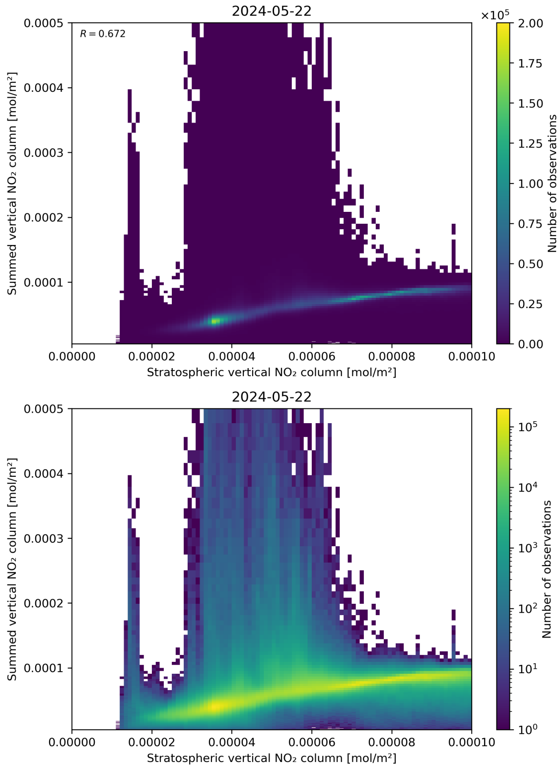
Figure 98: Scatter density plot of “Stratospheric vertical NO 2 column” against “Summed vertical NO 2 column” for 2024-05-21 to 2024-05-23.
