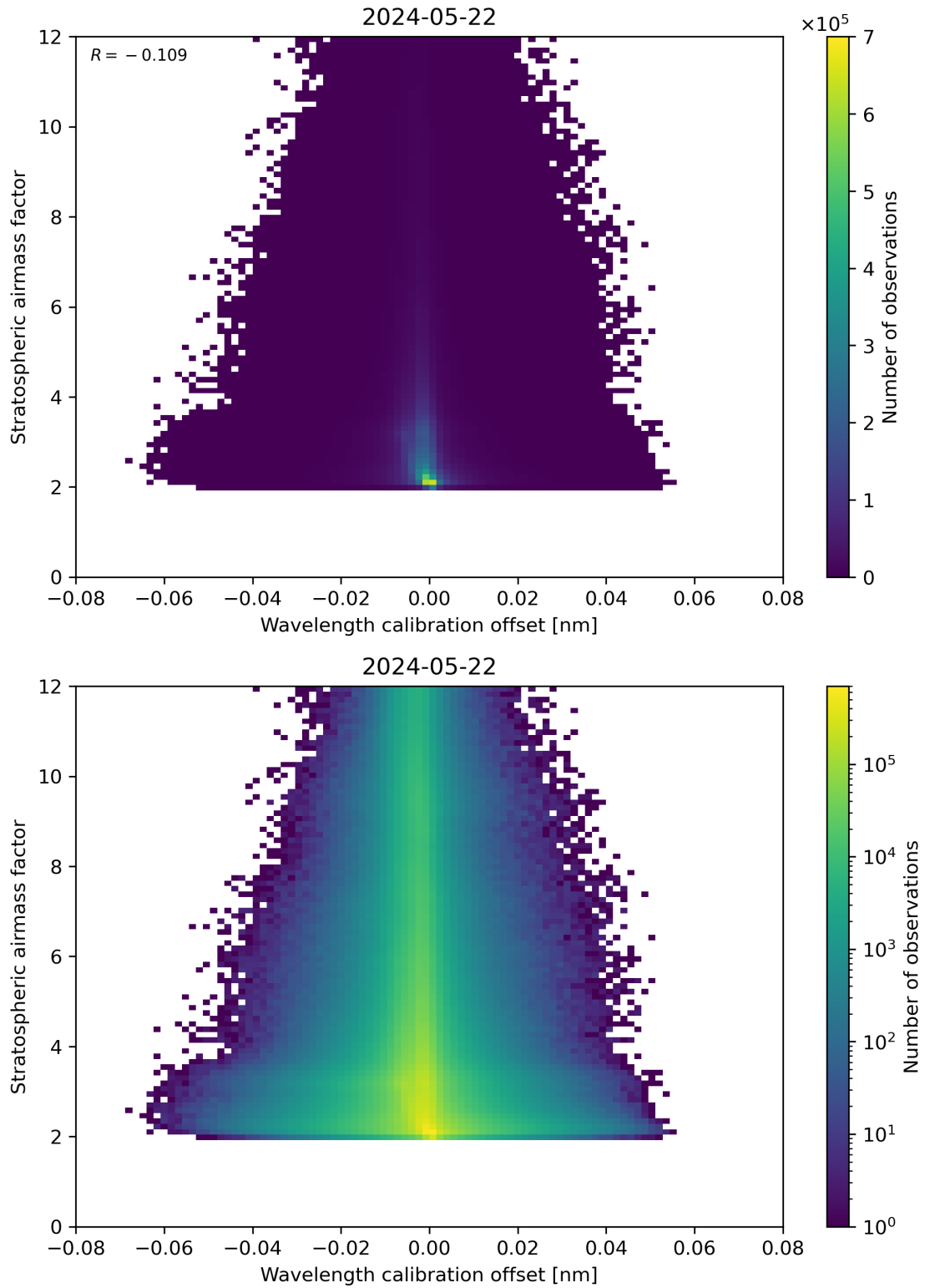
Figure 174: Scatter density plot of “Wavelength calibration offset” against “Stratospheric airmass factor” for 2024-05-21 to 2024-05-23.
