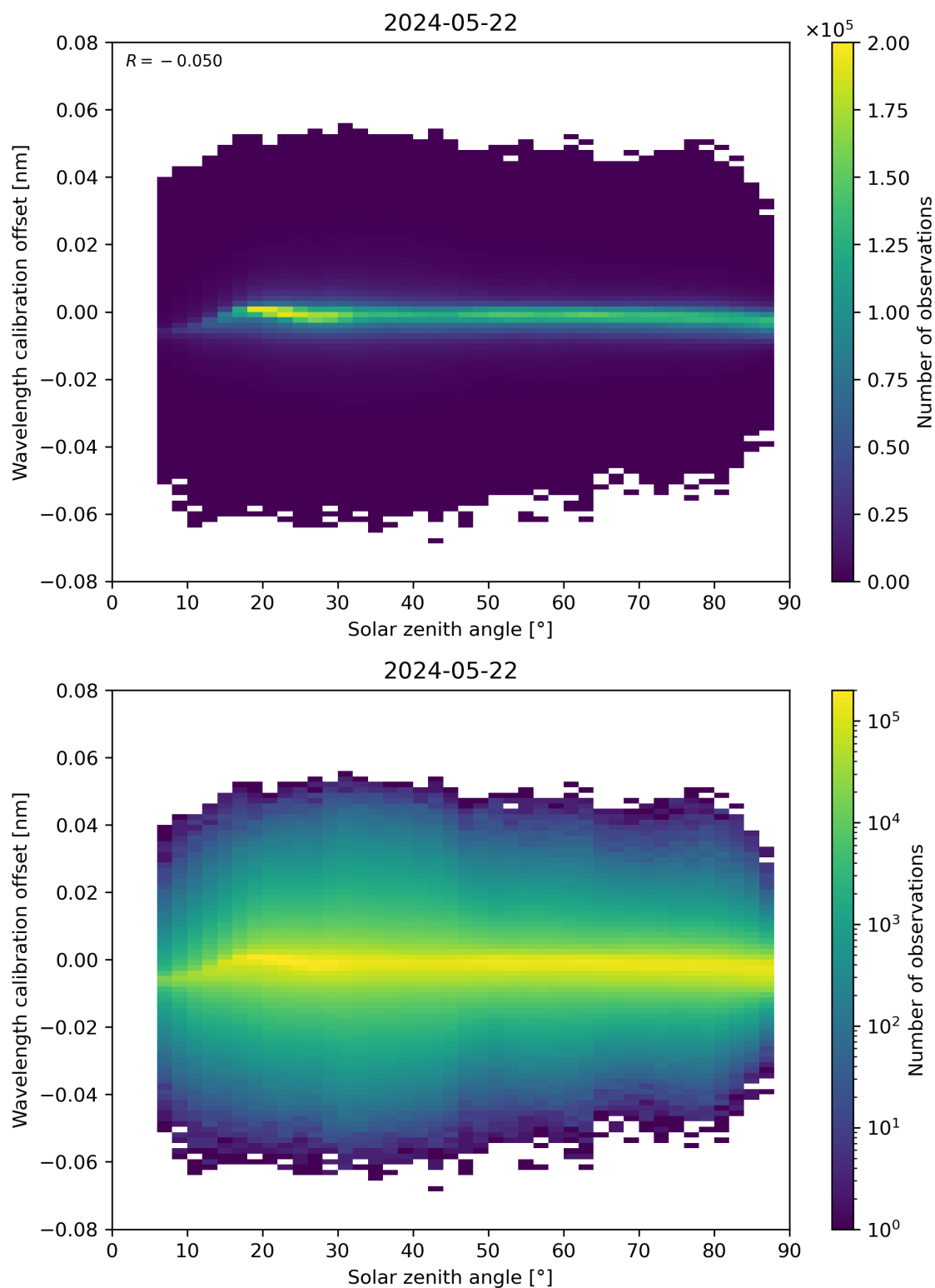
Figure 158: Scatter density plot of “Solar zenith angle” against “Wavelength calibration offset” for 2024-05-21 to 2024-05-23.
