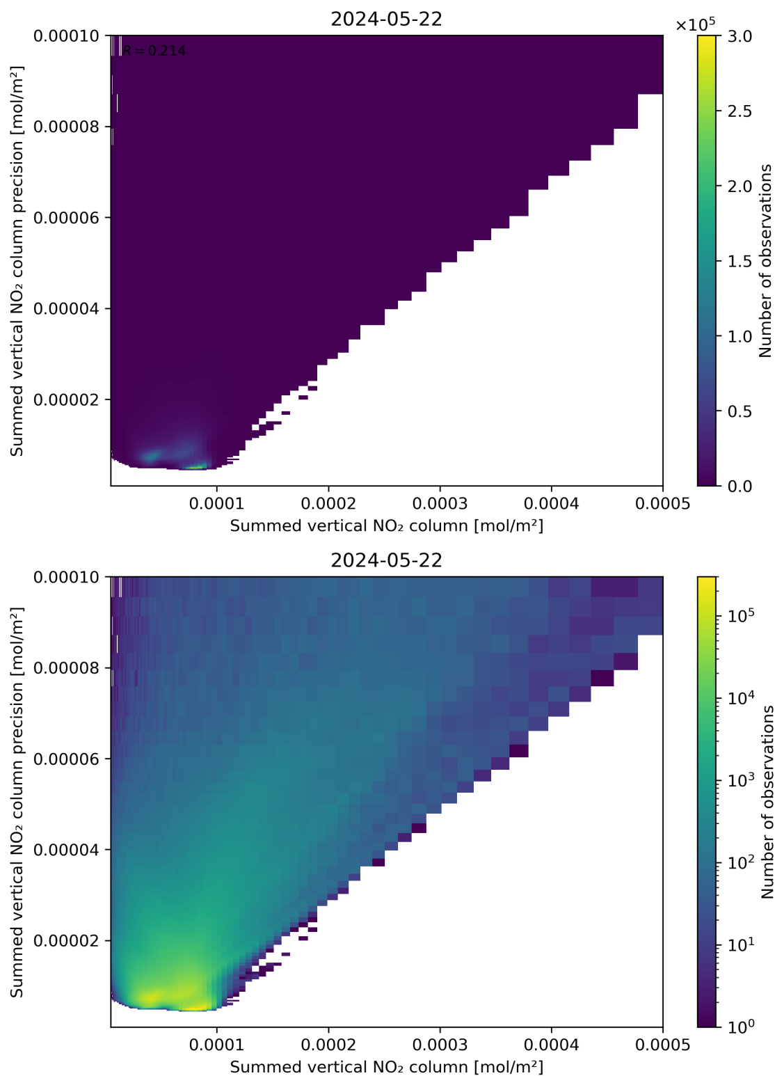
Figure 105: Scatter density plot of “Summed vertical NO 2 column” against “Summed vertical NO 2 column precision” for 2024-05-21 to 2024-05-23.
