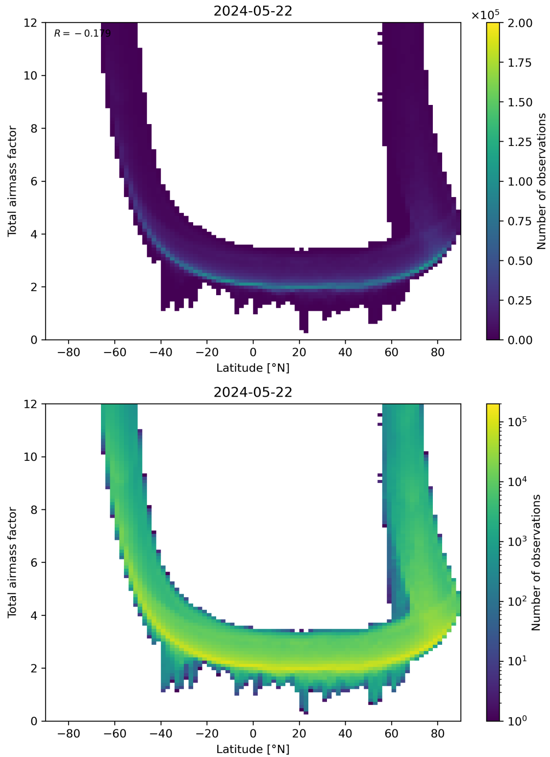
Figure 84: Scatter density plot of “Latitude” against “Total airmass factor” for 2024-05-21 to 2024-05-23.
