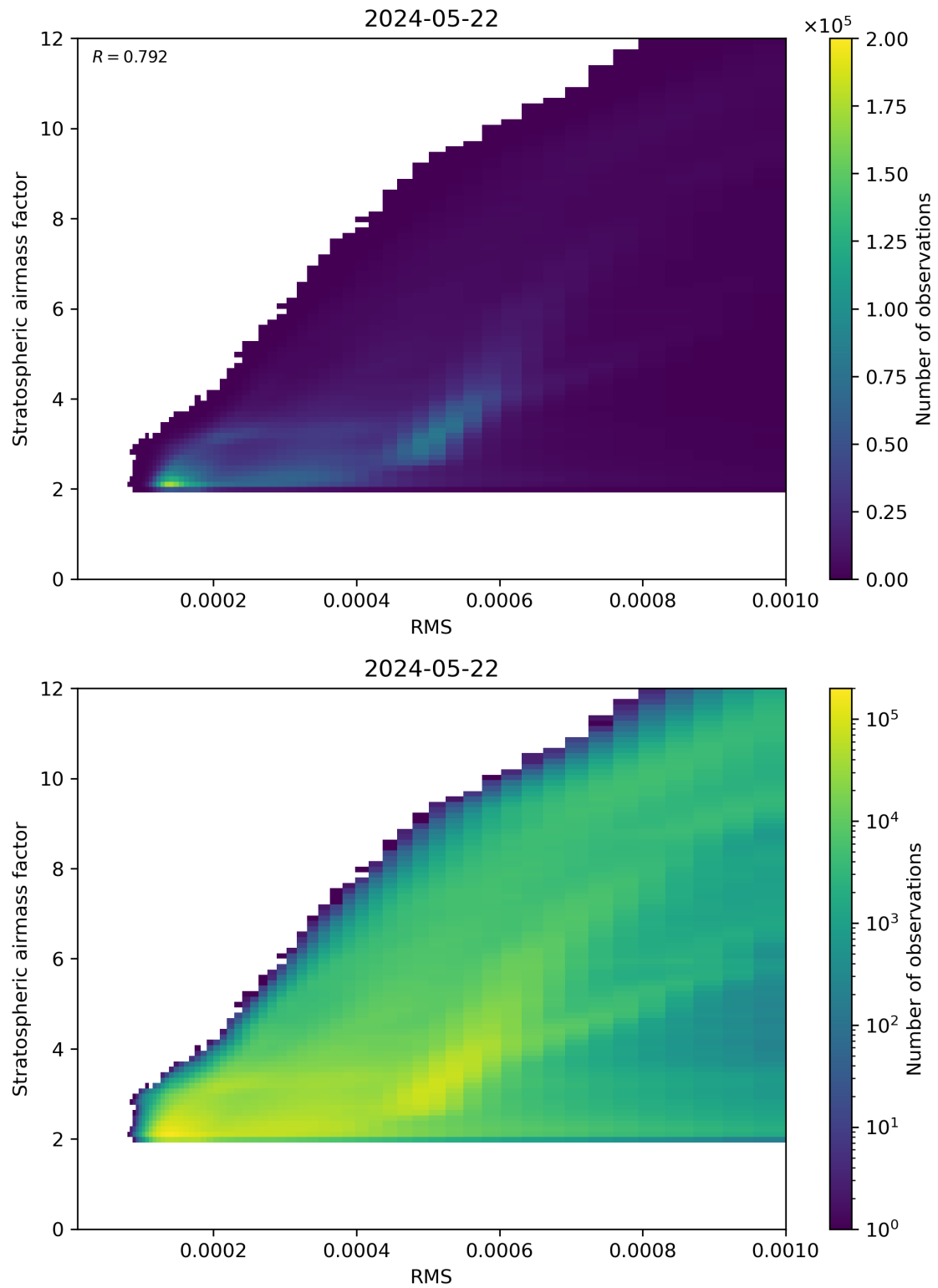
Figure 144: Scatter density plot of “RMS” against “Stratospheric airmass factor” for 2024-05-21 to 2024-05-23.
