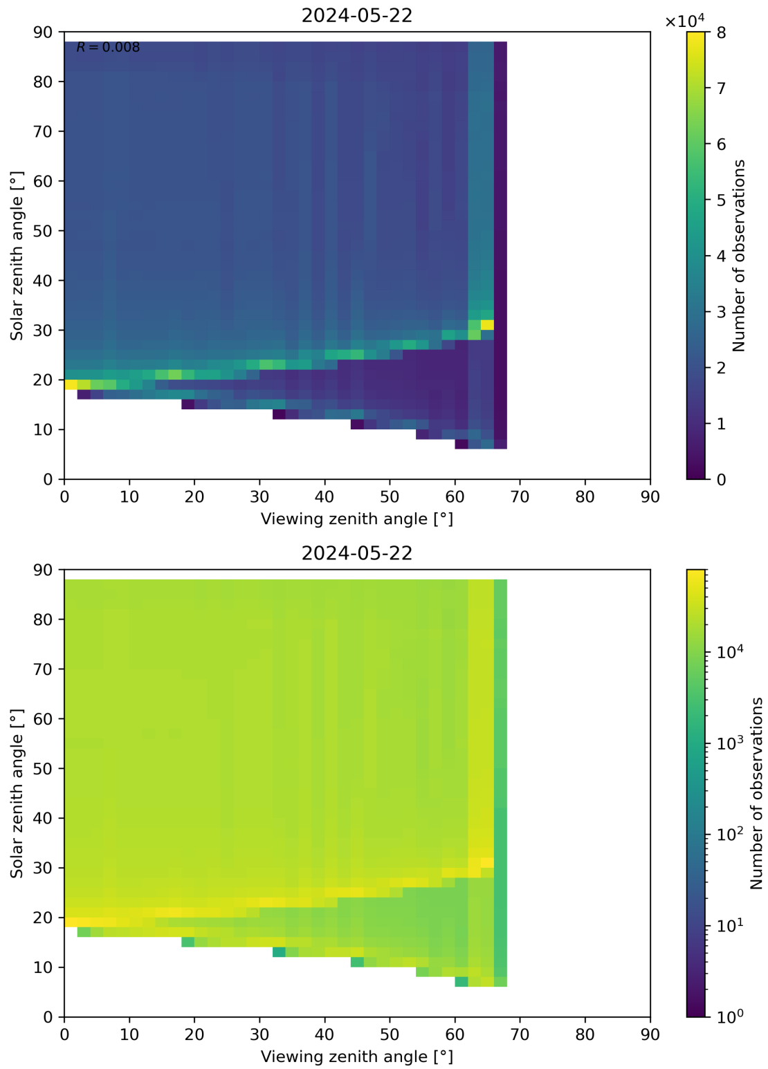
Figure 172: Scatter density plot of “Viewing zenith angle” against “Solar zenith angle” for 2024-05-21 to 2024-05-23.
