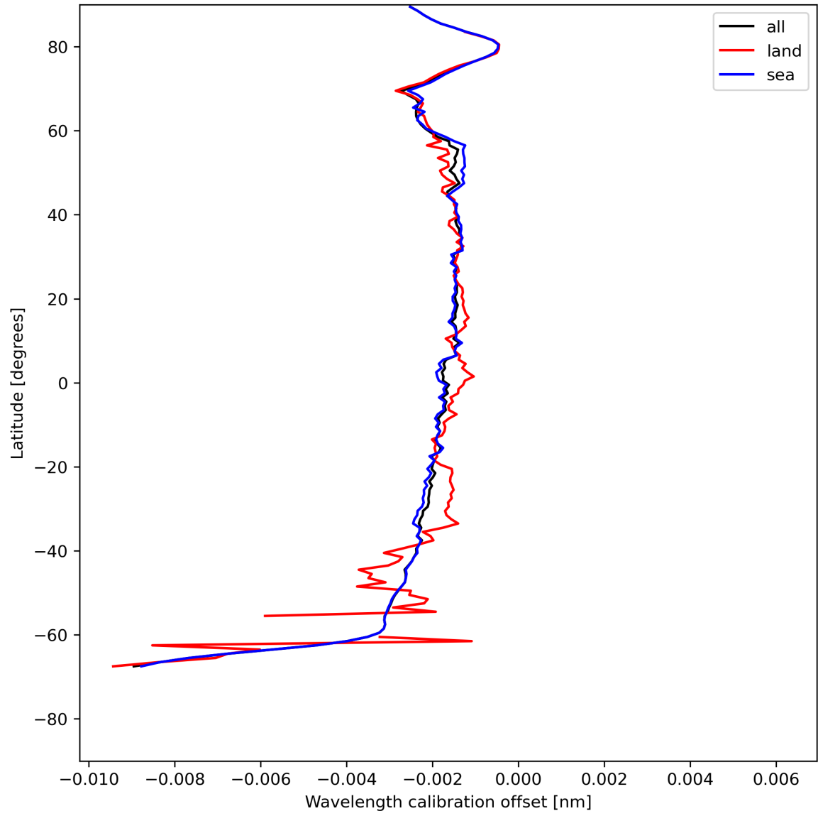
Figure 18: Zonal average of “Wavelength calibration offset” for 2024-05-21 to 2024-05-23.
