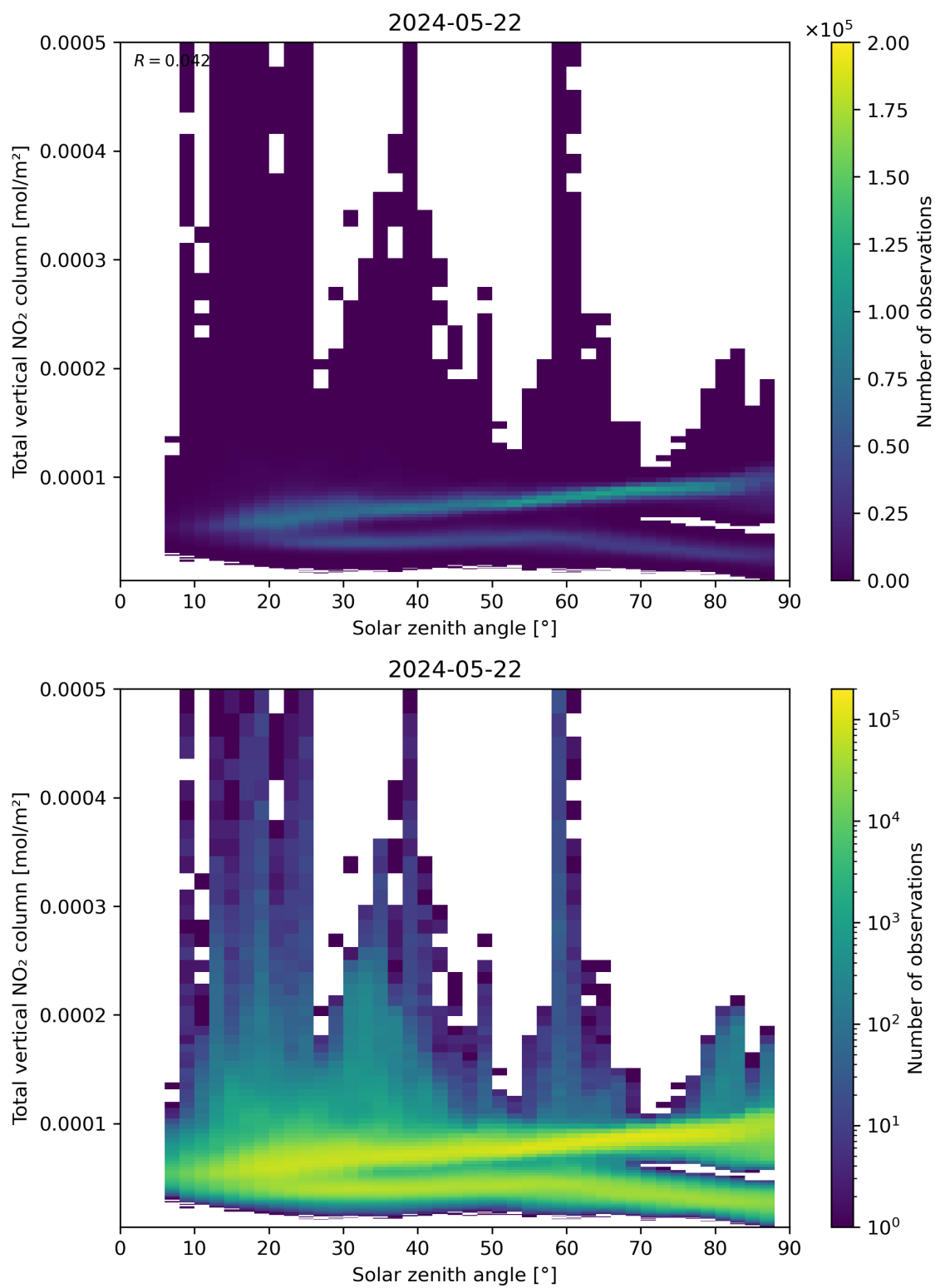
Figure 153: Scatter density plot of “Solar zenith angle” against “Total vertical NO 2 column” for 2024-05-21 to 2024-05-23.
