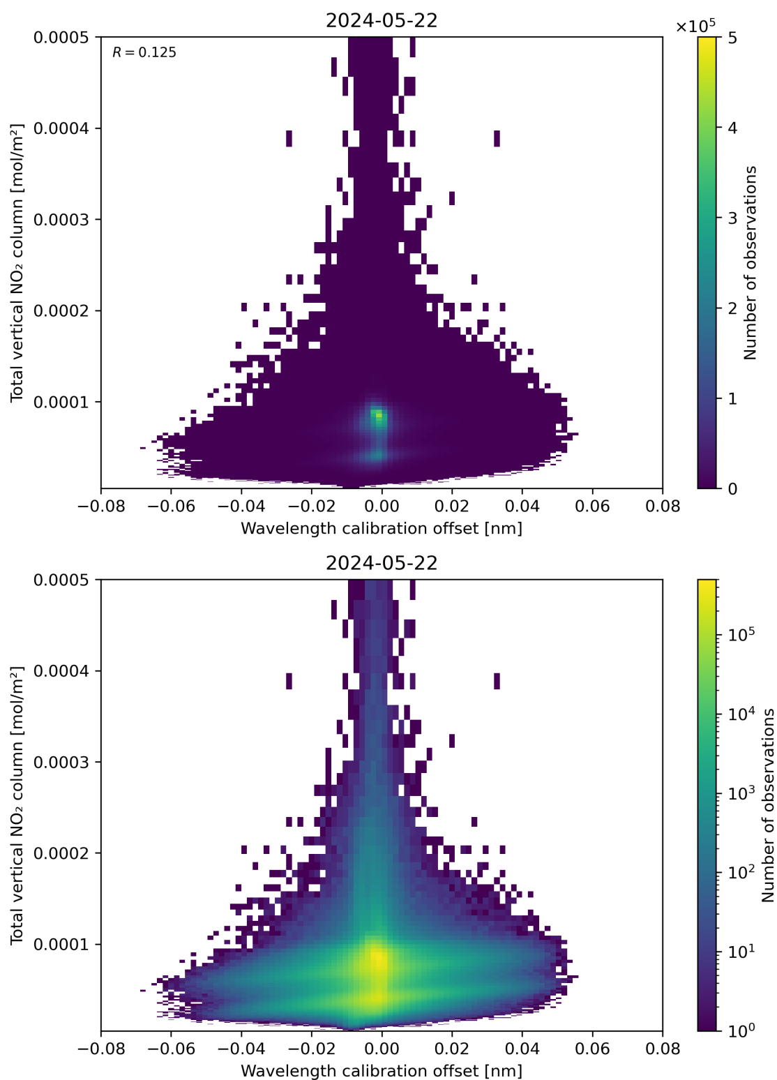
Figure 179: Scatter density plot of “Wavelength calibration offset” against “Total vertical NO 2 column” for 2024-05-21 to 2024-05-23.
