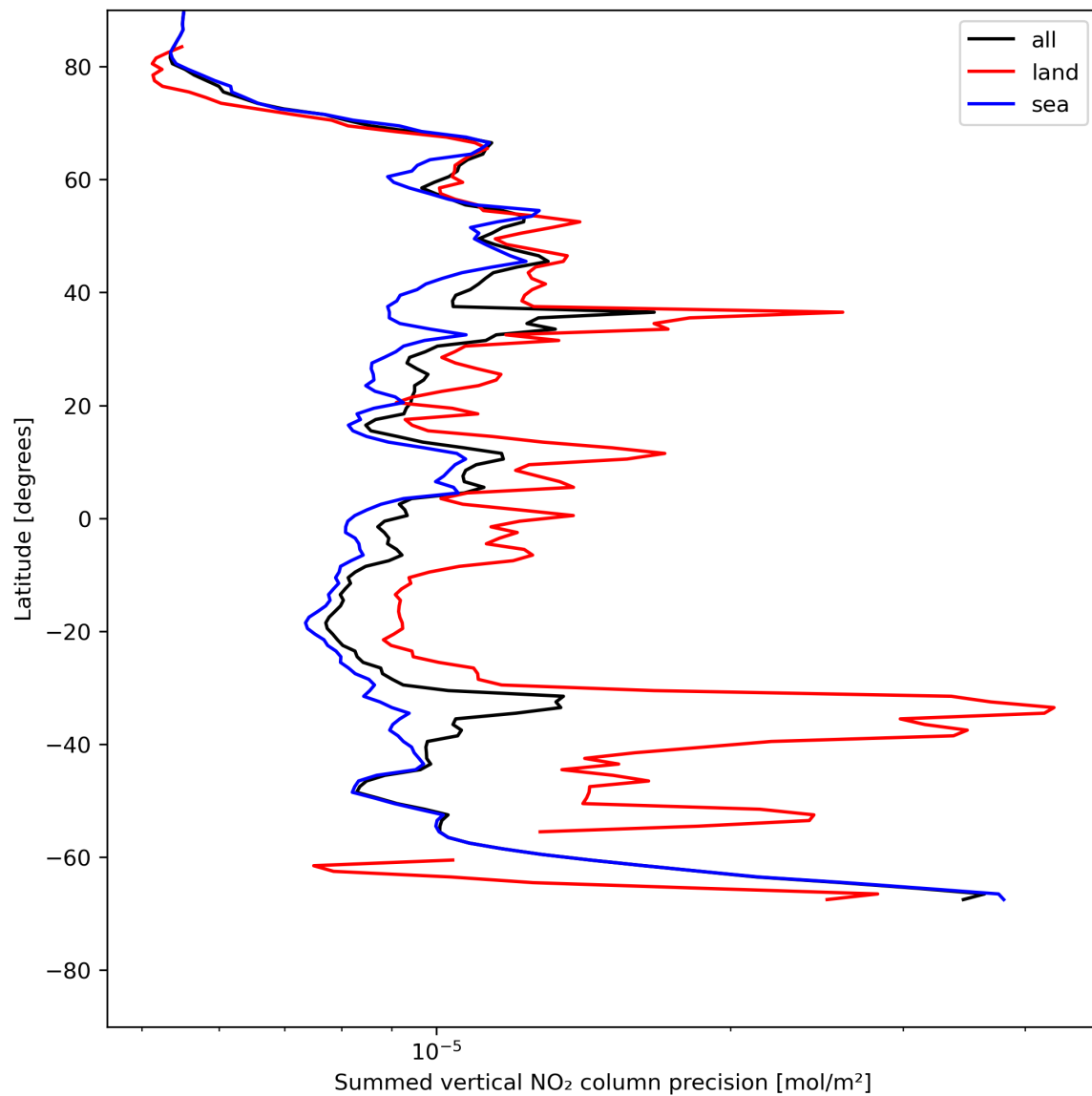
Figure 24: Zonal average of “Summed vertical NO 2 column precision” for 2024-05-21 to 2024-05-23.
