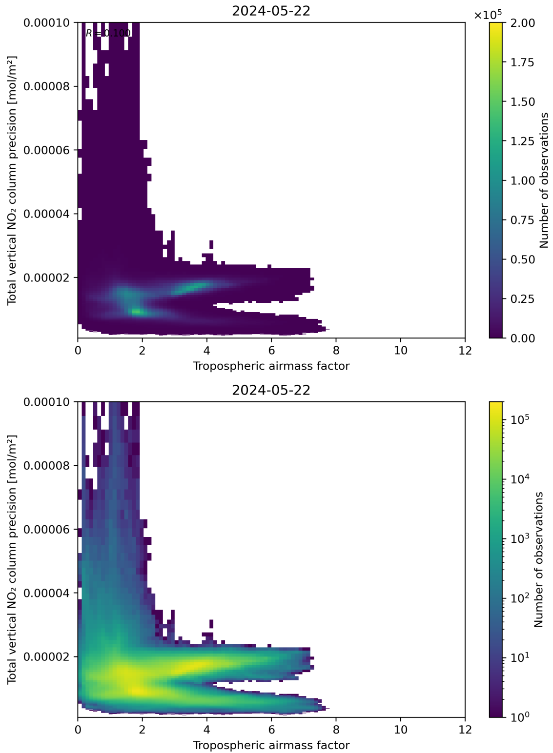
Figure 78: Scatter density plot of “Tropospheric air mass factor” against “Total vertical NO 2 column precision” for 2024-05-21 to 2024-05-23.
