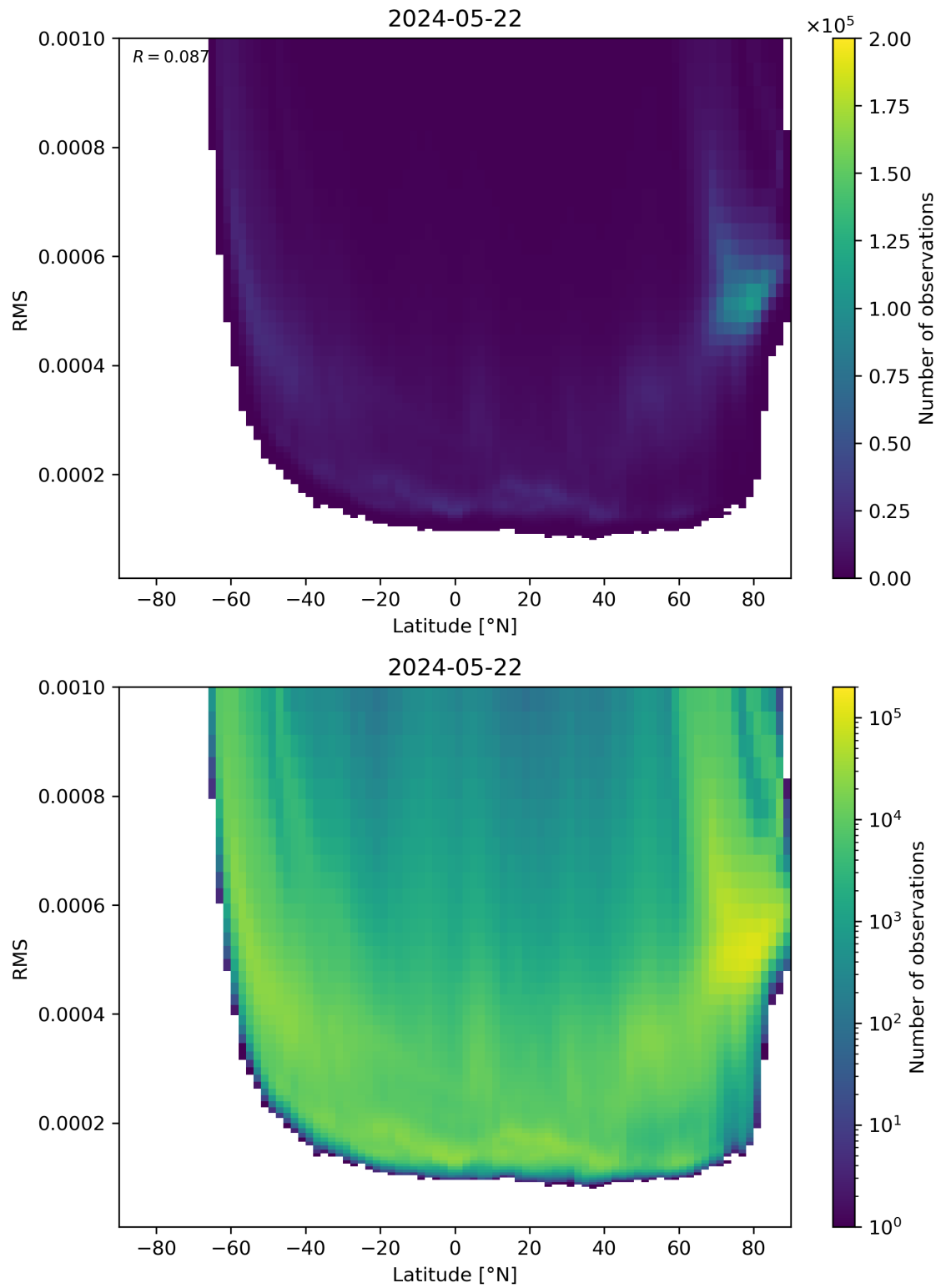
Figure 94: Scatter density plot of “Latitude” against “RMS” for 2024-05-21 to 2024-05-23.
