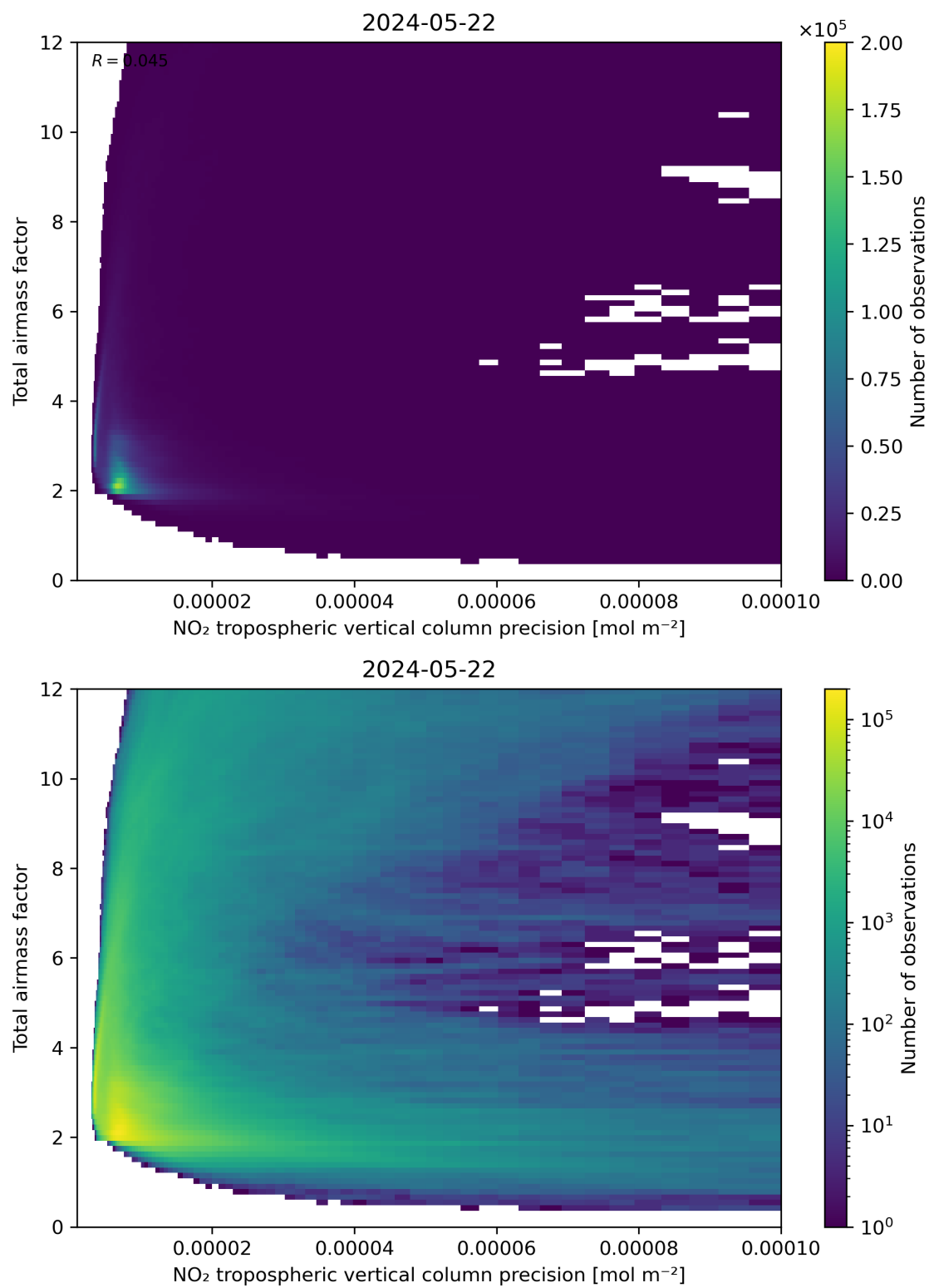
Figure 132: Scatter density plot of “NO 2 tropospheric vertical column precision” against “Total air mass factor” for 2024-05-21 to 2024-05-23.
