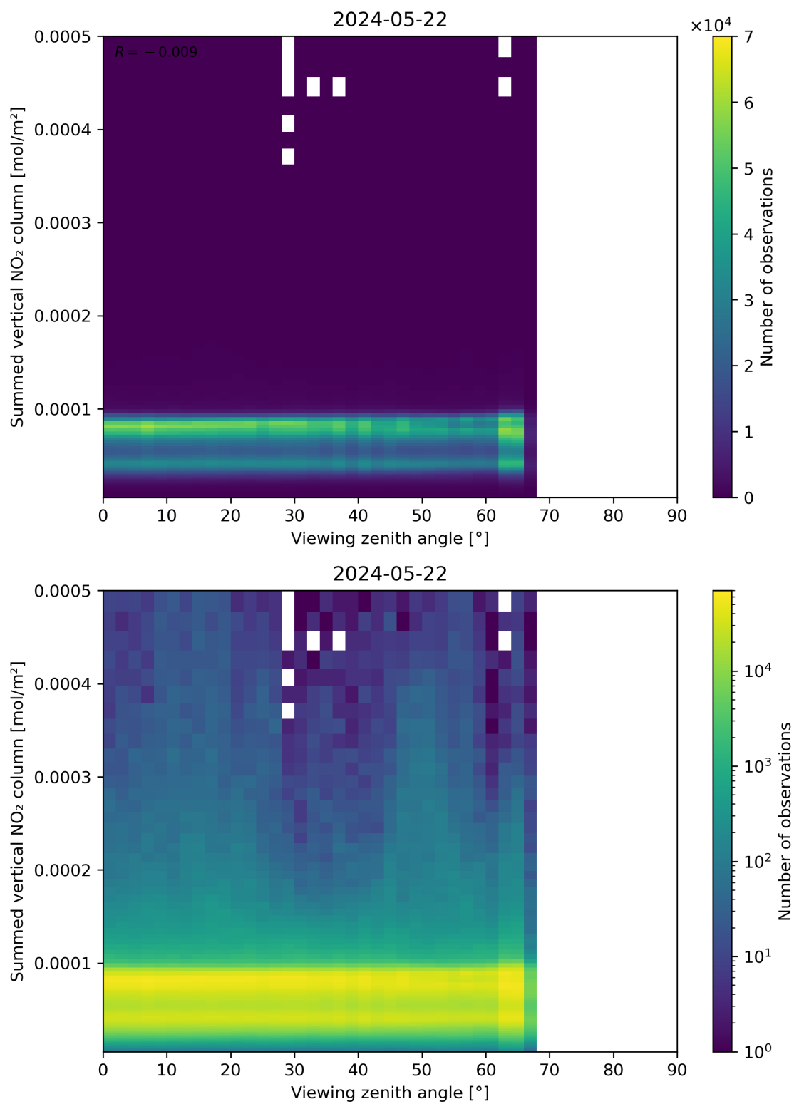
Figure 165: Scatter density plot of “Viewing zenith angle” against “Summed vertical NO 2 column” for 2024-05-21 to 2024-05-23.
