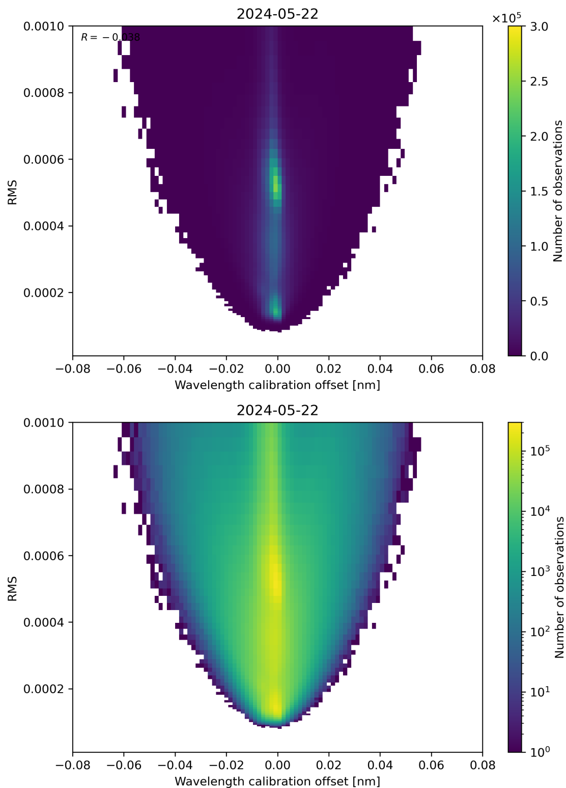
Figure 181: Scatter density plot of “Wavelength calibration offset” against “RMS” for 2024-05-21 to 2024-05-23.
