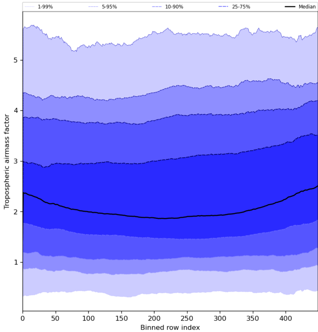
Figure 48: Along track statistics of “Tropospheric airmass factor” for 2024-05-21 to 2024-05-23
