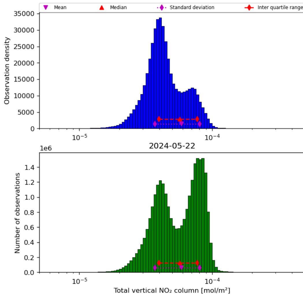
Figure 38: Histogram of “Total vertical NO 2 column” for 2024-05-21 to 2024-05-23
