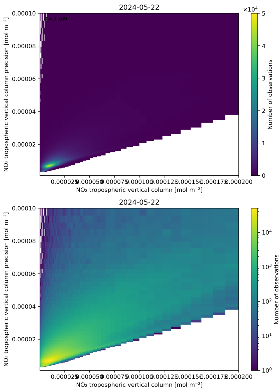
Figure 130: Scatter density plot of “NO 2 tropospheric vertical column” against “NO 2 tropospheric vertical column precision” for 2024-05-21 to 2024-05-23.
