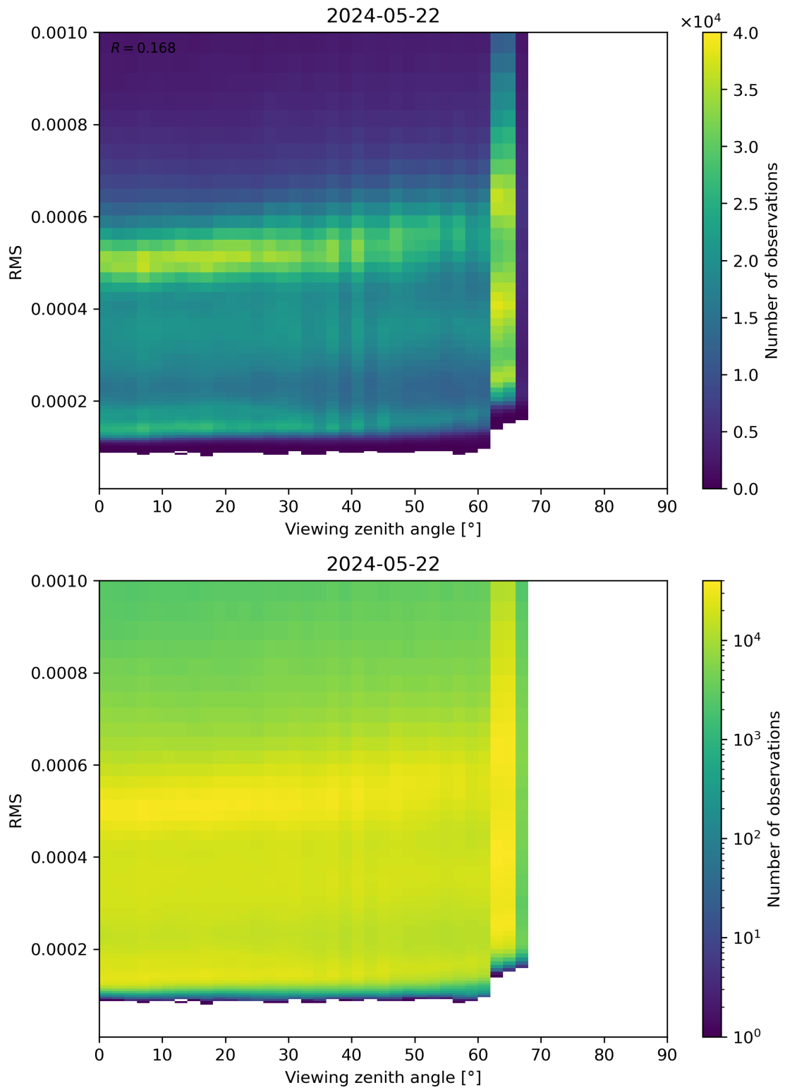
Figure 171: Scatter density plot of “Viewing zenith angle” against “RMS” for 2024-05-21 to 2024-05-23.
