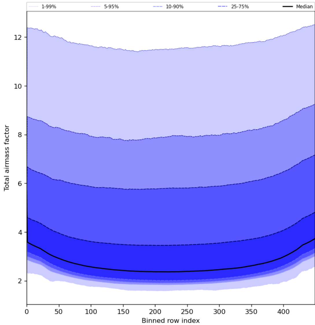
Figure 49: Along track statistics of “Total airmass factor” for 2024-05-21 to 2024-05-23
