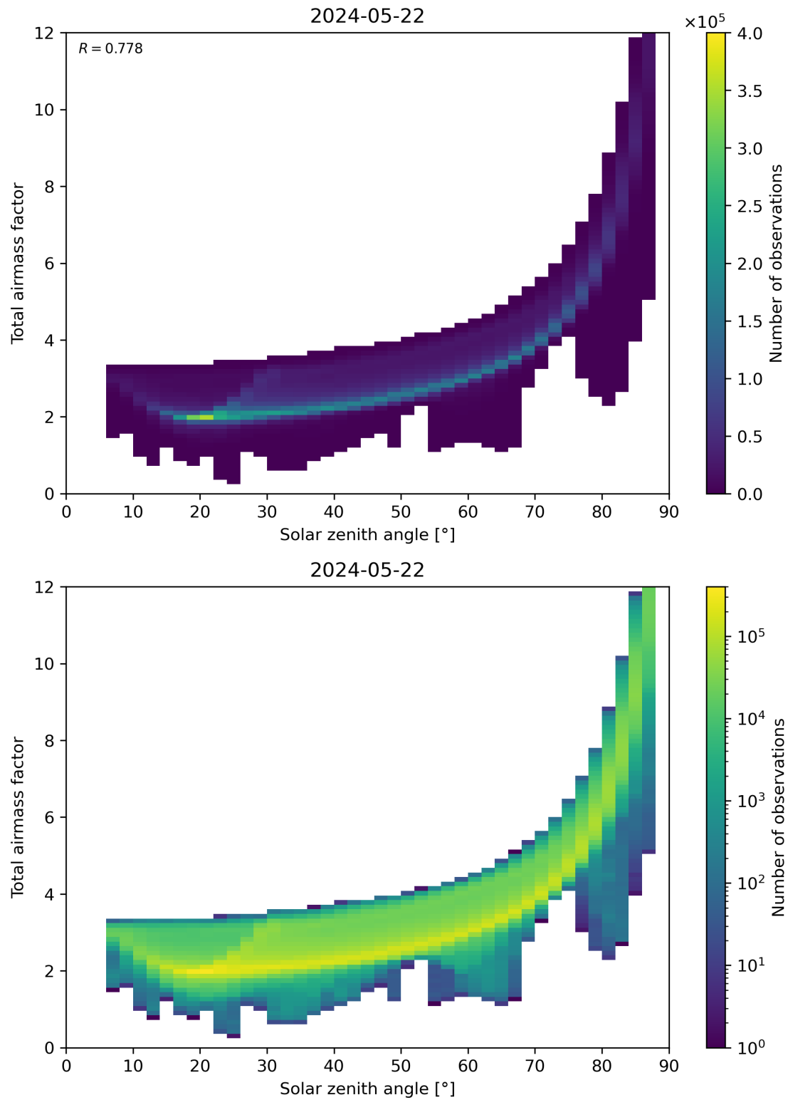
Figure 146: Scatter density plot of “Solar zenith angle” against “Total airmass factor” for 2024-05-21 to 2024-05-23.
