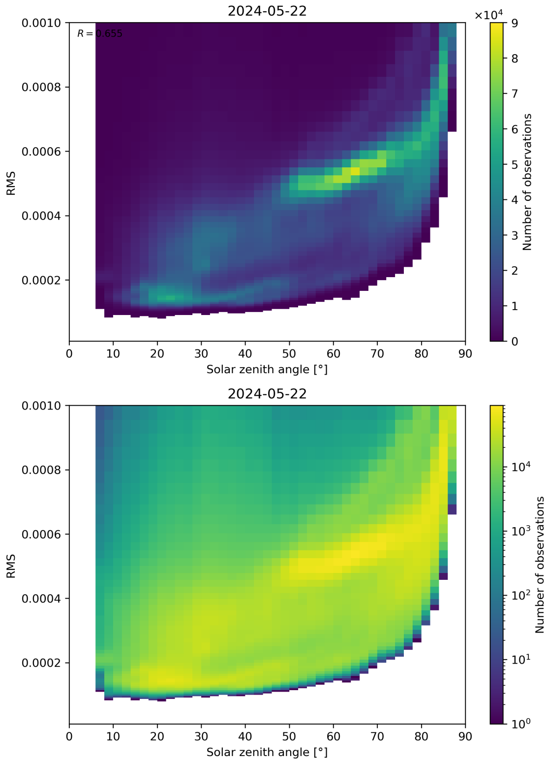
Figure 157: Scatter density plot of “Solar zenith angle” against “RMS” for 2024-05-21 to 2024-05-23.
