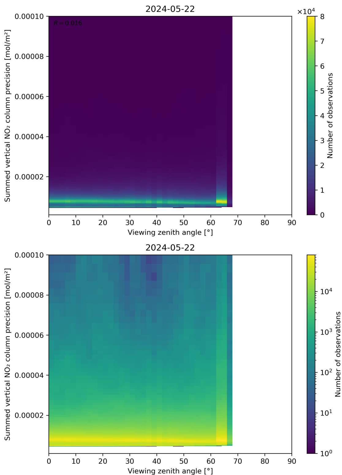
Figure 166: Scatter density plot of “Viewing zenith angle” against “Summed vertical NO 2 column precision” for 2024-05-21 to 2024-05-23.
