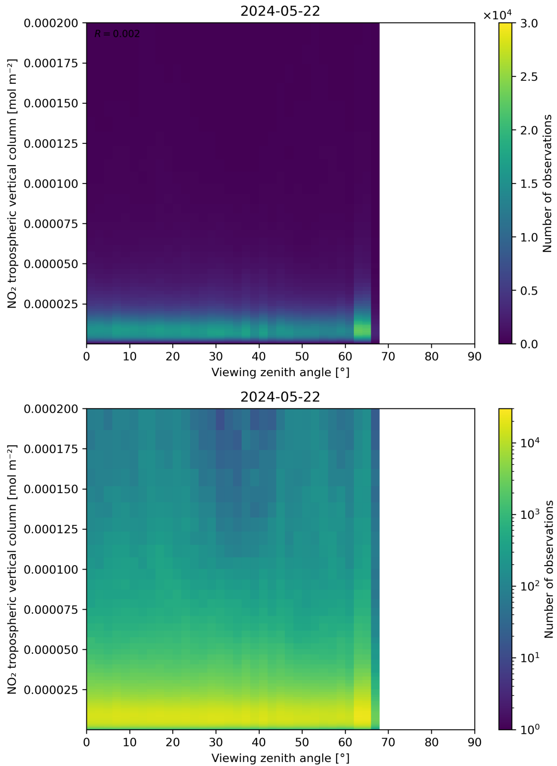
Figure 169: Scatter density plot of “Viewing zenith angle” against “NO 2 tropospheric vertical column” for 2024-05-21 to 2024-05-23.
