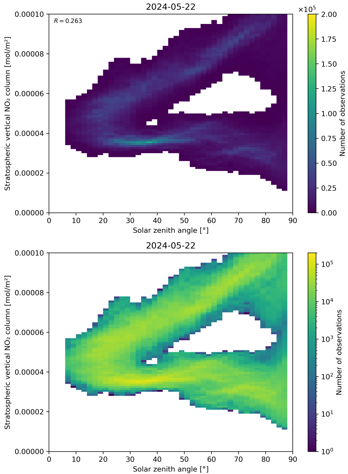
Figure 150: Scatter density plot of “Solar zenith angle” against “Stratospheric vertical NO 2 column” for 2024-05-21 to 2024-05-23.
