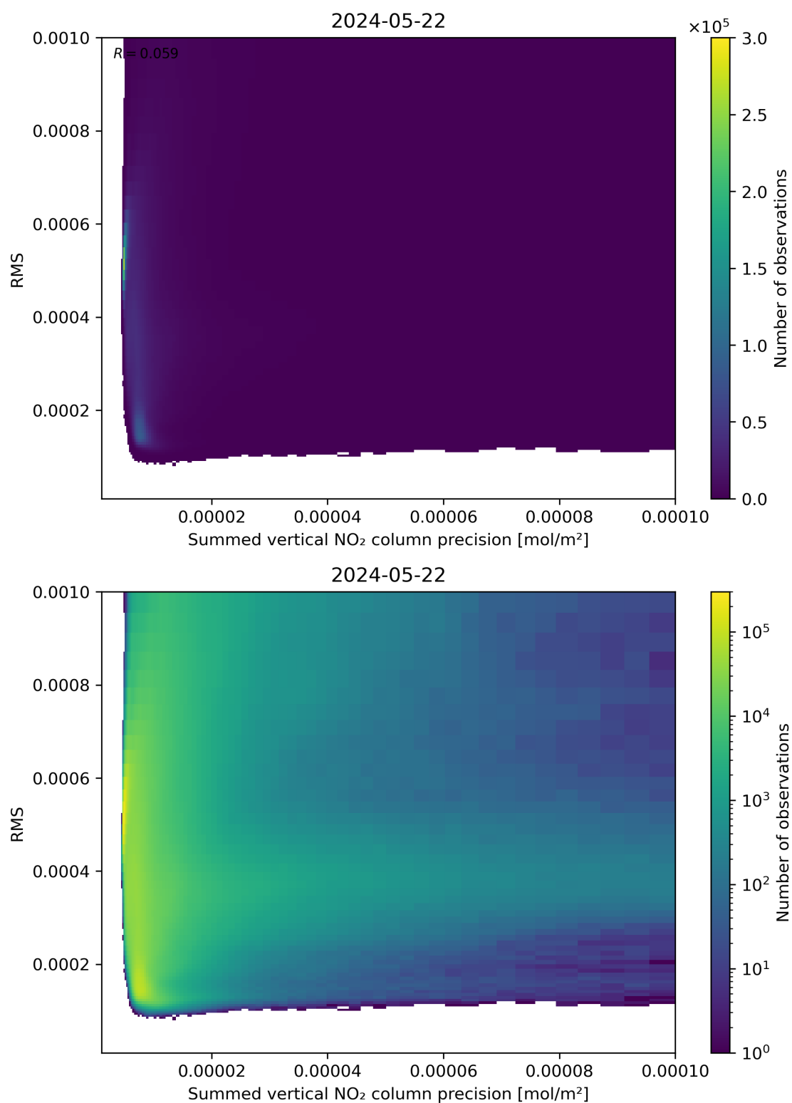
Figure 108: Scatter density plot of “Summed vertical NO 2 column precision” against “RMS” for 2024-05-21 to 2024-05-23.
