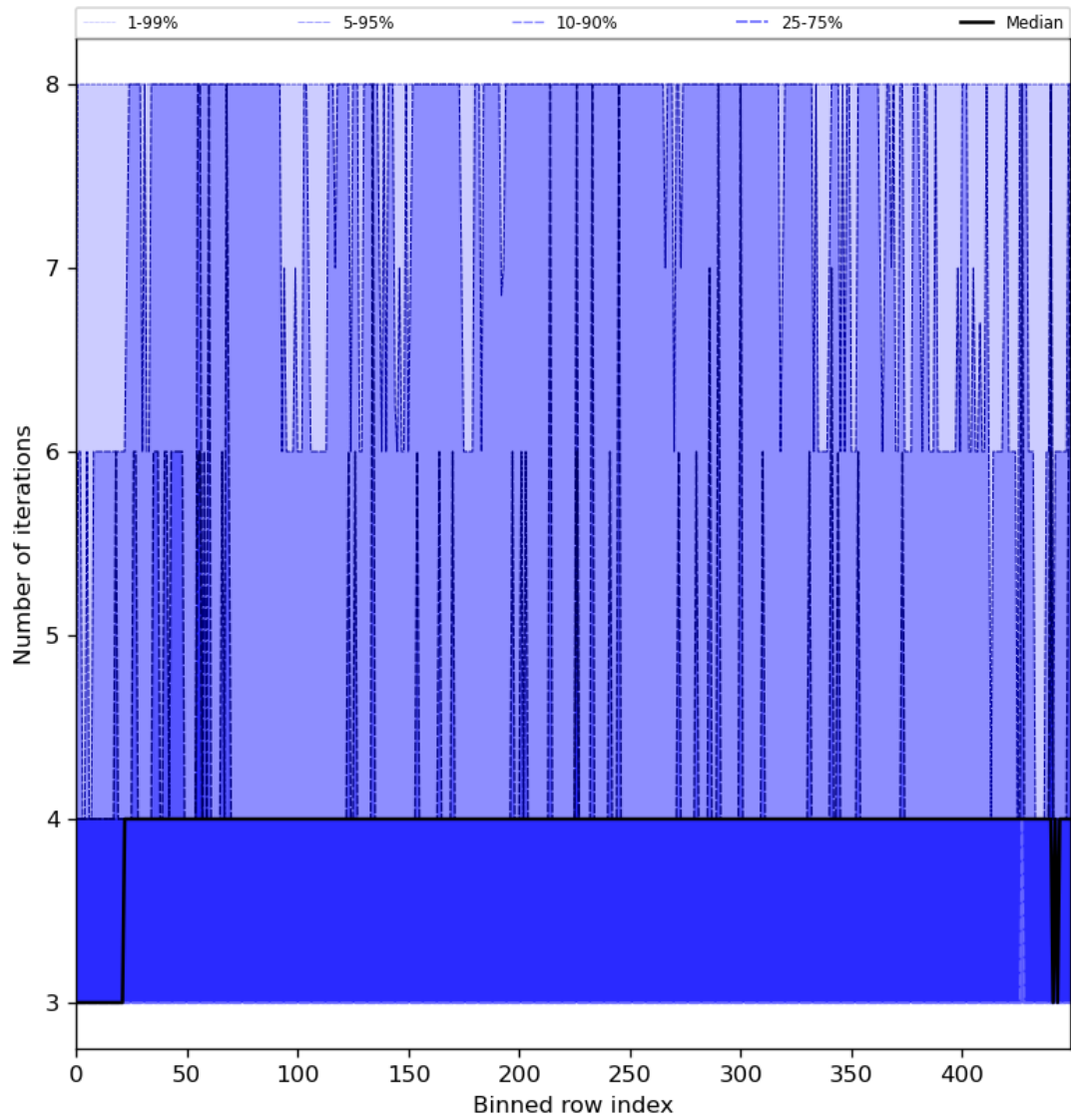
Figure 51: Along track statistics of “Number of iterations” for 2024-05-21 to 2024-05-23
