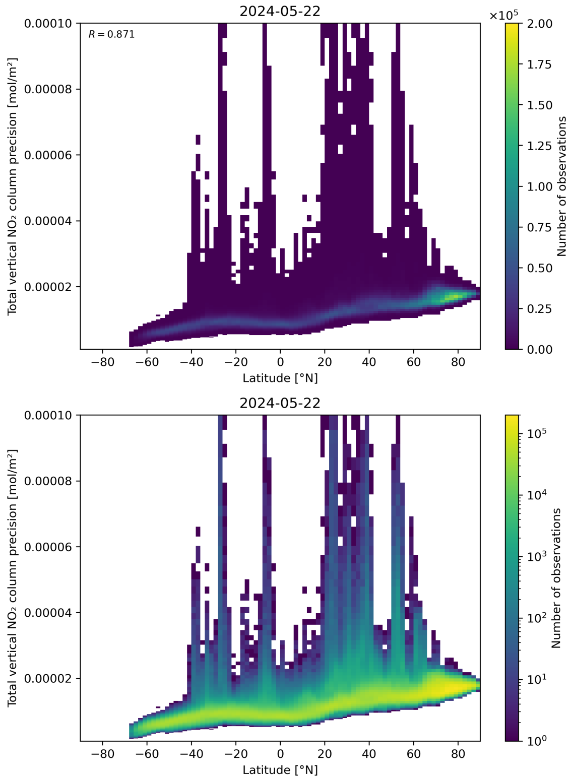
Figure 91: Scatter density plot of “Latitude” against “Total vertical NO 2 column precision” for 2024-05-21 to 2024-05-23.
