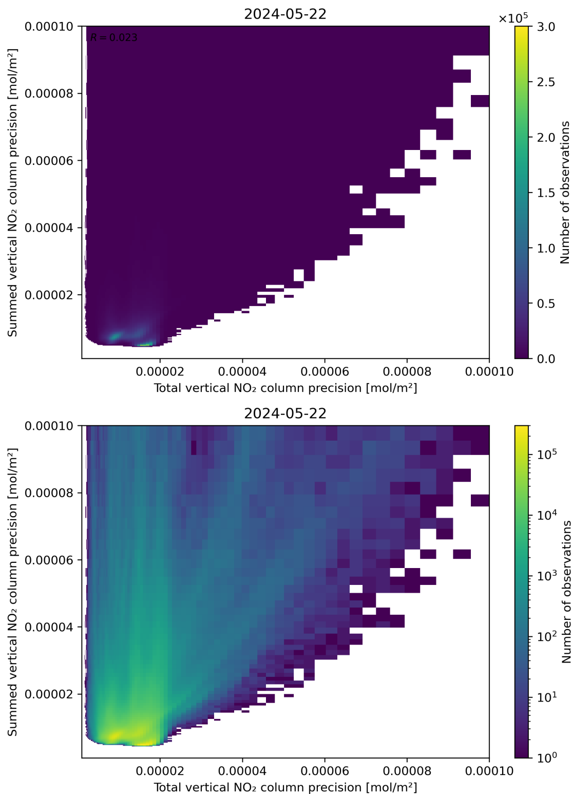
Figure 118: Scatter density plot of “Total vertical NO 2 column precision” against “Summed vertical NO 2 column precision” for 2024-05-21 to 2024-05-23.
