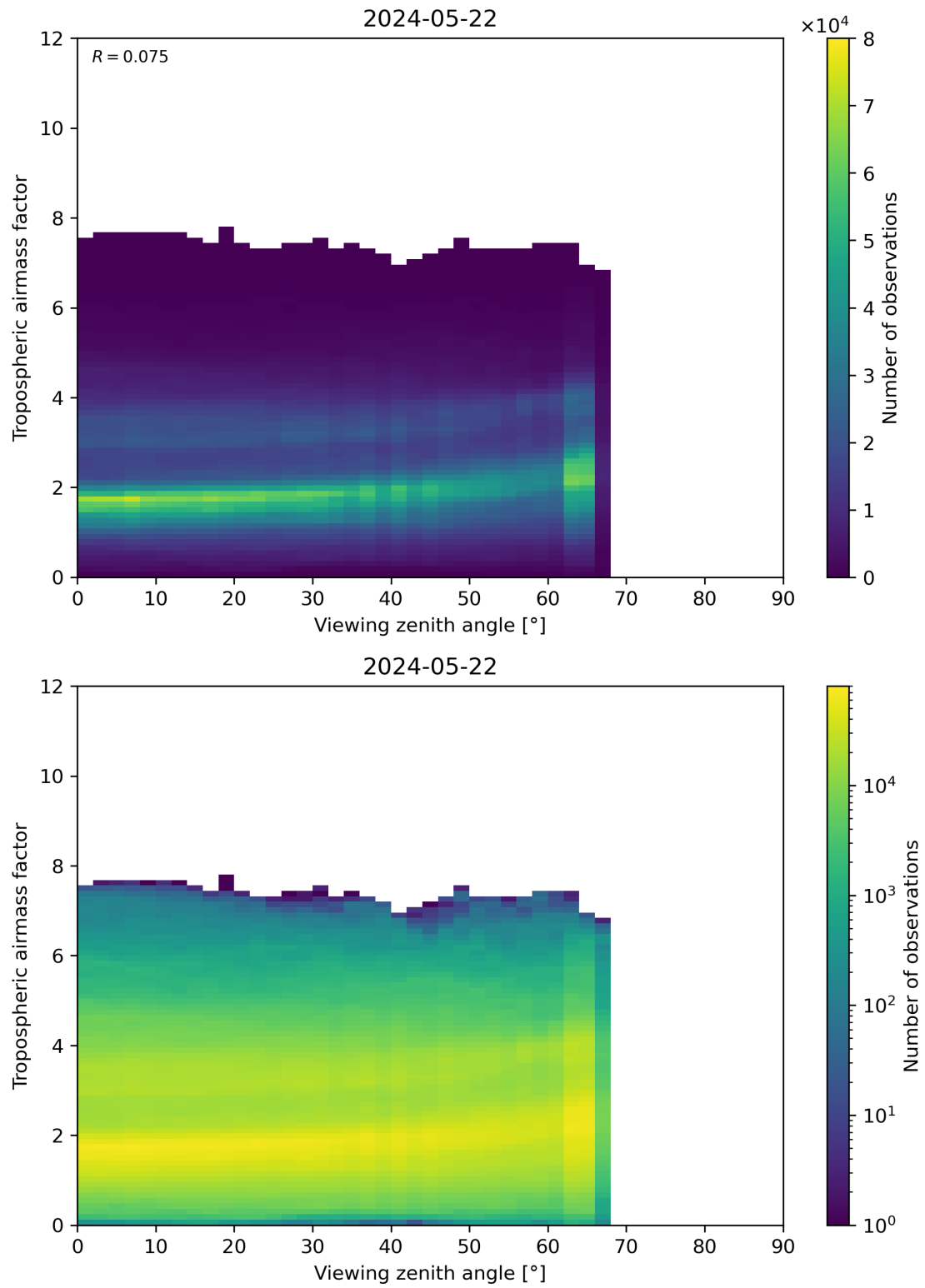
Figure 161: Scatter density plot of “Viewing zenith angle” against “Tropospheric airmass factor” for 2024-05-21 to 2024-05-23.
