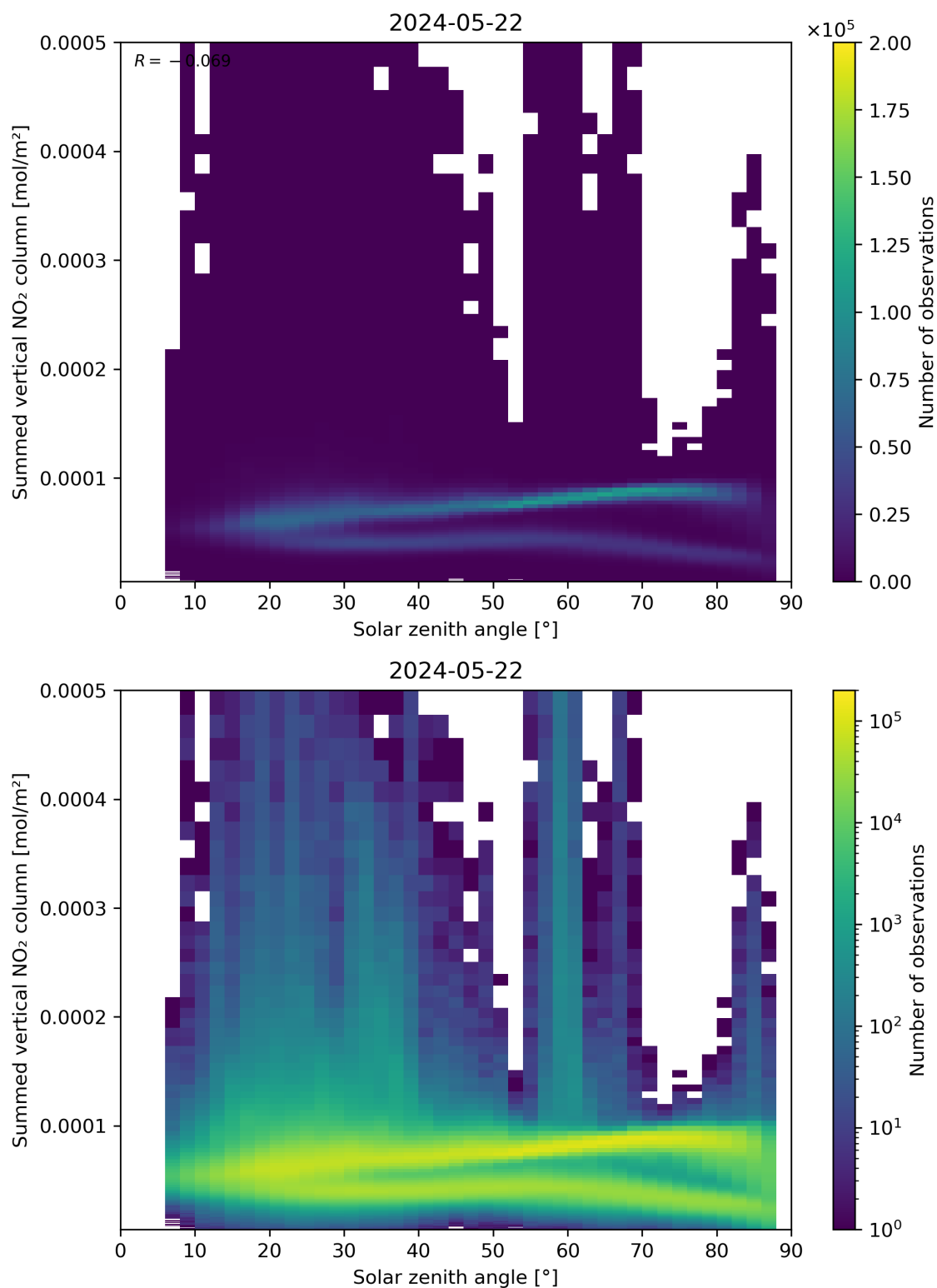
Figure 151: Scatter density plot of “Solar zenith angle” against “Summed vertical NO 2 column” for 2024-05-21 to 2024-05-23.
