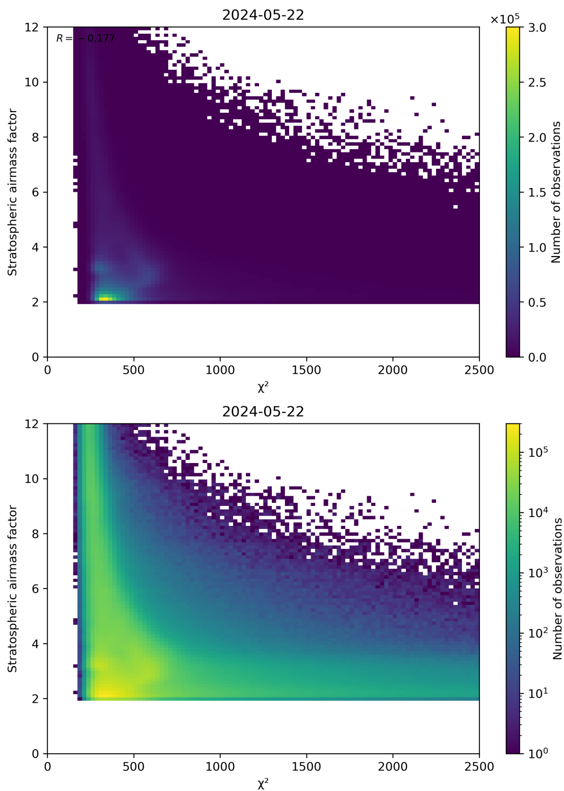
Figure 81: Scatter density plot of “ \chi^2 ” against “Stratospheric airmass factor” for 2024-05-21 to 2024-05-23.
