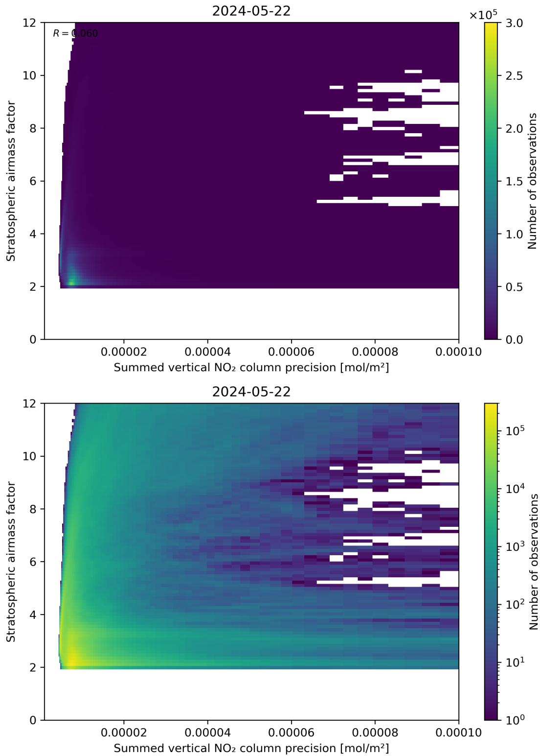
Figure 106: Scatter density plot of “Summed vertical NO 2 column precision” against “Stratospheric airmass factor” for 2024-05-21 to 2024-05-23.
