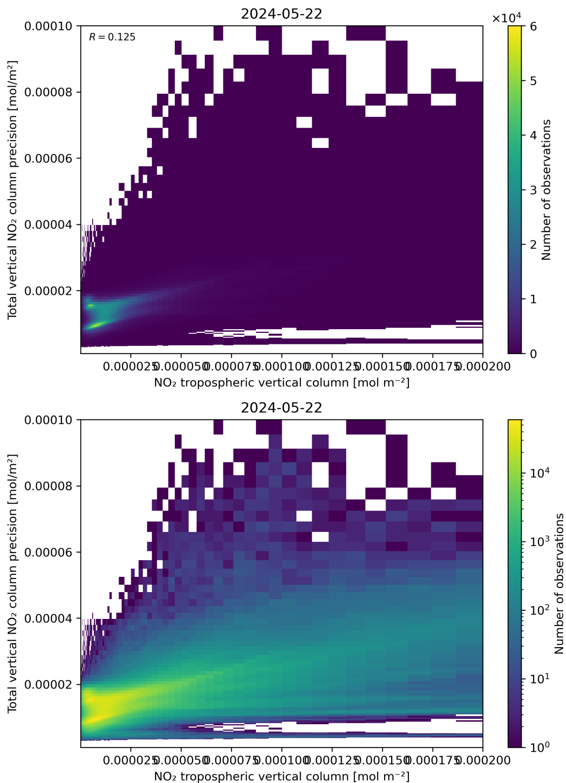
Figure 129: Scatter density plot of “NO 2 tropospheric vertical column” against “Total vertical NO 2 column precision” for 2024-05-21 to 2024-05-23.
