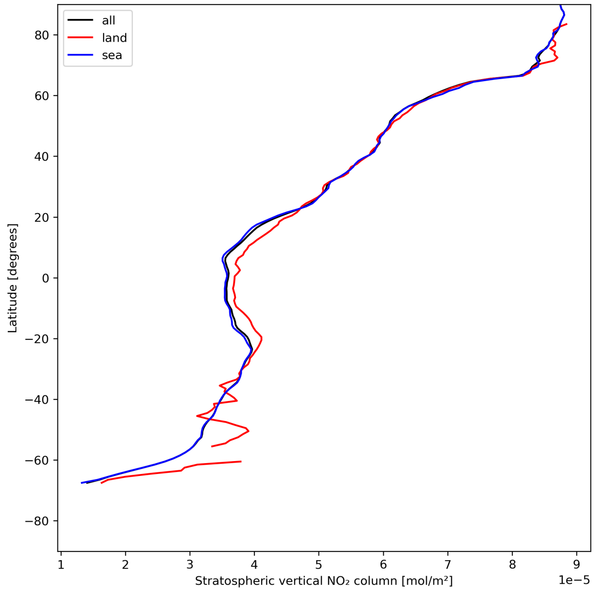
Figure 19: Zonal average of “Stratospheric vertical NO 2 column” for 2024-05-21 to 2024-05-23.
