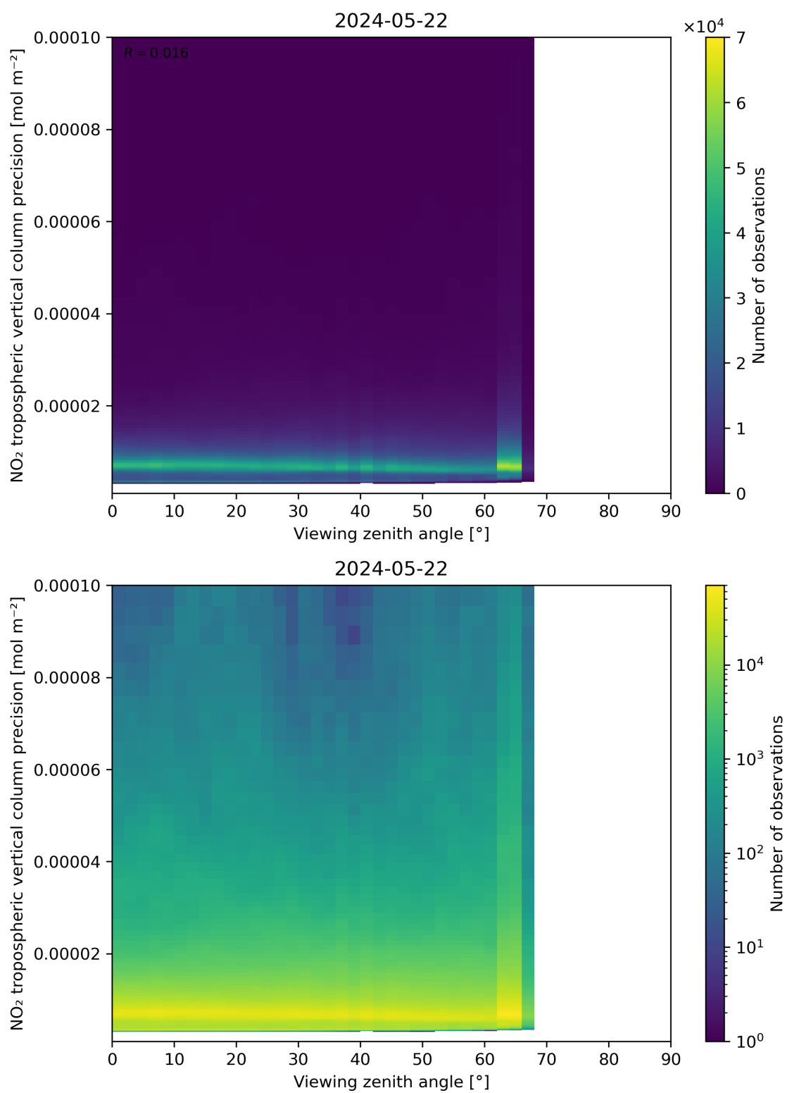
Figure 170: Scatter density plot of “Viewing zenith angle” against “NO 2 tropospheric vertical column precision” for 2024-05-21 to 2024-05-23.
