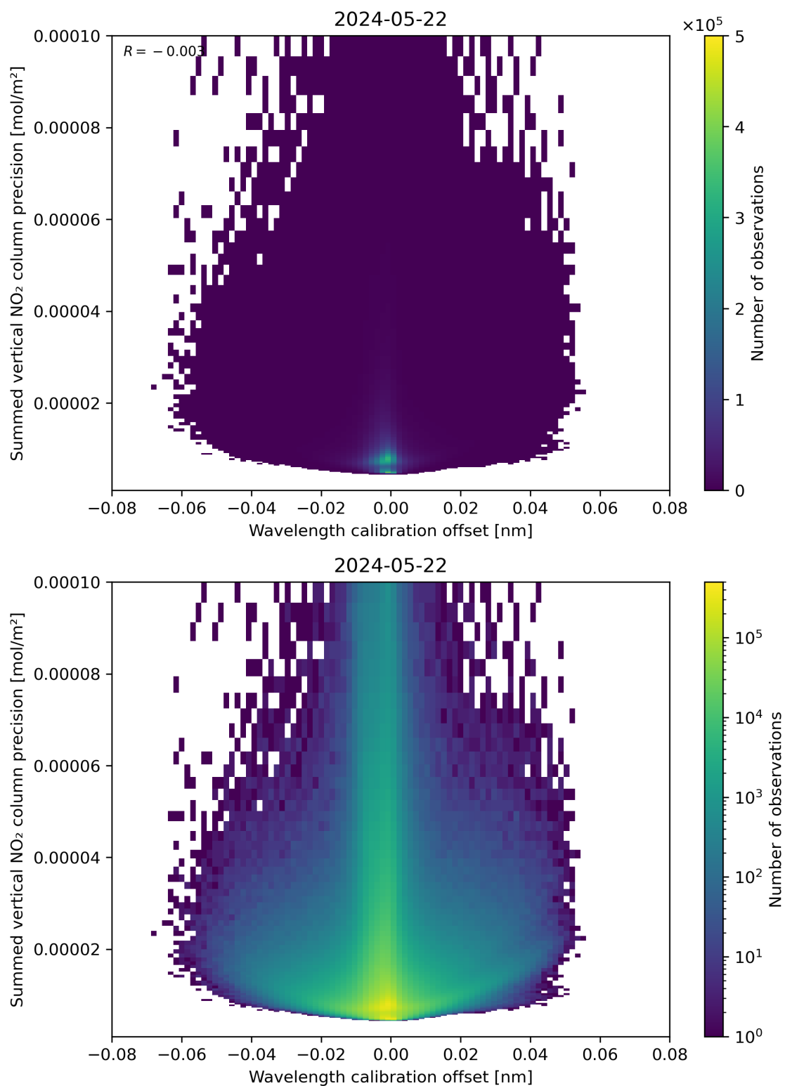
Figure 178: Scatter density plot of “Wavelength calibration offset” against “Summed vertical NO 2 column precision” for 2024-05-21 to 2024-05-23.
