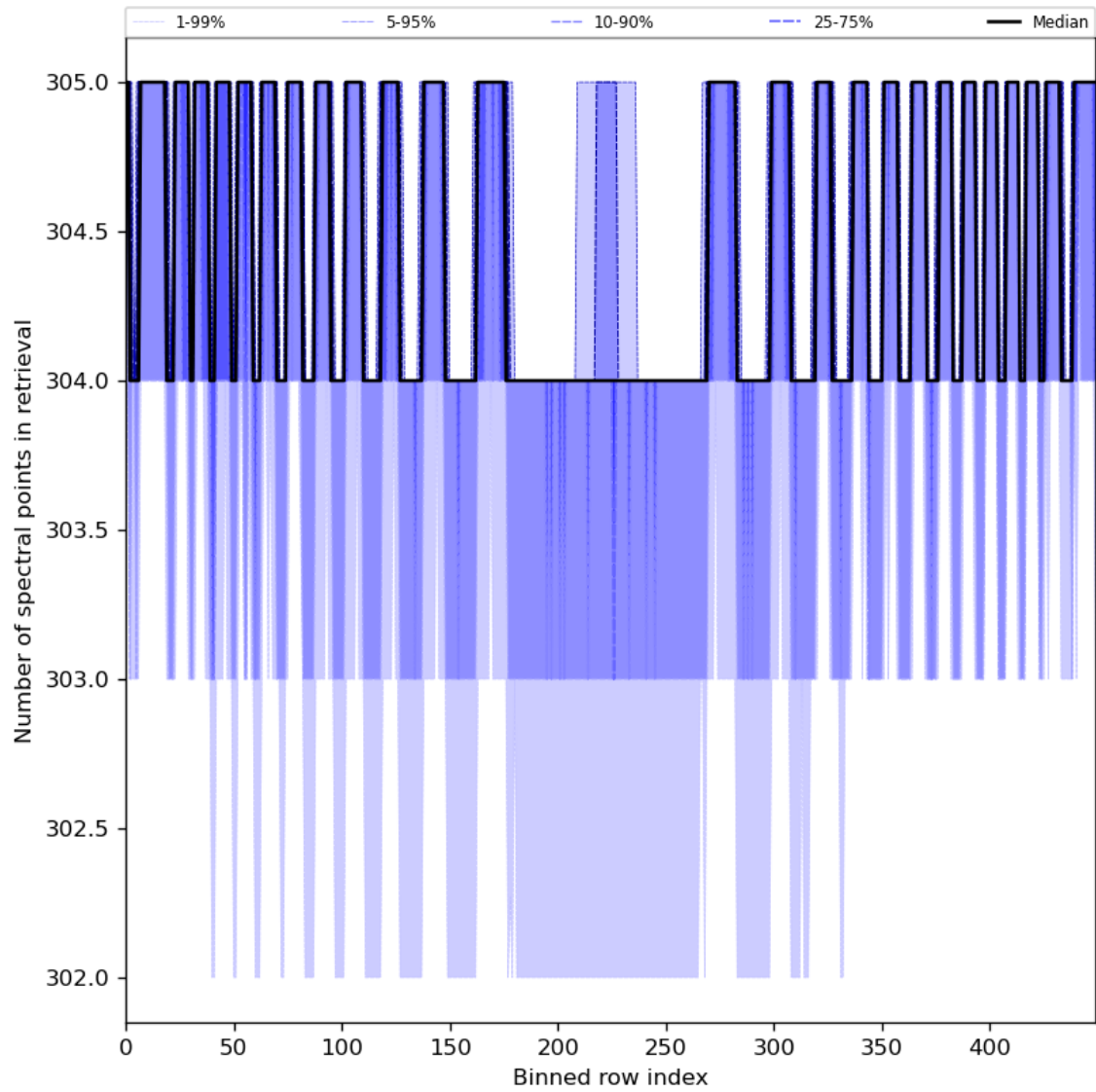
Figure 50: Along track statistics of “Number of spectral points in retrieval” for 2024-05-21 to 2024-05-23
