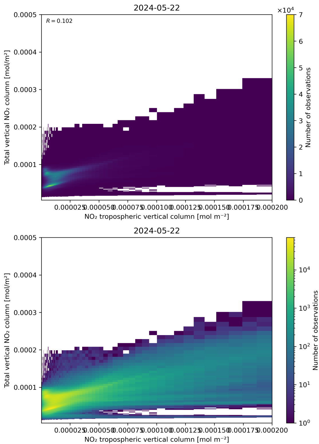
Figure 128: Scatter density plot of “NO 2 tropospheric vertical column” against “Total vertical NO 2 column” for 2024-05-21 to 2024-05-23.
