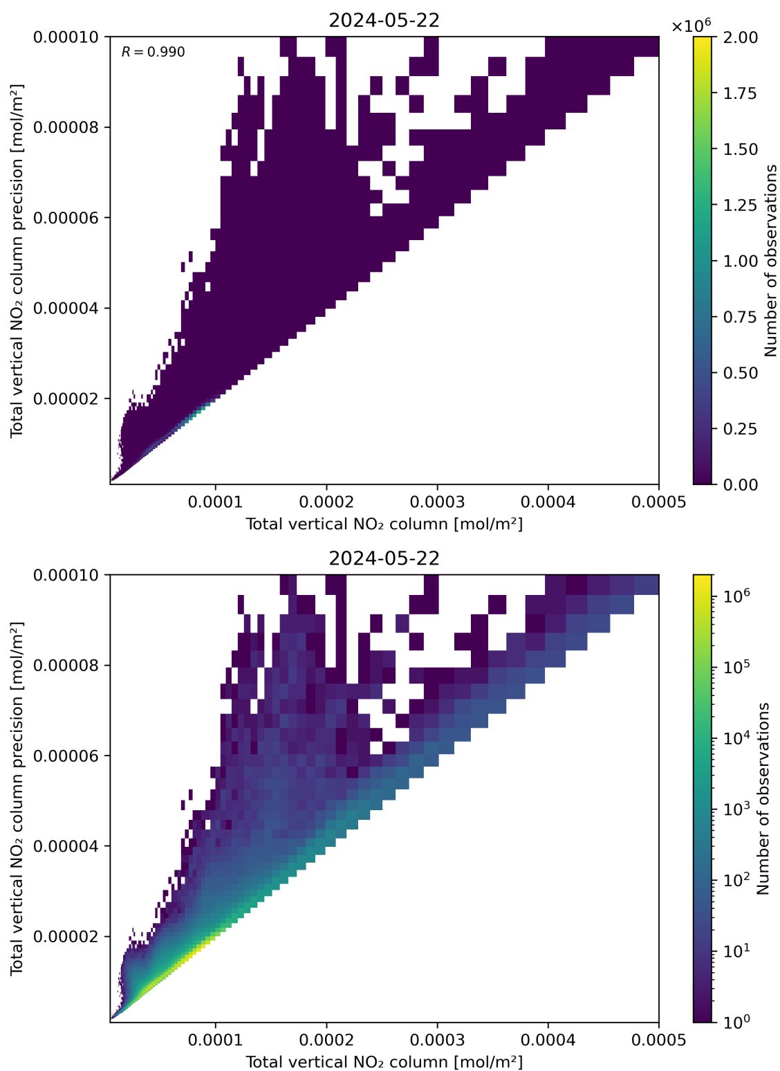
Figure 114: Scatter density plot of “Total vertical NO 2 column” against “Total vertical NO 2 column precision” for 2024-05-21 to 2024-05-23.
