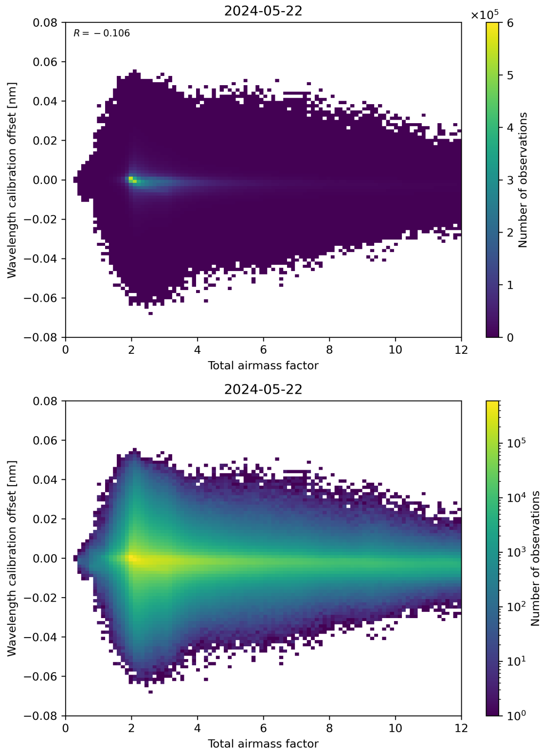
Figure 70: Scatter density plot of “Total airmass factor” against “Wavelength calibration offset” for 2024-05-21 to 2024-05-23.
