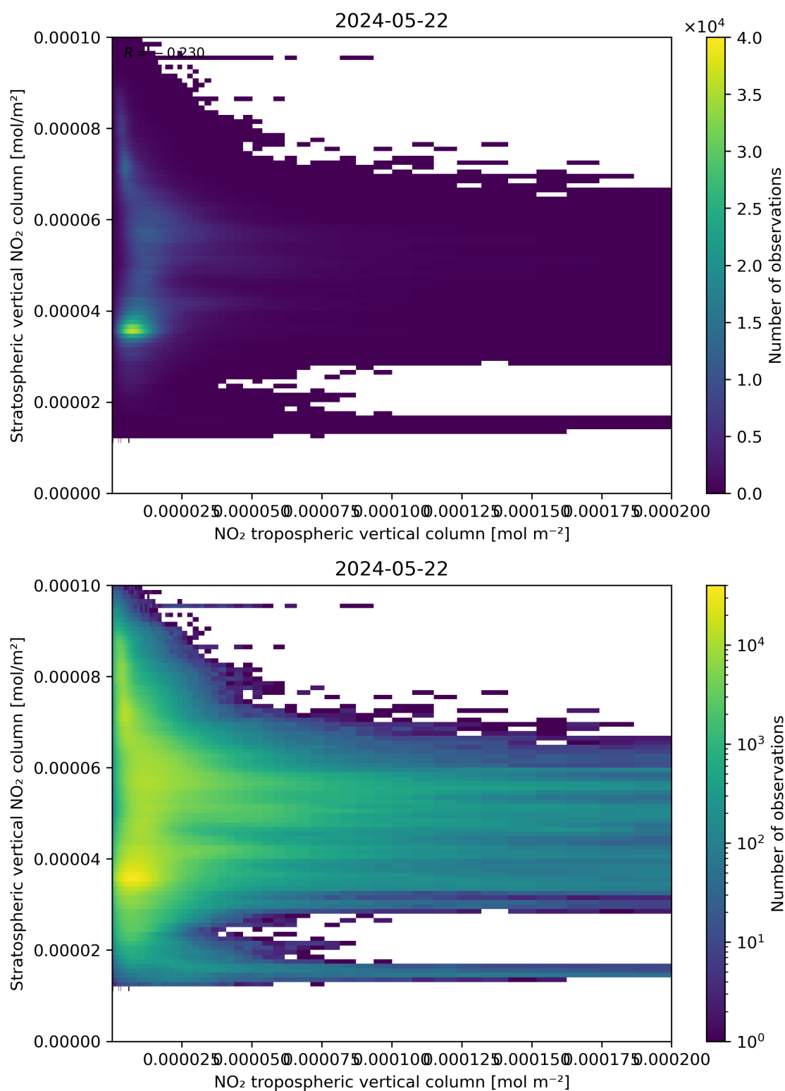
Figure 125: Scatter density plot of “NO 2 tropospheric vertical column” against “Stratospheric vertical NO 2 column” for 2024-05-21 to 2024-05-23.
