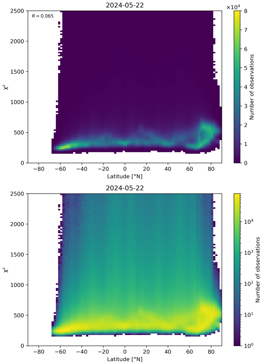
Figure 86: Scatter density plot of “Latitude” against “ \chi^2 ” for 2024-05-21 to 2024-05-23.
