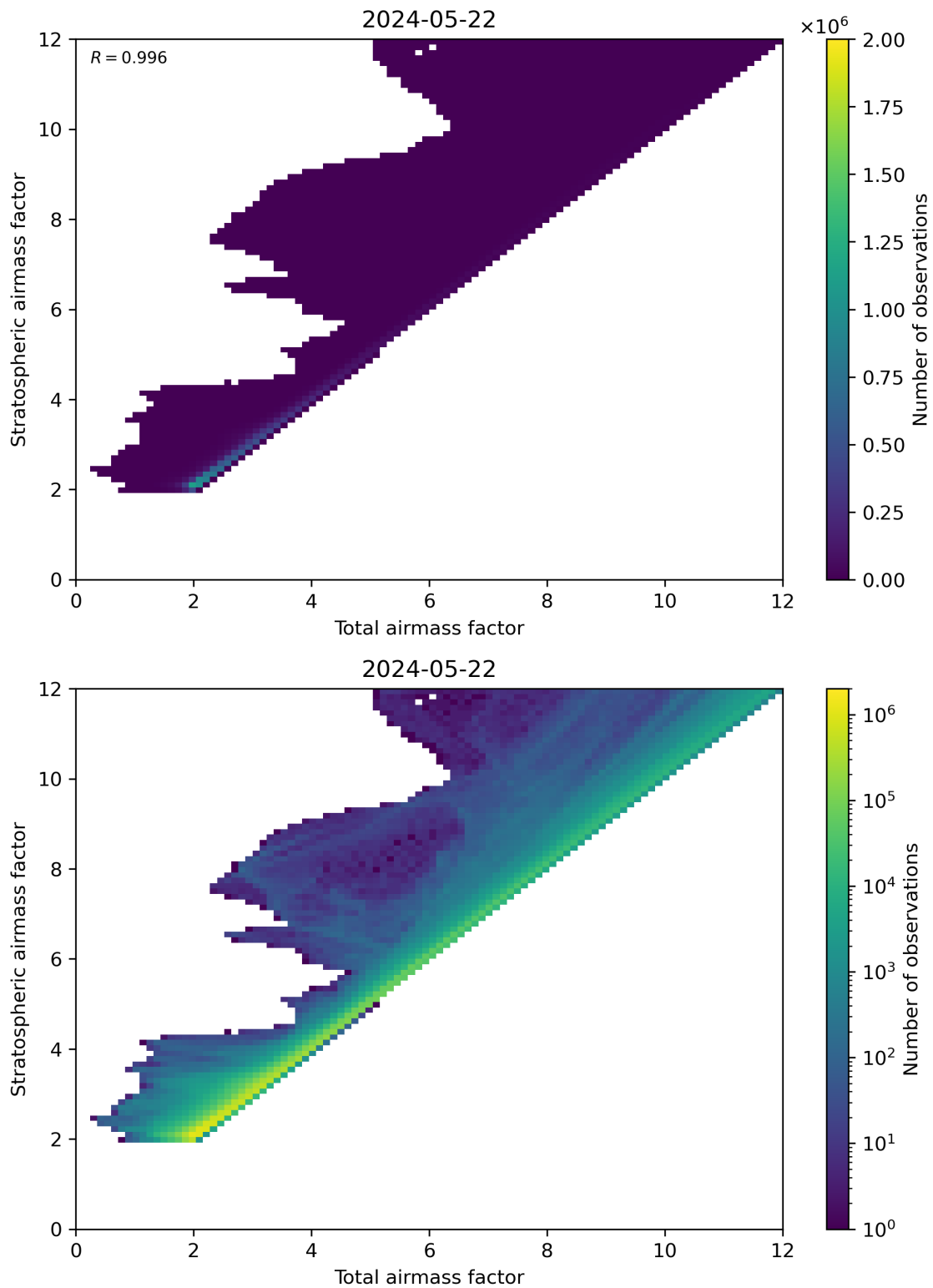
Figure 62: Scatter density plot of “Total airmass factor” against “Stratospheric airmass factor” for 2024-05-21 to 2024-05-23.
