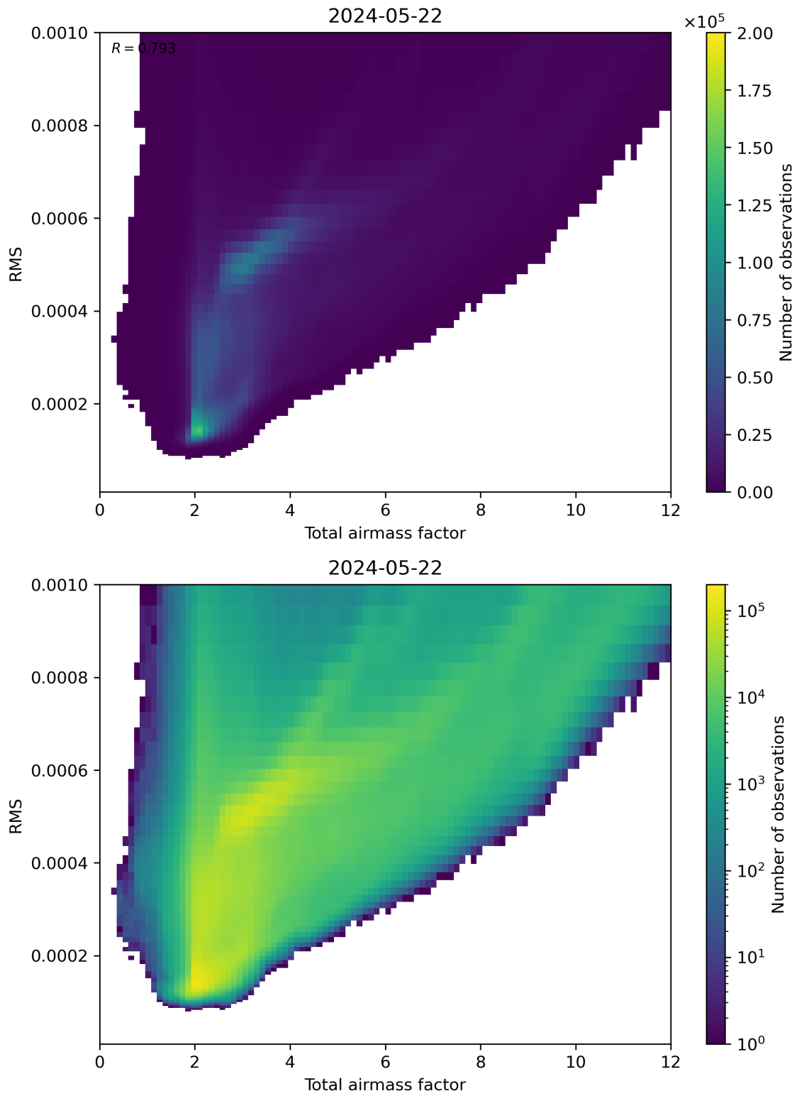
Figure 69: Scatter density plot of “Total airmass factor” against “RMS” for 2024-05-21 to 2024-05-23.
