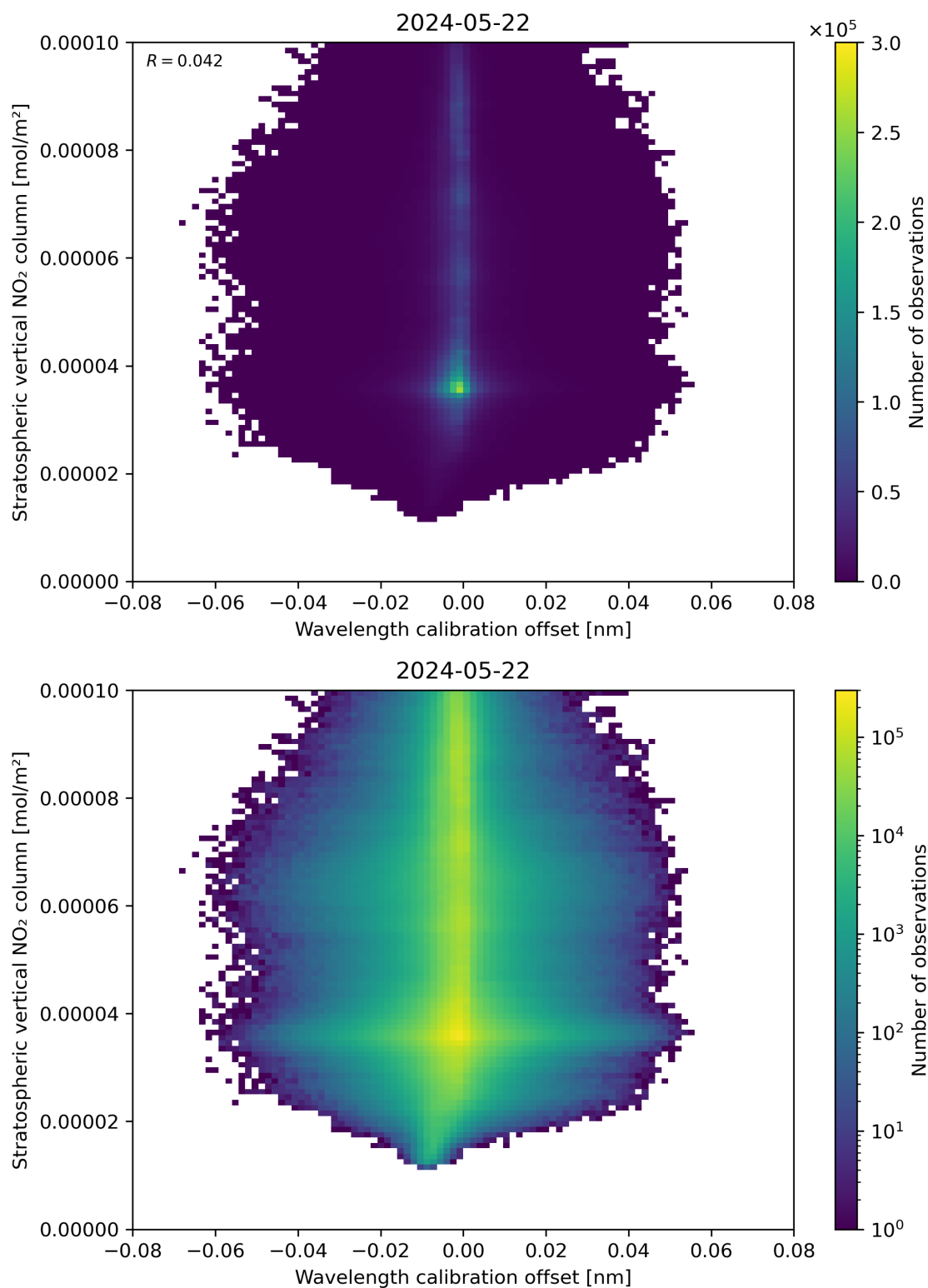
Figure 176: Scatter density plot of “Wavelength calibration offset” against “Stratospheric vertical NO 2 column” for 2024-05-21 to 2024-05-23.
