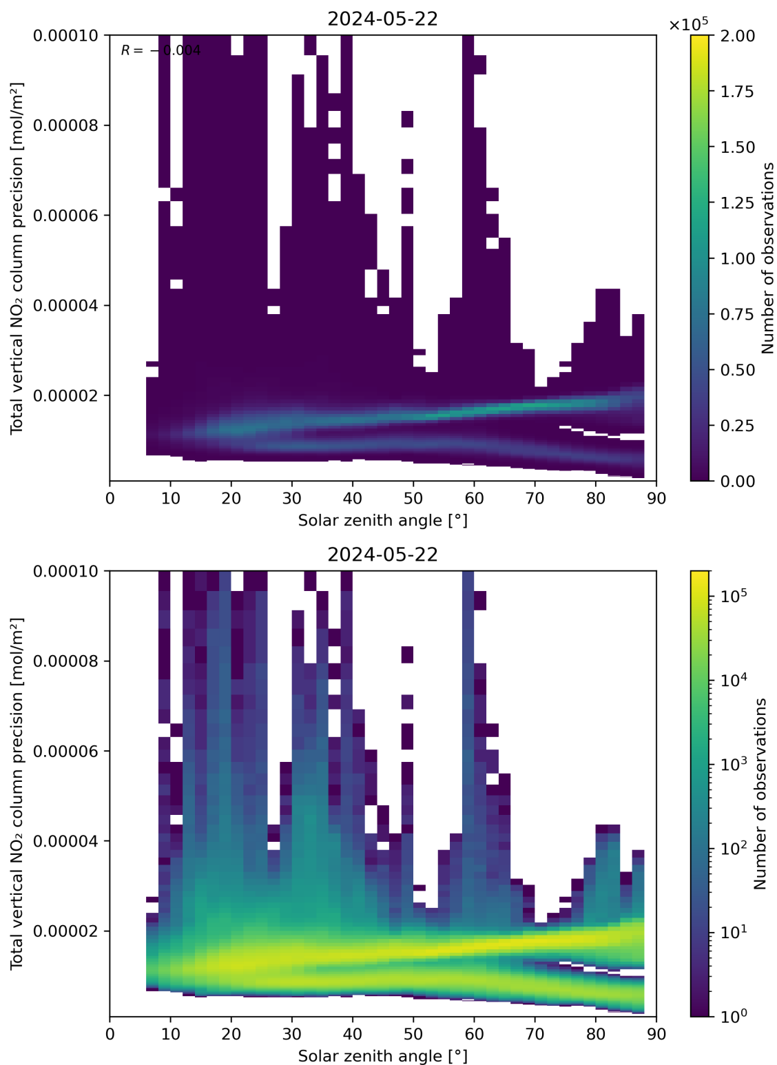
Figure 154: Scatter density plot of “Solar zenith angle” against “Total vertical NO 2 column precision” for 2024-05-21 to 2024-05-23.
