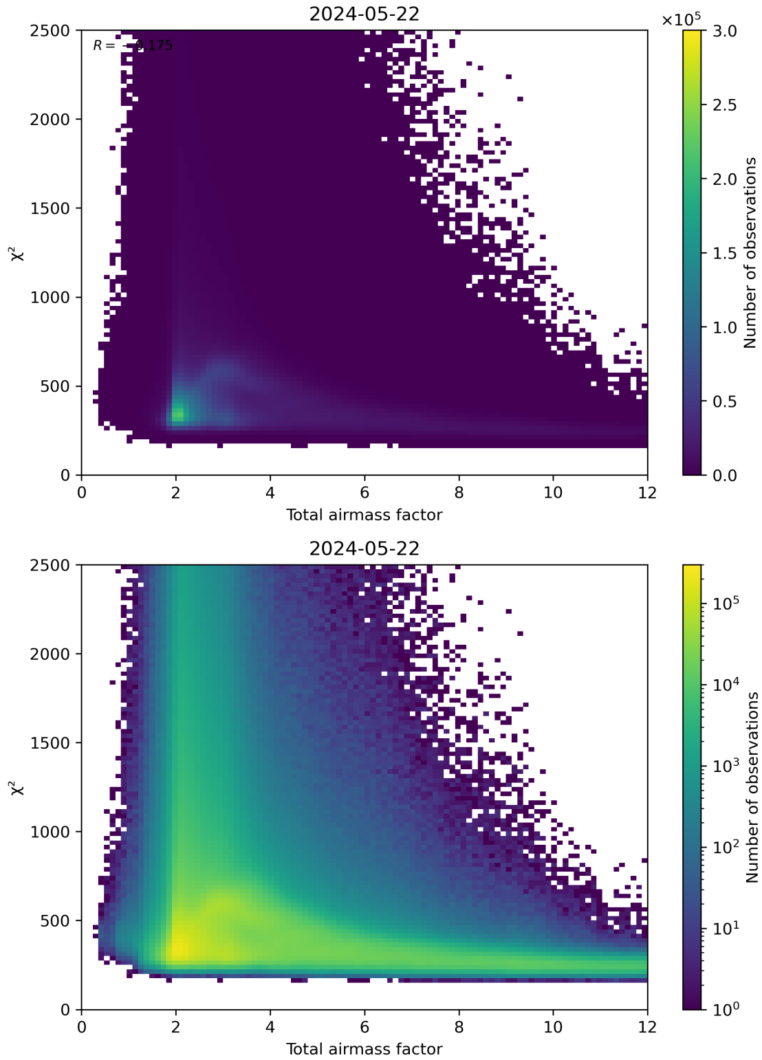
Figure 63: Scatter density plot of “Total airmass factor” against “ \chi^2 ” for 2024-05-21 to 2024-05-23.
