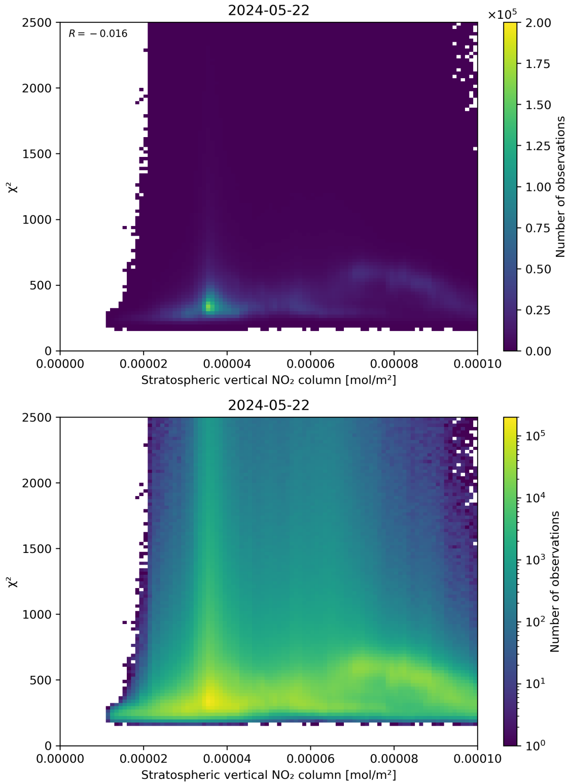
Figure 97: Scatter density plot of “Stratospheric vertical NO 2 column” against “ \chi^2 ” for 2024-05-21 to 2024-05-23.
