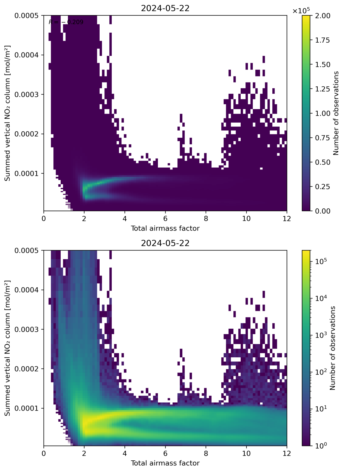
Figure 65: Scatter density plot of “Total airmass factor” against “Summed vertical NO 2 column” for 2024-05-21 to 2024-05-23.
