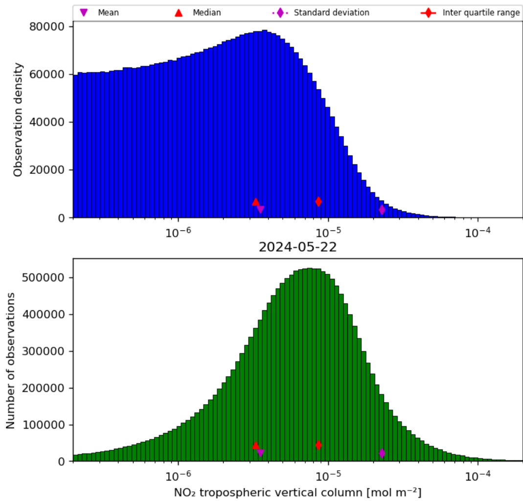
Figure 29: Histogram of “NO 2 tropospheric vertical column” for 2024-05-21 to 2024-05-23
