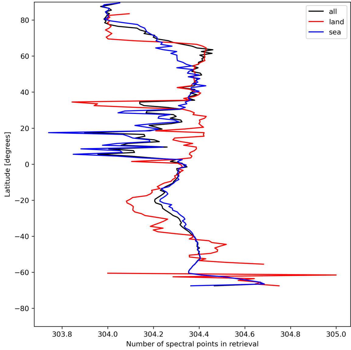
Figure 16: Zonal average of “Number of spectral points in retrieval” for 2024-05-21 to 2024-05-23.
