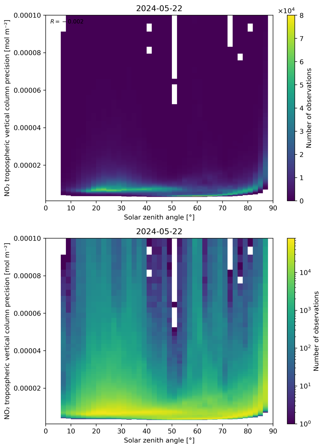
Figure 156: Scatter density plot of “Solar zenith angle” against “NO 2 tropospheric vertical column precision” for 2024-05-21 to 2024-05-23.
