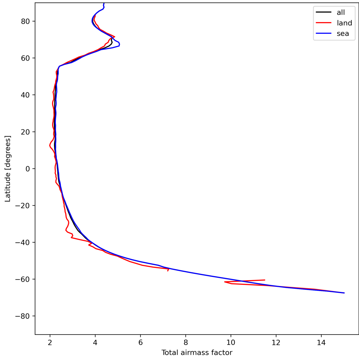
Figure 15: Zonal average of “Total airmass factor” for 2024-05-21 to 2024-05-23.
