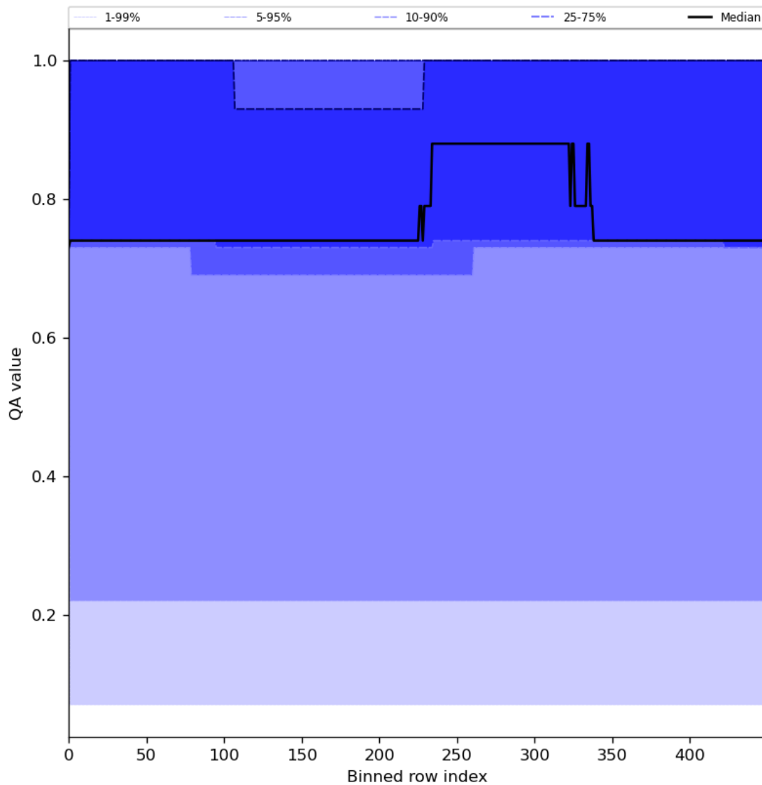
Figure 45: Along track statistics of “QA value” for 2024-05-21 to 2024-05-23
