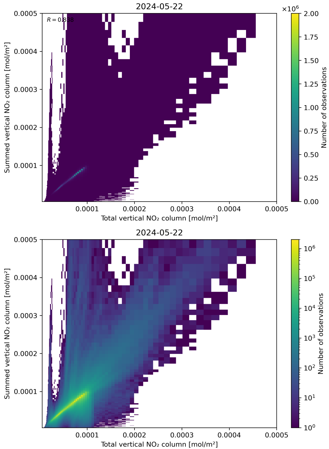
Figure 112: Scatter density plot of “Total vertical NO 2 column” against “Summed vertical NO 2 column” for 2024-05-21 to 2024-05-23.
