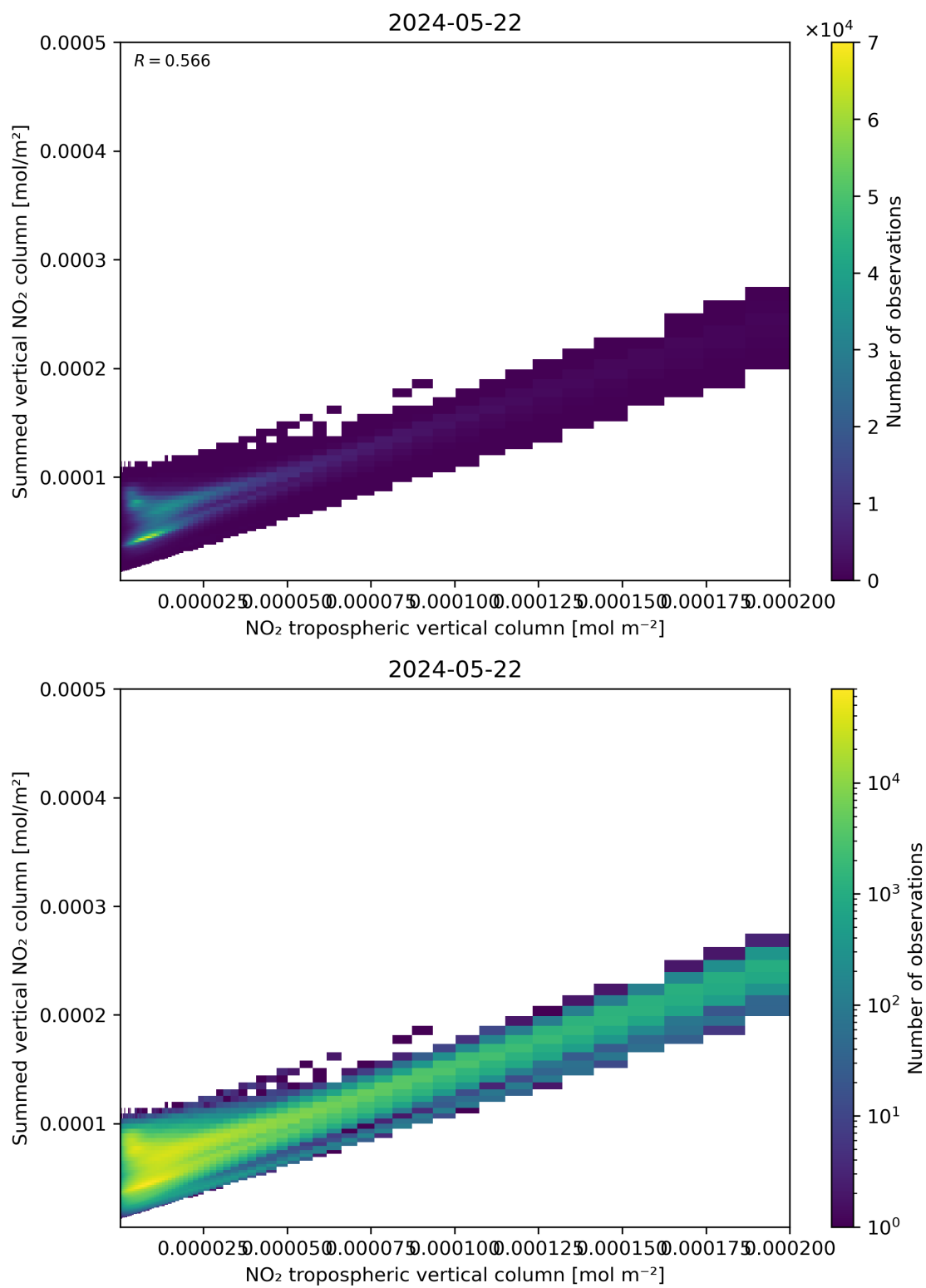
Figure 126: Scatter density plot of “NO 2 tropospheric vertical column” against “Summed vertical NO 2 column” for 2024-05-21 to 2024-05-23.
