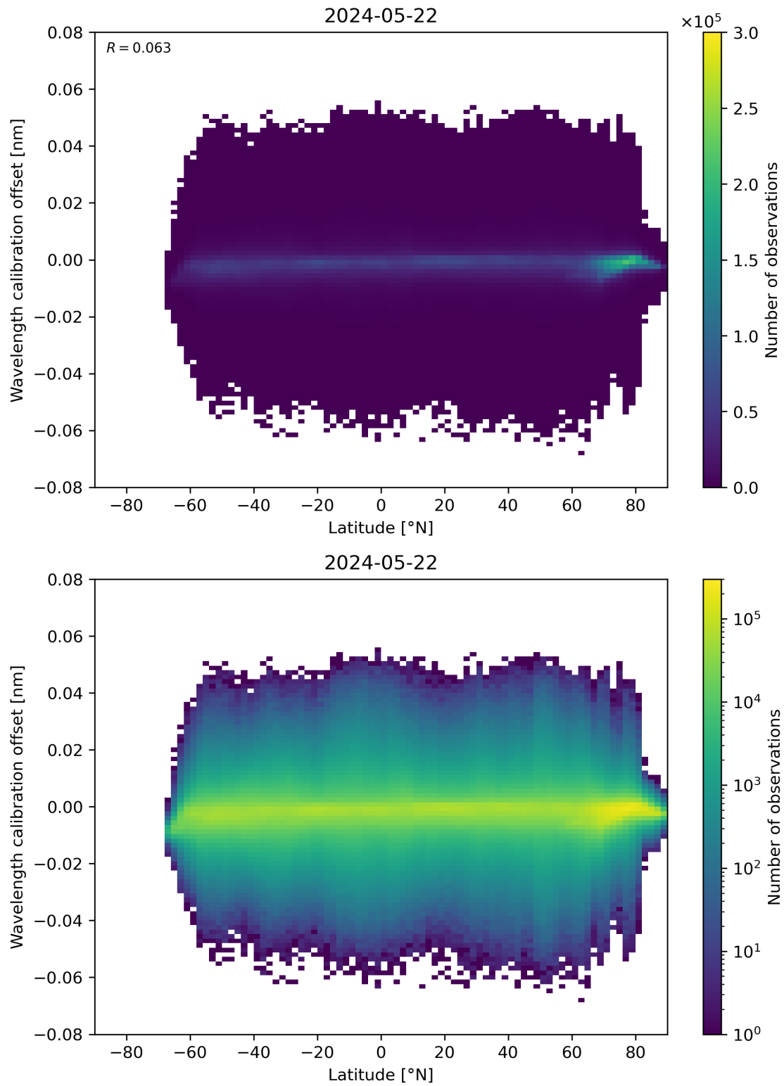
Figure 95: Scatter density plot of “Latitude” against “Wavelength calibration offset” for 2024-05-21 to 2024-05-23.
