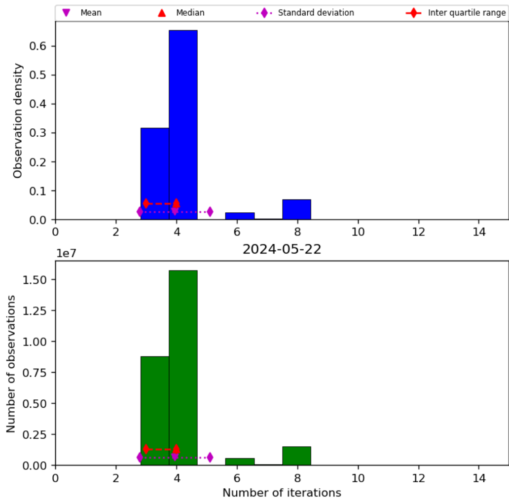
Figure 34: Histogram of “Number of iterations” for 2024-05-21 to 2024-05-23
