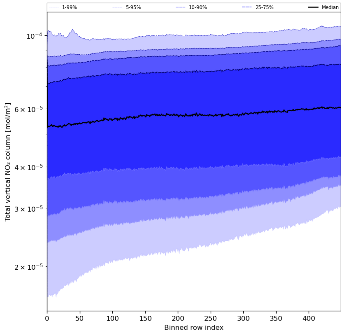
Figure 55: Along track statistics of “Total vertical NO 2 column” for 2024-05-21 to 2024-05-23
