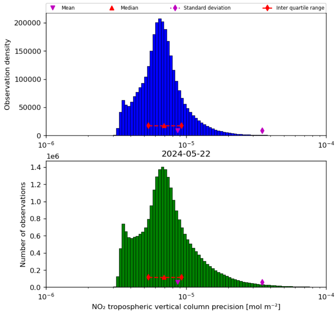
Figure 30: Histogram of “NO 2 tropospheric vertical column precision” for 2024-05-21 to 2024-05-23
