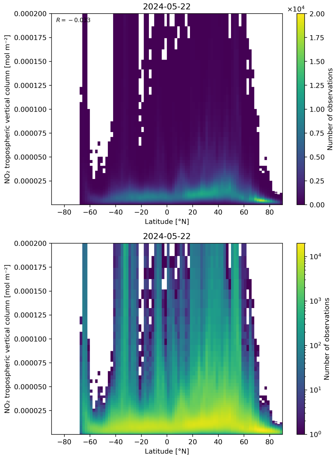
Figure 92: Scatter density plot of “Latitude” against “NO 2 tropospheric vertical column” for 2024-05-21 to 2024-05-23.
