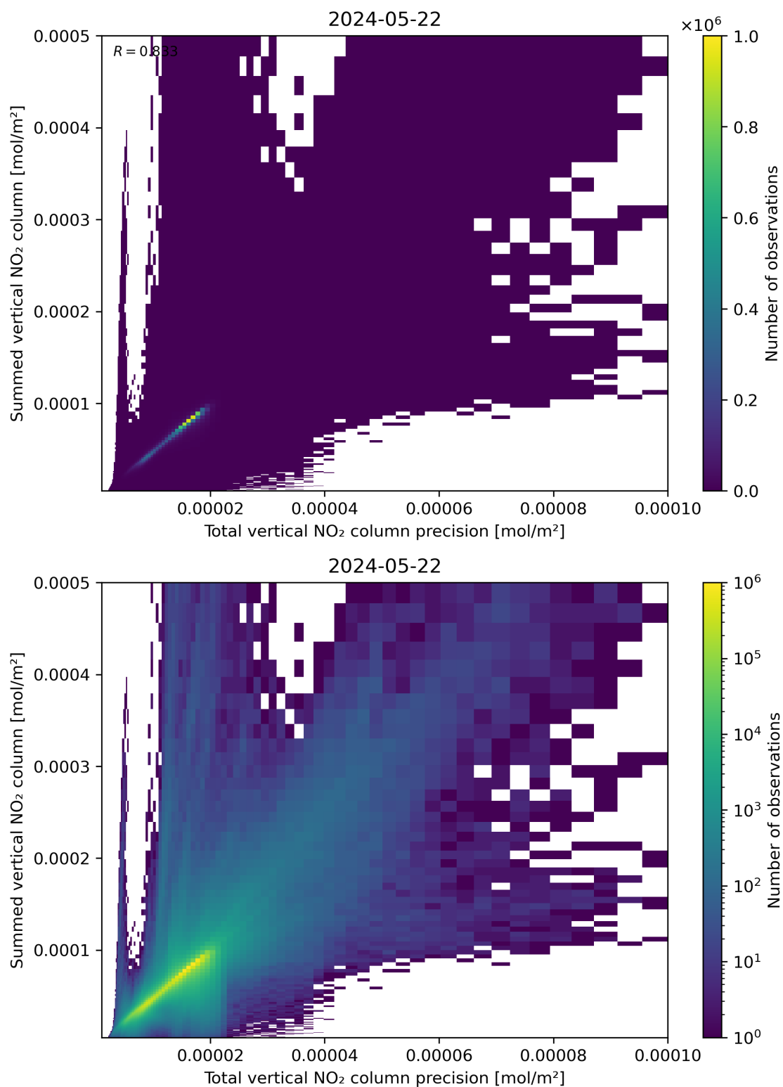
Figure 117: Scatter density plot of “Total vertical NO 2 column precision” against “Summed vertical NO 2 column” for 2024-05-21 to 2024-05-23.
