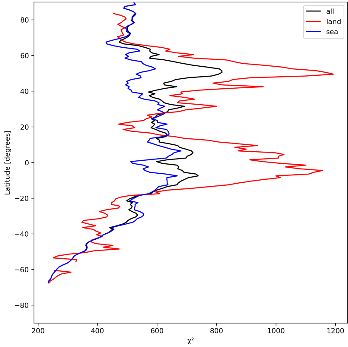
Figure 25: Zonal average of “ \chi^2 ” for 2024-05-21 to 2024-05-23.
