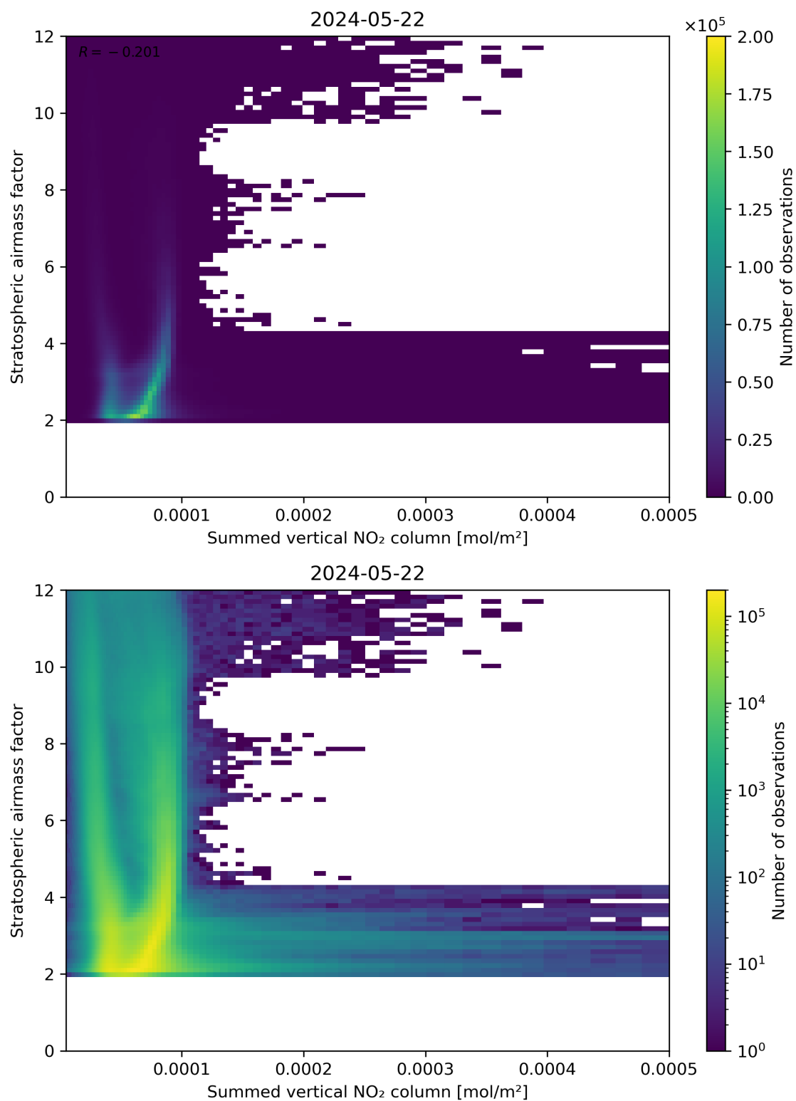
Figure 103: Scatter density plot of “Summed vertical NO 2 column” against “Stratospheric air mass factor” for 2024-05-21 to 2024-05-23.
