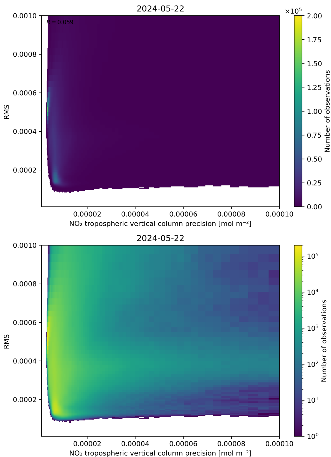
Figure 140: Scatter density plot of “NO 2 tropospheric vertical column precision” against “RMS” for 2024-05-21 to 2024-05-23.
