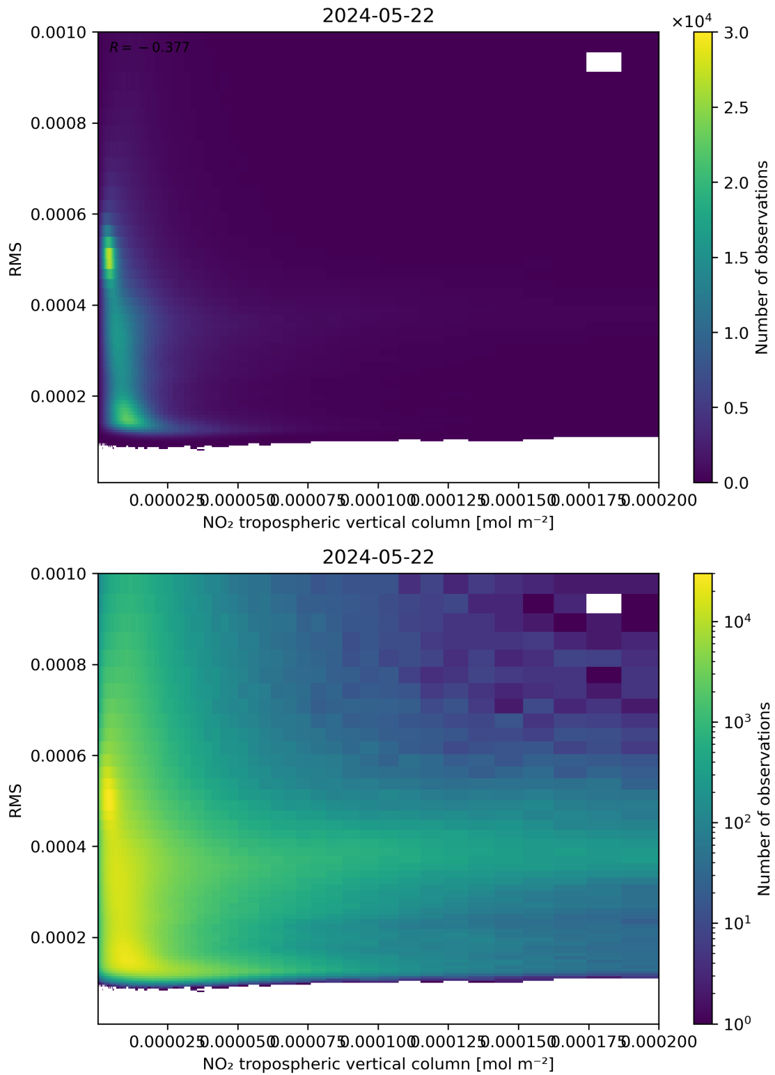
Figure 142: Scatter density plot of “NO 2 tropospheric vertical column” against “RMS” for 2024-05-21 to 2024-05-23.
