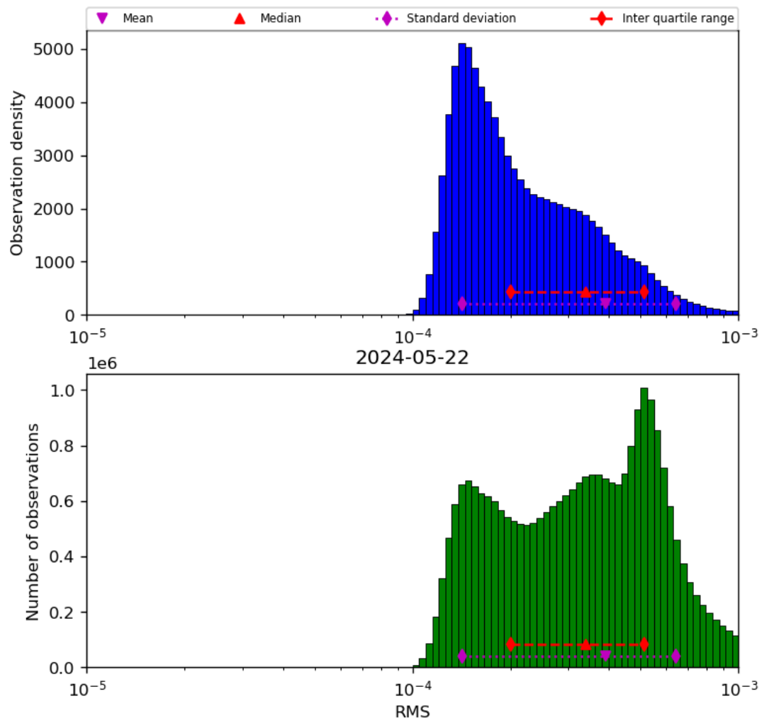
Figure 43: Histogram of “RMS” for 2024-05-21 to 2024-05-23
