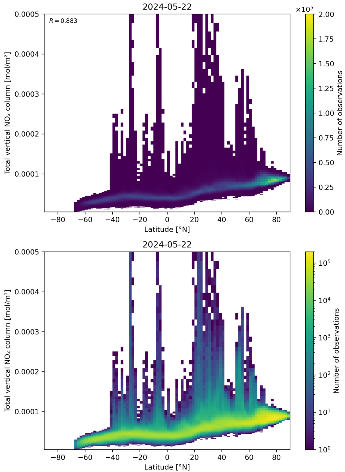
Figure 90: Scatter density plot of “Latitude” against “Total vertical NO 2 column” for 2024-05-21 to 2024-05-23.
