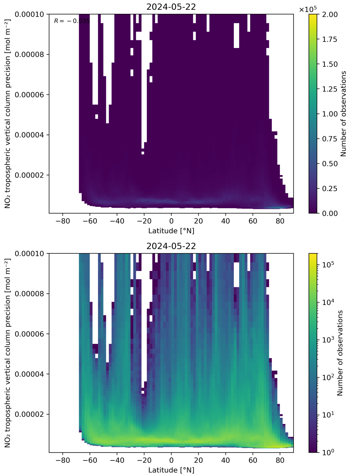
Figure 93: Scatter density plot of “Latitude” against “NO 2 tropospheric vertical column precision” for 2024-05-21 to 2024-05-23.
