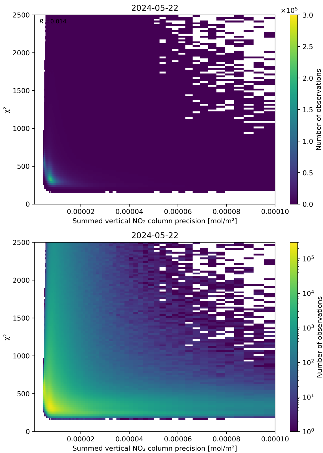
Figure 107: Scatter density plot of “Summed vertical NO 2 column precision” against “ \chi^2 ” for 2024-05-21 to 2024-05-23.
