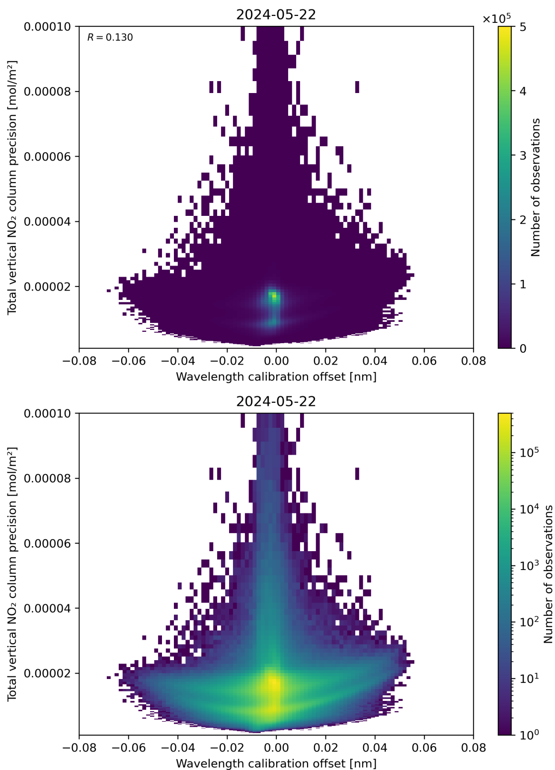
Figure 180: Scatter density plot of “Wavelength calibration offset” against “Total vertical NO 2 column precision” for 2024-05-21 to 2024-05-23.
