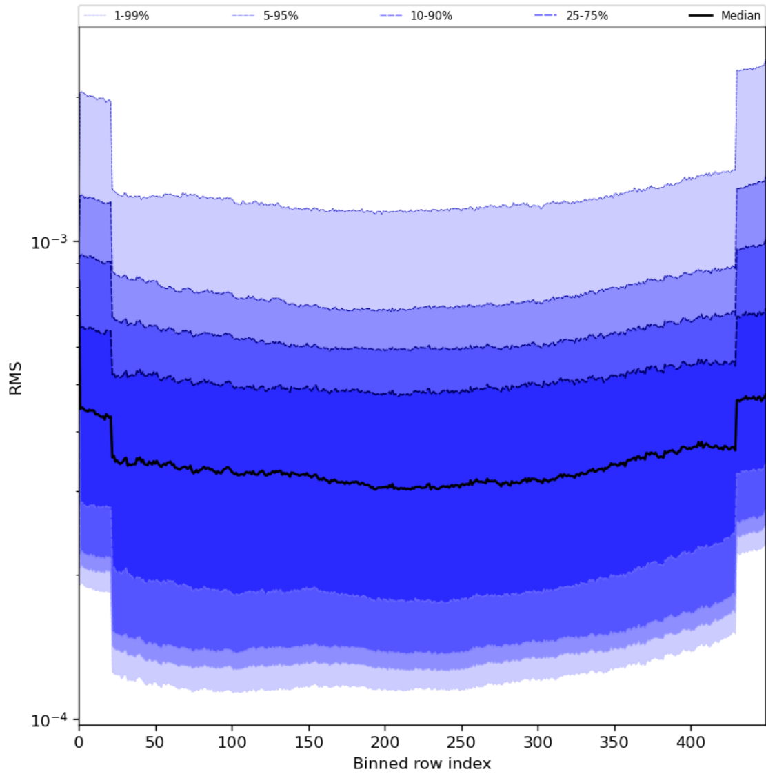
Figure 60: Along track statistics of “RMS” for 2024-05-21 to 2024-05-23
