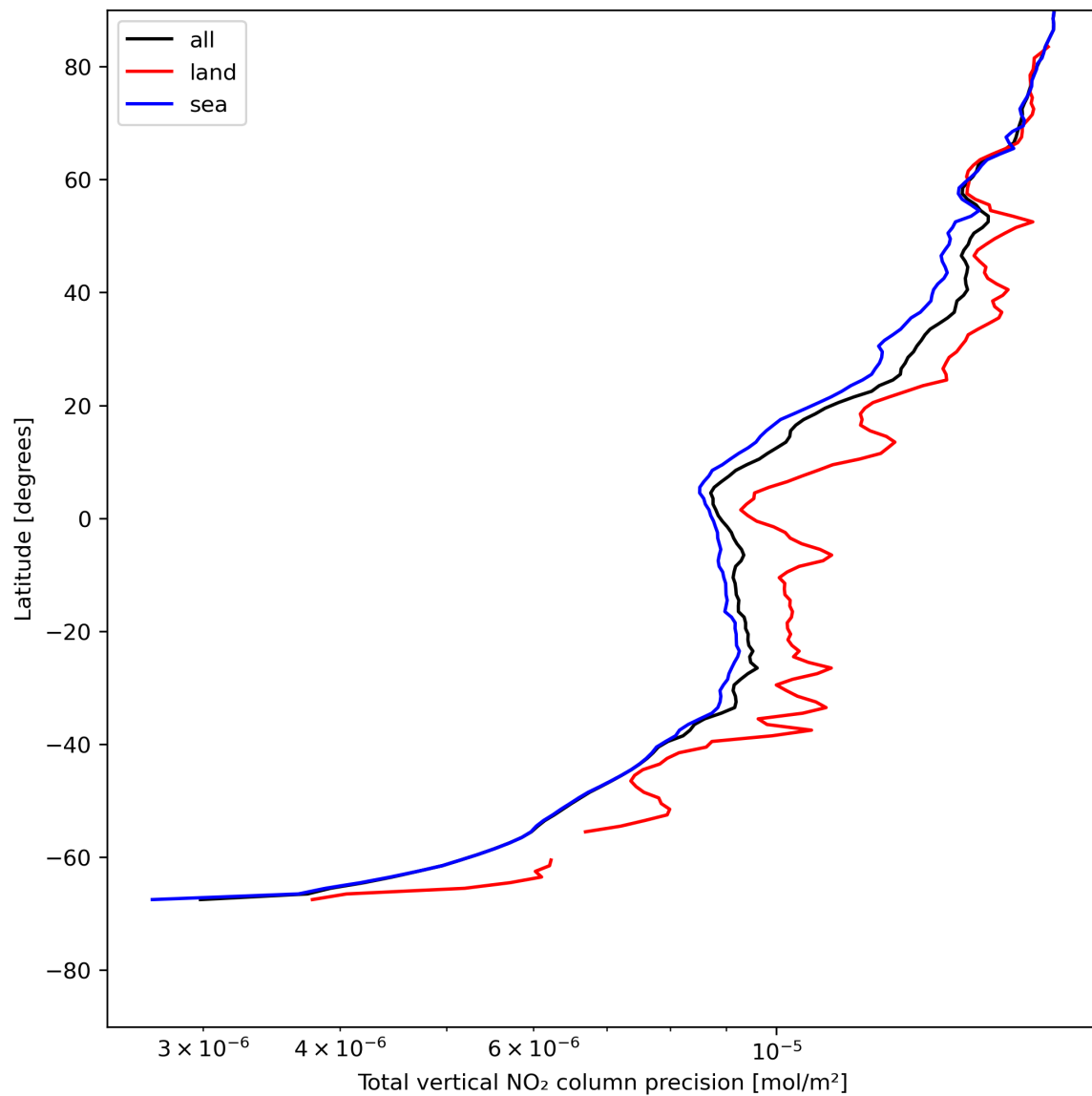
Figure 22: Zonal average of “Total vertical NO 2 column precision” for 2024-05-21 to 2024-05-23.
