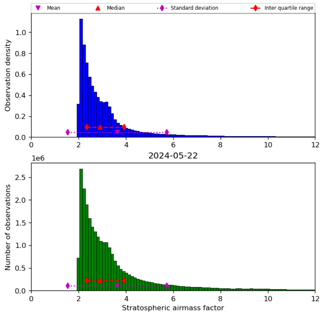
Figure 44: Histogram of “Stratospheric airmass factor” for 2024-05-21 to 2024-05-23
