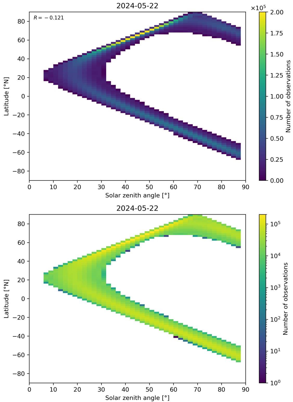
Figure 149: Scatter density plot of “Solar zenith angle” against “Latitude” for 2024-05-21 to 2024-05-23.
