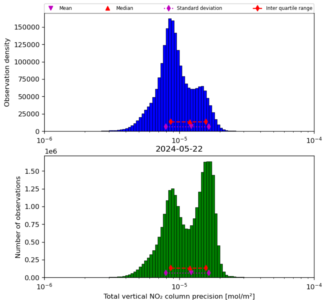
Figure 39: Histogram of “Total vertical NO 2 column precision” for 2024-05-21 to 2024-05-23
