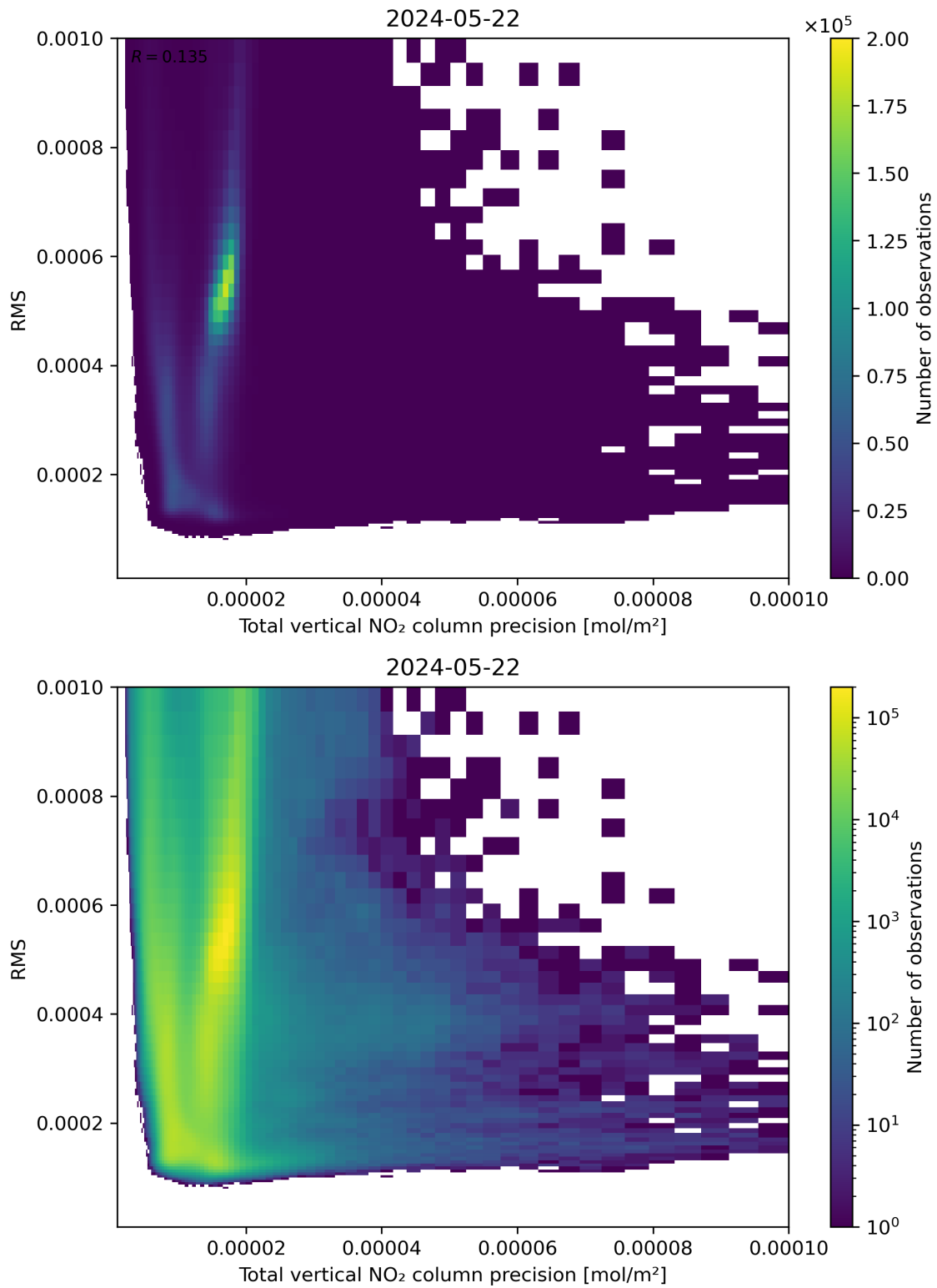
Figure 119: Scatter density plot of “Total vertical NO 2 column precision” against “RMS” for 2024-05-21 to 2024-05-23.
