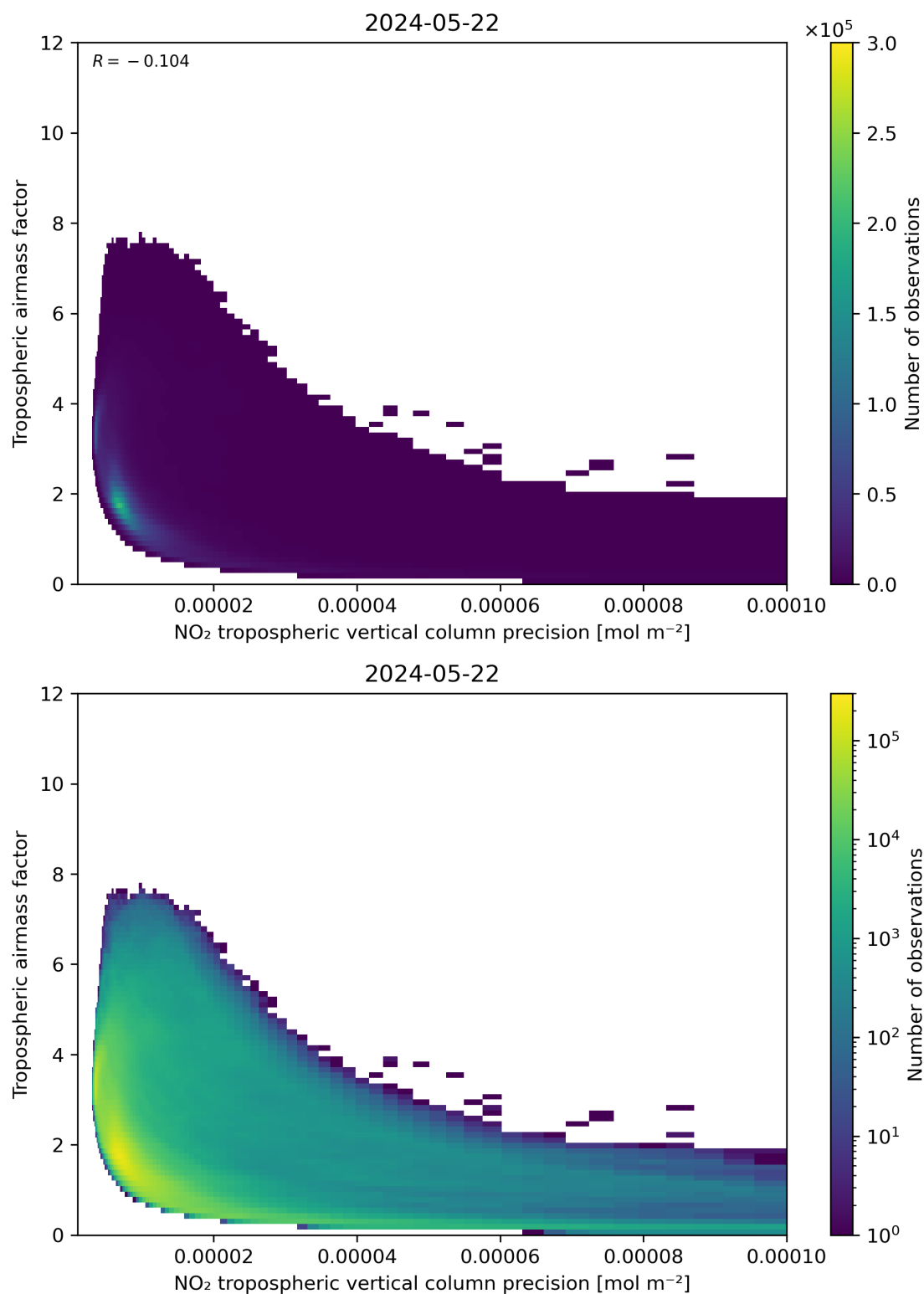
Figure 133: Scatter density plot of “NO 2 tropospheric vertical column precision” against “Tropospheric airmass factor” for 2024-05-21 to 2024-05-23.
