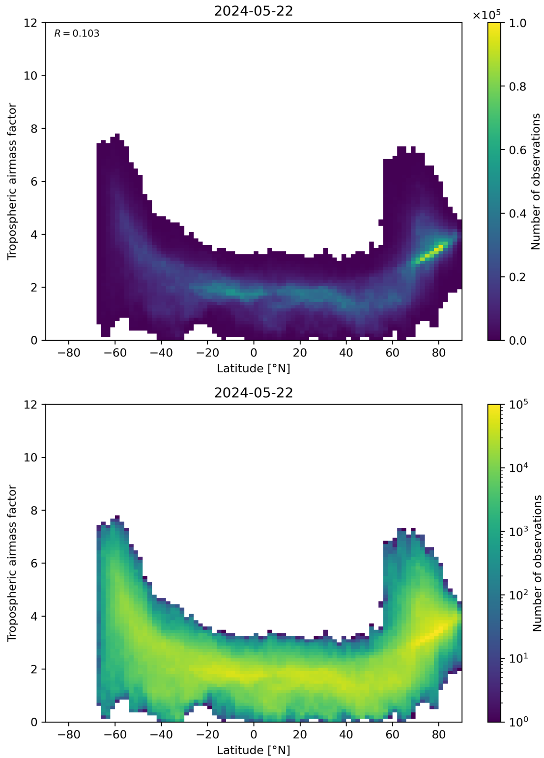
Figure 85: Scatter density plot of “Latitude” against “Tropospheric airmass factor” for 2024-05-21 to 2024-05-23.
