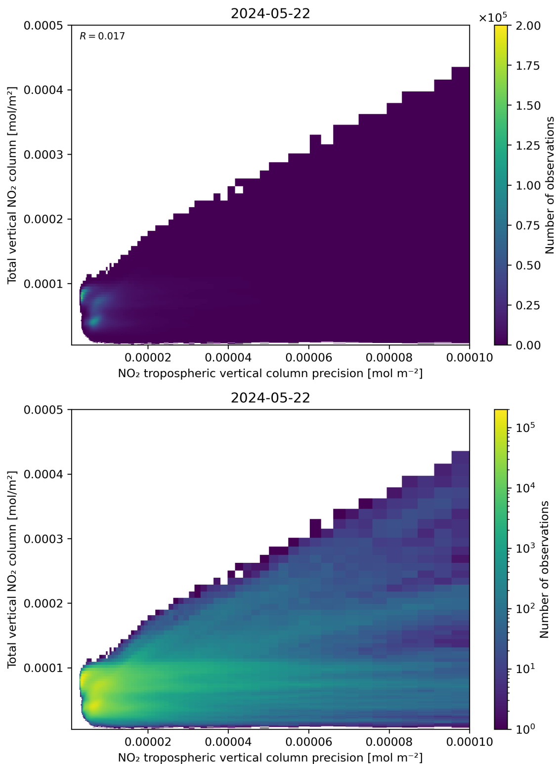
Figure 138: Scatter density plot of “NO 2 tropospheric vertical column precision” against “Total vertical NO 2 column” for 2024-05-21 to 2024-05-23.
