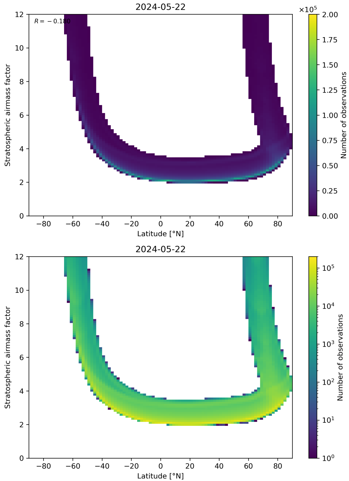
Figure 83: Scatter density plot of “Latitude” against “Stratospheric air mass factor” for 2024-05-21 to 2024-05-23.
