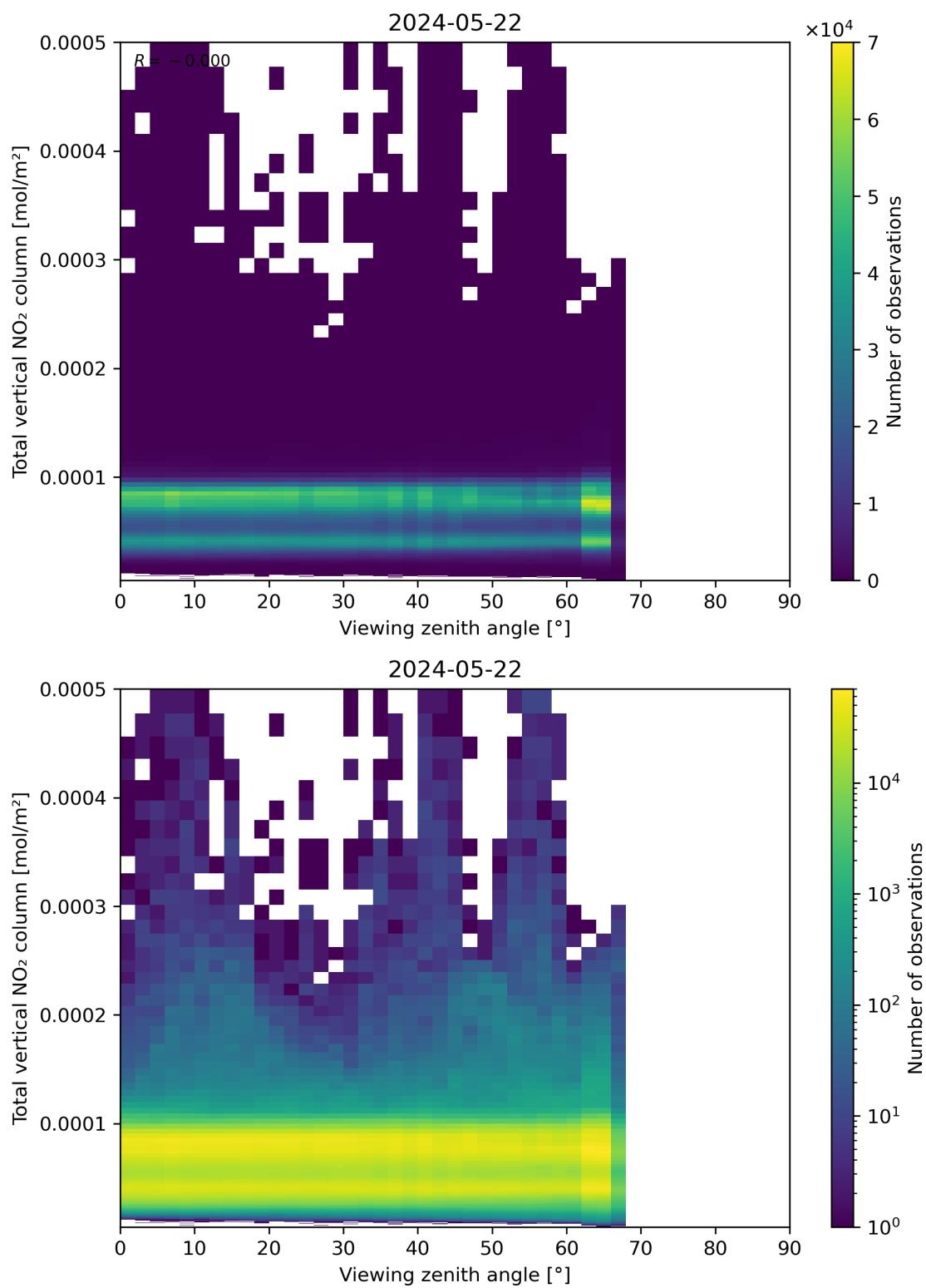
Figure 167: Scatter density plot of “Viewing zenith angle” against “Total vertical NO 2 column” for 2024-05-21 to 2024-05-23.
