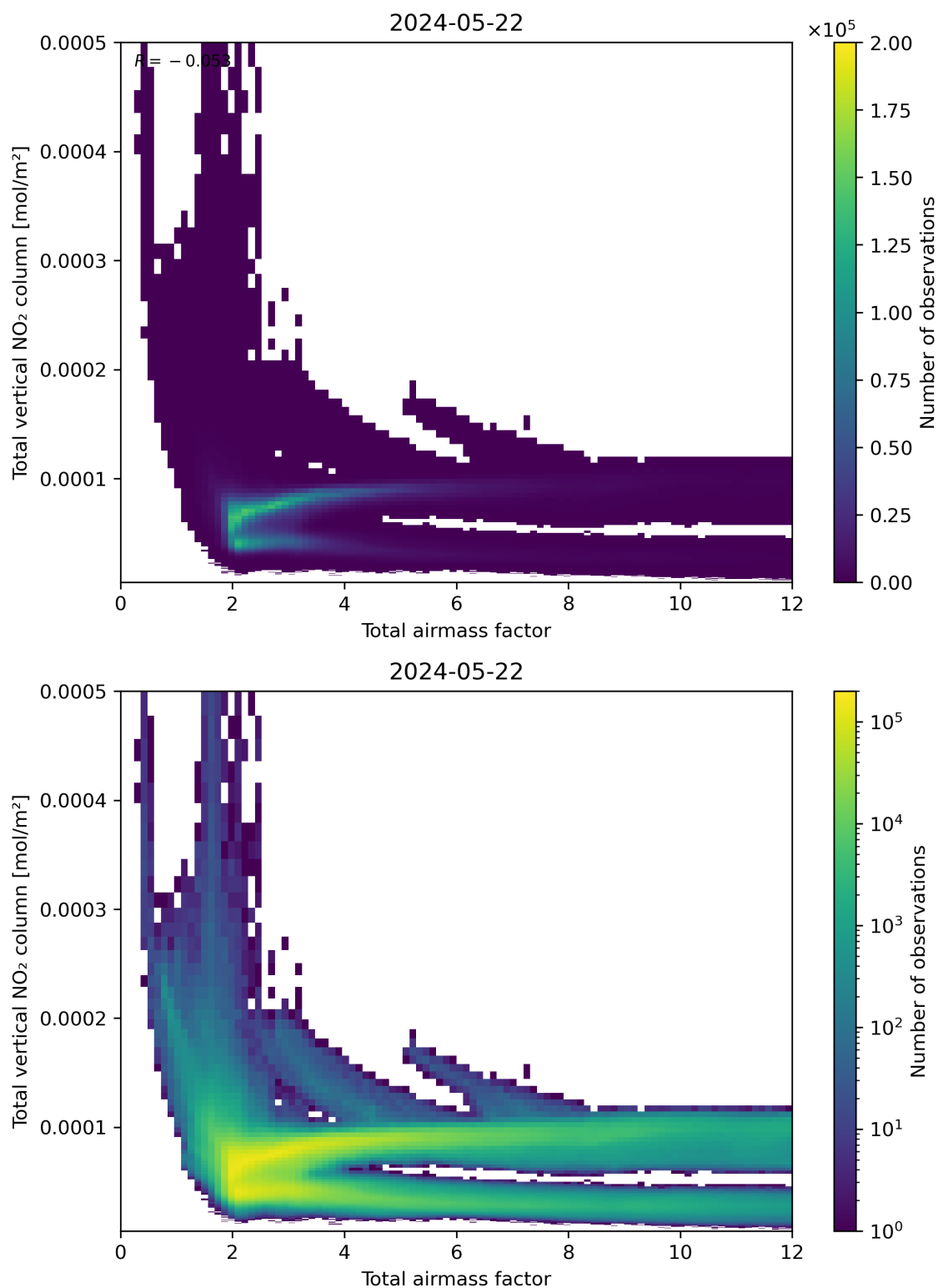
Figure 67: Scatter density plot of “Total airmass factor” against “Total vertical NO 2 column” for 2024-05-21 to 2024-05-23.
