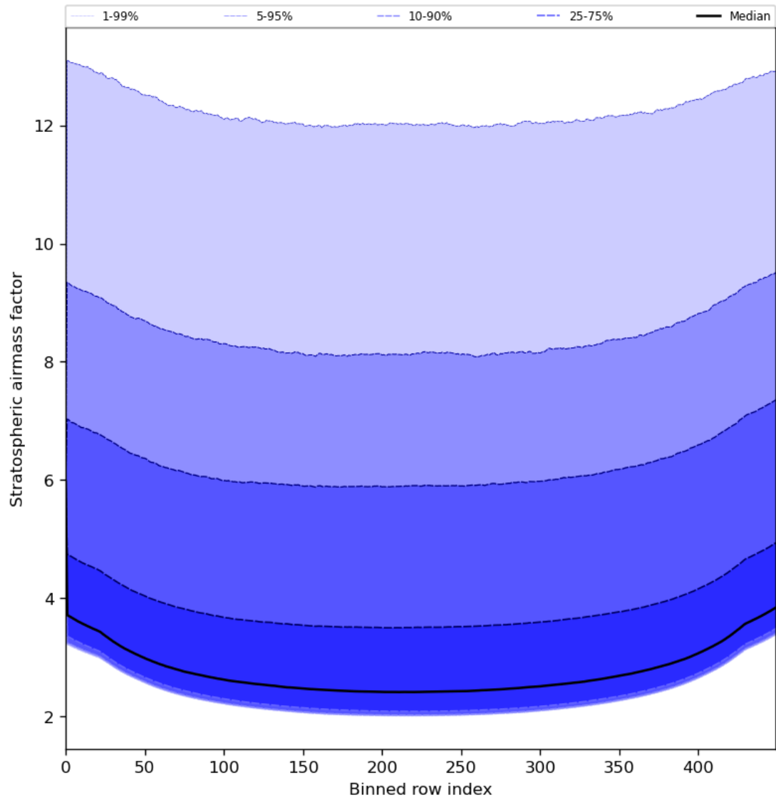
Figure 61: Along track statistics of “Stratospheric airmass factor” for 2024-05-21 to 2024-05-23
