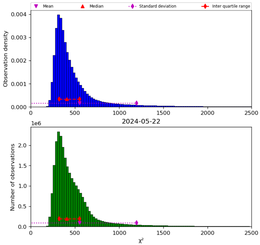
Figure 42: Histogram of “ \chi^2 ” for 2024-05-21 to 2024-05-23
