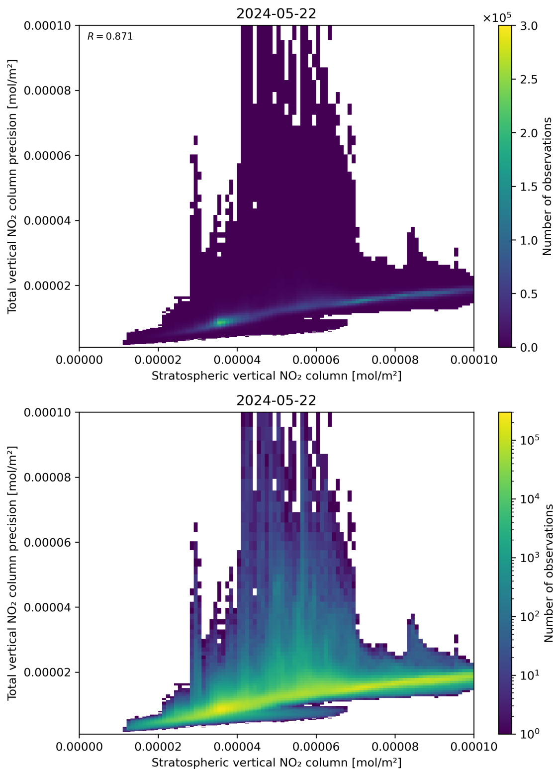
Figure 101: Scatter density plot of “Stratospheric vertical NO 2 column” against “Total vertical NO 2 column precision” for 2024-05-21 to 2024-05-23.
