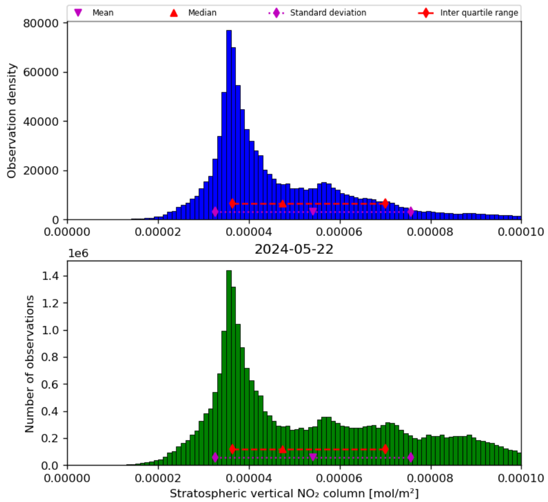
Figure 36: Histogram of “Stratospheric vertical NO 2 column” for 2024-05-21 to 2024-05-23
