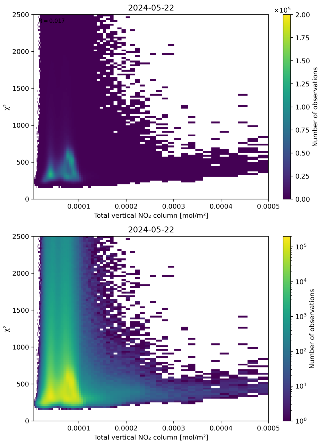
Figure 111: Scatter density plot of “Total vertical NO 2 column” against “ \chi^2 ” for 2024-05-21 to 2024-05-23.
