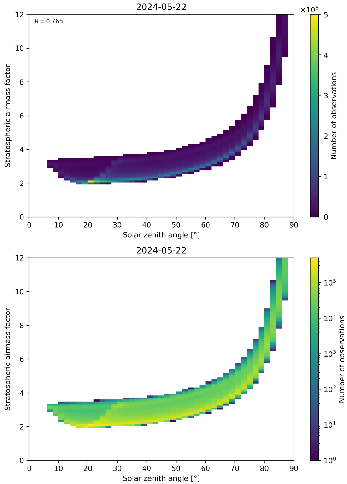
Figure 145: Scatter density plot of “Solar zenith angle” against “Stratospheric airmass factor” for 2024-05-21 to 2024-05-23.
