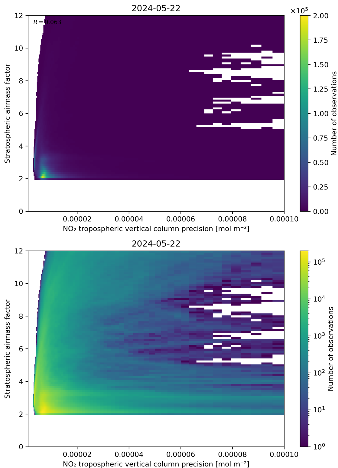
Figure 131: Scatter density plot of “NO 2 tropospheric vertical column precision” against “Stratospheric airmass factor” for 2024-05-21 to 2024-05-23.
