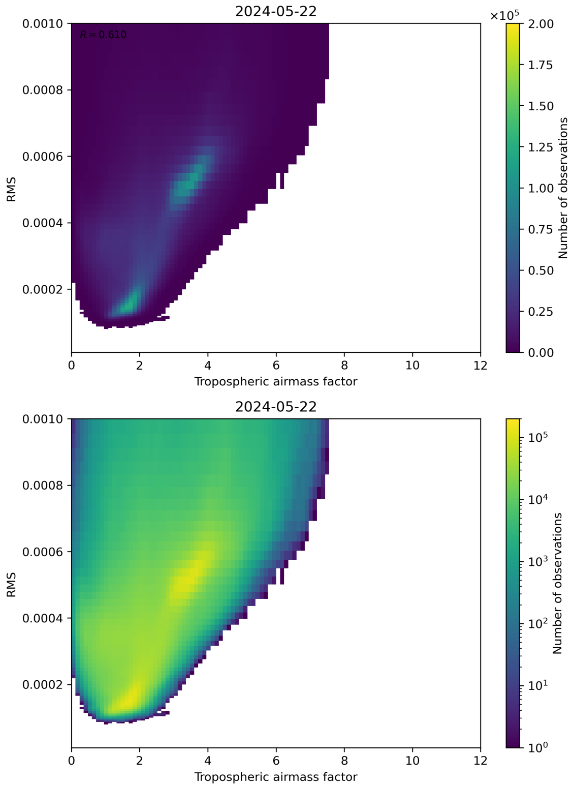
Figure 79: Scatter density plot of “Tropospheric airmass factor” against “RMS” for 2024-05-21 to 2024-05-23.
