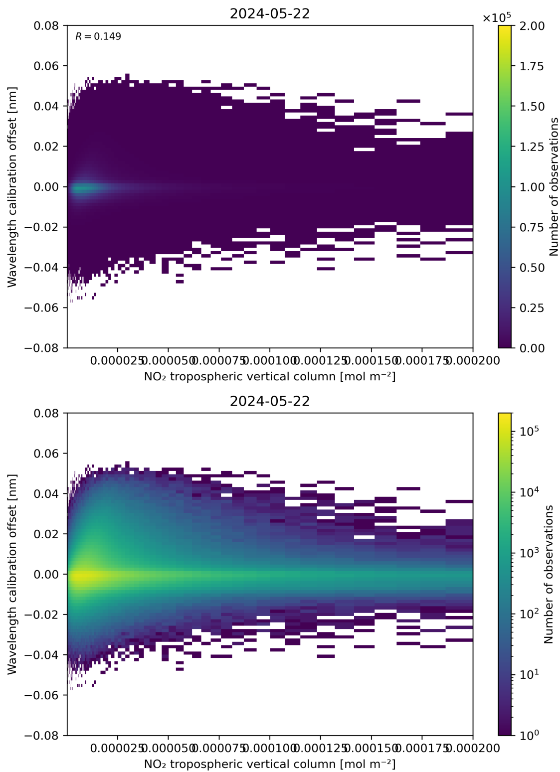
Figure 143: Scatter density plot of “NO 2 tropospheric vertical column” against “Wavelength calibration offset” for 2024-05-21 to 2024-05-23.
