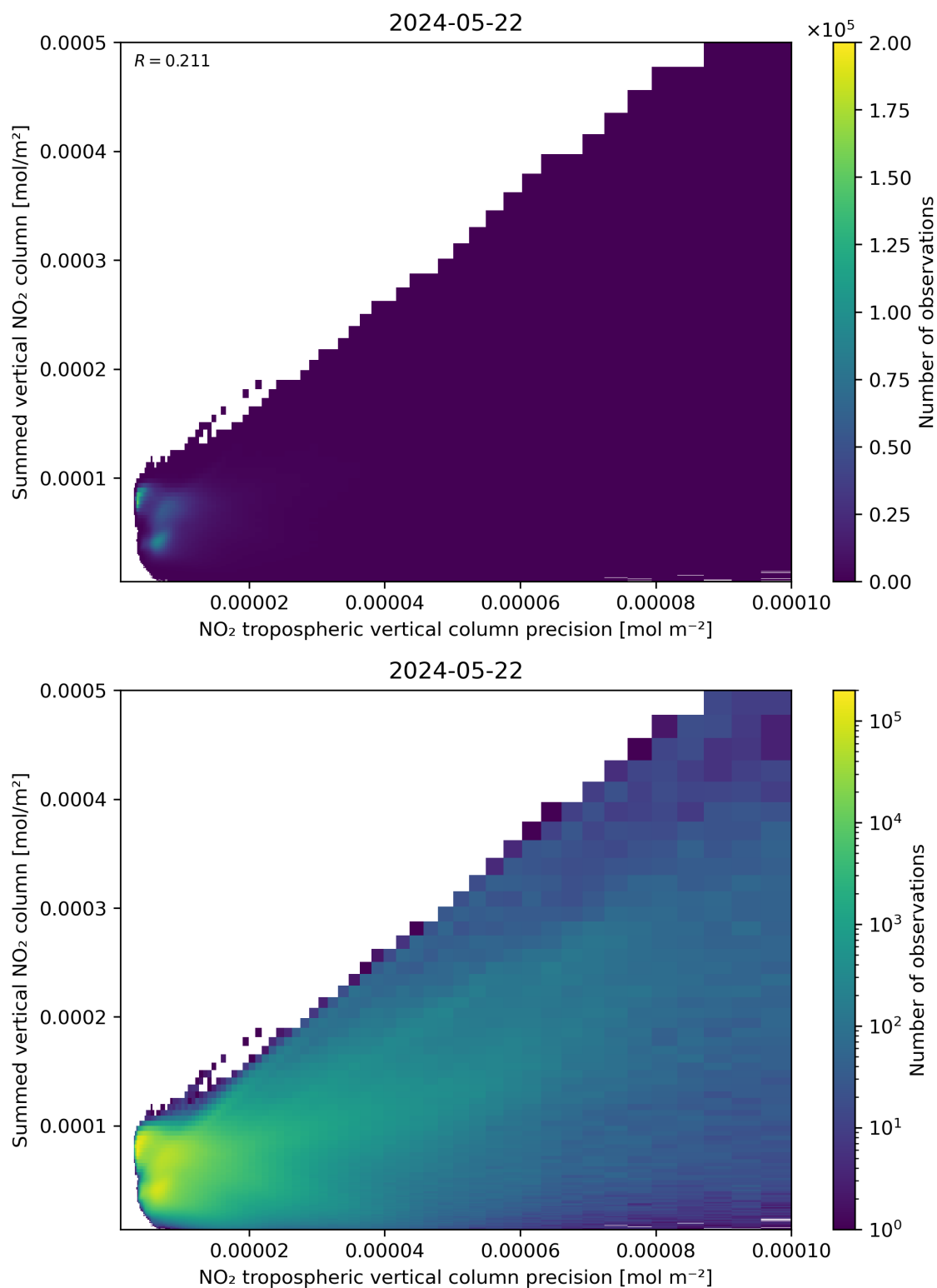
Figure 136: Scatter density plot of “NO 2 tropospheric vertical column precision” against “Summed vertical NO 2 column” for 2024-05-21 to 2024-05-23.
