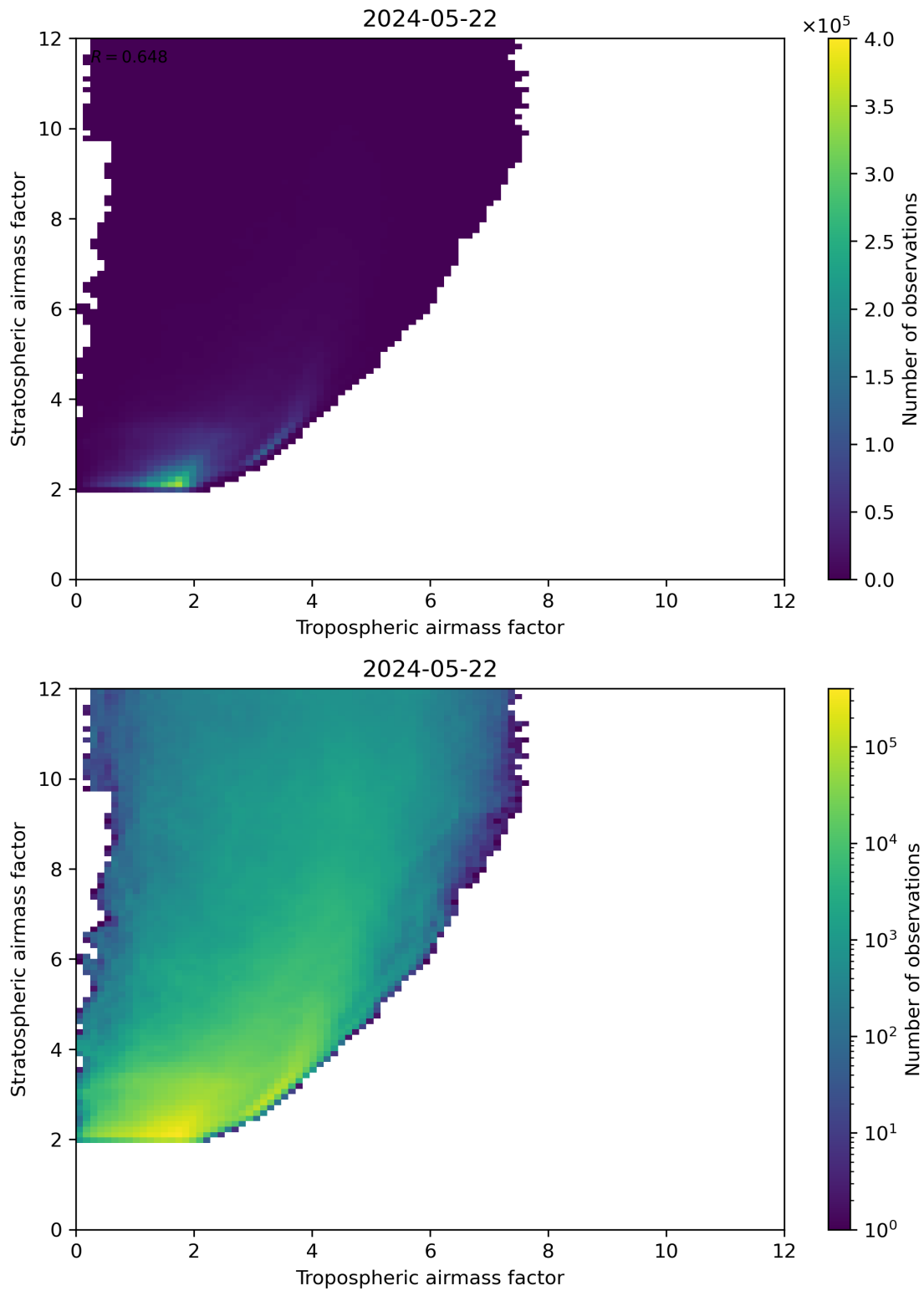
Figure 71: Scatter density plot of “Tropospheric airmass factor” against “Stratospheric airmass factor” for 2024-05-21 to 2024-05-23.
