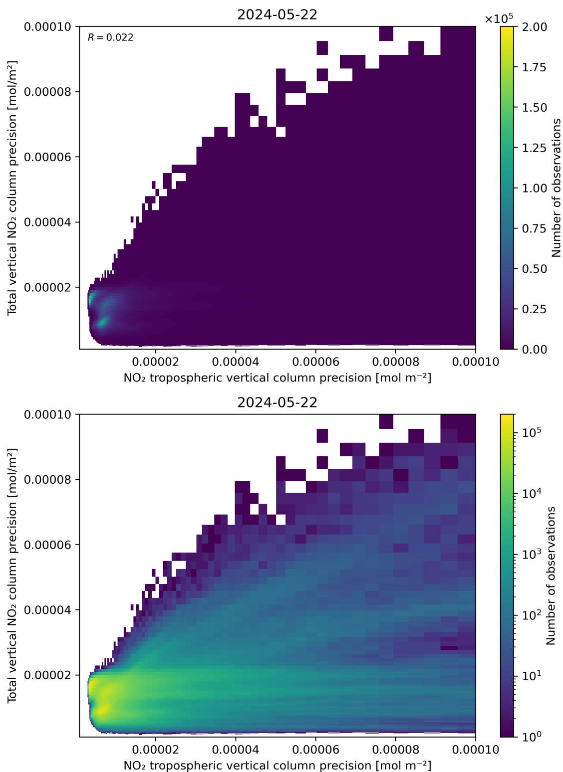
Figure 139: Scatter density plot of “NO 2 tropospheric vertical column precision” against “Total vertical NO 2 column precision” for 2024-05-21 to 2024-05-23.
