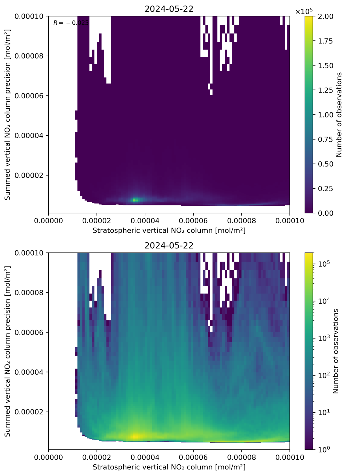
Figure 99: Scatter density plot of “Stratospheric vertical NO 2 column” against “Summed vertical NO 2 column precision” for 2024-05-21 to 2024-05-23.
