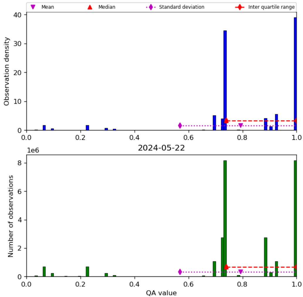
Figure 28: Histogram of “QA value” for 2024-05-21 to 2024-05-23
