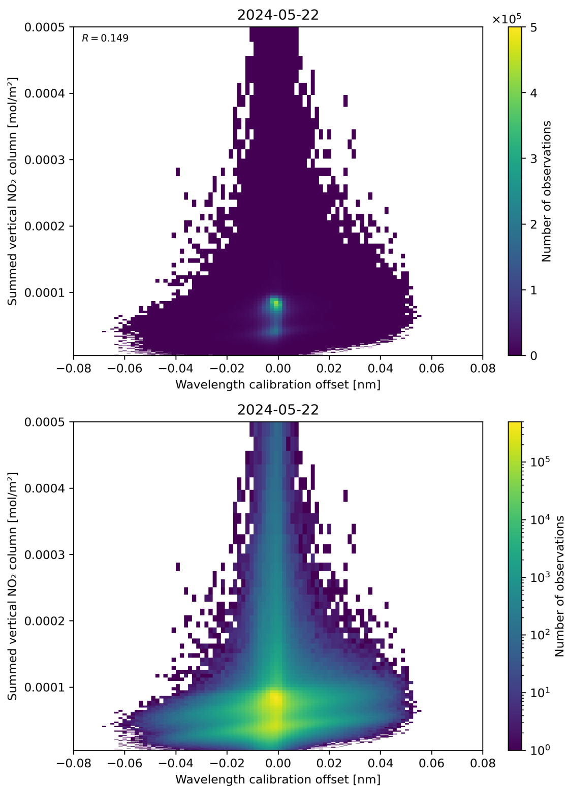
Figure 177: Scatter density plot of “Wavelength calibration offset” against “Summed vertical NO 2 column” for 2024-05-21 to 2024-05-23.
