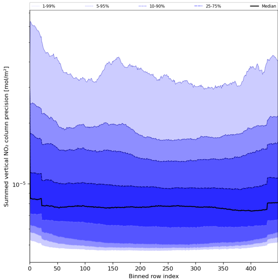
Figure 58: Along track statistics of “Summed vertical NO 2 column precision” for 2024-05-21 to 2024-05-23
