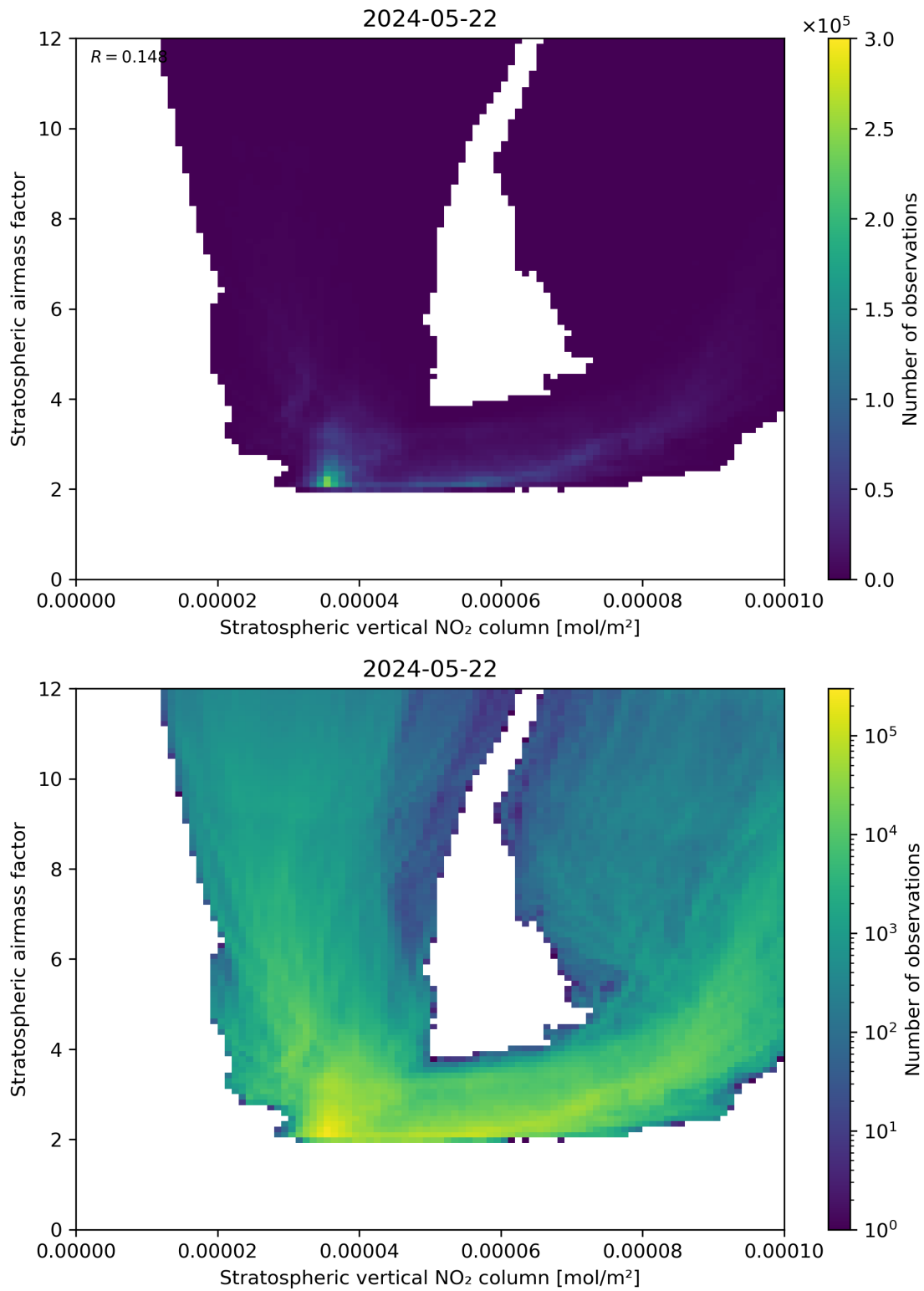
Figure 96: Scatter density plot of “Stratospheric vertical NO 2 column” against “Stratospheric airmass factor” for 2024-05-21 to 2024-05-23.
