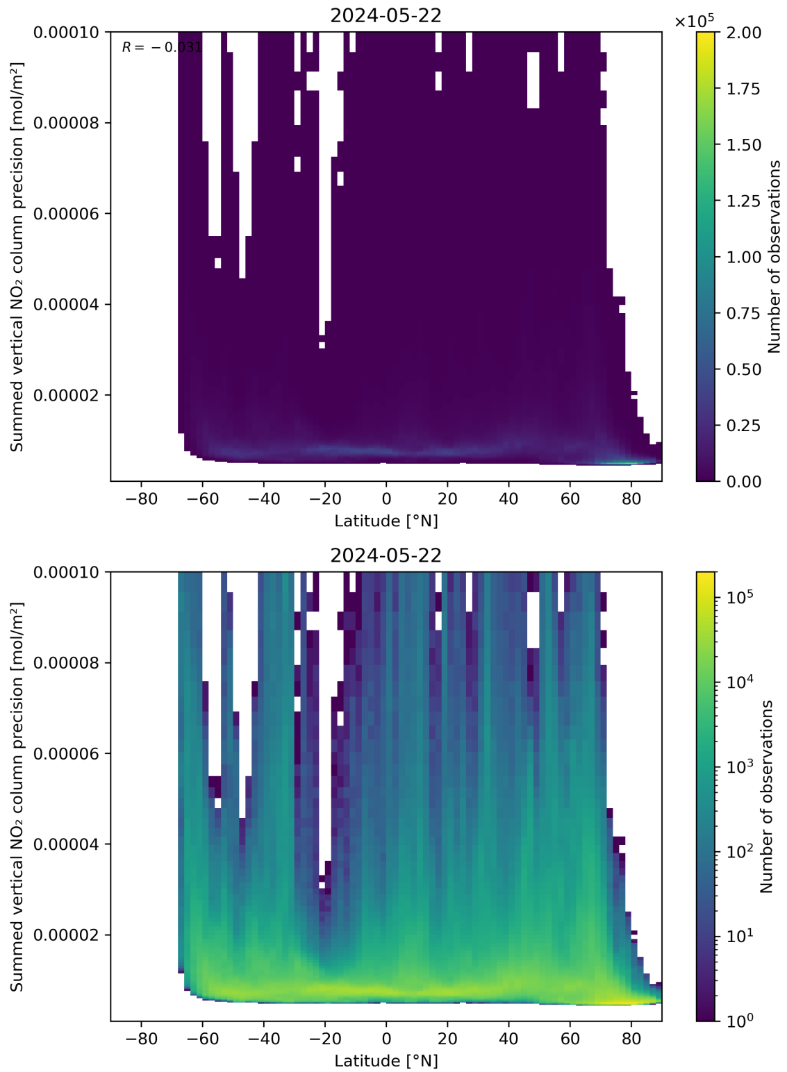
Figure 89: Scatter density plot of “Latitude” against “Summed vertical NO 2 column precision” for 2024-05-21 to 2024-05-23.
