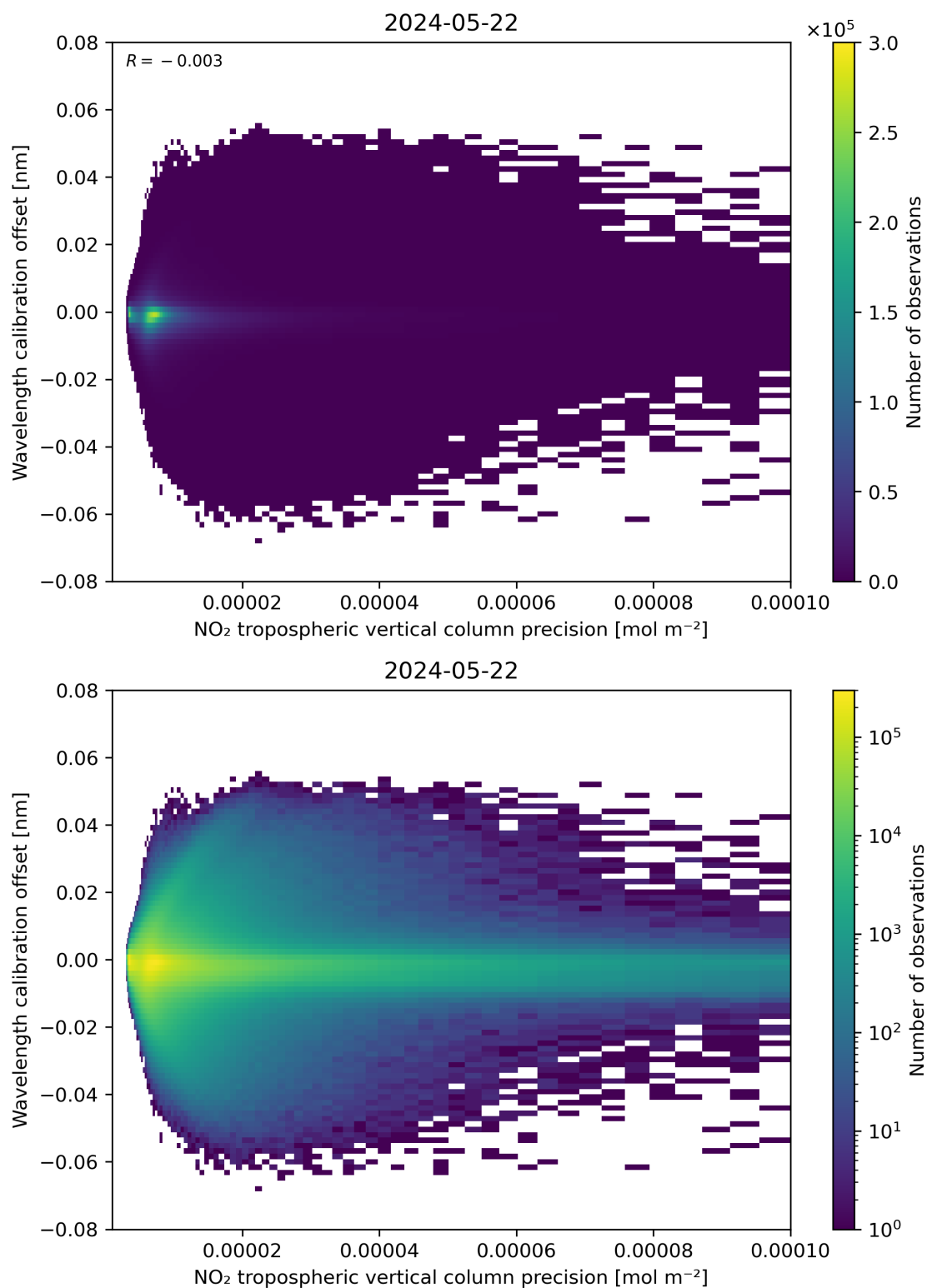
Figure 141: Scatter density plot of “NO 2 tropospheric vertical column precision” against “Wavelength calibration offset” for 2024-05-21 to 2024-05-23.
