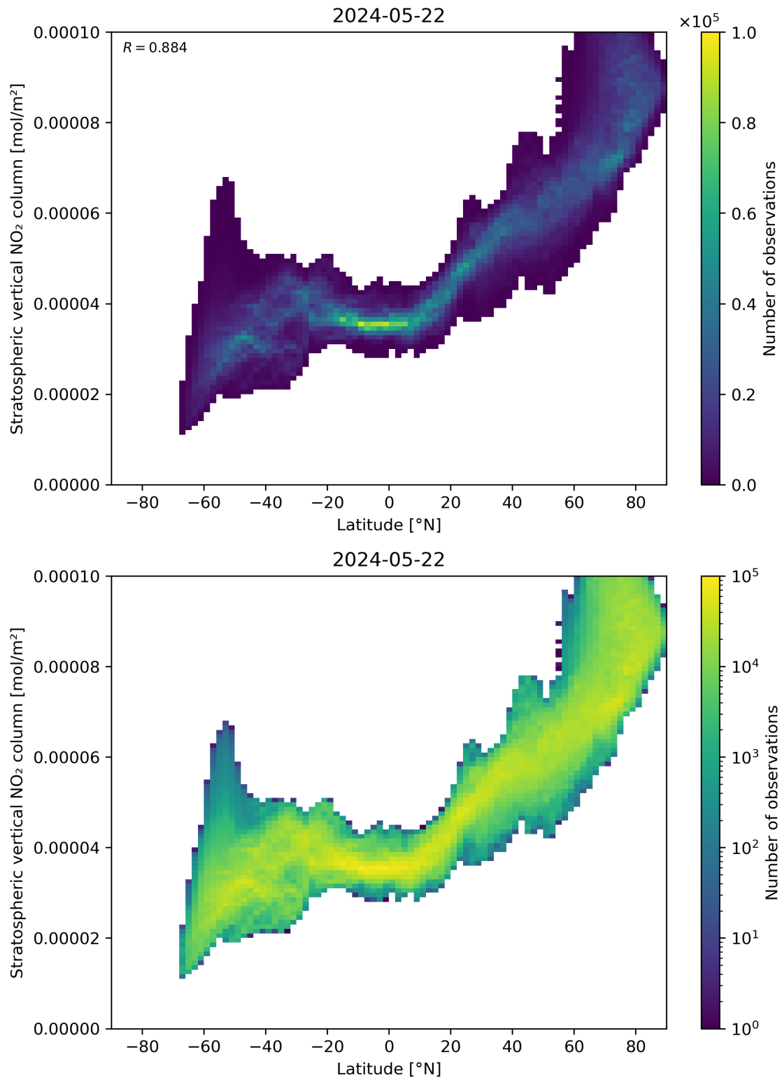
Figure 87: Scatter density plot of “Latitude” against “Stratospheric vertical NO 2 column” for 2024-05-21 to 2024-05-23.
