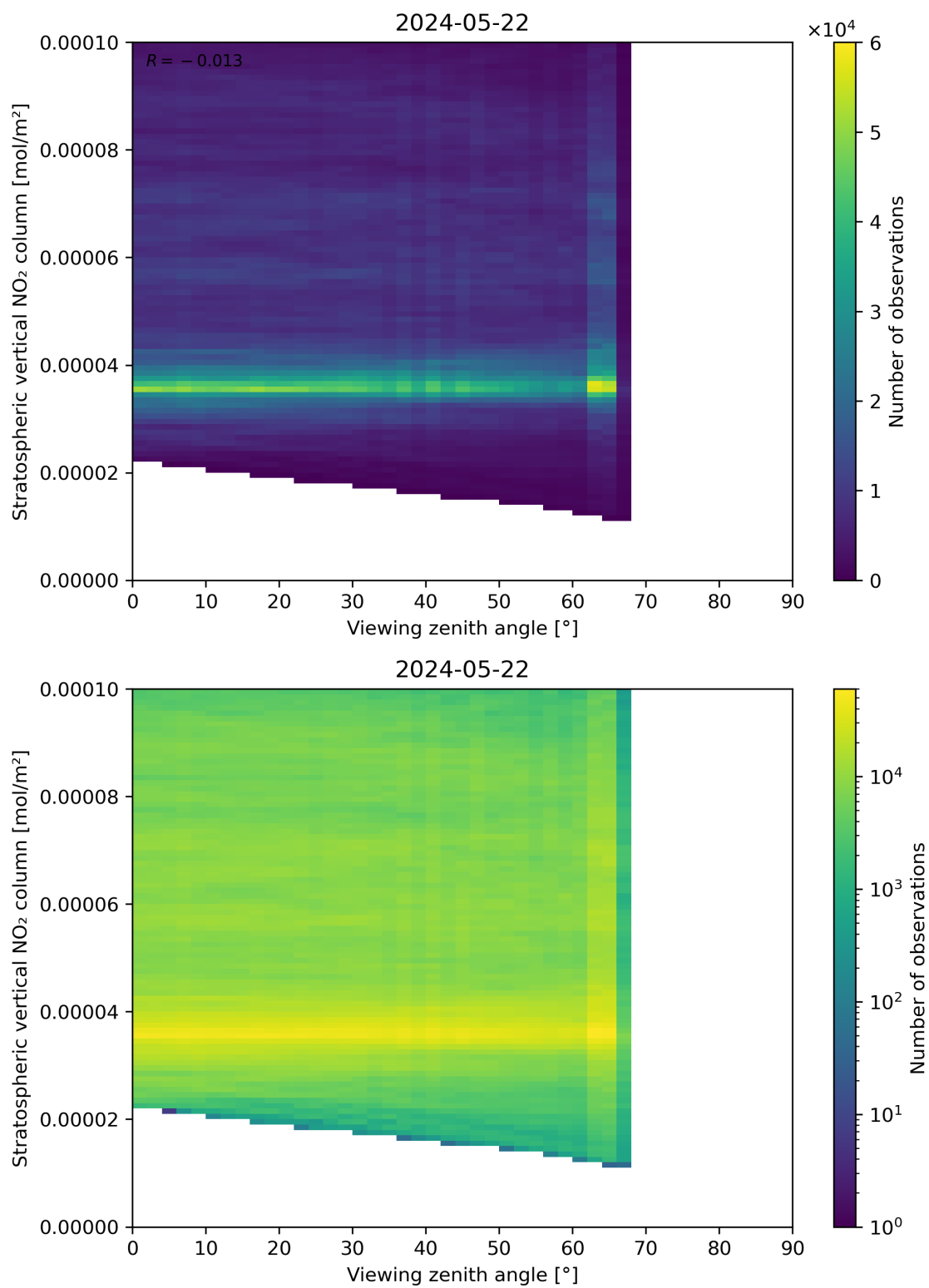
Figure 164: Scatter density plot of “Viewing zenith angle” against “Stratospheric vertical NO 2 column” for 2024-05-21 to 2024-05-23.
