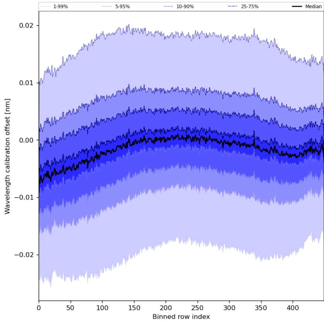
Figure 52: Along track statistics of “Wavelength calibration offset” for 2024-05-21 to 2024-05-23
