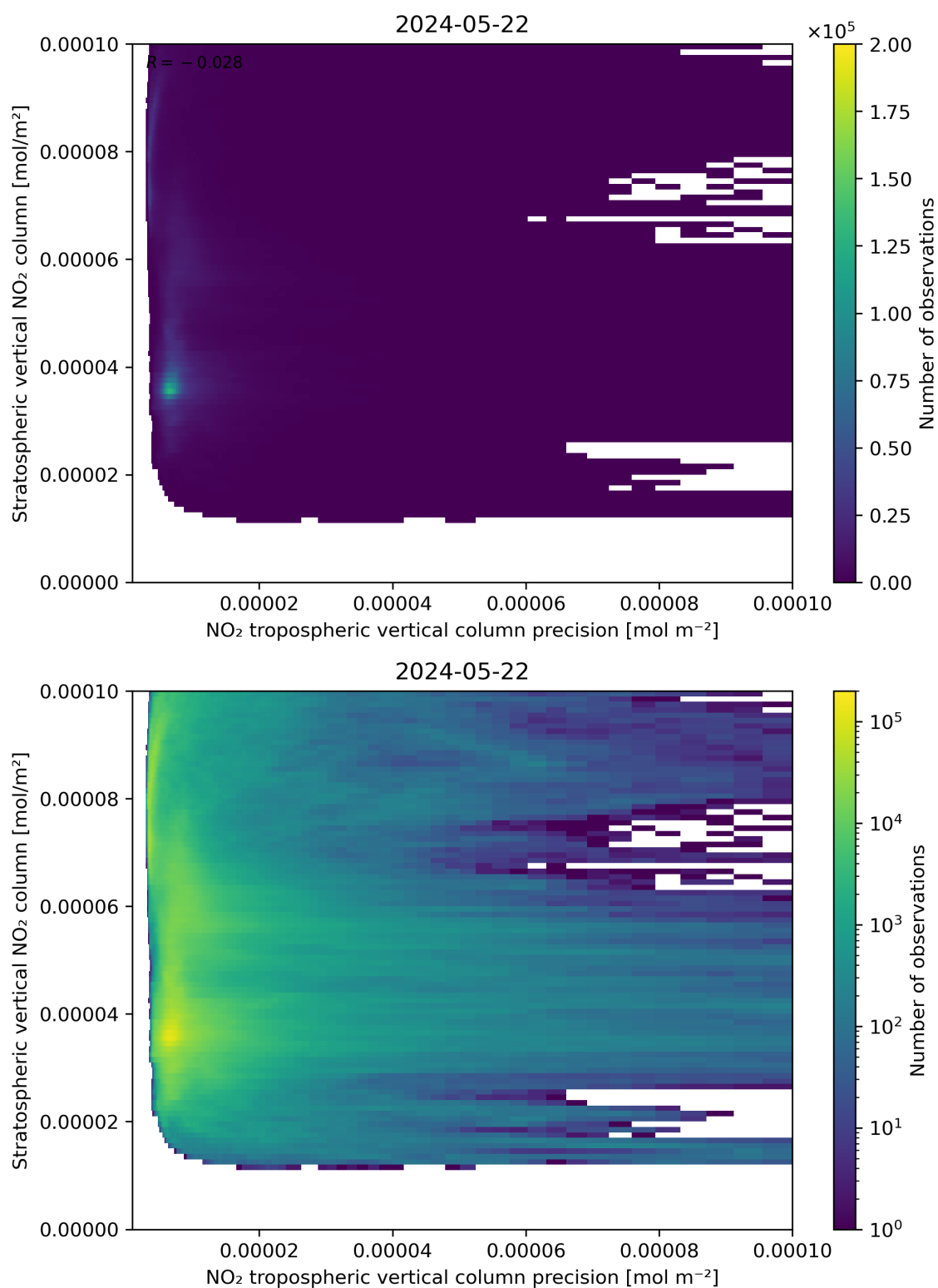
Figure 135: Scatter density plot of “NO 2 tropospheric vertical column precision” against “Stratospheric vertical NO 2 column” for 2024-05-21 to 2024-05-23.
