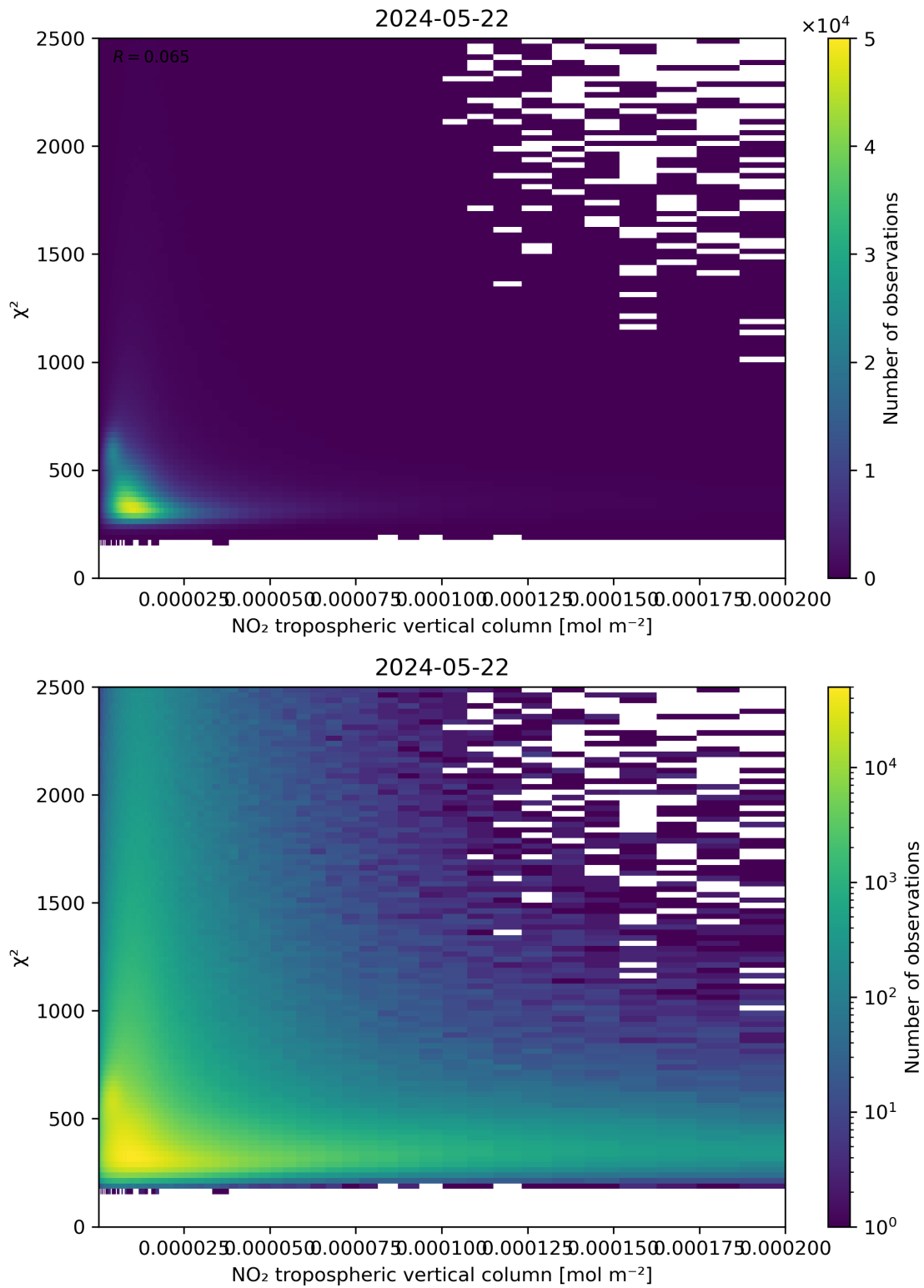
Figure 124: Scatter density plot of “NO 2 tropospheric vertical column” against “ \chi^2 ” for 2024-05-21 to 2024-05-23.
