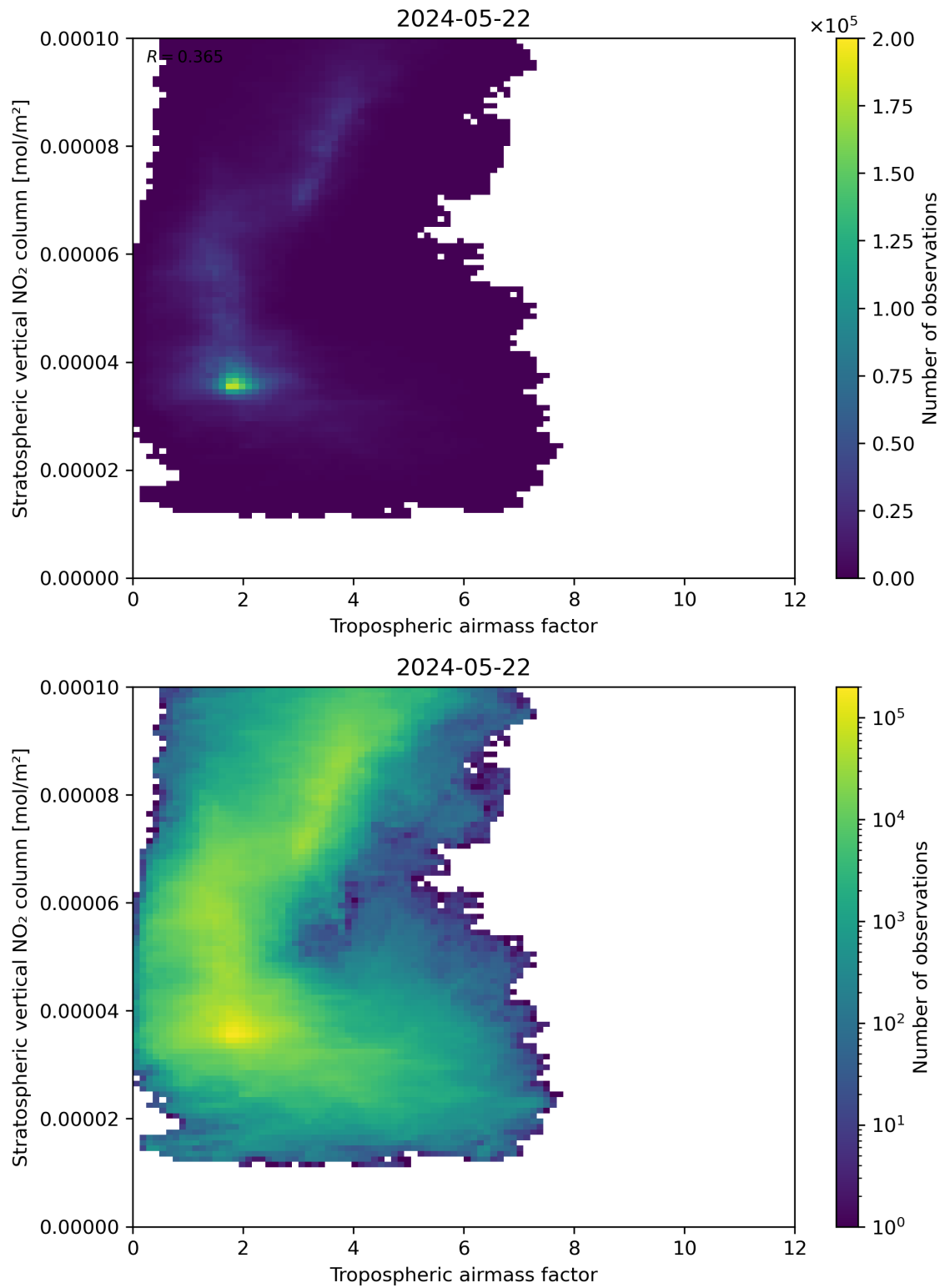
Figure 74: Scatter density plot of “Tropospheric air mass factor” against “Stratospheric vertical NO 2 column” for 2024-05-21 to 2024-05-23.
