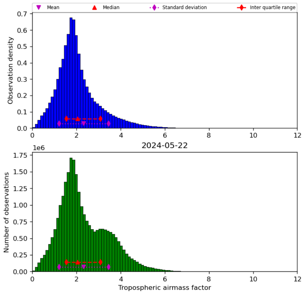
Figure 31: Histogram of “Tropospheric airmass factor” for 2024-05-21 to 2024-05-23
