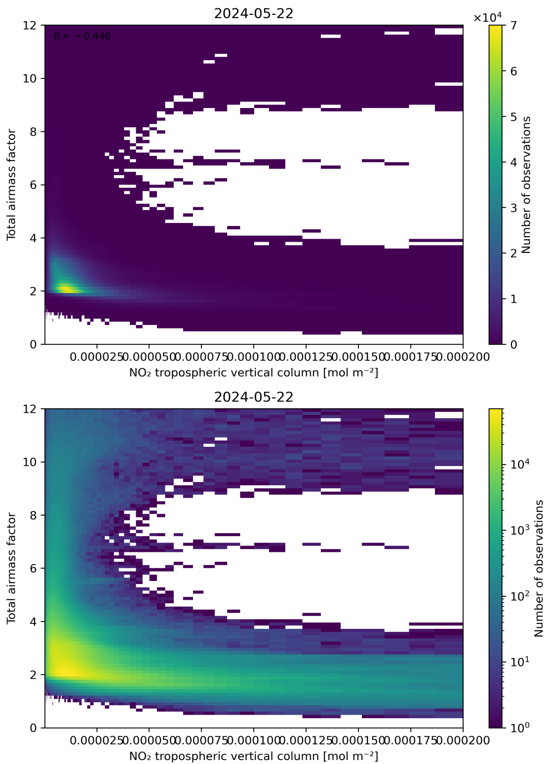
Figure 122: Scatter density plot of “NO 2 tropospheric vertical column” against “Total air mass factor” for 2024-05-21 to 2024-05-23.
