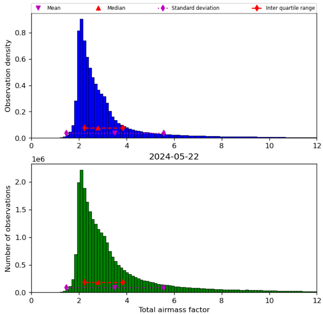
Figure 32: Histogram of “Total airmass factor” for 2024-05-21 to 2024-05-23
