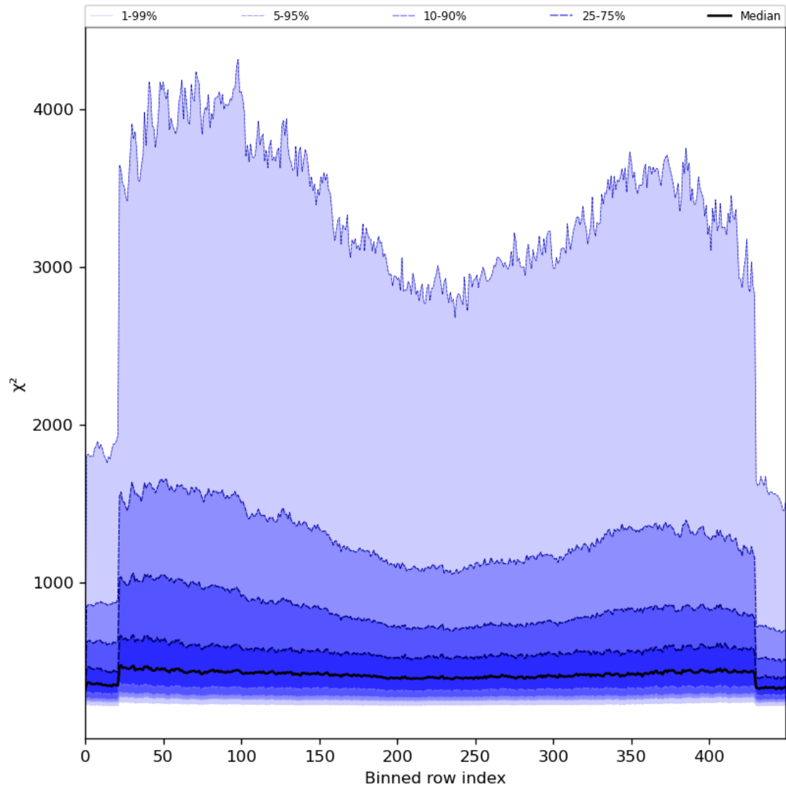
Figure 59: Along track statistics of “ \chi^2 ” for 2024-05-21 to 2024-05-23
