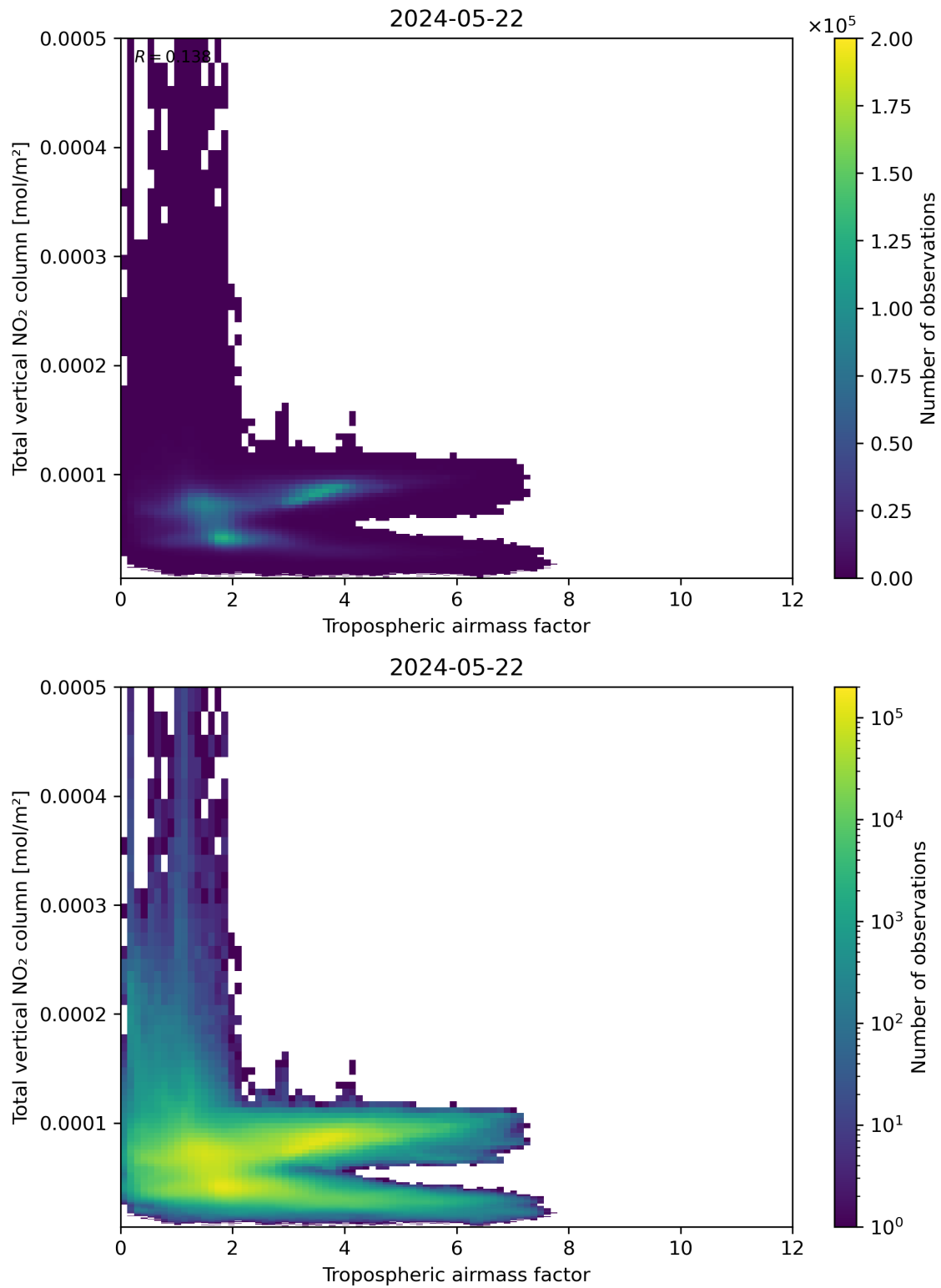
Figure 77: Scatter density plot of “Tropospheric airmass factor” against “Total vertical NO 2 column” for 2024-05-21 to 2024-05-23.
