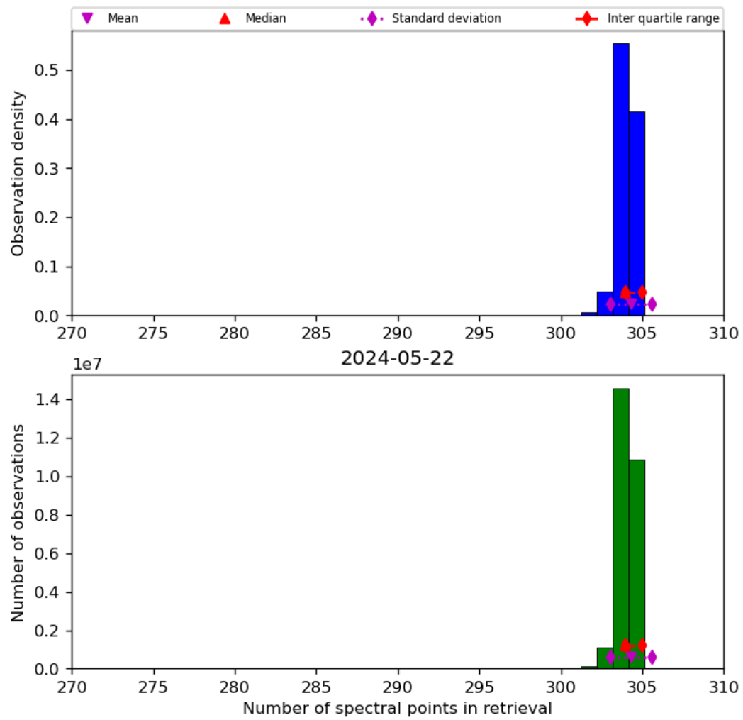
Figure 33: Histogram of “Number of spectral points in retrieval” for 2024-05-21 to 2024-05-23
