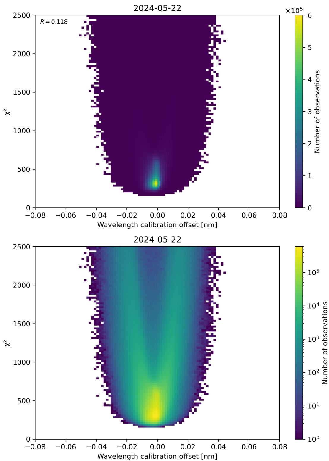
Figure 175: Scatter density plot of “Wavelength calibration offset” against “ \chi^2 ” for 2024-05-21 to 2024-05-23.
