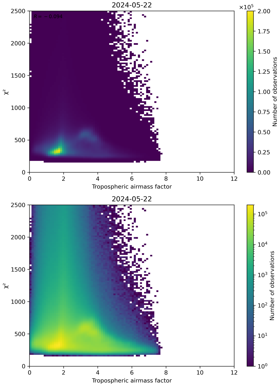
Figure 73: Scatter density plot of “Tropospheric airmass factor” against “ \chi^2 ” for 2024-05-21 to 2024-05-23.
