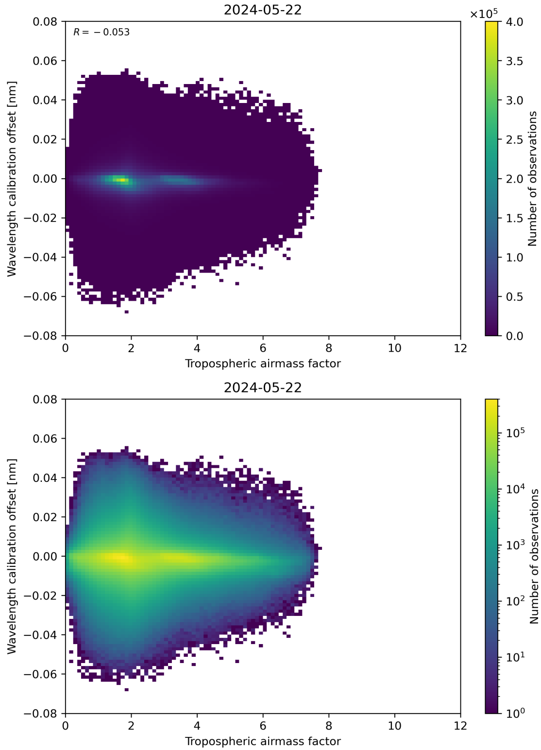
Figure 80: Scatter density plot of “Tropospheric airmass factor” against “Wavelength calibration offset” for 2024-05-21 to 2024-05-23.
