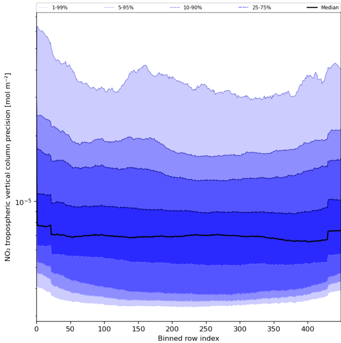
Figure 47: Along track statistics of “NO 2 tropospheric vertical column precision” for 2024-05-21 to 2024-05-23
