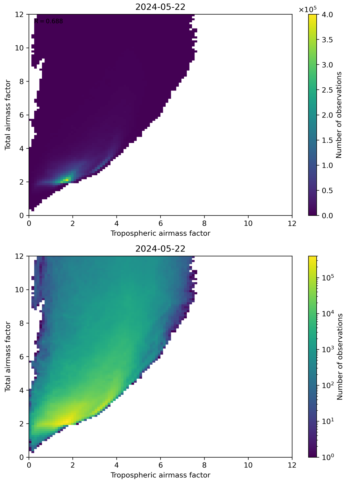
Figure 72: Scatter density plot of “Tropospheric airmass factor” against “Total airmass factor” for 2024-05-21 to 2024-05-23.
