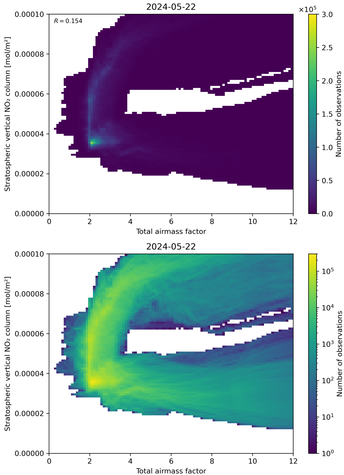
Figure 64: Scatter density plot of “Total airmass factor” against “Stratospheric vertical \text{NO}_2 column” for 2024-05-21 to 2024-05-23.
