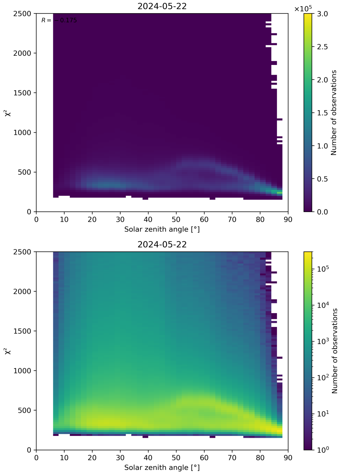
Figure 148: Scatter density plot of “Solar zenith angle” against “ \chi^2 ” for 2024-05-21 to 2024-05-23.
