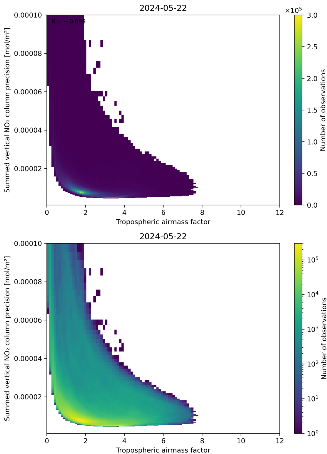
Figure 76: Scatter density plot of “Tropospheric air mass factor” against “Summed vertical NO 2 column precision” for 2024-05-21 to 2024-05-23.
