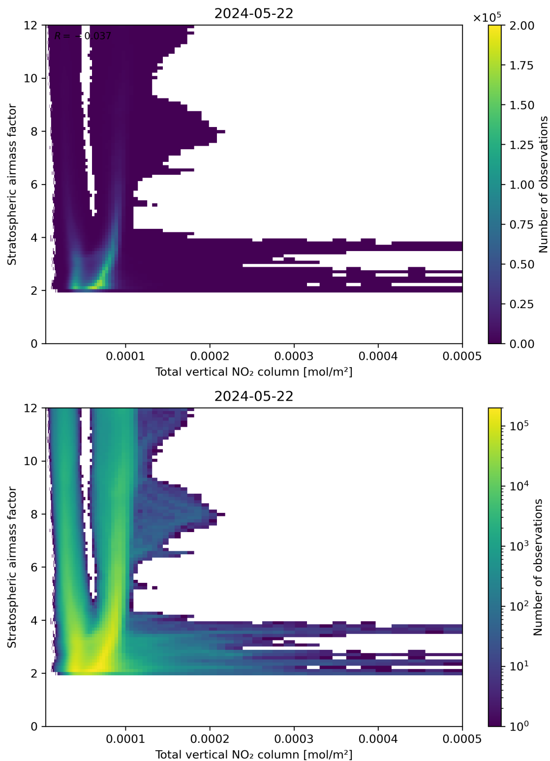
Figure 110: Scatter density plot of “Total vertical NO 2 column” against “Stratospheric airmass factor” for 2024-05-21 to 2024-05-23.
