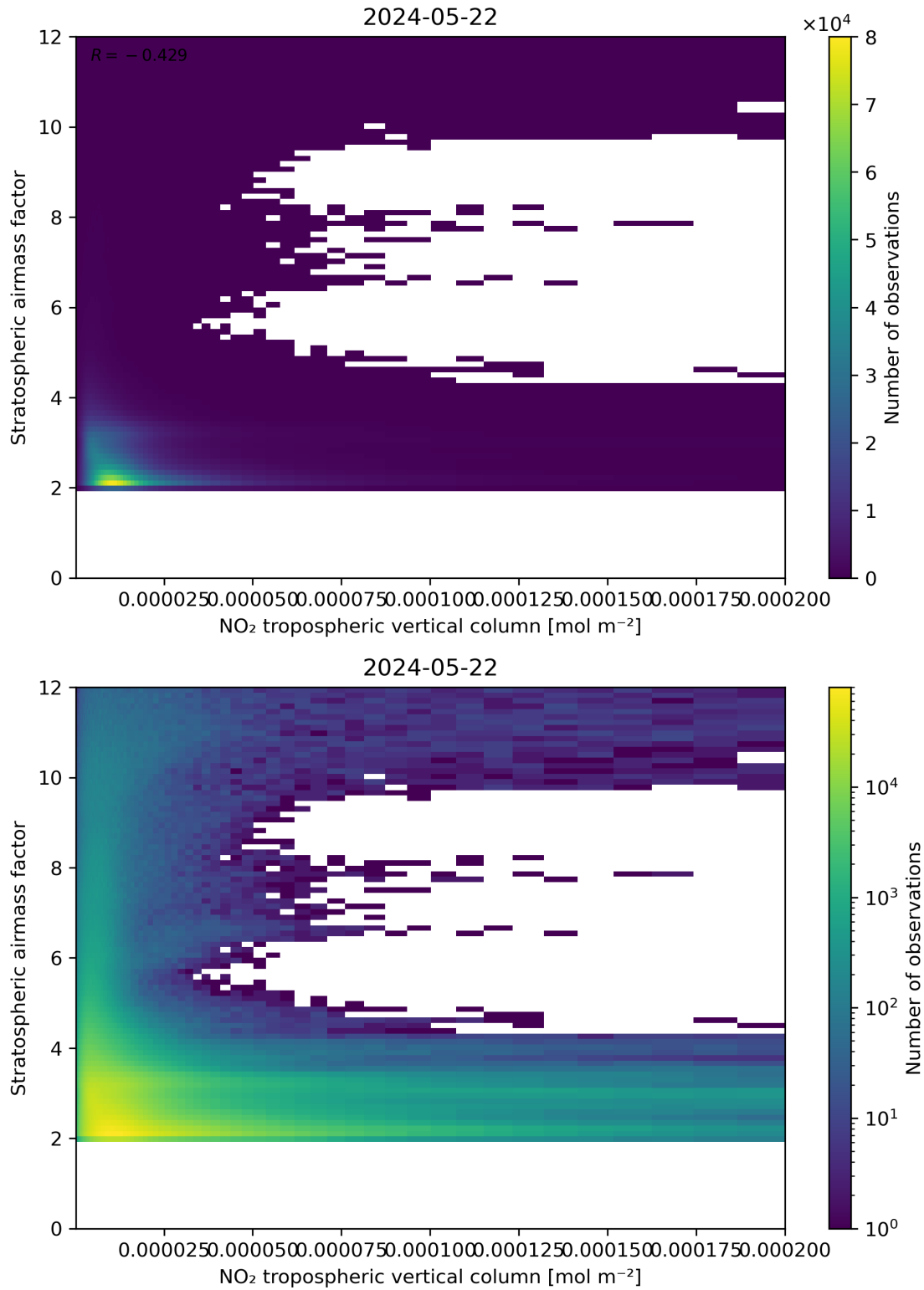
Figure 121: Scatter density plot of “NO 2 tropospheric vertical column” against “Stratospheric air mass factor” for 2024-05-21 to 2024-05-23.
