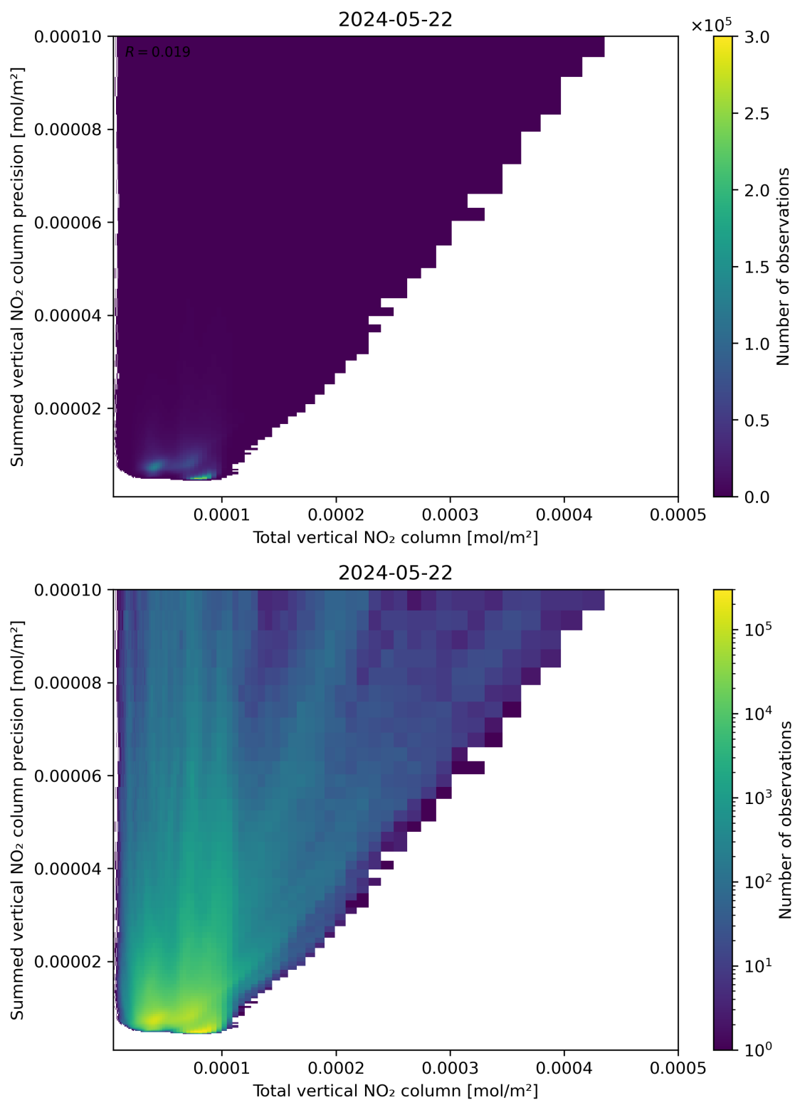
Figure 113: Scatter density plot of “Total vertical NO 2 column” against “Summed vertical NO 2 column precision” for 2024-05-21 to 2024-05-23.
