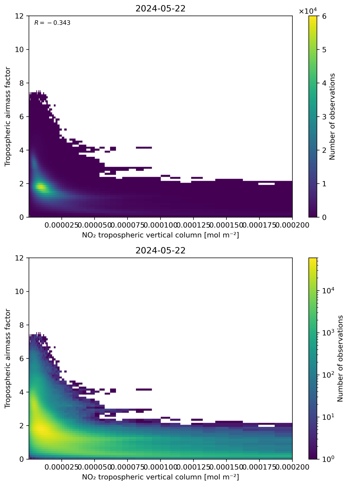
Figure 123: Scatter density plot of “NO 2 tropospheric vertical column” against “Tropospheric air mass factor” for 2024-05-21 to 2024-05-23.
