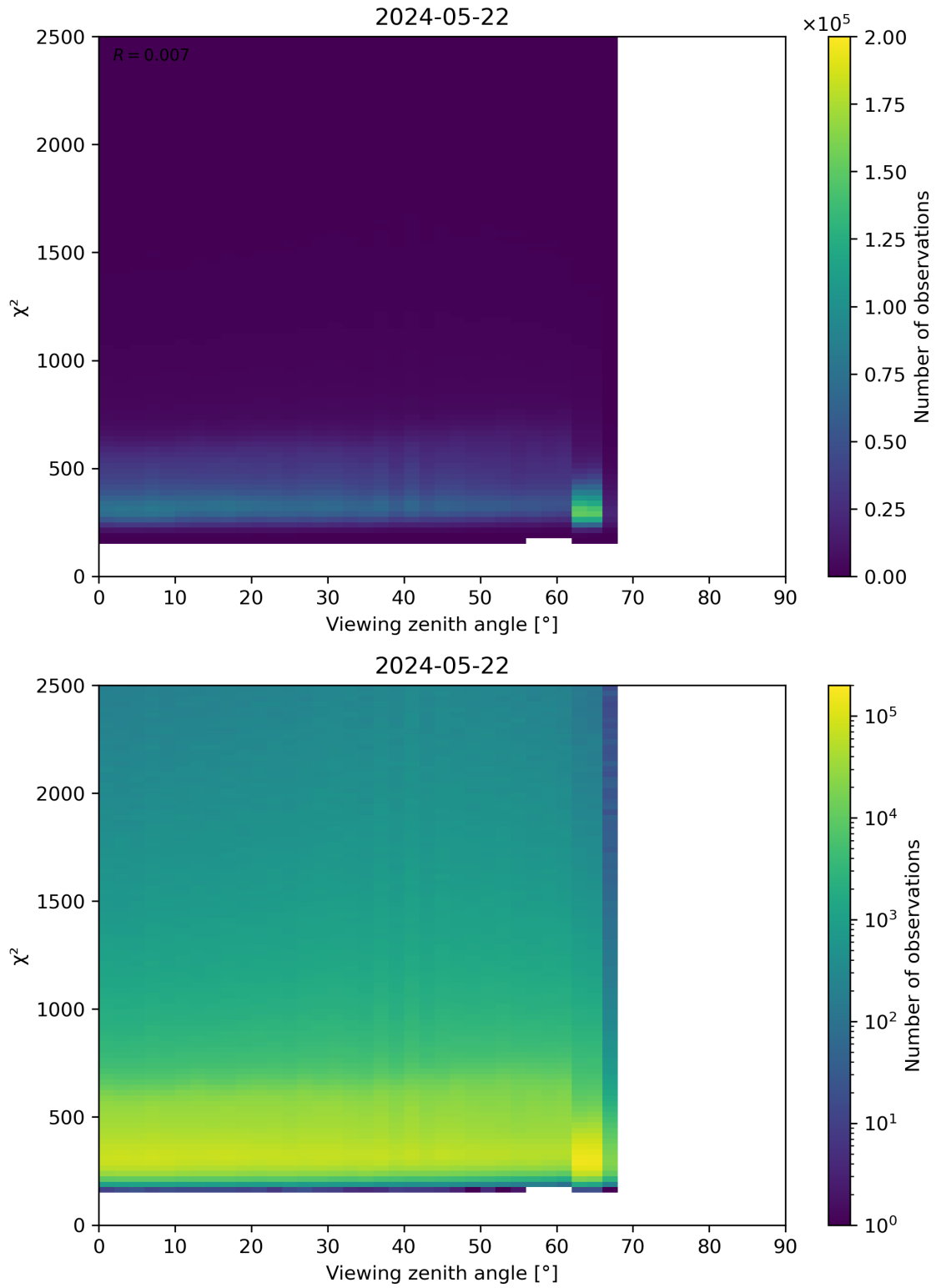
Figure 162: Scatter density plot of “Viewing zenith angle” against “ \chi^2 ” for 2024-05-21 to 2024-05-23.
