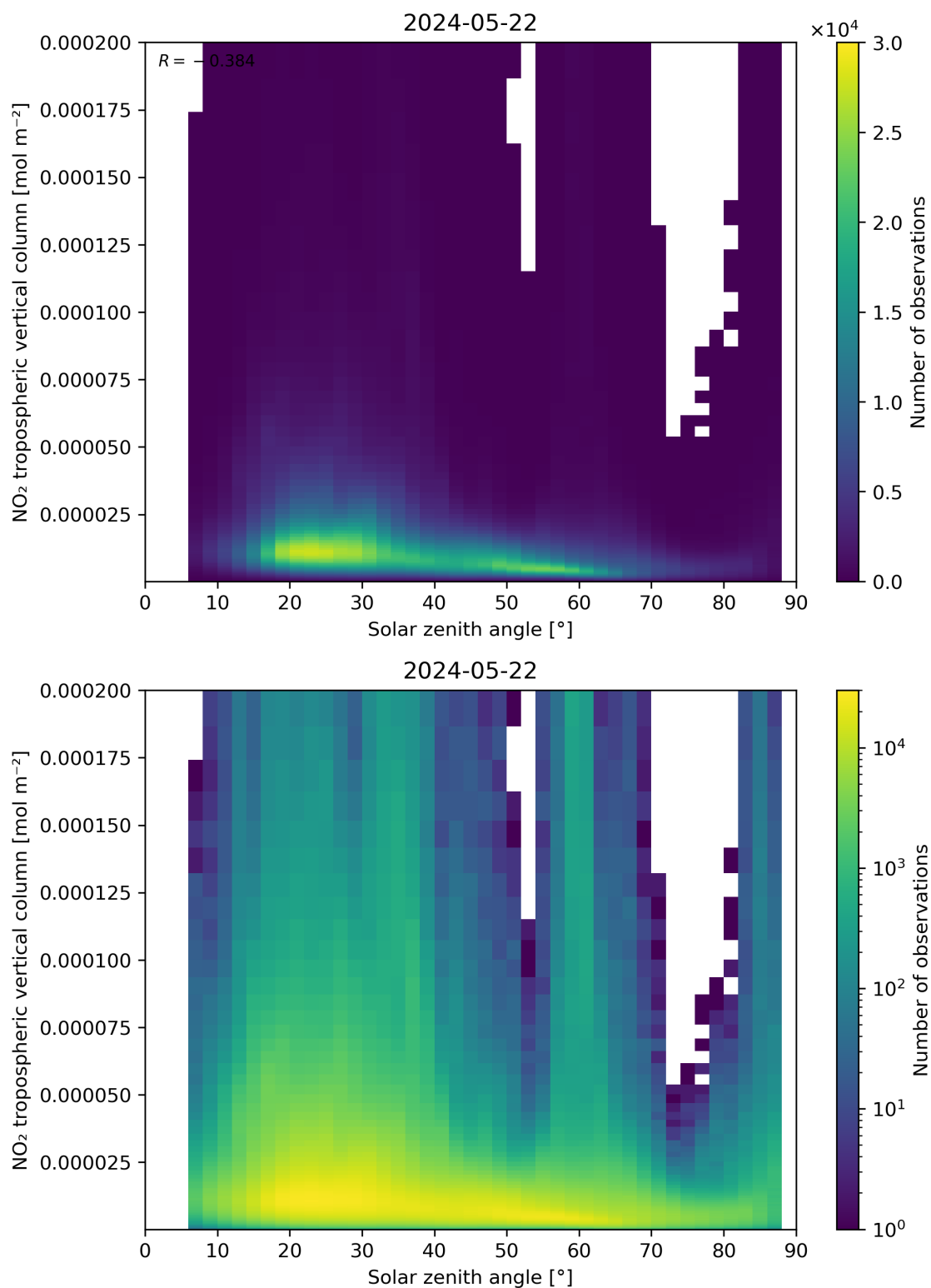
Figure 155: Scatter density plot of “Solar zenith angle” against “NO 2 tropospheric vertical column” for 2024-05-21 to 2024-05-23.
