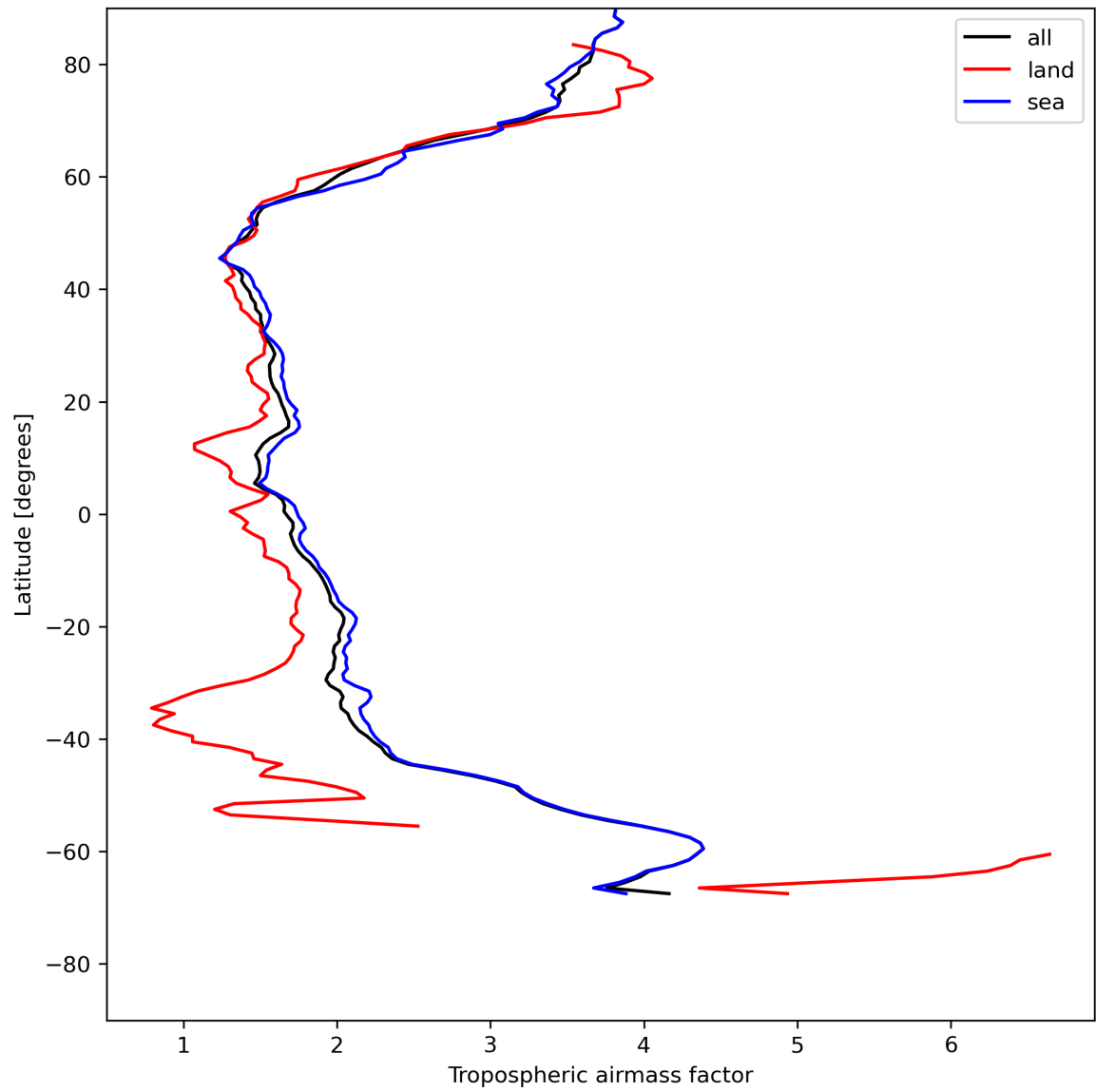
Figure 14: Zonal average of “Tropospheric airmass factor” for 2024-05-21 to 2024-05-23.
