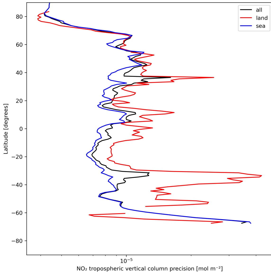
Figure 13: Zonal average of “NO 2 tropospheric vertical column precision” for 2024-05-21 to 2024-05-23.
