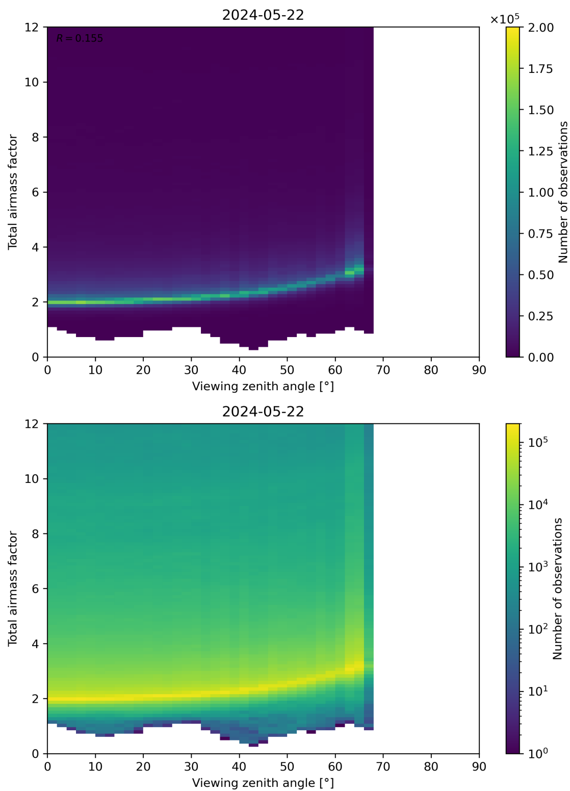
Figure 160: Scatter density plot of “Viewing zenith angle” against “Total airmass factor” for 2024-05-21 to 2024-05-23.
