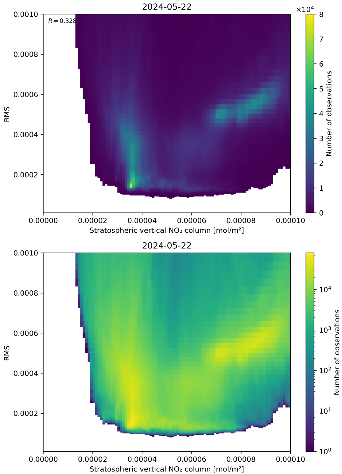
Figure 102: Scatter density plot of “Stratospheric vertical NO 2 column” against “RMS” for 2024-05-21 to 2024-05-23.
