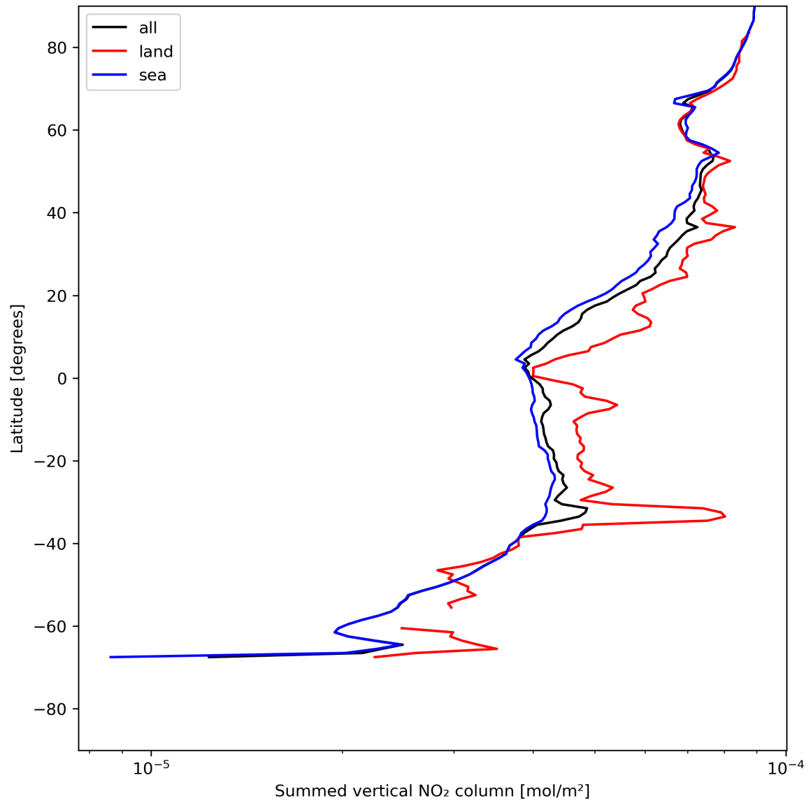
Figure 23: Zonal average of “Summed vertical NO 2 column” for 2024-05-21 to 2024-05-23.
