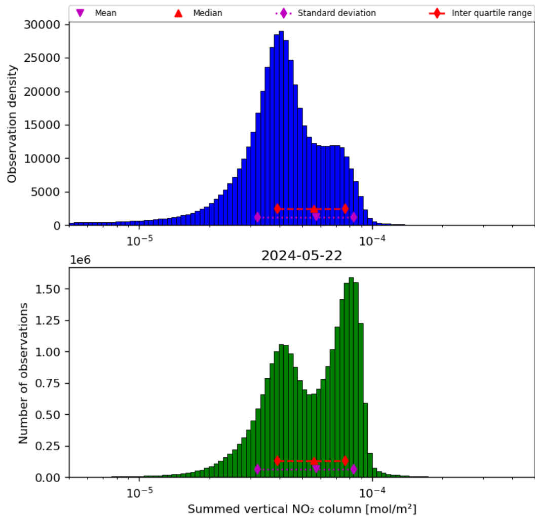
Figure 40: Histogram of “Summed vertical NO 2 column” for 2024-05-21 to 2024-05-23
