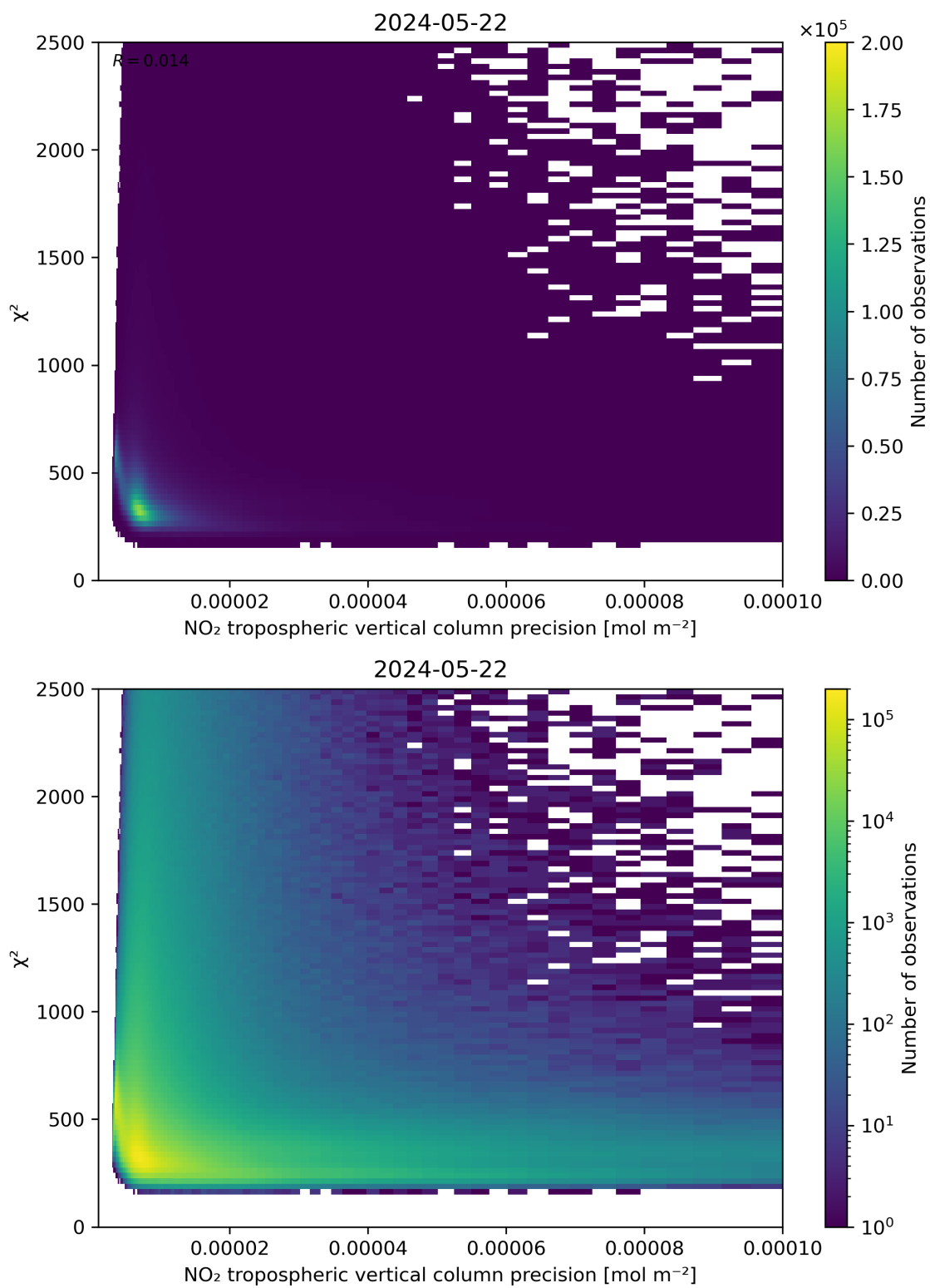
Figure 134: Scatter density plot of “NO 2 tropospheric vertical column precision” against “ \chi^2 ” for 2024-05-21 to 2024-05-23.
