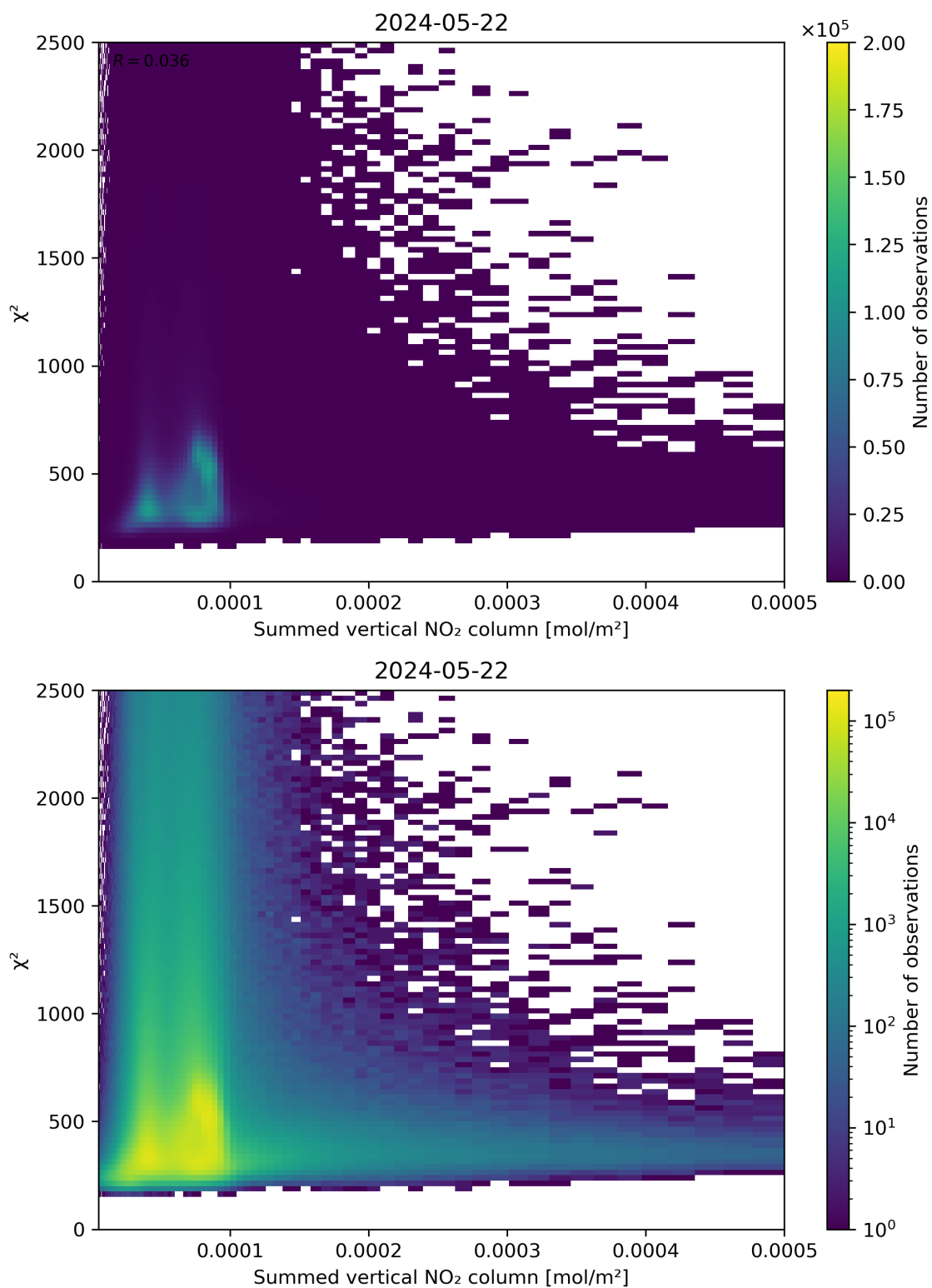
Figure 104: Scatter density plot of “Summed vertical NO 2 column” against “ \chi^2 ” for 2024-05-21 to 2024-05-23.
