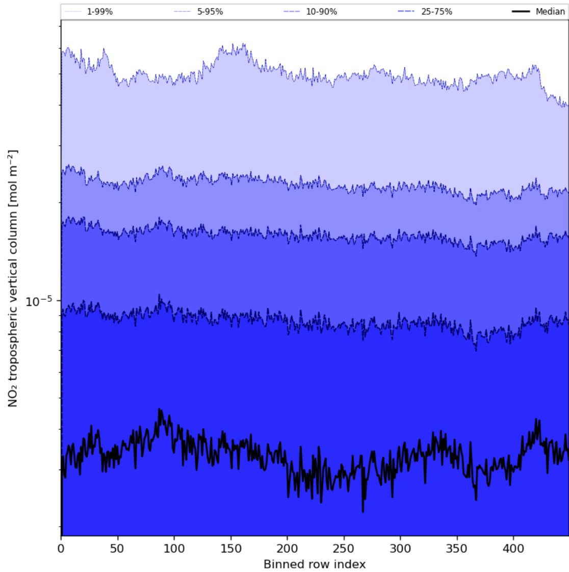
Figure 46: Along track statistics of “NO 2 tropospheric vertical column” for 2024-05-21 to 2024-05-23
