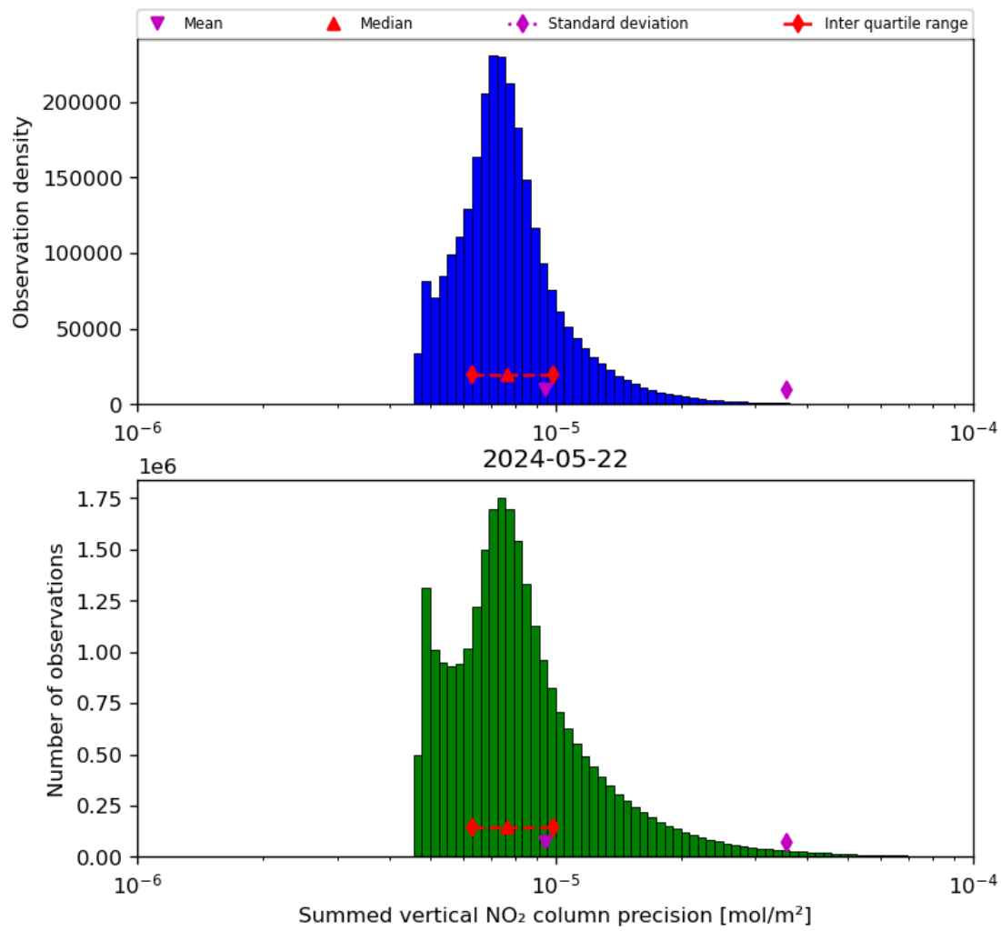
Figure 41: Histogram of "Summed vertical NO 2 column precision" for 2024-05-21 to 2024-05-23
