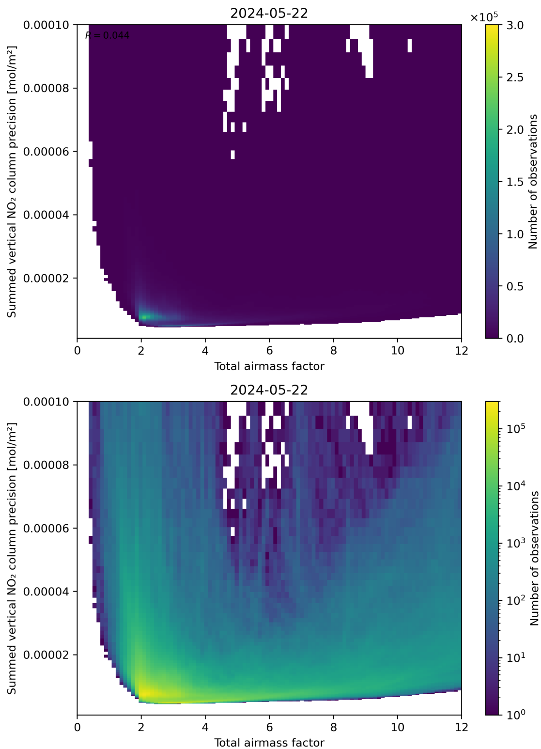
Figure 66: Scatter density plot of “Total airmass factor” against “Summed vertical NO 2 column precision” for 2024-05-21 to 2024-05-23.
