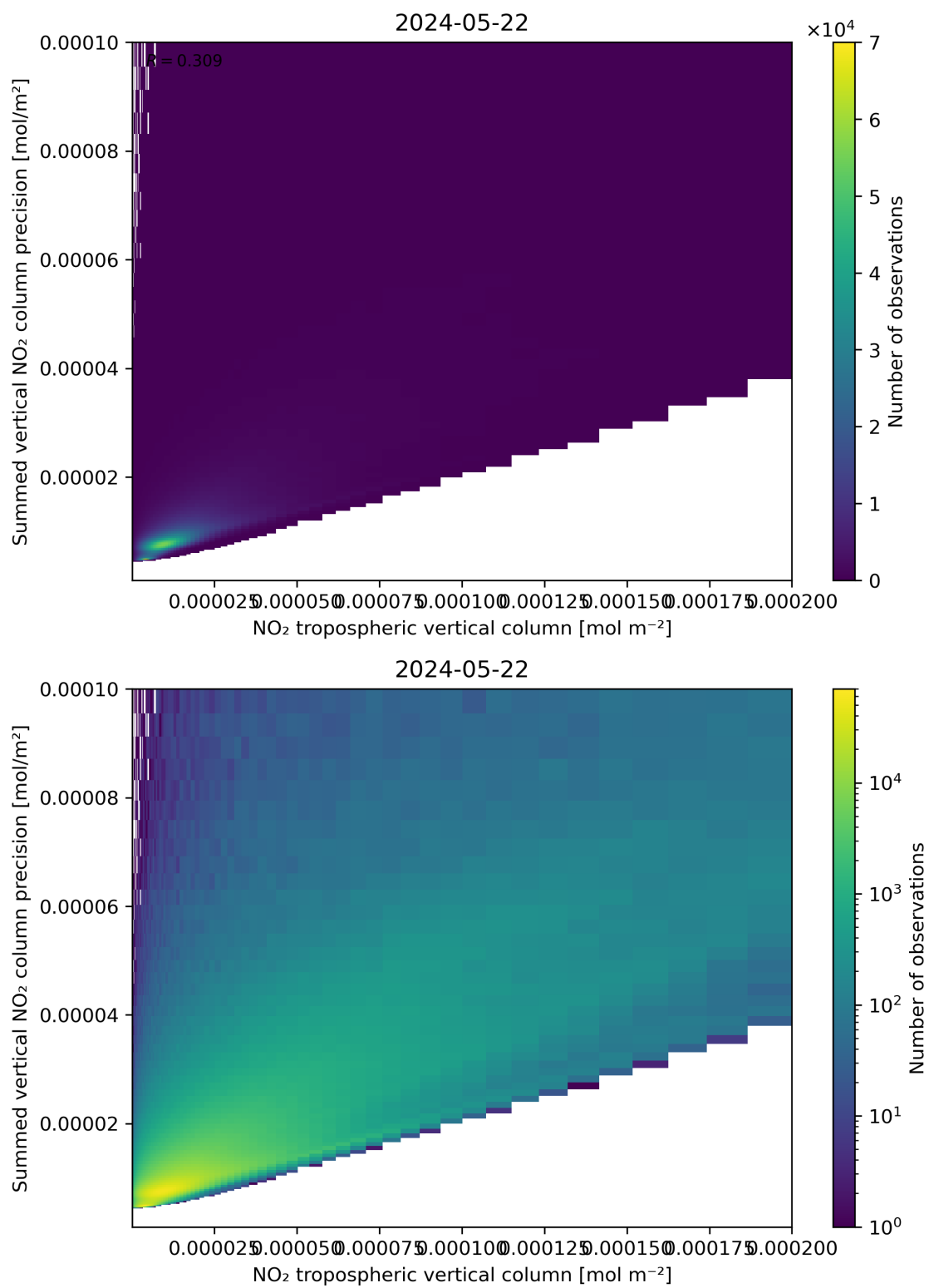
Figure 127: Scatter density plot of “NO 2 tropospheric vertical column” against “Summed vertical NO 2 column precision” for 2024-05-21 to 2024-05-23.
