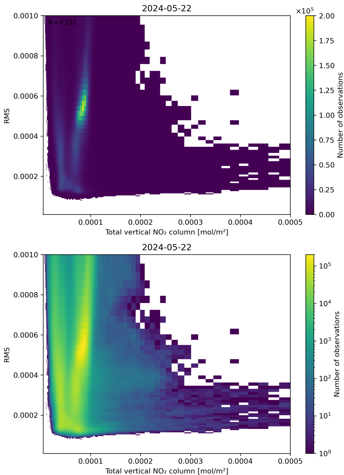
Figure 120: Scatter density plot of “Total vertical NO 2 column” against “RMS” for 2024-05-21 to 2024-05-23.
