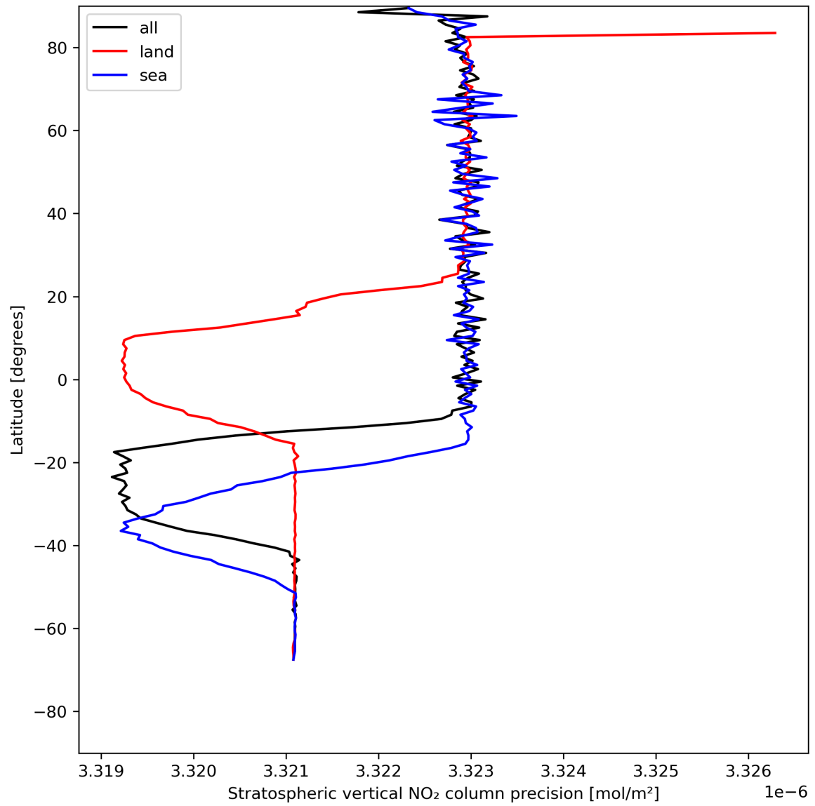
Figure 20: Zonal average of “Stratospheric vertical NO 2 column precision” for 2024-05-21 to 2024-05-23.
