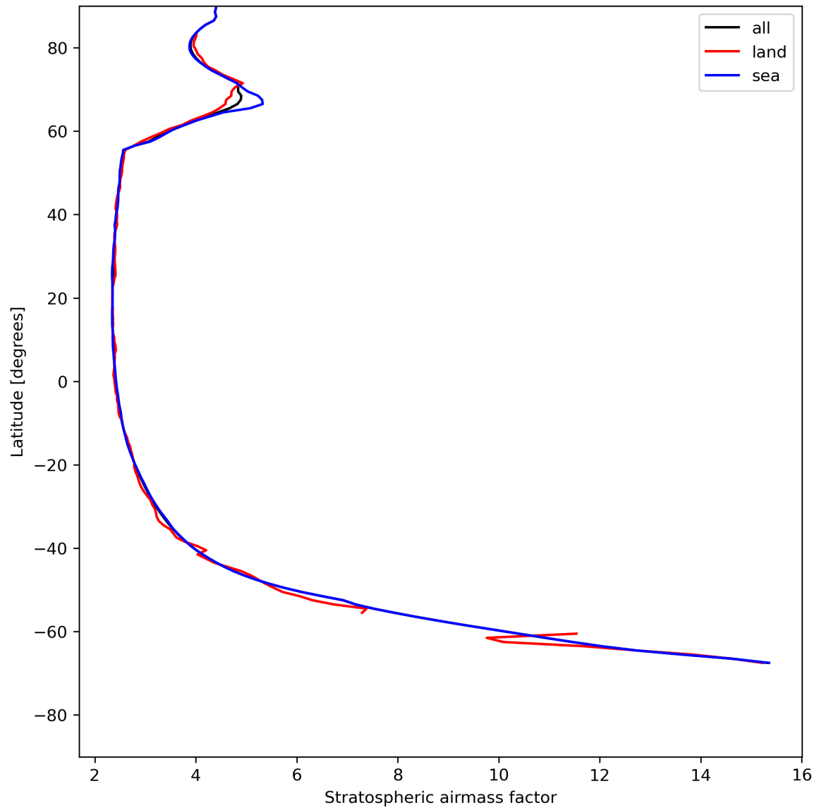
Figure 27: Zonal average of “Stratospheric airmass factor” for 2024-05-21 to 2024-05-23.
