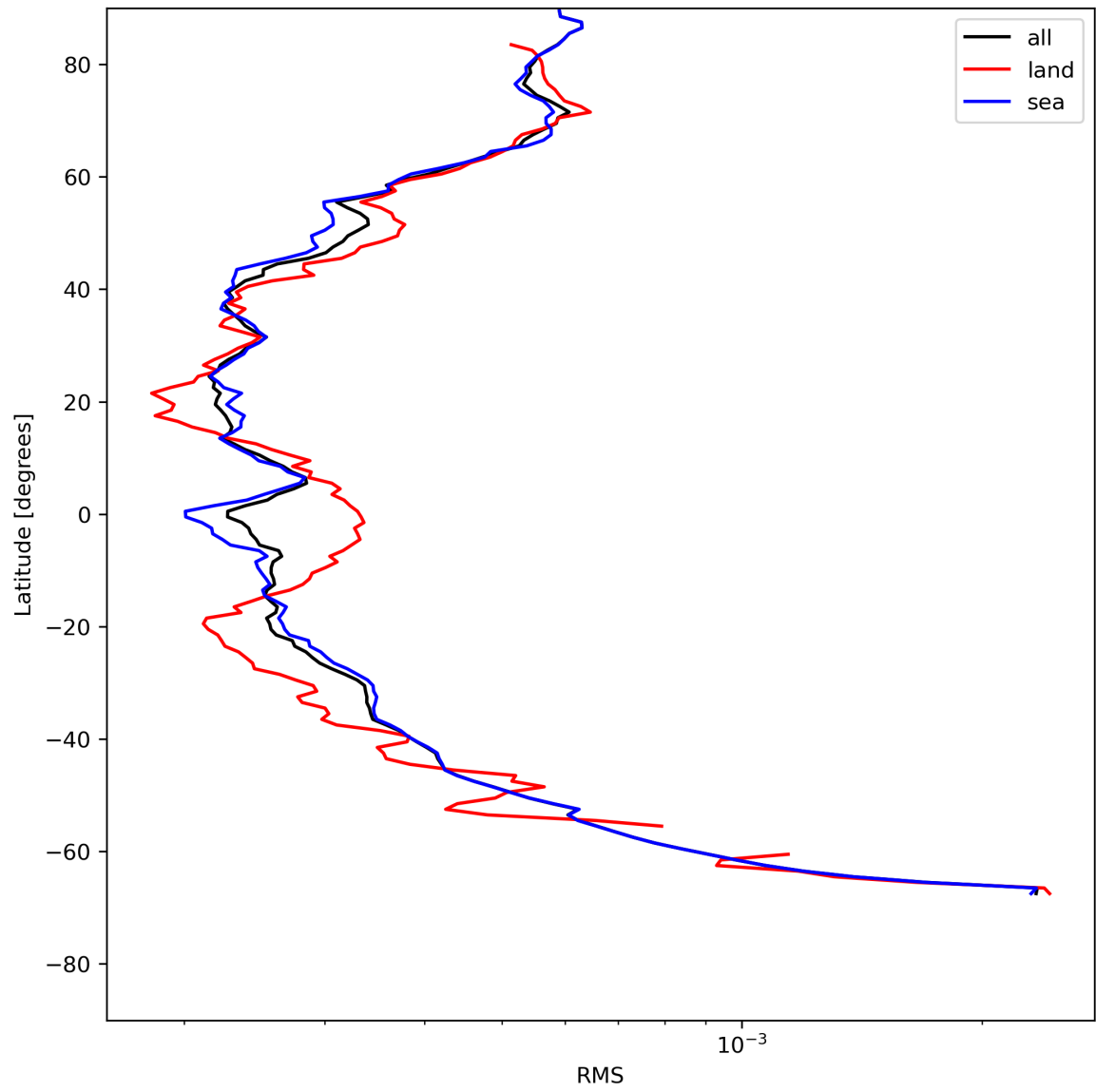
Figure 26: Zonal average of “RMS” for 2024-05-21 to 2024-05-23.
