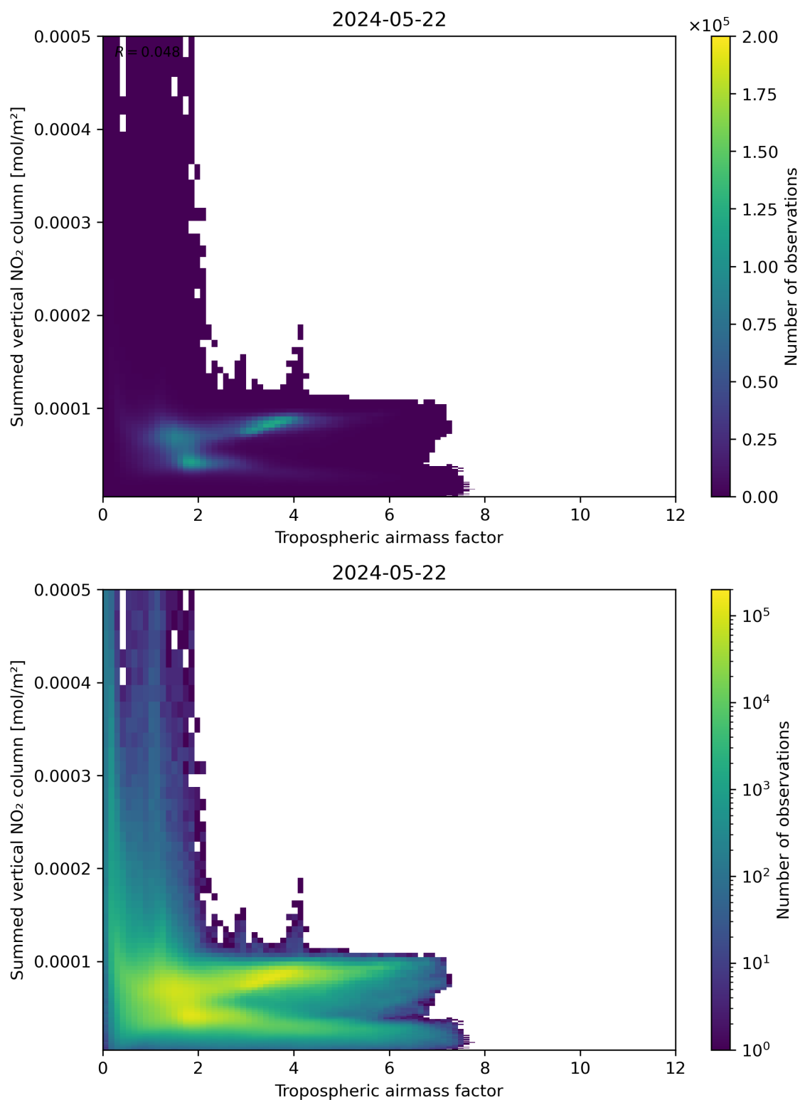
Figure 75: Scatter density plot of “Tropospheric airmass factor” against “Summed vertical NO 2 column” for 2024-05-21 to 2024-05-23.
