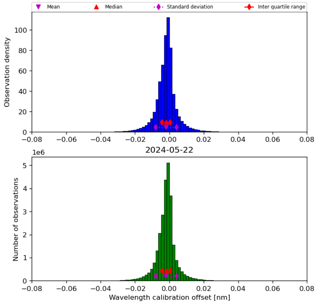
Figure 35: Histogram of “Wavelength calibration offset” for 2024-05-21 to 2024-05-23
