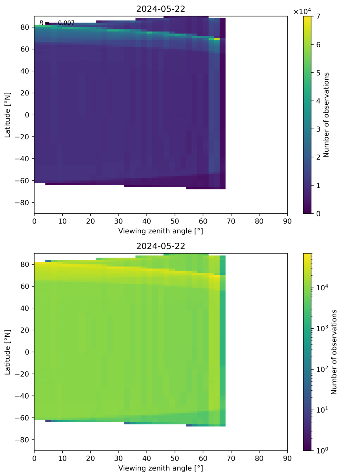
Figure 163: Scatter density plot of “Viewing zenith angle” against “Latitude” for 2024-05-21 to 2024-05-23.
