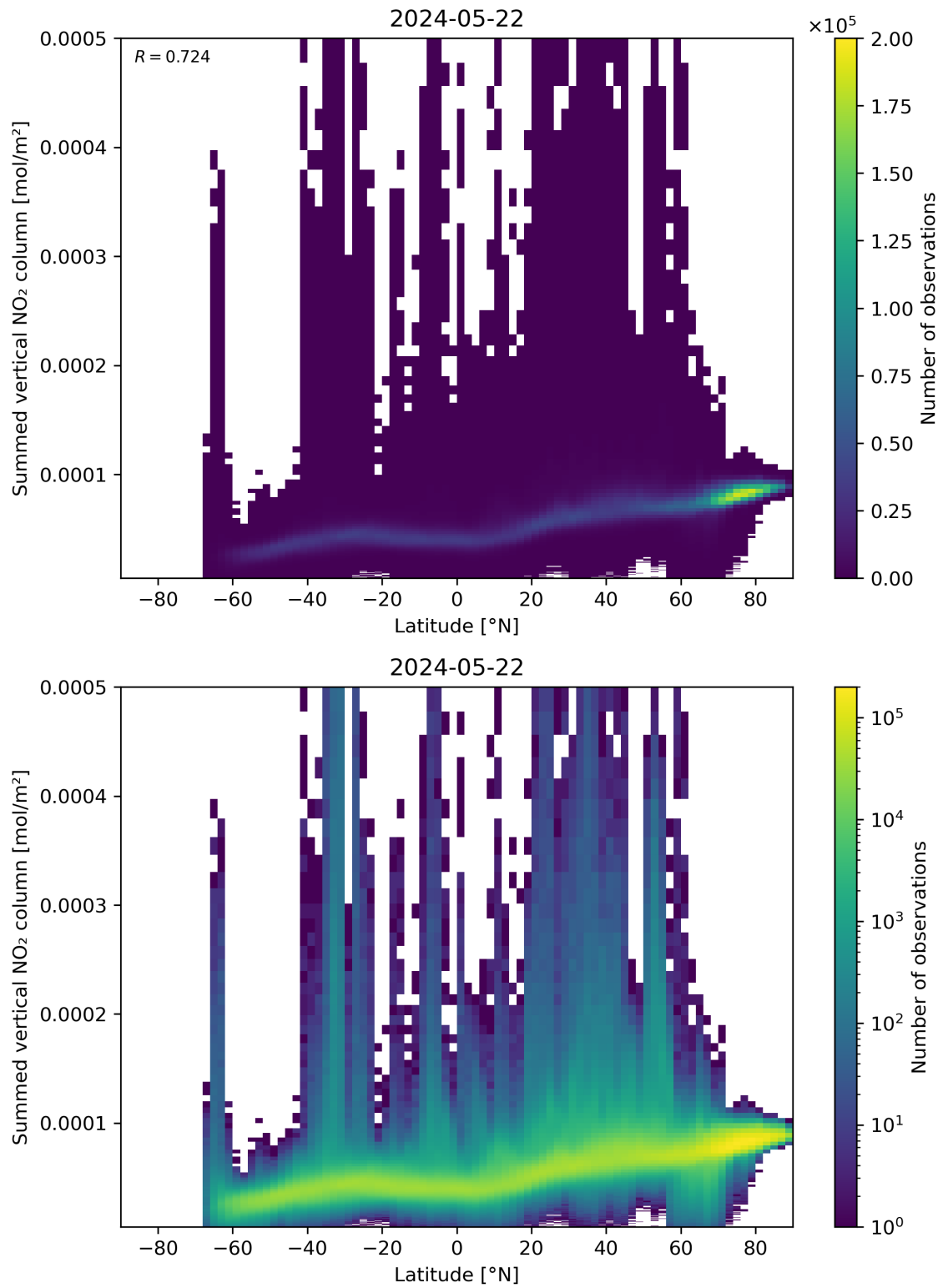
Figure 88: Scatter density plot of “Latitude” against “Summed vertical NO 2 column” for 2024-05-21 to 2024-05-23.
