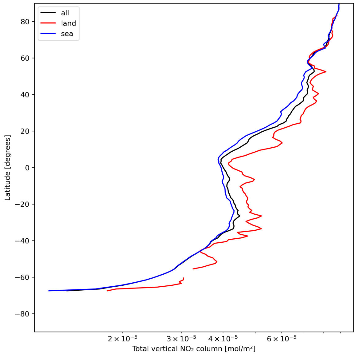
Figure 21: Zonal average of “Total vertical NO 2 column” for 2024-05-21 to 2024-05-23.
