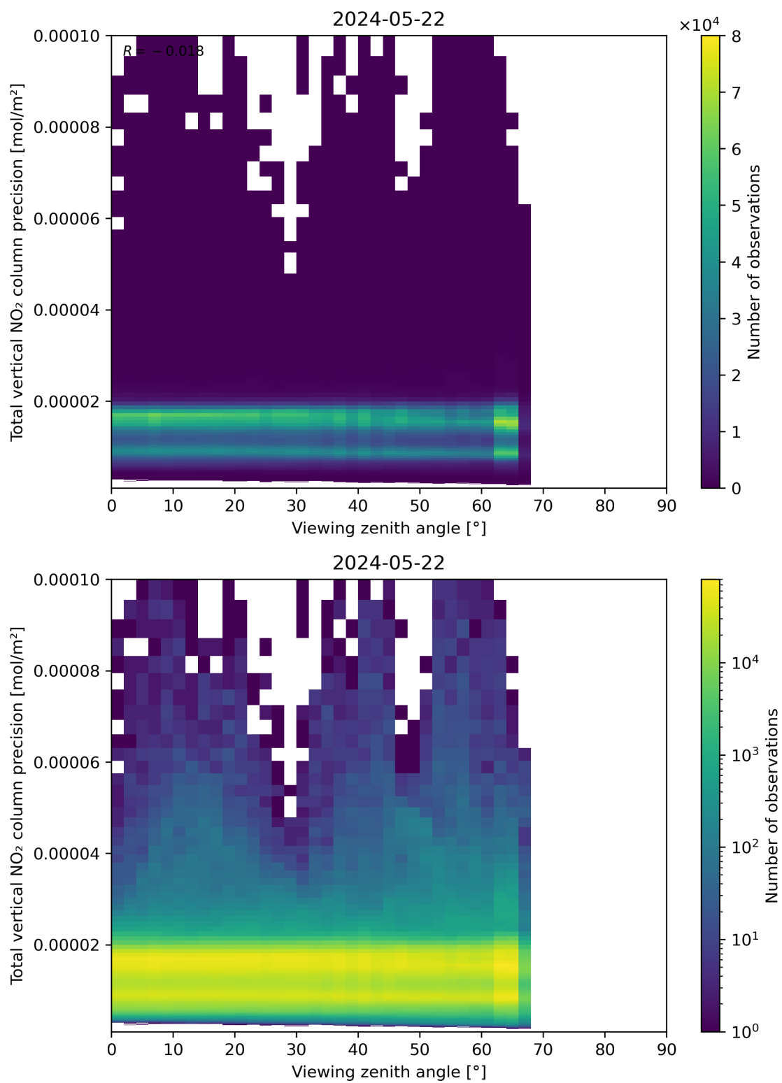
Figure 168: Scatter density plot of “Viewing zenith angle” against “Total vertical NO 2 column precision” for 2024-05-21 to 2024-05-23.
