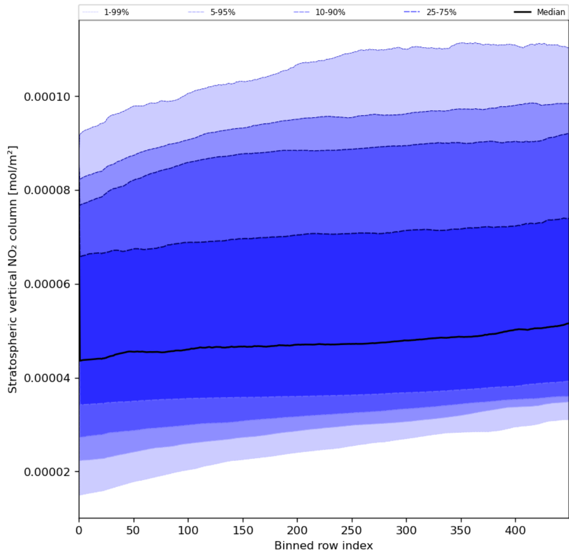
Figure 53: Along track statistics of “Stratospheric vertical NO 2 column” for 2024-05-21 to 2024-05-23
