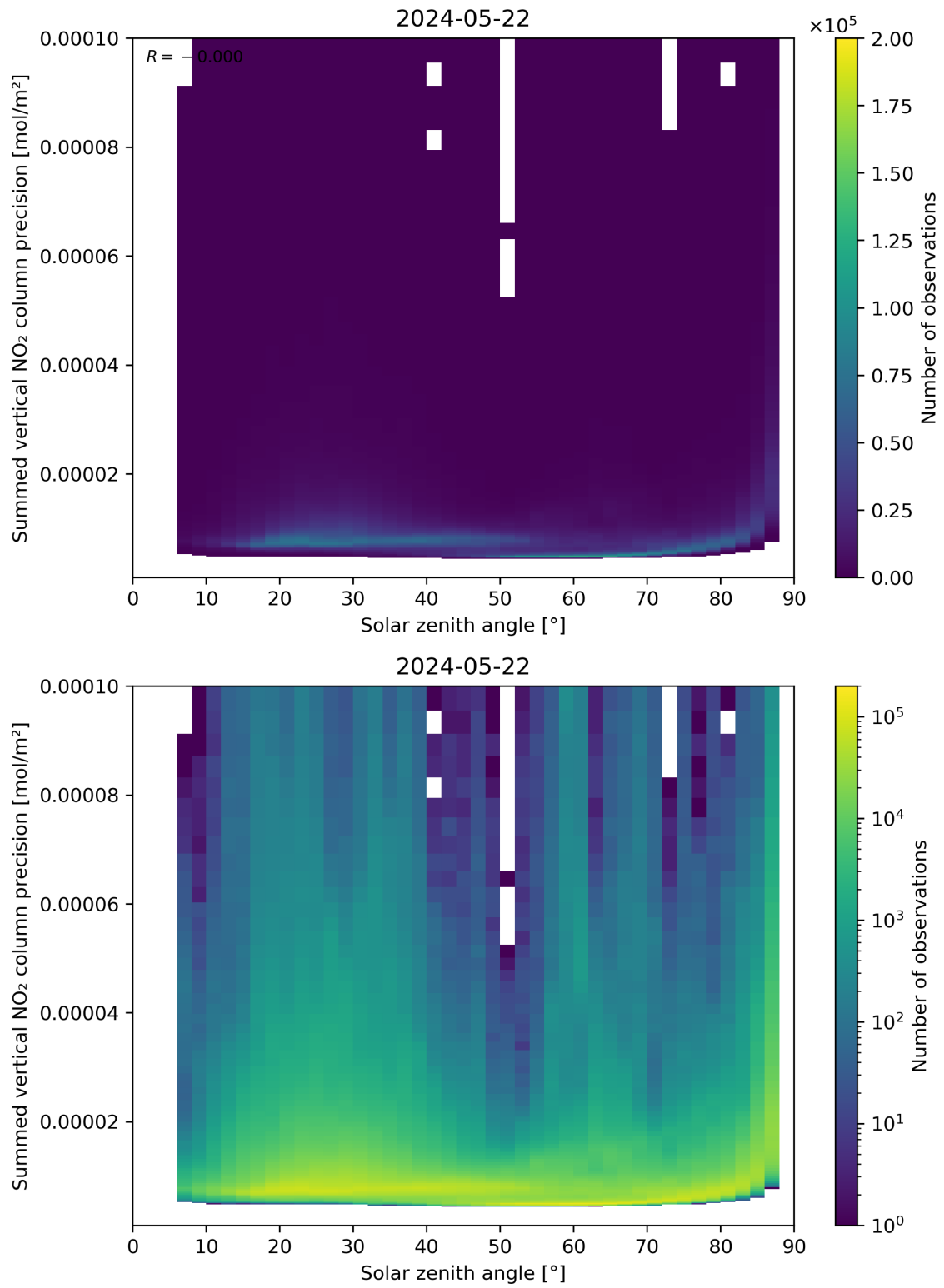
Figure 152: Scatter density plot of “Solar zenith angle” against “Summed vertical NO 2 column precision” for 2024-05-21 to 2024-05-23.
