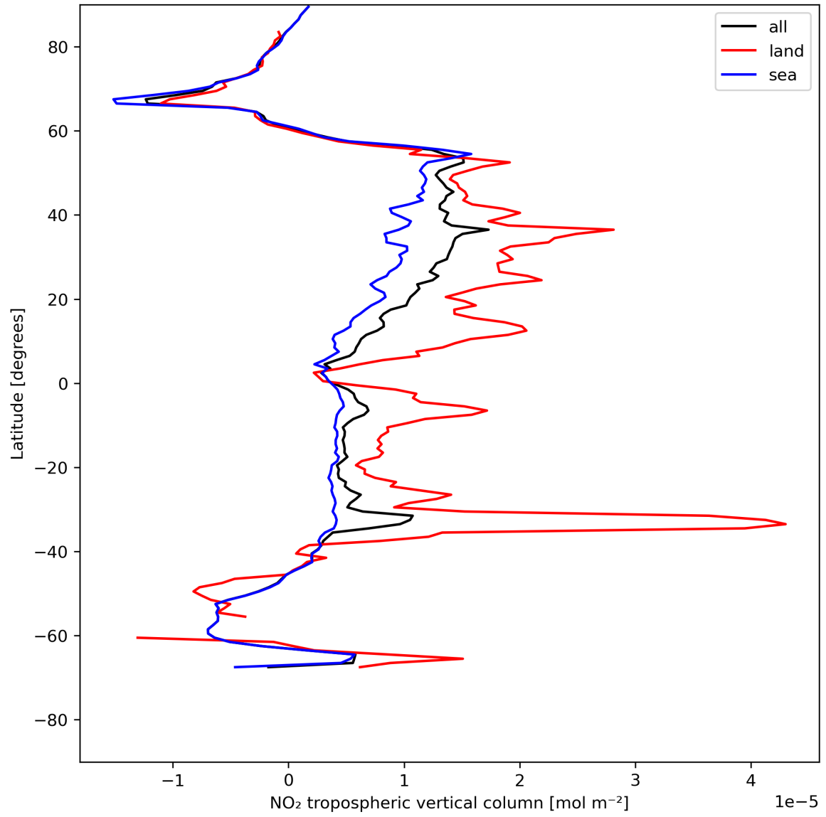
Figure 12: Zonal average of “NO 2 tropospheric vertical column” for 2024-05-21 to 2024-05-23.
