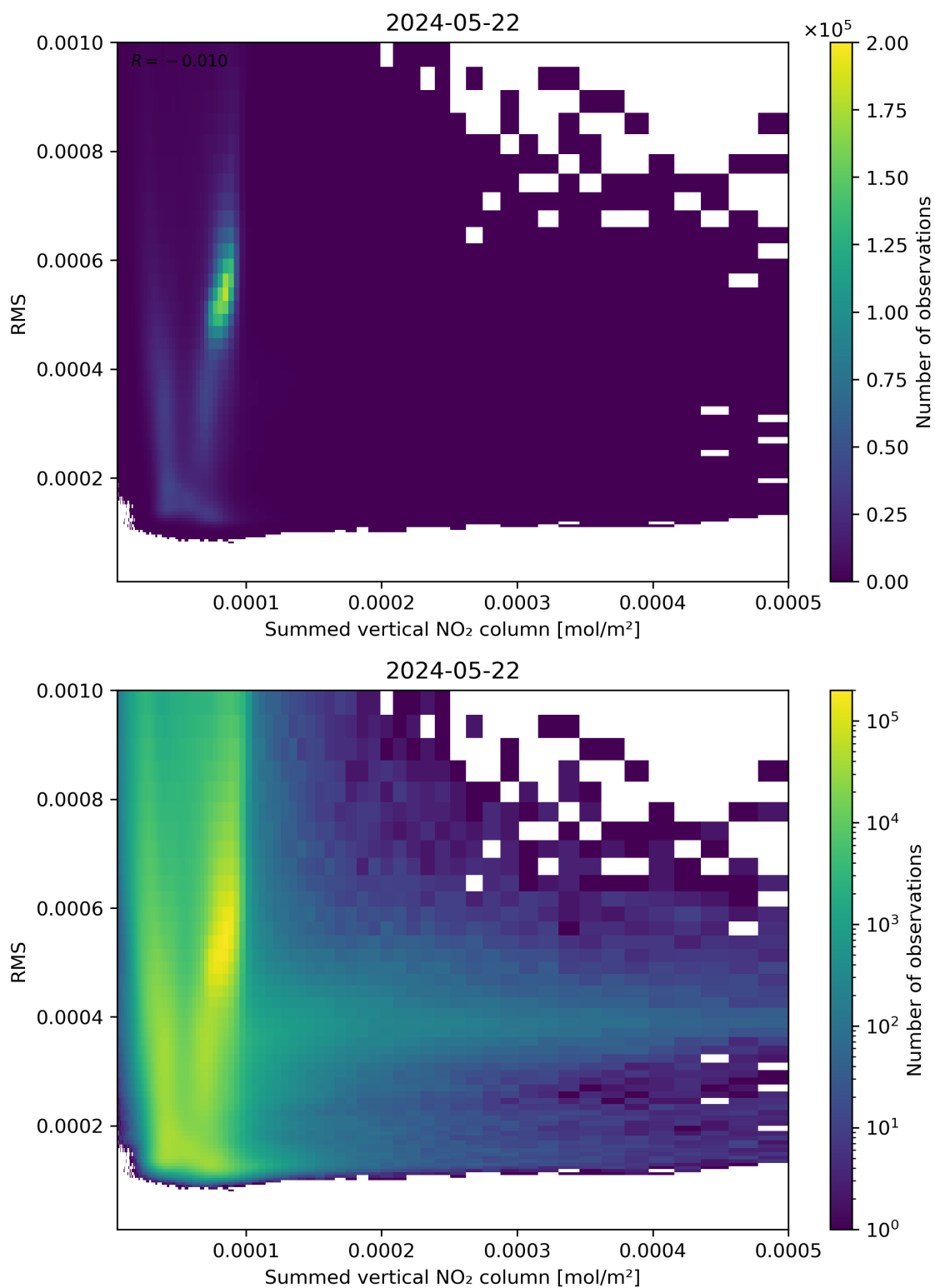
Figure 109: Scatter density plot of “Summed vertical NO 2 column” against “RMS” for 2024-05-21 to 2024-05-23.
