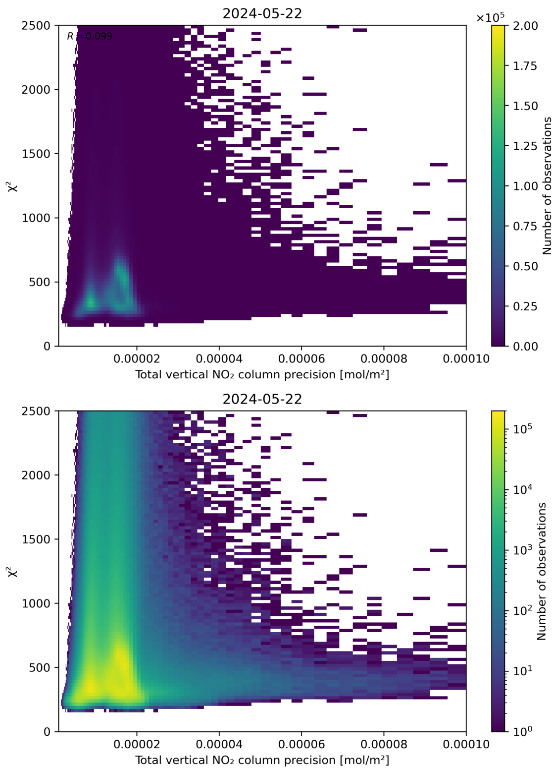
Figure 116: Scatter density plot of “Total vertical NO 2 column precision” against “ \chi^2 ” for 2024-05-21 to 2024-05-23.
