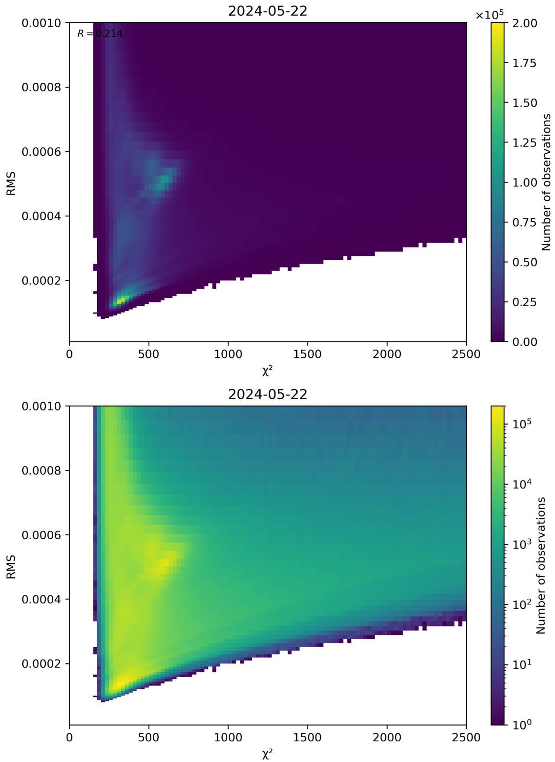
Figure 82: Scatter density plot of “ \chi^2 ” against “RMS” for 2024-05-21 to 2024-05-23.
