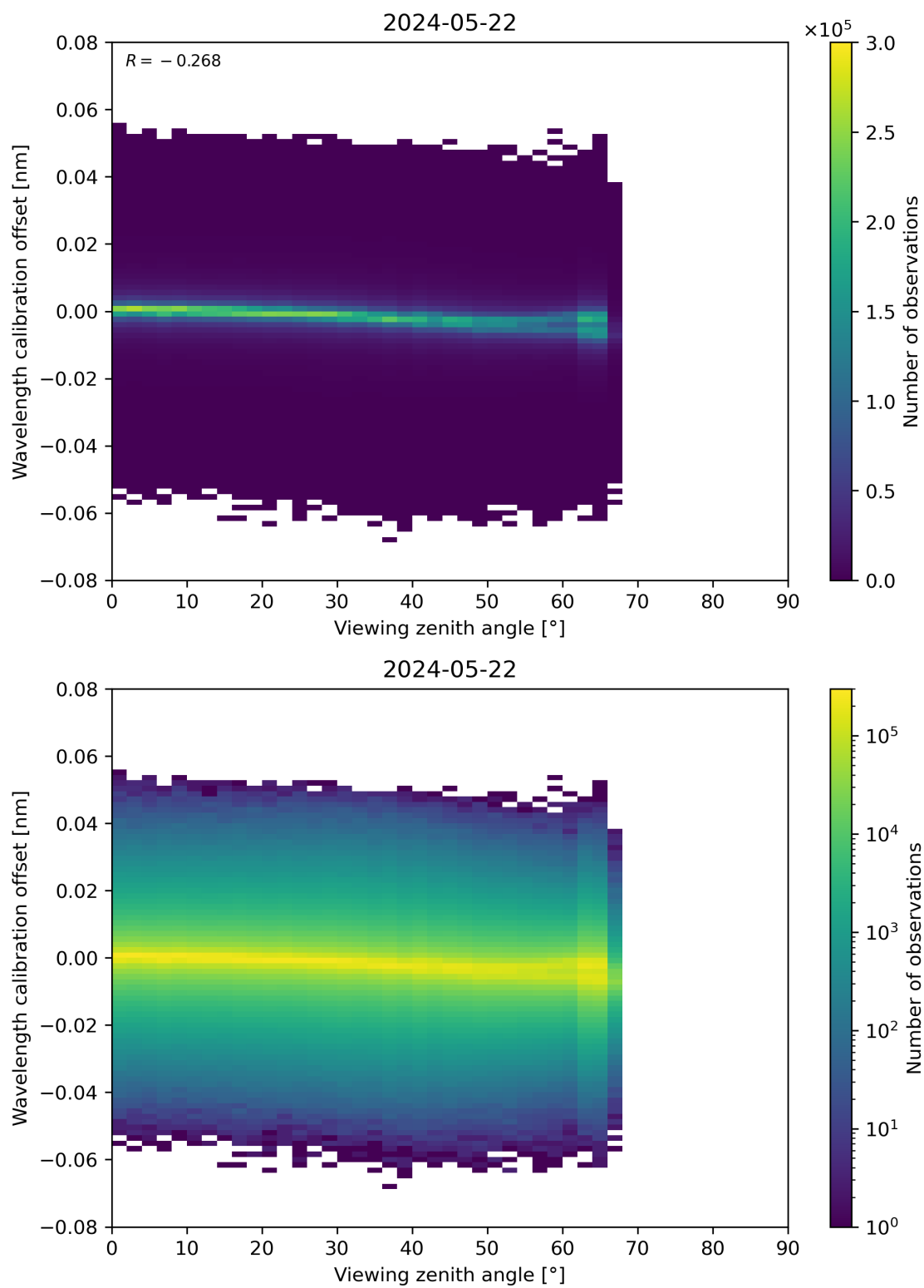
Figure 173: Scatter density plot of “Viewing zenith angle” against “Wavelength calibration offset” for 2024-05-21 to 2024-05-23.
