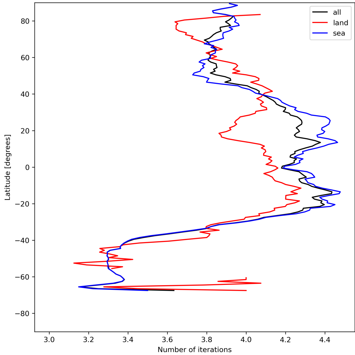
Figure 17: Zonal average of “Number of iterations” for 2024-05-21 to 2024-05-23.
