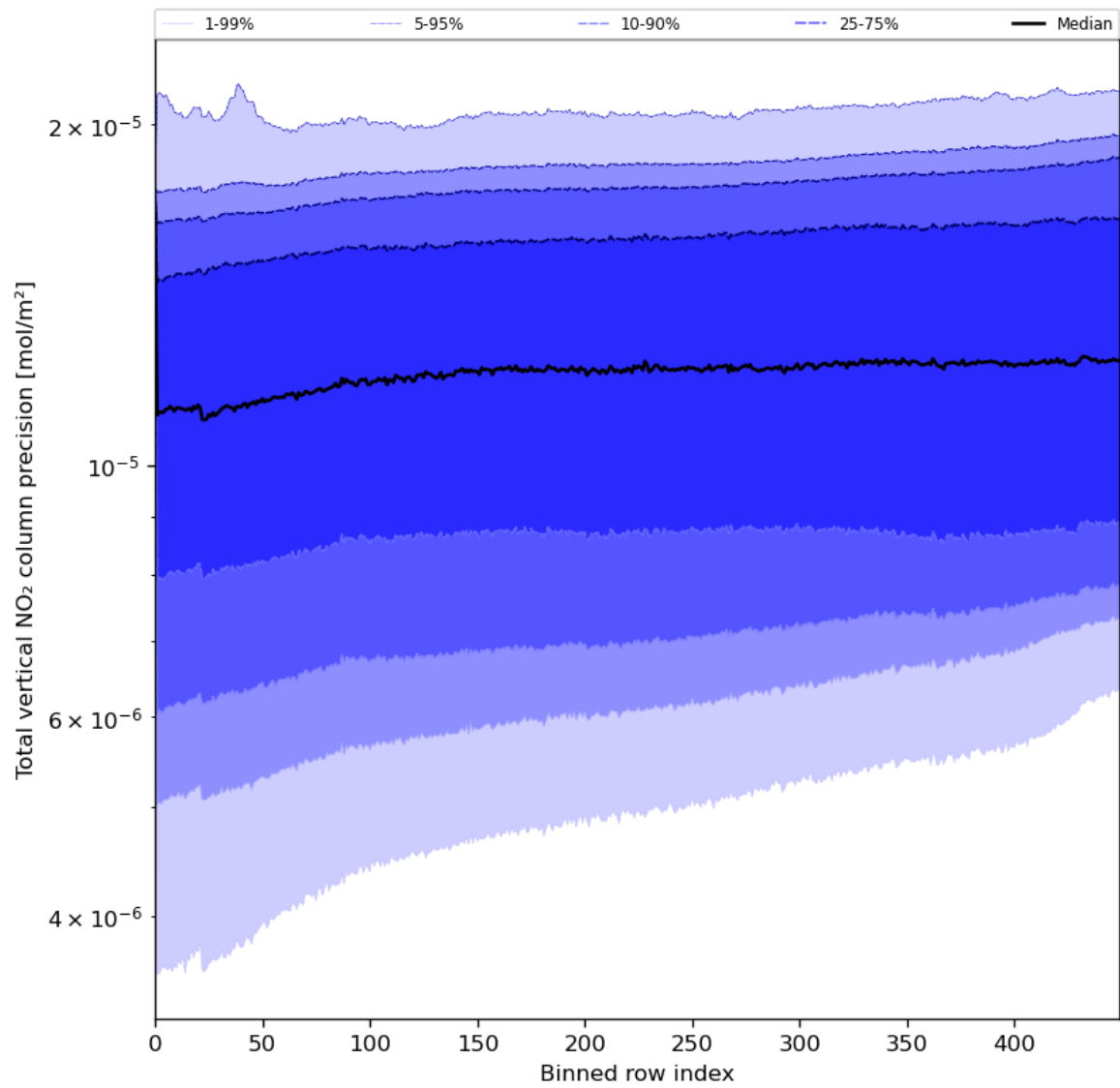
Figure 56: Along track statistics of “Total vertical NO 2 column precision” for 2024-05-21 to 2024-05-23
