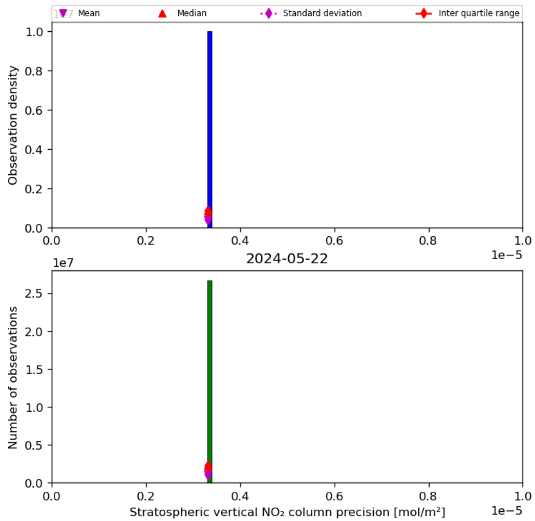
Figure 37: Histogram of “Stratospheric vertical NO 2 column precision” for 2024-05-21 to 2024-05-23
