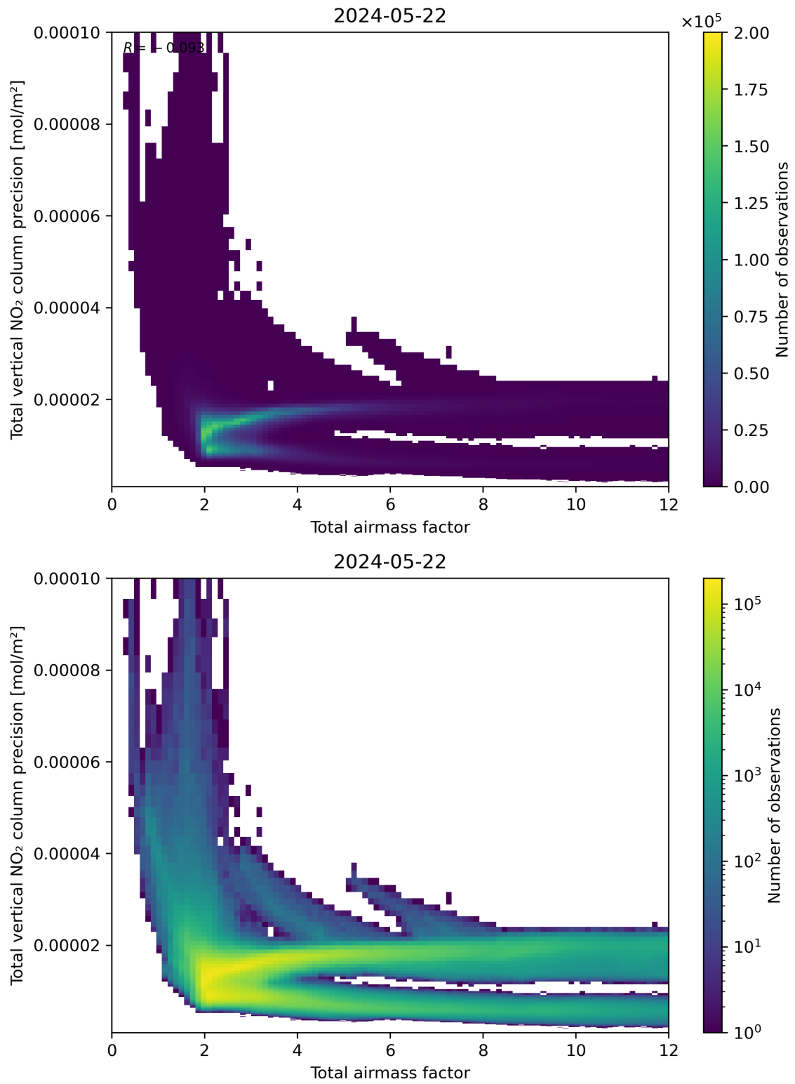
Figure 68: Scatter density plot of “Total airmass factor” against “Total vertical NO 2 column precision” for 2024-05-21 to 2024-05-23.
