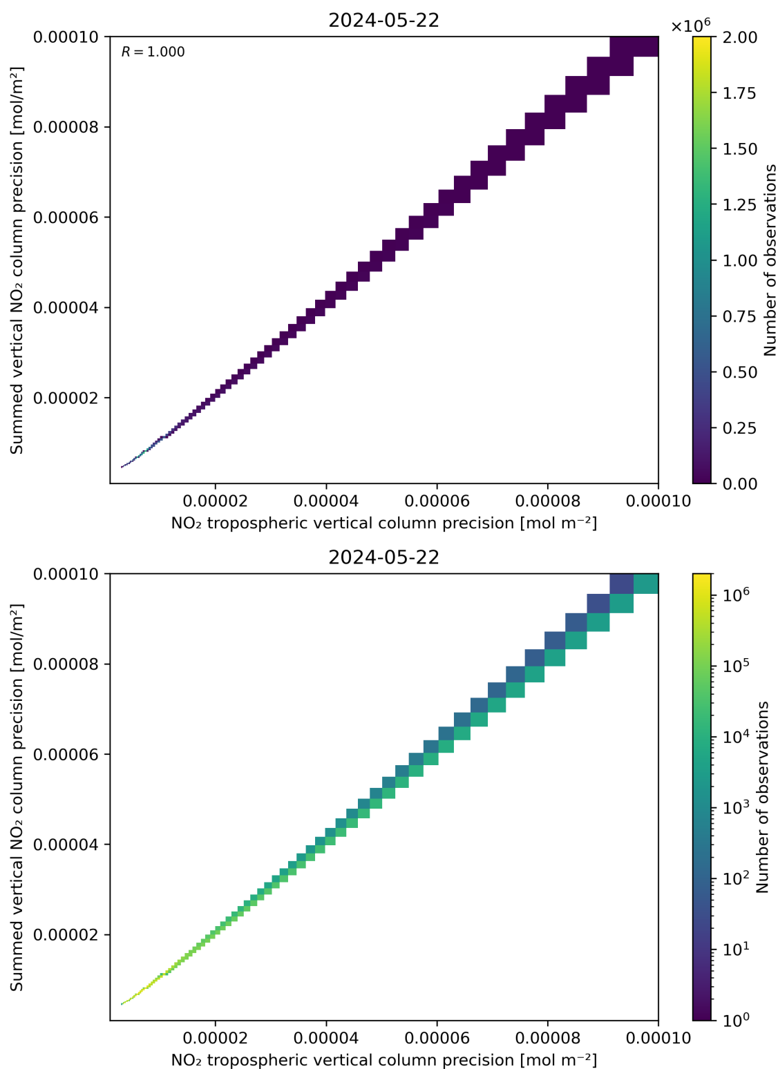
Figure 137: Scatter density plot of “NO 2 tropospheric vertical column precision” against “Summed vertical NO 2 column precision” for 2024-05-21 to 2024-05-23.
