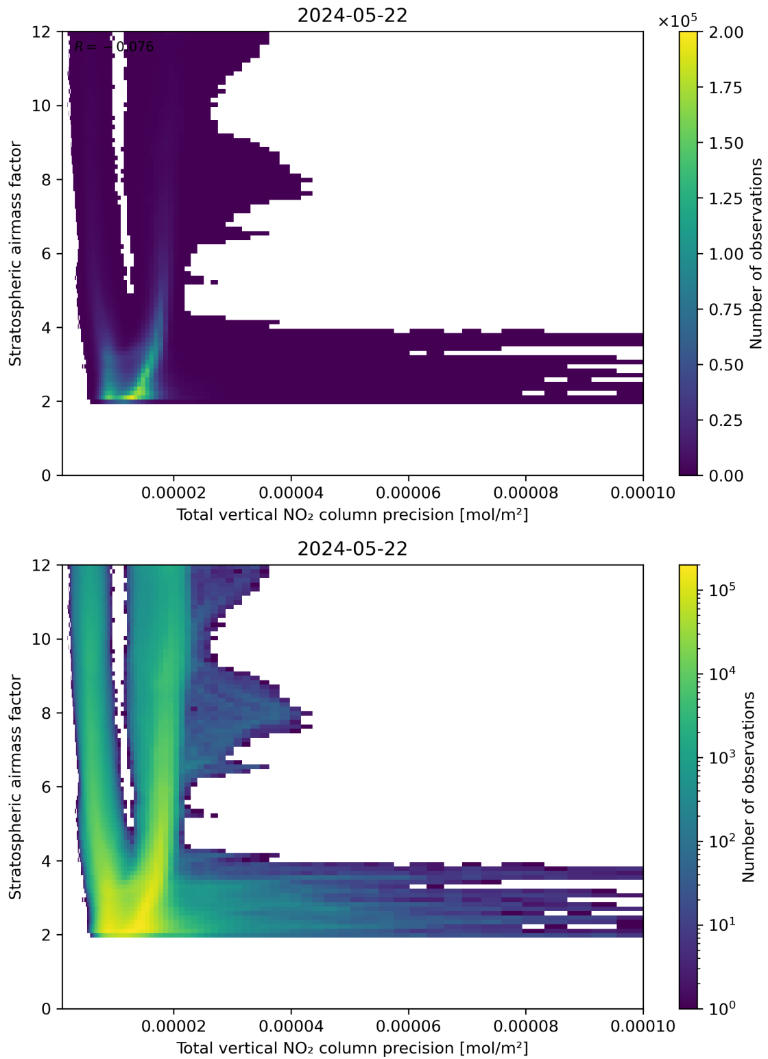
Figure 115: Scatter density plot of “Total vertical NO 2 column precision” against “Stratospheric air mass factor” for 2024-05-21 to 2024-05-23.
