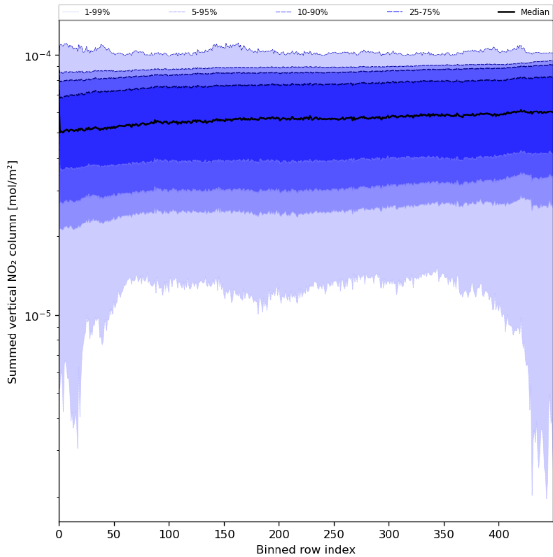
Figure 57: Along track statistics of “Summed vertical NO 2 column” for 2024-05-21 to 2024-05-23
