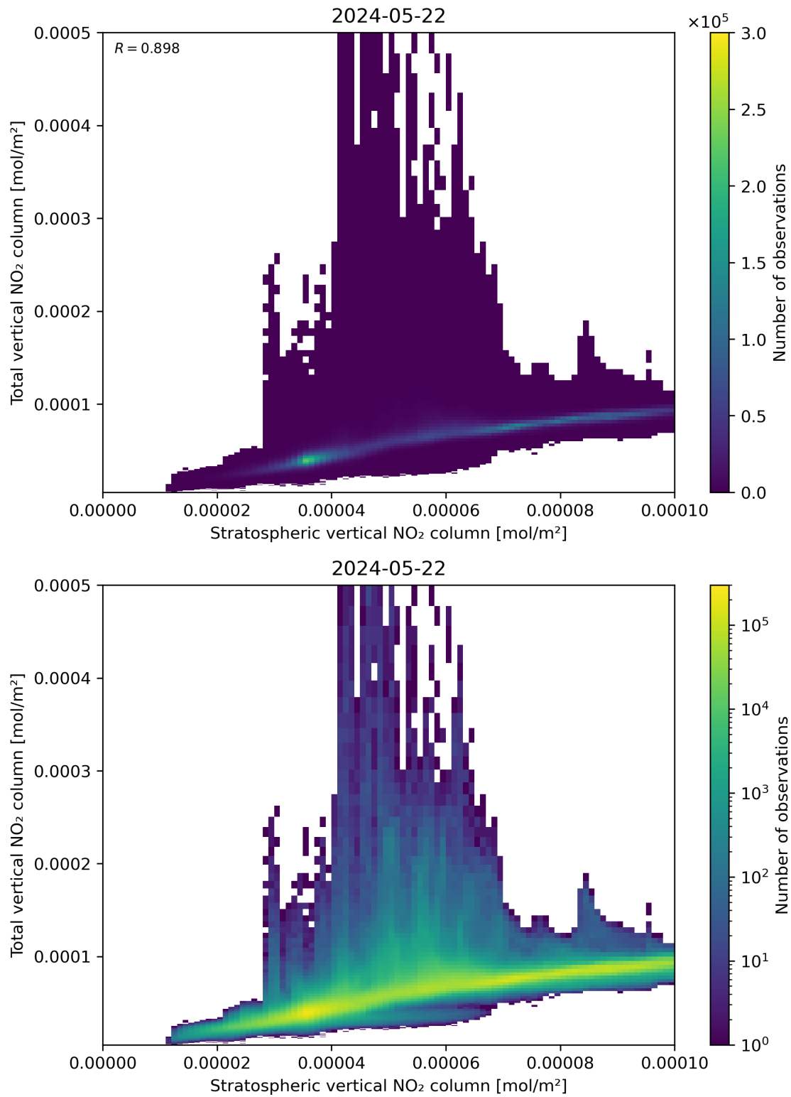
Figure 100: Scatter density plot of “Stratospheric vertical NO 2 column” against “Total vertical NO 2 column” for 2024-05-21 to 2024-05-23.
