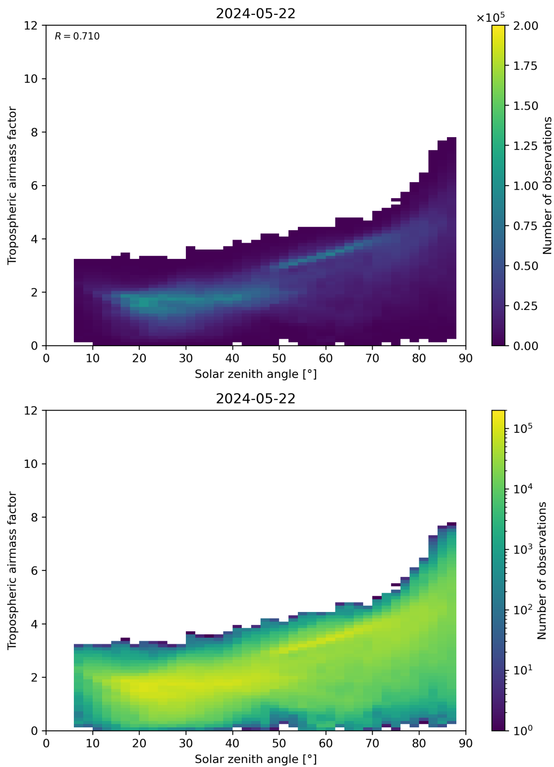
Figure 147: Scatter density plot of “Solar zenith angle” against “Tropospheric airmass factor” for 2024-05-21 to 2024-05-23.
