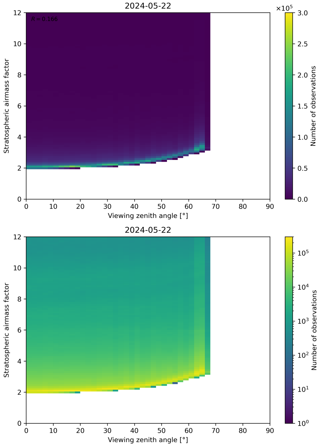
Figure 159: Scatter density plot of “Viewing zenith angle” against “Stratospheric airmass factor” for 2024-05-21 to 2024-05-23.
