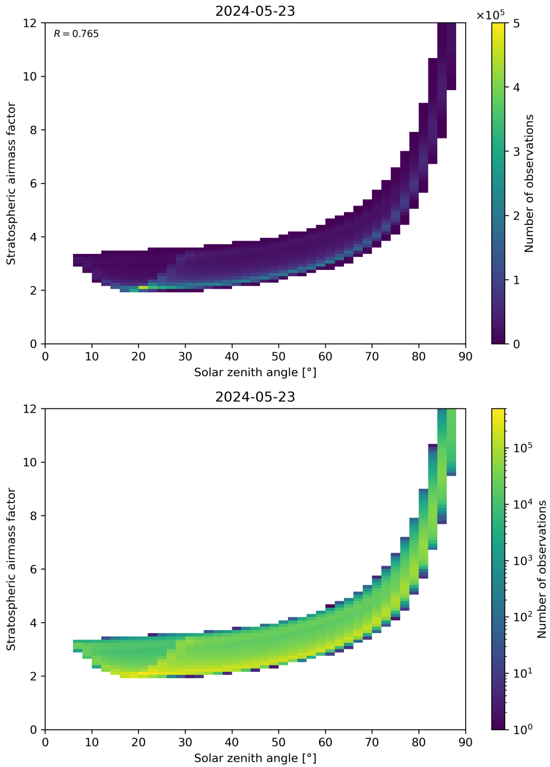
Figure 145: Scatter density plot of “Solar zenith angle” against “Stratospheric airmass factor” for 2024-05-23 to 2024-05-24.
