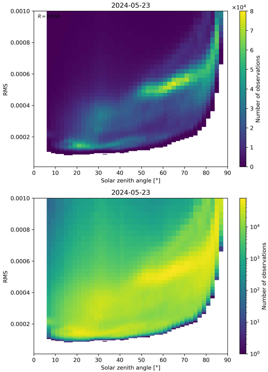
Figure 157: Scatter density plot of “Solar zenith angle” against “RMS” for 2024-05-23 to 2024-05-24.
