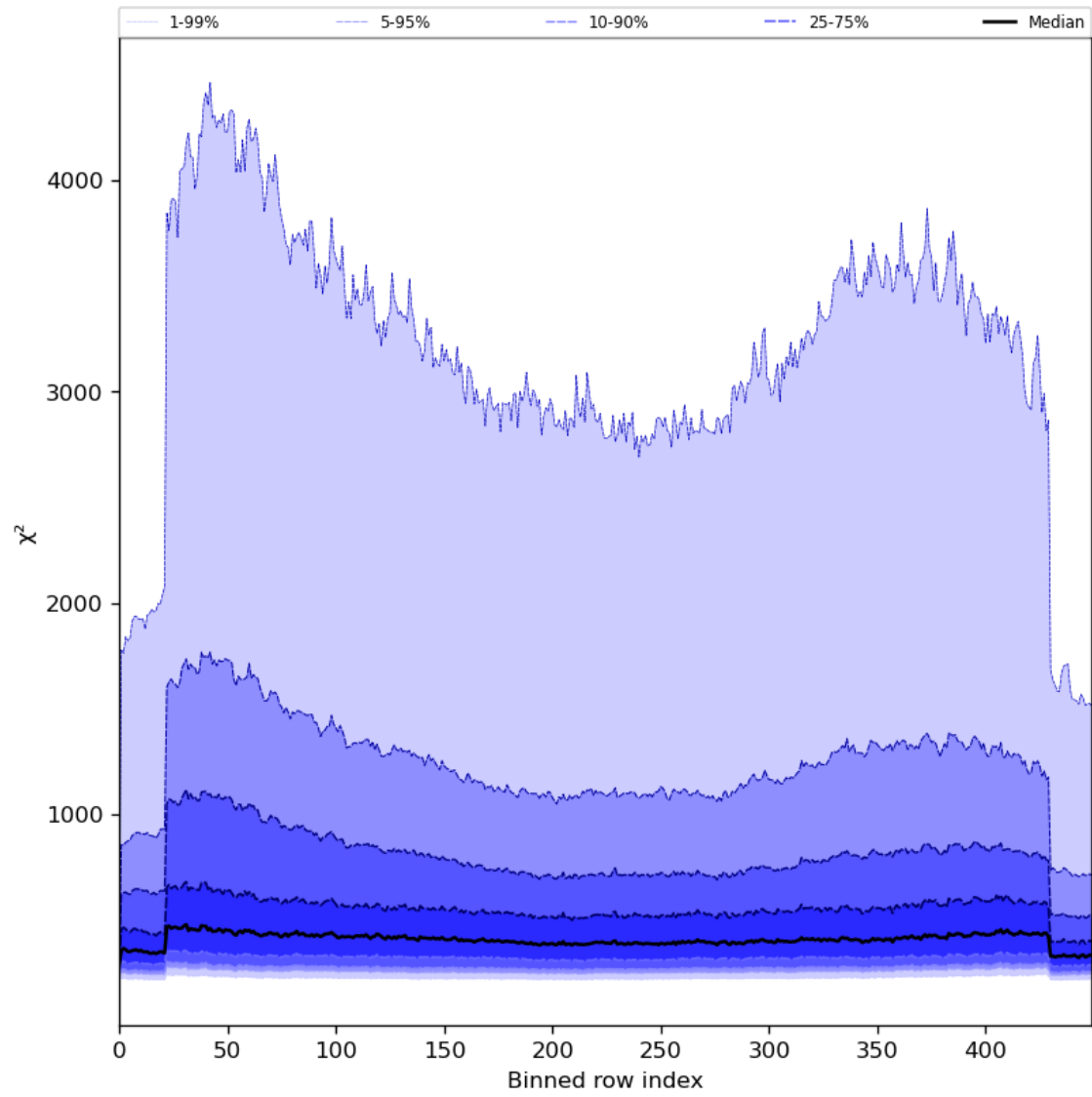
Figure 59: Along track statistics of “ \chi^2 ” for 2024-05-23 to 2024-05-24
