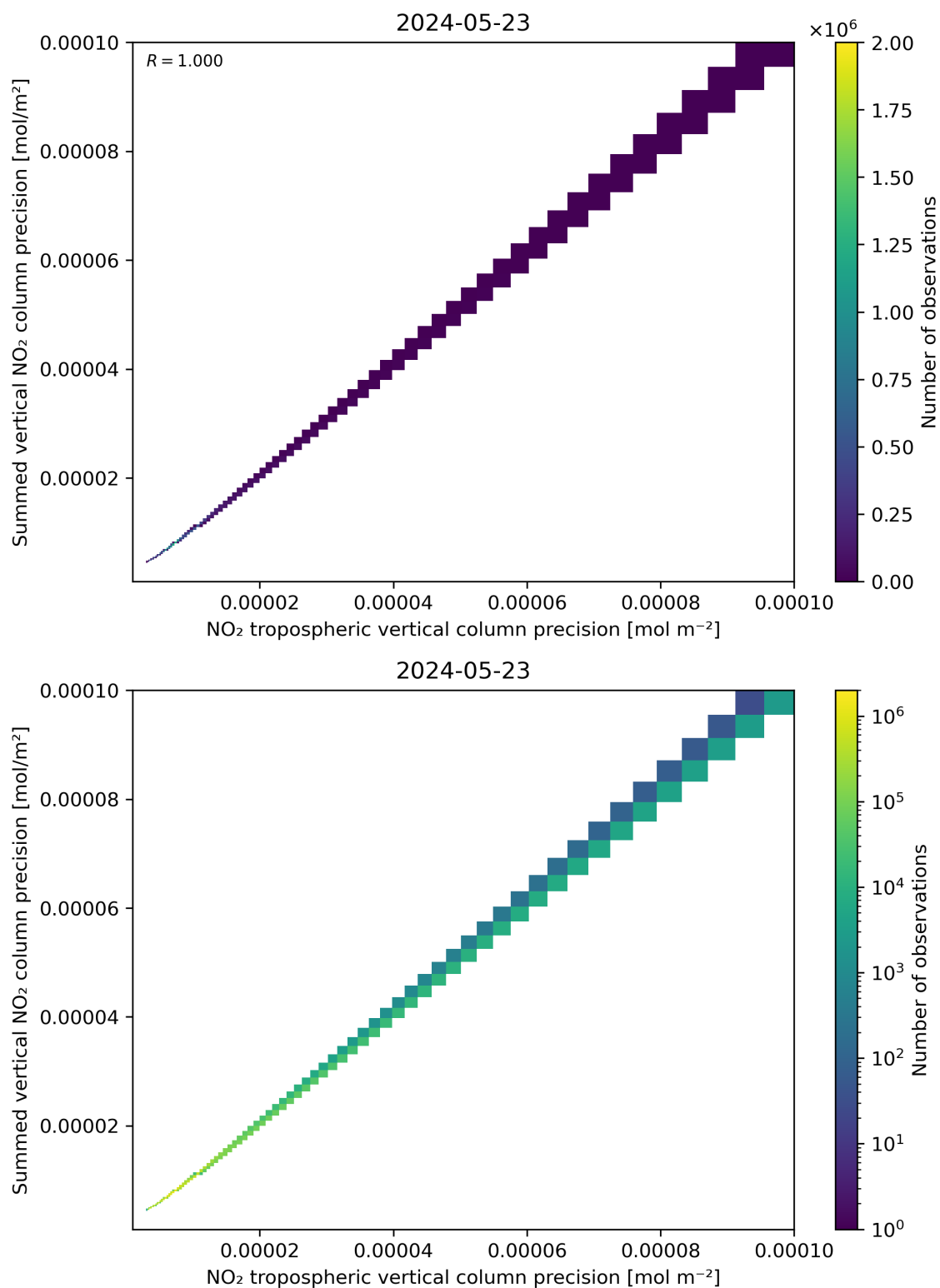
Figure 137: Scatter density plot of “NO 2 tropospheric vertical column precision” against “Summed vertical NO 2 column precision” for 2024-05-23 to 2024-05-24.
