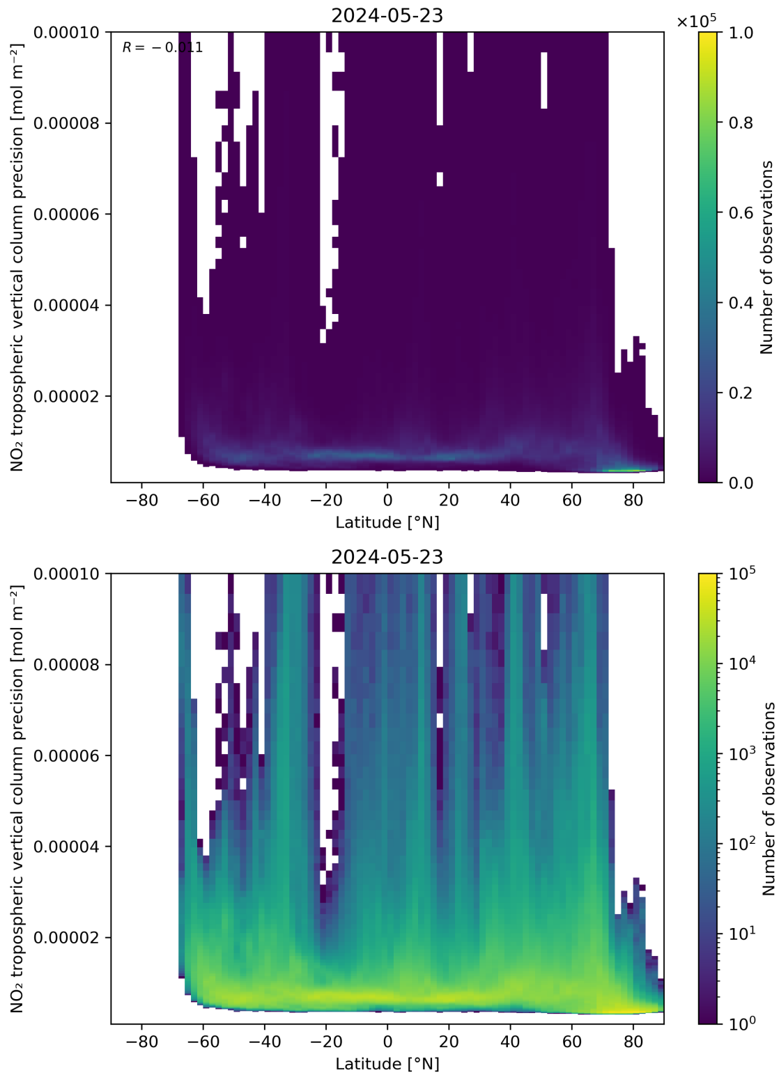
Figure 93: Scatter density plot of “Latitude” against “NO 2 tropospheric vertical column precision” for 2024-05-23 to 2024-05-24.
