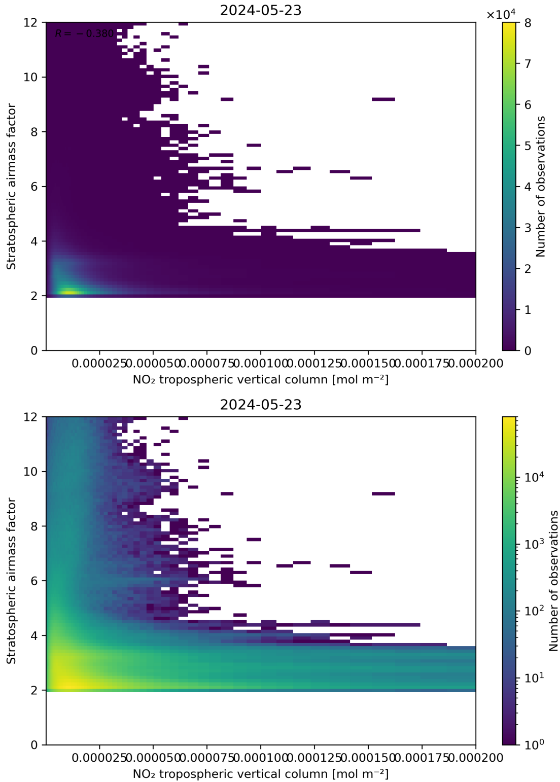
Figure 121: Scatter density plot of “NO 2 tropospheric vertical column” against “Stratospheric air mass factor” for 2024-05-23 to 2024-05-24.
