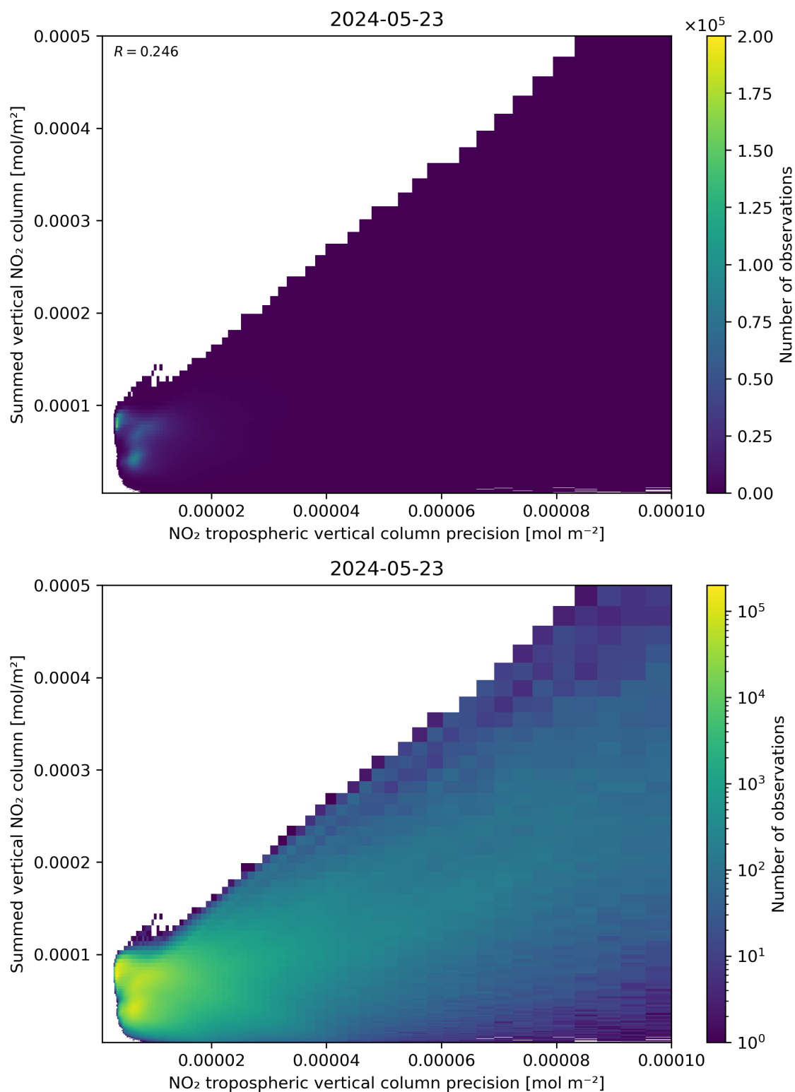
Figure 136: Scatter density plot of “NO 2 tropospheric vertical column precision” against “Summed vertical NO 2 column” for 2024-05-23 to 2024-05-24.
