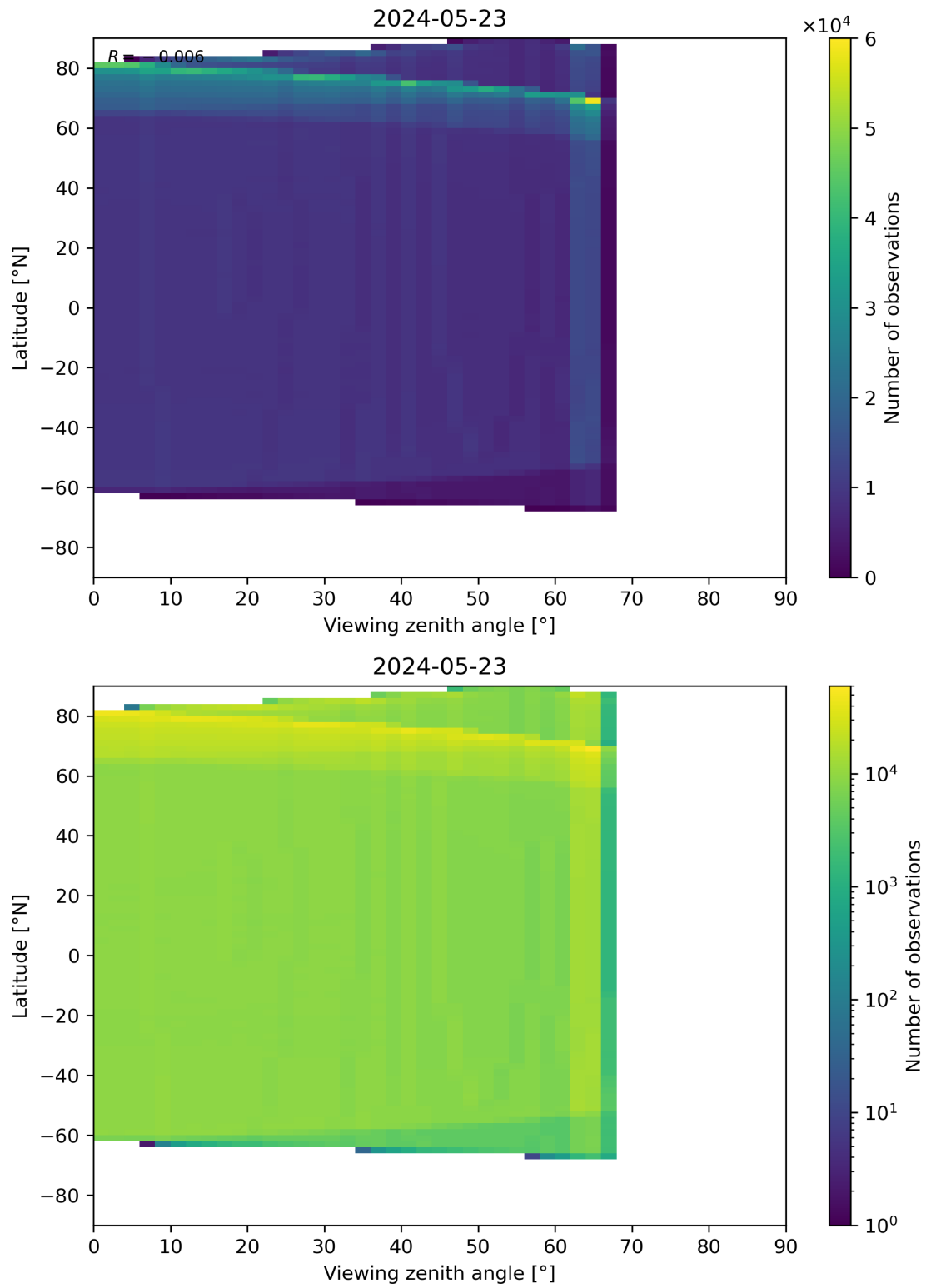
Figure 163: Scatter density plot of “Viewing zenith angle” against “Latitude” for 2024-05-23 to 2024-05-24.
