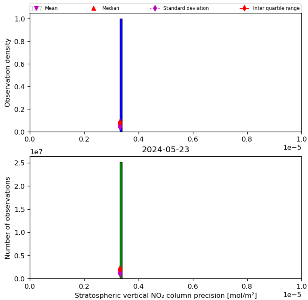
Figure 37: Histogram of “Stratospheric vertical NO 2 column precision” for 2024-05-23 to 2024-05-24
