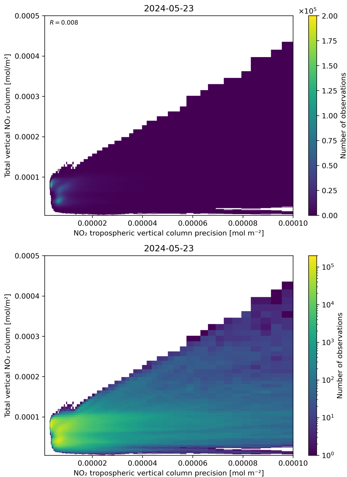
Figure 138: Scatter density plot of “NO 2 tropospheric vertical column precision” against “Total vertical NO 2 column” for 2024-05-23 to 2024-05-24.
