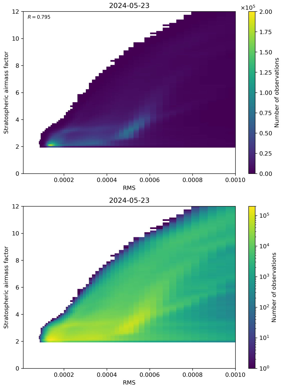
Figure 144: Scatter density plot of “RMS” against “Stratospheric airmass factor” for 2024-05-23 to 2024-05-24.
