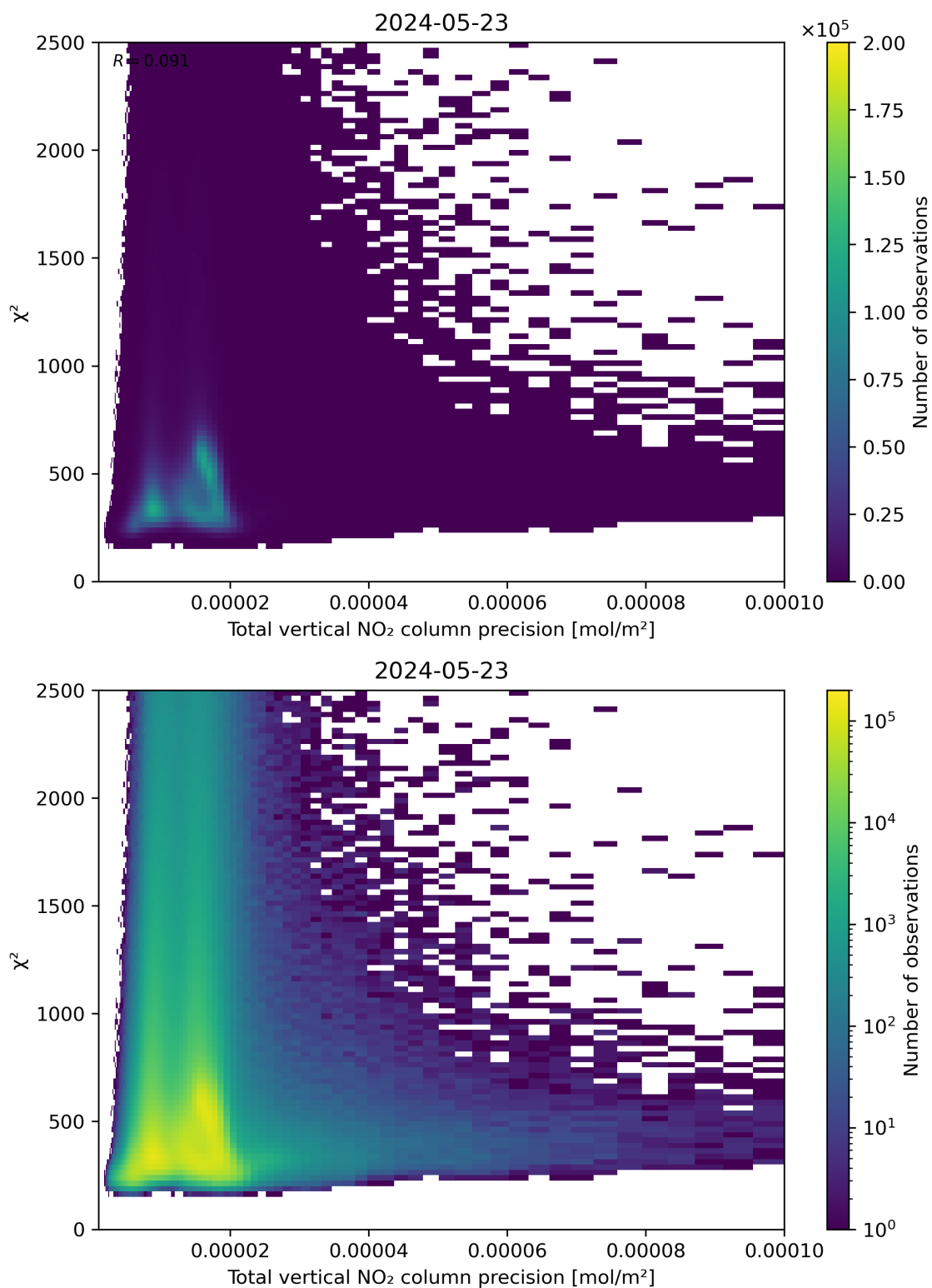
Figure 116: Scatter density plot of “Total vertical NO 2 column precision” against “ \chi^2 ” for 2024-05-23 to 2024-05-24.
