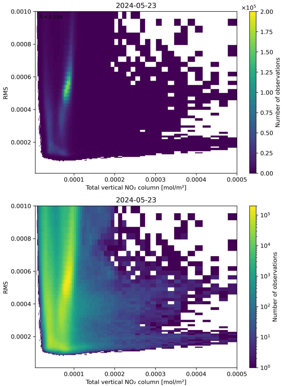
Figure 120: Scatter density plot of “Total vertical NO 2 column” against “RMS” for 2024-05-23 to 2024-05-24.
