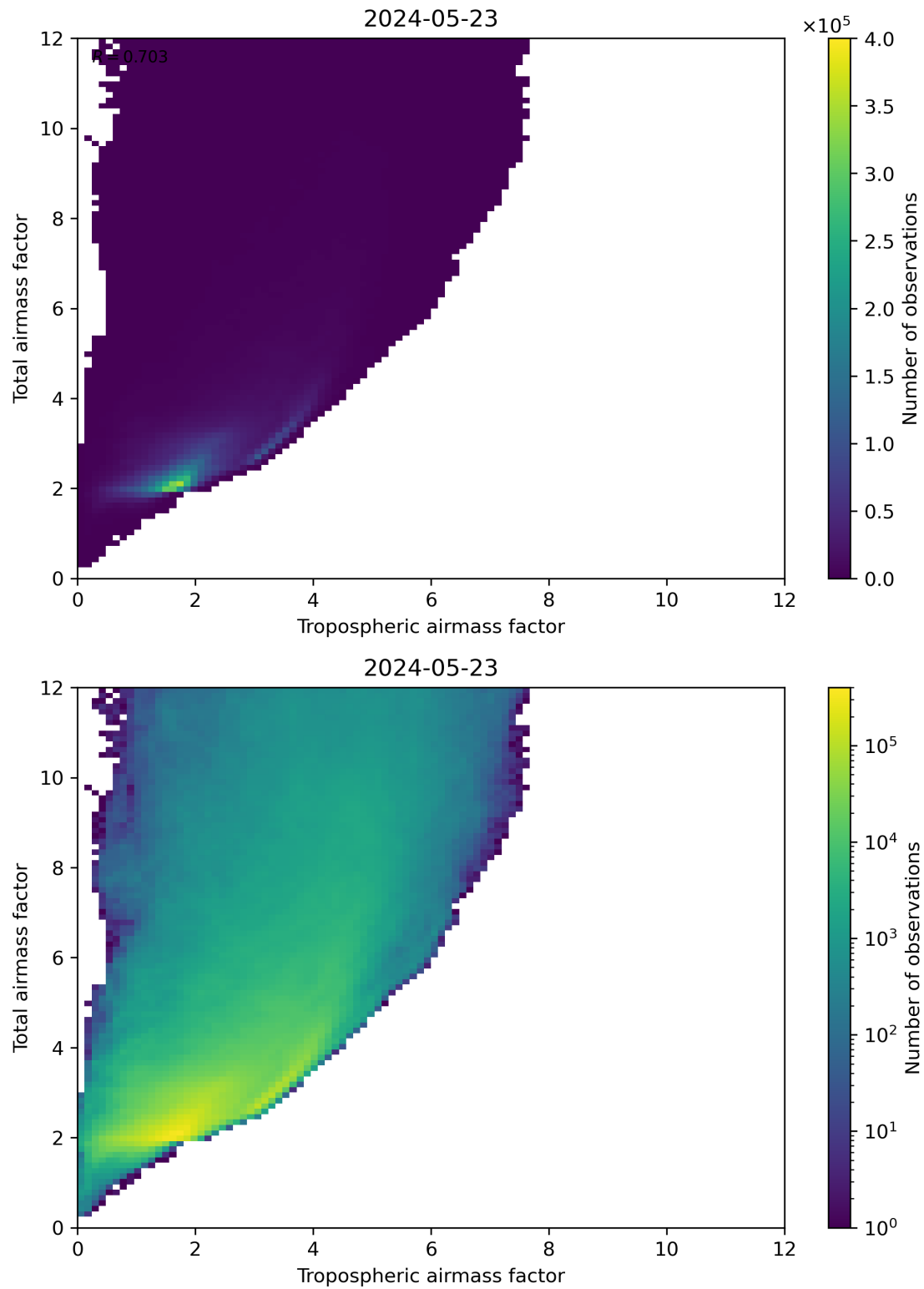
Figure 72: Scatter density plot of “Tropospheric airmass factor” against “Total airmass factor” for 2024-05-23 to 2024-05-24.
