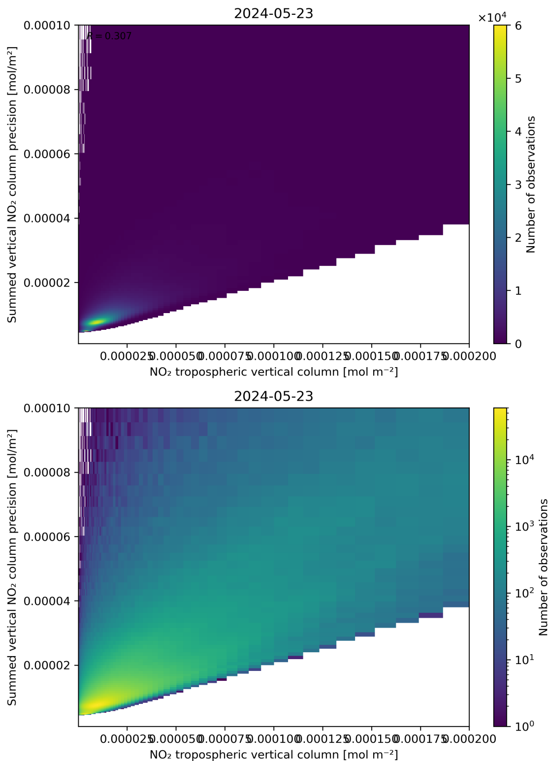
Figure 127: Scatter density plot of “NO 2 tropospheric vertical column” against “Summed vertical NO 2 column precision” for 2024-05-23 to 2024-05-24.
