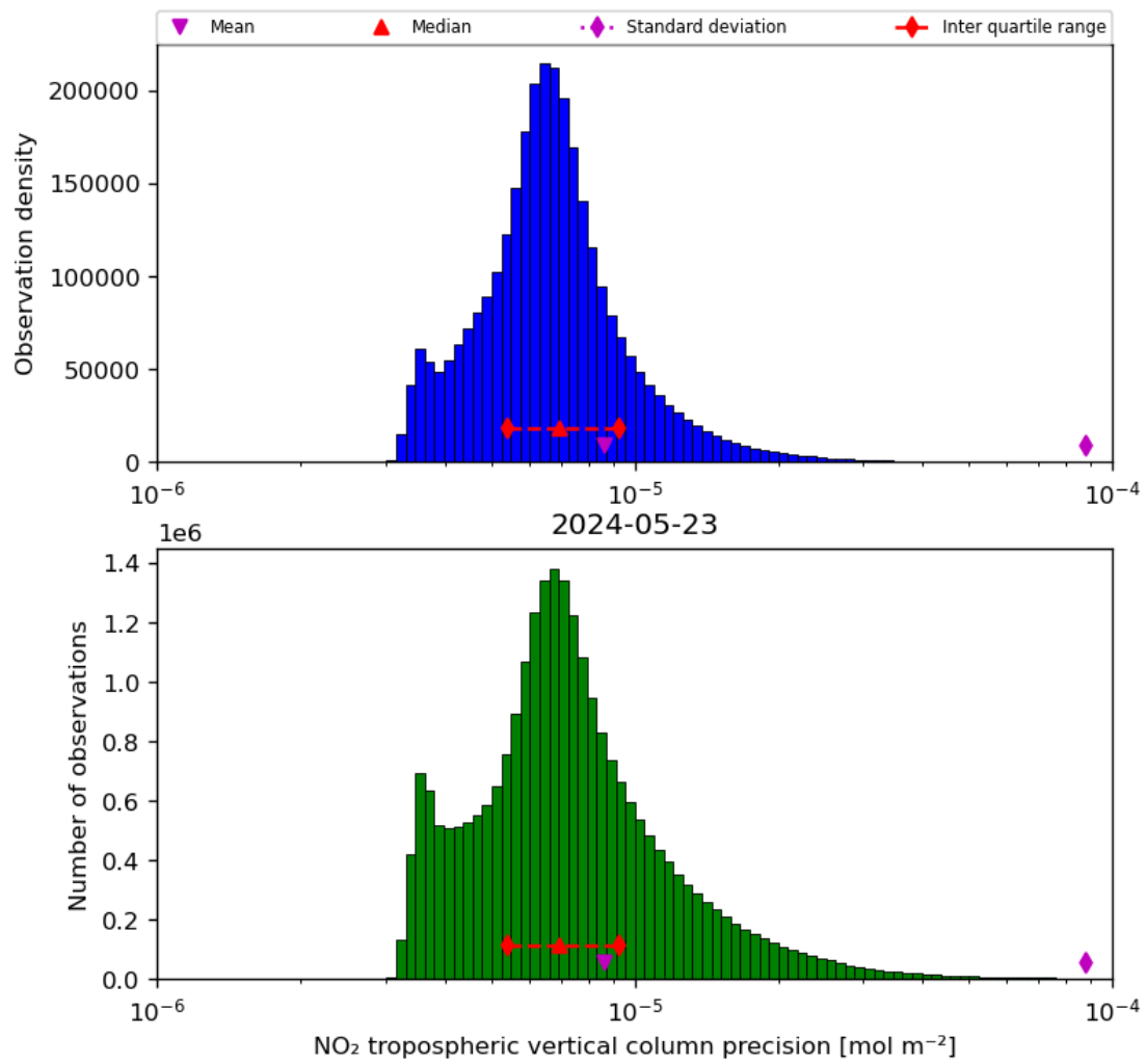
Figure 30: Histogram of “NO 2 tropospheric vertical column precision” for 2024-05-23 to 2024-05-24
