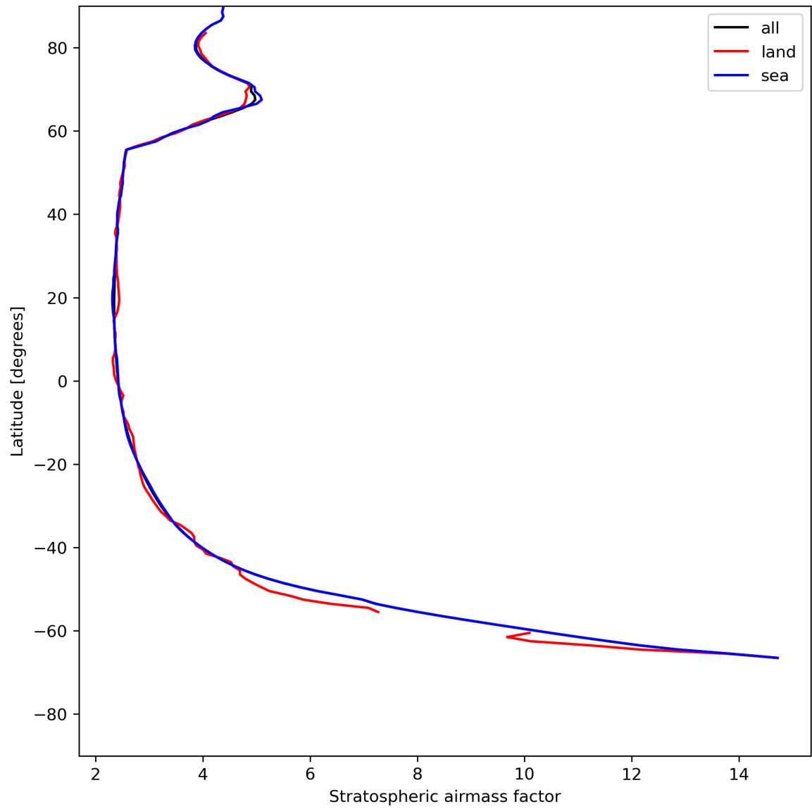
Figure 27: Zonal average of “Stratospheric airmass factor” for 2024-05-23 to 2024-05-24.
