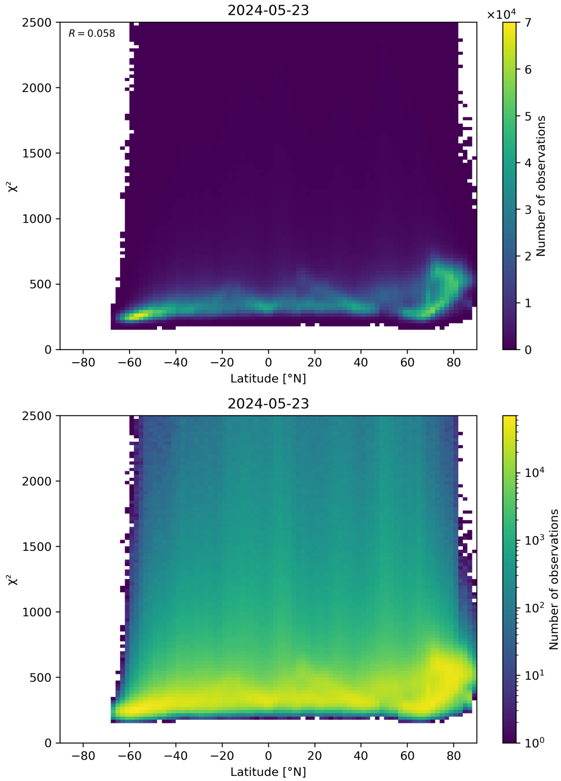
Figure 86: Scatter density plot of “Latitude” against “ \chi^2 ” for 2024-05-23 to 2024-05-24.
