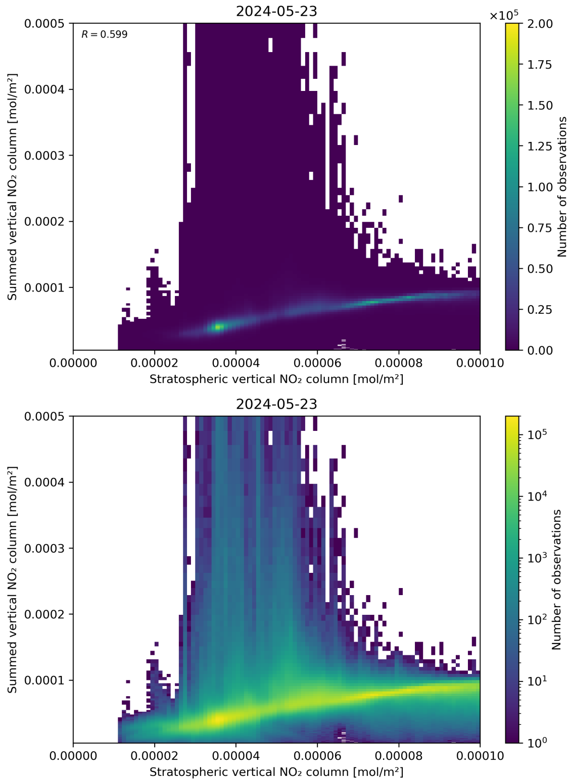
Figure 98: Scatter density plot of “Stratospheric vertical NO 2 column” against “Summed vertical NO 2 column” for 2024-05-23 to 2024-05-24.
