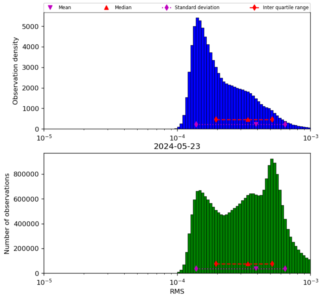
Figure 43: Histogram of “RMS” for 2024-05-23 to 2024-05-24
