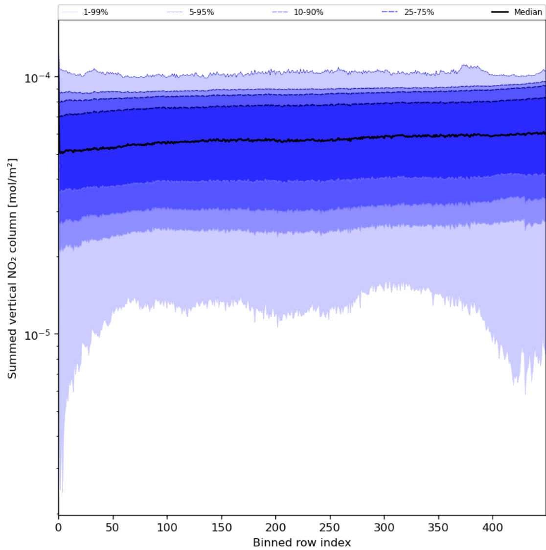
Figure 57: Along track statistics of “Summed vertical NO 2 column” for 2024-05-23 to 2024-05-24
