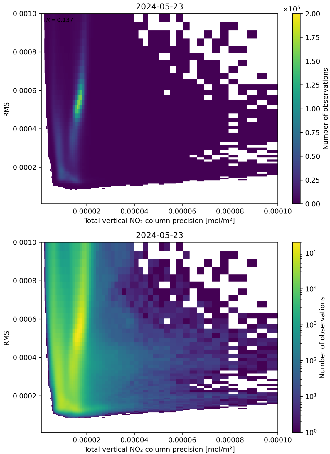
Figure 119: Scatter density plot of “Total vertical NO 2 column precision” against “RMS” for 2024-05-23 to 2024-05-24.
