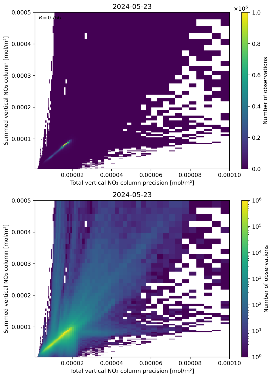
Figure 117: Scatter density plot of “Total vertical NO 2 column precision” against “Summed vertical NO 2 column” for 2024-05-23 to 2024-05-24.
