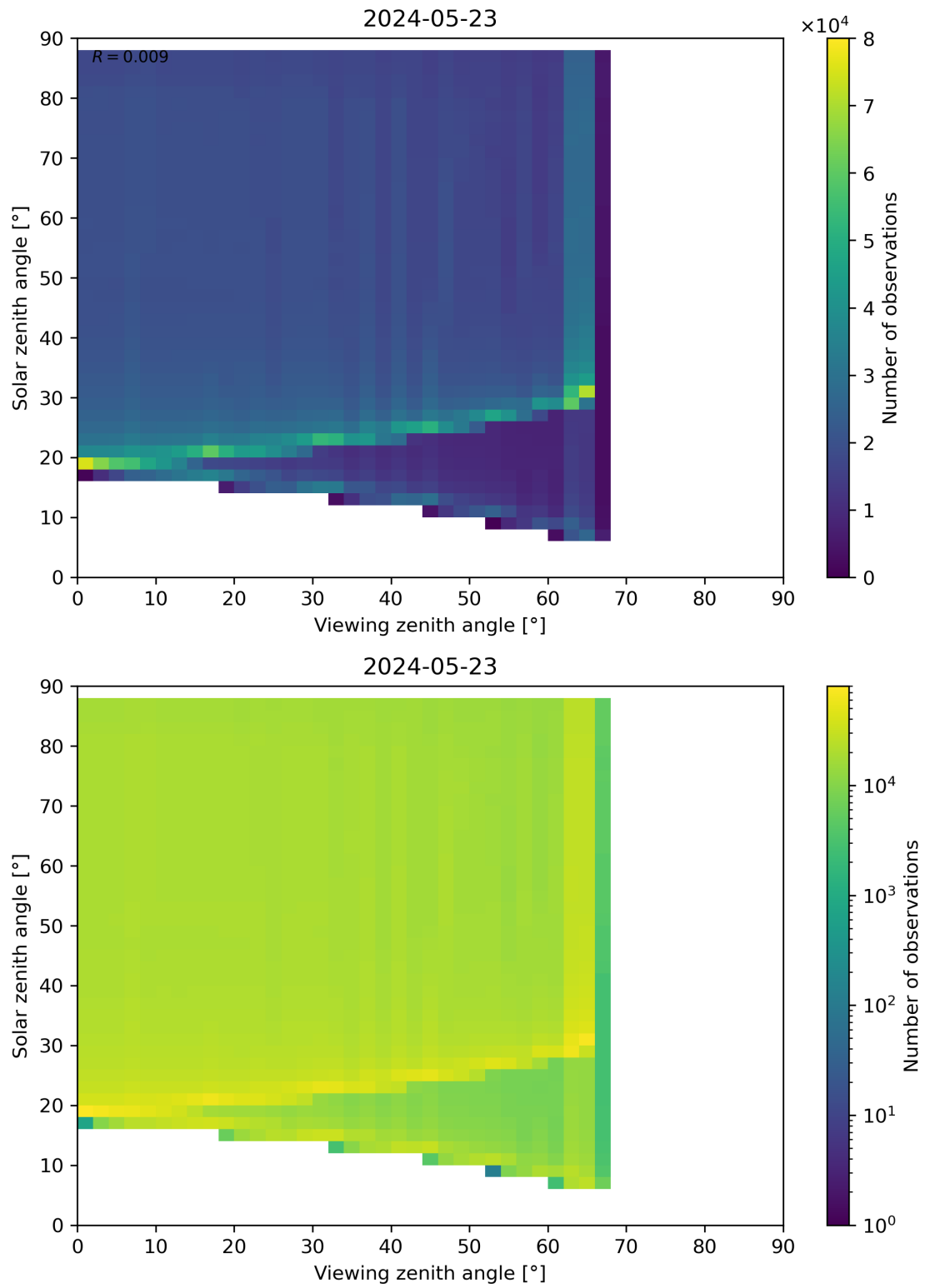
Figure 172: Scatter density plot of “Viewing zenith angle” against “Solar zenith angle” for 2024-05-23 to 2024-05-24.
