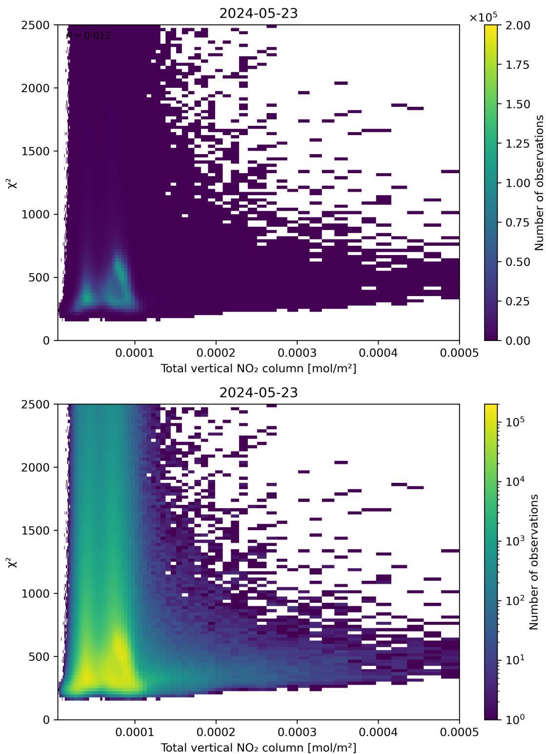
Figure 111: Scatter density plot of “Total vertical NO 2 column” against “ \chi^2 ” for 2024-05-23 to 2024-05-24.
