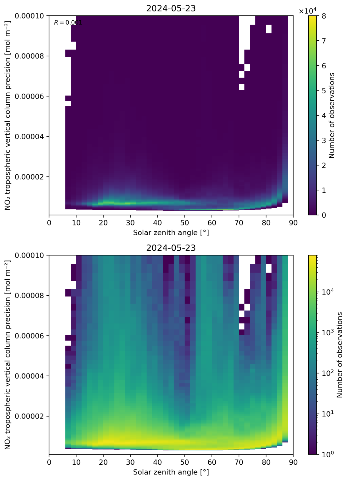
Figure 156: Scatter density plot of “Solar zenith angle” against “NO 2 tropospheric vertical column precision” for 2024-05-23 to 2024-05-24.
