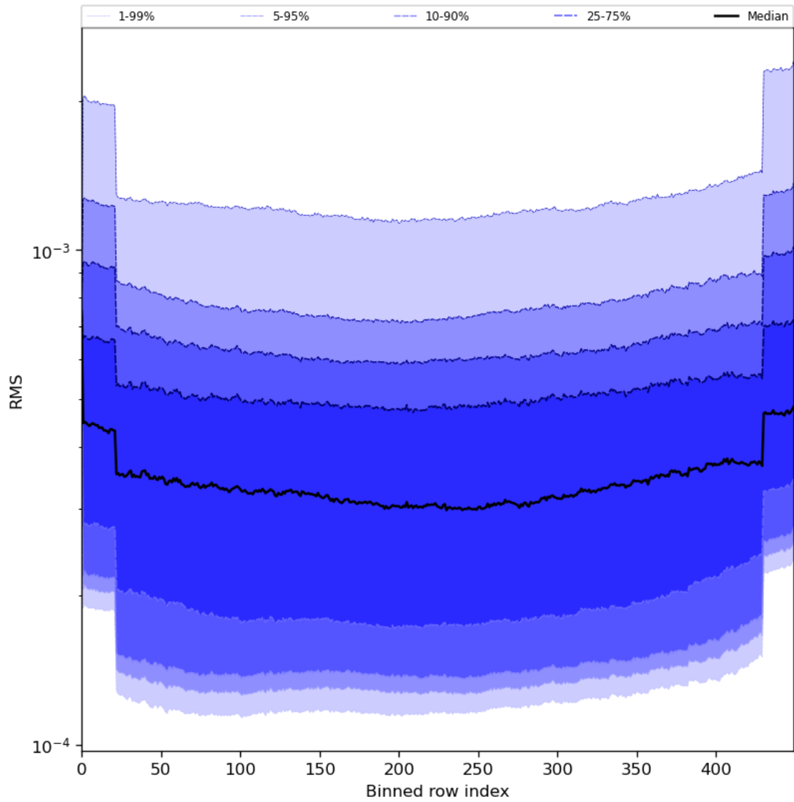
Figure 60: Along track statistics of “RMS” for 2024-05-23 to 2024-05-24
