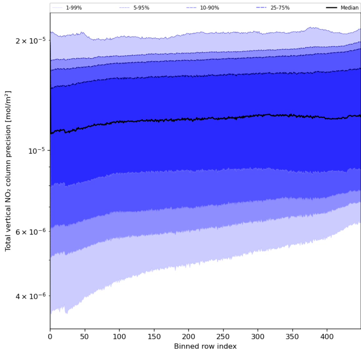
Figure 56: Along track statistics of “Total vertical NO 2 column precision” for 2024-05-23 to 2024-05-24
