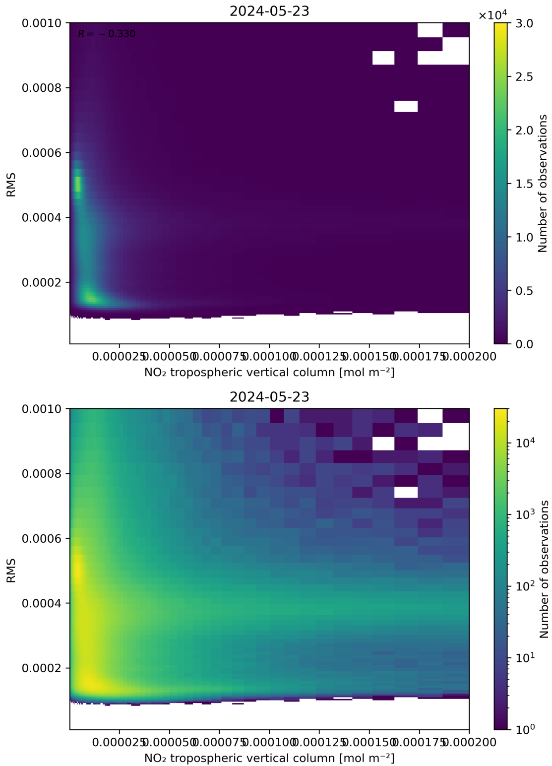
Figure 142: Scatter density plot of “NO 2 tropospheric vertical column” against “RMS” for 2024-05-23 to 2024-05-24.
