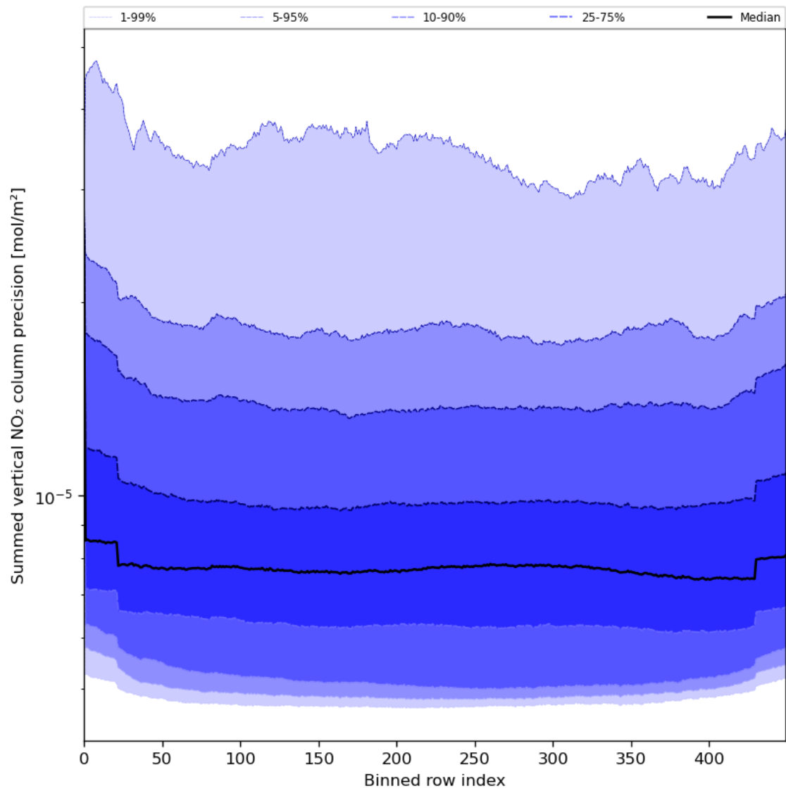
Figure 58: Along track statistics of “Summed vertical NO 2 column precision” for 2024-05-23 to 2024-05-24
