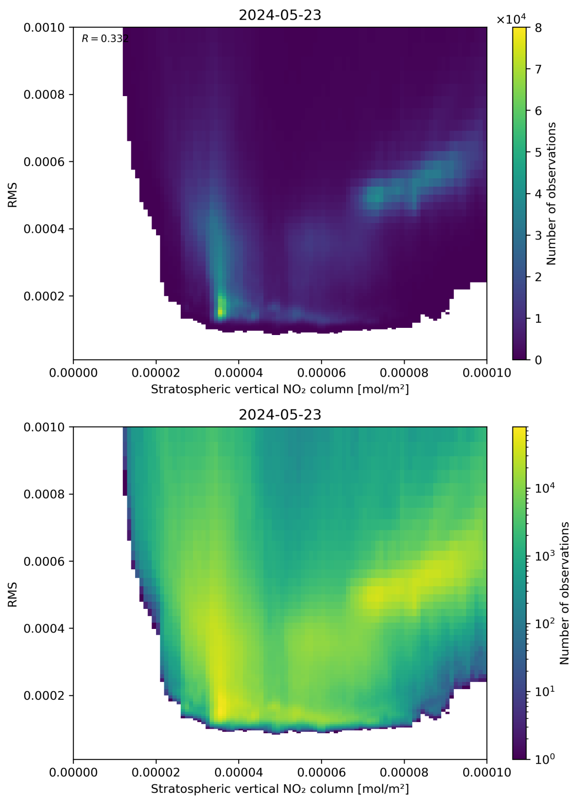
Figure 102: Scatter density plot of “Stratospheric vertical NO 2 column” against “RMS” for 2024-05-23 to 2024-05-24.
