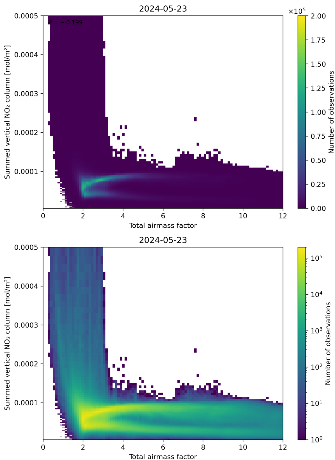
Figure 65: Scatter density plot of “Total airmass factor” against “Summed vertical NO 2 column” for 2024-05-23 to 2024-05-24.
