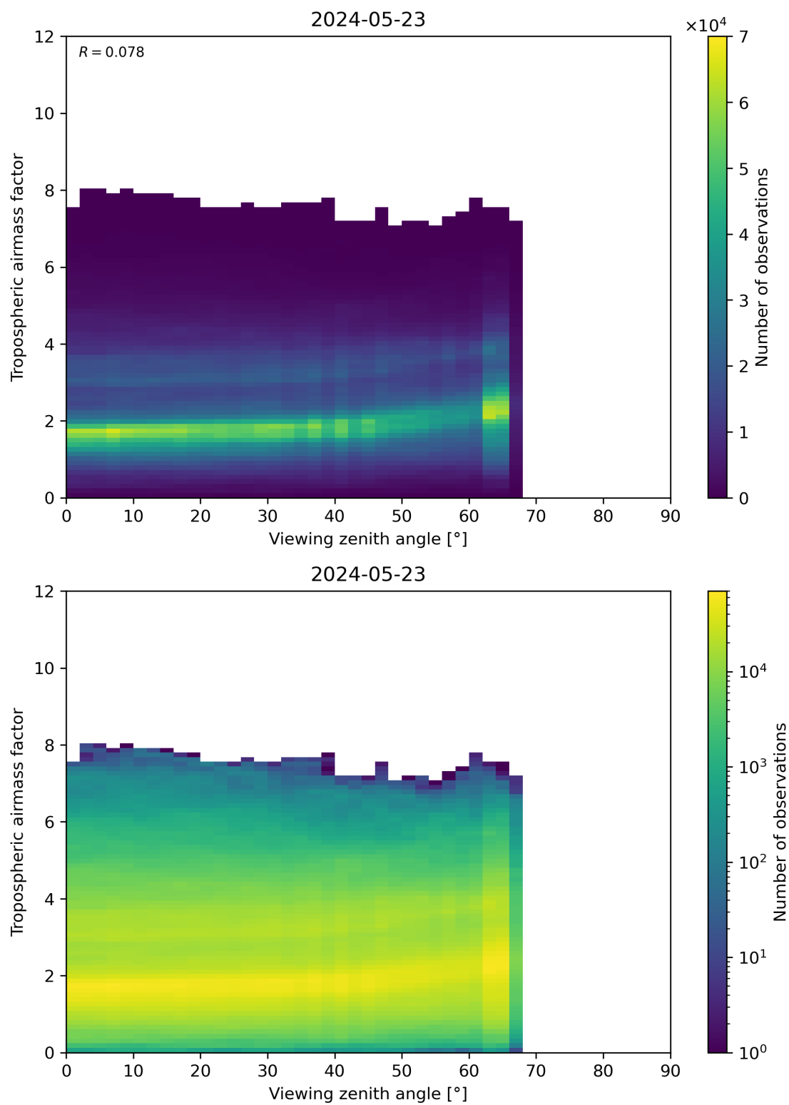
Figure 161: Scatter density plot of “Viewing zenith angle” against “Tropospheric airmass factor” for 2024-05-23 to 2024-05-24.
