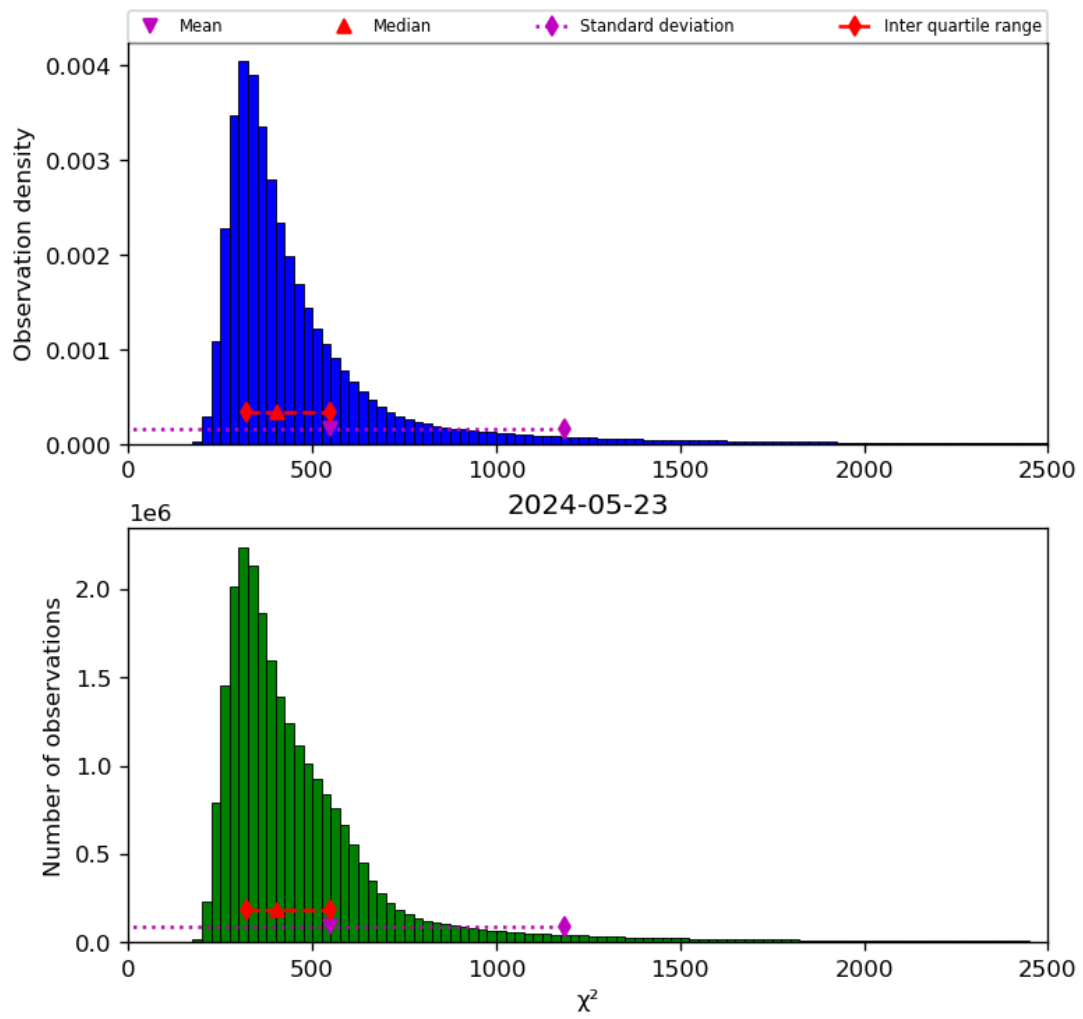
Figure 42: Histogram of " \chi^2 " for 2024-05-23 to 2024-05-24
