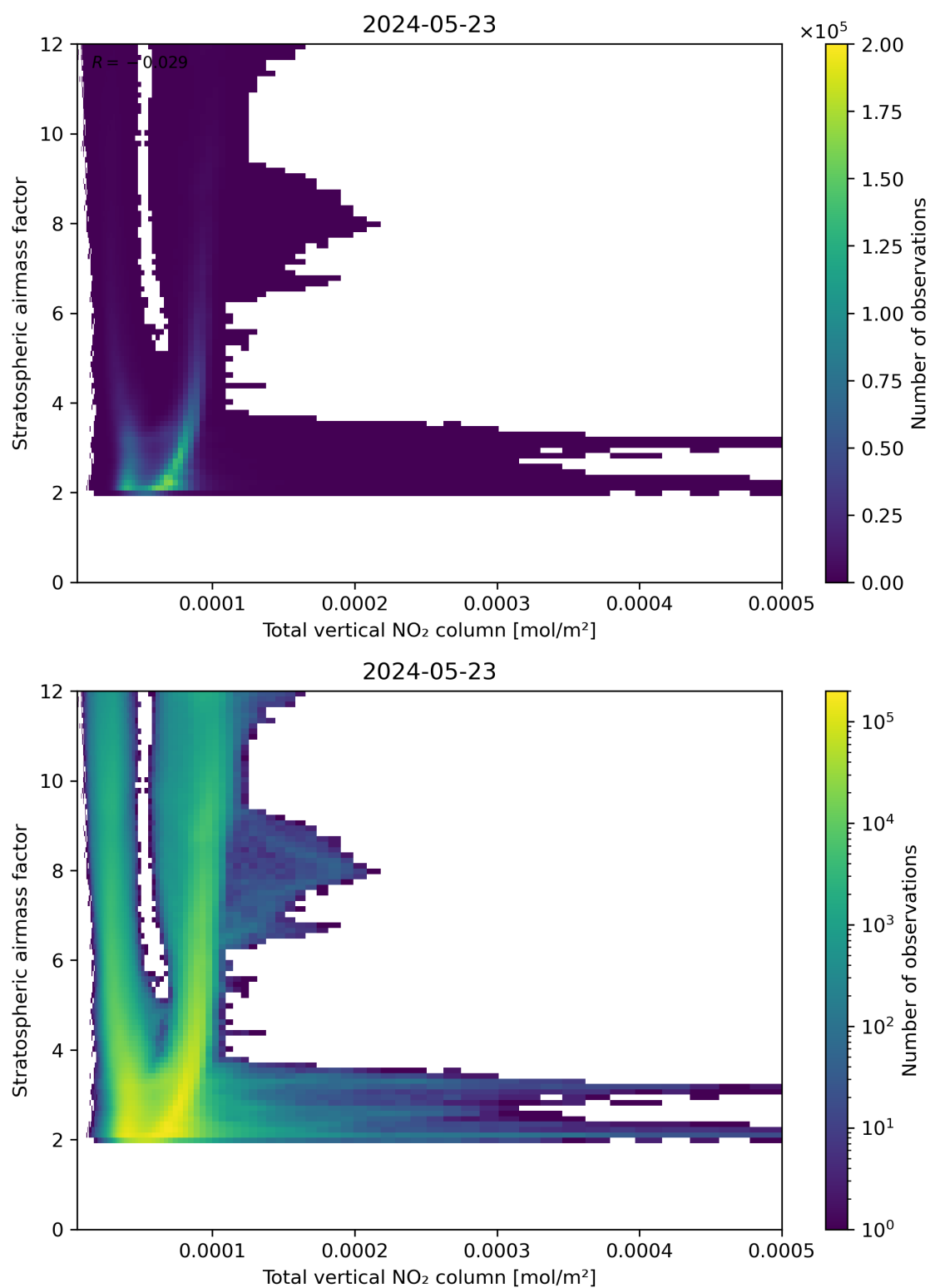
Figure 110: Scatter density plot of “Total vertical NO 2 column” against “Stratospheric air mass factor” for 2024-05-23 to 2024-05-24.
