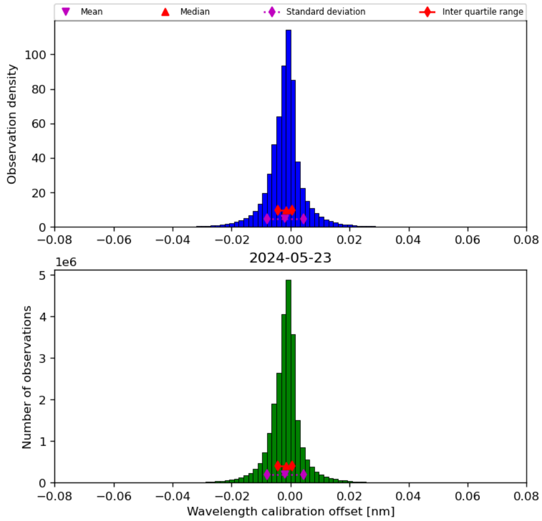
Figure 35: Histogram of “Wavelength calibration offset” for 2024-05-23 to 2024-05-24
