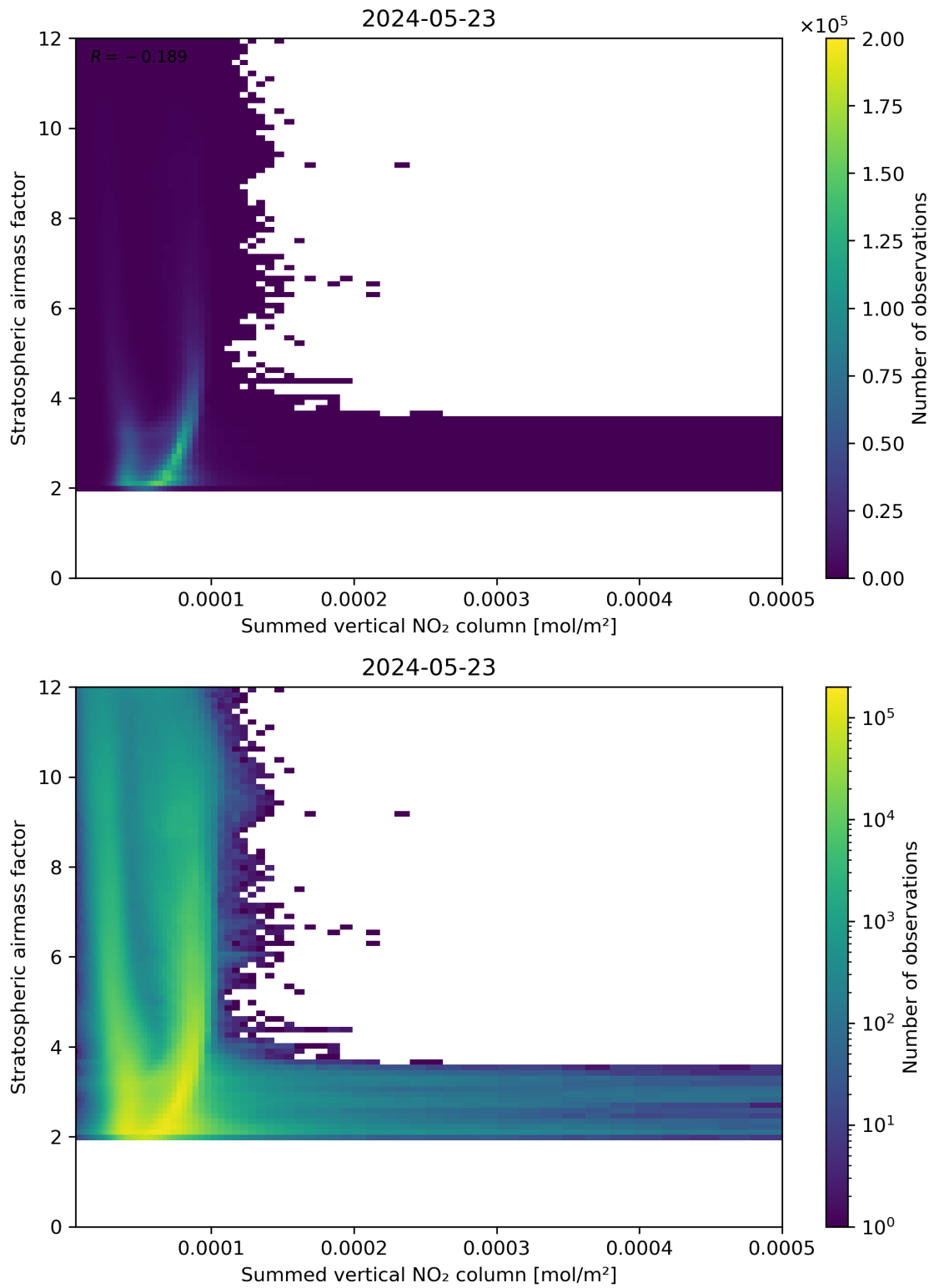
Figure 103: Scatter density plot of “Summed vertical NO 2 column” against “Stratospheric airmass factor” for 2024-05-23 to 2024-05-24.
