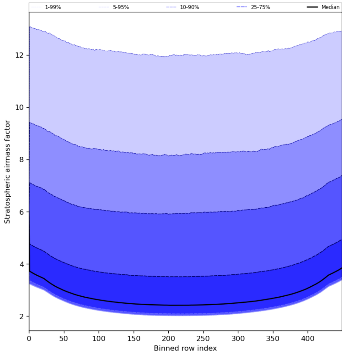
Figure 61: Along track statistics of “Stratospheric airmass factor” for 2024-05-23 to 2024-05-24
