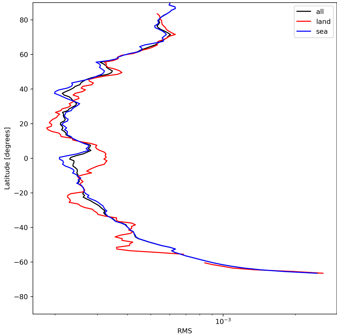
Figure 26: Zonal average of “RMS” for 2024-05-23 to 2024-05-24.
