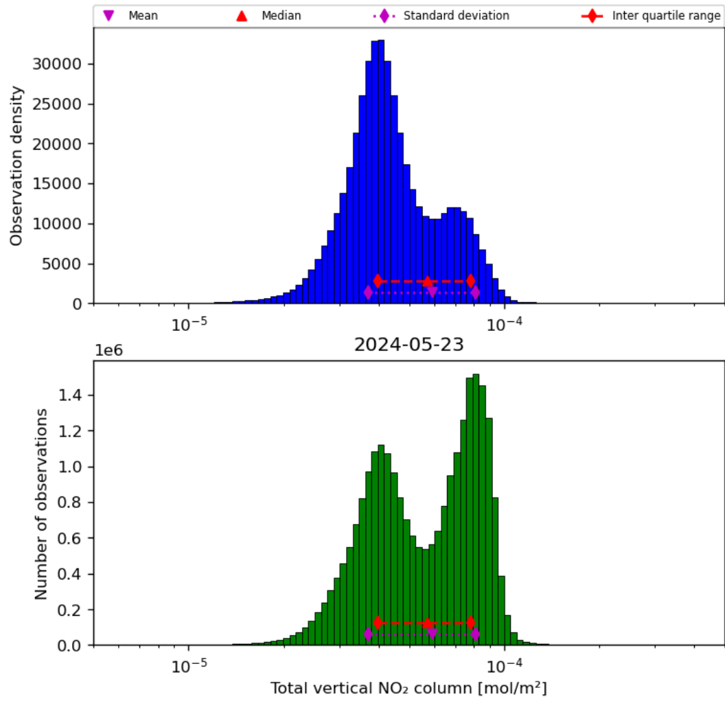
Figure 38: Histogram of "Total vertical NO 2 column" for 2024-05-23 to 2024-05-24
