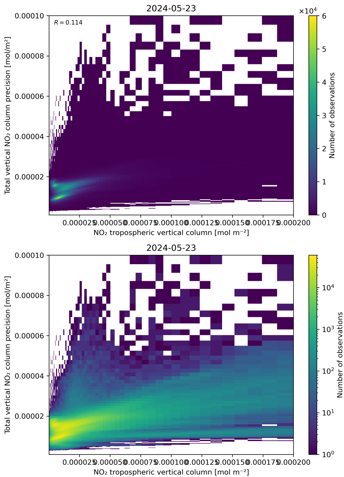
Figure 129: Scatter density plot of “NO 2 tropospheric vertical column” against “Total vertical NO 2 column precision” for 2024-05-23 to 2024-05-24.
