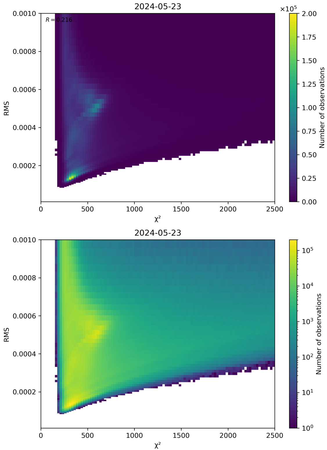
Figure 82: Scatter density plot of “ \chi^2 ” against “RMS” for 2024-05-23 to 2024-05-24.
