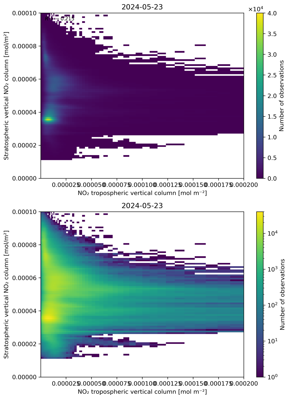
Figure 125: Scatter density plot of “NO 2 tropospheric vertical column” against “Stratospheric vertical NO 2 column” for 2024-05-23 to 2024-05-24.
