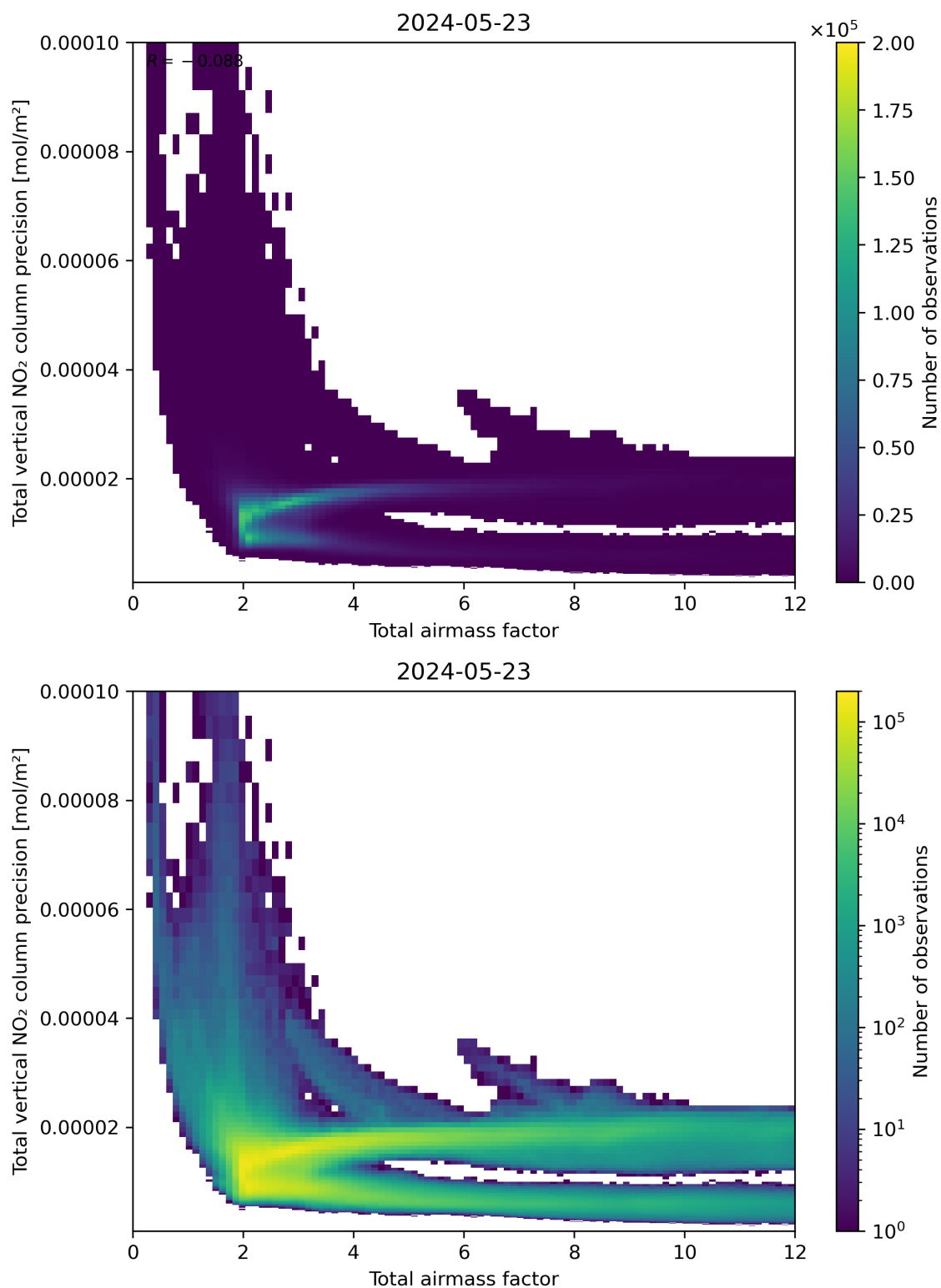
Figure 68: Scatter density plot of “Total airmass factor” against “Total vertical NO 2 column precision” for 2024-05-23 to 2024-05-24.
