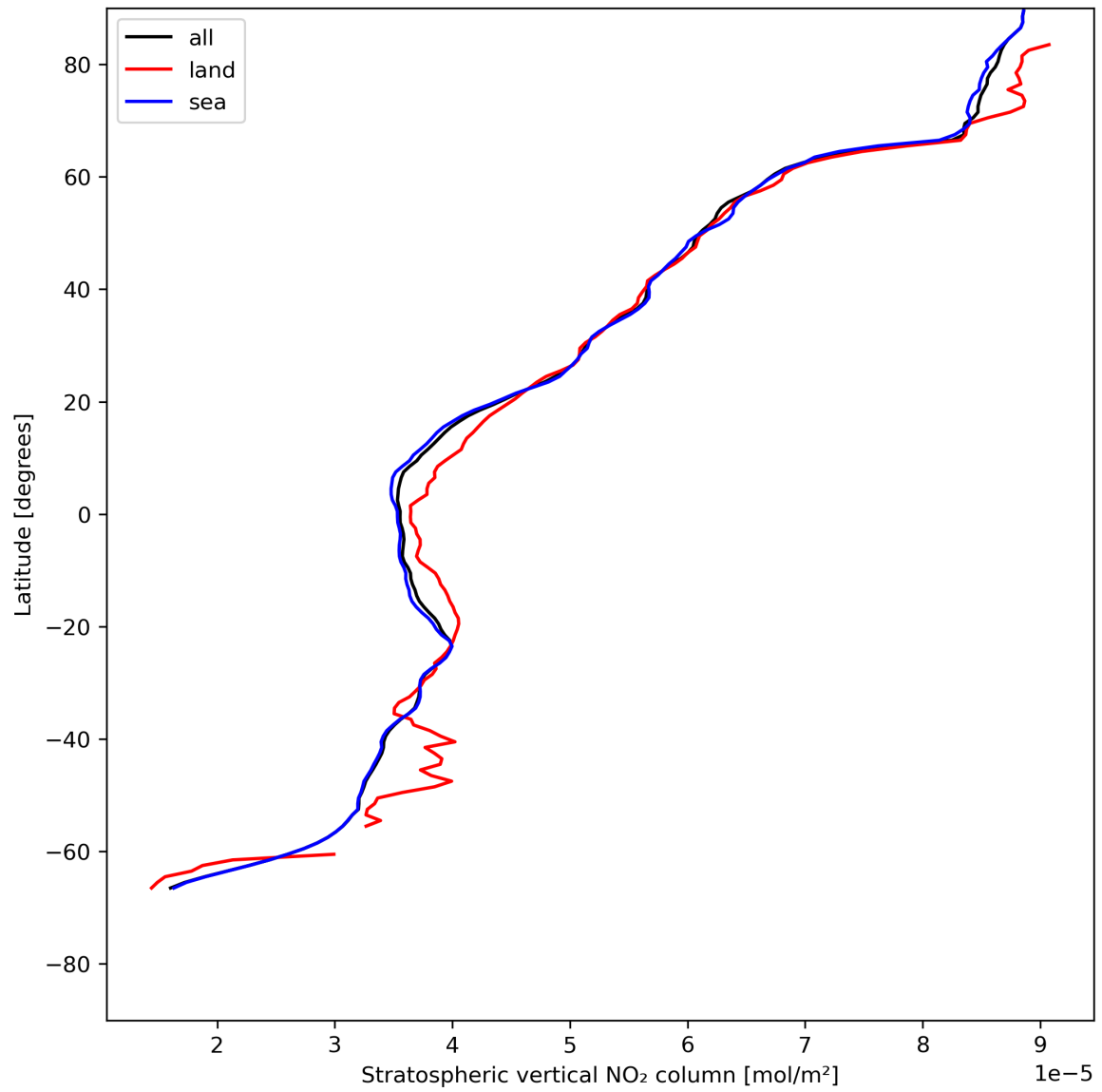
Figure 19: Zonal average of “Stratospheric vertical NO 2 column” for 2024-05-23 to 2024-05-24.
