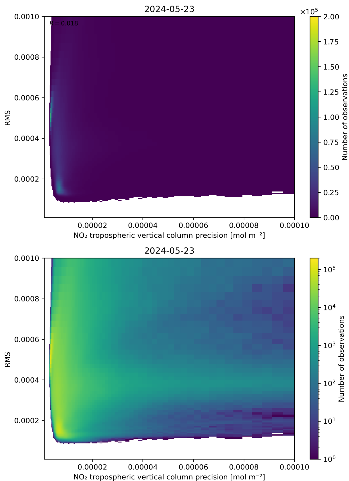
Figure 140: Scatter density plot of “NO 2 tropospheric vertical column precision” against “RMS” for 2024-05-23 to 2024-05-24.
