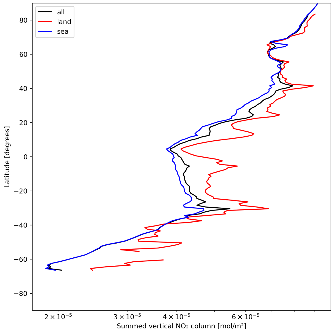
Figure 23: Zonal average of “Summed vertical NO 2 column” for 2024-05-23 to 2024-05-24.
