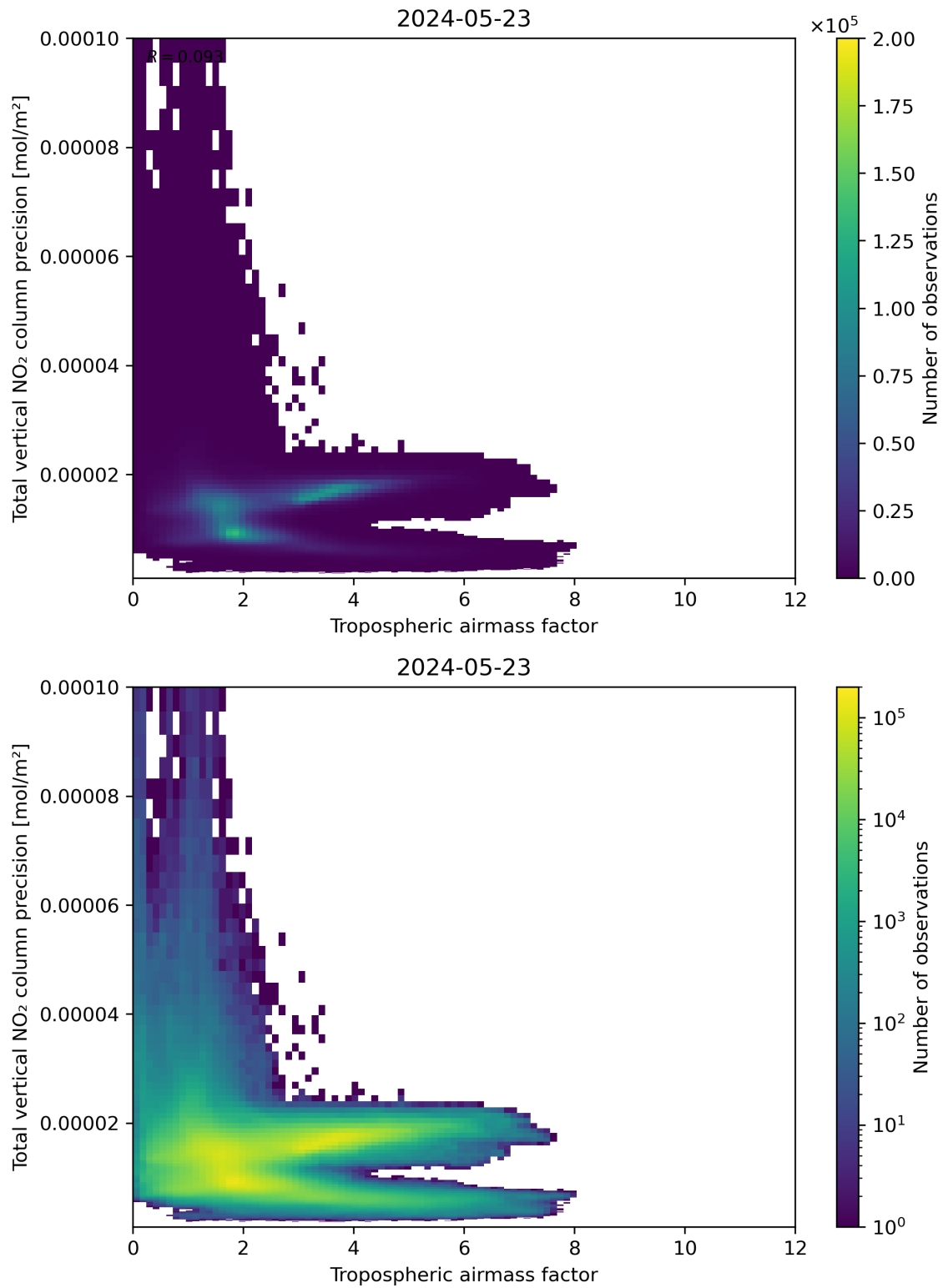
Figure 78: Scatter density plot of “Tropospheric air mass factor” against “Total vertical NO 2 column precision” for 2024-05-23 to 2024-05-24.
