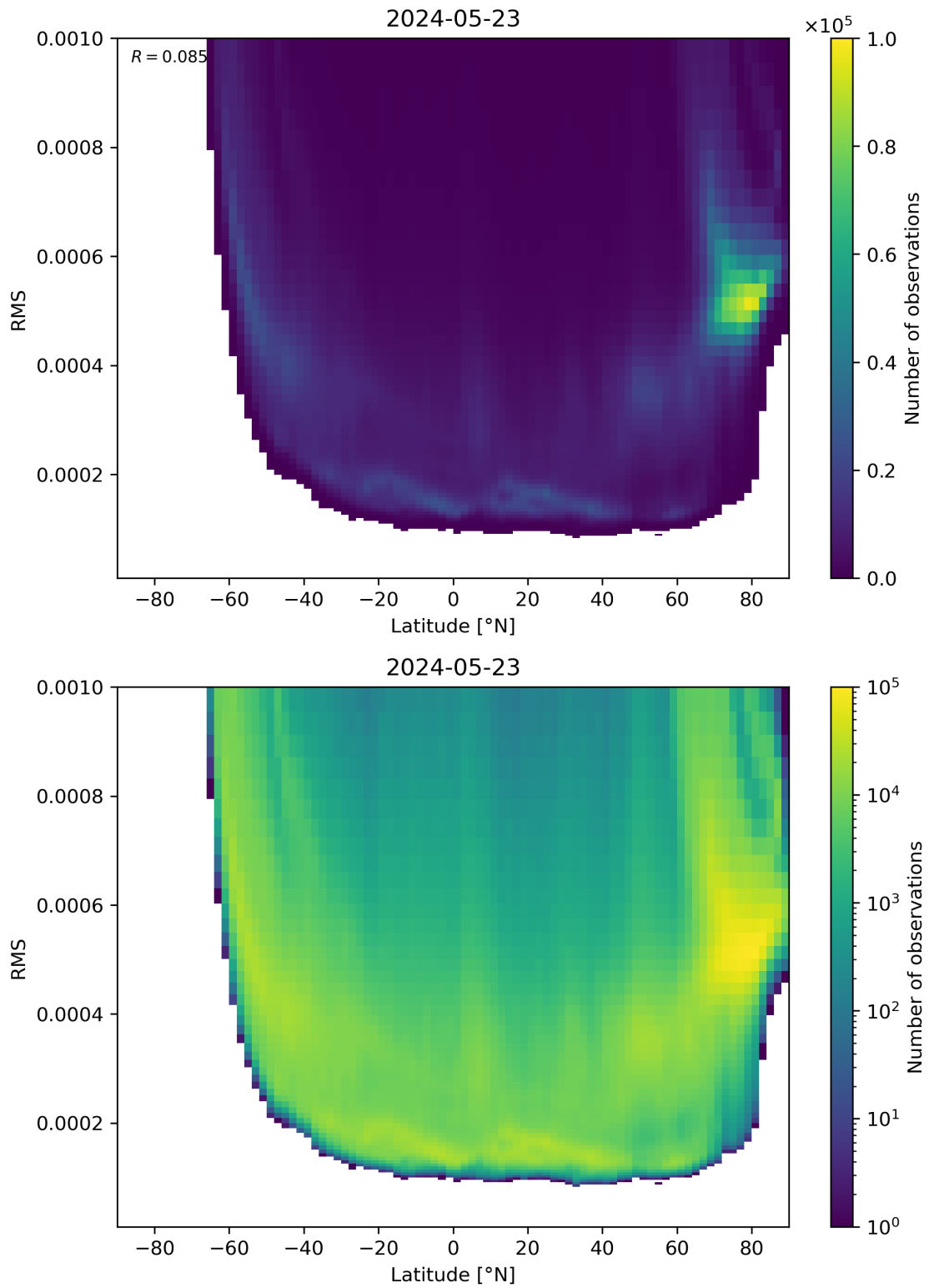
Figure 94: Scatter density plot of “Latitude” against “RMS” for 2024-05-23 to 2024-05-24.
