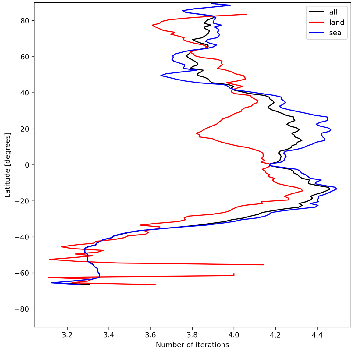
Figure 17: Zonal average of “Number of iterations” for 2024-05-23 to 2024-05-24.
