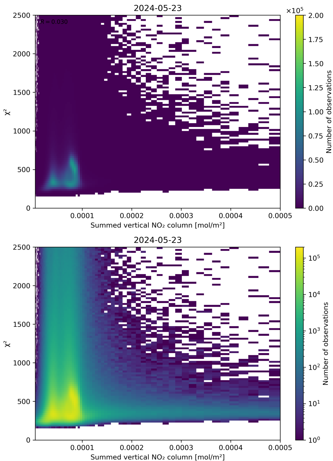
Figure 104: Scatter density plot of “Summed vertical NO 2 column” against “ \chi^2 ” for 2024-05-23 to 2024-05-24.
