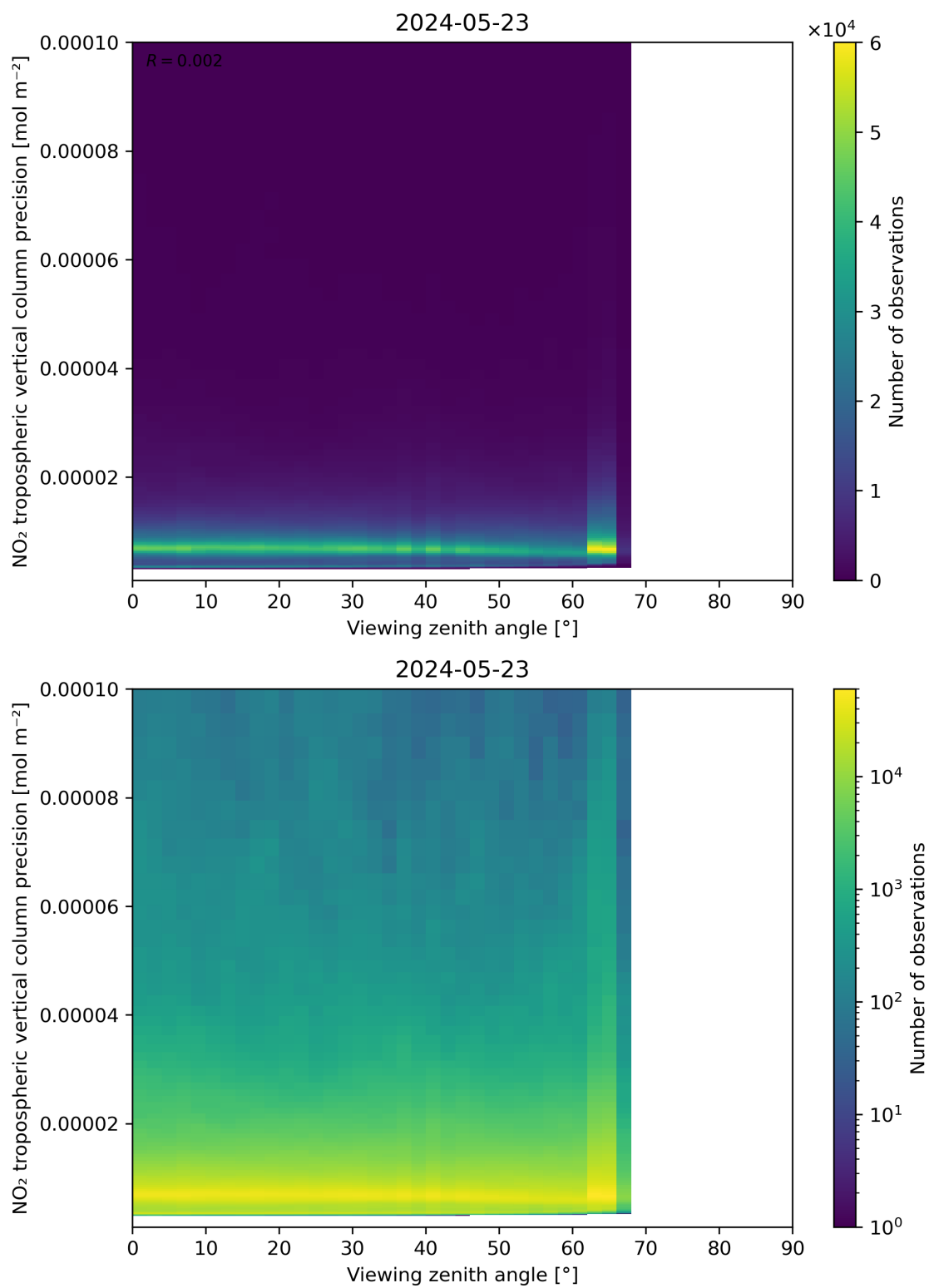
Figure 170: Scatter density plot of “Viewing zenith angle” against “NO 2 tropospheric vertical column precision” for 2024-05-23 to 2024-05-24.
