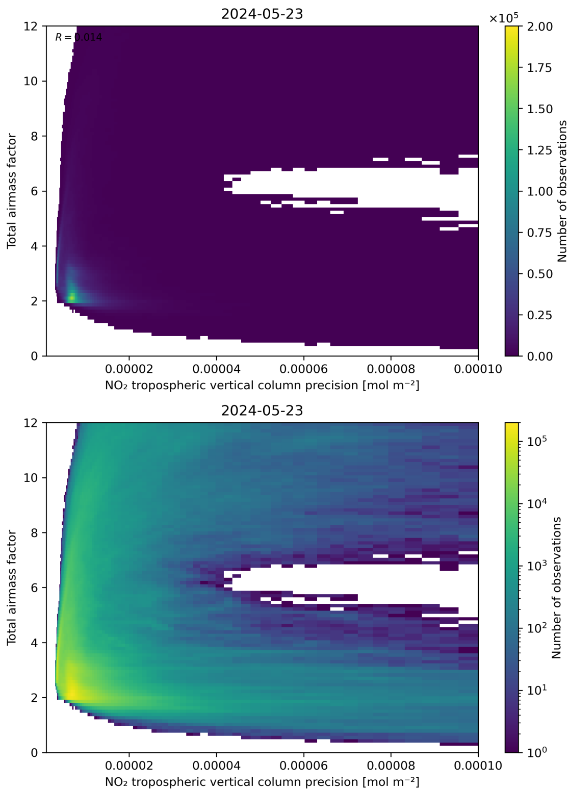
Figure 132: Scatter density plot of “NO 2 tropospheric vertical column precision” against “Total air mass factor” for 2024-05-23 to 2024-05-24.
