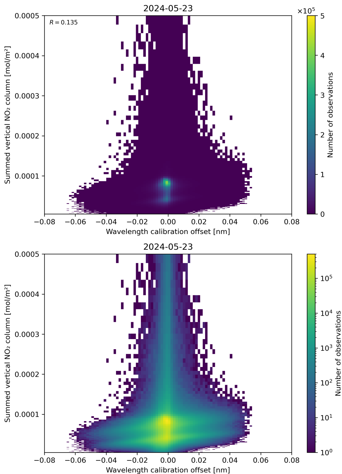
Figure 177: Scatter density plot of “Wavelength calibration offset” against “Summed vertical NO 2 column” for 2024-05-23 to 2024-05-24.
