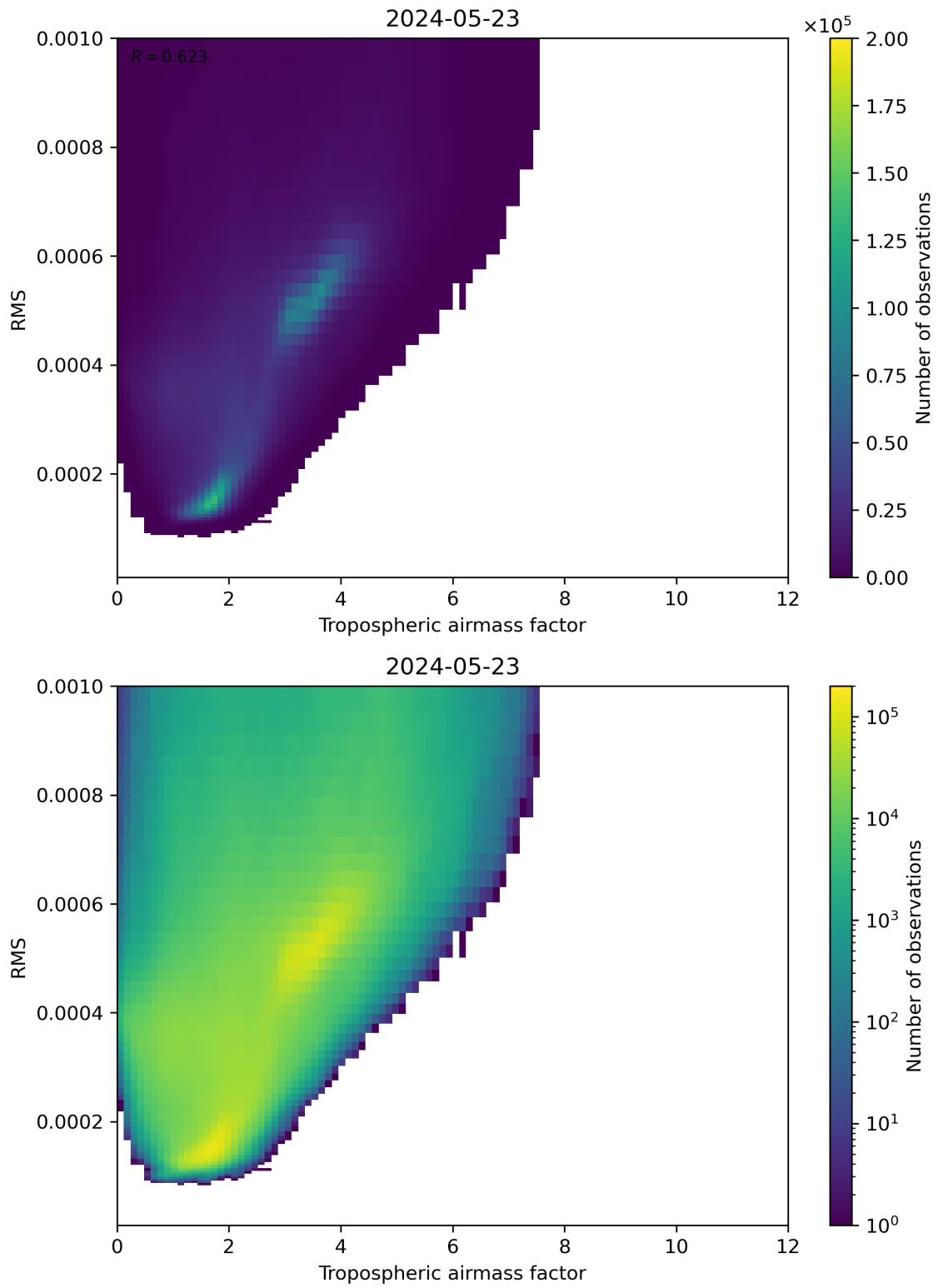
Figure 79: Scatter density plot of “Tropospheric airmass factor” against “RMS” for 2024-05-23 to 2024-05-24.
