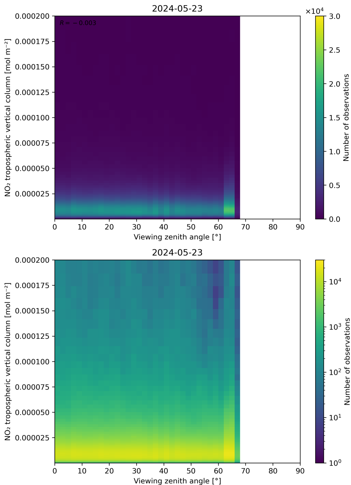
Figure 169: Scatter density plot of “Viewing zenith angle” against “NO 2 tropospheric vertical column” for 2024-05-23 to 2024-05-24.
