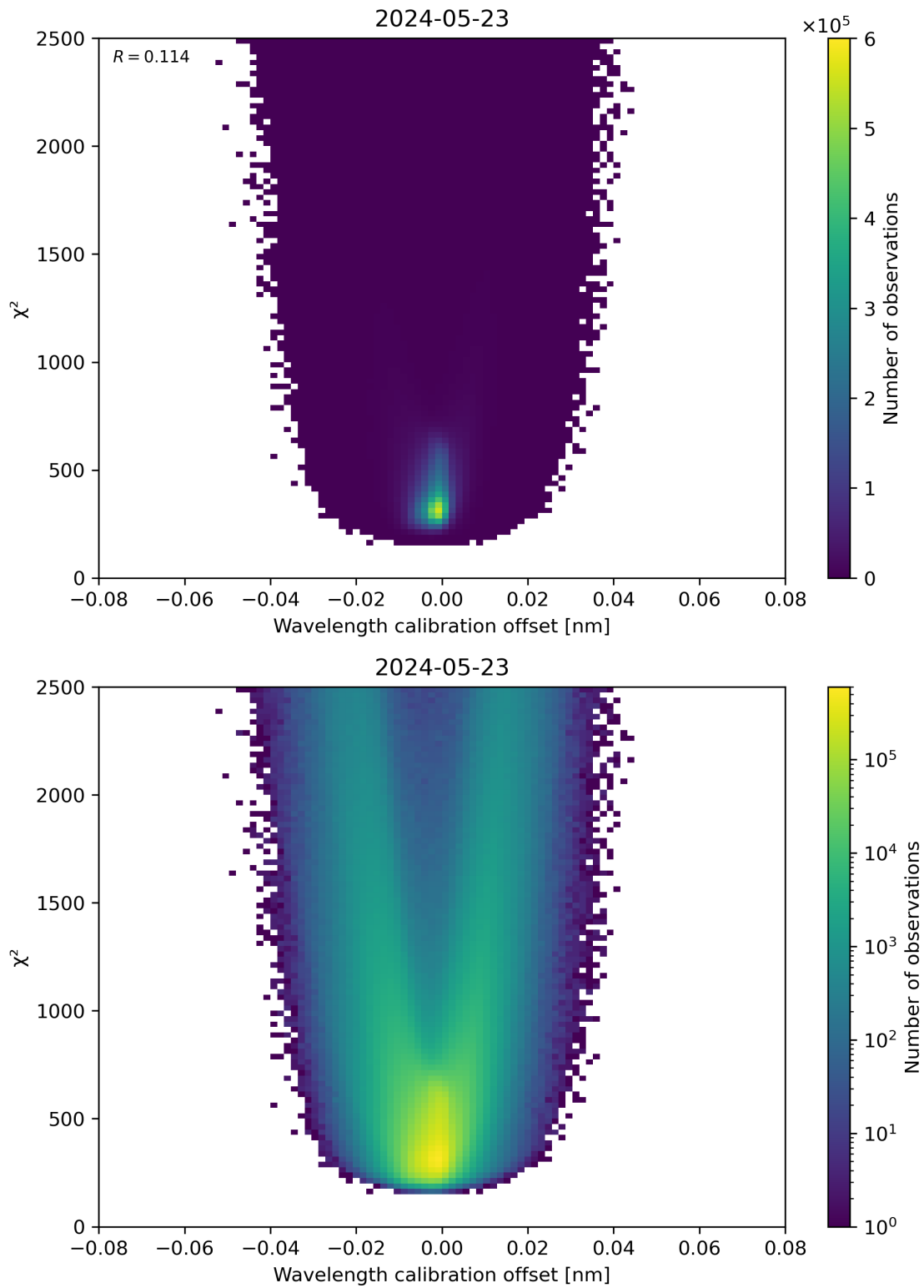
Figure 175: Scatter density plot of “Wavelength calibration offset” against “ \chi^2 ” for 2024-05-23 to 2024-05-24.
