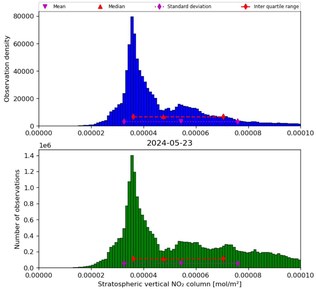
Figure 36: Histogram of “Stratospheric vertical NO 2 column” for 2024-05-23 to 2024-05-24
