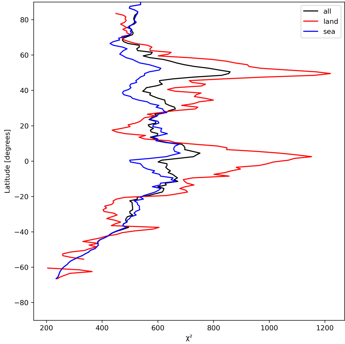
Figure 25: Zonal average of “ \chi^2 ” for 2024-05-23 to 2024-05-24.
