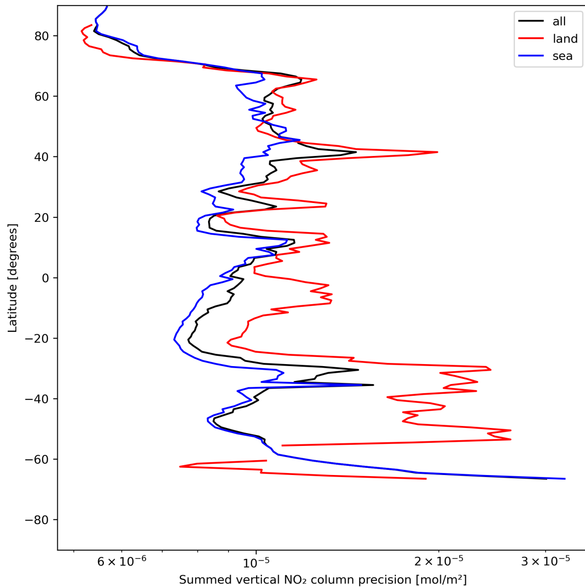
Figure 24: Zonal average of “Summed vertical NO 2 column precision” for 2024-05-23 to 2024-05-24.
