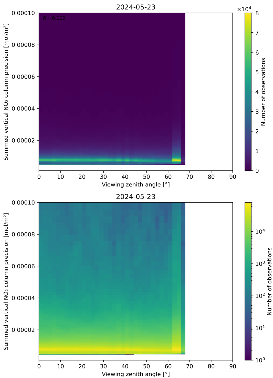
Figure 166: Scatter density plot of “Viewing zenith angle” against “Summed vertical NO 2 column precision” for 2024-05-23 to 2024-05-24.
