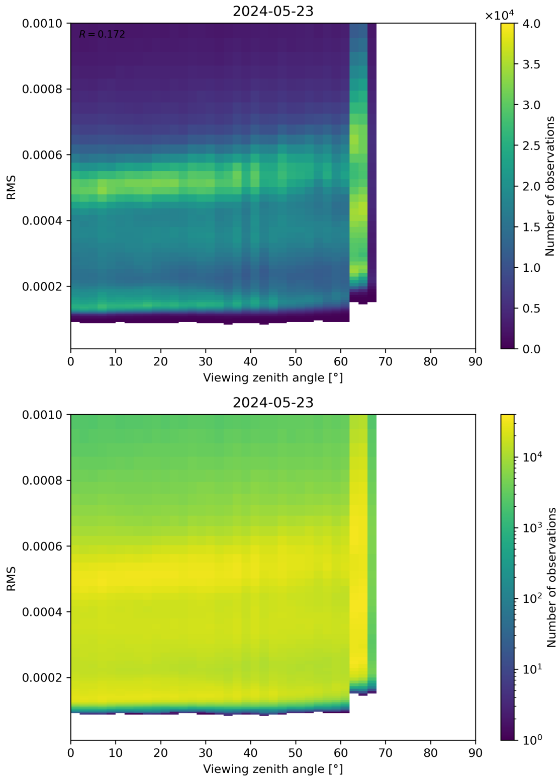
Figure 171: Scatter density plot of “Viewing zenith angle” against “RMS” for 2024-05-23 to 2024-05-24.
