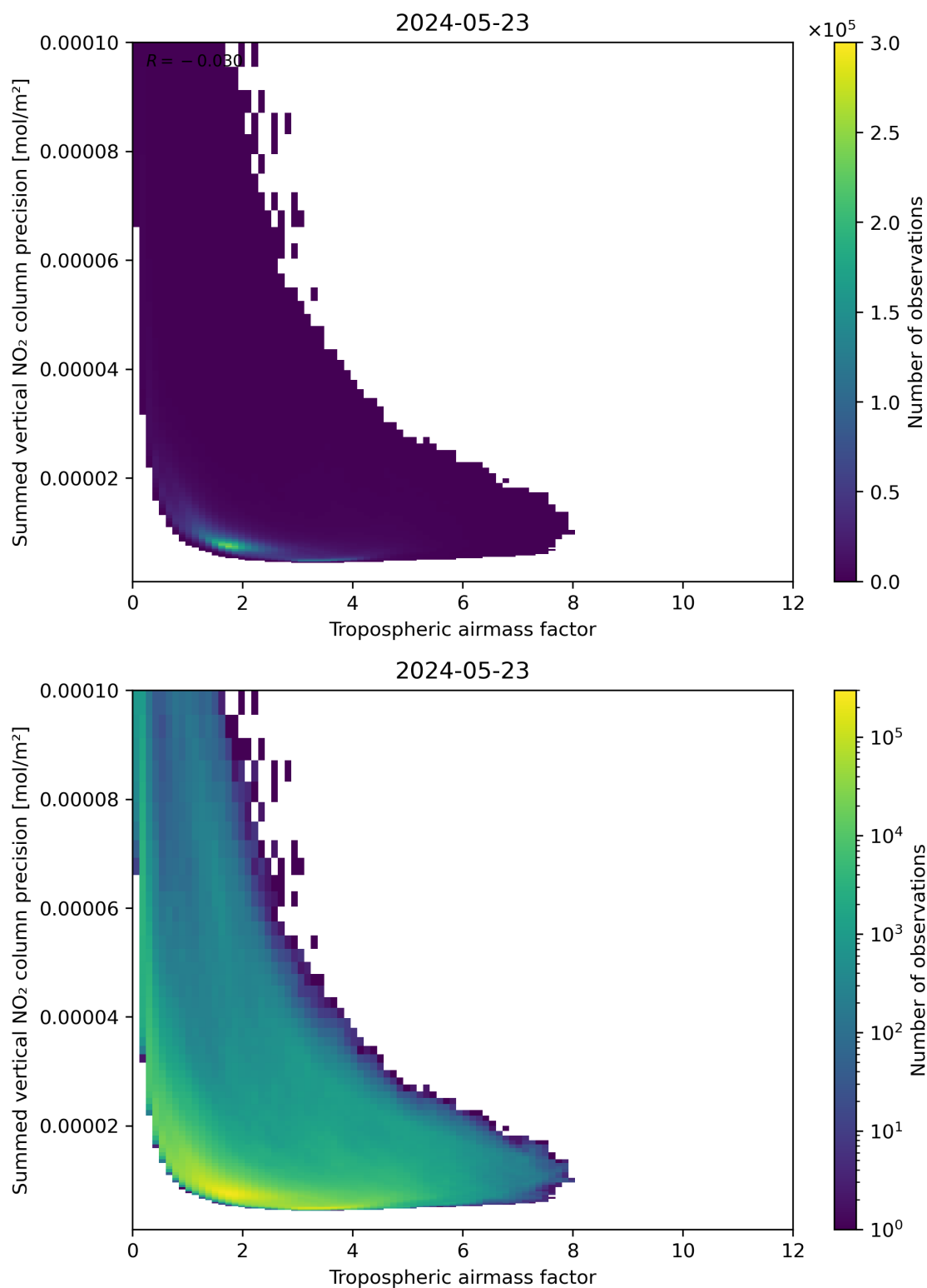
Figure 76: Scatter density plot of “Tropospheric air mass factor” against “Summed vertical NO 2 column precision” for 2024-05-23 to 2024-05-24.
