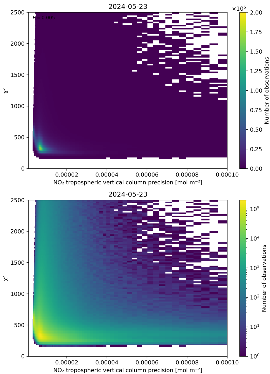
Figure 134: Scatter density plot of “NO 2 tropospheric vertical column precision” against “ \chi^2 ” for 2024-05-23 to 2024-05-24.
