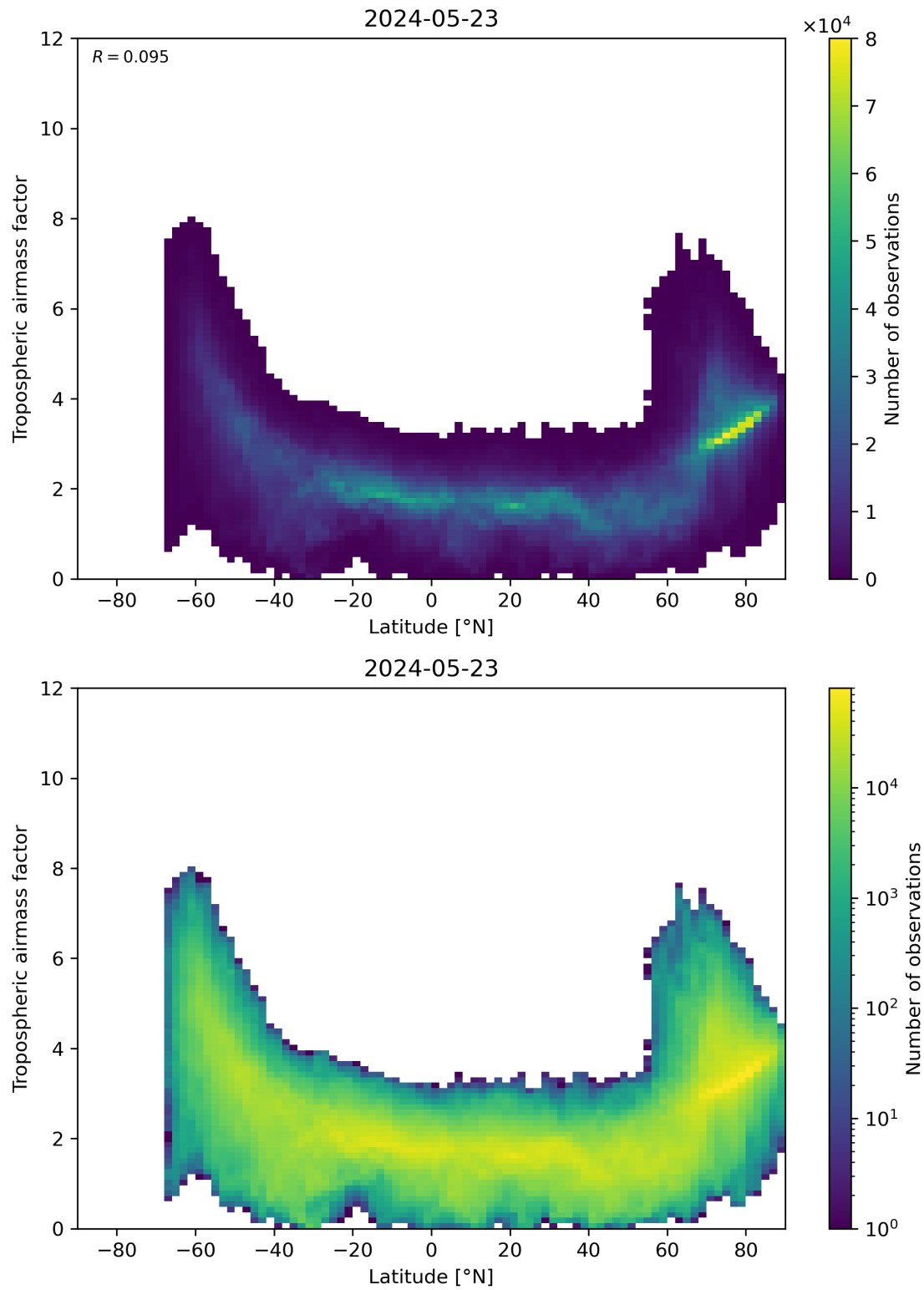
Figure 85: Scatter density plot of “Latitude” against “Tropospheric airmass factor” for 2024-05-23 to 2024-05-24.
