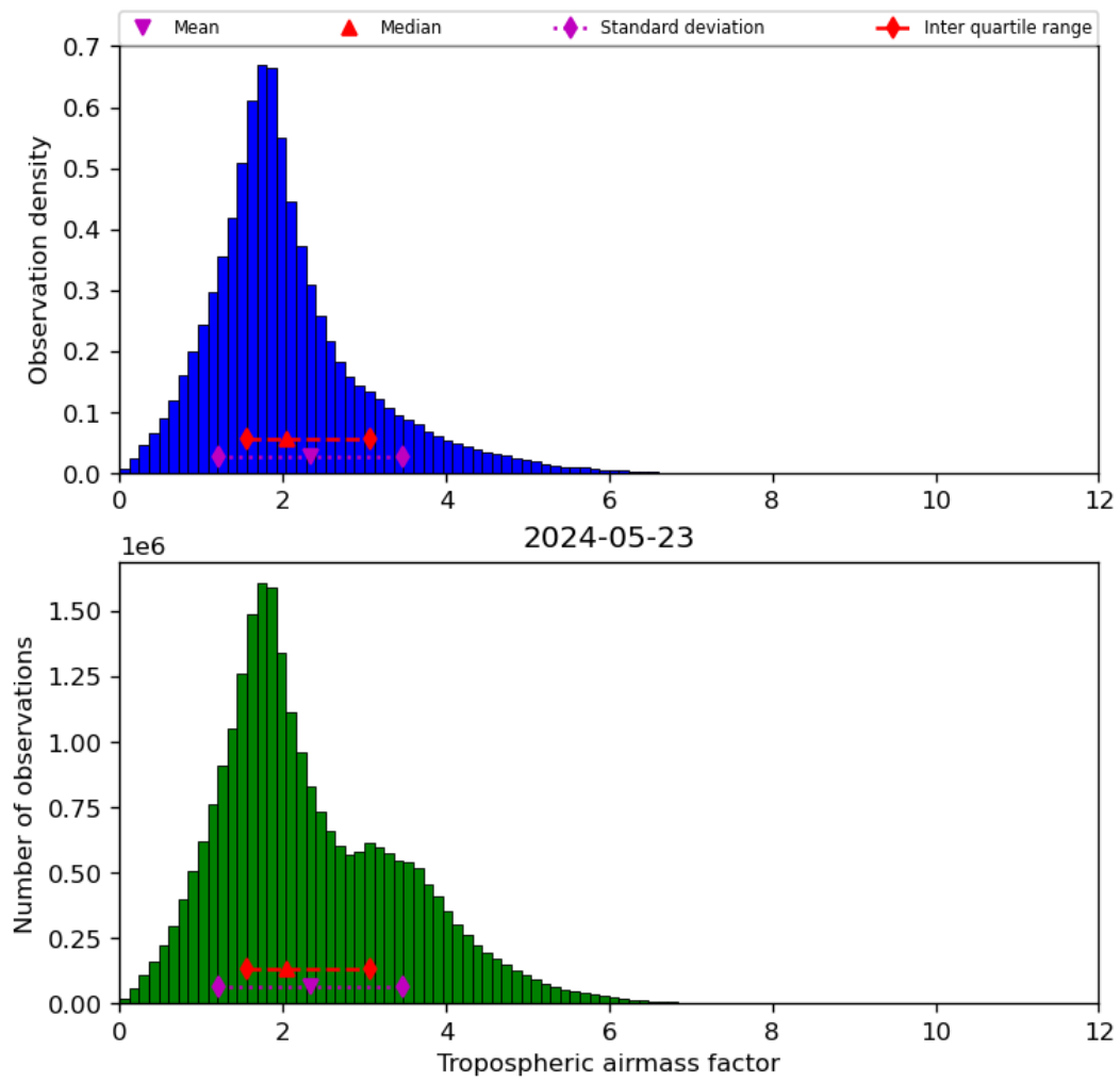
Figure 31: Histogram of “Tropospheric airmass factor” for 2024-05-23 to 2024-05-24
