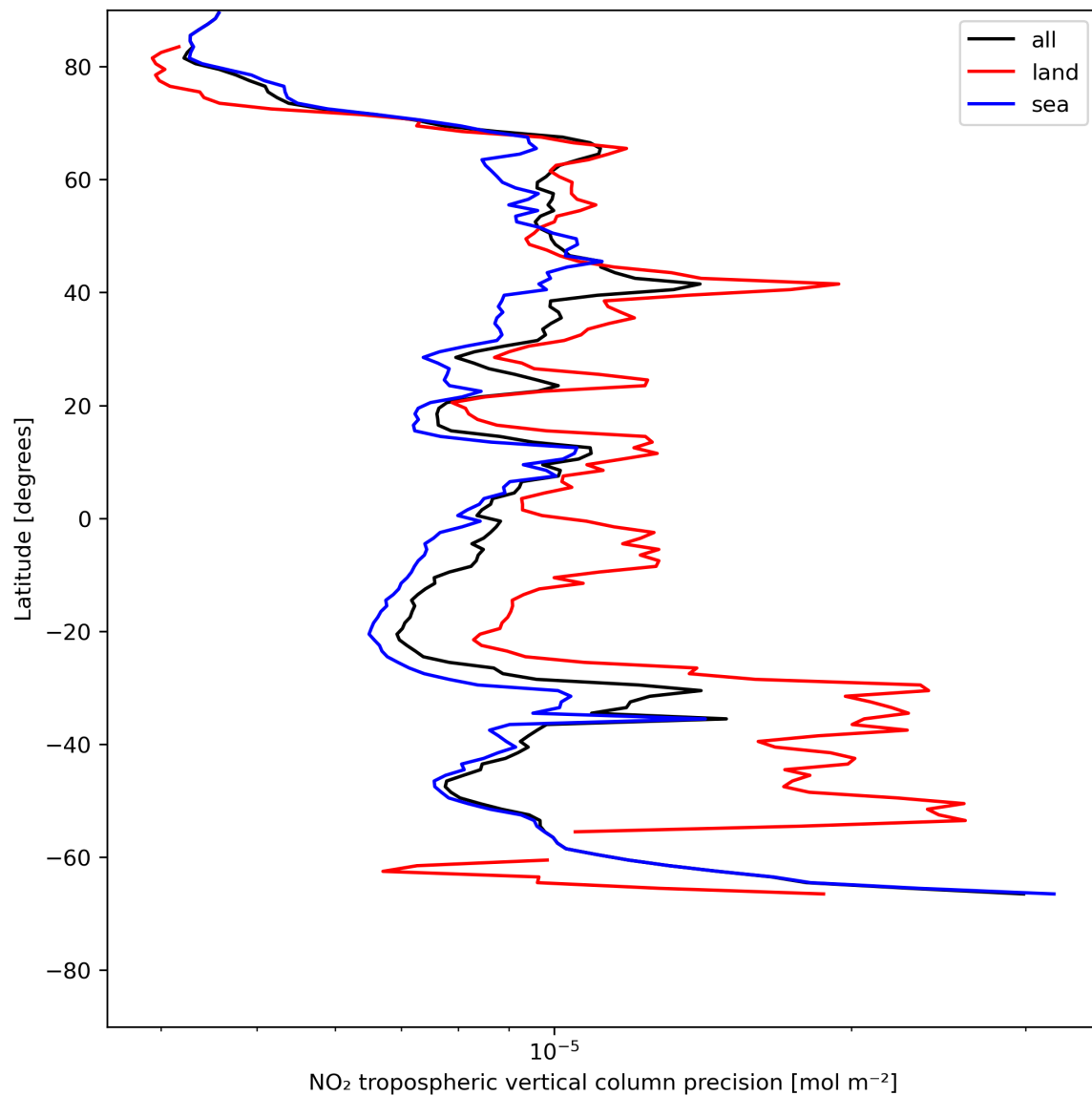
Figure 13: Zonal average of “NO 2 tropospheric vertical column precision” for 2024-05-23 to 2024-05-24.
