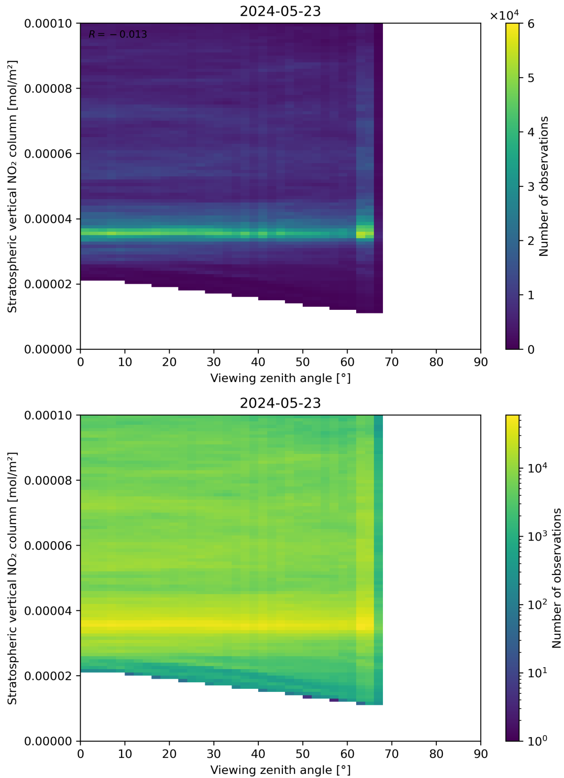
Figure 164: Scatter density plot of “Viewing zenith angle” against “Stratospheric vertical NO 2 column” for 2024-05-23 to 2024-05-24.
