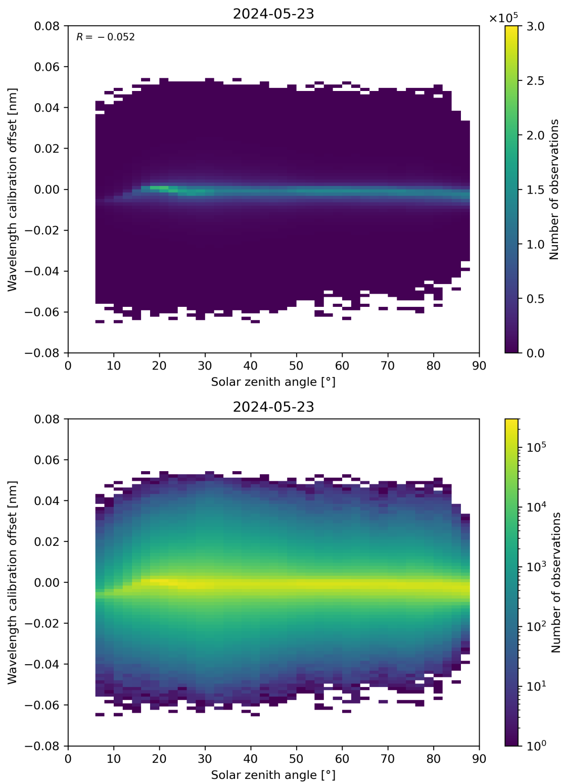
Figure 158: Scatter density plot of “Solar zenith angle” against “Wavelength calibration offset” for 2024-05-23 to 2024-05-24.
