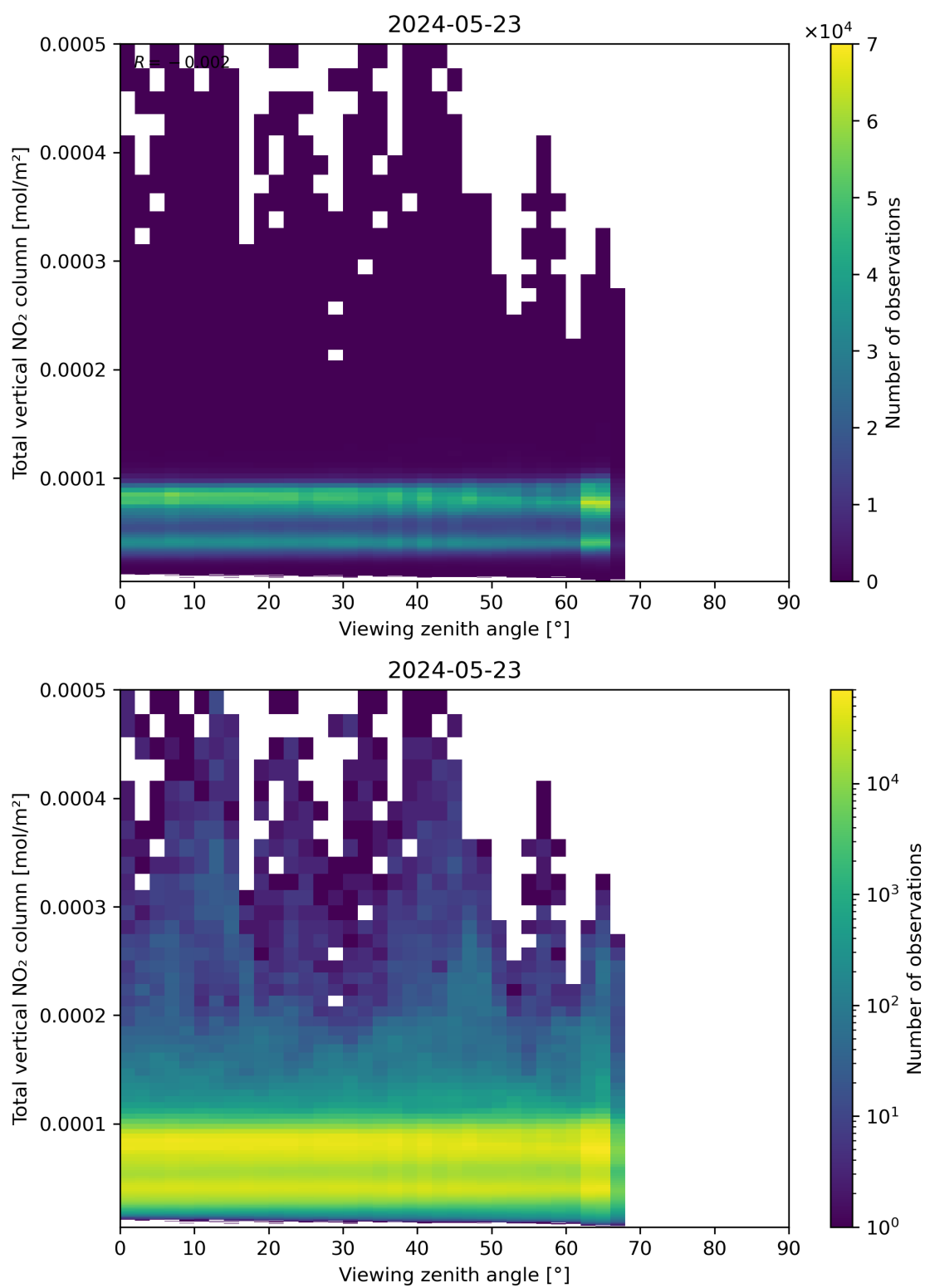
Figure 167: Scatter density plot of “Viewing zenith angle” against “Total vertical NO 2 column” for 2024-05-23 to 2024-05-24.
