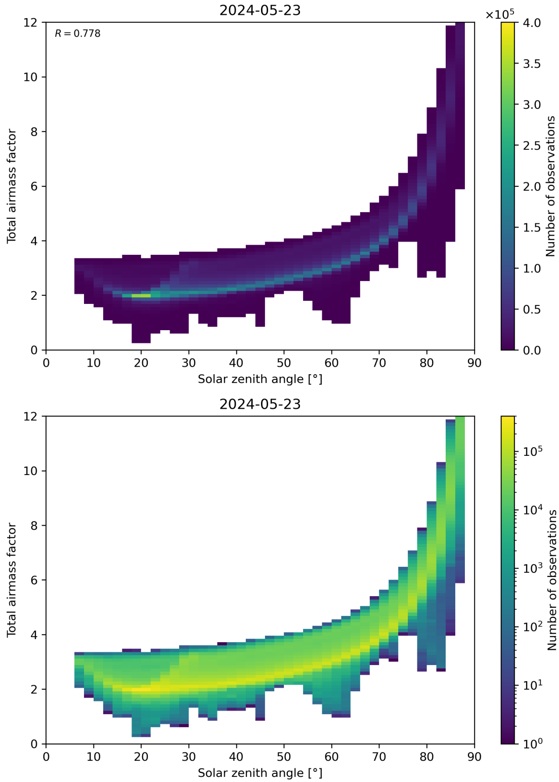
Figure 146: Scatter density plot of “Solar zenith angle” against “Total air mass factor” for 2024-05-23 to 2024-05-24.
