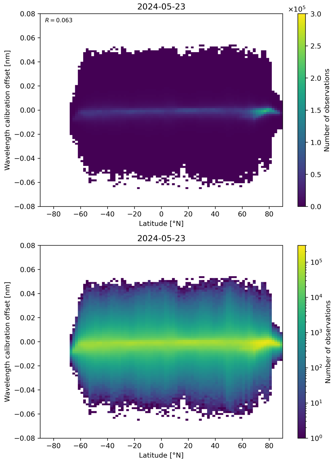
Figure 95: Scatter density plot of “Latitude” against “Wavelength calibration offset” for 2024-05-23 to 2024-05-24.
