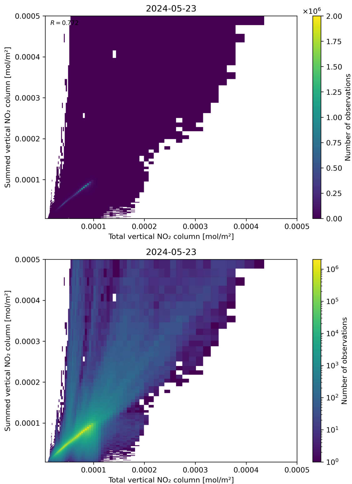
Figure 112: Scatter density plot of “Total vertical NO 2 column” against “Summed vertical NO 2 column” for 2024-05-23 to 2024-05-24.
