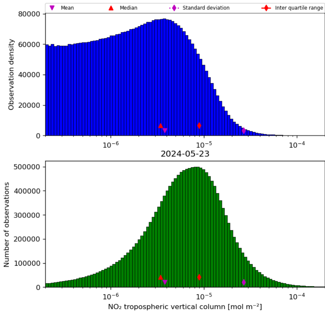
Figure 29: Histogram of “NO 2 tropospheric vertical column” for 2024-05-23 to 2024-05-24
