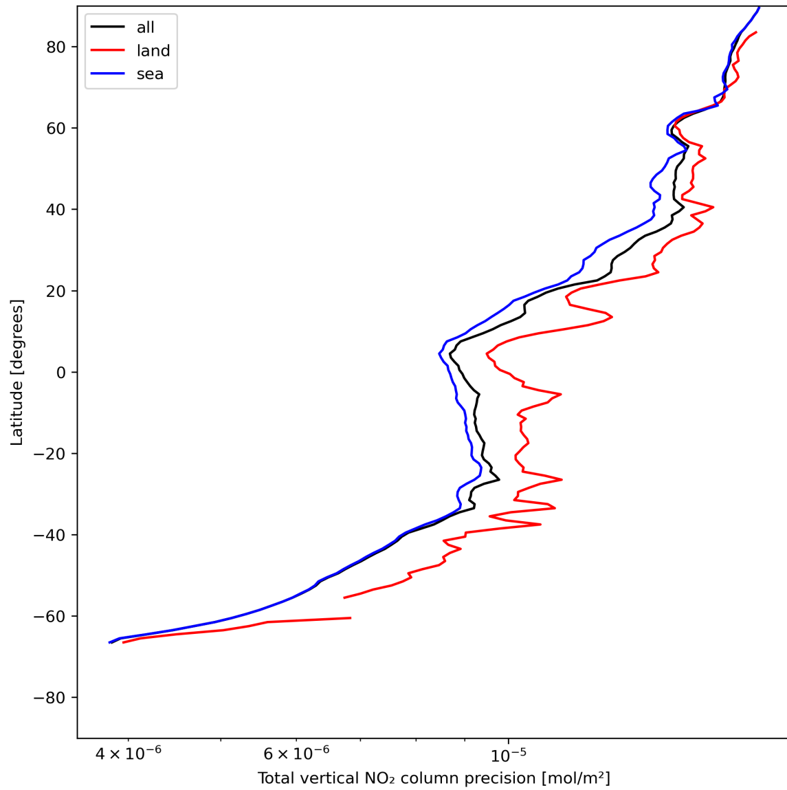
Figure 22: Zonal average of “Total vertical NO 2 column precision” for 2024-05-23 to 2024-05-24.
