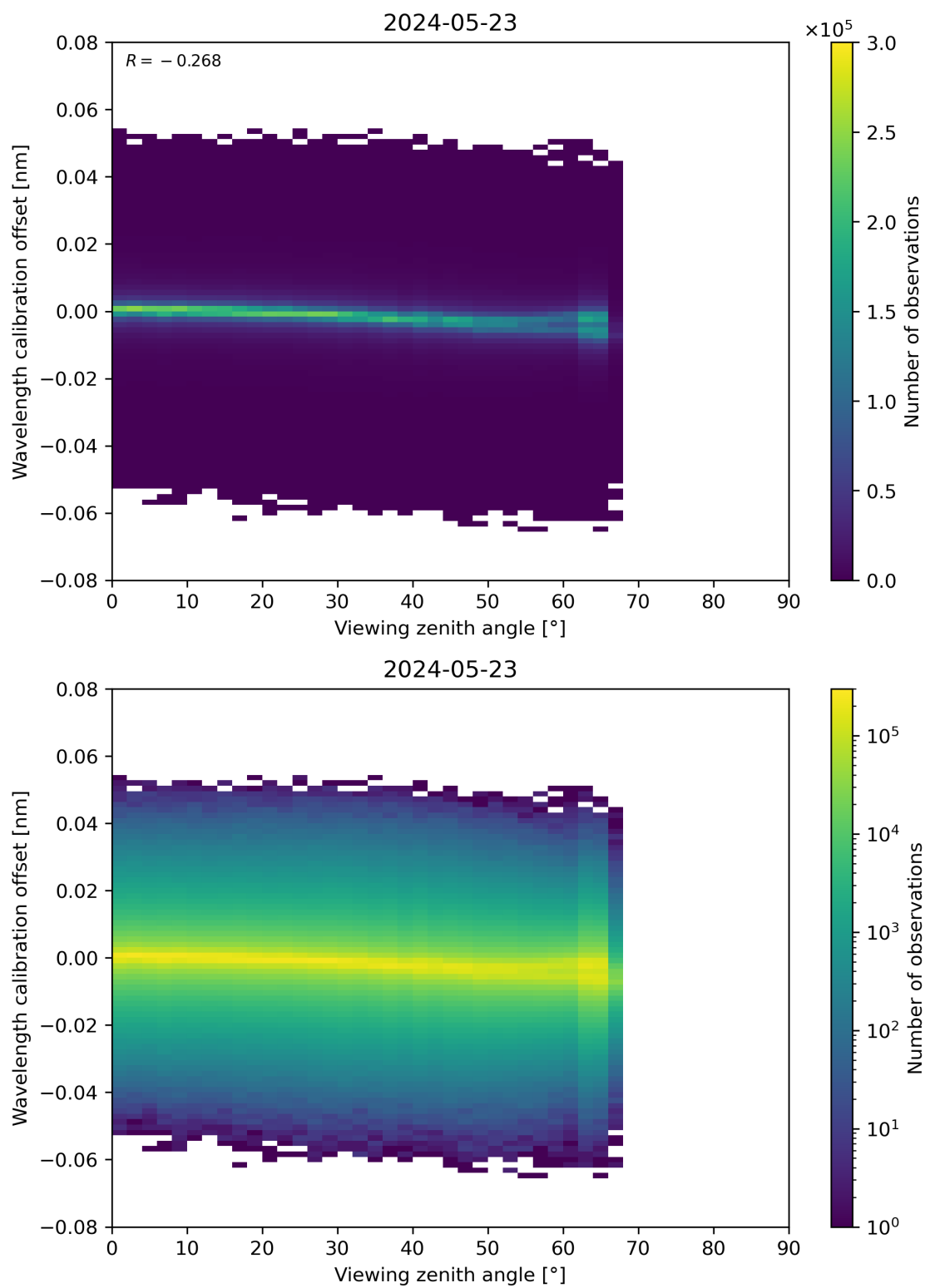
Figure 173: Scatter density plot of “Viewing zenith angle” against “Wavelength calibration offset” for 2024-05-23 to 2024-05-24.
