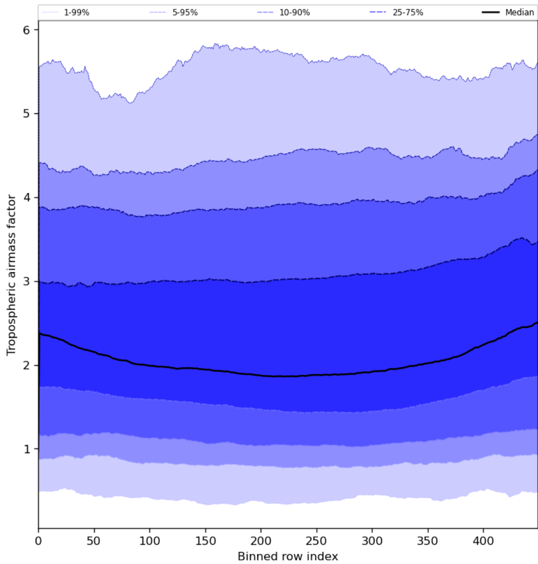
Figure 48: Along track statistics of “Tropospheric airmass factor” for 2024-05-23 to 2024-05-24
