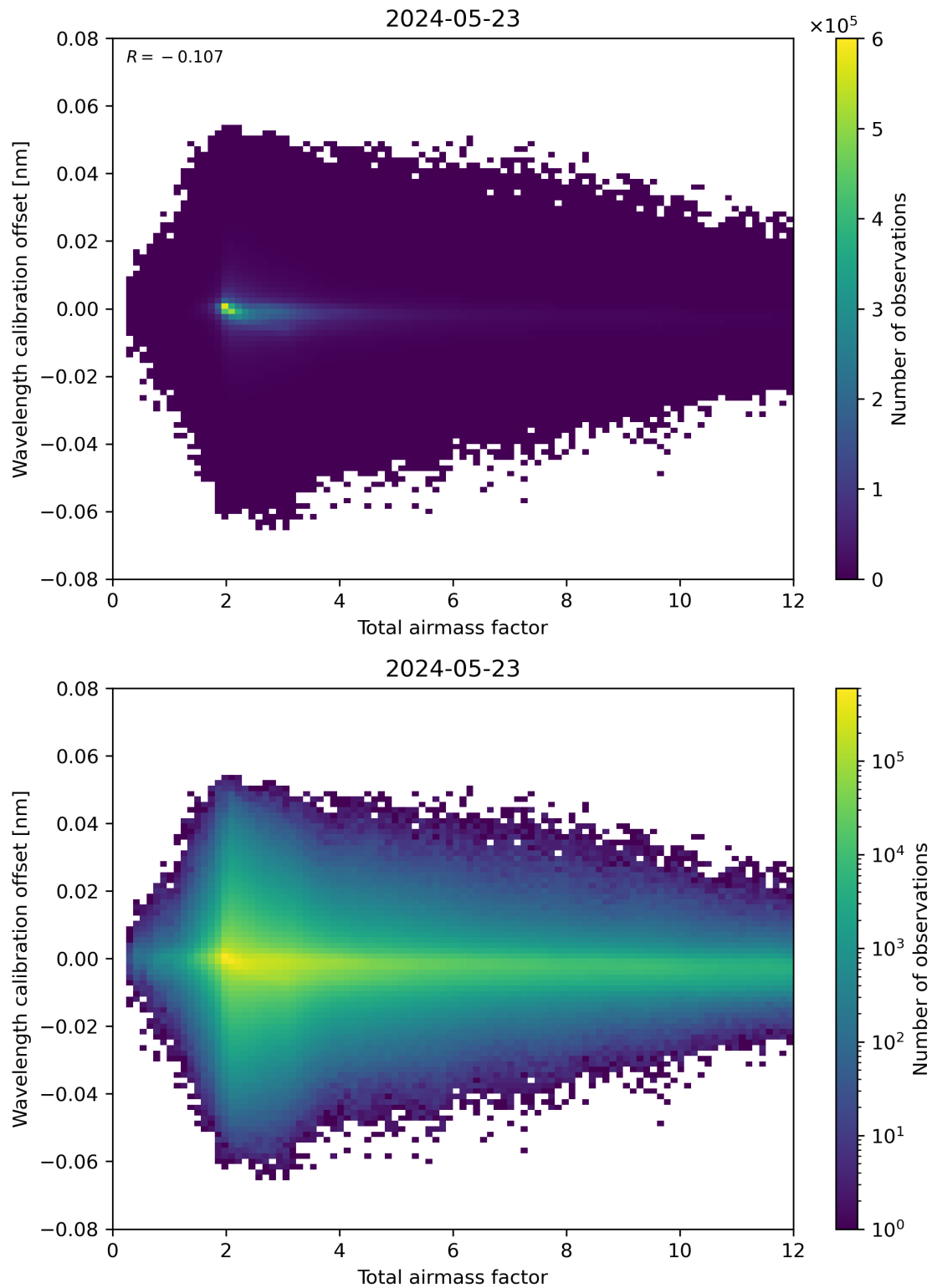
Figure 70: Scatter density plot of “Total airmass factor” against “Wavelength calibration offset” for 2024-05-23 to 2024-05-24.
