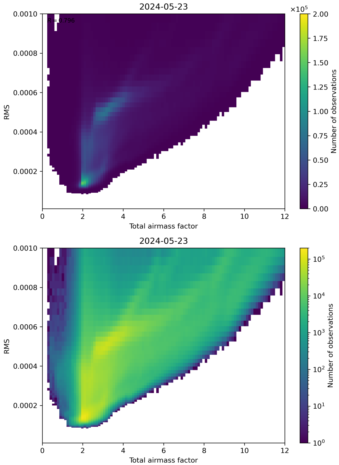
Figure 69: Scatter density plot of “Total airmass factor” against “RMS” for 2024-05-23 to 2024-05-24.
