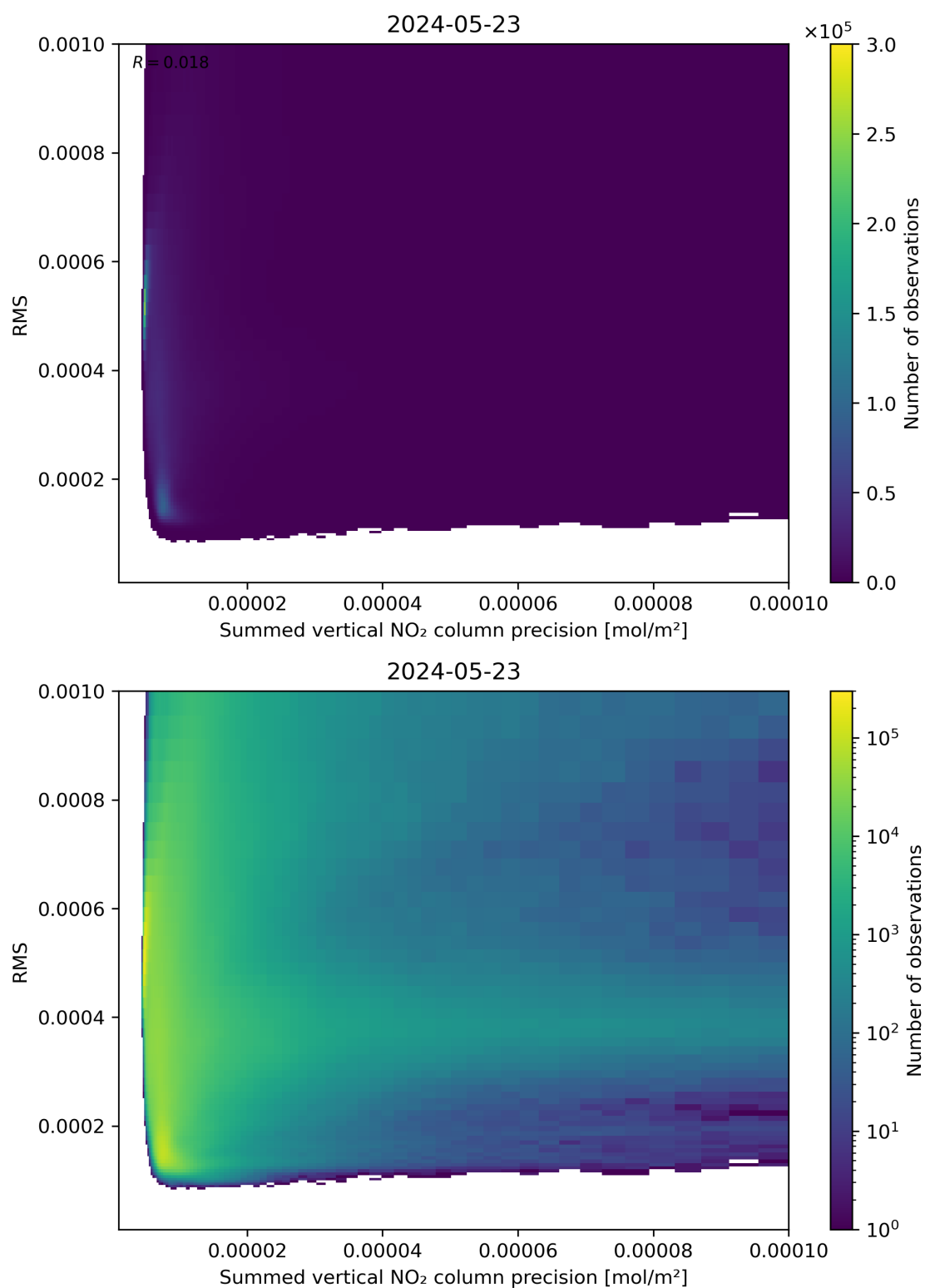
Figure 108: Scatter density plot of “Summed vertical NO 2 column precision” against “RMS” for 2024-05-23 to 2024-05-24.
