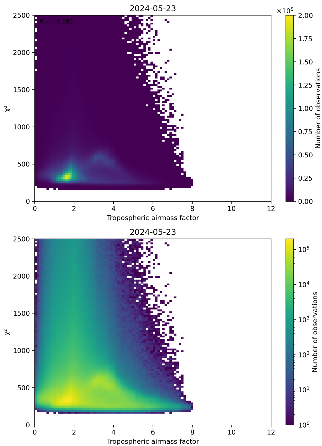
Figure 73: Scatter density plot of “Tropospheric airmass factor” against “ \chi^2 ” for 2024-05-23 to 2024-05-24.
