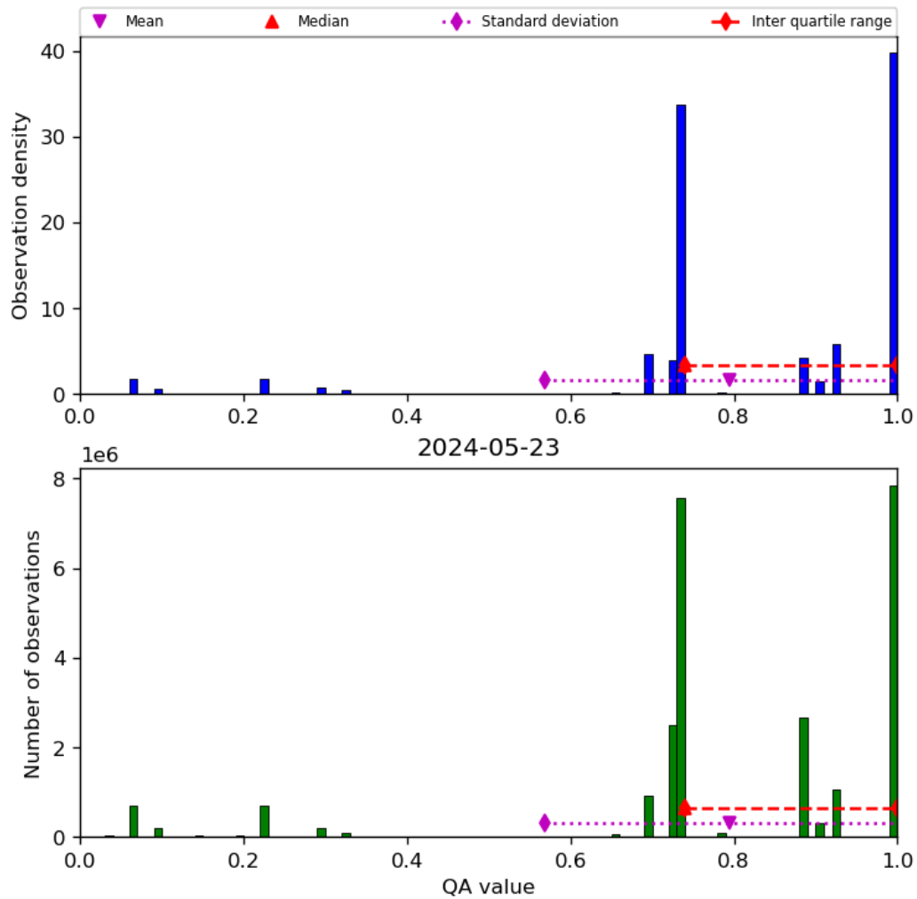
Figure 28: Histogram of “QA value” for 2024-05-23 to 2024-05-24
