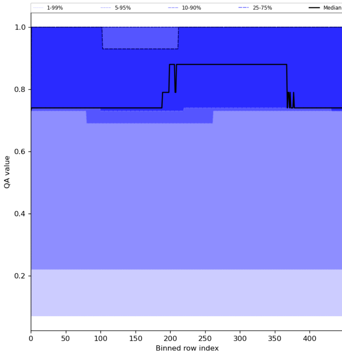
Figure 45: Along track statistics of “QA value” for 2024-05-23 to 2024-05-24
