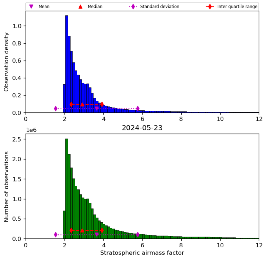
Figure 44: Histogram of “Stratospheric airmass factor” for 2024-05-23 to 2024-05-24
