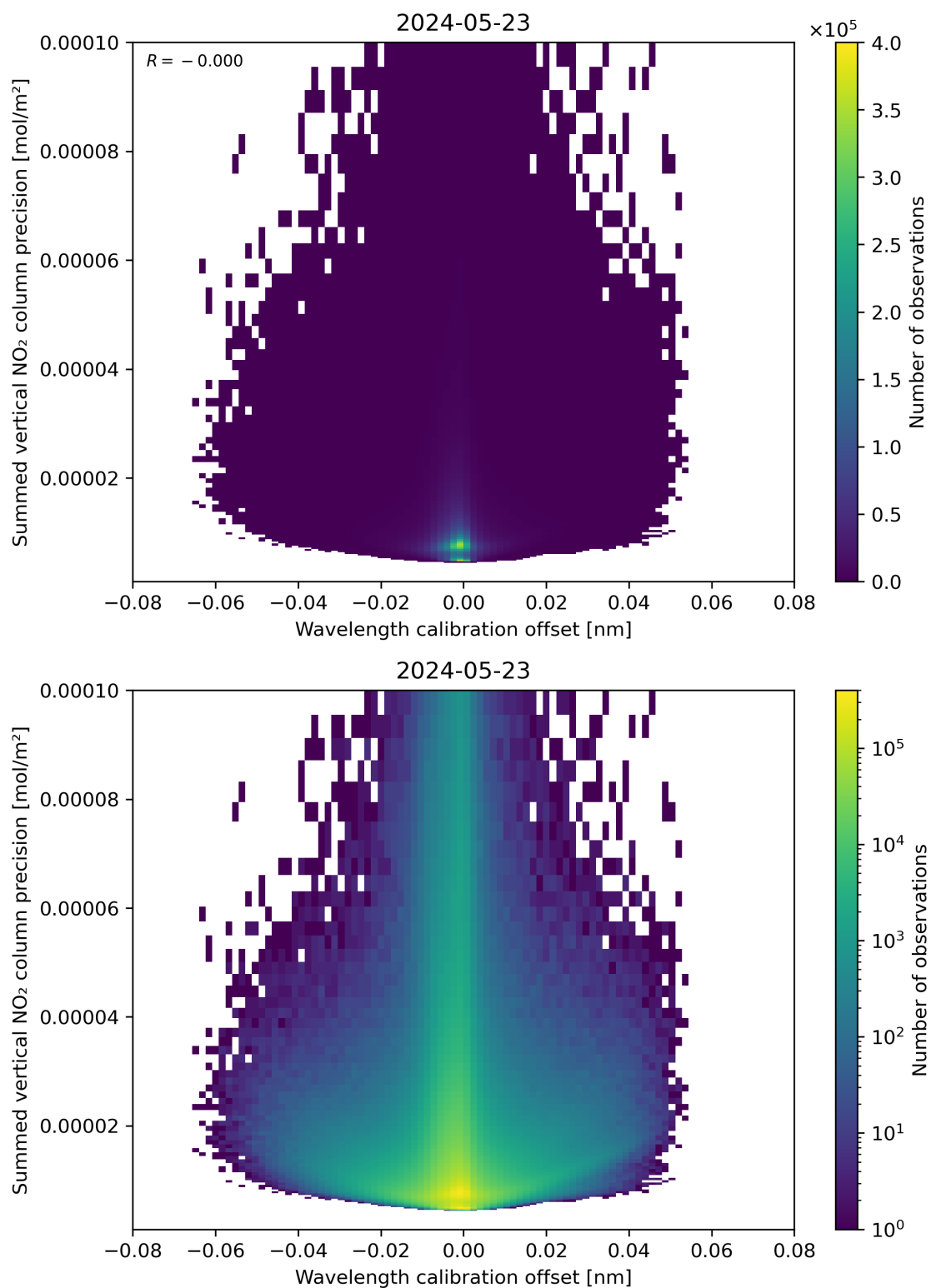
Figure 178: Scatter density plot of “Wavelength calibration offset” against “Summed vertical NO 2 column precision” for 2024-05-23 to 2024-05-24.
