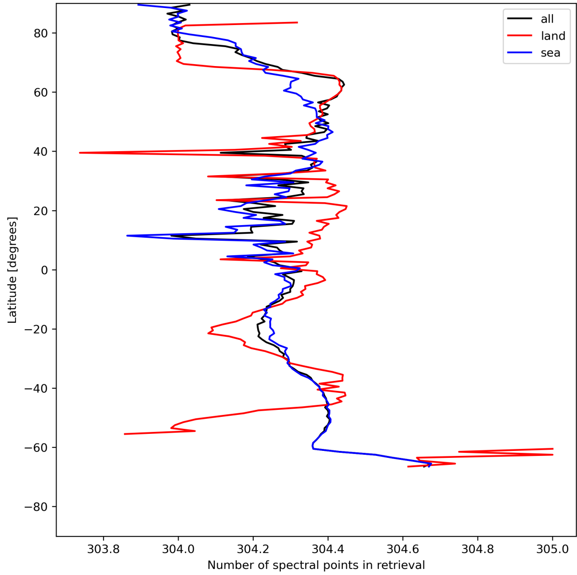
Figure 16: Zonal average of “Number of spectral points in retrieval” for 2024-05-23 to 2024-05-24.
