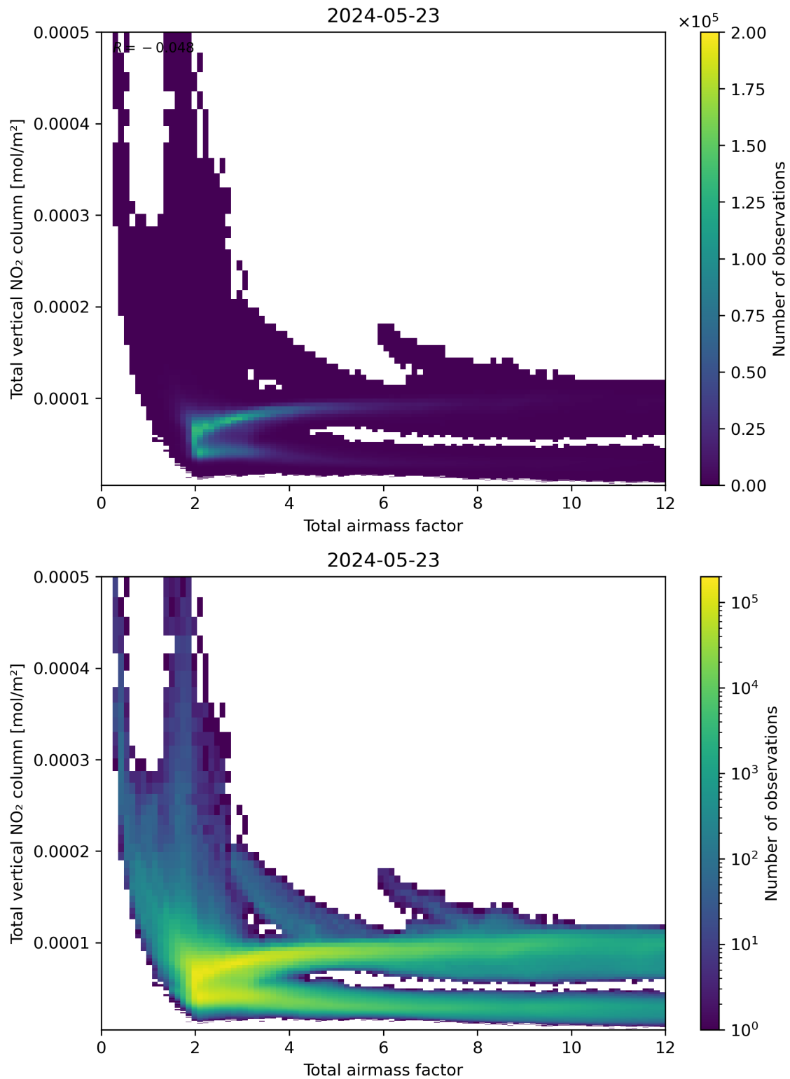
Figure 67: Scatter density plot of “Total airmass factor” against “Total vertical NO 2 column” for 2024-05-23 to 2024-05-24.
