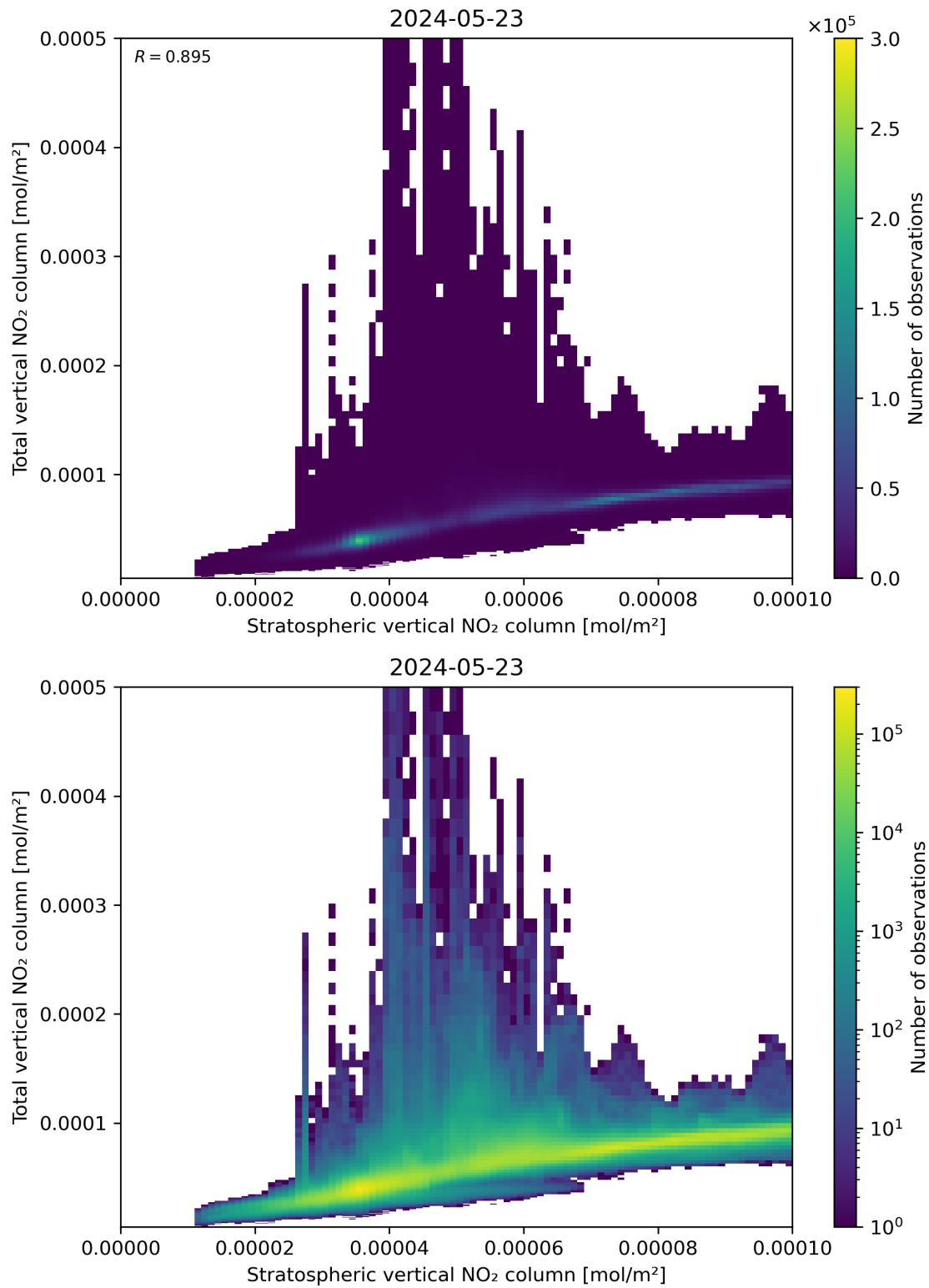
Figure 100: Scatter density plot of “Stratospheric vertical NO 2 column” against “Total vertical NO 2 column” for 2024-05-23 to 2024-05-24.
