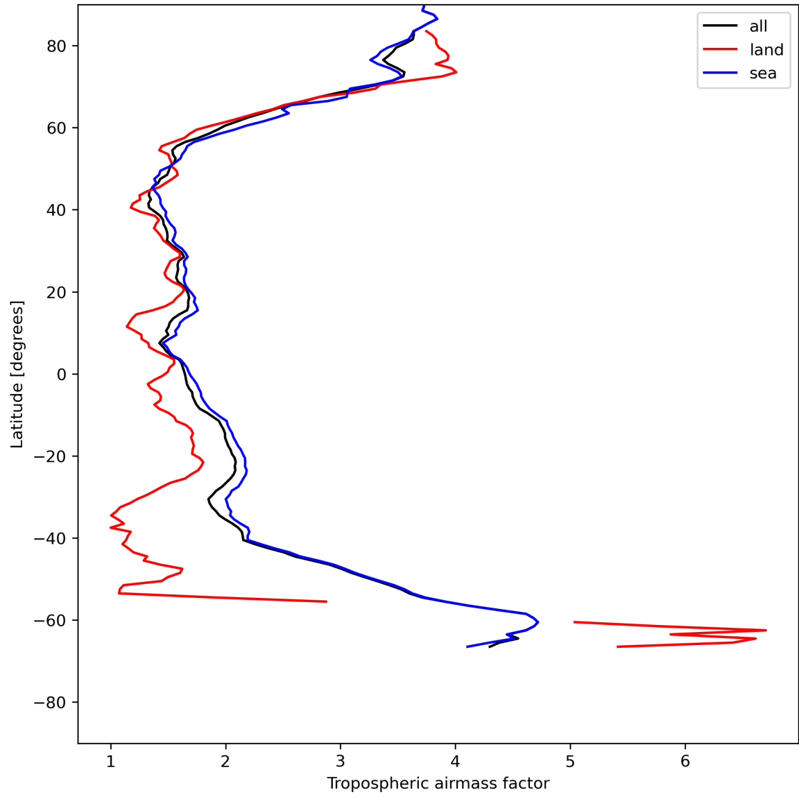
Figure 14: Zonal average of “Tropospheric airmass factor” for 2024-05-23 to 2024-05-24.
