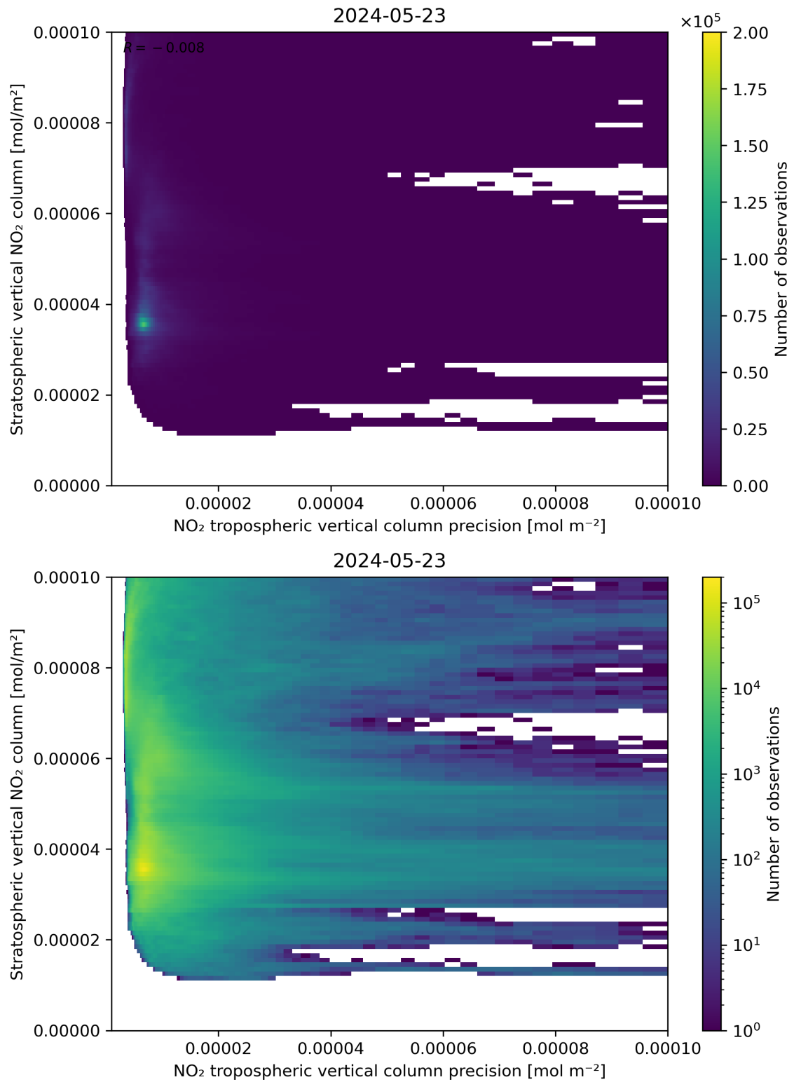
Figure 135: Scatter density plot of “NO 2 tropospheric vertical column precision” against “Stratospheric vertical NO 2 column” for 2024-05-23 to 2024-05-24.
