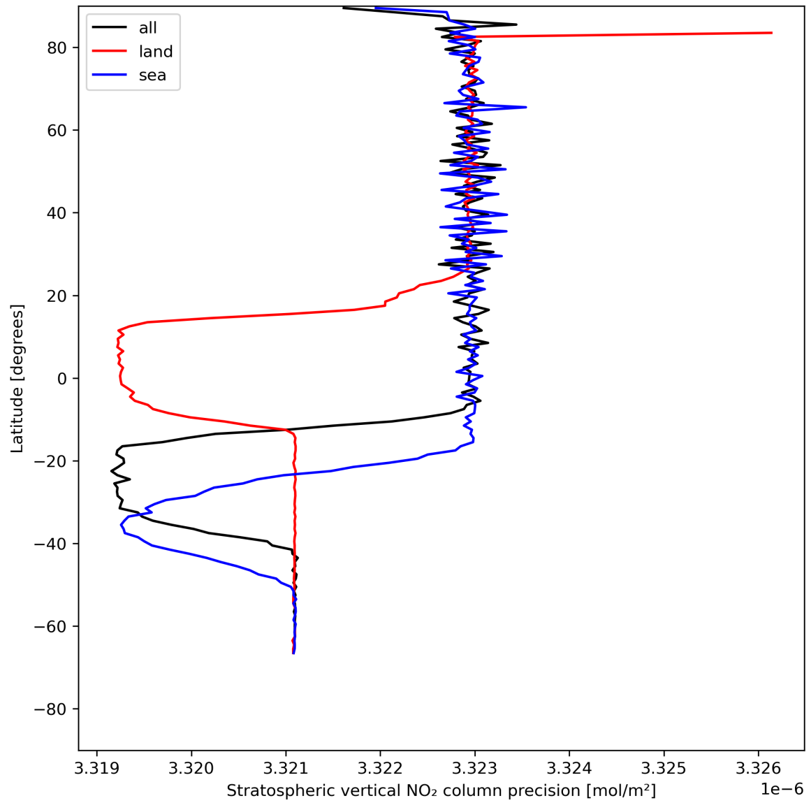
Figure 20: Zonal average of “Stratospheric vertical NO 2 column precision” for 2024-05-23 to 2024-05-24.
