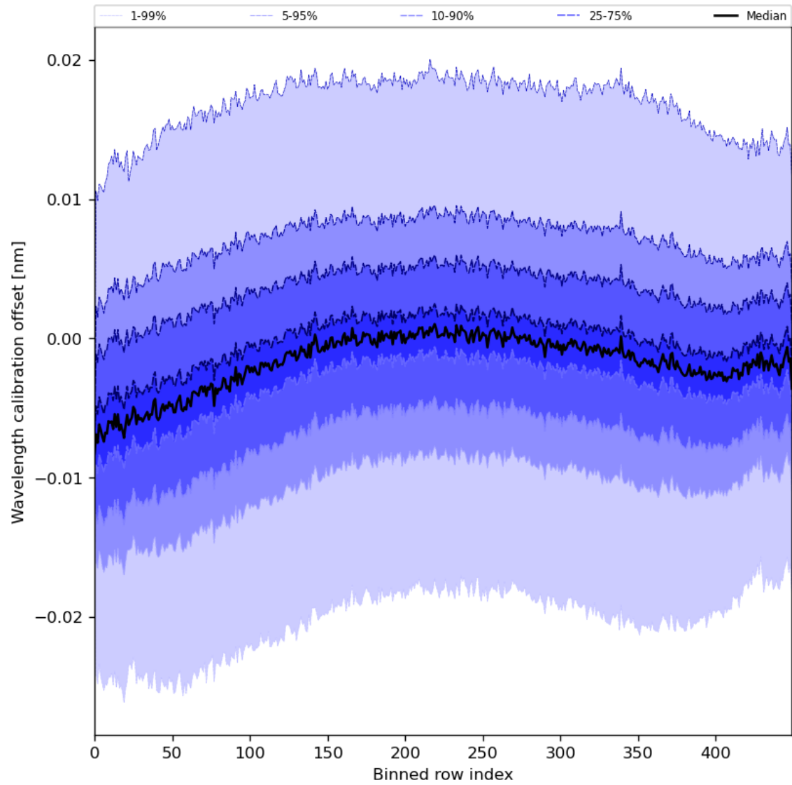
Figure 52: Along track statistics of “Wavelength calibration offset” for 2024-05-23 to 2024-05-24
