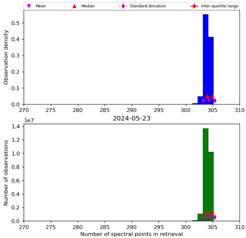
Figure 33: Histogram of “Number of spectral points in retrieval” for 2024-05-23 to 2024-05-24
