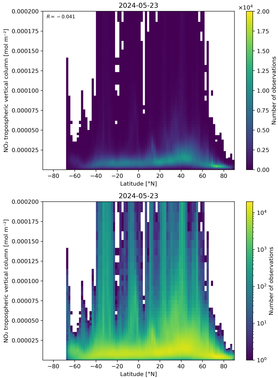
Figure 92: Scatter density plot of “Latitude” against “NO 2 tropospheric vertical column” for 2024-05-23 to 2024-05-24.
