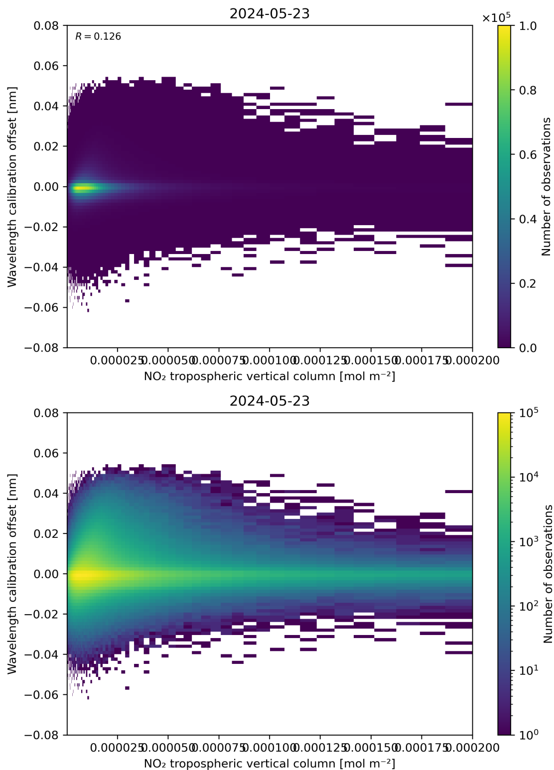
Figure 143: Scatter density plot of “NO 2 tropospheric vertical column” against “Wavelength calibration offset” for 2024-05-23 to 2024-05-24.
