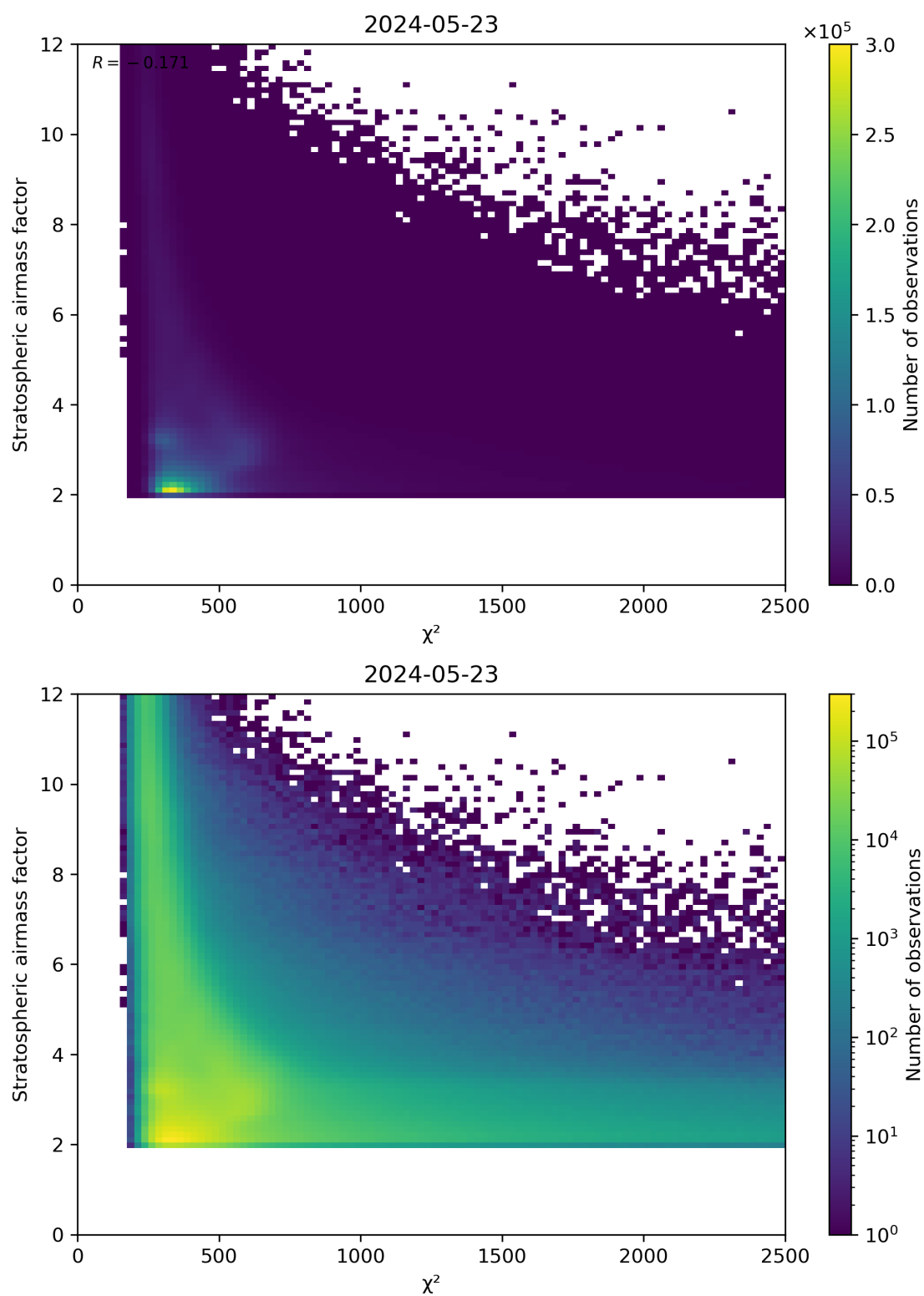
Figure 81: Scatter density plot of “ \chi^2 ” against “Stratospheric airmass factor” for 2024-05-23 to 2024-05-24.
