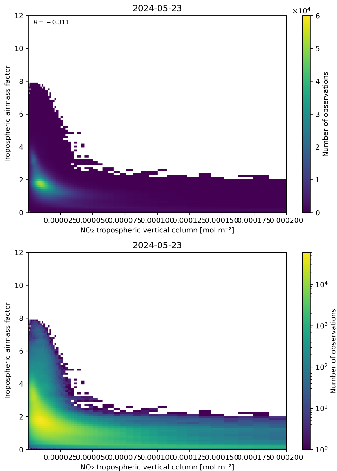
Figure 123: Scatter density plot of “NO 2 tropospheric vertical column” against “Tropospheric air mass factor” for 2024-05-23 to 2024-05-24.
