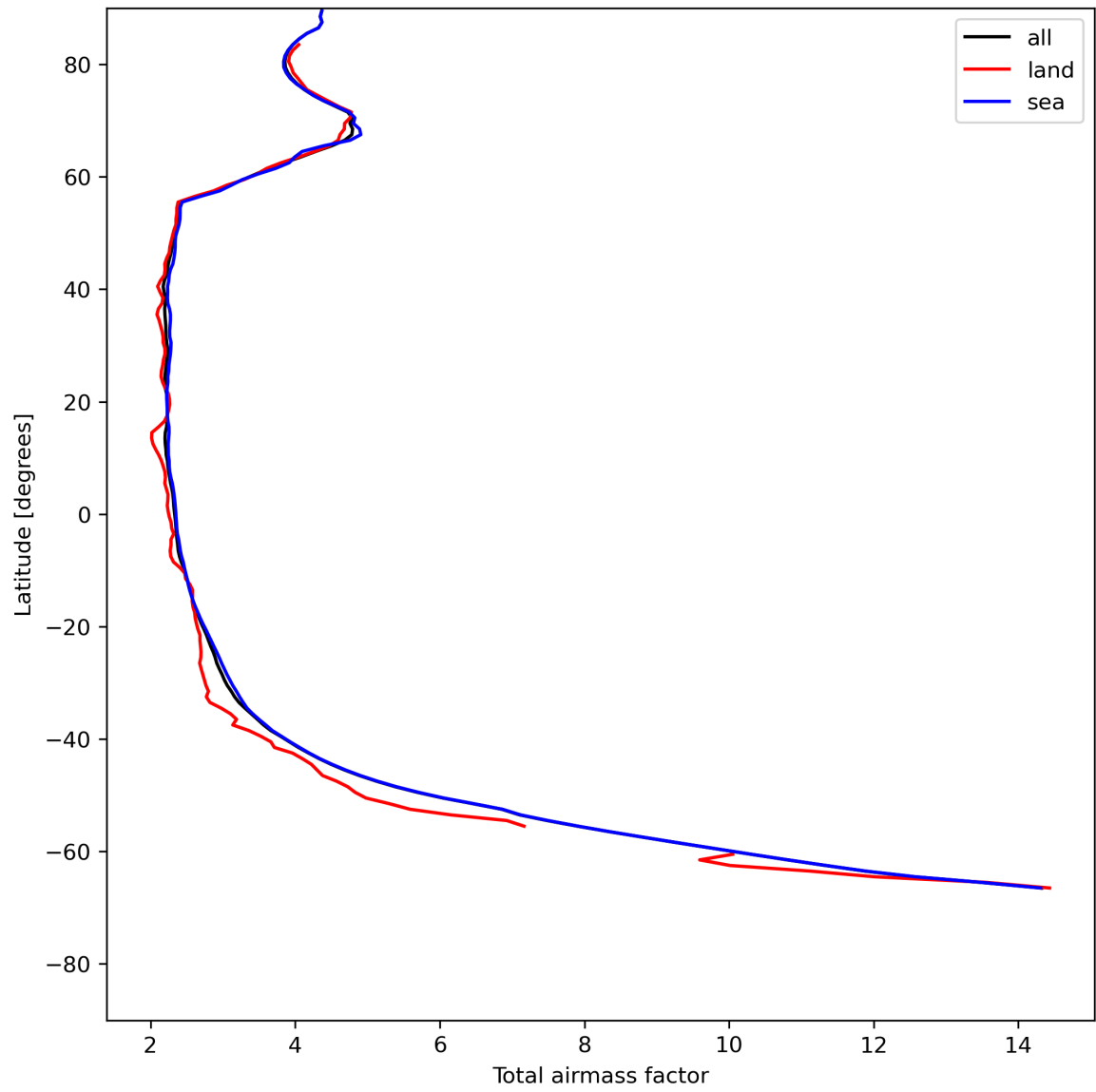
Figure 15: Zonal average of “Total airmass factor” for 2024-05-23 to 2024-05-24.
