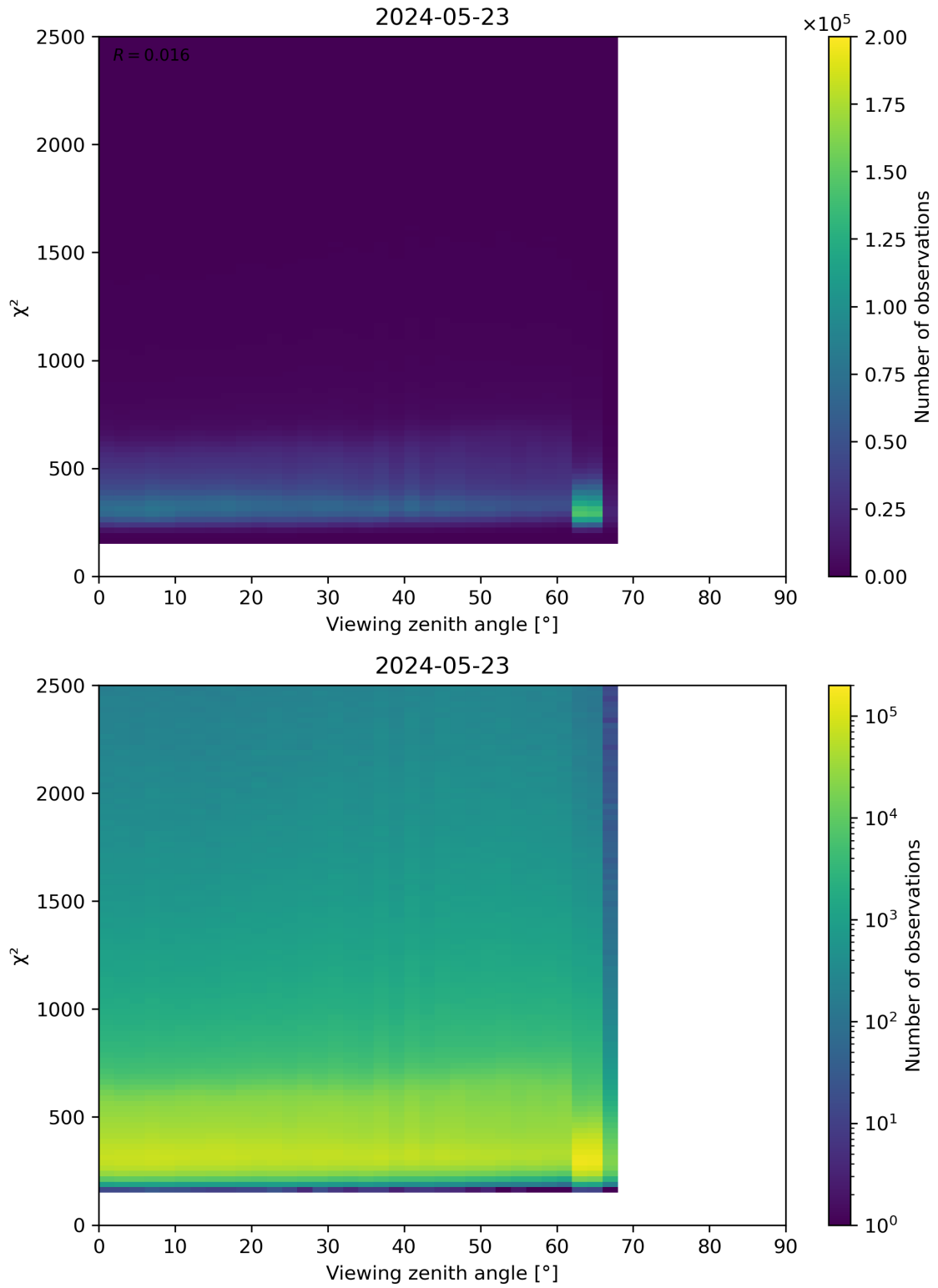
Figure 162: Scatter density plot of “Viewing zenith angle” against “ \chi^2 ” for 2024-05-23 to 2024-05-24.
