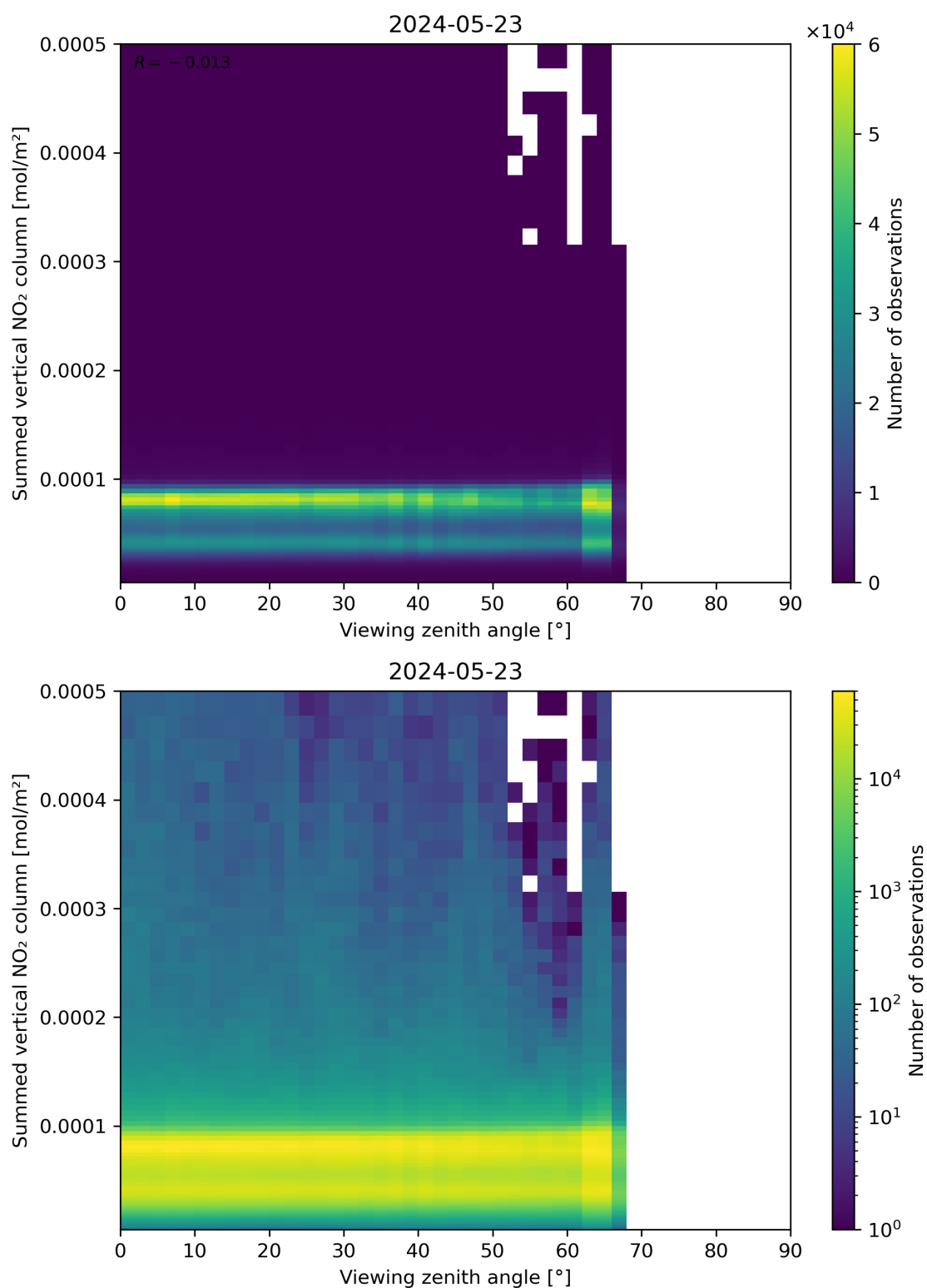
Figure 165: Scatter density plot of “Viewing zenith angle” against “Summed vertical NO 2 column” for 2024-05-23 to 2024-05-24.
