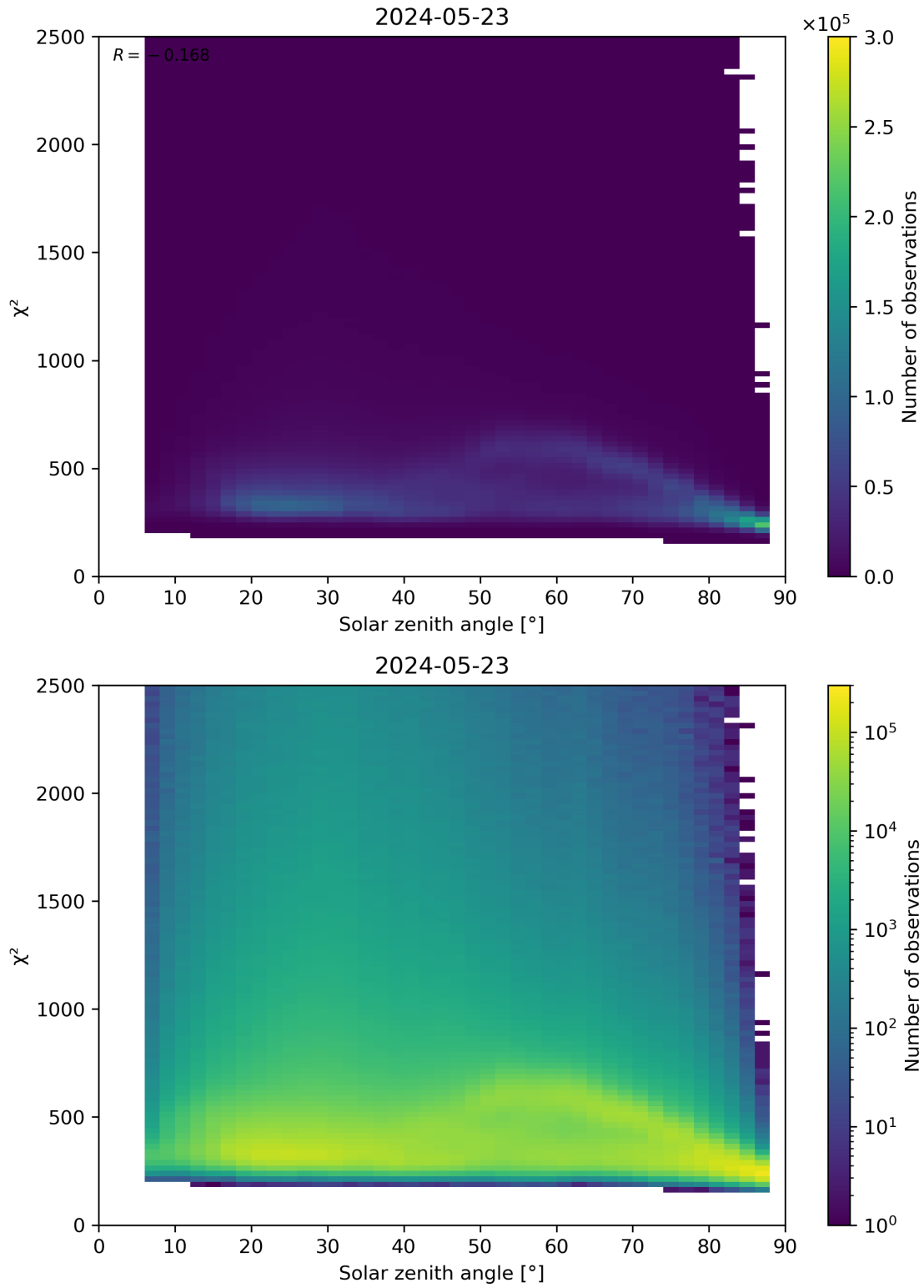
Figure 148: Scatter density plot of “Solar zenith angle” against “ \chi^2 ” for 2024-05-23 to 2024-05-24.
