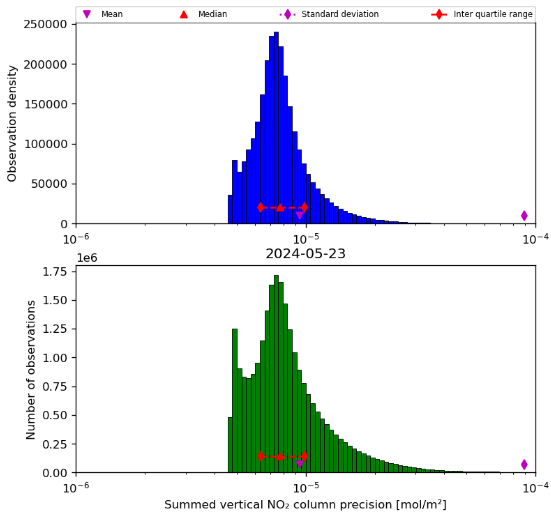
Figure 41: Histogram of “Summed vertical NO 2 column precision” for 2024-05-23 to 2024-05-24
