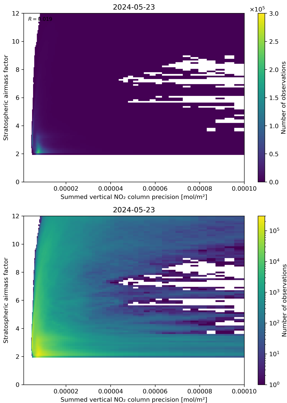
Figure 106: Scatter density plot of “Summed vertical NO 2 column precision” against “Stratospheric airmass factor” for 2024-05-23 to 2024-05-24.
