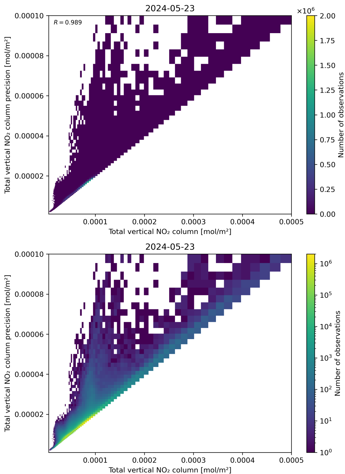
Figure 114: Scatter density plot of “Total vertical NO 2 column” against “Total vertical NO 2 column precision” for 2024-05-23 to 2024-05-24.
