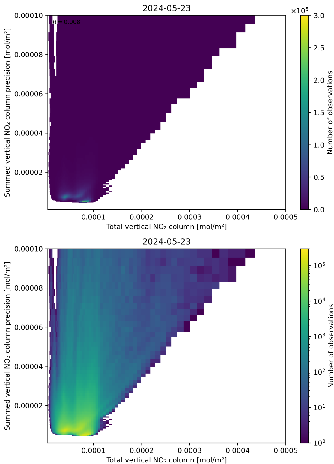
Figure 113: Scatter density plot of “Total vertical NO 2 column” against “Summed vertical NO 2 column precision” for 2024-05-23 to 2024-05-24.
