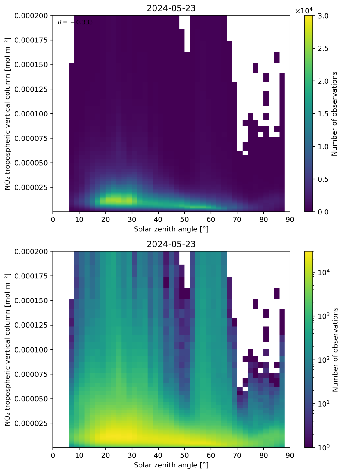
Figure 155: Scatter density plot of “Solar zenith angle” against “NO 2 tropospheric vertical column” for 2024-05-23 to 2024-05-24.
