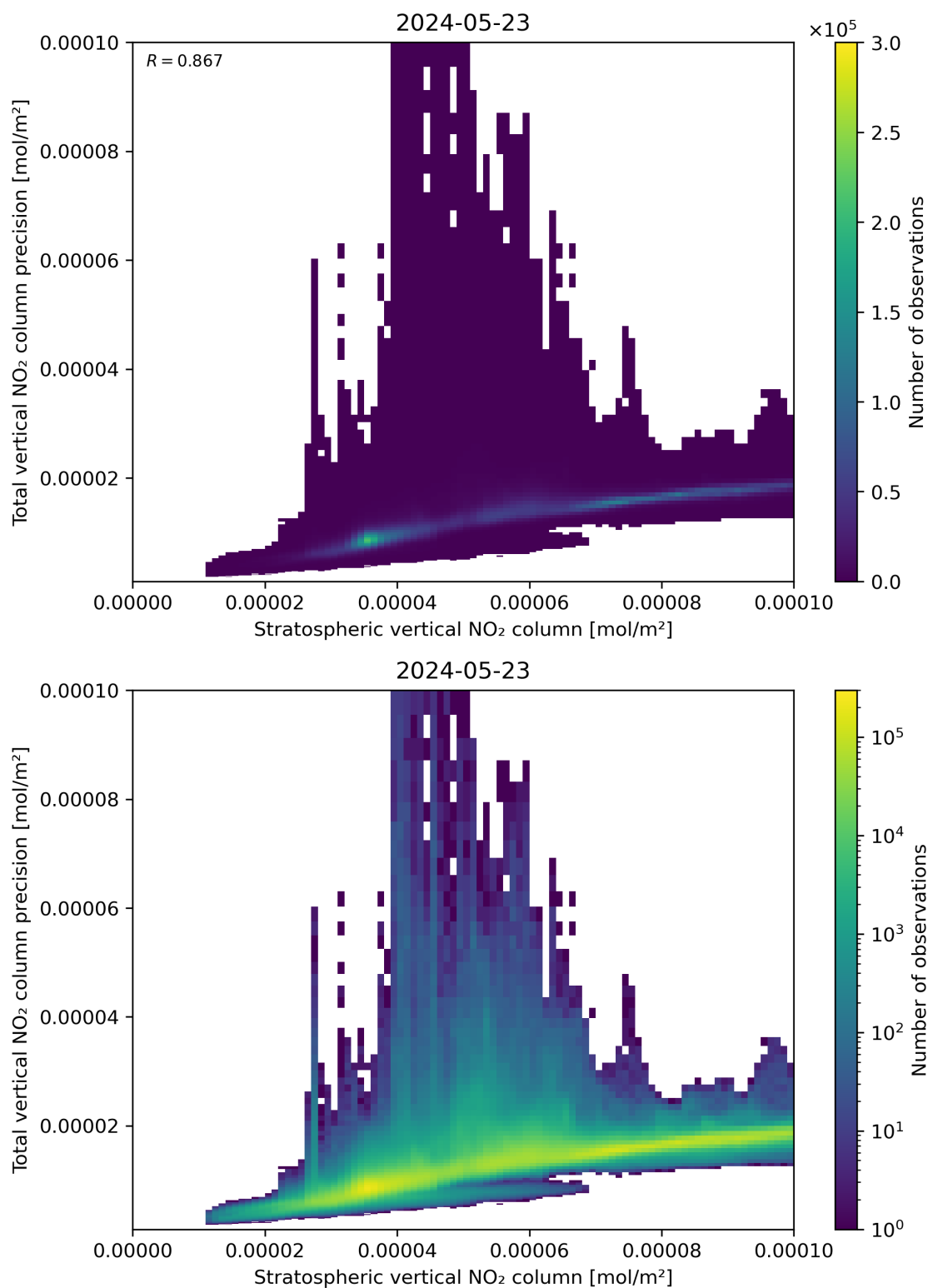
Figure 101: Scatter density plot of “Stratospheric vertical NO 2 column” against “Total vertical NO 2 column precision” for 2024-05-23 to 2024-05-24.
