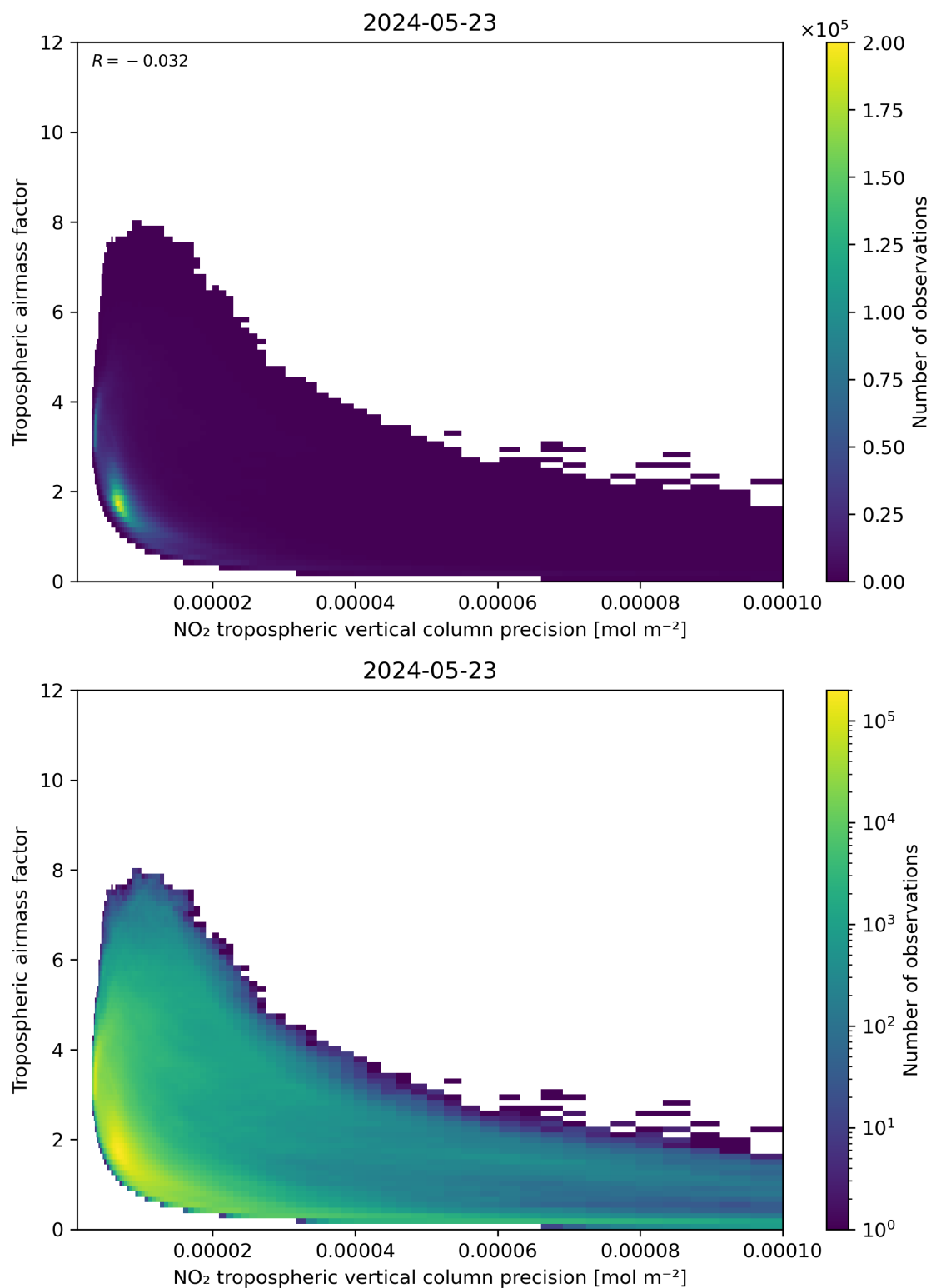
Figure 133: Scatter density plot of “NO 2 tropospheric vertical column precision” against “Tropospheric airmass factor” for 2024-05-23 to 2024-05-24.
