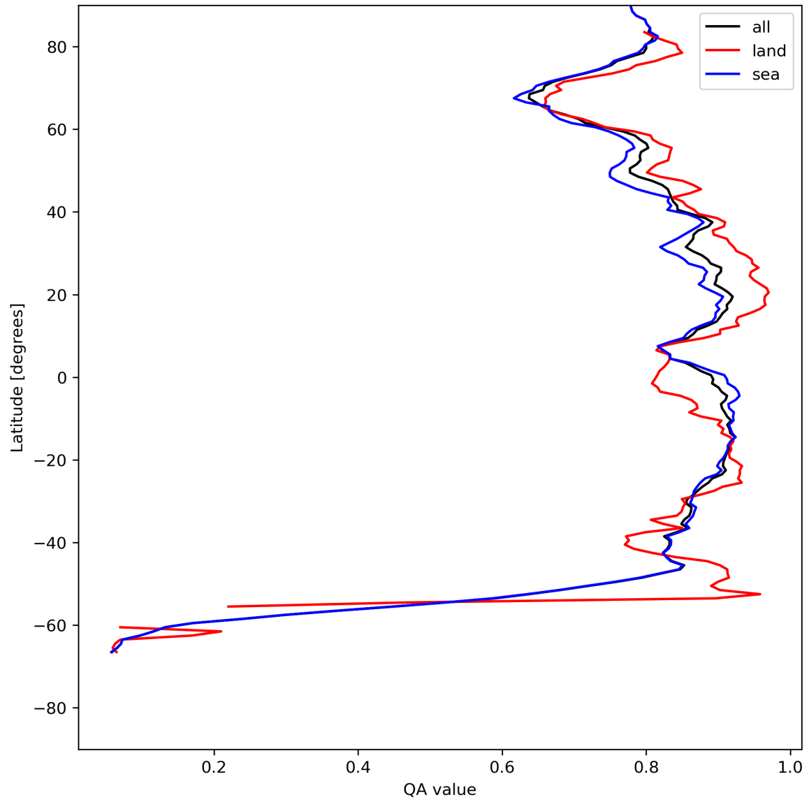
Figure 11: Zonal average of “QA value” for 2024-05-23 to 2024-05-24.
