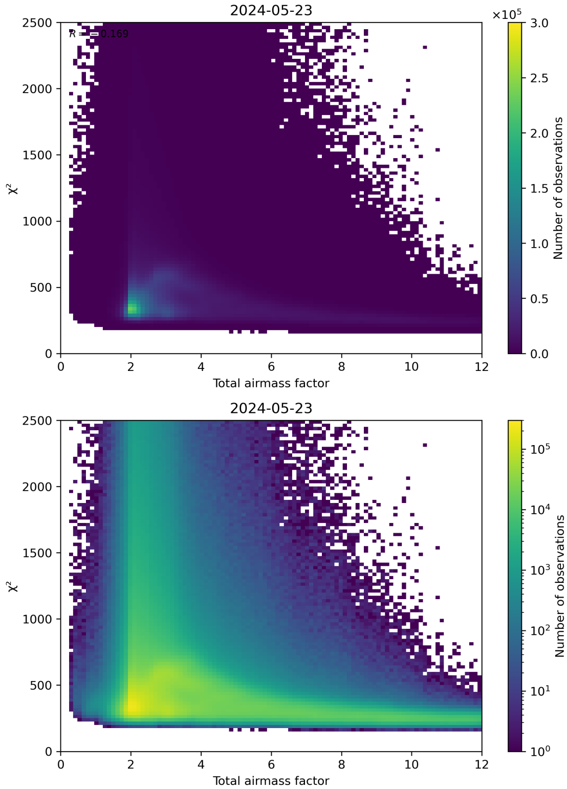
Figure 63: Scatter density plot of “Total airmass factor” against “ \chi^2 ” for 2024-05-23 to 2024-05-24.
