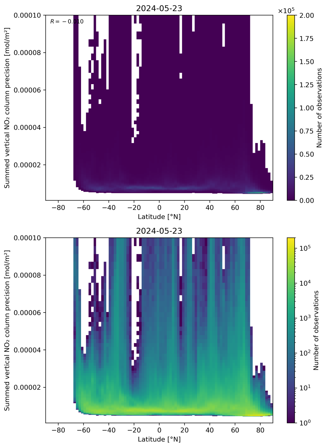
Figure 89: Scatter density plot of “Latitude” against “Summed vertical NO 2 column precision” for 2024-05-23 to 2024-05-24.
