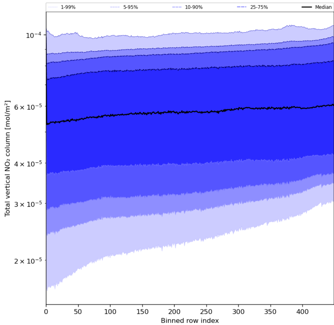
Figure 55: Along track statistics of “Total vertical NO 2 column” for 2024-05-23 to 2024-05-24
