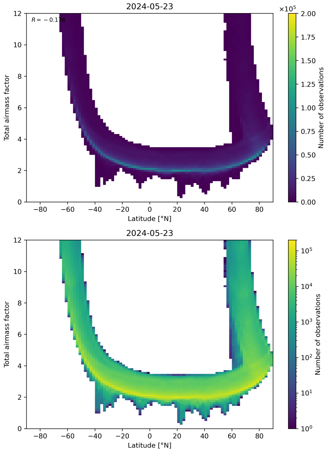
Figure 84: Scatter density plot of “Latitude” against “Total airmass factor” for 2024-05-23 to 2024-05-24.
