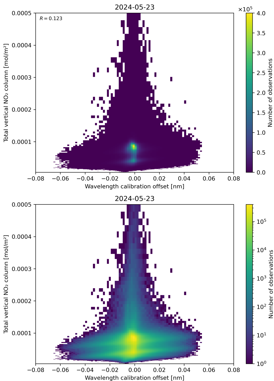
Figure 179: Scatter density plot of “Wavelength calibration offset” against “Total vertical NO 2 column” for 2024-05-23 to 2024-05-24.
