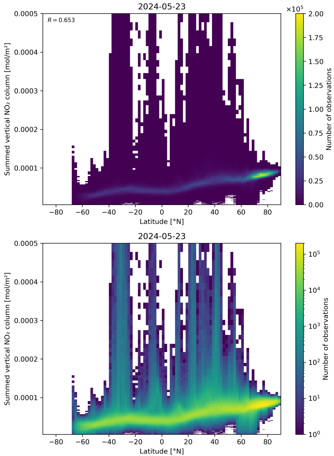
Figure 88: Scatter density plot of “Latitude” against “Summed vertical NO 2 column” for 2024-05-23 to 2024-05-24.
