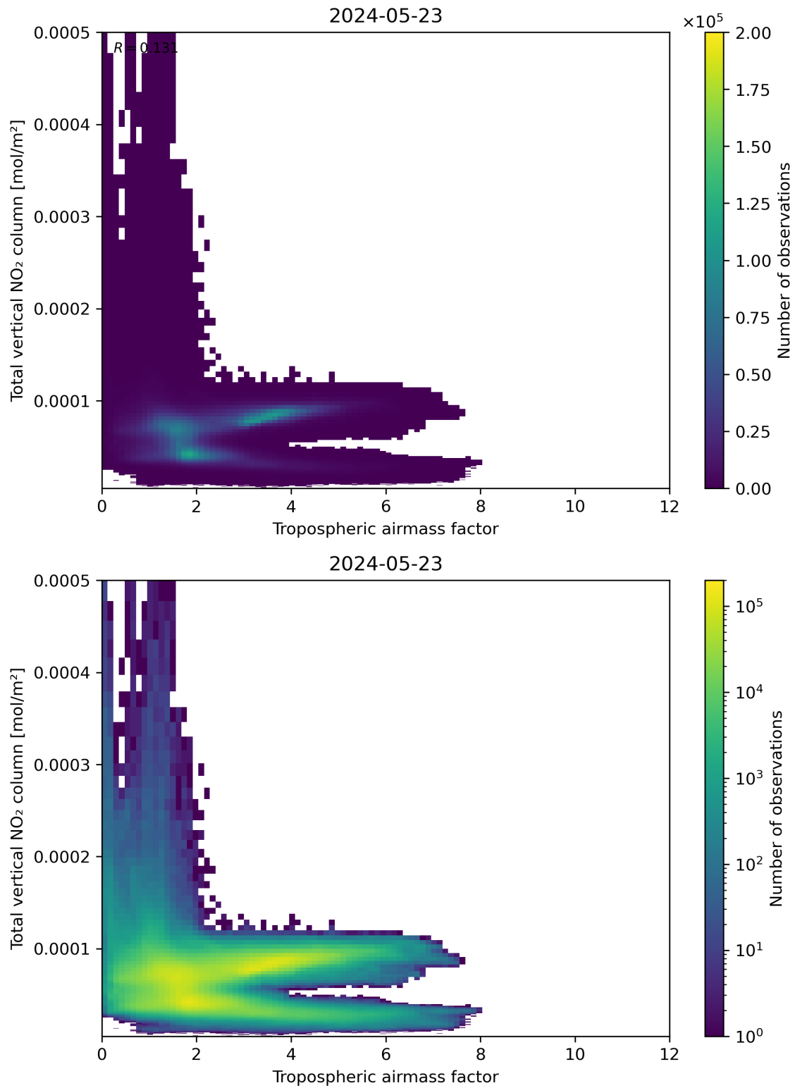
Figure 77: Scatter density plot of “Tropospheric airmass factor” against “Total vertical NO 2 column” for 2024-05-23 to 2024-05-24.
