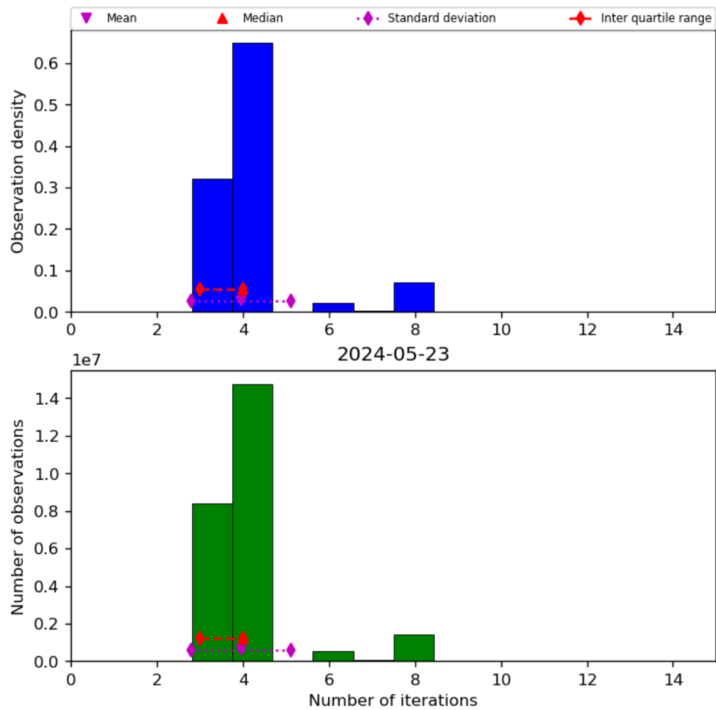
Figure 34: Histogram of “Number of iterations” for 2024-05-23 to 2024-05-24
