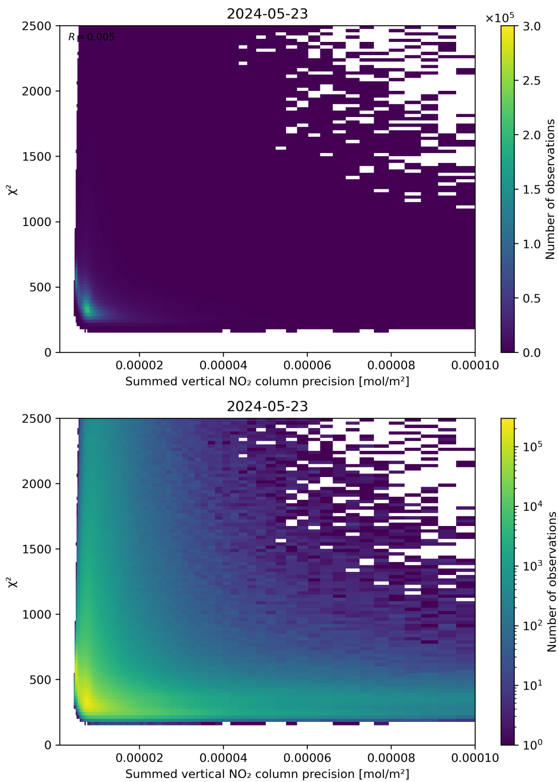
Figure 107: Scatter density plot of “Summed vertical NO 2 column precision” against “ \chi^2 ” for 2024-05-23 to 2024-05-24.
