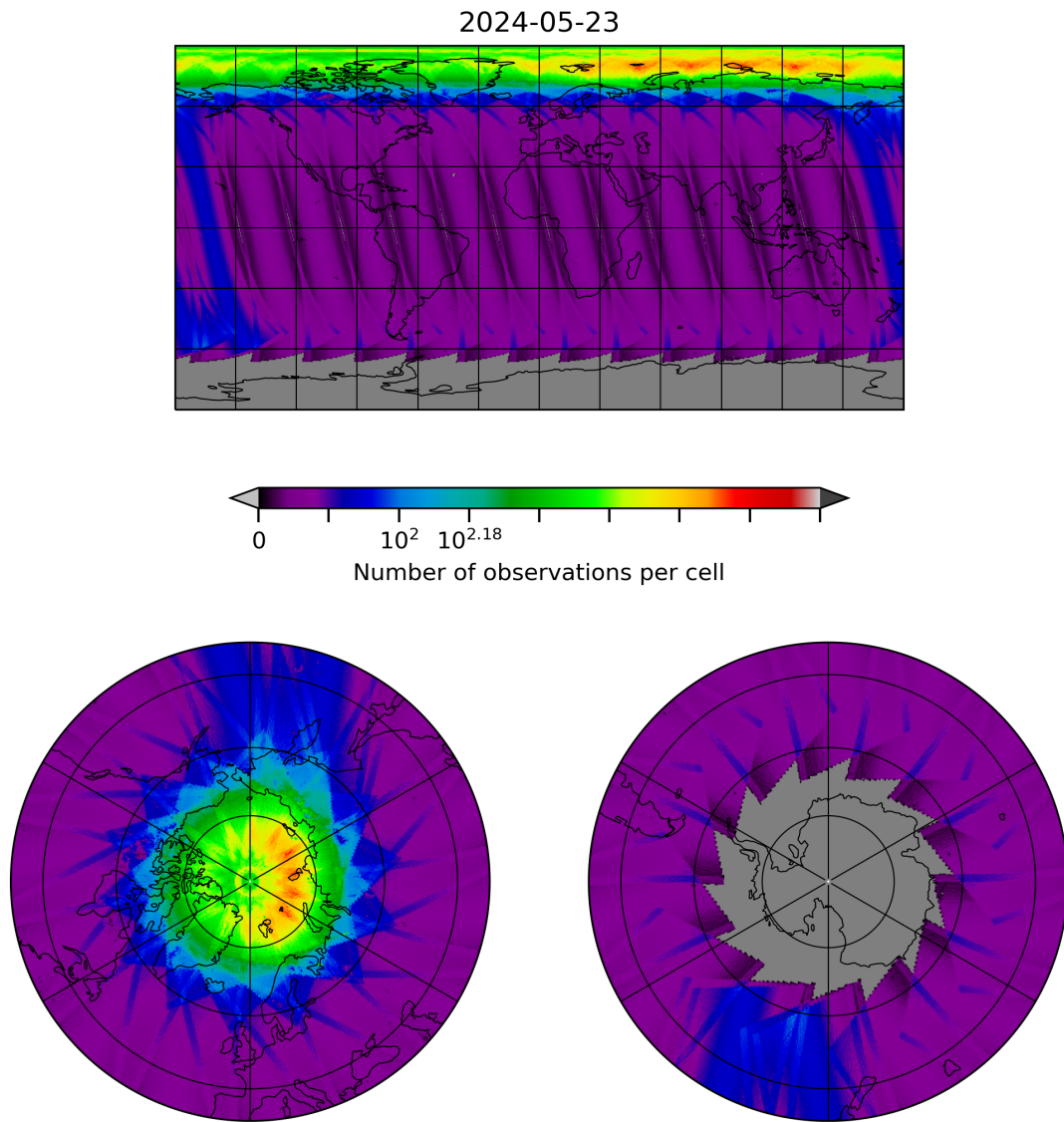
Figure 10: Map of the number of observations for 2024-05-23 to 2024-05-24
