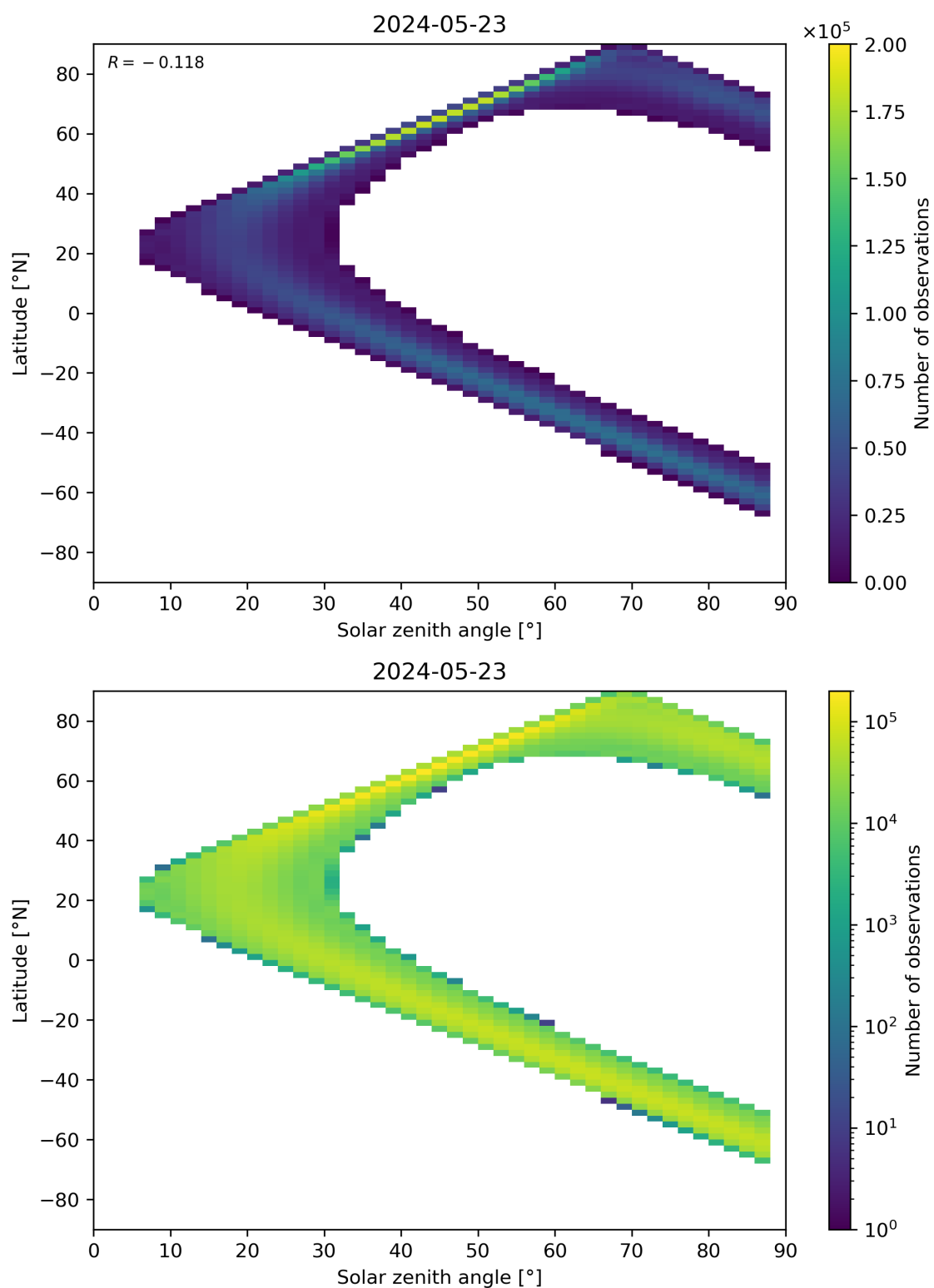
Figure 149: Scatter density plot of “Solar zenith angle” against “Latitude” for 2024-05-23 to 2024-05-24.
