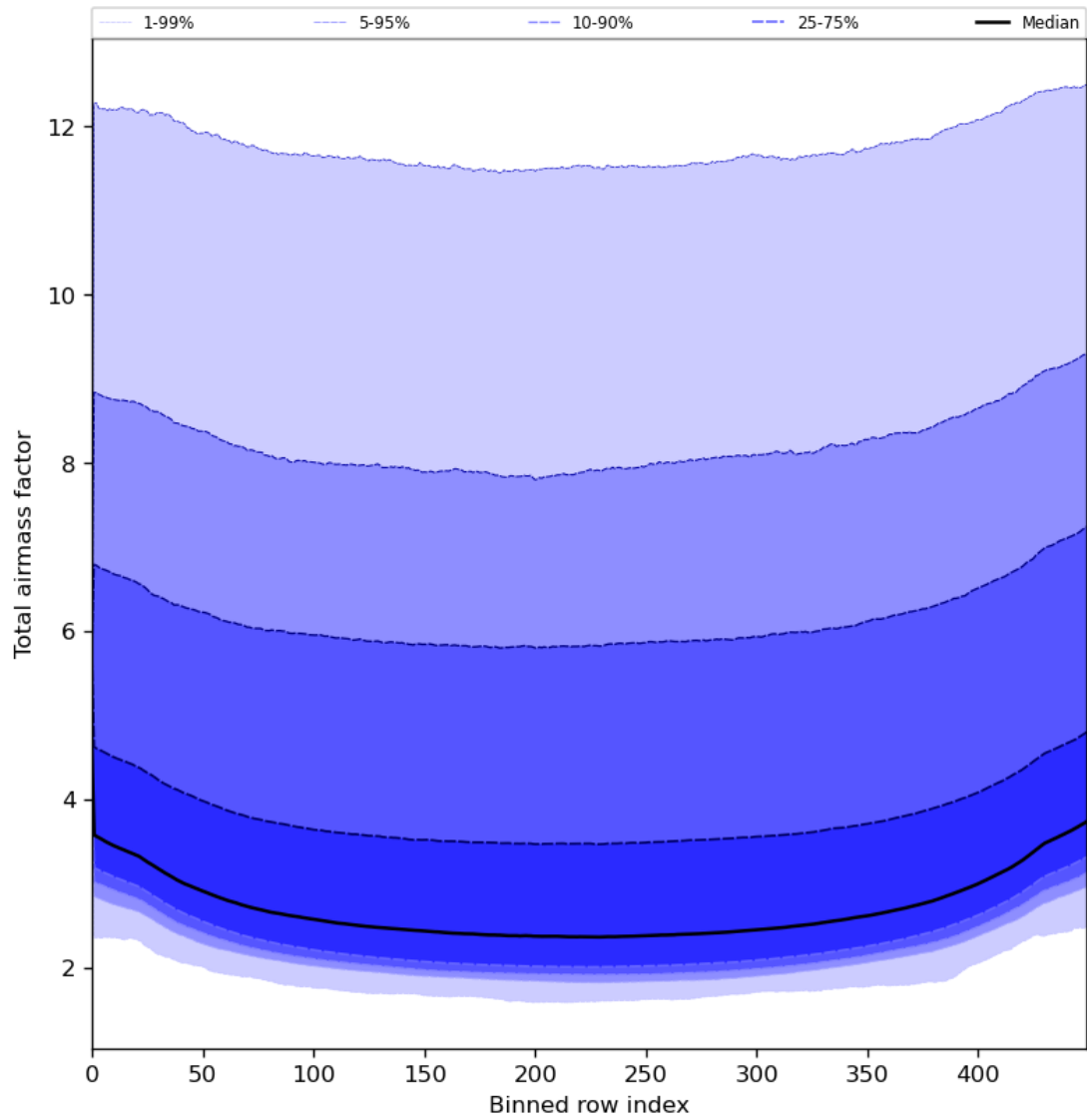
Figure 49: Along track statistics of “Total airmass factor” for 2024-05-23 to 2024-05-24
