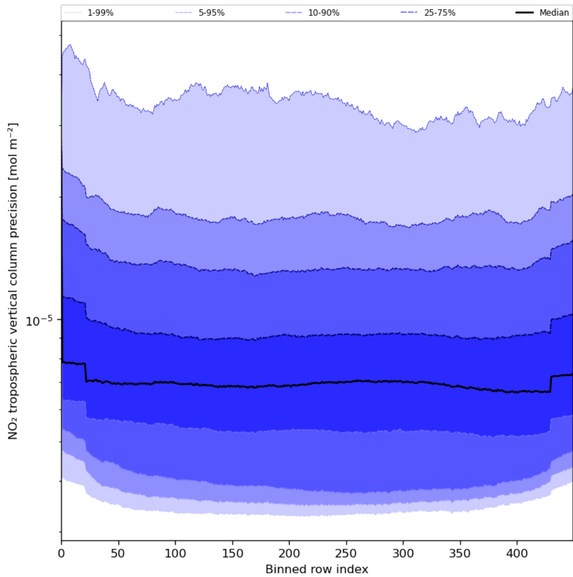
Figure 47: Along track statistics of “NO 2 tropospheric vertical column precision” for 2024-05-23 to 2024-05-24
