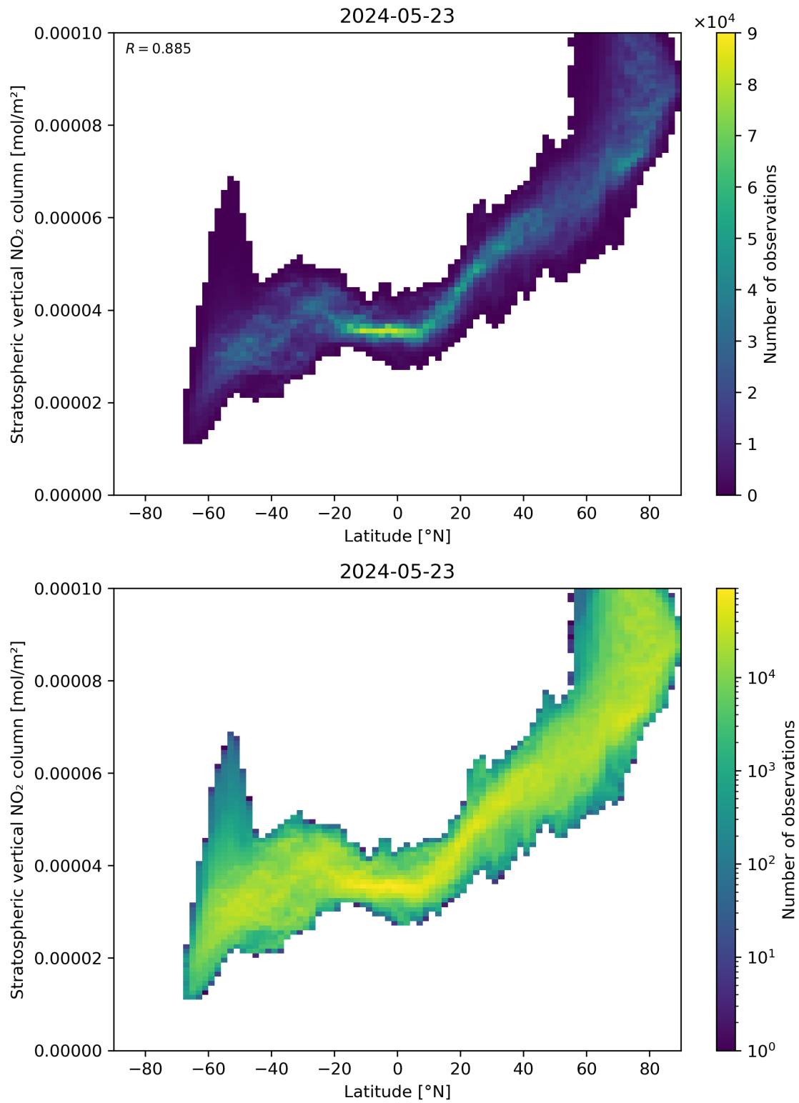
Figure 87: Scatter density plot of “Latitude” against “Stratospheric vertical NO 2 column” for 2024-05-23 to 2024-05-24.
