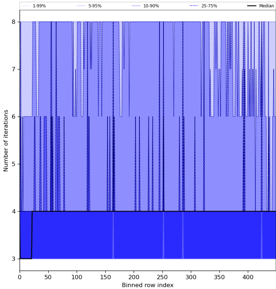
Figure 51: Along track statistics of “Number of iterations” for 2024-05-23 to 2024-05-24
