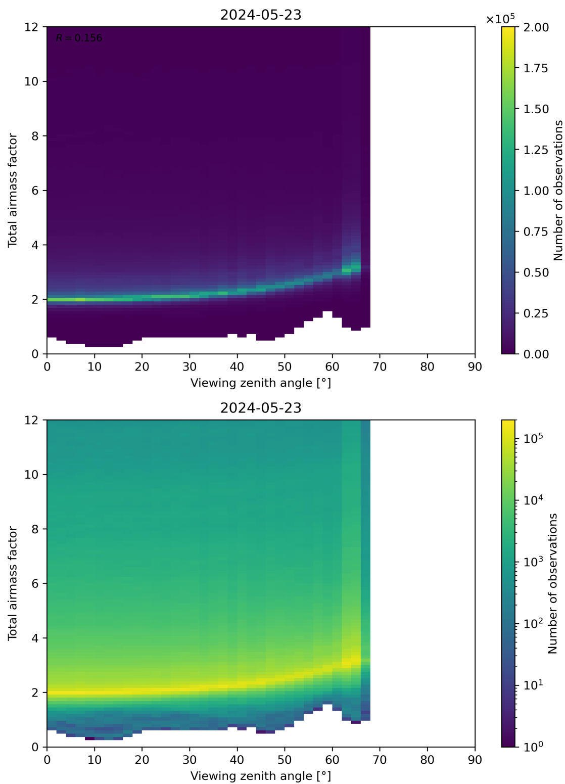
Figure 160: Scatter density plot of “Viewing zenith angle” against “Total airmass factor” for 2024-05-23 to 2024-05-24.
