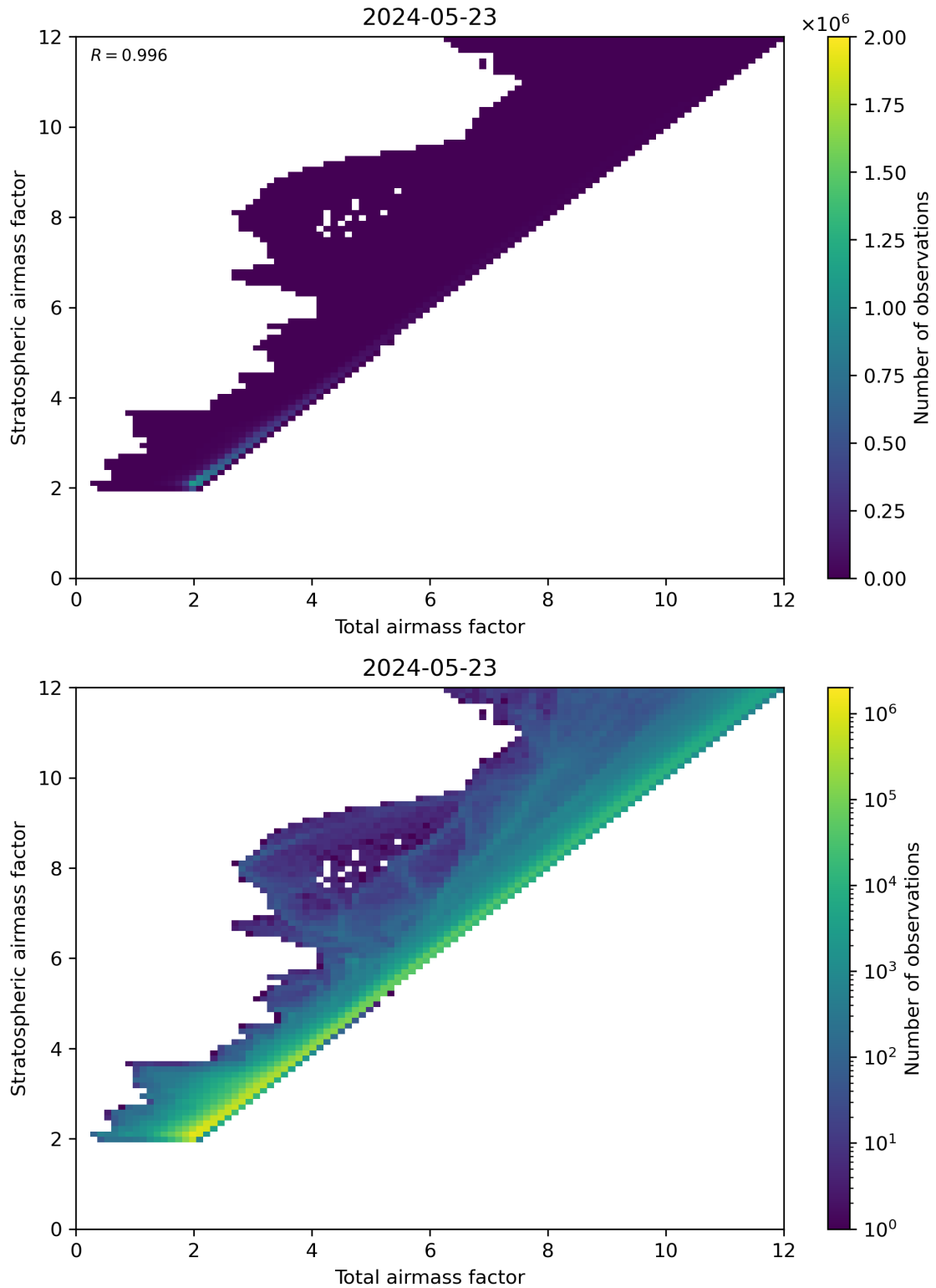
Figure 62: Scatter density plot of “Total airmass factor” against “Stratospheric airmass factor” for 2024-05-23 to 2024-05-24.
