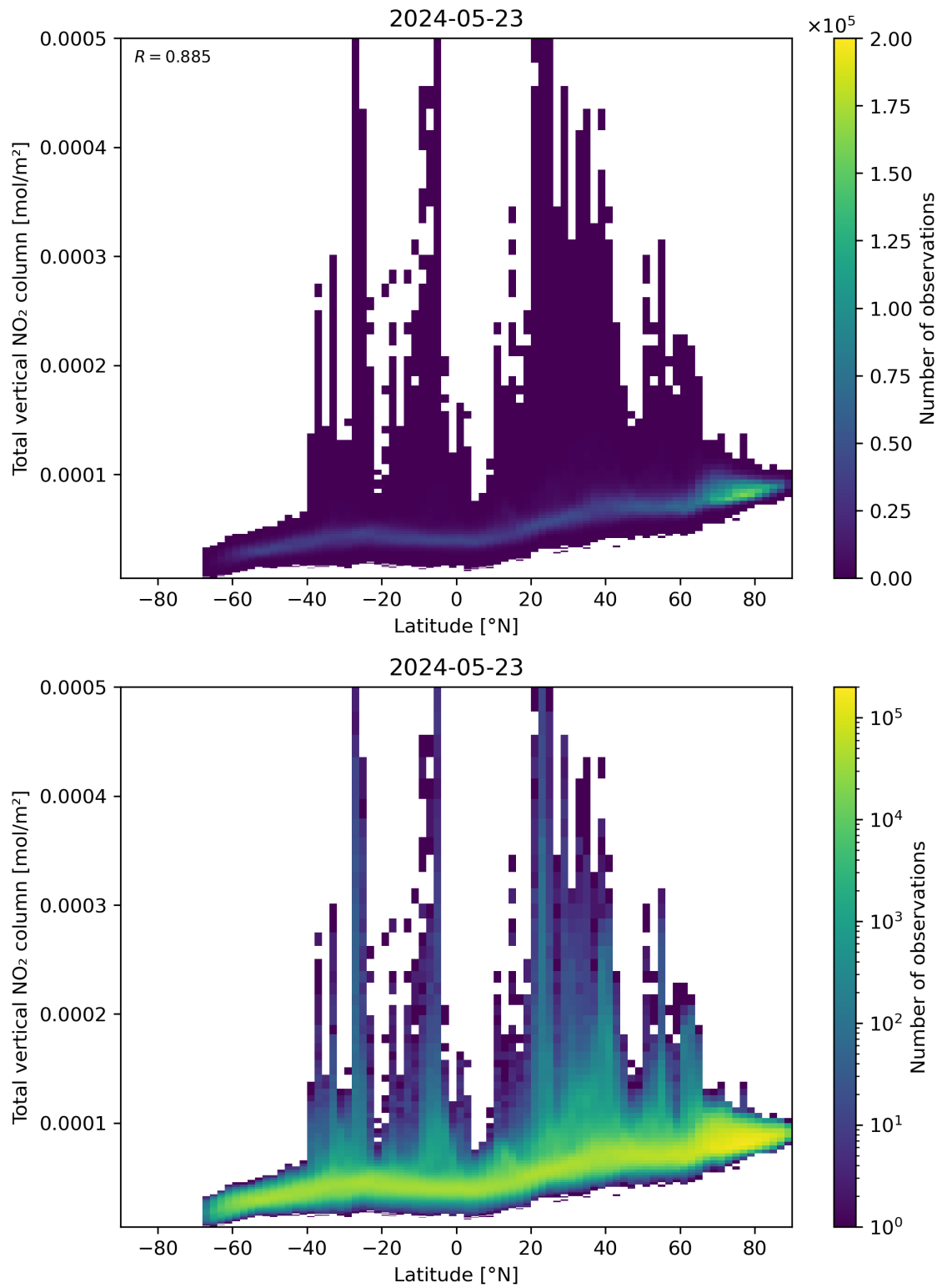
Figure 90: Scatter density plot of “Latitude” against “Total vertical NO 2 column” for 2024-05-23 to 2024-05-24.
