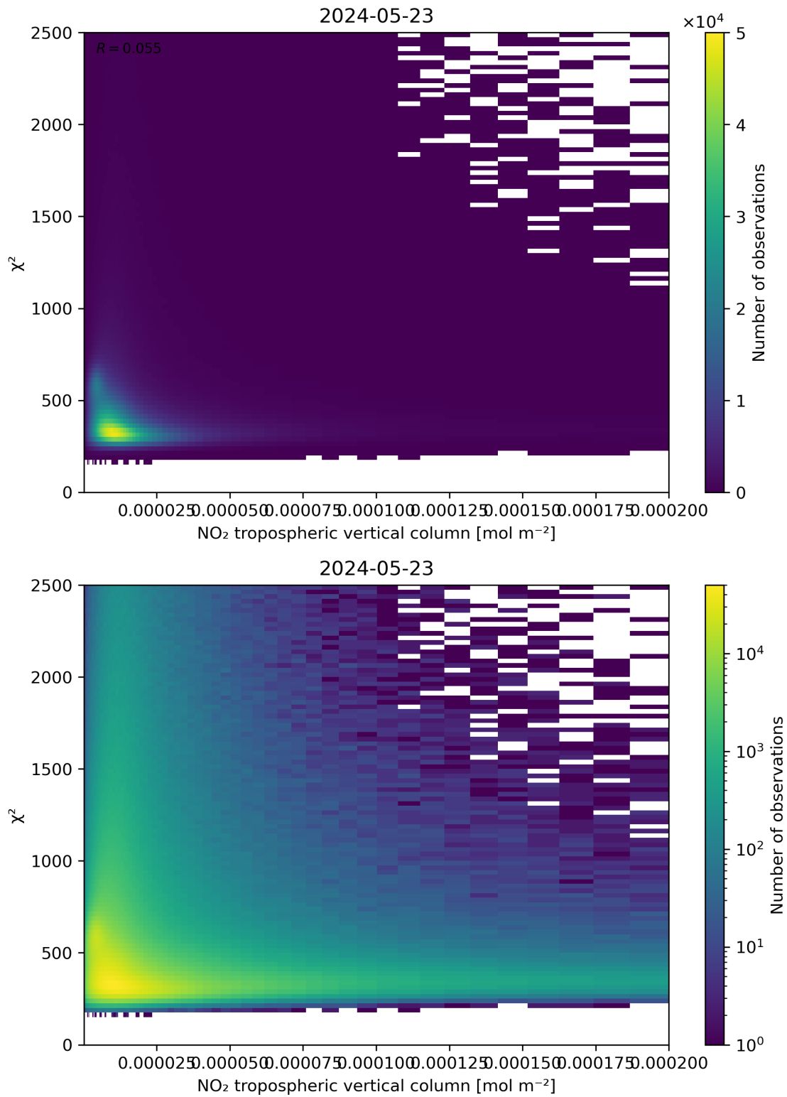
Figure 124: Scatter density plot of “NO 2 tropospheric vertical column” against “ \chi^2 ” for 2024-05-23 to 2024-05-24.
