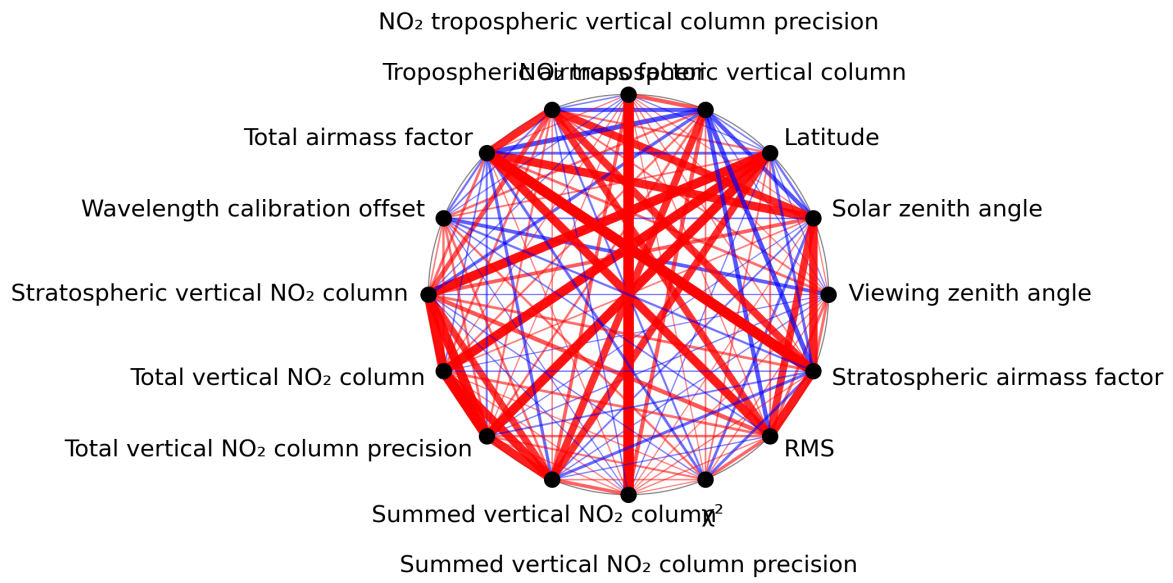
Figure 1: Map of correlation graph for 2024-05-23 to 2024-05-24.
