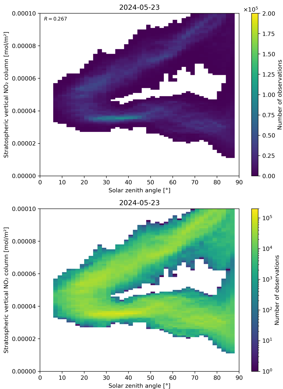
Figure 150: Scatter density plot of “Solar zenith angle” against “Stratospheric vertical NO 2 column” for 2024-05-23 to 2024-05-24.
