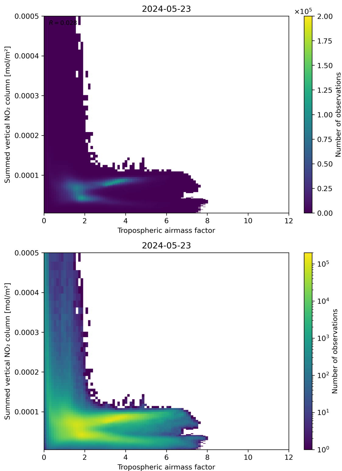
Figure 75: Scatter density plot of “Tropospheric air mass factor” against “Summed vertical NO 2 column” for 2024-05-23 to 2024-05-24.
