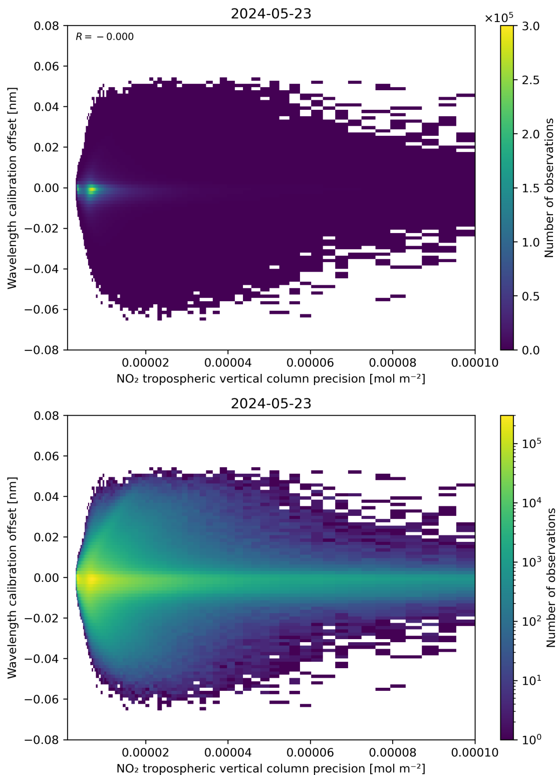
Figure 141: Scatter density plot of “NO 2 tropospheric vertical column precision” against “Wavelength calibration offset” for 2024-05-23 to 2024-05-24.
