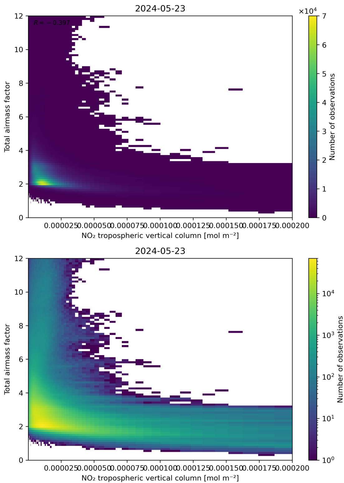
Figure 122: Scatter density plot of “NO 2 tropospheric vertical column” against “Total air mass factor” for 2024-05-23 to 2024-05-24.
