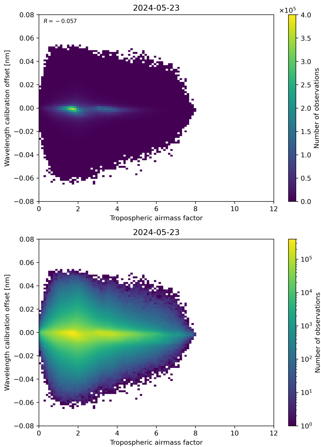
Figure 80: Scatter density plot of “Tropospheric airmass factor” against “Wavelength calibration offset” for 2024-05-23 to 2024-05-24.
