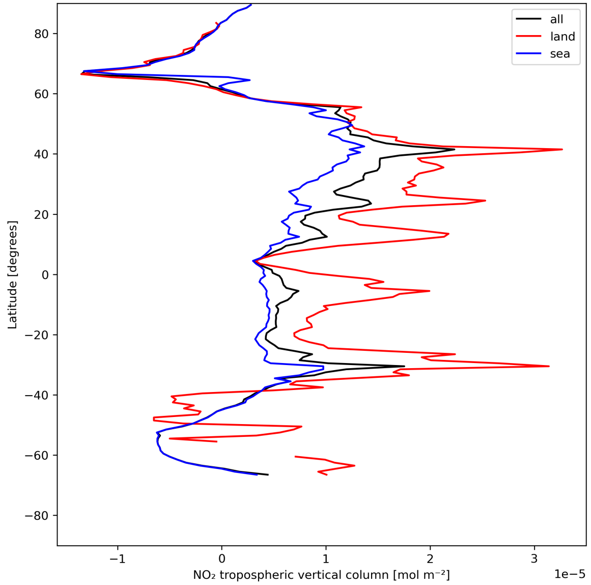
Figure 12: Zonal average of “NO 2 tropospheric vertical column” for 2024-05-23 to 2024-05-24.
