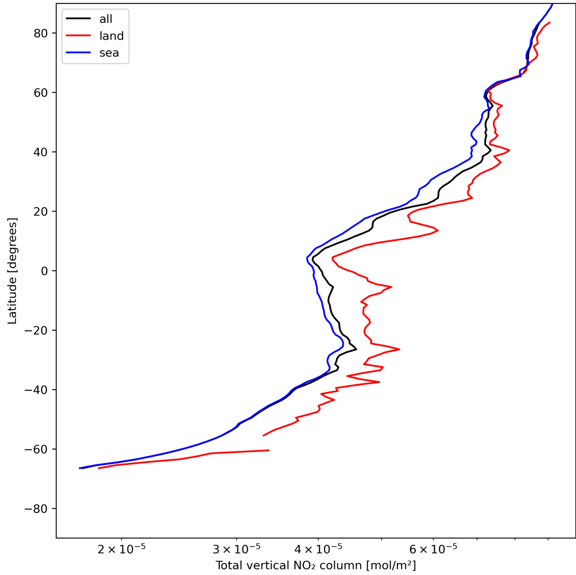
Figure 21: Zonal average of “Total vertical NO 2 column” for 2024-05-23 to 2024-05-24.
