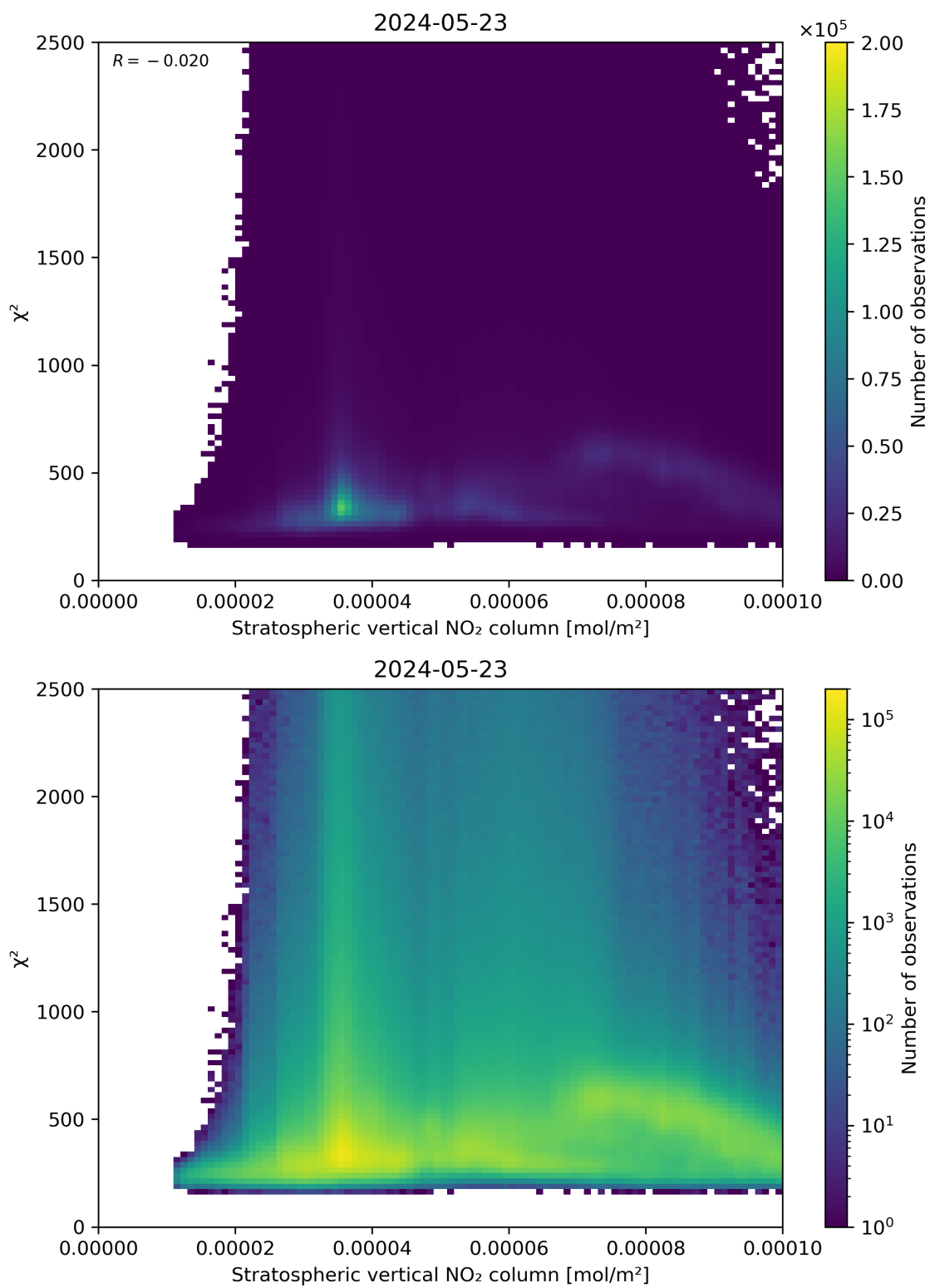
Figure 97: Scatter density plot of “Stratospheric vertical NO 2 column” against “ \chi^2 ” for 2024-05-23 to 2024-05-24.
