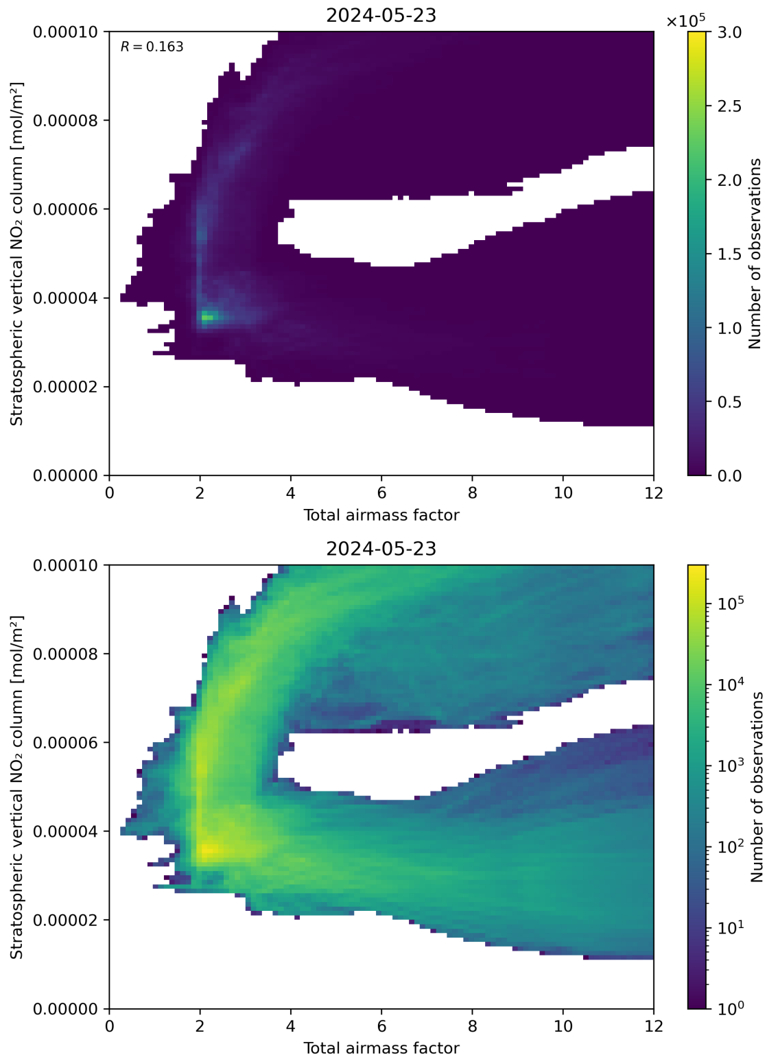
Figure 64: Scatter density plot of “Total airmass factor” against “Stratospheric vertical \text{NO}_2 column” for 2024-05-23 to 2024-05-24.
