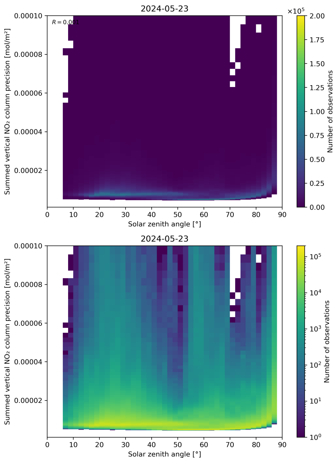
Figure 152: Scatter density plot of “Solar zenith angle” against “Summed vertical NO 2 column precision” for 2024-05-23 to 2024-05-24.
