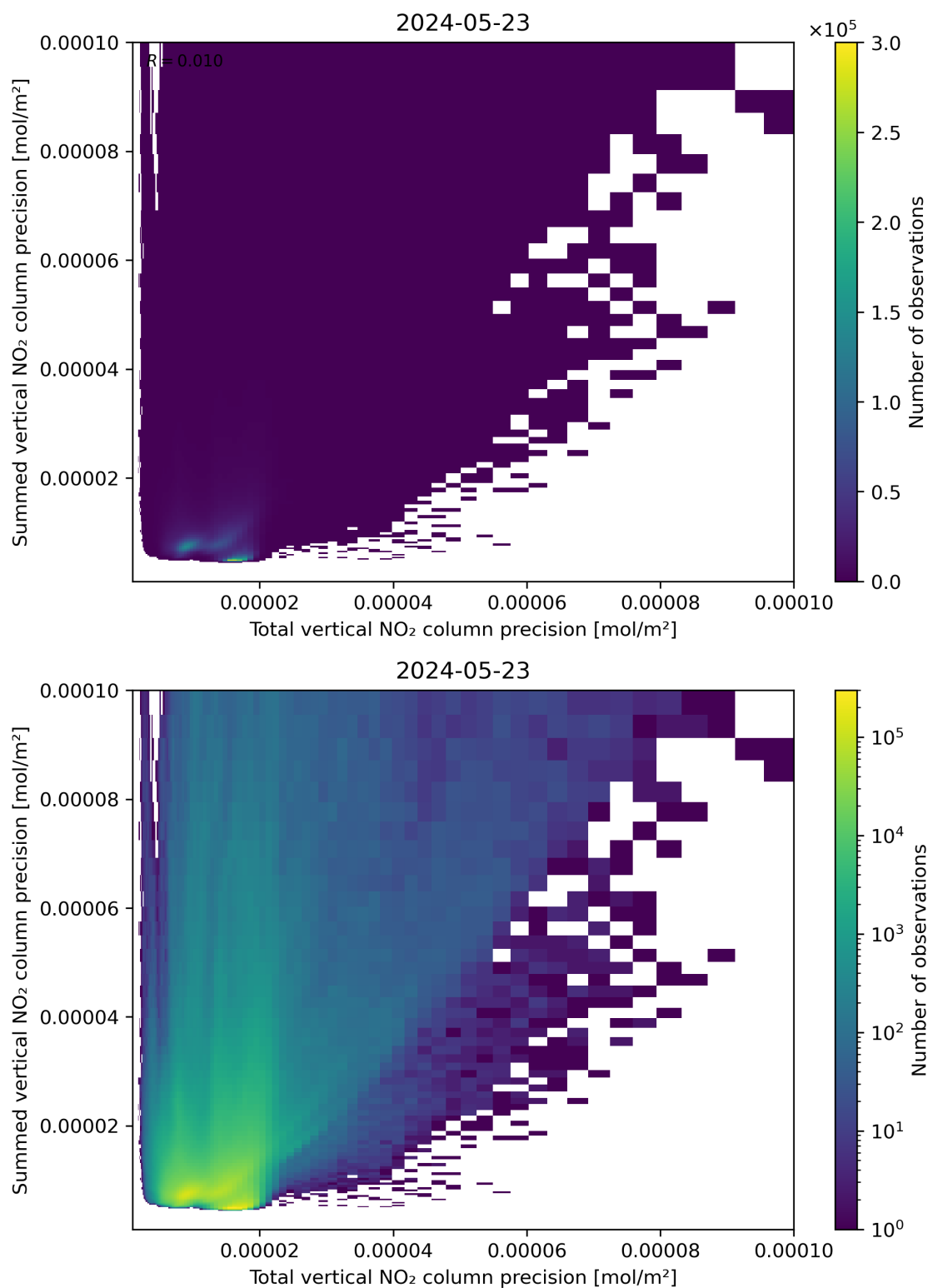
Figure 118: Scatter density plot of “Total vertical NO 2 column precision” against “Summed vertical NO 2 column precision” for 2024-05-23 to 2024-05-24.
