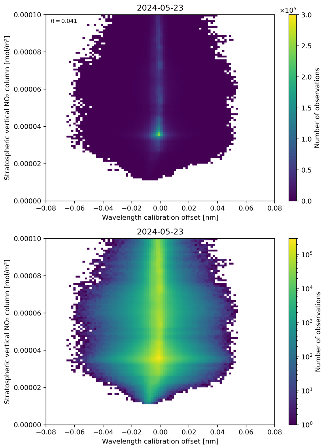
Figure 176: Scatter density plot of “Wavelength calibration offset” against “Stratospheric vertical NO 2 column” for 2024-05-23 to 2024-05-24.
