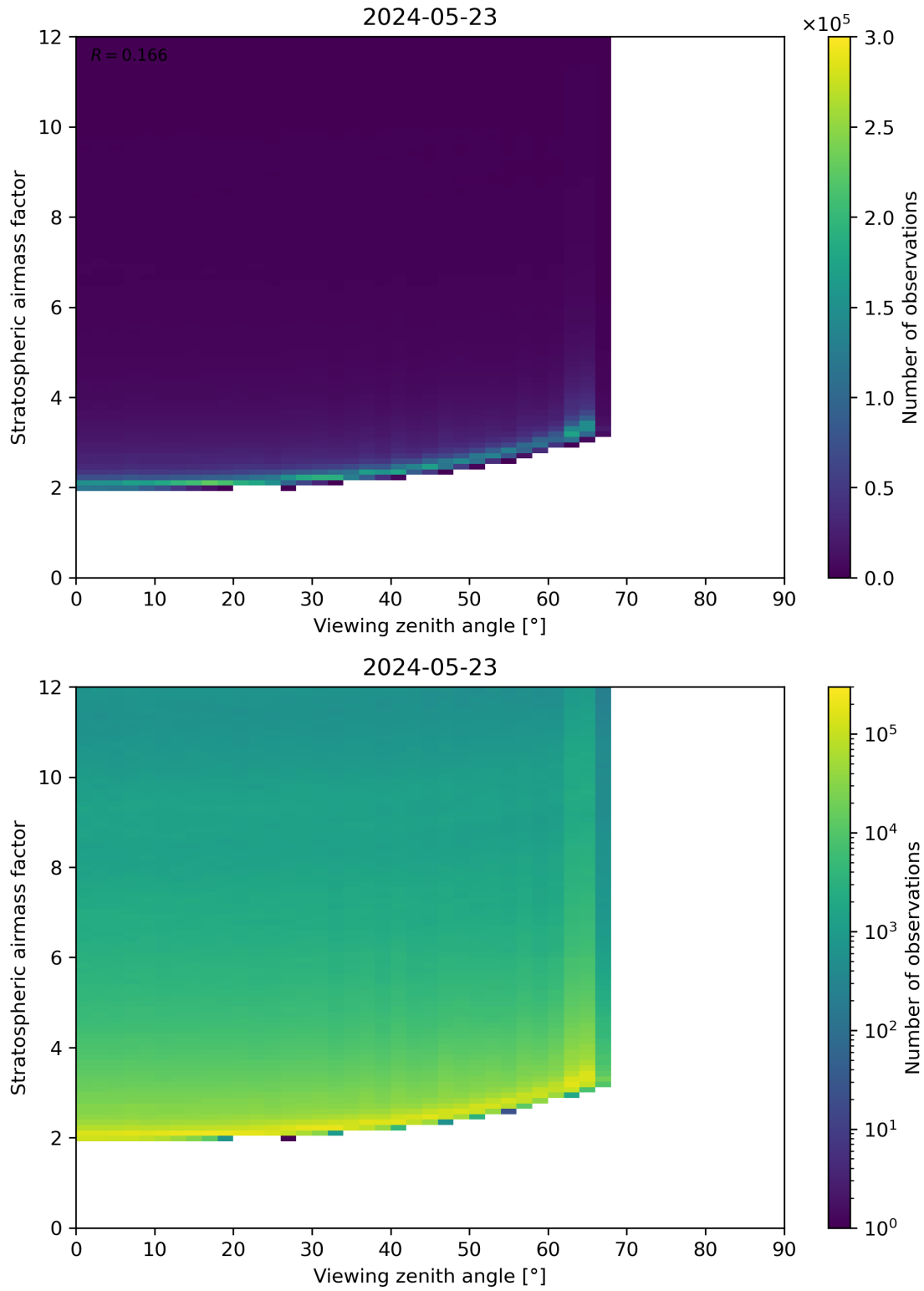
Figure 159: Scatter density plot of “Viewing zenith angle” against “Stratospheric airmass factor” for 2024-05-23 to 2024-05-24.
