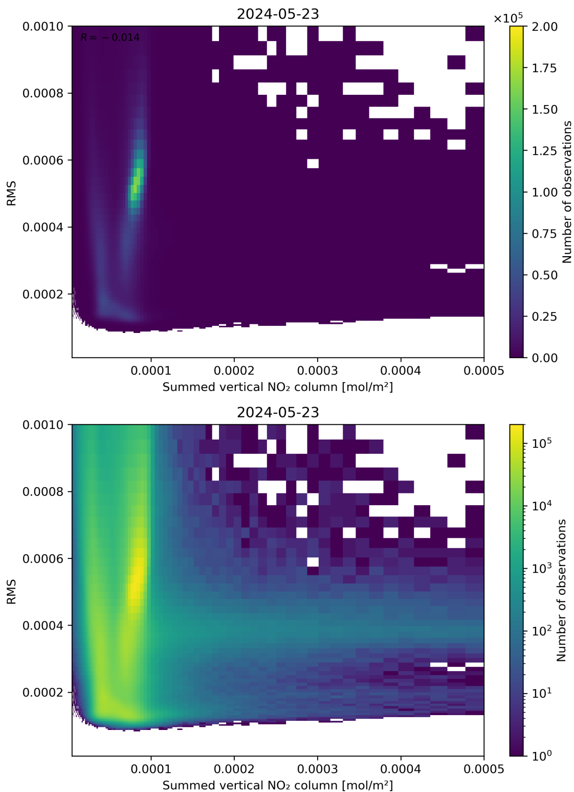
Figure 109: Scatter density plot of “Summed vertical NO 2 column” against “RMS” for 2024-05-23 to 2024-05-24.
