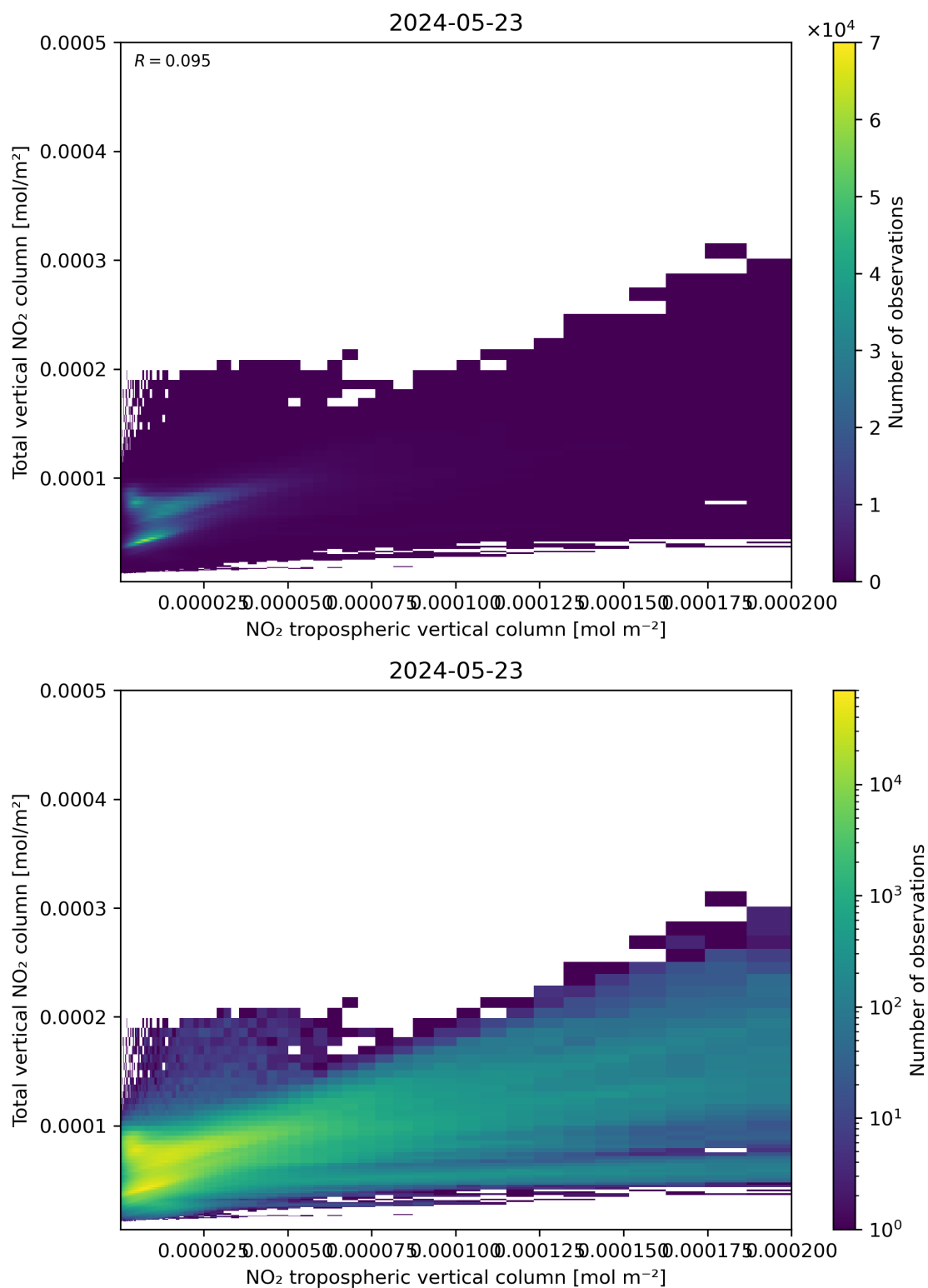
Figure 128: Scatter density plot of “NO 2 tropospheric vertical column” against “Total vertical NO 2 column” for 2024-05-23 to 2024-05-24.
