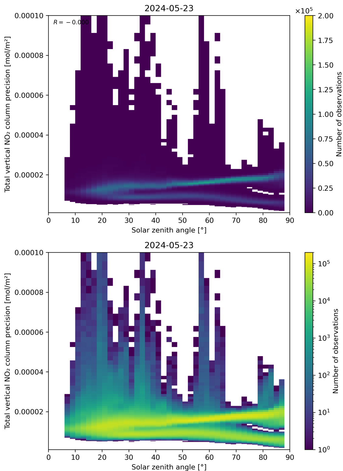
Figure 154: Scatter density plot of “Solar zenith angle” against “Total vertical NO 2 column precision” for 2024-05-23 to 2024-05-24.
