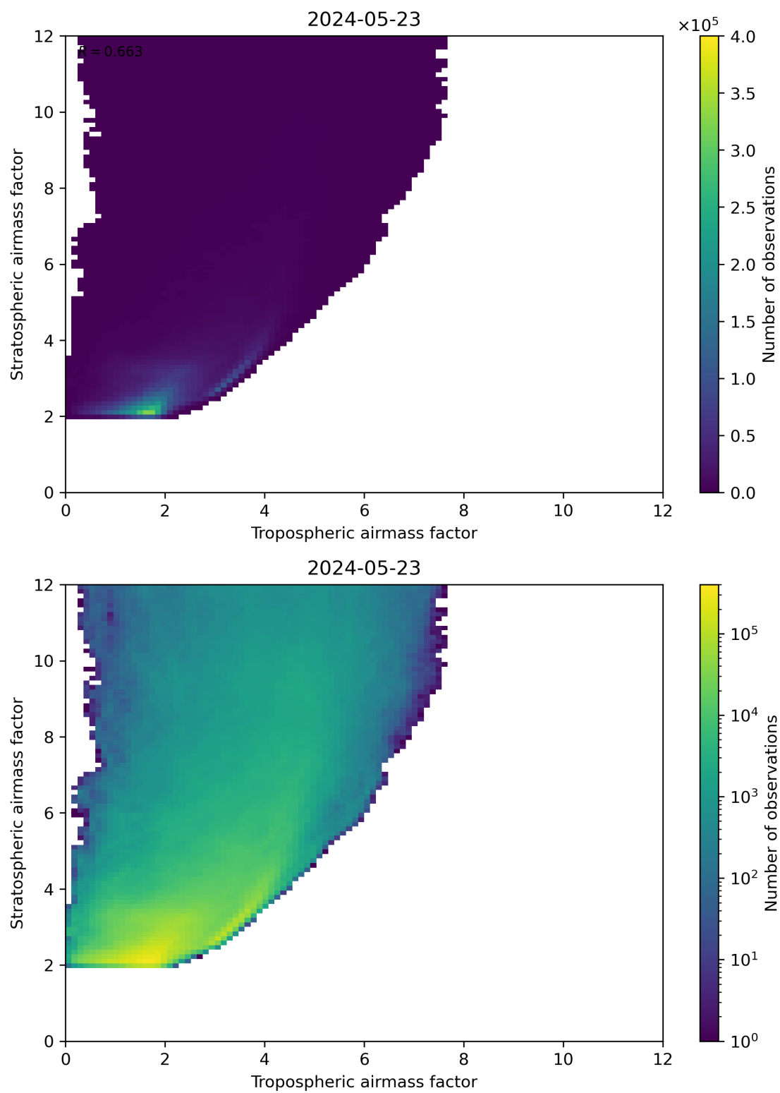
Figure 71: Scatter density plot of “Tropospheric airmass factor” against “Stratospheric airmass factor” for 2024-05-23 to 2024-05-24.
