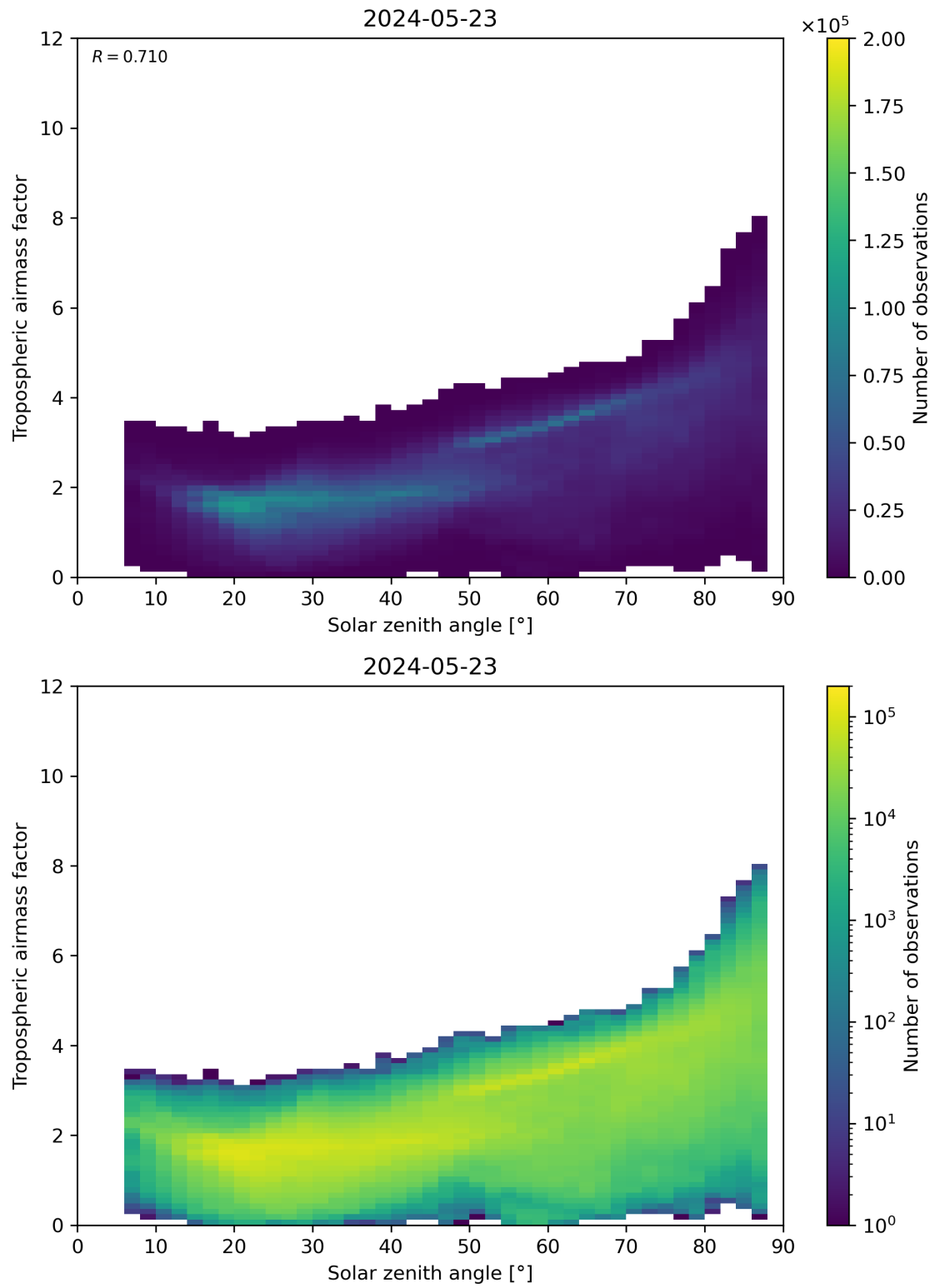
Figure 147: Scatter density plot of “Solar zenith angle” against “Tropospheric airmass factor” for 2024-05-23 to 2024-05-24.
