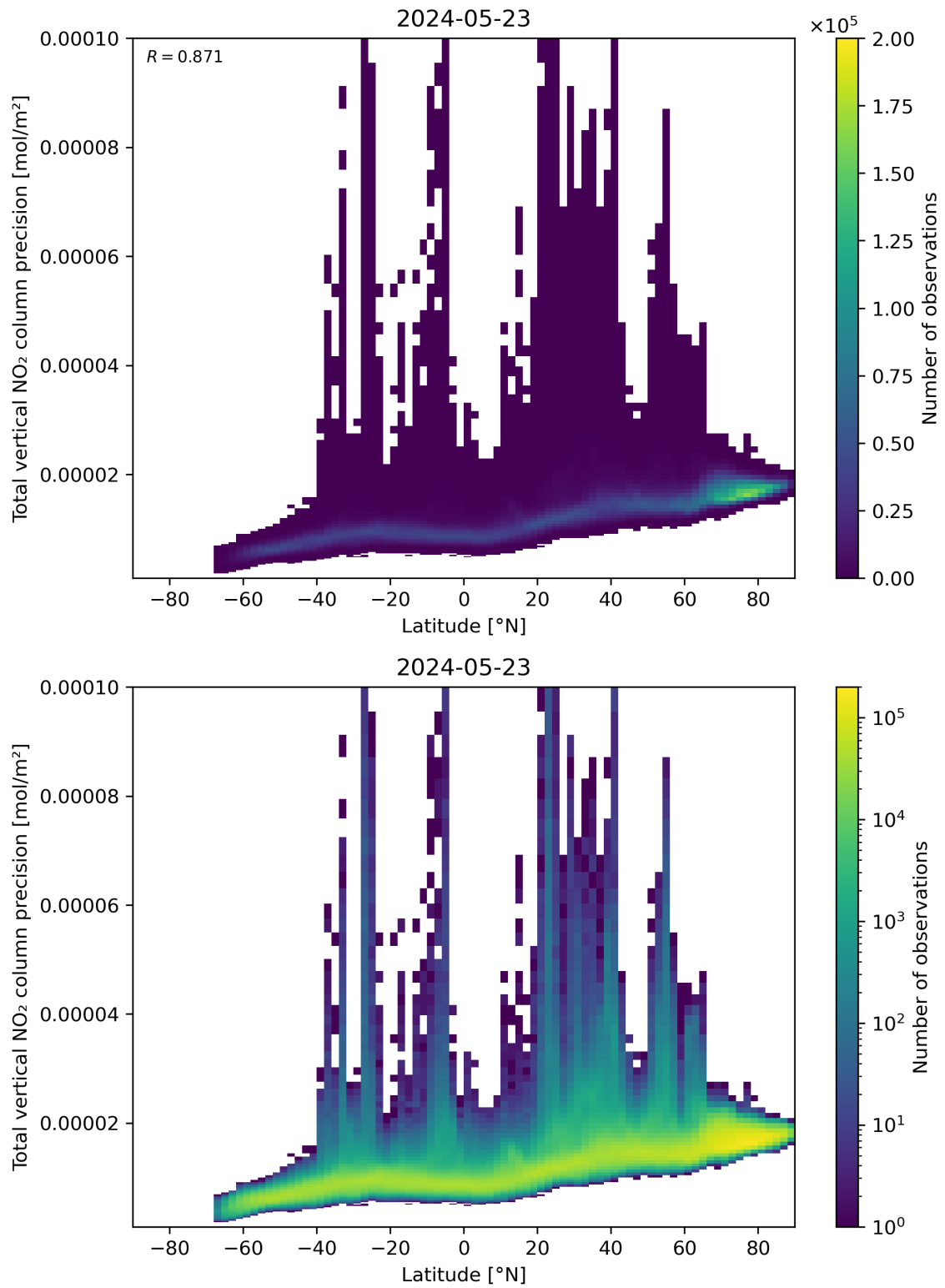
Figure 91: Scatter density plot of “Latitude” against “Total vertical NO 2 column precision” for 2024-05-23 to 2024-05-24.
