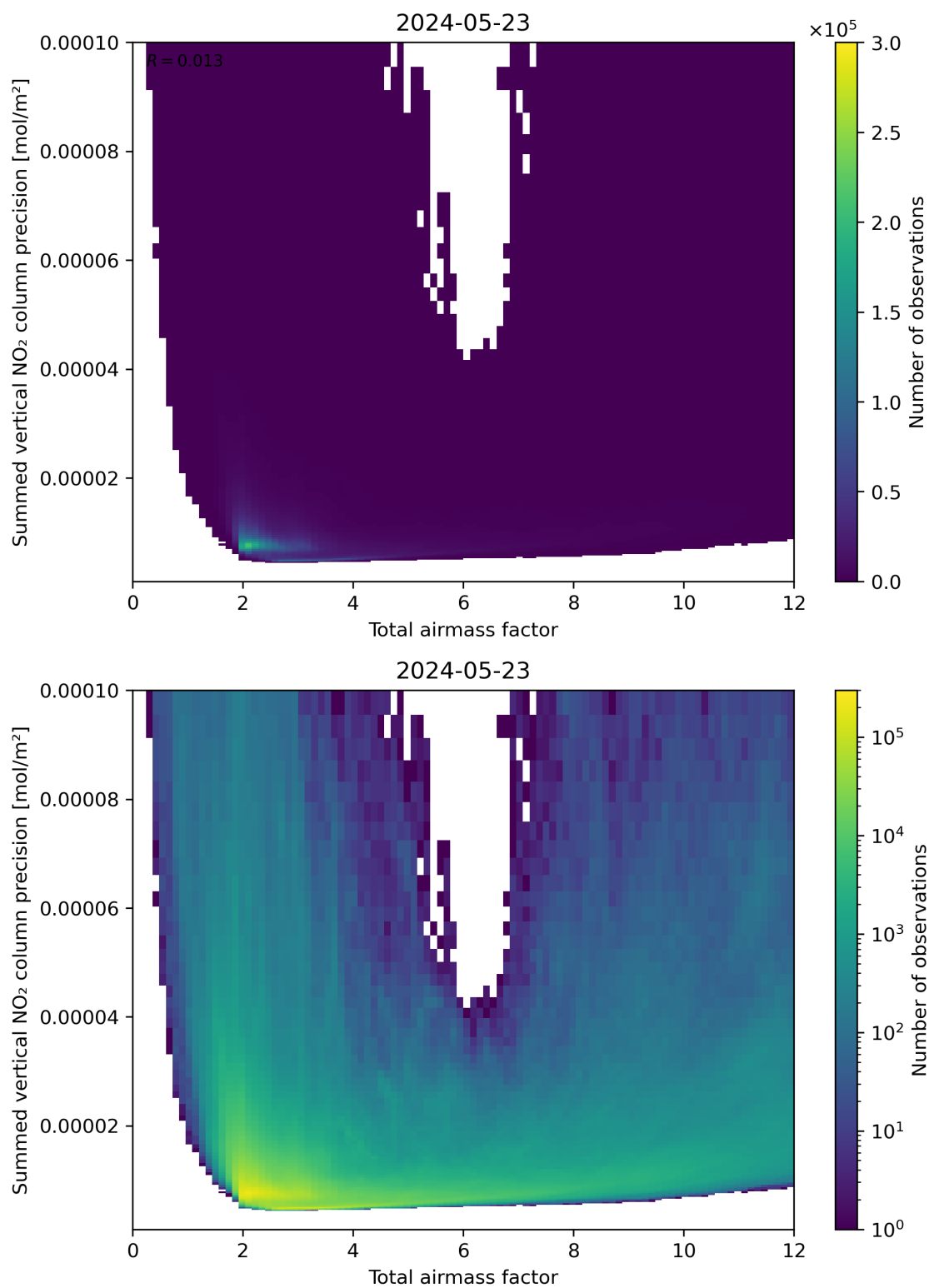
Figure 66: Scatter density plot of “Total airmass factor” against “Summed vertical NO 2 column precision” for 2024-05-23 to 2024-05-24.
