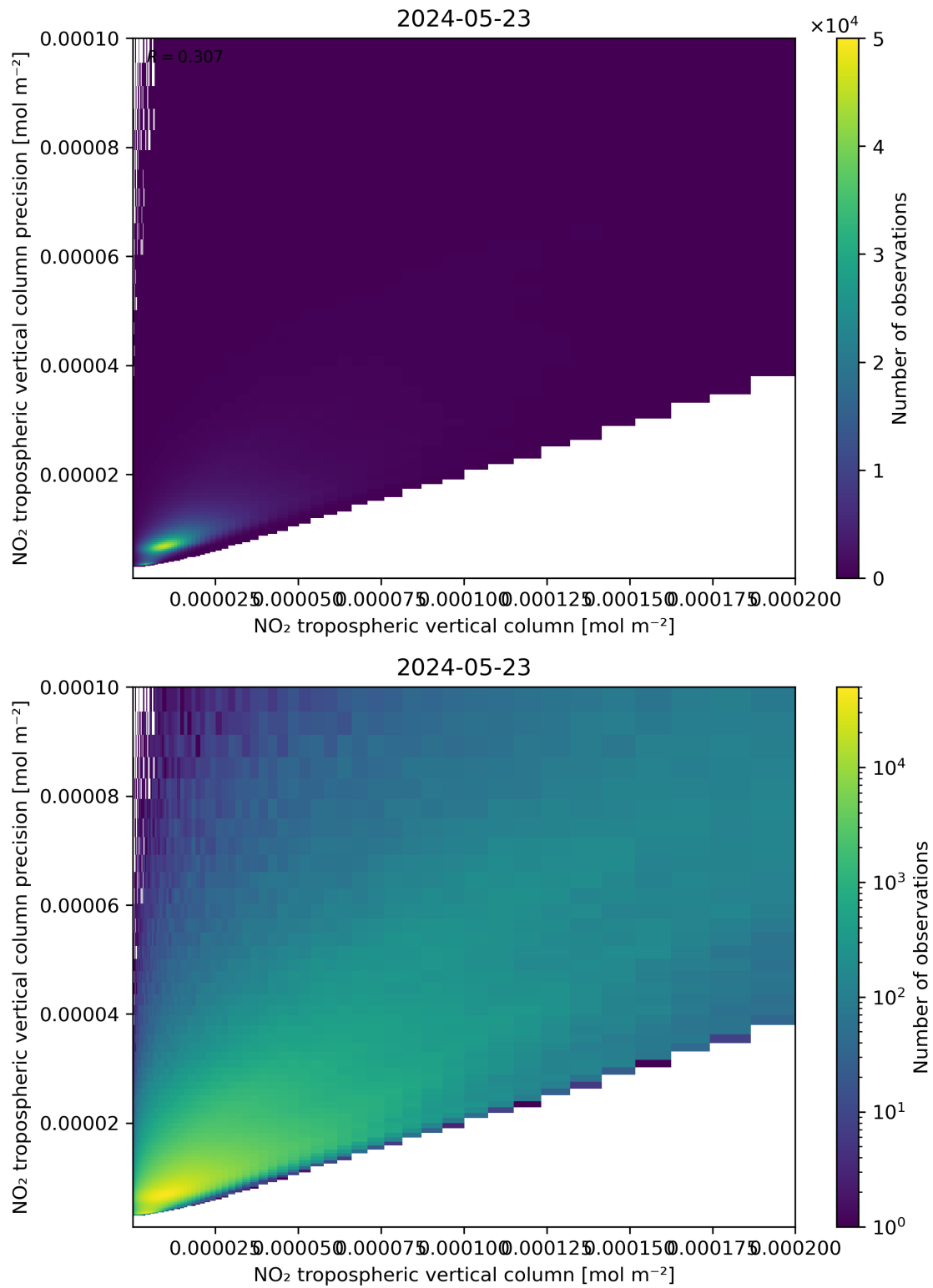
Figure 130: Scatter density plot of “NO 2 tropospheric vertical column” against “NO 2 tropospheric vertical column precision” for 2024-05-23 to 2024-05-24.
