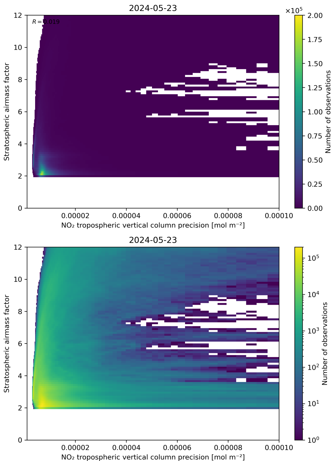
Figure 131: Scatter density plot of “NO 2 tropospheric vertical column precision” against “Stratospheric airmass factor” for 2024-05-23 to 2024-05-24.
