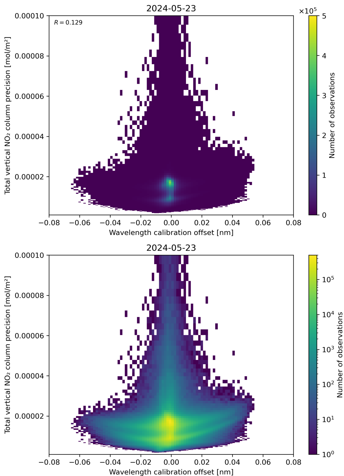
Figure 180: Scatter density plot of “Wavelength calibration offset” against “Total vertical NO 2 column precision” for 2024-05-23 to 2024-05-24.
