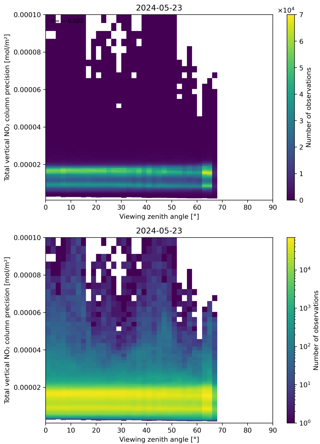
Figure 168: Scatter density plot of “Viewing zenith angle” against “Total vertical NO 2 column precision” for 2024-05-23 to 2024-05-24.
