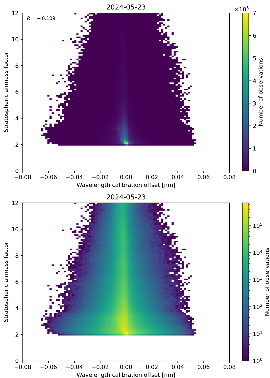
Figure 174: Scatter density plot of “Wavelength calibration offset” against “Stratospheric air mass factor” for 2024-05-23 to 2024-05-24.
