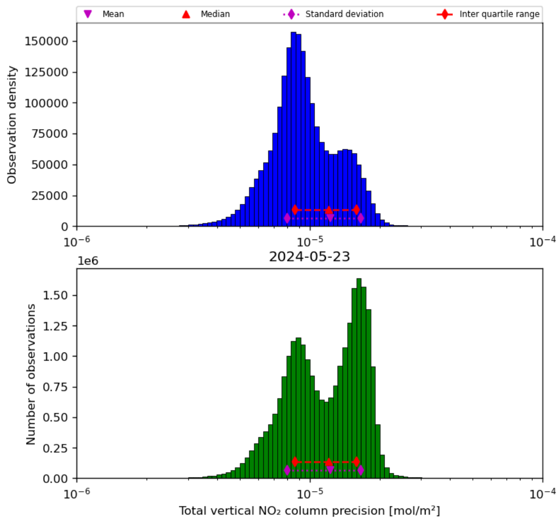
Figure 39: Histogram of “Total vertical NO 2 column precision” for 2024-05-23 to 2024-05-24
