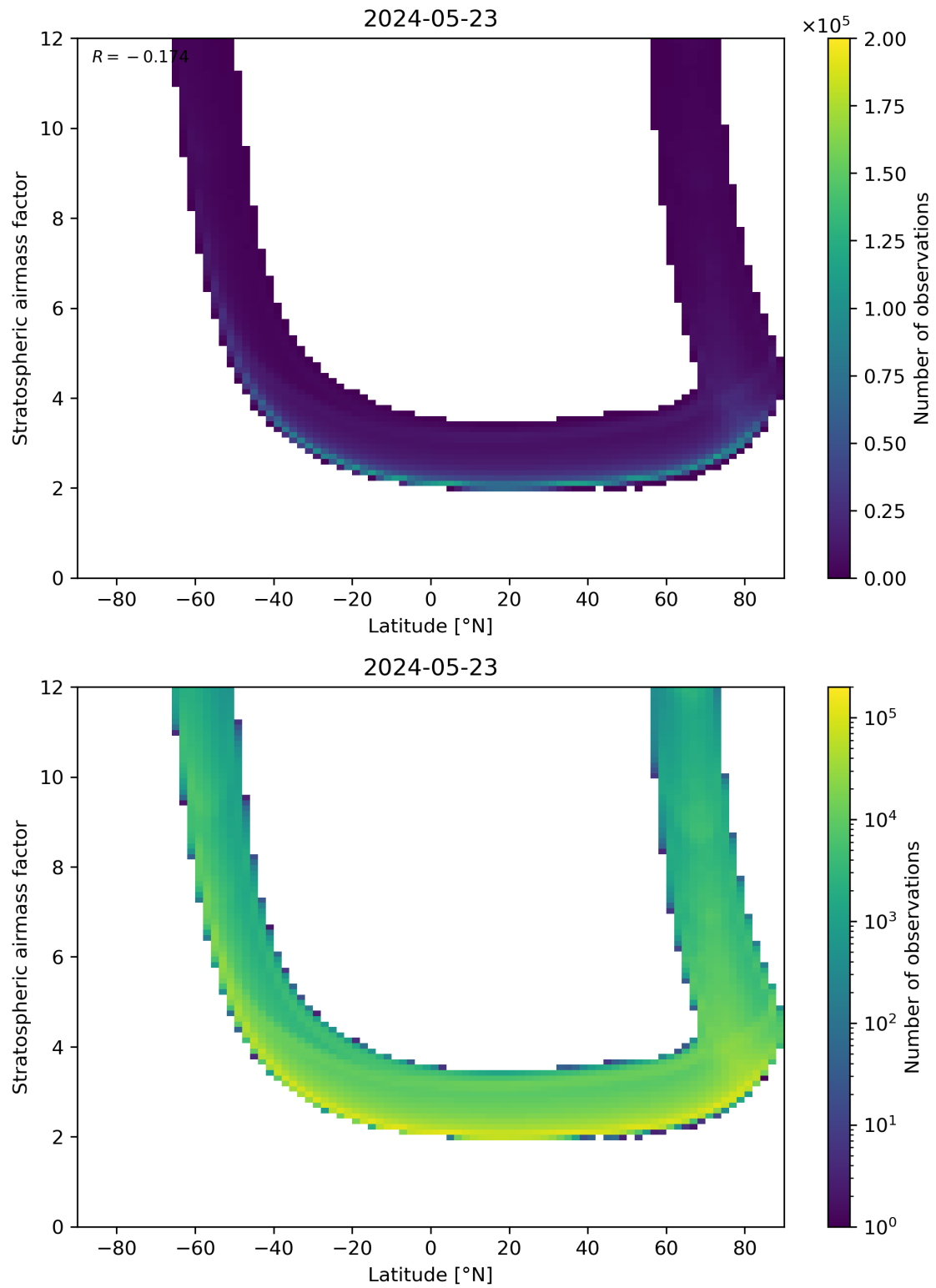
Figure 83: Scatter density plot of “Latitude” against “Stratospheric air mass factor” for 2024-05-23 to 2024-05-24.
