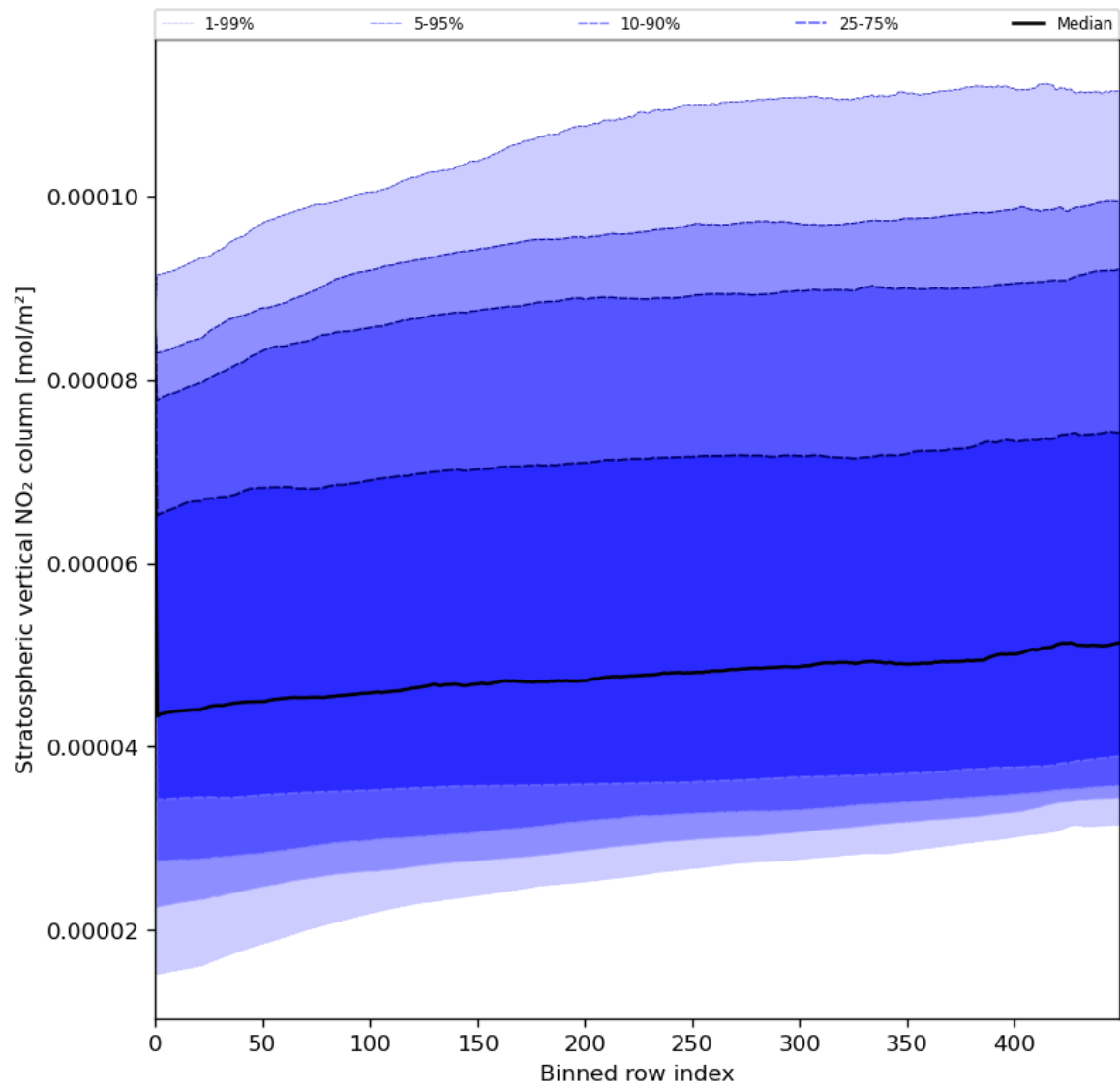
Figure 53: Along track statistics of “Stratospheric vertical NO 2 column” for 2024-05-23 to 2024-05-24
