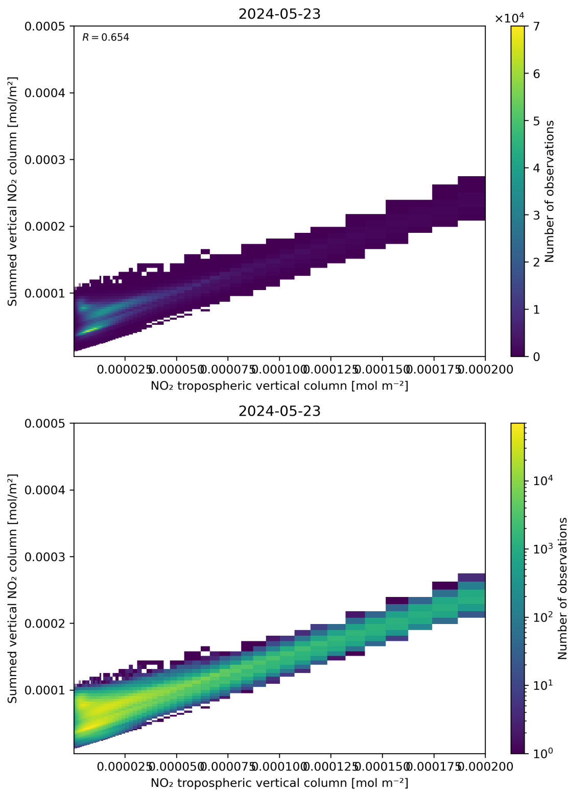
Figure 126: Scatter density plot of “NO 2 tropospheric vertical column” against “Summed vertical NO 2 column” for 2024-05-23 to 2024-05-24.
