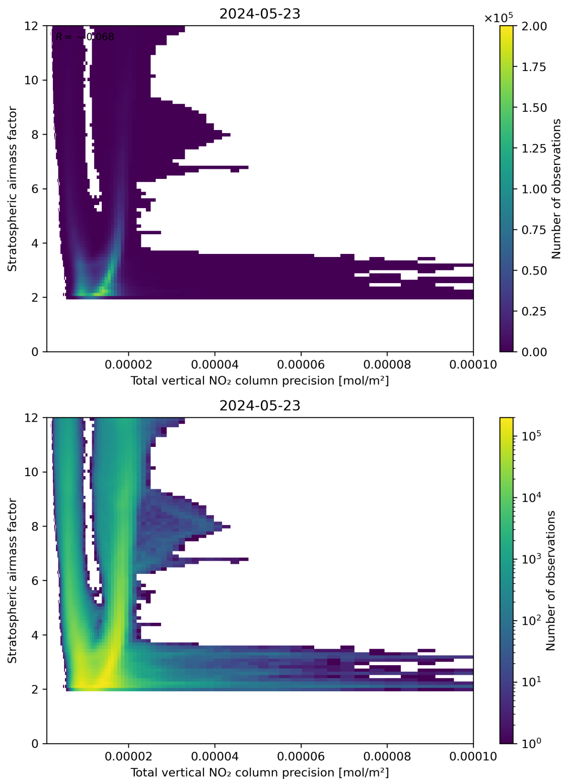
Figure 115: Scatter density plot of “Total vertical NO 2 column precision” against “Stratospheric air mass factor” for 2024-05-23 to 2024-05-24.
