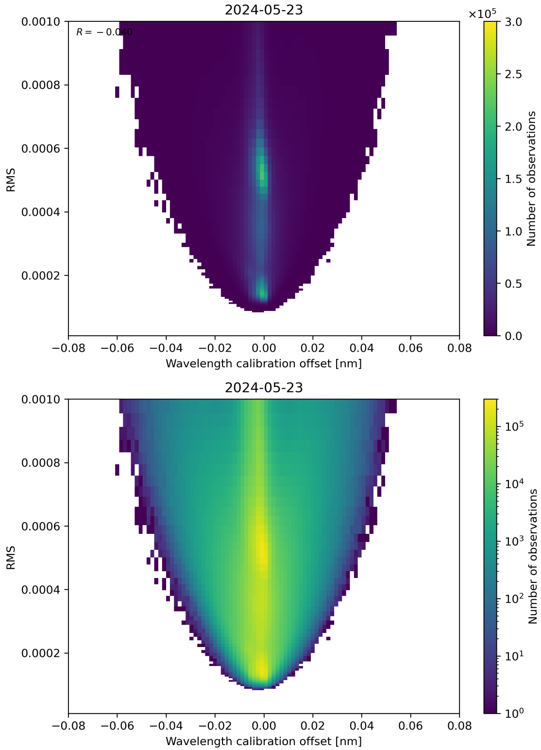
Figure 181: Scatter density plot of “Wavelength calibration offset” against “RMS” for 2024-05-23 to 2024-05-24.
