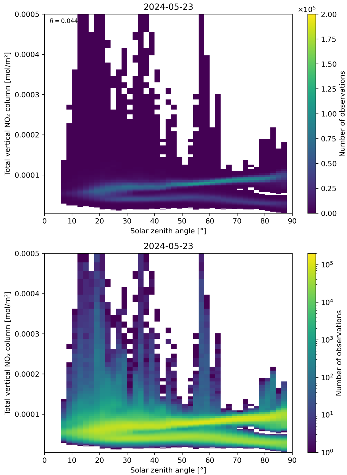
Figure 153: Scatter density plot of “Solar zenith angle” against “Total vertical NO 2 column” for 2024-05-23 to 2024-05-24.
