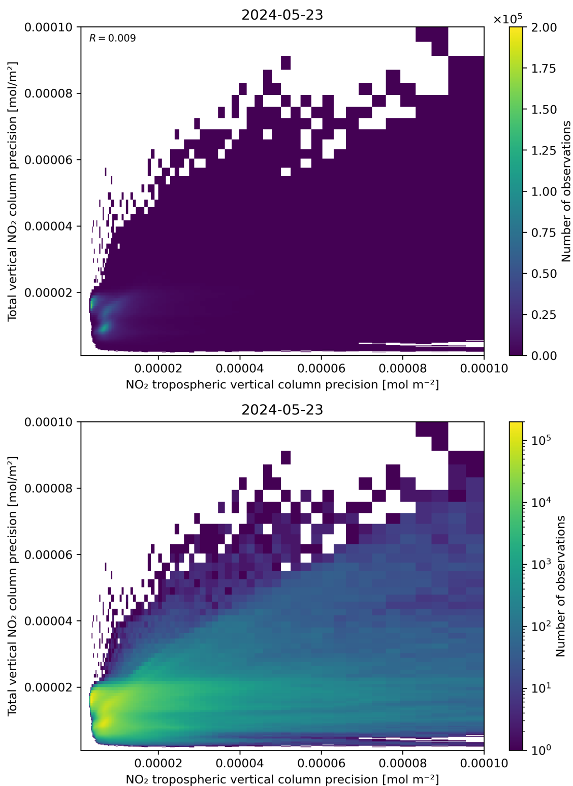
Figure 139: Scatter density plot of “NO 2 tropospheric vertical column precision” against “Total vertical NO 2 column precision” for 2024-05-23 to 2024-05-24.
