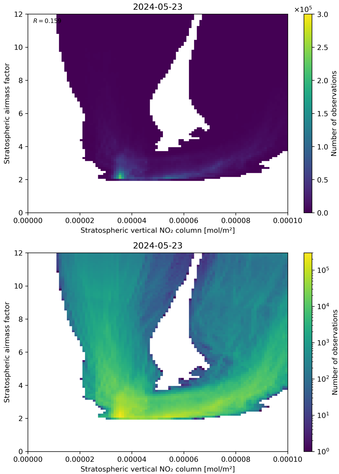
Figure 96: Scatter density plot of “Stratospheric vertical NO 2 column” against “Stratospheric airmass factor” for 2024-05-23 to 2024-05-24.
