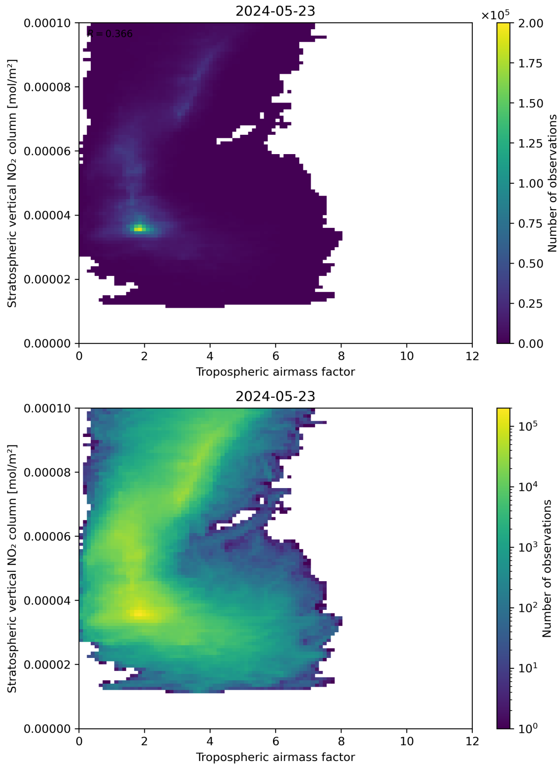
Figure 74: Scatter density plot of “Tropospheric air mass factor” against “Stratospheric vertical NO 2 column” for 2024-05-23 to 2024-05-24.
