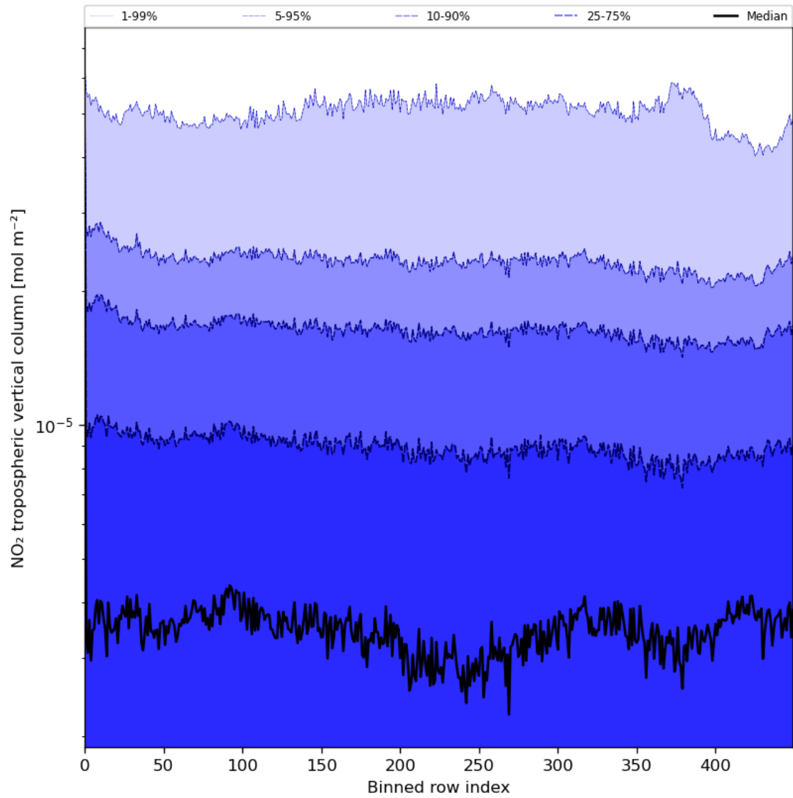
Figure 46: Along track statistics of “NO 2 tropospheric vertical column” for 2024-05-23 to 2024-05-24
