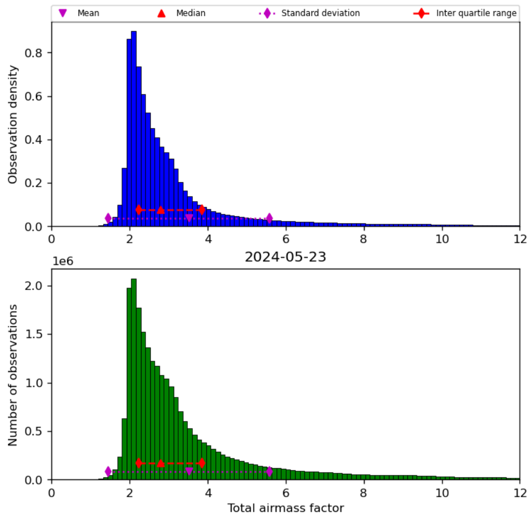
Figure 32: Histogram of “Total airmass factor” for 2024-05-23 to 2024-05-24
