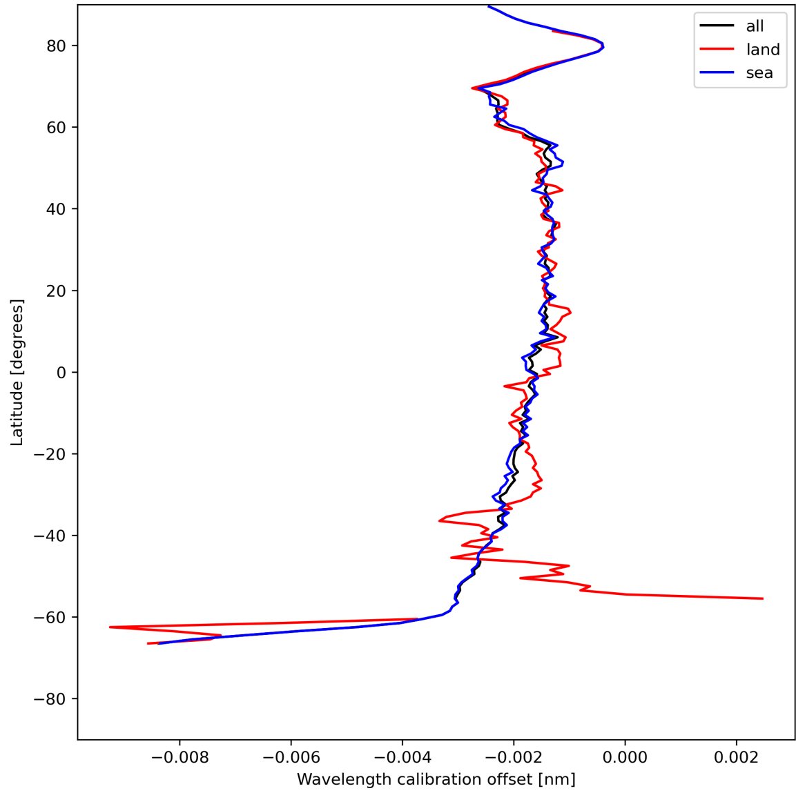
Figure 18: Zonal average of “Wavelength calibration offset” for 2024-05-23 to 2024-05-24.
