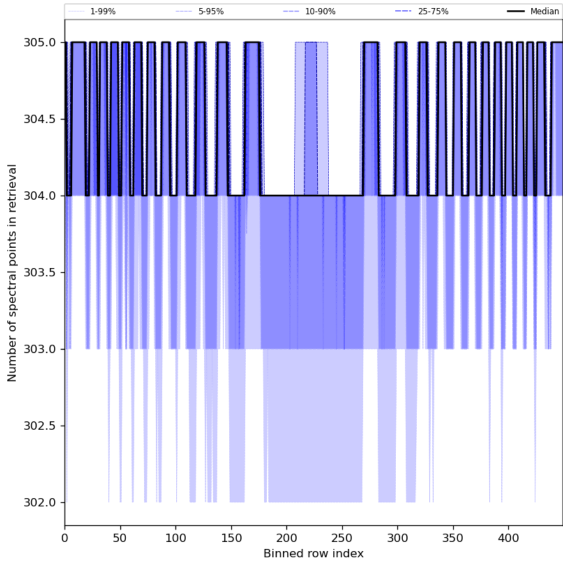
Figure 50: Along track statistics of “Number of spectral points in retrieval” for 2024-05-23 to 2024-05-24
