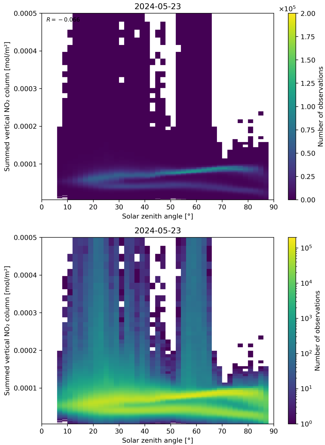
Figure 151: Scatter density plot of “Solar zenith angle” against “Summed vertical NO 2 column” for 2024-05-23 to 2024-05-24.
