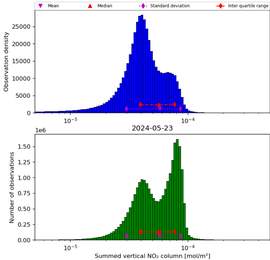
Figure 40: Histogram of “Summed vertical NO 2 column” for 2024-05-23 to 2024-05-24
