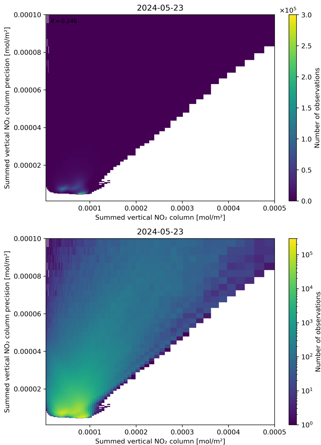
Figure 105: Scatter density plot of “Summed vertical NO 2 column” against “Summed vertical NO 2 column precision” for 2024-05-23 to 2024-05-24.
