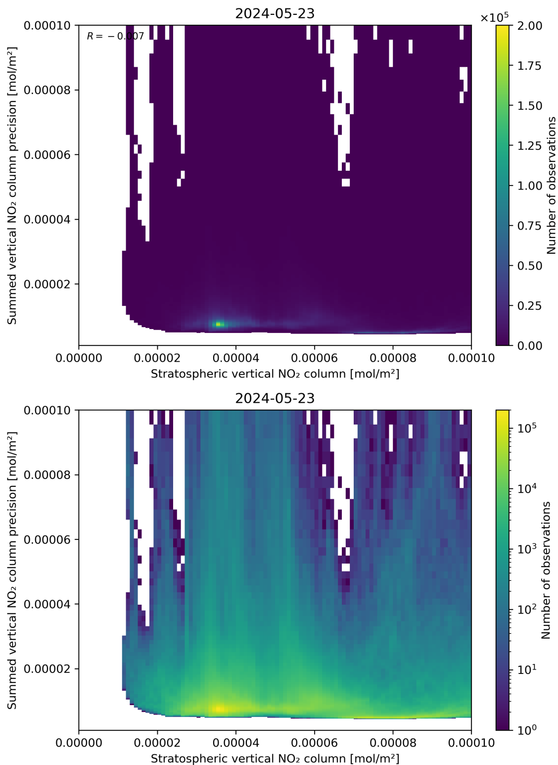
Figure 99: Scatter density plot of “Stratospheric vertical NO 2 column” against “Summed vertical NO 2 column precision” for 2024-05-23 to 2024-05-24.
