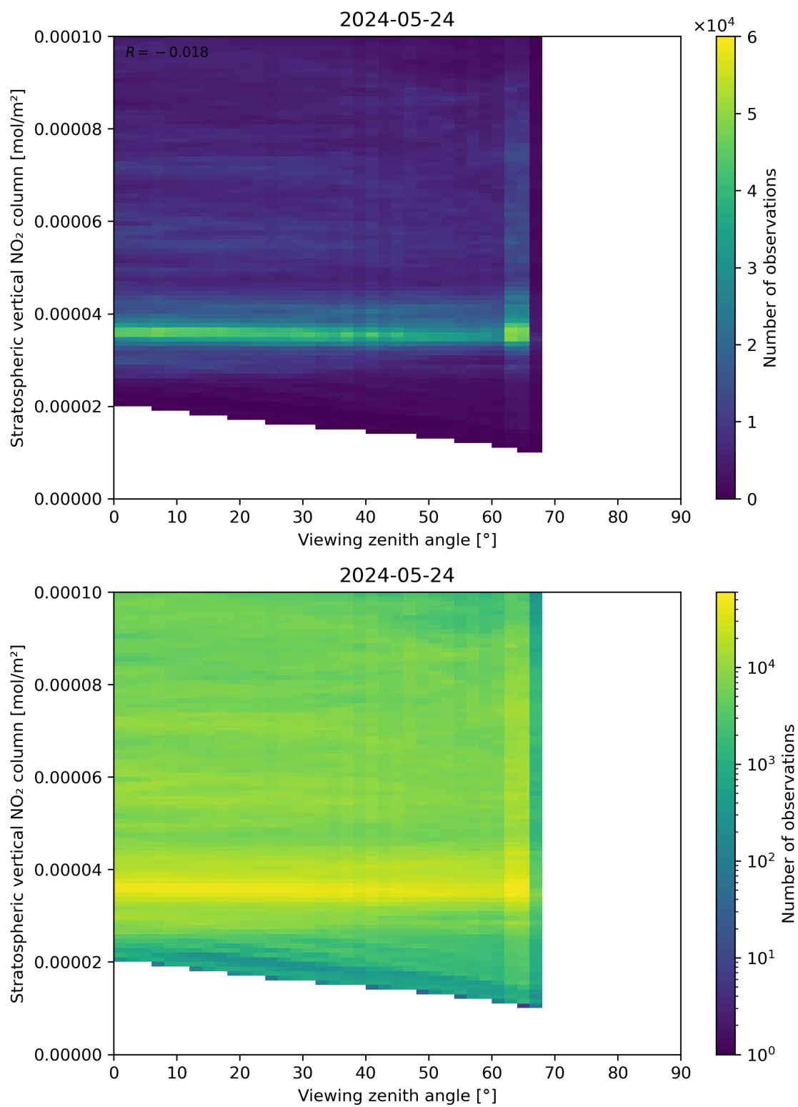
Figure 164: Scatter density plot of “Viewing zenith angle” against “Stratospheric vertical NO 2 column” for 2024-05-23 to 2024-05-25.
