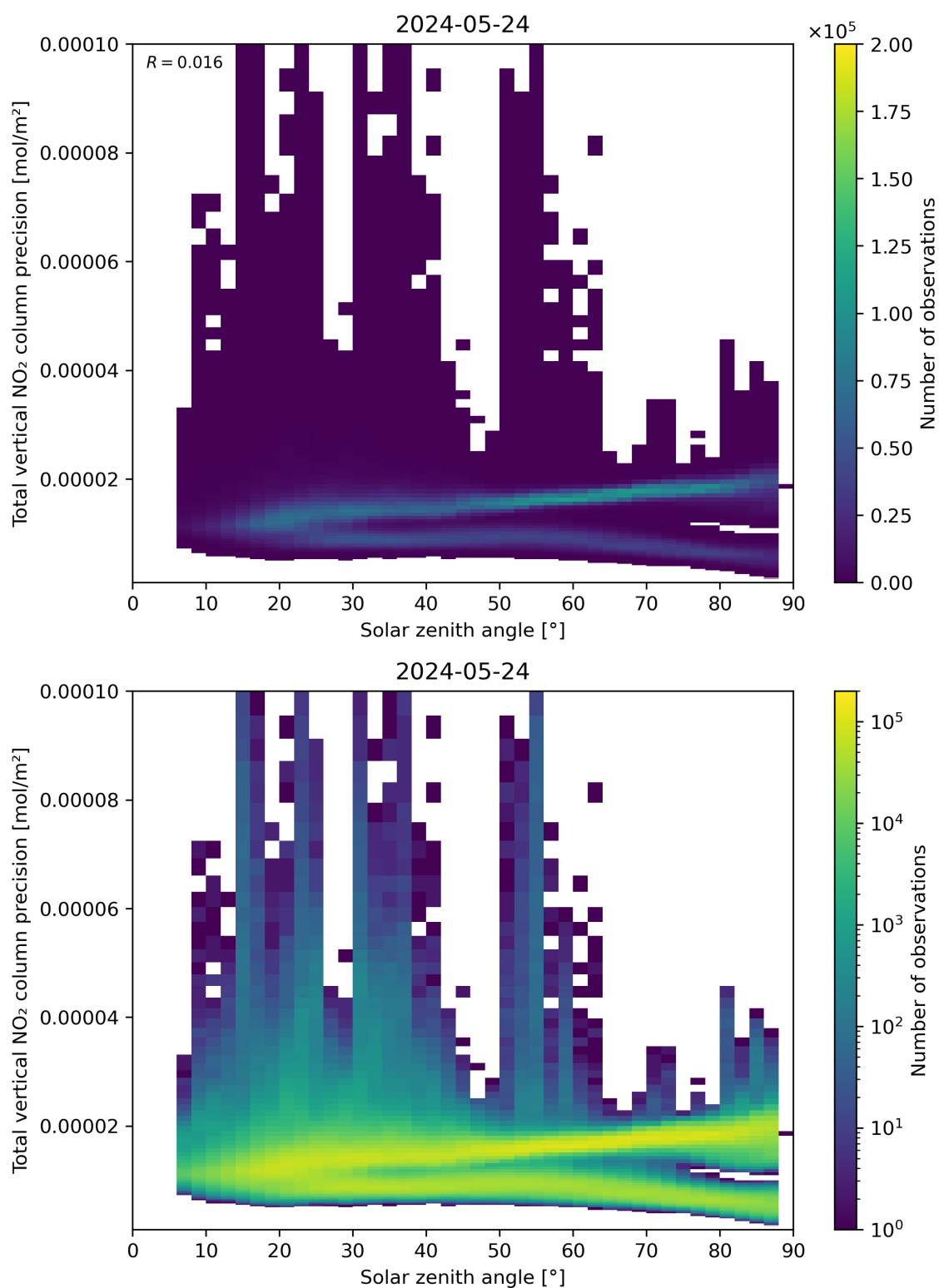
Figure 154: Scatter density plot of “Solar zenith angle” against “Total vertical NO 2 column precision” for 2024-05-23 to 2024-05-25.
