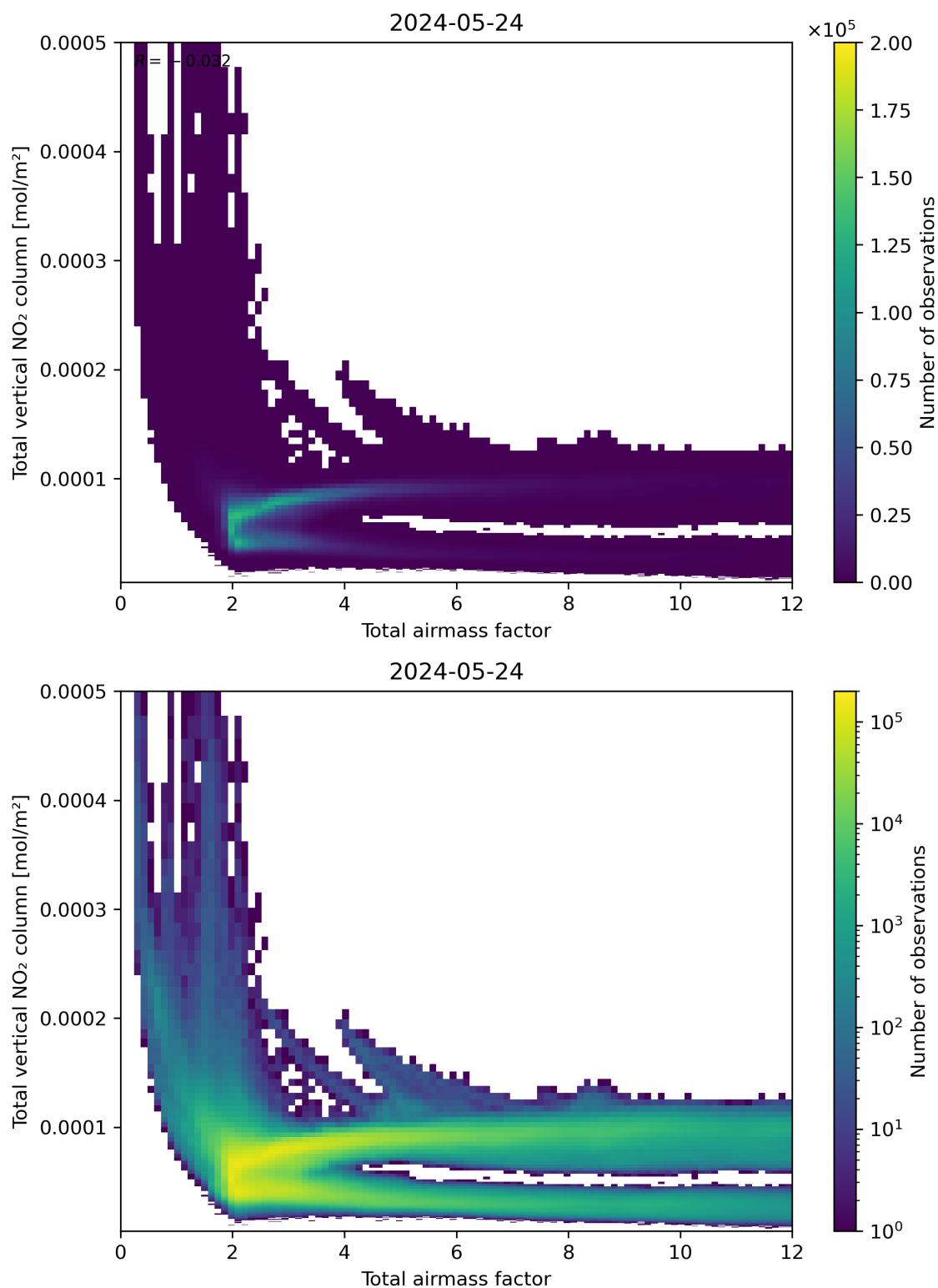
Figure 67: Scatter density plot of “Total airmass factor” against “Total vertical NO 2 column” for 2024-05-23 to 2024-05-25.
