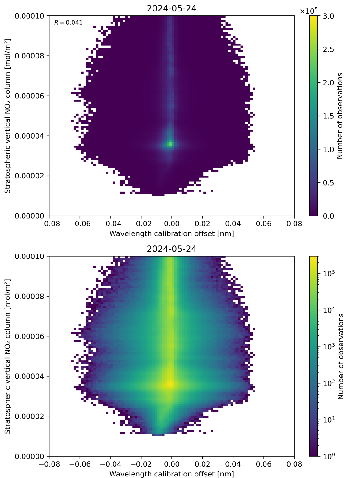
Figure 176: Scatter density plot of “Wavelength calibration offset” against “Stratospheric vertical NO 2 column” for 2024-05-23 to 2024-05-25.
