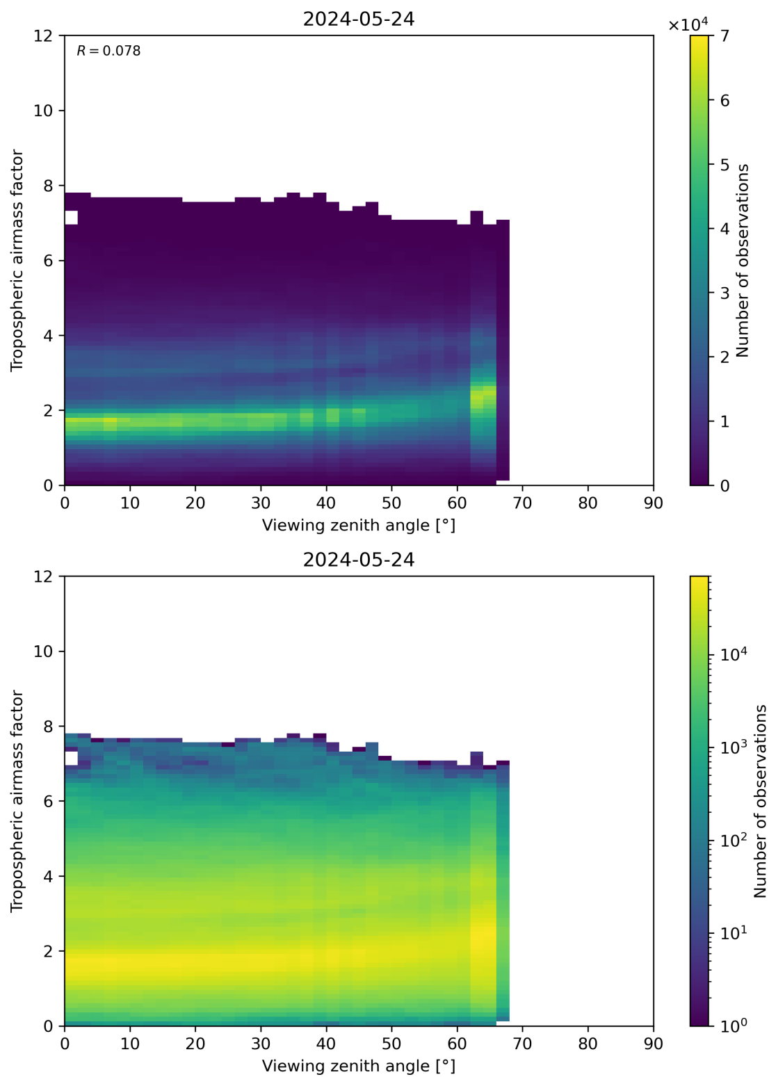
Figure 161: Scatter density plot of “Viewing zenith angle” against “Tropospheric airmass factor” for 2024-05-23 to 2024-05-25.
