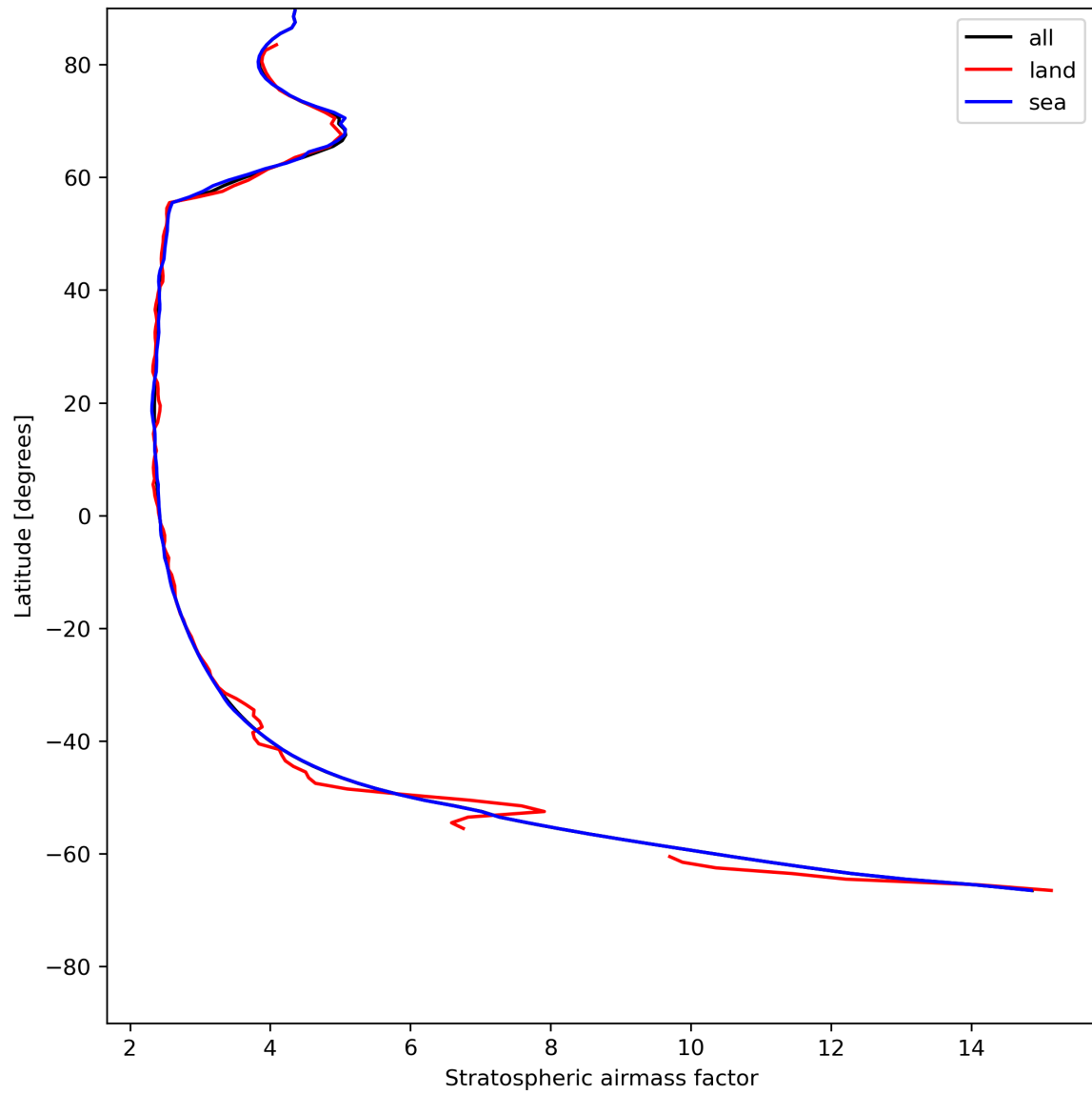
Figure 27: Zonal average of “Stratospheric air mass factor” for 2024-05-23 to 2024-05-25.
