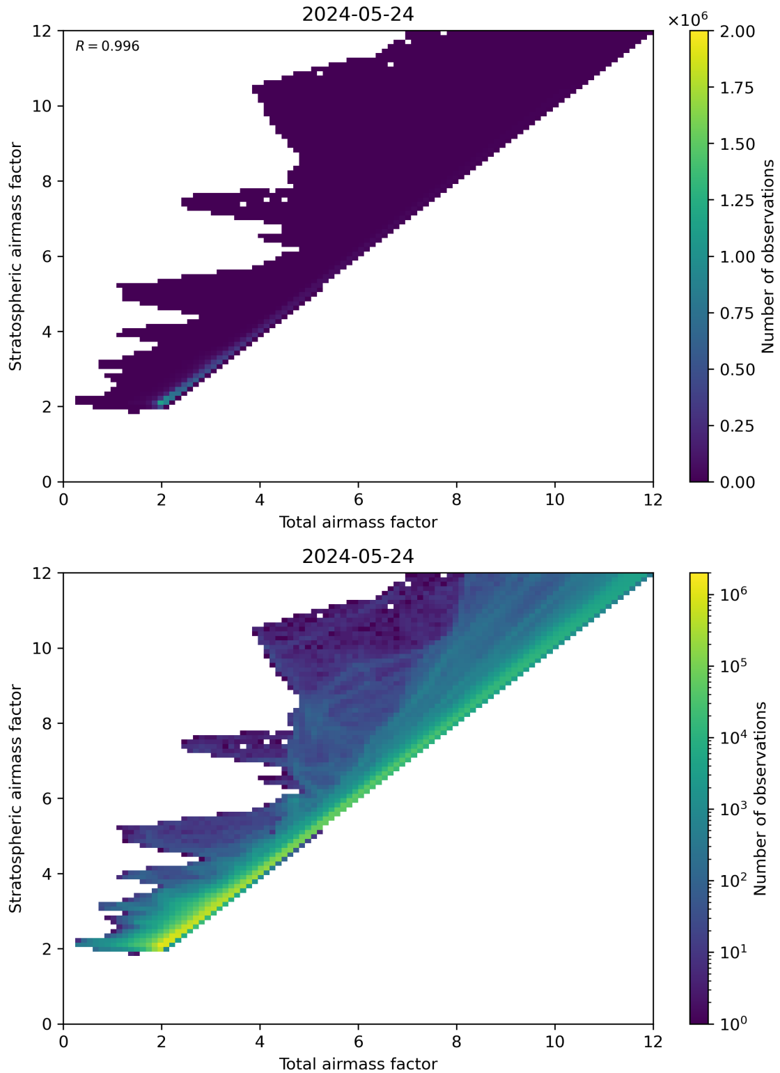
Figure 62: Scatter density plot of “Total airmass factor” against “Stratospheric airmass factor” for 2024-05-23 to 2024-05-25.
