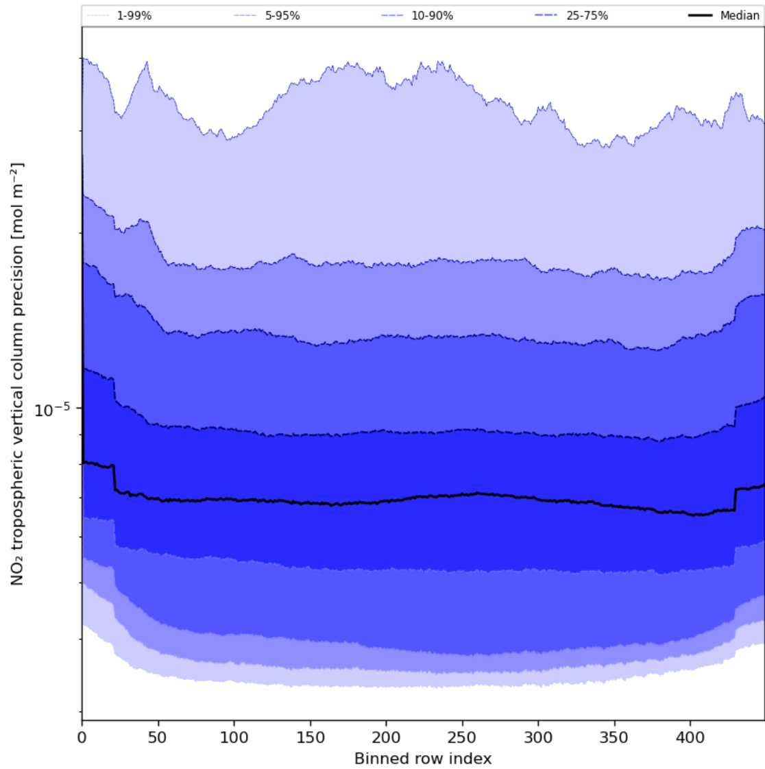
Figure 47: Along track statistics of “NO 2 tropospheric vertical column precision” for 2024-05-23 to 2024-05-25
