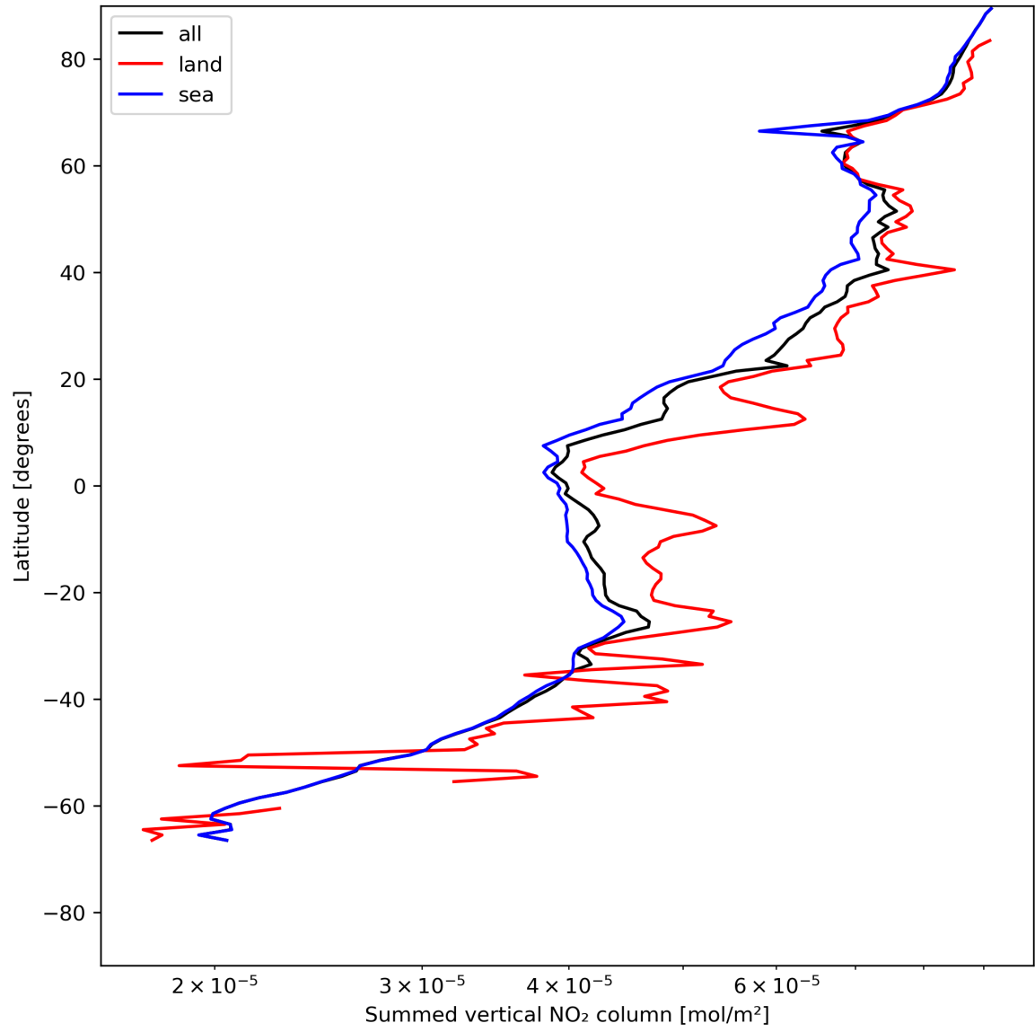
Figure 23: Zonal average of “Summed vertical NO 2 column” for 2024-05-23 to 2024-05-25.
