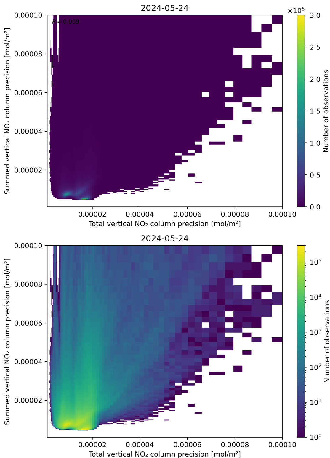
Figure 118: Scatter density plot of “Total vertical NO 2 column precision” against “Summed vertical NO 2 column precision” for 2024-05-23 to 2024-05-25.
