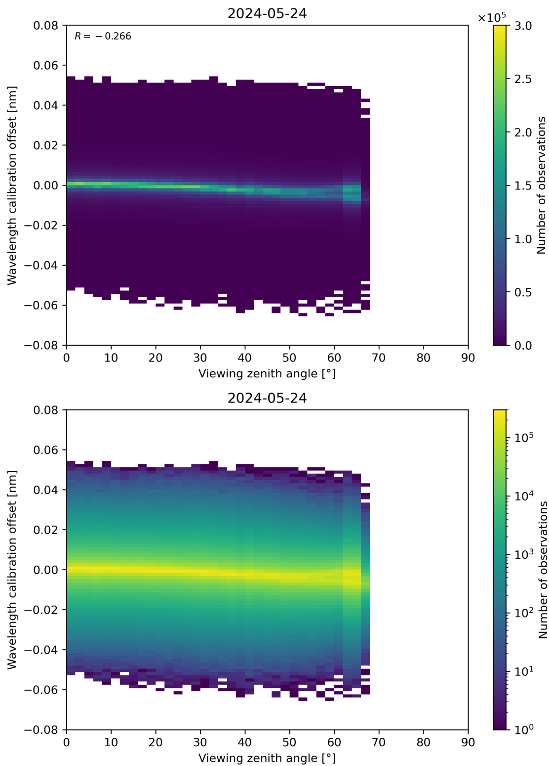
Figure 173: Scatter density plot of “Viewing zenith angle” against “Wavelength calibration offset” for 2024-05-23 to 2024-05-25.
