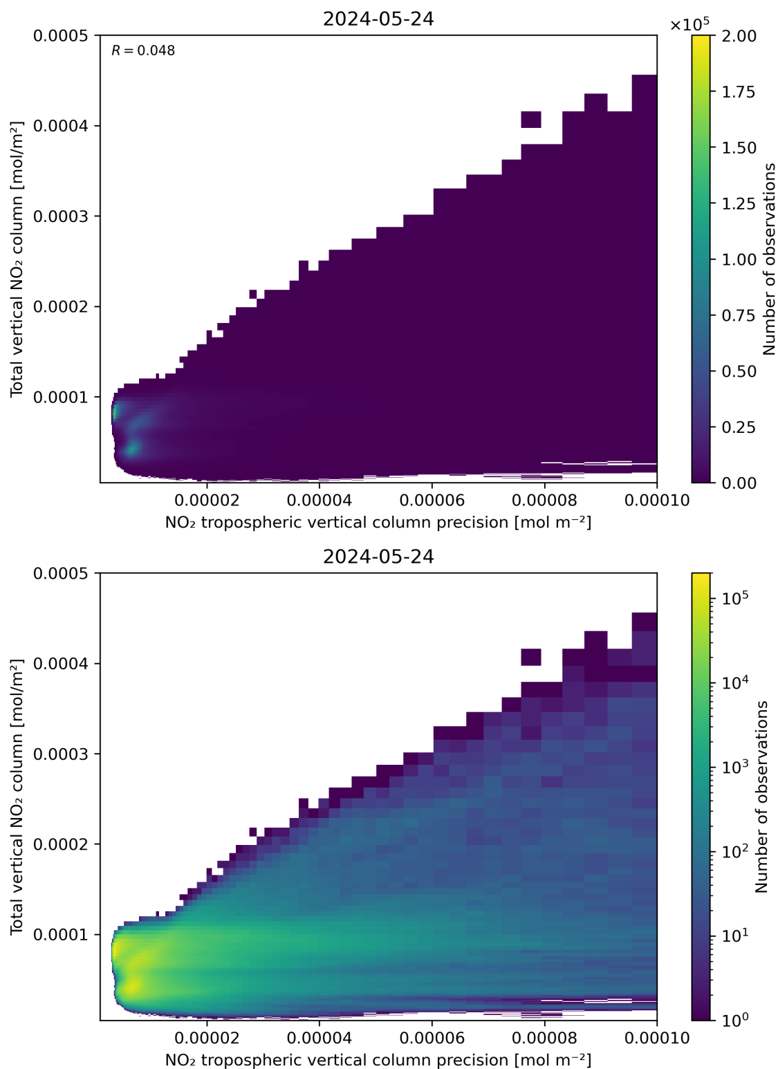
Figure 138: Scatter density plot of “NO 2 tropospheric vertical column precision” against “Total vertical NO 2 column” for 2024-05-23 to 2024-05-25.
