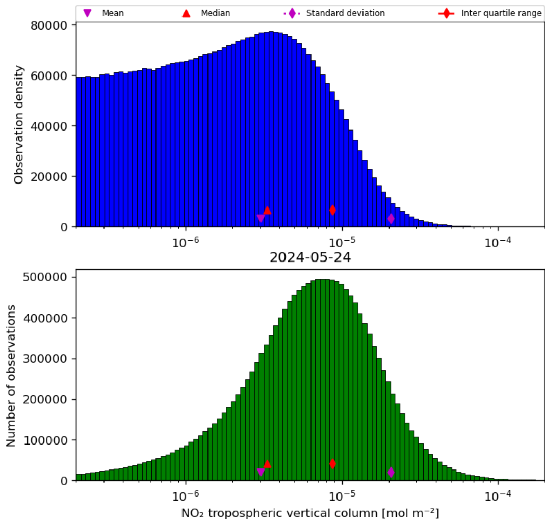
Figure 29: Histogram of “NO 2 tropospheric vertical column” for 2024-05-23 to 2024-05-25
