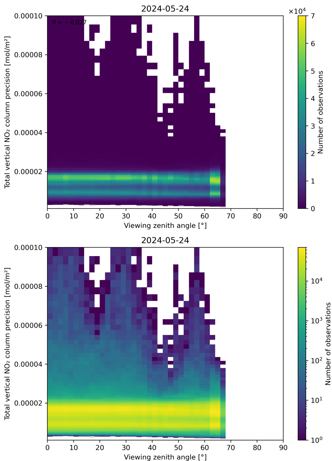
Figure 168: Scatter density plot of “Viewing zenith angle” against “Total vertical NO 2 column precision” for 2024-05-23 to 2024-05-25.
