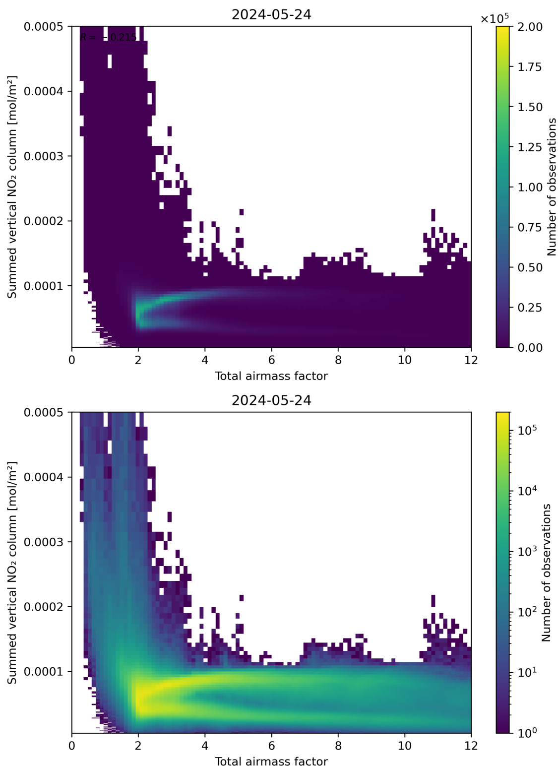
Figure 65: Scatter density plot of “Total airmass factor” against “Summed vertical NO 2 column” for 2024-05-23 to 2024-05-25.
