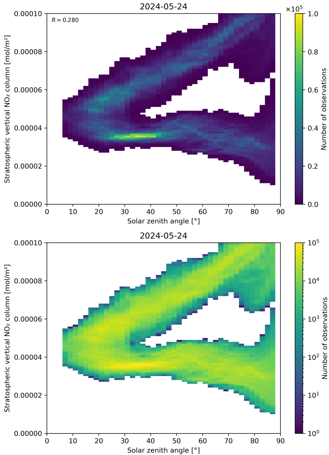
Figure 150: Scatter density plot of “Solar zenith angle” against “Stratospheric vertical NO 2 column” for 2024-05-23 to 2024-05-25.
