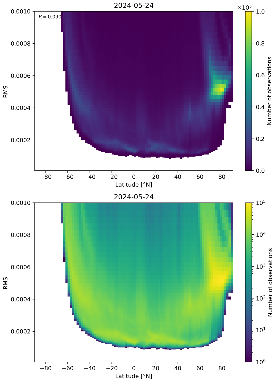
Figure 94: Scatter density plot of “Latitude” against “RMS” for 2024-05-23 to 2024-05-25.
