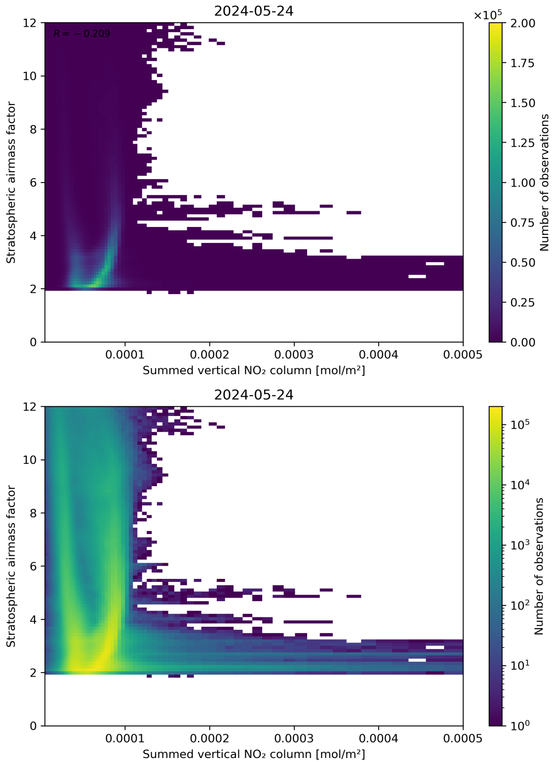
Figure 103: Scatter density plot of “Summed vertical NO 2 column” against “Stratospheric airmass factor” for 2024-05-23 to 2024-05-25.
