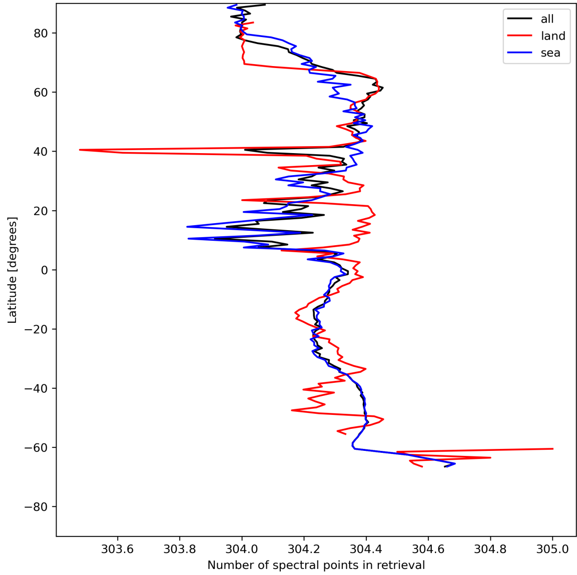
Figure 16: Zonal average of “Number of spectral points in retrieval” for 2024-05-23 to 2024-05-25.
