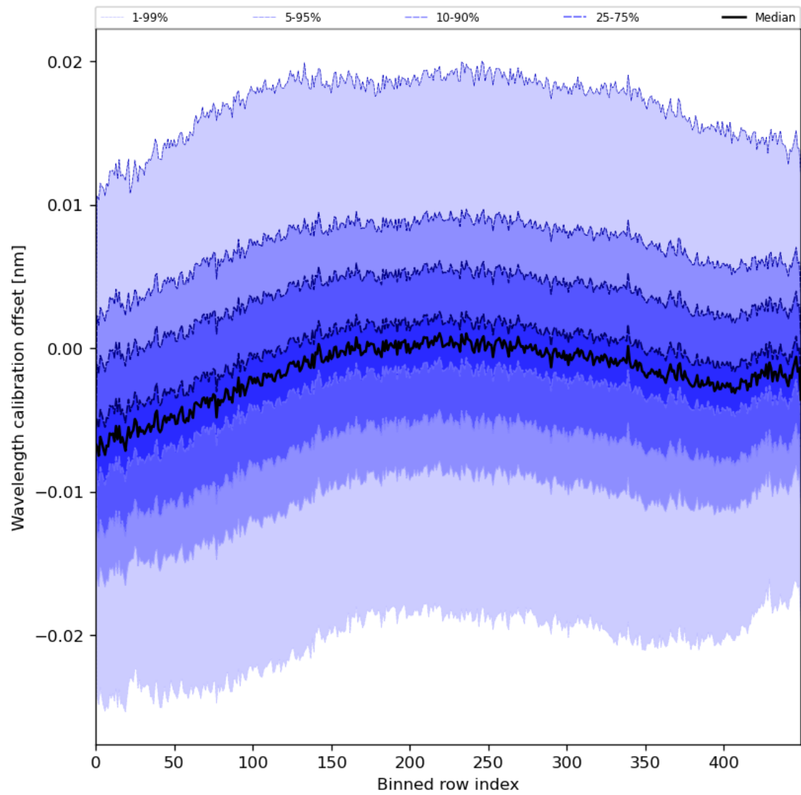
Figure 52: Along track statistics of “Wavelength calibration offset” for 2024-05-23 to 2024-05-25
