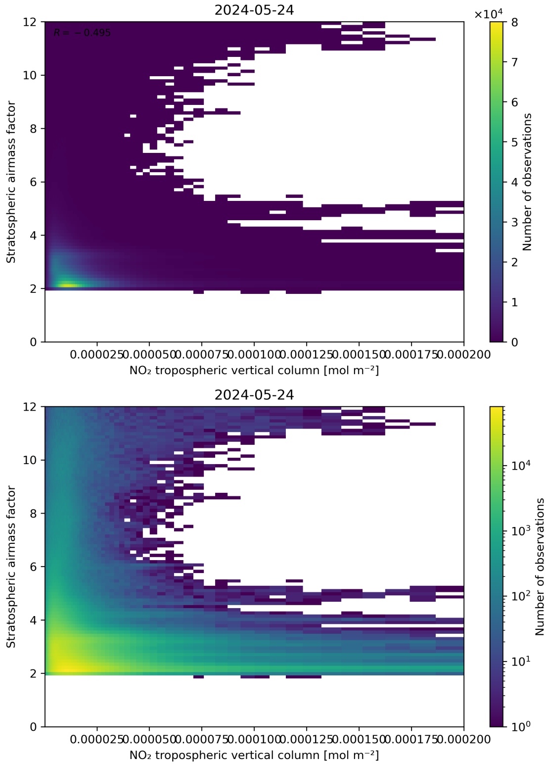
Figure 121: Scatter density plot of “NO 2 tropospheric vertical column” against “Stratospheric air mass factor” for 2024-05-23 to 2024-05-25.
