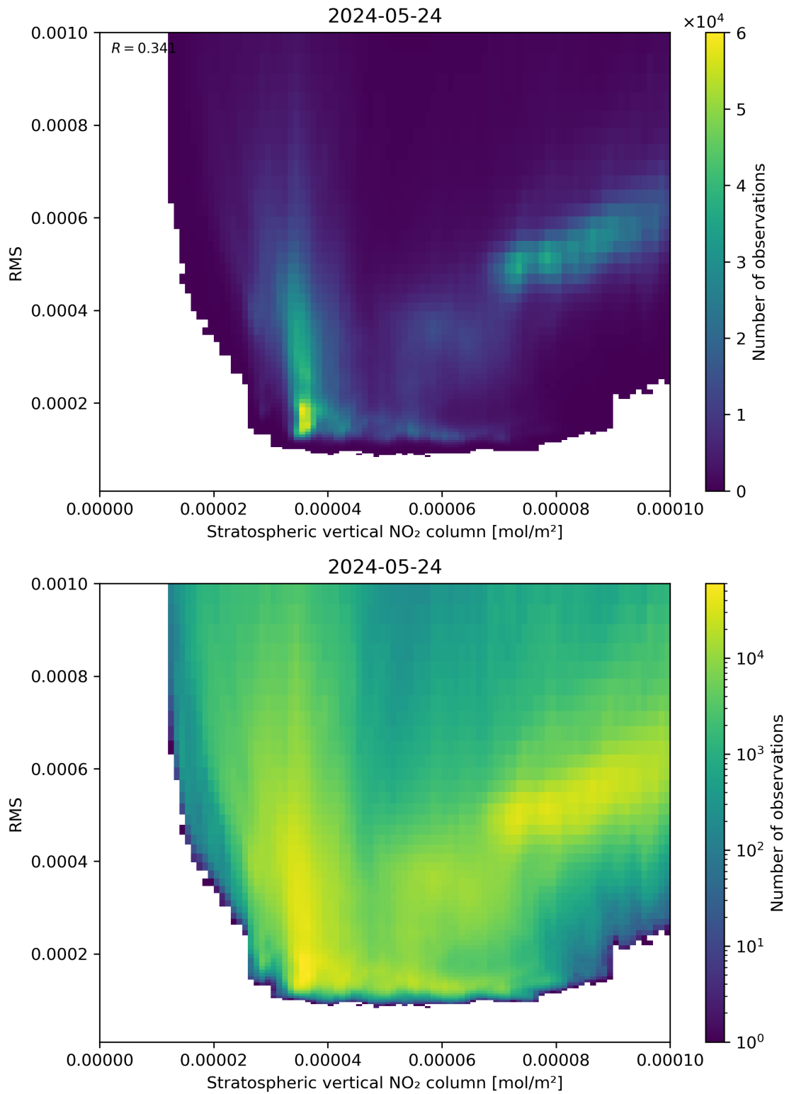
Figure 102: Scatter density plot of “Stratospheric vertical NO 2 column” against “RMS” for 2024-05-23 to 2024-05-25.
