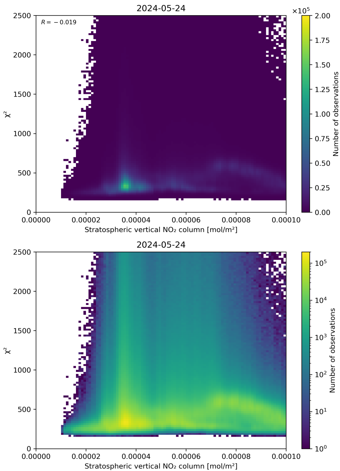
Figure 97: Scatter density plot of “Stratospheric vertical NO 2 column” against “ \chi^2 ” for 2024-05-23 to 2024-05-25.
