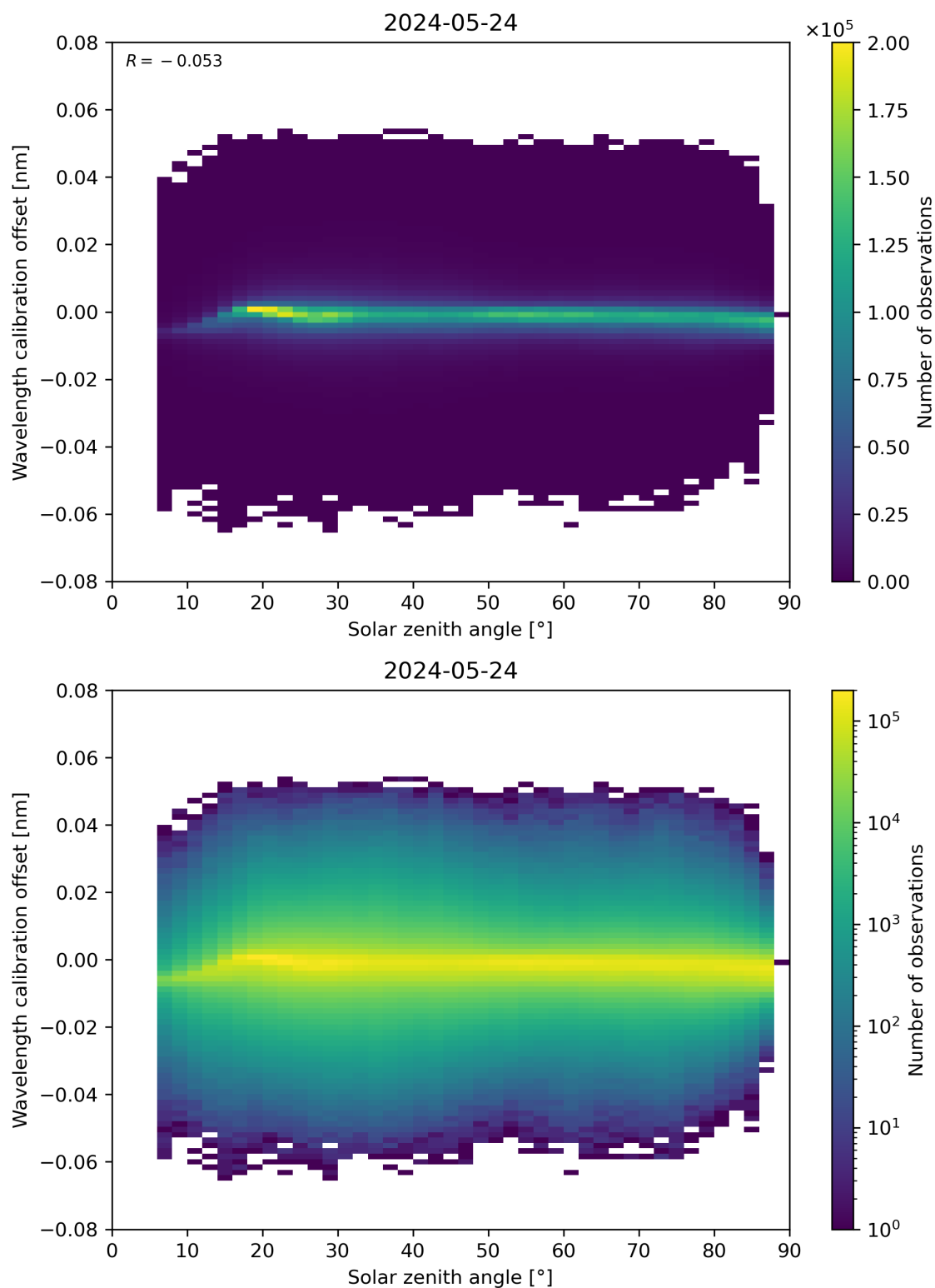
Figure 158: Scatter density plot of “Solar zenith angle” against “Wavelength calibration offset” for 2024-05-23 to 2024-05-25.
