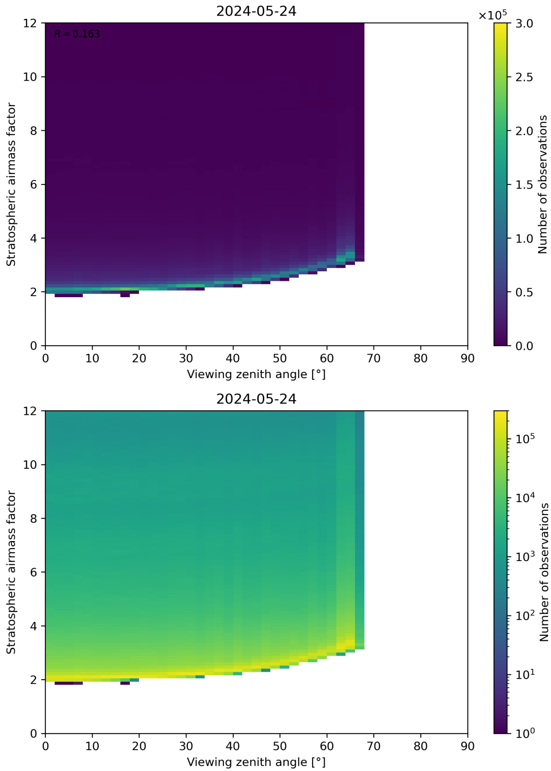
Figure 159: Scatter density plot of “Viewing zenith angle” against “Stratospheric airmass factor” for 2024-05-23 to 2024-05-25.
