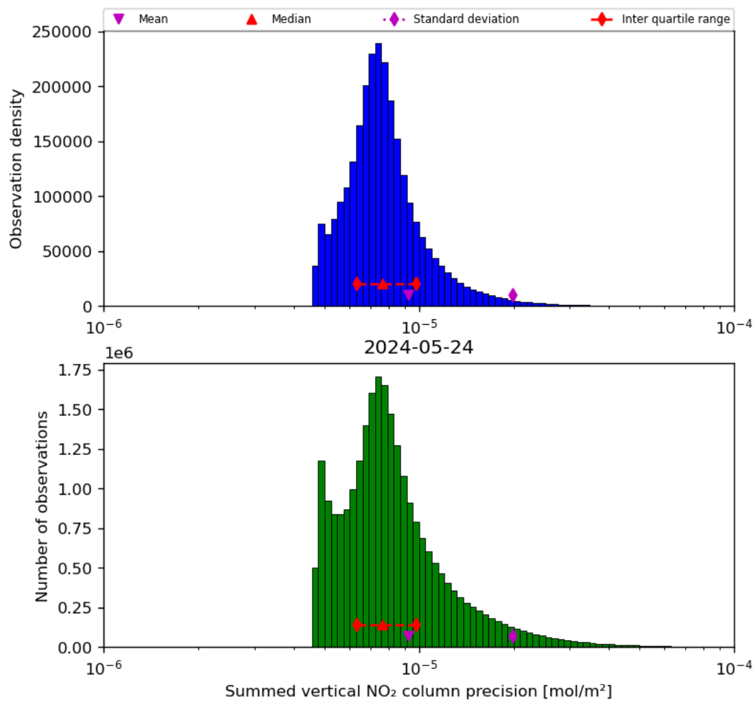
Figure 41: Histogram of “Summed vertical NO 2 column precision” for 2024-05-23 to 2024-05-25
