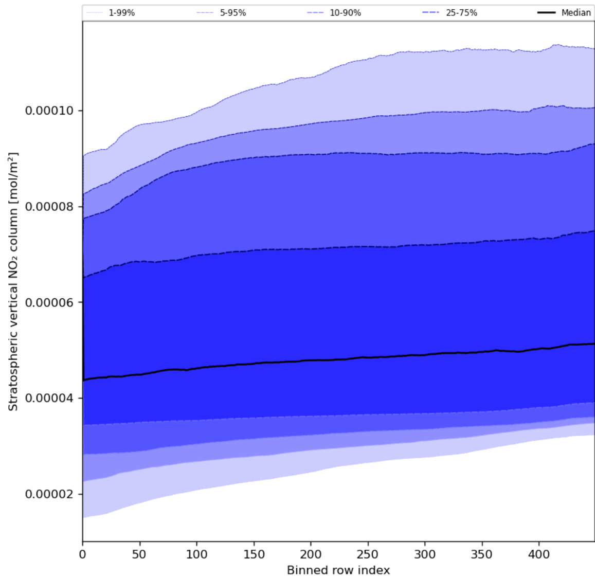
Figure 53: Along track statistics of “Stratospheric vertical NO 2 column” for 2024-05-23 to 2024-05-25
