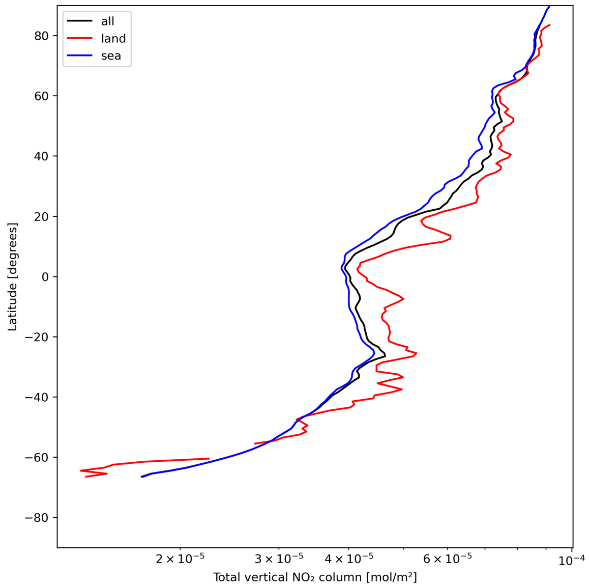
Figure 21: Zonal average of “Total vertical NO 2 column” for 2024-05-23 to 2024-05-25.
