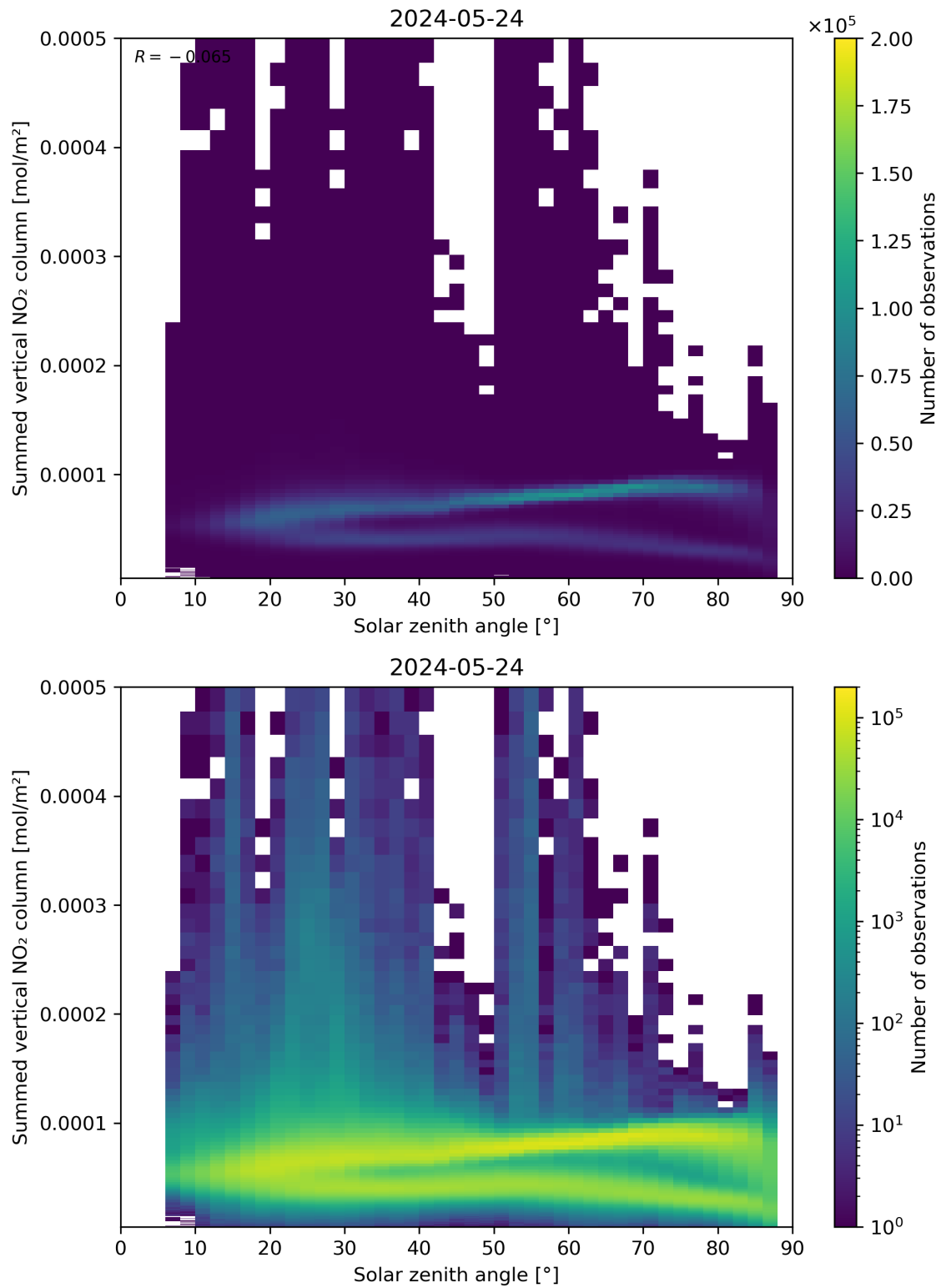
Figure 151: Scatter density plot of “Solar zenith angle” against “Summed vertical NO 2 column” for 2024-05-23 to 2024-05-25.
