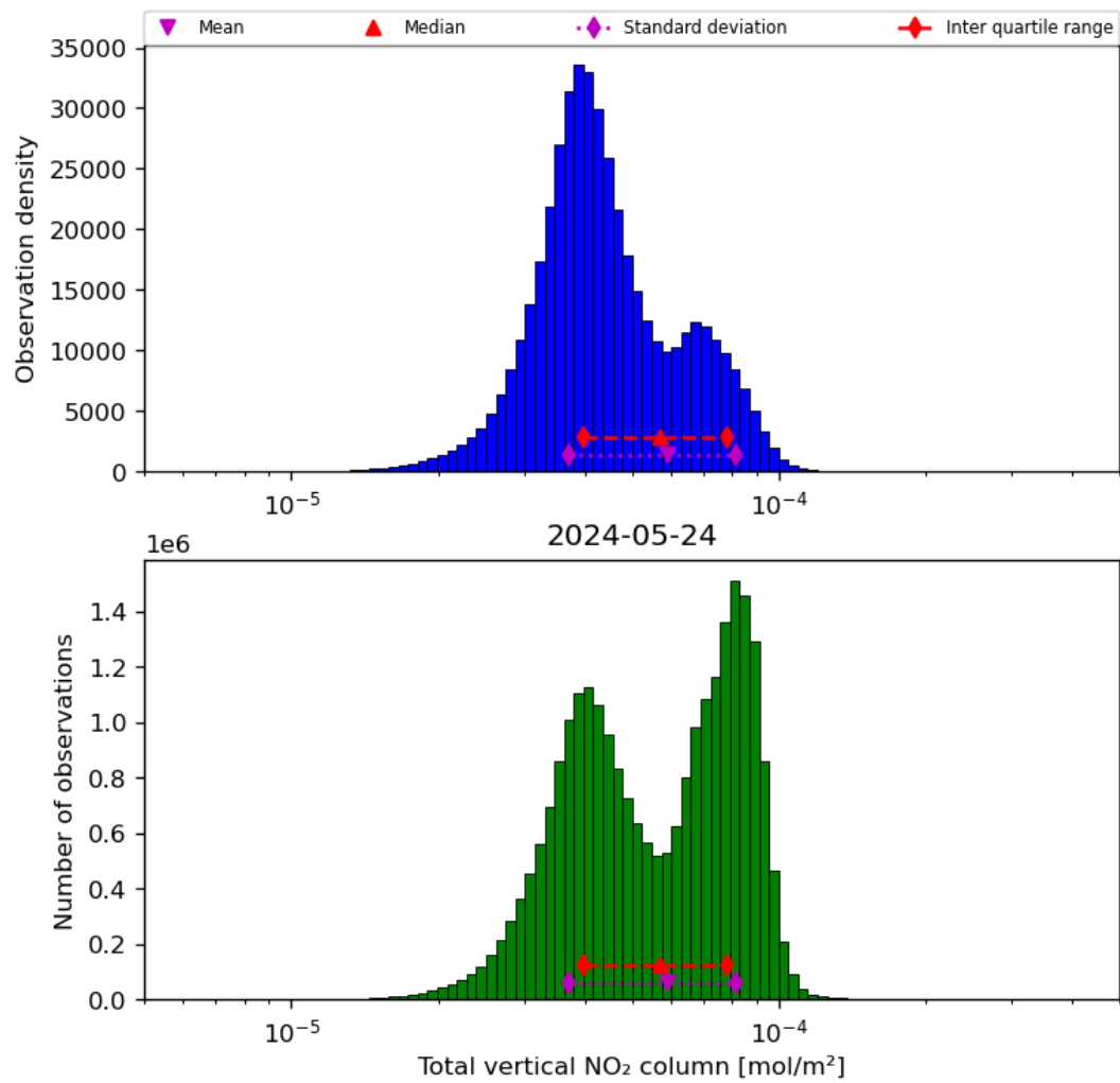
Figure 38: Histogram of “Total vertical NO 2 column” for 2024-05-23 to 2024-05-25
