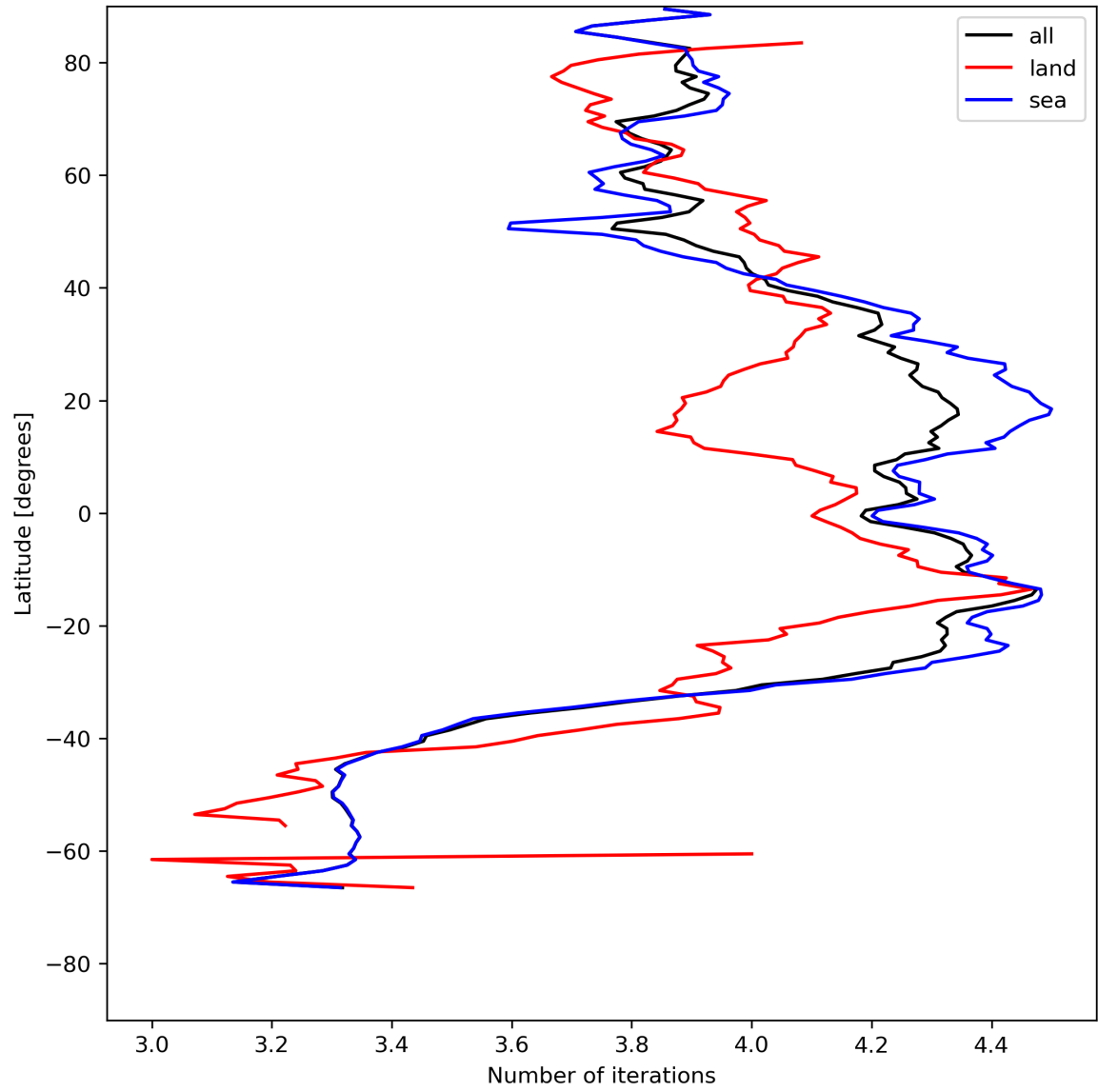
Figure 17: Zonal average of “Number of iterations” for 2024-05-23 to 2024-05-25.
