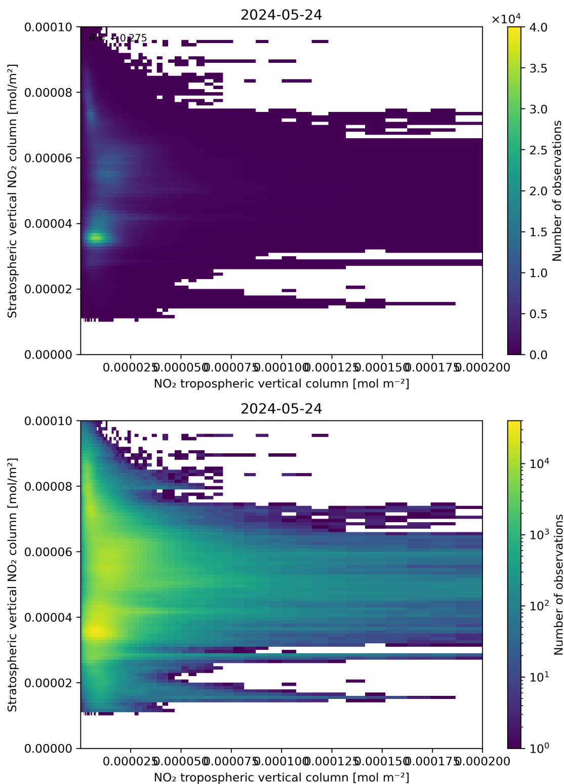
Figure 125: Scatter density plot of “NO 2 tropospheric vertical column” against “Stratospheric vertical NO 2 column” for 2024-05-23 to 2024-05-25.
