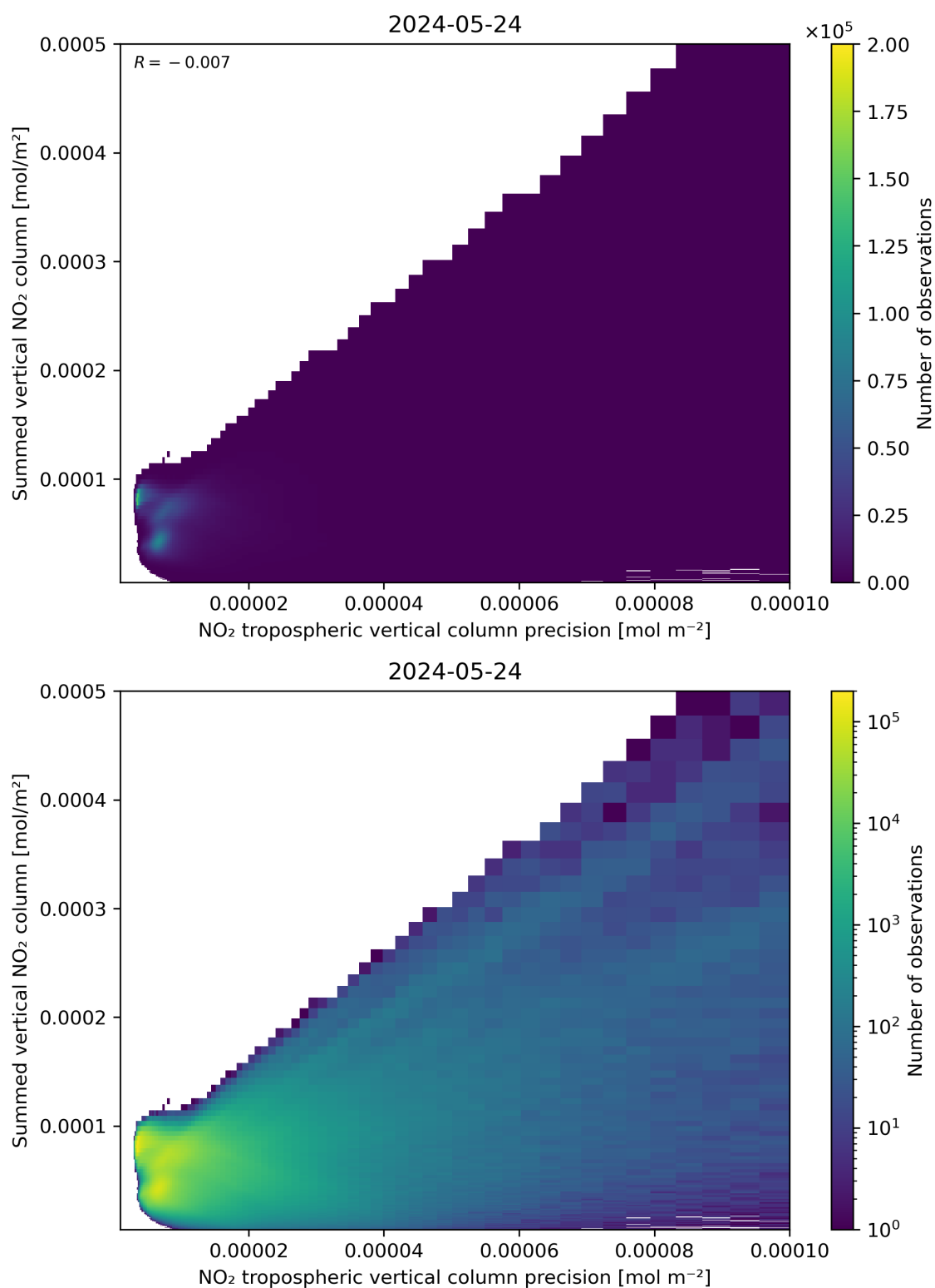
Figure 136: Scatter density plot of “NO 2 tropospheric vertical column precision” against “Summed vertical NO 2 column” for 2024-05-23 to 2024-05-25.
