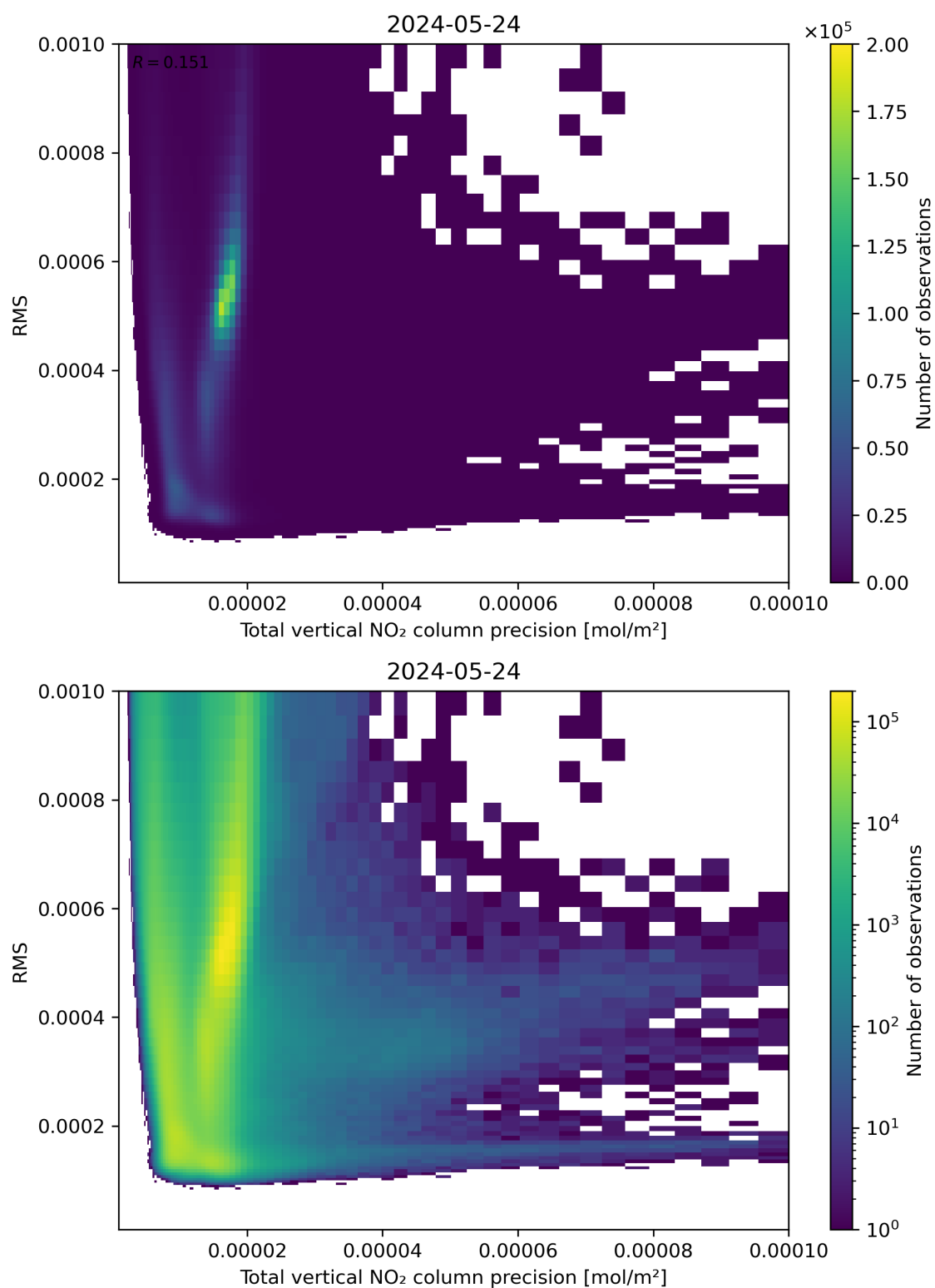
Figure 119: Scatter density plot of “Total vertical NO 2 column precision” against “RMS” for 2024-05-23 to 2024-05-25.
