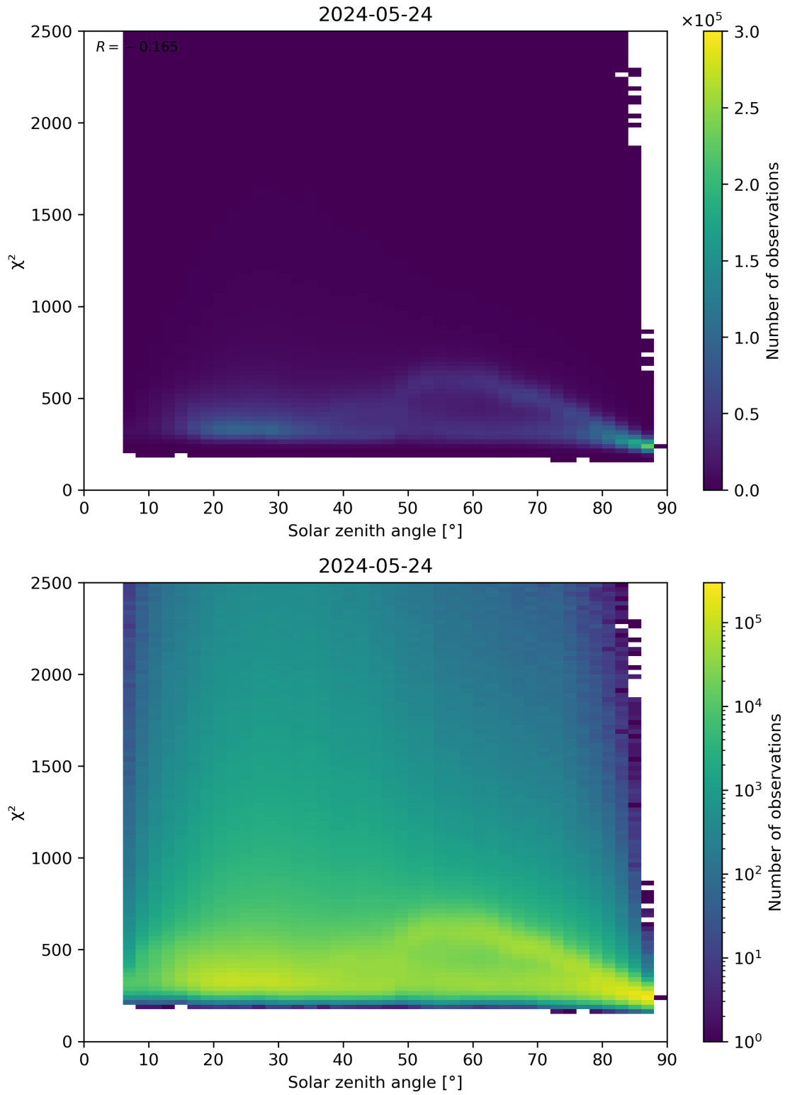
Figure 148: Scatter density plot of “Solar zenith angle” against “ \chi^2 ” for 2024-05-23 to 2024-05-25.
