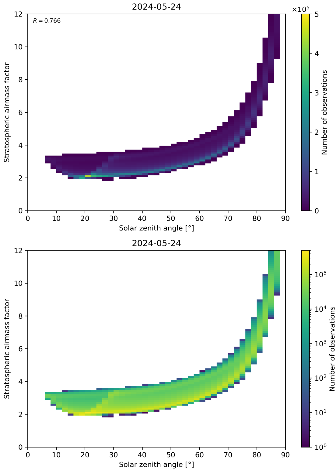
Figure 145: Scatter density plot of “Solar zenith angle” against “Stratospheric airmass factor” for 2024-05-23 to 2024-05-25.
