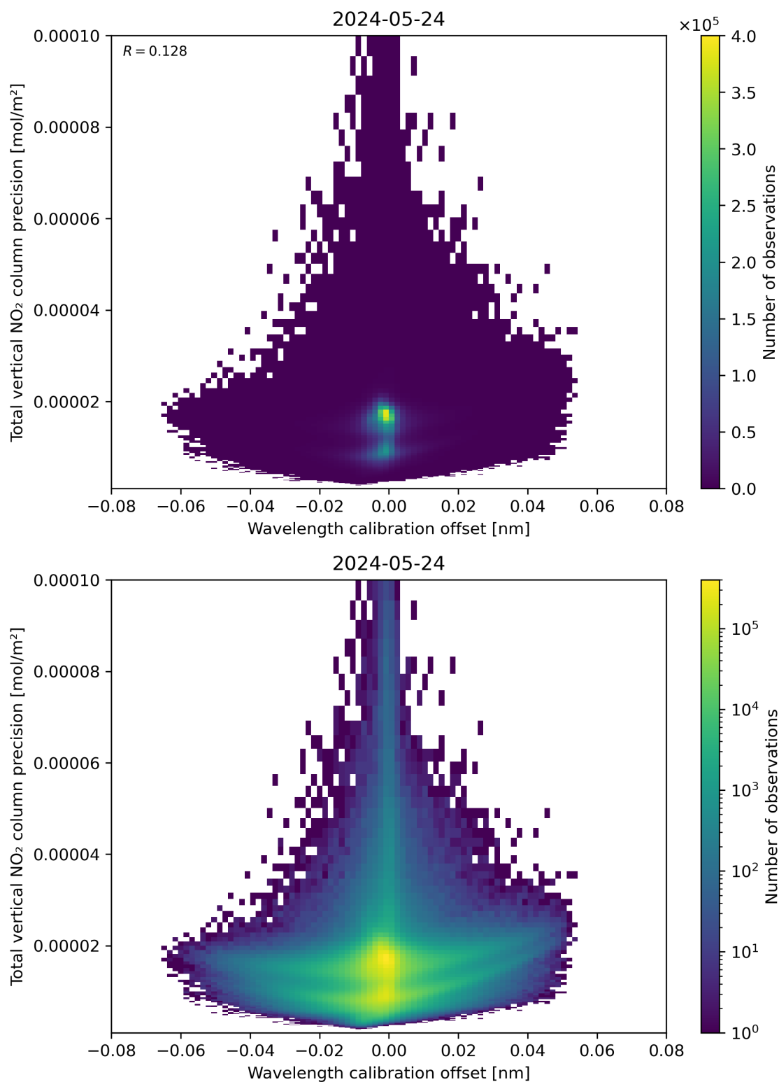
Figure 180: Scatter density plot of “Wavelength calibration offset” against “Total vertical NO 2 column precision” for 2024-05-23 to 2024-05-25.
