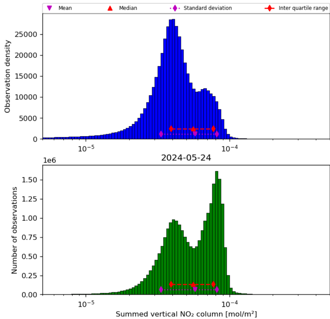
Figure 40: Histogram of “Summed vertical NO 2 column” for 2024-05-23 to 2024-05-25
