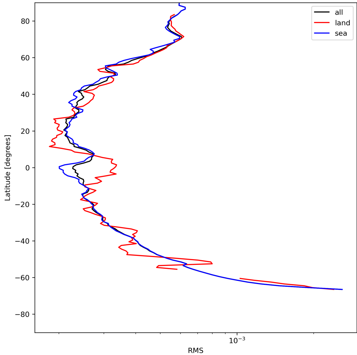
Figure 26: Zonal average of “RMS” for 2024-05-23 to 2024-05-25.
