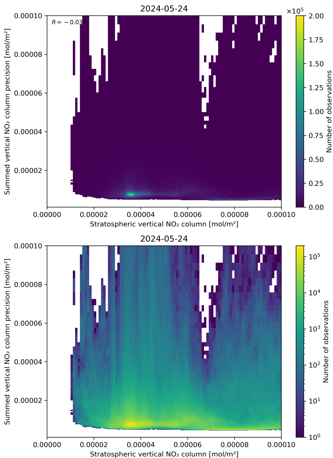
Figure 99: Scatter density plot of “Stratospheric vertical NO 2 column” against “Summed vertical NO 2 column precision” for 2024-05-23 to 2024-05-25.
