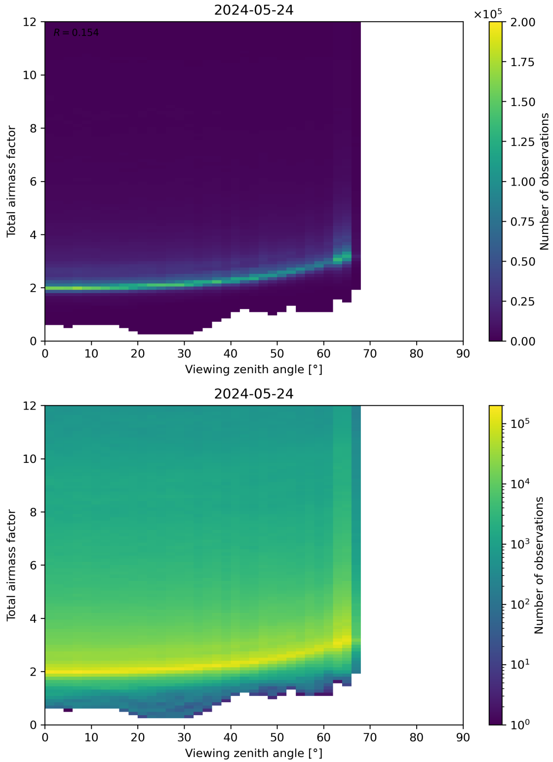
Figure 160: Scatter density plot of “Viewing zenith angle” against “Total airmass factor” for 2024-05-23 to 2024-05-25.
