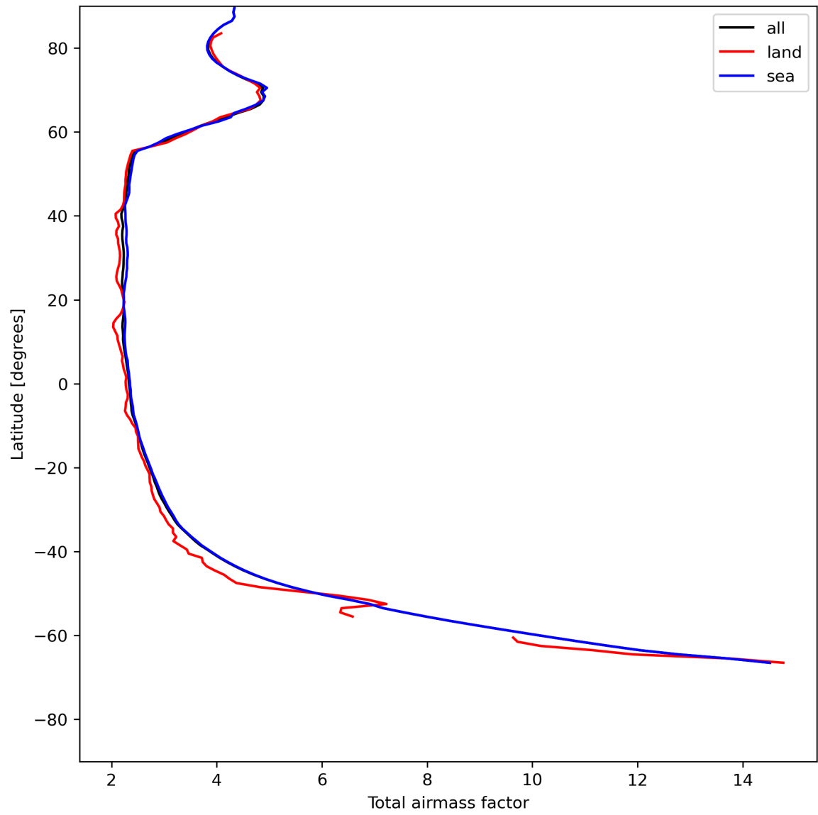
Figure 15: Zonal average of “Total airmass factor” for 2024-05-23 to 2024-05-25.
