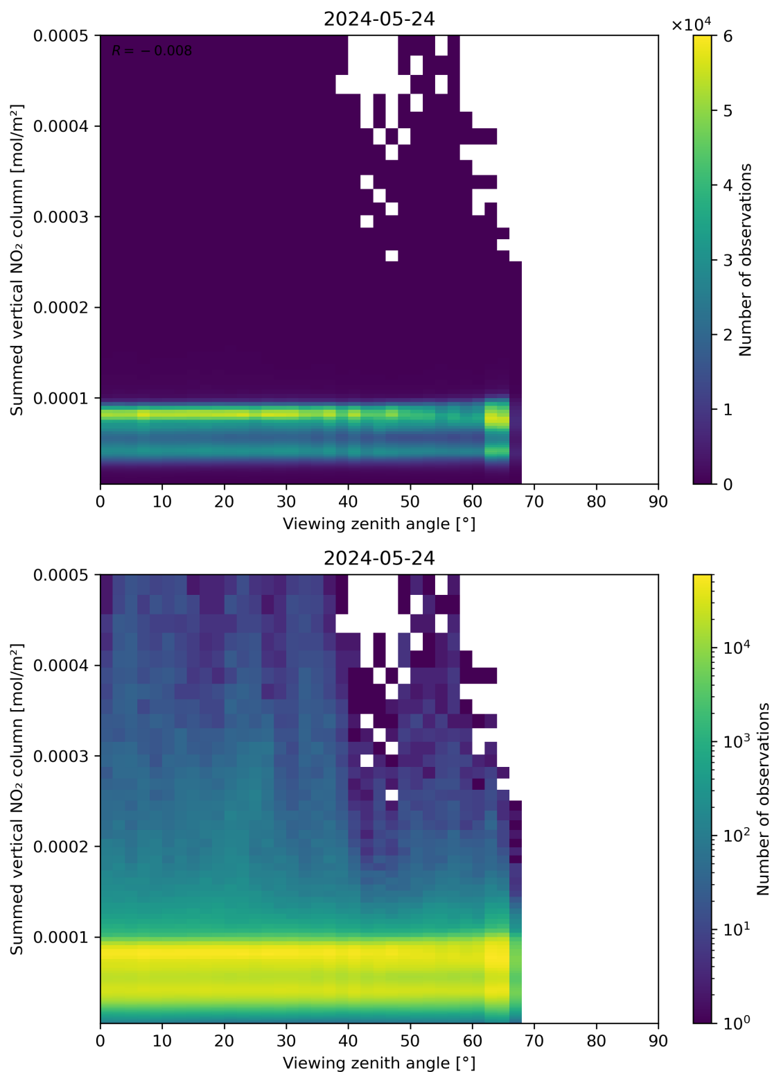
Figure 165: Scatter density plot of “Viewing zenith angle” against “Summed vertical NO 2 column” for 2024-05-23 to 2024-05-25.
