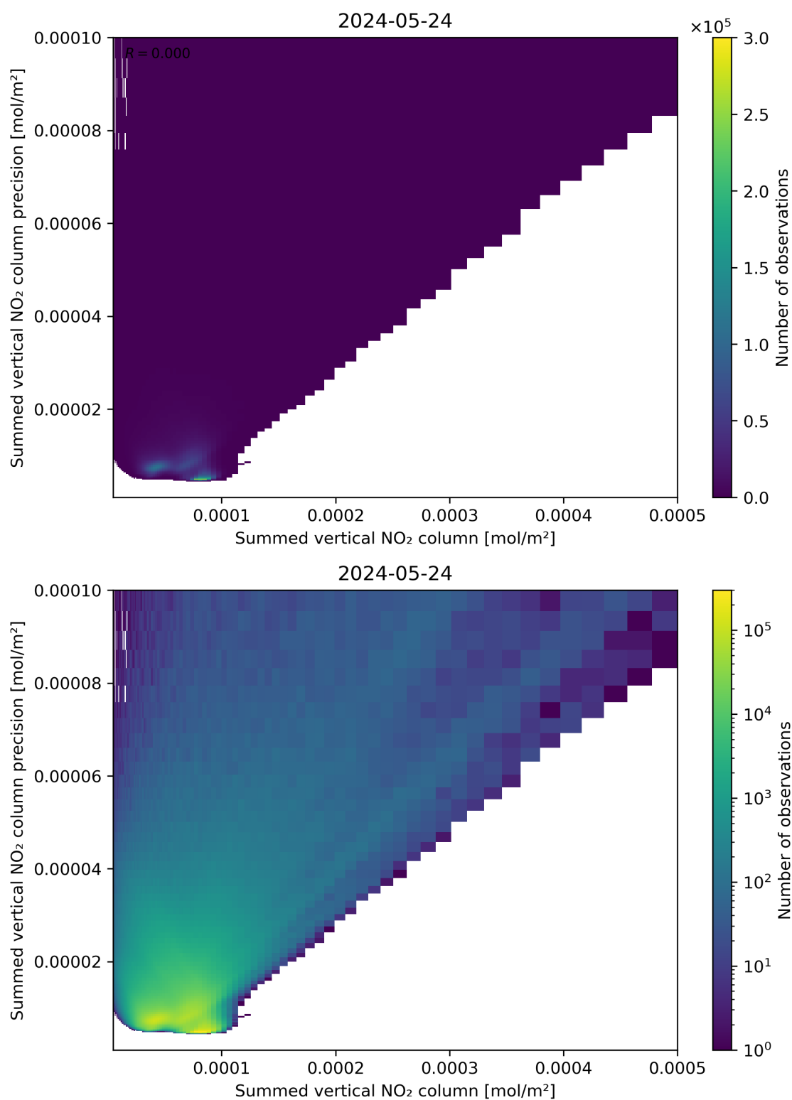
Figure 105: Scatter density plot of “Summed vertical NO 2 column” against “Summed vertical NO 2 column precision” for 2024-05-23 to 2024-05-25.
