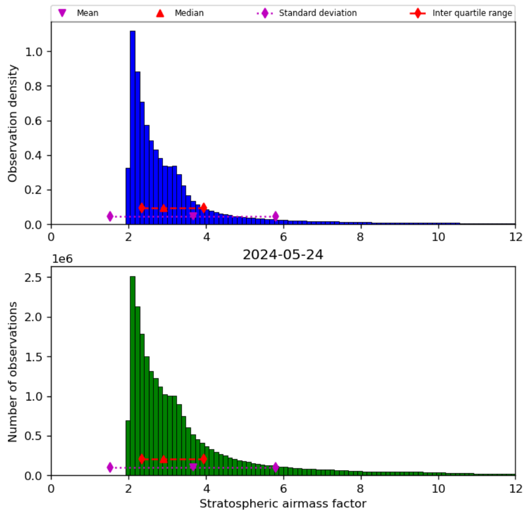
Figure 44: Histogram of “Stratospheric airmass factor” for 2024-05-23 to 2024-05-25
