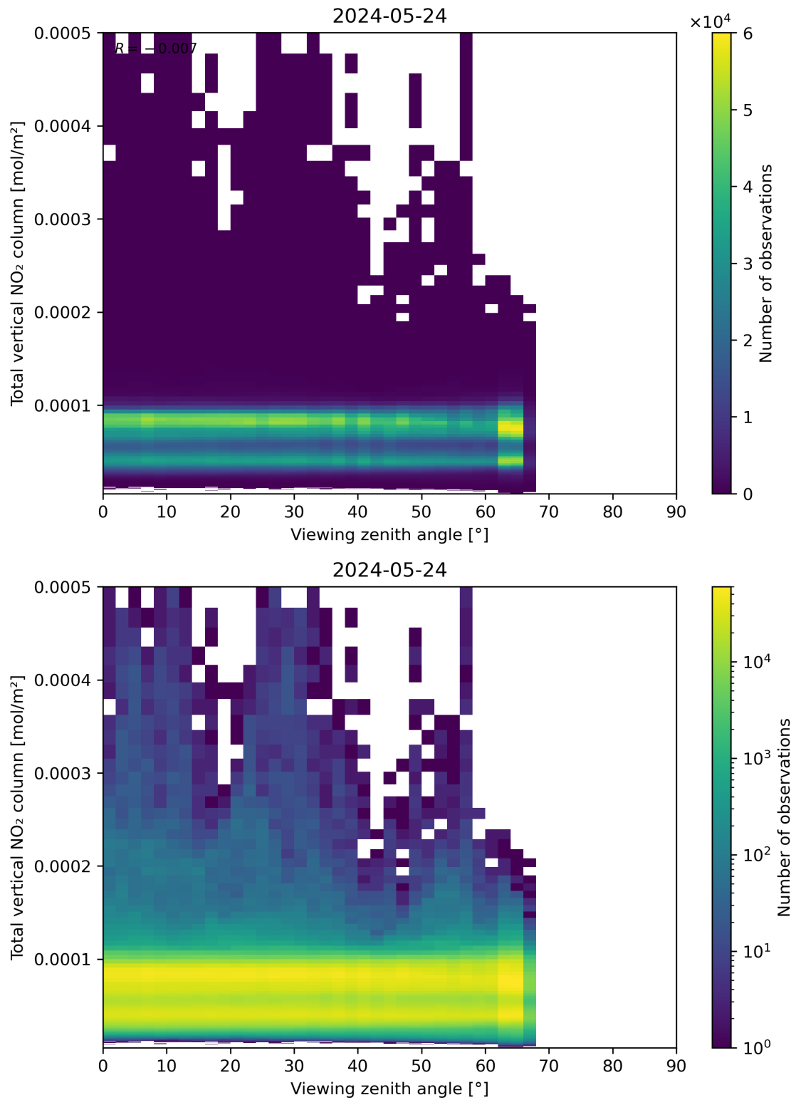
Figure 167: Scatter density plot of “Viewing zenith angle” against “Total vertical NO 2 column” for 2024-05-23 to 2024-05-25.
