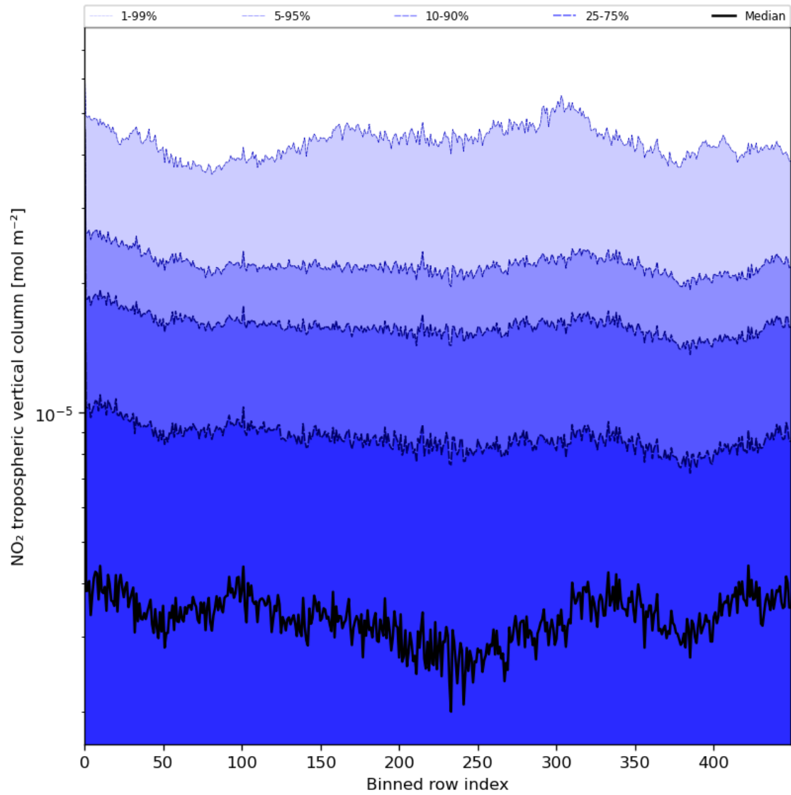
Figure 46: Along track statistics of “NO 2 tropospheric vertical column” for 2024-05-23 to 2024-05-25
