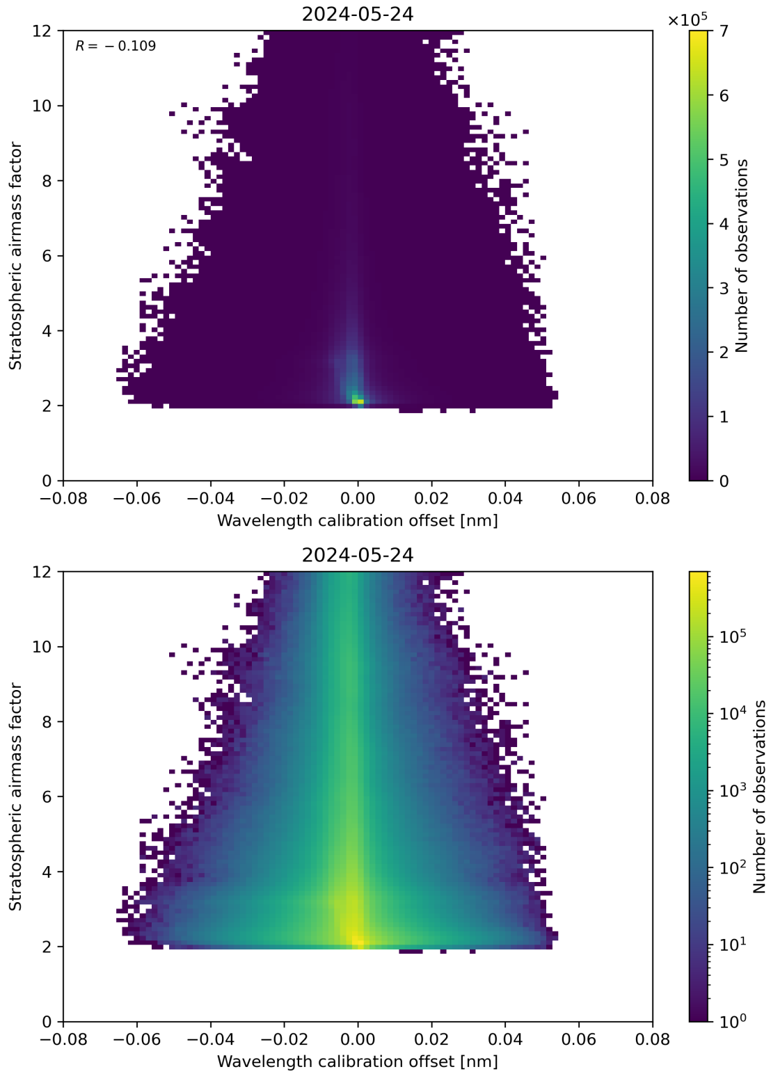
Figure 174: Scatter density plot of “Wavelength calibration offset” against “Stratospheric airmass factor” for 2024-05-23 to 2024-05-25.
