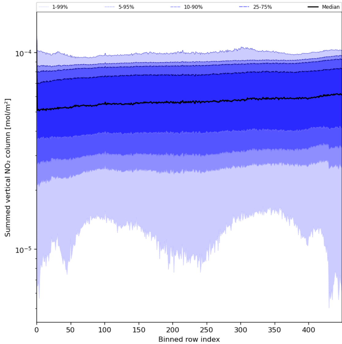
Figure 57: Along track statistics of “Summed vertical NO 2 column” for 2024-05-23 to 2024-05-25
