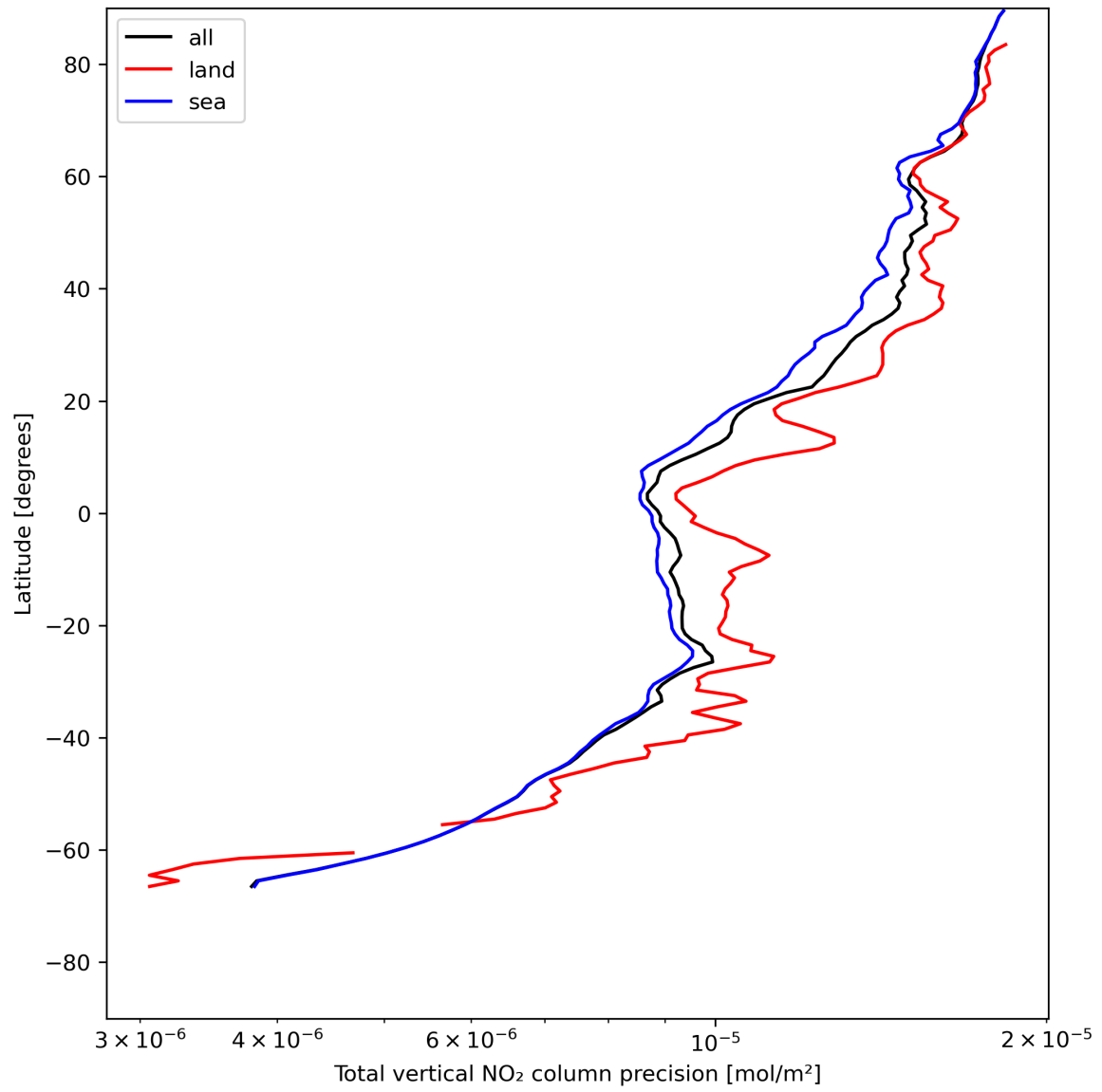
Figure 22: Zonal average of “Total vertical NO 2 column precision” for 2024-05-23 to 2024-05-25.
