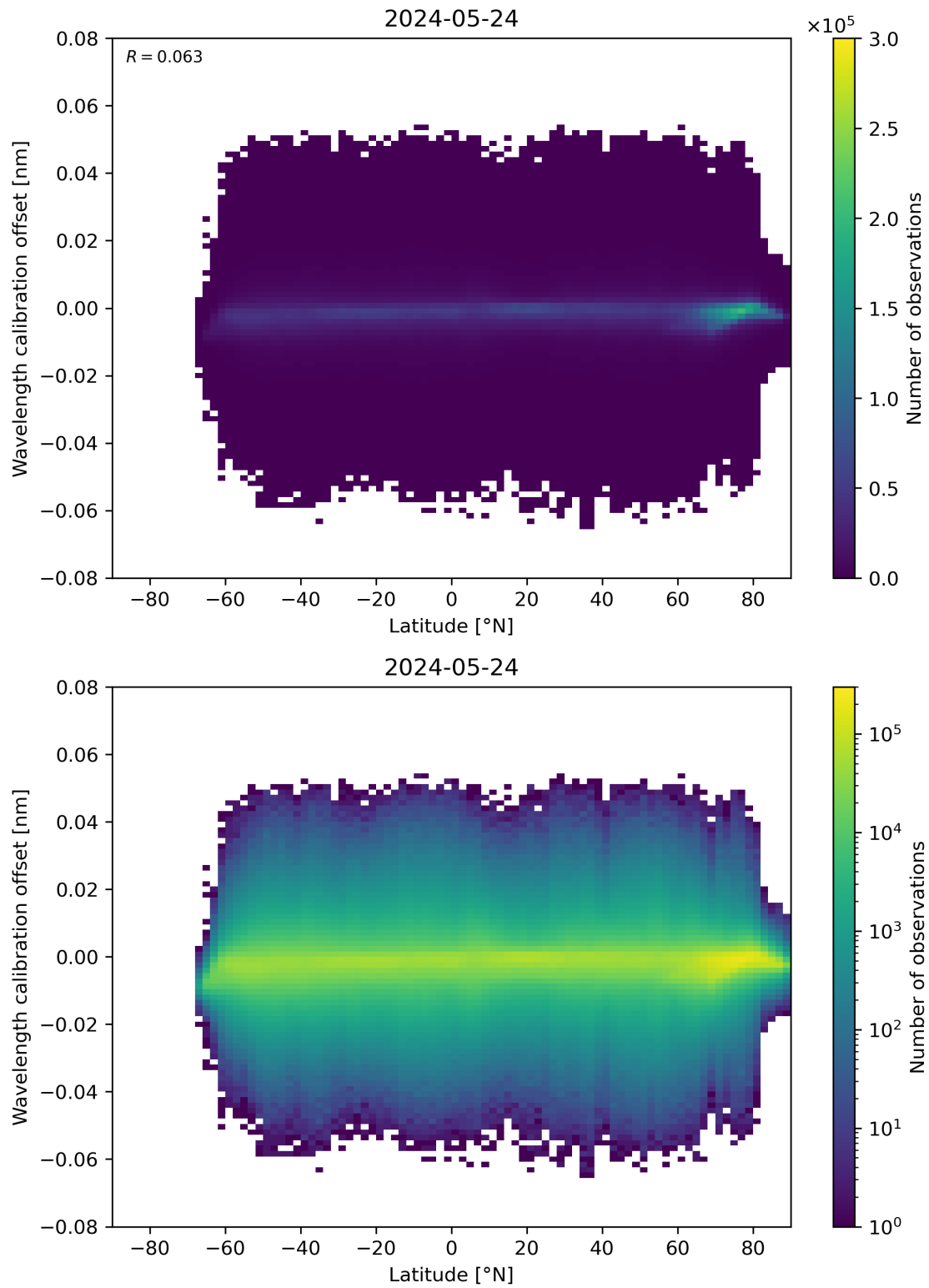
Figure 95: Scatter density plot of “Latitude” against “Wavelength calibration offset” for 2024-05-23 to 2024-05-25.
