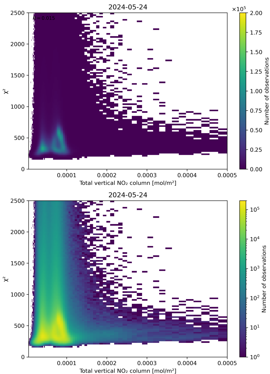
Figure 111: Scatter density plot of “Total vertical NO 2 column” against “ \chi^2 ” for 2024-05-23 to 2024-05-25.
