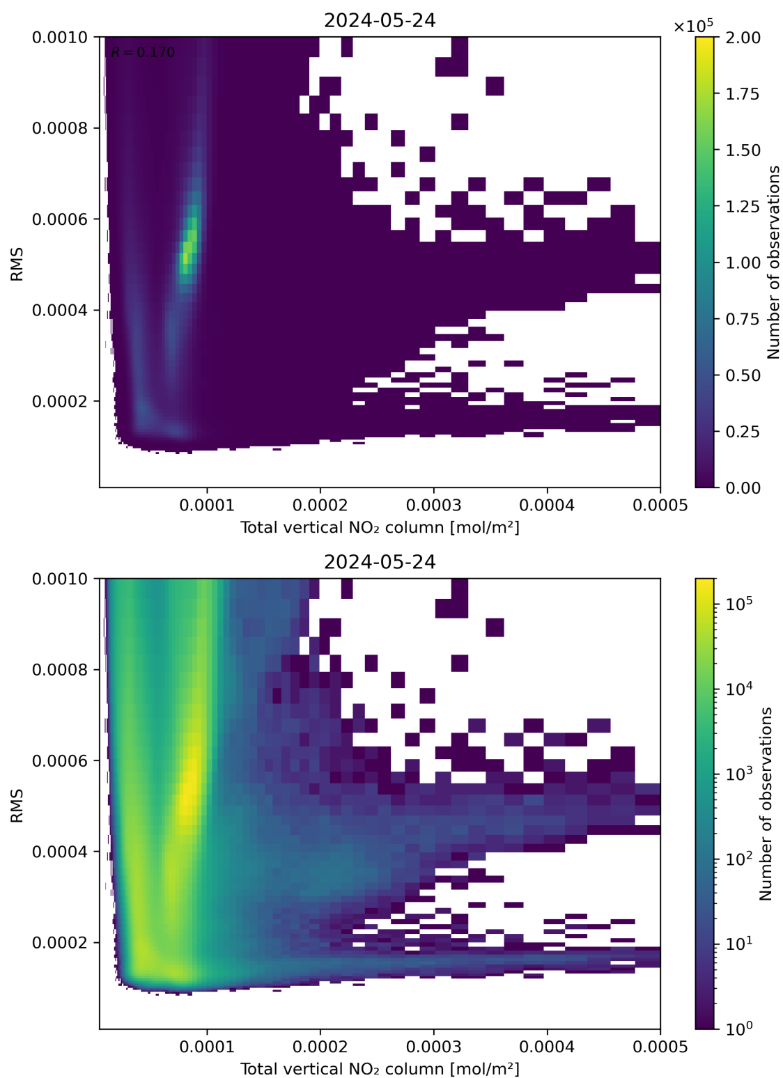
Figure 120: Scatter density plot of “Total vertical NO 2 column” against “RMS” for 2024-05-23 to 2024-05-25.
