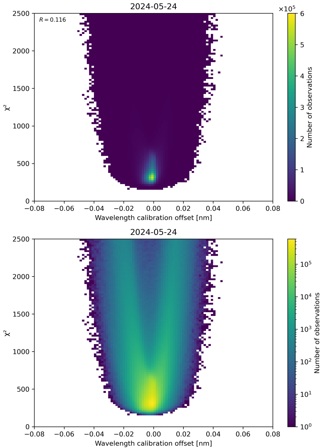
Figure 175: Scatter density plot of “Wavelength calibration offset” against “ \chi^2 ” for 2024-05-23 to 2024-05-25.
