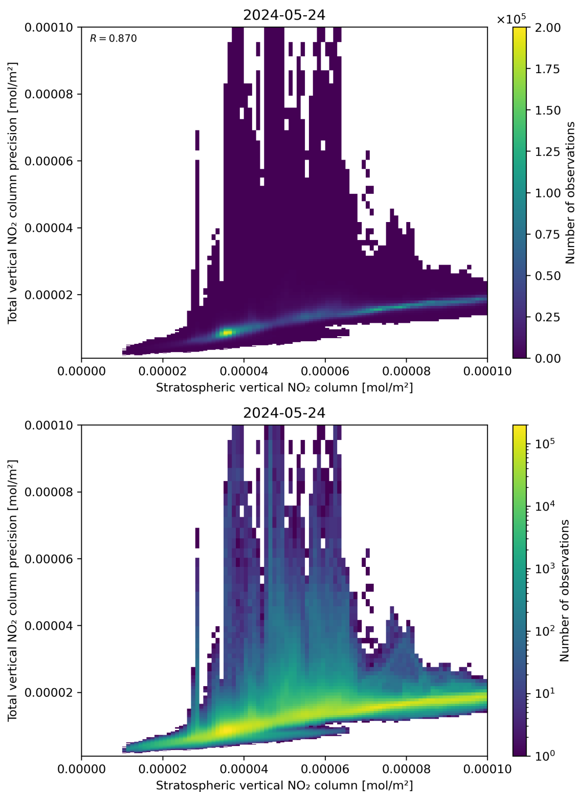
Figure 101: Scatter density plot of “Stratospheric vertical NO 2 column” against “Total vertical NO 2 column precision” for 2024-05-23 to 2024-05-25.
