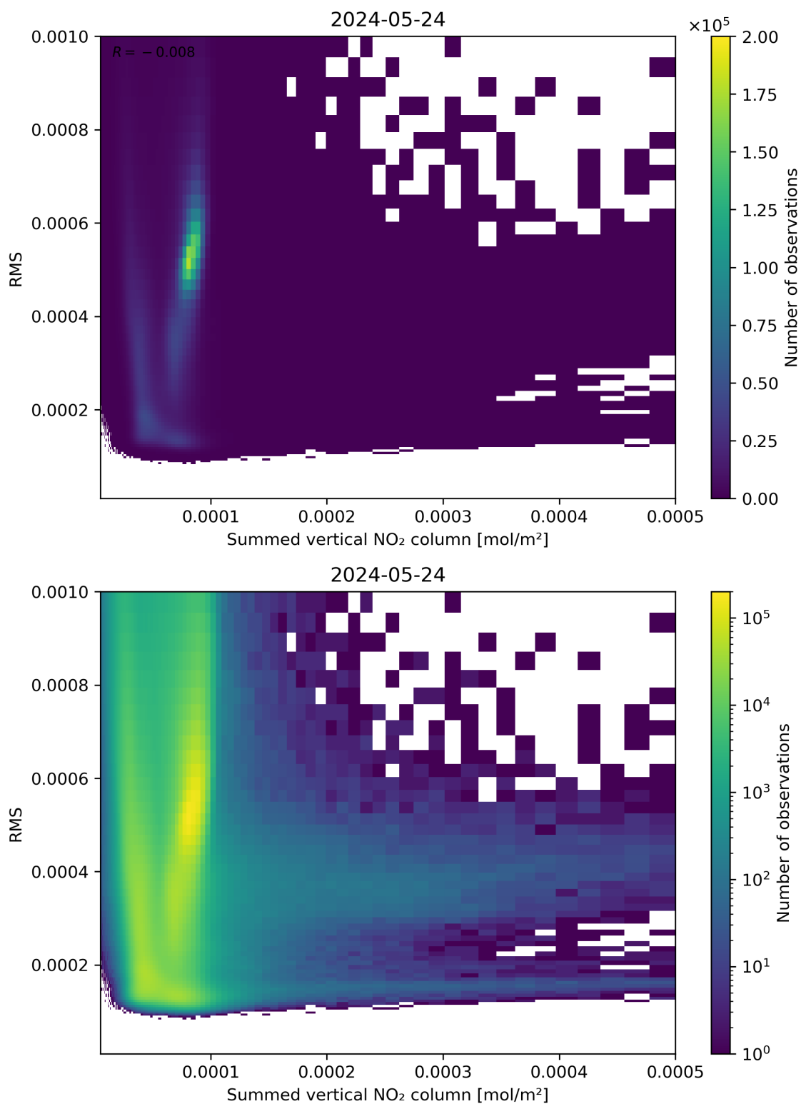
Figure 109: Scatter density plot of “Summed vertical NO 2 column” against “RMS” for 2024-05-23 to 2024-05-25.
