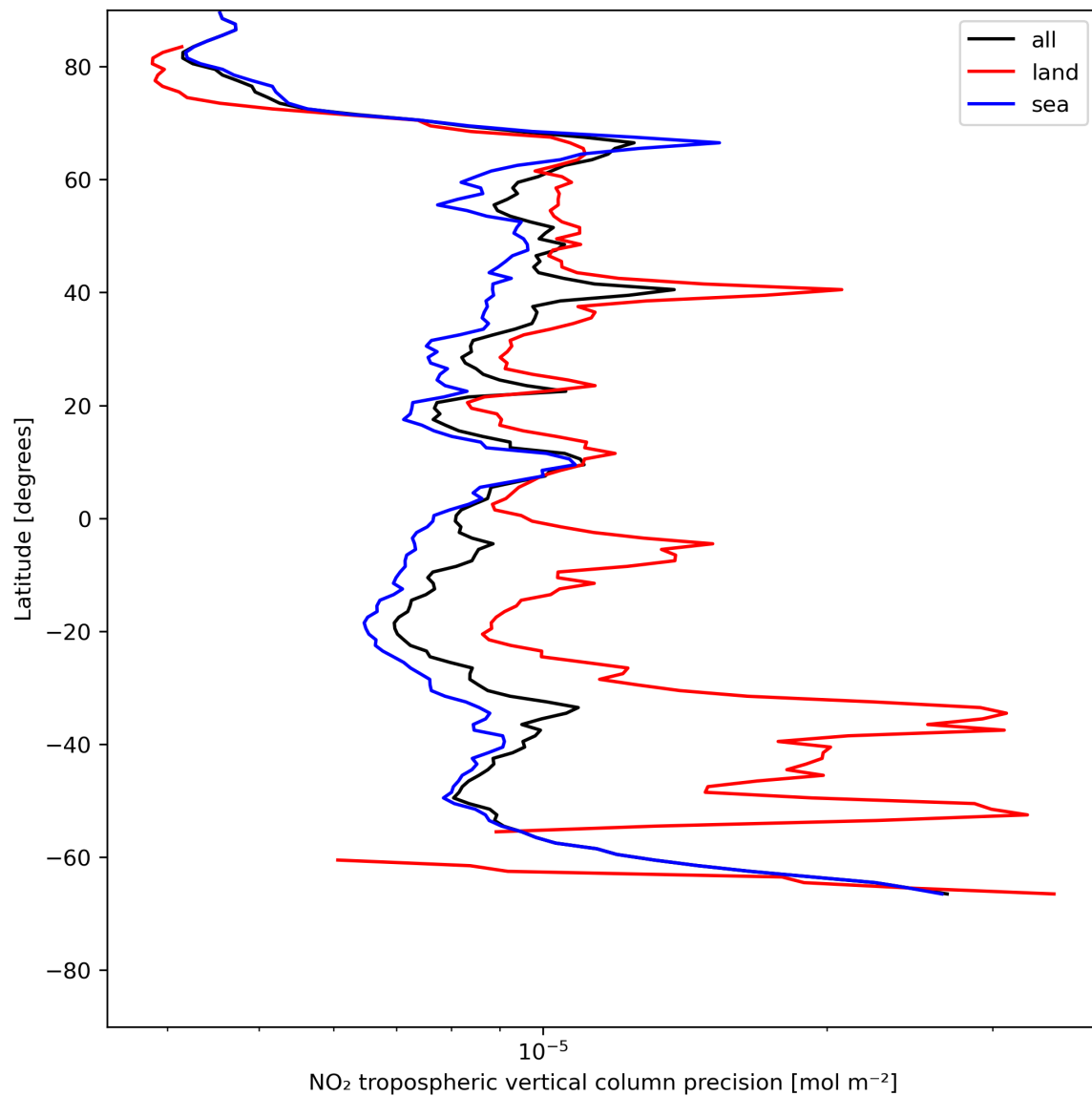
Figure 13: Zonal average of “NO 2 tropospheric vertical column precision” for 2024-05-23 to 2024-05-25.
