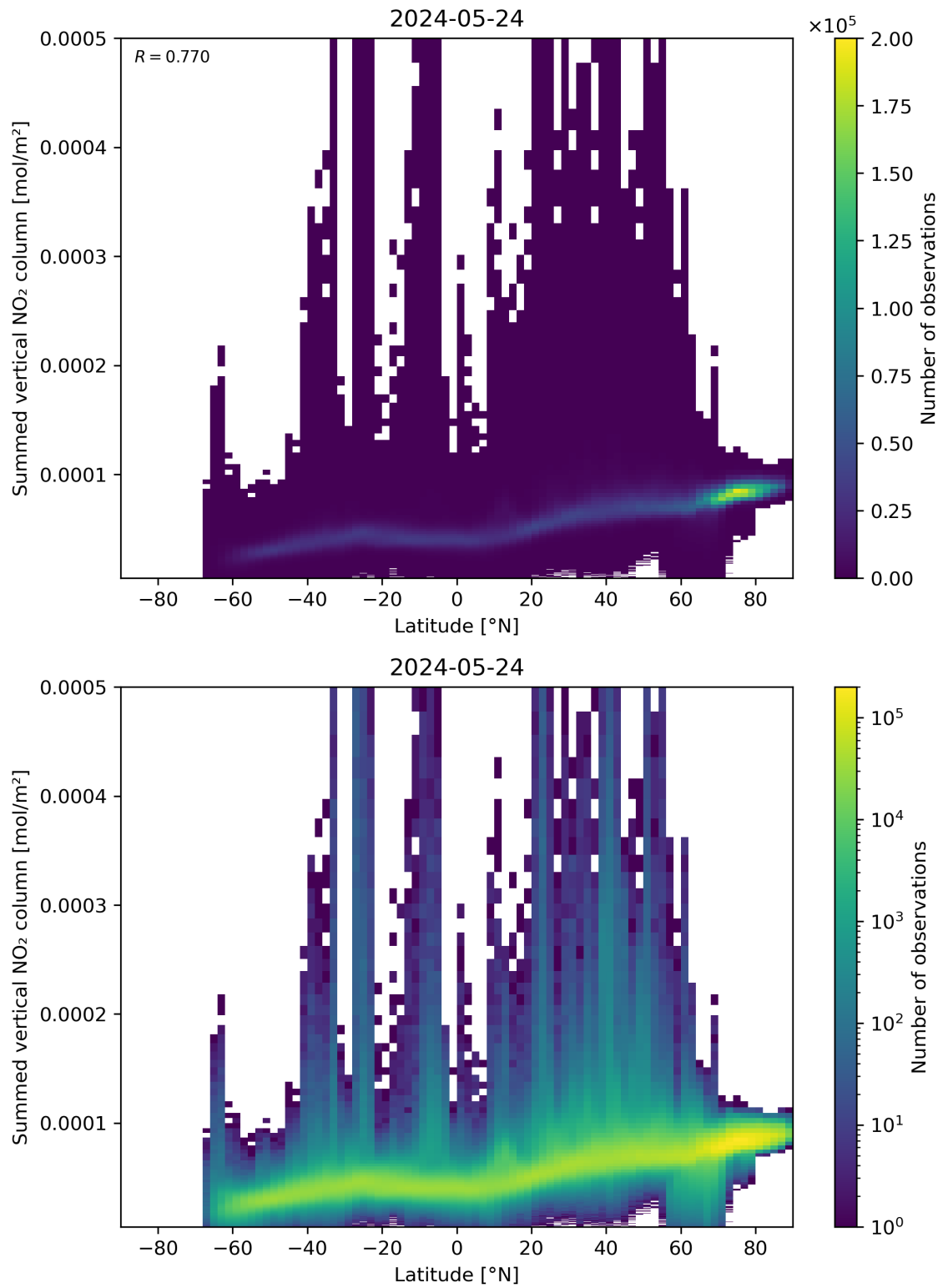
Figure 88: Scatter density plot of “Latitude” against “Summed vertical NO 2 column” for 2024-05-23 to 2024-05-25.
