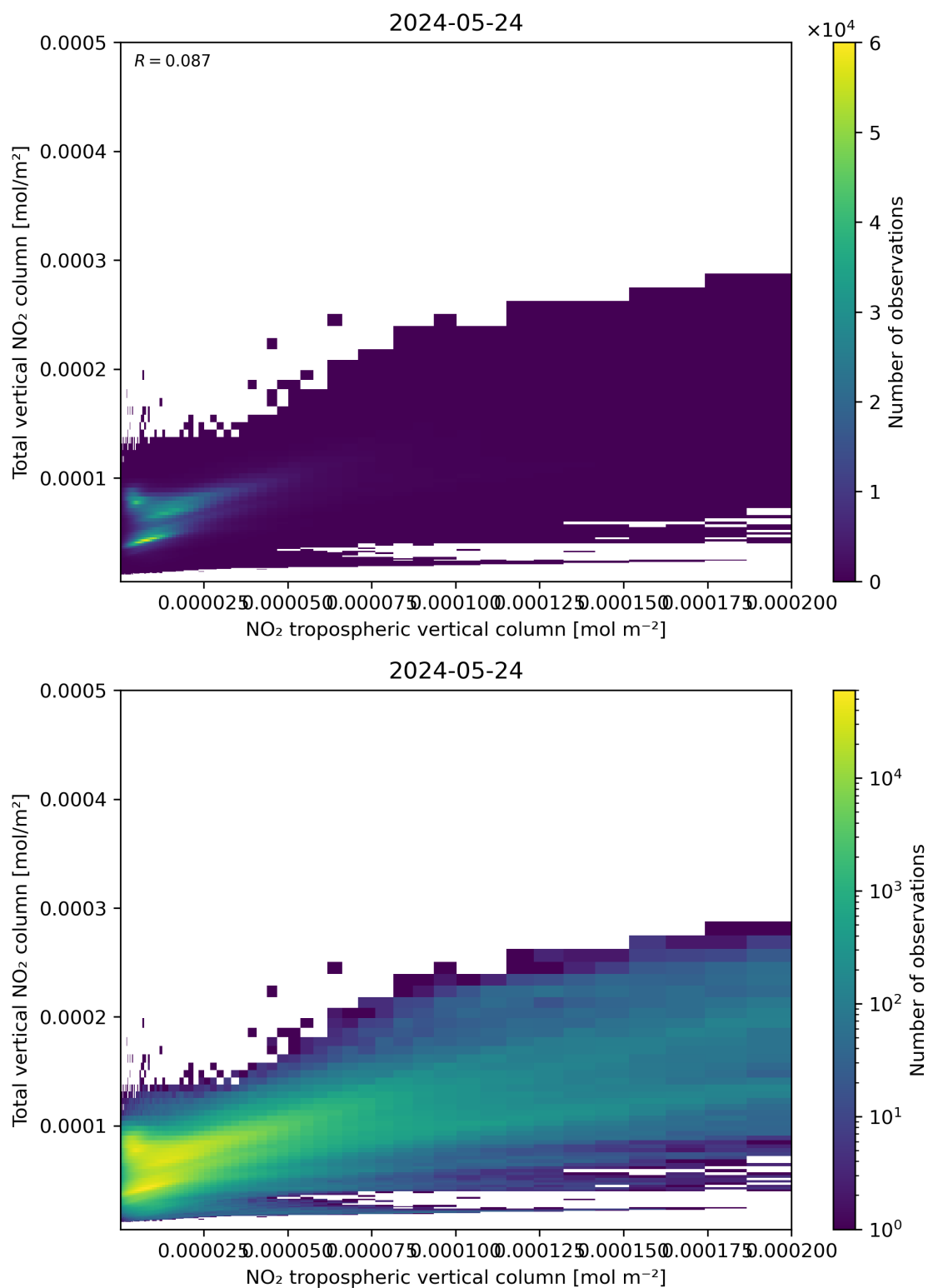
Figure 128: Scatter density plot of “NO 2 tropospheric vertical column” against “Total vertical NO 2 column” for 2024-05-23 to 2024-05-25.
