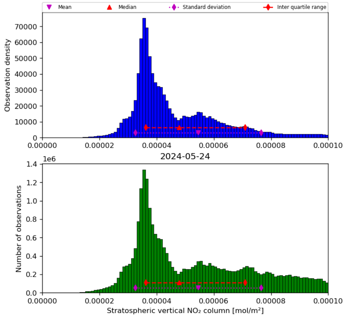
Figure 36: Histogram of “Stratospheric vertical NO 2 column” for 2024-05-23 to 2024-05-25
