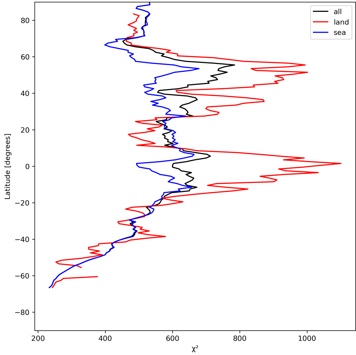
Figure 25: Zonal average of “ \chi^2 ” for 2024-05-23 to 2024-05-25.
