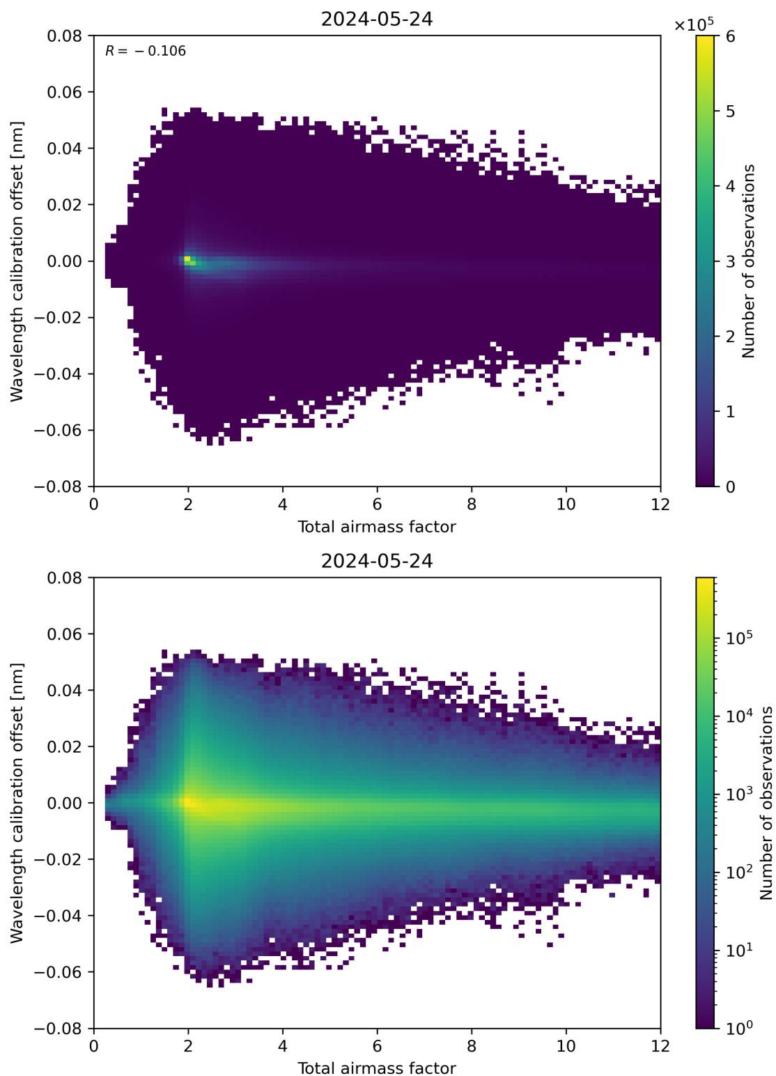
Figure 70: Scatter density plot of “Total airmass factor” against “Wavelength calibration offset” for 2024-05-23 to 2024-05-25.
