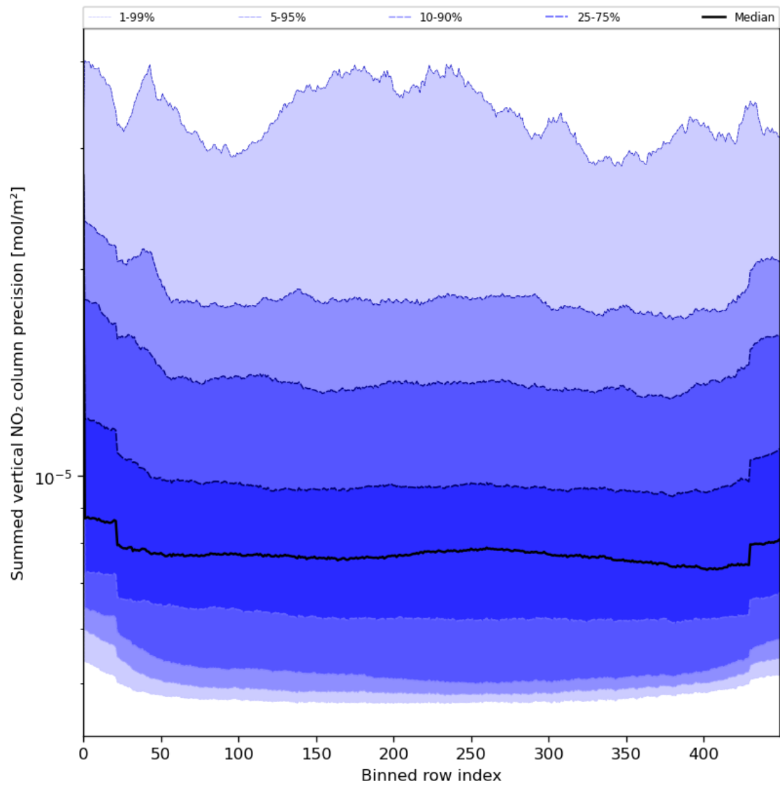
Figure 58: Along track statistics of “Summed vertical NO 2 column precision” for 2024-05-23 to 2024-05-25
