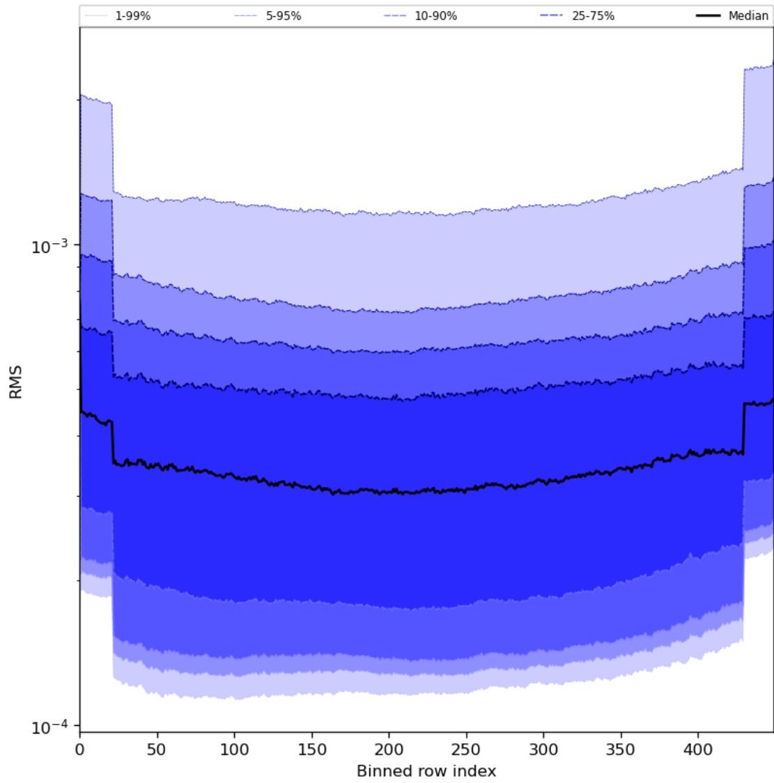
Figure 60: Along track statistics of “RMS” for 2024-05-23 to 2024-05-25
