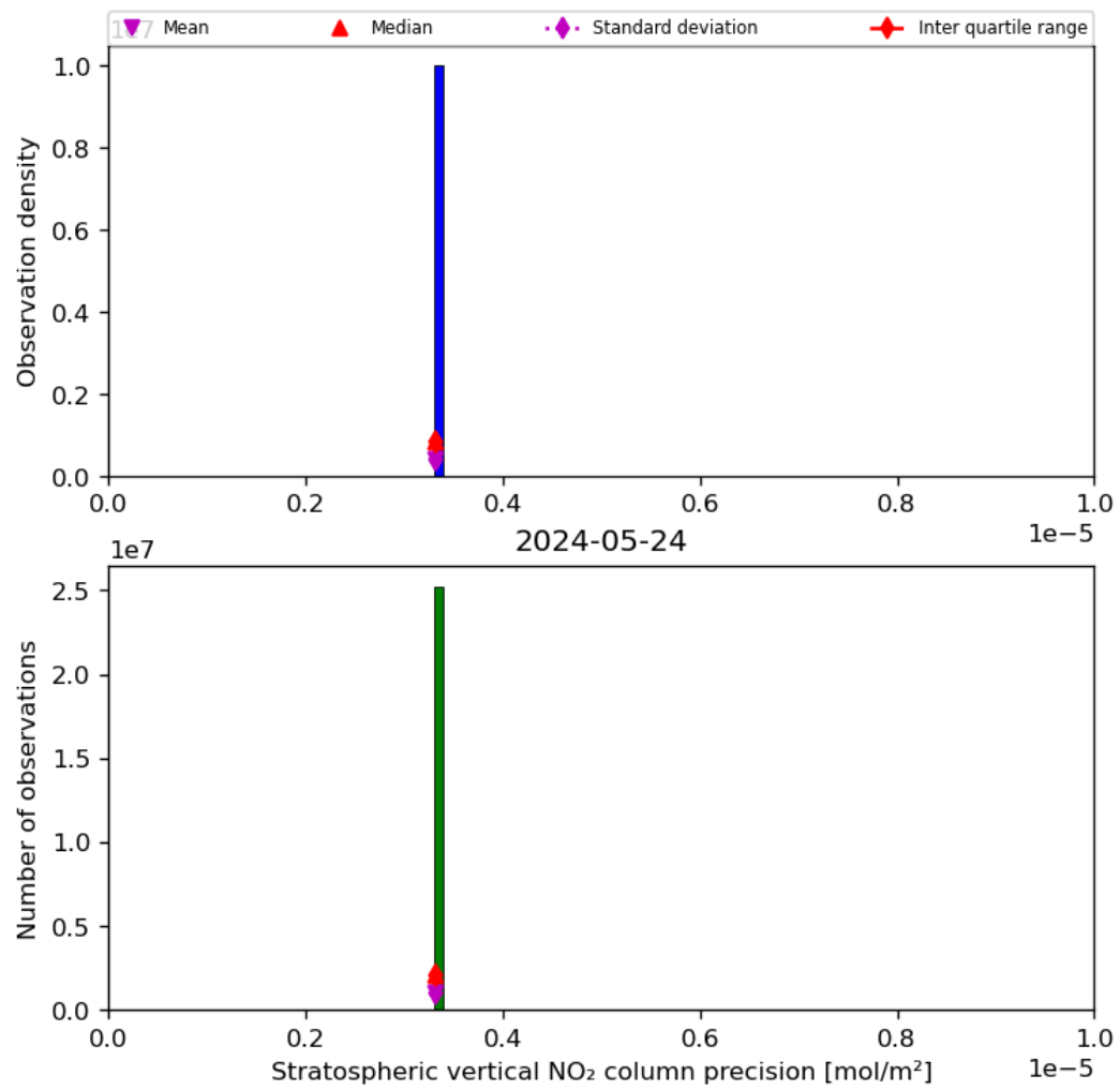
Figure 37: Histogram of “Stratospheric vertical NO 2 column precision” for 2024-05-23 to 2024-05-25
