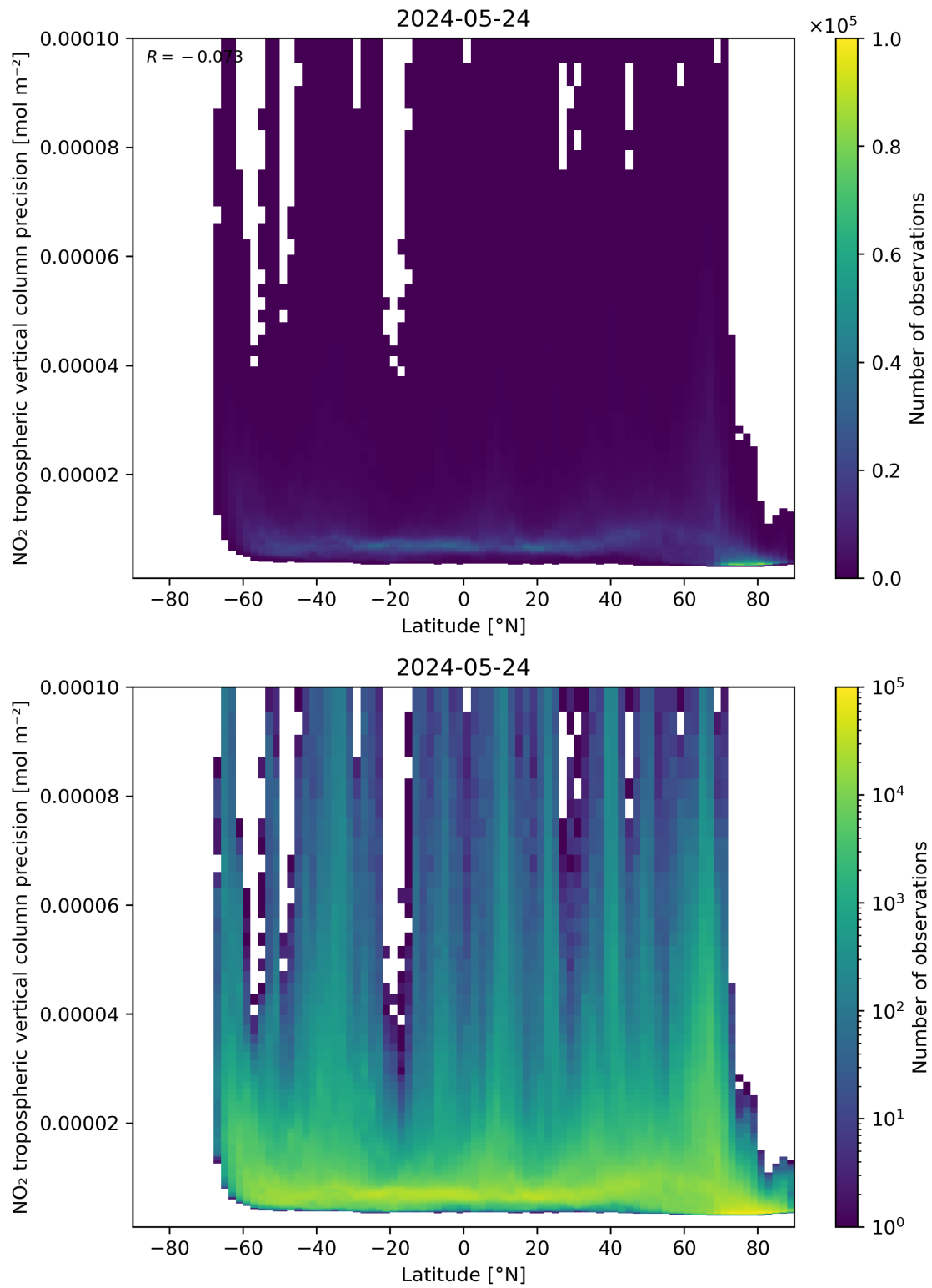
Figure 93: Scatter density plot of “Latitude” against “NO 2 tropospheric vertical column precision” for 2024-05-23 to 2024-05-25.
