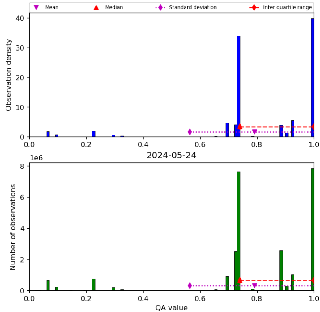
Figure 28: Histogram of “QA value” for 2024-05-23 to 2024-05-25
