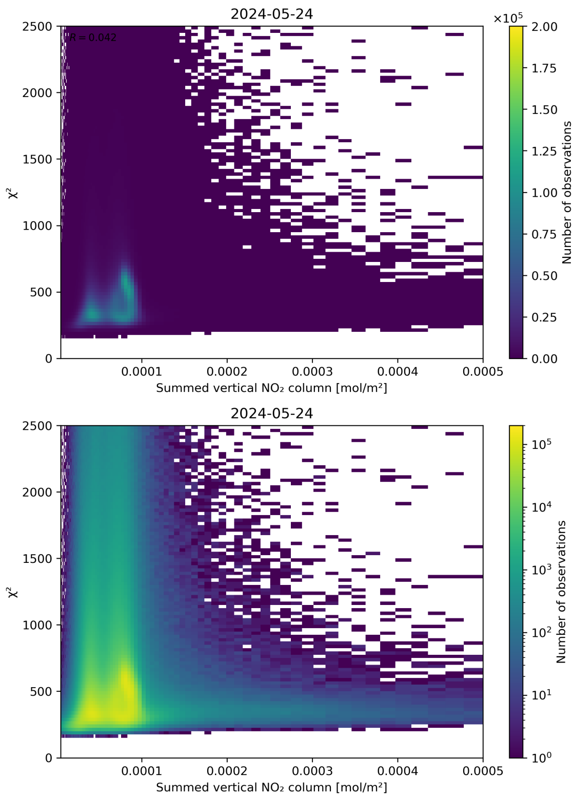
Figure 104: Scatter density plot of “Summed vertical NO 2 column” against “ \chi^2 ” for 2024-05-23 to 2024-05-25.
