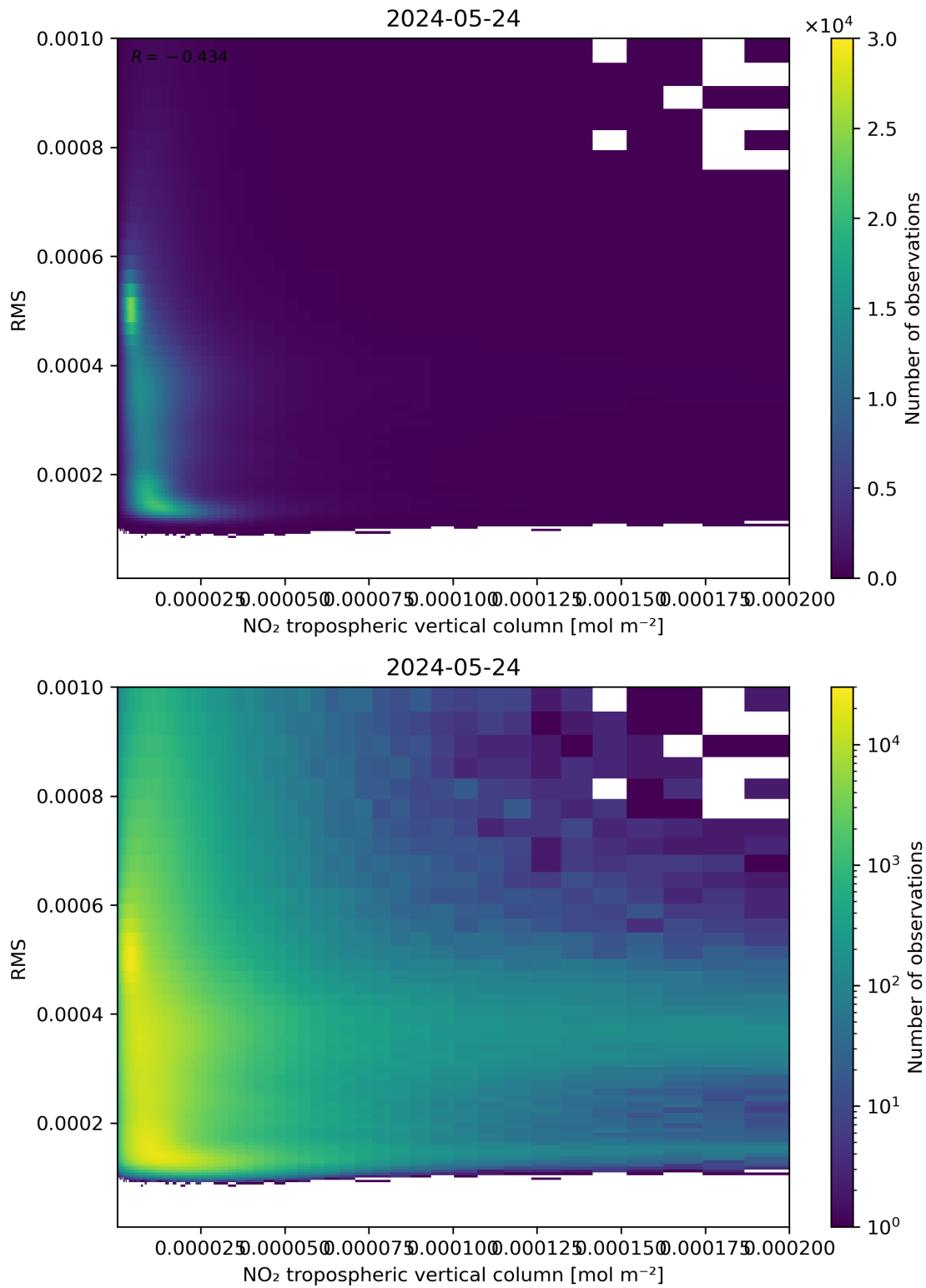
Figure 142: Scatter density plot of “NO 2 tropospheric vertical column” against “RMS” for 2024-05-23 to 2024-05-25.
