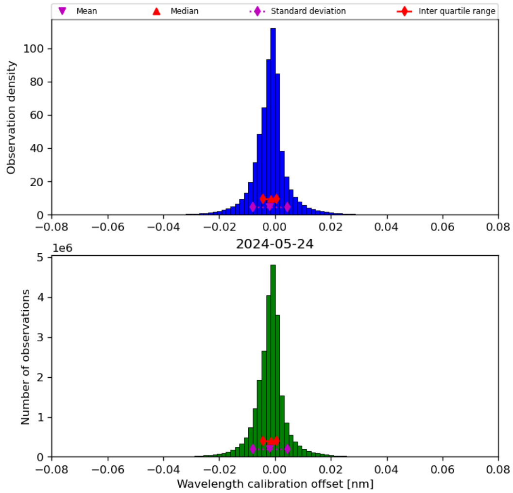
Figure 35: Histogram of “Wavelength calibration offset” for 2024-05-23 to 2024-05-25
