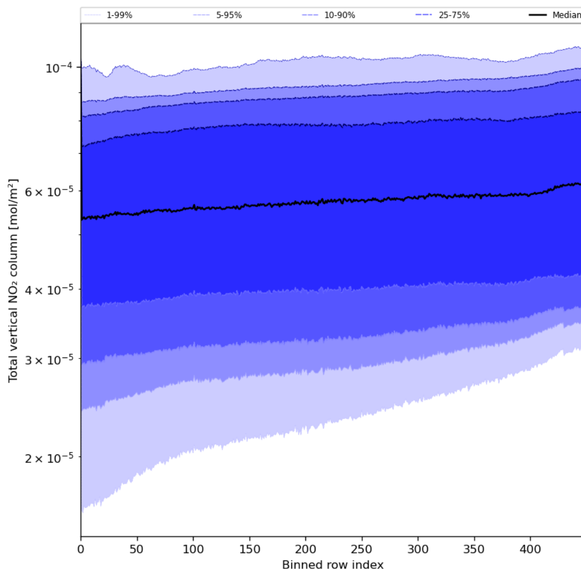
Figure 55: Along track statistics of “Total vertical NO 2 column” for 2024-05-23 to 2024-05-25
