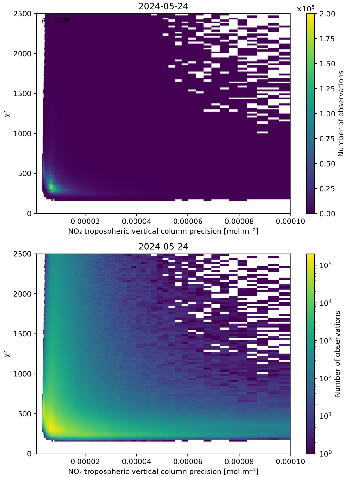
Figure 134: Scatter density plot of “NO 2 tropospheric vertical column precision” against “ \chi^2 ” for 2024-05-23 to 2024-05-25.
