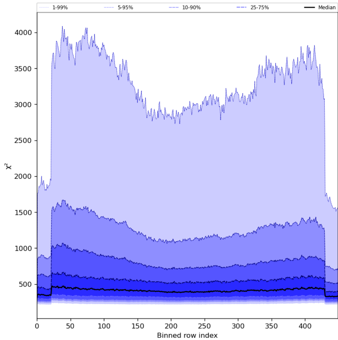
Figure 59: Along track statistics of “ \chi^2 ” for 2024-05-23 to 2024-05-25
