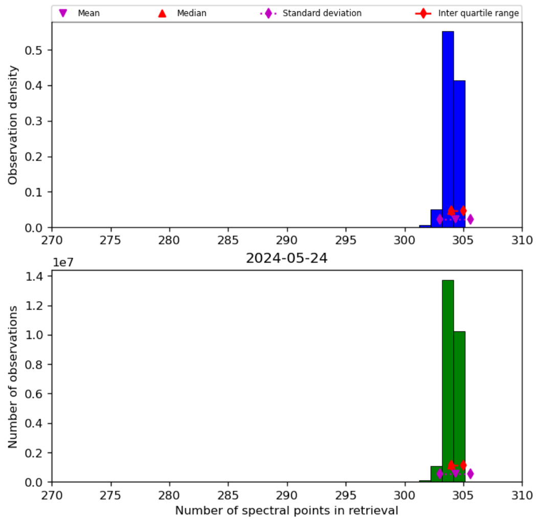
Figure 33: Histogram of “Number of spectral points in retrieval” for 2024-05-23 to 2024-05-25
