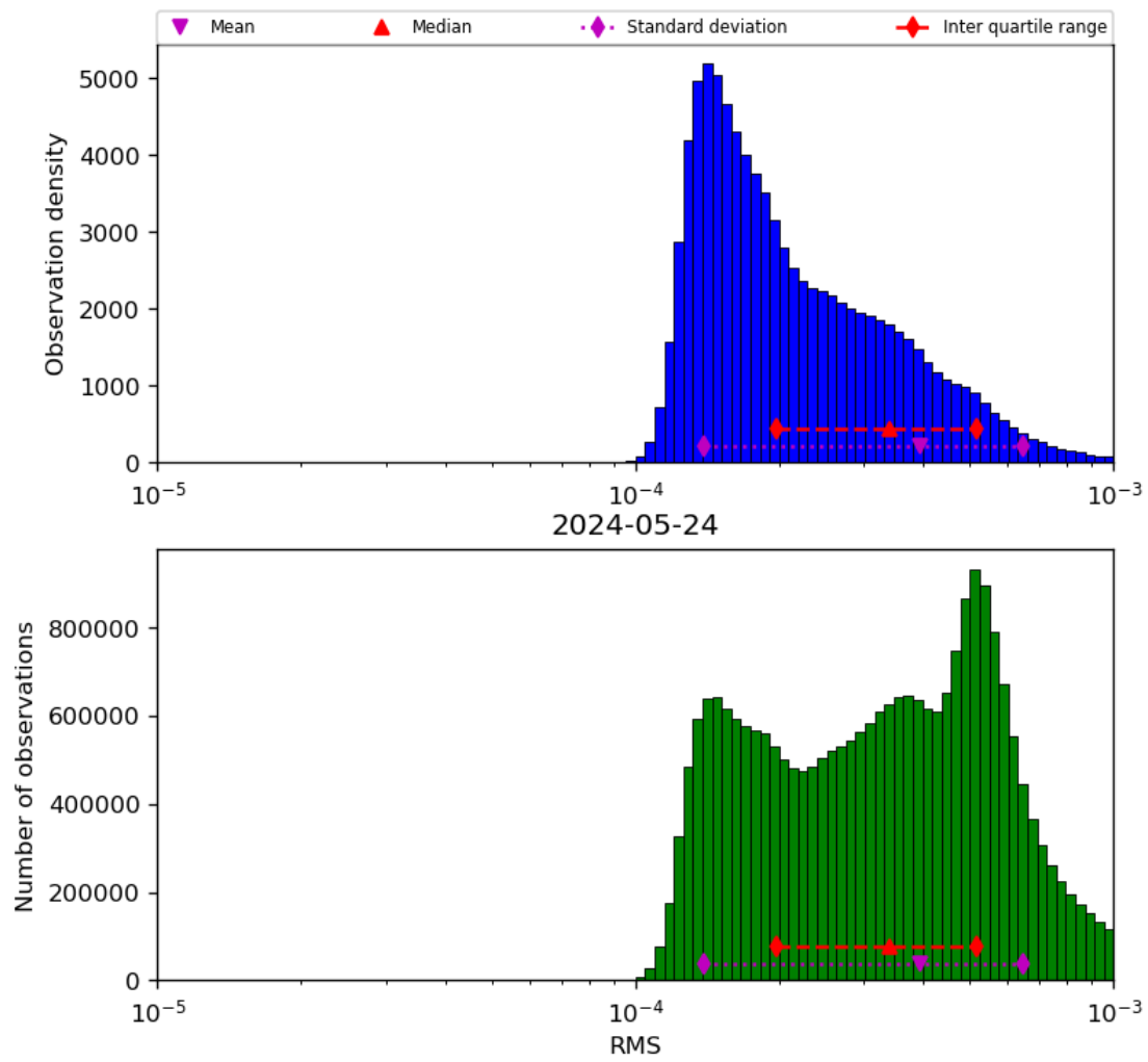
Figure 43: Histogram of “RMS” for 2024-05-23 to 2024-05-25
