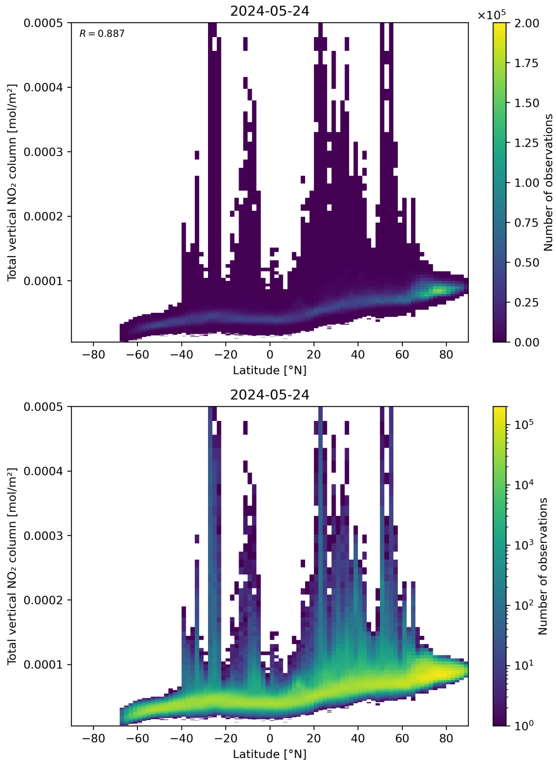
Figure 90: Scatter density plot of “Latitude” against “Total vertical NO 2 column” for 2024-05-23 to 2024-05-25.
