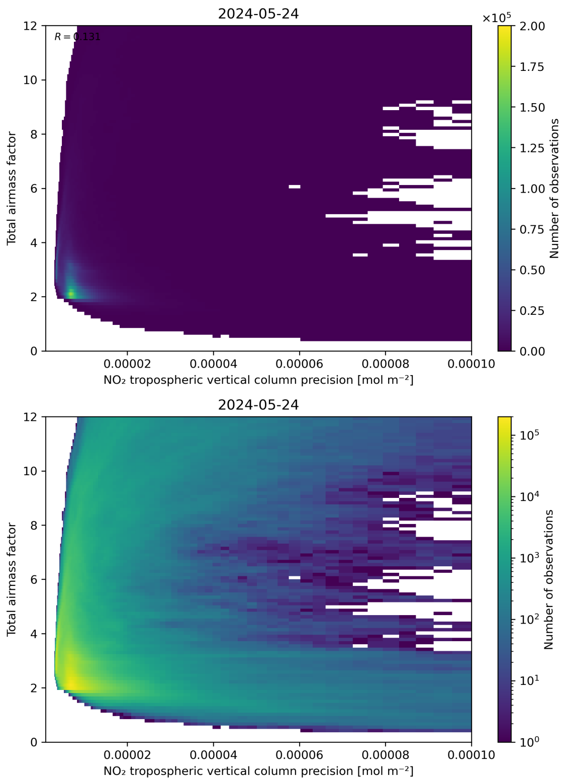
Figure 132: Scatter density plot of “NO 2 tropospheric vertical column precision” against “Total air mass factor” for 2024-05-23 to 2024-05-25.
