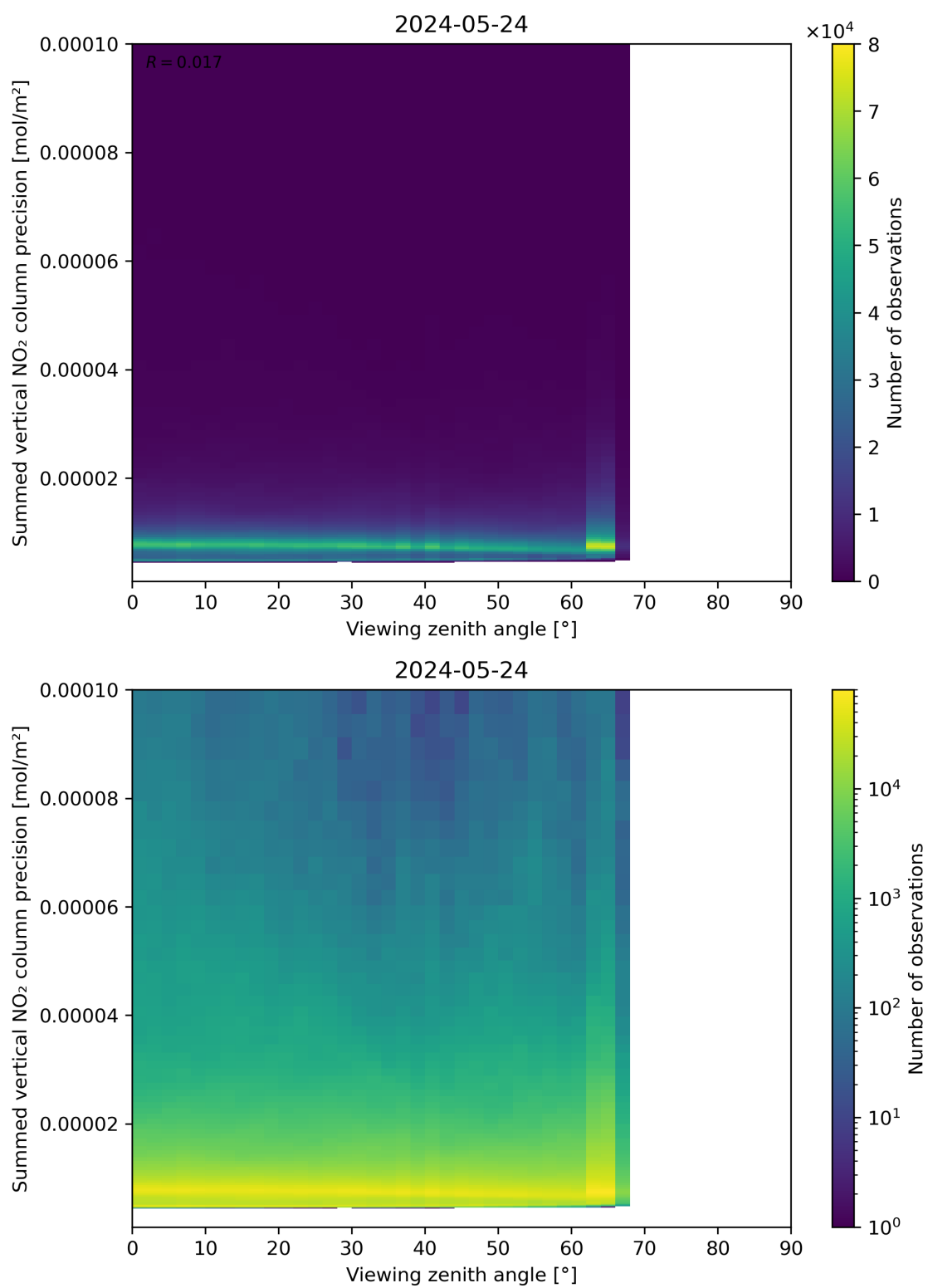
Figure 166: Scatter density plot of “Viewing zenith angle” against “Summed vertical NO 2 column precision” for 2024-05-23 to 2024-05-25.
