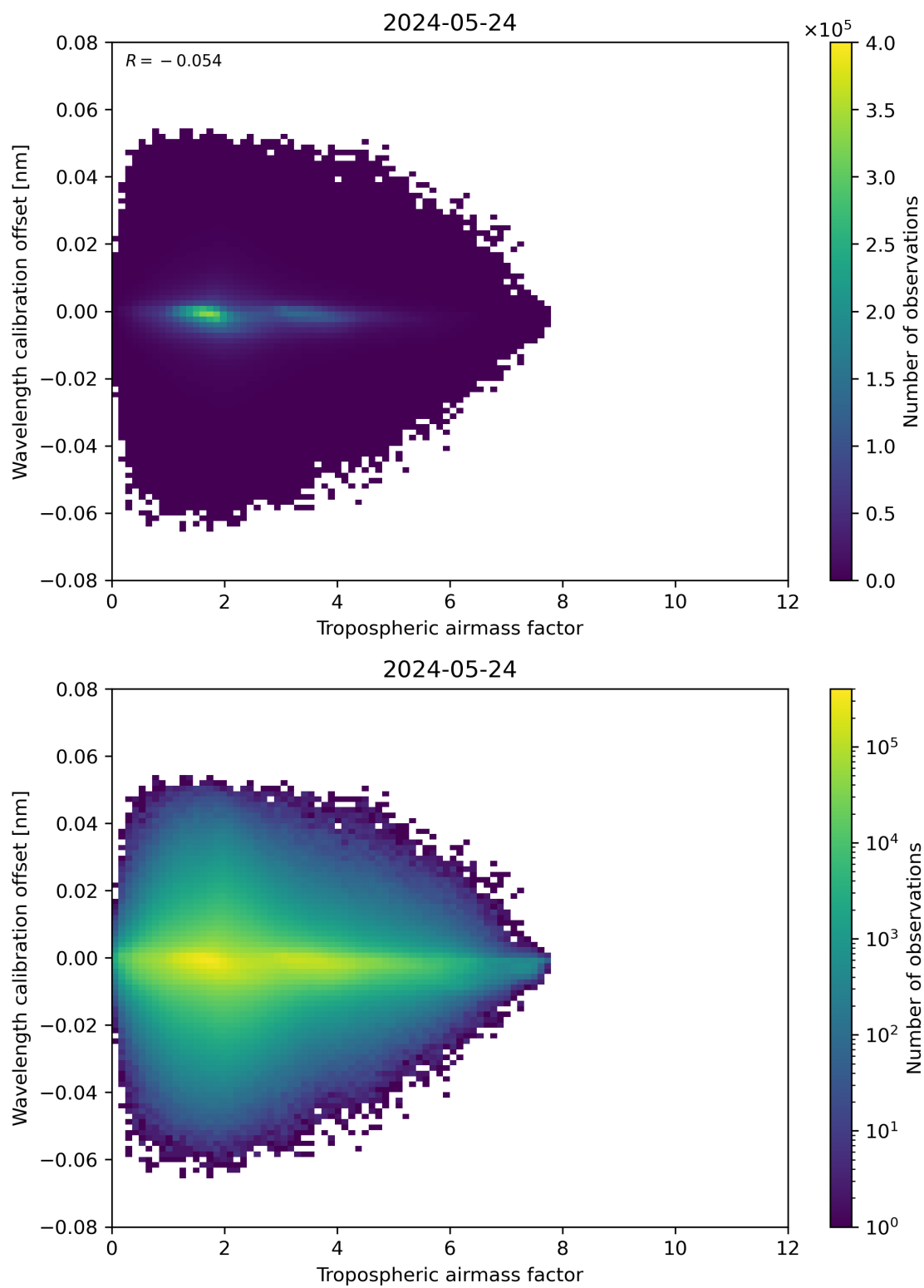
Figure 80: Scatter density plot of “Tropospheric air mass factor” against “Wavelength calibration offset” for 2024-05-23 to 2024-05-25.
