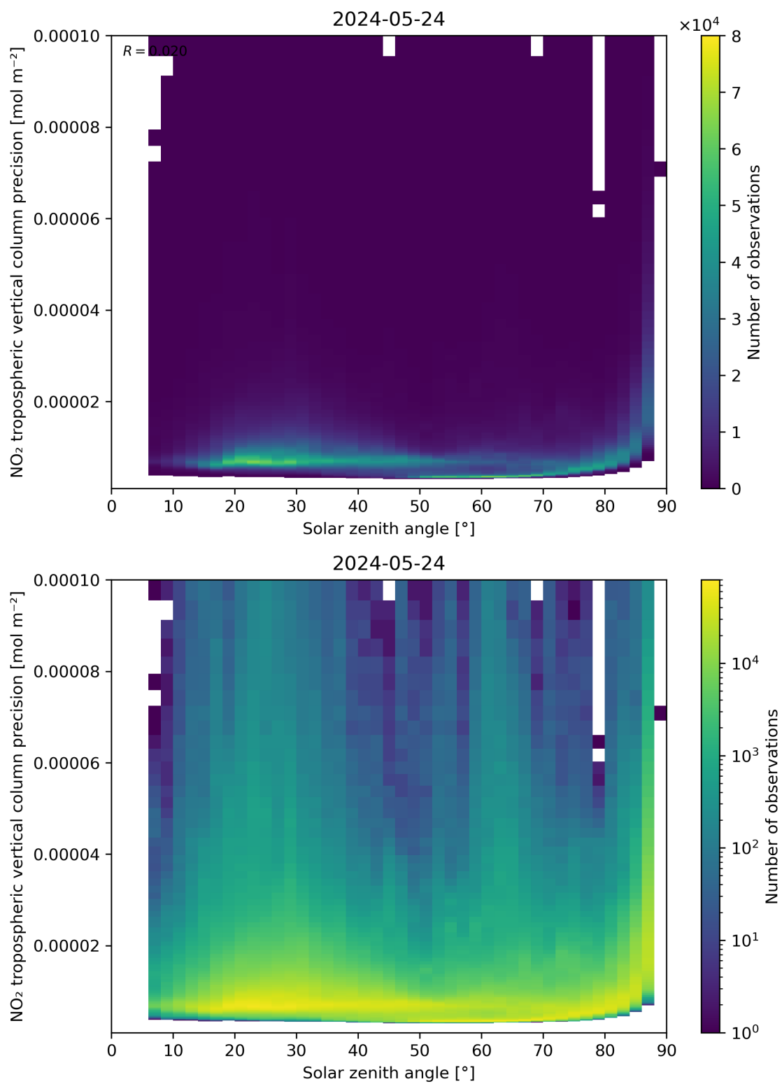
Figure 156: Scatter density plot of “Solar zenith angle” against “NO 2 tropospheric vertical column precision” for 2024-05-23 to 2024-05-25.
