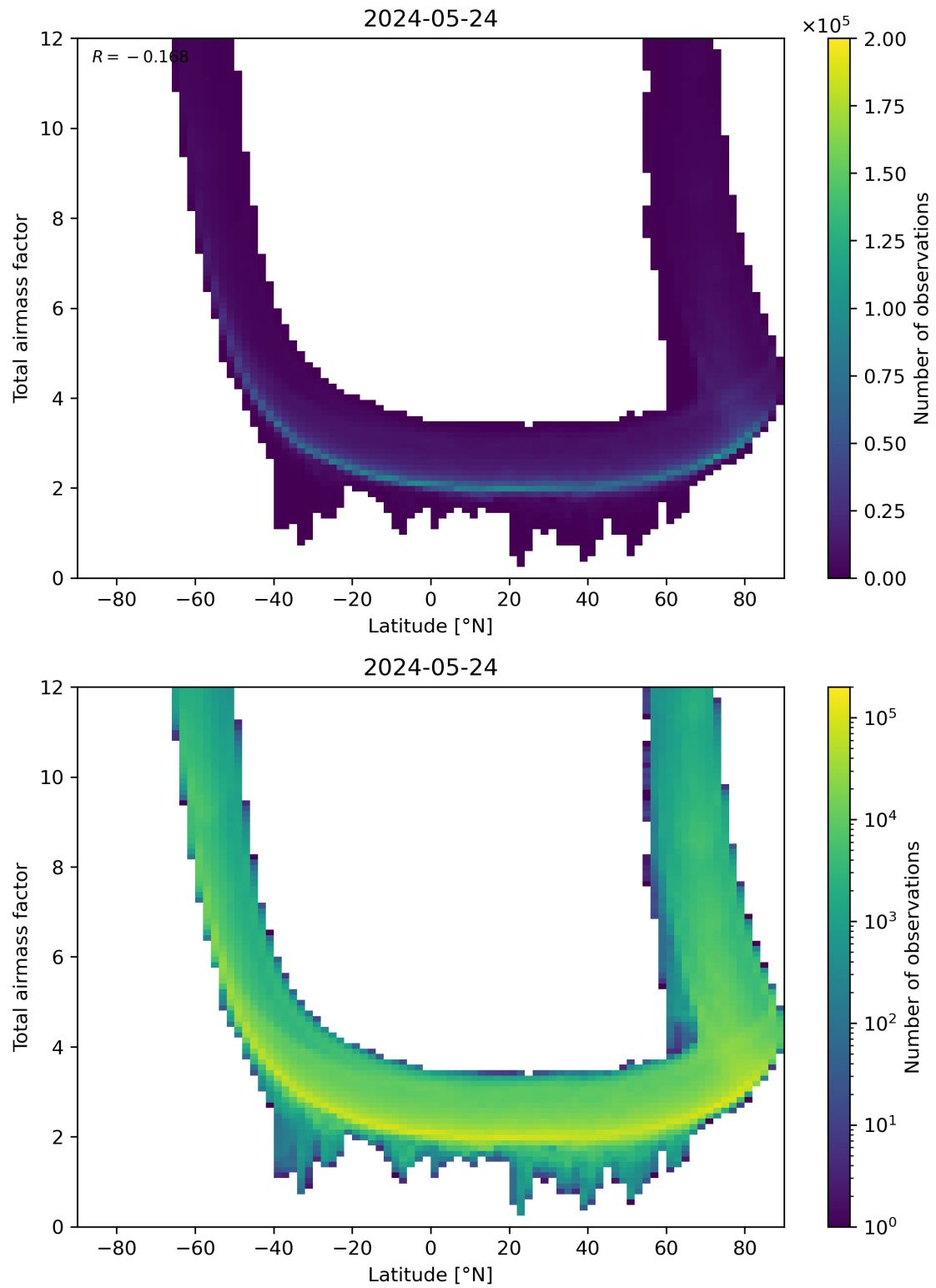
Figure 84: Scatter density plot of “Latitude” against “Total airmass factor” for 2024-05-23 to 2024-05-25.
