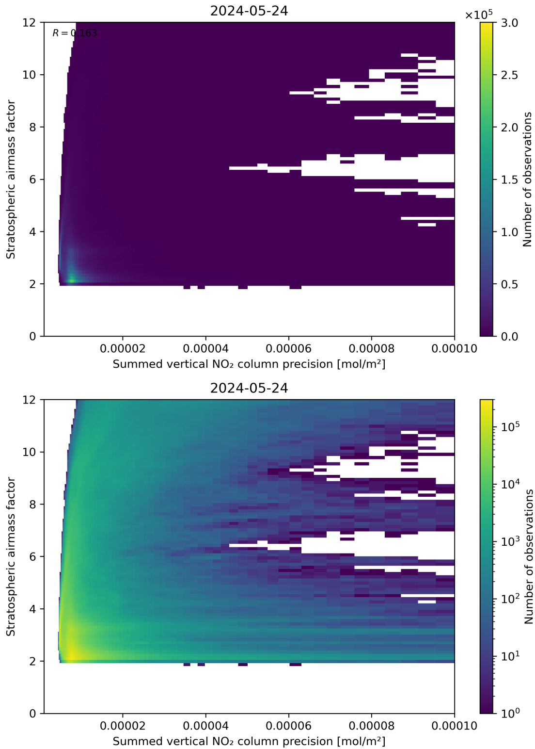
Figure 106: Scatter density plot of “Summed vertical NO 2 column precision” against “Stratospheric airmass factor” for 2024-05-23 to 2024-05-25.
