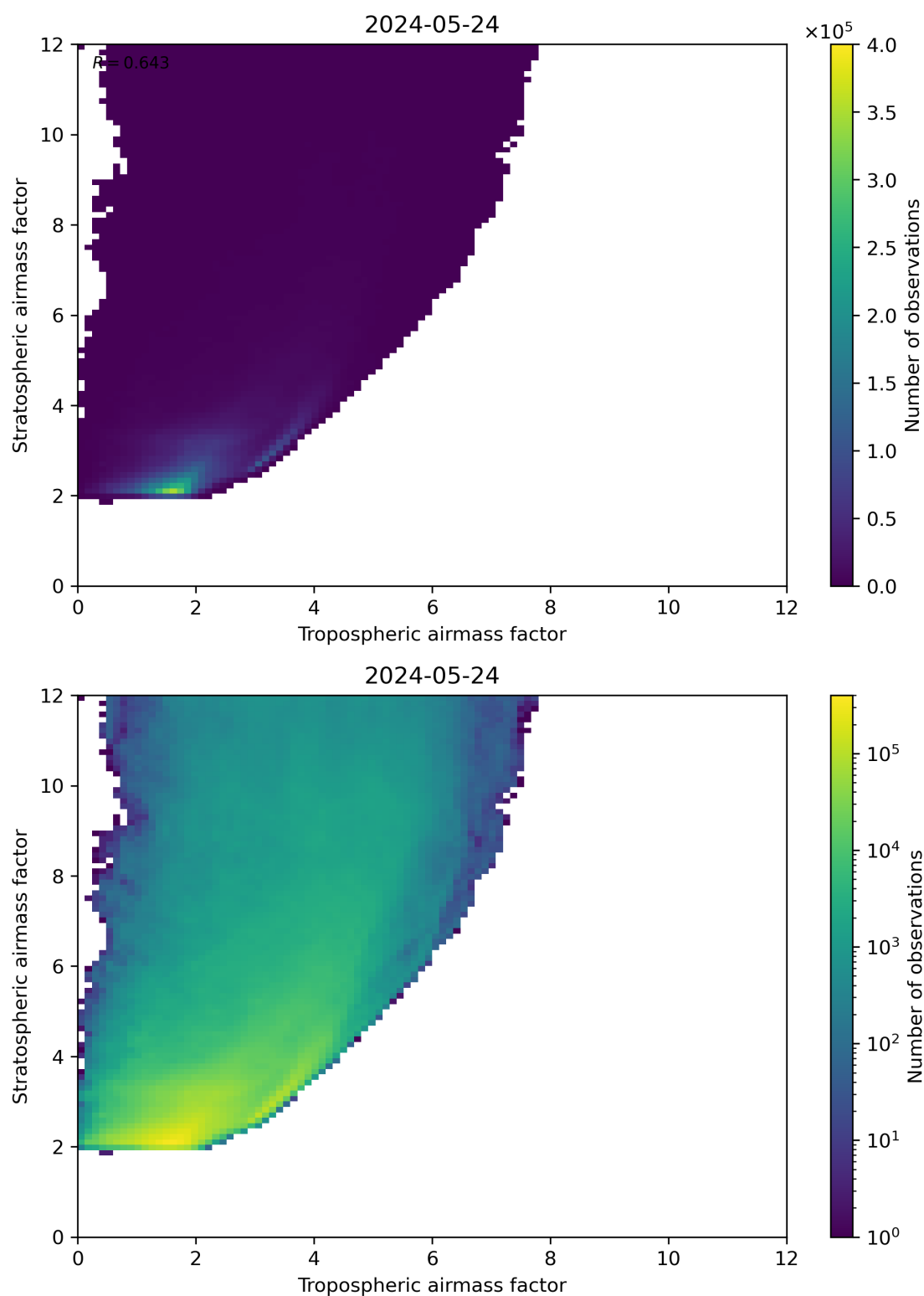
Figure 71: Scatter density plot of “Tropospheric airmass factor” against “Stratospheric airmass factor” for 2024-05-23 to 2024-05-25.
