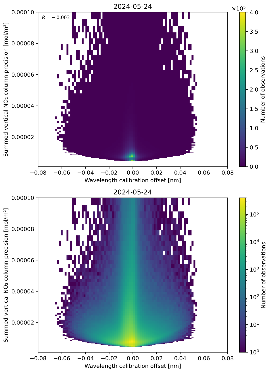
Figure 178: Scatter density plot of “Wavelength calibration offset” against “Summed vertical NO 2 column precision” for 2024-05-23 to 2024-05-25.
