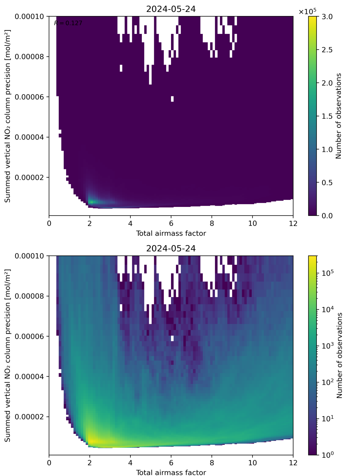
Figure 66: Scatter density plot of “Total airmass factor” against “Summed vertical NO 2 column precision” for 2024-05-23 to 2024-05-25.
