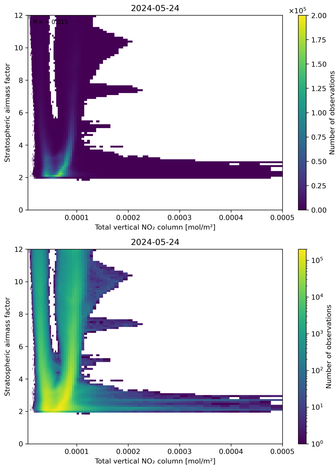
Figure 110: Scatter density plot of “Total vertical NO 2 column” against “Stratospheric airmass factor” for 2024-05-23 to 2024-05-25.
