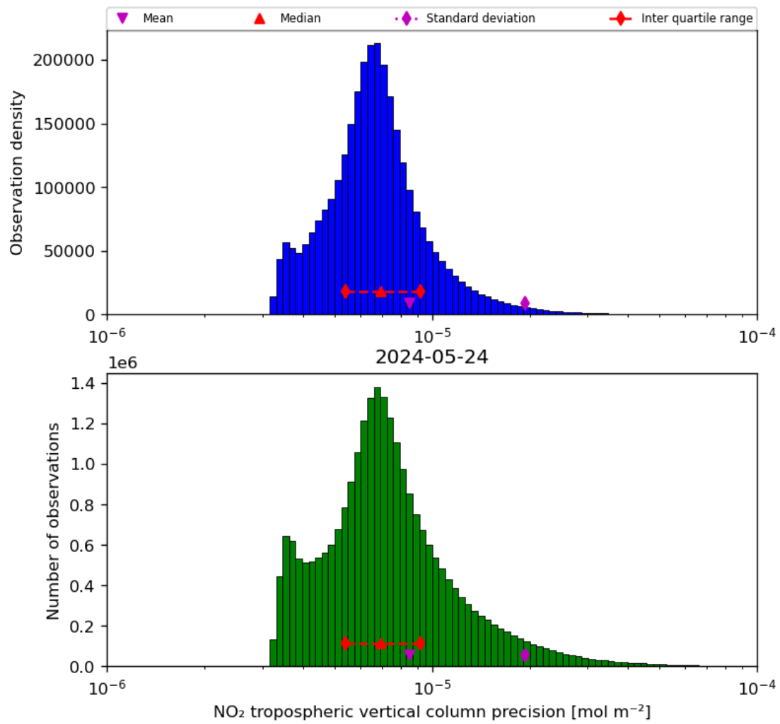
Figure 30: Histogram of “NO 2 tropospheric vertical column precision” for 2024-05-23 to 2024-05-25
