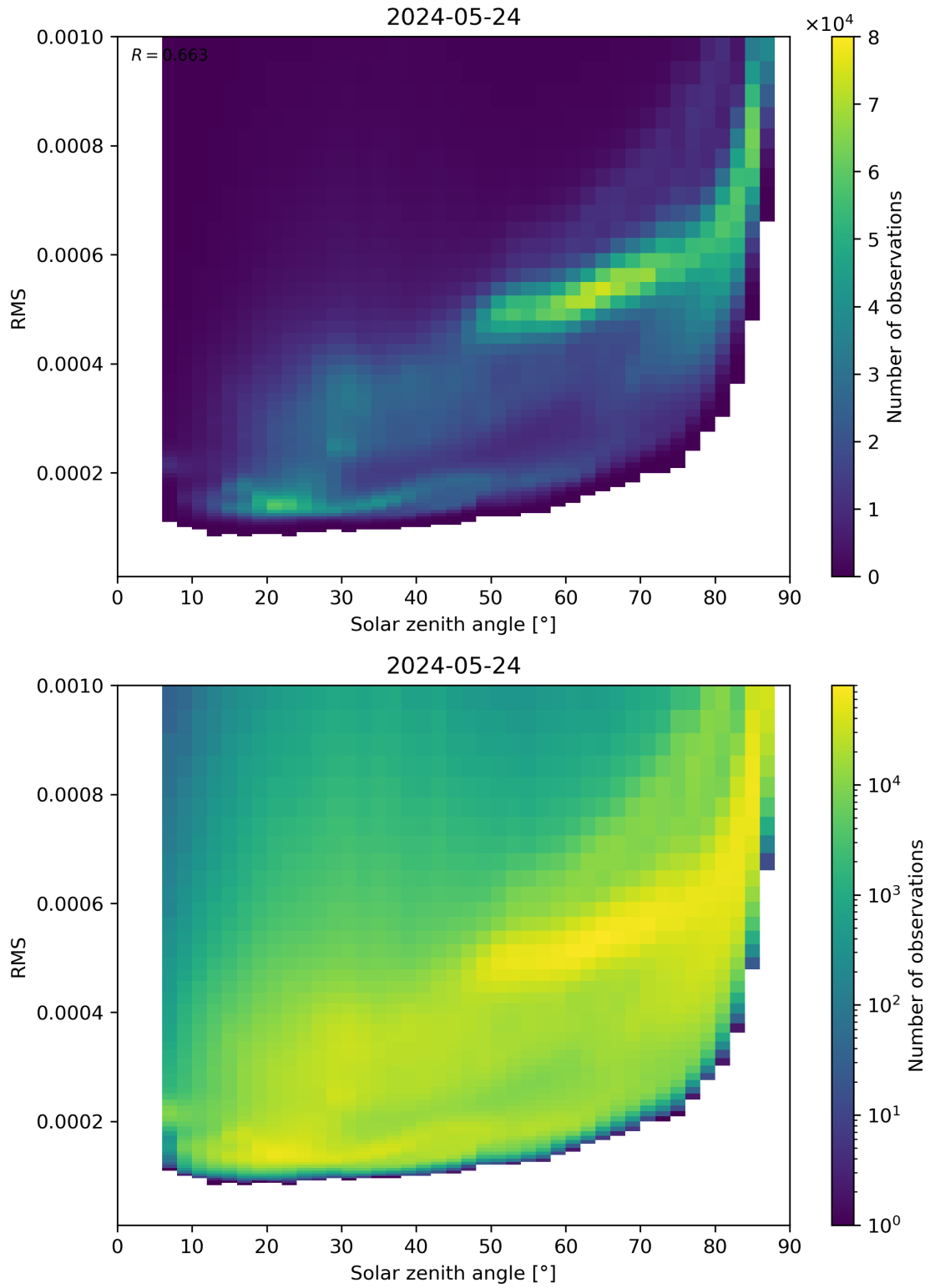
Figure 157: Scatter density plot of “Solar zenith angle” against “RMS” for 2024-05-23 to 2024-05-25.
