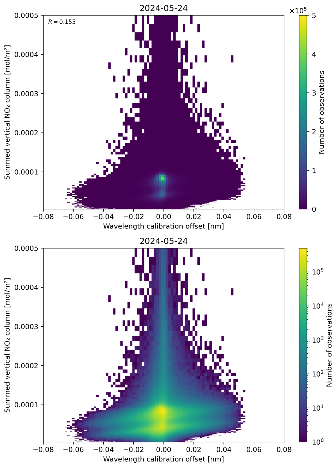
Figure 177: Scatter density plot of “Wavelength calibration offset” against “Summed vertical NO 2 column” for 2024-05-23 to 2024-05-25.
