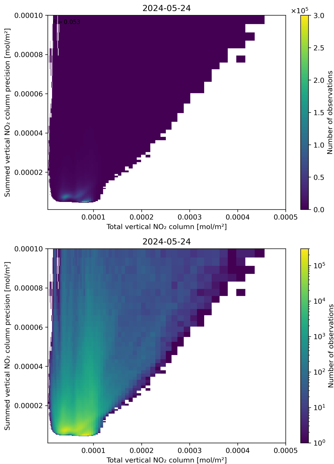
Figure 113: Scatter density plot of “Total vertical NO 2 column” against “Summed vertical NO 2 column precision” for 2024-05-23 to 2024-05-25.
