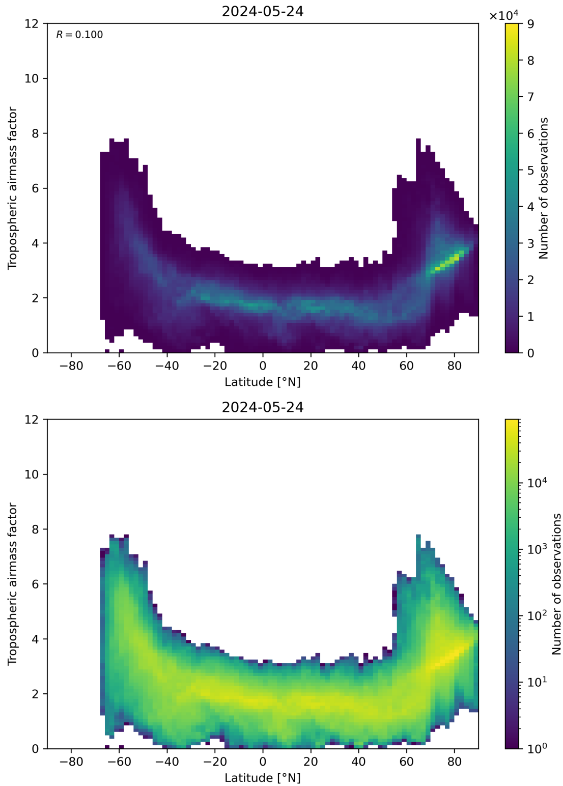
Figure 85: Scatter density plot of “Latitude” against “Tropospheric air mass factor” for 2024-05-23 to 2024-05-25.
