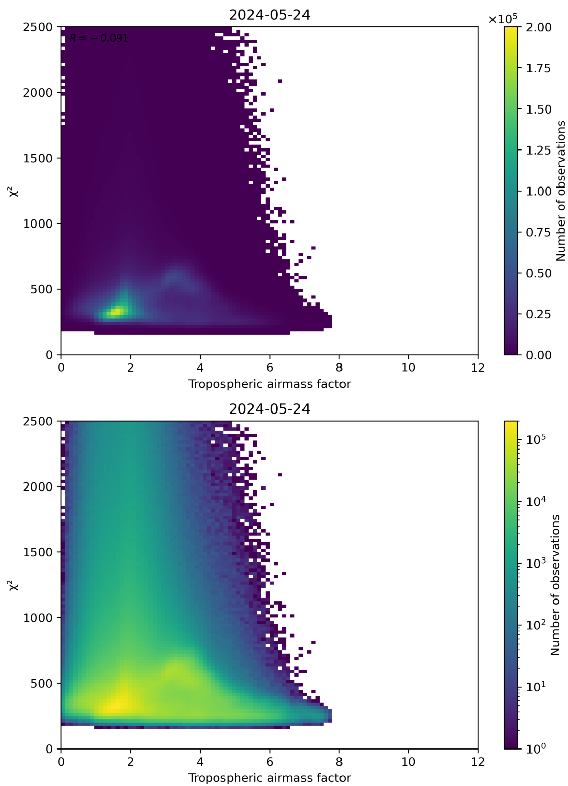
Figure 73: Scatter density plot of “Tropospheric airmass factor” against “ \chi^2 ” for 2024-05-23 to 2024-05-25.
