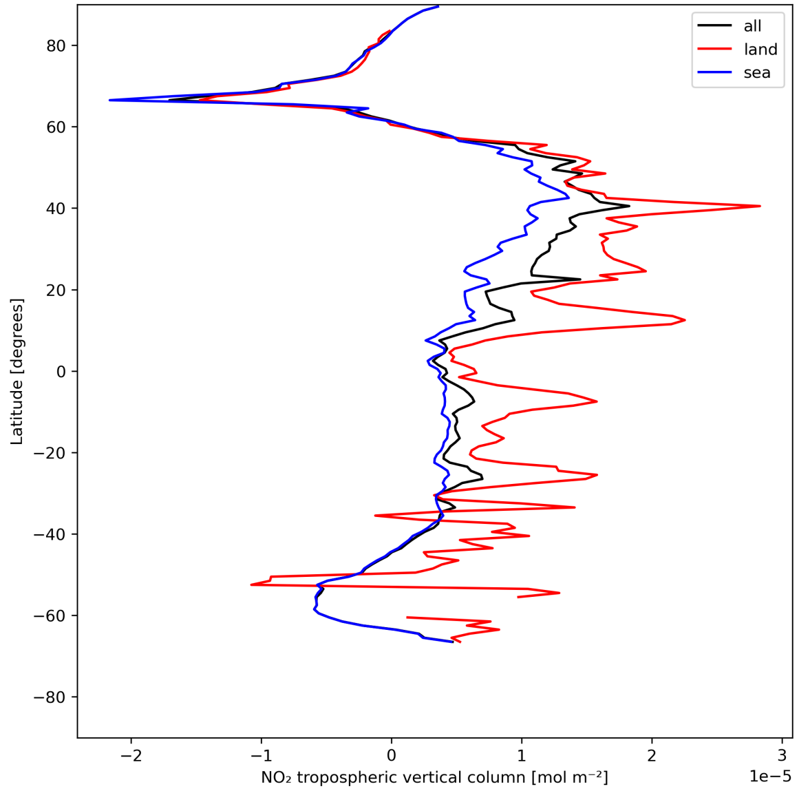
Figure 12: Zonal average of “NO 2 tropospheric vertical column” for 2024-05-23 to 2024-05-25.
