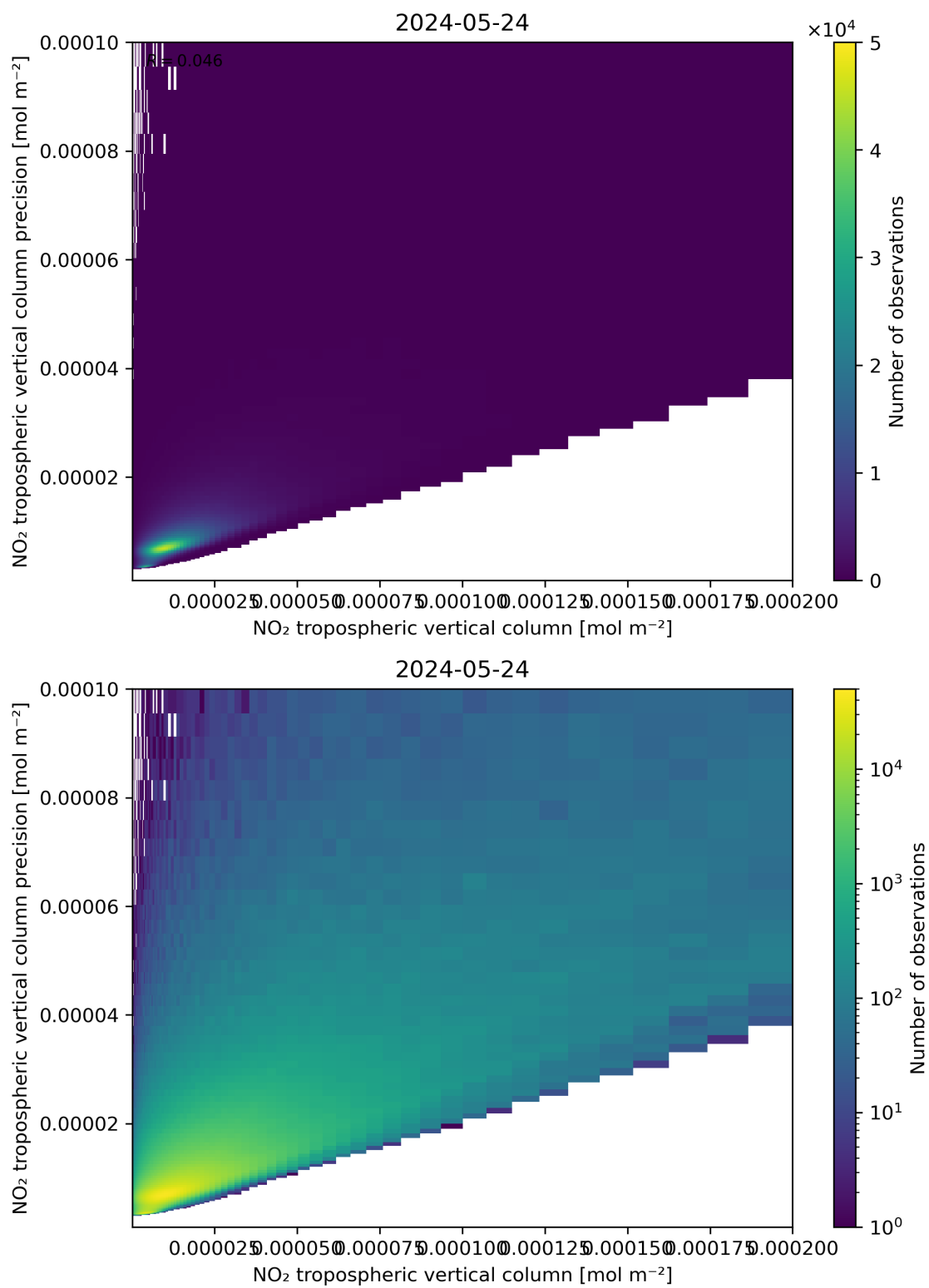
Figure 130: Scatter density plot of “NO 2 tropospheric vertical column” against “NO 2 tropospheric vertical column precision” for 2024-05-23 to 2024-05-25.
