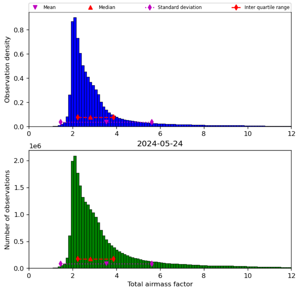
Figure 32: Histogram of “Total airmass factor” for 2024-05-23 to 2024-05-25
