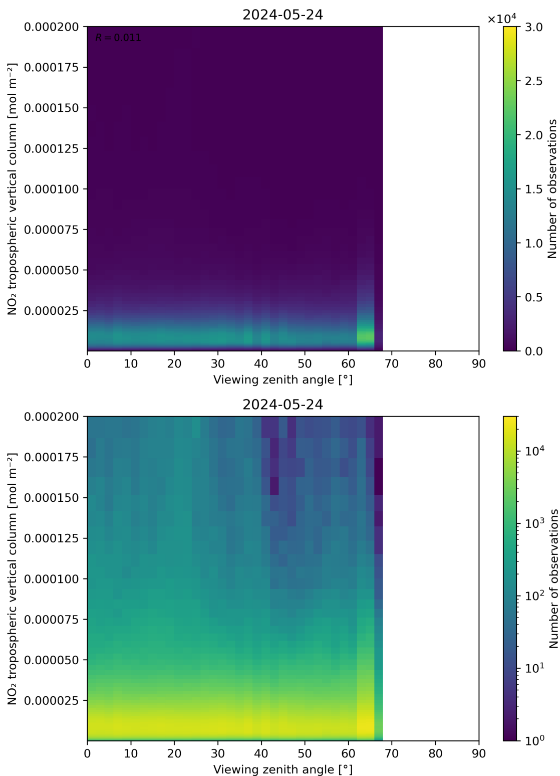
Figure 169: Scatter density plot of “Viewing zenith angle” against “NO 2 tropospheric vertical column” for 2024-05-23 to 2024-05-25.
