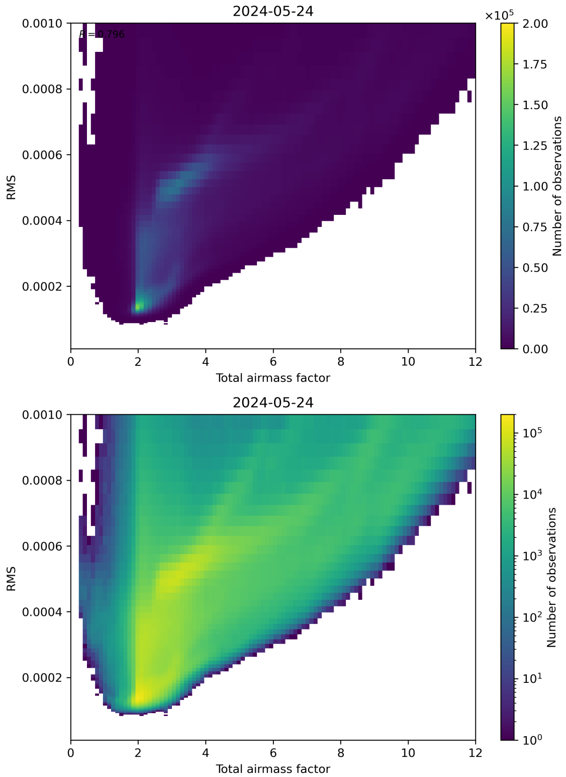
Figure 69: Scatter density plot of “Total airmass factor” against “RMS” for 2024-05-23 to 2024-05-25.
