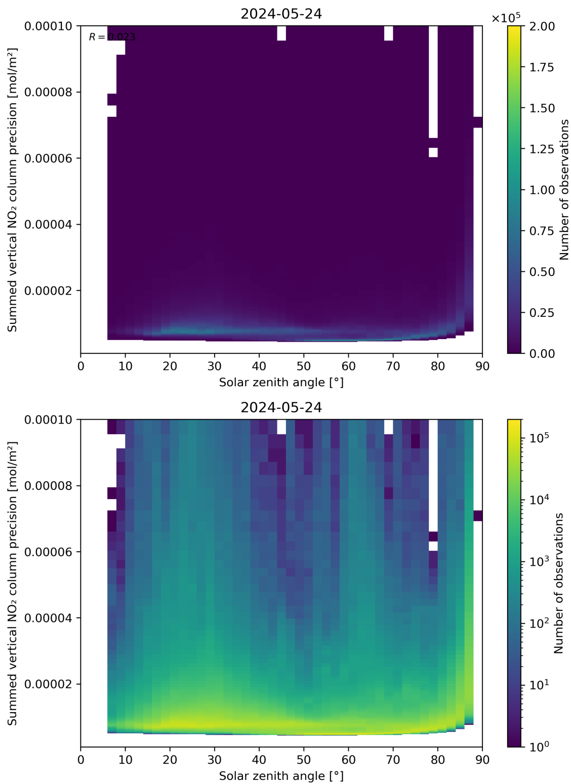
Figure 152: Scatter density plot of “Solar zenith angle” against “Summed vertical NO 2 column precision” for 2024-05-23 to 2024-05-25.
