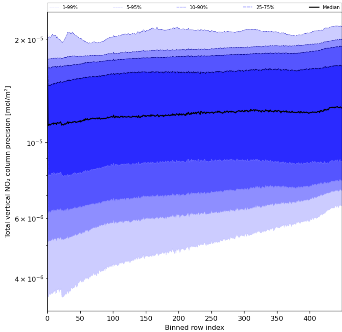
Figure 56: Along track statistics of “Total vertical NO 2 column precision” for 2024-05-23 to 2024-05-25
