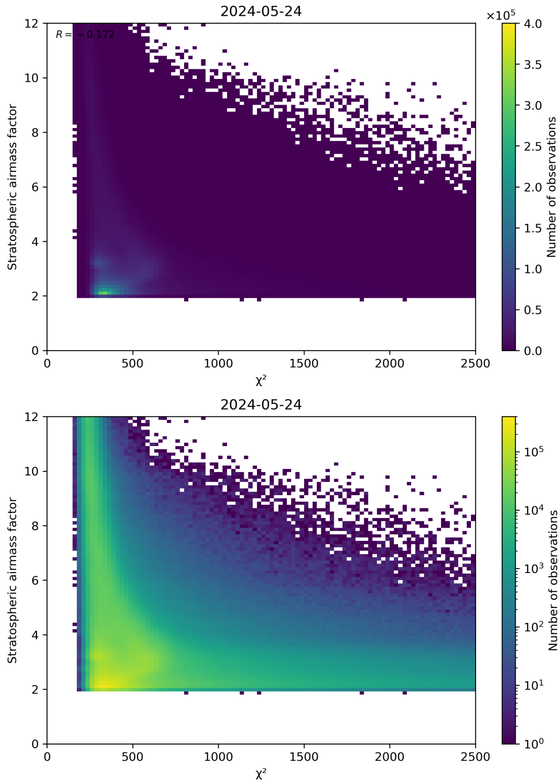
Figure 81: Scatter density plot of “ \chi^2 ” against “Stratospheric airmass factor” for 2024-05-23 to 2024-05-25.
