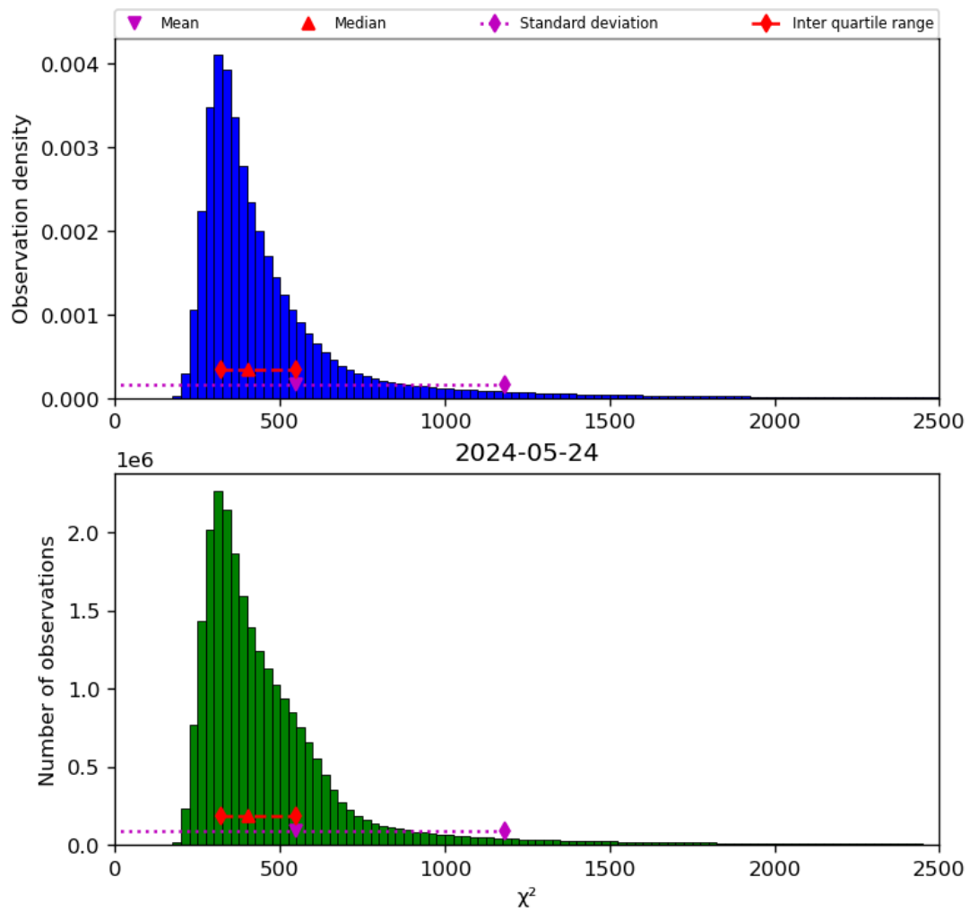
Figure 42: Histogram of “ \chi^2 ” for 2024-05-23 to 2024-05-25
