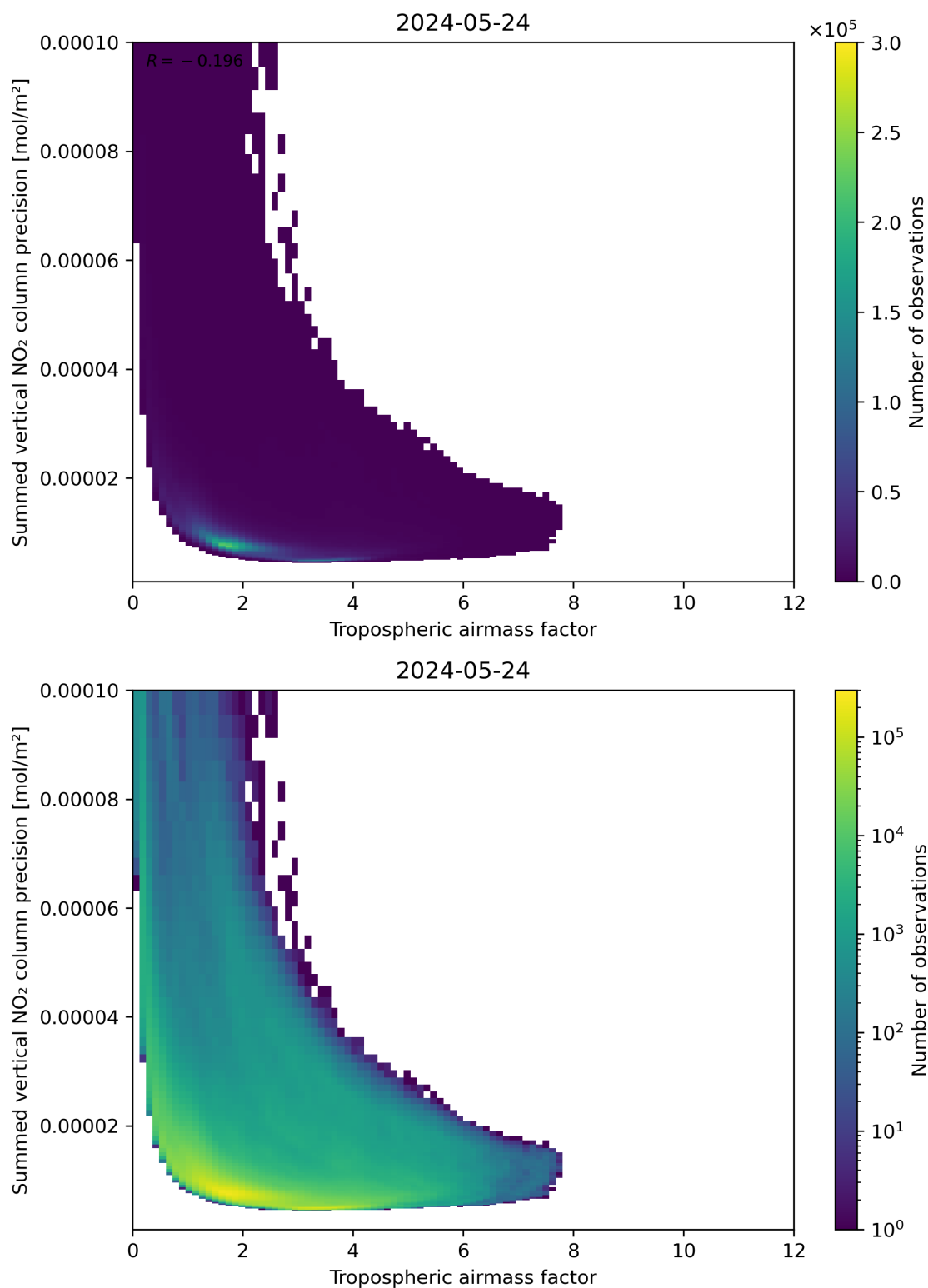
Figure 76: Scatter density plot of “Tropospheric air mass factor” against “Summed vertical NO 2 column precision” for 2024-05-23 to 2024-05-25.
