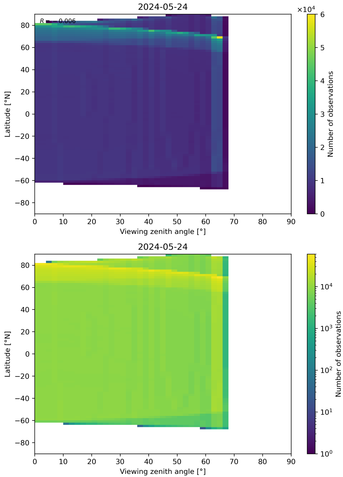
Figure 163: Scatter density plot of “Viewing zenith angle” against “Latitude” for 2024-05-23 to 2024-05-25.
