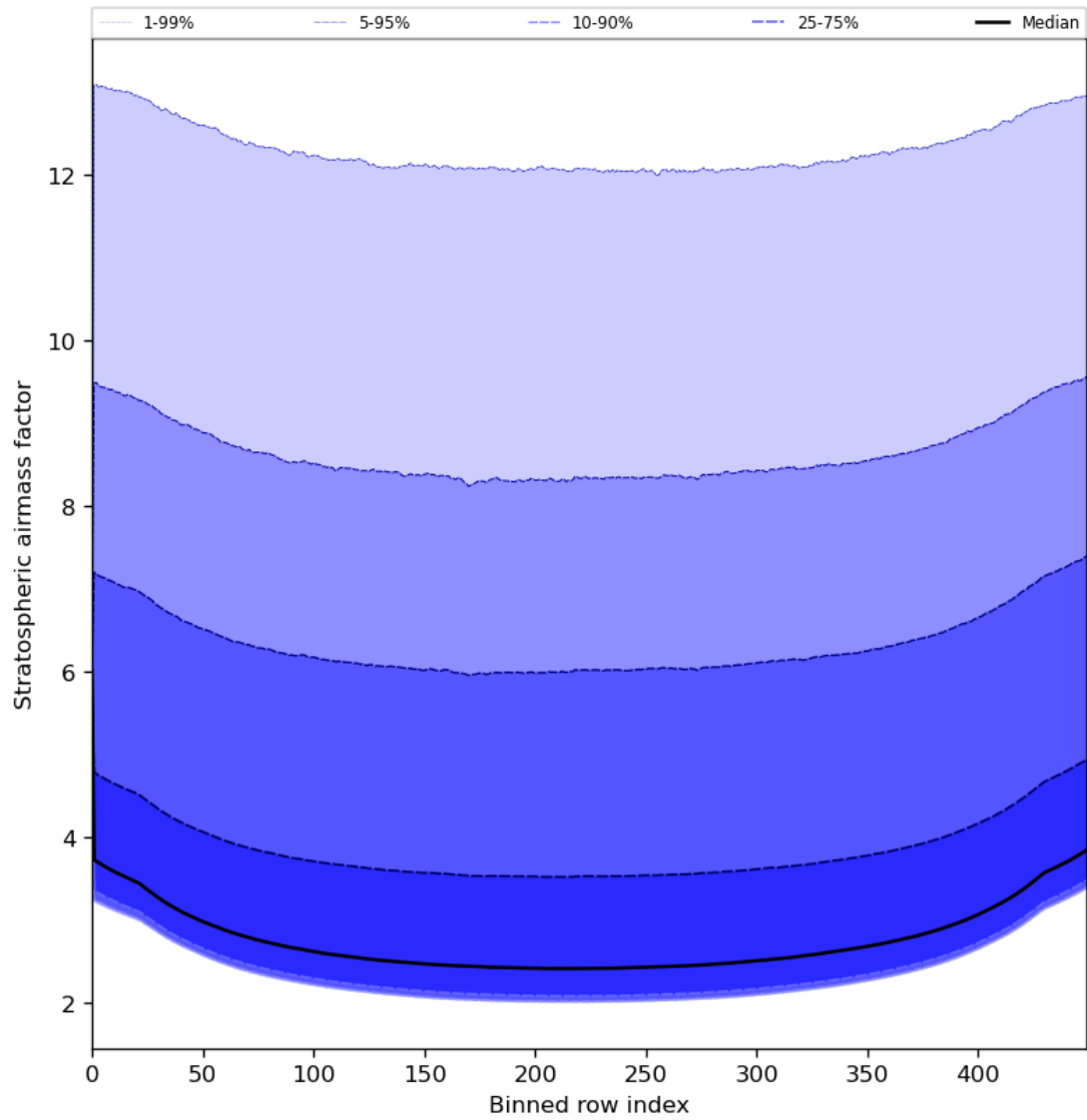
Figure 61: Along track statistics of “Stratospheric airmass factor” for 2024-05-23 to 2024-05-25
