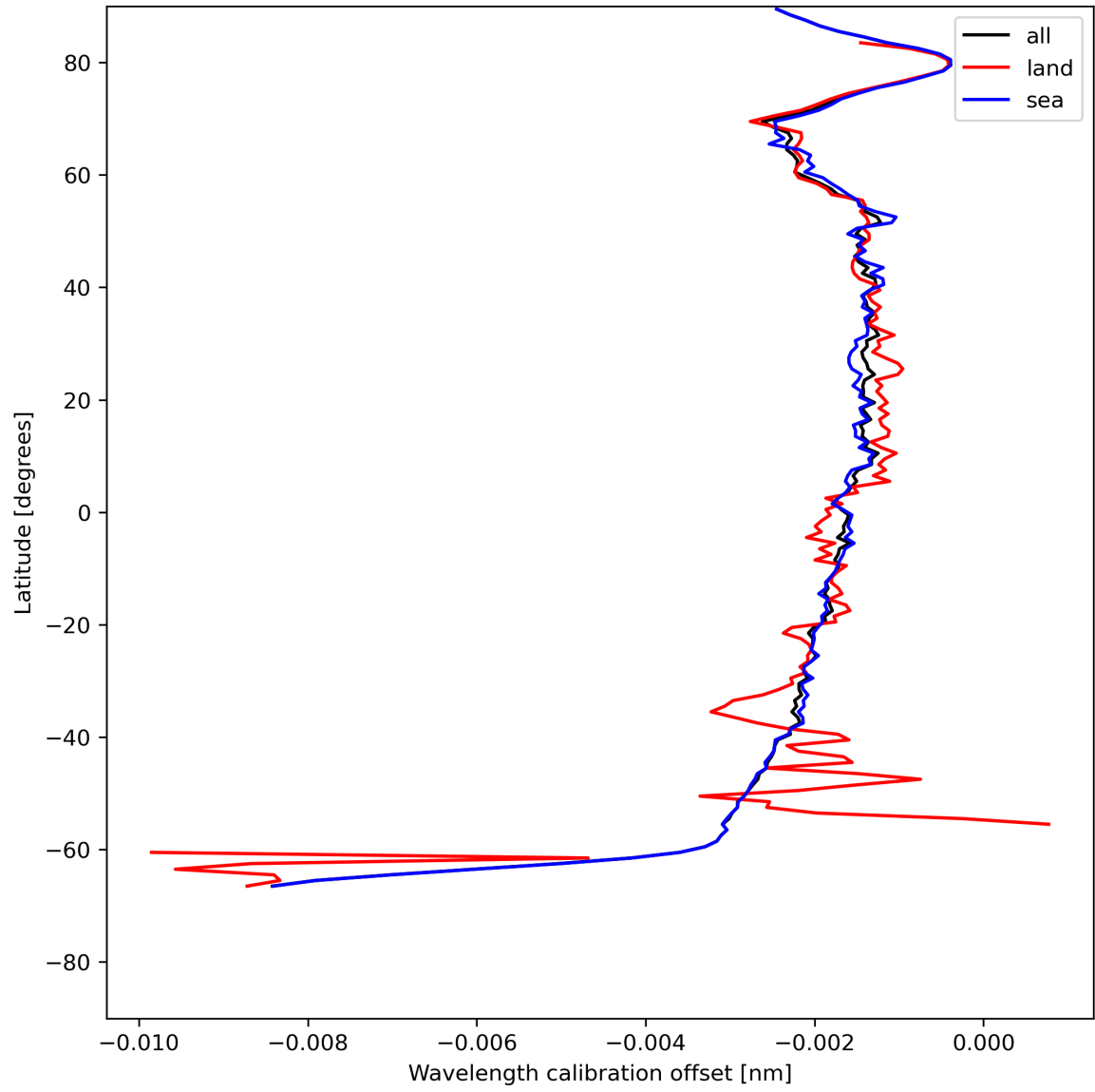
Figure 18: Zonal average of “Wavelength calibration offset” for 2024-05-23 to 2024-05-25.
