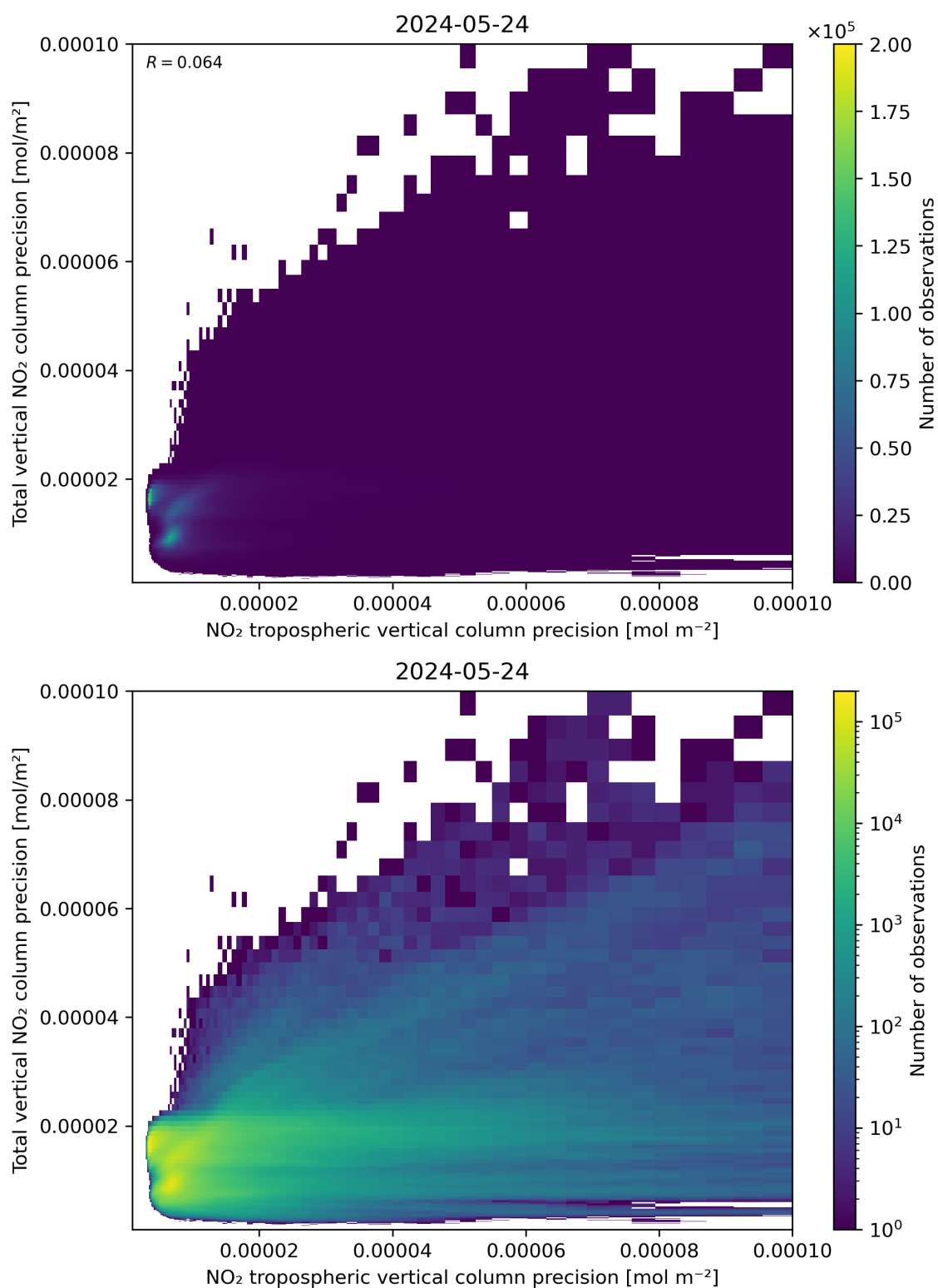
Figure 139: Scatter density plot of “NO 2 tropospheric vertical column precision” against “Total vertical NO 2 column precision” for 2024-05-23 to 2024-05-25.
