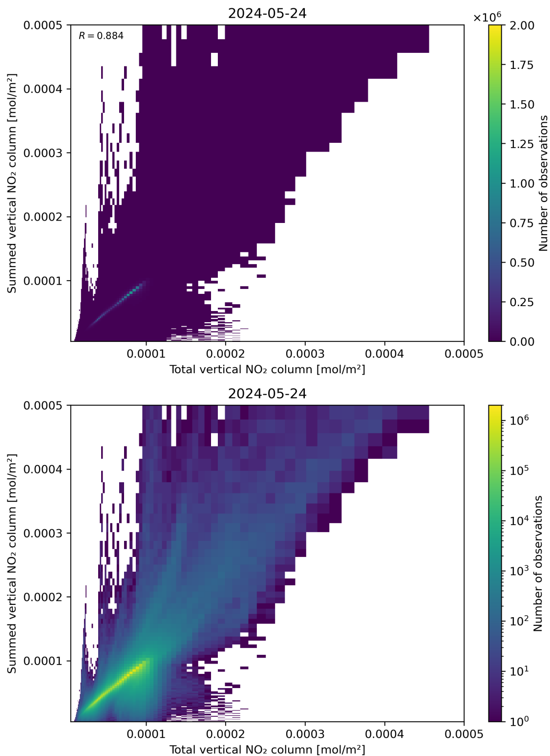
Figure 112: Scatter density plot of “Total vertical NO 2 column” against “Summed vertical NO 2 column” for 2024-05-23 to 2024-05-25.
