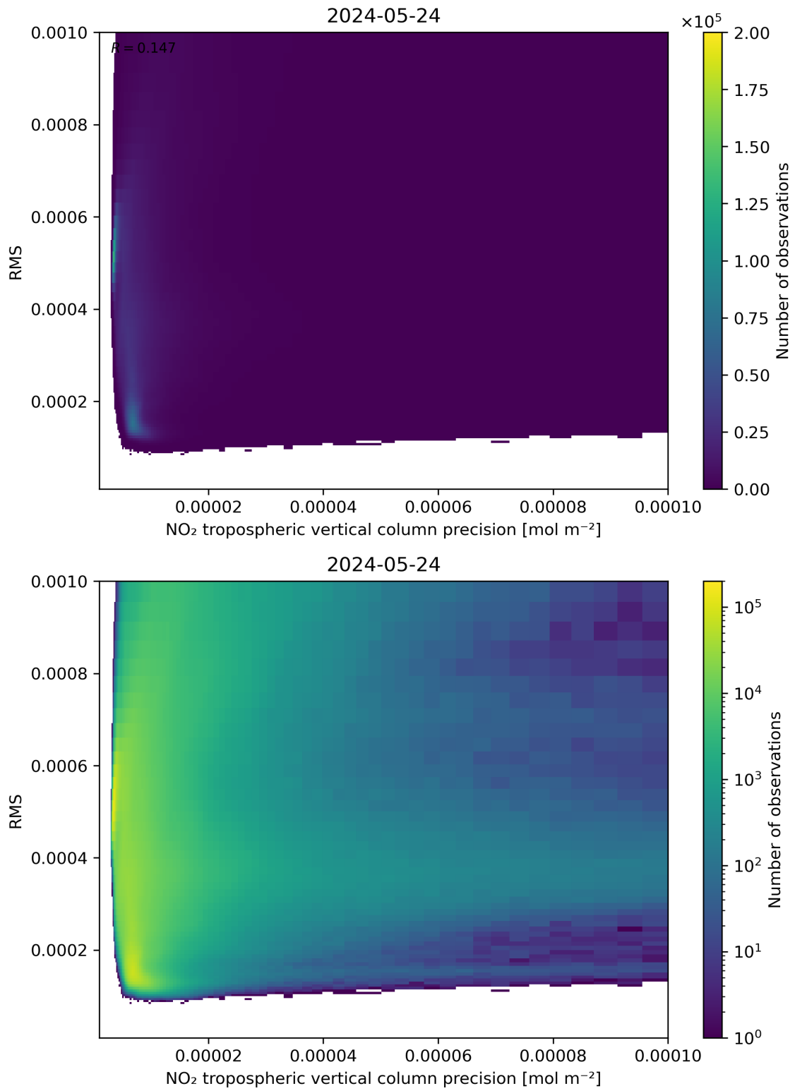
Figure 140: Scatter density plot of “NO 2 tropospheric vertical column precision” against “RMS” for 2024-05-23 to 2024-05-25.
