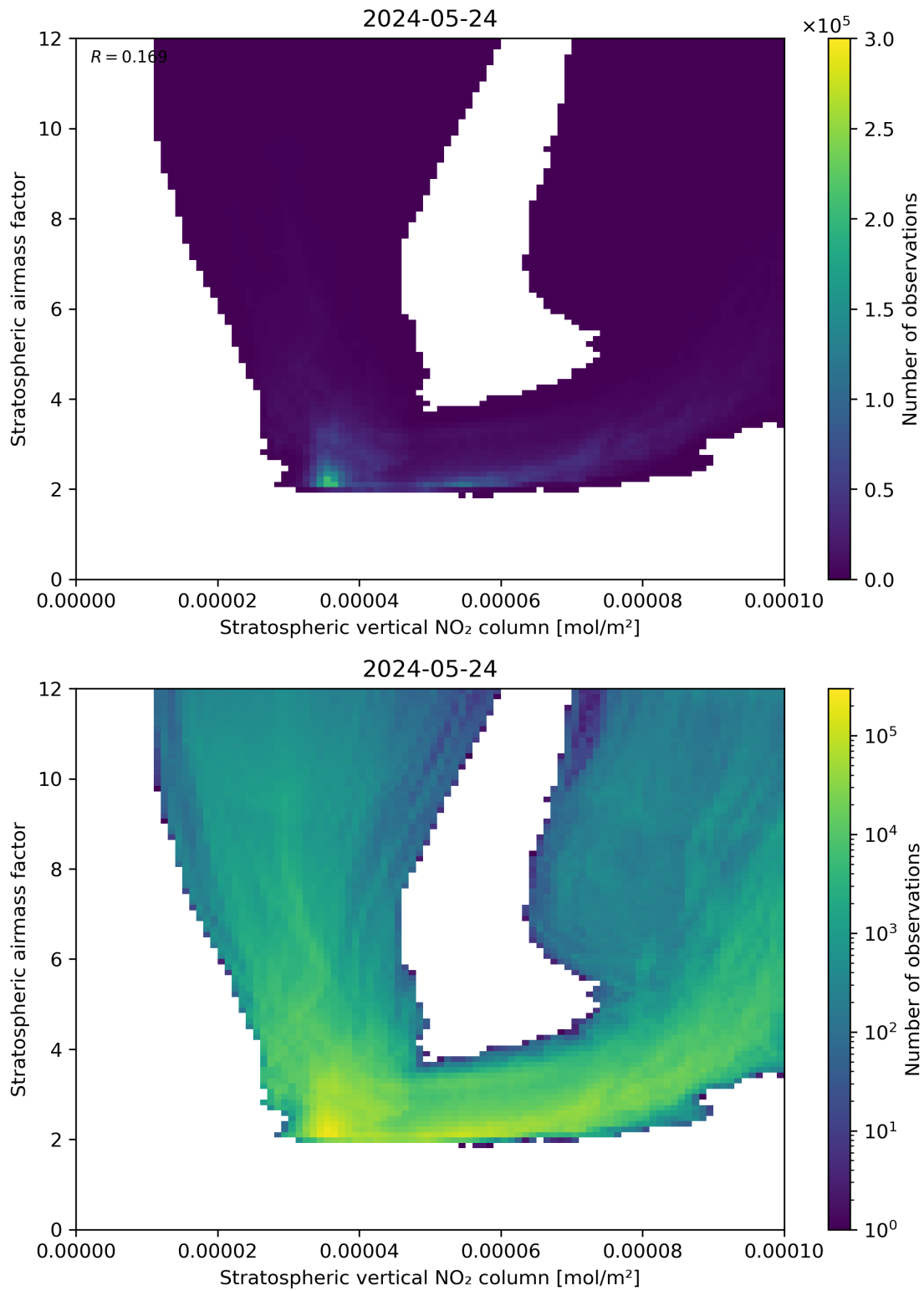
Figure 96: Scatter density plot of “Stratospheric vertical NO 2 column” against “Stratospheric airmass factor” for 2024-05-23 to 2024-05-25.
