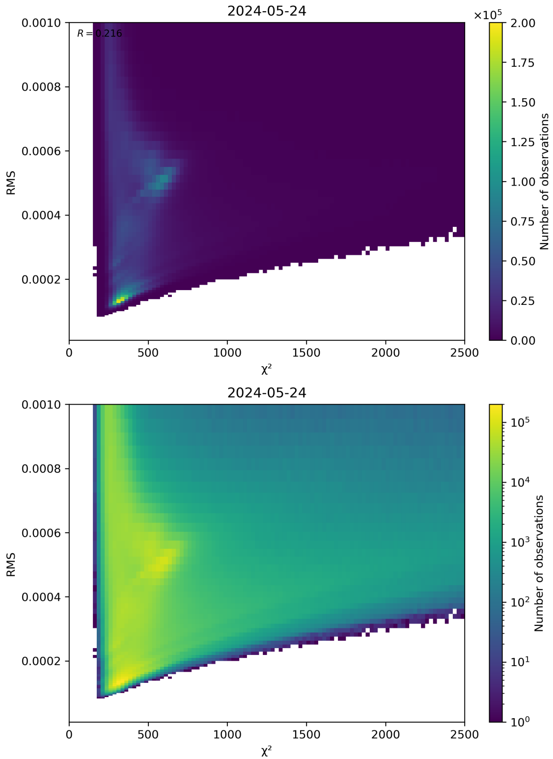
Figure 82: Scatter density plot of “ \chi^2 ” against “RMS” for 2024-05-23 to 2024-05-25.
