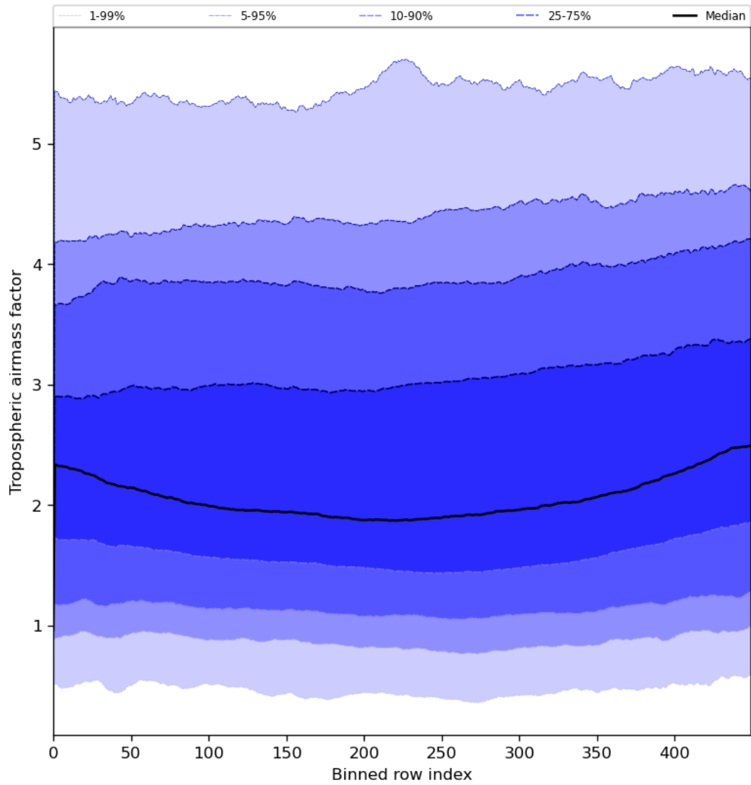
Figure 48: Along track statistics of “Tropospheric airmass factor” for 2024-05-23 to 2024-05-25
