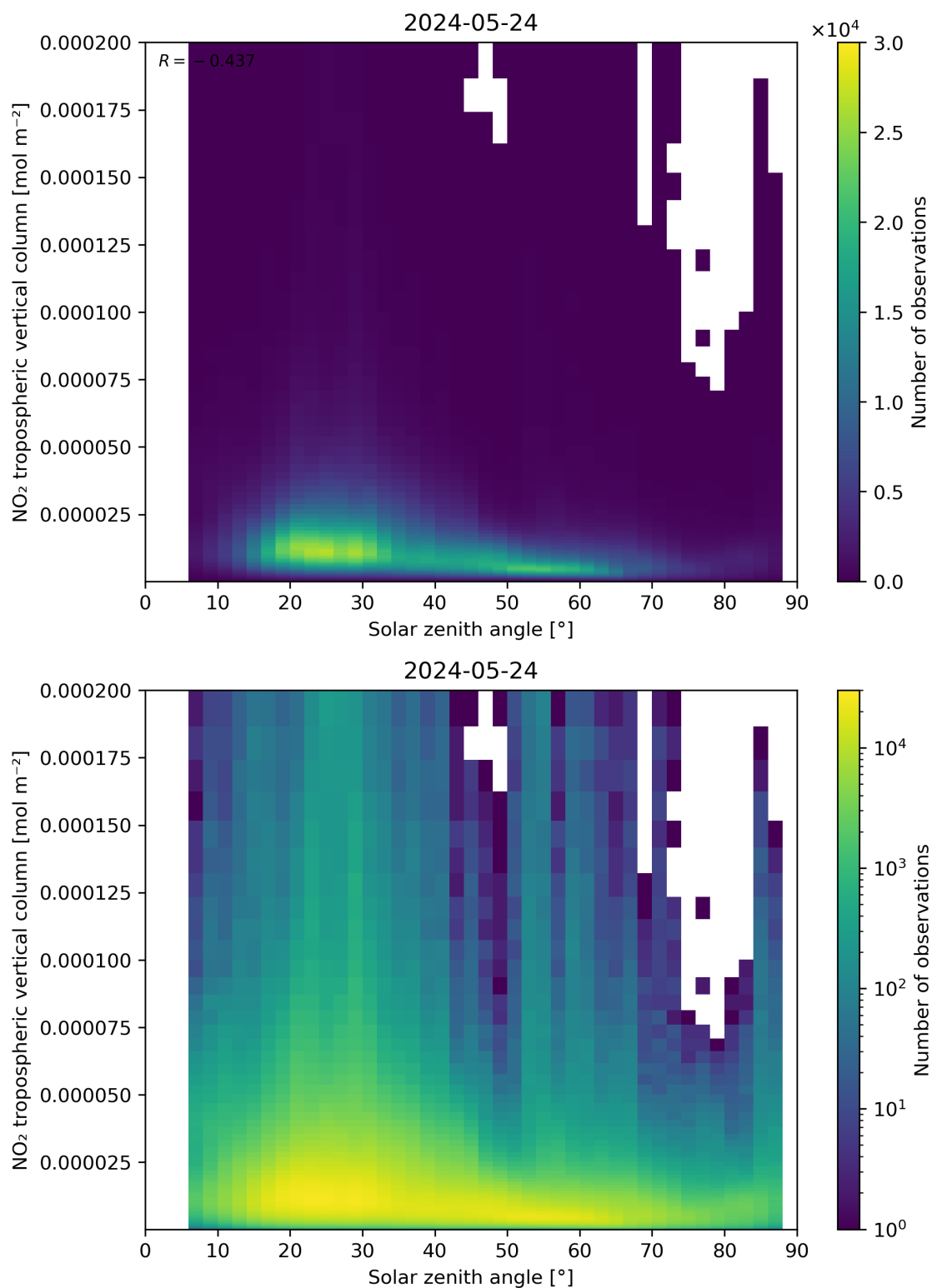
Figure 155: Scatter density plot of “Solar zenith angle” against “NO 2 tropospheric vertical column” for 2024-05-23 to 2024-05-25.
