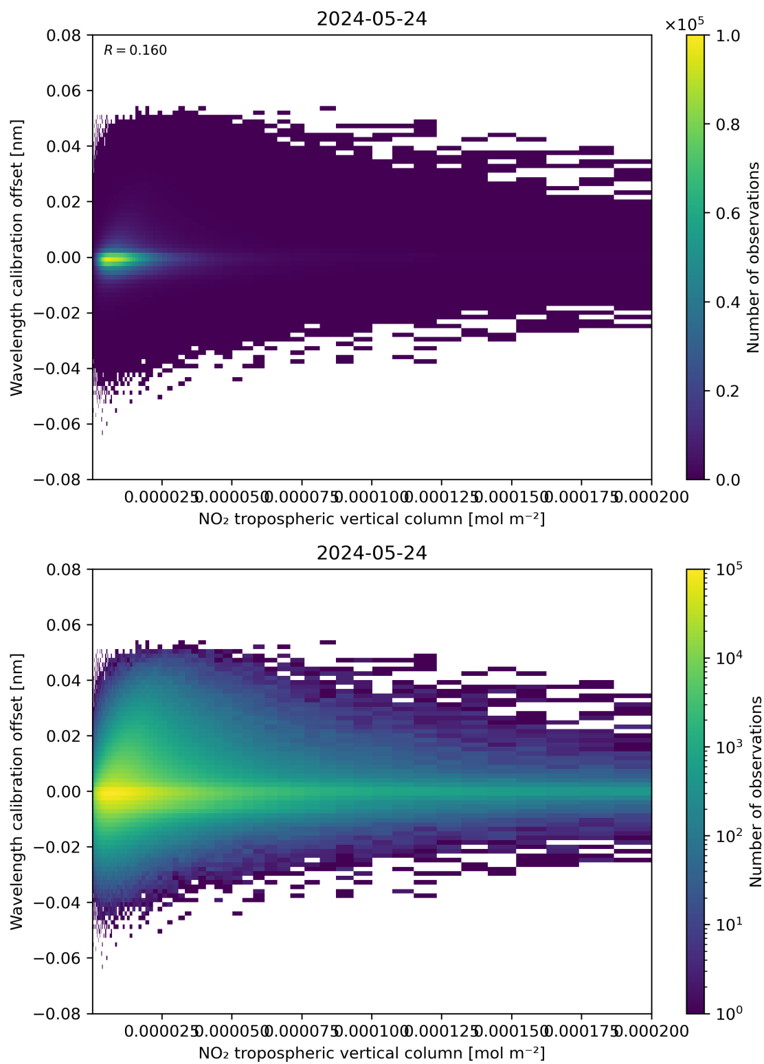
Figure 143: Scatter density plot of “NO 2 tropospheric vertical column” against “Wavelength calibration offset” for 2024-05-23 to 2024-05-25.
