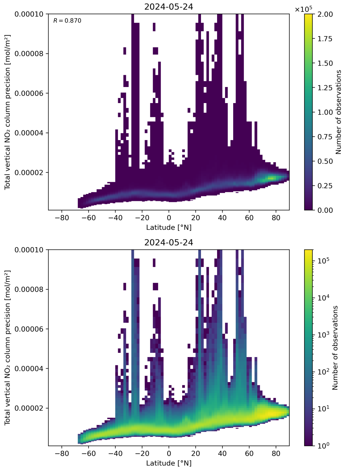
Figure 91: Scatter density plot of “Latitude” against “Total vertical NO 2 column precision” for 2024-05-23 to 2024-05-25.
