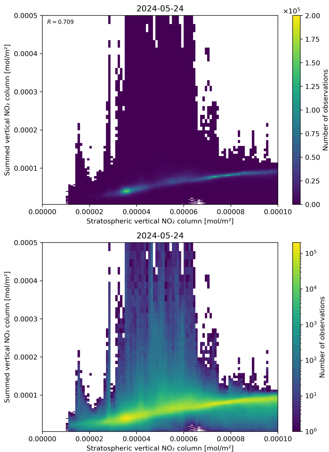
Figure 98: Scatter density plot of “Stratospheric vertical NO 2 column” against “Summed vertical NO 2 column” for 2024-05-23 to 2024-05-25.
