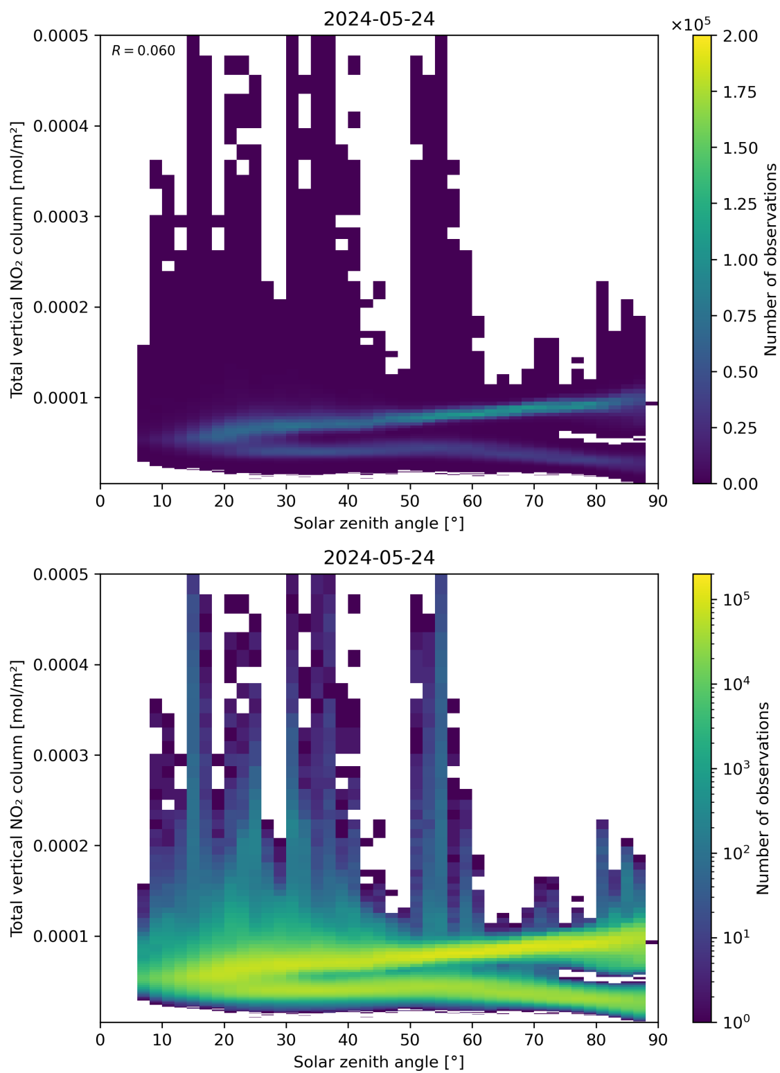
Figure 153: Scatter density plot of “Solar zenith angle” against “Total vertical \text{NO}_2 column” for 2024-05-23 to 2024-05-25.
