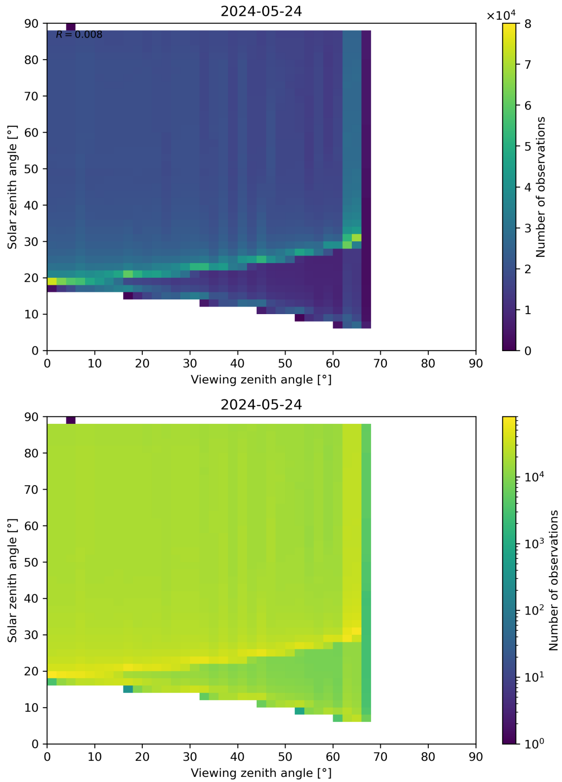
Figure 172: Scatter density plot of “Viewing zenith angle” against “Solar zenith angle” for 2024-05-23 to 2024-05-25.
