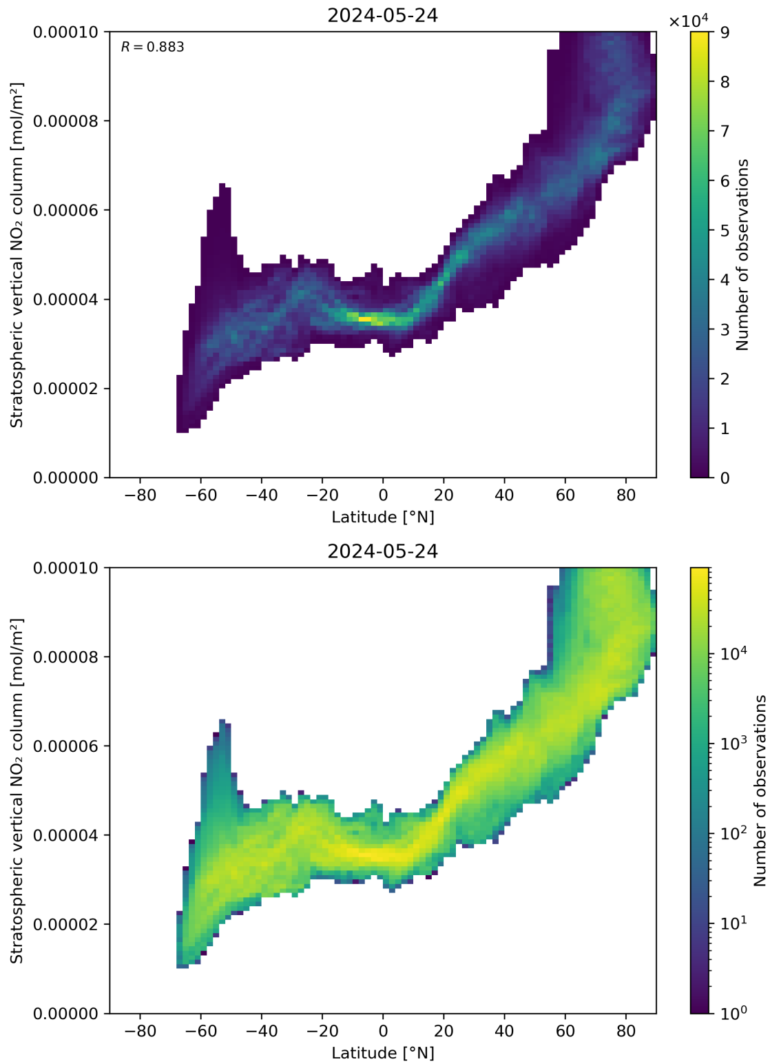
Figure 87: Scatter density plot of “Latitude” against “Stratospheric vertical NO 2 column” for 2024-05-23 to 2024-05-25.
