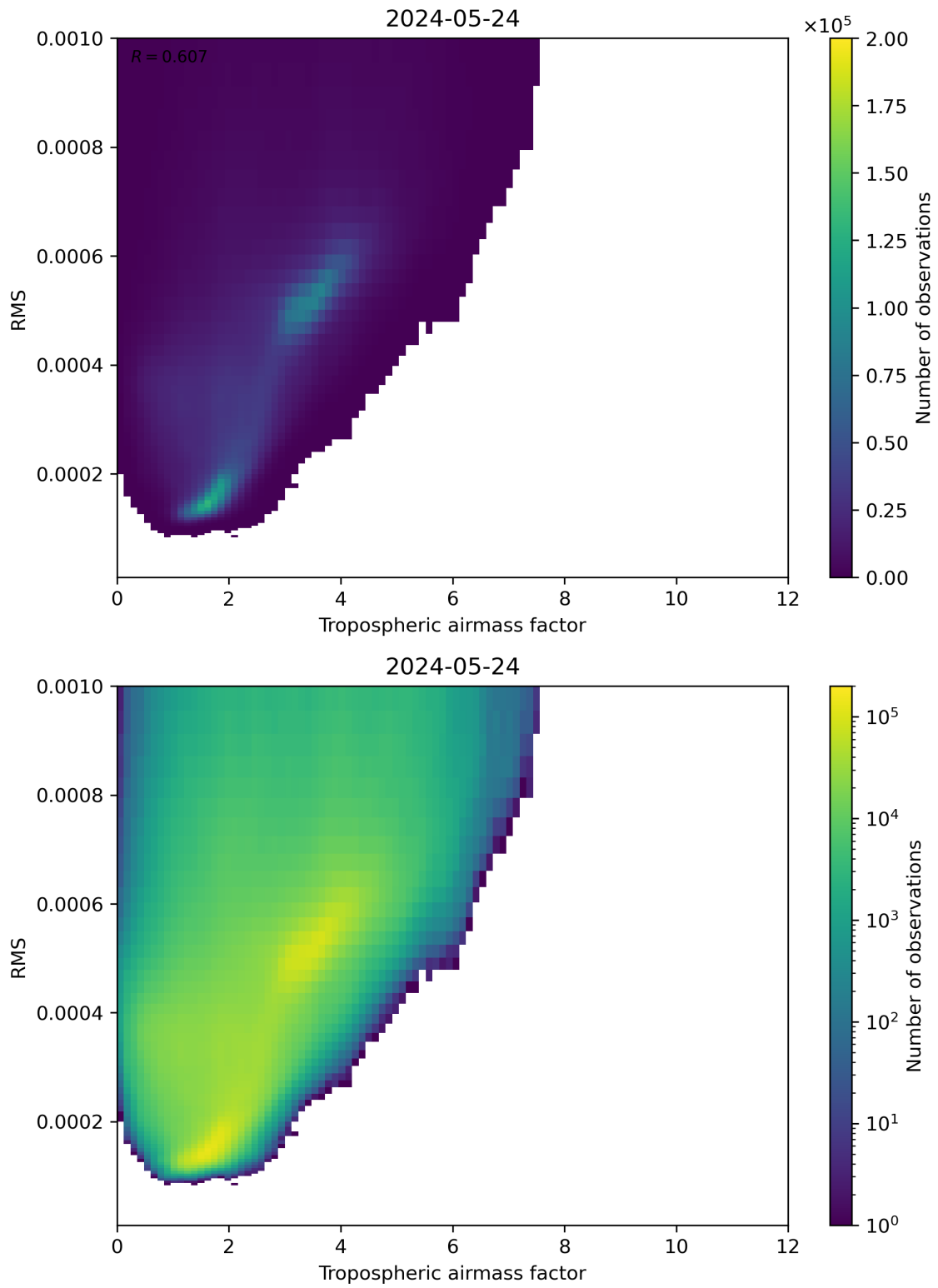
Figure 79: Scatter density plot of “Tropospheric airmass factor” against “RMS” for 2024-05-23 to 2024-05-25.
