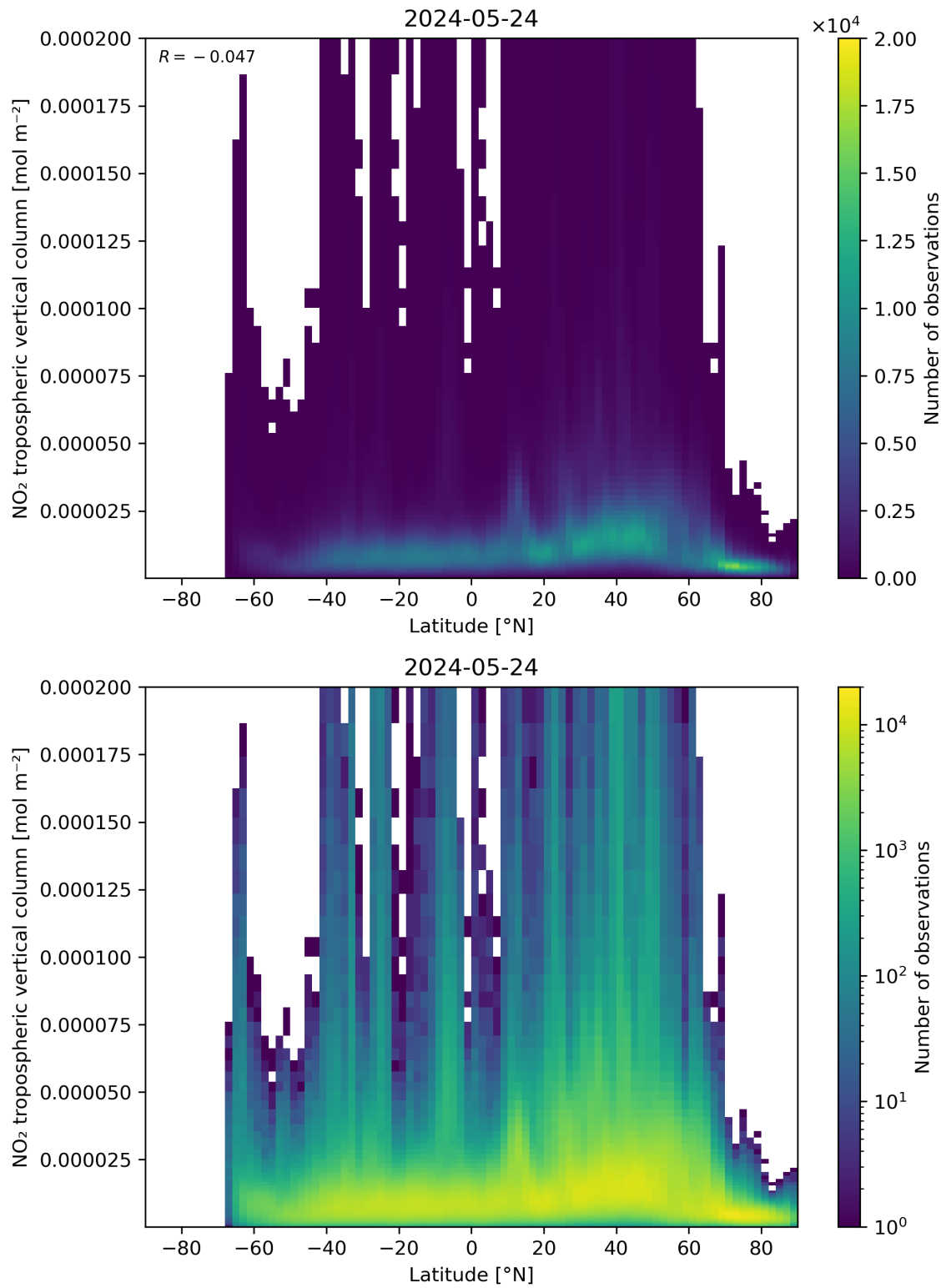
Figure 92: Scatter density plot of “Latitude” against “NO 2 tropospheric vertical column” for 2024-05-23 to 2024-05-25.
