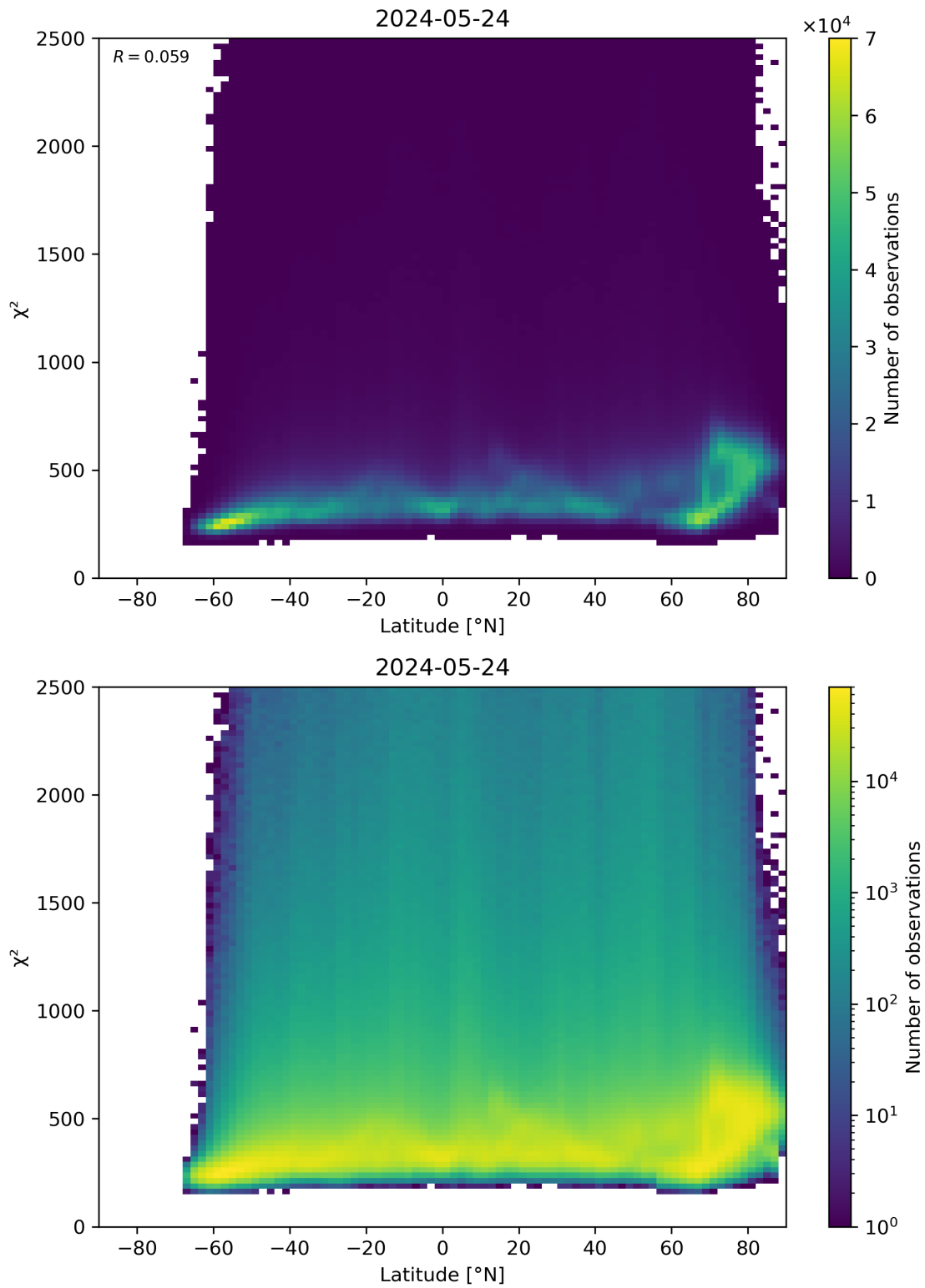
Figure 86: Scatter density plot of “Latitude” against “ \chi^2 ” for 2024-05-23 to 2024-05-25.
