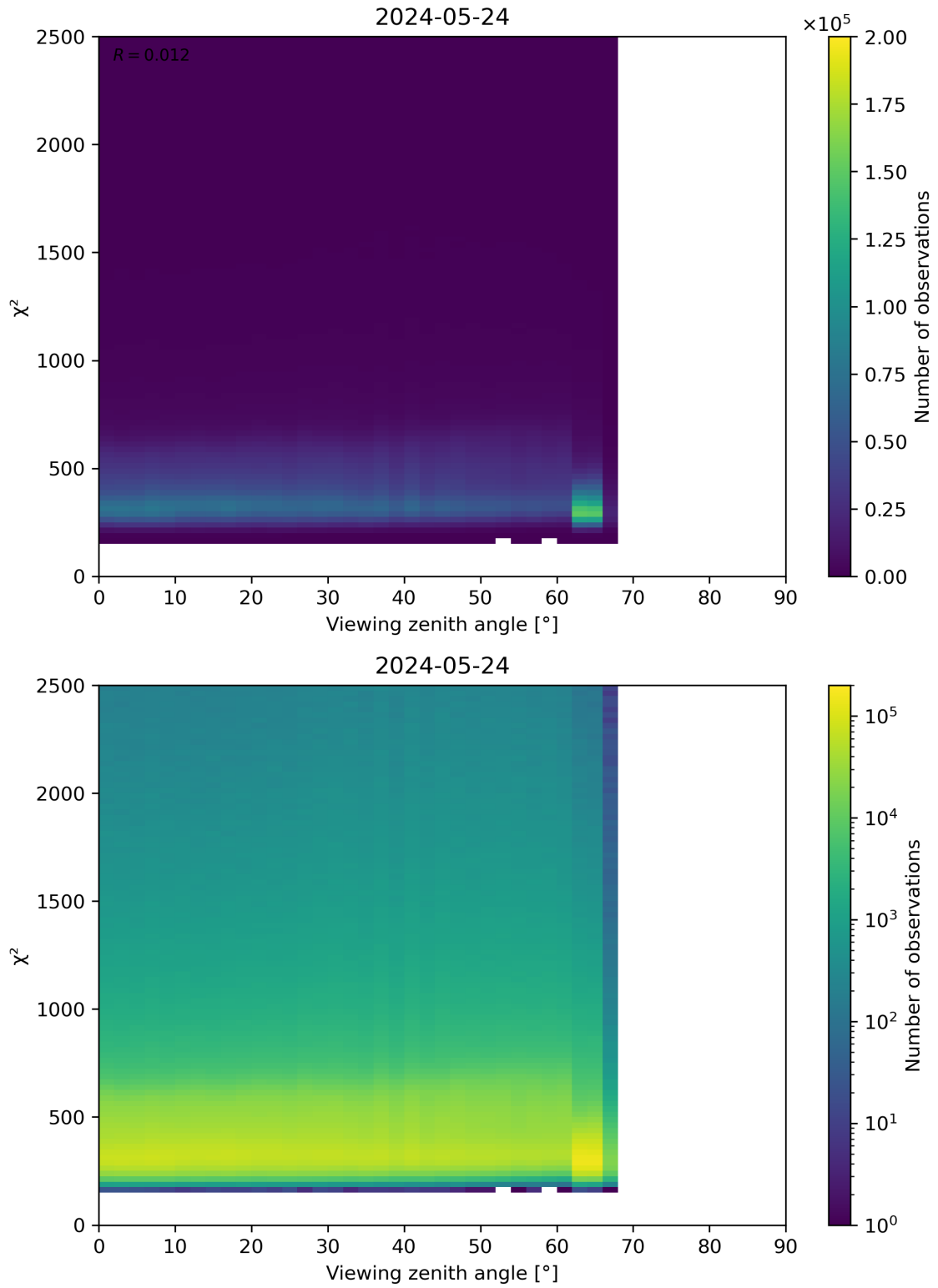
Figure 162: Scatter density plot of “Viewing zenith angle” against “ \chi^2 ” for 2024-05-23 to 2024-05-25.
