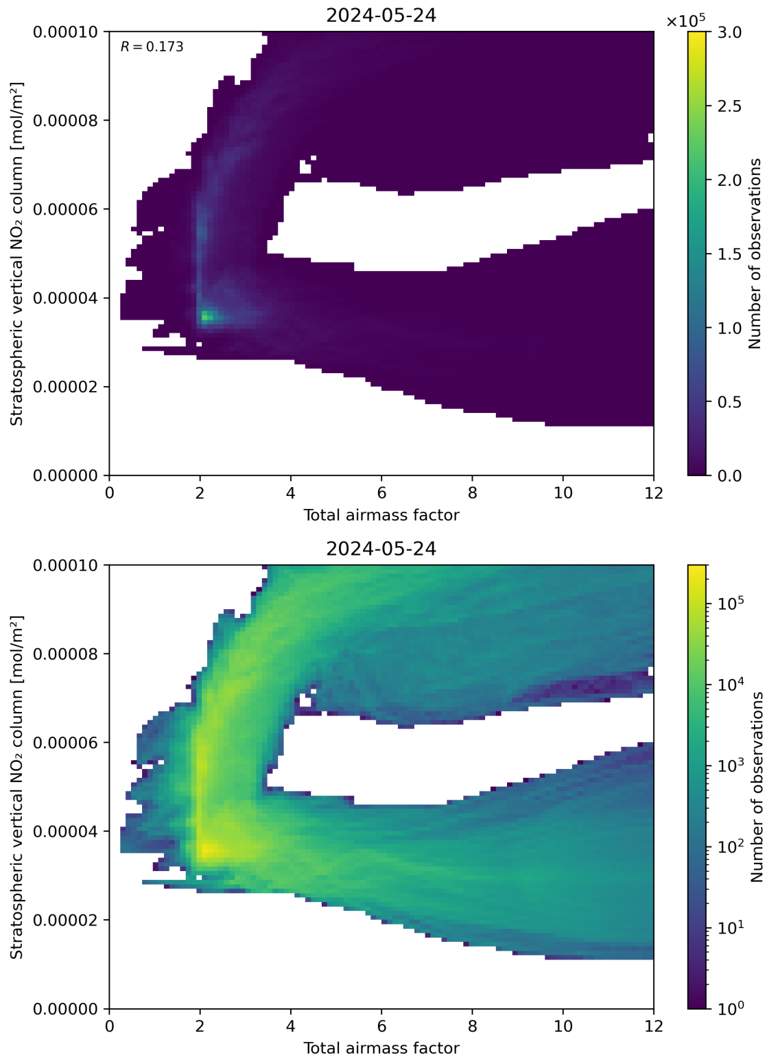
Figure 64: Scatter density plot of “Total airmass factor” against “Stratospheric vertical NO 2 column” for 2024-05-23 to 2024-05-25.
