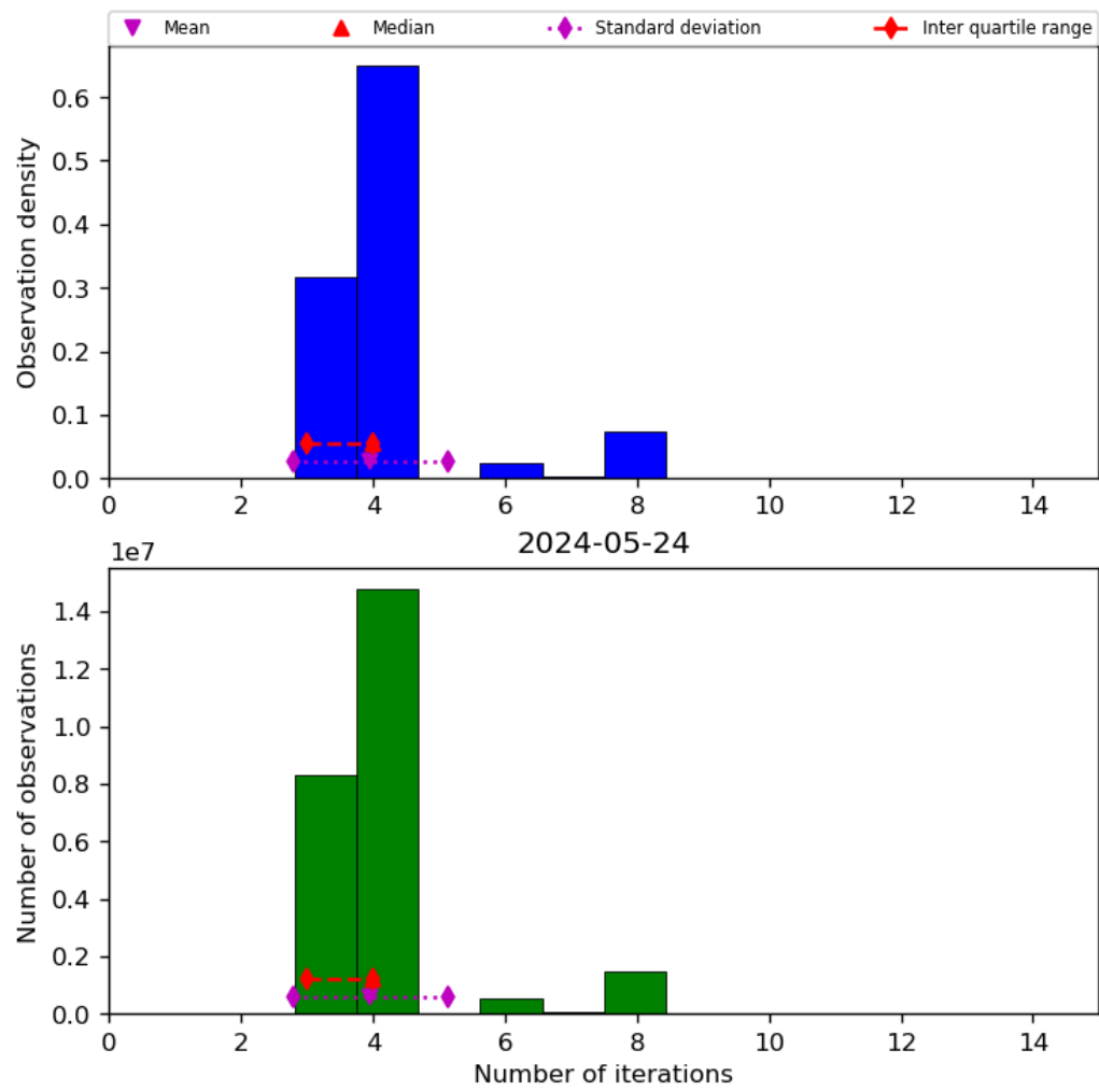
Figure 34: Histogram of “Number of iterations” for 2024-05-23 to 2024-05-25
