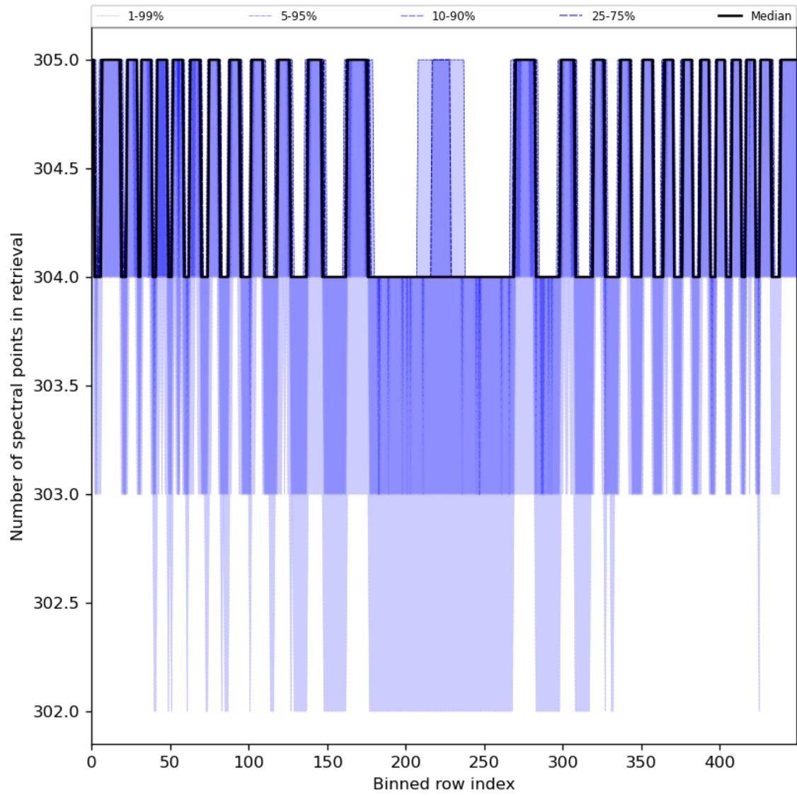
Figure 50: Along track statistics of “Number of spectral points in retrieval” for 2024-05-23 to 2024-05-25
