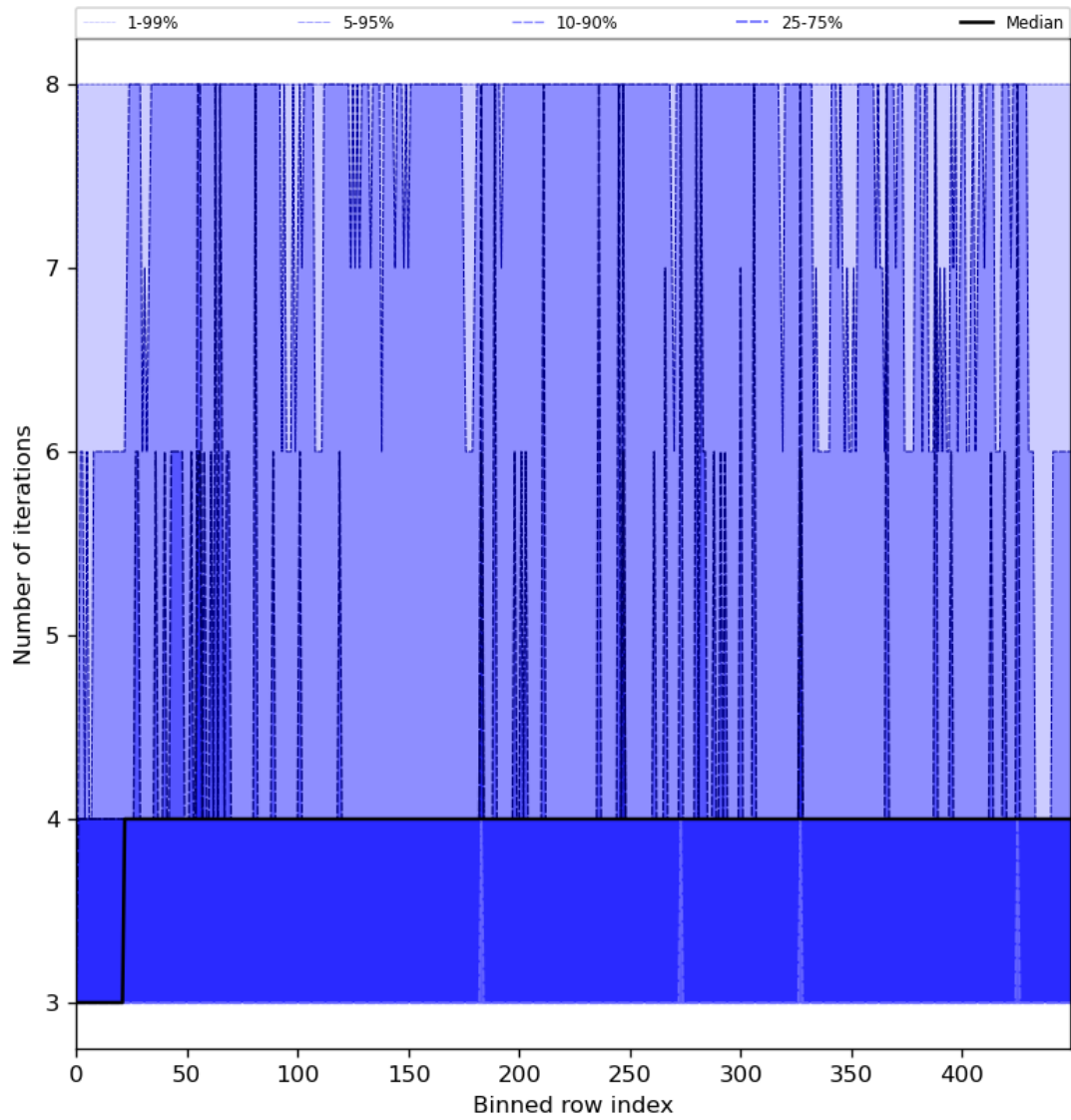
Figure 51: Along track statistics of “Number of iterations” for 2024-05-23 to 2024-05-25
