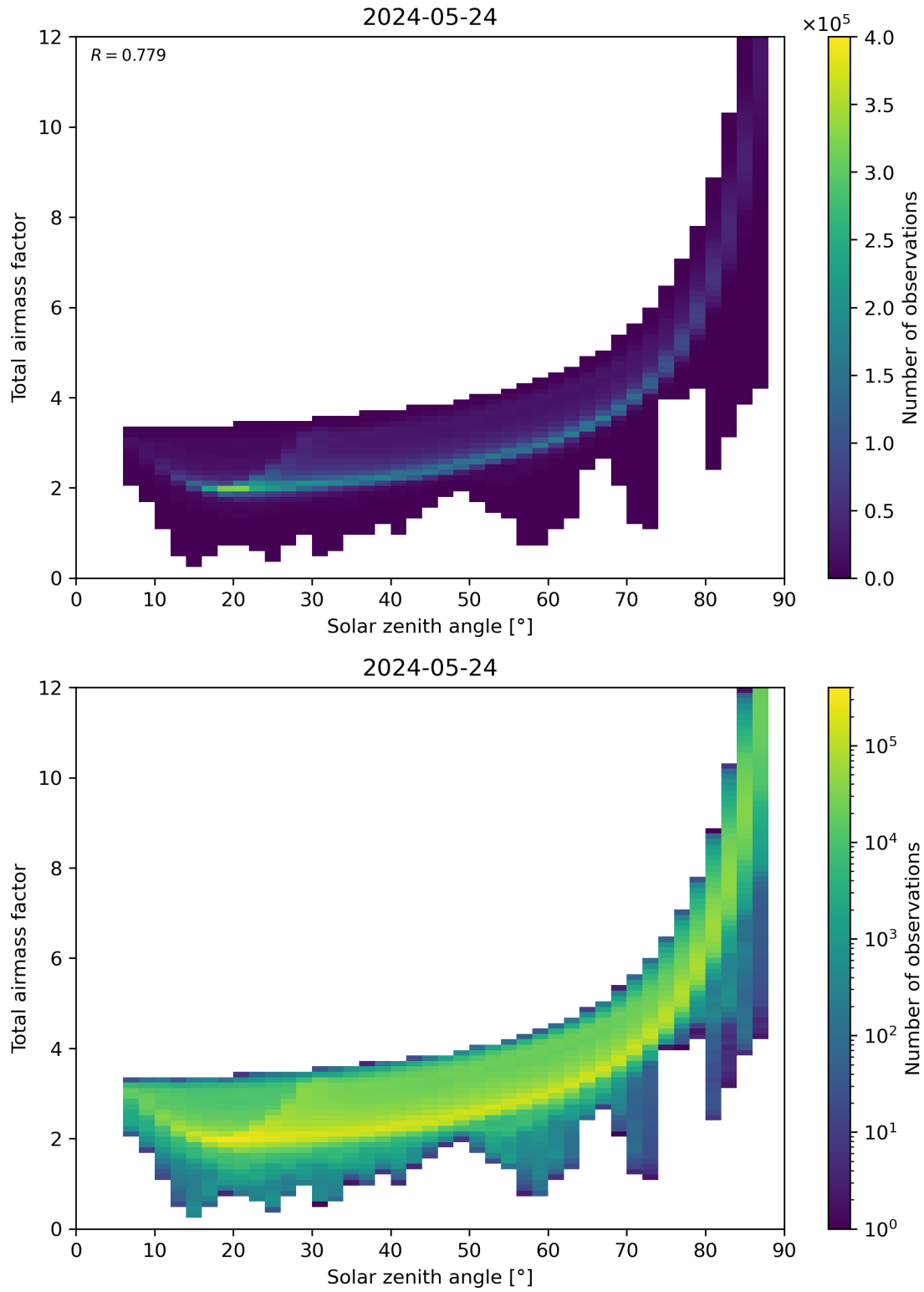
Figure 146: Scatter density plot of “Solar zenith angle” against “Total air mass factor” for 2024-05-23 to 2024-05-25.
