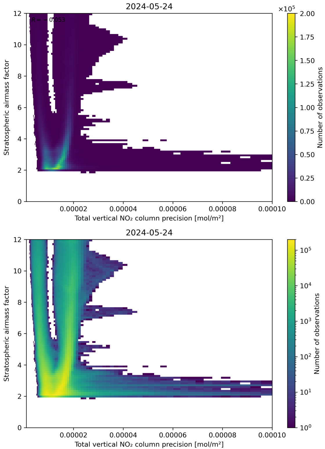
Figure 115: Scatter density plot of “Total vertical NO 2 column precision” against “Stratospheric air mass factor” for 2024-05-23 to 2024-05-25.
