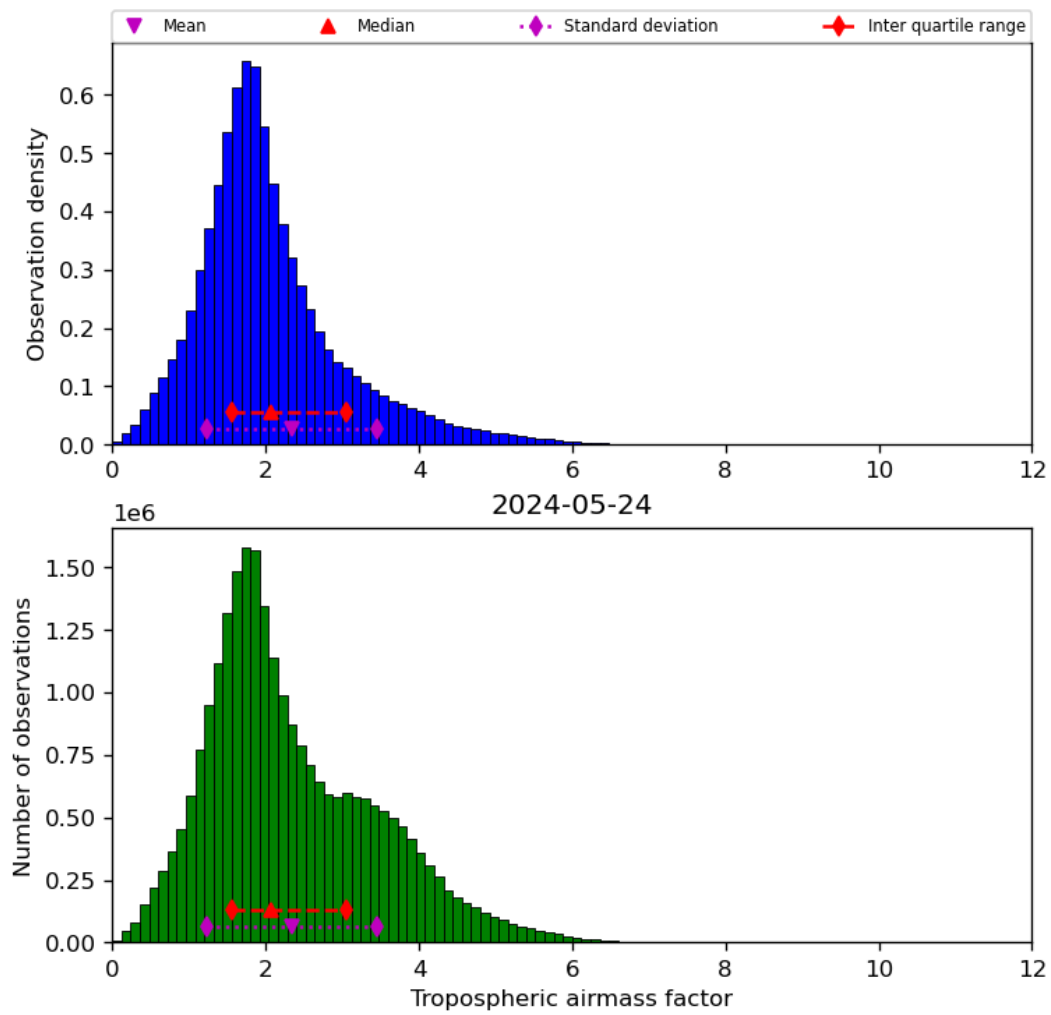
Figure 31: Histogram of “Tropospheric airmass factor” for 2024-05-23 to 2024-05-25
