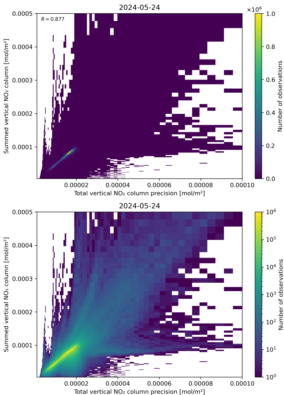
Figure 117: Scatter density plot of “Total vertical NO 2 column precision” against “Summed vertical NO 2 column” for 2024-05-23 to 2024-05-25.
