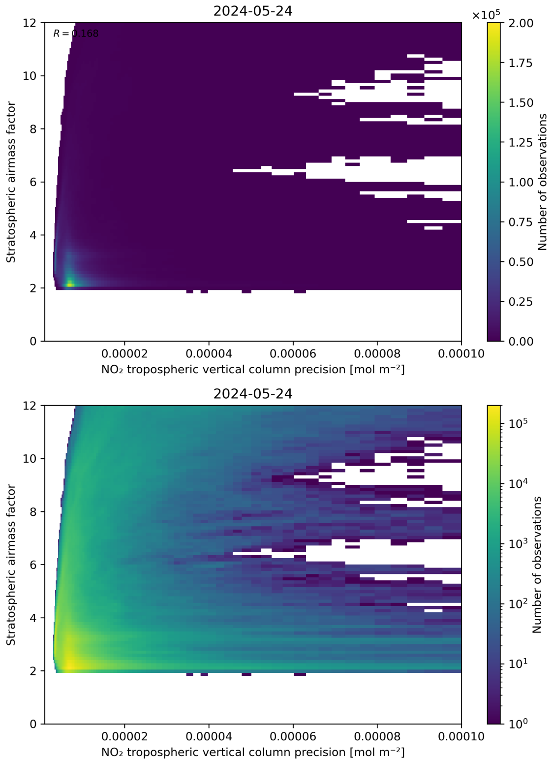
Figure 131: Scatter density plot of “NO 2 tropospheric vertical column precision” against “Stratospheric airmass factor” for 2024-05-23 to 2024-05-25.
