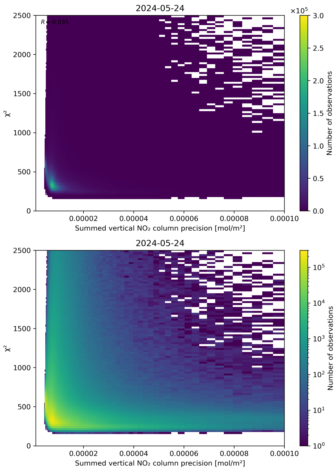
Figure 107: Scatter density plot of “Summed vertical NO 2 column precision” against “ \chi^2 ” for 2024-05-23 to 2024-05-25.
