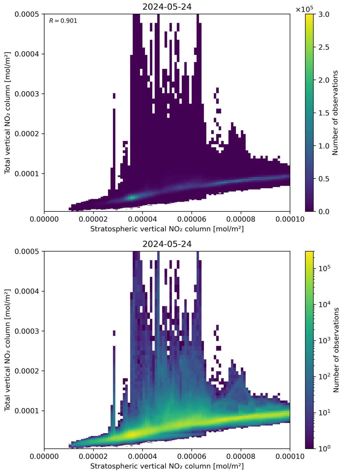
Figure 100: Scatter density plot of “Stratospheric vertical NO 2 column” against “Total vertical NO 2 column” for 2024-05-23 to 2024-05-25.
