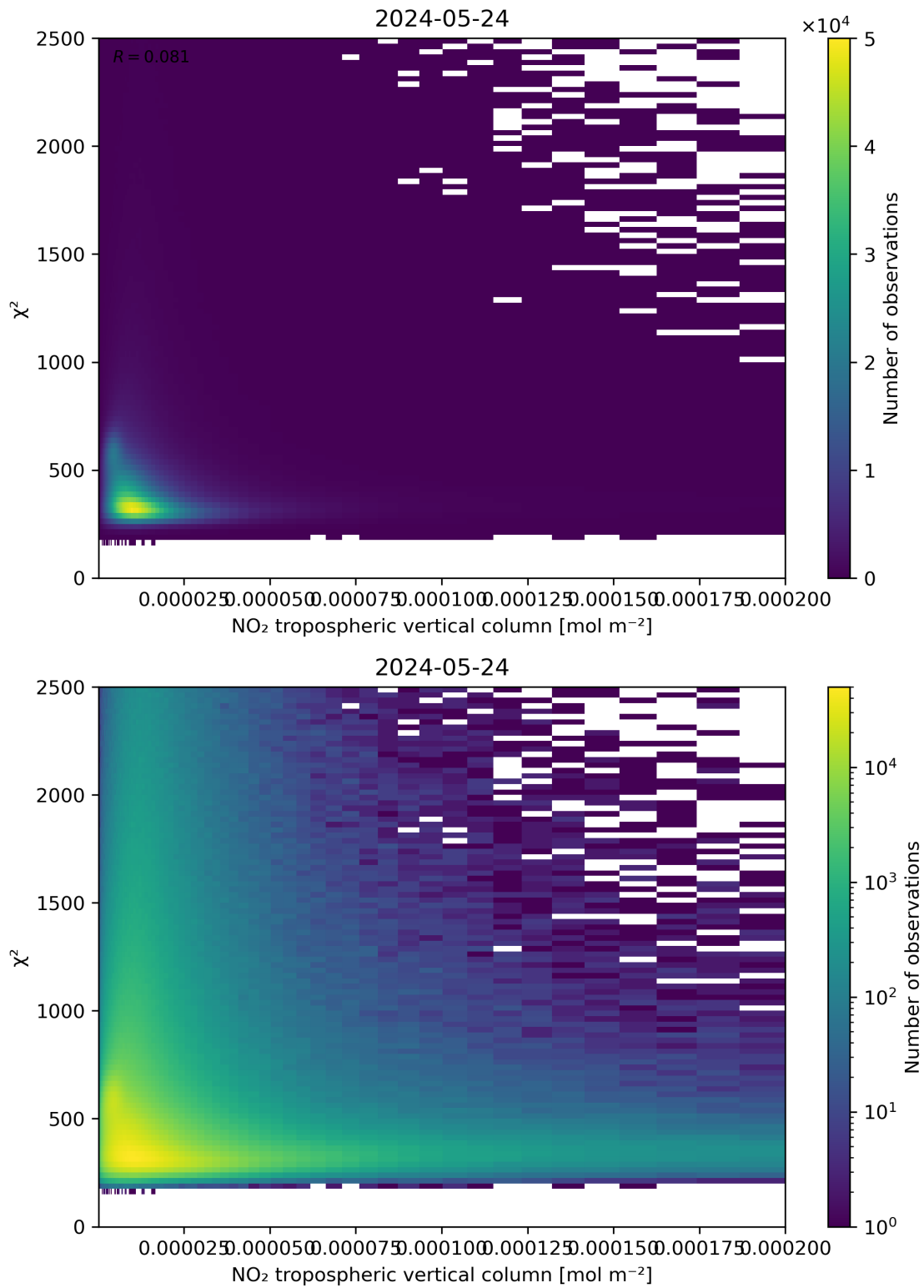
Figure 124: Scatter density plot of “NO 2 tropospheric vertical column” against “ \chi^2 ” for 2024-05-23 to 2024-05-25.
