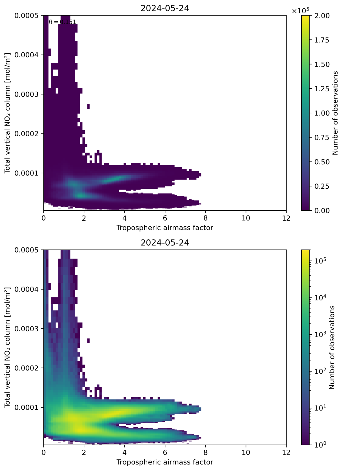
Figure 77: Scatter density plot of “Tropospheric airmass factor” against “Total vertical NO 2 column” for 2024-05-23 to 2024-05-25.
