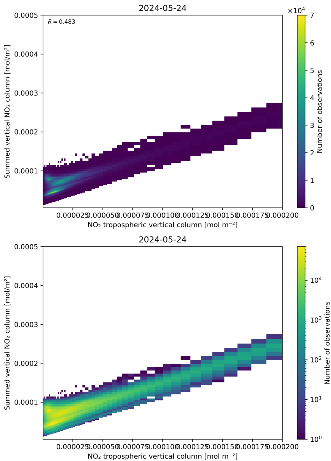
Figure 126: Scatter density plot of “NO 2 tropospheric vertical column” against “Summed vertical NO 2 column” for 2024-05-23 to 2024-05-25.
