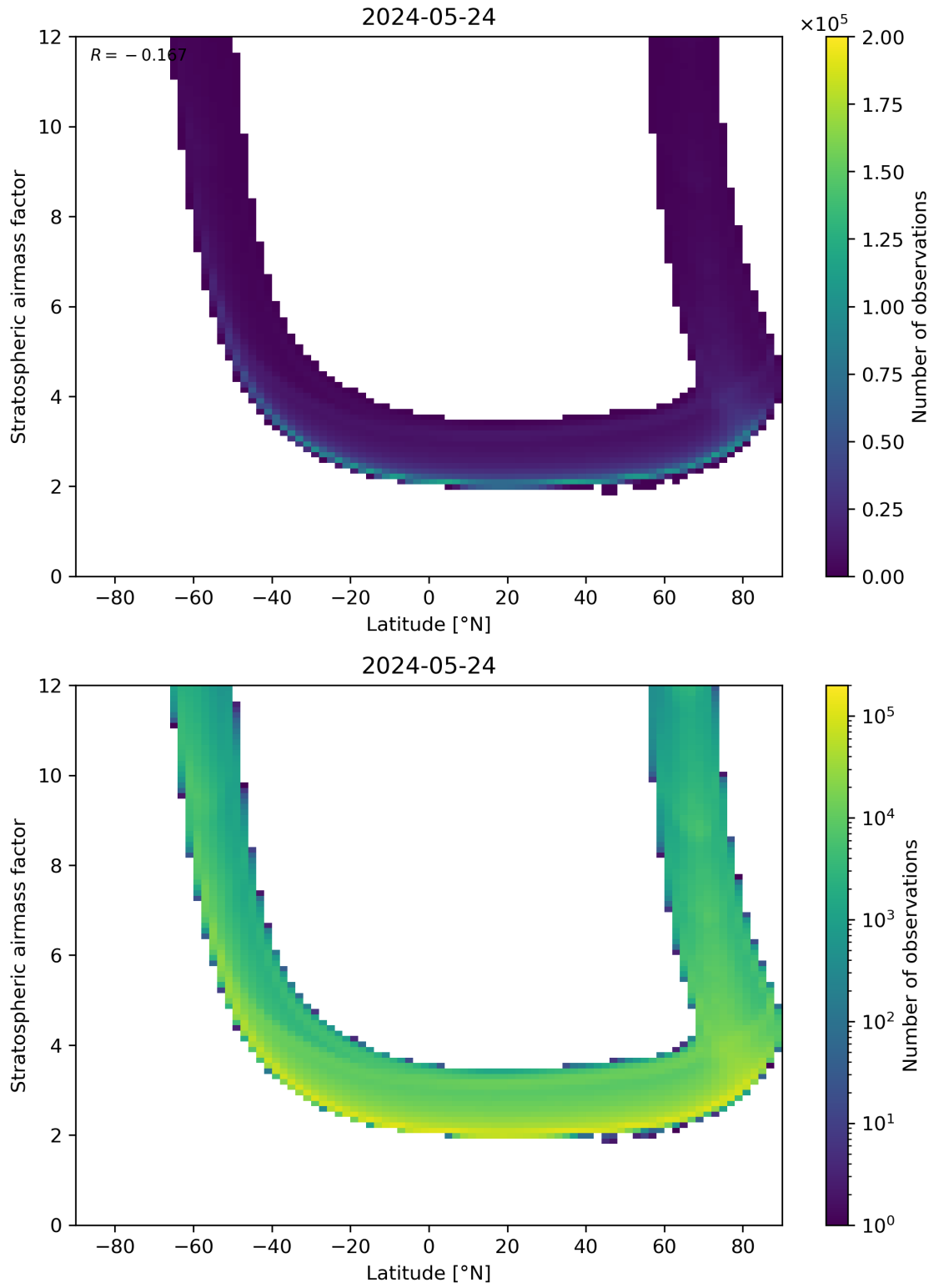
Figure 83: Scatter density plot of “Latitude” against “Stratospheric air mass factor” for 2024-05-23 to 2024-05-25.
