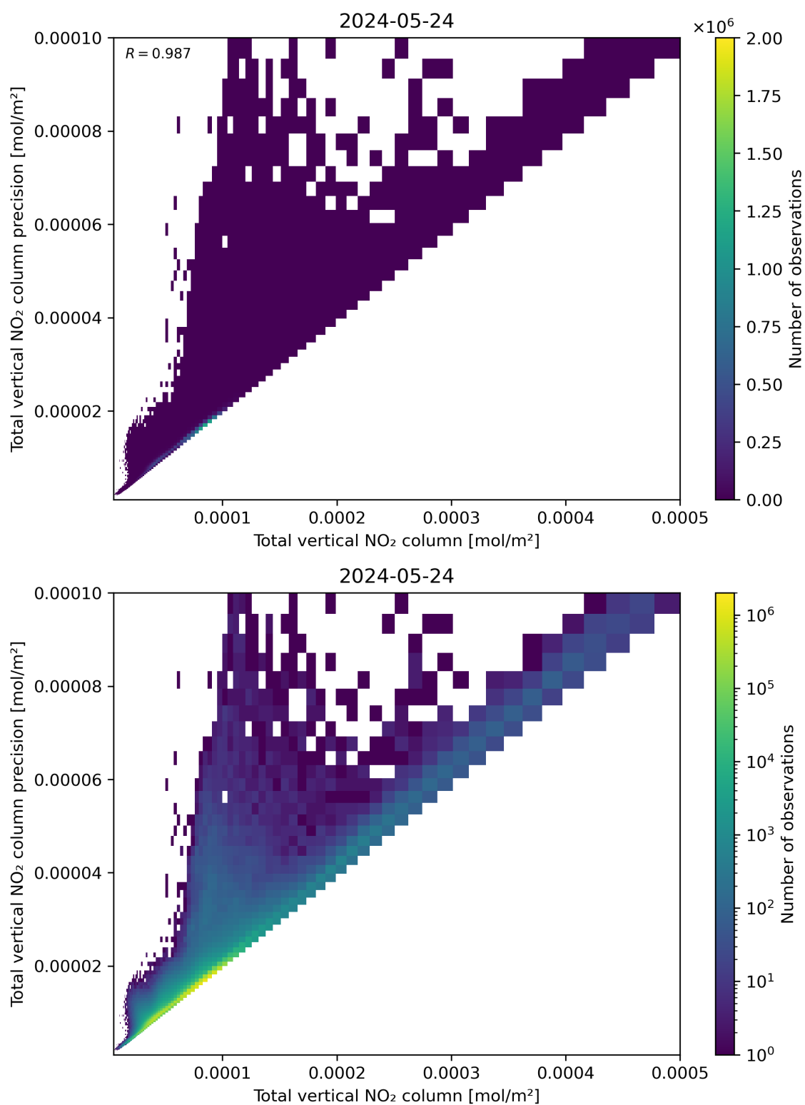
Figure 114: Scatter density plot of “Total vertical NO 2 column” against “Total vertical NO 2 column precision” for 2024-05-23 to 2024-05-25.
