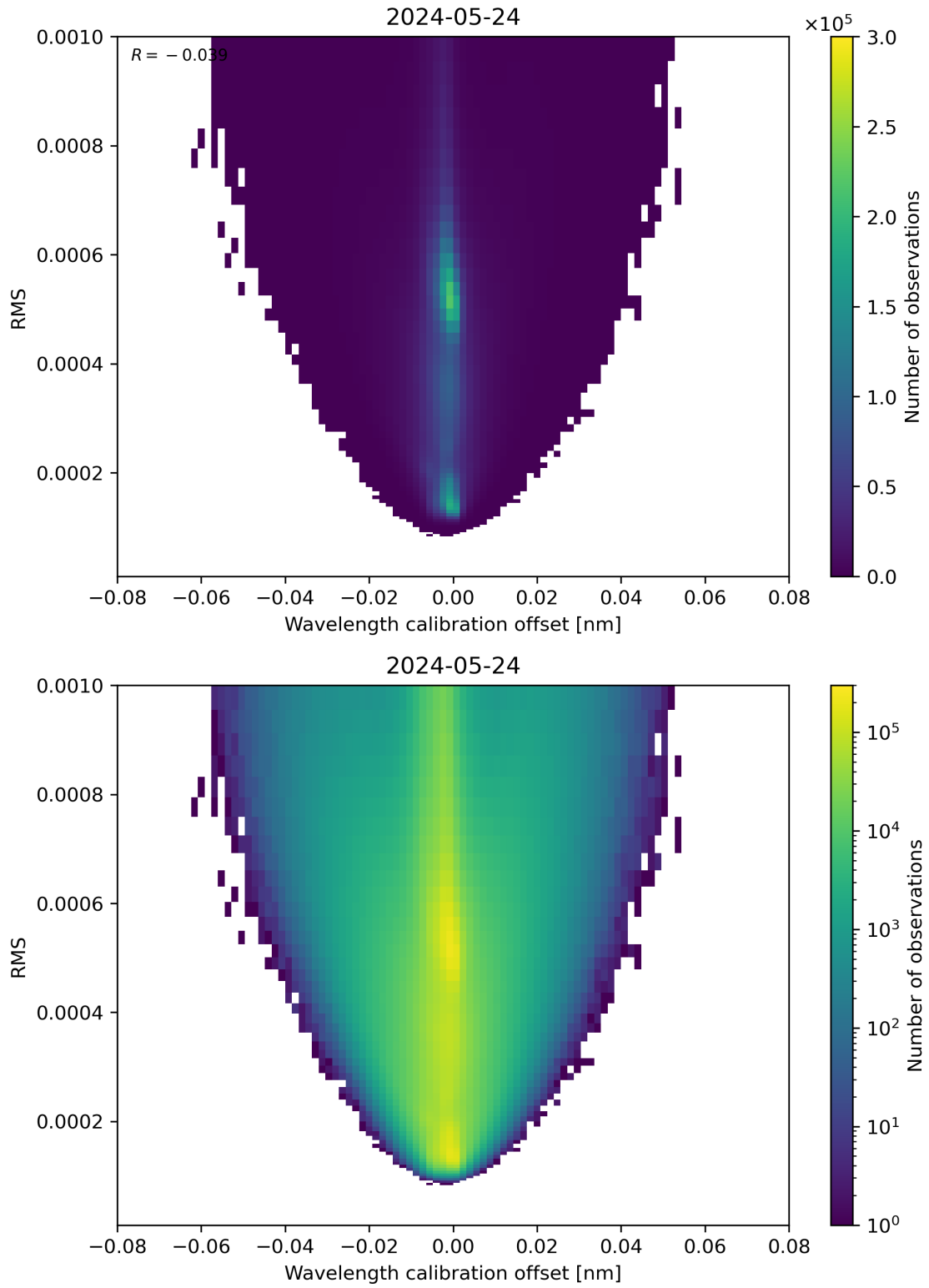
Figure 181: Scatter density plot of “Wavelength calibration offset” against “RMS” for 2024-05-23 to 2024-05-25.
