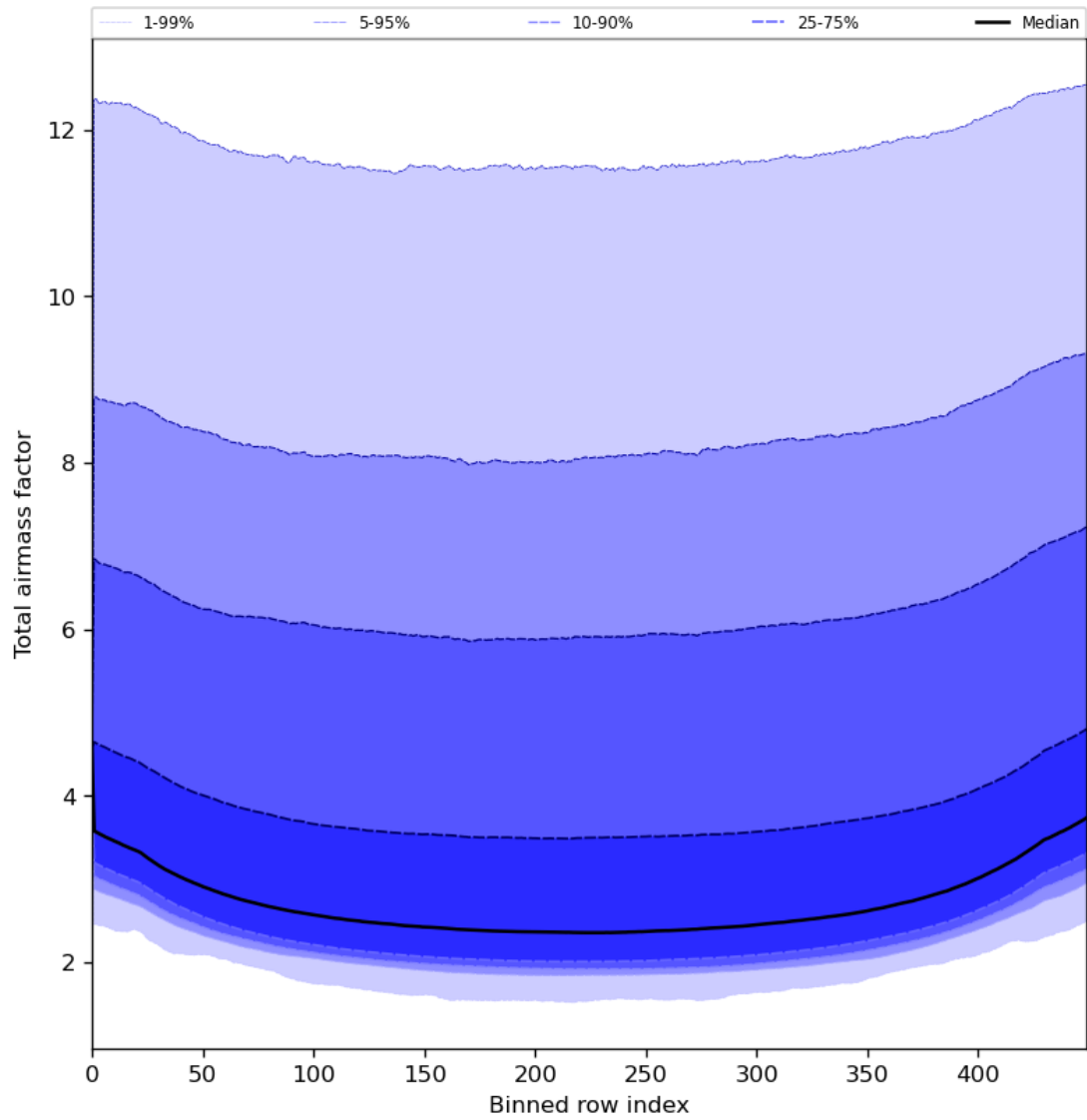
Figure 49: Along track statistics of “Total airmass factor” for 2024-05-23 to 2024-05-25
