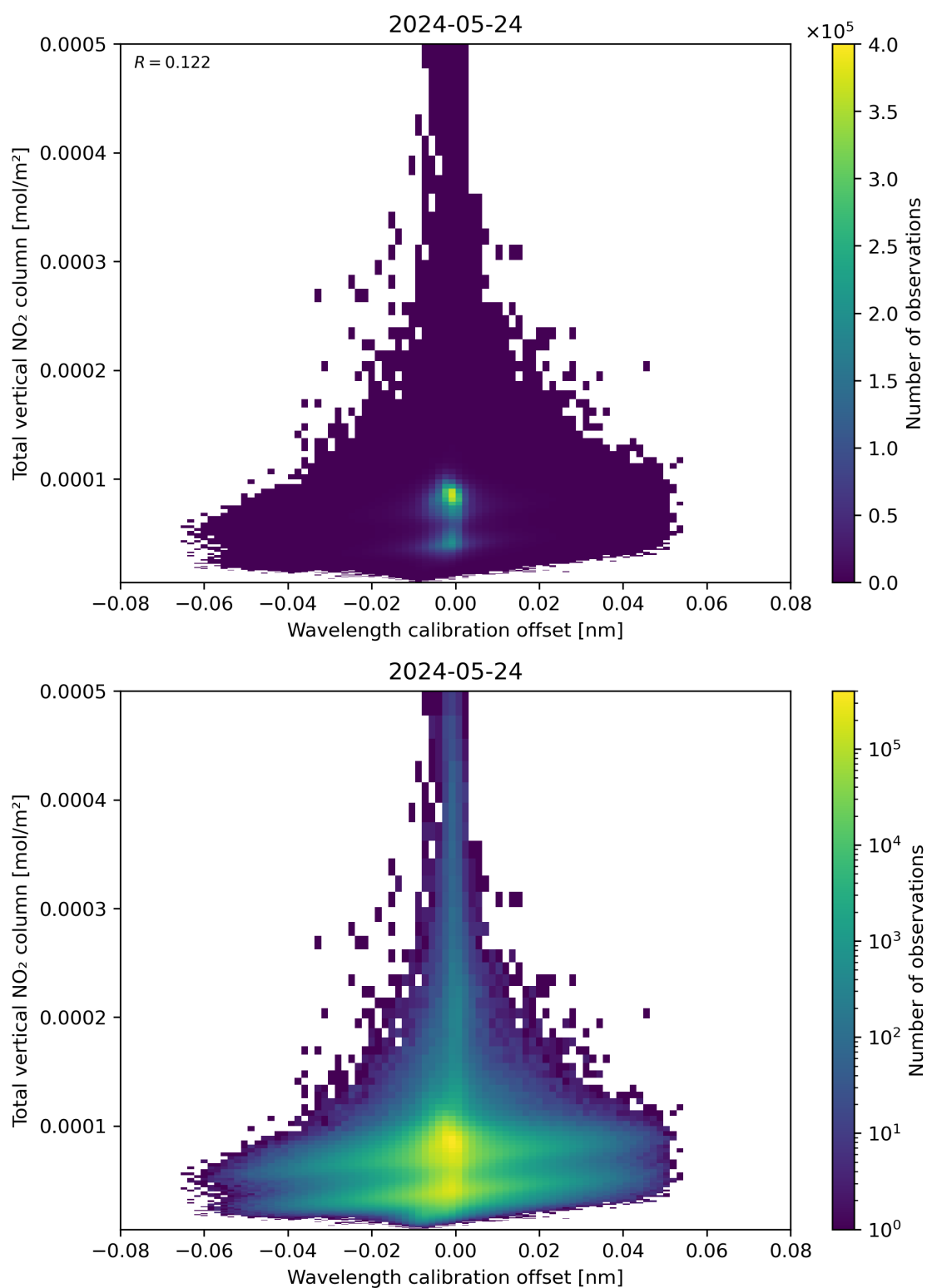
Figure 179: Scatter density plot of “Wavelength calibration offset” against “Total vertical NO 2 column” for 2024-05-23 to 2024-05-25.
