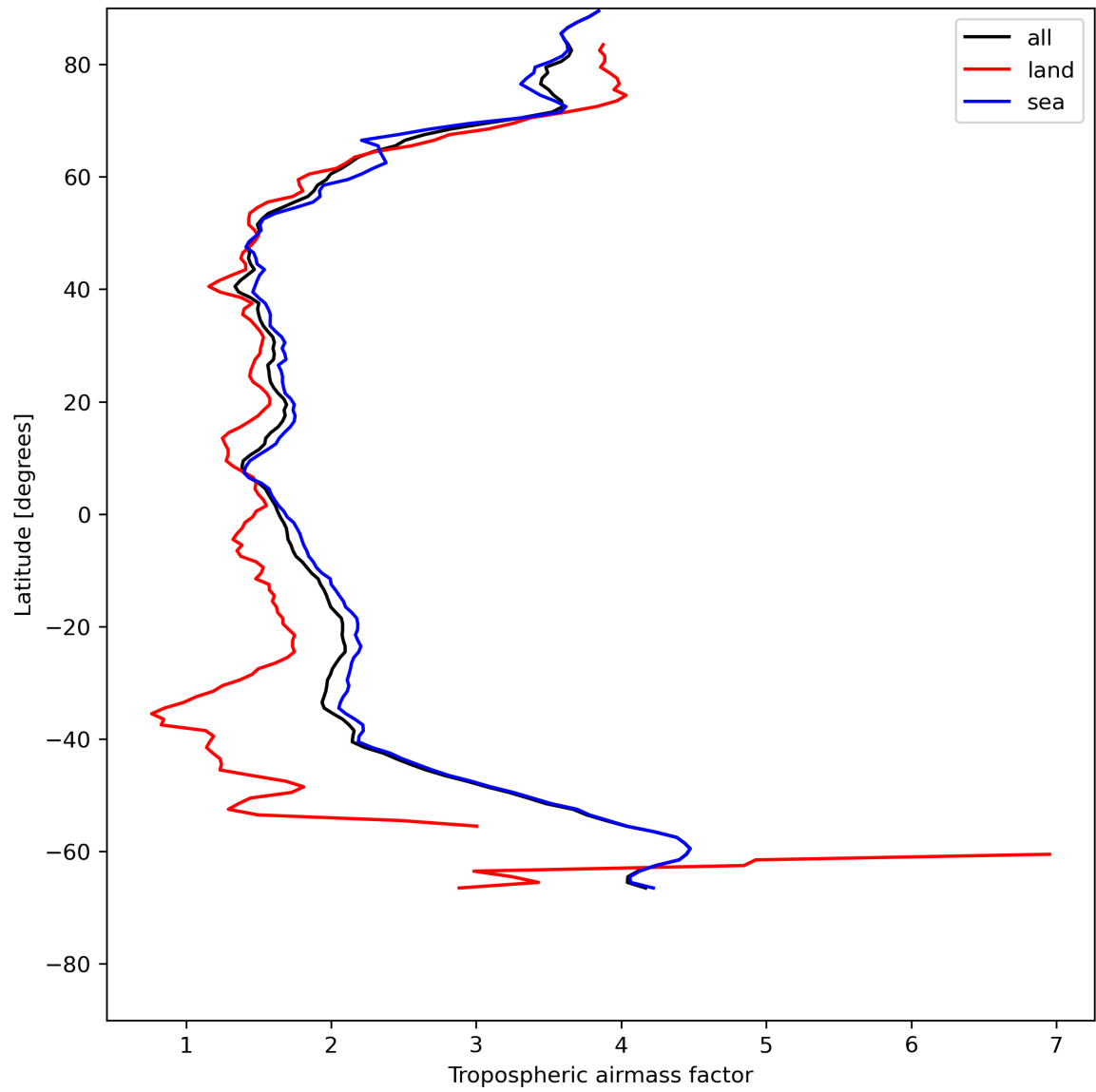
Figure 14: Zonal average of “Tropospheric airmass factor” for 2024-05-23 to 2024-05-25.
