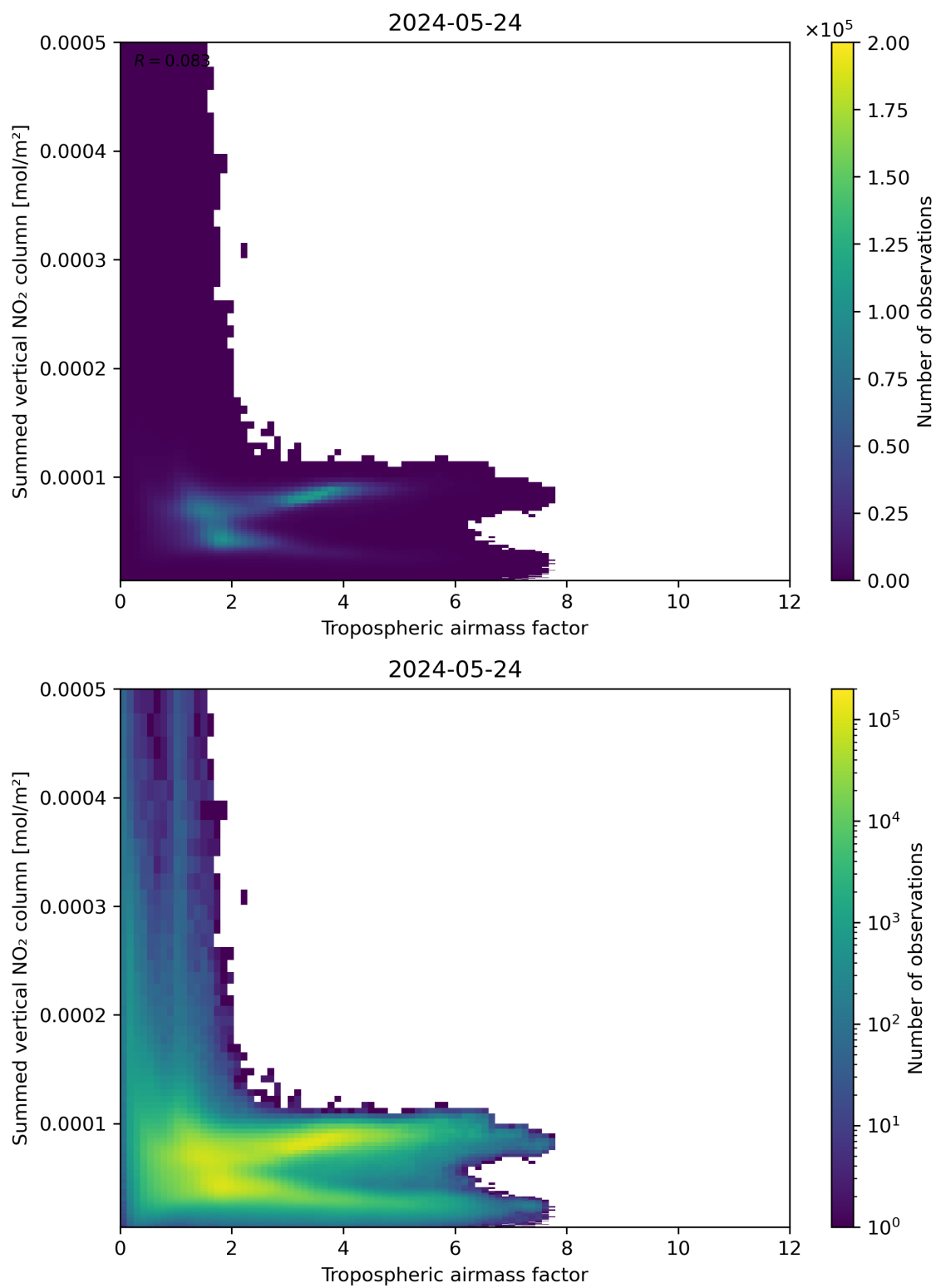
Figure 75: Scatter density plot of “Tropospheric airmass factor” against “Summed vertical NO 2 column” for 2024-05-23 to 2024-05-25.
