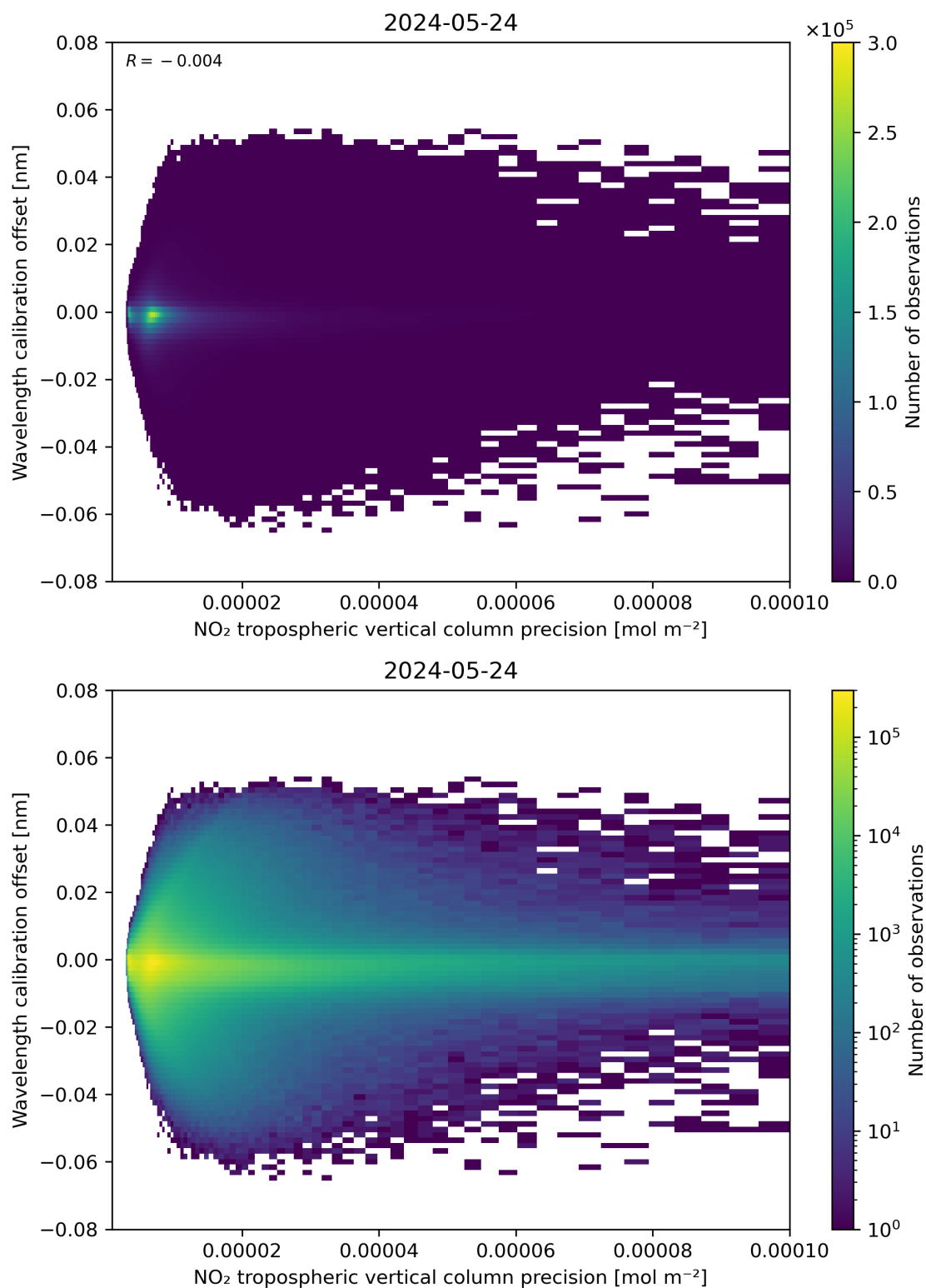
Figure 141: Scatter density plot of “NO 2 tropospheric vertical column precision” against “Wavelength calibration offset” for 2024-05-23 to 2024-05-25.
