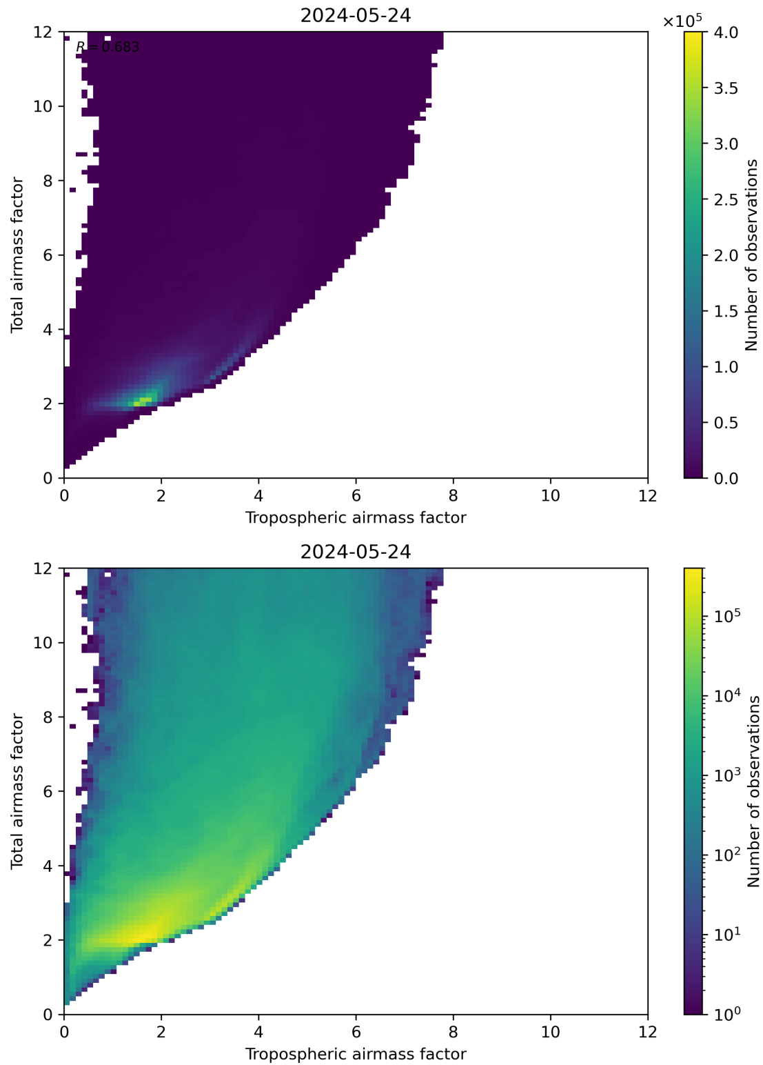
Figure 72: Scatter density plot of “Tropospheric airmass factor” against “Total airmass factor” for 2024-05-23 to 2024-05-25.
