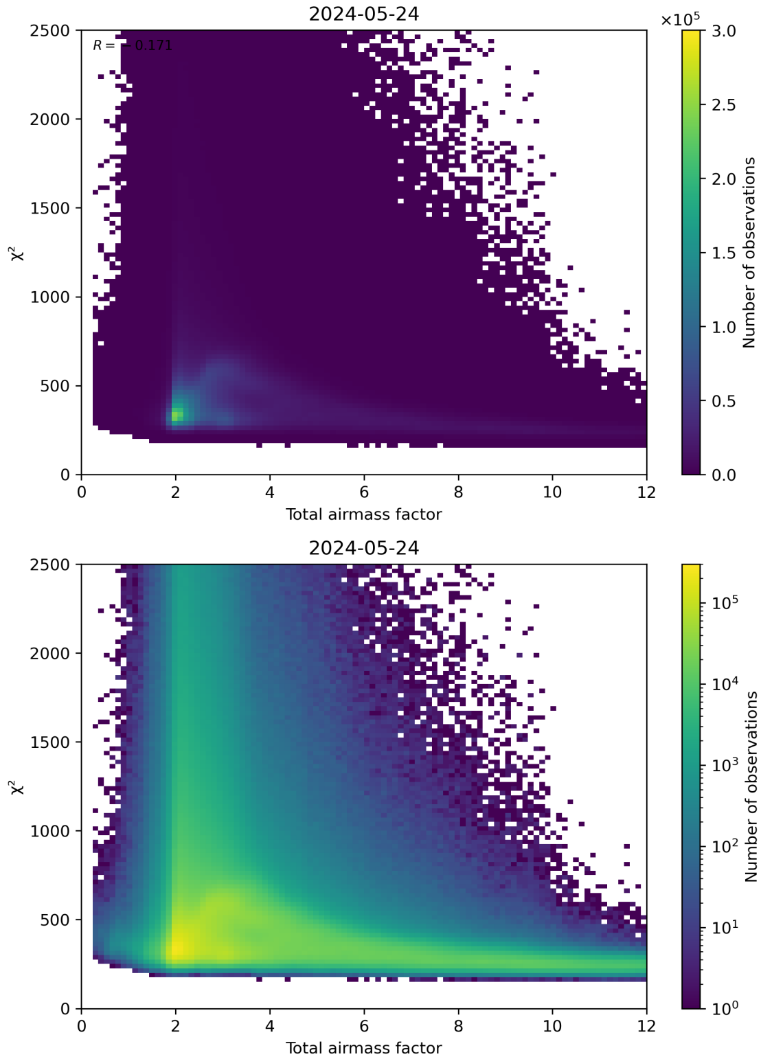
Figure 63: Scatter density plot of “Total airmass factor” against “ \chi^2 ” for 2024-05-23 to 2024-05-25.
