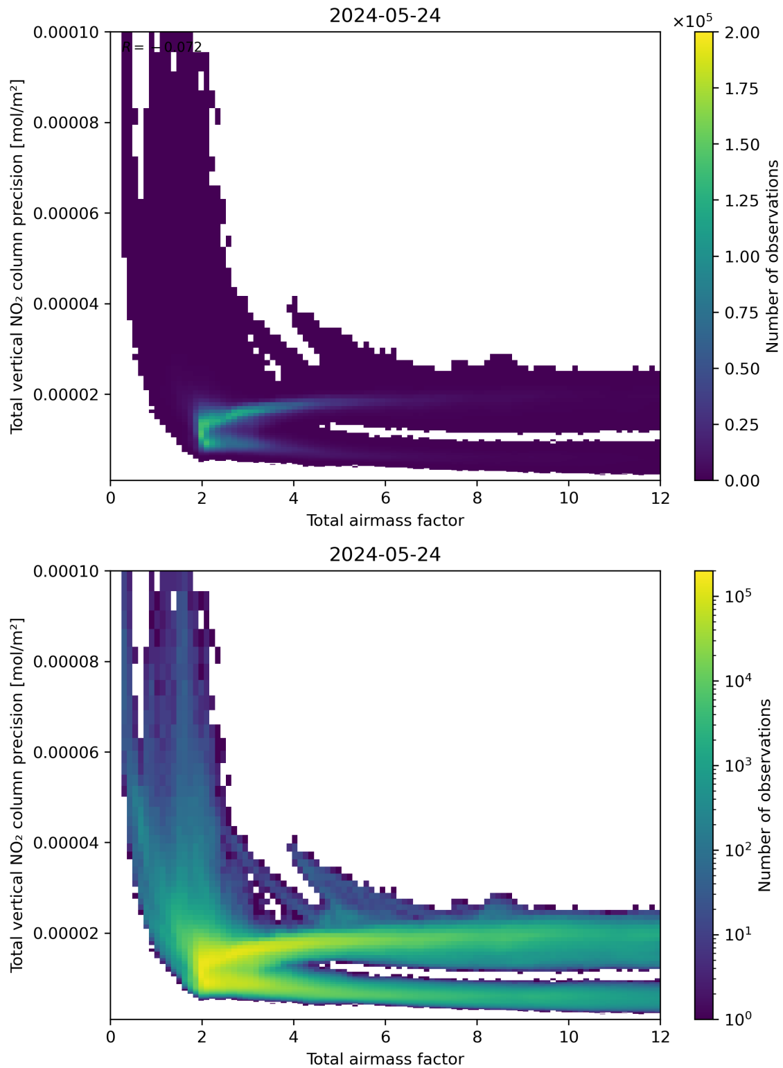
Figure 68: Scatter density plot of “Total airmass factor” against “Total vertical NO 2 column precision” for 2024-05-23 to 2024-05-25.
