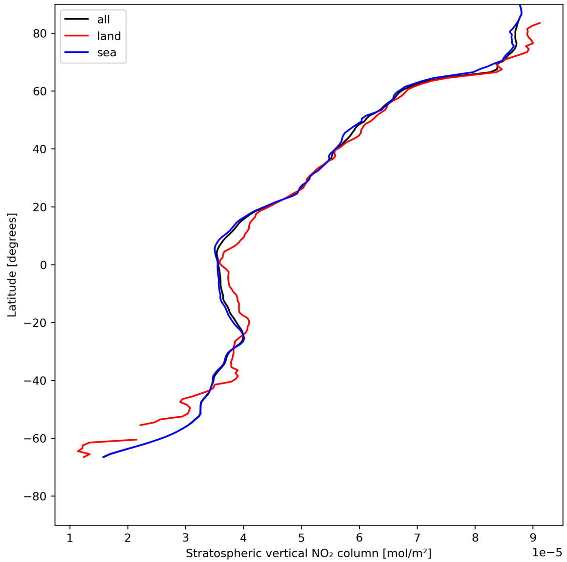
Figure 19: Zonal average of “Stratospheric vertical NO 2 column” for 2024-05-23 to 2024-05-25.
