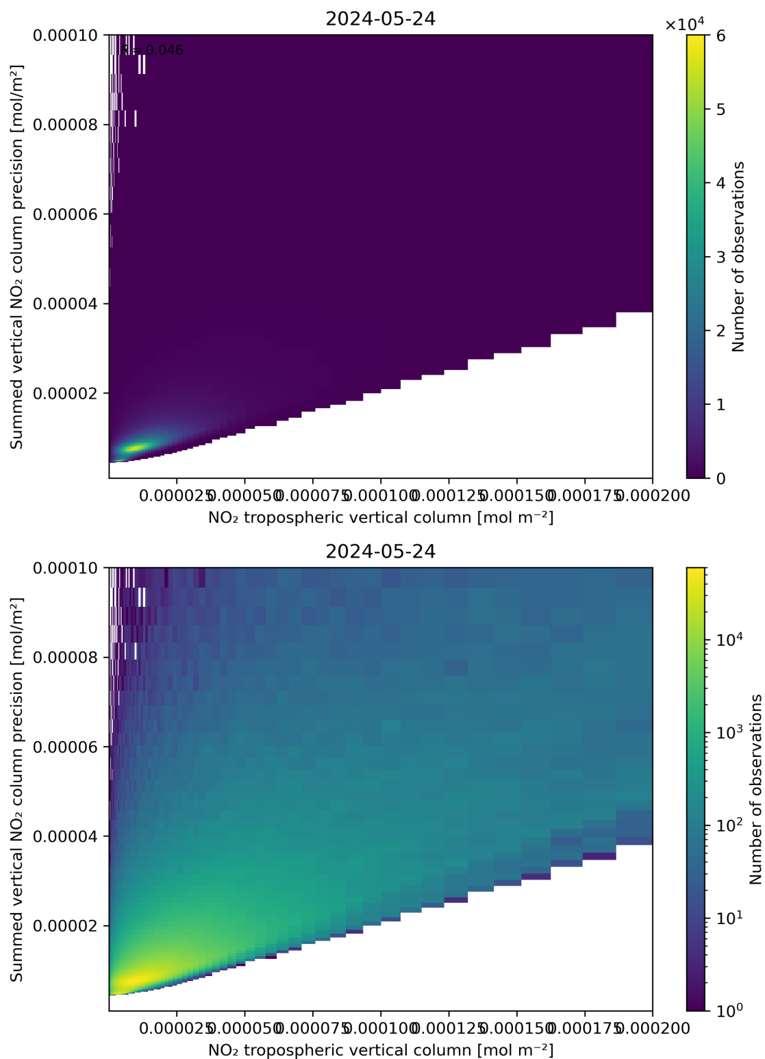
Figure 127: Scatter density plot of “NO 2 tropospheric vertical column” against “Summed vertical NO 2 column precision” for 2024-05-23 to 2024-05-25.
