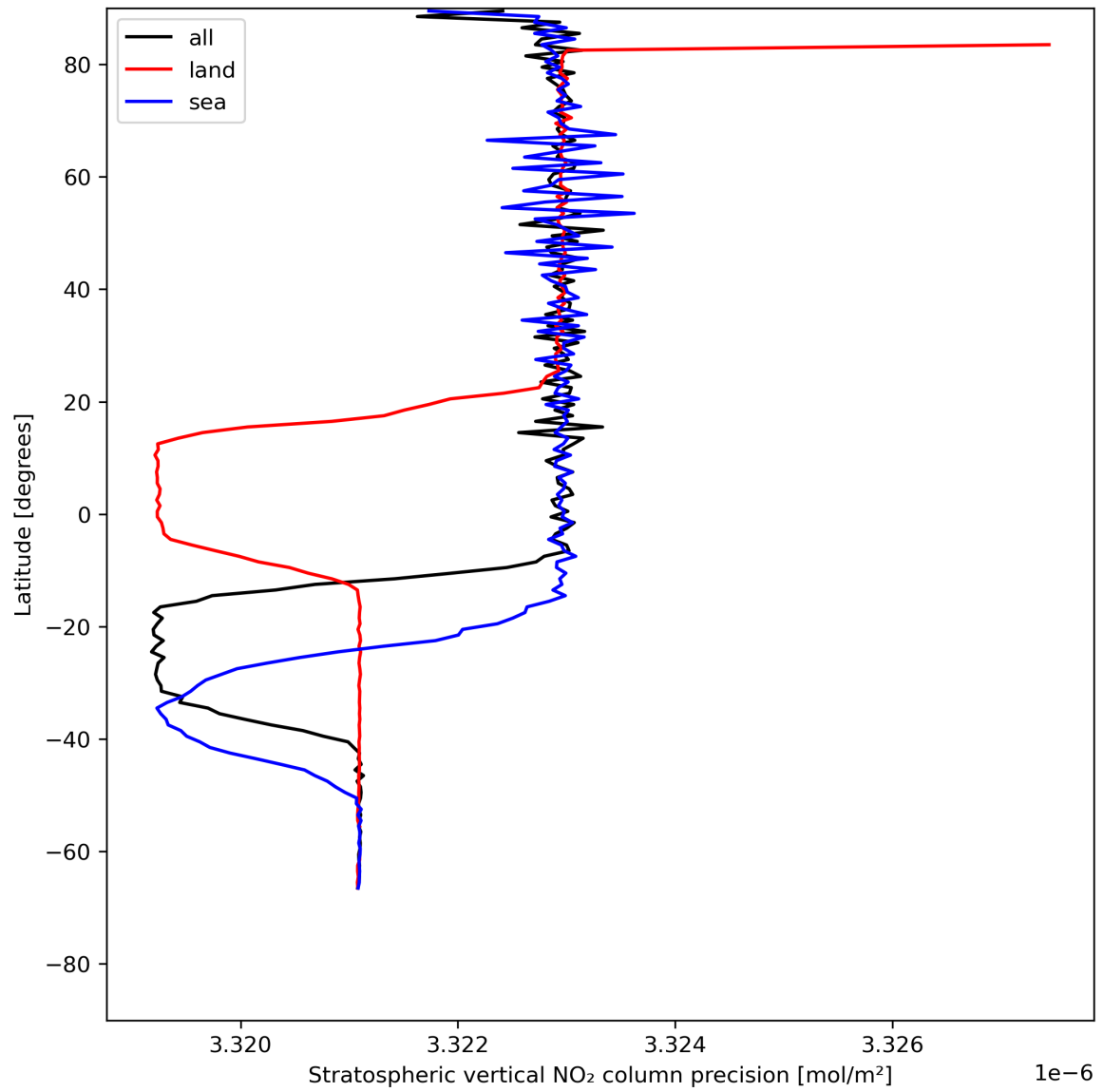
Figure 20: Zonal average of “Stratospheric vertical NO 2 column precision” for 2024-05-23 to 2024-05-25.
