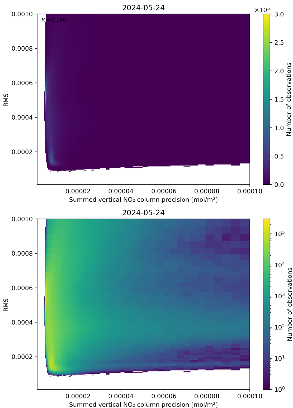
Figure 108: Scatter density plot of “Summed vertical NO 2 column precision” against “RMS” for 2024-05-23 to 2024-05-25.
