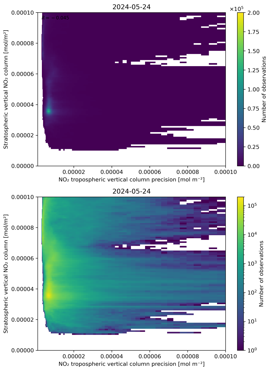
Figure 135: Scatter density plot of “NO 2 tropospheric vertical column precision” against “Stratospheric vertical NO 2 column” for 2024-05-23 to 2024-05-25.
