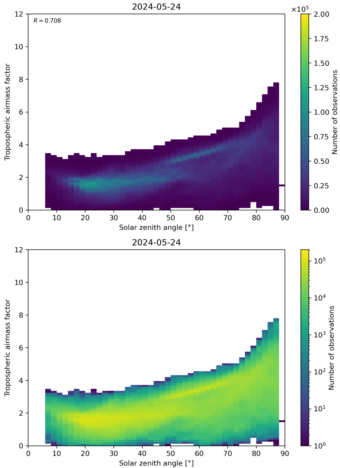
Figure 147: Scatter density plot of “Solar zenith angle” against “Tropospheric airmass factor” for 2024-05-23 to 2024-05-25.
