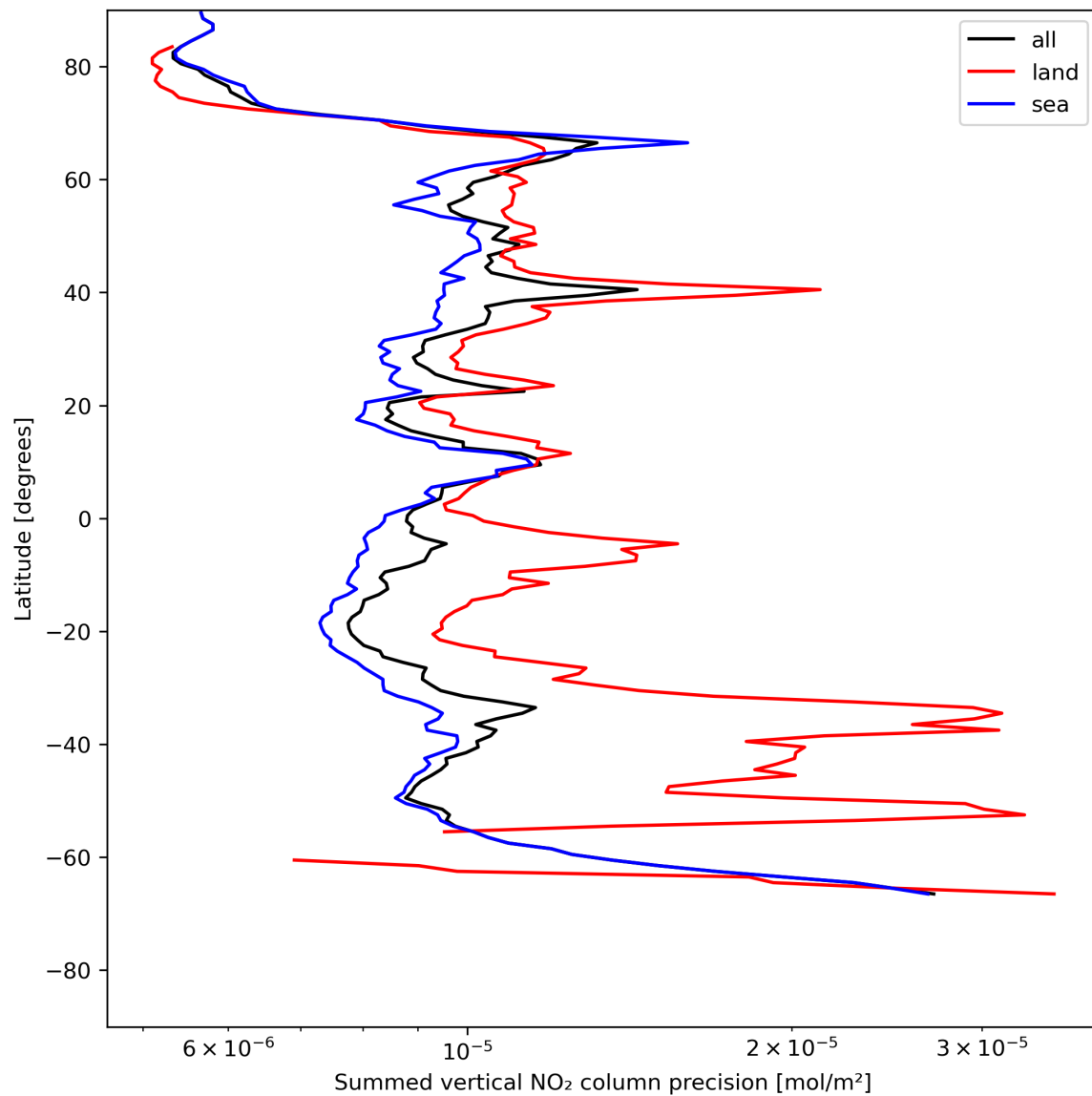
Figure 24: Zonal average of “Summed vertical NO 2 column precision” for 2024-05-23 to 2024-05-25.
