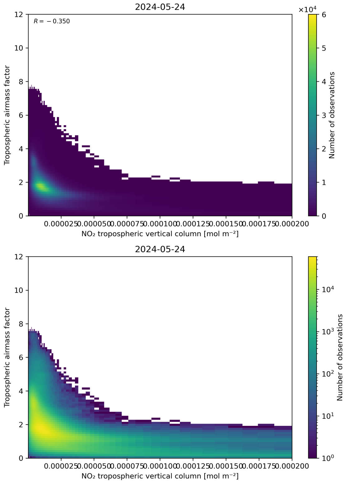
Figure 123: Scatter density plot of “NO 2 tropospheric vertical column” against “Tropospheric airmass factor” for 2024-05-23 to 2024-05-25.
