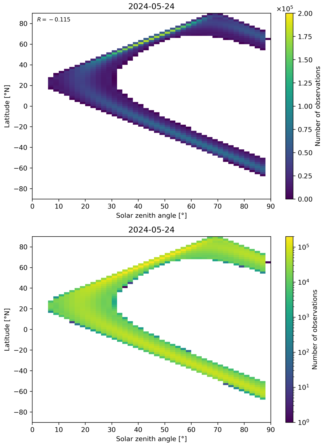
Figure 149: Scatter density plot of “Solar zenith angle” against “Latitude” for 2024-05-23 to 2024-05-25.
