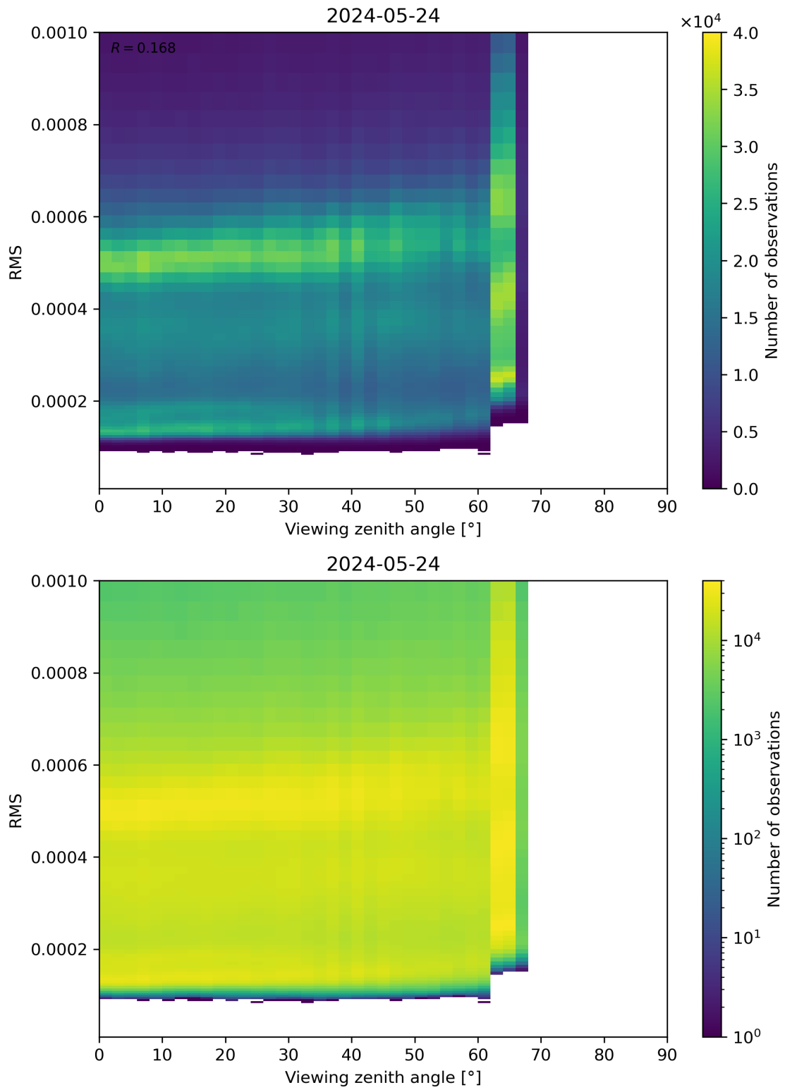
Figure 171: Scatter density plot of “Viewing zenith angle” against “RMS” for 2024-05-23 to 2024-05-25.
