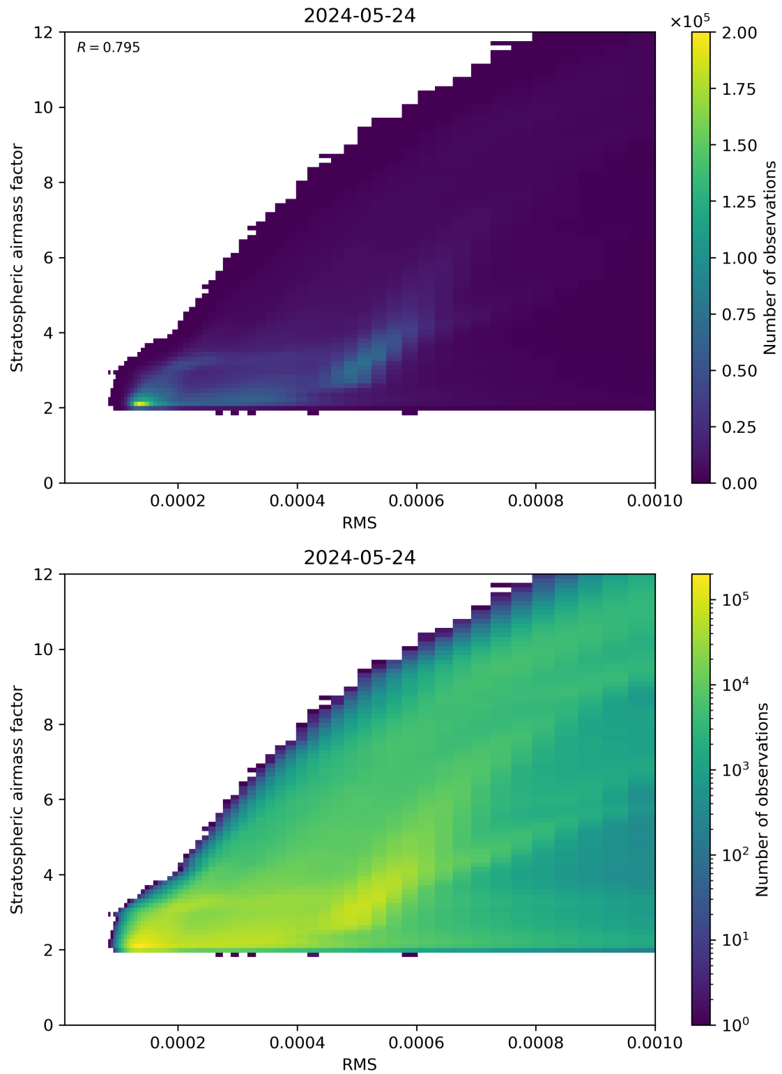
Figure 144: Scatter density plot of “RMS” against “Stratospheric airmass factor” for 2024-05-23 to 2024-05-25.
