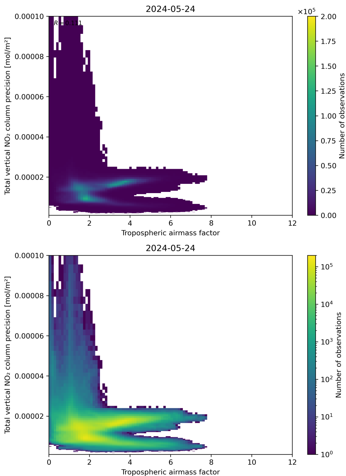
Figure 78: Scatter density plot of “Tropospheric air mass factor” against “Total vertical NO 2 column precision” for 2024-05-23 to 2024-05-25.
