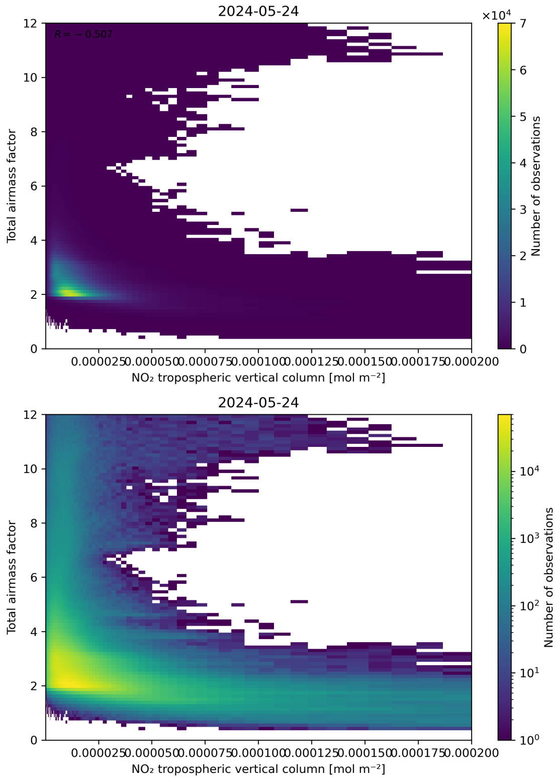
Figure 122: Scatter density plot of “NO 2 tropospheric vertical column” against “Total air mass factor” for 2024-05-23 to 2024-05-25.
