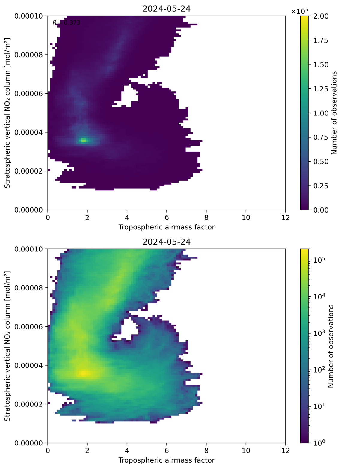
Figure 74: Scatter density plot of “Tropospheric airmass factor” against “Stratospheric vertical NO 2 column” for 2024-05-23 to 2024-05-25.
