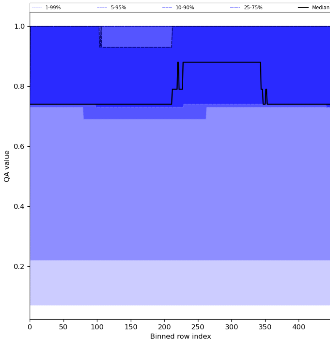
Figure 45: Along track statistics of “QA value” for 2024-05-23 to 2024-05-25
