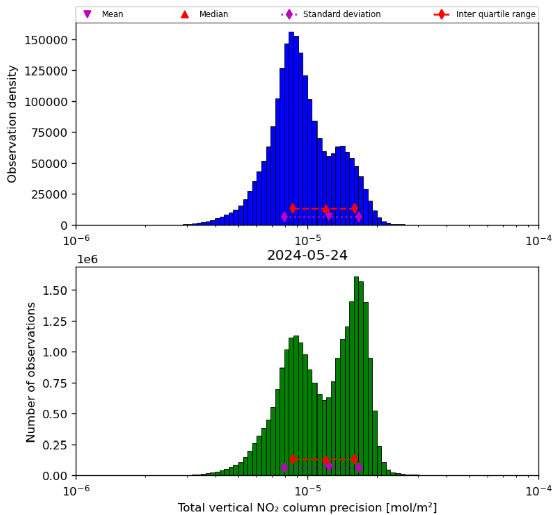
Figure 39: Histogram of “Total vertical NO 2 column precision” for 2024-05-23 to 2024-05-25
