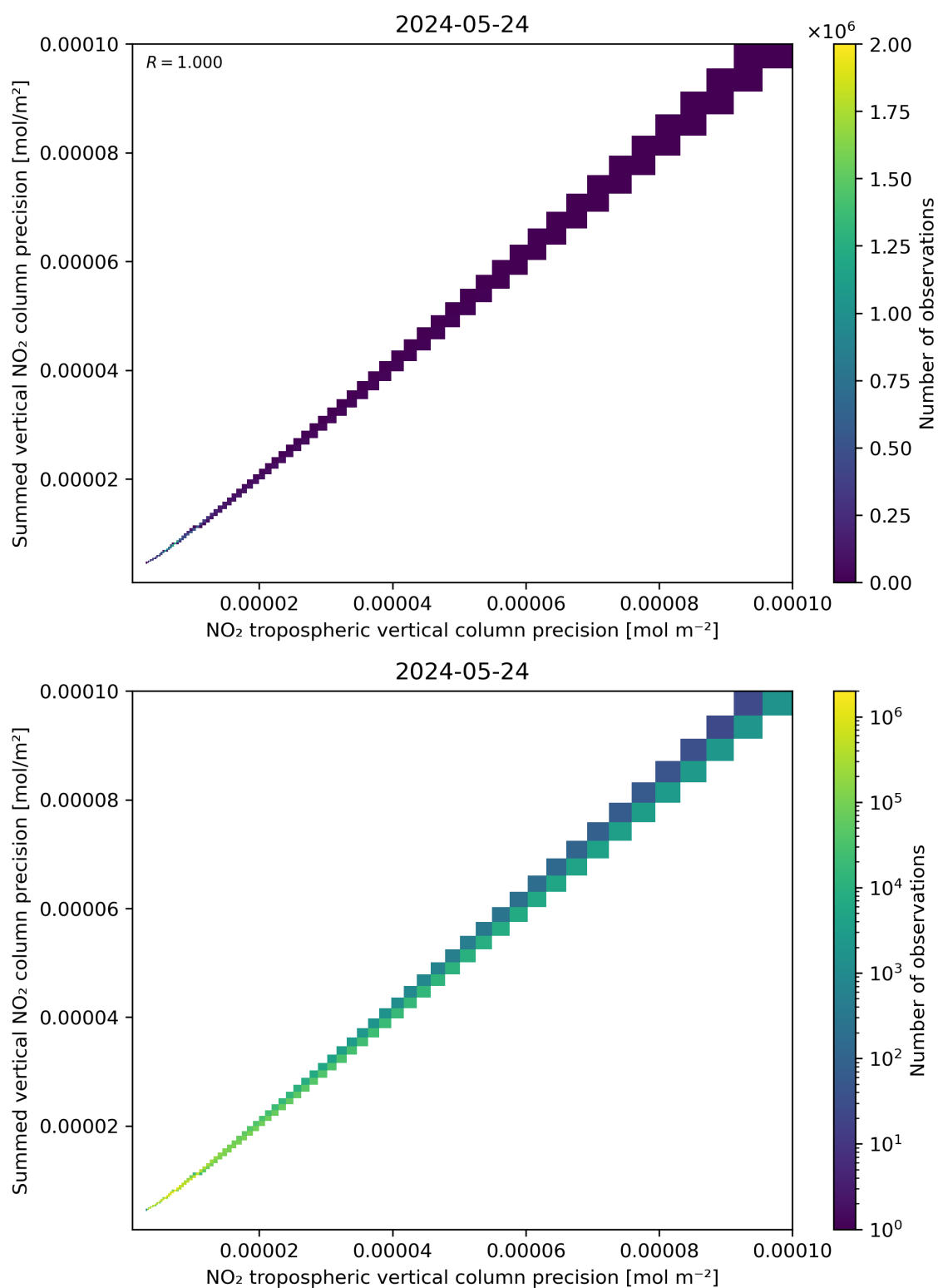
Figure 137: Scatter density plot of “NO 2 tropospheric vertical column precision” against “Summed vertical NO 2 column precision” for 2024-05-23 to 2024-05-25.
