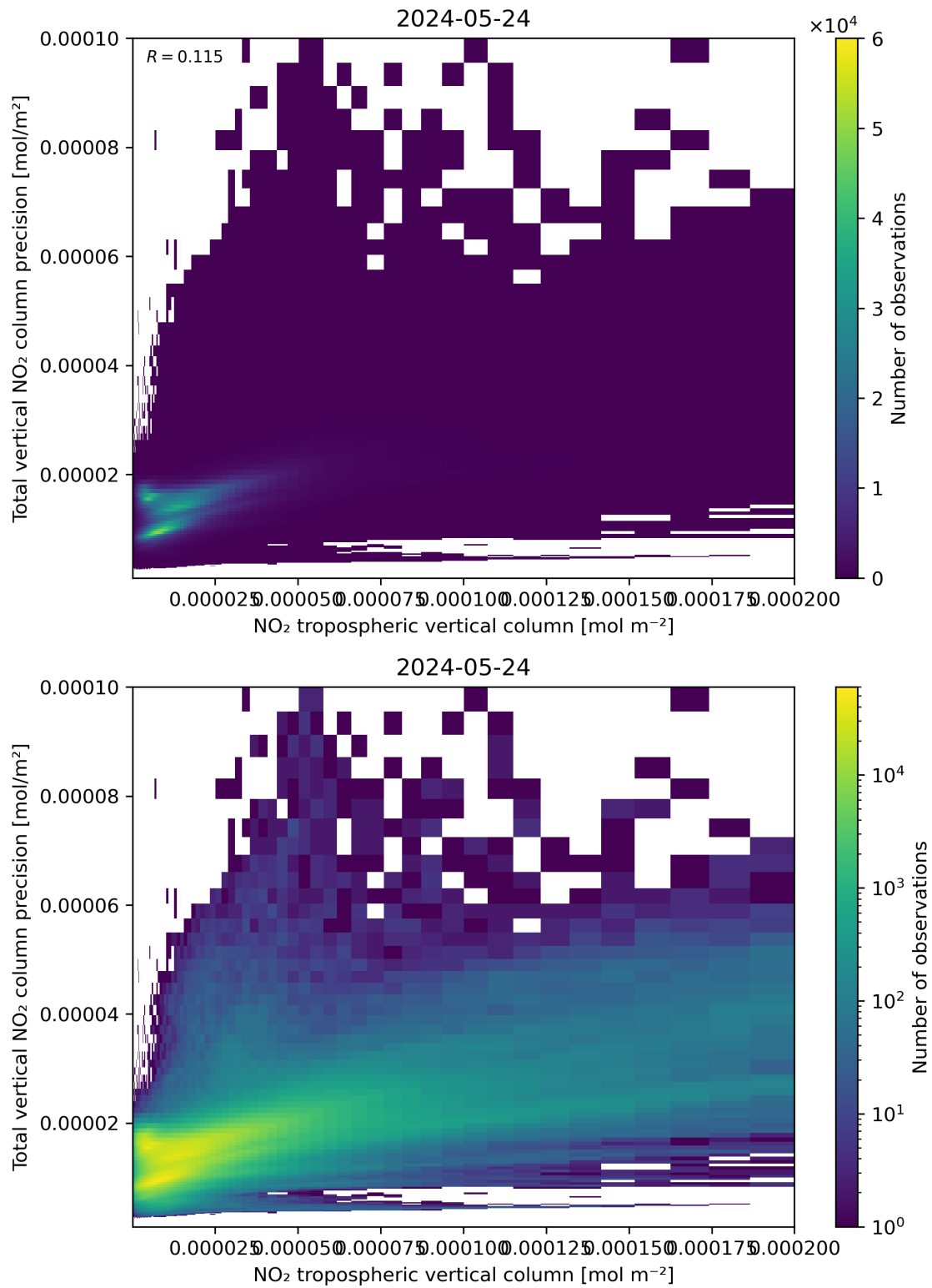
Figure 129: Scatter density plot of “NO 2 tropospheric vertical column” against “Total vertical NO 2 column precision” for 2024-05-23 to 2024-05-25.
