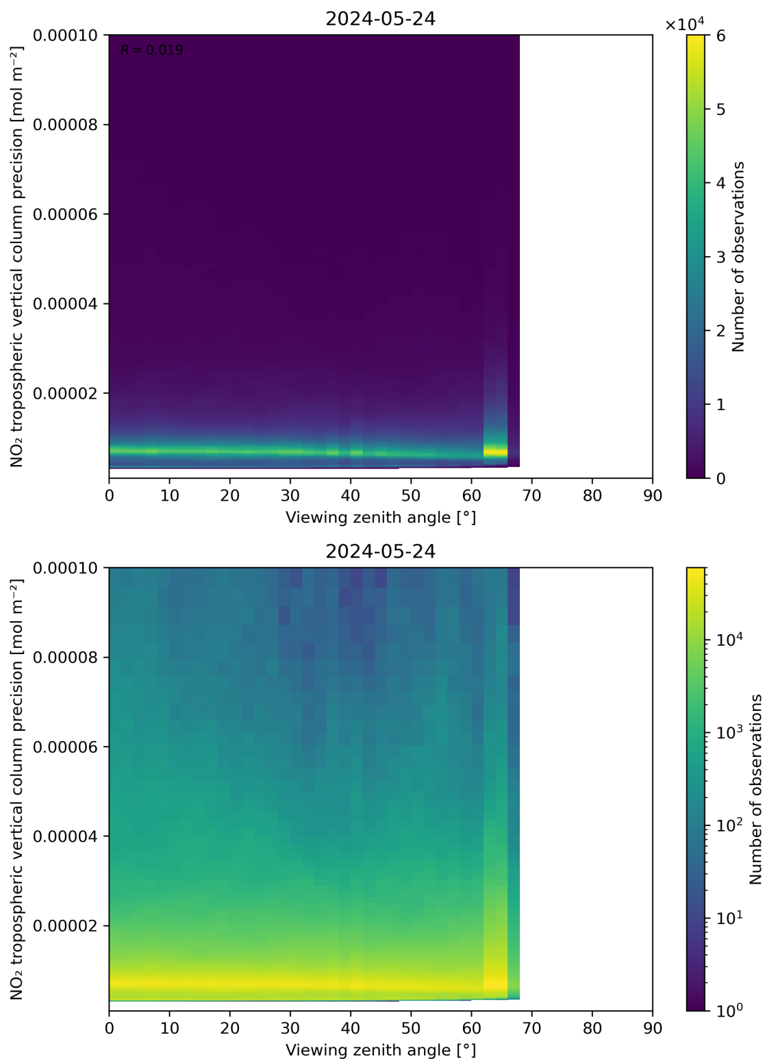
Figure 170: Scatter density plot of “Viewing zenith angle” against “NO 2 tropospheric vertical column precision” for 2024-05-23 to 2024-05-25.
