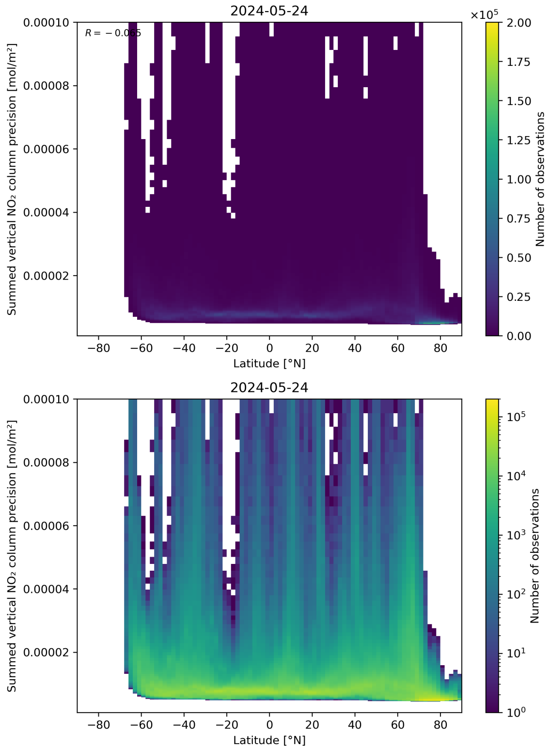
Figure 89: Scatter density plot of “Latitude” against “Summed vertical NO 2 column precision” for 2024-05-23 to 2024-05-25.
