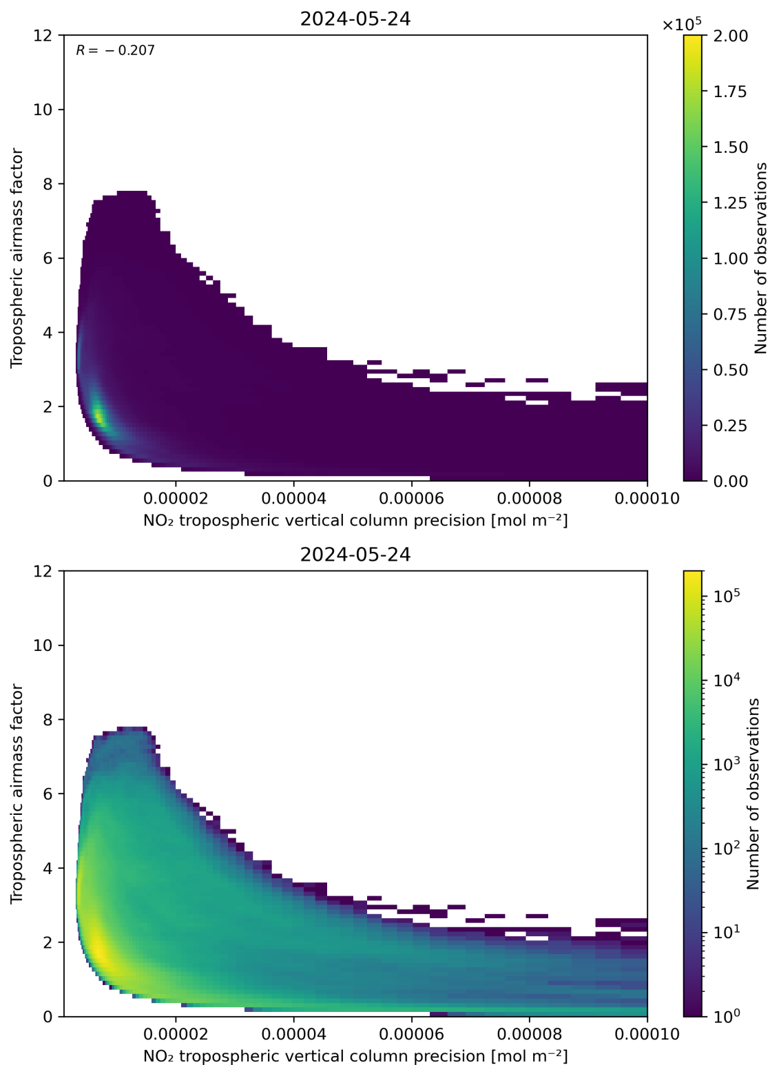
Figure 133: Scatter density plot of “NO 2 tropospheric vertical column precision” against “Tropospheric airmass factor” for 2024-05-23 to 2024-05-25.
