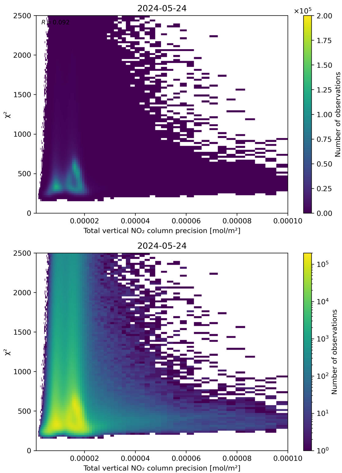
Figure 116: Scatter density plot of “Total vertical NO 2 column precision” against “ \chi^2 ” for 2024-05-23 to 2024-05-25.
