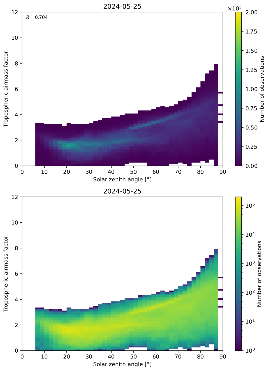
Figure 147: Scatter density plot of “Solar zenith angle” against “Tropospheric airmass factor” for 2024-05-24 to 2024-05-26.
