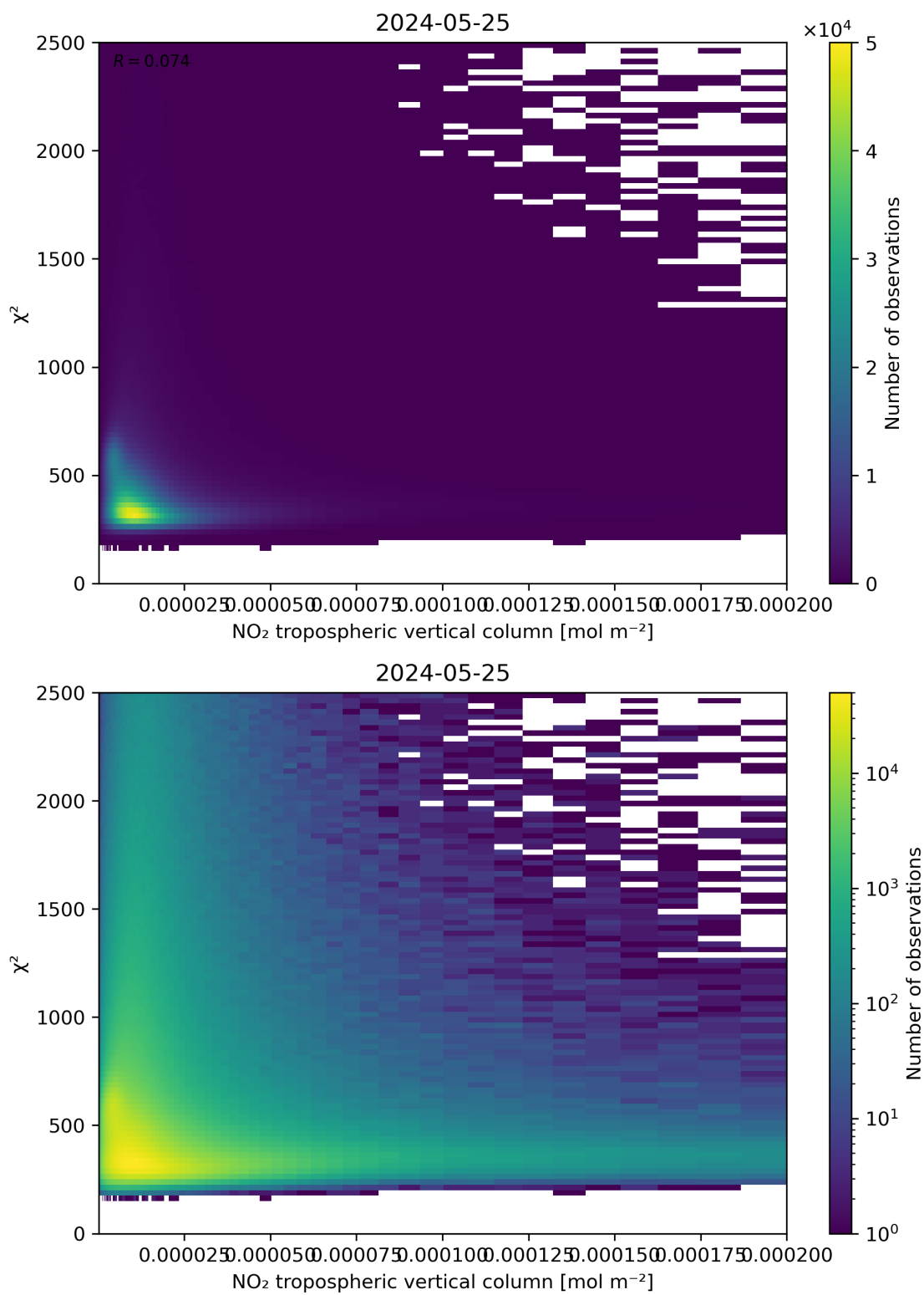
Figure 124: Scatter density plot of “NO 2 tropospheric vertical column” against “ \chi^2 ” for 2024-05-24 to 2024-05-26.
