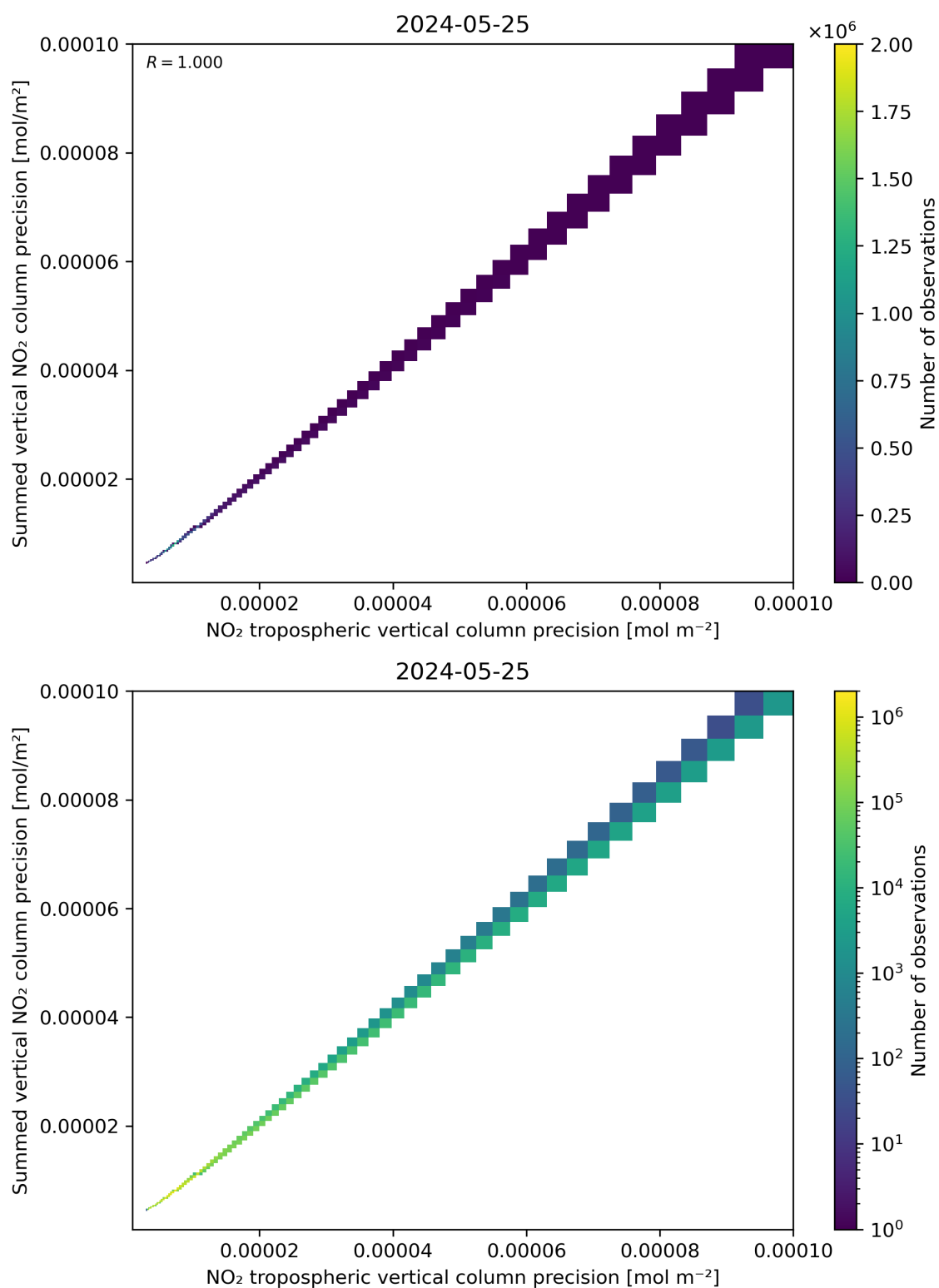
Figure 137: Scatter density plot of “NO 2 tropospheric vertical column precision” against “Summed vertical NO 2 column precision” for 2024-05-24 to 2024-05-26.
