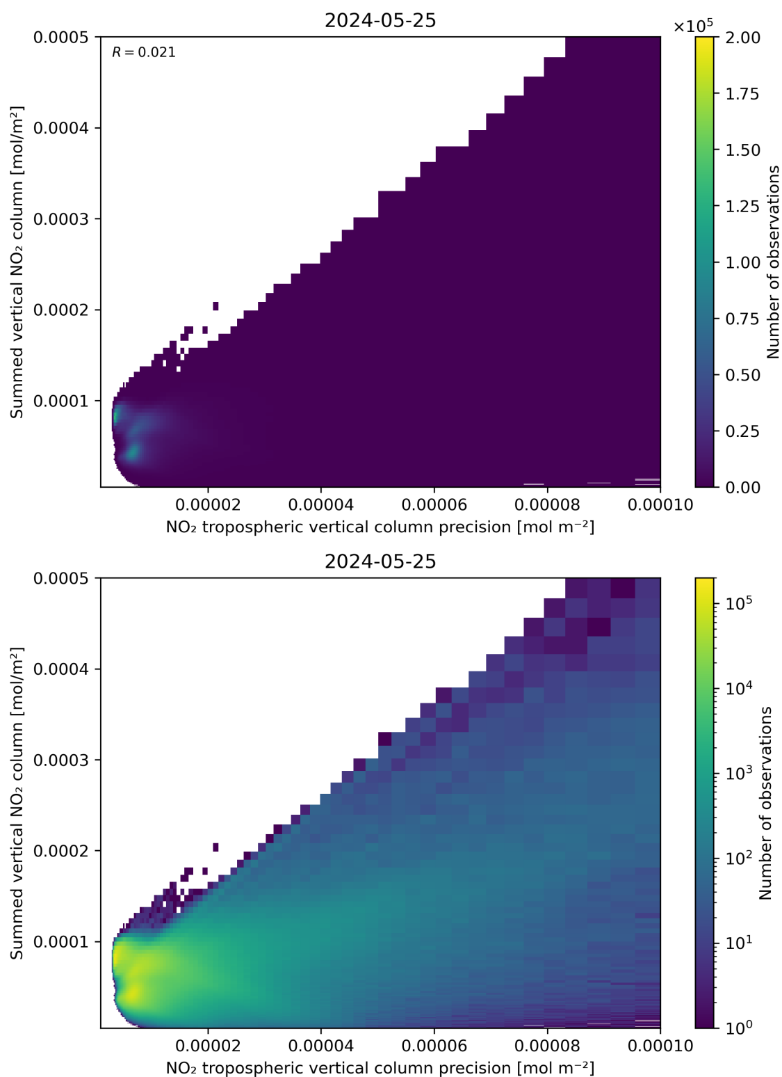
Figure 136: Scatter density plot of “NO 2 tropospheric vertical column precision” against “Summed vertical NO 2 column” for 2024-05-24 to 2024-05-26.
