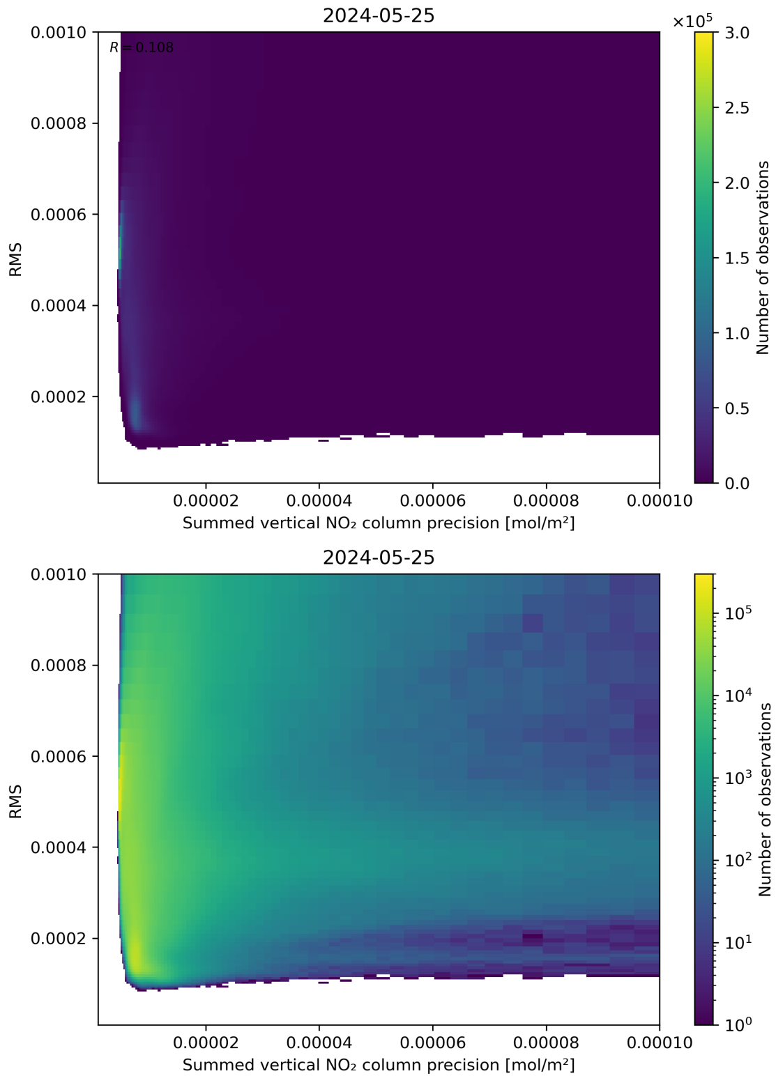
Figure 108: Scatter density plot of “Summed vertical NO 2 column precision” against “RMS” for 2024-05-24 to 2024-05-26.
