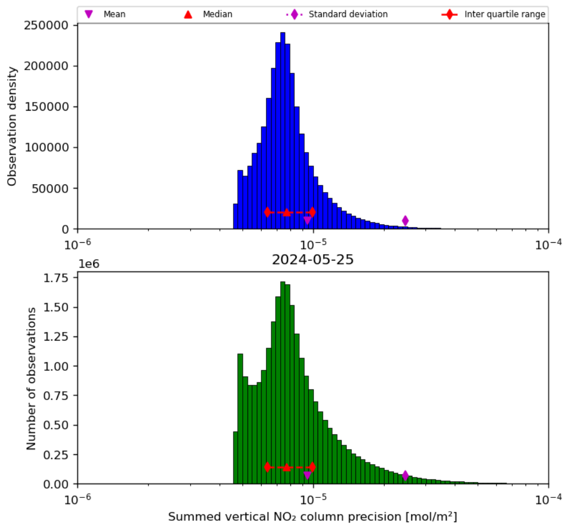
Figure 41: Histogram of "Summed vertical NO 2 column precision" for 2024-05-24 to 2024-05-26
