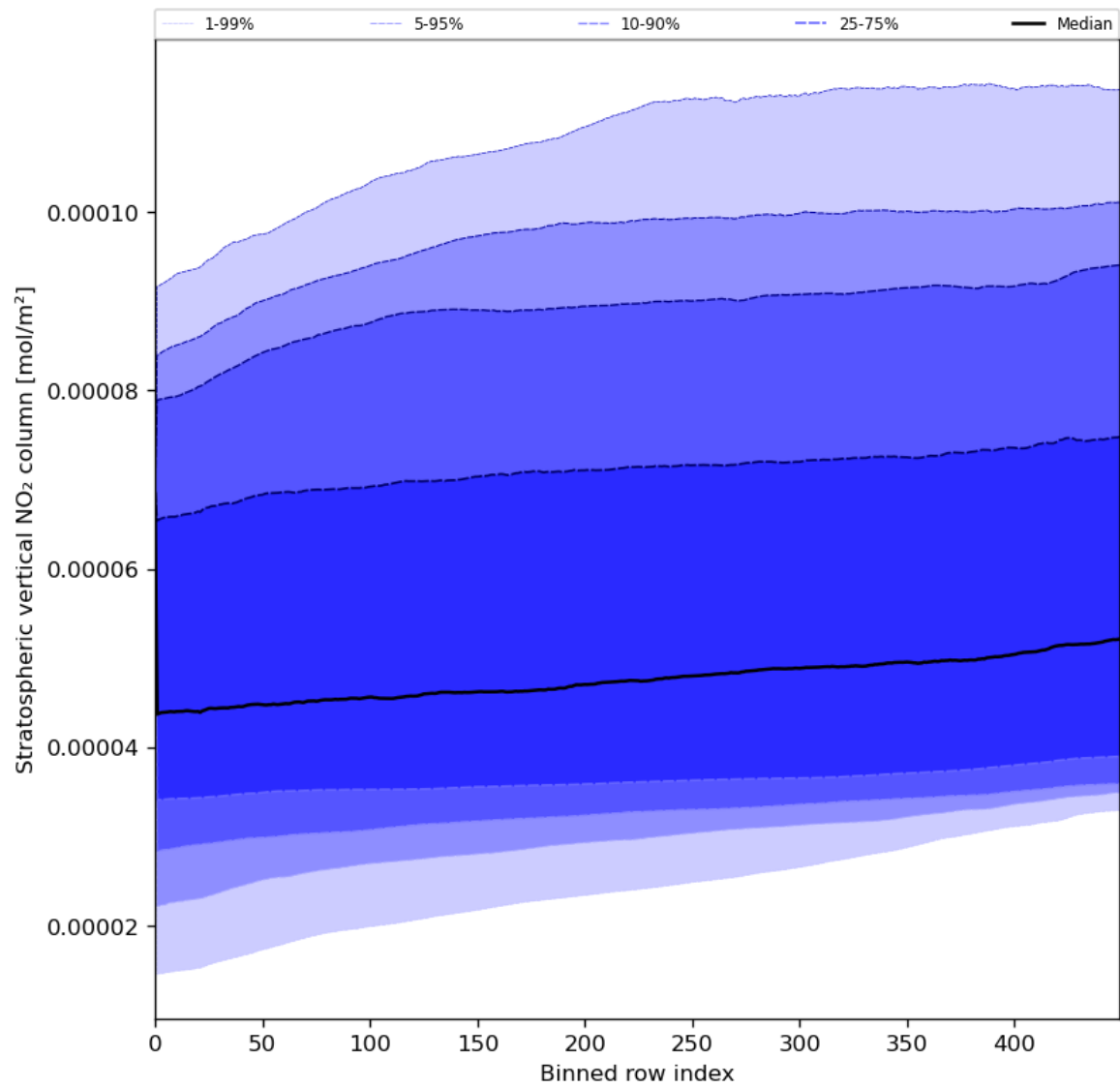
Figure 53: Along track statistics of “Stratospheric vertical NO 2 column” for 2024-05-24 to 2024-05-26
