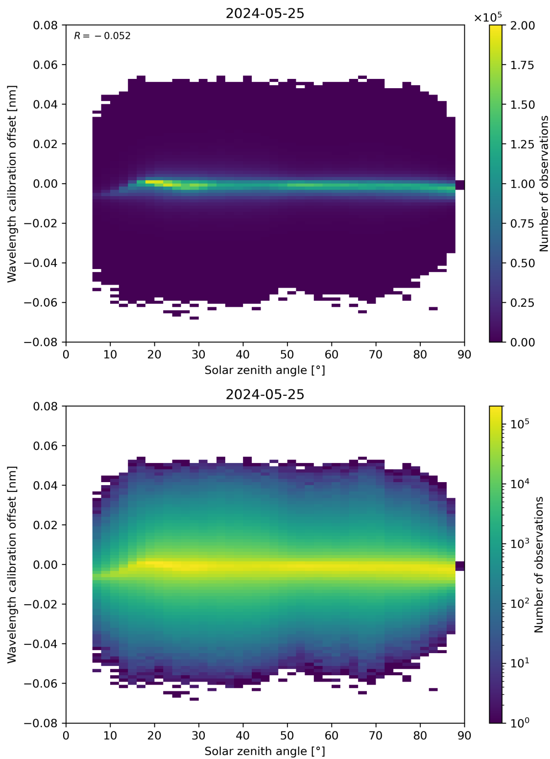
Figure 158: Scatter density plot of “Solar zenith angle” against “Wavelength calibration offset” for 2024-05-24 to 2024-05-26.
