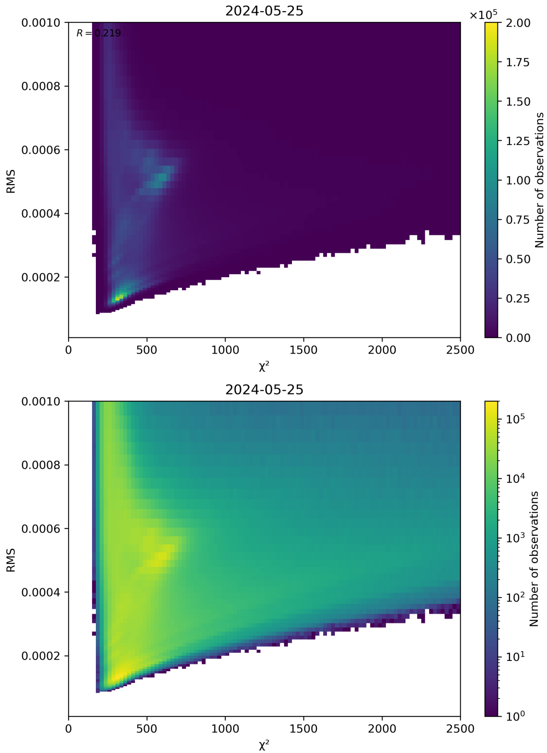
Figure 82: Scatter density plot of “ \chi^2 ” against “RMS” for 2024-05-24 to 2024-05-26.
