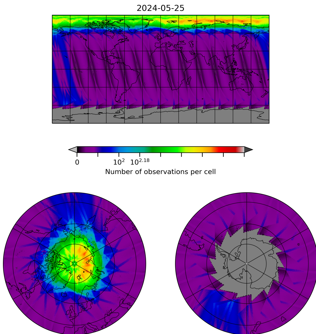
Figure 10: Map of the number of observations for 2024-05-24 to 2024-05-26
