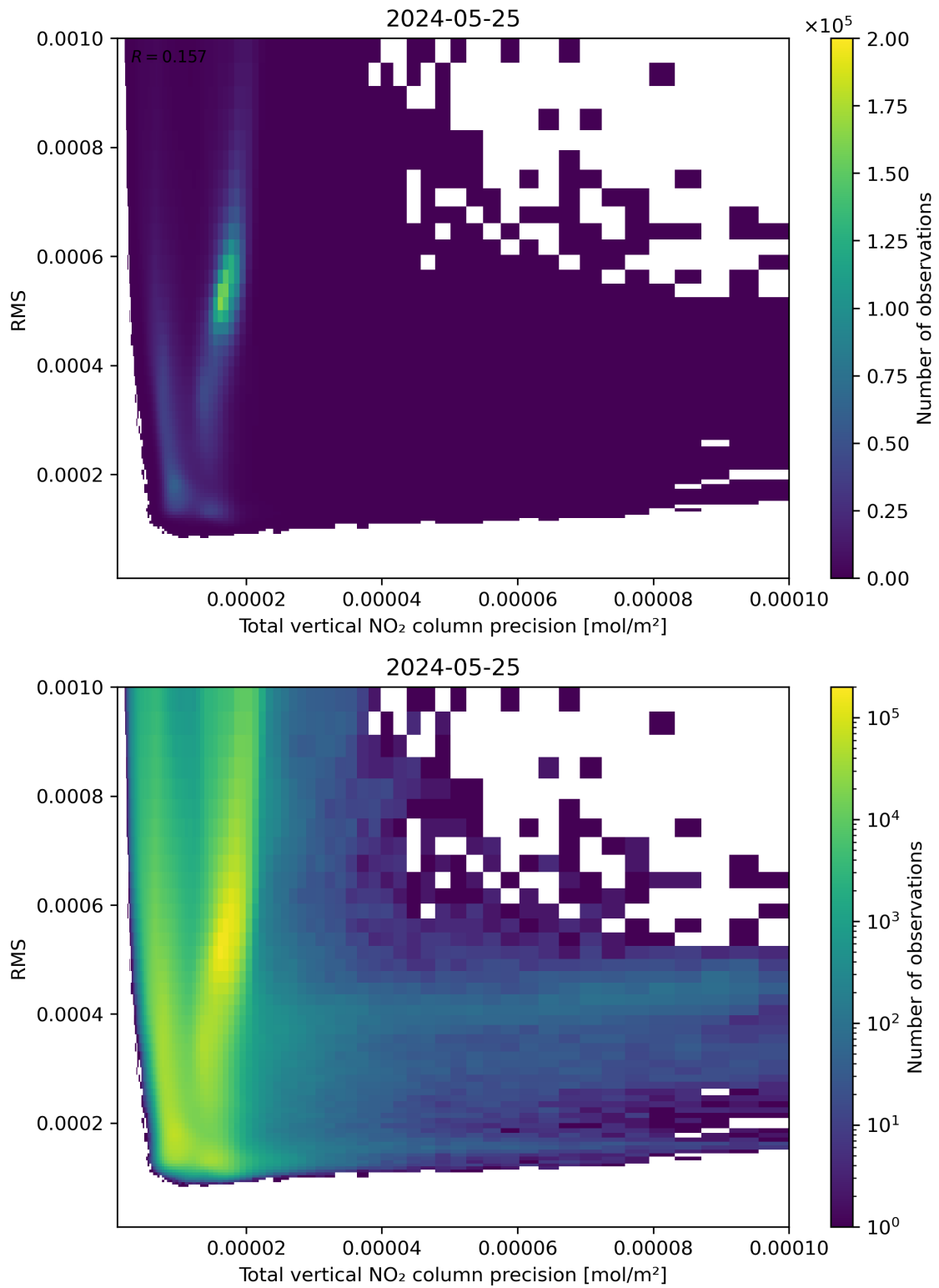
Figure 119: Scatter density plot of “Total vertical NO 2 column precision” against “RMS” for 2024-05-24 to 2024-05-26.
