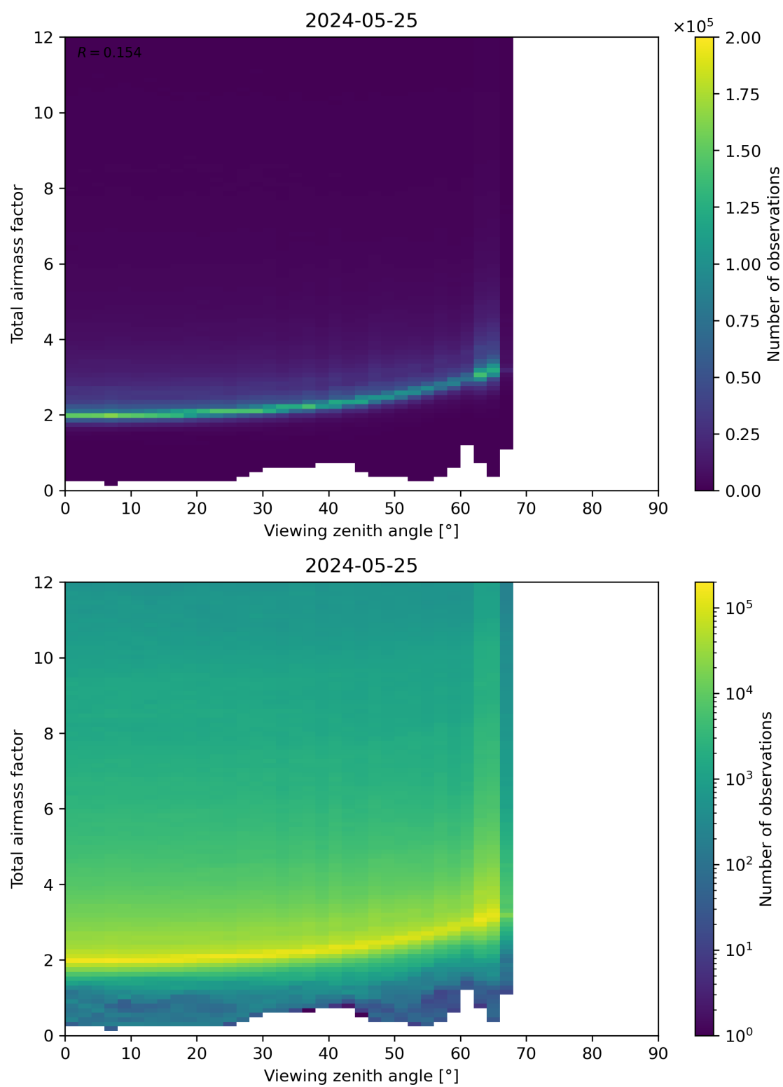
Figure 160: Scatter density plot of “Viewing zenith angle” against “Total airmass factor” for 2024-05-24 to 2024-05-26.
