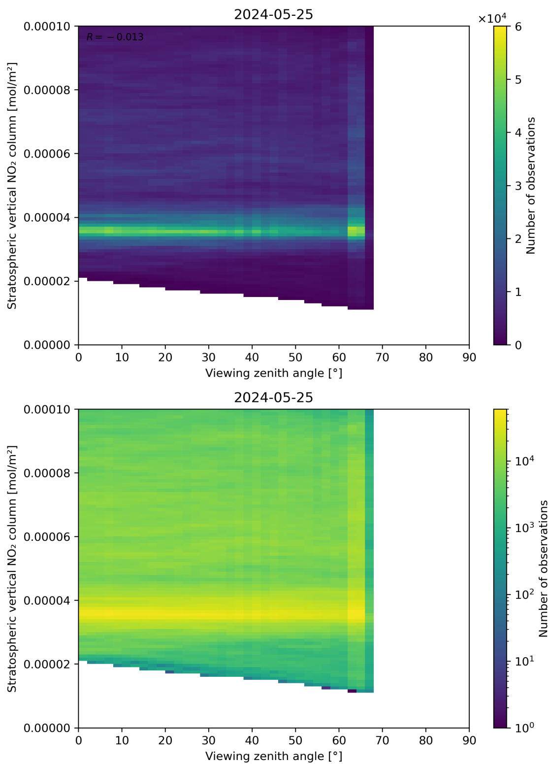
Figure 164: Scatter density plot of “Viewing zenith angle” against “Stratospheric vertical NO 2 column” for 2024-05-24 to 2024-05-26.
