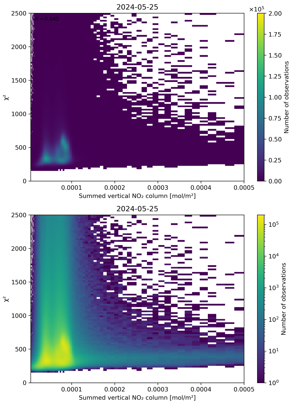
Figure 104: Scatter density plot of “Summed vertical NO 2 column” against “ \chi^2 ” for 2024-05-24 to 2024-05-26.
