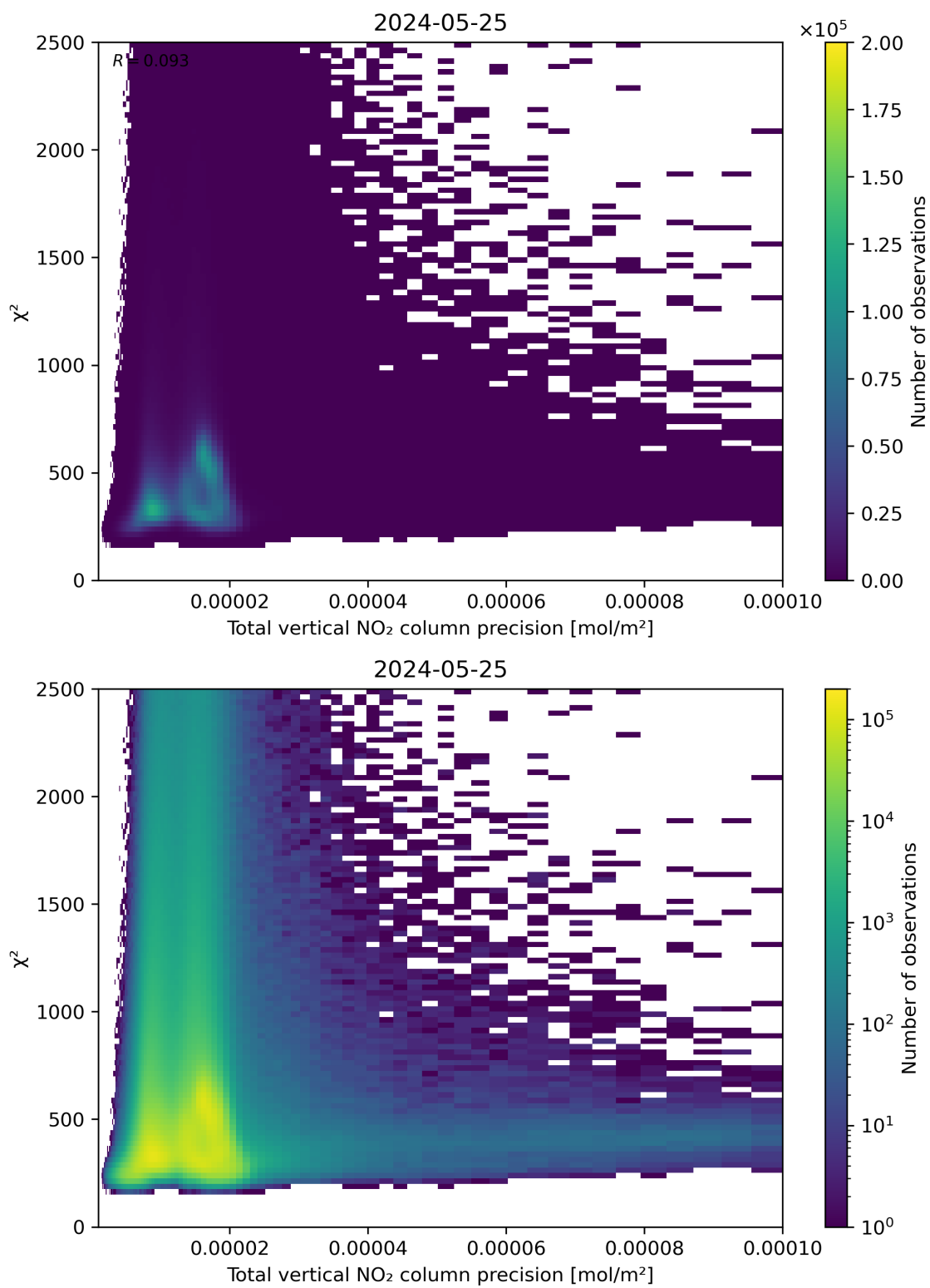
Figure 116: Scatter density plot of “Total vertical NO 2 column precision” against “ \chi^2 ” for 2024-05-24 to 2024-05-26.
