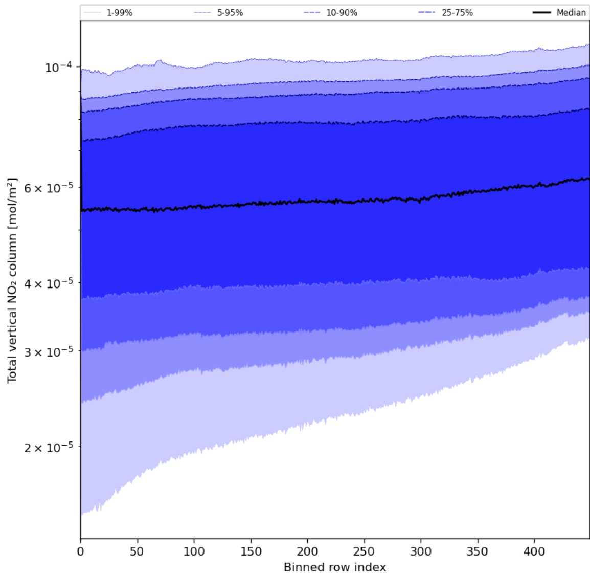
Figure 55: Along track statistics of “Total vertical NO 2 column” for 2024-05-24 to 2024-05-26
