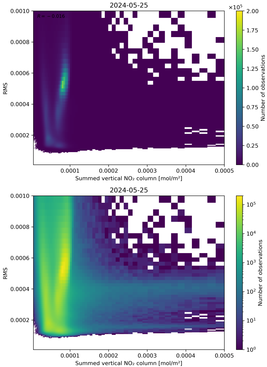
Figure 109: Scatter density plot of “Summed vertical NO 2 column” against “RMS” for 2024-05-24 to 2024-05-26.
