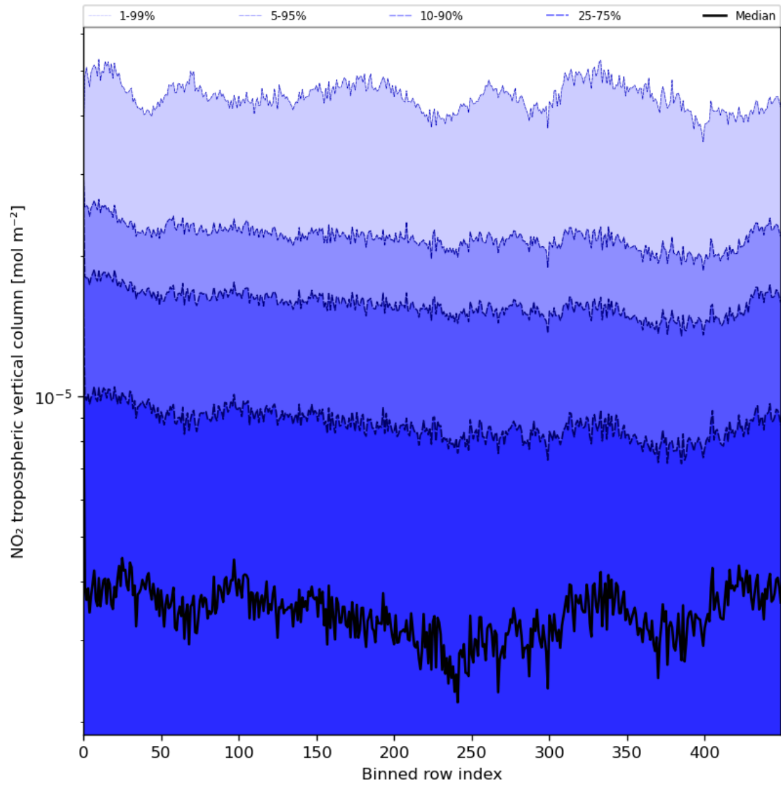
Figure 46: Along track statistics of “NO 2 tropospheric vertical column” for 2024-05-24 to 2024-05-26
