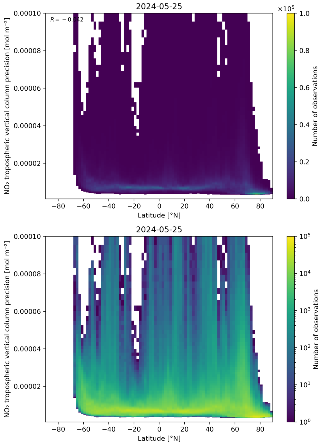
Figure 93: Scatter density plot of “Latitude” against “NO 2 tropospheric vertical column precision” for 2024-05-24 to 2024-05-26.
