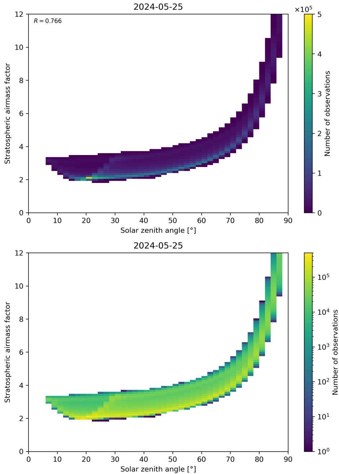
Figure 145: Scatter density plot of “Solar zenith angle” against “Stratospheric airmass factor” for 2024-05-24 to 2024-05-26.
