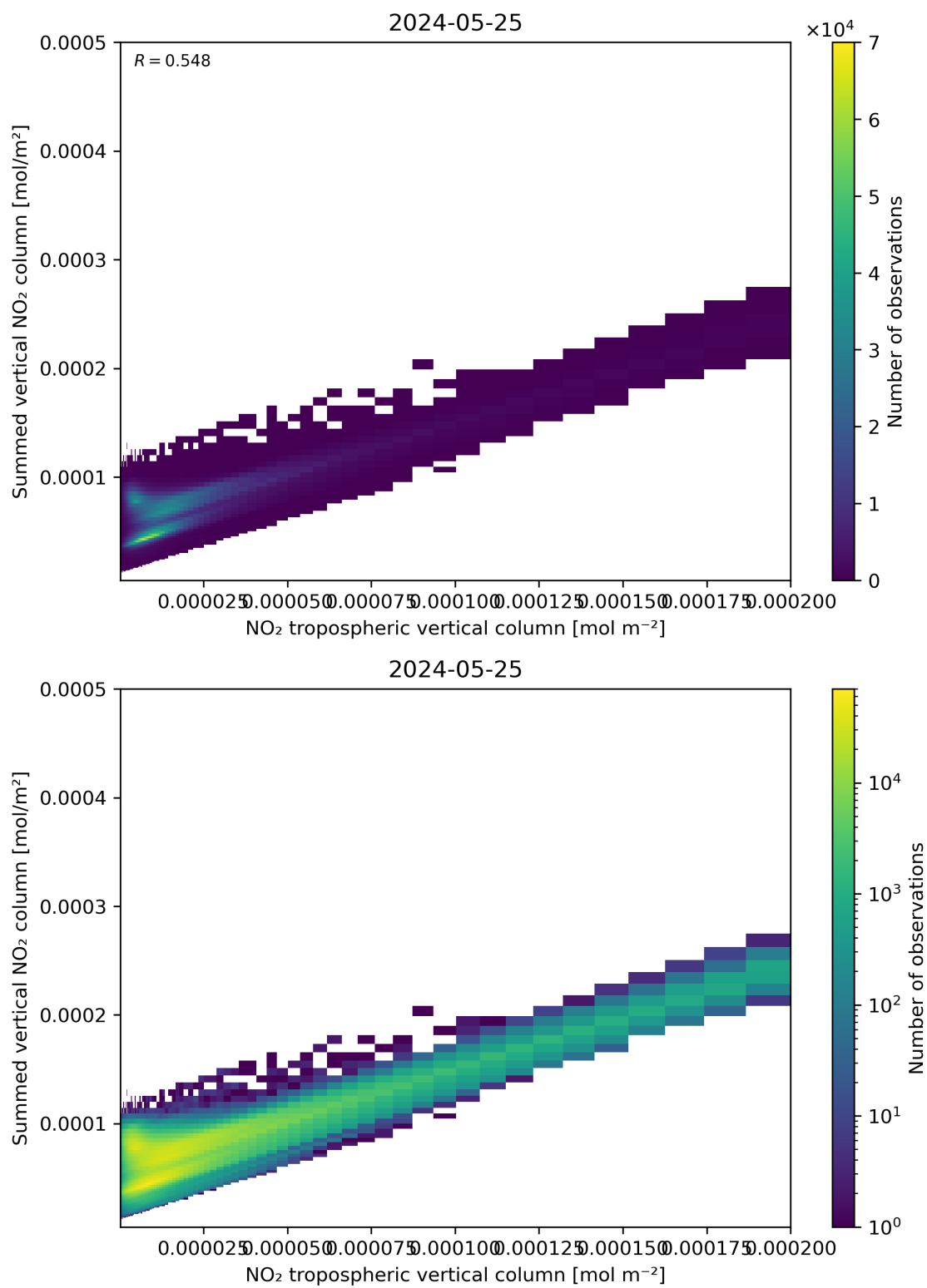
Figure 126: Scatter density plot of “NO 2 tropospheric vertical column” against “Summed vertical NO 2 column” for 2024-05-24 to 2024-05-26.
