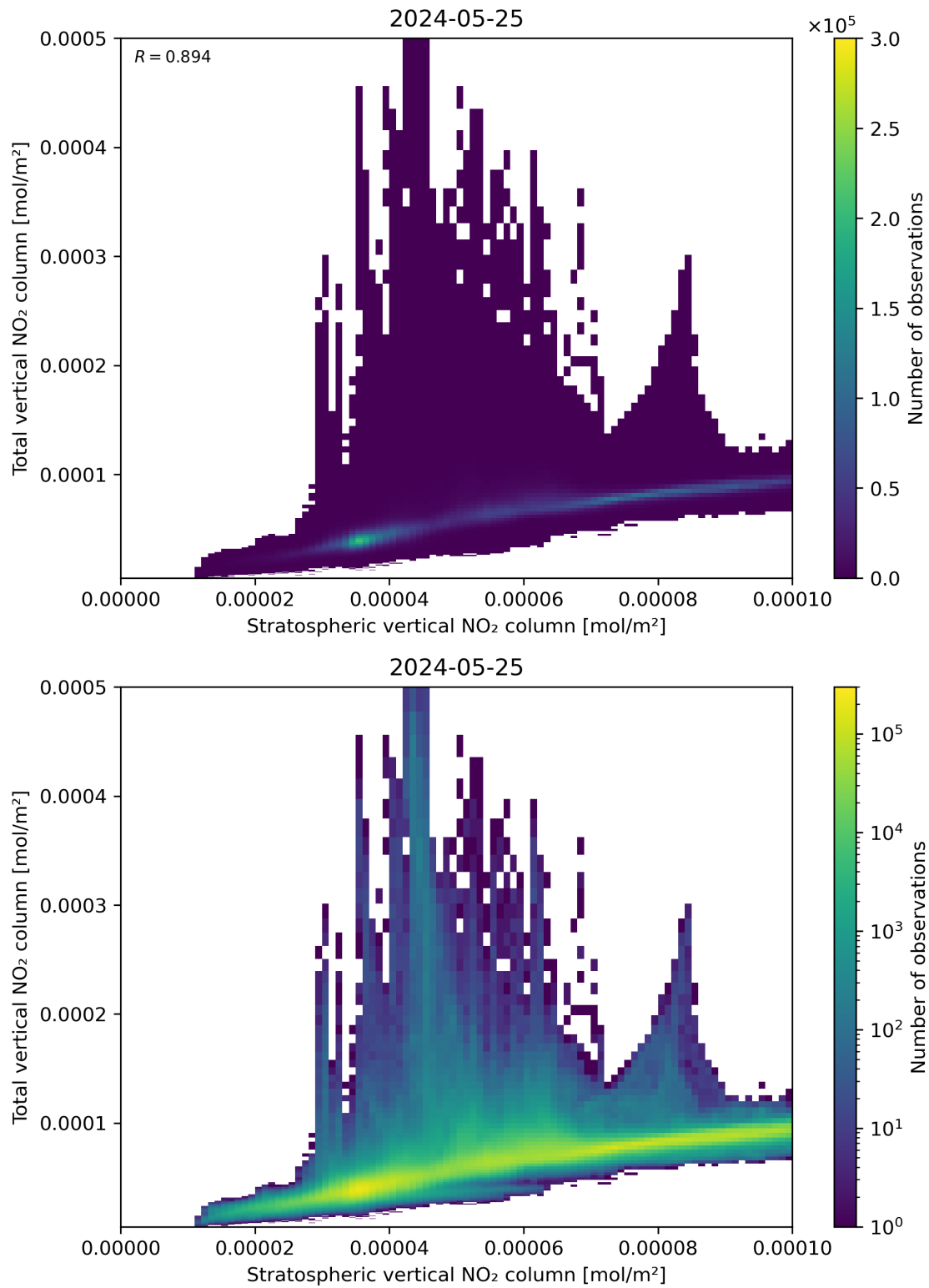
Figure 100: Scatter density plot of “Stratospheric vertical NO 2 column” against “Total vertical NO 2 column” for 2024-05-24 to 2024-05-26.
