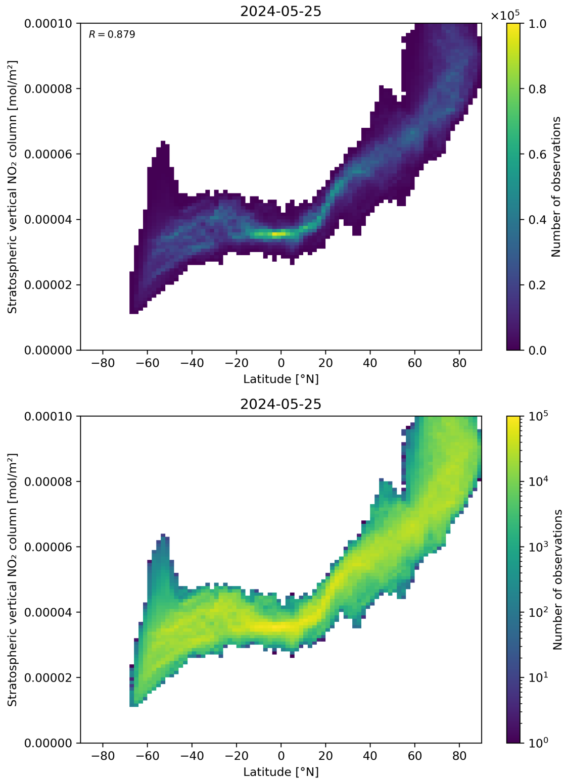
Figure 87: Scatter density plot of “Latitude” against “Stratospheric vertical NO 2 column” for 2024-05-24 to 2024-05-26.
