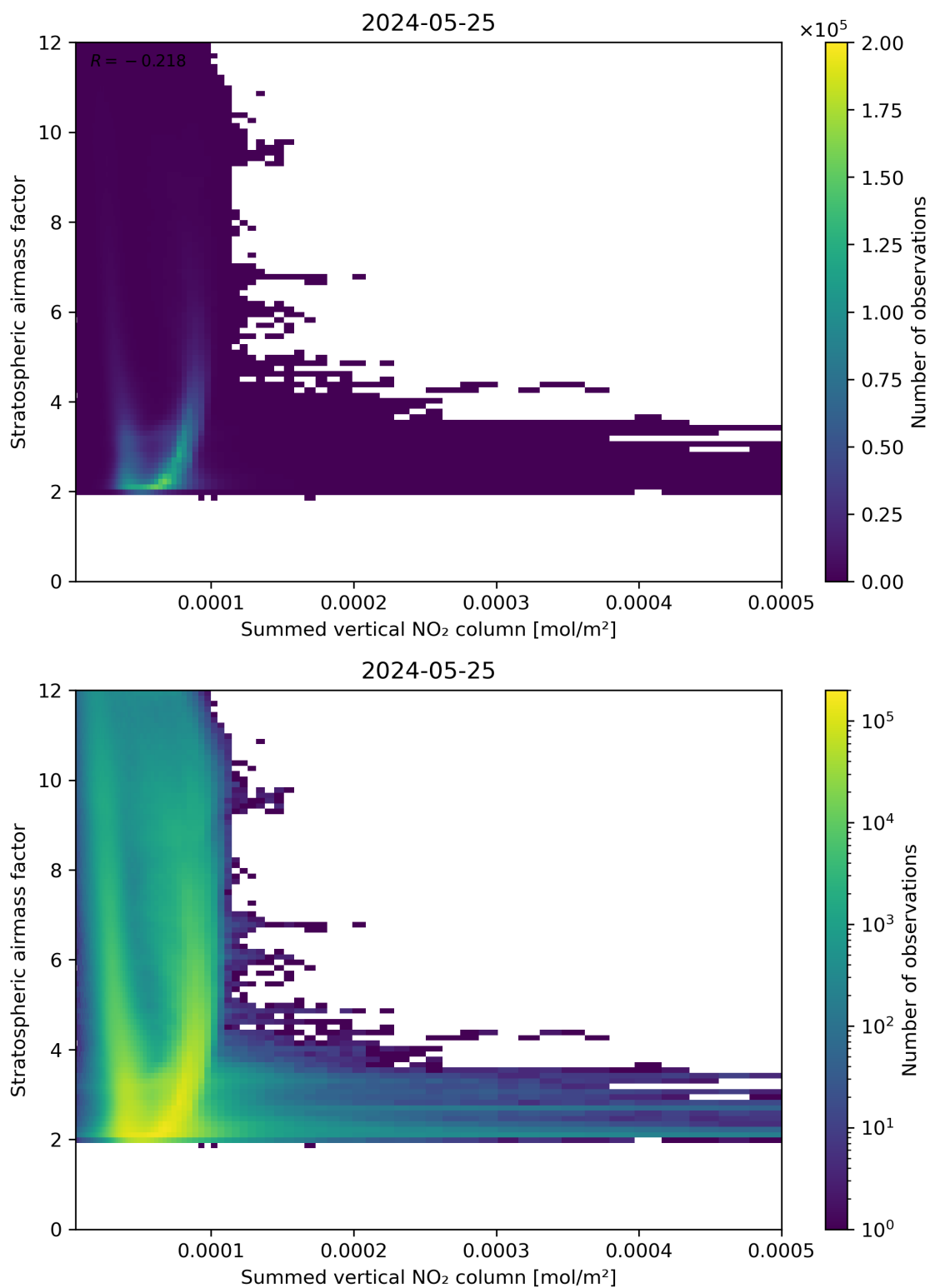
Figure 103: Scatter density plot of “Summed vertical NO 2 column” against “Stratospheric air mass factor” for 2024-05-24 to 2024-05-26.
