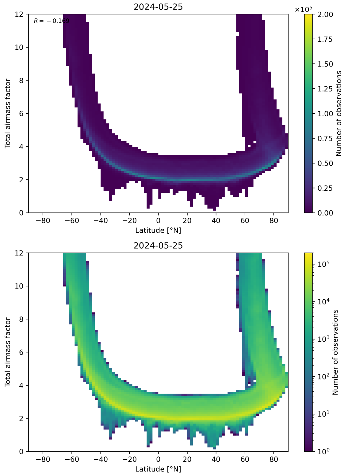
Figure 84: Scatter density plot of “Latitude” against “Total airmass factor” for 2024-05-24 to 2024-05-26.
