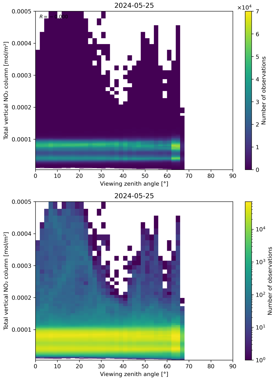
Figure 167: Scatter density plot of “Viewing zenith angle” against “Total vertical NO 2 column” for 2024-05-24 to 2024-05-26.
