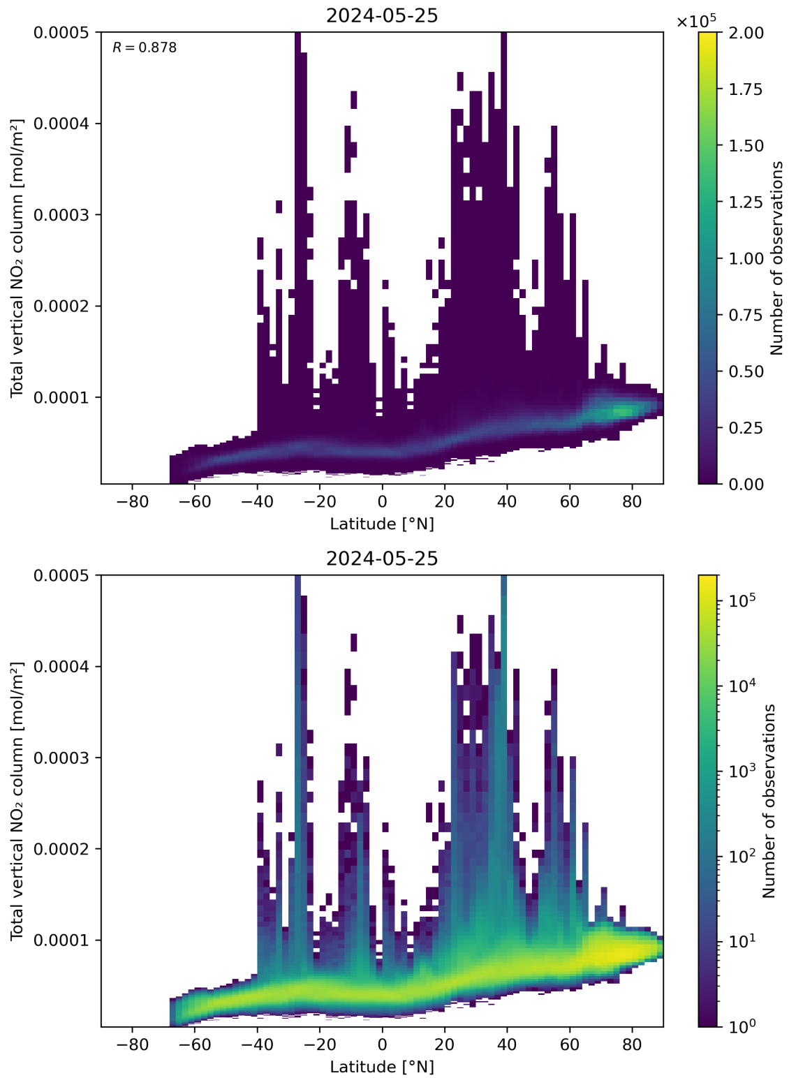
Figure 90: Scatter density plot of “Latitude” against “Total vertical NO 2 column” for 2024-05-24 to 2024-05-26.
