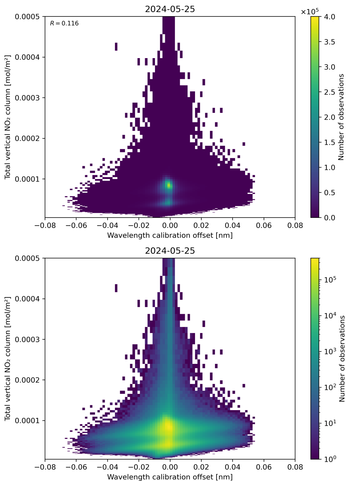
Figure 179: Scatter density plot of “Wavelength calibration offset” against “Total vertical NO 2 column” for 2024-05-24 to 2024-05-26.
