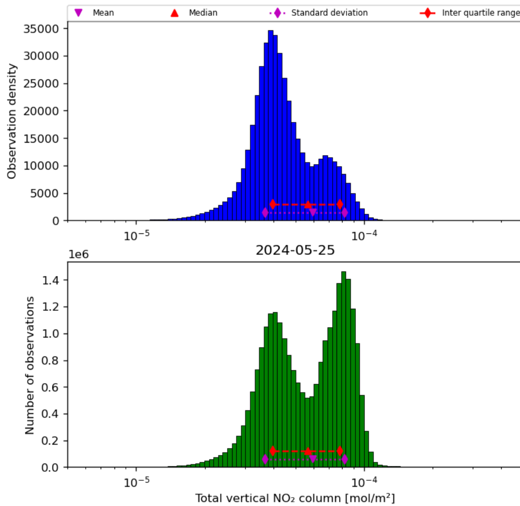
Figure 38: Histogram of “Total vertical NO 2 column” for 2024-05-24 to 2024-05-26
