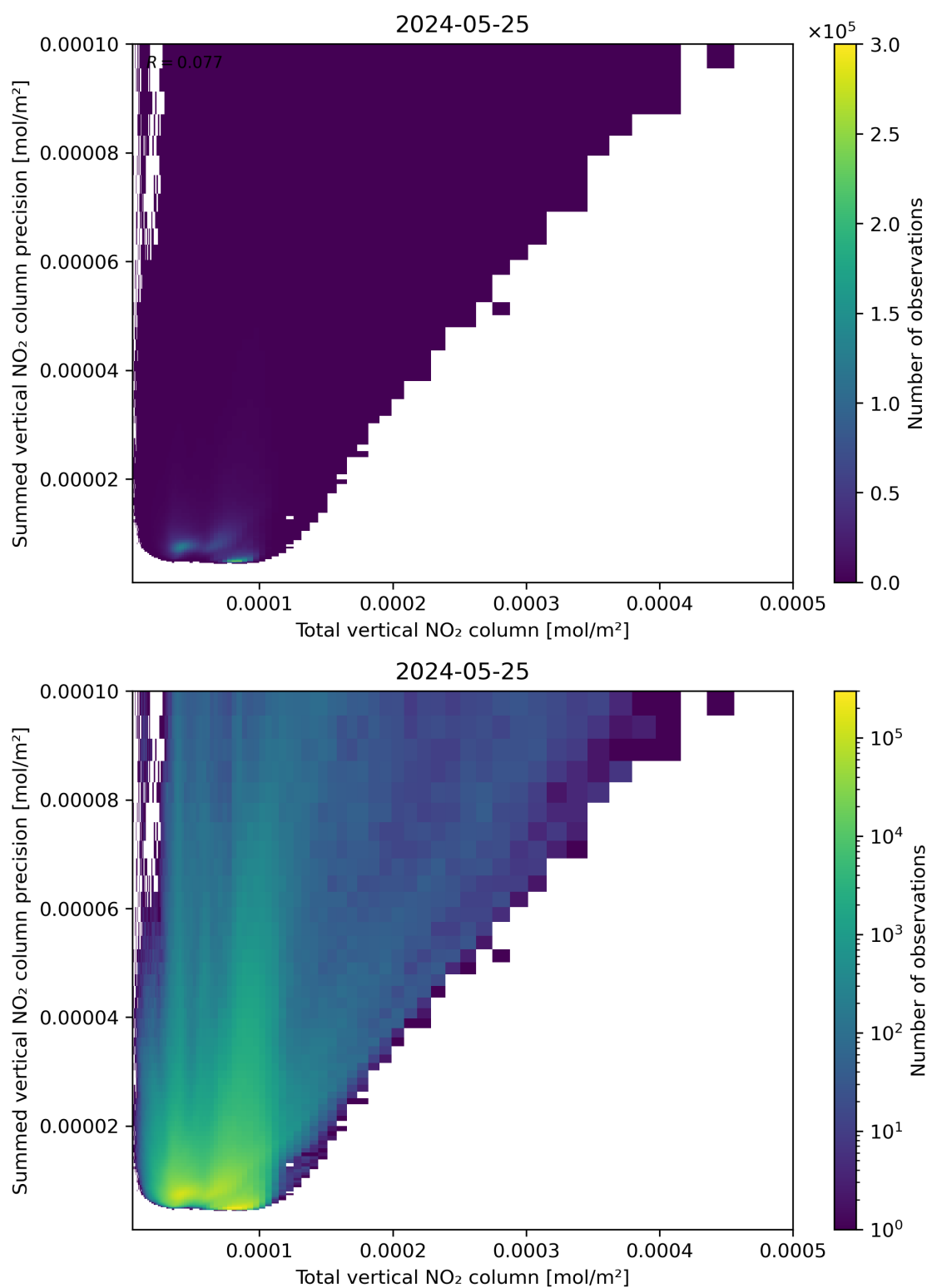
Figure 113: Scatter density plot of “Total vertical NO 2 column” against “Summed vertical NO 2 column precision” for 2024-05-24 to 2024-05-26.
