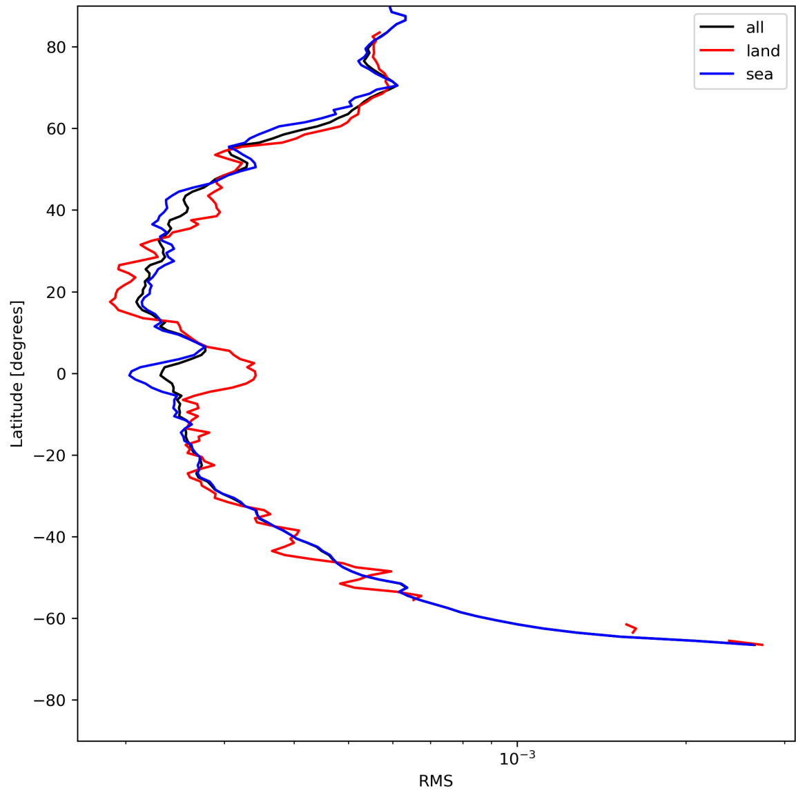
Figure 26: Zonal average of “RMS” for 2024-05-24 to 2024-05-26.
