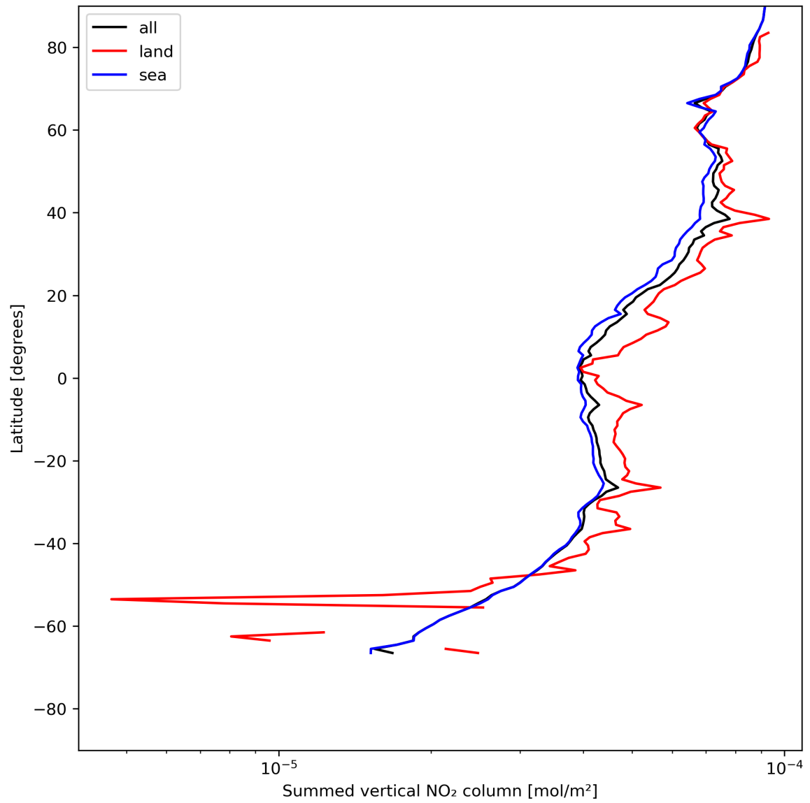
Figure 23: Zonal average of “Summed vertical NO 2 column” for 2024-05-24 to 2024-05-26.
