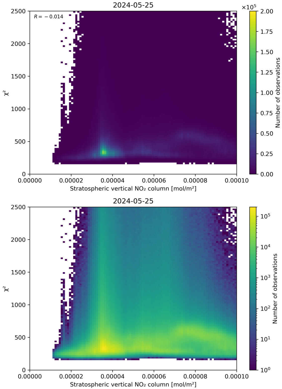
Figure 97: Scatter density plot of “Stratospheric vertical NO 2 column” against “ \chi^2 ” for 2024-05-24 to 2024-05-26.
