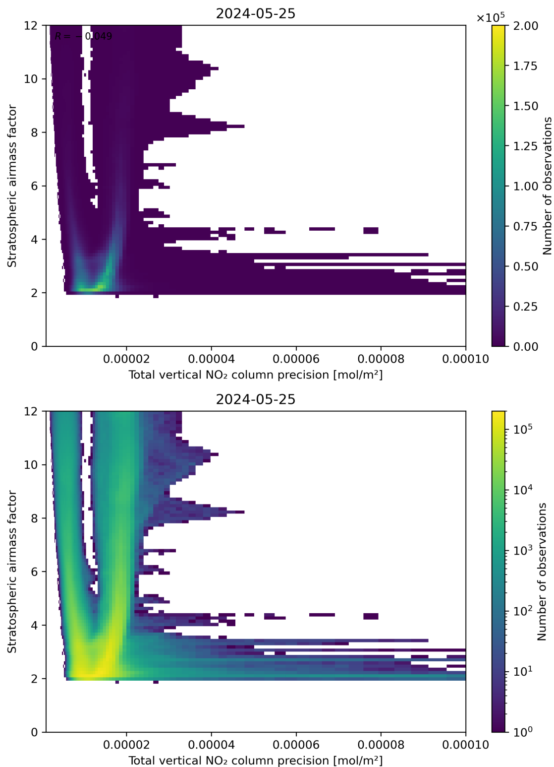
Figure 115: Scatter density plot of “Total vertical NO 2 column precision” against “Stratospheric air mass factor” for 2024-05-24 to 2024-05-26.
