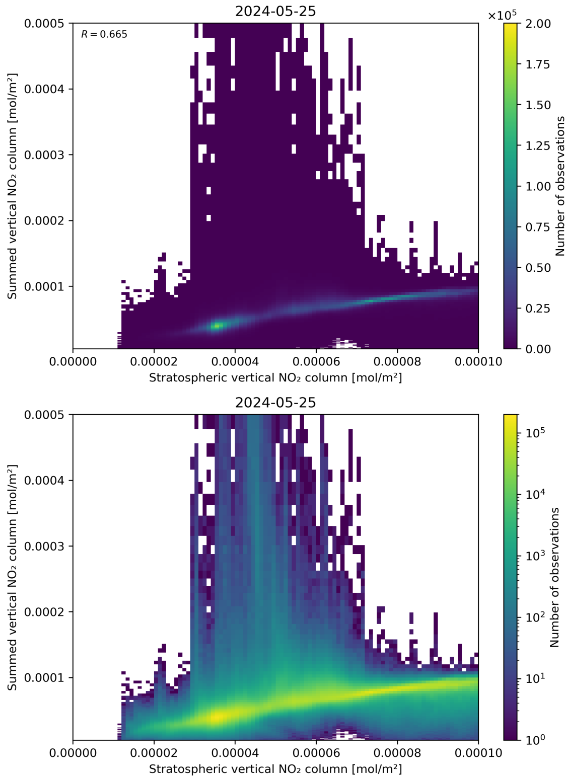
Figure 98: Scatter density plot of “Stratospheric vertical NO 2 column” against “Summed vertical NO 2 column” for 2024-05-24 to 2024-05-26.
