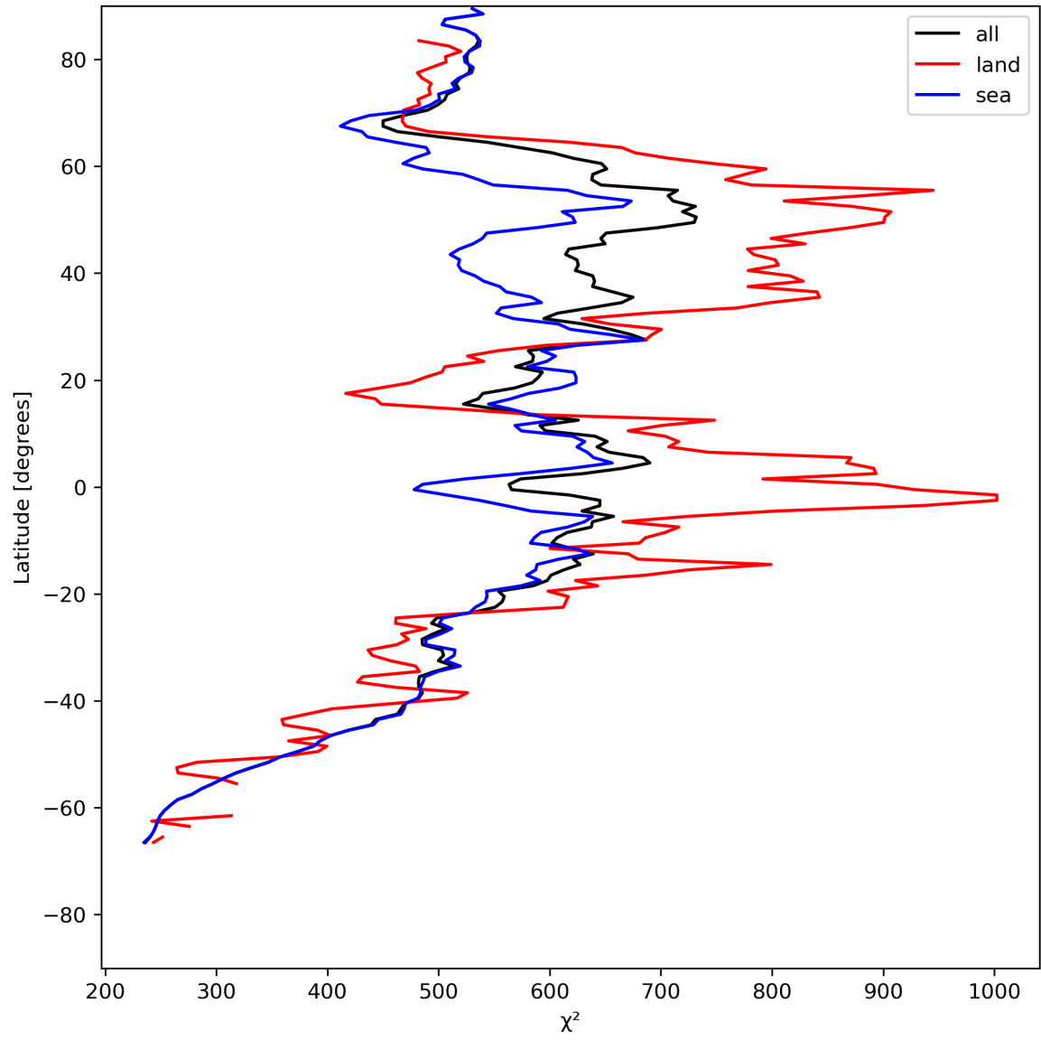
Figure 25: Zonal average of “ \chi^2 ” for 2024-05-24 to 2024-05-26.
