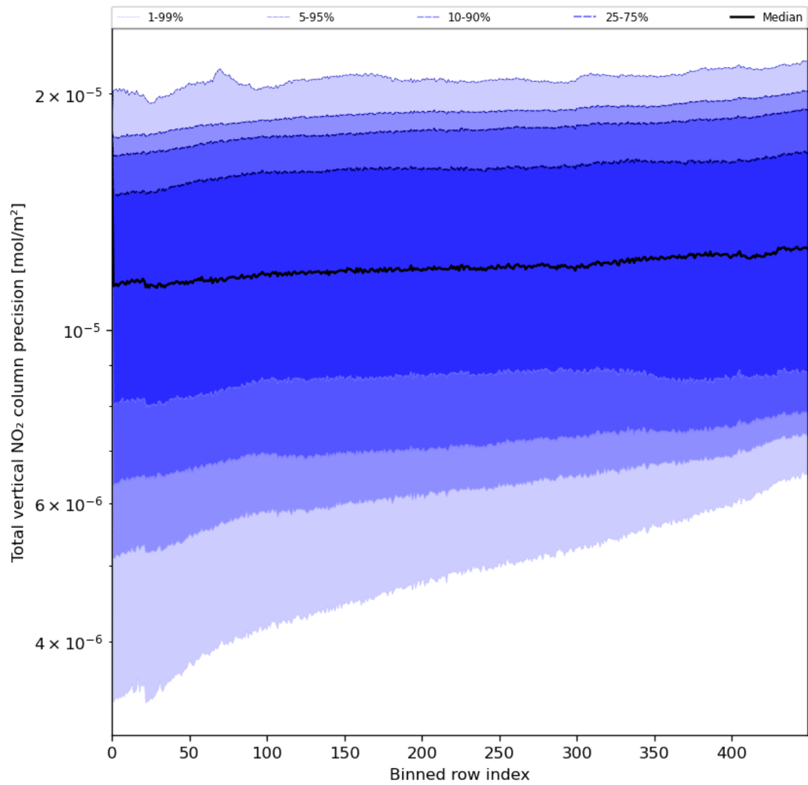
Figure 56: Along track statistics of "Total vertical NO 2 column precision" for 2024-05-24 to 2024-05-26
