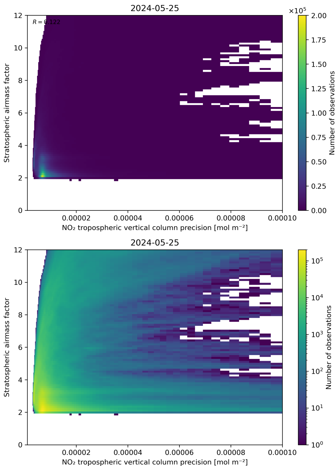
Figure 131: Scatter density plot of “NO 2 tropospheric vertical column precision” against “Stratospheric airmass factor” for 2024-05-24 to 2024-05-26.
