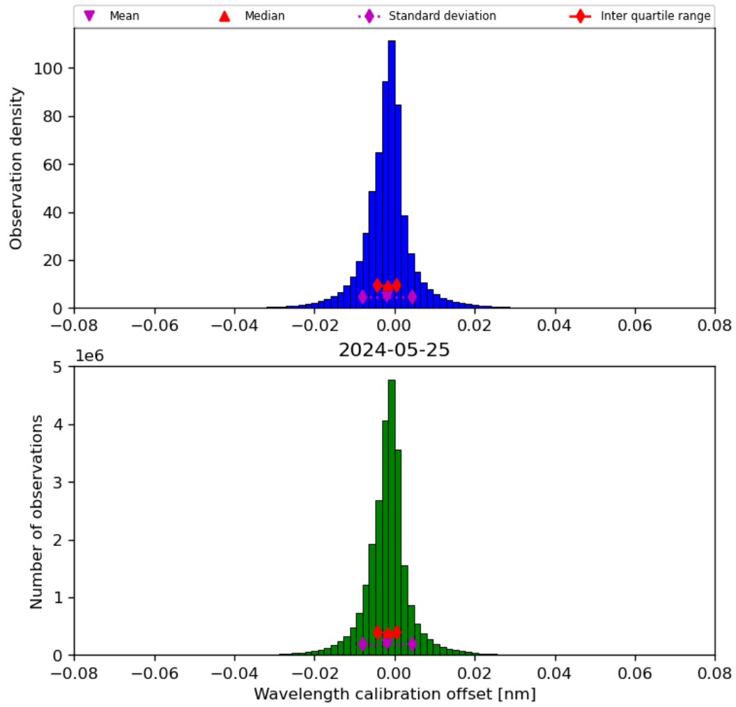
Figure 35: Histogram of “Wavelength calibration offset” for 2024-05-24 to 2024-05-26
