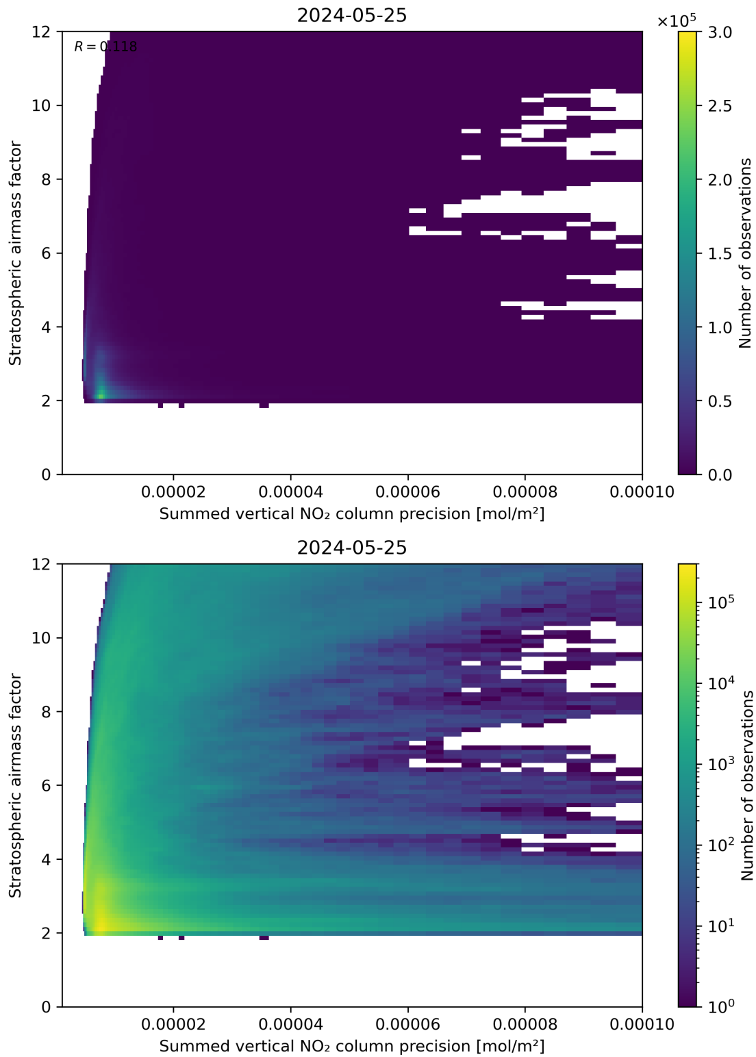
Figure 106: Scatter density plot of “Summed vertical NO 2 column precision” against “Stratospheric airmass factor” for 2024-05-24 to 2024-05-26.
