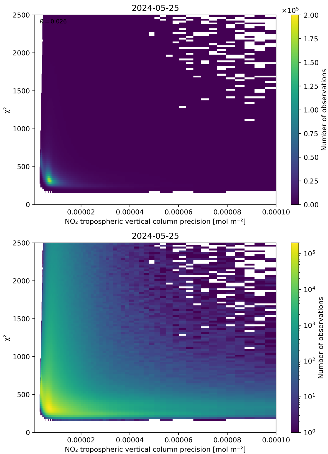
Figure 134: Scatter density plot of “NO 2 tropospheric vertical column precision” against “ \chi^2 ” for 2024-05-24 to 2024-05-26.
