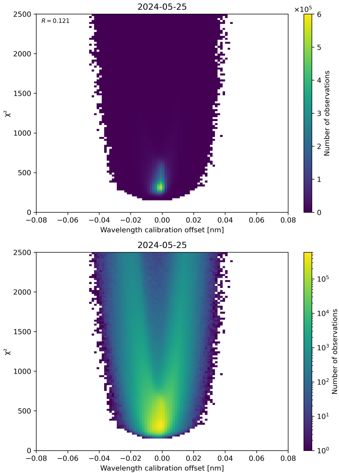
Figure 175: Scatter density plot of “Wavelength calibration offset” against “ \chi^2 ” for 2024-05-24 to 2024-05-26.
