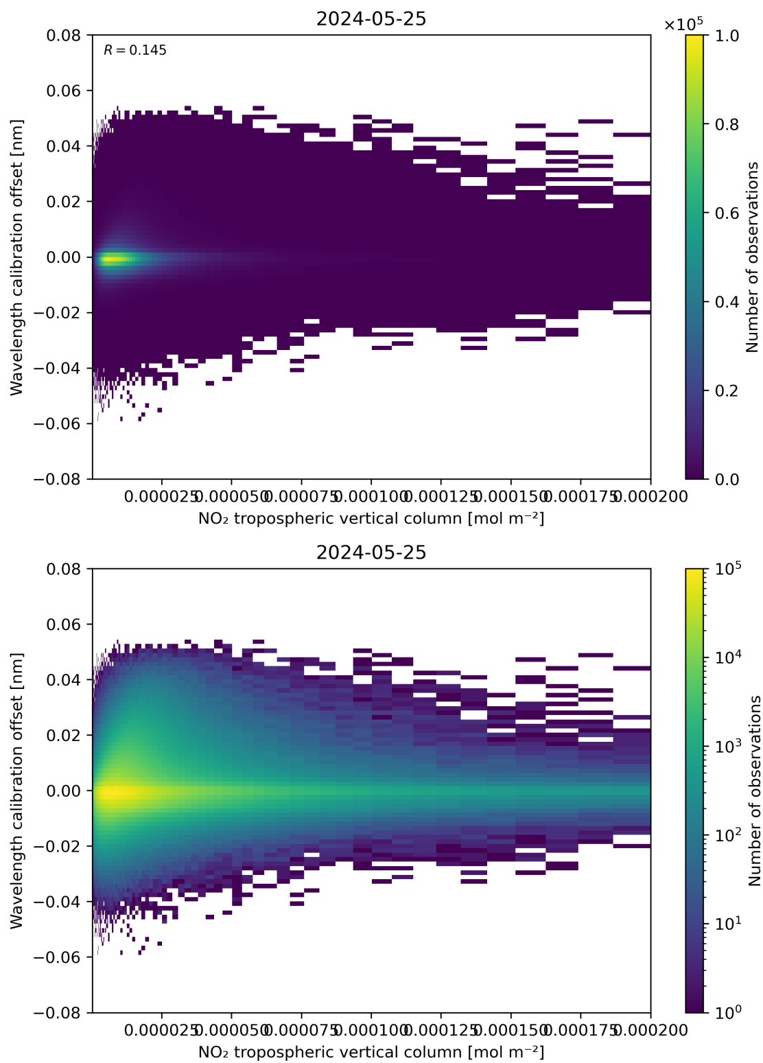
Figure 143: Scatter density plot of “NO 2 tropospheric vertical column” against “Wavelength calibration offset” for 2024-05-24 to 2024-05-26.
