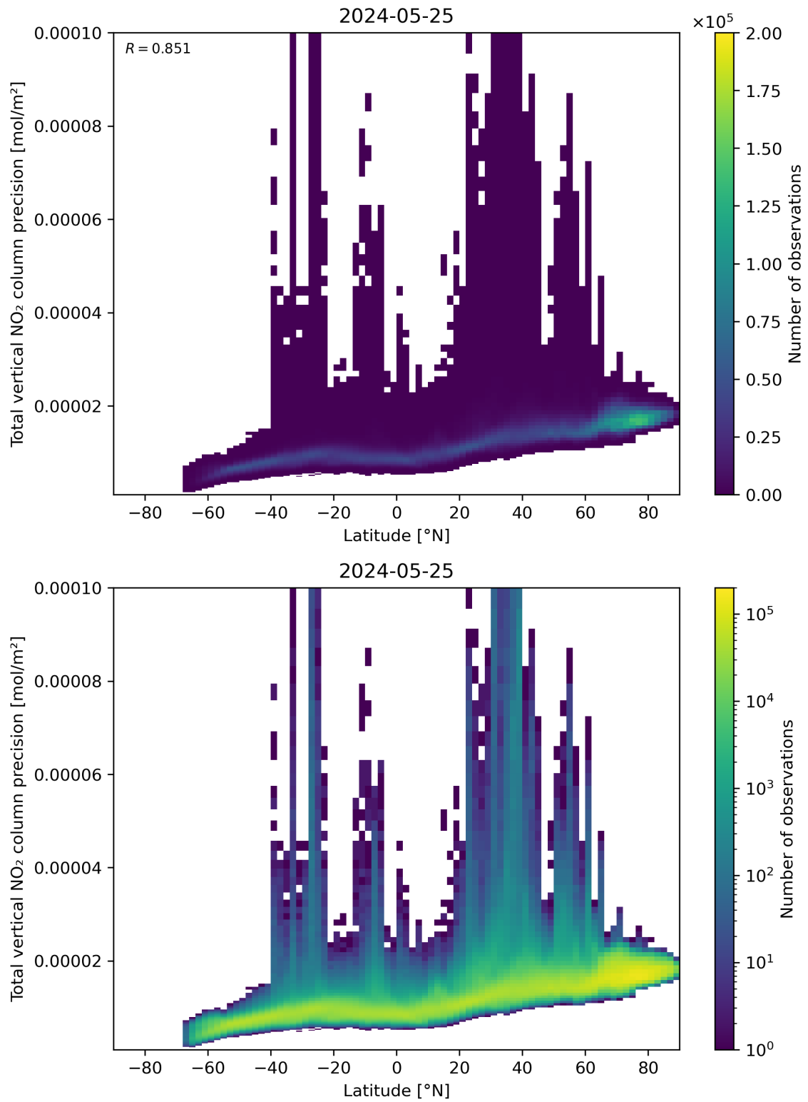
Figure 91: Scatter density plot of “Latitude” against “Total vertical NO 2 column precision” for 2024-05-24 to 2024-05-26.
