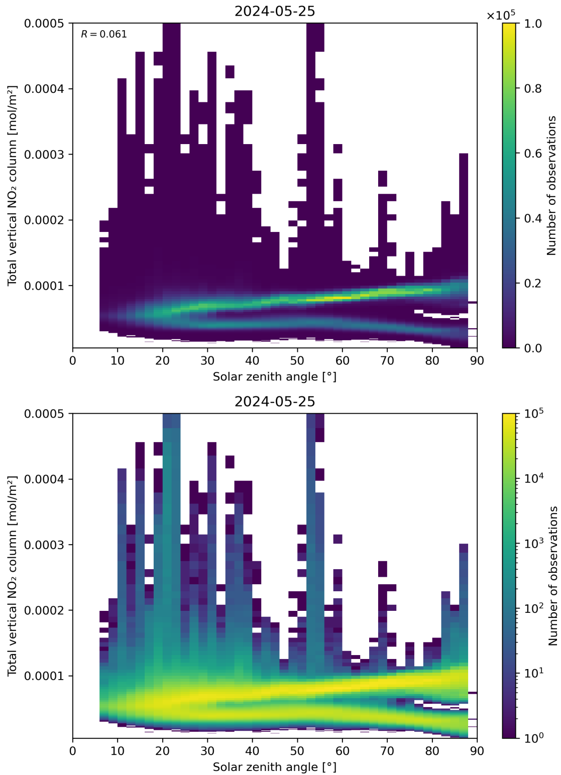
Figure 153: Scatter density plot of “Solar zenith angle” against “Total vertical NO 2 column” for 2024-05-24 to 2024-05-26.
