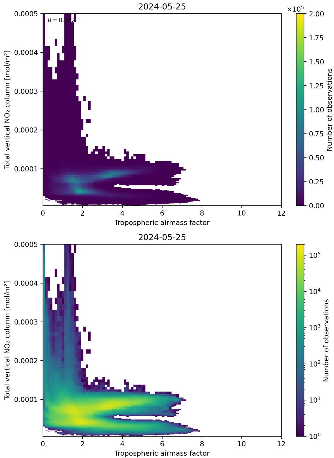
Figure 77: Scatter density plot of “Tropospheric airmass factor” against “Total vertical NO 2 column” for 2024-05-24 to 2024-05-26.
