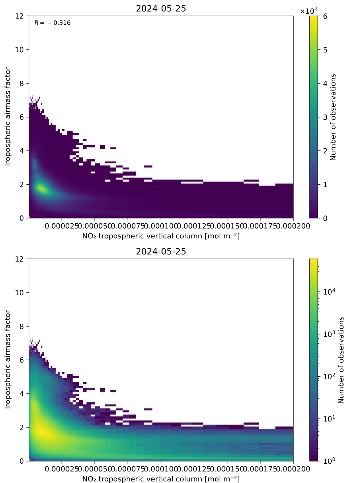
Figure 123: Scatter density plot of “NO 2 tropospheric vertical column” against “Tropospheric air mass factor” for 2024-05-24 to 2024-05-26.
