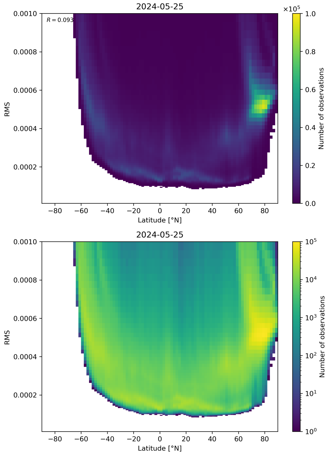
Figure 94: Scatter density plot of “Latitude” against “RMS” for 2024-05-24 to 2024-05-26.
