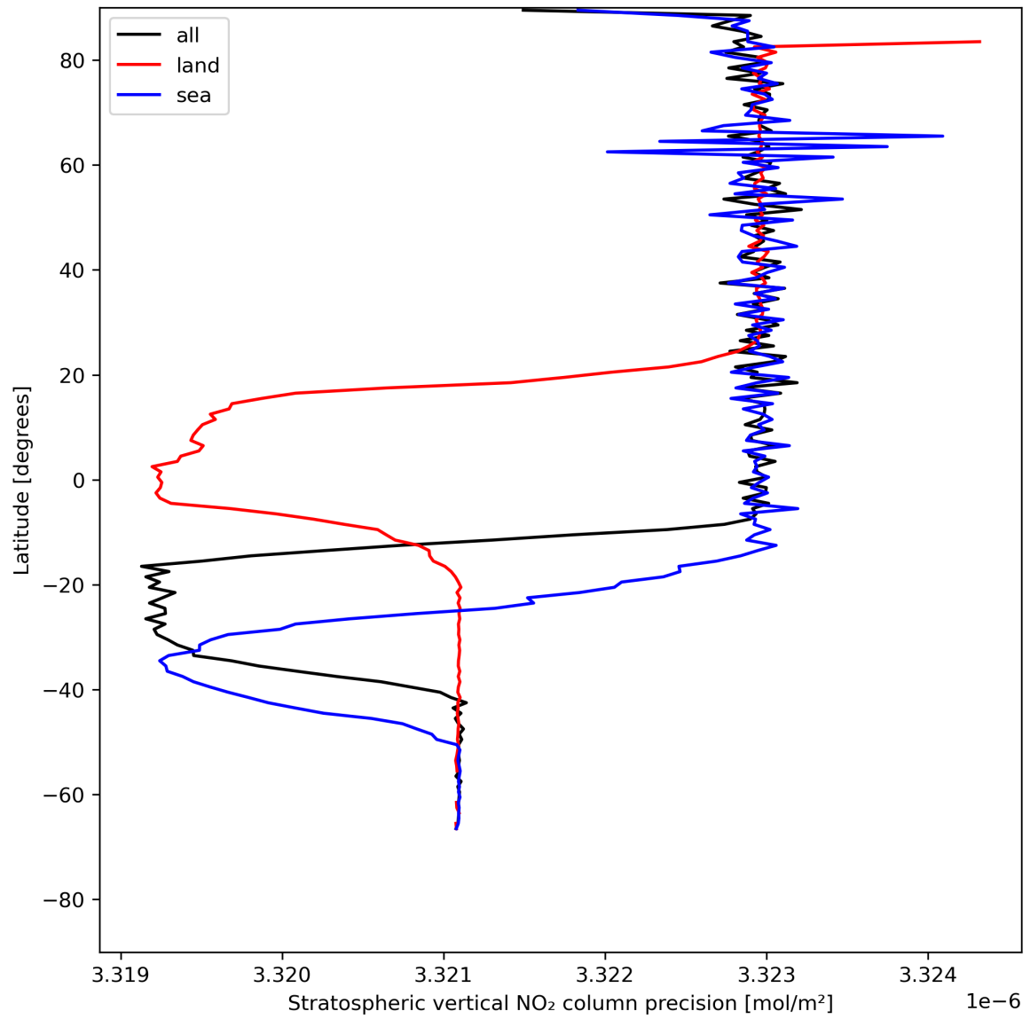
Figure 20: Zonal average of “Stratospheric vertical NO 2 column precision” for 2024-05-24 to 2024-05-26.
