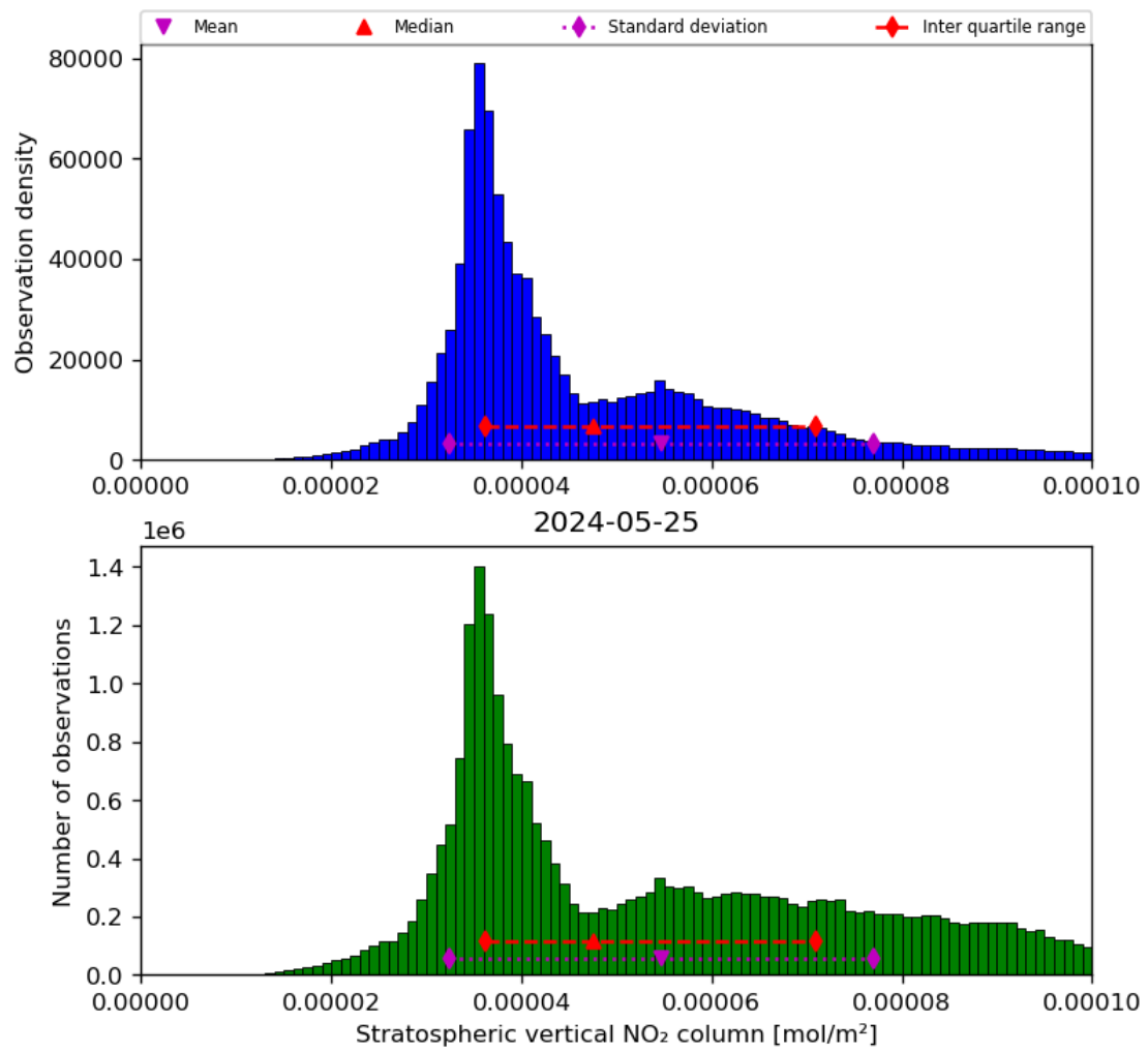
Figure 36: Histogram of “Stratospheric vertical NO 2 column” for 2024-05-24 to 2024-05-26
