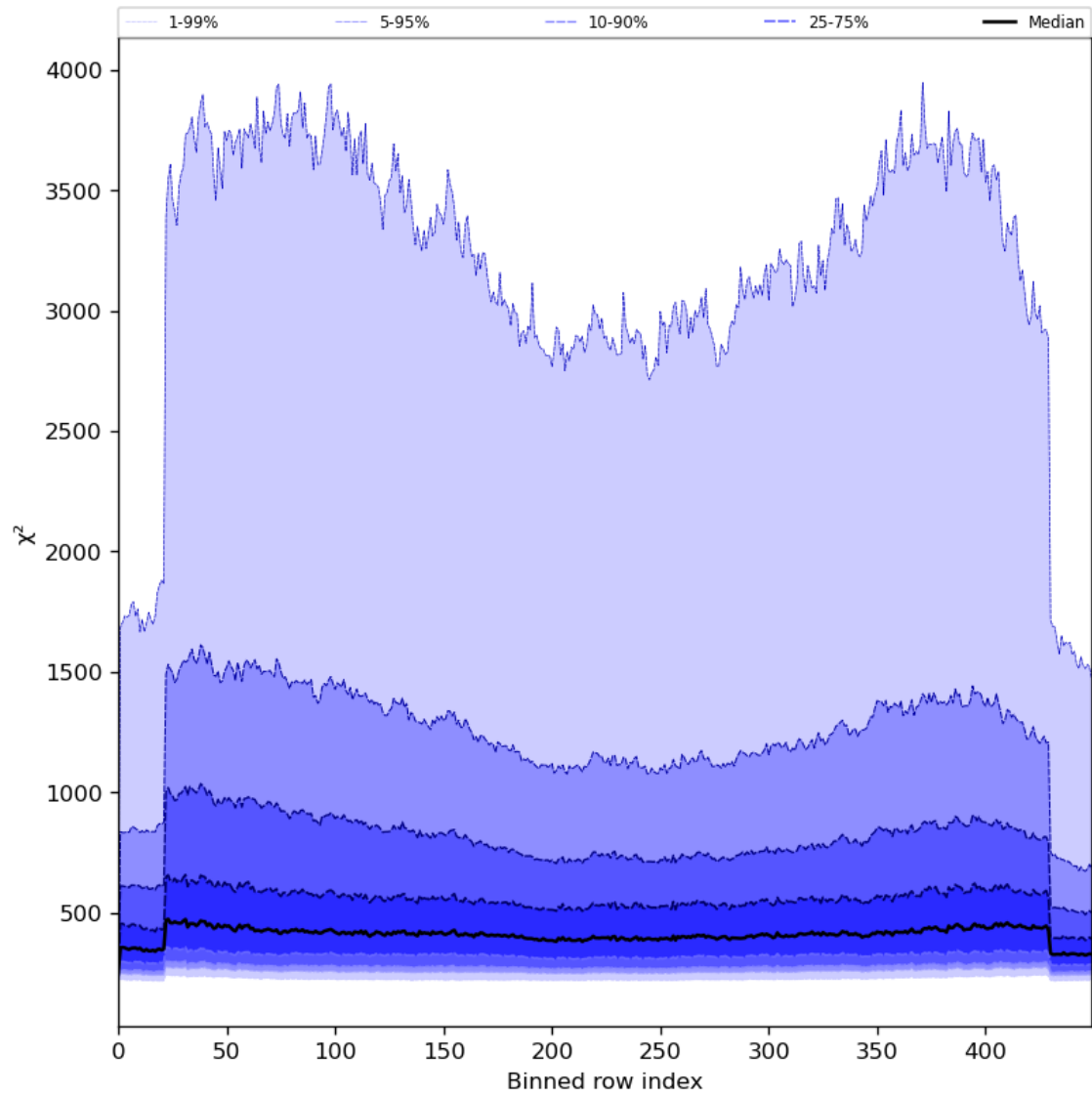
Figure 59: Along track statistics of “ \chi^2 ” for 2024-05-24 to 2024-05-26
