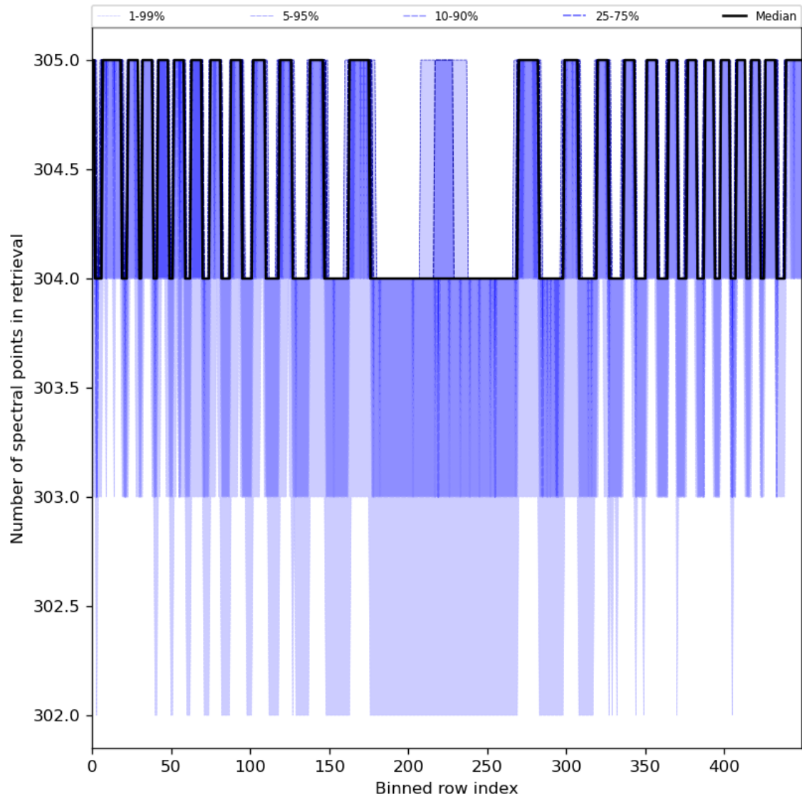
Figure 50: Along track statistics of “Number of spectral points in retrieval” for 2024-05-24 to 2024-05-26
