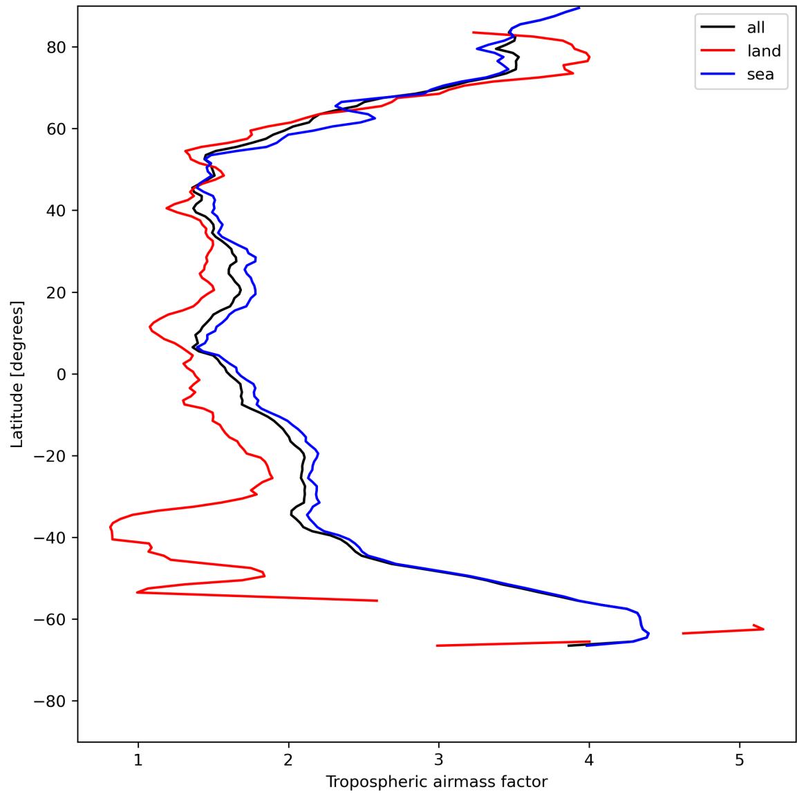
Figure 14: Zonal average of “Tropospheric air mass factor” for 2024-05-24 to 2024-05-26.
