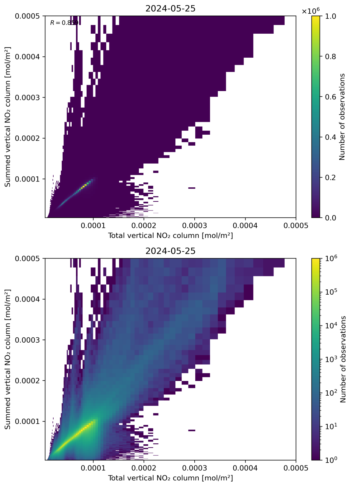
Figure 112: Scatter density plot of “Total vertical NO 2 column” against “Summed vertical NO 2 column” for 2024-05-24 to 2024-05-26.
