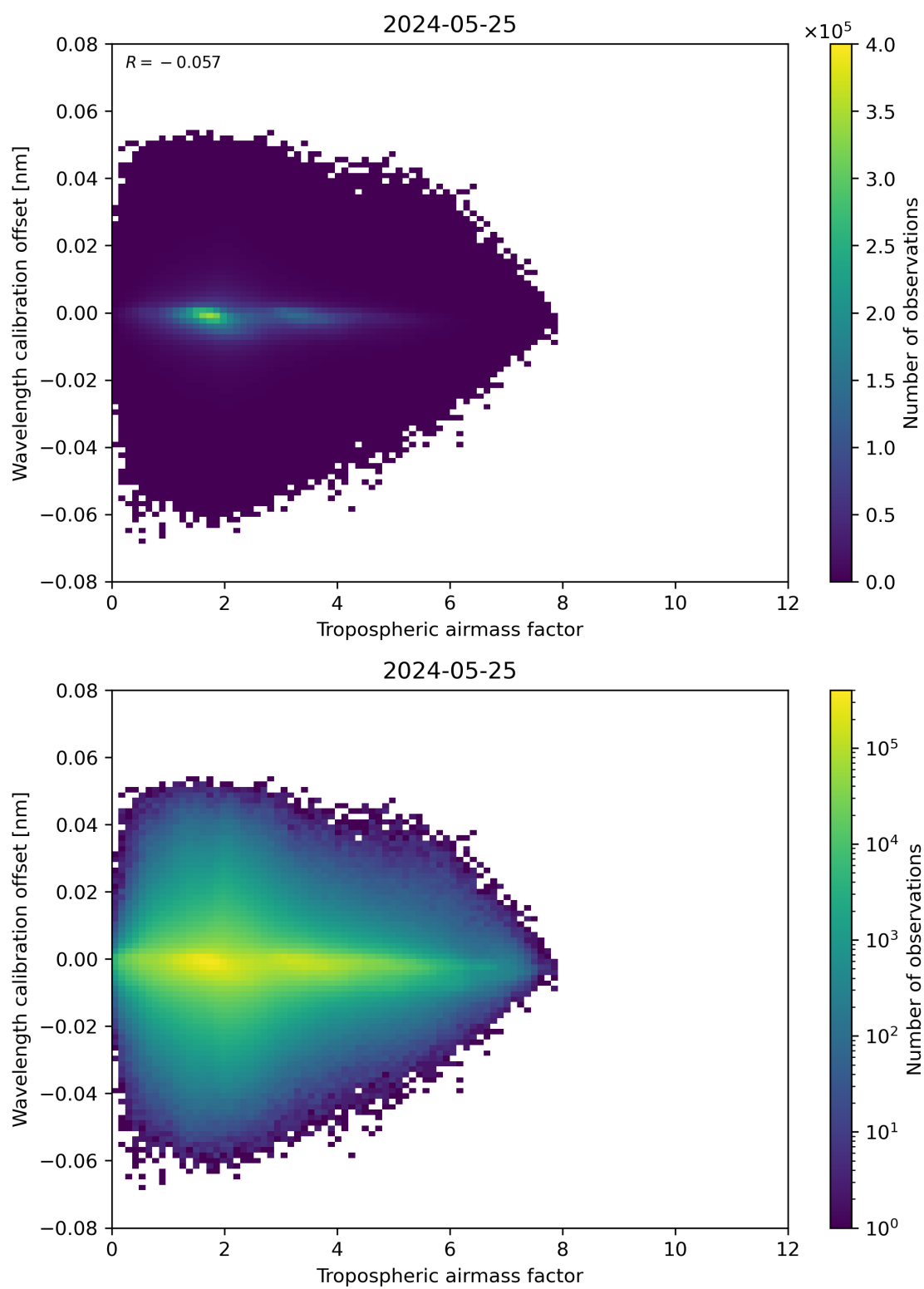
Figure 80: Scatter density plot of “Tropospheric air mass factor” against “Wavelength calibration offset” for 2024-05-24 to 2024-05-26.
