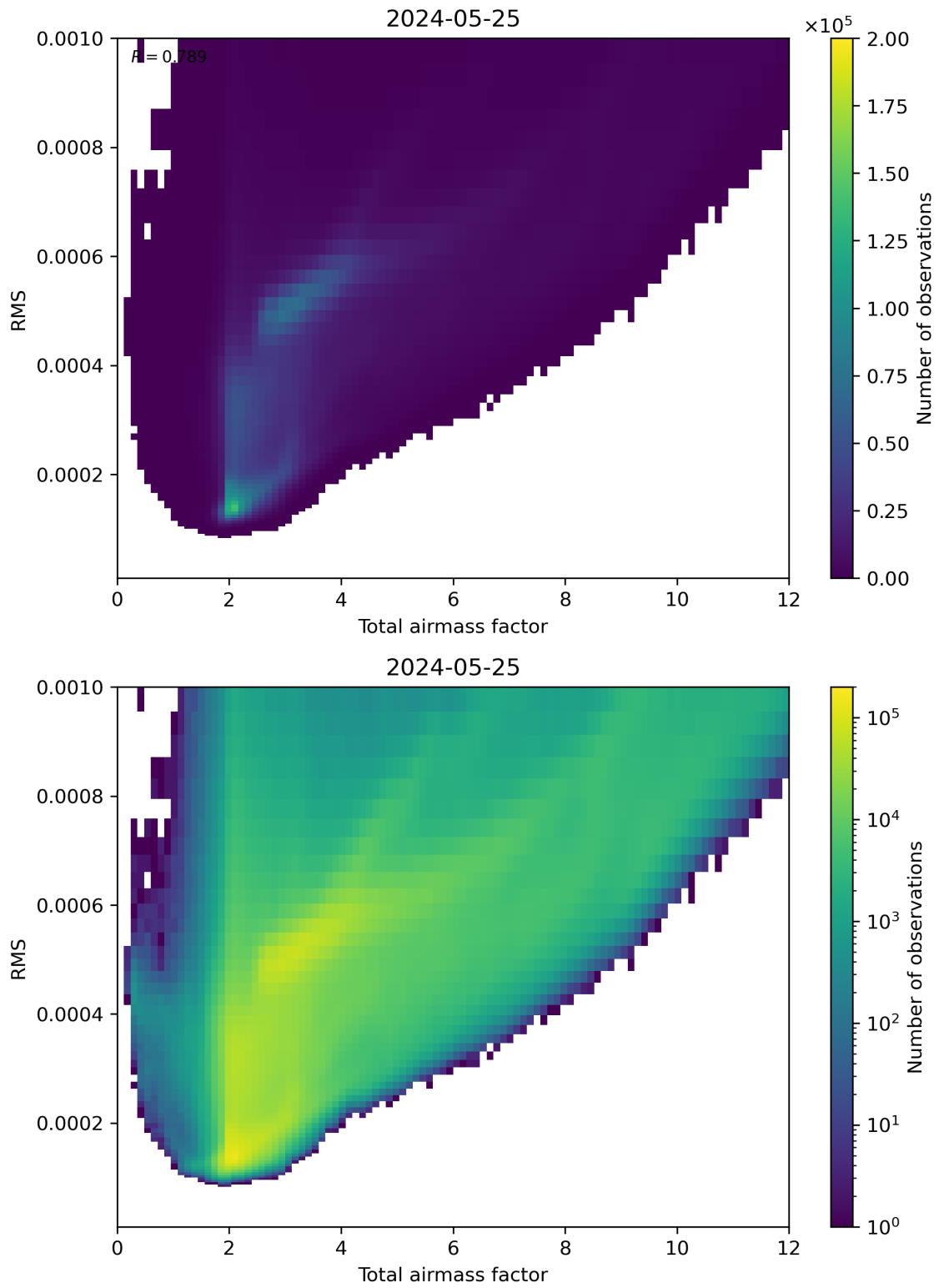
Figure 69: Scatter density plot of “Total airmass factor” against “RMS” for 2024-05-24 to 2024-05-26.
