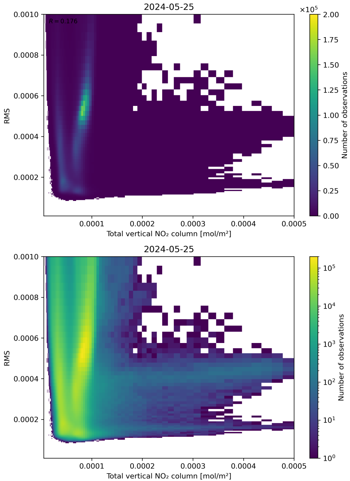
Figure 120: Scatter density plot of “Total vertical NO 2 column” against “RMS” for 2024-05-24 to 2024-05-26.
