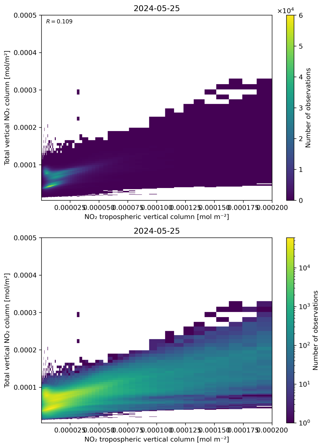
Figure 128: Scatter density plot of “NO 2 tropospheric vertical column” against “Total vertical NO 2 column” for 2024-05-24 to 2024-05-26.
