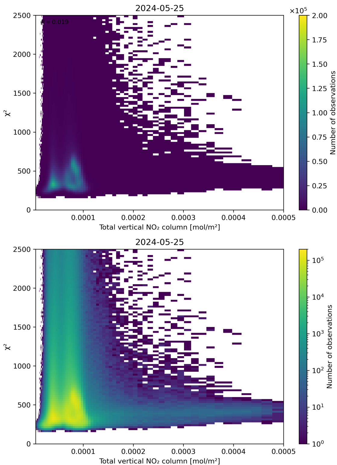
Figure 111: Scatter density plot of “Total vertical NO 2 column” against “ \chi^2 ” for 2024-05-24 to 2024-05-26.
