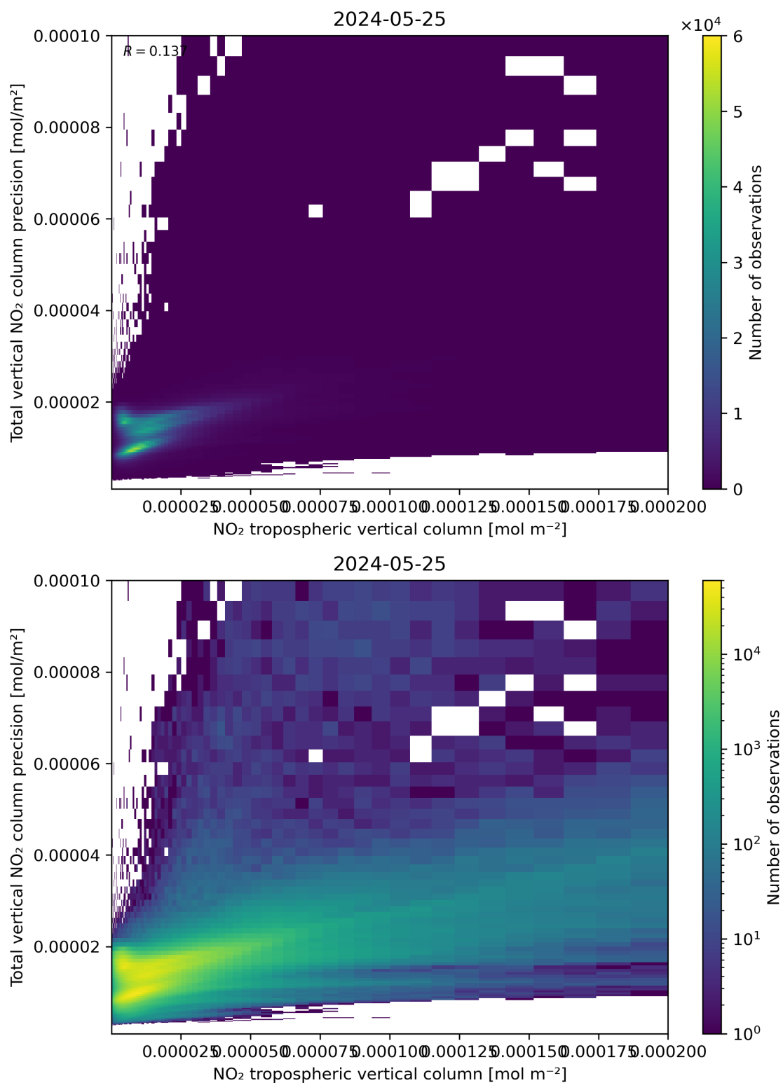
Figure 129: Scatter density plot of “NO 2 tropospheric vertical column” against “Total vertical NO 2 column precision” for 2024-05-24 to 2024-05-26.
