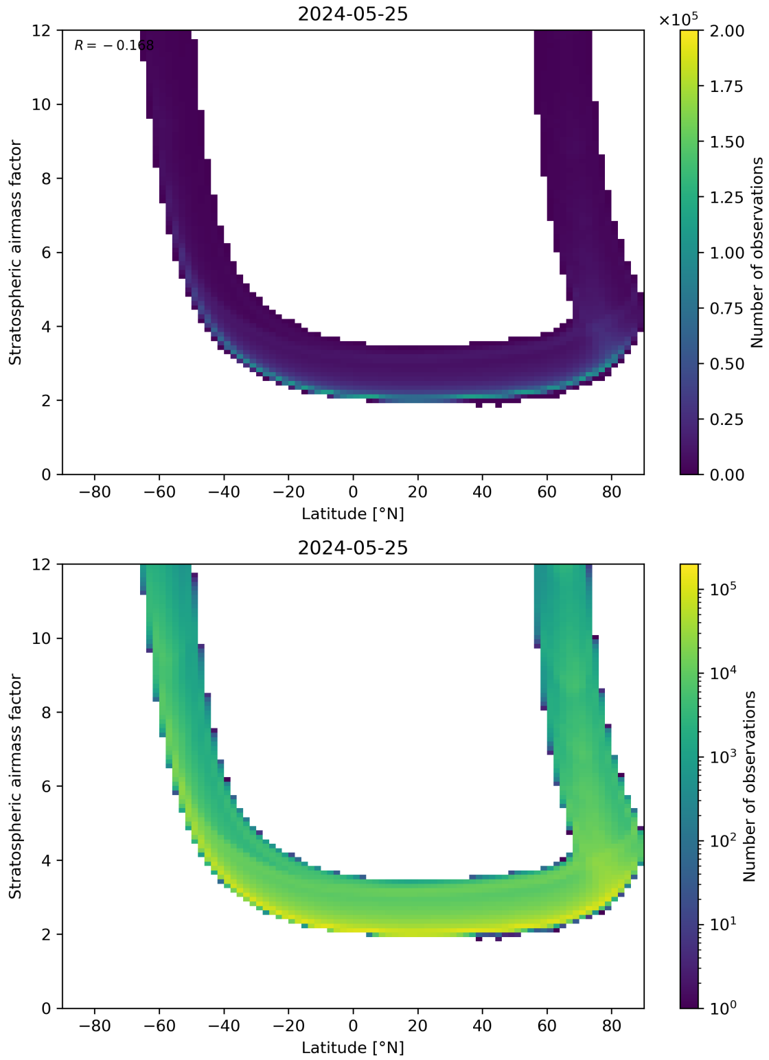
Figure 83: Scatter density plot of “Latitude” against “Stratospheric air mass factor” for 2024-05-24 to 2024-05-26.
