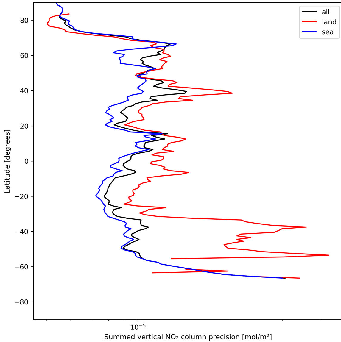
Figure 24: Zonal average of “Summed vertical NO 2 column precision” for 2024-05-24 to 2024-05-26.
