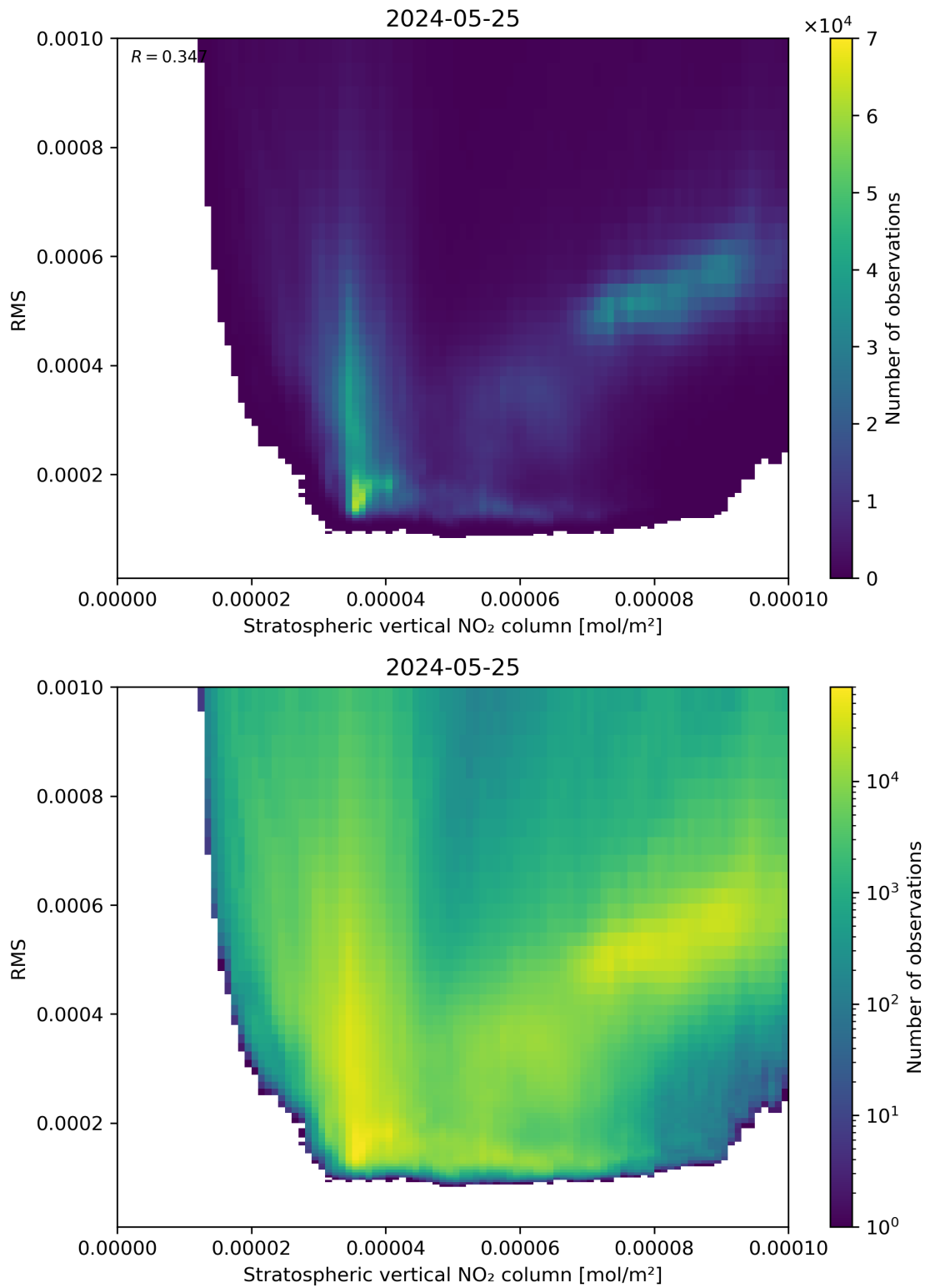
Figure 102: Scatter density plot of “Stratospheric vertical NO 2 column” against “RMS” for 2024-05-24 to 2024-05-26.
