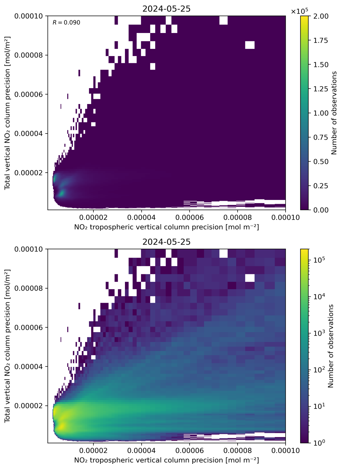
Figure 139: Scatter density plot of “NO 2 tropospheric vertical column precision” against “Total vertical NO 2 column precision” for 2024-05-24 to 2024-05-26.
