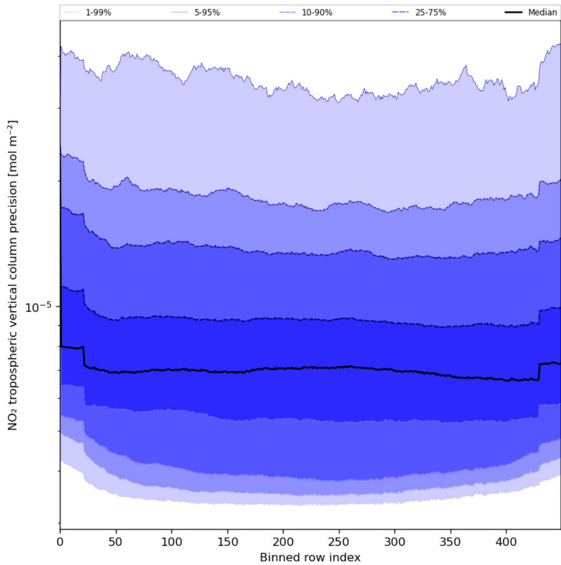
Figure 47: Along track statistics of “NO 2 tropospheric vertical column precision” for 2024-05-24 to 2024-05-26
