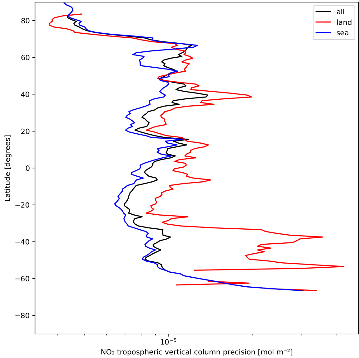
Figure 13: Zonal average of “NO 2 tropospheric vertical column precision” for 2024-05-24 to 2024-05-26.
