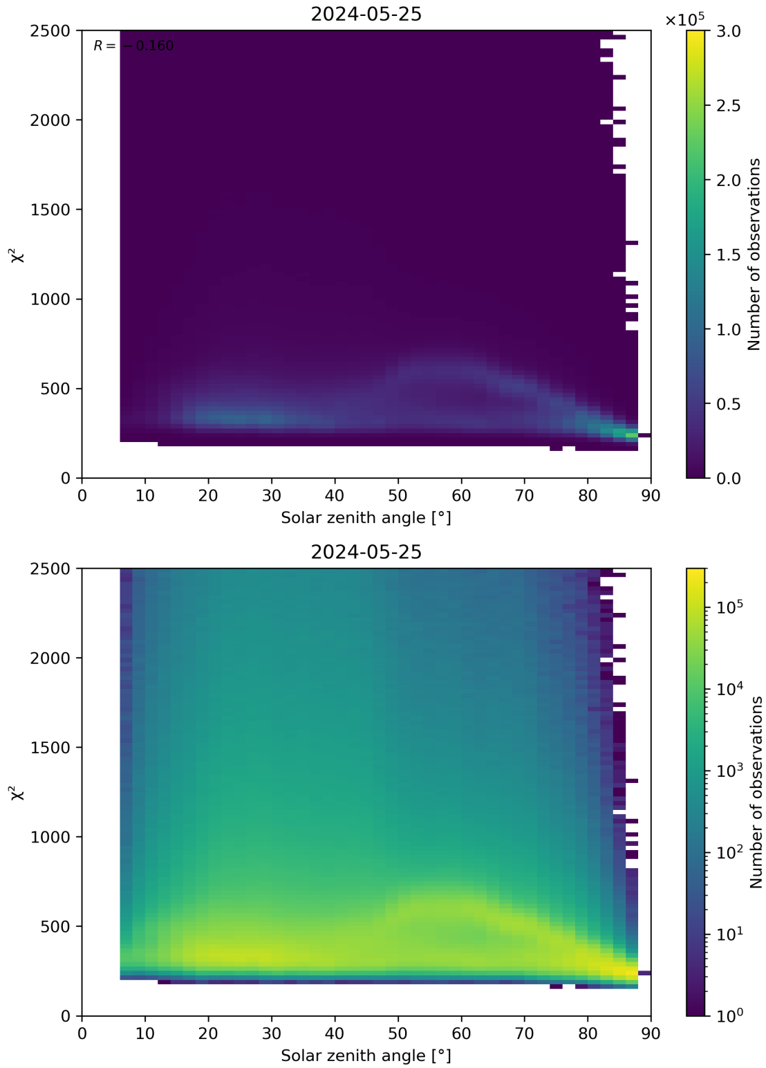
Figure 148: Scatter density plot of “Solar zenith angle” against “ \chi^2 ” for 2024-05-24 to 2024-05-26.
