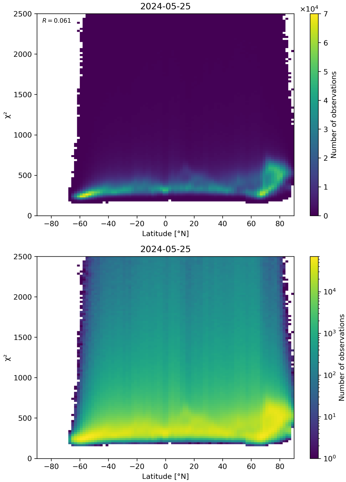
Figure 86: Scatter density plot of “Latitude” against “ \chi^2 ” for 2024-05-24 to 2024-05-26.
