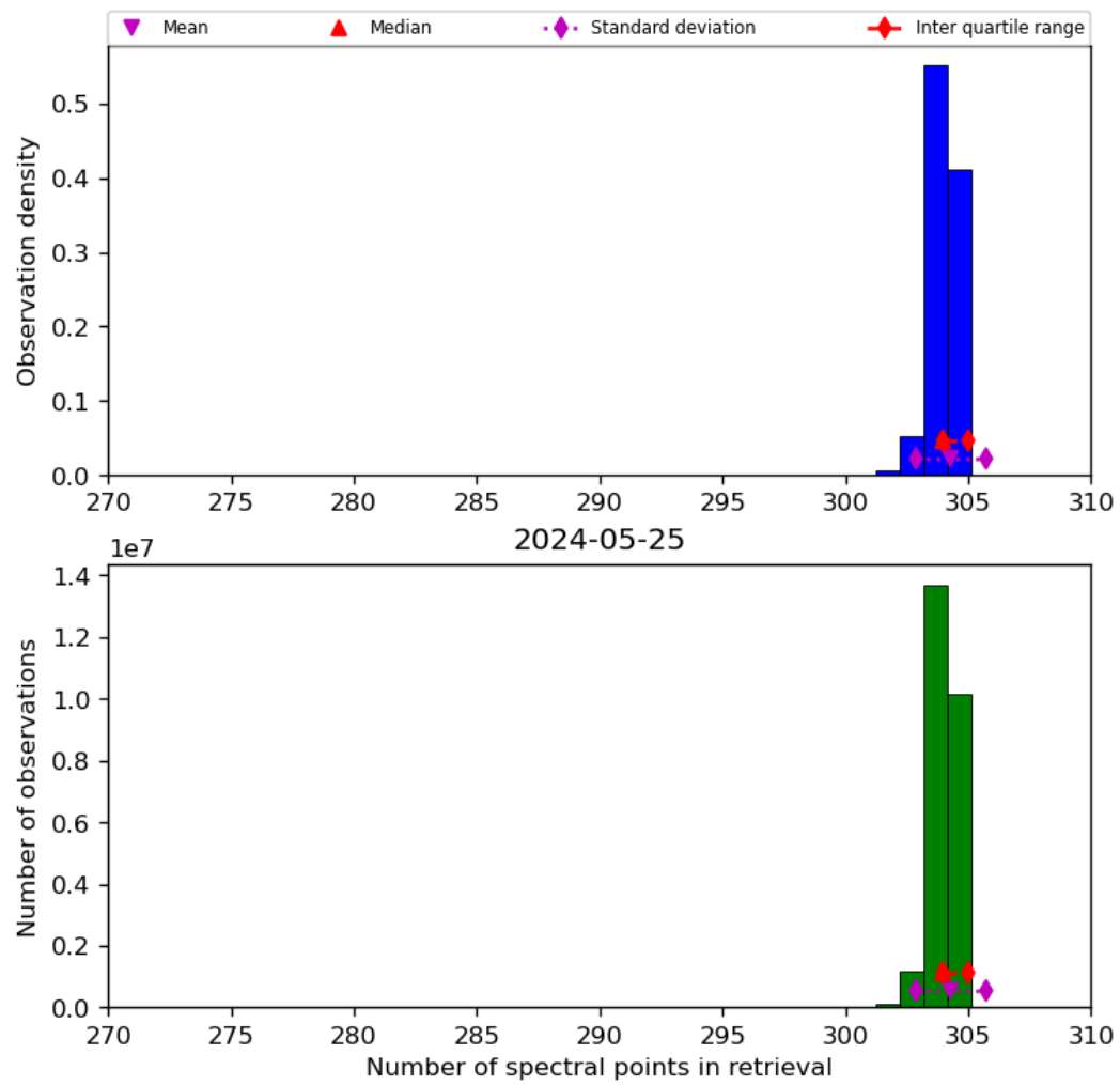
Figure 33: Histogram of “Number of spectral points in retrieval” for 2024-05-24 to 2024-05-26
