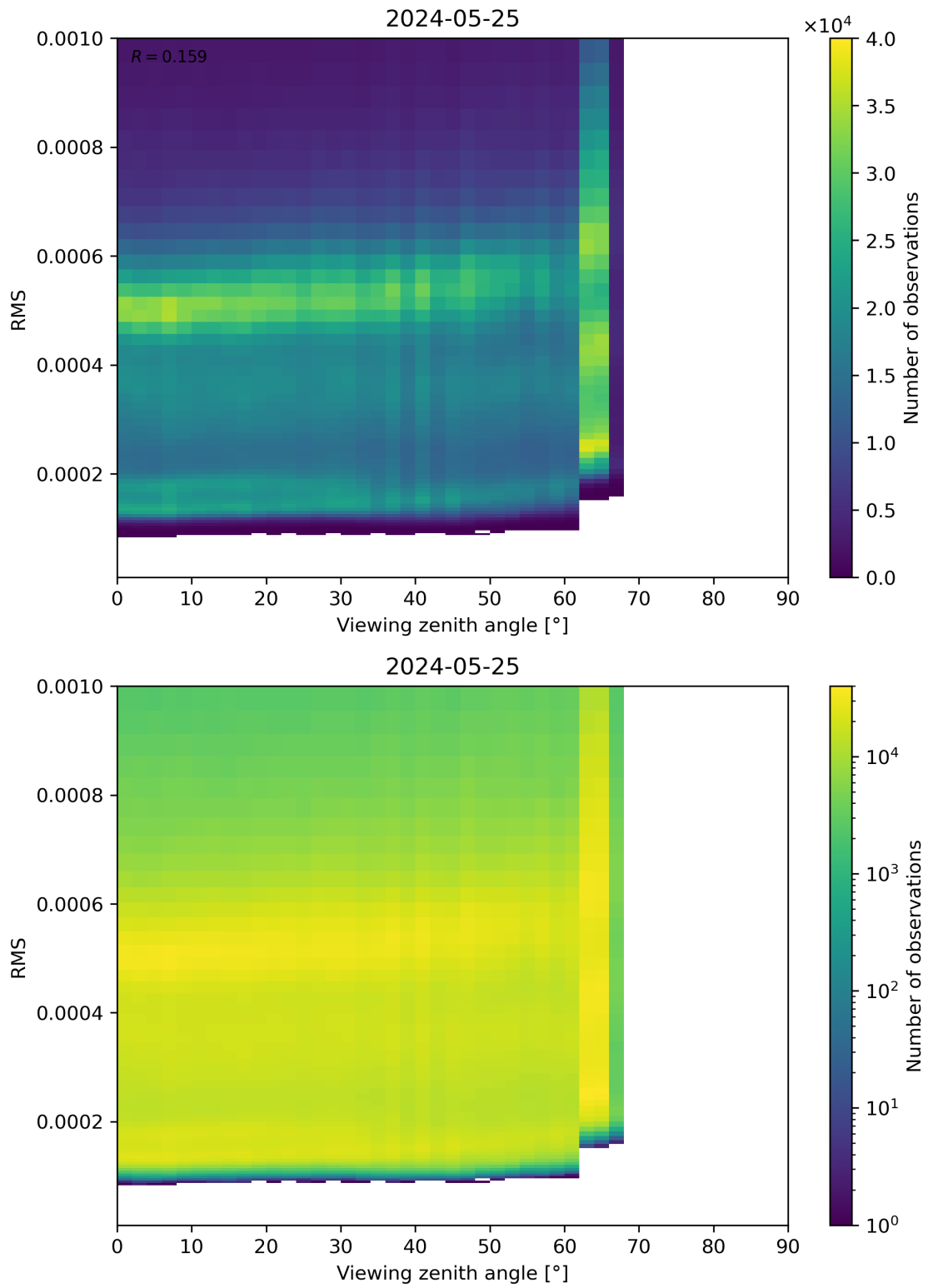
Figure 171: Scatter density plot of “Viewing zenith angle” against “RMS” for 2024-05-24 to 2024-05-26.
