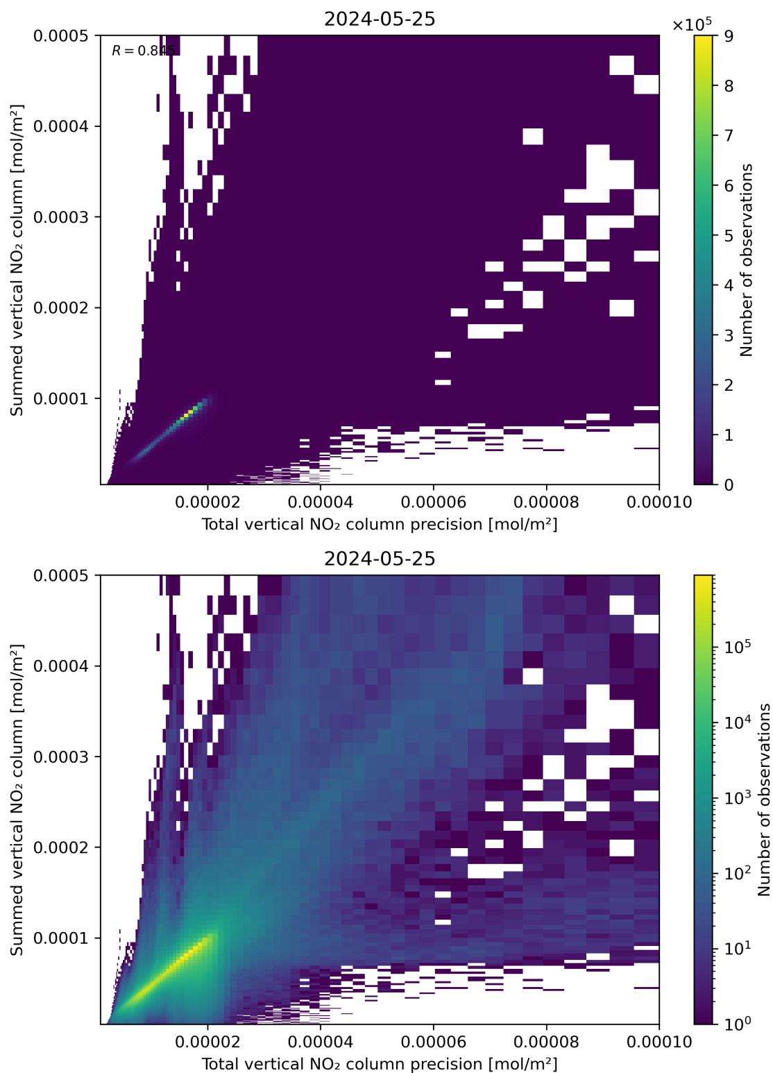
Figure 117: Scatter density plot of “Total vertical NO 2 column precision” against “Summed vertical NO 2 column” for 2024-05-24 to 2024-05-26.
