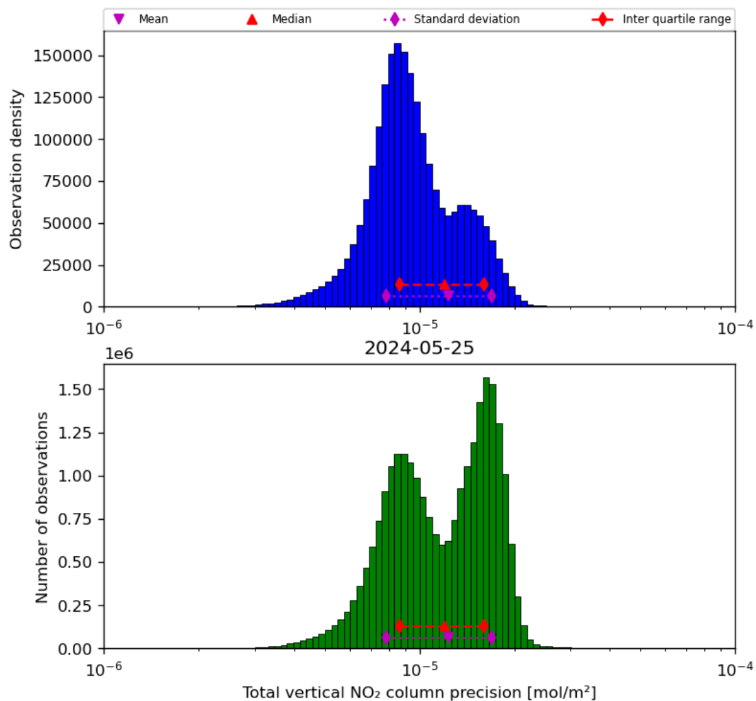
Figure 39: Histogram of “Total vertical NO 2 column precision” for 2024-05-24 to 2024-05-26
