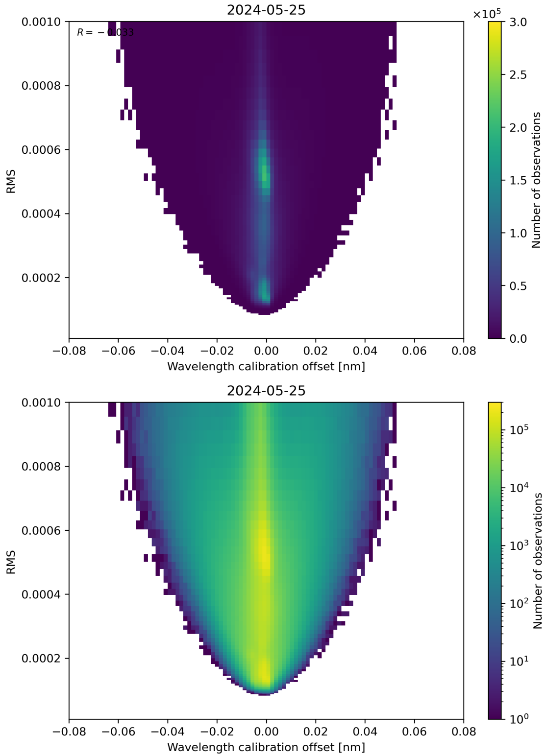
Figure 181: Scatter density plot of “Wavelength calibration offset” against “RMS” for 2024-05-24 to 2024-05-26.
