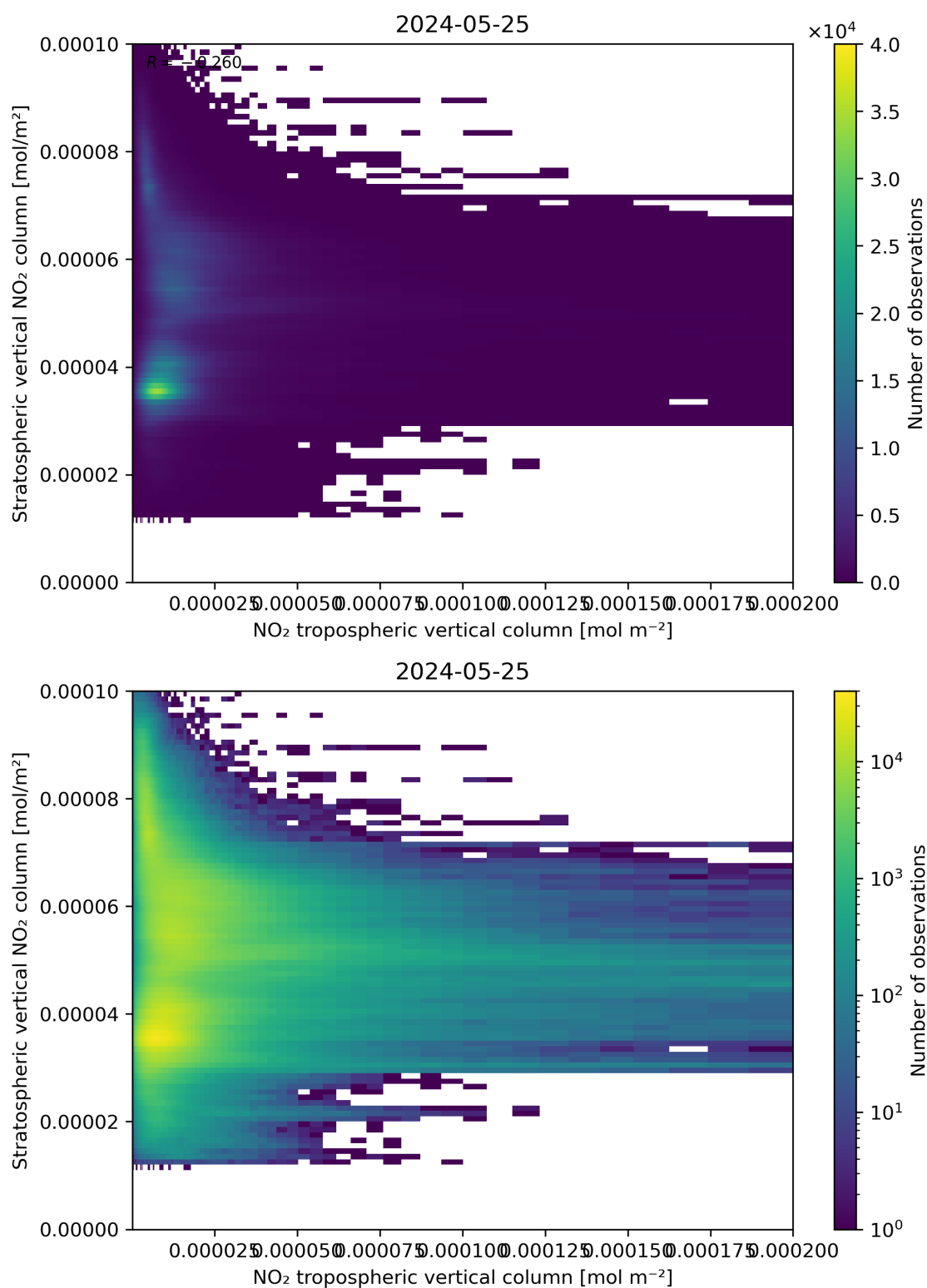
Figure 125: Scatter density plot of “NO 2 tropospheric vertical column” against “Stratospheric vertical NO 2 column” for 2024-05-24 to 2024-05-26.
