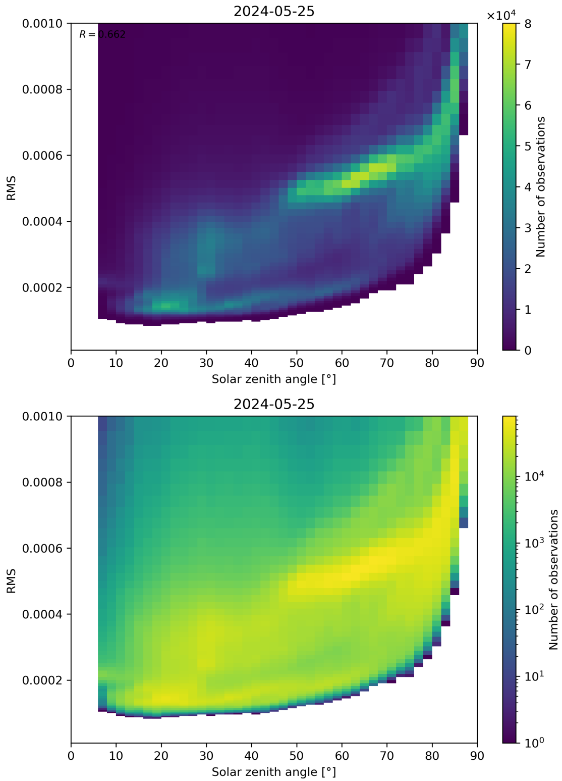
Figure 157: Scatter density plot of “Solar zenith angle” against “RMS” for 2024-05-24 to 2024-05-26.
