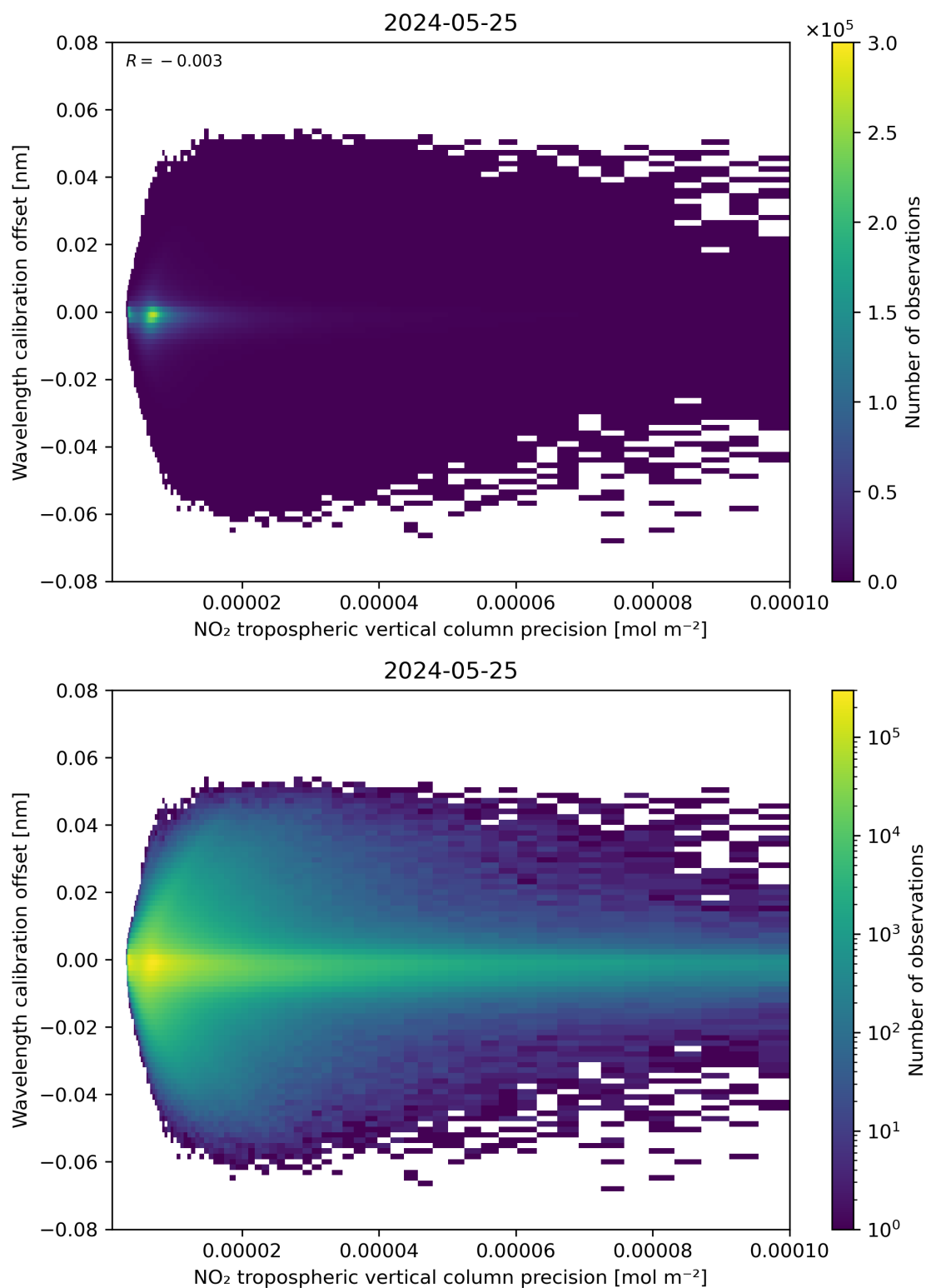
Figure 141: Scatter density plot of “NO 2 tropospheric vertical column precision” against “Wavelength calibration offset” for 2024-05-24 to 2024-05-26.
