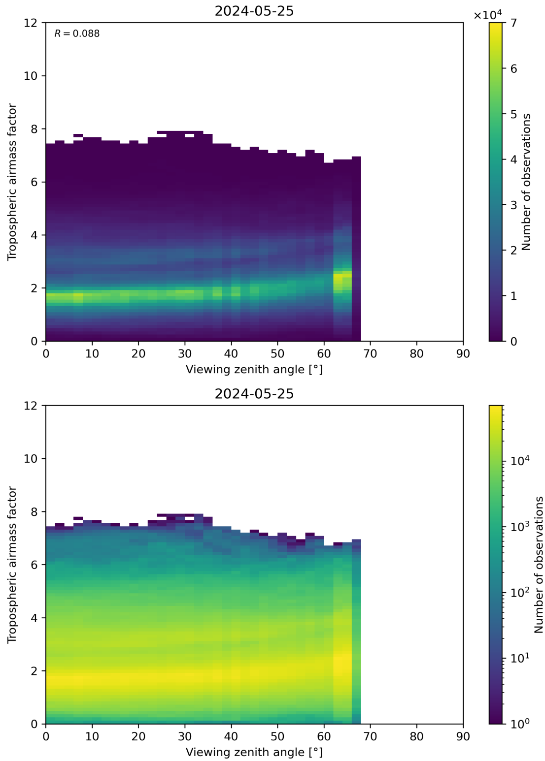
Figure 161: Scatter density plot of “Viewing zenith angle” against “Tropospheric airmass factor” for 2024-05-24 to 2024-05-26.
