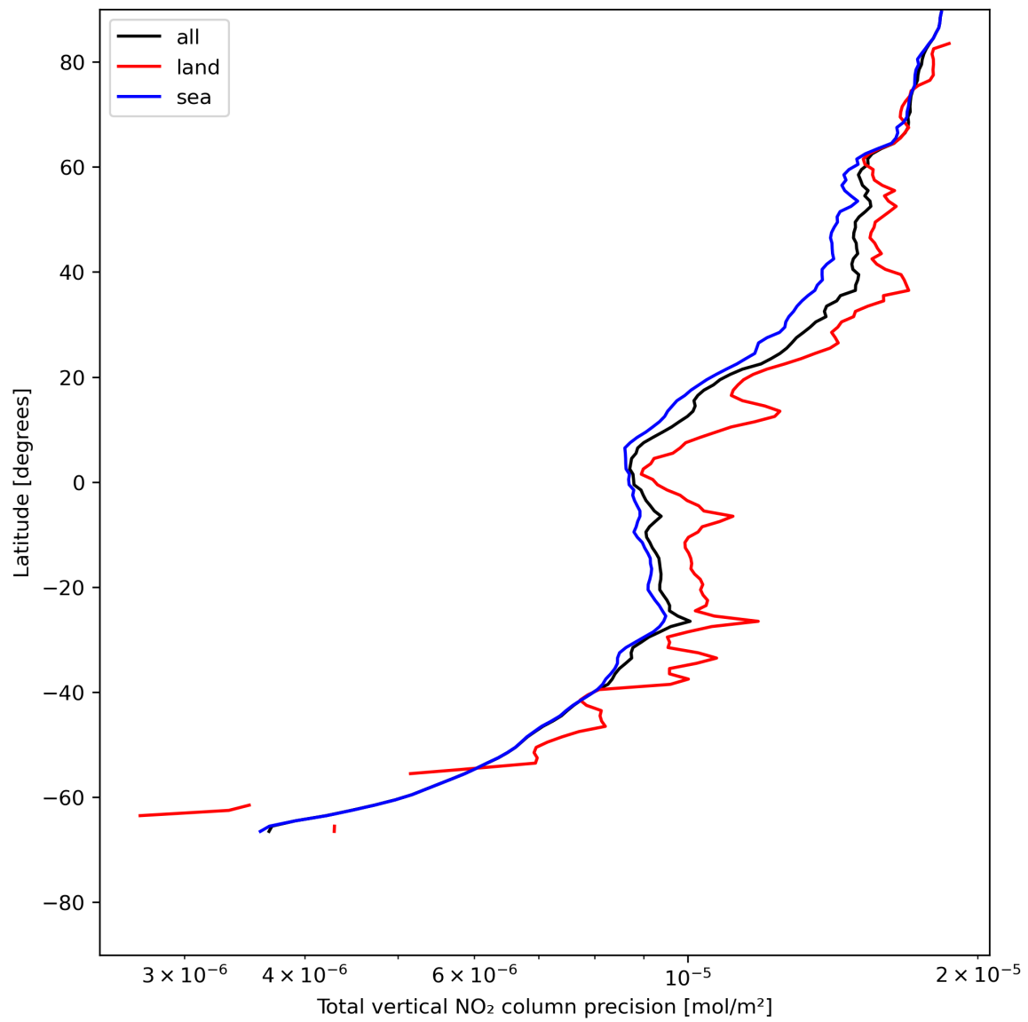
Figure 22: Zonal average of “Total vertical NO 2 column precision” for 2024-05-24 to 2024-05-26.
