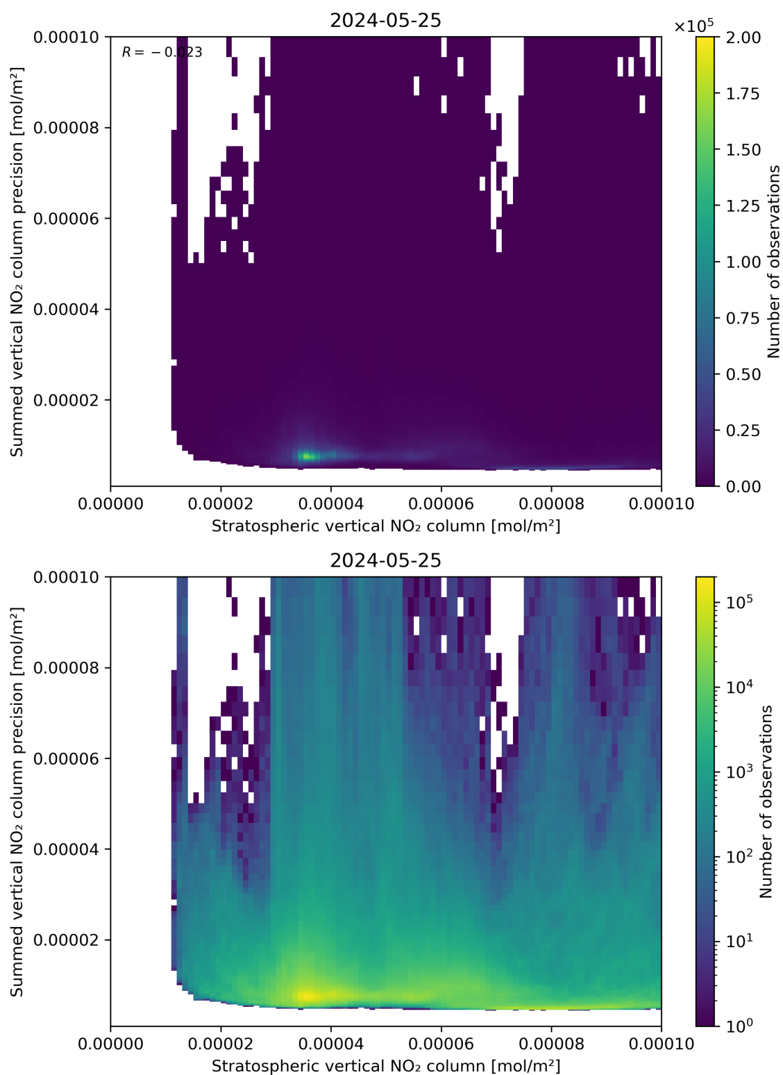
Figure 99: Scatter density plot of “Stratospheric vertical NO 2 column” against “Summed vertical NO 2 column precision” for 2024-05-24 to 2024-05-26.
