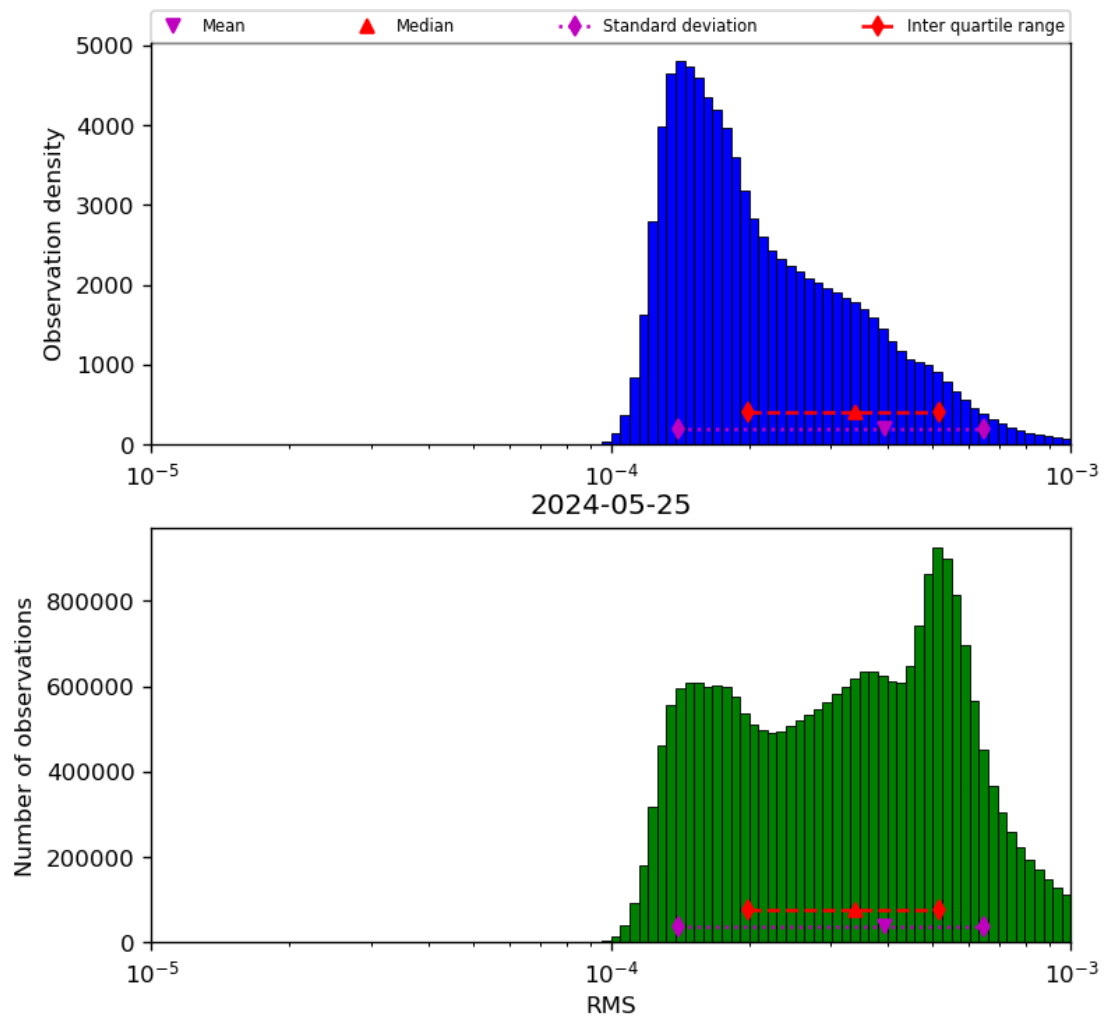
Figure 43: Histogram of “RMS” for 2024-05-24 to 2024-05-26
