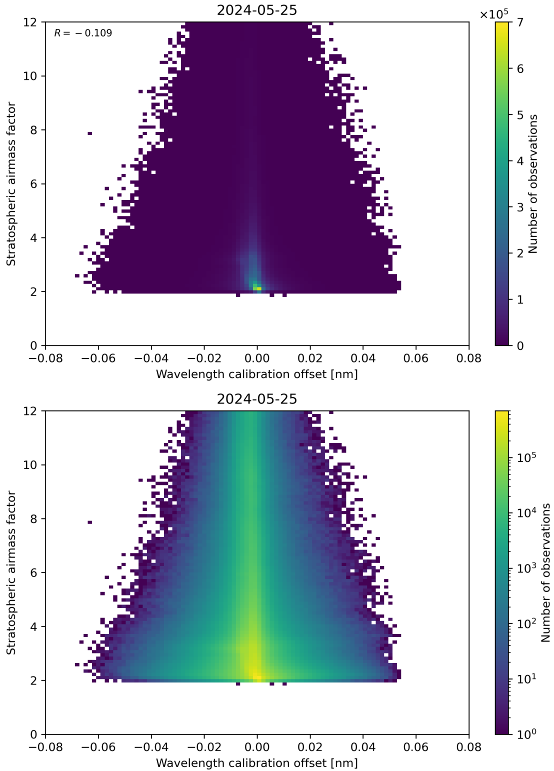
Figure 174: Scatter density plot of “Wavelength calibration offset” against “Stratospheric airmass factor” for 2024-05-24 to 2024-05-26.
