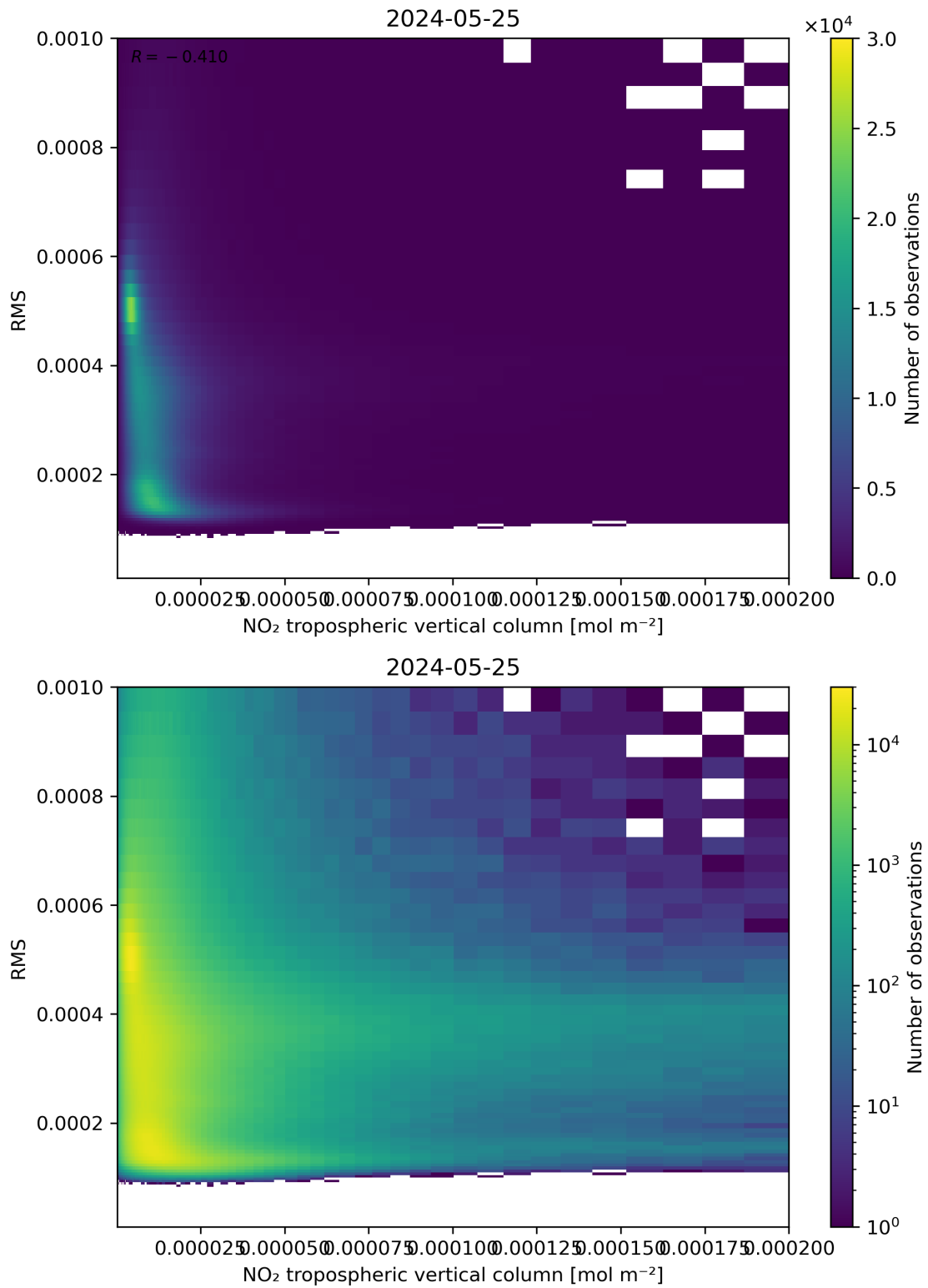
Figure 142: Scatter density plot of “NO 2 tropospheric vertical column” against “RMS” for 2024-05-24 to 2024-05-26.
