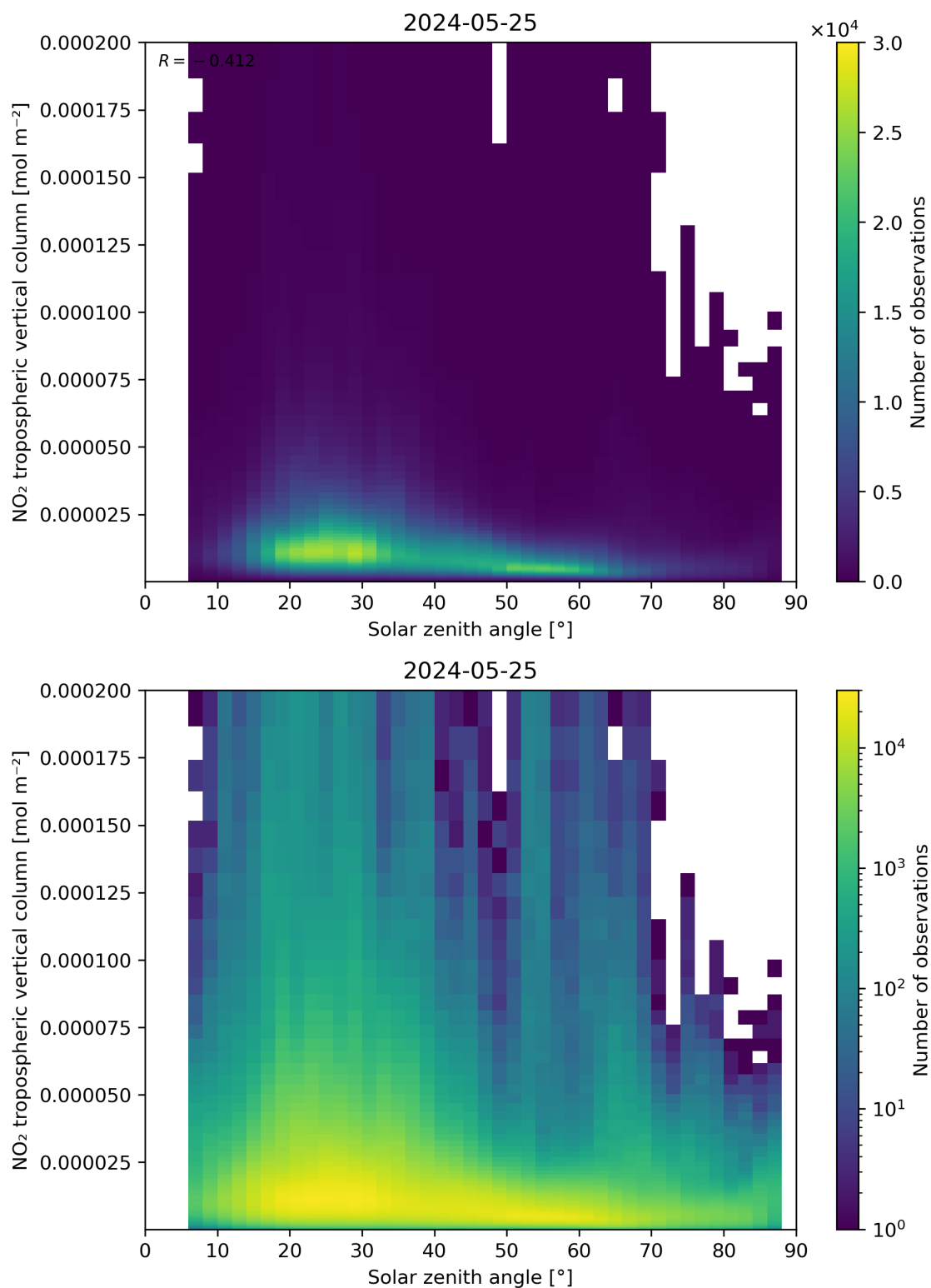
Figure 155: Scatter density plot of “Solar zenith angle” against “NO 2 tropospheric vertical column” for 2024-05-24 to 2024-05-26.
