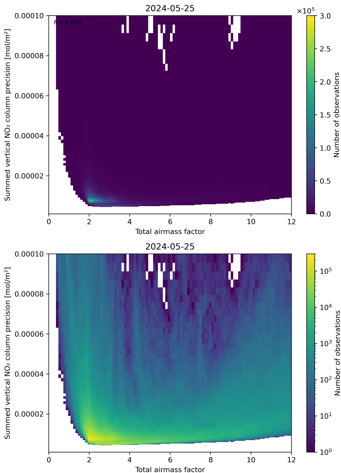
Figure 66: Scatter density plot of “Total airmass factor” against “Summed vertical NO 2 column precision” for 2024-05-24 to 2024-05-26.
