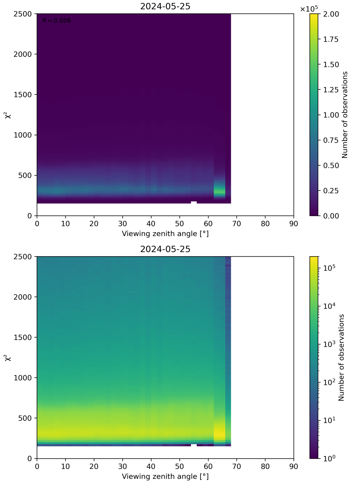
Figure 162: Scatter density plot of “Viewing zenith angle” against “ \chi^2 ” for 2024-05-24 to 2024-05-26.
