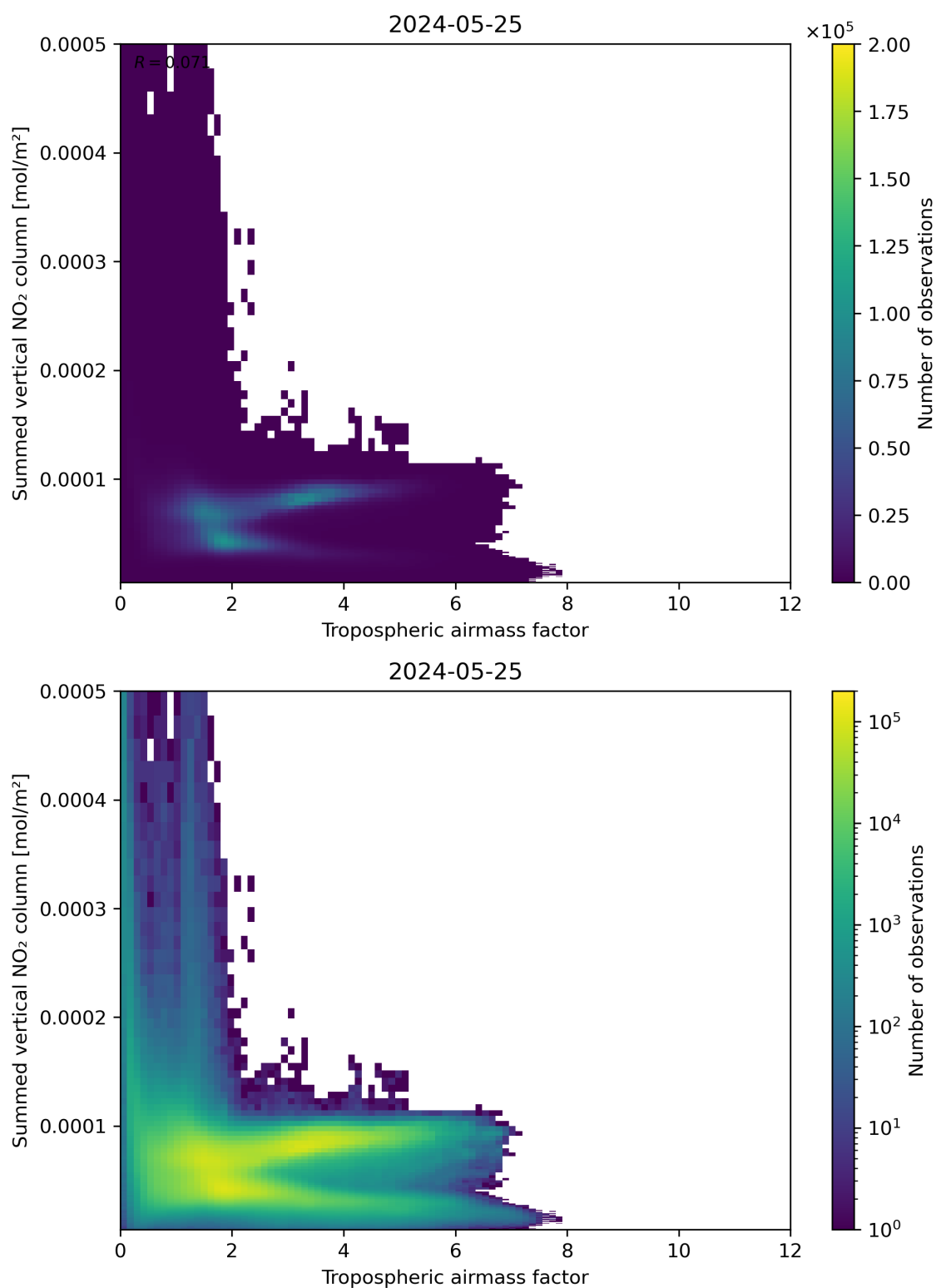
Figure 75: Scatter density plot of “Tropospheric air mass factor” against “Summed vertical NO 2 column” for 2024-05-24 to 2024-05-26.
