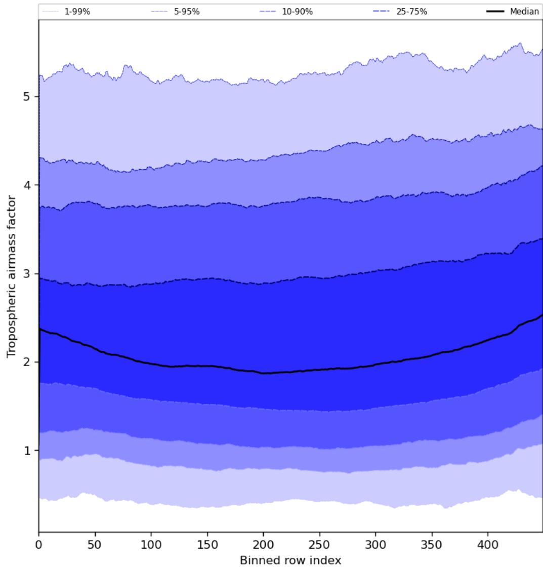
Figure 48: Along track statistics of “Tropospheric airmass factor” for 2024-05-24 to 2024-05-26
