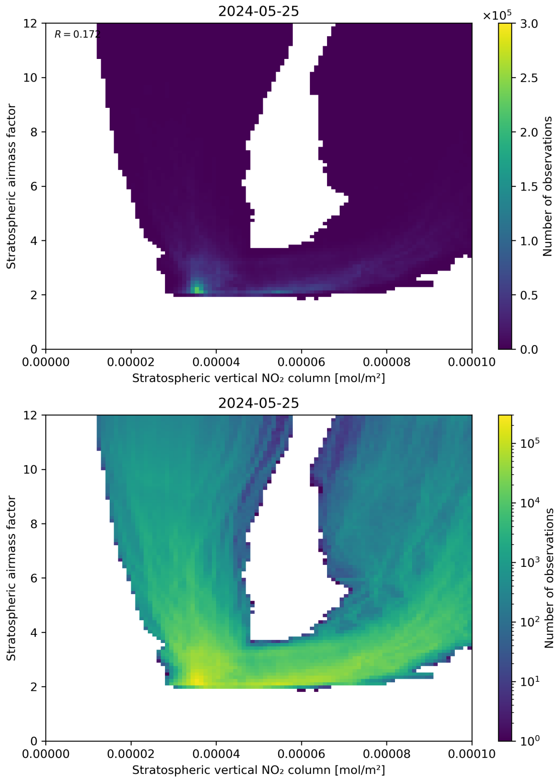
Figure 96: Scatter density plot of “Stratospheric vertical NO 2 column” against “Stratospheric airmass factor” for 2024-05-24 to 2024-05-26.
