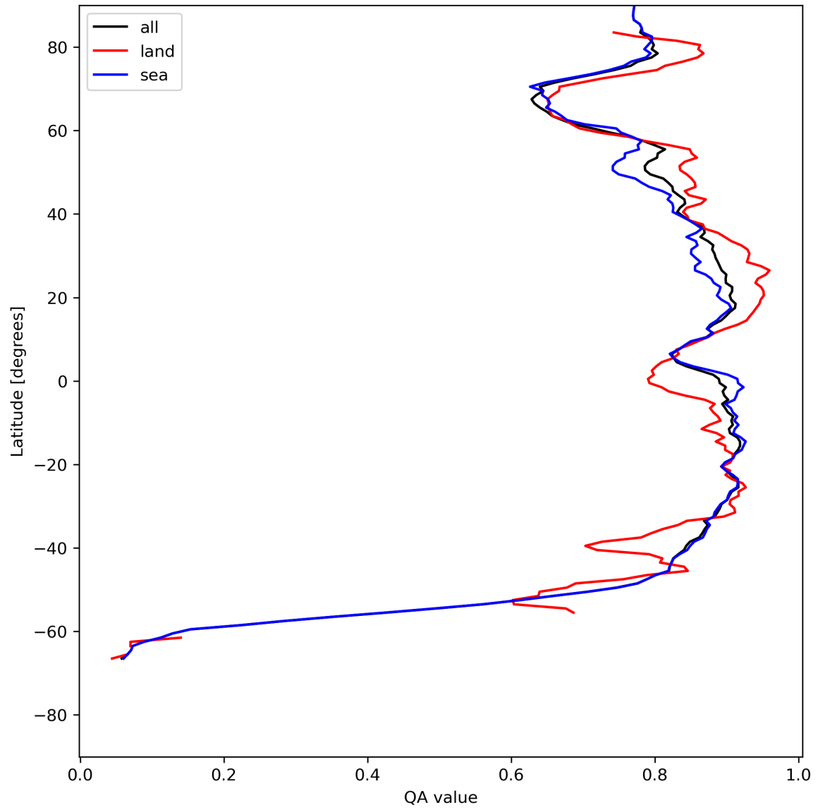
Figure 11: Zonal average of “QA value” for 2024-05-24 to 2024-05-26.
