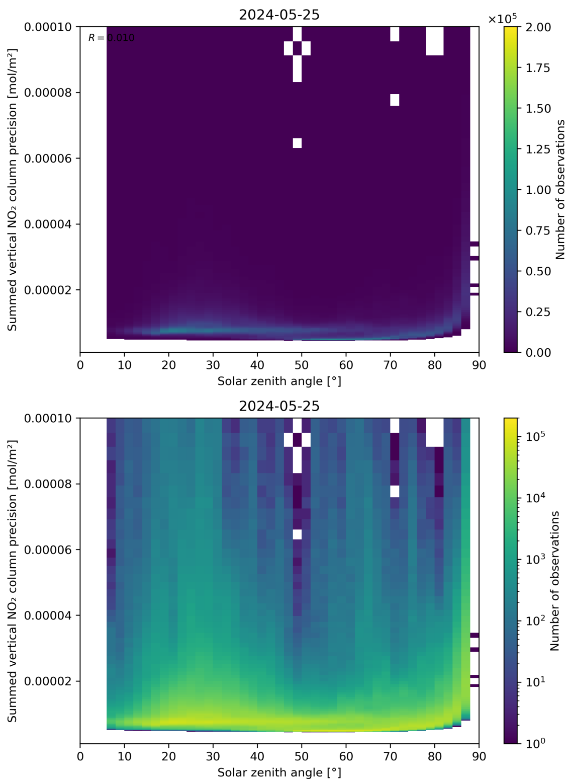
Figure 152: Scatter density plot of “Solar zenith angle” against “Summed vertical NO 2 column precision” for 2024-05-24 to 2024-05-26.
