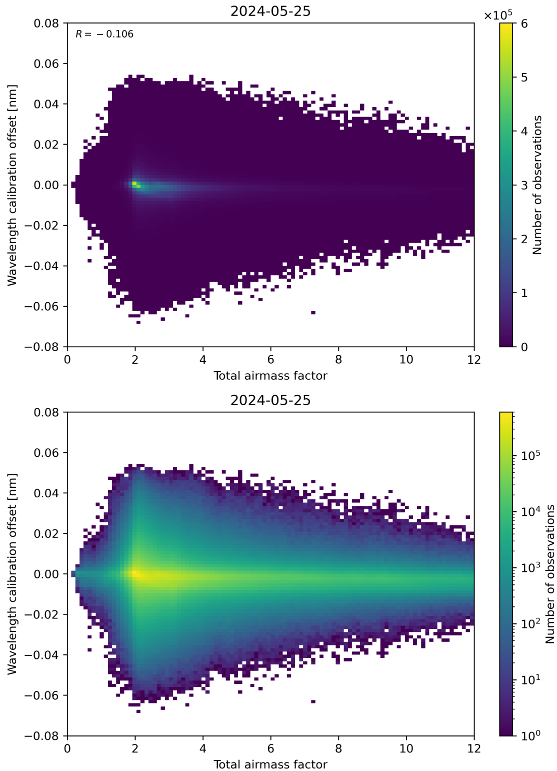
Figure 70: Scatter density plot of “Total airmass factor” against “Wavelength calibration offset” for 2024-05-24 to 2024-05-26.
