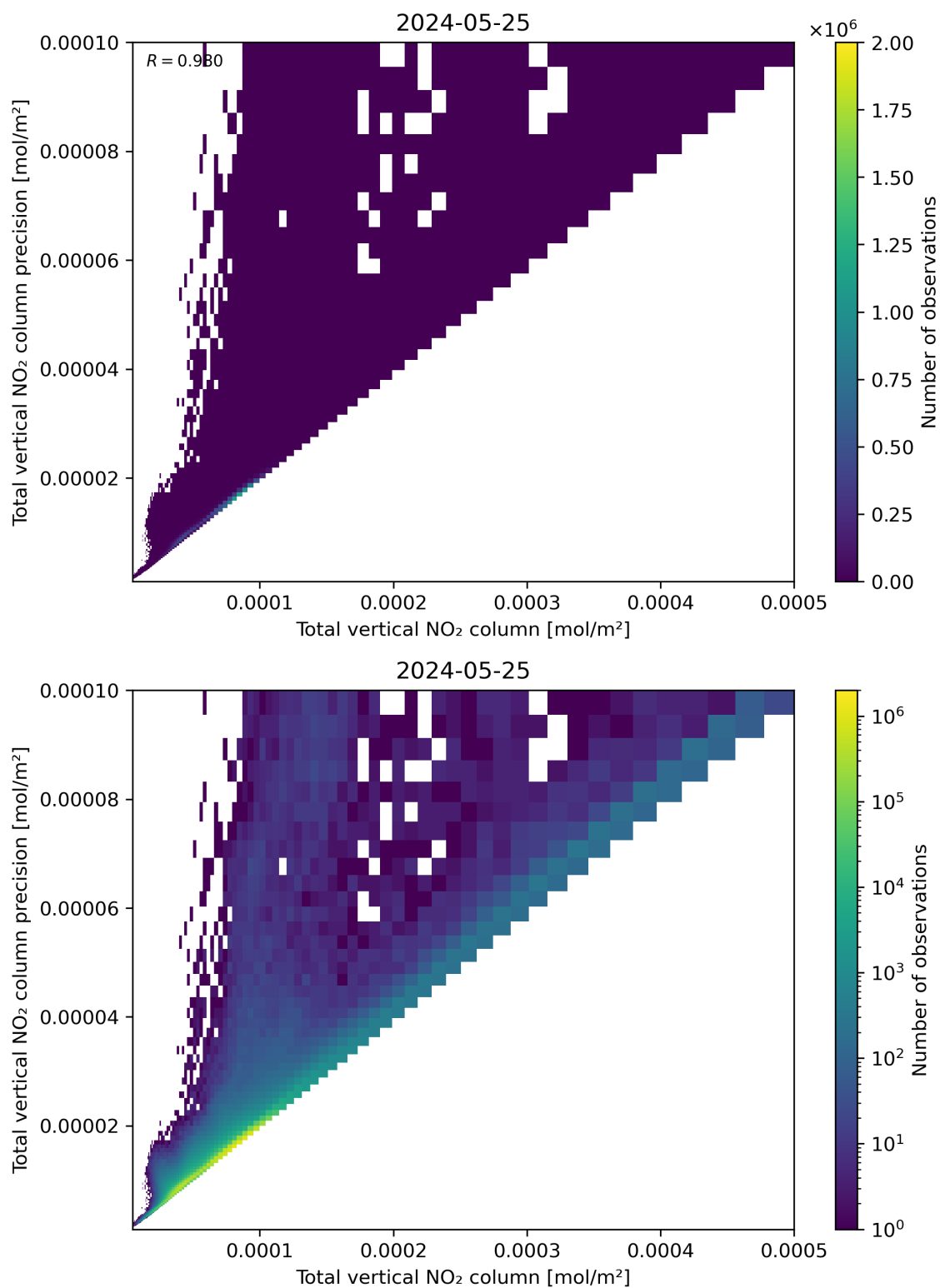
Figure 114: Scatter density plot of “Total vertical NO 2 column” against “Total vertical NO 2 column precision” for 2024-05-24 to 2024-05-26.
