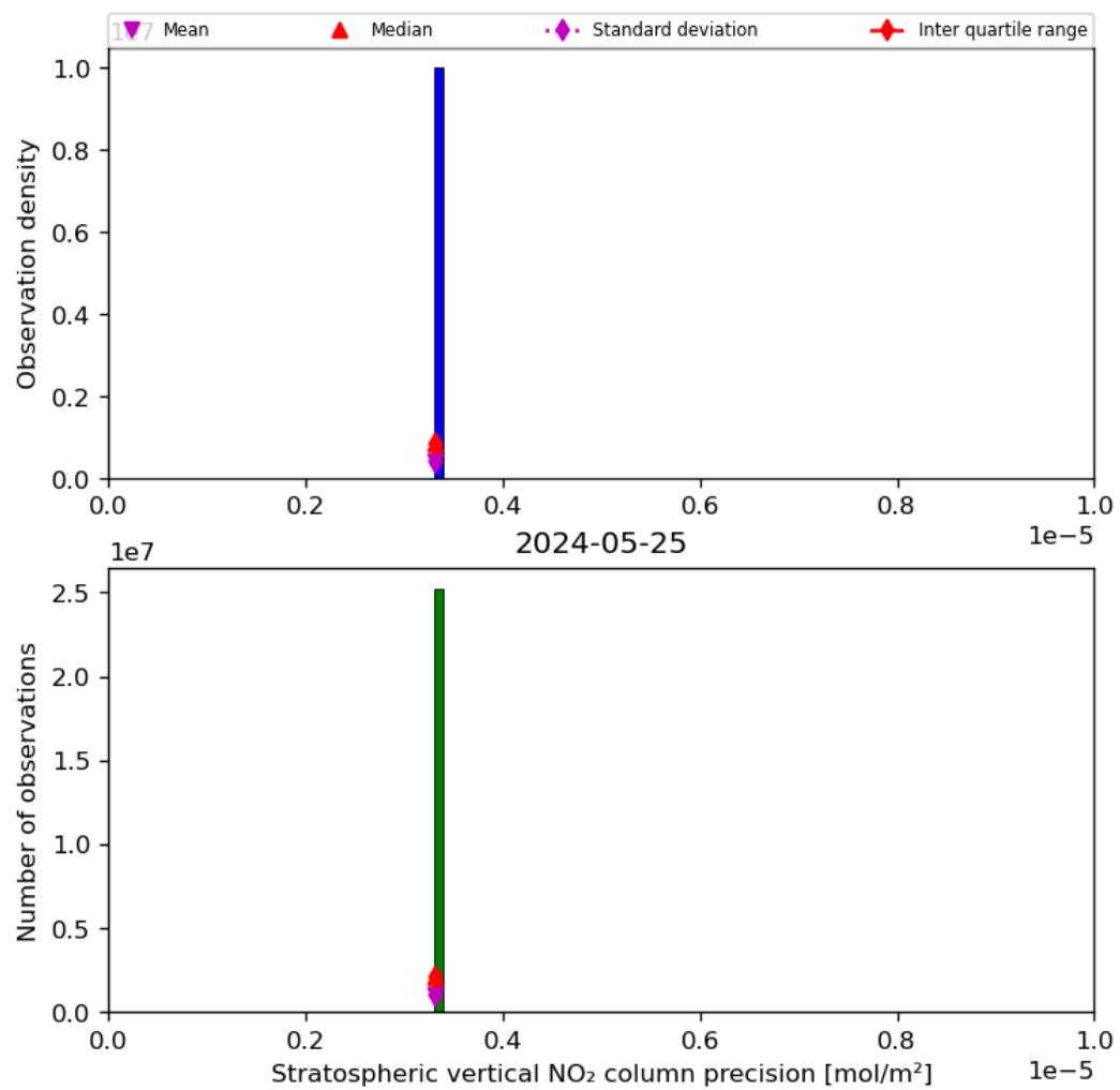
Figure 37: Histogram of “Stratospheric vertical NO 2 column precision” for 2024-05-24 to 2024-05-26
