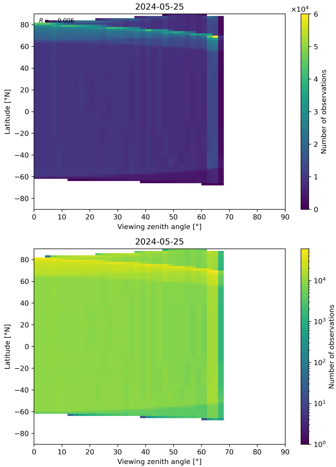
Figure 163: Scatter density plot of “Viewing zenith angle” against “Latitude” for 2024-05-24 to 2024-05-26.
