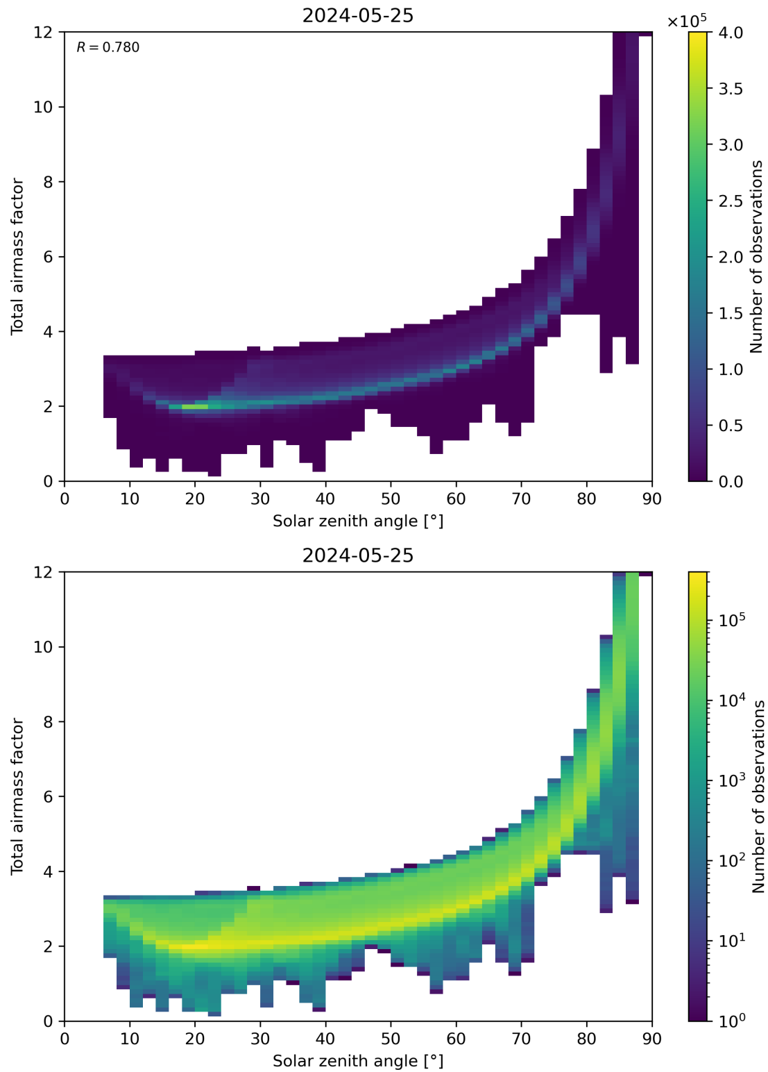
Figure 146: Scatter density plot of “Solar zenith angle” against “Total air mass factor” for 2024-05-24 to 2024-05-26.
