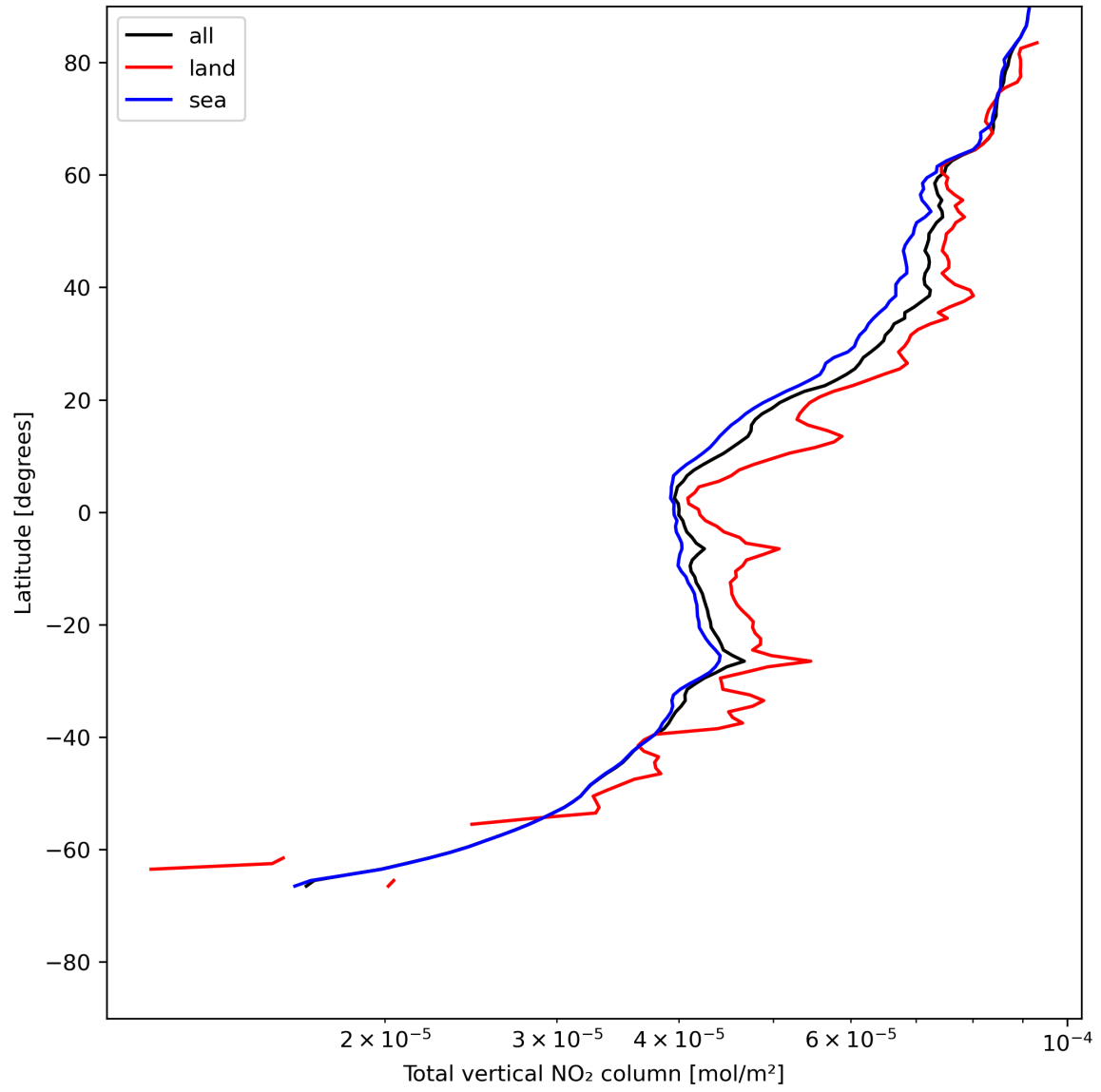
Figure 21: Zonal average of “Total vertical NO 2 column” for 2024-05-24 to 2024-05-26.
