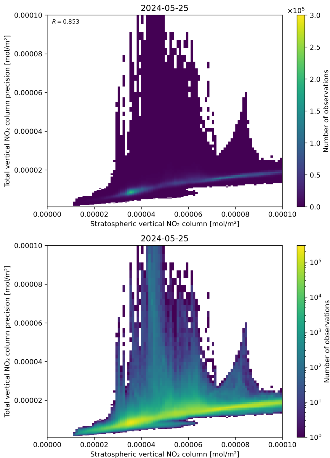
Figure 101: Scatter density plot of “Stratospheric vertical NO 2 column” against “Total vertical NO 2 column precision” for 2024-05-24 to 2024-05-26.
