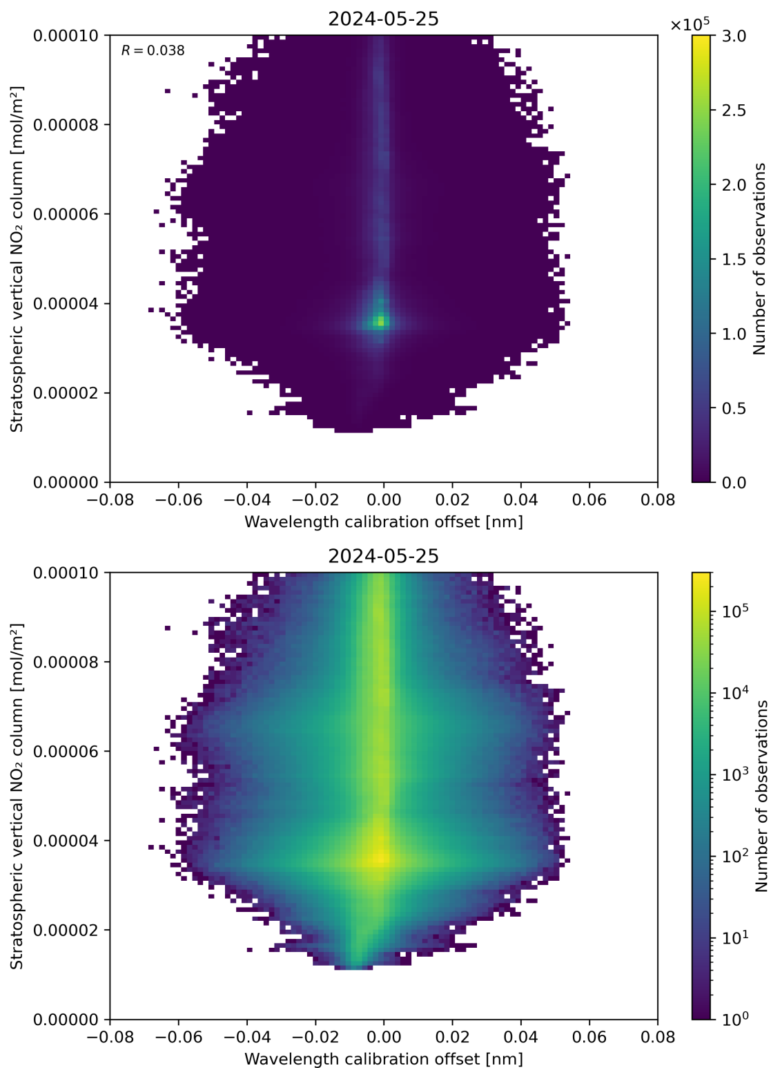
Figure 176: Scatter density plot of “Wavelength calibration offset” against “Stratospheric vertical NO 2 column” for 2024-05-24 to 2024-05-26.
