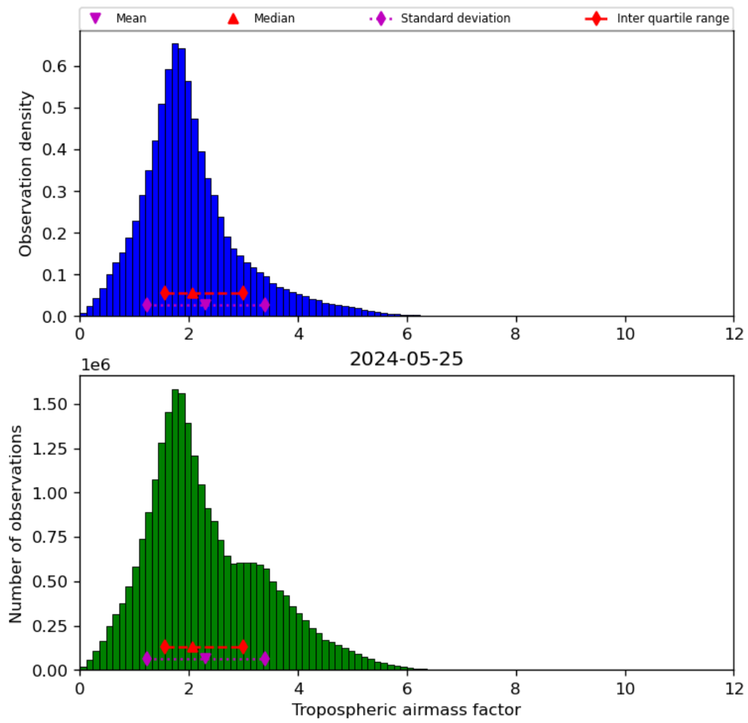
Figure 31: Histogram of “Tropospheric airmass factor” for 2024-05-24 to 2024-05-26
