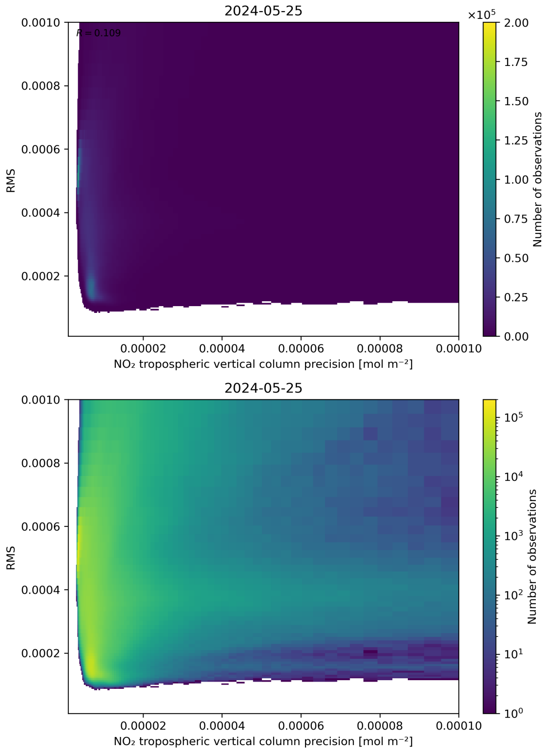
Figure 140: Scatter density plot of “NO 2 tropospheric vertical column precision” against “RMS” for 2024-05-24 to 2024-05-26.
