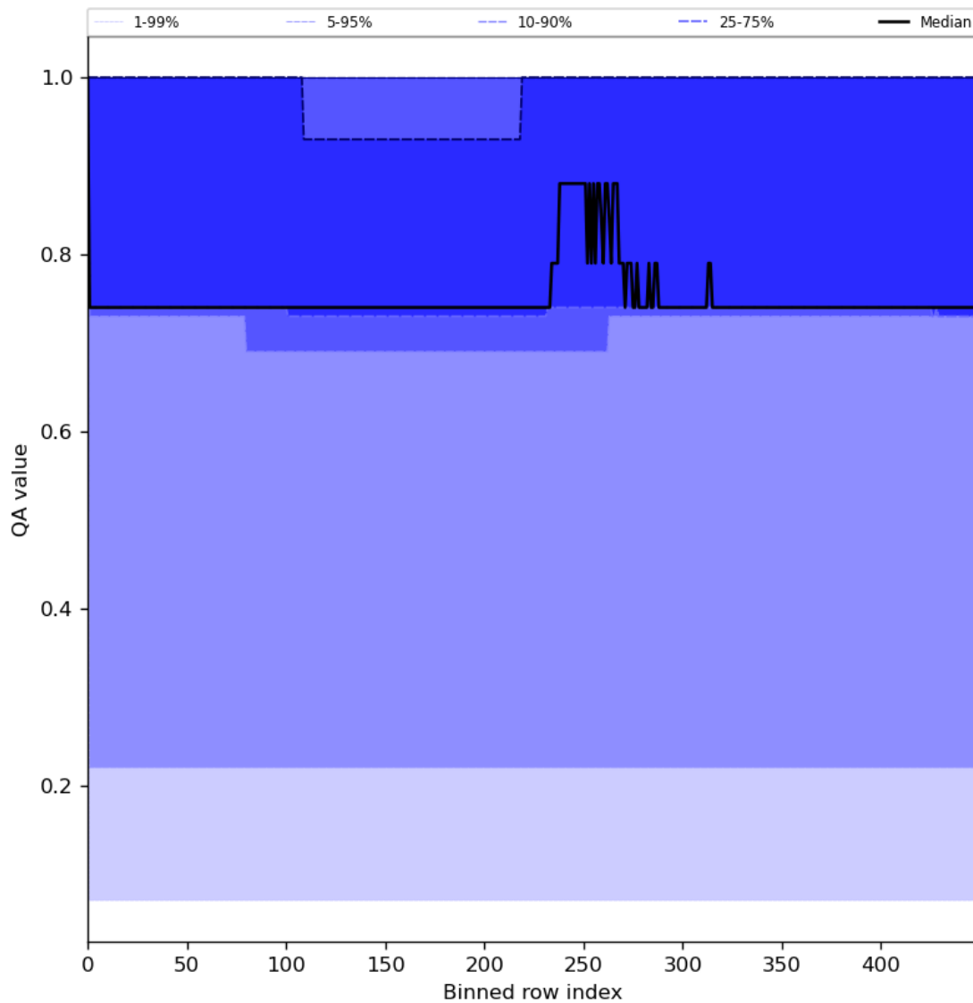
Figure 45: Along track statistics of “QA value” for 2024-05-24 to 2024-05-26
