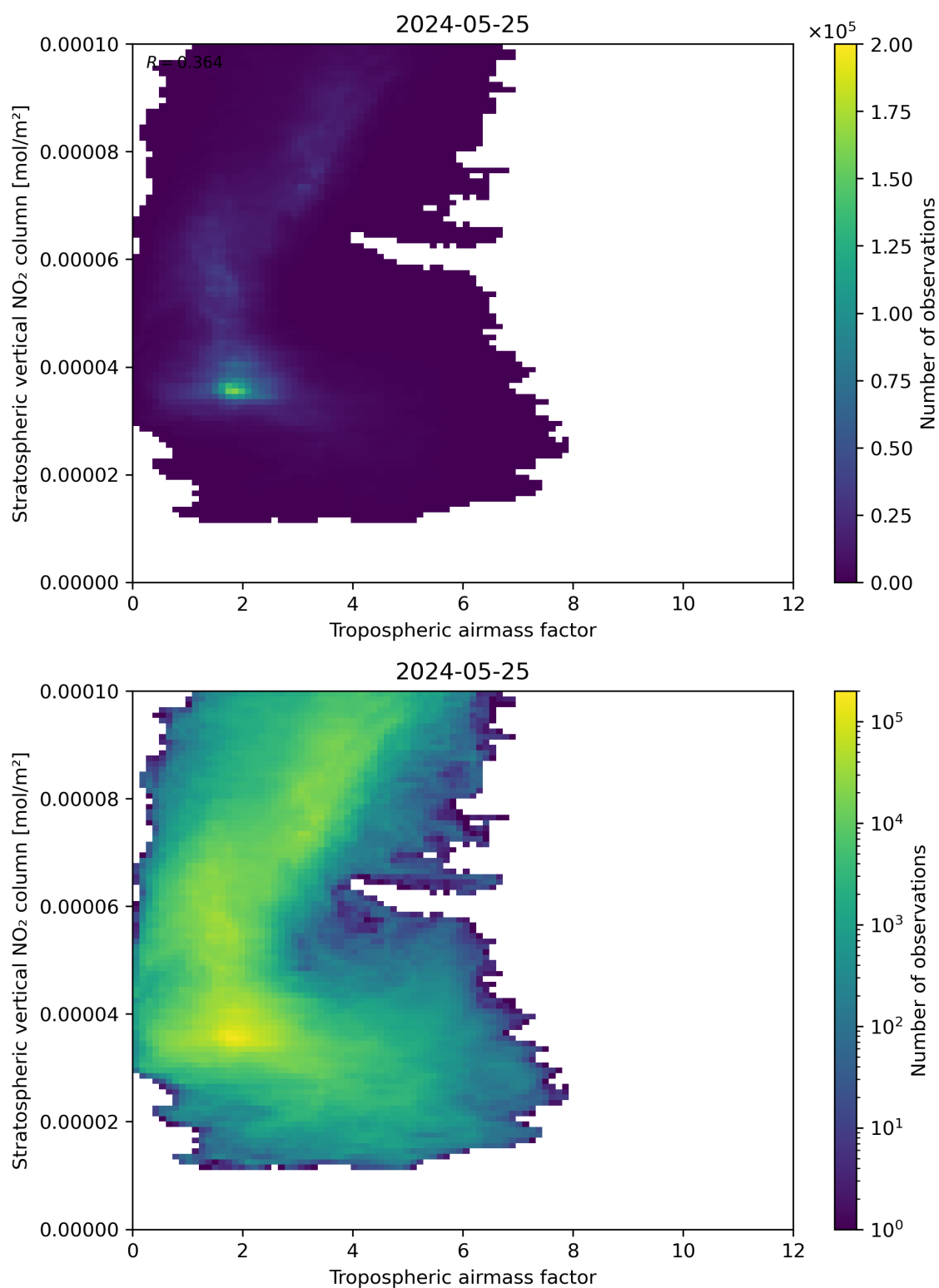
Figure 74: Scatter density plot of “Tropospheric air mass factor” against “Stratospheric vertical NO 2 column” for 2024-05-24 to 2024-05-26.
