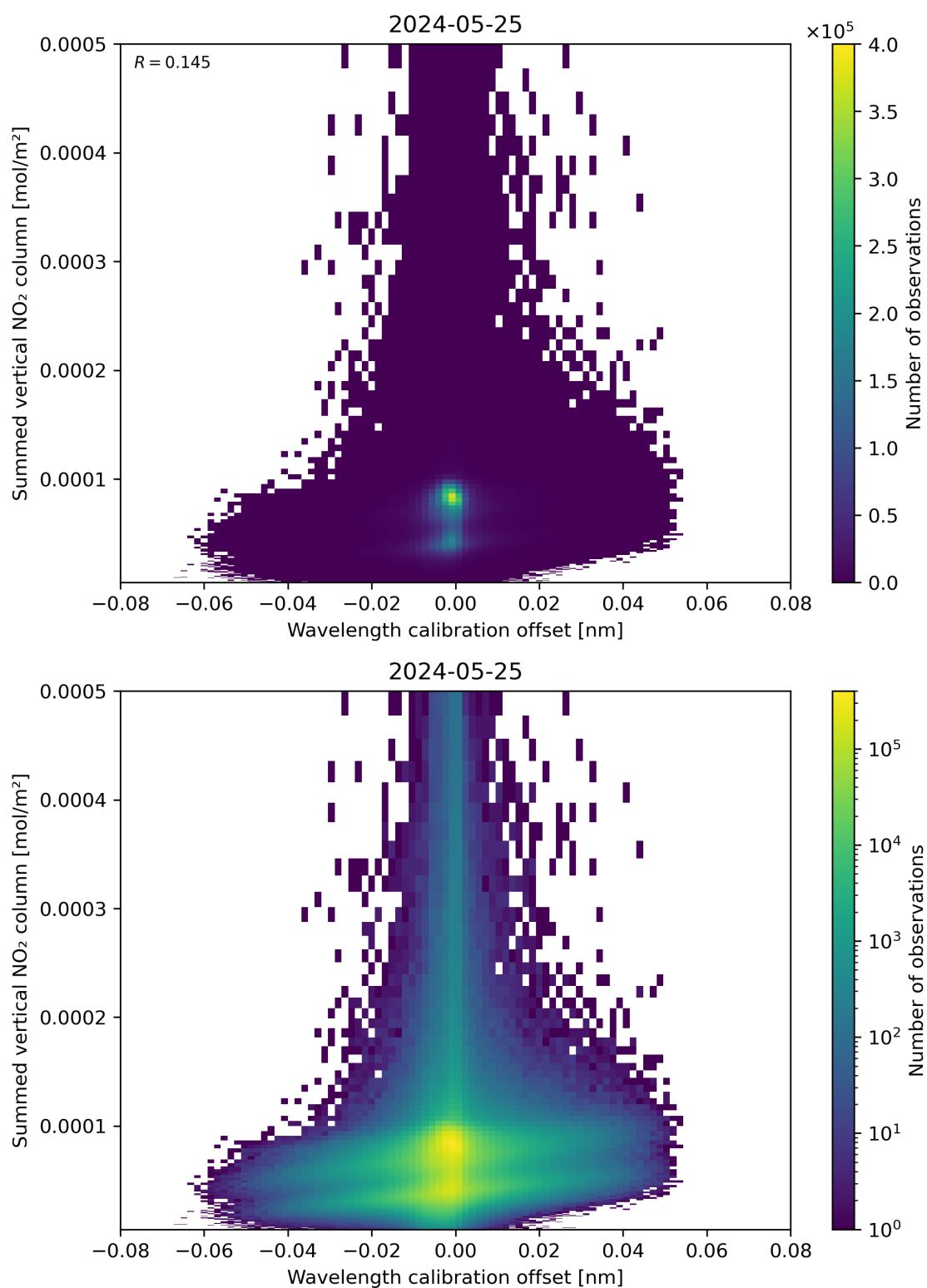
Figure 177: Scatter density plot of “Wavelength calibration offset” against “Summed vertical NO 2 column” for 2024-05-24 to 2024-05-26.
