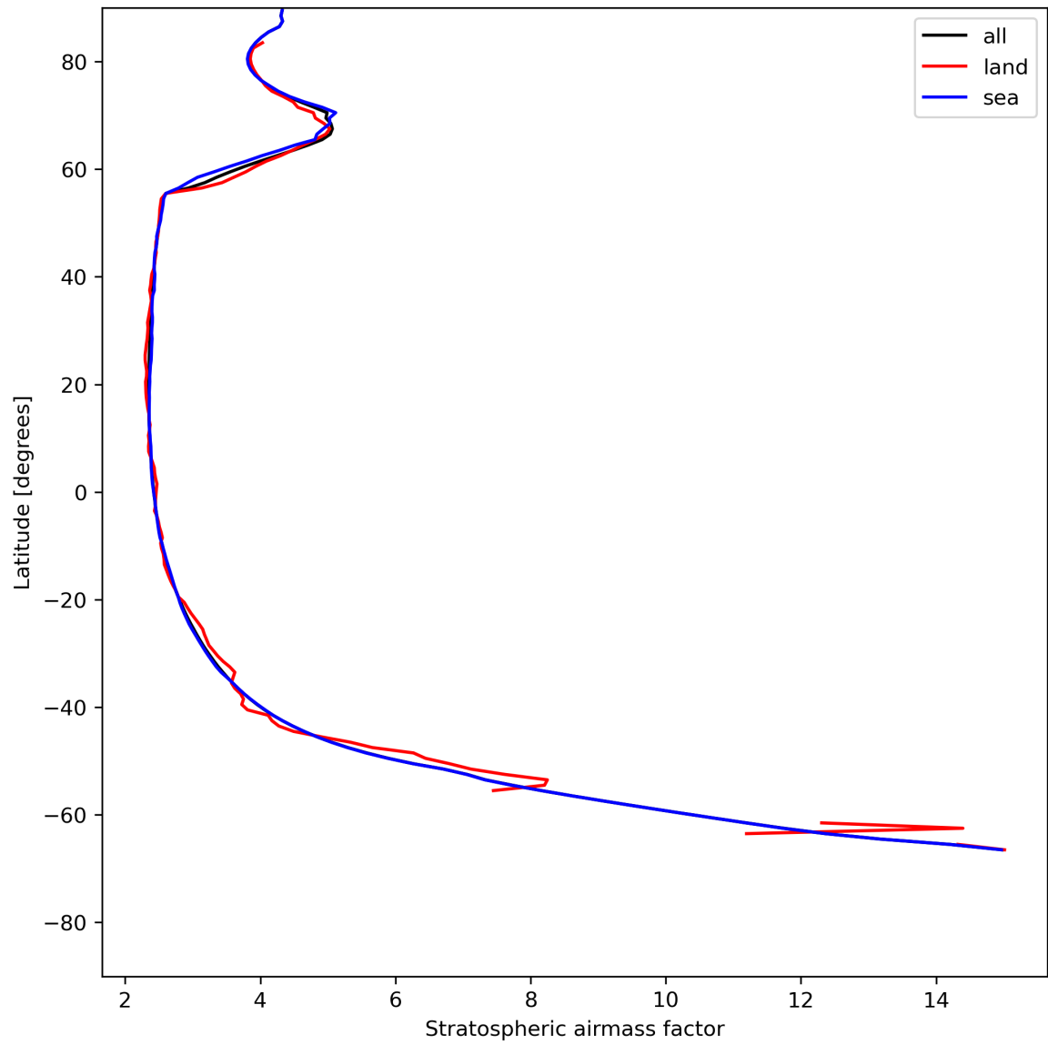
Figure 27: Zonal average of “Stratospheric airmass factor” for 2024-05-24 to 2024-05-26.
