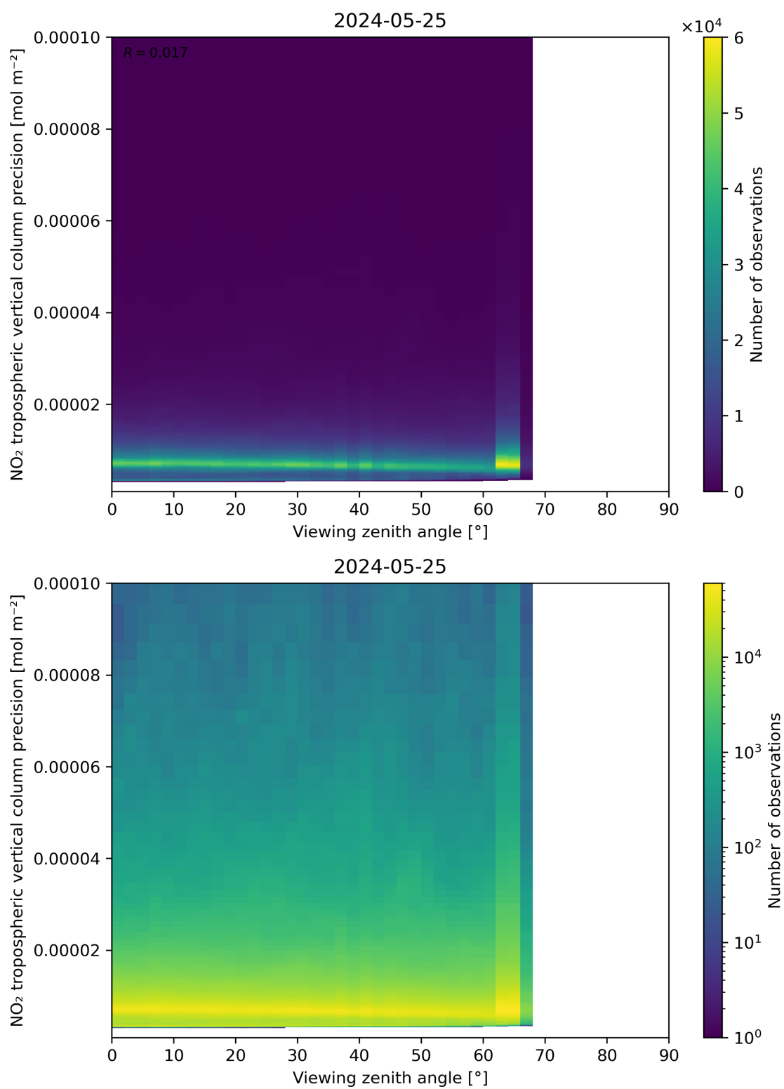
Figure 170: Scatter density plot of “Viewing zenith angle” against “NO 2 tropospheric vertical column precision” for 2024-05-24 to 2024-05-26.
