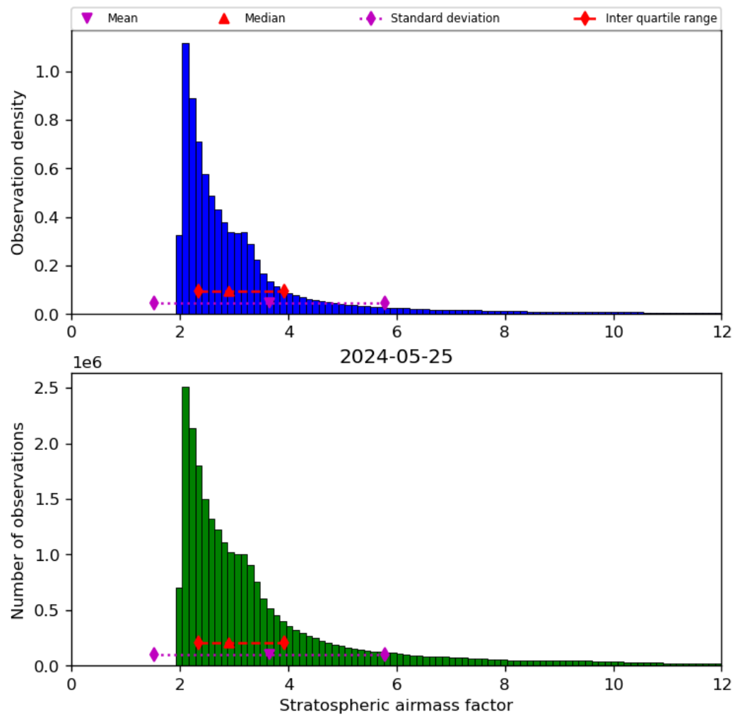
Figure 44: Histogram of “Stratospheric airmass factor” for 2024-05-24 to 2024-05-26
