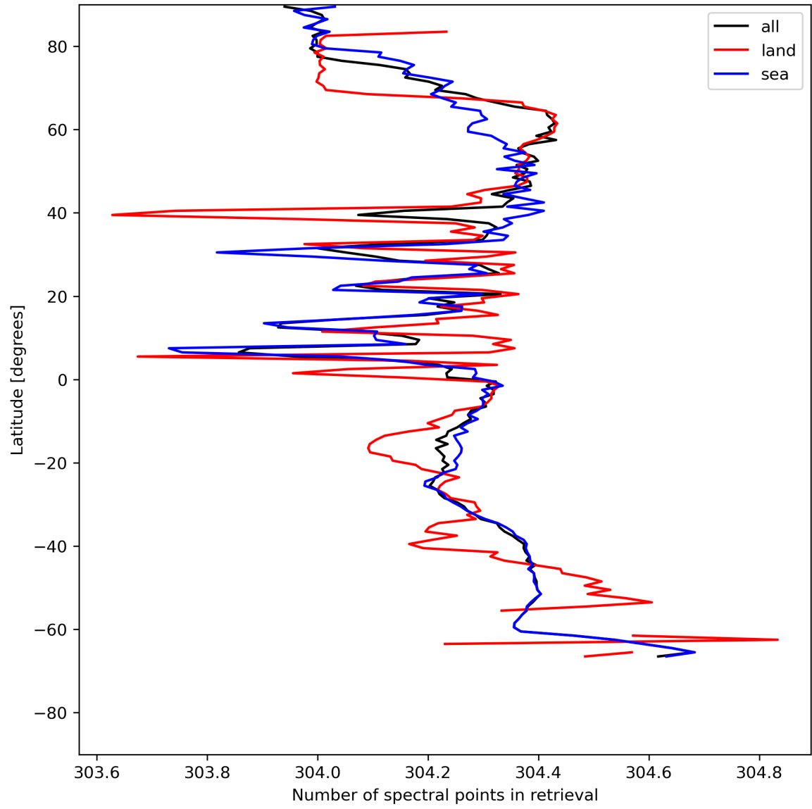
Figure 16: Zonal average of “Number of spectral points in retrieval” for 2024-05-24 to 2024-05-26.
