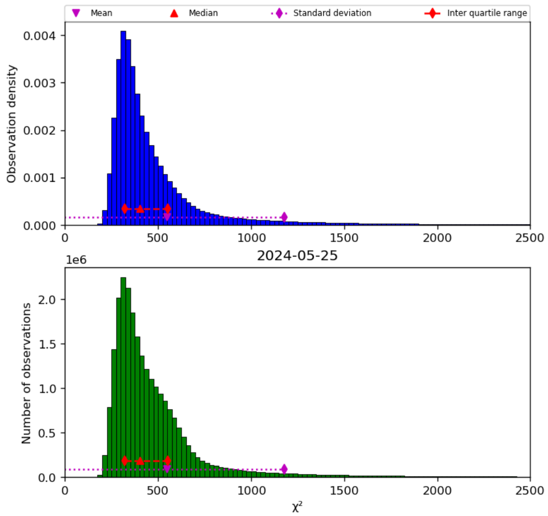
Figure 42: Histogram of “ \chi^2 ” for 2024-05-24 to 2024-05-26
