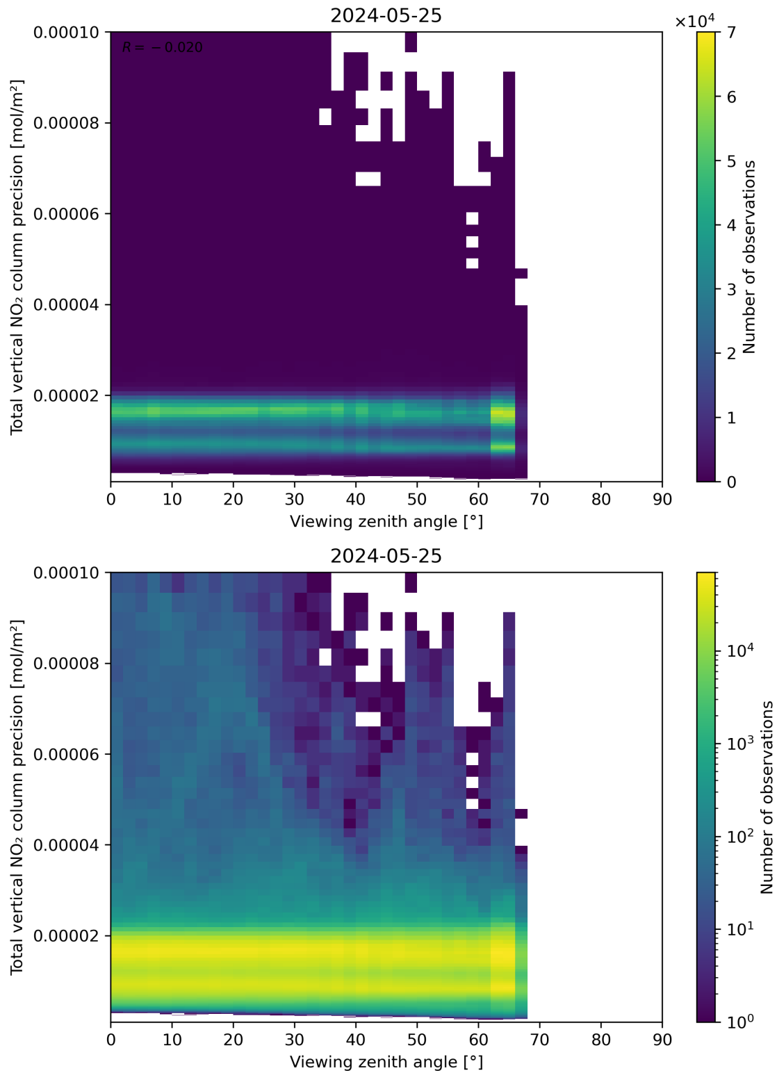
Figure 168: Scatter density plot of “Viewing zenith angle” against “Total vertical NO 2 column precision” for 2024-05-24 to 2024-05-26.
