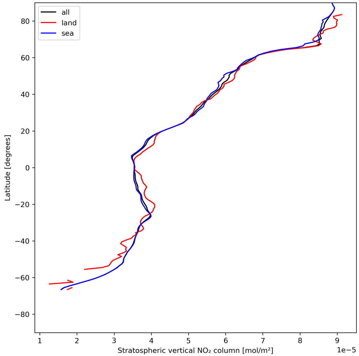
Figure 19: Zonal average of “Stratospheric vertical NO 2 column” for 2024-05-24 to 2024-05-26.
