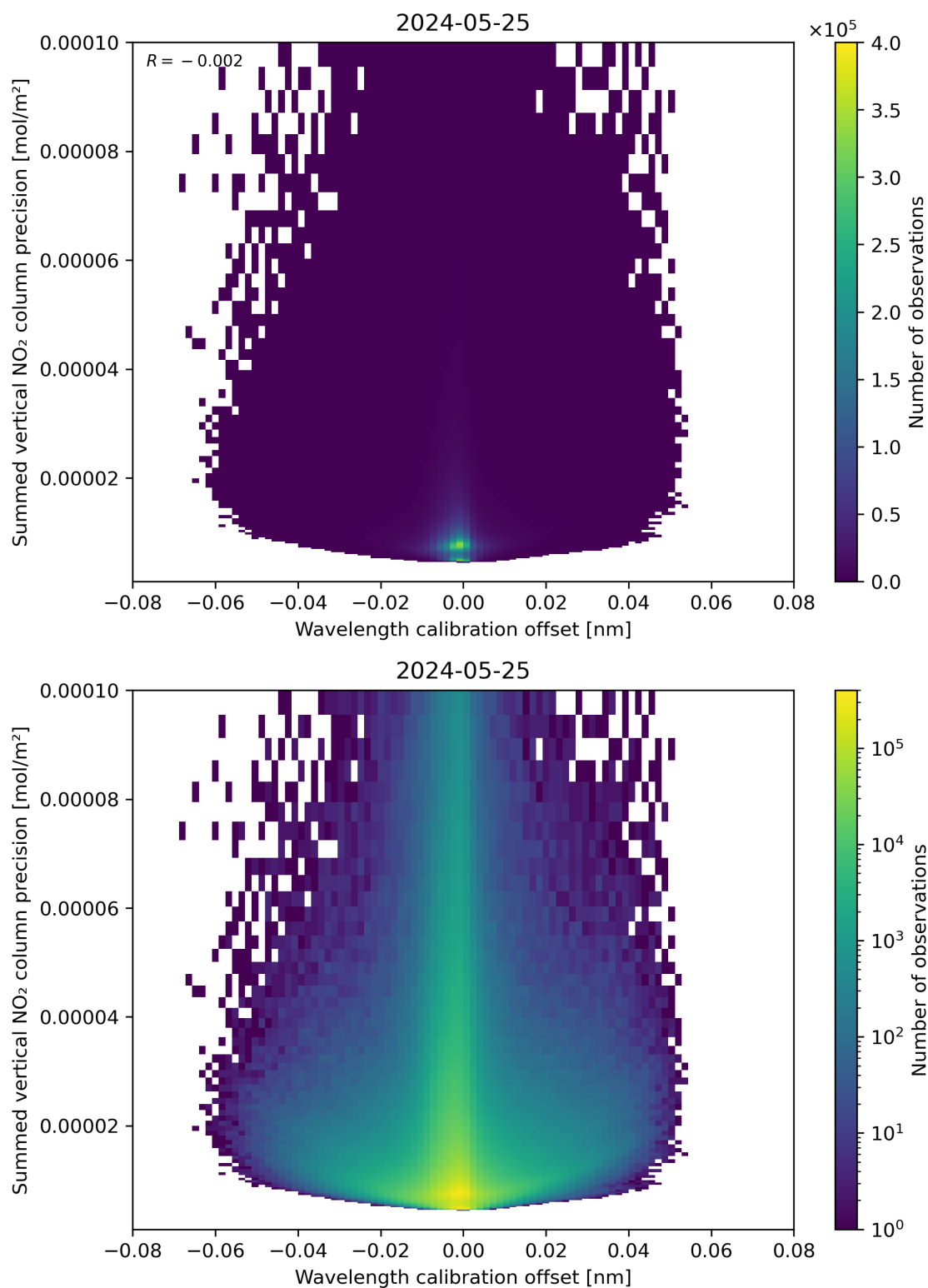
Figure 178: Scatter density plot of “Wavelength calibration offset” against “Summed vertical NO 2 column precision” for 2024-05-24 to 2024-05-26.
