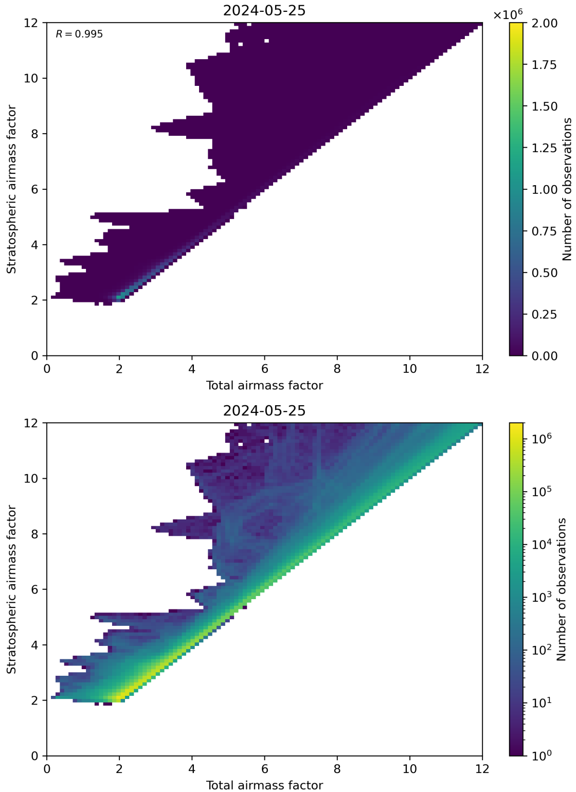
Figure 62: Scatter density plot of “Total airmass factor” against “Stratospheric airmass factor” for 2024-05-24 to 2024-05-26.
