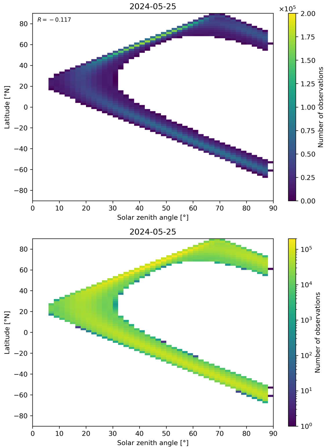
Figure 149: Scatter density plot of “Solar zenith angle” against “Latitude” for 2024-05-24 to 2024-05-26.
