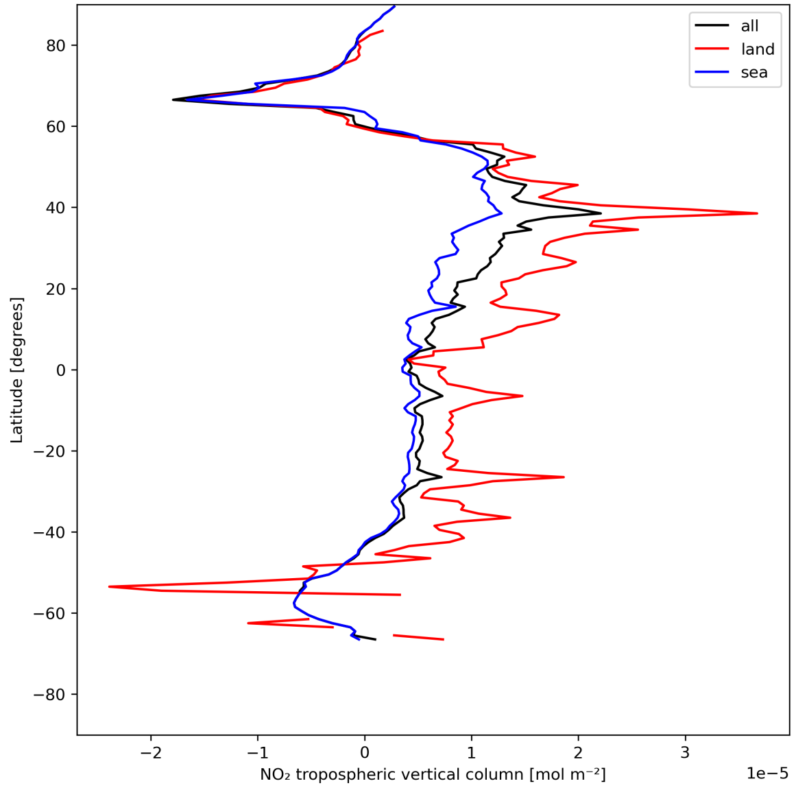
Figure 12: Zonal average of “NO 2 tropospheric vertical column” for 2024-05-24 to 2024-05-26.
