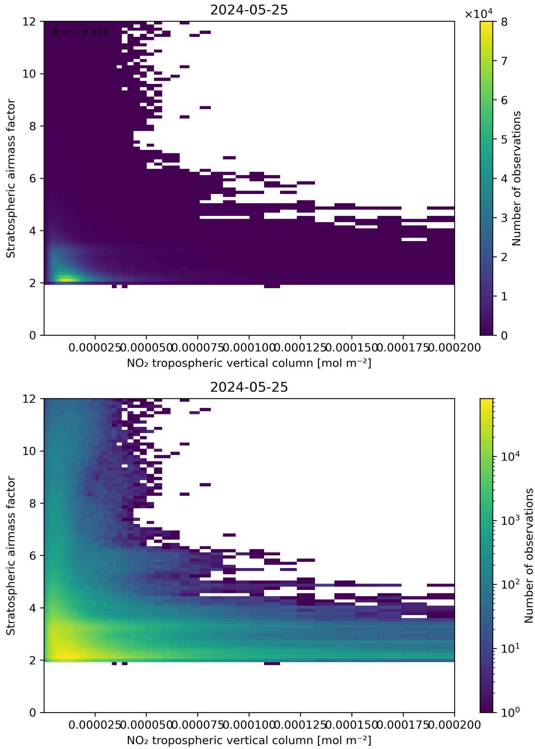
Figure 121: Scatter density plot of “NO 2 tropospheric vertical column” against “Stratospheric airmass factor” for 2024-05-24 to 2024-05-26.
