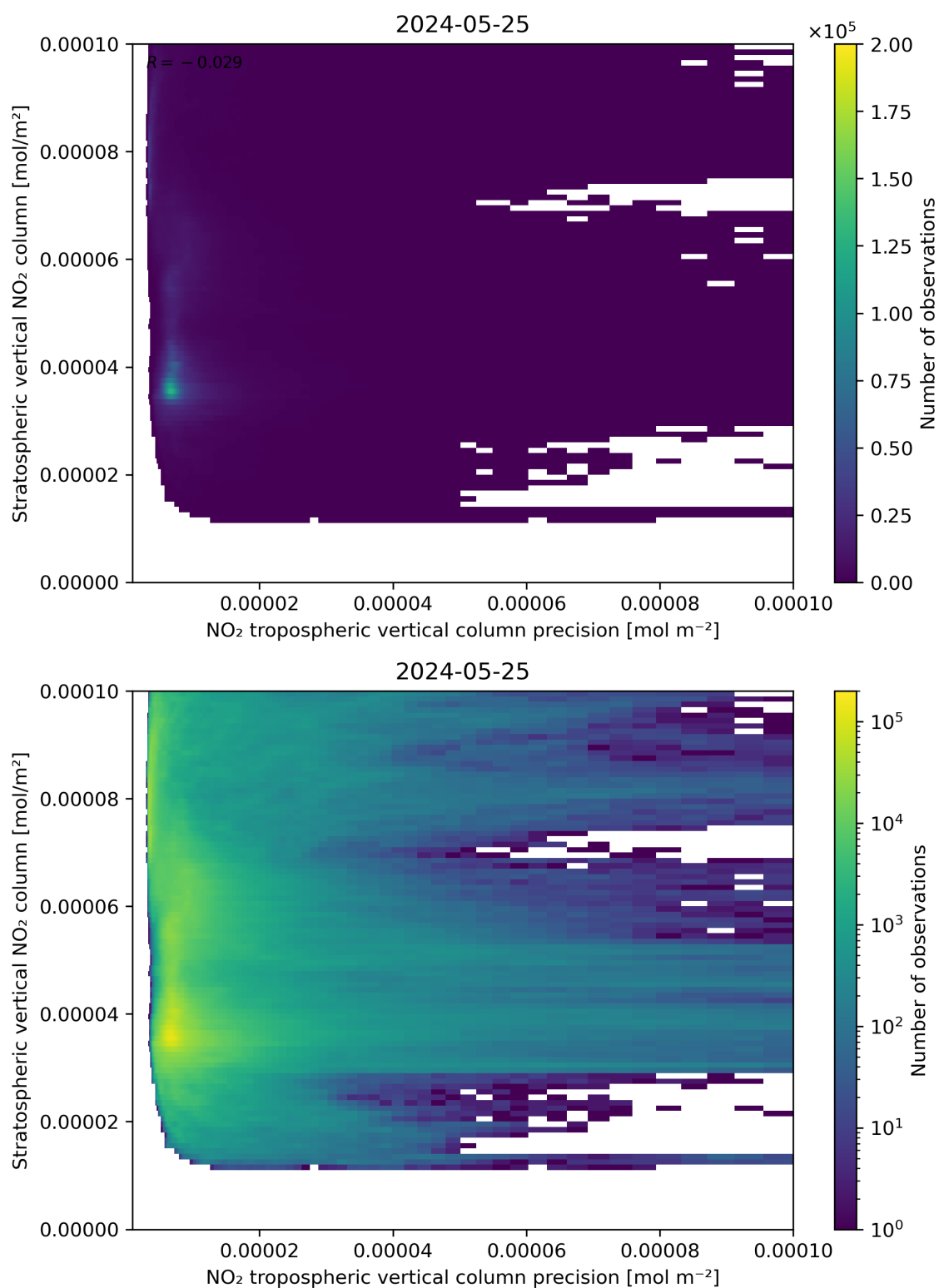
Figure 135: Scatter density plot of “NO 2 tropospheric vertical column precision” against “Stratospheric vertical NO 2 column” for 2024-05-24 to 2024-05-26.
