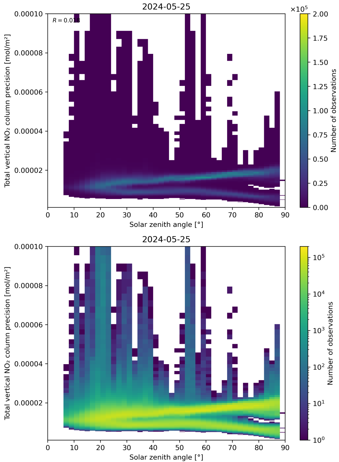
Figure 154: Scatter density plot of “Solar zenith angle” against “Total vertical NO 2 column precision” for 2024-05-24 to 2024-05-26.
