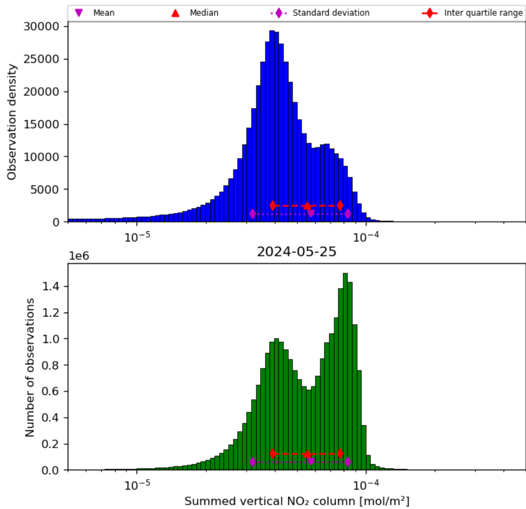
Figure 40: Histogram of “Summed vertical NO 2 column” for 2024-05-24 to 2024-05-26
