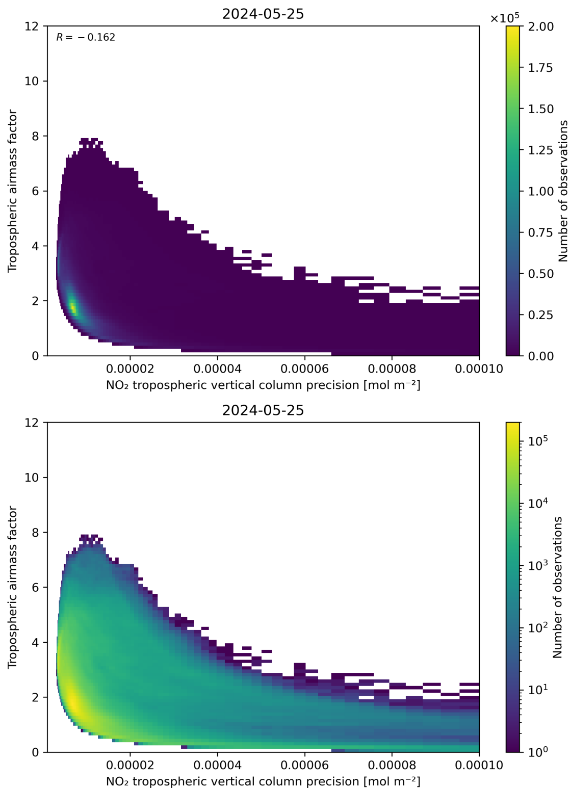
Figure 133: Scatter density plot of “NO 2 tropospheric vertical column precision” against “Tropospheric airmass factor” for 2024-05-24 to 2024-05-26.
