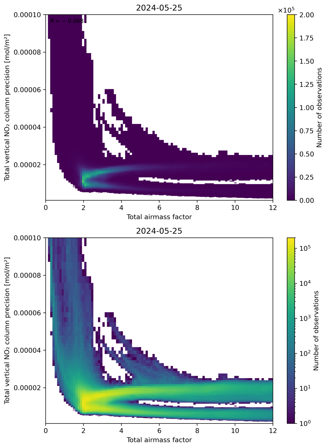
Figure 68: Scatter density plot of “Total airmass factor” against “Total vertical NO 2 column precision” for 2024-05-24 to 2024-05-26.
