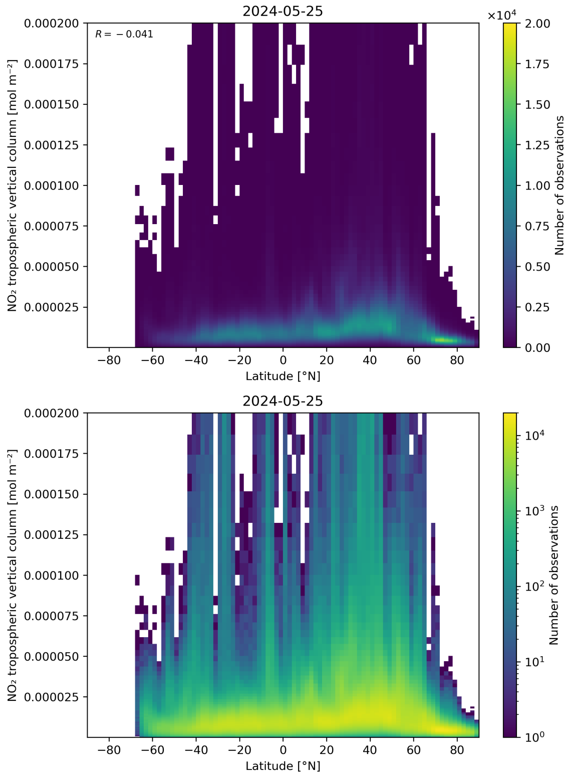
Figure 92: Scatter density plot of “Latitude” against “NO 2 tropospheric vertical column” for 2024-05-24 to 2024-05-26.
