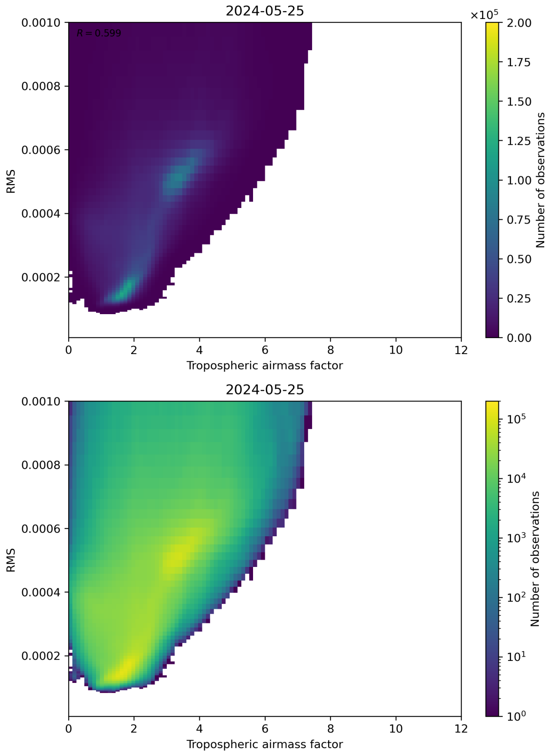
Figure 79: Scatter density plot of “Tropospheric airmass factor” against “RMS” for 2024-05-24 to 2024-05-26.
