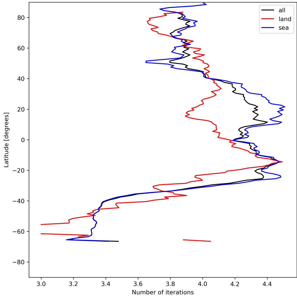
Figure 17: Zonal average of “Number of iterations” for 2024-05-24 to 2024-05-26.
