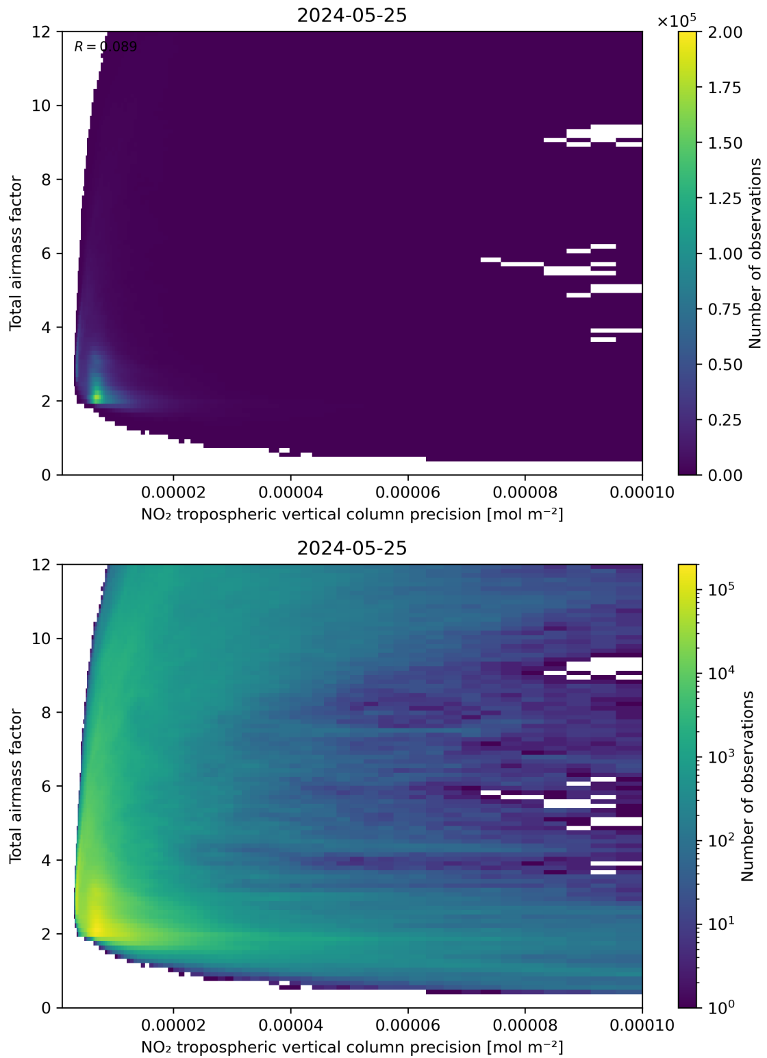
Figure 132: Scatter density plot of “NO 2 tropospheric vertical column precision” against “Total air mass factor” for 2024-05-24 to 2024-05-26.
