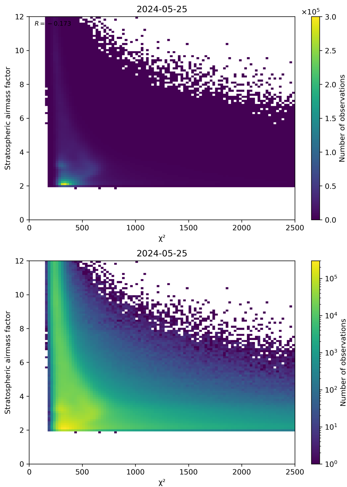
Figure 81: Scatter density plot of “ \chi^2 ” against “Stratospheric airmass factor” for 2024-05-24 to 2024-05-26.
