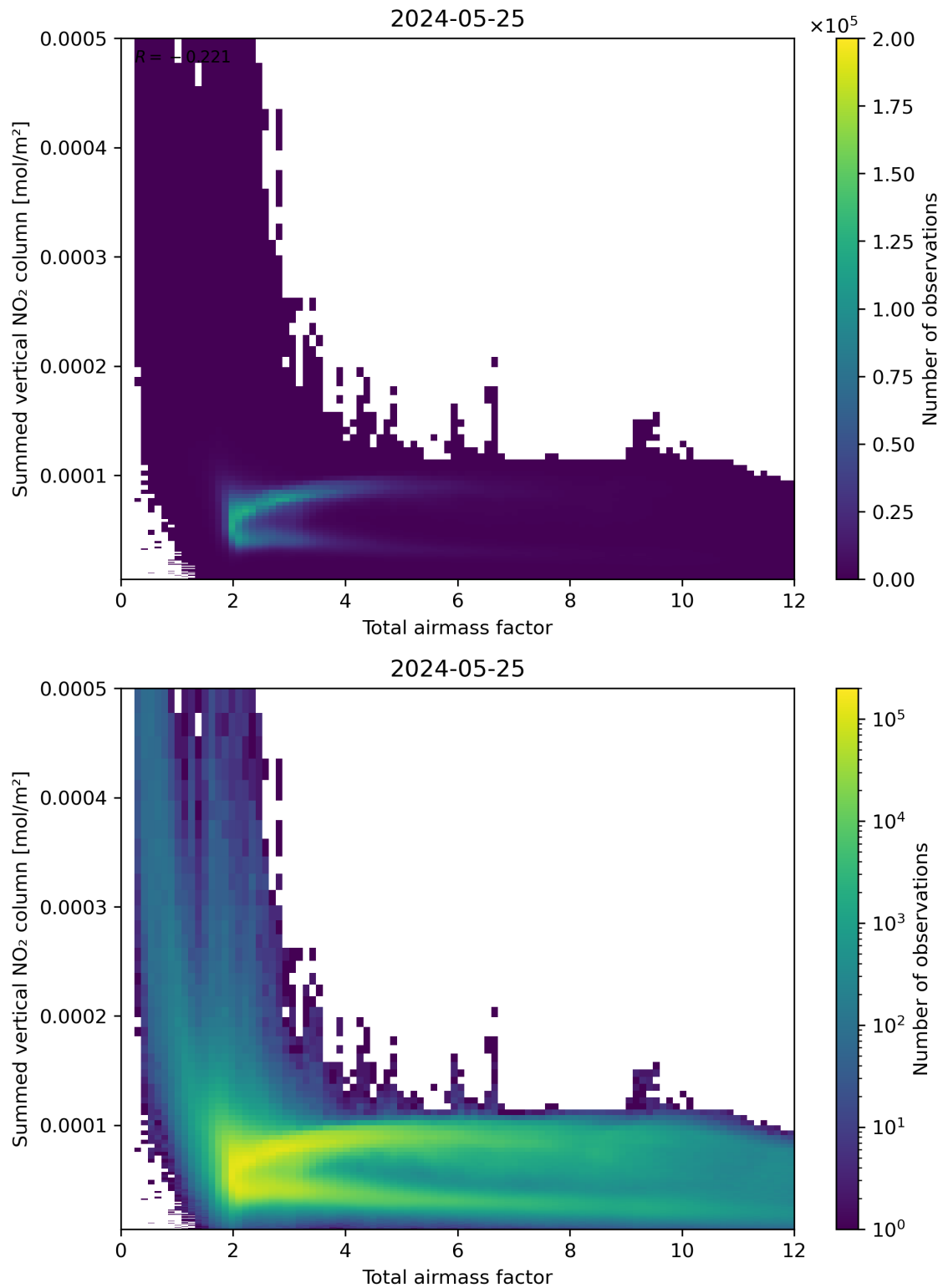
Figure 65: Scatter density plot of “Total airmass factor” against “Summed vertical NO 2 column” for 2024-05-24 to 2024-05-26.
