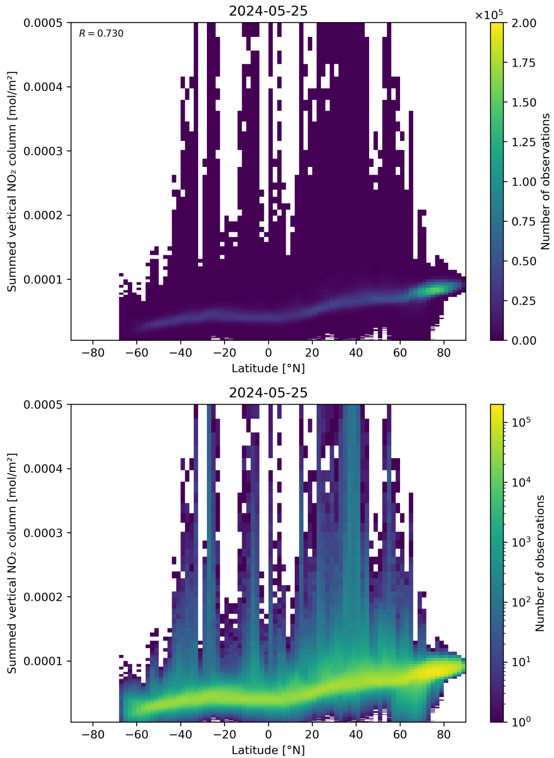
Figure 88: Scatter density plot of “Latitude” against “Summed vertical NO 2 column” for 2024-05-24 to 2024-05-26.
