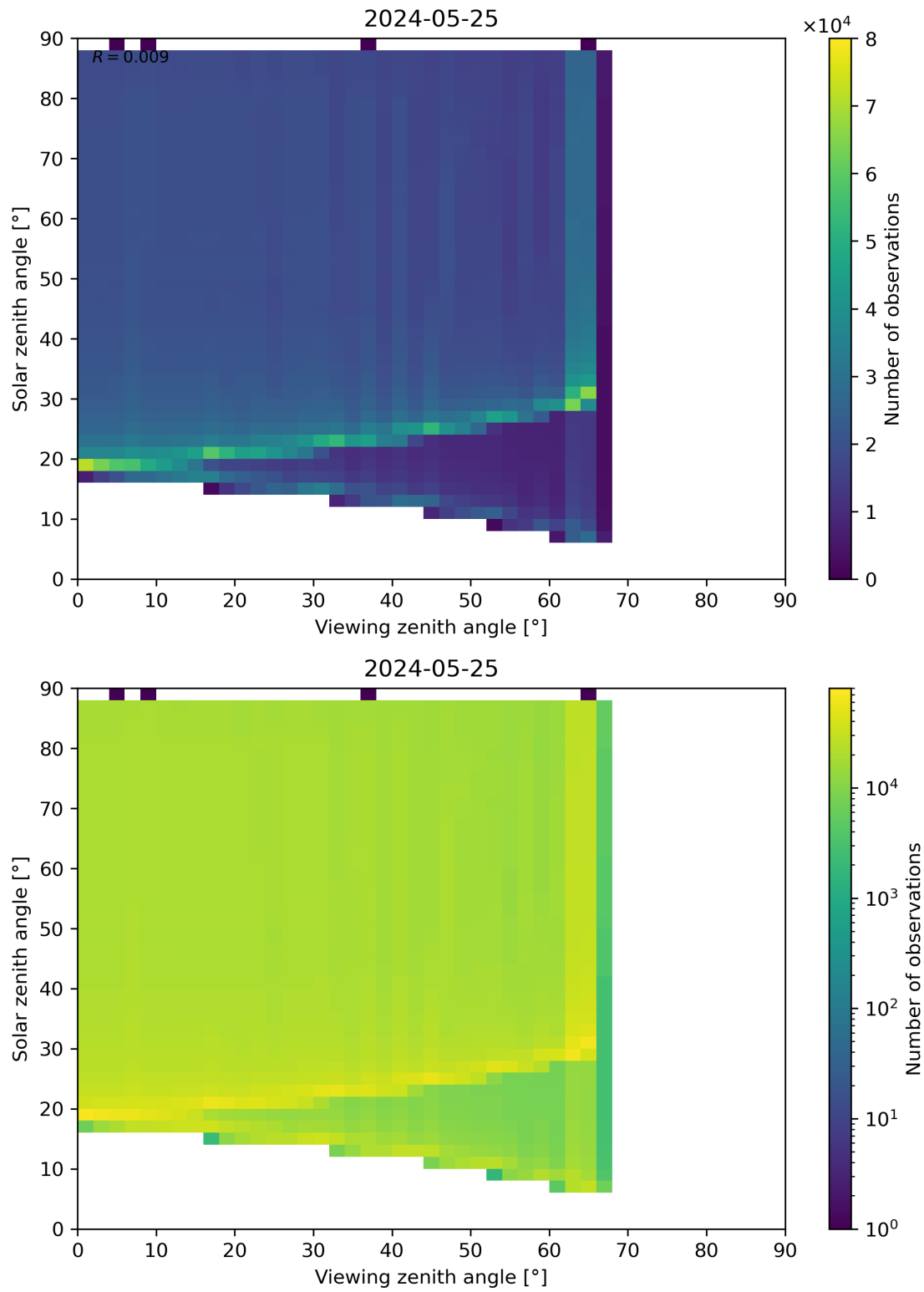
Figure 172: Scatter density plot of “Viewing zenith angle” against “Solar zenith angle” for 2024-05-24 to 2024-05-26.
