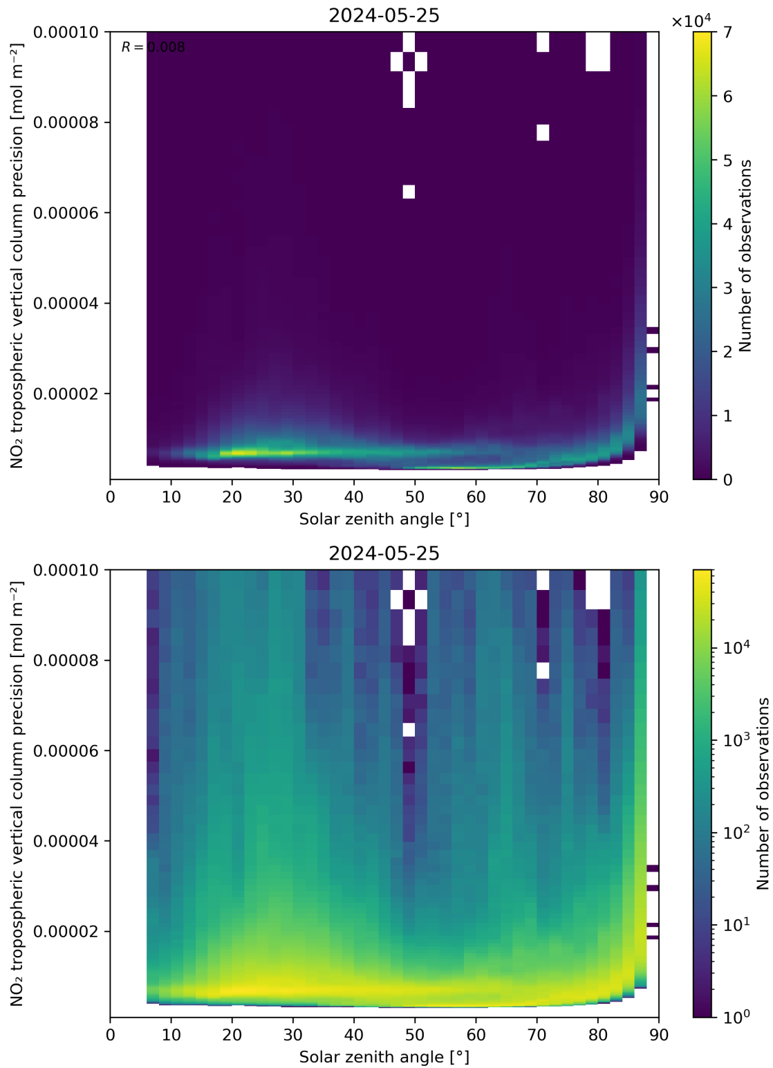
Figure 156: Scatter density plot of “Solar zenith angle” against “NO 2 tropospheric vertical column precision” for 2024-05-24 to 2024-05-26.
