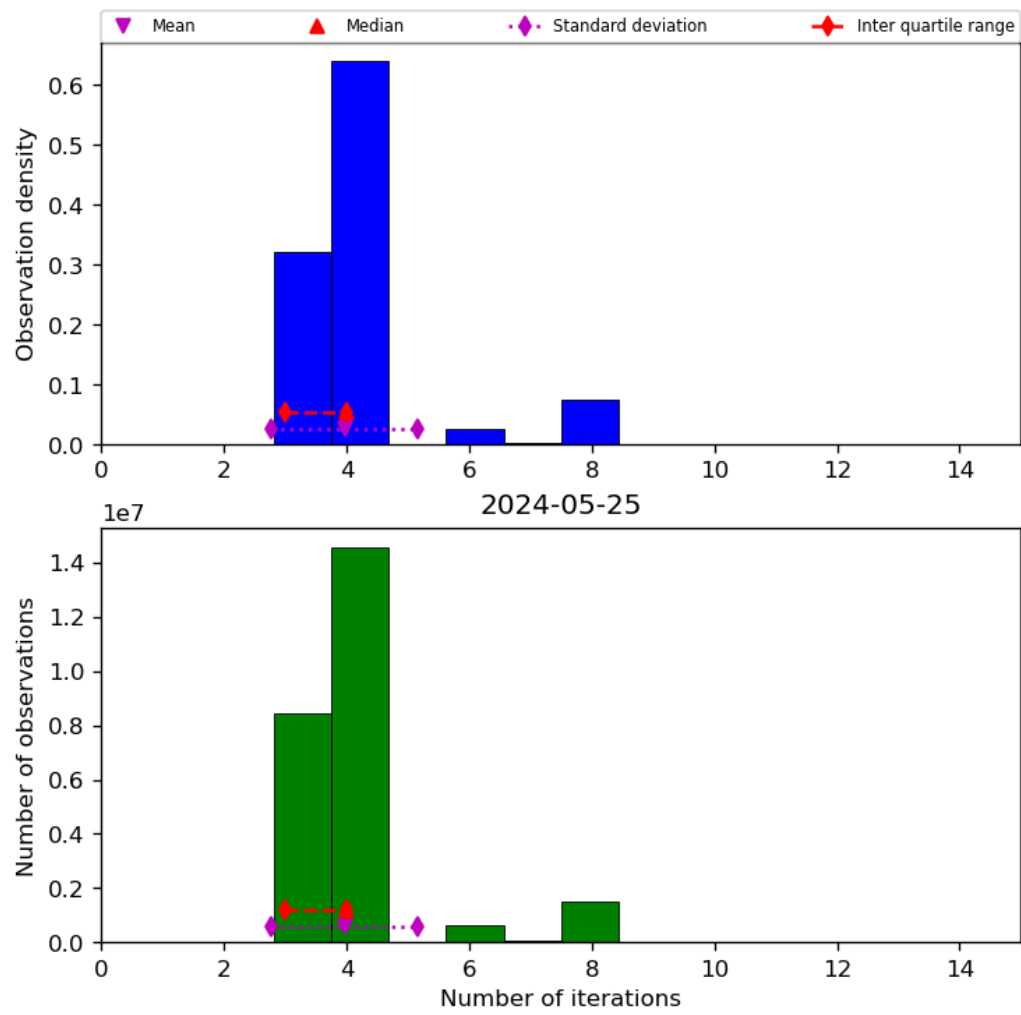
Figure 34: Histogram of “Number of iterations” for 2024-05-24 to 2024-05-26
