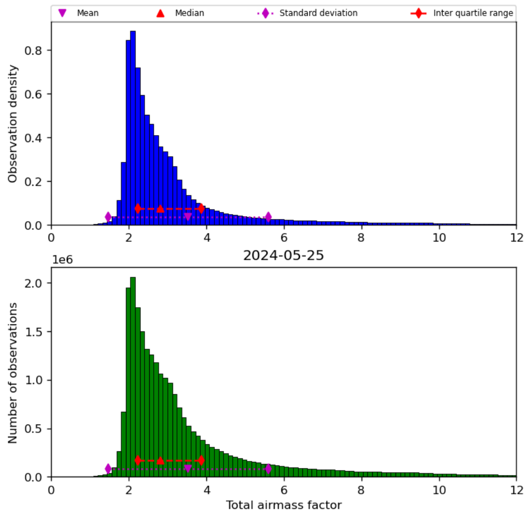
Figure 32: Histogram of “Total airmass factor” for 2024-05-24 to 2024-05-26
