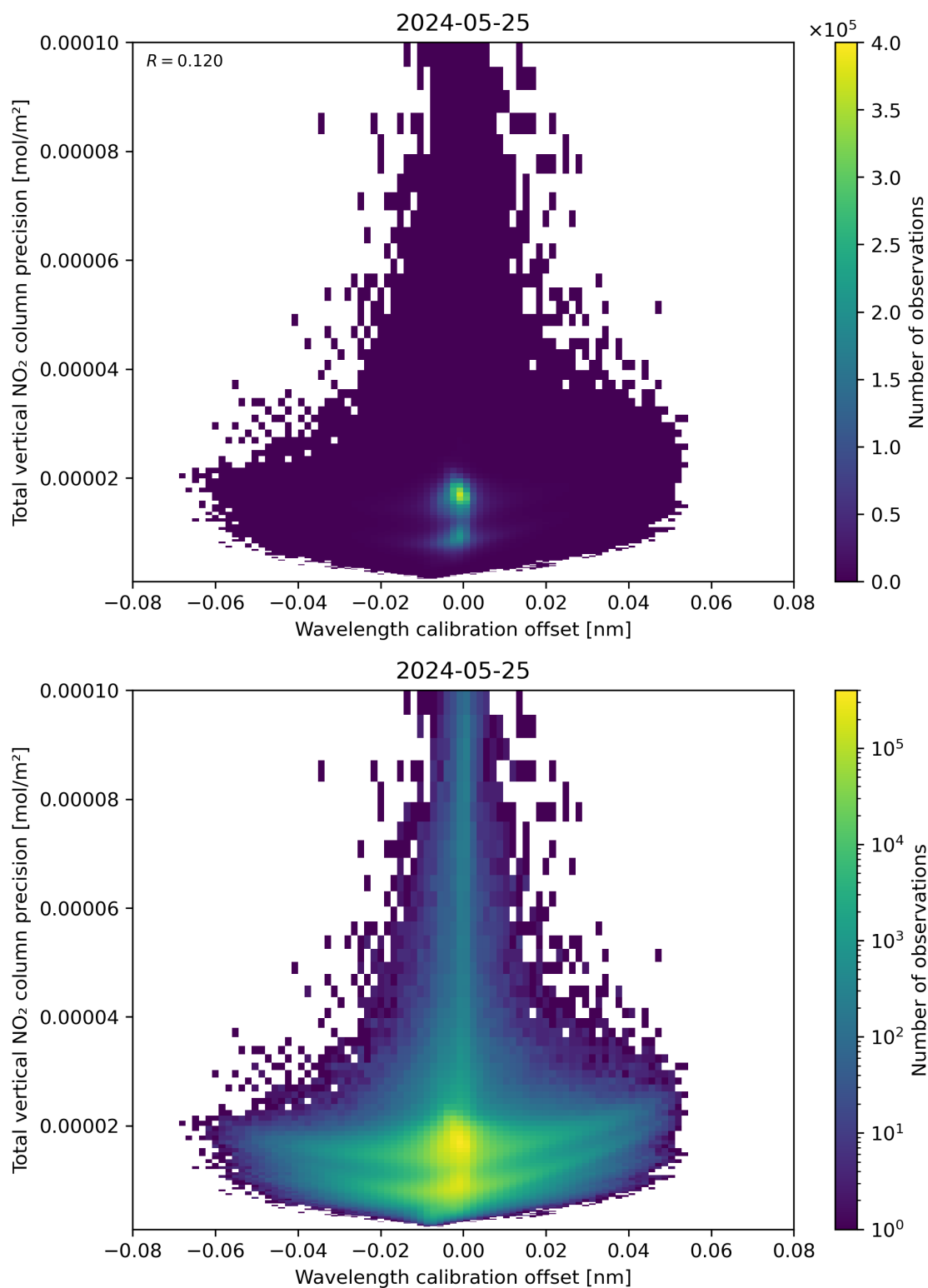
Figure 180: Scatter density plot of “Wavelength calibration offset” against “Total vertical NO 2 column precision” for 2024-05-24 to 2024-05-26.
