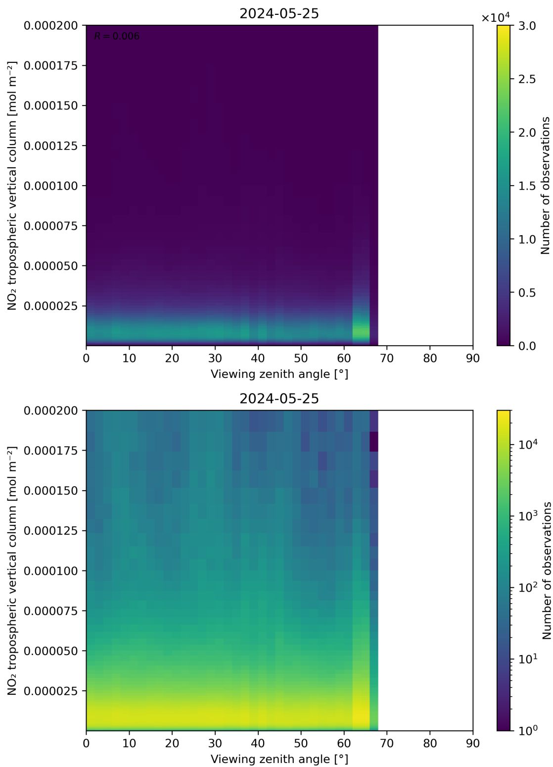
Figure 169: Scatter density plot of “Viewing zenith angle” against “NO 2 tropospheric vertical column” for 2024-05-24 to 2024-05-26.
