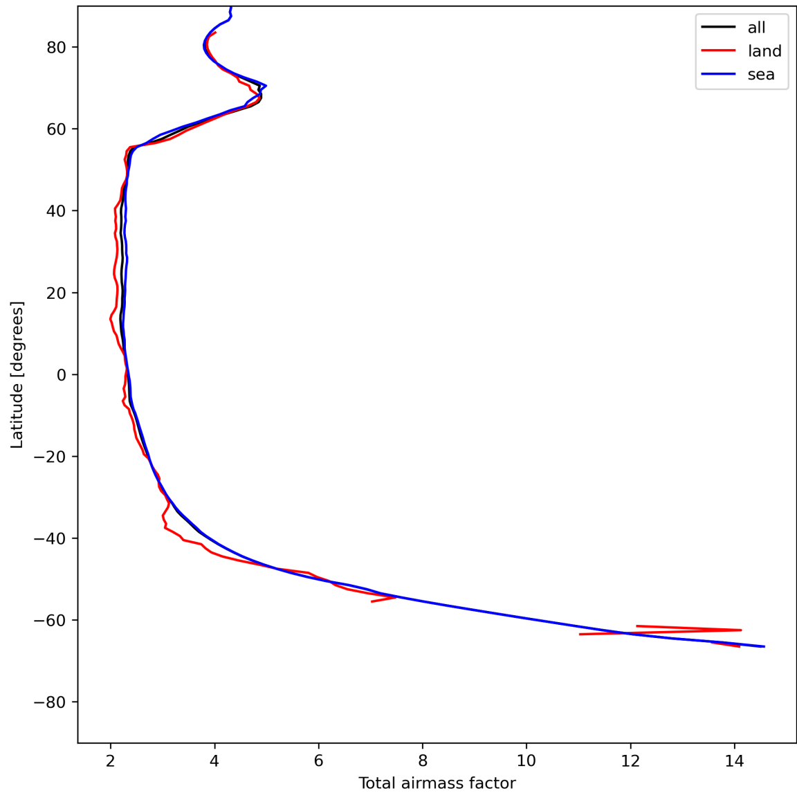
Figure 15: Zonal average of “Total airmass factor” for 2024-05-24 to 2024-05-26.
