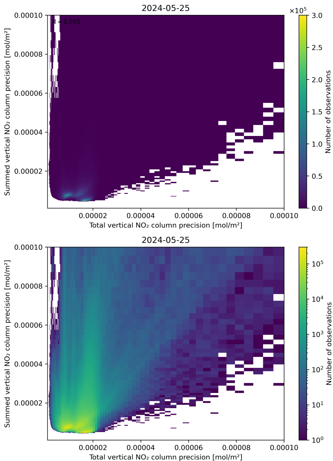
Figure 118: Scatter density plot of “Total vertical NO 2 column precision” against “Summed vertical NO 2 column precision” for 2024-05-24 to 2024-05-26.
