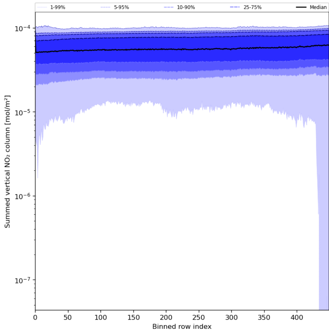
Figure 57: Along track statistics of “Summed vertical NO 2 column” for 2024-05-24 to 2024-05-26
