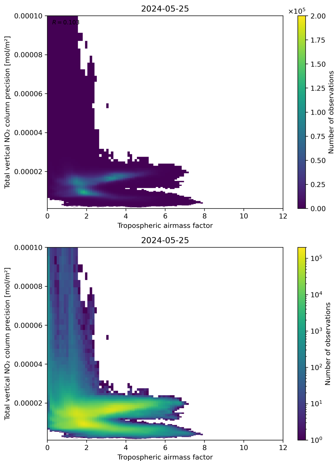
Figure 78: Scatter density plot of “Tropospheric air mass factor” against “Total vertical NO 2 column precision” for 2024-05-24 to 2024-05-26.
