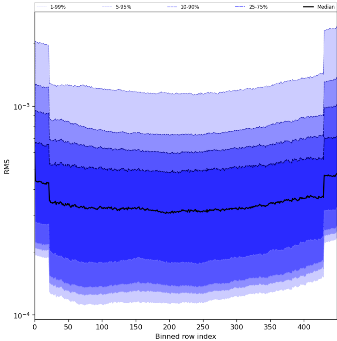
Figure 60: Along track statistics of “RMS” for 2024-05-24 to 2024-05-26
