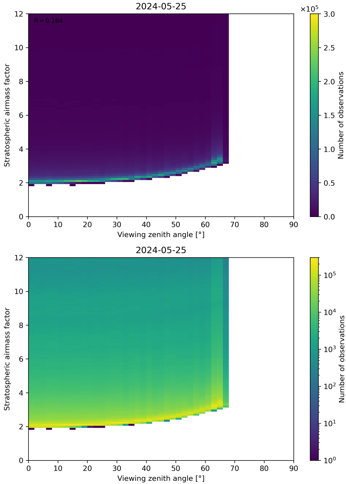
Figure 159: Scatter density plot of “Viewing zenith angle” against “Stratospheric airmass factor” for 2024-05-24 to 2024-05-26.
