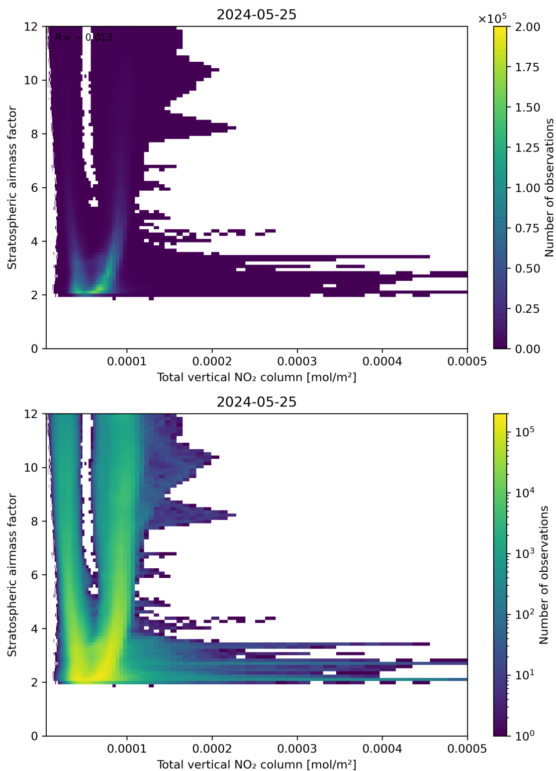
Figure 110: Scatter density plot of “Total vertical NO 2 column” against “Stratospheric airmass factor” for 2024-05-24 to 2024-05-26.
