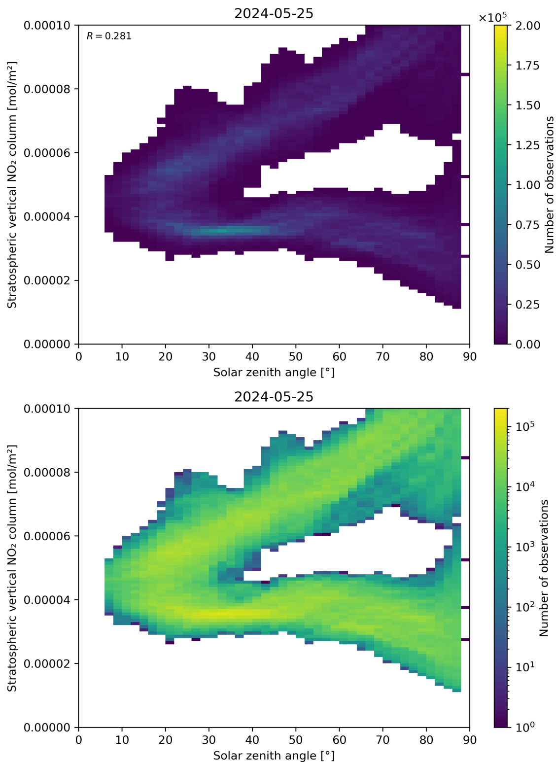
Figure 150: Scatter density plot of “Solar zenith angle” against “Stratospheric vertical NO 2 column” for 2024-05-24 to 2024-05-26.
