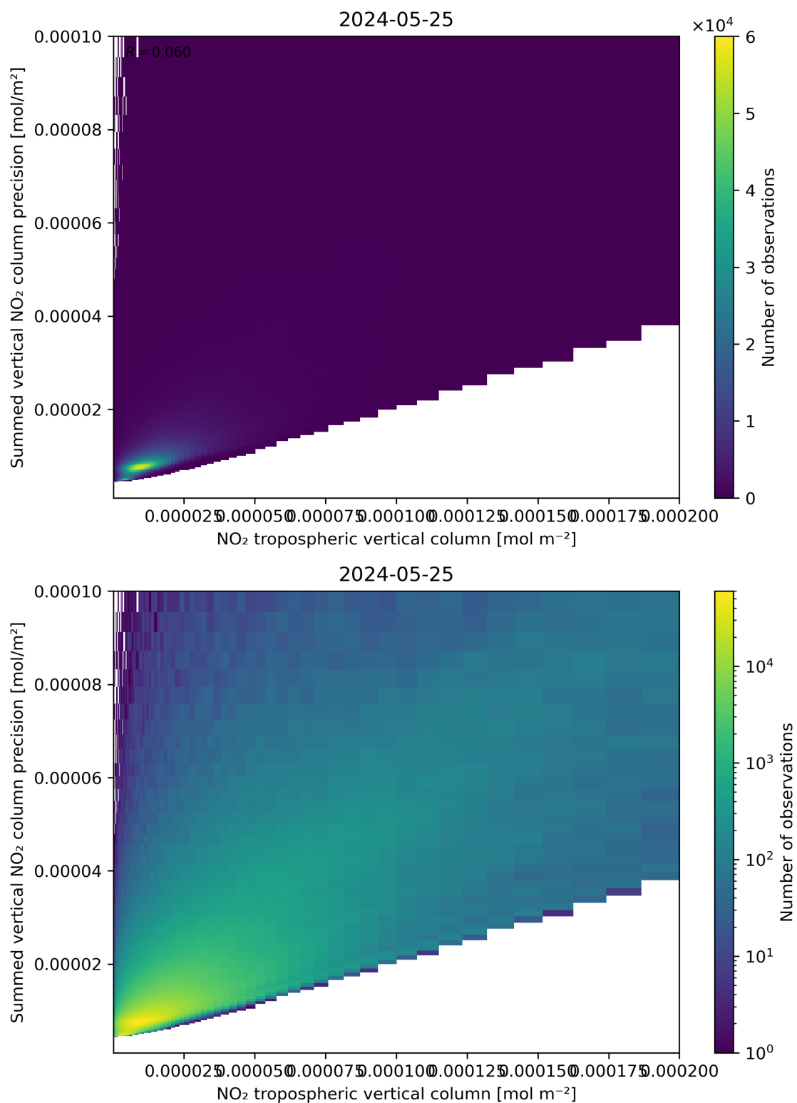
Figure 127: Scatter density plot of “NO 2 tropospheric vertical column” against “Summed vertical NO 2 column precision” for 2024-05-24 to 2024-05-26.
