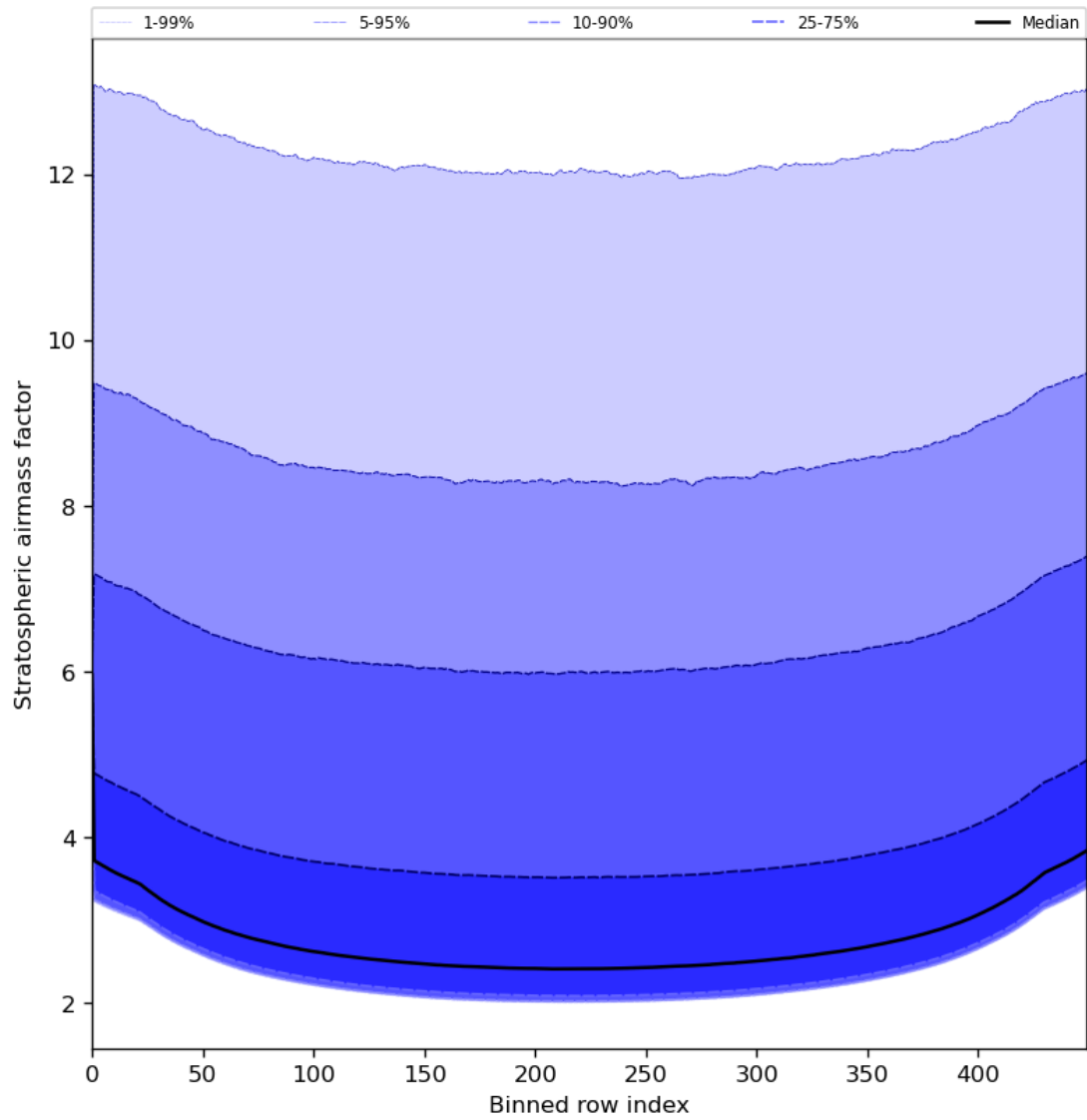
Figure 61: Along track statistics of “Stratospheric airmass factor” for 2024-05-24 to 2024-05-26
