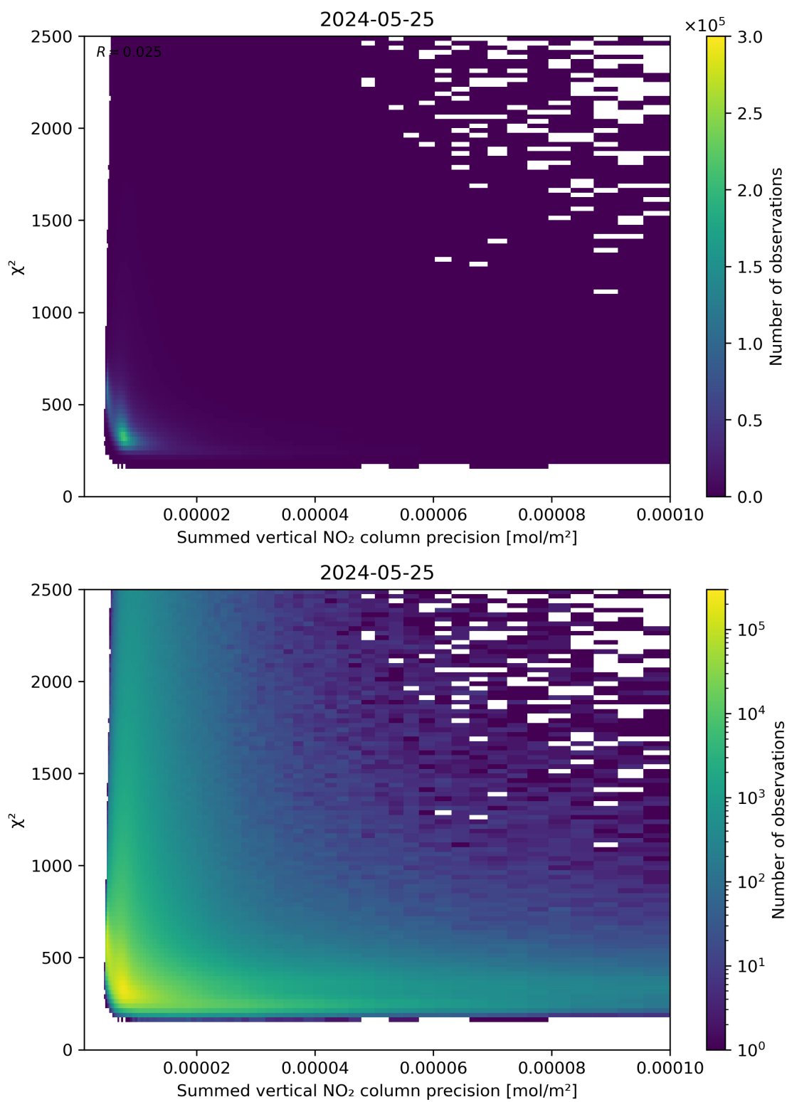
Figure 107: Scatter density plot of “Summed vertical NO 2 column precision” against “ \chi^2 ” for 2024-05-24 to 2024-05-26.
