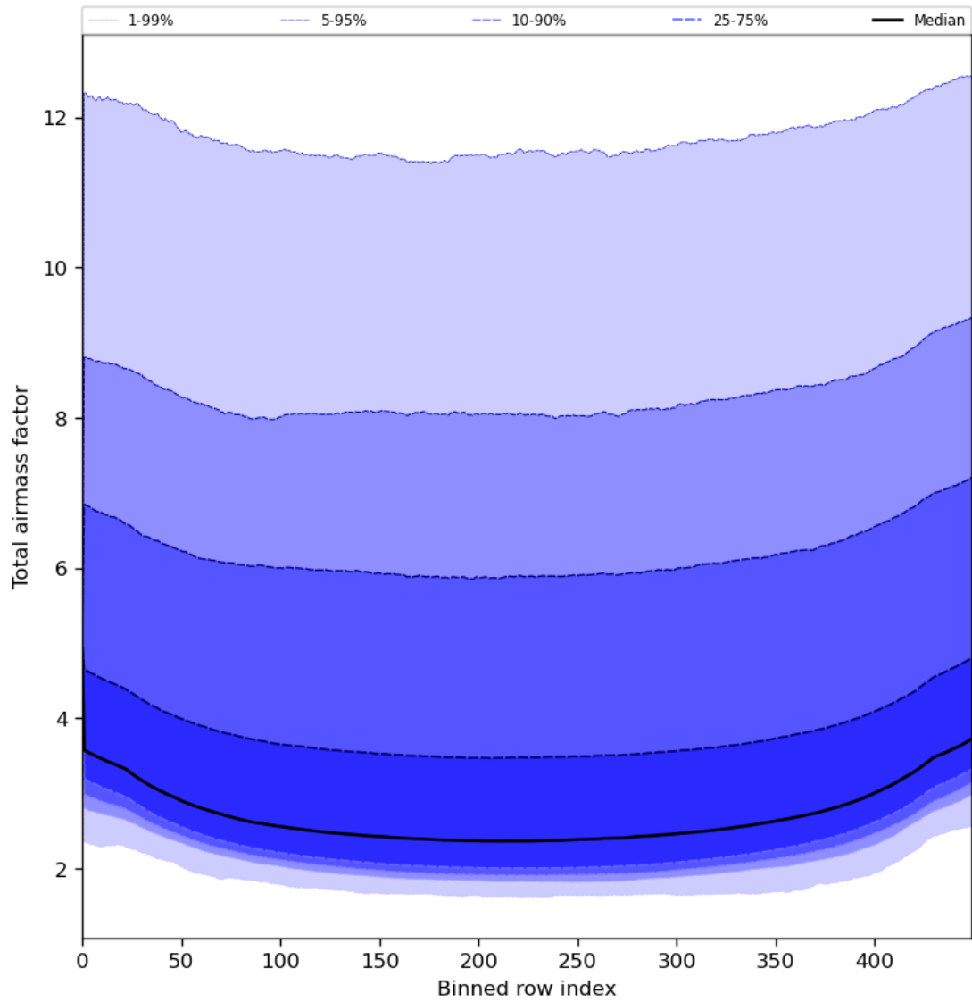
Figure 49: Along track statistics of “Total airmass factor” for 2024-05-24 to 2024-05-26
