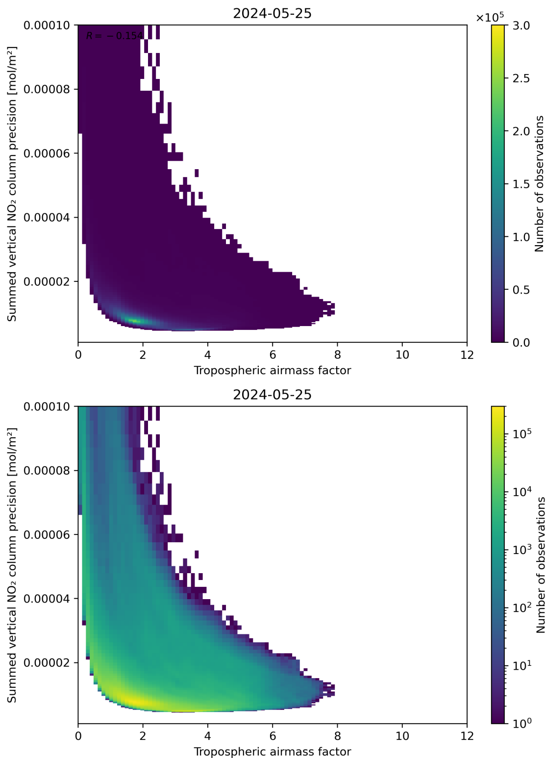
Figure 76: Scatter density plot of “Tropospheric air mass factor” against “Summed vertical NO 2 column precision” for 2024-05-24 to 2024-05-26.
