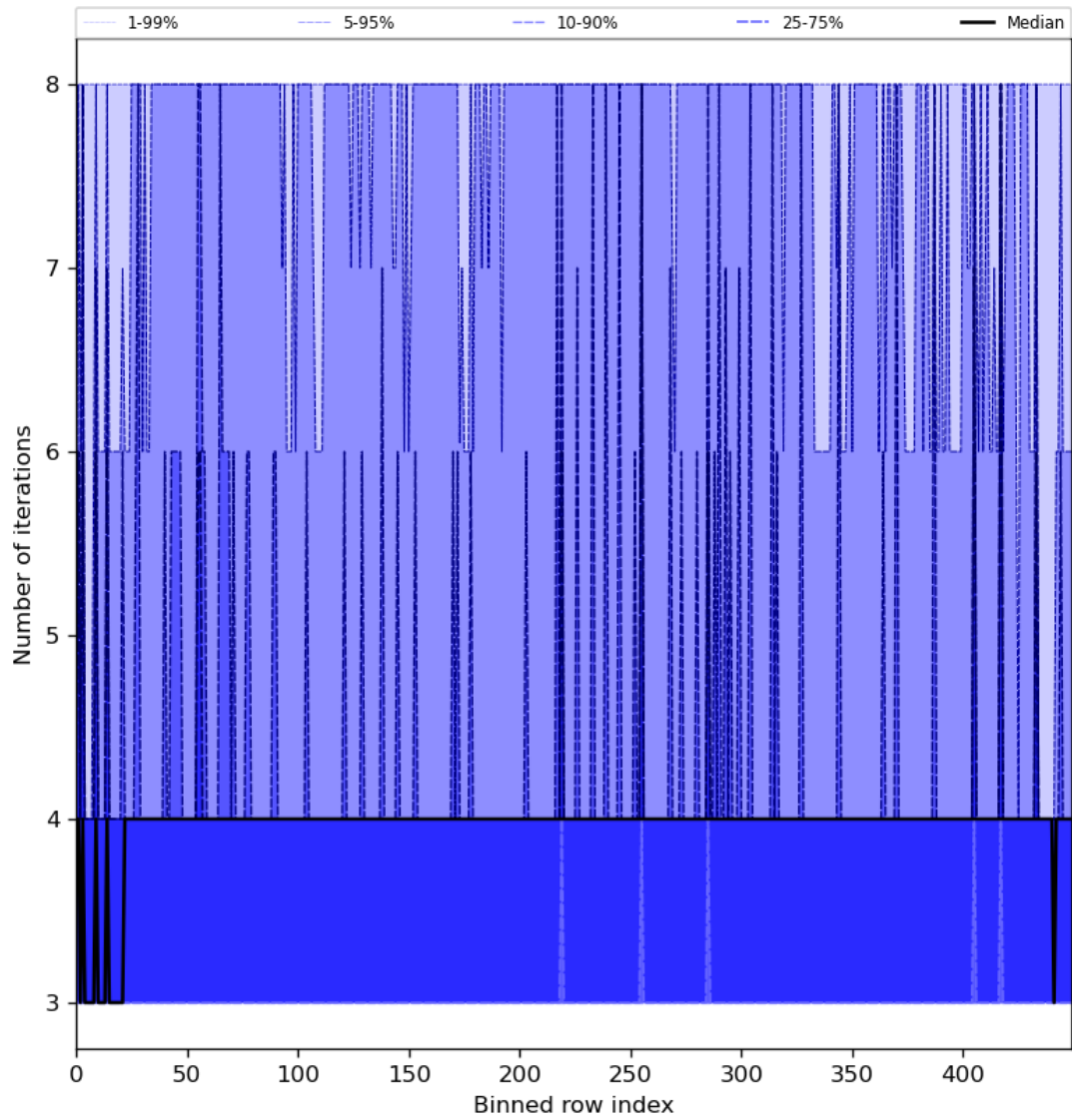
Figure 51: Along track statistics of “Number of iterations” for 2024-05-24 to 2024-05-26
