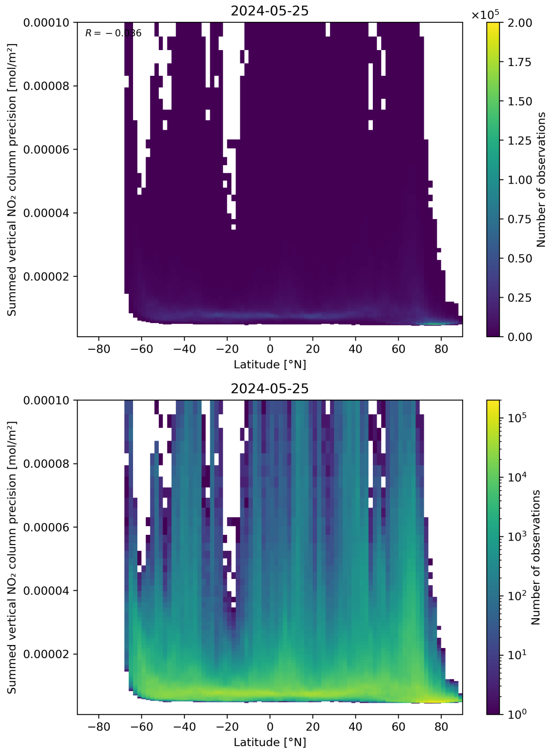
Figure 89: Scatter density plot of “Latitude” against “Summed vertical NO 2 column precision” for 2024-05-24 to 2024-05-26.
