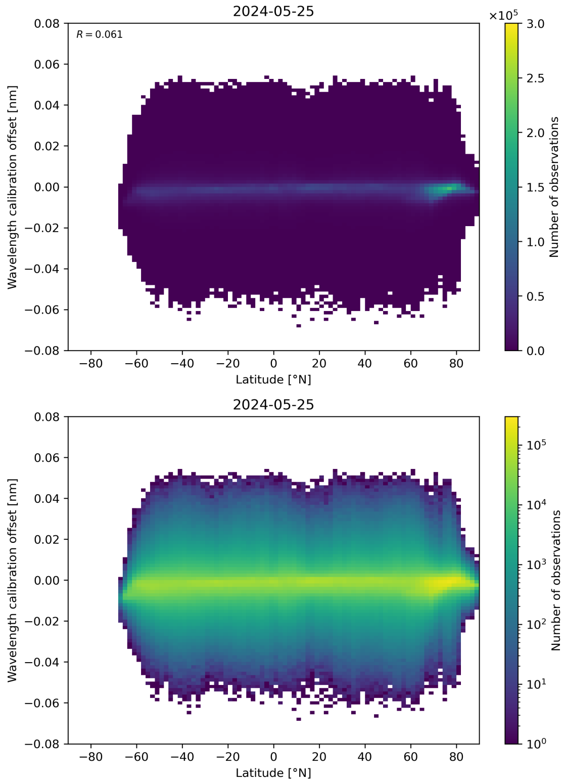
Figure 95: Scatter density plot of “Latitude” against “Wavelength calibration offset” for 2024-05-24 to 2024-05-26.
