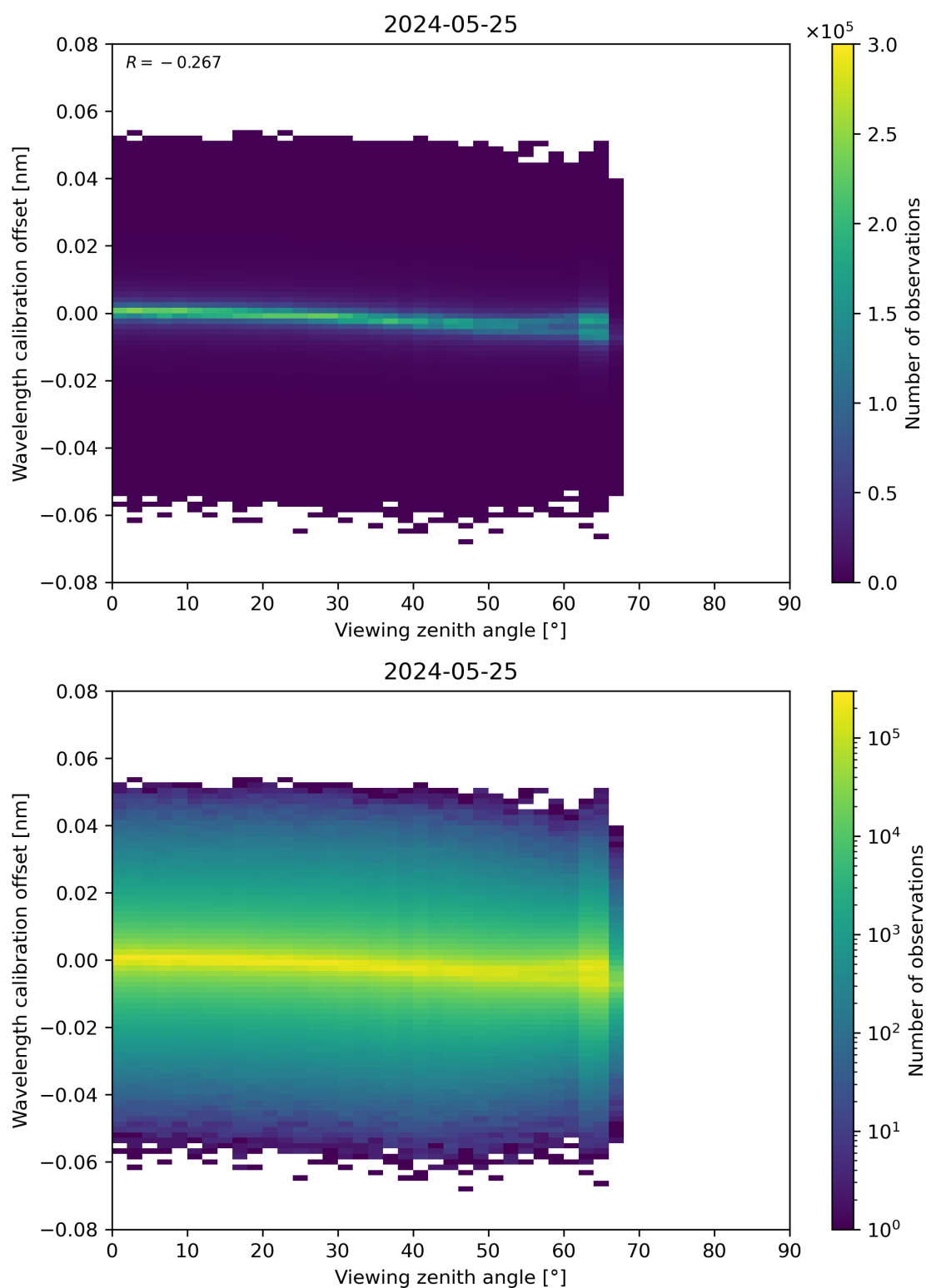
Figure 173: Scatter density plot of “Viewing zenith angle” against “Wavelength calibration offset” for 2024-05-24 to 2024-05-26.
