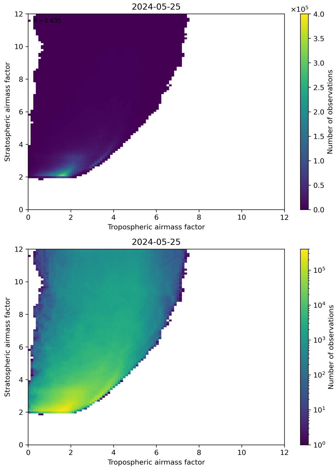
Figure 71: Scatter density plot of “Tropospheric airmass factor” against “Stratospheric airmass factor” for 2024-05-24 to 2024-05-26.
