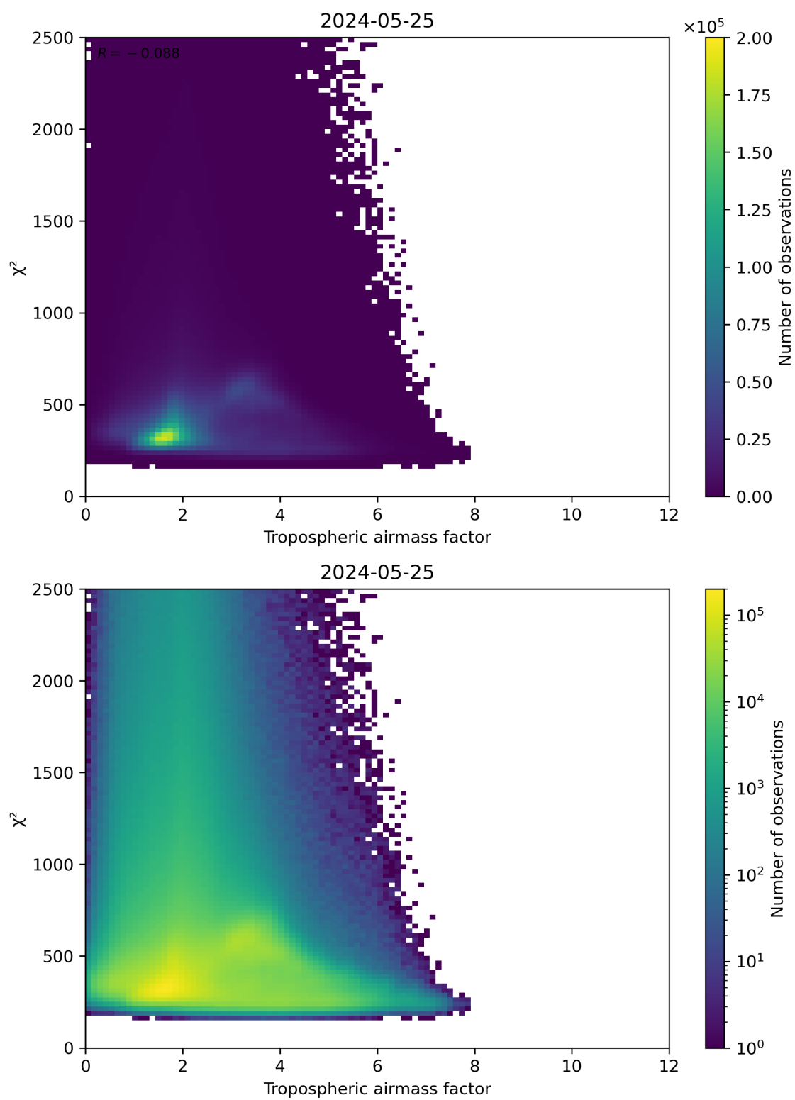
Figure 73: Scatter density plot of “Tropospheric airmass factor” against “ \chi^2 ” for 2024-05-24 to 2024-05-26.
