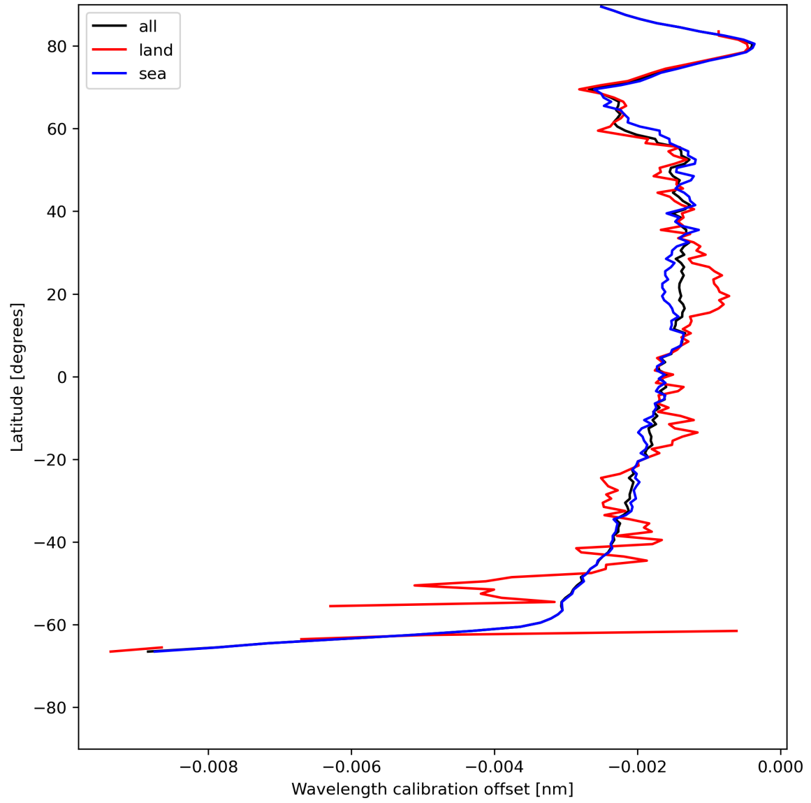
Figure 18: Zonal average of “Wavelength calibration offset” for 2024-05-24 to 2024-05-26.
