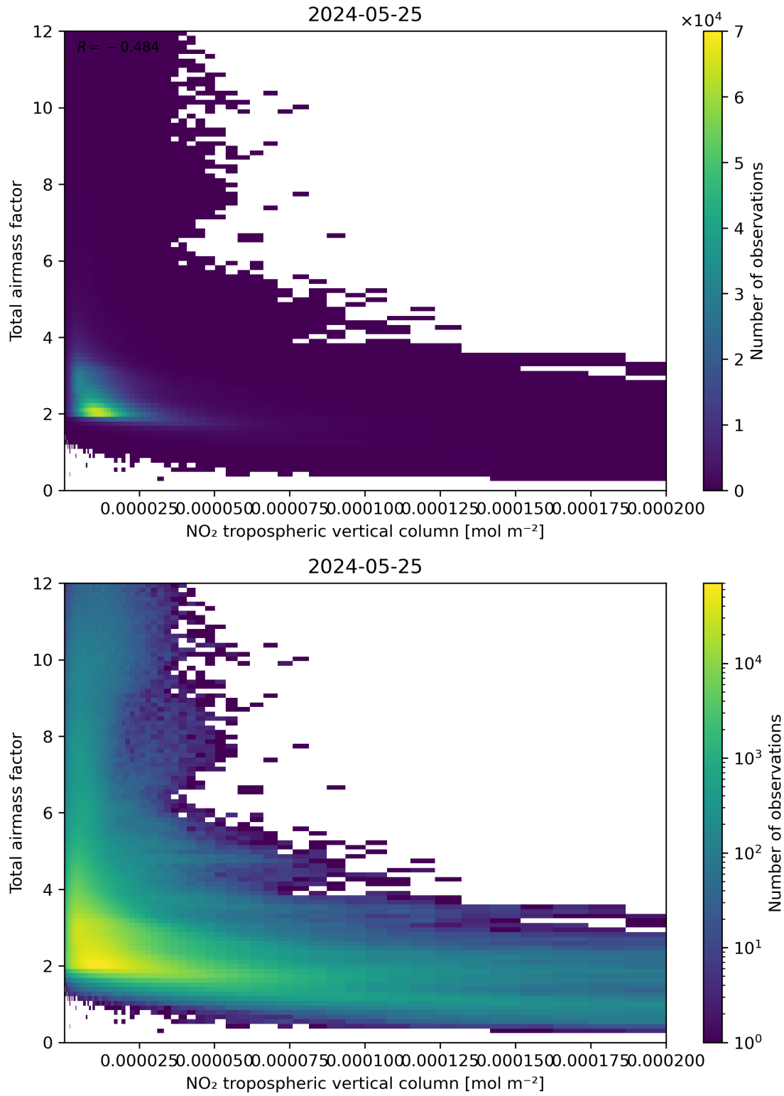
Figure 122: Scatter density plot of “NO 2 tropospheric vertical column” against “Total air mass factor” for 2024-05-24 to 2024-05-26.
