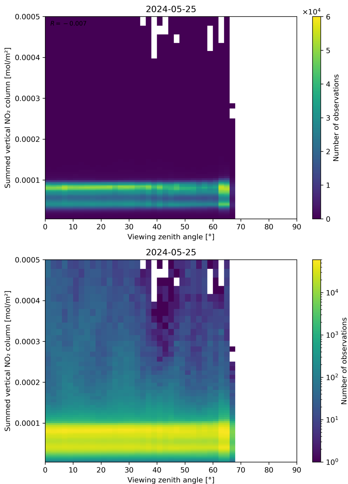
Figure 165: Scatter density plot of “Viewing zenith angle” against “Summed vertical NO 2 column” for 2024-05-24 to 2024-05-26.
