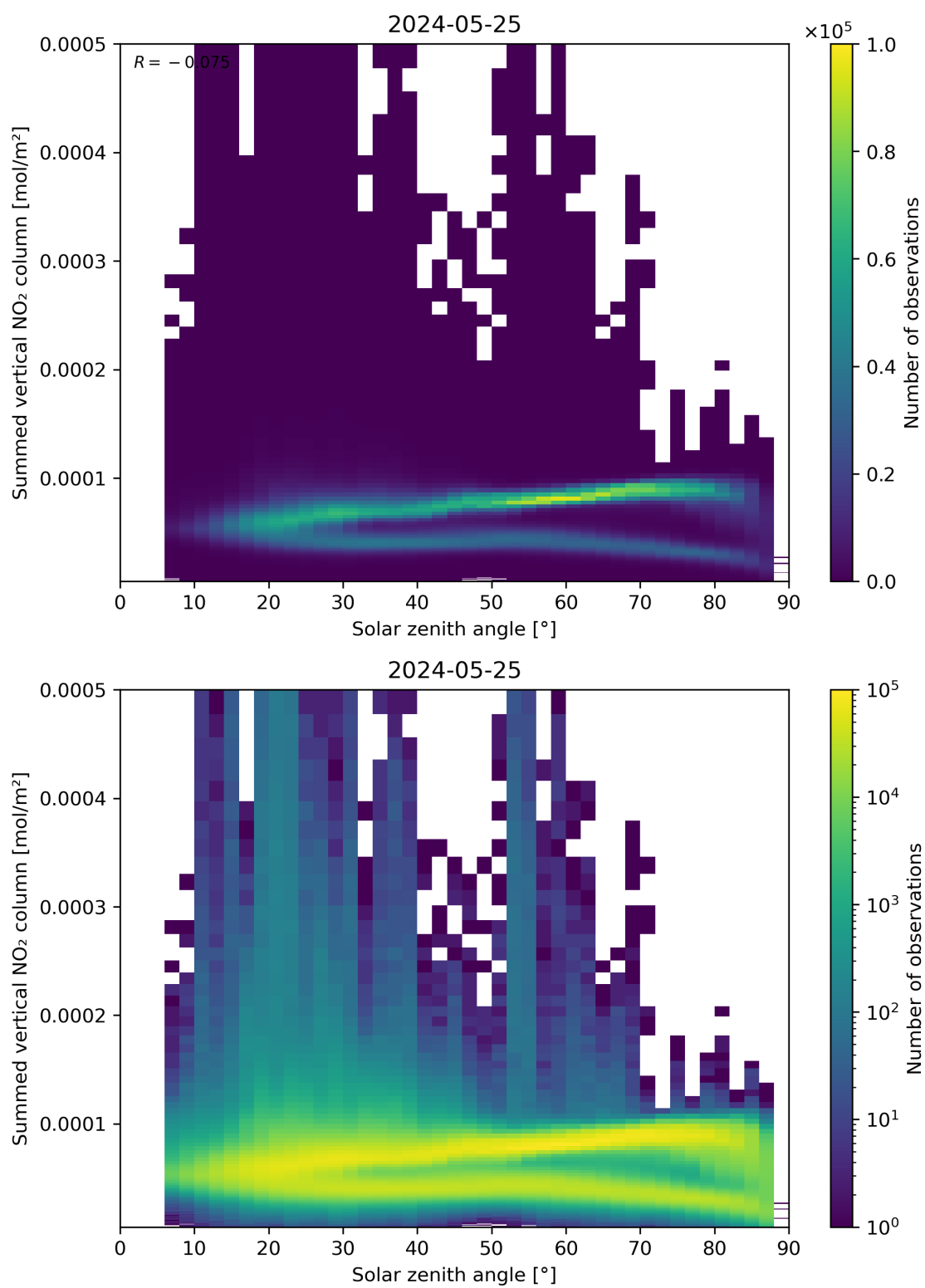
Figure 151: Scatter density plot of “Solar zenith angle” against “Summed vertical NO 2 column” for 2024-05-24 to 2024-05-26.
