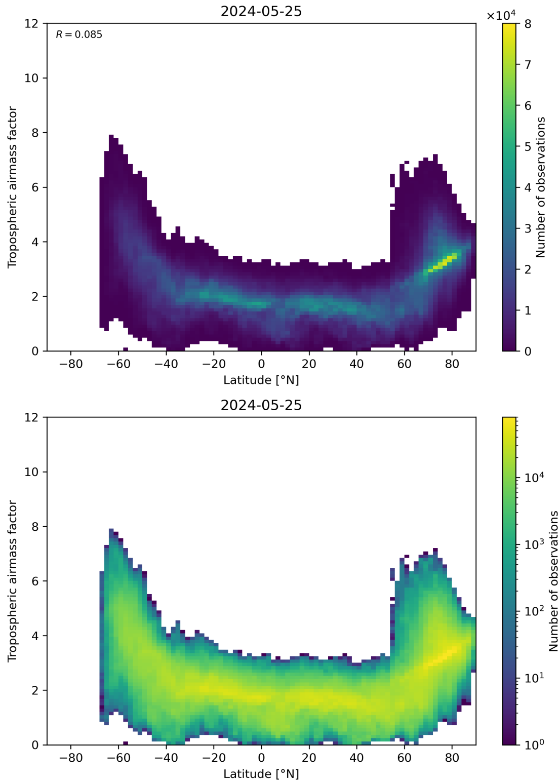
Figure 85: Scatter density plot of “Latitude” against “Tropospheric air mass factor” for 2024-05-24 to 2024-05-26.
