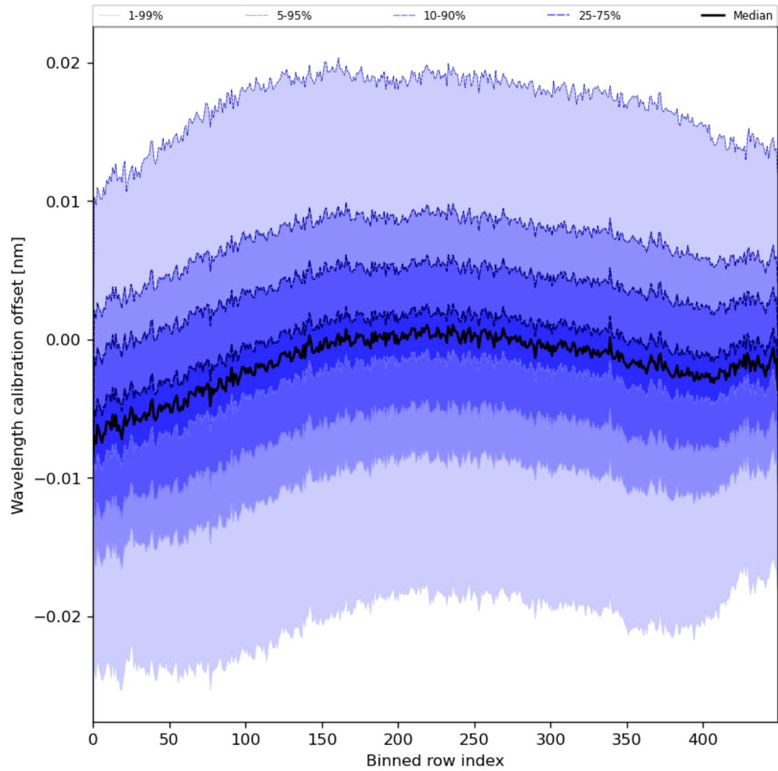
Figure 52: Along track statistics of “Wavelength calibration offset” for 2024-05-24 to 2024-05-26
