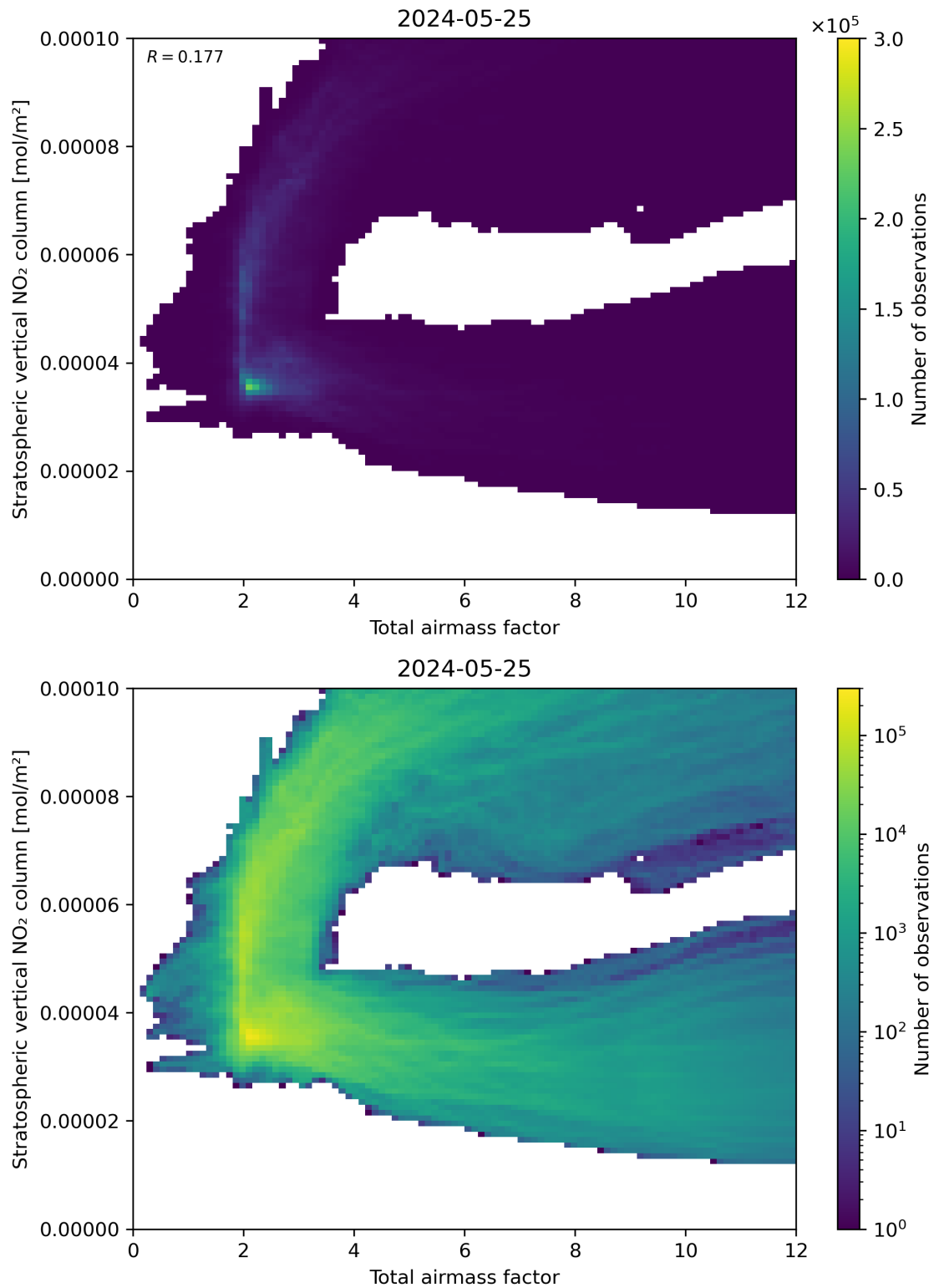
Figure 64: Scatter density plot of “Total airmass factor” against “Stratospheric vertical NO 2 column” for 2024-05-24 to 2024-05-26.
