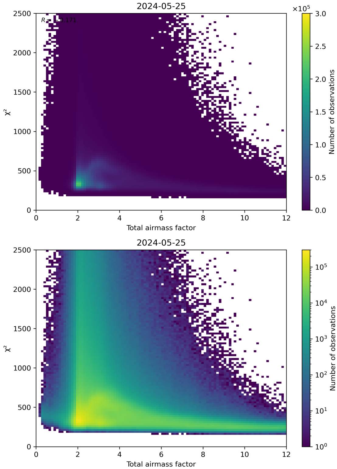
Figure 63: Scatter density plot of “Total airmass factor” against “ \chi^2 ” for 2024-05-24 to 2024-05-26.
