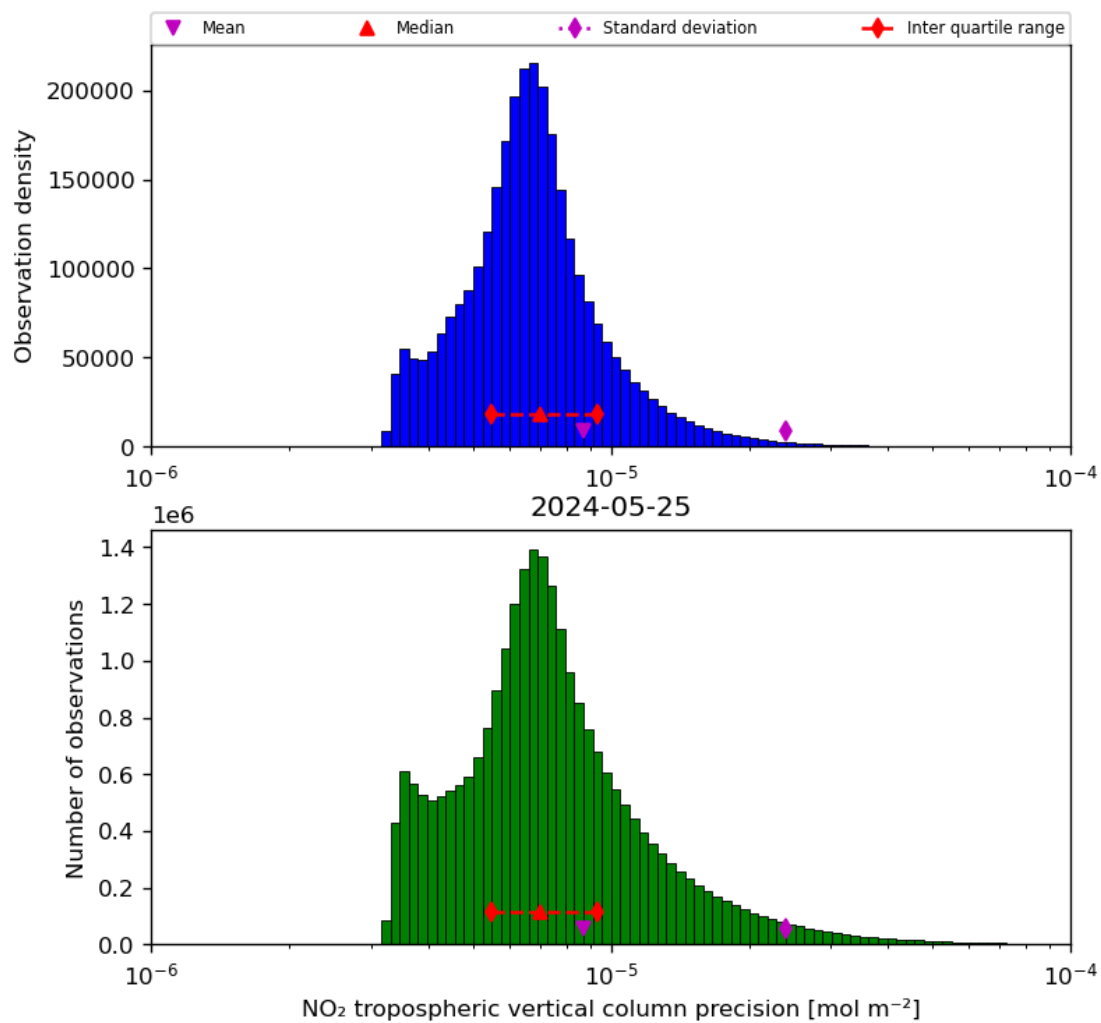
Figure 30: Histogram of “NO 2 tropospheric vertical column precision” for 2024-05-24 to 2024-05-26
