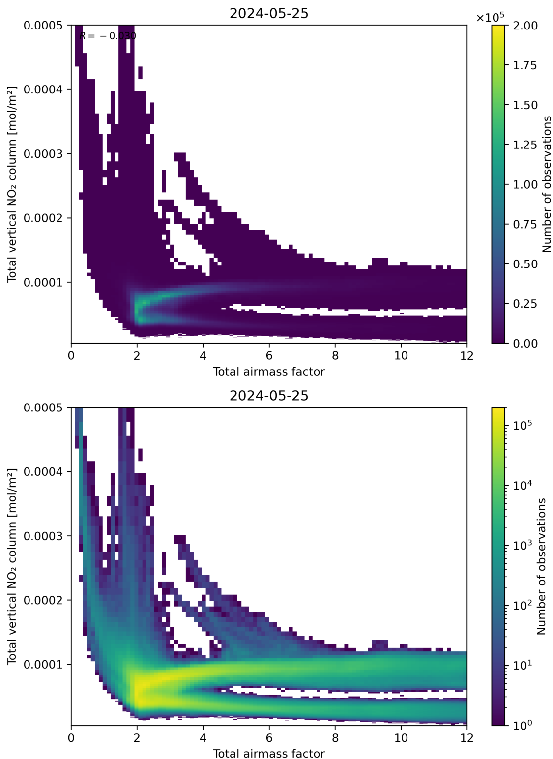
Figure 67: Scatter density plot of “Total airmass factor” against “Total vertical NO 2 column” for 2024-05-24 to 2024-05-26.
