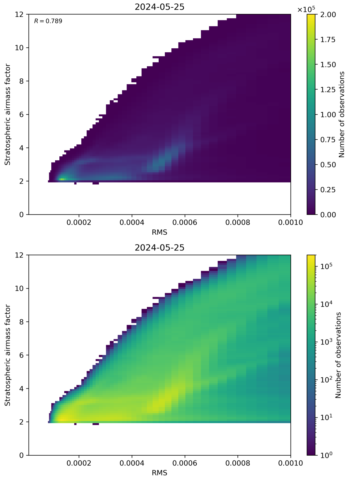
Figure 144: Scatter density plot of “RMS” against “Stratospheric airmass factor” for 2024-05-24 to 2024-05-26.
