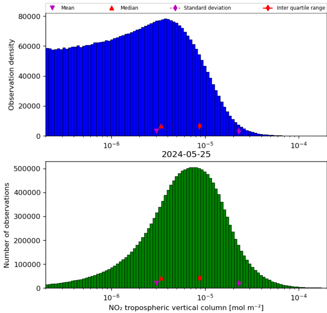
Figure 29: Histogram of “NO 2 tropospheric vertical column” for 2024-05-24 to 2024-05-26
