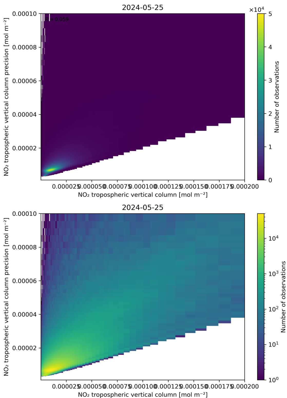
Figure 130: Scatter density plot of “NO 2 tropospheric vertical column” against “NO 2 tropospheric vertical column precision” for 2024-05-24 to 2024-05-26.
