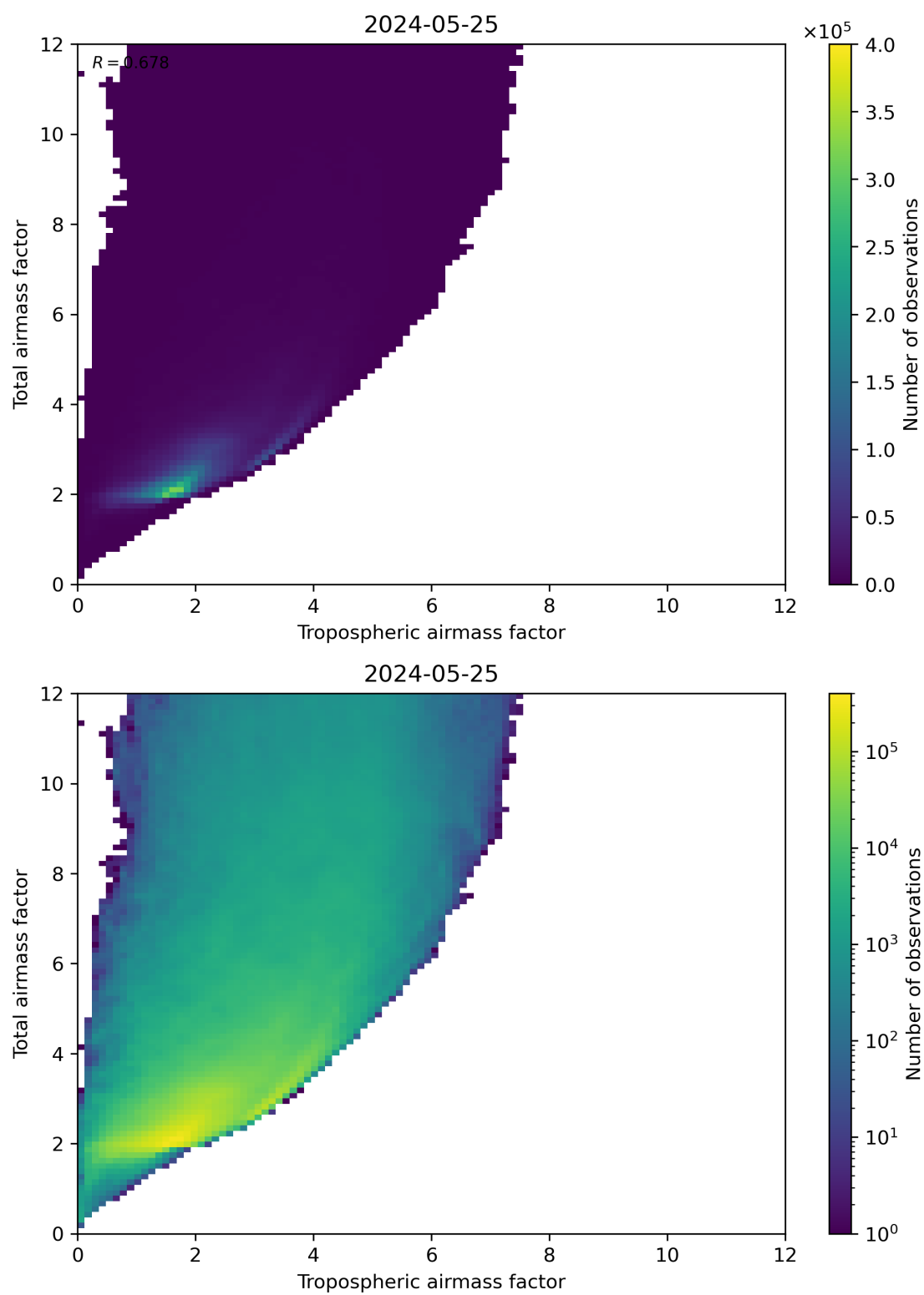
Figure 72: Scatter density plot of “Tropospheric airmass factor” against “Total airmass factor” for 2024-05-24 to 2024-05-26.
