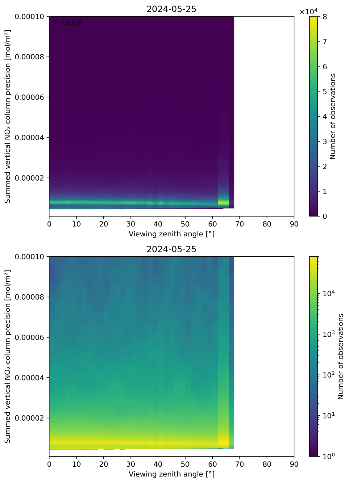
Figure 166: Scatter density plot of “Viewing zenith angle” against “Summed vertical NO 2 column precision” for 2024-05-24 to 2024-05-26.
