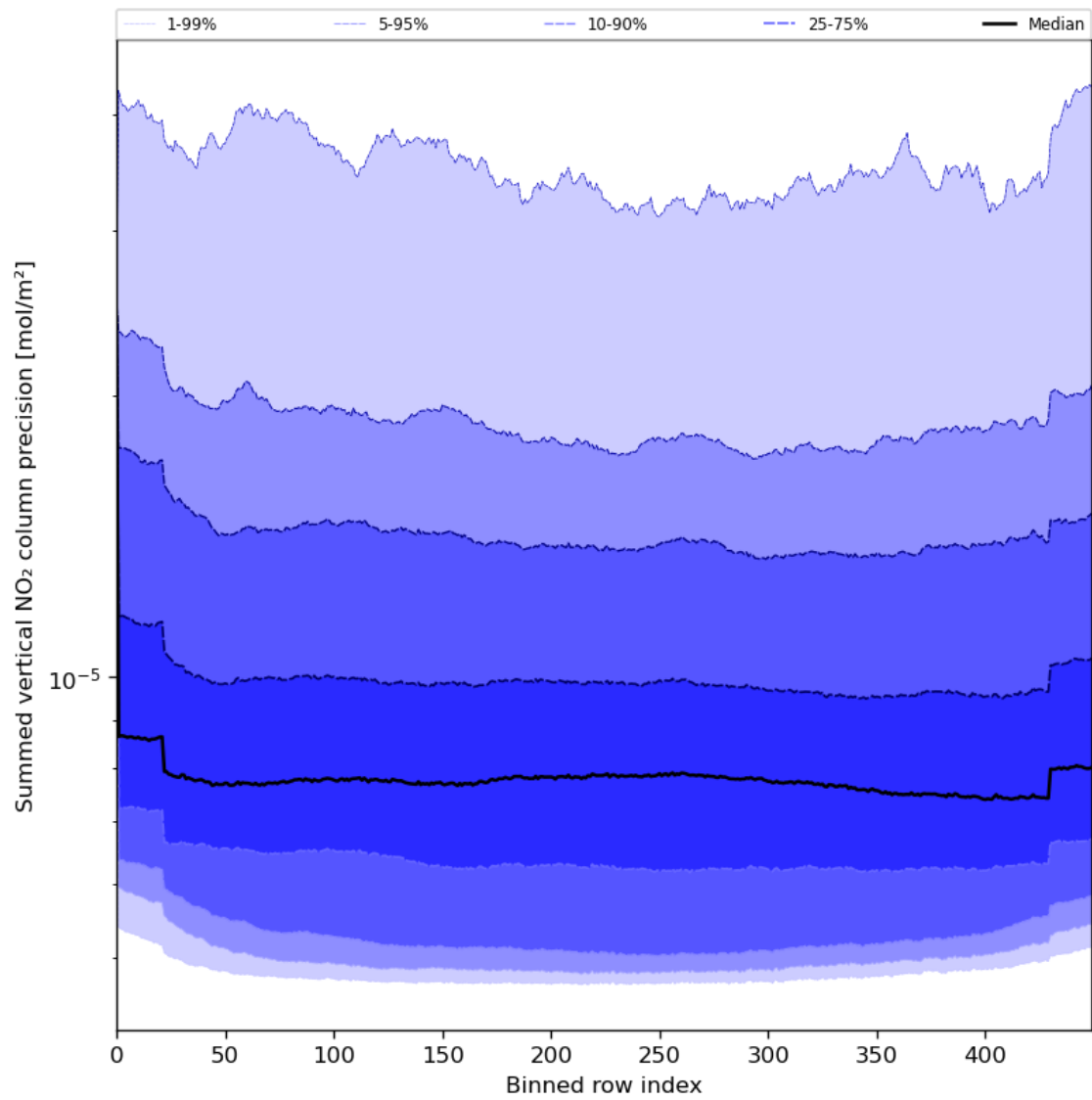
Figure 58: Along track statistics of “Summed vertical NO 2 column precision” for 2024-05-24 to 2024-05-26
