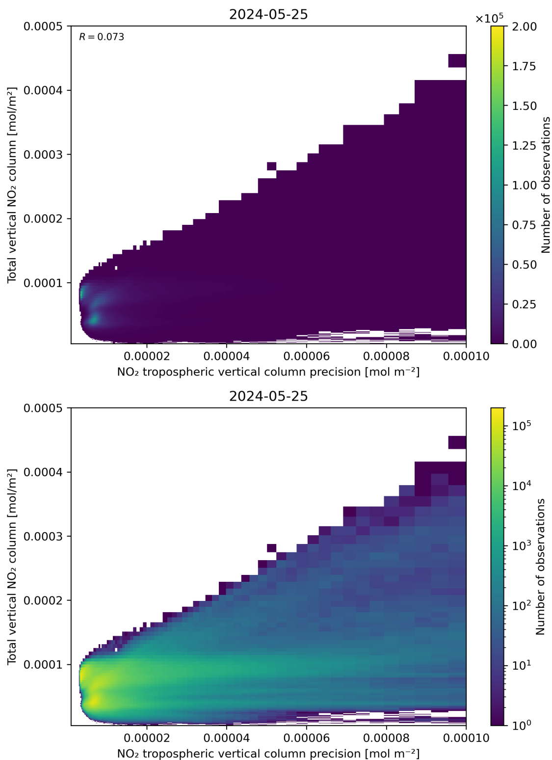
Figure 138: Scatter density plot of “NO 2 tropospheric vertical column precision” against “Total vertical NO 2 column” for 2024-05-24 to 2024-05-26.
