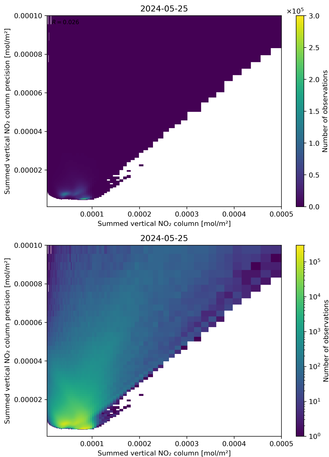
Figure 105: Scatter density plot of “Summed vertical NO 2 column” against “Summed vertical NO 2 column precision” for 2024-05-24 to 2024-05-26.
