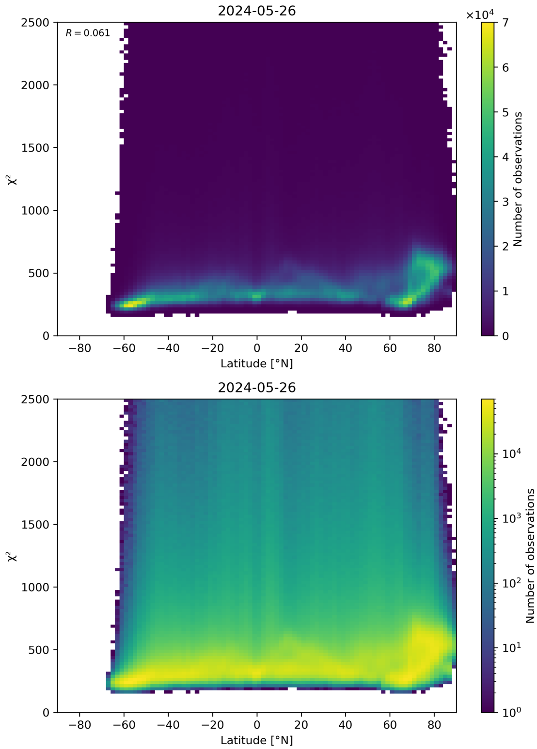
Figure 86: Scatter density plot of “Latitude” against “ \chi^2 ” for 2024-05-25 to 2024-05-27.
