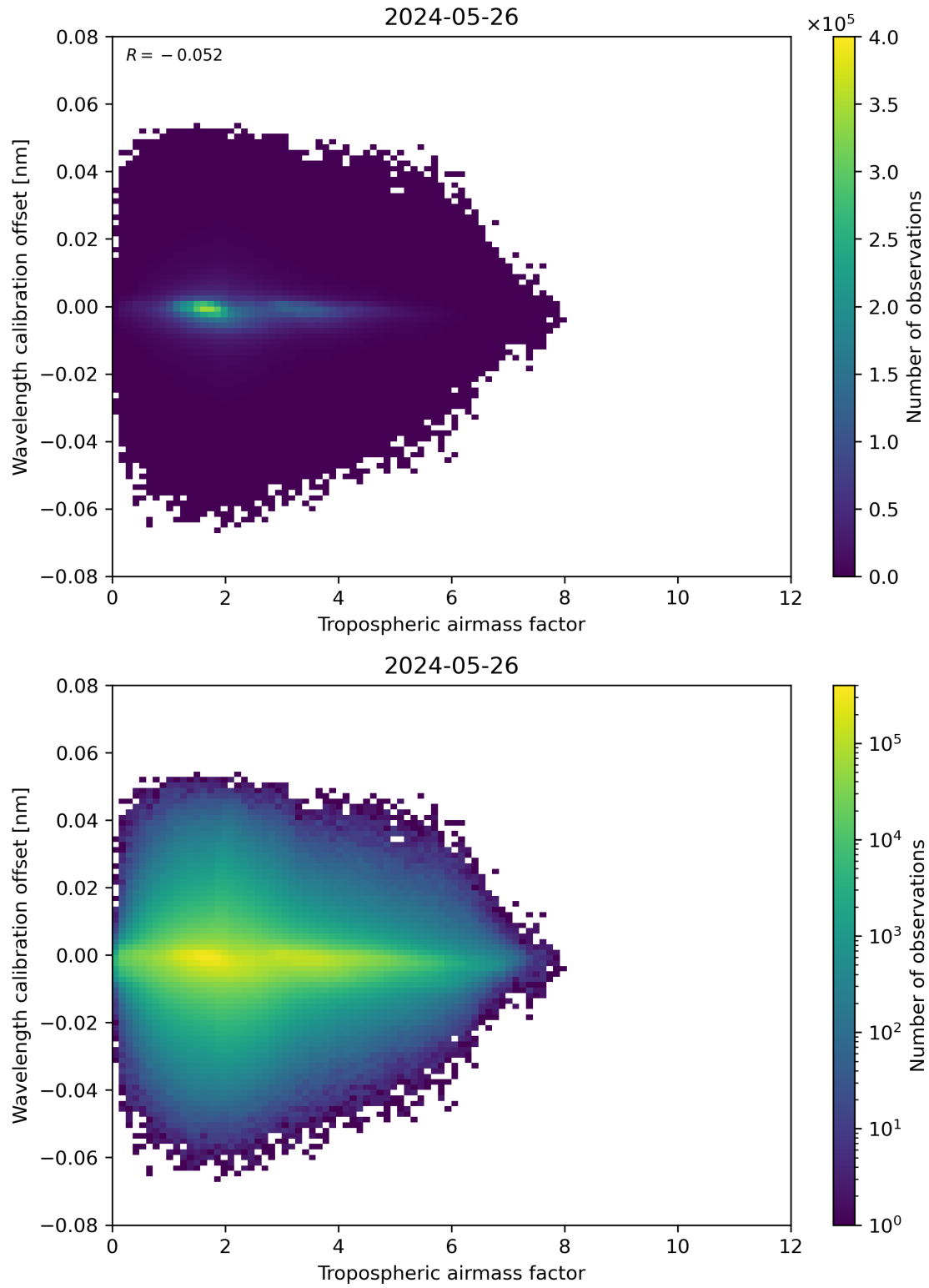
Figure 80: Scatter density plot of “Tropospheric airmass factor” against “Wavelength calibration offset” for 2024-05-25 to 2024-05-27.
