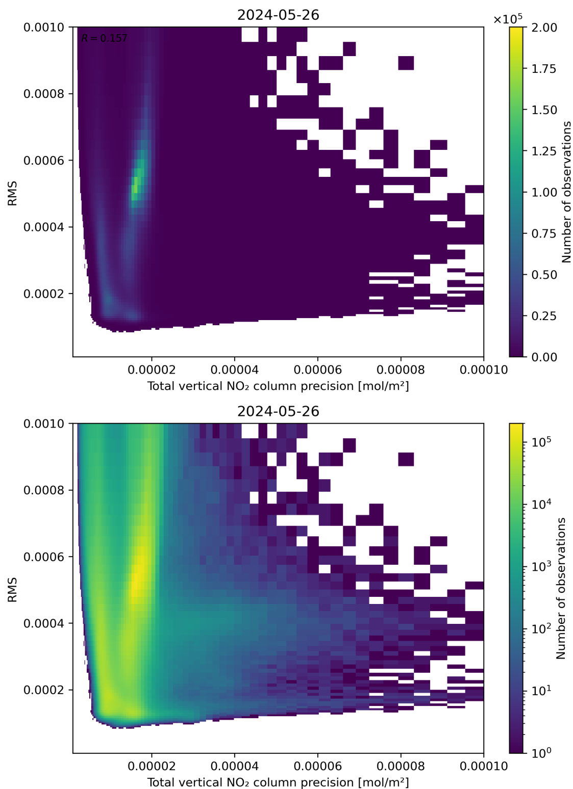
Figure 119: Scatter density plot of “Total vertical NO 2 column precision” against “RMS” for 2024-05-25 to 2024-05-27.
