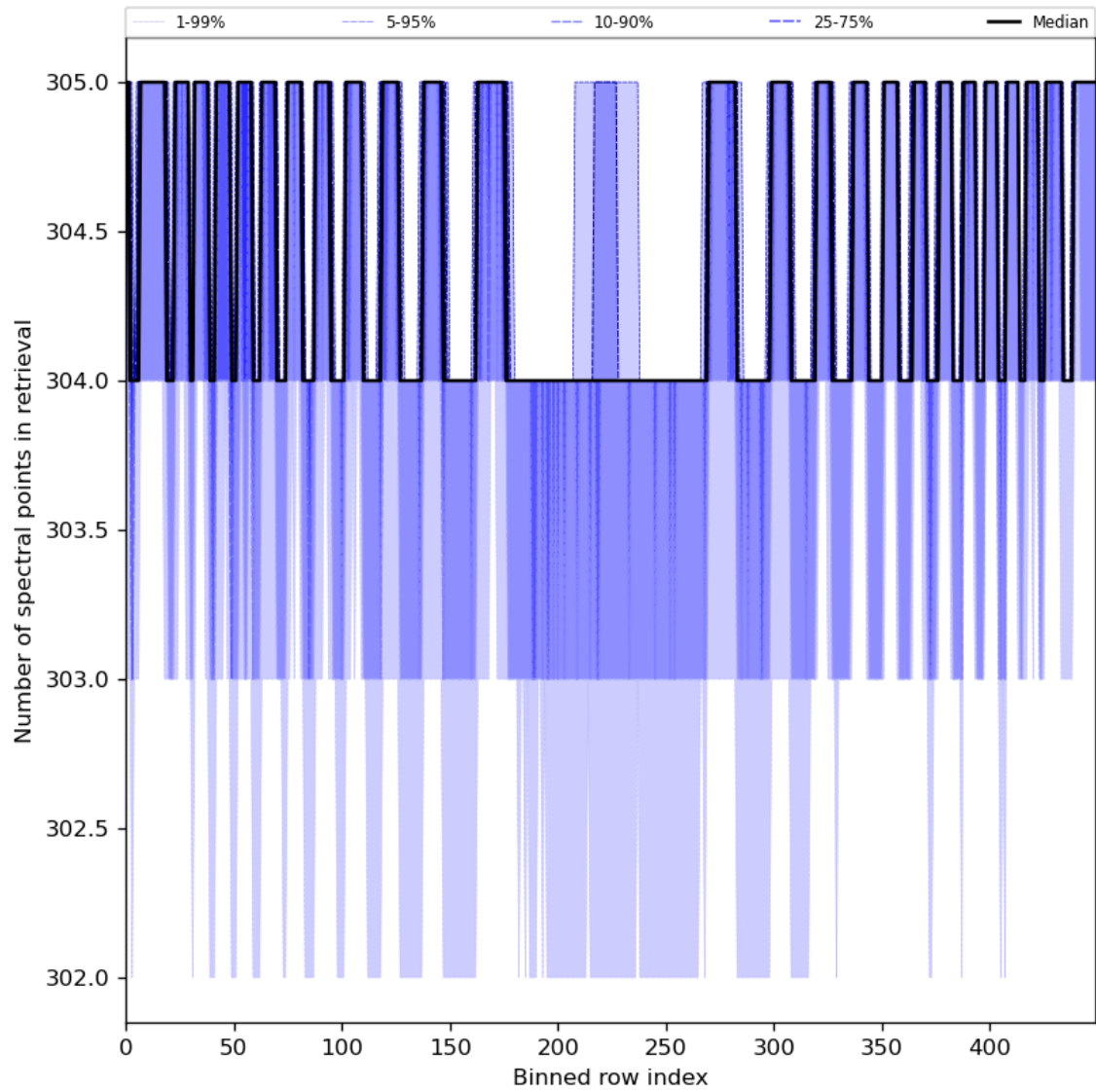
Figure 50: Along track statistics of “Number of spectral points in retrieval” for 2024-05-25 to 2024-05-27
