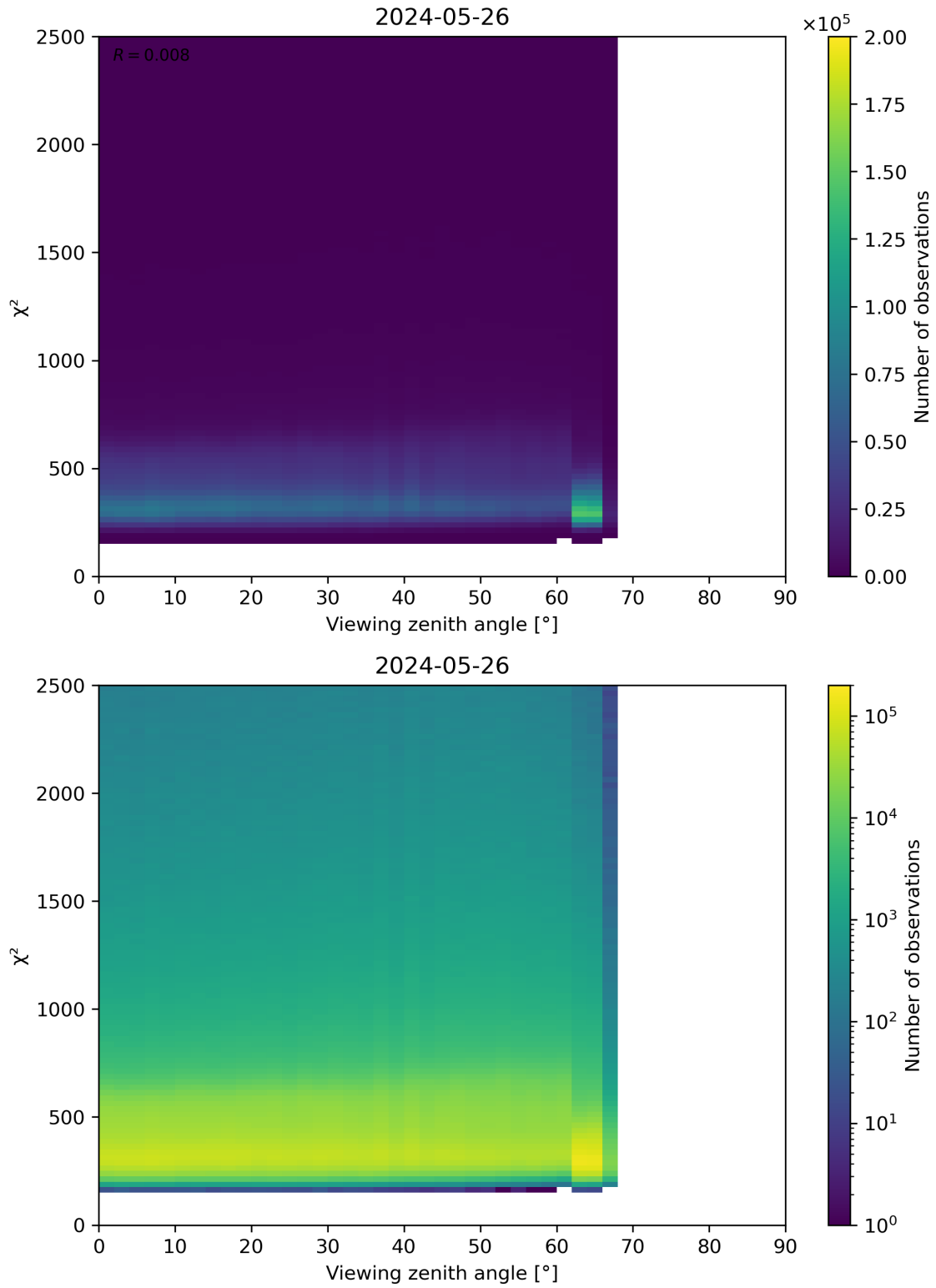
Figure 162: Scatter density plot of “Viewing zenith angle” against “ \chi^2 ” for 2024-05-25 to 2024-05-27.
