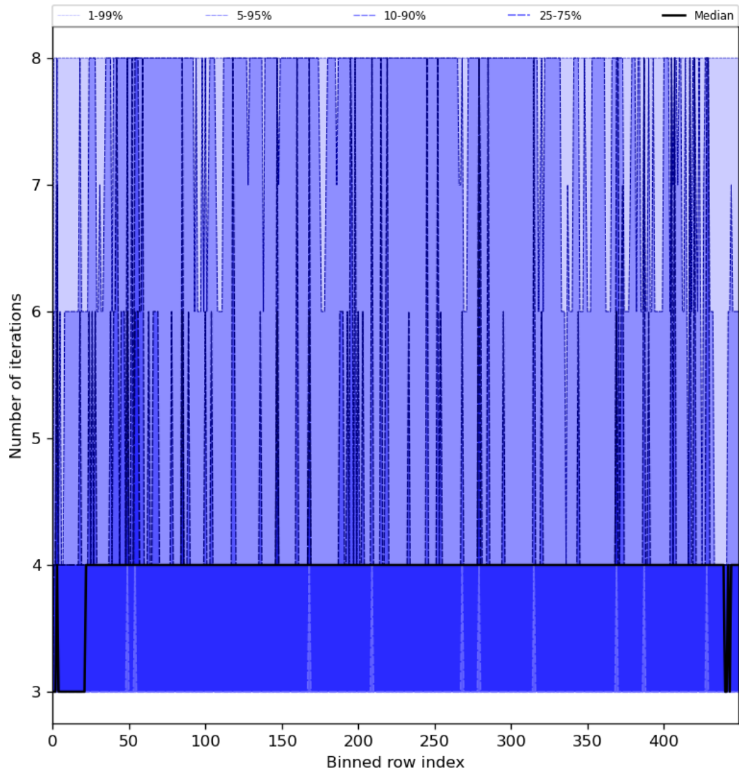
Figure 51: Along track statistics of “Number of iterations” for 2024-05-25 to 2024-05-27
