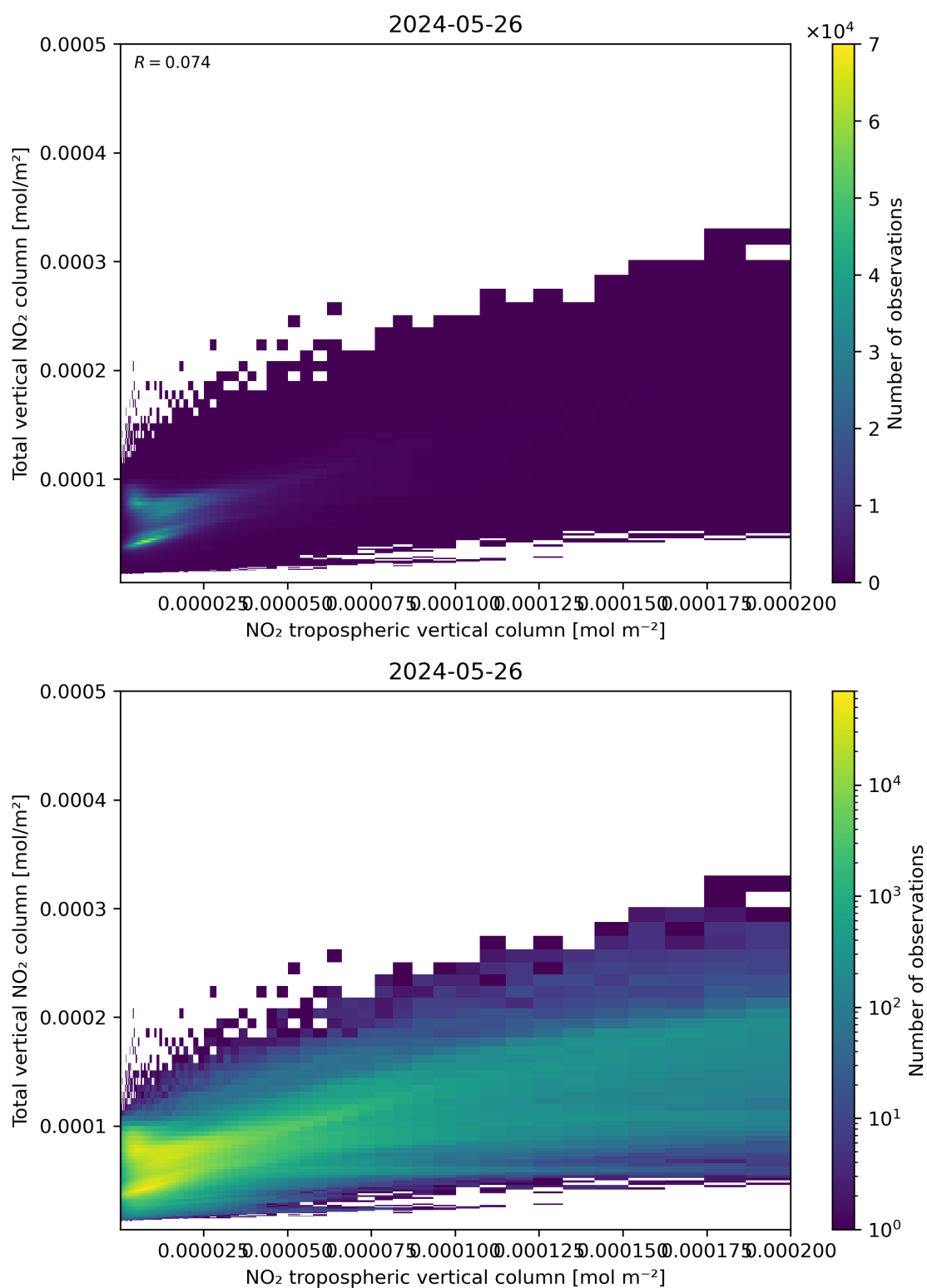
Figure 128: Scatter density plot of “NO 2 tropospheric vertical column” against “Total vertical NO 2 column” for 2024-05-25 to 2024-05-27.
