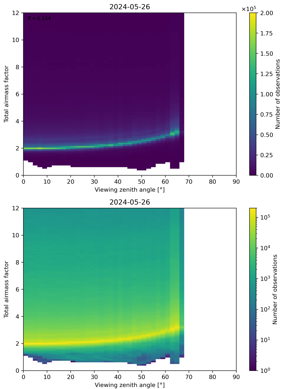
Figure 160: Scatter density plot of “Viewing zenith angle” against “Total airmass factor” for 2024-05-25 to 2024-05-27.
