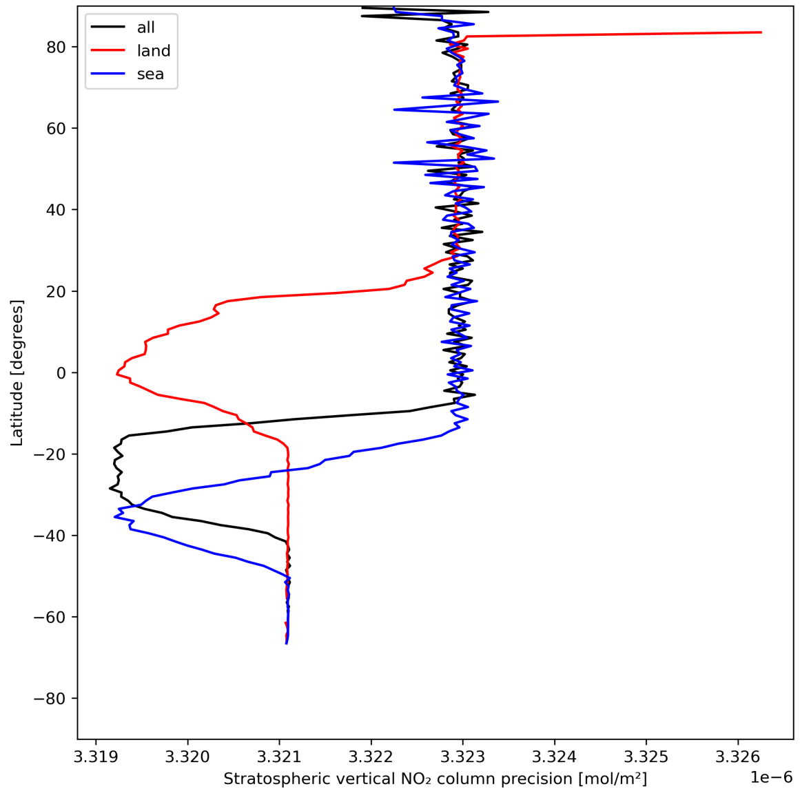
Figure 20: Zonal average of “Stratospheric vertical NO 2 column precision” for 2024-05-25 to 2024-05-27.
