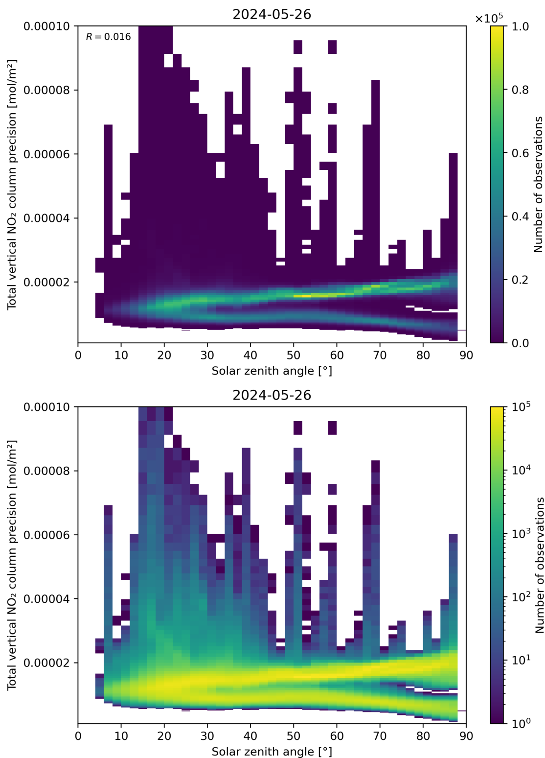
Figure 154: Scatter density plot of “Solar zenith angle” against “Total vertical NO 2 column precision” for 2024-05-25 to 2024-05-27.
