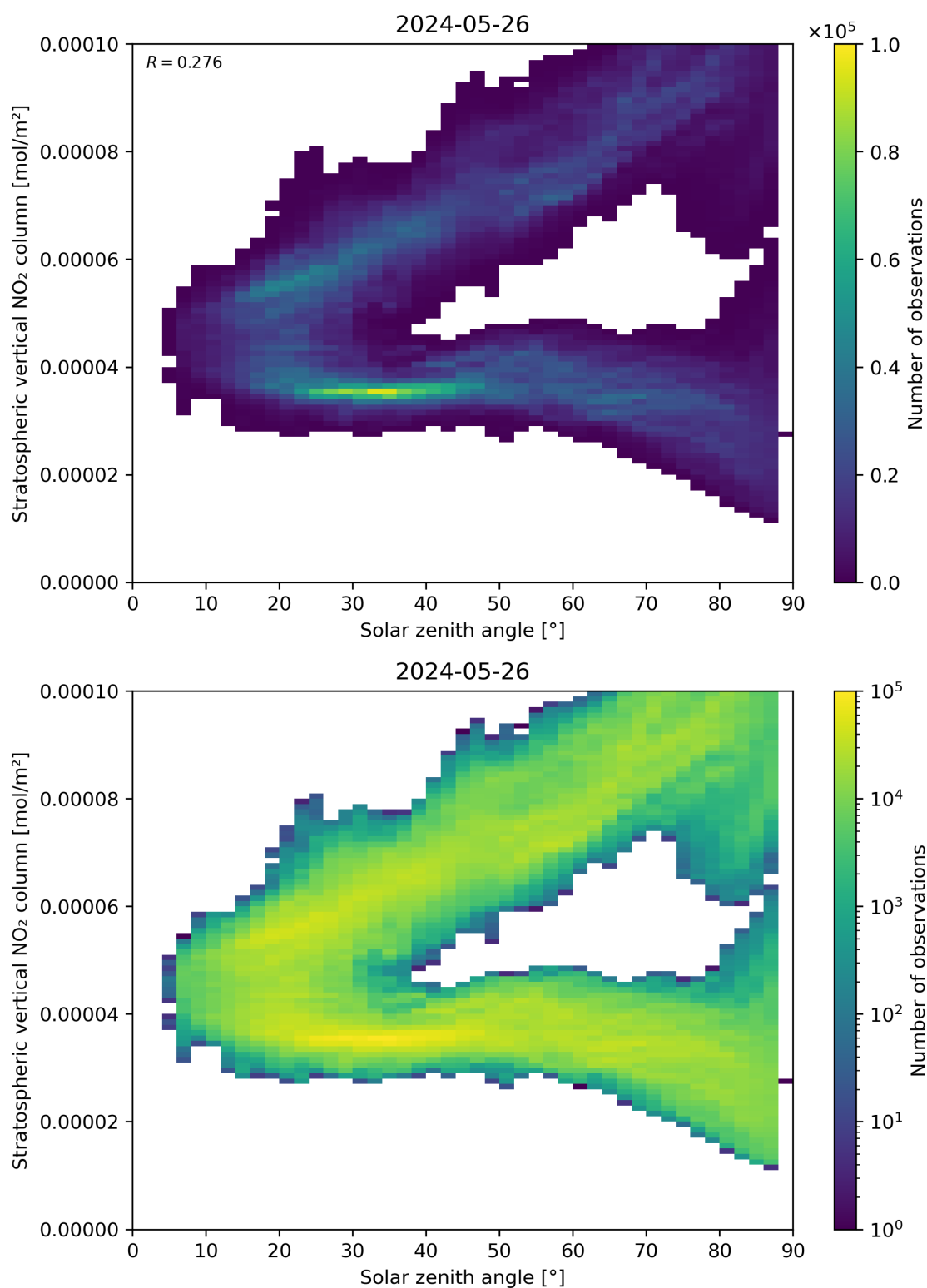
Figure 150: Scatter density plot of “Solar zenith angle” against “Stratospheric vertical \text{NO}_2 column” for 2024-05-25 to 2024-05-27.
