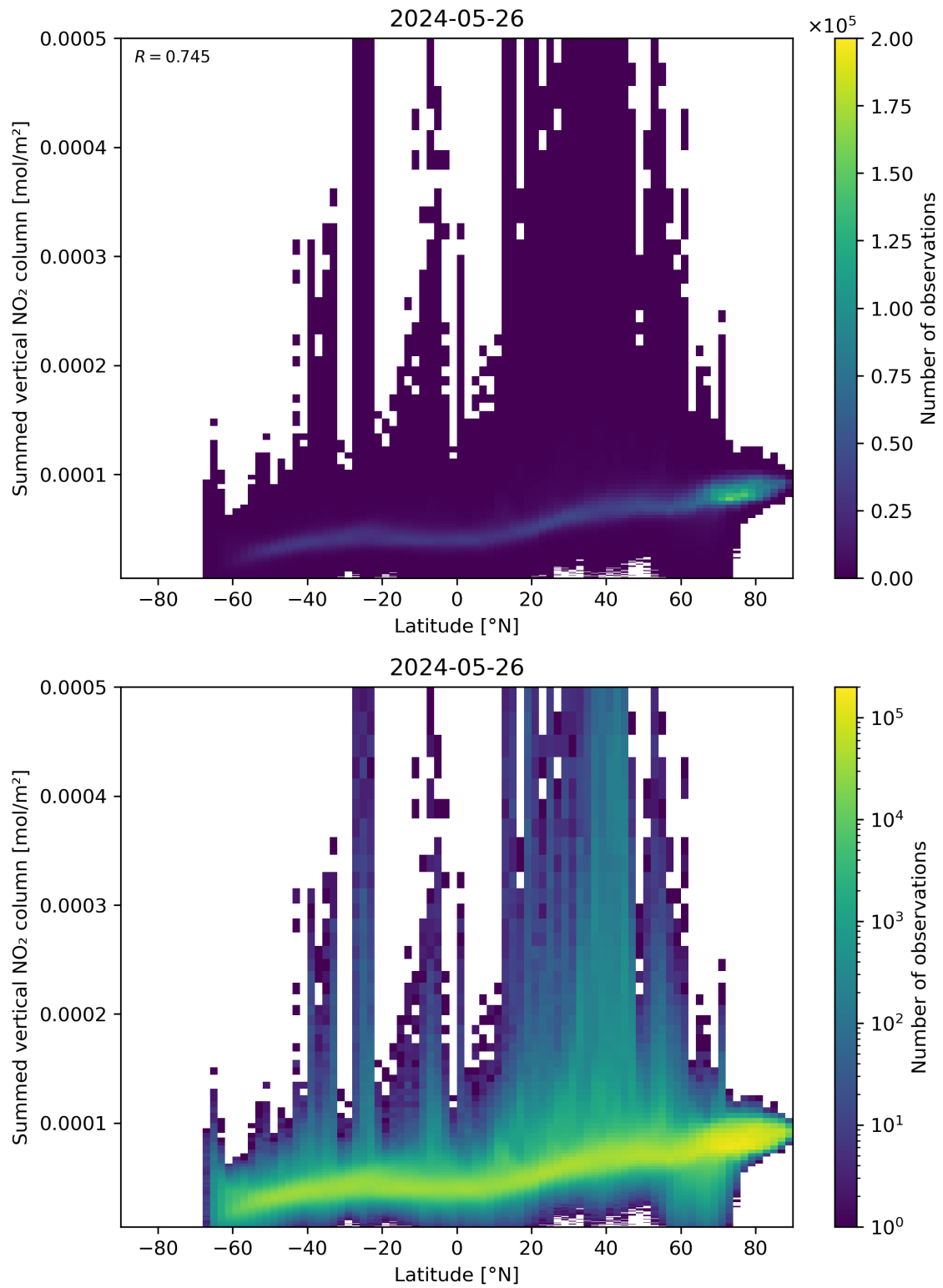
Figure 88: Scatter density plot of “Latitude” against “Summed vertical NO 2 column” for 2024-05-25 to 2024-05-27.
