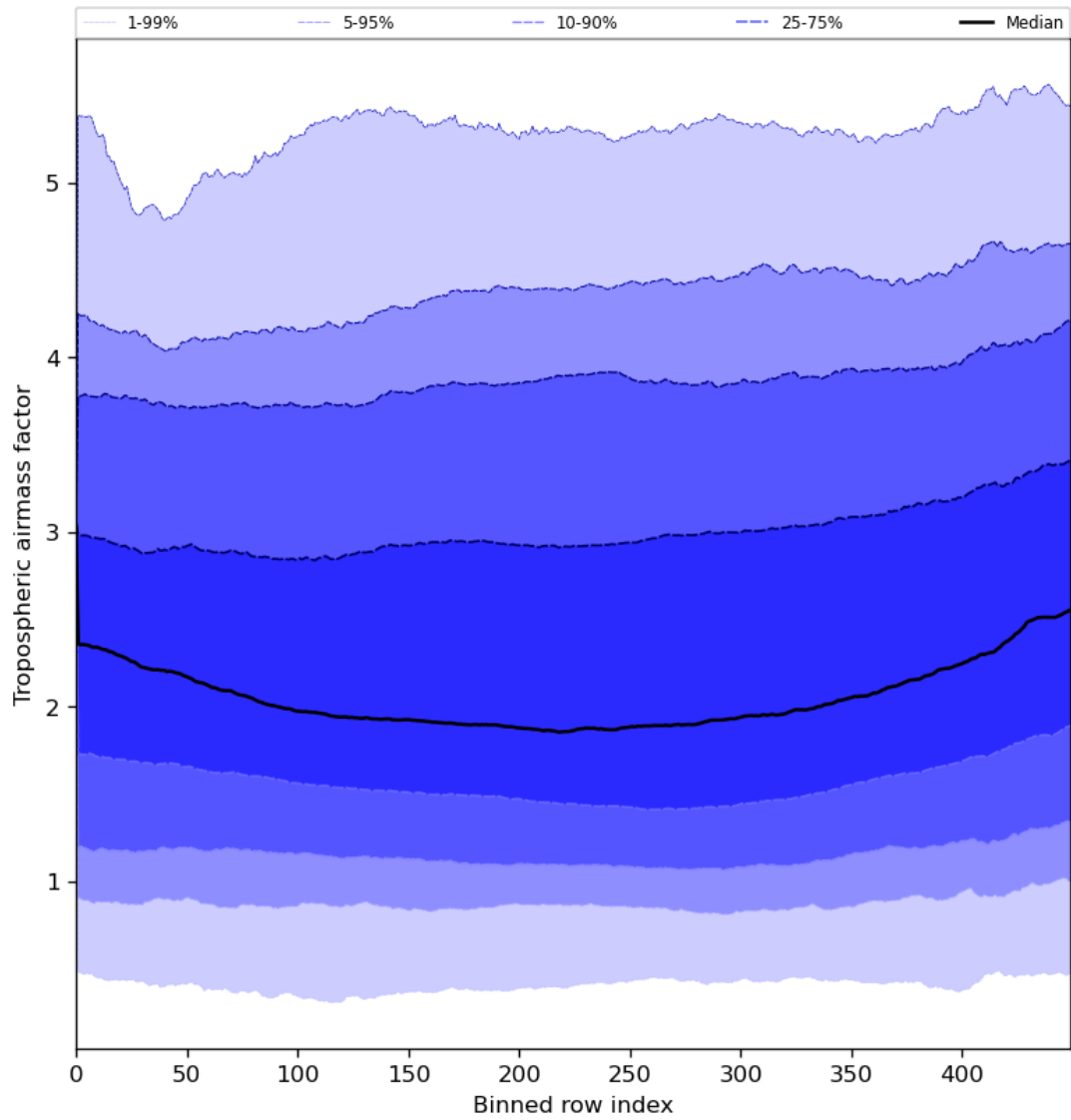
Figure 48: Along track statistics of “Tropospheric airmass factor” for 2024-05-25 to 2024-05-27
