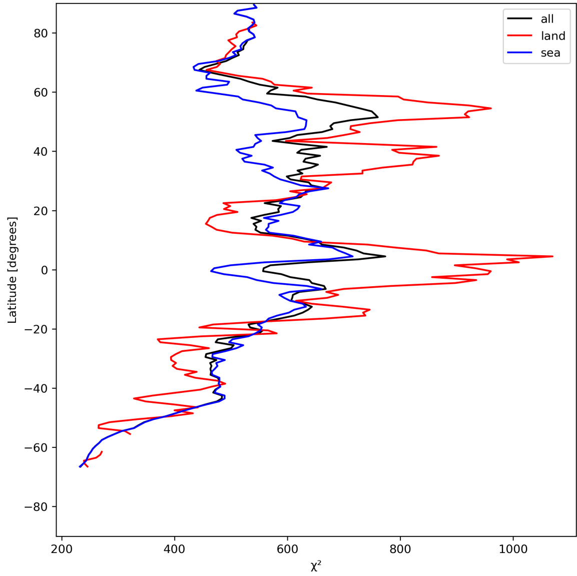
Figure 25: Zonal average of “ \chi^2 ” for 2024-05-25 to 2024-05-27.
