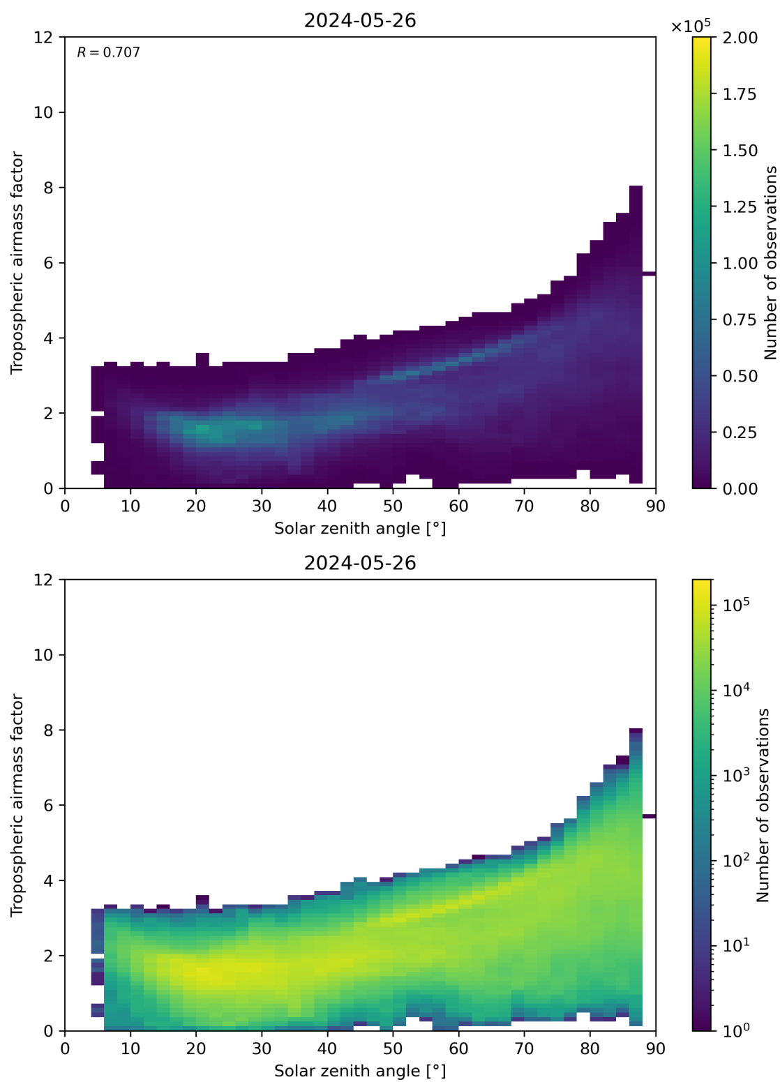
Figure 147: Scatter density plot of “Solar zenith angle” against “Tropospheric airmass factor” for 2024-05-25 to 2024-05-27.
