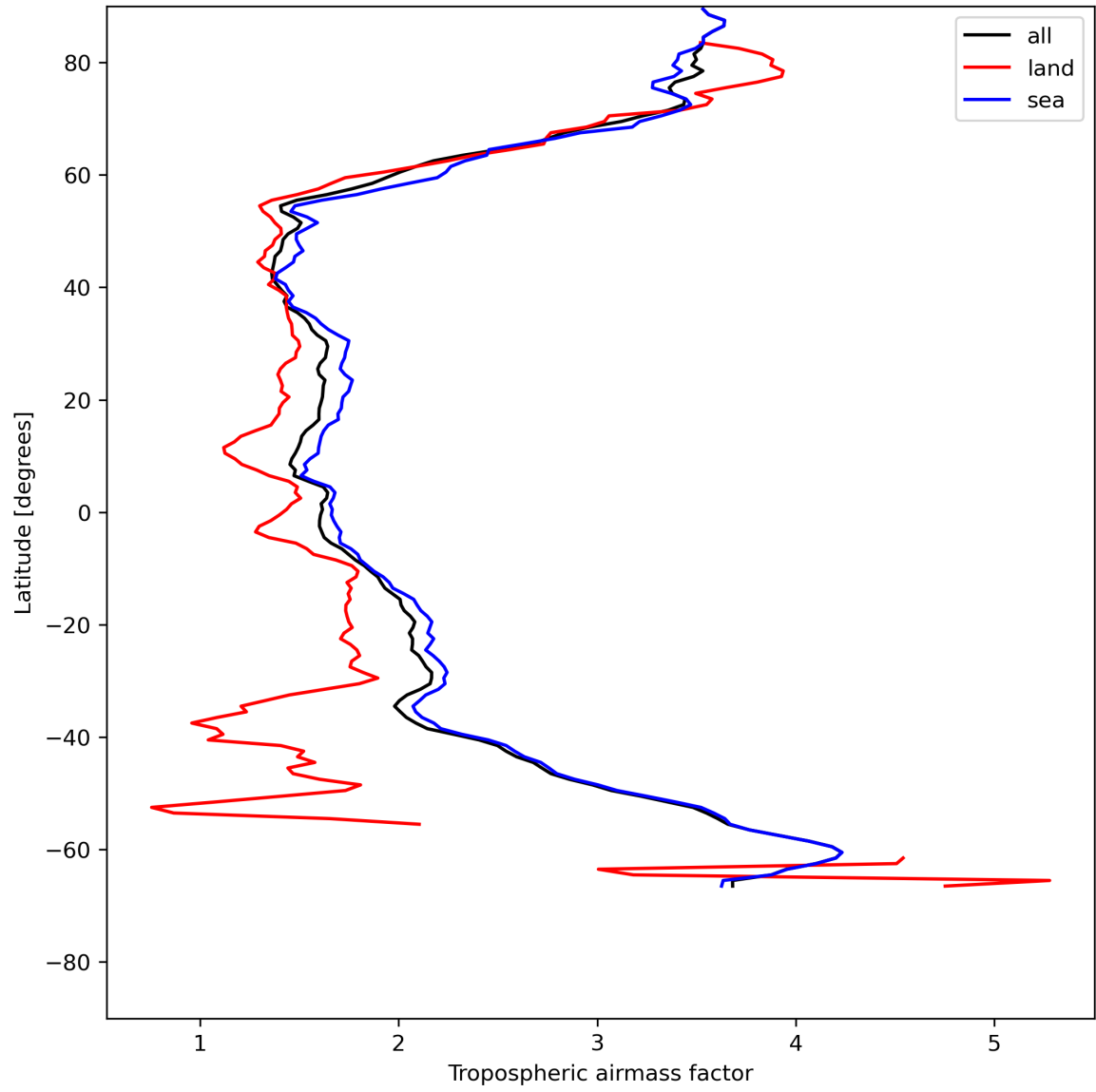
Figure 14: Zonal average of “Tropospheric airmass factor” for 2024-05-25 to 2024-05-27.
