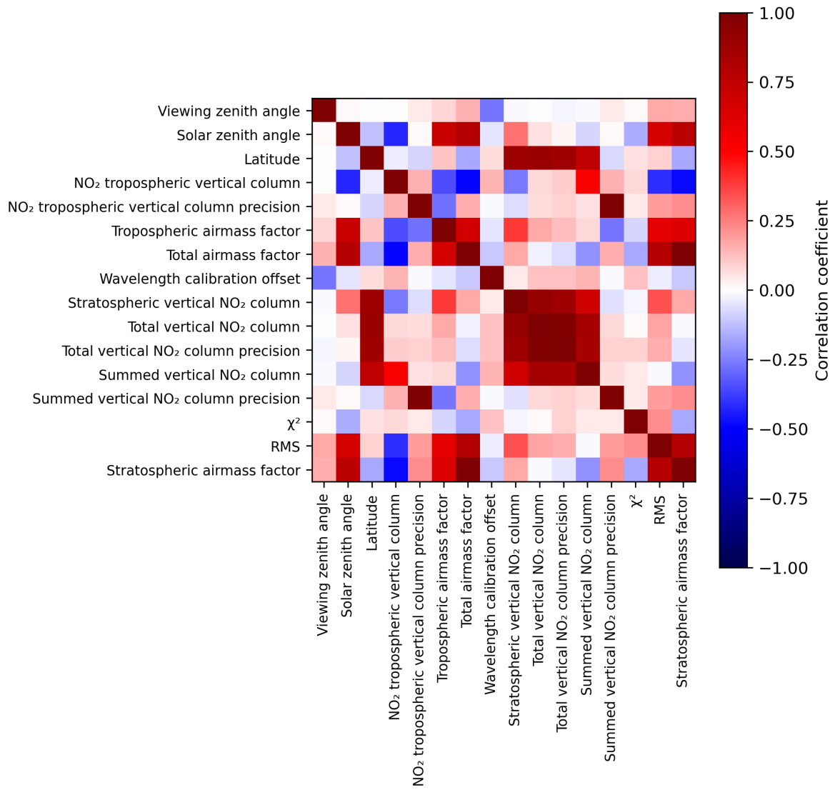
Figure 2: Map of correlation matrix for 2024-05-25 to 2024-05-27.
