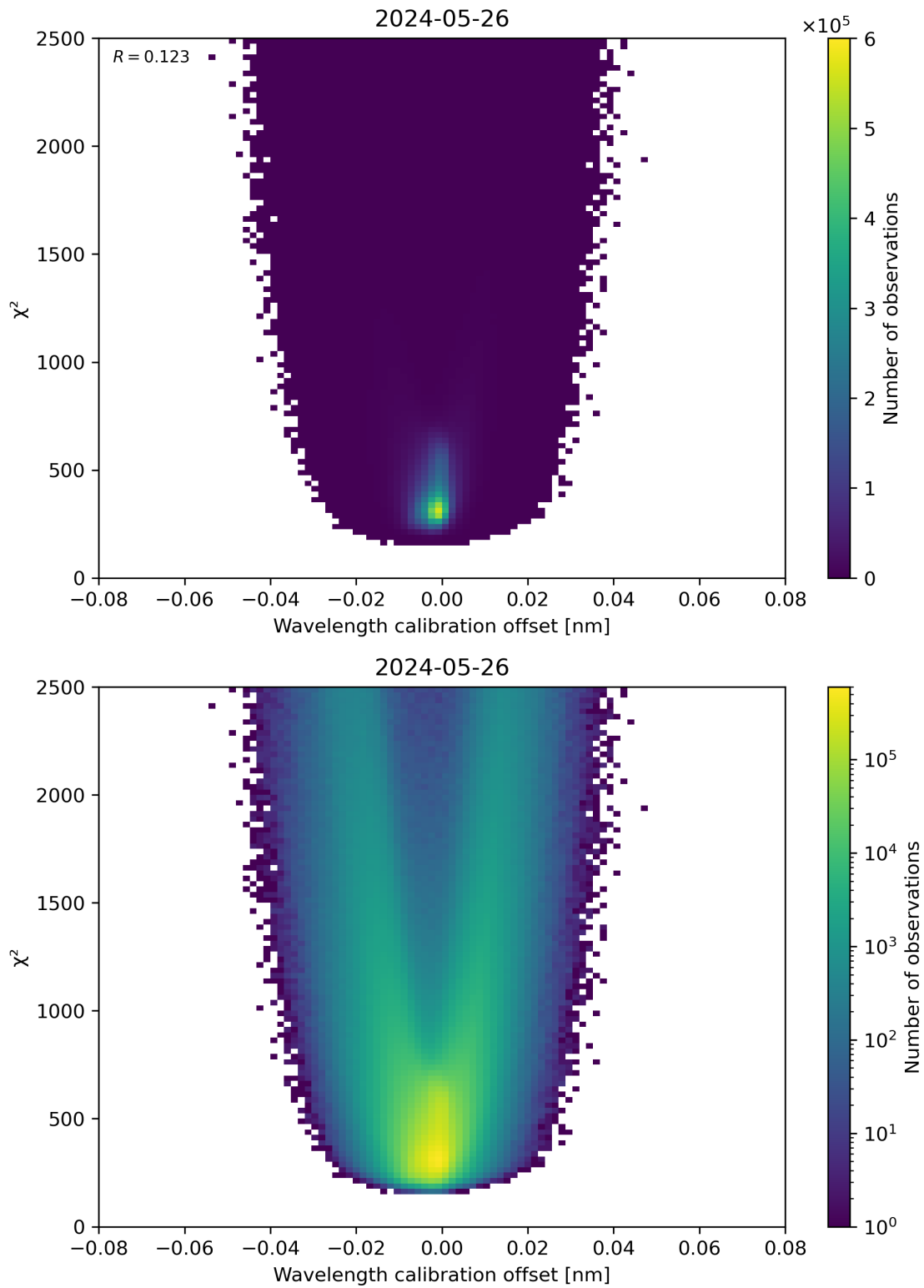
Figure 175: Scatter density plot of “Wavelength calibration offset” against “ \chi^2 ” for 2024-05-25 to 2024-05-27.
