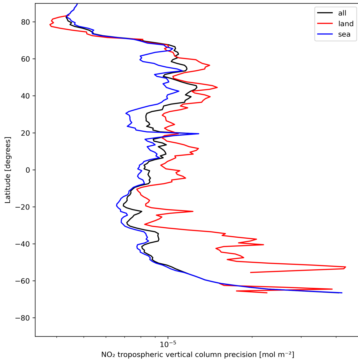
Figure 13: Zonal average of “NO 2 tropospheric vertical column precision” for 2024-05-25 to 2024-05-27.
