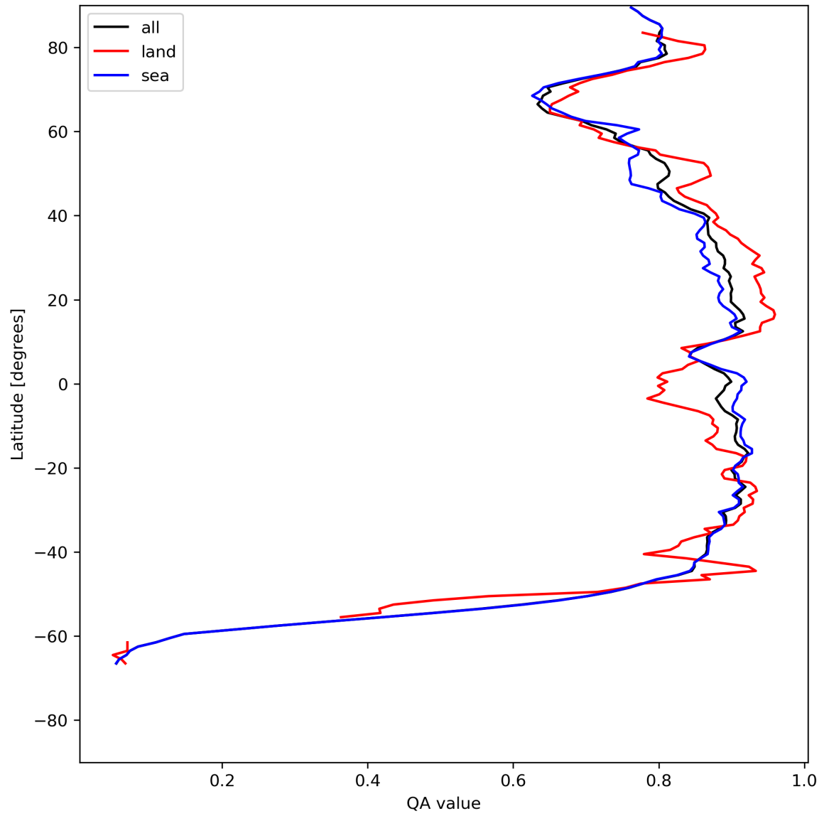
Figure 11: Zonal average of “QA value” for 2024-05-25 to 2024-05-27.
