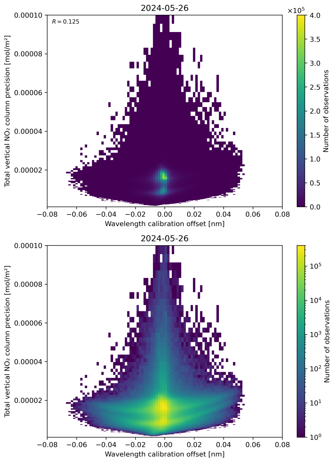
Figure 180: Scatter density plot of “Wavelength calibration offset” against “Total vertical NO 2 column precision” for 2024-05-25 to 2024-05-27.
