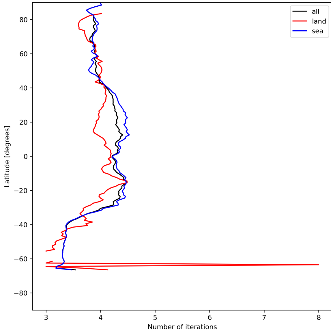
Figure 17: Zonal average of “Number of iterations” for 2024-05-25 to 2024-05-27.
