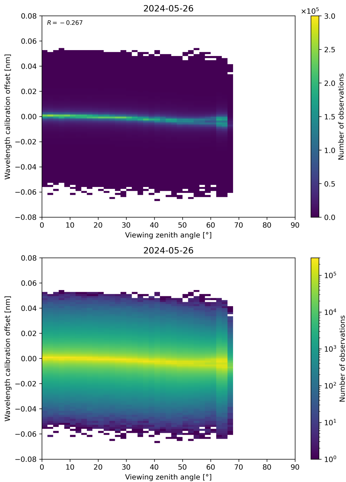
Figure 173: Scatter density plot of “Viewing zenith angle” against “Wavelength calibration offset” for 2024-05-25 to 2024-05-27.
