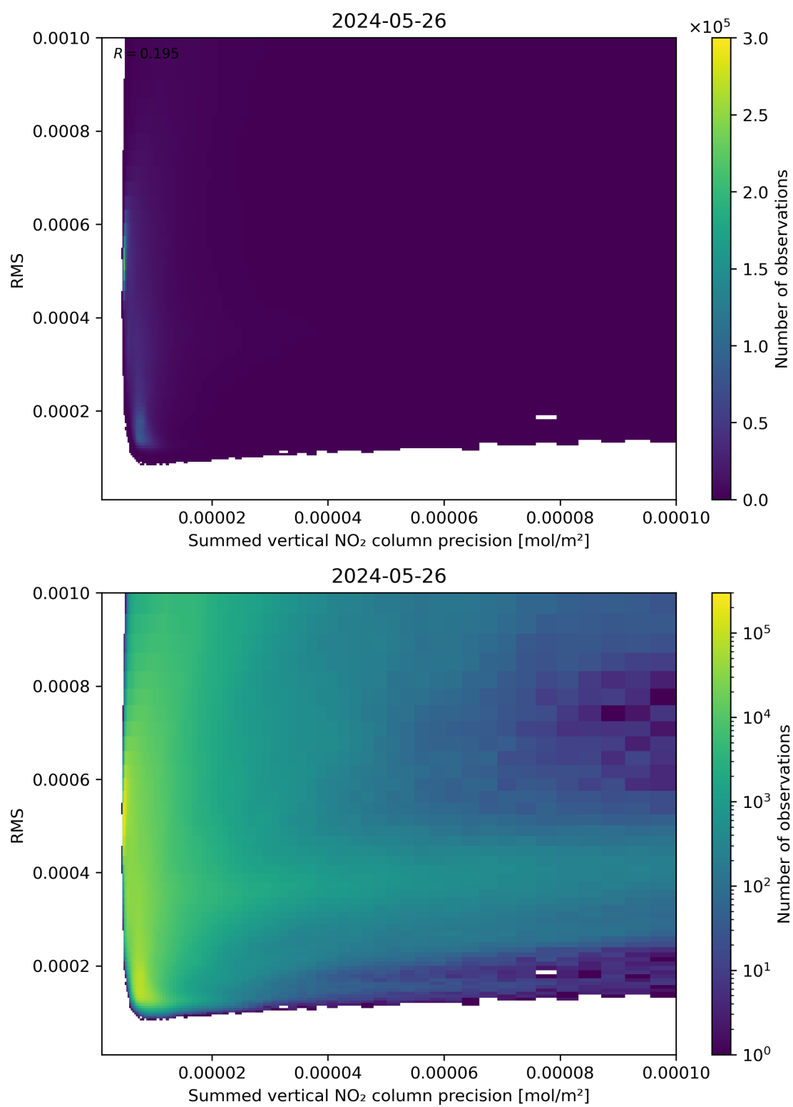
Figure 108: Scatter density plot of “Summed vertical NO 2 column precision” against “RMS” for 2024-05-25 to 2024-05-27.
