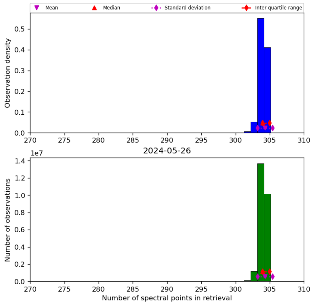
Figure 33: Histogram of “Number of spectral points in retrieval” for 2024-05-25 to 2024-05-27
