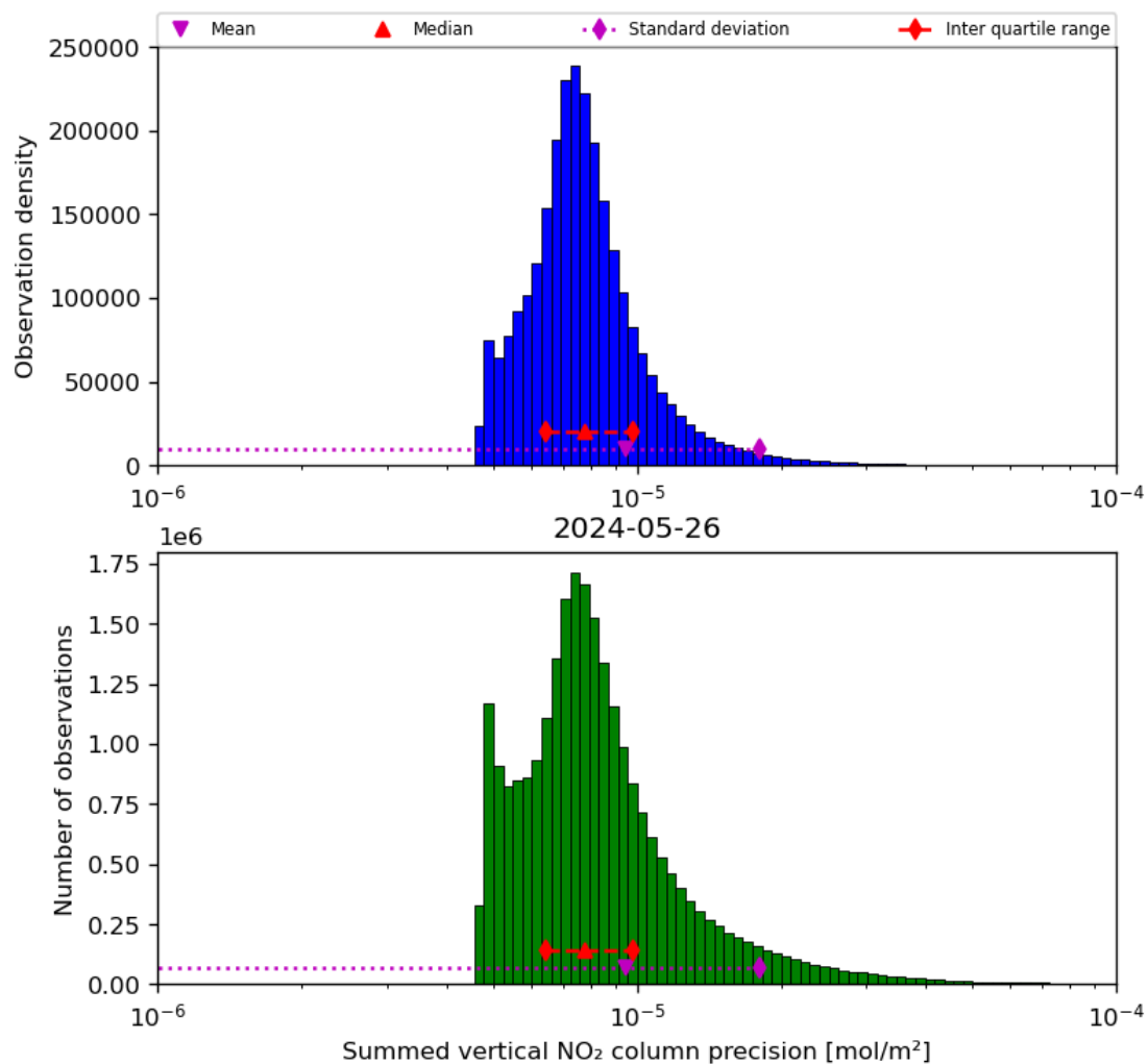
Figure 41: Histogram of "Summed vertical NO 2 column precision" for 2024-05-25 to 2024-05-27
