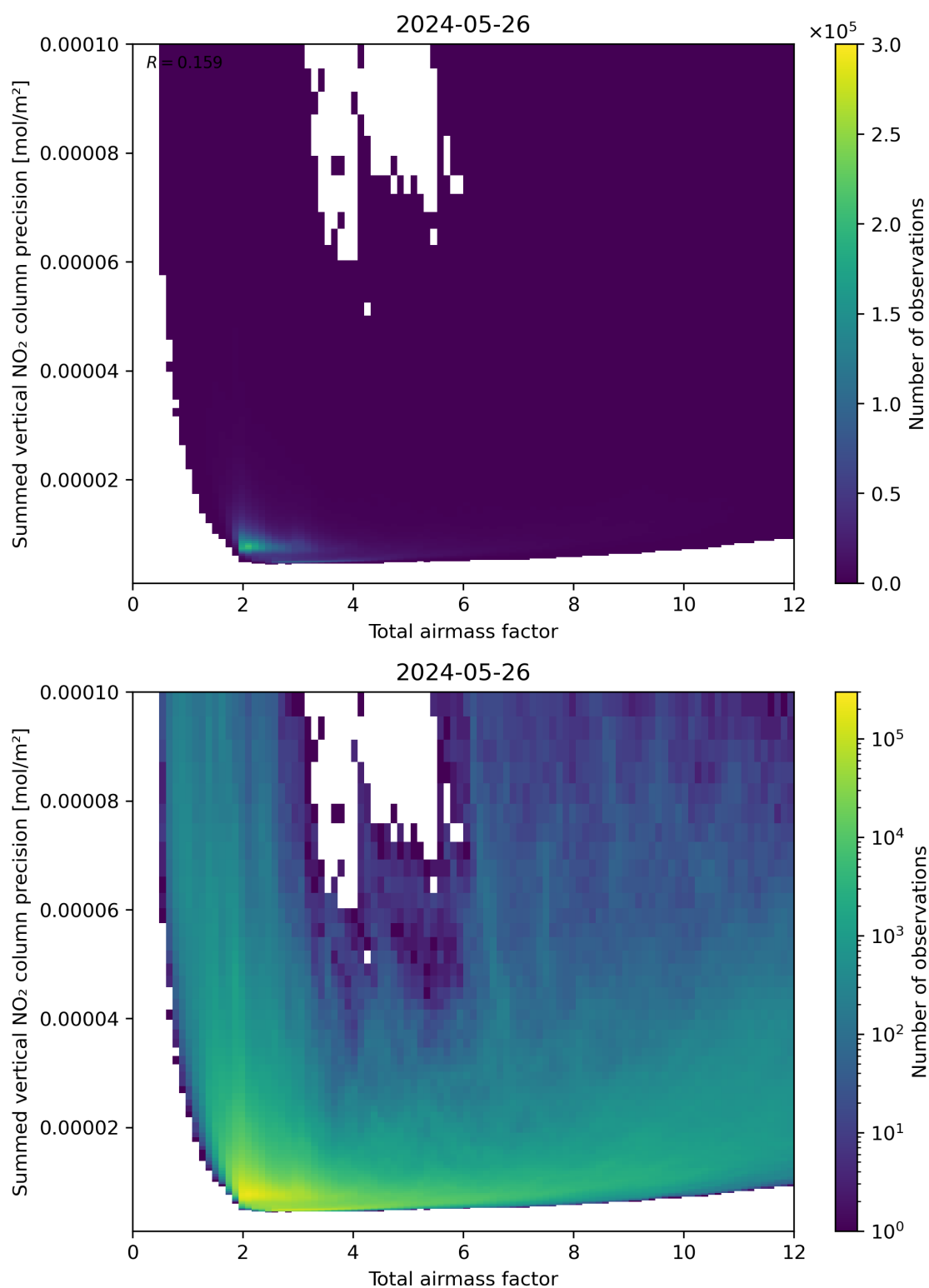
Figure 66: Scatter density plot of “Total airmass factor” against “Summed vertical NO 2 column precision” for 2024-05-25 to 2024-05-27.
