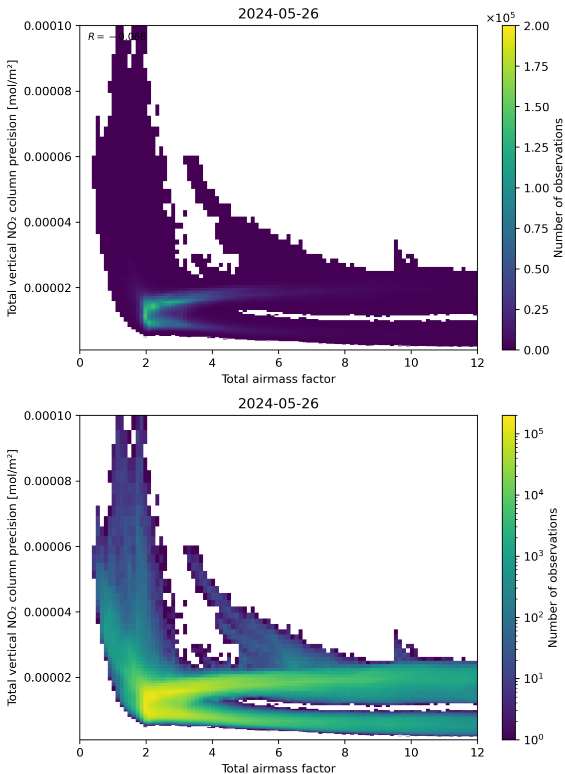
Figure 68: Scatter density plot of “Total airmass factor” against “Total vertical NO 2 column precision” for 2024-05-25 to 2024-05-27.
