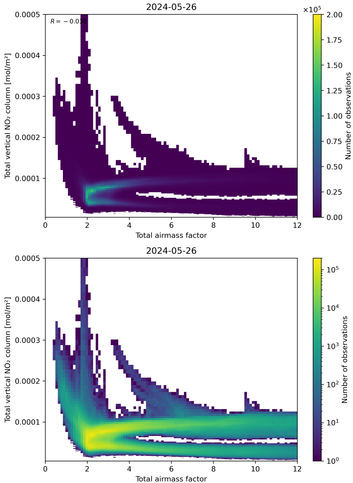
Figure 67: Scatter density plot of “Total airmass factor” against “Total vertical NO 2 column” for 2024-05-25 to 2024-05-27.
