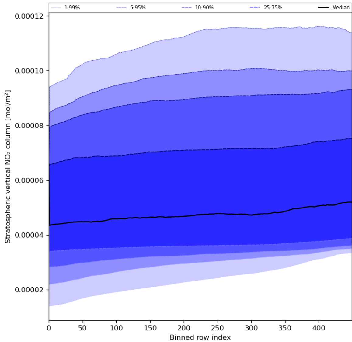
Figure 53: Along track statistics of “Stratospheric vertical NO 2 column” for 2024-05-25 to 2024-05-27
