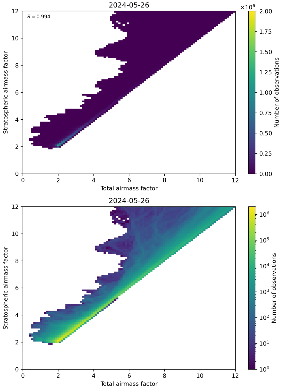
Figure 62: Scatter density plot of “Total airmass factor” against “Stratospheric airmass factor” for 2024-05-25 to 2024-05-27.
