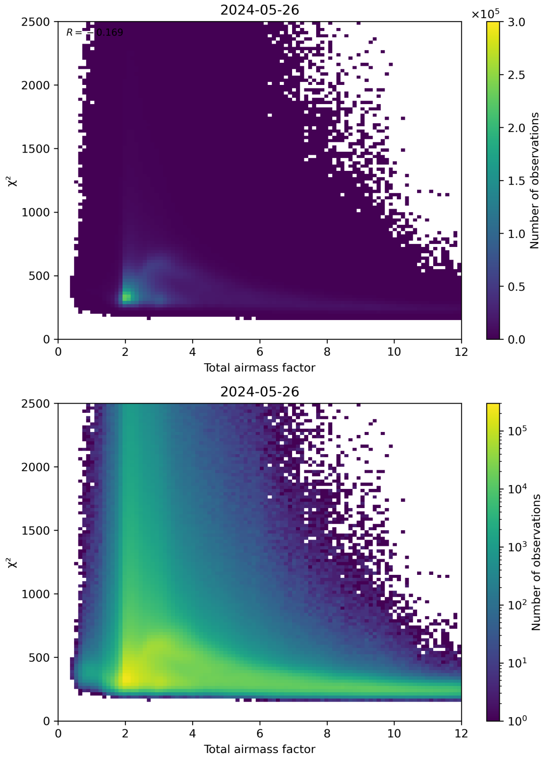
Figure 63: Scatter density plot of “Total airmass factor” against “ \chi^2 ” for 2024-05-25 to 2024-05-27.
