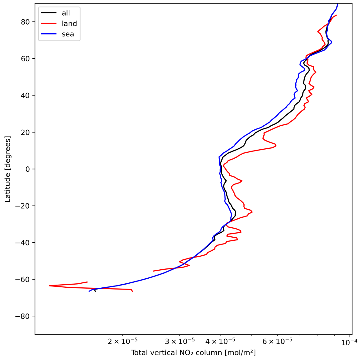
Figure 21: Zonal average of “Total vertical NO 2 column” for 2024-05-25 to 2024-05-27.
