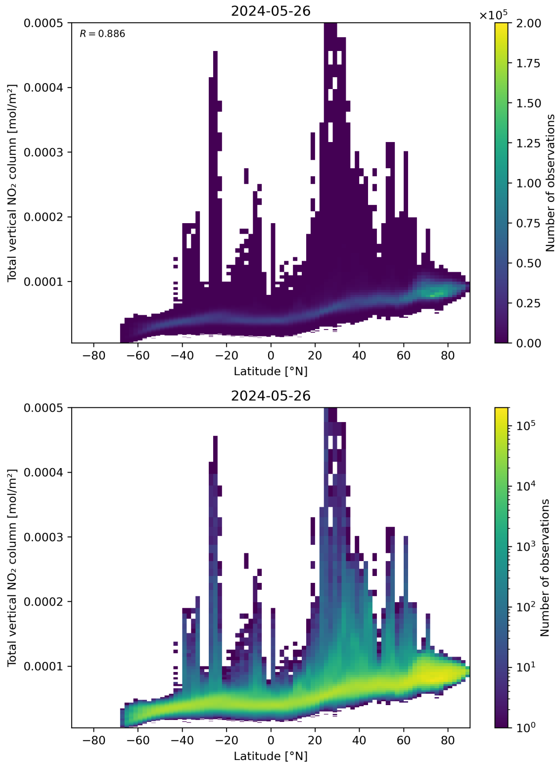
Figure 90: Scatter density plot of “Latitude” against “Total vertical NO 2 column” for 2024-05-25 to 2024-05-27.
