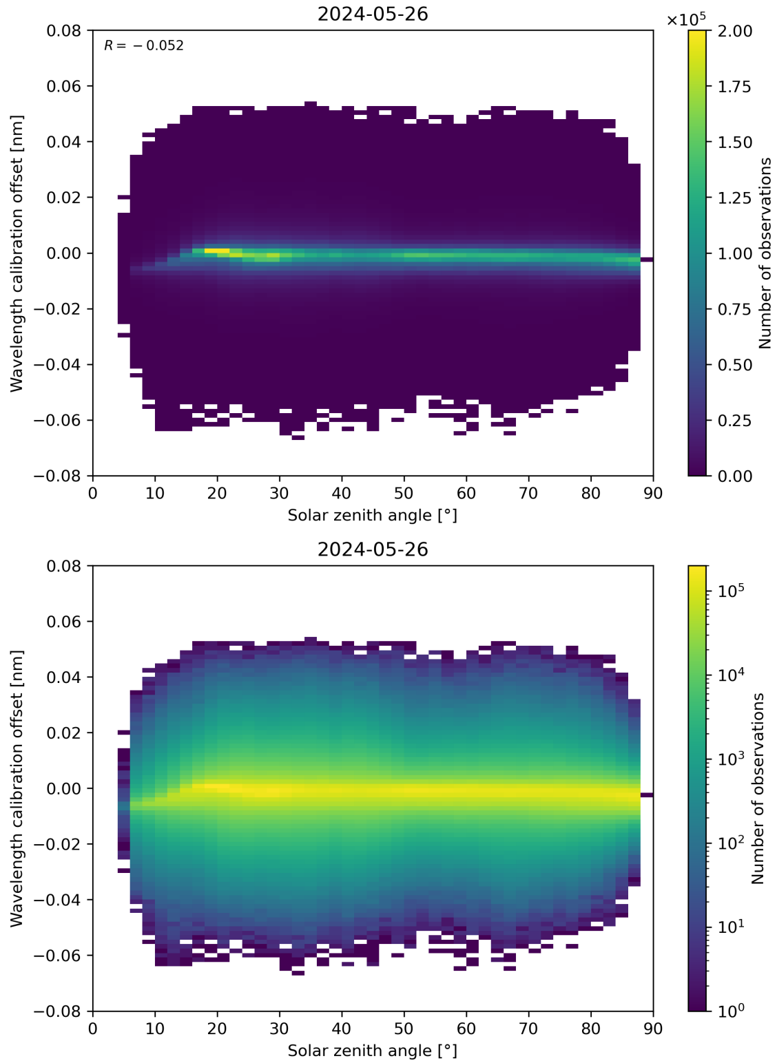
Figure 158: Scatter density plot of “Solar zenith angle” against “Wavelength calibration offset” for 2024-05-25 to 2024-05-27.
