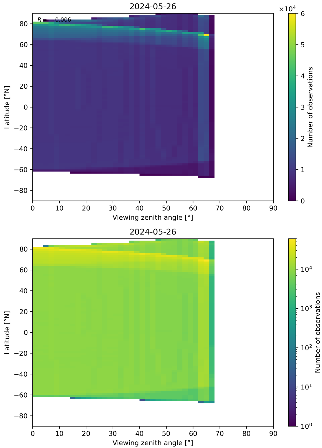
Figure 163: Scatter density plot of “Viewing zenith angle” against “Latitude” for 2024-05-25 to 2024-05-27.
