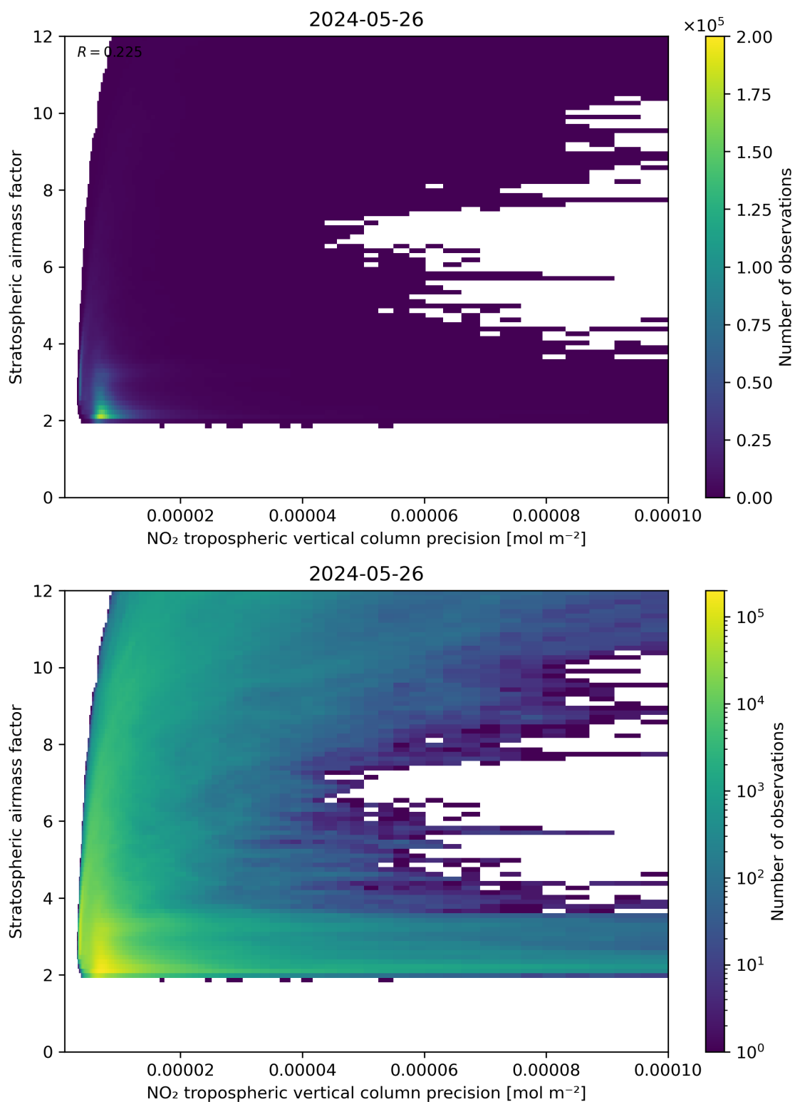
Figure 131: Scatter density plot of “NO 2 tropospheric vertical column precision” against “Stratospheric airmass factor” for 2024-05-25 to 2024-05-27.
