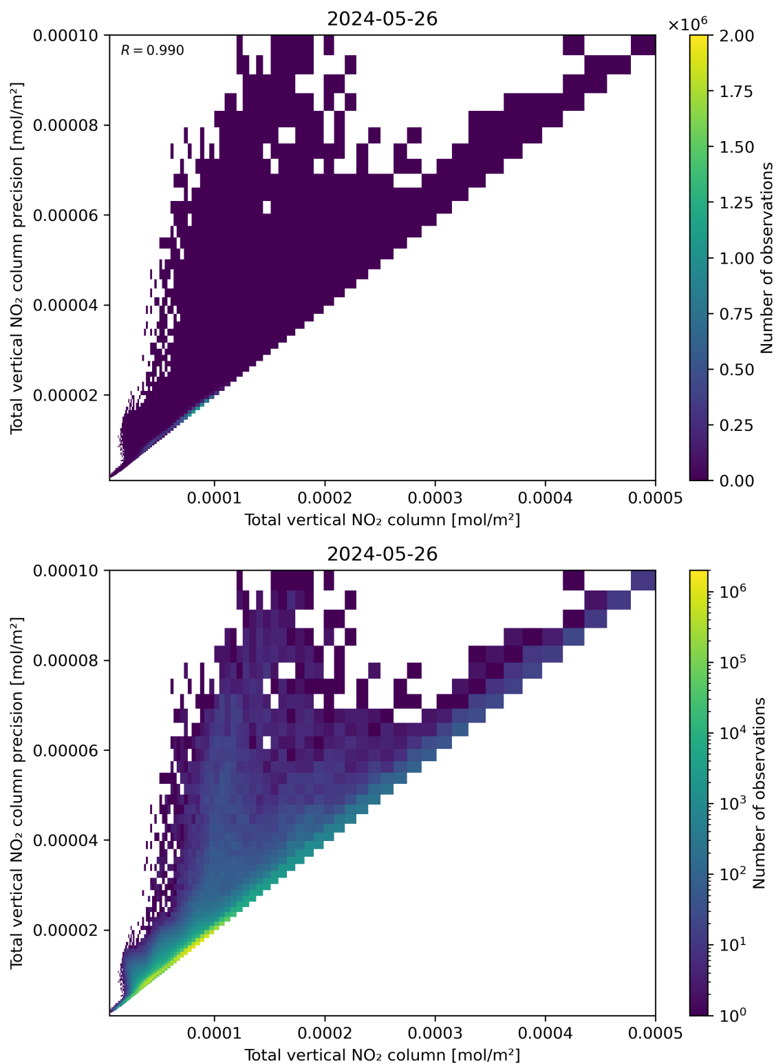
Figure 114: Scatter density plot of “Total vertical NO 2 column” against “Total vertical NO 2 column precision” for 2024-05-25 to 2024-05-27.
