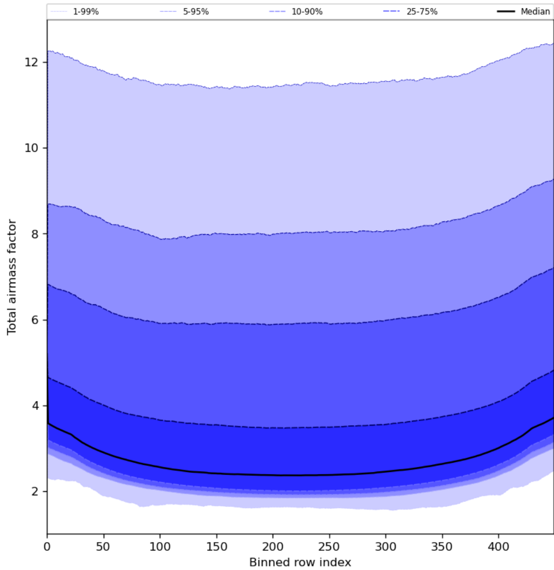
Figure 49: Along track statistics of “Total airmass factor” for 2024-05-25 to 2024-05-27
