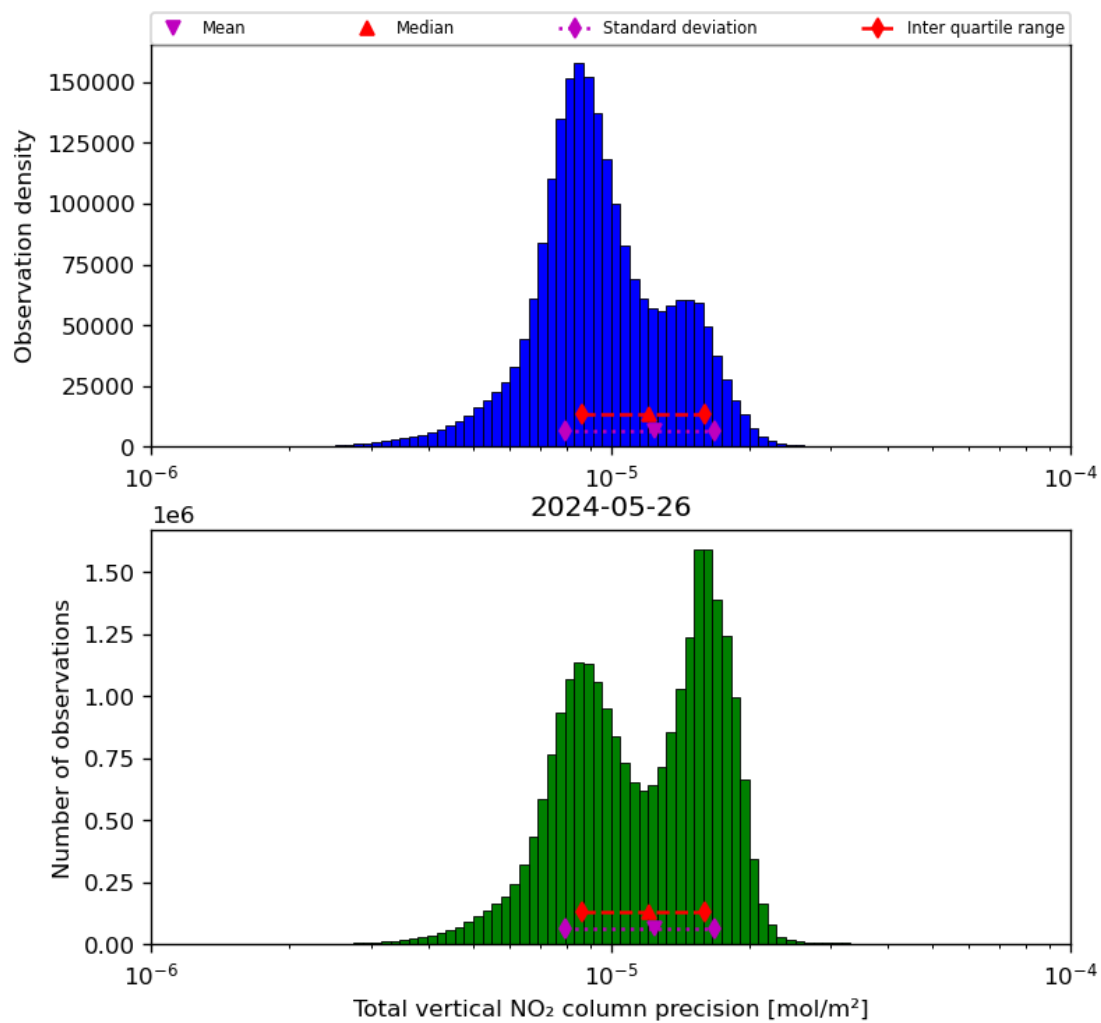
Figure 39: Histogram of “Total vertical NO 2 column precision” for 2024-05-25 to 2024-05-27
