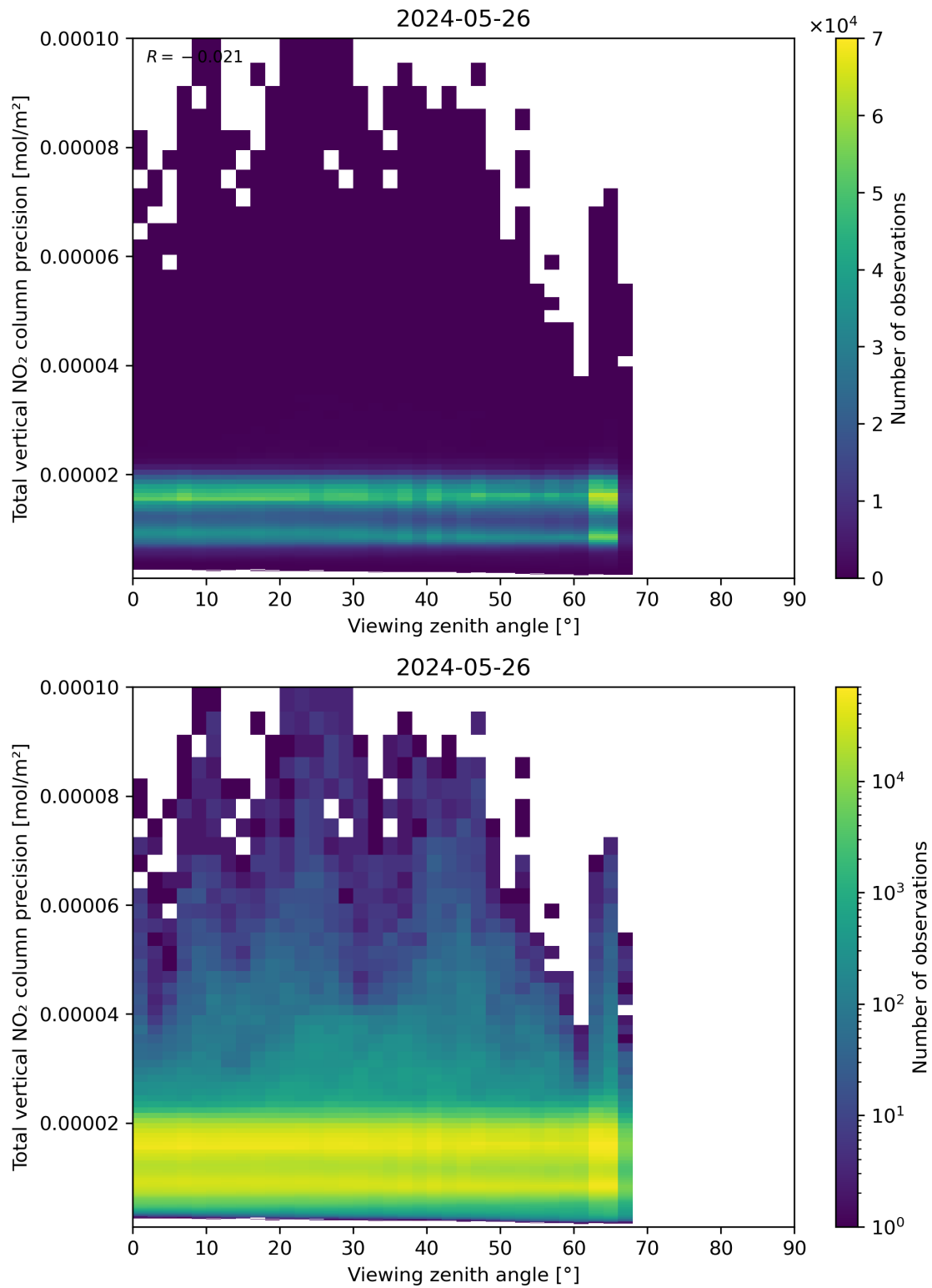
Figure 168: Scatter density plot of “Viewing zenith angle” against “Total vertical NO 2 column precision” for 2024-05-25 to 2024-05-27.
