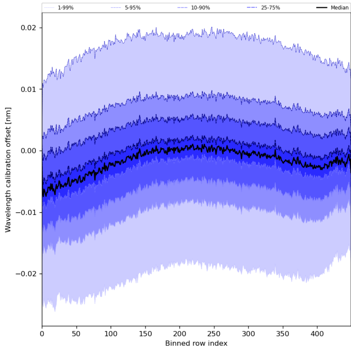
Figure 52: Along track statistics of “Wavelength calibration offset” for 2024-05-25 to 2024-05-27
