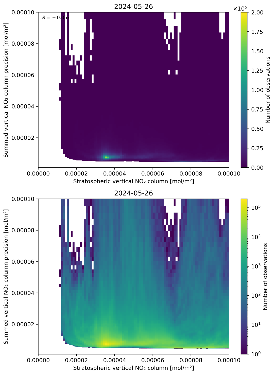
Figure 99: Scatter density plot of “Stratospheric vertical NO 2 column” against “Summed vertical NO 2 column precision” for 2024-05-25 to 2024-05-27.
