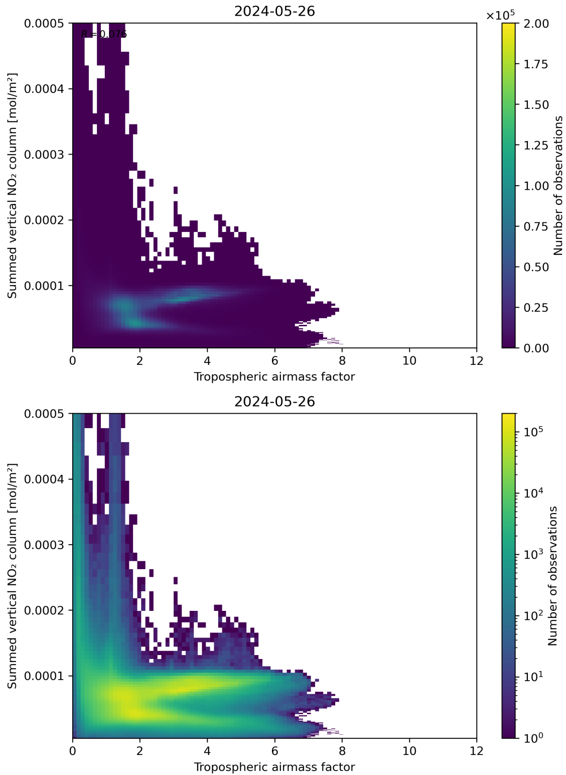
Figure 75: Scatter density plot of “Tropospheric airmass factor” against “Summed vertical NO 2 column” for 2024-05-25 to 2024-05-27.
