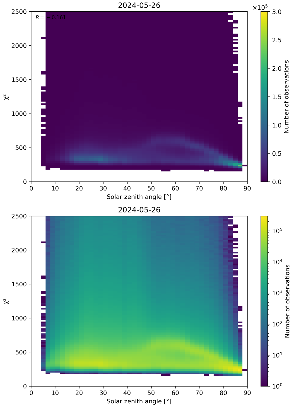
Figure 148: Scatter density plot of “Solar zenith angle” against “ \chi^2 ” for 2024-05-25 to 2024-05-27.
