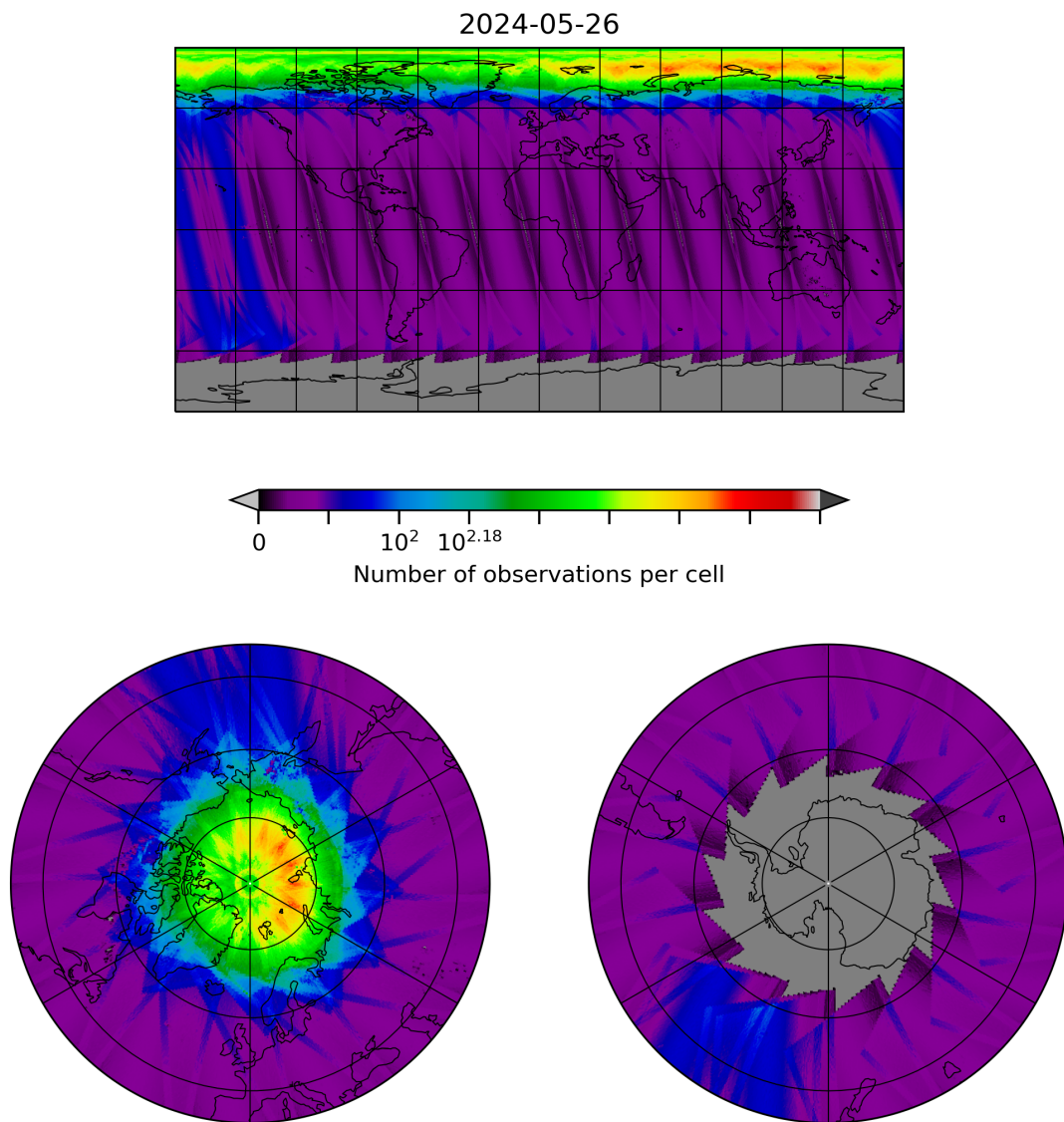
Figure 10: Map of the number of observations for 2024-05-25 to 2024-05-27
