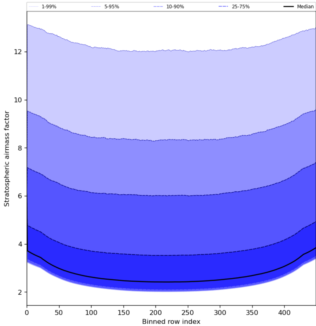
Figure 61: Along track statistics of “Stratospheric airmass factor” for 2024-05-25 to 2024-05-27
