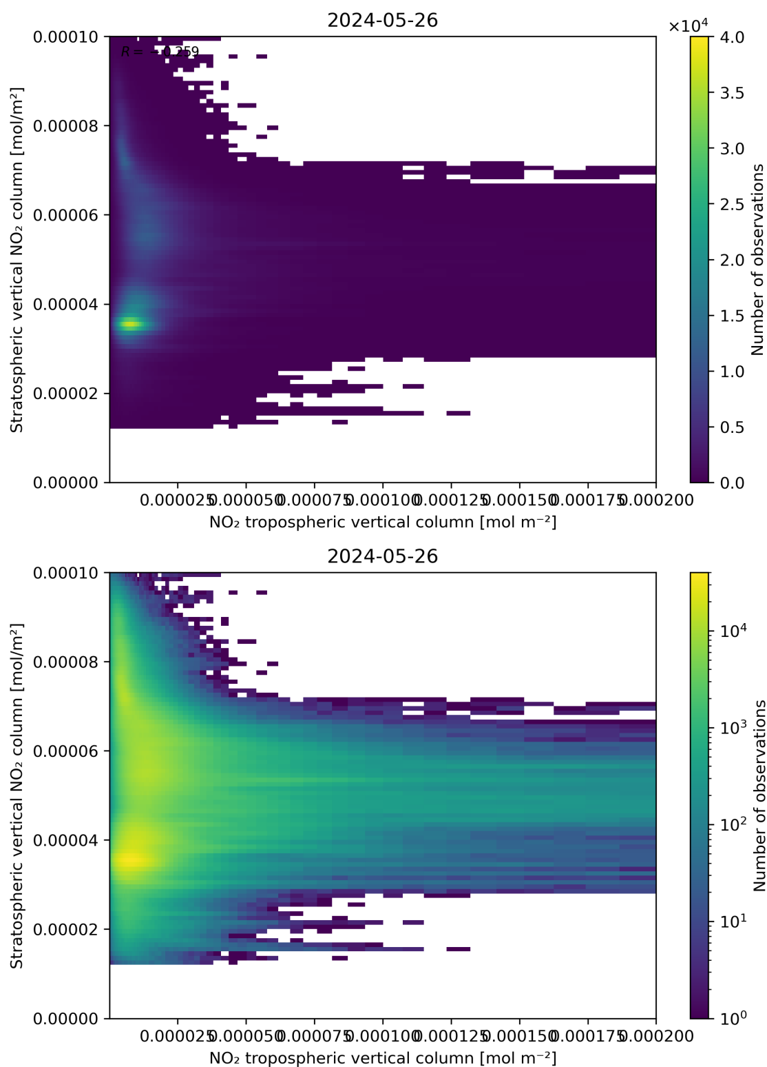
Figure 125: Scatter density plot of “NO 2 tropospheric vertical column” against “Stratospheric vertical NO 2 column” for 2024-05-25 to 2024-05-27.
