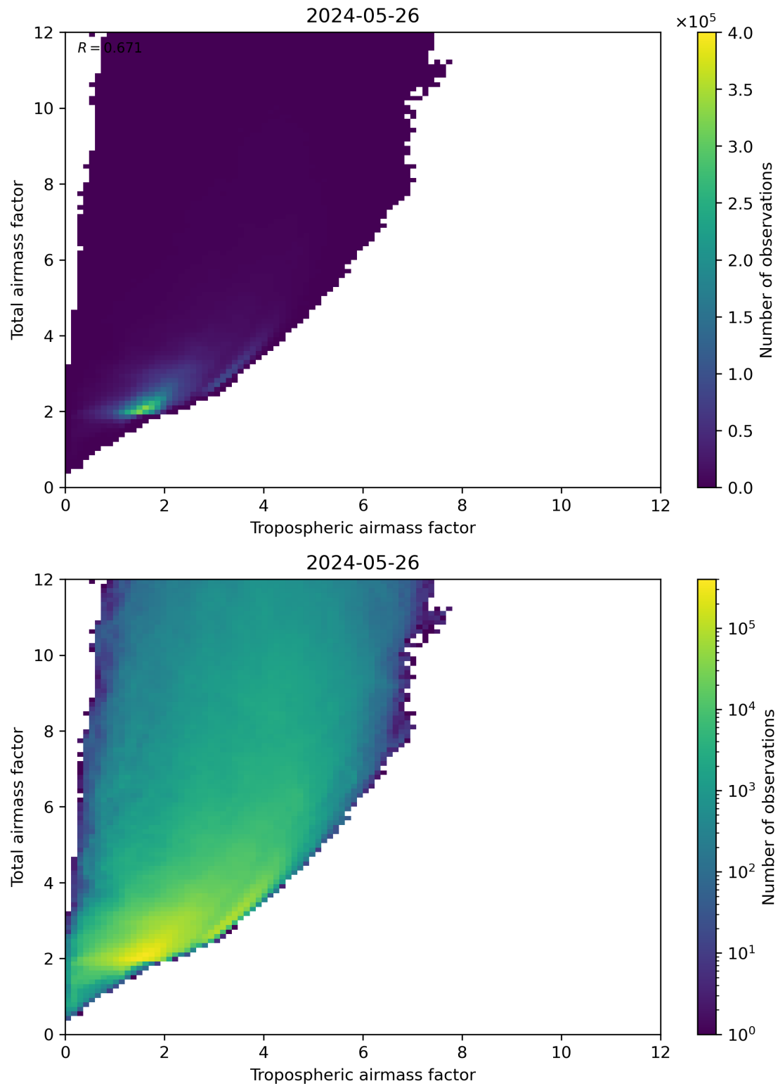
Figure 72: Scatter density plot of “Tropospheric airmass factor” against “Total airmass factor” for 2024-05-25 to 2024-05-27.
