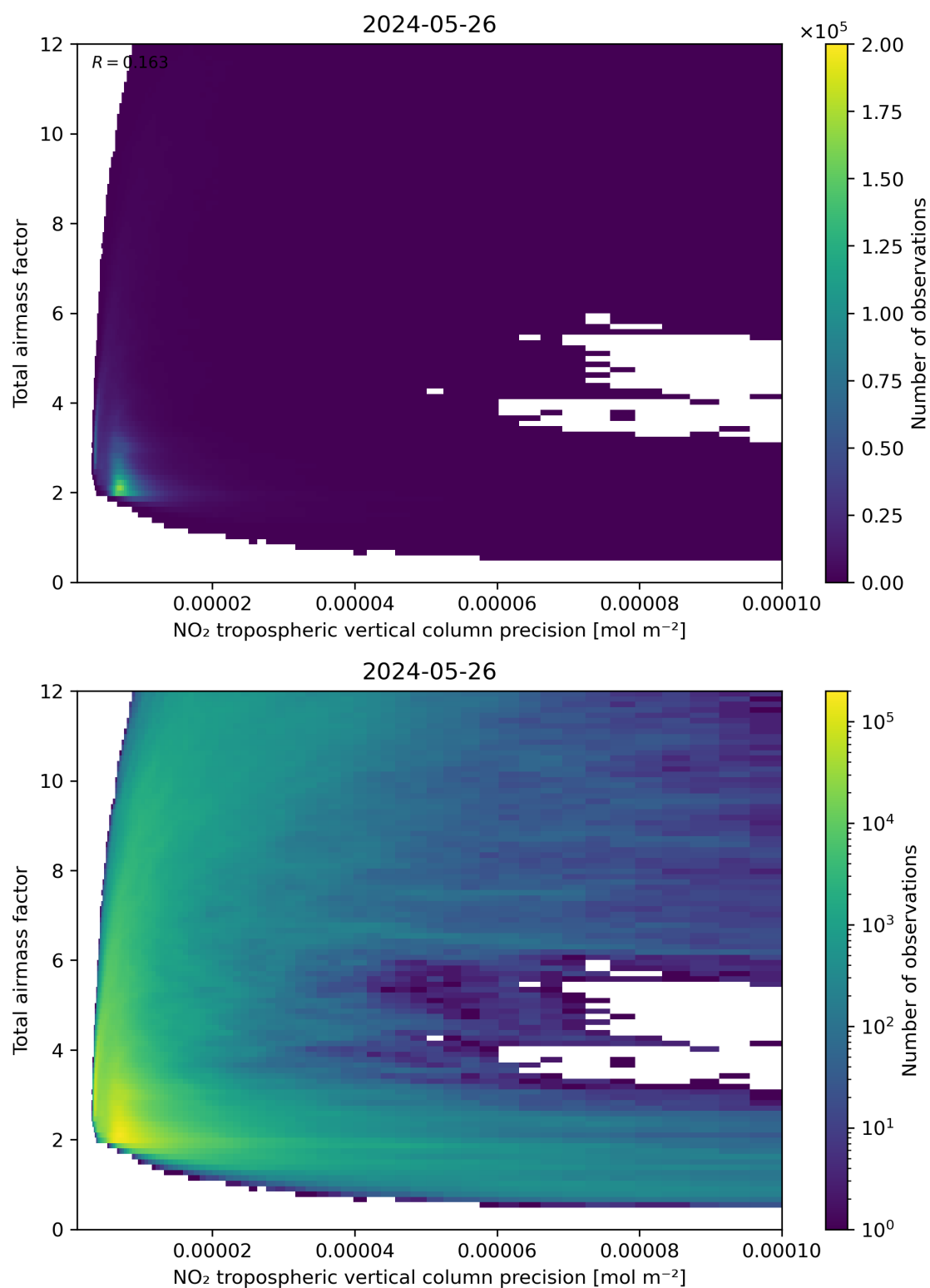
Figure 132: Scatter density plot of “NO 2 tropospheric vertical column precision” against “Total air mass factor” for 2024-05-25 to 2024-05-27.
