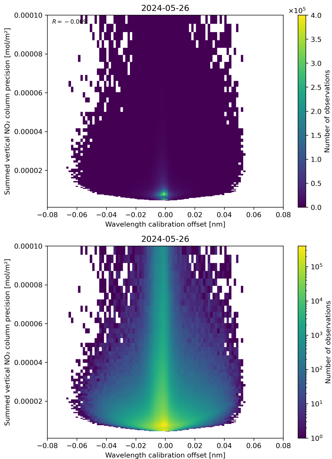
Figure 178: Scatter density plot of “Wavelength calibration offset” against “Summed vertical NO 2 column precision” for 2024-05-25 to 2024-05-27.
