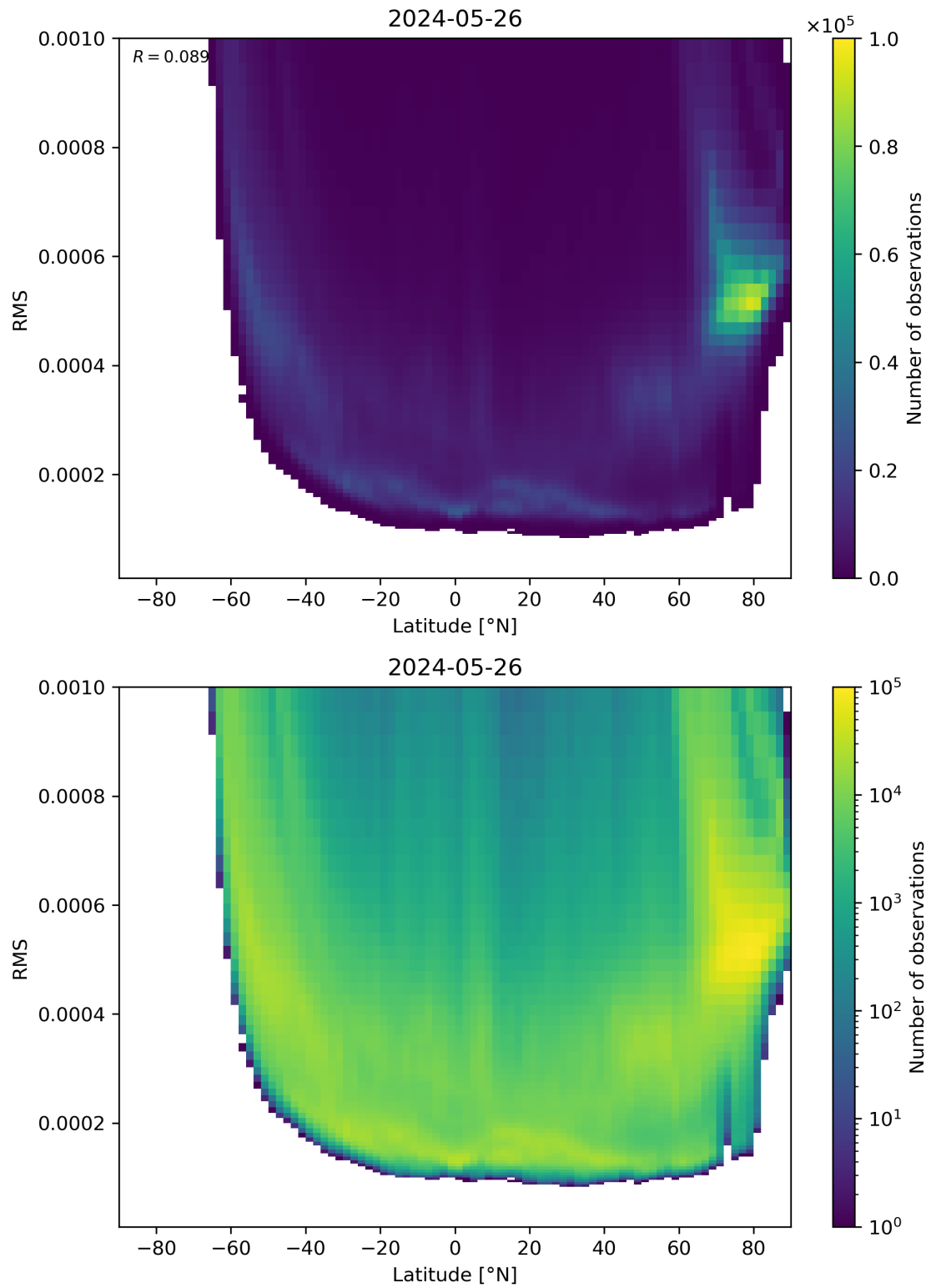
Figure 94: Scatter density plot of “Latitude” against “RMS” for 2024-05-25 to 2024-05-27.
