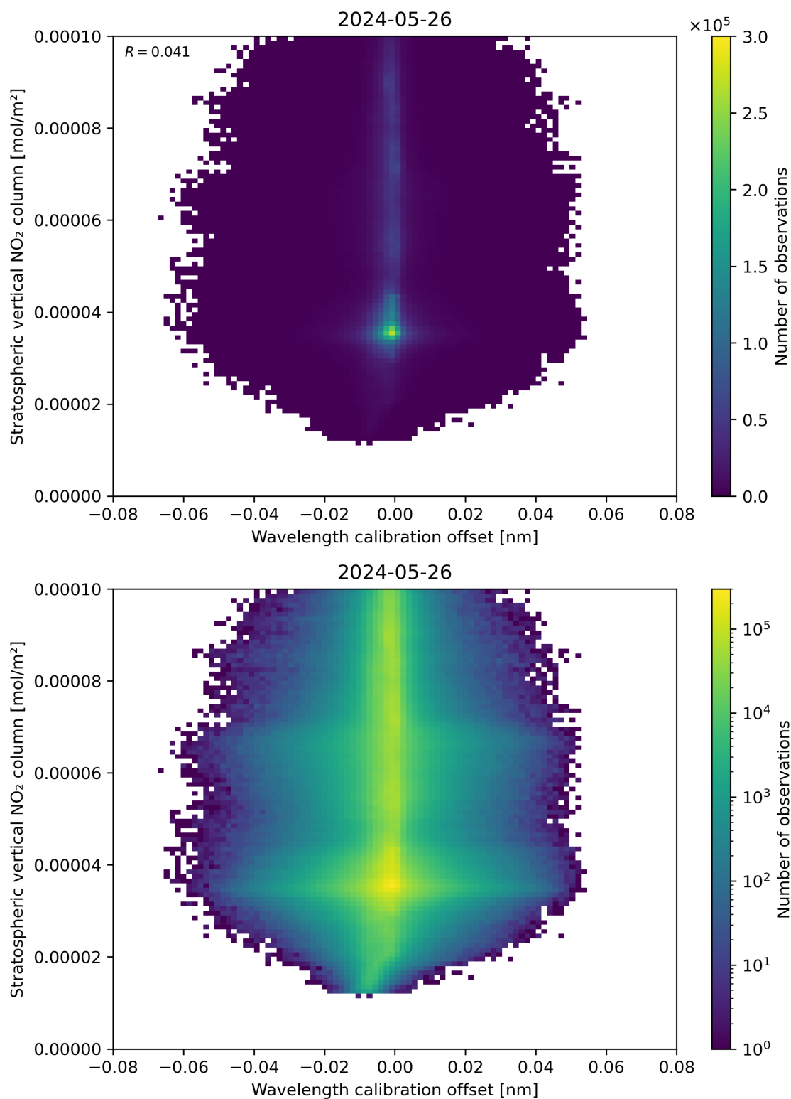
Figure 176: Scatter density plot of “Wavelength calibration offset” against “Stratospheric vertical NO 2 column” for 2024-05-25 to 2024-05-27.
