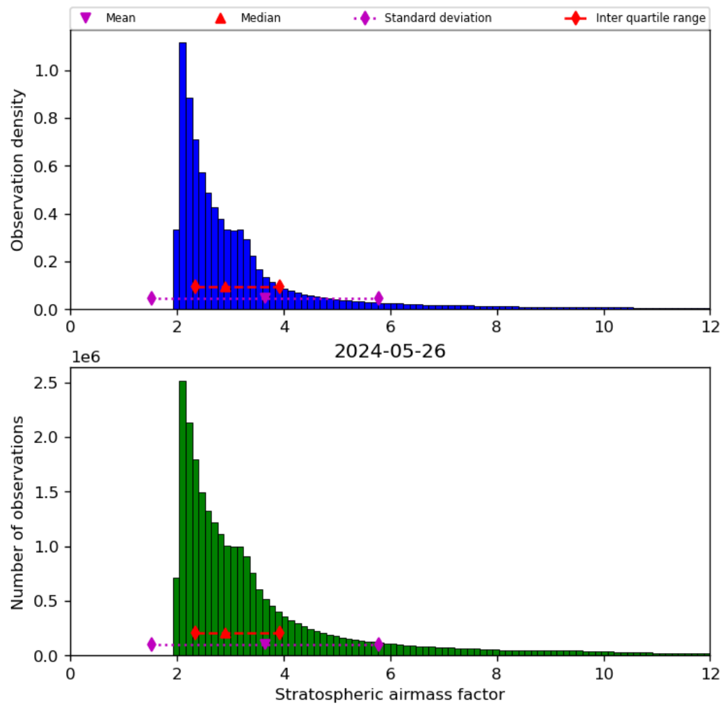
Figure 44: Histogram of “Stratospheric airmass factor” for 2024-05-25 to 2024-05-27
