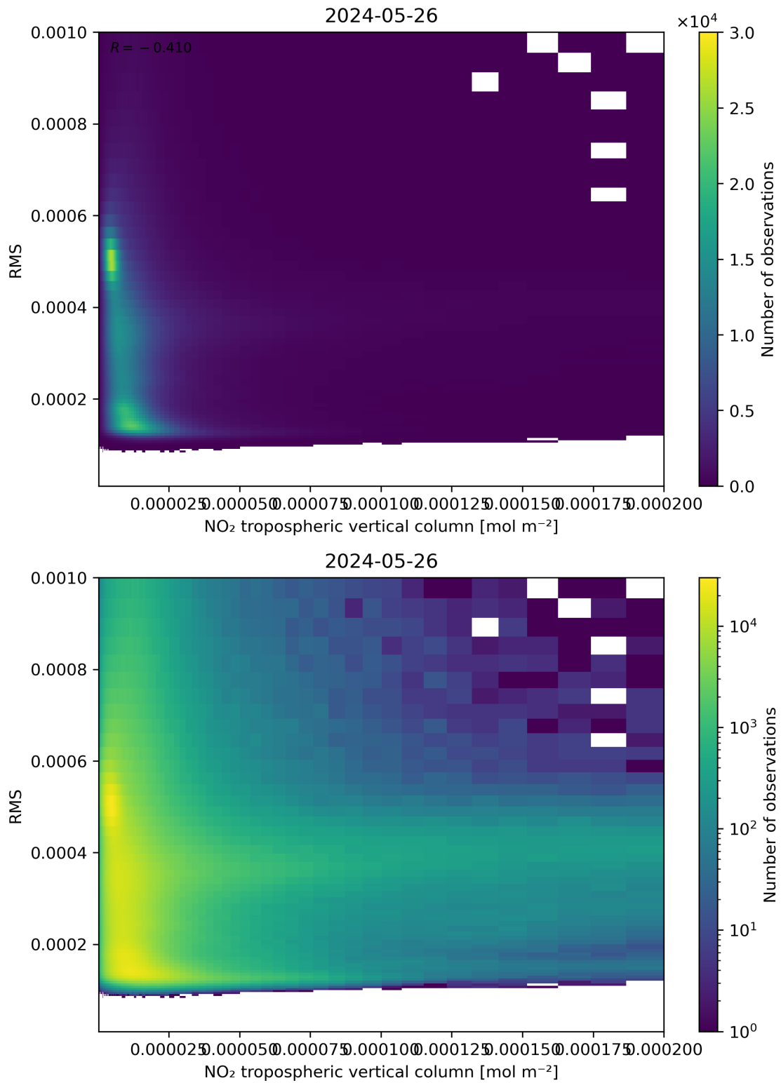
Figure 142: Scatter density plot of “NO 2 tropospheric vertical column” against “RMS” for 2024-05-25 to 2024-05-27.
