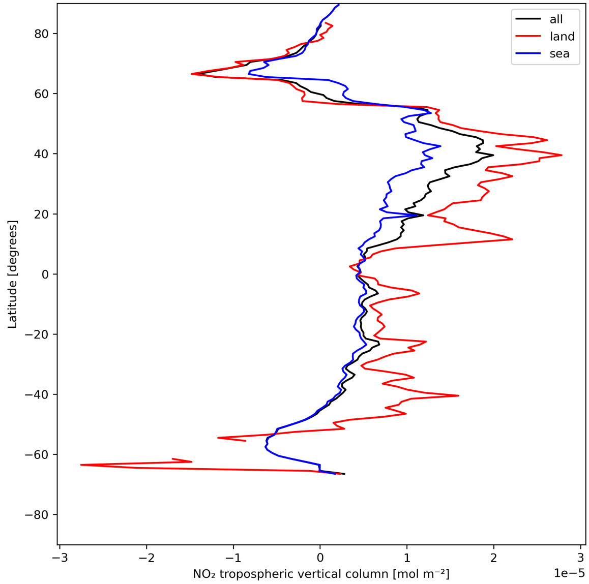
Figure 12: Zonal average of “NO 2 tropospheric vertical column” for 2024-05-25 to 2024-05-27.
