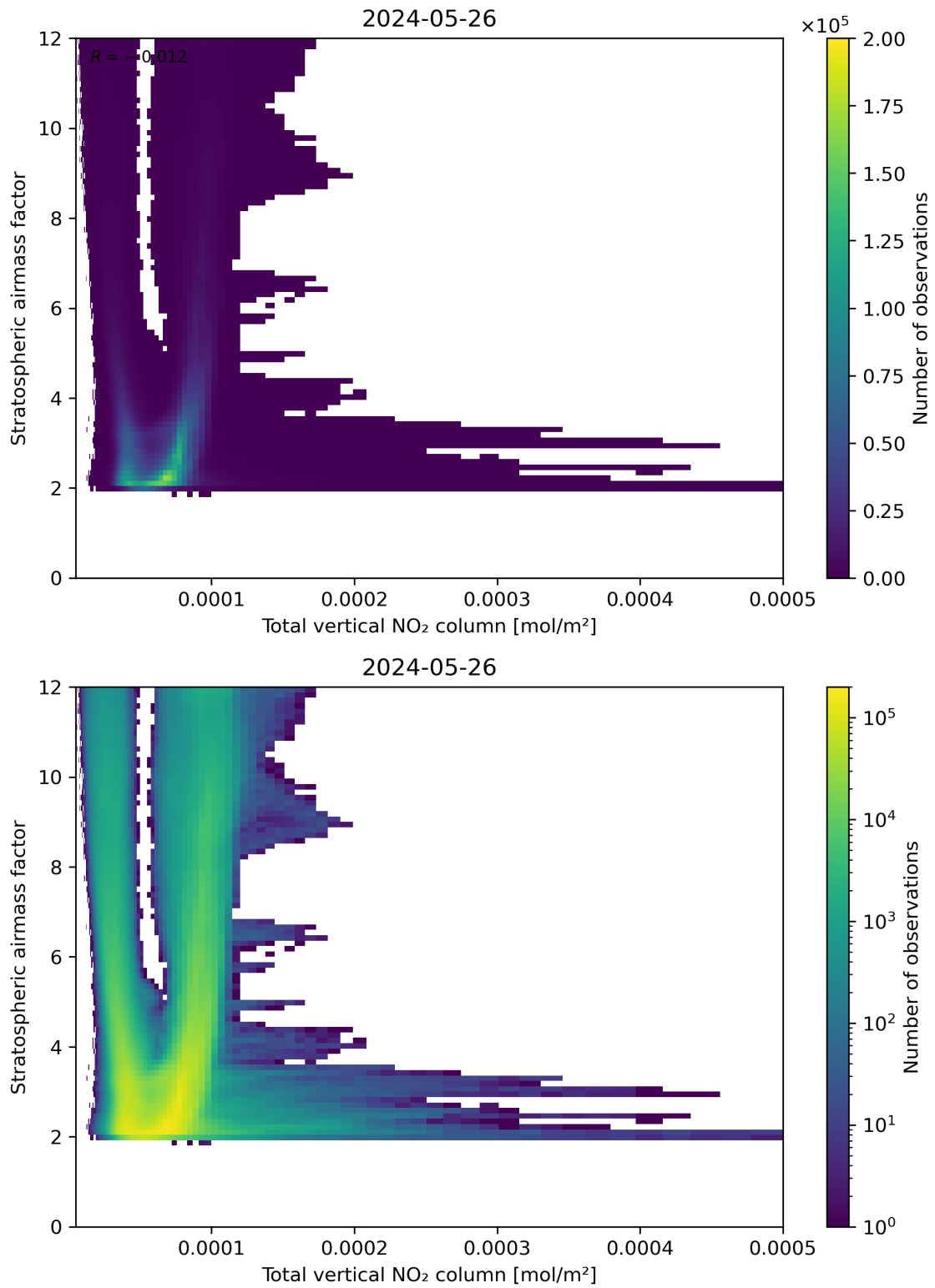
Figure 110: Scatter density plot of “Total vertical NO 2 column” against “Stratospheric airmass factor” for 2024-05-25 to 2024-05-27.
