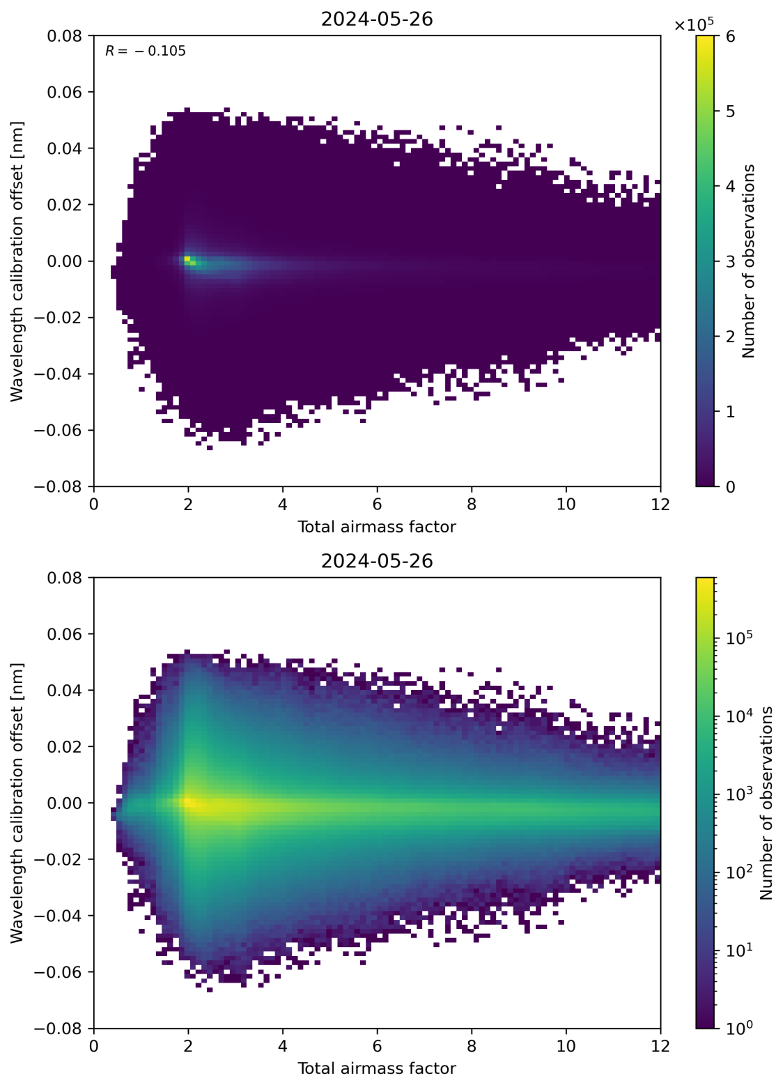
Figure 70: Scatter density plot of “Total airmass factor” against “Wavelength calibration offset” for 2024-05-25 to 2024-05-27.
