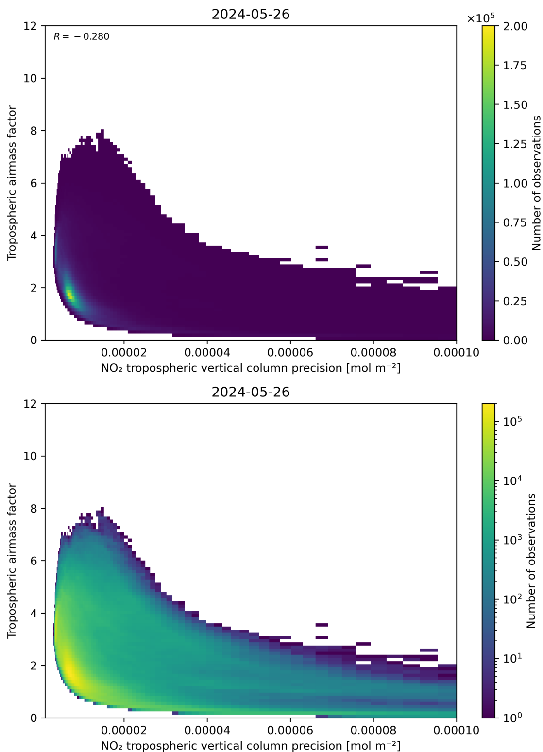
Figure 133: Scatter density plot of “NO 2 tropospheric vertical column precision” against “Tropospheric airmass factor” for 2024-05-25 to 2024-05-27.
