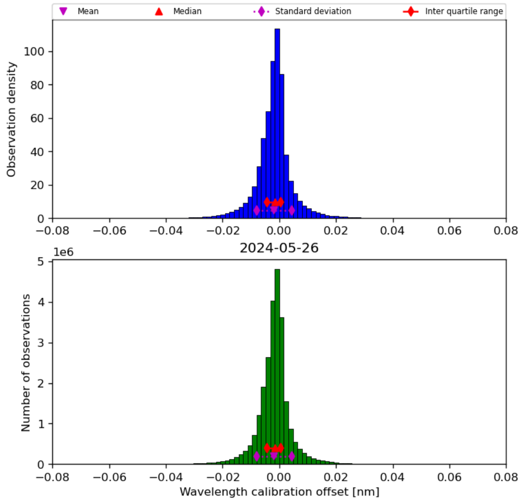
Figure 35: Histogram of “Wavelength calibration offset” for 2024-05-25 to 2024-05-27
