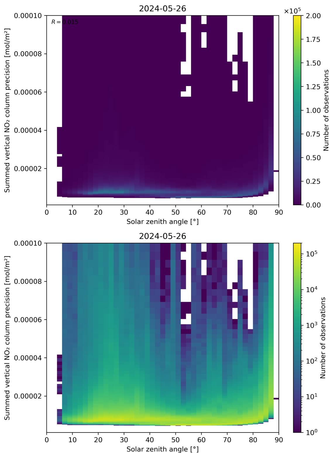
Figure 152: Scatter density plot of “Solar zenith angle” against “Summed vertical NO 2 column precision” for 2024-05-25 to 2024-05-27.
