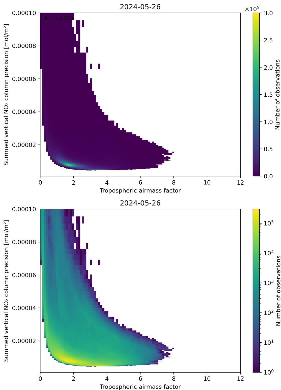
Figure 76: Scatter density plot of “Tropospheric air mass factor” against “Summed vertical NO 2 column precision” for 2024-05-25 to 2024-05-27.
