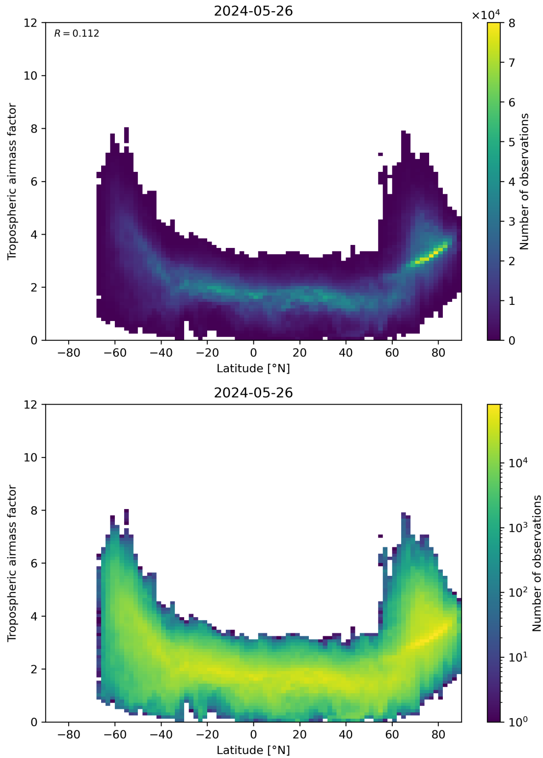
Figure 85: Scatter density plot of “Latitude” against “Tropospheric airmass factor” for 2024-05-25 to 2024-05-27.
