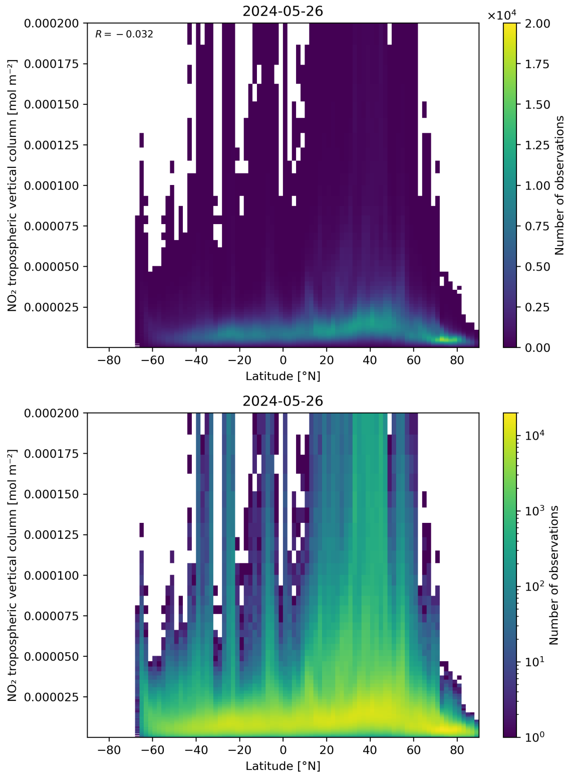
Figure 92: Scatter density plot of “Latitude” against “NO 2 tropospheric vertical column” for 2024-05-25 to 2024-05-27.
