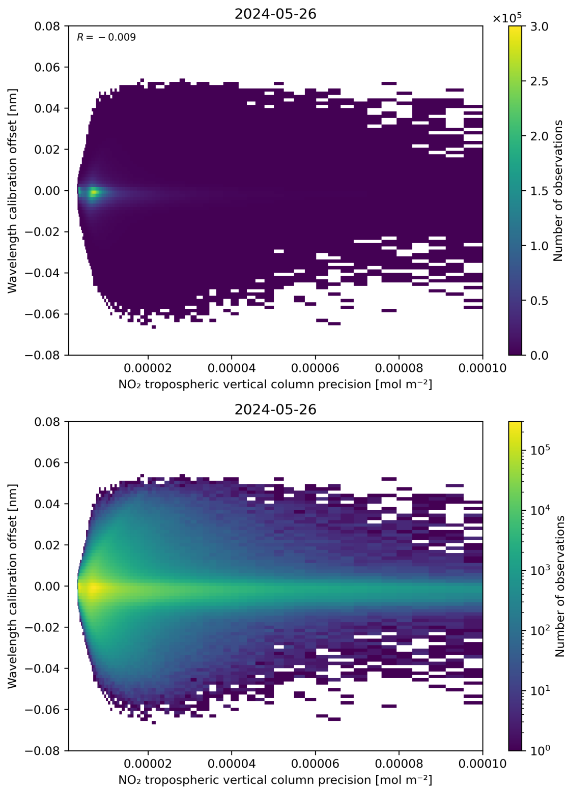
Figure 141: Scatter density plot of “NO 2 tropospheric vertical column precision” against “Wavelength calibration offset” for 2024-05-25 to 2024-05-27.
