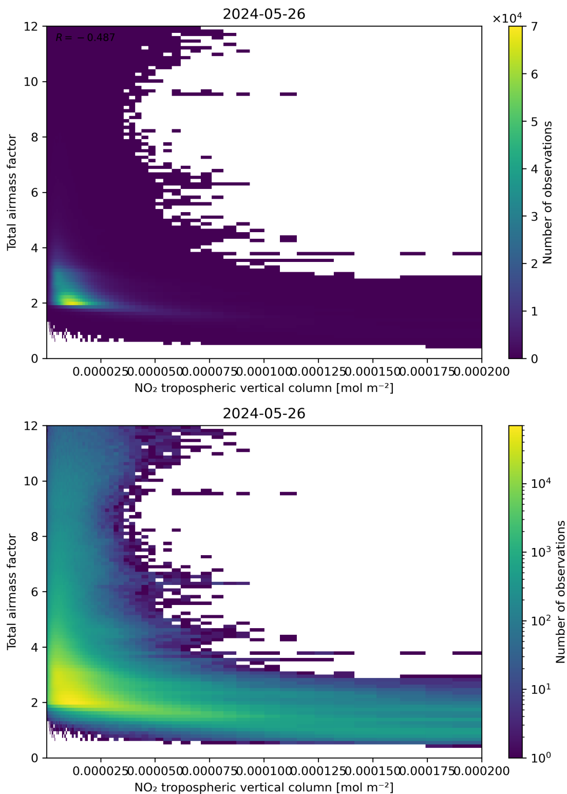
Figure 122: Scatter density plot of “NO 2 tropospheric vertical column” against “Total air mass factor” for 2024-05-25 to 2024-05-27.
