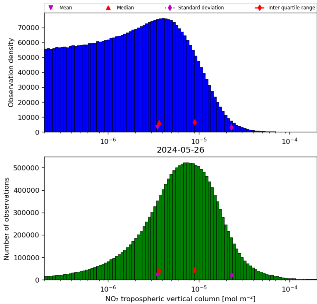
Figure 29: Histogram of “NO 2 tropospheric vertical column” for 2024-05-25 to 2024-05-27
