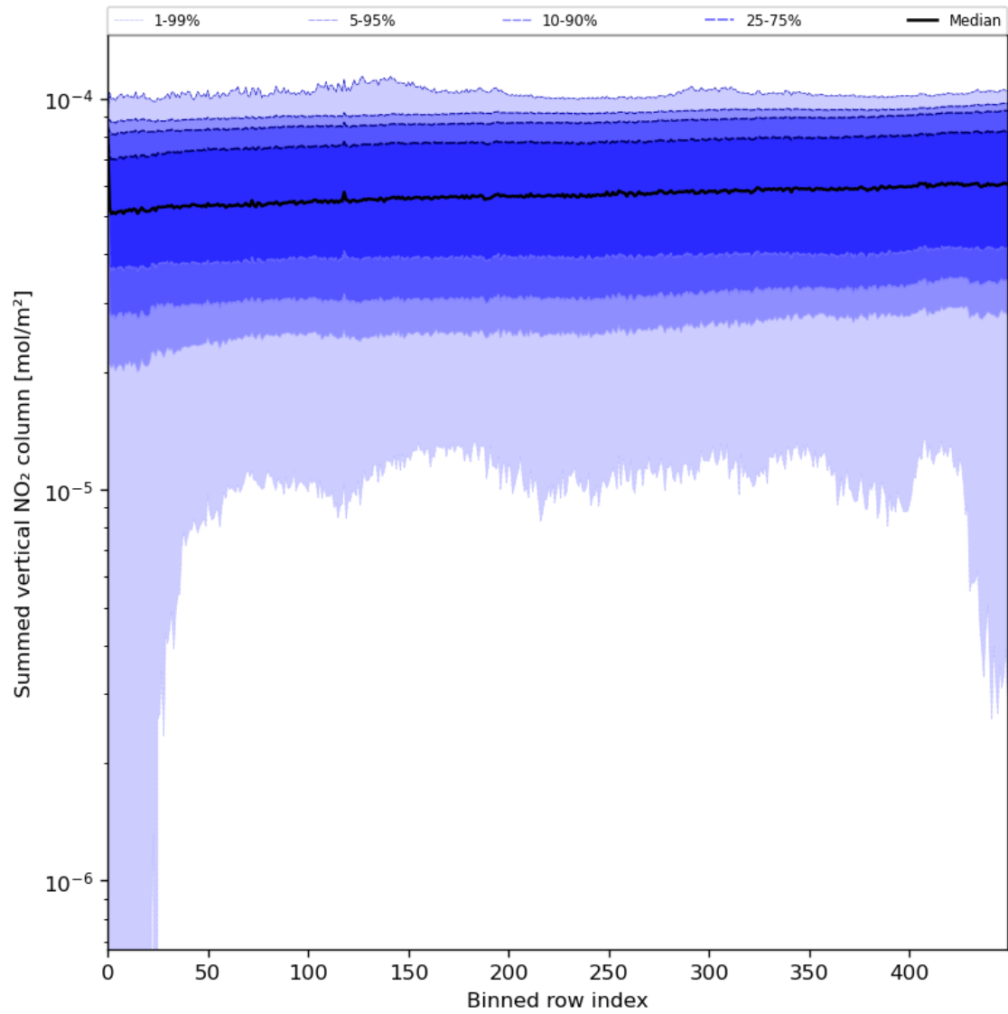
Figure 57: Along track statistics of “Summed vertical NO 2 column” for 2024-05-25 to 2024-05-27
