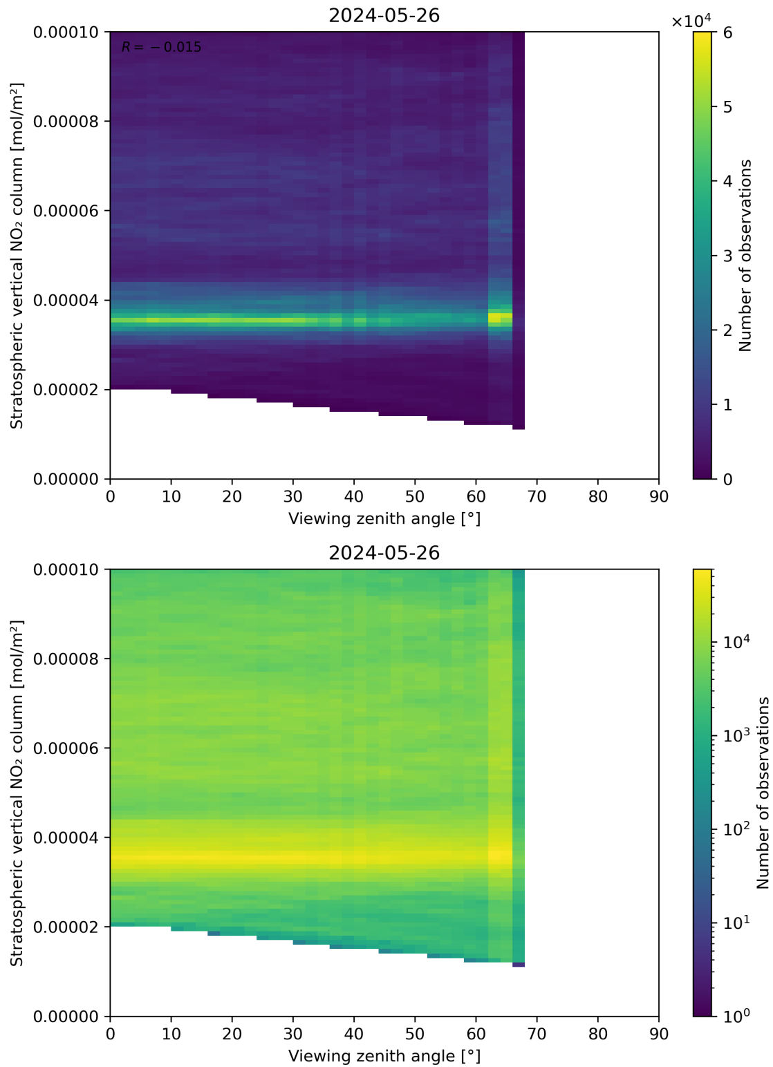
Figure 164: Scatter density plot of “Viewing zenith angle” against “Stratospheric vertical NO 2 column” for 2024-05-25 to 2024-05-27.
