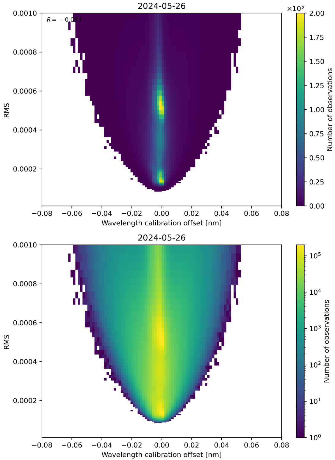
Figure 181: Scatter density plot of “Wavelength calibration offset” against “RMS” for 2024-05-25 to 2024-05-27.
