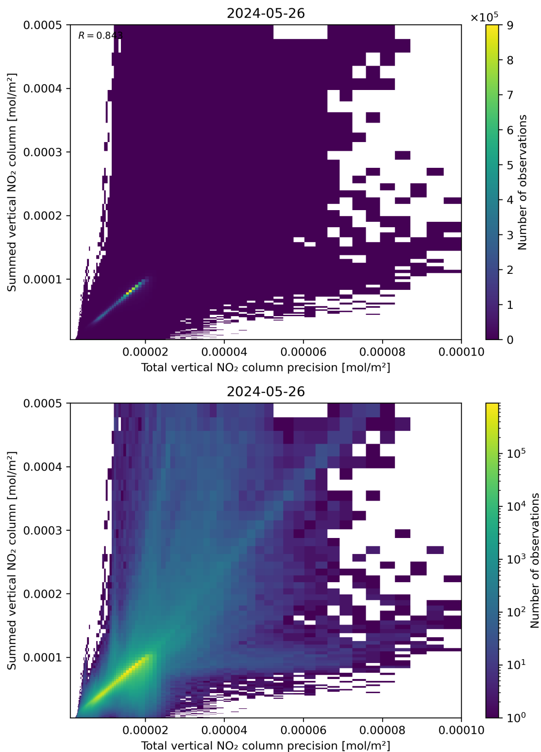
Figure 117: Scatter density plot of “Total vertical NO 2 column precision” against “Summed vertical NO 2 column” for 2024-05-25 to 2024-05-27.
