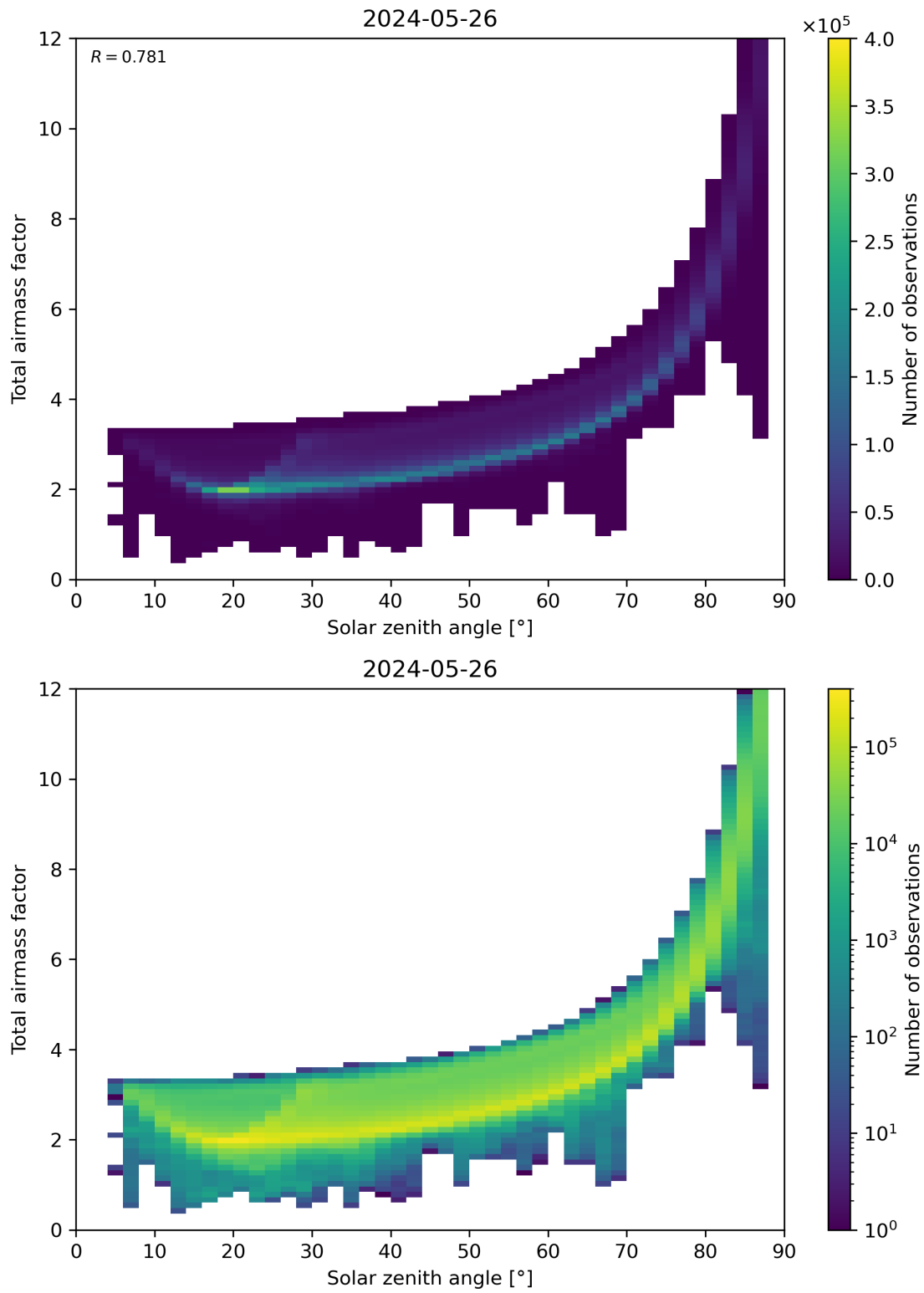
Figure 146: Scatter density plot of “Solar zenith angle” against “Total air mass factor” for 2024-05-25 to 2024-05-27.
