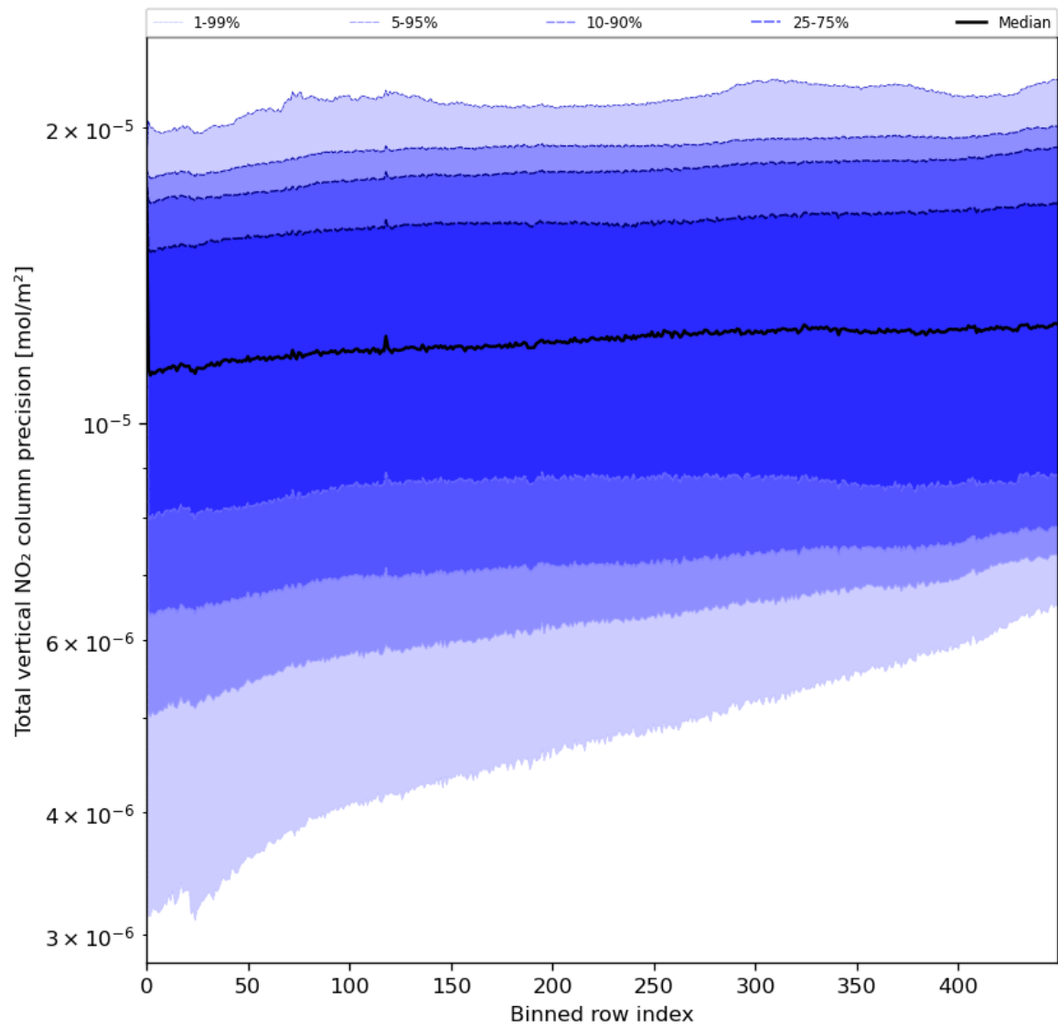
Figure 56: Along track statistics of “Total vertical NO 2 column precision” for 2024-05-25 to 2024-05-27
