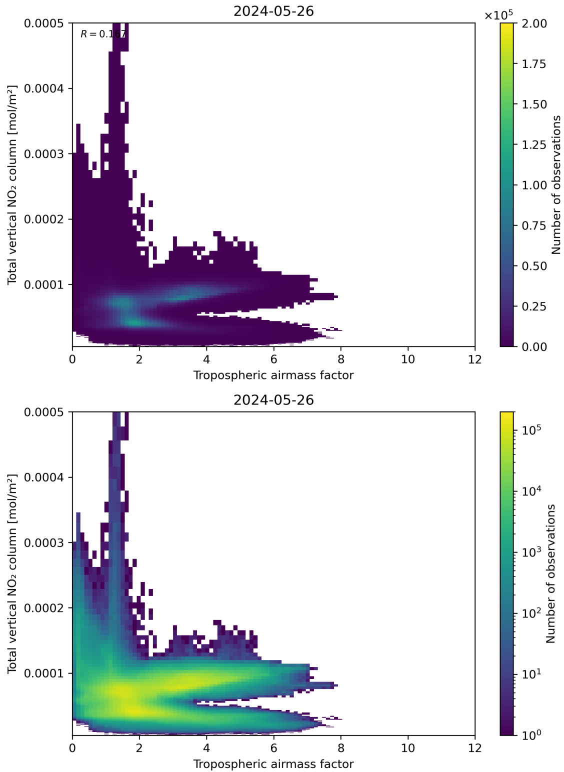
Figure 77: Scatter density plot of “Tropospheric airmass factor” against “Total vertical NO 2 column” for 2024-05-25 to 2024-05-27.
