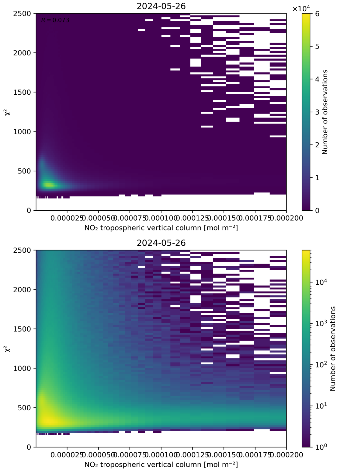
Figure 124: Scatter density plot of “NO 2 tropospheric vertical column” against “ \chi^2 ” for 2024-05-25 to 2024-05-27.
