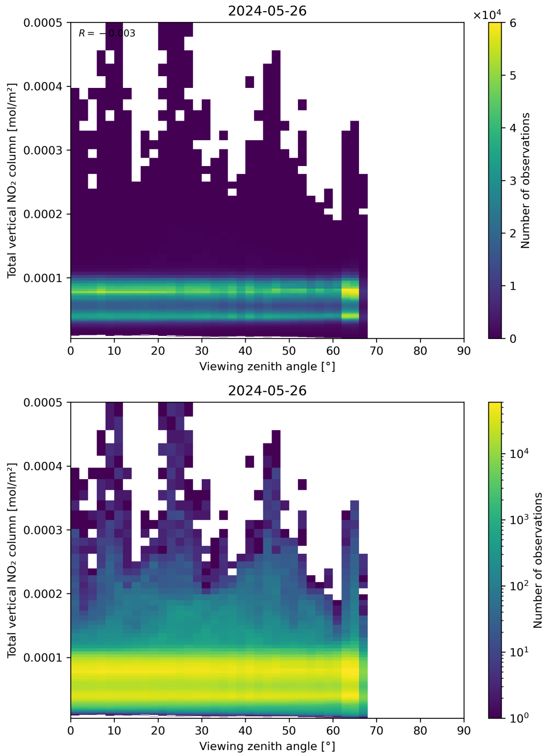
Figure 167: Scatter density plot of “Viewing zenith angle” against “Total vertical NO 2 column” for 2024-05-25 to 2024-05-27.
