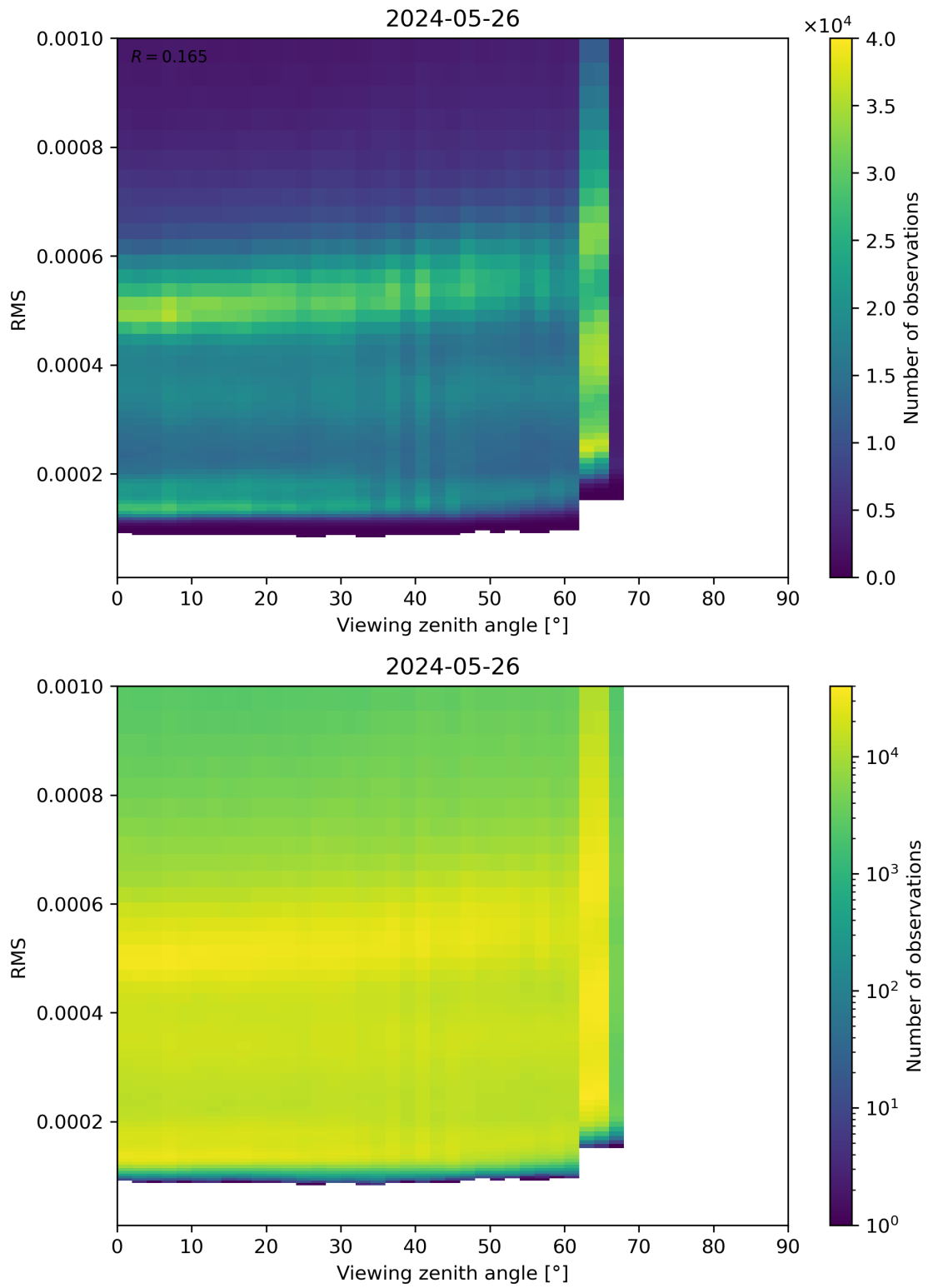
Figure 171: Scatter density plot of “Viewing zenith angle” against “RMS” for 2024-05-25 to 2024-05-27.
