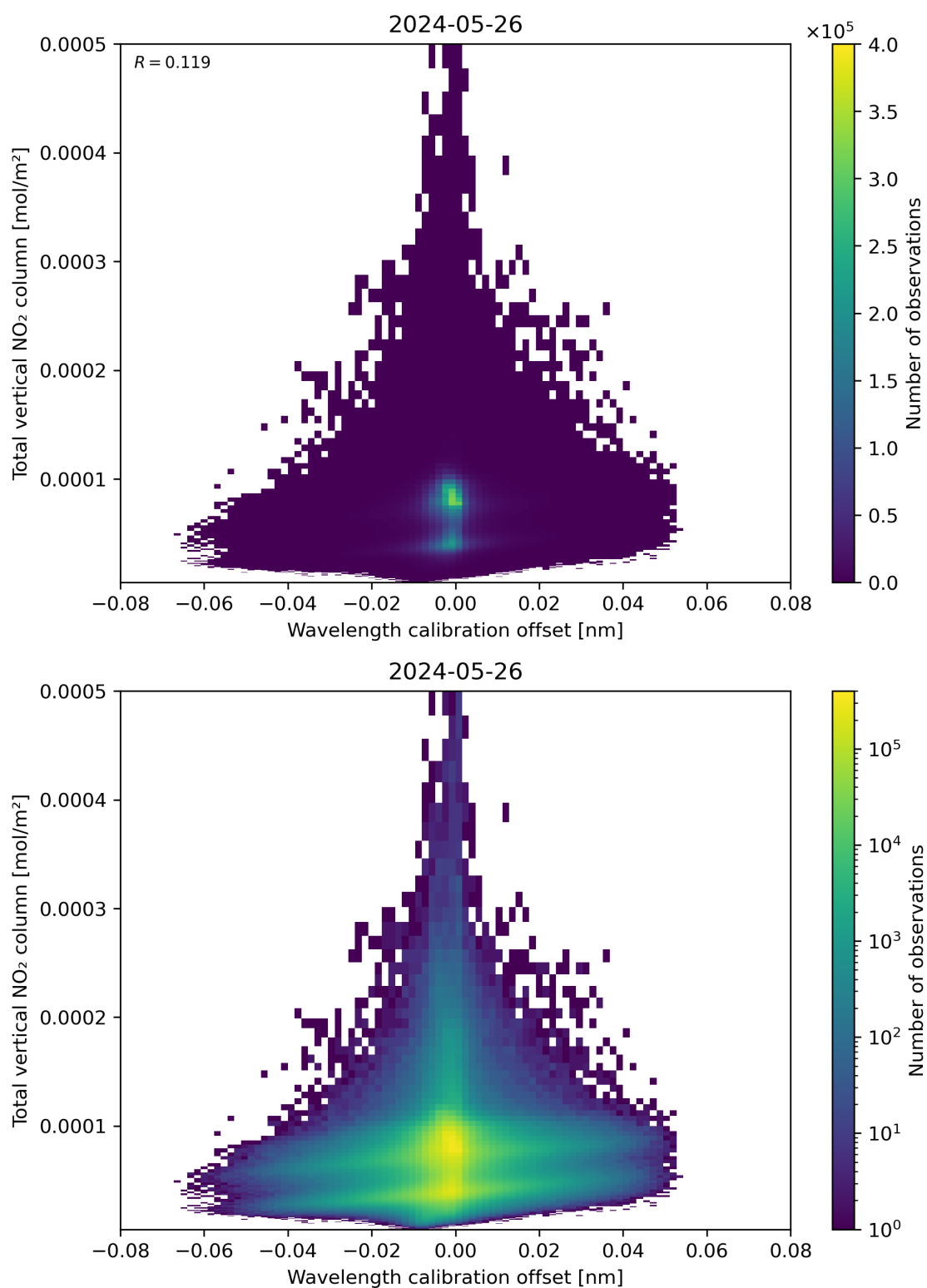
Figure 179: Scatter density plot of “Wavelength calibration offset” against “Total vertical NO 2 column” for 2024-05-25 to 2024-05-27.
