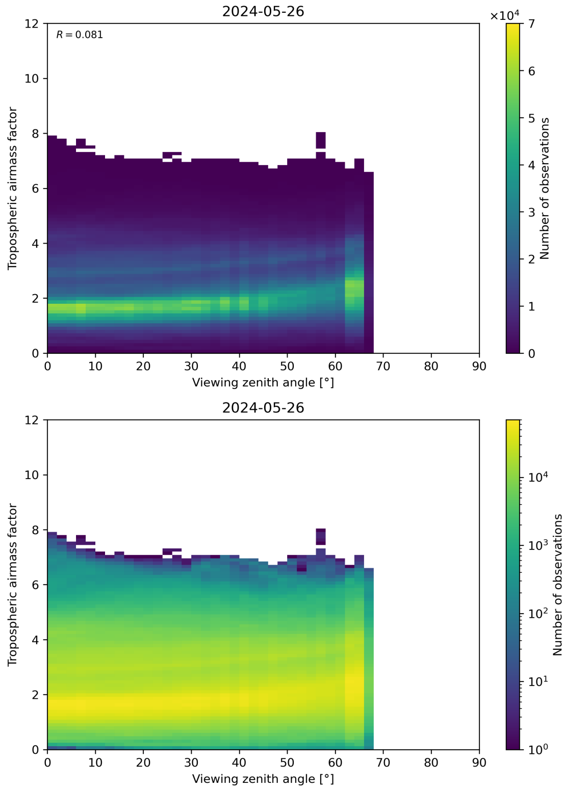
Figure 161: Scatter density plot of “Viewing zenith angle” against “Tropospheric airmass factor” for 2024-05-25 to 2024-05-27.
