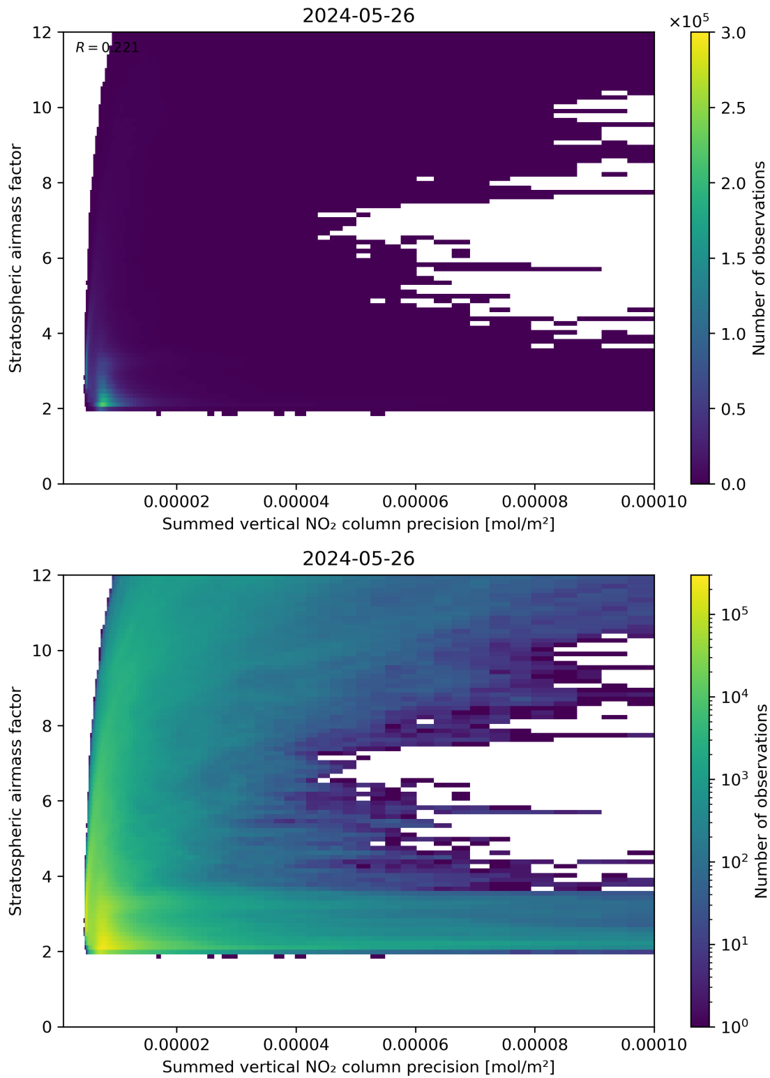
Figure 106: Scatter density plot of “Summed vertical NO 2 column precision” against “Stratospheric airmass factor” for 2024-05-25 to 2024-05-27.
