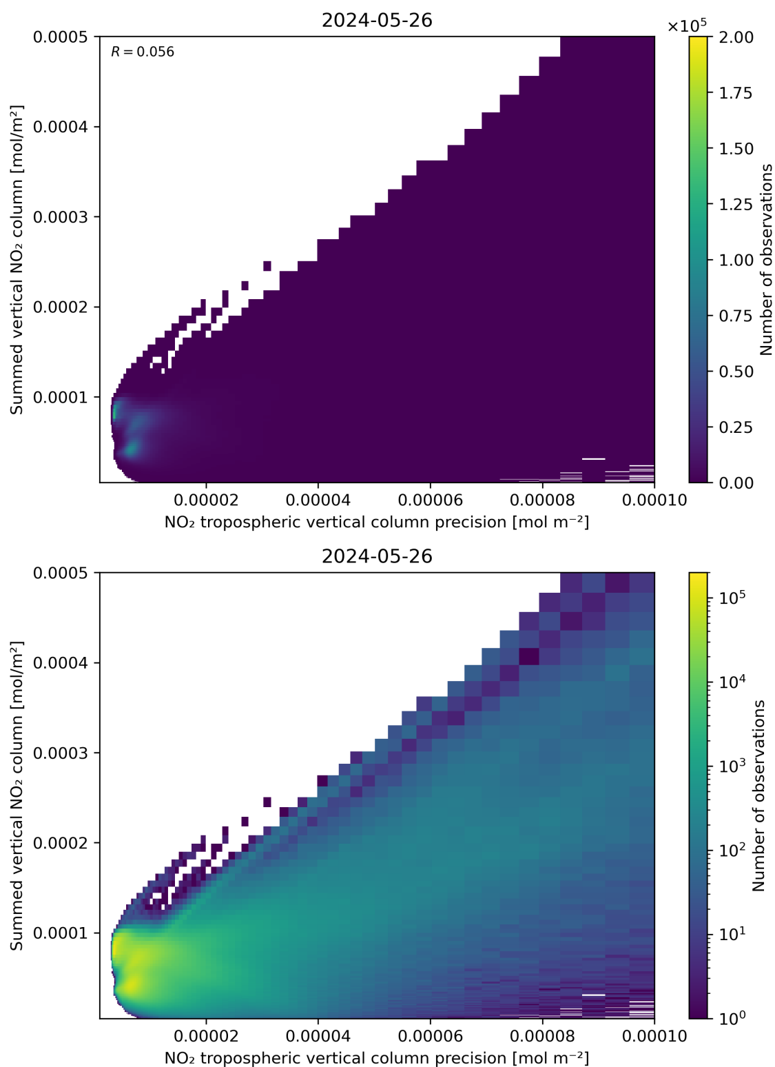
Figure 136: Scatter density plot of “NO 2 tropospheric vertical column precision” against “Summed vertical NO 2 column” for 2024-05-25 to 2024-05-27.
