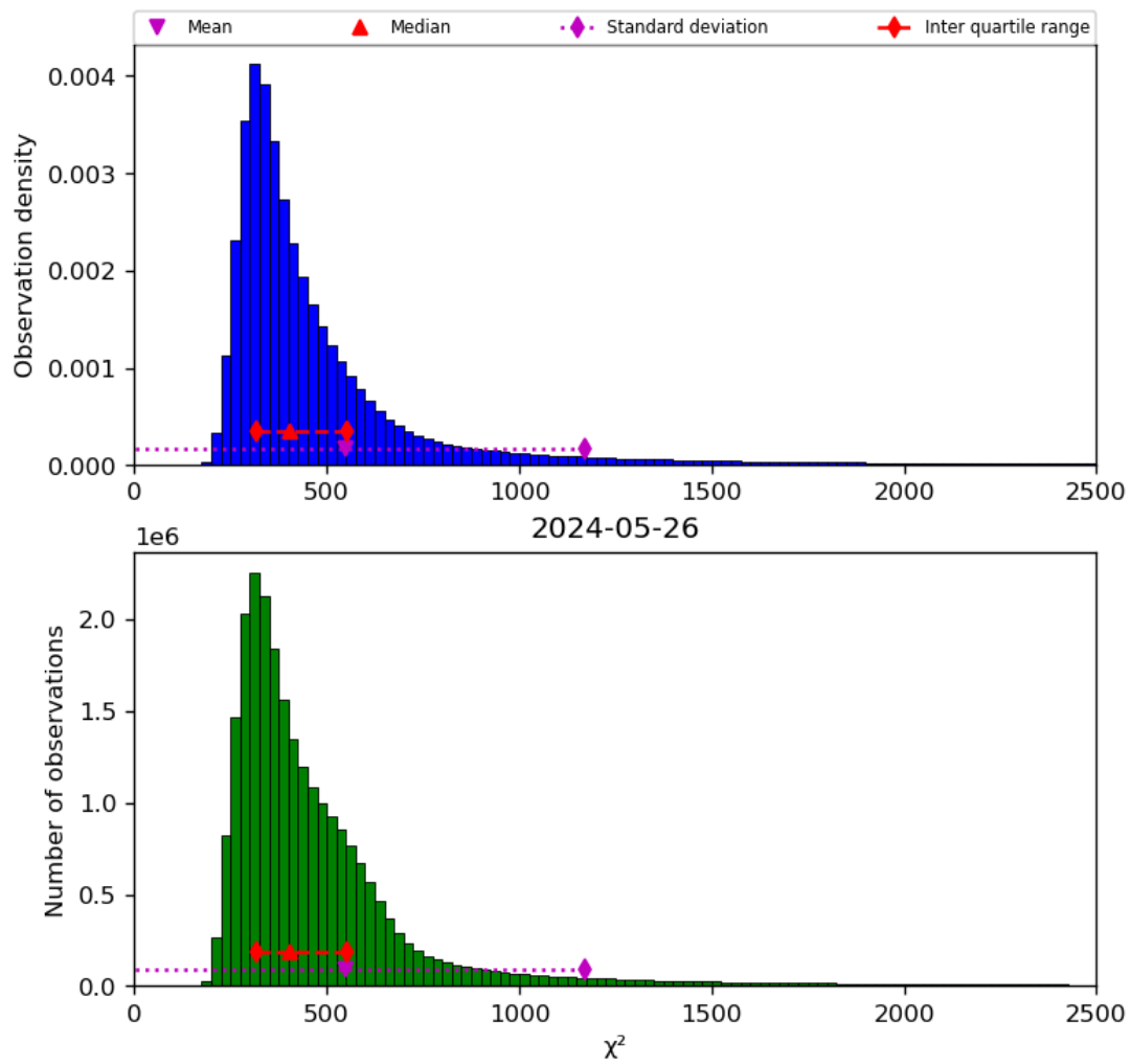
Figure 42: Histogram of " \chi^2 " for 2024-05-25 to 2024-05-27
