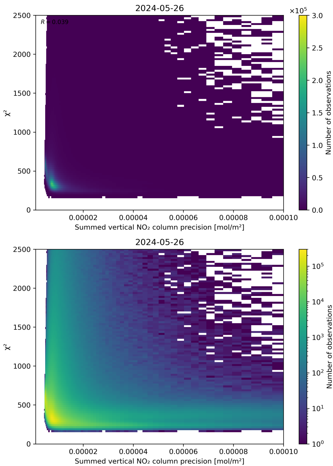
Figure 107: Scatter density plot of “Summed vertical NO 2 column precision” against “ \chi^2 ” for 2024-05-25 to 2024-05-27.
