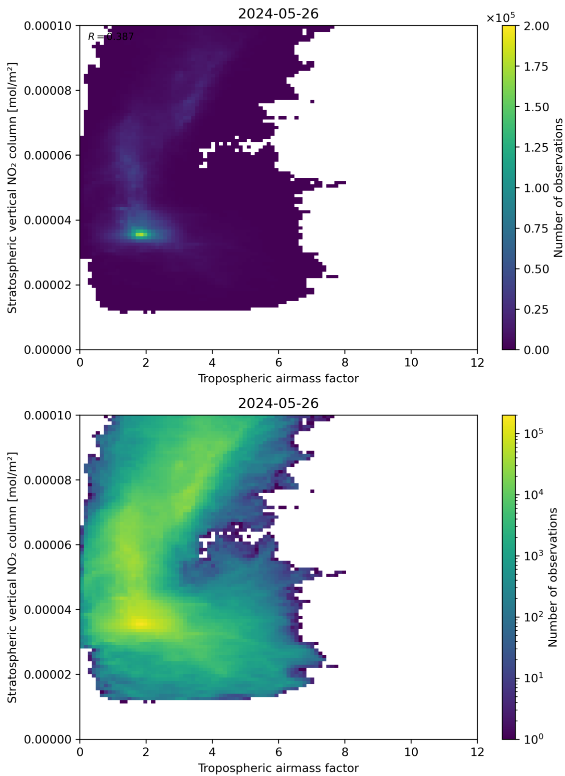
Figure 74: Scatter density plot of “Tropospheric air mass factor” against “Stratospheric vertical NO 2 column” for 2024-05-25 to 2024-05-27.
