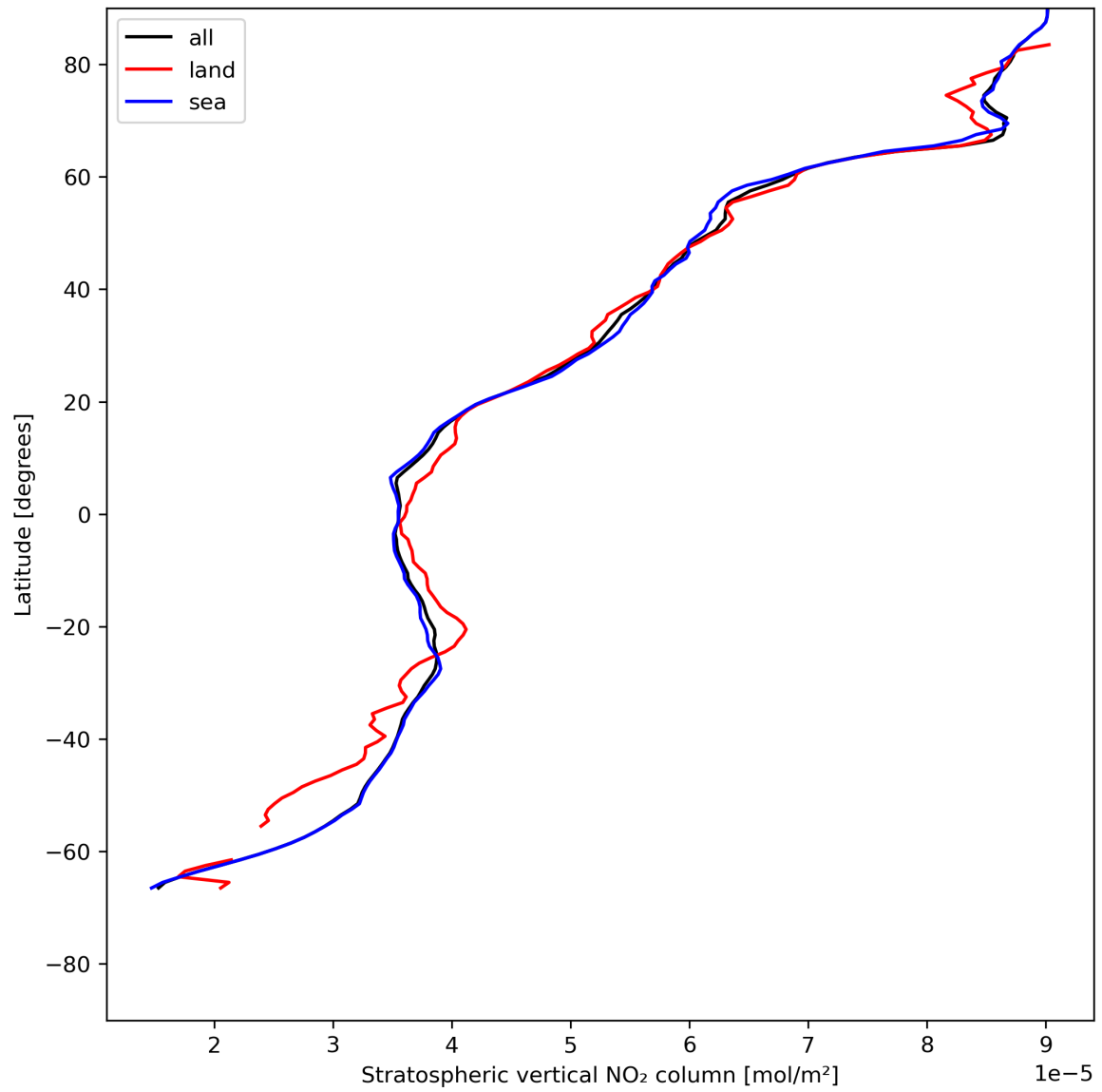
Figure 19: Zonal average of “Stratospheric vertical NO 2 column” for 2024-05-25 to 2024-05-27.
