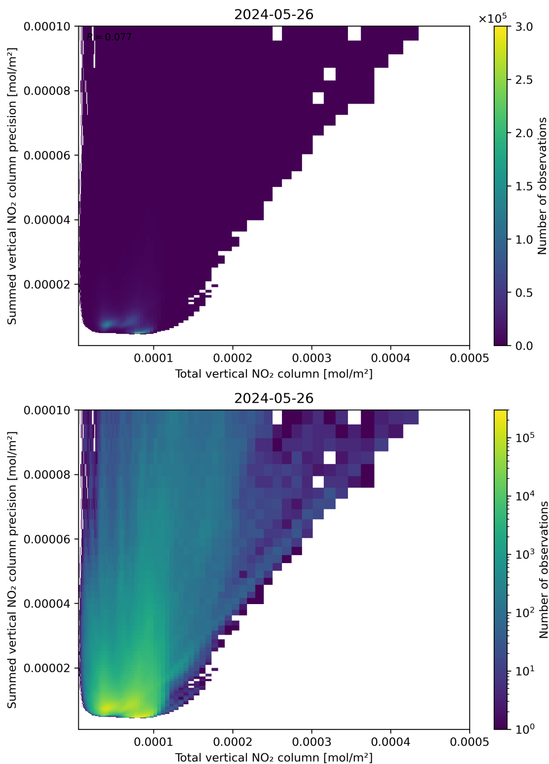
Figure 113: Scatter density plot of “Total vertical NO 2 column” against “Summed vertical NO 2 column precision” for 2024-05-25 to 2024-05-27.
