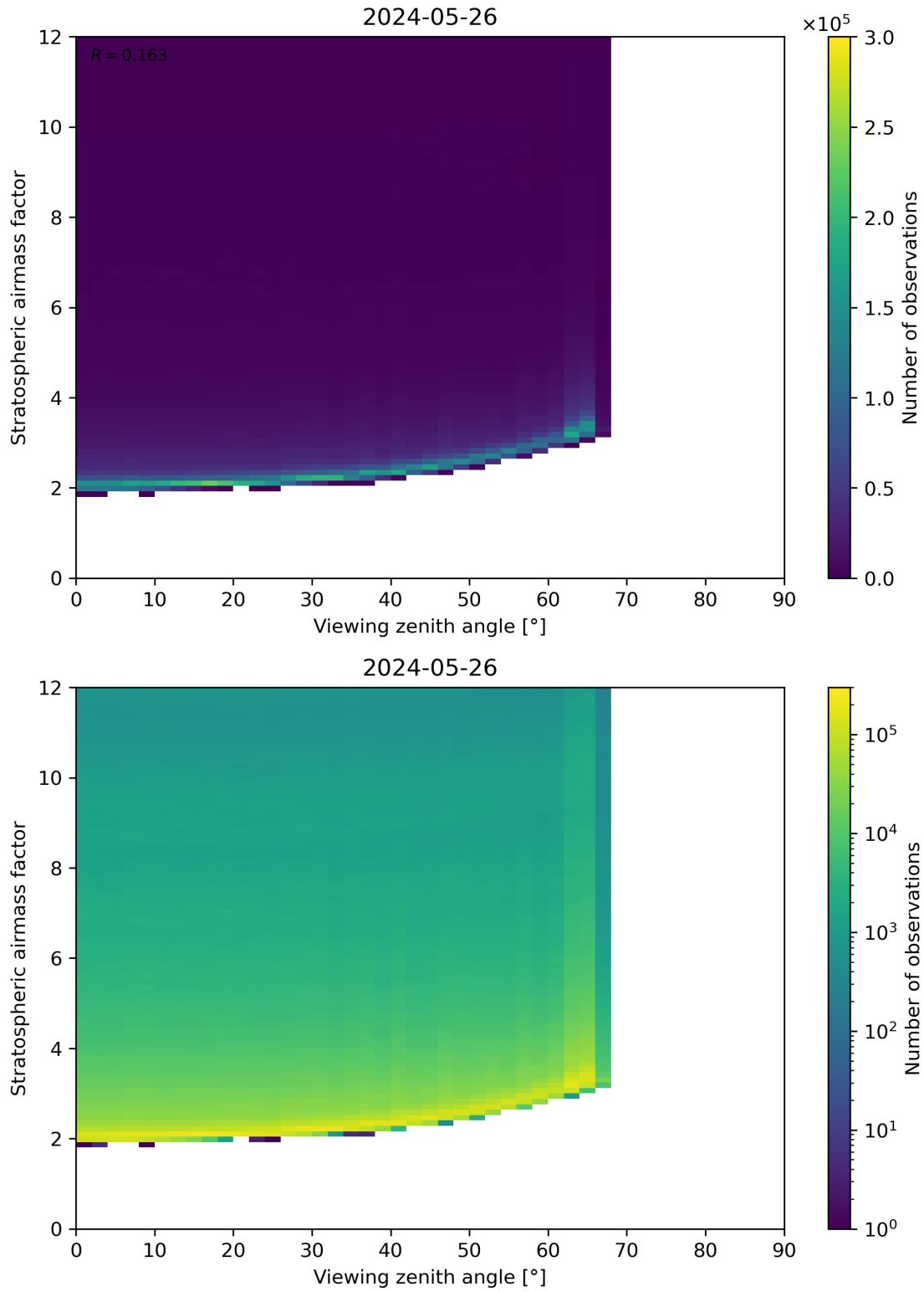
Figure 159: Scatter density plot of “Viewing zenith angle” against “Stratospheric airmass factor” for 2024-05-25 to 2024-05-27.
