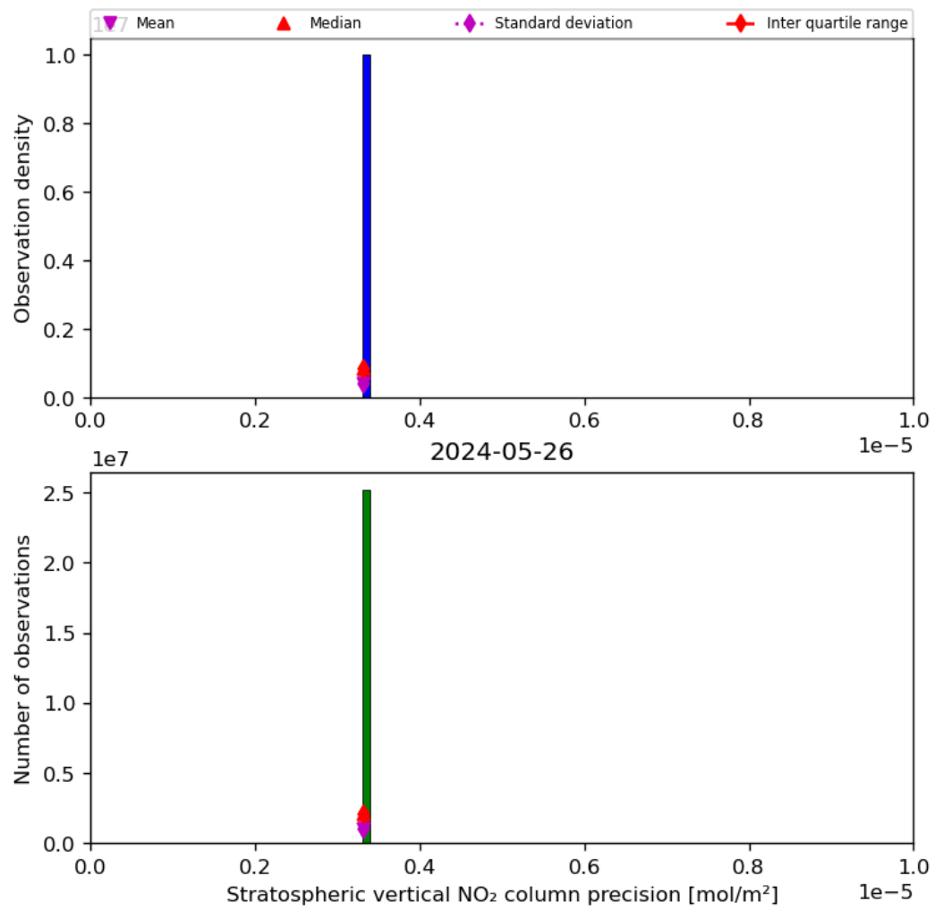
Figure 37: Histogram of “Stratospheric vertical NO 2 column precision” for 2024-05-25 to 2024-05-27
