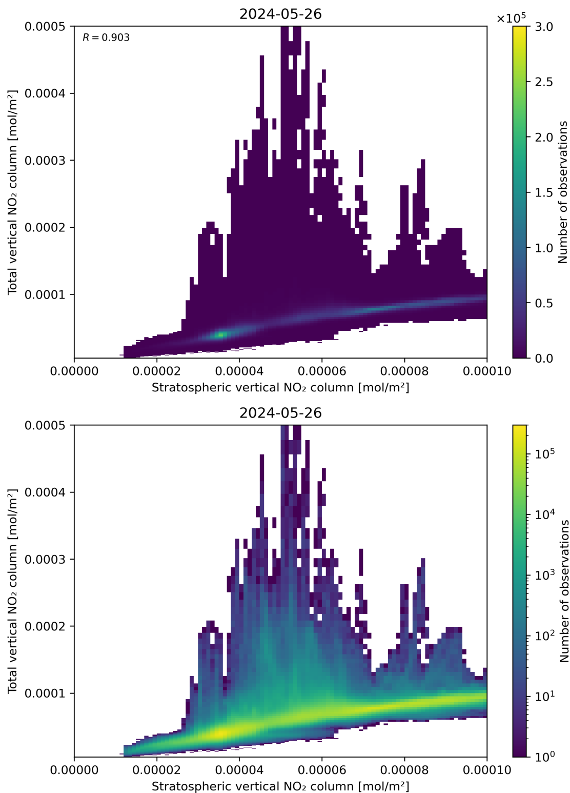
Figure 100: Scatter density plot of “Stratospheric vertical NO 2 column” against “Total vertical NO 2 column” for 2024-05-25 to 2024-05-27.
