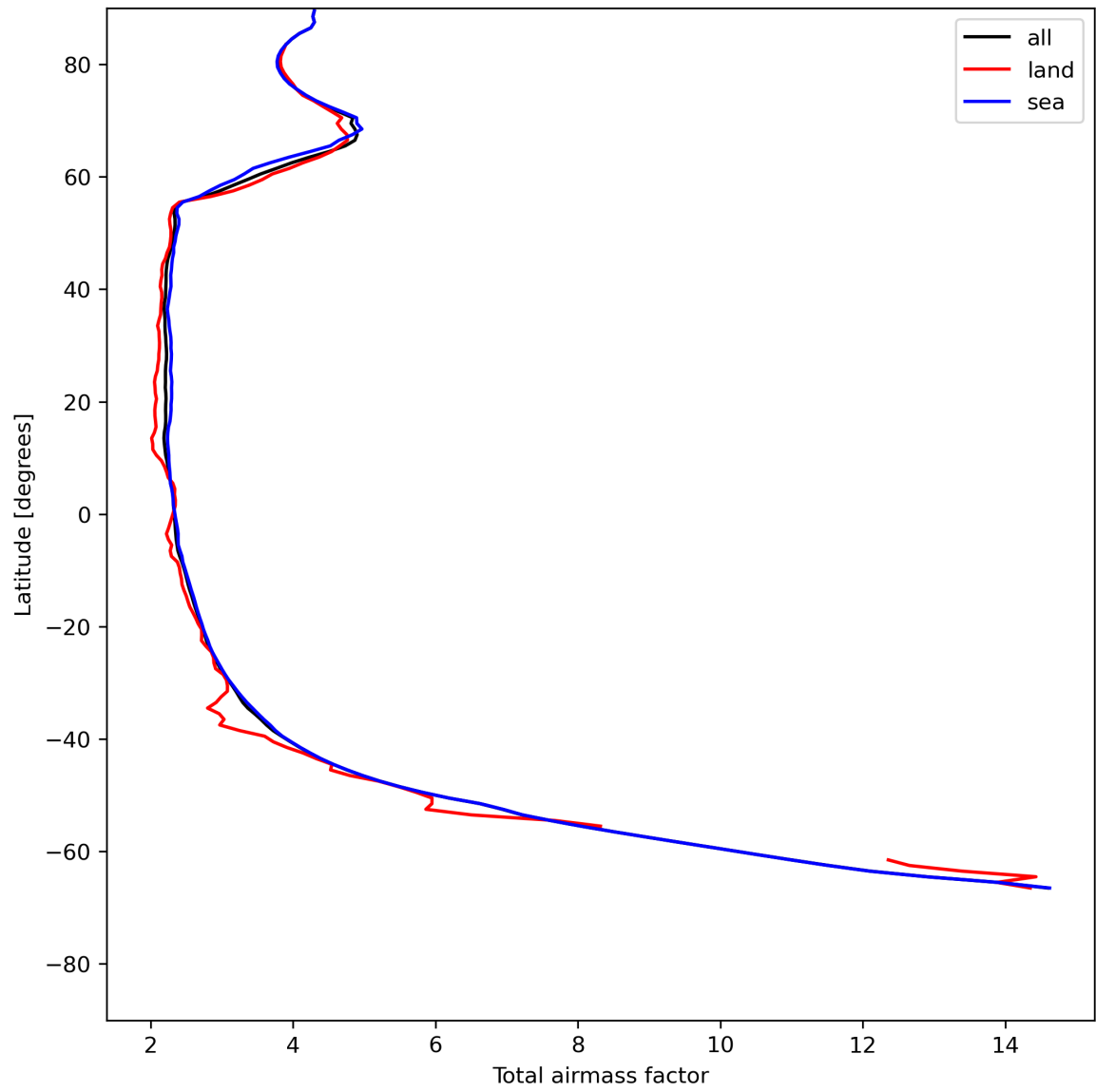
Figure 15: Zonal average of “Total airmass factor” for 2024-05-25 to 2024-05-27.
