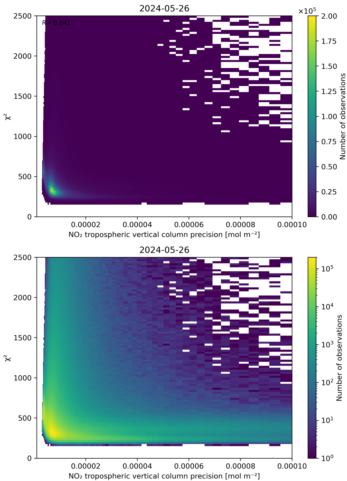
Figure 134: Scatter density plot of “NO 2 tropospheric vertical column precision” against “ \chi^2 ” for 2024-05-25 to 2024-05-27.
