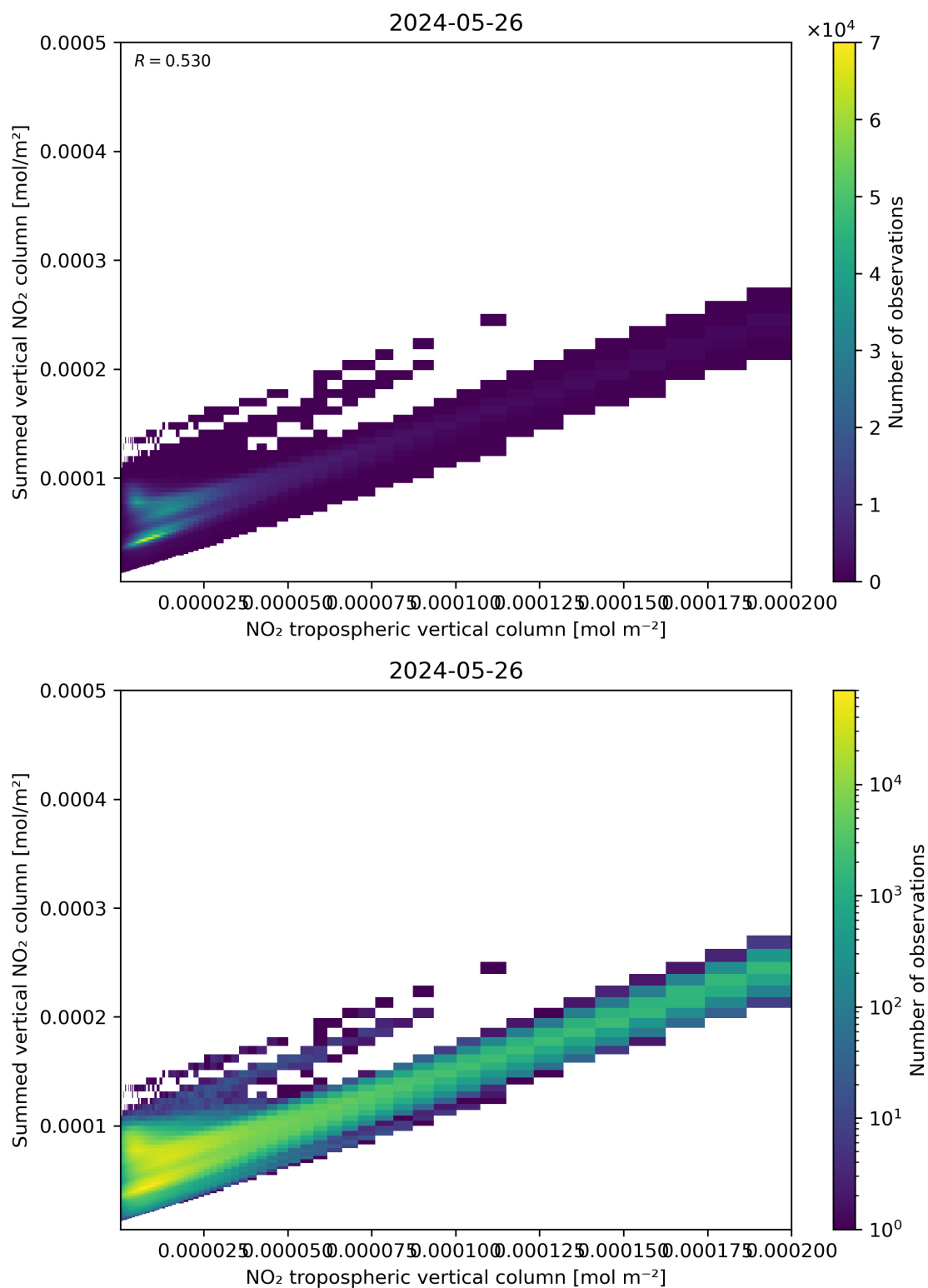
Figure 126: Scatter density plot of “NO 2 tropospheric vertical column” against “Summed vertical NO 2 column” for 2024-05-25 to 2024-05-27.
