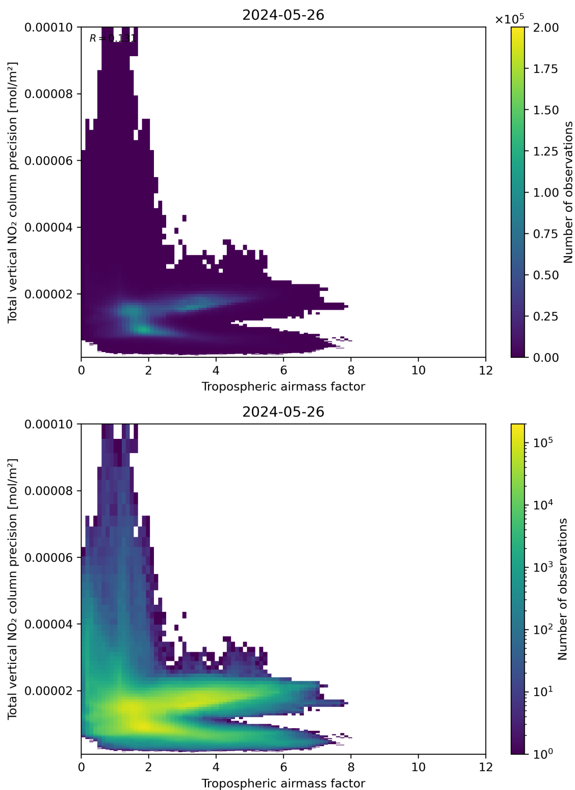
Figure 78: Scatter density plot of “Tropospheric air mass factor” against “Total vertical NO 2 column precision” for 2024-05-25 to 2024-05-27.
