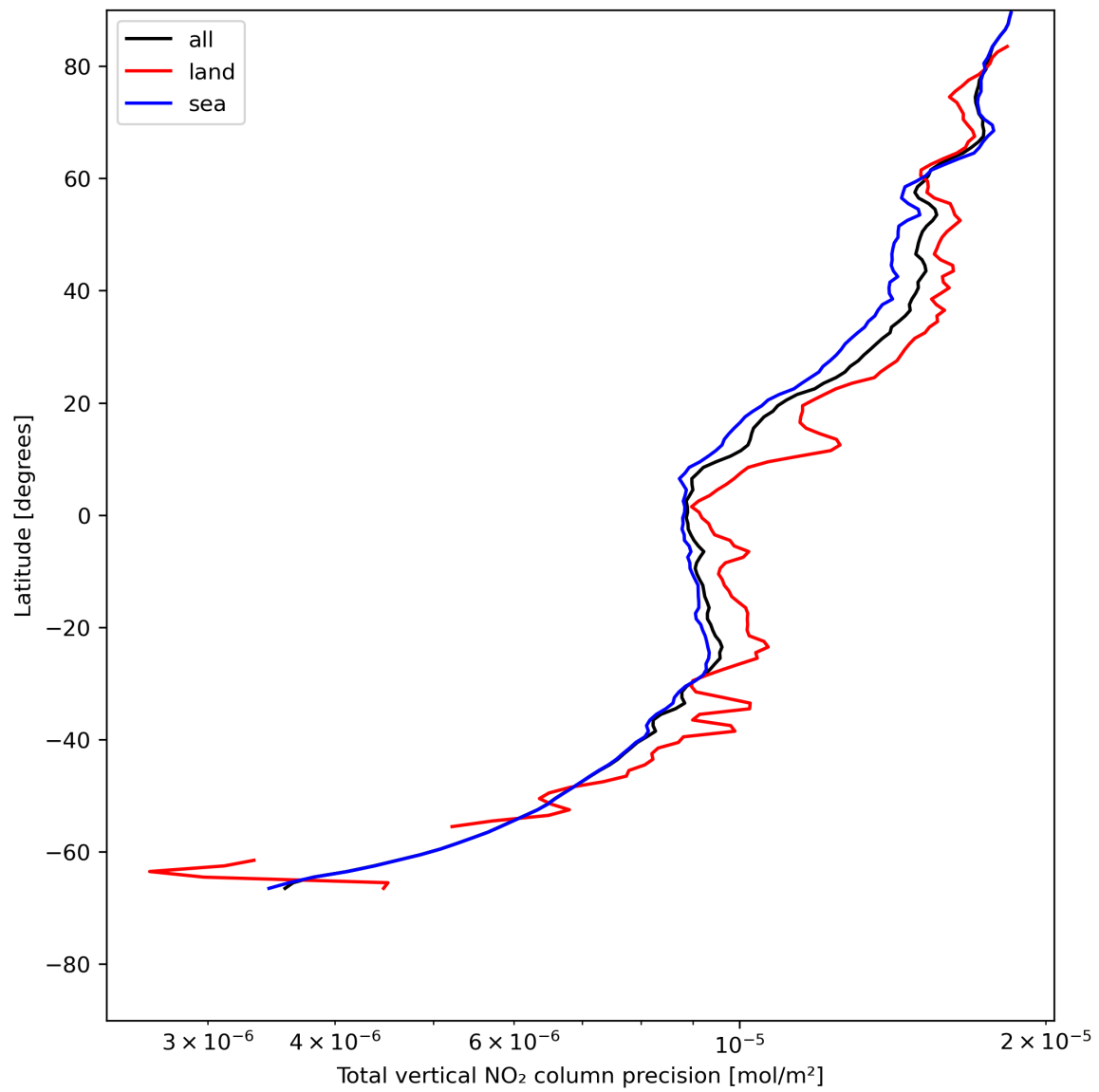
Figure 22: Zonal average of “Total vertical NO 2 column precision” for 2024-05-25 to 2024-05-27.
