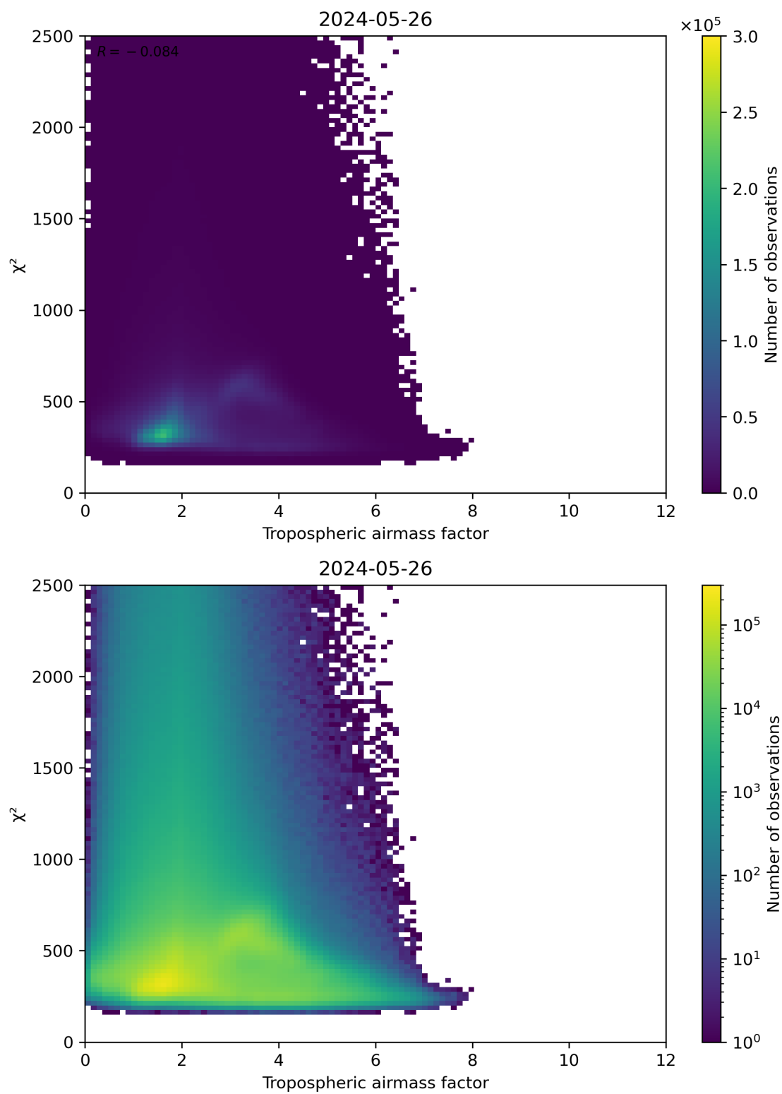
Figure 73: Scatter density plot of “Tropospheric airmass factor” against “ \chi^2 ” for 2024-05-25 to 2024-05-27.
