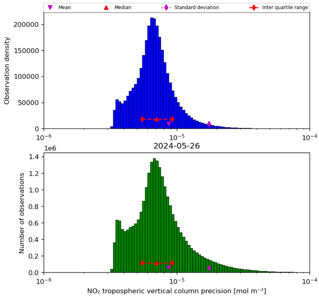
Figure 30: Histogram of “NO 2 tropospheric vertical column precision” for 2024-05-25 to 2024-05-27
