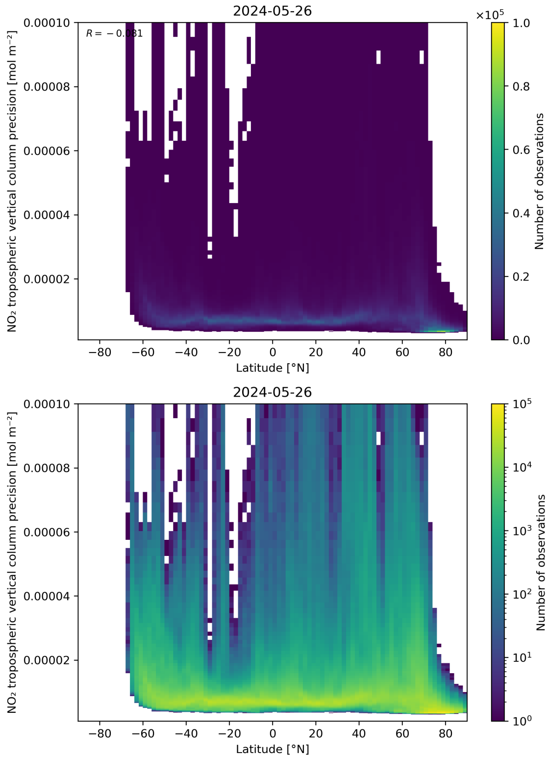
Figure 93: Scatter density plot of “Latitude” against “NO 2 tropospheric vertical column precision” for 2024-05-25 to 2024-05-27.
