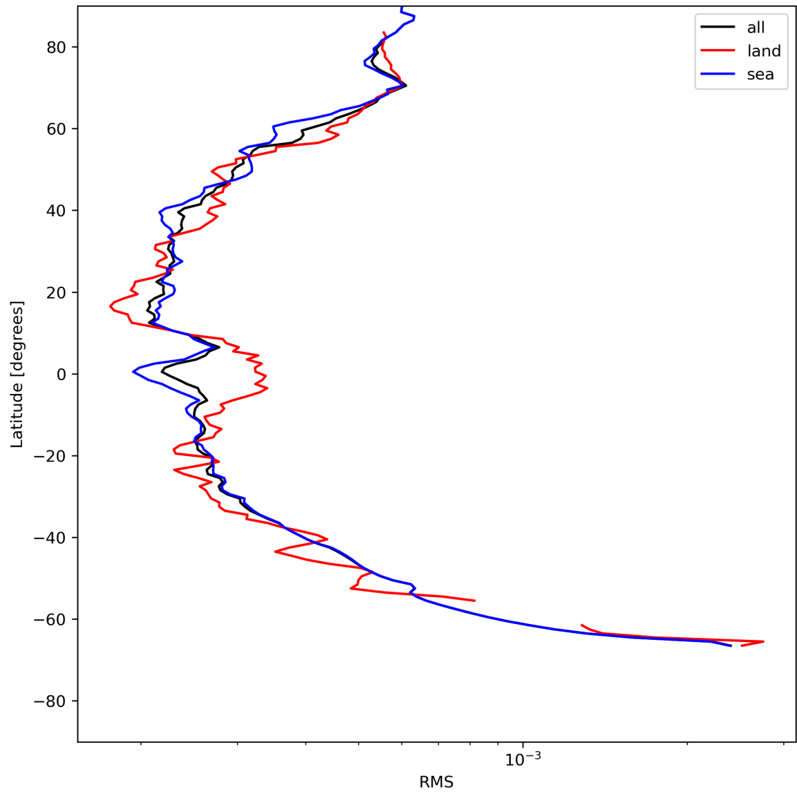
Figure 26: Zonal average of “RMS” for 2024-05-25 to 2024-05-27.
