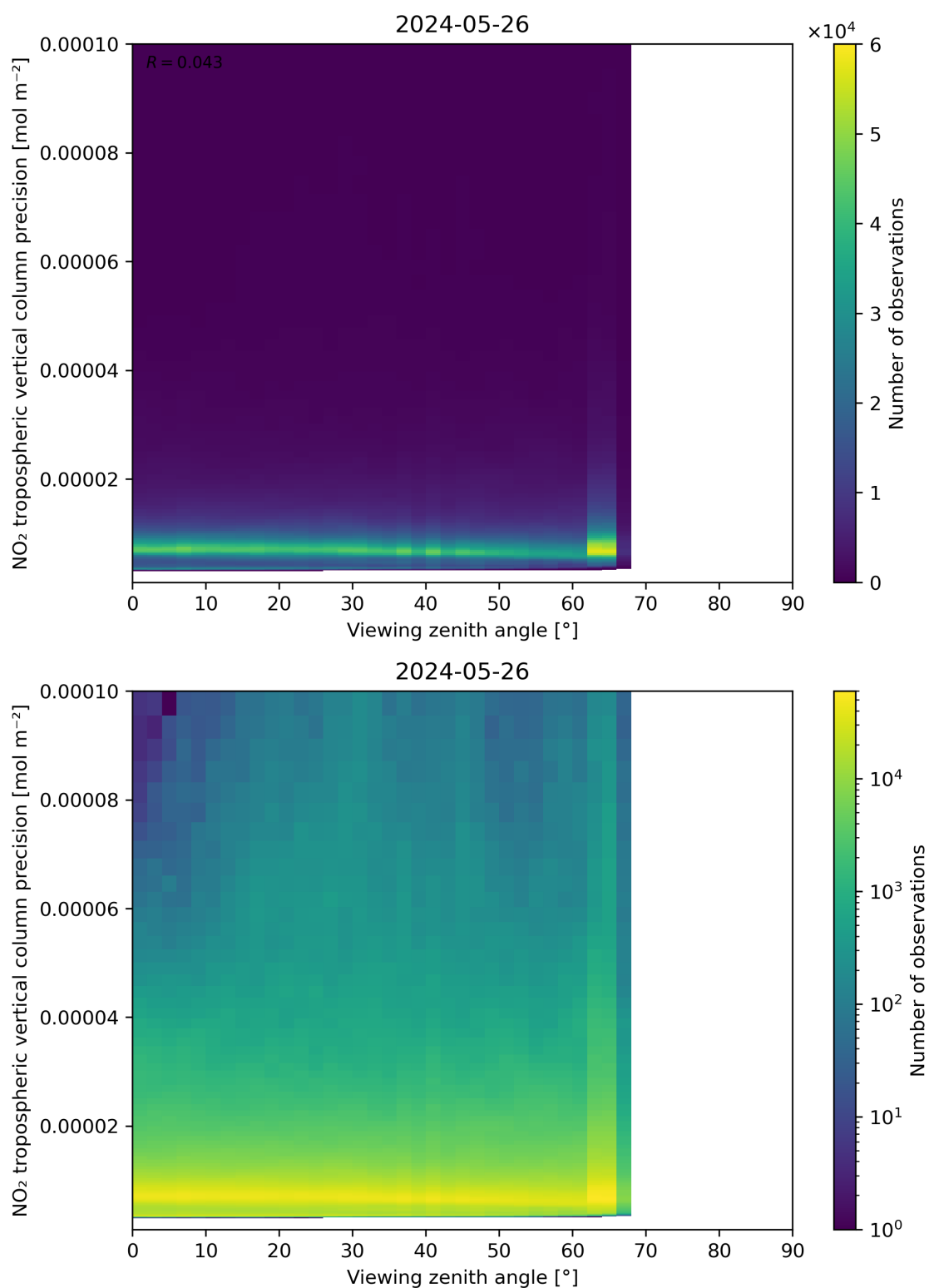
Figure 170: Scatter density plot of “Viewing zenith angle” against “NO 2 tropospheric vertical column precision” for 2024-05-25 to 2024-05-27.
