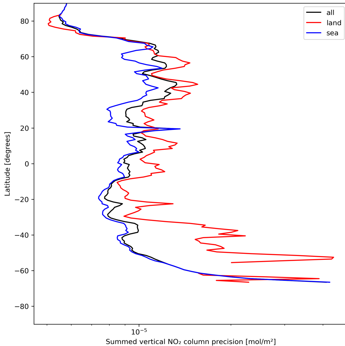
Figure 24: Zonal average of “Summed vertical NO 2 column precision” for 2024-05-25 to 2024-05-27.
