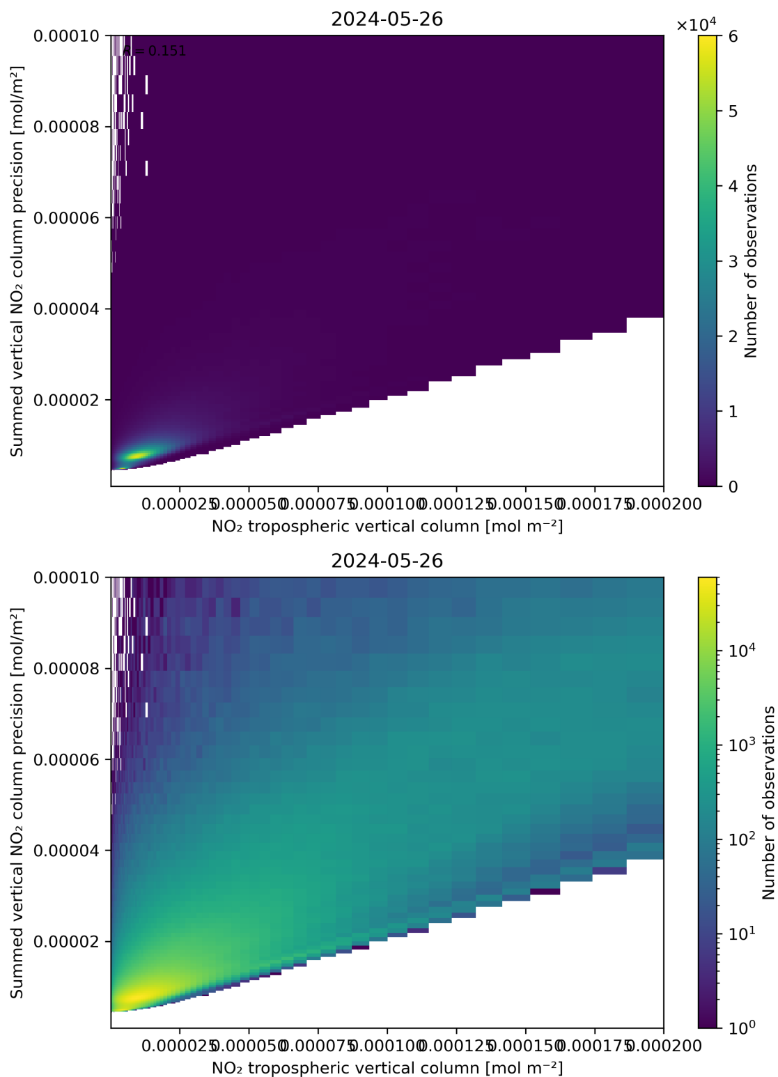
Figure 127: Scatter density plot of “NO 2 tropospheric vertical column” against “Summed vertical NO 2 column precision” for 2024-05-25 to 2024-05-27.
