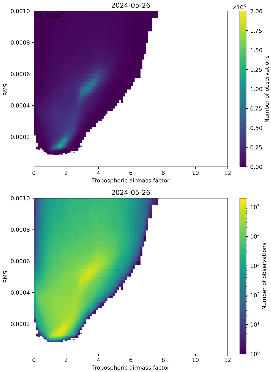
Figure 79: Scatter density plot of “Tropospheric airmass factor” against “RMS” for 2024-05-25 to 2024-05-27.
