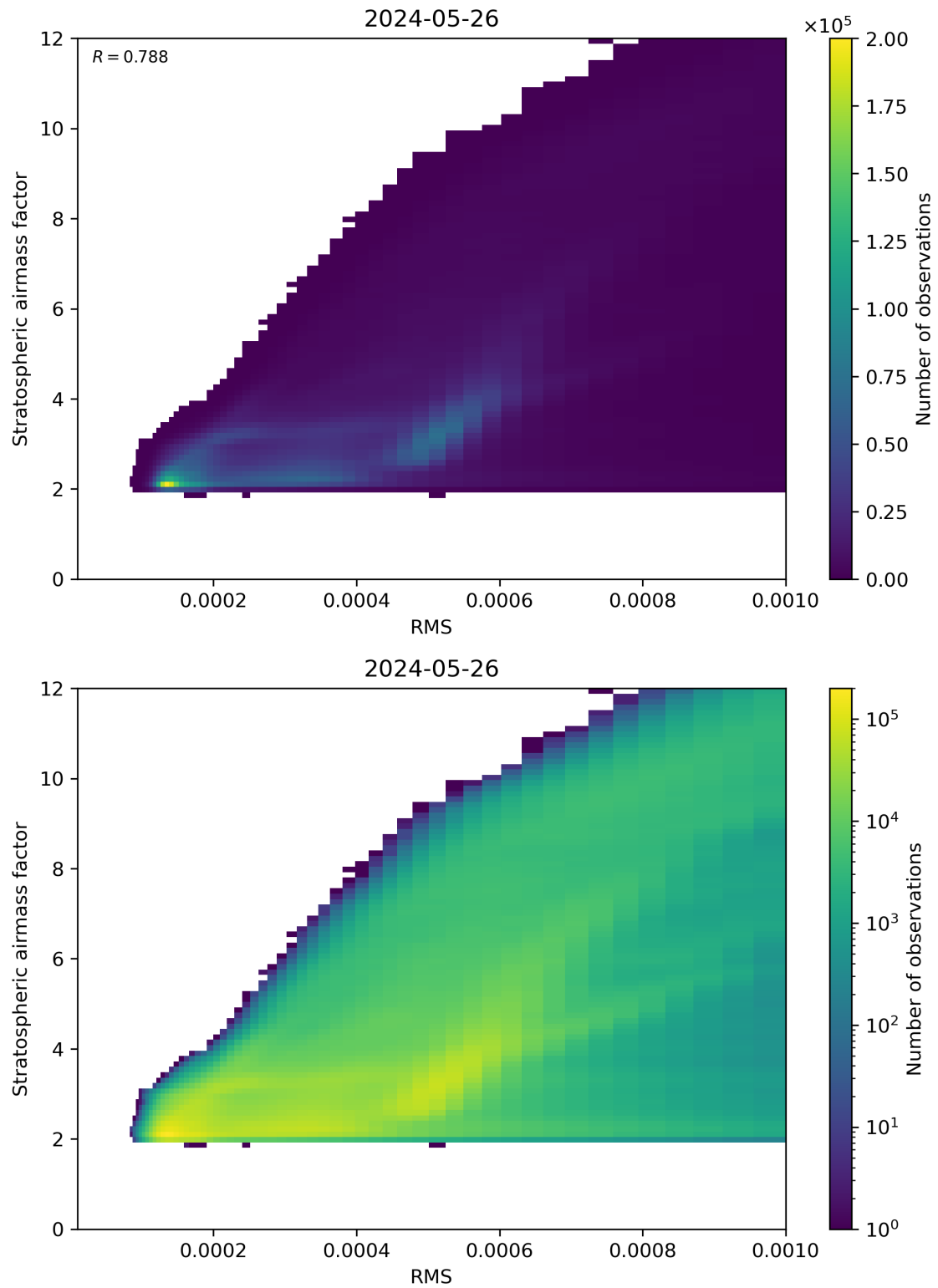
Figure 144: Scatter density plot of “RMS” against “Stratospheric airmass factor” for 2024-05-25 to 2024-05-27.
