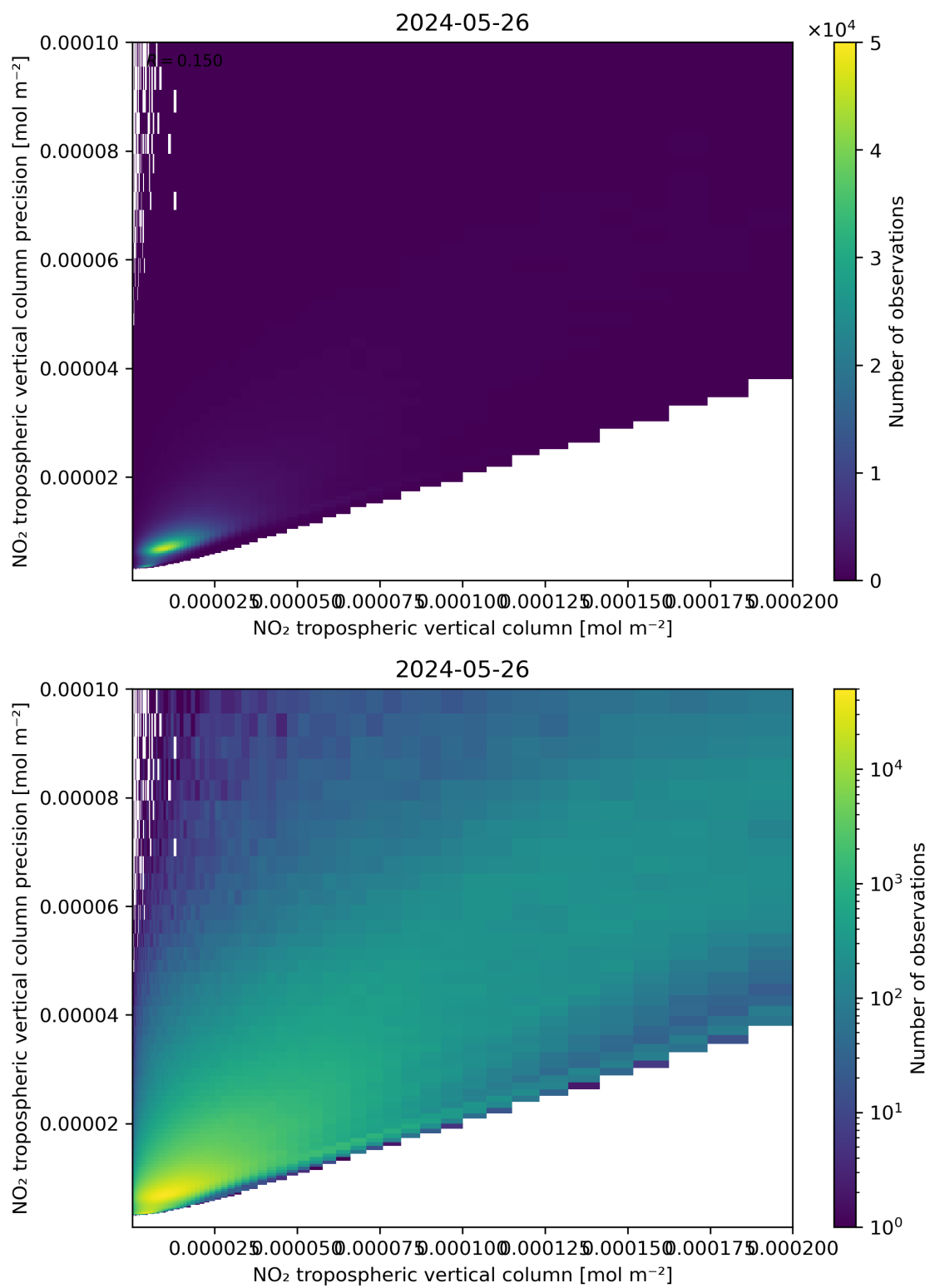
Figure 130: Scatter density plot of “NO 2 tropospheric vertical column” against “NO 2 tropospheric vertical column precision” for 2024-05-25 to 2024-05-27.
