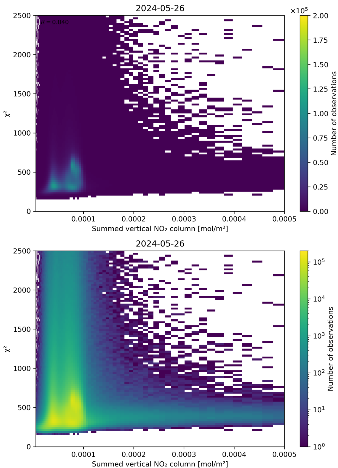
Figure 104: Scatter density plot of “Summed vertical NO 2 column” against “ \chi^2 ” for 2024-05-25 to 2024-05-27.
