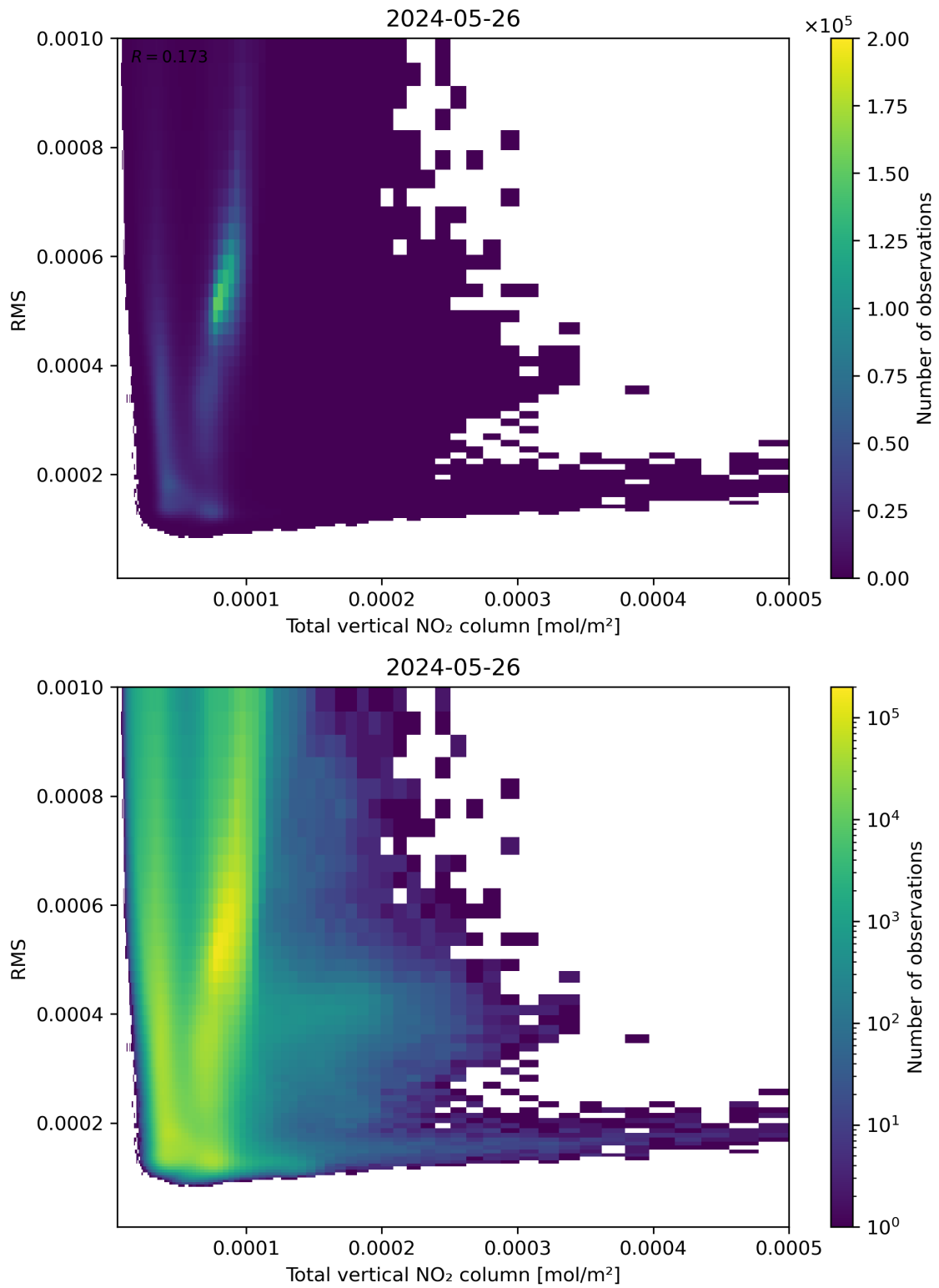
Figure 120: Scatter density plot of “Total vertical NO 2 column” against “RMS” for 2024-05-25 to 2024-05-27.
