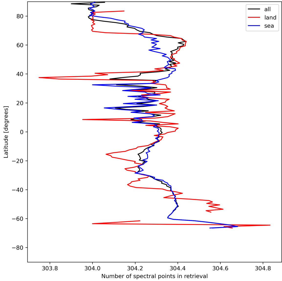
Figure 16: Zonal average of “Number of spectral points in retrieval” for 2024-05-25 to 2024-05-27.
