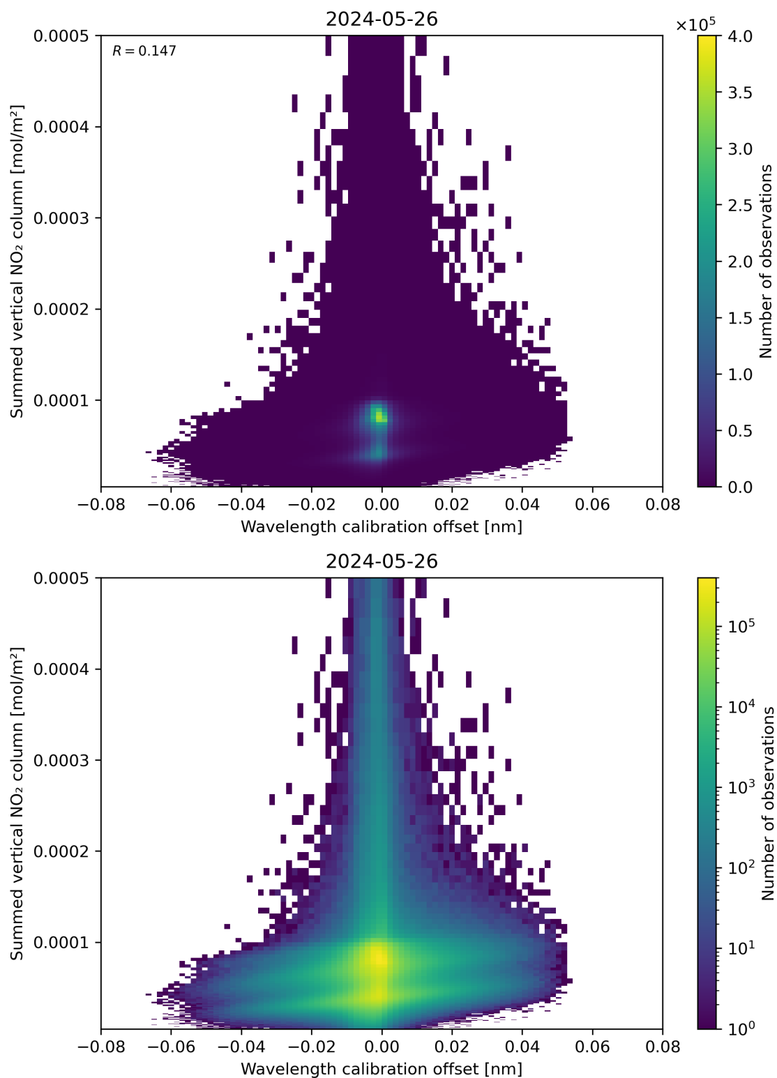
Figure 177: Scatter density plot of “Wavelength calibration offset” against “Summed vertical NO 2 column” for 2024-05-25 to 2024-05-27.
