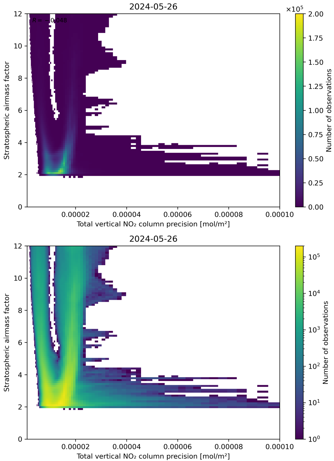
Figure 115: Scatter density plot of “Total vertical NO 2 column precision” against “Stratospheric airmass factor” for 2024-05-25 to 2024-05-27.
