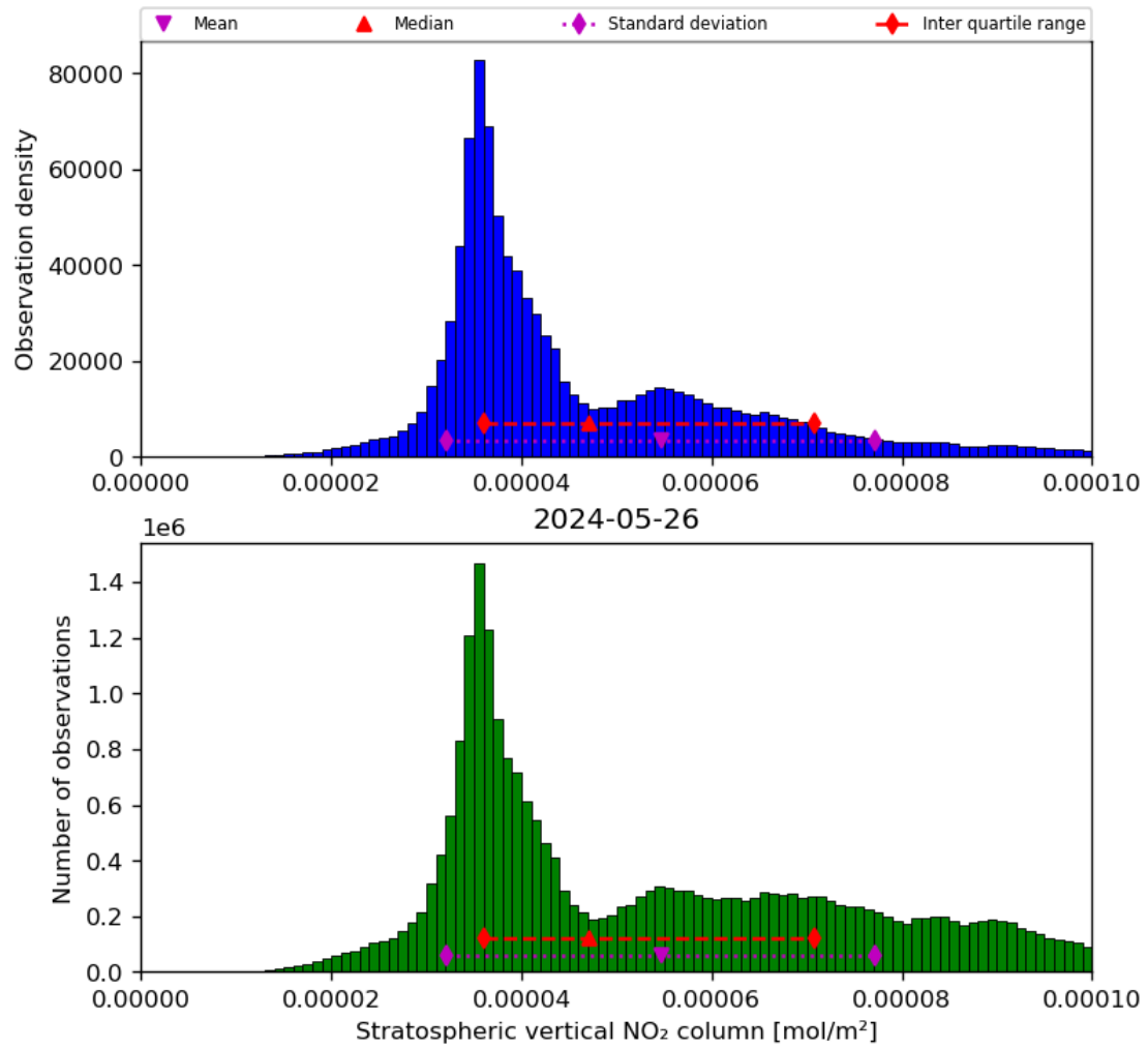
Figure 36: Histogram of “Stratospheric vertical NO 2 column” for 2024-05-25 to 2024-05-27
