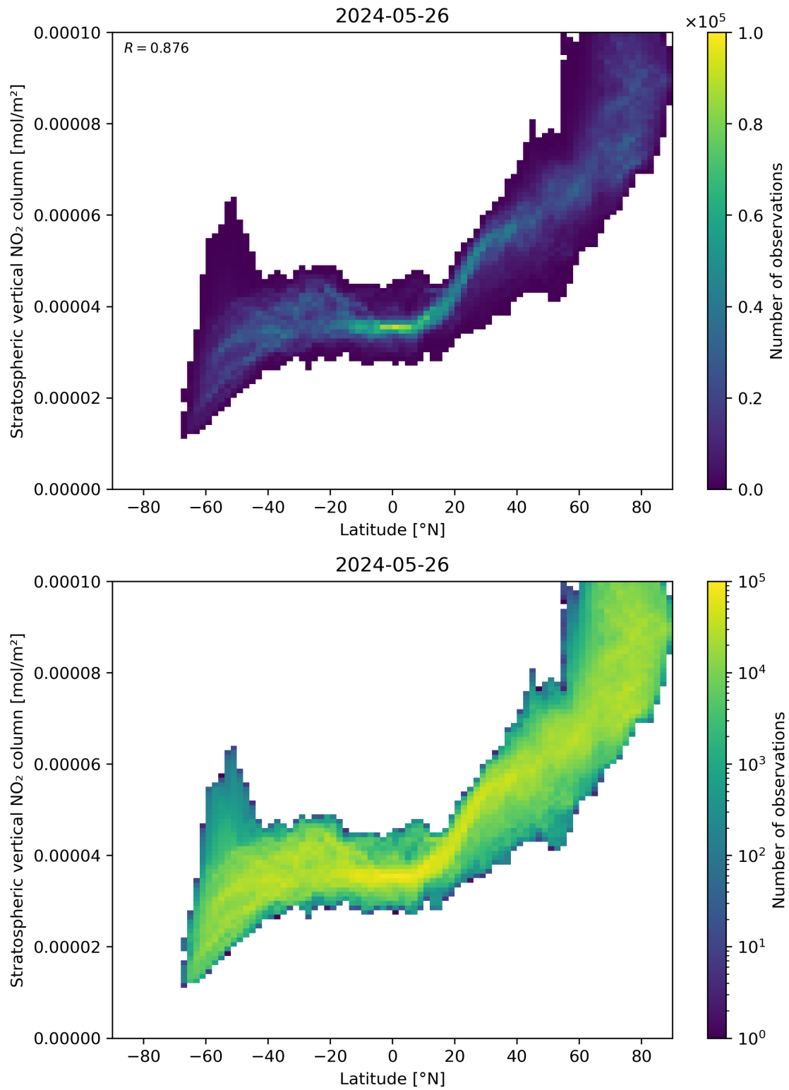
Figure 87: Scatter density plot of “Latitude” against “Stratospheric vertical NO 2 column” for 2024-05-25 to 2024-05-27.
