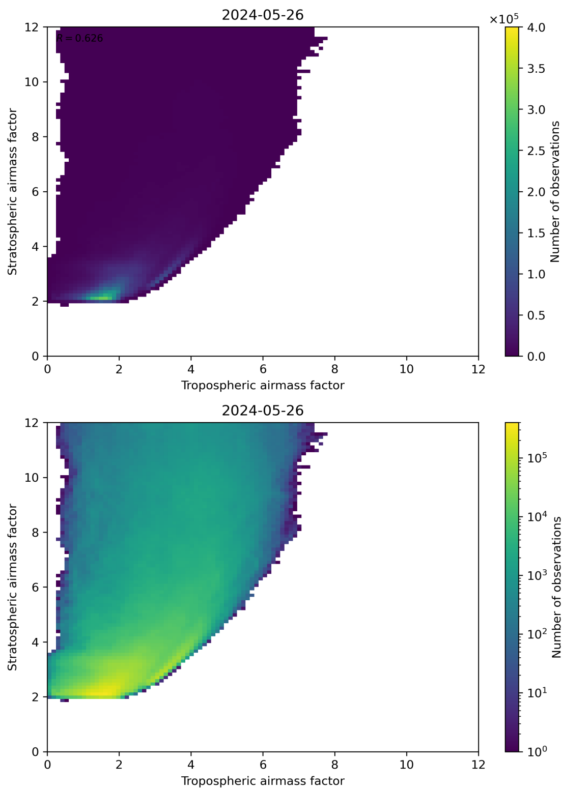
Figure 71: Scatter density plot of “Tropospheric airmass factor” against “Stratospheric airmass factor” for 2024-05-25 to 2024-05-27.
