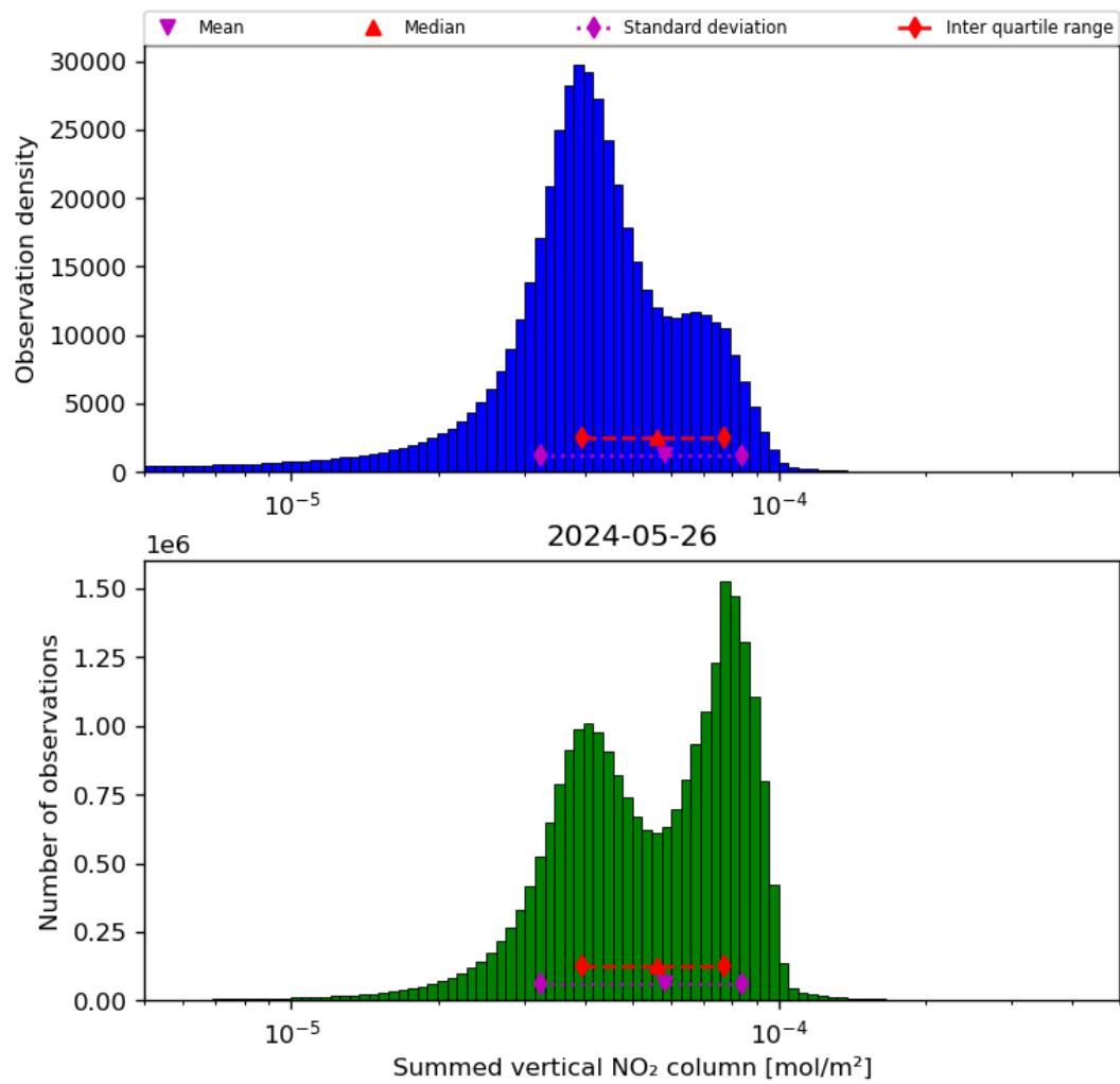
Figure 40: Histogram of "Summed vertical NO 2 column" for 2024-05-25 to 2024-05-27
