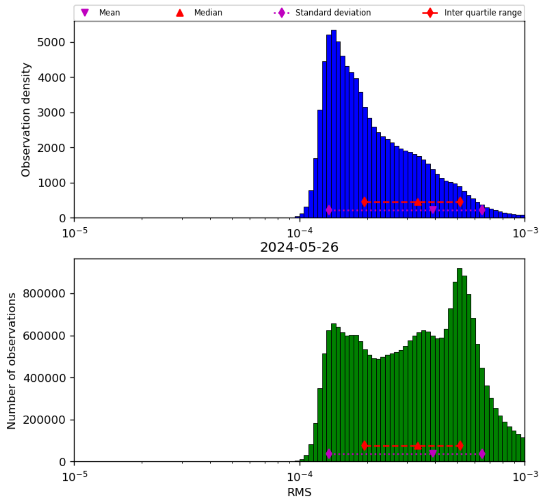
Figure 43: Histogram of “RMS” for 2024-05-25 to 2024-05-27
