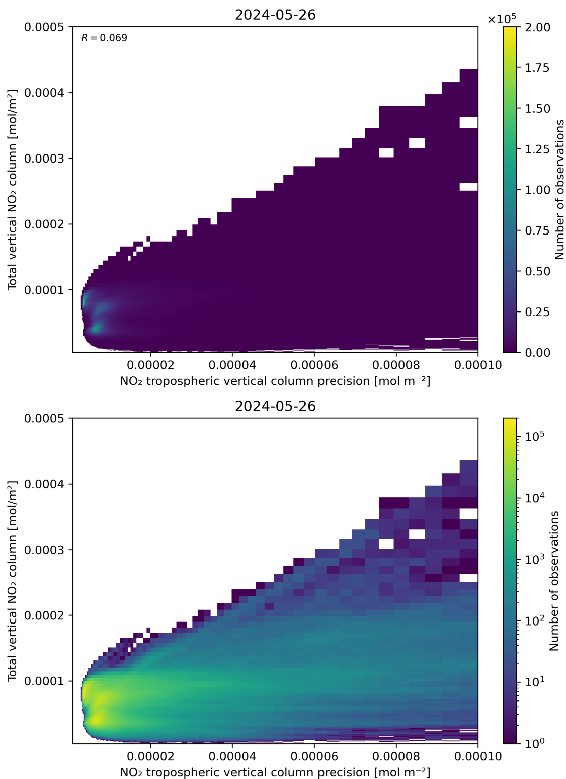
Figure 138: Scatter density plot of “NO 2 tropospheric vertical column precision” against “Total vertical NO 2 column” for 2024-05-25 to 2024-05-27.
