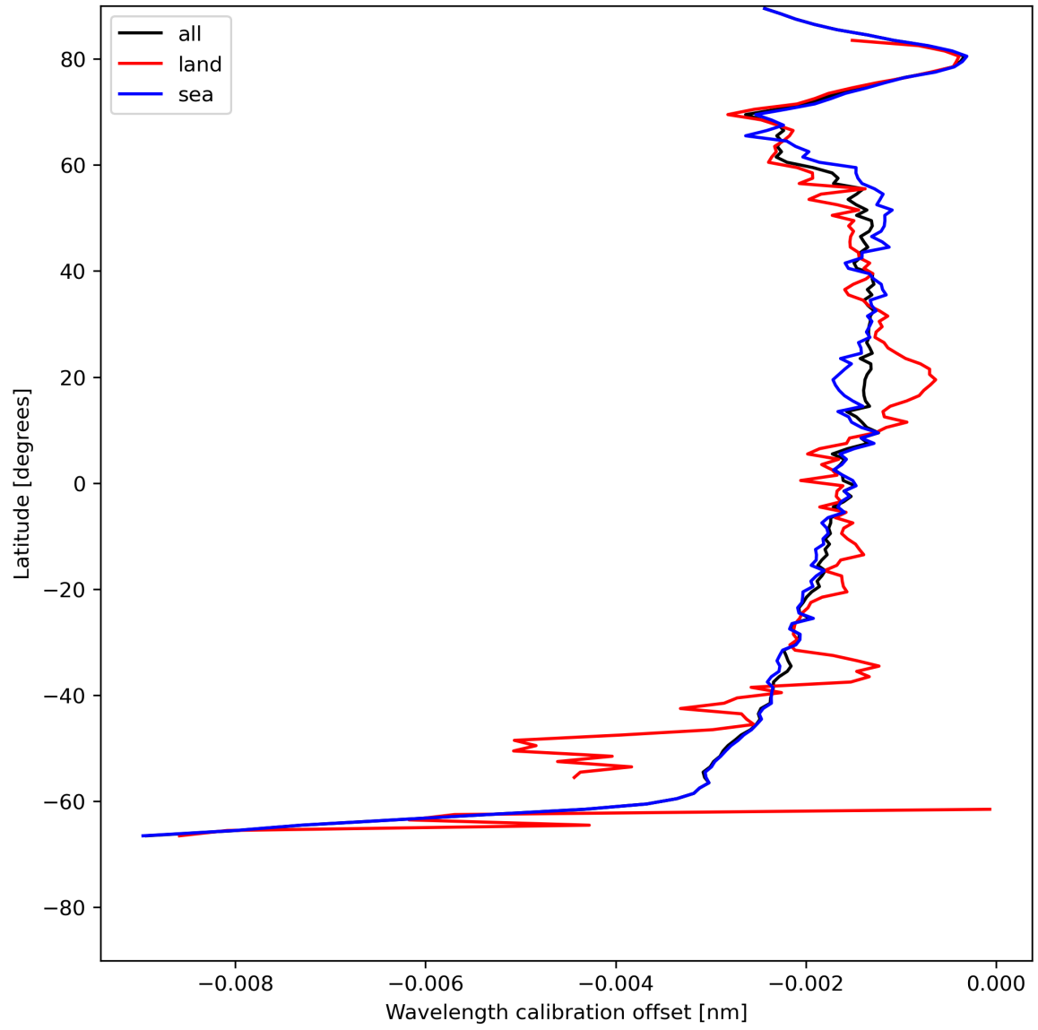
Figure 18: Zonal average of “Wavelength calibration offset” for 2024-05-25 to 2024-05-27.
