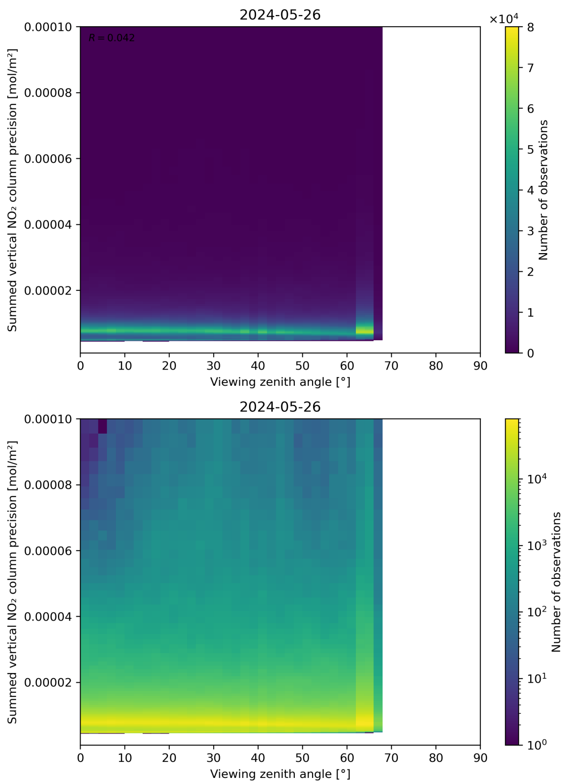
Figure 166: Scatter density plot of “Viewing zenith angle” against “Summed vertical NO 2 column precision” for 2024-05-25 to 2024-05-27.
