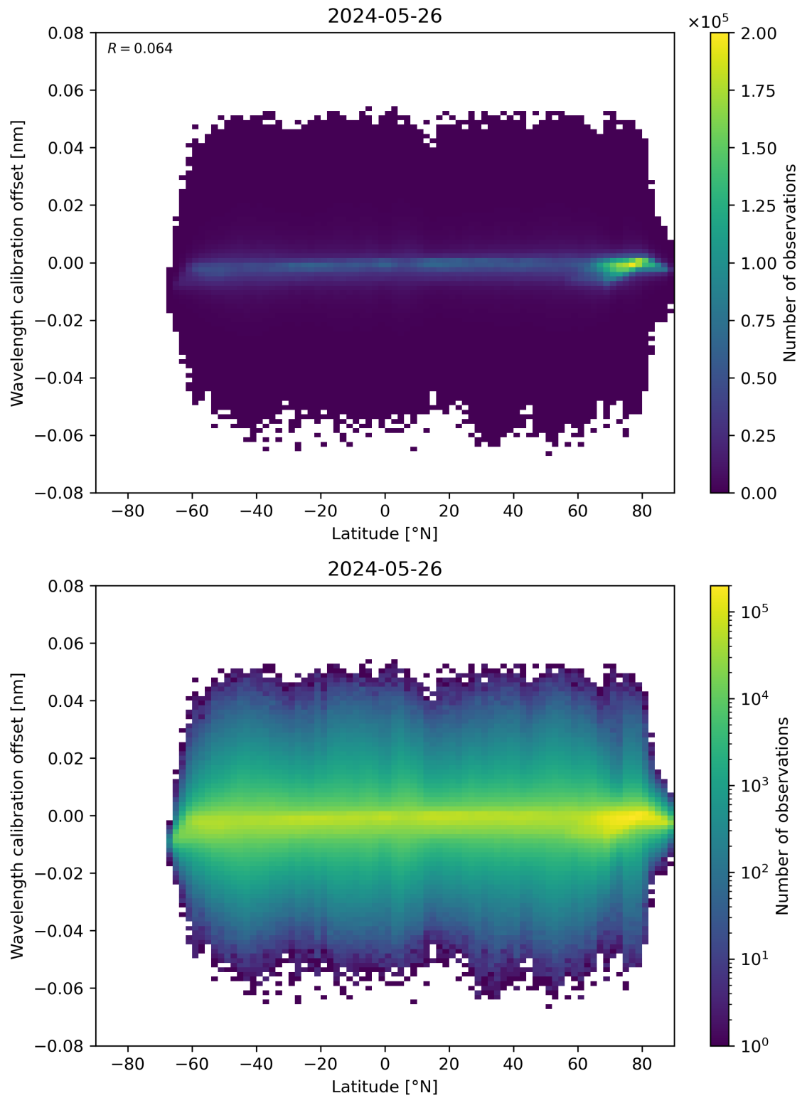
Figure 95: Scatter density plot of “Latitude” against “Wavelength calibration offset” for 2024-05-25 to 2024-05-27.
