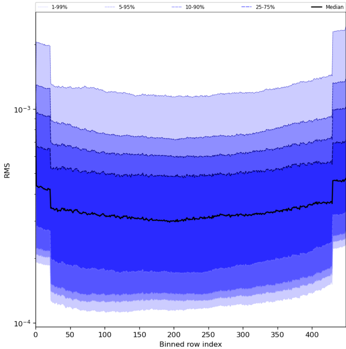
Figure 60: Along track statistics of “RMS” for 2024-05-25 to 2024-05-27
