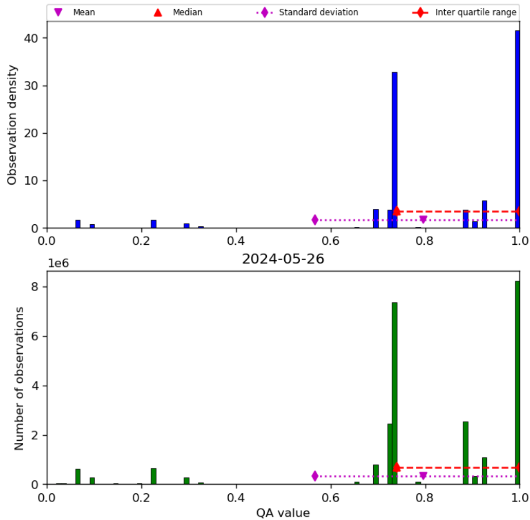
Figure 28: Histogram of “QA value” for 2024-05-25 to 2024-05-27
