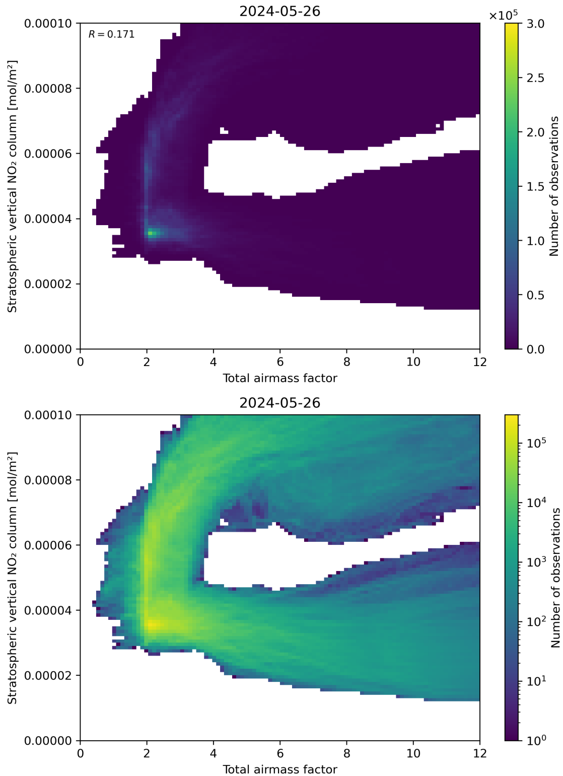
Figure 64: Scatter density plot of “Total airmass factor” against “Stratospheric vertical NO 2 column” for 2024-05-25 to 2024-05-27.
