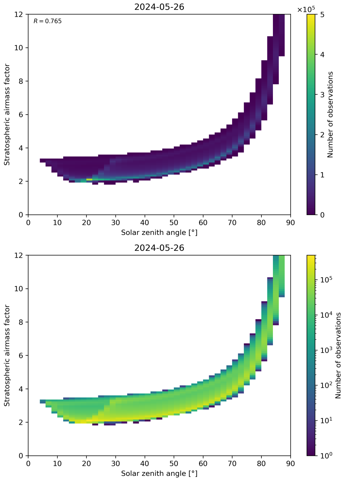
Figure 145: Scatter density plot of “Solar zenith angle” against “Stratospheric airmass factor” for 2024-05-25 to 2024-05-27.
