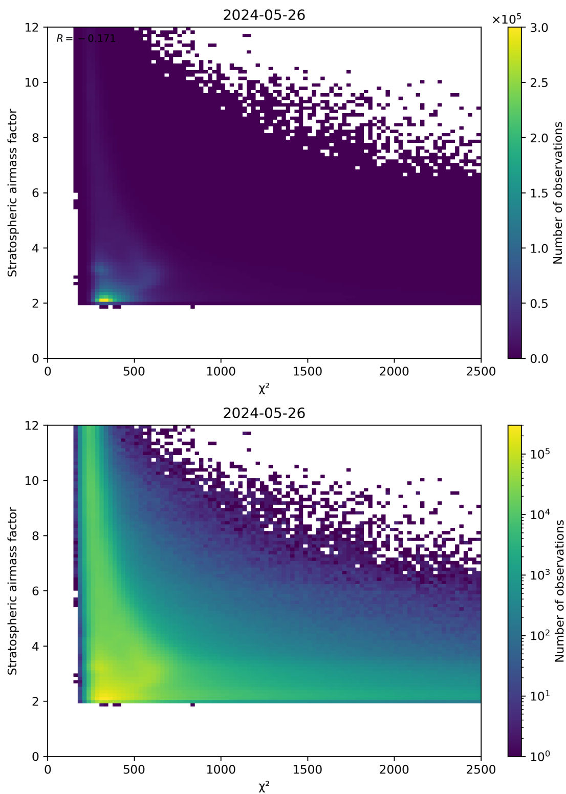
Figure 81: Scatter density plot of “ \chi^2 ” against “Stratospheric air mass factor” for 2024-05-25 to 2024-05-27.
