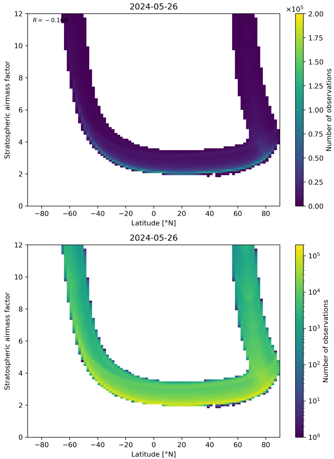
Figure 83: Scatter density plot of “Latitude” against “Stratospheric air mass factor” for 2024-05-25 to 2024-05-27.
