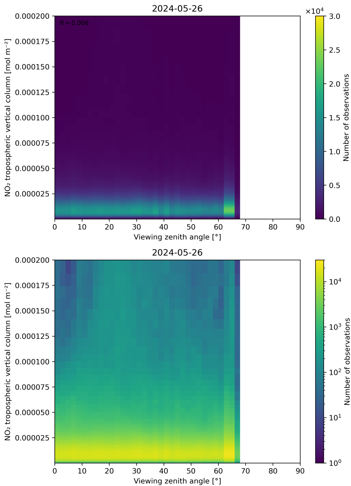
Figure 169: Scatter density plot of “Viewing zenith angle” against “NO 2 tropospheric vertical column” for 2024-05-25 to 2024-05-27.
