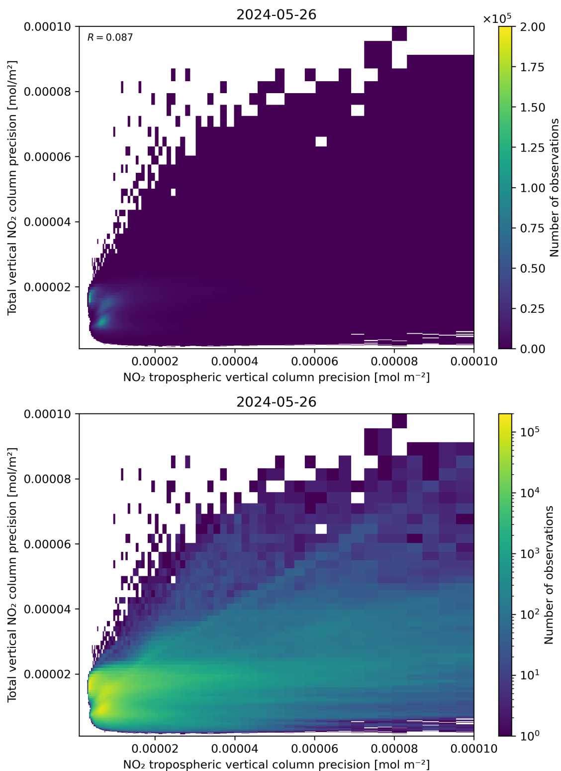
Figure 139: Scatter density plot of “NO 2 tropospheric vertical column precision” against “Total vertical NO 2 column precision” for 2024-05-25 to 2024-05-27.
