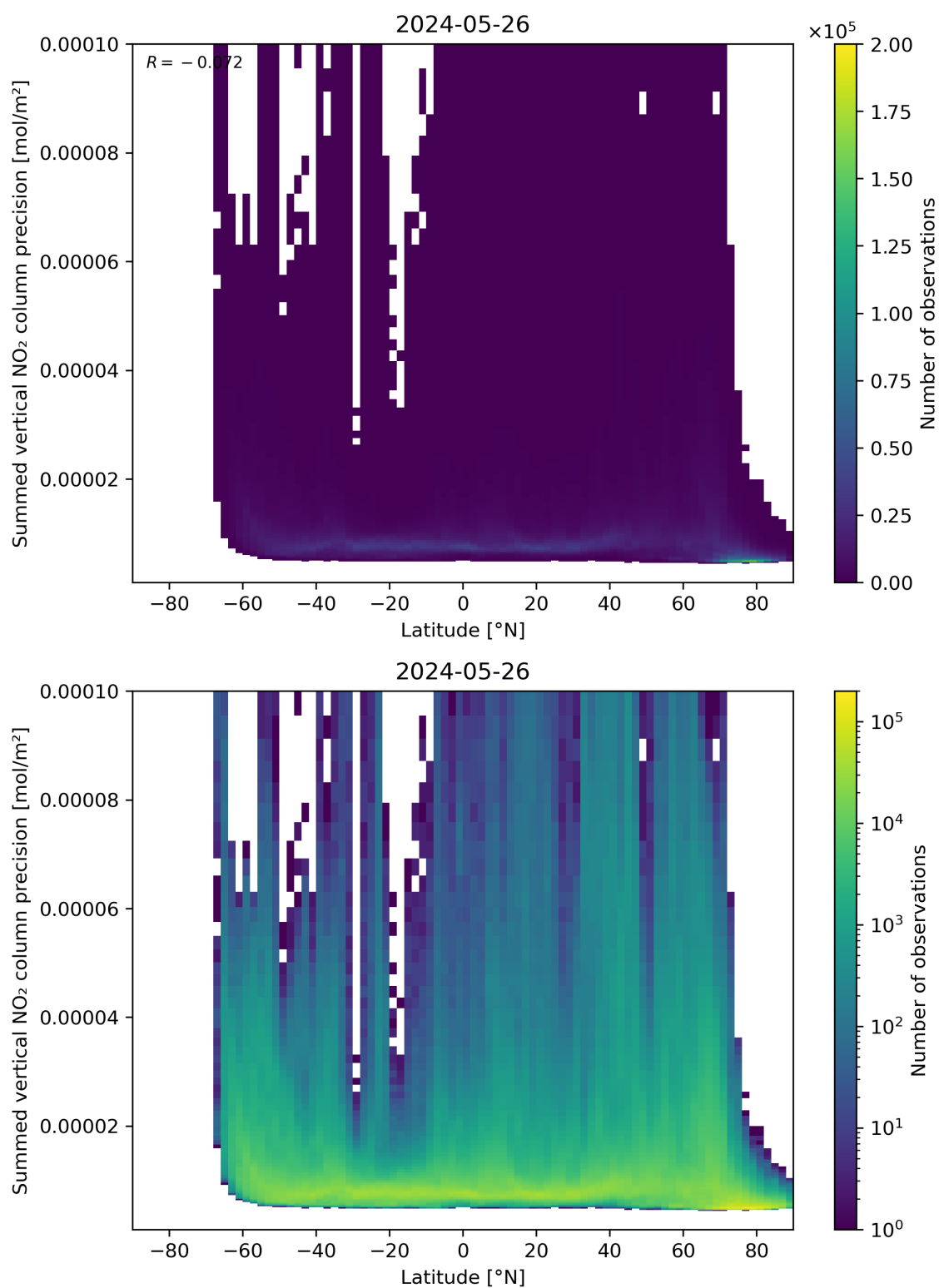
Figure 89: Scatter density plot of “Latitude” against “Summed vertical NO 2 column precision” for 2024-05-25 to 2024-05-27.
