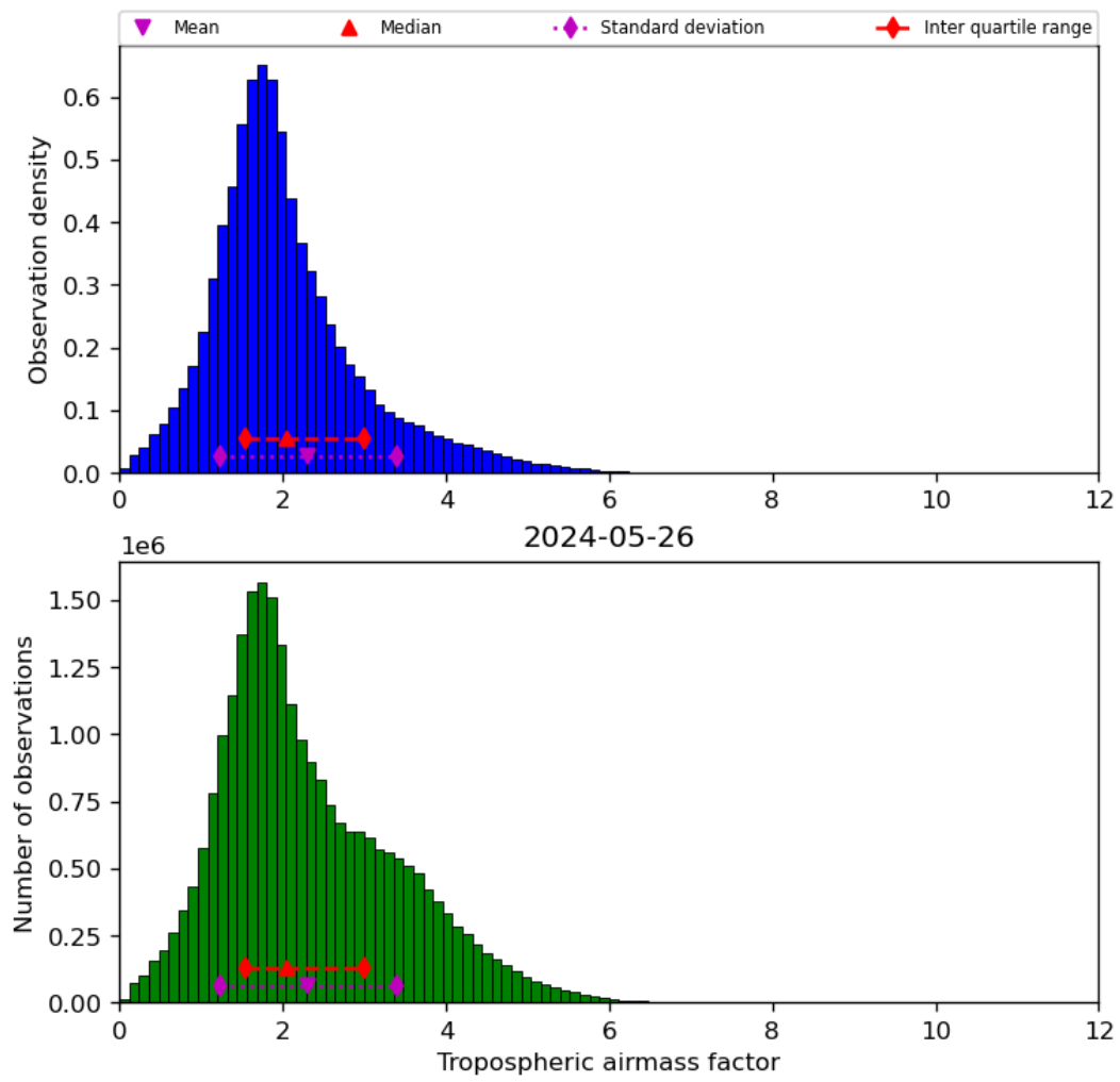
Figure 31: Histogram of “Tropospheric airmass factor” for 2024-05-25 to 2024-05-27
