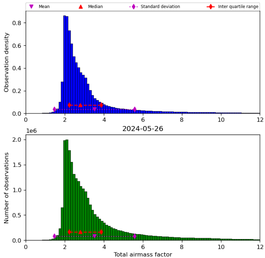
Figure 32: Histogram of “Total airmass factor” for 2024-05-25 to 2024-05-27
