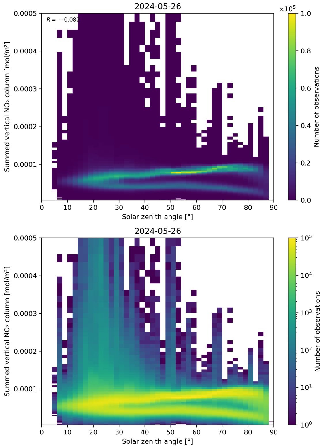
Figure 151: Scatter density plot of “Solar zenith angle” against “Summed vertical NO 2 column” for 2024-05-25 to 2024-05-27.
