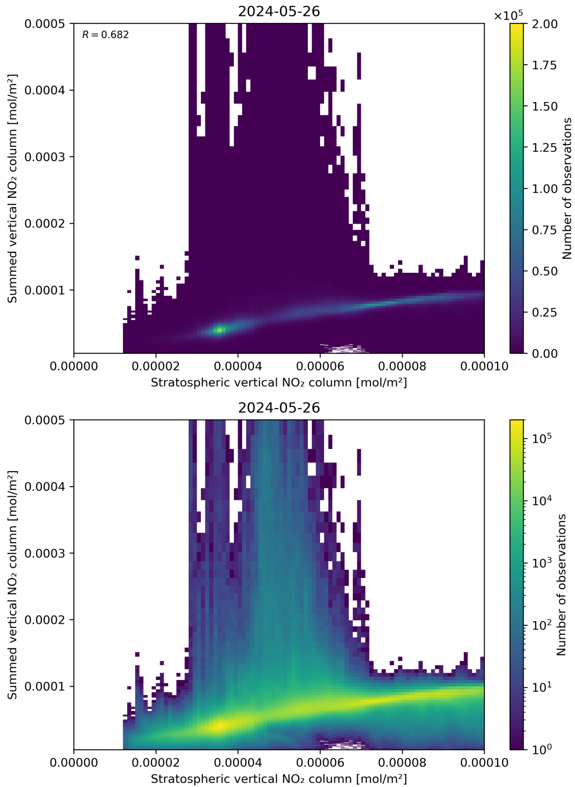
Figure 98: Scatter density plot of “Stratospheric vertical NO 2 column” against “Summed vertical NO 2 column” for 2024-05-25 to 2024-05-27.
