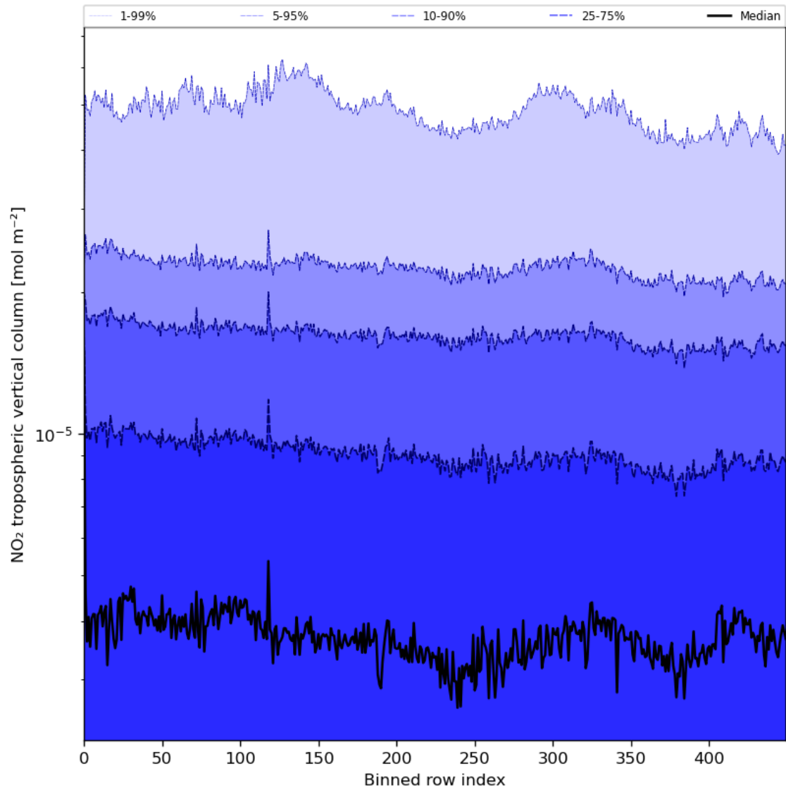
Figure 46: Along track statistics of “NO 2 tropospheric vertical column” for 2024-05-25 to 2024-05-27
