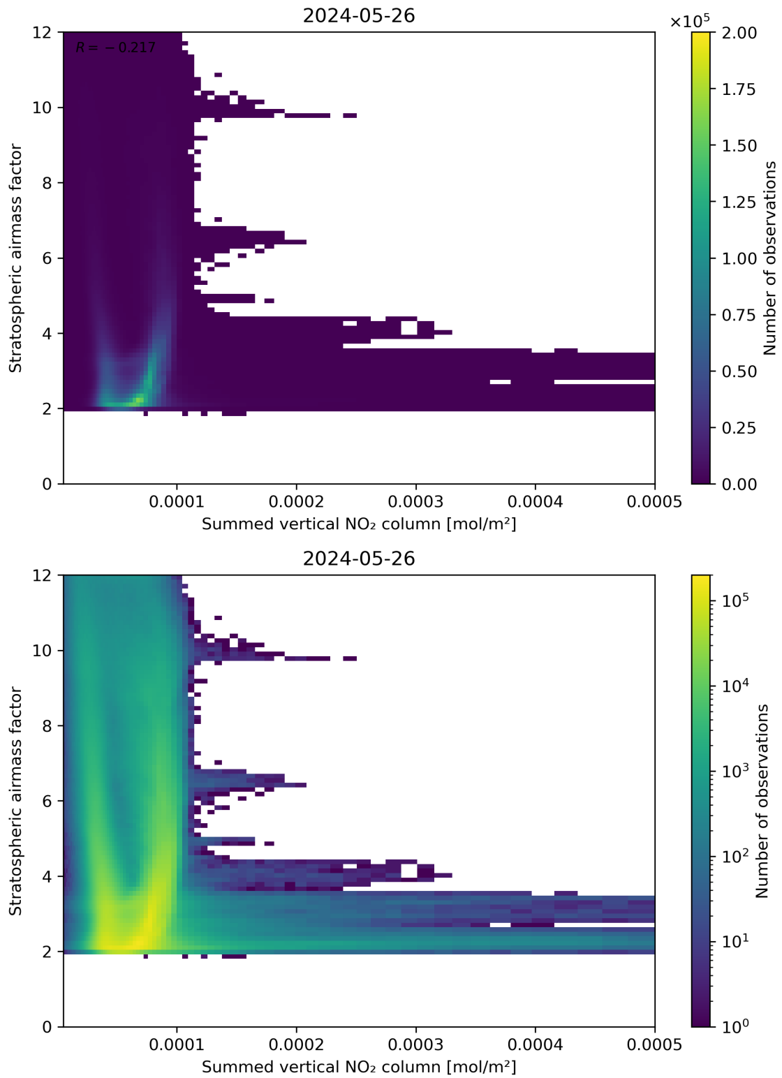
Figure 103: Scatter density plot of “Summed vertical NO 2 column” against “Stratospheric air mass factor” for 2024-05-25 to 2024-05-27.
