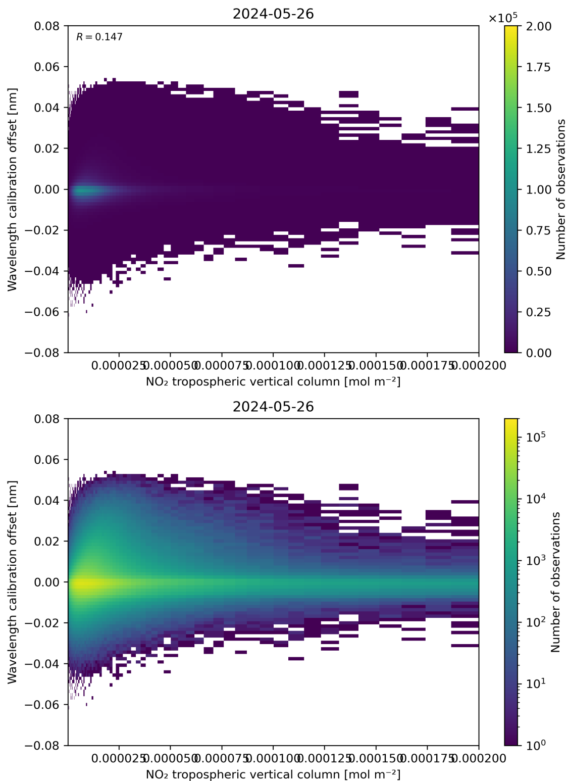
Figure 143: Scatter density plot of “NO 2 tropospheric vertical column” against “Wavelength calibration offset” for 2024-05-25 to 2024-05-27.
