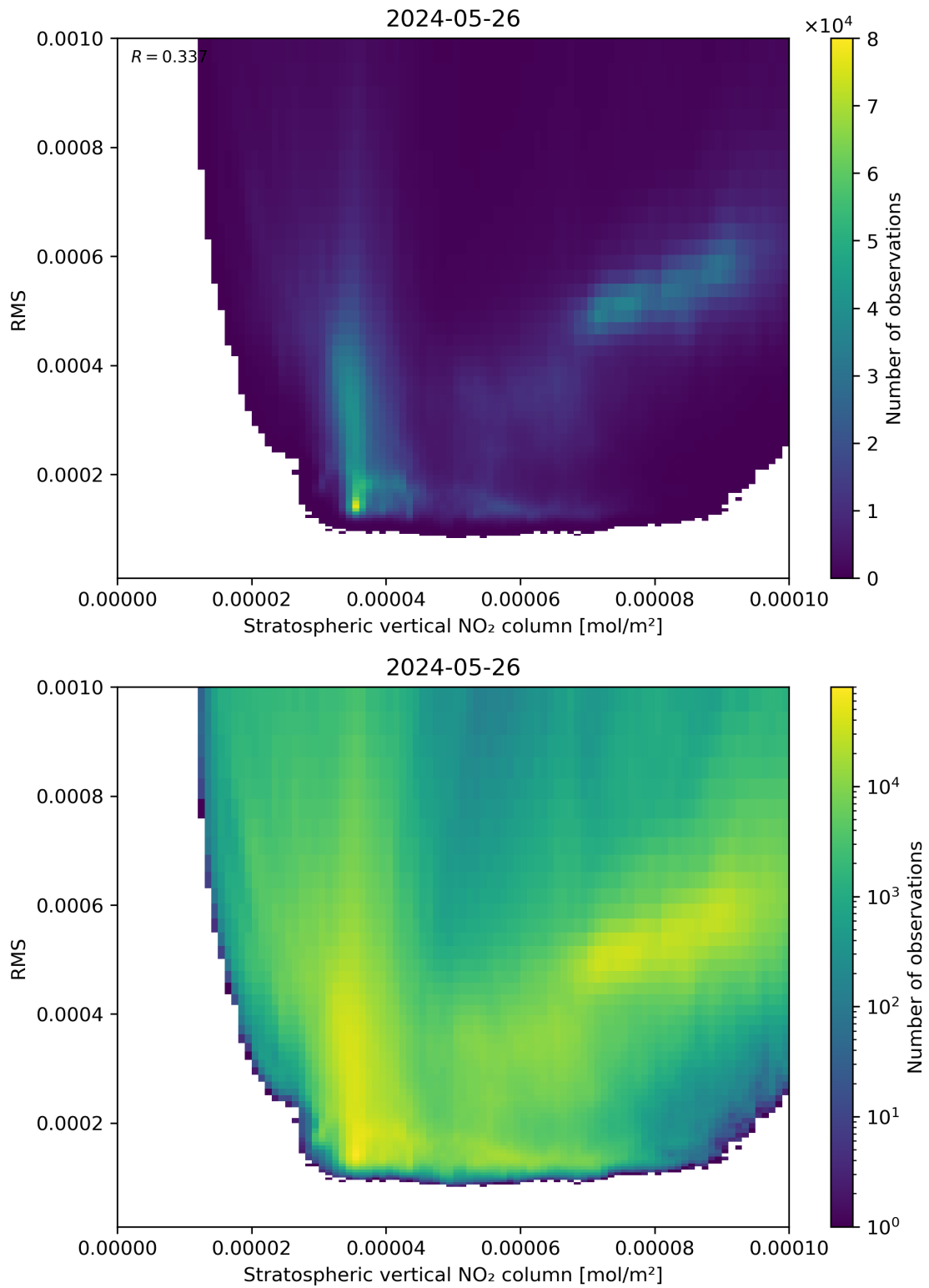
Figure 102: Scatter density plot of “Stratospheric vertical NO 2 column” against “RMS” for 2024-05-25 to 2024-05-27.
