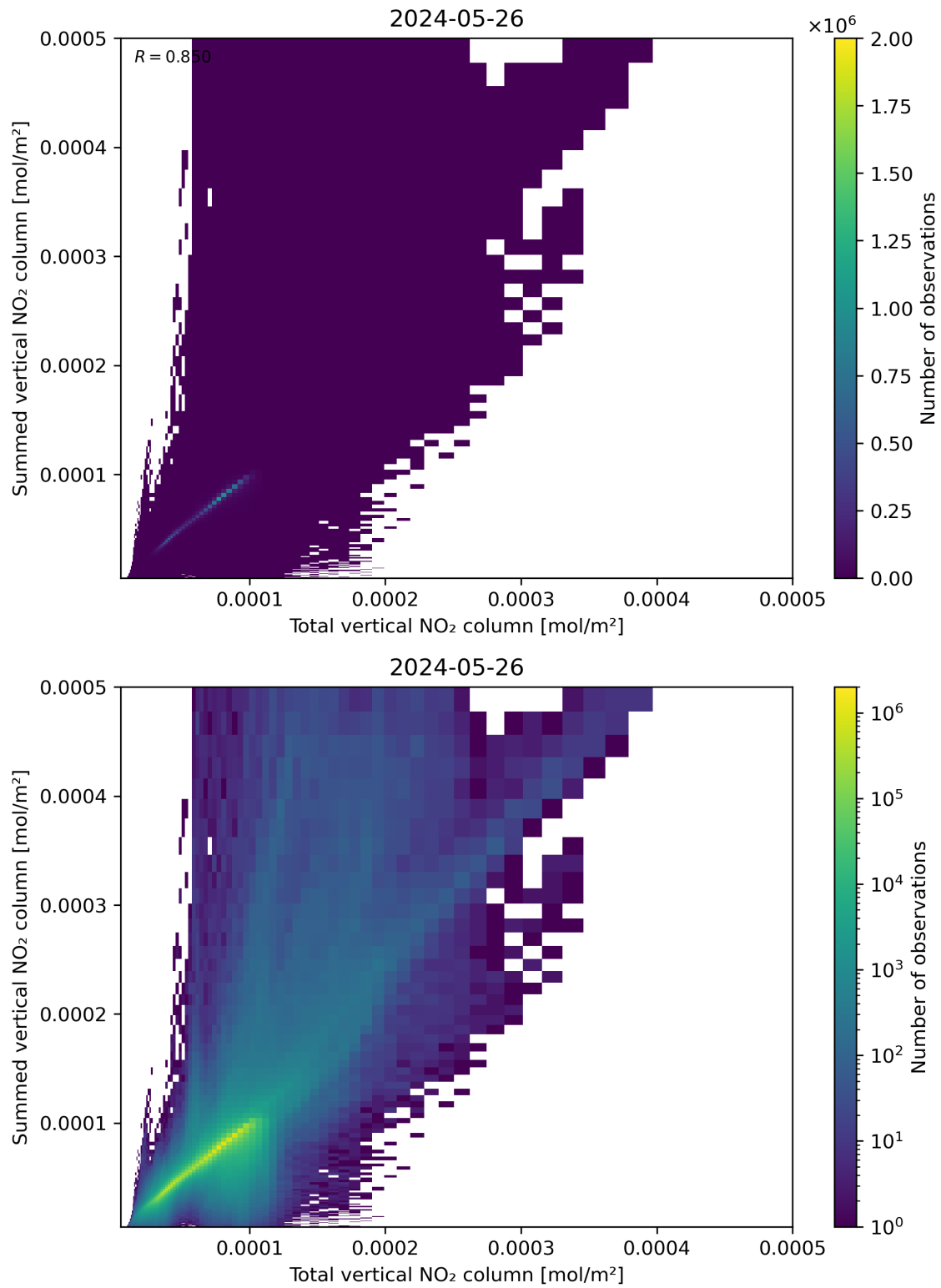
Figure 112: Scatter density plot of “Total vertical NO 2 column” against “Summed vertical NO 2 column” for 2024-05-25 to 2024-05-27.
