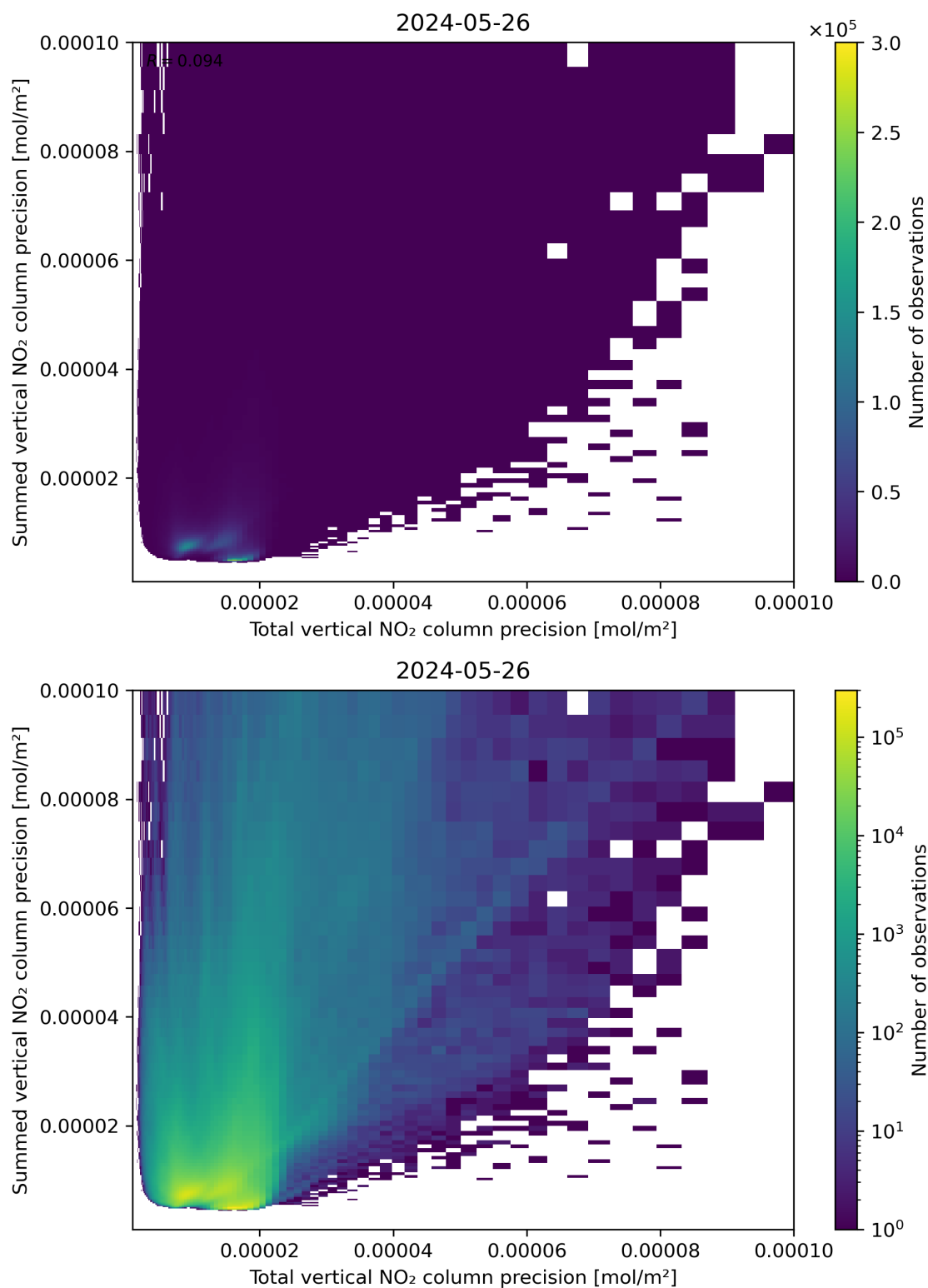
Figure 118: Scatter density plot of “Total vertical NO 2 column precision” against “Summed vertical NO 2 column precision” for 2024-05-25 to 2024-05-27.
