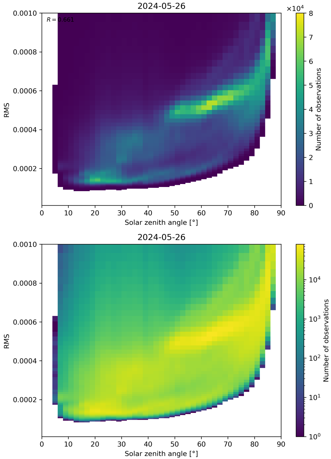
Figure 157: Scatter density plot of “Solar zenith angle” against “RMS” for 2024-05-25 to 2024-05-27.
