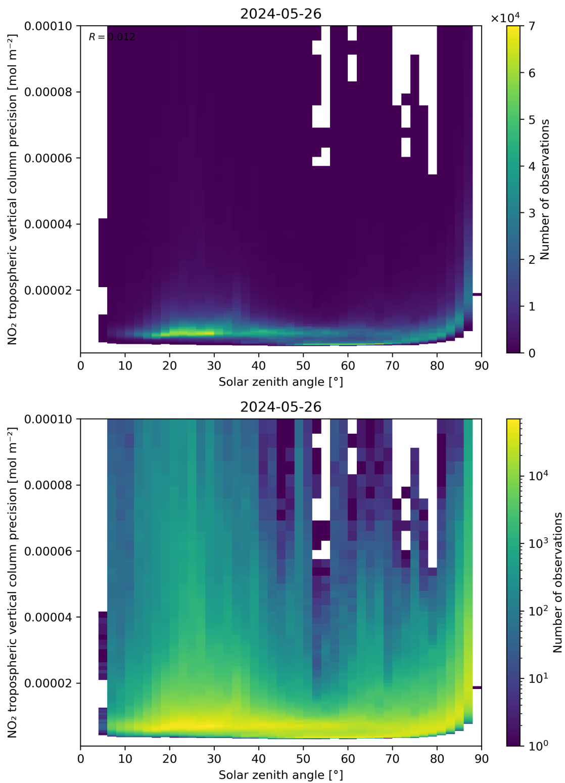
Figure 156: Scatter density plot of “Solar zenith angle” against “NO 2 tropospheric vertical column precision” for 2024-05-25 to 2024-05-27.
