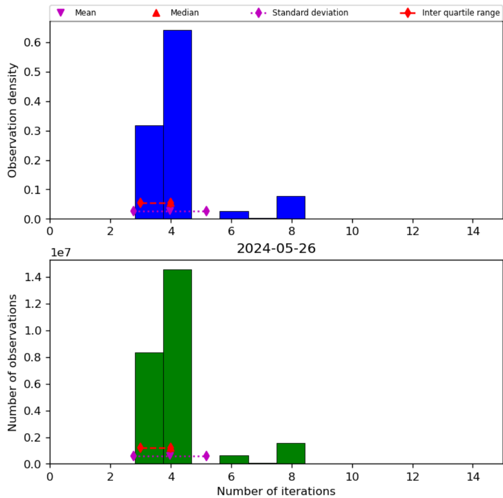
Figure 34: Histogram of “Number of iterations” for 2024-05-25 to 2024-05-27
