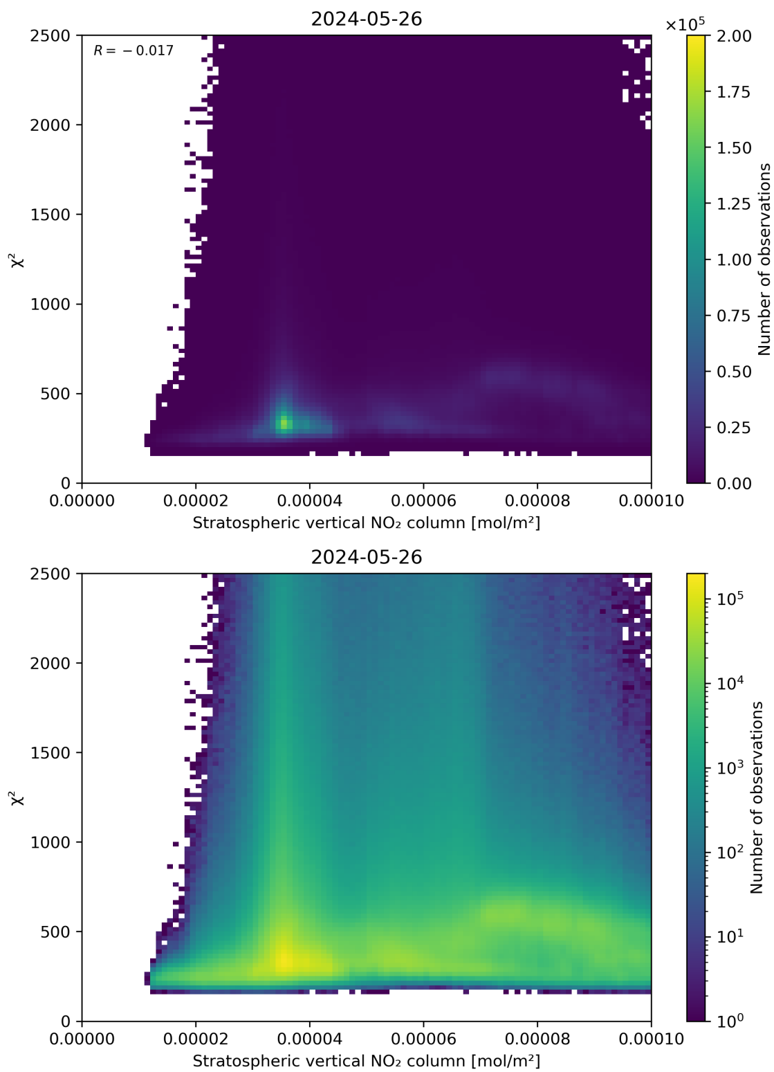
Figure 97: Scatter density plot of “Stratospheric vertical NO 2 column” against “ \chi^2 ” for 2024-05-25 to 2024-05-27.
