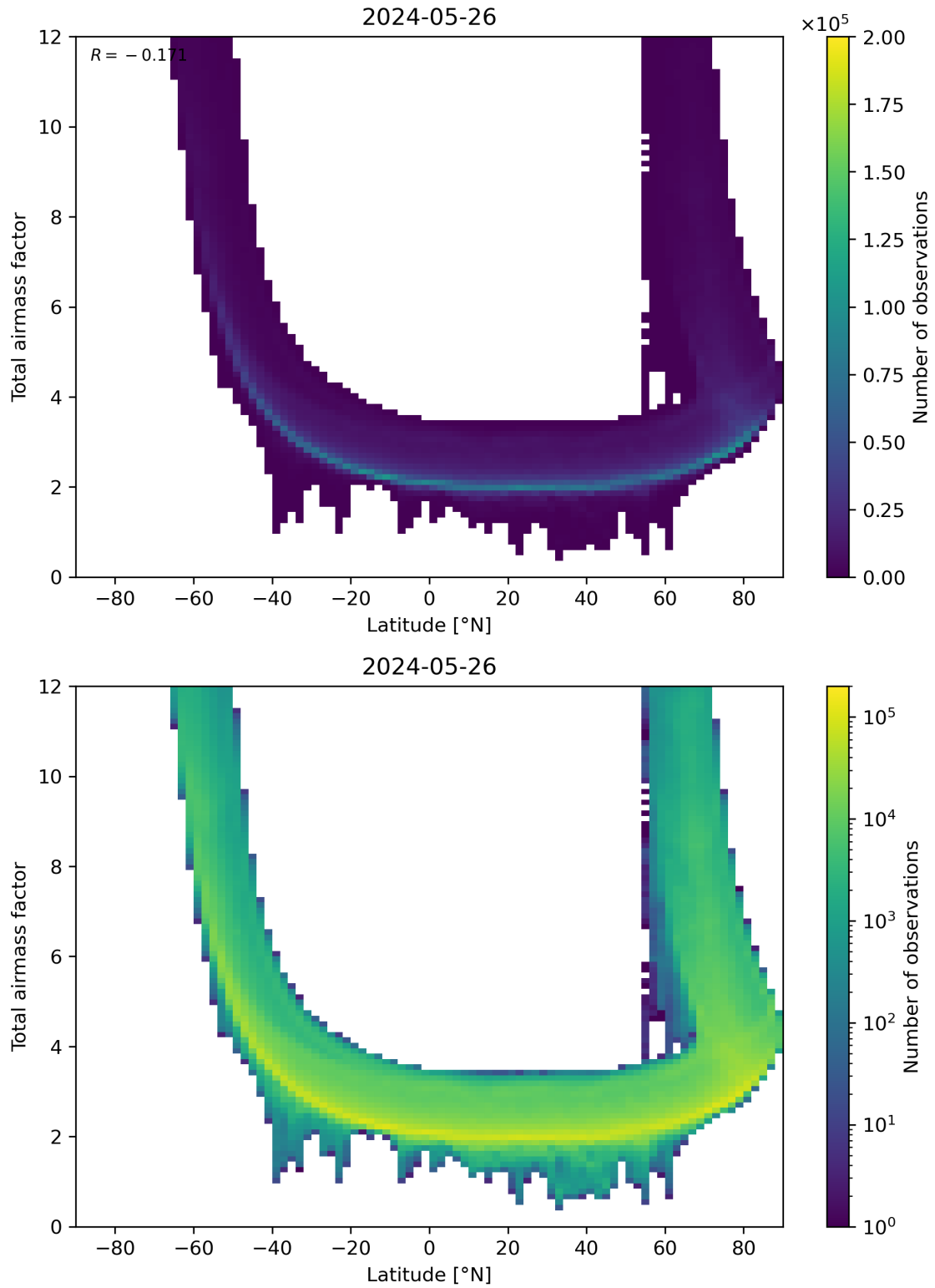
Figure 84: Scatter density plot of “Latitude” against “Total airmass factor” for 2024-05-25 to 2024-05-27.
