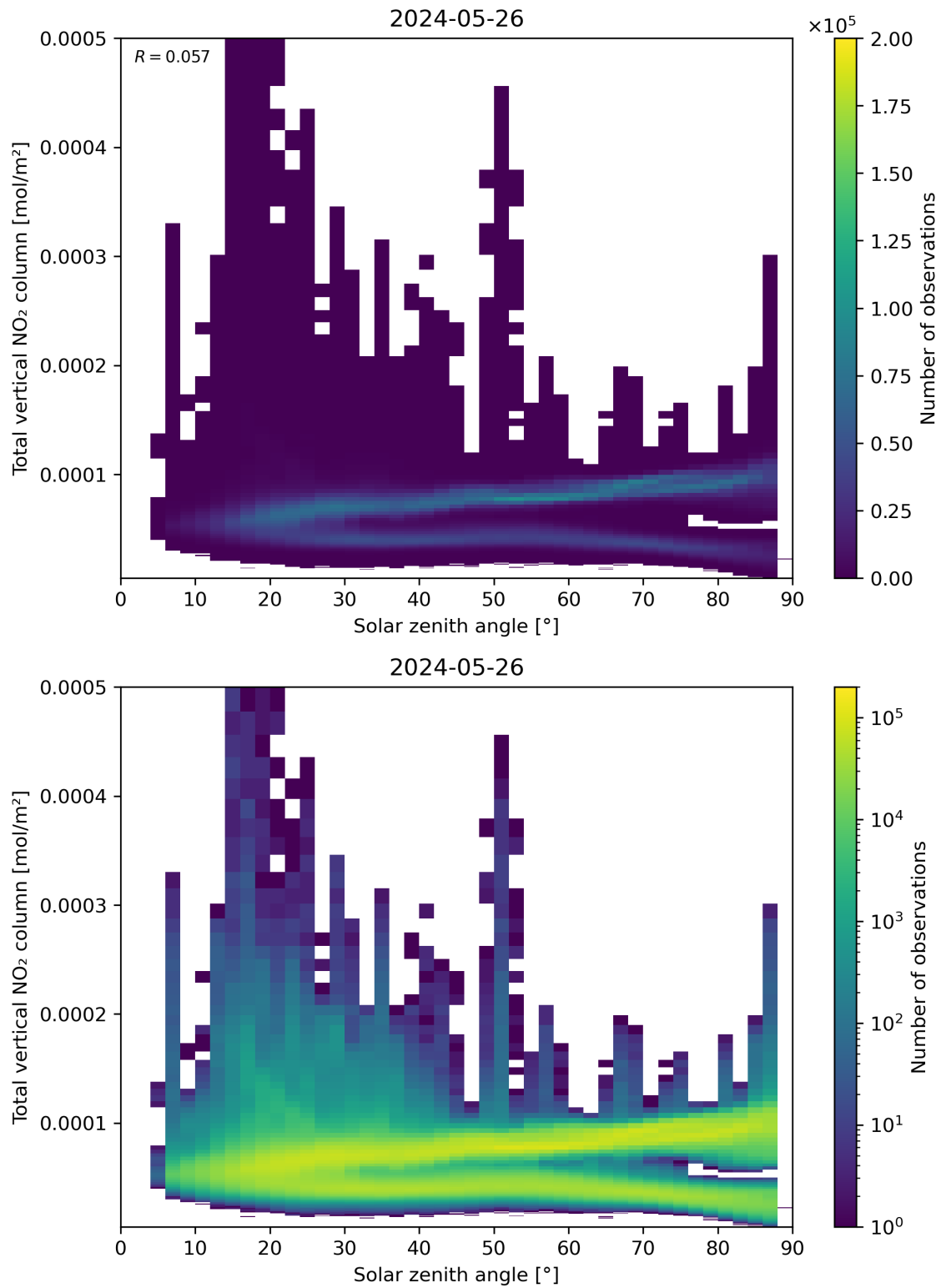
Figure 153: Scatter density plot of “Solar zenith angle” against “Total vertical NO 2 column” for 2024-05-25 to 2024-05-27.
