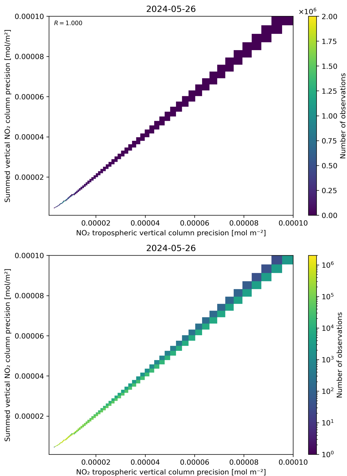
Figure 137: Scatter density plot of “NO 2 tropospheric vertical column precision” against “Summed vertical NO 2 column precision” for 2024-05-25 to 2024-05-27.
