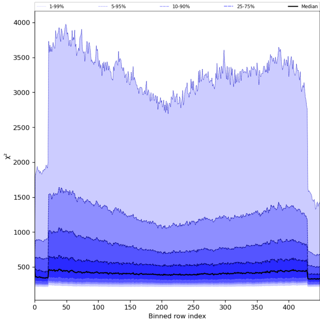
Figure 59: Along track statistics of “ \chi^2 ” for 2024-05-25 to 2024-05-27
