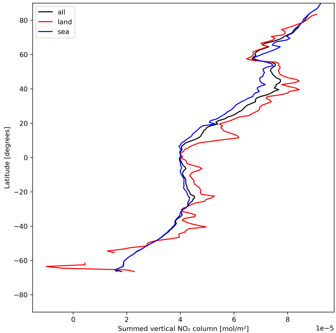
Figure 23: Zonal average of “Summed vertical NO 2 column” for 2024-05-25 to 2024-05-27.
