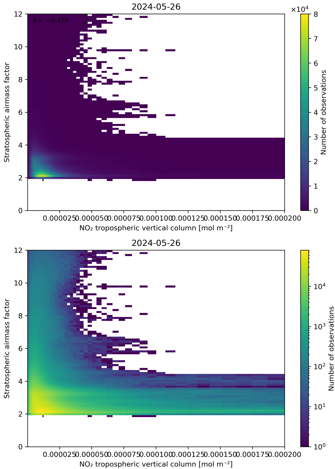
Figure 121: Scatter density plot of “NO 2 tropospheric vertical column” against “Stratospheric air mass factor” for 2024-05-25 to 2024-05-27.
