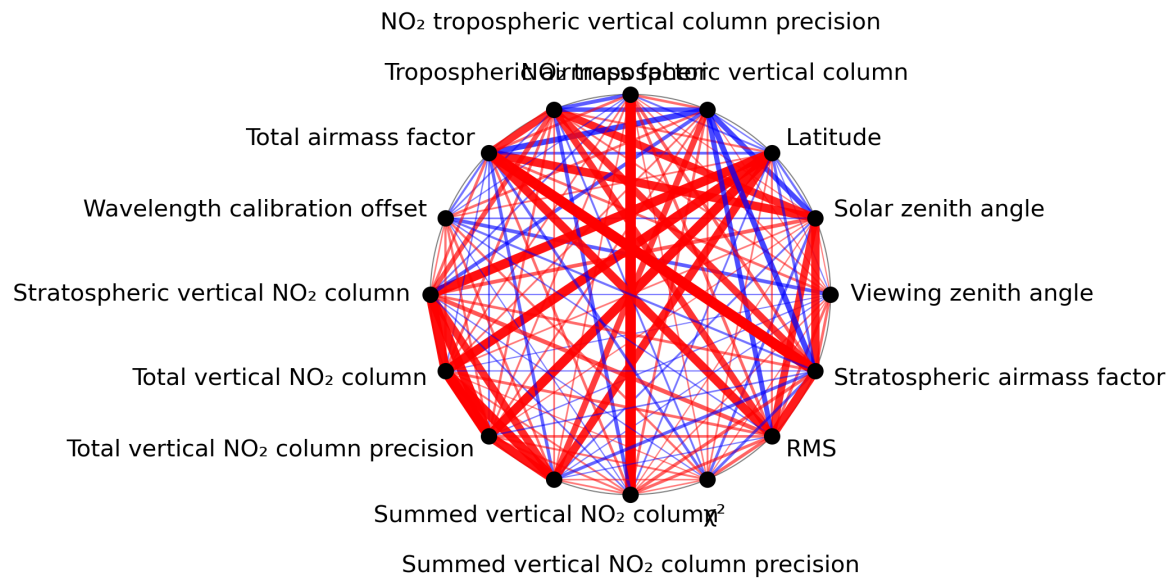
Figure 1: Map of correlation graph for 2024-05-25 to 2024-05-27.
