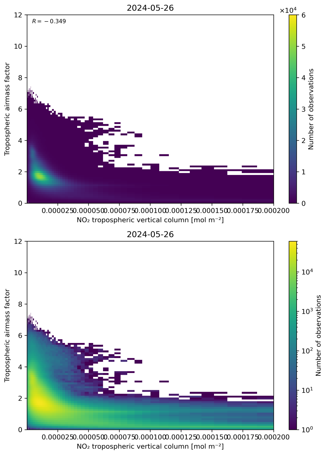
Figure 123: Scatter density plot of “NO 2 tropospheric vertical column” against “Tropospheric airmass factor” for 2024-05-25 to 2024-05-27.
