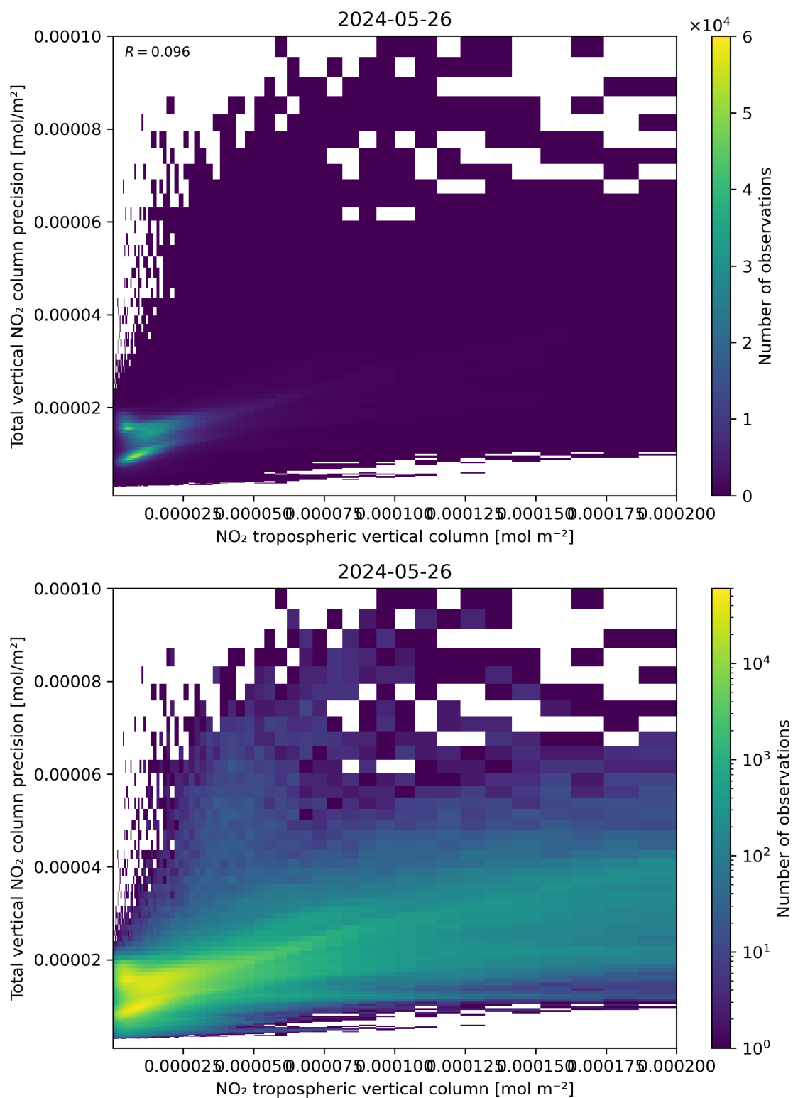
Figure 129: Scatter density plot of “NO 2 tropospheric vertical column” against “Total vertical NO 2 column precision” for 2024-05-25 to 2024-05-27.
