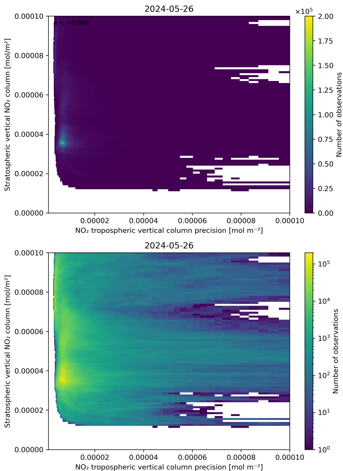
Figure 135: Scatter density plot of “NO 2 tropospheric vertical column precision” against “Stratospheric vertical NO 2 column” for 2024-05-25 to 2024-05-27.
