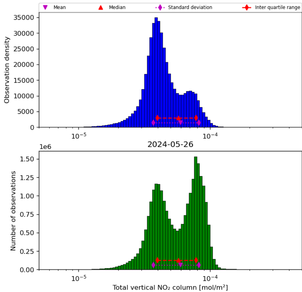
Figure 38: Histogram of “Total vertical NO 2 column” for 2024-05-25 to 2024-05-27
