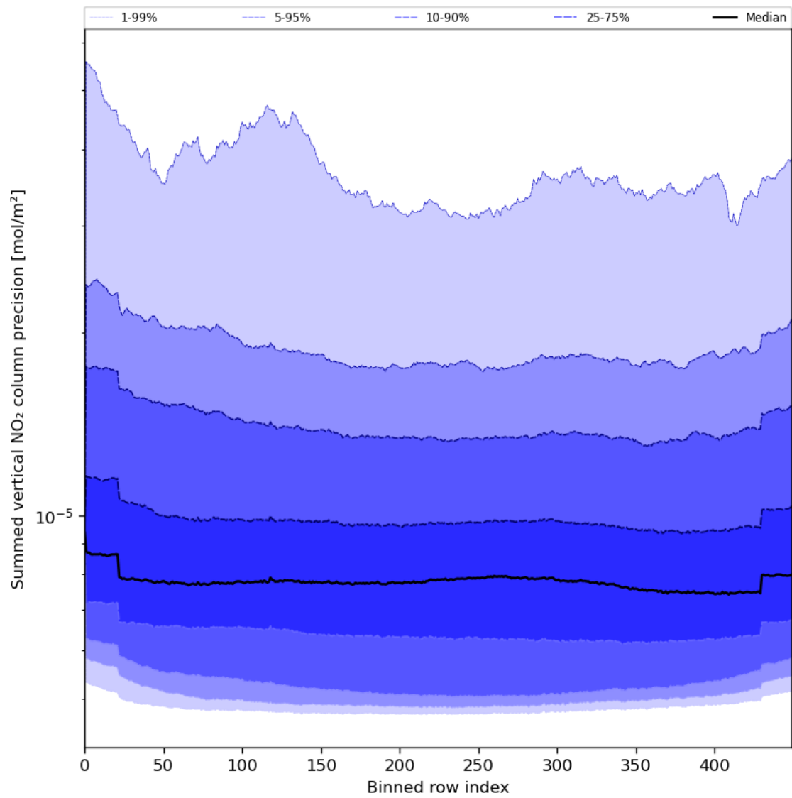
Figure 58: Along track statistics of “Summed vertical NO 2 column precision” for 2024-05-25 to 2024-05-27
