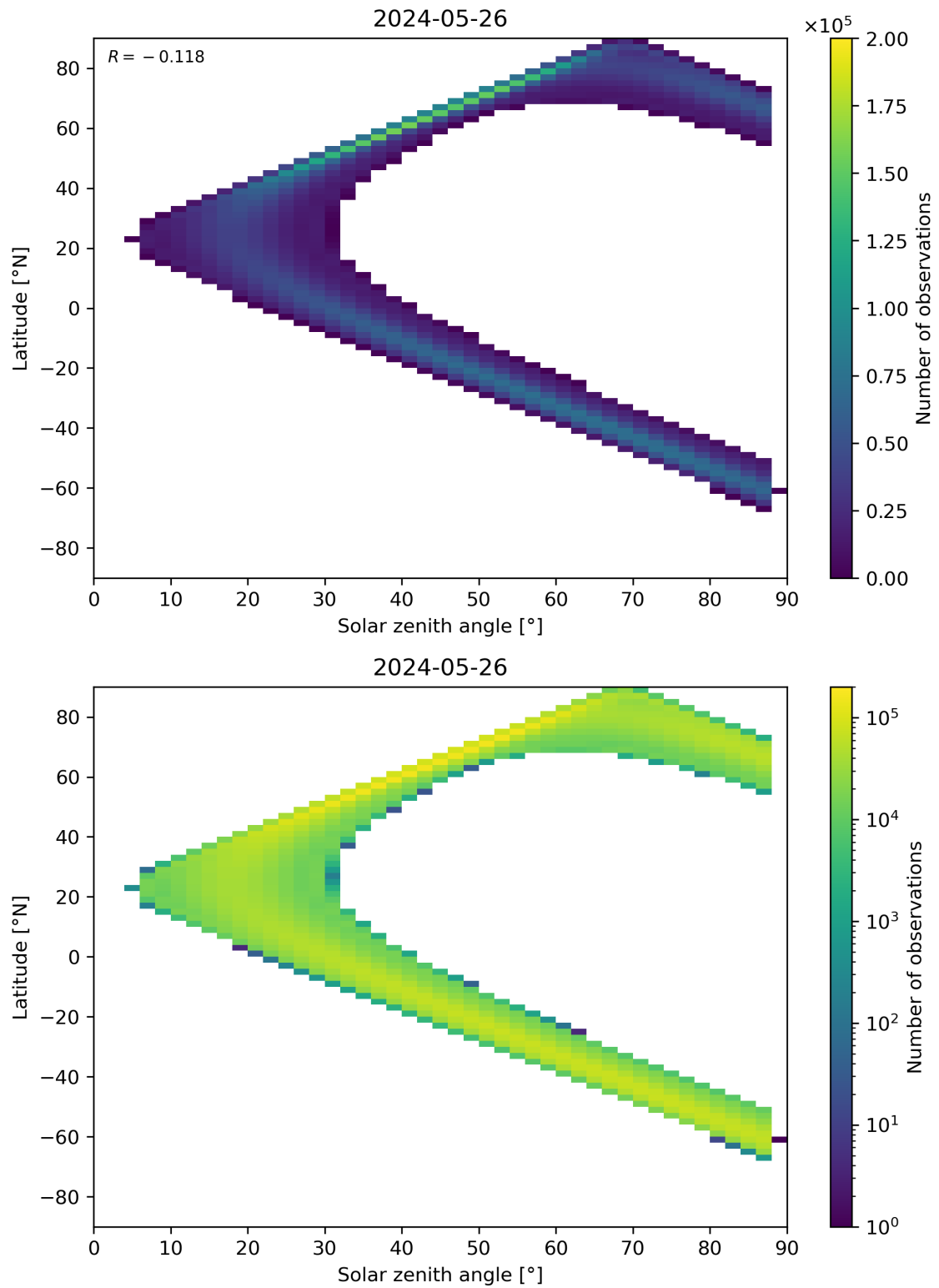
Figure 149: Scatter density plot of “Solar zenith angle” against “Latitude” for 2024-05-25 to 2024-05-27.
