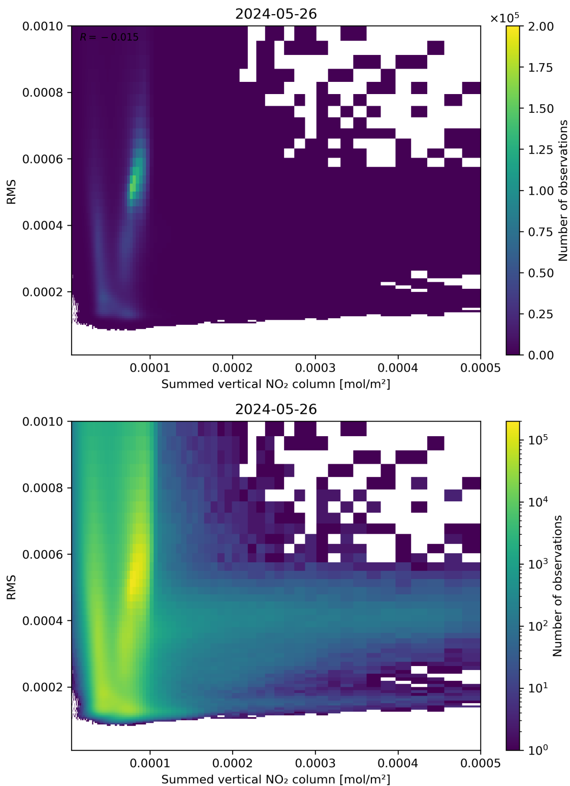
Figure 109: Scatter density plot of “Summed vertical NO 2 column” against “RMS” for 2024-05-25 to 2024-05-27.
