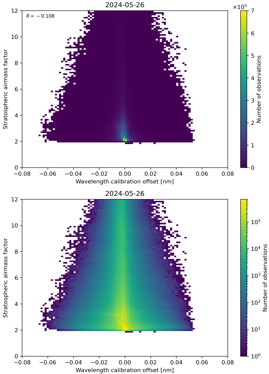
Figure 174: Scatter density plot of “Wavelength calibration offset” against “Stratospheric airmass factor” for 2024-05-25 to 2024-05-27.
