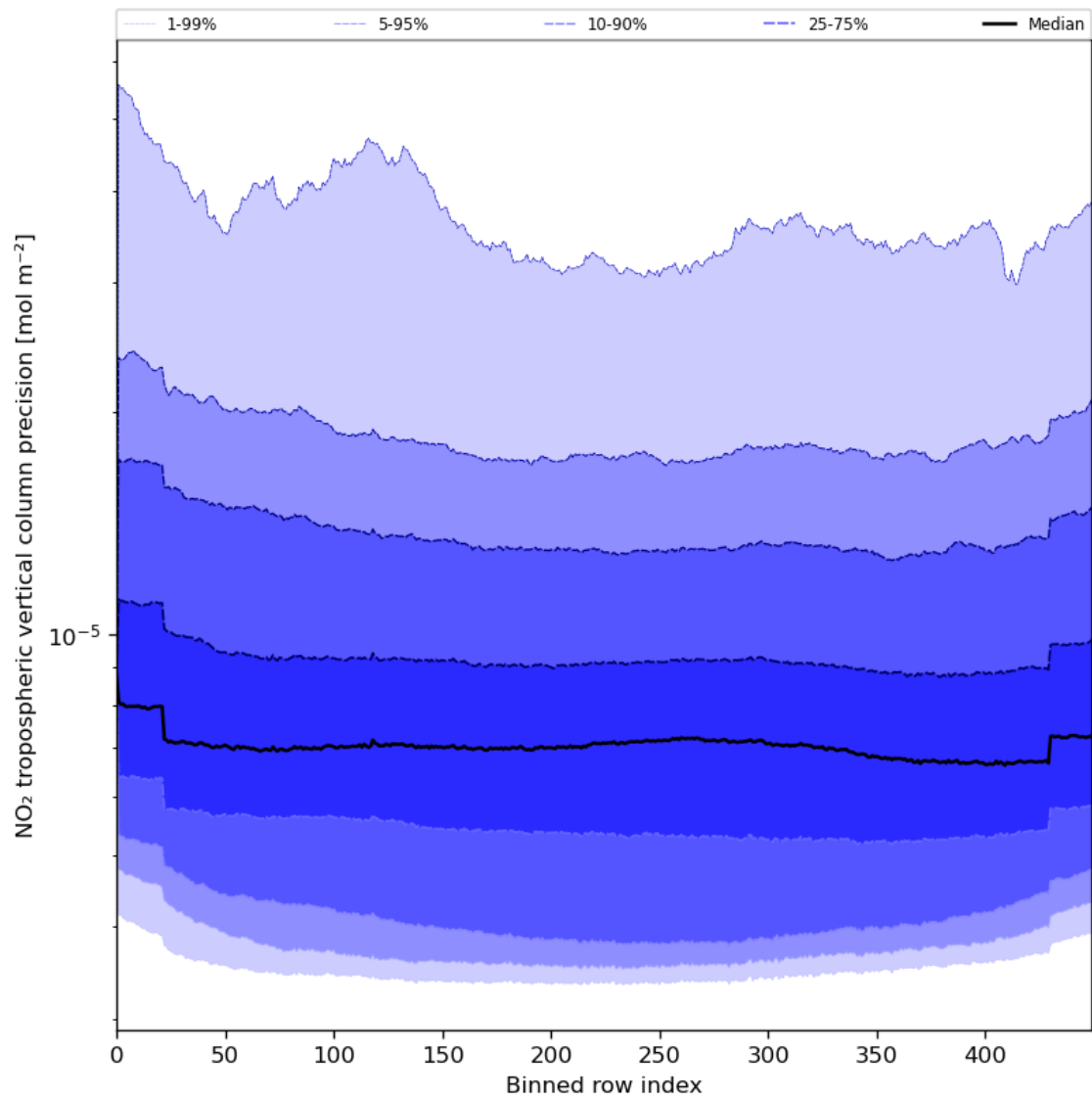
Figure 47: Along track statistics of “NO 2 tropospheric vertical column precision” for 2024-05-25 to 2024-05-27
