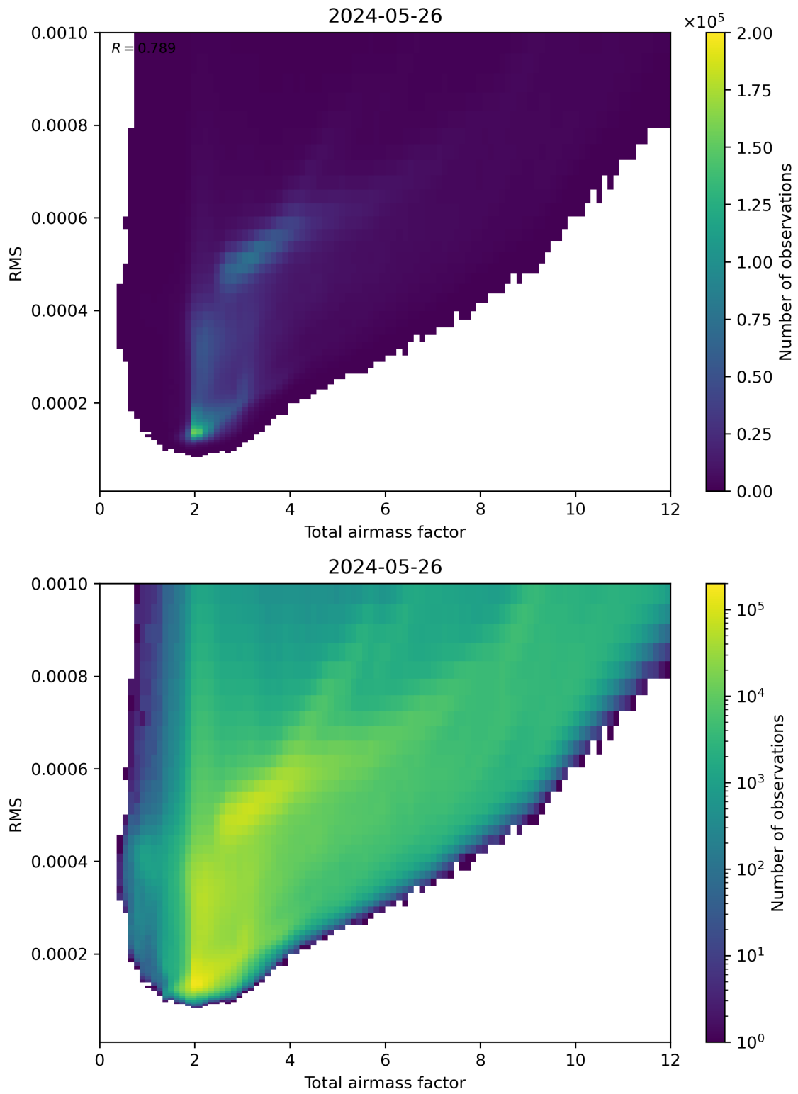
Figure 69: Scatter density plot of “Total airmass factor” against “RMS” for 2024-05-25 to 2024-05-27.
