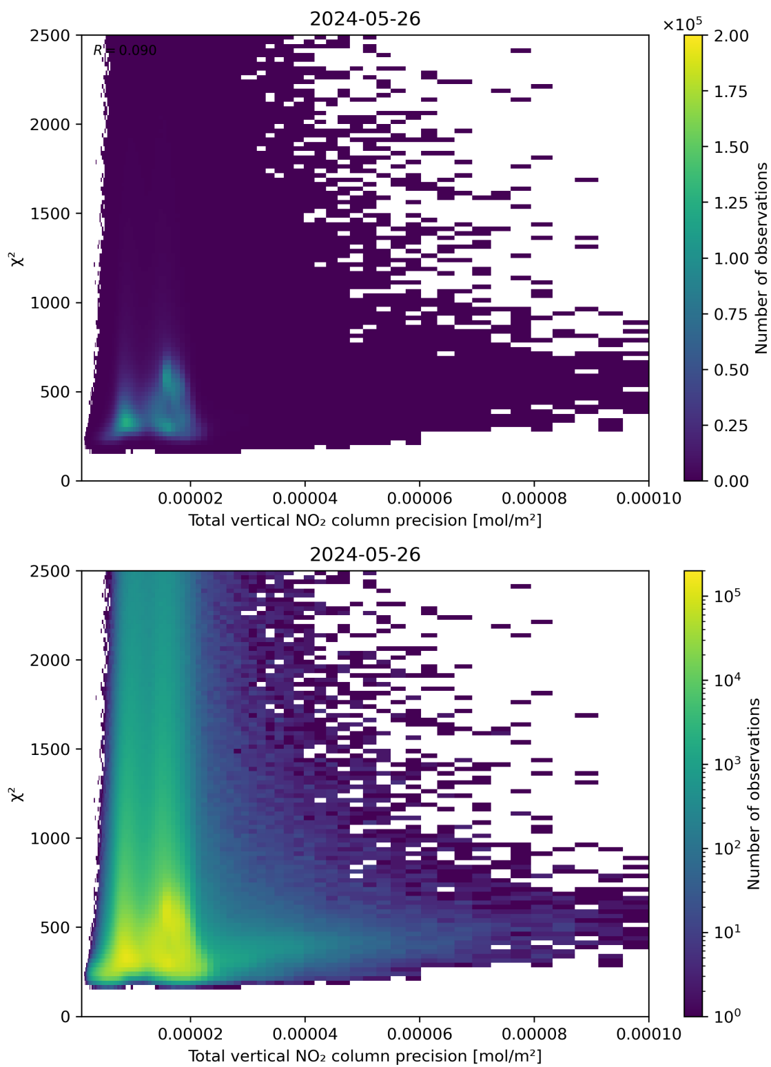
Figure 116: Scatter density plot of “Total vertical NO 2 column precision” against “ \chi^2 ” for 2024-05-25 to 2024-05-27.
