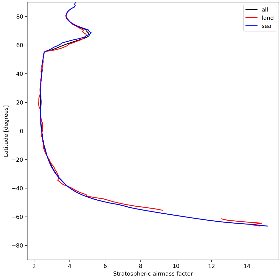
Figure 27: Zonal average of “Stratospheric airmass factor” for 2024-05-25 to 2024-05-27.
