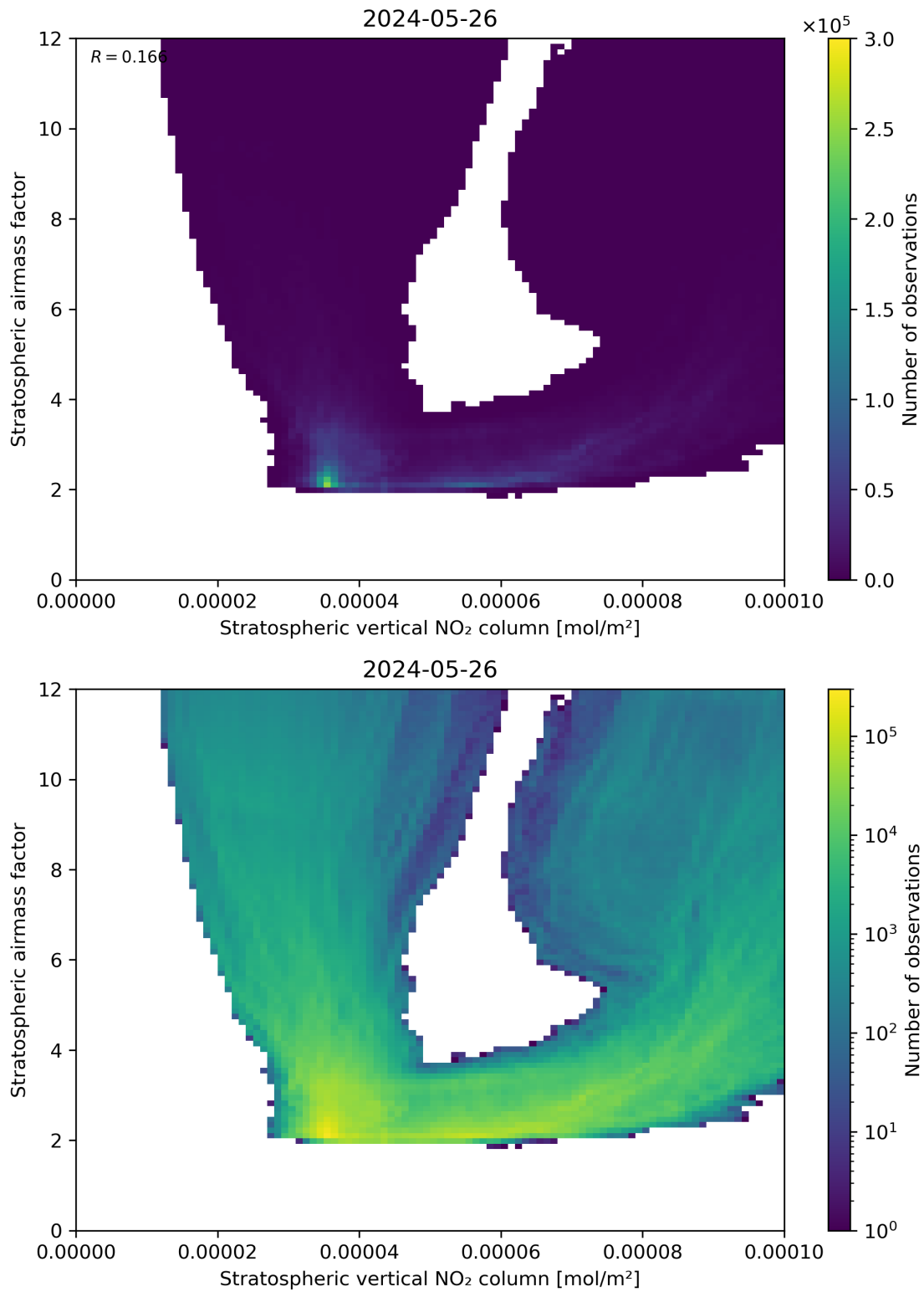
Figure 96: Scatter density plot of “Stratospheric vertical NO 2 column” against “Stratospheric airmass factor” for 2024-05-25 to 2024-05-27.
