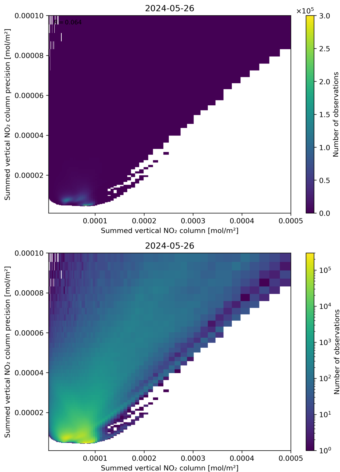
Figure 105: Scatter density plot of “Summed vertical NO 2 column” against “Summed vertical NO 2 column precision” for 2024-05-25 to 2024-05-27.
