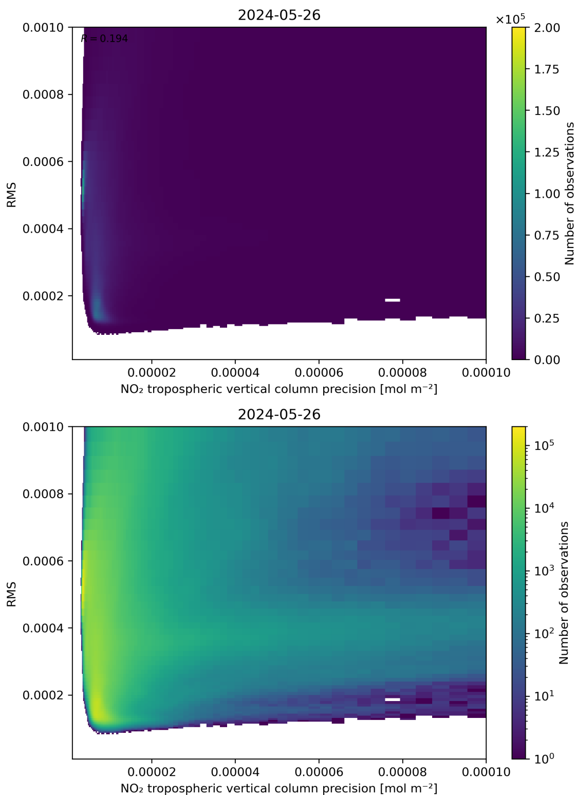
Figure 140: Scatter density plot of “NO 2 tropospheric vertical column precision” against “RMS” for 2024-05-25 to 2024-05-27.
