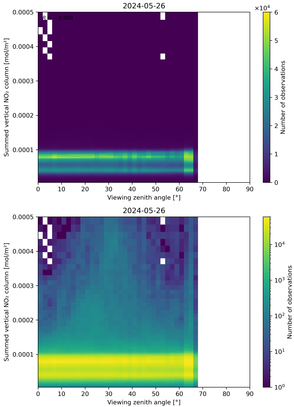
Figure 165: Scatter density plot of “Viewing zenith angle” against “Summed vertical NO 2 column” for 2024-05-25 to 2024-05-27.
