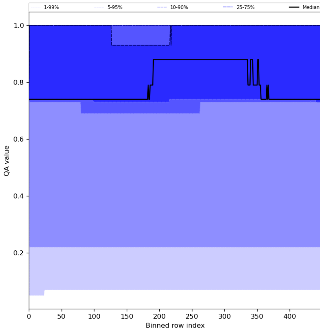
Figure 45: Along track statistics of “QA value” for 2024-05-25 to 2024-05-27
