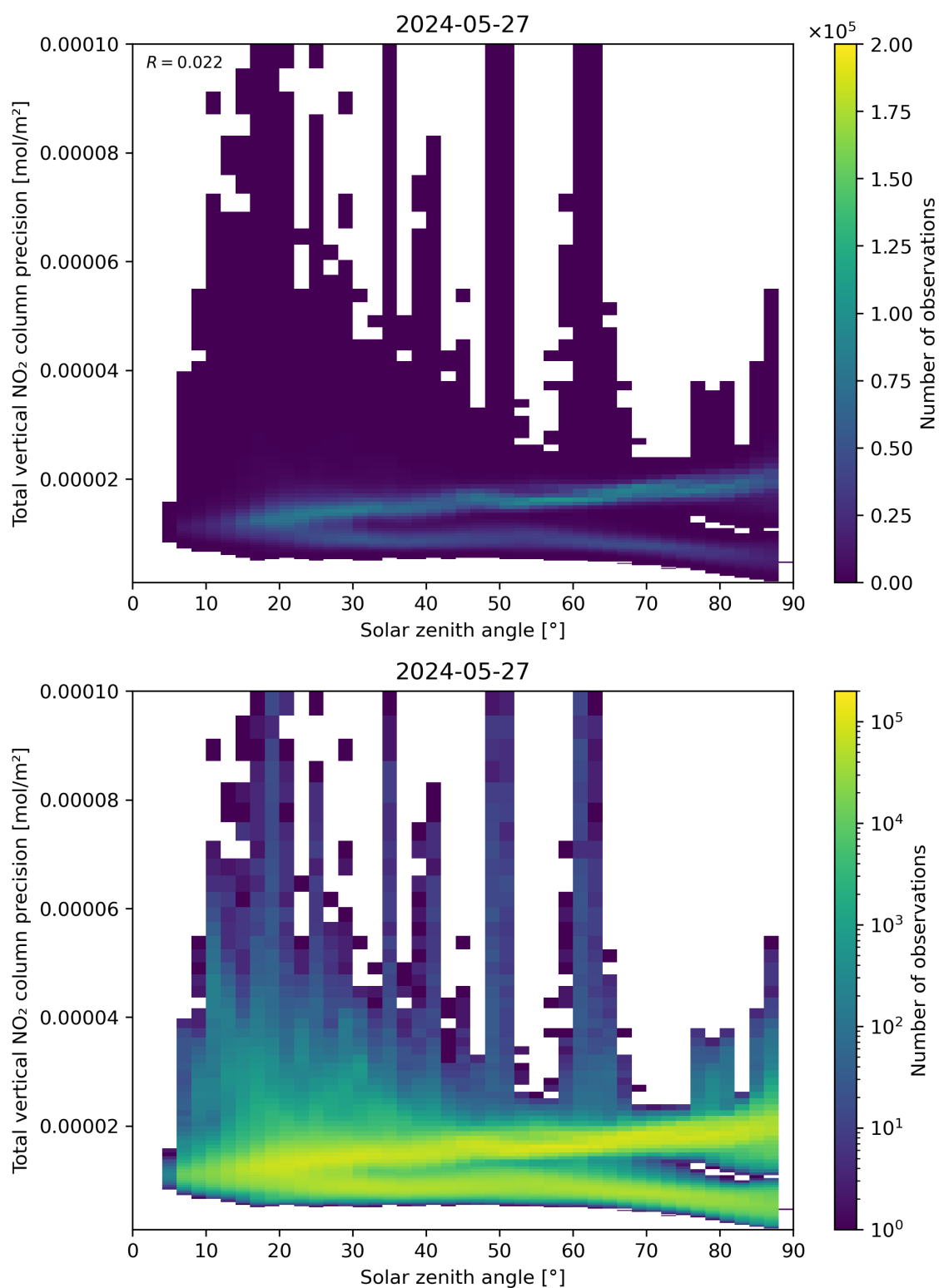
Figure 154: Scatter density plot of “Solar zenith angle” against “Total vertical NO 2 column precision” for 2024-05-26 to 2024-05-28.
