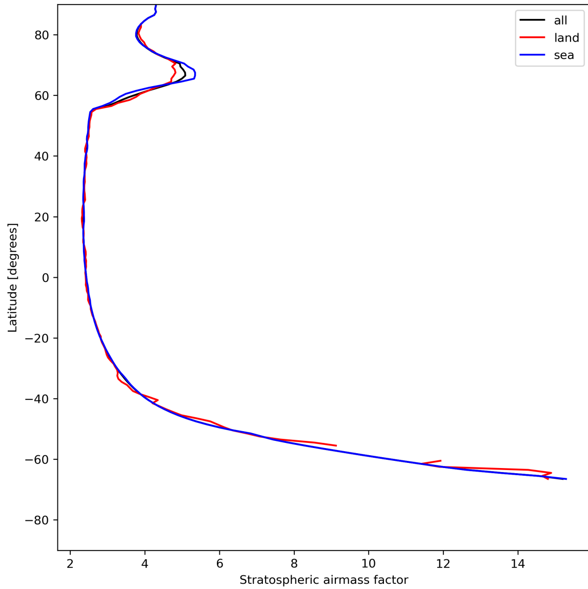
Figure 27: Zonal average of “Stratospheric airmass factor” for 2024-05-26 to 2024-05-28.
