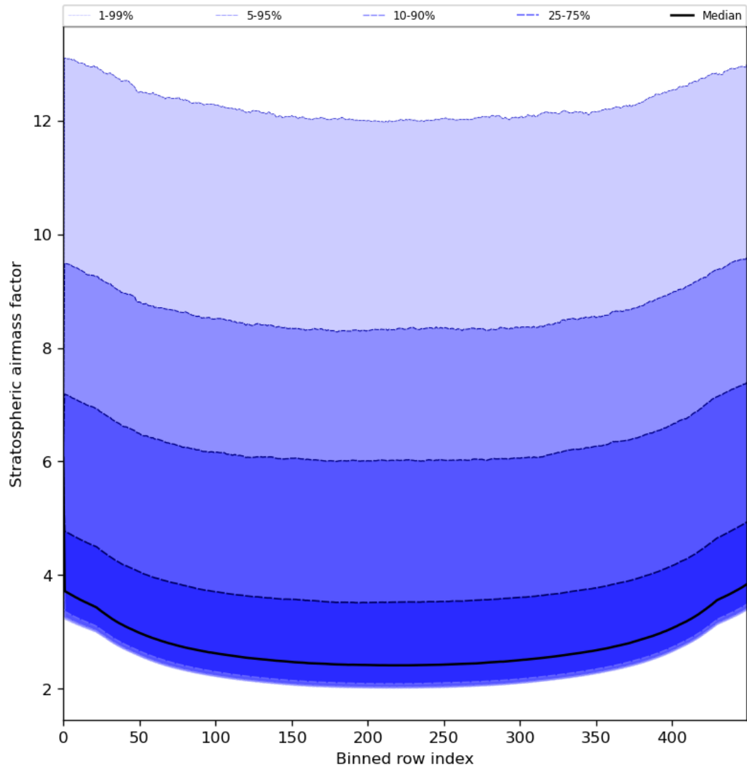
Figure 61: Along track statistics of “Stratospheric airmass factor” for 2024-05-26 to 2024-05-28
