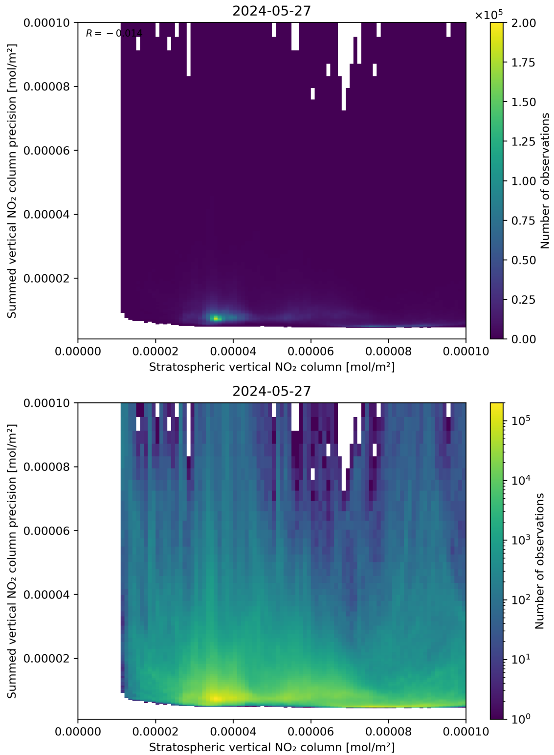
Figure 99: Scatter density plot of “Stratospheric vertical NO 2 column” against “Summed vertical NO 2 column precision” for 2024-05-26 to 2024-05-28.
