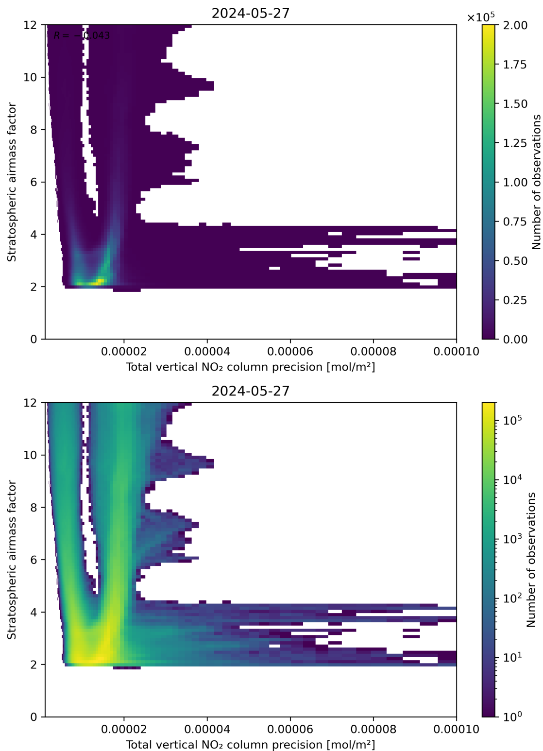
Figure 115: Scatter density plot of “Total vertical NO 2 column precision” against “Stratospheric air mass factor” for 2024-05-26 to 2024-05-28.
