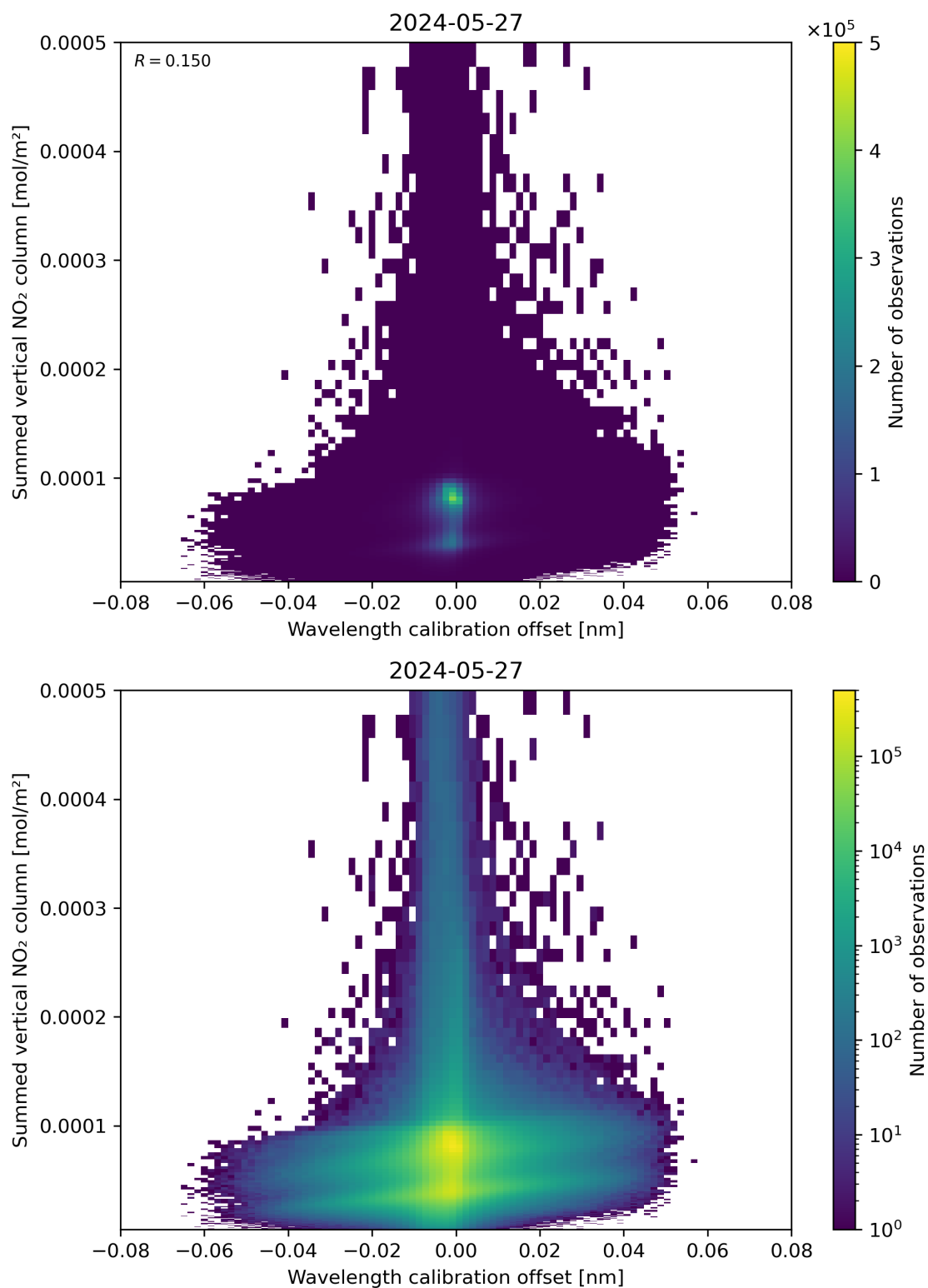
Figure 177: Scatter density plot of “Wavelength calibration offset” against “Summed vertical NO 2 column” for 2024-05-26 to 2024-05-28.
