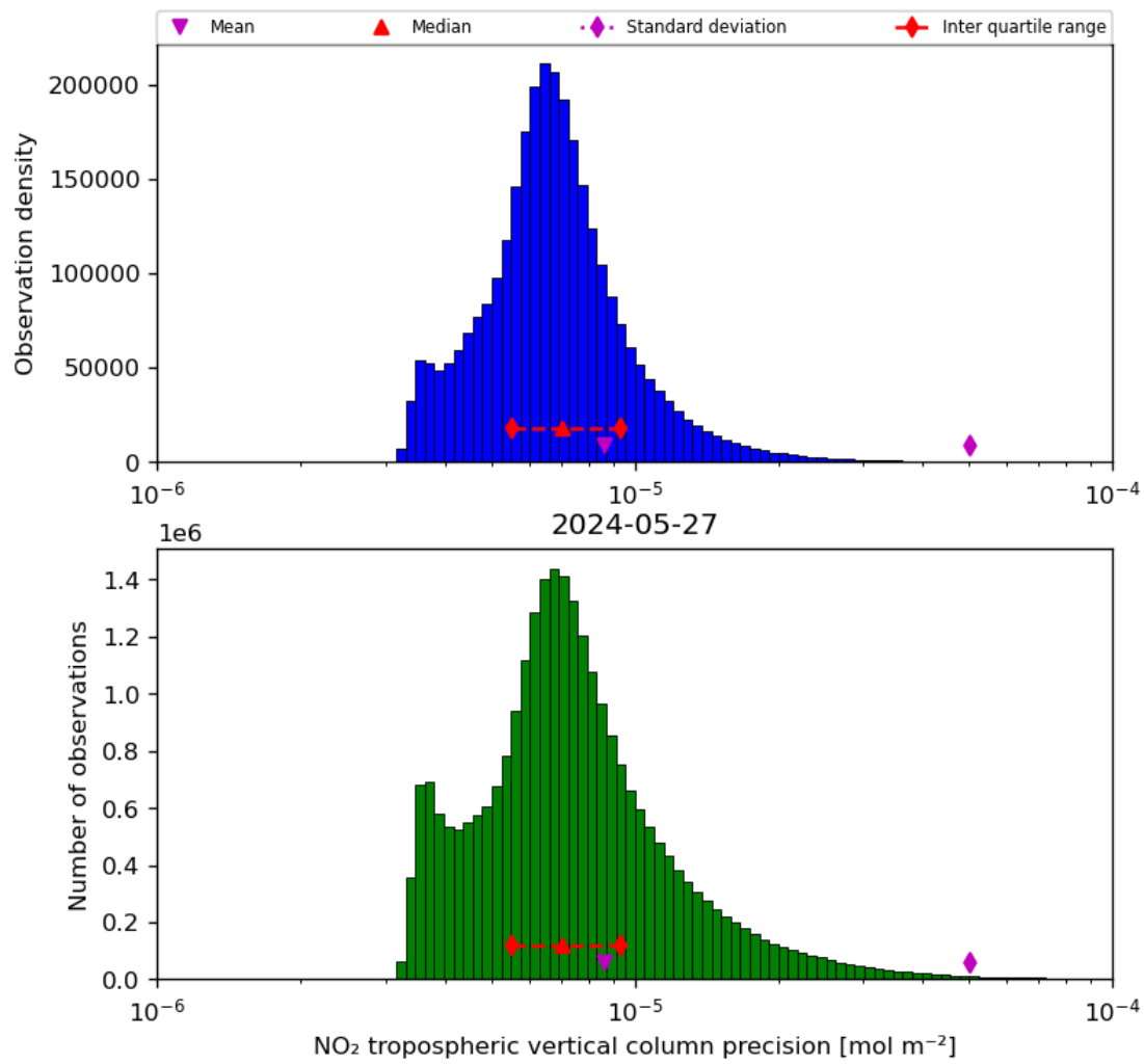
Figure 30: Histogram of “NO 2 tropospheric vertical column precision” for 2024-05-26 to 2024-05-28
