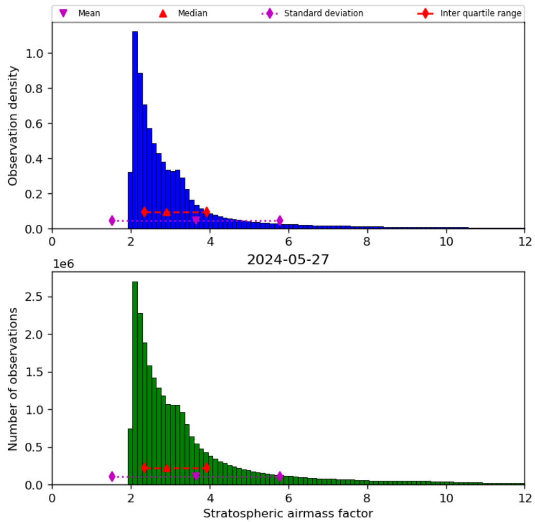
Figure 44: Histogram of “Stratospheric airmass factor” for 2024-05-26 to 2024-05-28
