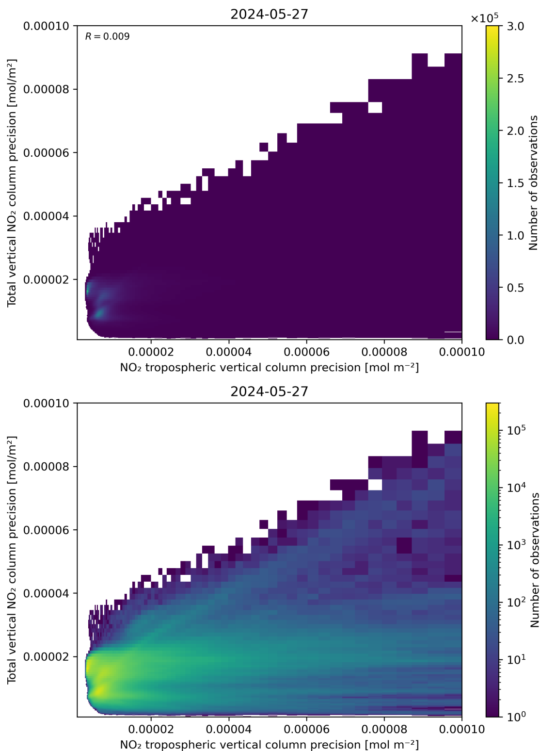
Figure 139: Scatter density plot of “NO 2 tropospheric vertical column precision” against “Total vertical NO 2 column precision” for 2024-05-26 to 2024-05-28.
