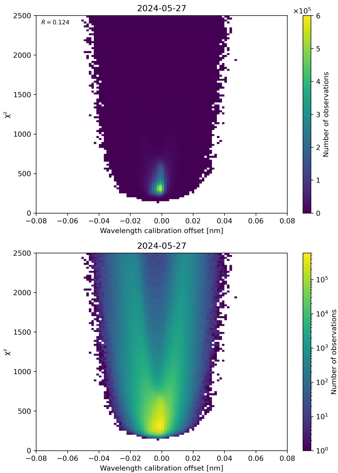
Figure 175: Scatter density plot of “Wavelength calibration offset” against “ \chi^2 ” for 2024-05-26 to 2024-05-28.
