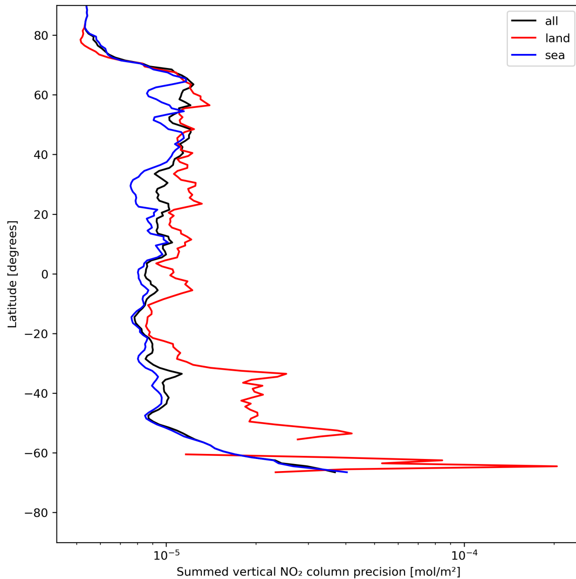
Figure 24: Zonal average of “Summed vertical NO 2 column precision” for 2024-05-26 to 2024-05-28.
