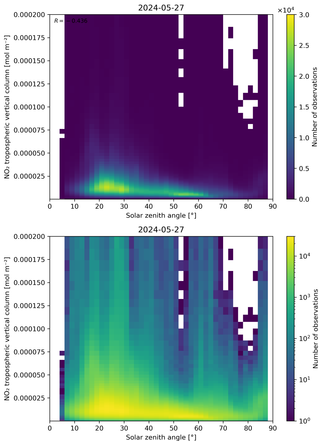
Figure 155: Scatter density plot of “Solar zenith angle” against “NO 2 tropospheric vertical column” for 2024-05-26 to 2024-05-28.
