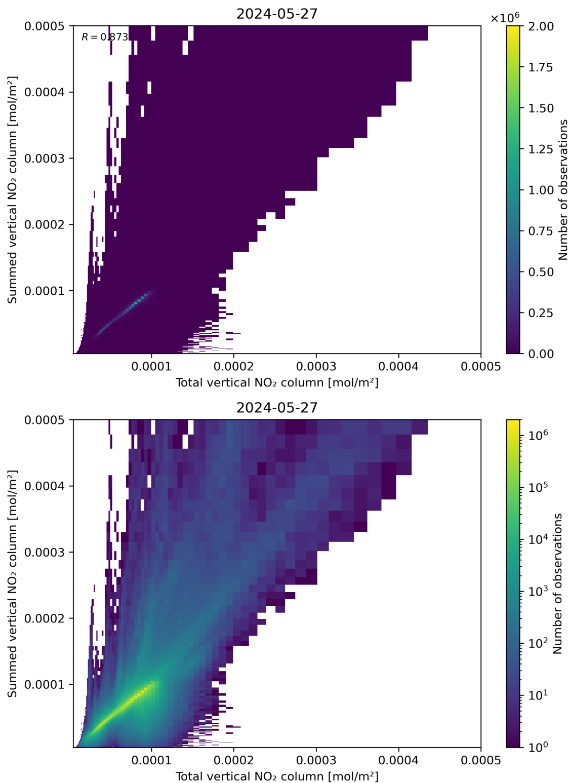
Figure 112: Scatter density plot of “Total vertical NO 2 column” against “Summed vertical NO 2 column” for 2024-05-26 to 2024-05-28.
