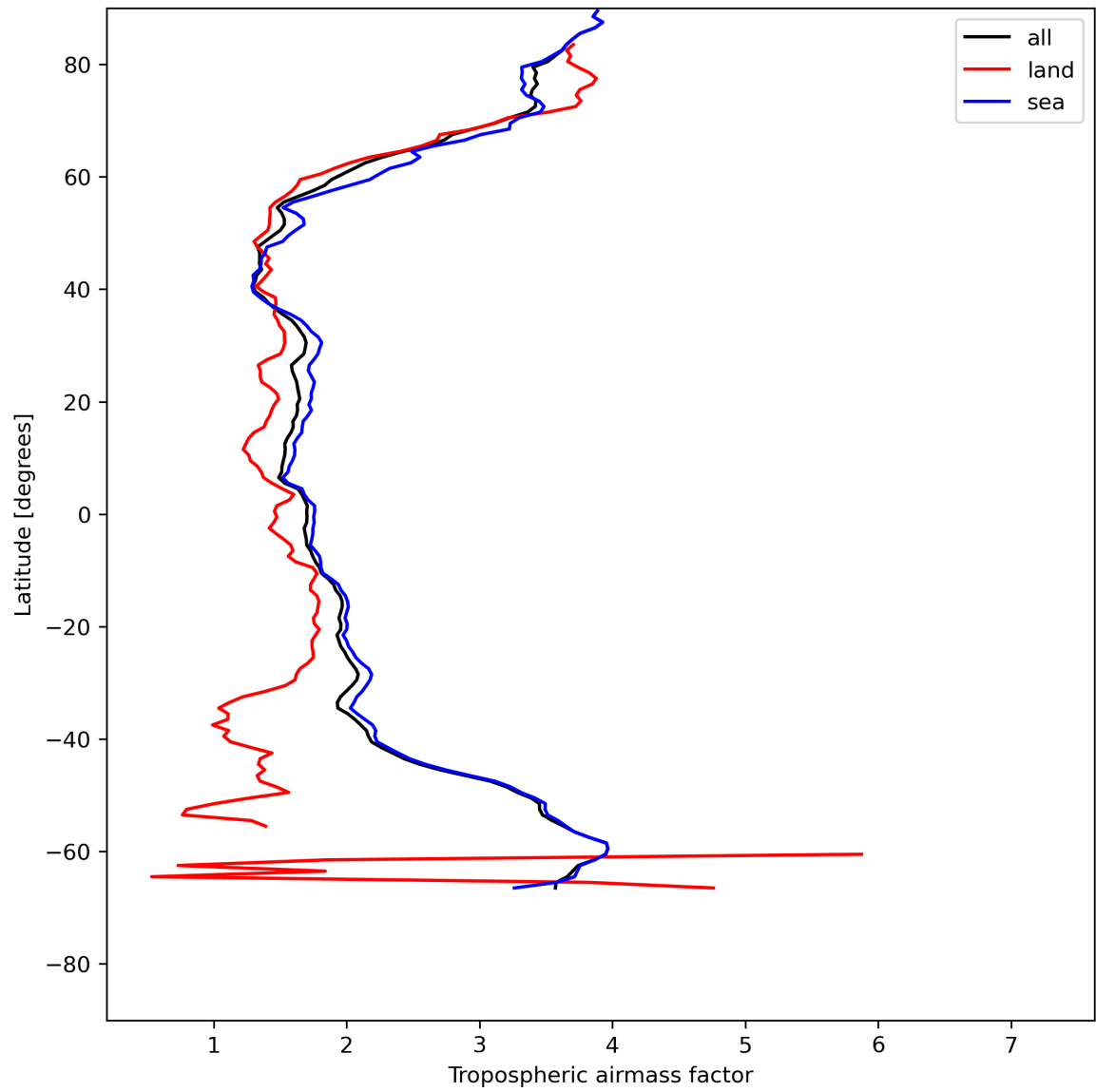
Figure 14: Zonal average of “Tropospheric airmass factor” for 2024-05-26 to 2024-05-28.
