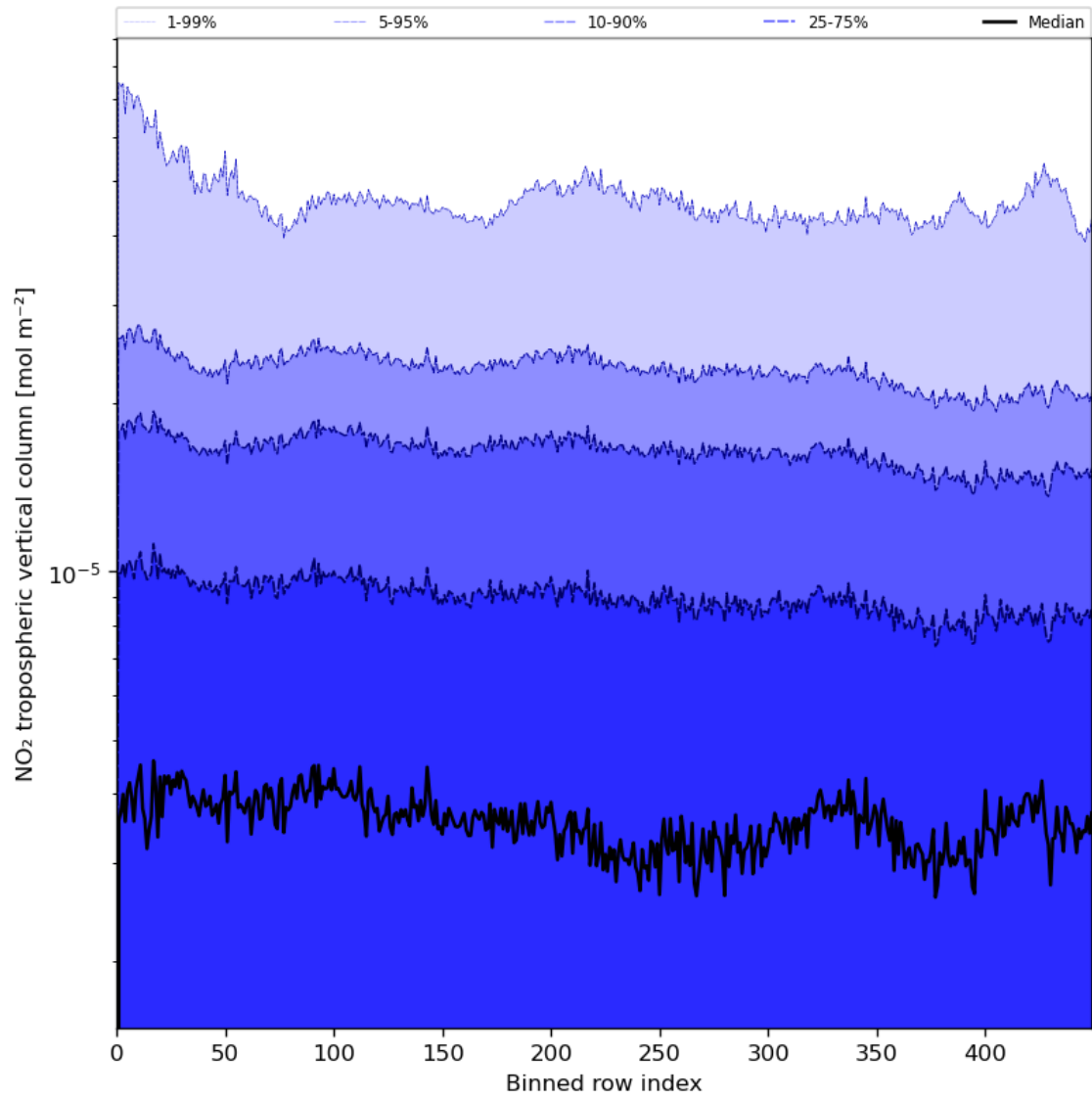
Figure 46: Along track statistics of “NO 2 tropospheric vertical column” for 2024-05-26 to 2024-05-28
