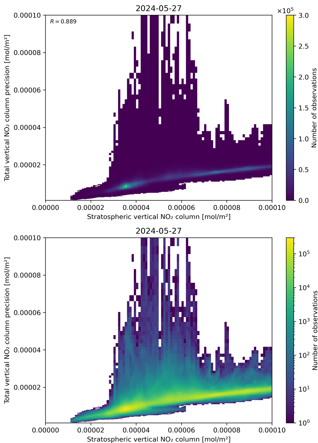
Figure 101: Scatter density plot of “Stratospheric vertical NO 2 column” against “Total vertical NO 2 column precision” for 2024-05-26 to 2024-05-28.
