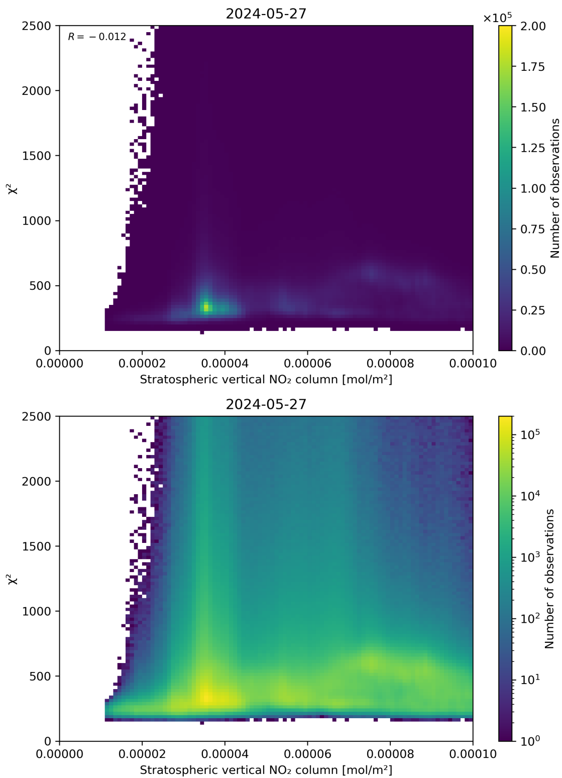
Figure 97: Scatter density plot of “Stratospheric vertical NO 2 column” against “ \chi^2 ” for 2024-05-26 to 2024-05-28.
