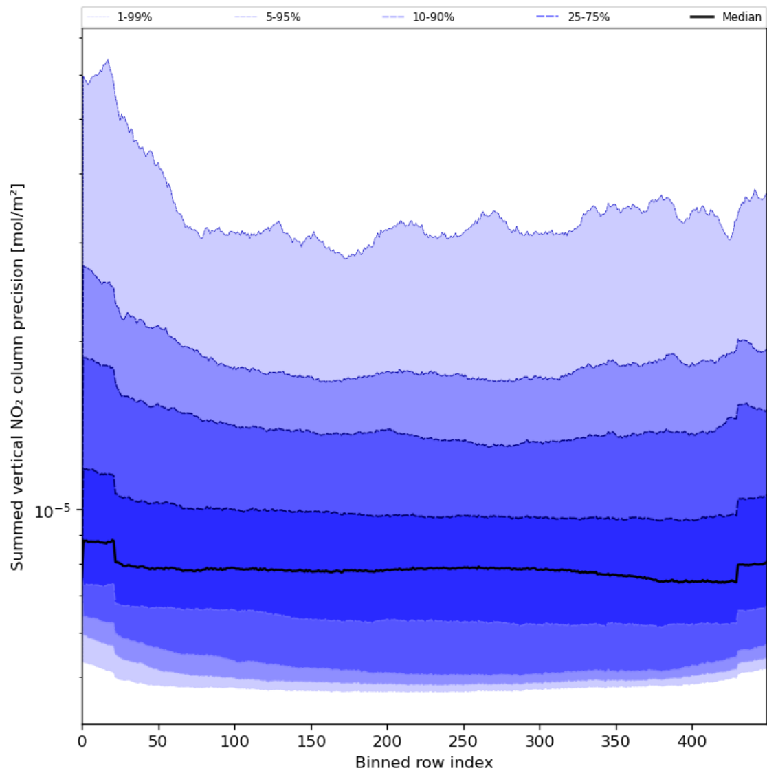
Figure 58: Along track statistics of “Summed vertical NO 2 column precision” for 2024-05-26 to 2024-05-28
