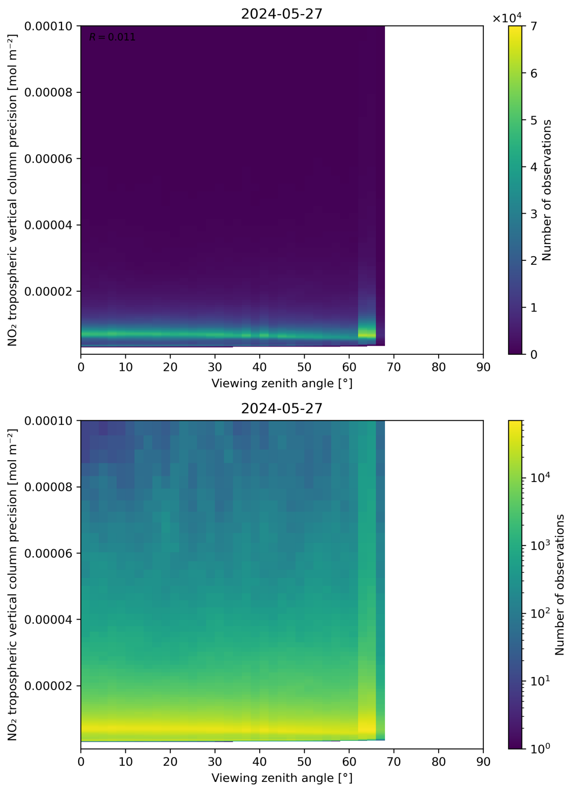
Figure 170: Scatter density plot of “Viewing zenith angle” against “NO 2 tropospheric vertical column precision” for 2024-05-26 to 2024-05-28.
