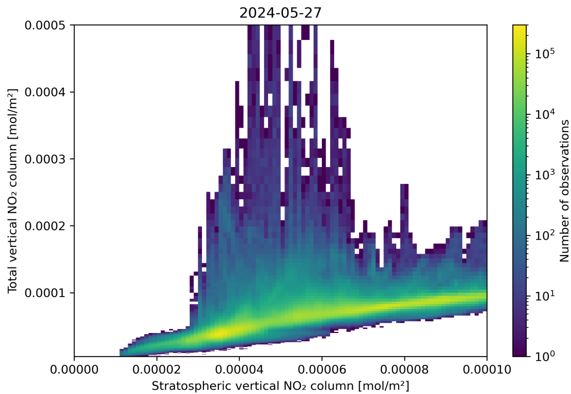
Figure 100: Scatter density plot of “Stratospheric vertical NO 2 column” against “Total vertical NO 2 column” for 2024-05-26 to 2024-05-28.
