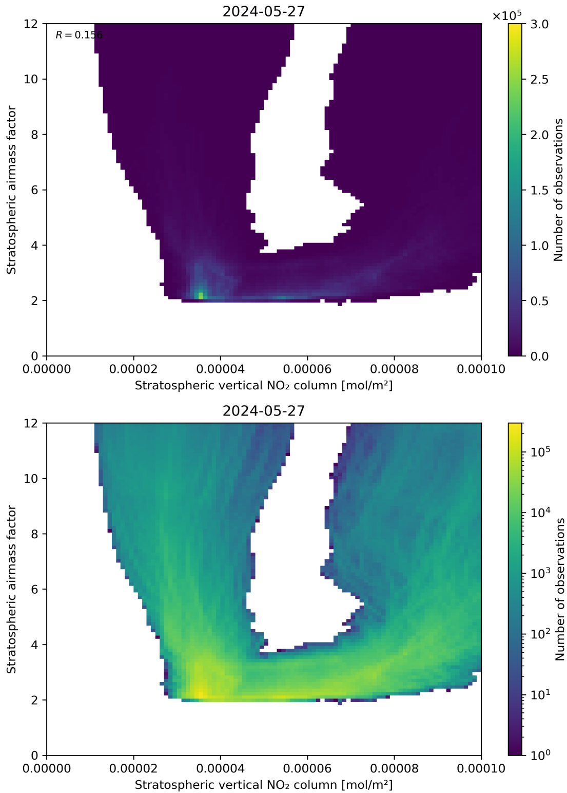
Figure 96: Scatter density plot of “Stratospheric vertical NO 2 column” against “Stratospheric airmass factor” for 2024-05-26 to 2024-05-28.
