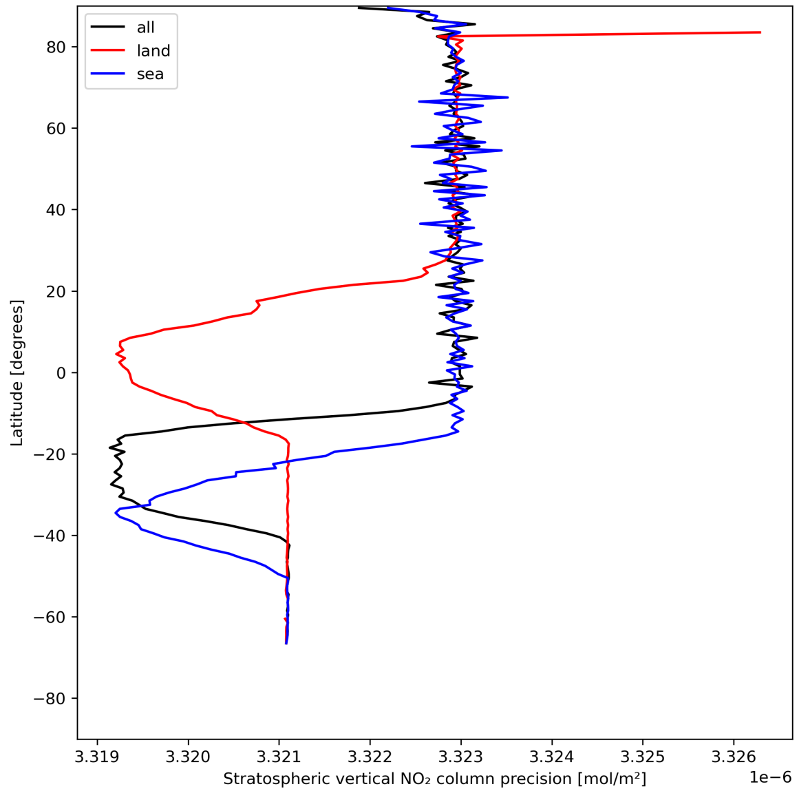
Figure 20: Zonal average of “Stratospheric vertical NO 2 column precision” for 2024-05-26 to 2024-05-28.
