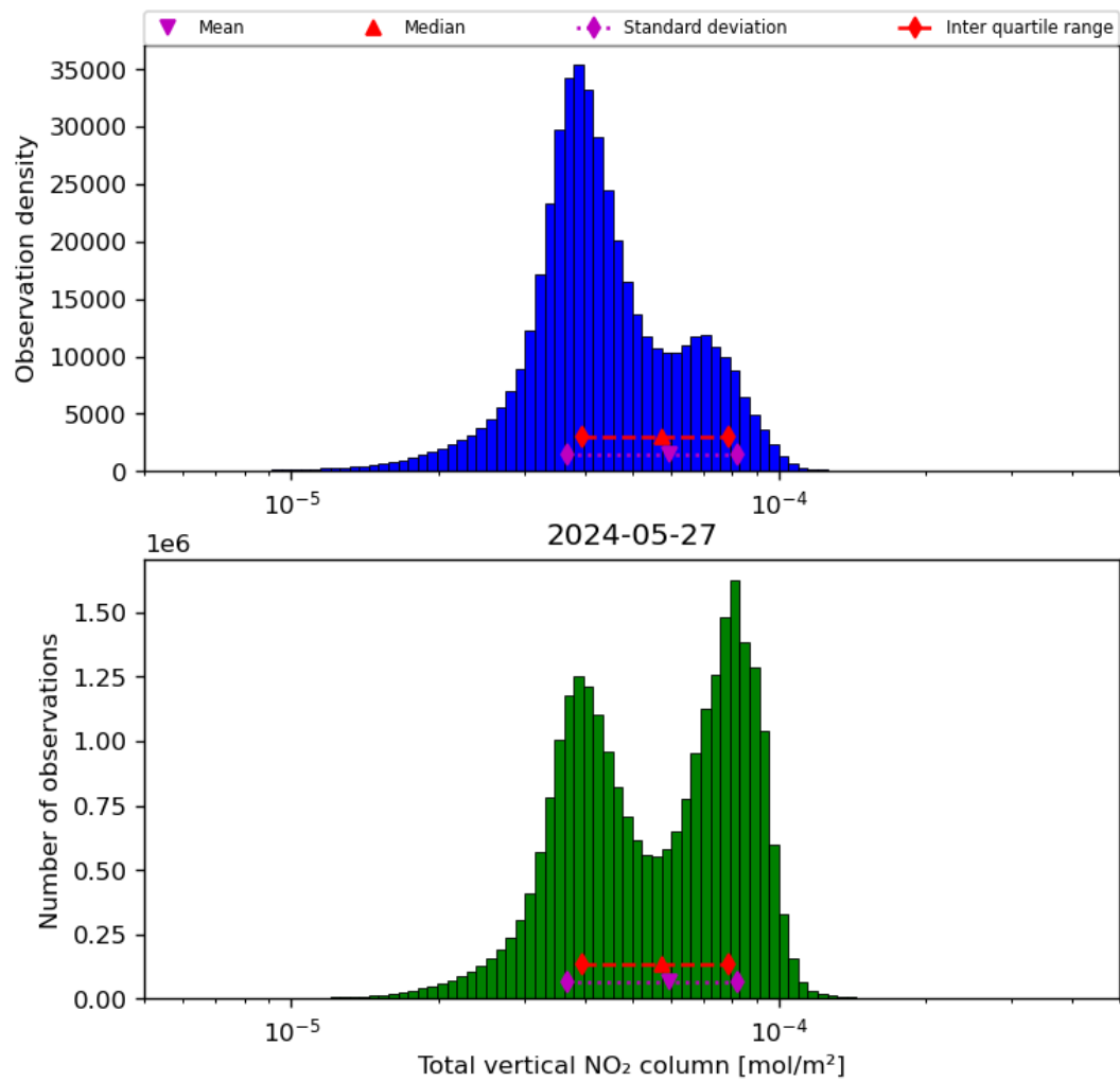
Figure 38: Histogram of “Total vertical NO 2 column” for 2024-05-26 to 2024-05-28
