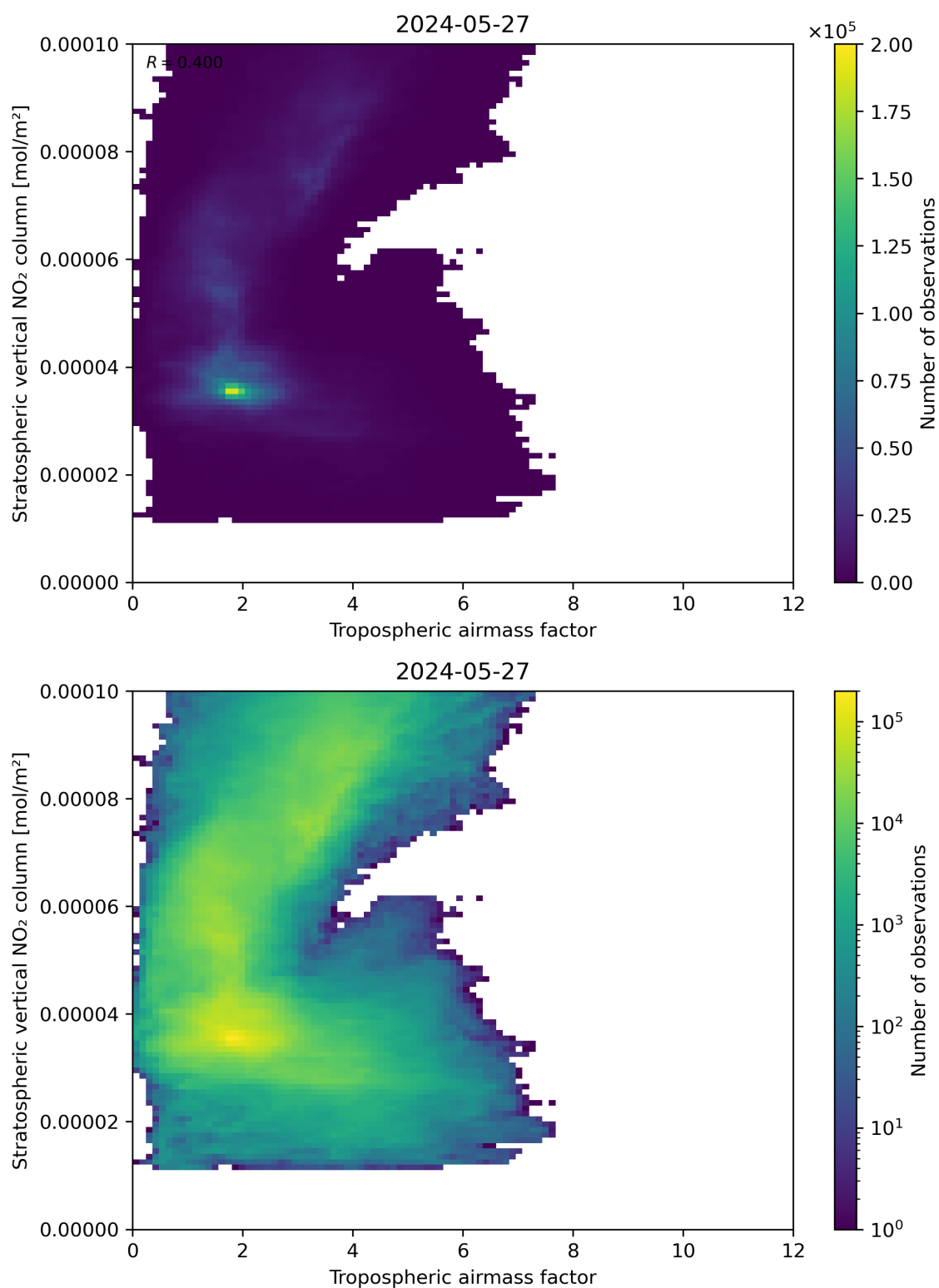
Figure 74: Scatter density plot of “Tropospheric air mass factor” against “Stratospheric vertical NO 2 column” for 2024-05-26 to 2024-05-28.
