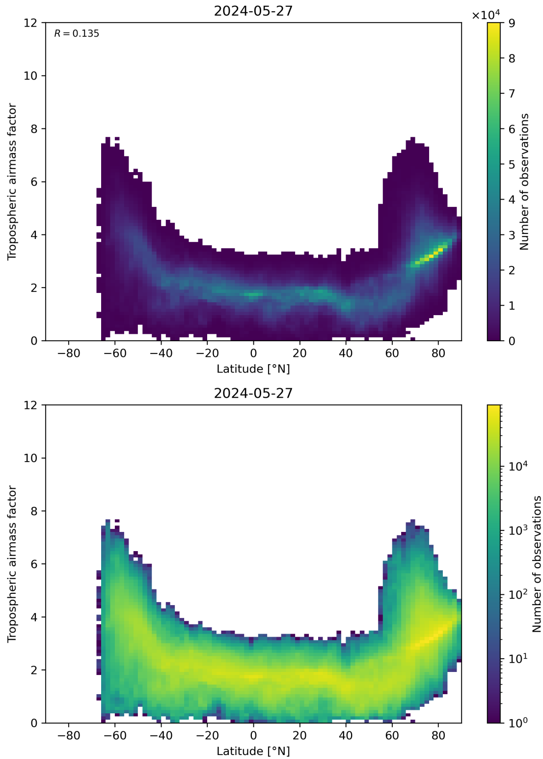
Figure 85: Scatter density plot of “Latitude” against “Tropospheric air mass factor” for 2024-05-26 to 2024-05-28.
