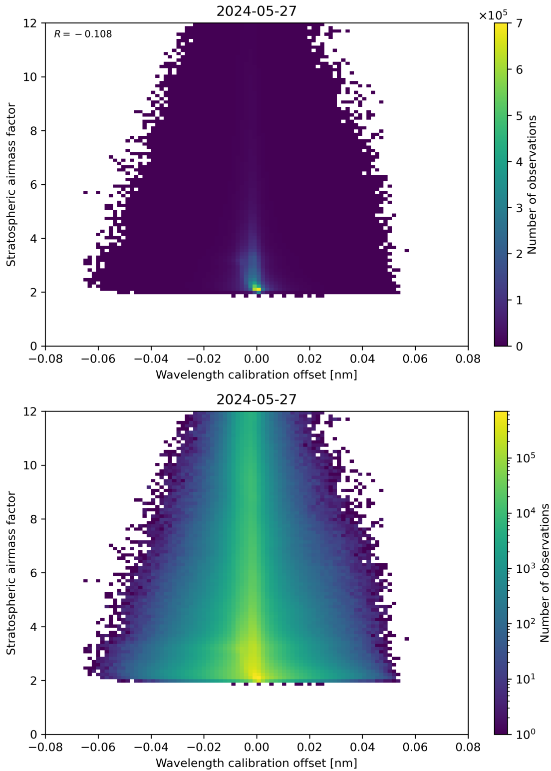
Figure 174: Scatter density plot of “Wavelength calibration offset” against “Stratospheric airmass factor” for 2024-05-26 to 2024-05-28.
