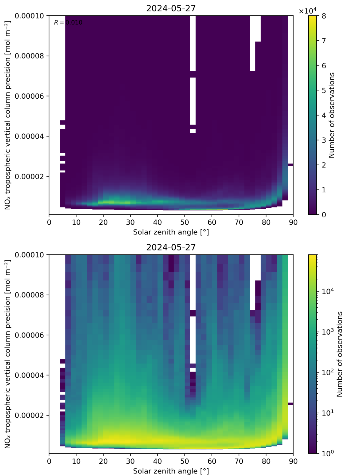
Figure 156: Scatter density plot of “Solar zenith angle” against “NO 2 tropospheric vertical column precision” for 2024-05-26 to 2024-05-28.
