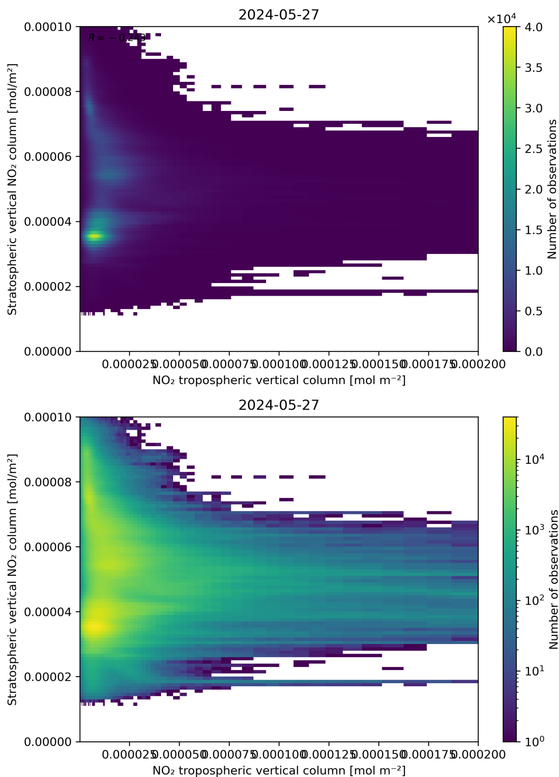
Figure 125: Scatter density plot of “NO 2 tropospheric vertical column” against “Stratospheric vertical NO 2 column” for 2024-05-26 to 2024-05-28.
