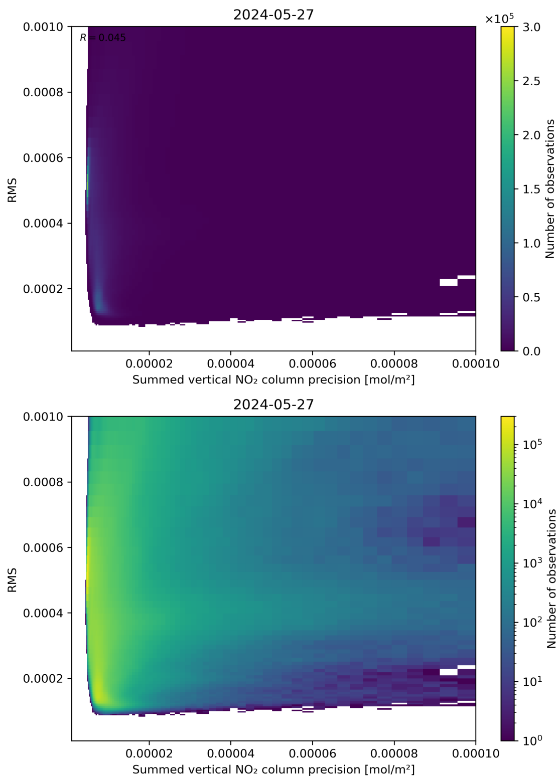
Figure 108: Scatter density plot of “Summed vertical NO 2 column precision” against “RMS” for 2024-05-26 to 2024-05-28.
