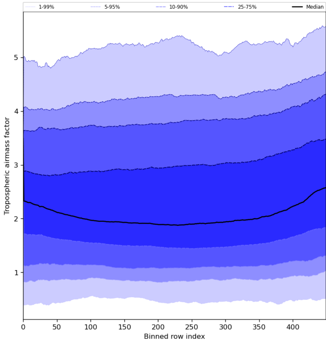
Figure 48: Along track statistics of “Tropospheric airmass factor” for 2024-05-26 to 2024-05-28
