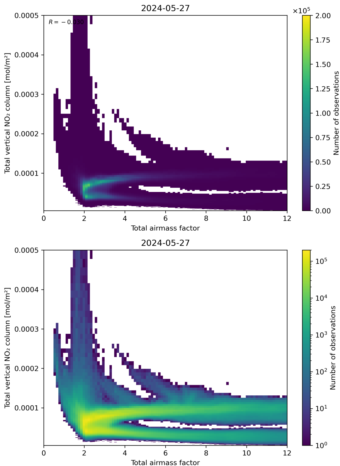
Figure 67: Scatter density plot of “Total airmass factor” against “Total vertical NO 2 column” for 2024-05-26 to 2024-05-28.
