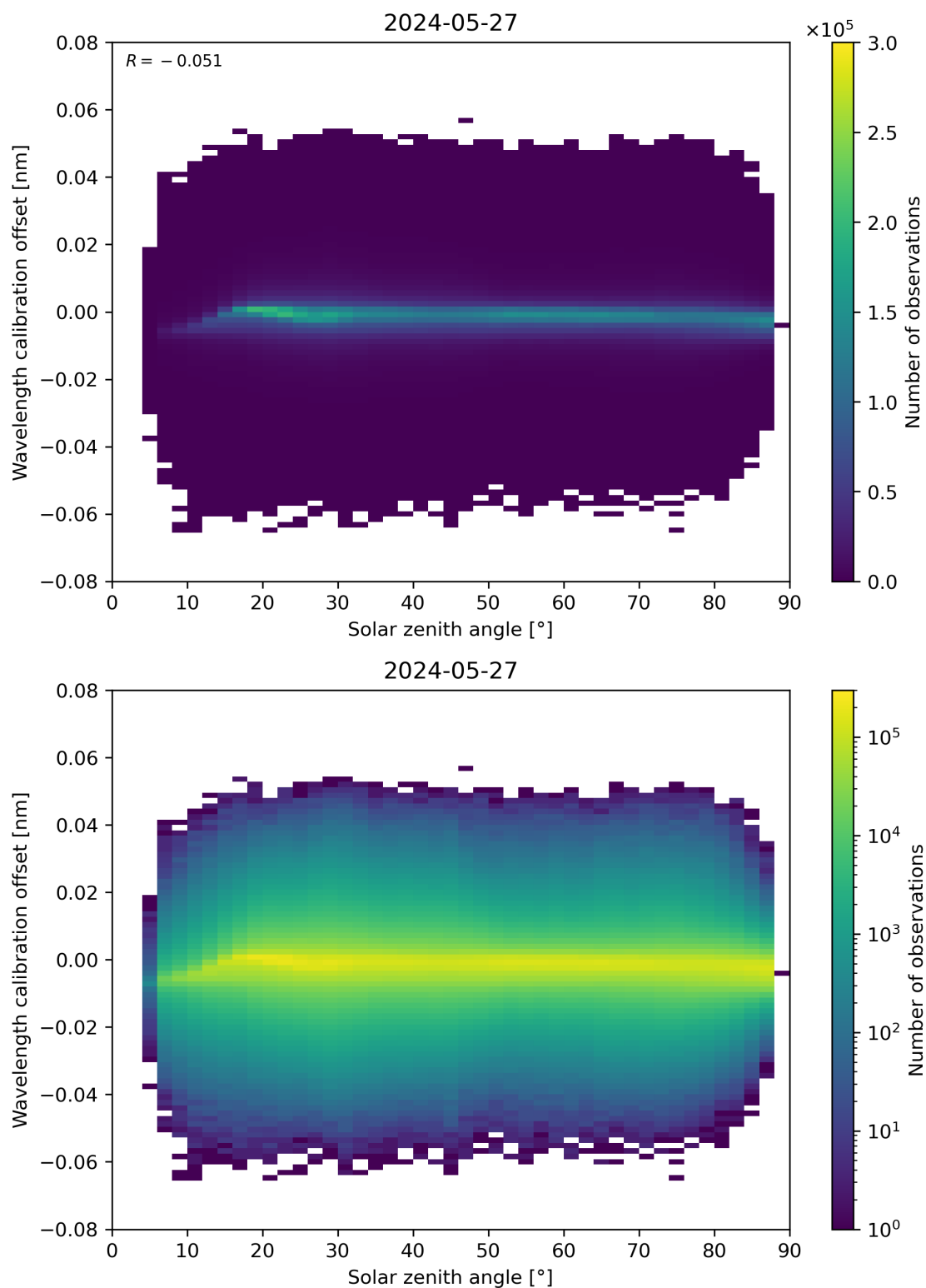
Figure 158: Scatter density plot of “Solar zenith angle” against “Wavelength calibration offset” for 2024-05-26 to 2024-05-28.
