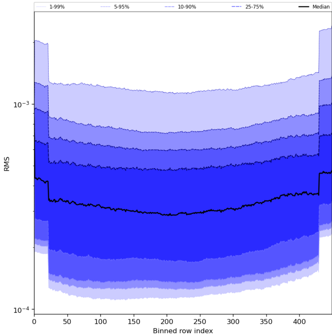
Figure 60: Along track statistics of “RMS” for 2024-05-26 to 2024-05-28
