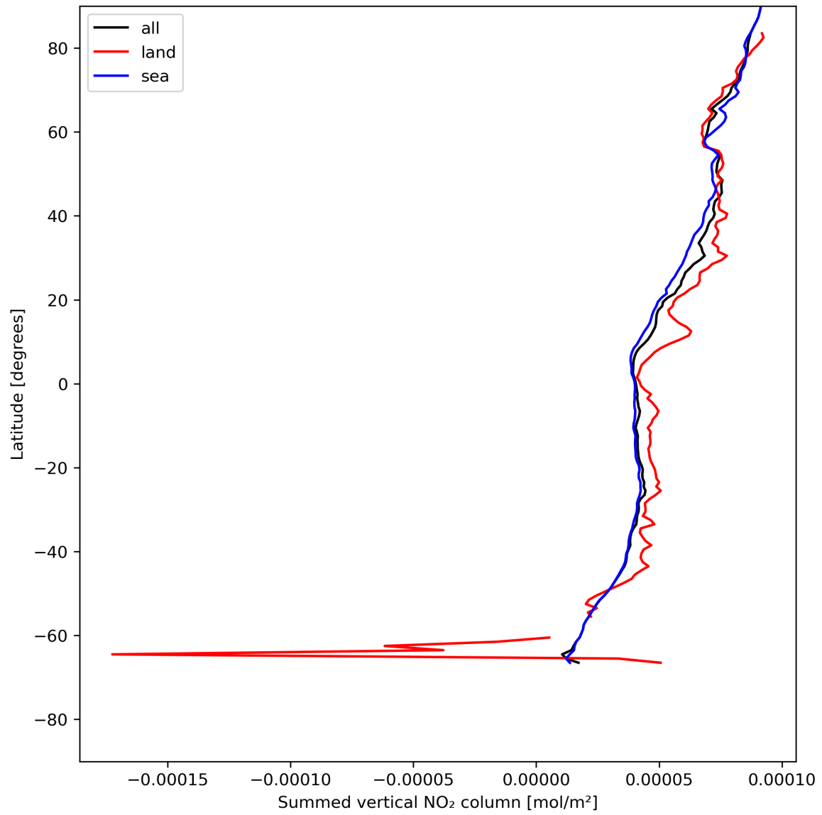
Figure 23: Zonal average of “Summed vertical NO 2 column” for 2024-05-26 to 2024-05-28.
