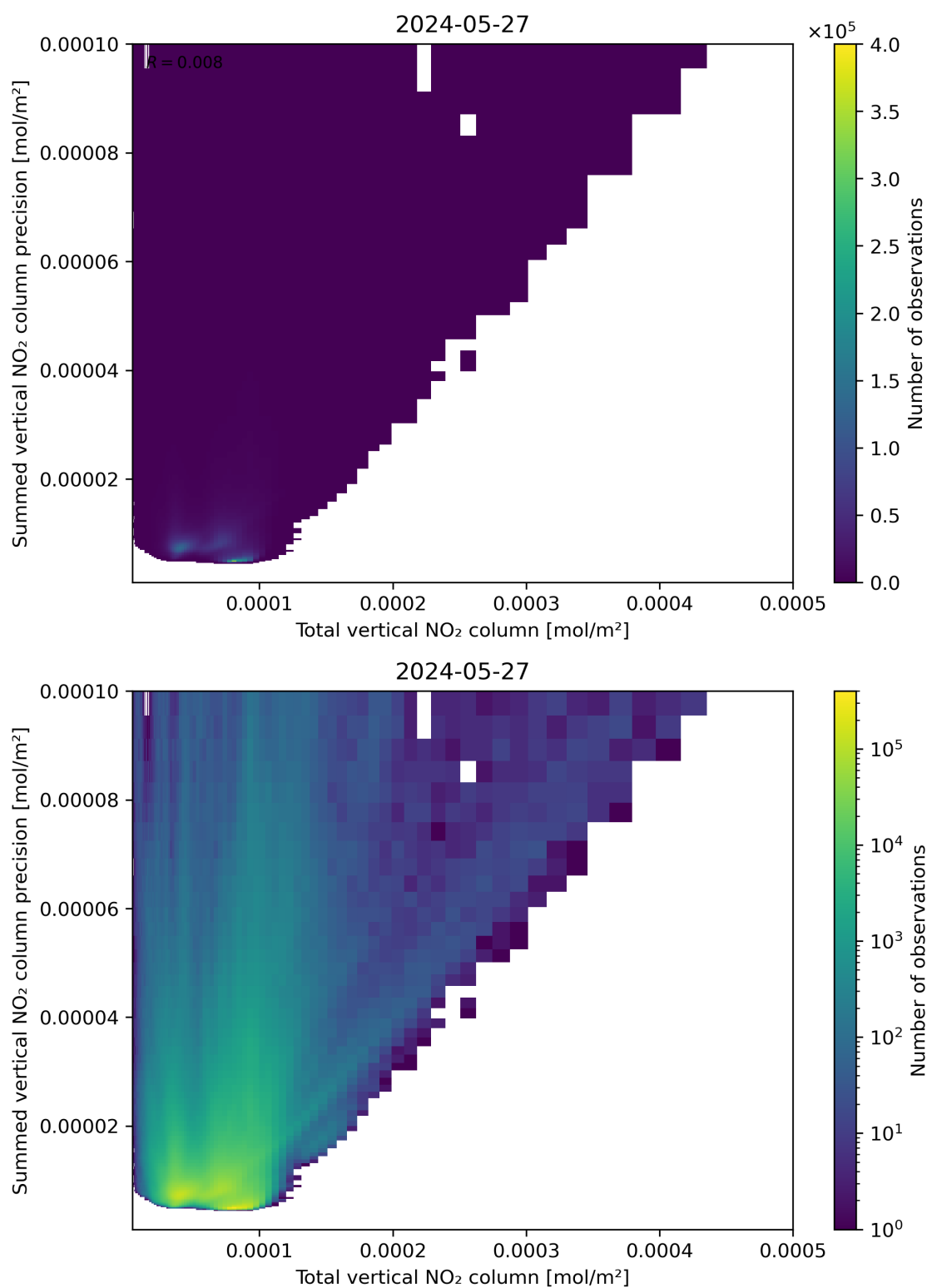
Figure 113: Scatter density plot of “Total vertical NO 2 column” against “Summed vertical NO 2 column precision” for 2024-05-26 to 2024-05-28.
