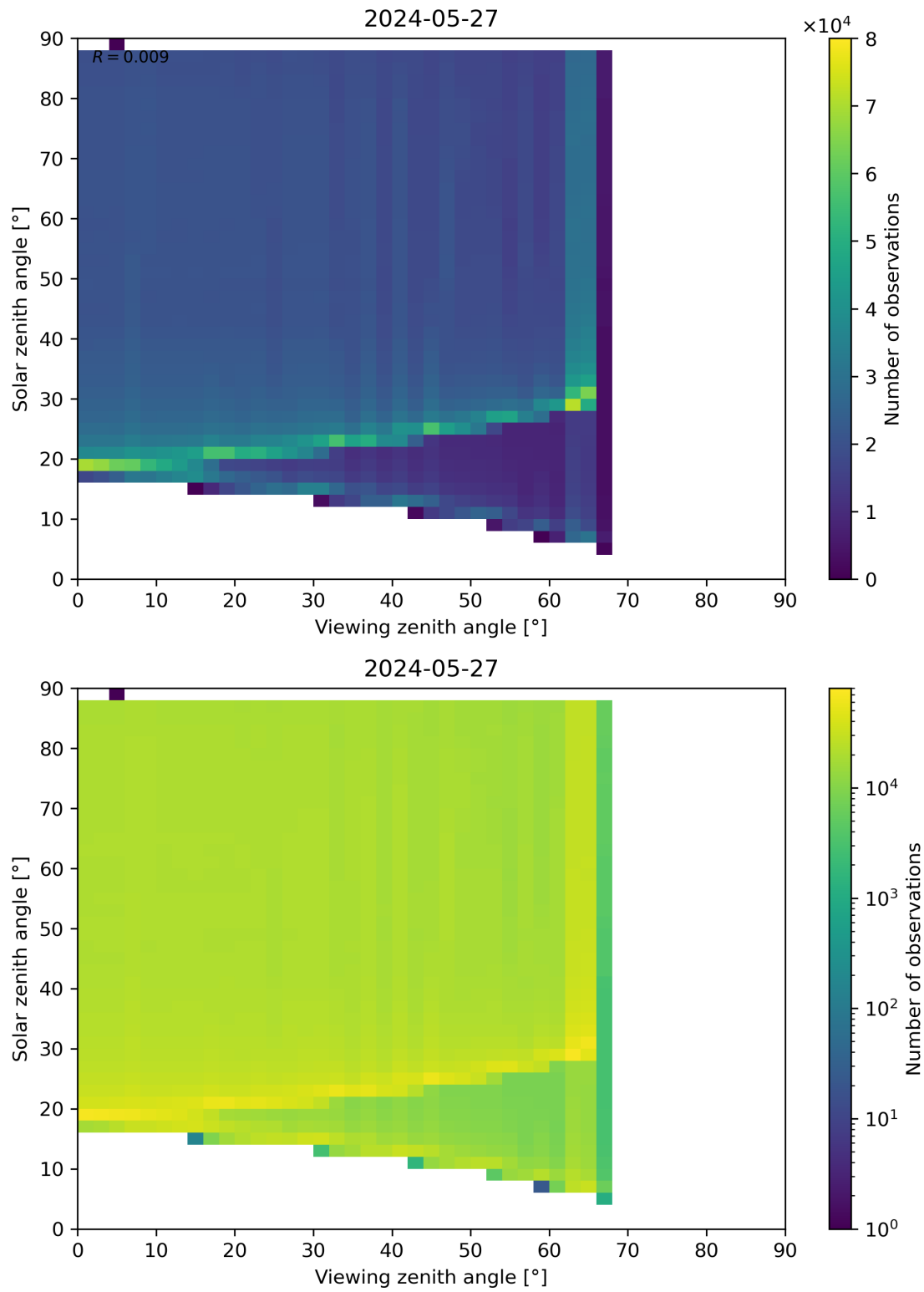
Figure 172: Scatter density plot of “Viewing zenith angle” against “Solar zenith angle” for 2024-05-26 to 2024-05-28.
