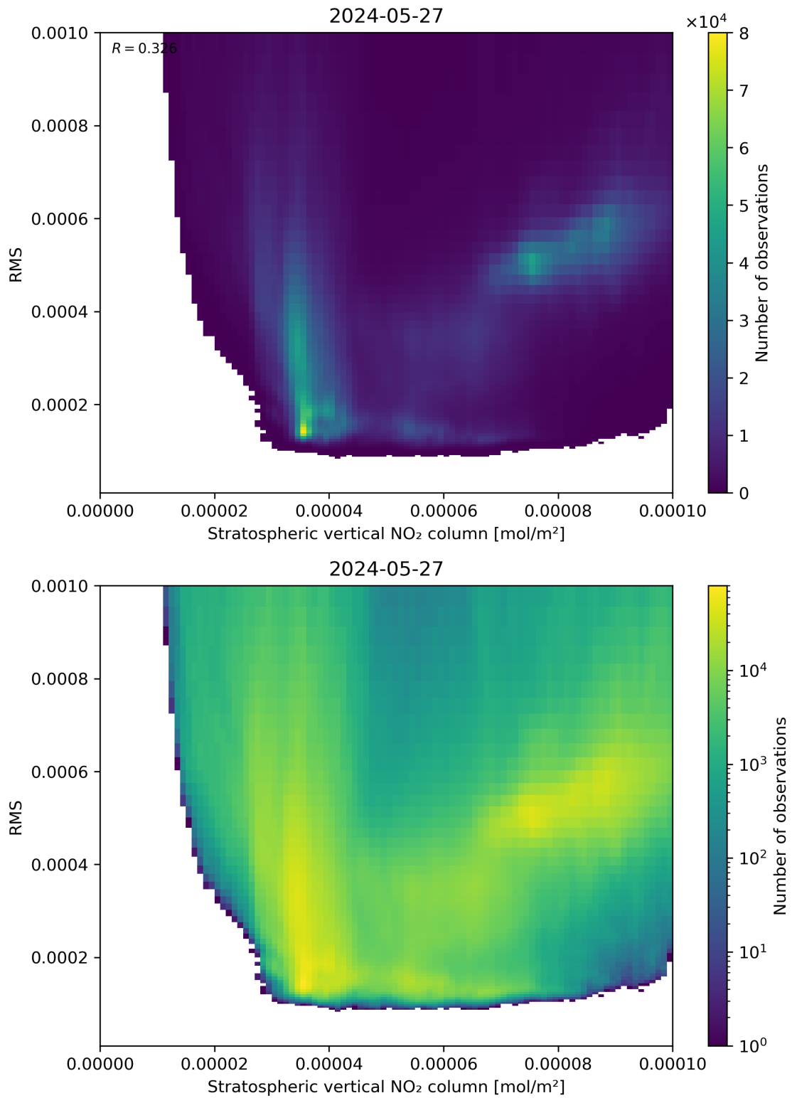
Figure 102: Scatter density plot of “Stratospheric vertical NO 2 column” against “RMS” for 2024-05-26 to 2024-05-28.
