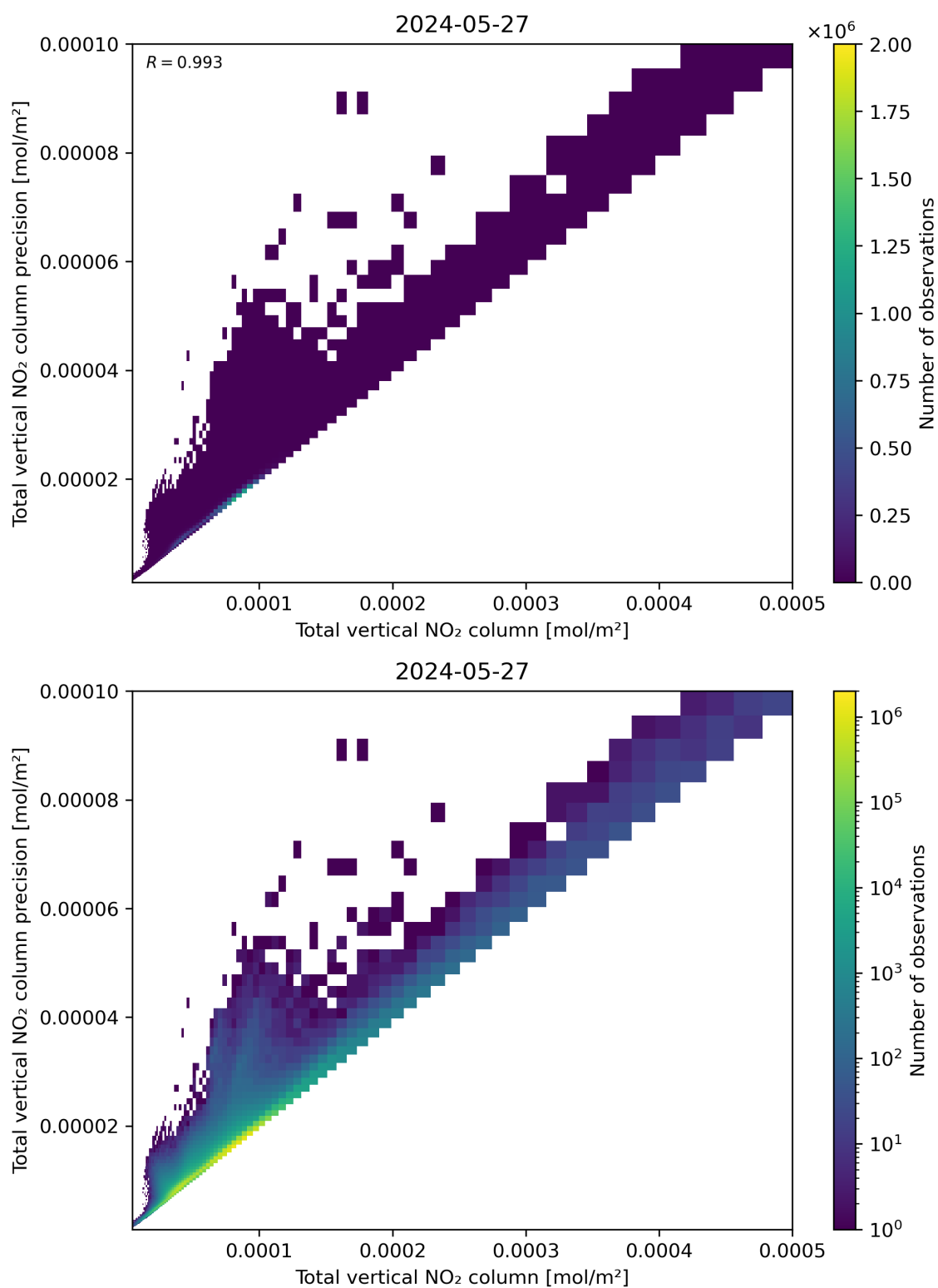
Figure 114: Scatter density plot of “Total vertical NO 2 column” against “Total vertical NO 2 column precision” for 2024-05-26 to 2024-05-28.
