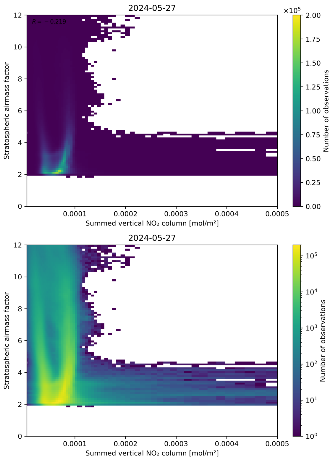
Figure 103: Scatter density plot of “Summed vertical NO 2 column” against “Stratospheric airmass factor” for 2024-05-26 to 2024-05-28.
