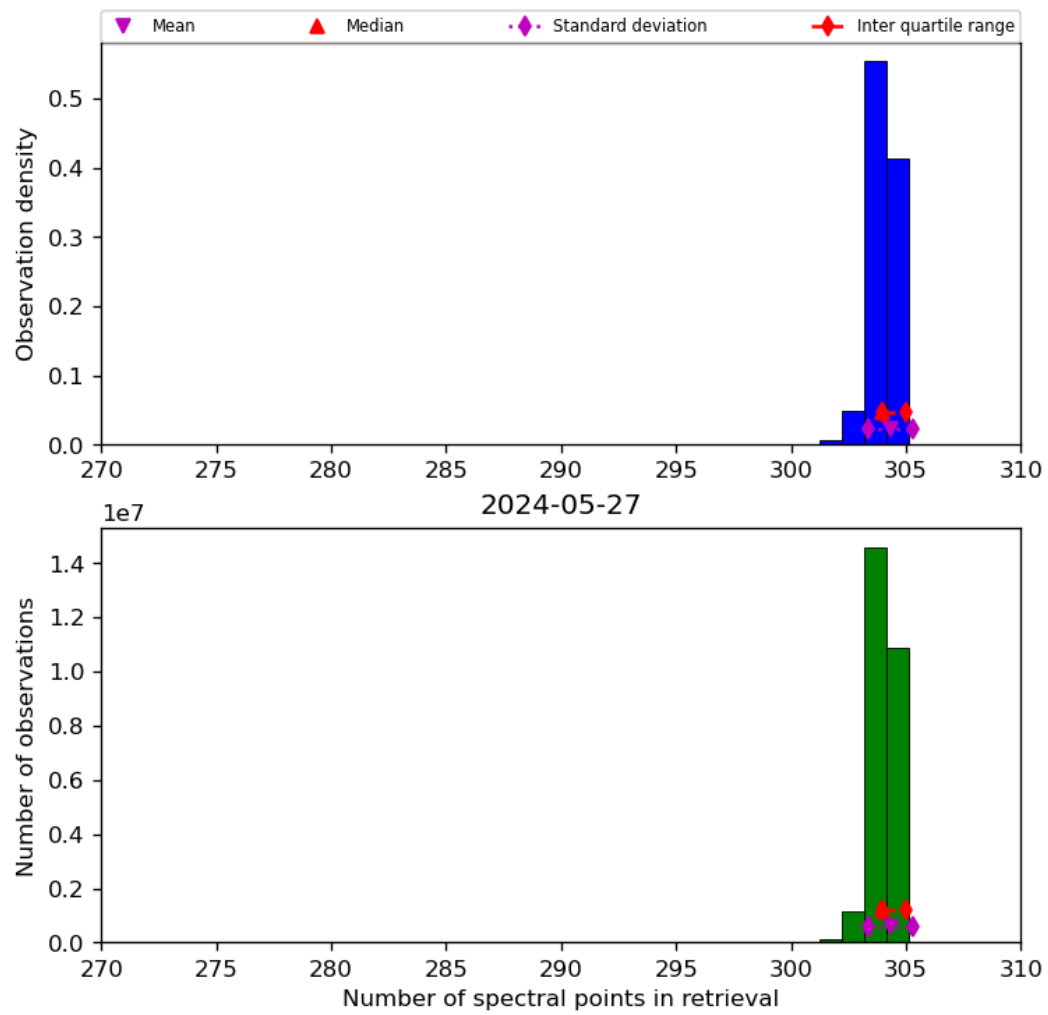
Figure 33: Histogram of “Number of spectral points in retrieval” for 2024-05-26 to 2024-05-28
