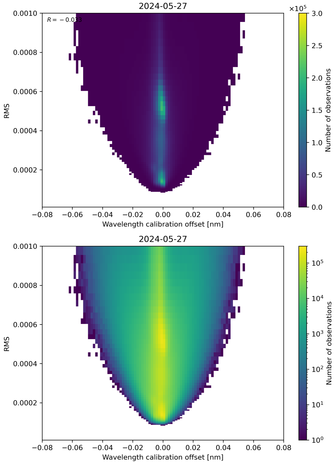
Figure 181: Scatter density plot of “Wavelength calibration offset” against “RMS” for 2024-05-26 to 2024-05-28.
