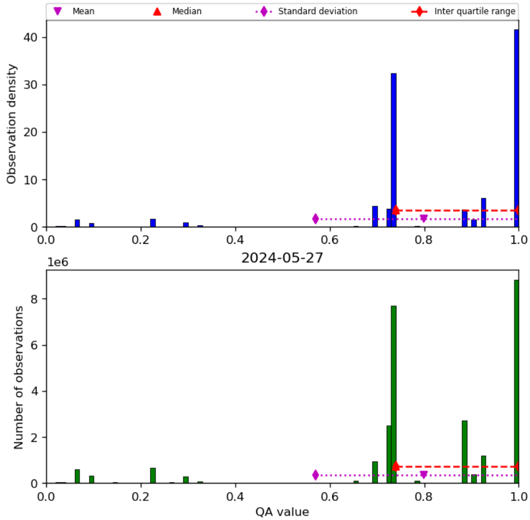
Figure 28: Histogram of “QA value” for 2024-05-26 to 2024-05-28
