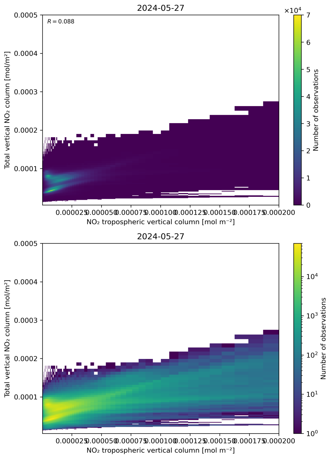
Figure 128: Scatter density plot of “NO 2 tropospheric vertical column” against “Total vertical NO 2 column” for 2024-05-26 to 2024-05-28.
