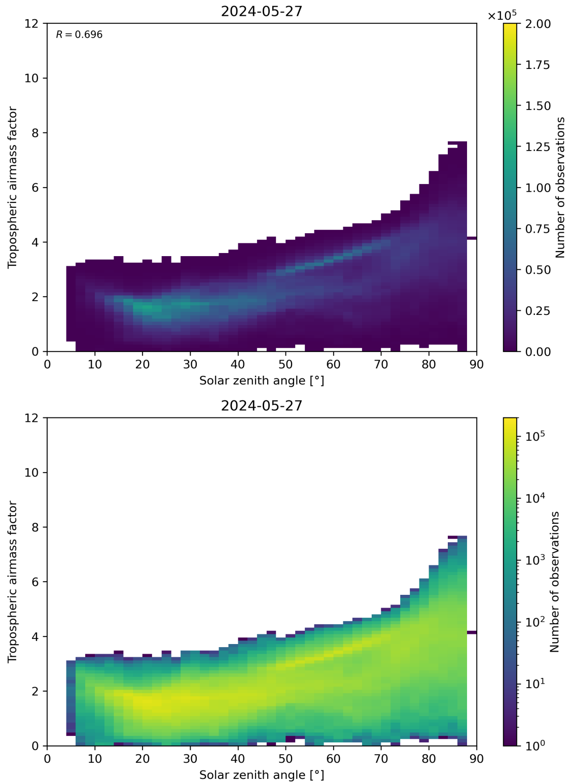
Figure 147: Scatter density plot of “Solar zenith angle” against “Tropospheric airmass factor” for 2024-05-26 to 2024-05-28.
