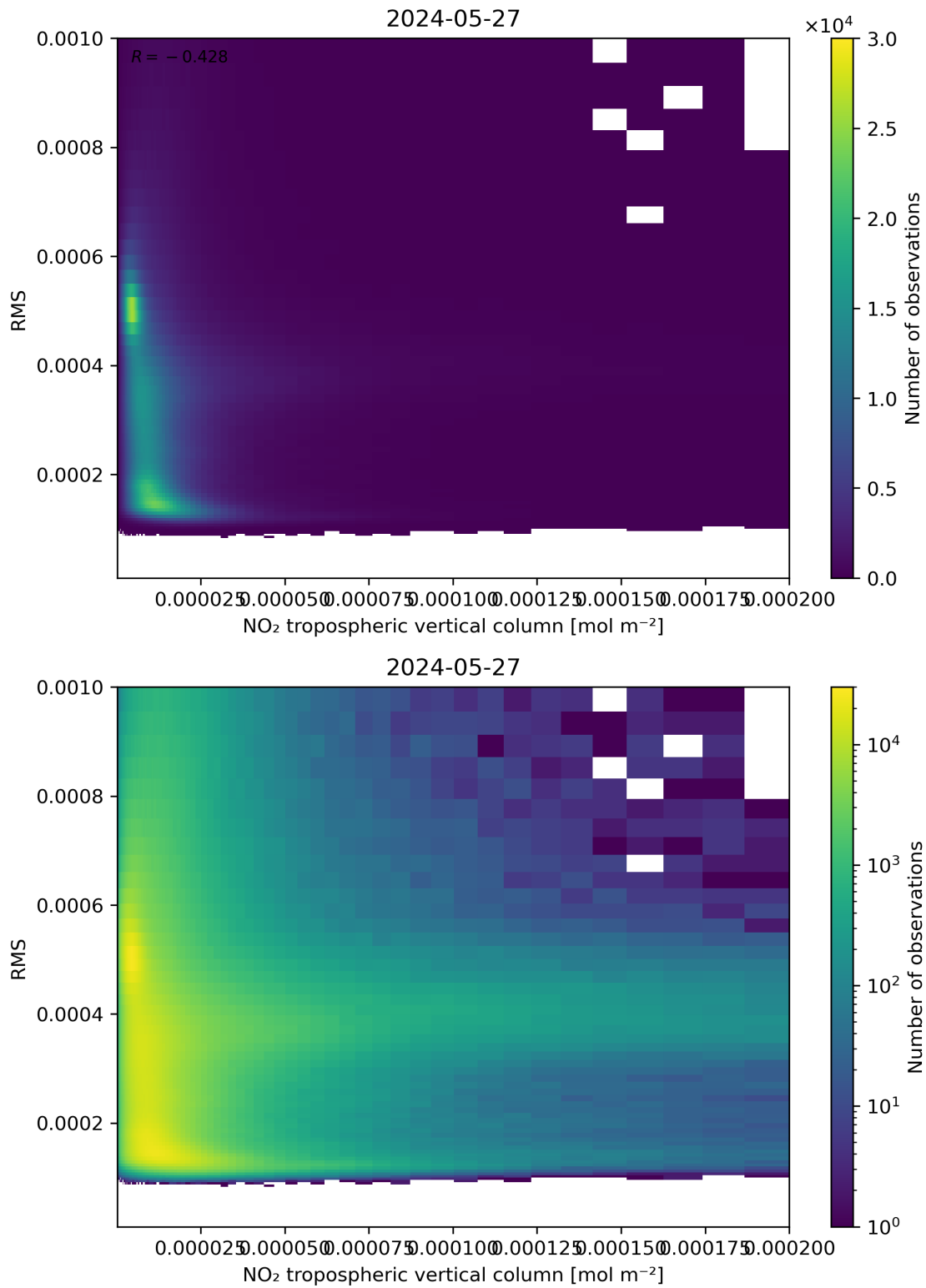
Figure 142: Scatter density plot of “NO 2 tropospheric vertical column” against “RMS” for 2024-05-26 to 2024-05-28.
