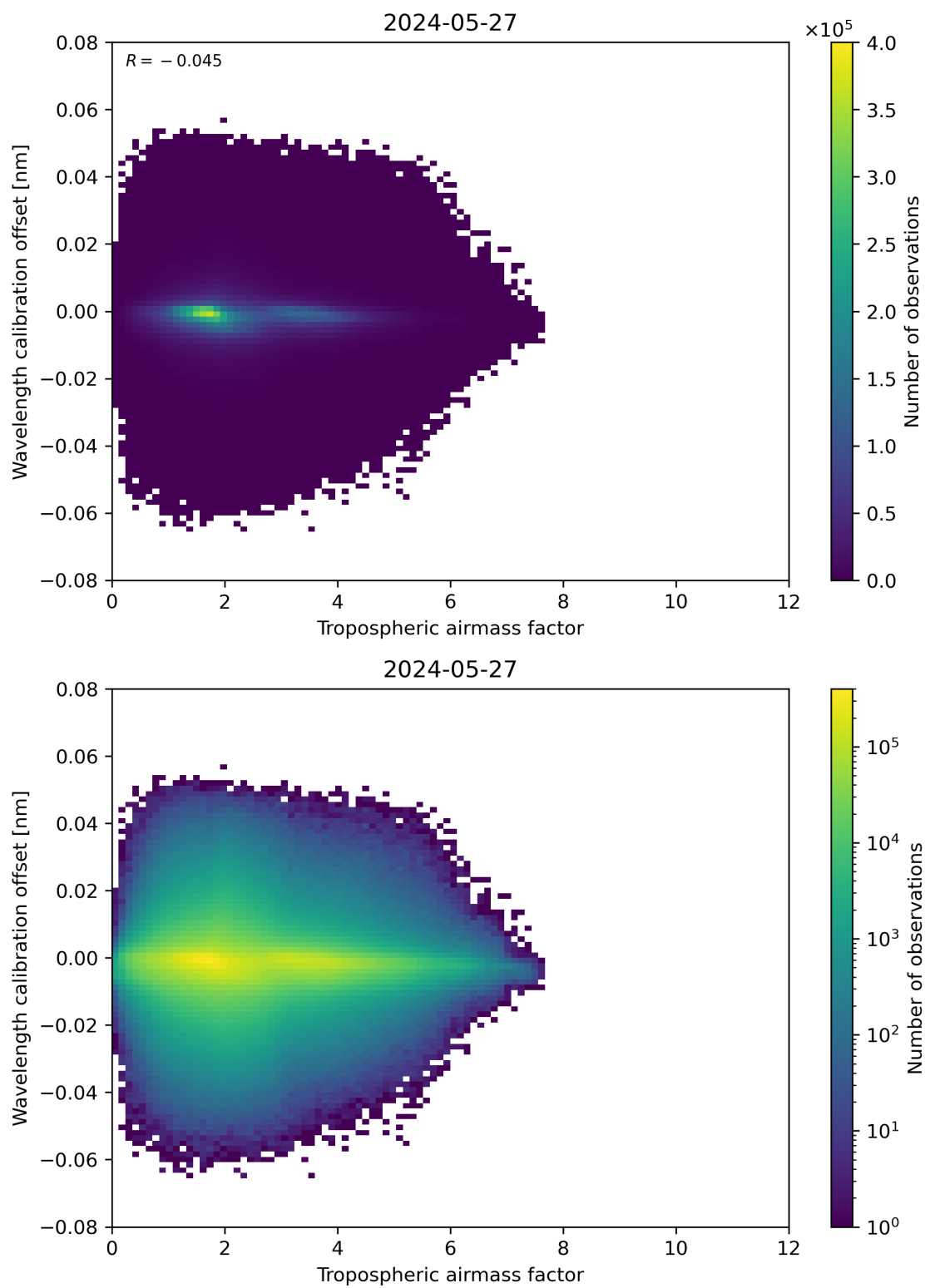
Figure 80: Scatter density plot of “Tropospheric airmass factor” against “Wavelength calibration offset” for 2024-05-26 to 2024-05-28.
