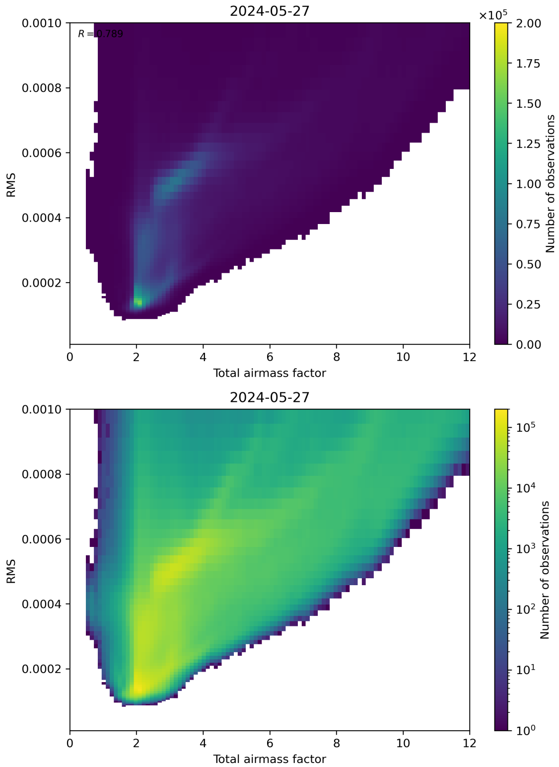
Figure 69: Scatter density plot of “Total airmass factor” against “RMS” for 2024-05-26 to 2024-05-28.
