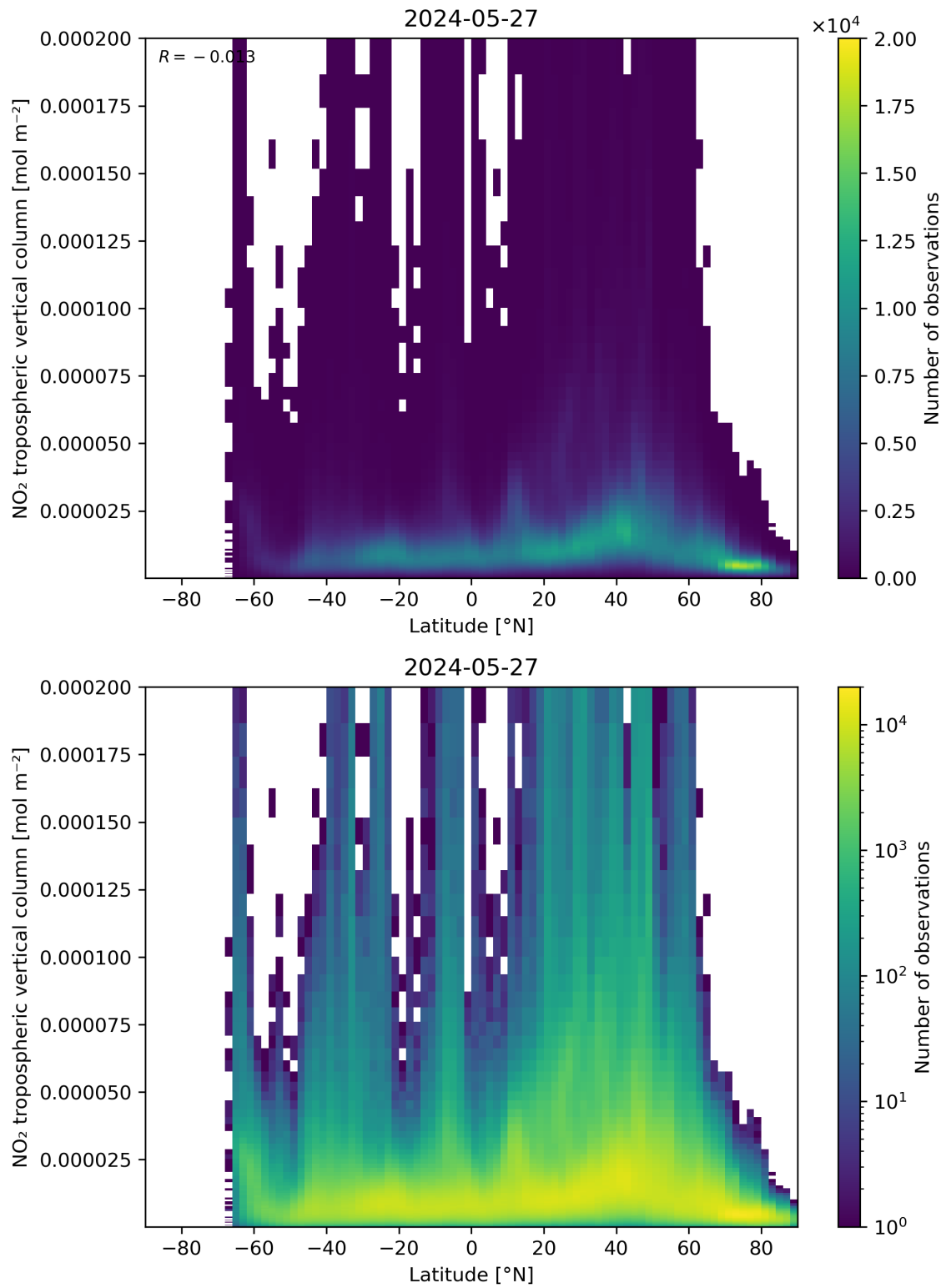
Figure 92: Scatter density plot of “Latitude” against “NO 2 tropospheric vertical column” for 2024-05-26 to 2024-05-28.
