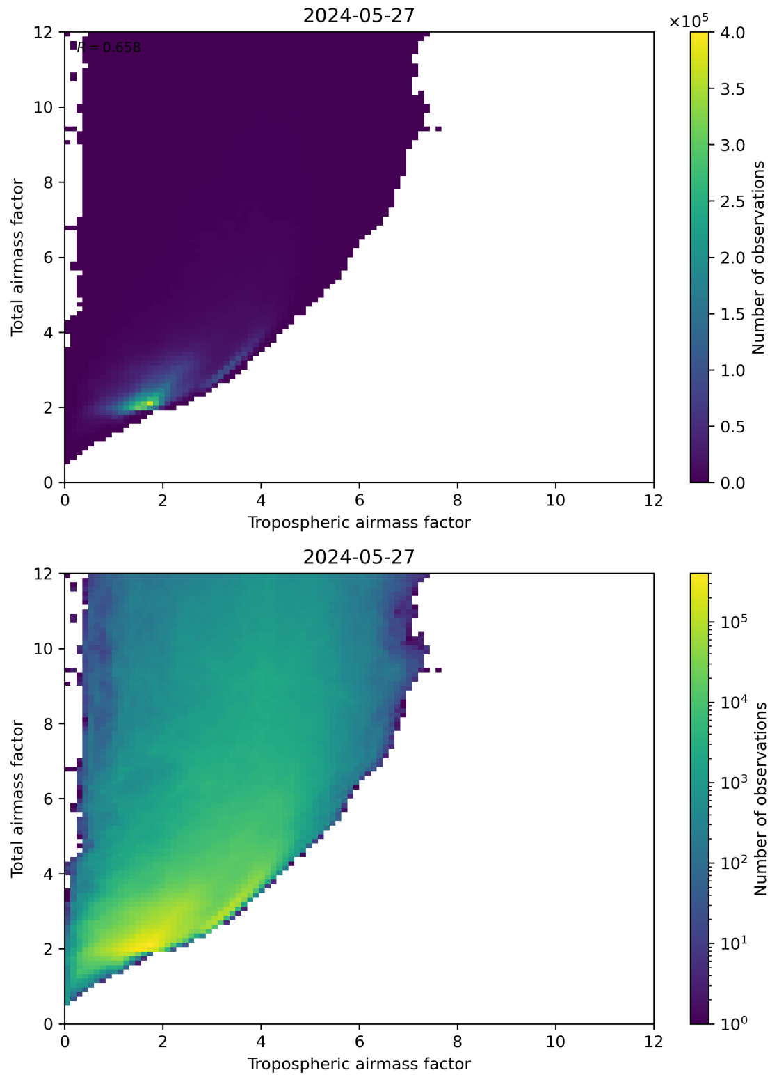
Figure 72: Scatter density plot of “Tropospheric airmass factor” against “Total airmass factor” for 2024-05-26 to 2024-05-28.
