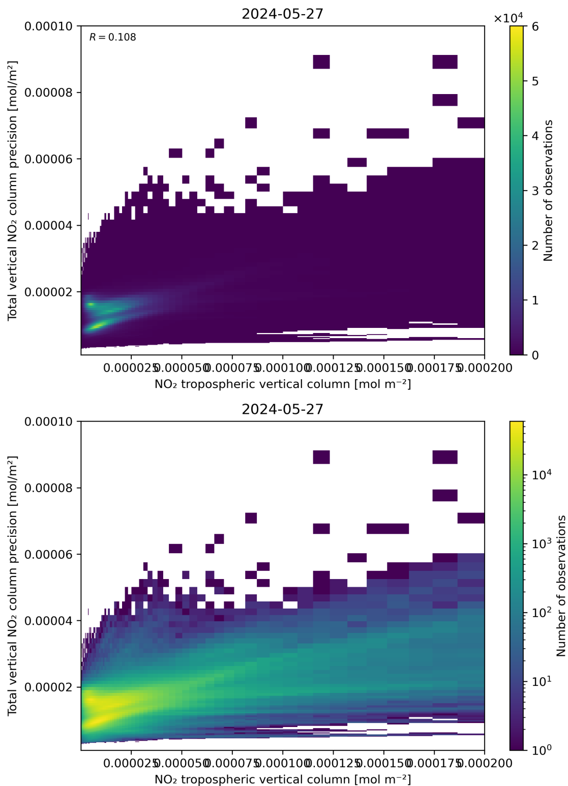
Figure 129: Scatter density plot of “NO 2 tropospheric vertical column” against “Total vertical NO 2 column precision” for 2024-05-26 to 2024-05-28.
