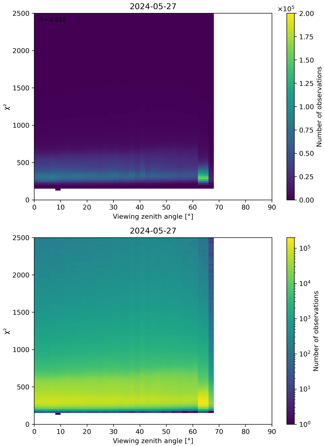
Figure 162: Scatter density plot of “Viewing zenith angle” against “ \chi^2 ” for 2024-05-26 to 2024-05-28.
