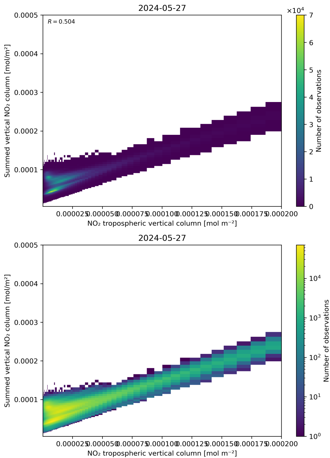
Figure 126: Scatter density plot of “NO 2 tropospheric vertical column” against “Summed vertical NO 2 column” for 2024-05-26 to 2024-05-28.
