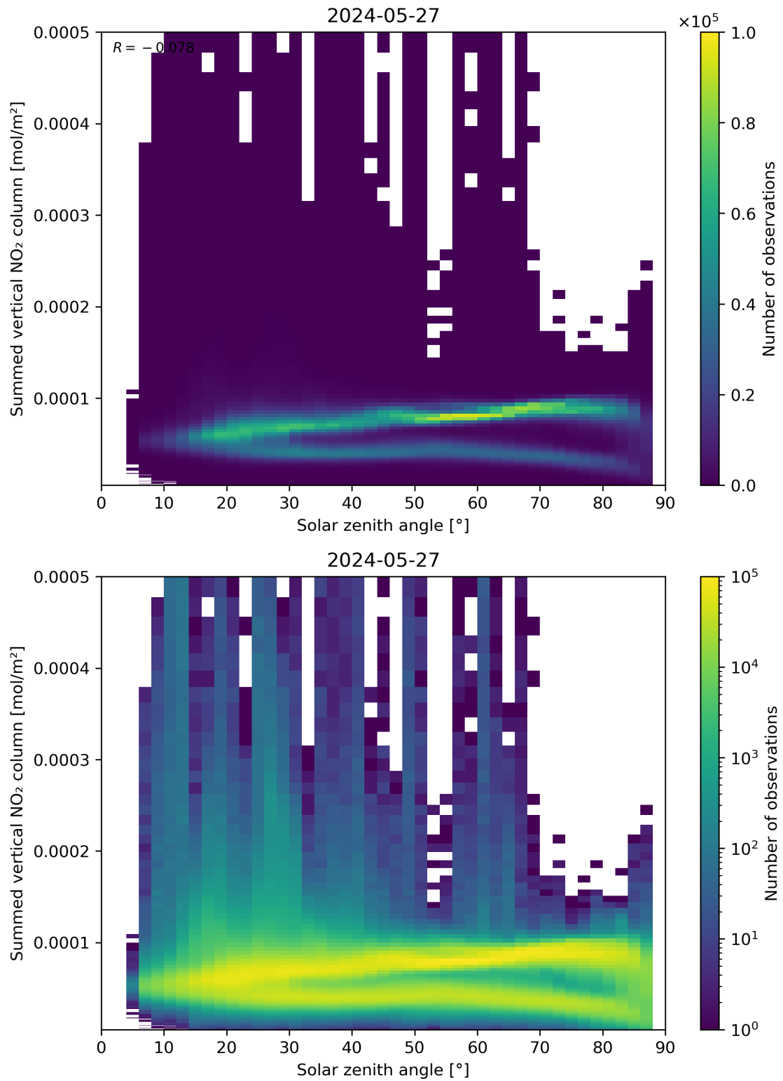
Figure 151: Scatter density plot of “Solar zenith angle” against “Summed vertical NO 2 column” for 2024-05-26 to 2024-05-28.
