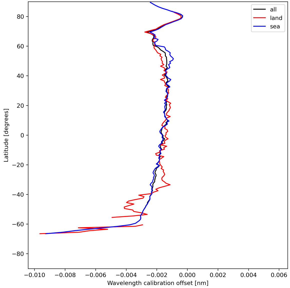
Figure 18: Zonal average of “Wavelength calibration offset” for 2024-05-26 to 2024-05-28.
