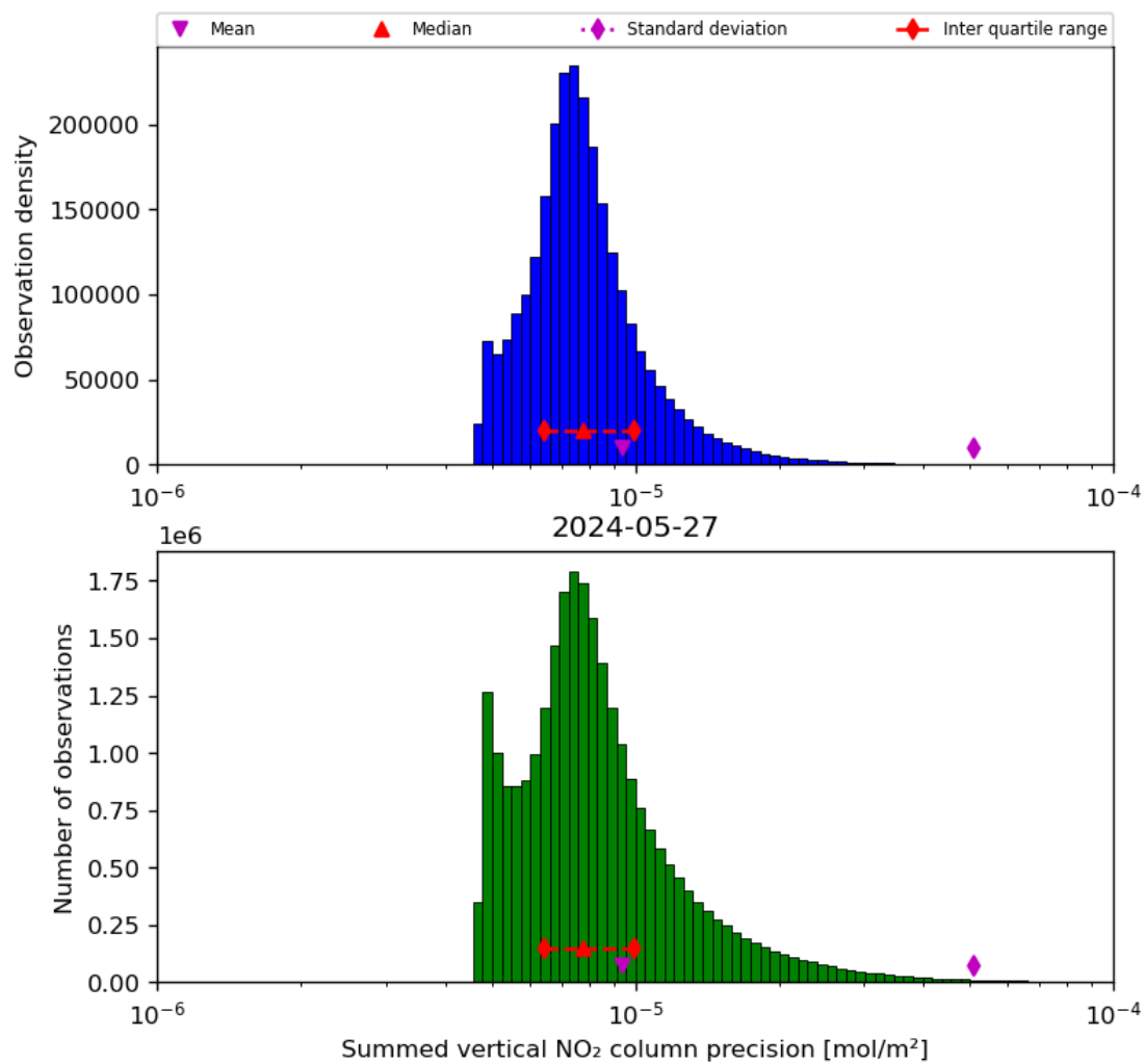
Figure 41: Histogram of “Summed vertical NO 2 column precision” for 2024-05-26 to 2024-05-28
