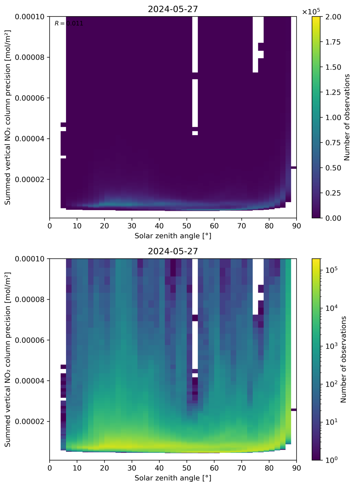
Figure 152: Scatter density plot of “Solar zenith angle” against “Summed vertical NO 2 column precision” for 2024-05-26 to 2024-05-28.
