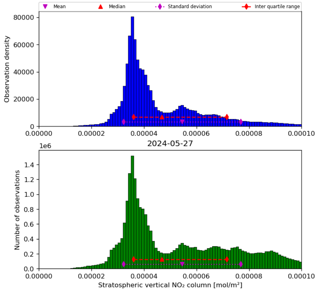
Figure 36: Histogram of “Stratospheric vertical NO 2 column” for 2024-05-26 to 2024-05-28
