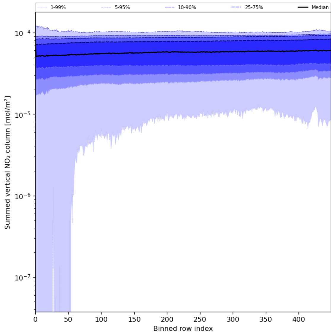
Figure 57: Along track statistics of “Summed vertical NO 2 column” for 2024-05-26 to 2024-05-28
