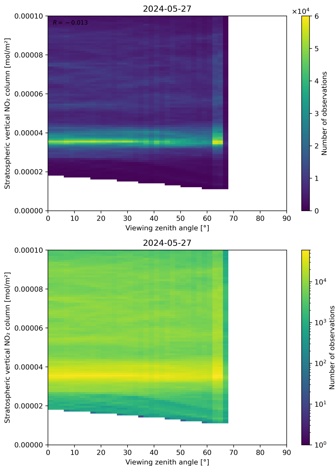
Figure 164: Scatter density plot of “Viewing zenith angle” against “Stratospheric vertical NO 2 column” for 2024-05-26 to 2024-05-28.
