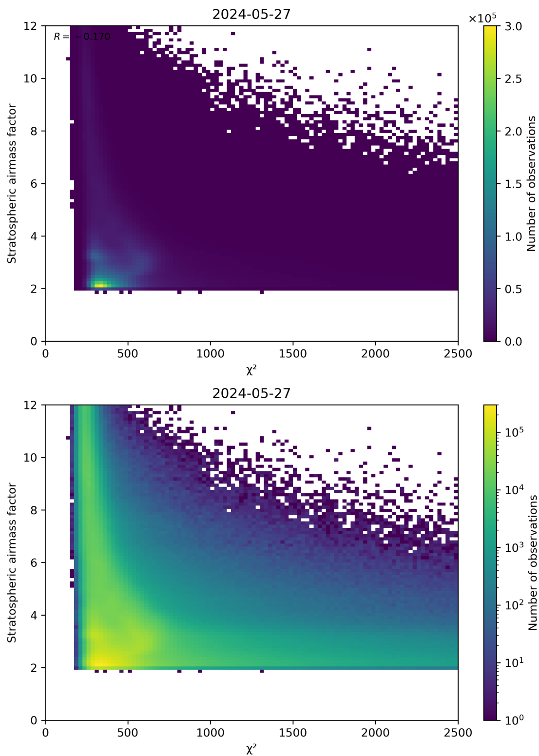
Figure 81: Scatter density plot of “ \chi^2 ” against “Stratospheric airmass factor” for 2024-05-26 to 2024-05-28.
