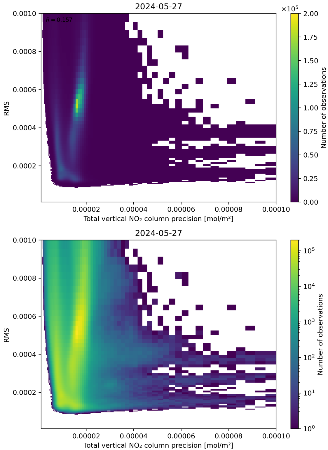
Figure 119: Scatter density plot of “Total vertical NO 2 column precision” against “RMS” for 2024-05-26 to 2024-05-28.
