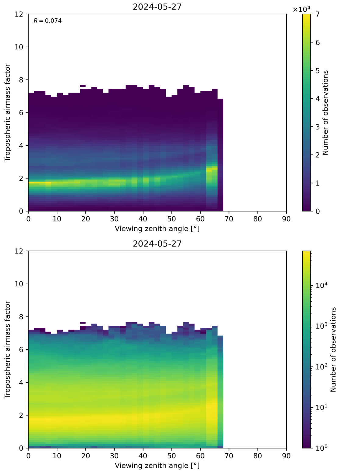
Figure 161: Scatter density plot of “Viewing zenith angle” against “Tropospheric airmass factor” for 2024-05-26 to 2024-05-28.
