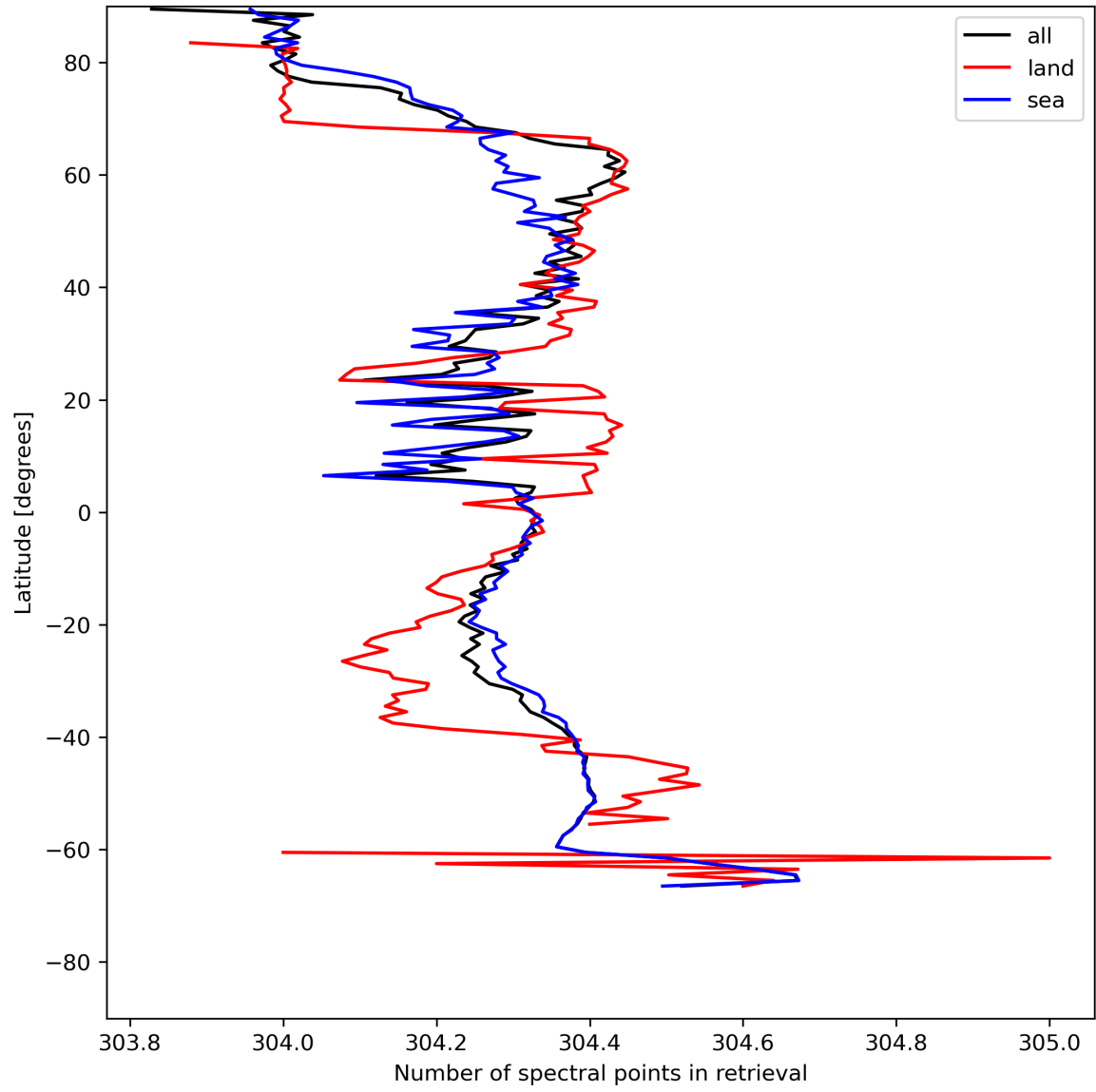
Figure 16: Zonal average of “Number of spectral points in retrieval” for 2024-05-26 to 2024-05-28.
