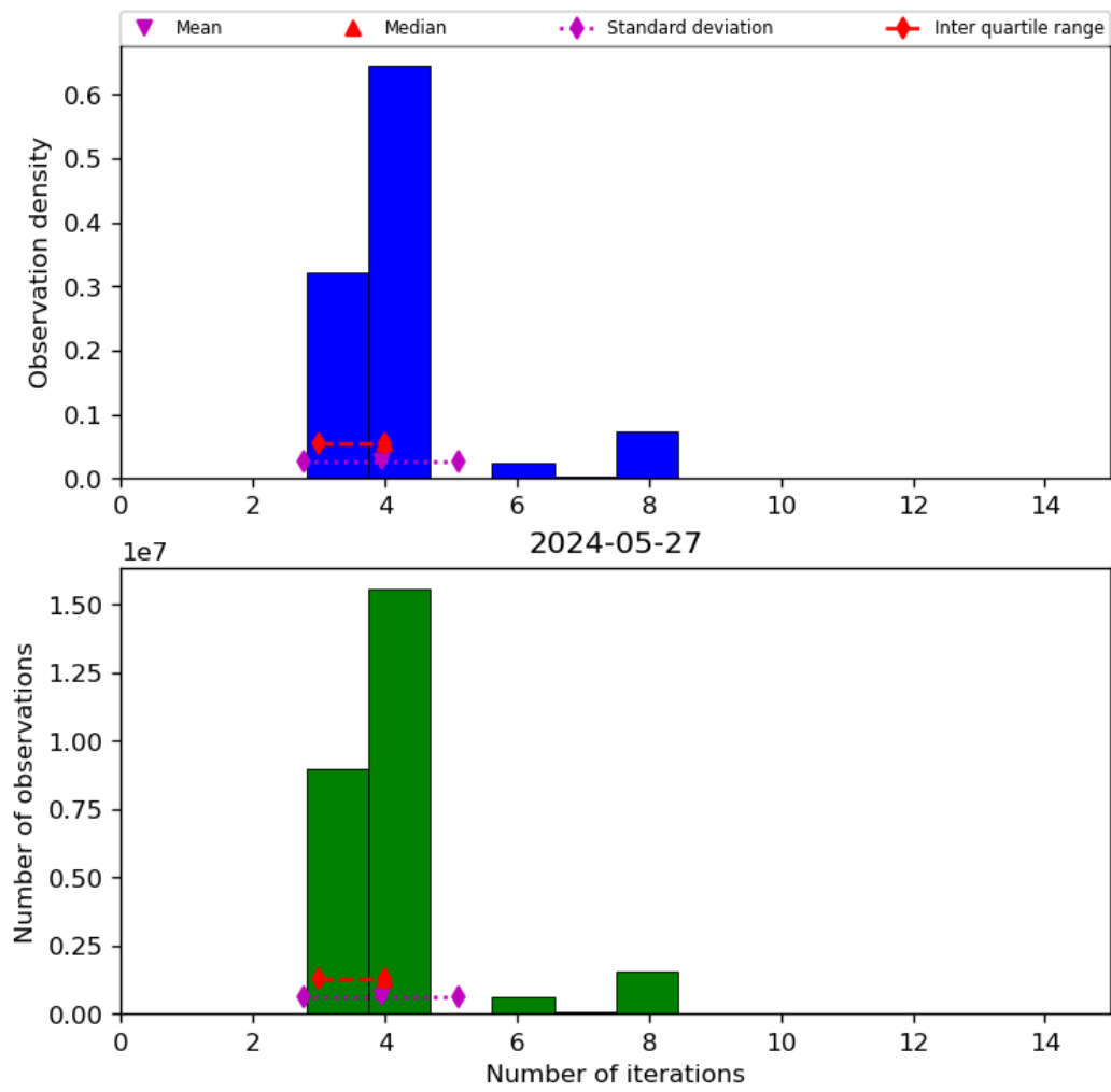
Figure 34: Histogram of “Number of iterations” for 2024-05-26 to 2024-05-28
