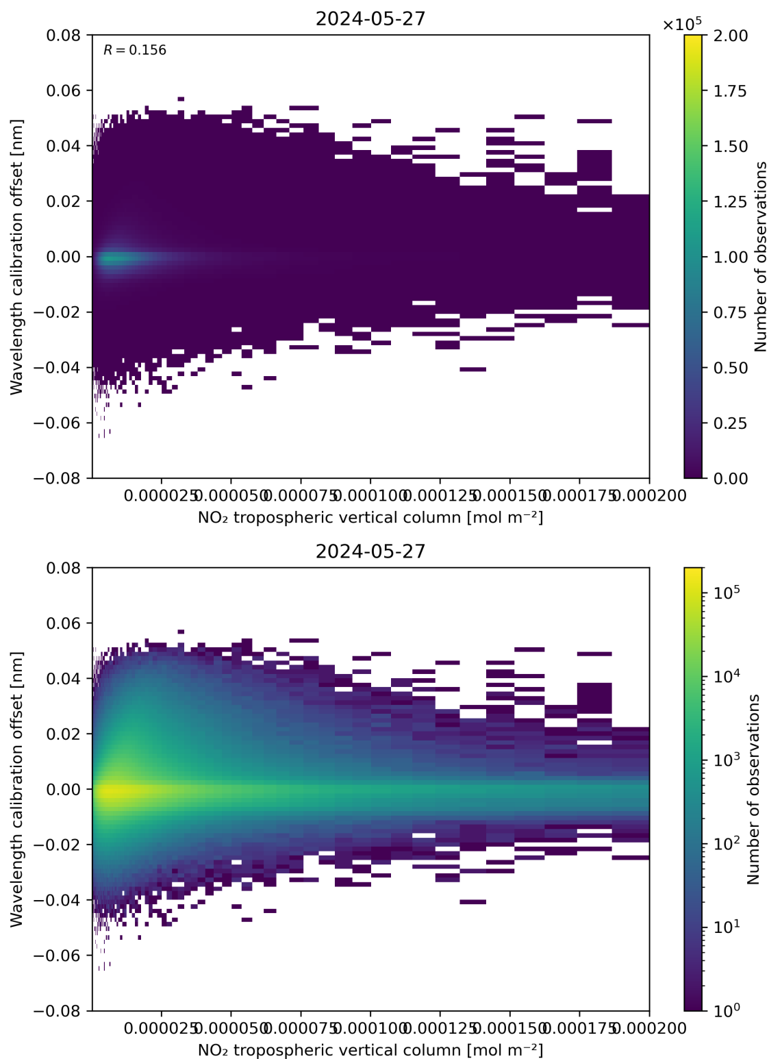
Figure 143: Scatter density plot of “NO 2 tropospheric vertical column” against “Wavelength calibration offset” for 2024-05-26 to 2024-05-28.
