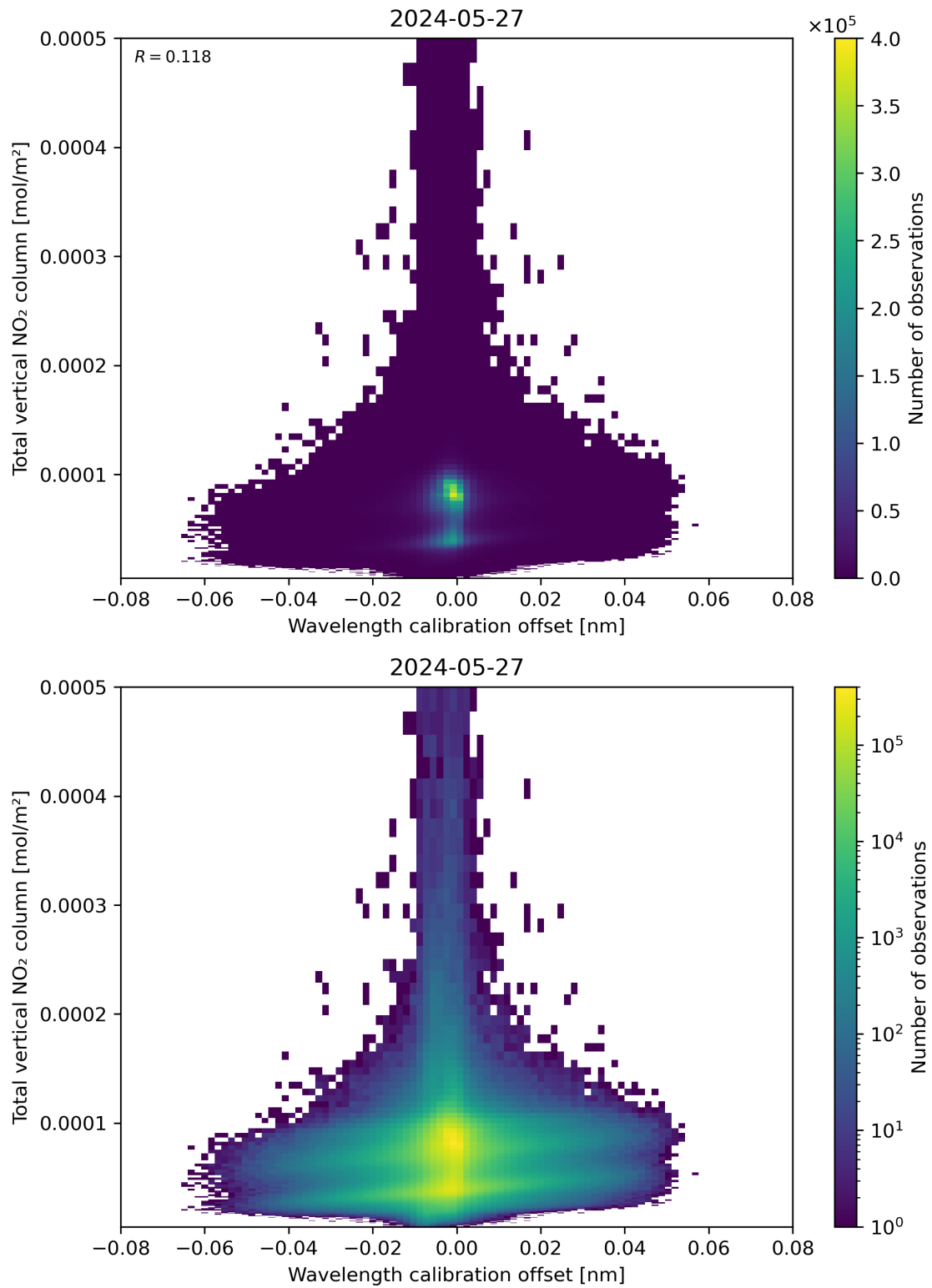
Figure 179: Scatter density plot of “Wavelength calibration offset” against “Total vertical NO 2 column” for 2024-05-26 to 2024-05-28.
