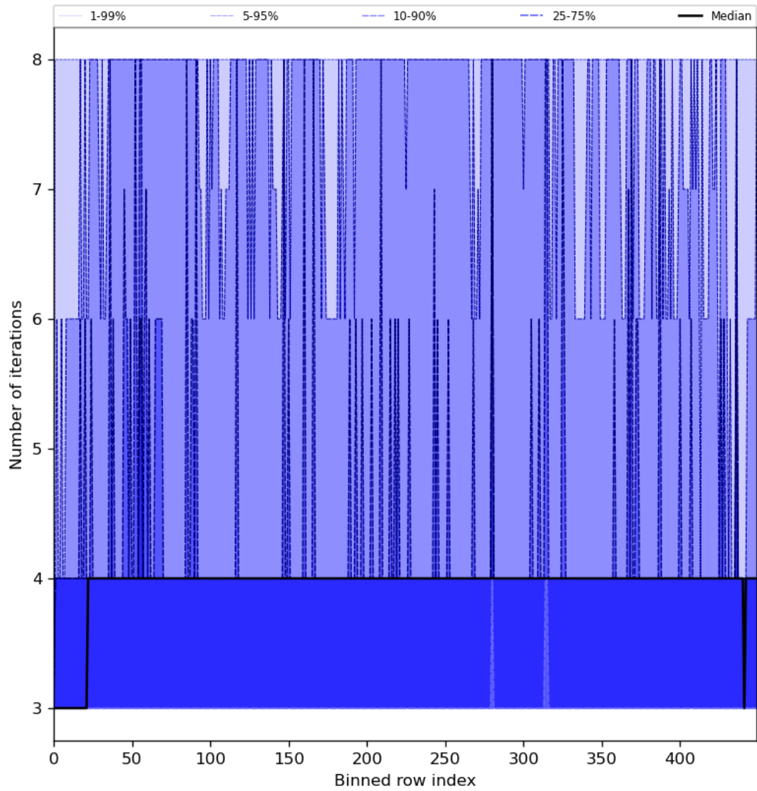
Figure 51: Along track statistics of “Number of iterations” for 2024-05-26 to 2024-05-28
