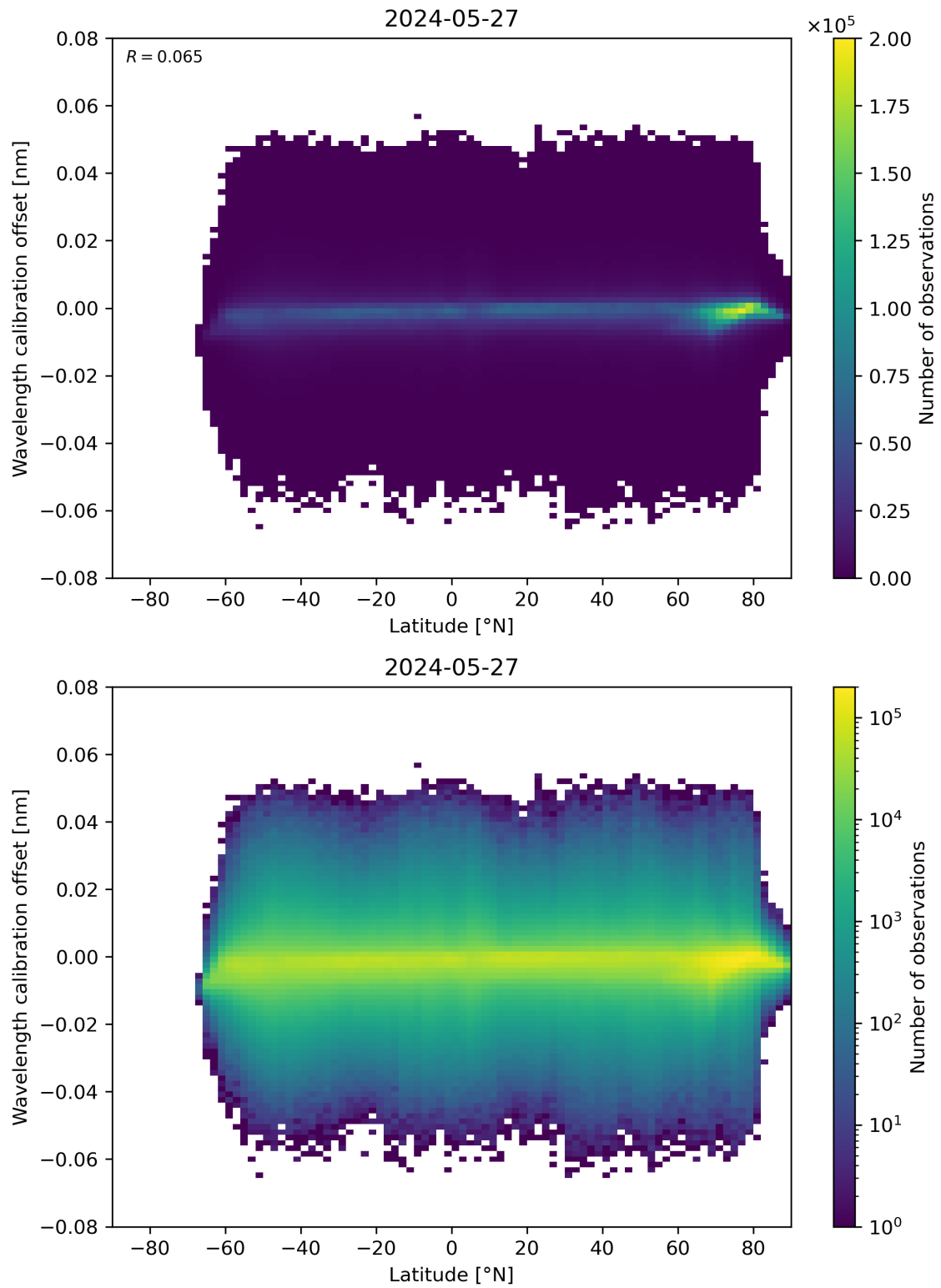
Figure 95: Scatter density plot of “Latitude” against “Wavelength calibration offset” for 2024-05-26 to 2024-05-28.
