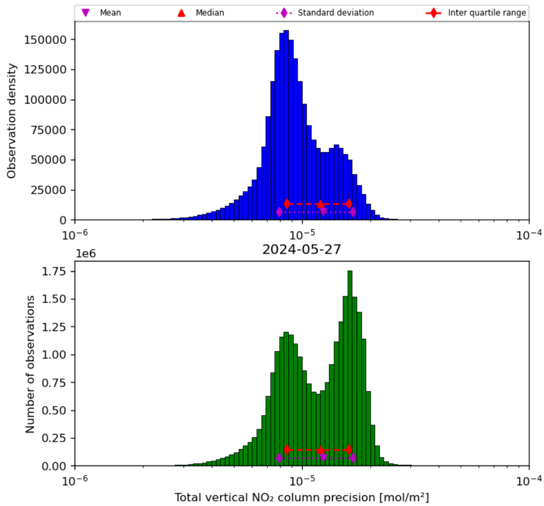
Figure 39: Histogram of “Total vertical NO 2 column precision” for 2024-05-26 to 2024-05-28
