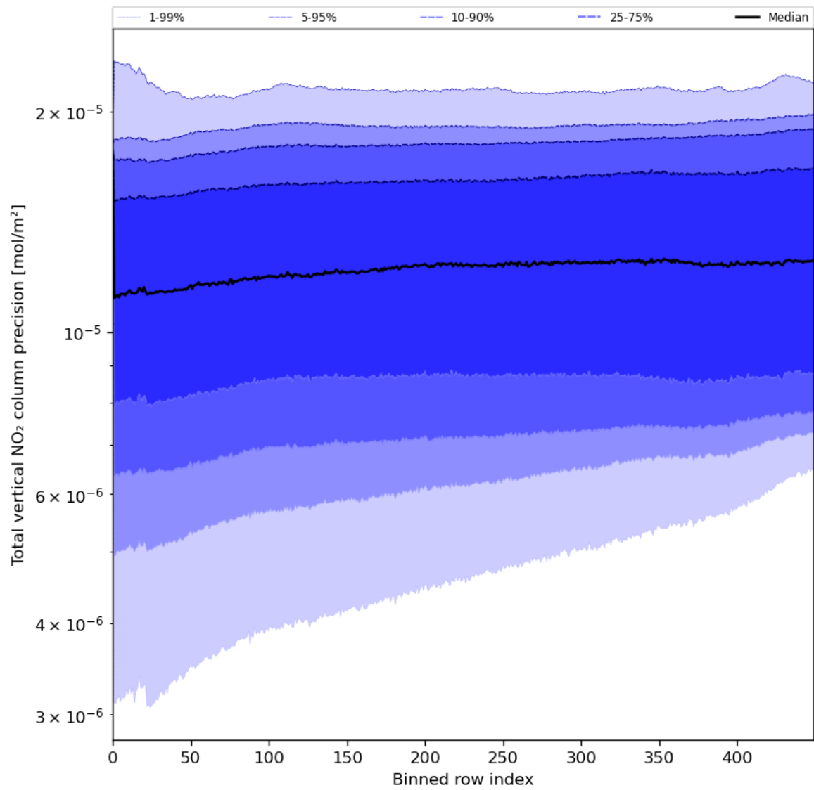
Figure 56: Along track statistics of “Total vertical NO 2 column precision” for 2024-05-26 to 2024-05-28
