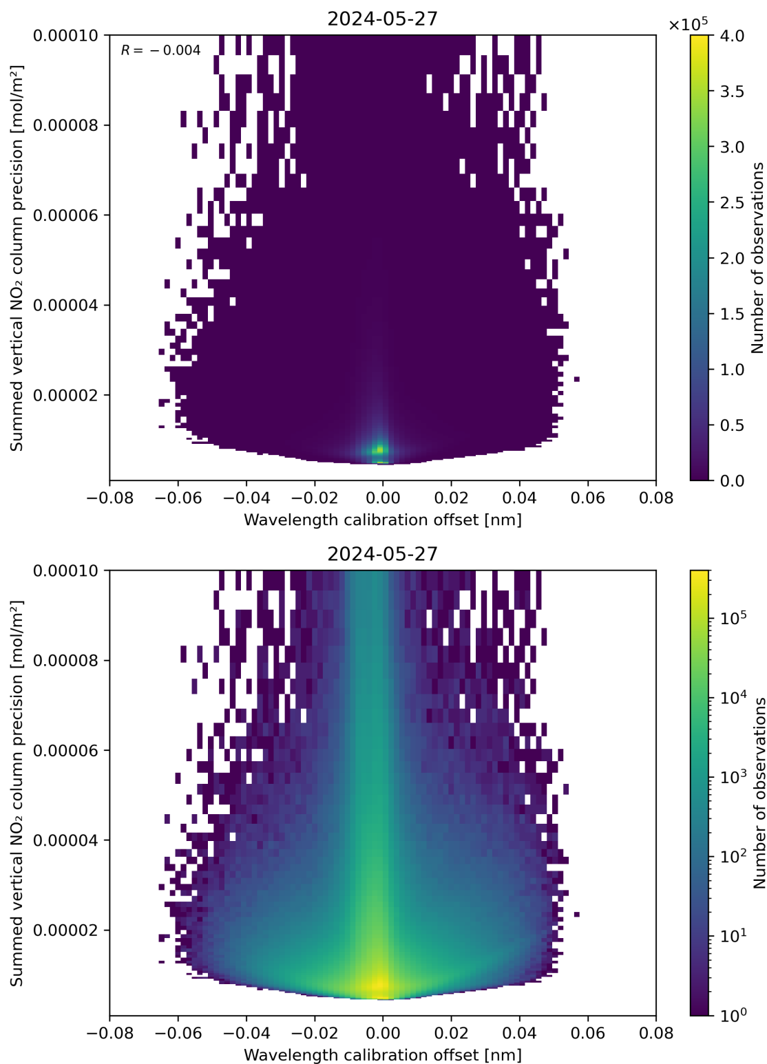
Figure 178: Scatter density plot of “Wavelength calibration offset” against “Summed vertical NO 2 column precision” for 2024-05-26 to 2024-05-28.
