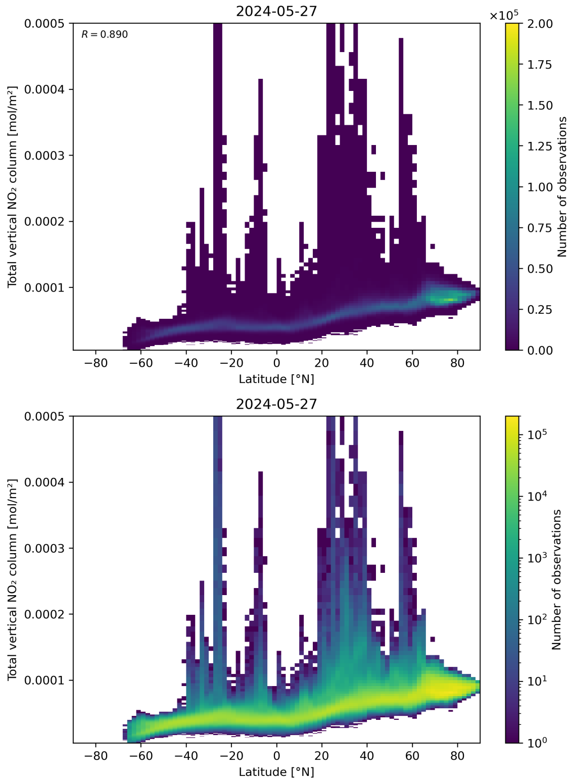
Figure 90: Scatter density plot of “Latitude” against “Total vertical NO 2 column” for 2024-05-26 to 2024-05-28.
