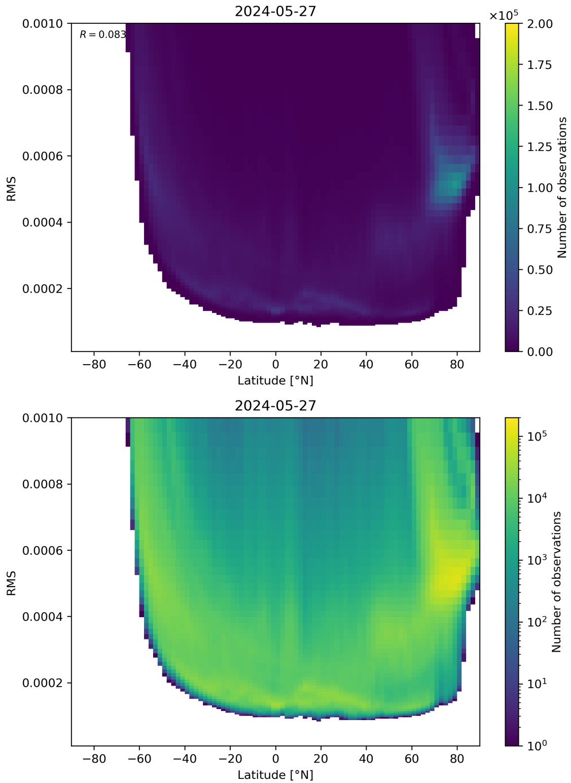
Figure 94: Scatter density plot of “Latitude” against “RMS” for 2024-05-26 to 2024-05-28.
