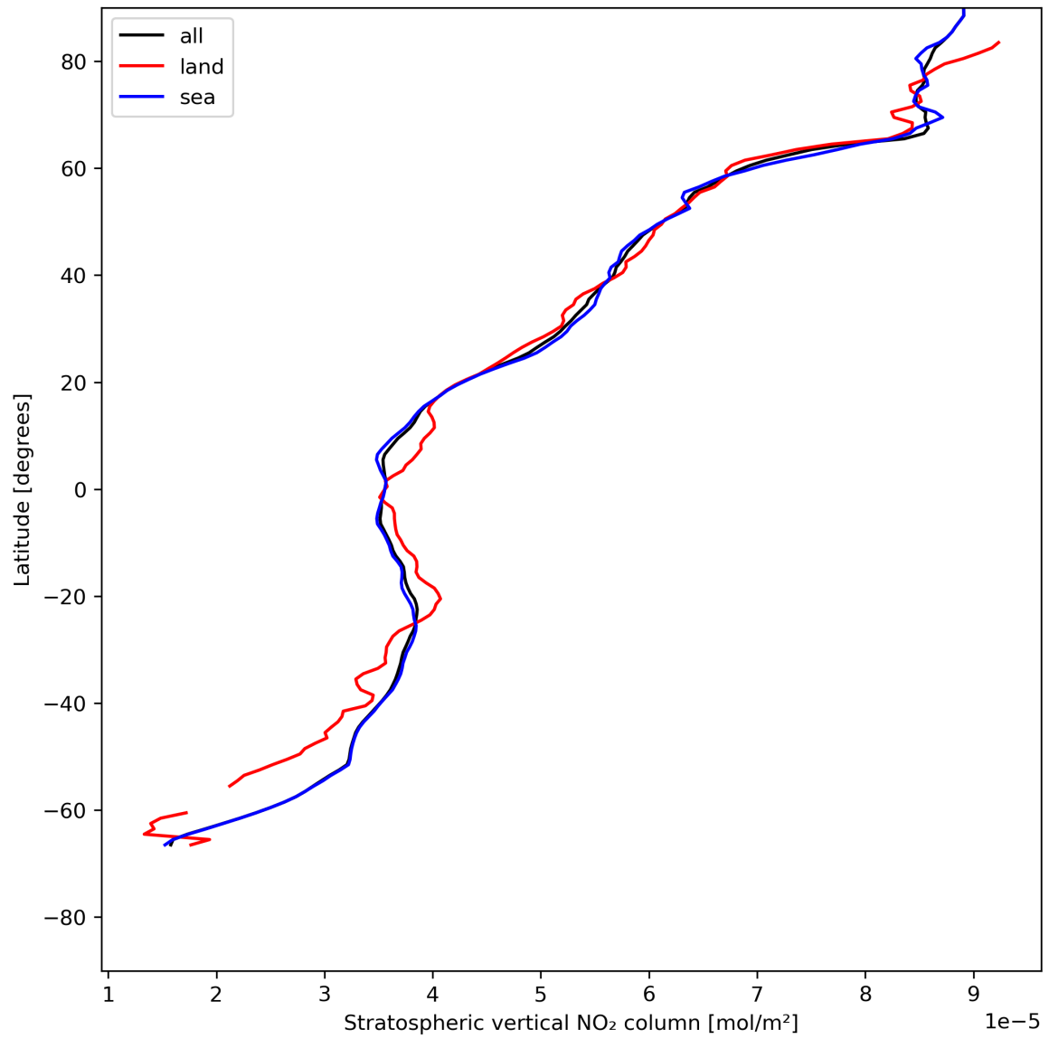
Figure 19: Zonal average of “Stratospheric vertical NO 2 column” for 2024-05-26 to 2024-05-28.
