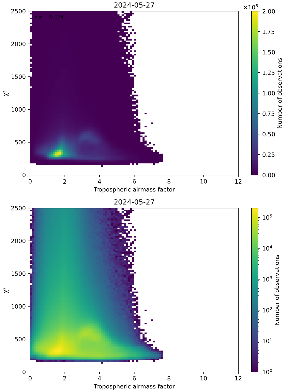
Figure 73: Scatter density plot of “Tropospheric airmass factor” against “ \chi^2 ” for 2024-05-26 to 2024-05-28.
