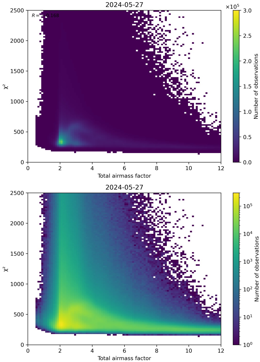
Figure 63: Scatter density plot of “Total airmass factor” against “ \chi^2 ” for 2024-05-26 to 2024-05-28.
