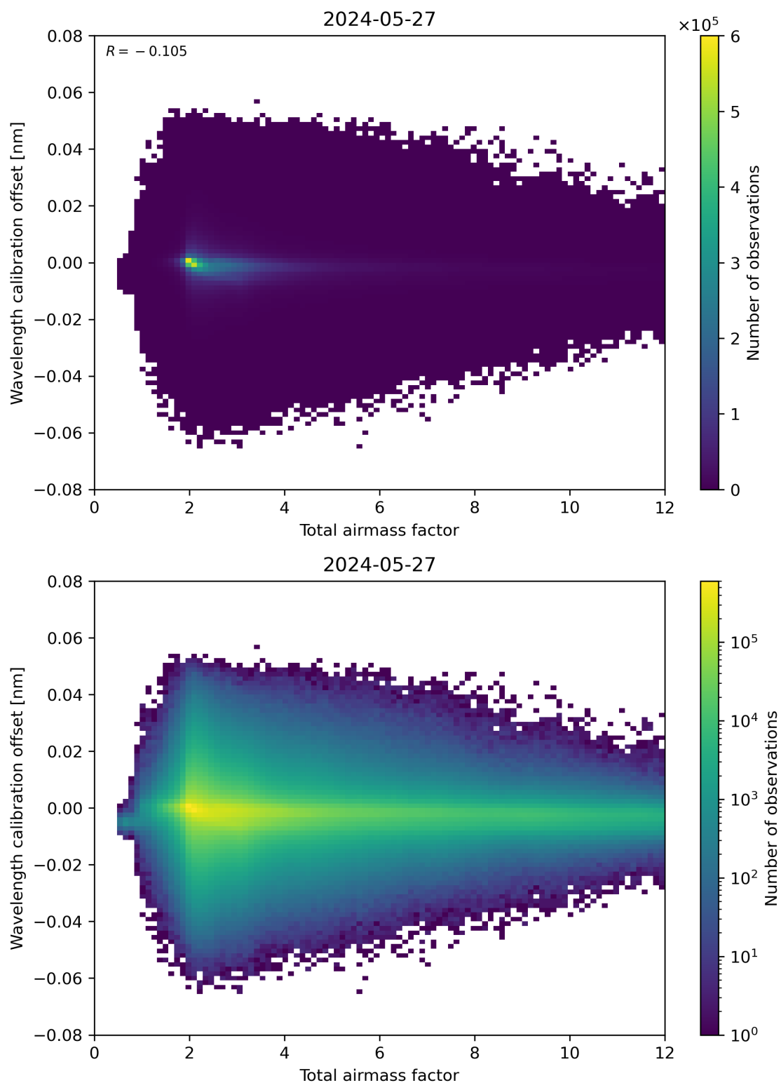
Figure 70: Scatter density plot of “Total airmass factor” against “Wavelength calibration offset” for 2024-05-26 to 2024-05-28.
