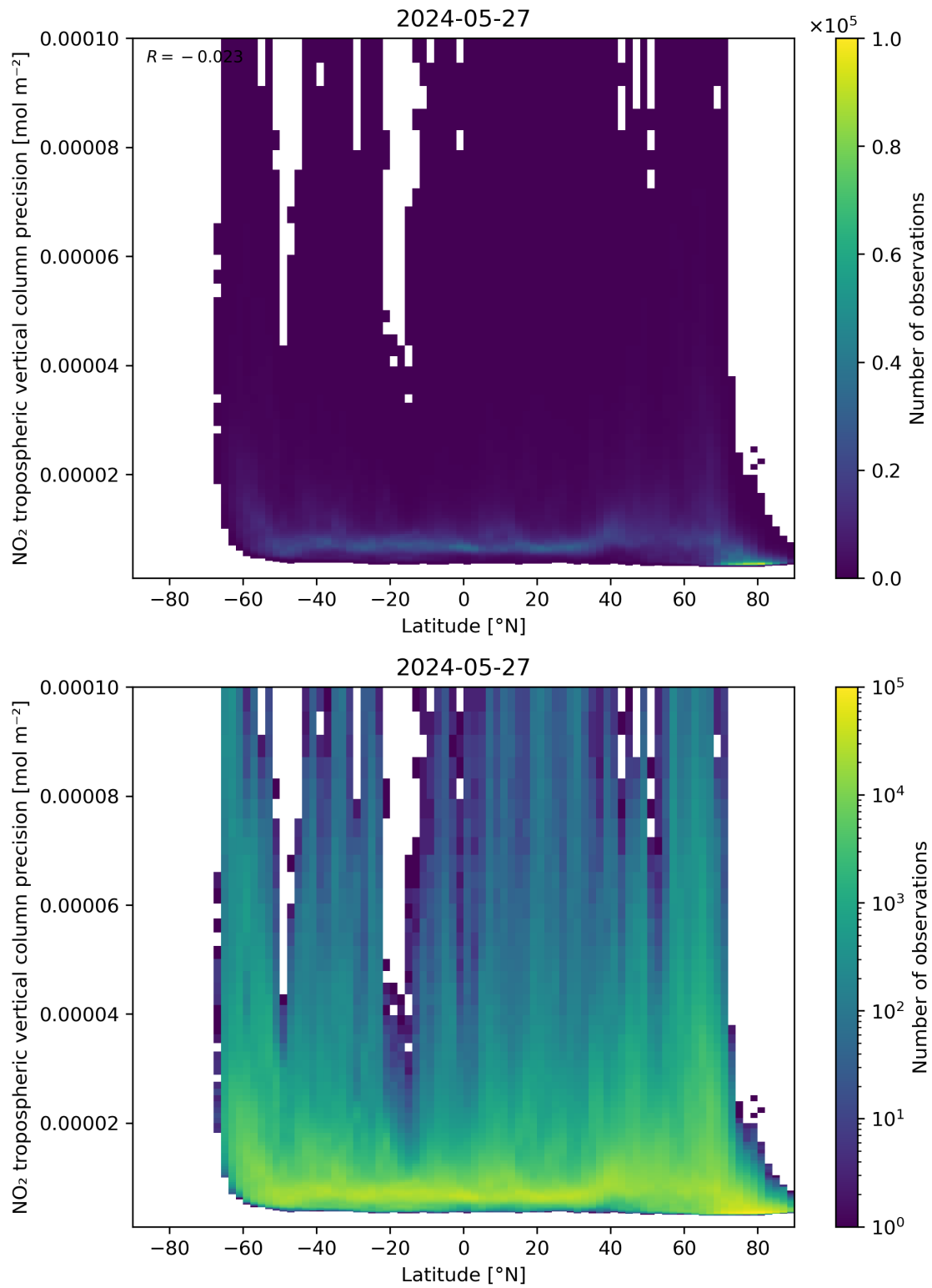
Figure 93: Scatter density plot of “Latitude” against “NO 2 tropospheric vertical column precision” for 2024-05-26 to 2024-05-28.
