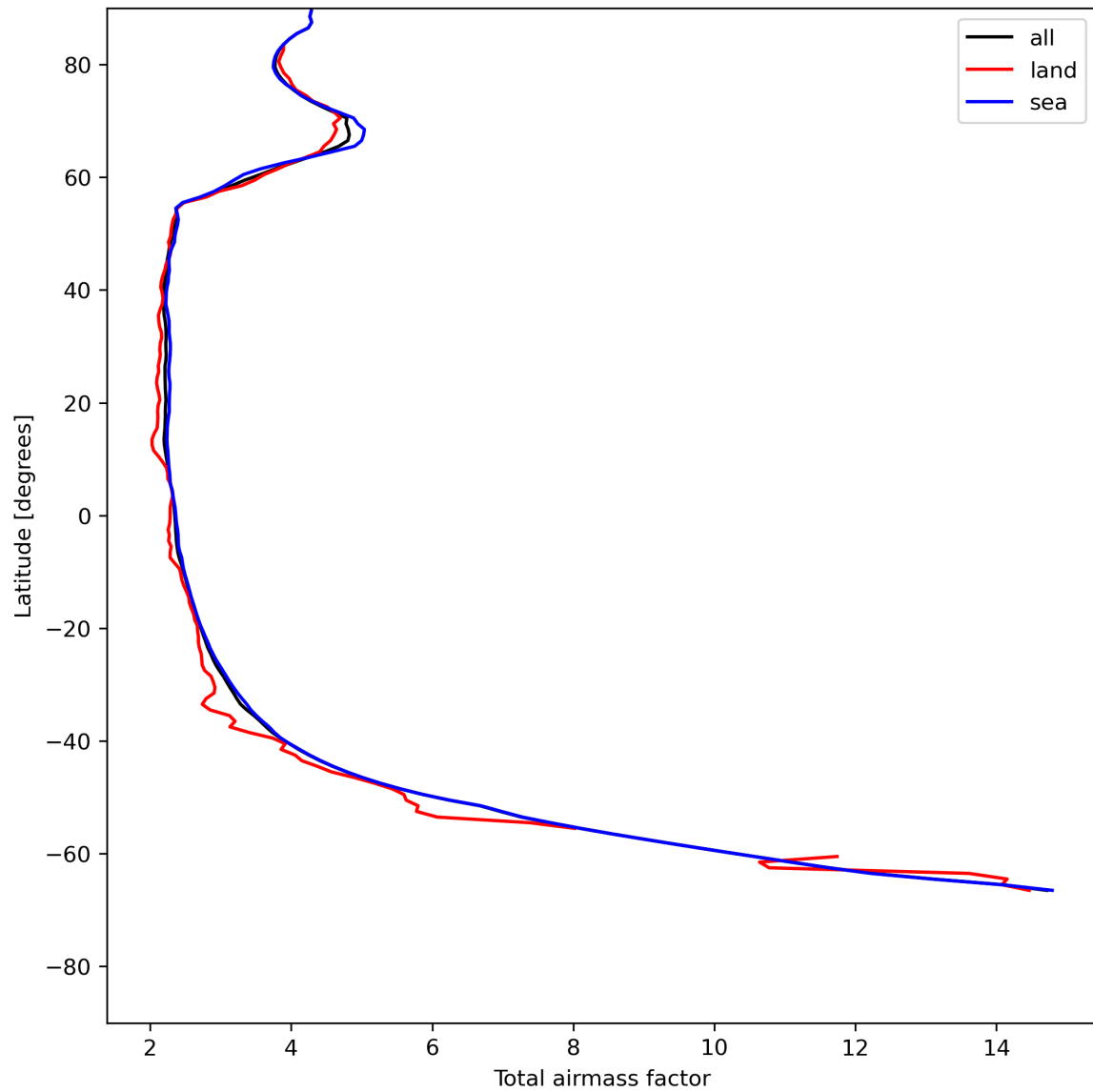
Figure 15: Zonal average of “Total airmass factor” for 2024-05-26 to 2024-05-28.
