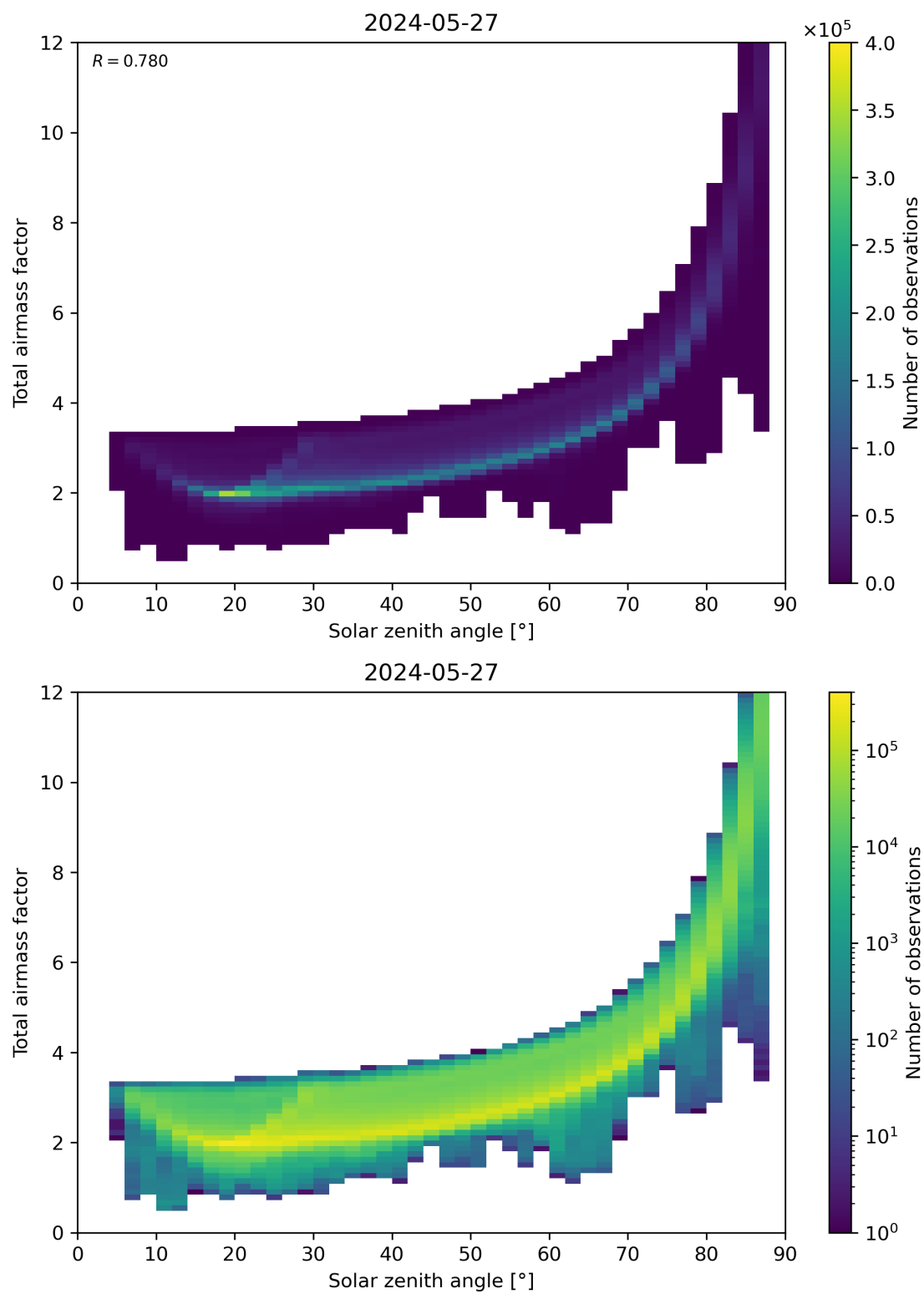
Figure 146: Scatter density plot of “Solar zenith angle” against “Total air mass factor” for 2024-05-26 to 2024-05-28.
