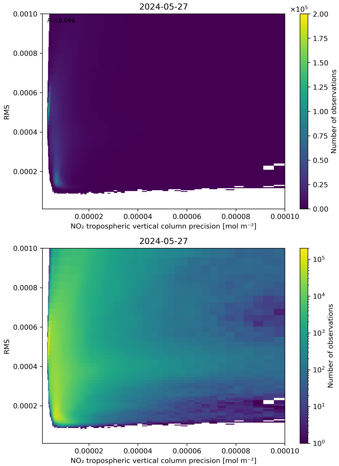
Figure 140: Scatter density plot of “NO 2 tropospheric vertical column precision” against “RMS” for 2024-05-26 to 2024-05-28.
