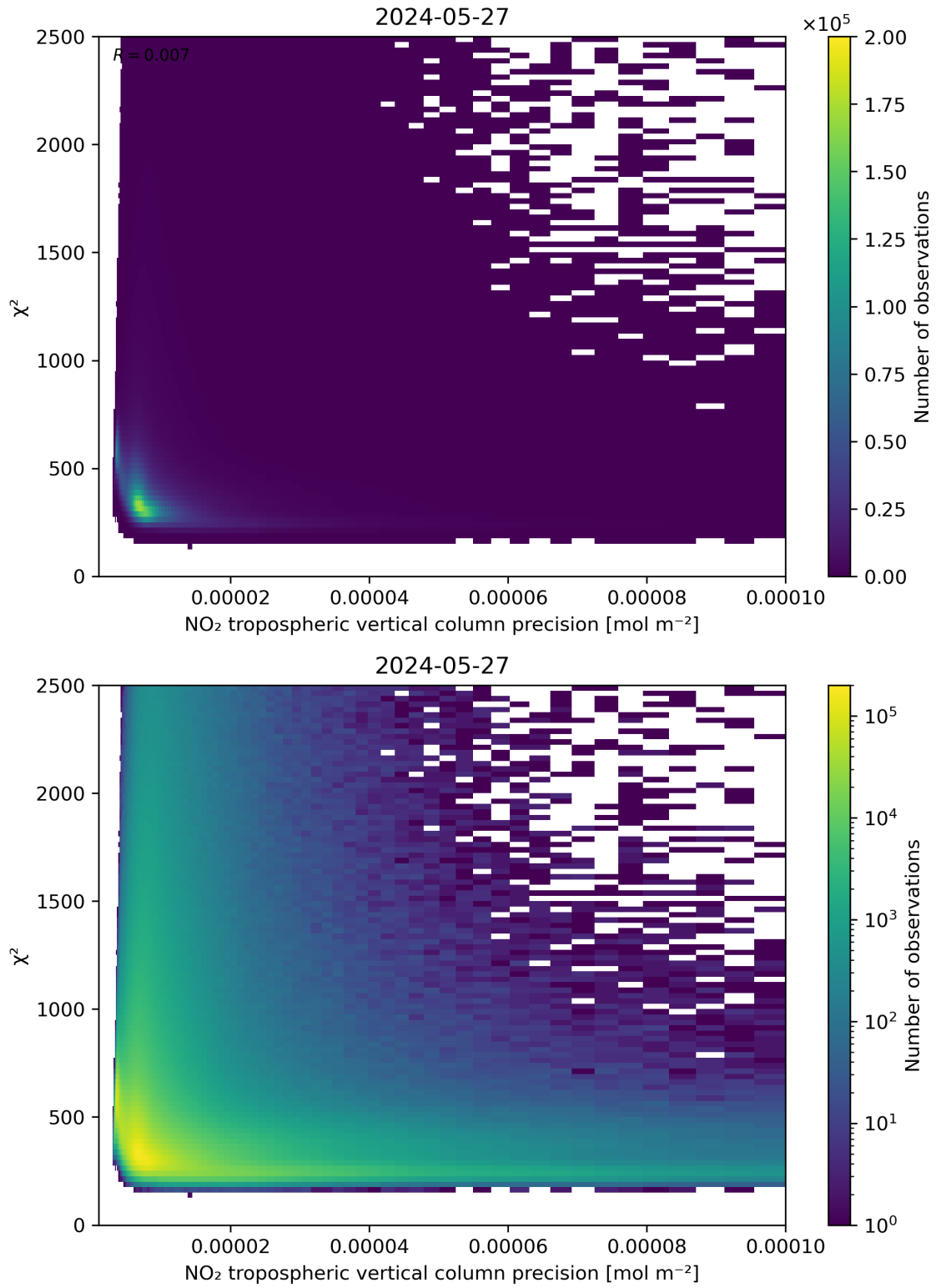
Figure 134: Scatter density plot of “NO 2 tropospheric vertical column precision” against “ \chi^2 ” for 2024-05-26 to 2024-05-28.
