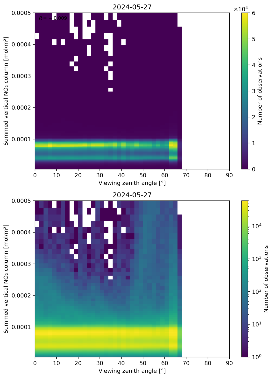
Figure 165: Scatter density plot of “Viewing zenith angle” against “Summed vertical NO 2 column” for 2024-05-26 to 2024-05-28.
