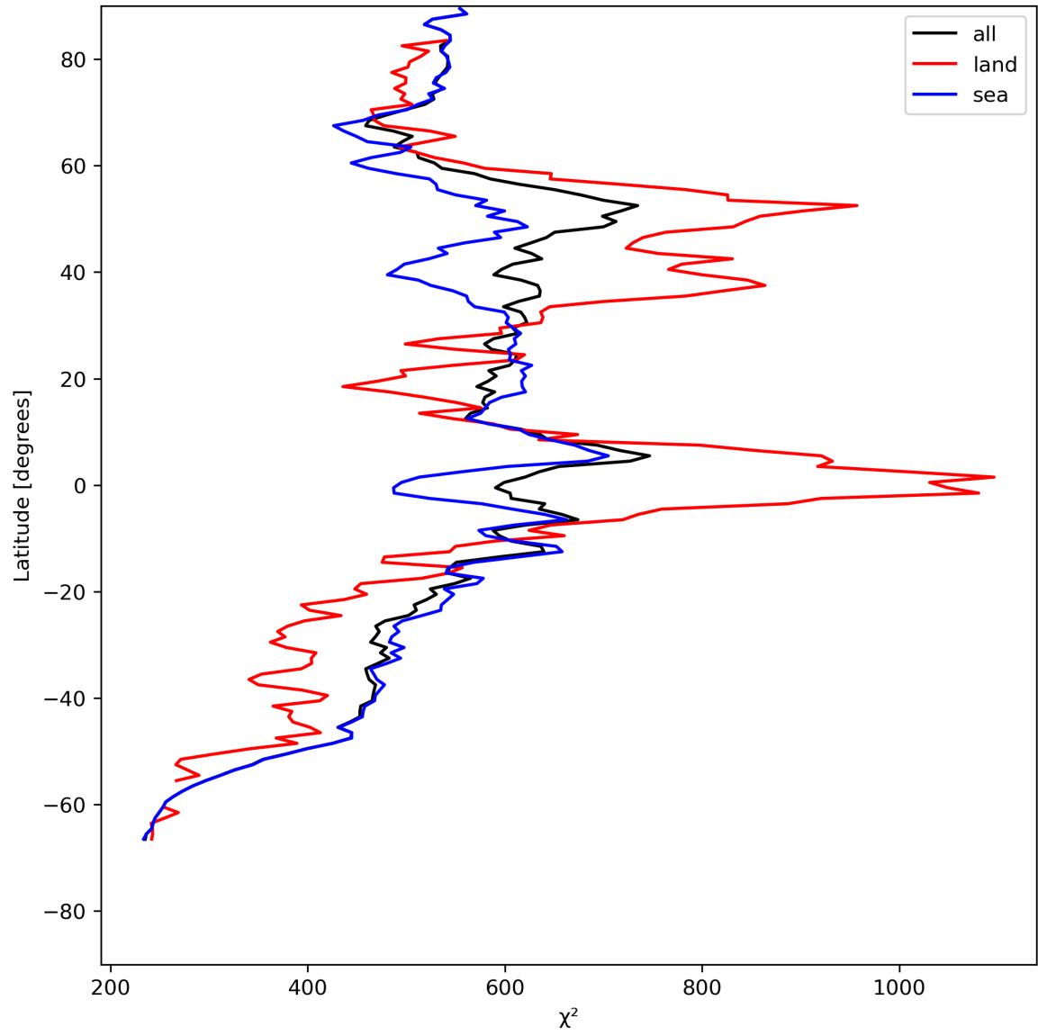
Figure 25: Zonal average of “ \chi^2 ” for 2024-05-26 to 2024-05-28.
