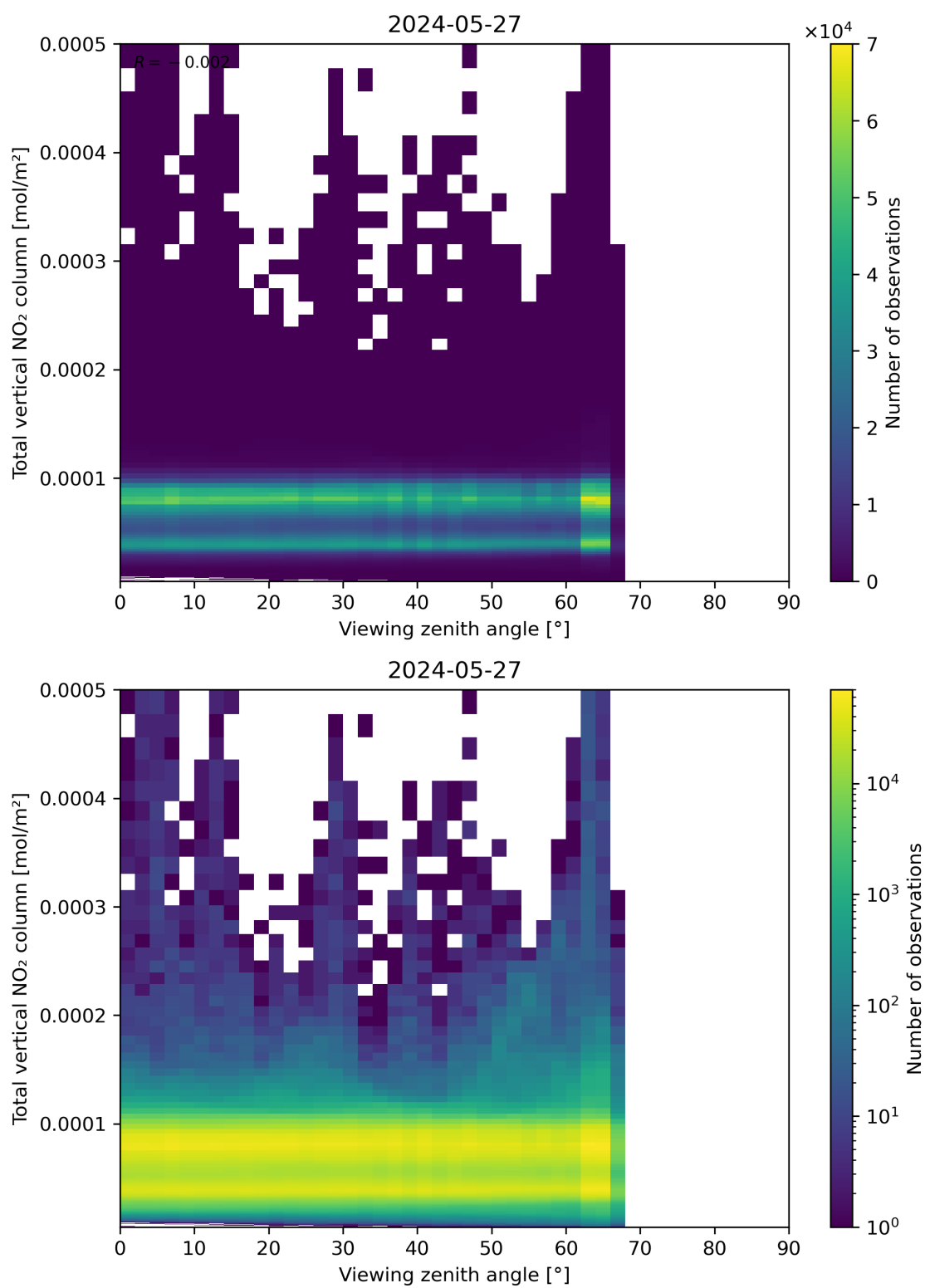
Figure 167: Scatter density plot of “Viewing zenith angle” against “Total vertical NO 2 column” for 2024-05-26 to 2024-05-28.
