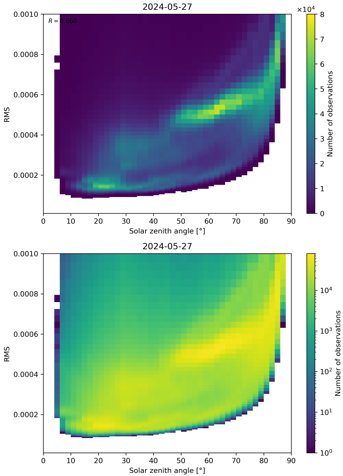
Figure 157: Scatter density plot of “Solar zenith angle” against “RMS” for 2024-05-26 to 2024-05-28.
