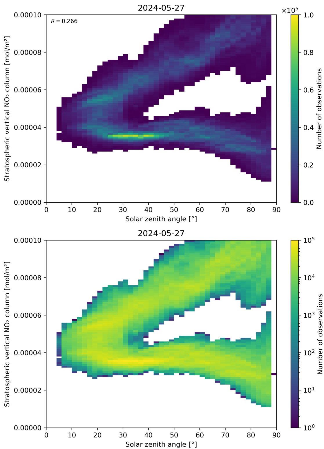
Figure 150: Scatter density plot of “Solar zenith angle” against “Stratospheric vertical NO 2 column” for 2024-05-26 to 2024-05-28.
