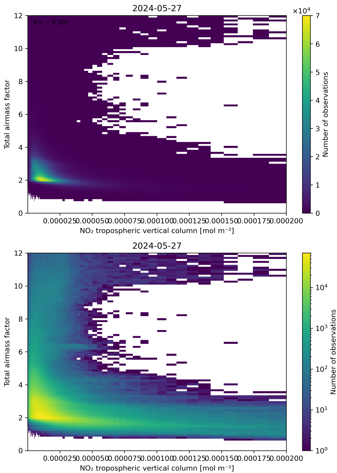
Figure 122: Scatter density plot of “NO 2 tropospheric vertical column” against “Total air mass factor” for 2024-05-26 to 2024-05-28.
