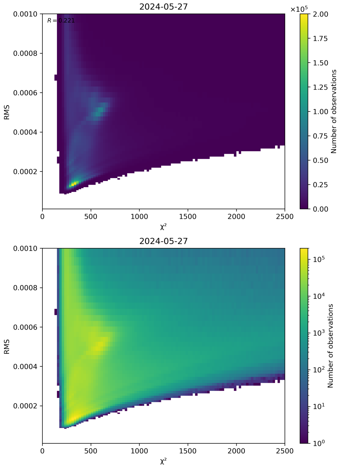
Figure 82: Scatter density plot of “ \chi^2 ” against “RMS” for 2024-05-26 to 2024-05-28.
