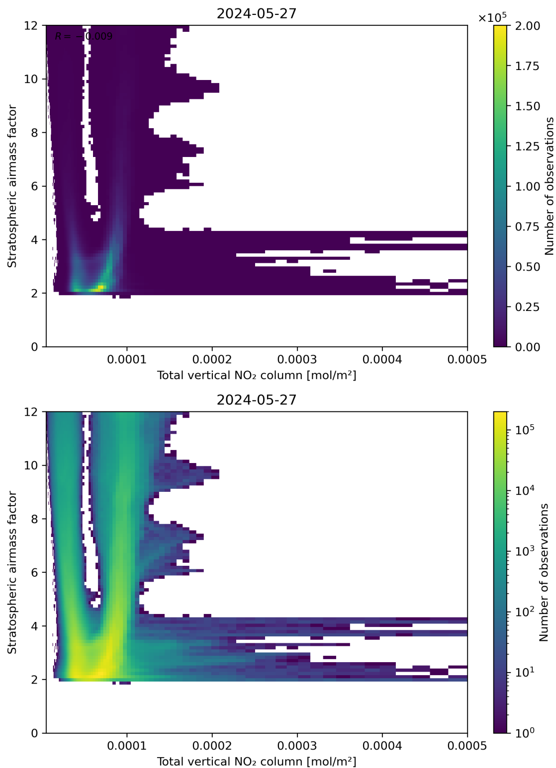
Figure 110: Scatter density plot of “Total vertical NO 2 column” against “Stratospheric airmass factor” for 2024-05-26 to 2024-05-28.
