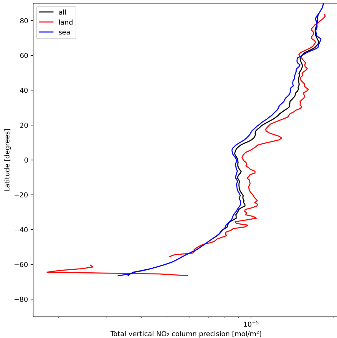
Figure 22: Zonal average of “Total vertical NO 2 column precision” for 2024-05-26 to 2024-05-28.
