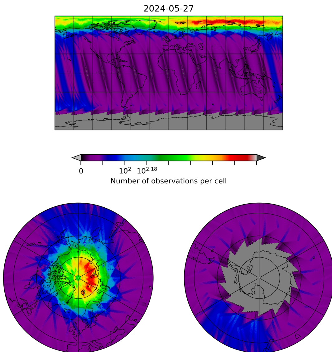
Figure 10: Map of the number of observations for 2024-05-26 to 2024-05-28
