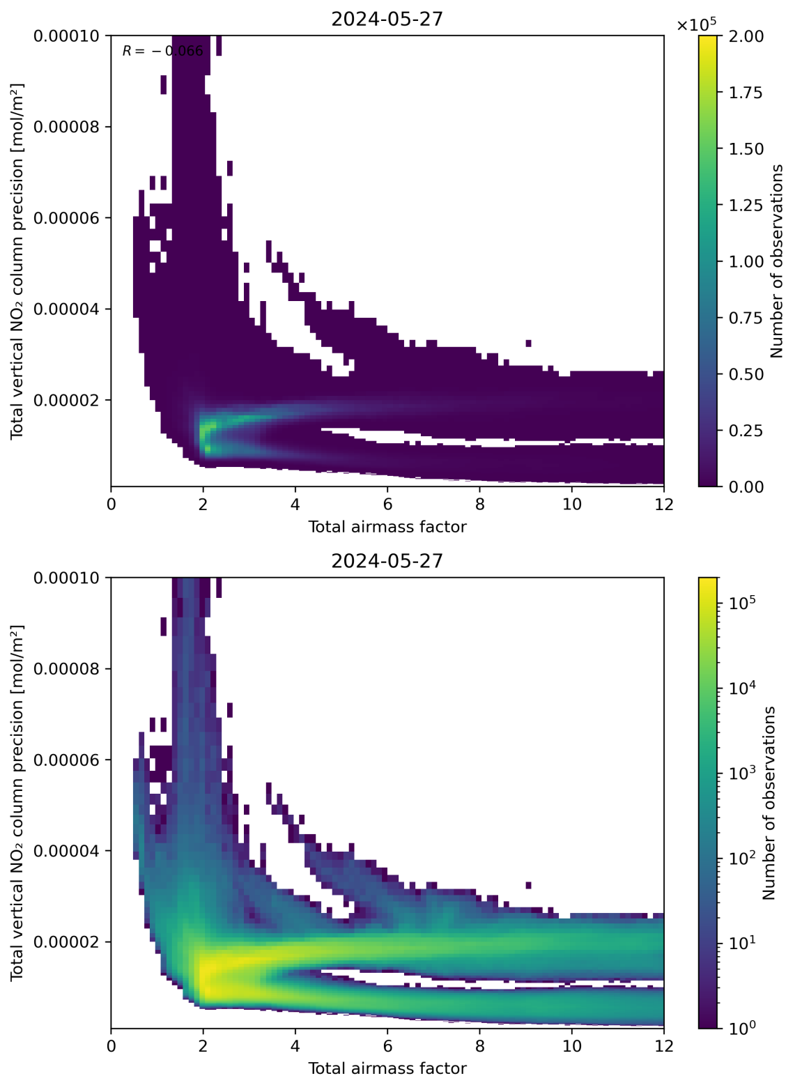
Figure 68: Scatter density plot of “Total airmass factor” against “Total vertical NO 2 column precision” for 2024-05-26 to 2024-05-28.
