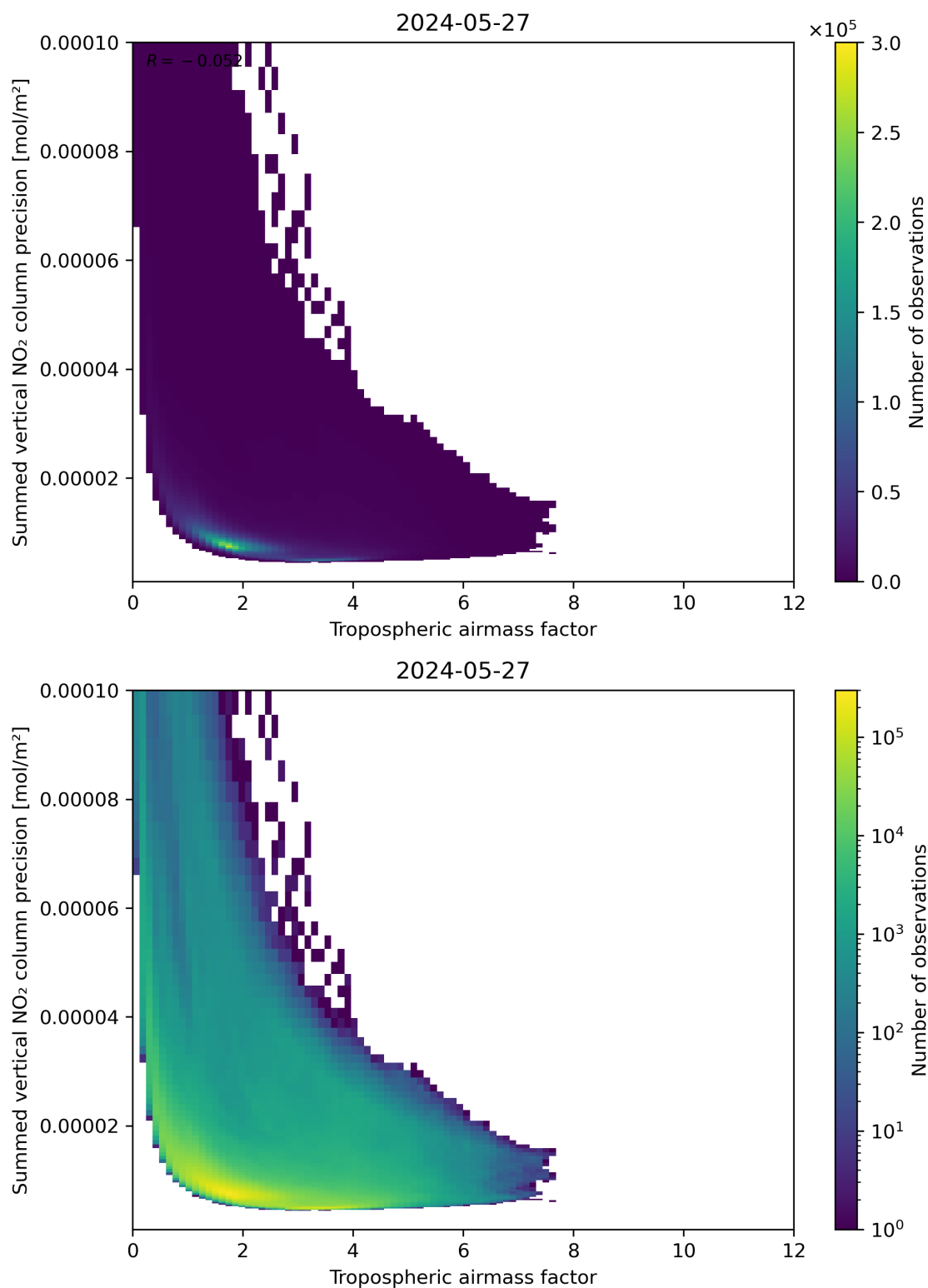
Figure 76: Scatter density plot of “Tropospheric air mass factor” against “Summed vertical NO 2 column precision” for 2024-05-26 to 2024-05-28.
