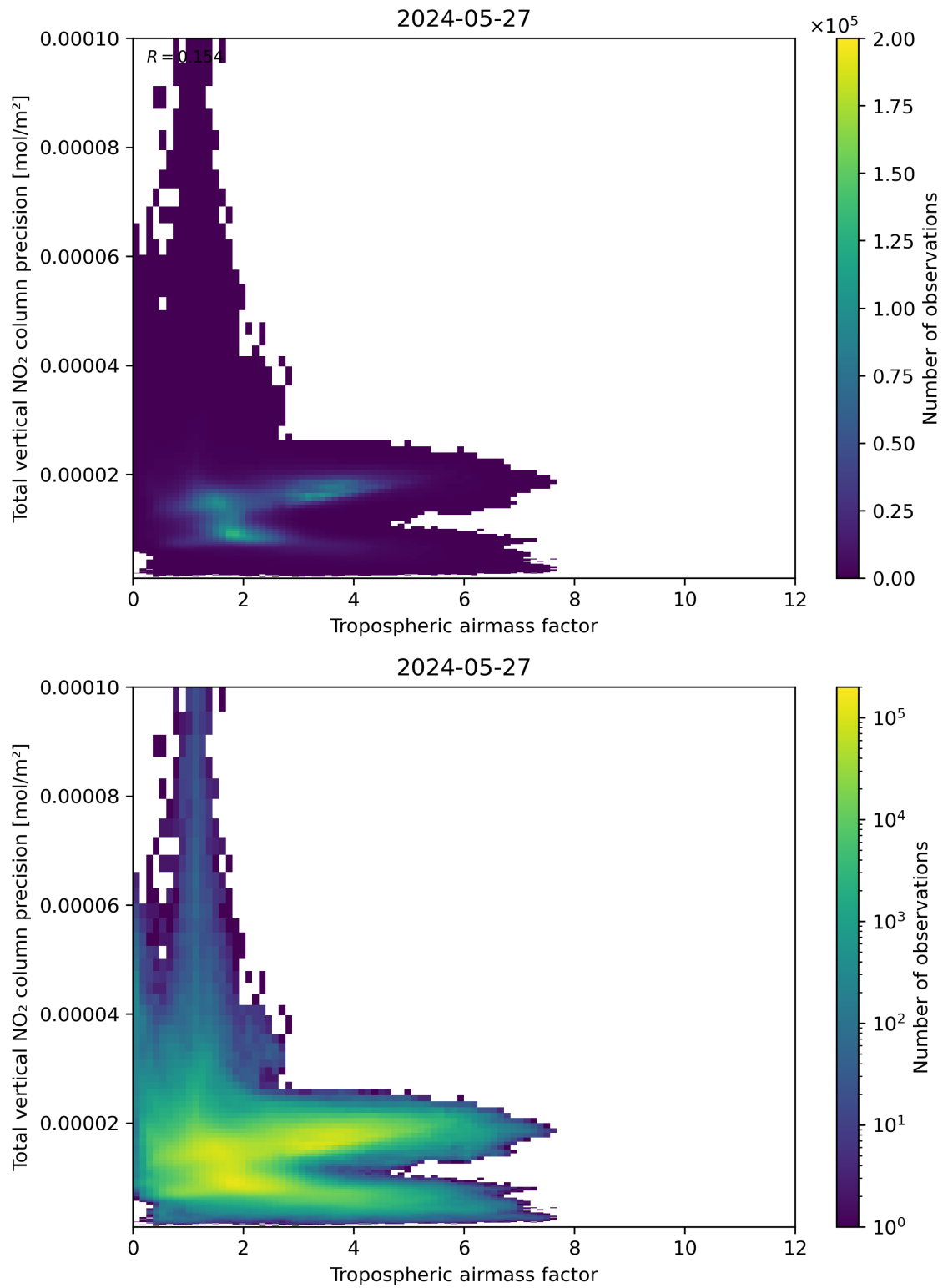
Figure 78: Scatter density plot of “Tropospheric air mass factor” against “Total vertical NO 2 column precision” for 2024-05-26 to 2024-05-28.
