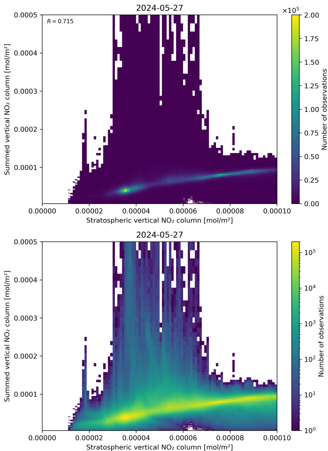
Figure 98: Scatter density plot of “Stratospheric vertical NO 2 column” against “Summed vertical NO 2 column” for 2024-05-26 to 2024-05-28.
