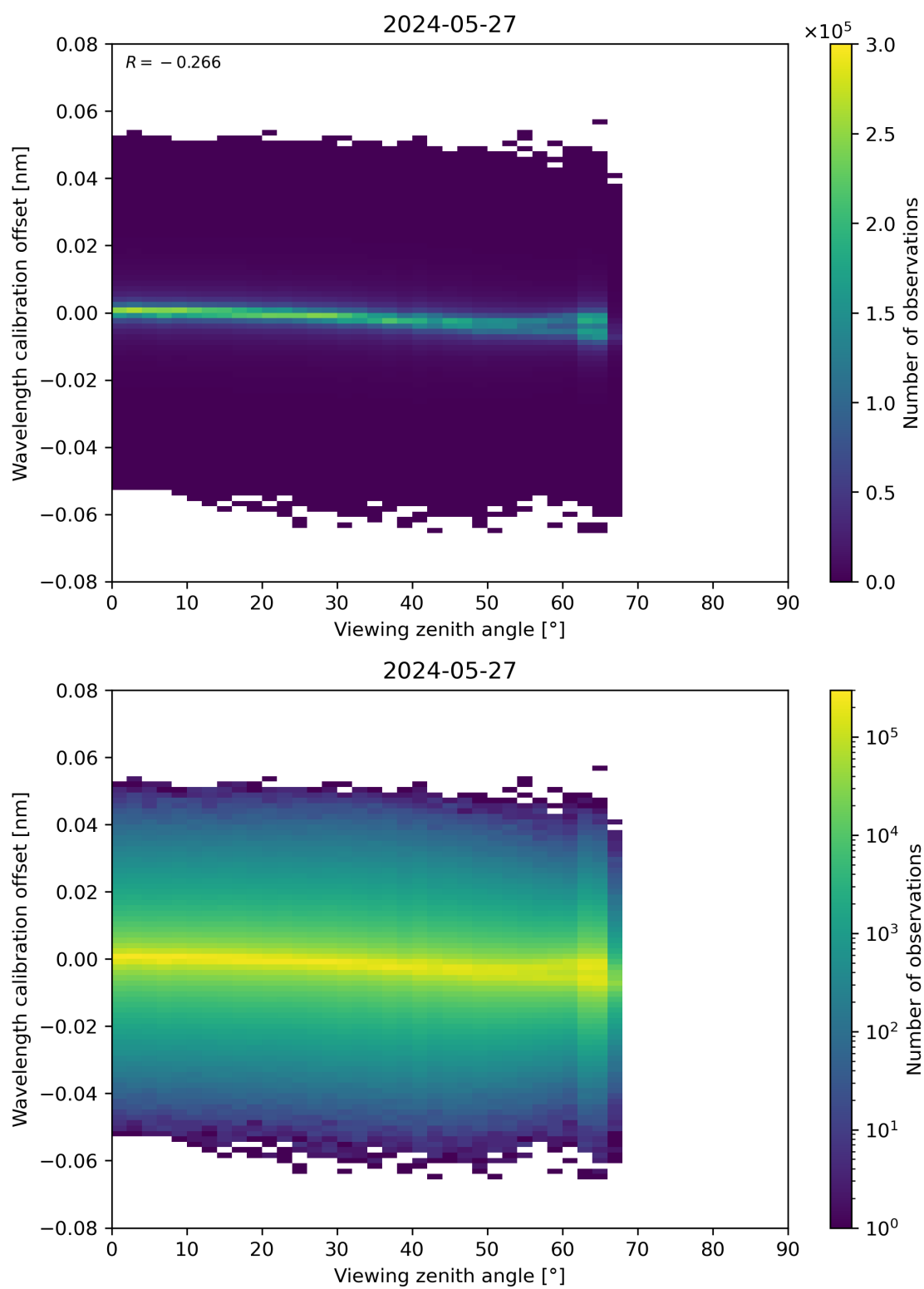
Figure 173: Scatter density plot of “Viewing zenith angle” against “Wavelength calibration offset” for 2024-05-26 to 2024-05-28.
