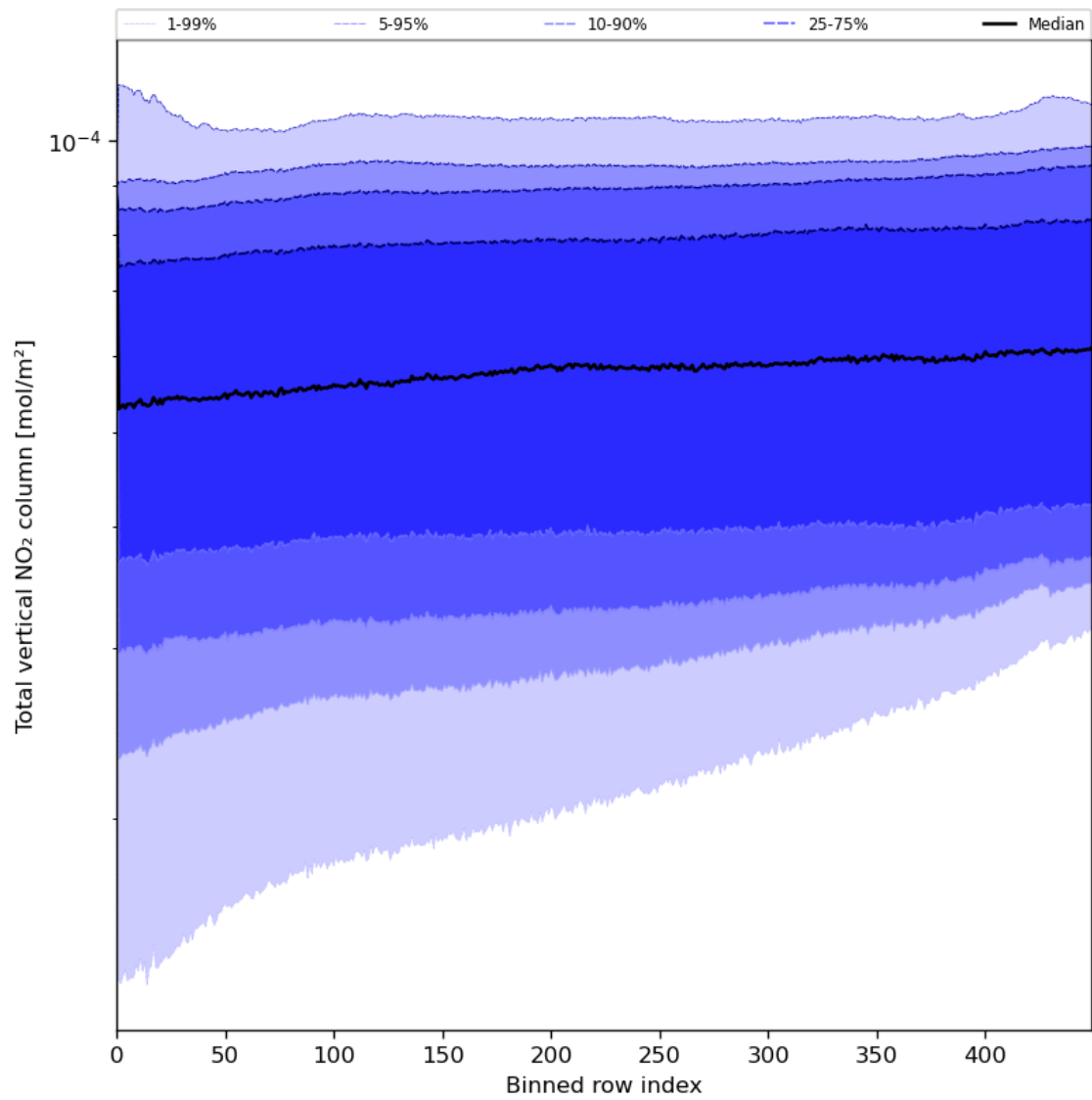
Figure 55: Along track statistics of “Total vertical NO 2 column” for 2024-05-26 to 2024-05-28
