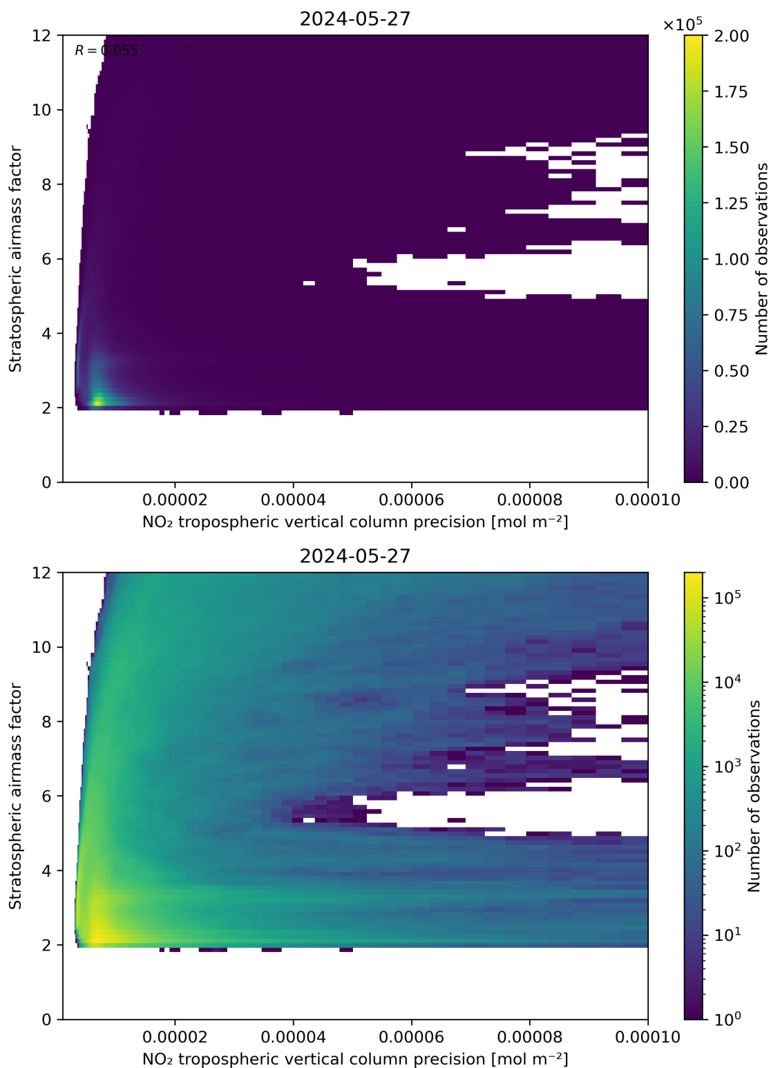
Figure 131: Scatter density plot of “NO 2 tropospheric vertical column precision” against “Stratospheric airmass factor” for 2024-05-26 to 2024-05-28.
