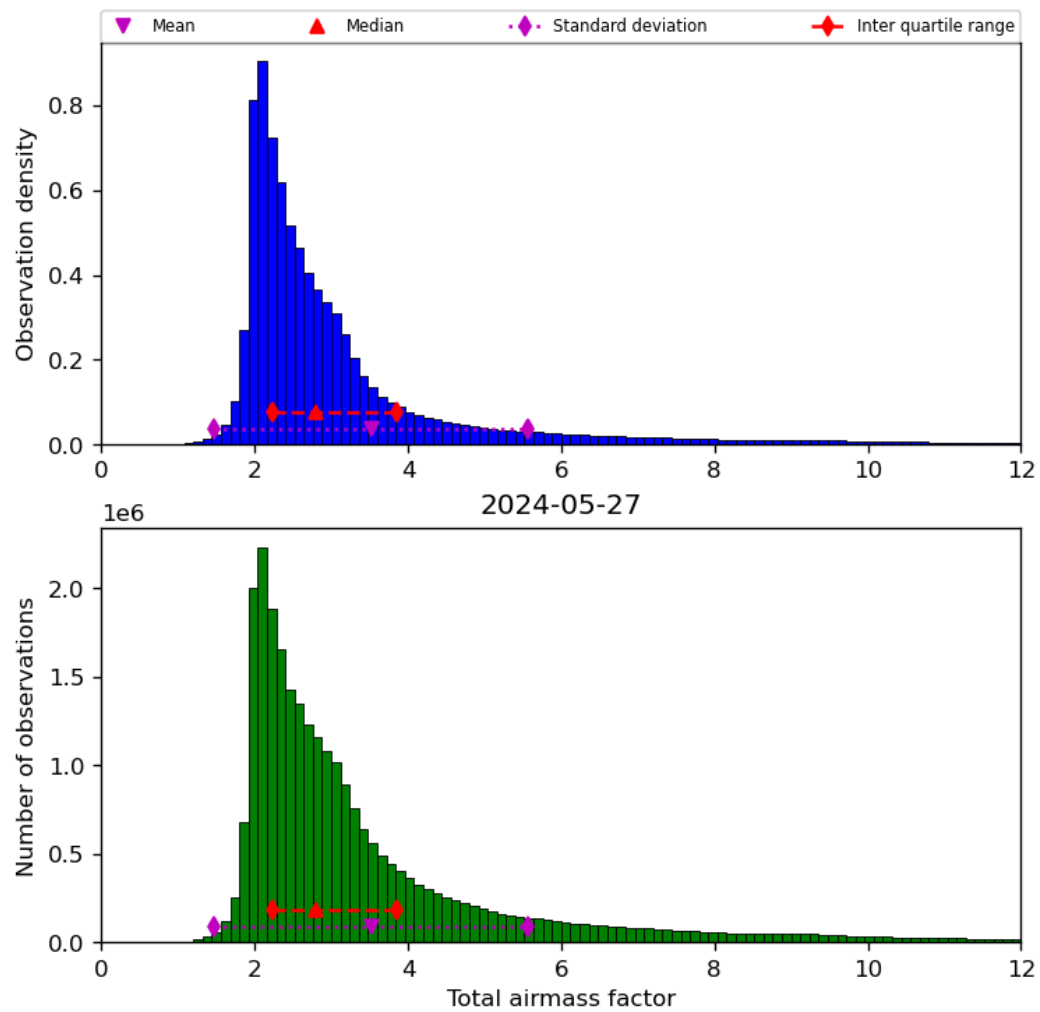
Figure 32: Histogram of “Total airmass factor” for 2024-05-26 to 2024-05-28
