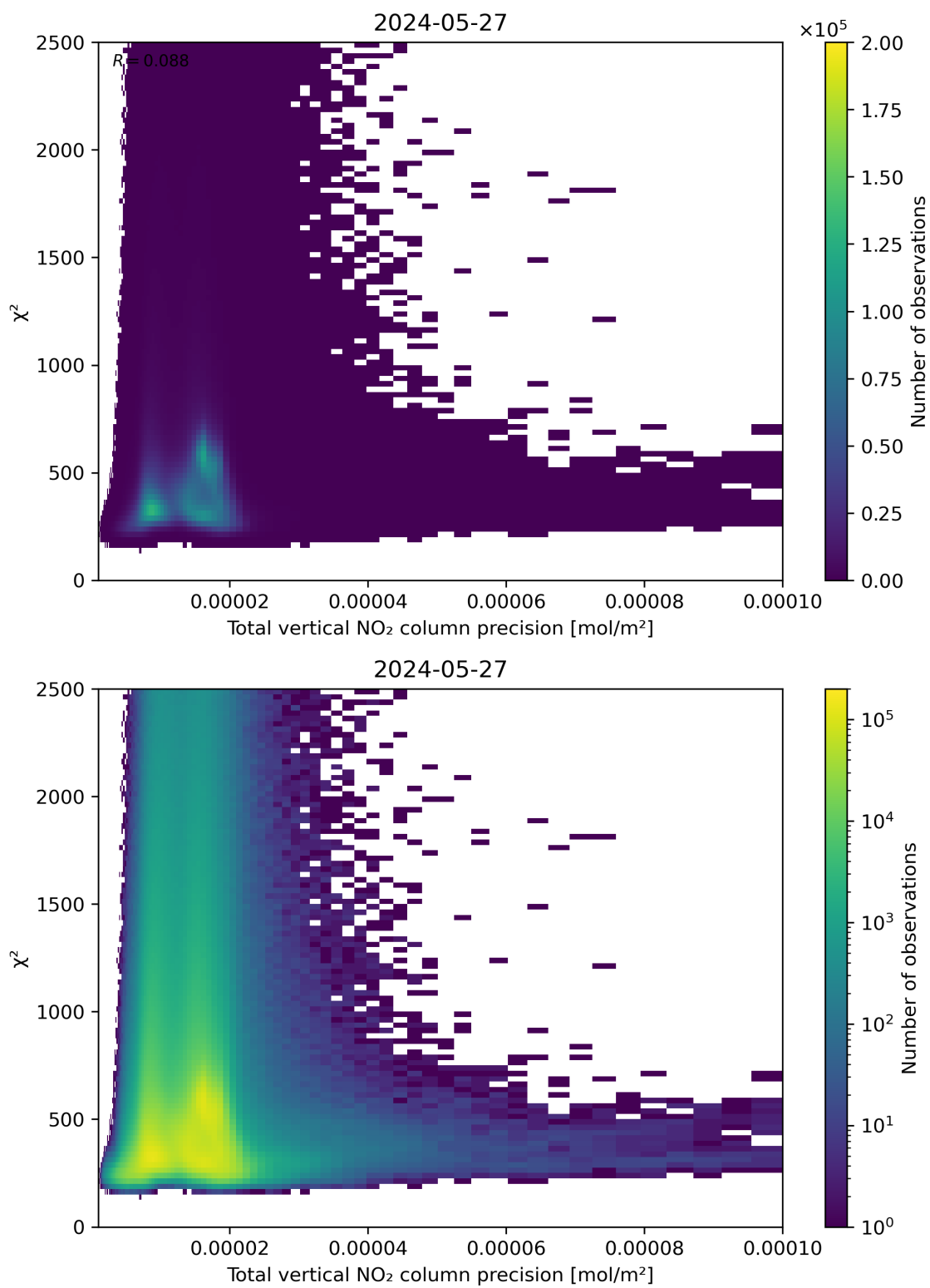
Figure 116: Scatter density plot of “Total vertical NO 2 column precision” against “ \chi^2 ” for 2024-05-26 to 2024-05-28.
