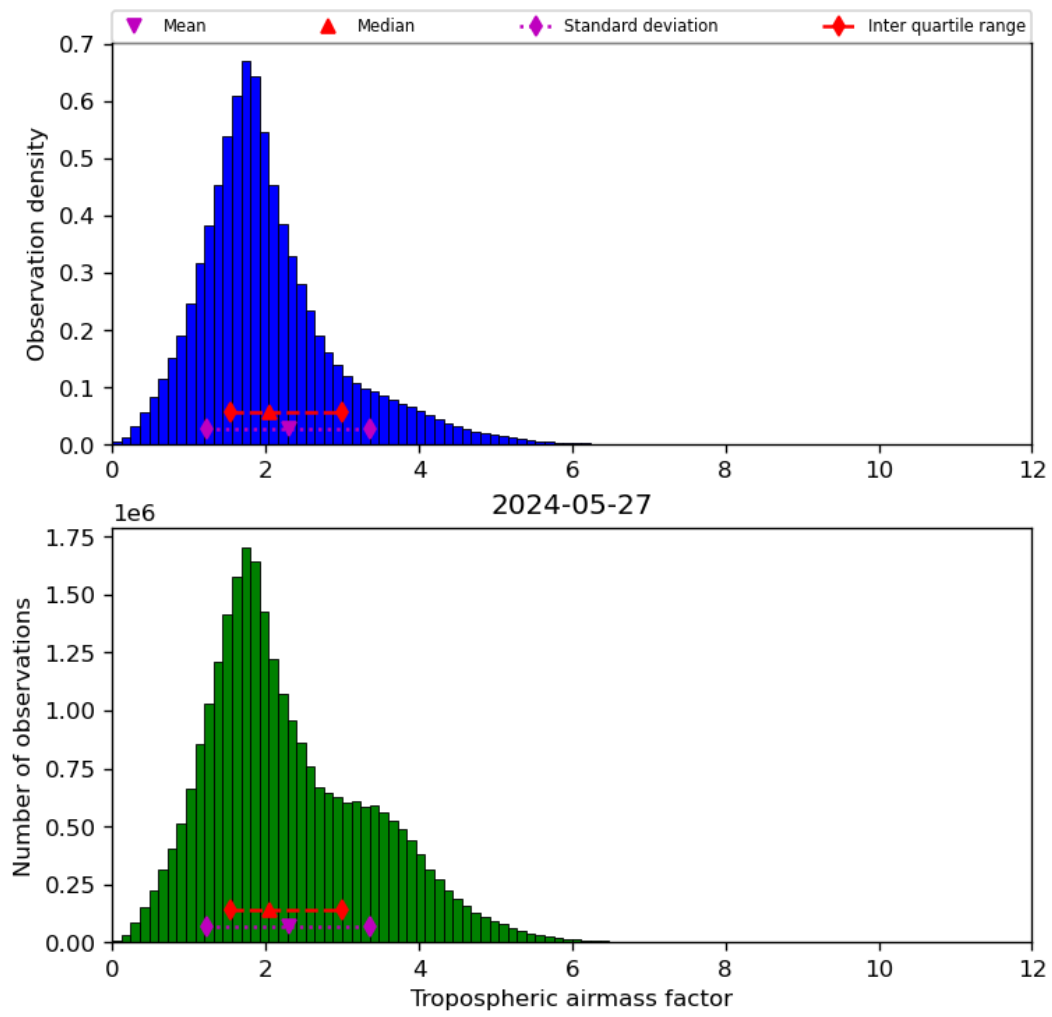
Figure 31: Histogram of “Tropospheric airmass factor” for 2024-05-26 to 2024-05-28
