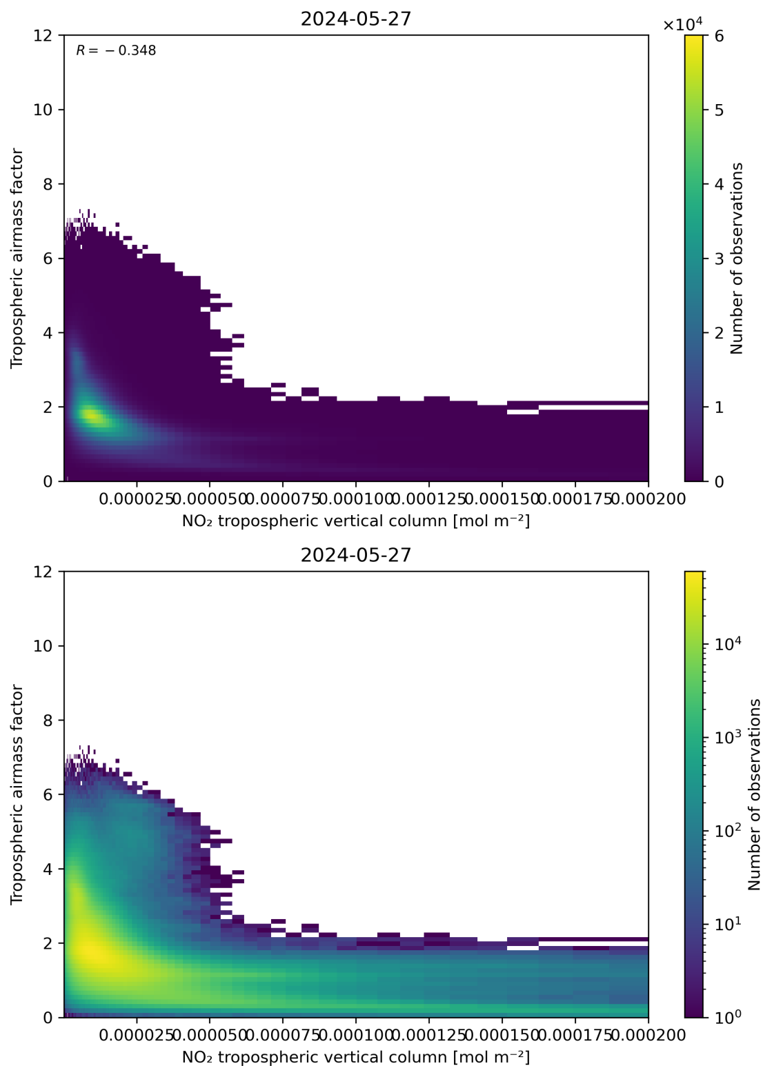
Figure 123: Scatter density plot of “NO 2 tropospheric vertical column” against “Tropospheric airmass factor” for 2024-05-26 to 2024-05-28.
