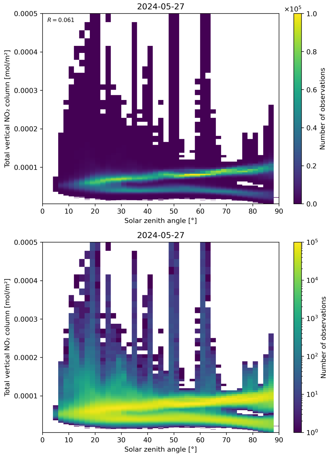
Figure 153: Scatter density plot of “Solar zenith angle” against “Total vertical NO 2 column” for 2024-05-26 to 2024-05-28.
