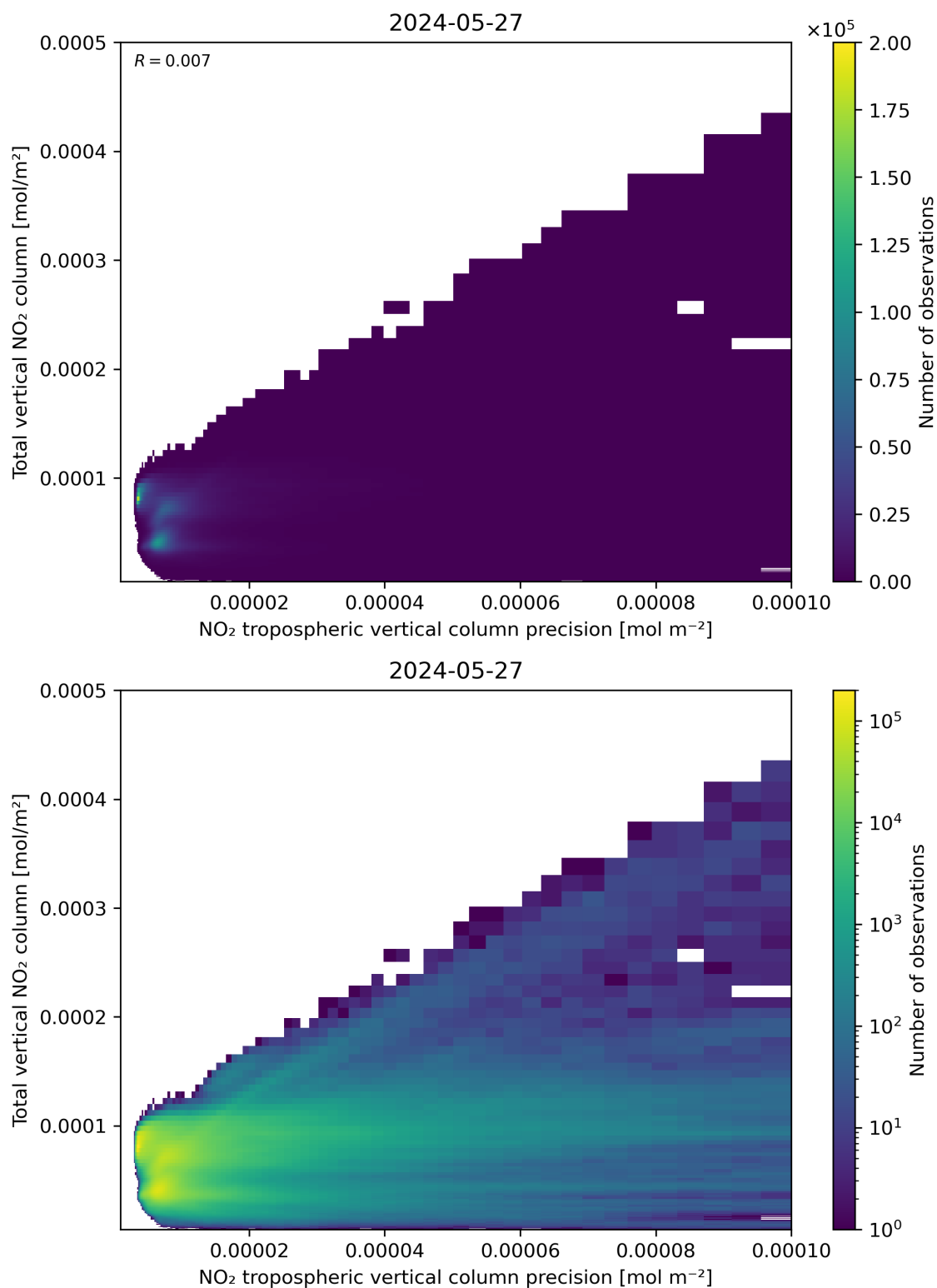
Figure 138: Scatter density plot of “NO 2 tropospheric vertical column precision” against “Total vertical NO 2 column” for 2024-05-26 to 2024-05-28.
