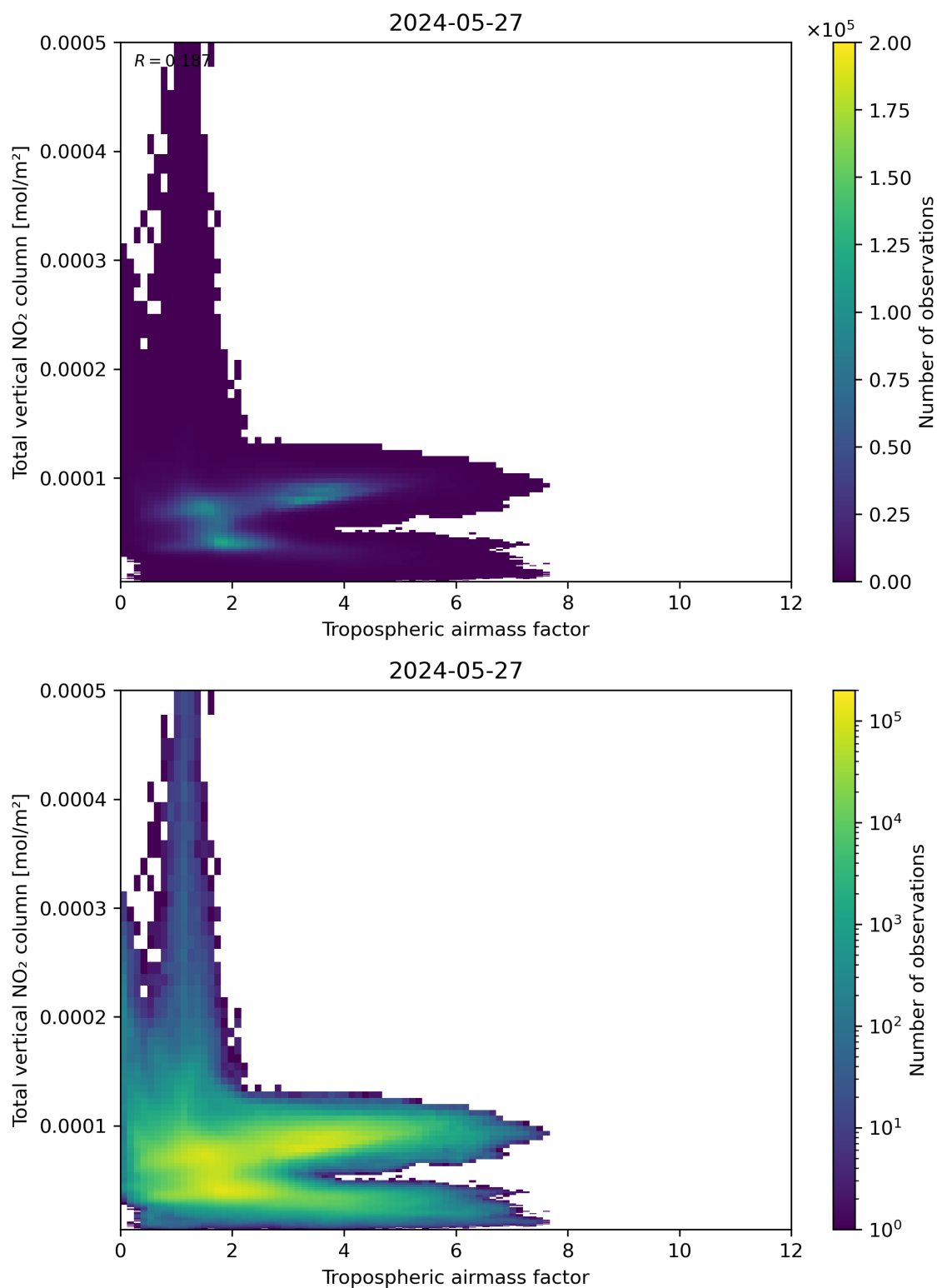
Figure 77: Scatter density plot of “Tropospheric airmass factor” against “Total vertical NO 2 column” for 2024-05-26 to 2024-05-28.
