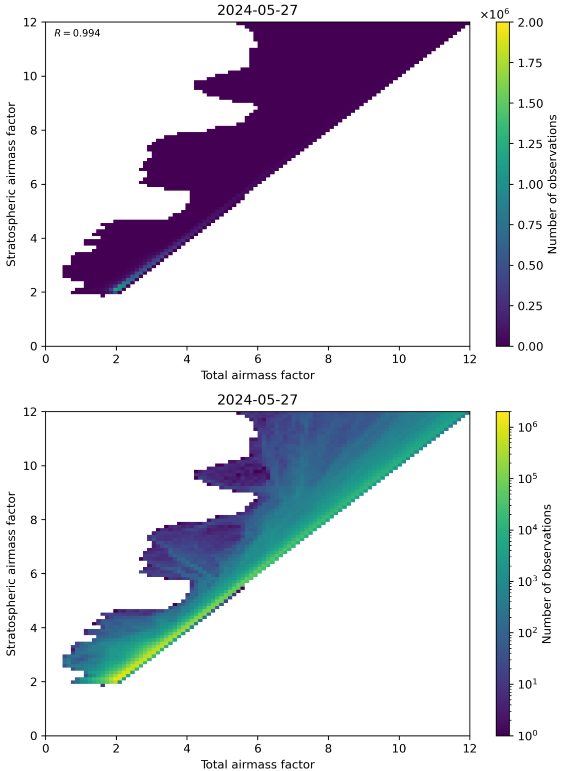
Figure 62: Scatter density plot of “Total airmass factor” against “Stratospheric airmass factor” for 2024-05-26 to 2024-05-28.
