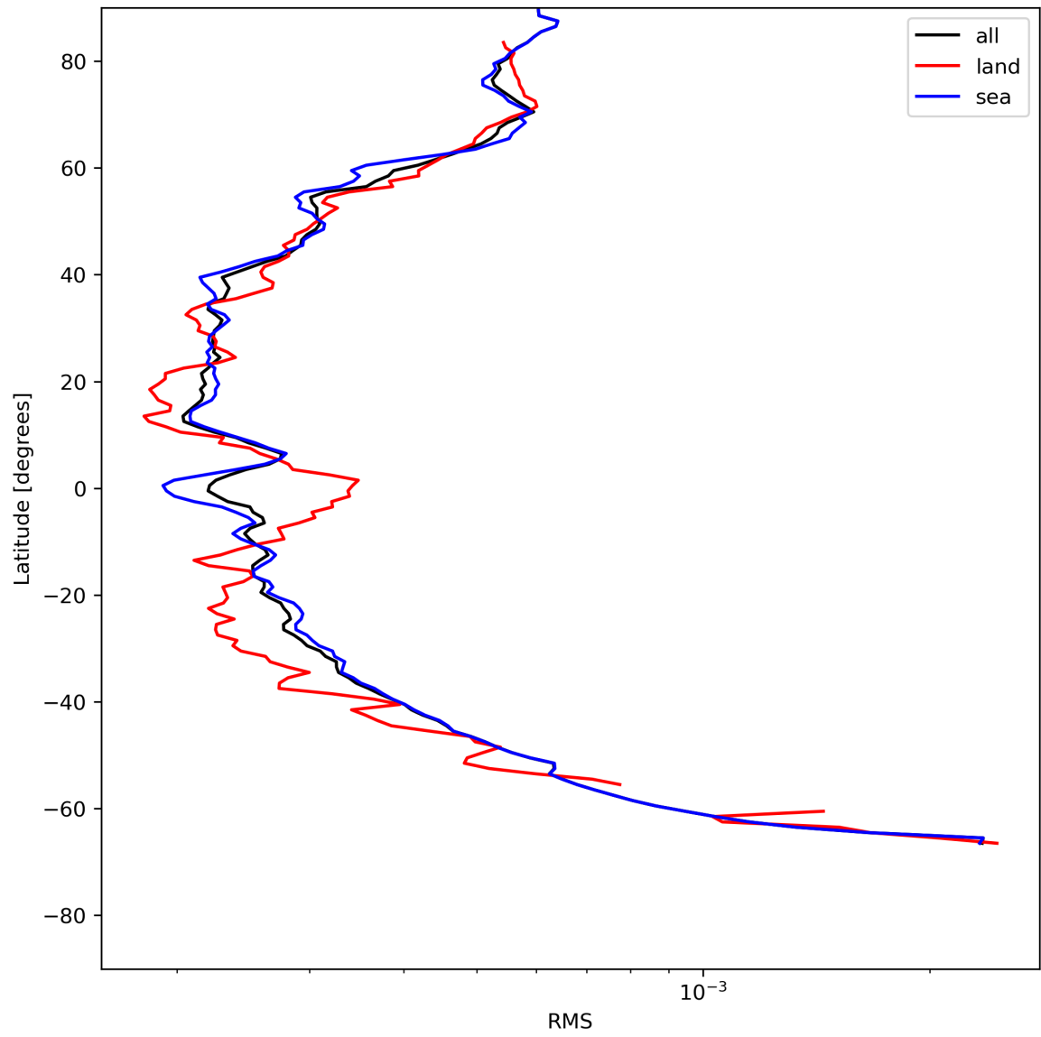
Figure 26: Zonal average of “RMS” for 2024-05-26 to 2024-05-28.
