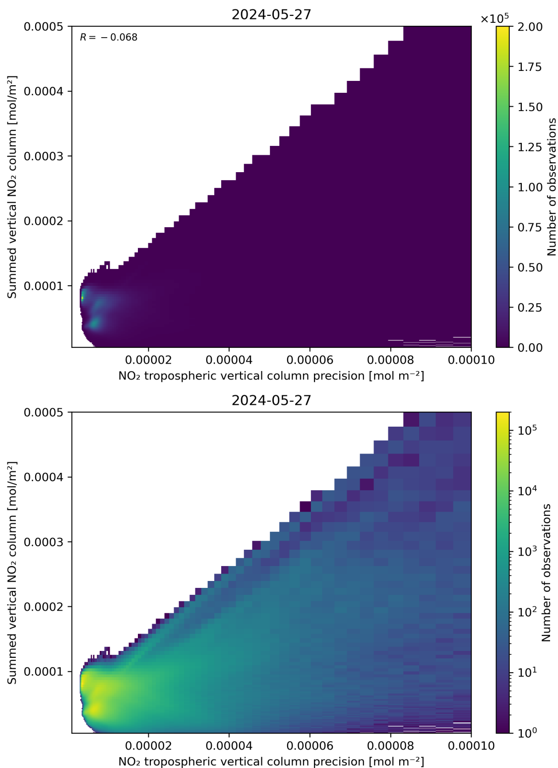
Figure 136: Scatter density plot of “NO 2 tropospheric vertical column precision” against “Summed vertical NO 2 column” for 2024-05-26 to 2024-05-28.
