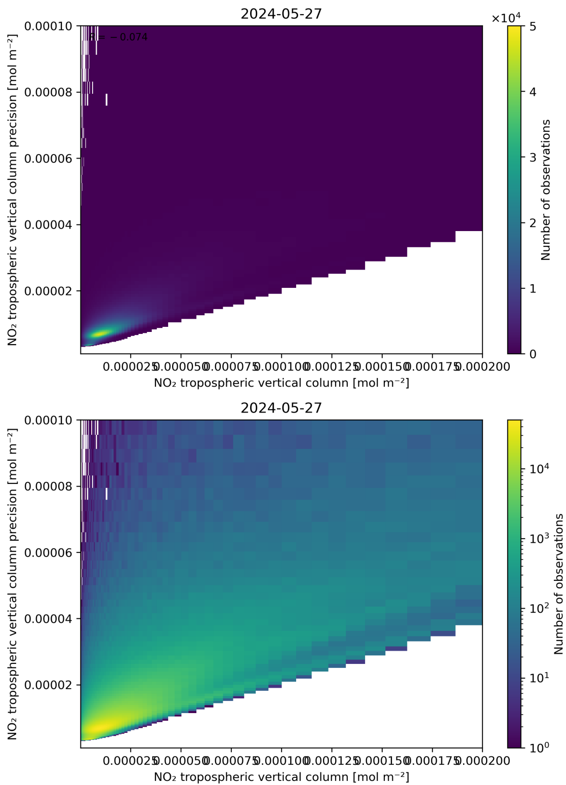
Figure 130: Scatter density plot of “NO 2 tropospheric vertical column” against “NO 2 tropospheric vertical column precision” for 2024-05-26 to 2024-05-28.
