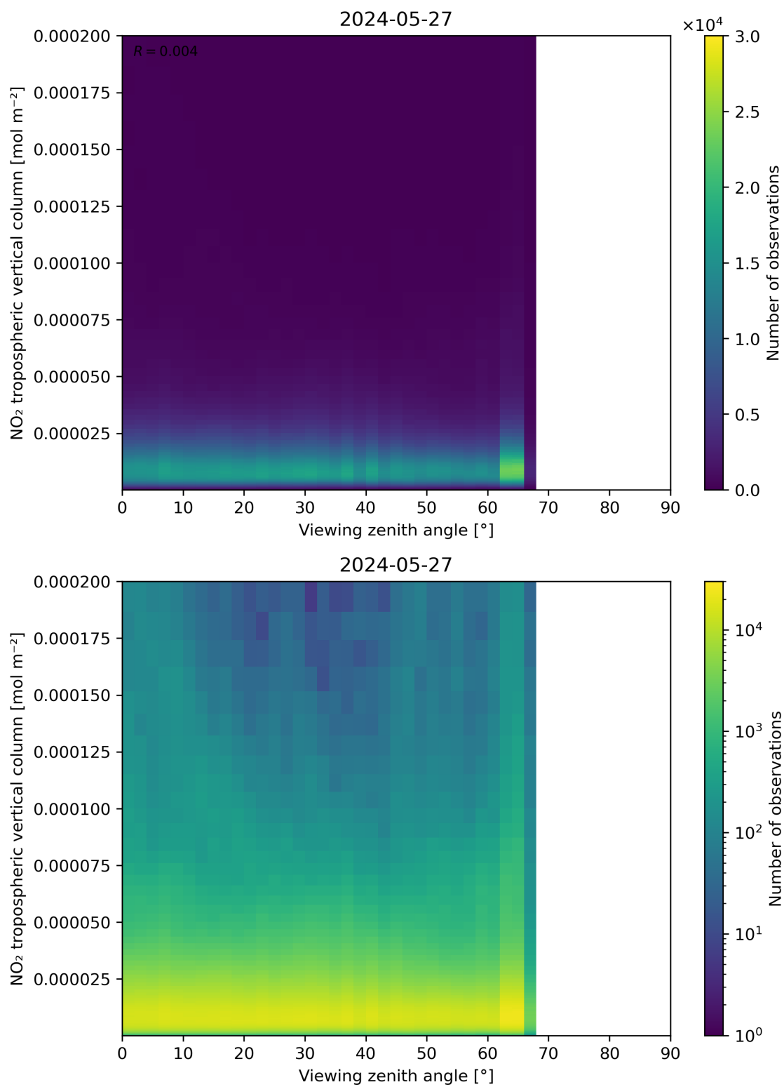
Figure 169: Scatter density plot of “Viewing zenith angle” against “NO 2 tropospheric vertical column” for 2024-05-26 to 2024-05-28.
