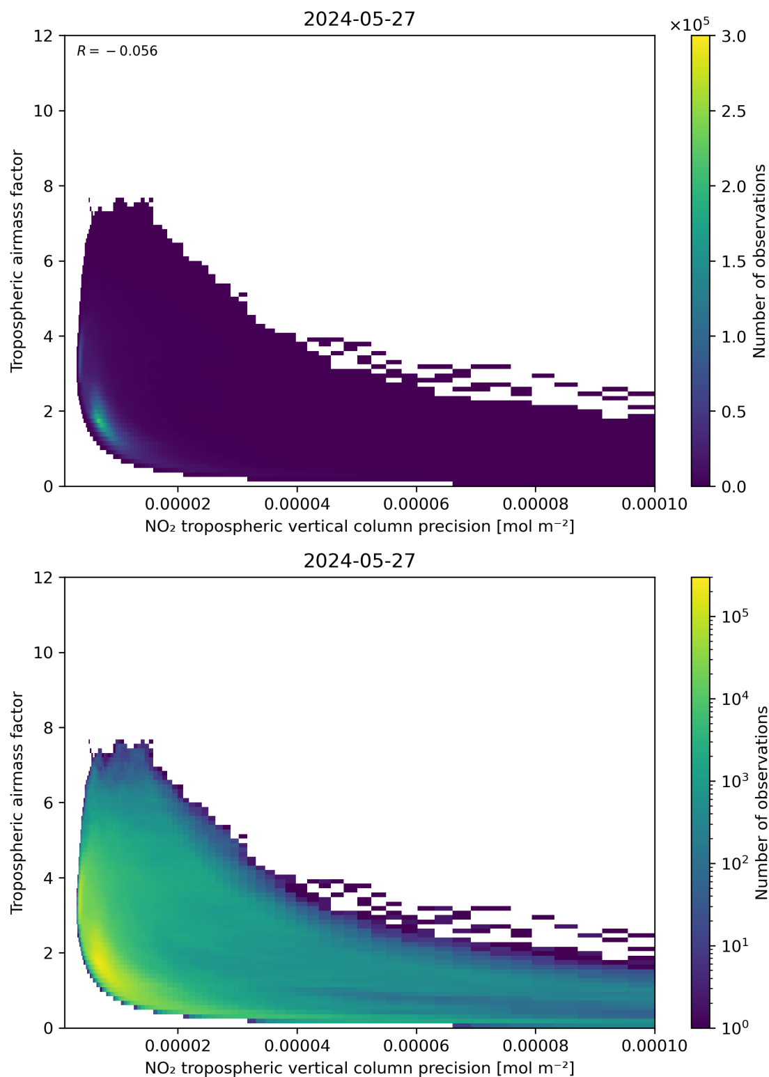
Figure 133: Scatter density plot of “NO 2 tropospheric vertical column precision” against “Tropospheric airmass factor” for 2024-05-26 to 2024-05-28.
