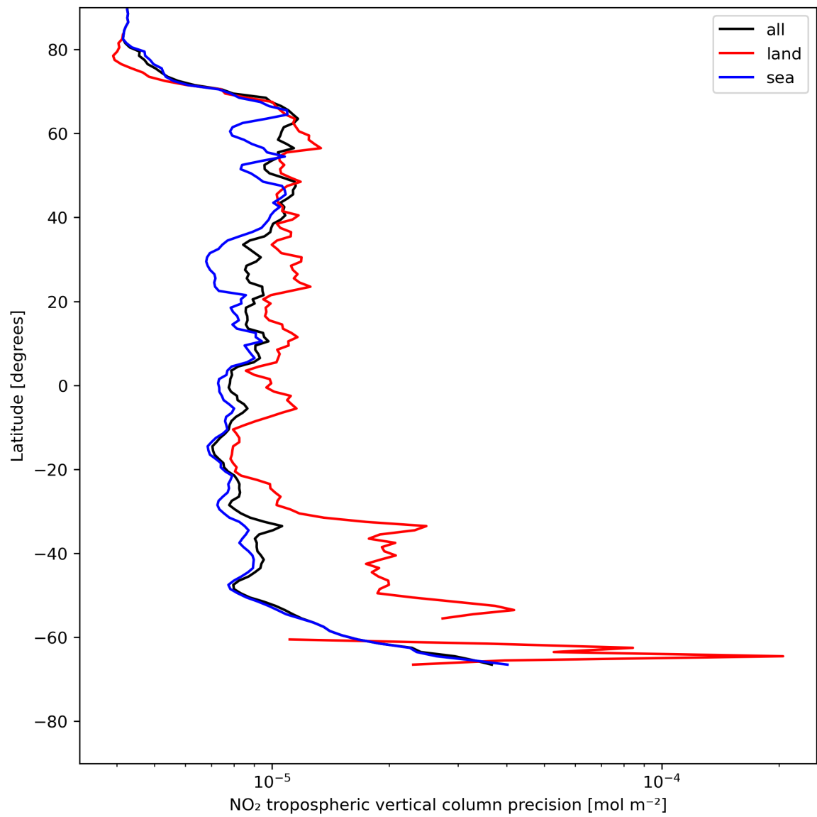
Figure 13: Zonal average of “NO 2 tropospheric vertical column precision” for 2024-05-26 to 2024-05-28.
