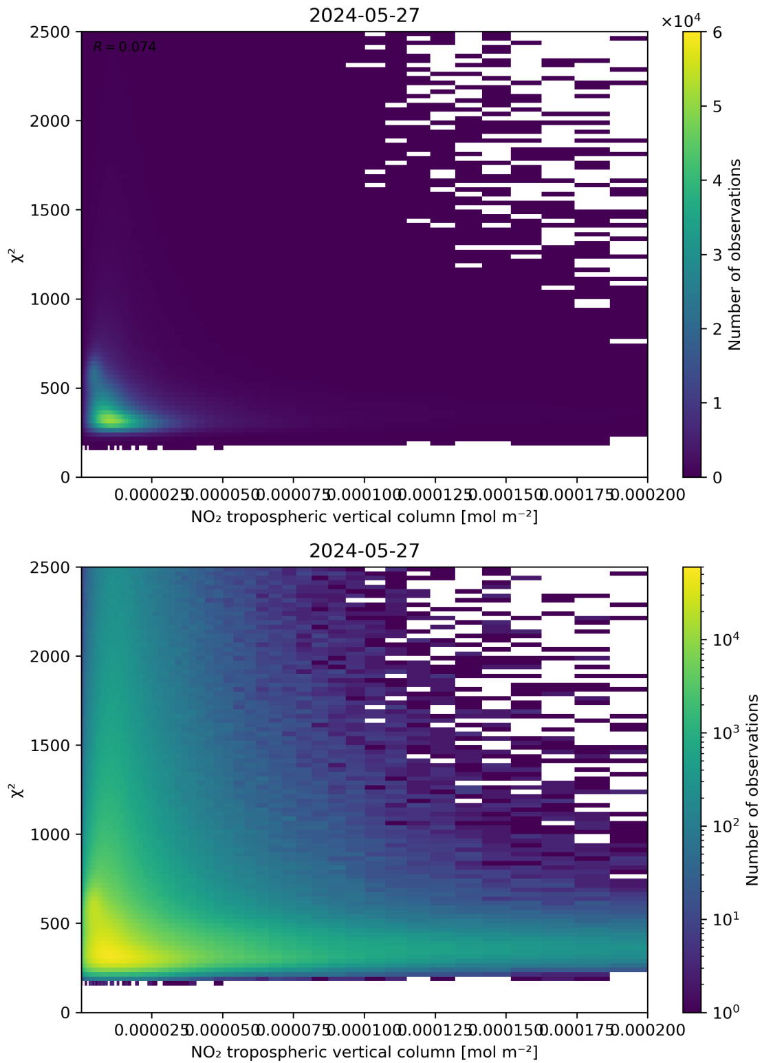
Figure 124: Scatter density plot of “NO 2 tropospheric vertical column” against “ \chi^2 ” for 2024-05-26 to 2024-05-28.
