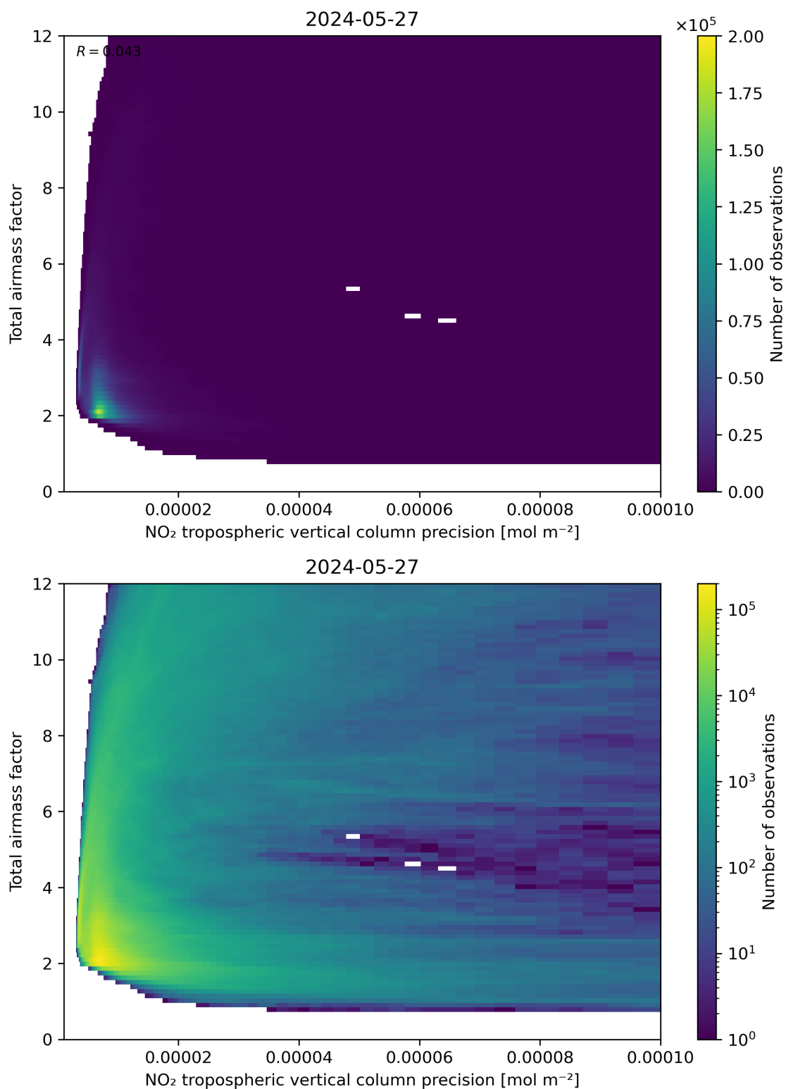
Figure 132: Scatter density plot of “NO 2 tropospheric vertical column precision” against “Total air mass factor” for 2024-05-26 to 2024-05-28.
