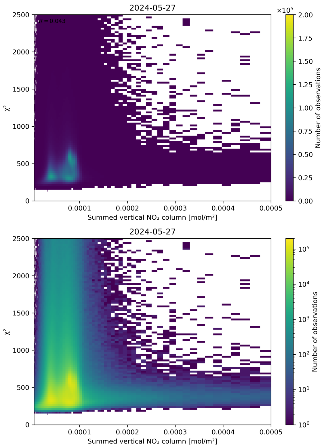
Figure 104: Scatter density plot of “Summed vertical NO 2 column” against “ \chi^2 ” for 2024-05-26 to 2024-05-28.
