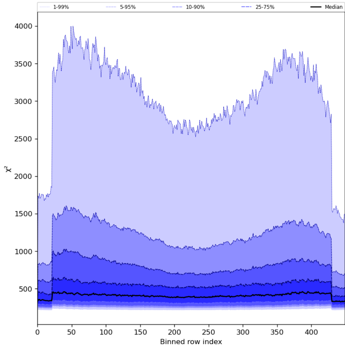
Figure 59: Along track statistics of “ \chi^2 ” for 2024-05-26 to 2024-05-28
