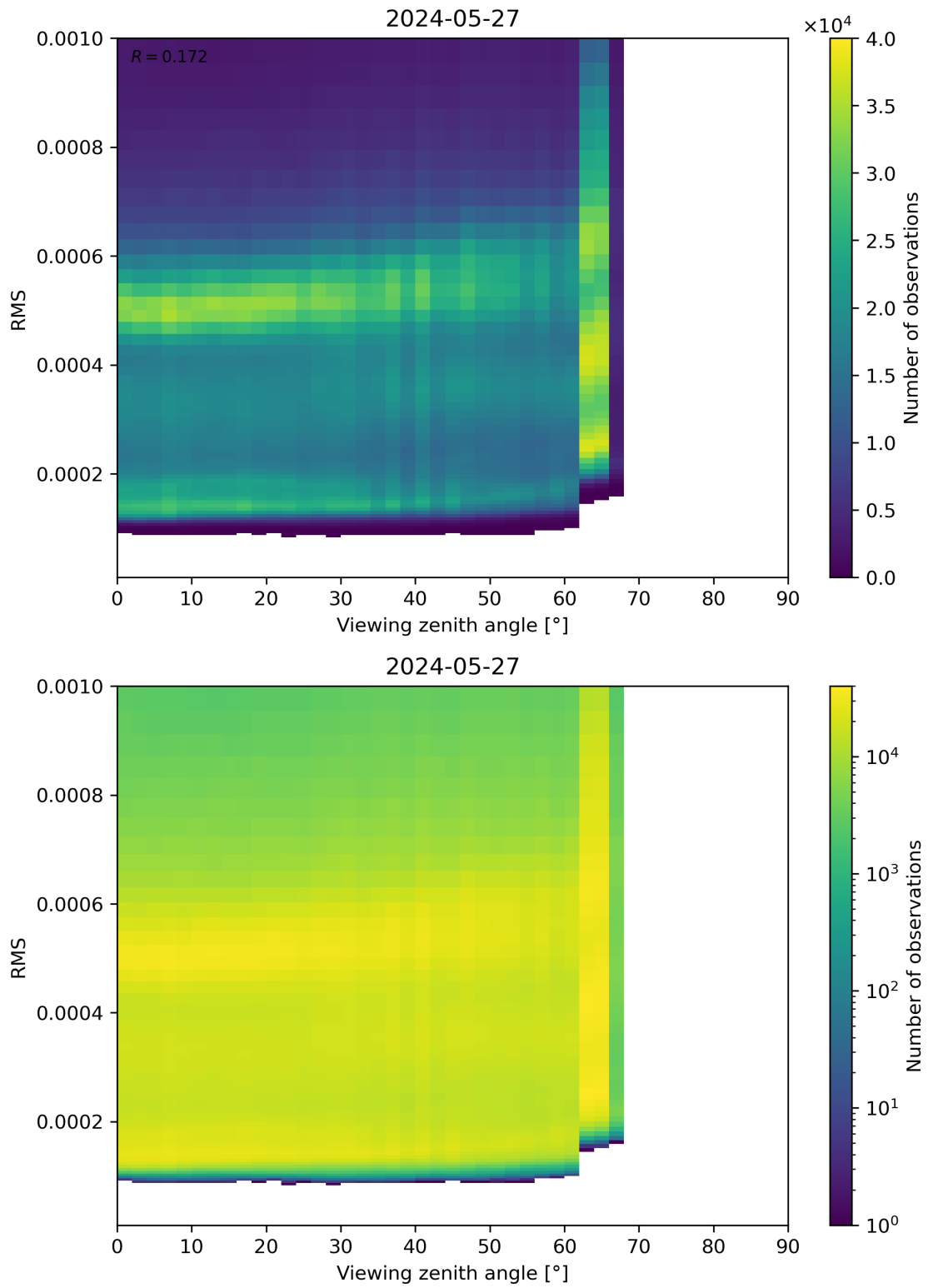
Figure 171: Scatter density plot of “Viewing zenith angle” against “RMS” for 2024-05-26 to 2024-05-28.
