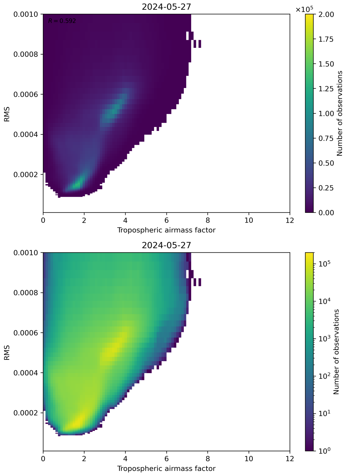
Figure 79: Scatter density plot of “Tropospheric airmass factor” against “RMS” for 2024-05-26 to 2024-05-28.
