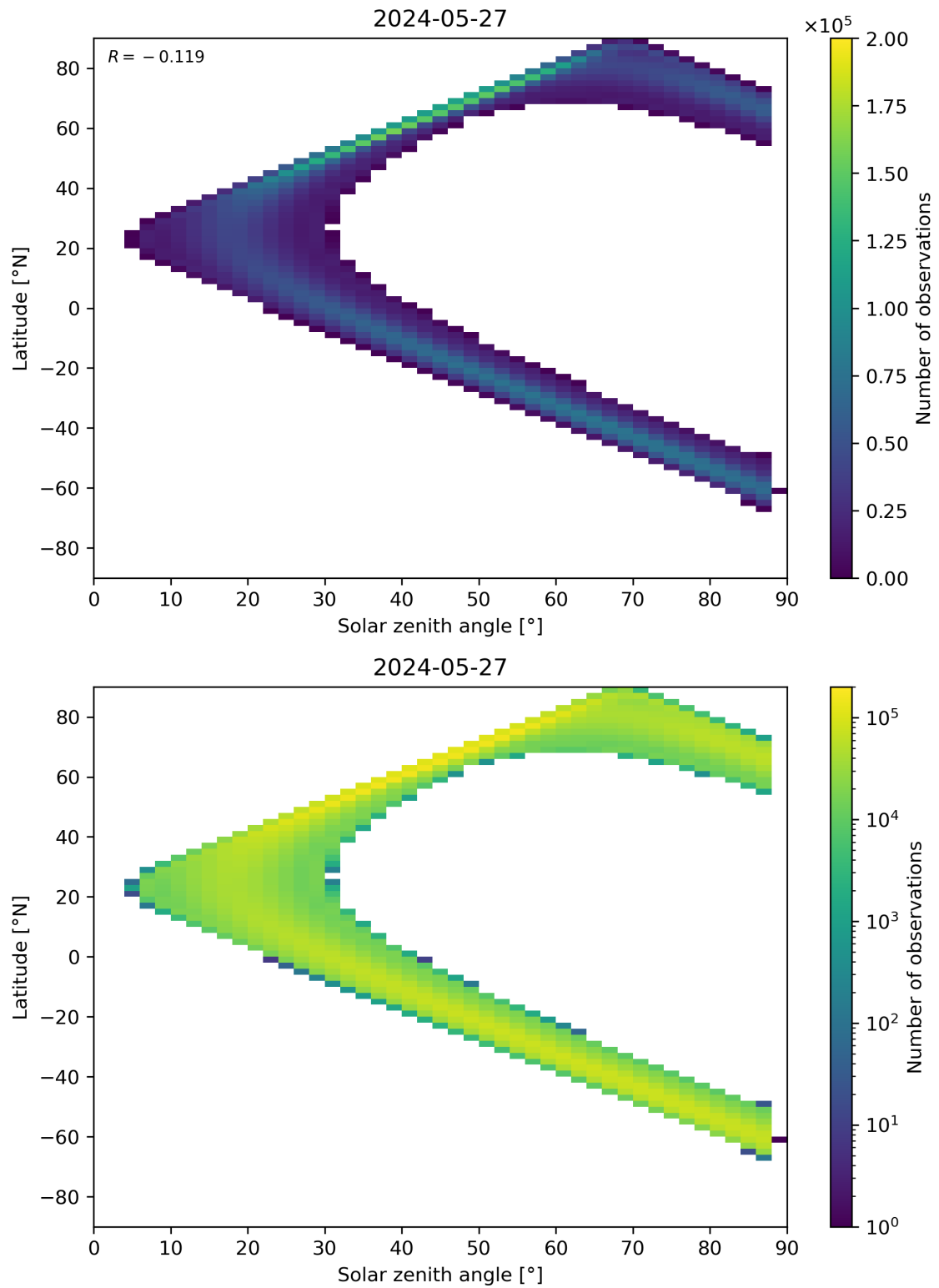
Figure 149: Scatter density plot of “Solar zenith angle” against “Latitude” for 2024-05-26 to 2024-05-28.
