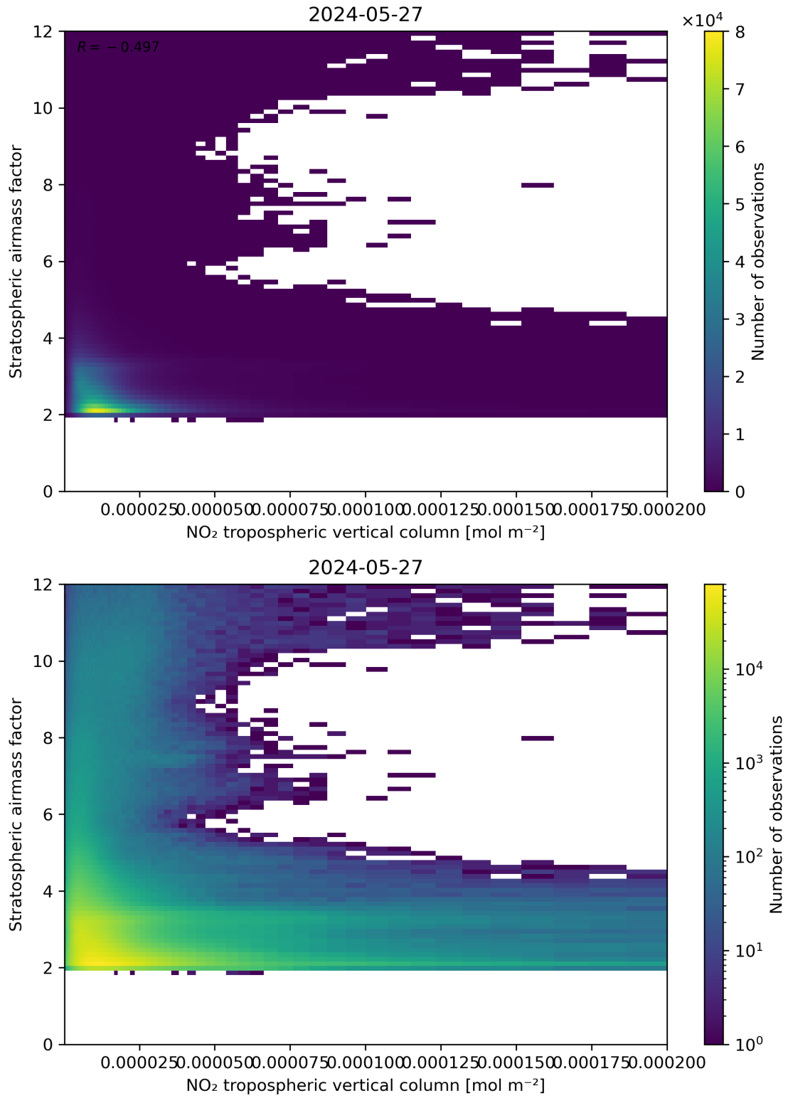
Figure 121: Scatter density plot of “NO 2 tropospheric vertical column” against “Stratospheric air mass factor” for 2024-05-26 to 2024-05-28.
