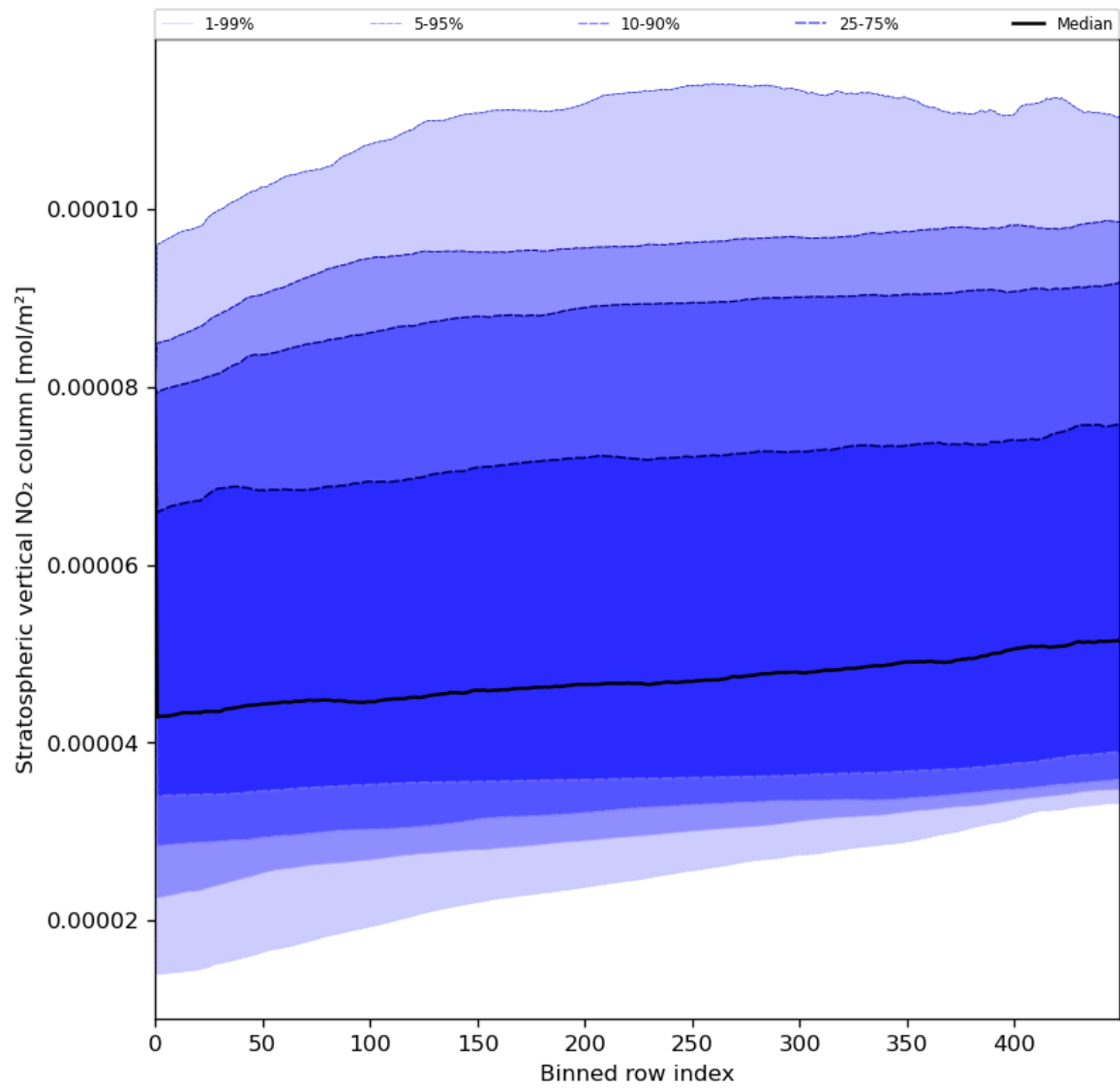
Figure 53: Along track statistics of “Stratospheric vertical NO 2 column” for 2024-05-26 to 2024-05-28
