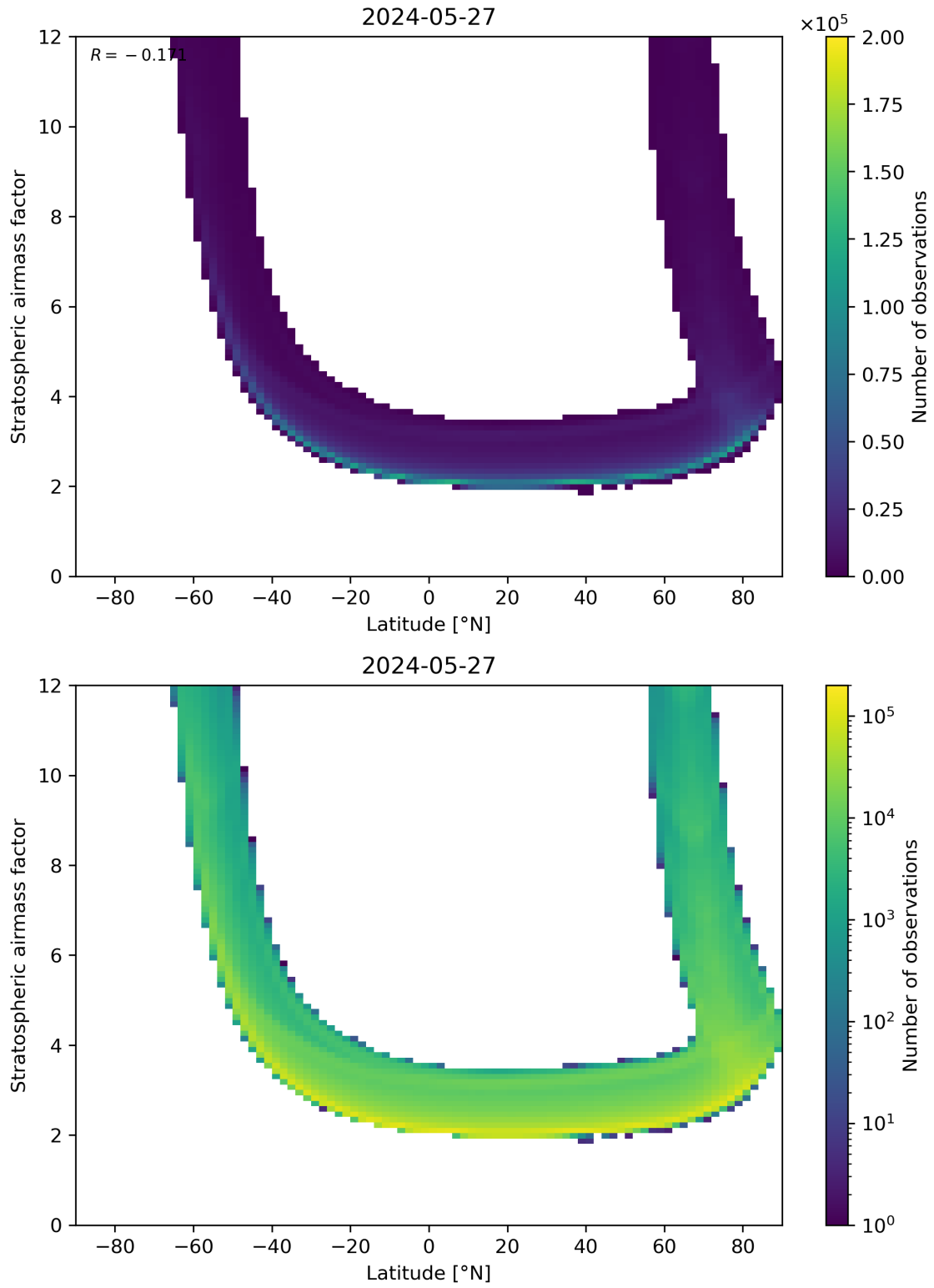
Figure 83: Scatter density plot of “Latitude” against “Stratospheric air mass factor” for 2024-05-26 to 2024-05-28.
