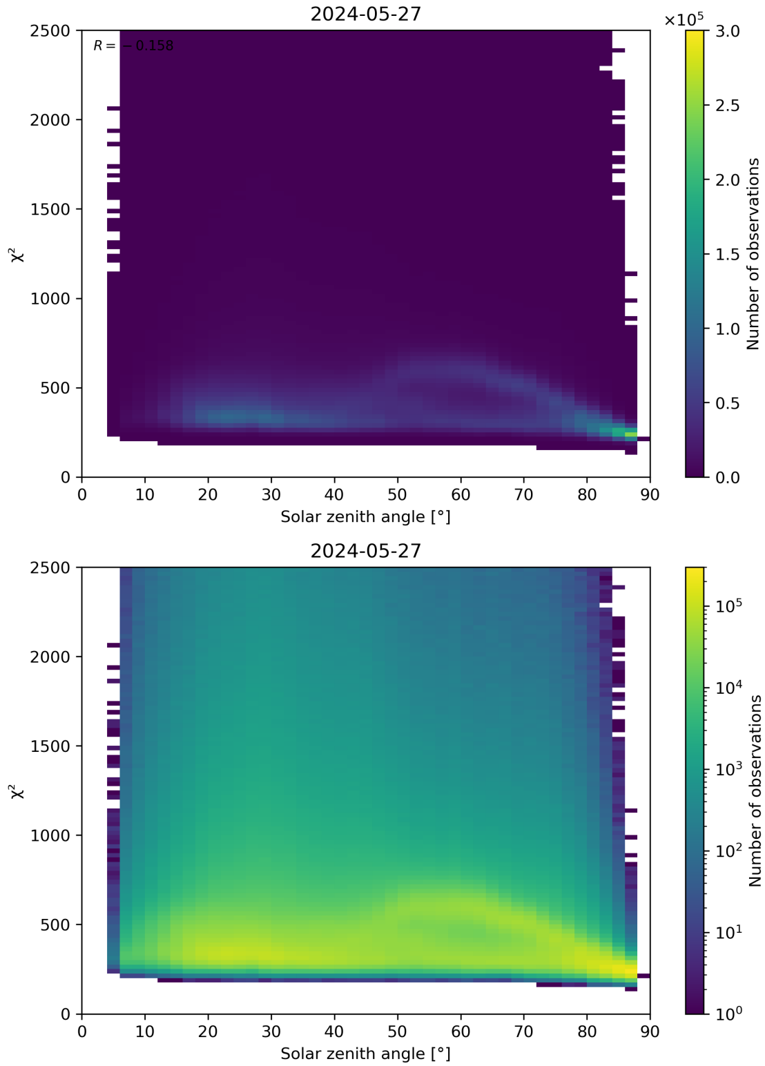
Figure 148: Scatter density plot of “Solar zenith angle” against “ \chi^2 ” for 2024-05-26 to 2024-05-28.
