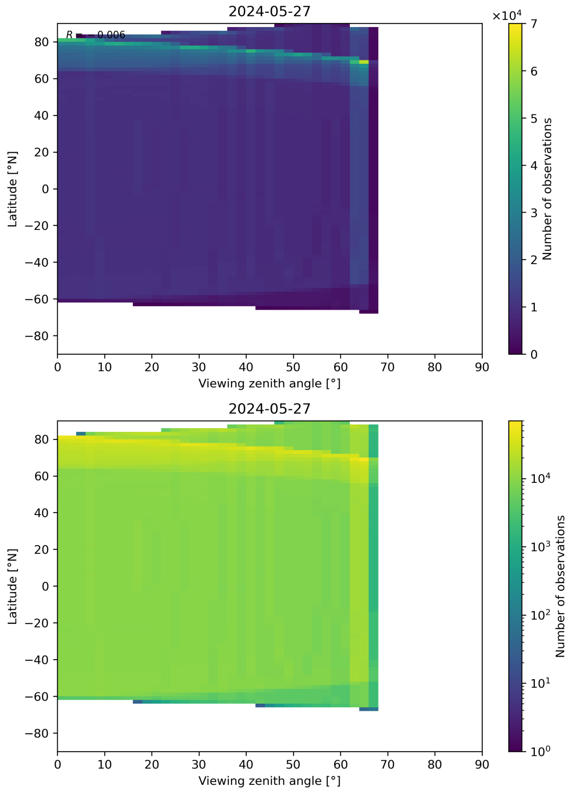
Figure 163: Scatter density plot of “Viewing zenith angle” against “Latitude” for 2024-05-26 to 2024-05-28.
