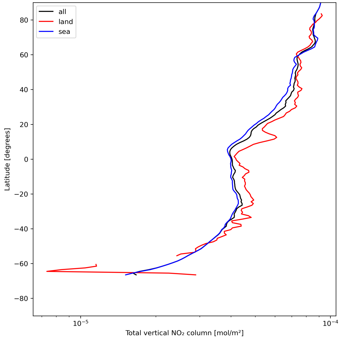
Figure 21: Zonal average of “Total vertical NO 2 column” for 2024-05-26 to 2024-05-28.
