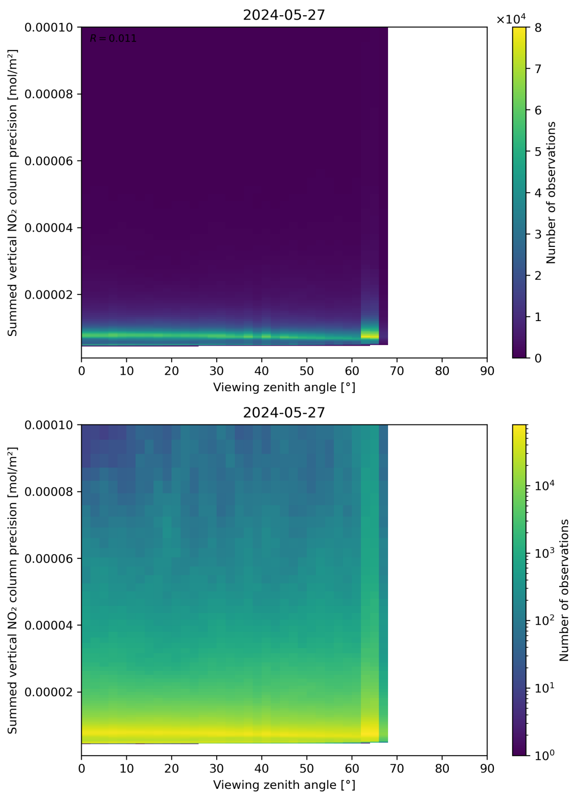
Figure 166: Scatter density plot of “Viewing zenith angle” against “Summed vertical NO 2 column precision” for 2024-05-26 to 2024-05-28.
