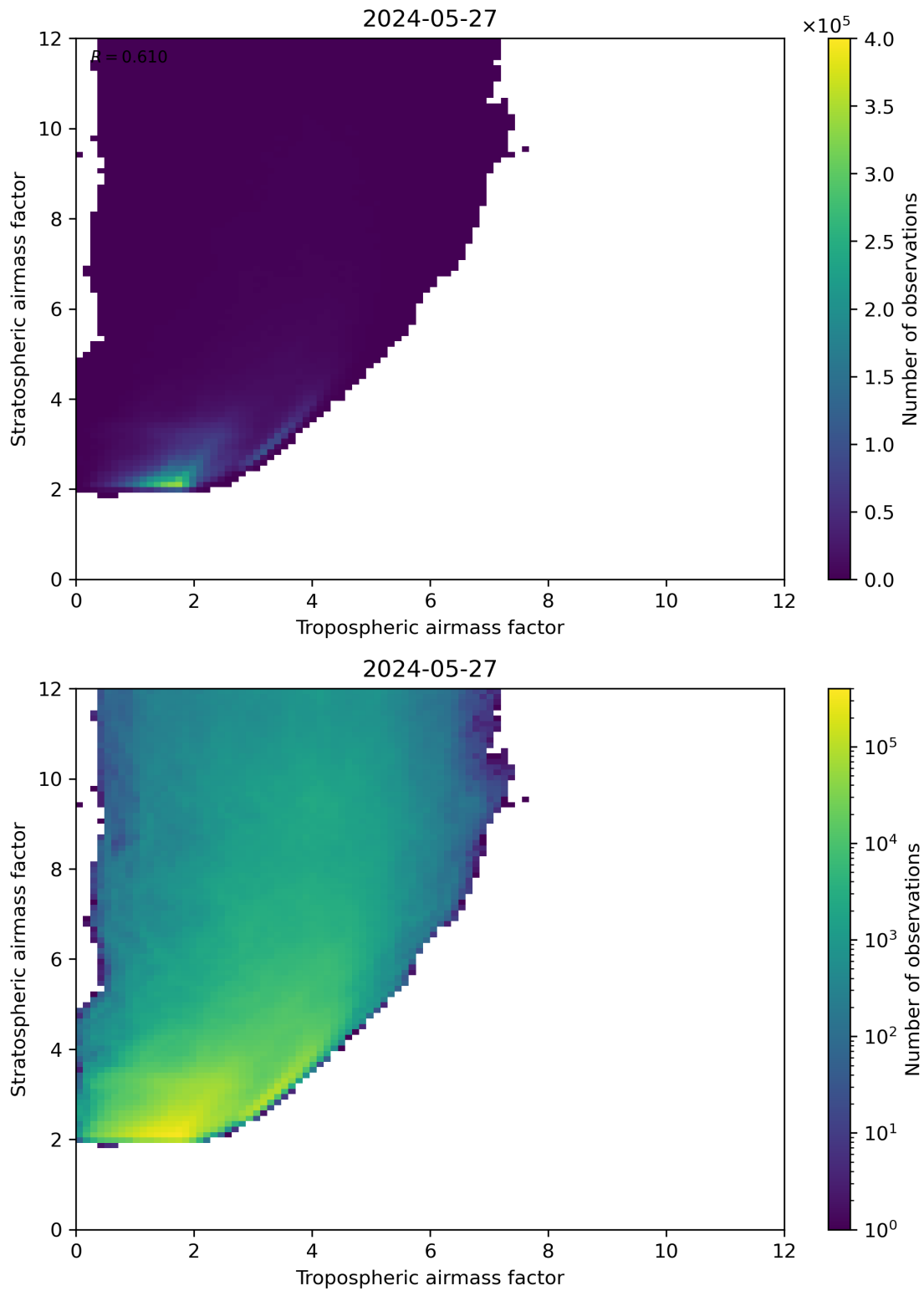
Figure 71: Scatter density plot of “Tropospheric airmass factor” against “Stratospheric airmass factor” for 2024-05-26 to 2024-05-28.
