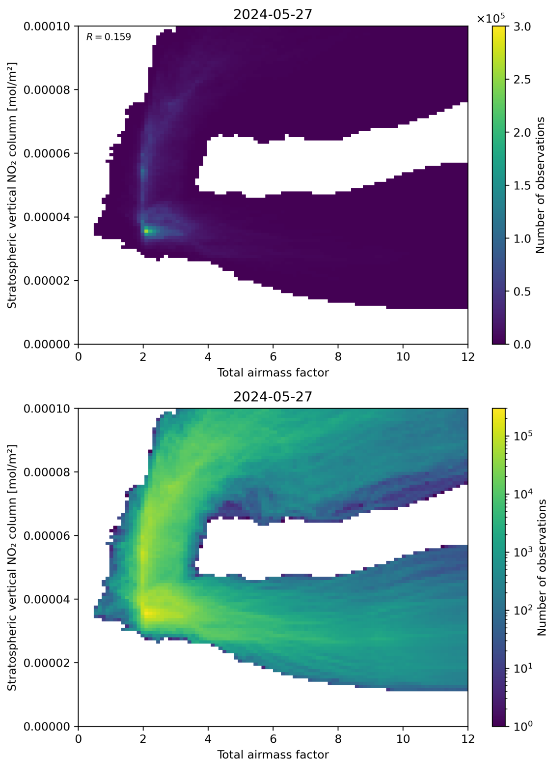
Figure 64: Scatter density plot of “Total airmass factor” against “Stratospheric vertical \text{NO}_2 column” for 2024-05-26 to 2024-05-28.
