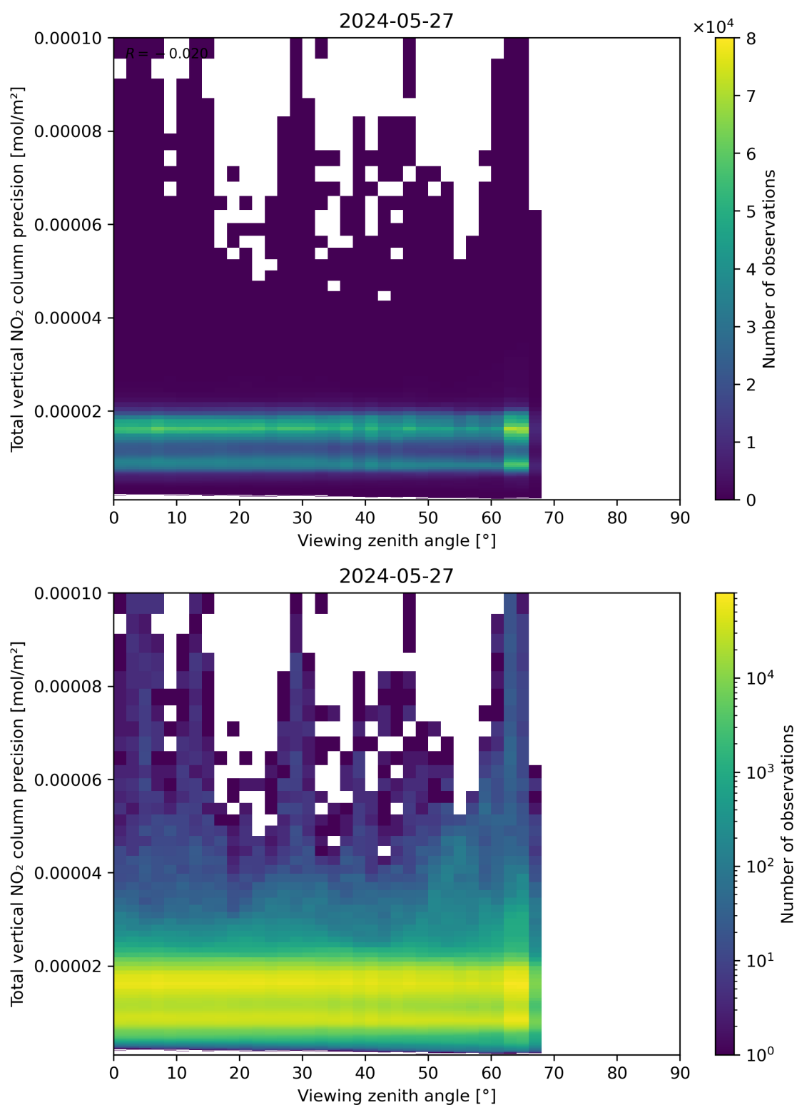
Figure 168: Scatter density plot of “Viewing zenith angle” against “Total vertical NO 2 column precision” for 2024-05-26 to 2024-05-28.
