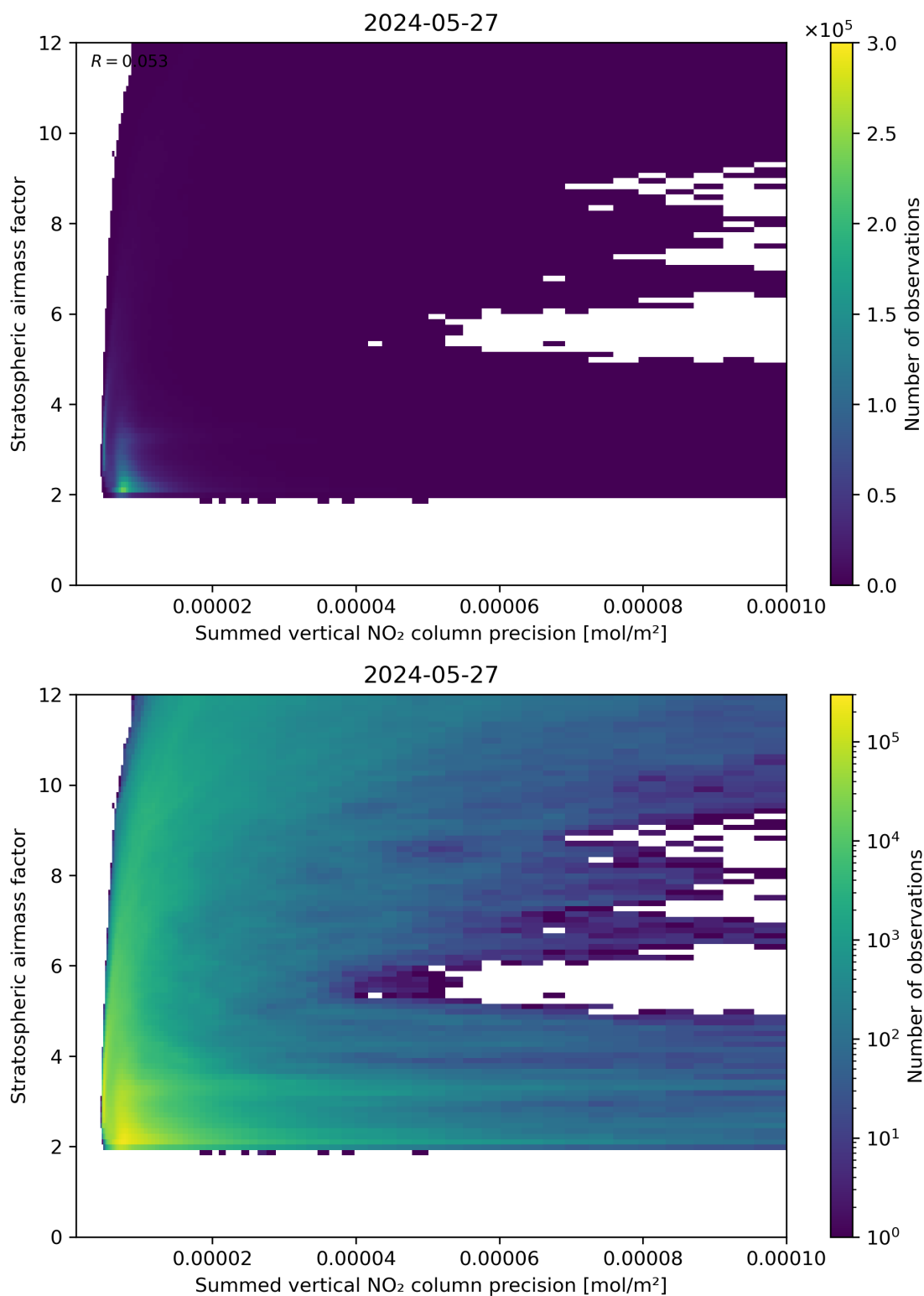
Figure 106: Scatter density plot of “Summed vertical NO 2 column precision” against “Stratospheric airmass factor” for 2024-05-26 to 2024-05-28.
