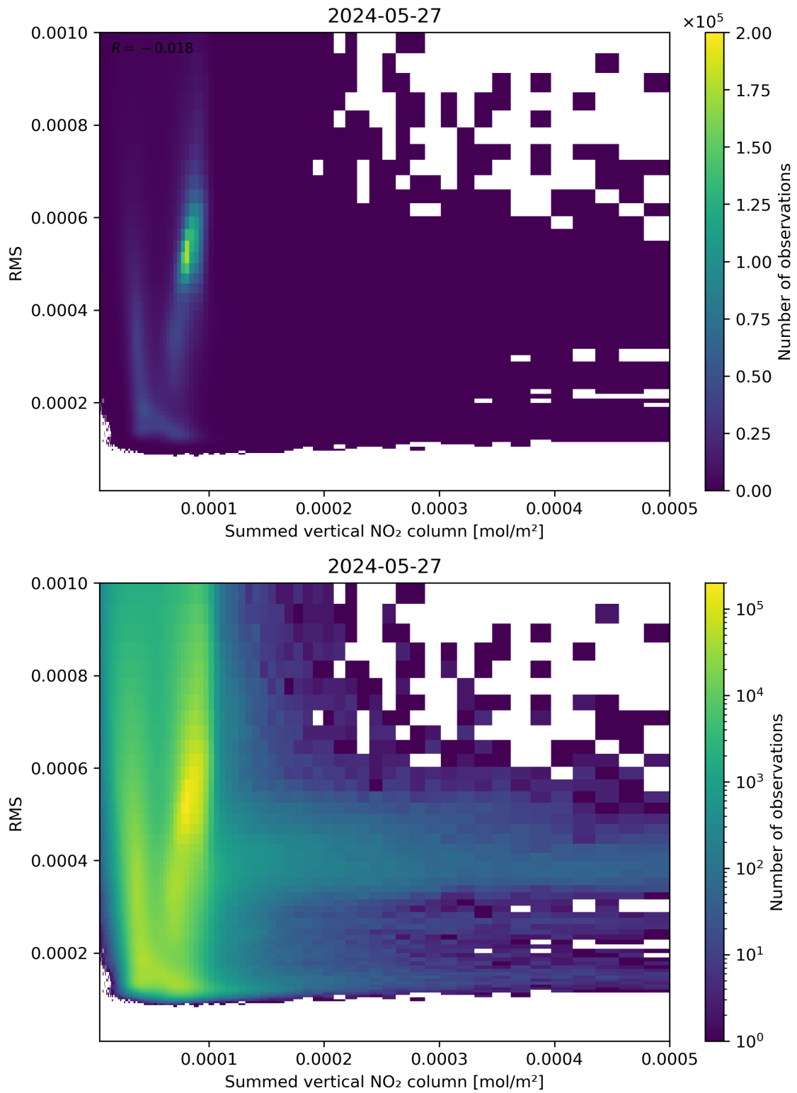
Figure 109: Scatter density plot of “Summed vertical NO 2 column” against “RMS” for 2024-05-26 to 2024-05-28.
