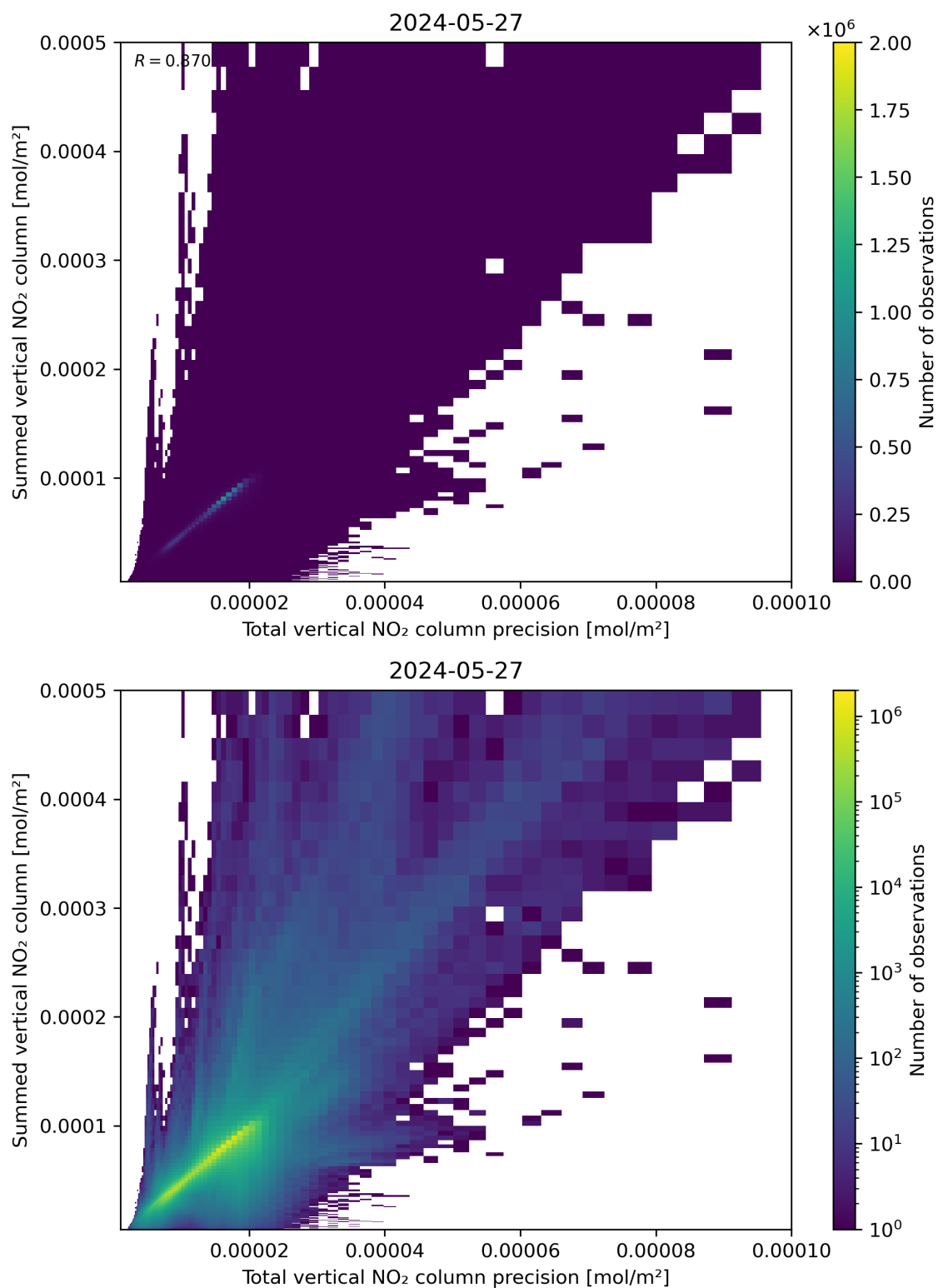
Figure 117: Scatter density plot of “Total vertical NO 2 column precision” against “Summed vertical NO 2 column” for 2024-05-26 to 2024-05-28.
