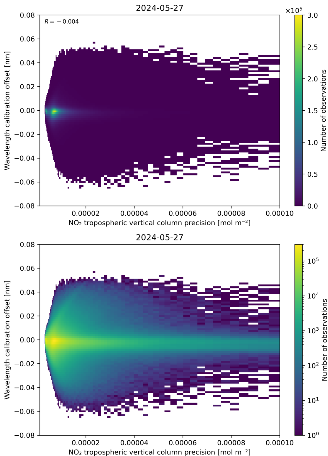
Figure 141: Scatter density plot of “NO 2 tropospheric vertical column precision” against “Wavelength calibration offset” for 2024-05-26 to 2024-05-28.
