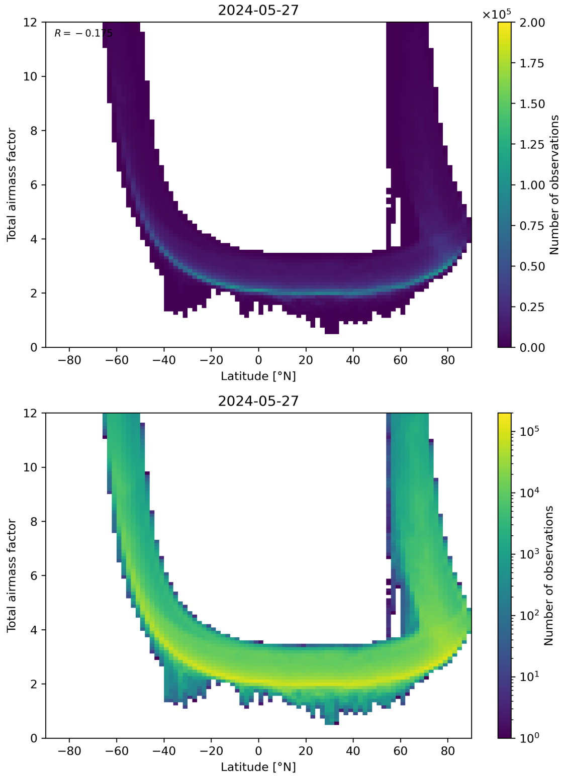
Figure 84: Scatter density plot of “Latitude” against “Total airmass factor” for 2024-05-26 to 2024-05-28.
