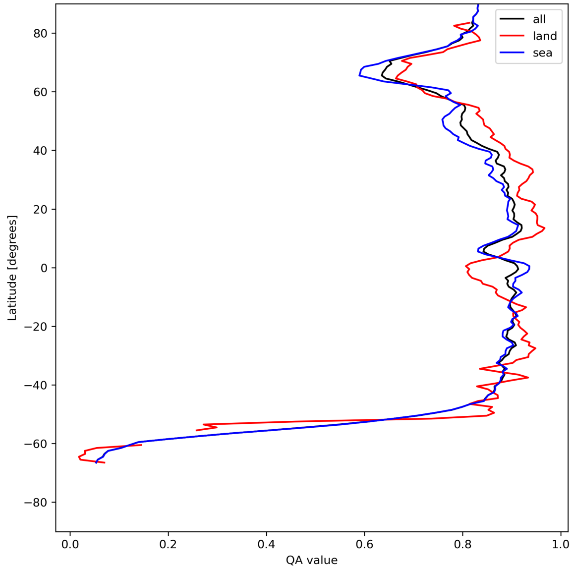
Figure 11: Zonal average of “QA value” for 2024-05-26 to 2024-05-28.
