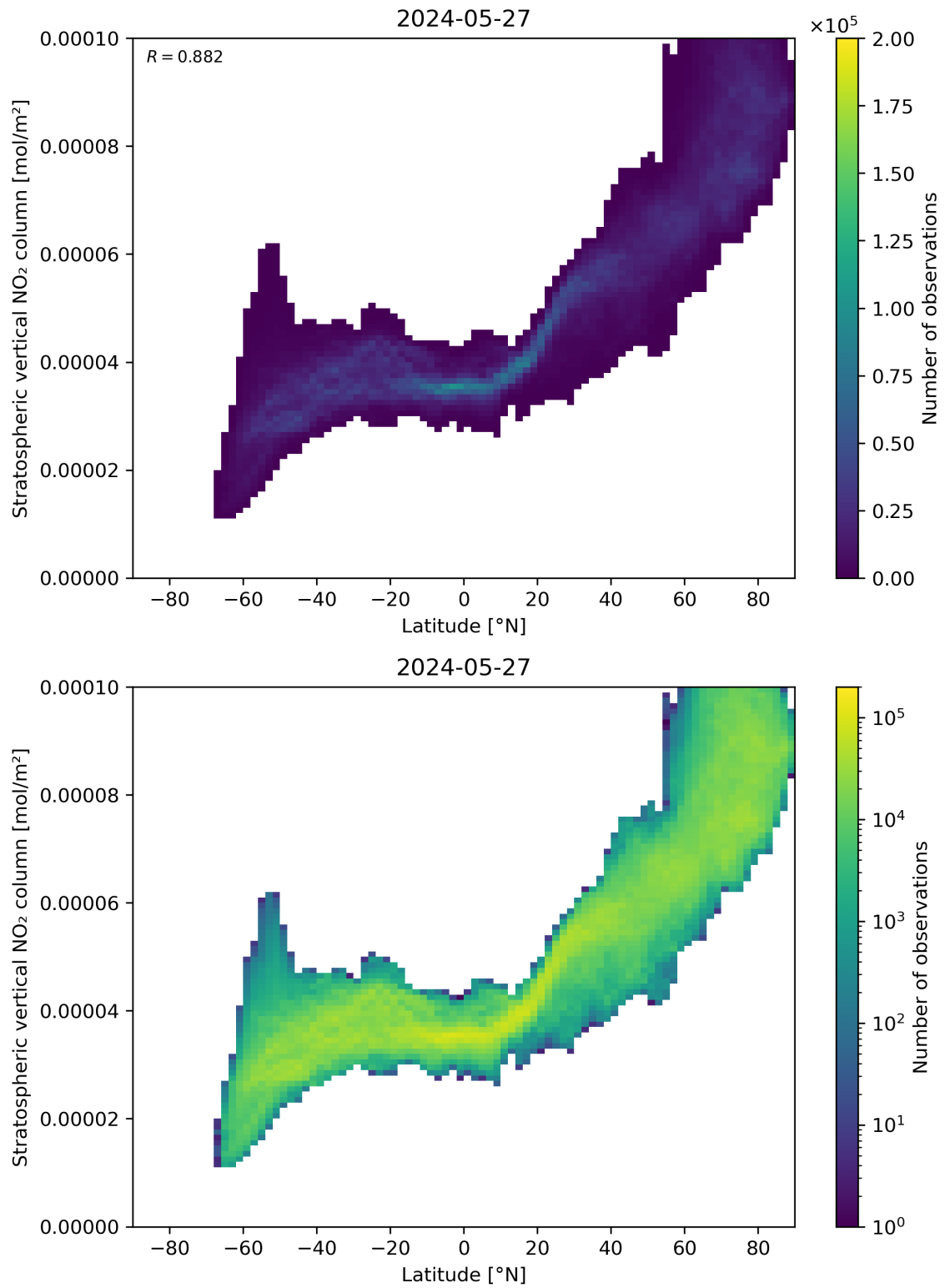
Figure 87: Scatter density plot of “Latitude” against “Stratospheric vertical \text{NO}_2 column” for 2024-05-26 to 2024-05-28.
