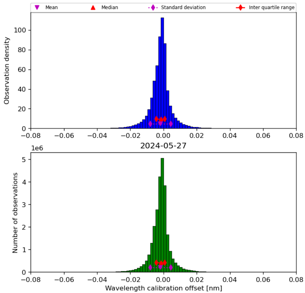
Figure 35: Histogram of “Wavelength calibration offset” for 2024-05-26 to 2024-05-28
