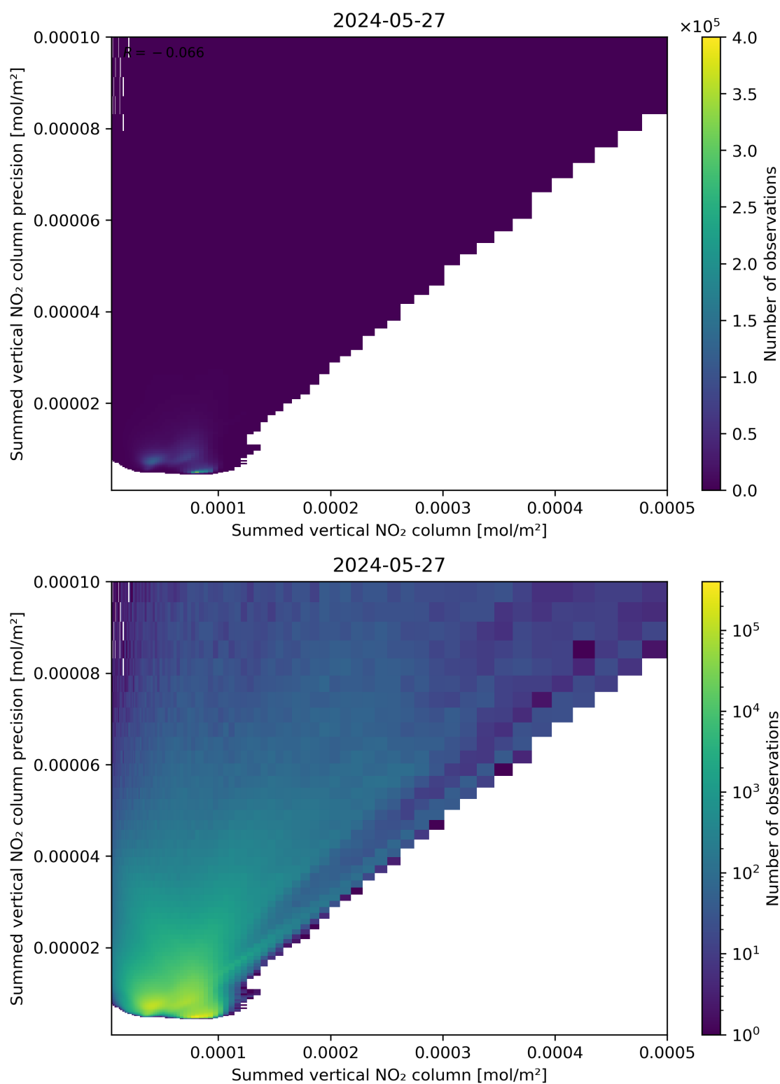
Figure 105: Scatter density plot of “Summed vertical NO 2 column” against “Summed vertical NO 2 column precision” for 2024-05-26 to 2024-05-28.
