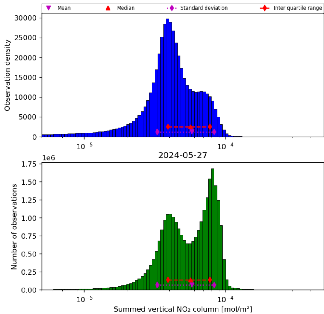
Figure 40: Histogram of “Summed vertical NO 2 column” for 2024-05-26 to 2024-05-28
