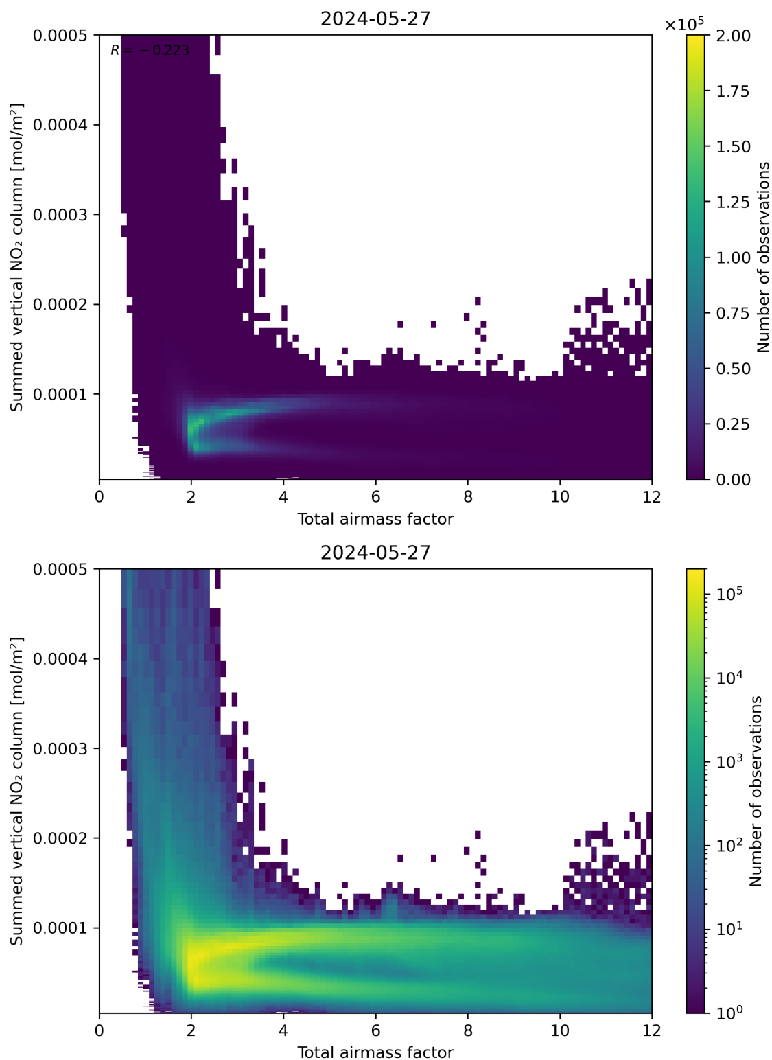
Figure 65: Scatter density plot of “Total airmass factor” against “Summed vertical NO 2 column” for 2024-05-26 to 2024-05-28.
