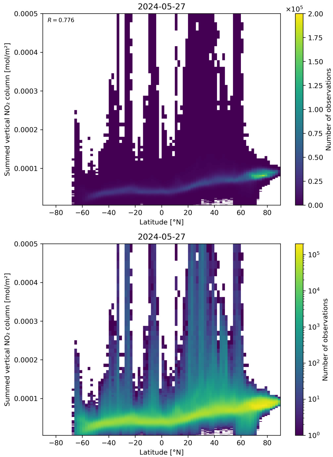
Figure 88: Scatter density plot of “Latitude” against “Summed vertical NO 2 column” for 2024-05-26 to 2024-05-28.
