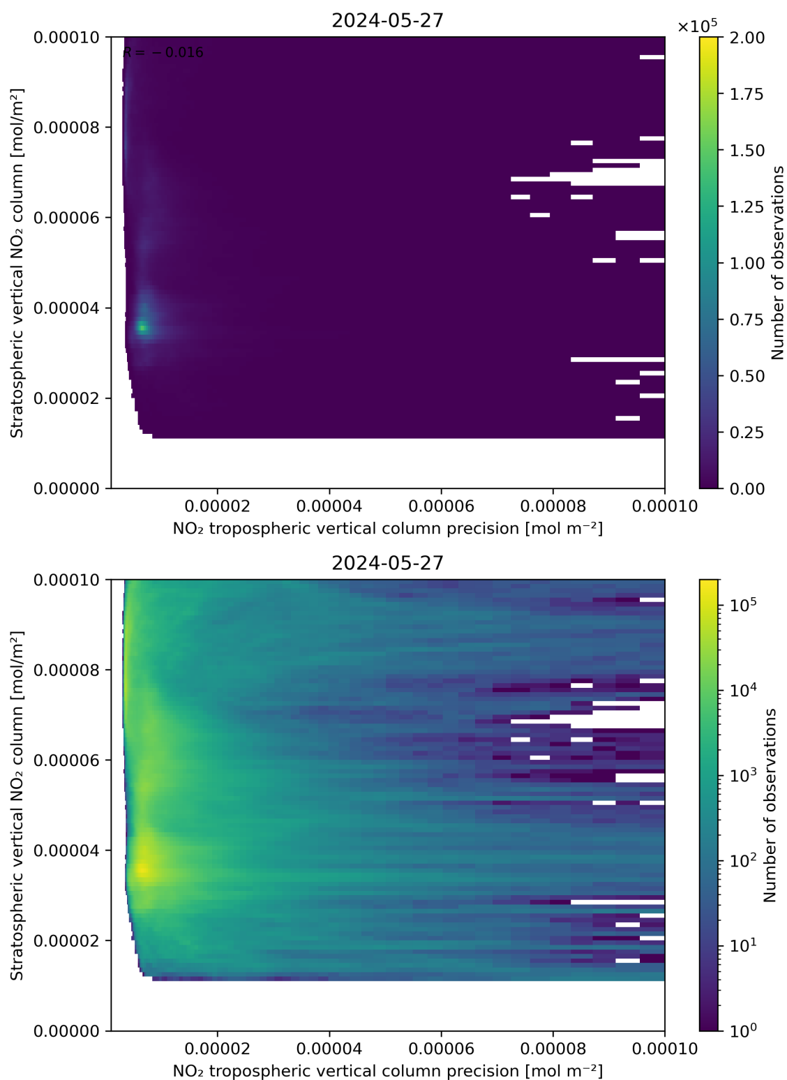
Figure 135: Scatter density plot of “NO 2 tropospheric vertical column precision” against “Stratospheric vertical NO 2 column” for 2024-05-26 to 2024-05-28.
