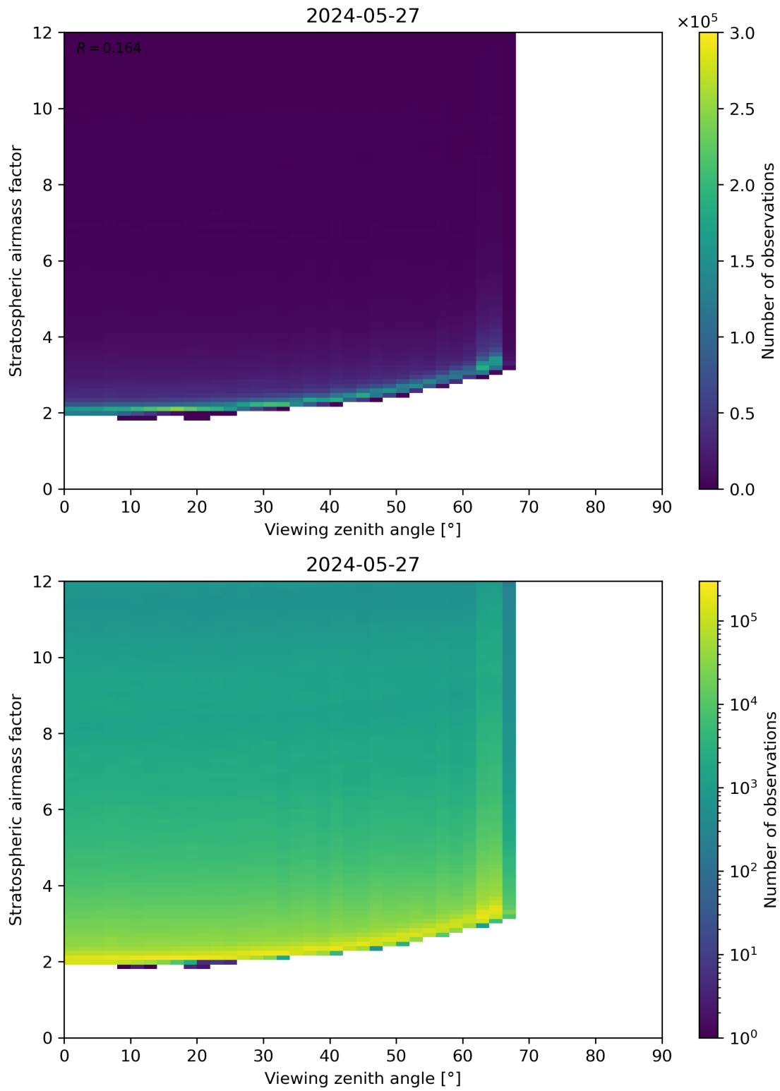
Figure 159: Scatter density plot of “Viewing zenith angle” against “Stratospheric airmass factor” for 2024-05-26 to 2024-05-28.
