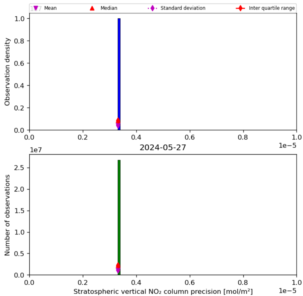
Figure 37: Histogram of “Stratospheric vertical NO 2 column precision” for 2024-05-26 to 2024-05-28
