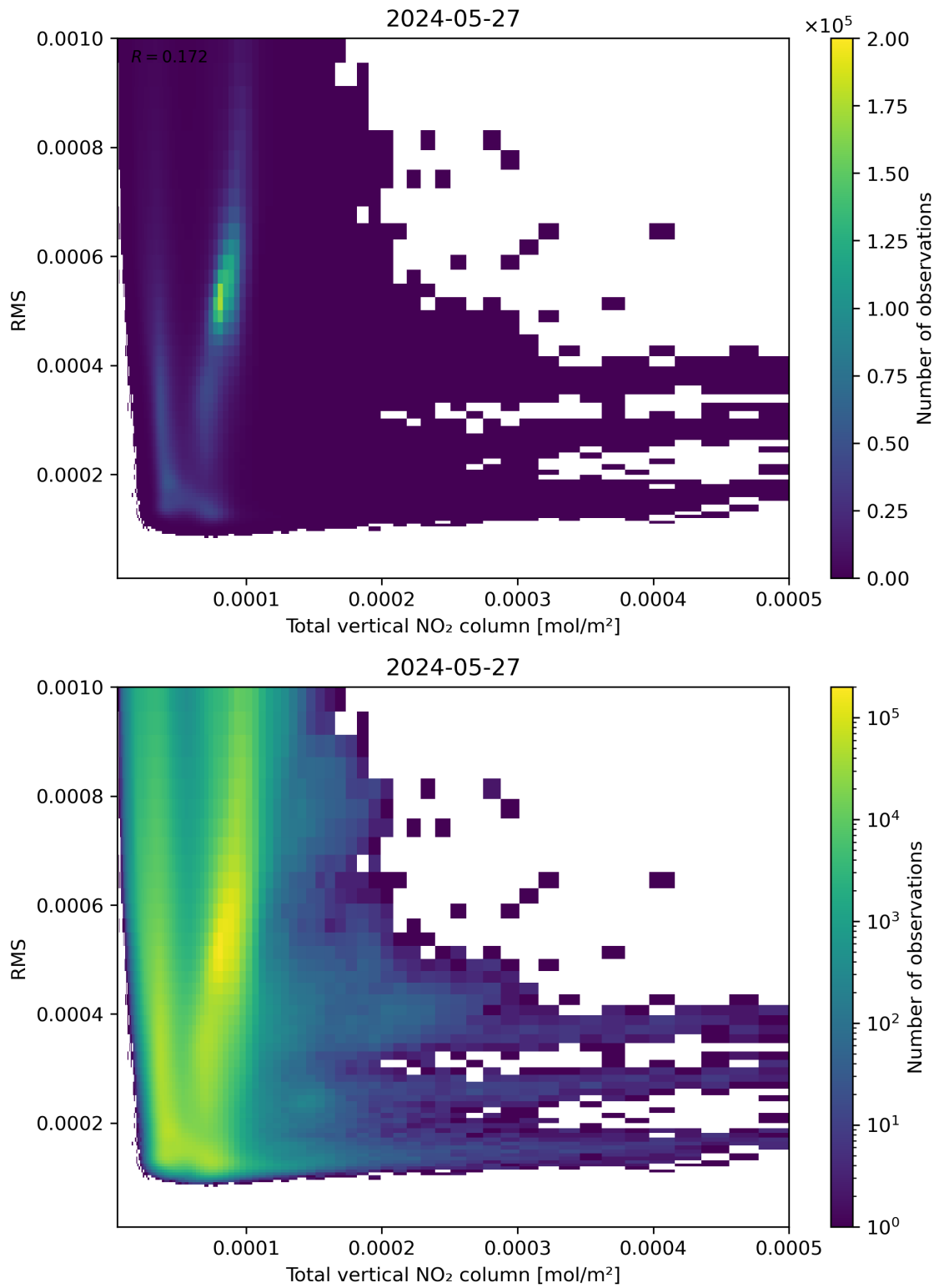
Figure 120: Scatter density plot of “Total vertical NO 2 column” against “RMS” for 2024-05-26 to 2024-05-28.
