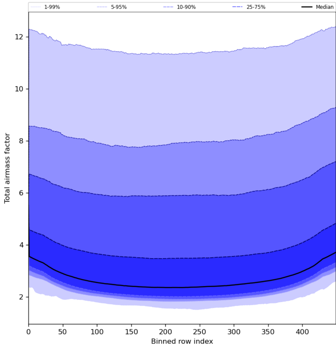
Figure 49: Along track statistics of “Total airmass factor” for 2024-05-26 to 2024-05-28
