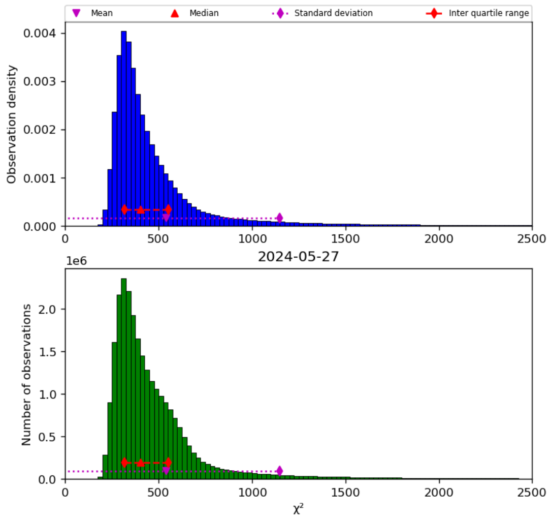
Figure 42: Histogram of “ \chi^2 ” for 2024-05-26 to 2024-05-28
