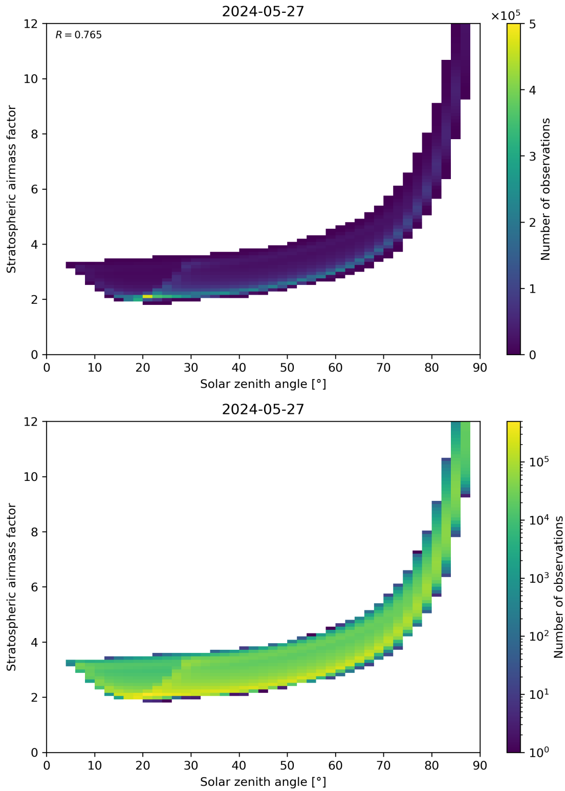
Figure 145: Scatter density plot of “Solar zenith angle” against “Stratospheric airmass factor” for 2024-05-26 to 2024-05-28.
