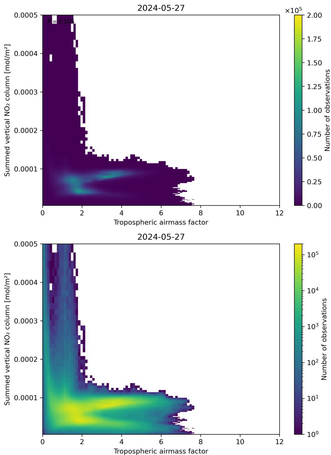
Figure 75: Scatter density plot of “Tropospheric airmass factor” against “Summed vertical NO 2 column” for 2024-05-26 to 2024-05-28.
