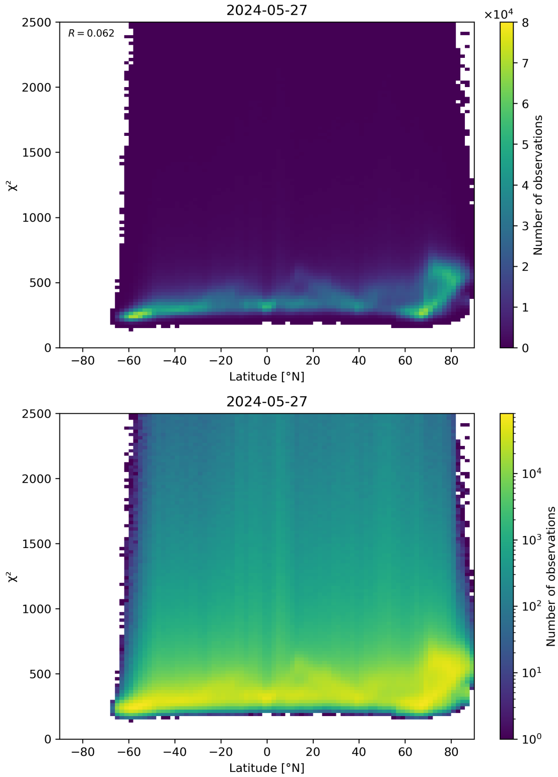
Figure 86: Scatter density plot of “Latitude” against “ \chi^2 ” for 2024-05-26 to 2024-05-28.
