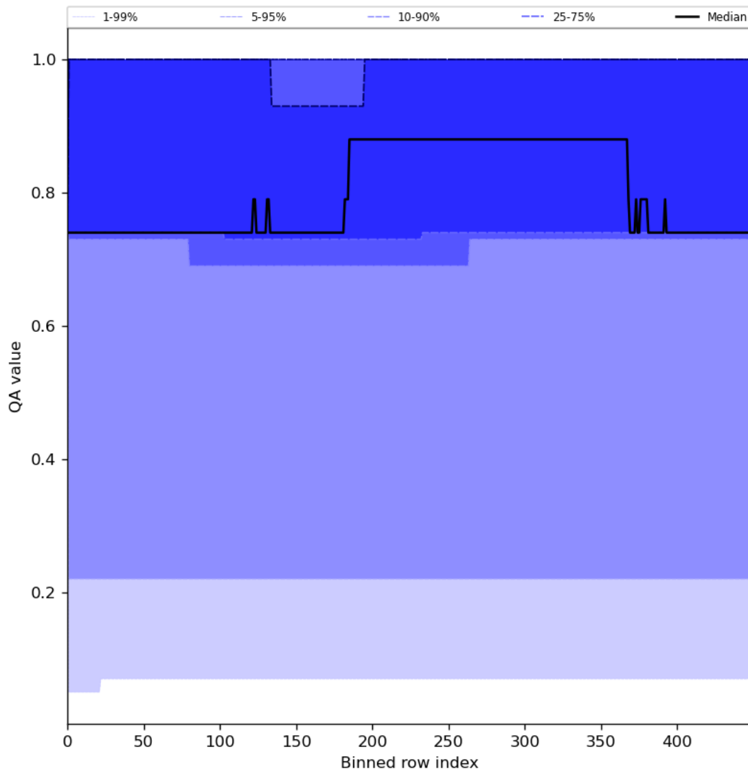
Figure 45: Along track statistics of "QA value" for 2024-05-26 to 2024-05-28
