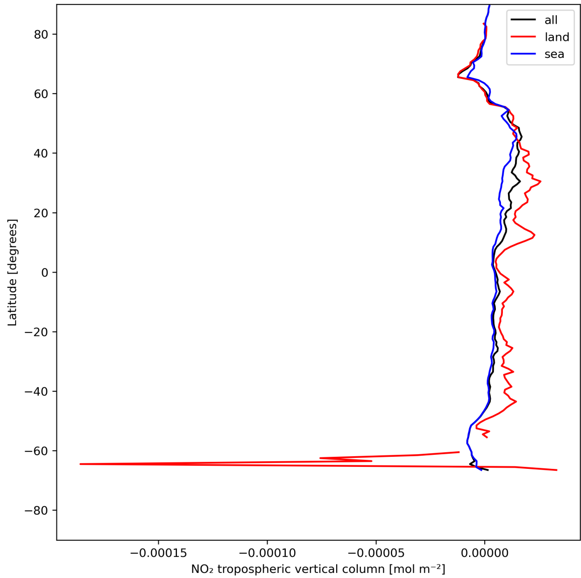
Figure 12: Zonal average of “NO 2 tropospheric vertical column” for 2024-05-26 to 2024-05-28.
