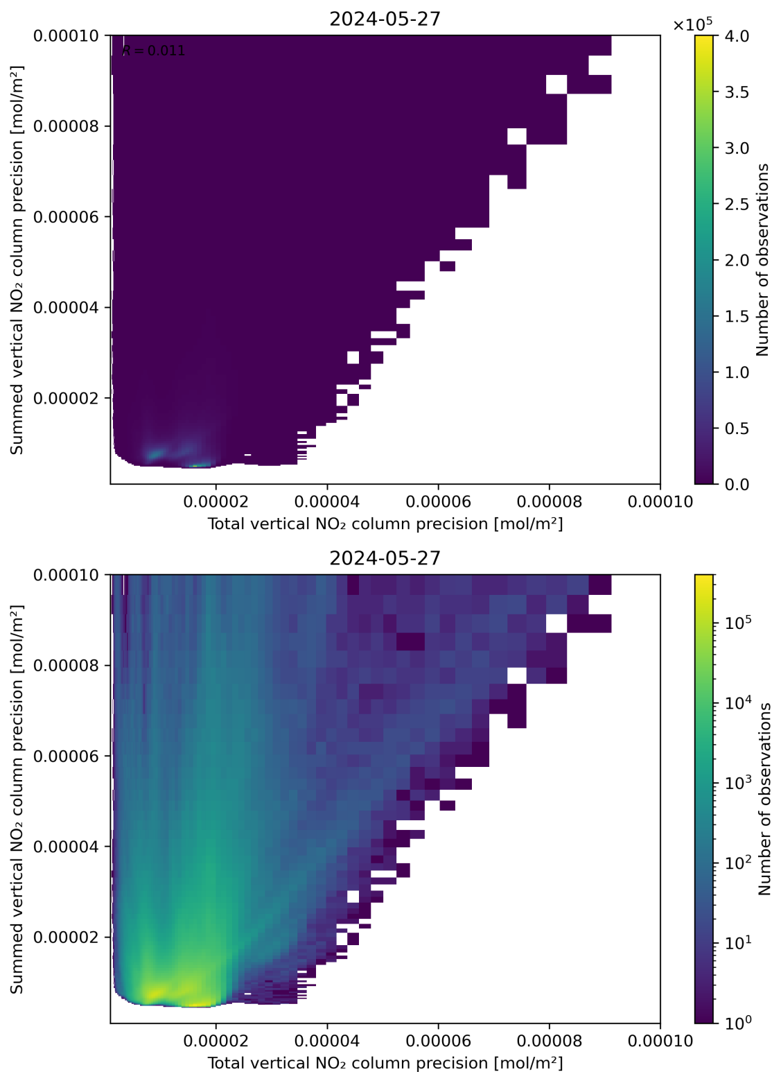
Figure 118: Scatter density plot of “Total vertical NO 2 column precision” against “Summed vertical NO 2 column precision” for 2024-05-26 to 2024-05-28.
