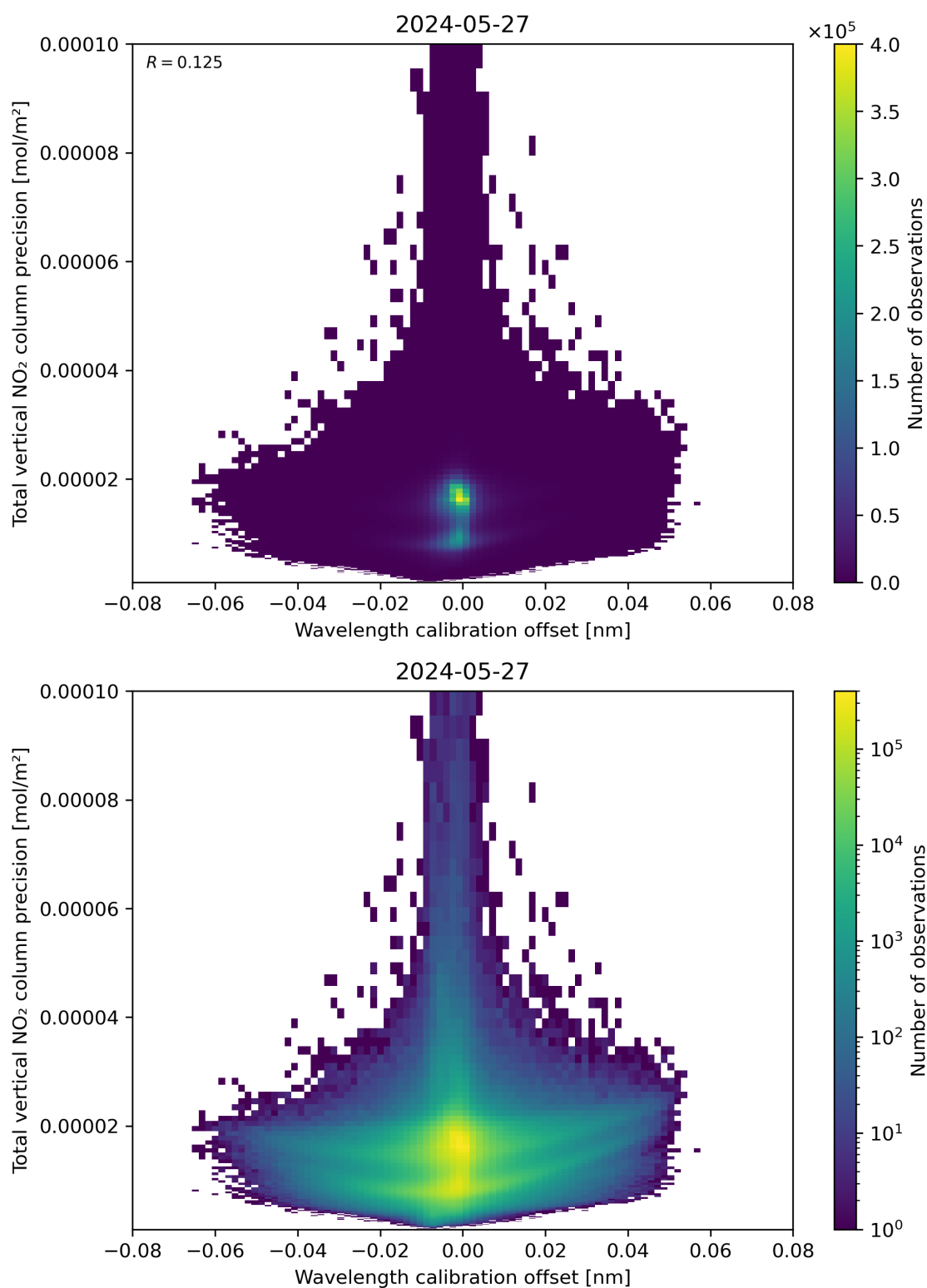
Figure 180: Scatter density plot of “Wavelength calibration offset” against “Total vertical NO 2 column precision” for 2024-05-26 to 2024-05-28.
