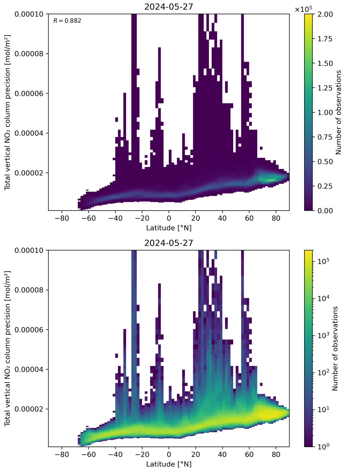
Figure 91: Scatter density plot of “Latitude” against “Total vertical NO 2 column precision” for 2024-05-26 to 2024-05-28.
