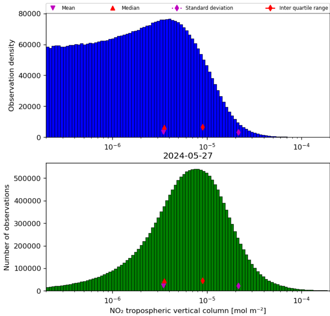
Figure 29: Histogram of “NO 2 tropospheric vertical column” for 2024-05-26 to 2024-05-28
