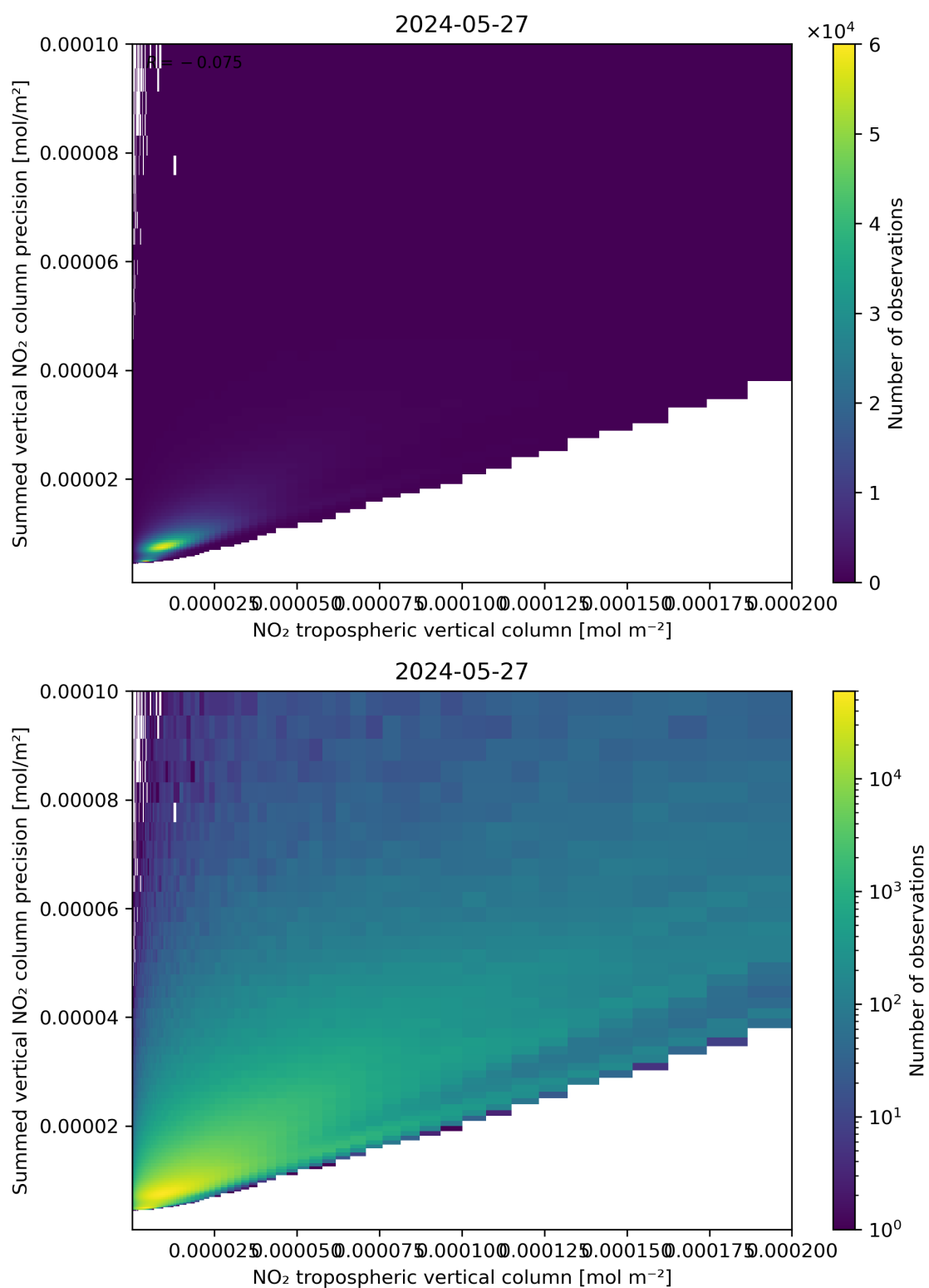
Figure 127: Scatter density plot of “NO 2 tropospheric vertical column” against “Summed vertical NO 2 column precision” for 2024-05-26 to 2024-05-28.
