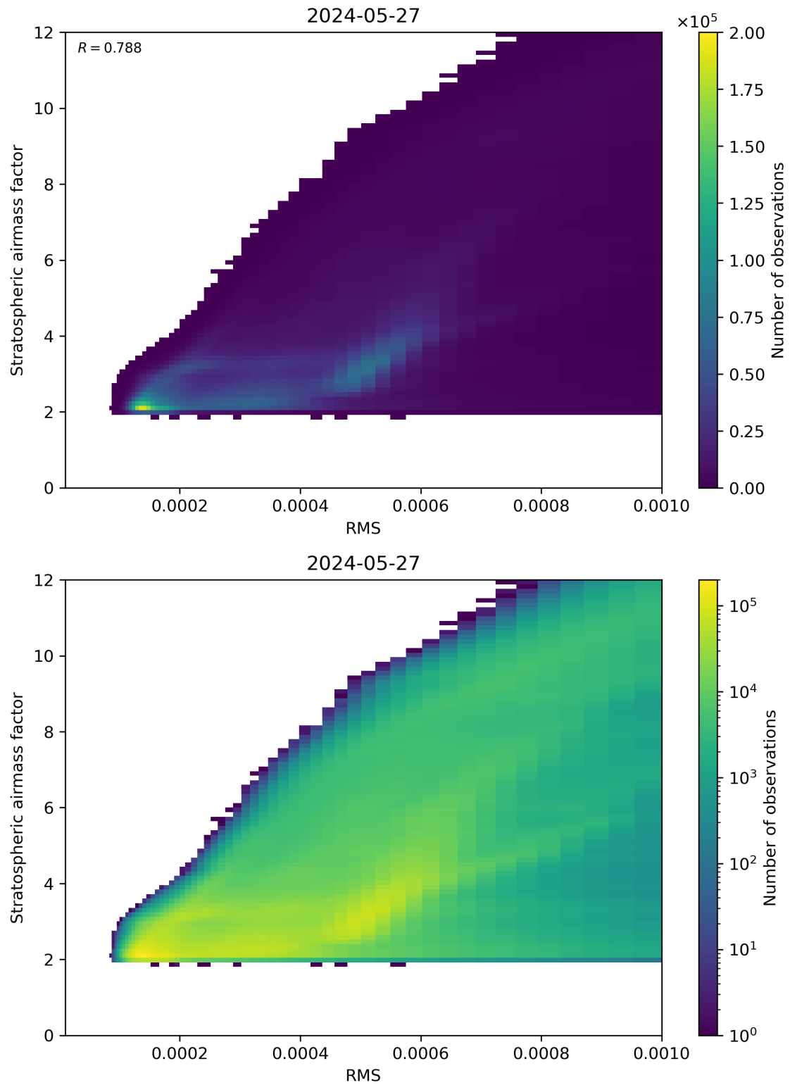
Figure 144: Scatter density plot of “RMS” against “Stratospheric airmass factor” for 2024-05-26 to 2024-05-28.
