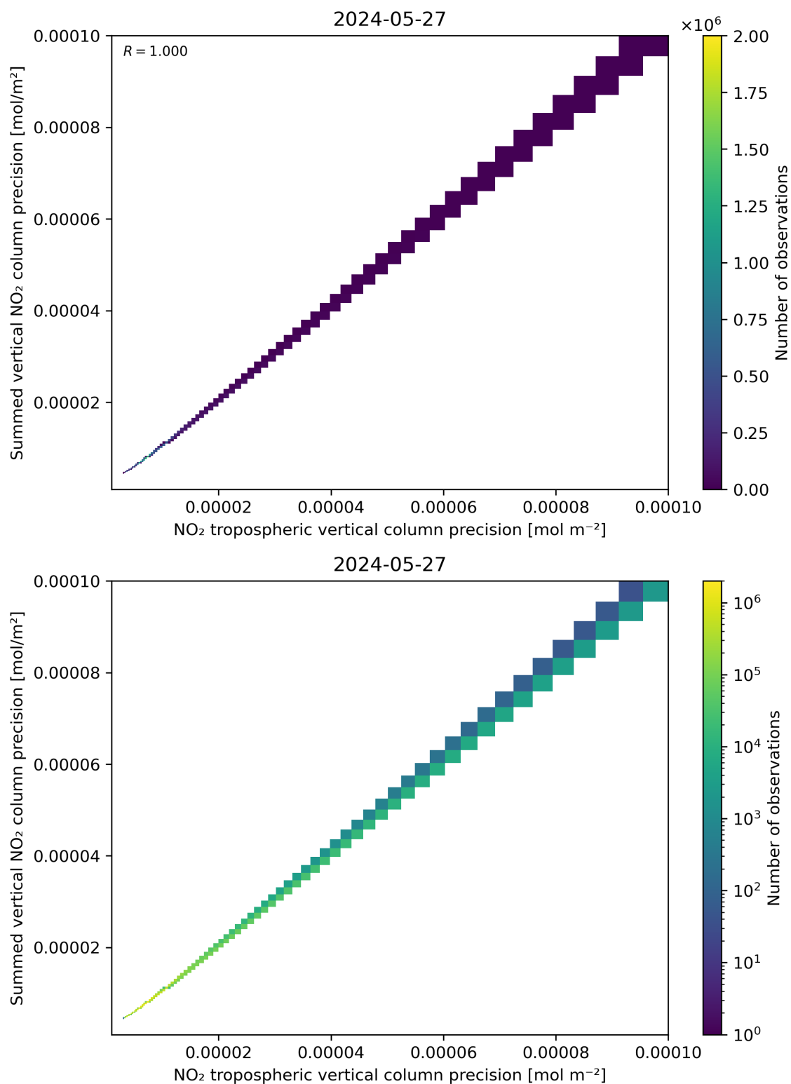
Figure 137: Scatter density plot of “NO 2 tropospheric vertical column precision” against “Summed vertical NO 2 column precision” for 2024-05-26 to 2024-05-28.
