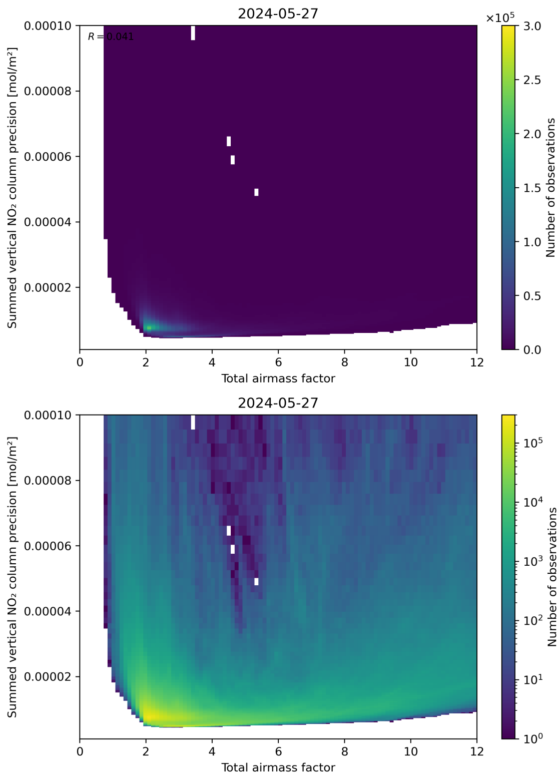
Figure 66: Scatter density plot of “Total airmass factor” against “Summed vertical NO 2 column precision” for 2024-05-26 to 2024-05-28.
