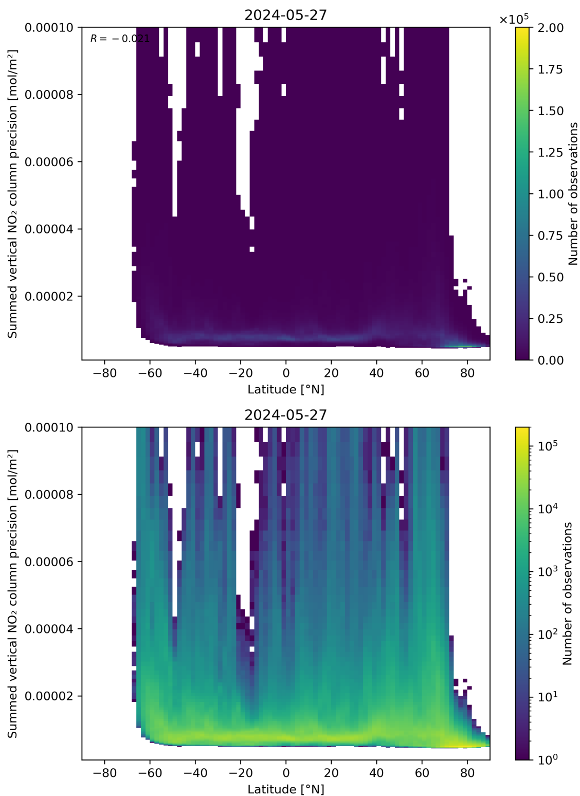
Figure 89: Scatter density plot of “Latitude” against “Summed vertical NO 2 column precision” for 2024-05-26 to 2024-05-28.
