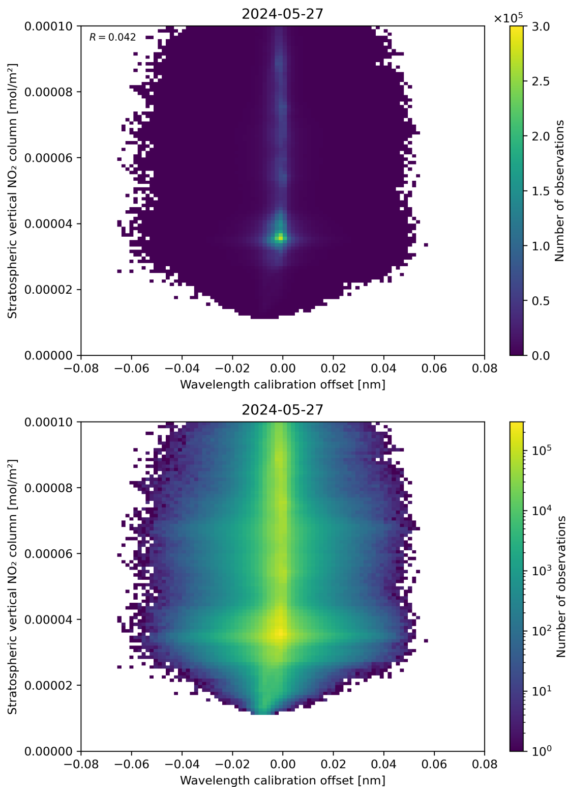
Figure 176: Scatter density plot of “Wavelength calibration offset” against “Stratospheric vertical NO 2 column” for 2024-05-26 to 2024-05-28.
