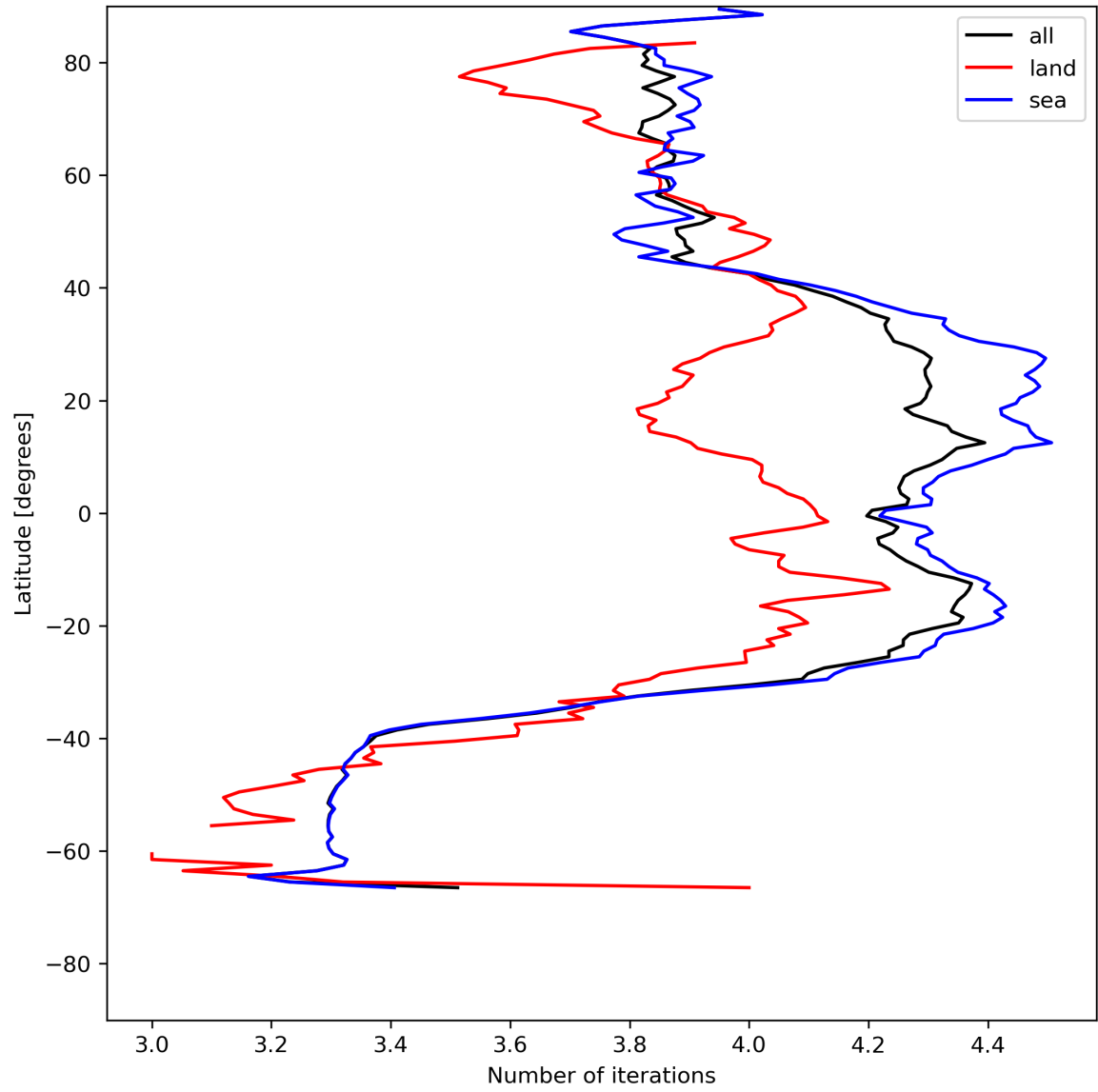
Figure 17: Zonal average of “Number of iterations” for 2024-05-26 to 2024-05-28.
