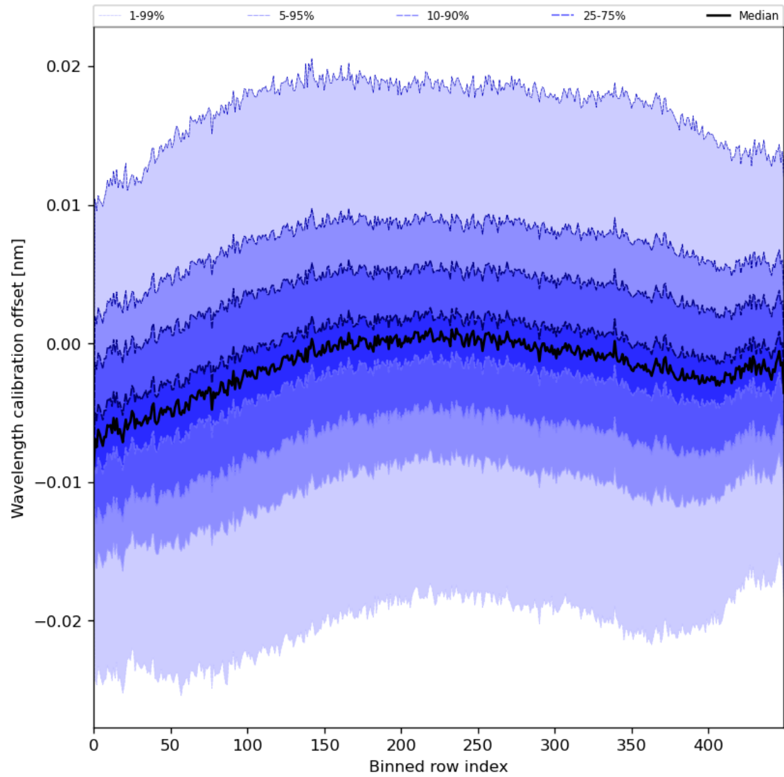
Figure 52: Along track statistics of “Wavelength calibration offset” for 2024-05-26 to 2024-05-28
