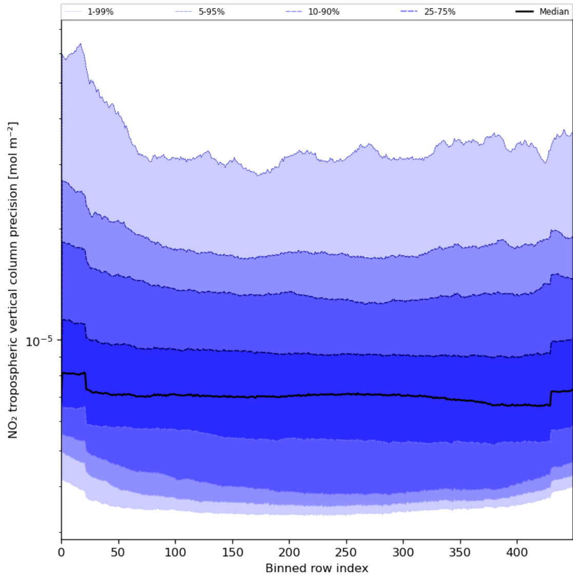
Figure 47: Along track statistics of “NO 2 tropospheric vertical column precision” for 2024-05-26 to 2024-05-28
