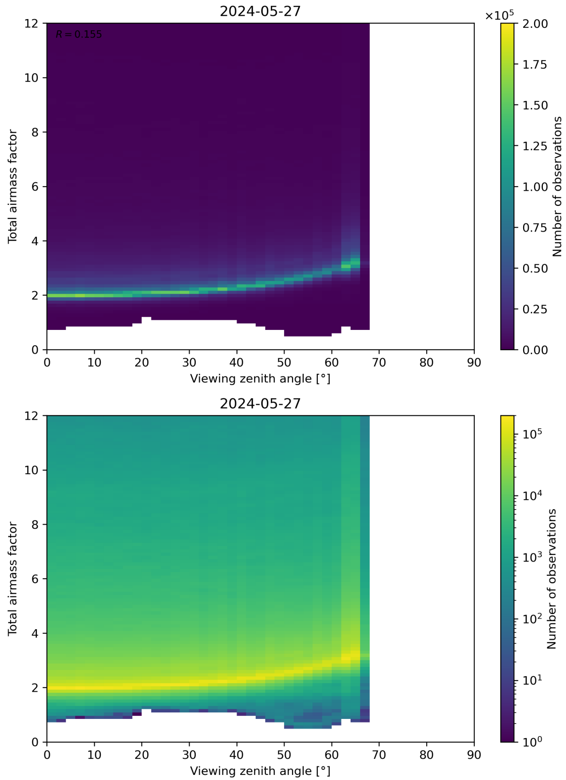
Figure 160: Scatter density plot of “Viewing zenith angle” against “Total airmass factor” for 2024-05-26 to 2024-05-28.
