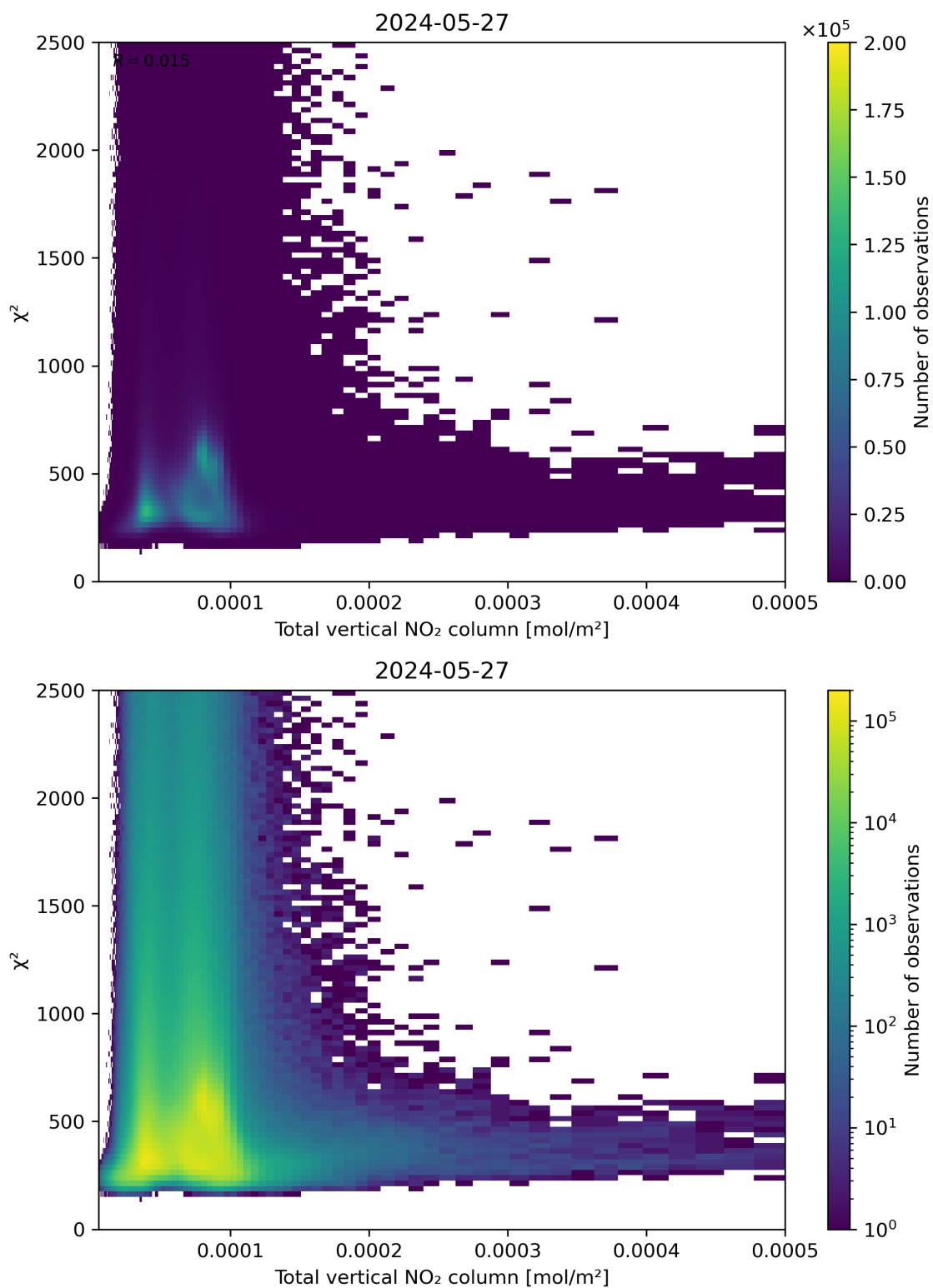
Figure 111: Scatter density plot of “Total vertical NO 2 column” against “ \chi^2 ” for 2024-05-26 to 2024-05-28.
