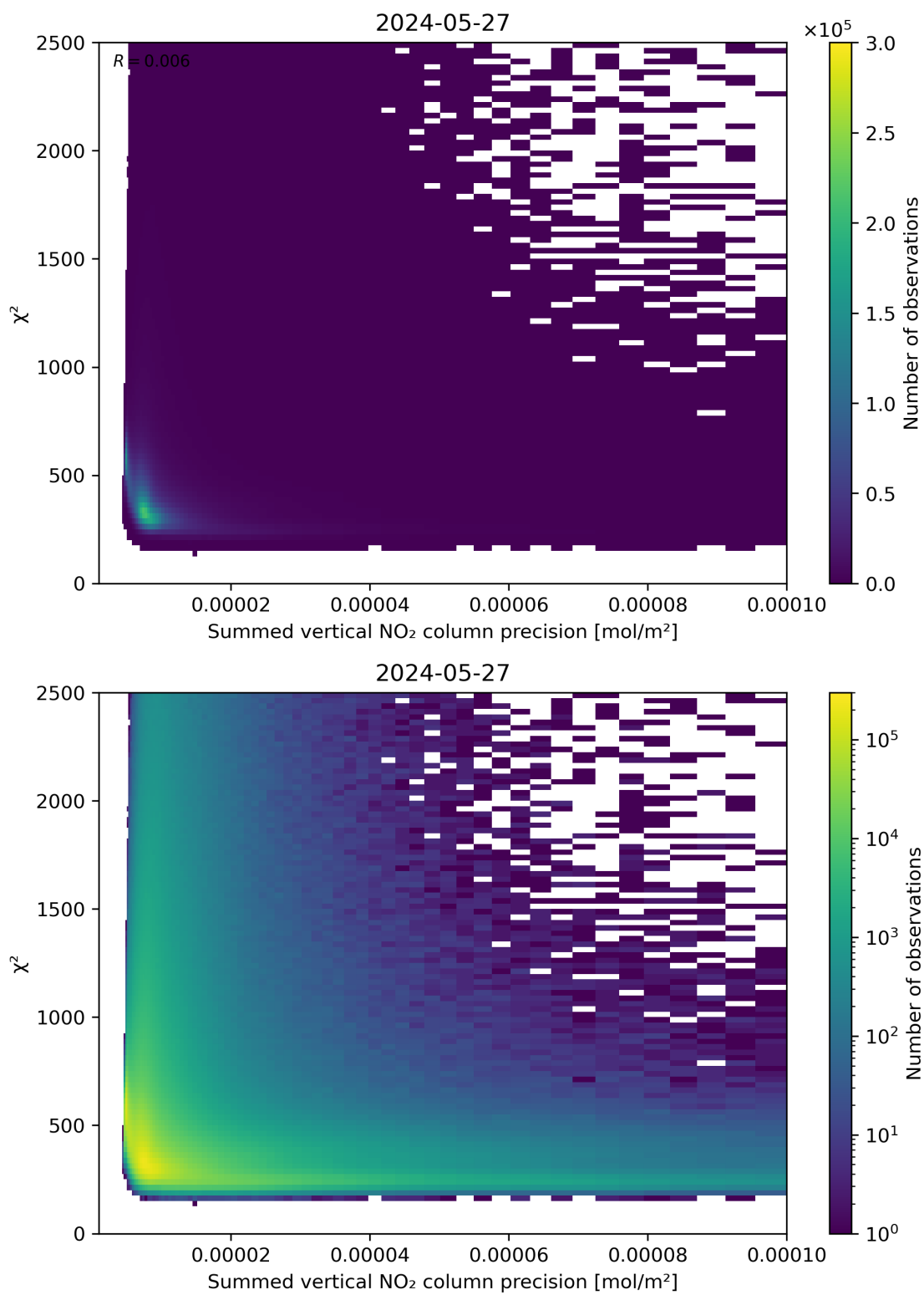
Figure 107: Scatter density plot of “Summed vertical NO 2 column precision” against “ \chi^2 ” for 2024-05-26 to 2024-05-28.
