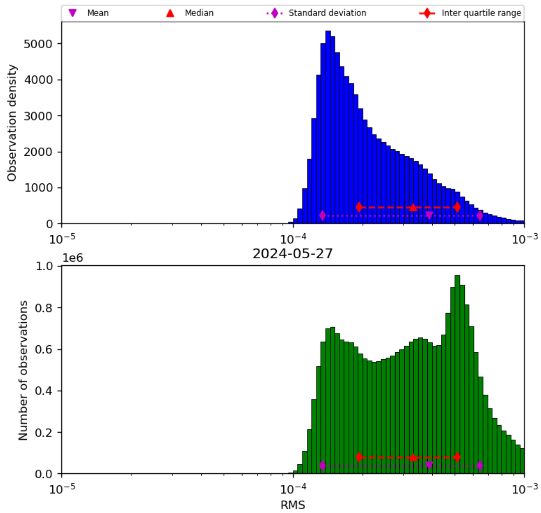
Figure 43: Histogram of “RMS” for 2024-05-26 to 2024-05-28
