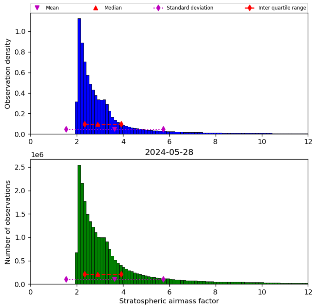
Figure 44: Histogram of “Stratospheric airmass factor” for 2024-05-28 to 2024-05-29
