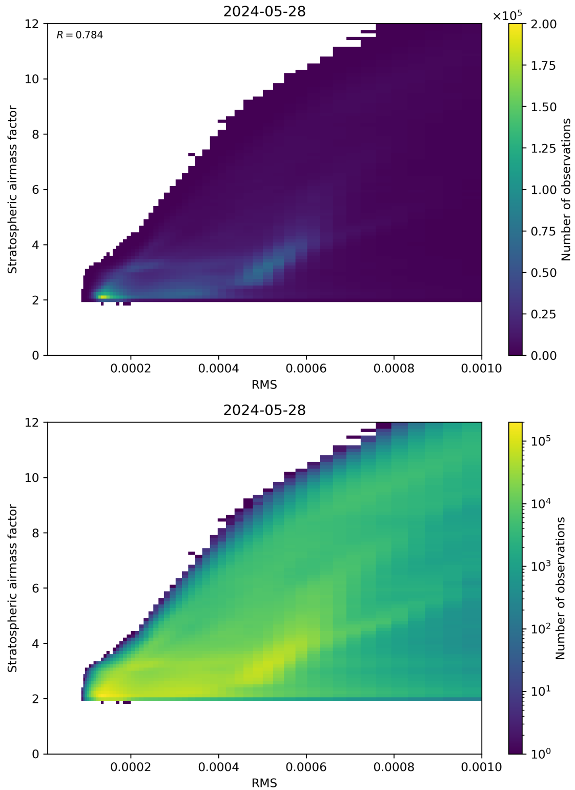
Figure 144: Scatter density plot of “RMS” against “Stratospheric airmass factor” for 2024-05-28 to 2024-05-29.
