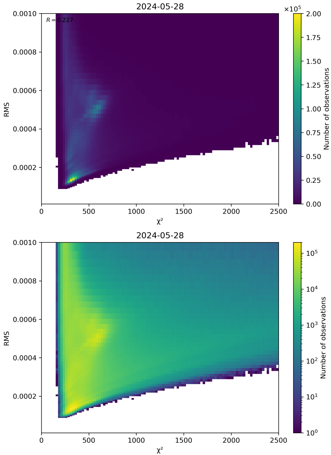
Figure 82: Scatter density plot of “ \chi^2 ” against “RMS” for 2024-05-28 to 2024-05-29.
