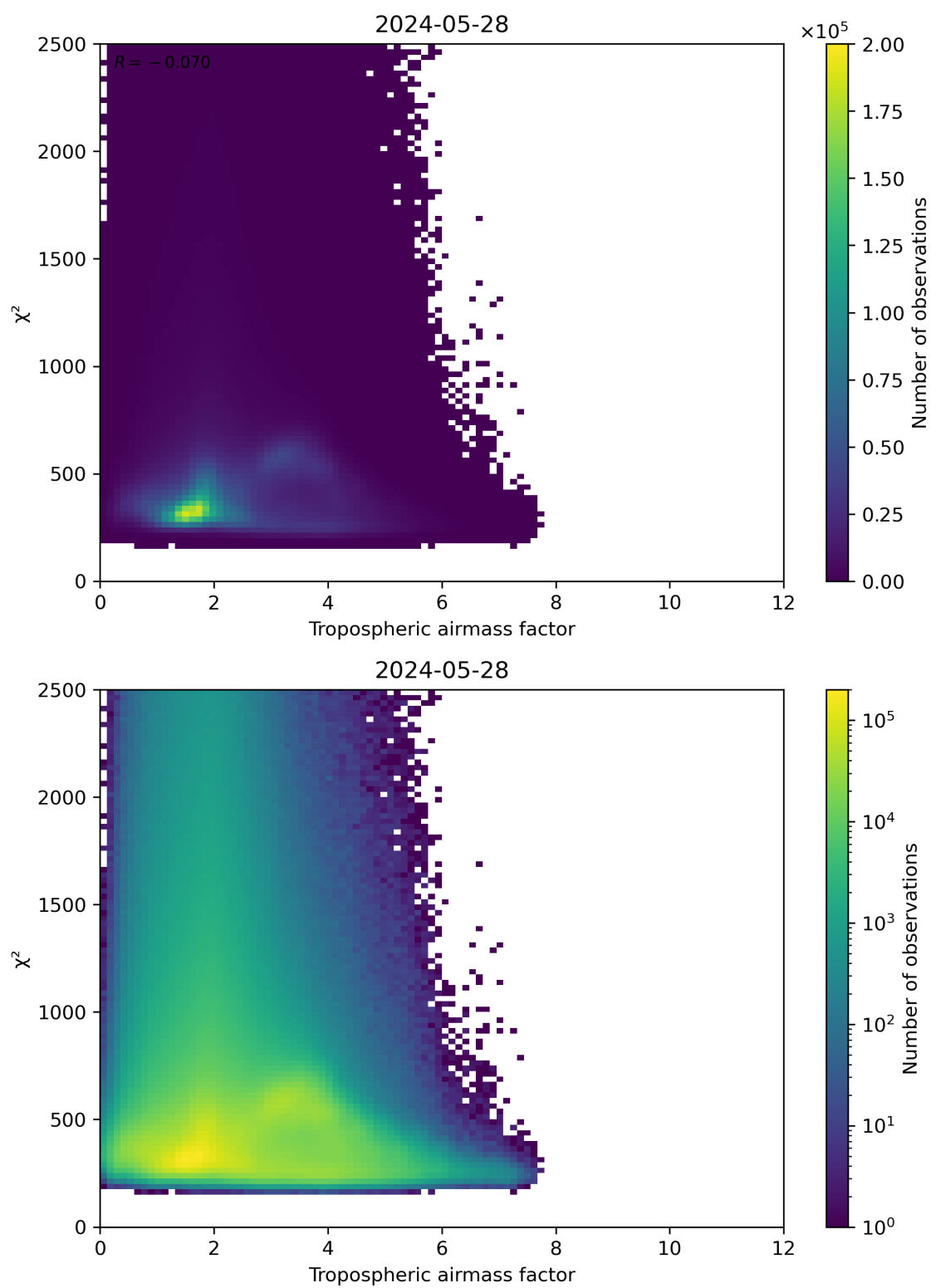
Figure 73: Scatter density plot of “Tropospheric airmass factor” against “ \chi^2 ” for 2024-05-28 to 2024-05-29.
