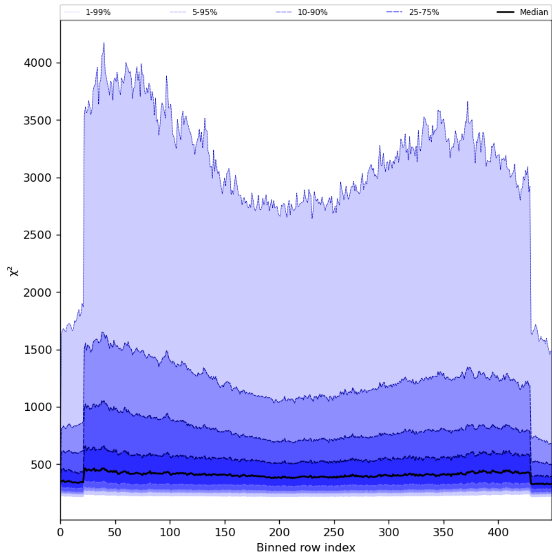
Figure 59: Along track statistics of “ \chi^2 ” for 2024-05-28 to 2024-05-29
