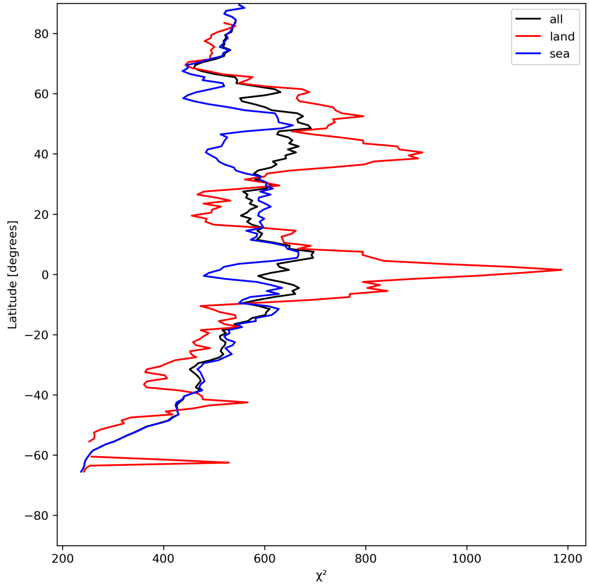
Figure 25: Zonal average of “ \chi^2 ” for 2024-05-28 to 2024-05-29.
