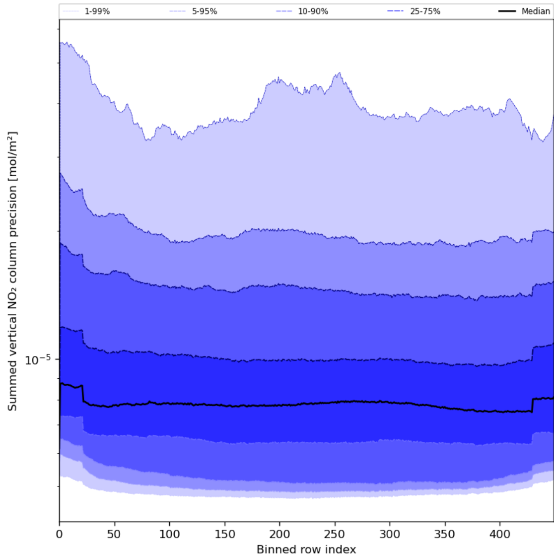
Figure 58: Along track statistics of “Summed vertical NO 2 column precision” for 2024-05-28 to 2024-05-29
