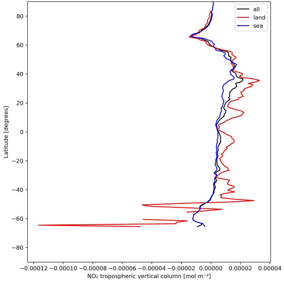
Figure 12: Zonal average of “NO 2 tropospheric vertical column” for 2024-05-28 to 2024-05-29.
