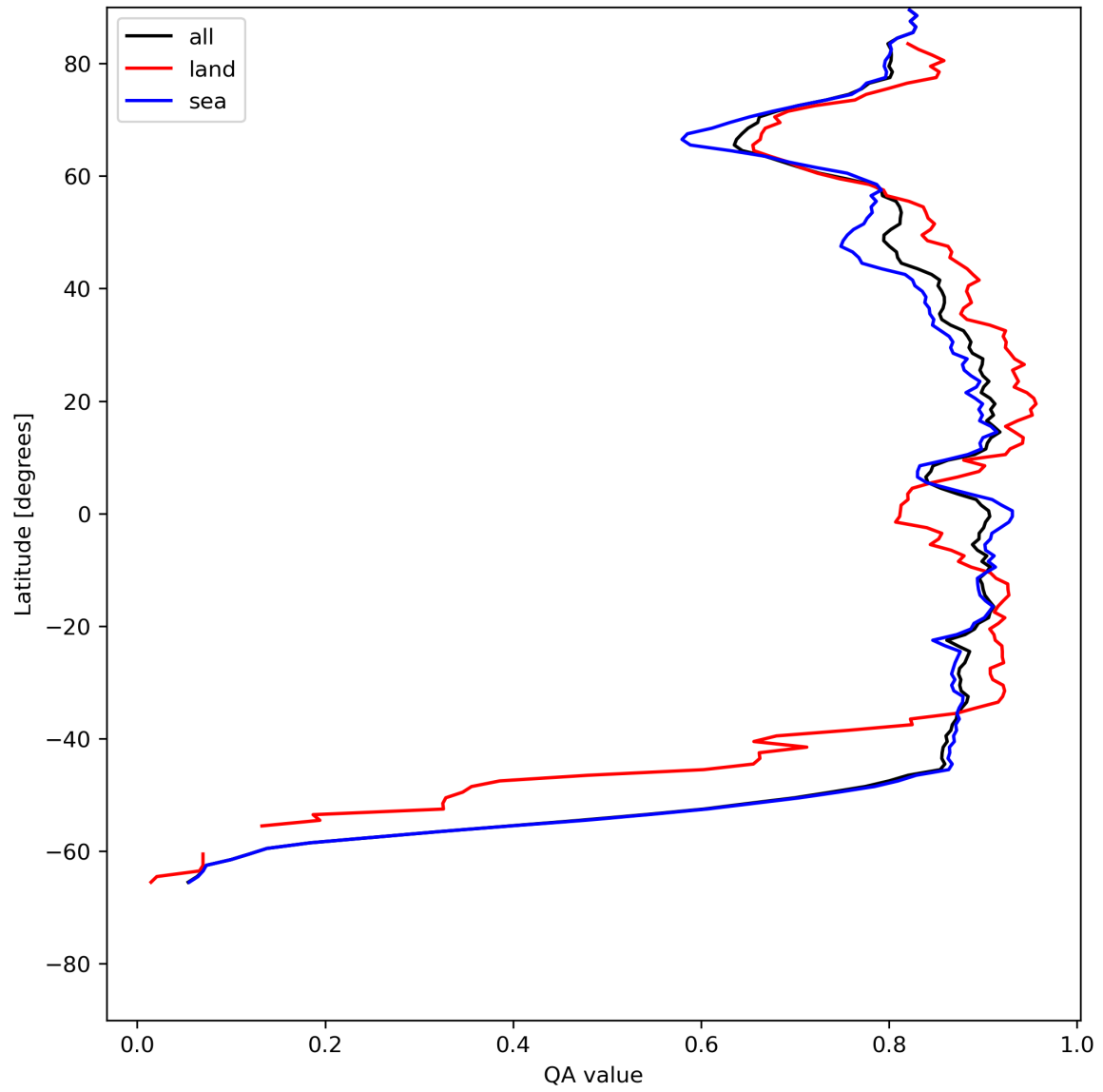
Figure 11: Zonal average of “QA value” for 2024-05-28 to 2024-05-29.
