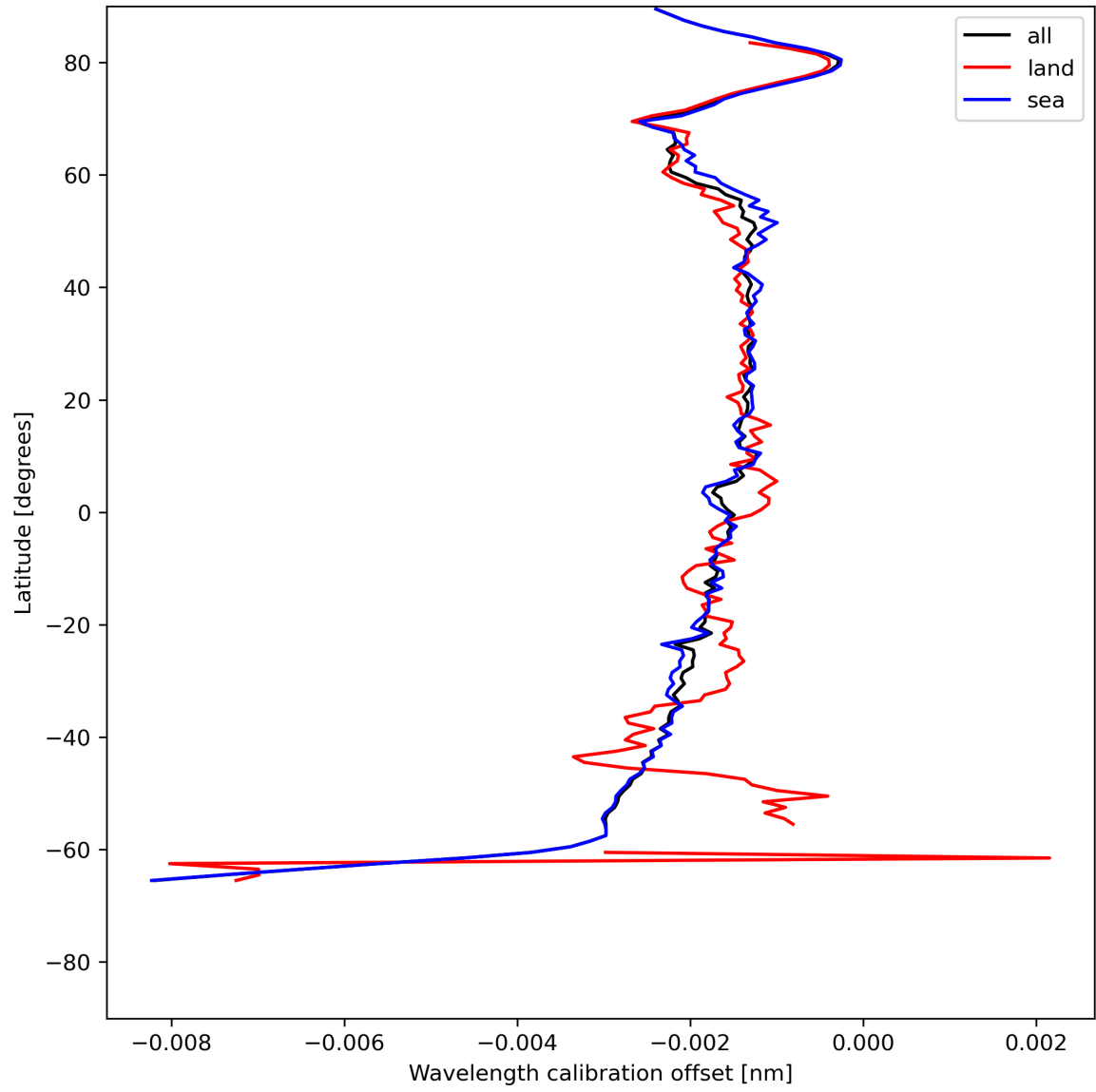
Figure 18: Zonal average of “Wavelength calibration offset” for 2024-05-28 to 2024-05-29.
