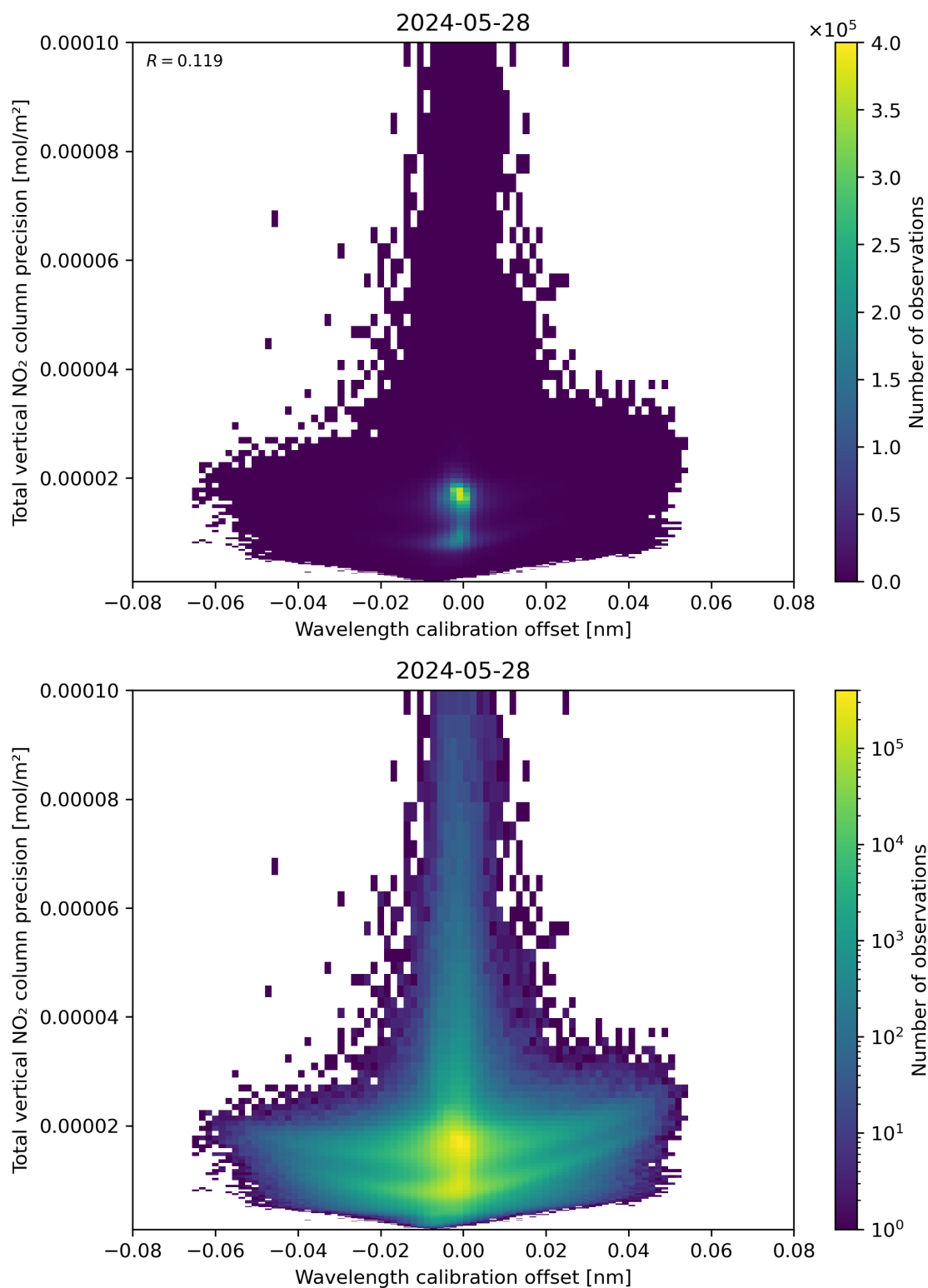
Figure 180: Scatter density plot of “Wavelength calibration offset” against “Total vertical NO 2 column precision” for 2024-05-28 to 2024-05-29.
