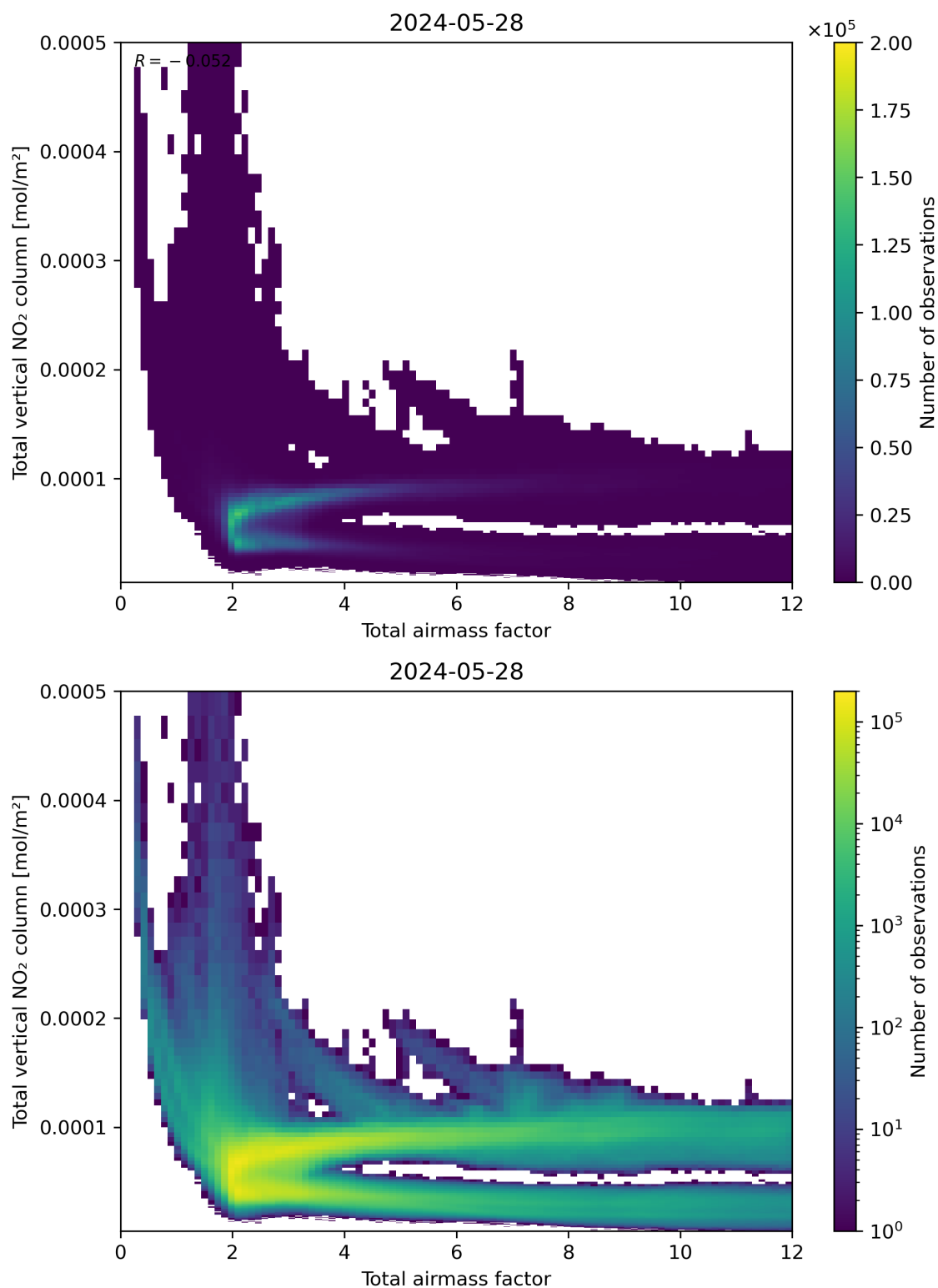
Figure 67: Scatter density plot of “Total airmass factor” against “Total vertical NO 2 column” for 2024-05-28 to 2024-05-29.
