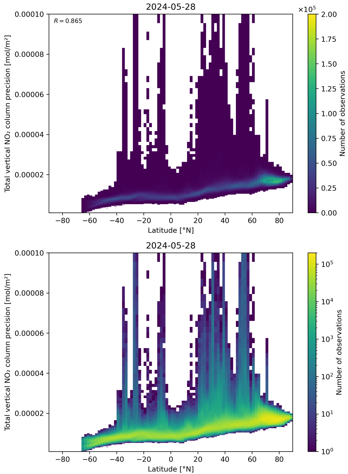
Figure 91: Scatter density plot of “Latitude” against “Total vertical NO 2 column precision” for 2024-05-28 to 2024-05-29.
