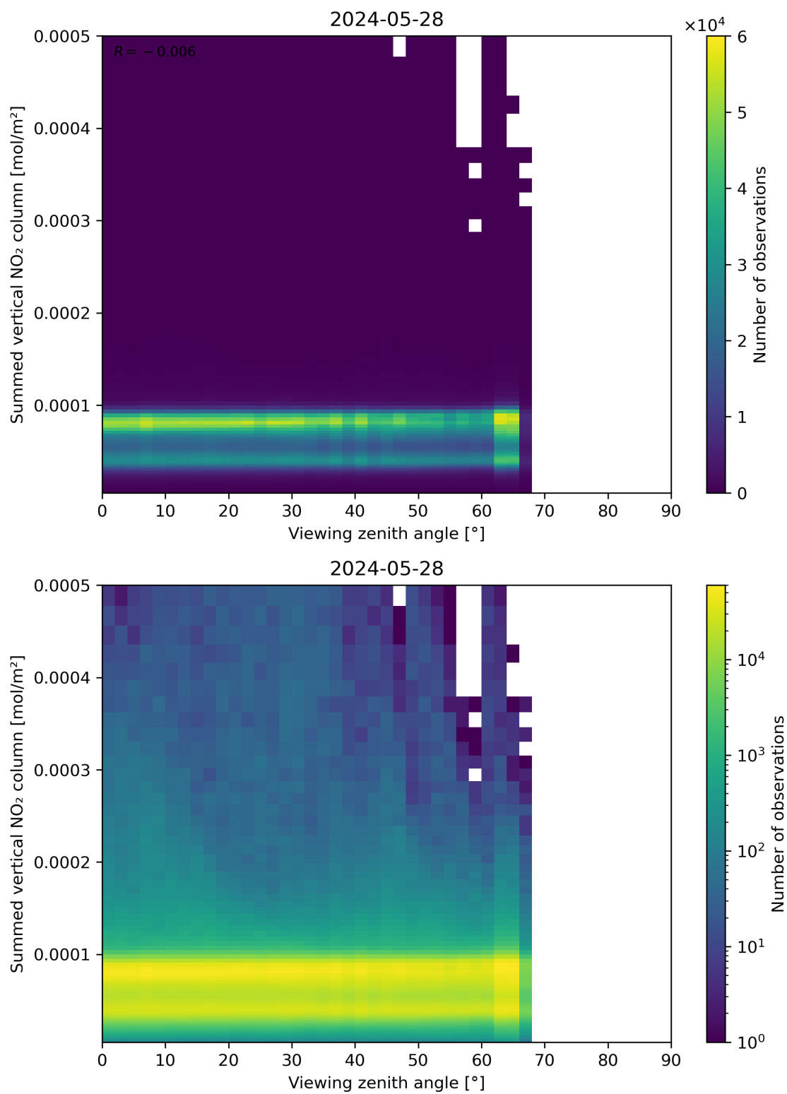
Figure 165: Scatter density plot of “Viewing zenith angle” against “Summed vertical NO 2 column” for 2024-05-28 to 2024-05-29.
