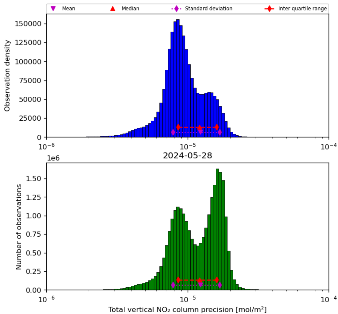
Figure 39: Histogram of “Total vertical NO 2 column precision” for 2024-05-28 to 2024-05-29
