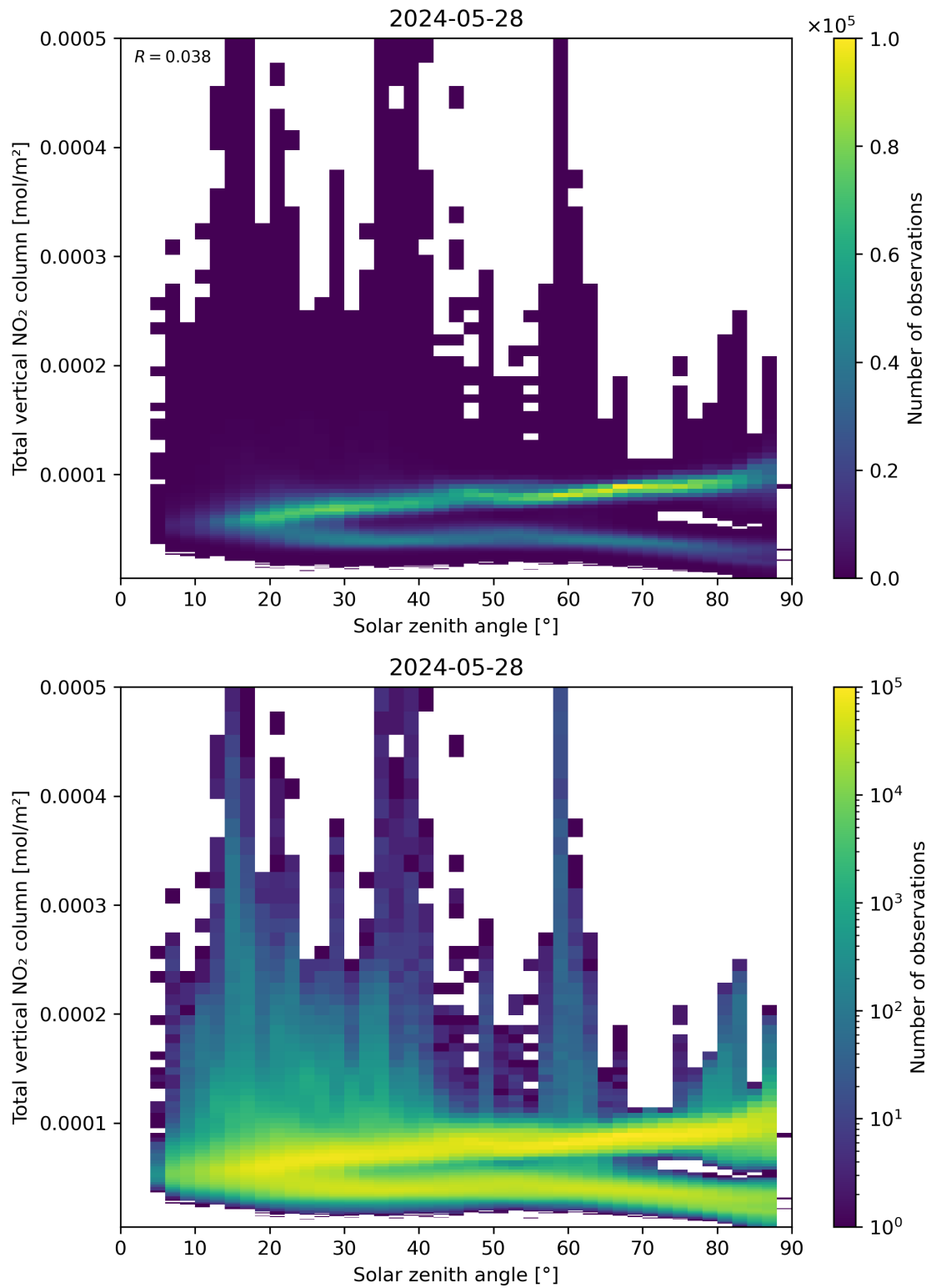
Figure 153: Scatter density plot of “Solar zenith angle” against “Total vertical NO 2 column” for 2024-05-28 to 2024-05-29.
