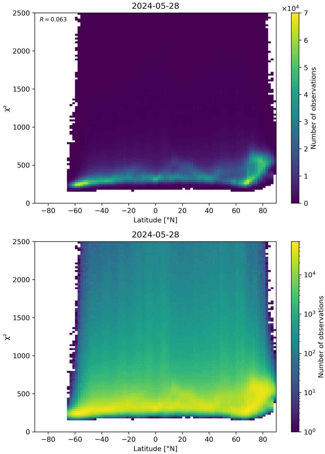
Figure 86: Scatter density plot of “Latitude” against “ \chi^2 ” for 2024-05-28 to 2024-05-29.
