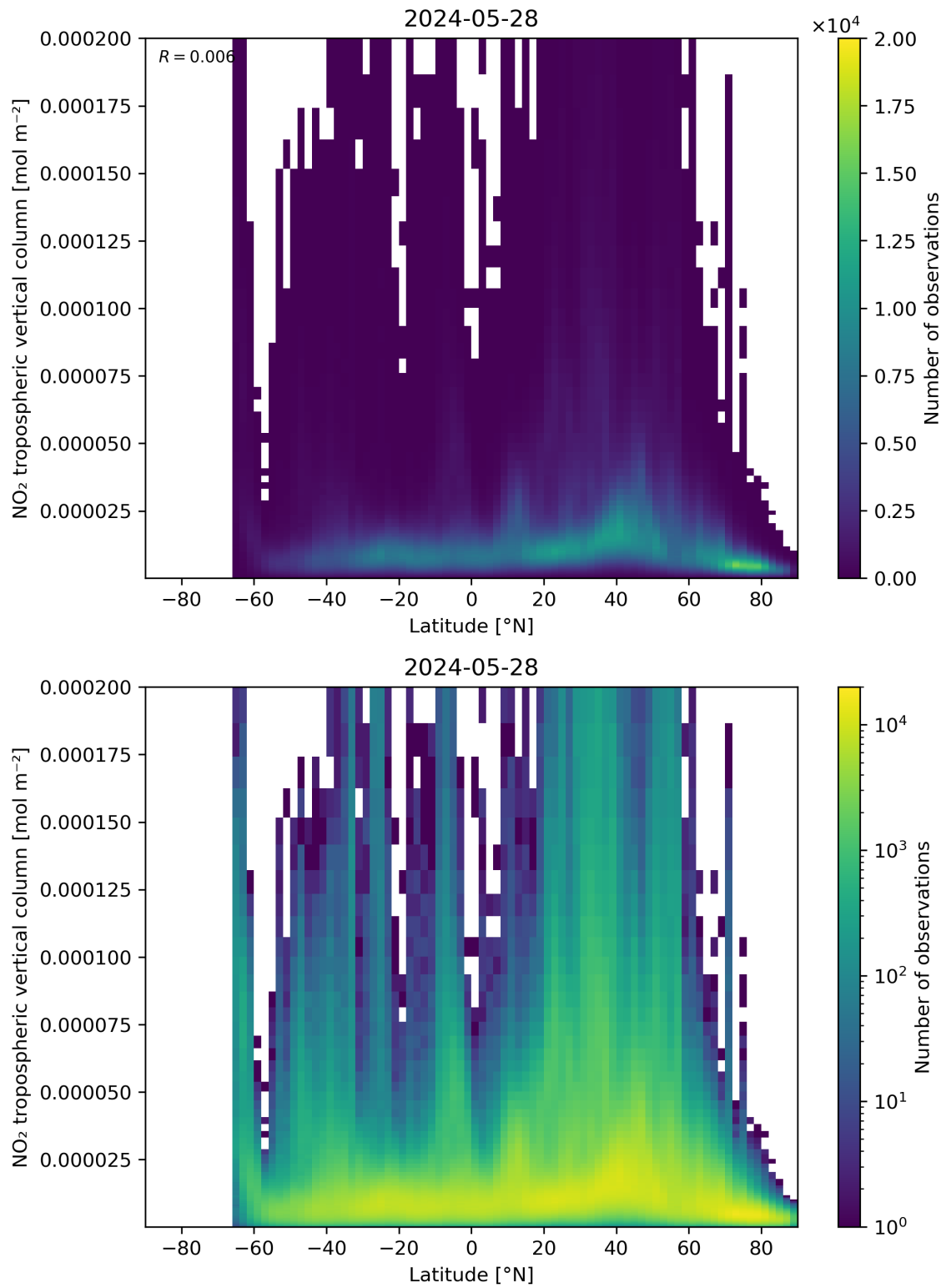
Figure 92: Scatter density plot of “Latitude” against “NO 2 tropospheric vertical column” for 2024-05-28 to 2024-05-29.
