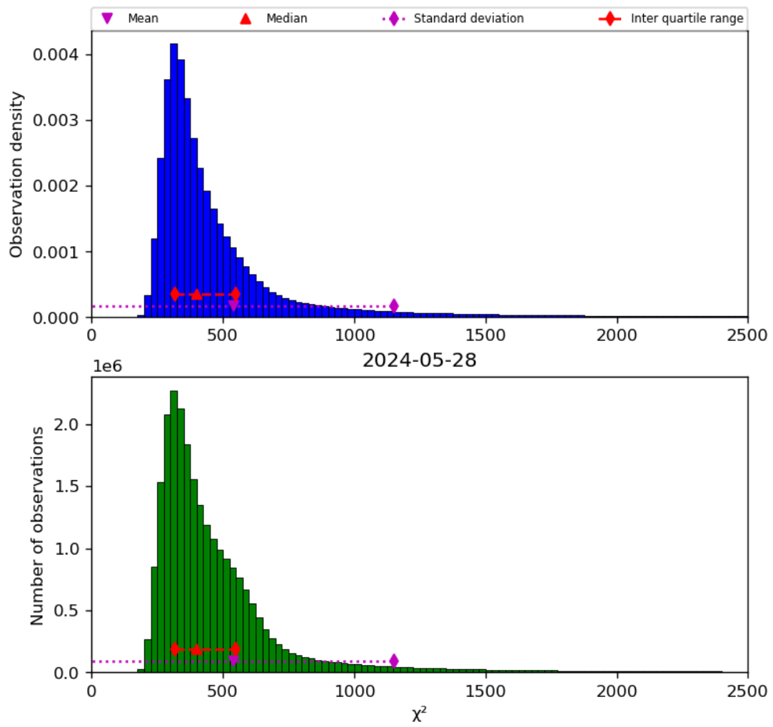
Figure 42: Histogram of “ \chi^2 ” for 2024-05-28 to 2024-05-29
