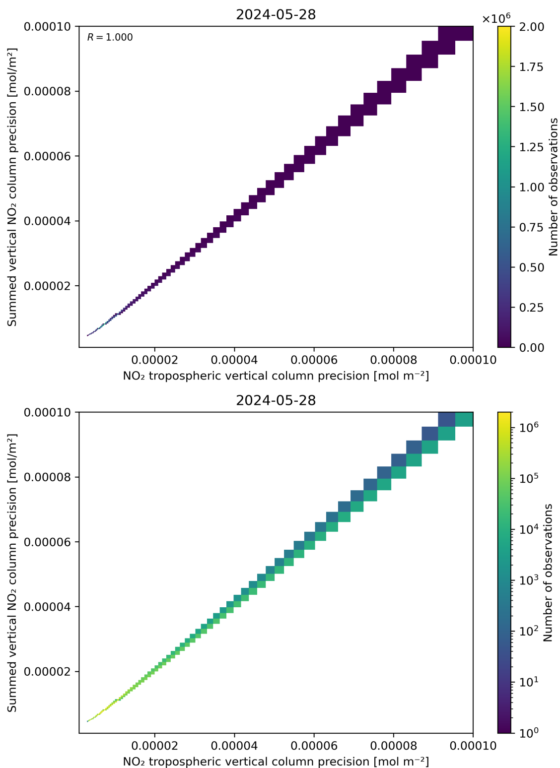
Figure 137: Scatter density plot of “NO 2 tropospheric vertical column precision” against “Summed vertical NO 2 column precision” for 2024-05-28 to 2024-05-29.
