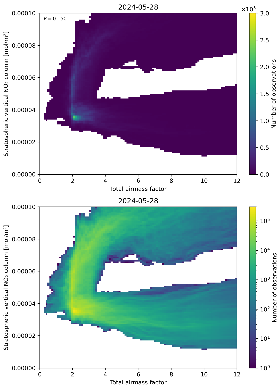
Figure 64: Scatter density plot of “Total airmass factor” against “Stratospheric vertical \text{NO}_2 column” for 2024-05-28 to 2024-05-29.
