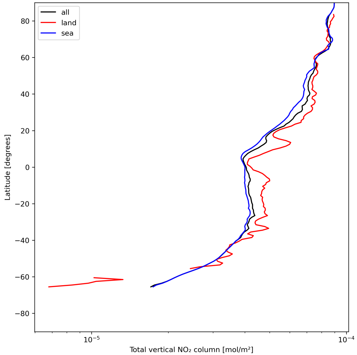
Figure 21: Zonal average of “Total vertical NO 2 column” for 2024-05-28 to 2024-05-29.
