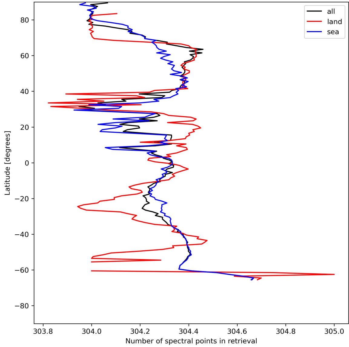
Figure 16: Zonal average of “Number of spectral points in retrieval” for 2024-05-28 to 2024-05-29.
