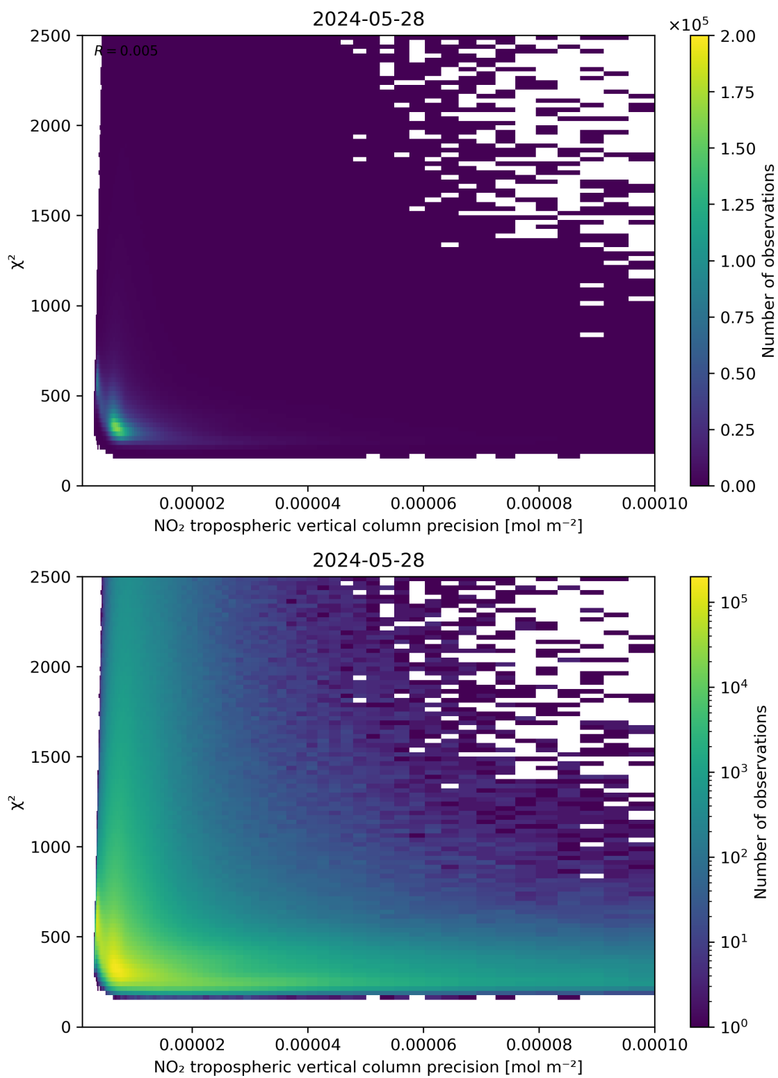
Figure 134: Scatter density plot of “NO 2 tropospheric vertical column precision” against “ \chi^2 ” for 2024-05-28 to 2024-05-29.
