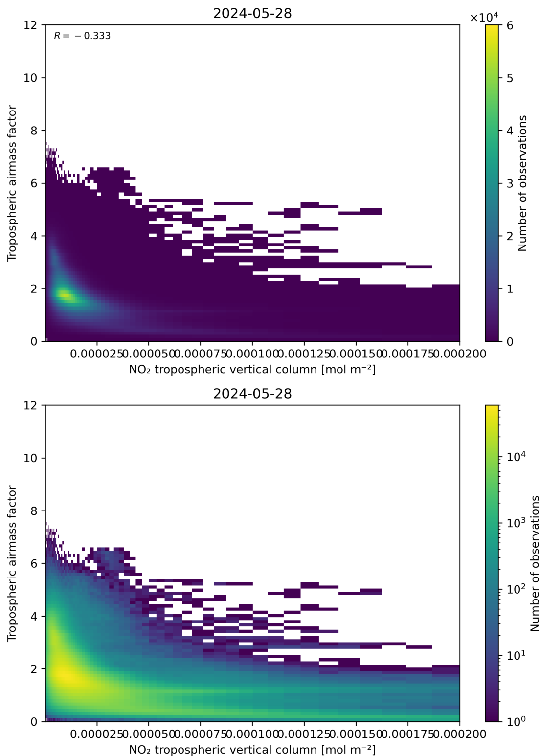
Figure 123: Scatter density plot of “NO 2 tropospheric vertical column” against “Tropospheric air mass factor” for 2024-05-28 to 2024-05-29.
