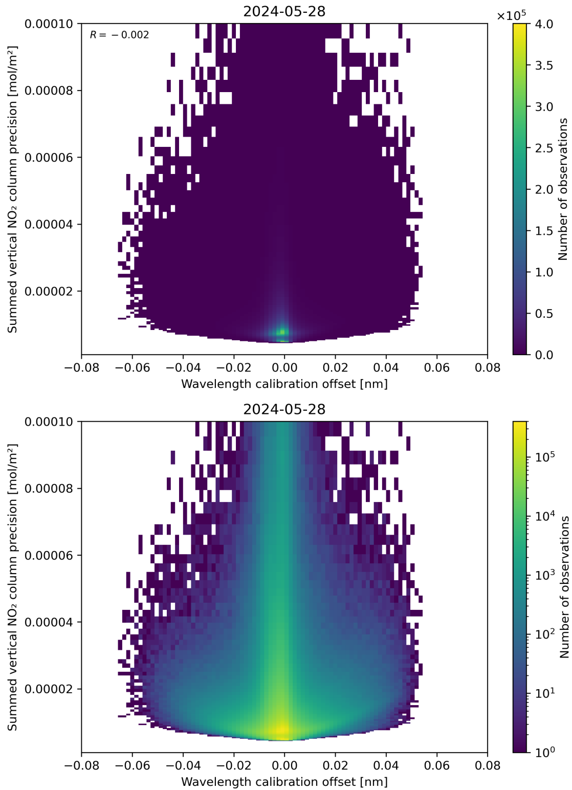
Figure 178: Scatter density plot of “Wavelength calibration offset” against “Summed vertical NO 2 column precision” for 2024-05-28 to 2024-05-29.
