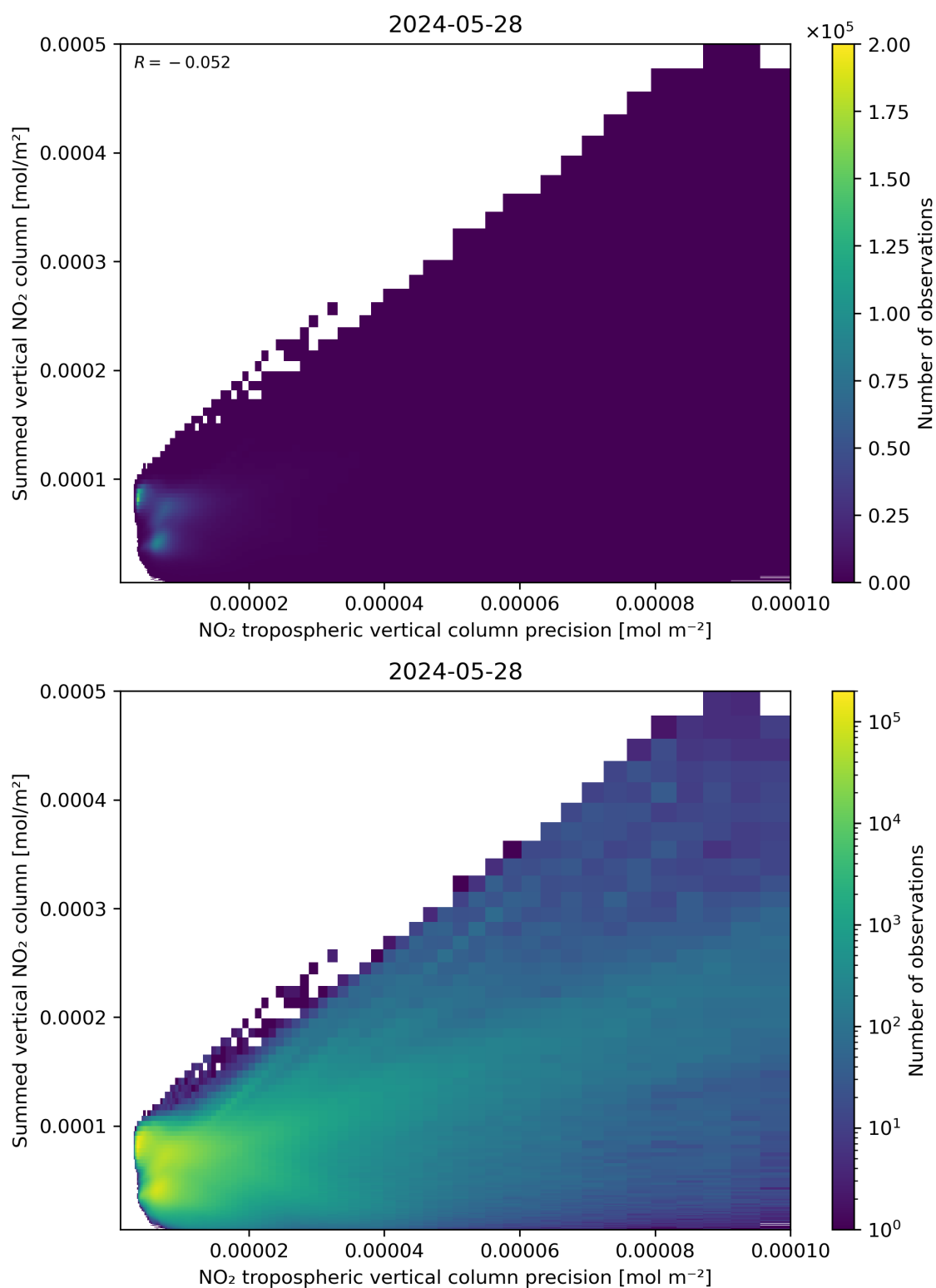
Figure 136: Scatter density plot of “NO 2 tropospheric vertical column precision” against “Summed vertical NO 2 column” for 2024-05-28 to 2024-05-29.
