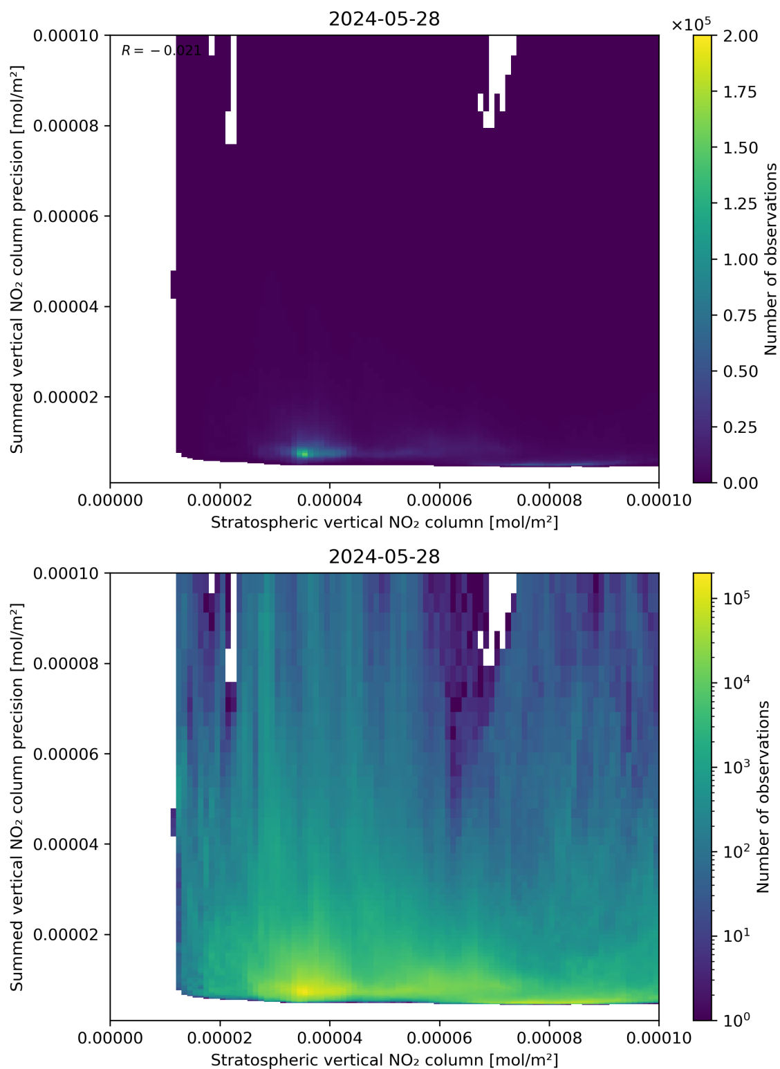
Figure 99: Scatter density plot of “Stratospheric vertical NO 2 column” against “Summed vertical NO 2 column precision” for 2024-05-28 to 2024-05-29.
