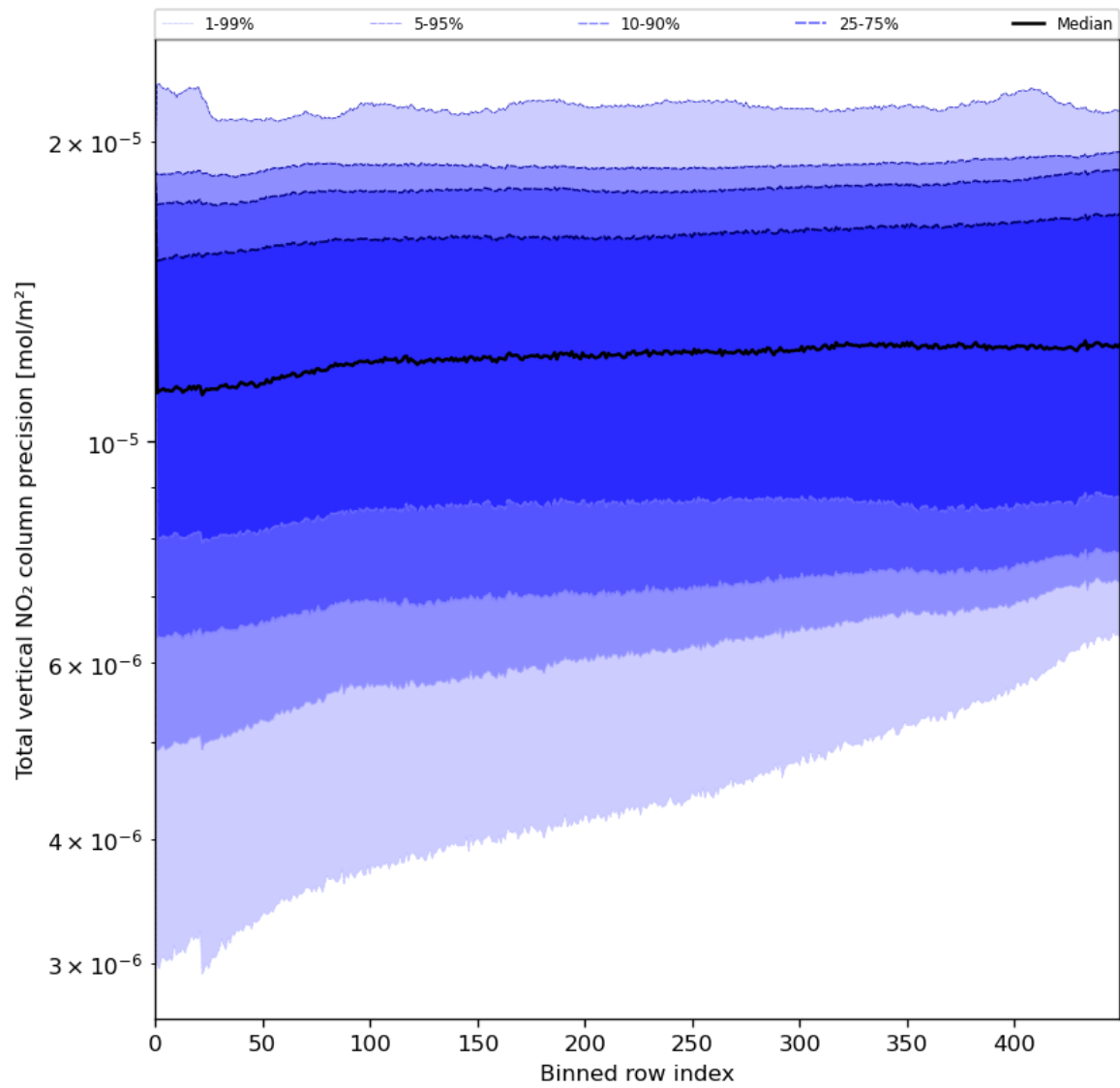
Figure 56: Along track statistics of “Total vertical NO 2 column precision” for 2024-05-28 to 2024-05-29
