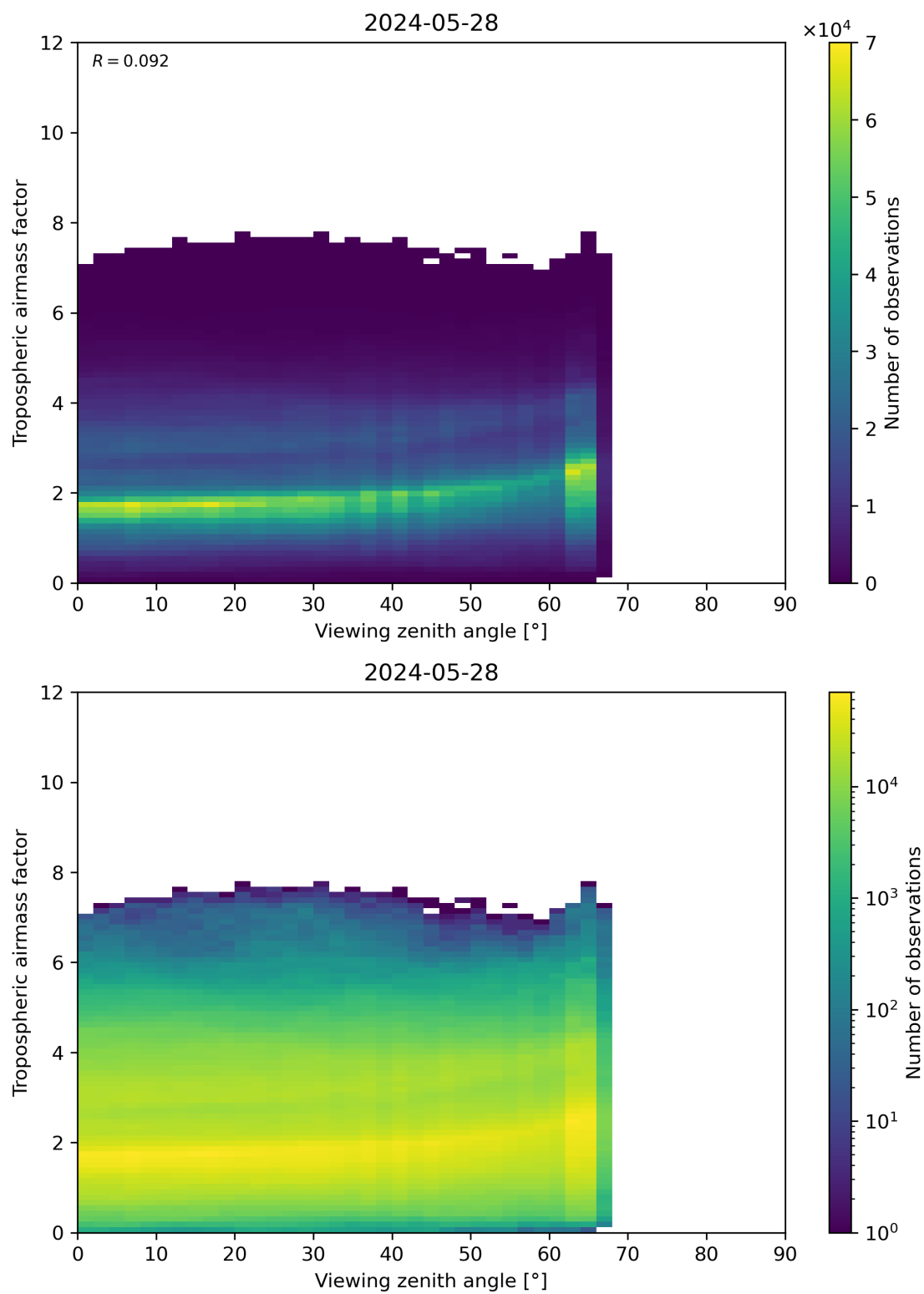
Figure 161: Scatter density plot of “Viewing zenith angle” against “Tropospheric airmass factor” for 2024-05-28 to 2024-05-29.
