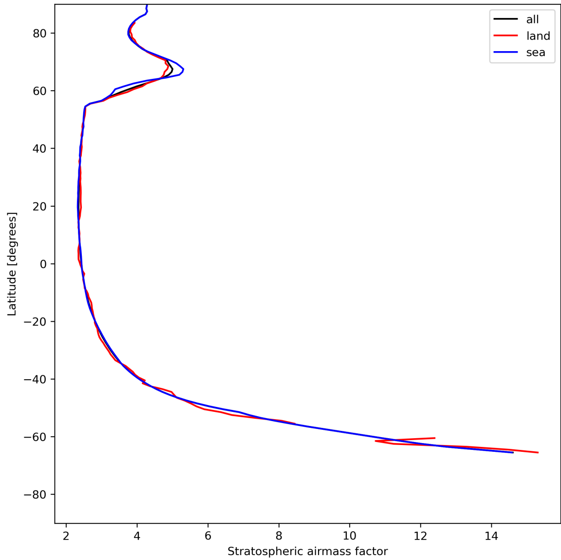
Figure 27: Zonal average of “Stratospheric airmass factor” for 2024-05-28 to 2024-05-29.
