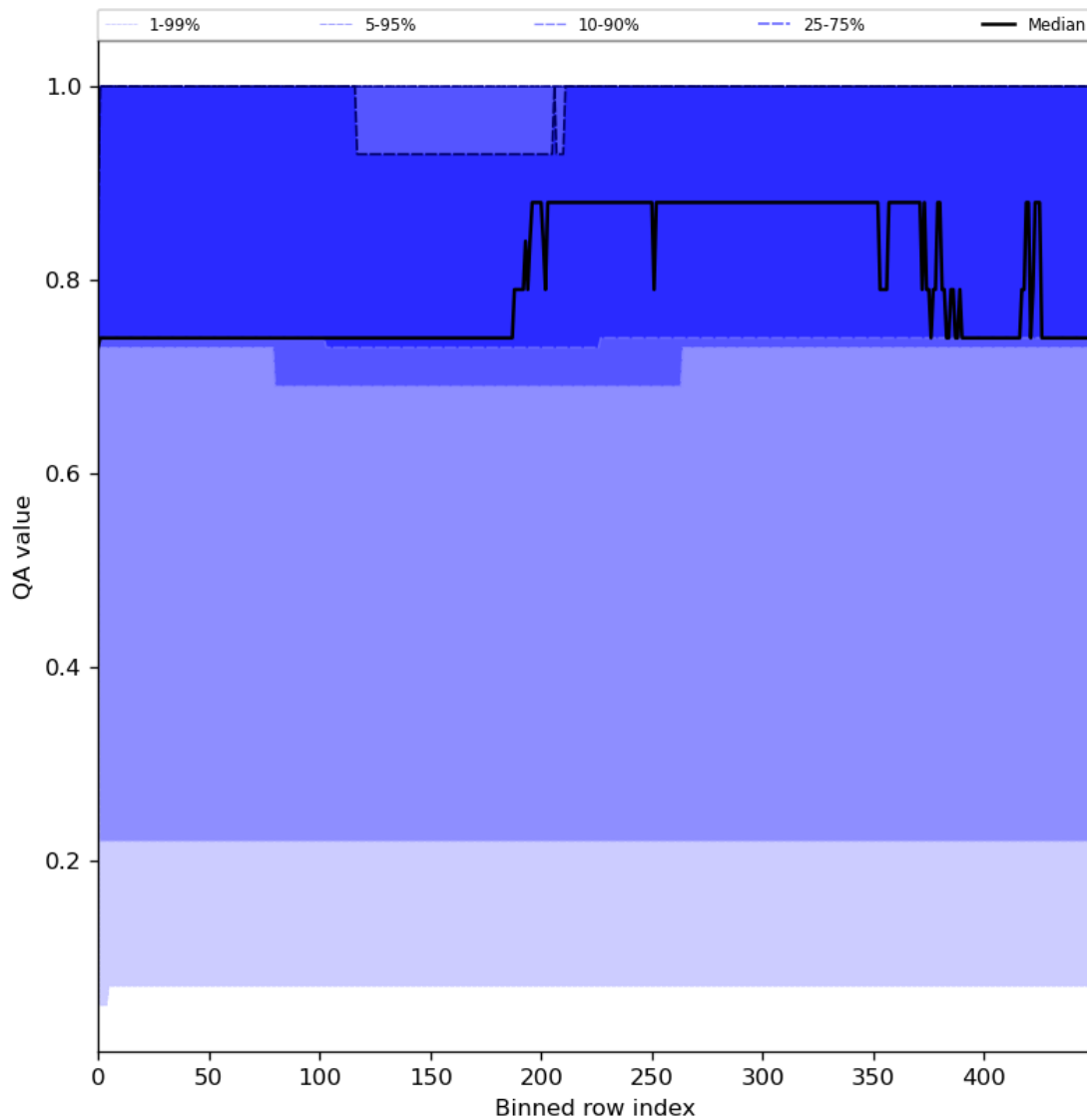
Figure 45: Along track statistics of “QA value” for 2024-05-28 to 2024-05-29
