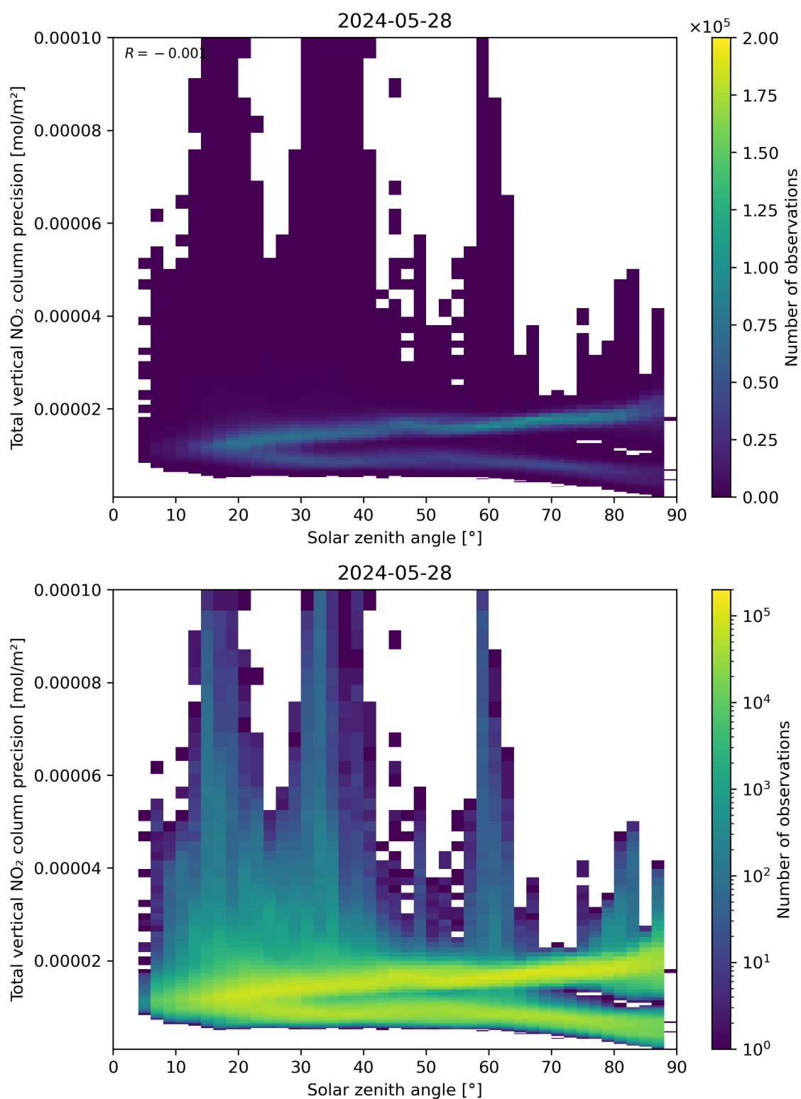
Figure 154: Scatter density plot of “Solar zenith angle” against “Total vertical NO 2 column precision” for 2024-05-28 to 2024-05-29.
