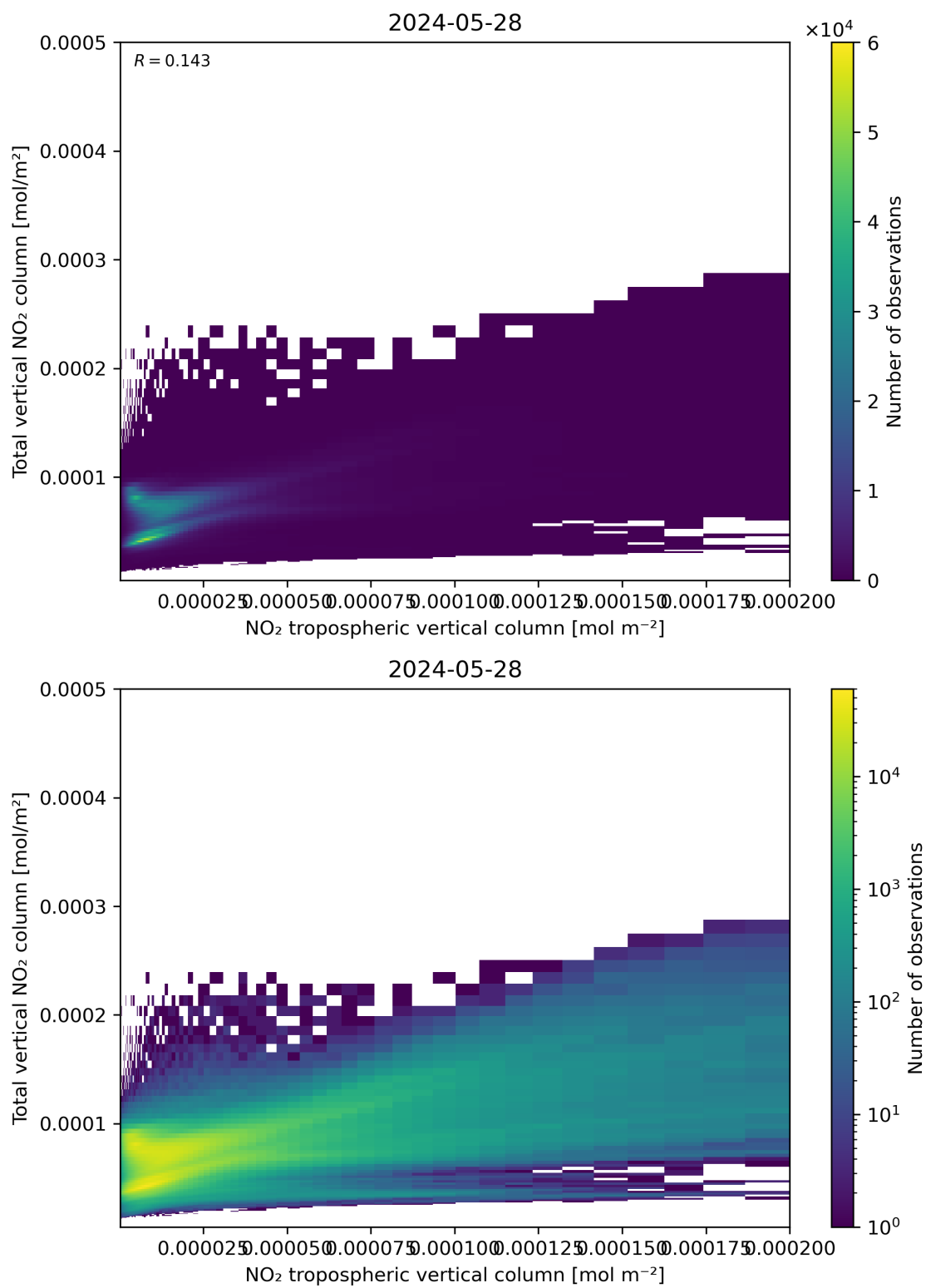
Figure 128: Scatter density plot of “NO 2 tropospheric vertical column” against “Total vertical NO 2 column” for 2024-05-28 to 2024-05-29.
