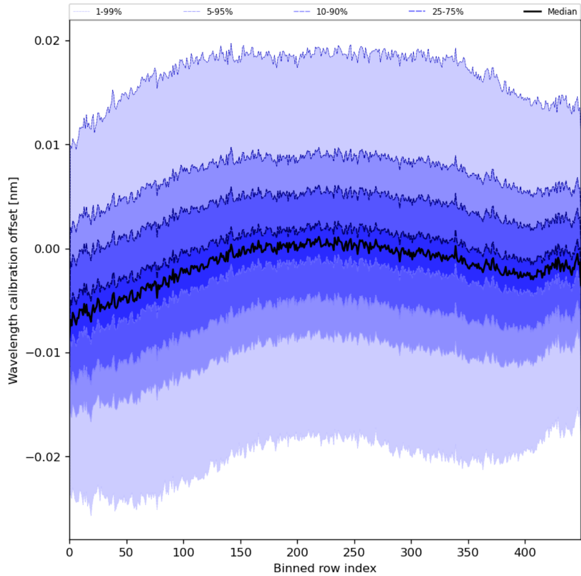
Figure 52: Along track statistics of “Wavelength calibration offset” for 2024-05-28 to 2024-05-29
