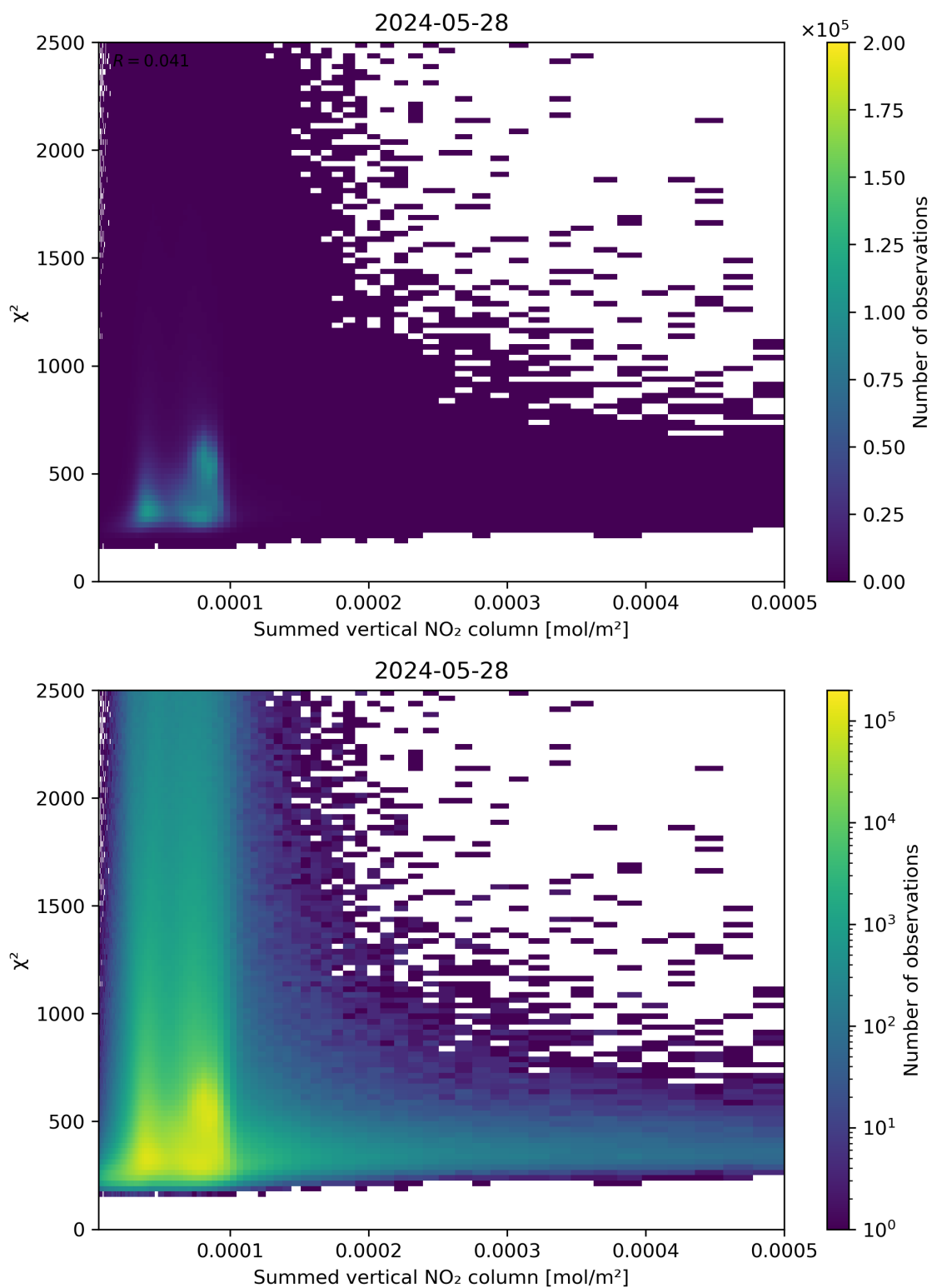
Figure 104: Scatter density plot of “Summed vertical NO 2 column” against “ \chi^2 ” for 2024-05-28 to 2024-05-29.
