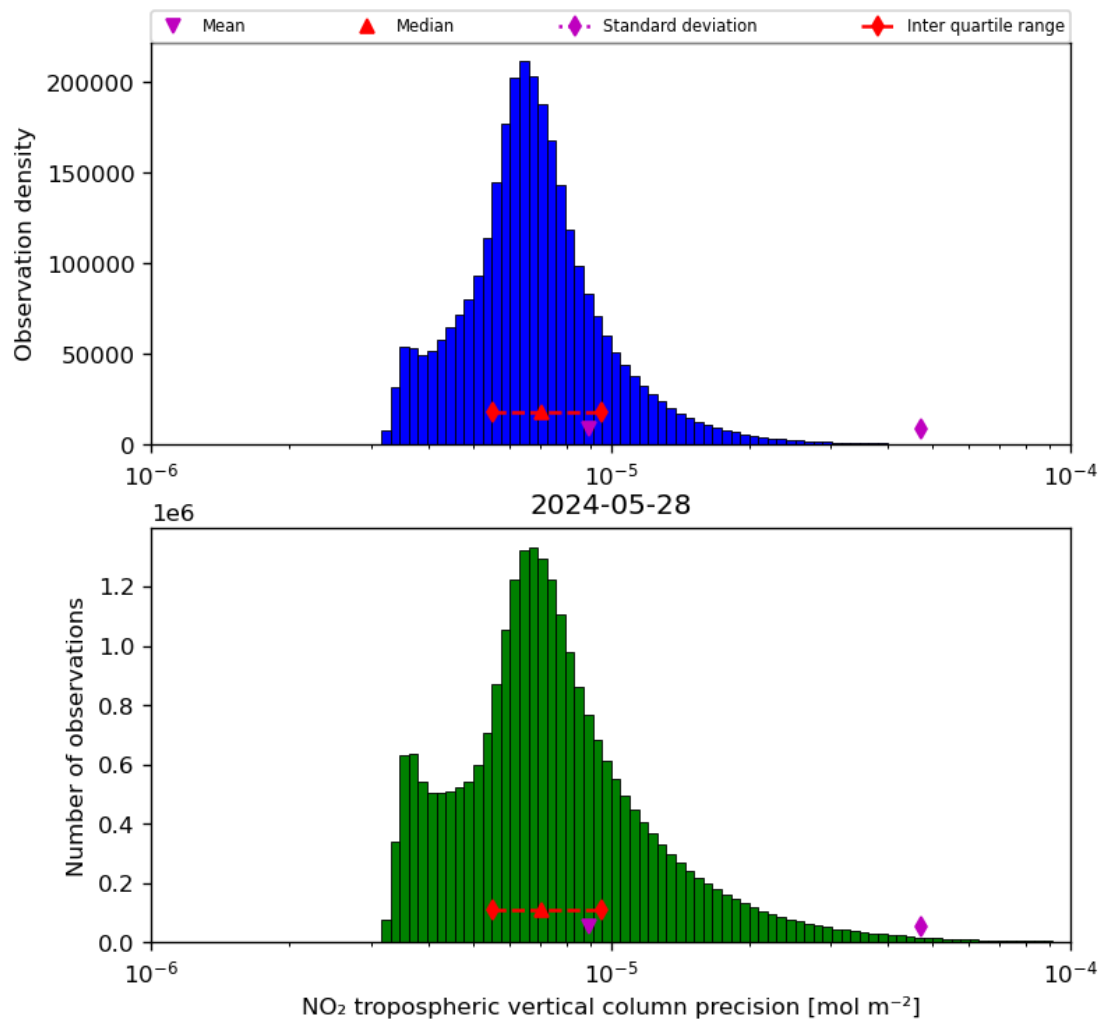
Figure 30: Histogram of “NO 2 tropospheric vertical column precision” for 2024-05-28 to 2024-05-29
