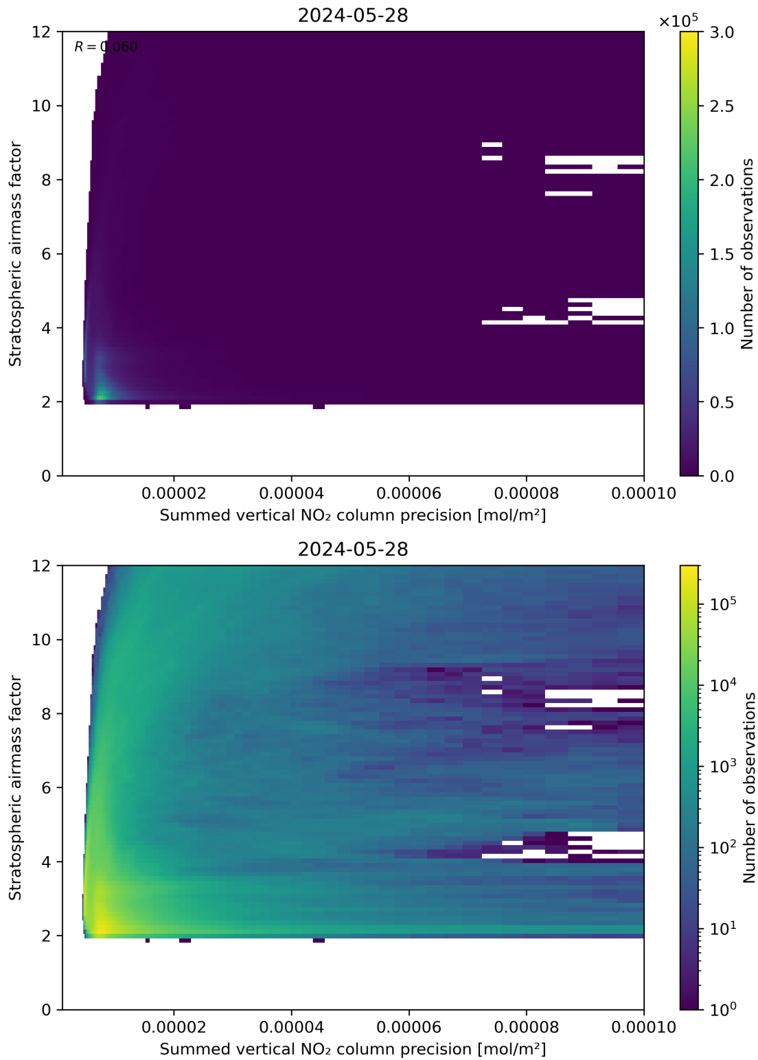
Figure 106: Scatter density plot of “Summed vertical NO 2 column precision” against “Stratospheric airmass factor” for 2024-05-28 to 2024-05-29.
