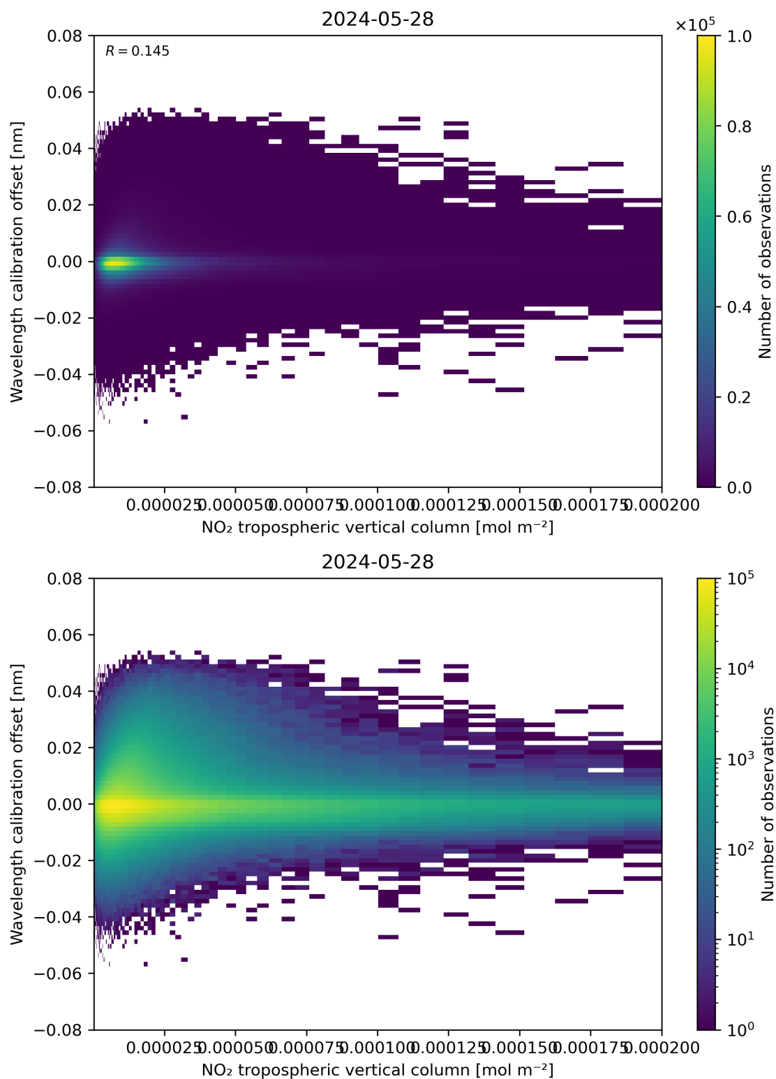
Figure 143: Scatter density plot of “NO 2 tropospheric vertical column” against “Wavelength calibration offset” for 2024-05-28 to 2024-05-29.
