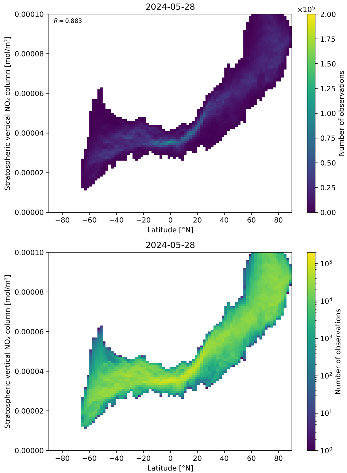
Figure 87: Scatter density plot of “Latitude” against “Stratospheric vertical NO 2 column” for 2024-05-28 to 2024-05-29.
