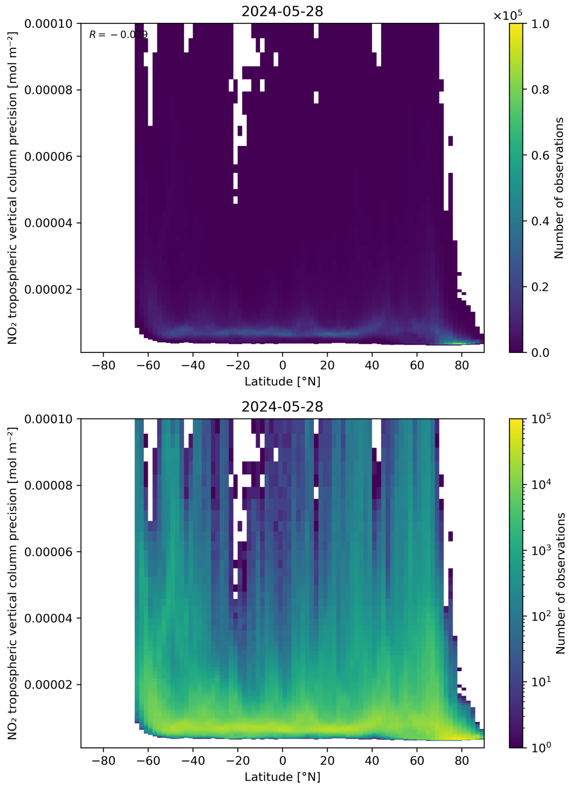
Figure 93: Scatter density plot of “Latitude” against “NO 2 tropospheric vertical column precision” for 2024-05-28 to 2024-05-29.
