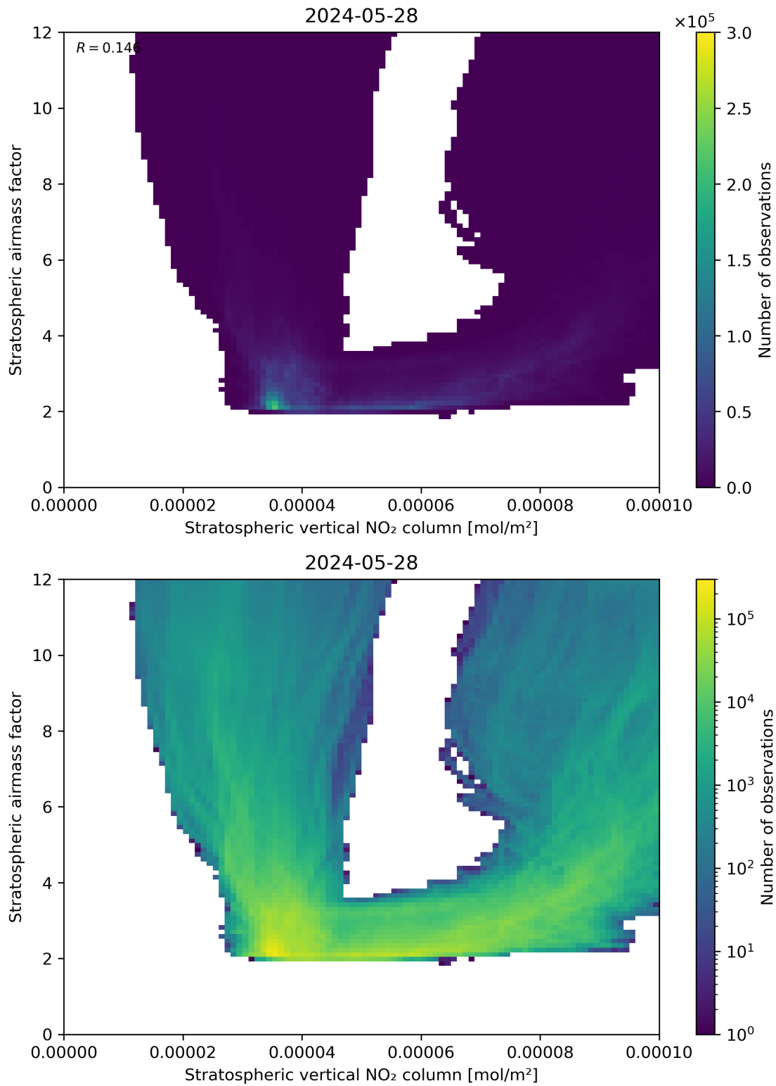
Figure 96: Scatter density plot of “Stratospheric vertical NO 2 column” against “Stratospheric airmass factor” for 2024-05-28 to 2024-05-29.
