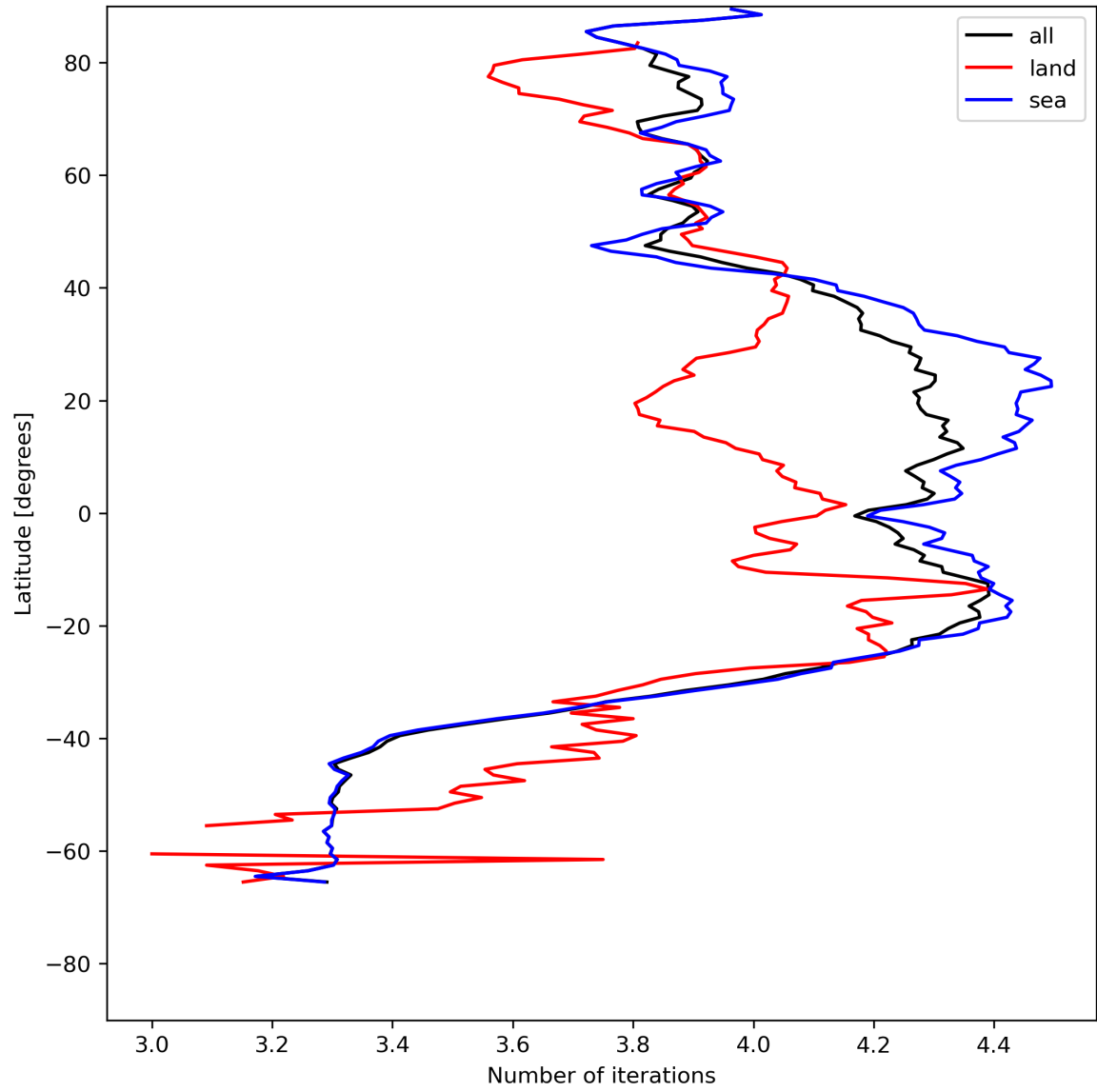
Figure 17: Zonal average of “Number of iterations” for 2024-05-28 to 2024-05-29.
