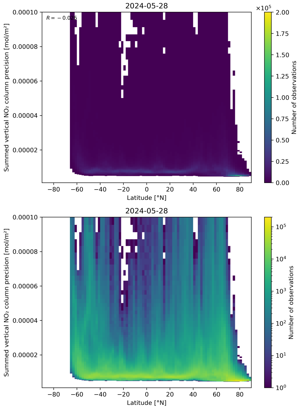
Figure 89: Scatter density plot of “Latitude” against “Summed vertical NO 2 column precision” for 2024-05-28 to 2024-05-29.
