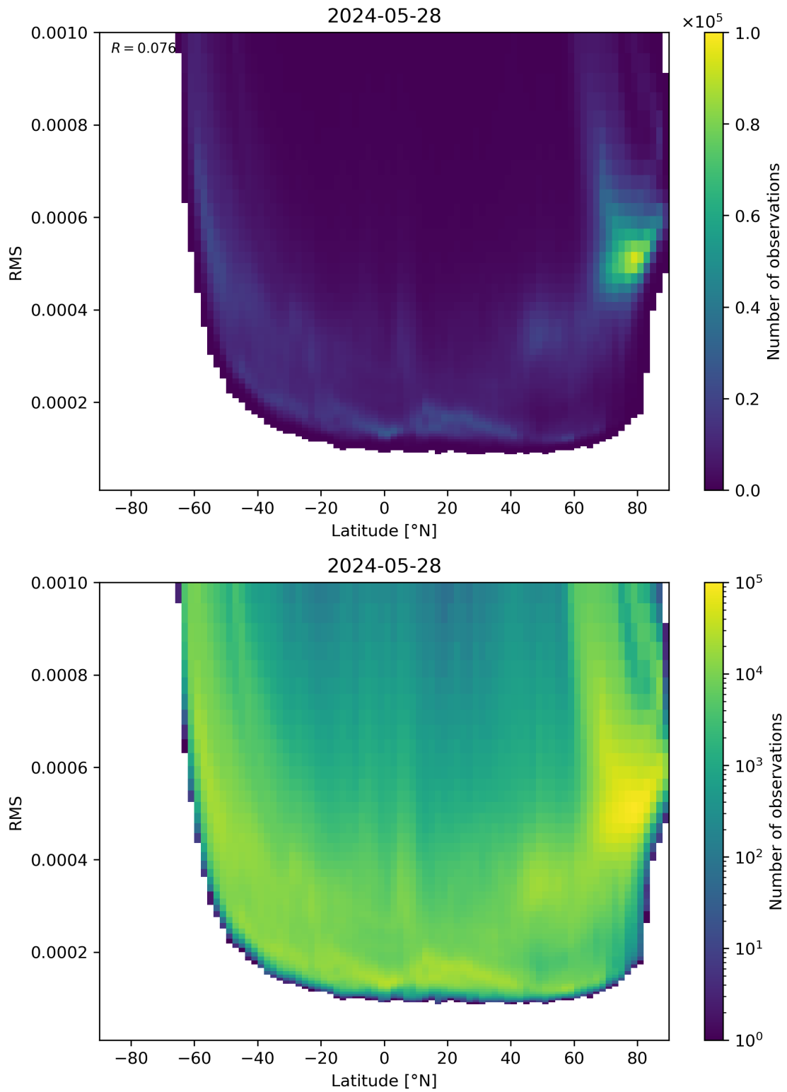
Figure 94: Scatter density plot of “Latitude” against “RMS” for 2024-05-28 to 2024-05-29.
