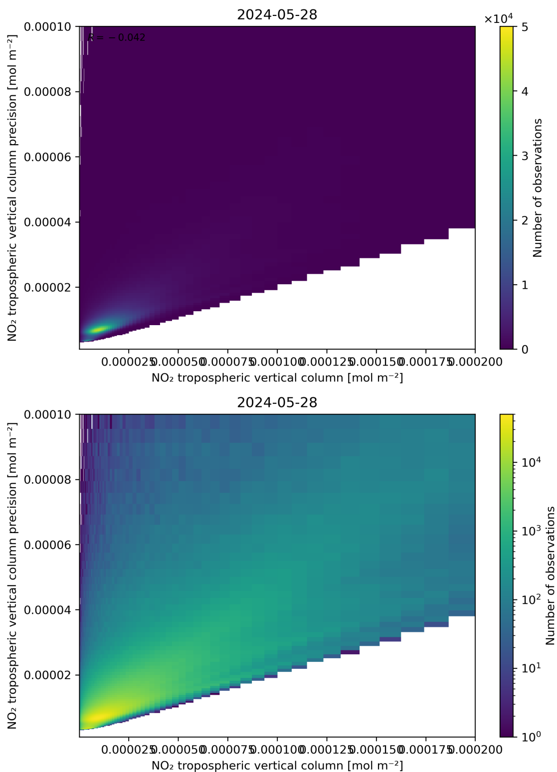
Figure 130: Scatter density plot of “NO 2 tropospheric vertical column” against “NO 2 tropospheric vertical column precision” for 2024-05-28 to 2024-05-29.
