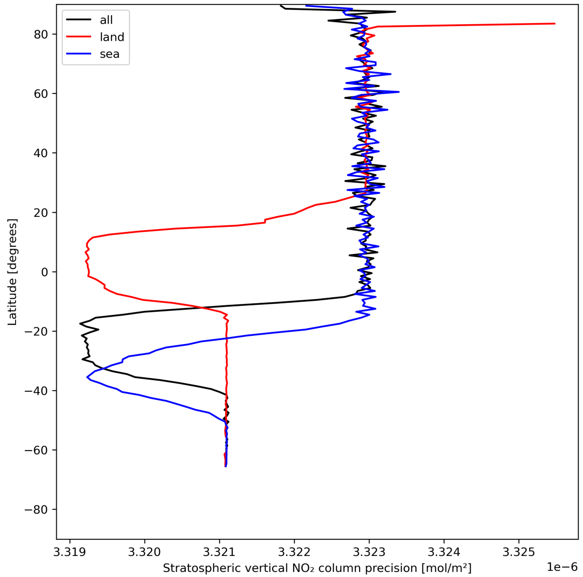
Figure 20: Zonal average of “Stratospheric vertical NO 2 column precision” for 2024-05-28 to 2024-05-29.
