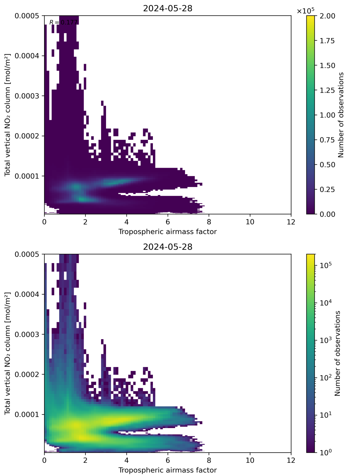
Figure 77: Scatter density plot of “Tropospheric airmass factor” against “Total vertical NO 2 column” for 2024-05-28 to 2024-05-29.
