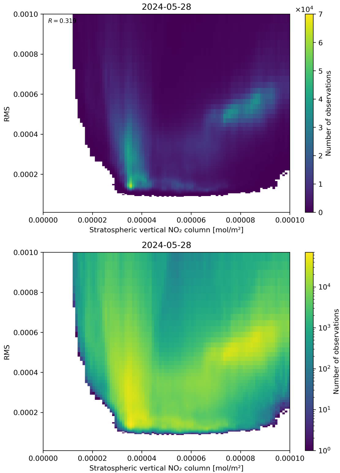
Figure 102: Scatter density plot of “Stratospheric vertical NO 2 column” against “RMS” for 2024-05-28 to 2024-05-29.
