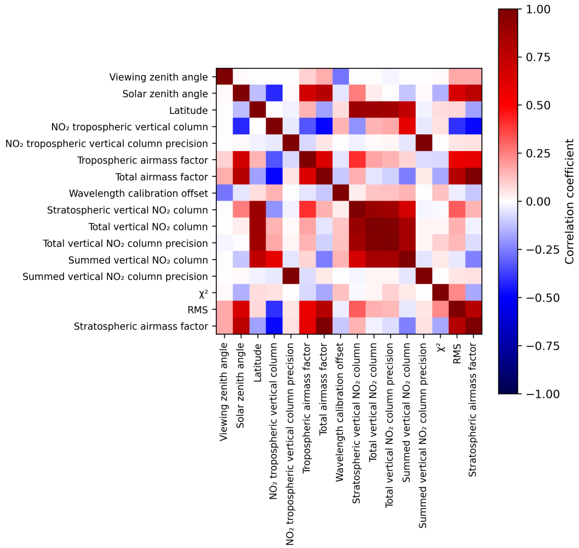
Figure 2: Map of correlation matrix for 2024-05-28 to 2024-05-29.
