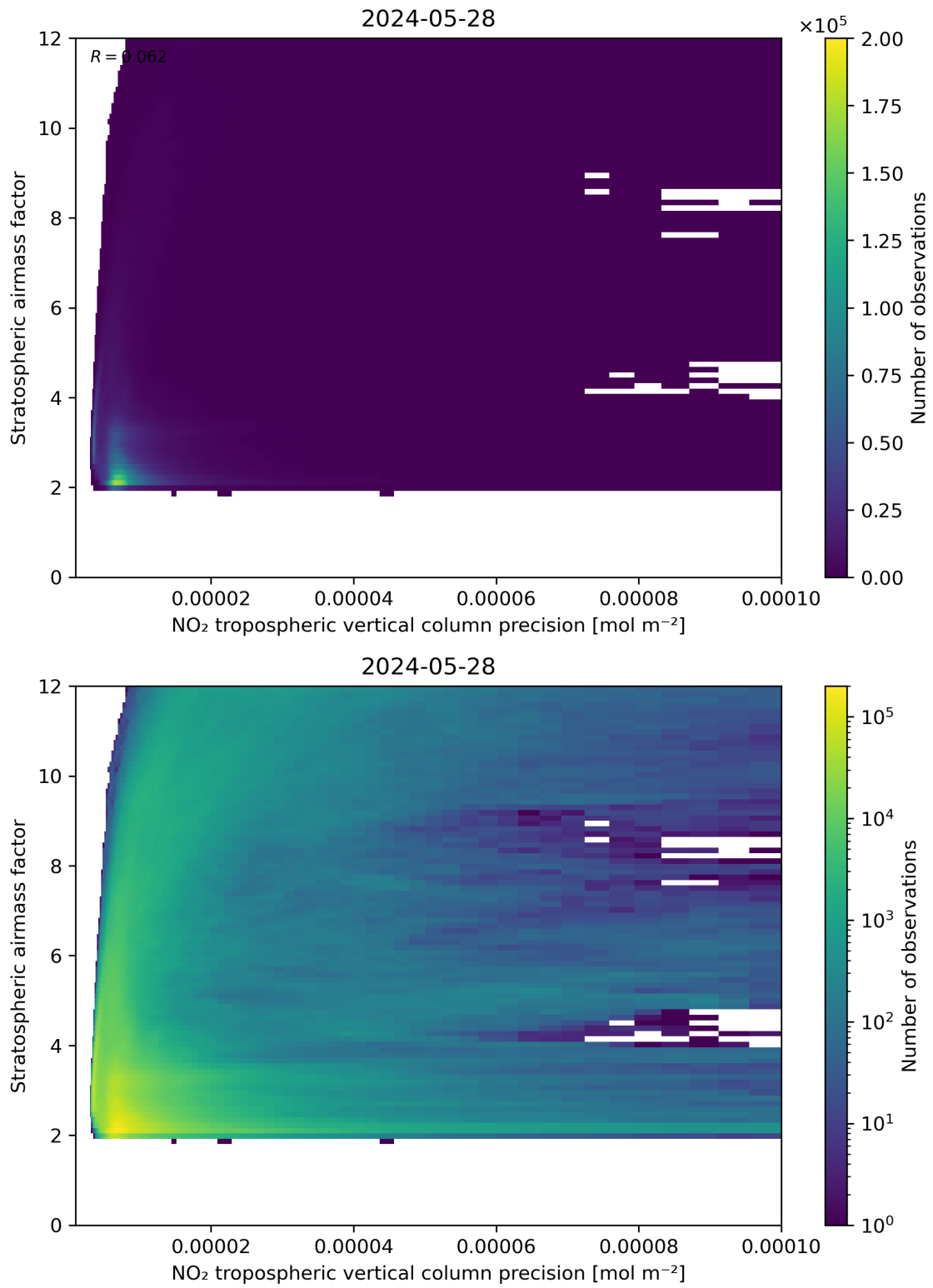
Figure 131: Scatter density plot of “NO 2 tropospheric vertical column precision” against “Stratospheric airmass factor” for 2024-05-28 to 2024-05-29.
