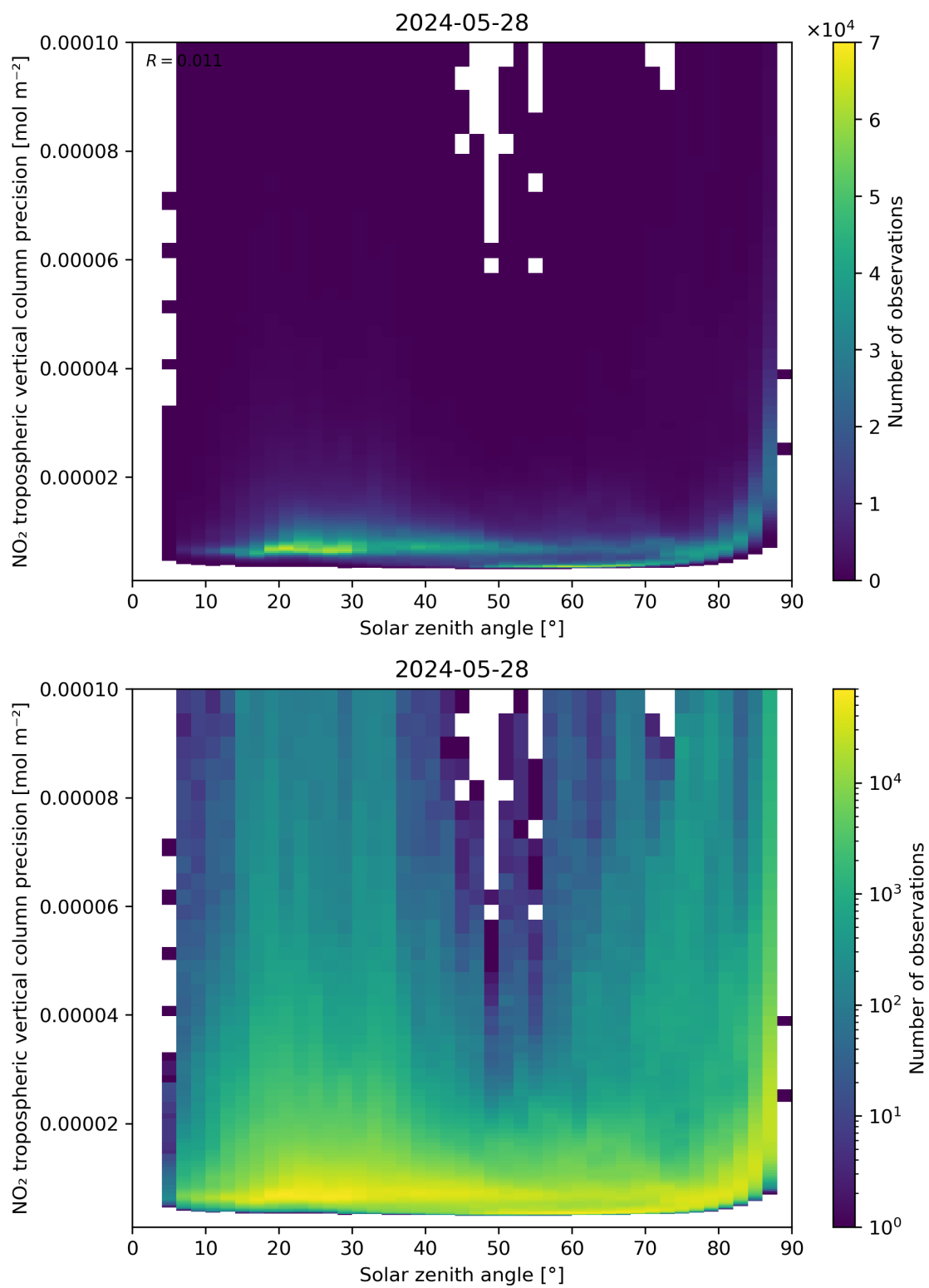
Figure 156: Scatter density plot of “Solar zenith angle” against “NO 2 tropospheric vertical column precision” for 2024-05-28 to 2024-05-29.
