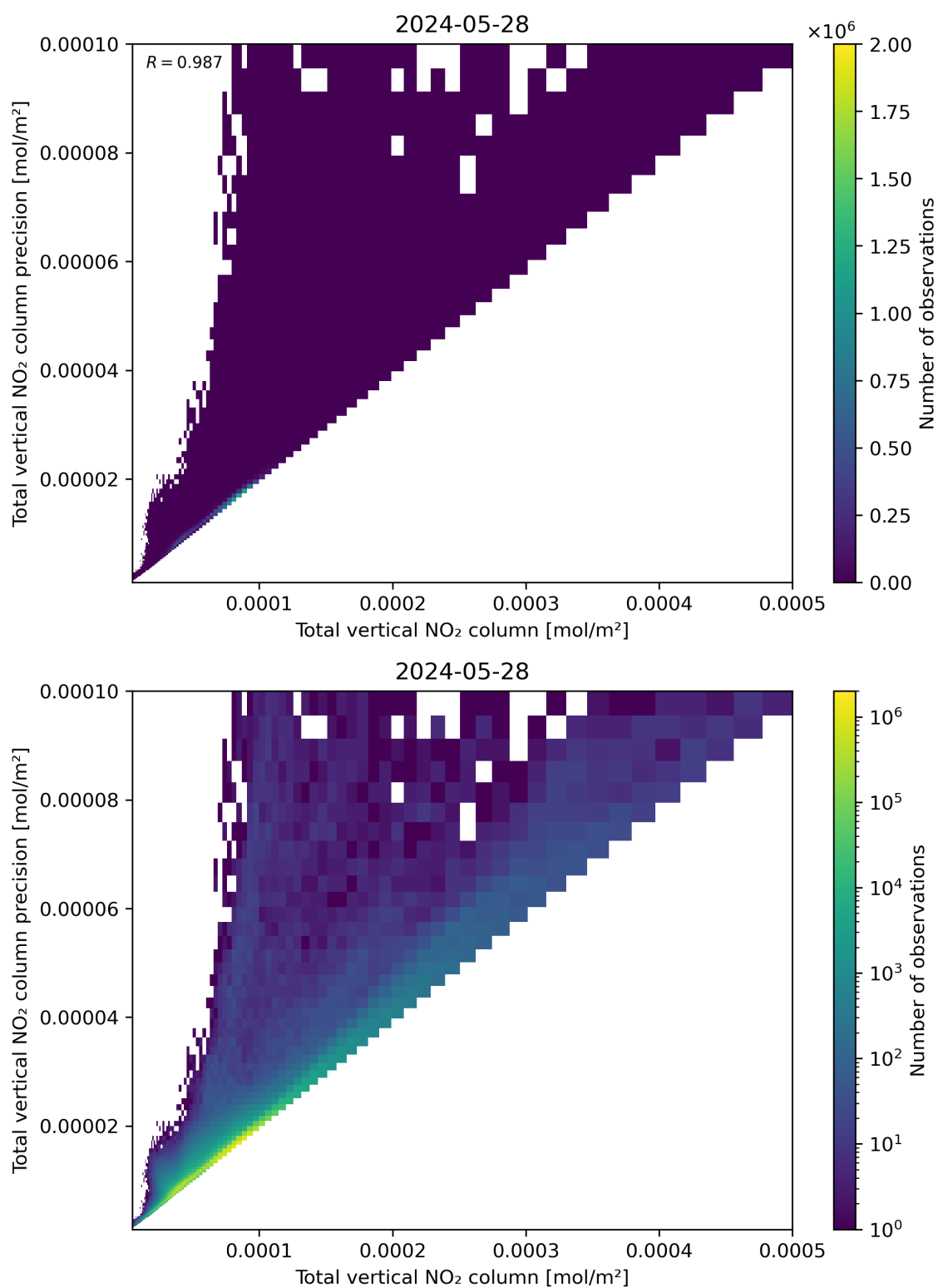
Figure 114: Scatter density plot of “Total vertical NO 2 column” against “Total vertical NO 2 column precision” for 2024-05-28 to 2024-05-29.
