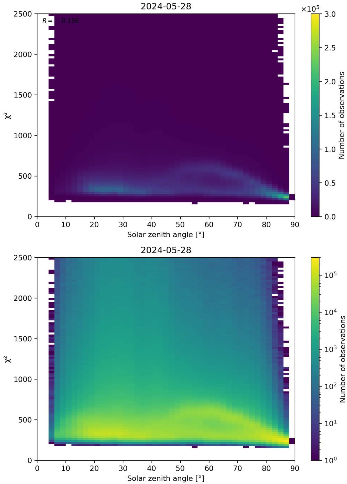
Figure 148: Scatter density plot of “Solar zenith angle” against “ \chi^2 ” for 2024-05-28 to 2024-05-29.
