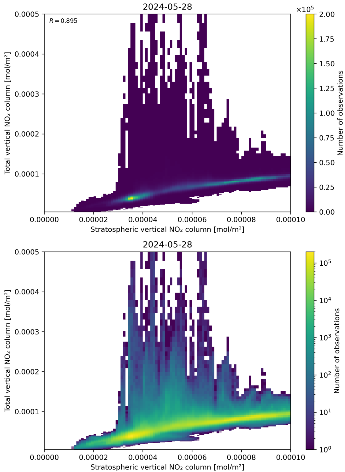
Figure 100: Scatter density plot of “Stratospheric vertical NO 2 column” against “Total vertical NO 2 column” for 2024-05-28 to 2024-05-29.
