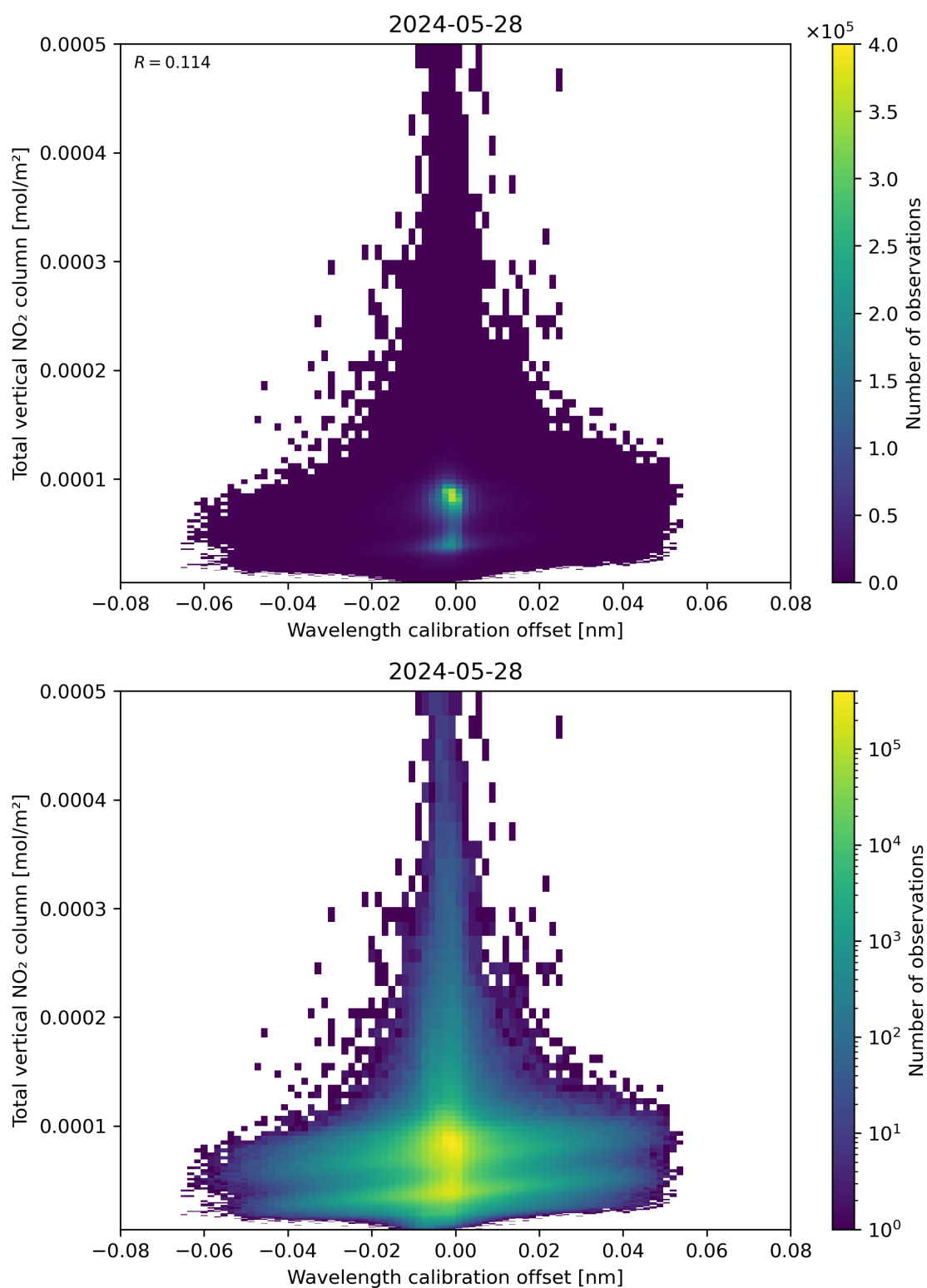
Figure 179: Scatter density plot of “Wavelength calibration offset” against “Total vertical NO 2 column” for 2024-05-28 to 2024-05-29.
