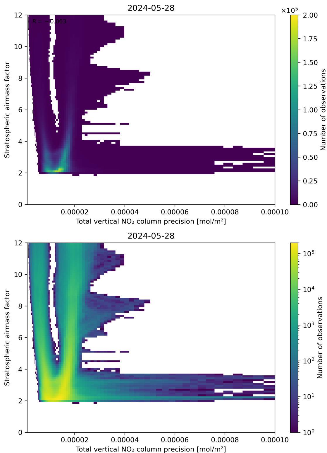
Figure 115: Scatter density plot of “Total vertical NO 2 column precision” against “Stratospheric air mass factor” for 2024-05-28 to 2024-05-29.
