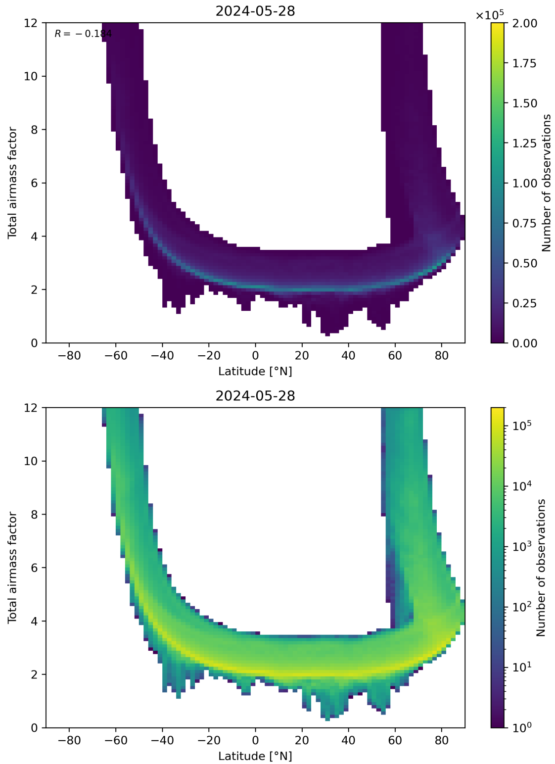
Figure 84: Scatter density plot of “Latitude” against “Total airmass factor” for 2024-05-28 to 2024-05-29.
