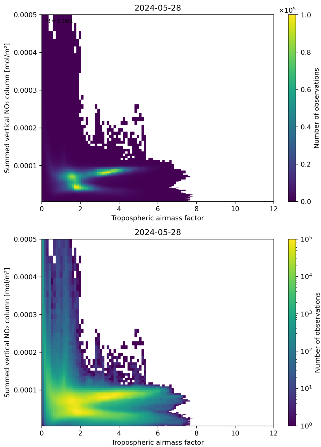
Figure 75: Scatter density plot of “Tropospheric airmass factor” against “Summed vertical NO 2 column” for 2024-05-28 to 2024-05-29.
