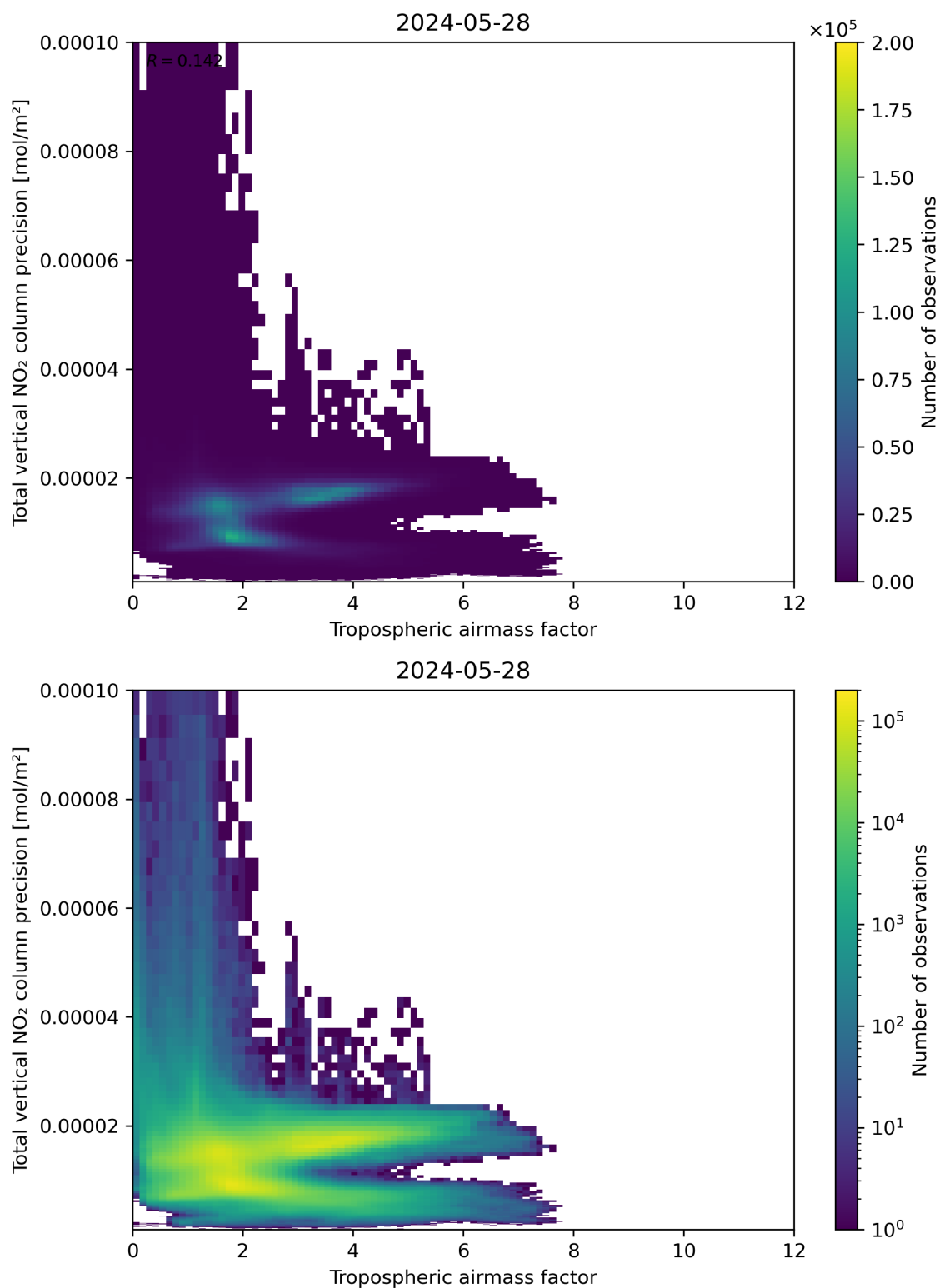
Figure 78: Scatter density plot of “Tropospheric air mass factor” against “Total vertical NO 2 column precision” for 2024-05-28 to 2024-05-29.
