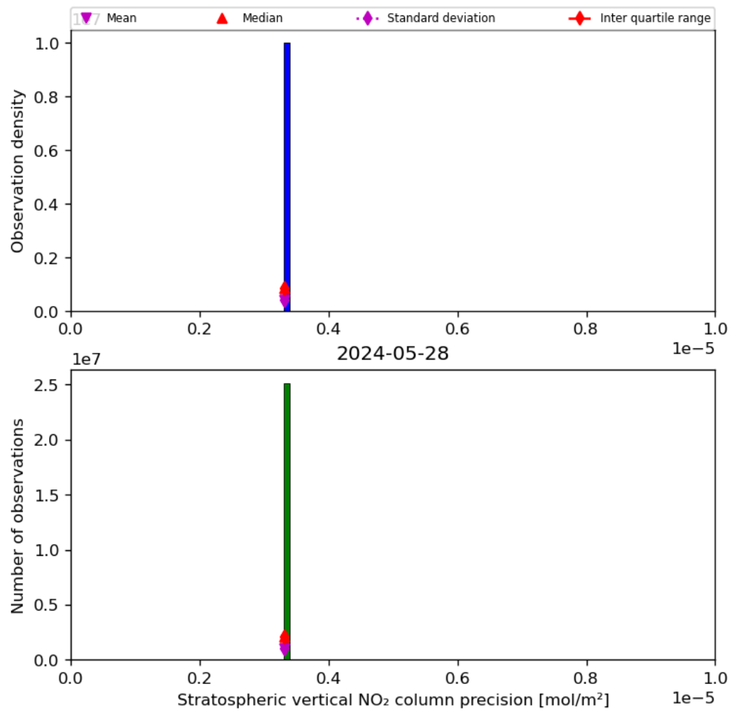
Figure 37: Histogram of “Stratospheric vertical NO 2 column precision” for 2024-05-28 to 2024-05-29
