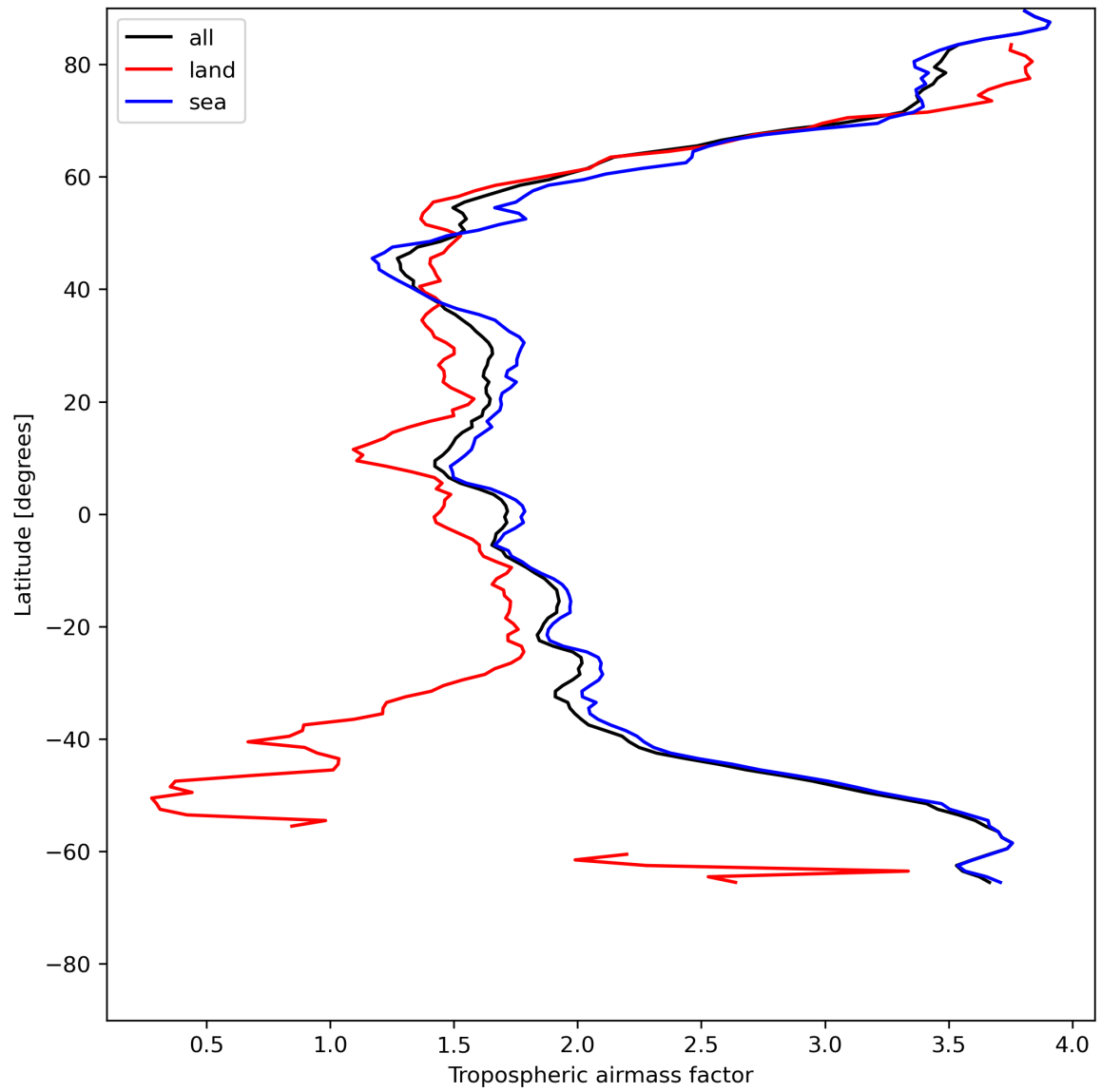
Figure 14: Zonal average of “Tropospheric air mass factor” for 2024-05-28 to 2024-05-29.
