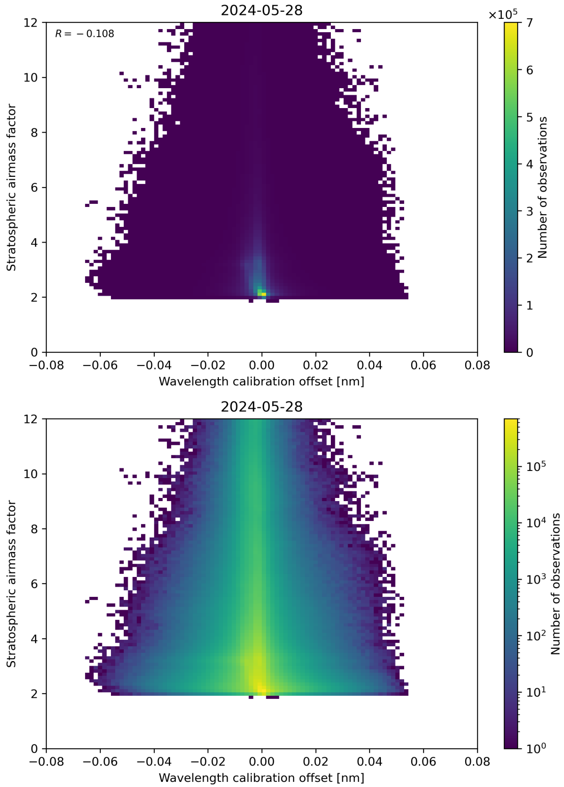
Figure 174: Scatter density plot of “Wavelength calibration offset” against “Stratospheric airmass factor” for 2024-05-28 to 2024-05-29.
