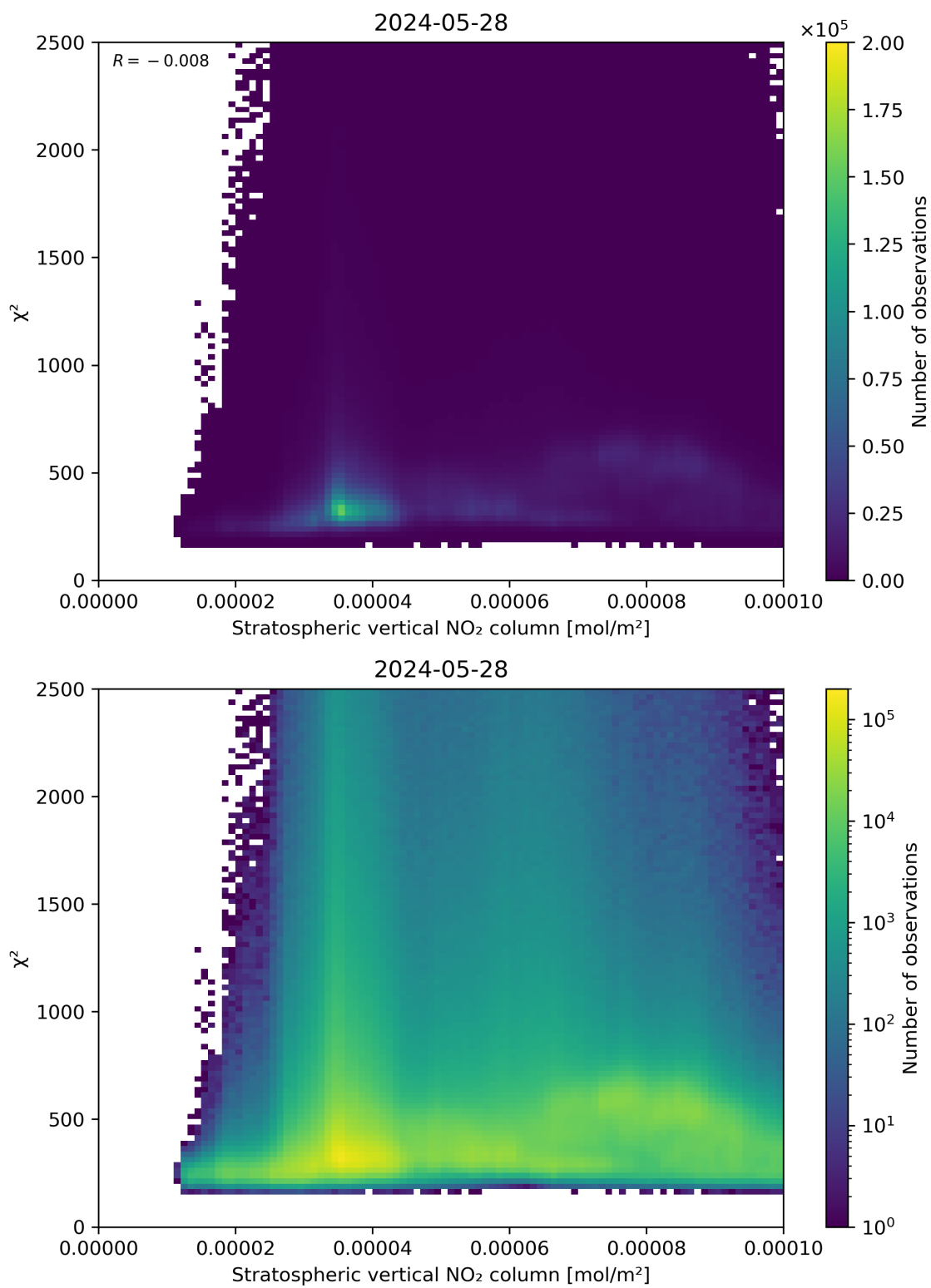
Figure 97: Scatter density plot of “Stratospheric vertical NO 2 column” against “ \chi^2 ” for 2024-05-28 to 2024-05-29.
