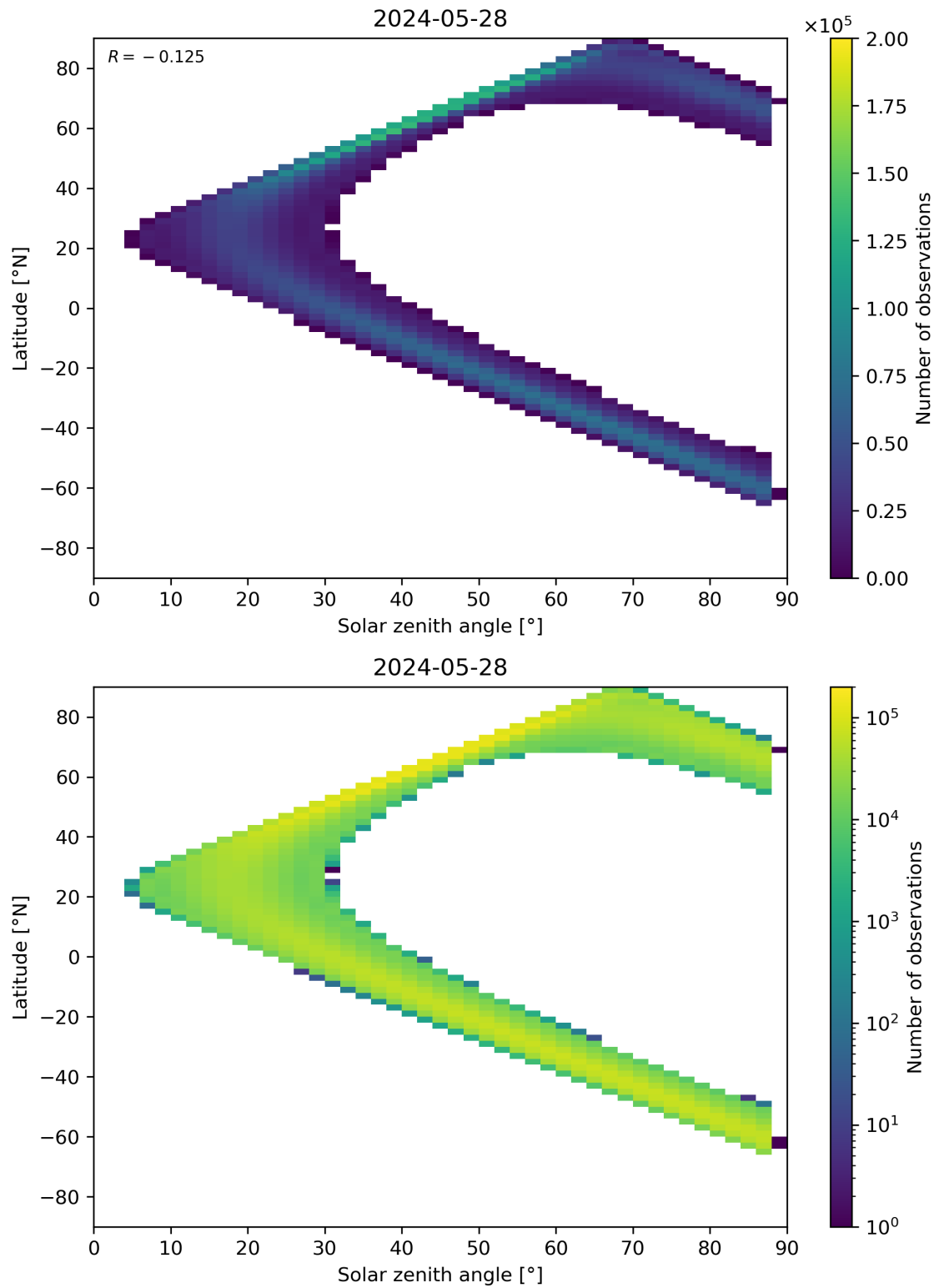
Figure 149: Scatter density plot of “Solar zenith angle” against “Latitude” for 2024-05-28 to 2024-05-29.
