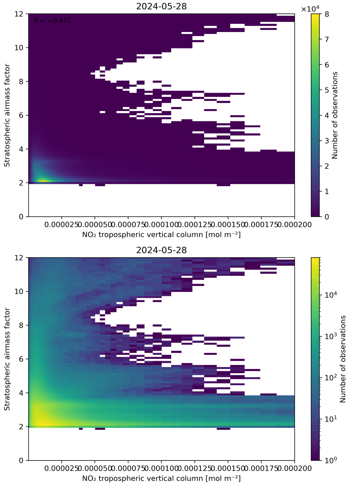
Figure 121: Scatter density plot of “NO 2 tropospheric vertical column” against “Stratospheric air mass factor” for 2024-05-28 to 2024-05-29.
