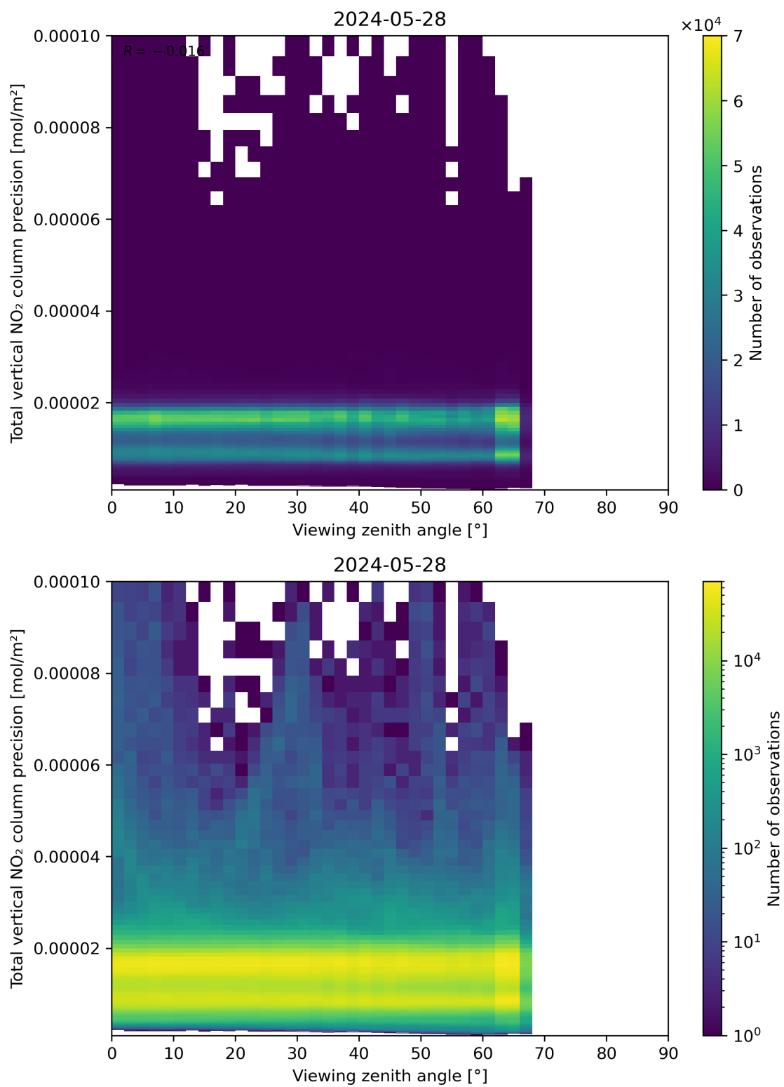
Figure 168: Scatter density plot of “Viewing zenith angle” against “Total vertical NO 2 column precision” for 2024-05-28 to 2024-05-29.
