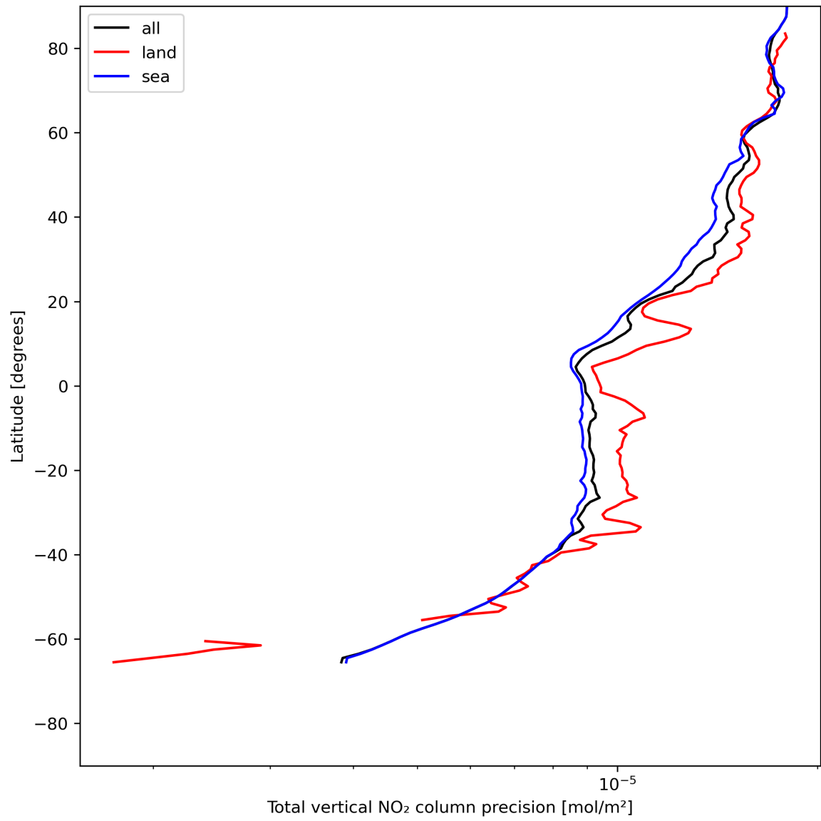
Figure 22: Zonal average of “Total vertical NO 2 column precision” for 2024-05-28 to 2024-05-29.
