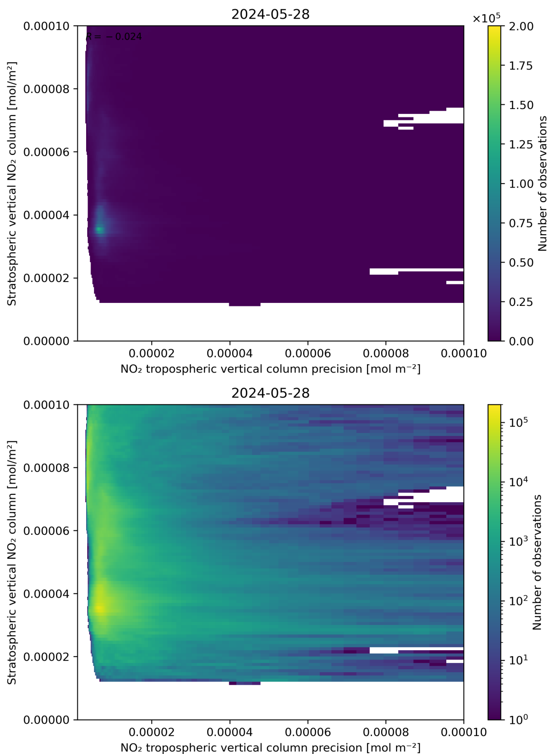
Figure 135: Scatter density plot of “NO 2 tropospheric vertical column precision” against “Stratospheric vertical NO 2 column” for 2024-05-28 to 2024-05-29.
