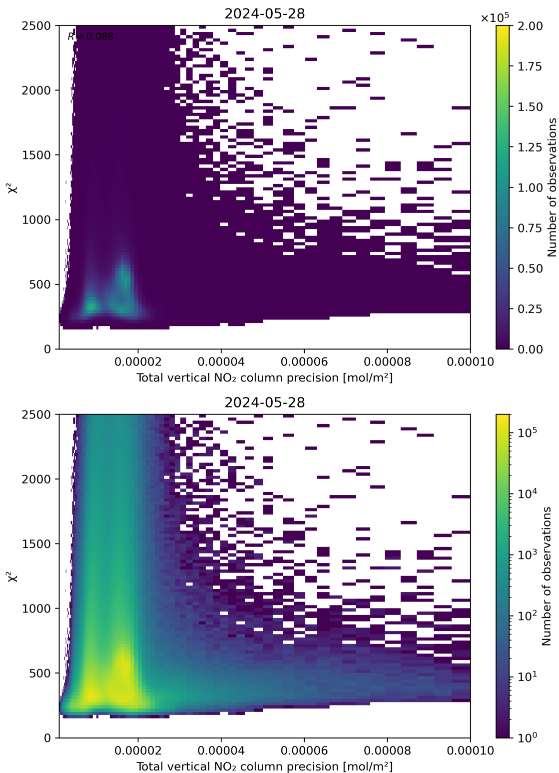
Figure 116: Scatter density plot of “Total vertical NO 2 column precision” against “ \chi^2 ” for 2024-05-28 to 2024-05-29.
