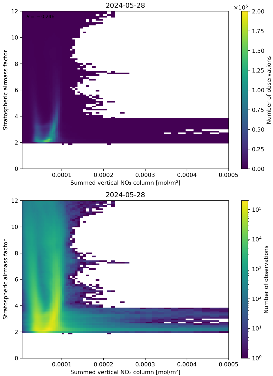
Figure 103: Scatter density plot of “Summed vertical NO 2 column” against “Stratospheric air mass factor” for 2024-05-28 to 2024-05-29.
