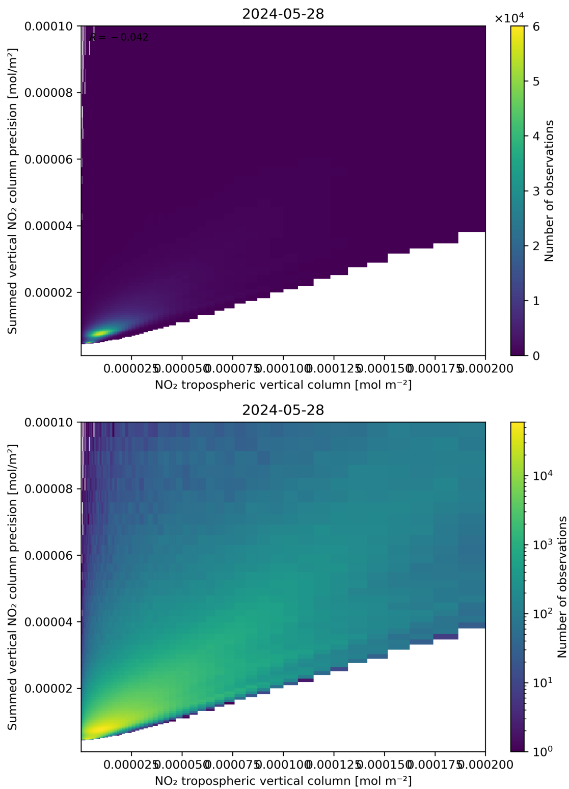
Figure 127: Scatter density plot of “NO 2 tropospheric vertical column” against “Summed vertical NO 2 column precision” for 2024-05-28 to 2024-05-29.
