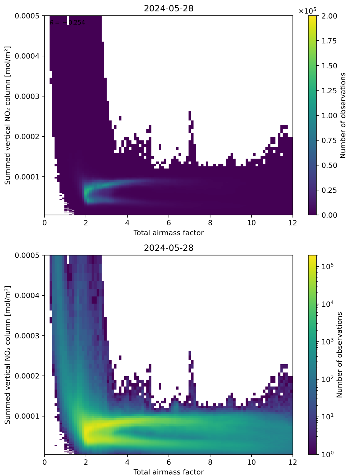
Figure 65: Scatter density plot of “Total airmass factor” against “Summed vertical NO 2 column” for 2024-05-28 to 2024-05-29.
