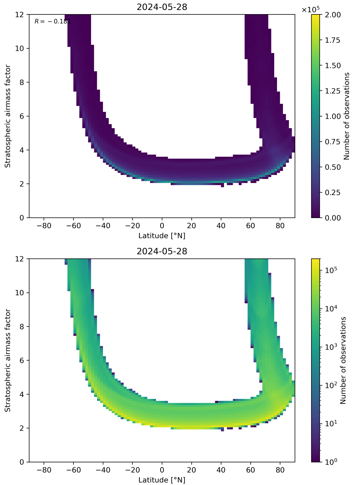
Figure 83: Scatter density plot of “Latitude” against “Stratospheric air mass factor” for 2024-05-28 to 2024-05-29.
