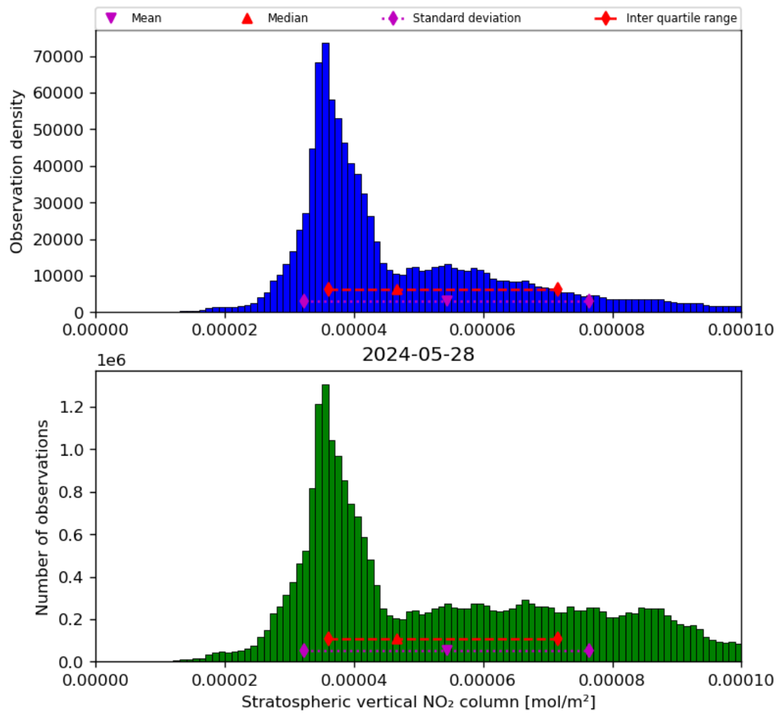
Figure 36: Histogram of “Stratospheric vertical NO 2 column” for 2024-05-28 to 2024-05-29
