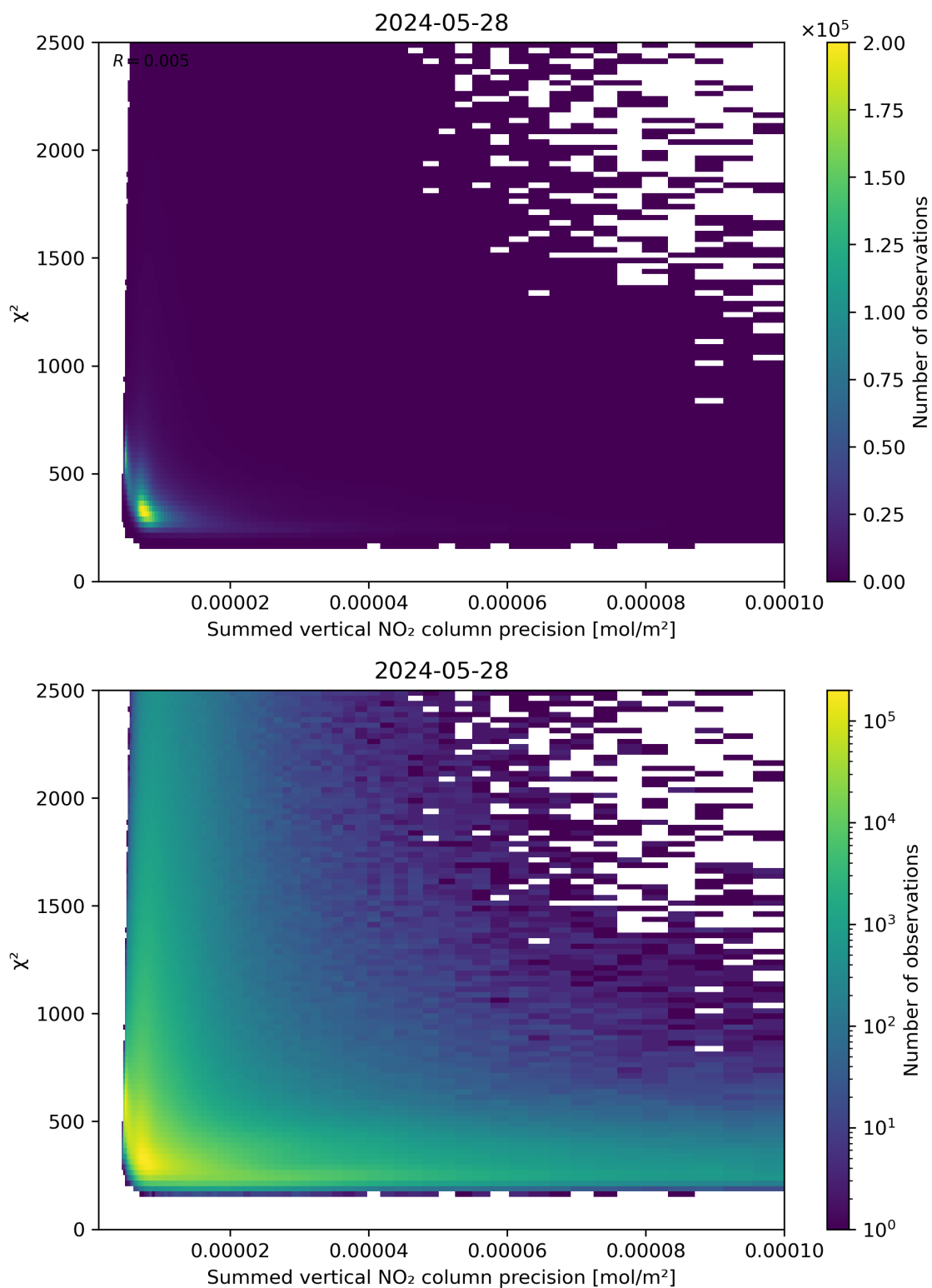
Figure 107: Scatter density plot of “Summed vertical NO 2 column precision” against “ \chi^2 ” for 2024-05-28 to 2024-05-29.
