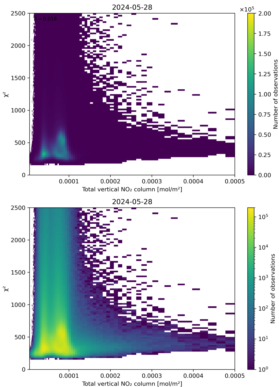
Figure 111: Scatter density plot of “Total vertical NO 2 column” against “ \chi^2 ” for 2024-05-28 to 2024-05-29.
