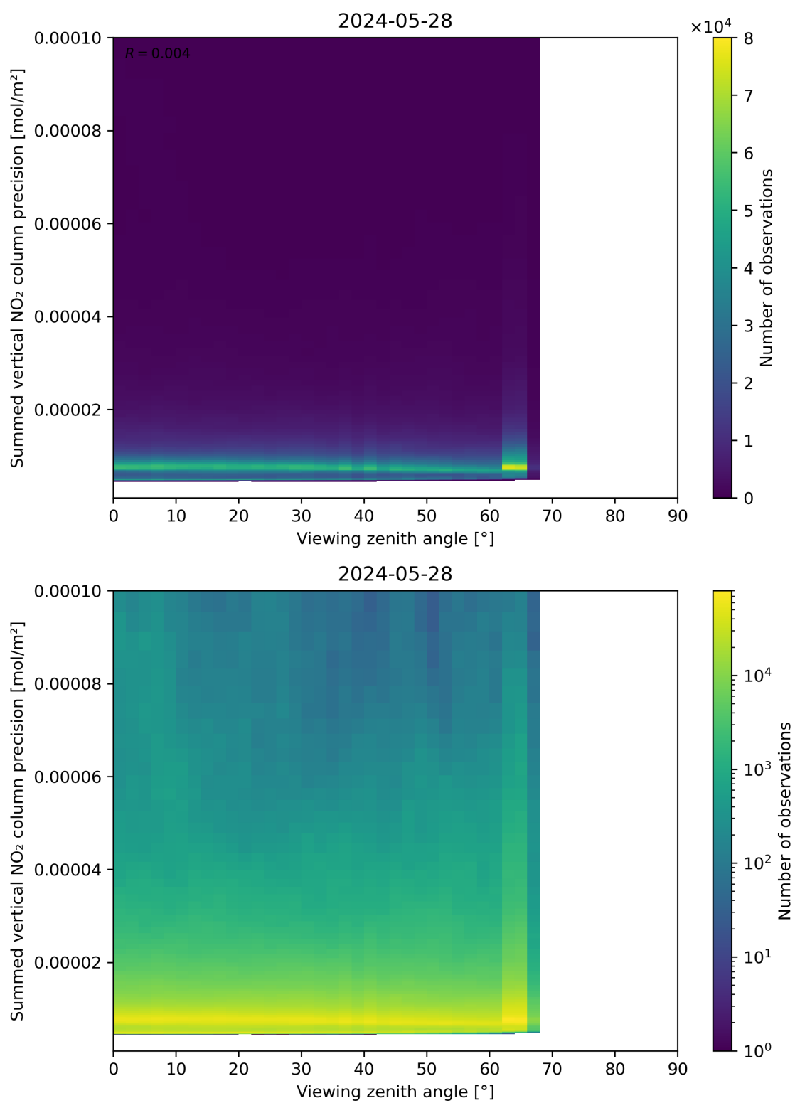
Figure 166: Scatter density plot of “Viewing zenith angle” against “Summed vertical NO 2 column precision” for 2024-05-28 to 2024-05-29.
