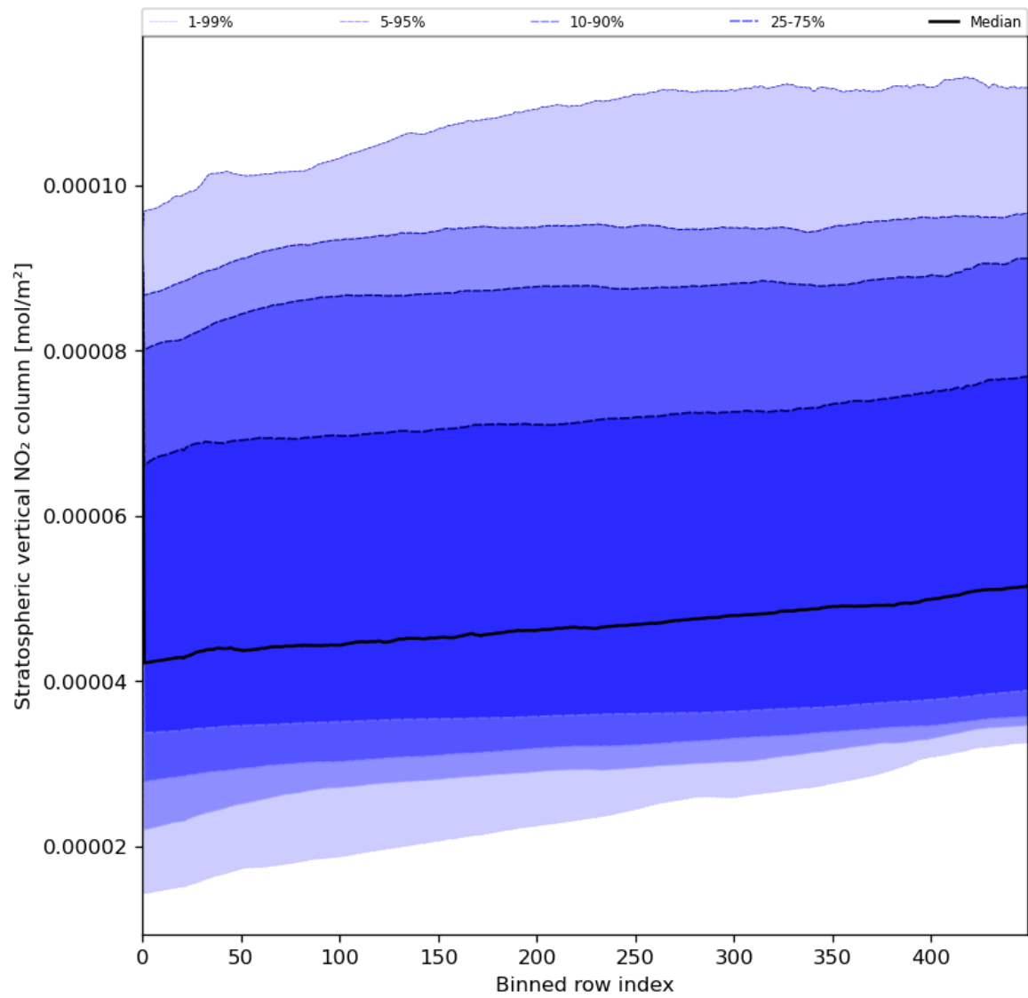
Figure 53: Along track statistics of “Stratospheric vertical NO 2 column” for 2024-05-28 to 2024-05-29
