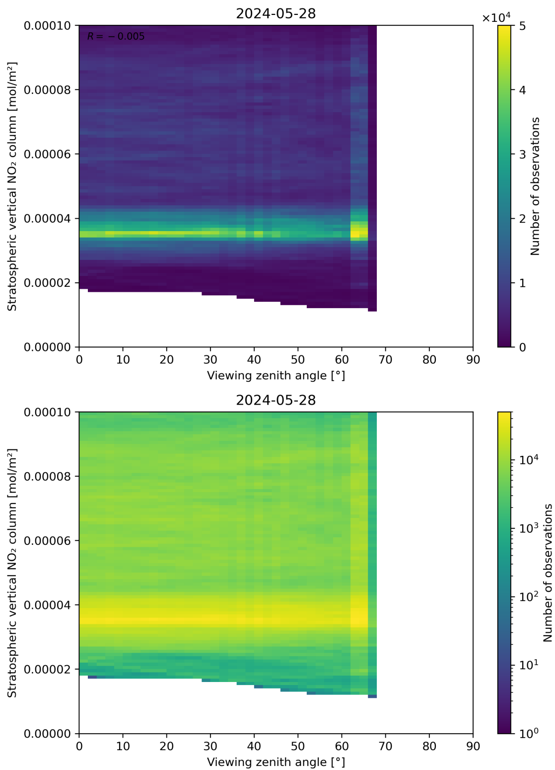
Figure 164: Scatter density plot of “Viewing zenith angle” against “Stratospheric vertical NO 2 column” for 2024-05-28 to 2024-05-29.
