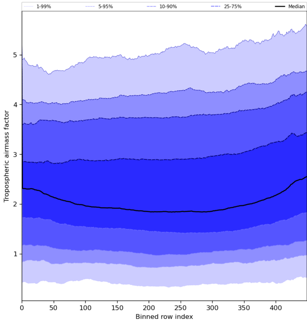
Figure 48: Along track statistics of “Tropospheric airmass factor” for 2024-05-28 to 2024-05-29
