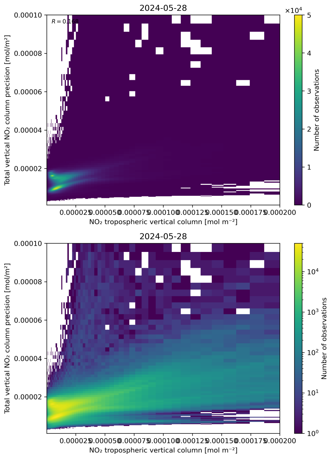
Figure 129: Scatter density plot of “NO 2 tropospheric vertical column” against “Total vertical NO 2 column precision” for 2024-05-28 to 2024-05-29.
