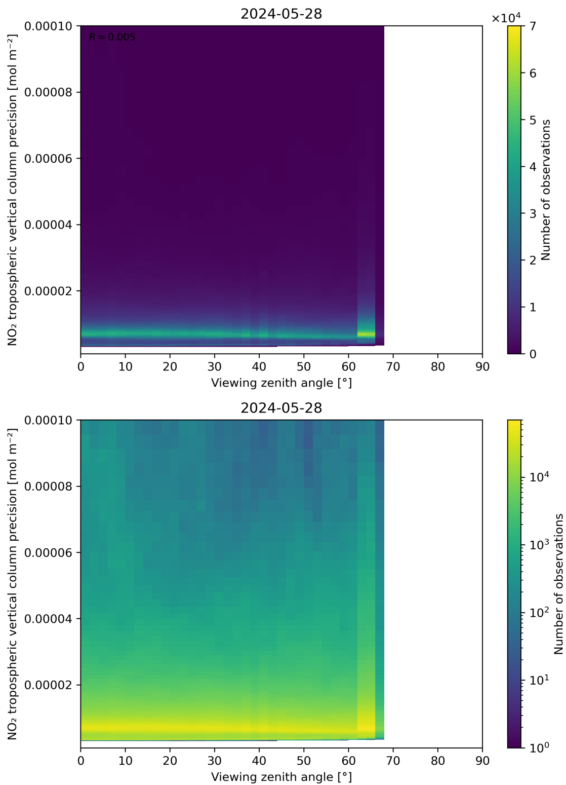
Figure 170: Scatter density plot of “Viewing zenith angle” against “NO 2 tropospheric vertical column precision” for 2024-05-28 to 2024-05-29.
