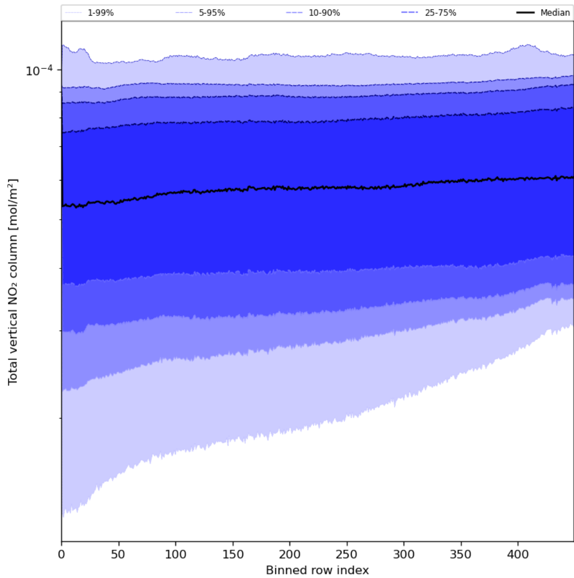
Figure 55: Along track statistics of “Total vertical NO 2 column” for 2024-05-28 to 2024-05-29
