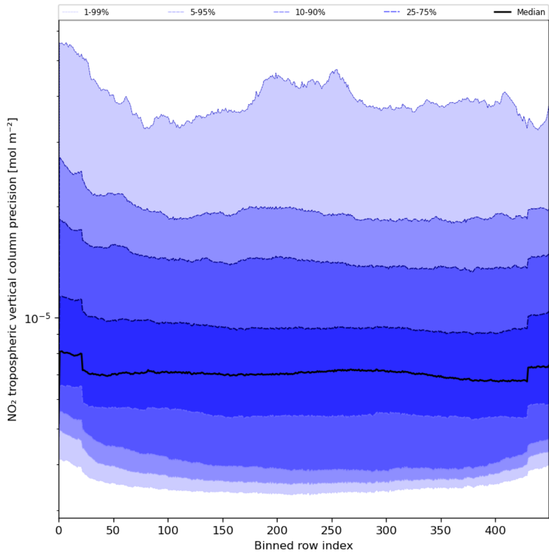
Figure 47: Along track statistics of “NO 2 tropospheric vertical column precision” for 2024-05-28 to 2024-05-29
