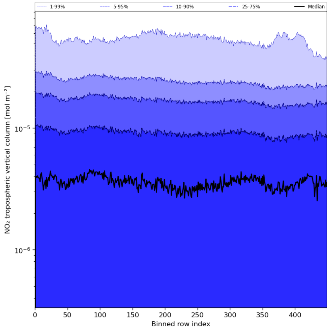
Figure 46: Along track statistics of “NO 2 tropospheric vertical column” for 2024-05-28 to 2024-05-29
