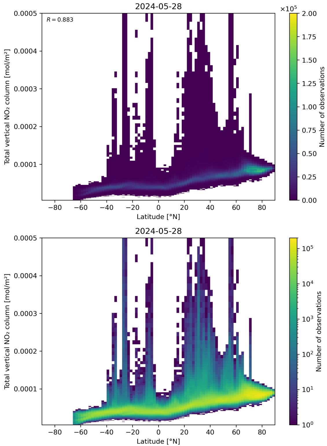
Figure 90: Scatter density plot of “Latitude” against “Total vertical NO 2 column” for 2024-05-28 to 2024-05-29.
