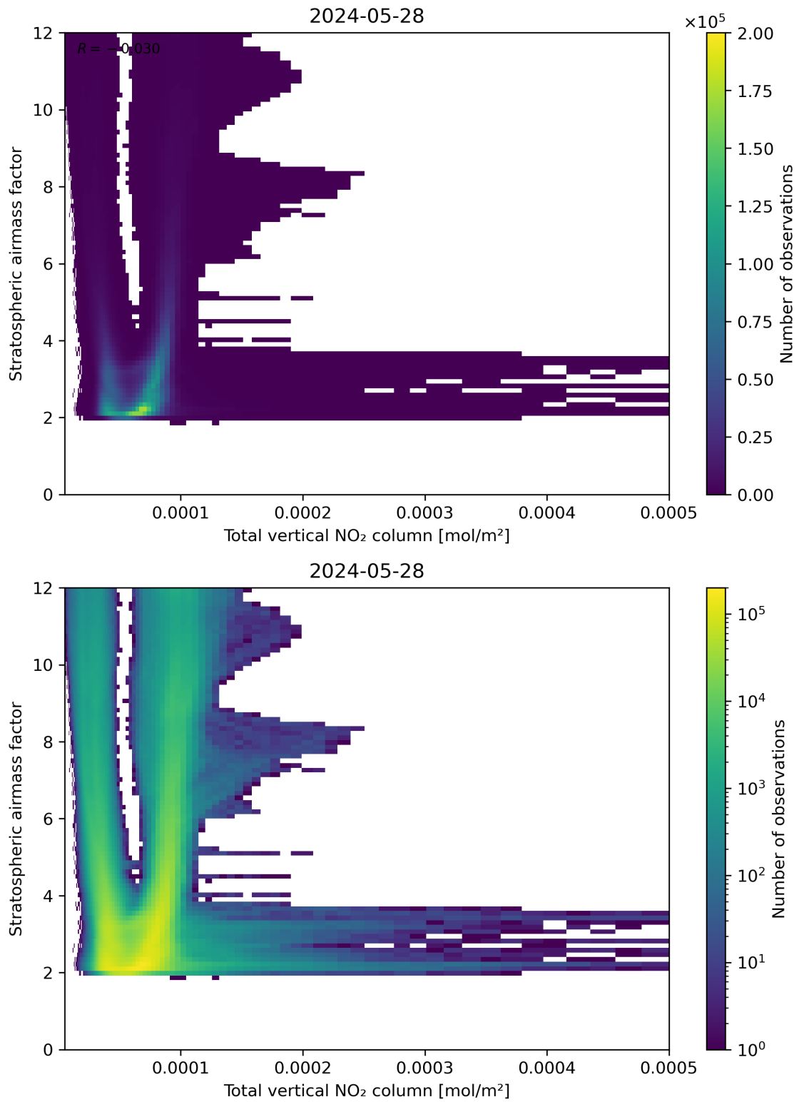
Figure 110: Scatter density plot of “Total vertical NO 2 column” against “Stratospheric airmass factor” for 2024-05-28 to 2024-05-29.
