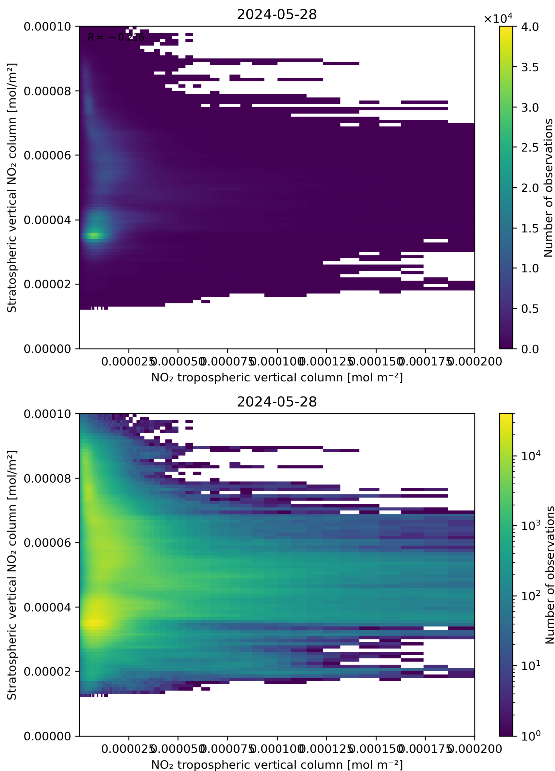
Figure 125: Scatter density plot of “NO 2 tropospheric vertical column” against “Stratospheric vertical NO 2 column” for 2024-05-28 to 2024-05-29.
