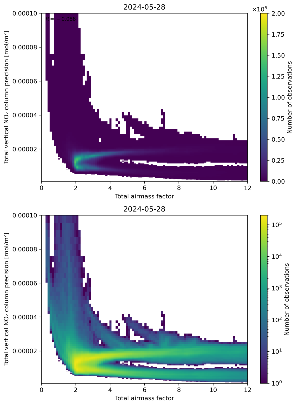
Figure 68: Scatter density plot of “Total airmass factor” against “Total vertical NO 2 column precision” for 2024-05-28 to 2024-05-29.
