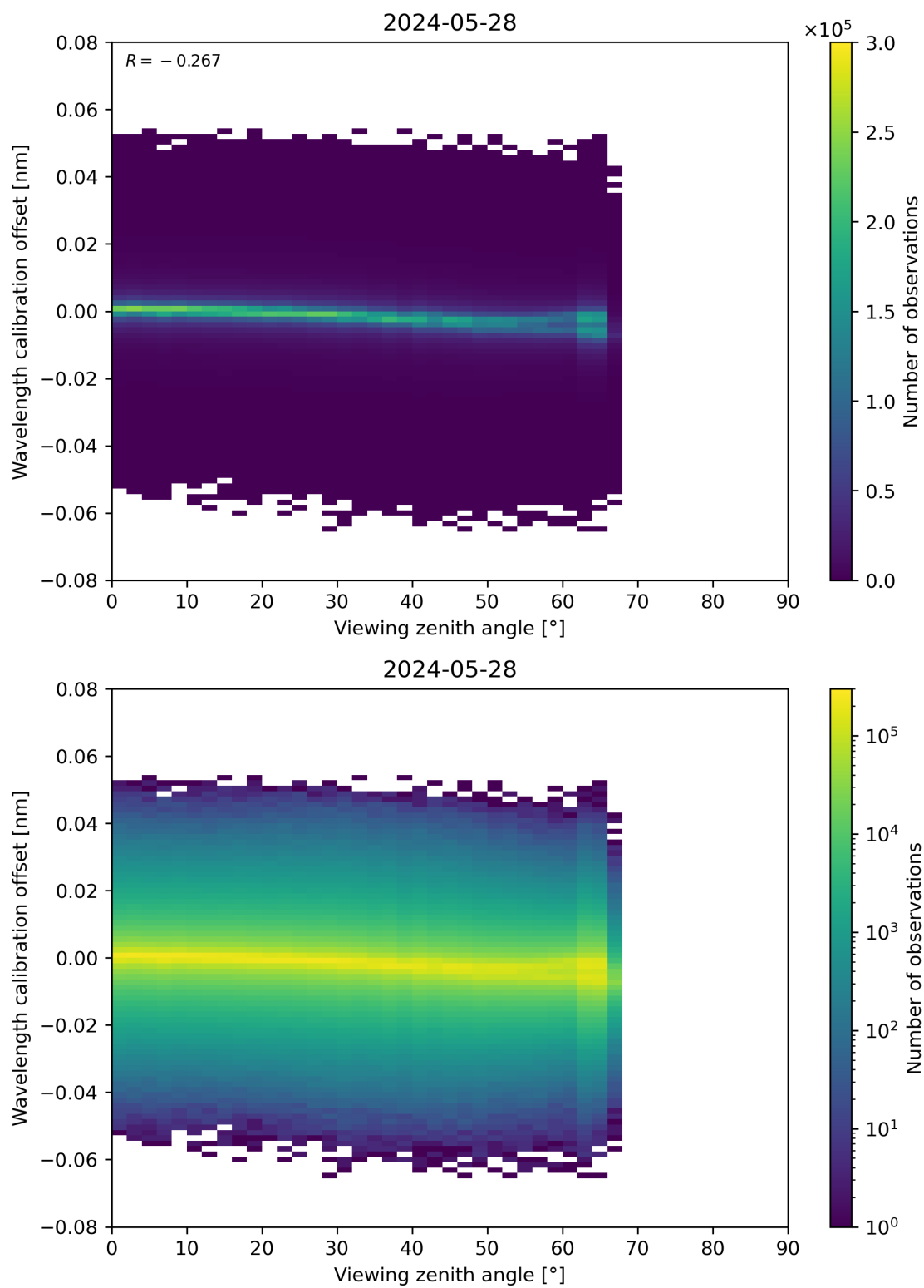
Figure 173: Scatter density plot of “Viewing zenith angle” against “Wavelength calibration offset” for 2024-05-28 to 2024-05-29.
