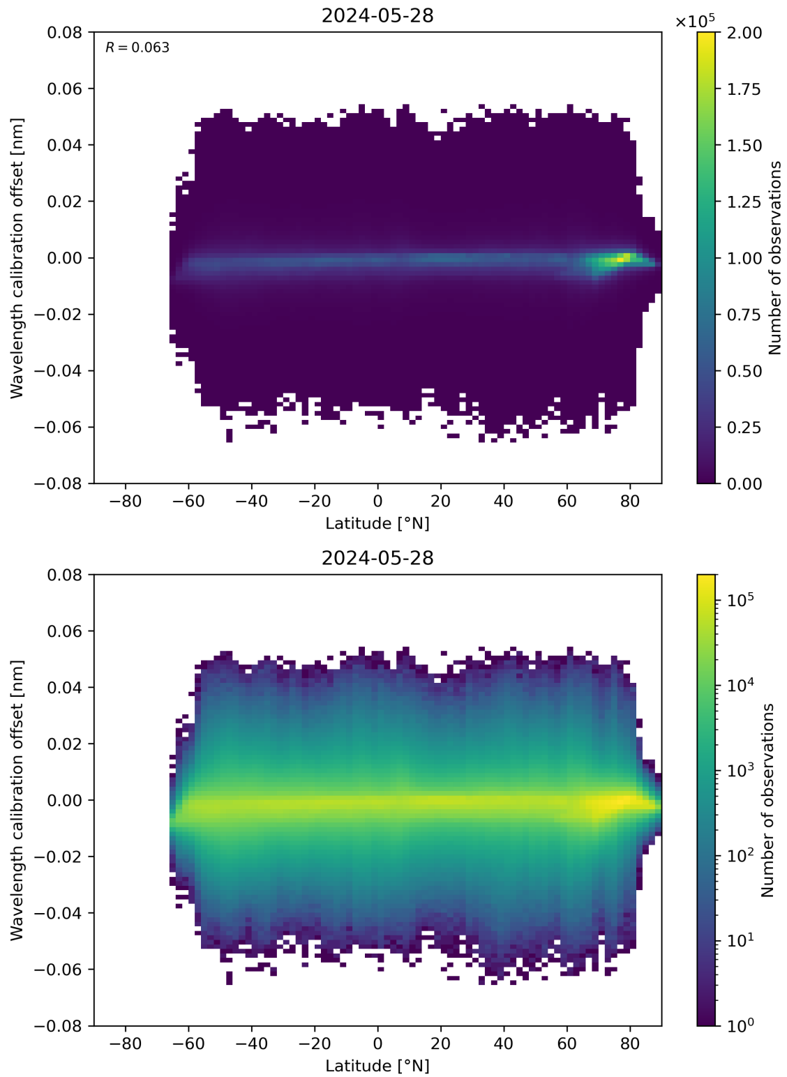
Figure 95: Scatter density plot of “Latitude” against “Wavelength calibration offset” for 2024-05-28 to 2024-05-29.
