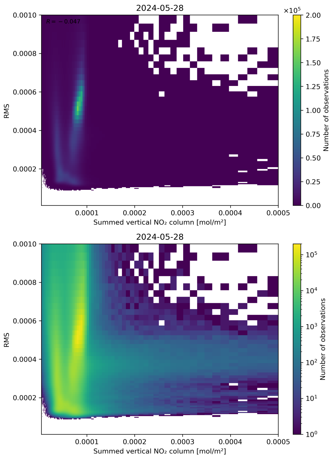
Figure 109: Scatter density plot of “Summed vertical NO 2 column” against “RMS” for 2024-05-28 to 2024-05-29.
