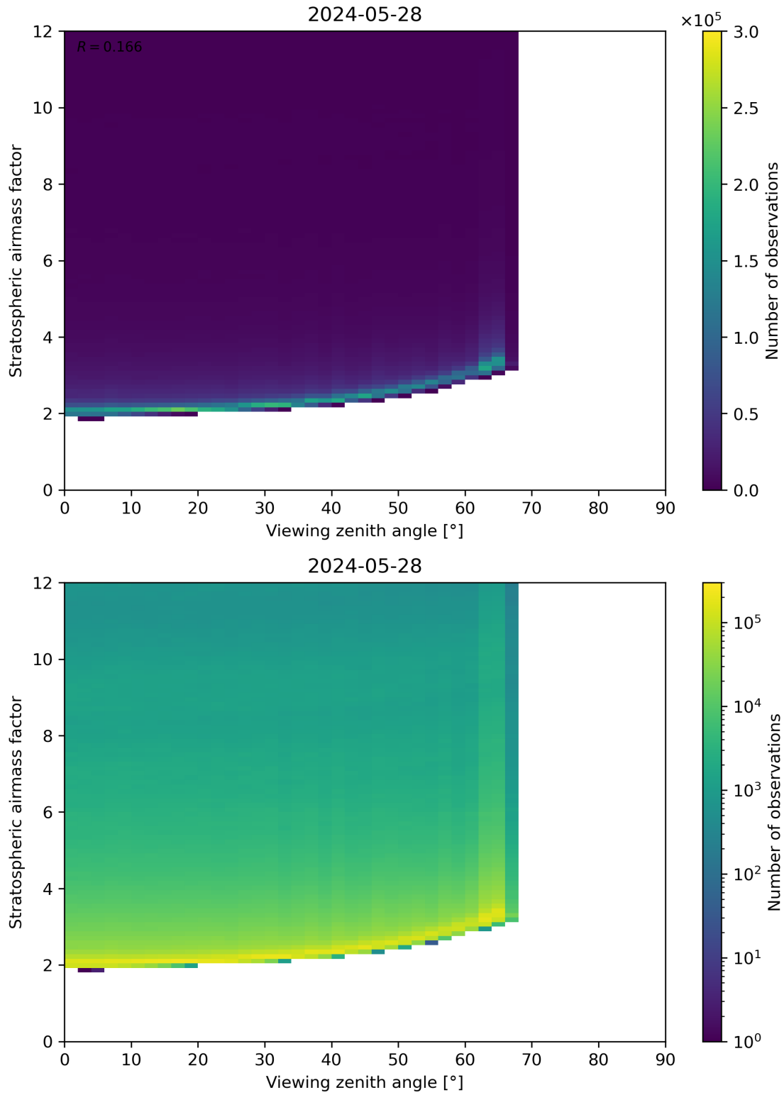
Figure 159: Scatter density plot of “Viewing zenith angle” against “Stratospheric airmass factor” for 2024-05-28 to 2024-05-29.
