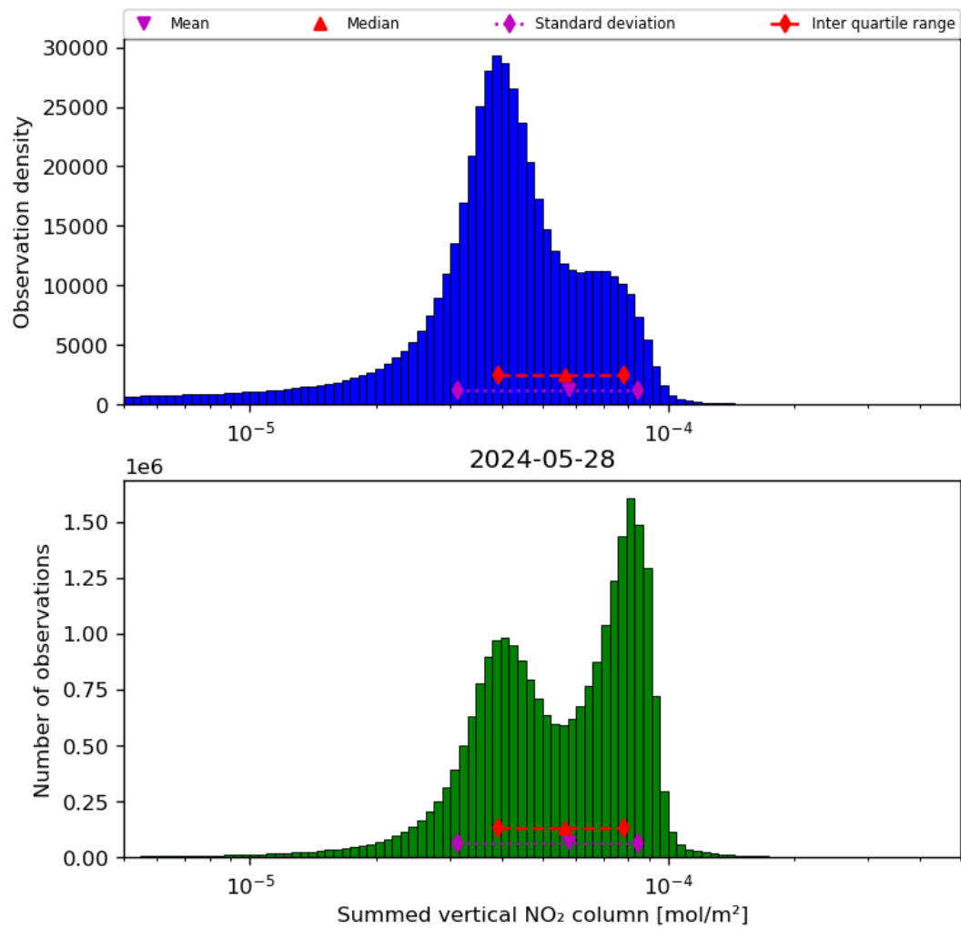
Figure 40: Histogram of “Summed vertical NO 2 column” for 2024-05-28 to 2024-05-29
