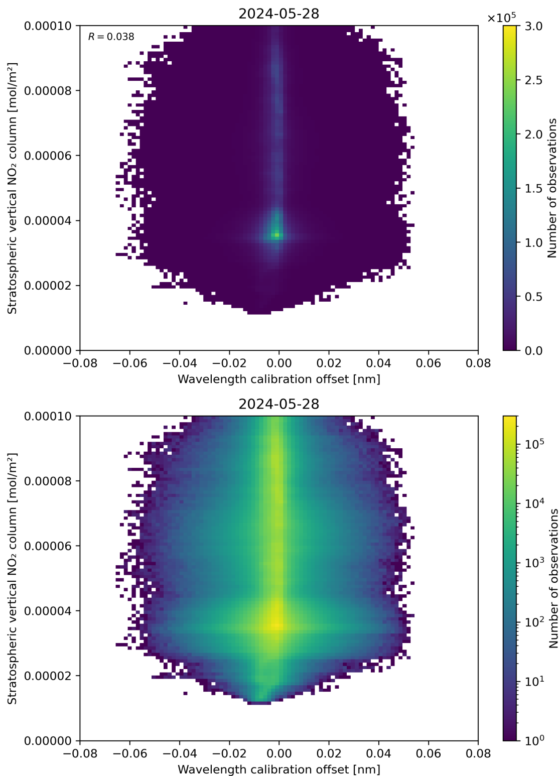
Figure 176: Scatter density plot of “Wavelength calibration offset” against “Stratospheric vertical \text{NO}_2 column” for 2024-05-28 to 2024-05-29.
