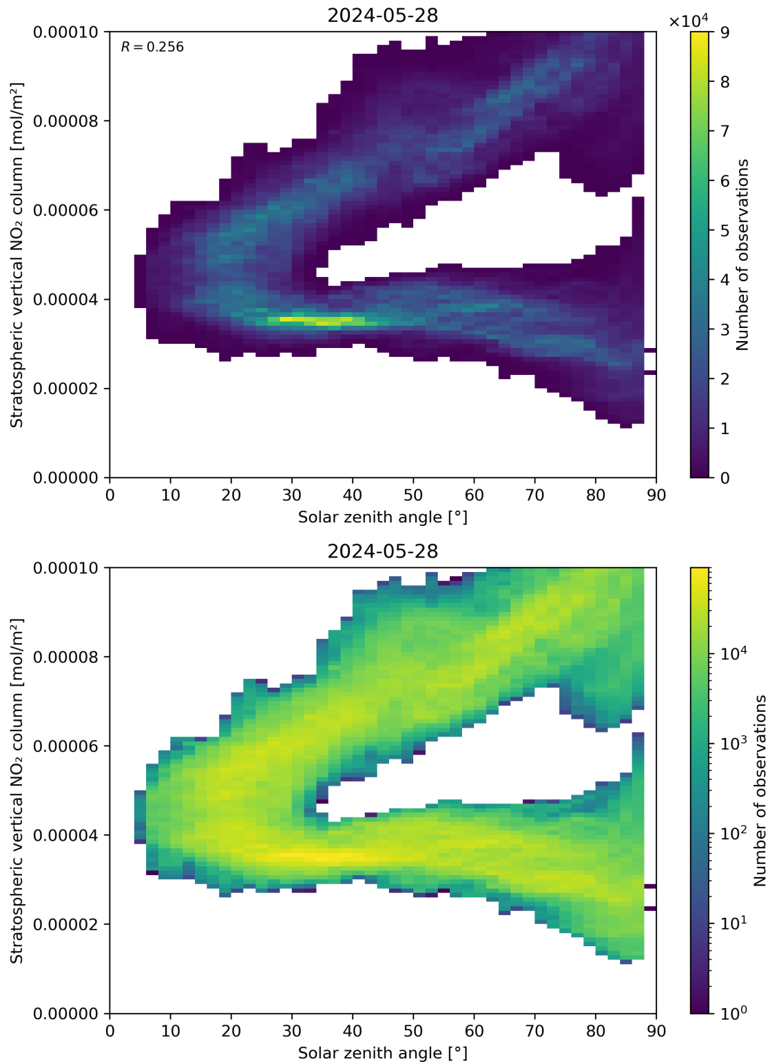
Figure 150: Scatter density plot of “Solar zenith angle” against “Stratospheric vertical NO 2 column” for 2024-05-28 to 2024-05-29.
