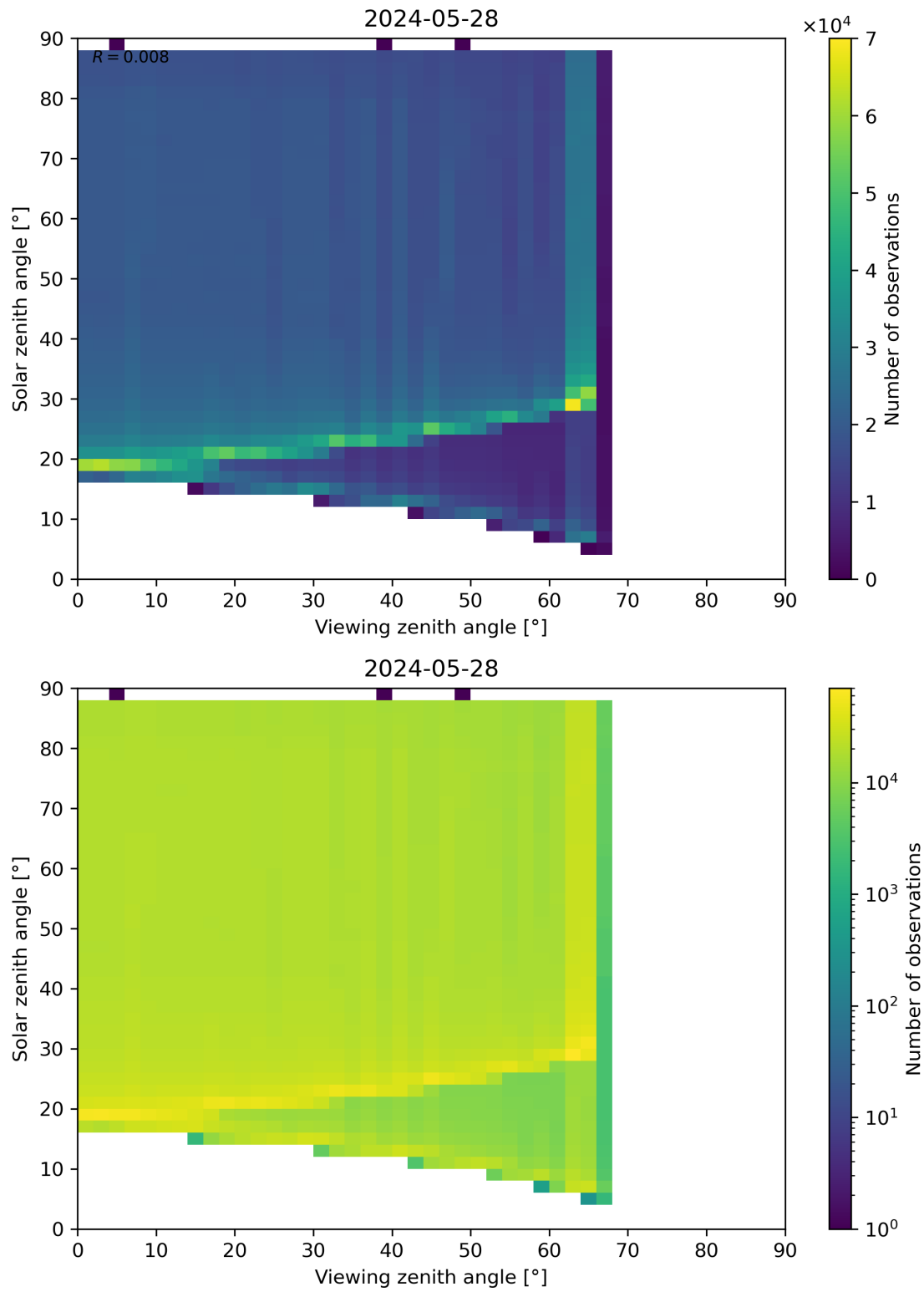
Figure 172: Scatter density plot of “Viewing zenith angle” against “Solar zenith angle” for 2024-05-28 to 2024-05-29.
