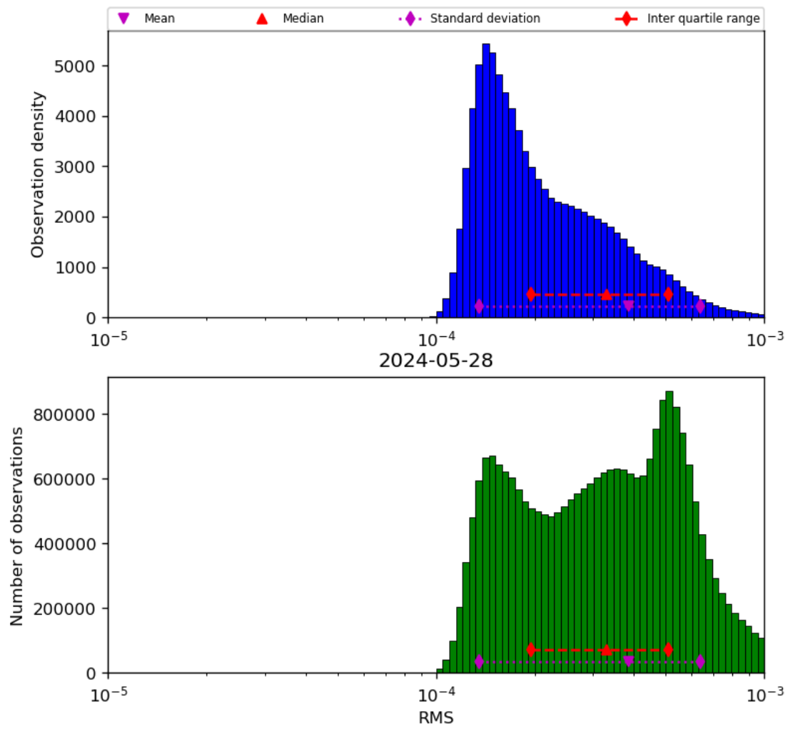
Figure 43: Histogram of “RMS” for 2024-05-28 to 2024-05-29
