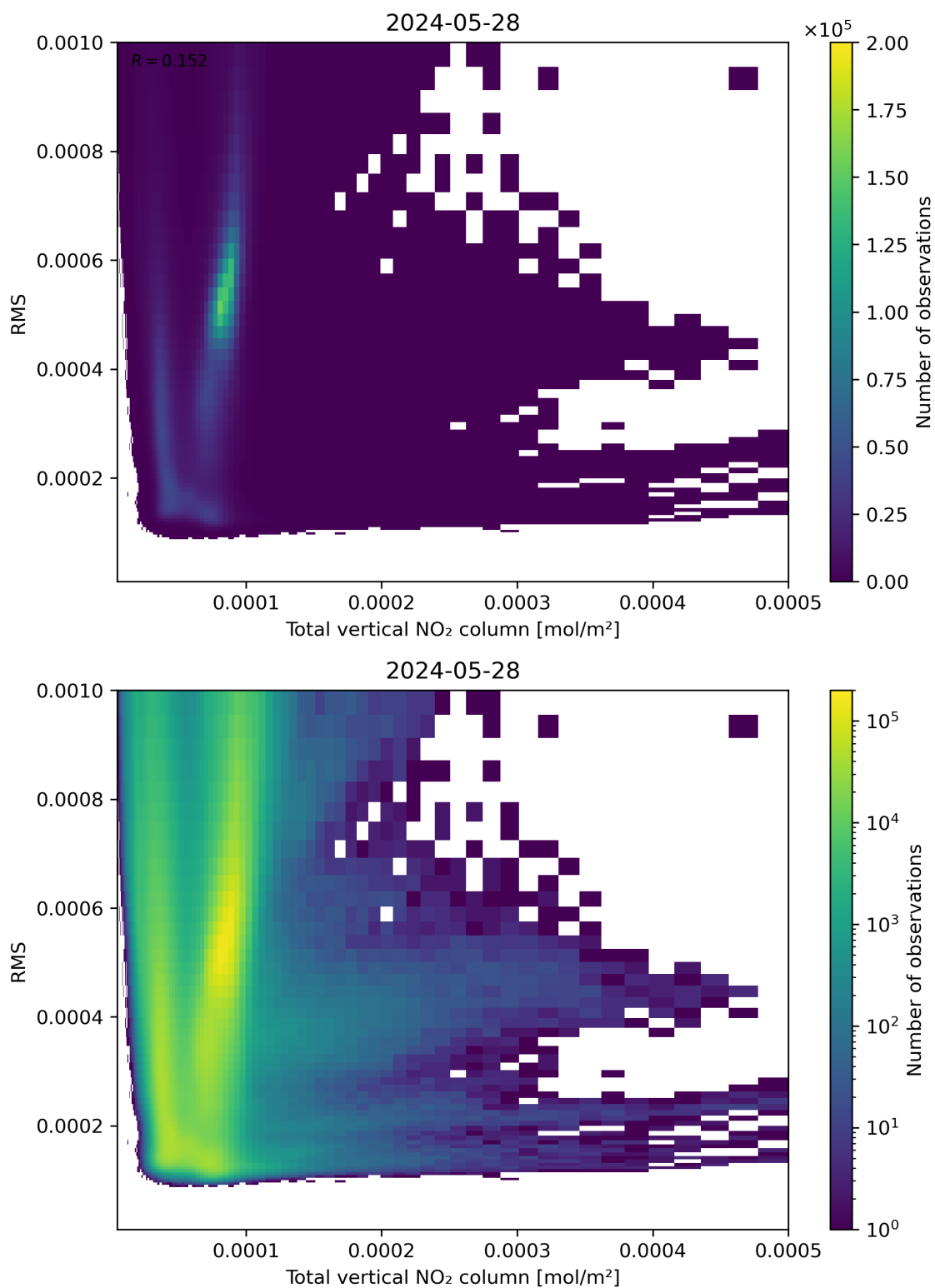
Figure 120: Scatter density plot of “Total vertical NO 2 column” against “RMS” for 2024-05-28 to 2024-05-29.
