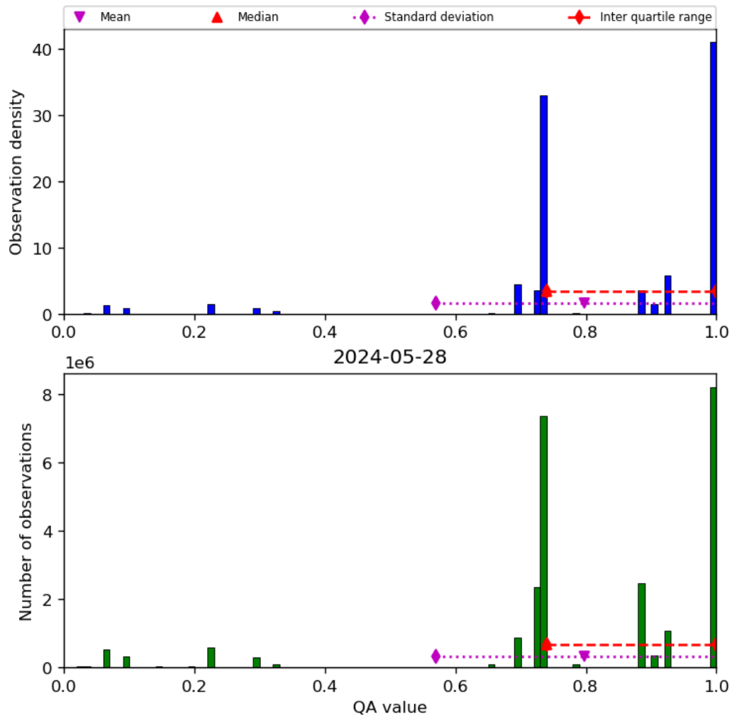
Figure 28: Histogram of “QA value” for 2024-05-28 to 2024-05-29
