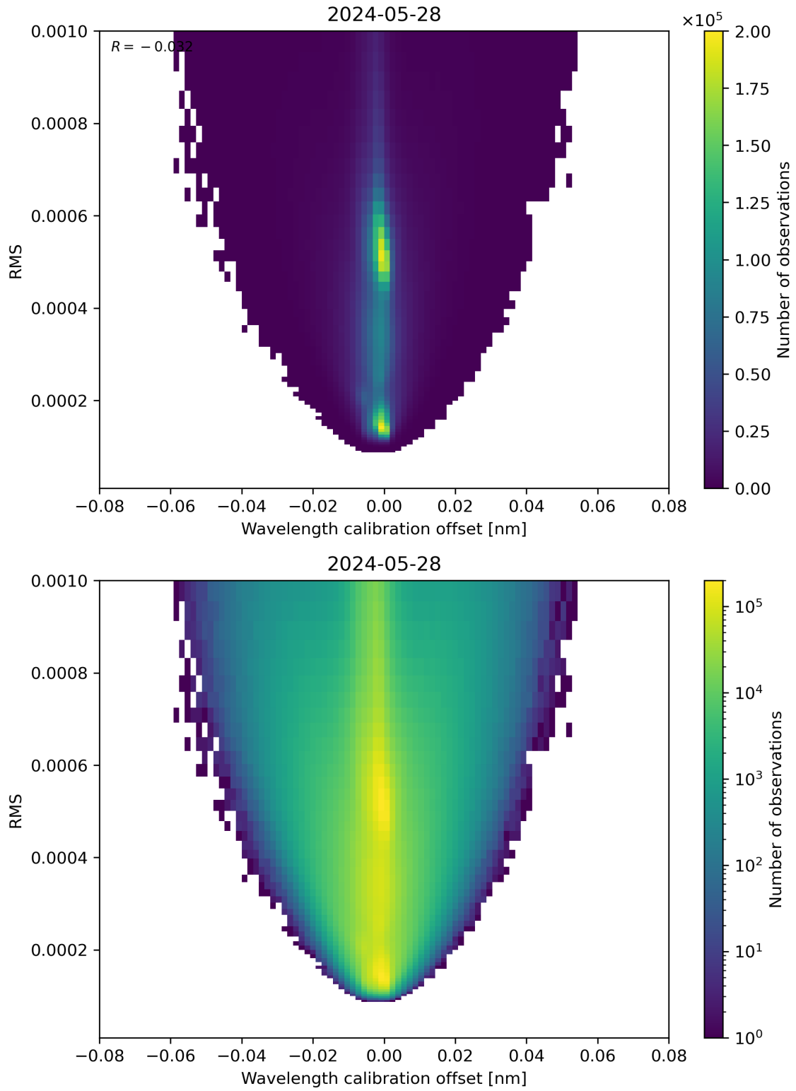
Figure 181: Scatter density plot of “Wavelength calibration offset” against “RMS” for 2024-05-28 to 2024-05-29.
