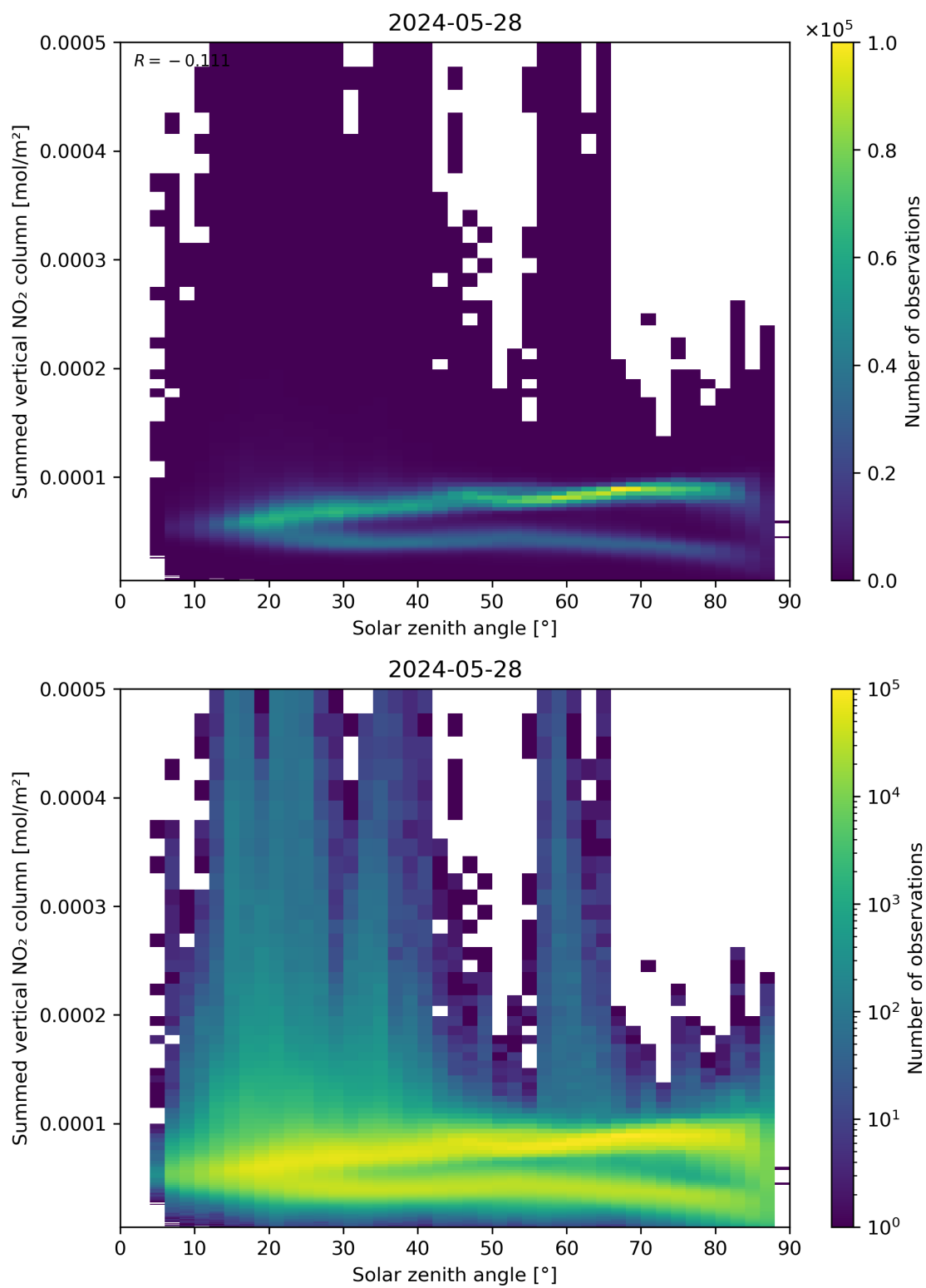
Figure 151: Scatter density plot of “Solar zenith angle” against “Summed vertical NO 2 column” for 2024-05-28 to 2024-05-29.
