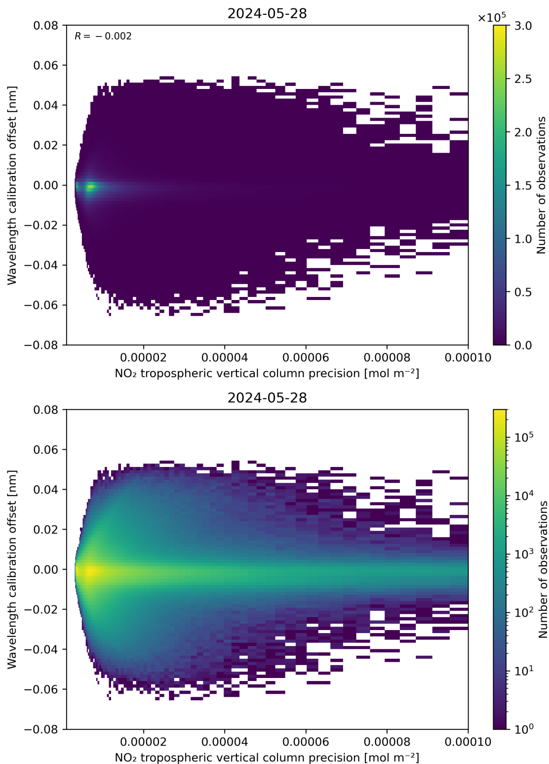
Figure 141: Scatter density plot of “NO 2 tropospheric vertical column precision” against “Wavelength calibration offset” for 2024-05-28 to 2024-05-29.
