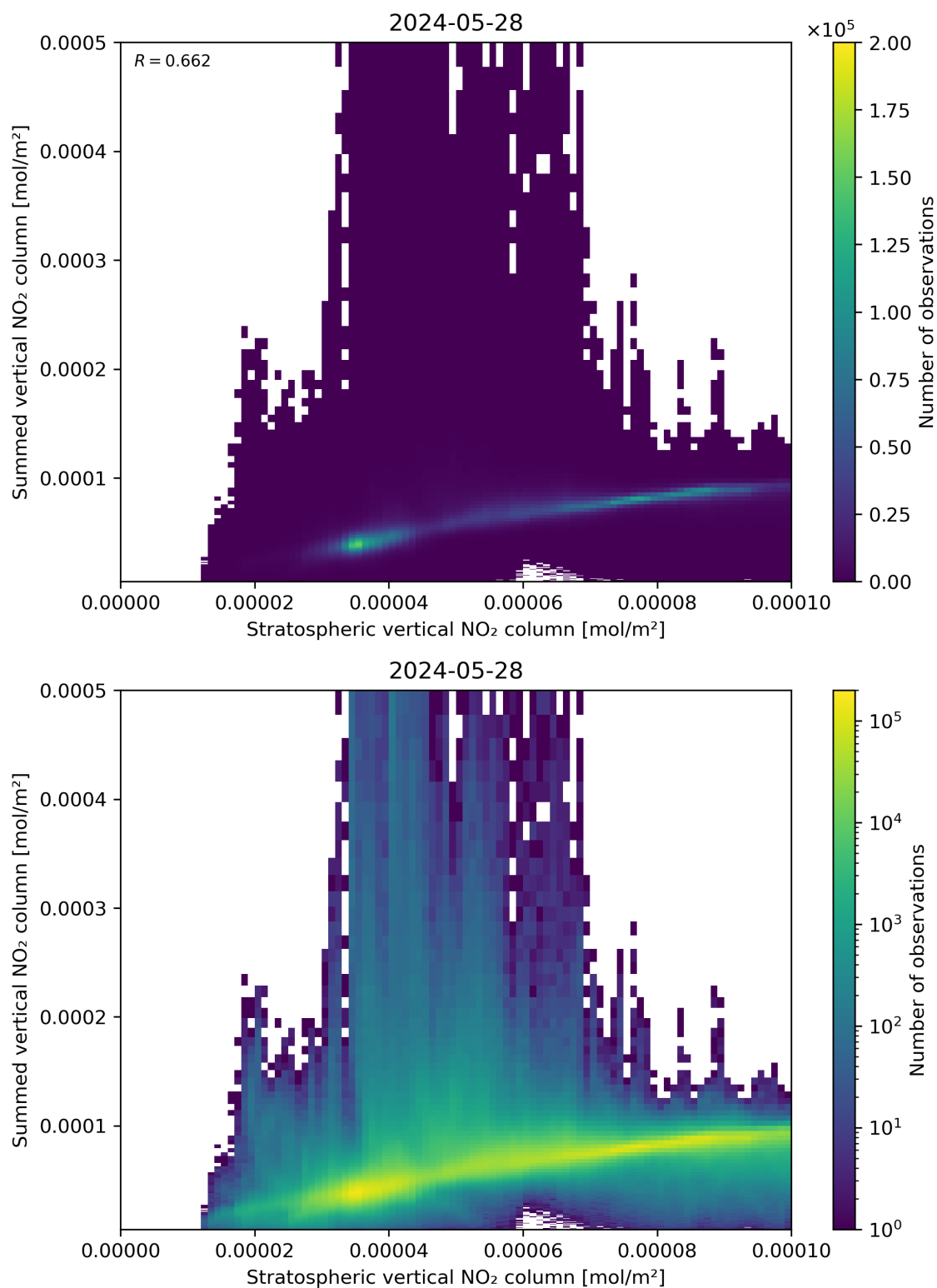
Figure 98: Scatter density plot of “Stratospheric vertical NO 2 column” against “Summed vertical NO 2 column” for 2024-05-28 to 2024-05-29.
