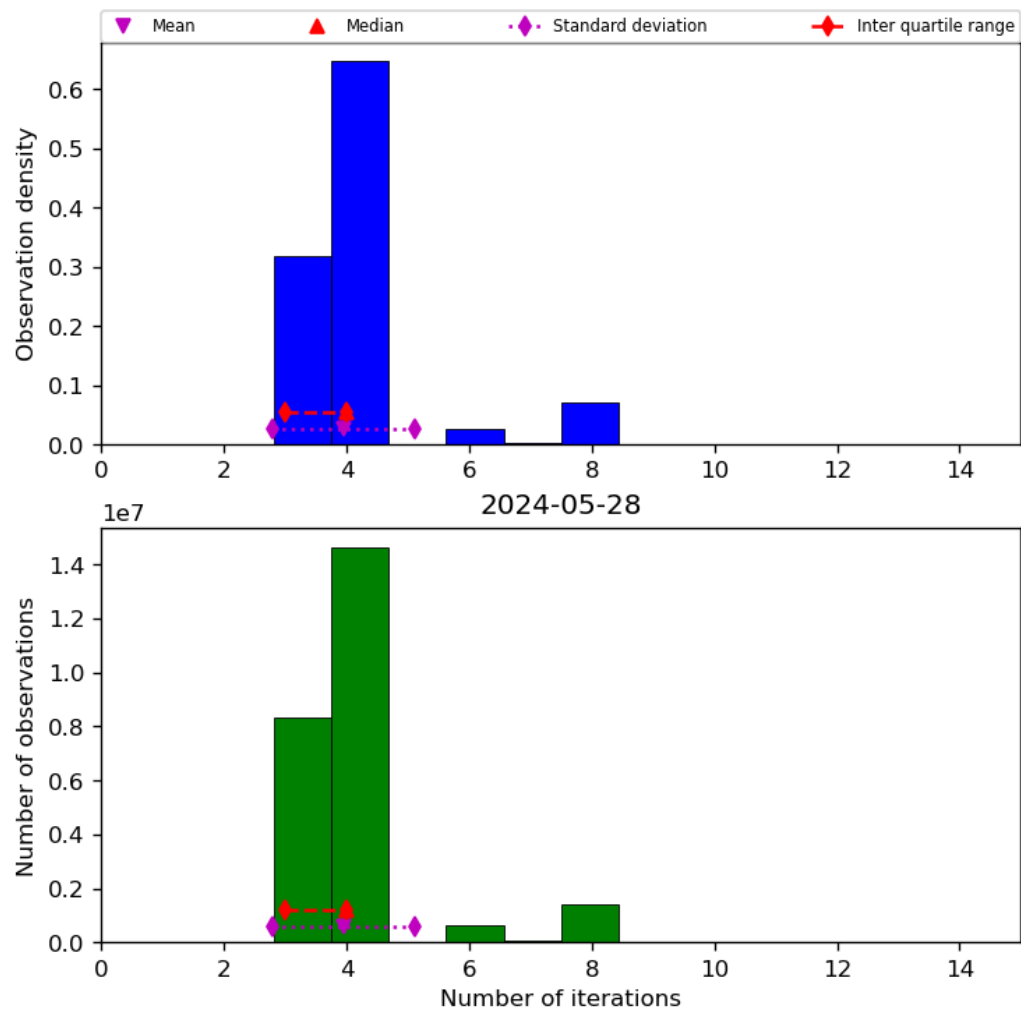
Figure 34: Histogram of “Number of iterations” for 2024-05-28 to 2024-05-29
