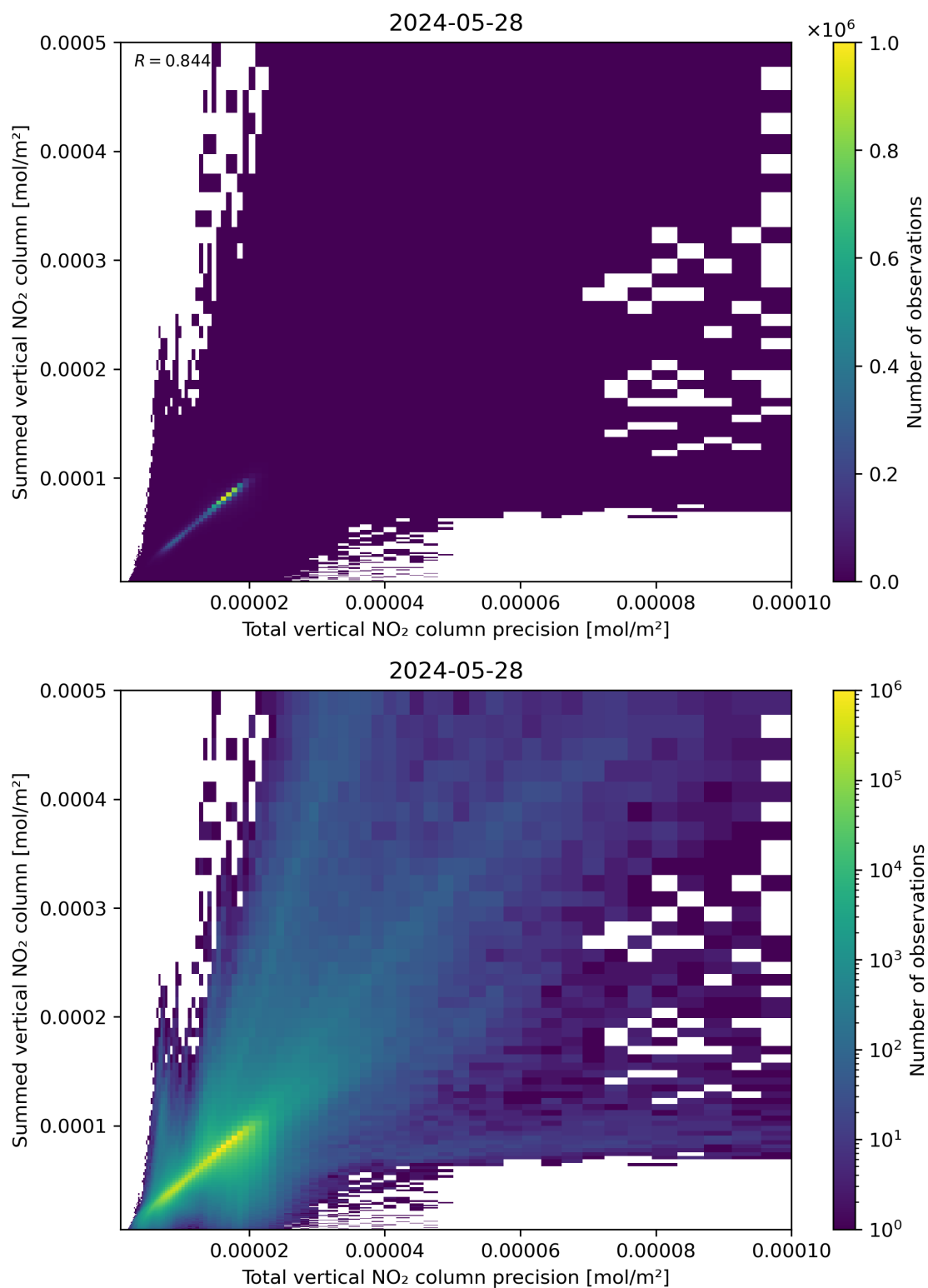
Figure 117: Scatter density plot of “Total vertical NO 2 column precision” against “Summed vertical NO 2 column” for 2024-05-28 to 2024-05-29.
