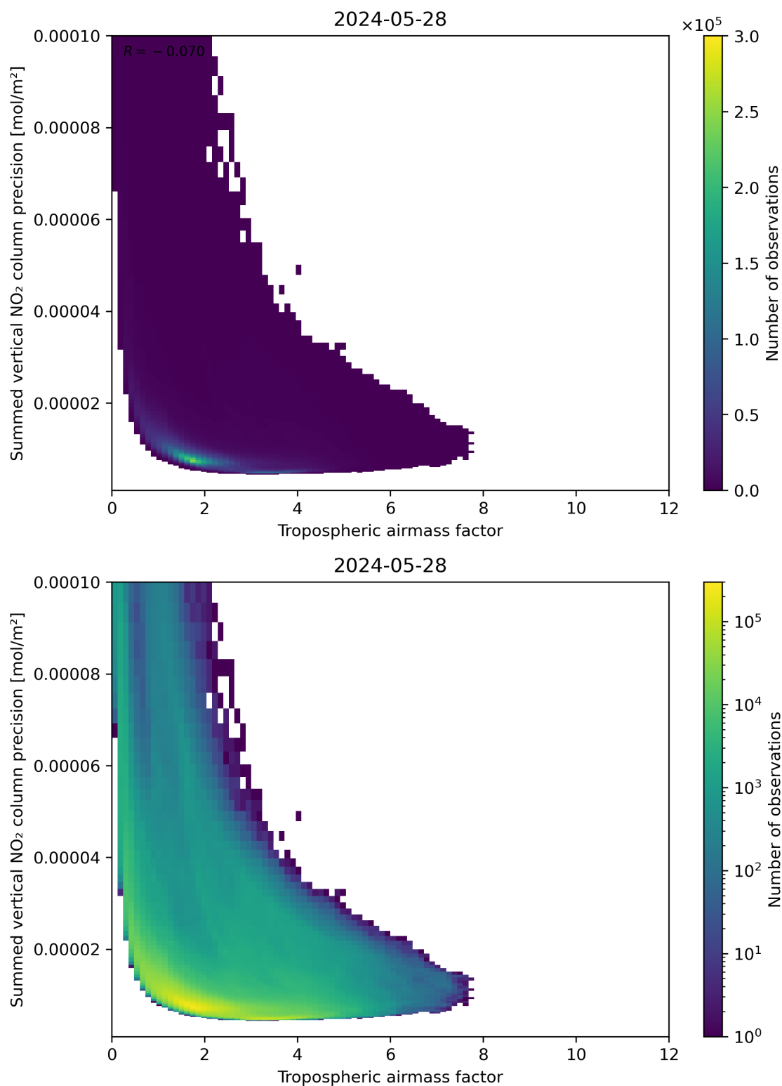
Figure 76: Scatter density plot of “Tropospheric air mass factor” against “Summed vertical NO 2 column precision” for 2024-05-28 to 2024-05-29.
