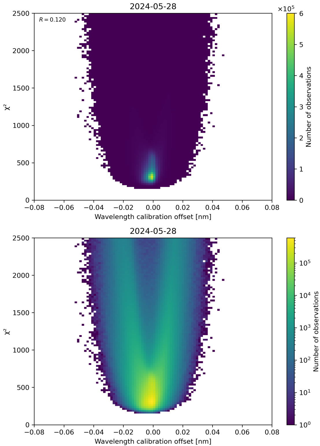
Figure 175: Scatter density plot of “Wavelength calibration offset” against “ \chi^2 ” for 2024-05-28 to 2024-05-29.
