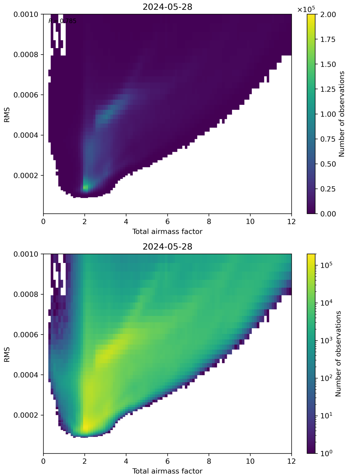
Figure 69: Scatter density plot of “Total airmass factor” against “RMS” for 2024-05-28 to 2024-05-29.
