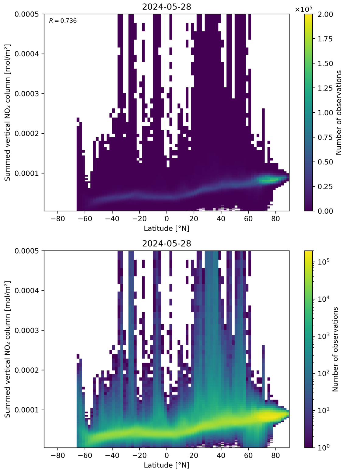
Figure 88: Scatter density plot of “Latitude” against “Summed vertical NO 2 column” for 2024-05-28 to 2024-05-29.
