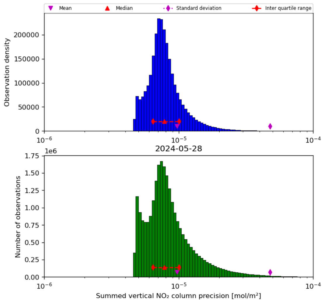
Figure 41: Histogram of “Summed vertical NO 2 column precision” for 2024-05-28 to 2024-05-29
