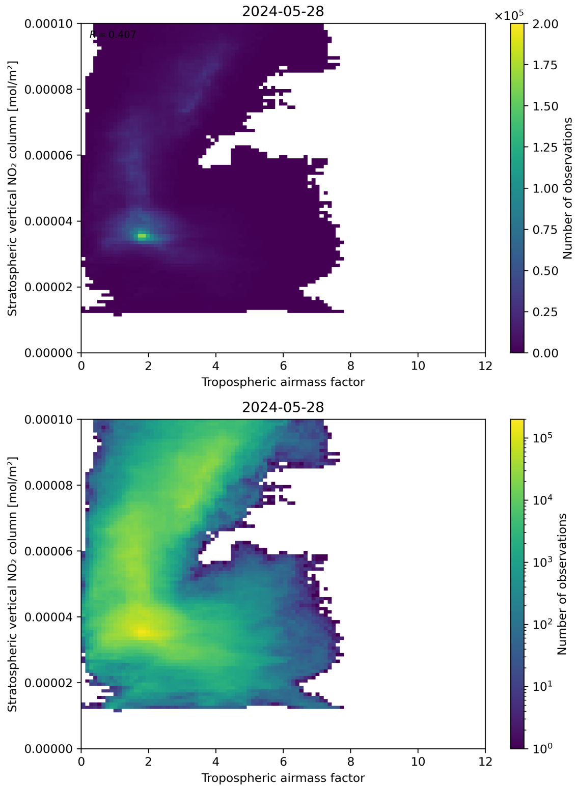
Figure 74: Scatter density plot of “Tropospheric air mass factor” against “Stratospheric vertical NO 2 column” for 2024-05-28 to 2024-05-29.
