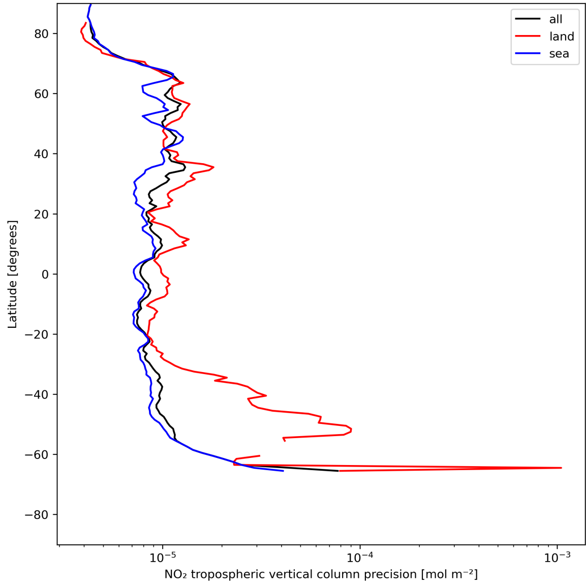
Figure 13: Zonal average of “NO 2 tropospheric vertical column precision” for 2024-05-28 to 2024-05-29.
