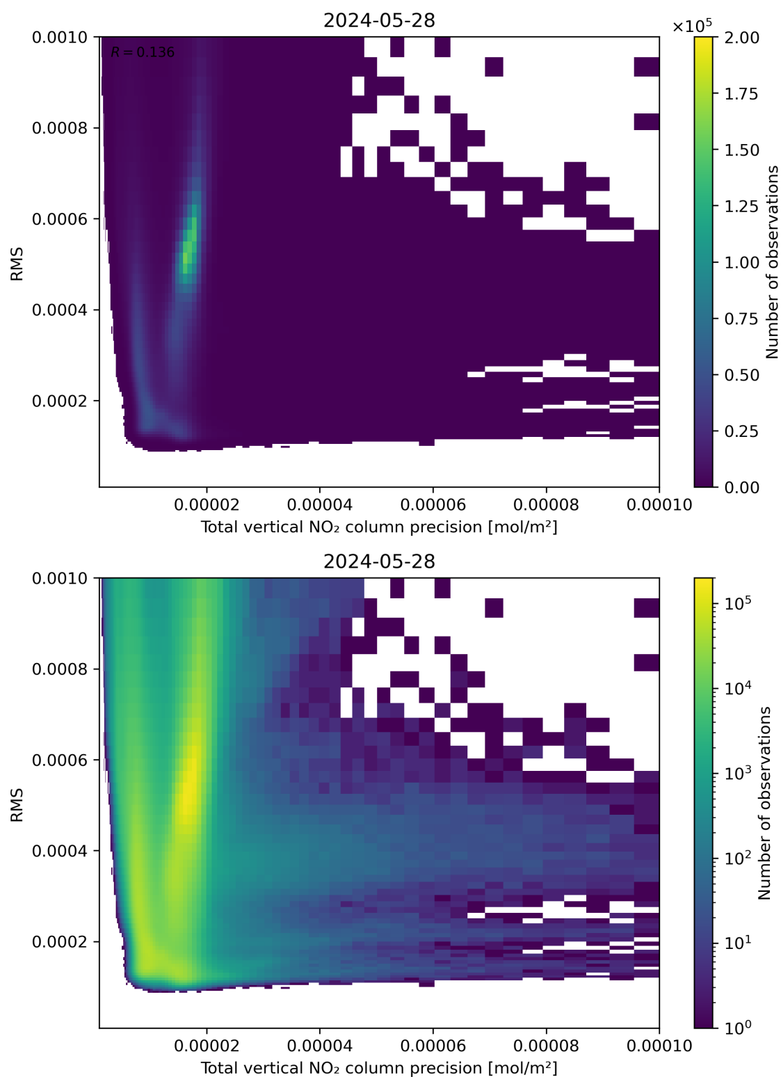
Figure 119: Scatter density plot of “Total vertical NO 2 column precision” against “RMS” for 2024-05-28 to 2024-05-29.
