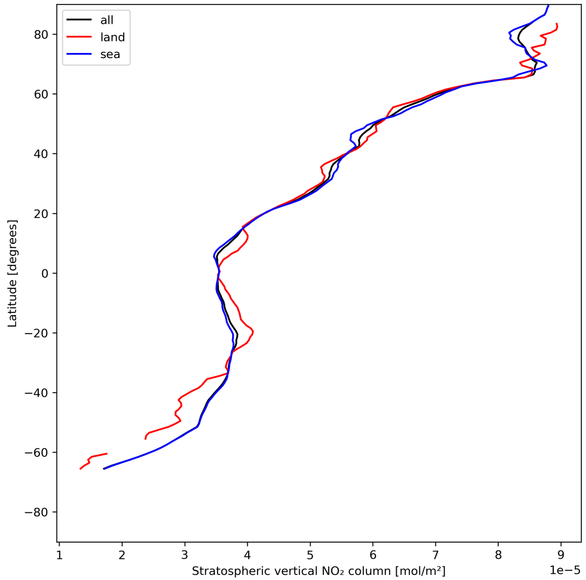
Figure 19: Zonal average of “Stratospheric vertical NO 2 column” for 2024-05-28 to 2024-05-29.
