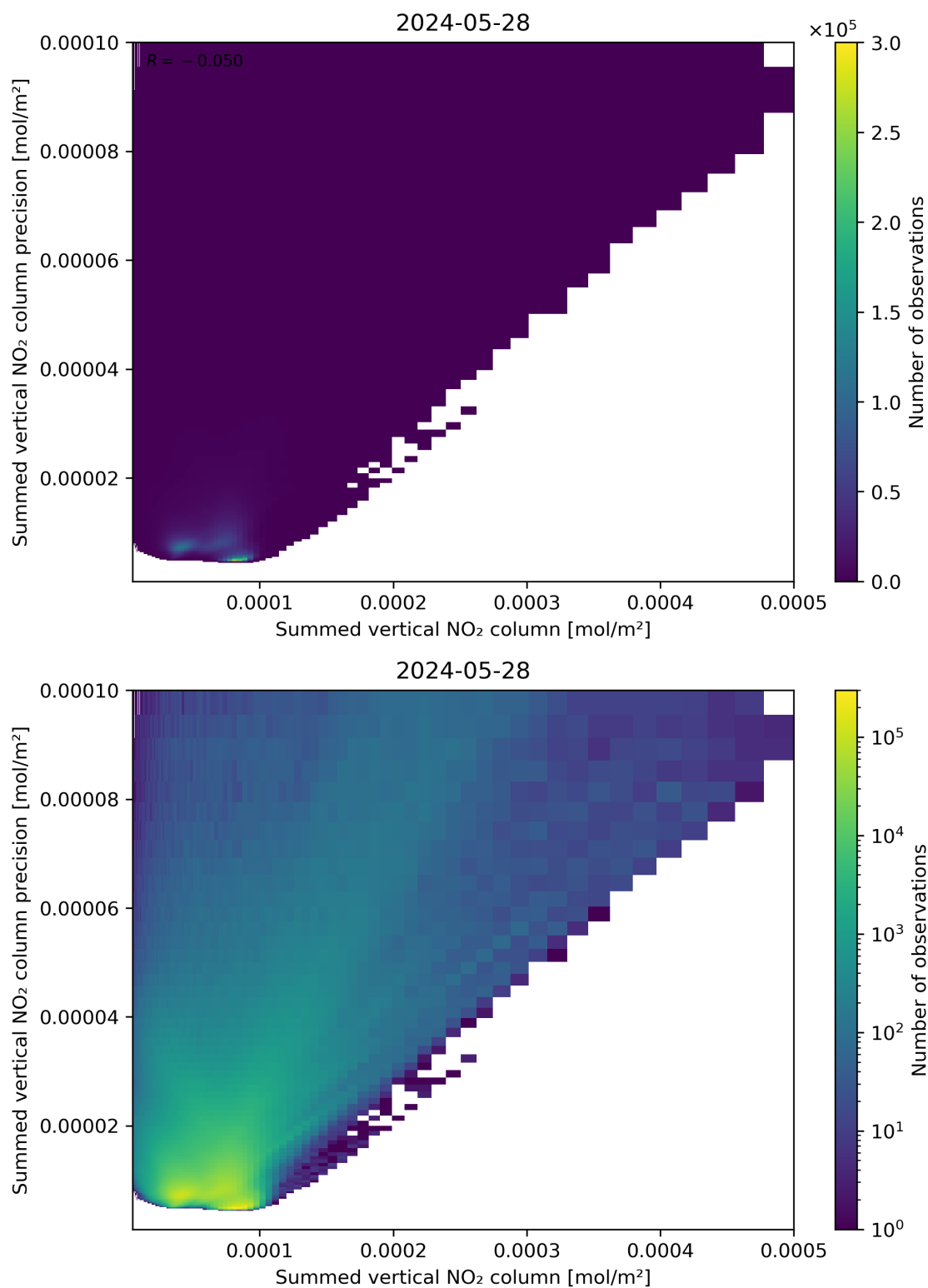
Figure 105: Scatter density plot of “Summed vertical NO 2 column” against “Summed vertical NO 2 column precision” for 2024-05-28 to 2024-05-29.
