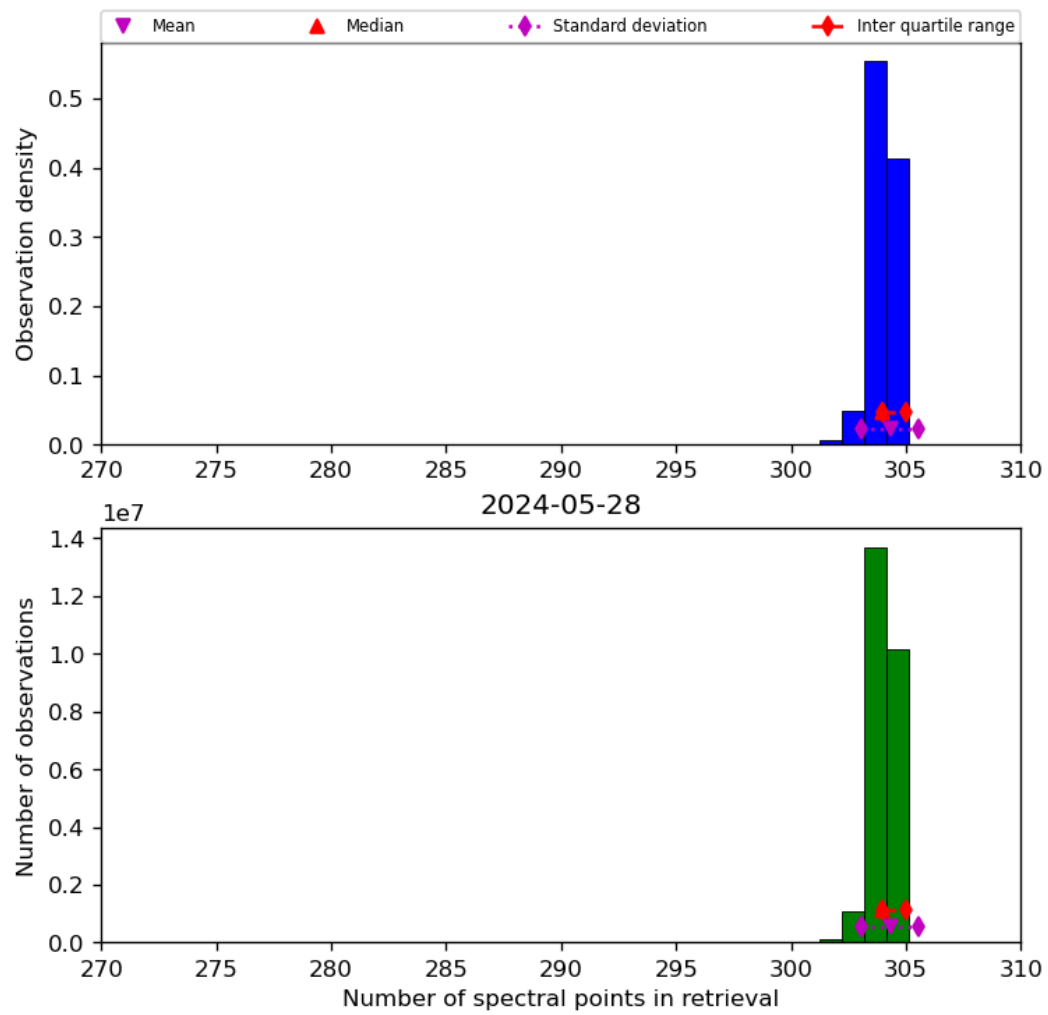
Figure 33: Histogram of “Number of spectral points in retrieval” for 2024-05-28 to 2024-05-29
