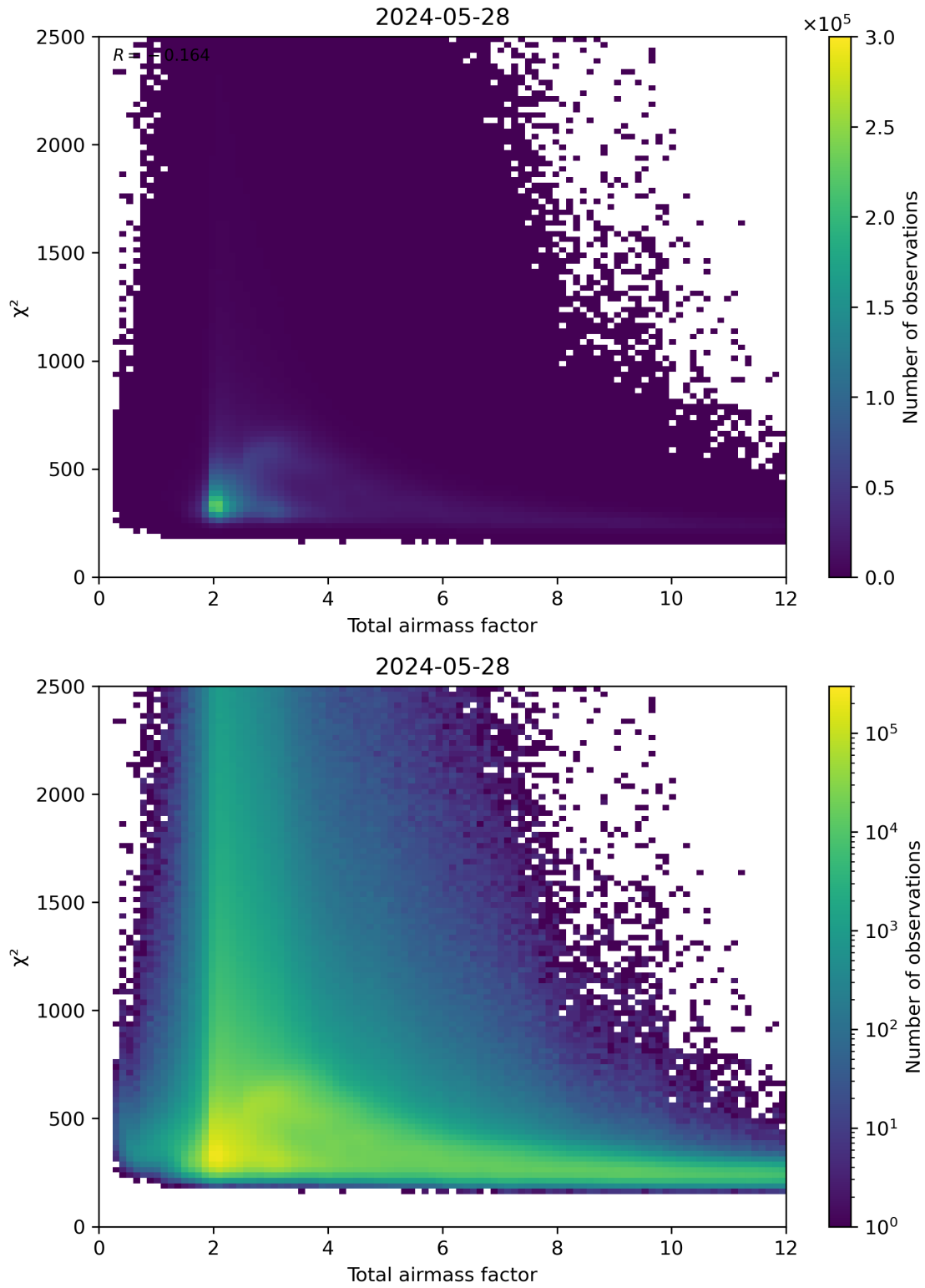
Figure 63: Scatter density plot of “Total airmass factor” against “ \chi^2 ” for 2024-05-28 to 2024-05-29.
