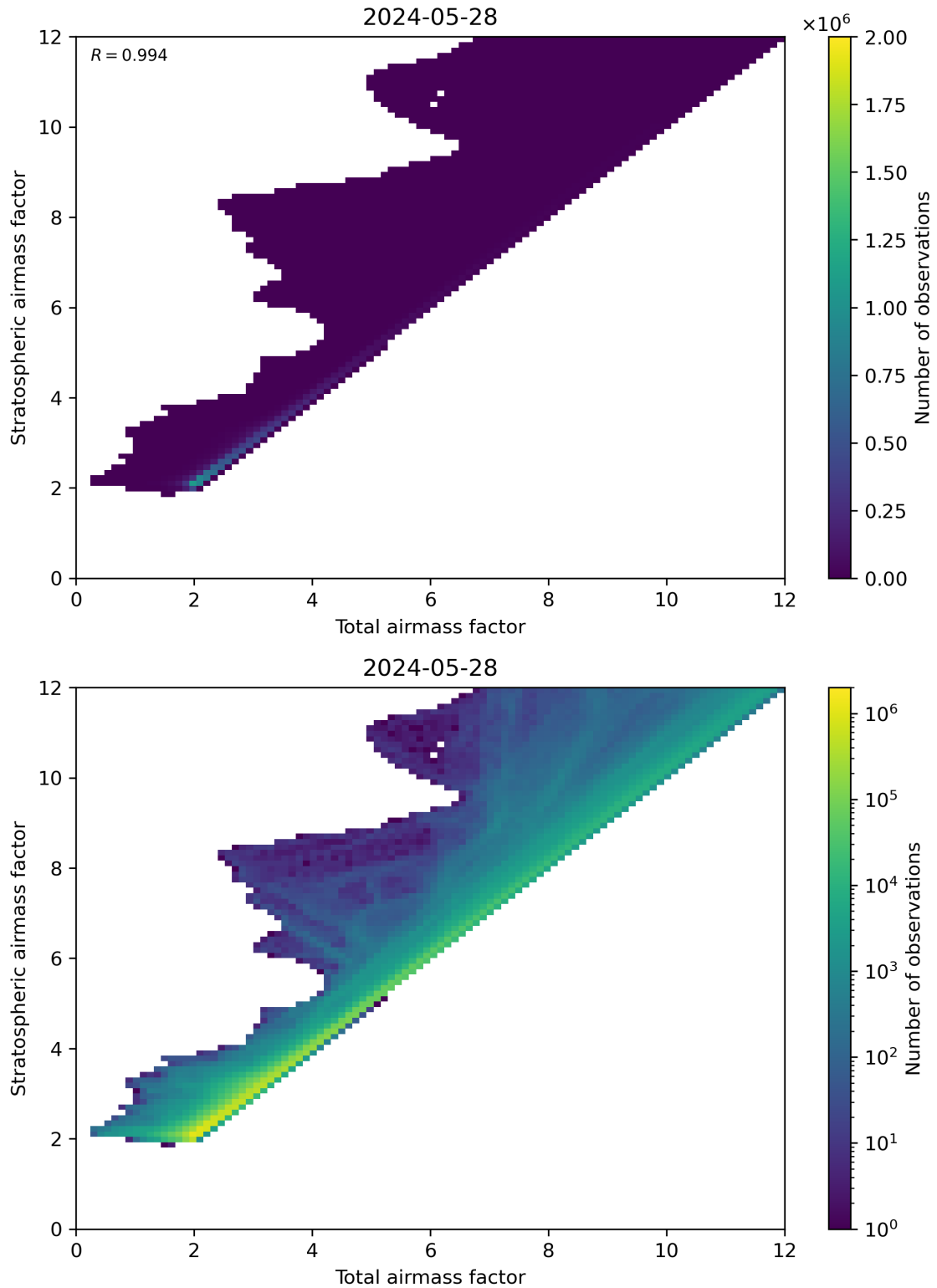
Figure 62: Scatter density plot of “Total airmass factor” against “Stratospheric airmass factor” for 2024-05-28 to 2024-05-29.
