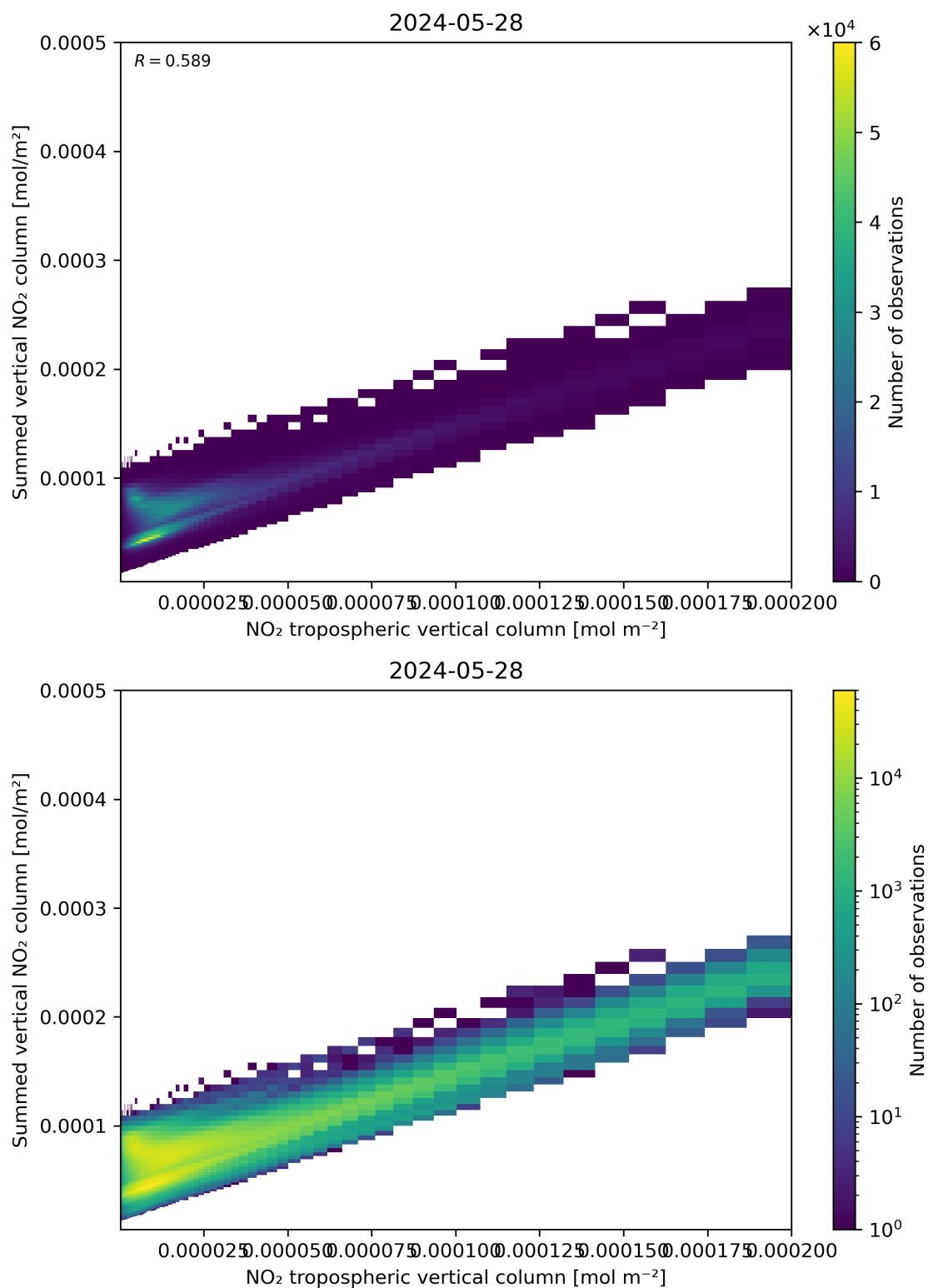
Figure 126: Scatter density plot of “NO 2 tropospheric vertical column” against “Summed vertical NO 2 column” for 2024-05-28 to 2024-05-29.
