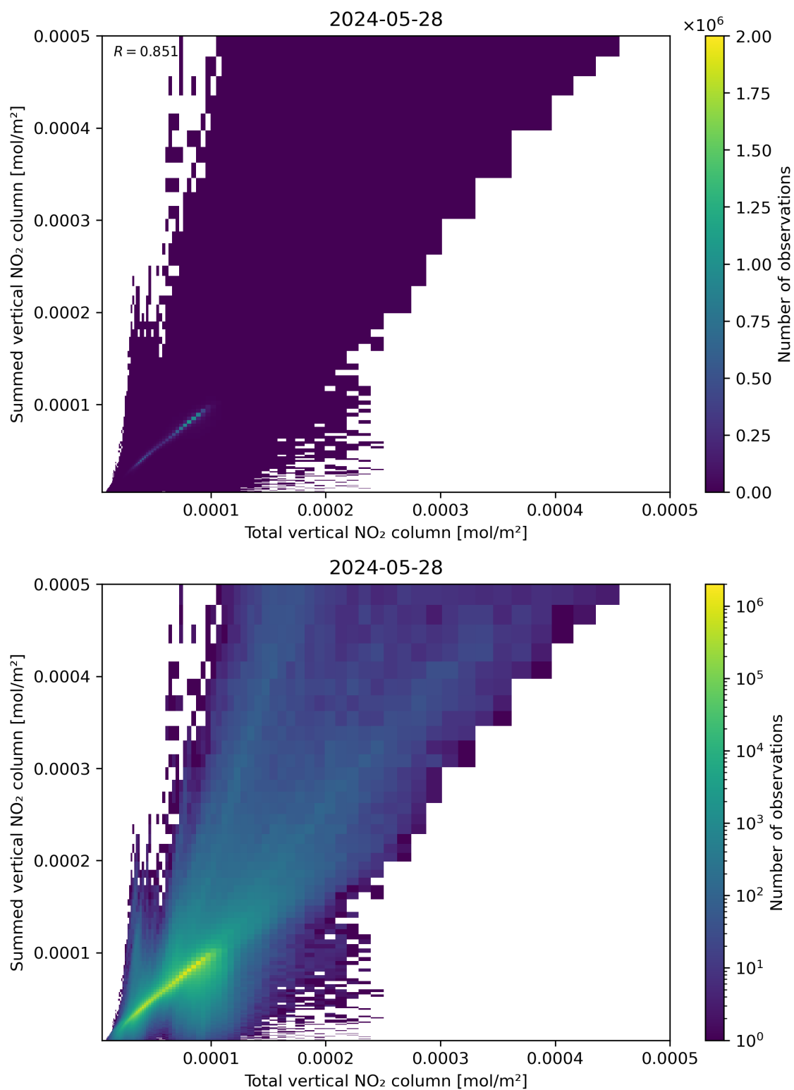
Figure 112: Scatter density plot of “Total vertical NO 2 column” against “Summed vertical NO 2 column” for 2024-05-28 to 2024-05-29.
