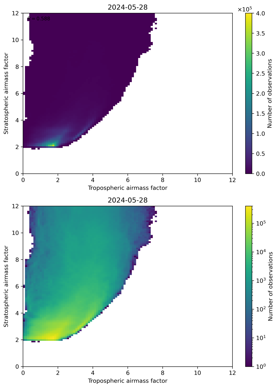
Figure 71: Scatter density plot of “Tropospheric airmass factor” against “Stratospheric airmass factor” for 2024-05-28 to 2024-05-29.
