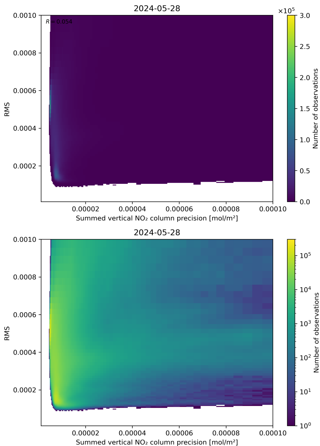
Figure 108: Scatter density plot of “Summed vertical NO 2 column precision” against “RMS” for 2024-05-28 to 2024-05-29.
