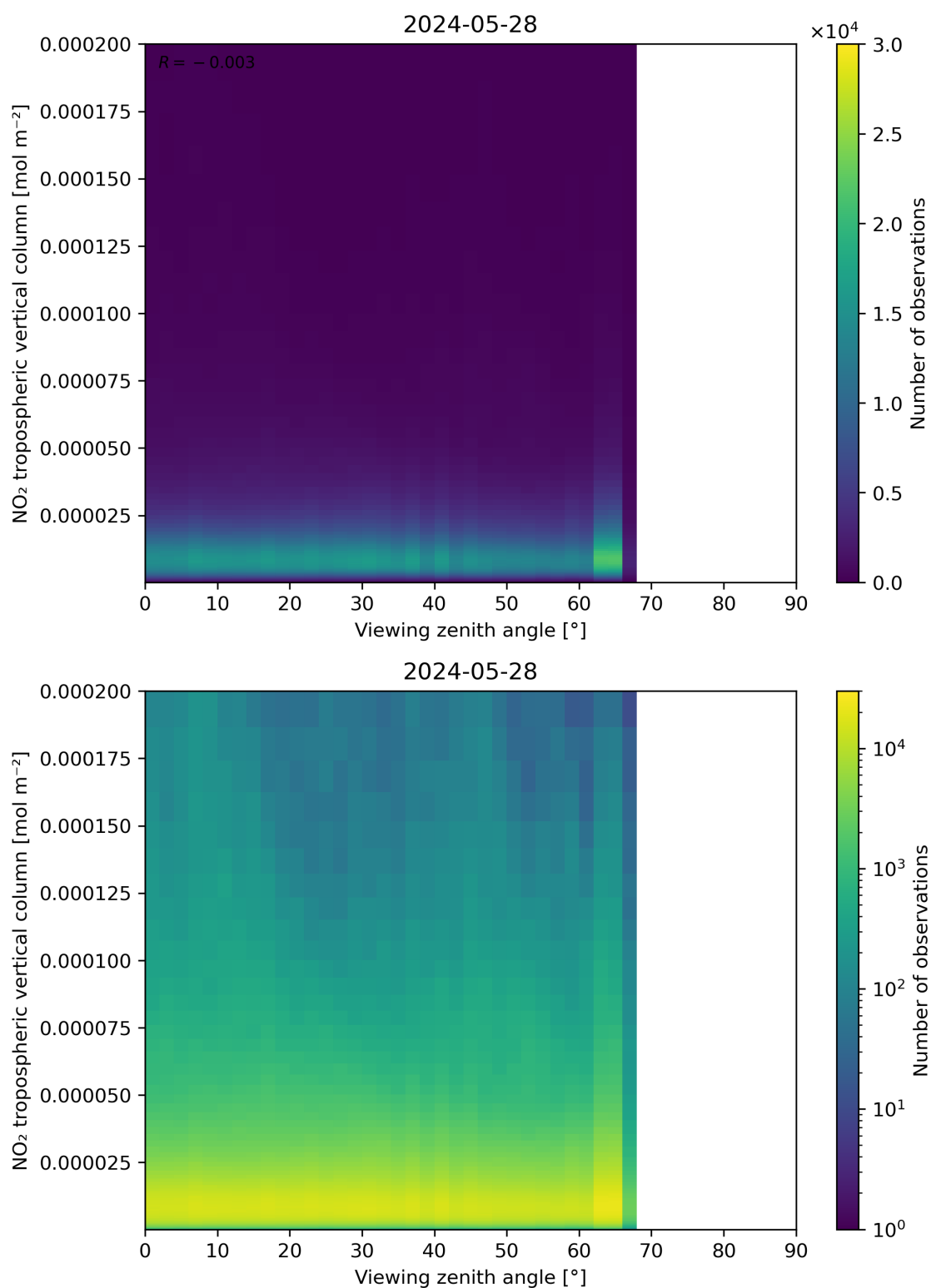
Figure 169: Scatter density plot of “Viewing zenith angle” against “NO 2 tropospheric vertical column” for 2024-05-28 to 2024-05-29.
