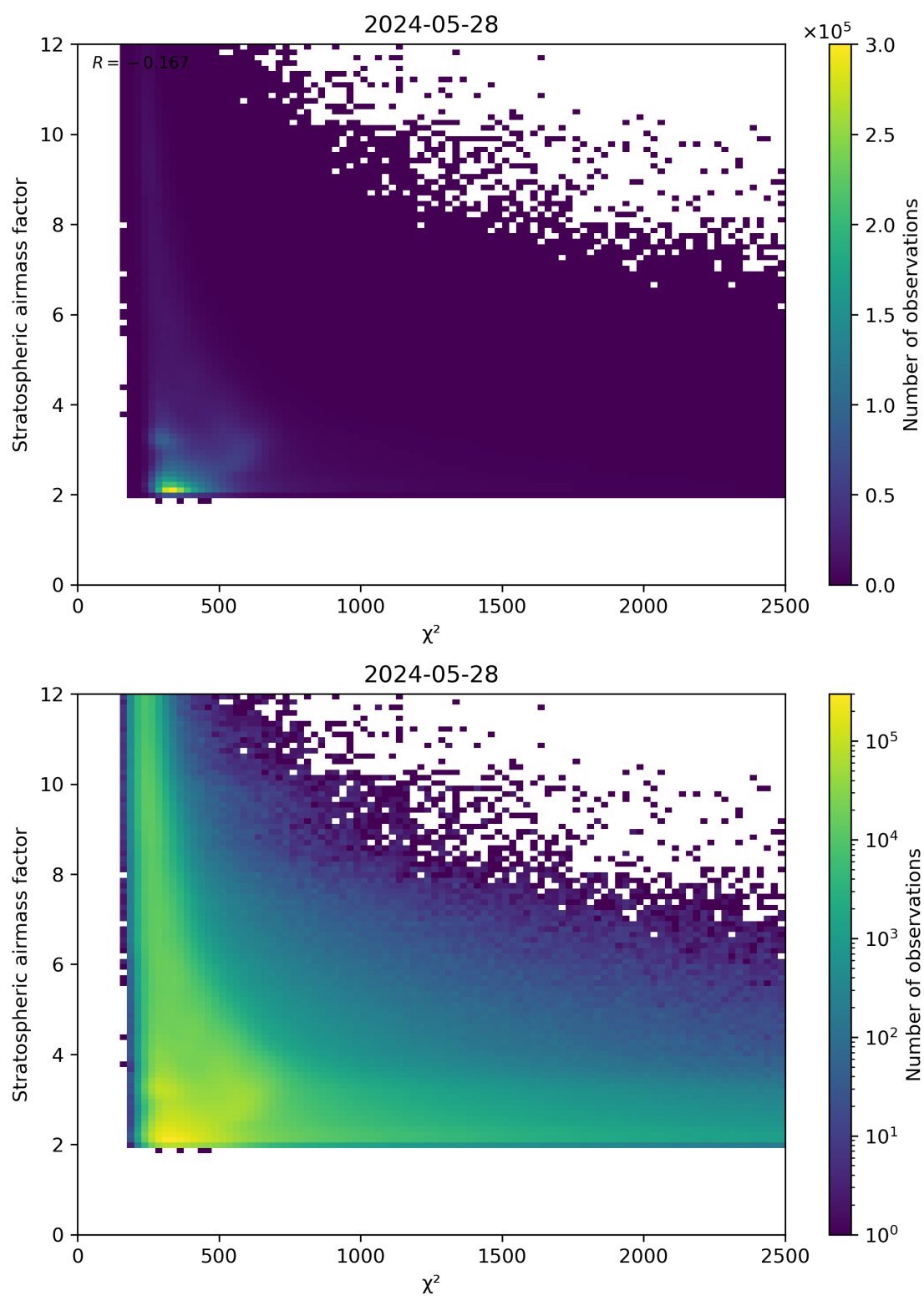
Figure 81: Scatter density plot of “ \chi^2 ” against “Stratospheric airmass factor” for 2024-05-28 to 2024-05-29.
