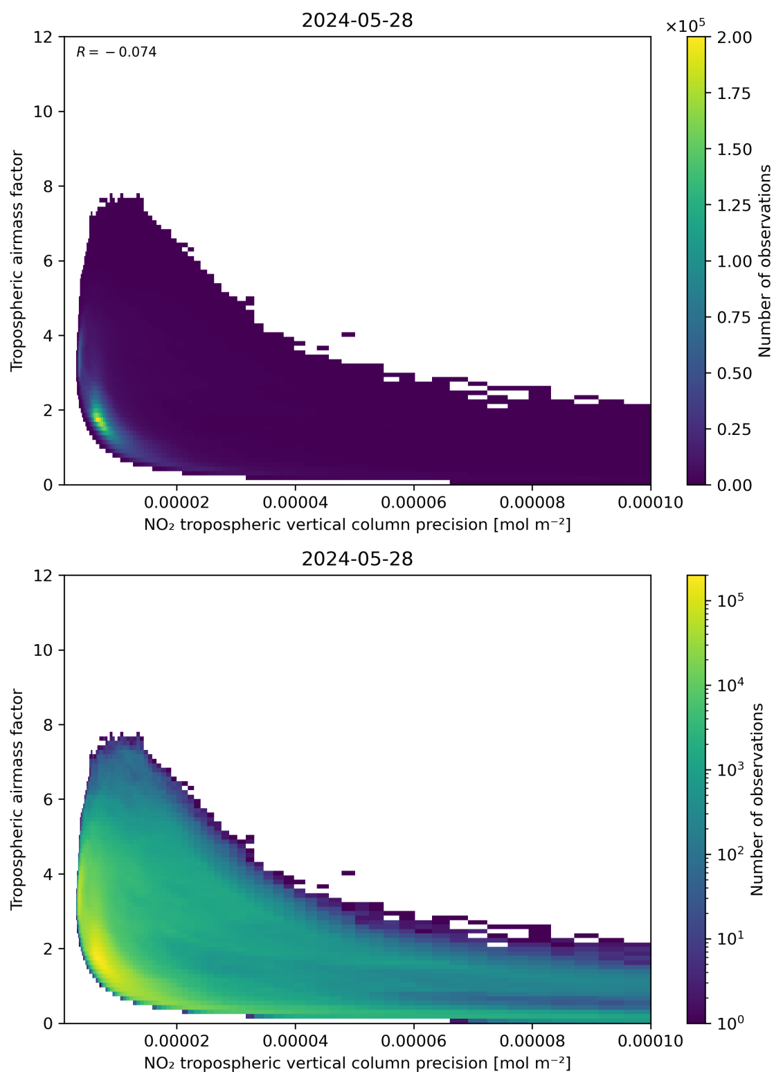
Figure 133: Scatter density plot of “NO 2 tropospheric vertical column precision” against “Tropospheric airmass factor” for 2024-05-28 to 2024-05-29.
