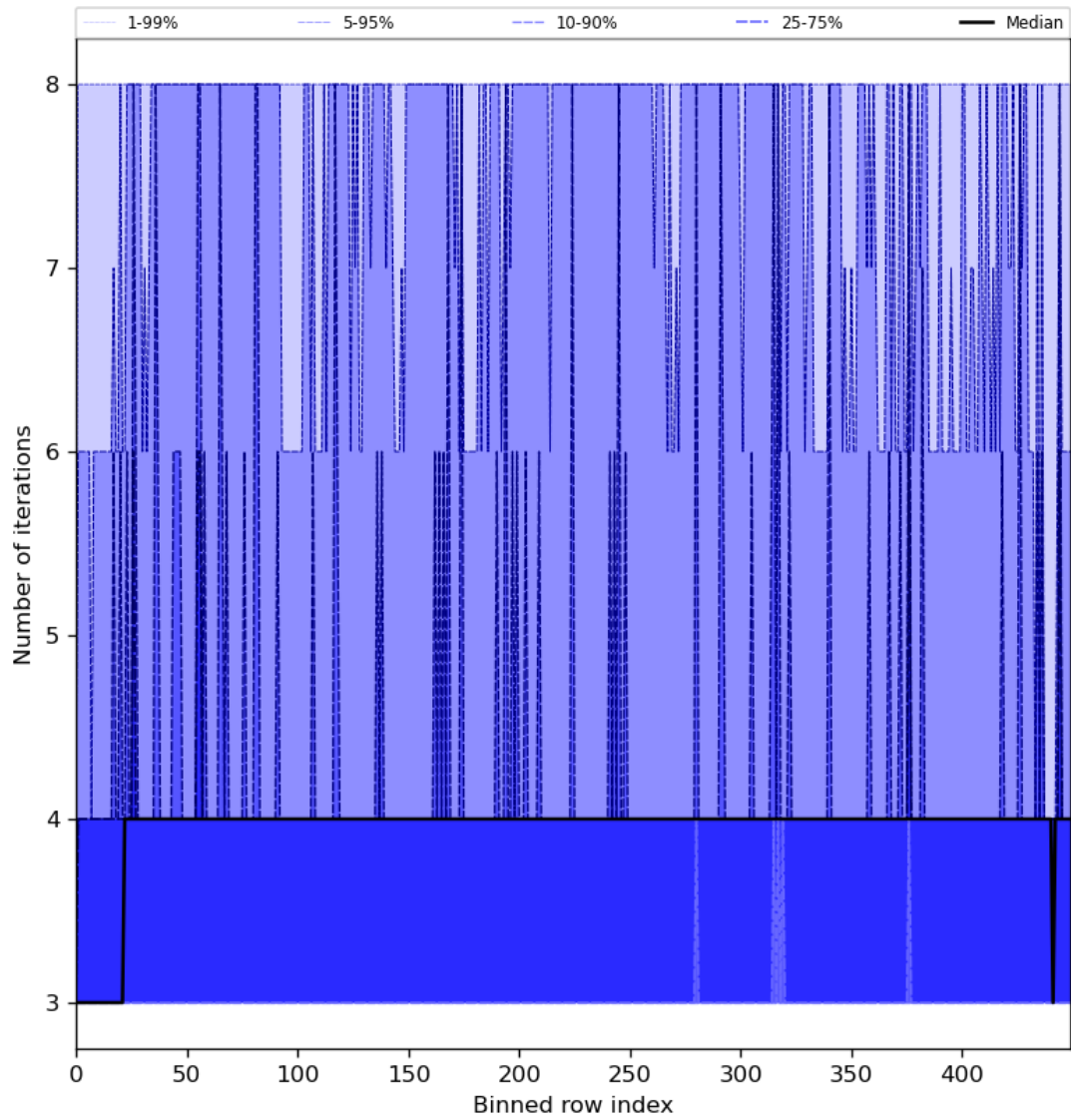
Figure 51: Along track statistics of “Number of iterations” for 2024-05-28 to 2024-05-29
