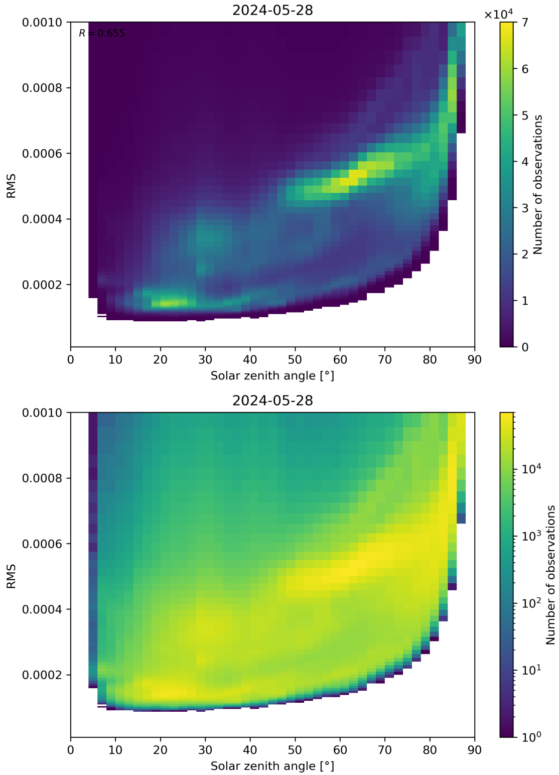
Figure 157: Scatter density plot of “Solar zenith angle” against “RMS” for 2024-05-28 to 2024-05-29.
