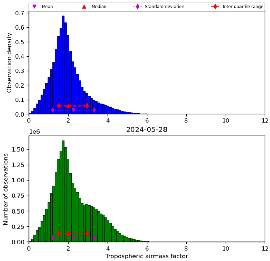
Figure 31: Histogram of “Tropospheric airmass factor” for 2024-05-28 to 2024-05-29
