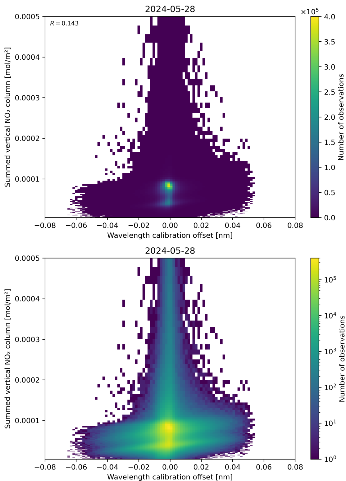
Figure 177: Scatter density plot of “Wavelength calibration offset” against “Summed vertical NO 2 column” for 2024-05-28 to 2024-05-29.
