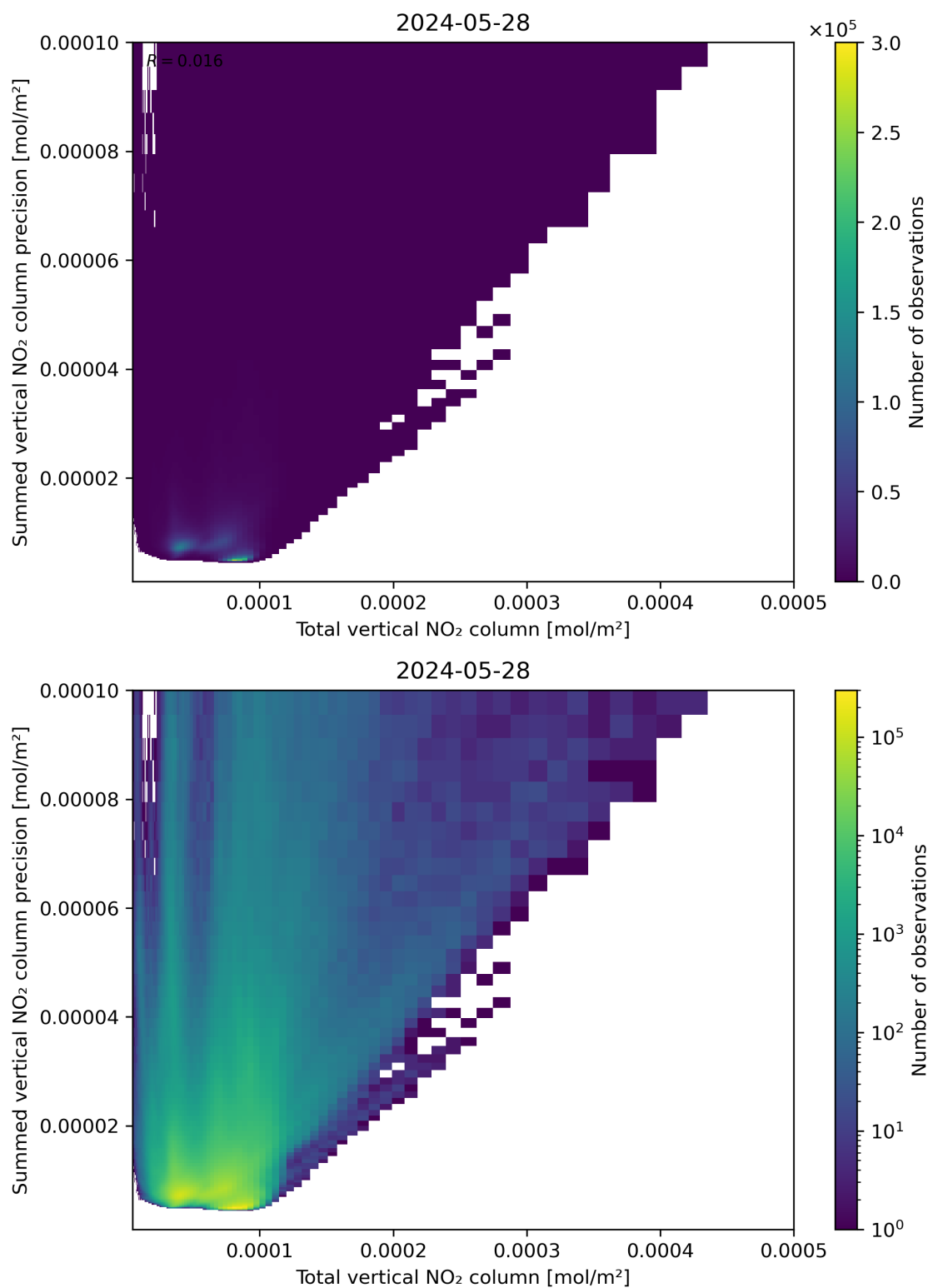
Figure 113: Scatter density plot of “Total vertical NO 2 column” against “Summed vertical NO 2 column precision” for 2024-05-28 to 2024-05-29.
