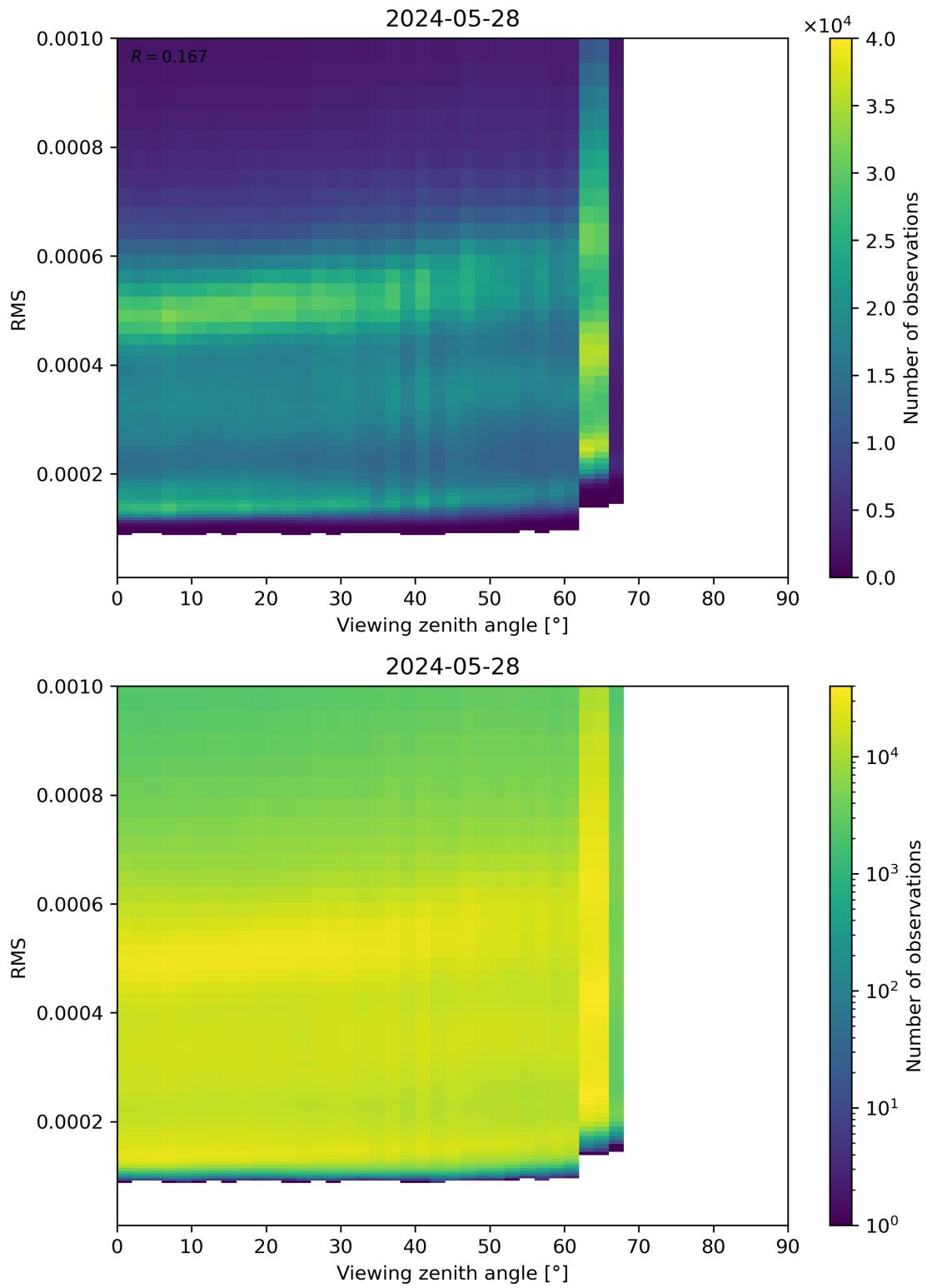
Figure 171: Scatter density plot of “Viewing zenith angle” against “RMS” for 2024-05-28 to 2024-05-29.
