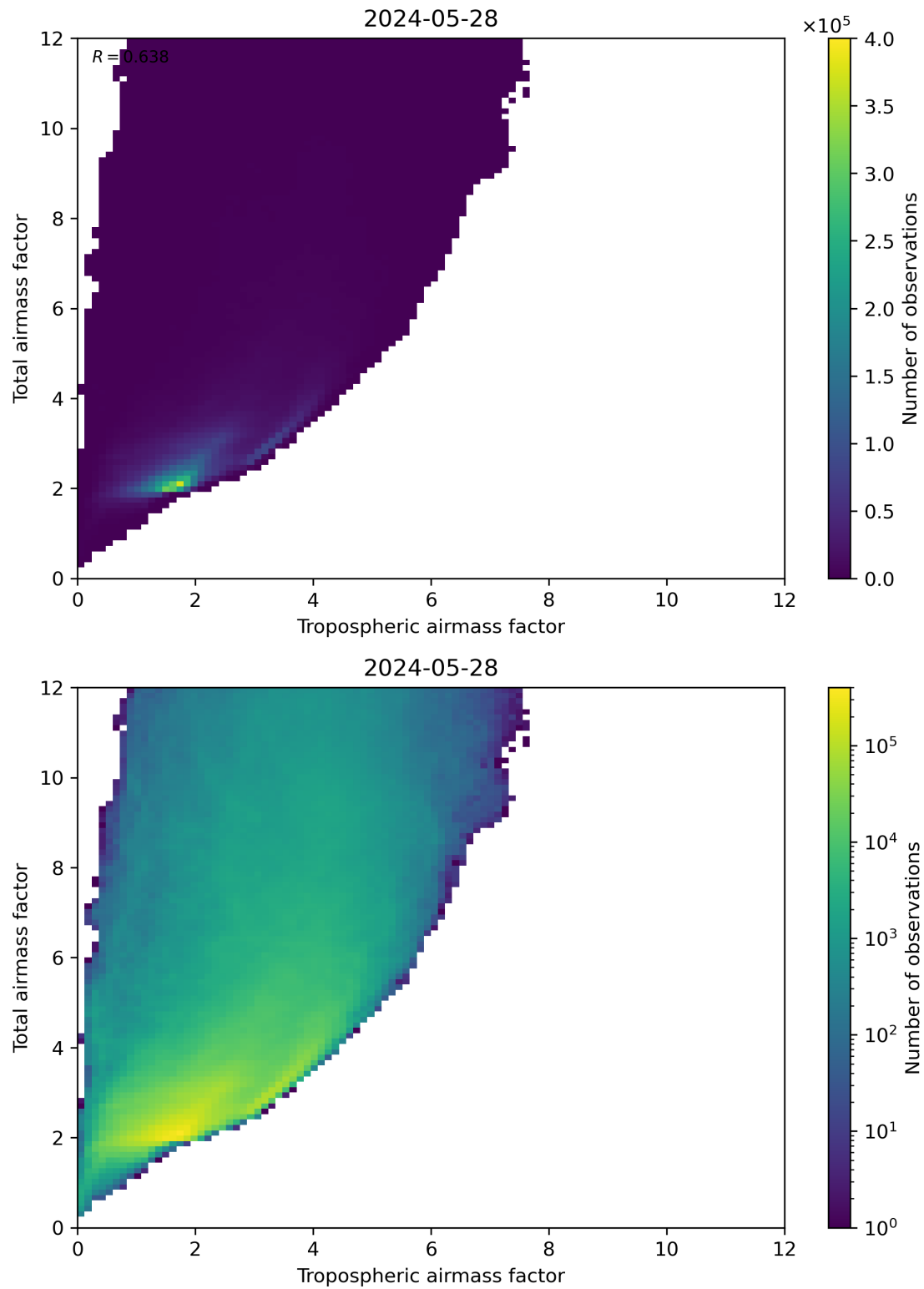
Figure 72: Scatter density plot of “Tropospheric airmass factor” against “Total airmass factor” for 2024-05-28 to 2024-05-29.
