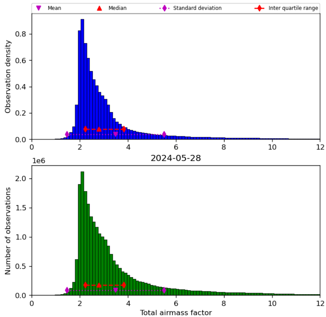
Figure 32: Histogram of “Total airmass factor” for 2024-05-28 to 2024-05-29
