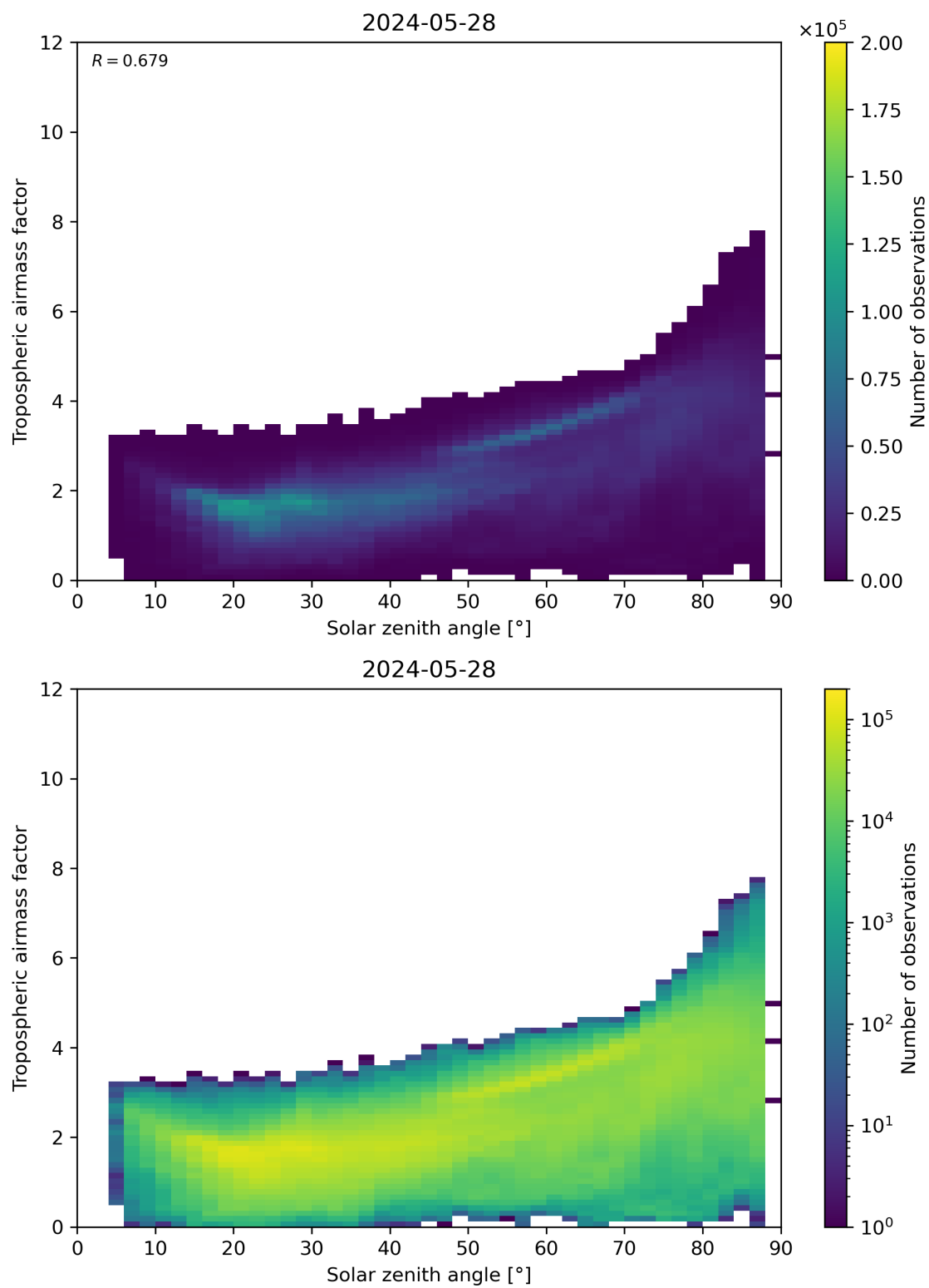
Figure 147: Scatter density plot of “Solar zenith angle” against “Tropospheric airmass factor” for 2024-05-28 to 2024-05-29.
