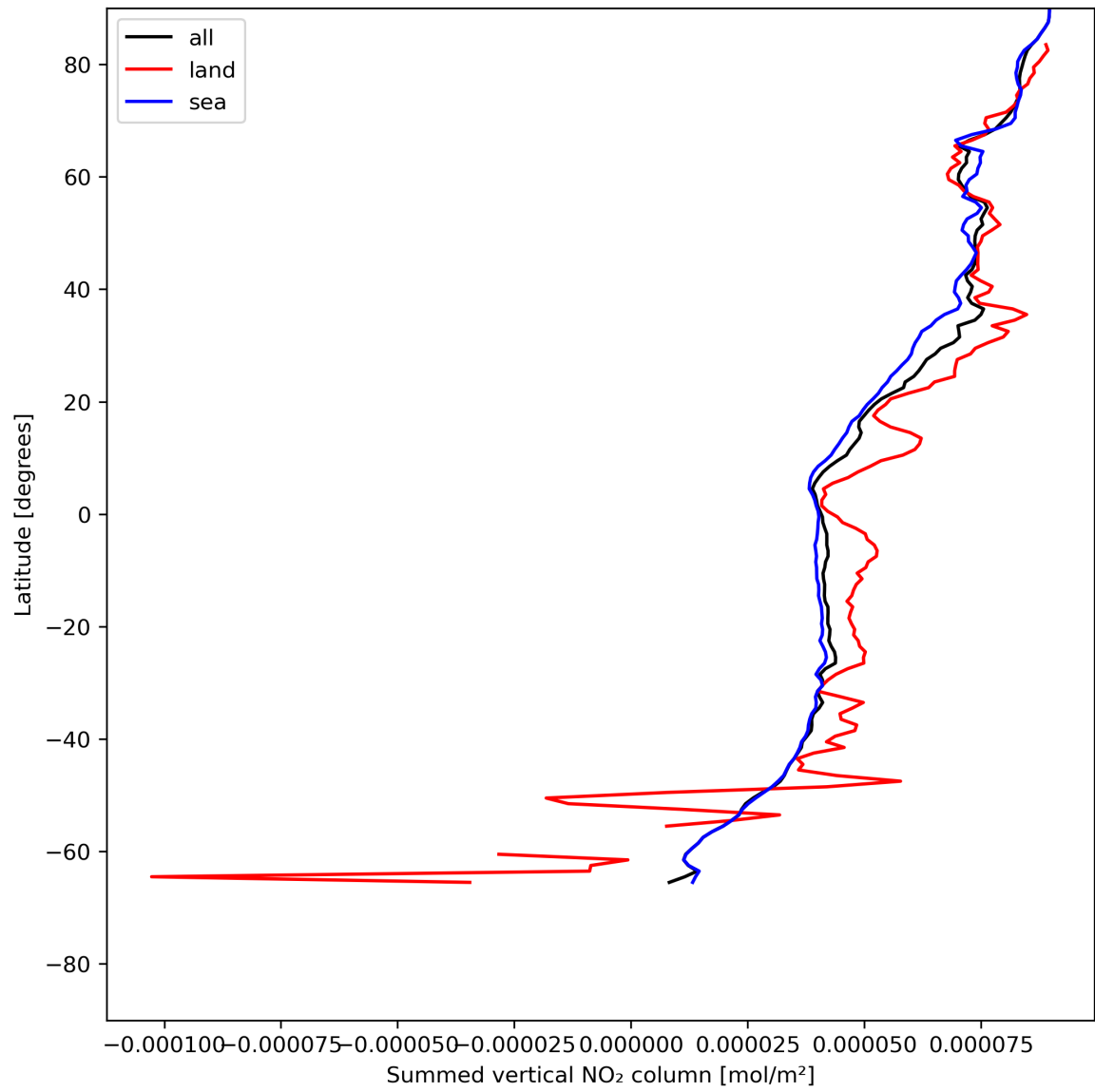
Figure 23: Zonal average of “Summed vertical NO 2 column” for 2024-05-28 to 2024-05-29.
