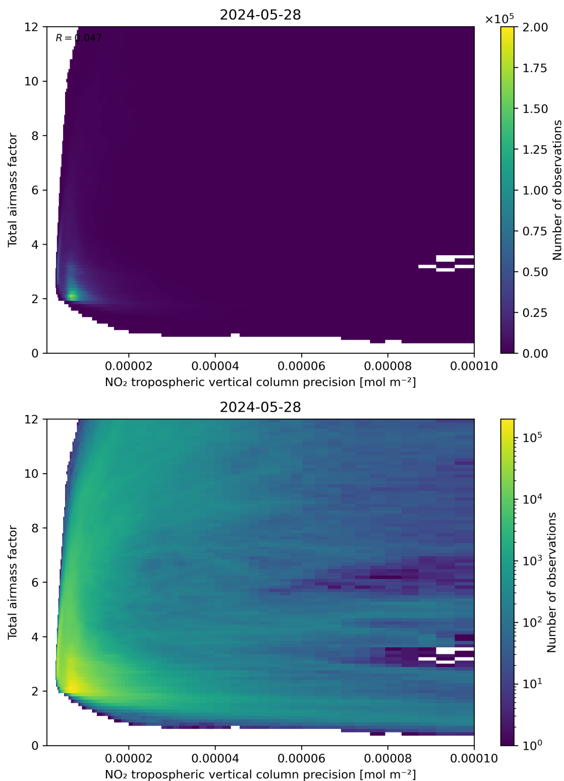
Figure 132: Scatter density plot of “NO 2 tropospheric vertical column precision” against “Total air mass factor” for 2024-05-28 to 2024-05-29.
