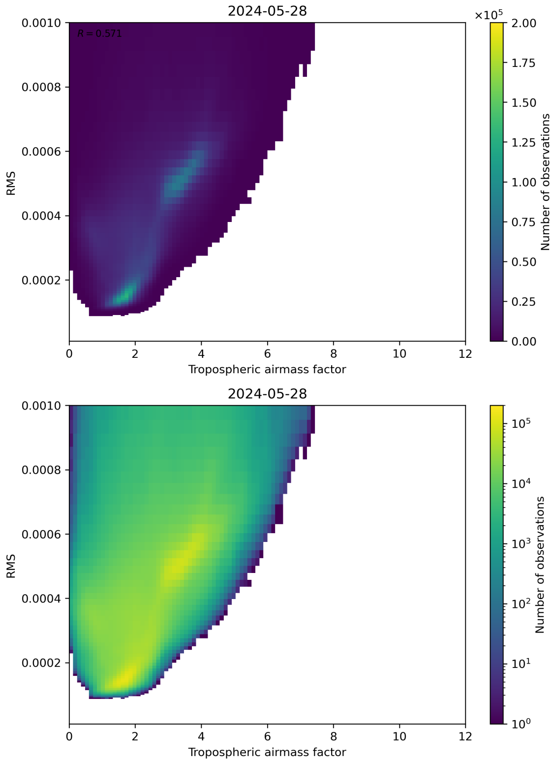
Figure 79: Scatter density plot of “Tropospheric airmass factor” against “RMS” for 2024-05-28 to 2024-05-29.
