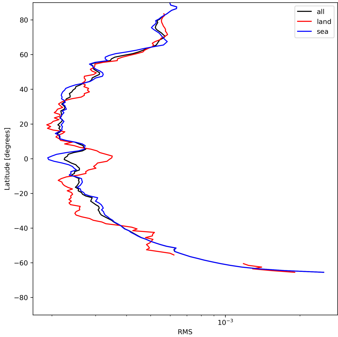
Figure 26: Zonal average of “RMS” for 2024-05-28 to 2024-05-29.
