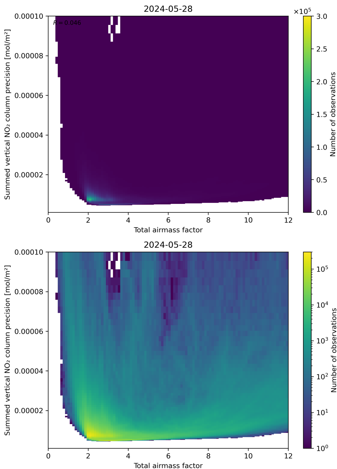
Figure 66: Scatter density plot of “Total airmass factor” against “Summed vertical NO 2 column precision” for 2024-05-28 to 2024-05-29.
