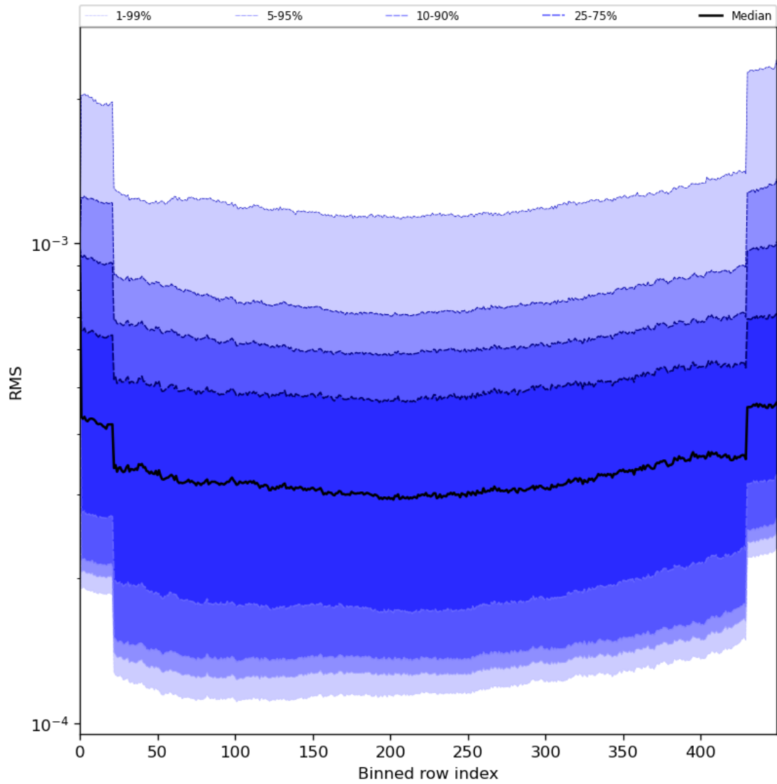
Figure 60: Along track statistics of “RMS” for 2024-05-28 to 2024-05-29
