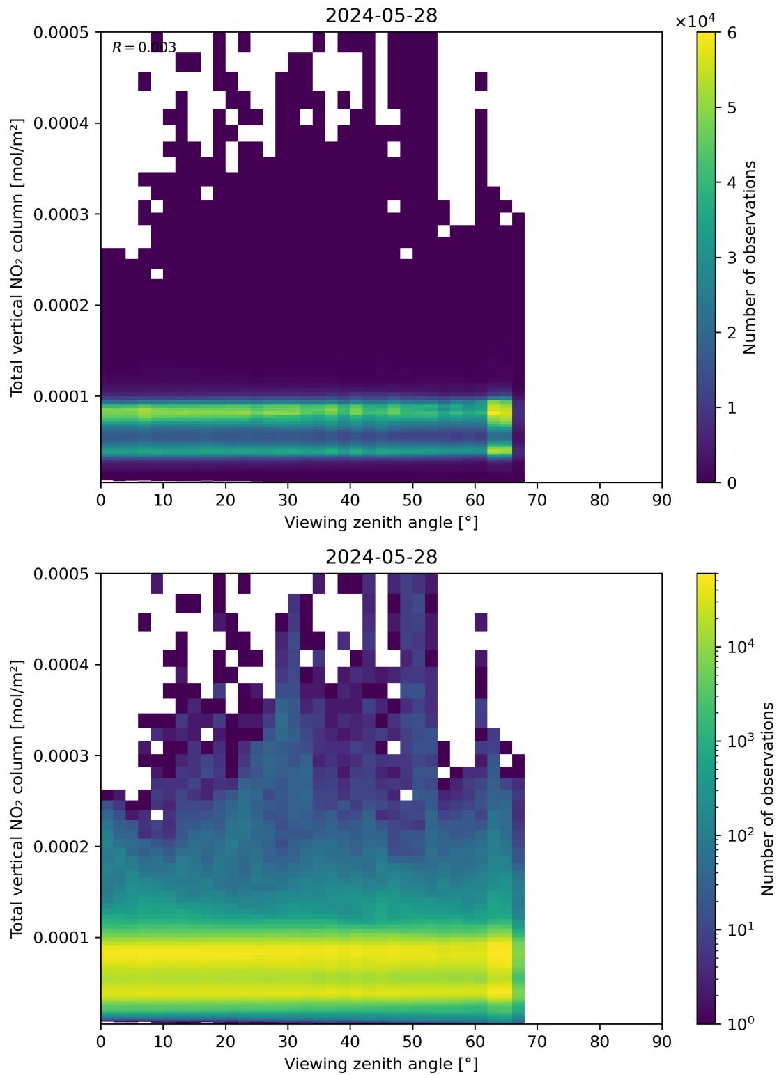
Figure 167: Scatter density plot of “Viewing zenith angle” against “Total vertical NO 2 column” for 2024-05-28 to 2024-05-29.
