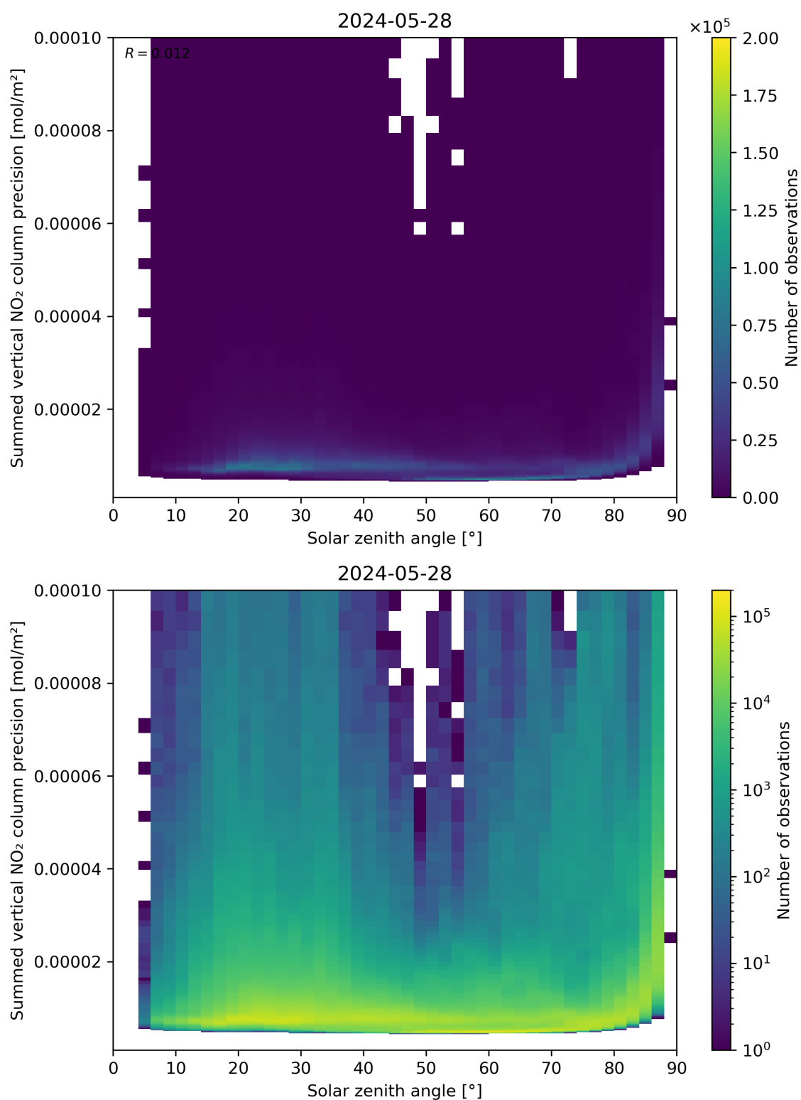
Figure 152: Scatter density plot of “Solar zenith angle” against “Summed vertical NO 2 column precision” for 2024-05-28 to 2024-05-29.
