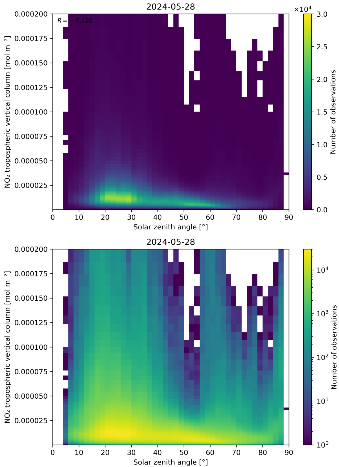
Figure 155: Scatter density plot of “Solar zenith angle” against “NO 2 tropospheric vertical column” for 2024-05-28 to 2024-05-29.
