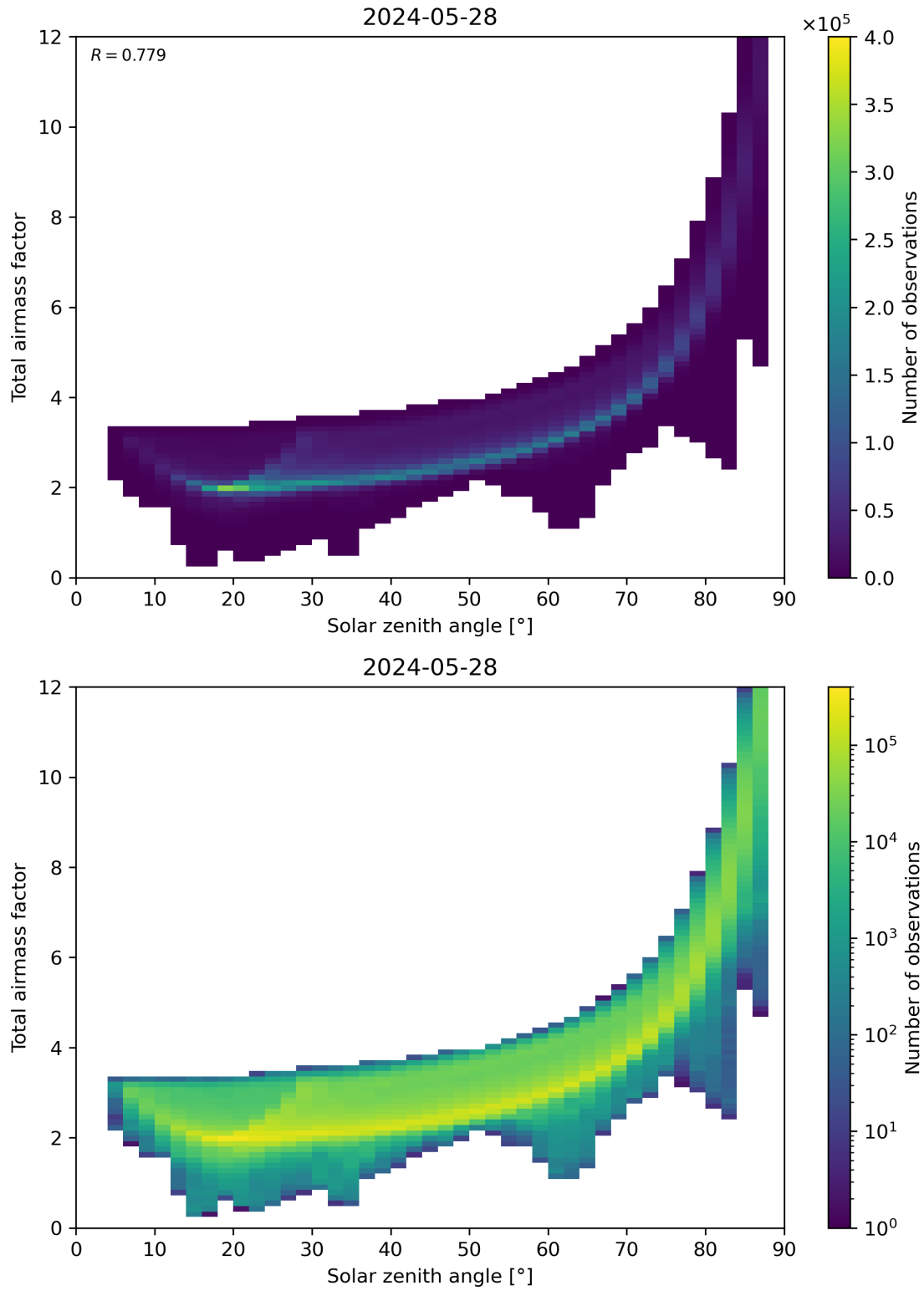
Figure 146: Scatter density plot of “Solar zenith angle” against “Total air mass factor” for 2024-05-28 to 2024-05-29.
