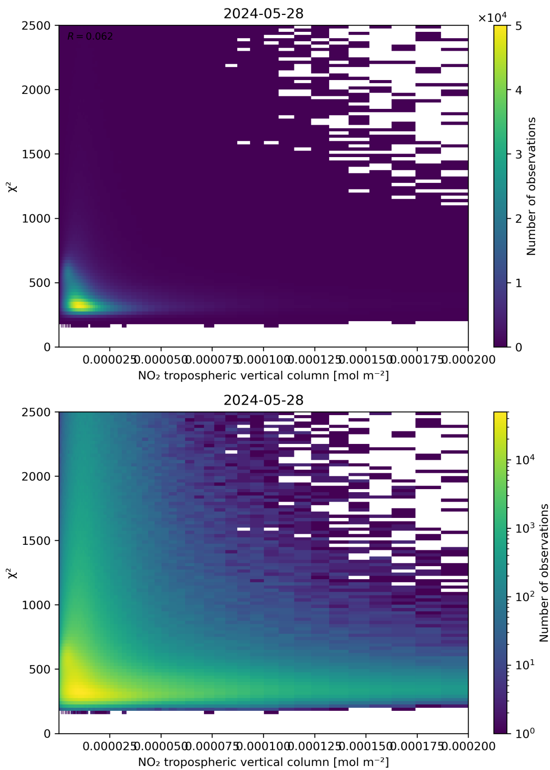
Figure 124: Scatter density plot of “NO 2 tropospheric vertical column” against “ \chi^2 ” for 2024-05-28 to 2024-05-29.
