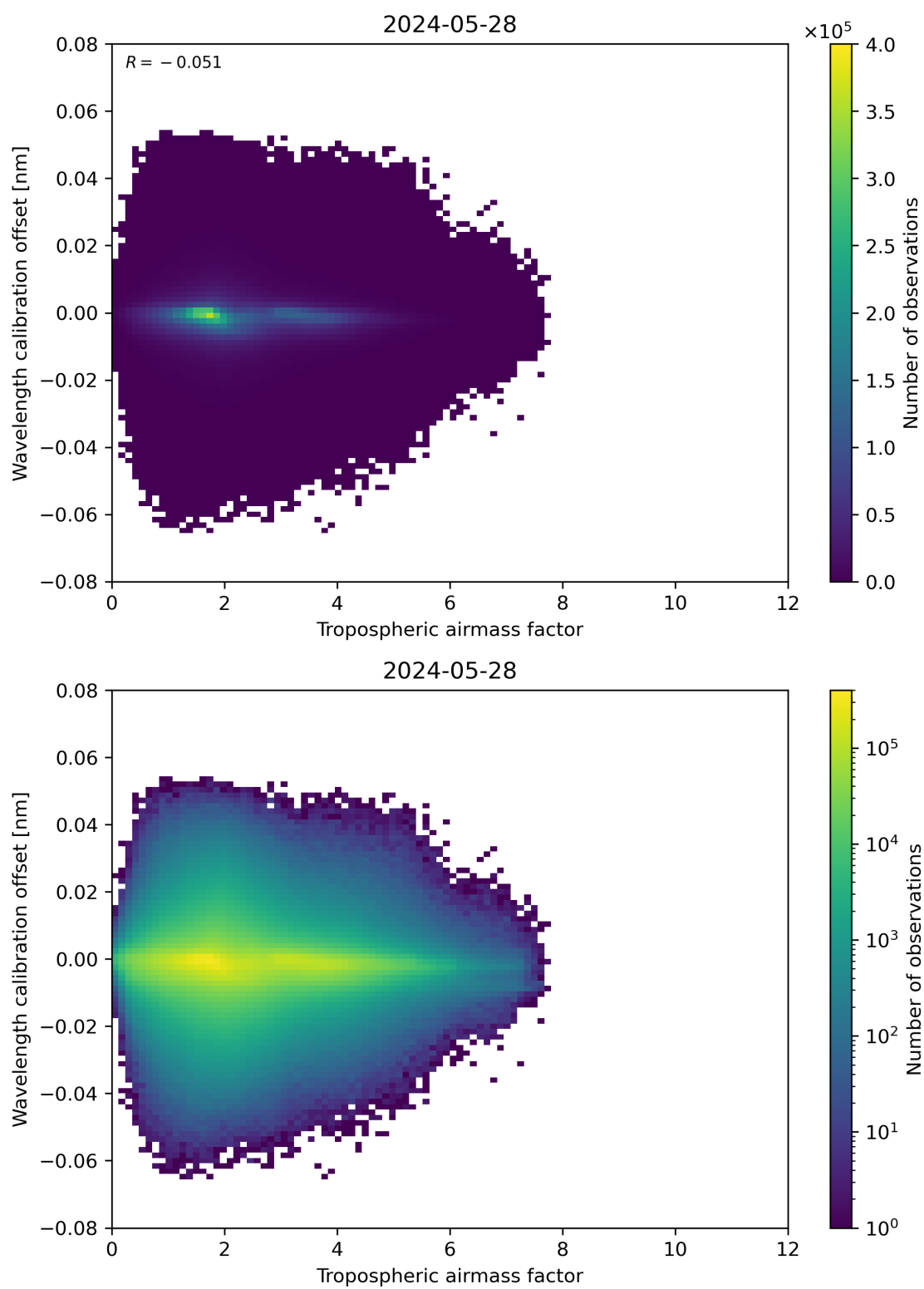
Figure 80: Scatter density plot of “Tropospheric air mass factor” against “Wavelength calibration offset” for 2024-05-28 to 2024-05-29.
