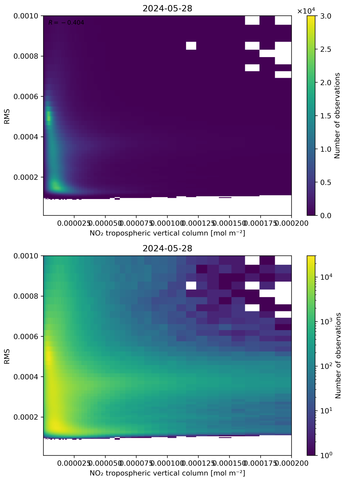
Figure 142: Scatter density plot of “NO 2 tropospheric vertical column” against “RMS” for 2024-05-28 to 2024-05-29.
