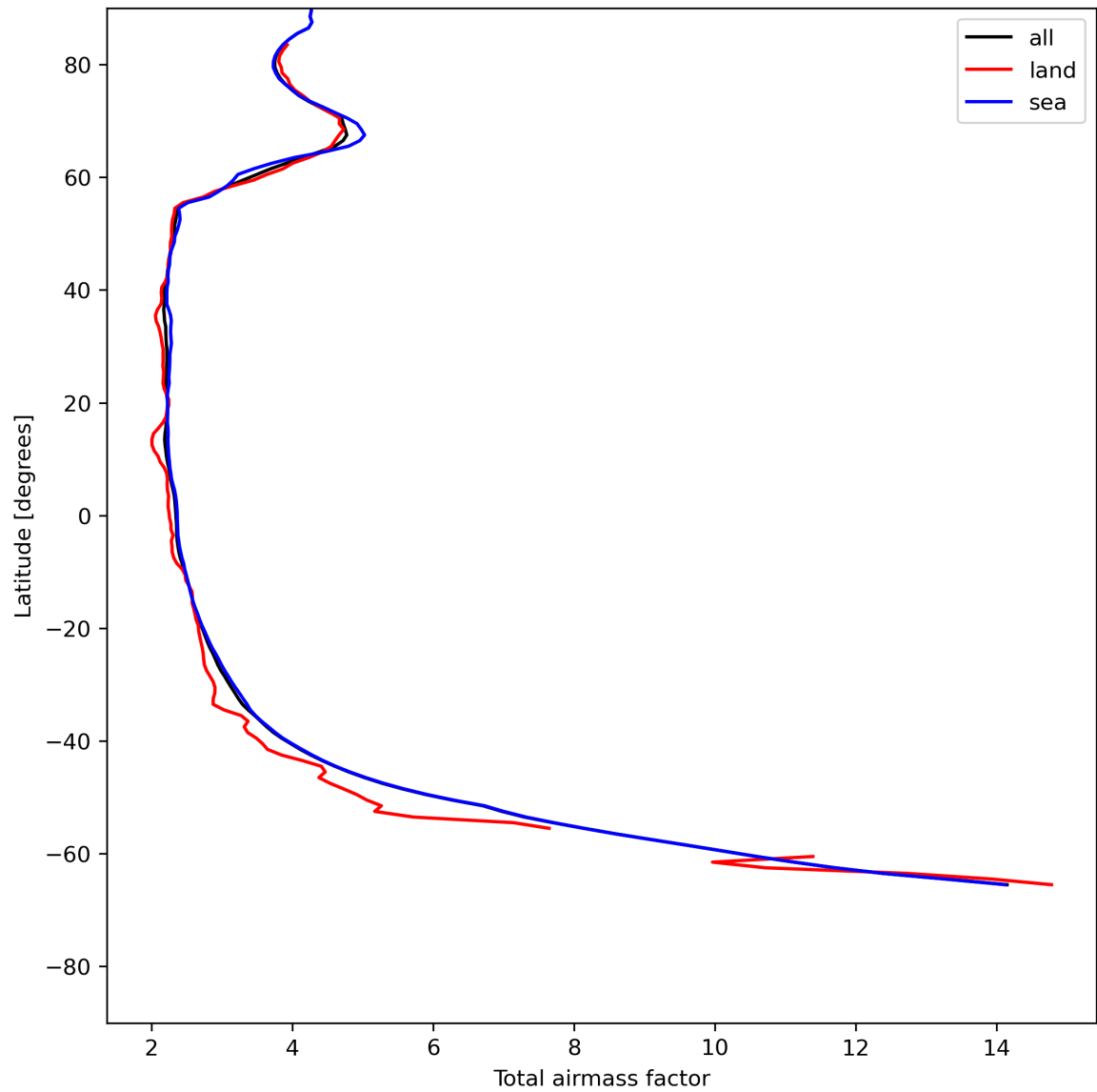
Figure 15: Zonal average of “Total airmass factor” for 2024-05-28 to 2024-05-29.
