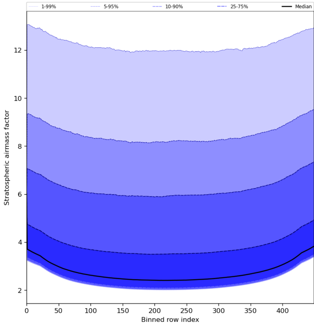
Figure 61: Along track statistics of “Stratospheric airmass factor” for 2024-05-28 to 2024-05-29
