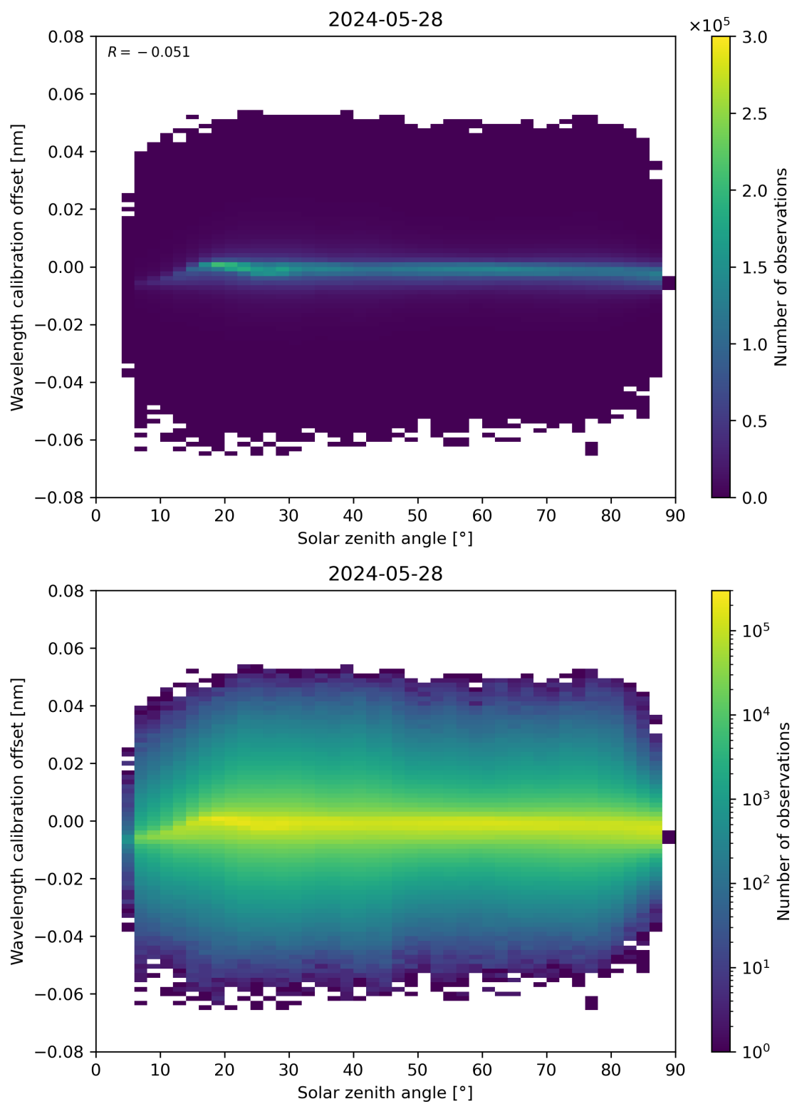
Figure 158: Scatter density plot of “Solar zenith angle” against “Wavelength calibration offset” for 2024-05-28 to 2024-05-29.
