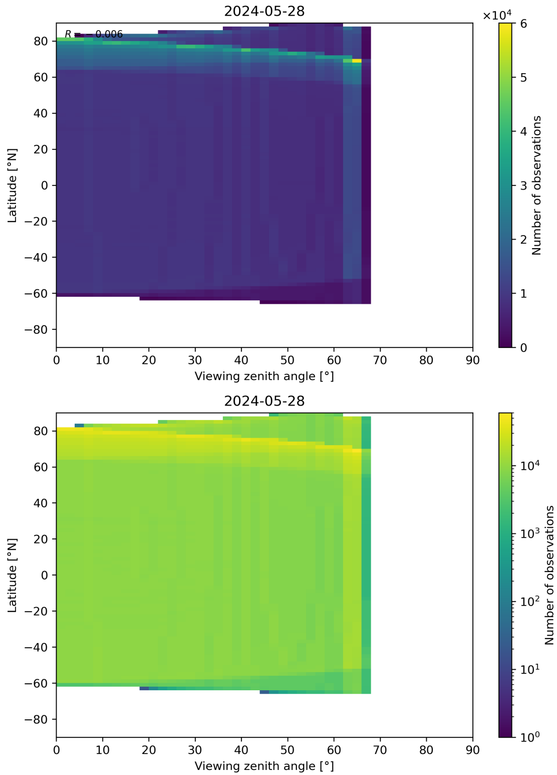
Figure 163: Scatter density plot of “Viewing zenith angle” against “Latitude” for 2024-05-28 to 2024-05-29.
