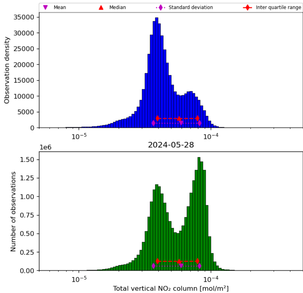
Figure 38: Histogram of “Total vertical NO 2 column” for 2024-05-28 to 2024-05-29
