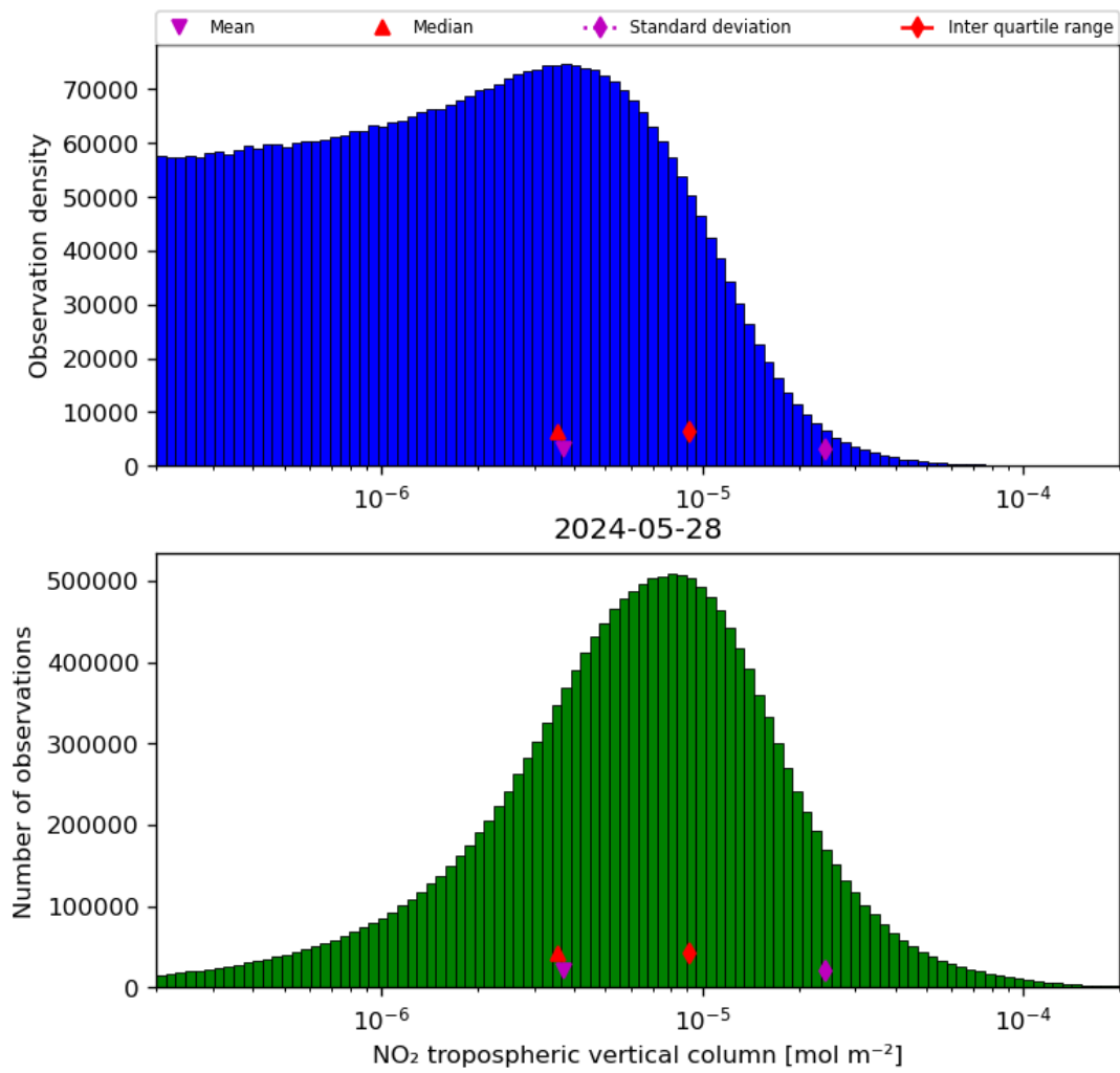
Figure 29: Histogram of “NO 2 tropospheric vertical column” for 2024-05-28 to 2024-05-29
