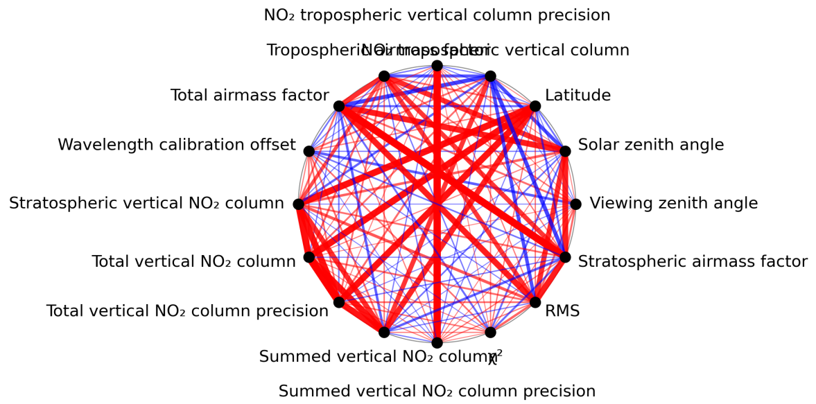
Figure 1: Map of correlation graph for 2024-05-28 to 2024-05-29.
