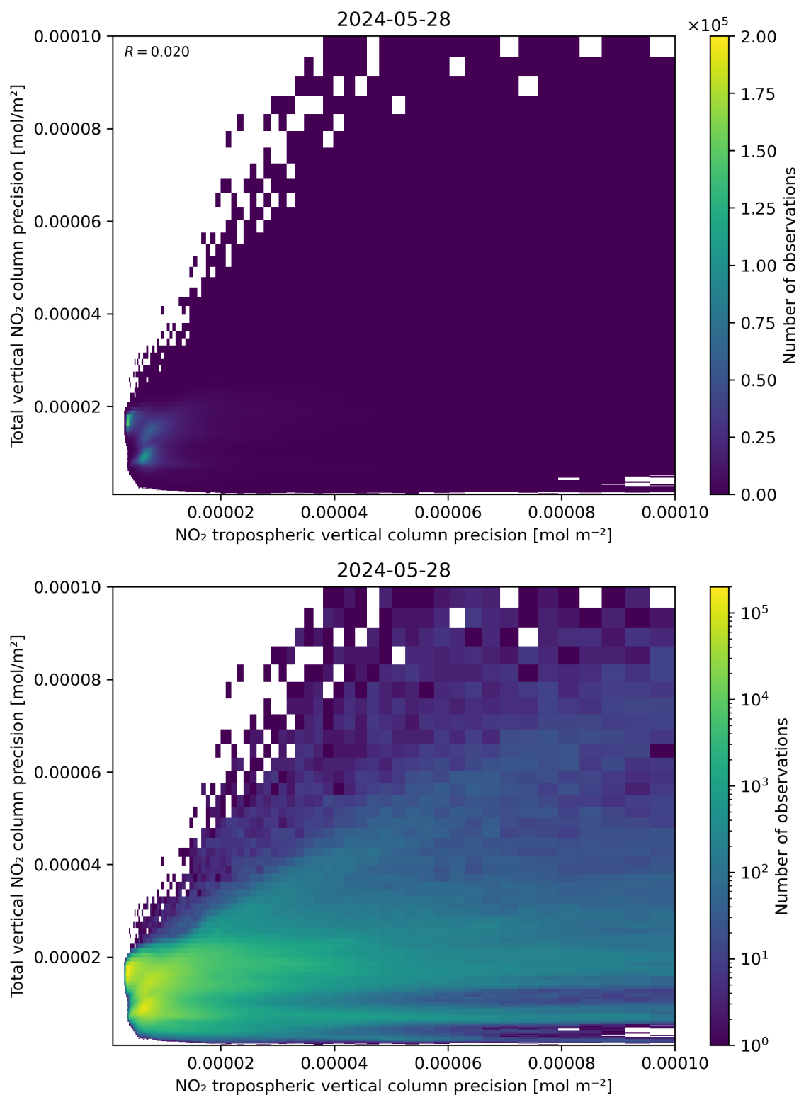
Figure 139: Scatter density plot of “NO 2 tropospheric vertical column precision” against “Total vertical NO 2 column precision” for 2024-05-28 to 2024-05-29.
