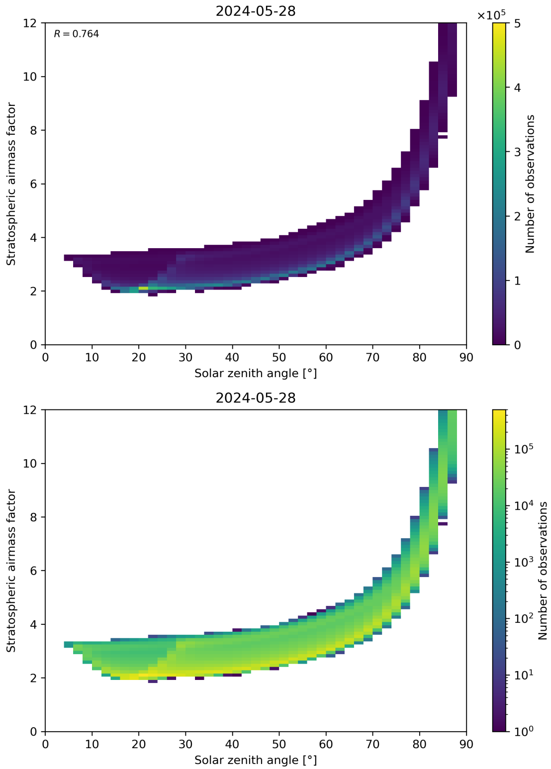
Figure 145: Scatter density plot of “Solar zenith angle” against “Stratospheric airmass factor” for 2024-05-28 to 2024-05-29.
