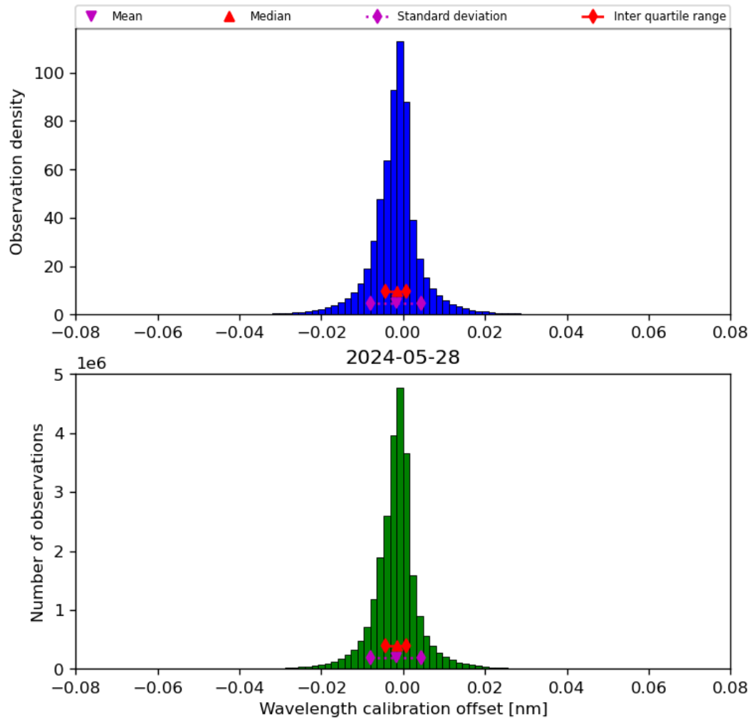
Figure 35: Histogram of “Wavelength calibration offset” for 2024-05-28 to 2024-05-29
