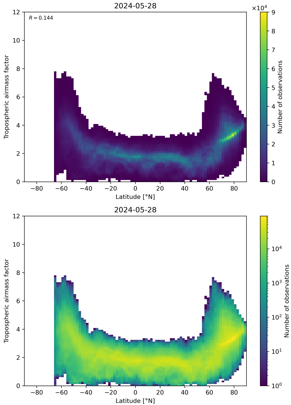
Figure 85: Scatter density plot of “Latitude” against “Tropospheric air mass factor” for 2024-05-28 to 2024-05-29.
