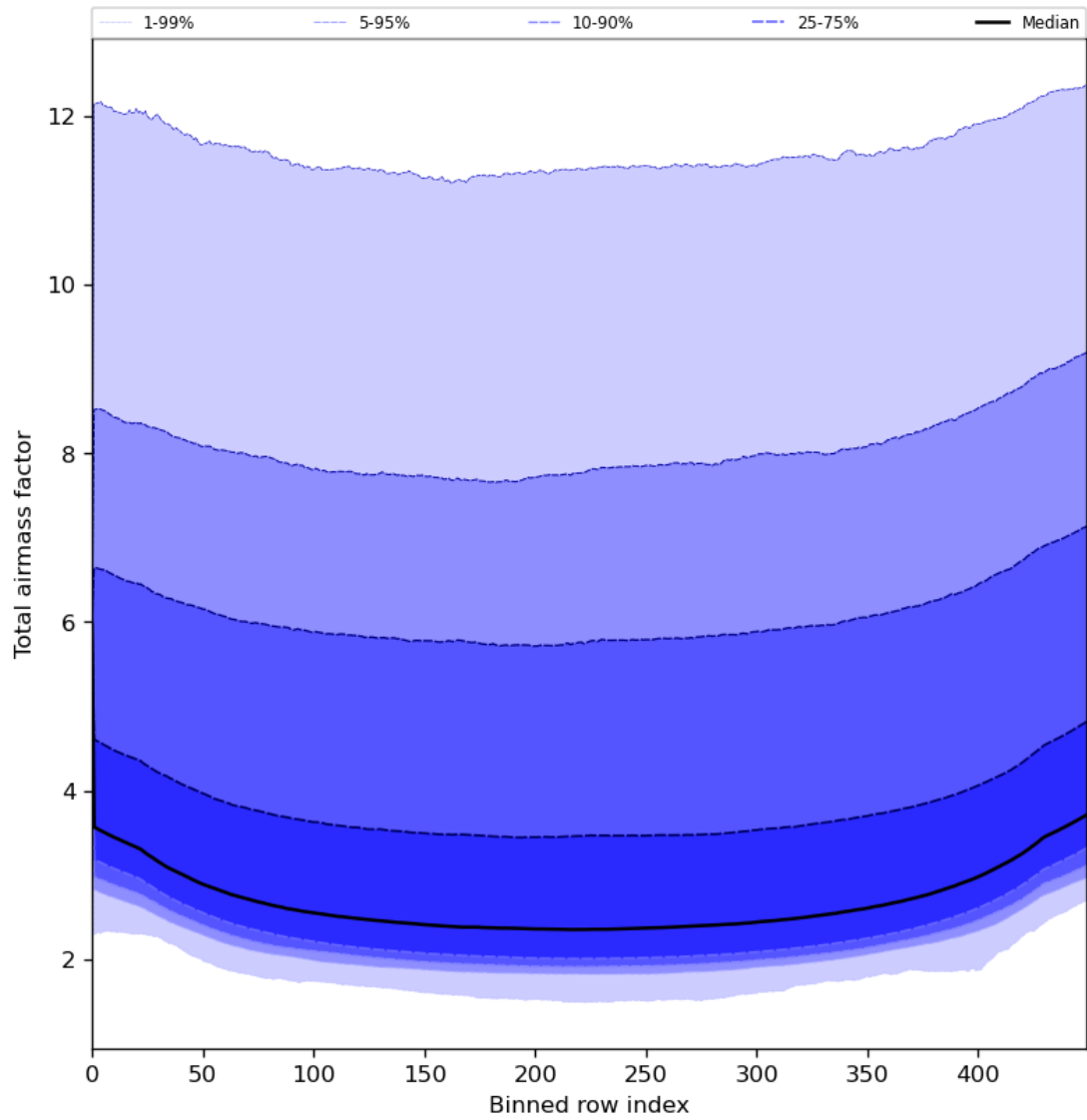
Figure 49: Along track statistics of “Total airmass factor” for 2024-05-28 to 2024-05-29
