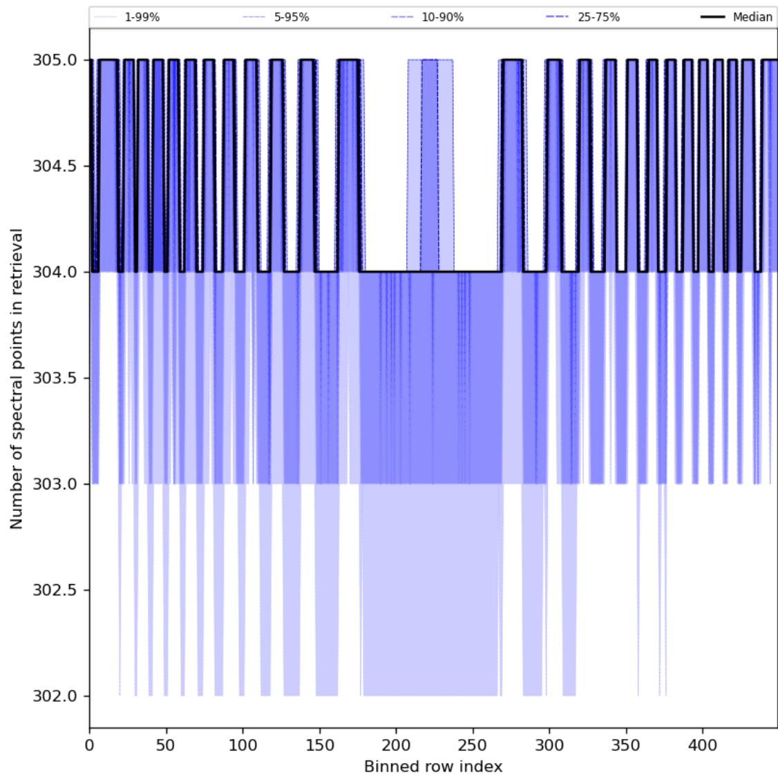
Figure 50: Along track statistics of “Number of spectral points in retrieval” for 2024-05-28 to 2024-05-29
