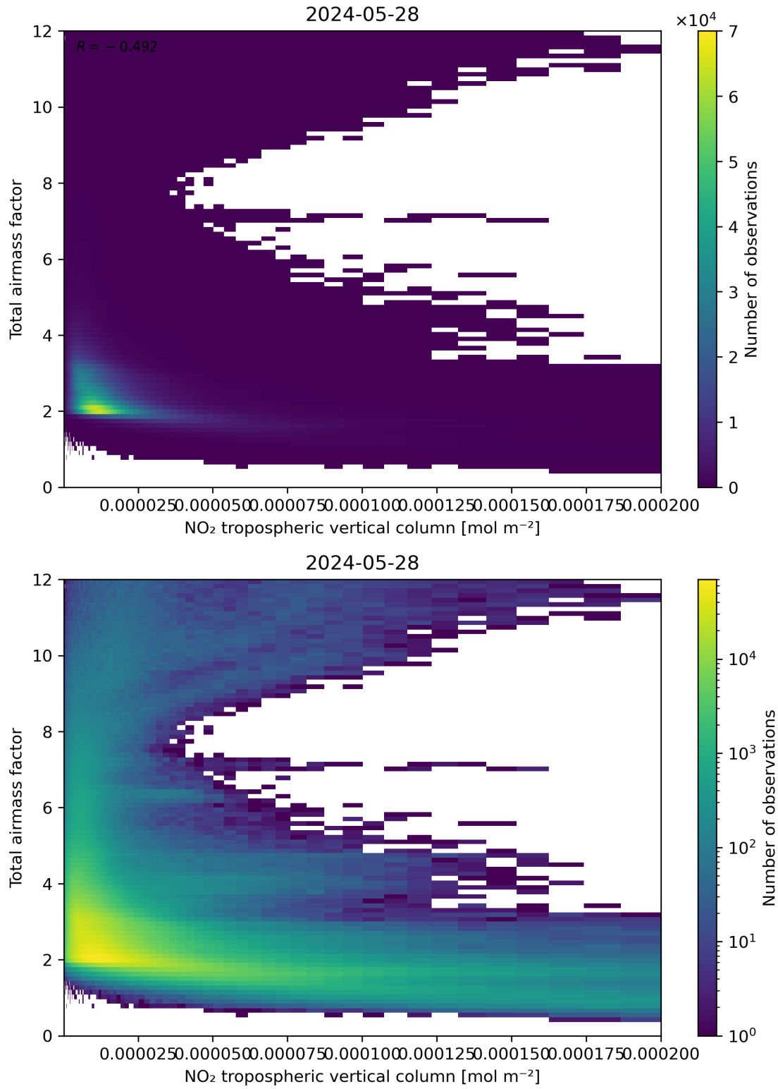
Figure 122: Scatter density plot of “NO 2 tropospheric vertical column” against “Total air mass factor” for 2024-05-28 to 2024-05-29.
