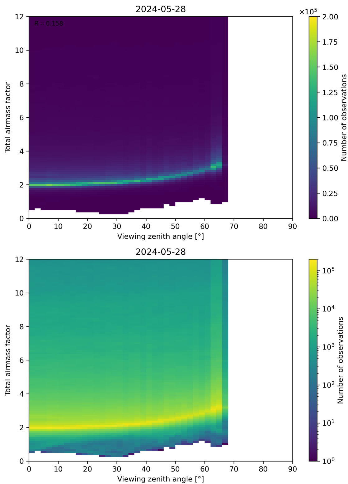
Figure 160: Scatter density plot of “Viewing zenith angle” against “Total airmass factor” for 2024-05-28 to 2024-05-29.
