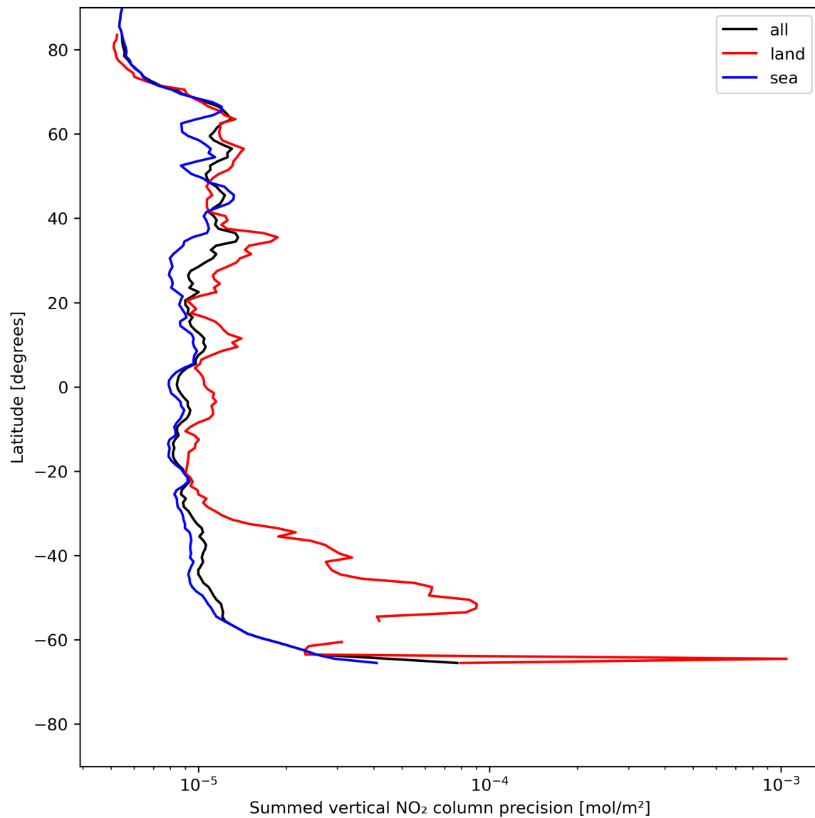
Figure 24: Zonal average of “Summed vertical NO 2 column precision” for 2024-05-28 to 2024-05-29.
