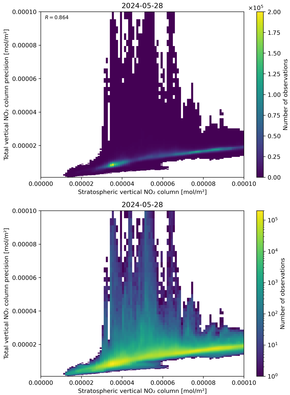
Figure 101: Scatter density plot of “Stratospheric vertical NO 2 column” against “Total vertical NO 2 column precision” for 2024-05-28 to 2024-05-29.
