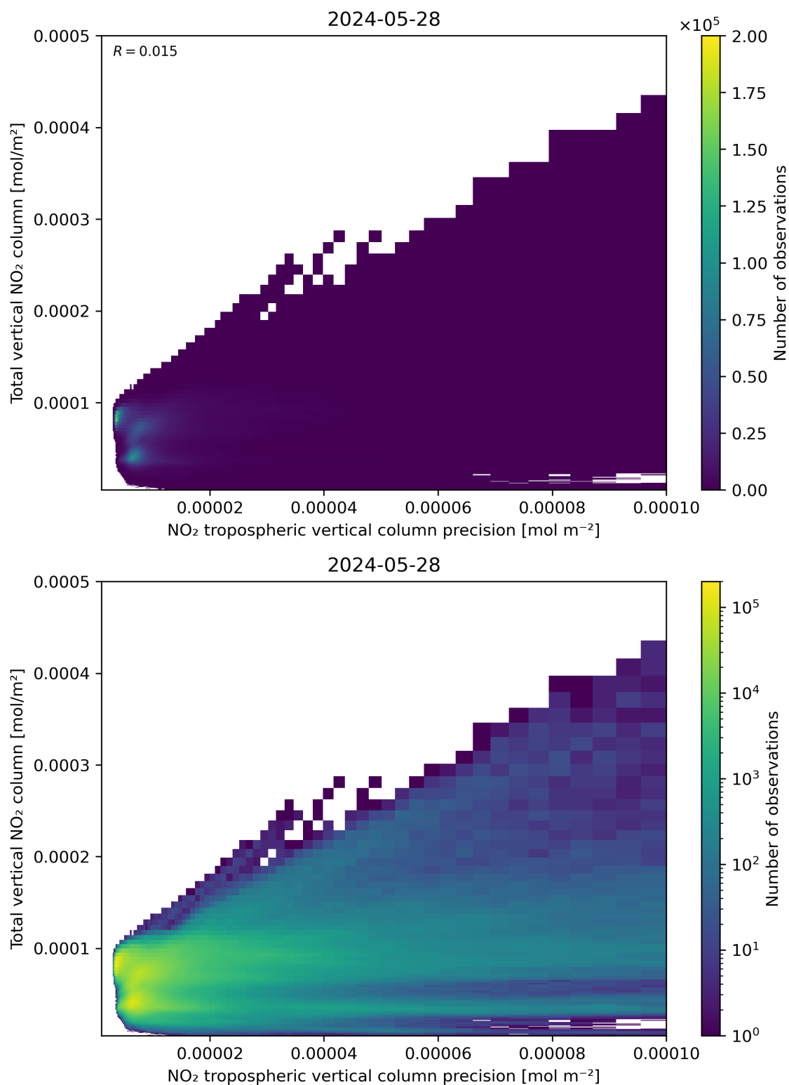
Figure 138: Scatter density plot of “NO 2 tropospheric vertical column precision” against “Total vertical NO 2 column” for 2024-05-28 to 2024-05-29.
