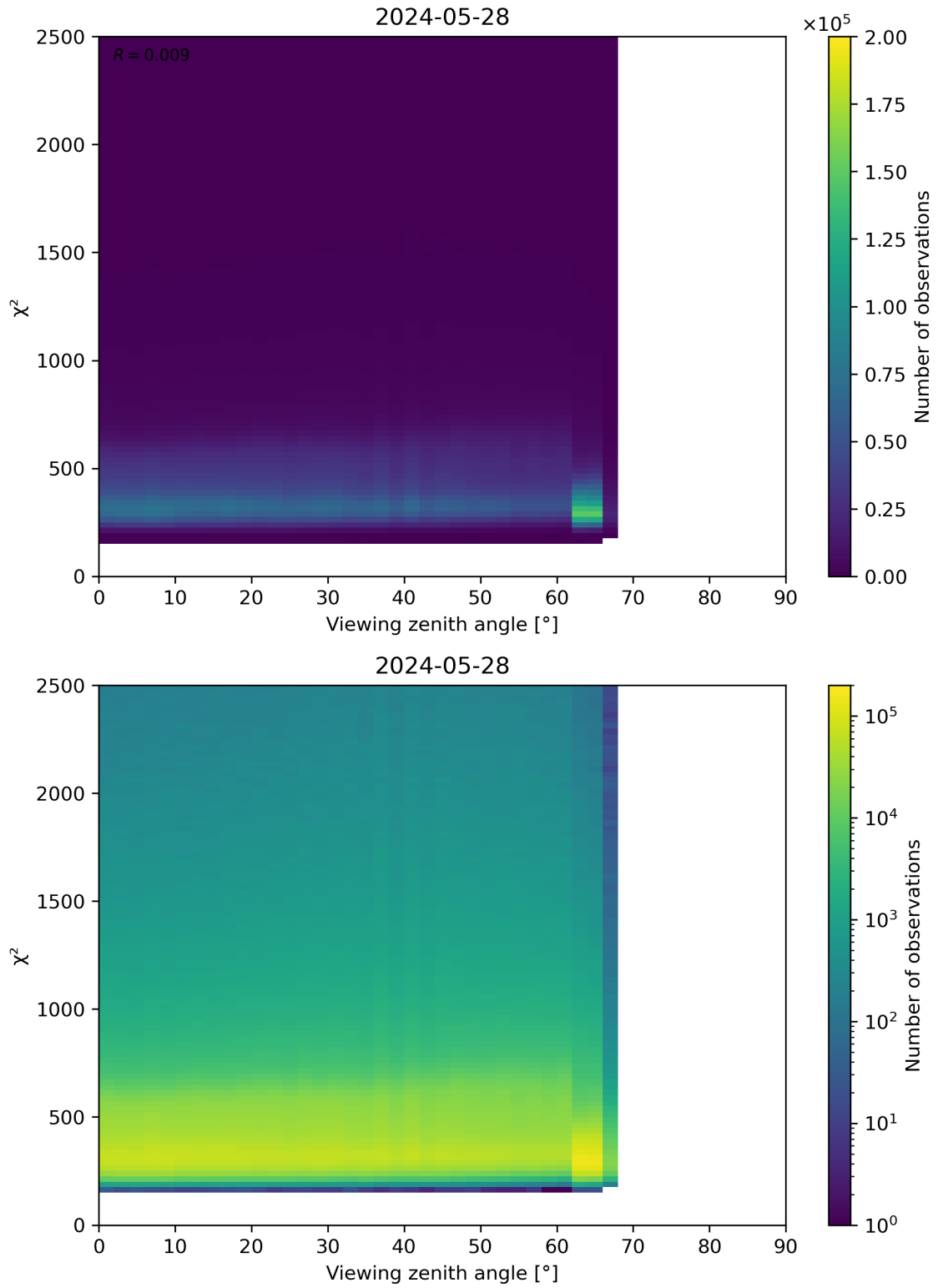
Figure 162: Scatter density plot of “Viewing zenith angle” against “ \chi^2 ” for 2024-05-28 to 2024-05-29.
