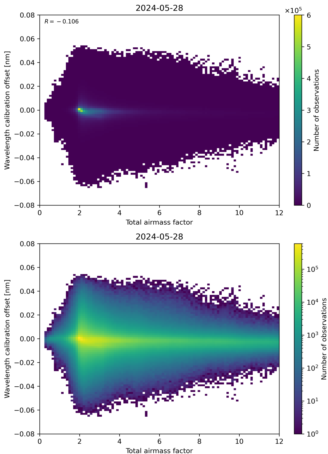
Figure 70: Scatter density plot of “Total airmass factor” against “Wavelength calibration offset” for 2024-05-28 to 2024-05-29.
