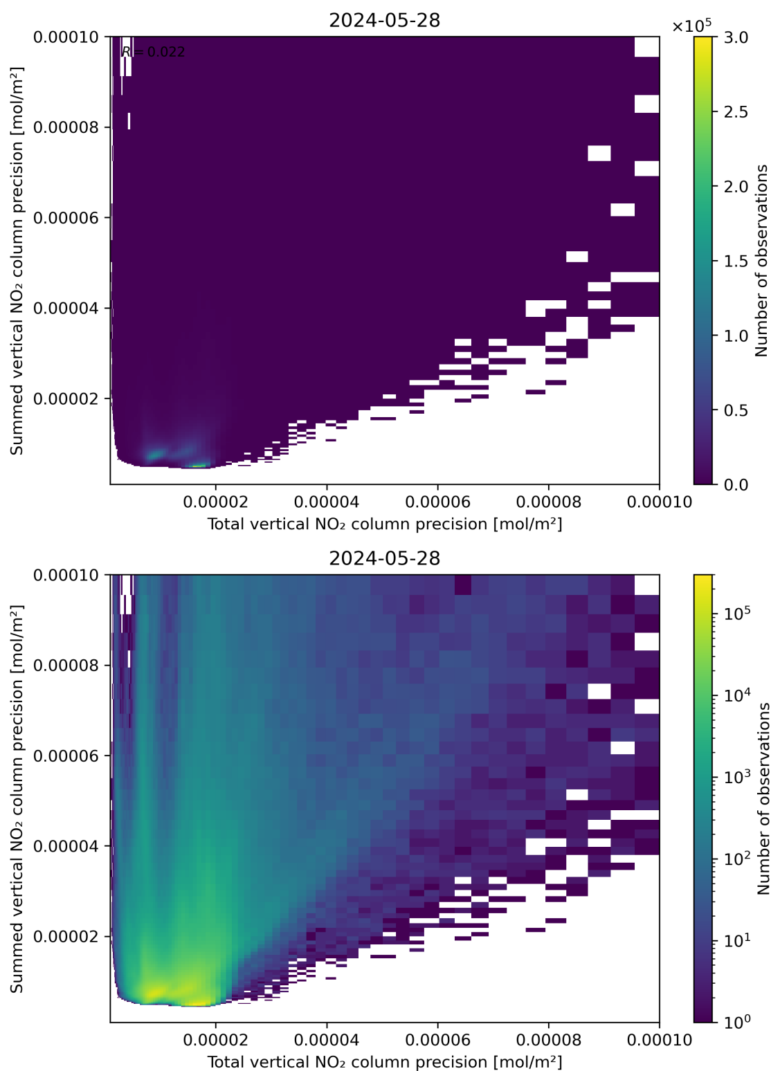
Figure 118: Scatter density plot of “Total vertical NO 2 column precision” against “Summed vertical NO 2 column precision” for 2024-05-28 to 2024-05-29.
