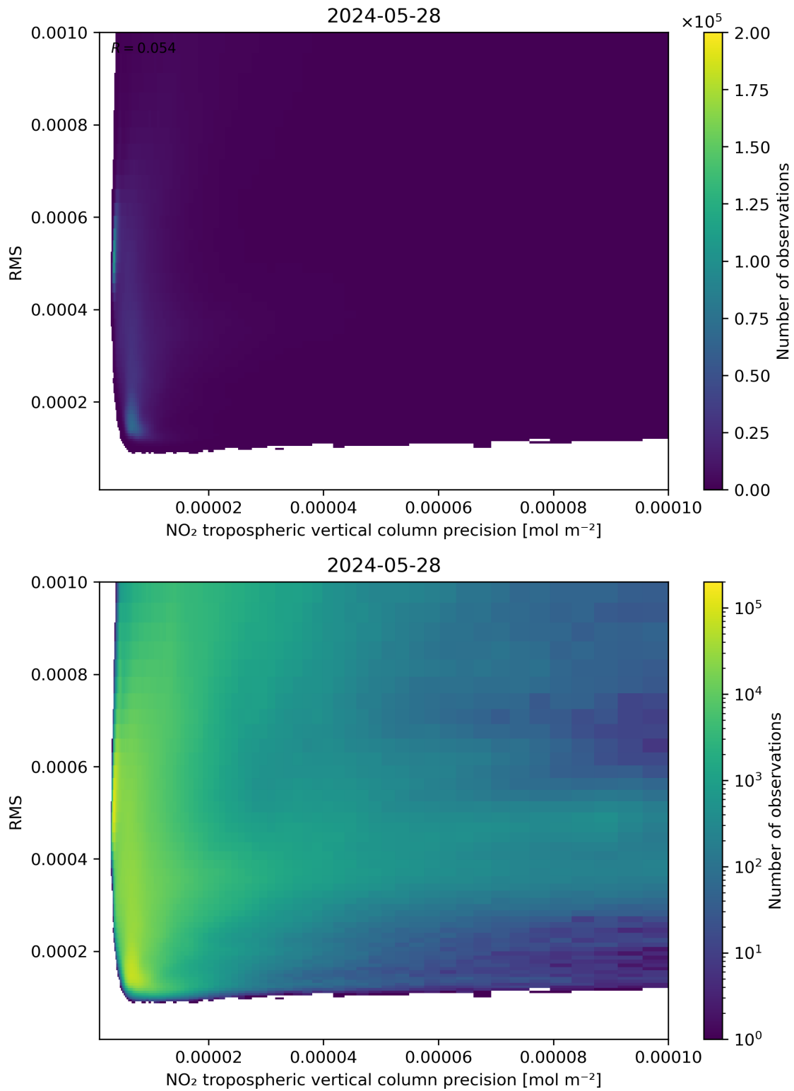
Figure 140: Scatter density plot of “NO 2 tropospheric vertical column precision” against “RMS” for 2024-05-28 to 2024-05-29.
