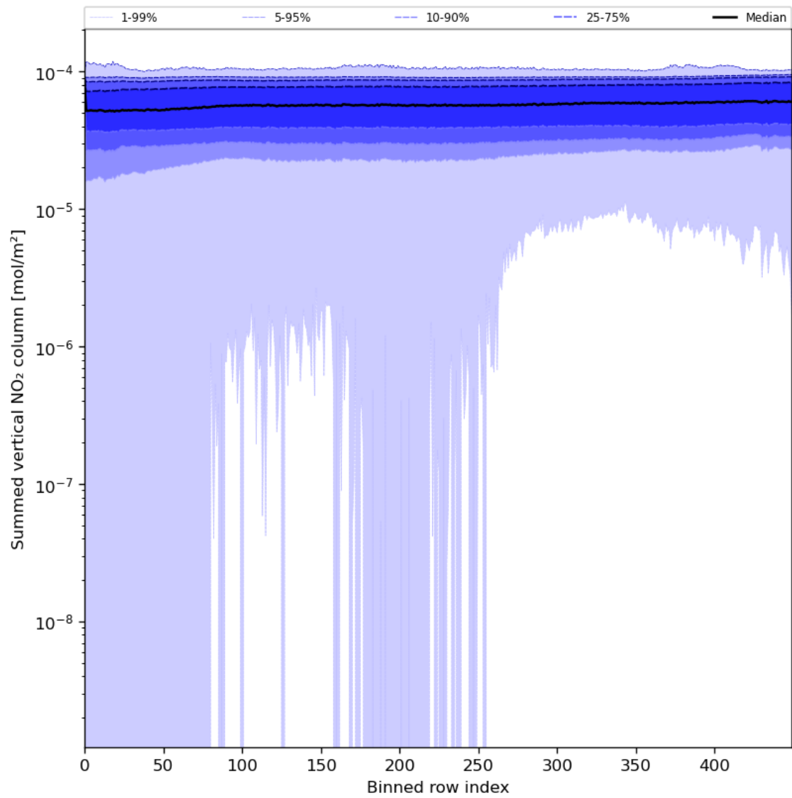
Figure 57: Along track statistics of “Summed vertical NO 2 column” for 2024-05-28 to 2024-05-29
