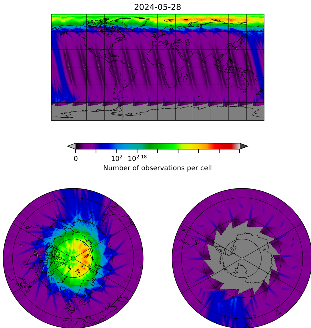
Figure 10: Map of the number of observations for 2024-05-28 to 2024-05-29
