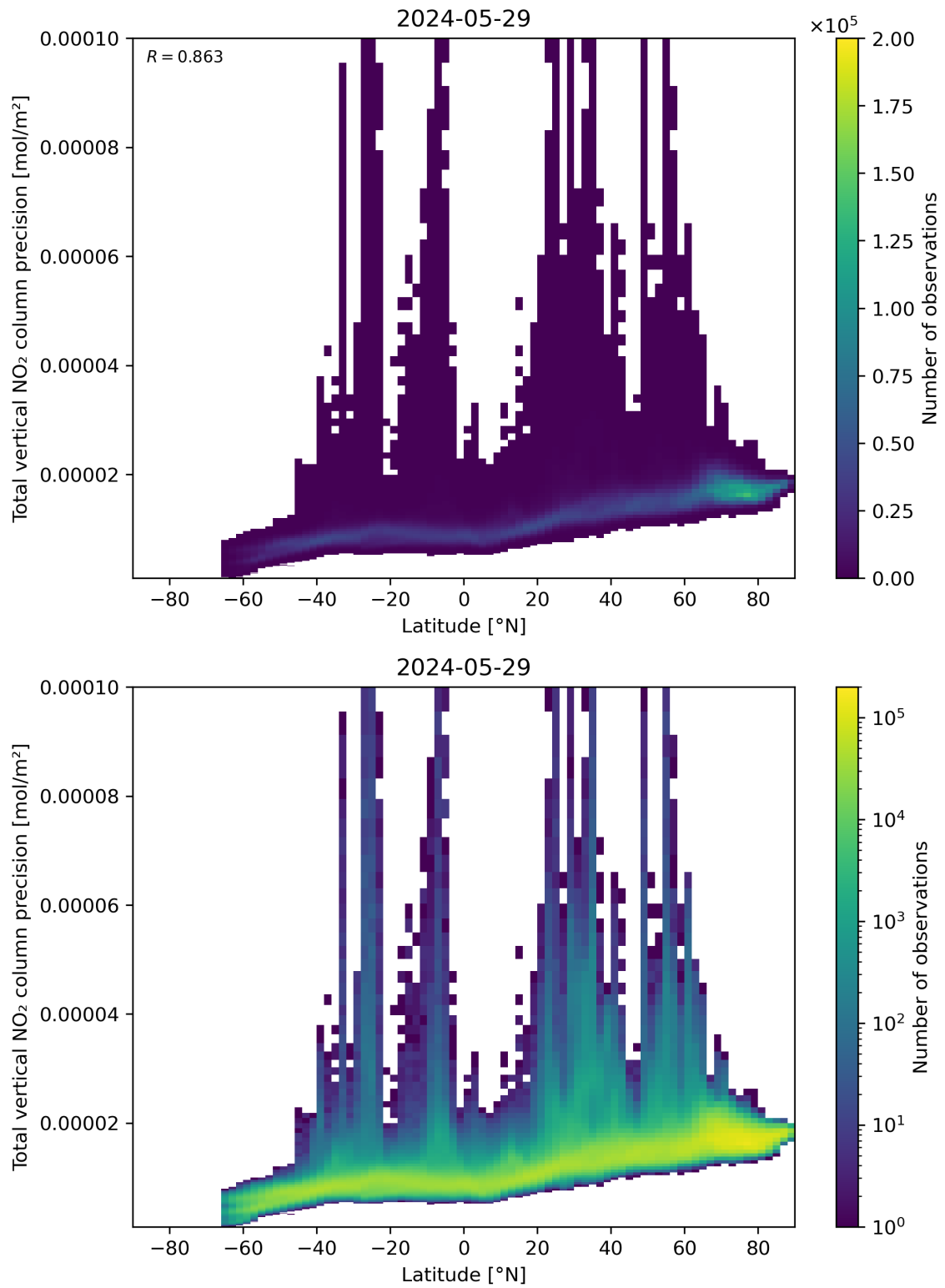
Figure 91: Scatter density plot of “Latitude” against “Total vertical NO 2 column precision” for 2024-05-28 to 2024-05-30.
