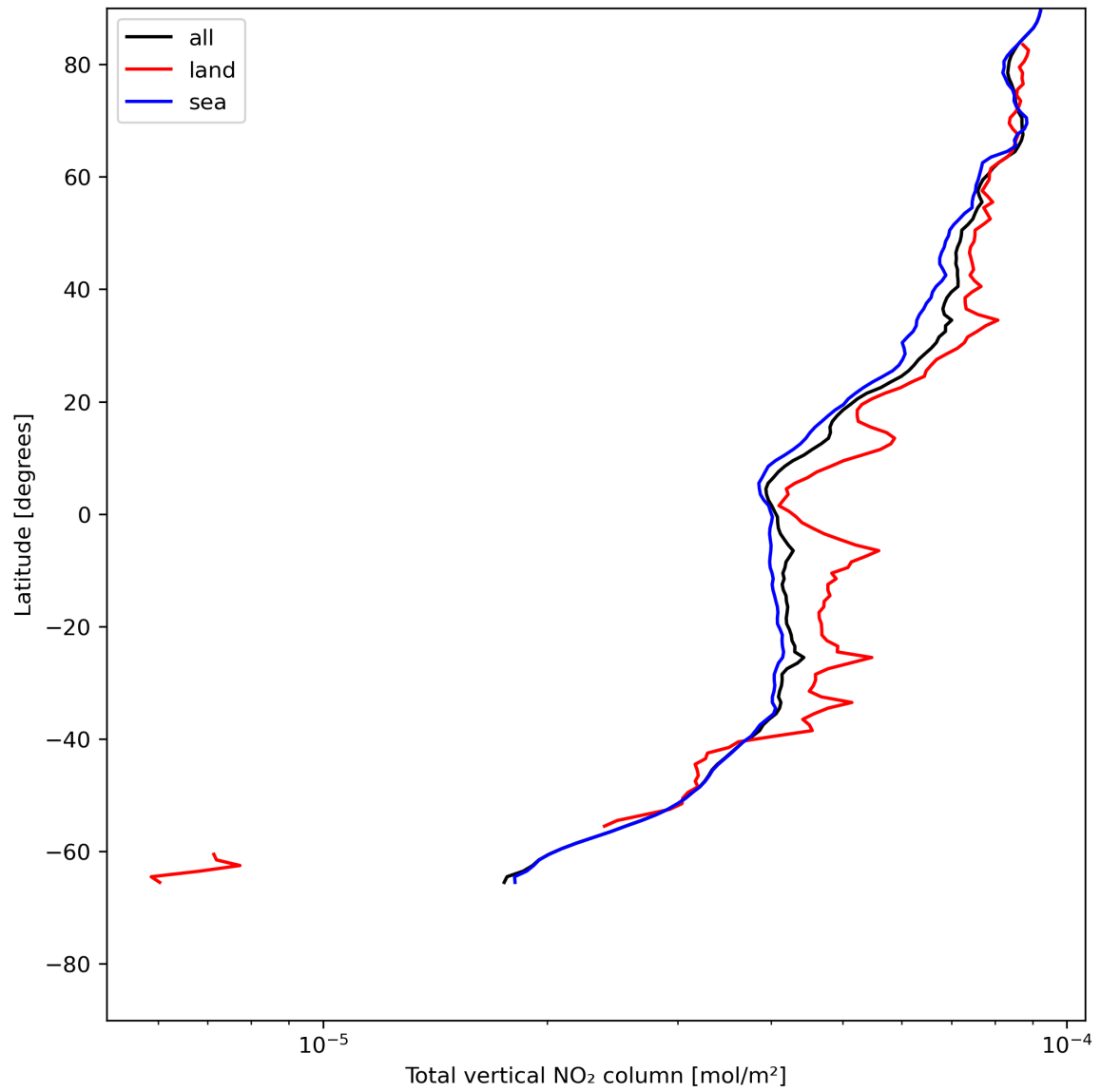
Figure 21: Zonal average of “Total vertical NO 2 column” for 2024-05-28 to 2024-05-30.
