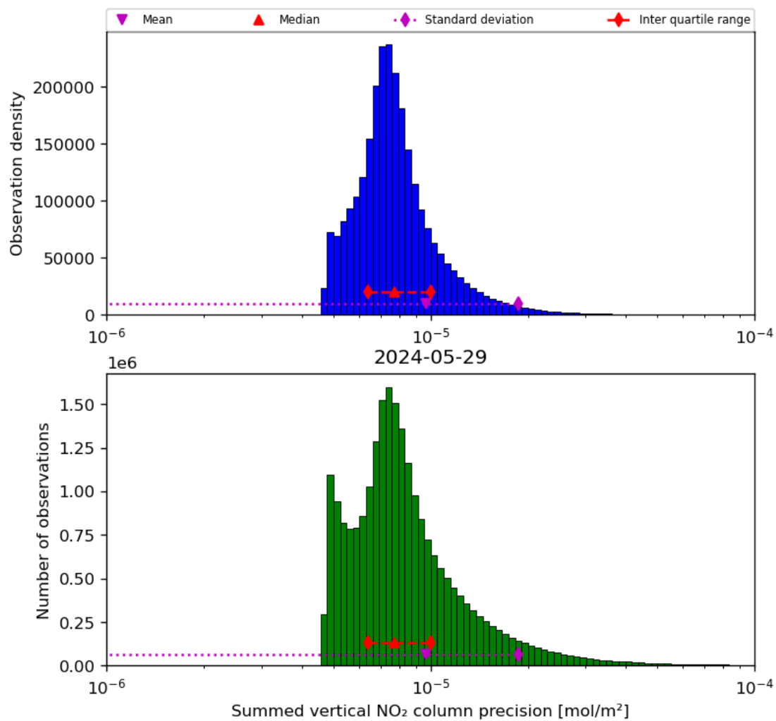
Figure 41: Histogram of "Summed vertical NO 2 column precision" for 2024-05-28 to 2024-05-30
