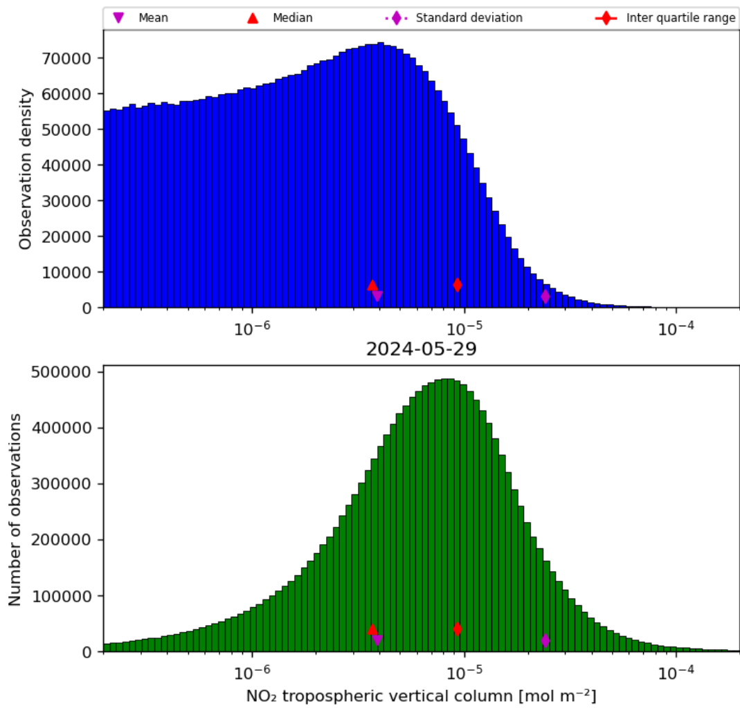
Figure 29: Histogram of “NO 2 tropospheric vertical column” for 2024-05-28 to 2024-05-30
