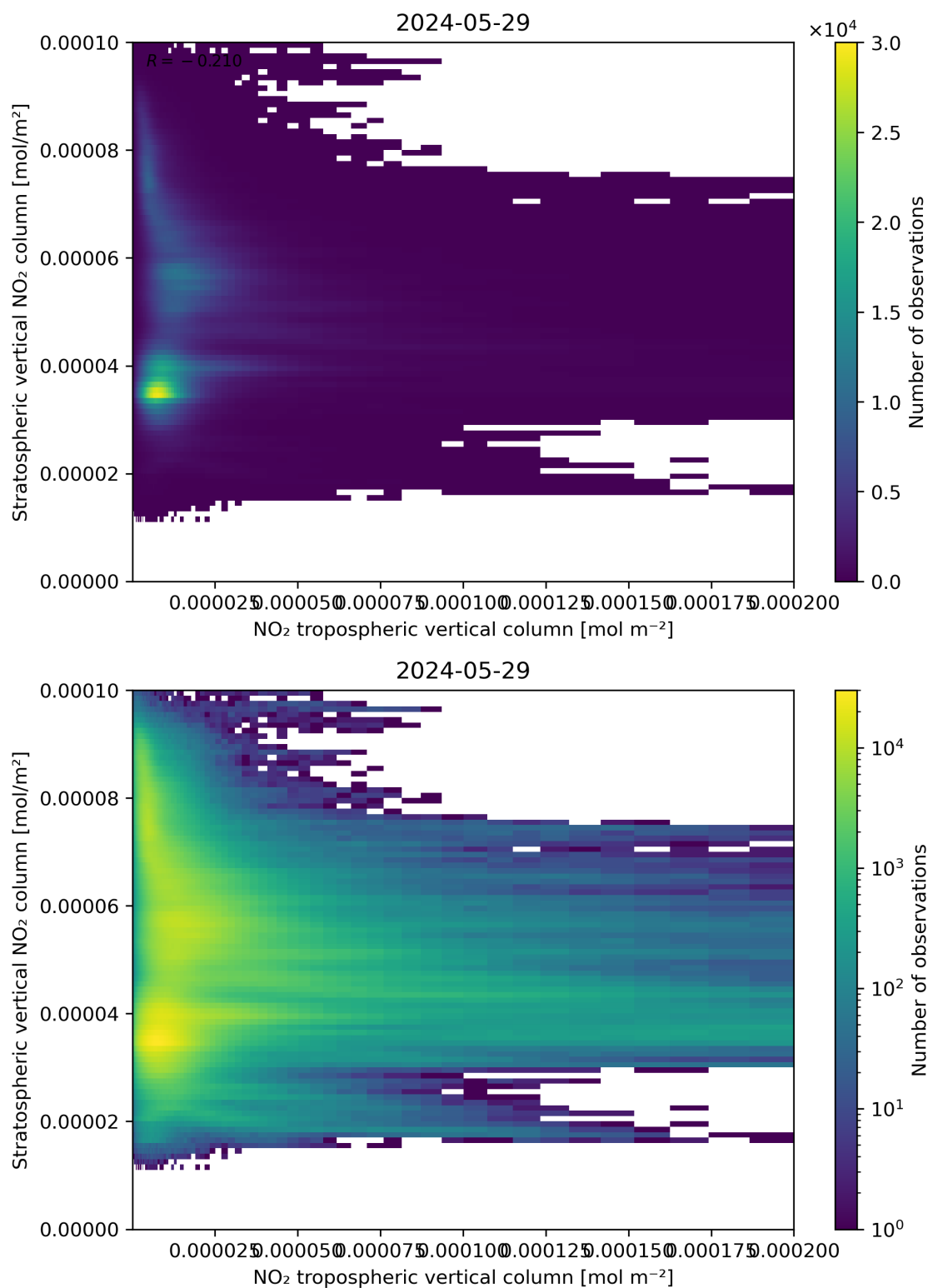
Figure 125: Scatter density plot of “NO 2 tropospheric vertical column” against “Stratospheric vertical NO 2 column” for 2024-05-28 to 2024-05-30.
