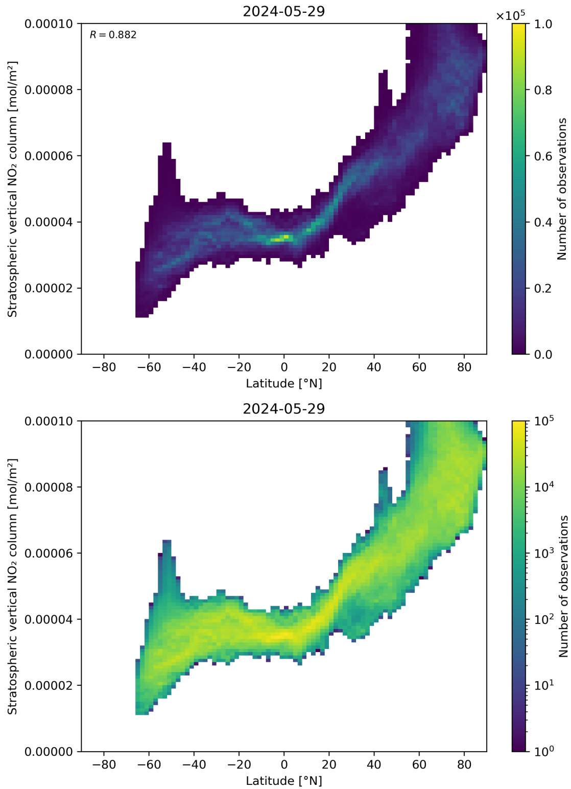
Figure 87: Scatter density plot of “Latitude” against “Stratospheric vertical NO 2 column” for 2024-05-28 to 2024-05-30.
