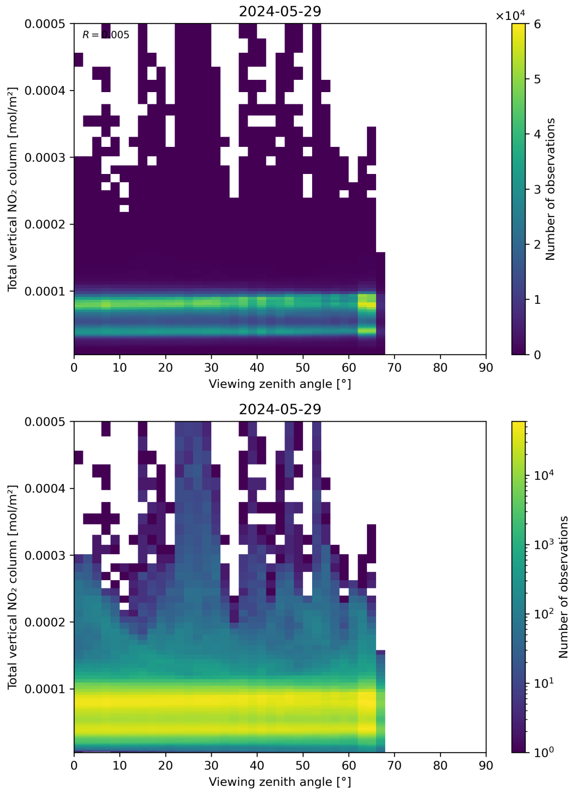
Figure 167: Scatter density plot of “Viewing zenith angle” against “Total vertical NO 2 column” for 2024-05-28 to 2024-05-30.
