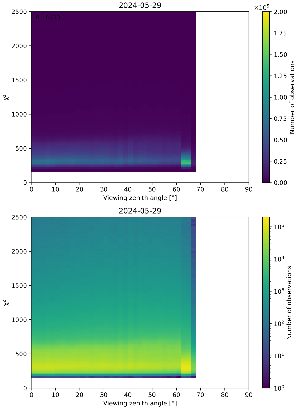
Figure 162: Scatter density plot of “Viewing zenith angle” against “ \chi^2 ” for 2024-05-28 to 2024-05-30.
