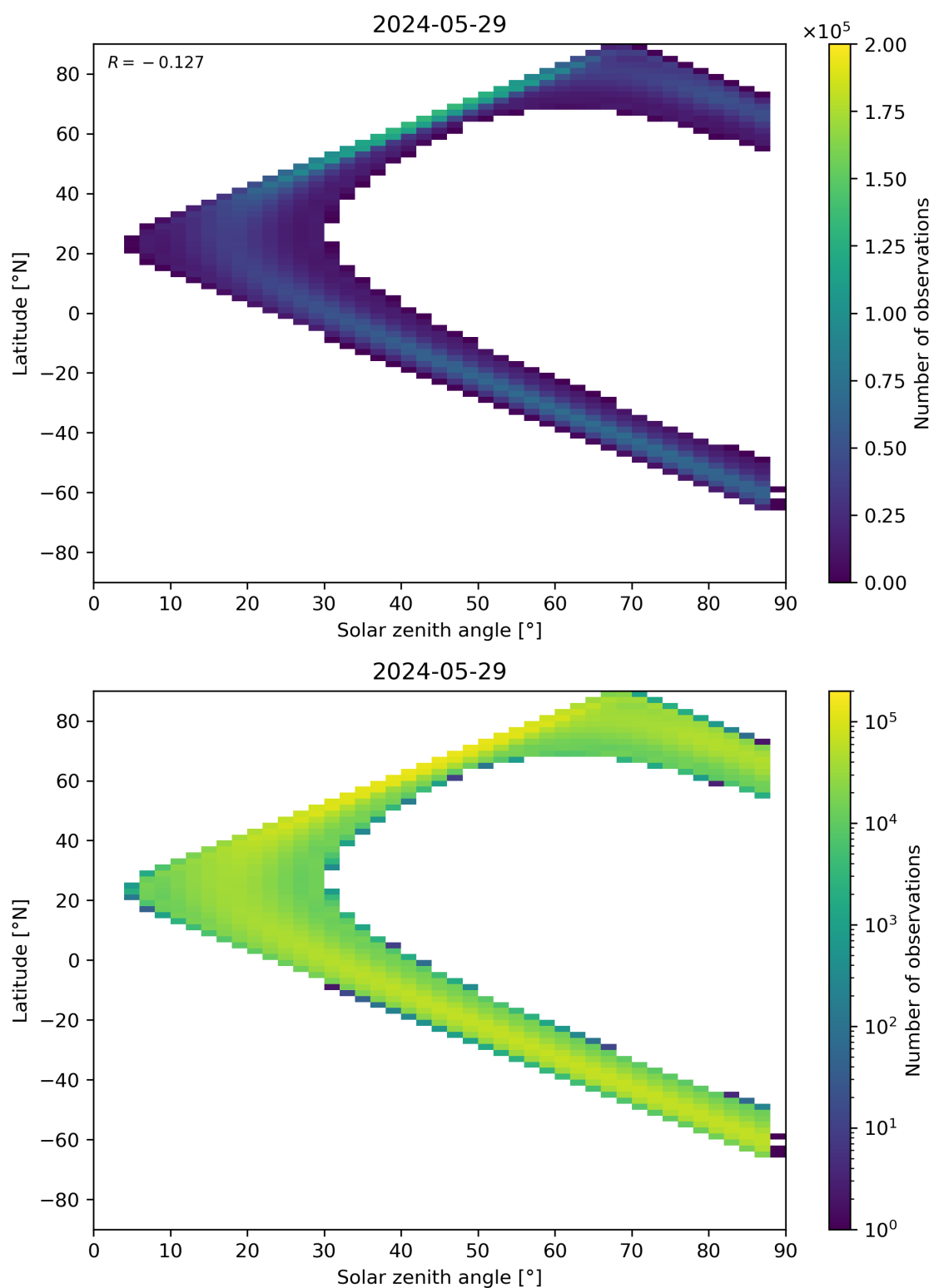
Figure 149: Scatter density plot of “Solar zenith angle” against “Latitude” for 2024-05-28 to 2024-05-30.
