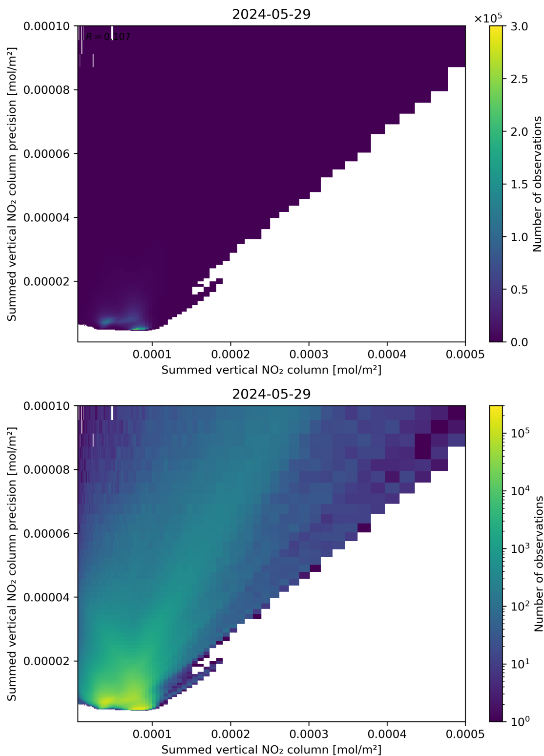
Figure 105: Scatter density plot of “Summed vertical NO 2 column” against “Summed vertical NO 2 column precision” for 2024-05-28 to 2024-05-30.
