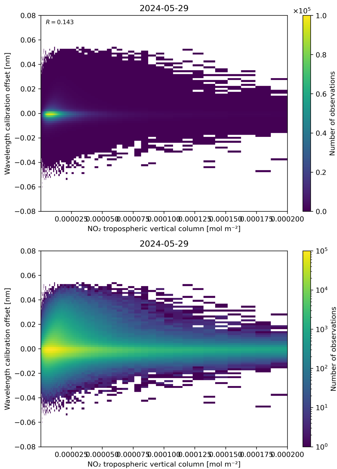
Figure 143: Scatter density plot of “NO 2 tropospheric vertical column” against “Wavelength calibration offset” for 2024-05-28 to 2024-05-30.
