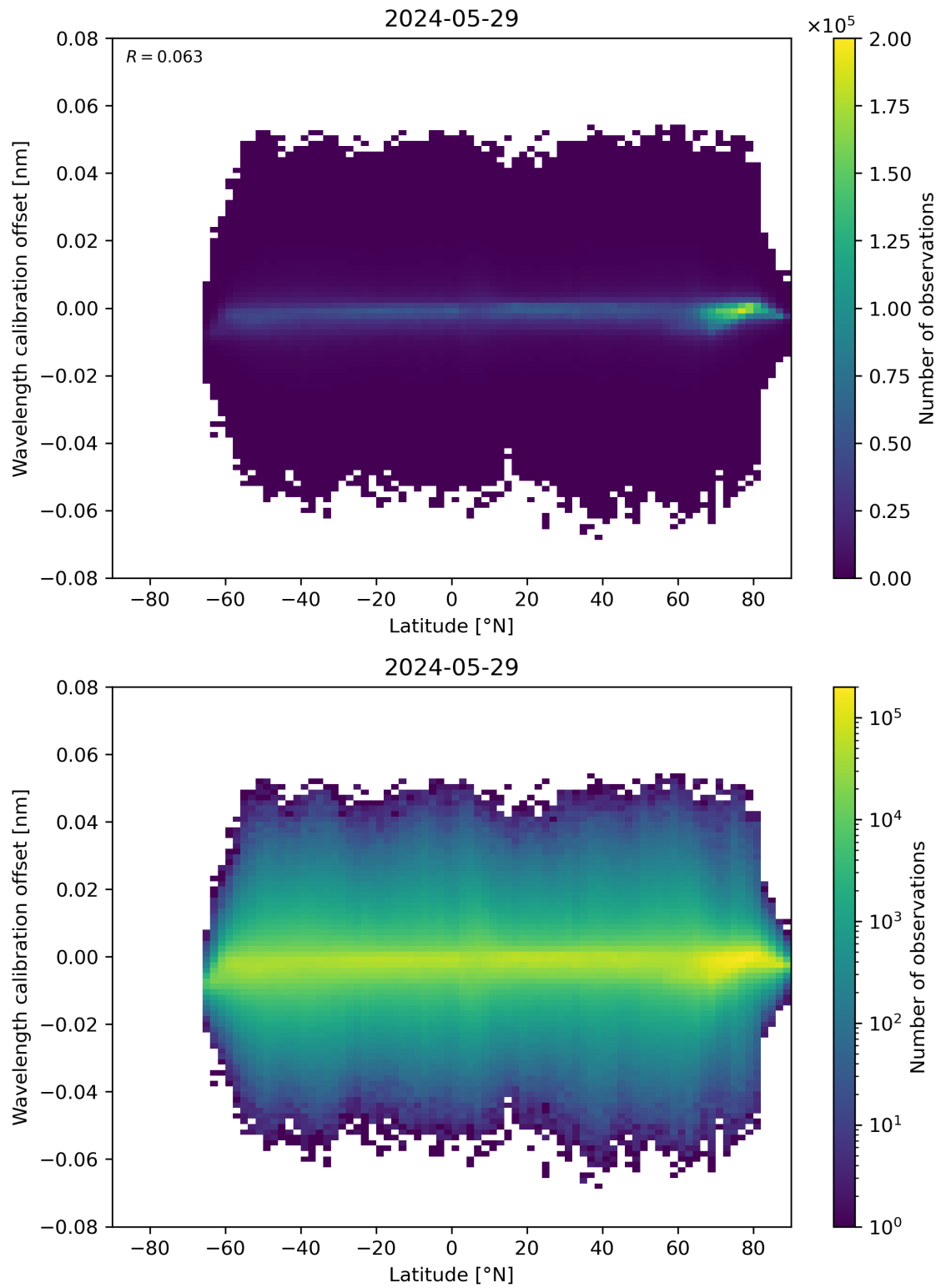
Figure 95: Scatter density plot of “Latitude” against “Wavelength calibration offset” for 2024-05-28 to 2024-05-30.
