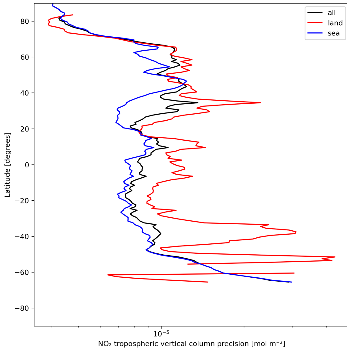
Figure 13: Zonal average of “NO 2 tropospheric vertical column precision” for 2024-05-28 to 2024-05-30.
