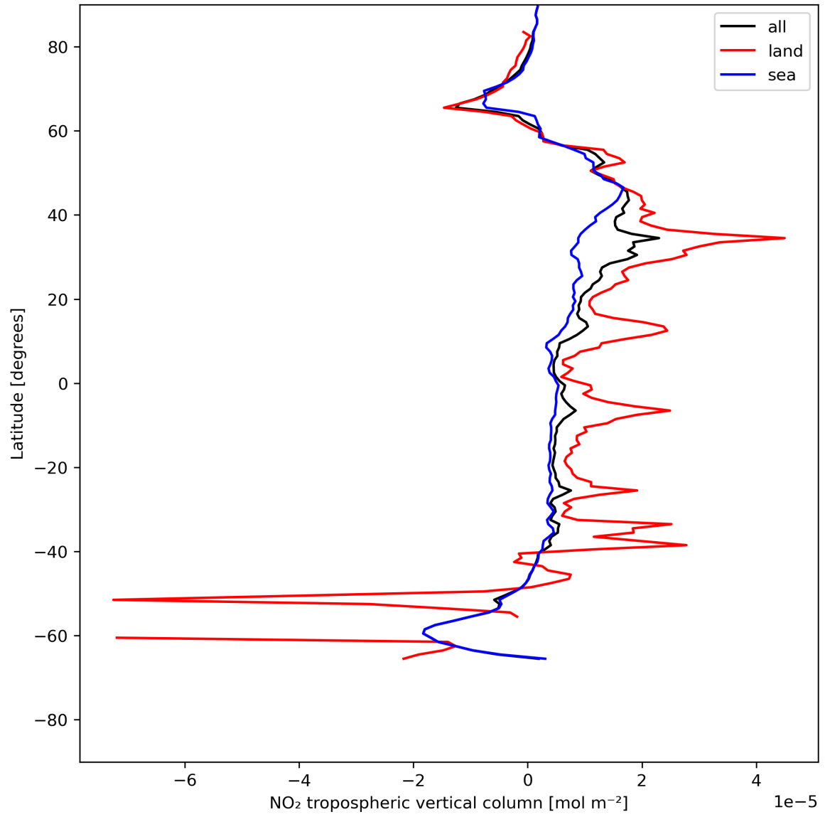
Figure 12: Zonal average of “NO 2 tropospheric vertical column” for 2024-05-28 to 2024-05-30.
