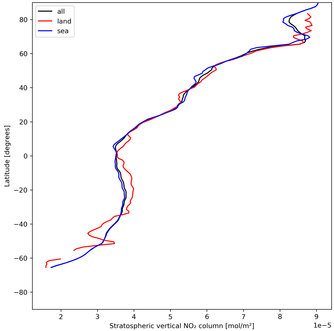
Figure 19: Zonal average of “Stratospheric vertical NO 2 column” for 2024-05-28 to 2024-05-30.
