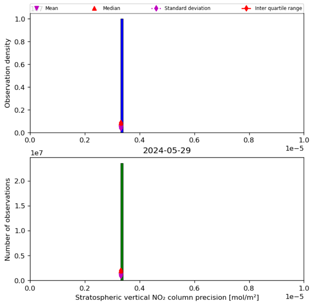
Figure 37: Histogram of “Stratospheric vertical NO 2 column precision” for 2024-05-28 to 2024-05-30
