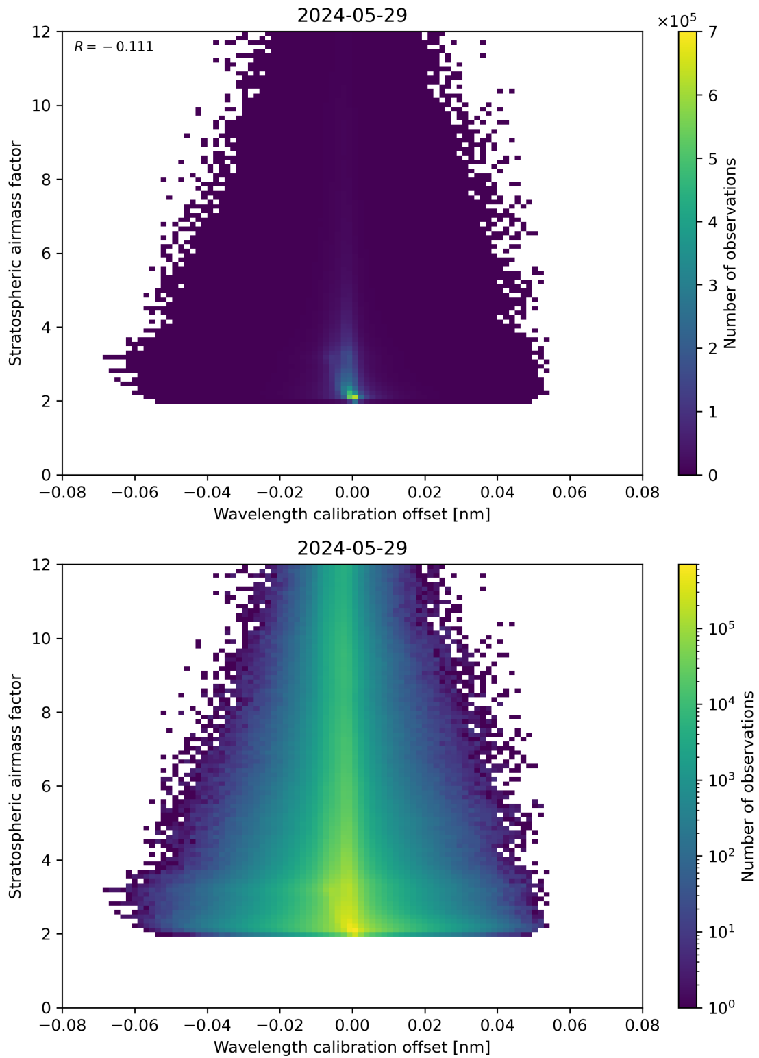
Figure 174: Scatter density plot of “Wavelength calibration offset” against “Stratospheric air mass factor” for 2024-05-28 to 2024-05-30.
