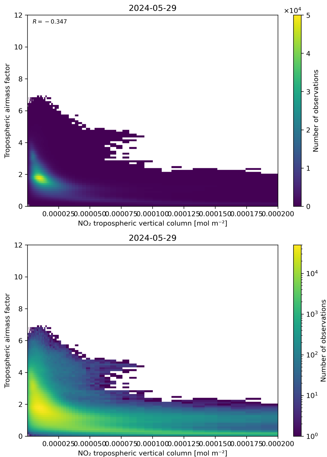
Figure 123: Scatter density plot of “NO 2 tropospheric vertical column” against “Tropospheric air mass factor” for 2024-05-28 to 2024-05-30.
