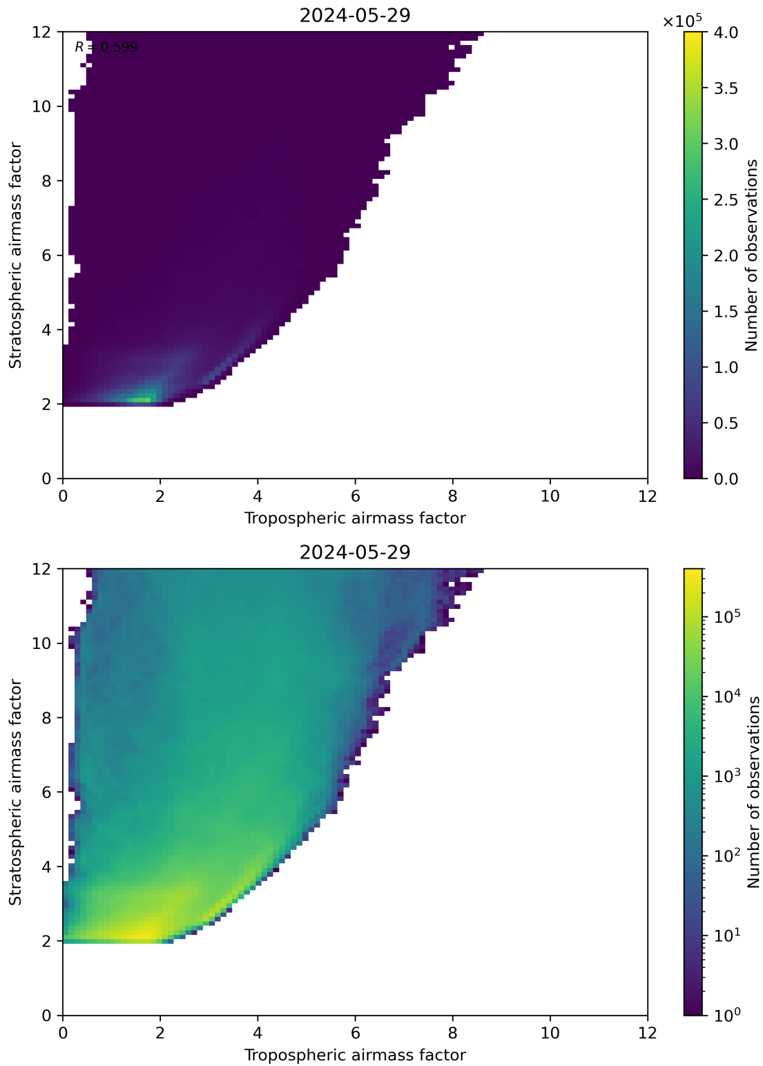
Figure 71: Scatter density plot of “Tropospheric airmass factor” against “Stratospheric airmass factor” for 2024-05-28 to 2024-05-30.
