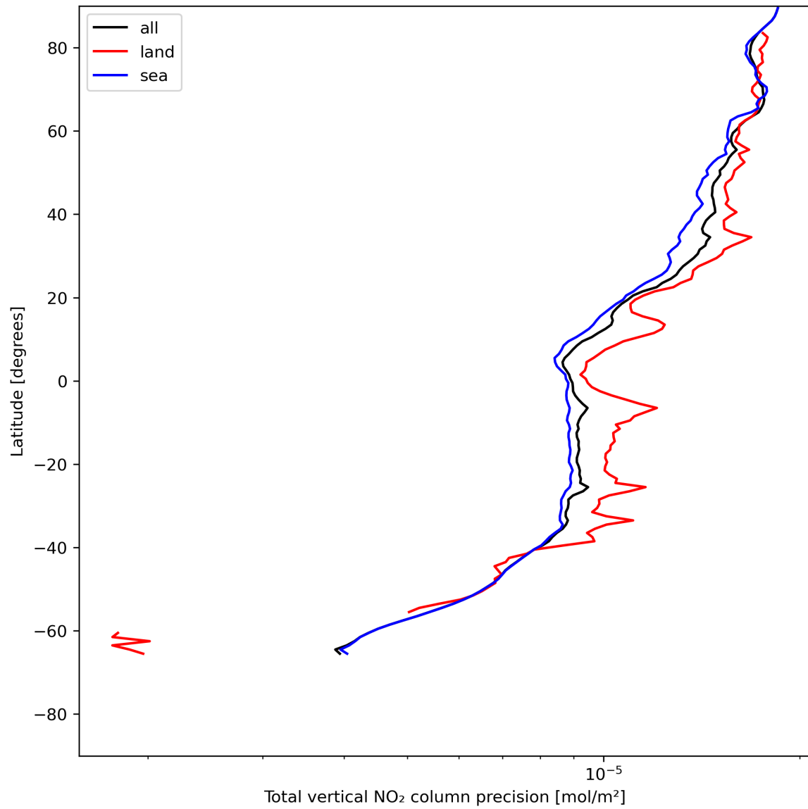
Figure 22: Zonal average of “Total vertical NO 2 column precision” for 2024-05-28 to 2024-05-30.
