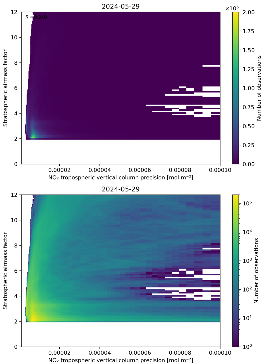
Figure 131: Scatter density plot of “NO 2 tropospheric vertical column precision” against “Stratospheric airmass factor” for 2024-05-28 to 2024-05-30.
