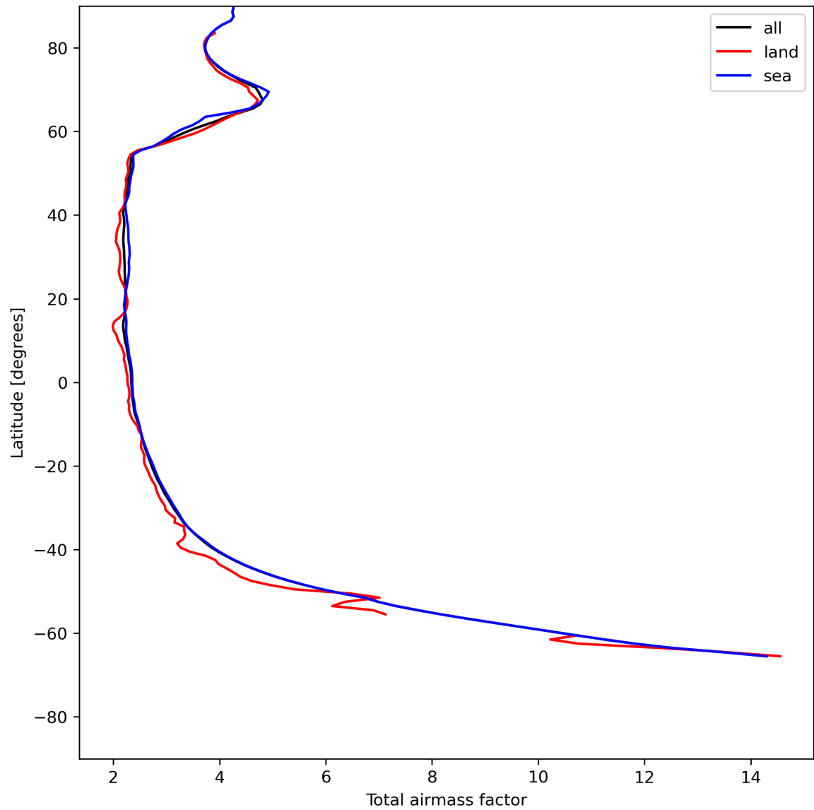
Figure 15: Zonal average of “Total airmass factor” for 2024-05-28 to 2024-05-30.
