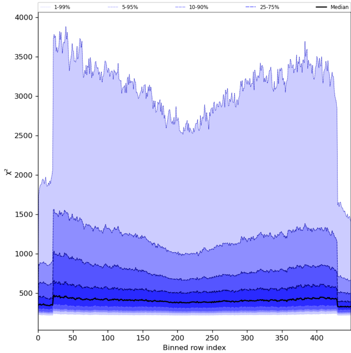
Figure 59: Along track statistics of “ \chi^2 ” for 2024-05-28 to 2024-05-30
