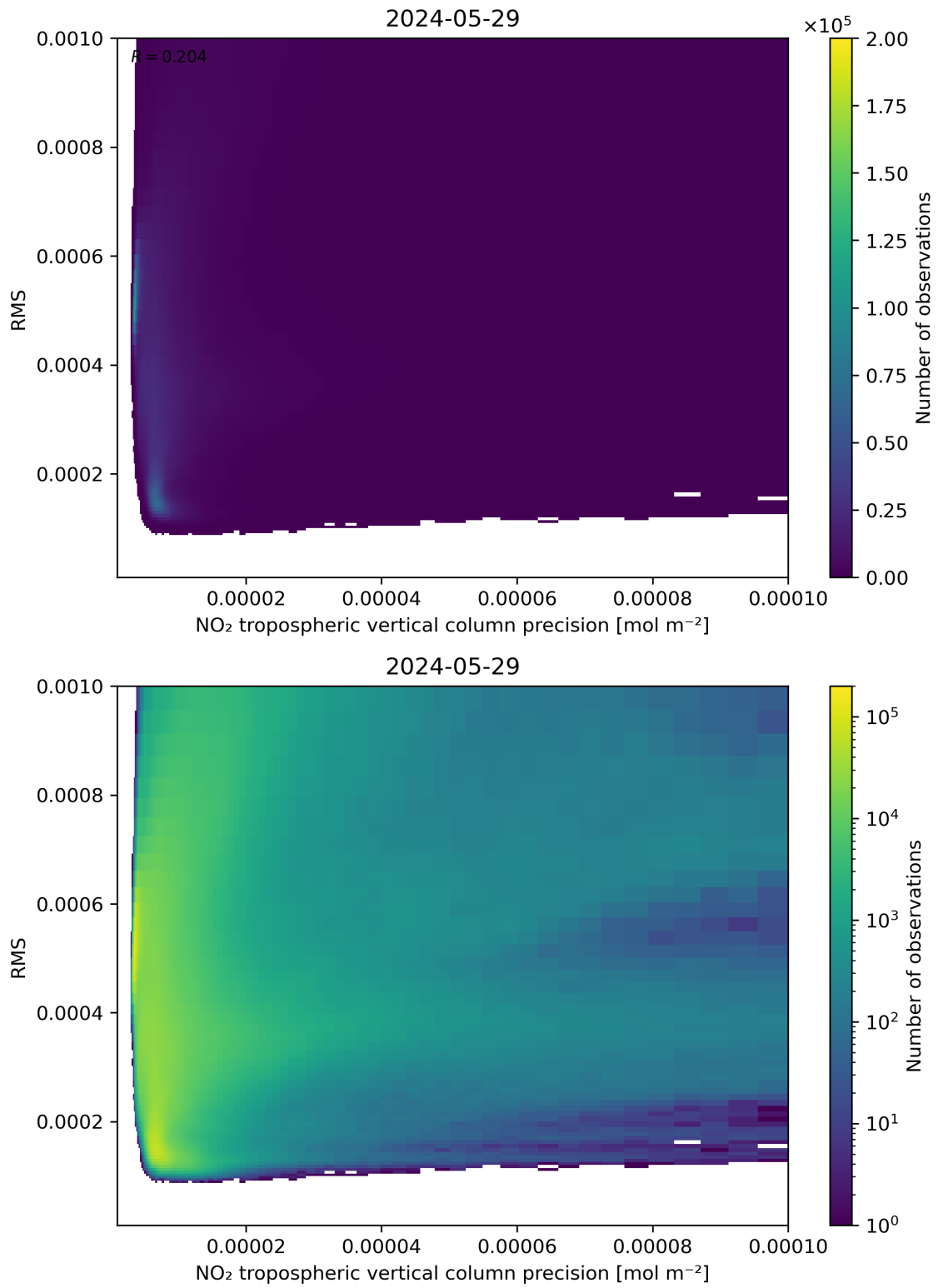
Figure 140: Scatter density plot of “NO 2 tropospheric vertical column precision” against “RMS” for 2024-05-28 to 2024-05-30.
