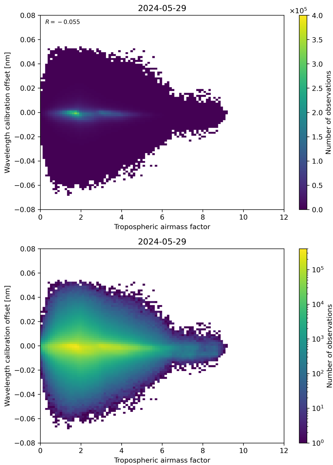
Figure 80: Scatter density plot of “Tropospheric airmass factor” against “Wavelength calibration offset” for 2024-05-28 to 2024-05-30.
