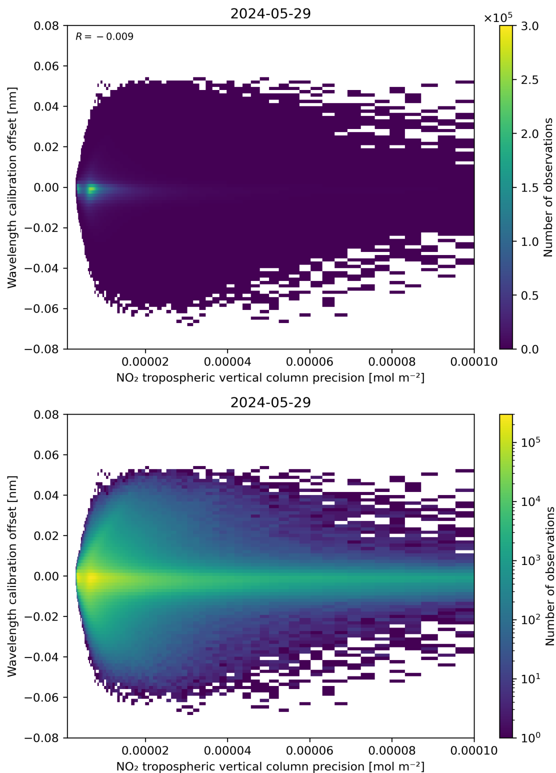
Figure 141: Scatter density plot of “NO 2 tropospheric vertical column precision” against “Wavelength calibration offset” for 2024-05-28 to 2024-05-30.
