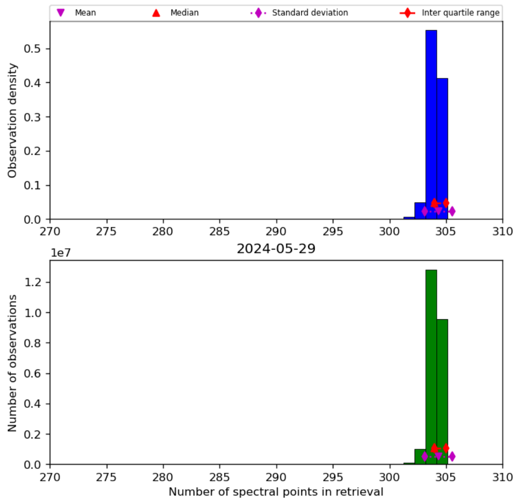
Figure 33: Histogram of “Number of spectral points in retrieval” for 2024-05-28 to 2024-05-30
