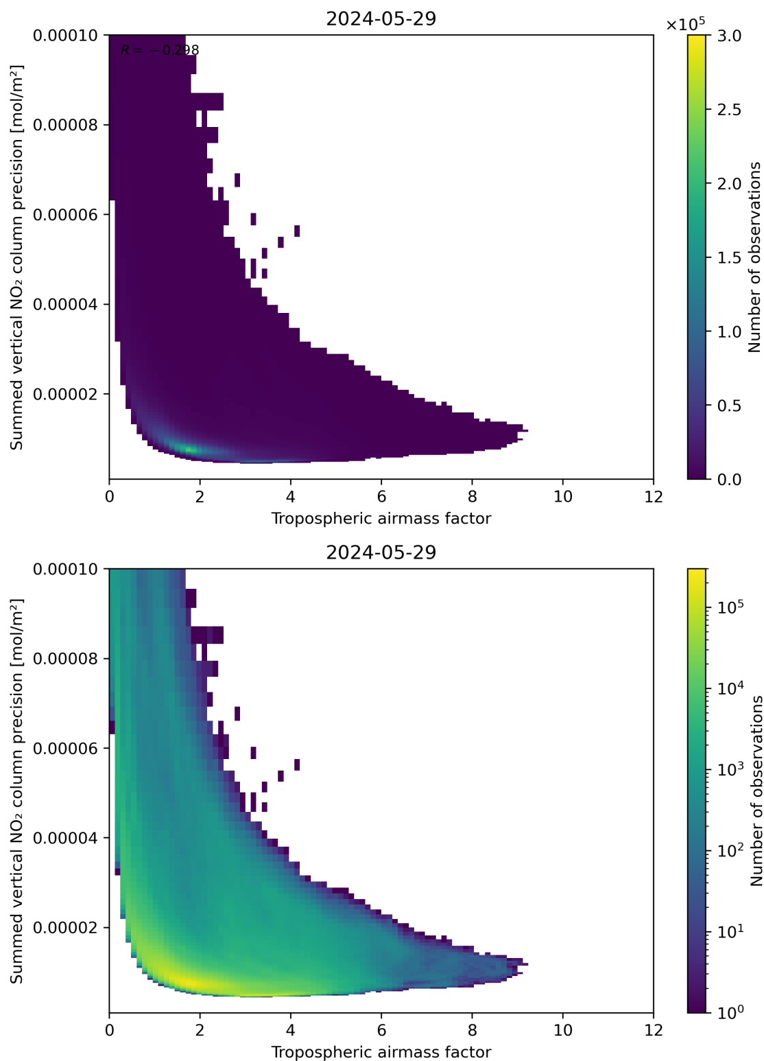
Figure 76: Scatter density plot of “Tropospheric air mass factor” against “Summed vertical NO 2 column precision” for 2024-05-28 to 2024-05-30.
