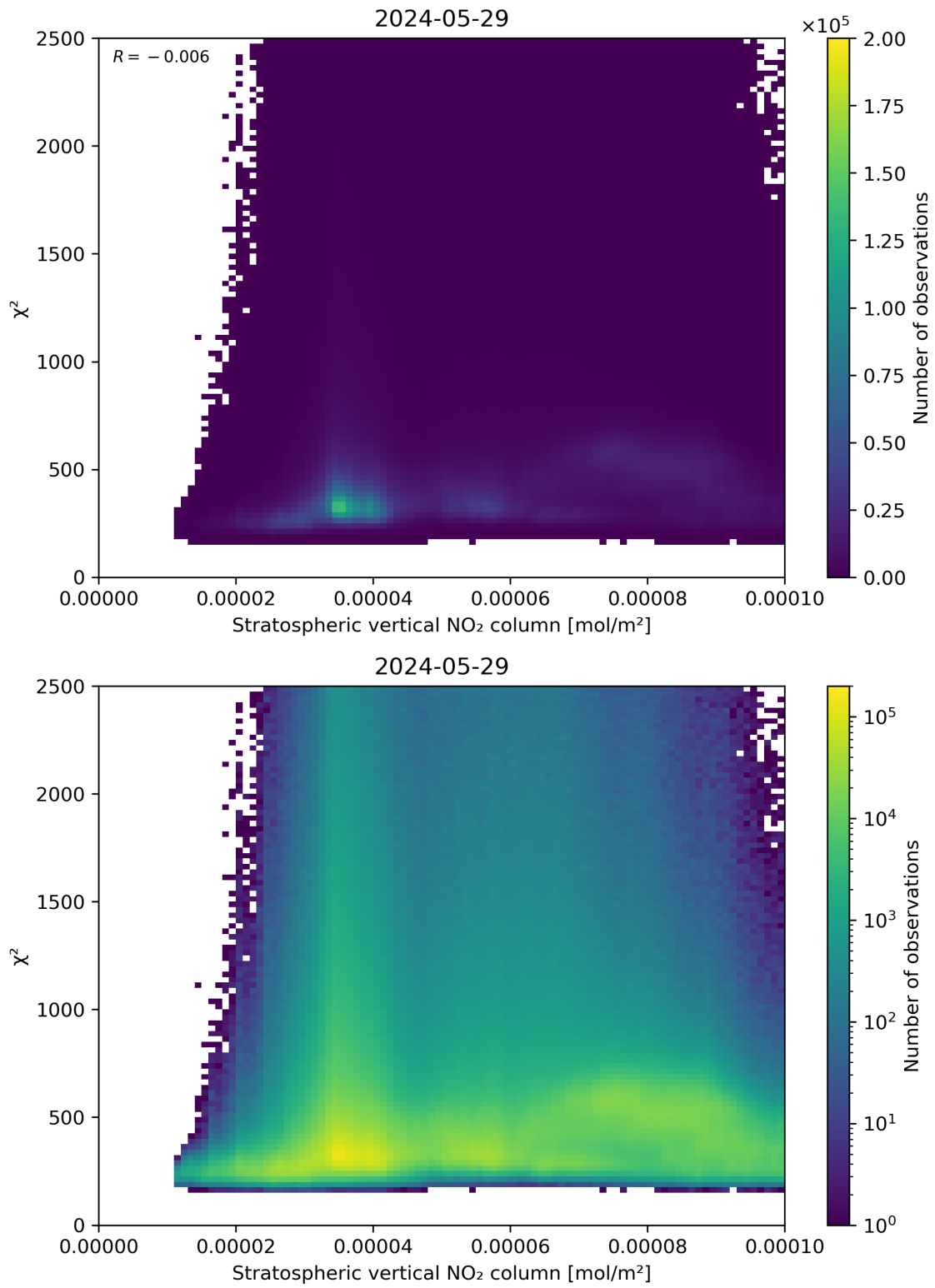
Figure 97: Scatter density plot of “Stratospheric vertical NO 2 column” against “ \chi^2 ” for 2024-05-28 to 2024-05-30.
