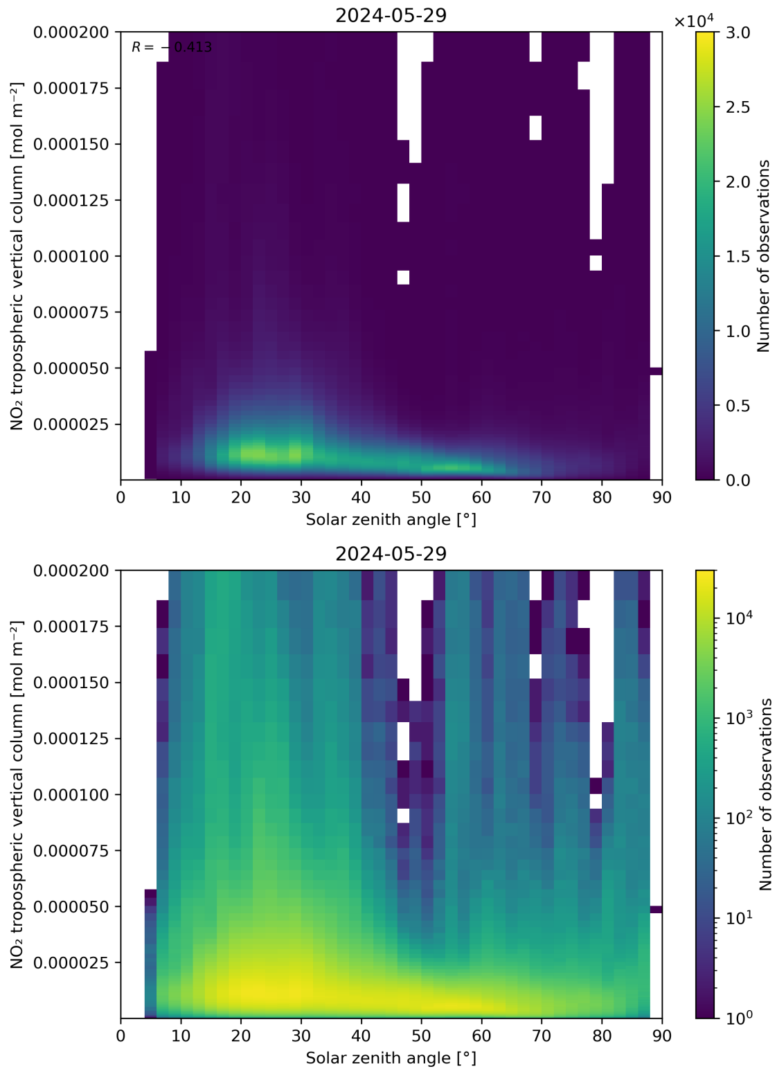
Figure 155: Scatter density plot of “Solar zenith angle” against “NO 2 tropospheric vertical column” for 2024-05-28 to 2024-05-30.
