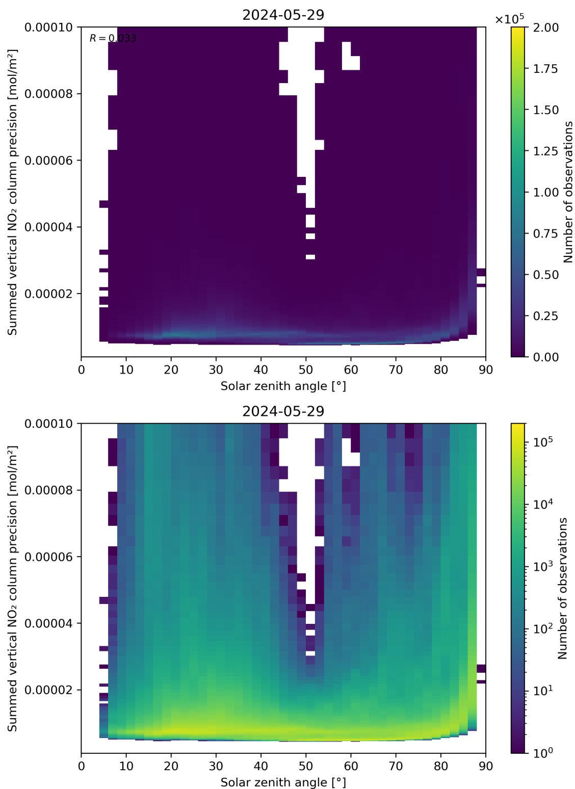
Figure 152: Scatter density plot of “Solar zenith angle” against “Summed vertical NO 2 column precision” for 2024-05-28 to 2024-05-30.
