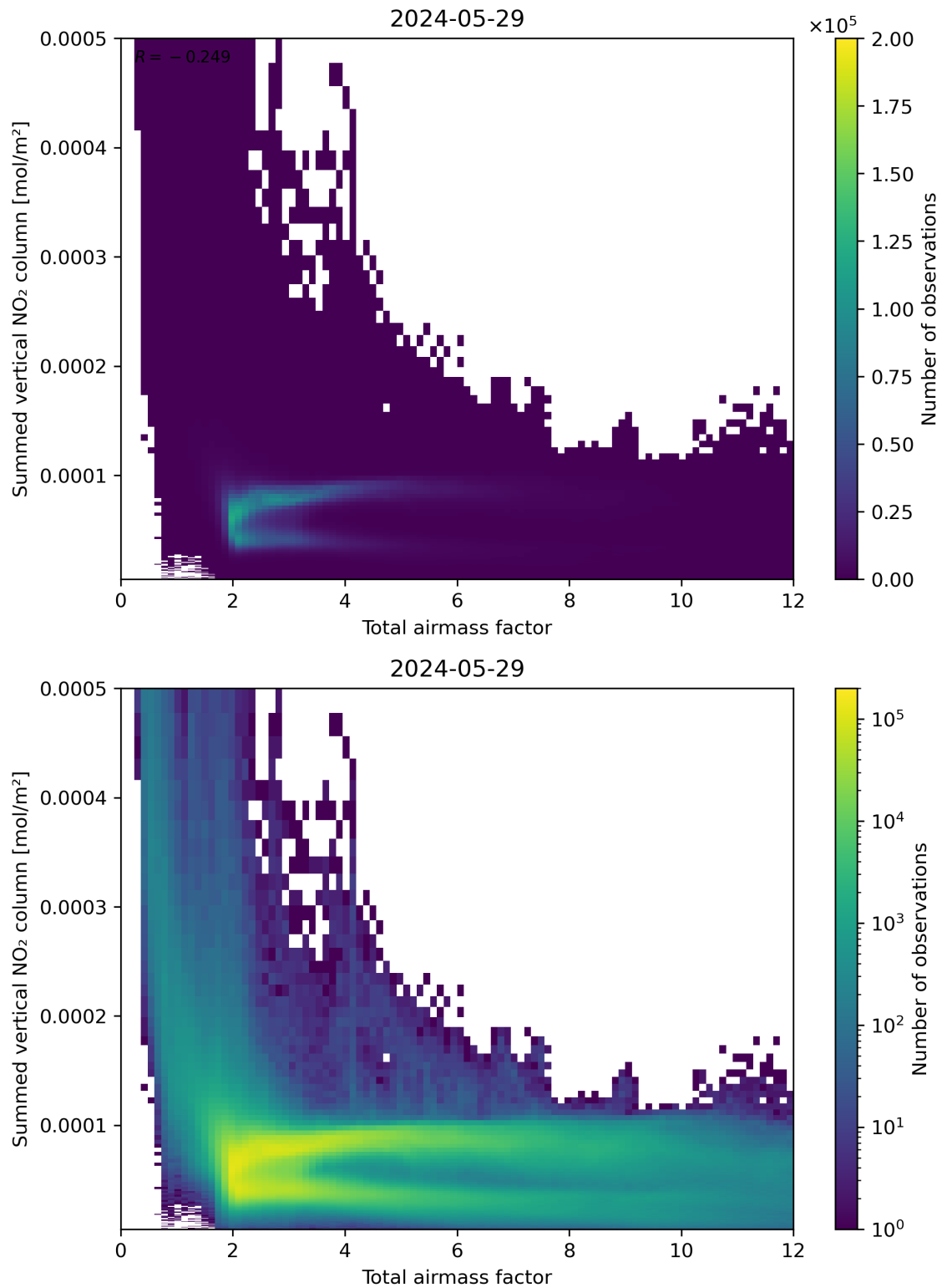
Figure 65: Scatter density plot of “Total airmass factor” against “Summed vertical NO 2 column” for 2024-05-28 to 2024-05-30.
