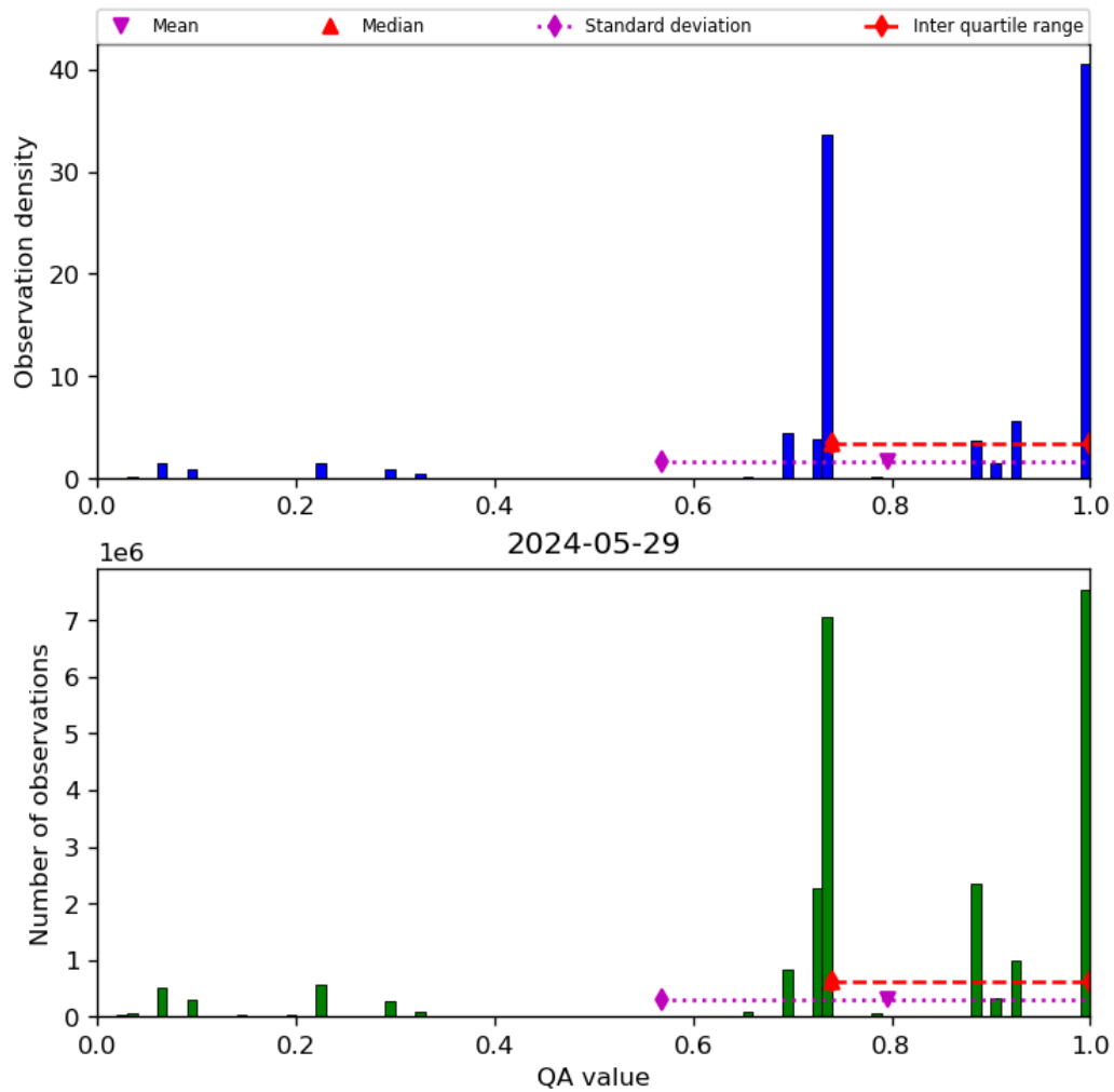
Figure 28: Histogram of “QA value” for 2024-05-28 to 2024-05-30
