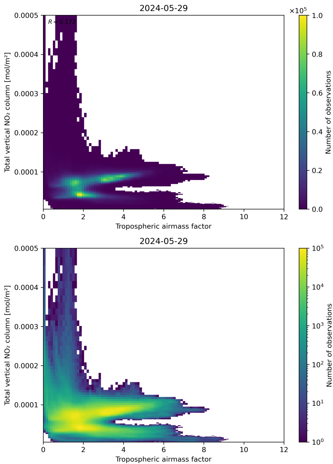
Figure 77: Scatter density plot of “Tropospheric airmass factor” against “Total vertical NO 2 column” for 2024-05-28 to 2024-05-30.
