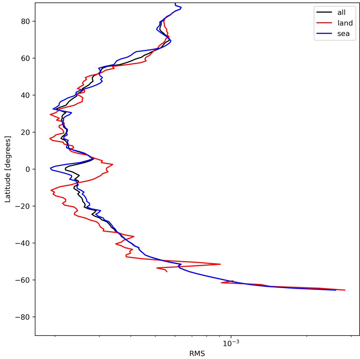
Figure 26: Zonal average of “RMS” for 2024-05-28 to 2024-05-30.
