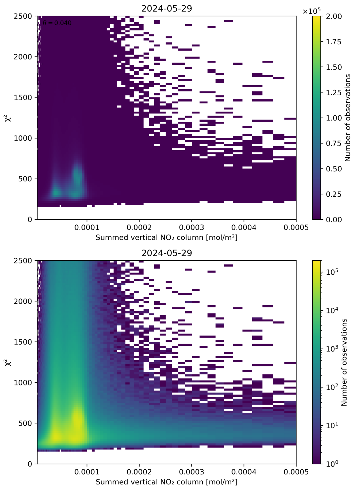
Figure 104: Scatter density plot of “Summed vertical NO 2 column” against “ \chi^2 ” for 2024-05-28 to 2024-05-30.
