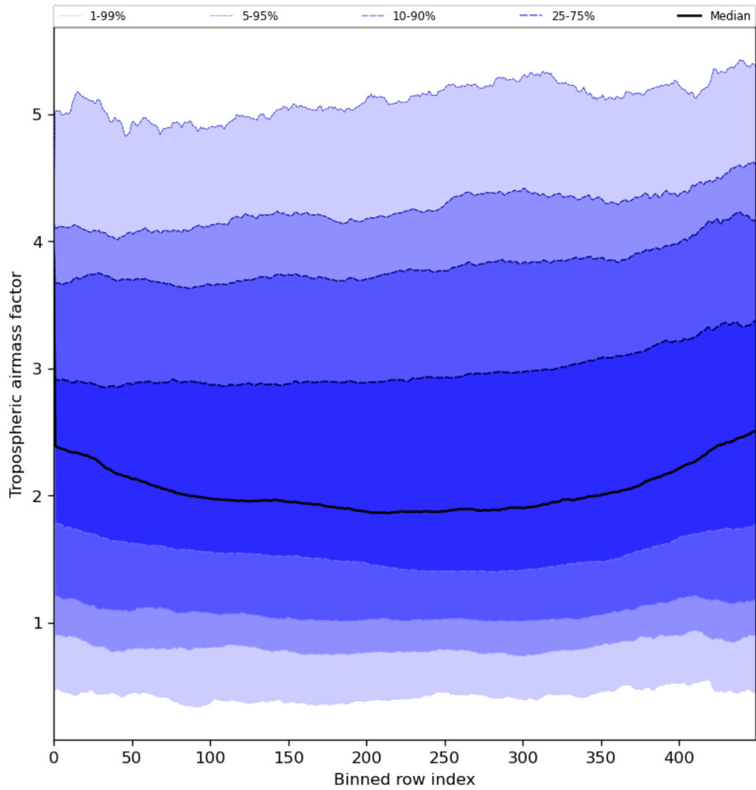
Figure 48: Along track statistics of “Tropospheric airmass factor” for 2024-05-28 to 2024-05-30
