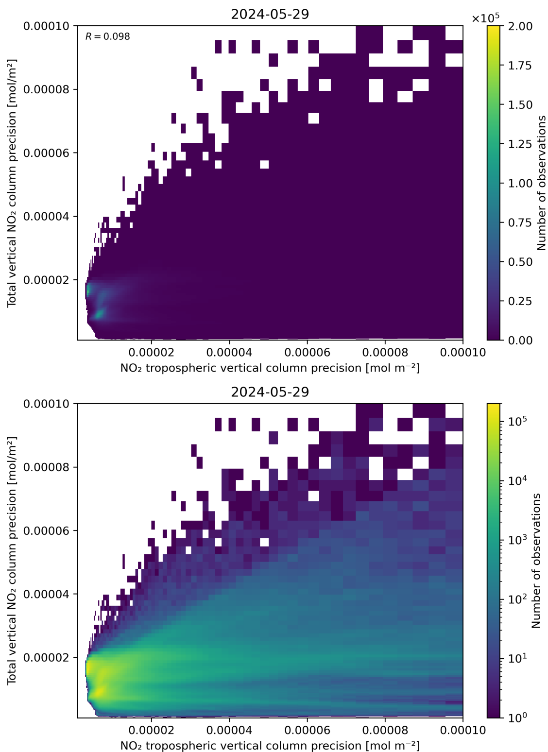
Figure 139: Scatter density plot of “NO 2 tropospheric vertical column precision” against “Total vertical NO 2 column precision” for 2024-05-28 to 2024-05-30.
