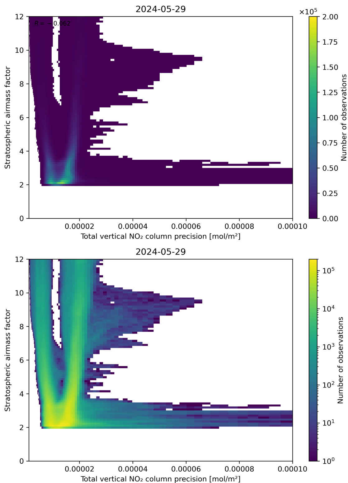
Figure 115: Scatter density plot of “Total vertical NO 2 column precision” against “Stratospheric airmass factor” for 2024-05-28 to 2024-05-30.
