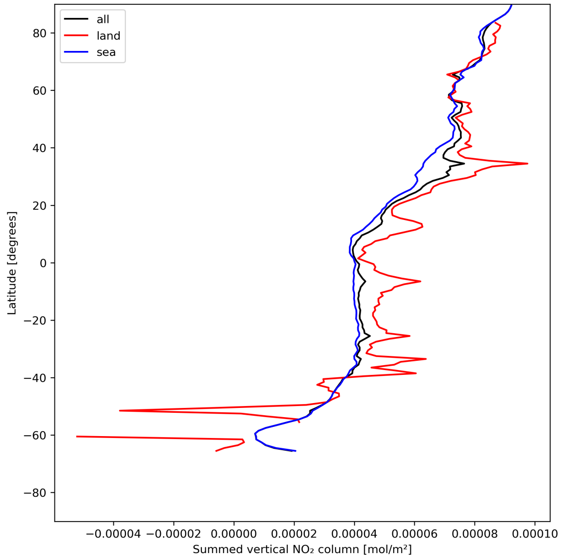
Figure 23: Zonal average of “Summed vertical NO 2 column” for 2024-05-28 to 2024-05-30.
