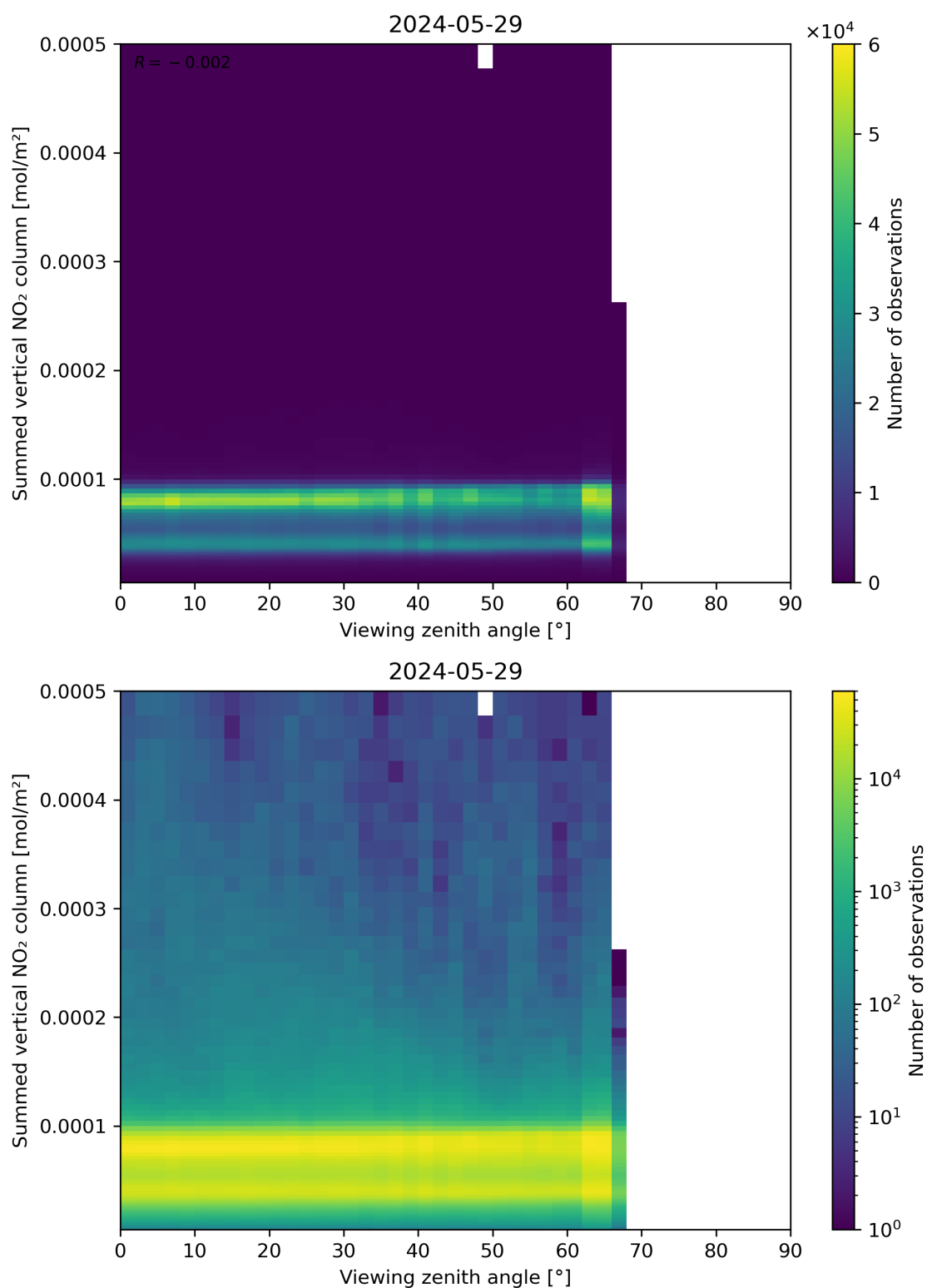
Figure 165: Scatter density plot of “Viewing zenith angle” against “Summed vertical NO 2 column” for 2024-05-28 to 2024-05-30.
