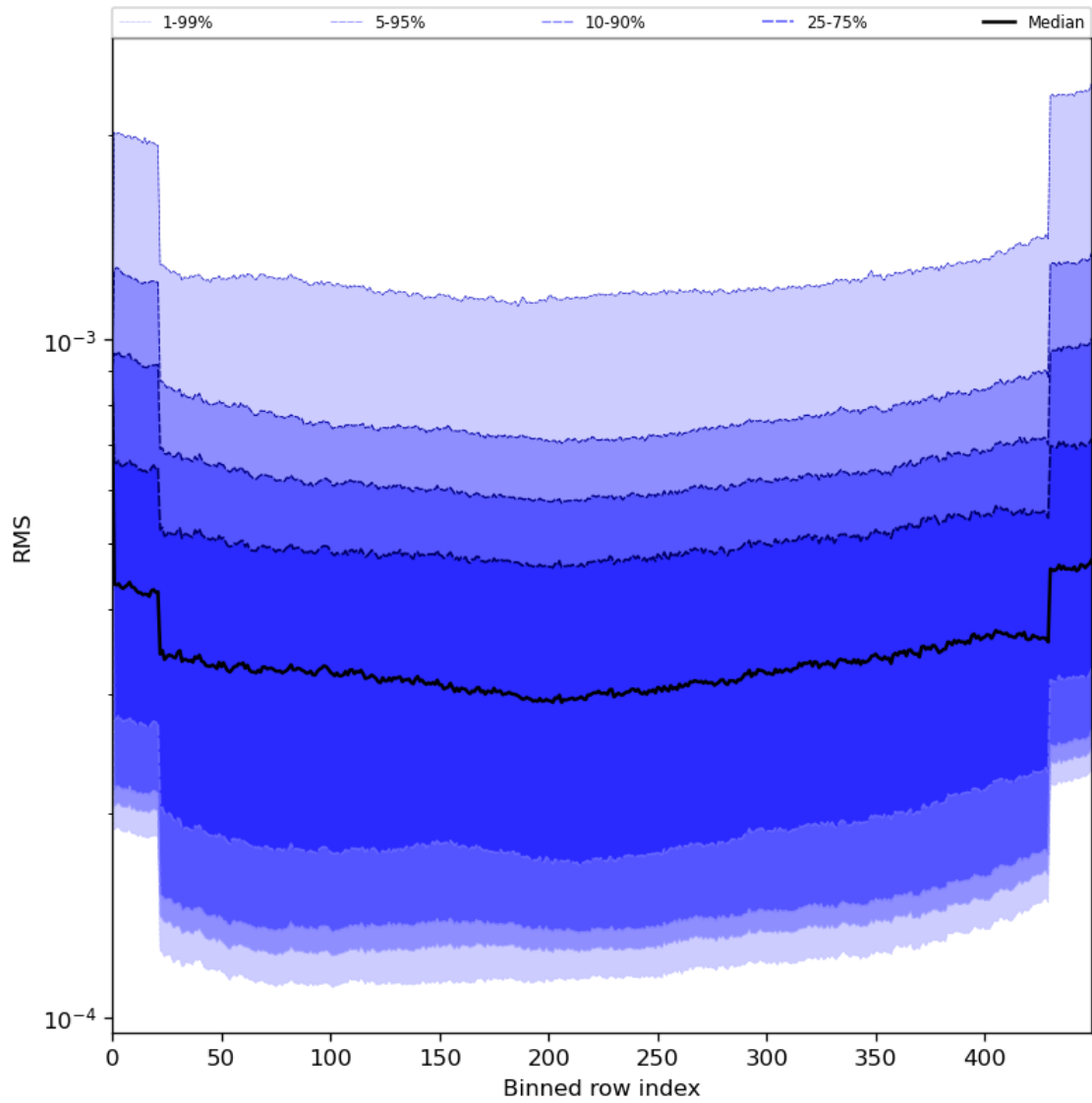
Figure 60: Along track statistics of “RMS” for 2024-05-28 to 2024-05-30
