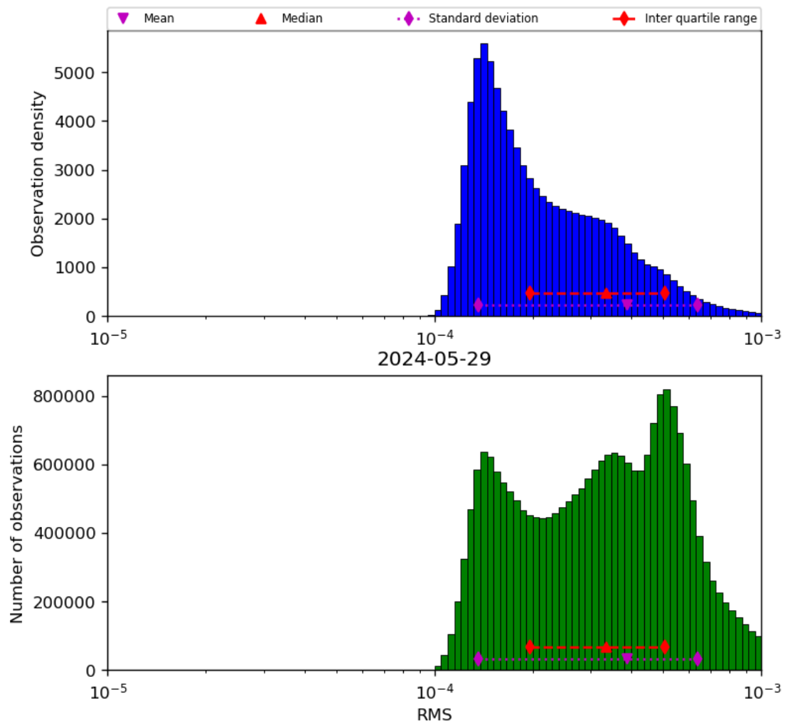
Figure 43: Histogram of “RMS” for 2024-05-28 to 2024-05-30
