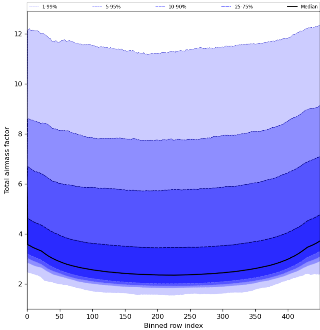
Figure 49: Along track statistics of “Total airmass factor” for 2024-05-28 to 2024-05-30
