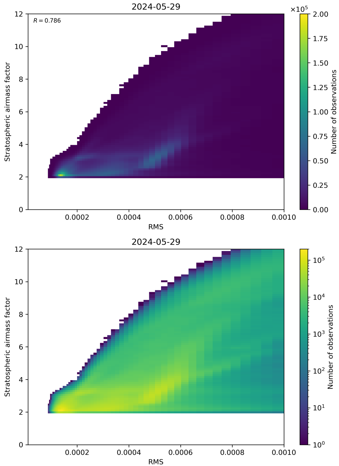
Figure 144: Scatter density plot of “RMS” against “Stratospheric airmass factor” for 2024-05-28 to 2024-05-30.
