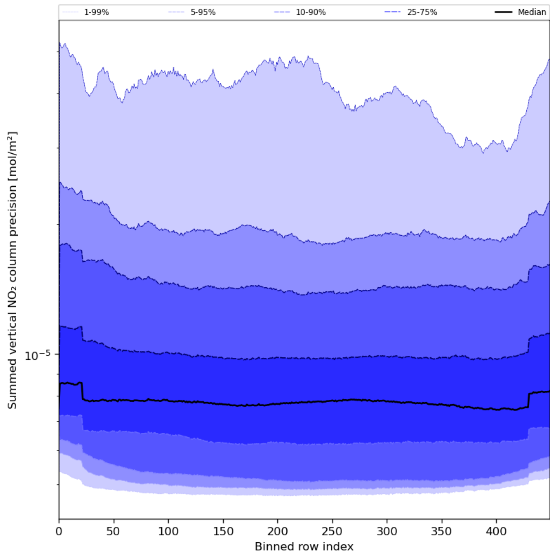
Figure 58: Along track statistics of “Summed vertical NO 2 column precision” for 2024-05-28 to 2024-05-30
