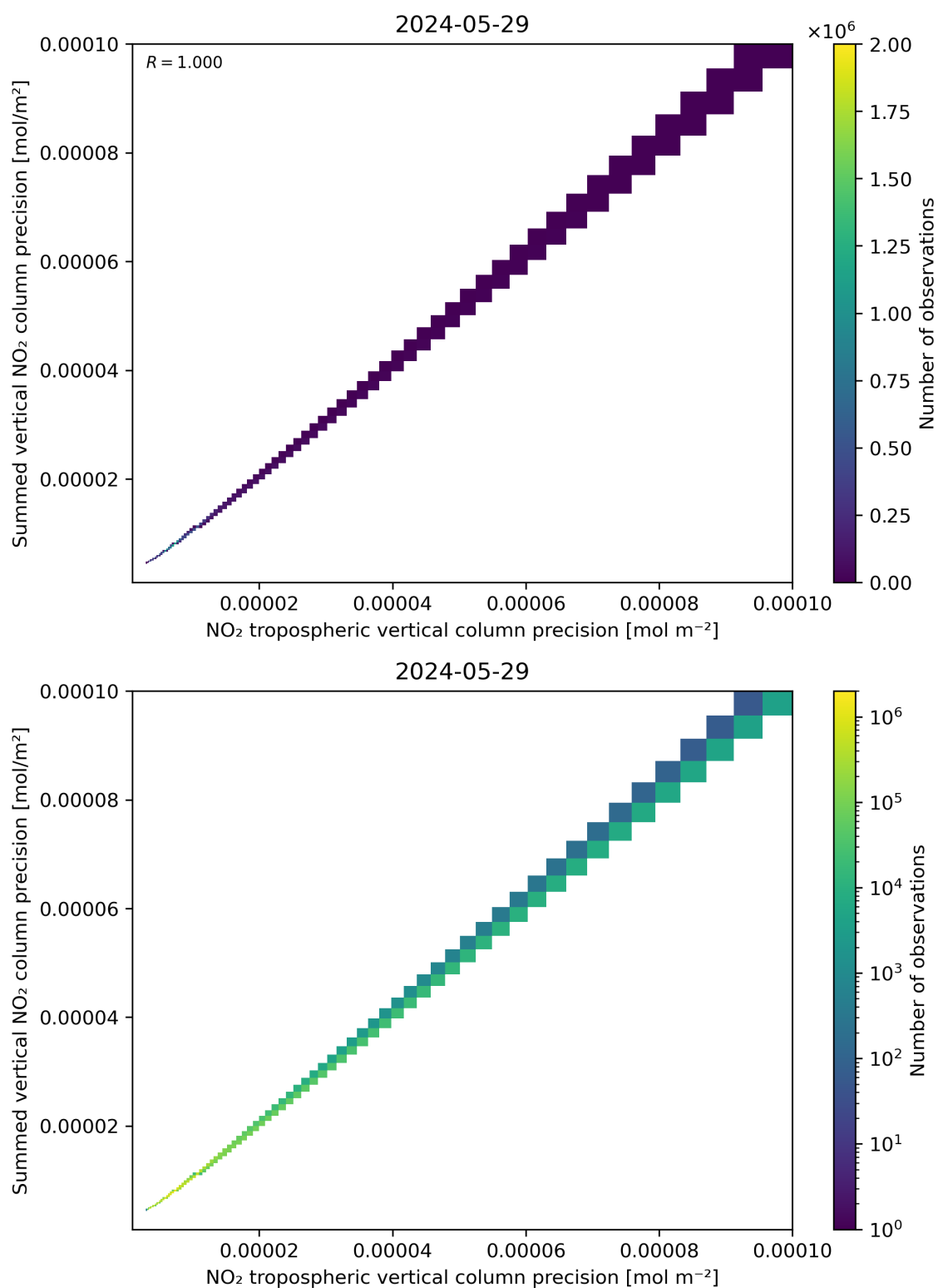
Figure 137: Scatter density plot of “NO 2 tropospheric vertical column precision” against “Summed vertical NO 2 column precision” for 2024-05-28 to 2024-05-30.
