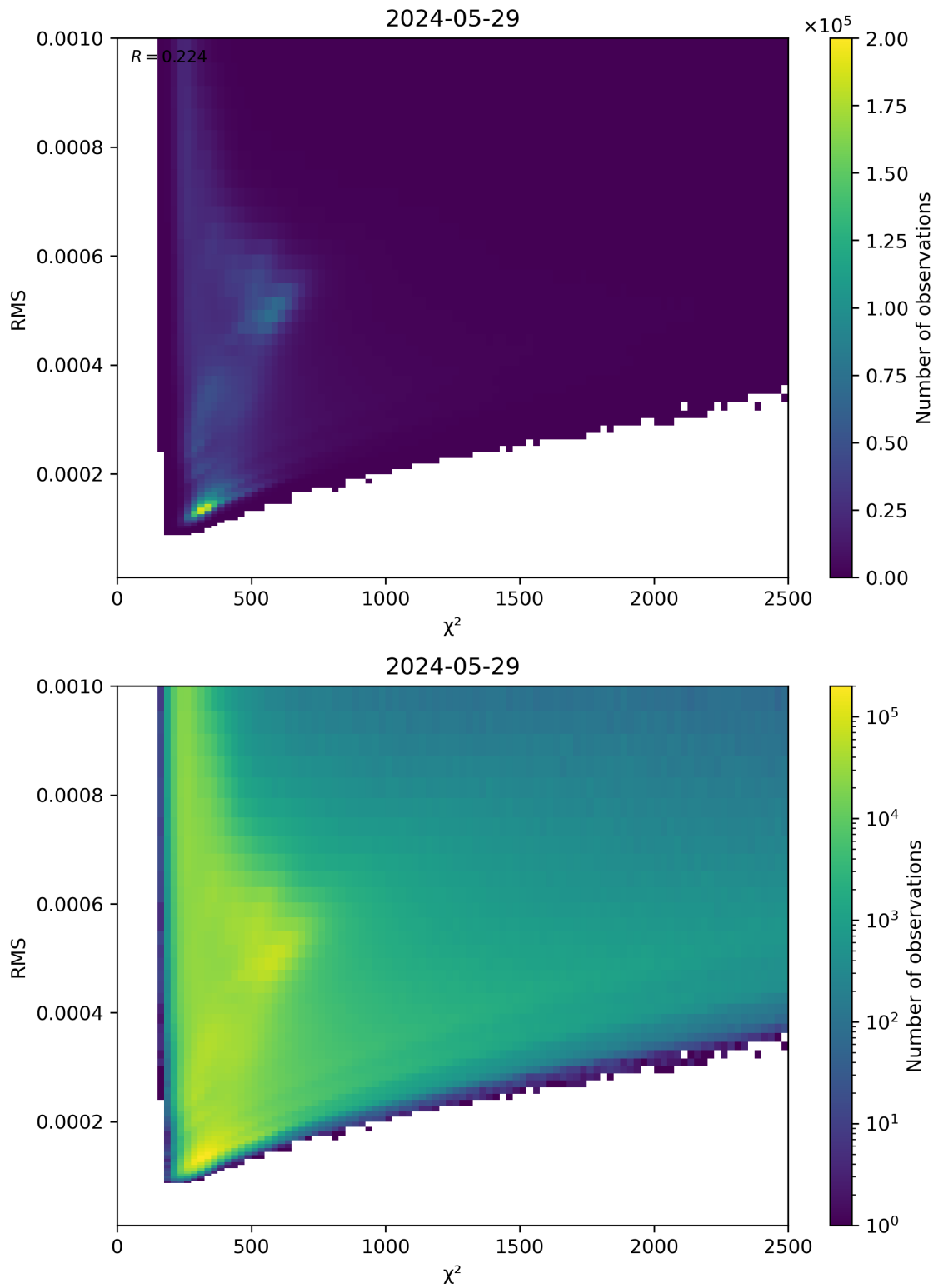
Figure 82: Scatter density plot of “ \chi^2 ” against “RMS” for 2024-05-28 to 2024-05-30.
