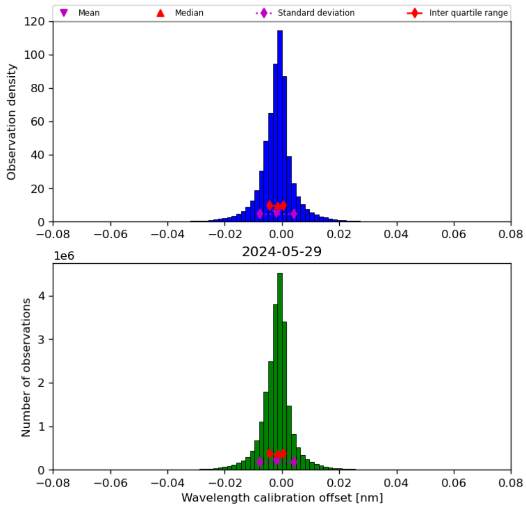
Figure 35: Histogram of “Wavelength calibration offset” for 2024-05-28 to 2024-05-30
