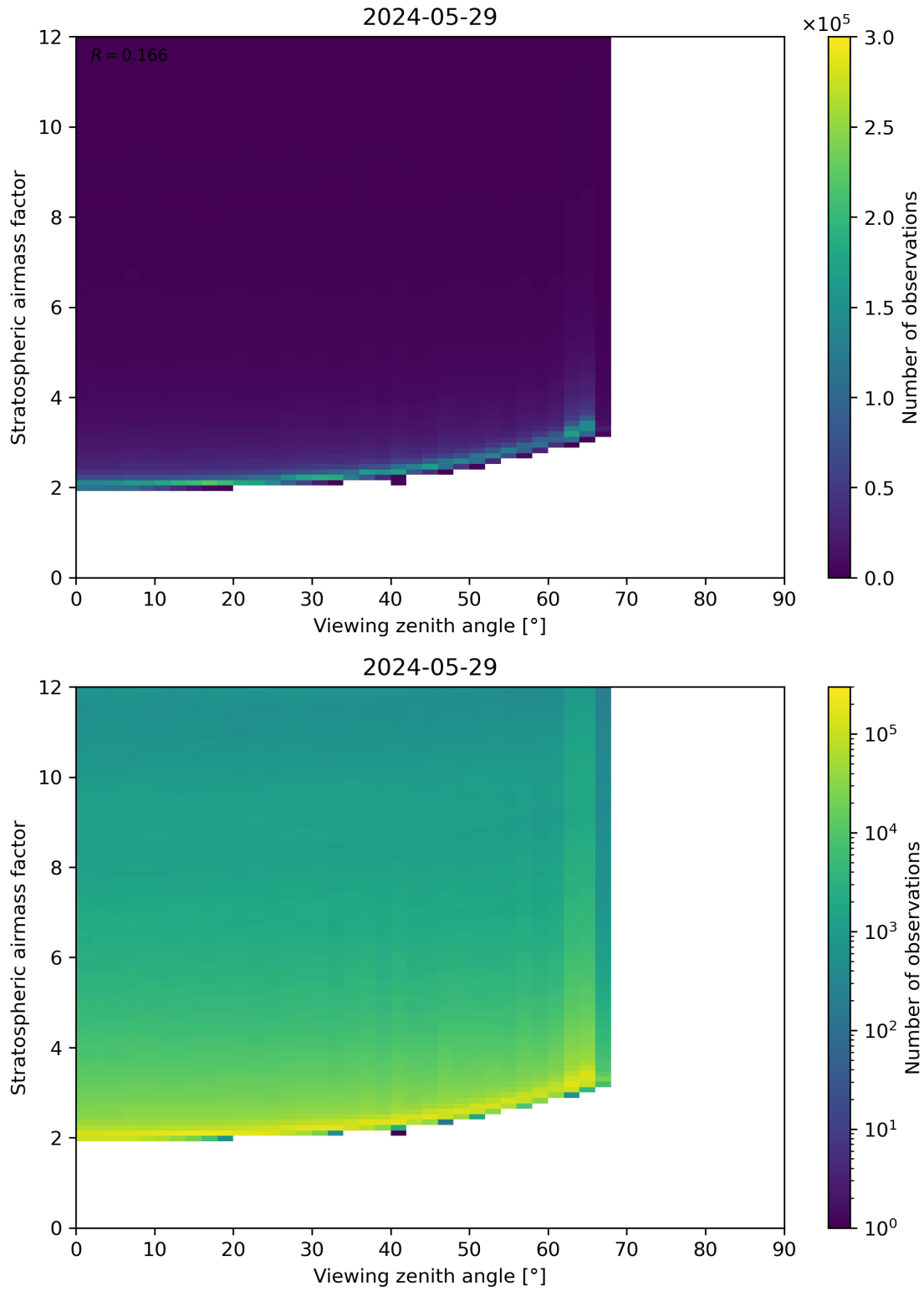
Figure 159: Scatter density plot of “Viewing zenith angle” against “Stratospheric airmass factor” for 2024-05-28 to 2024-05-30.
