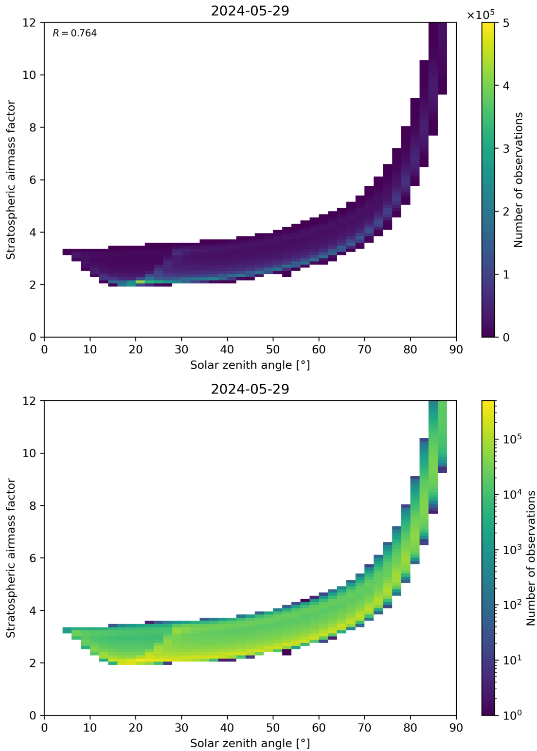
Figure 145: Scatter density plot of “Solar zenith angle” against “Stratospheric airmass factor” for 2024-05-28 to 2024-05-30.
