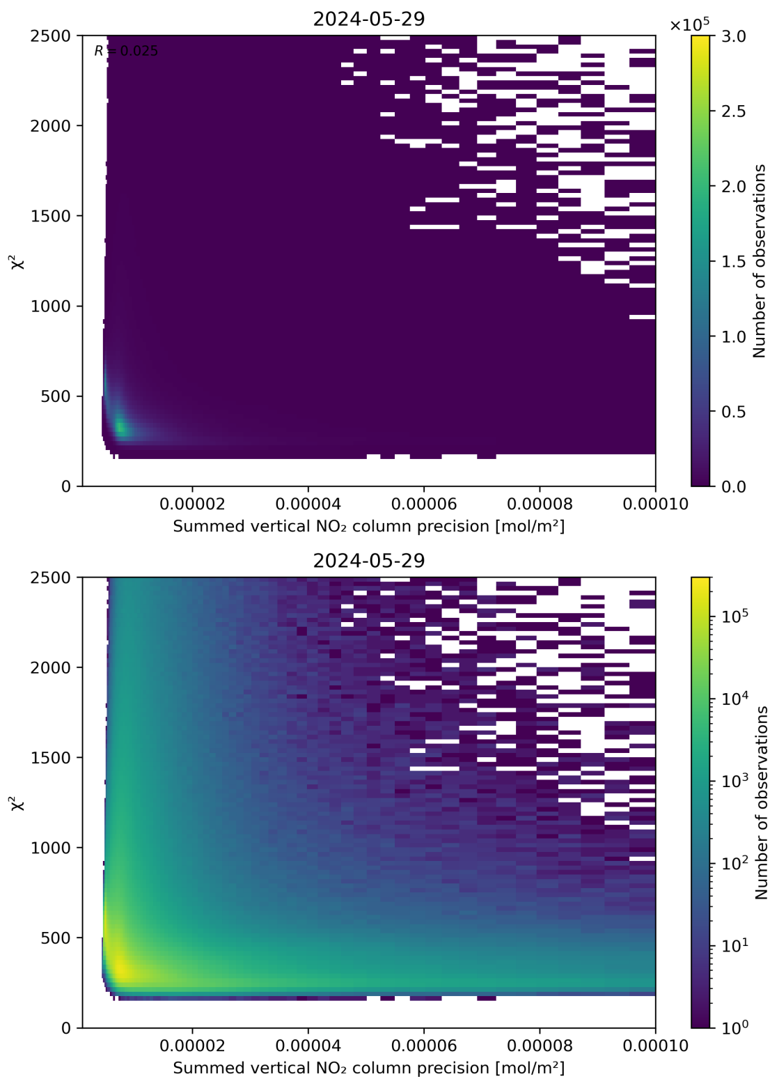
Figure 107: Scatter density plot of “Summed vertical NO 2 column precision” against “ \chi^2 ” for 2024-05-28 to 2024-05-30.
