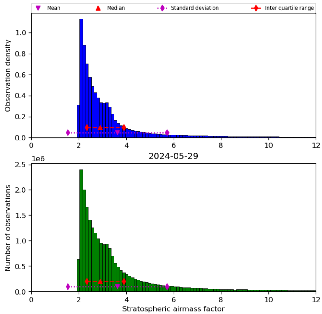
Figure 44: Histogram of “Stratospheric airmass factor” for 2024-05-28 to 2024-05-30
