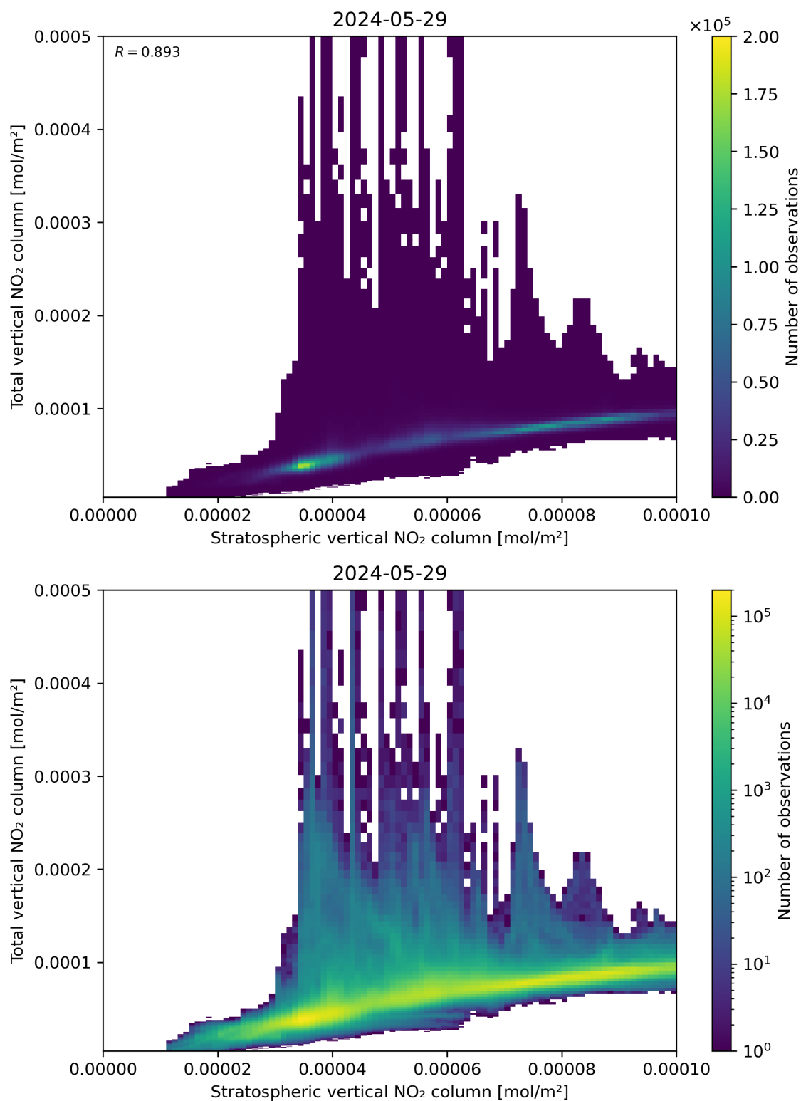
Figure 100: Scatter density plot of “Stratospheric vertical NO 2 column” against “Total vertical NO 2 column” for 2024-05-28 to 2024-05-30.
