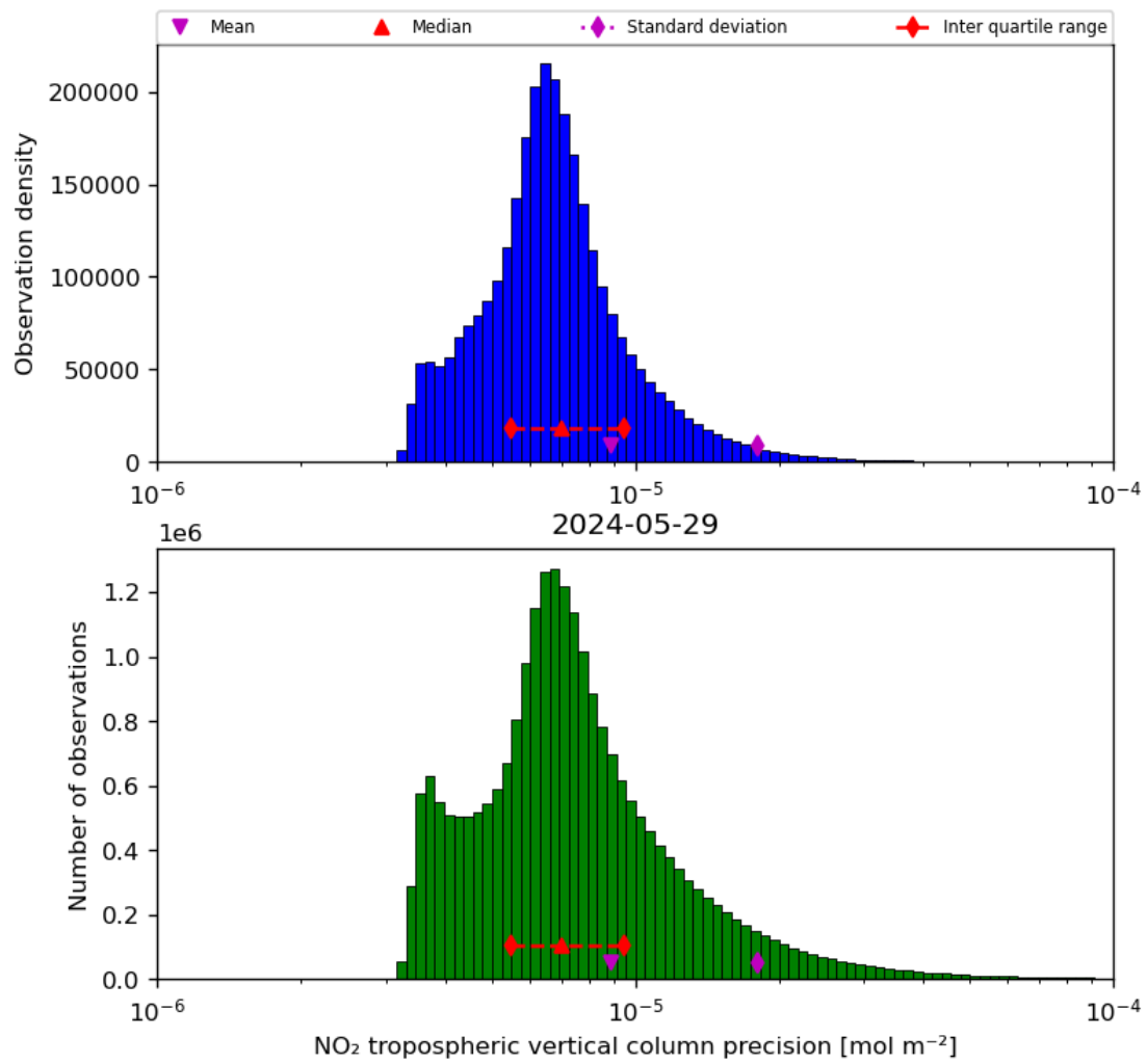
Figure 30: Histogram of “NO 2 tropospheric vertical column precision” for 2024-05-28 to 2024-05-30
