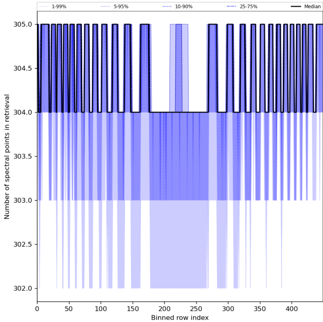
Figure 50: Along track statistics of “Number of spectral points in retrieval” for 2024-05-28 to 2024-05-30
