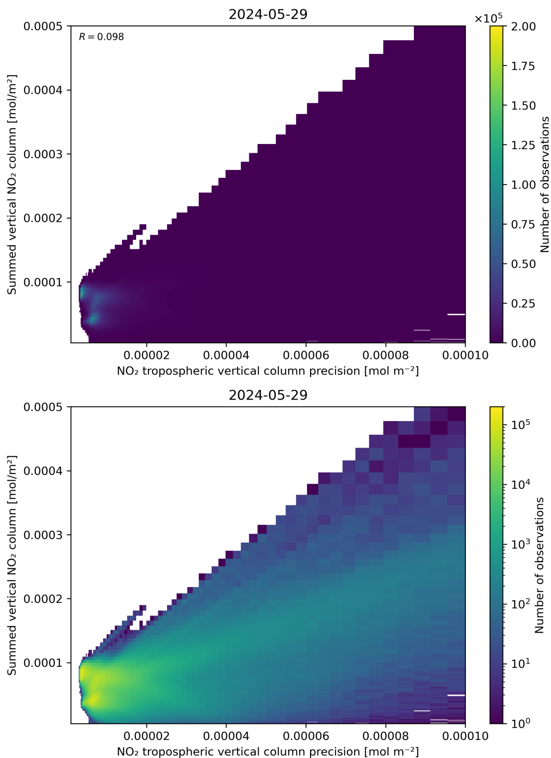
Figure 136: Scatter density plot of “NO 2 tropospheric vertical column precision” against “Summed vertical NO 2 column” for 2024-05-28 to 2024-05-30.
