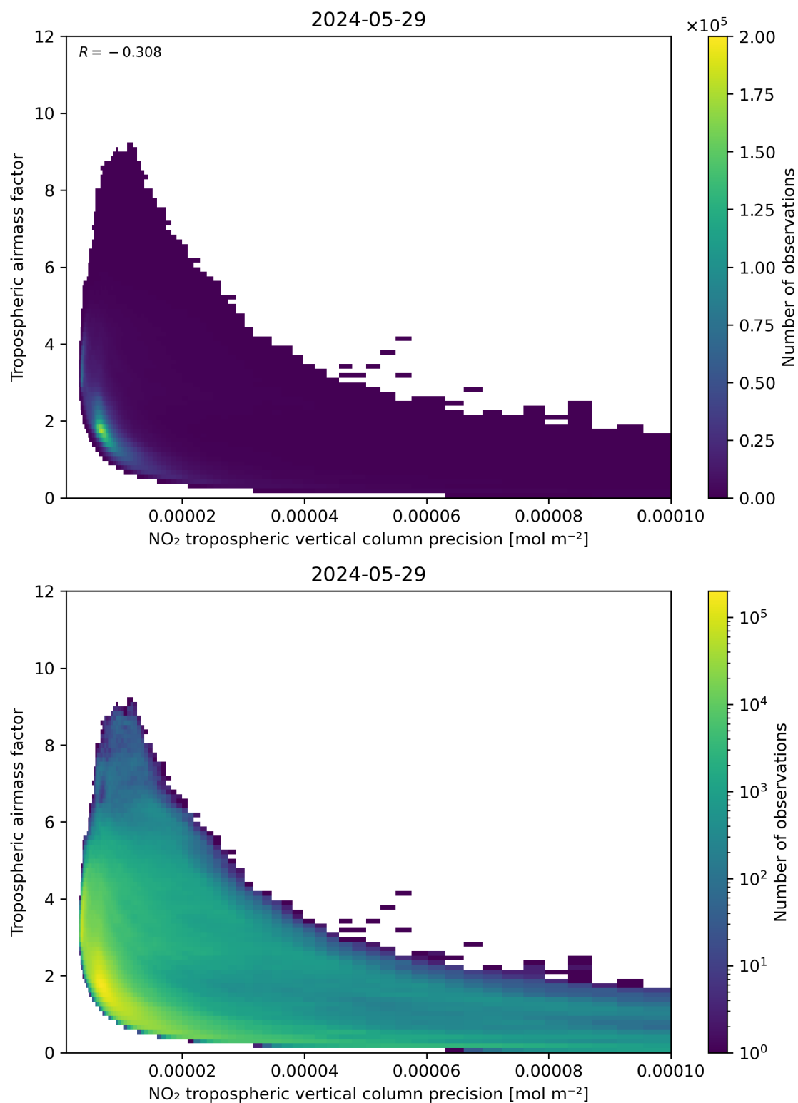
Figure 133: Scatter density plot of “NO 2 tropospheric vertical column precision” against “Tropospheric airmass factor” for 2024-05-28 to 2024-05-30.
