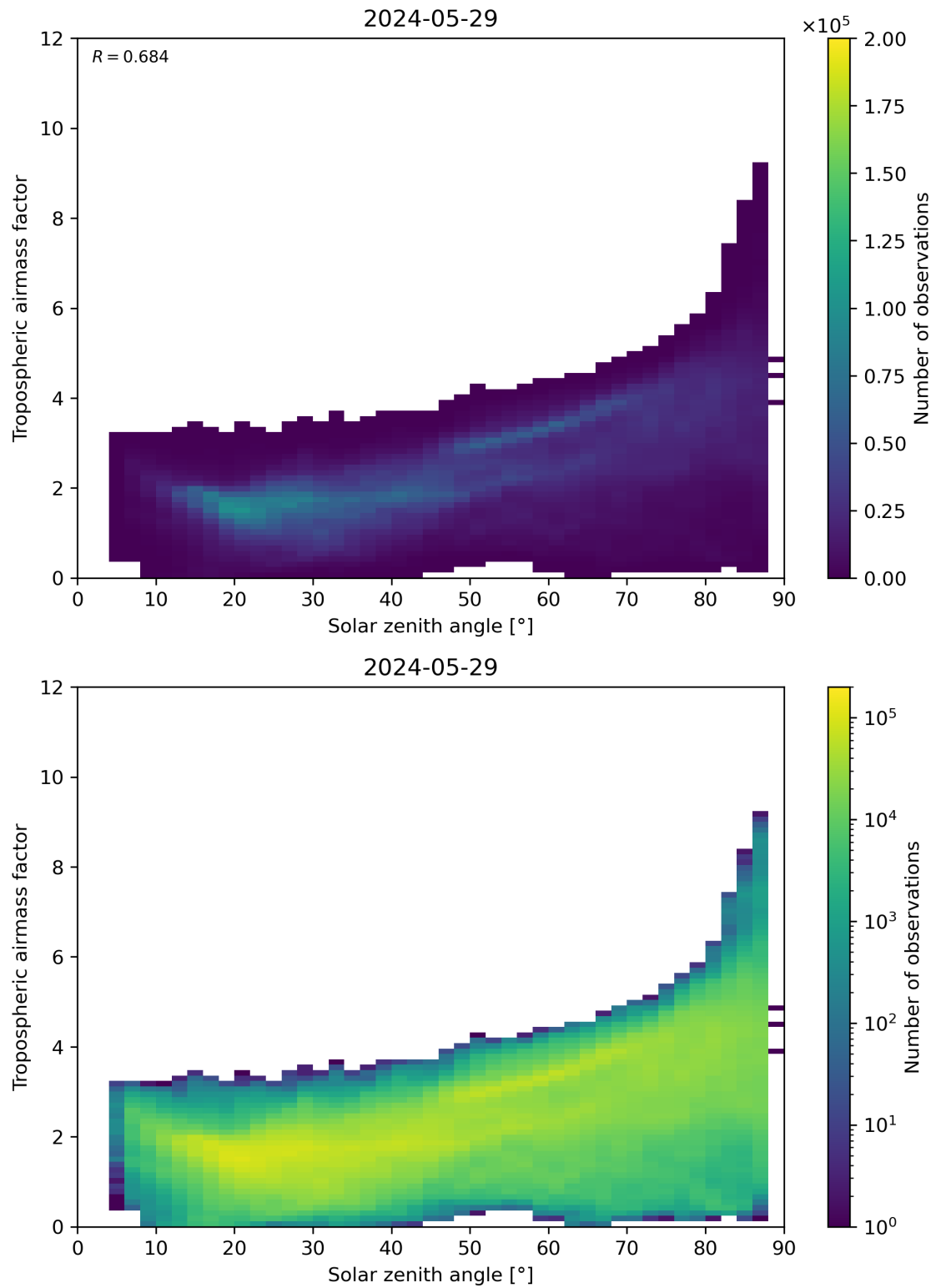
Figure 147: Scatter density plot of “Solar zenith angle” against “Tropospheric airmass factor” for 2024-05-28 to 2024-05-30.
