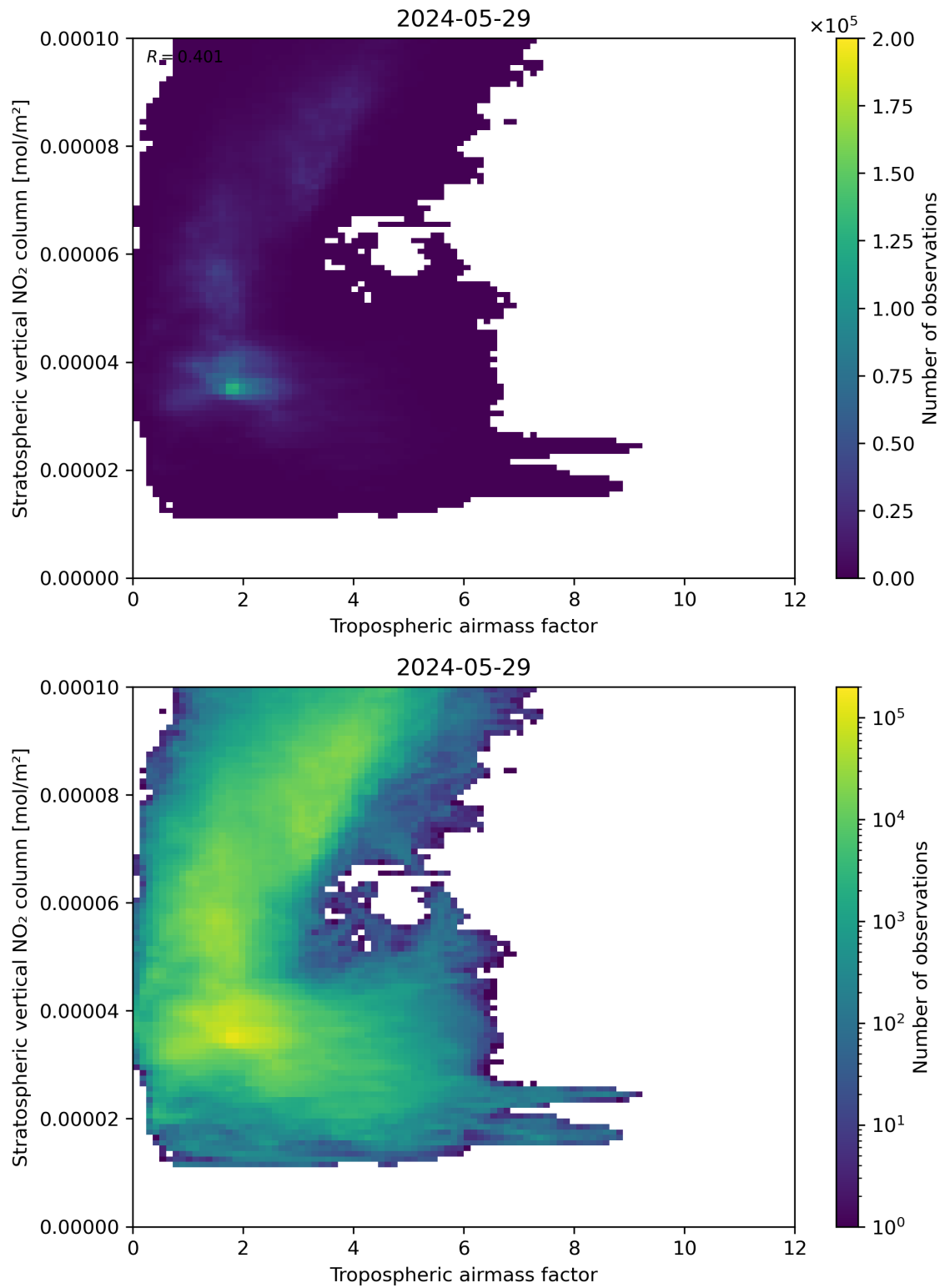
Figure 74: Scatter density plot of “Tropospheric air mass factor” against “Stratospheric vertical NO 2 column” for 2024-05-28 to 2024-05-30.
