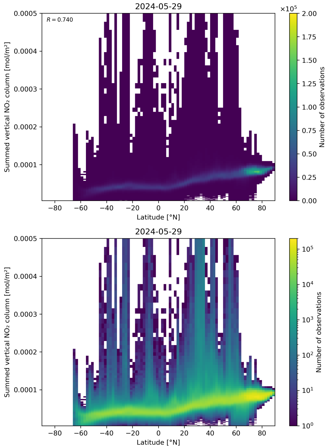
Figure 88: Scatter density plot of “Latitude” against “Summed vertical NO 2 column” for 2024-05-28 to 2024-05-30.
