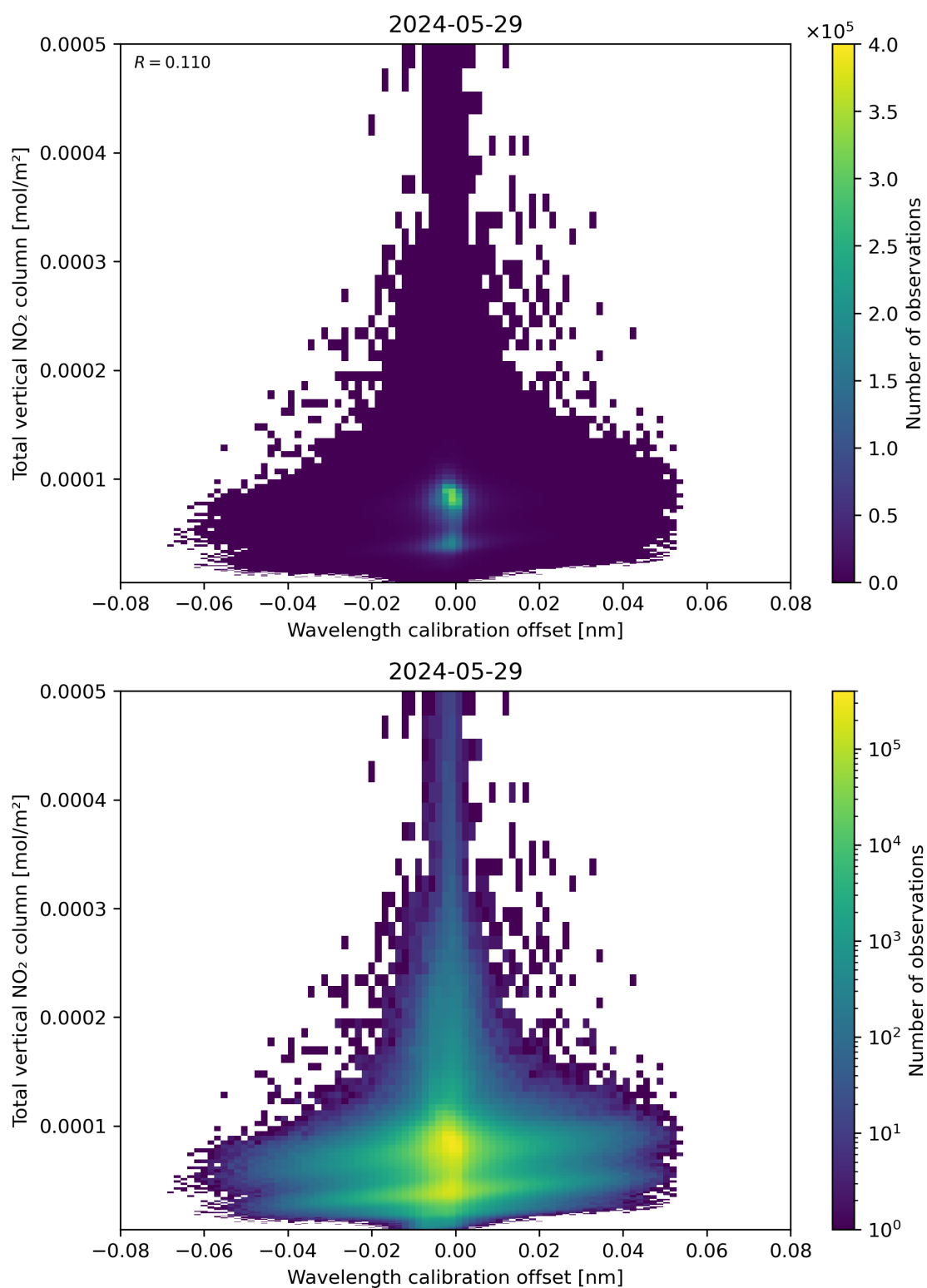
Figure 179: Scatter density plot of “Wavelength calibration offset” against “Total vertical NO 2 column” for 2024-05-28 to 2024-05-30.
