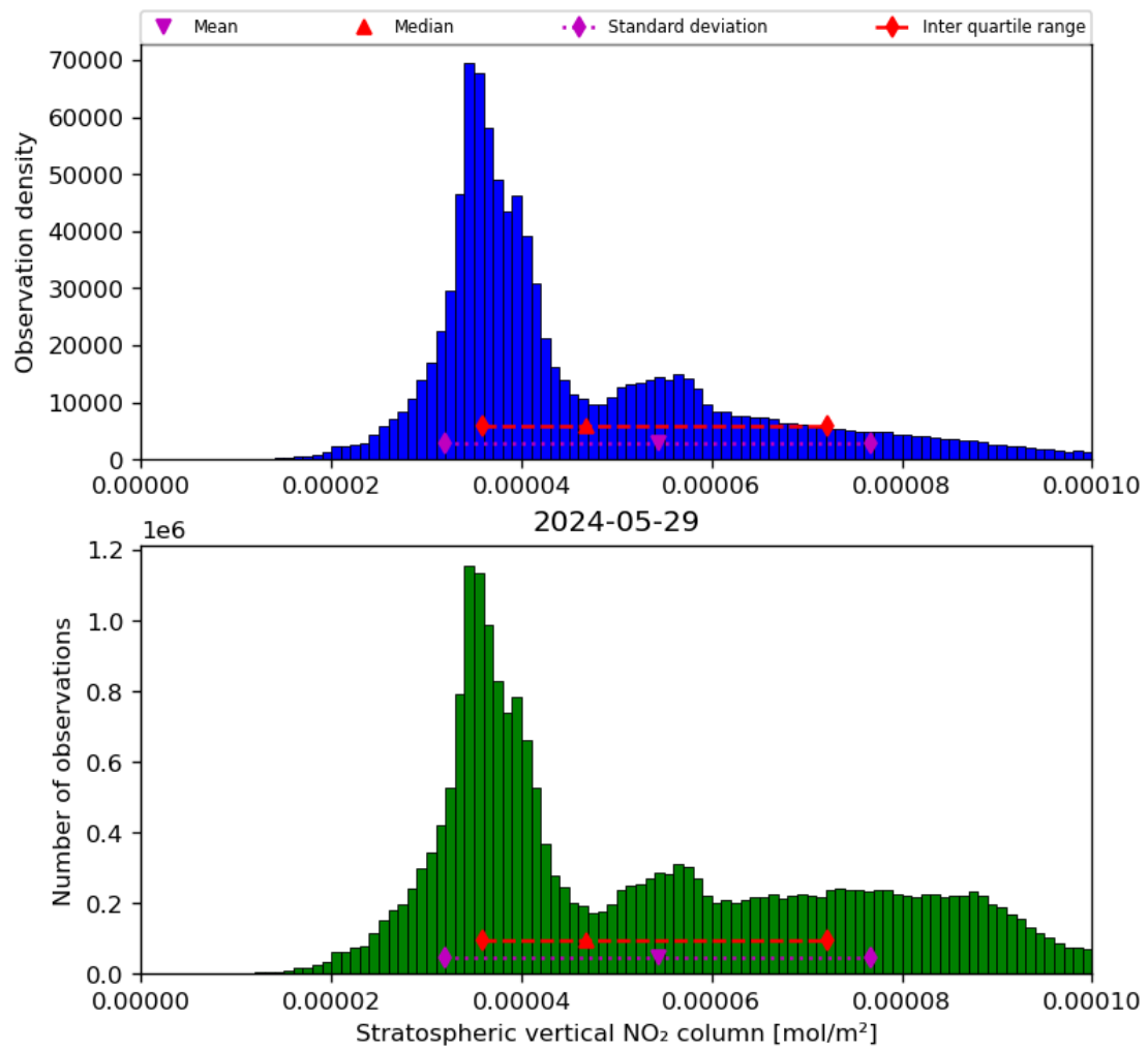
Figure 36: Histogram of “Stratospheric vertical NO 2 column” for 2024-05-28 to 2024-05-30
