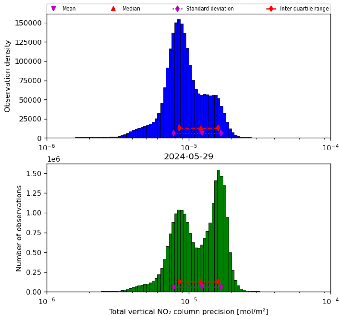
Figure 39: Histogram of “Total vertical NO 2 column precision” for 2024-05-28 to 2024-05-30
