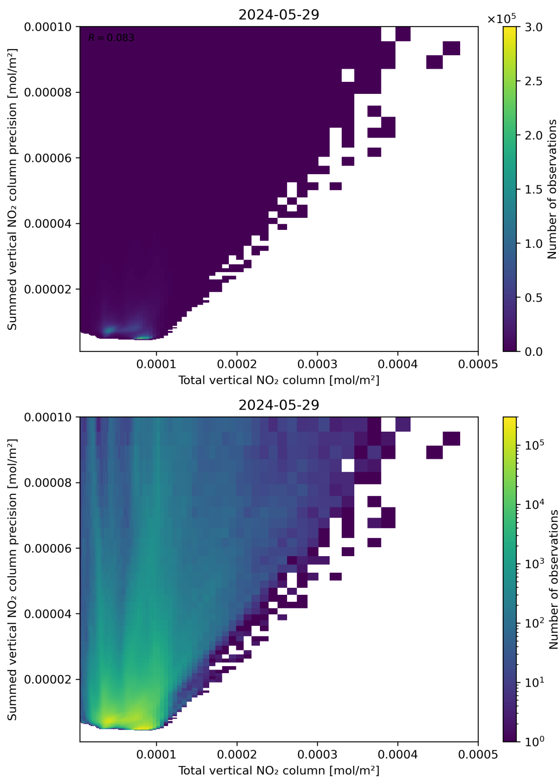
Figure 113: Scatter density plot of “Total vertical NO 2 column” against “Summed vertical NO 2 column precision” for 2024-05-28 to 2024-05-30.
