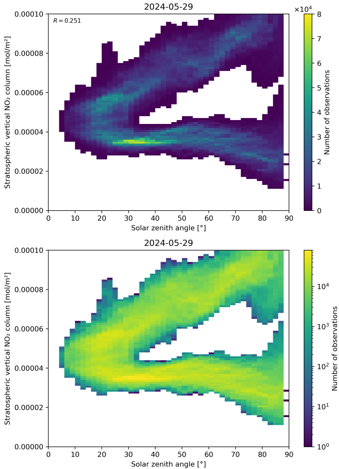
Figure 150: Scatter density plot of “Solar zenith angle” against “Stratospheric vertical NO 2 column” for 2024-05-28 to 2024-05-30.
