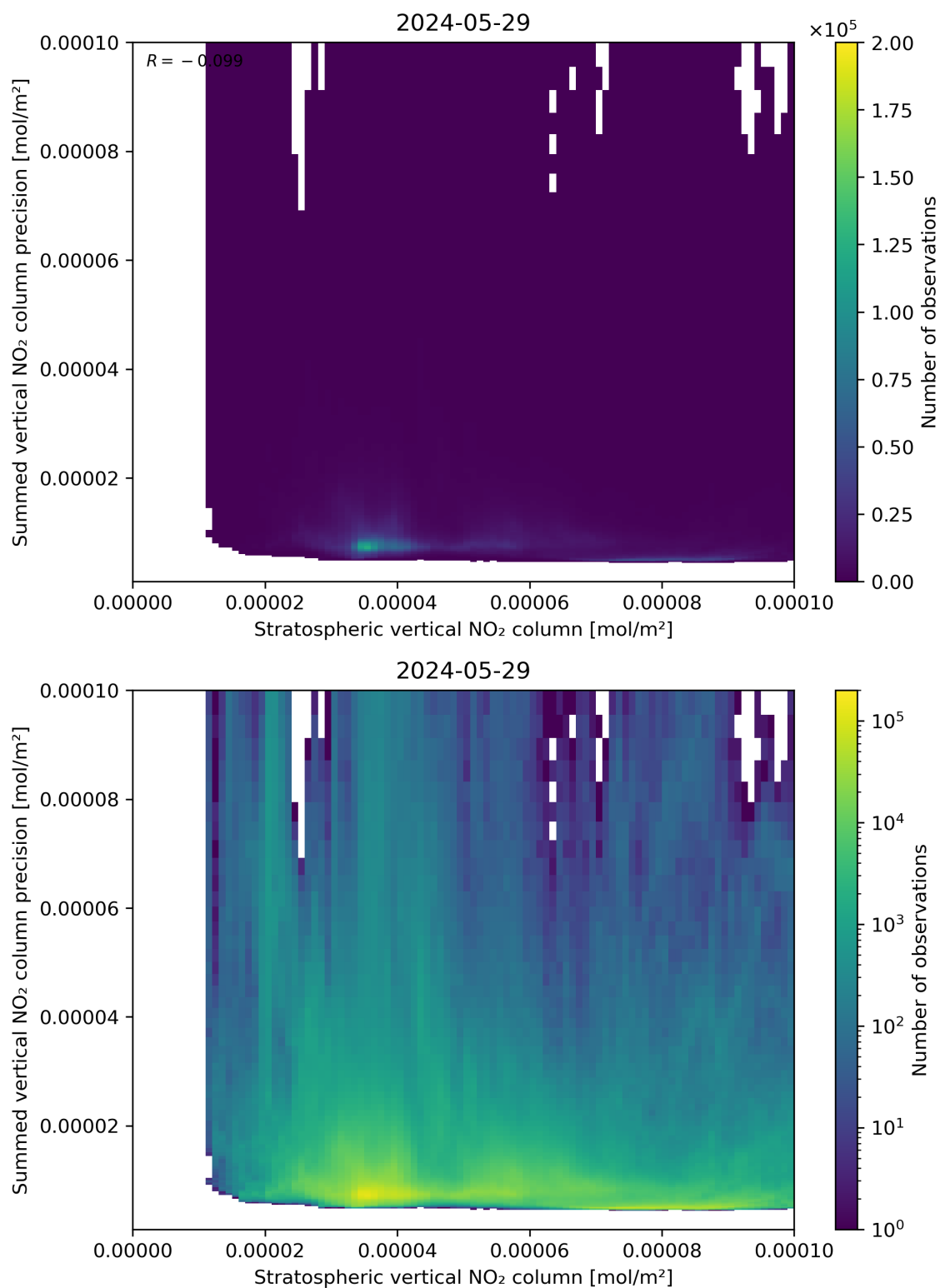
Figure 99: Scatter density plot of “Stratospheric vertical NO 2 column” against “Summed vertical NO 2 column precision” for 2024-05-28 to 2024-05-30.
