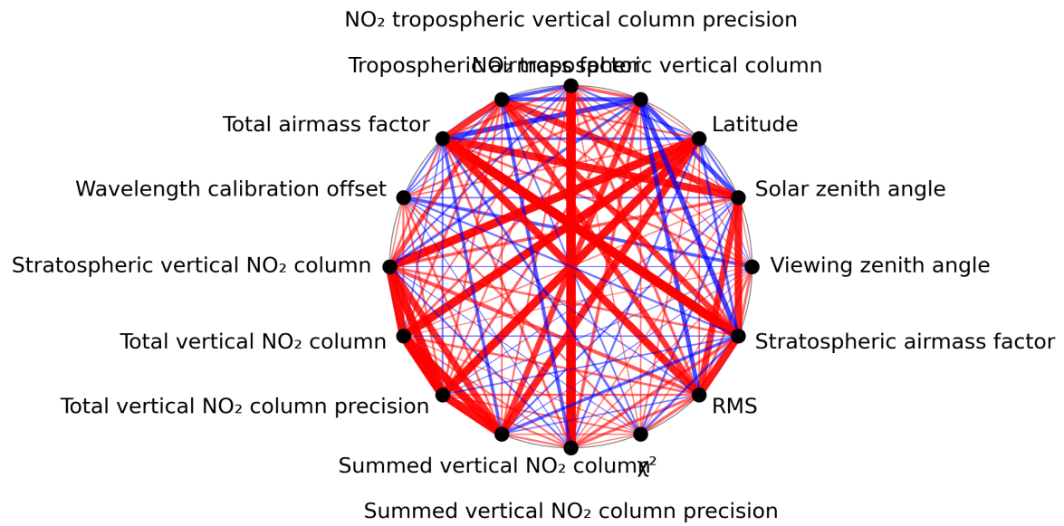
Figure 1: Map of correlation graph for 2024-05-28 to 2024-05-30.
