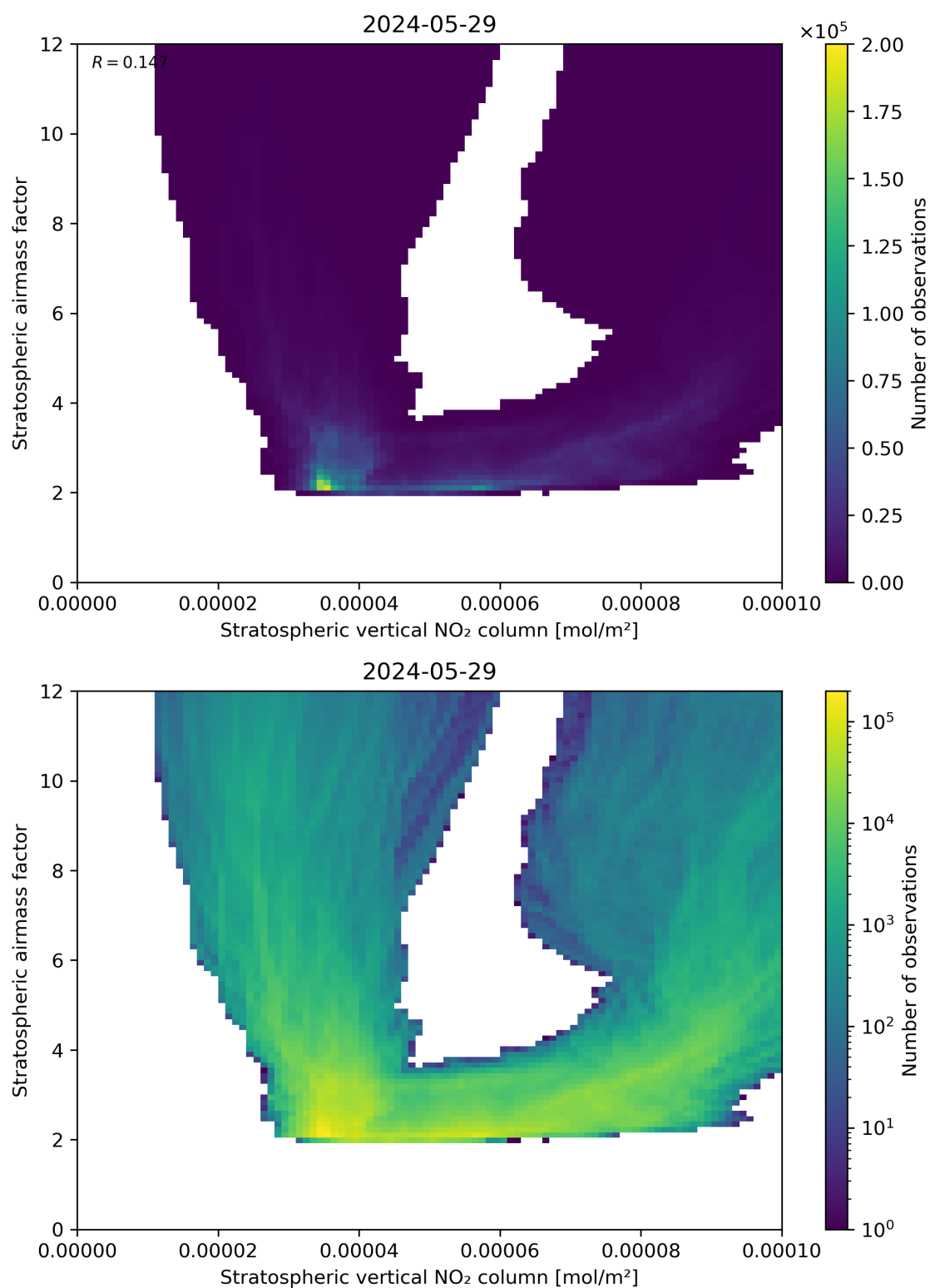
Figure 96: Scatter density plot of “Stratospheric vertical NO 2 column” against “Stratospheric airmass factor” for 2024-05-28 to 2024-05-30.
