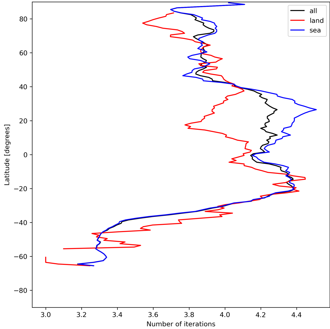
Figure 17: Zonal average of “Number of iterations” for 2024-05-28 to 2024-05-30.
