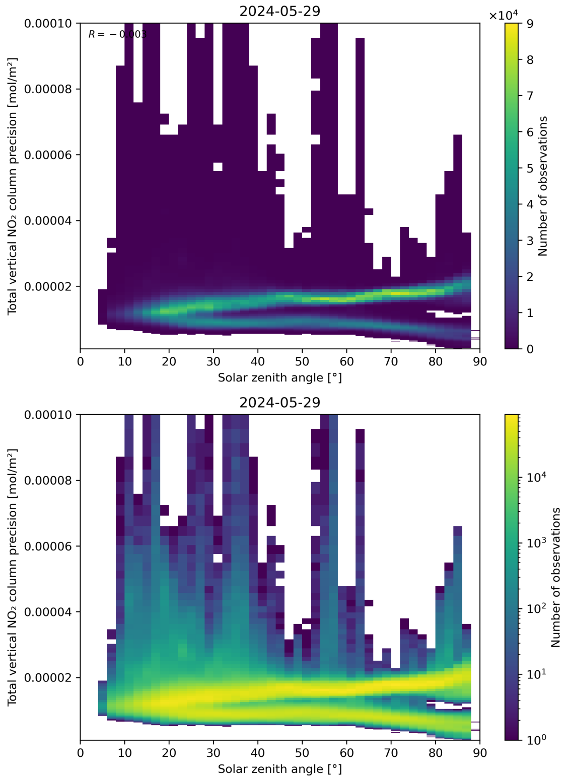
Figure 154: Scatter density plot of “Solar zenith angle” against “Total vertical NO 2 column precision” for 2024-05-28 to 2024-05-30.
