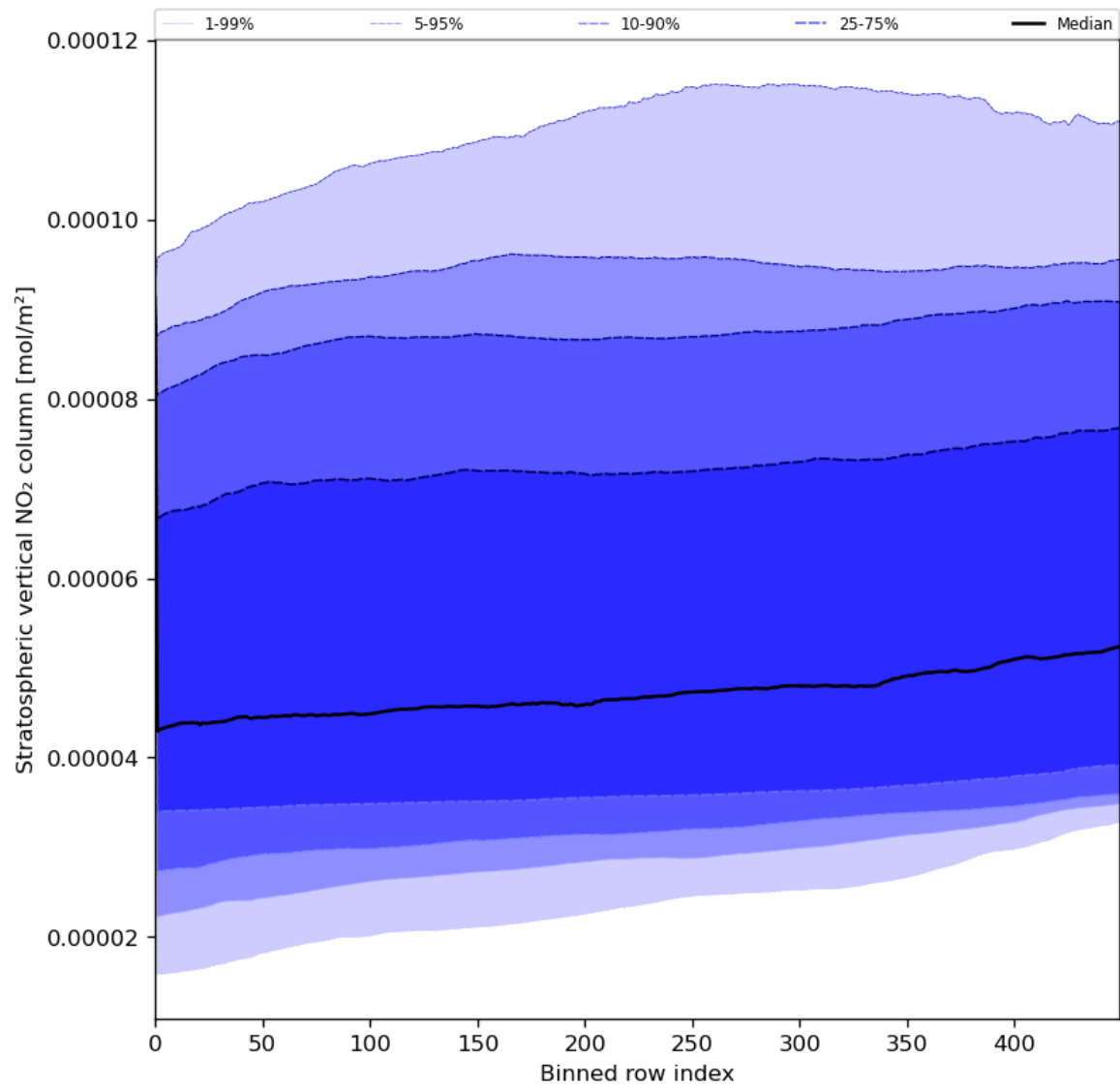
Figure 53: Along track statistics of “Stratospheric vertical NO 2 column” for 2024-05-28 to 2024-05-30
