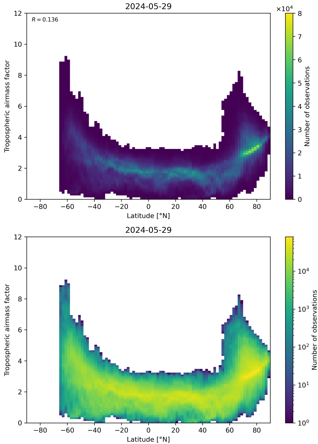
Figure 85: Scatter density plot of “Latitude” against “Tropospheric airmass factor” for 2024-05-28 to 2024-05-30.
