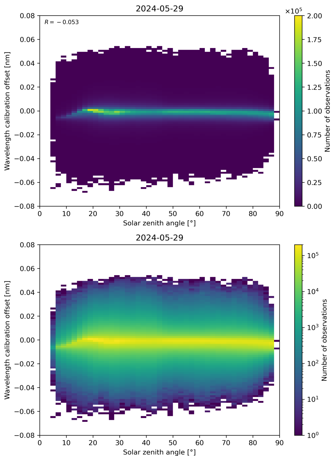
Figure 158: Scatter density plot of “Solar zenith angle” against “Wavelength calibration offset” for 2024-05-28 to 2024-05-30.
