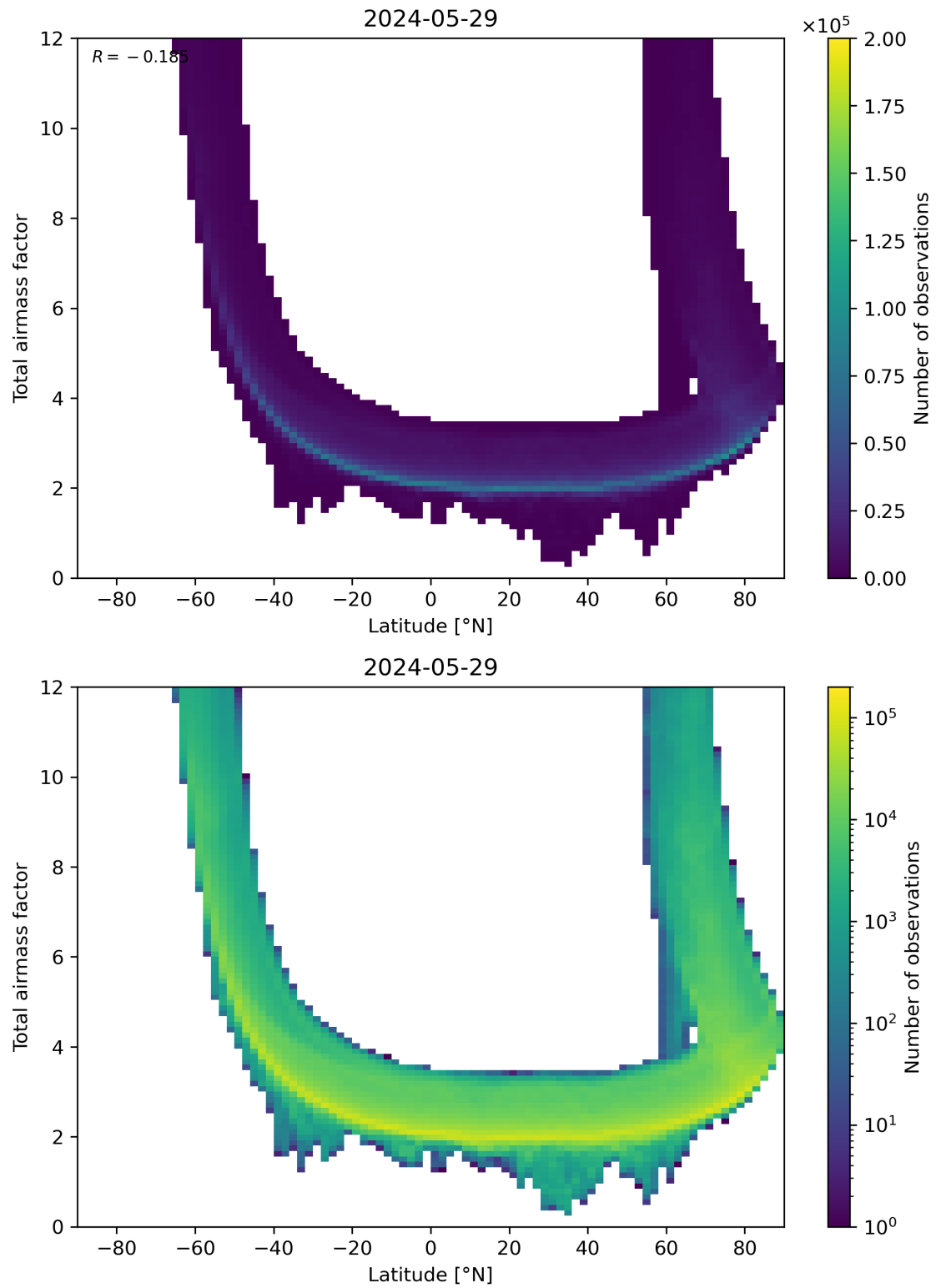
Figure 84: Scatter density plot of “Latitude” against “Total airmass factor” for 2024-05-28 to 2024-05-30.
