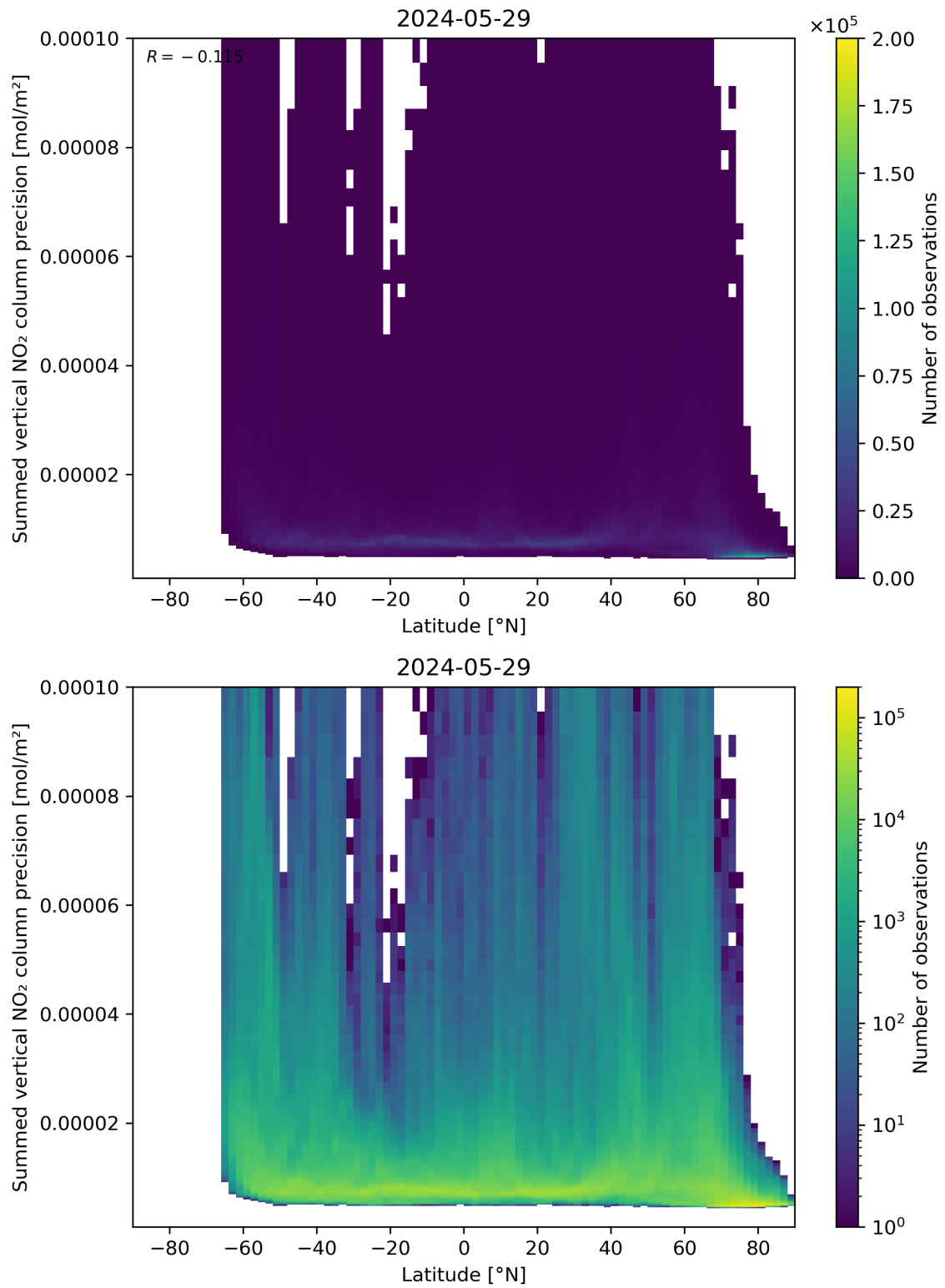
Figure 89: Scatter density plot of “Latitude” against “Summed vertical NO 2 column precision” for 2024-05-28 to 2024-05-30.
