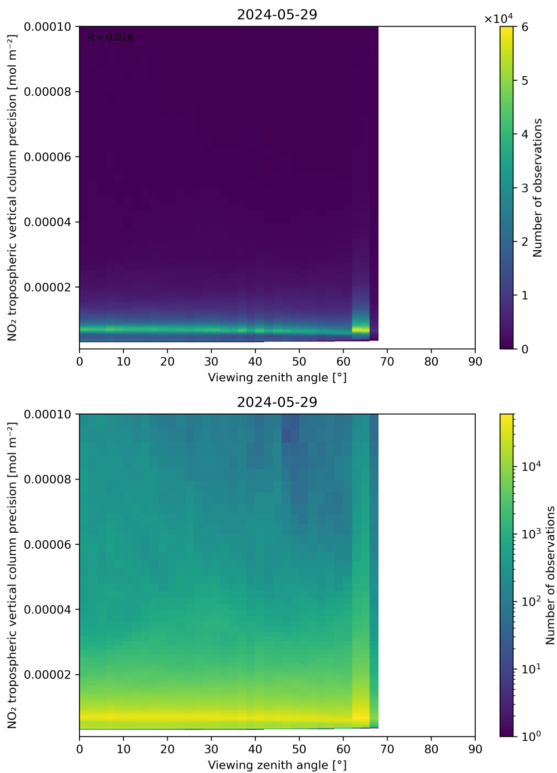
Figure 170: Scatter density plot of “Viewing zenith angle” against “NO 2 tropospheric vertical column precision” for 2024-05-28 to 2024-05-30.
