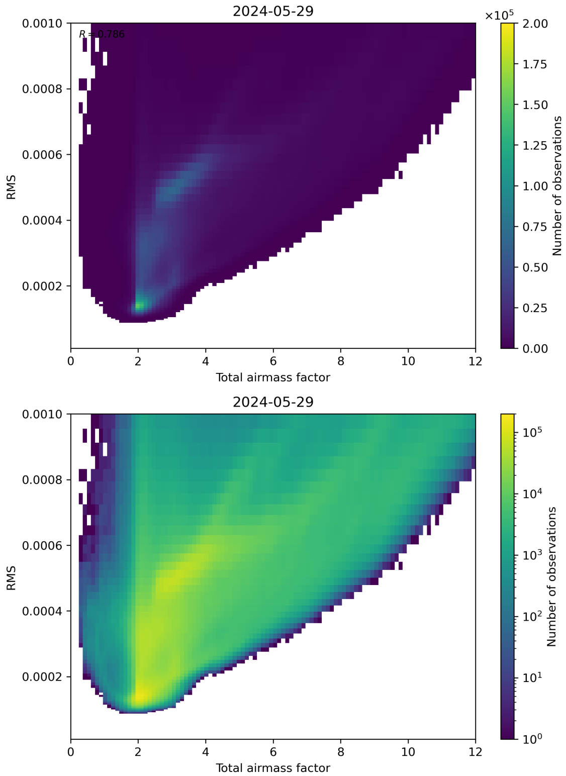
Figure 69: Scatter density plot of “Total airmass factor” against “RMS” for 2024-05-28 to 2024-05-30.
