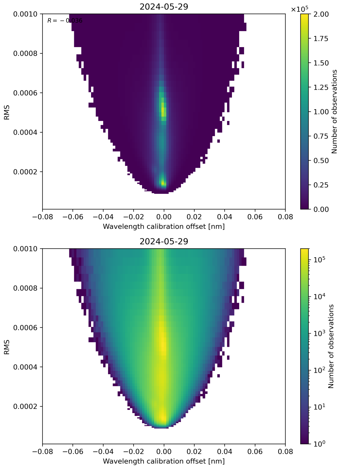
Figure 181: Scatter density plot of “Wavelength calibration offset” against “RMS” for 2024-05-28 to 2024-05-30.
