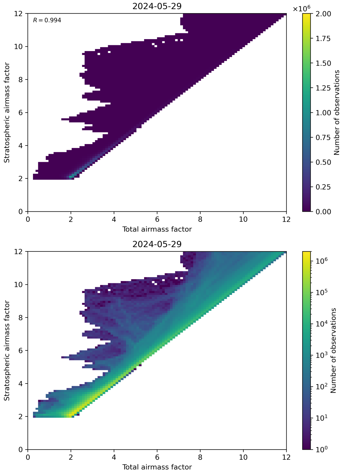
Figure 62: Scatter density plot of “Total airmass factor” against “Stratospheric airmass factor” for 2024-05-28 to 2024-05-30.
