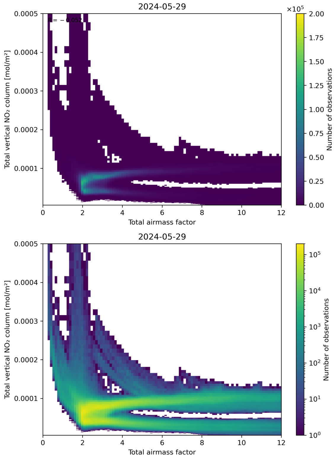
Figure 67: Scatter density plot of “Total airmass factor” against “Total vertical NO 2 column” for 2024-05-28 to 2024-05-30.
