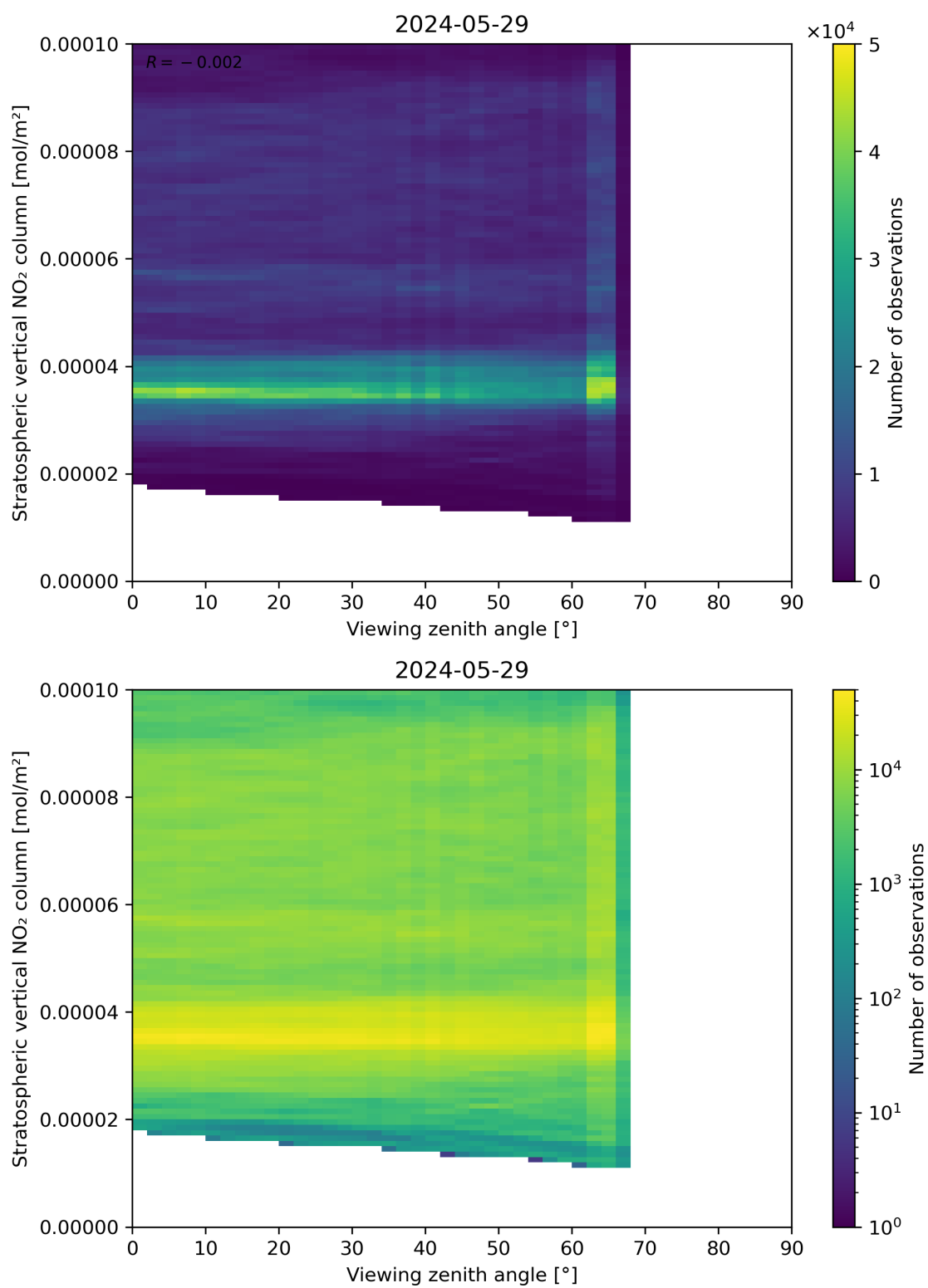
Figure 164: Scatter density plot of “Viewing zenith angle” against “Stratospheric vertical NO 2 column” for 2024-05-28 to 2024-05-30.
