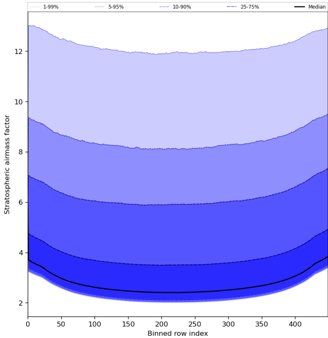
Figure 61: Along track statistics of “Stratospheric airmass factor” for 2024-05-28 to 2024-05-30
