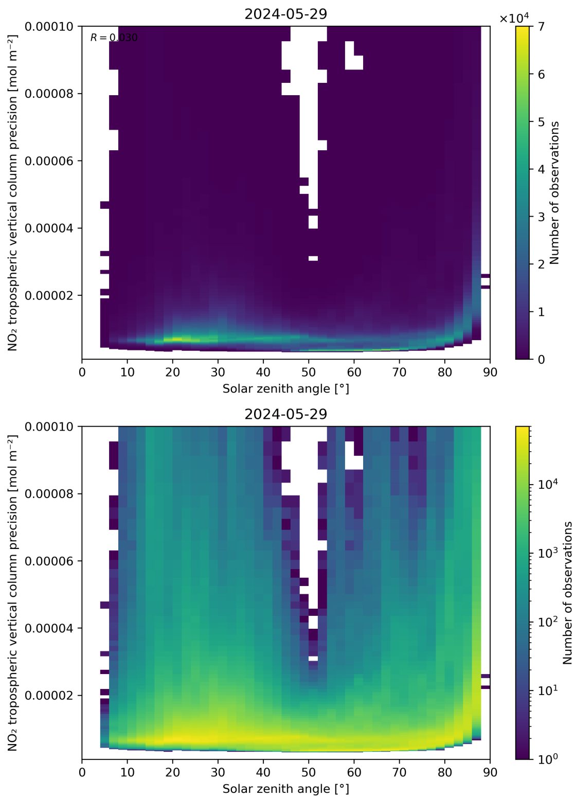
Figure 156: Scatter density plot of “Solar zenith angle” against “NO 2 tropospheric vertical column precision” for 2024-05-28 to 2024-05-30.
