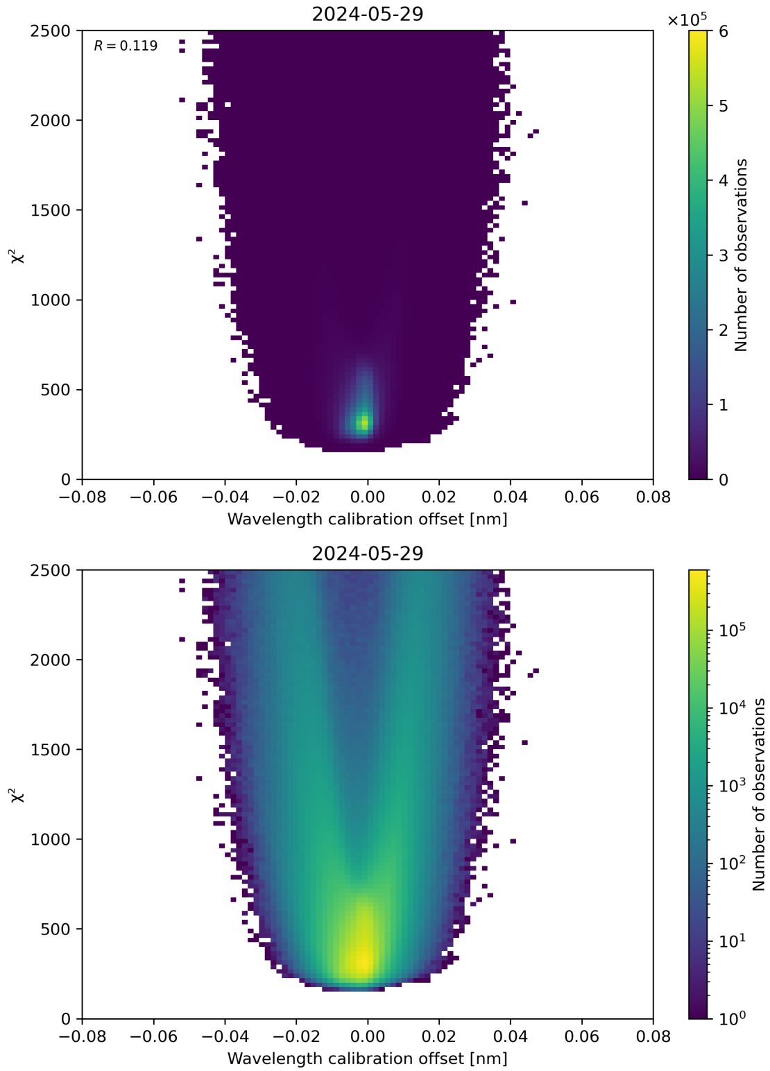
Figure 175: Scatter density plot of “Wavelength calibration offset” against “ \chi^2 ” for 2024-05-28 to 2024-05-30.
