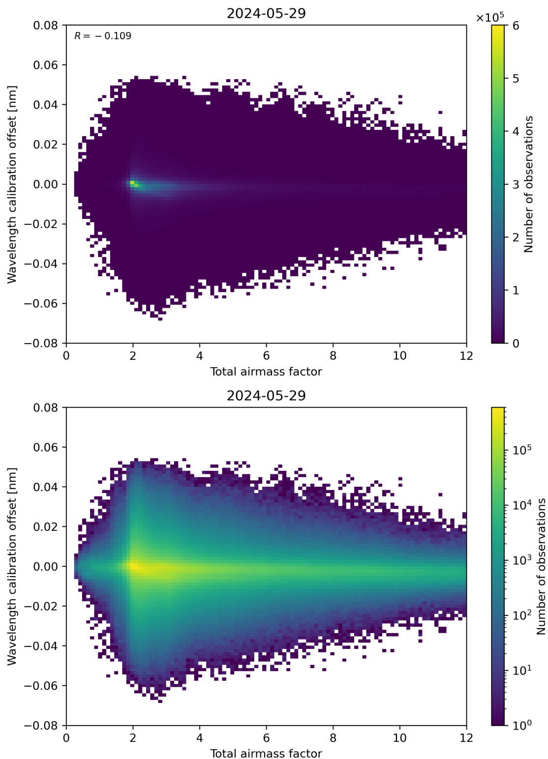
Figure 70: Scatter density plot of “Total airmass factor” against “Wavelength calibration offset” for 2024-05-28 to 2024-05-30.
