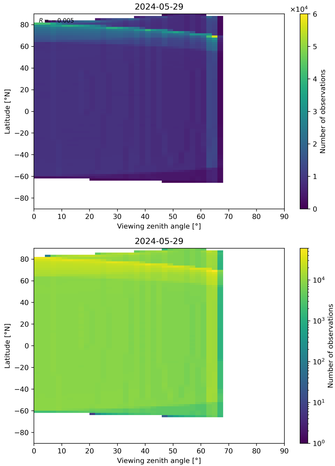
Figure 163: Scatter density plot of “Viewing zenith angle” against “Latitude” for 2024-05-28 to 2024-05-30.
