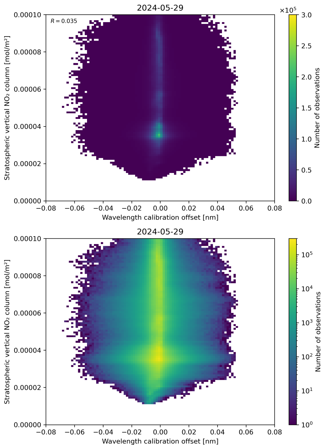
Figure 176: Scatter density plot of “Wavelength calibration offset” against “Stratospheric vertical NO 2 column” for 2024-05-28 to 2024-05-30.
