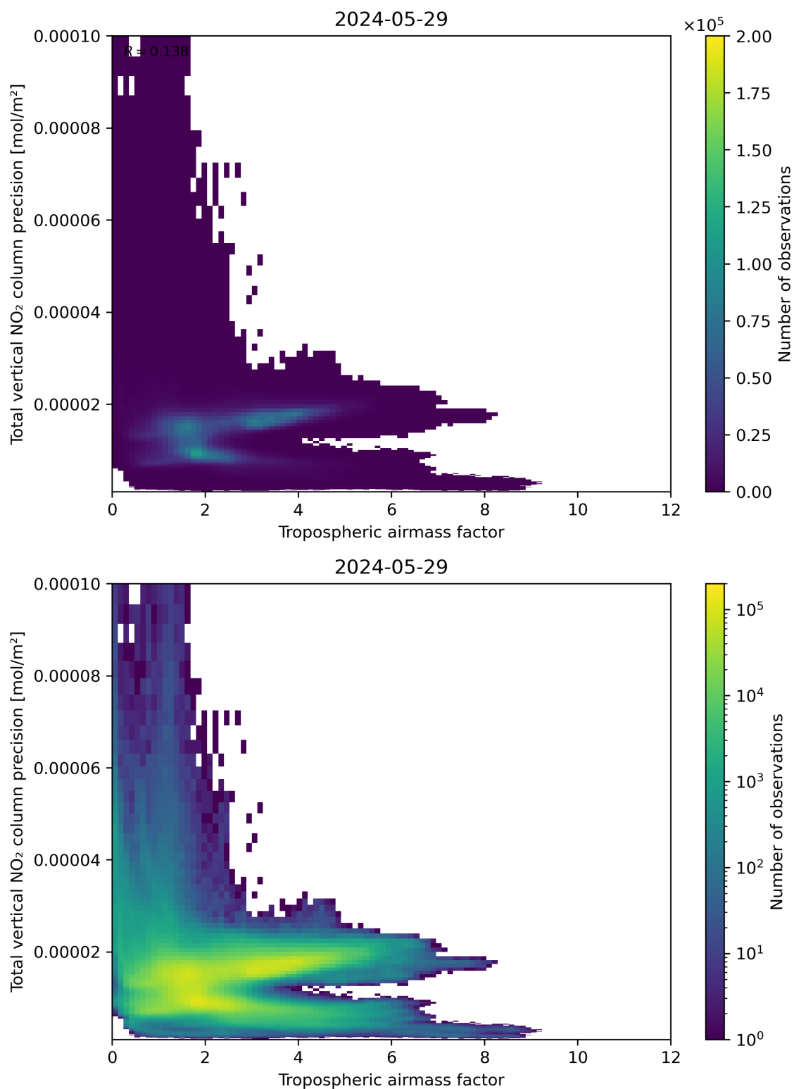
Figure 78: Scatter density plot of “Tropospheric air mass factor” against “Total vertical NO 2 column precision” for 2024-05-28 to 2024-05-30.
