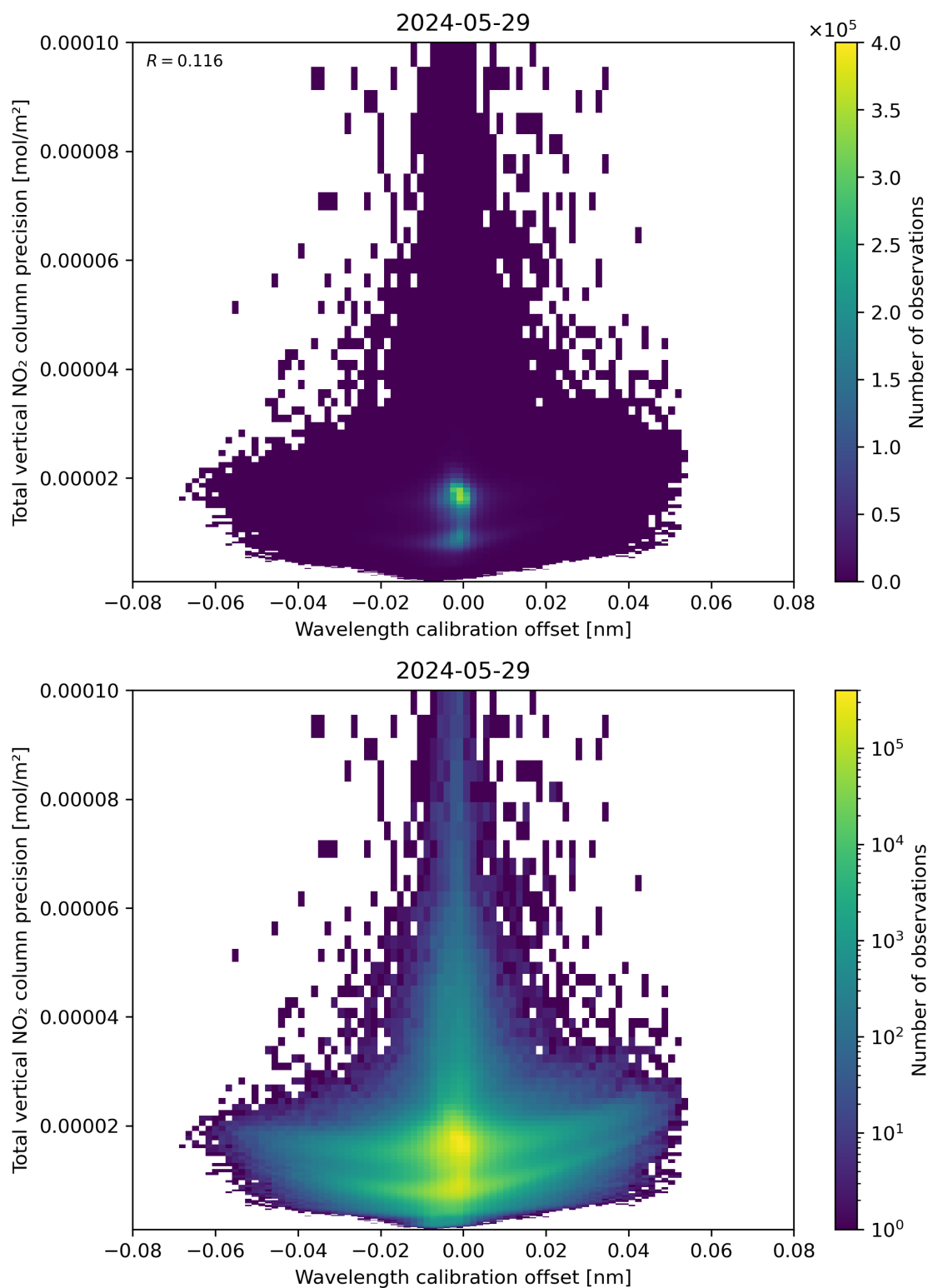
Figure 180: Scatter density plot of “Wavelength calibration offset” against “Total vertical NO 2 column precision” for 2024-05-28 to 2024-05-30.
