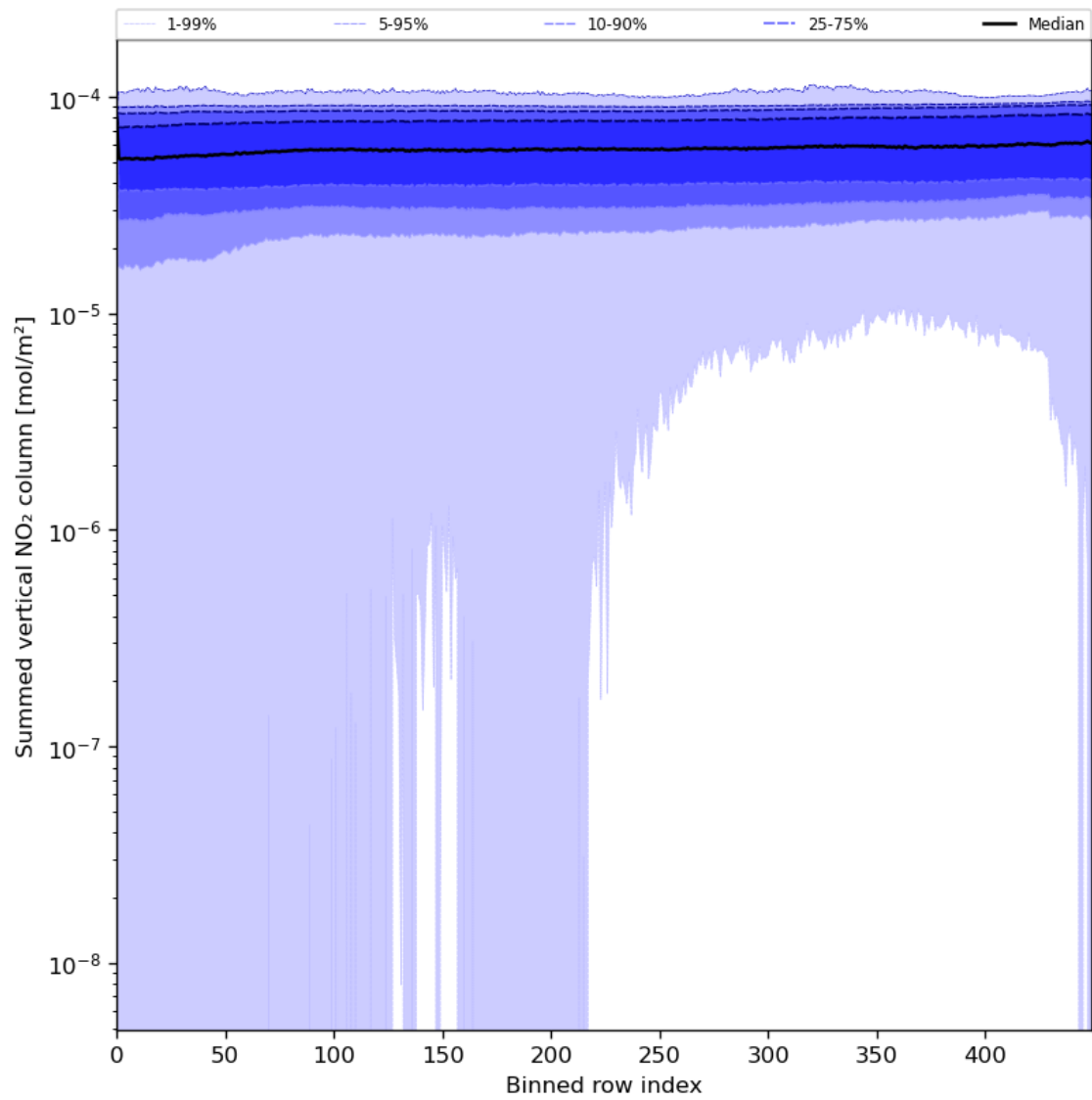
Figure 57: Along track statistics of “Summed vertical NO 2 column” for 2024-05-28 to 2024-05-30
