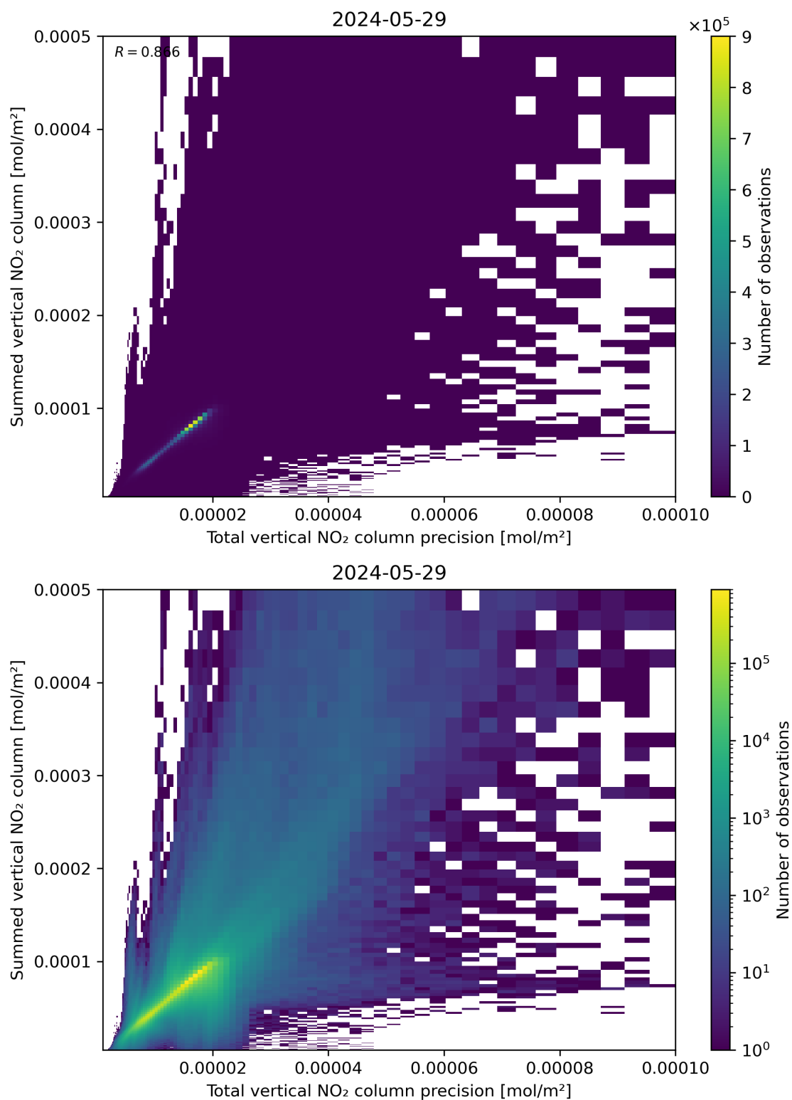
Figure 117: Scatter density plot of “Total vertical NO 2 column precision” against “Summed vertical NO 2 column” for 2024-05-28 to 2024-05-30.
