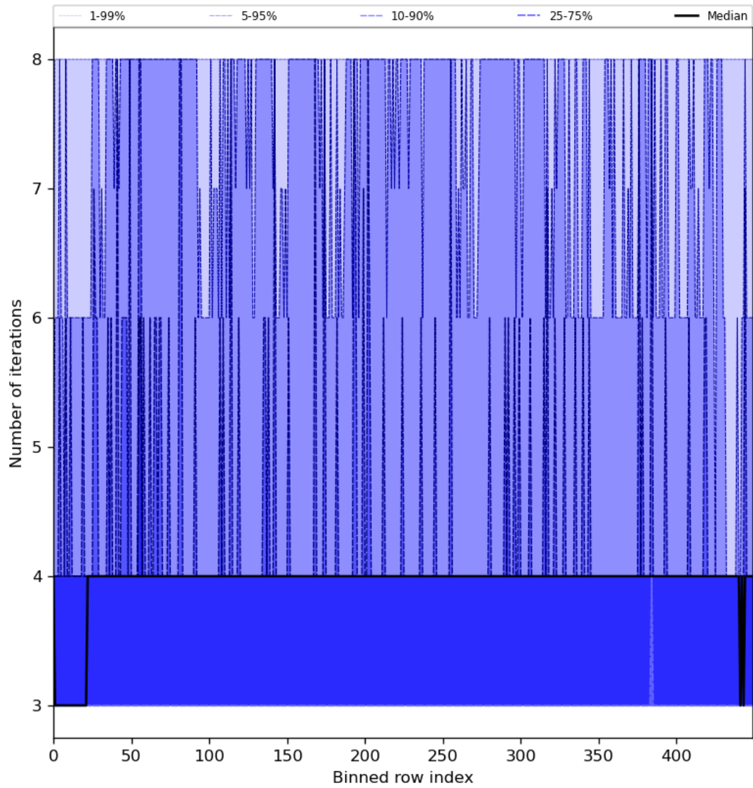
Figure 51: Along track statistics of “Number of iterations” for 2024-05-28 to 2024-05-30
