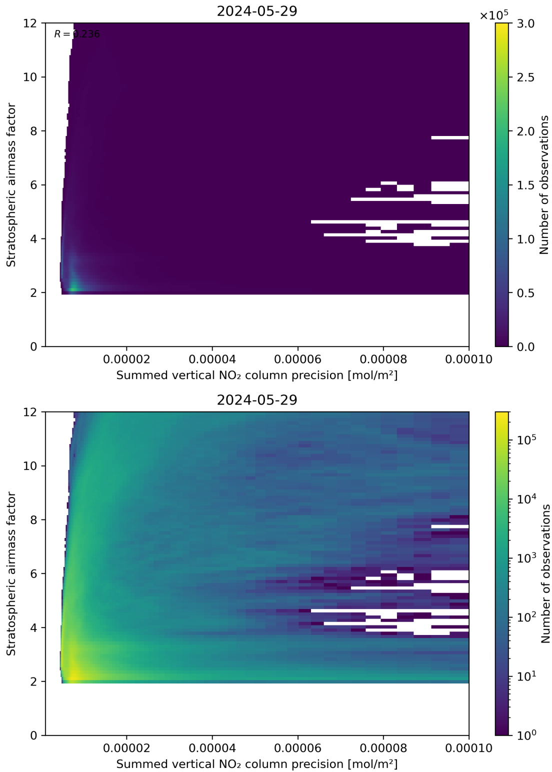
Figure 106: Scatter density plot of “Summed vertical NO 2 column precision” against “Stratospheric airmass factor” for 2024-05-28 to 2024-05-30.
