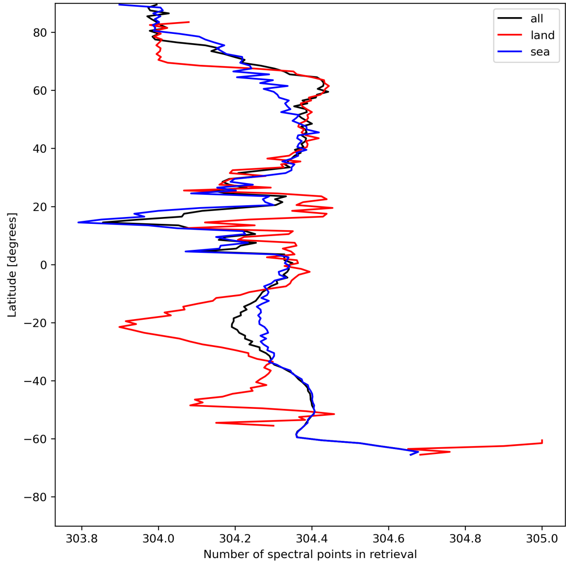
Figure 16: Zonal average of “Number of spectral points in retrieval” for 2024-05-28 to 2024-05-30.
