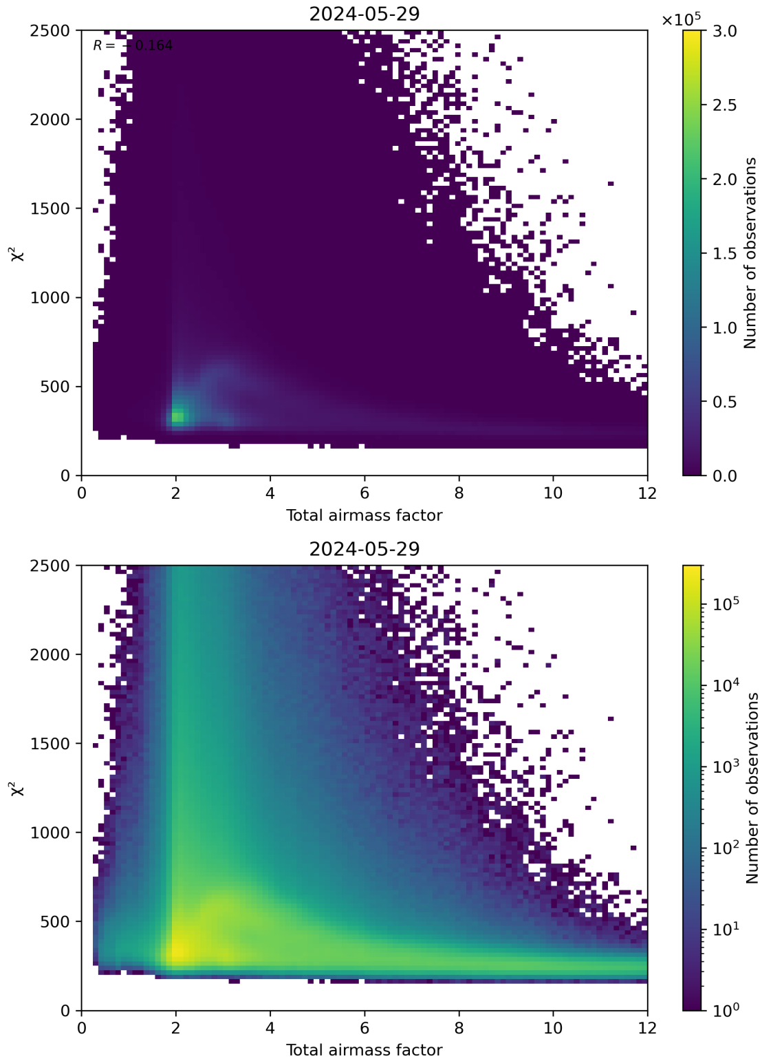
Figure 63: Scatter density plot of “Total airmass factor” against “ \chi^2 ” for 2024-05-28 to 2024-05-30.
