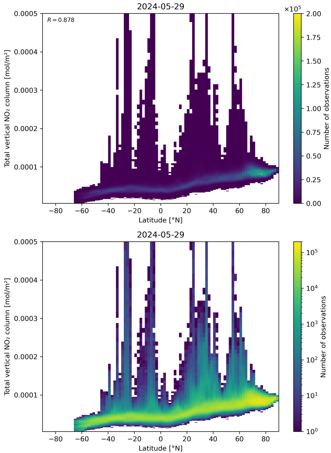
Figure 90: Scatter density plot of “Latitude” against “Total vertical NO 2 column” for 2024-05-28 to 2024-05-30.
