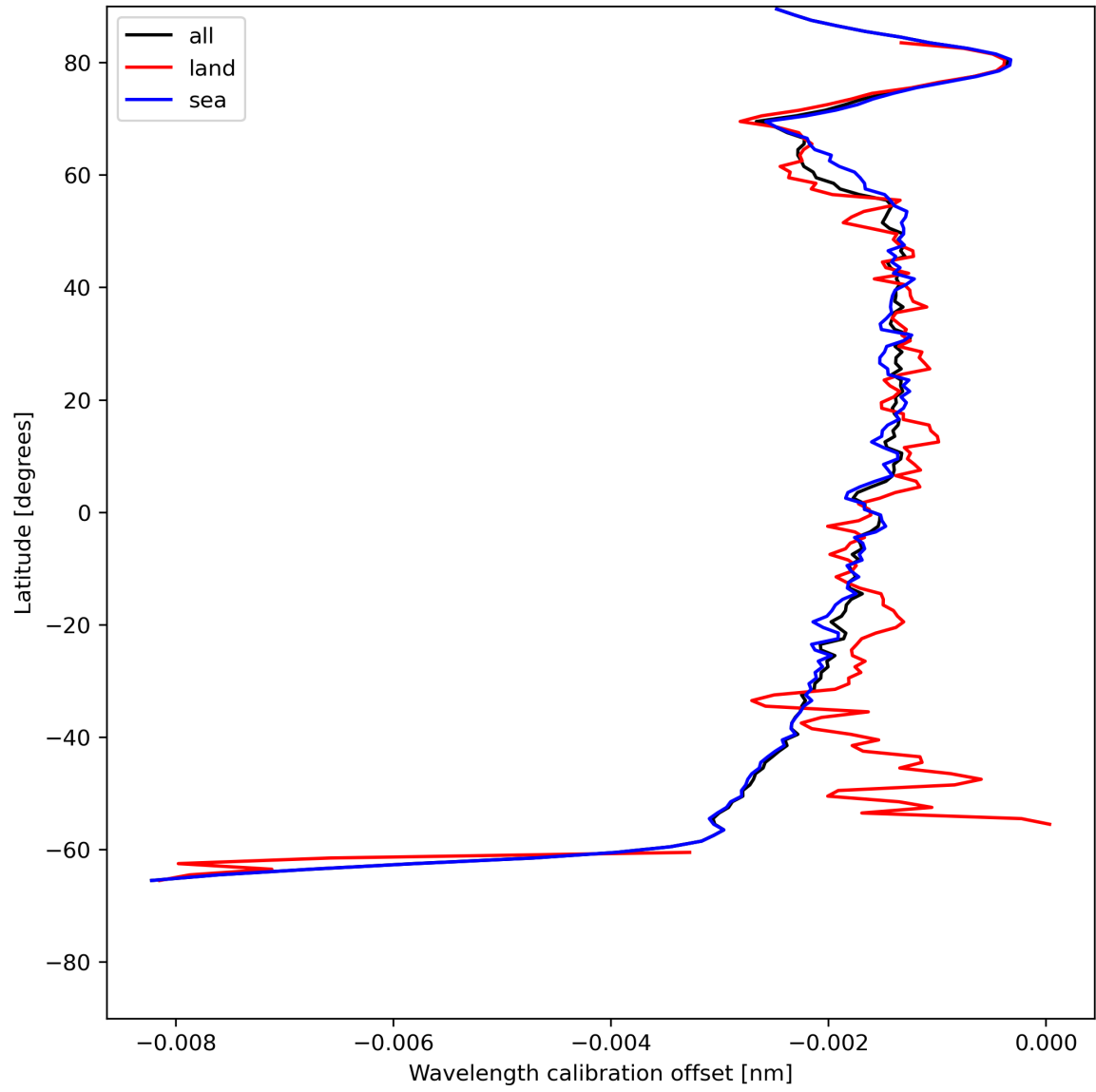
Figure 18: Zonal average of “Wavelength calibration offset” for 2024-05-28 to 2024-05-30.
