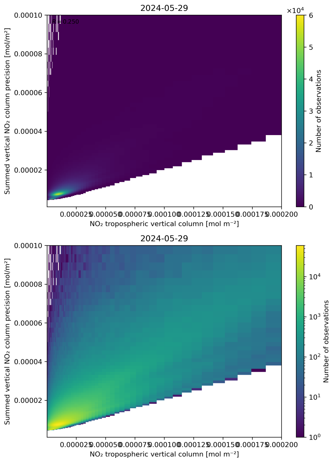
Figure 127: Scatter density plot of “NO 2 tropospheric vertical column” against “Summed vertical NO 2 column precision” for 2024-05-28 to 2024-05-30.
