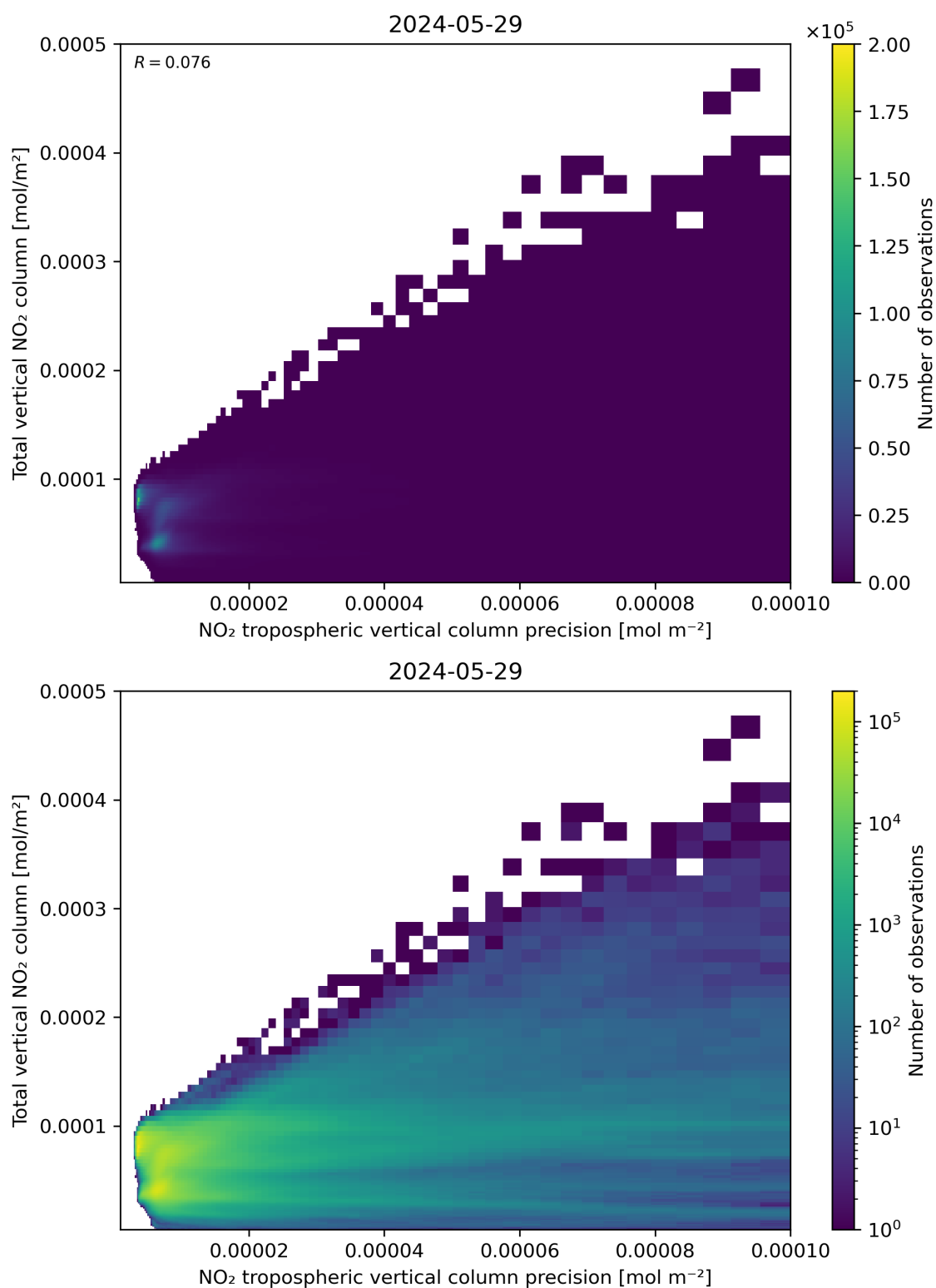
Figure 138: Scatter density plot of “NO 2 tropospheric vertical column precision” against “Total vertical NO 2 column” for 2024-05-28 to 2024-05-30.
