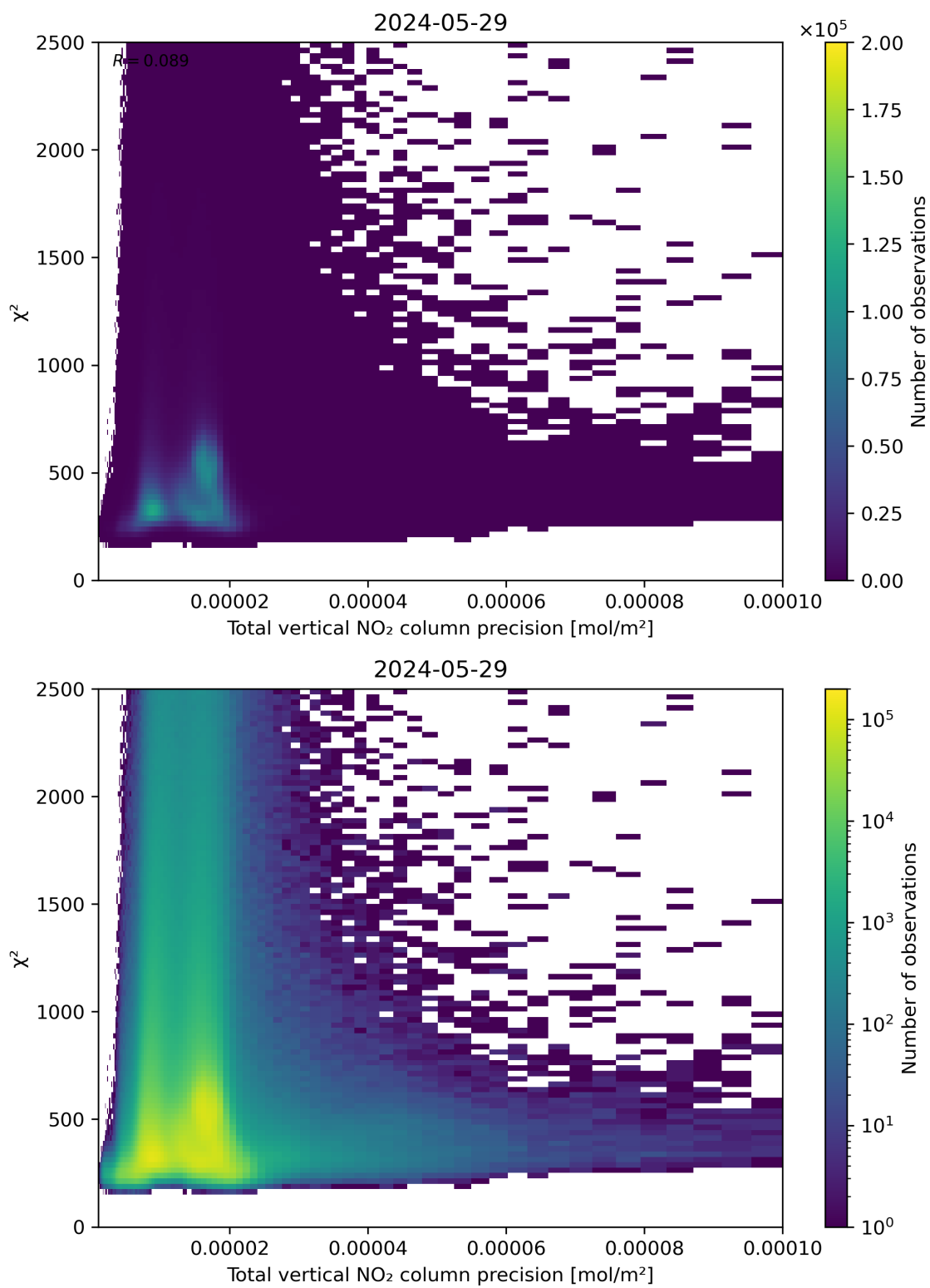
Figure 116: Scatter density plot of “Total vertical NO 2 column precision” against “ \chi^2 ” for 2024-05-28 to 2024-05-30.
