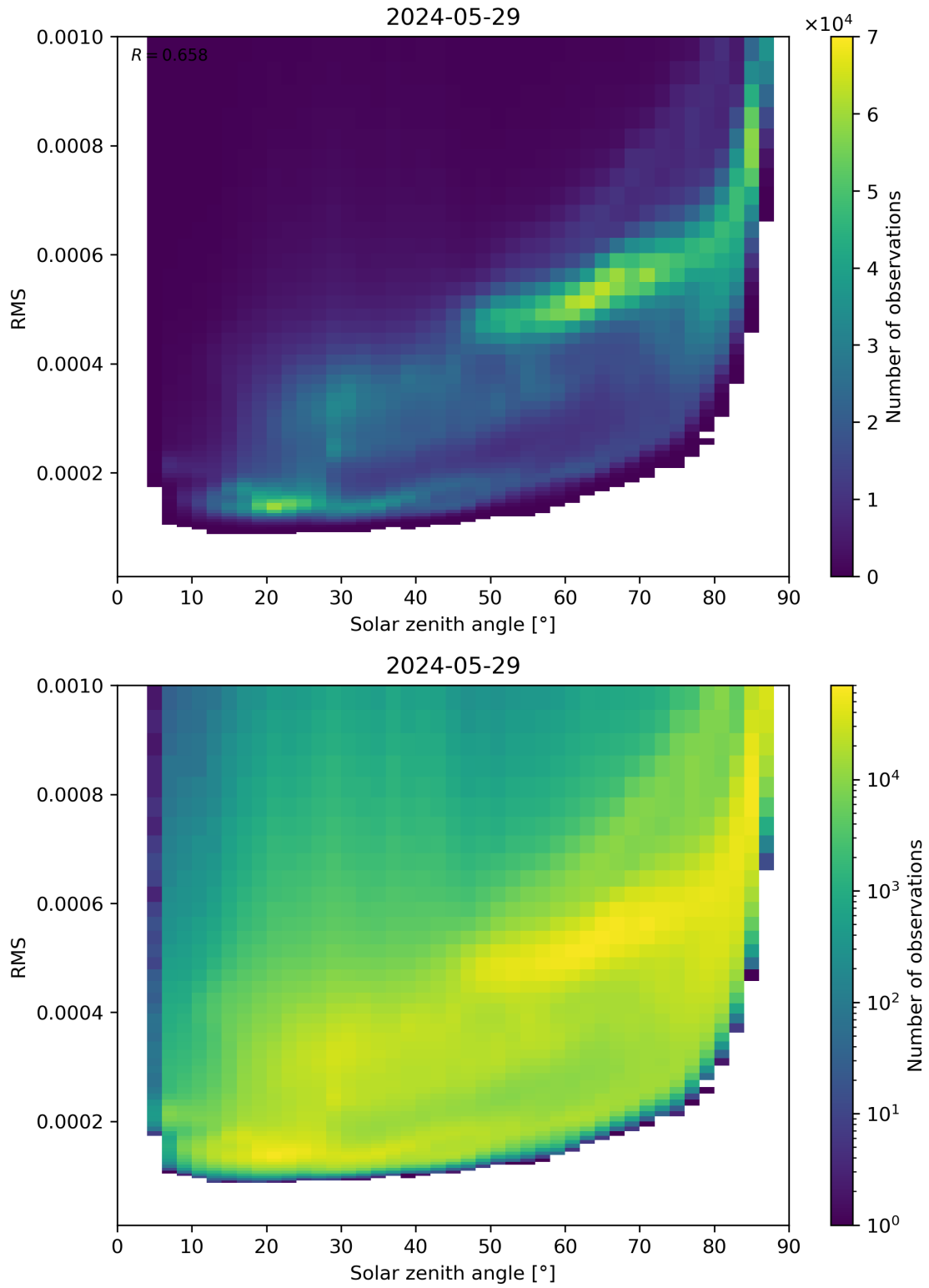
Figure 157: Scatter density plot of “Solar zenith angle” against “RMS” for 2024-05-28 to 2024-05-30.
