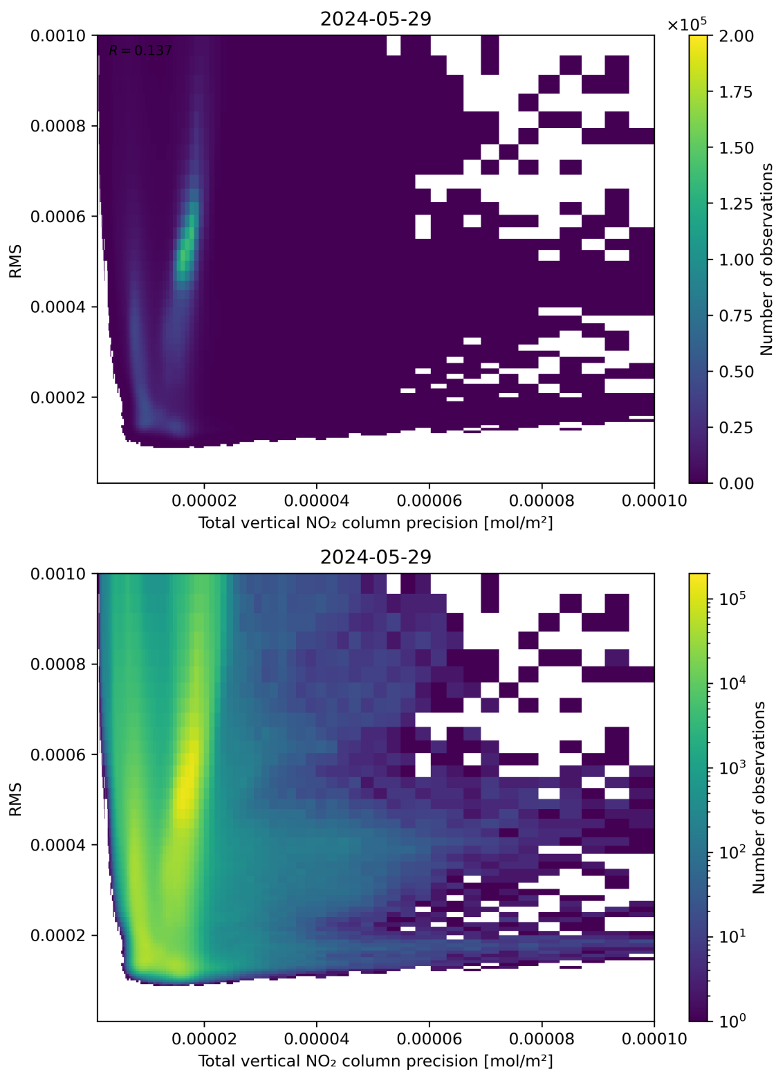
Figure 119: Scatter density plot of “Total vertical NO 2 column precision” against “RMS” for 2024-05-28 to 2024-05-30.
