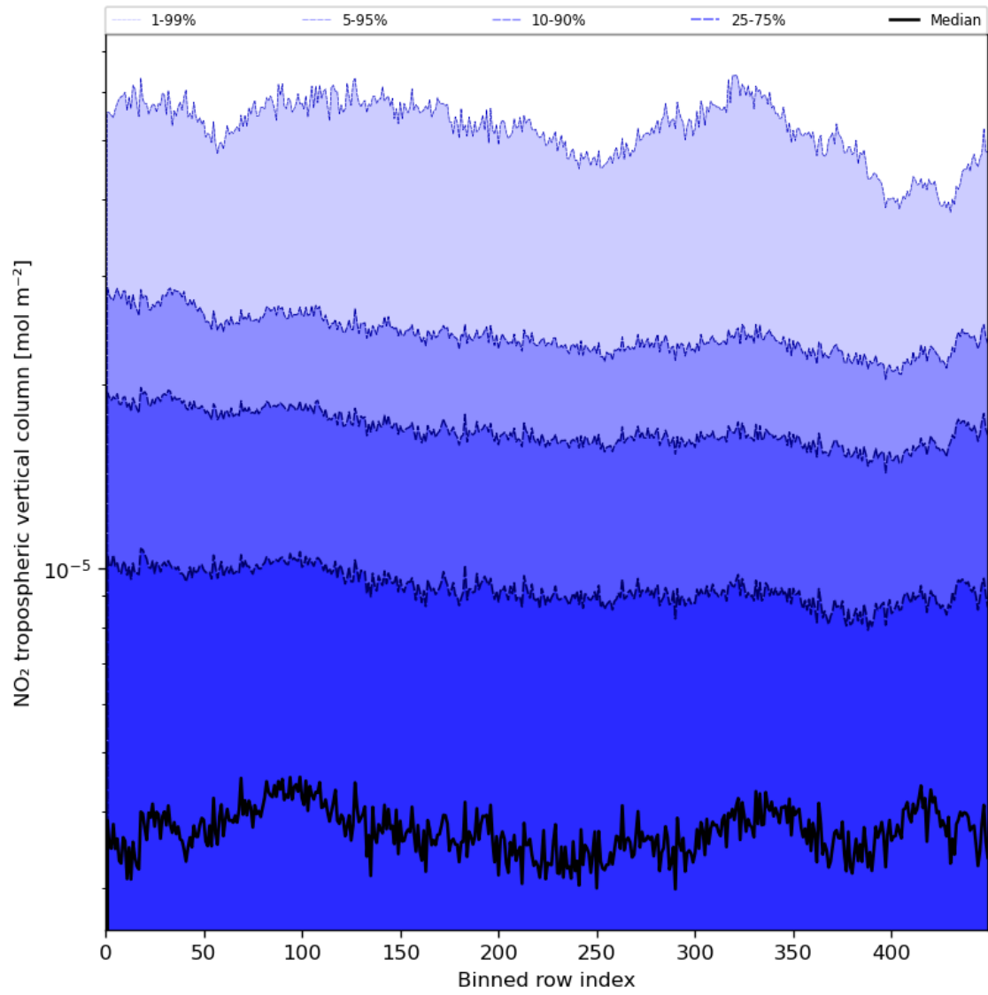
Figure 46: Along track statistics of “NO 2 tropospheric vertical column” for 2024-05-28 to 2024-05-30
