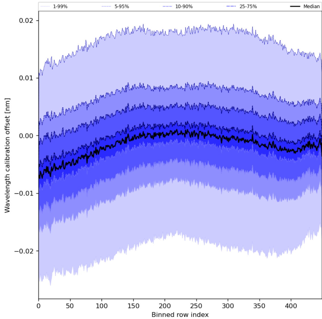
Figure 52: Along track statistics of “Wavelength calibration offset” for 2024-05-28 to 2024-05-30
