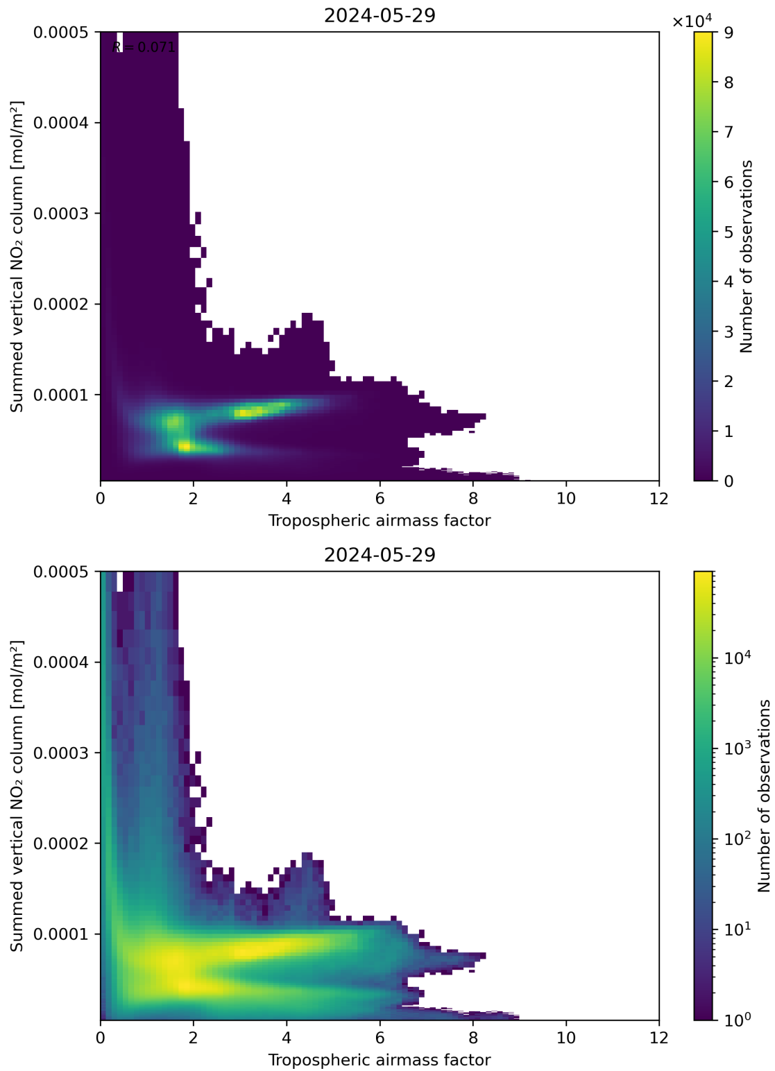
Figure 75: Scatter density plot of “Tropospheric air mass factor” against “Summed vertical NO 2 column” for 2024-05-28 to 2024-05-30.
