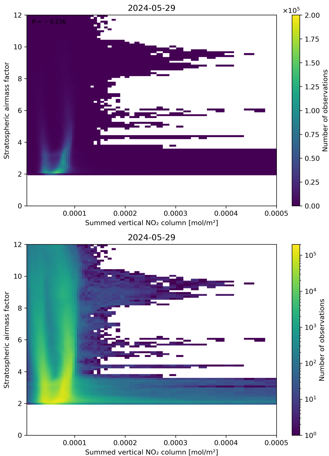
Figure 103: Scatter density plot of “Summed vertical NO 2 column” against “Stratospheric air mass factor” for 2024-05-28 to 2024-05-30.
