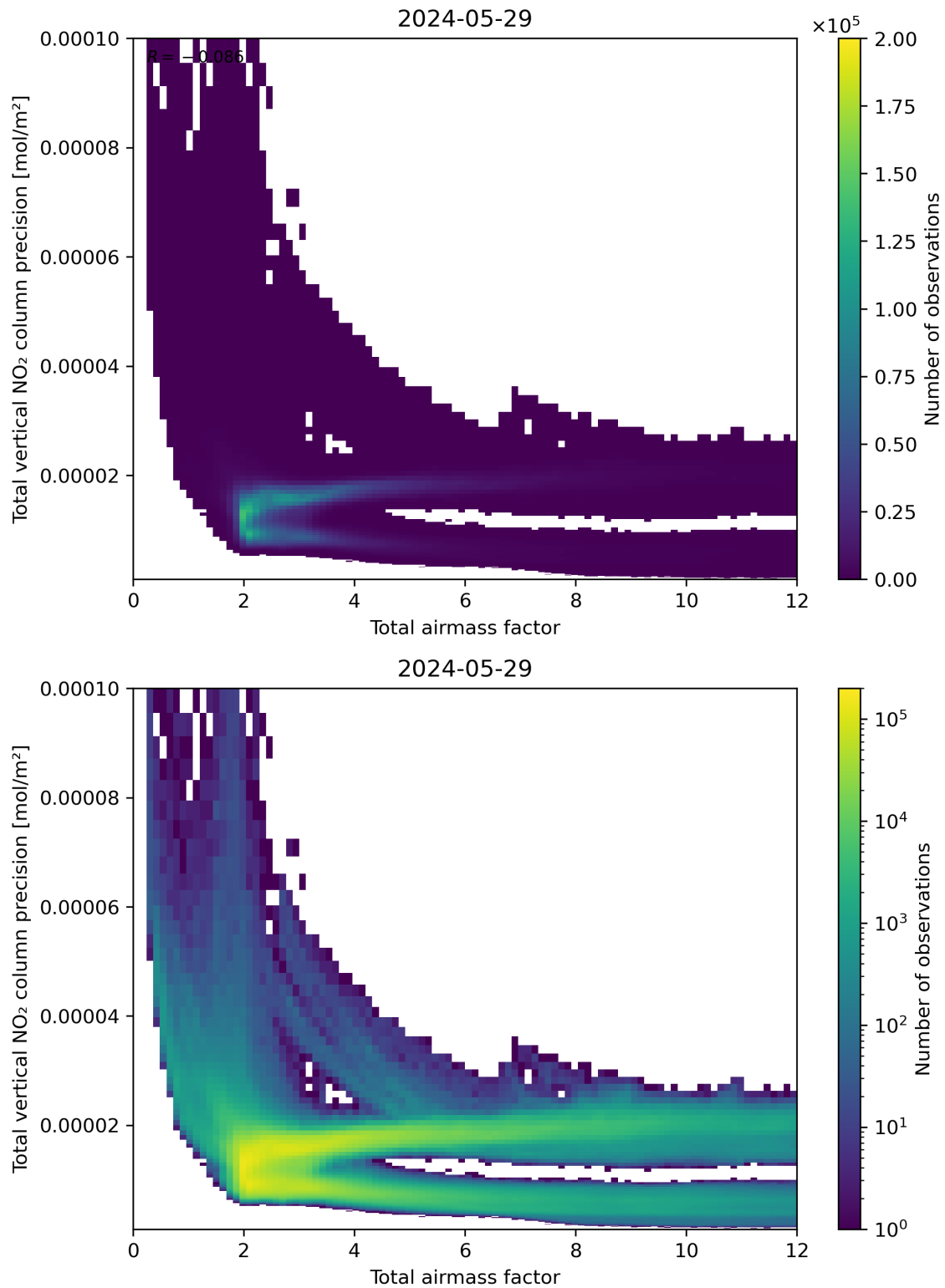
Figure 68: Scatter density plot of “Total airmass factor” against “Total vertical NO 2 column precision” for 2024-05-28 to 2024-05-30.
