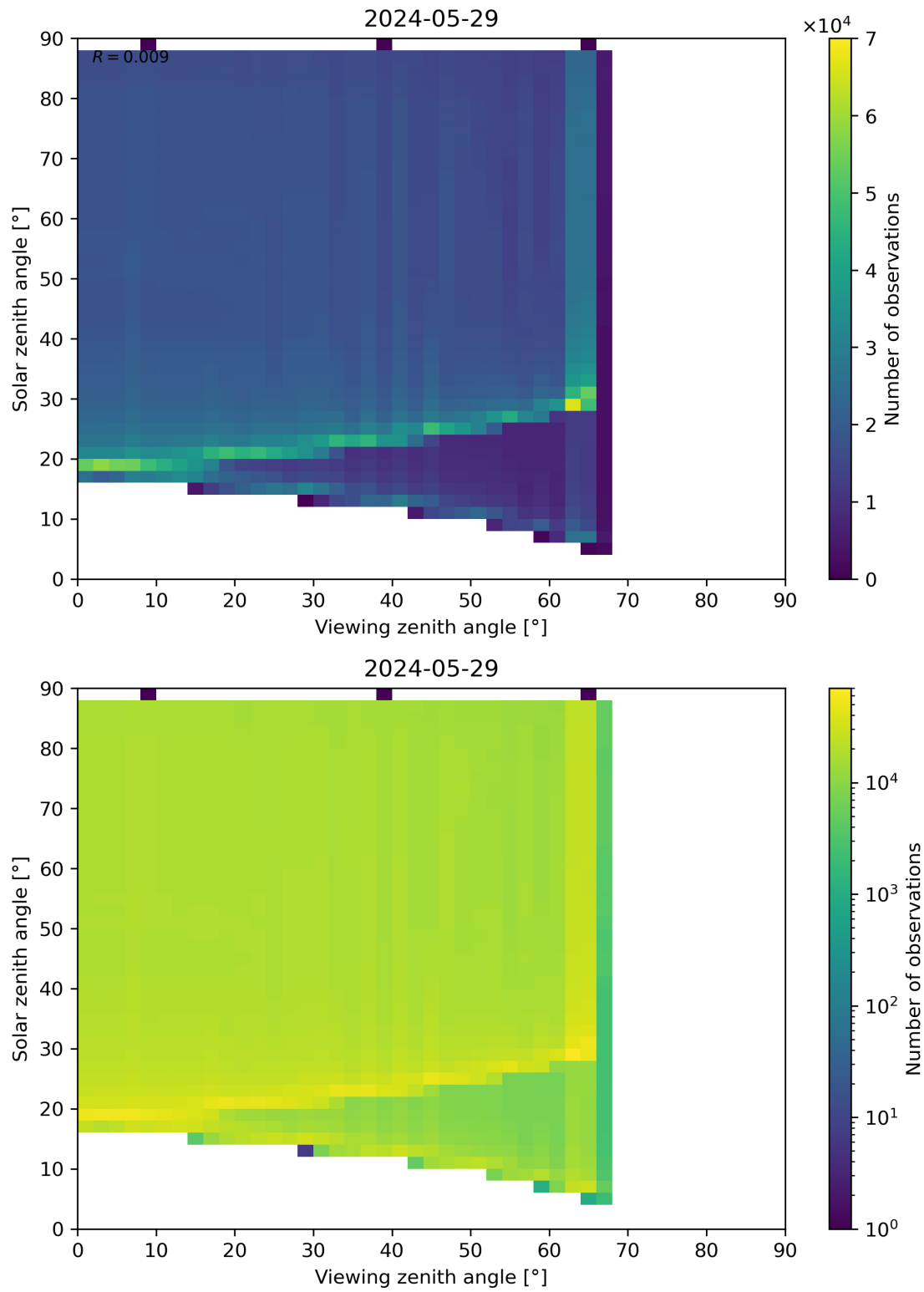
Figure 172: Scatter density plot of “Viewing zenith angle” against “Solar zenith angle” for 2024-05-28 to 2024-05-30.
