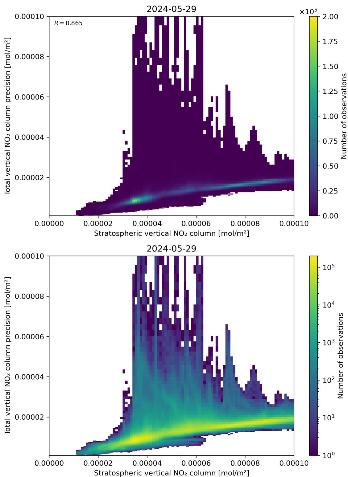
Figure 101: Scatter density plot of “Stratospheric vertical NO 2 column” against “Total vertical NO 2 column precision” for 2024-05-28 to 2024-05-30.
