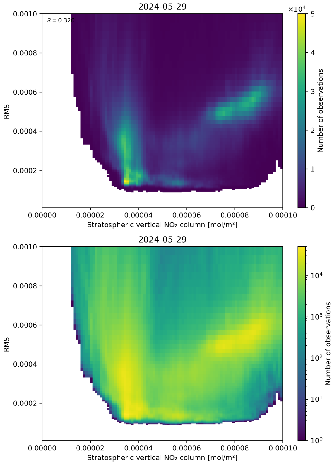
Figure 102: Scatter density plot of “Stratospheric vertical NO 2 column” against “RMS” for 2024-05-28 to 2024-05-30.
