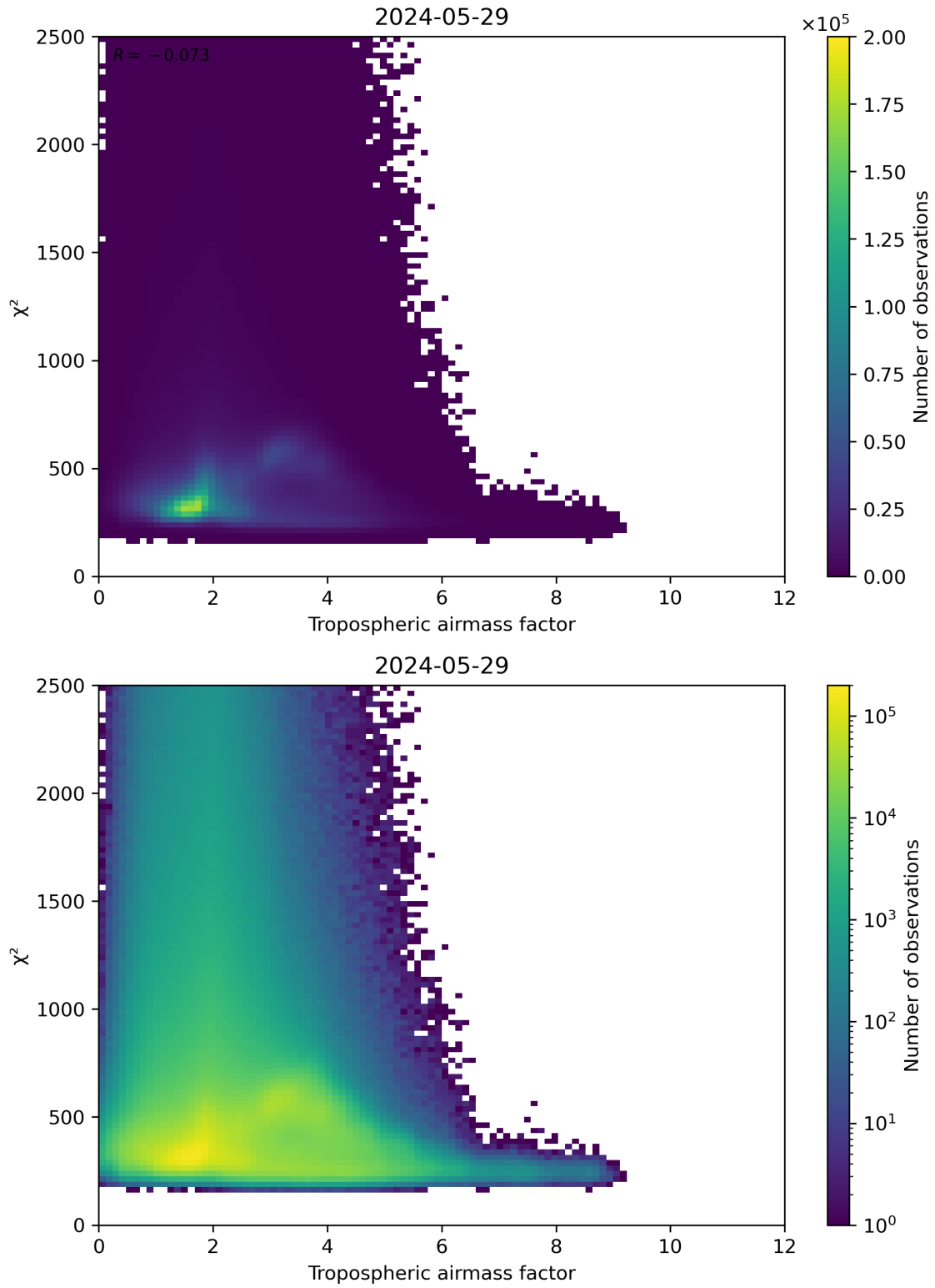
Figure 73: Scatter density plot of “Tropospheric airmass factor” against “ \chi^2 ” for 2024-05-28 to 2024-05-30.
