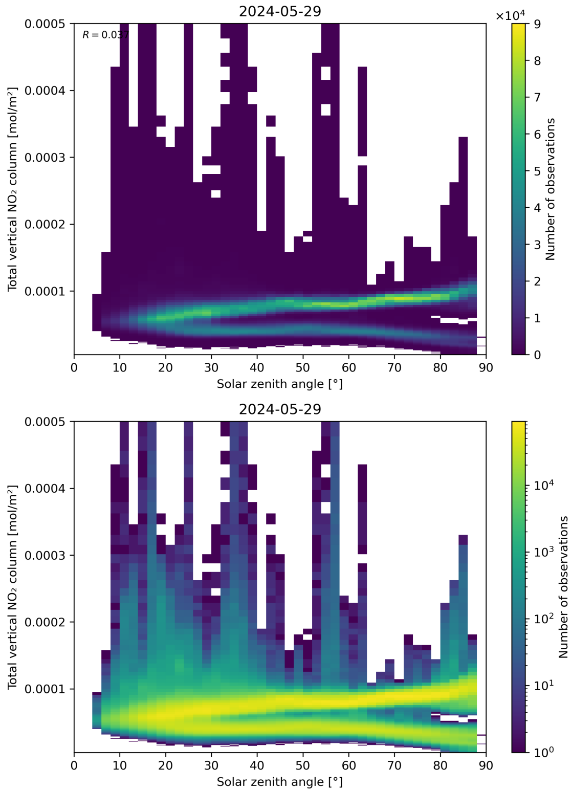
Figure 153: Scatter density plot of “Solar zenith angle” against “Total vertical NO 2 column” for 2024-05-28 to 2024-05-30.
