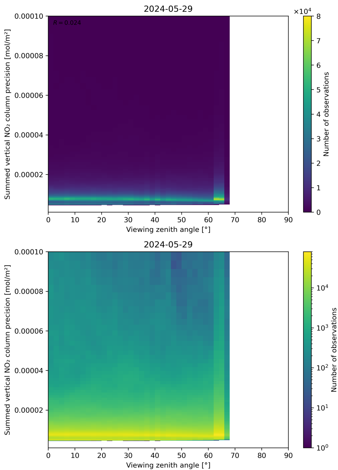
Figure 166: Scatter density plot of “Viewing zenith angle” against “Summed vertical NO 2 column precision” for 2024-05-28 to 2024-05-30.
