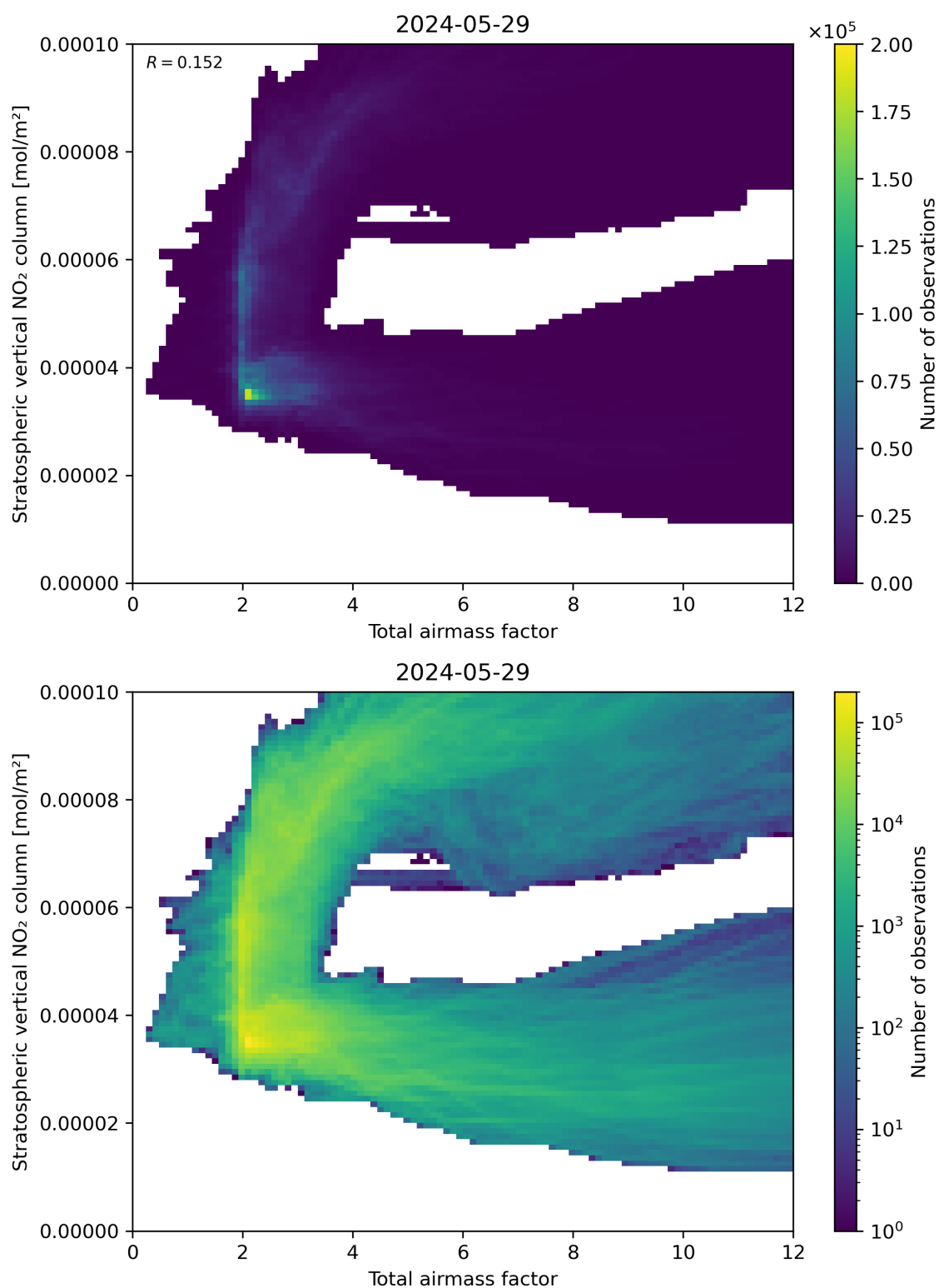
Figure 64: Scatter density plot of “Total airmass factor” against “Stratospheric vertical NO 2 column” for 2024-05-28 to 2024-05-30.
