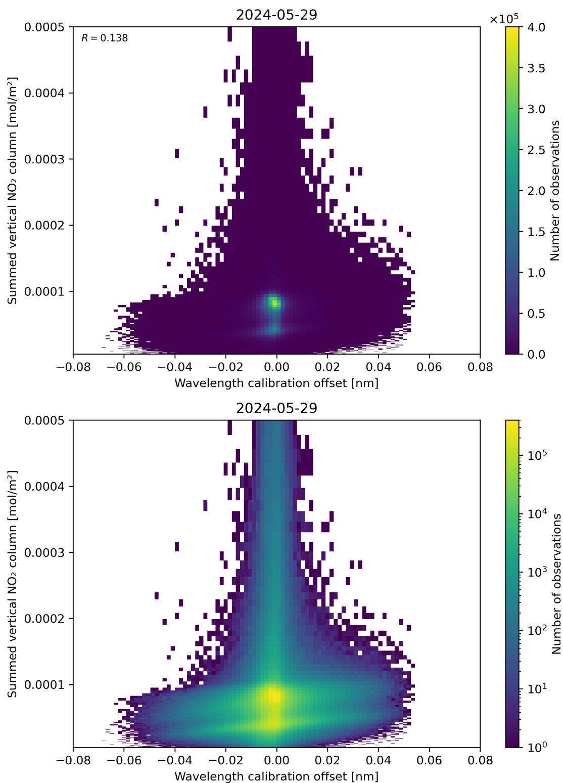
Figure 177: Scatter density plot of “Wavelength calibration offset” against “Summed vertical NO 2 column” for 2024-05-28 to 2024-05-30.
