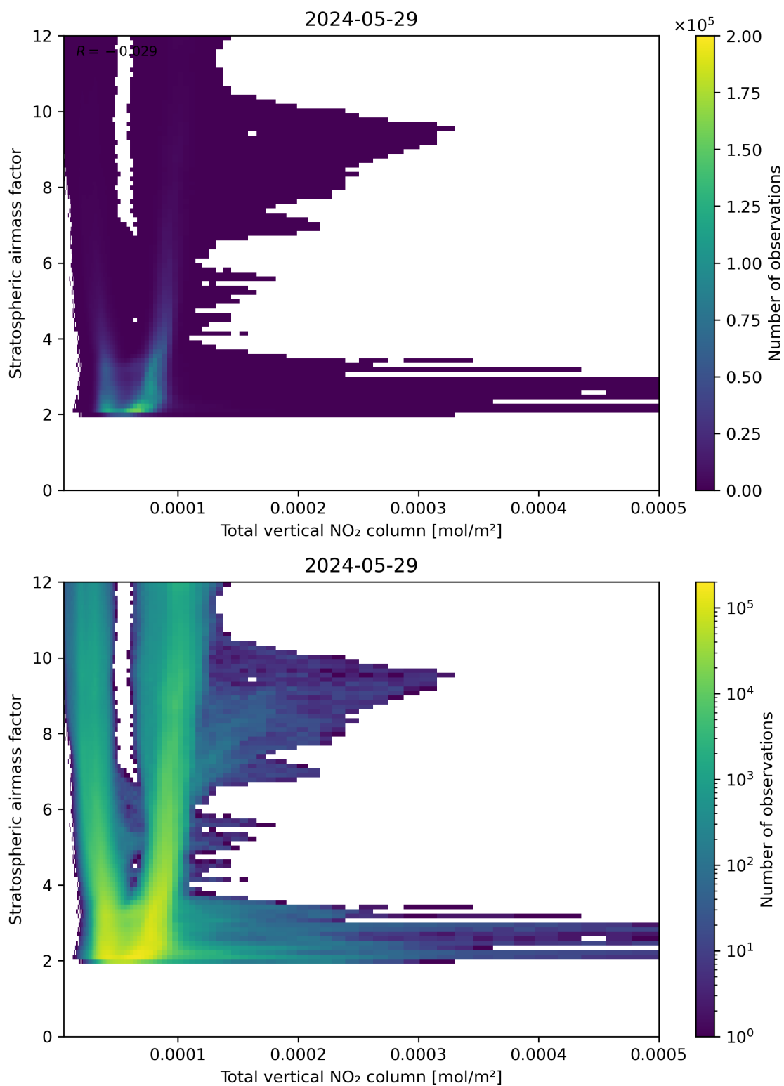
Figure 110: Scatter density plot of “Total vertical NO 2 column” against “Stratospheric airmass factor” for 2024-05-28 to 2024-05-30.
