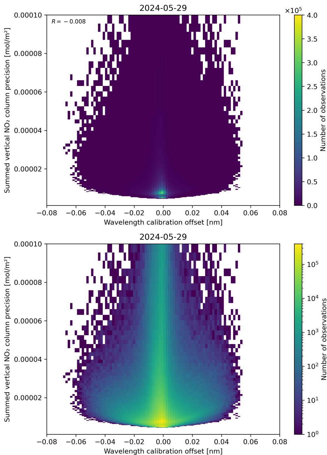
Figure 178: Scatter density plot of “Wavelength calibration offset” against “Summed vertical NO 2 column precision” for 2024-05-28 to 2024-05-30.
