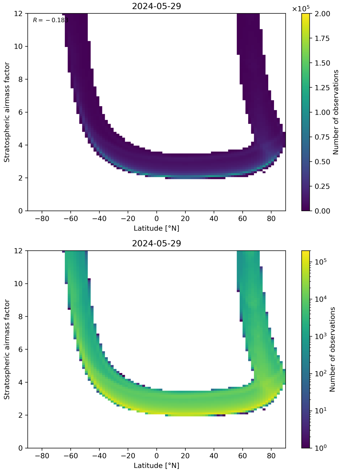
Figure 83: Scatter density plot of “Latitude” against “Stratospheric air mass factor” for 2024-05-28 to 2024-05-30.
