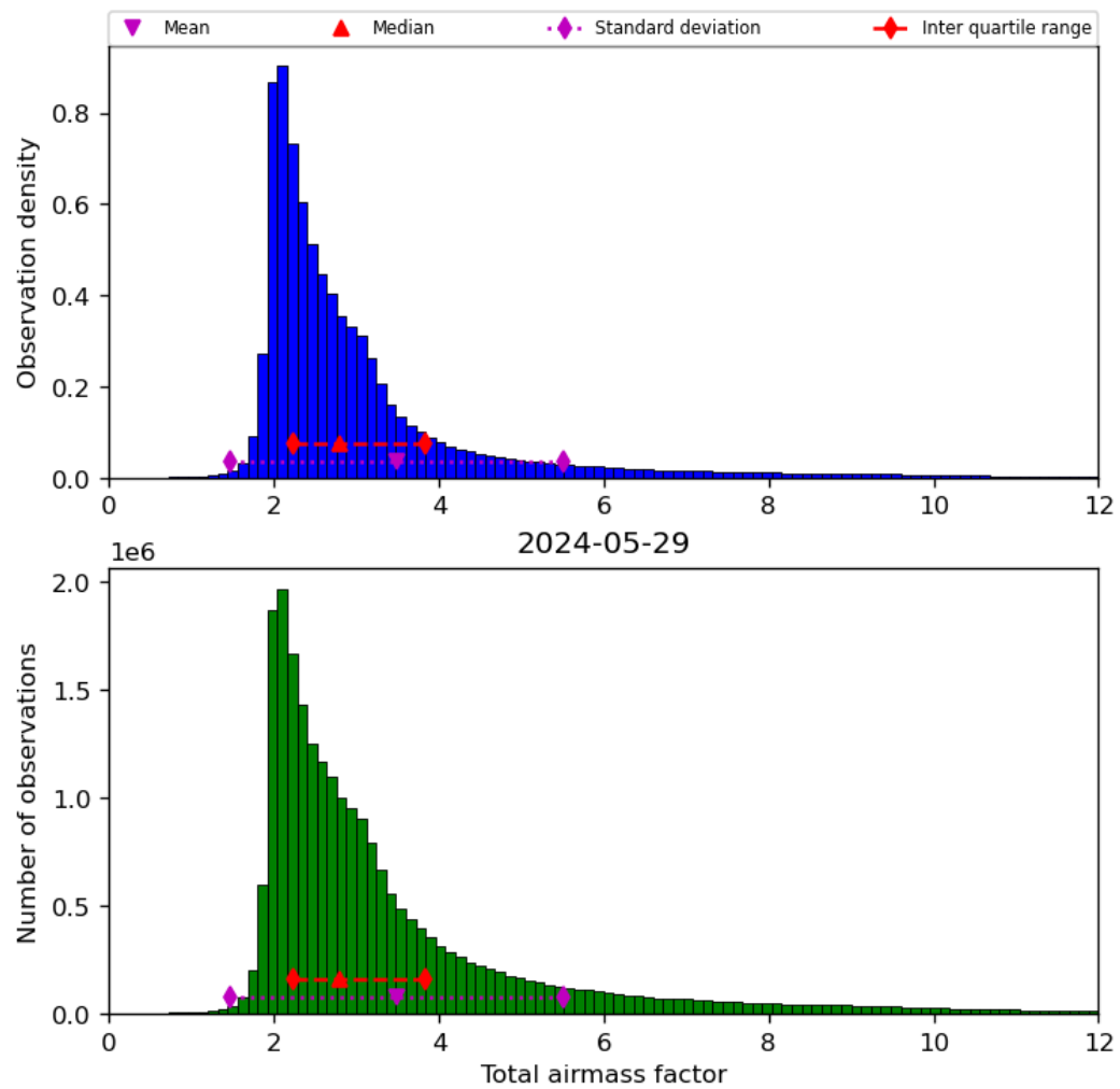
Figure 32: Histogram of “Total airmass factor” for 2024-05-28 to 2024-05-30
