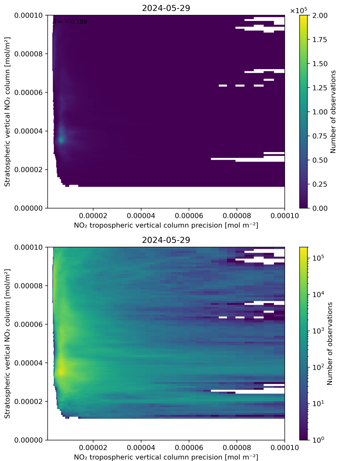
Figure 135: Scatter density plot of “ \text{NO}_2 tropospheric vertical column precision” against “Stratospheric vertical \text{NO}_2 column” for 2024-05-28 to 2024-05-30.
