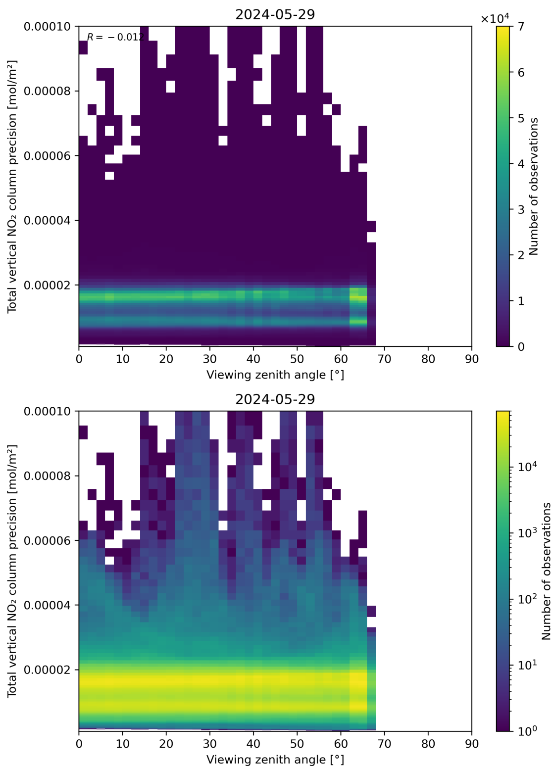
Figure 168: Scatter density plot of “Viewing zenith angle” against “Total vertical NO 2 column precision” for 2024-05-28 to 2024-05-30.
