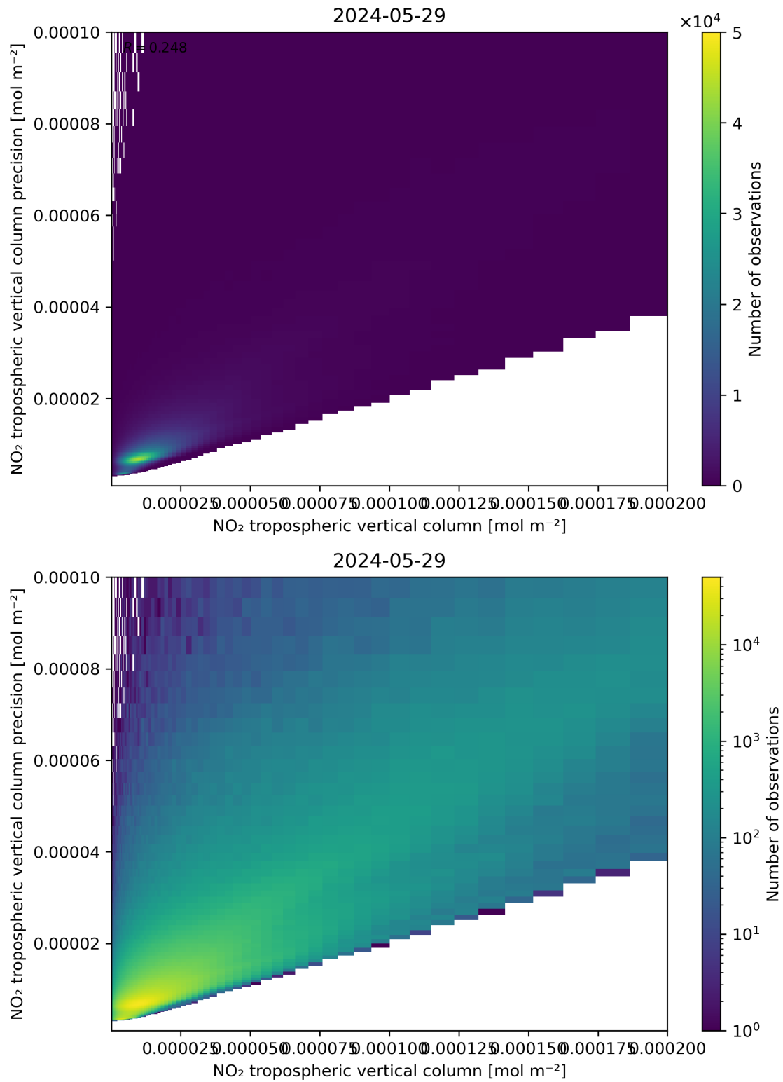
Figure 130: Scatter density plot of “NO 2 tropospheric vertical column” against “NO 2 tropospheric vertical column precision” for 2024-05-28 to 2024-05-30.
