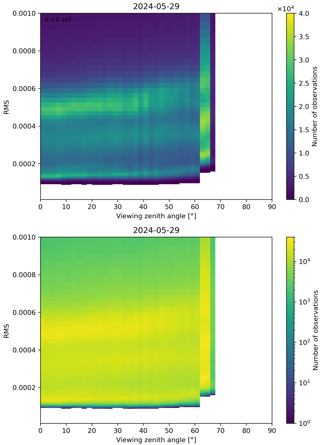
Figure 171: Scatter density plot of “Viewing zenith angle” against “RMS” for 2024-05-28 to 2024-05-30.
