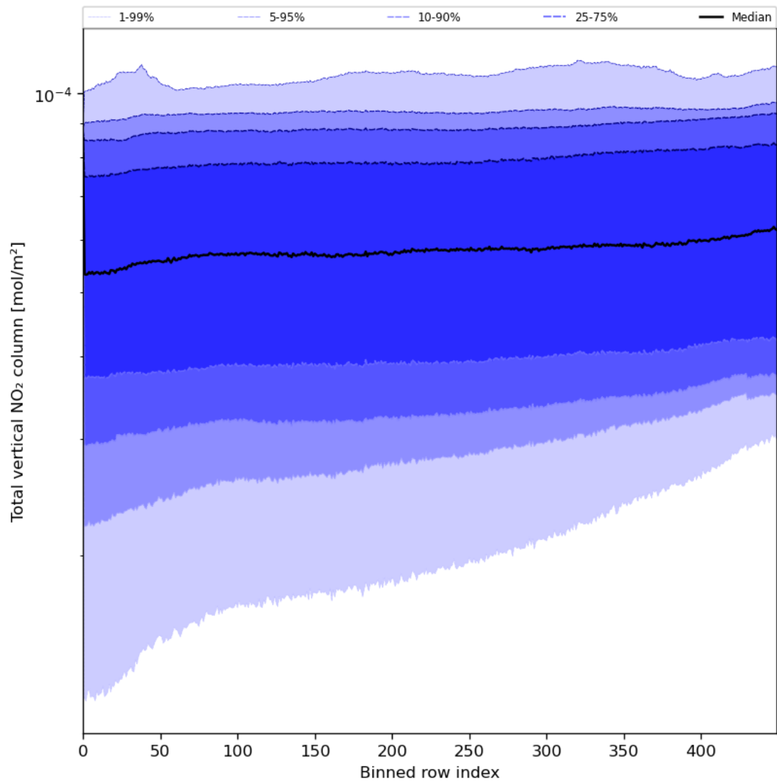
Figure 55: Along track statistics of “Total vertical NO 2 column” for 2024-05-28 to 2024-05-30
