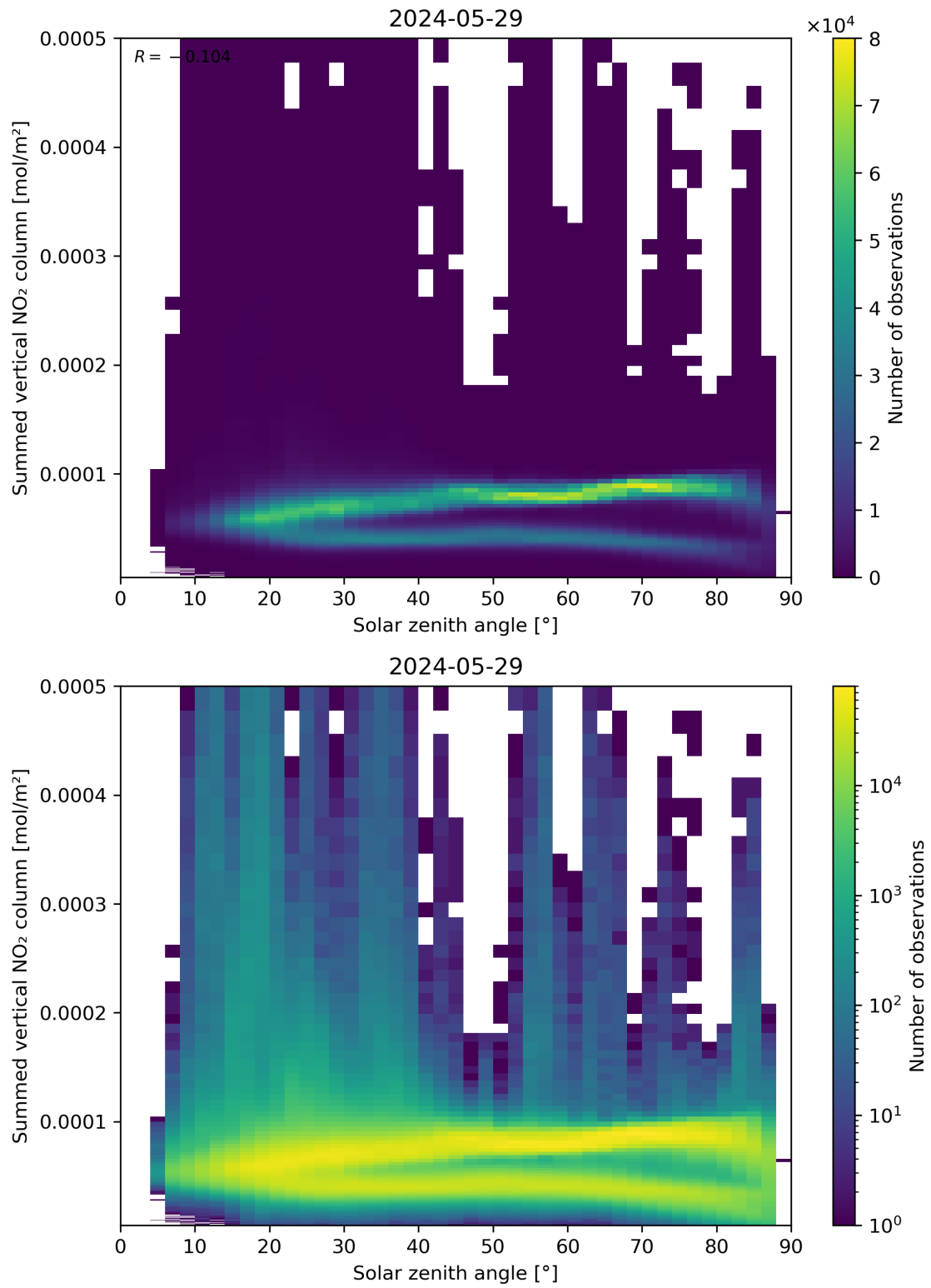
Figure 151: Scatter density plot of “Solar zenith angle” against “Summed vertical NO 2 column” for 2024-05-28 to 2024-05-30.
