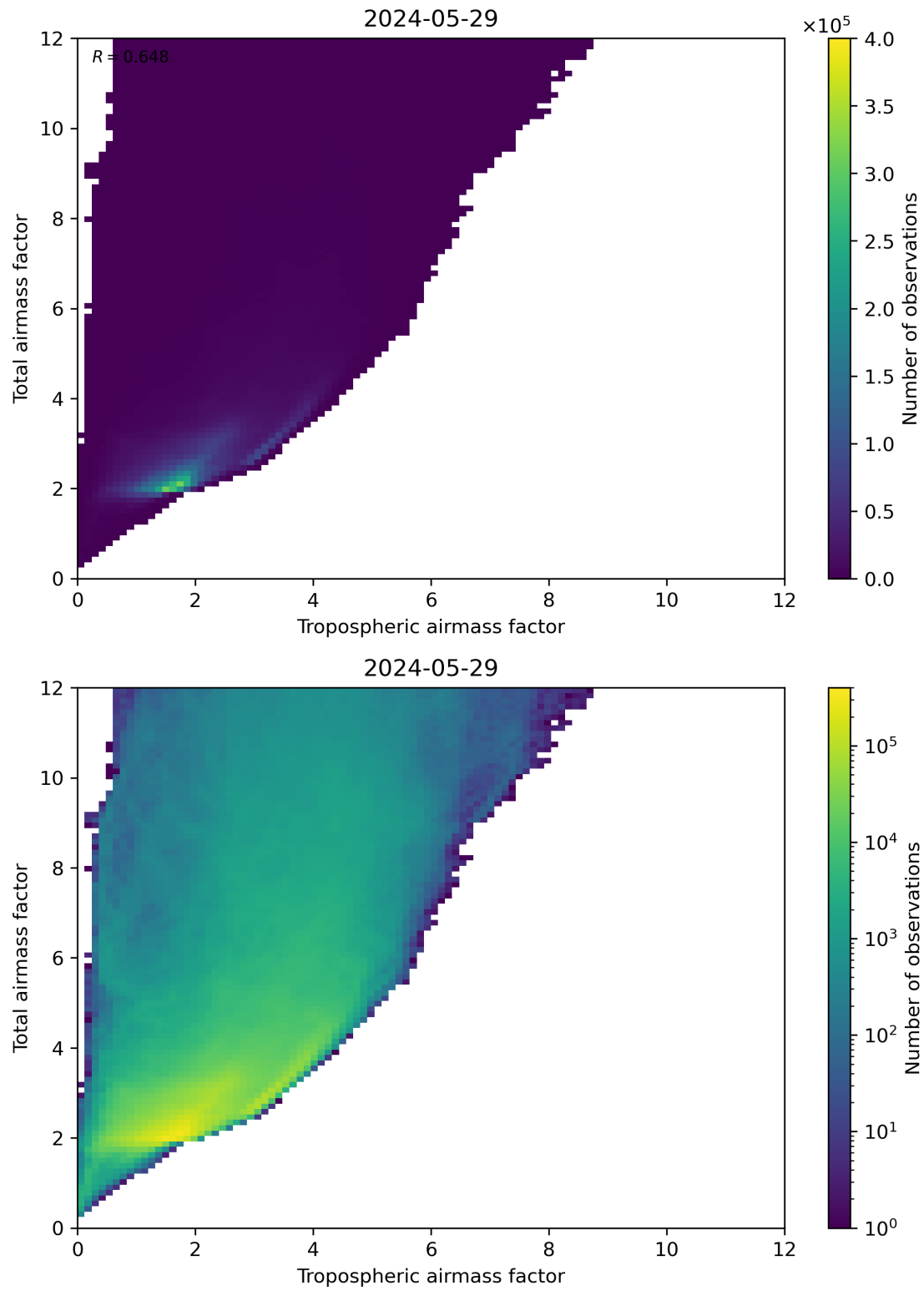
Figure 72: Scatter density plot of “Tropospheric airmass factor” against “Total airmass factor” for 2024-05-28 to 2024-05-30.
