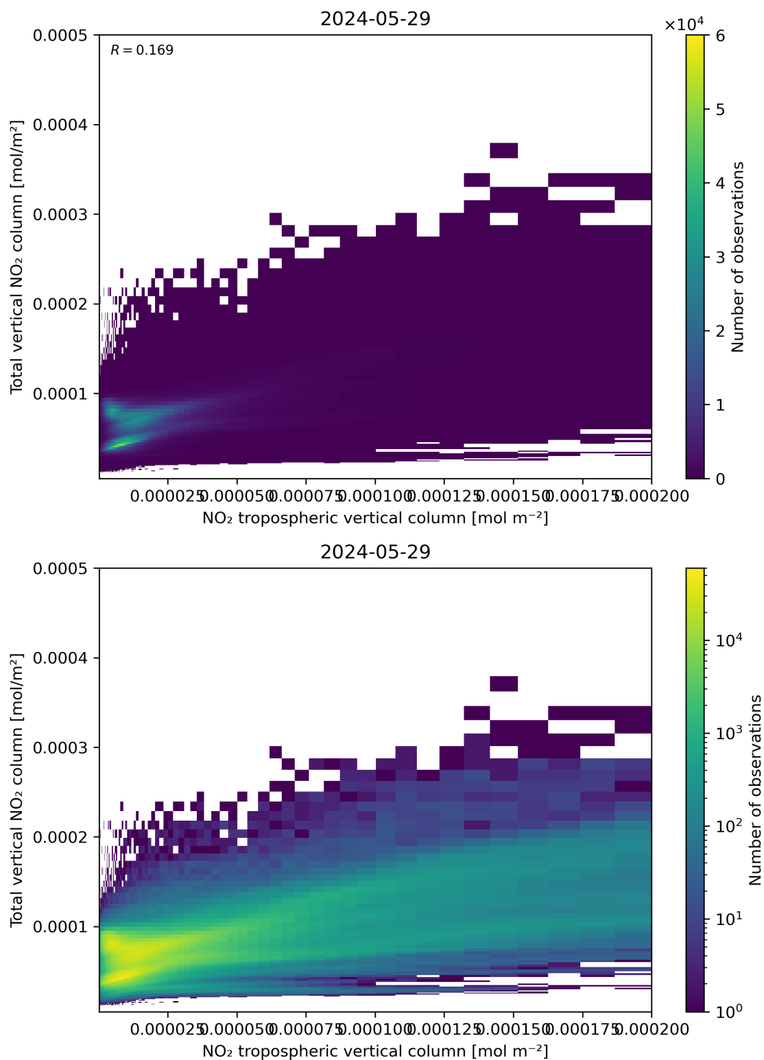
Figure 128: Scatter density plot of “NO 2 tropospheric vertical column” against “Total vertical NO 2 column” for 2024-05-28 to 2024-05-30.
