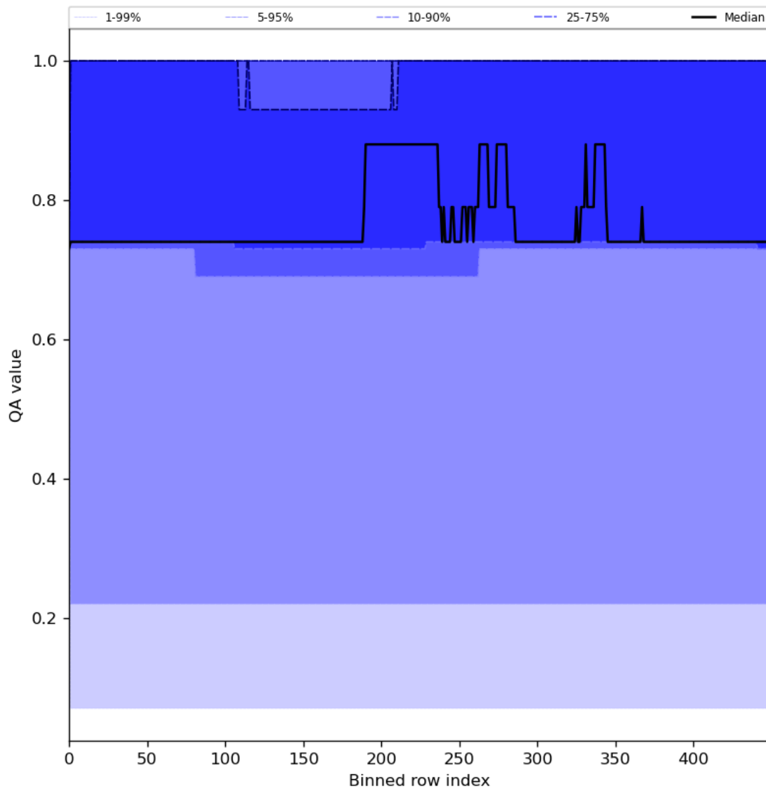
Figure 45: Along track statistics of “QA value” for 2024-05-28 to 2024-05-30
