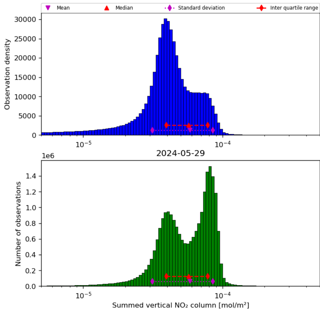
Figure 40: Histogram of "Summed vertical NO 2 column" for 2024-05-28 to 2024-05-30
