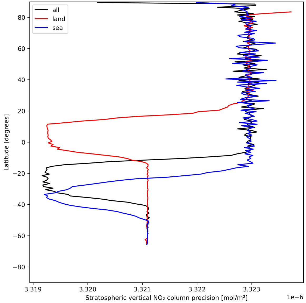
Figure 20: Zonal average of “Stratospheric vertical NO 2 column precision” for 2024-05-28 to 2024-05-30.
