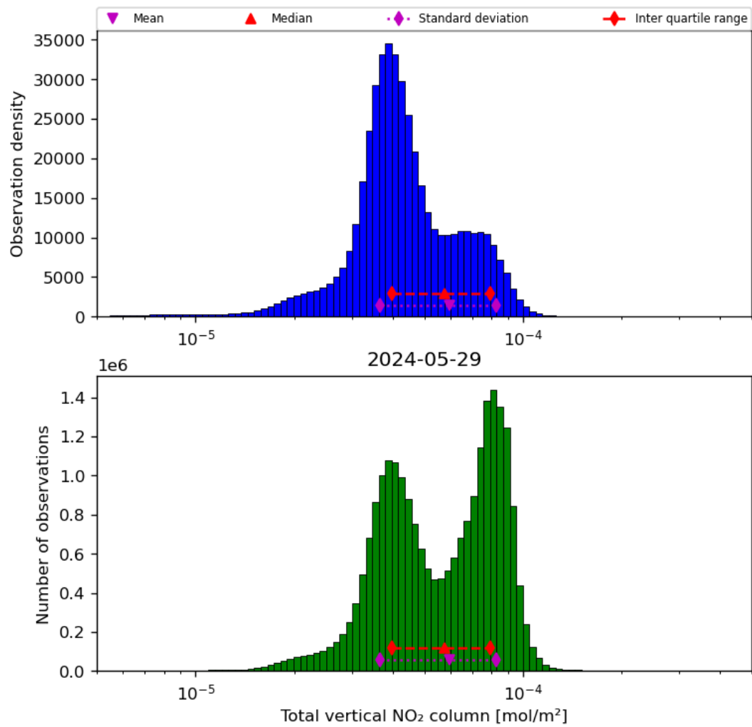
Figure 38: Histogram of “Total vertical NO 2 column” for 2024-05-28 to 2024-05-30
