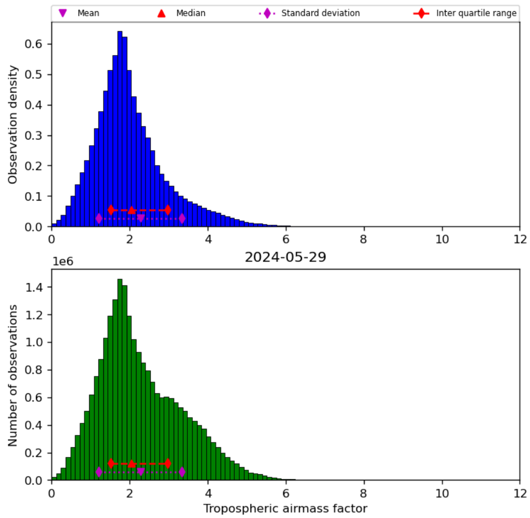
Figure 31: Histogram of “Tropospheric airmass factor” for 2024-05-28 to 2024-05-30
