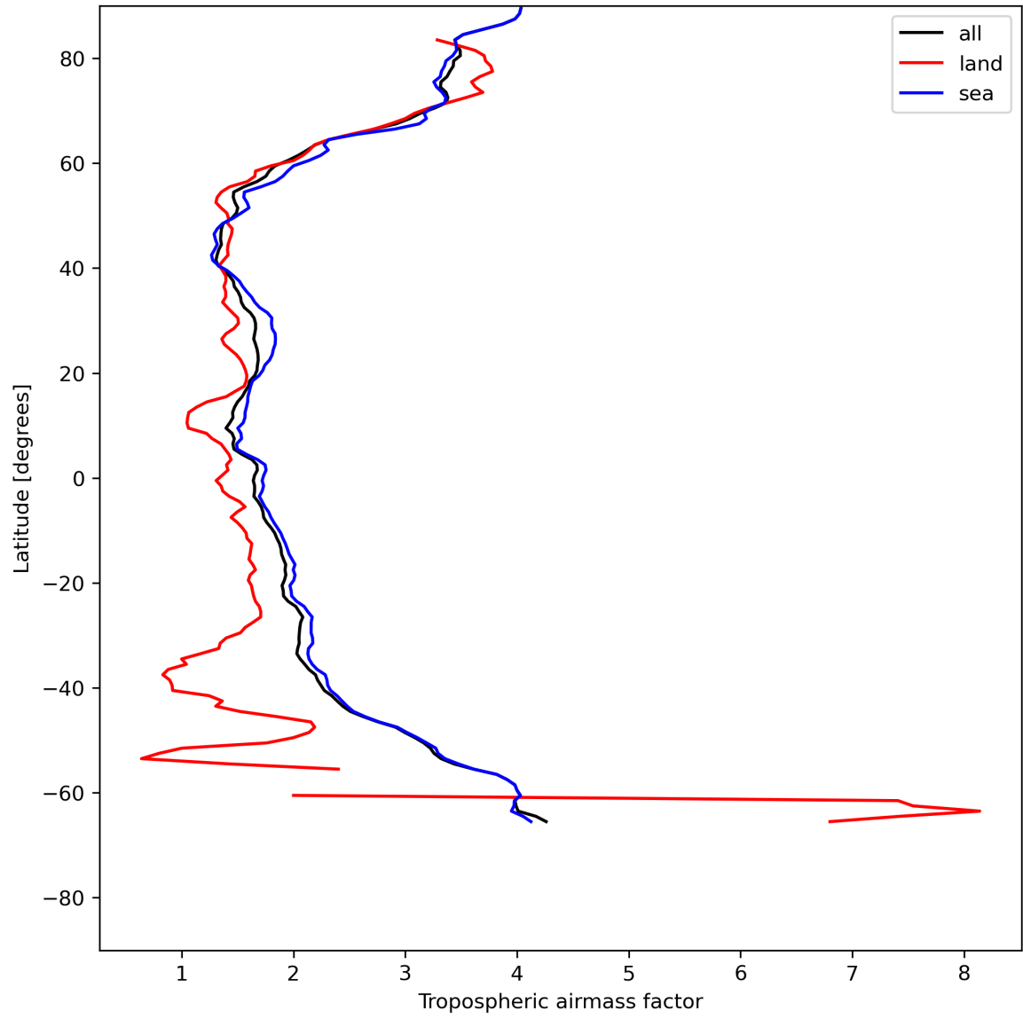
Figure 14: Zonal average of “Tropospheric airmass factor” for 2024-05-28 to 2024-05-30.
