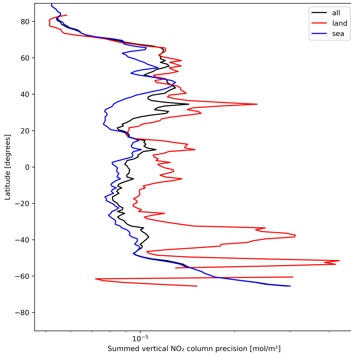
Figure 24: Zonal average of “Summed vertical NO 2 column precision” for 2024-05-28 to 2024-05-30.
