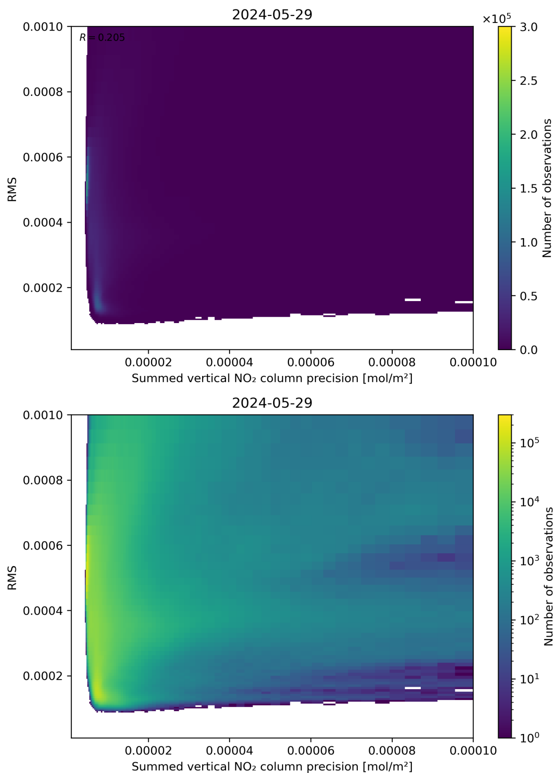
Figure 108: Scatter density plot of “Summed vertical NO 2 column precision” against “RMS” for 2024-05-28 to 2024-05-30.
