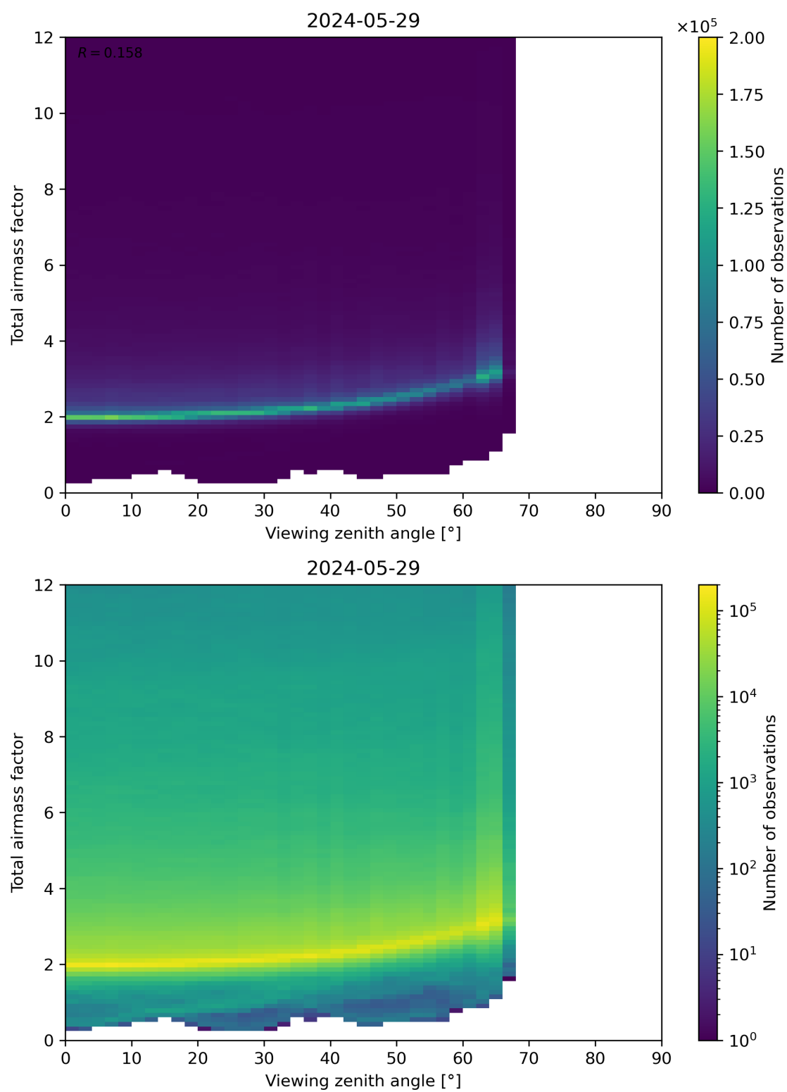
Figure 160: Scatter density plot of “Viewing zenith angle” against “Total airmass factor” for 2024-05-28 to 2024-05-30.
