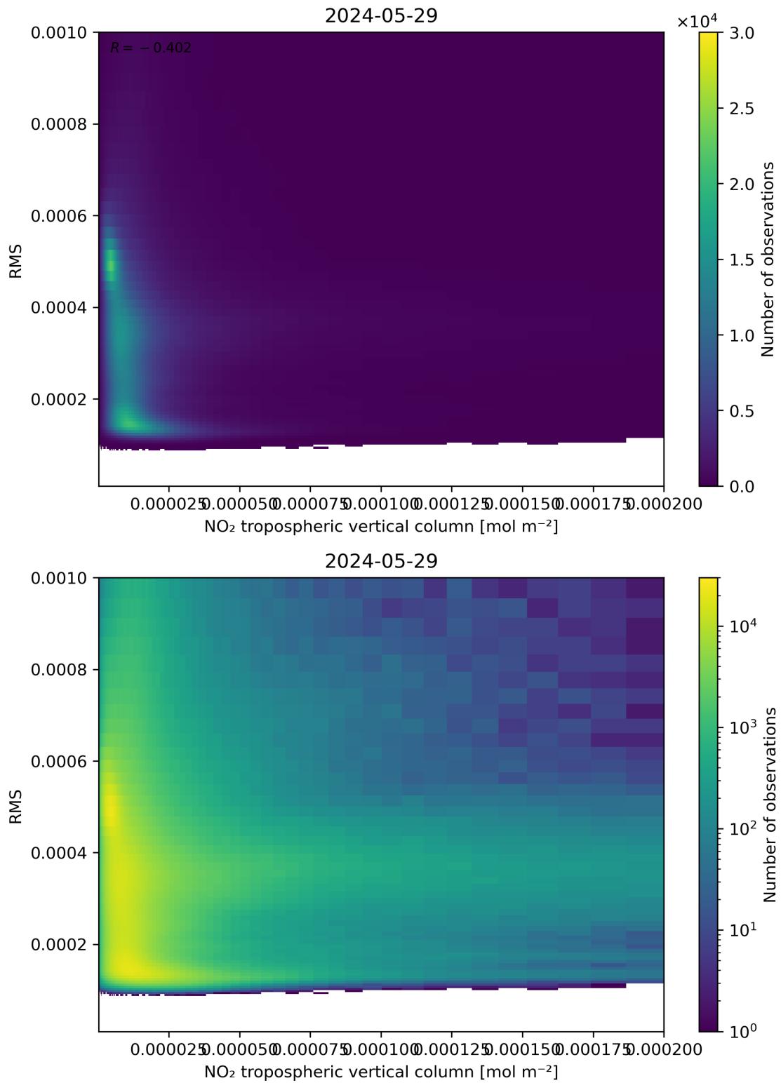
Figure 142: Scatter density plot of “NO 2 tropospheric vertical column” against “RMS” for 2024-05-28 to 2024-05-30.
