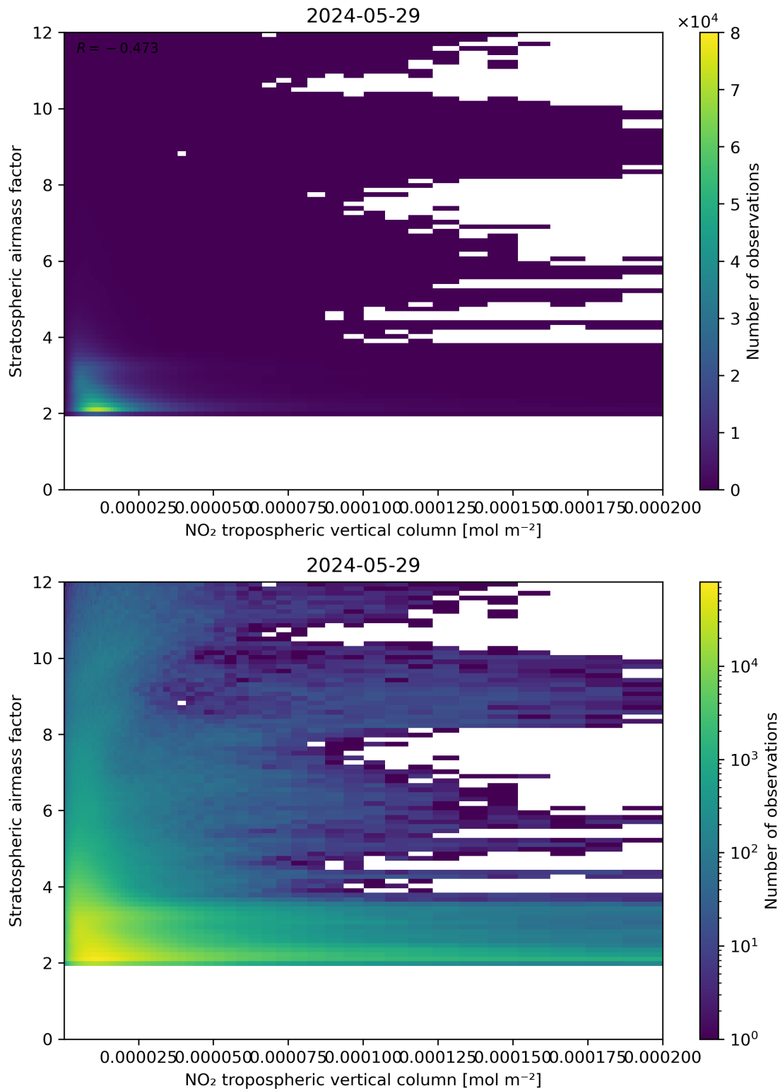
Figure 121: Scatter density plot of “NO 2 tropospheric vertical column” against “Stratospheric air mass factor” for 2024-05-28 to 2024-05-30.
