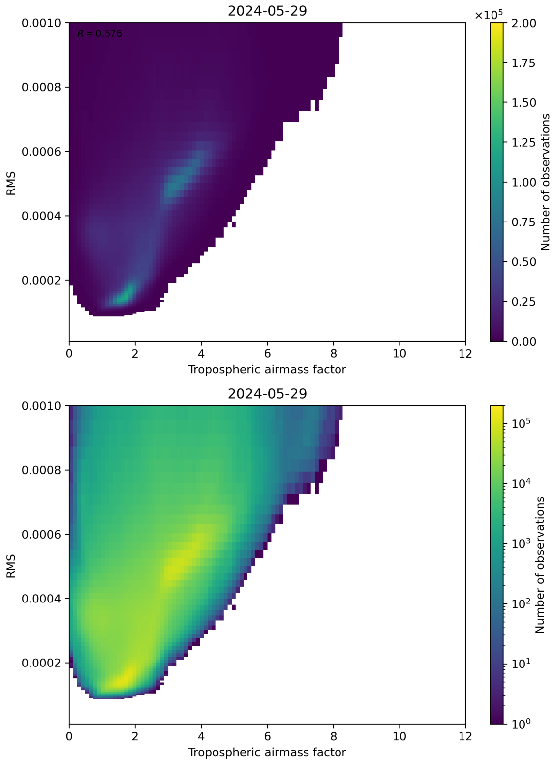
Figure 79: Scatter density plot of “Tropospheric airmass factor” against “RMS” for 2024-05-28 to 2024-05-30.
