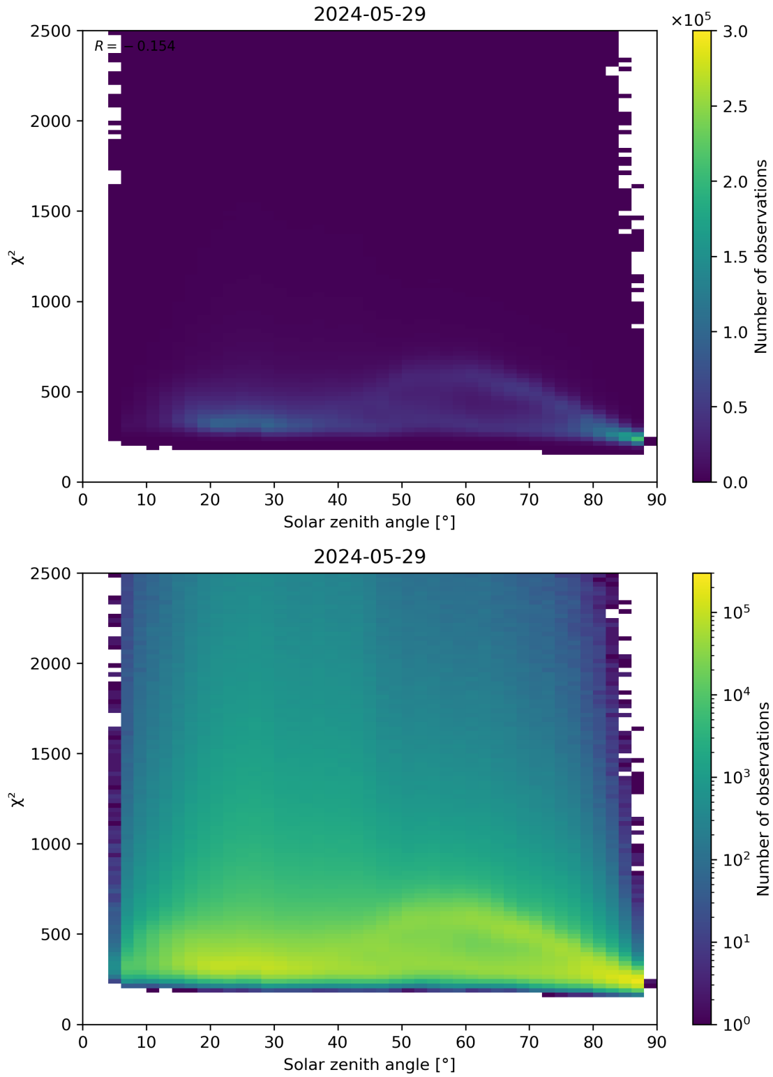
Figure 148: Scatter density plot of “Solar zenith angle” against “ \chi^2 ” for 2024-05-28 to 2024-05-30.
