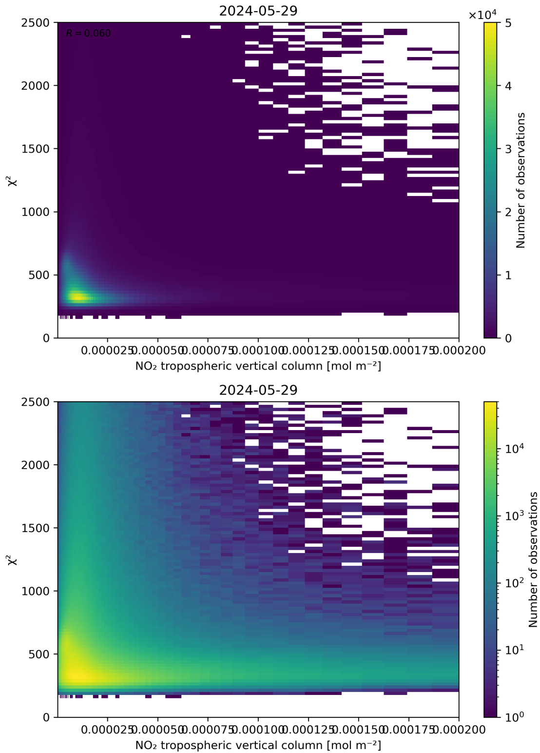
Figure 124: Scatter density plot of “NO 2 tropospheric vertical column” against “ \chi^2 ” for 2024-05-28 to 2024-05-30.
