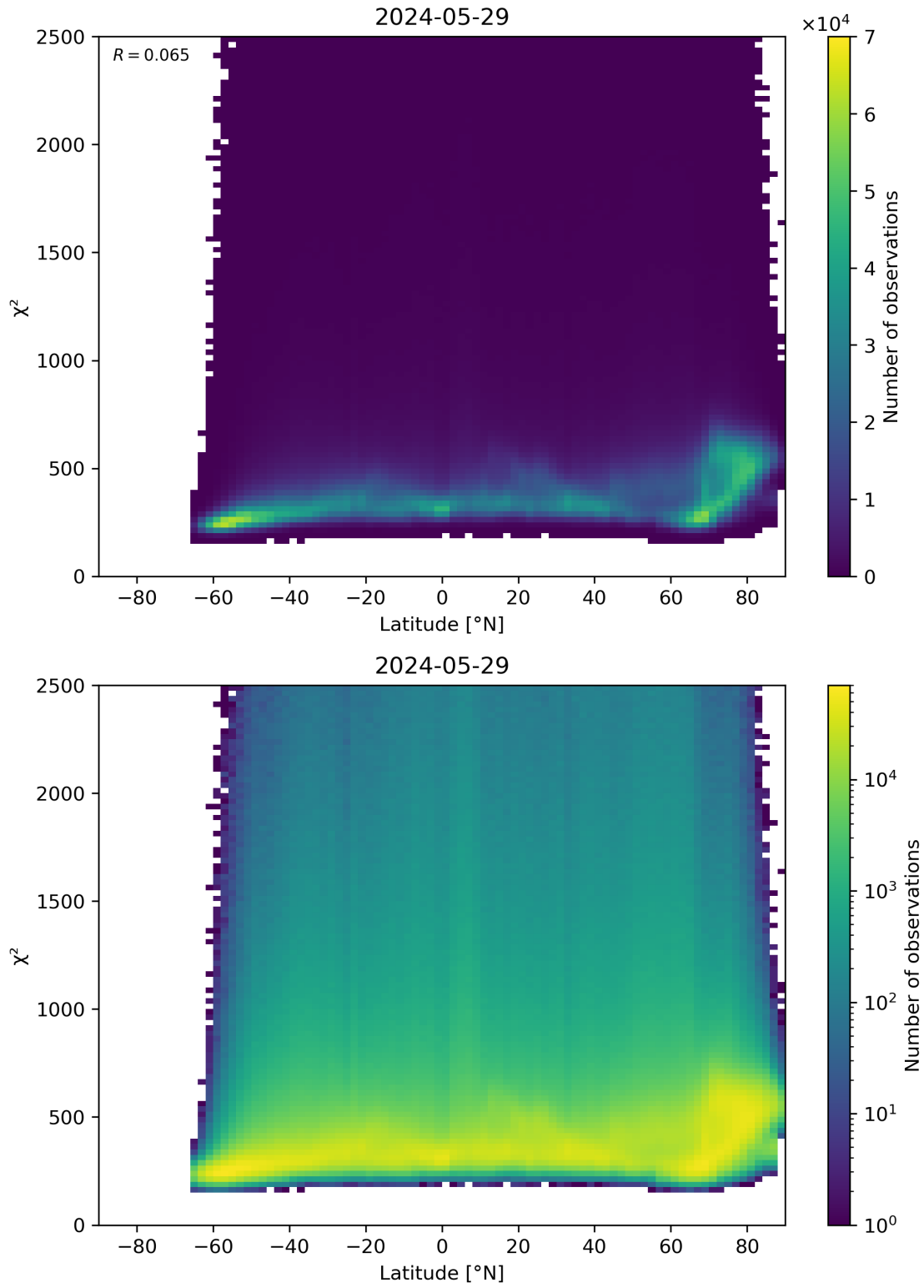
Figure 86: Scatter density plot of “Latitude” against “ \chi^2 ” for 2024-05-28 to 2024-05-30.
