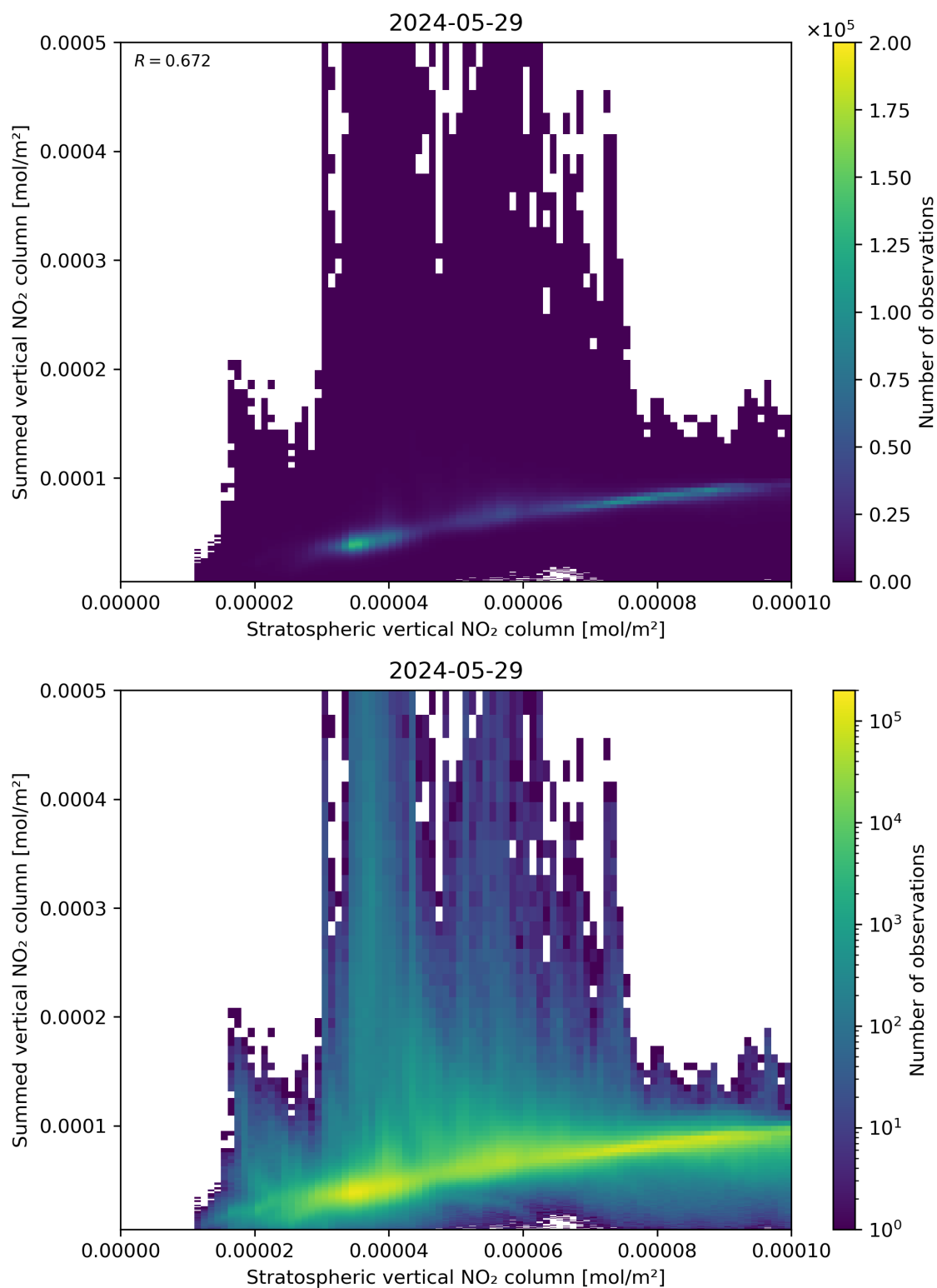
Figure 98: Scatter density plot of “Stratospheric vertical NO 2 column” against “Summed vertical NO 2 column” for 2024-05-28 to 2024-05-30.
