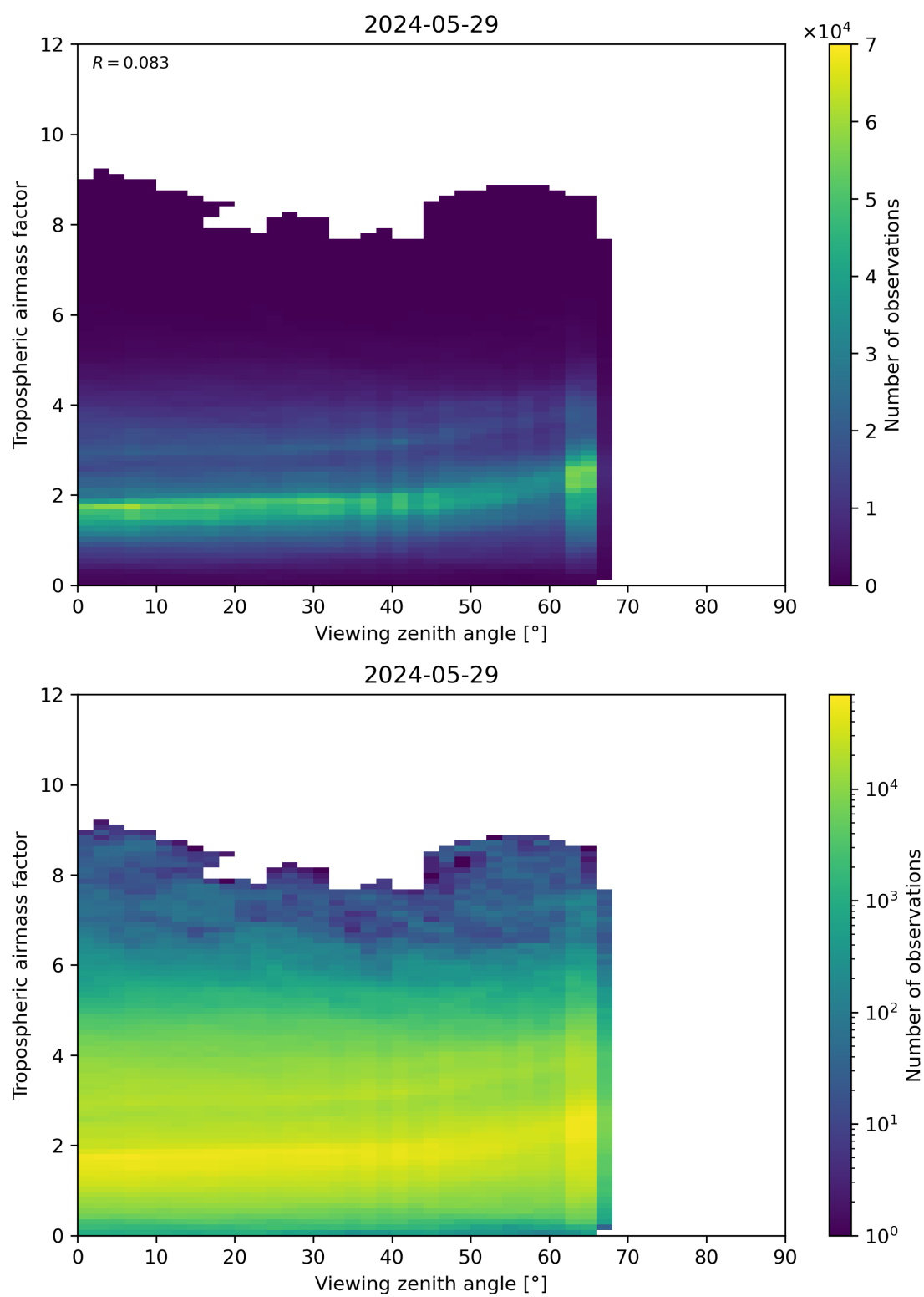
Figure 161: Scatter density plot of “Viewing zenith angle” against “Tropospheric airmass factor” for 2024-05-28 to 2024-05-30.
