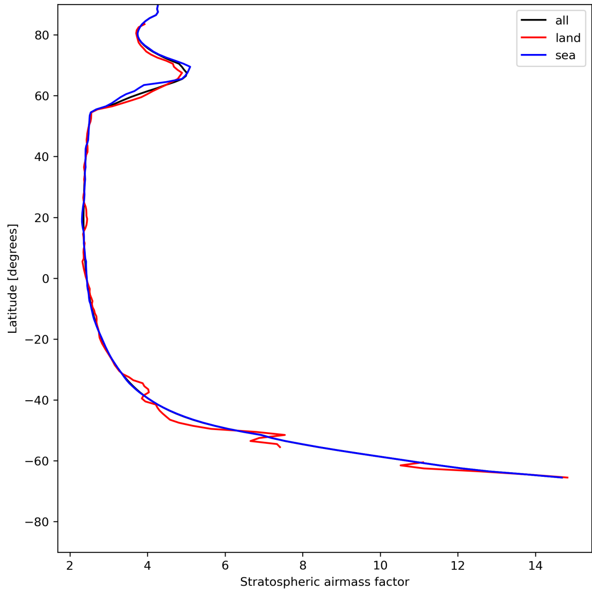
Figure 27: Zonal average of “Stratospheric airmass factor” for 2024-05-28 to 2024-05-30.
