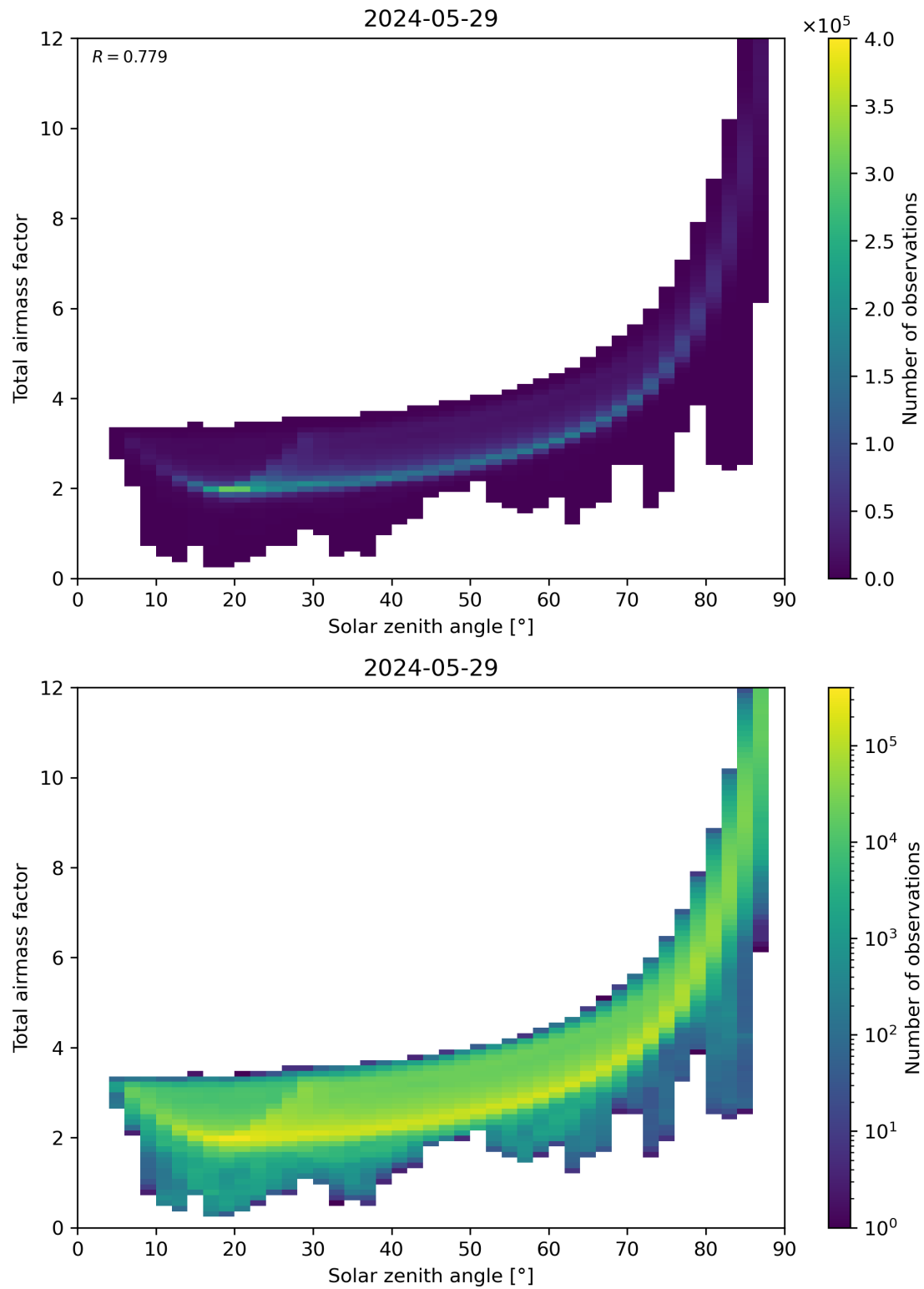
Figure 146: Scatter density plot of “Solar zenith angle” against “Total air mass factor” for 2024-05-28 to 2024-05-30.
