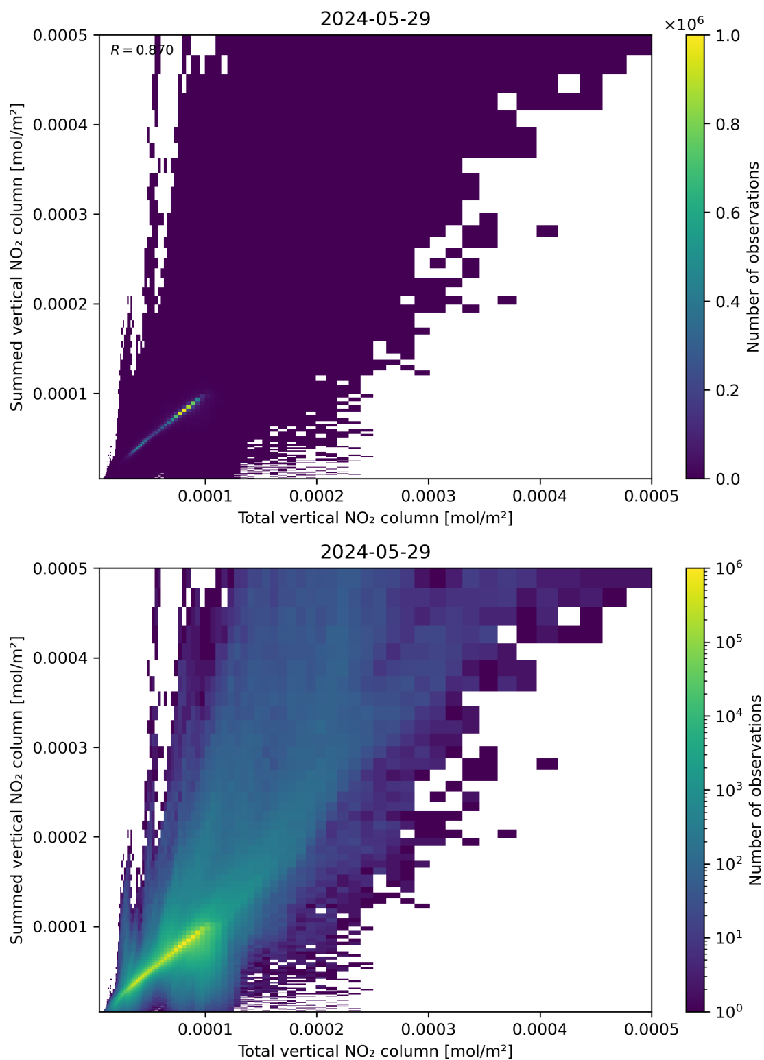
Figure 112: Scatter density plot of “Total vertical NO 2 column” against “Summed vertical NO 2 column” for 2024-05-28 to 2024-05-30.
