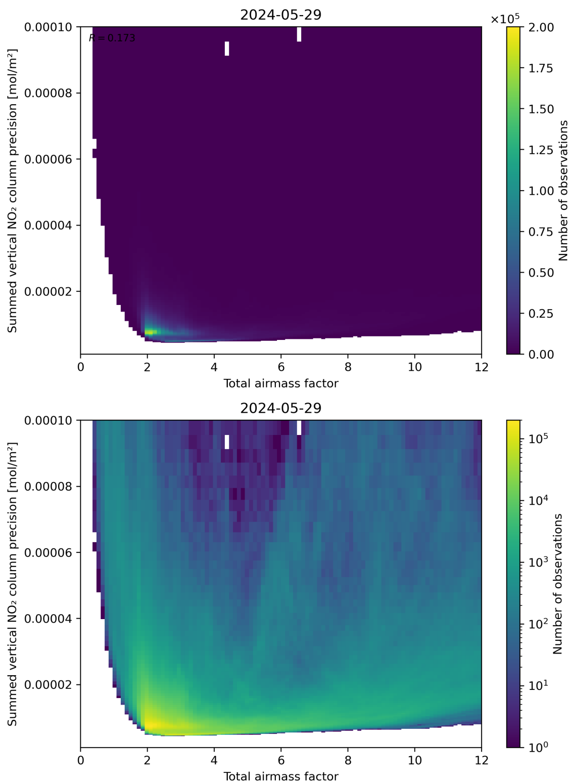
Figure 66: Scatter density plot of “Total airmass factor” against “Summed vertical NO 2 column precision” for 2024-05-28 to 2024-05-30.
