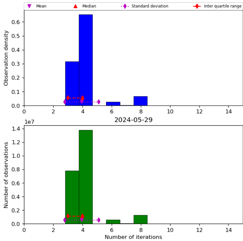
Figure 34: Histogram of “Number of iterations” for 2024-05-28 to 2024-05-30
