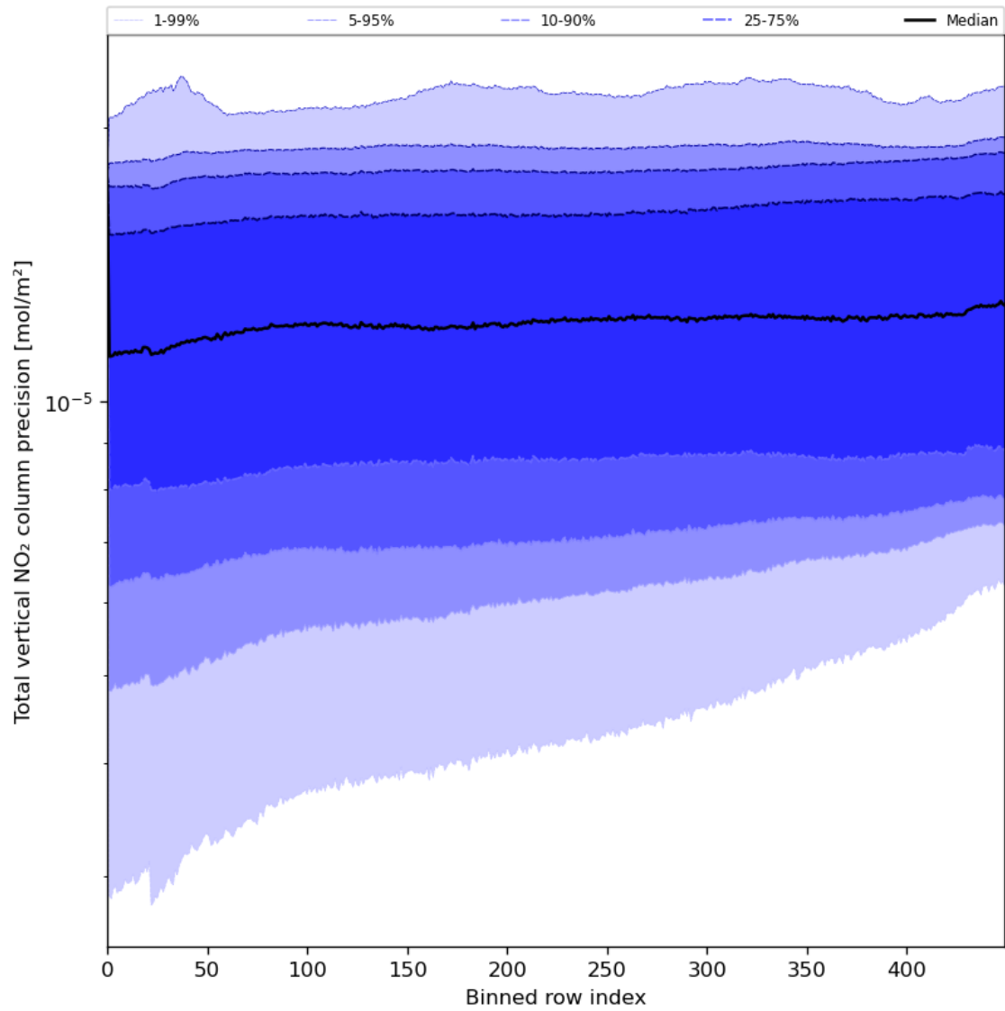
Figure 56: Along track statistics of “Total vertical NO 2 column precision” for 2024-05-28 to 2024-05-30
