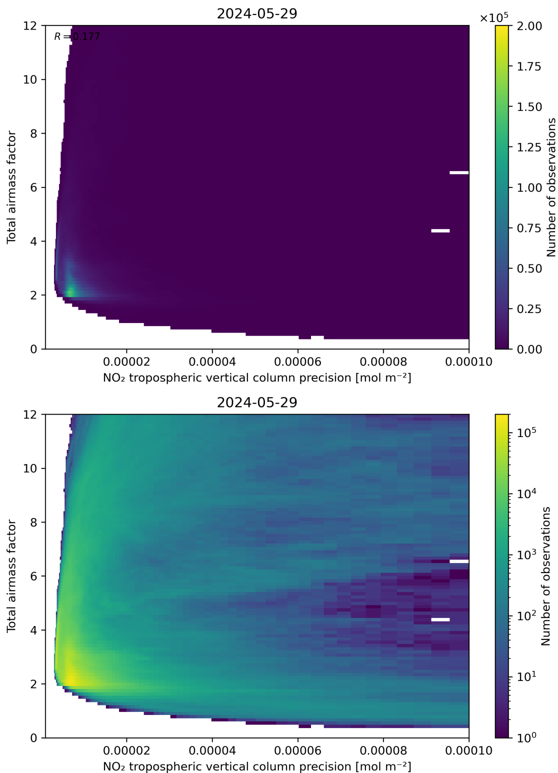
Figure 132: Scatter density plot of “NO 2 tropospheric vertical column precision” against “Total air mass factor” for 2024-05-28 to 2024-05-30.
