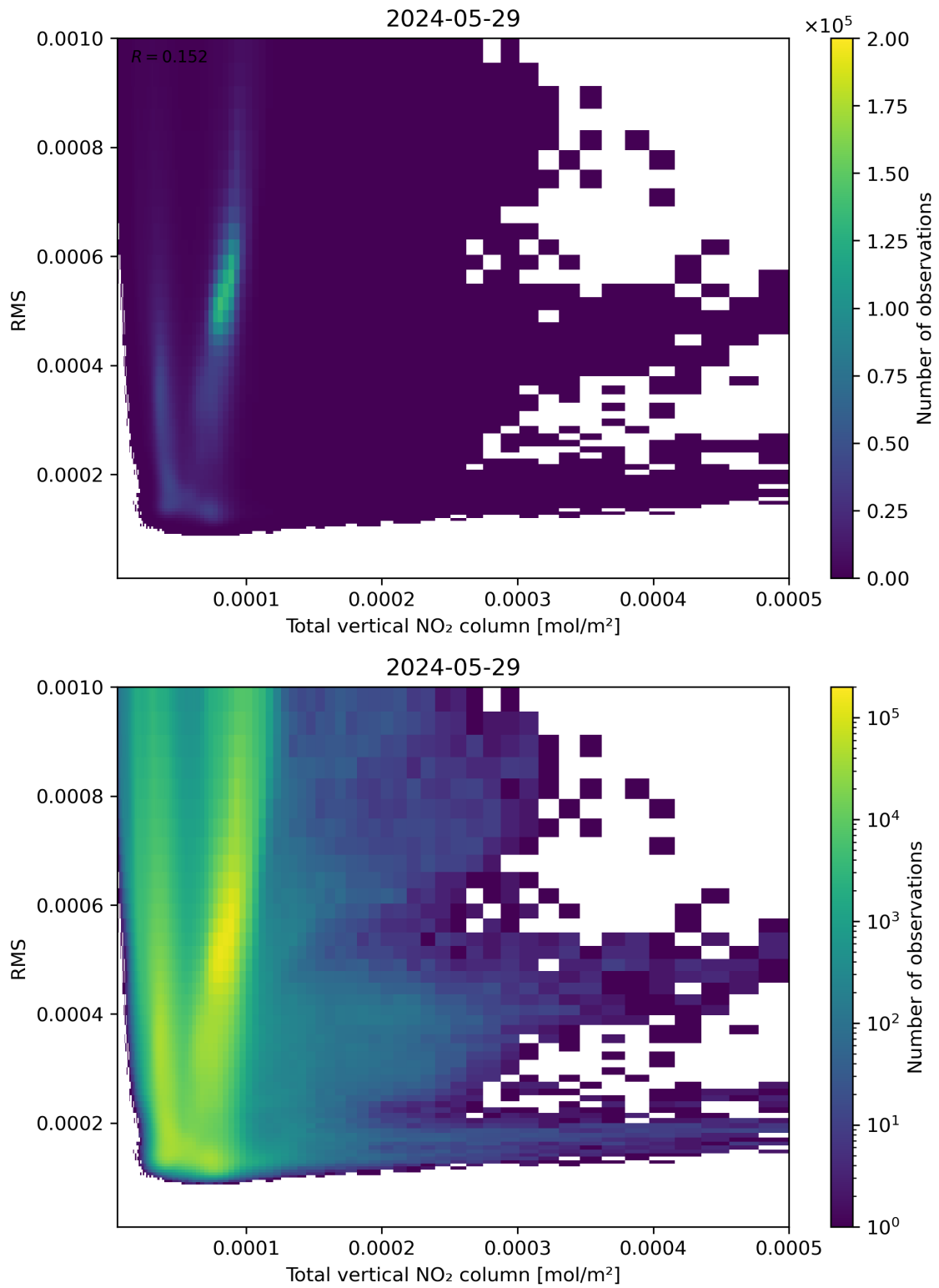
Figure 120: Scatter density plot of “Total vertical NO 2 column” against “RMS” for 2024-05-28 to 2024-05-30.
