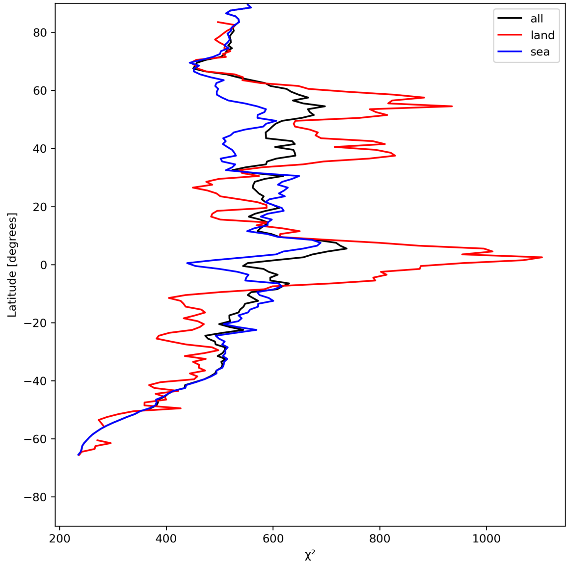
Figure 25: Zonal average of “ \chi^2 ” for 2024-05-28 to 2024-05-30.
