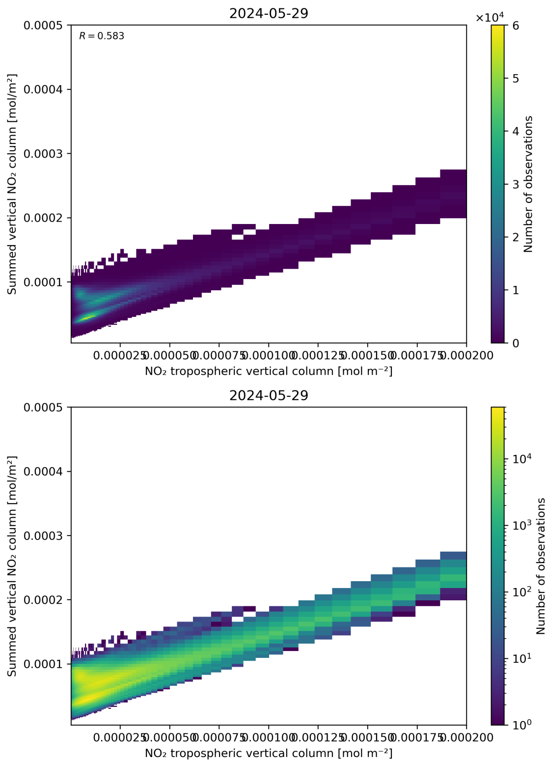
Figure 126: Scatter density plot of “NO 2 tropospheric vertical column” against “Summed vertical NO 2 column” for 2024-05-28 to 2024-05-30.
