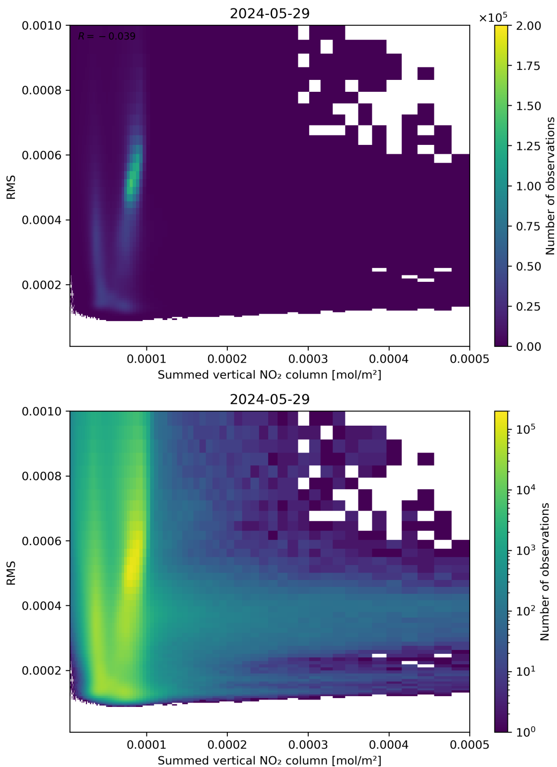
Figure 109: Scatter density plot of “Summed vertical NO 2 column” against “RMS” for 2024-05-28 to 2024-05-30.
