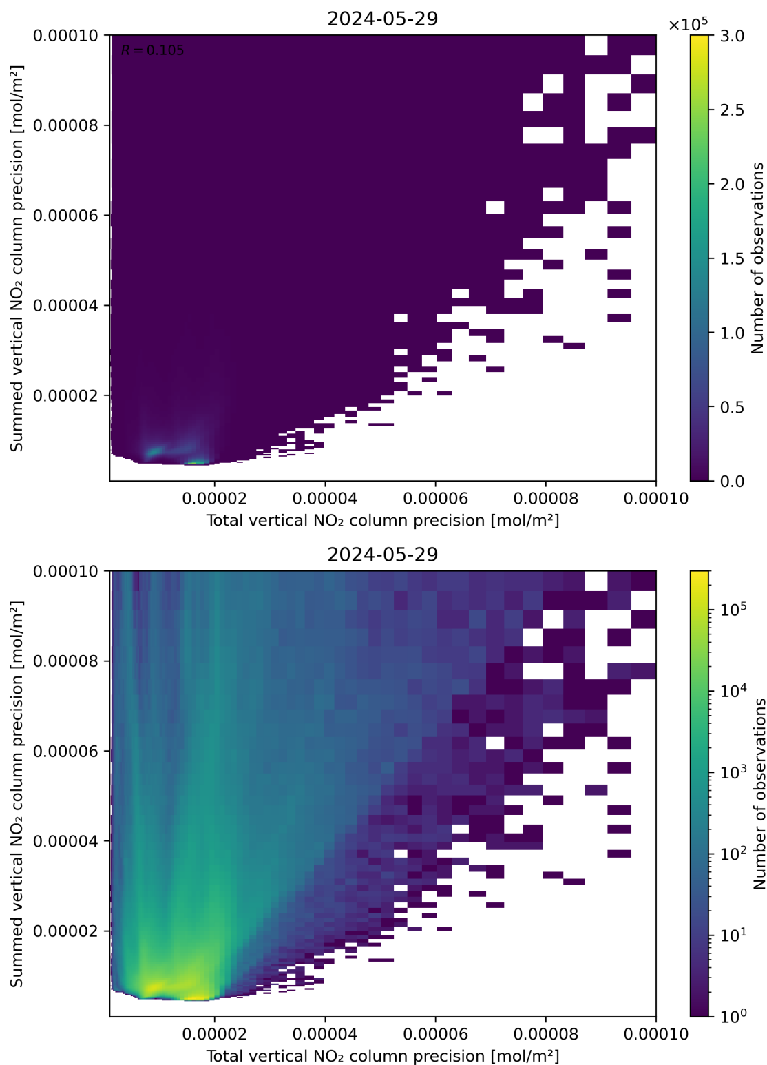
Figure 118: Scatter density plot of “Total vertical NO 2 column precision” against “Summed vertical NO 2 column precision” for 2024-05-28 to 2024-05-30.
