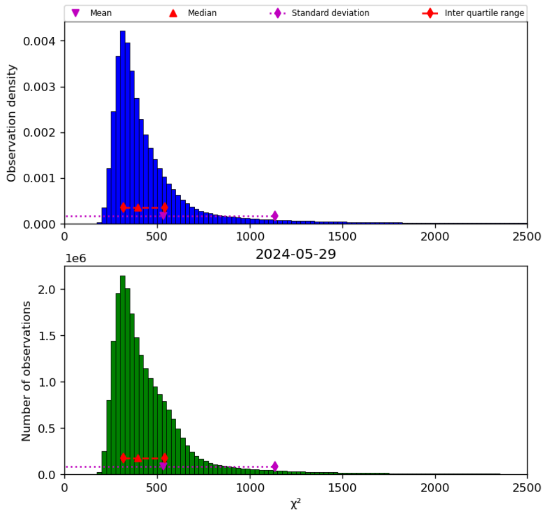
Figure 42: Histogram of “ \chi^2 ” for 2024-05-28 to 2024-05-30
