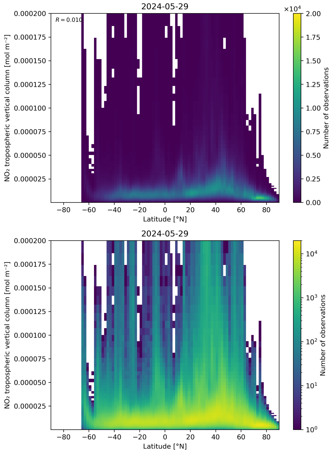
Figure 92: Scatter density plot of “Latitude” against “NO 2 tropospheric vertical column” for 2024-05-28 to 2024-05-30.
