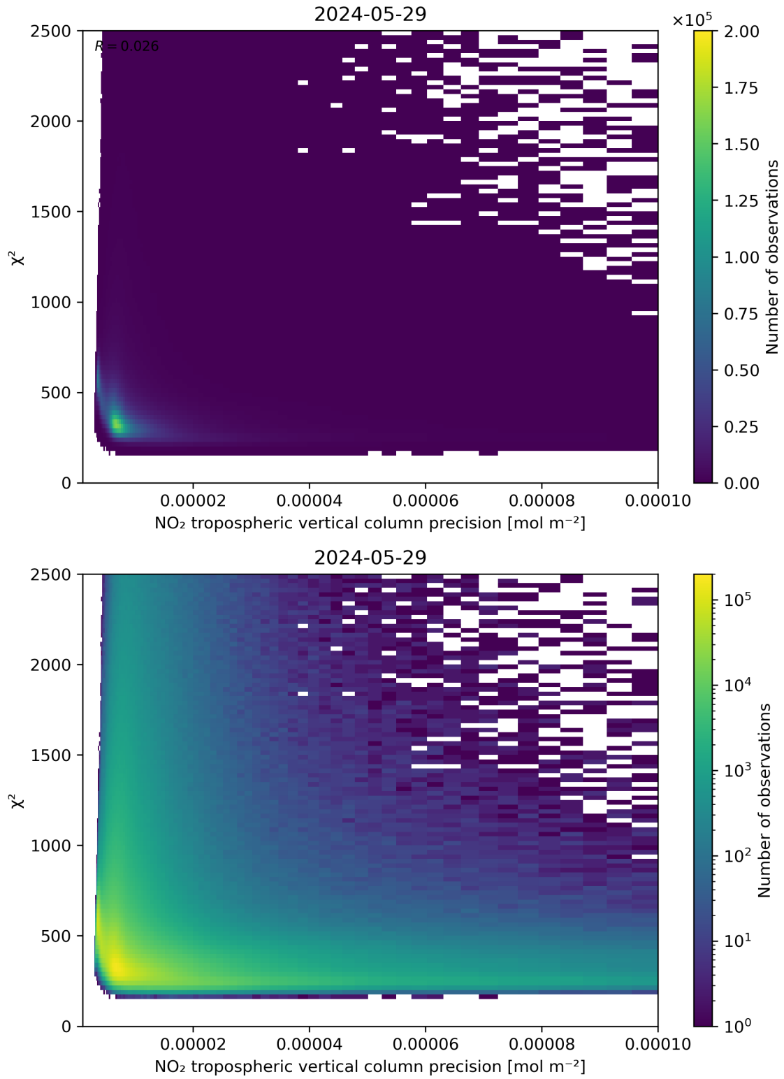
Figure 134: Scatter density plot of “NO 2 tropospheric vertical column precision” against “ \chi^2 ” for 2024-05-28 to 2024-05-30.
