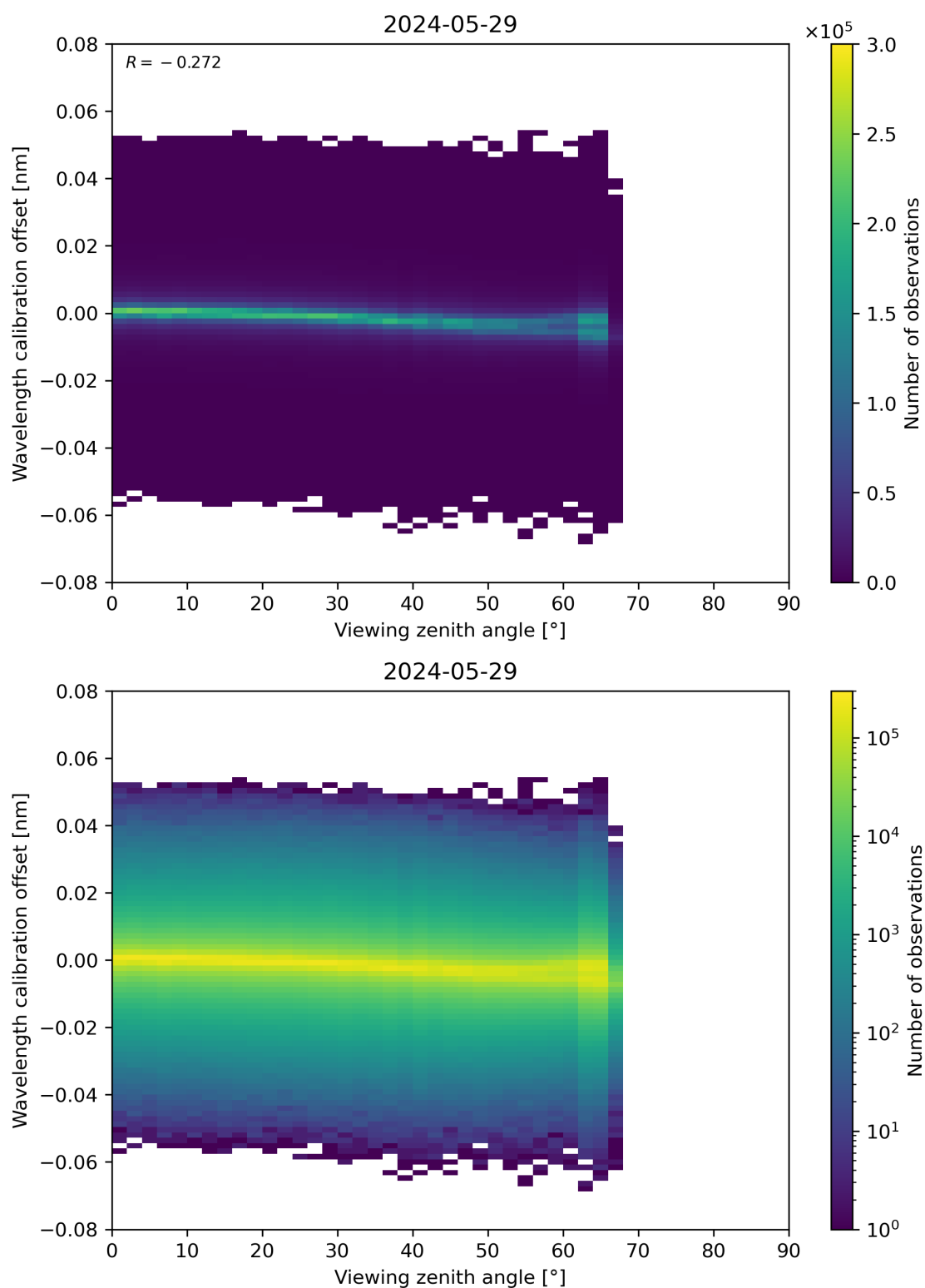
Figure 173: Scatter density plot of “Viewing zenith angle” against “Wavelength calibration offset” for 2024-05-28 to 2024-05-30.
