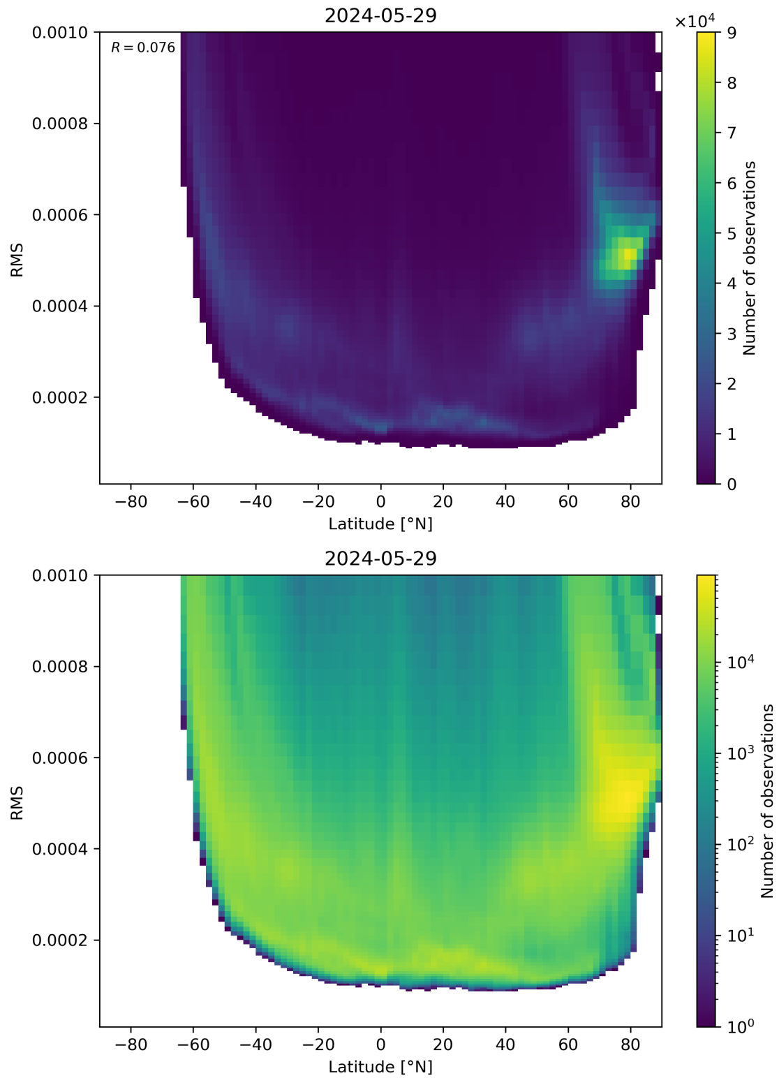
Figure 94: Scatter density plot of “Latitude” against “RMS” for 2024-05-28 to 2024-05-30.
