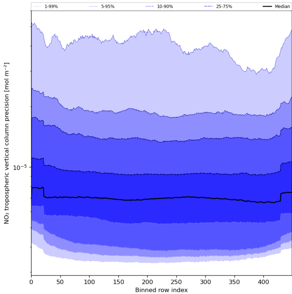
Figure 47: Along track statistics of “NO 2 tropospheric vertical column precision” for 2024-05-28 to 2024-05-30
