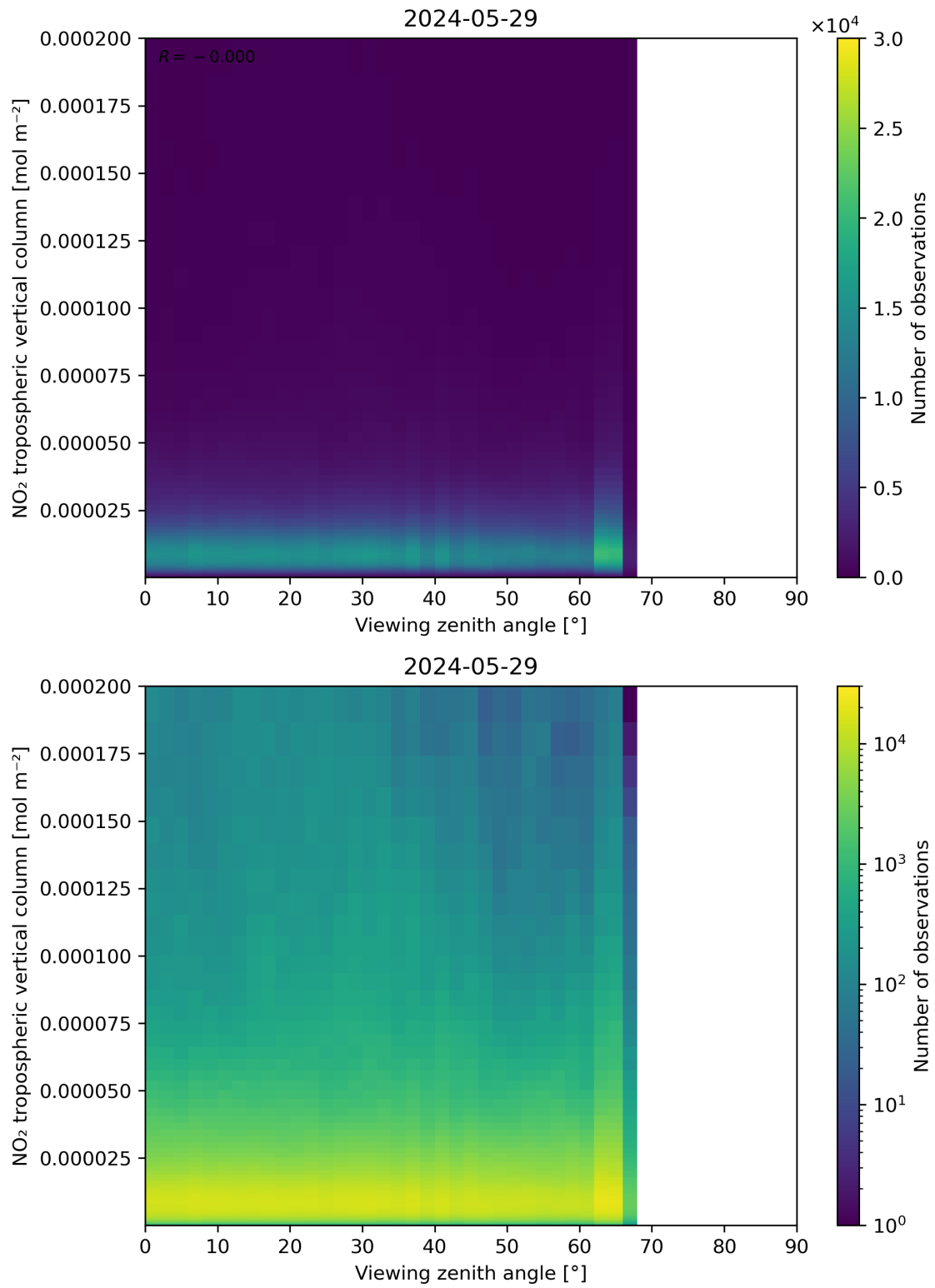
Figure 169: Scatter density plot of “Viewing zenith angle” against “NO 2 tropospheric vertical column” for 2024-05-28 to 2024-05-30.
