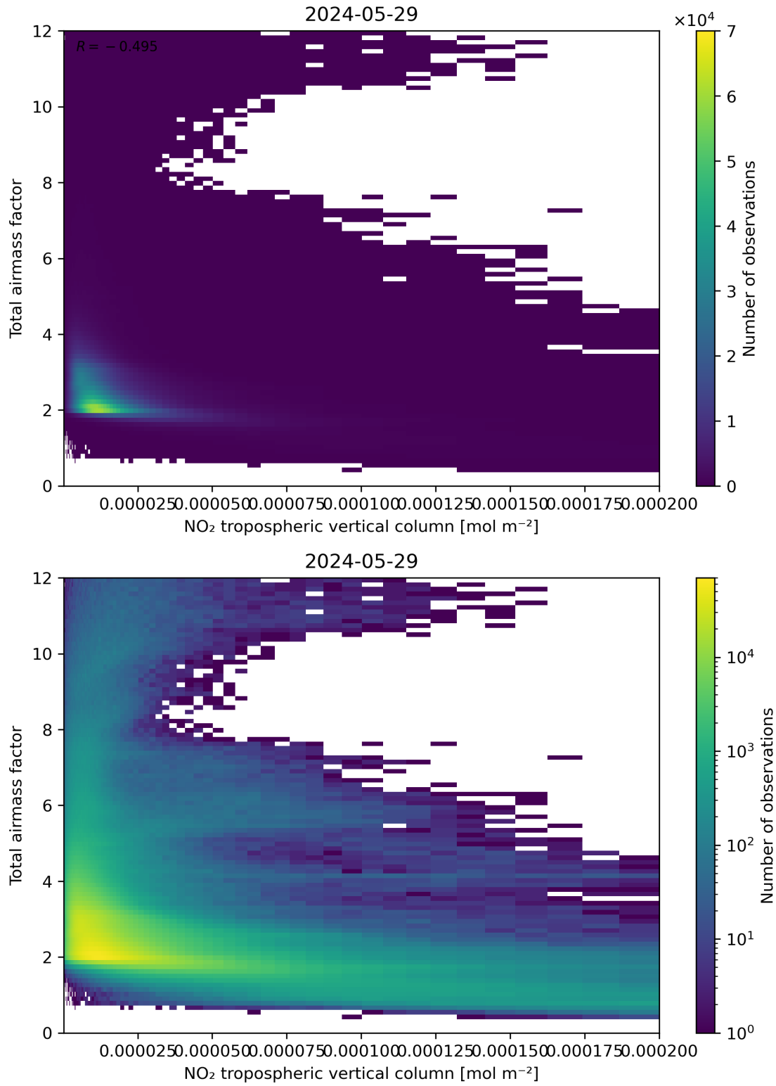
Figure 122: Scatter density plot of “NO 2 tropospheric vertical column” against “Total air mass factor” for 2024-05-28 to 2024-05-30.
