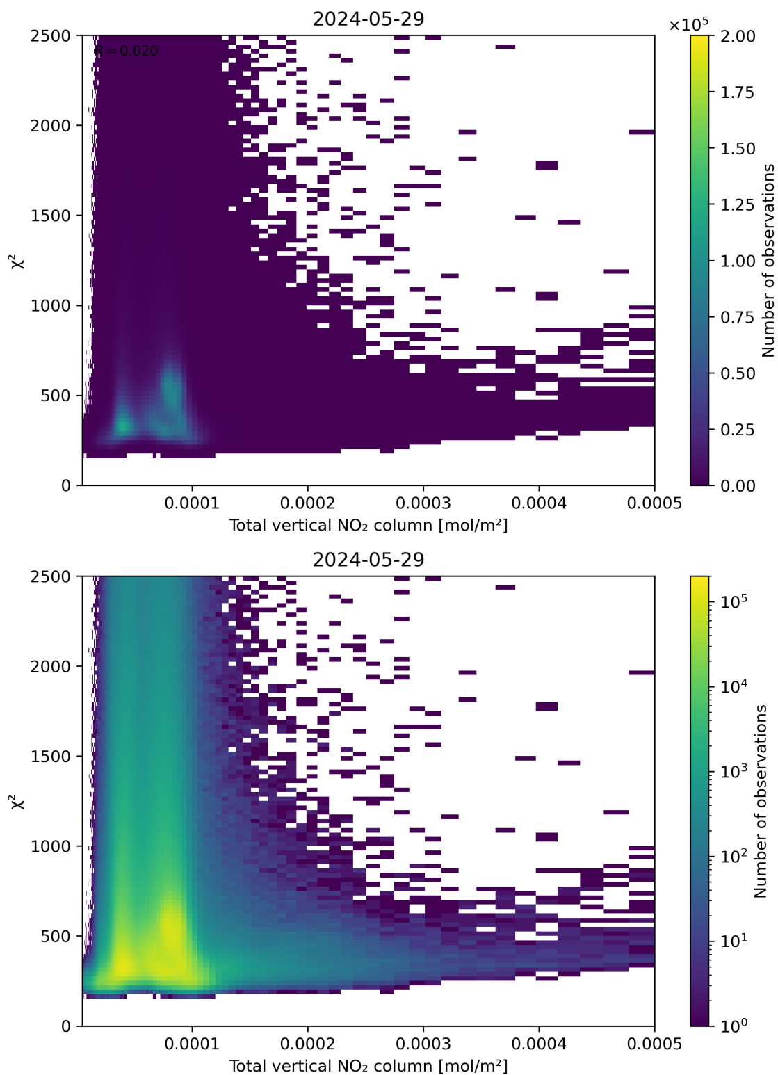
Figure 111: Scatter density plot of “Total vertical NO 2 column” against “ \chi^2 ” for 2024-05-28 to 2024-05-30.
