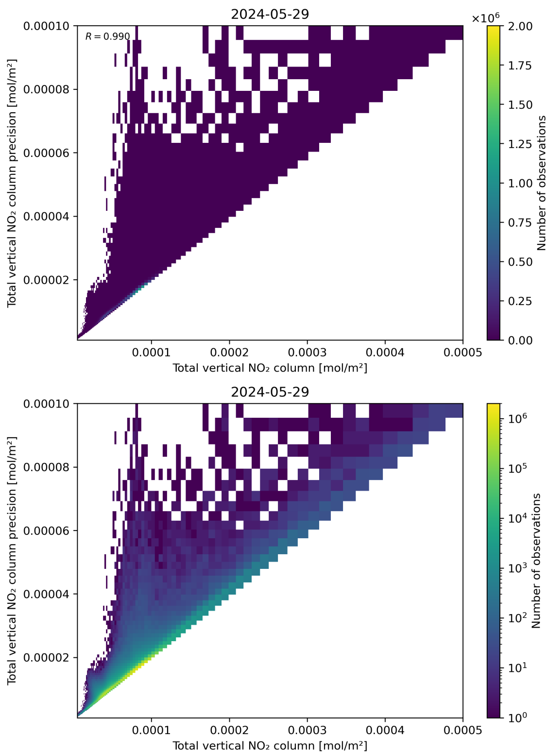
Figure 114: Scatter density plot of “Total vertical NO 2 column” against “Total vertical NO 2 column precision” for 2024-05-28 to 2024-05-30.
