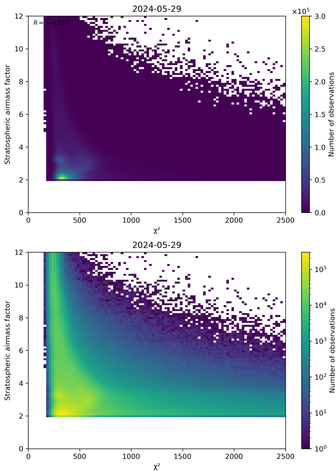
Figure 81: Scatter density plot of “ \chi^2 ” against “Stratospheric airmass factor” for 2024-05-28 to 2024-05-30.
