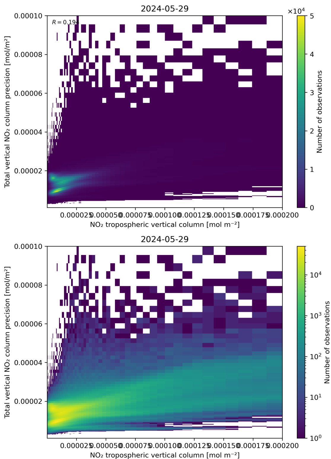
Figure 129: Scatter density plot of “NO 2 tropospheric vertical column” against “Total vertical NO 2 column precision” for 2024-05-28 to 2024-05-30.
