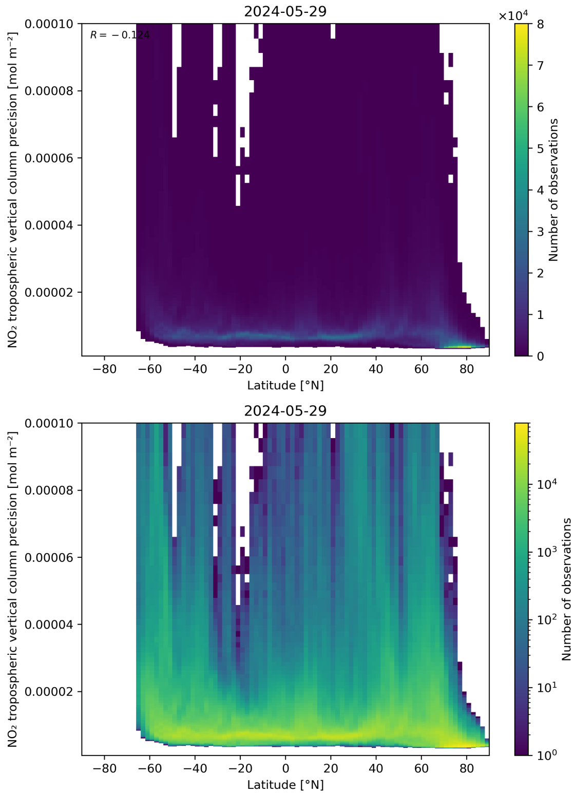
Figure 93: Scatter density plot of “Latitude” against “NO 2 tropospheric vertical column precision” for 2024-05-28 to 2024-05-30.
