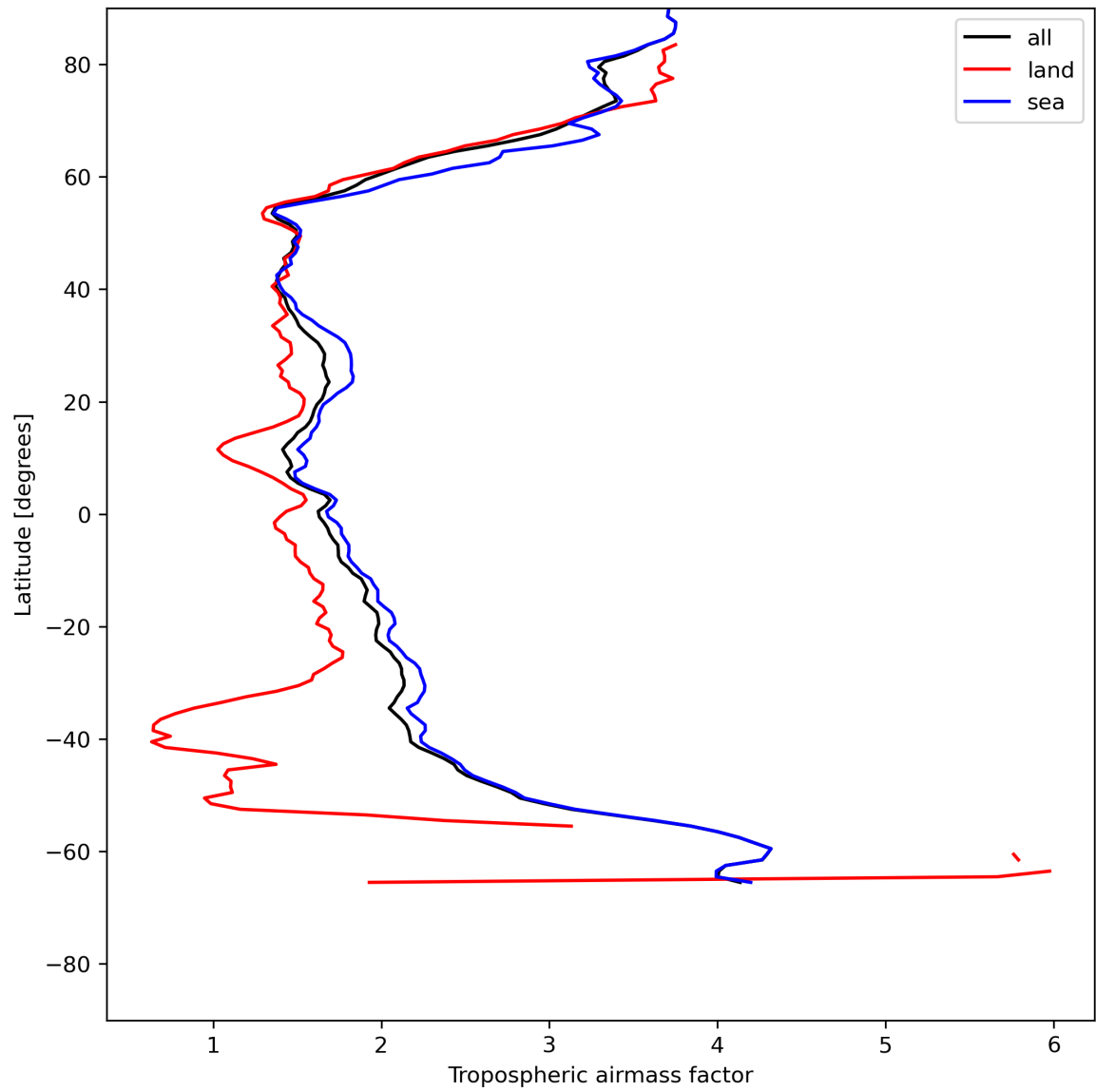
Figure 14: Zonal average of “Tropospheric airmass factor” for 2024-05-29 to 2024-05-31.
