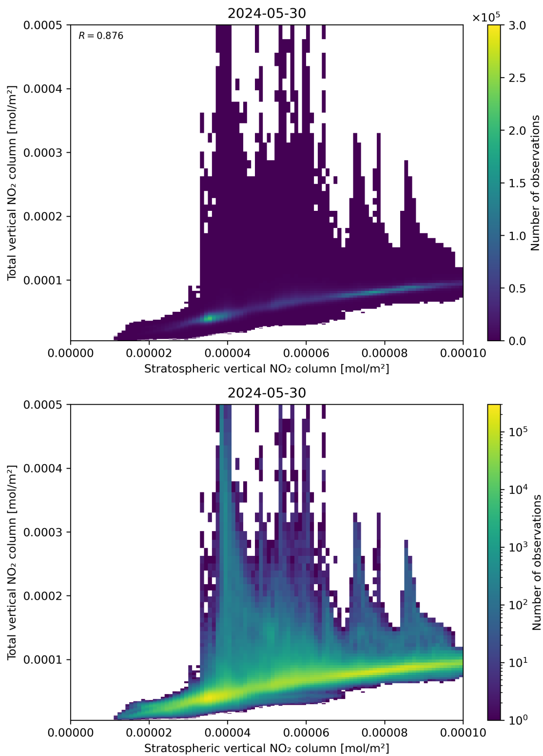
Figure 100: Scatter density plot of “Stratospheric vertical NO 2 column” against “Total vertical NO 2 column” for 2024-05-29 to 2024-05-31.
