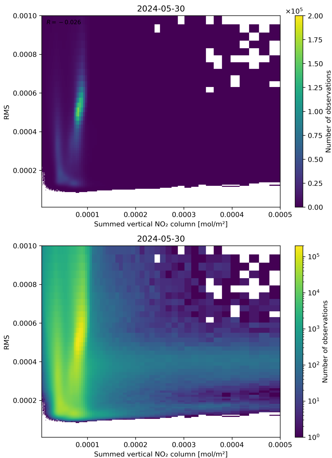
Figure 109: Scatter density plot of “Summed vertical NO 2 column” against “RMS” for 2024-05-29 to 2024-05-31.
