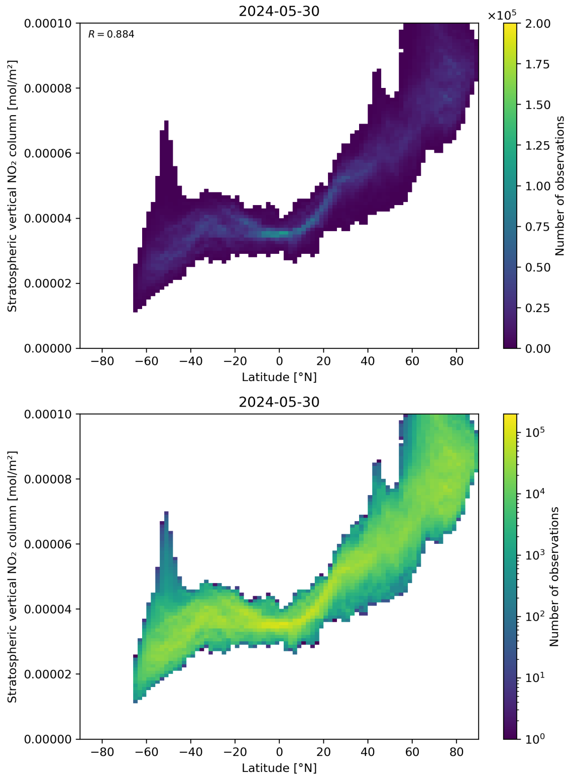
Figure 87: Scatter density plot of “Latitude” against “Stratospheric vertical NO 2 column” for 2024-05-29 to 2024-05-31.
