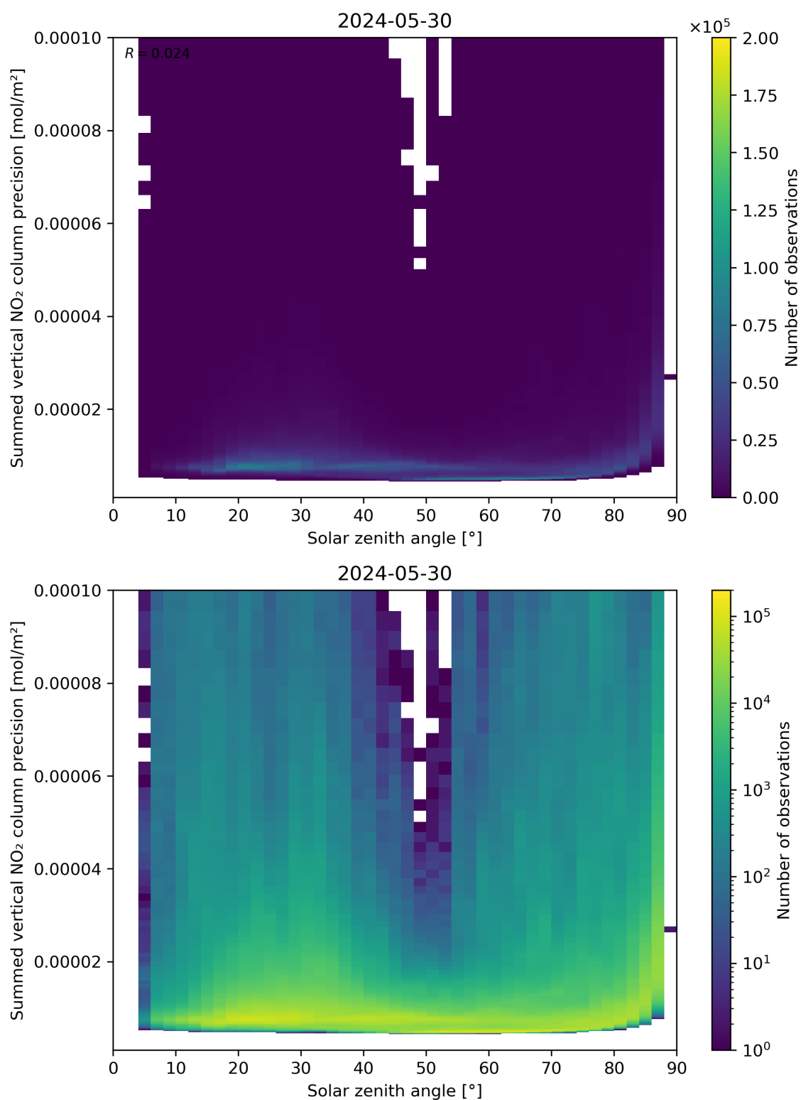
Figure 152: Scatter density plot of “Solar zenith angle” against “Summed vertical NO 2 column precision” for 2024-05-29 to 2024-05-31.
