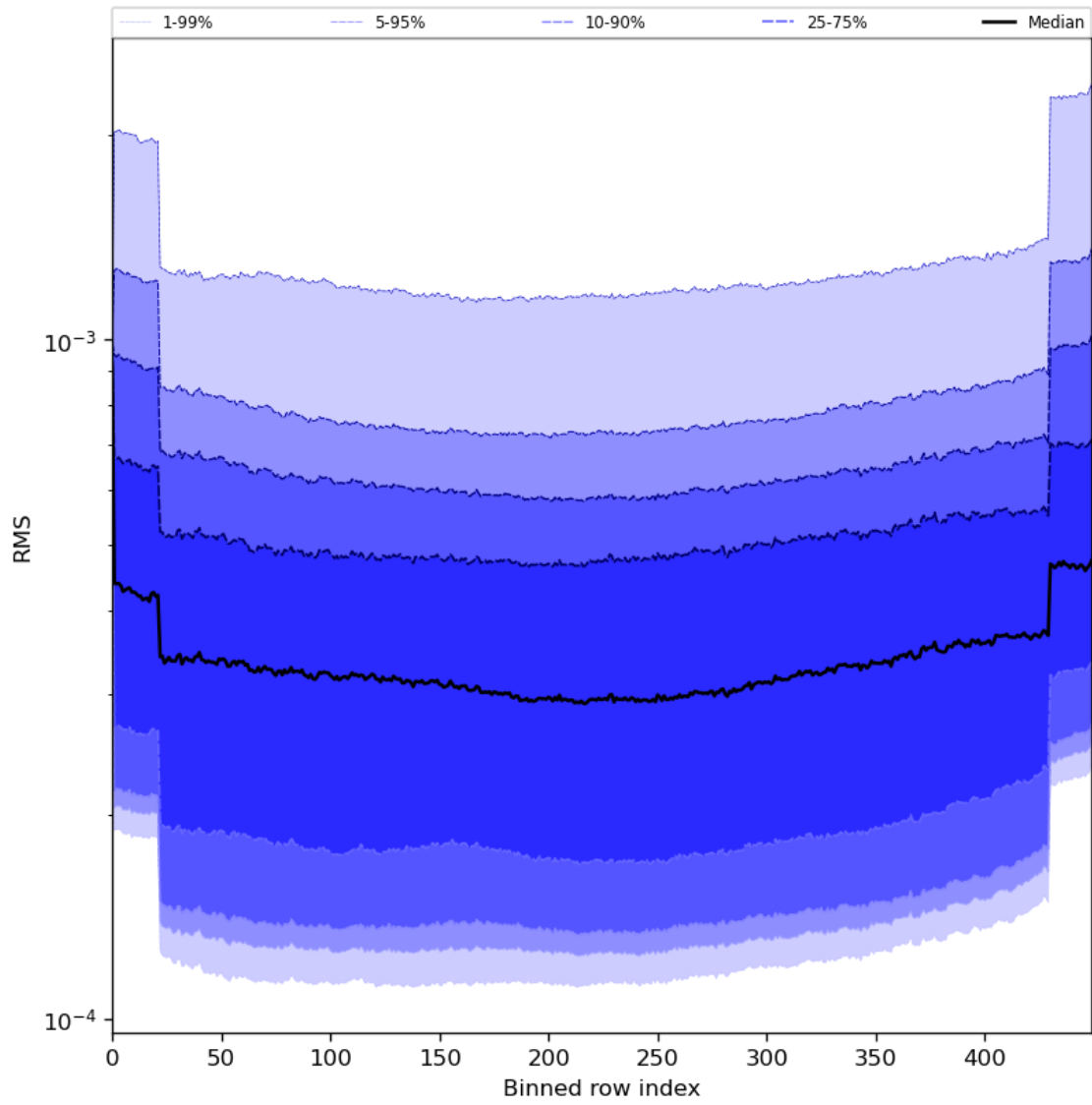
Figure 60: Along track statistics of “RMS” for 2024-05-29 to 2024-05-31
