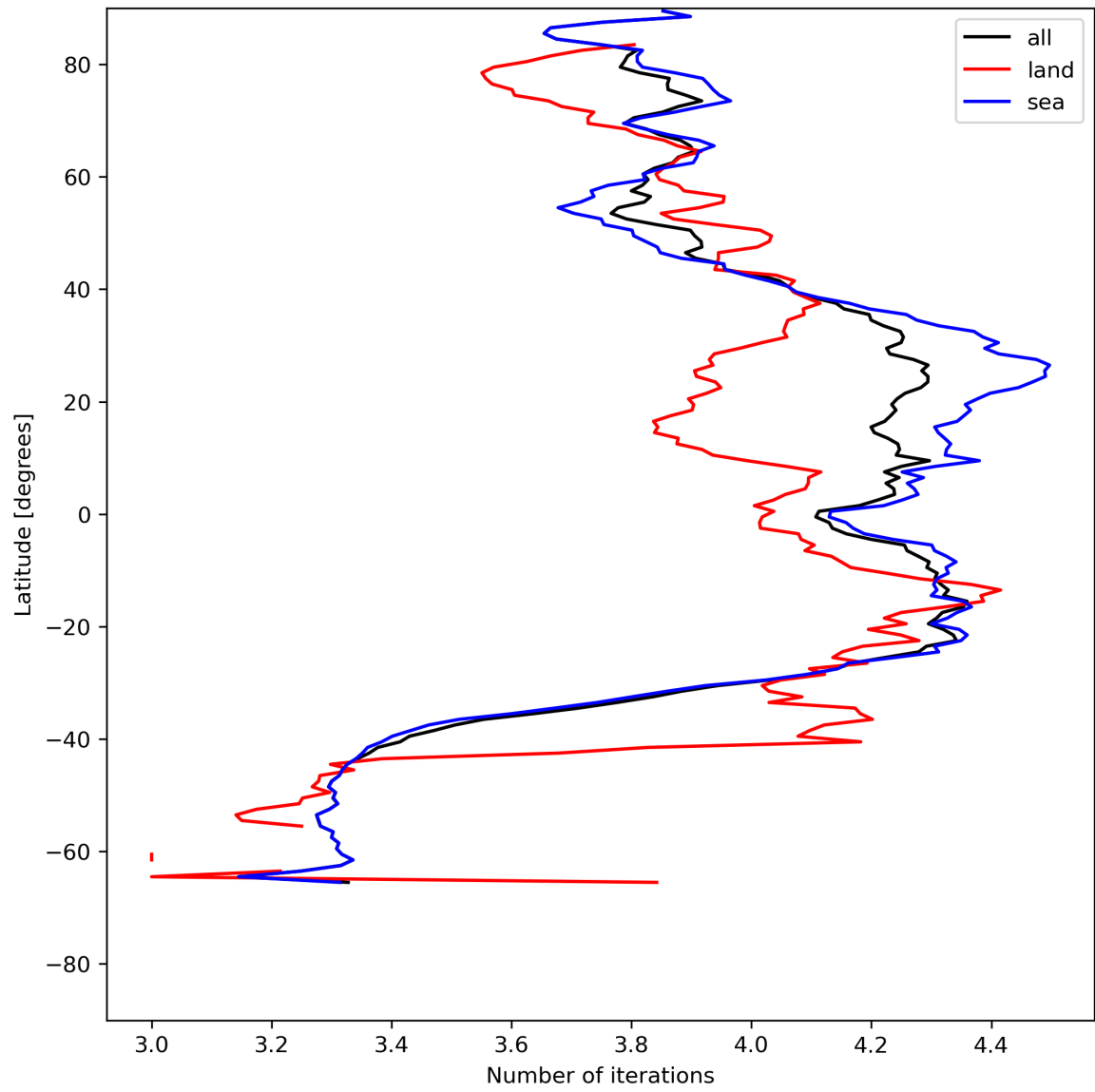
Figure 17: Zonal average of “Number of iterations” for 2024-05-29 to 2024-05-31.
