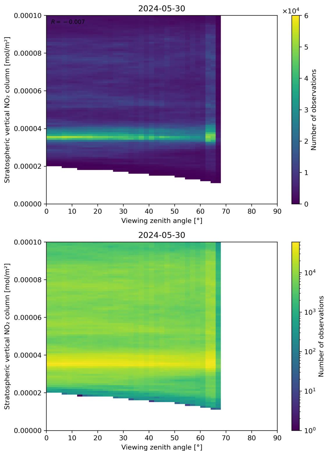
Figure 164: Scatter density plot of “Viewing zenith angle” against “Stratospheric vertical NO 2 column” for 2024-05-29 to 2024-05-31.
