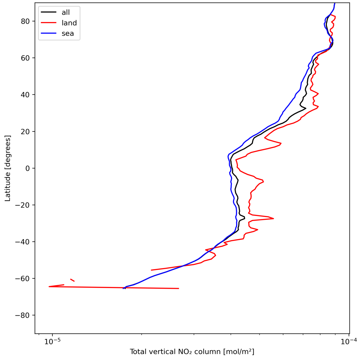
Figure 21: Zonal average of “Total vertical NO 2 column” for 2024-05-29 to 2024-05-31.
