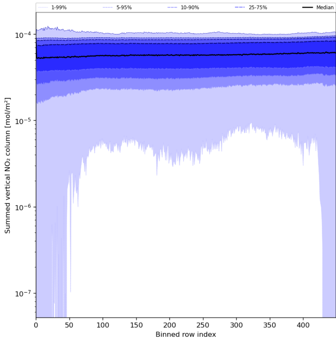
Figure 57: Along track statistics of “Summed vertical NO 2 column” for 2024-05-29 to 2024-05-31
