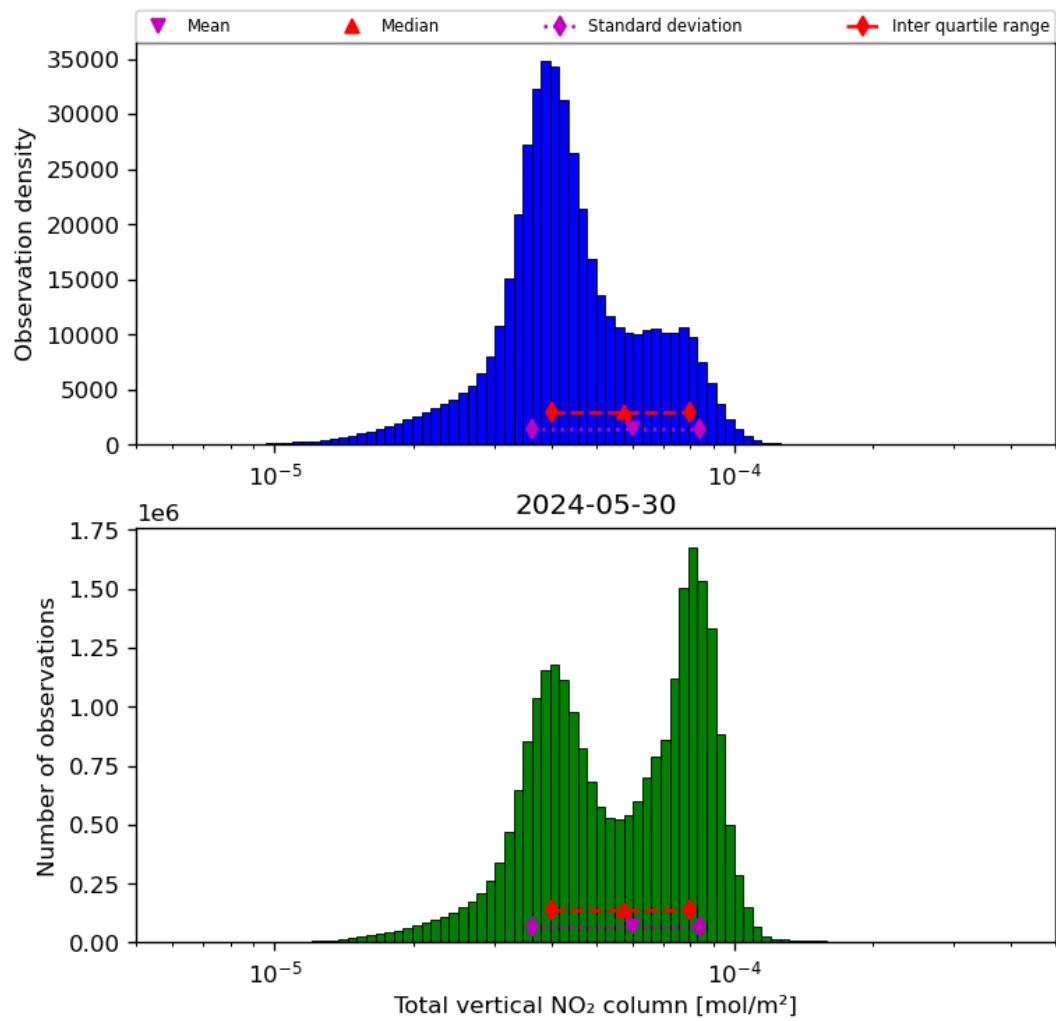
Figure 38: Histogram of “Total vertical NO 2 column” for 2024-05-29 to 2024-05-31
