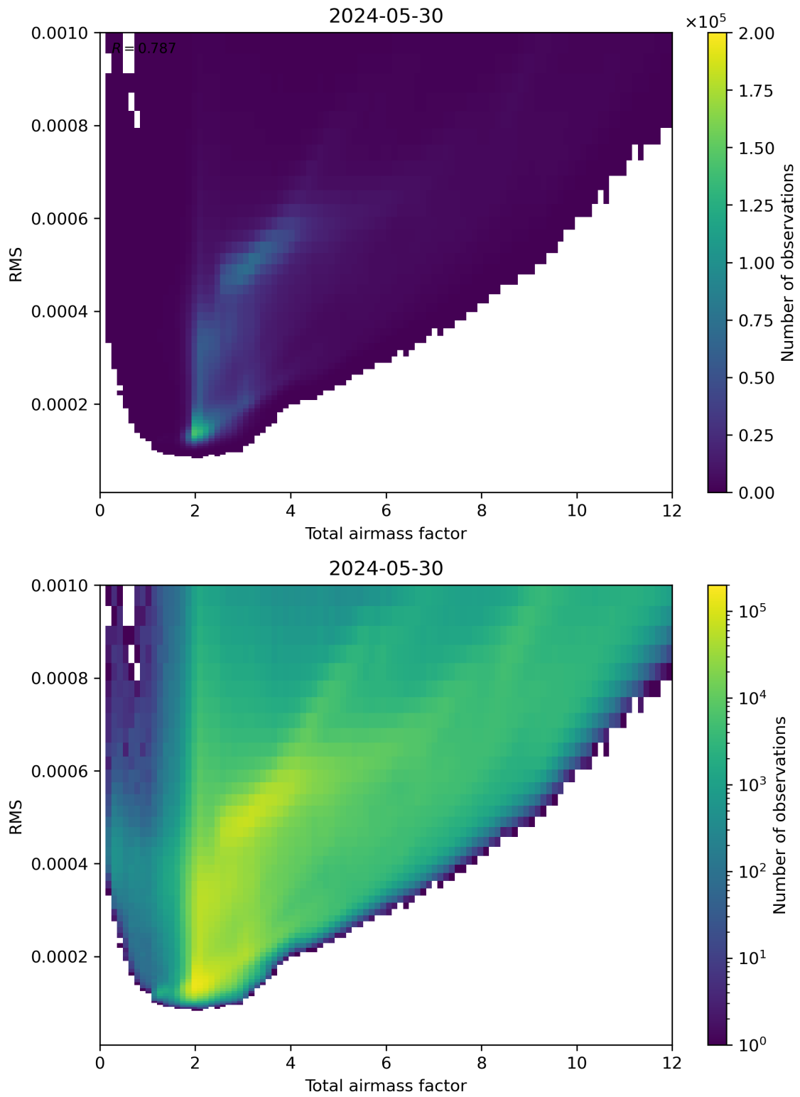
Figure 69: Scatter density plot of “Total airmass factor” against “RMS” for 2024-05-29 to 2024-05-31.
