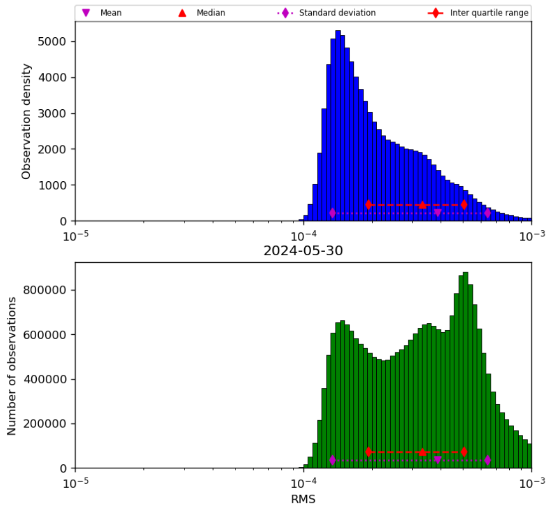
Figure 43: Histogram of “RMS” for 2024-05-29 to 2024-05-31
