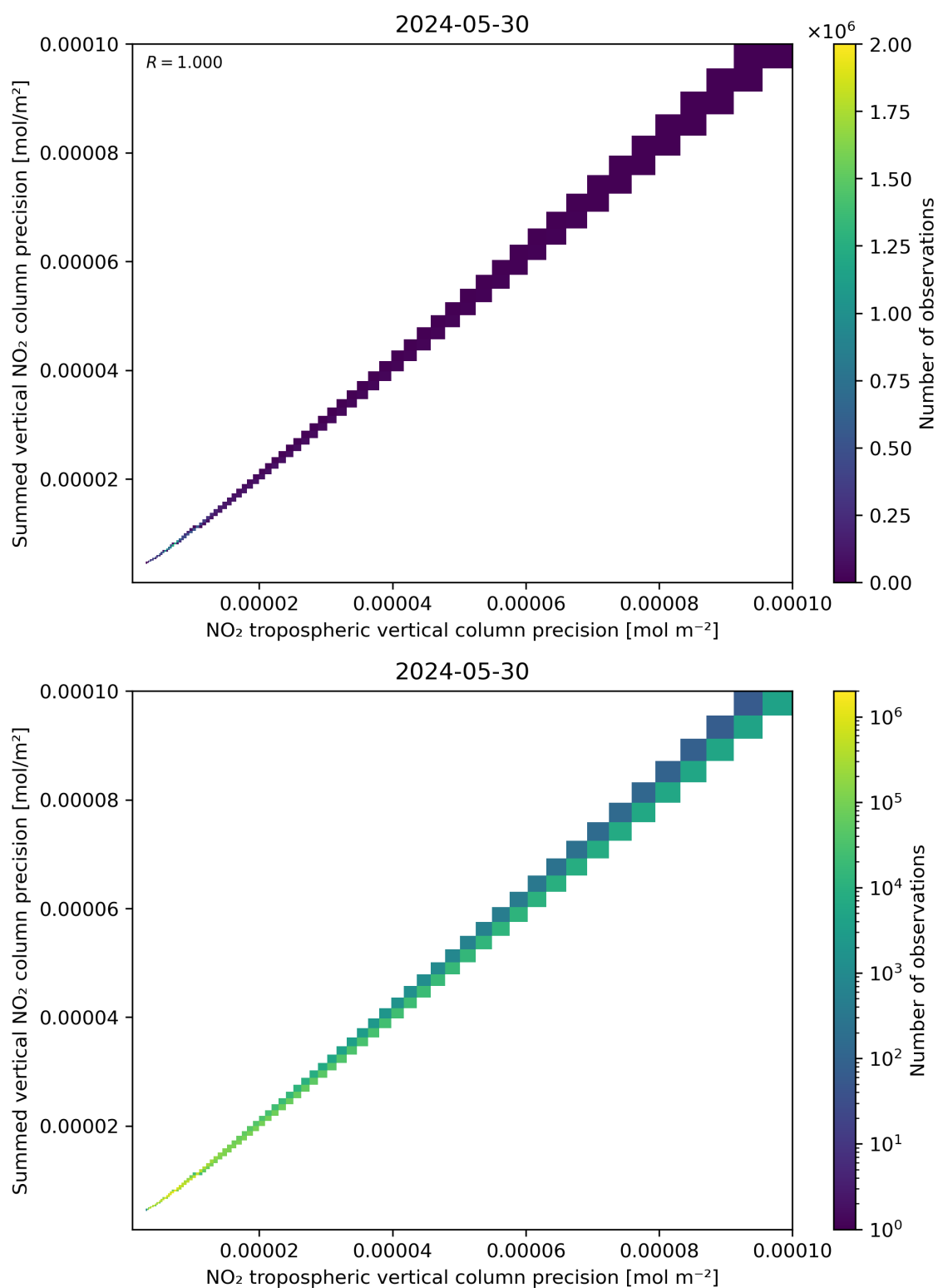
Figure 137: Scatter density plot of “NO 2 tropospheric vertical column precision” against “Summed vertical NO 2 column precision” for 2024-05-29 to 2024-05-31.
