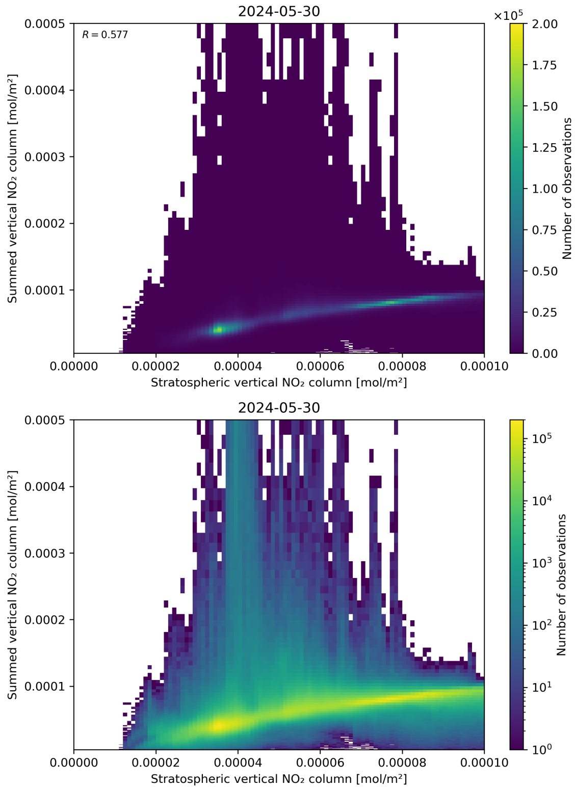
Figure 98: Scatter density plot of “Stratospheric vertical NO 2 column” against “Summed vertical NO 2 column” for 2024-05-29 to 2024-05-31.
