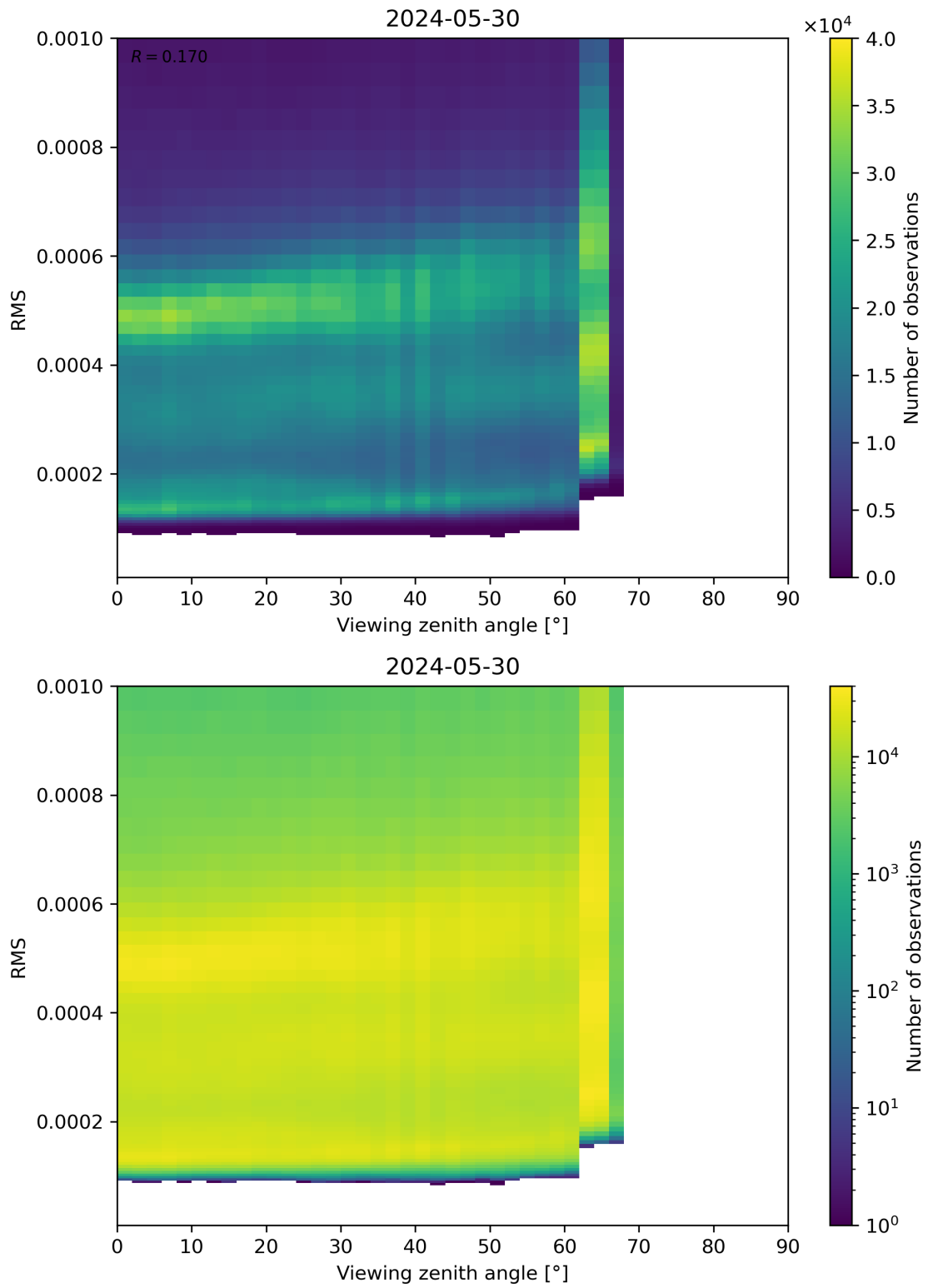
Figure 171: Scatter density plot of “Viewing zenith angle” against “RMS” for 2024-05-29 to 2024-05-31.
