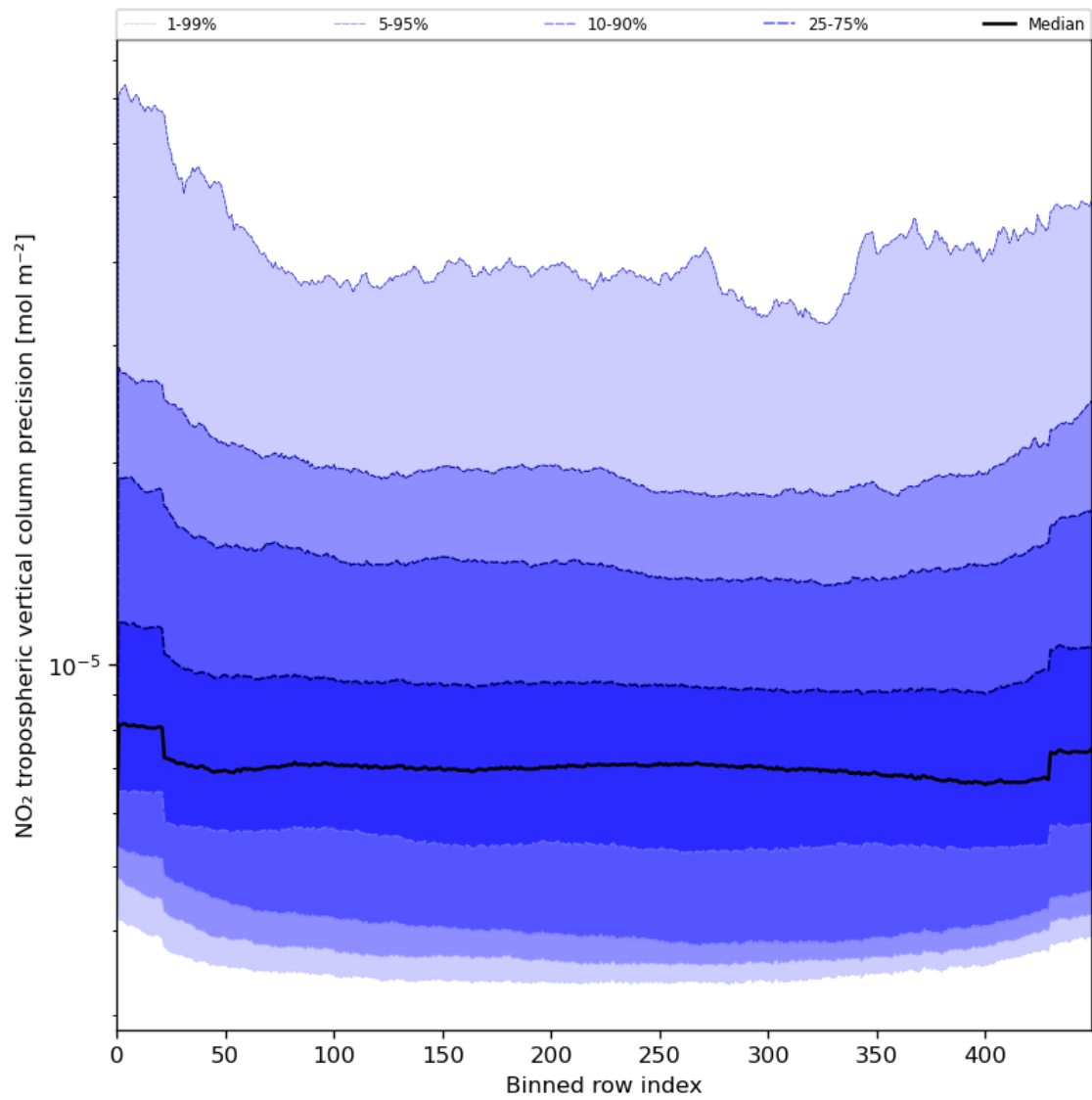
Figure 47: Along track statistics of “NO 2 tropospheric vertical column precision” for 2024-05-29 to 2024-05-31
