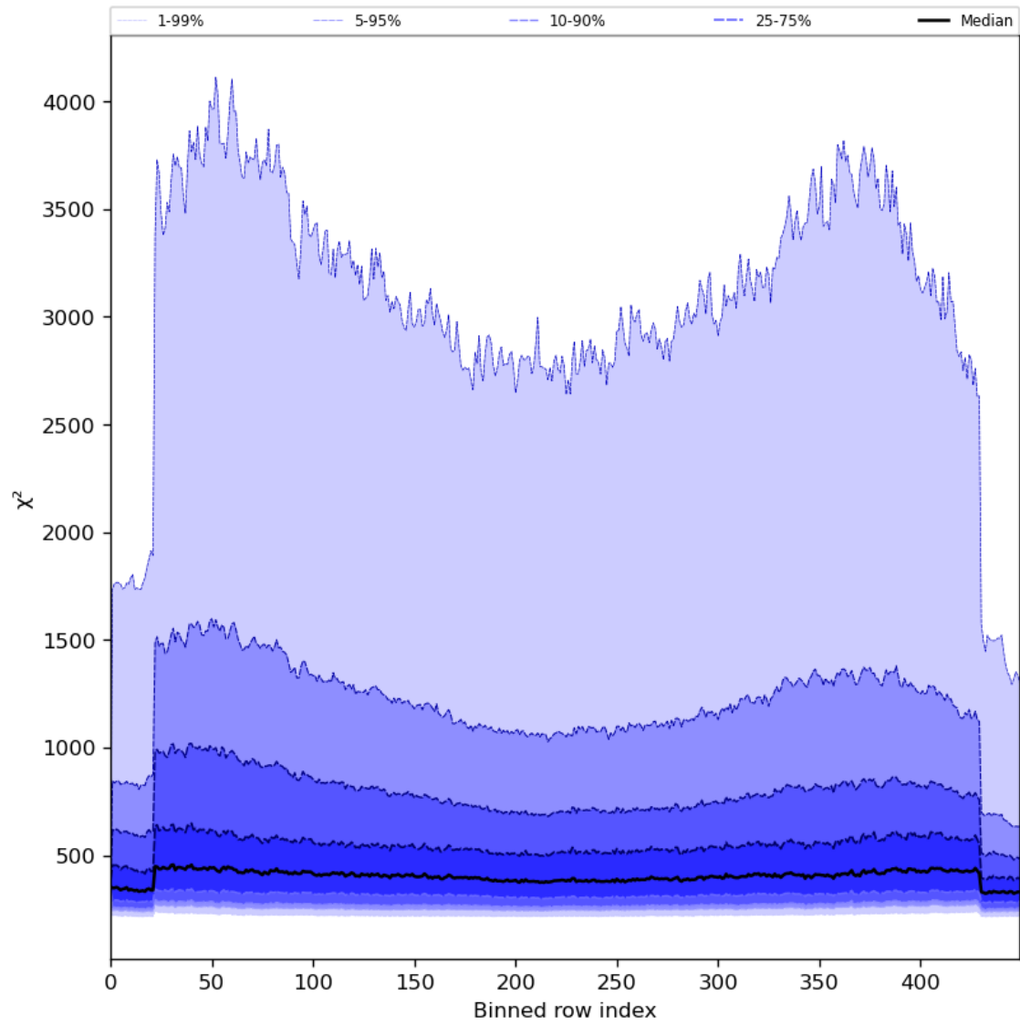
Figure 59: Along track statistics of “ \chi^2 ” for 2024-05-29 to 2024-05-31
