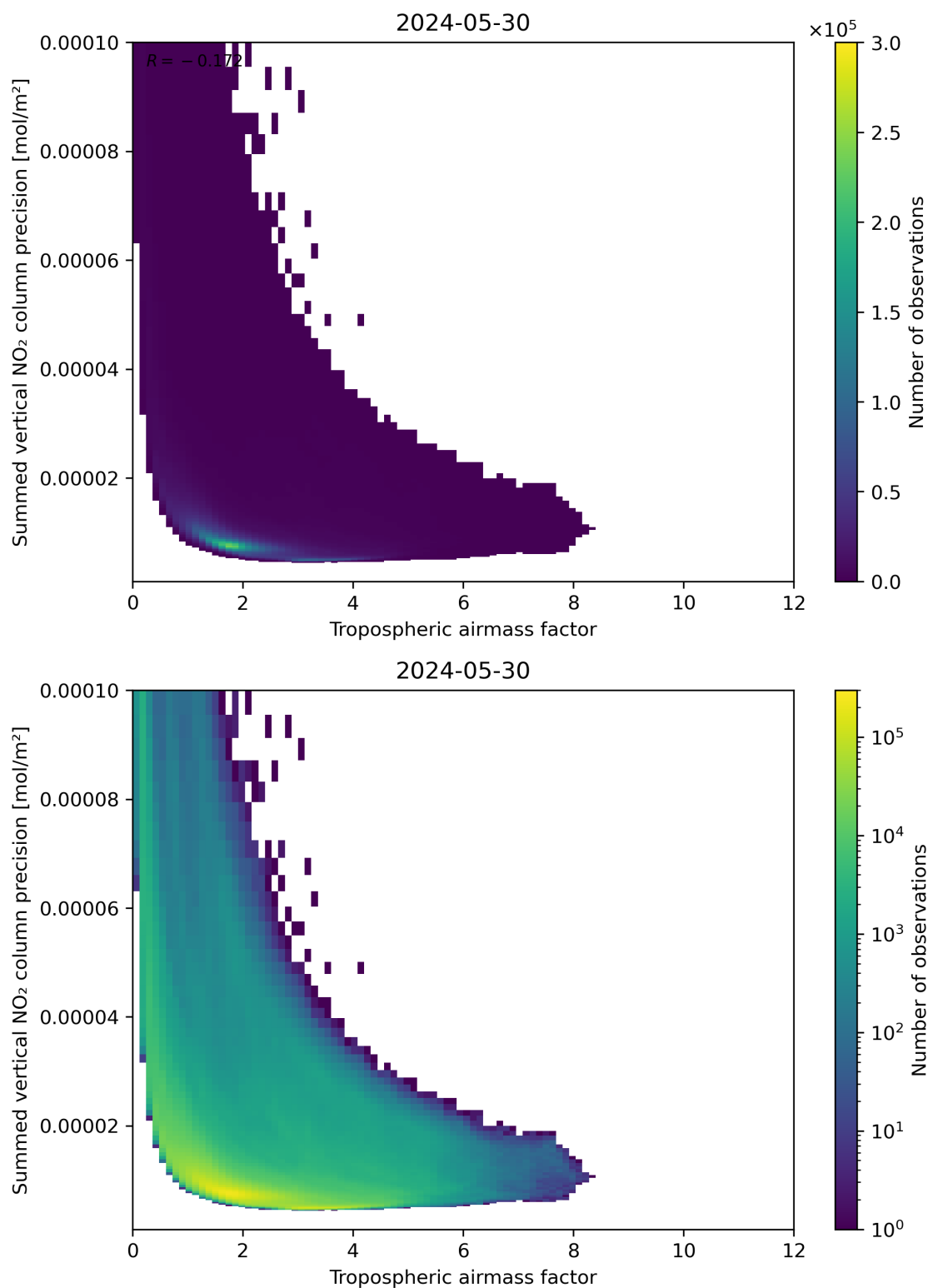
Figure 76: Scatter density plot of “Tropospheric air mass factor” against “Summed vertical NO 2 column precision” for 2024-05-29 to 2024-05-31.
