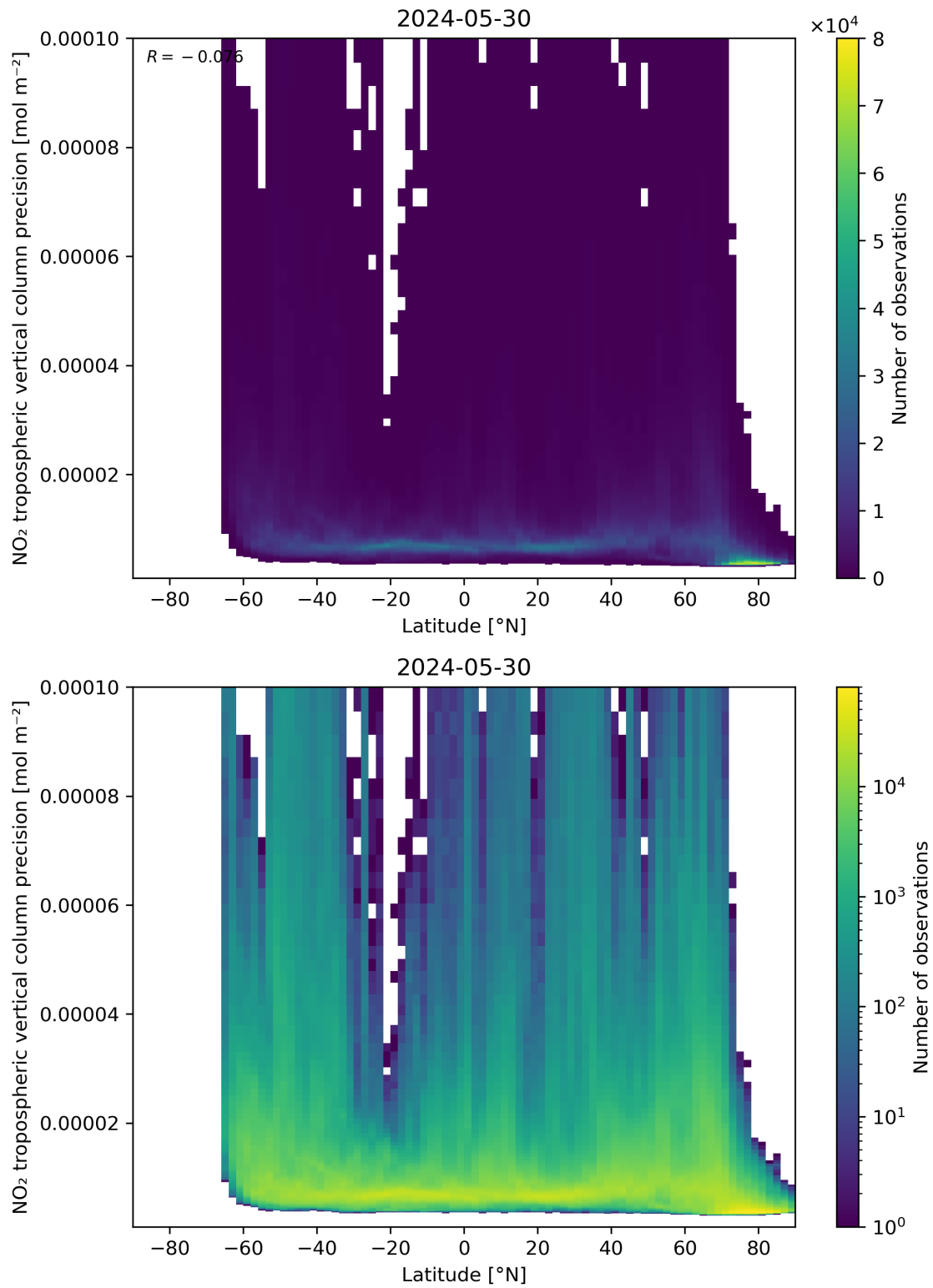
Figure 93: Scatter density plot of “Latitude” against “NO 2 tropospheric vertical column precision” for 2024-05-29 to 2024-05-31.
