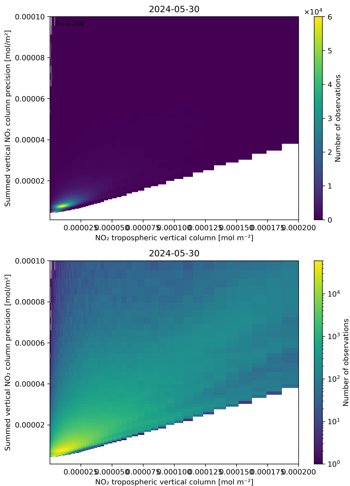
Figure 127: Scatter density plot of “NO 2 tropospheric vertical column” against “Summed vertical NO 2 column precision” for 2024-05-29 to 2024-05-31.
