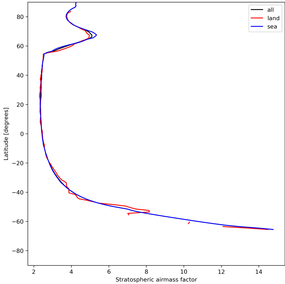
Figure 27: Zonal average of “Stratospheric airmass factor” for 2024-05-29 to 2024-05-31.
