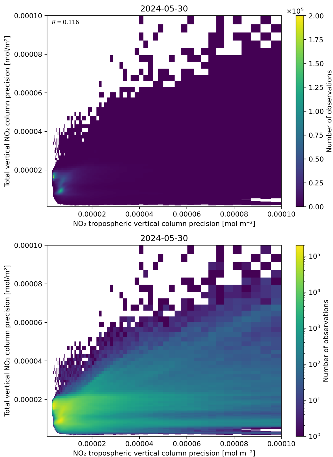
Figure 139: Scatter density plot of “NO 2 tropospheric vertical column precision” against “Total vertical NO 2 column precision” for 2024-05-29 to 2024-05-31.
