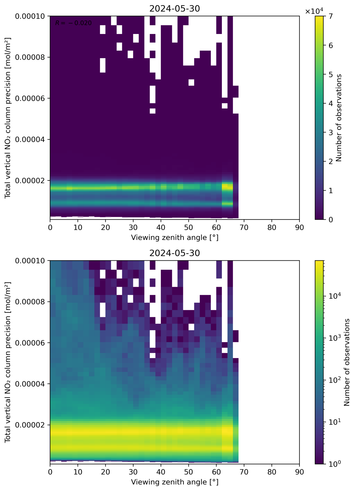
Figure 168: Scatter density plot of “Viewing zenith angle” against “Total vertical NO 2 column precision” for 2024-05-29 to 2024-05-31.
