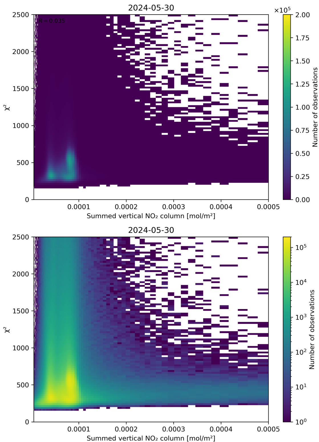
Figure 104: Scatter density plot of “Summed vertical NO 2 column” against “ \chi^2 ” for 2024-05-29 to 2024-05-31.
