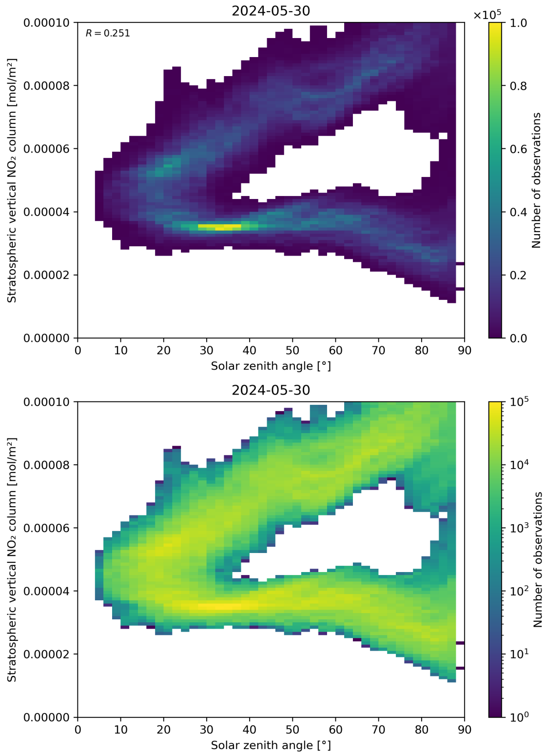
Figure 150: Scatter density plot of “Solar zenith angle” against “Stratospheric vertical NO 2 column” for 2024-05-29 to 2024-05-31.
