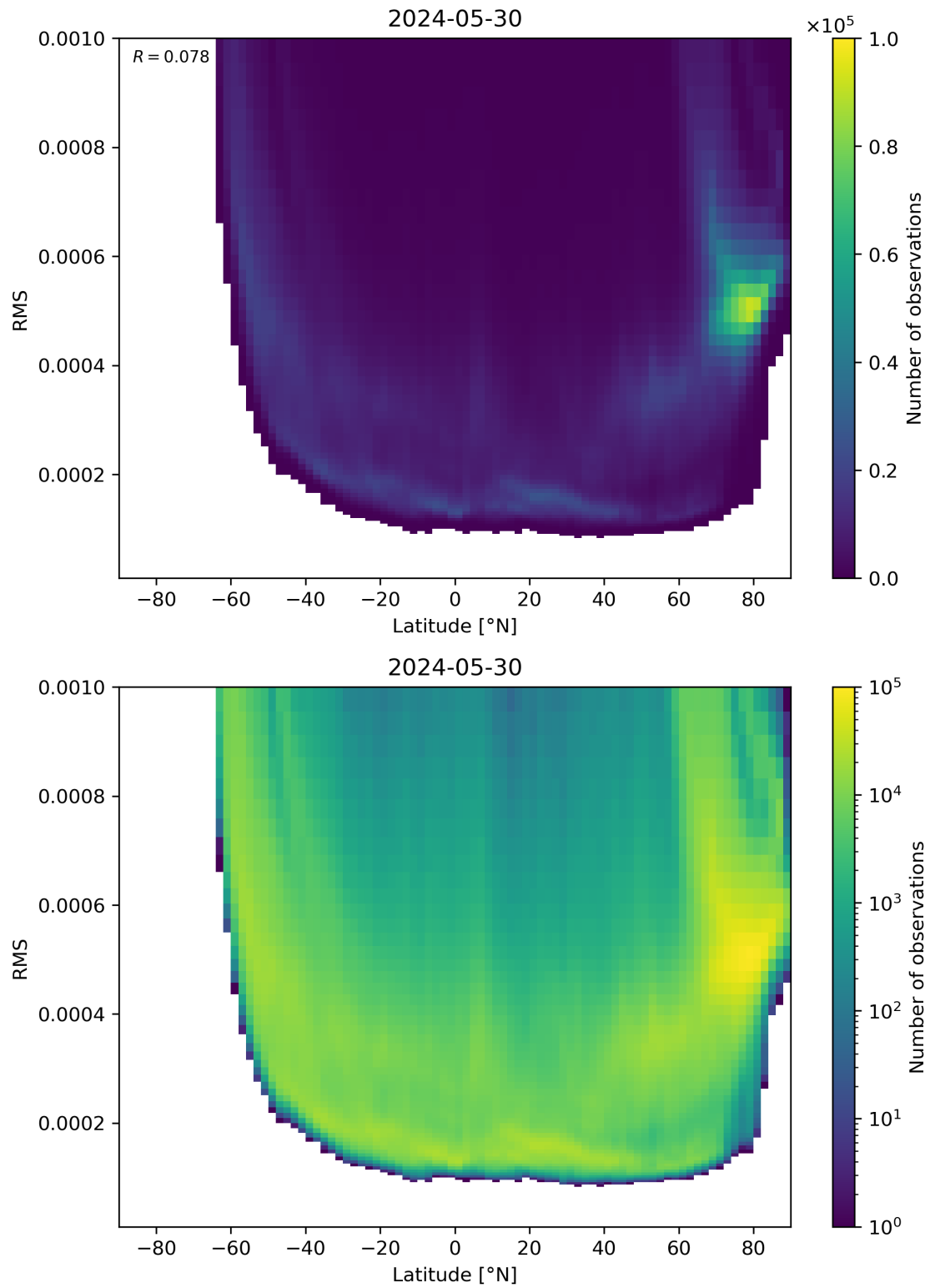
Figure 94: Scatter density plot of “Latitude” against “RMS” for 2024-05-29 to 2024-05-31.
