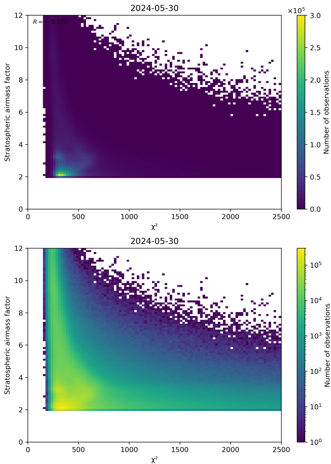
Figure 81: Scatter density plot of “ \chi^2 ” against “Stratospheric airmass factor” for 2024-05-29 to 2024-05-31.
