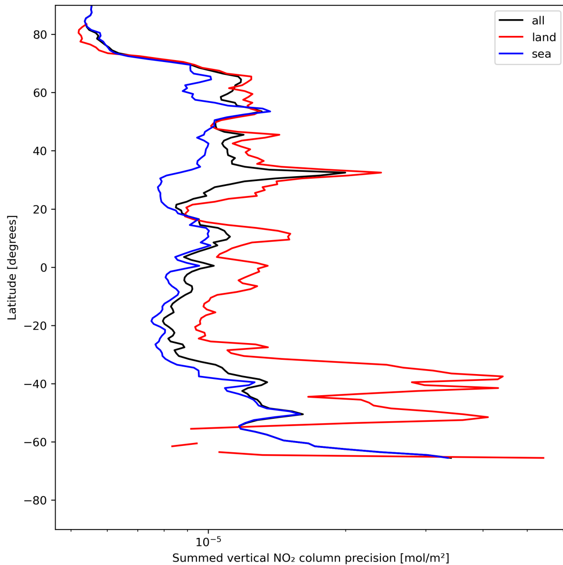
Figure 24: Zonal average of “Summed vertical NO 2 column precision” for 2024-05-29 to 2024-05-31.
