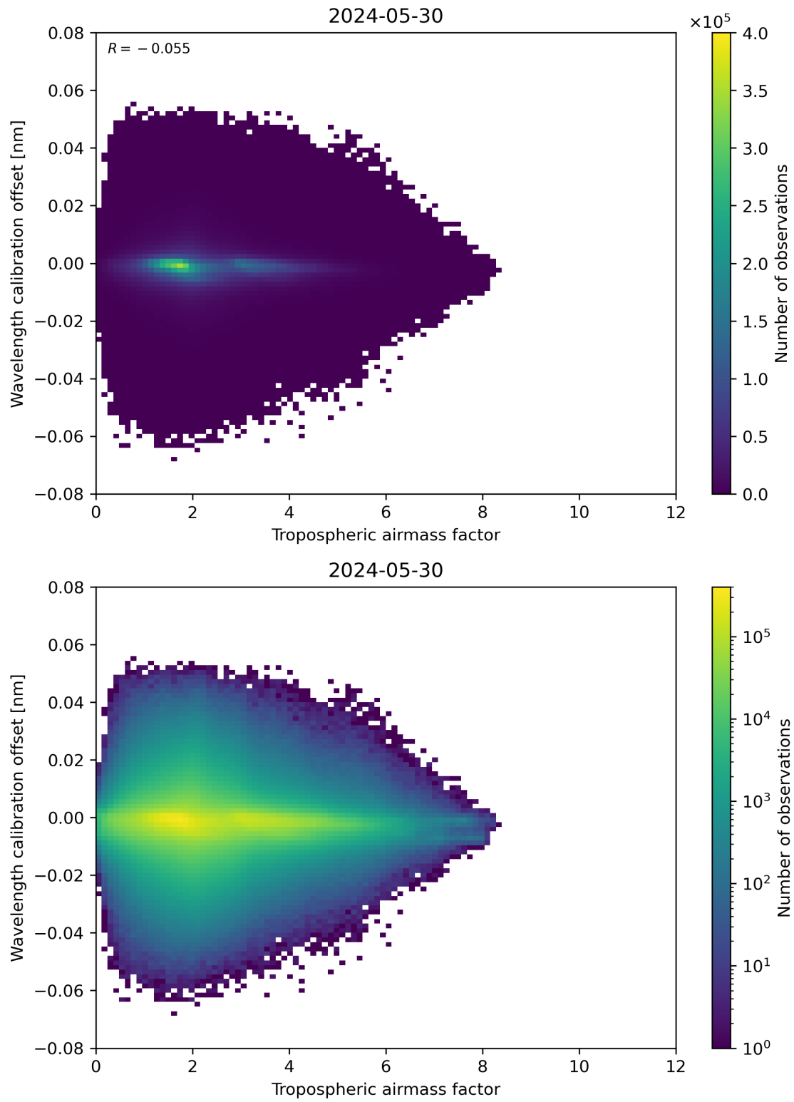
Figure 80: Scatter density plot of “Tropospheric airmass factor” against “Wavelength calibration offset” for 2024-05-29 to 2024-05-31.
