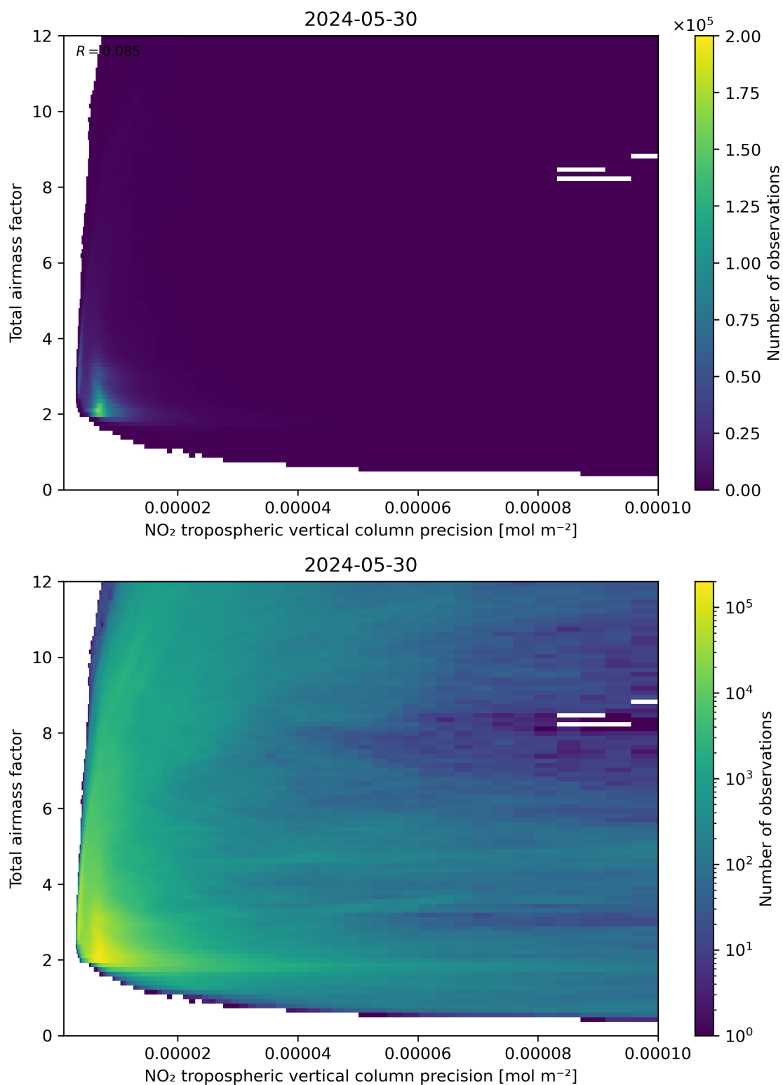
Figure 132: Scatter density plot of “NO 2 tropospheric vertical column precision” against “Total air mass factor” for 2024-05-29 to 2024-05-31.
