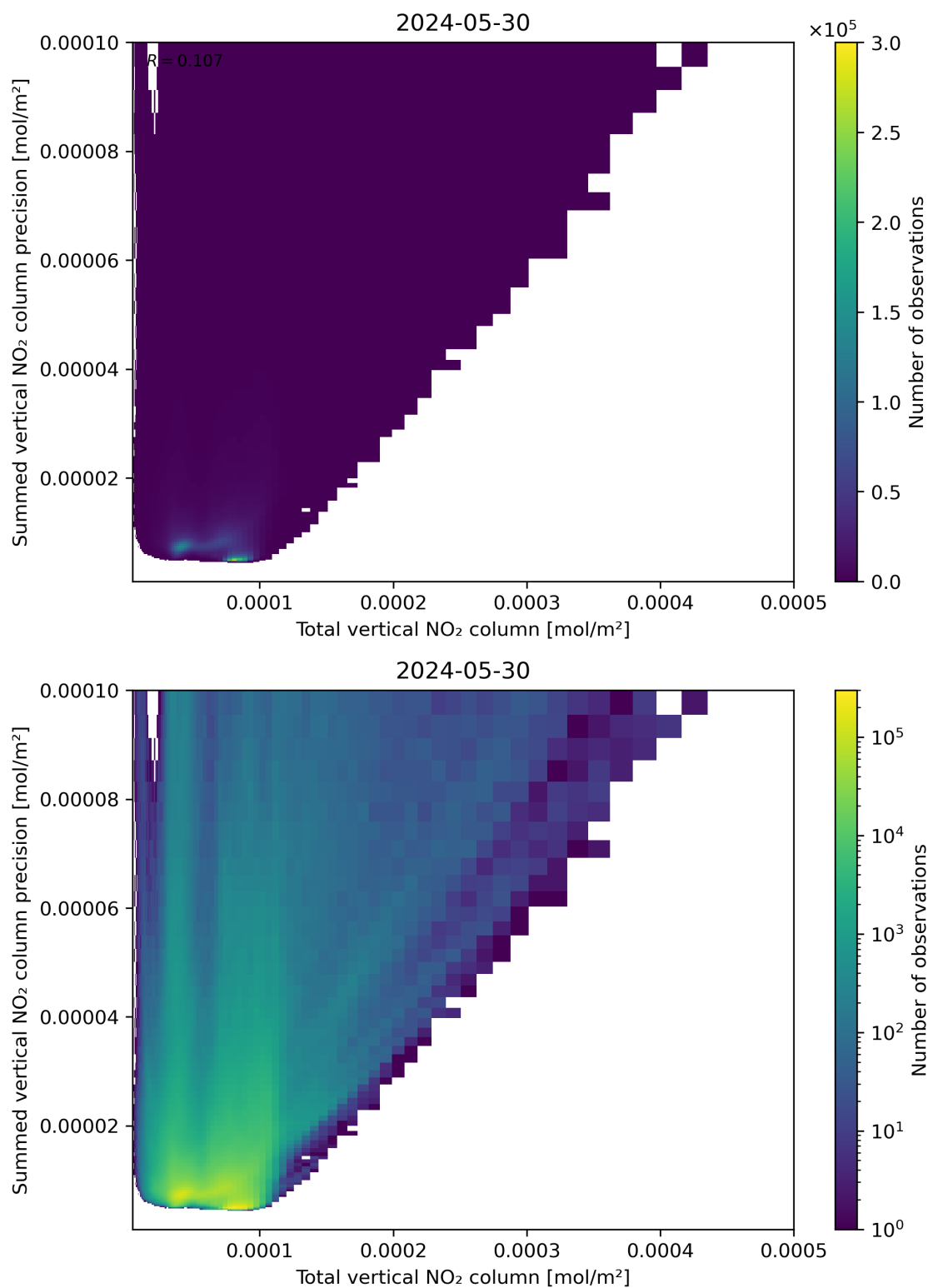
Figure 113: Scatter density plot of “Total vertical NO 2 column” against “Summed vertical NO 2 column precision” for 2024-05-29 to 2024-05-31.
