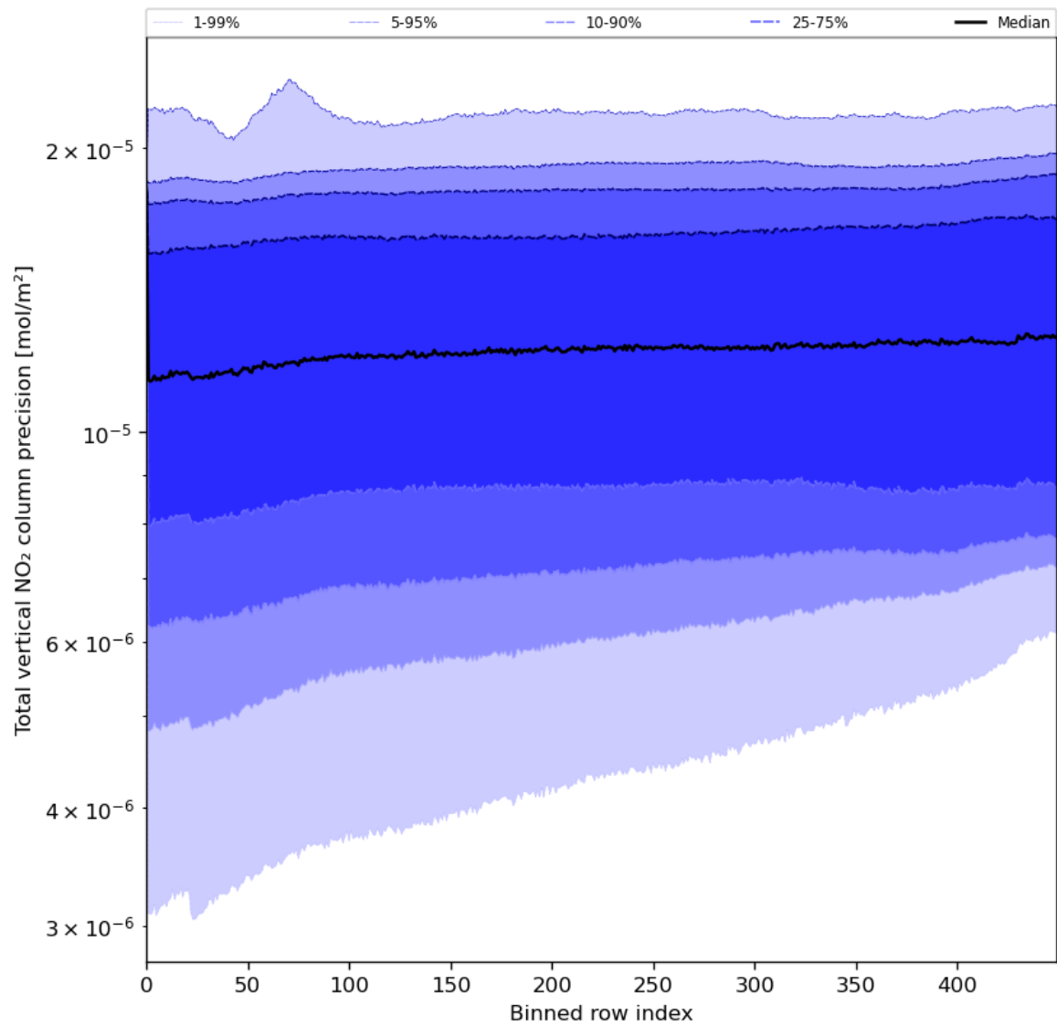
Figure 56: Along track statistics of “Total vertical NO 2 column precision” for 2024-05-29 to 2024-05-31
