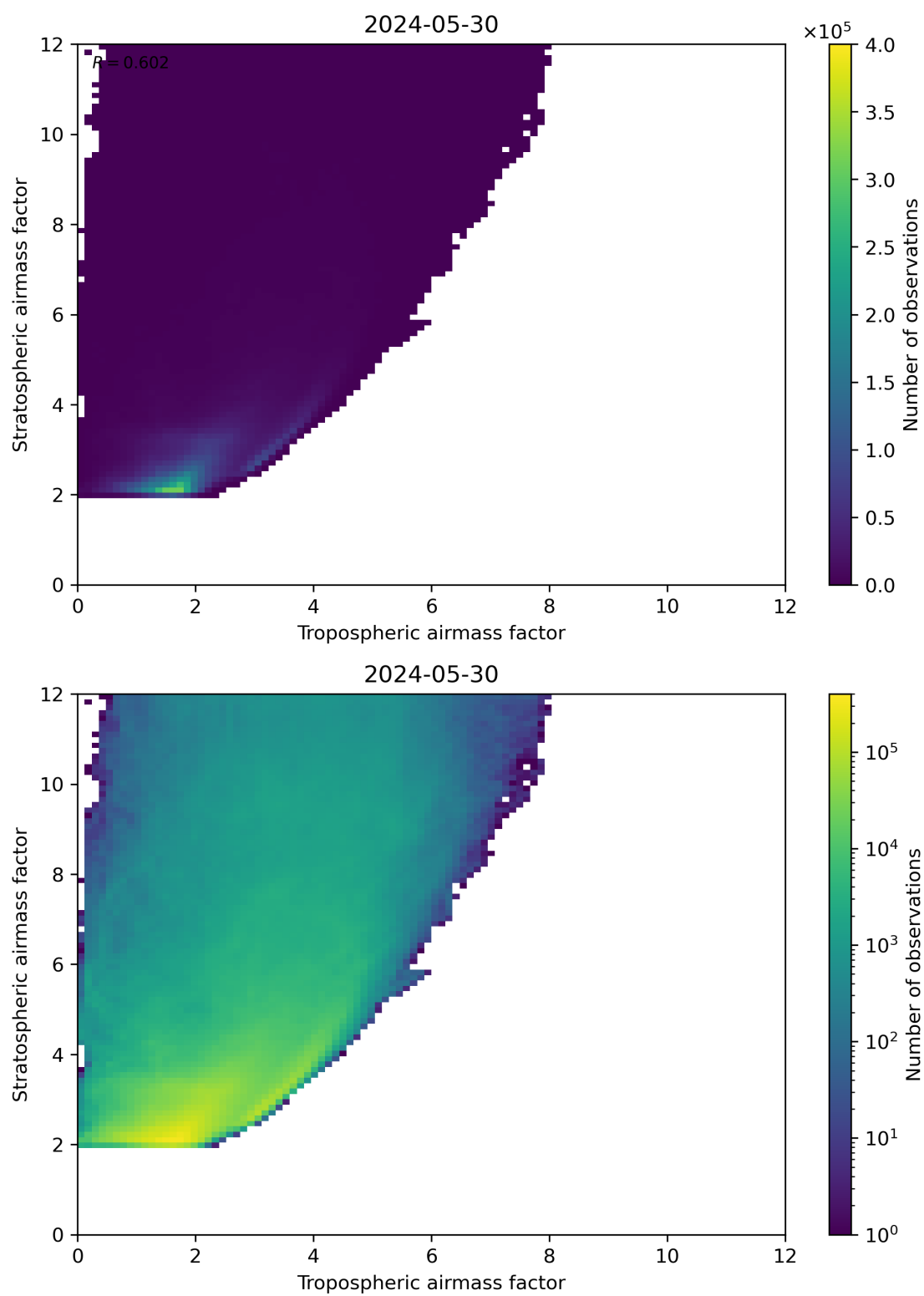
Figure 71: Scatter density plot of “Tropospheric airmass factor” against “Stratospheric airmass factor” for 2024-05-29 to 2024-05-31.
