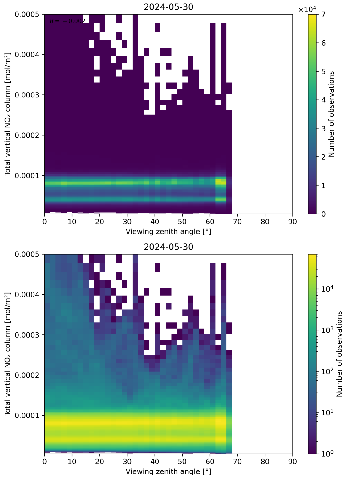
Figure 167: Scatter density plot of “Viewing zenith angle” against “Total vertical NO 2 column” for 2024-05-29 to 2024-05-31.
