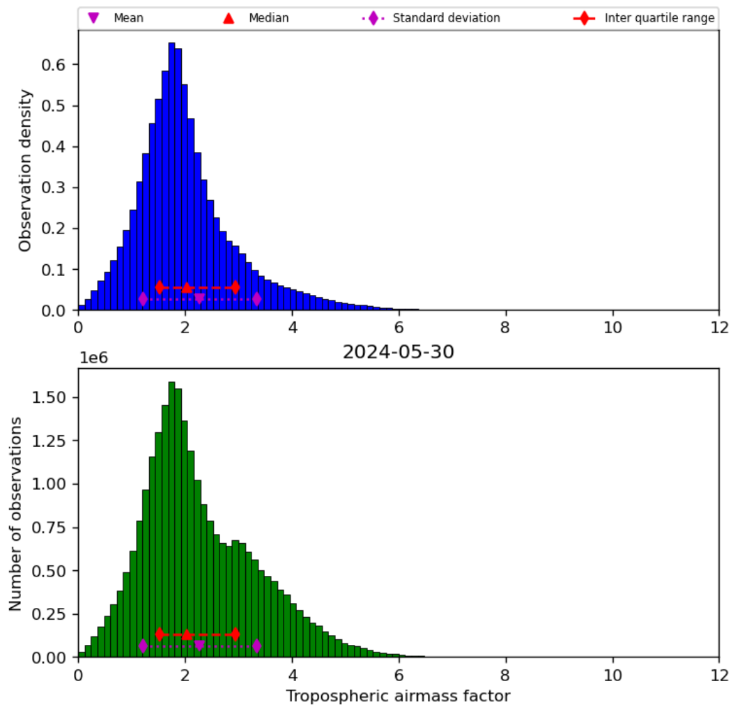
Figure 31: Histogram of “Tropospheric airmass factor” for 2024-05-29 to 2024-05-31
