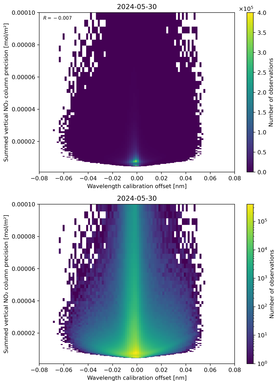
Figure 178: Scatter density plot of “Wavelength calibration offset” against “Summed vertical NO 2 column precision” for 2024-05-29 to 2024-05-31.
