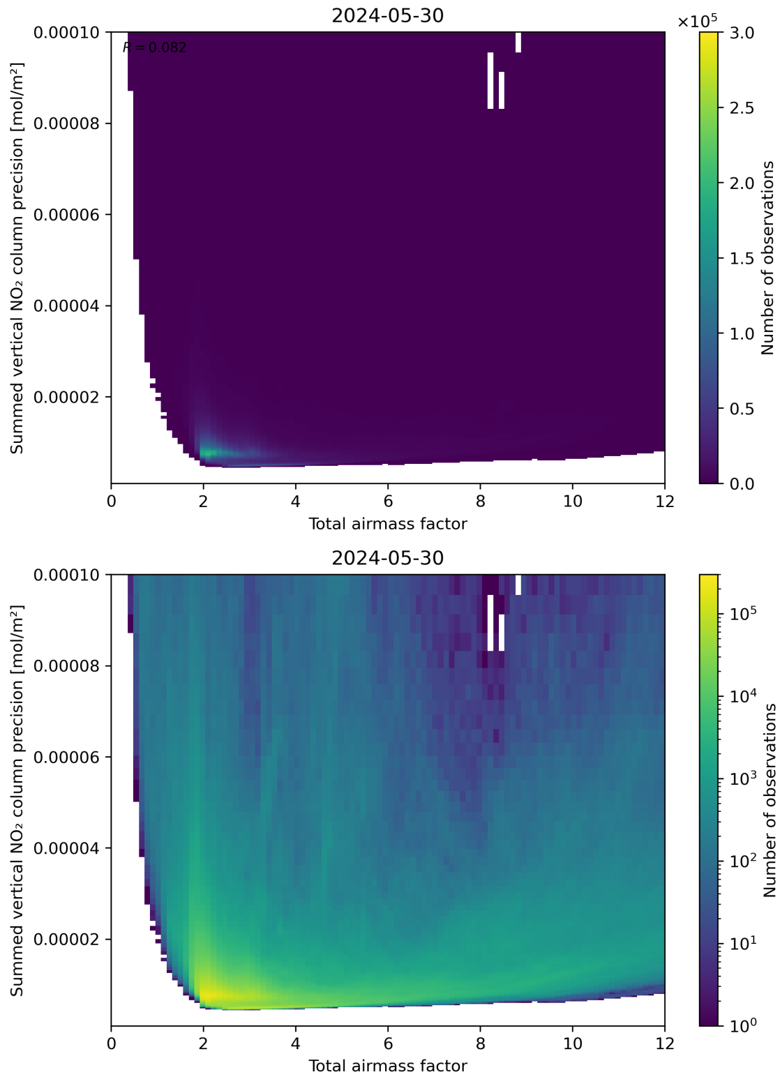
Figure 66: Scatter density plot of “Total airmass factor” against “Summed vertical NO 2 column precision” for 2024-05-29 to 2024-05-31.
