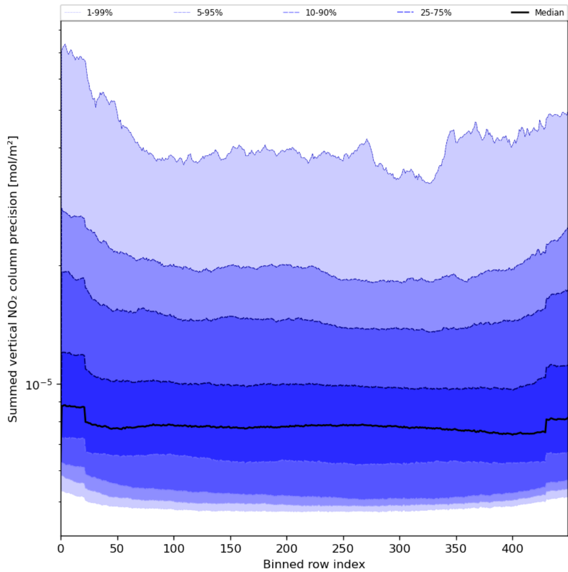
Figure 58: Along track statistics of “Summed vertical NO 2 column precision” for 2024-05-29 to 2024-05-31
