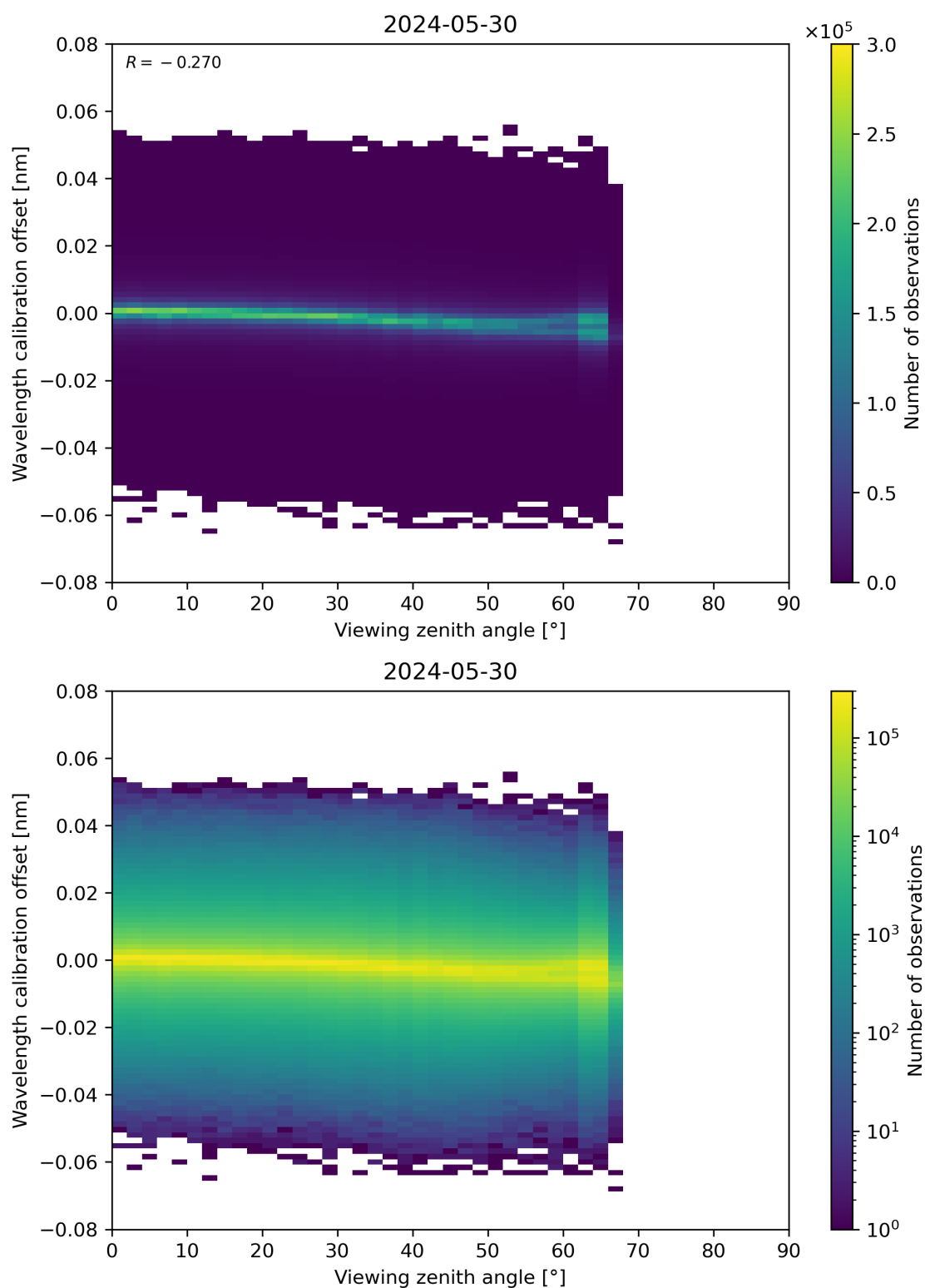
Figure 173: Scatter density plot of “Viewing zenith angle” against “Wavelength calibration offset” for 2024-05-29 to 2024-05-31.
