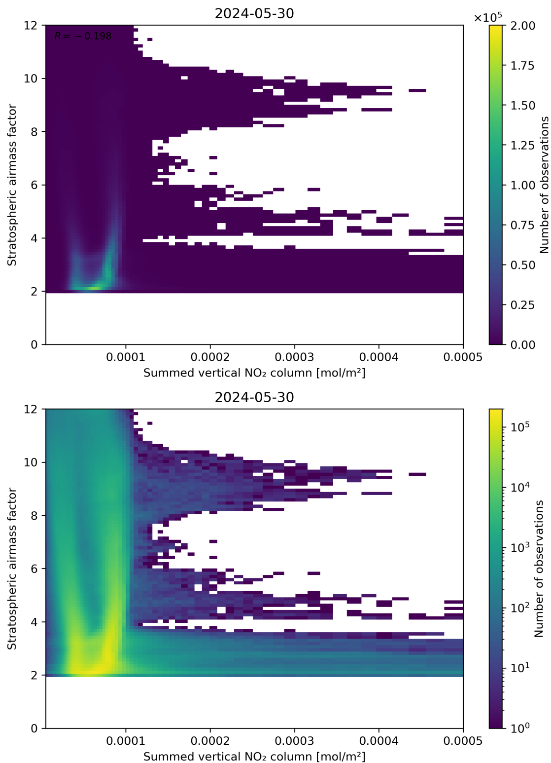
Figure 103: Scatter density plot of “Summed vertical NO 2 column” against “Stratospheric air mass factor” for 2024-05-29 to 2024-05-31.
