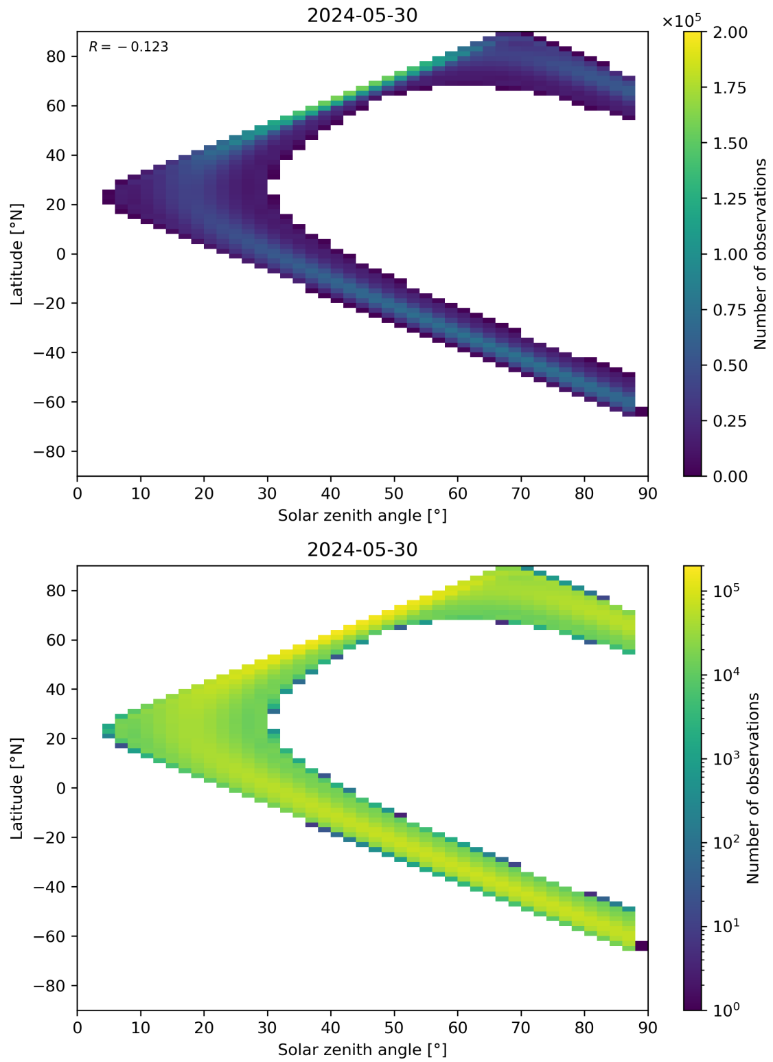
Figure 149: Scatter density plot of “Solar zenith angle” against “Latitude” for 2024-05-29 to 2024-05-31.
