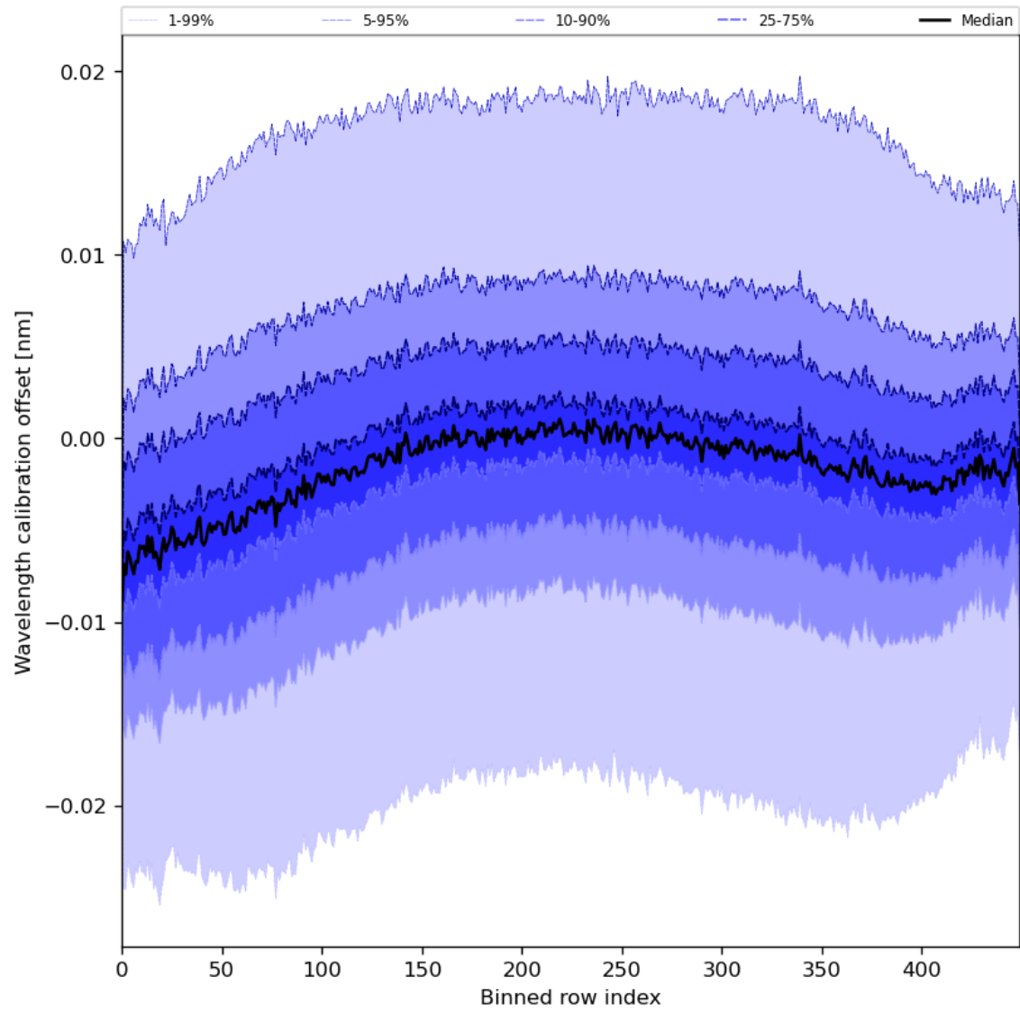
Figure 52: Along track statistics of “Wavelength calibration offset” for 2024-05-29 to 2024-05-31
