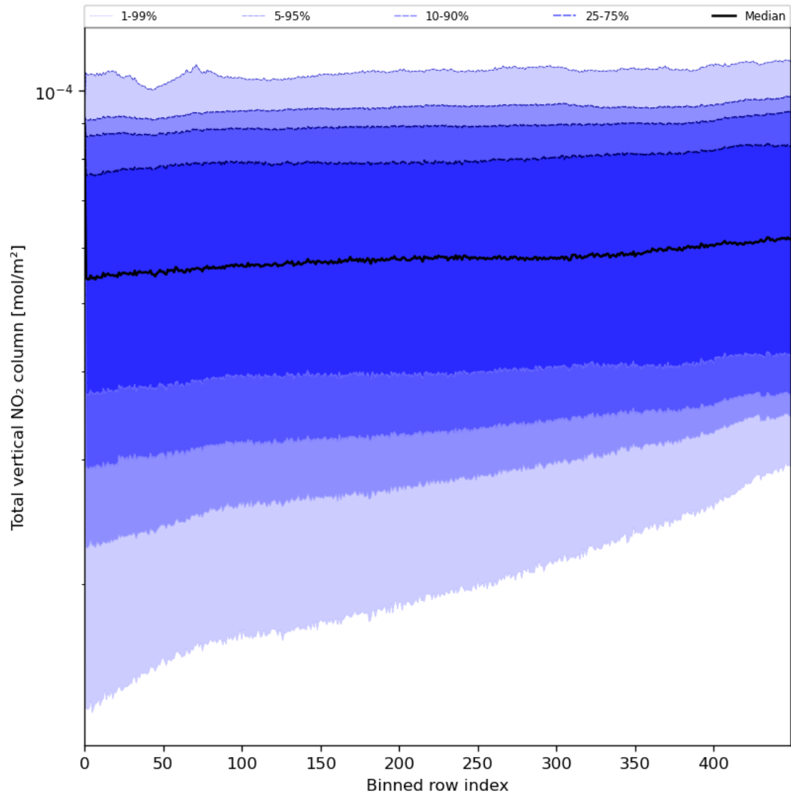
Figure 55: Along track statistics of “Total vertical NO 2 column” for 2024-05-29 to 2024-05-31
