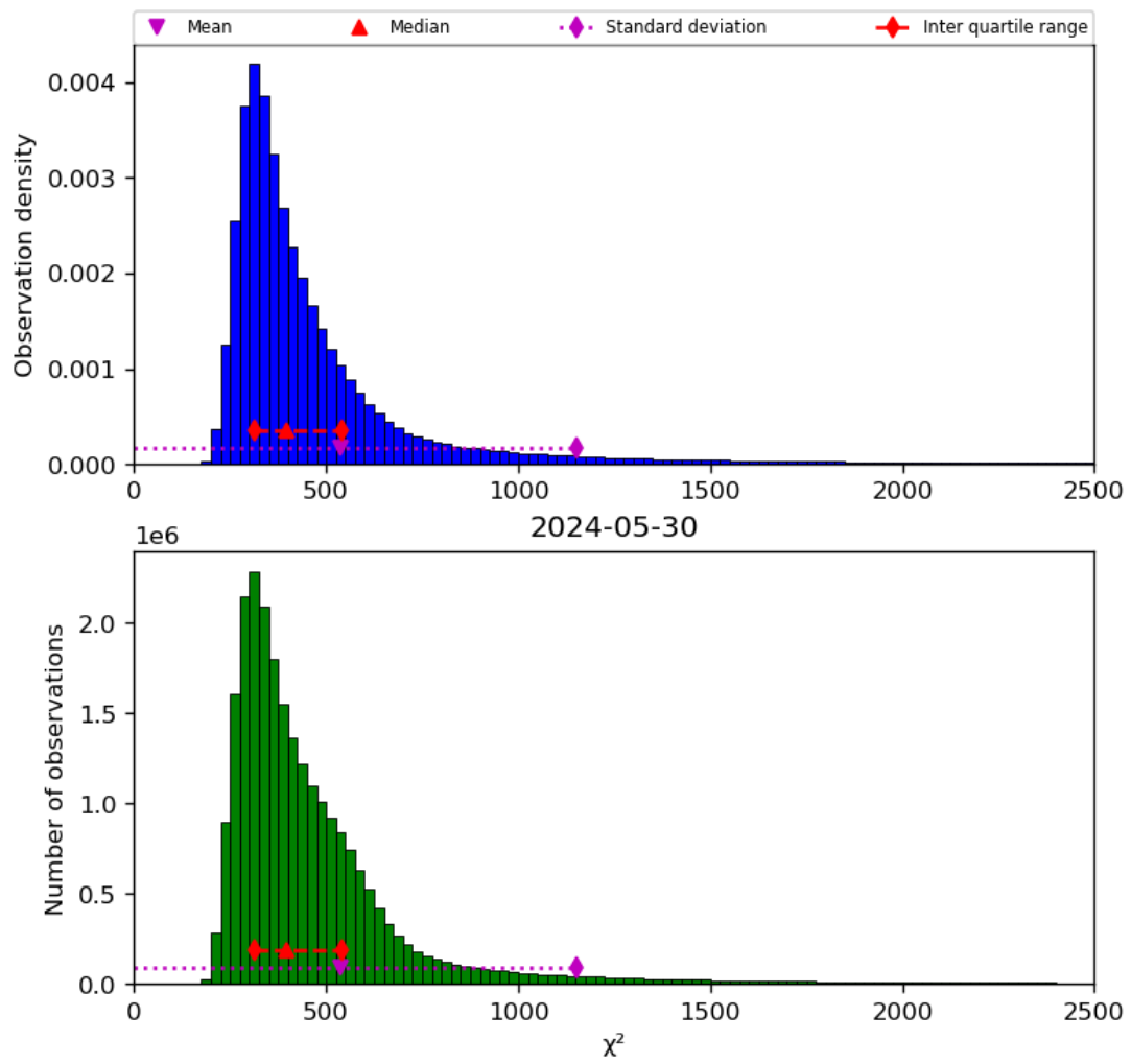
Figure 42: Histogram of “ \chi^2 ” for 2024-05-29 to 2024-05-31
