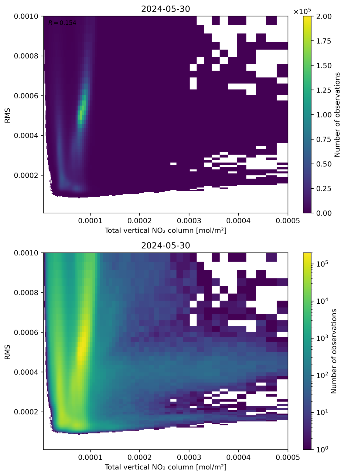
Figure 120: Scatter density plot of “Total vertical NO 2 column” against “RMS” for 2024-05-29 to 2024-05-31.
