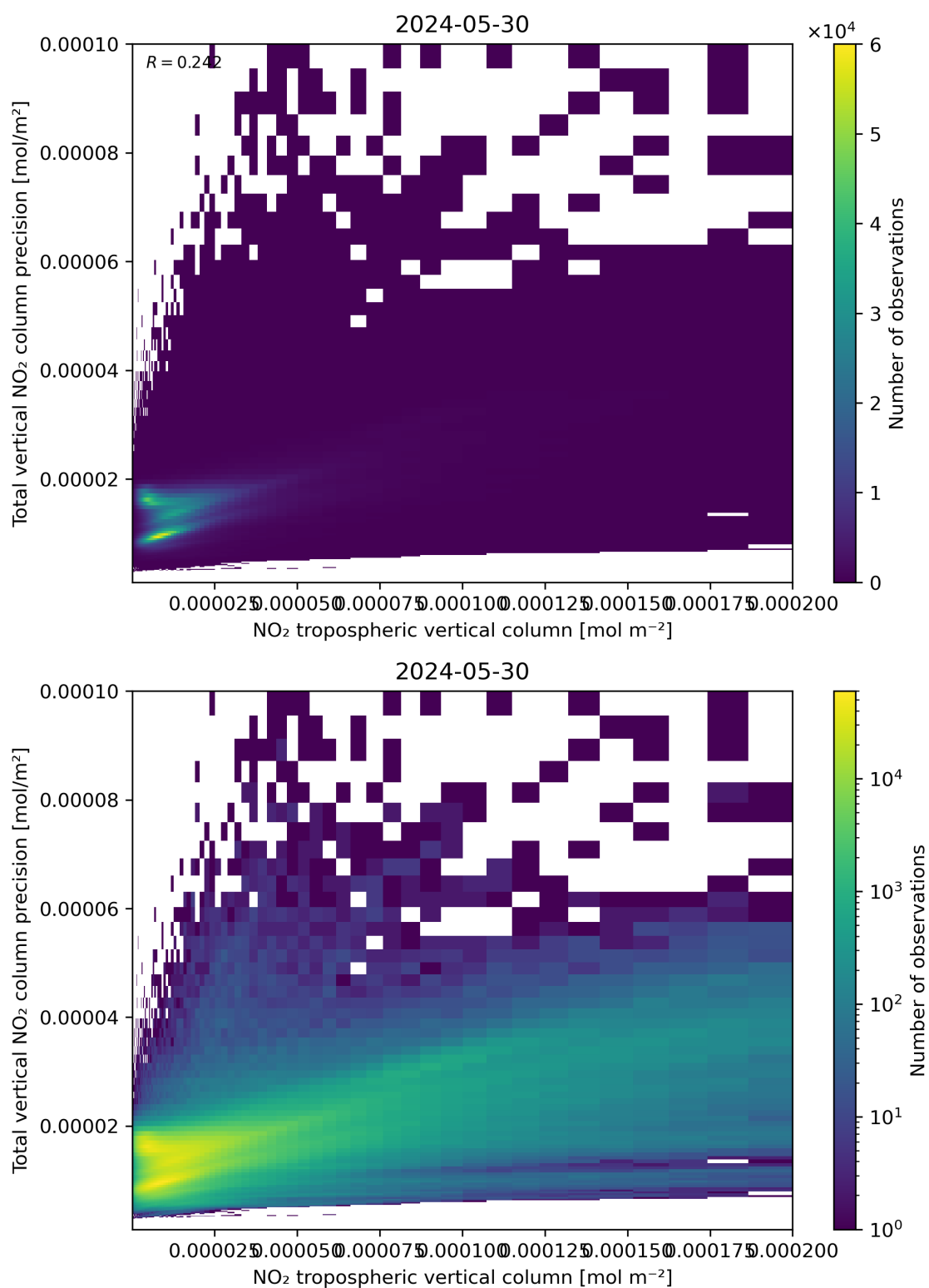
Figure 129: Scatter density plot of “NO 2 tropospheric vertical column” against “Total vertical NO 2 column precision” for 2024-05-29 to 2024-05-31.
