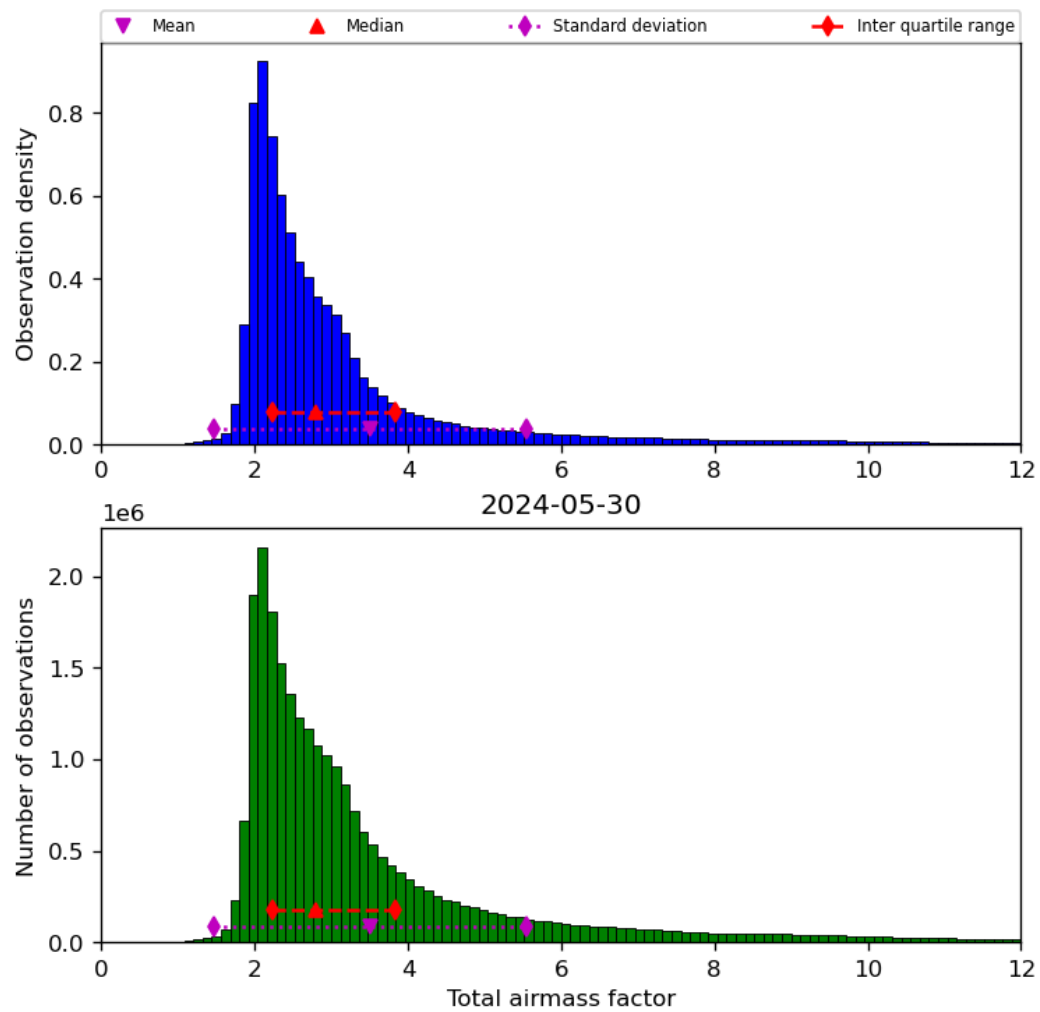
Figure 32: Histogram of “Total airmass factor” for 2024-05-29 to 2024-05-31
