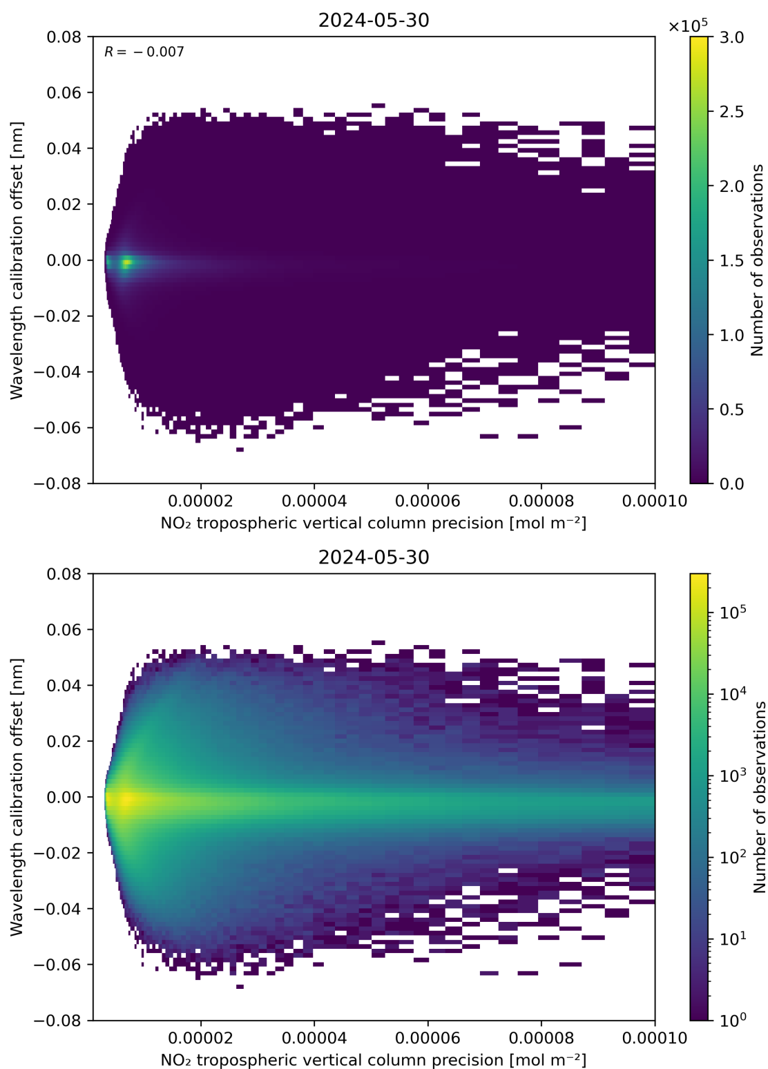
Figure 141: Scatter density plot of “NO 2 tropospheric vertical column precision” against “Wavelength calibration offset” for 2024-05-29 to 2024-05-31.
