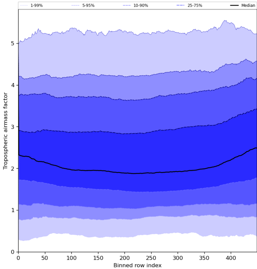
Figure 48: Along track statistics of “Tropospheric airmass factor” for 2024-05-29 to 2024-05-31
