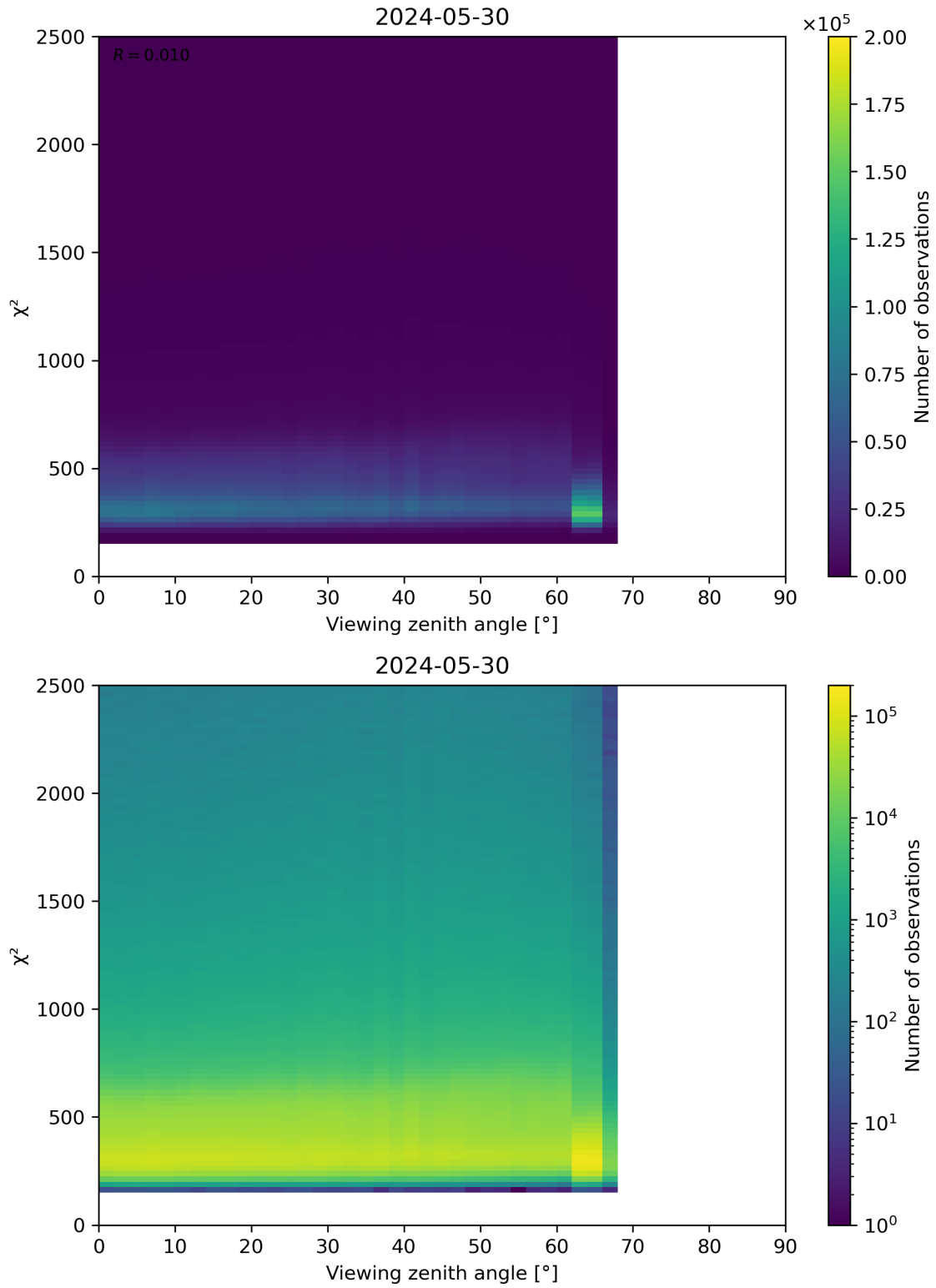
Figure 162: Scatter density plot of “Viewing zenith angle” against “ \chi^2 ” for 2024-05-29 to 2024-05-31.
