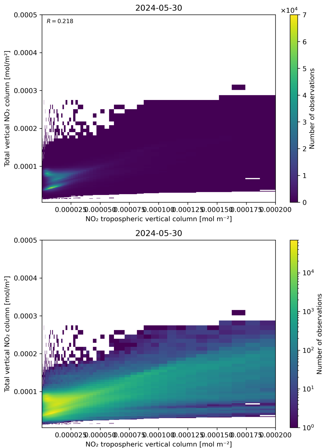
Figure 128: Scatter density plot of “NO 2 tropospheric vertical column” against “Total vertical NO 2 column” for 2024-05-29 to 2024-05-31.
