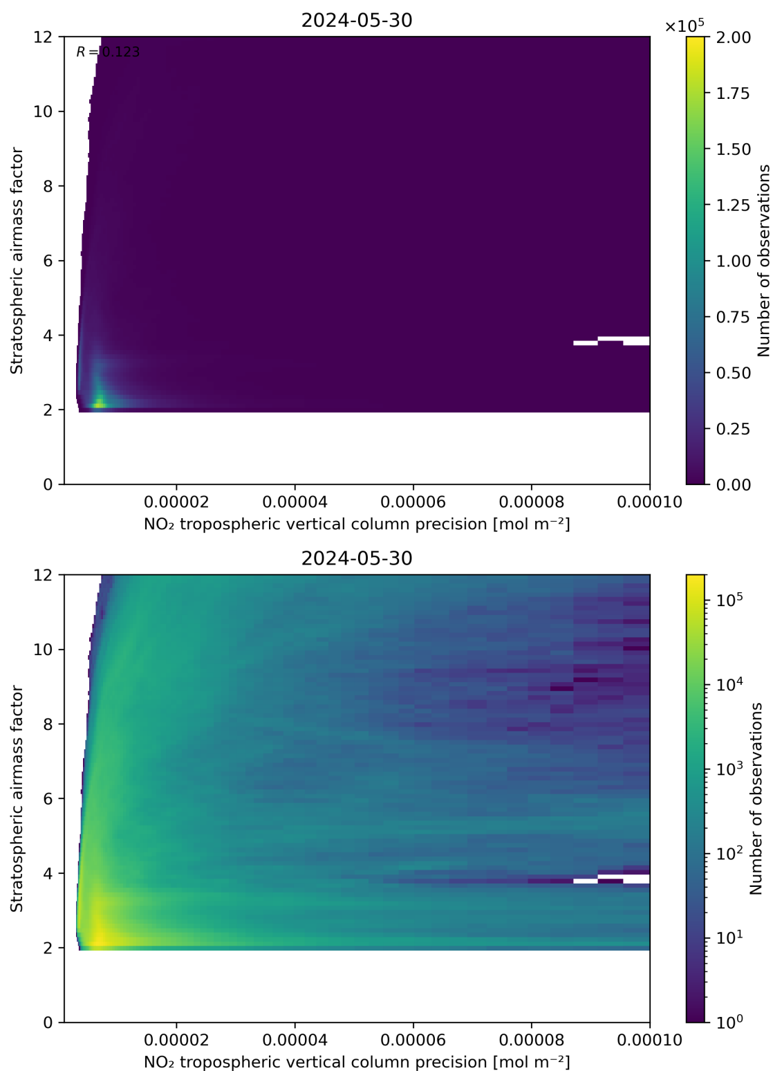
Figure 131: Scatter density plot of “NO 2 tropospheric vertical column precision” against “Stratospheric airmass factor” for 2024-05-29 to 2024-05-31.
