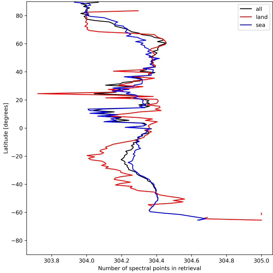
Figure 16: Zonal average of “Number of spectral points in retrieval” for 2024-05-29 to 2024-05-31.
