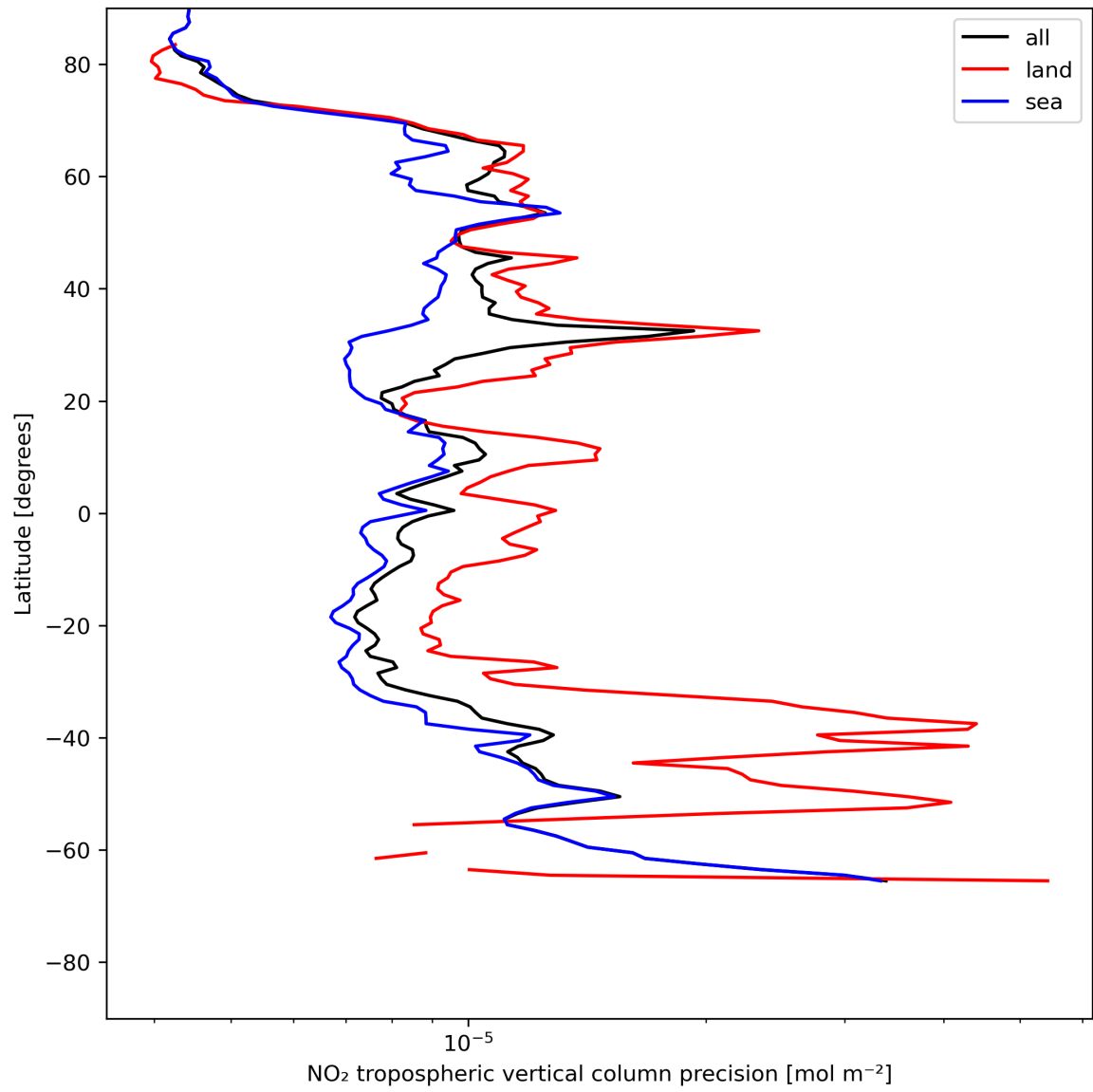
Figure 13: Zonal average of “NO 2 tropospheric vertical column precision” for 2024-05-29 to 2024-05-31.
