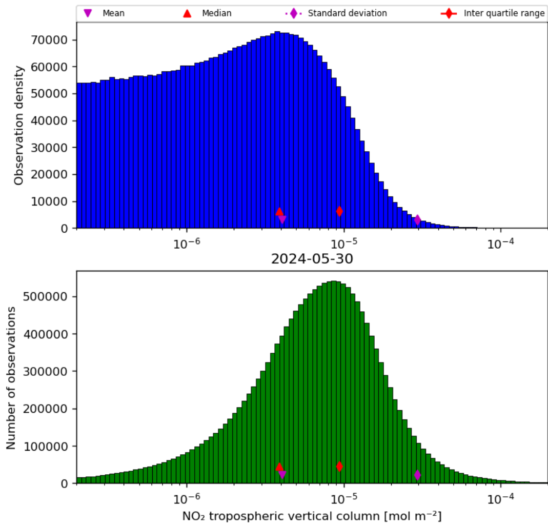
Figure 29: Histogram of “NO 2 tropospheric vertical column” for 2024-05-29 to 2024-05-31
