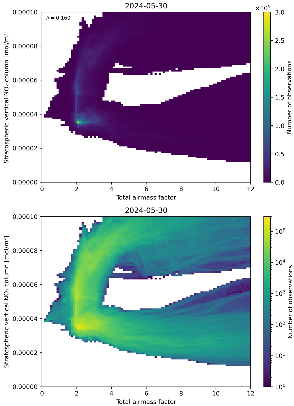
Figure 64: Scatter density plot of “Total airmass factor” against “Stratospheric vertical NO 2 column” for 2024-05-29 to 2024-05-31.
