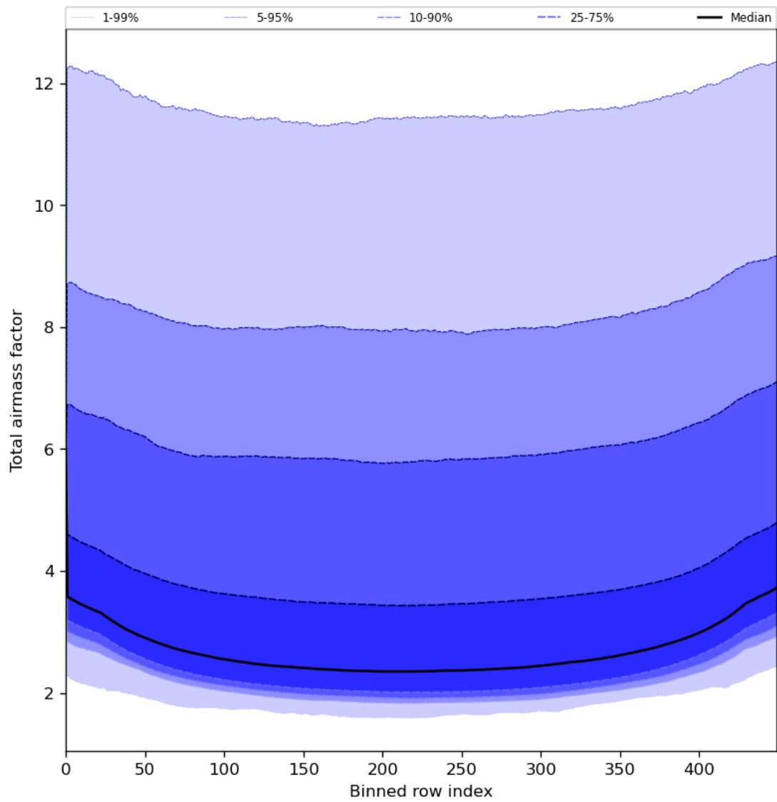
Figure 49: Along track statistics of “Total airmass factor” for 2024-05-29 to 2024-05-31
