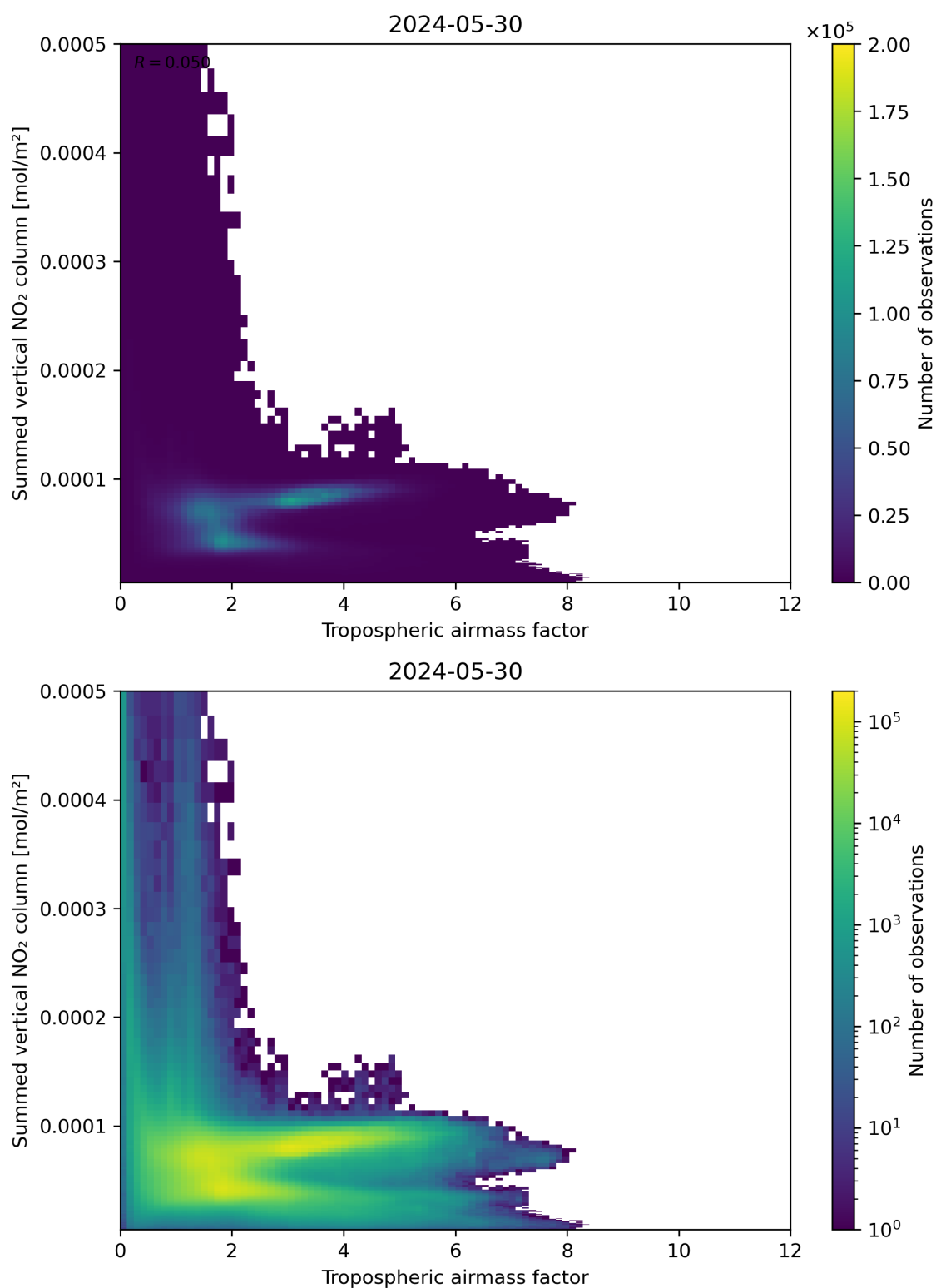
Figure 75: Scatter density plot of “Tropospheric air mass factor” against “Summed vertical NO 2 column” for 2024-05-29 to 2024-05-31.
