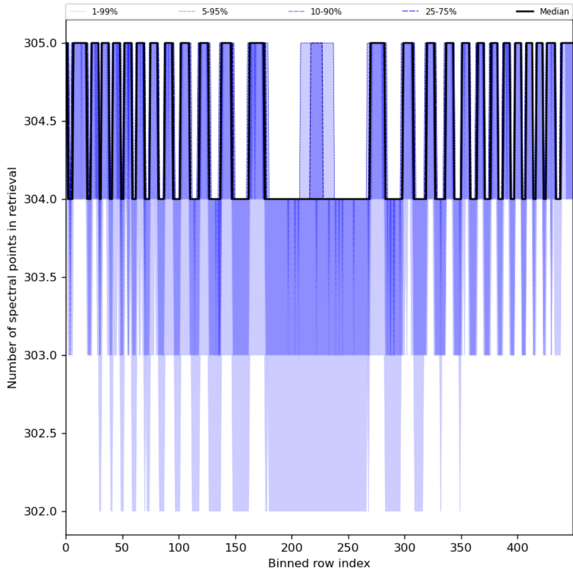
Figure 50: Along track statistics of “Number of spectral points in retrieval” for 2024-05-29 to 2024-05-31
