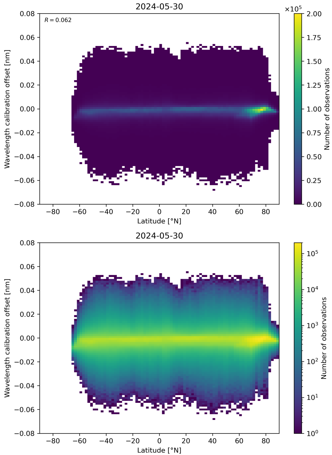
Figure 95: Scatter density plot of “Latitude” against “Wavelength calibration offset” for 2024-05-29 to 2024-05-31.
