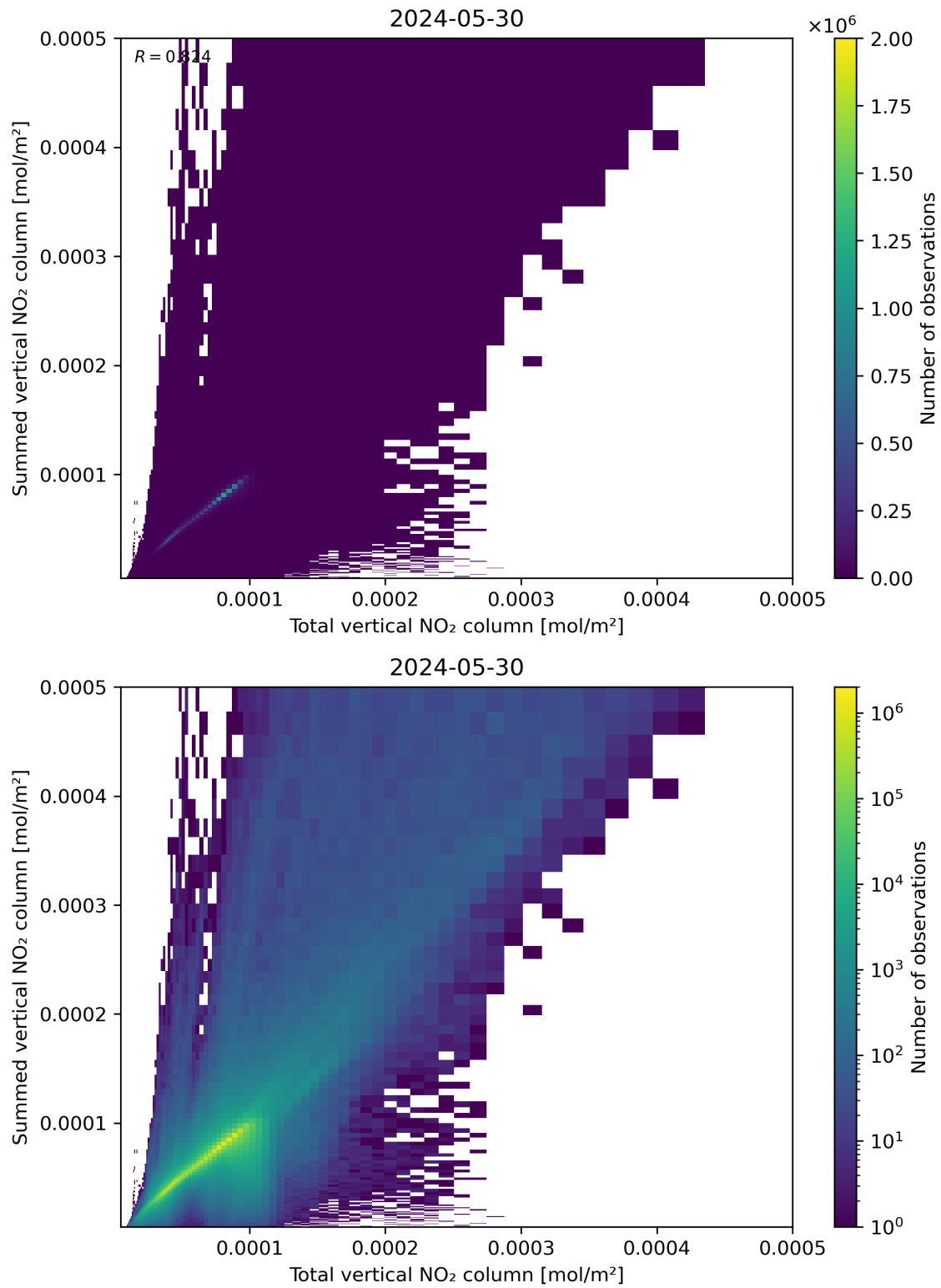
Figure 112: Scatter density plot of “Total vertical NO 2 column” against “Summed vertical NO 2 column” for 2024-05-29 to 2024-05-31.
