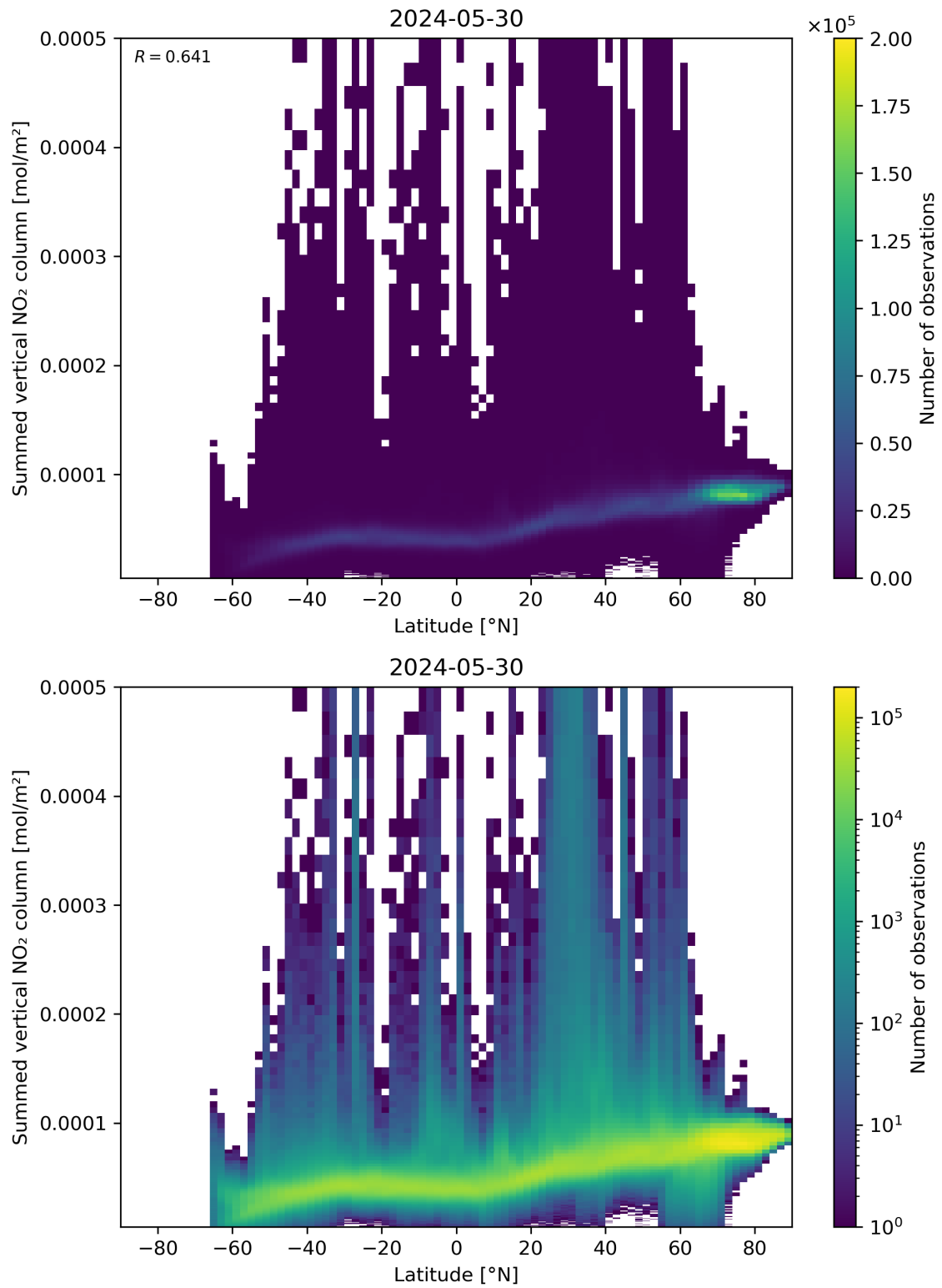
Figure 88: Scatter density plot of “Latitude” against “Summed vertical NO 2 column” for 2024-05-29 to 2024-05-31.
