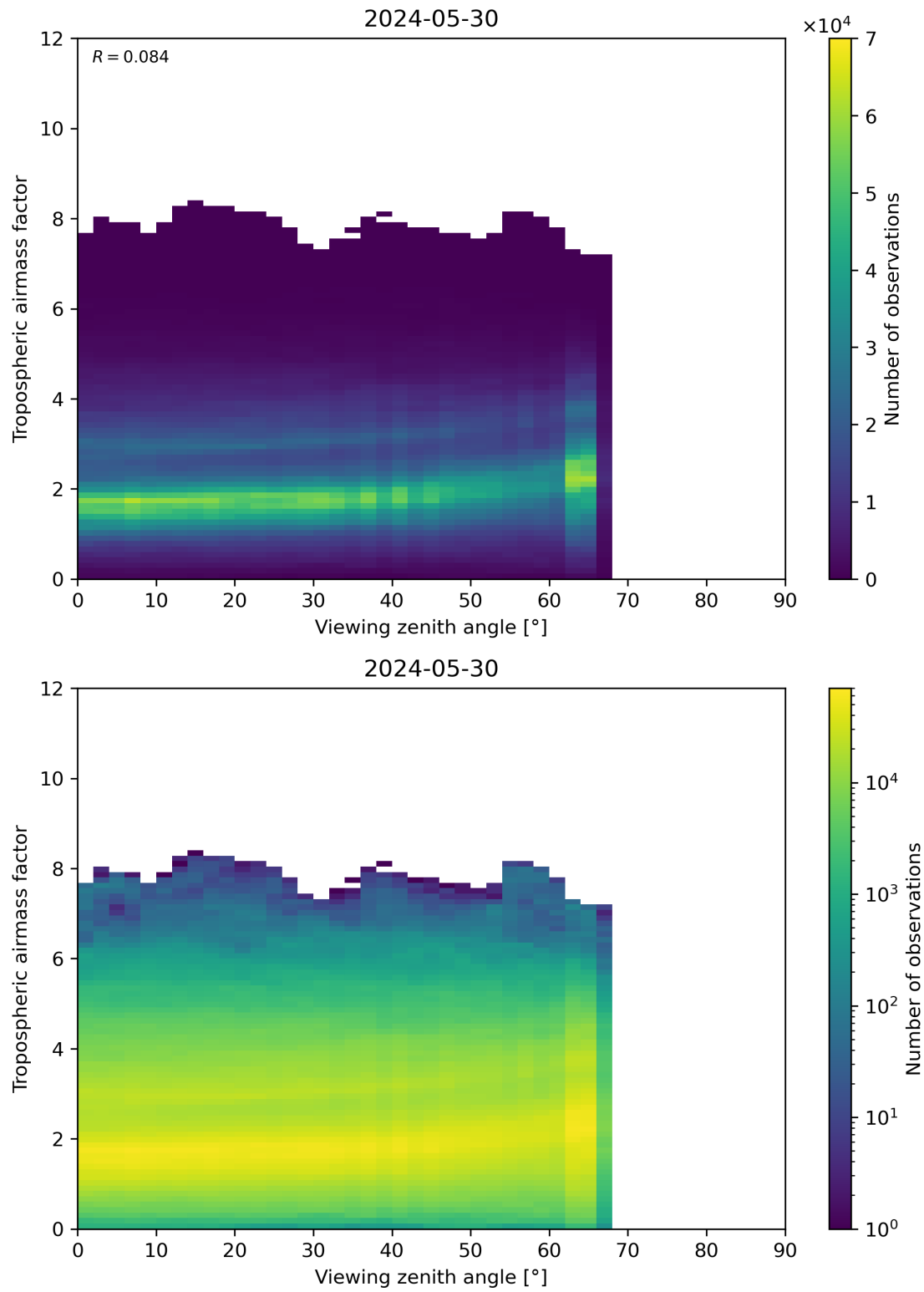
Figure 161: Scatter density plot of “Viewing zenith angle” against “Tropospheric airmass factor” for 2024-05-29 to 2024-05-31.
