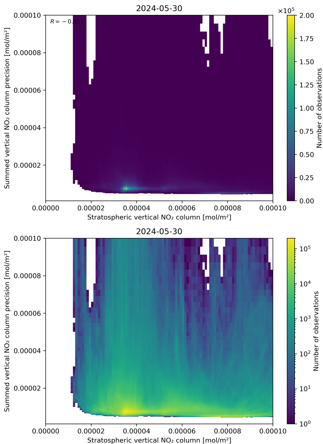
Figure 99: Scatter density plot of “Stratospheric vertical NO 2 column” against “Summed vertical NO 2 column precision” for 2024-05-29 to 2024-05-31.
