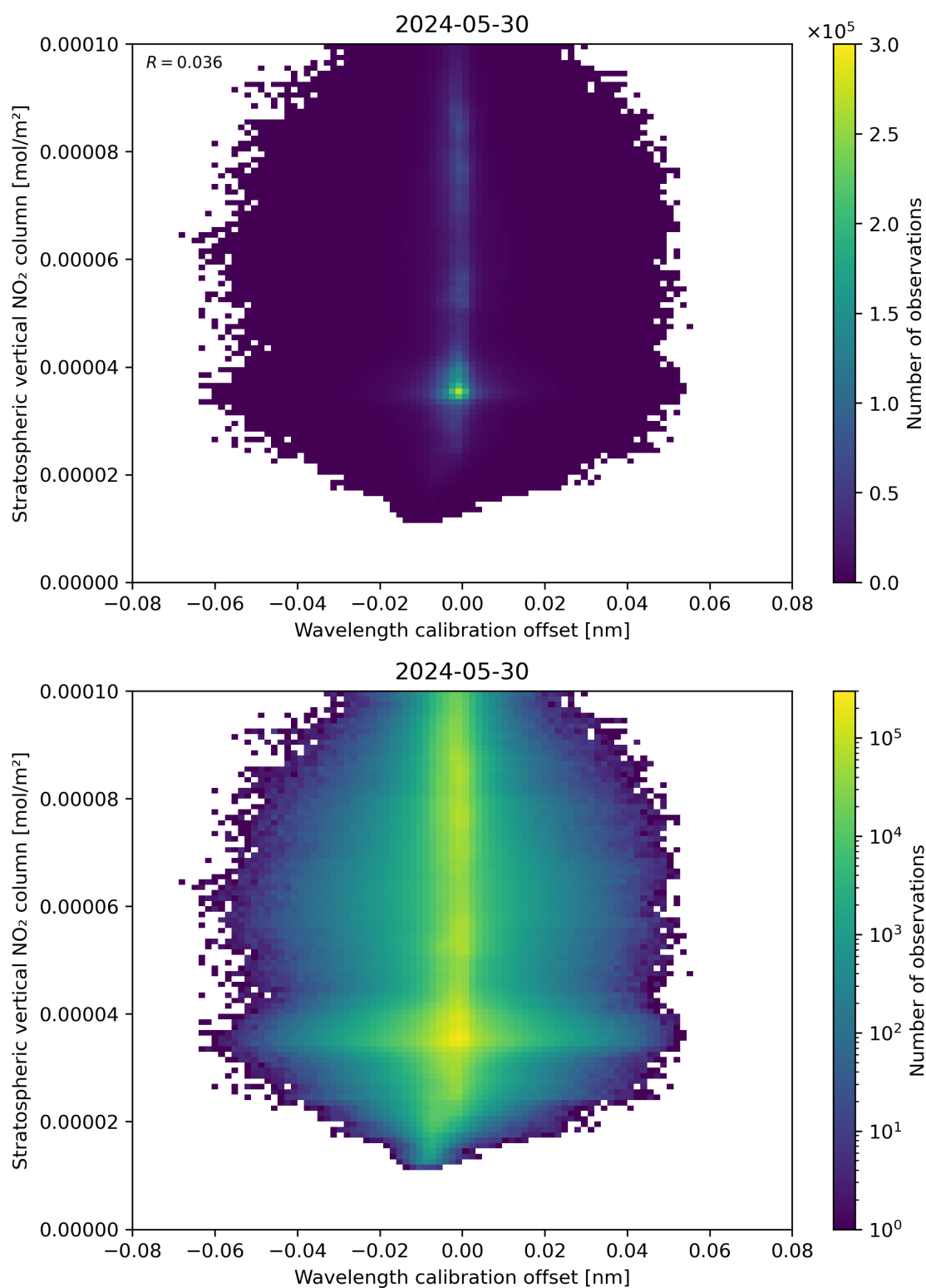
Figure 176: Scatter density plot of “Wavelength calibration offset” against “Stratospheric vertical NO 2 column” for 2024-05-29 to 2024-05-31.
