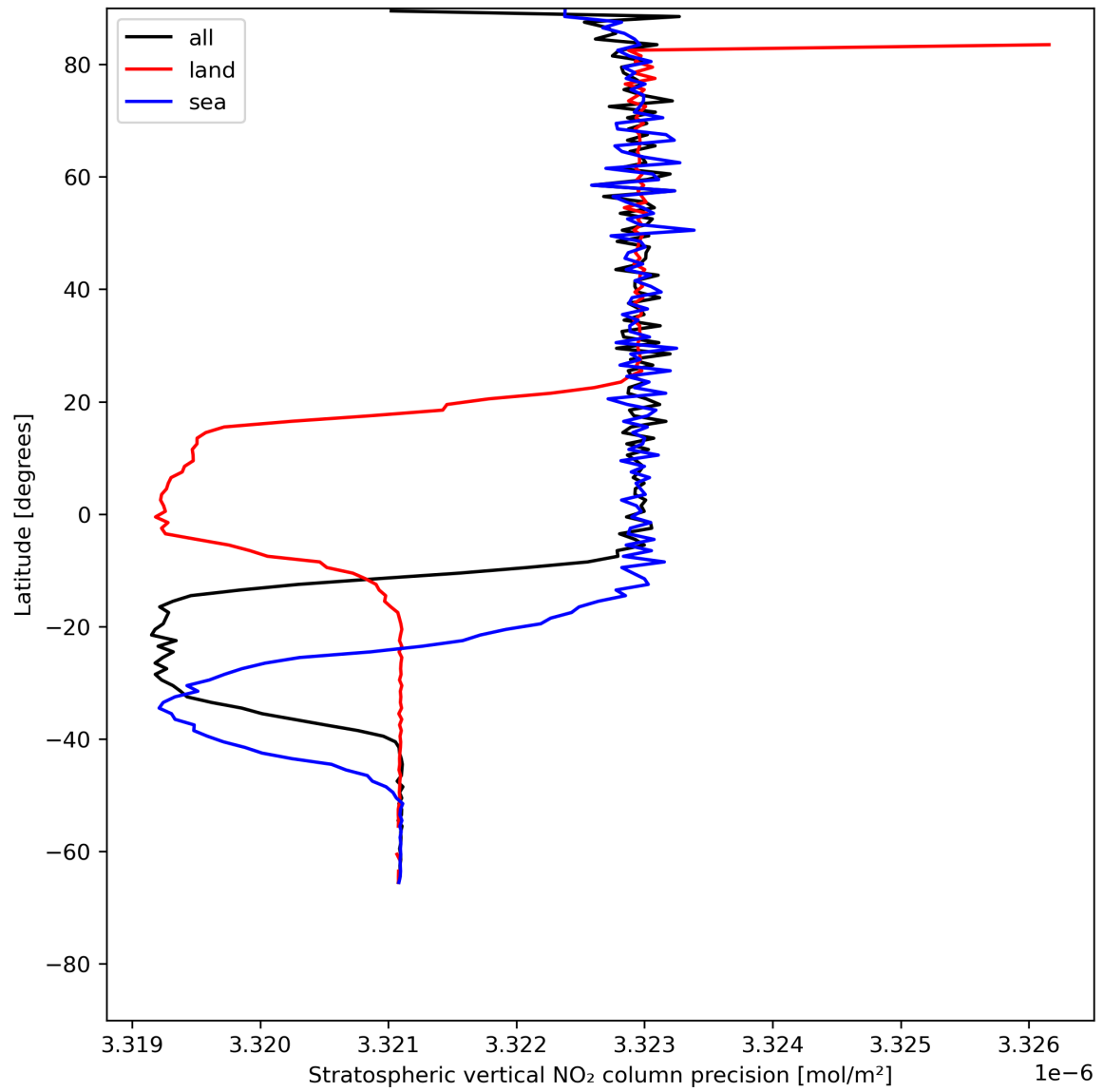
Figure 20: Zonal average of “Stratospheric vertical NO 2 column precision” for 2024-05-29 to 2024-05-31.
