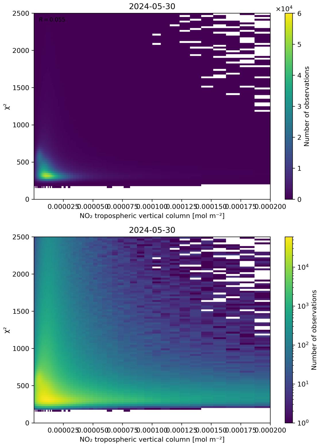
Figure 124: Scatter density plot of “NO 2 tropospheric vertical column” against “ \chi^2 ” for 2024-05-29 to 2024-05-31.
