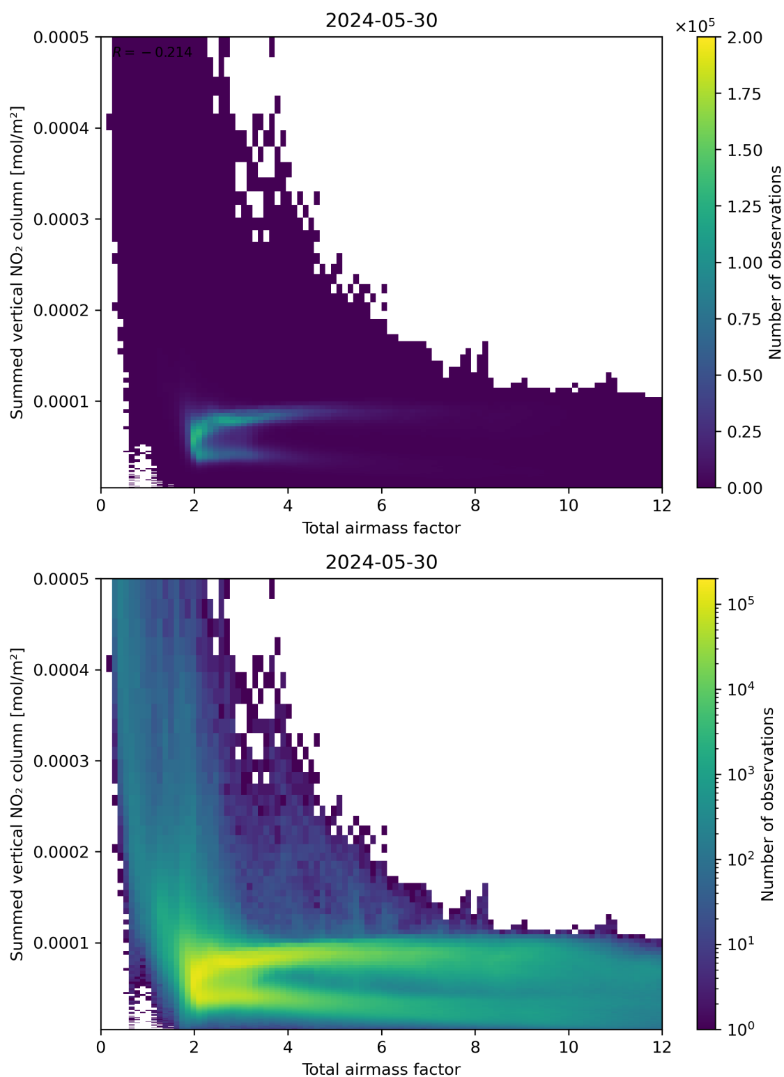
Figure 65: Scatter density plot of “Total airmass factor” against “Summed vertical NO 2 column” for 2024-05-29 to 2024-05-31.
