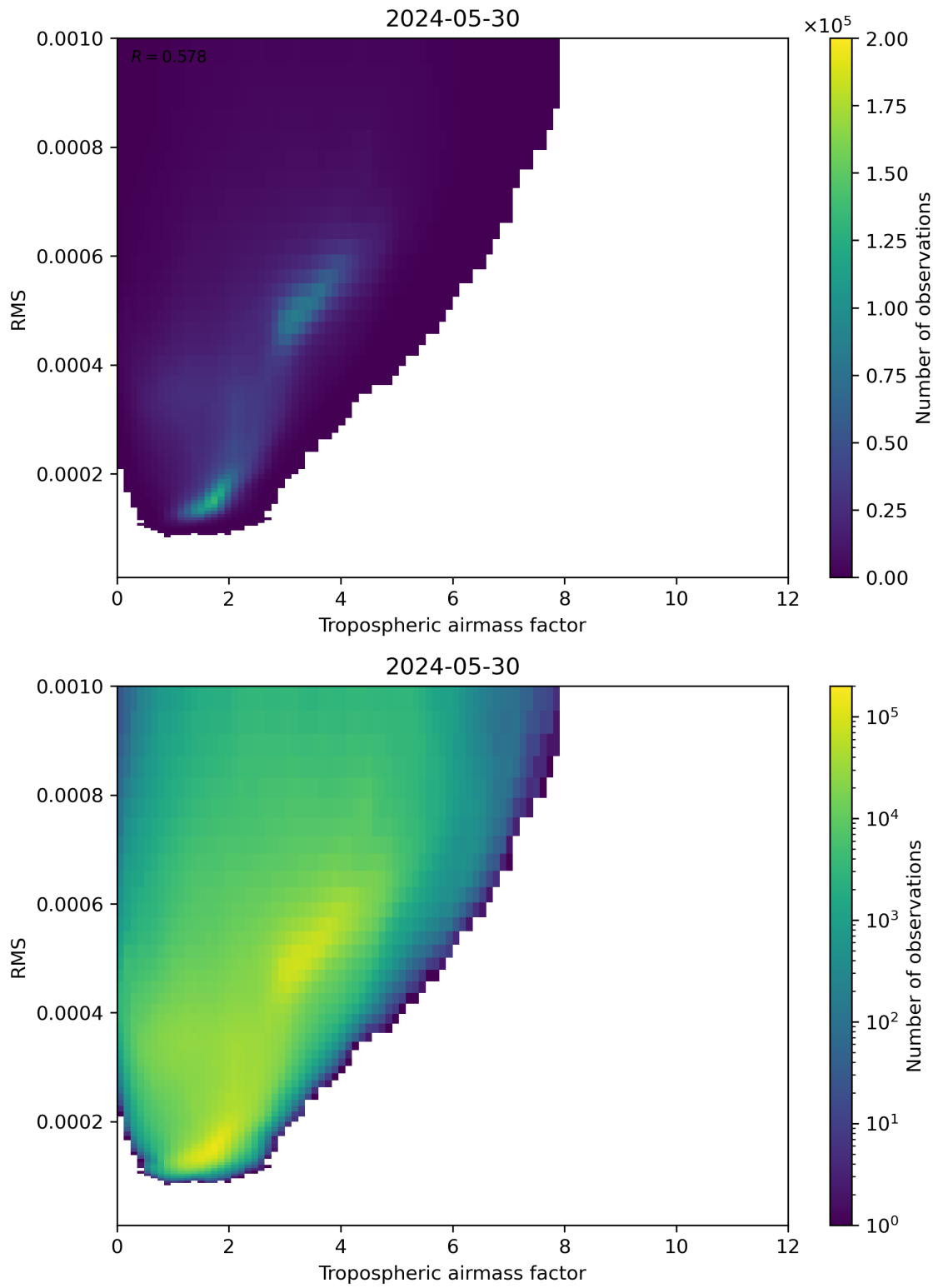
Figure 79: Scatter density plot of “Tropospheric airmass factor” against “RMS” for 2024-05-29 to 2024-05-31.
