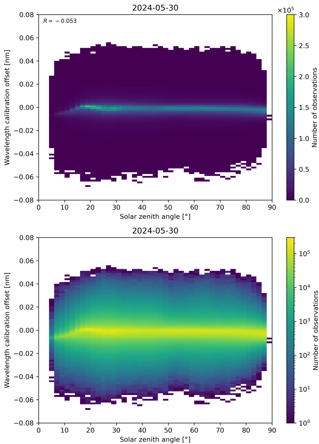
Figure 158: Scatter density plot of “Solar zenith angle” against “Wavelength calibration offset” for 2024-05-29 to 2024-05-31.
