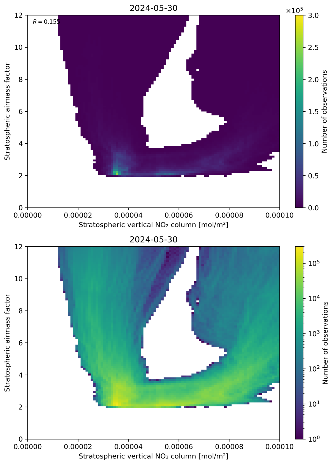
Figure 96: Scatter density plot of “Stratospheric vertical NO 2 column” against “Stratospheric airmass factor” for 2024-05-29 to 2024-05-31.
