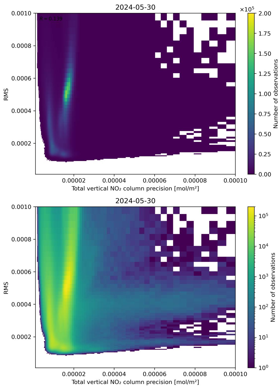
Figure 119: Scatter density plot of “Total vertical NO 2 column precision” against “RMS” for 2024-05-29 to 2024-05-31.
