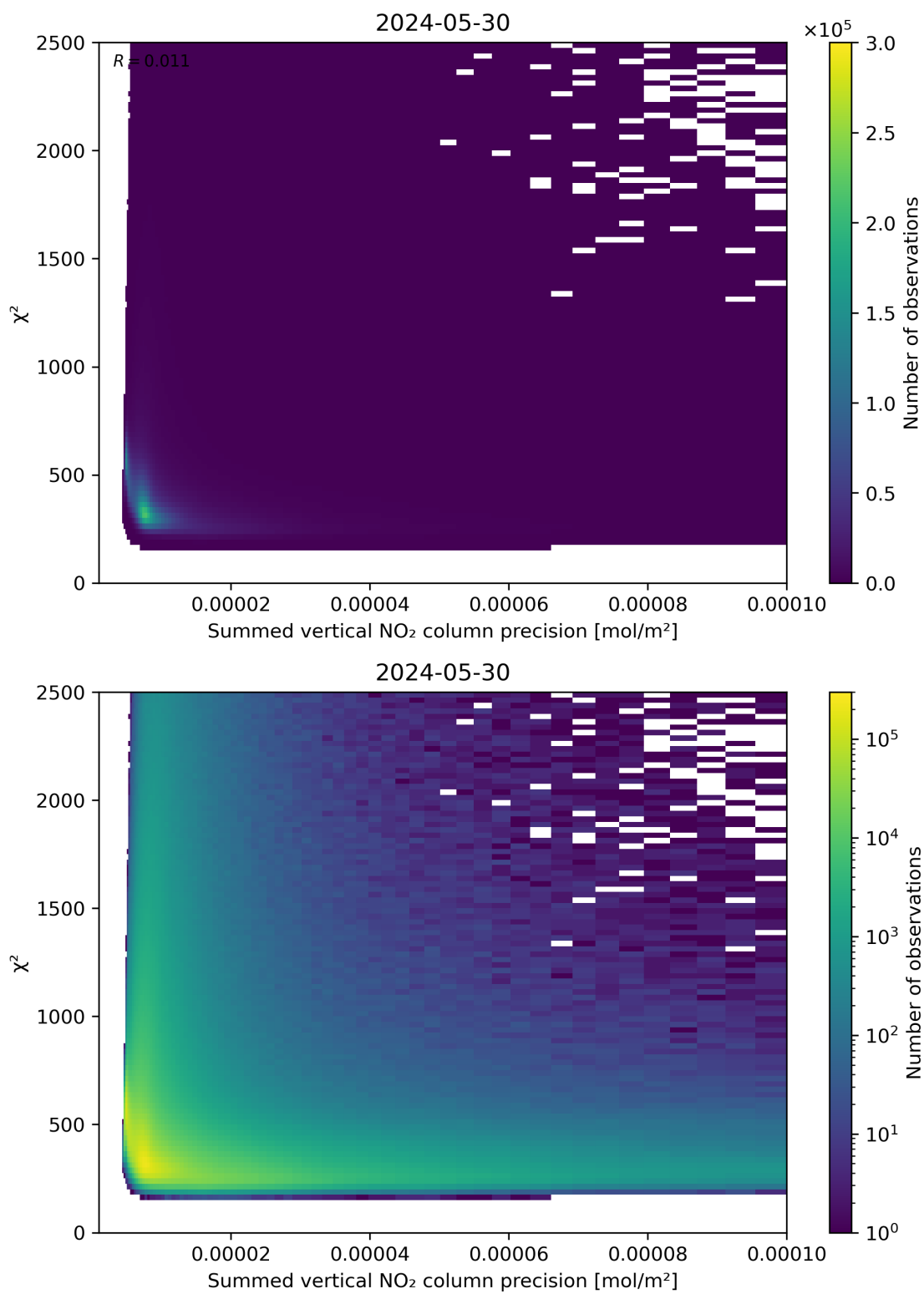
Figure 107: Scatter density plot of “Summed vertical NO 2 column precision” against “ \chi^2 ” for 2024-05-29 to 2024-05-31.
