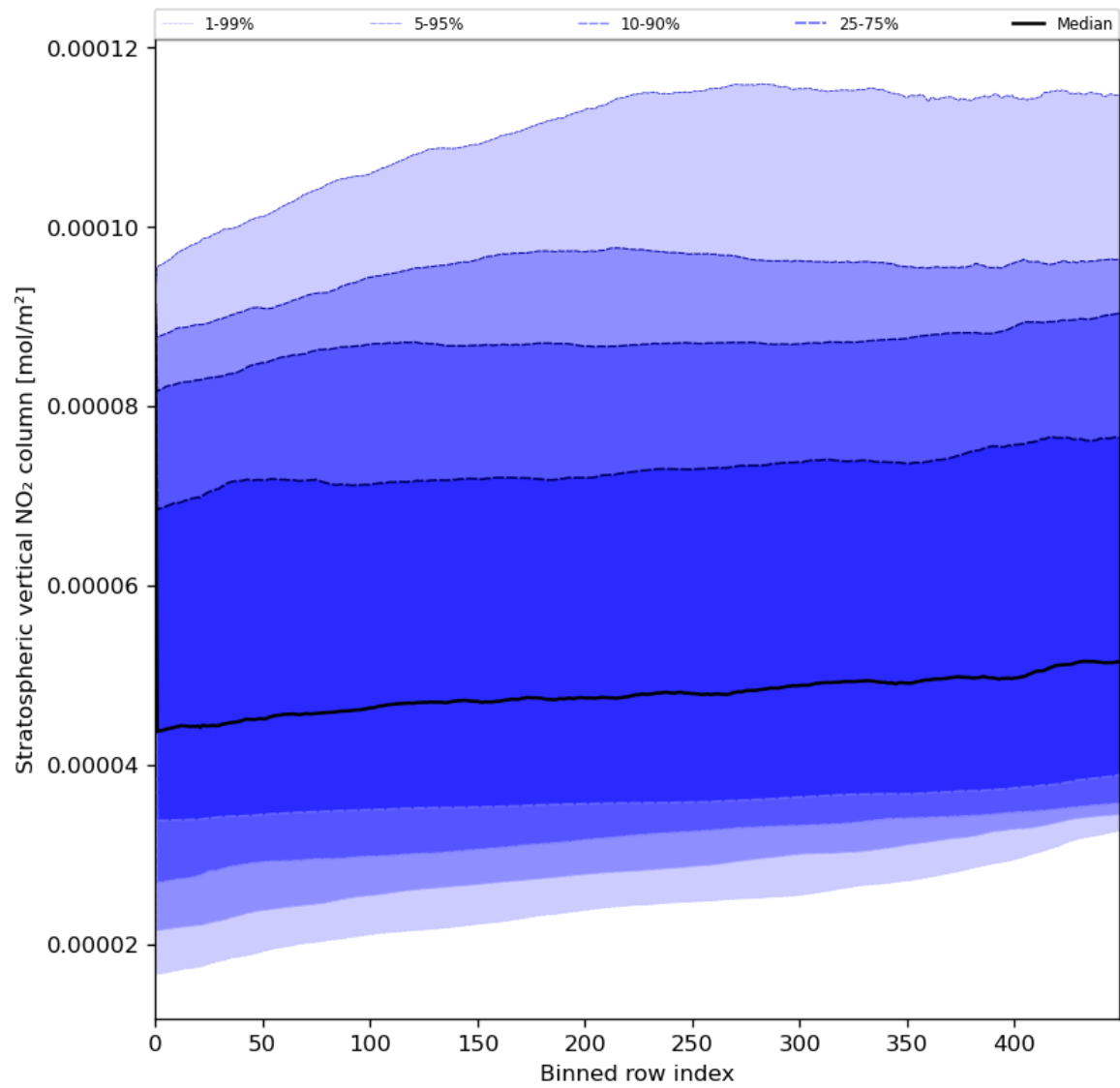
Figure 53: Along track statistics of “Stratospheric vertical NO 2 column” for 2024-05-29 to 2024-05-31
