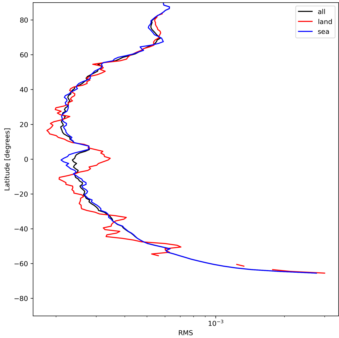
Figure 26: Zonal average of “RMS” for 2024-05-29 to 2024-05-31.
