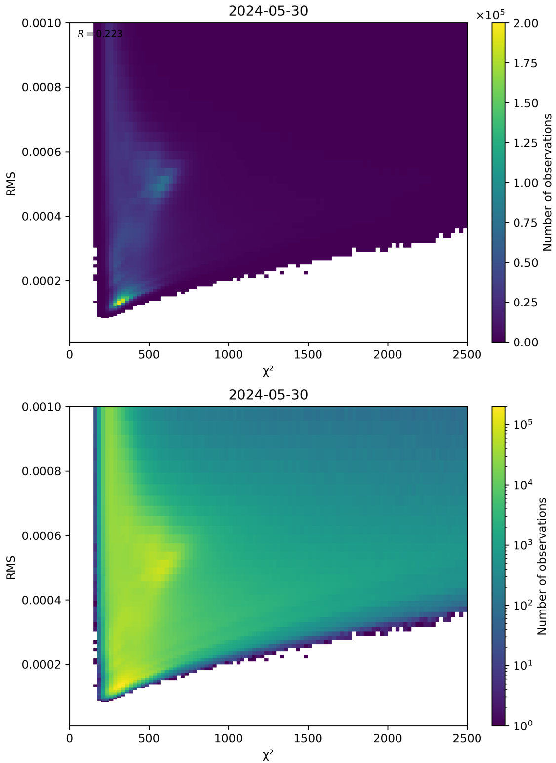
Figure 82: Scatter density plot of “ \chi^2 ” against “RMS” for 2024-05-29 to 2024-05-31.
