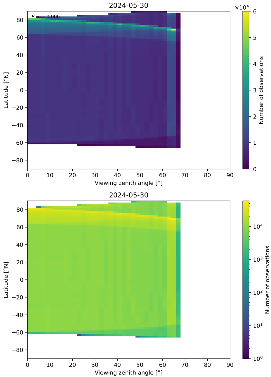
Figure 163: Scatter density plot of “Viewing zenith angle” against “Latitude” for 2024-05-29 to 2024-05-31.
