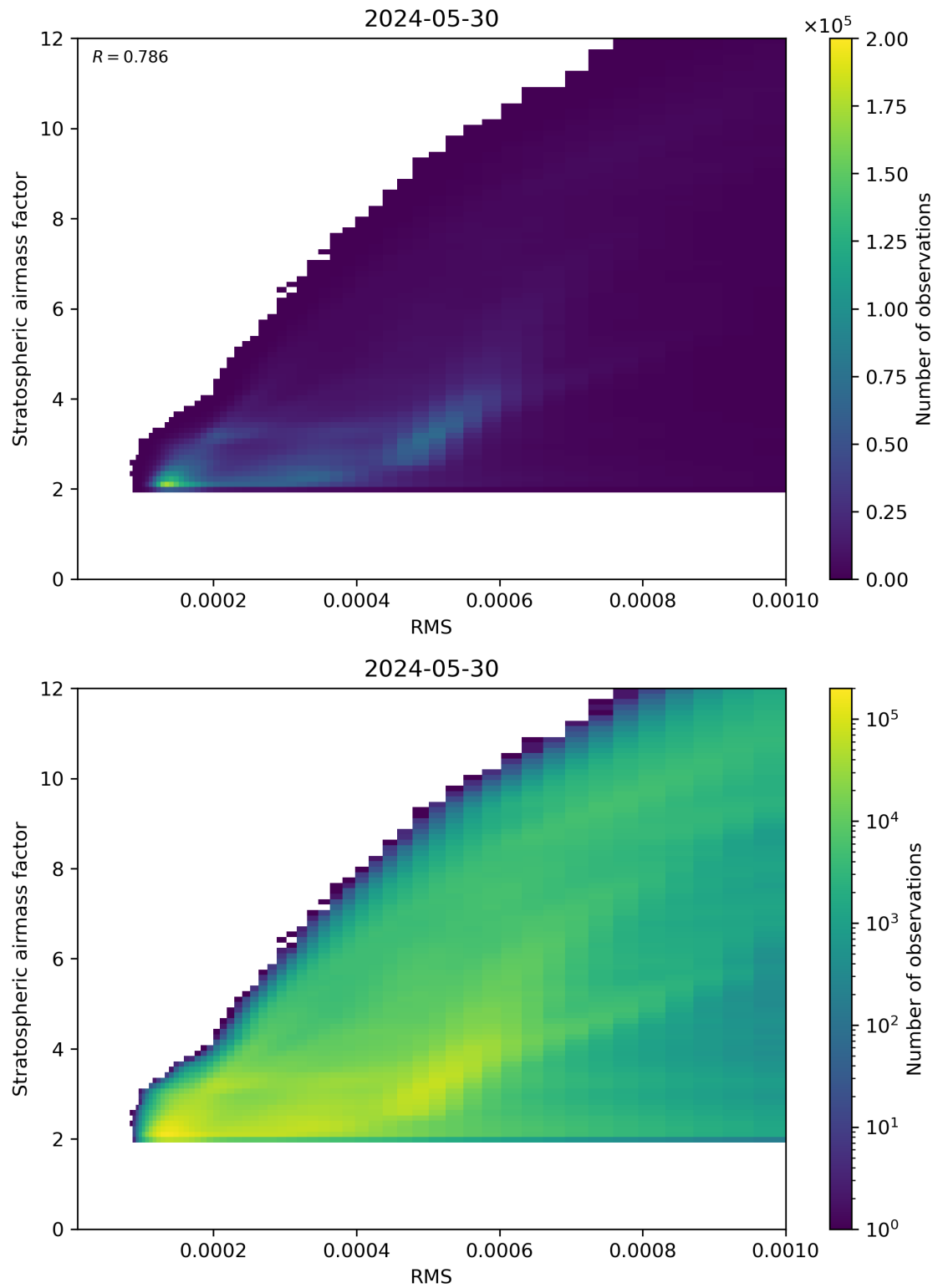
Figure 144: Scatter density plot of “RMS” against “Stratospheric airmass factor” for 2024-05-29 to 2024-05-31.
