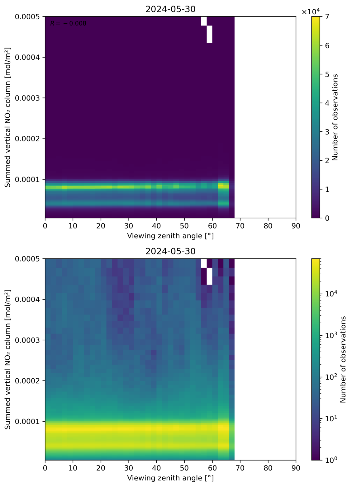
Figure 165: Scatter density plot of “Viewing zenith angle” against “Summed vertical NO 2 column” for 2024-05-29 to 2024-05-31.
