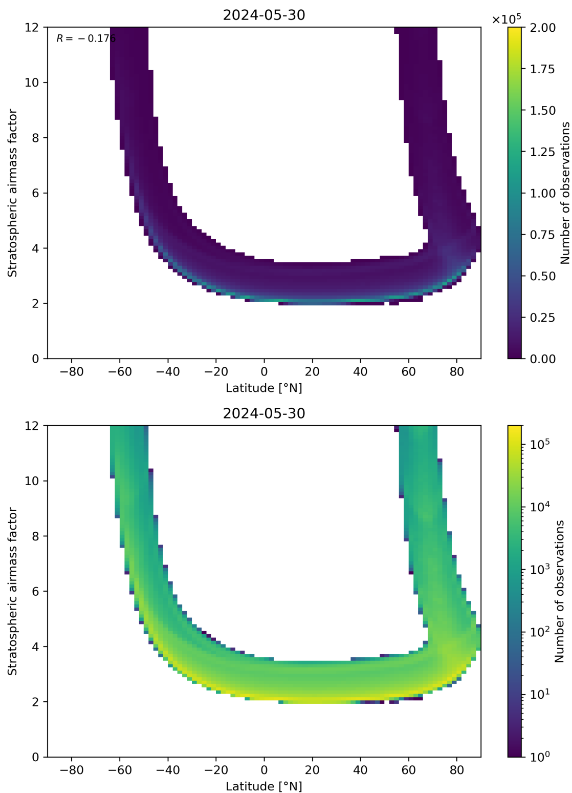
Figure 83: Scatter density plot of “Latitude” against “Stratospheric airmass factor” for 2024-05-29 to 2024-05-31.
