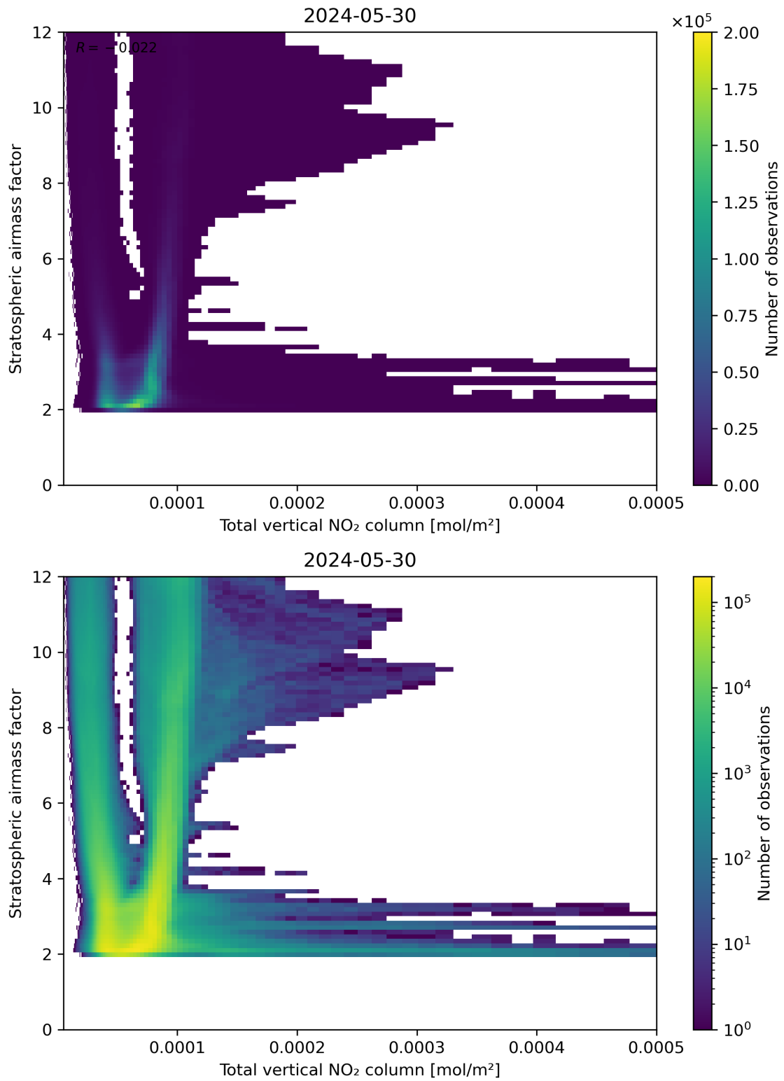
Figure 110: Scatter density plot of “Total vertical NO 2 column” against “Stratospheric airmass factor” for 2024-05-29 to 2024-05-31.
