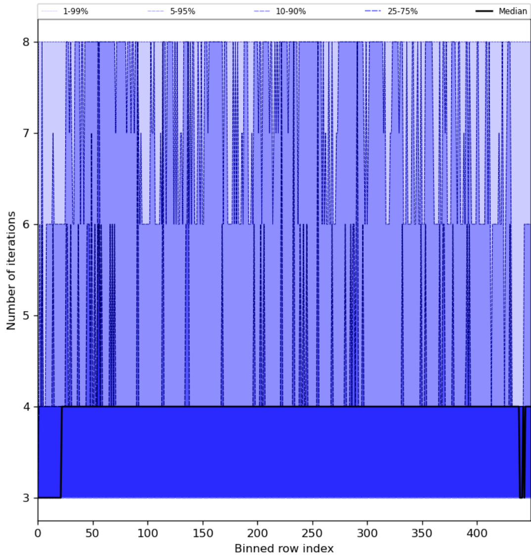
Figure 51: Along track statistics of “Number of iterations” for 2024-05-29 to 2024-05-31
