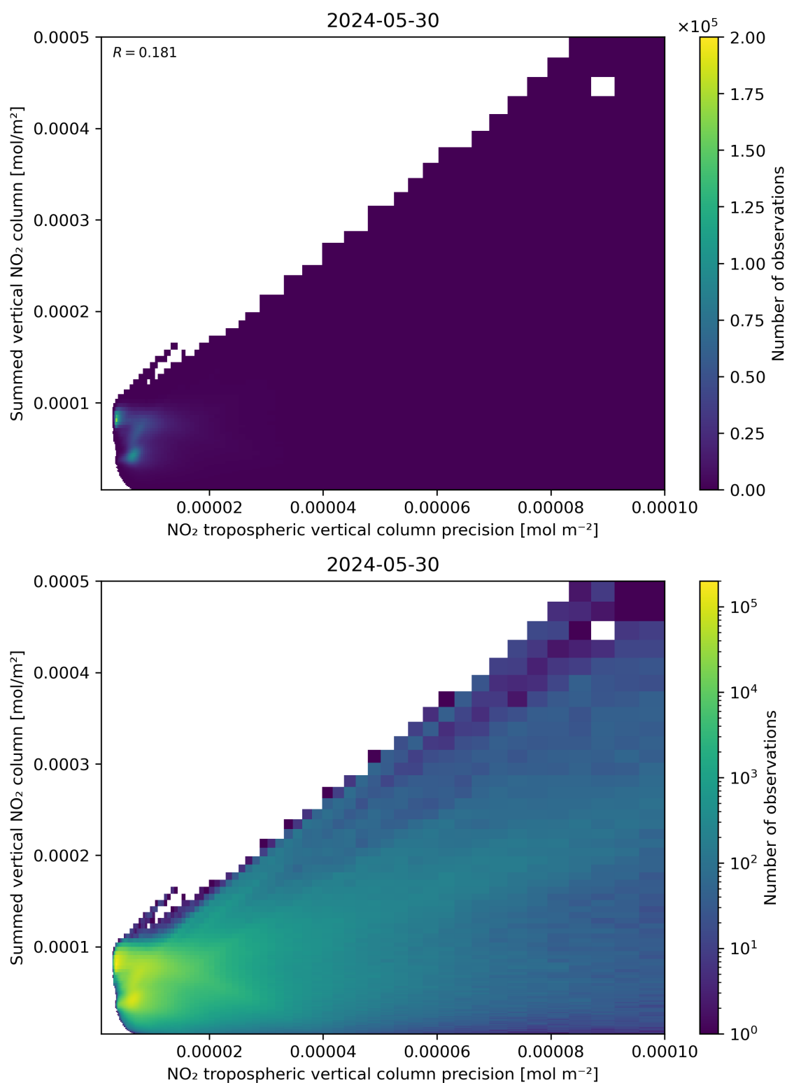
Figure 136: Scatter density plot of “NO 2 tropospheric vertical column precision” against “Summed vertical NO 2 column” for 2024-05-29 to 2024-05-31.
