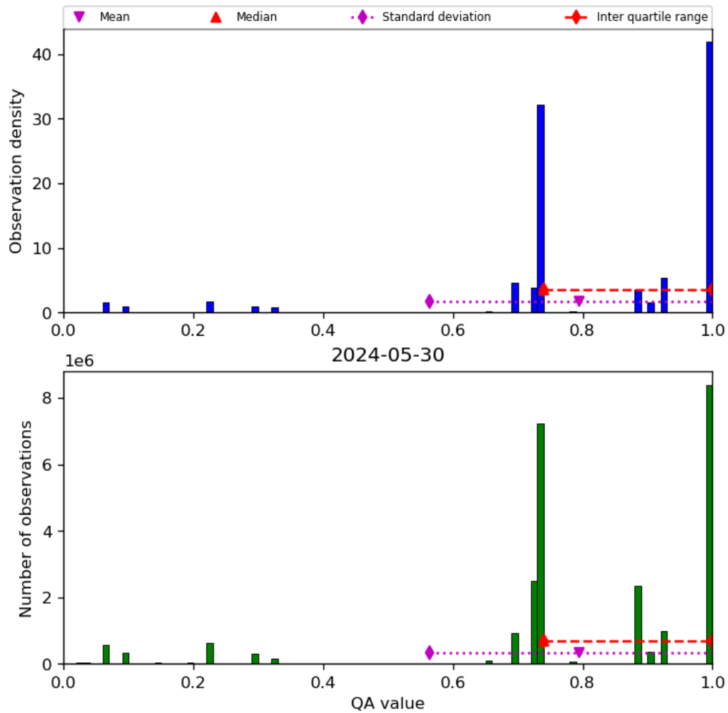
Figure 28: Histogram of “QA value” for 2024-05-29 to 2024-05-31
