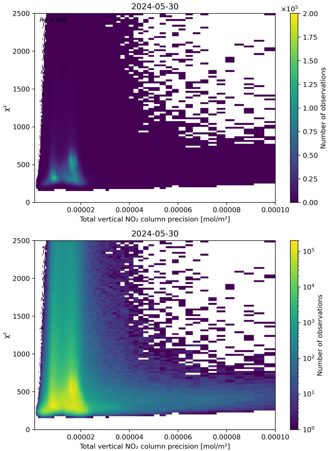
Figure 116: Scatter density plot of “Total vertical NO 2 column precision” against “ \chi^2 ” for 2024-05-29 to 2024-05-31.
