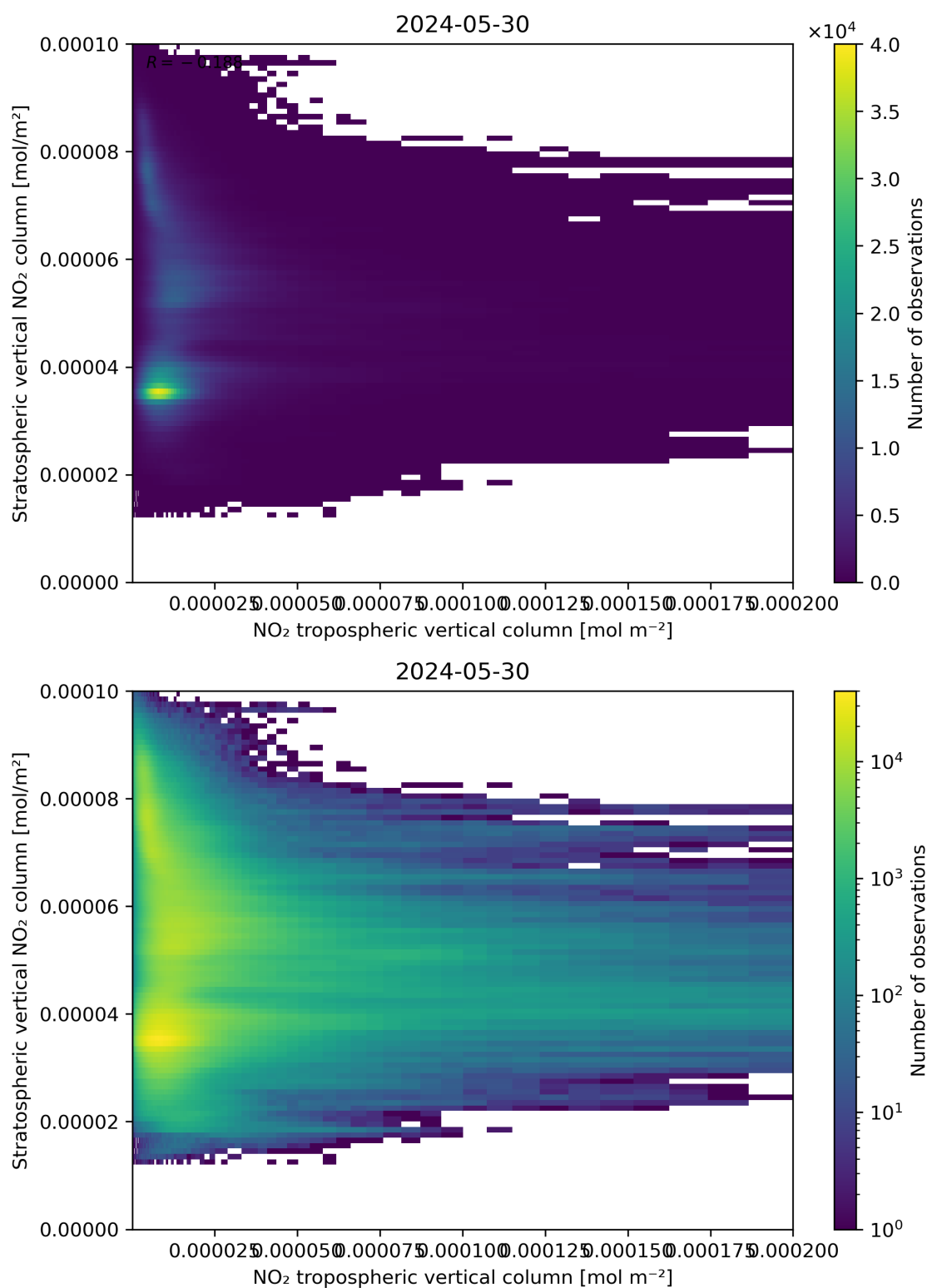
Figure 125: Scatter density plot of “NO 2 tropospheric vertical column” against “Stratospheric vertical NO 2 column” for 2024-05-29 to 2024-05-31.
