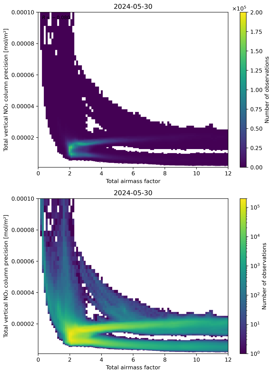
Figure 68: Scatter density plot of “Total airmass factor” against “Total vertical NO 2 column precision” for 2024-05-29 to 2024-05-31.
