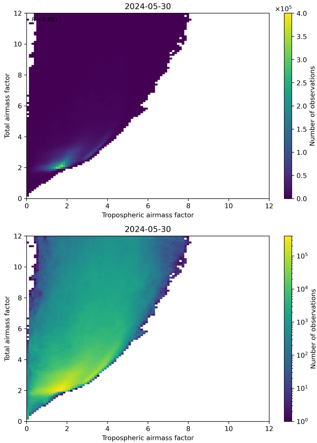
Figure 72: Scatter density plot of “Tropospheric airmass factor” against “Total airmass factor” for 2024-05-29 to 2024-05-31.
