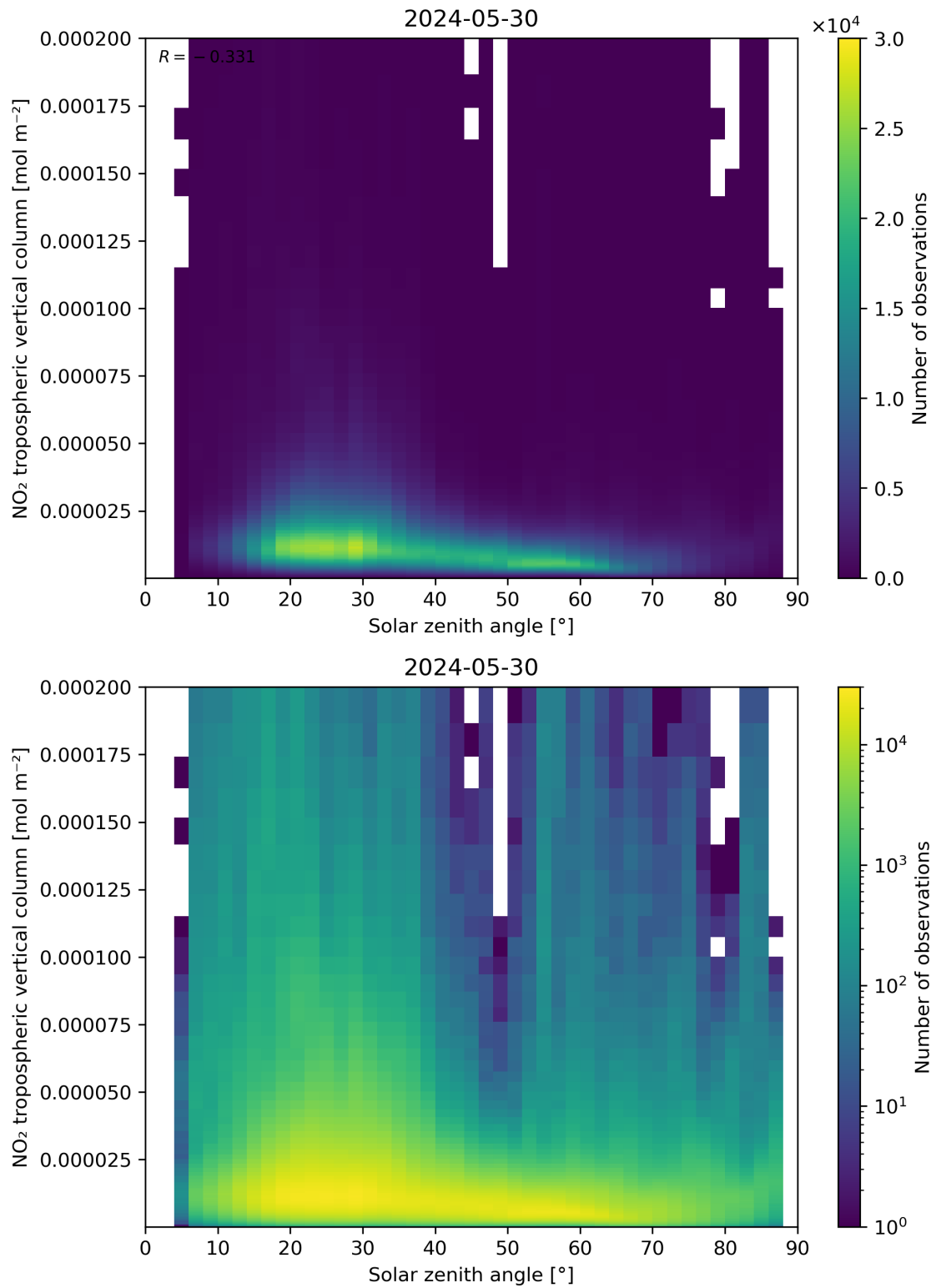
Figure 155: Scatter density plot of “Solar zenith angle” against “NO 2 tropospheric vertical column” for 2024-05-29 to 2024-05-31.
