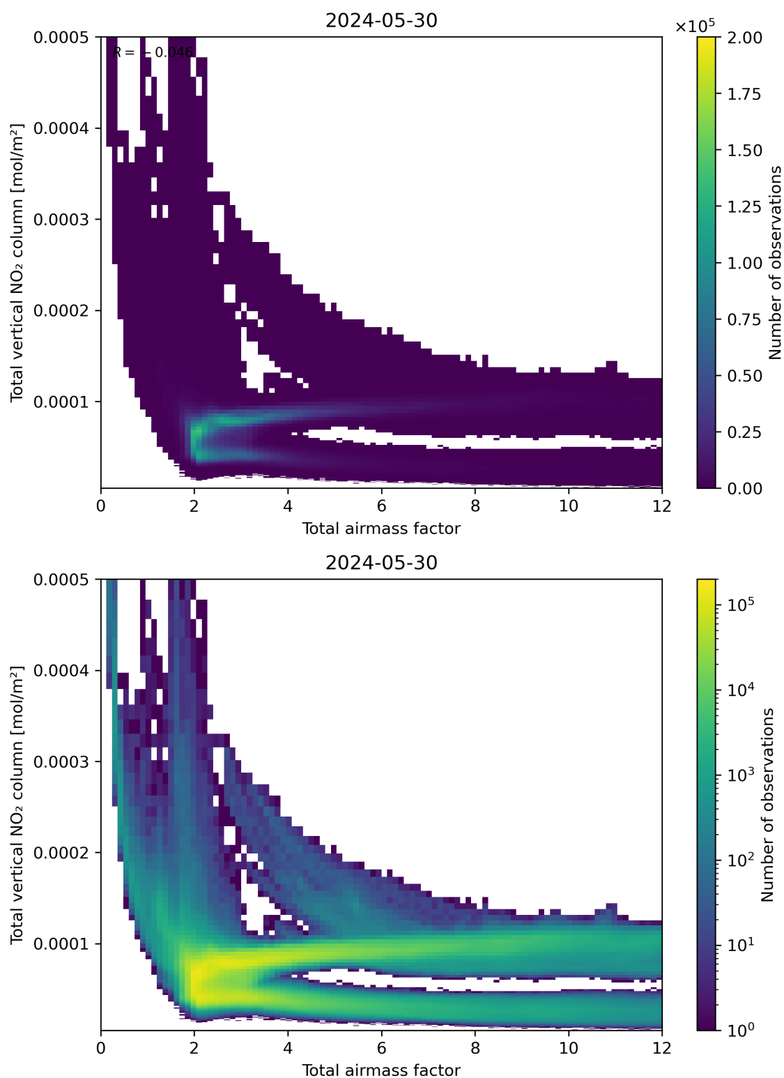
Figure 67: Scatter density plot of “Total airmass factor” against “Total vertical NO 2 column” for 2024-05-29 to 2024-05-31.
