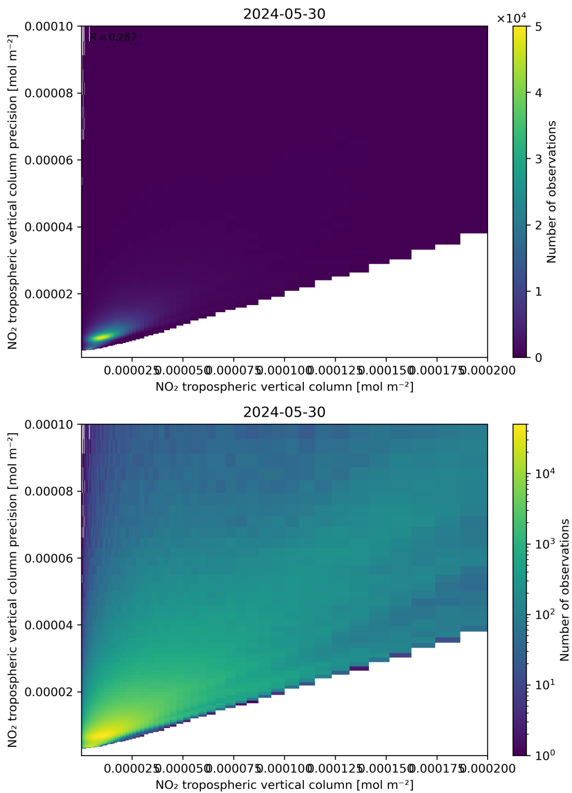
Figure 130: Scatter density plot of “NO 2 tropospheric vertical column” against “NO 2 tropospheric vertical column precision” for 2024-05-29 to 2024-05-31.
