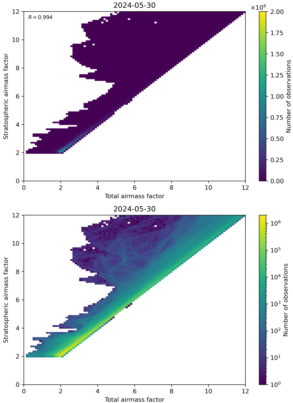
Figure 62: Scatter density plot of “Total airmass factor” against “Stratospheric airmass factor” for 2024-05-29 to 2024-05-31.
