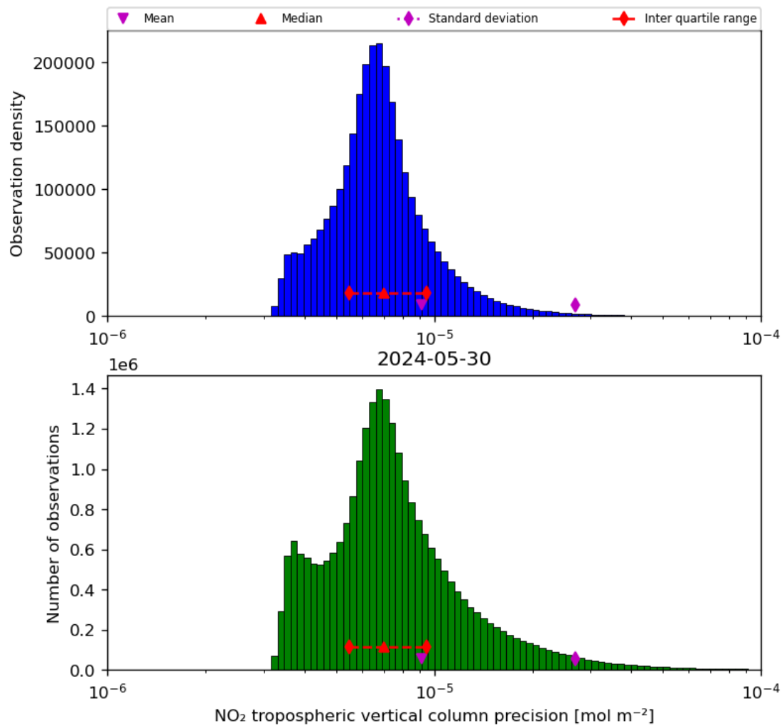
Figure 30: Histogram of “NO 2 tropospheric vertical column precision” for 2024-05-29 to 2024-05-31
