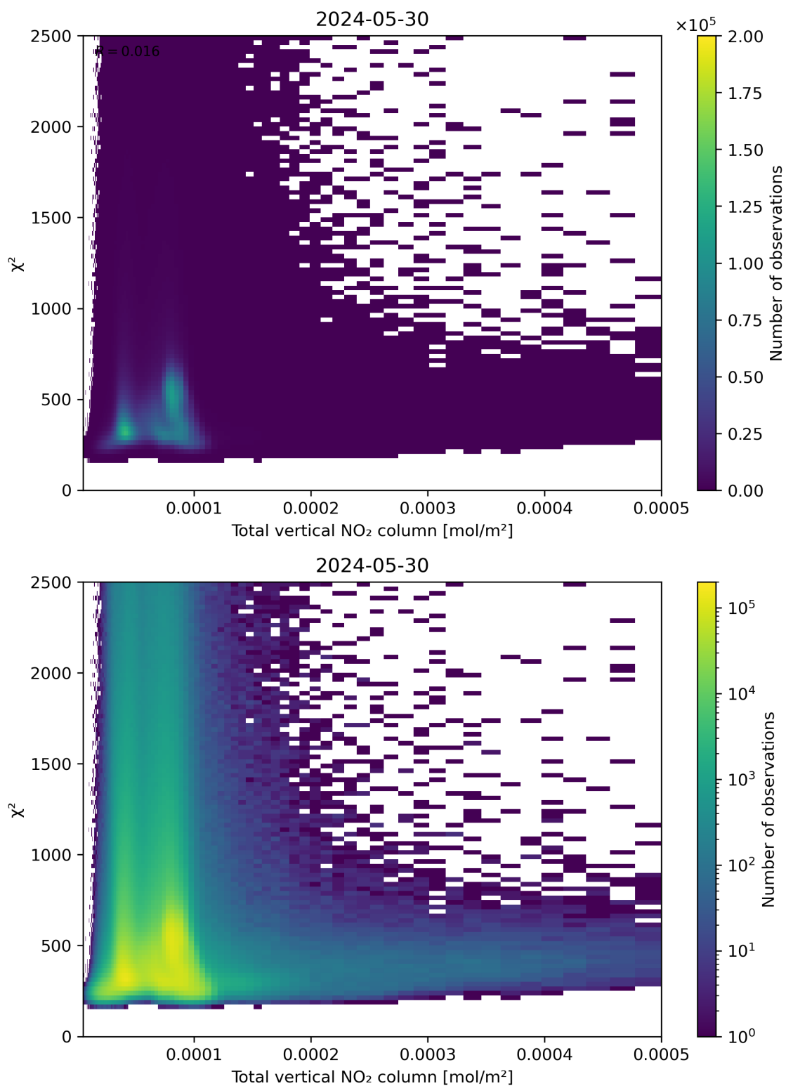
Figure 111: Scatter density plot of “Total vertical NO 2 column” against “ \chi^2 ” for 2024-05-29 to 2024-05-31.
