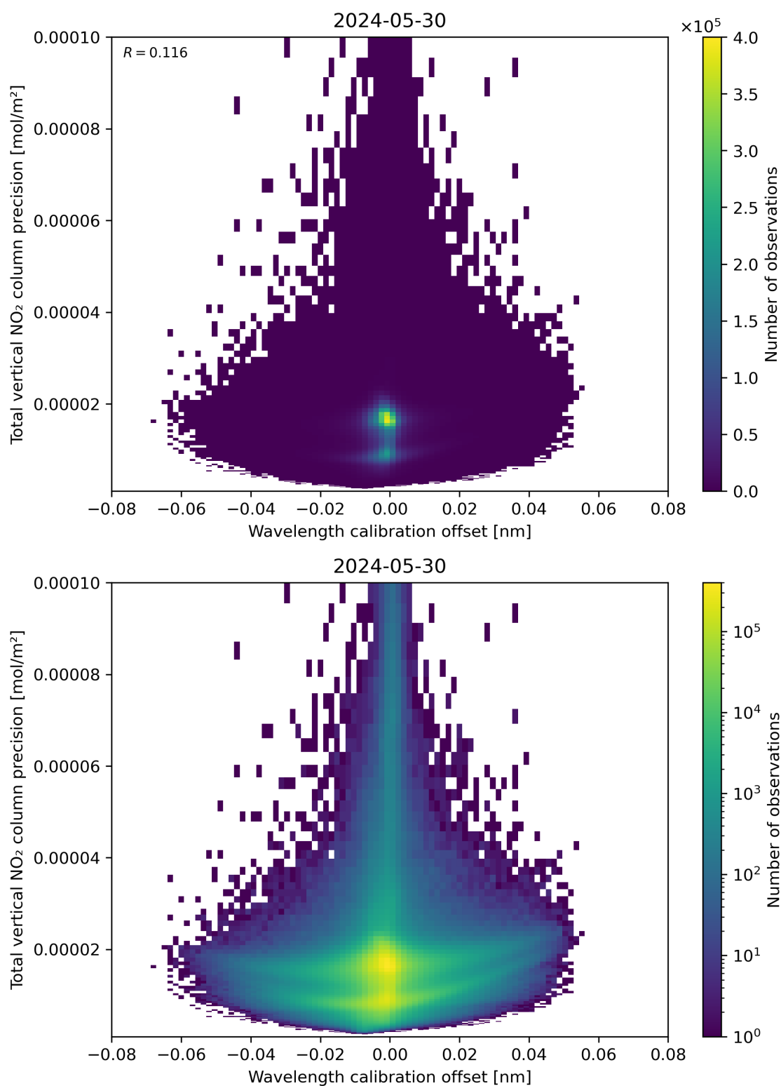
Figure 180: Scatter density plot of “Wavelength calibration offset” against “Total vertical NO 2 column precision” for 2024-05-29 to 2024-05-31.
