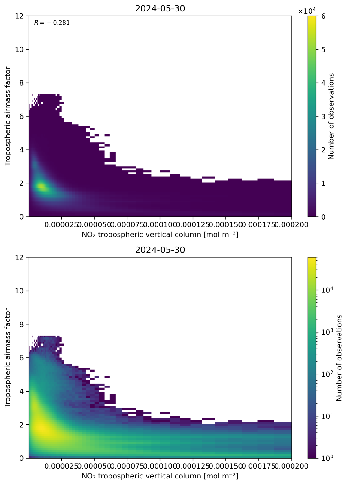
Figure 123: Scatter density plot of “NO 2 tropospheric vertical column” against “Tropospheric airmass factor” for 2024-05-29 to 2024-05-31.
