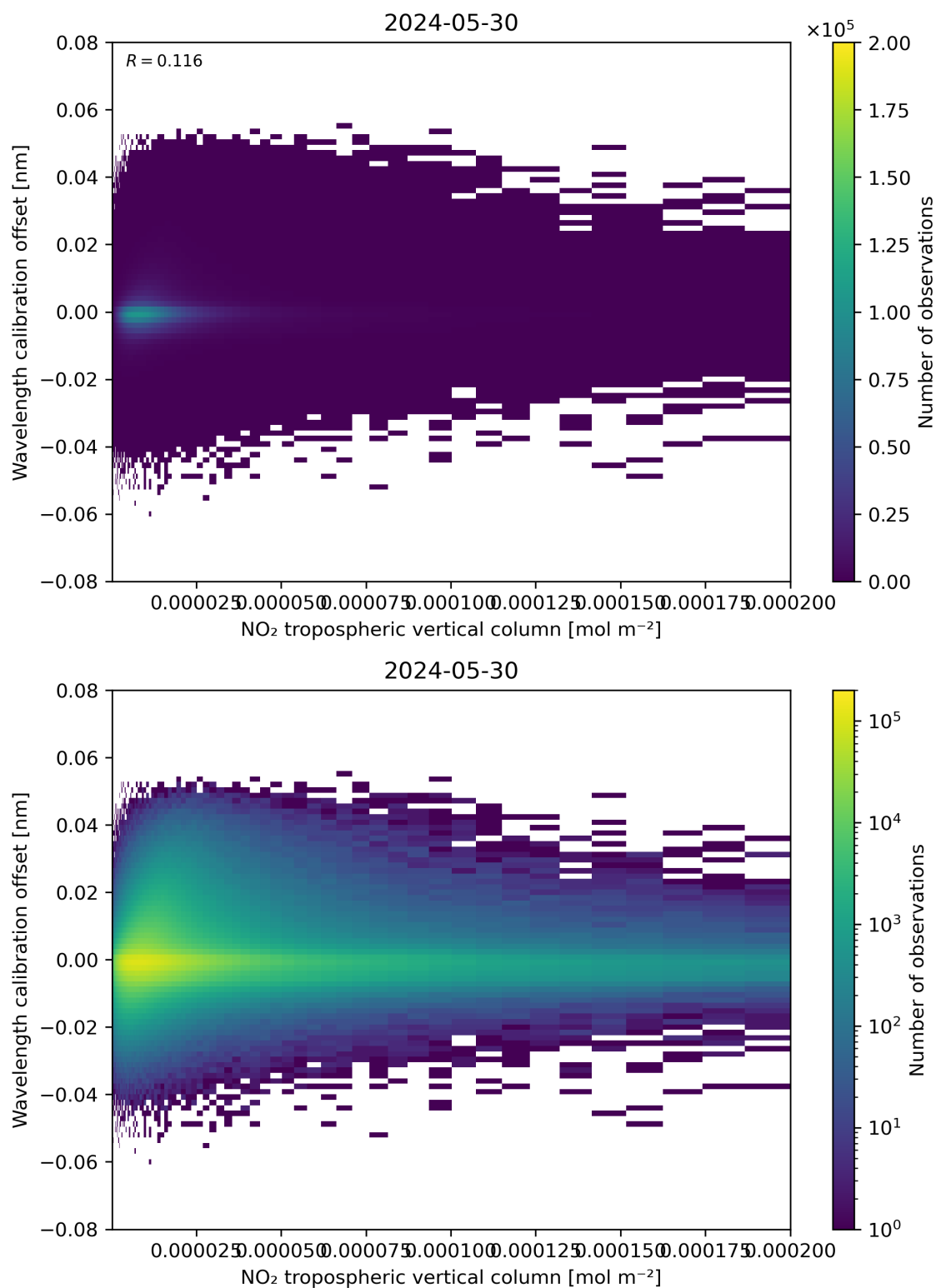
Figure 143: Scatter density plot of “NO 2 tropospheric vertical column” against “Wavelength calibration offset” for 2024-05-29 to 2024-05-31.
