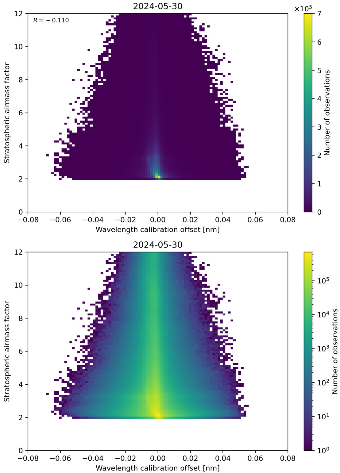
Figure 174: Scatter density plot of “Wavelength calibration offset” against “Stratospheric airmass factor” for 2024-05-29 to 2024-05-31.
