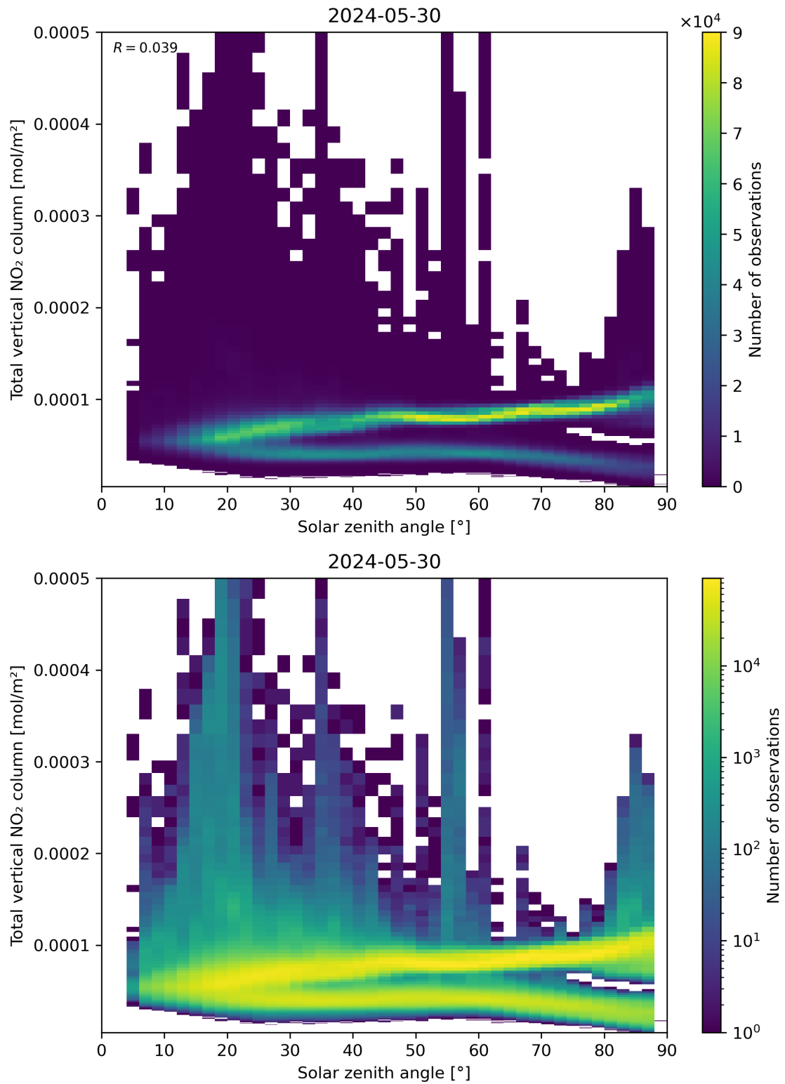
Figure 153: Scatter density plot of “Solar zenith angle” against “Total vertical NO 2 column” for 2024-05-29 to 2024-05-31.
