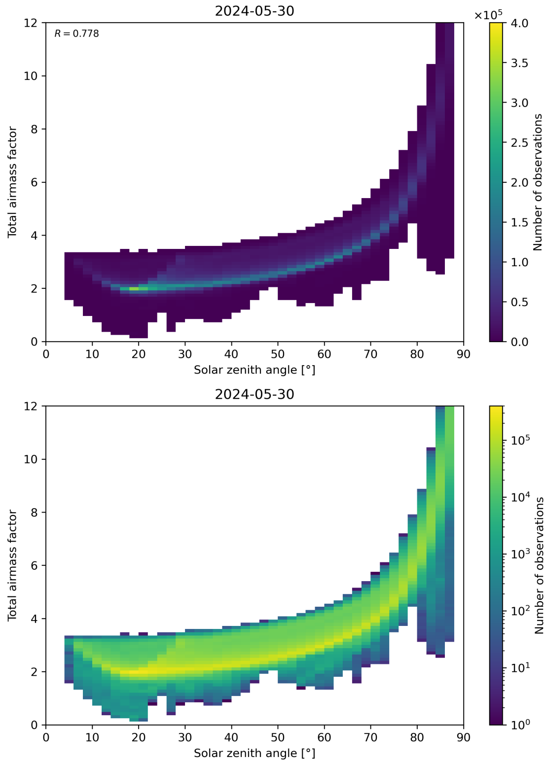
Figure 146: Scatter density plot of “Solar zenith angle” against “Total air mass factor” for 2024-05-29 to 2024-05-31.
