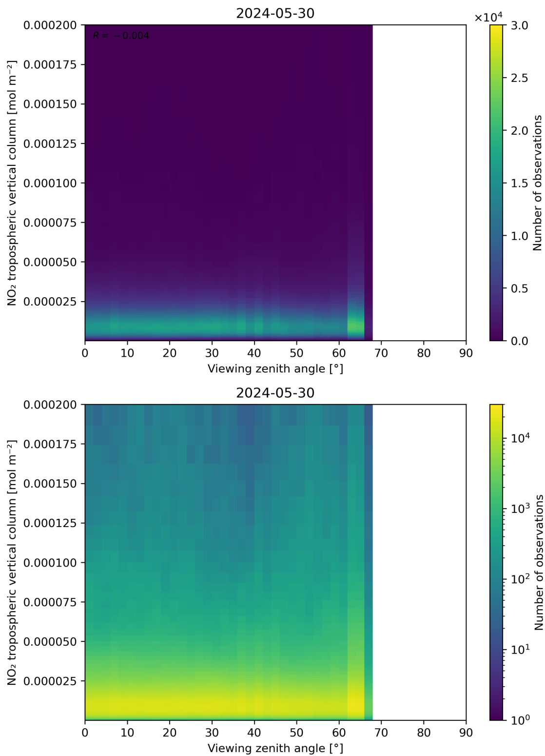
Figure 169: Scatter density plot of “Viewing zenith angle” against “NO 2 tropospheric vertical column” for 2024-05-29 to 2024-05-31.
