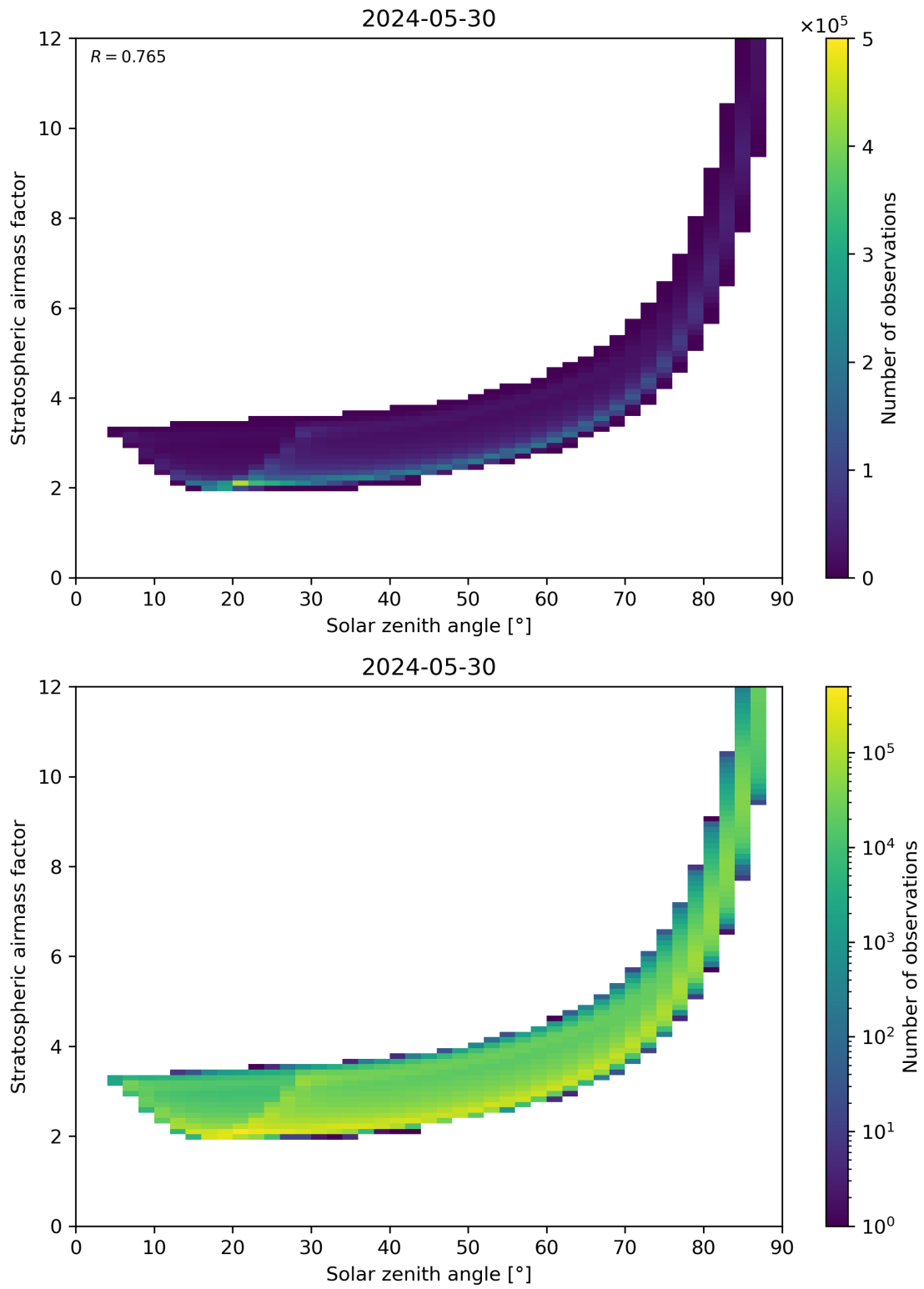
Figure 145: Scatter density plot of “Solar zenith angle” against “Stratospheric airmass factor” for 2024-05-29 to 2024-05-31.
