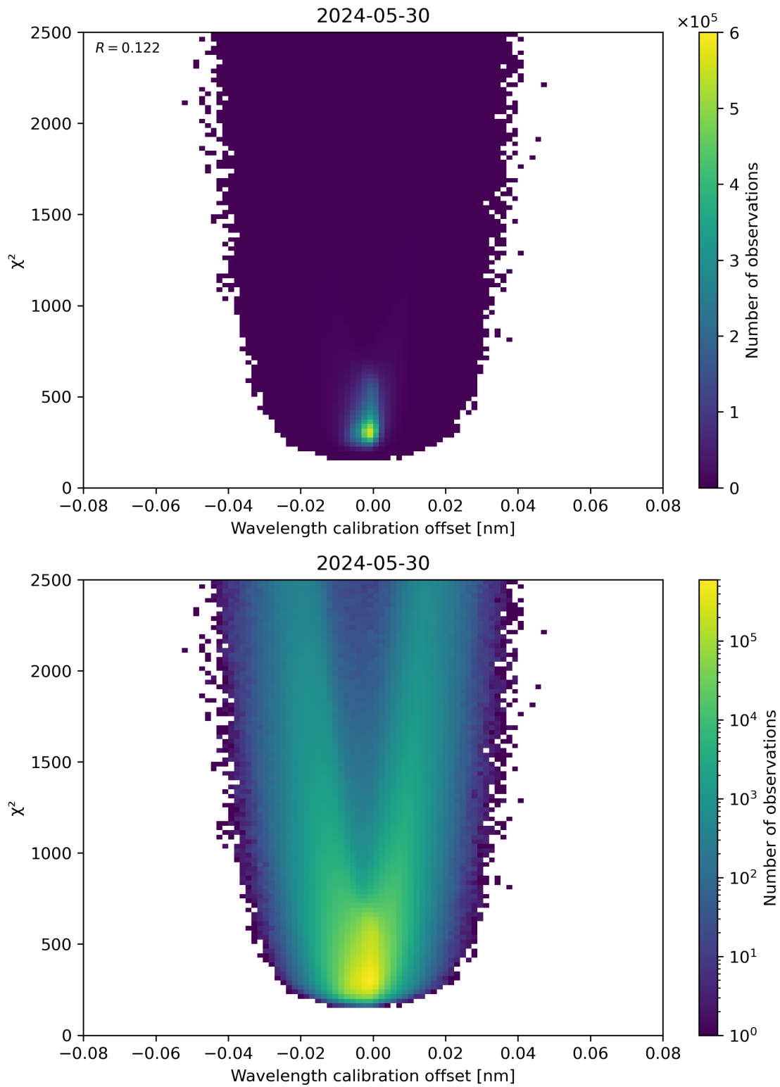
Figure 175: Scatter density plot of “Wavelength calibration offset” against “ \chi^2 ” for 2024-05-29 to 2024-05-31.
