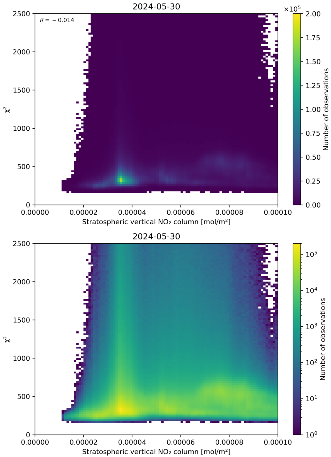
Figure 97: Scatter density plot of “Stratospheric vertical NO 2 column” against “ \chi^2 ” for 2024-05-29 to 2024-05-31.
