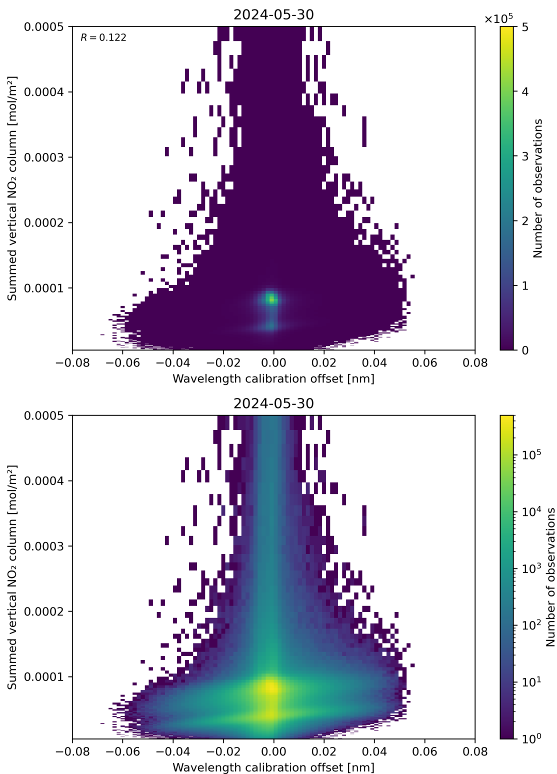
Figure 177: Scatter density plot of “Wavelength calibration offset” against “Summed vertical NO 2 column” for 2024-05-29 to 2024-05-31.
