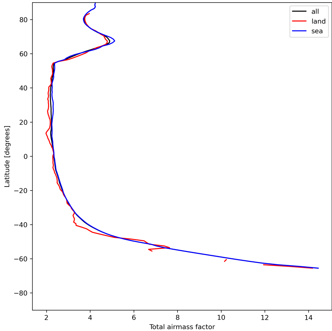
Figure 15: Zonal average of “Total airmass factor” for 2024-05-29 to 2024-05-31.
