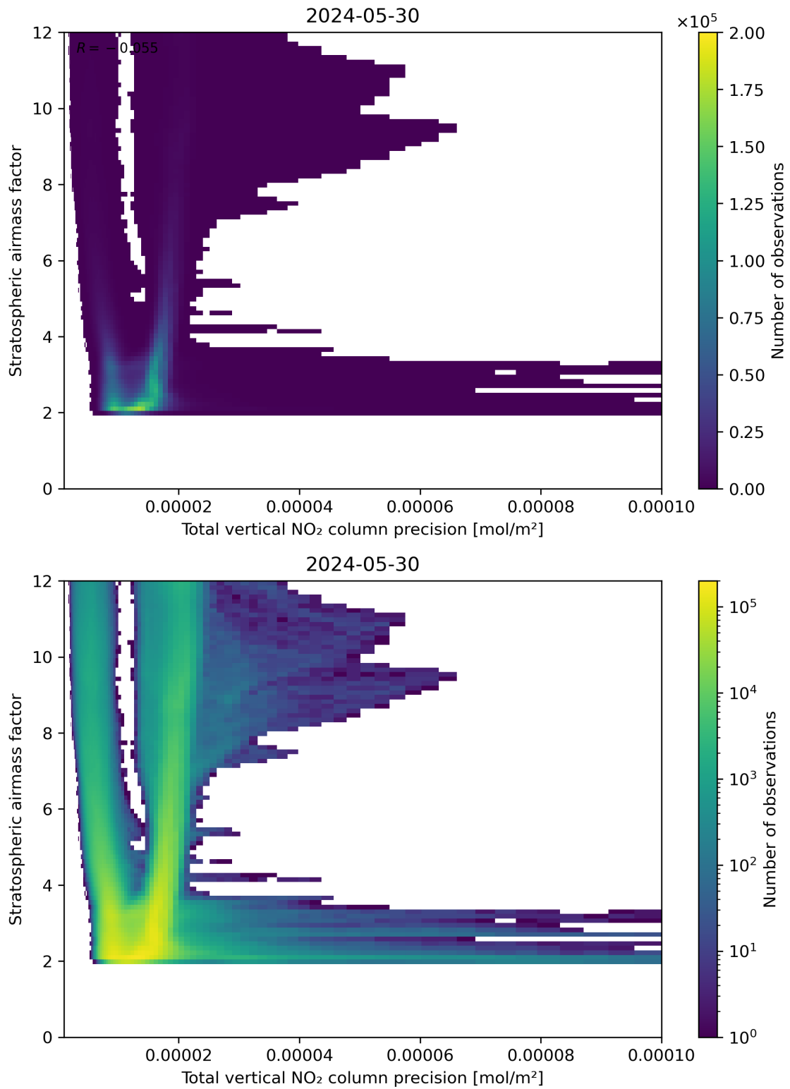
Figure 115: Scatter density plot of “Total vertical NO 2 column precision” against “Stratospheric air mass factor” for 2024-05-29 to 2024-05-31.
