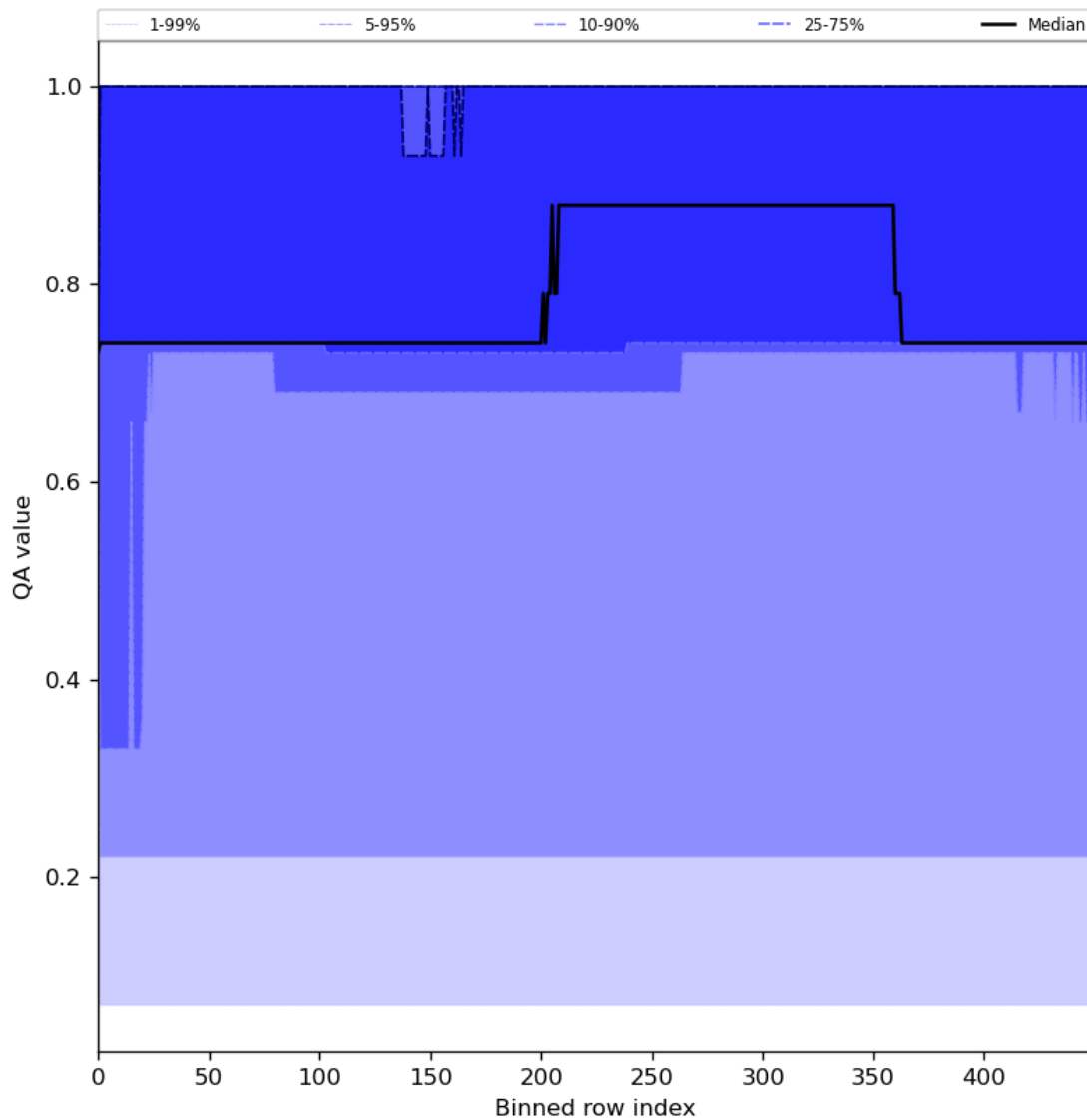
Figure 45: Along track statistics of “QA value” for 2024-05-29 to 2024-05-31
