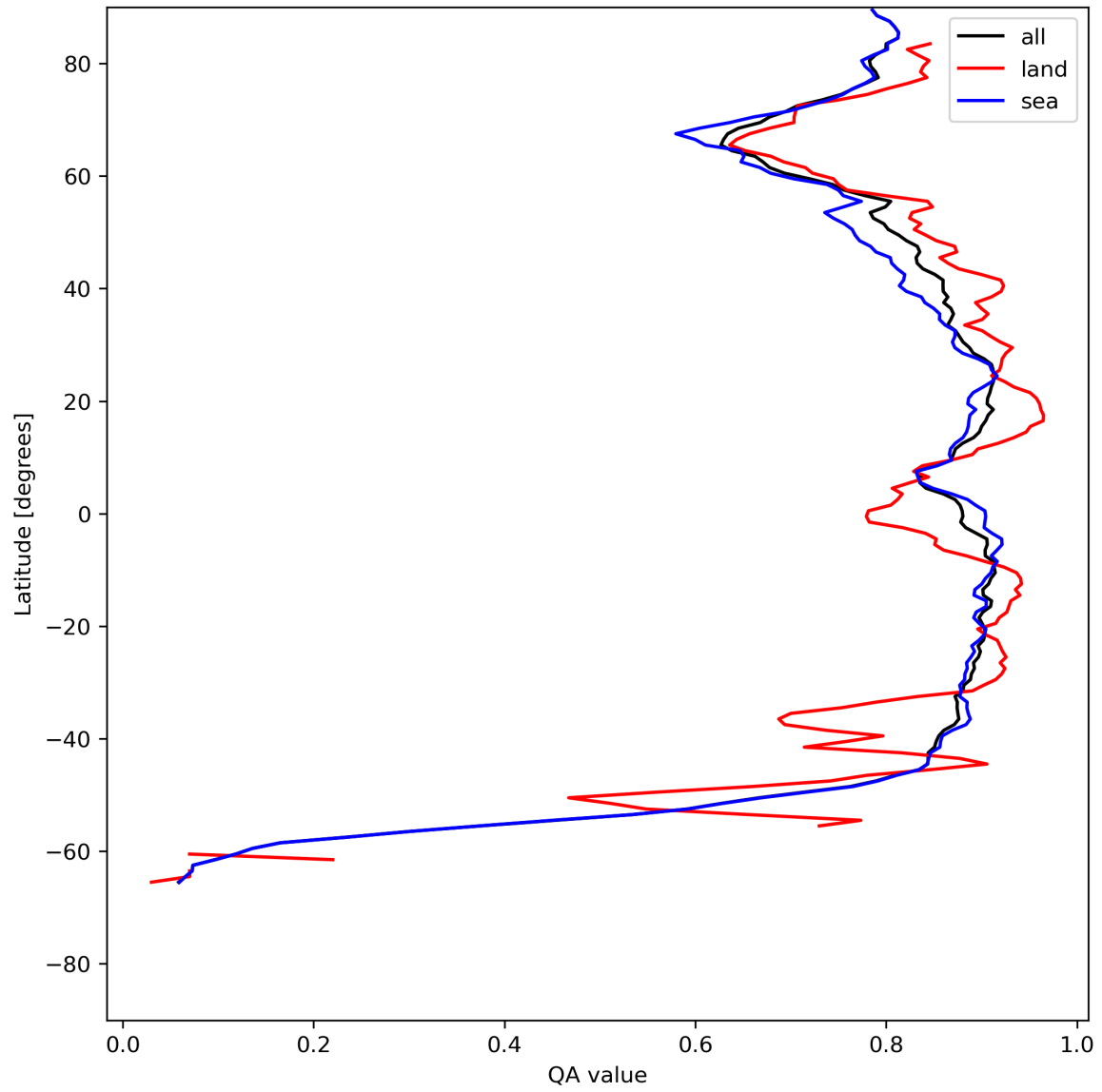
Figure 11: Zonal average of “QA value” for 2024-05-29 to 2024-05-31.
