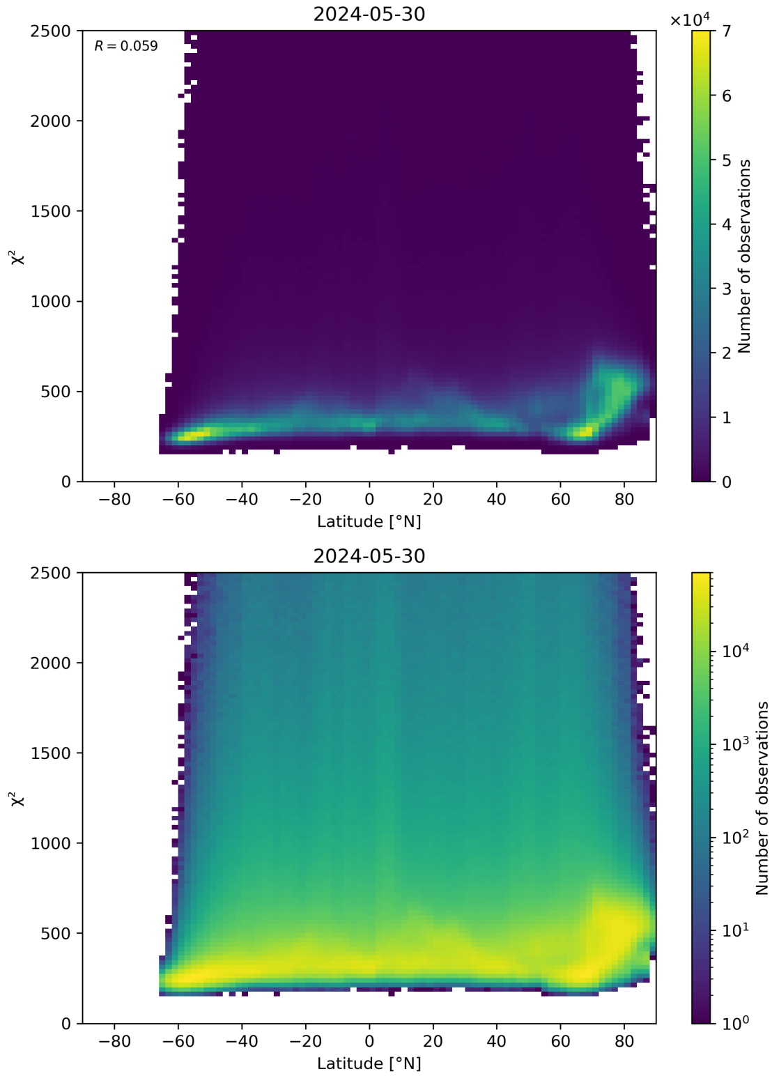
Figure 86: Scatter density plot of “Latitude” against “ \chi^2 ” for 2024-05-29 to 2024-05-31.
