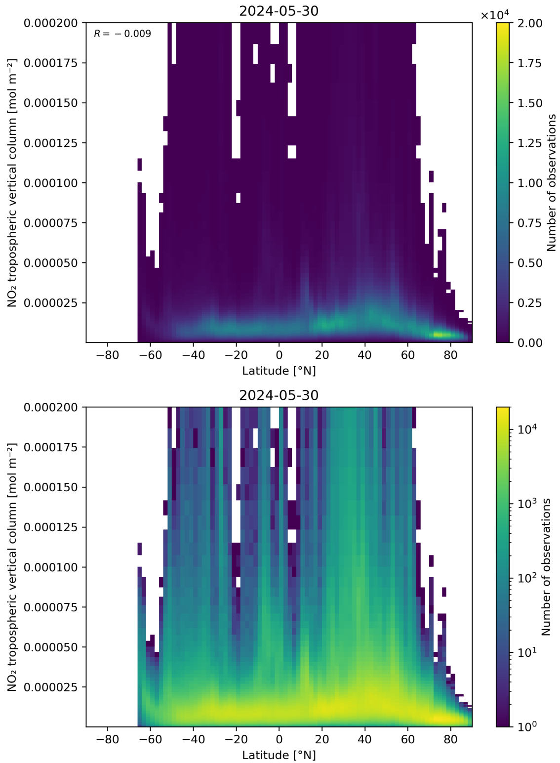
Figure 92: Scatter density plot of “Latitude” against “NO 2 tropospheric vertical column” for 2024-05-29 to 2024-05-31.
