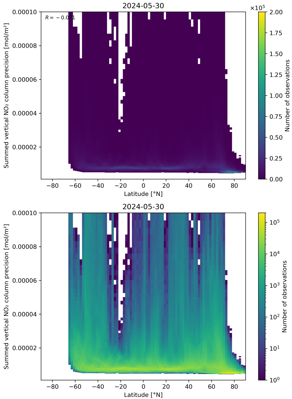
Figure 89: Scatter density plot of “Latitude” against “Summed vertical NO 2 column precision” for 2024-05-29 to 2024-05-31.
