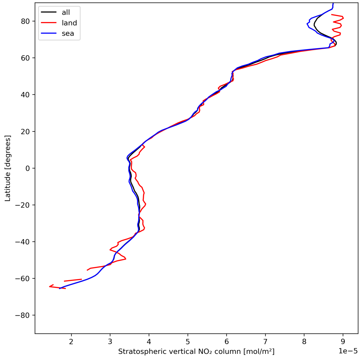
Figure 19: Zonal average of “Stratospheric vertical NO 2 column” for 2024-05-29 to 2024-05-31.
