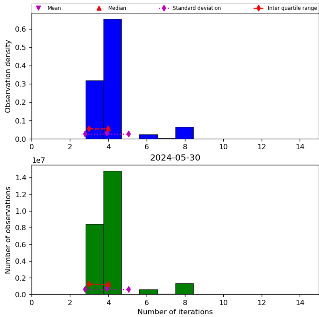
Figure 34: Histogram of “Number of iterations” for 2024-05-29 to 2024-05-31
