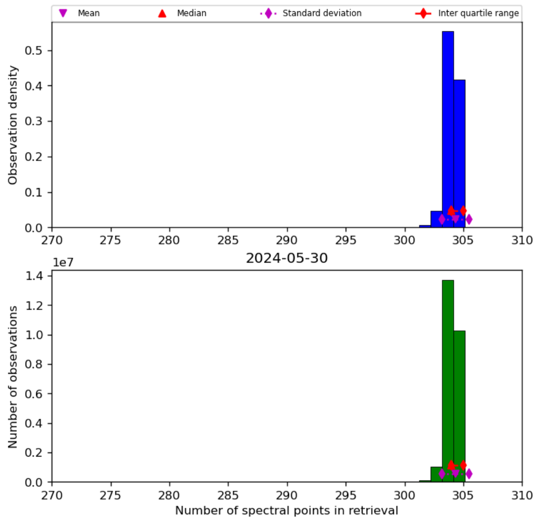
Figure 33: Histogram of “Number of spectral points in retrieval” for 2024-05-29 to 2024-05-31
