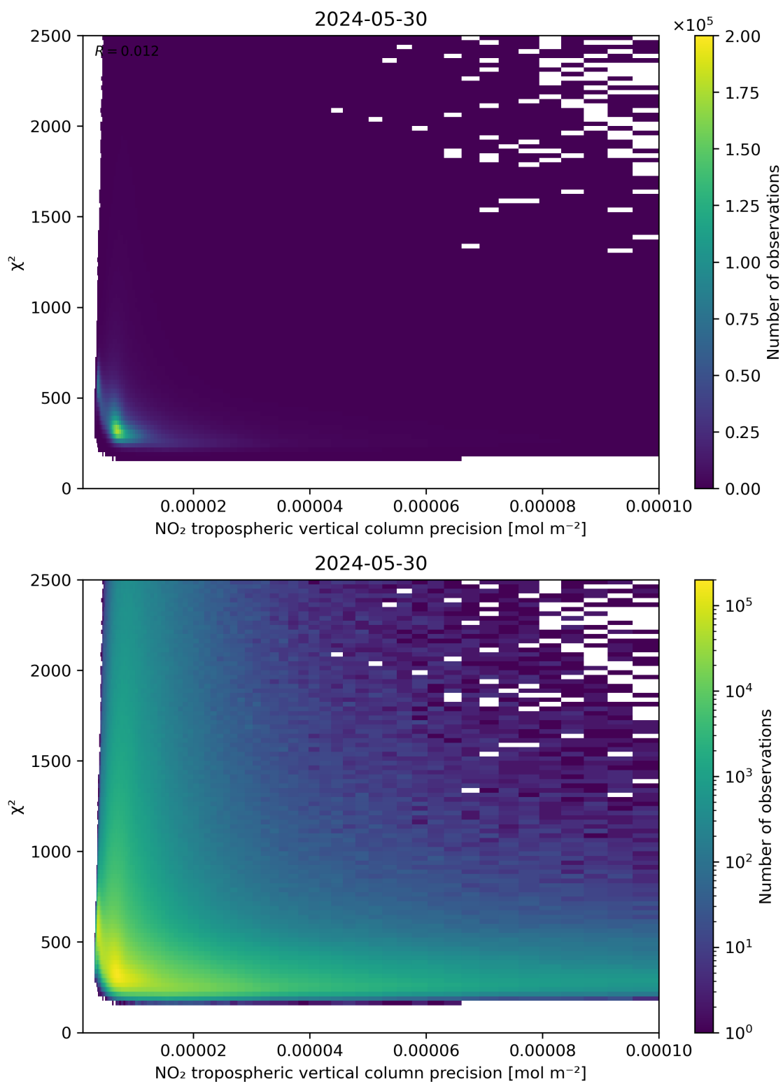
Figure 134: Scatter density plot of “NO 2 tropospheric vertical column precision” against “ \chi^2 ” for 2024-05-29 to 2024-05-31.
