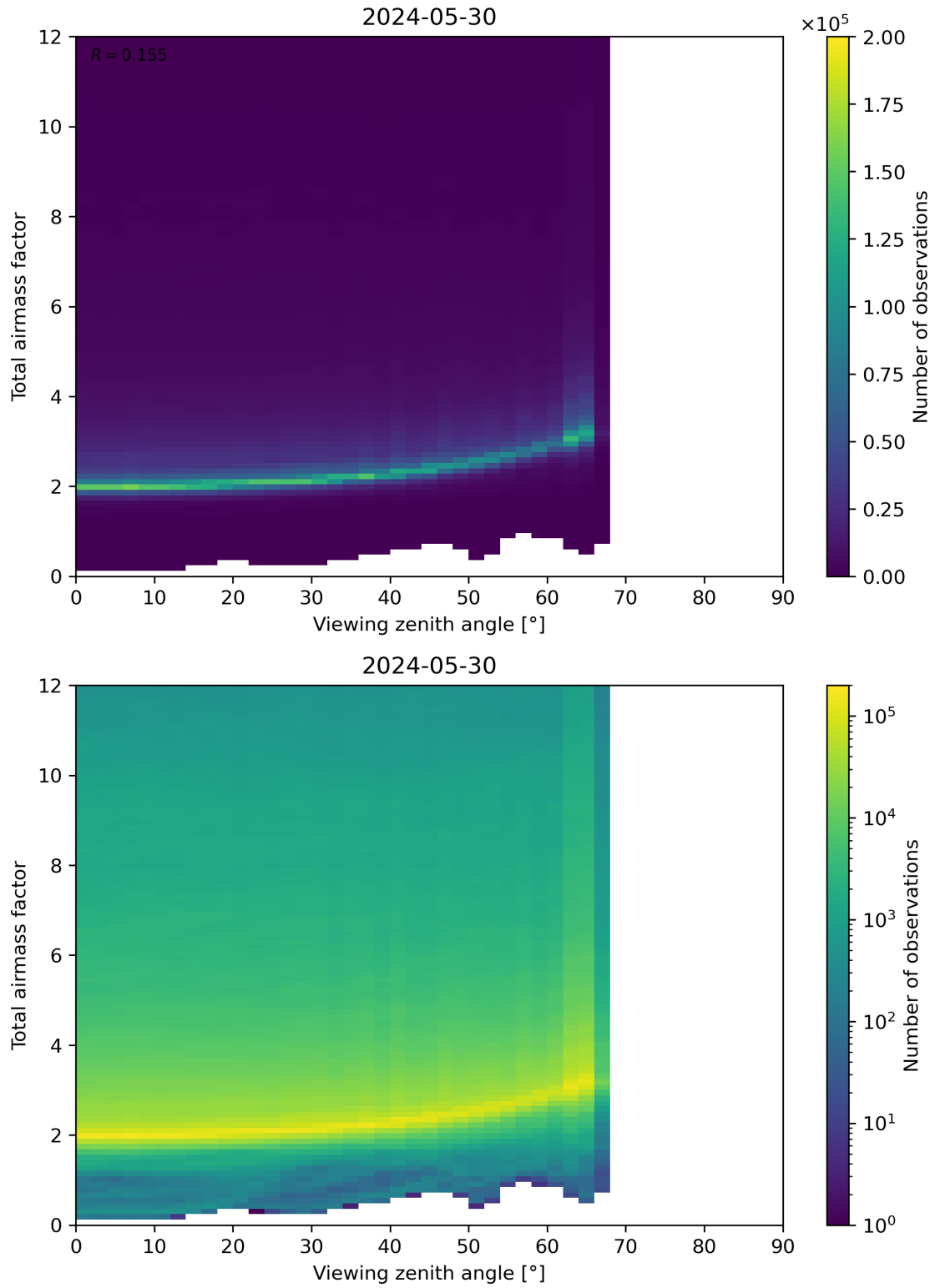
Figure 160: Scatter density plot of “Viewing zenith angle” against “Total airmass factor” for 2024-05-29 to 2024-05-31.
