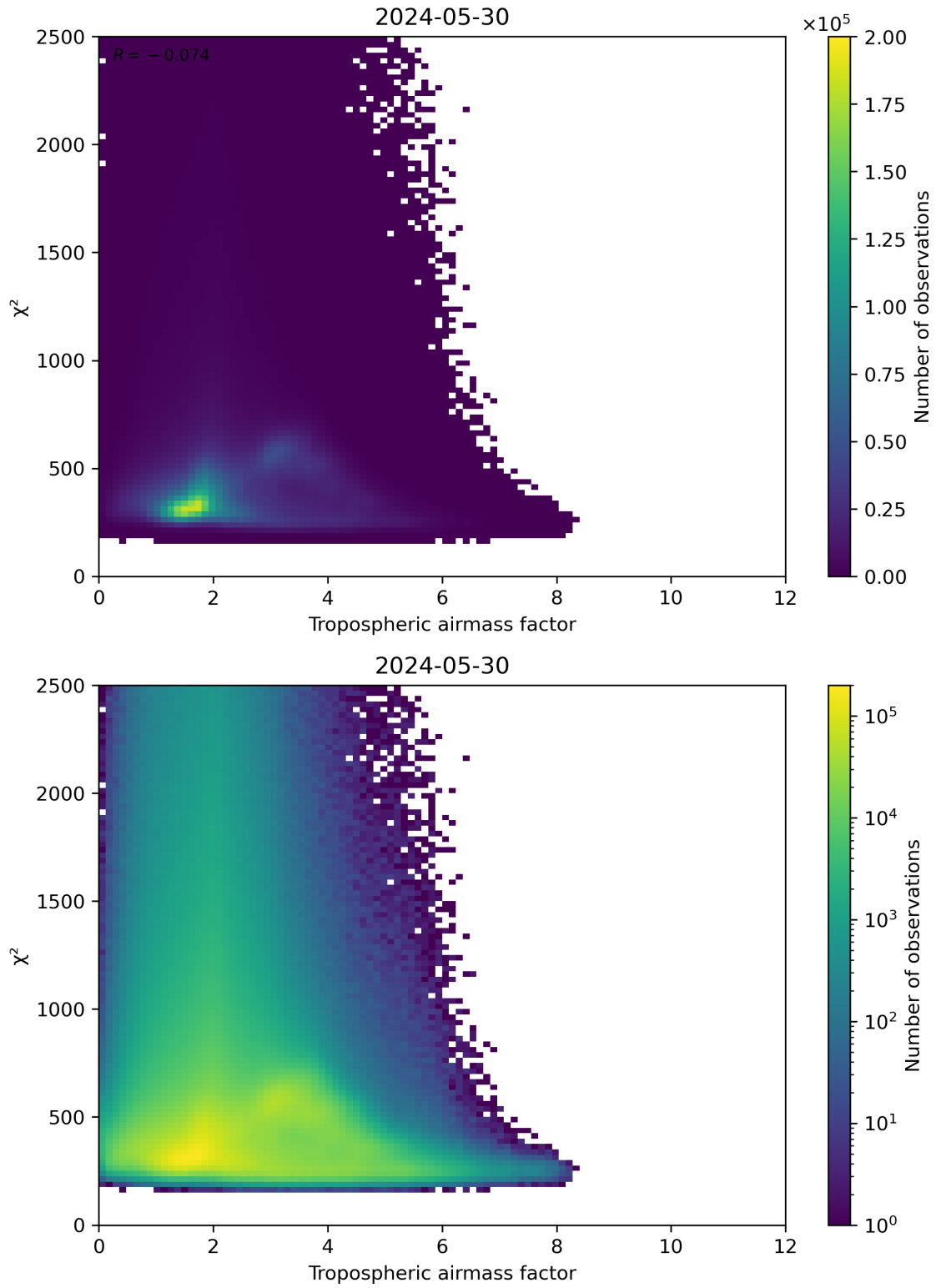
Figure 73: Scatter density plot of “Tropospheric airmass factor” against “ \chi^2 ” for 2024-05-29 to 2024-05-31.
