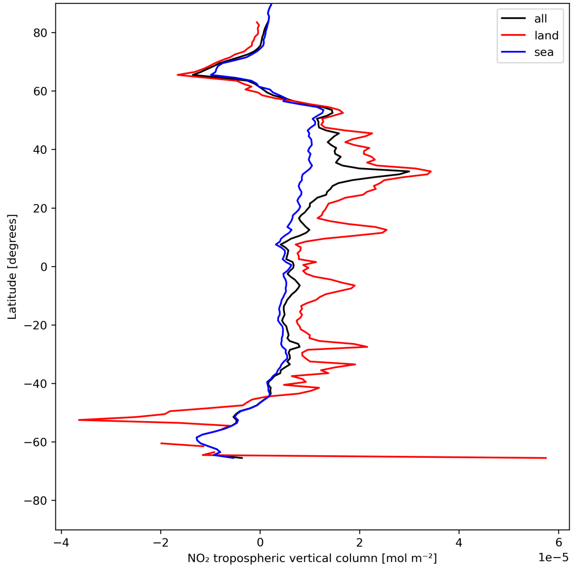
Figure 12: Zonal average of “NO 2 tropospheric vertical column” for 2024-05-29 to 2024-05-31.
