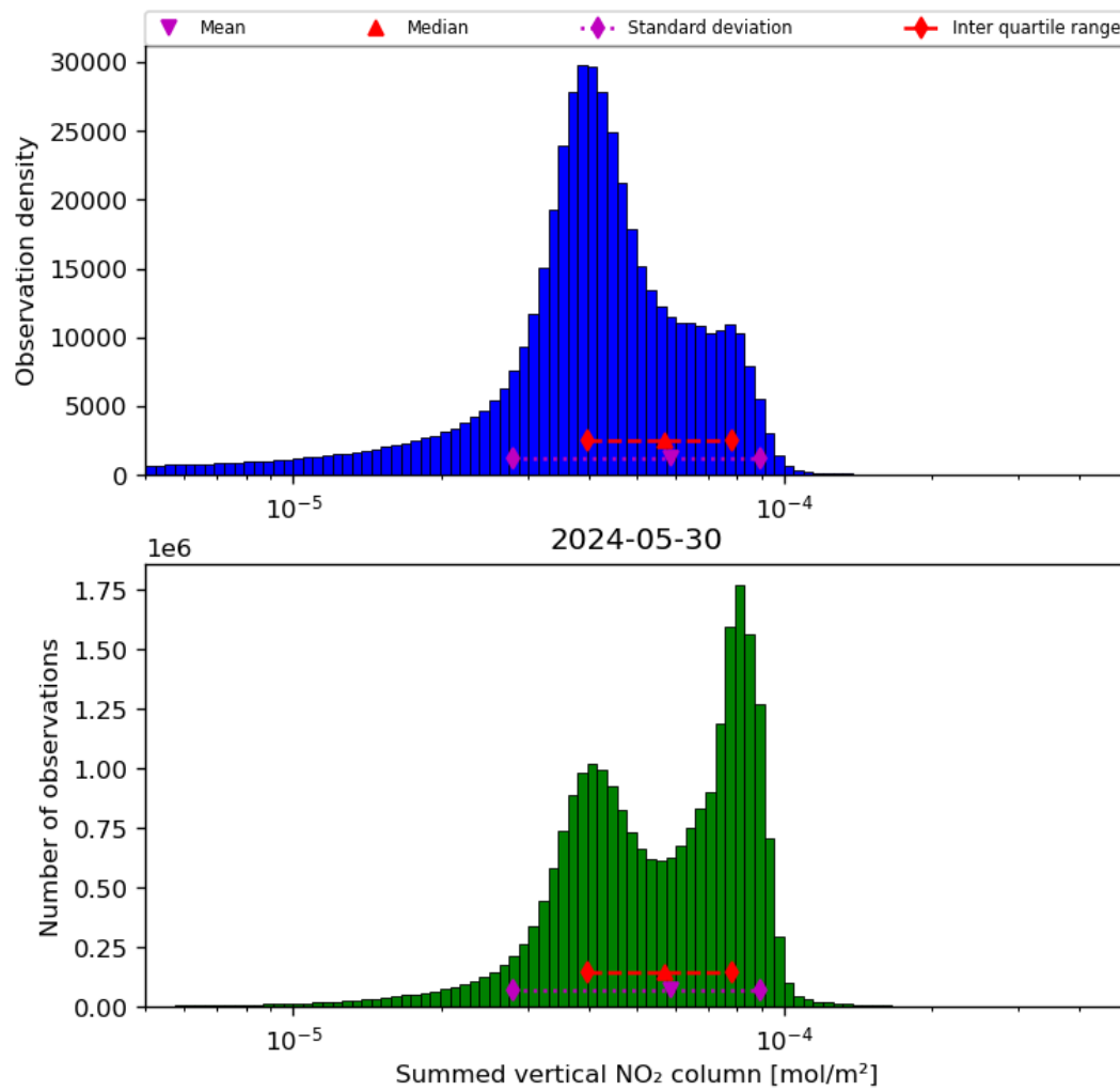
Figure 40: Histogram of “Summed vertical NO 2 column” for 2024-05-29 to 2024-05-31
