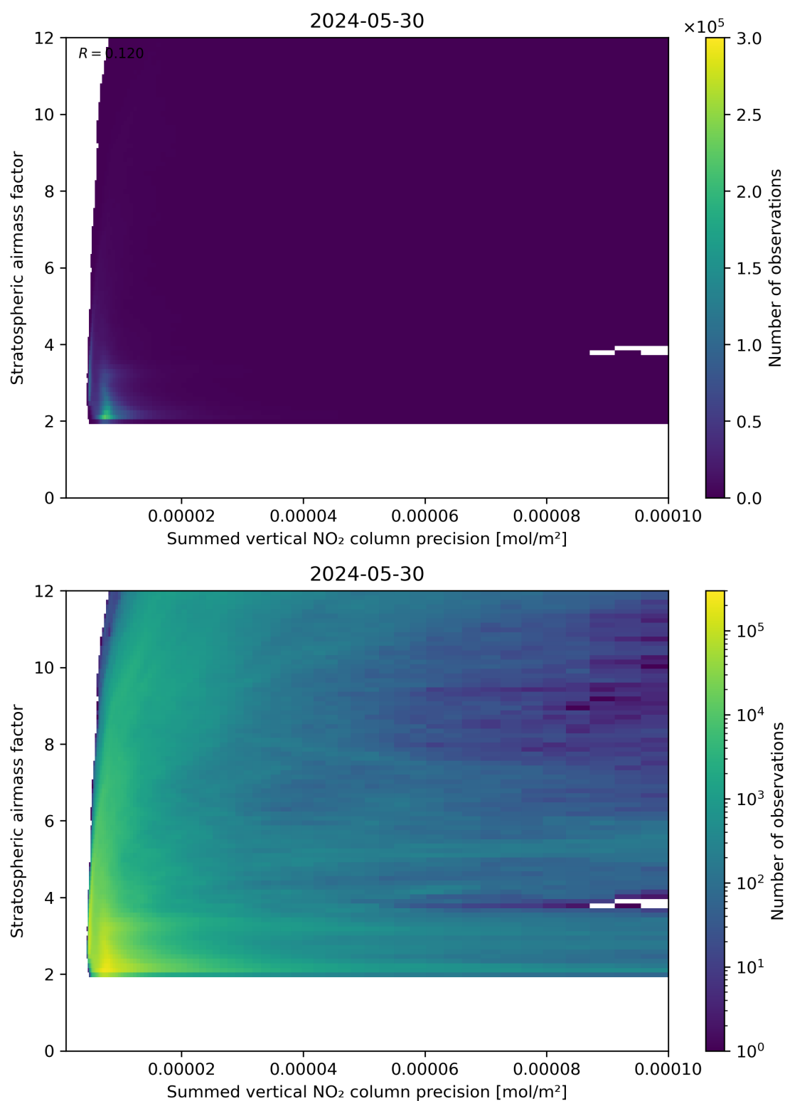
Figure 106: Scatter density plot of “Summed vertical NO 2 column precision” against “Stratospheric airmass factor” for 2024-05-29 to 2024-05-31.
