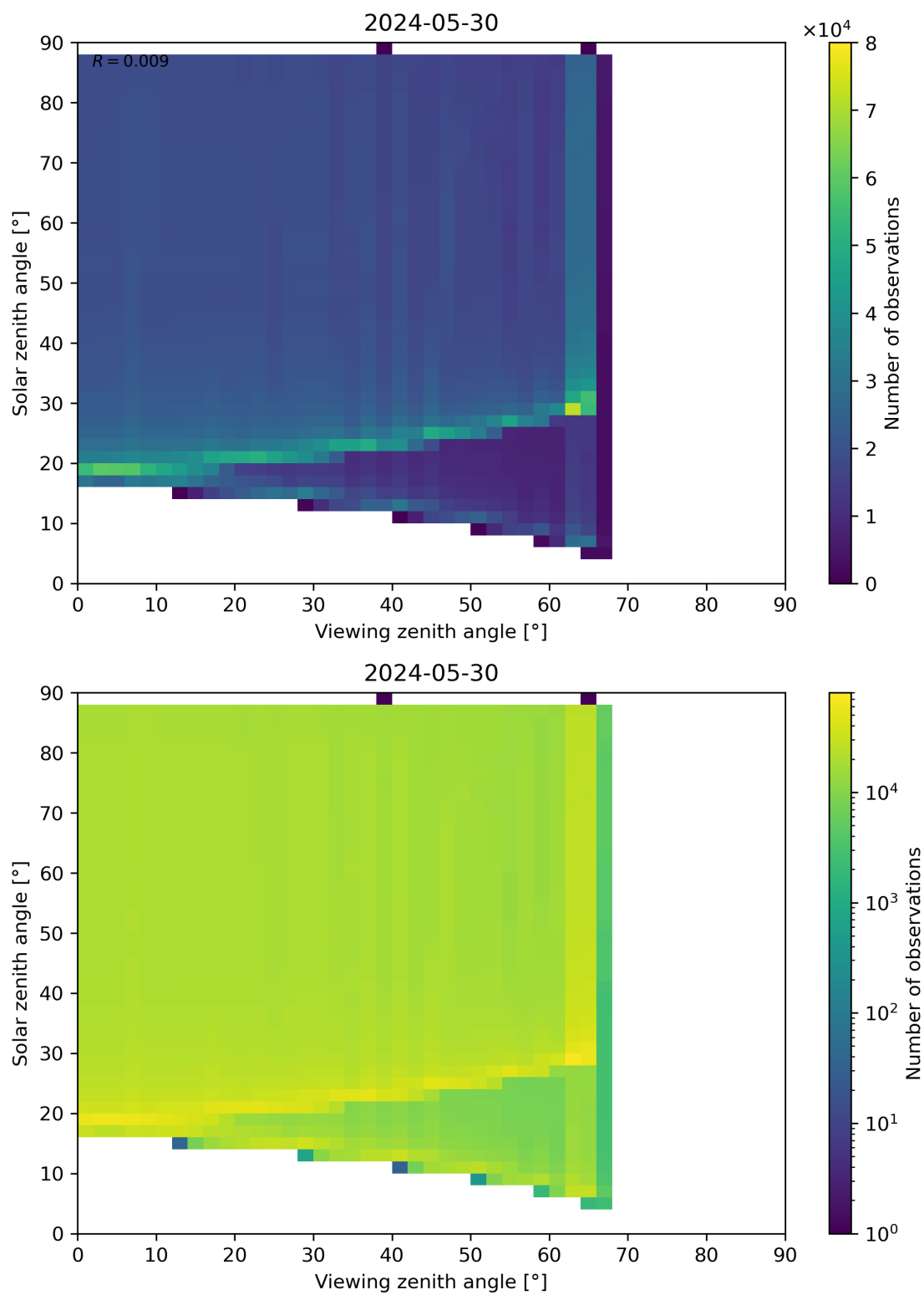
Figure 172: Scatter density plot of “Viewing zenith angle” against “Solar zenith angle” for 2024-05-29 to 2024-05-31.
