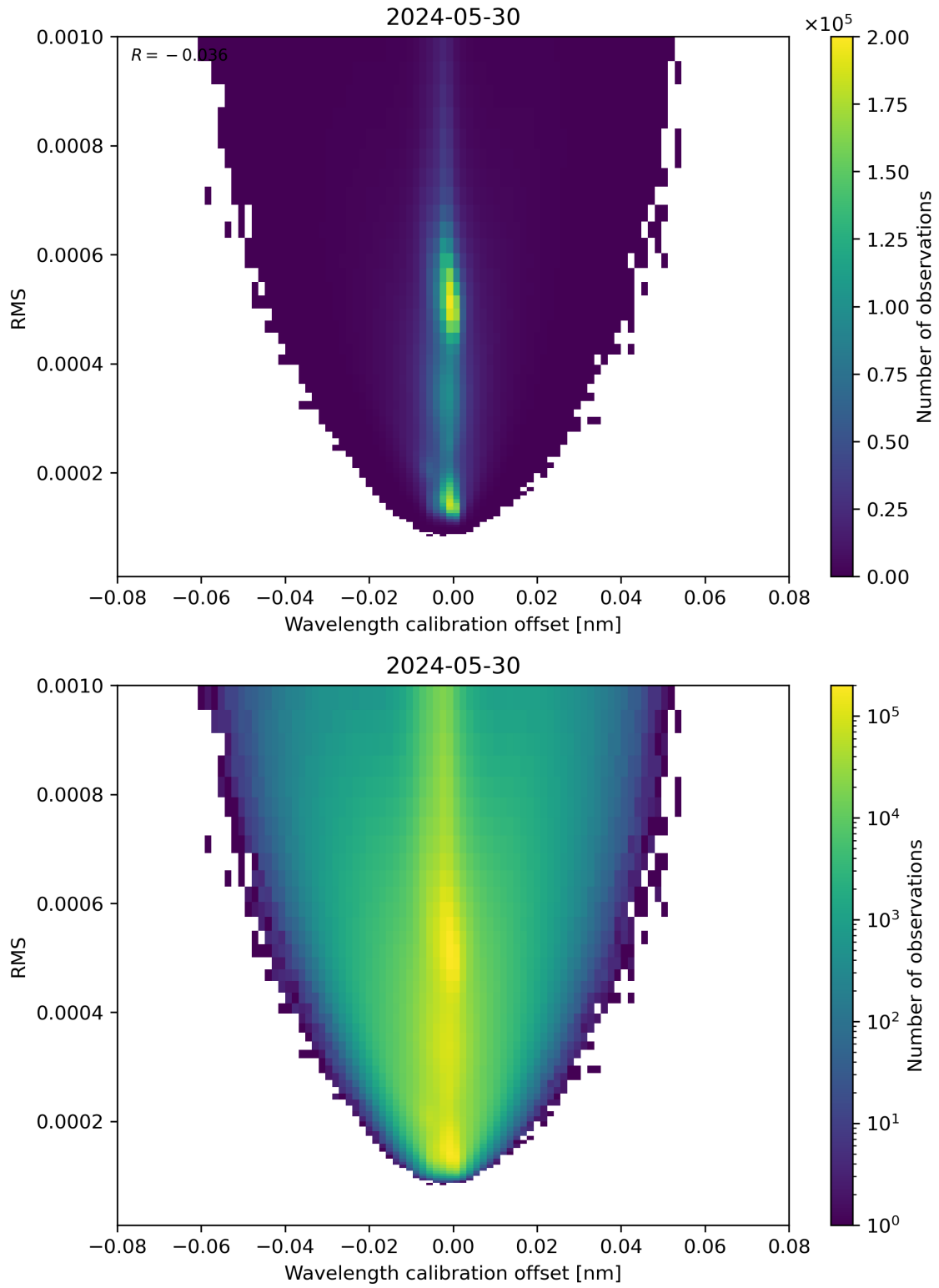
Figure 181: Scatter density plot of “Wavelength calibration offset” against “RMS” for 2024-05-29 to 2024-05-31.
