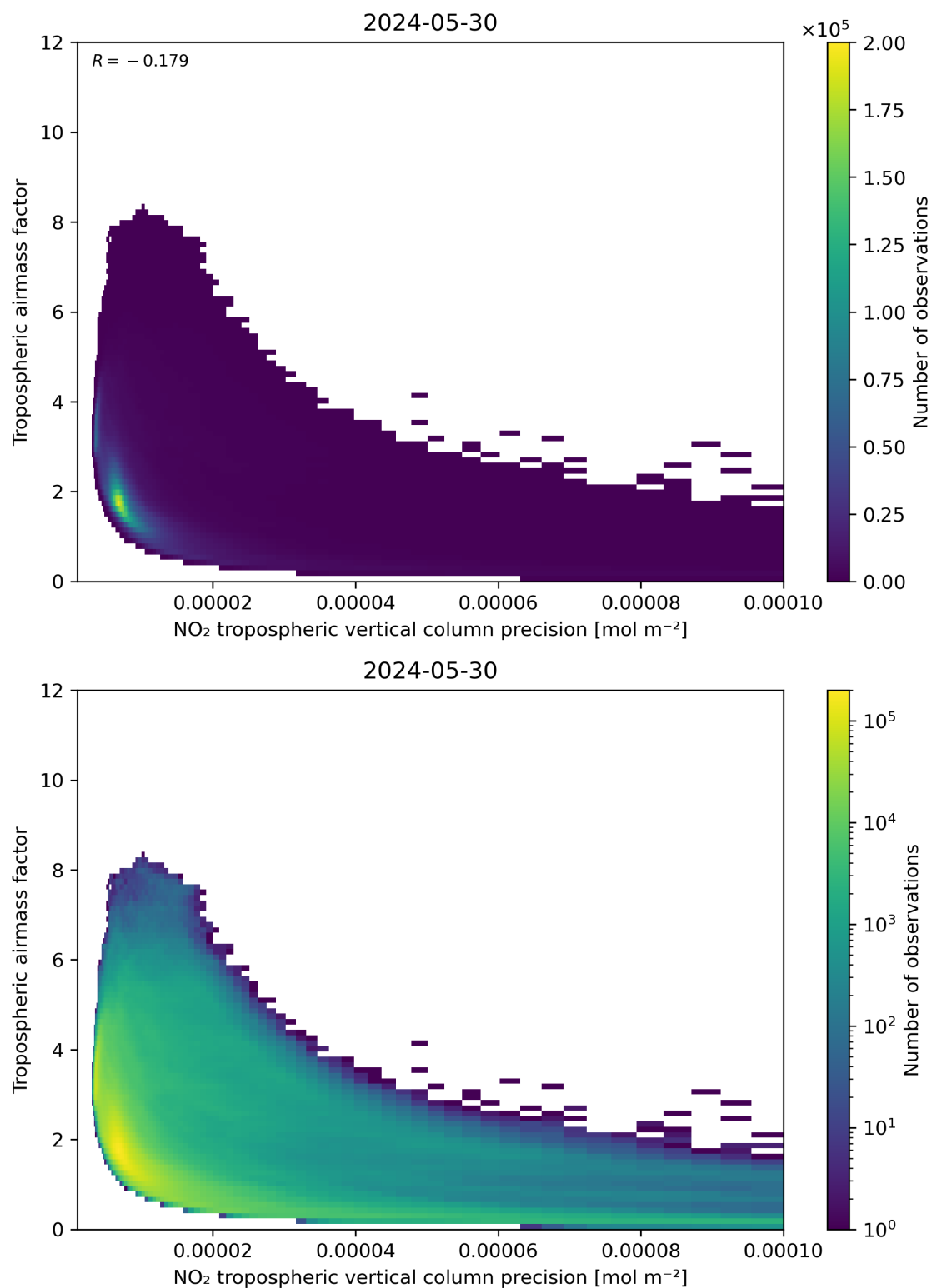
Figure 133: Scatter density plot of “NO 2 tropospheric vertical column precision” against “Tropospheric air mass factor” for 2024-05-29 to 2024-05-31.
