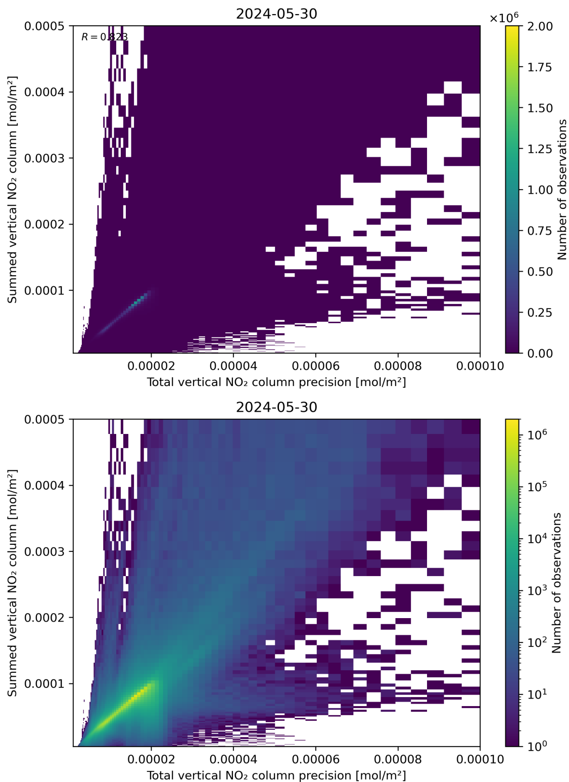
Figure 117: Scatter density plot of “Total vertical NO 2 column precision” against “Summed vertical NO 2 column” for 2024-05-29 to 2024-05-31.
