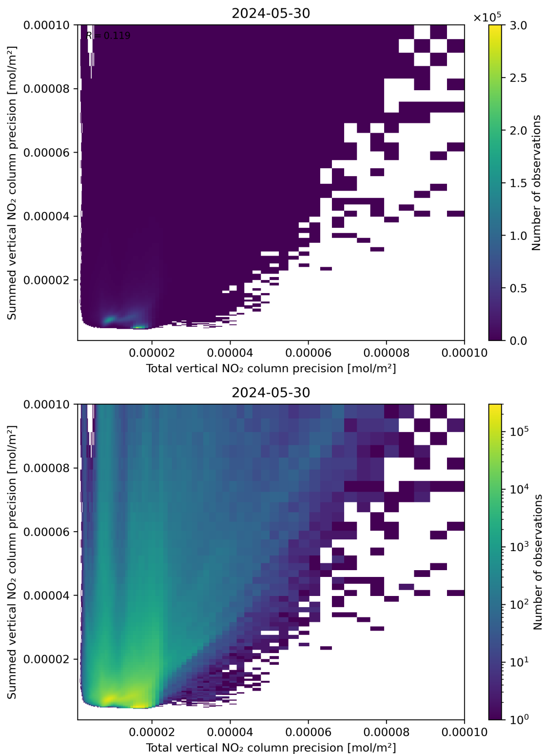
Figure 118: Scatter density plot of “Total vertical NO 2 column precision” against “Summed vertical NO 2 column precision” for 2024-05-29 to 2024-05-31.
