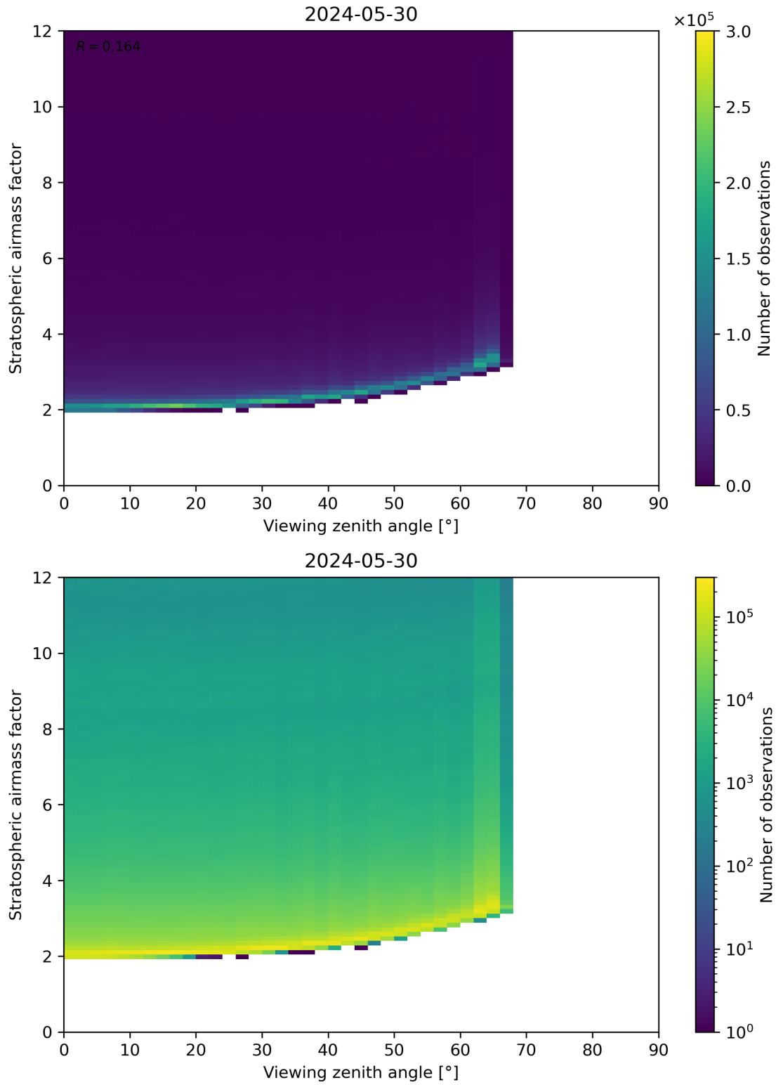
Figure 159: Scatter density plot of “Viewing zenith angle” against “Stratospheric airmass factor” for 2024-05-29 to 2024-05-31.
