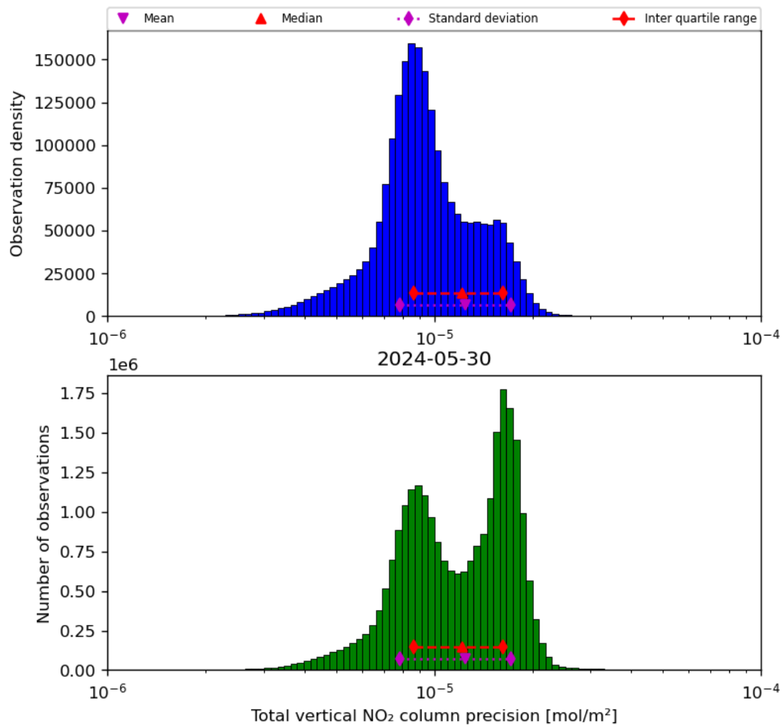
Figure 39: Histogram of “Total vertical NO 2 column precision” for 2024-05-29 to 2024-05-31
