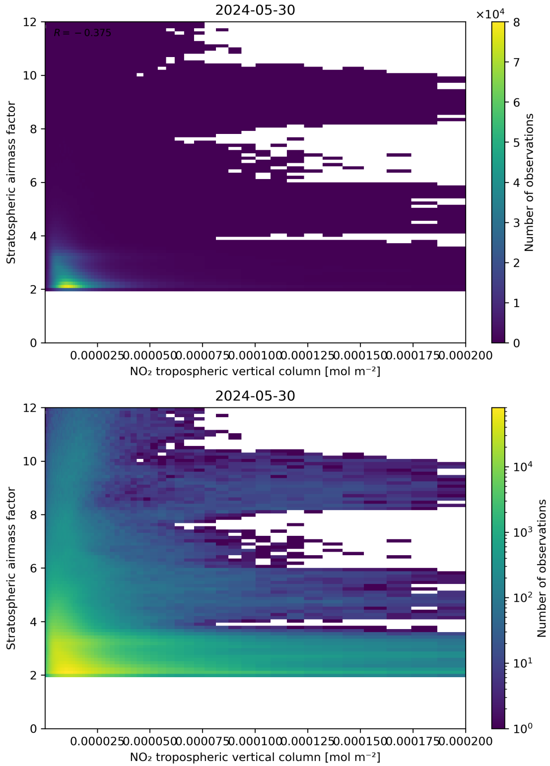
Figure 121: Scatter density plot of “NO 2 tropospheric vertical column” against “Stratospheric air mass factor” for 2024-05-29 to 2024-05-31.
