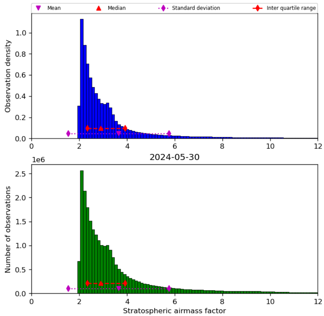
Figure 44: Histogram of “Stratospheric airmass factor” for 2024-05-29 to 2024-05-31
