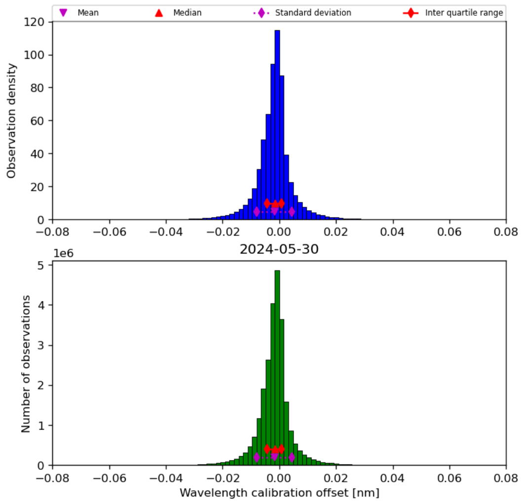
Figure 35: Histogram of “Wavelength calibration offset” for 2024-05-29 to 2024-05-31
