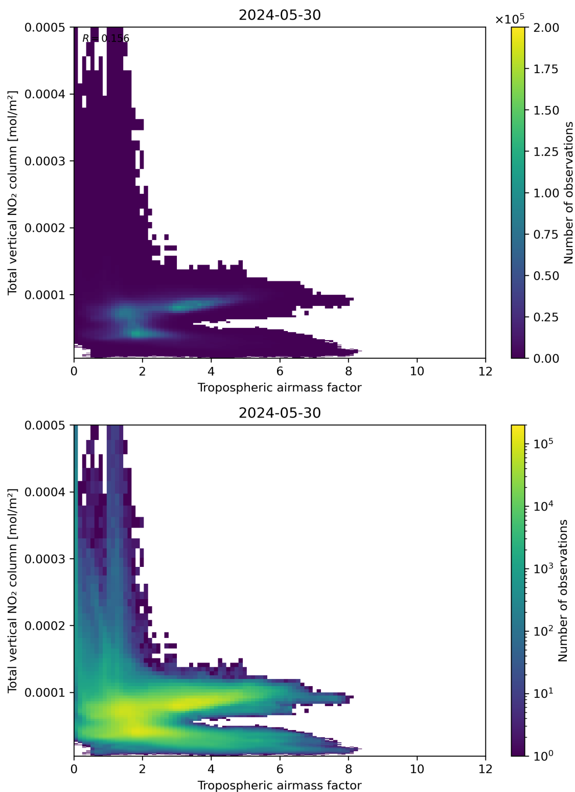
Figure 77: Scatter density plot of “Tropospheric airmass factor” against “Total vertical NO 2 column” for 2024-05-29 to 2024-05-31.
