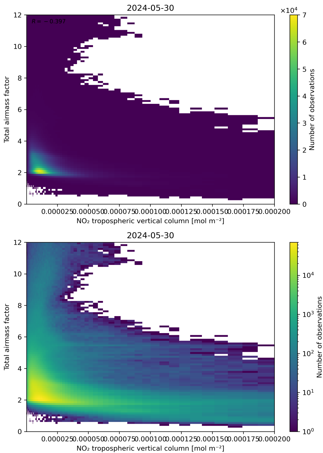
Figure 122: Scatter density plot of “NO 2 tropospheric vertical column” against “Total air mass factor” for 2024-05-29 to 2024-05-31.
