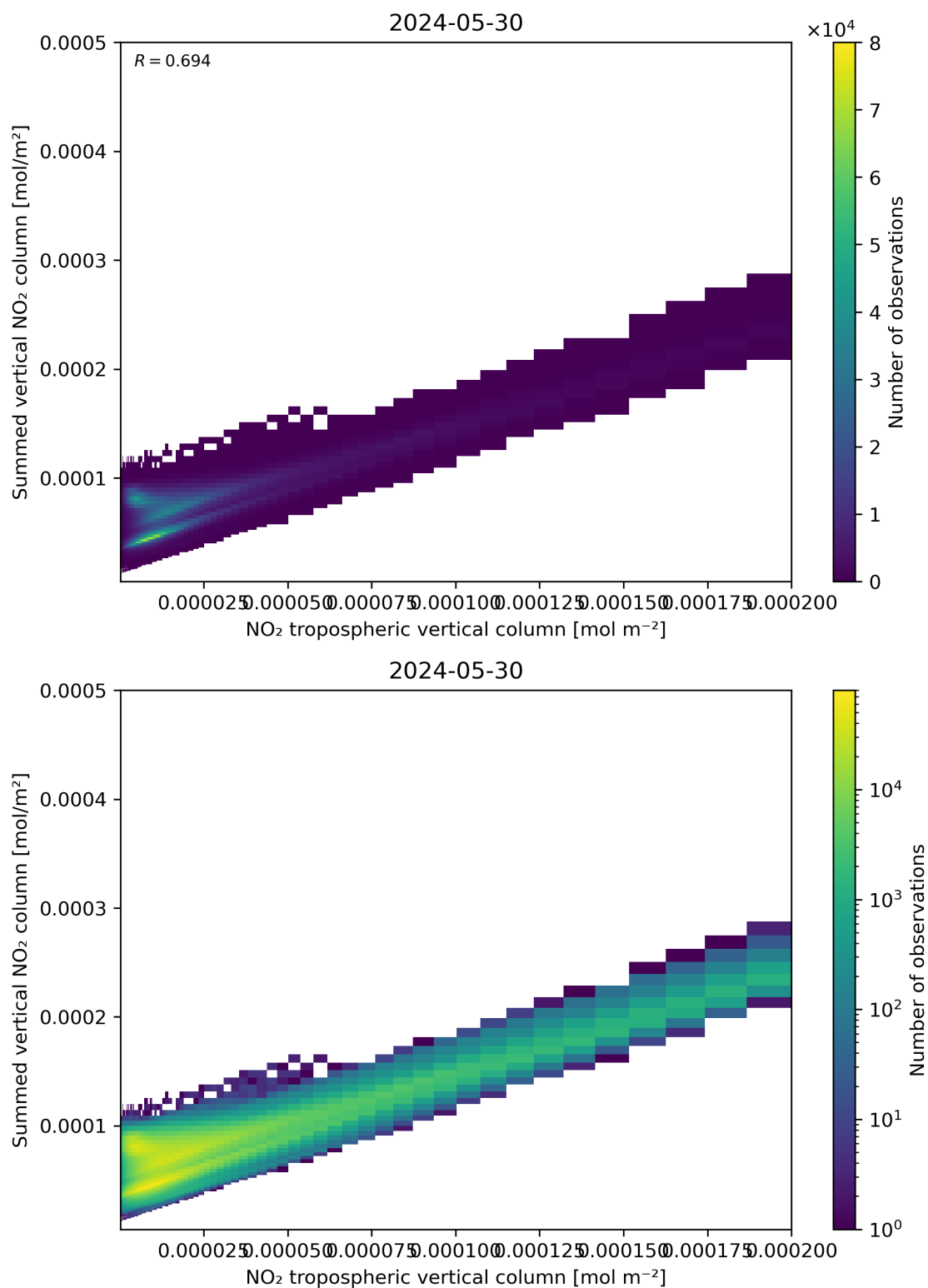
Figure 126: Scatter density plot of “NO 2 tropospheric vertical column” against “Summed vertical NO 2 column” for 2024-05-29 to 2024-05-31.
