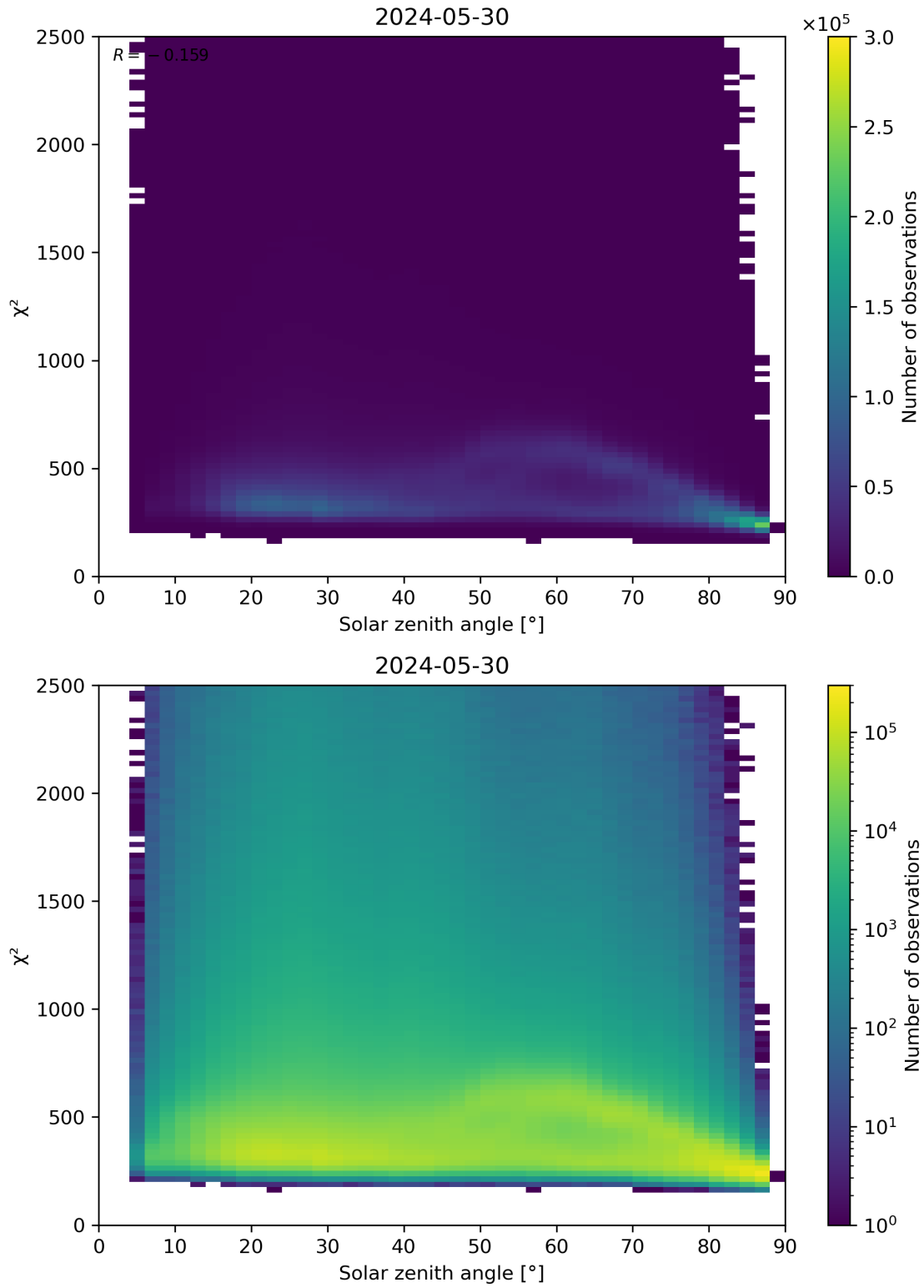
Figure 148: Scatter density plot of “Solar zenith angle” against “ \chi^2 ” for 2024-05-29 to 2024-05-31.
