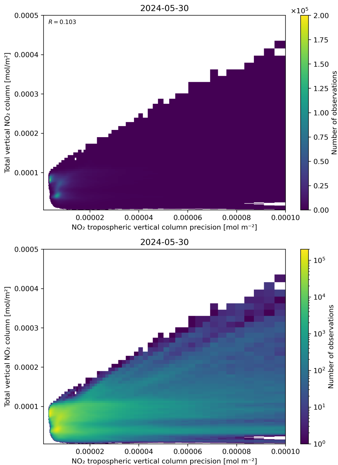
Figure 138: Scatter density plot of “NO 2 tropospheric vertical column precision” against “Total vertical NO 2 column” for 2024-05-29 to 2024-05-31.
