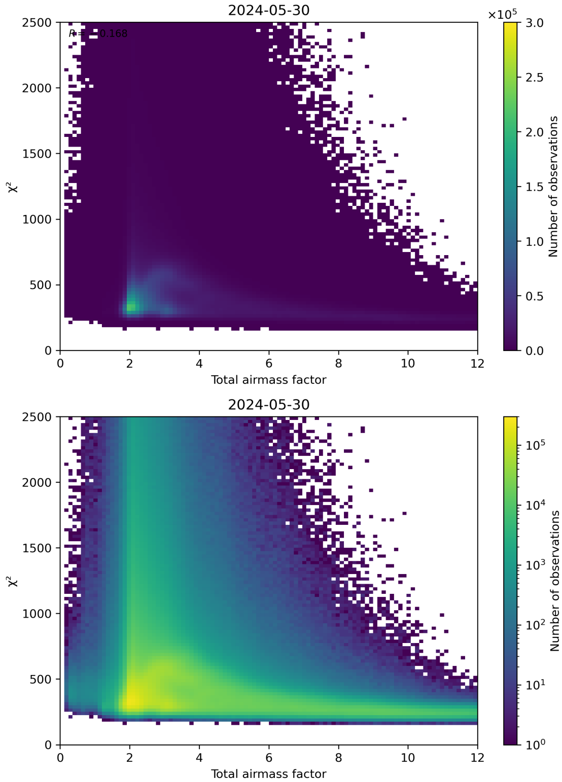
Figure 63: Scatter density plot of “Total airmass factor” against “ \chi^2 ” for 2024-05-29 to 2024-05-31.
