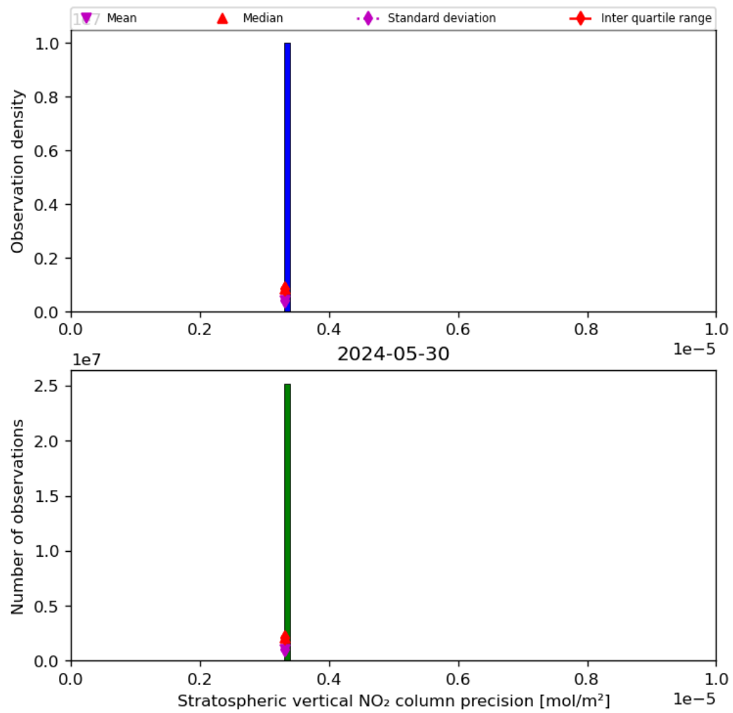
Figure 37: Histogram of “Stratospheric vertical NO 2 column precision” for 2024-05-29 to 2024-05-31
