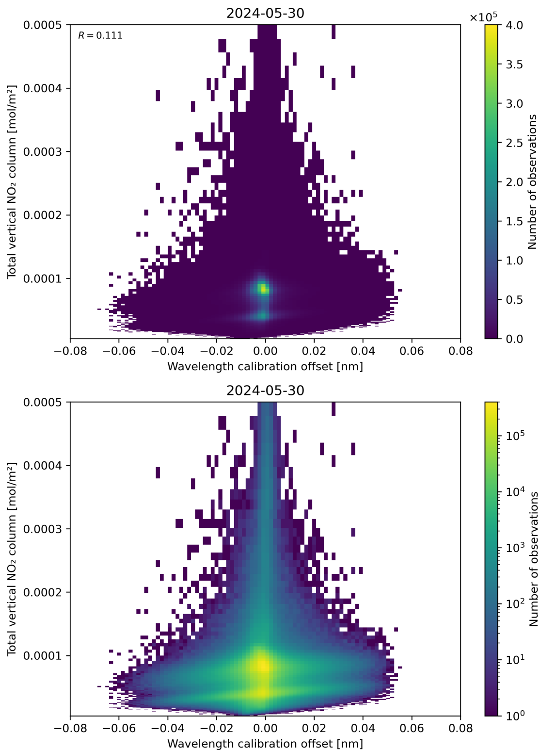
Figure 179: Scatter density plot of “Wavelength calibration offset” against “Total vertical NO 2 column” for 2024-05-29 to 2024-05-31.
