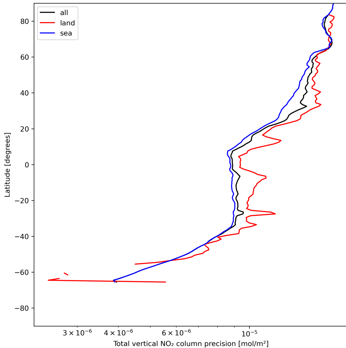
Figure 22: Zonal average of “Total vertical NO 2 column precision” for 2024-05-29 to 2024-05-31.
