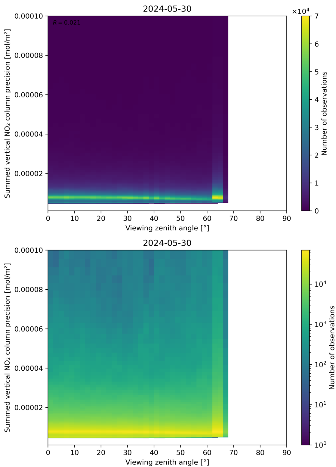
Figure 166: Scatter density plot of “Viewing zenith angle” against “Summed vertical NO 2 column precision” for 2024-05-29 to 2024-05-31.
