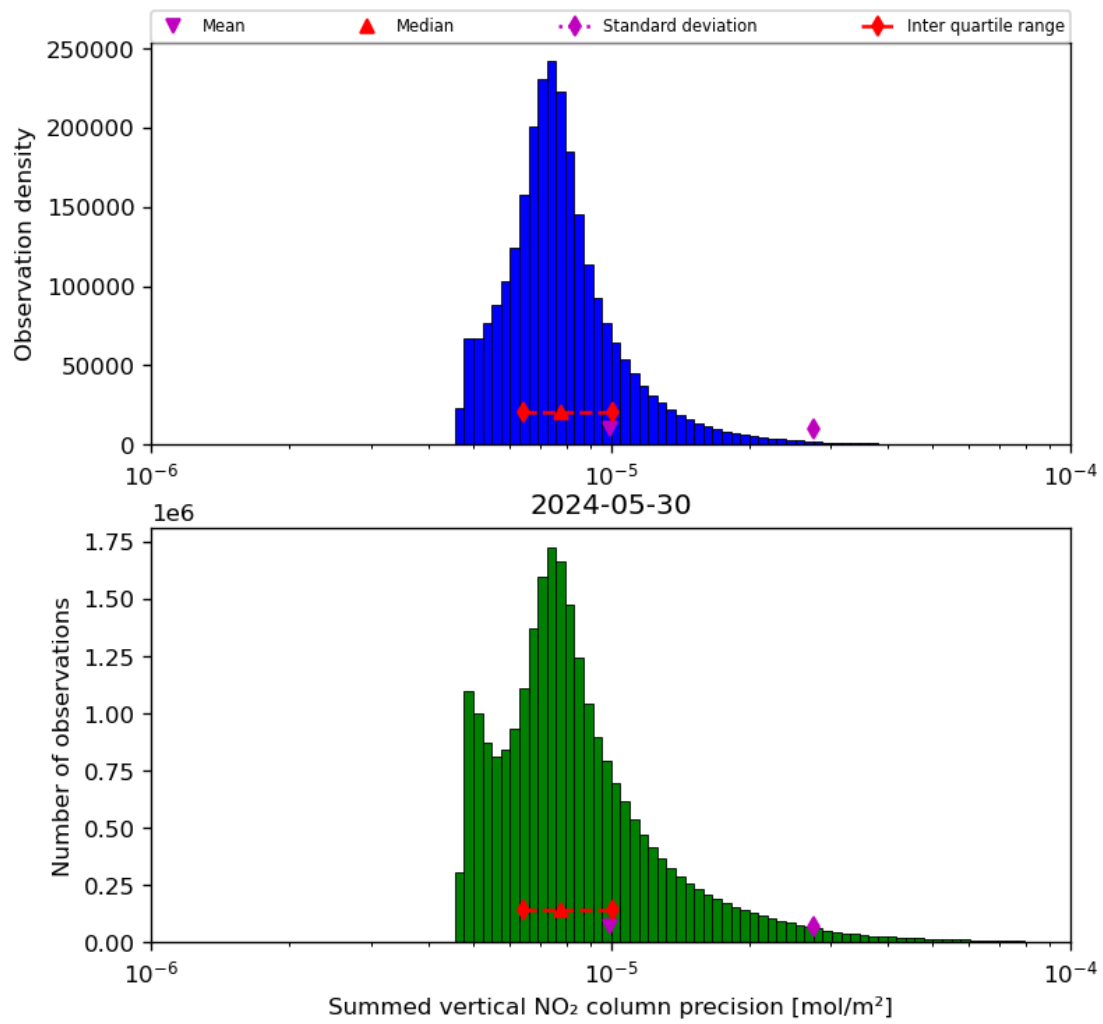
Figure 41: Histogram of "Summed vertical NO 2 column precision" for 2024-05-29 to 2024-05-31
