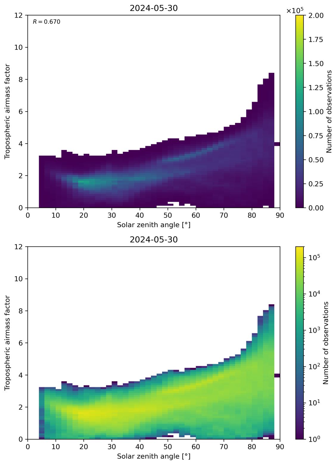
Figure 147: Scatter density plot of “Solar zenith angle” against “Tropospheric airmass factor” for 2024-05-29 to 2024-05-31.
