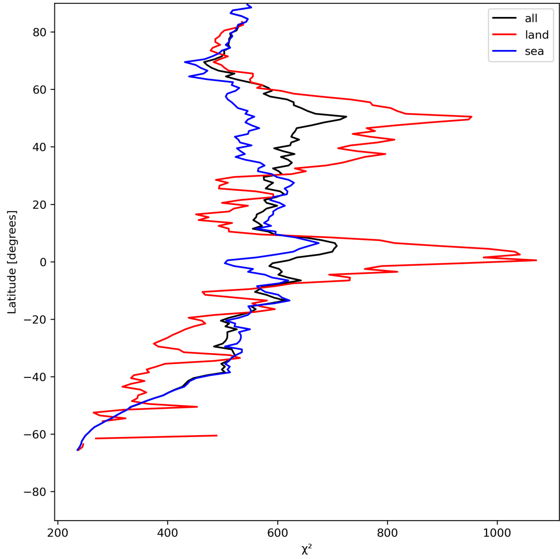
Figure 25: Zonal average of “ \chi^2 ” for 2024-05-29 to 2024-05-31.
