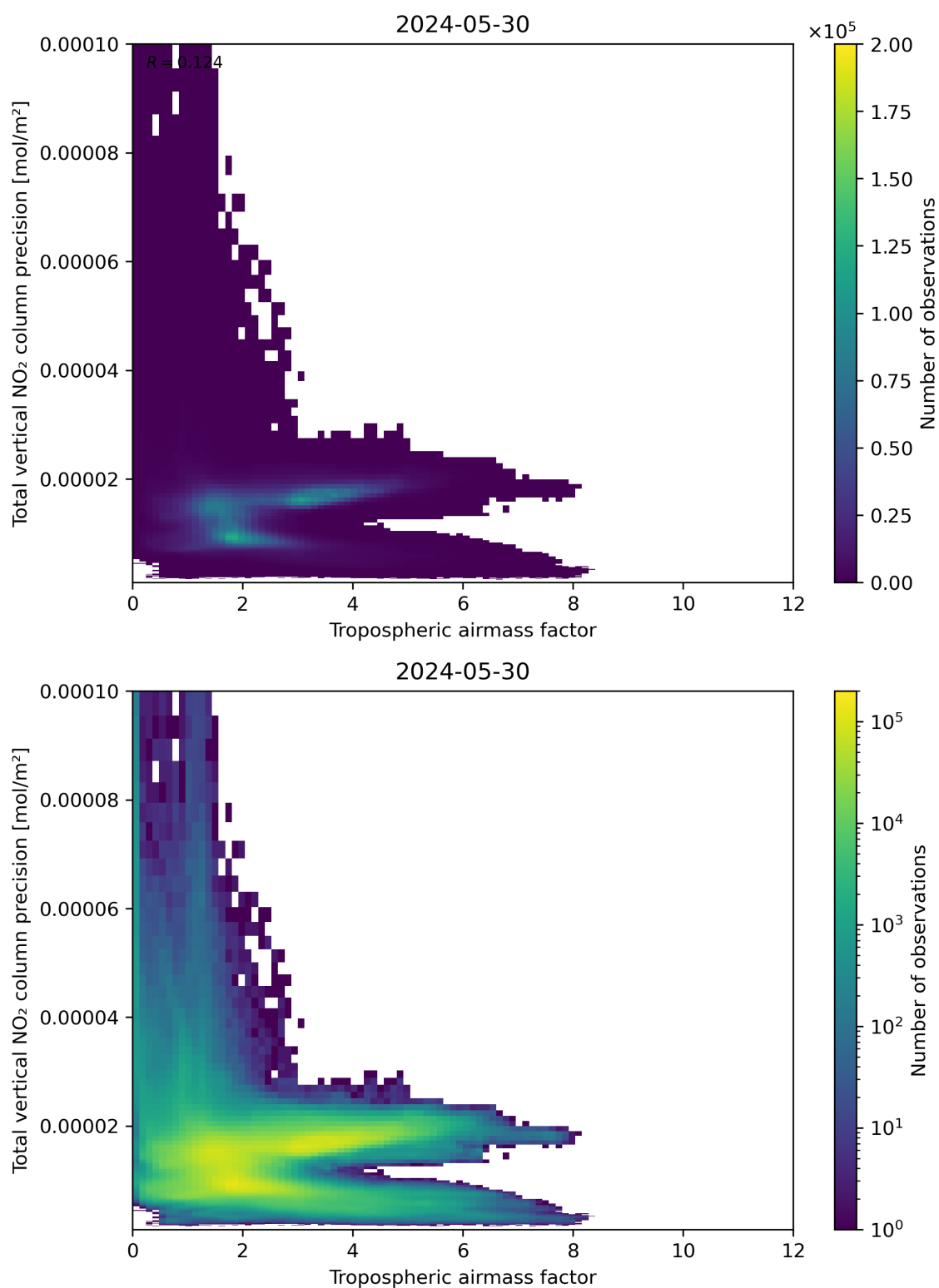
Figure 78: Scatter density plot of “Tropospheric air mass factor” against “Total vertical NO 2 column precision” for 2024-05-29 to 2024-05-31.
