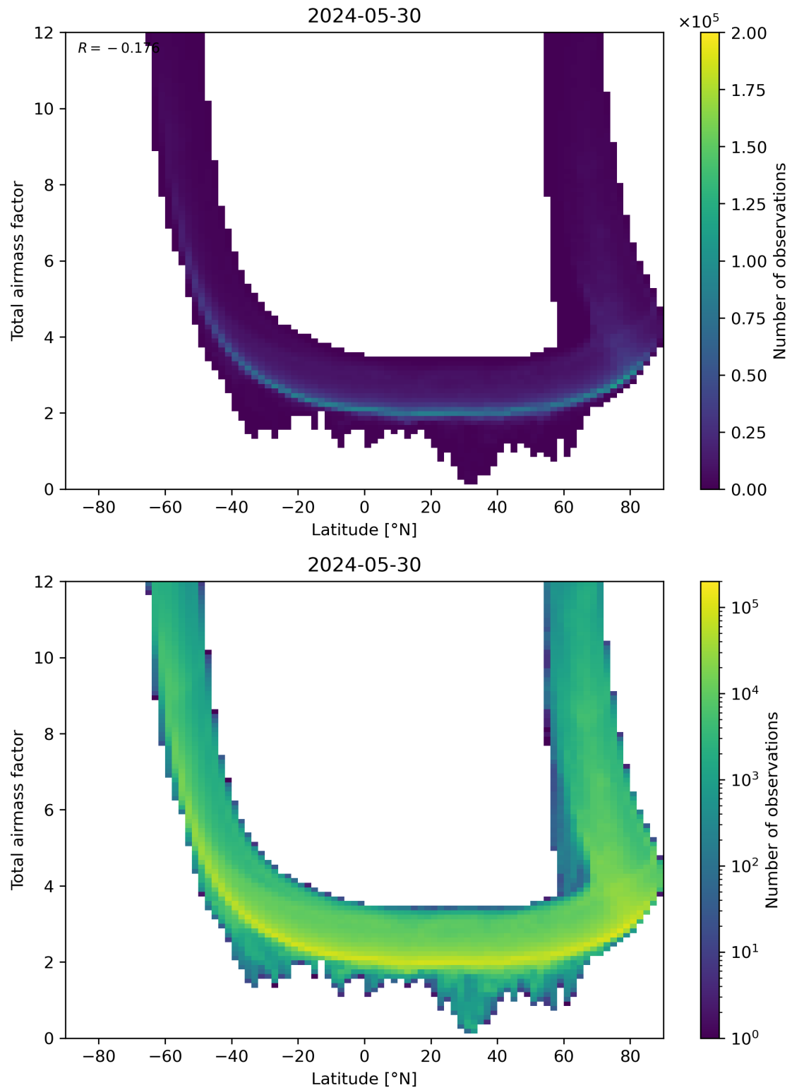
Figure 84: Scatter density plot of “Latitude” against “Total airmass factor” for 2024-05-29 to 2024-05-31.
