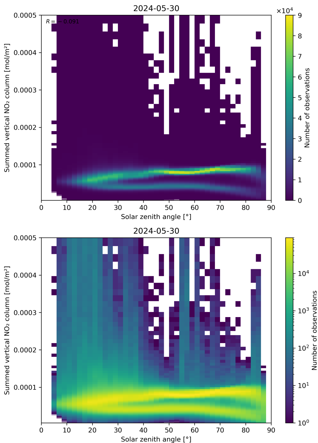
Figure 151: Scatter density plot of “Solar zenith angle” against “Summed vertical NO 2 column” for 2024-05-29 to 2024-05-31.
