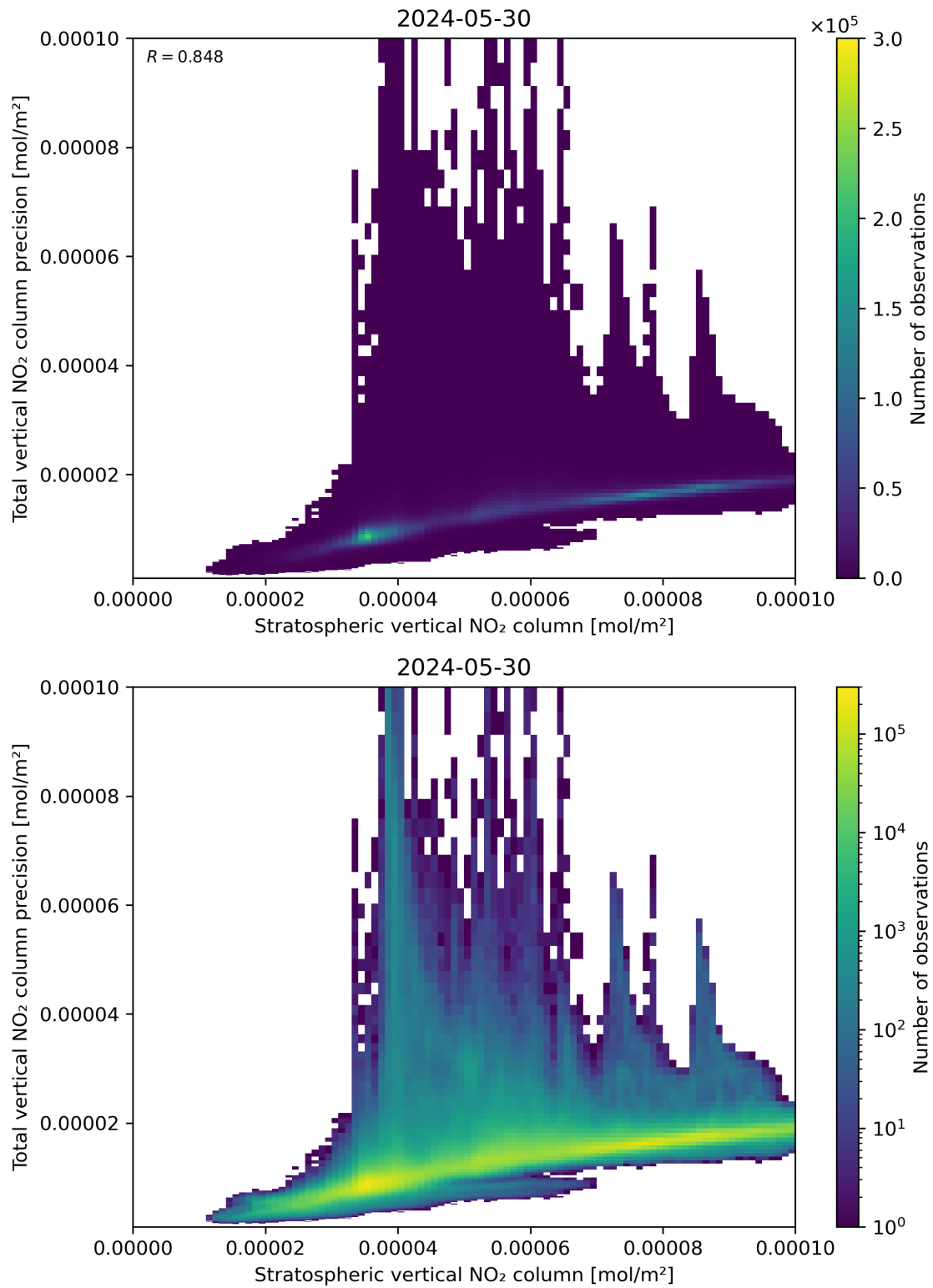
Figure 101: Scatter density plot of “Stratospheric vertical NO 2 column” against “Total vertical NO 2 column precision” for 2024-05-29 to 2024-05-31.
