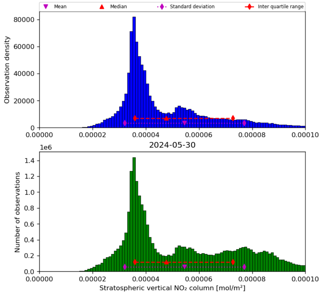
Figure 36: Histogram of “Stratospheric vertical NO 2 column” for 2024-05-29 to 2024-05-31
