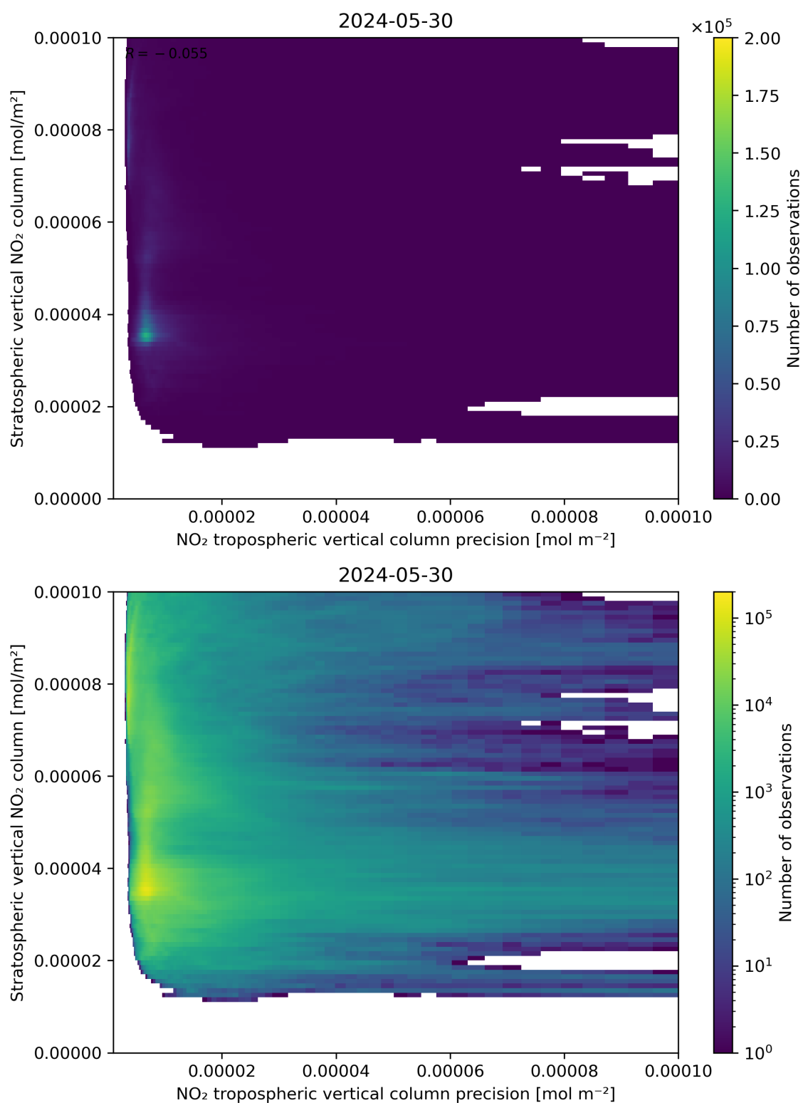
Figure 135: Scatter density plot of “NO 2 tropospheric vertical column precision” against “Stratospheric vertical NO 2 column” for 2024-05-29 to 2024-05-31.
