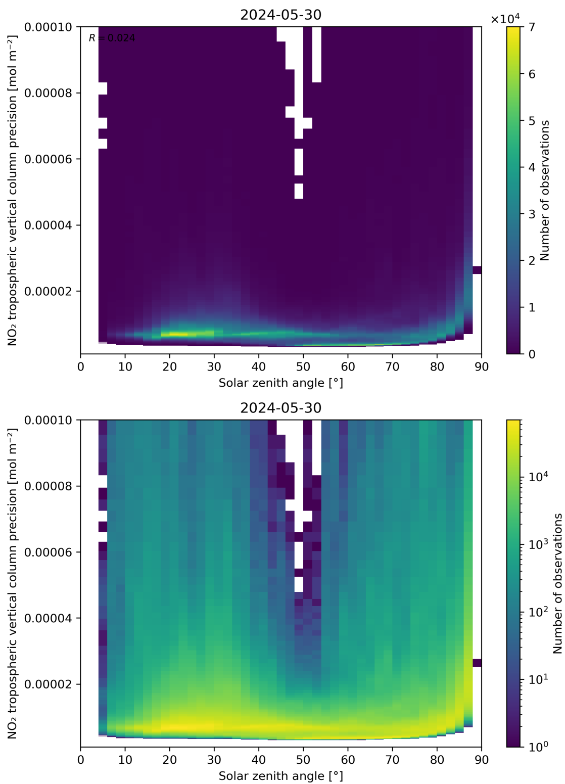
Figure 156: Scatter density plot of “Solar zenith angle” against “NO 2 tropospheric vertical column precision” for 2024-05-29 to 2024-05-31.
