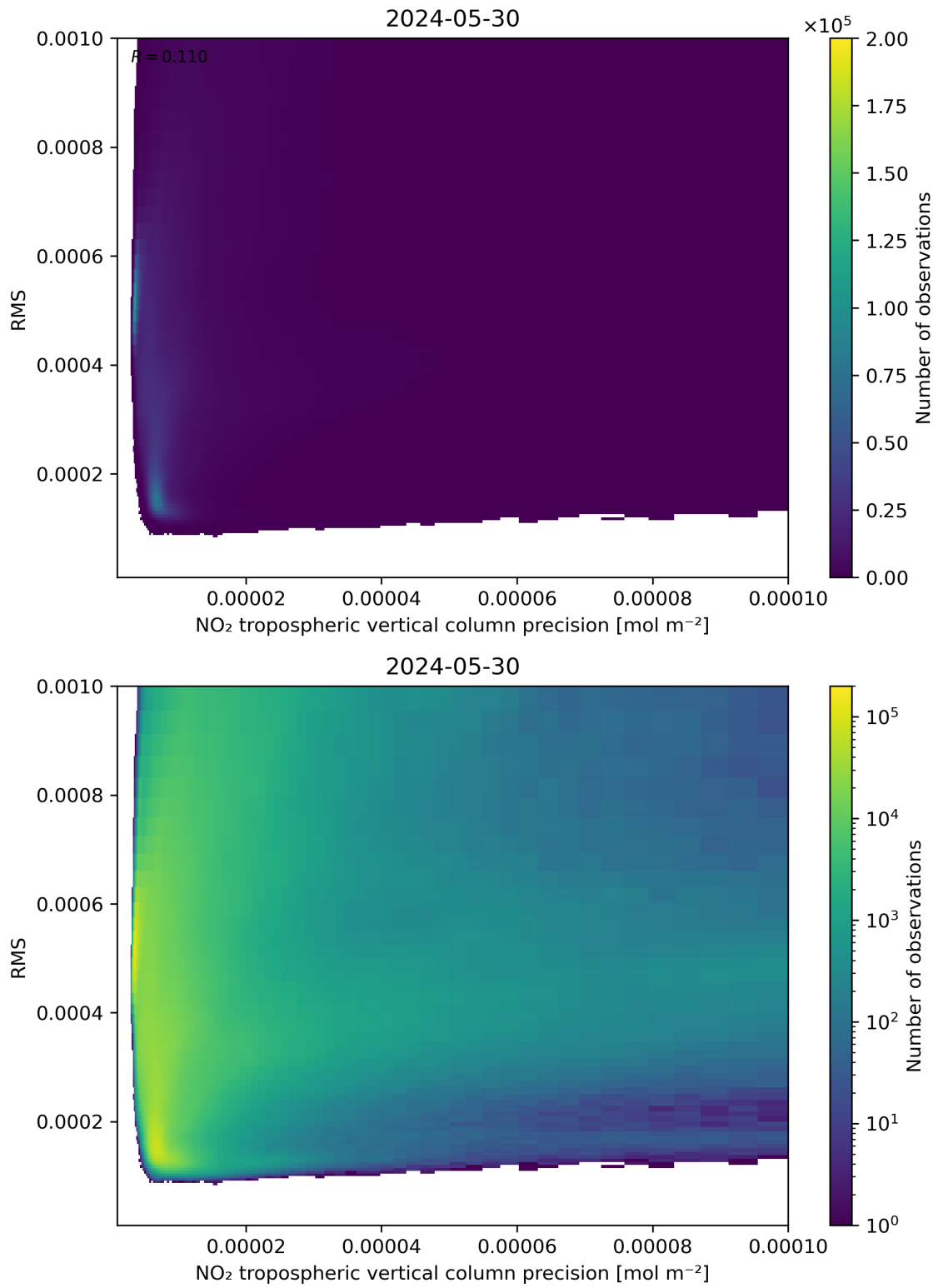
Figure 140: Scatter density plot of “NO 2 tropospheric vertical column precision” against “RMS” for 2024-05-29 to 2024-05-31.
