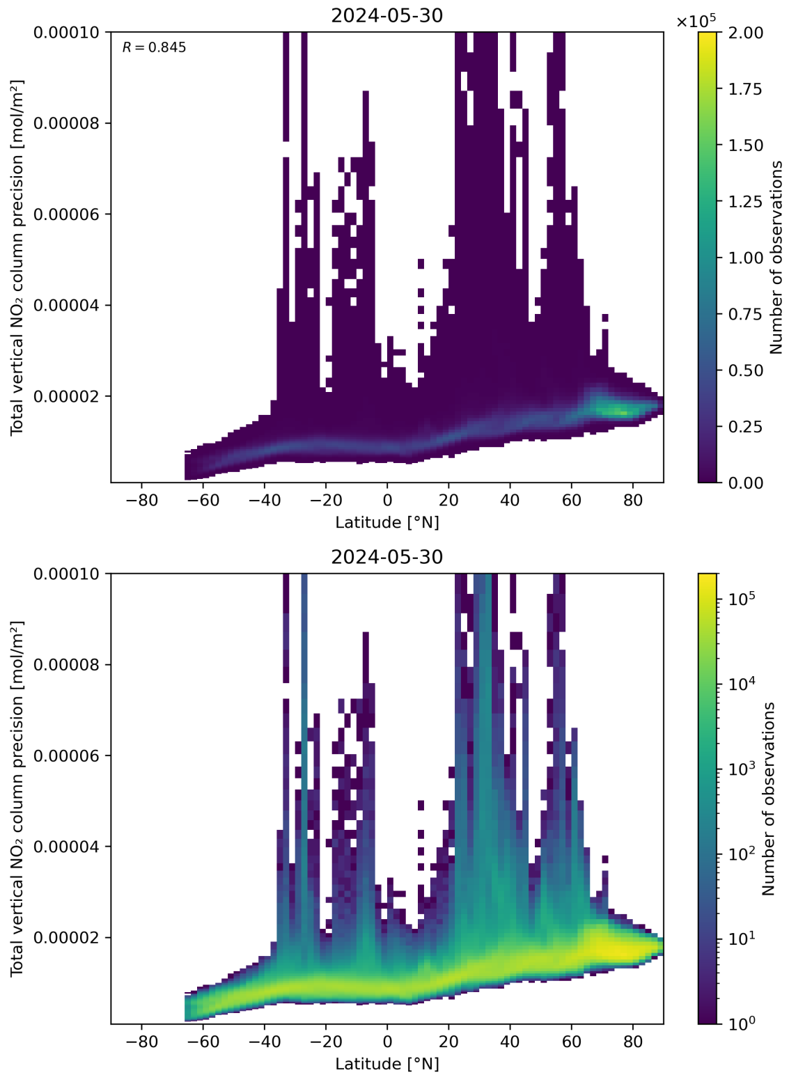
Figure 91: Scatter density plot of “Latitude” against “Total vertical NO 2 column precision” for 2024-05-29 to 2024-05-31.
