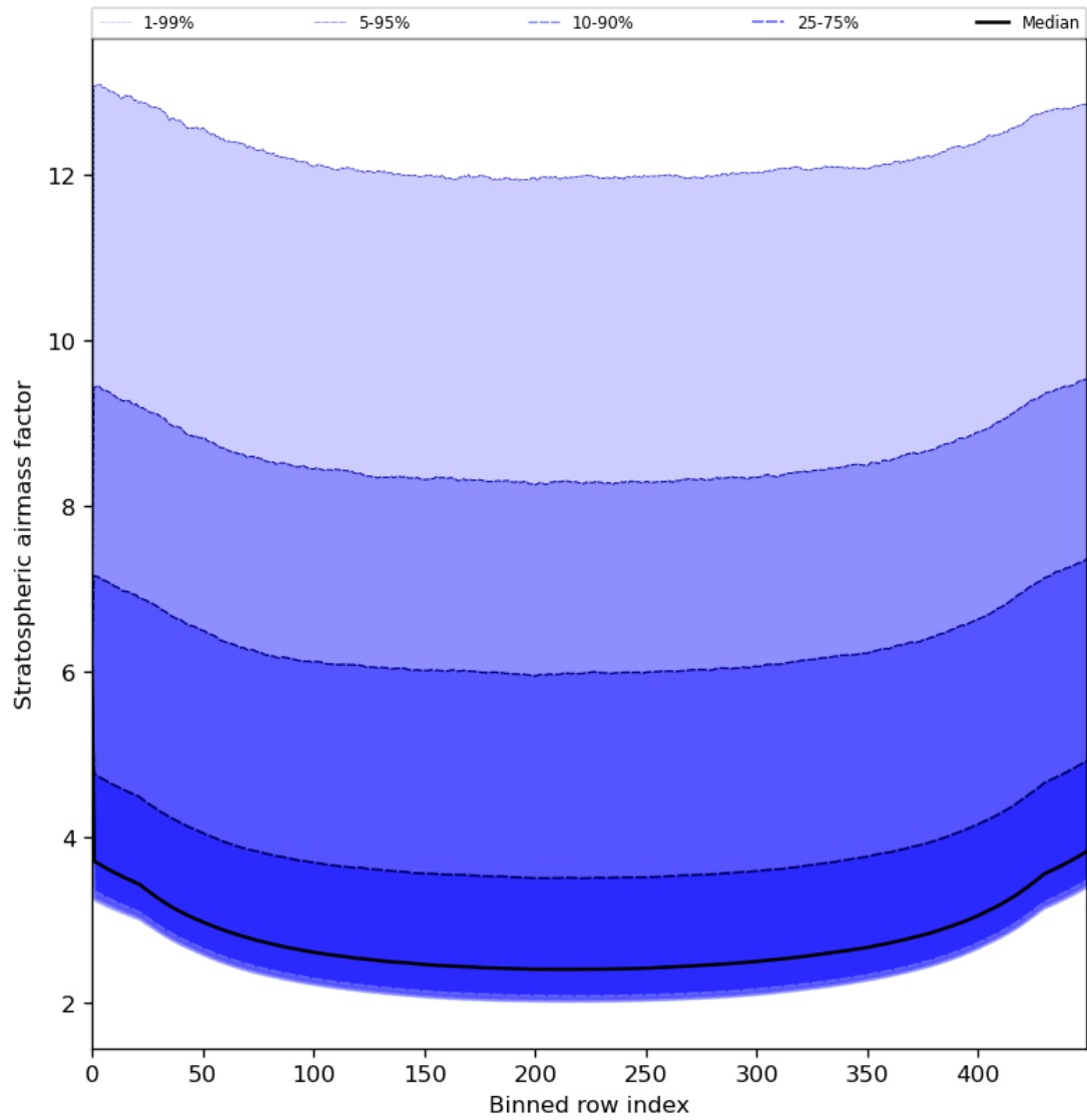
Figure 61: Along track statistics of “Stratospheric airmass factor” for 2024-05-29 to 2024-05-31
