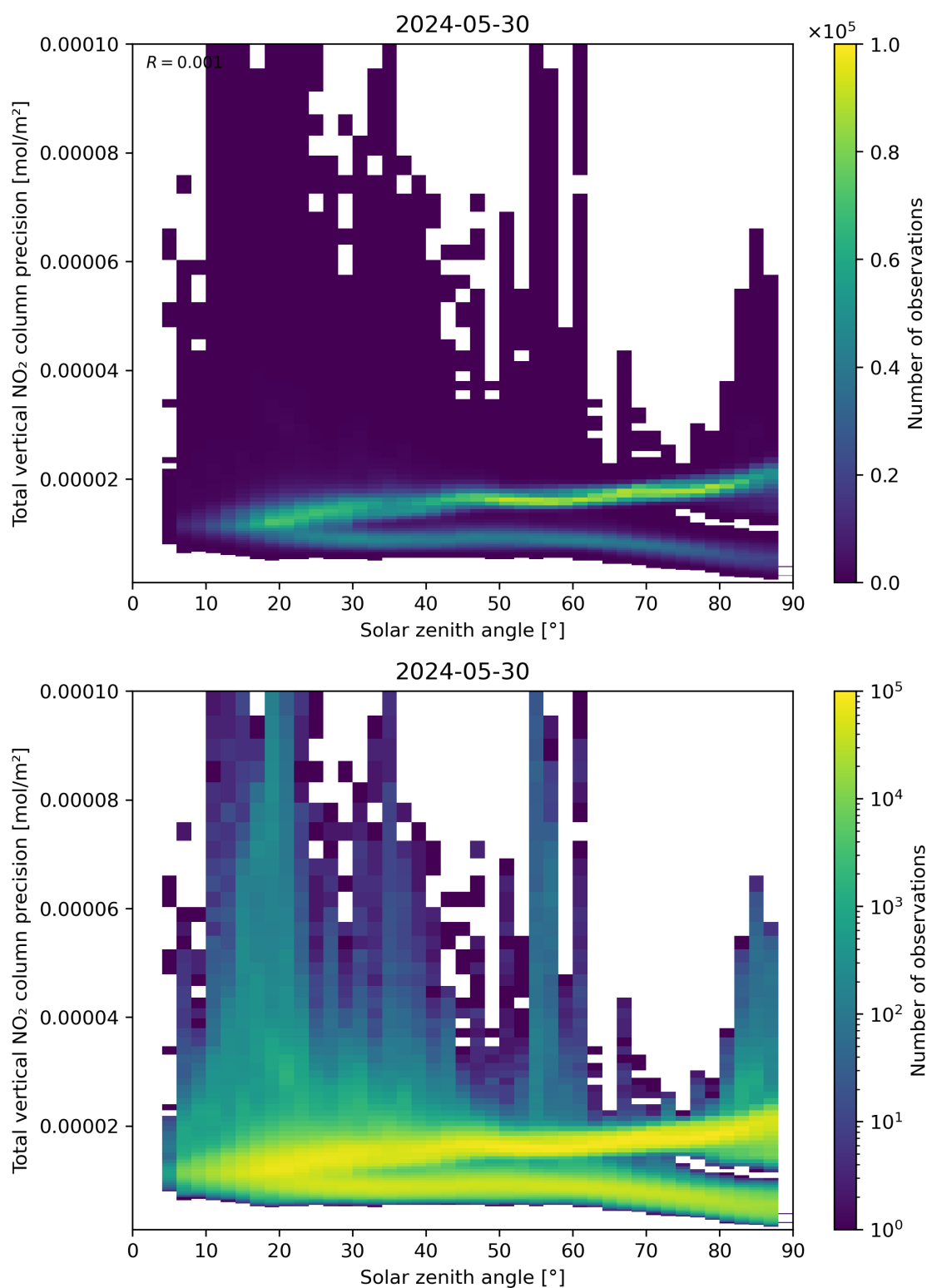
Figure 154: Scatter density plot of “Solar zenith angle” against “Total vertical NO 2 column precision” for 2024-05-29 to 2024-05-31.
