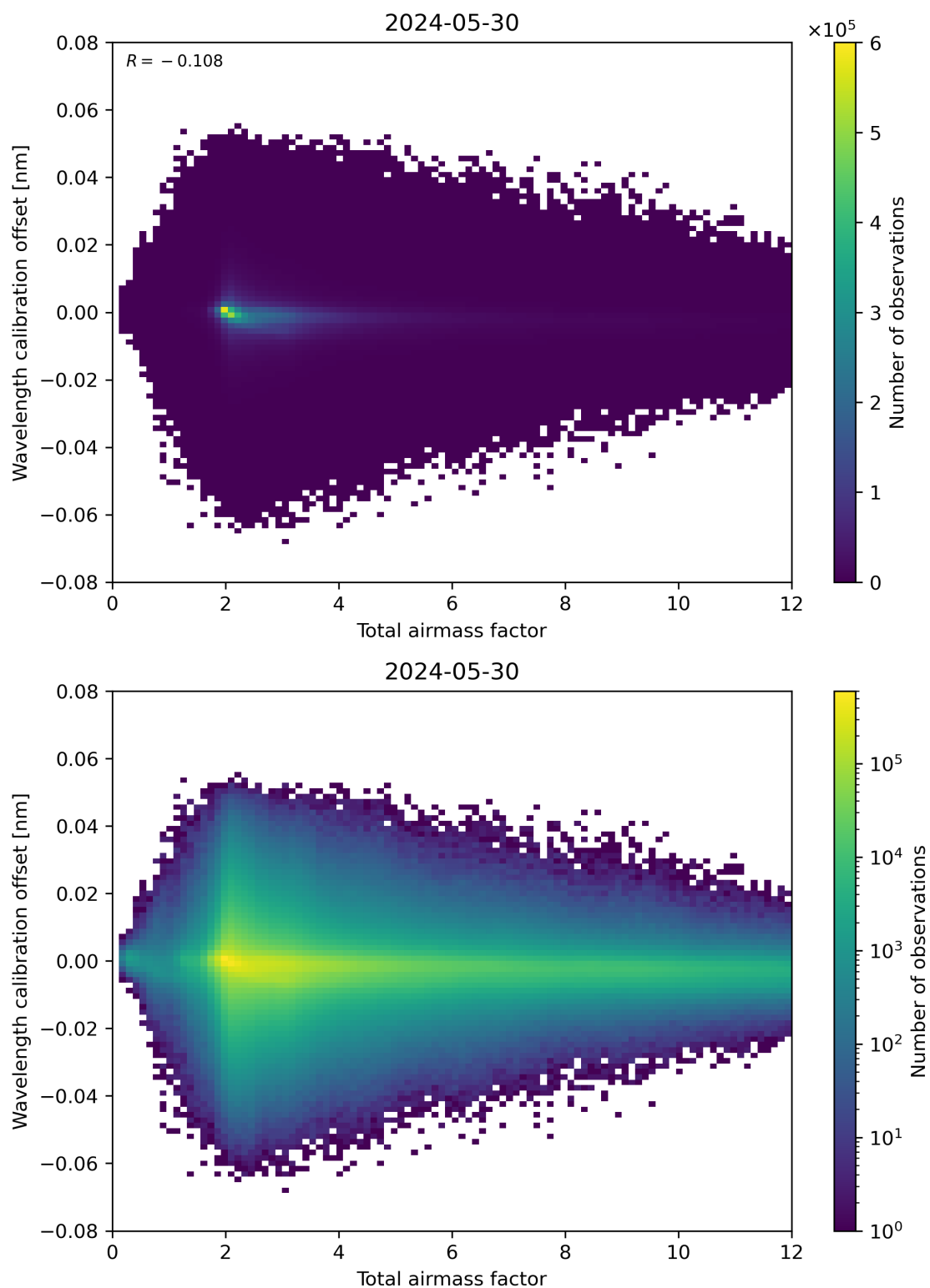
Figure 70: Scatter density plot of “Total airmass factor” against “Wavelength calibration offset” for 2024-05-29 to 2024-05-31.
