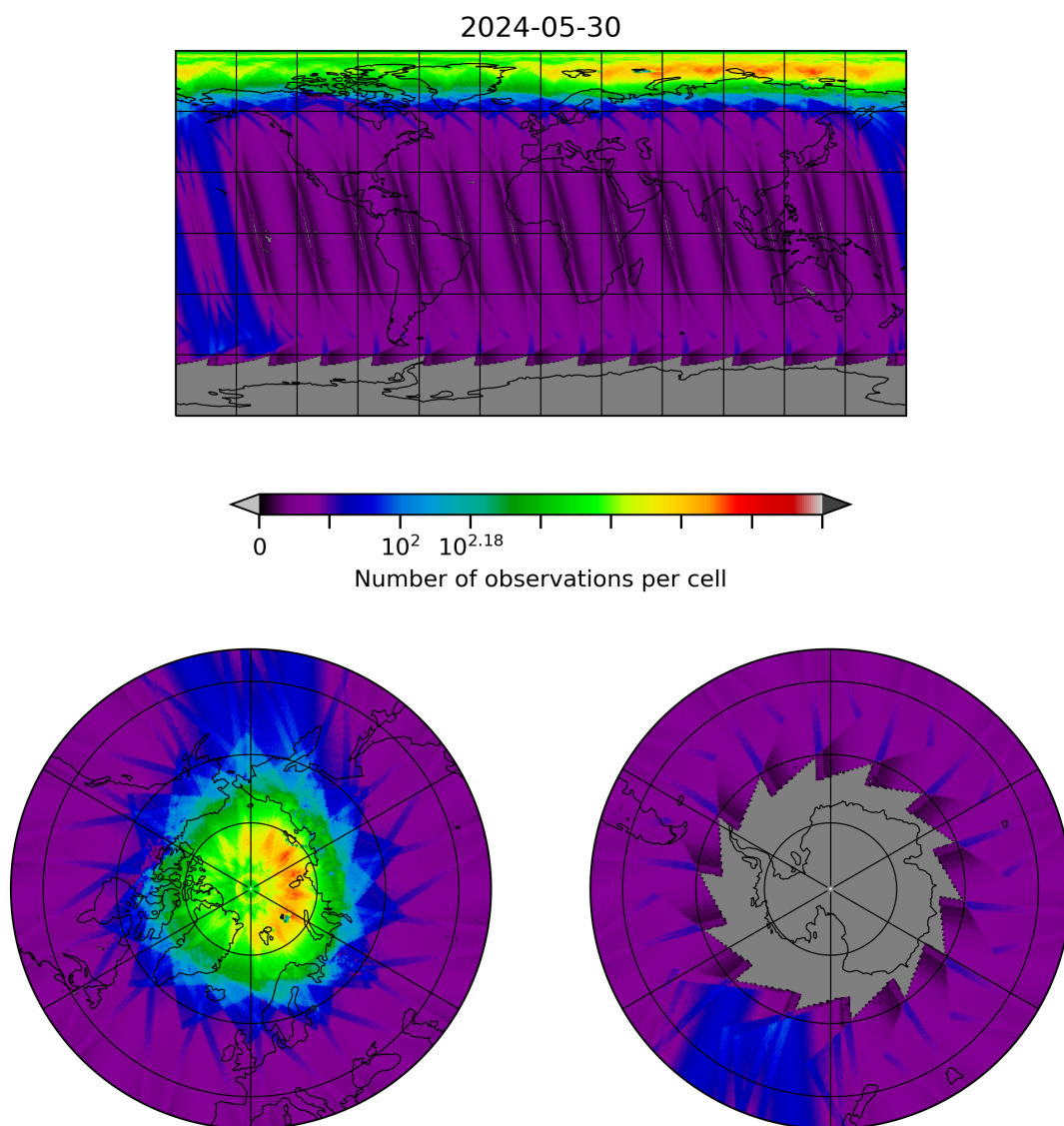
Figure 10: Map of the number of observations for 2024-05-29 to 2024-05-31
