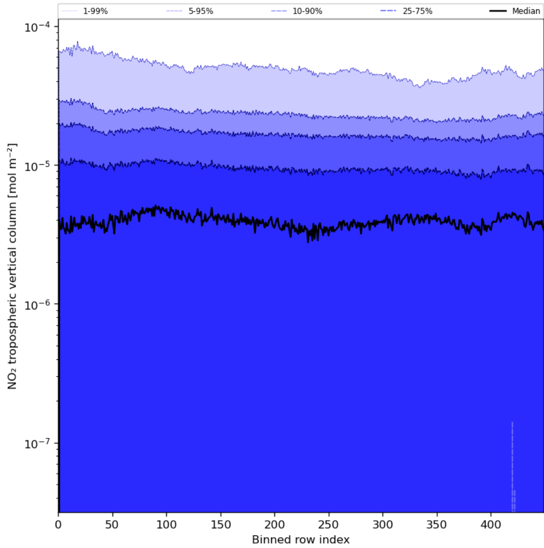
Figure 46: Along track statistics of “NO 2 tropospheric vertical column” for 2024-05-29 to 2024-05-31
