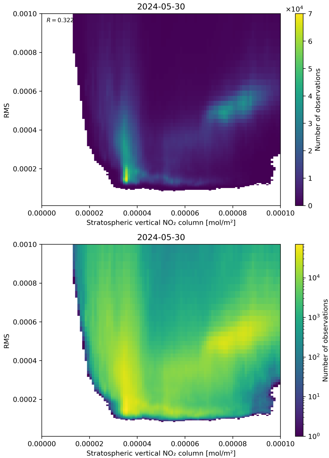
Figure 102: Scatter density plot of “Stratospheric vertical NO 2 column” against “RMS” for 2024-05-29 to 2024-05-31.
