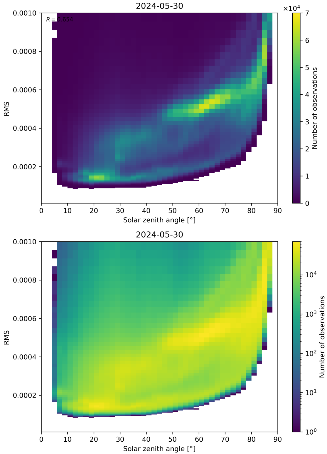
Figure 157: Scatter density plot of “Solar zenith angle” against “RMS” for 2024-05-29 to 2024-05-31.
