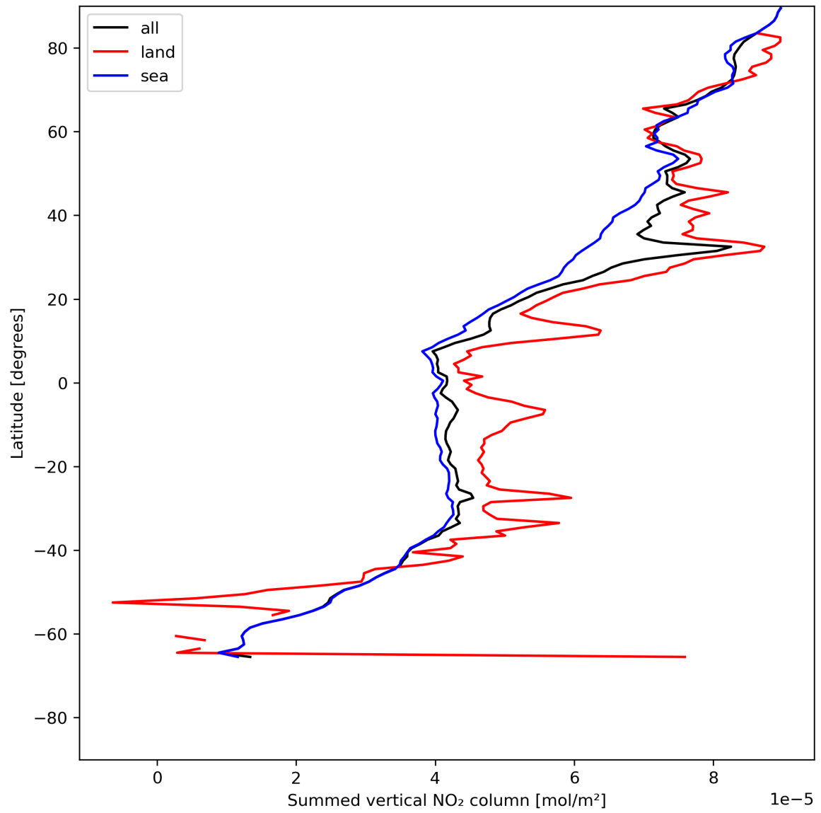
Figure 23: Zonal average of “Summed vertical NO 2 column” for 2024-05-29 to 2024-05-31.
