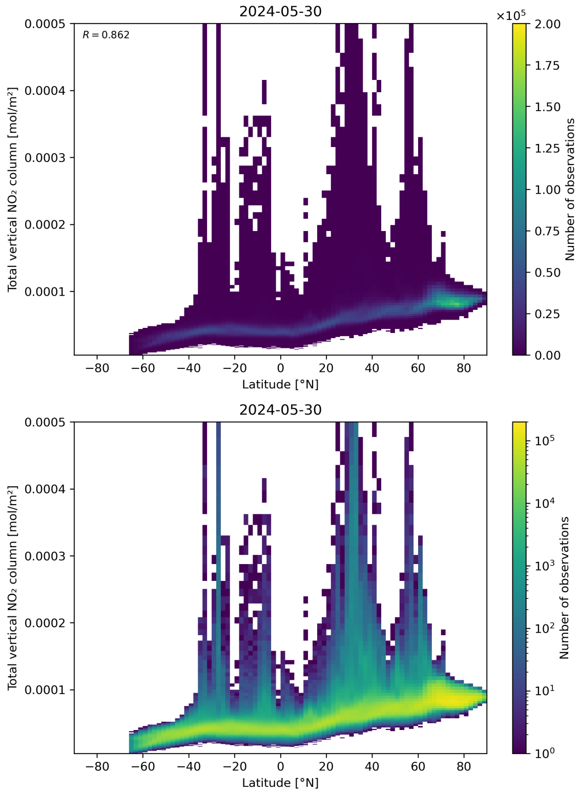
Figure 90: Scatter density plot of “Latitude” against “Total vertical NO 2 column” for 2024-05-29 to 2024-05-31.
