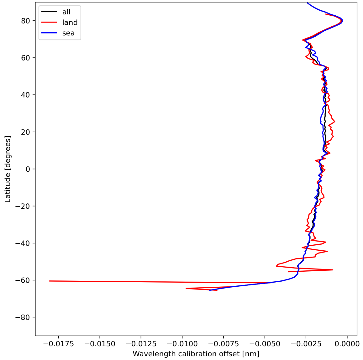
Figure 18: Zonal average of “Wavelength calibration offset” for 2024-05-29 to 2024-05-31.
