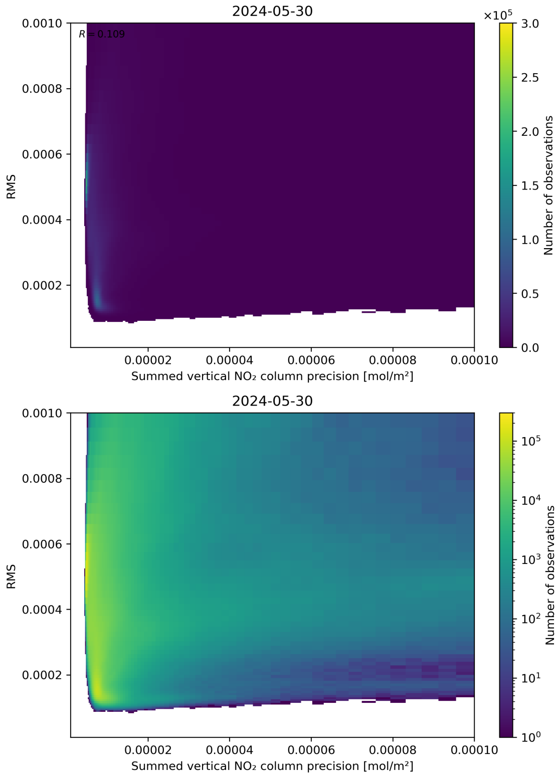
Figure 108: Scatter density plot of “Summed vertical NO 2 column precision” against “RMS” for 2024-05-29 to 2024-05-31.
