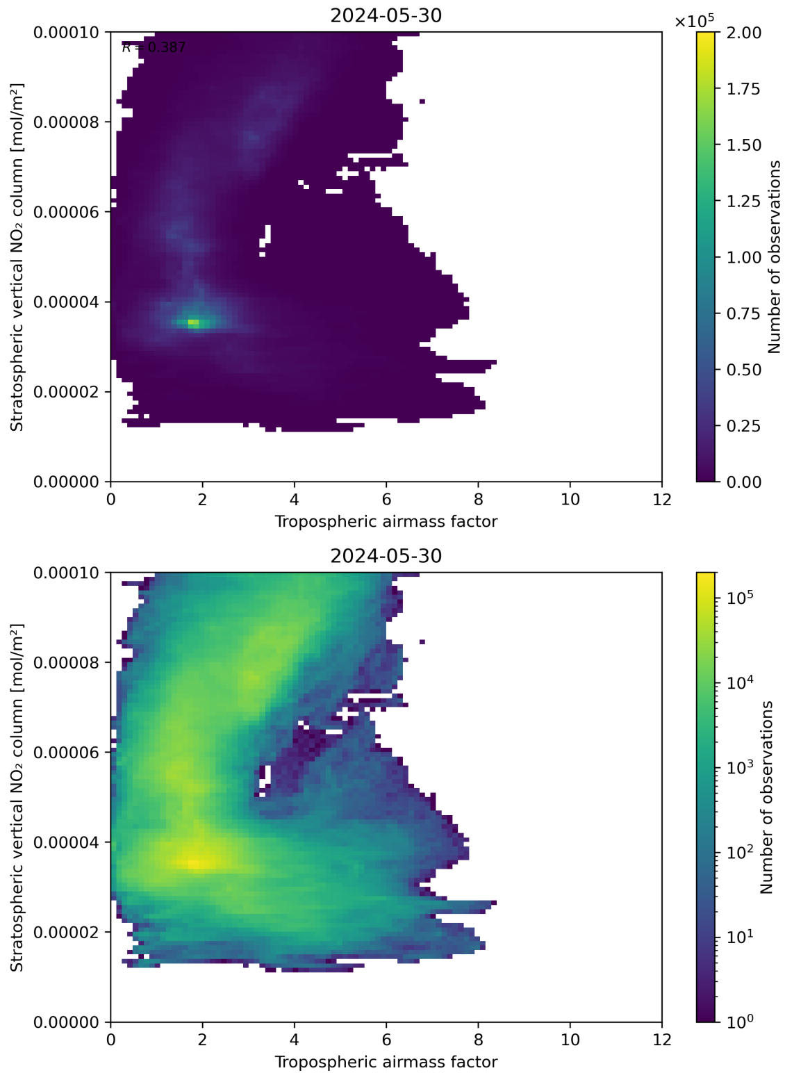
Figure 74: Scatter density plot of “Tropospheric air mass factor” against “Stratospheric vertical NO 2 column” for 2024-05-29 to 2024-05-31.
