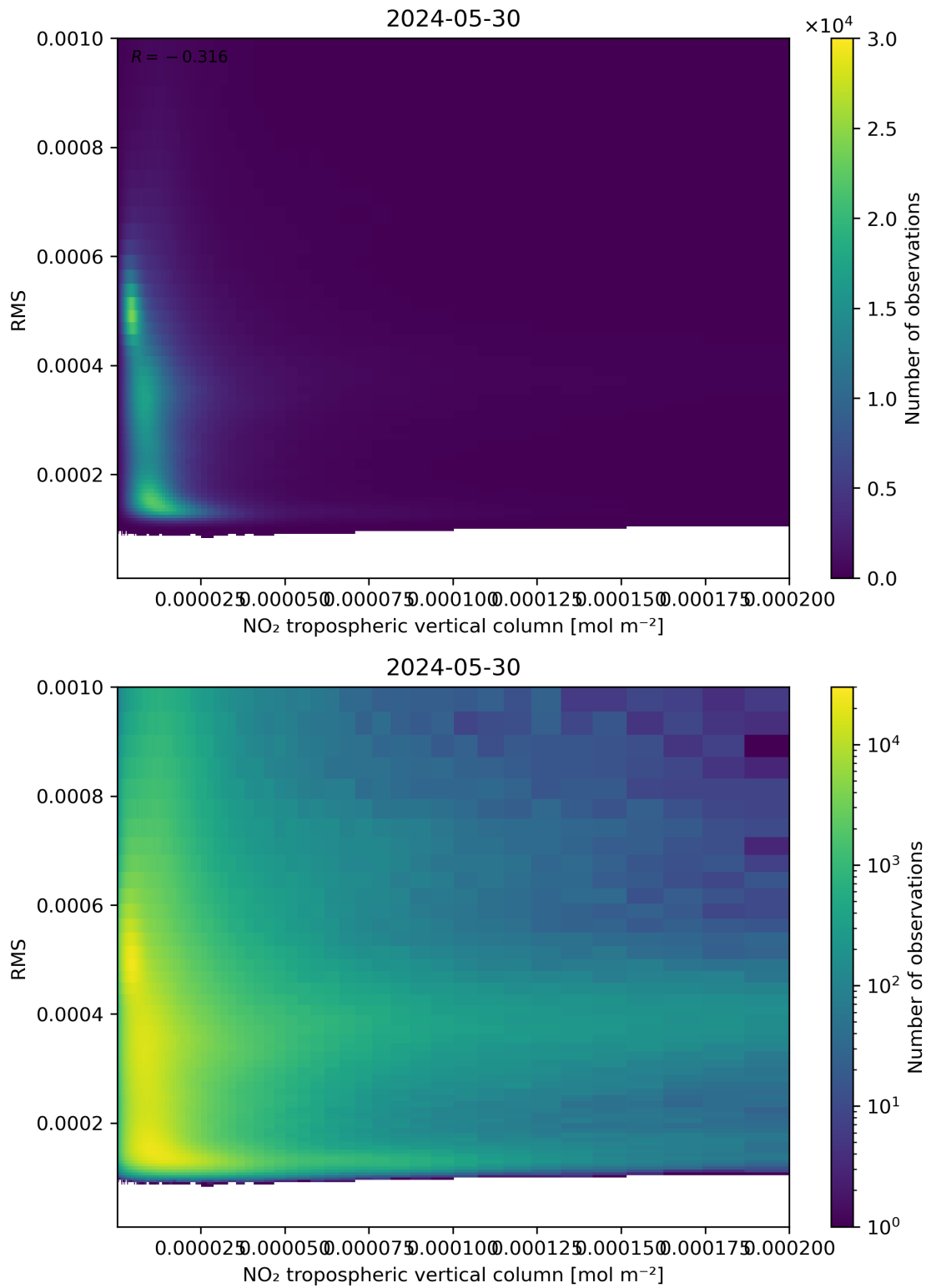
Figure 142: Scatter density plot of “NO 2 tropospheric vertical column” against “RMS” for 2024-05-29 to 2024-05-31.
