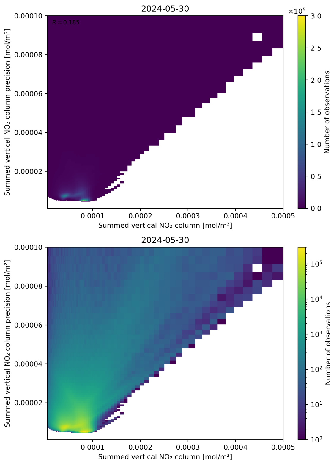
Figure 105: Scatter density plot of “Summed vertical NO 2 column” against “Summed vertical NO 2 column precision” for 2024-05-29 to 2024-05-31.
