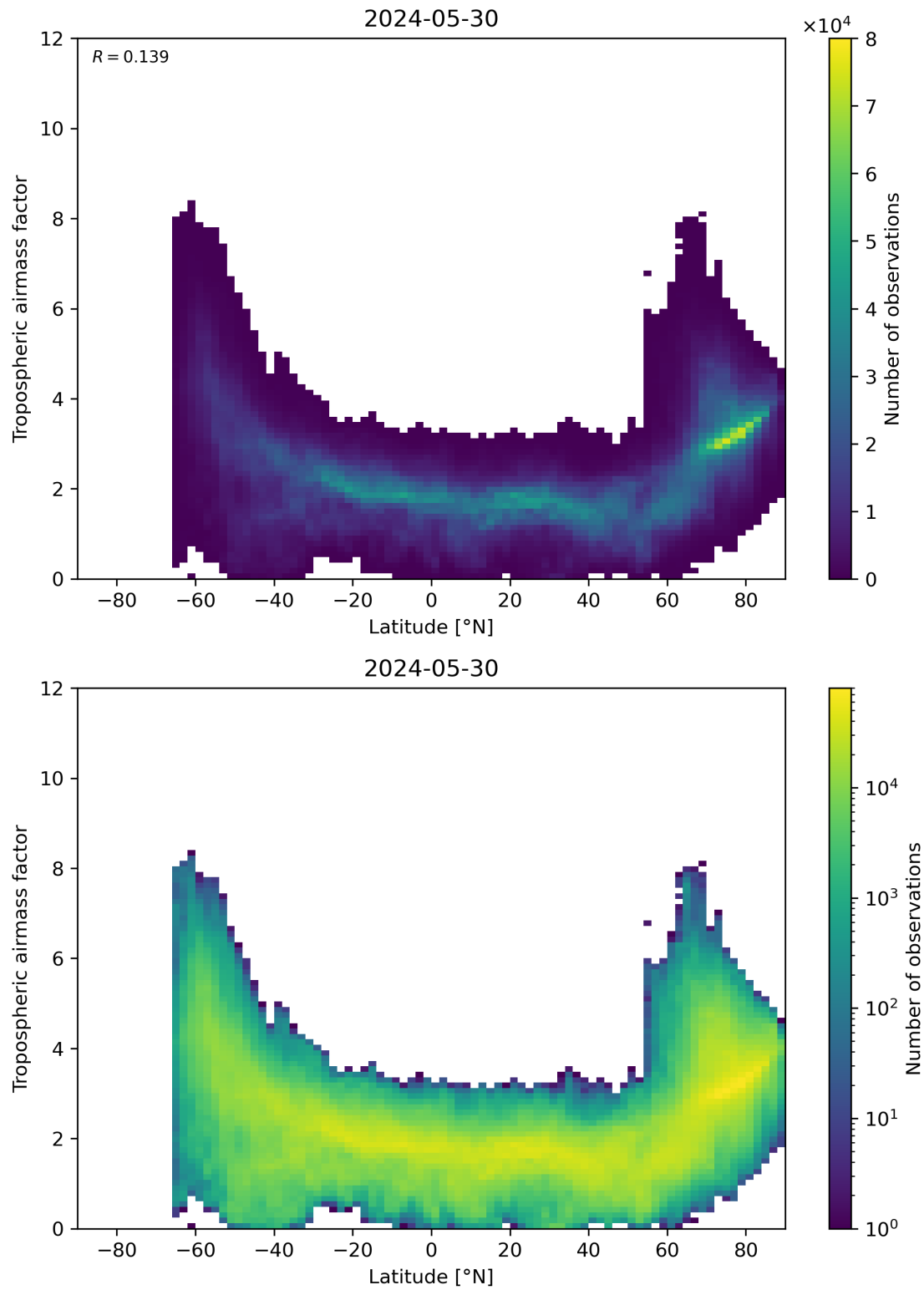
Figure 85: Scatter density plot of “Latitude” against “Tropospheric airmass factor” for 2024-05-29 to 2024-05-31.
