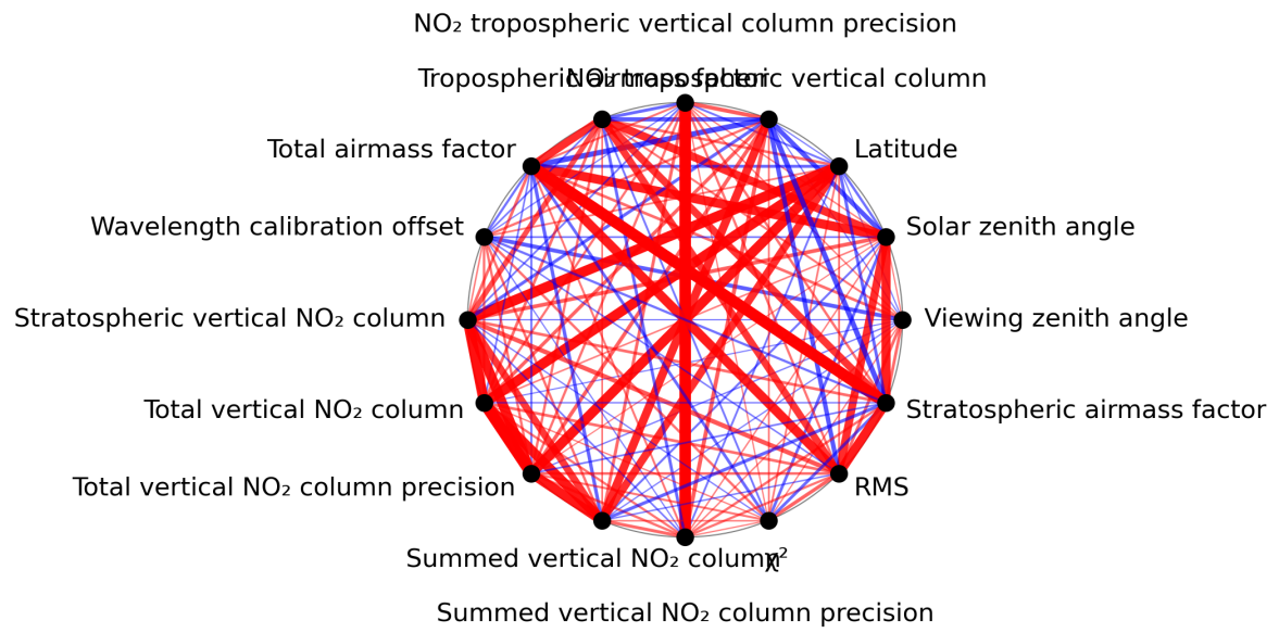
Figure 1: Map of correlation graph for 2024-05-29 to 2024-05-31.
