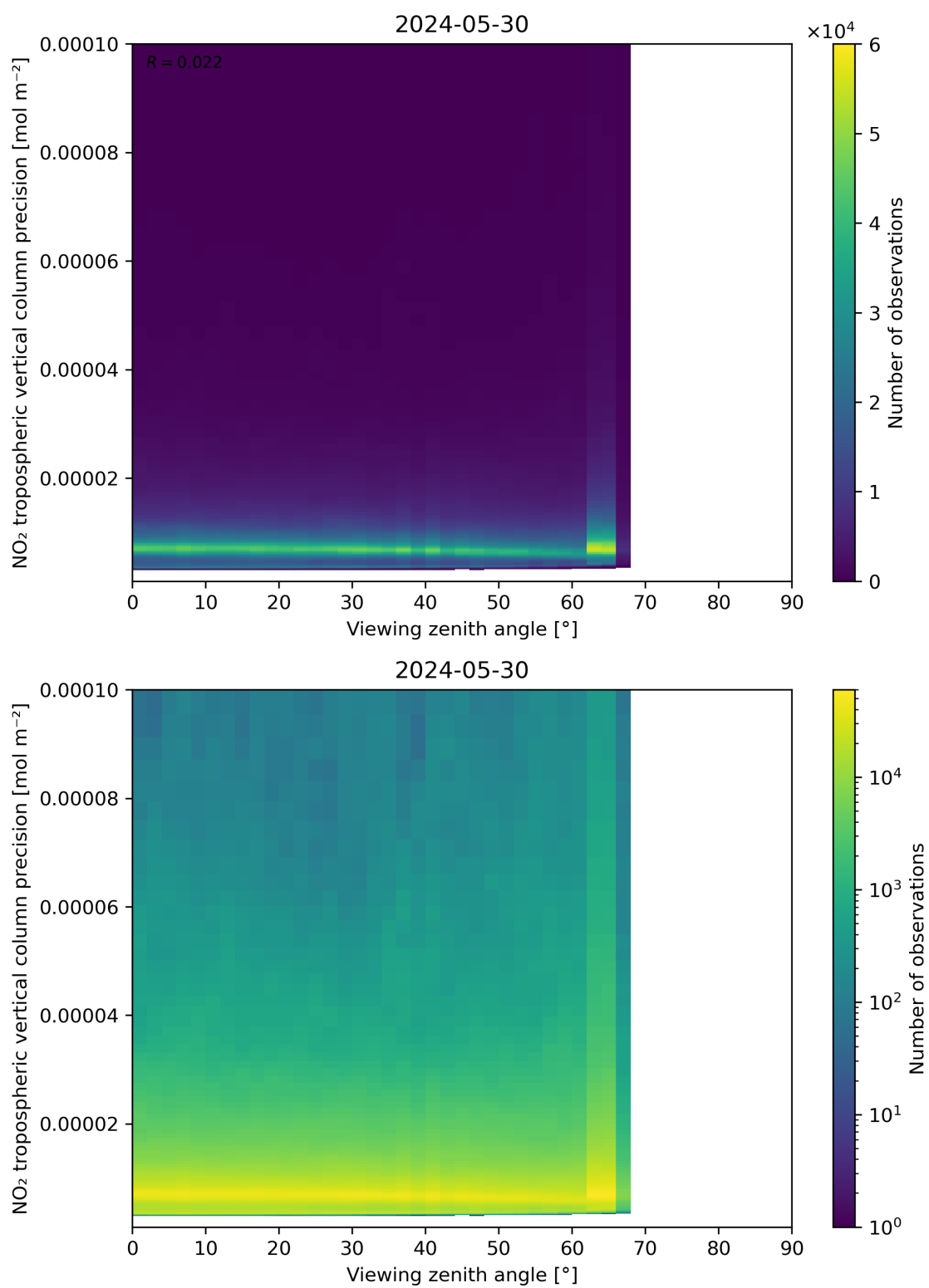
Figure 170: Scatter density plot of “Viewing zenith angle” against “NO 2 tropospheric vertical column precision” for 2024-05-29 to 2024-05-31.
