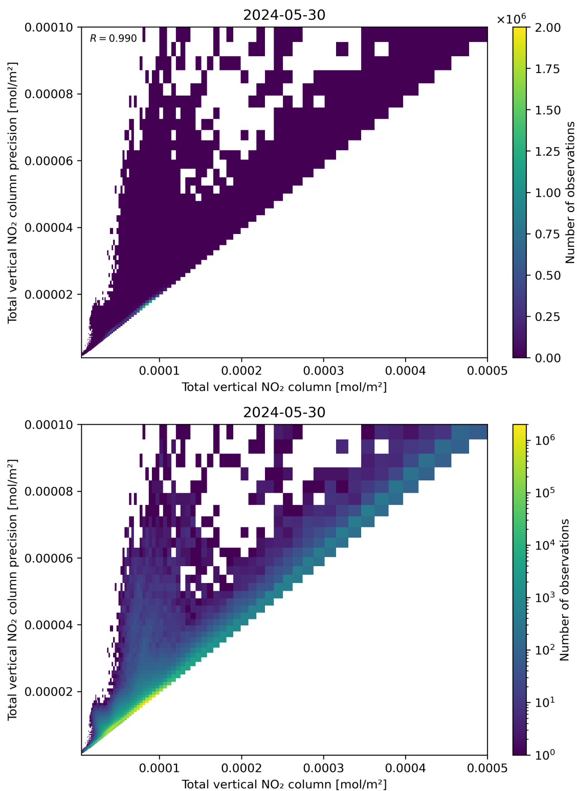
Figure 114: Scatter density plot of “Total vertical NO 2 column” against “Total vertical NO 2 column precision” for 2024-05-29 to 2024-05-31.
