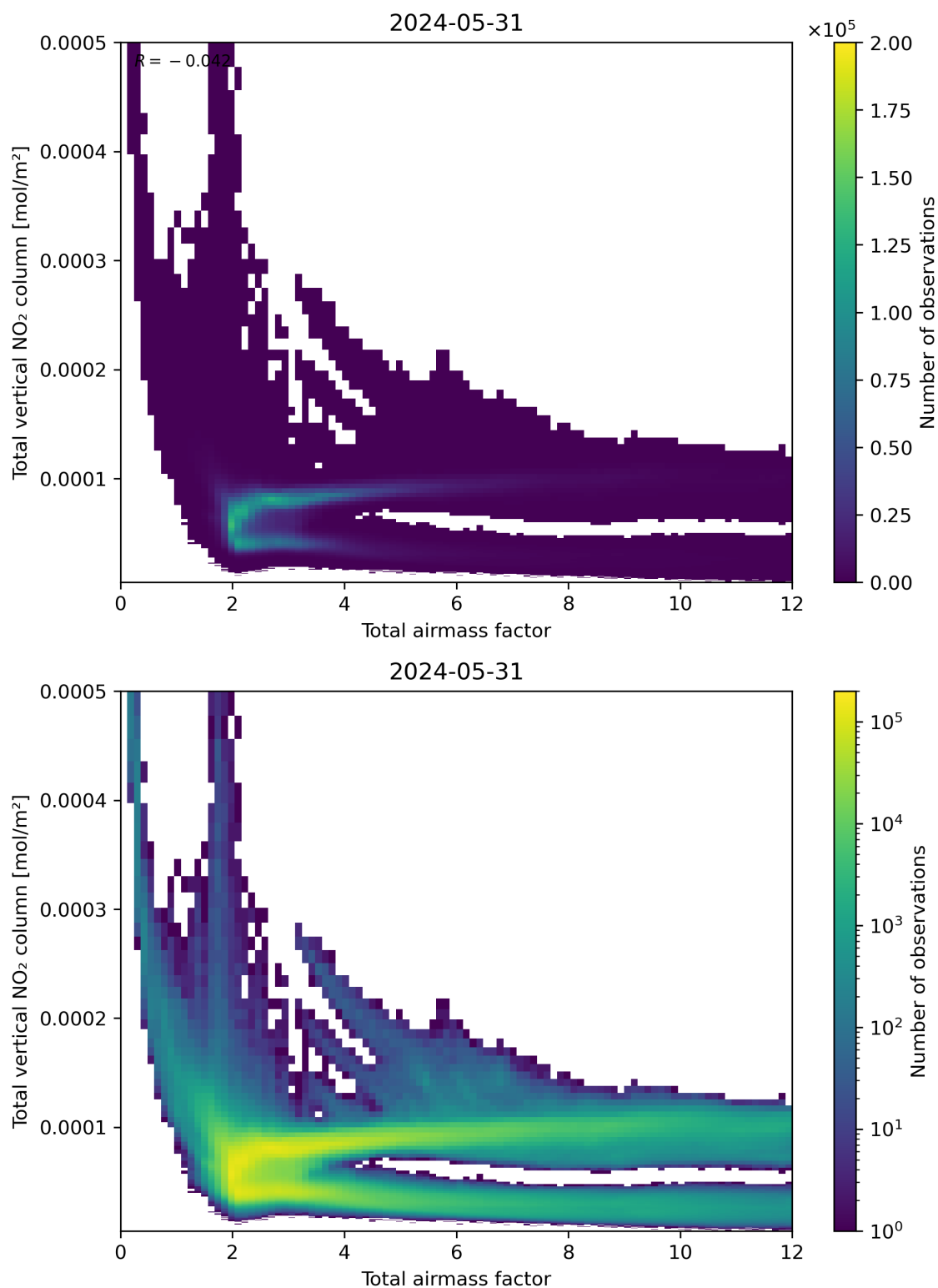
Figure 67: Scatter density plot of “Total airmass factor” against “Total vertical NO 2 column” for 2024-05-30 to 2024-06-01.
