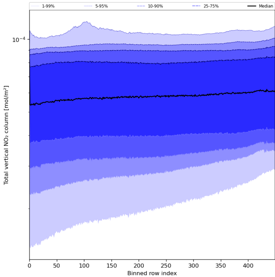
Figure 55: Along track statistics of “Total vertical NO 2 column” for 2024-05-30 to 2024-06-01
