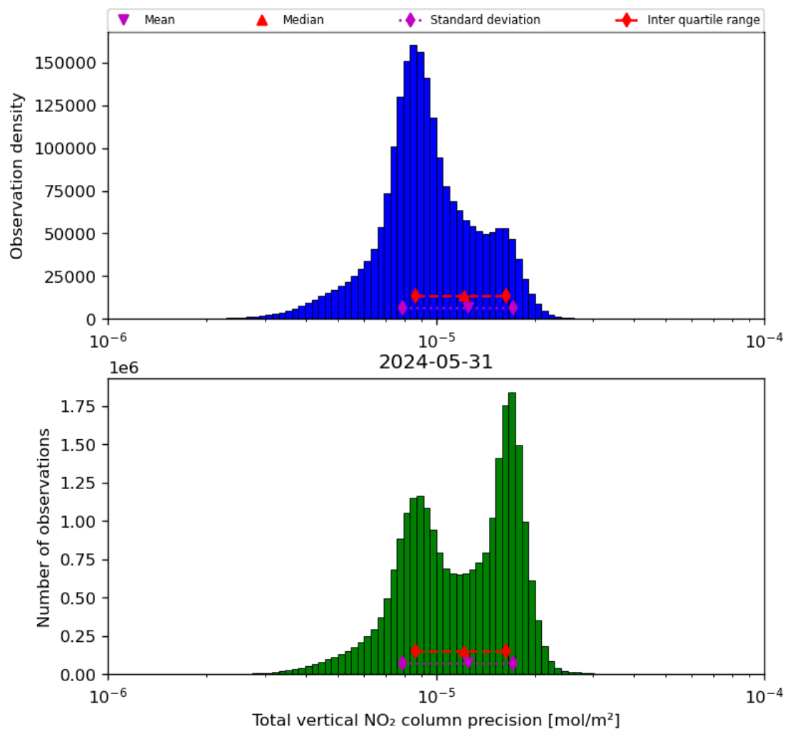
Figure 39: Histogram of “Total vertical NO 2 column precision” for 2024-05-30 to 2024-06-01
