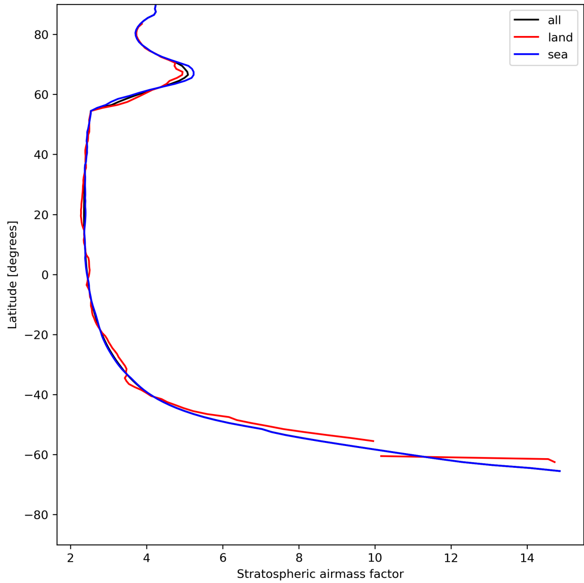
Figure 27: Zonal average of “Stratospheric airmass factor” for 2024-05-30 to 2024-06-01.
