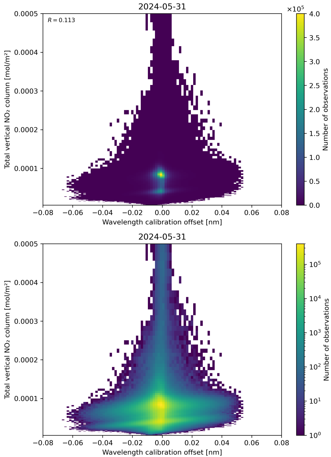
Figure 179: Scatter density plot of “Wavelength calibration offset” against “Total vertical NO 2 column” for 2024-05-30 to 2024-06-01.
