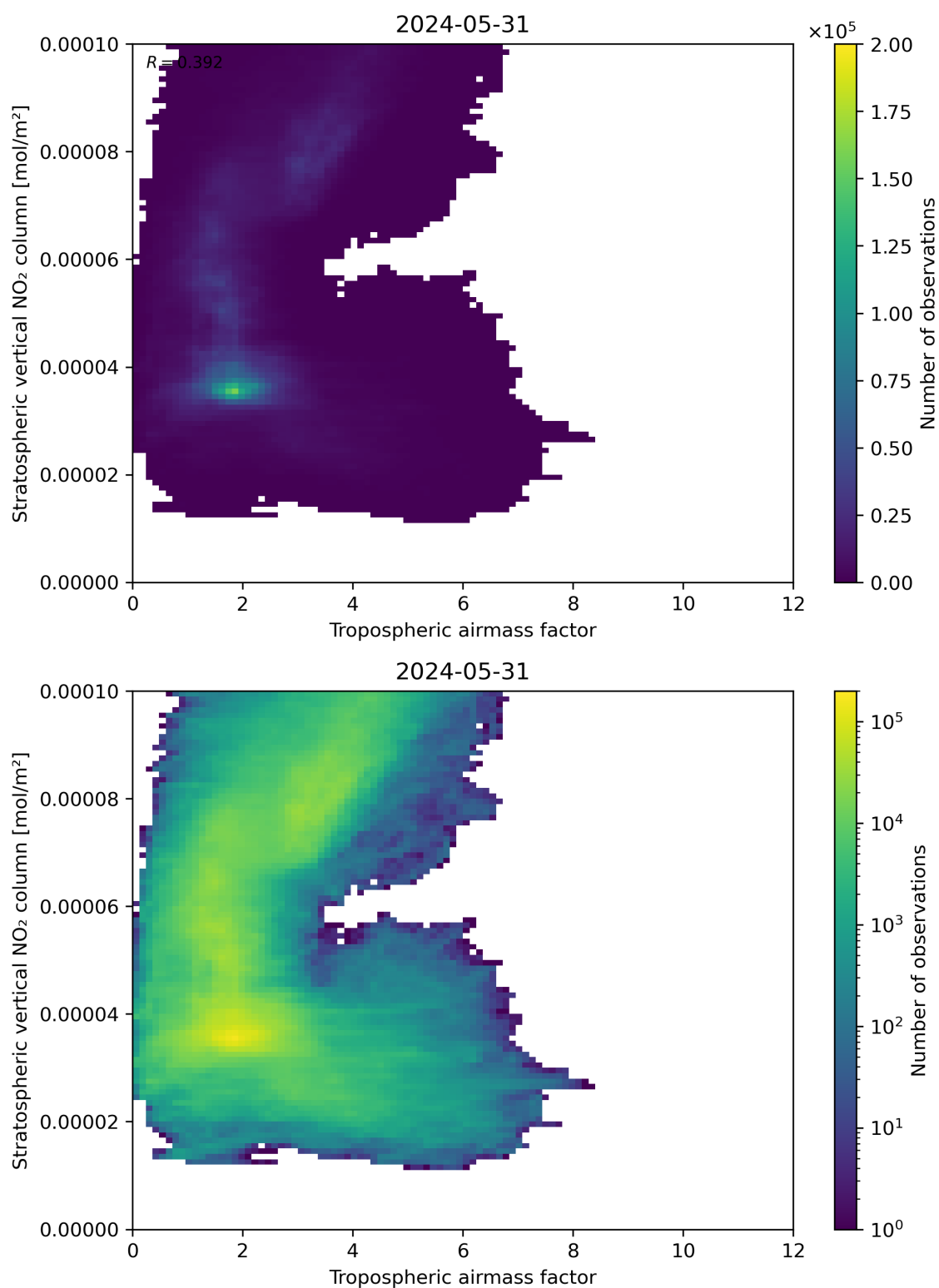
Figure 74: Scatter density plot of “Tropospheric airmass factor” against “Stratospheric vertical NO 2 column” for 2024-05-30 to 2024-06-01.
