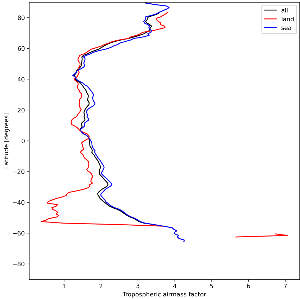
Figure 14: Zonal average of “Tropospheric airmass factor” for 2024-05-30 to 2024-06-01.
