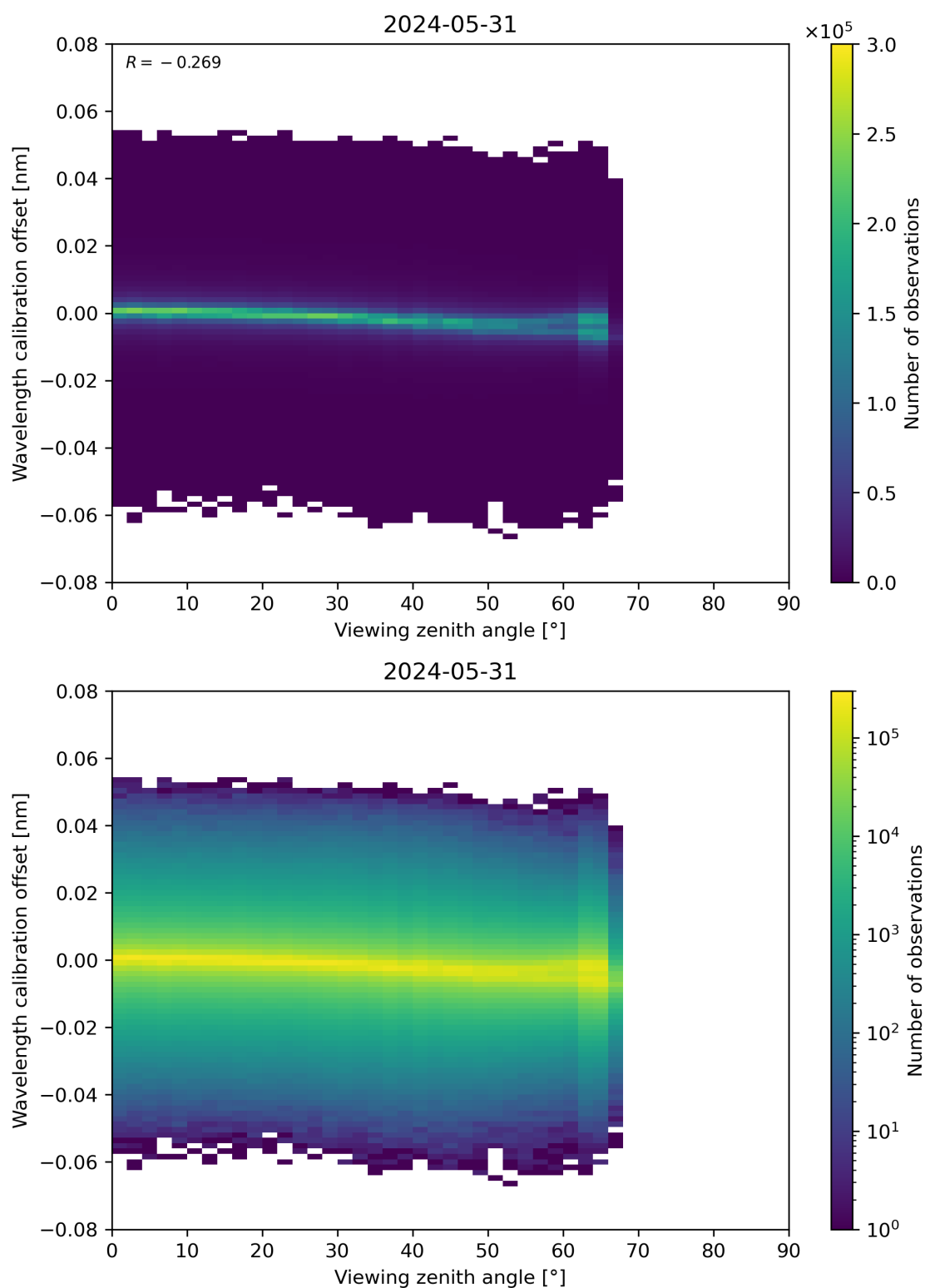
Figure 173: Scatter density plot of “Viewing zenith angle” against “Wavelength calibration offset” for 2024-05-30 to 2024-06-01.
