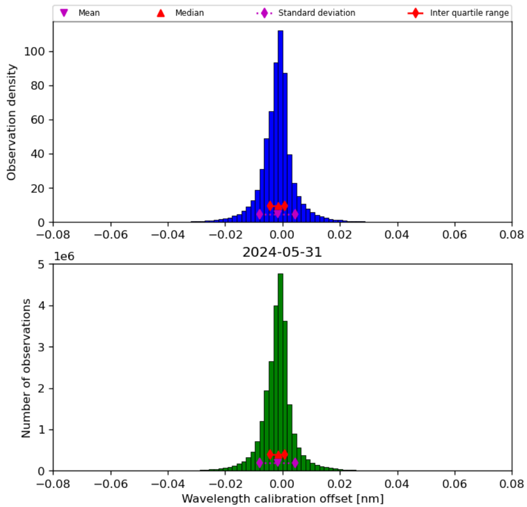
Figure 35: Histogram of “Wavelength calibration offset” for 2024-05-30 to 2024-06-01
