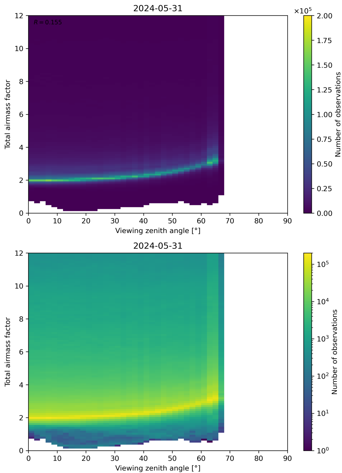
Figure 160: Scatter density plot of “Viewing zenith angle” against “Total airmass factor” for 2024-05-30 to 2024-06-01.
