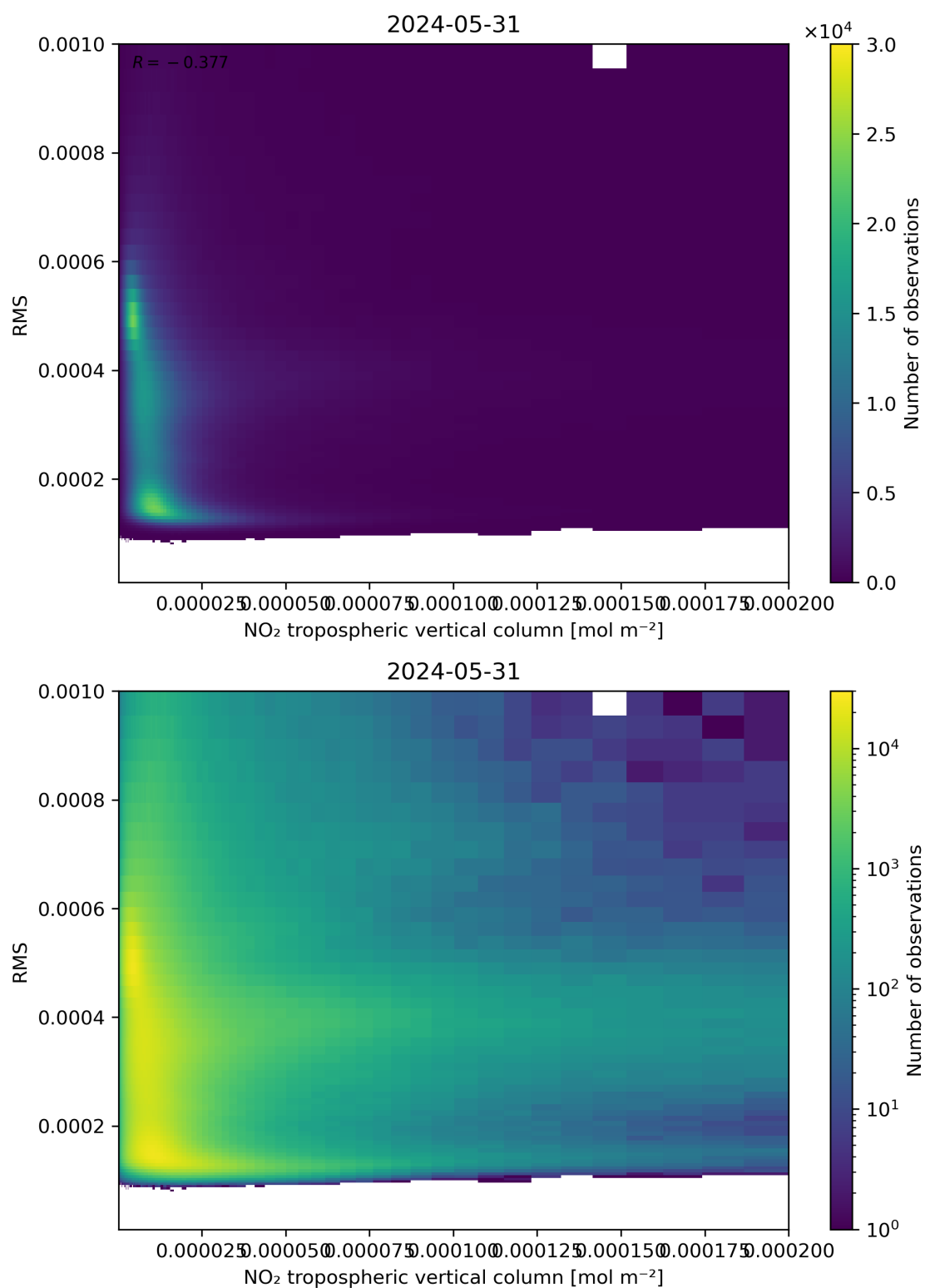
Figure 142: Scatter density plot of “NO 2 tropospheric vertical column” against “RMS” for 2024-05-30 to 2024-06-01.
