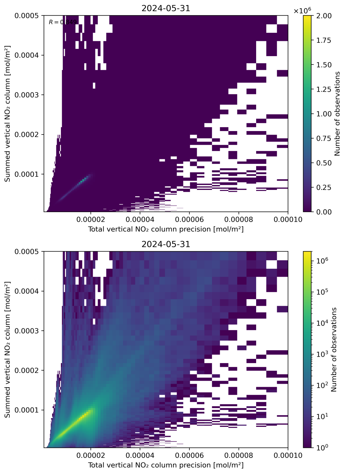
Figure 117: Scatter density plot of “Total vertical NO 2 column precision” against “Summed vertical NO 2 column” for 2024-05-30 to 2024-06-01.
