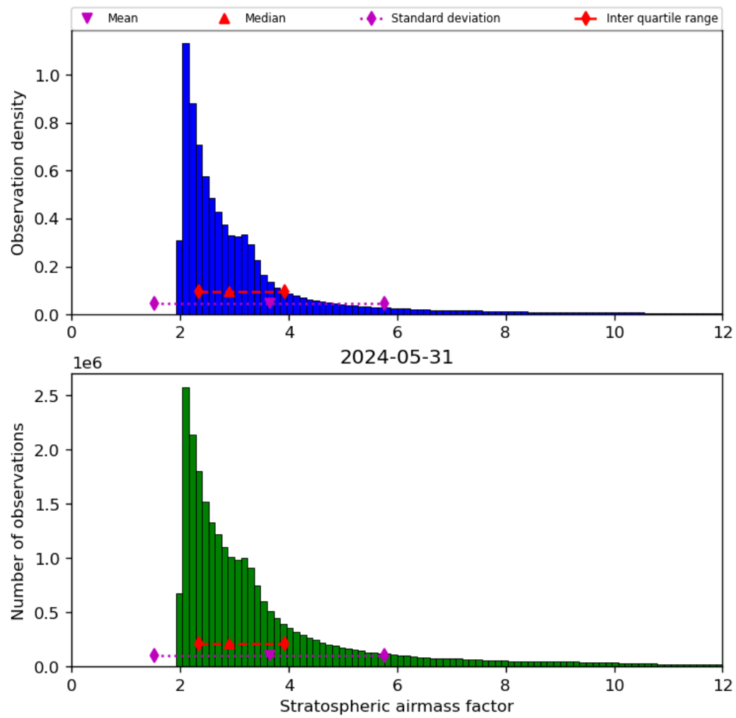
Figure 44: Histogram of “Stratospheric airmass factor” for 2024-05-30 to 2024-06-01
