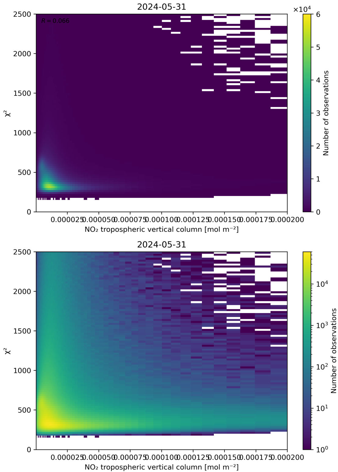
Figure 124: Scatter density plot of “NO 2 tropospheric vertical column” against “ \chi^2 ” for 2024-05-30 to 2024-06-01.
