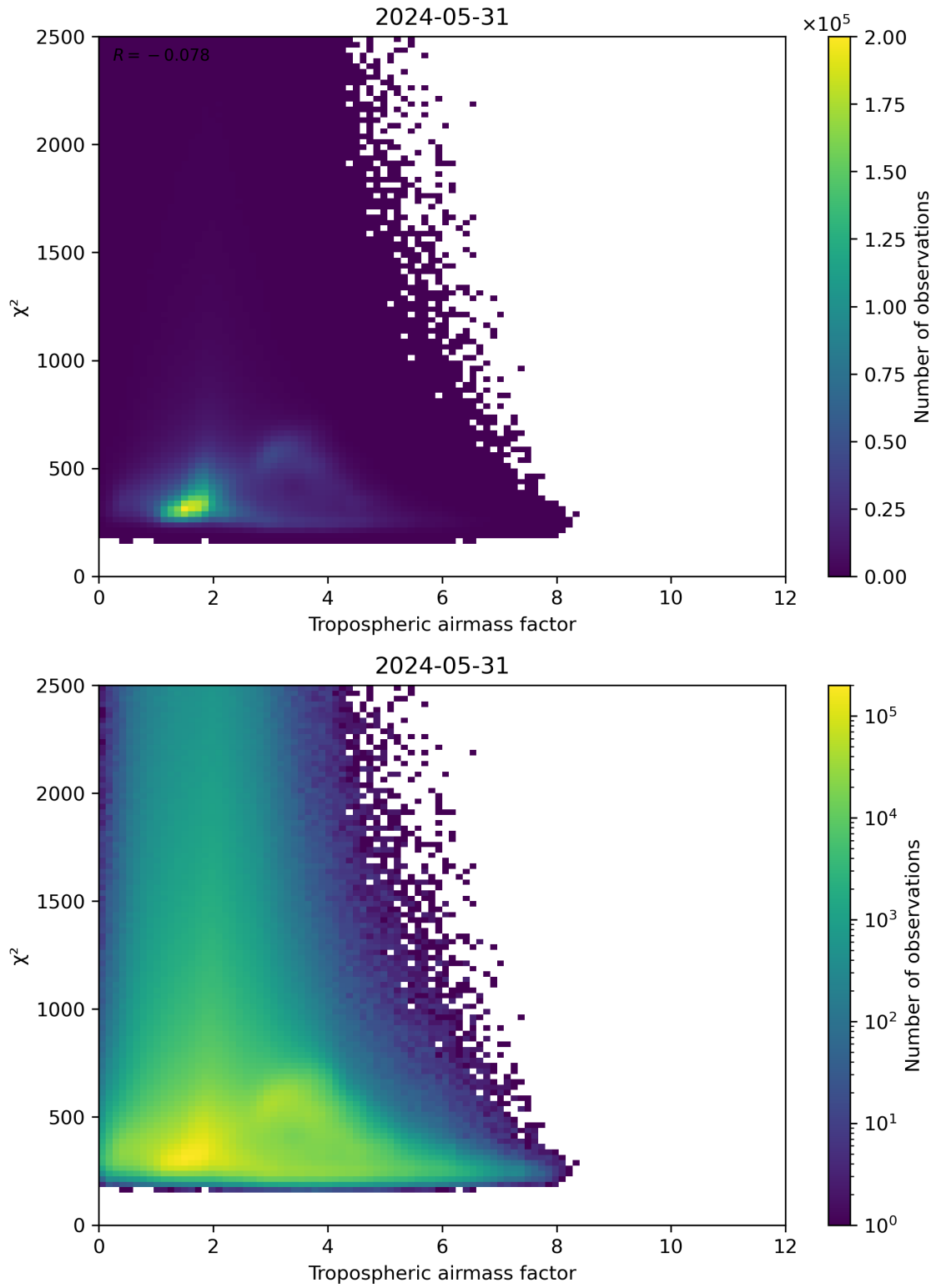
Figure 73: Scatter density plot of “Tropospheric airmass factor” against “ \chi^2 ” for 2024-05-30 to 2024-06-01.
