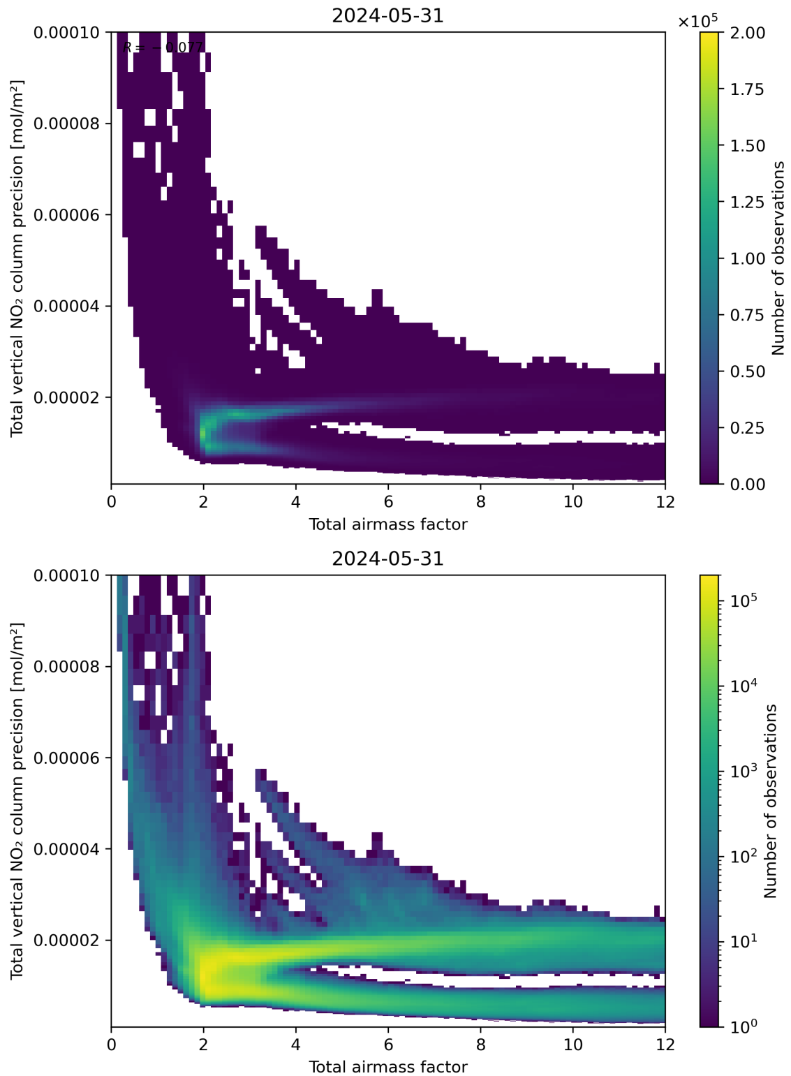
Figure 68: Scatter density plot of “Total airmass factor” against “Total vertical NO 2 column precision” for 2024-05-30 to 2024-06-01.
