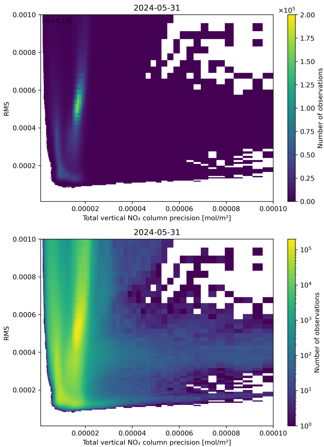
Figure 119: Scatter density plot of “Total vertical NO 2 column precision” against “RMS” for 2024-05-30 to 2024-06-01.
