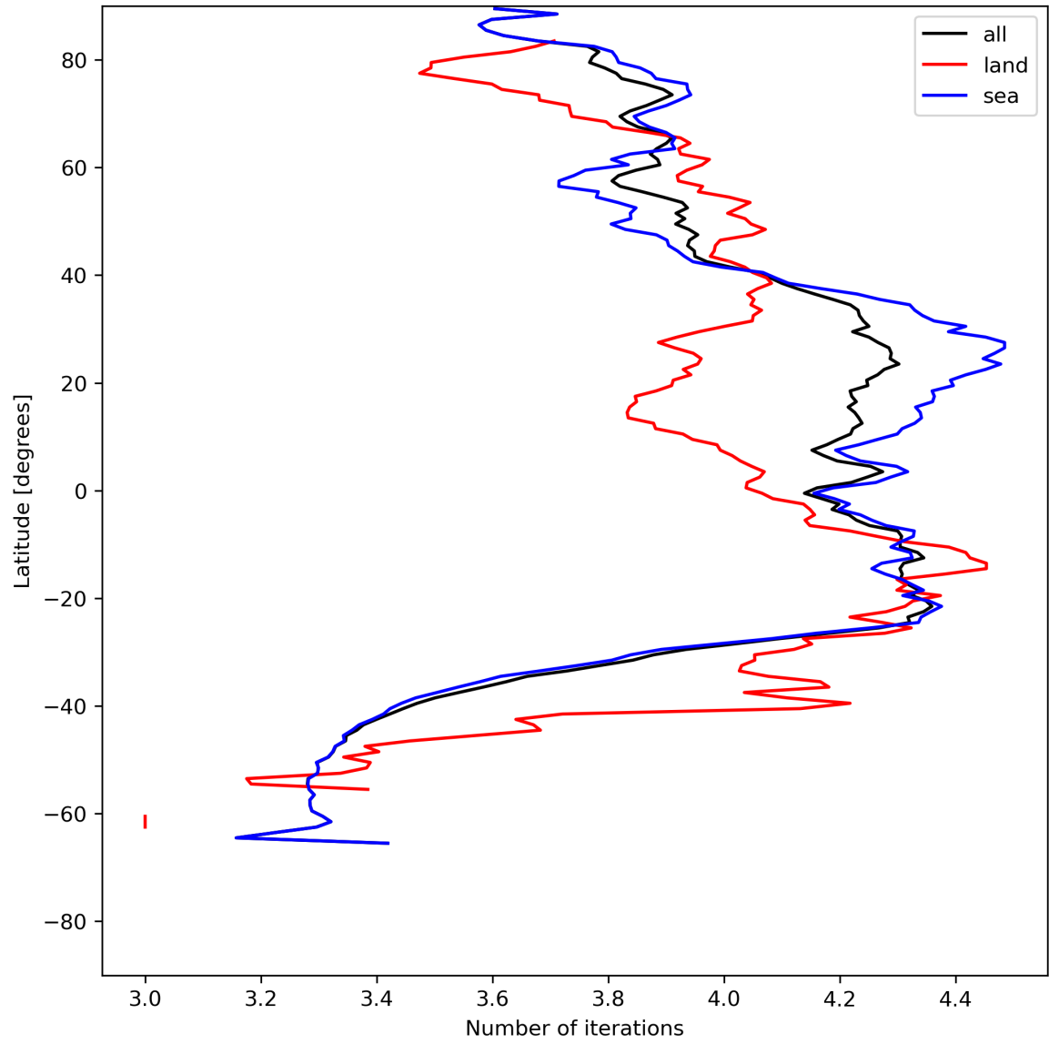
Figure 17: Zonal average of “Number of iterations” for 2024-05-30 to 2024-06-01.
