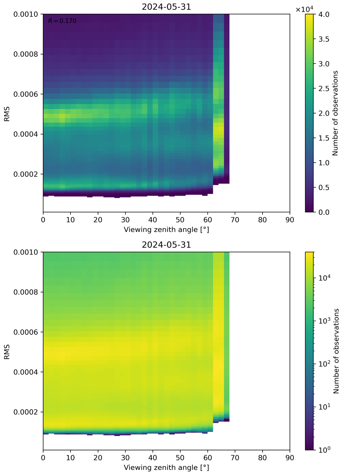
Figure 171: Scatter density plot of “Viewing zenith angle” against “RMS” for 2024-05-30 to 2024-06-01.
