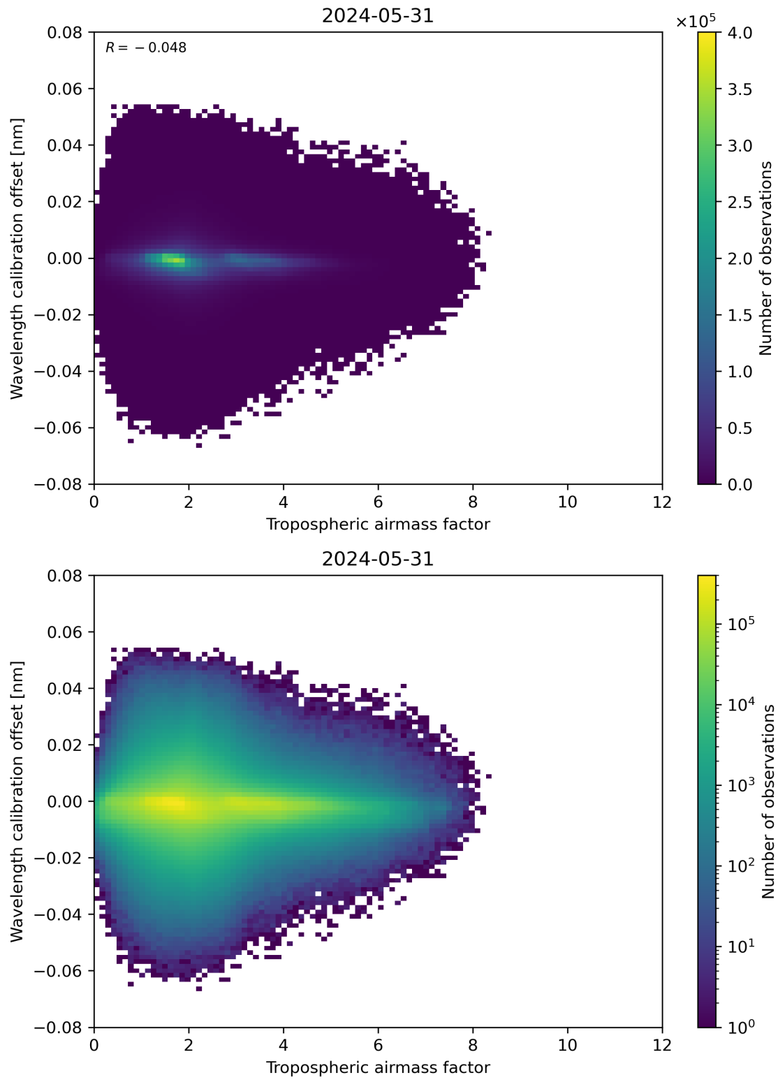
Figure 80: Scatter density plot of “Tropospheric air mass factor” against “Wavelength calibration offset” for 2024-05-30 to 2024-06-01.
