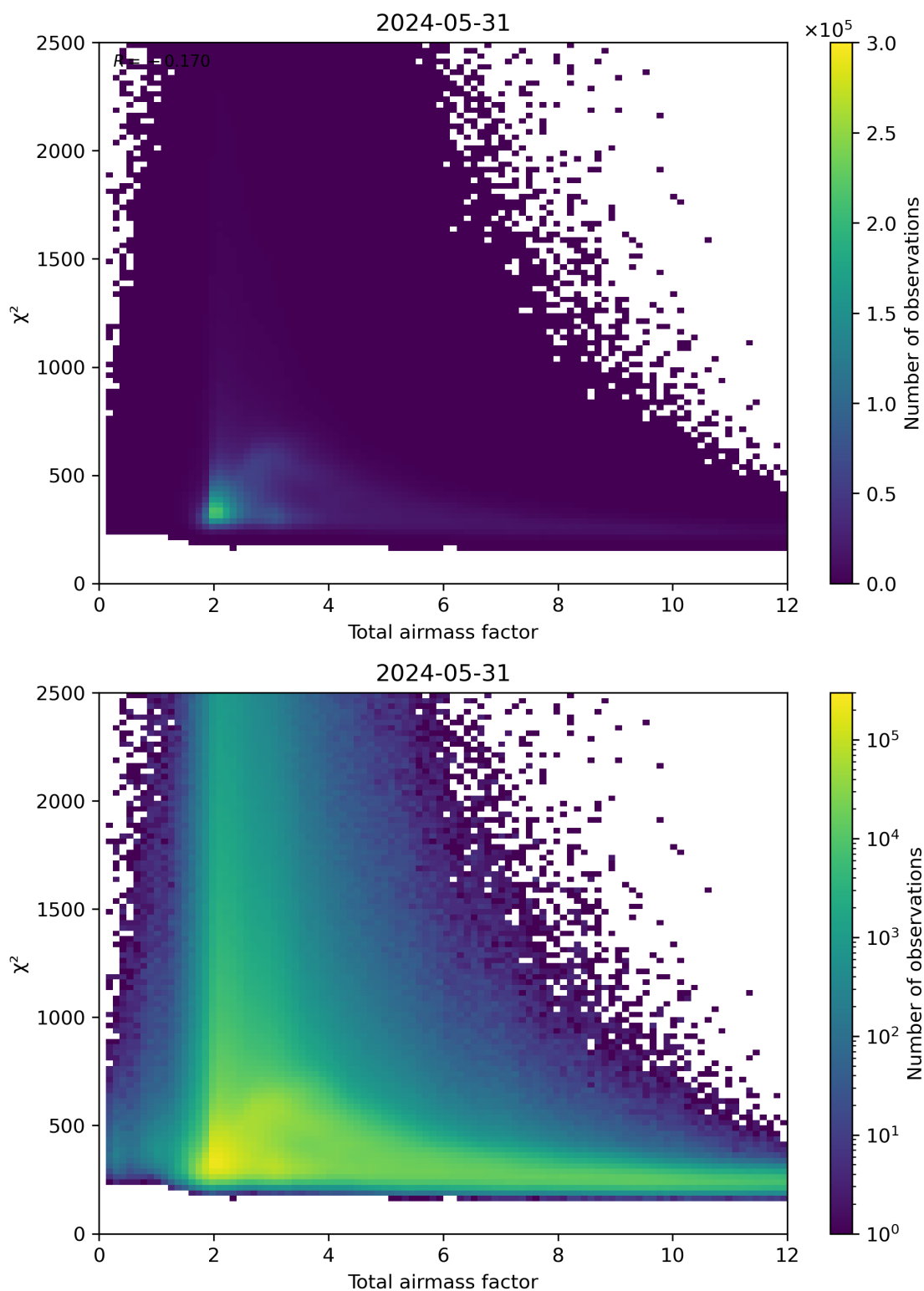
Figure 63: Scatter density plot of “Total airmass factor” against “ \chi^2 ” for 2024-05-30 to 2024-06-01.
