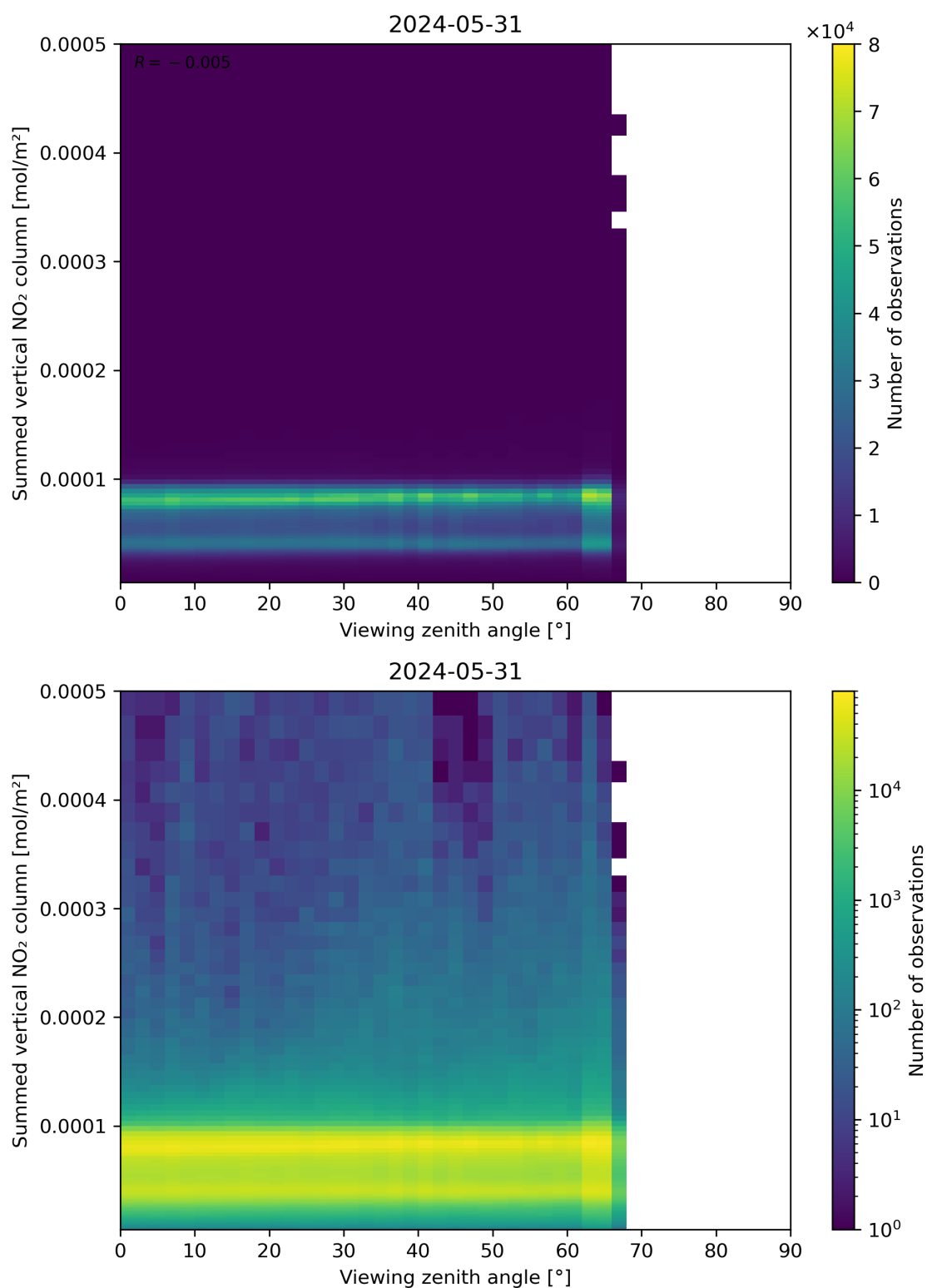
Figure 165: Scatter density plot of “Viewing zenith angle” against “Summed vertical NO 2 column” for 2024-05-30 to 2024-06-01.
