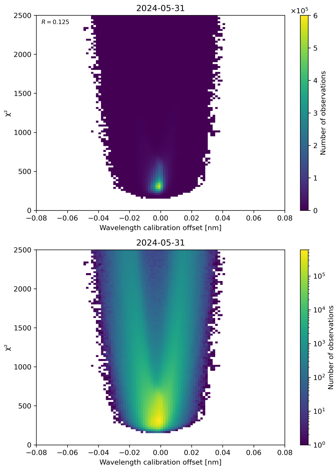
Figure 175: Scatter density plot of “Wavelength calibration offset” against “ \chi^2 ” for 2024-05-30 to 2024-06-01.
