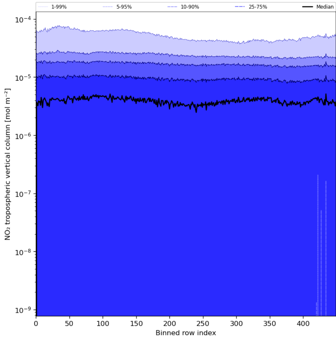
Figure 46: Along track statistics of “NO 2 tropospheric vertical column” for 2024-05-30 to 2024-06-01
