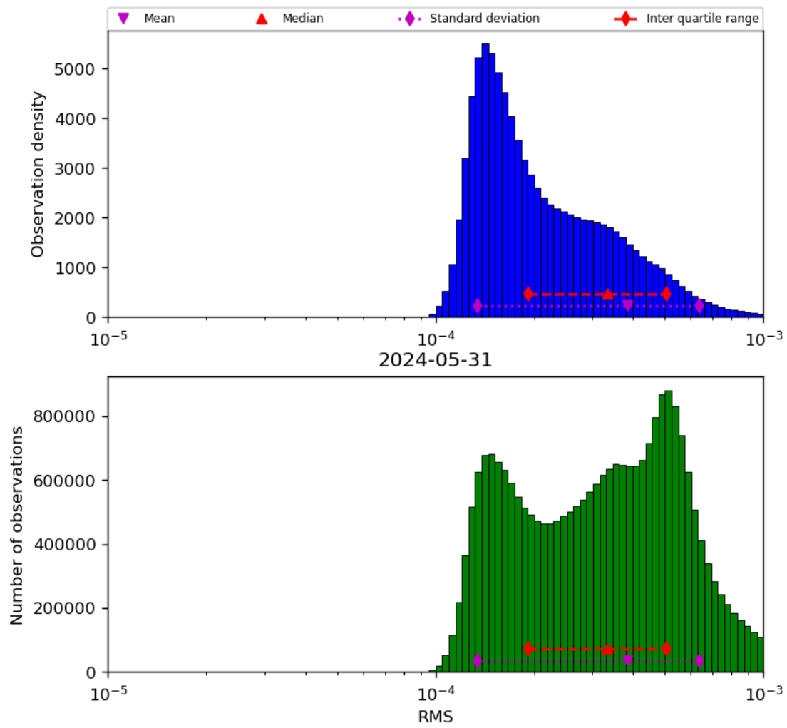
Figure 43: Histogram of “RMS” for 2024-05-30 to 2024-06-01
