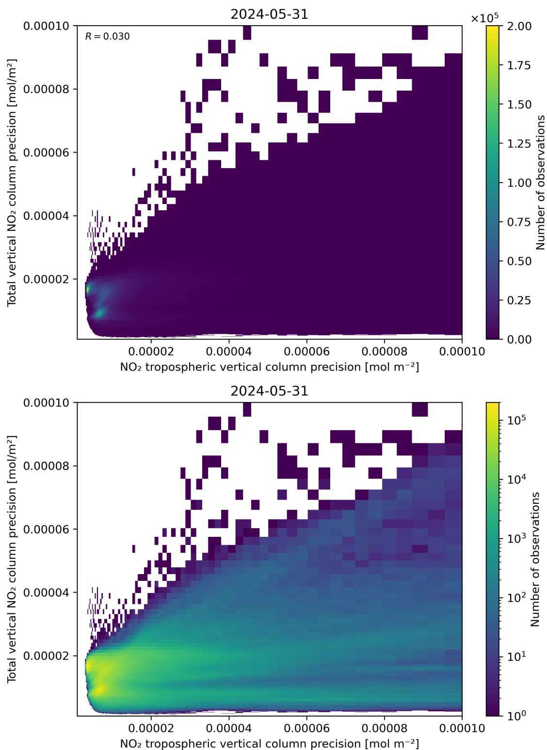
Figure 139: Scatter density plot of “NO 2 tropospheric vertical column precision” against “Total vertical NO 2 column precision” for 2024-05-30 to 2024-06-01.
