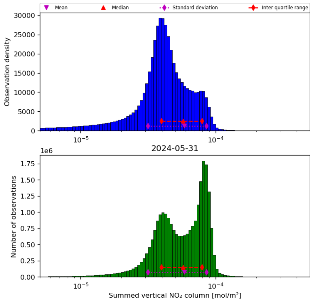
Figure 40: Histogram of “Summed vertical NO 2 column” for 2024-05-30 to 2024-06-01
