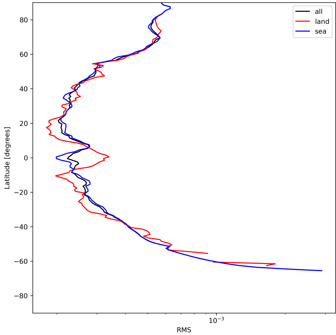
Figure 26: Zonal average of “RMS” for 2024-05-30 to 2024-06-01.
