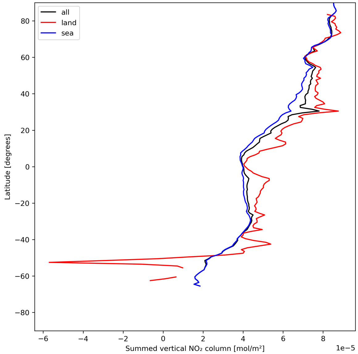
Figure 23: Zonal average of “Summed vertical NO 2 column” for 2024-05-30 to 2024-06-01.
