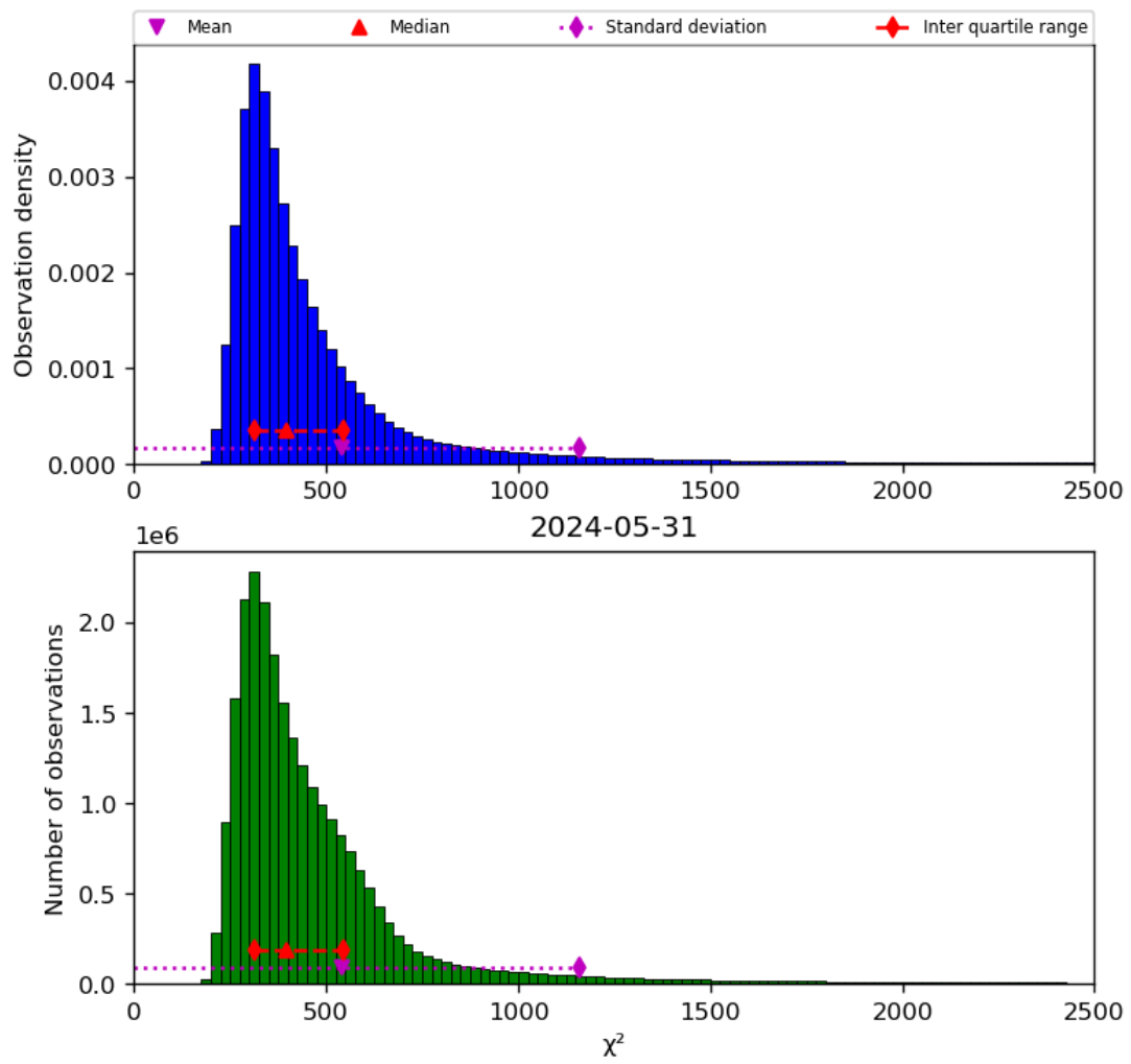
Figure 42: Histogram of “ \chi^2 ” for 2024-05-30 to 2024-06-01
