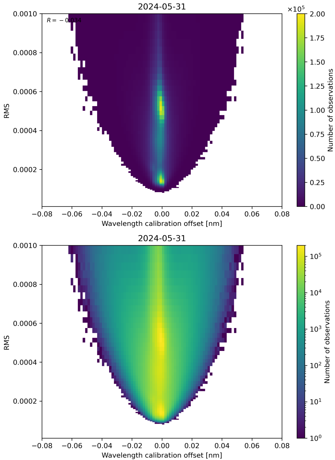
Figure 181: Scatter density plot of “Wavelength calibration offset” against “RMS” for 2024-05-30 to 2024-06-01.
