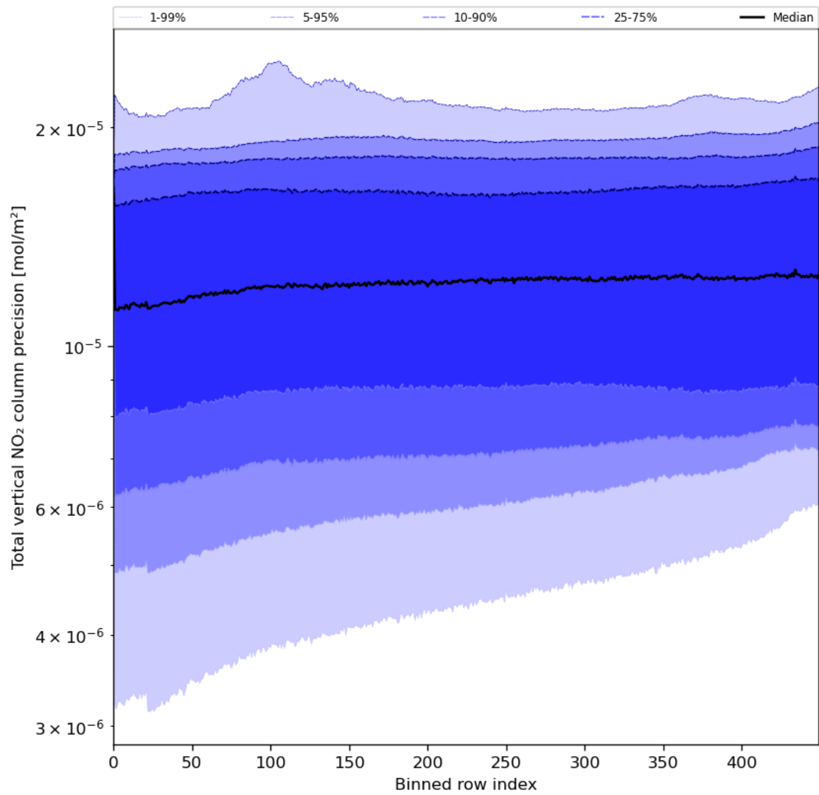
Figure 56: Along track statistics of “Total vertical NO 2 column precision” for 2024-05-30 to 2024-06-01
