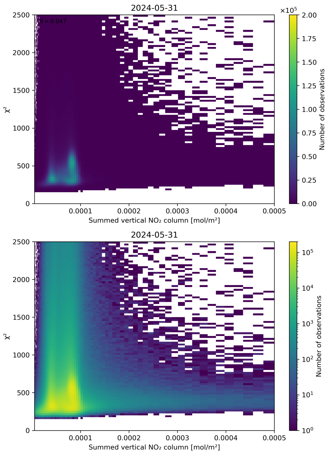
Figure 104: Scatter density plot of “Summed vertical NO 2 column” against “ \chi^2 ” for 2024-05-30 to 2024-06-01.
