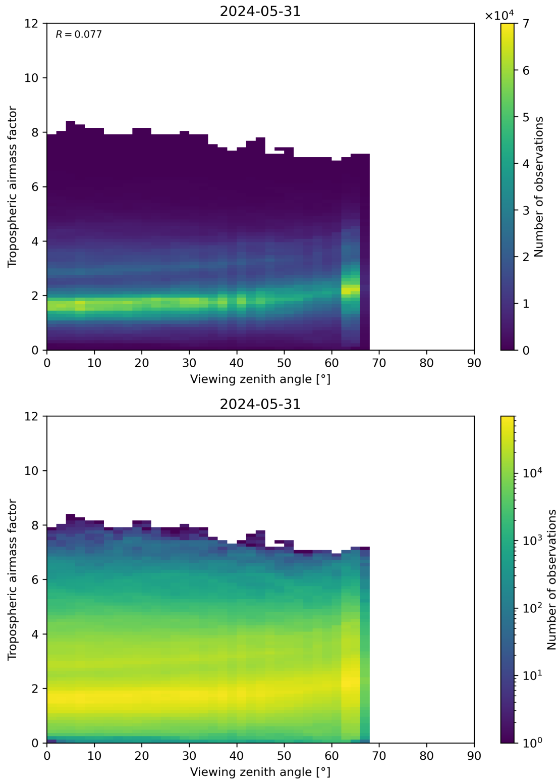
Figure 161: Scatter density plot of “Viewing zenith angle” against “Tropospheric airmass factor” for 2024-05-30 to 2024-06-01.
