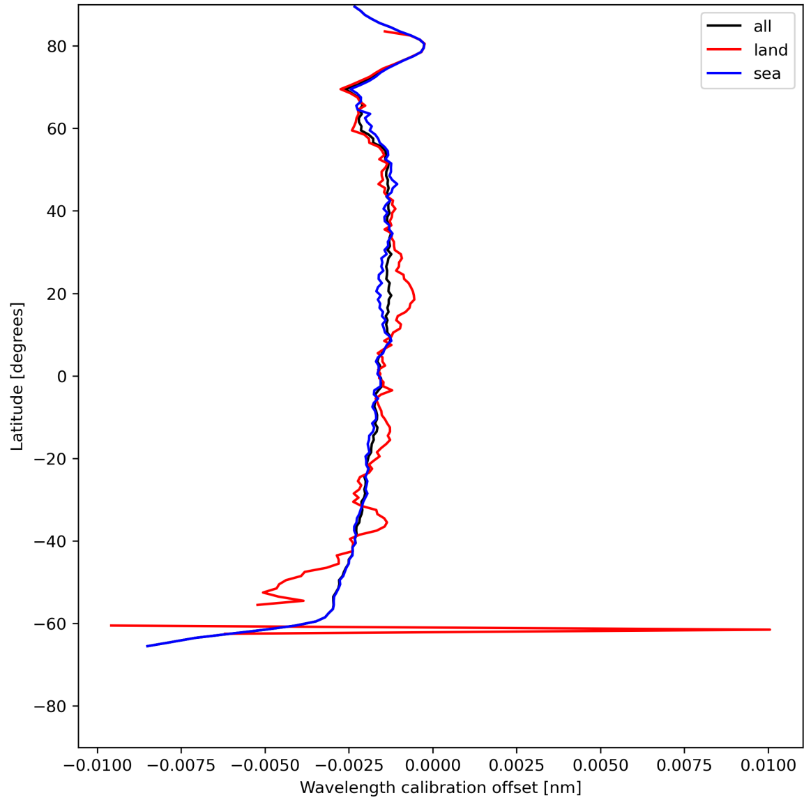
Figure 18: Zonal average of “Wavelength calibration offset” for 2024-05-30 to 2024-06-01.
