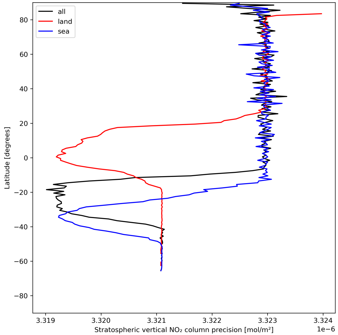
Figure 20: Zonal average of “Stratospheric vertical NO 2 column precision” for 2024-05-30 to 2024-06-01.
