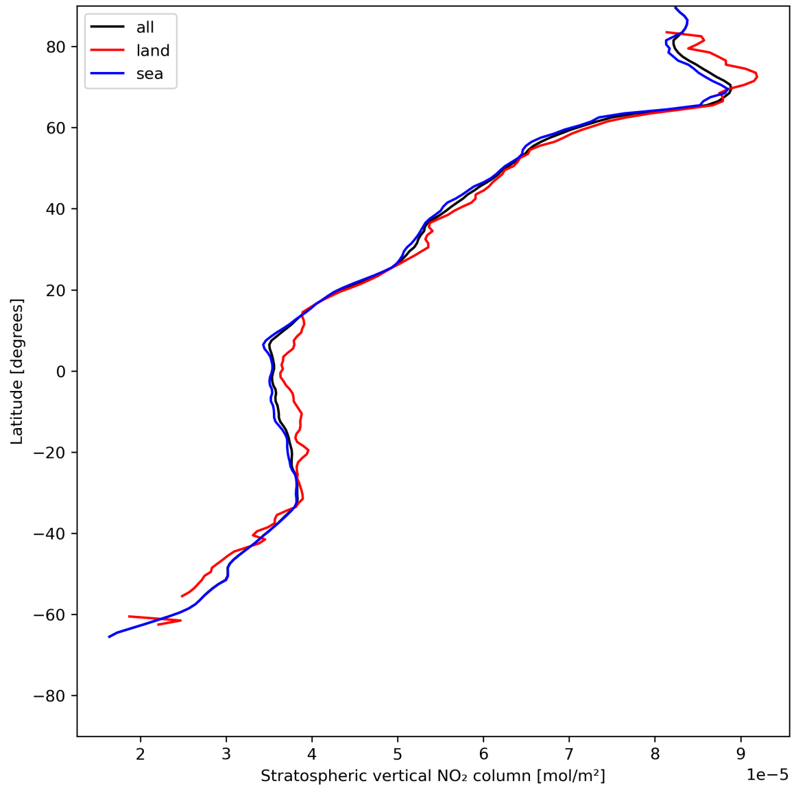
Figure 19: Zonal average of “Stratospheric vertical NO 2 column” for 2024-05-30 to 2024-06-01.
