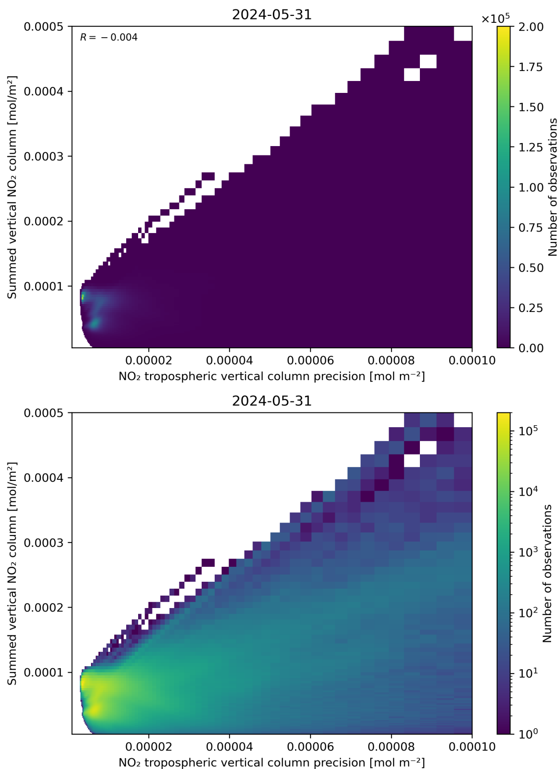
Figure 136: Scatter density plot of “NO 2 tropospheric vertical column precision” against “Summed vertical NO 2 column” for 2024-05-30 to 2024-06-01.
