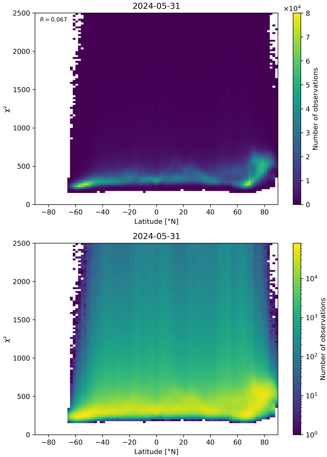
Figure 86: Scatter density plot of “Latitude” against “ \chi^2 ” for 2024-05-30 to 2024-06-01.
