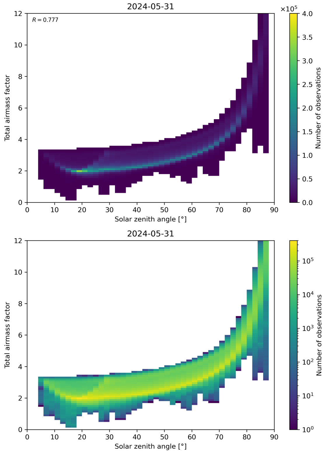
Figure 146: Scatter density plot of “Solar zenith angle” against “Total air mass factor” for 2024-05-30 to 2024-06-01.
