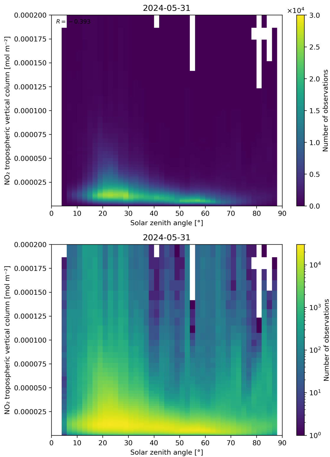
Figure 155: Scatter density plot of “Solar zenith angle” against “NO 2 tropospheric vertical column” for 2024-05-30 to 2024-06-01.
