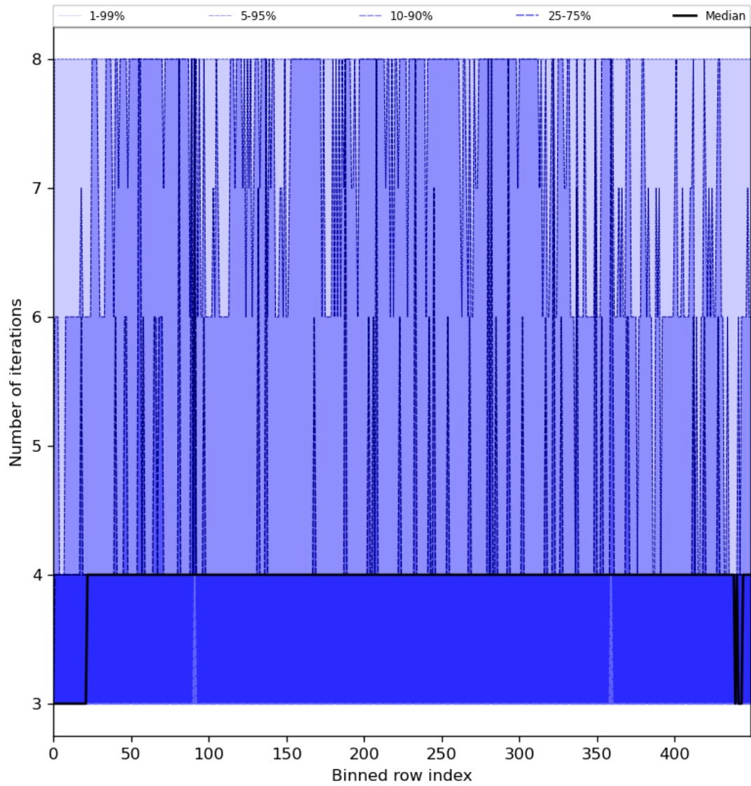
Figure 51: Along track statistics of “Number of iterations” for 2024-05-30 to 2024-06-01
