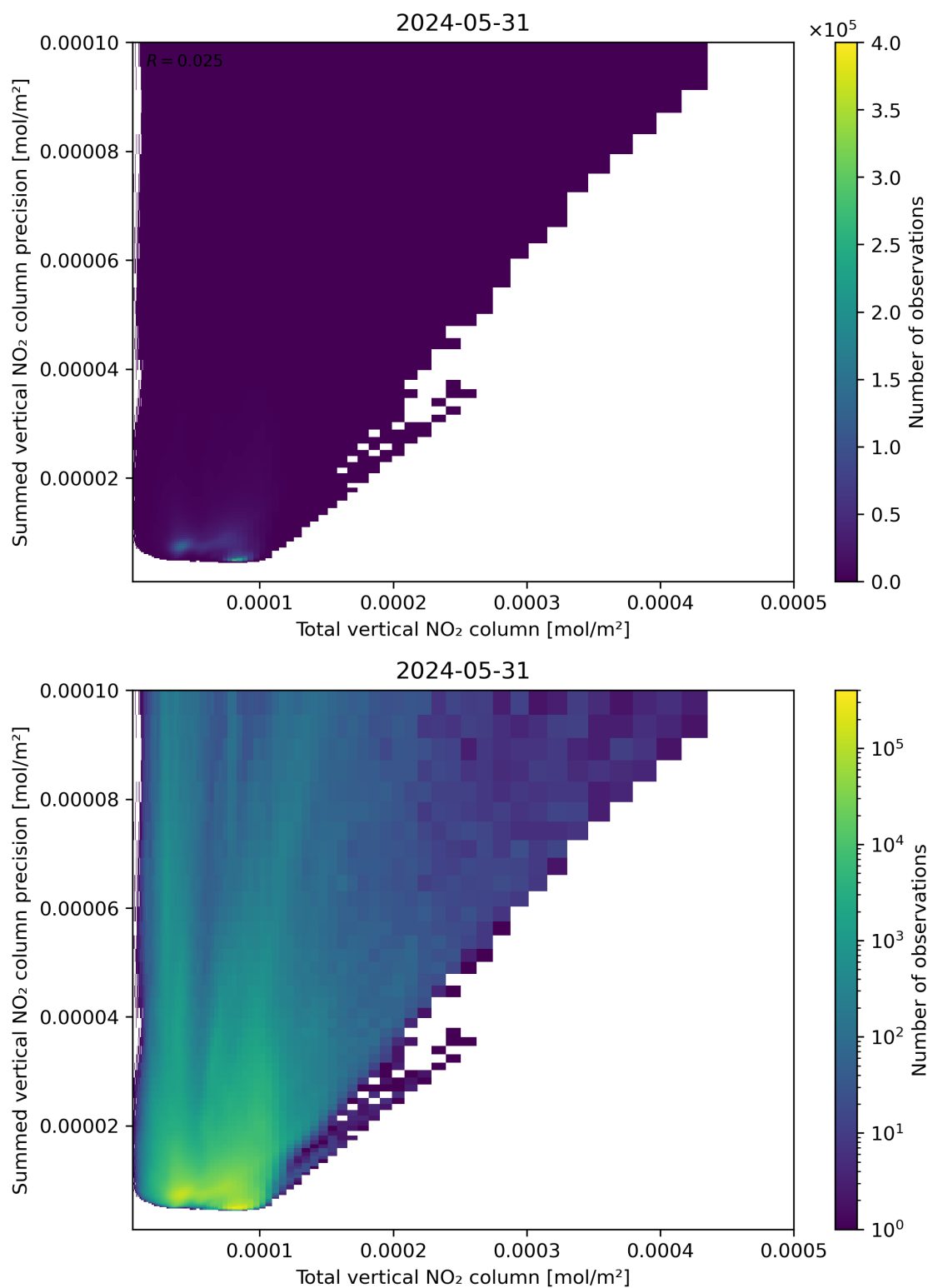
Figure 113: Scatter density plot of “Total vertical NO 2 column” against “Summed vertical NO 2 column precision” for 2024-05-30 to 2024-06-01.
