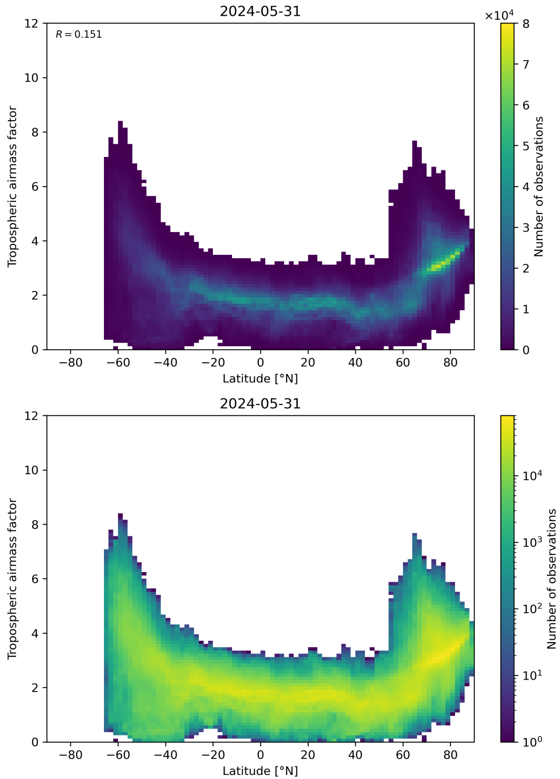
Figure 85: Scatter density plot of “Latitude” against “Tropospheric airmass factor” for 2024-05-30 to 2024-06-01.
