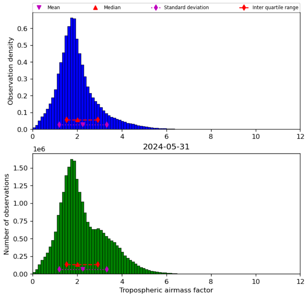
Figure 31: Histogram of “Tropospheric airmass factor” for 2024-05-30 to 2024-06-01
