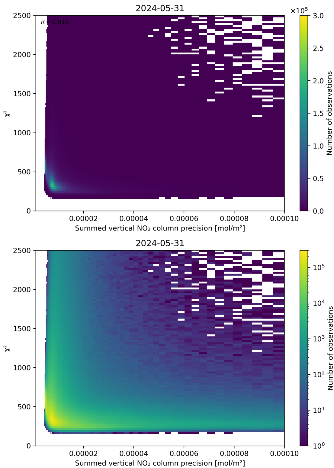
Figure 107: Scatter density plot of “Summed vertical NO 2 column precision” against “ \chi^2 ” for 2024-05-30 to 2024-06-01.
