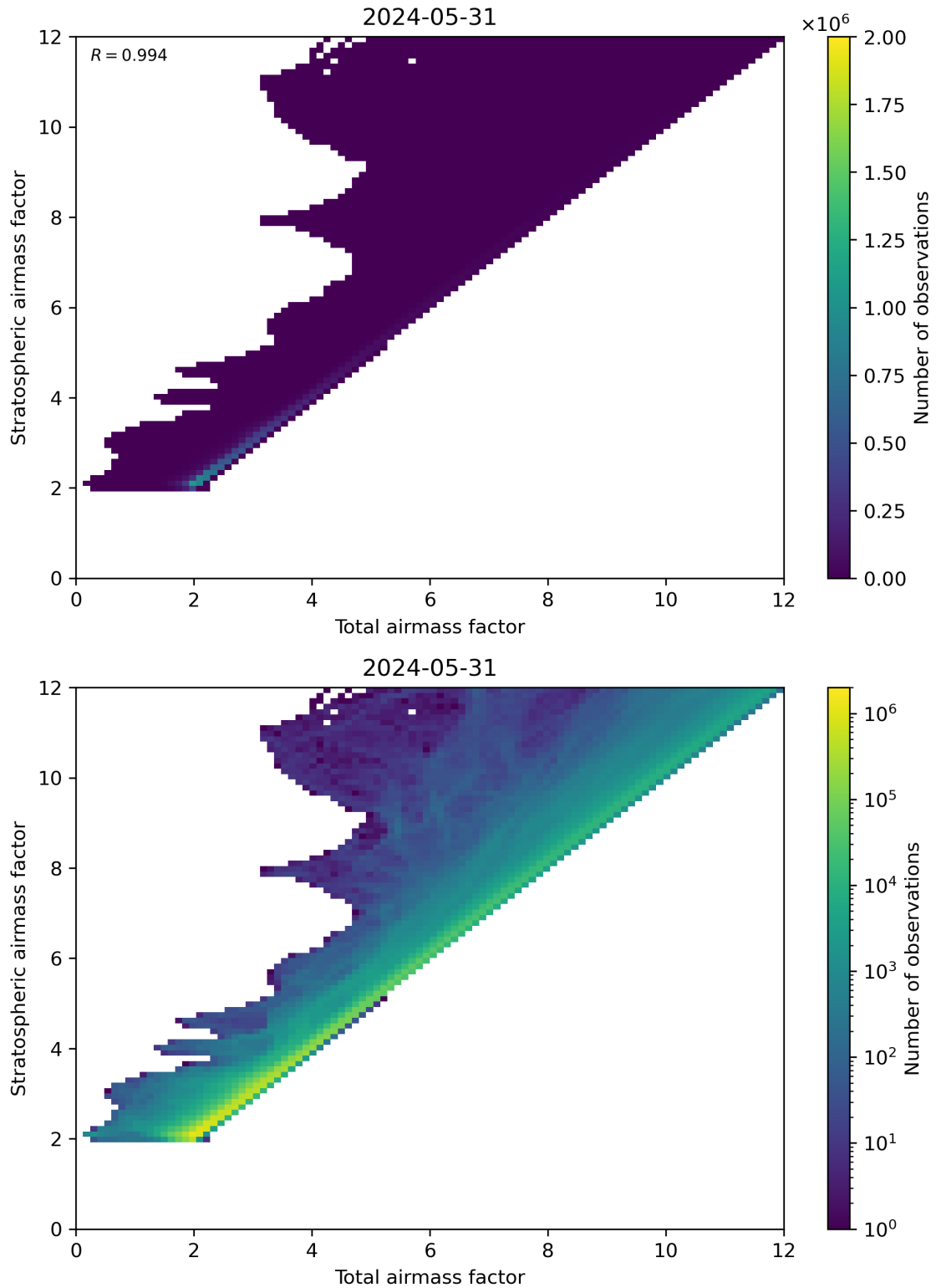
Figure 62: Scatter density plot of “Total airmass factor” against “Stratospheric airmass factor” for 2024-05-30 to 2024-06-01.
