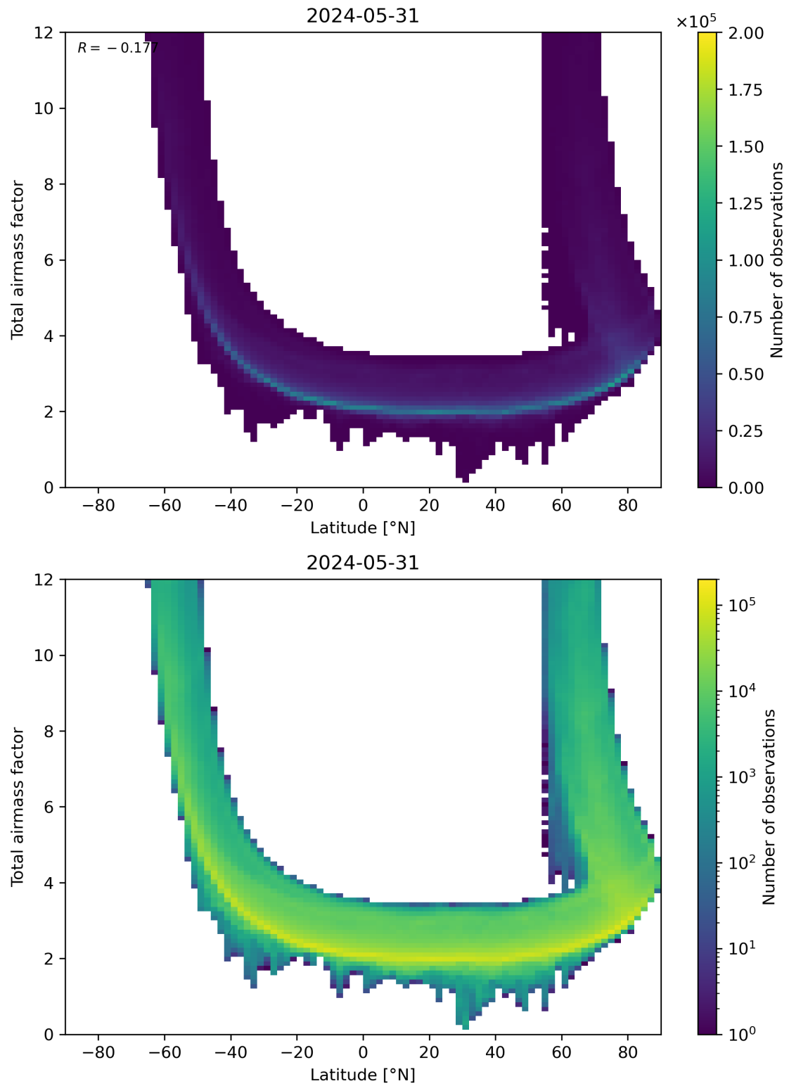
Figure 84: Scatter density plot of “Latitude” against “Total airmass factor” for 2024-05-30 to 2024-06-01.
