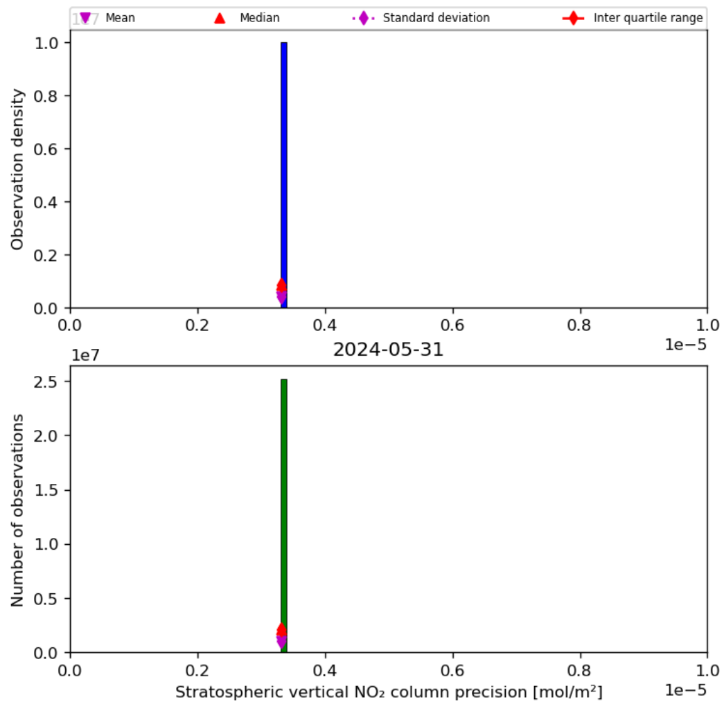
Figure 37: Histogram of “Stratospheric vertical NO 2 column precision” for 2024-05-30 to 2024-06-01
