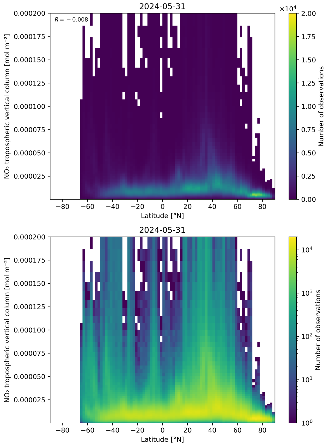
Figure 92: Scatter density plot of “Latitude” against “NO 2 tropospheric vertical column” for 2024-05-30 to 2024-06-01.
