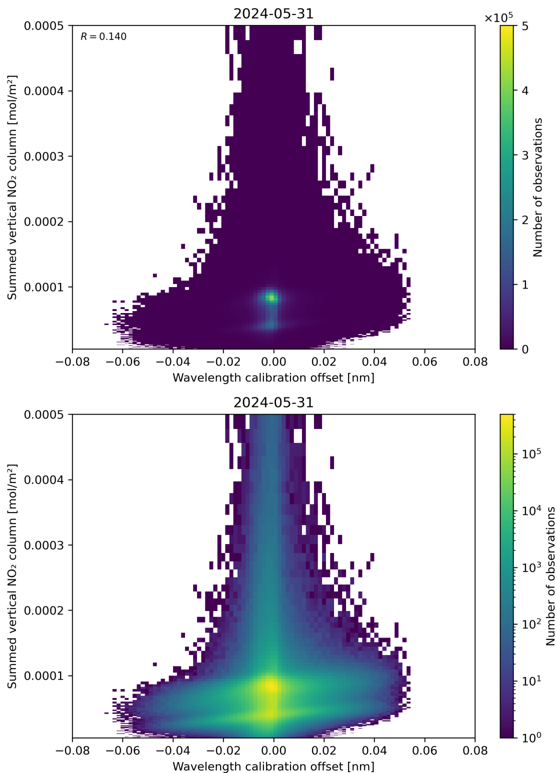
Figure 177: Scatter density plot of “Wavelength calibration offset” against “Summed vertical NO 2 column” for 2024-05-30 to 2024-06-01.
