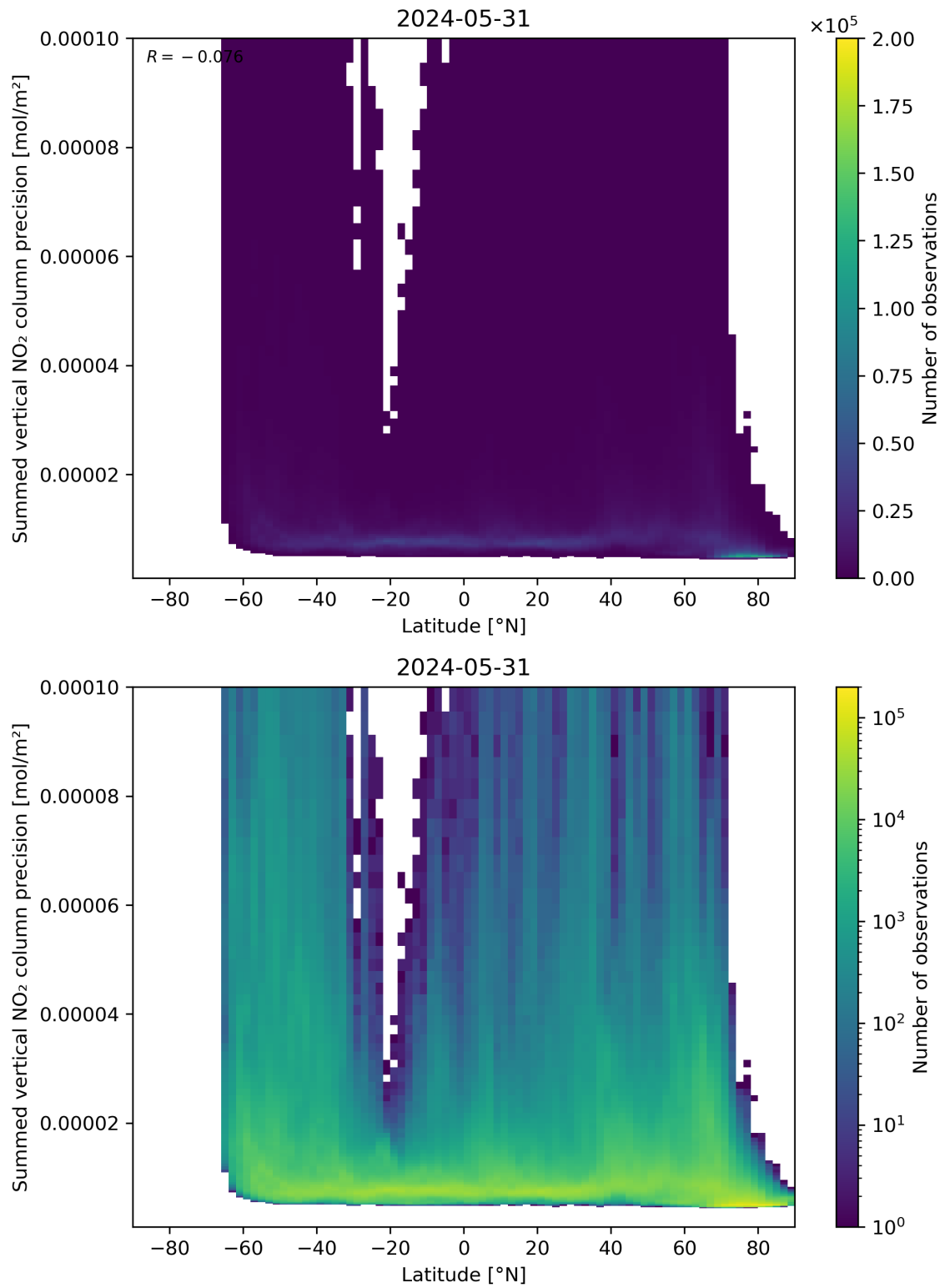
Figure 89: Scatter density plot of “Latitude” against “Summed vertical NO 2 column precision” for 2024-05-30 to 2024-06-01.
