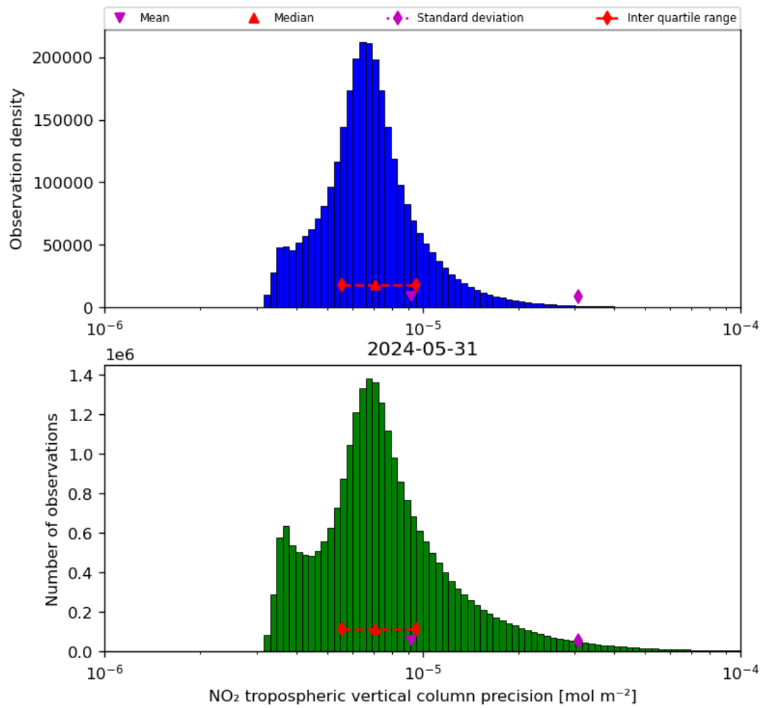
Figure 30: Histogram of “NO 2 tropospheric vertical column precision” for 2024-05-30 to 2024-06-01
