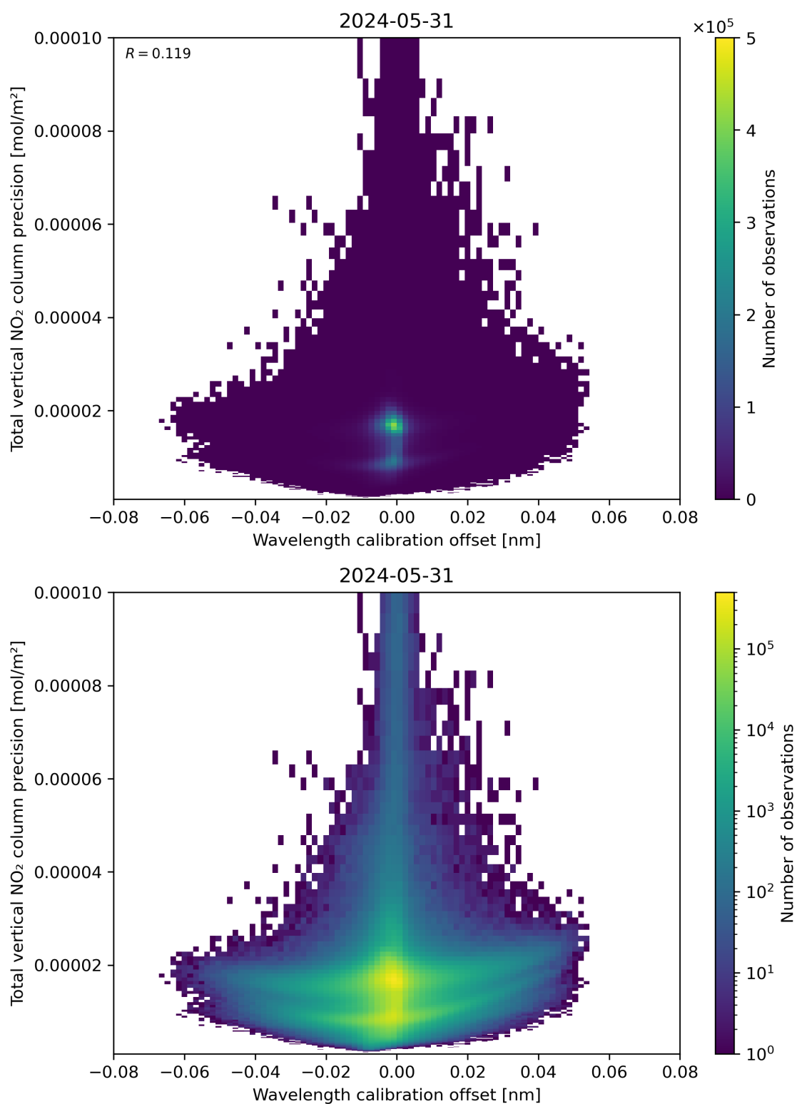
Figure 180: Scatter density plot of “Wavelength calibration offset” against “Total vertical NO 2 column precision” for 2024-05-30 to 2024-06-01.
