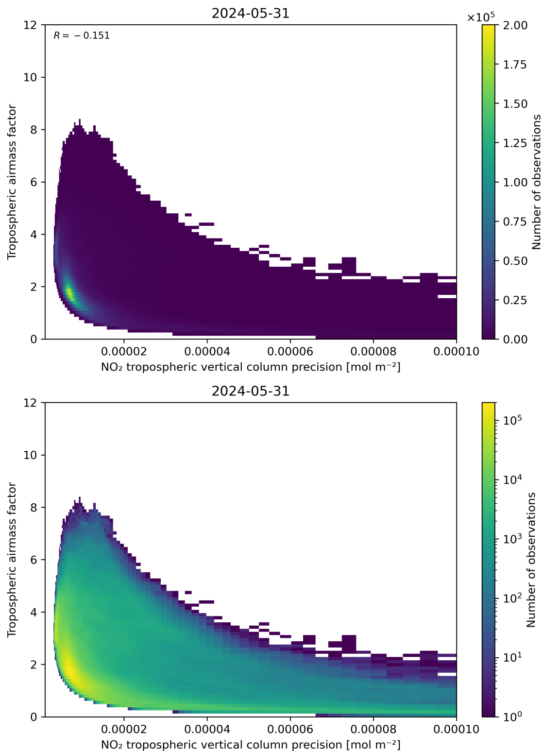
Figure 133: Scatter density plot of “NO 2 tropospheric vertical column precision” against “Tropospheric airmass factor” for 2024-05-30 to 2024-06-01.
