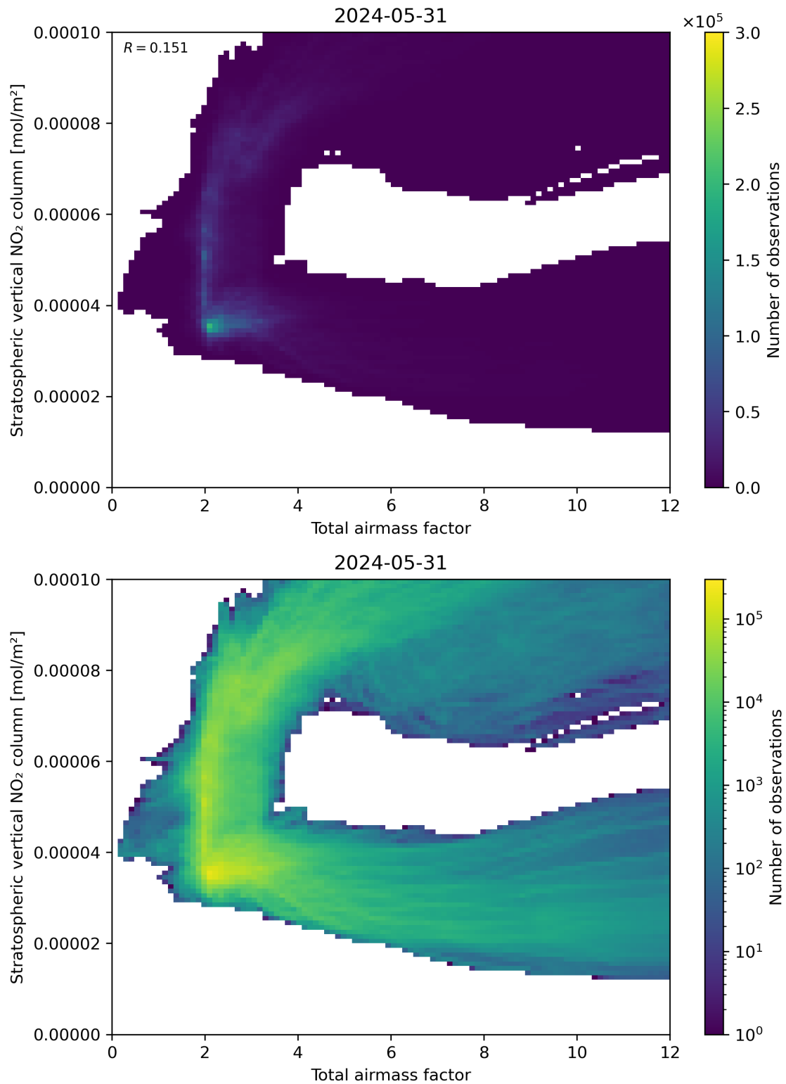
Figure 64: Scatter density plot of “Total airmass factor” against “Stratospheric vertical NO 2 column” for 2024-05-30 to 2024-06-01.
