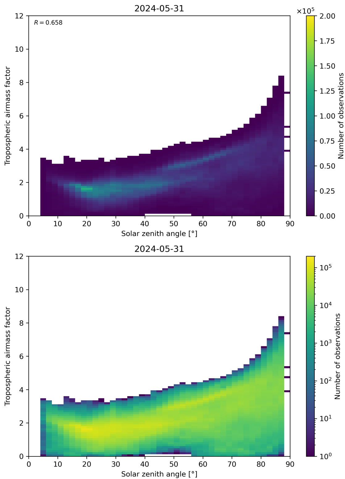
Figure 147: Scatter density plot of “Solar zenith angle” against “Tropospheric airmass factor” for 2024-05-30 to 2024-06-01.
