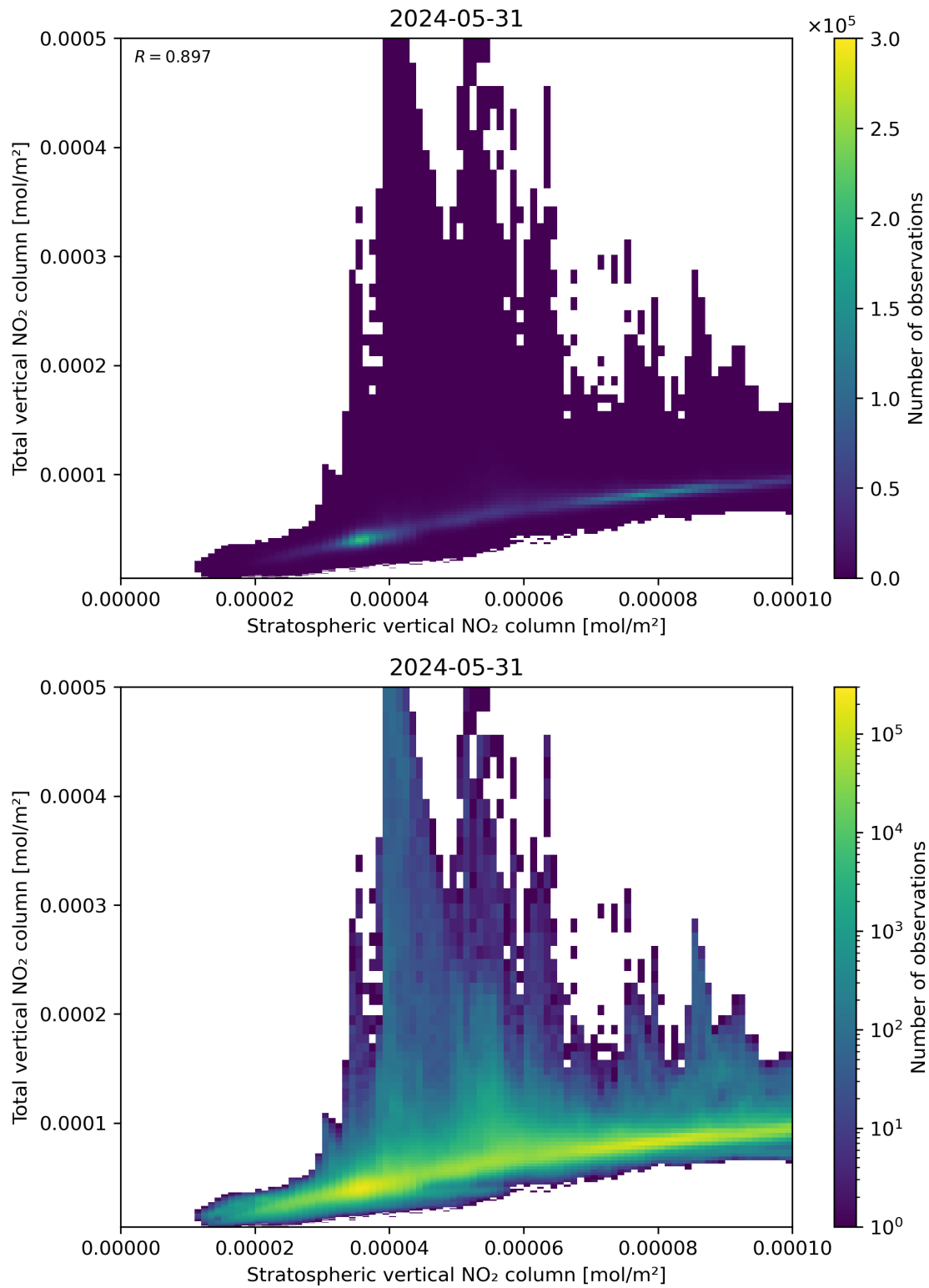
Figure 100: Scatter density plot of “Stratospheric vertical NO 2 column” against “Total vertical NO 2 column” for 2024-05-30 to 2024-06-01.
