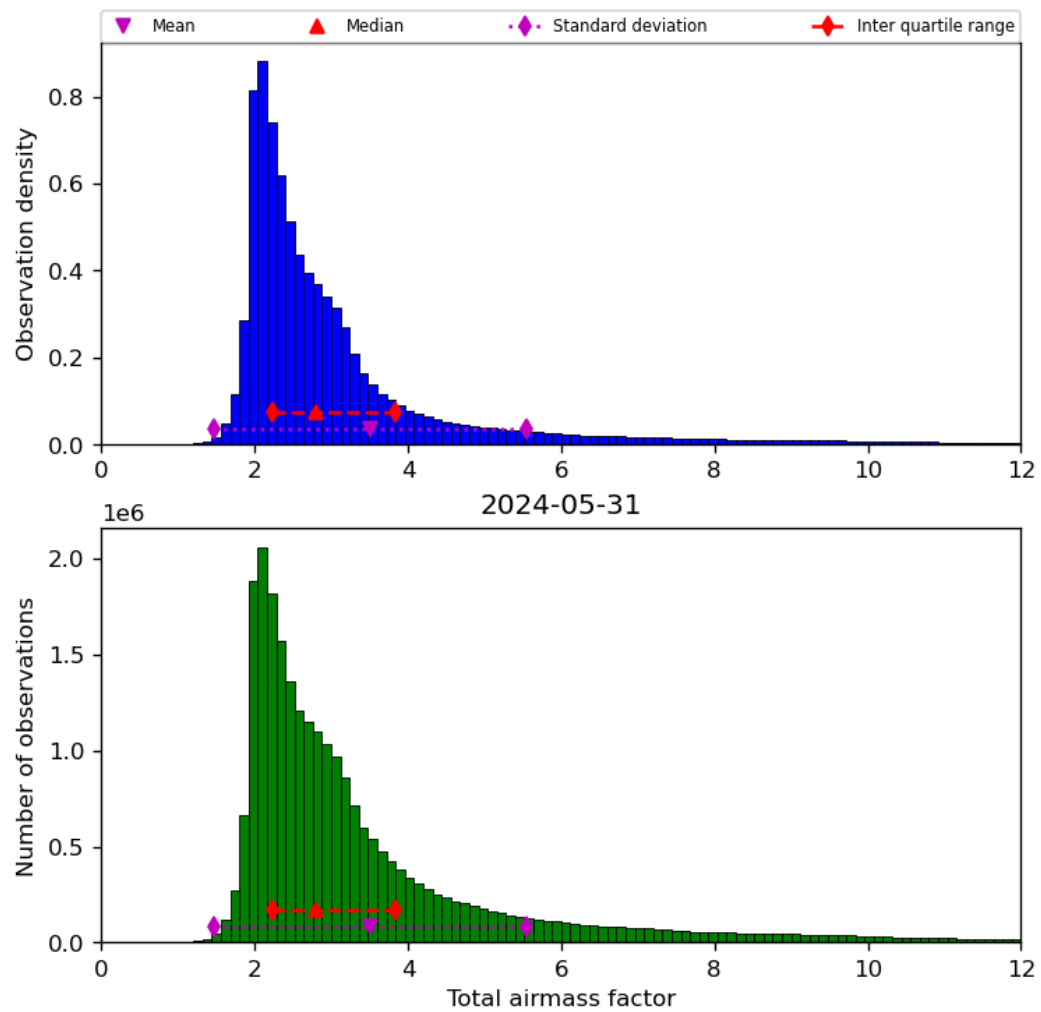
Figure 32: Histogram of “Total airmass factor” for 2024-05-30 to 2024-06-01
