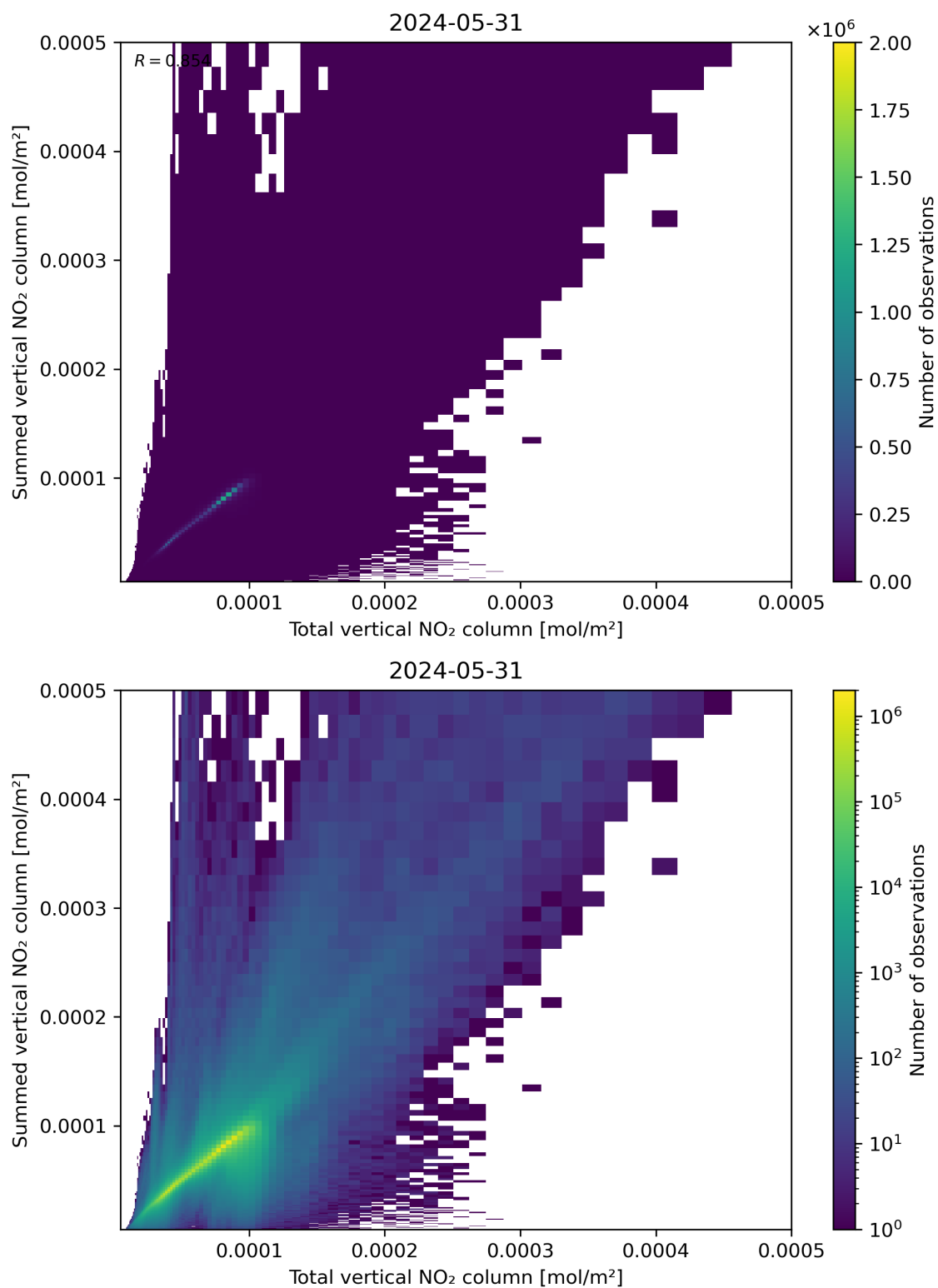
Figure 112: Scatter density plot of “Total vertical NO 2 column” against “Summed vertical NO 2 column” for 2024-05-30 to 2024-06-01.
