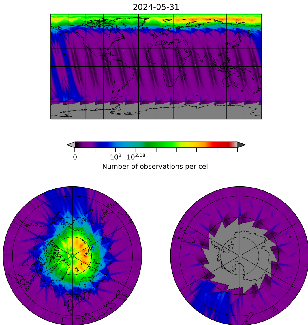
Figure 10: Map of the number of observations for 2024-05-30 to 2024-06-01
