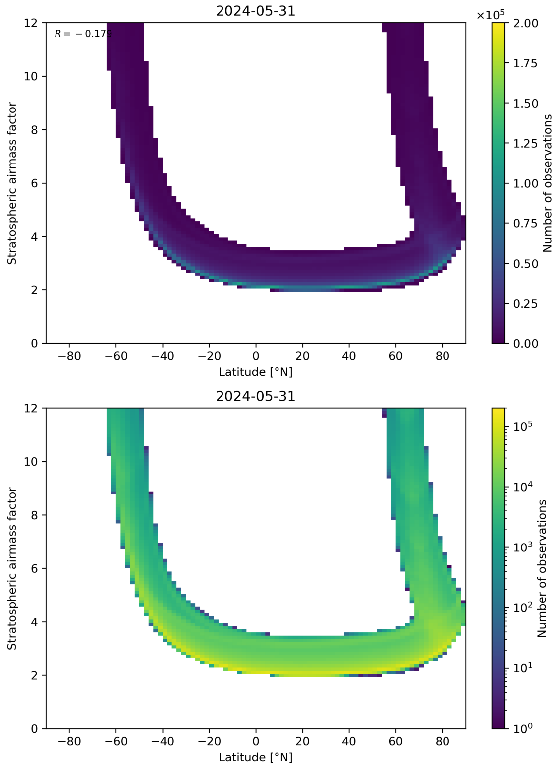
Figure 83: Scatter density plot of “Latitude” against “Stratospheric air mass factor” for 2024-05-30 to 2024-06-01.
