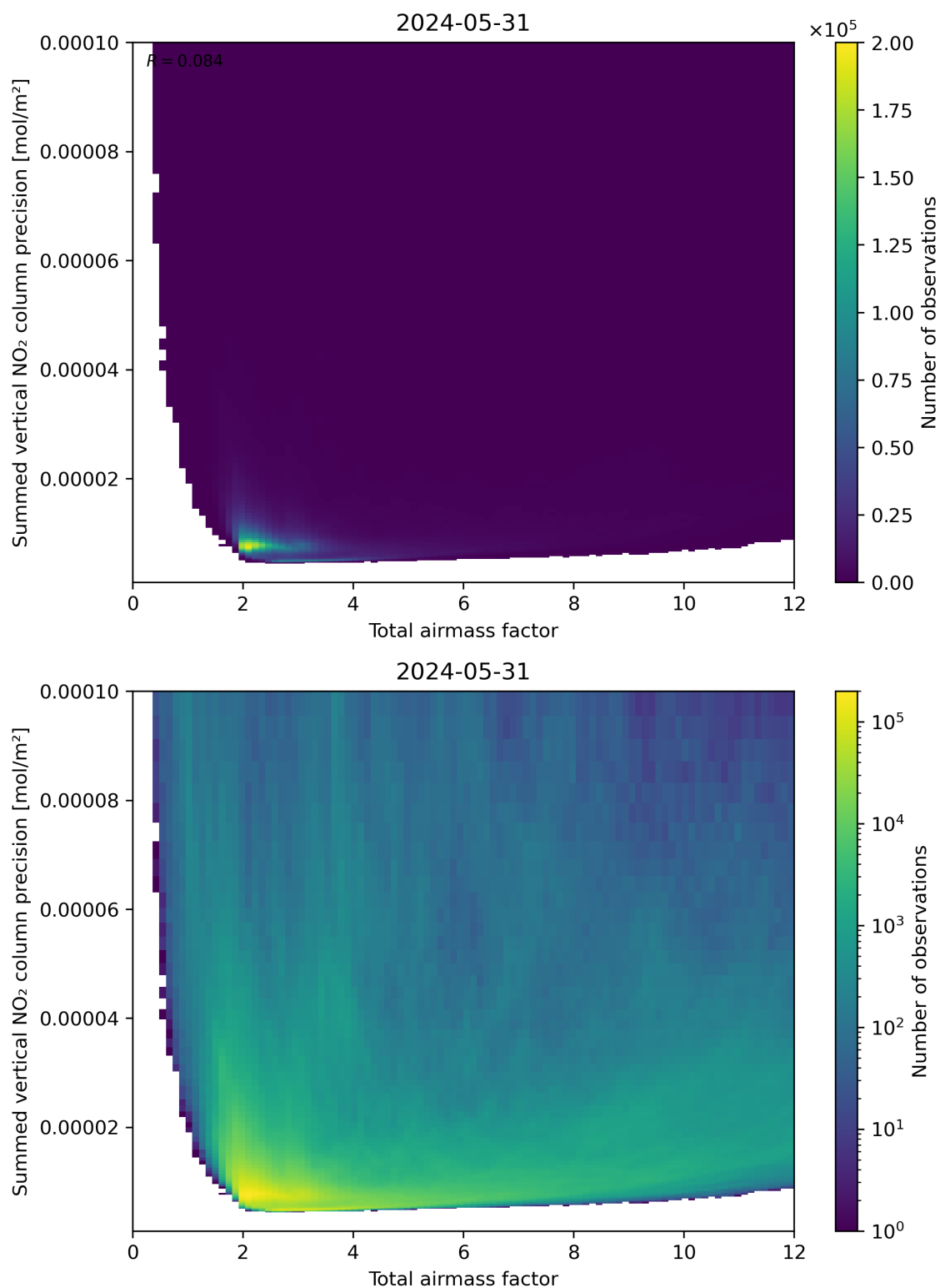
Figure 66: Scatter density plot of “Total airmass factor” against “Summed vertical NO 2 column precision” for 2024-05-30 to 2024-06-01.
