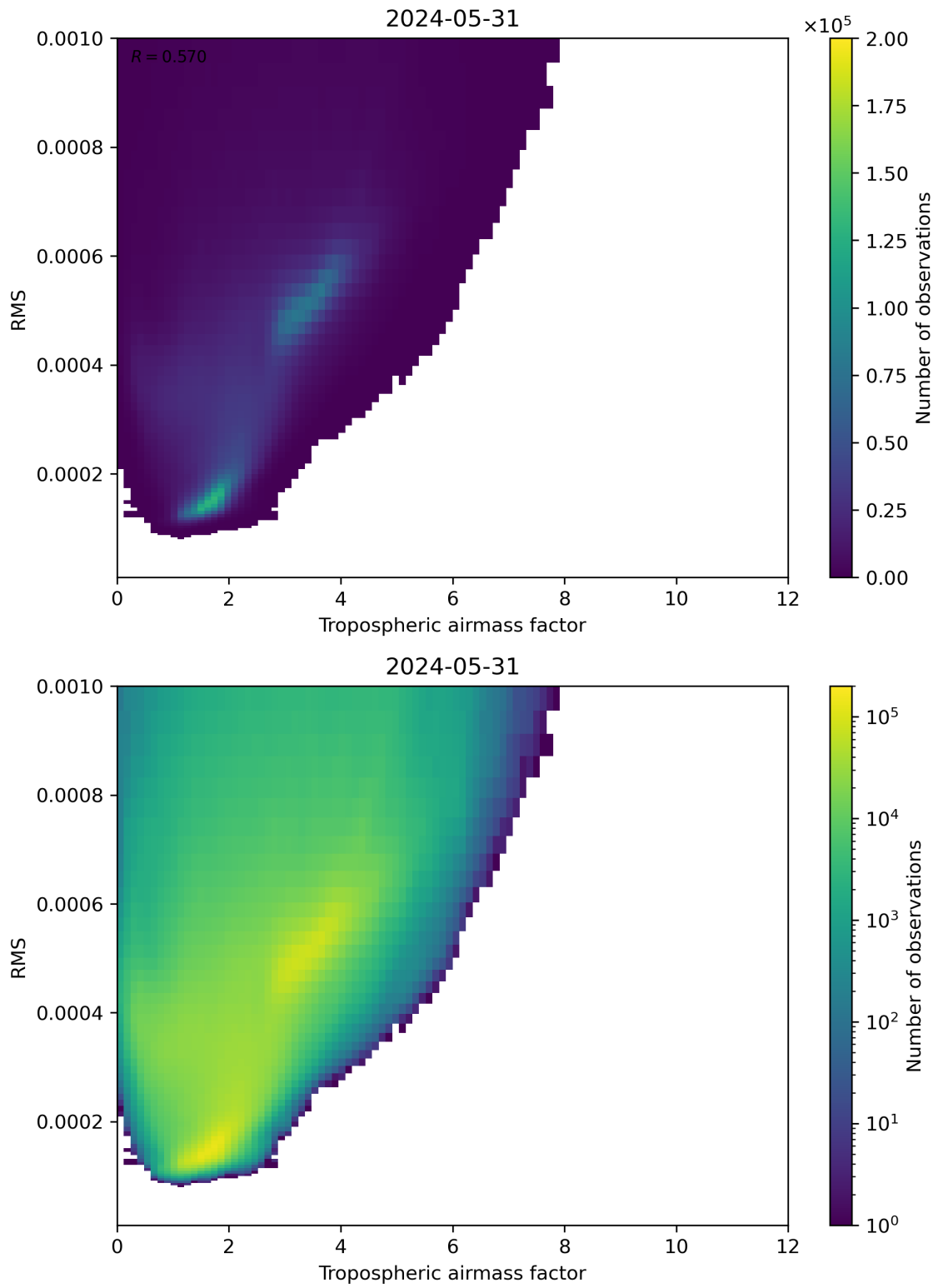
Figure 79: Scatter density plot of “Tropospheric airmass factor” against “RMS” for 2024-05-30 to 2024-06-01.
