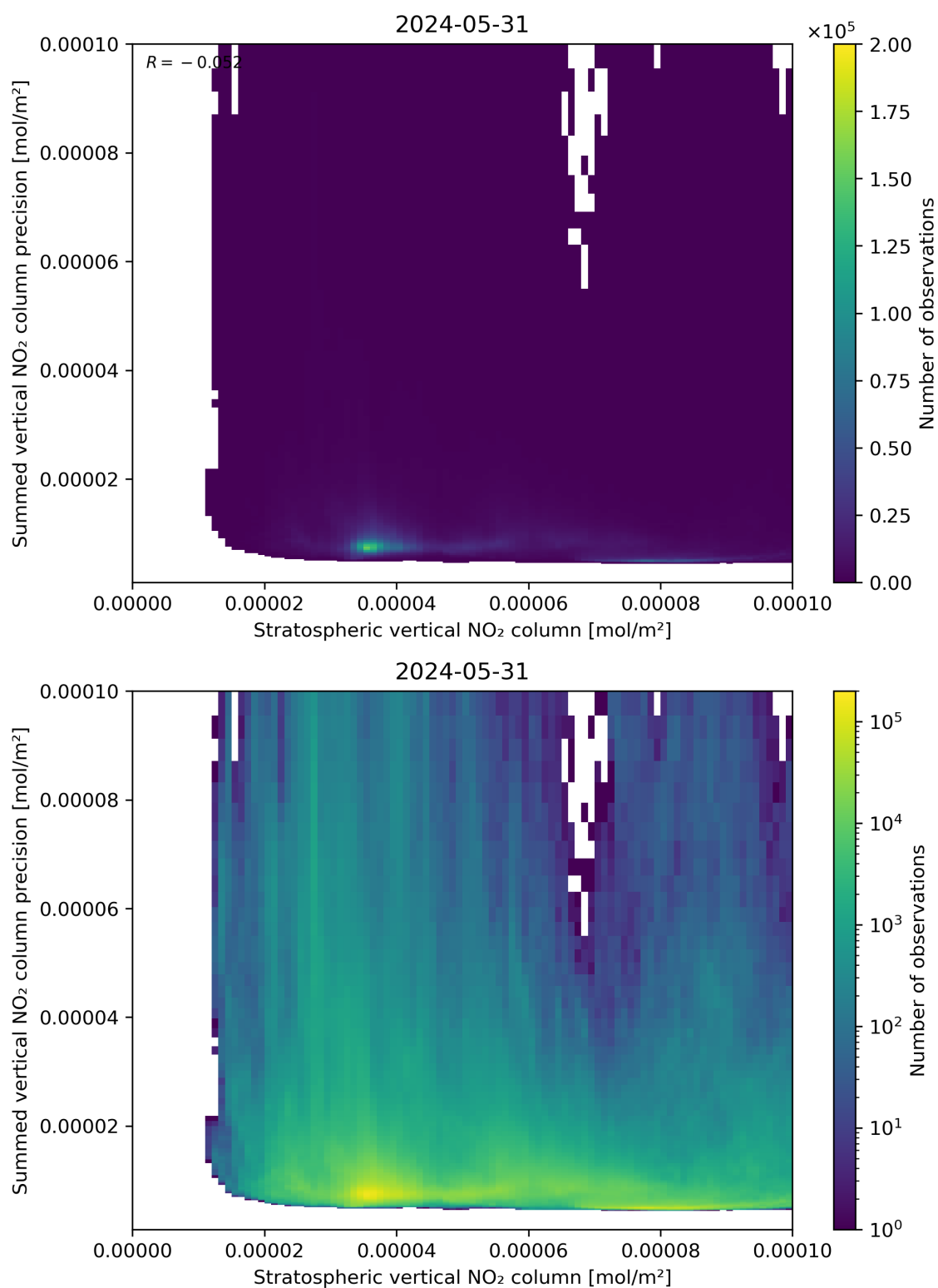
Figure 99: Scatter density plot of “Stratospheric vertical NO 2 column” against “Summed vertical NO 2 column precision” for 2024-05-30 to 2024-06-01.
