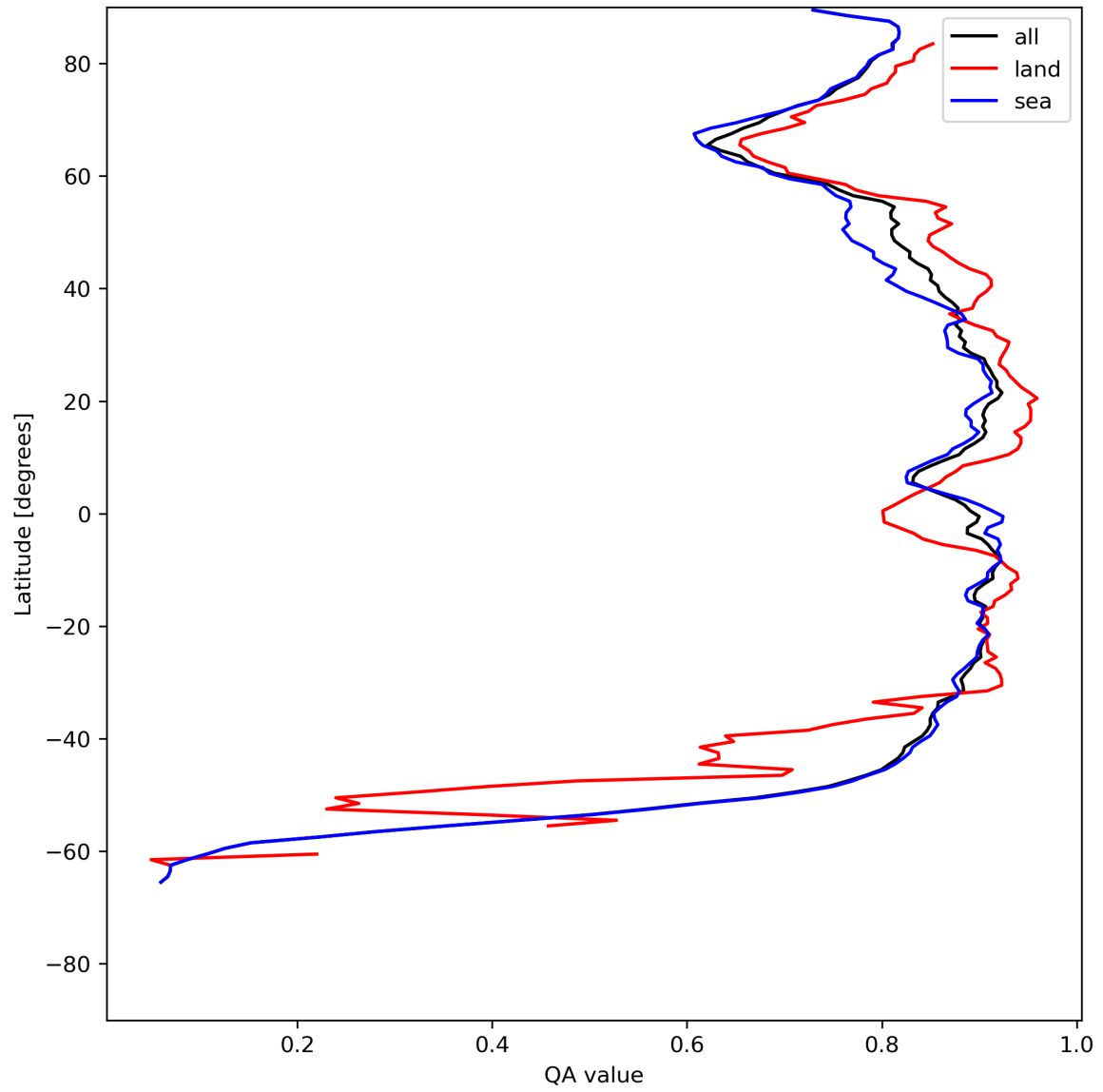
Figure 11: Zonal average of “QA value” for 2024-05-30 to 2024-06-01.
