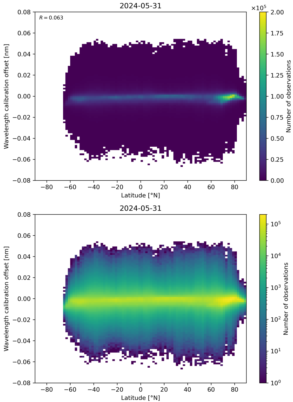
Figure 95: Scatter density plot of “Latitude” against “Wavelength calibration offset” for 2024-05-30 to 2024-06-01.
