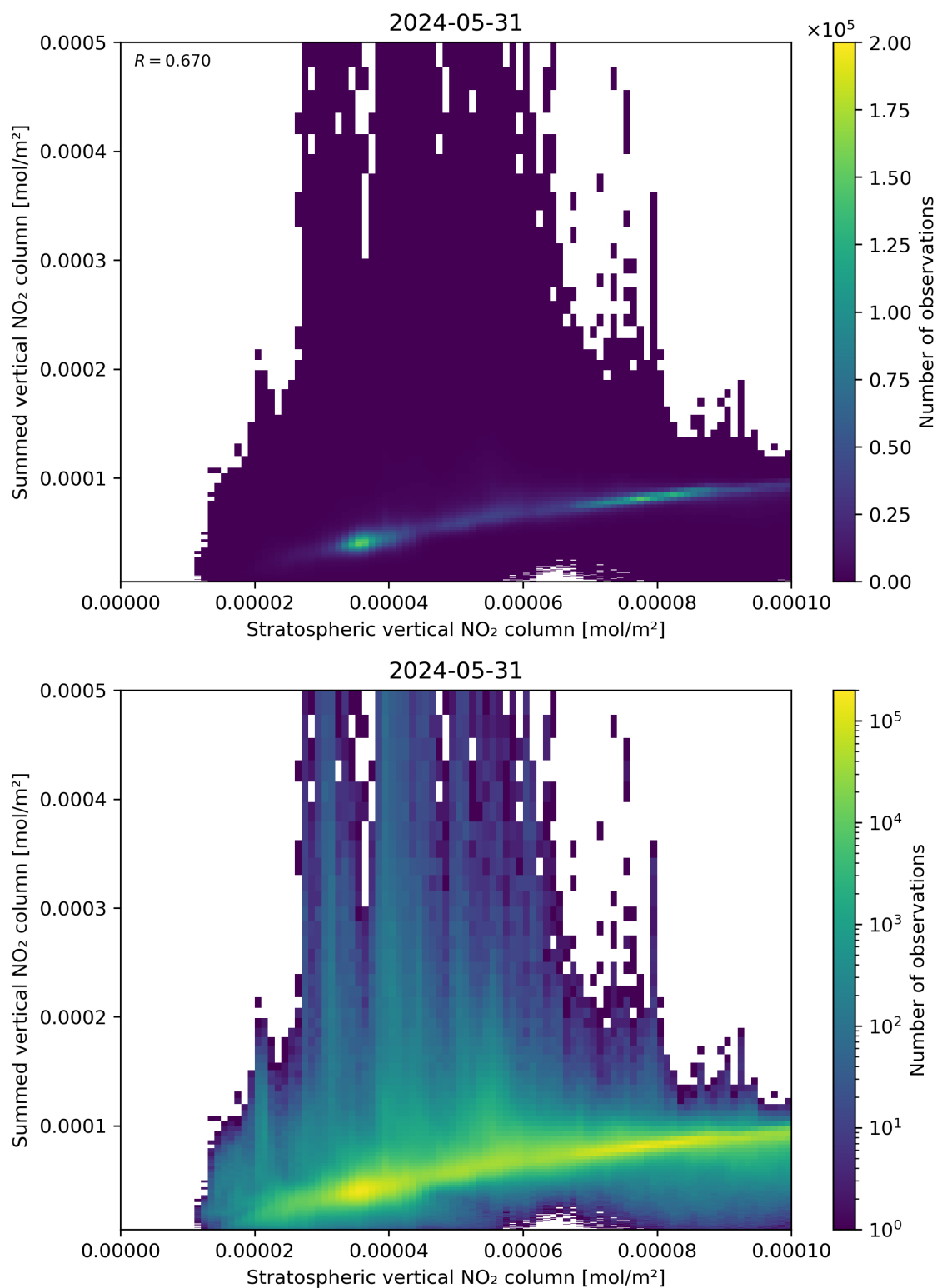
Figure 98: Scatter density plot of “Stratospheric vertical NO 2 column” against “Summed vertical NO 2 column” for 2024-05-30 to 2024-06-01.
