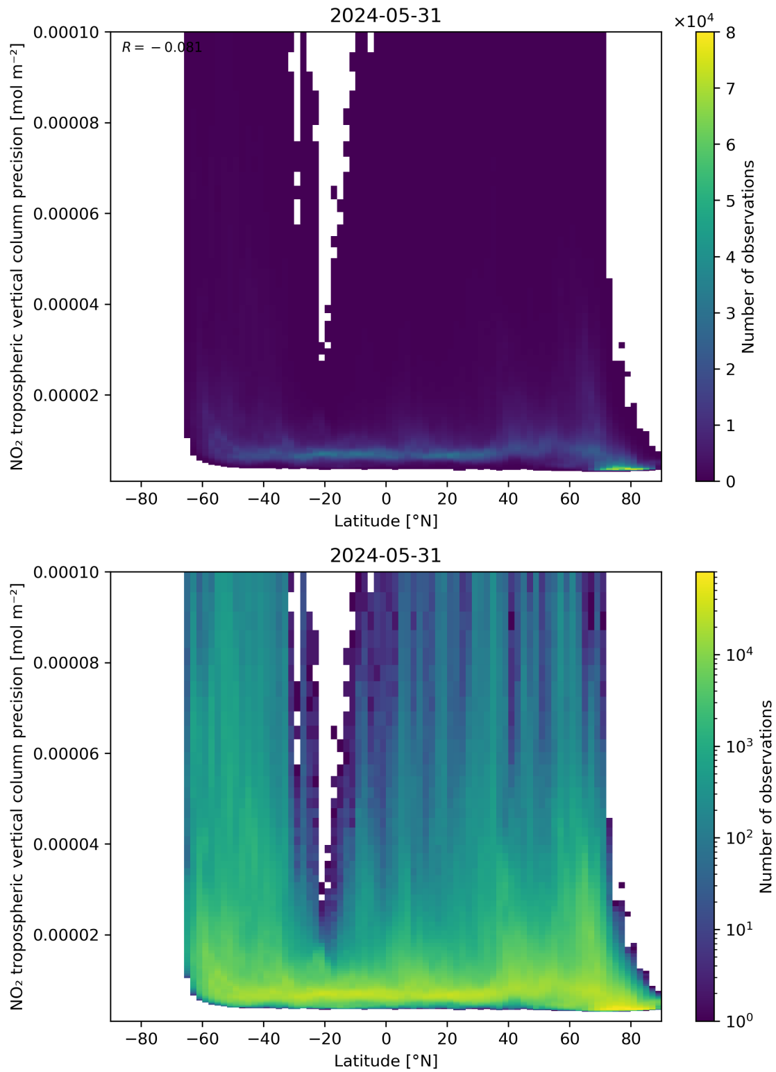
Figure 93: Scatter density plot of “Latitude” against “NO 2 tropospheric vertical column precision” for 2024-05-30 to 2024-06-01.
