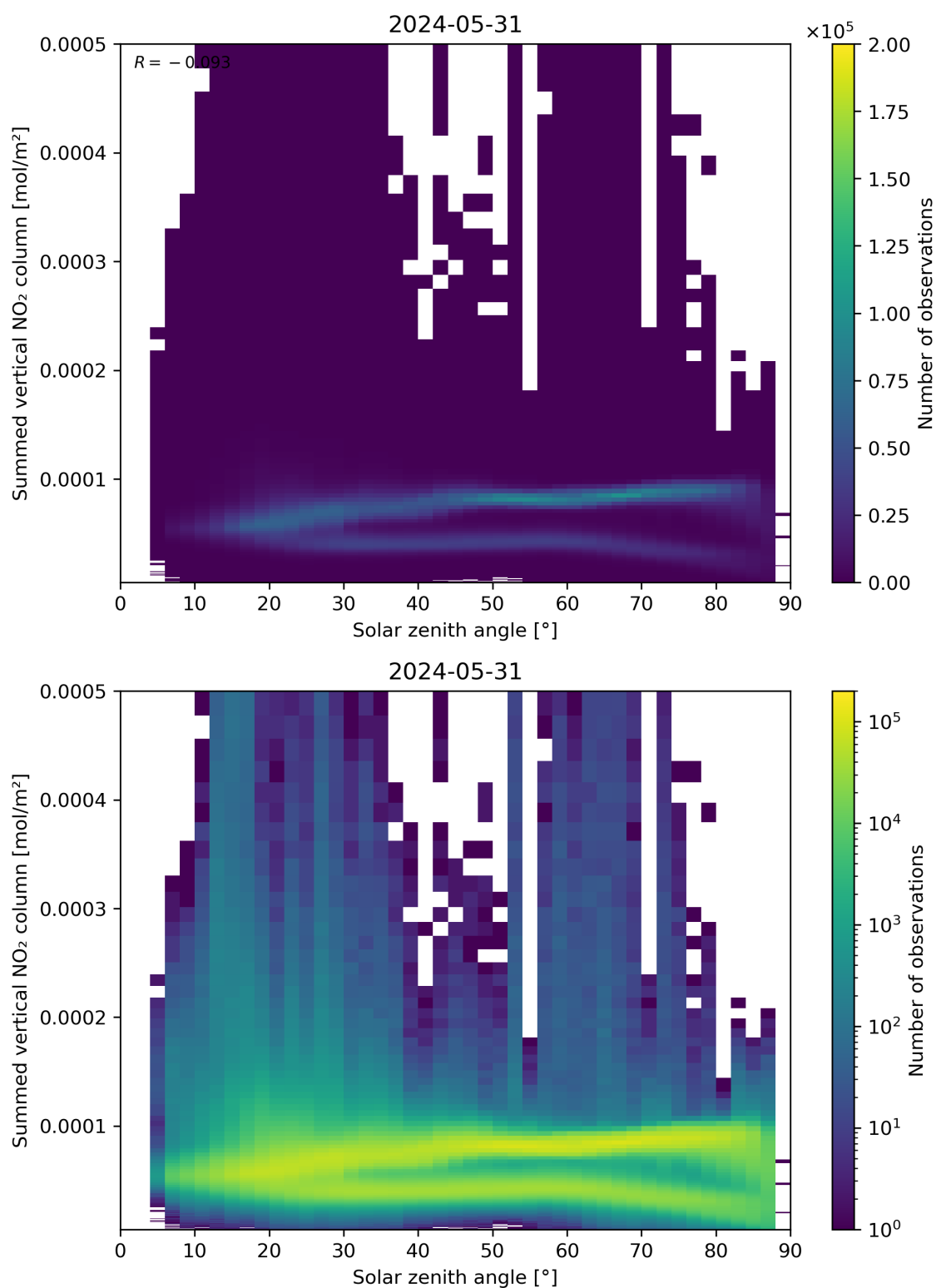
Figure 151: Scatter density plot of “Solar zenith angle” against “Summed vertical NO 2 column” for 2024-05-30 to 2024-06-01.
