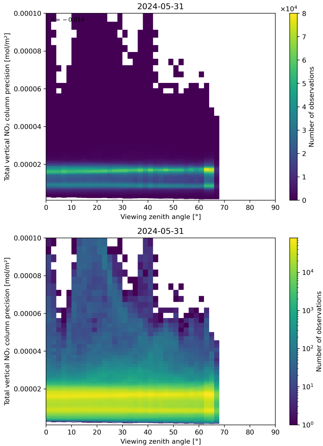
Figure 168: Scatter density plot of “Viewing zenith angle” against “Total vertical NO 2 column precision” for 2024-05-30 to 2024-06-01.
