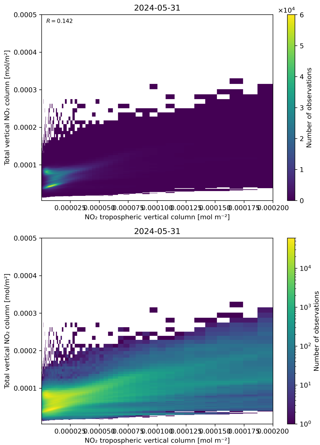
Figure 128: Scatter density plot of “NO 2 tropospheric vertical column” against “Total vertical NO 2 column” for 2024-05-30 to 2024-06-01.
