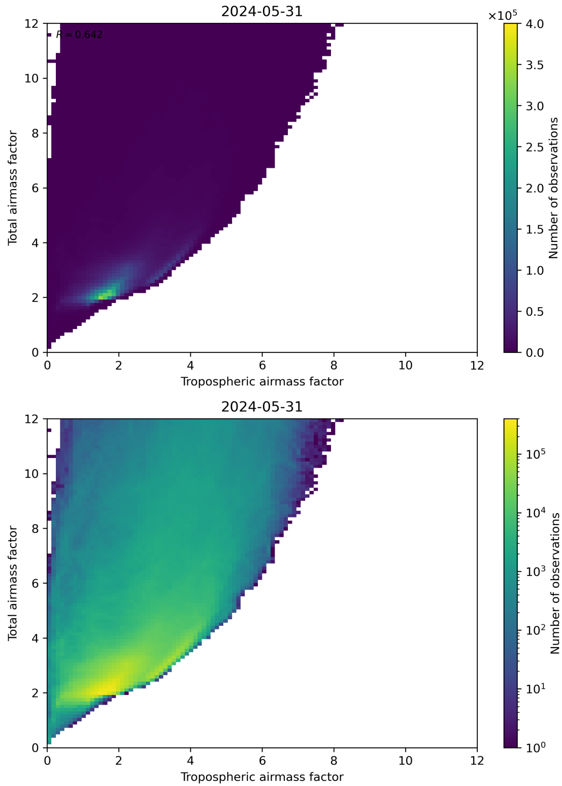
Figure 72: Scatter density plot of “Tropospheric airmass factor” against “Total airmass factor” for 2024-05-30 to 2024-06-01.
