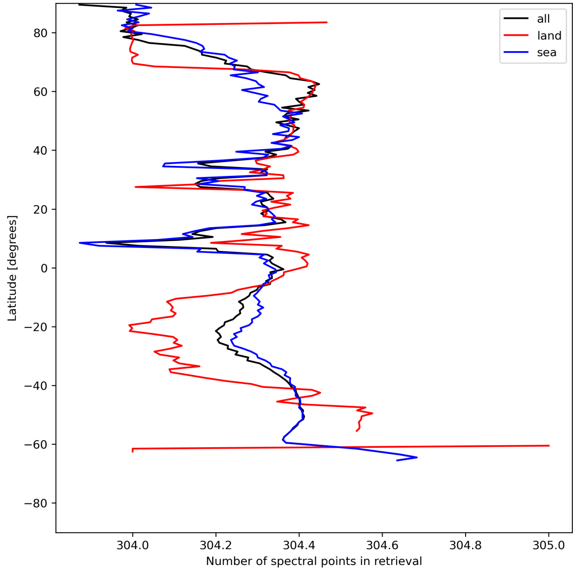
Figure 16: Zonal average of “Number of spectral points in retrieval” for 2024-05-30 to 2024-06-01.
