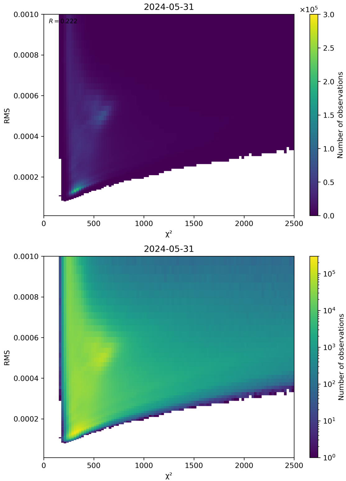
Figure 82: Scatter density plot of “ \chi^2 ” against “RMS” for 2024-05-30 to 2024-06-01.
