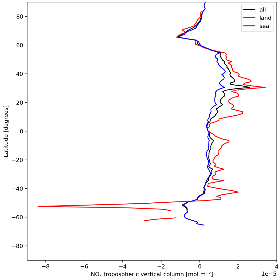
Figure 12: Zonal average of “NO 2 tropospheric vertical column” for 2024-05-30 to 2024-06-01.
