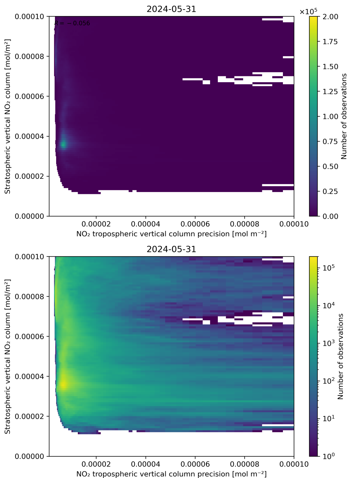
Figure 135: Scatter density plot of “NO 2 tropospheric vertical column precision” against “Stratospheric vertical NO 2 column” for 2024-05-30 to 2024-06-01.
