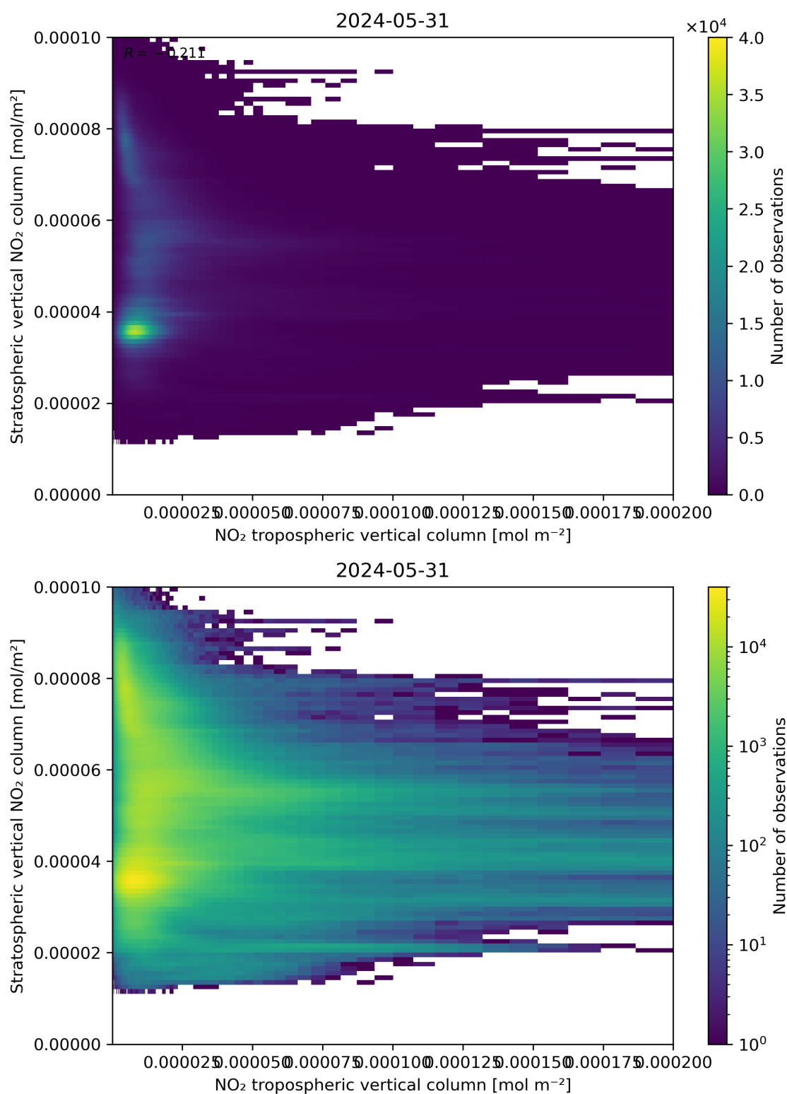
Figure 125: Scatter density plot of “NO 2 tropospheric vertical column” against “Stratospheric vertical NO 2 column” for 2024-05-30 to 2024-06-01.
