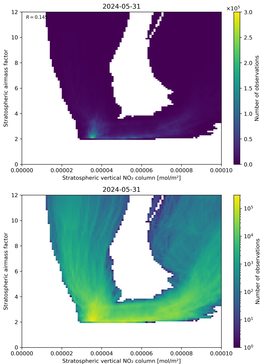
Figure 96: Scatter density plot of “Stratospheric vertical NO 2 column” against “Stratospheric airmass factor” for 2024-05-30 to 2024-06-01.
