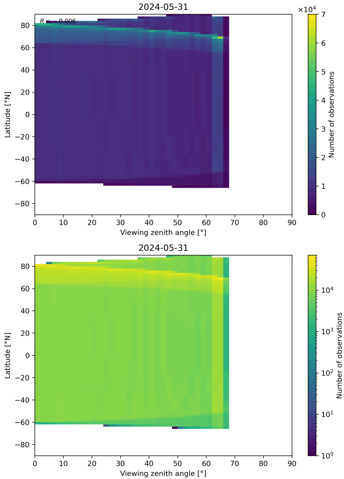
Figure 163: Scatter density plot of “Viewing zenith angle” against “Latitude” for 2024-05-30 to 2024-06-01.
