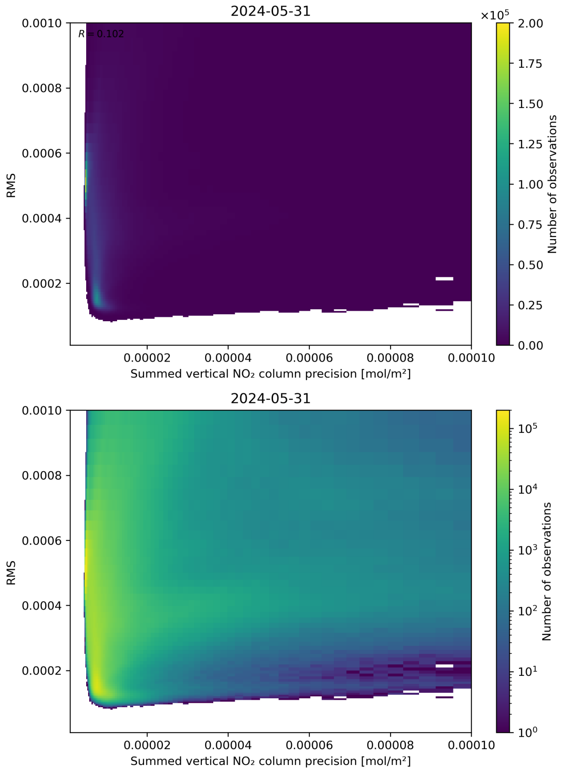
Figure 108: Scatter density plot of “Summed vertical NO 2 column precision” against “RMS” for 2024-05-30 to 2024-06-01.
