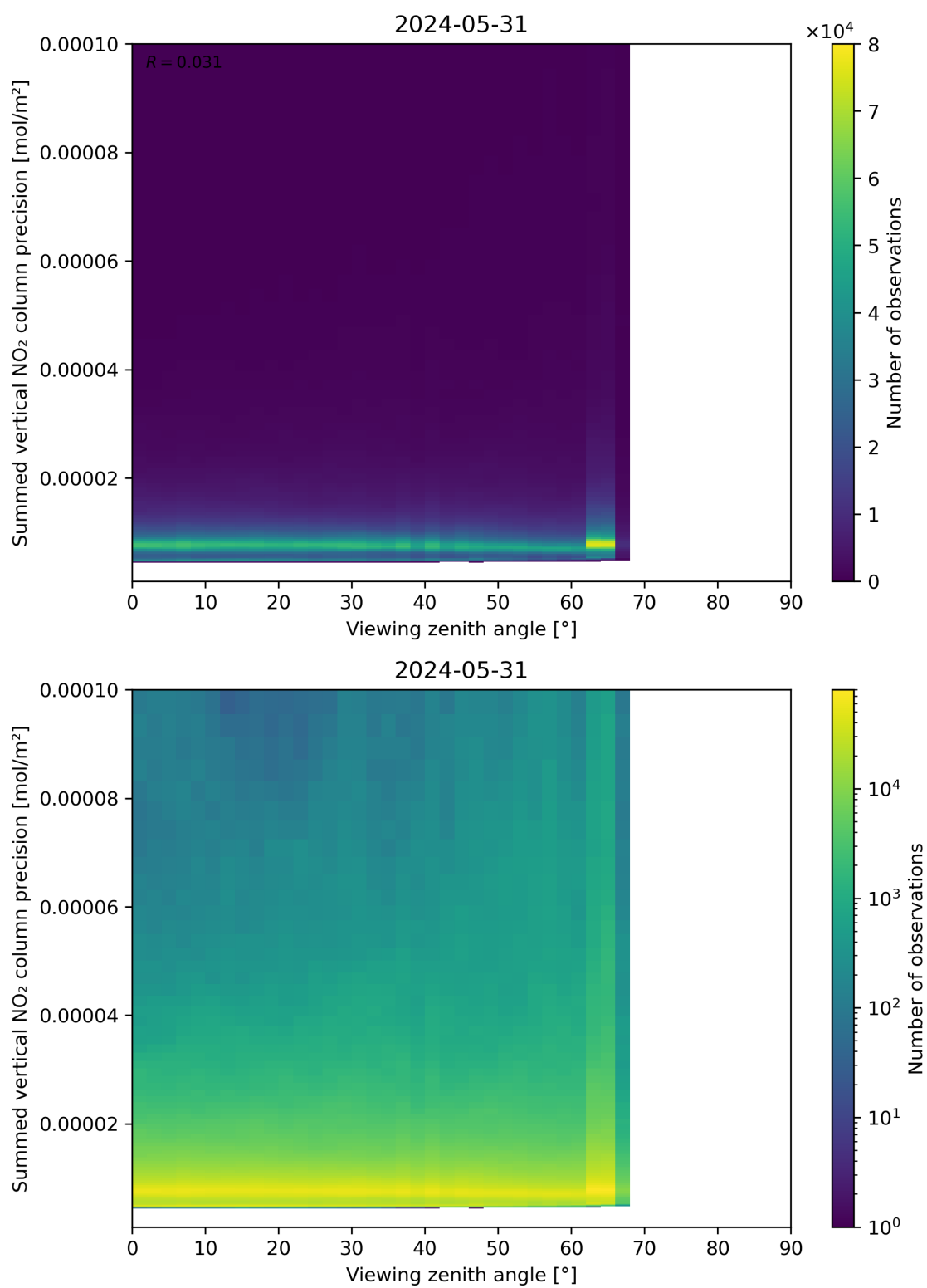
Figure 166: Scatter density plot of “Viewing zenith angle” against “Summed vertical NO 2 column precision” for 2024-05-30 to 2024-06-01.
