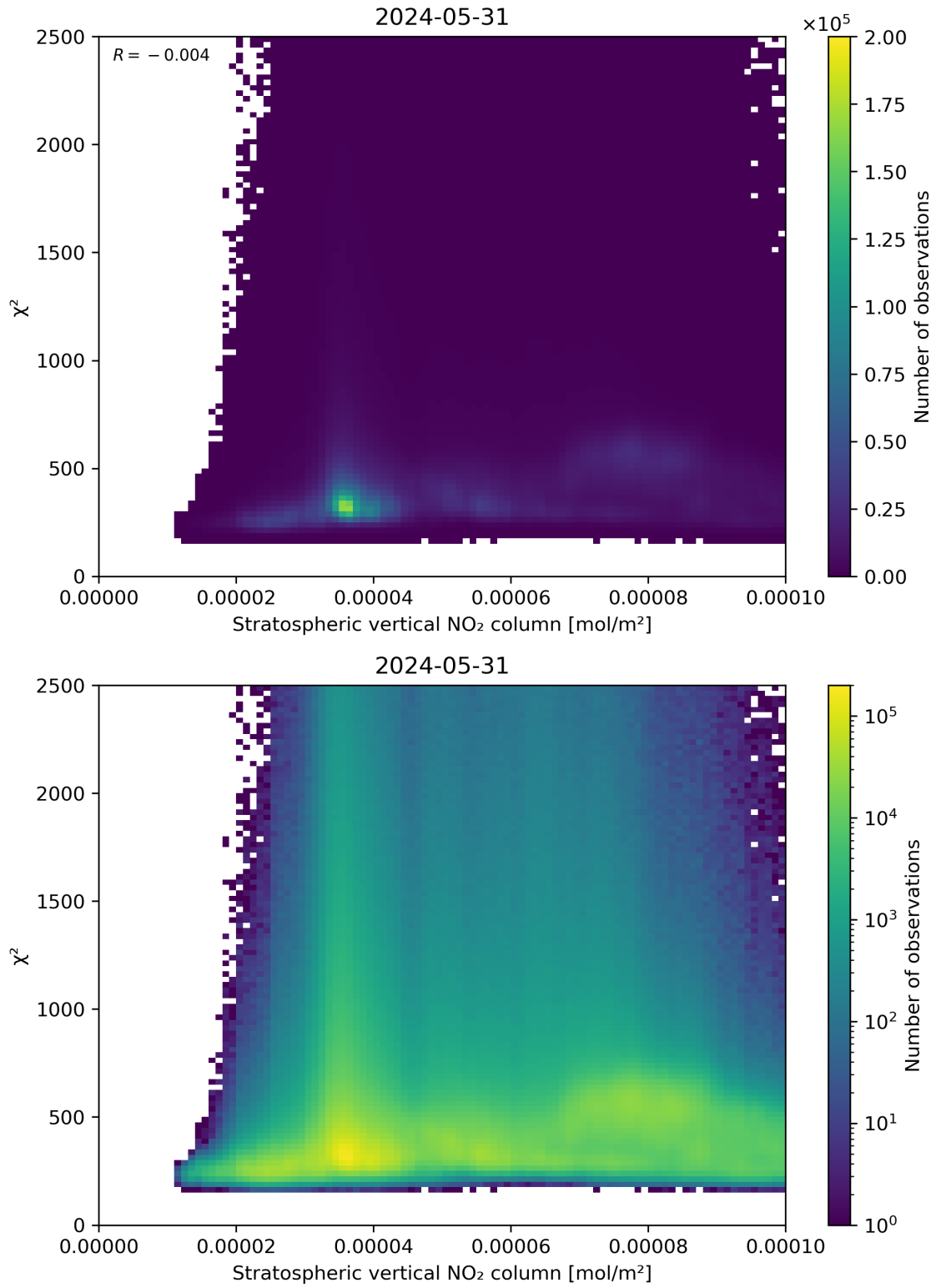
Figure 97: Scatter density plot of “Stratospheric vertical NO 2 column” against “ \chi^2 ” for 2024-05-30 to 2024-06-01.
