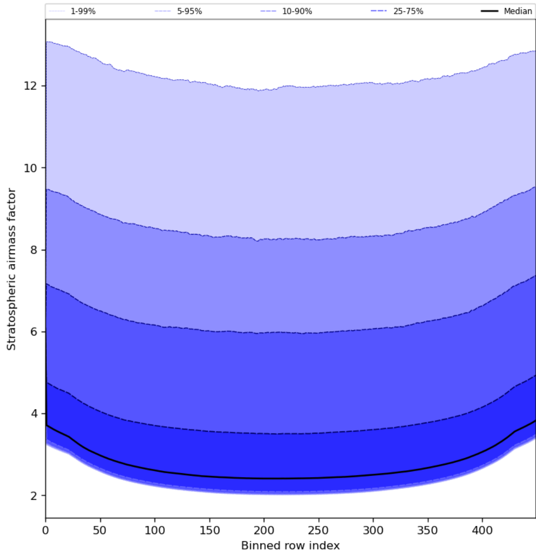
Figure 61: Along track statistics of “Stratospheric airmass factor” for 2024-05-30 to 2024-06-01
