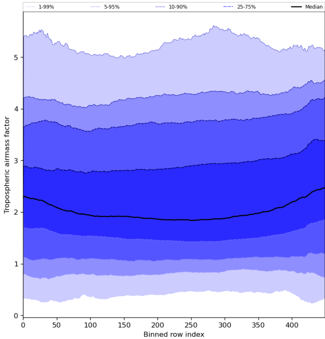
Figure 48: Along track statistics of “Tropospheric airmass factor” for 2024-05-30 to 2024-06-01
