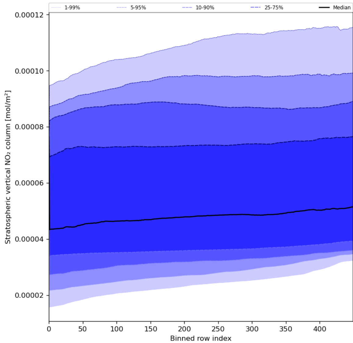
Figure 53: Along track statistics of “Stratospheric vertical NO 2 column” for 2024-05-30 to 2024-06-01
