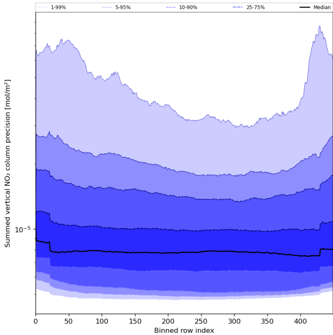
Figure 58: Along track statistics of “Summed vertical NO 2 column precision” for 2024-05-30 to 2024-06-01
