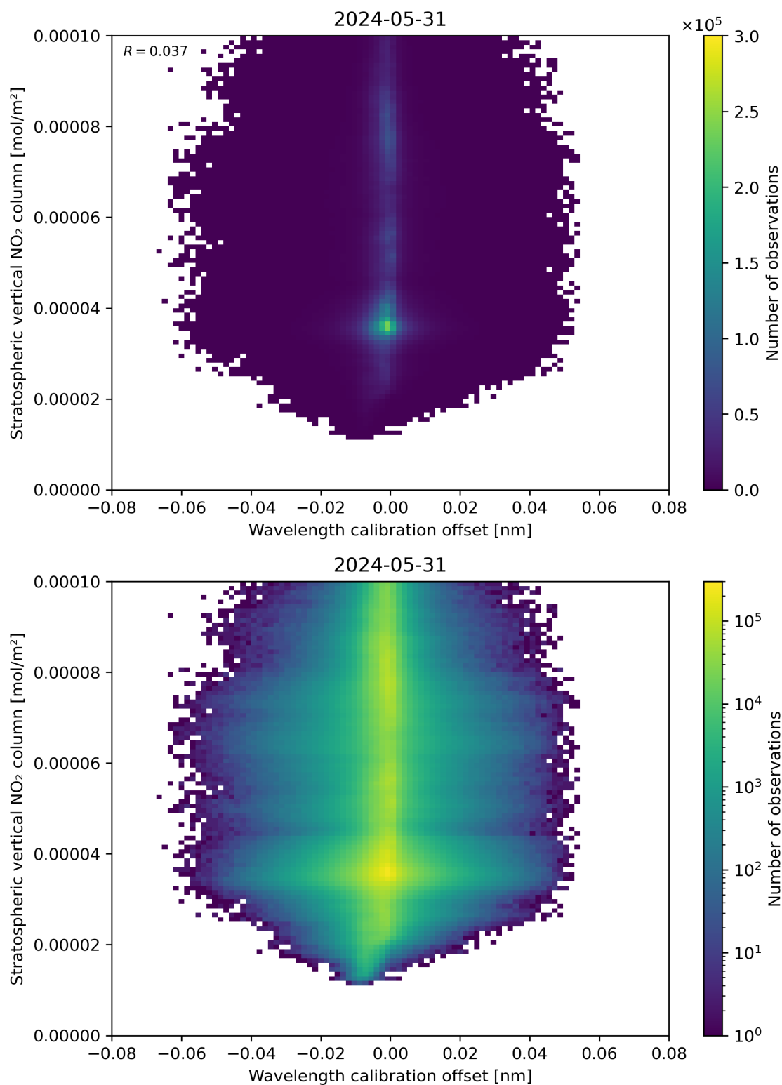
Figure 176: Scatter density plot of “Wavelength calibration offset” against “Stratospheric vertical NO 2 column” for 2024-05-30 to 2024-06-01.
