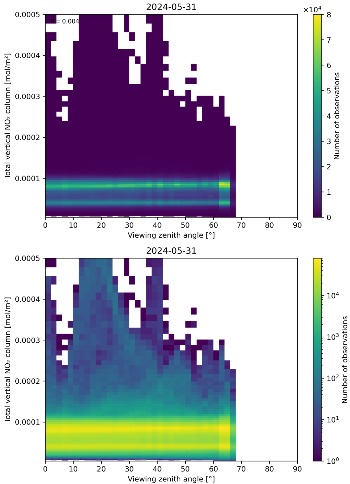
Figure 167: Scatter density plot of “Viewing zenith angle” against “Total vertical NO 2 column” for 2024-05-30 to 2024-06-01.
