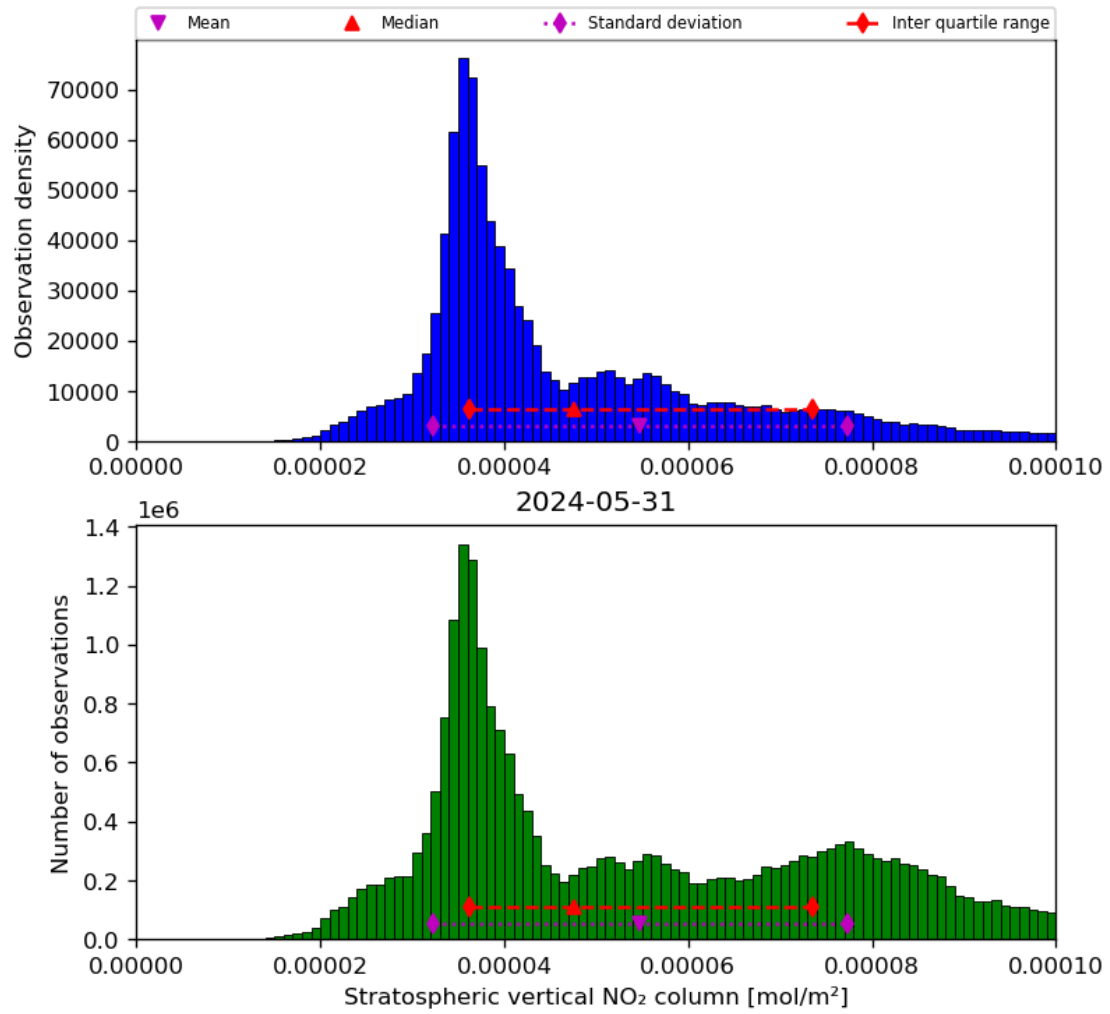
Figure 36: Histogram of “Stratospheric vertical NO 2 column” for 2024-05-30 to 2024-06-01
