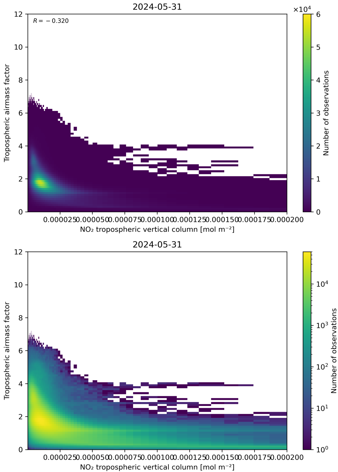
Figure 123: Scatter density plot of “NO 2 tropospheric vertical column” against “Tropospheric air mass factor” for 2024-05-30 to 2024-06-01.
