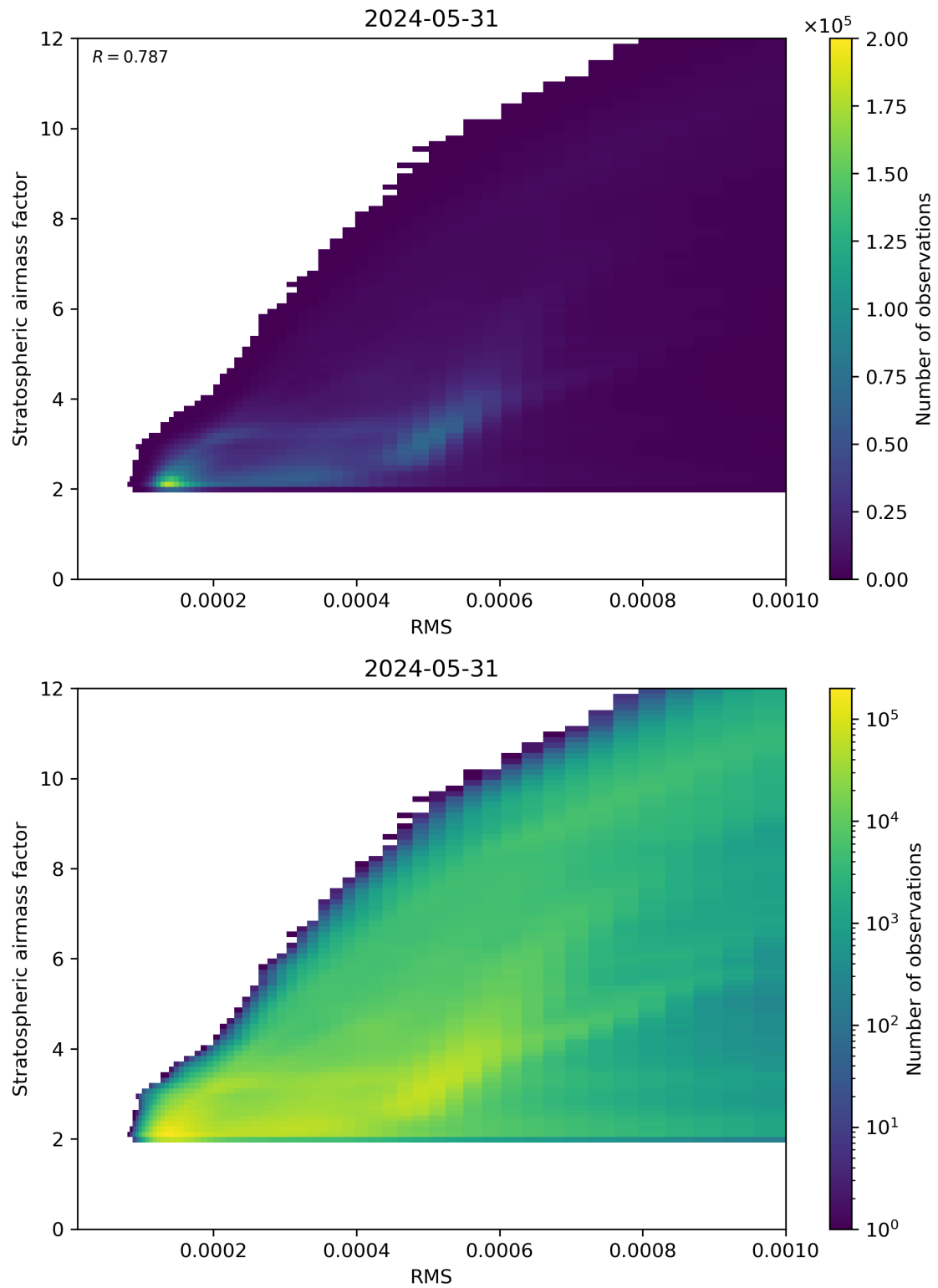
Figure 144: Scatter density plot of “RMS” against “Stratospheric airmass factor” for 2024-05-30 to 2024-06-01.
