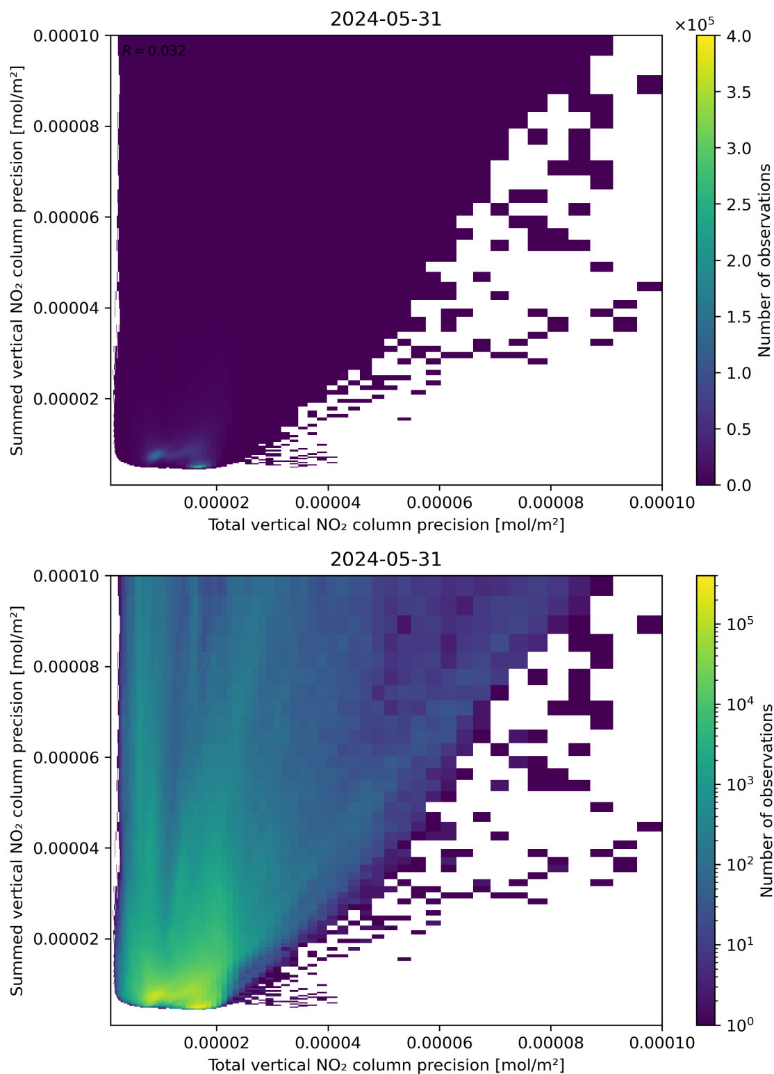
Figure 118: Scatter density plot of “Total vertical NO 2 column precision” against “Summed vertical NO 2 column precision” for 2024-05-30 to 2024-06-01.
