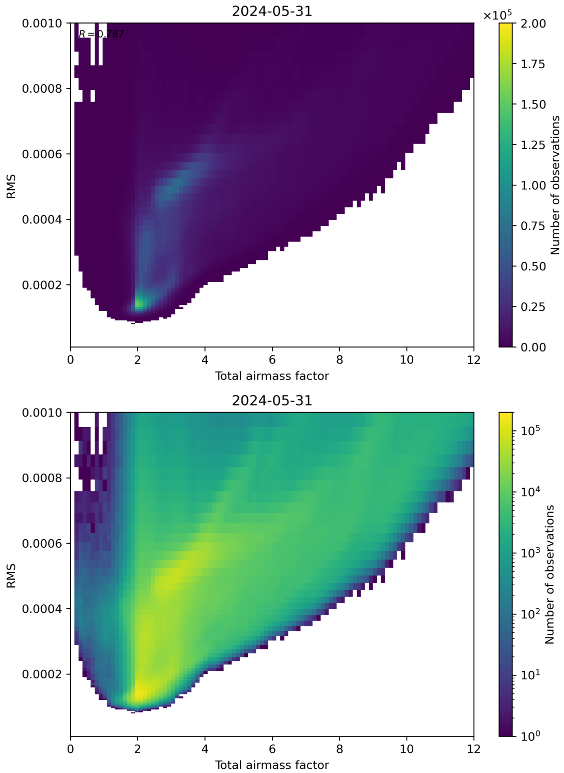
Figure 69: Scatter density plot of “Total airmass factor” against “RMS” for 2024-05-30 to 2024-06-01.
