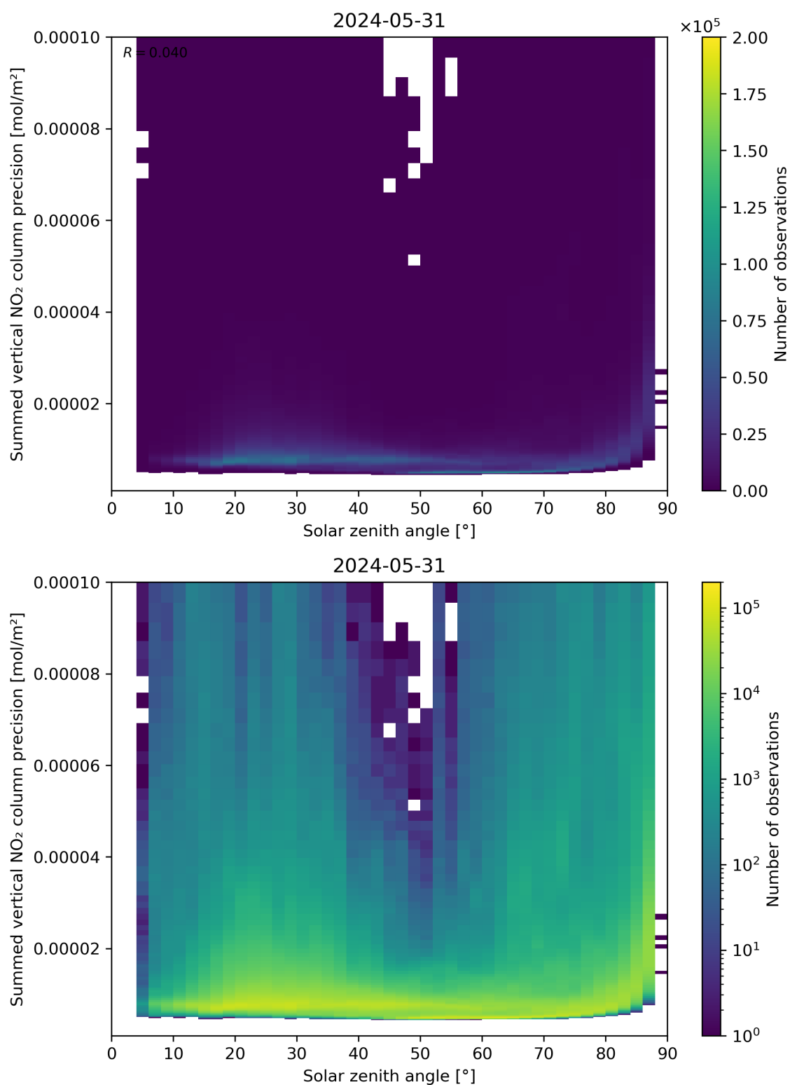
Figure 152: Scatter density plot of “Solar zenith angle” against “Summed vertical NO 2 column precision” for 2024-05-30 to 2024-06-01.
