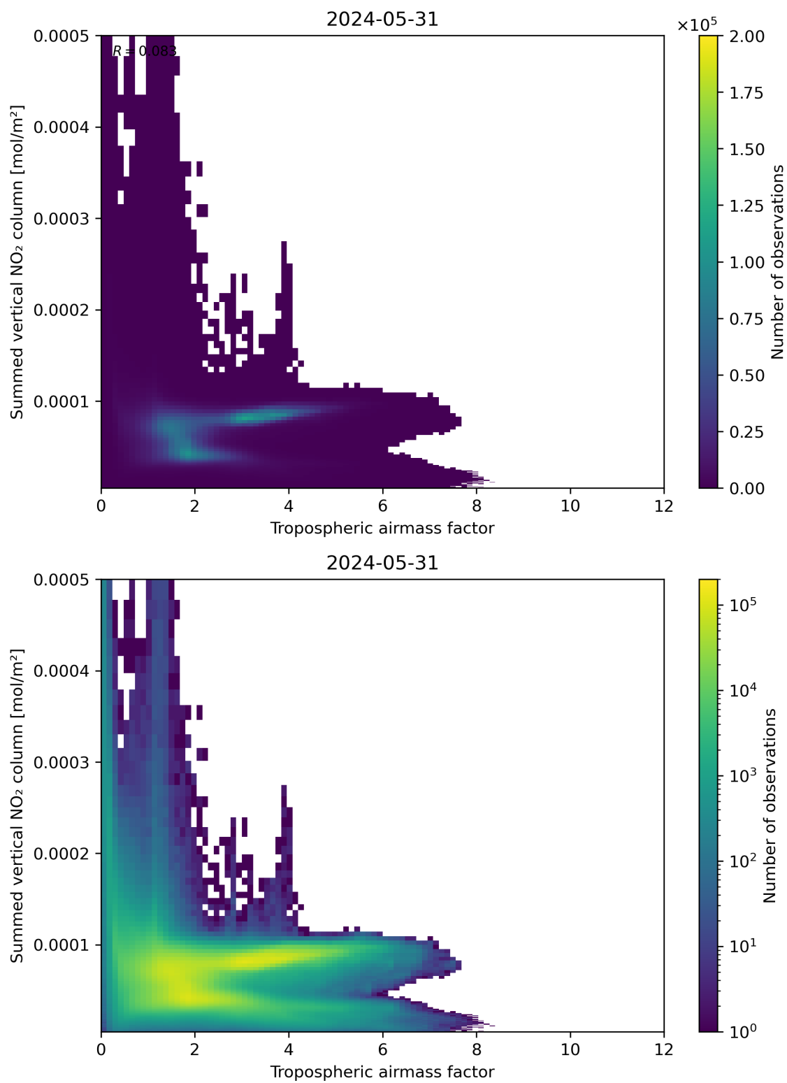
Figure 75: Scatter density plot of “Tropospheric airmass factor” against “Summed vertical NO 2 column” for 2024-05-30 to 2024-06-01.
