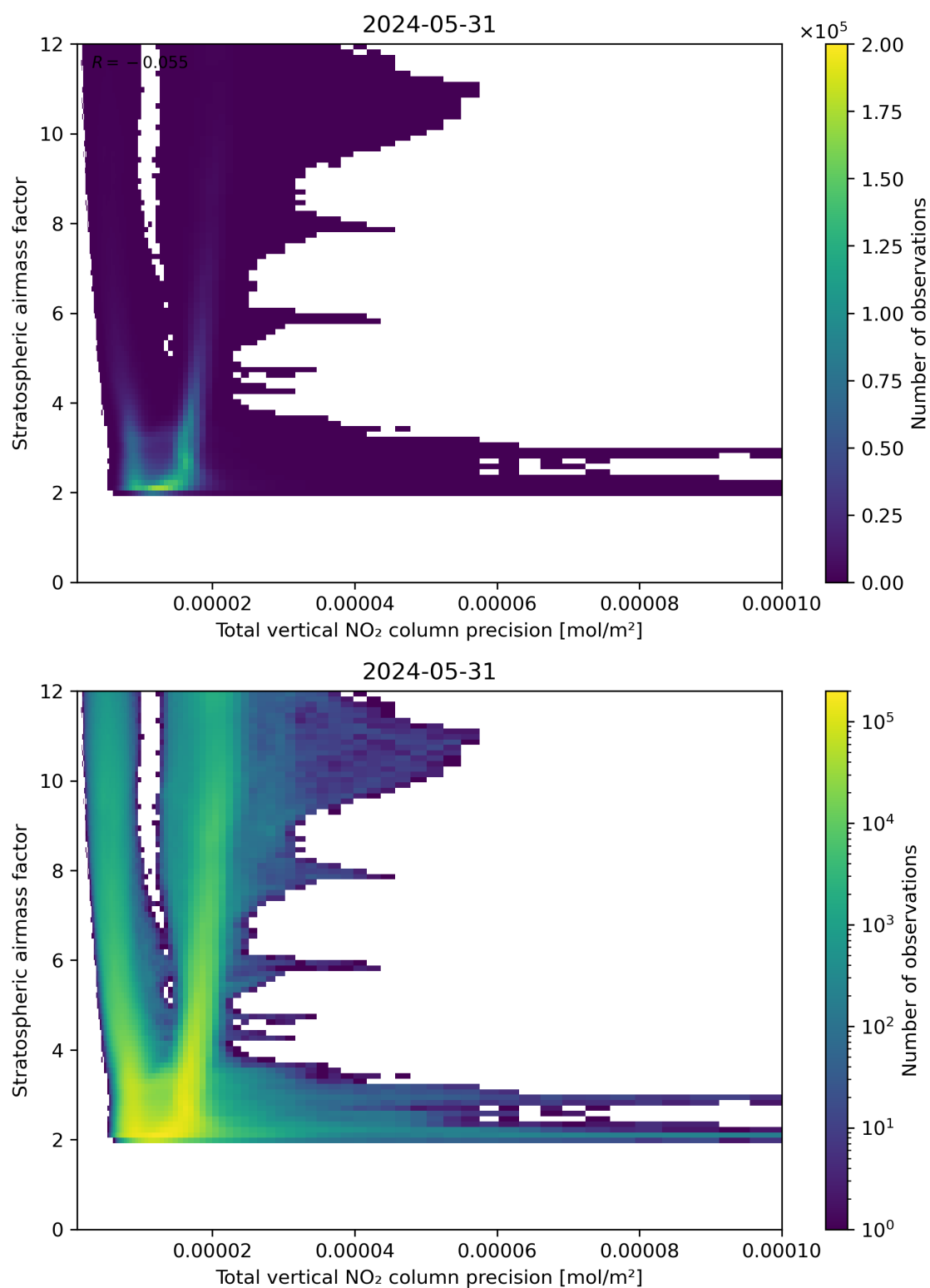
Figure 115: Scatter density plot of “Total vertical NO 2 column precision” against “Stratospheric air mass factor” for 2024-05-30 to 2024-06-01.
