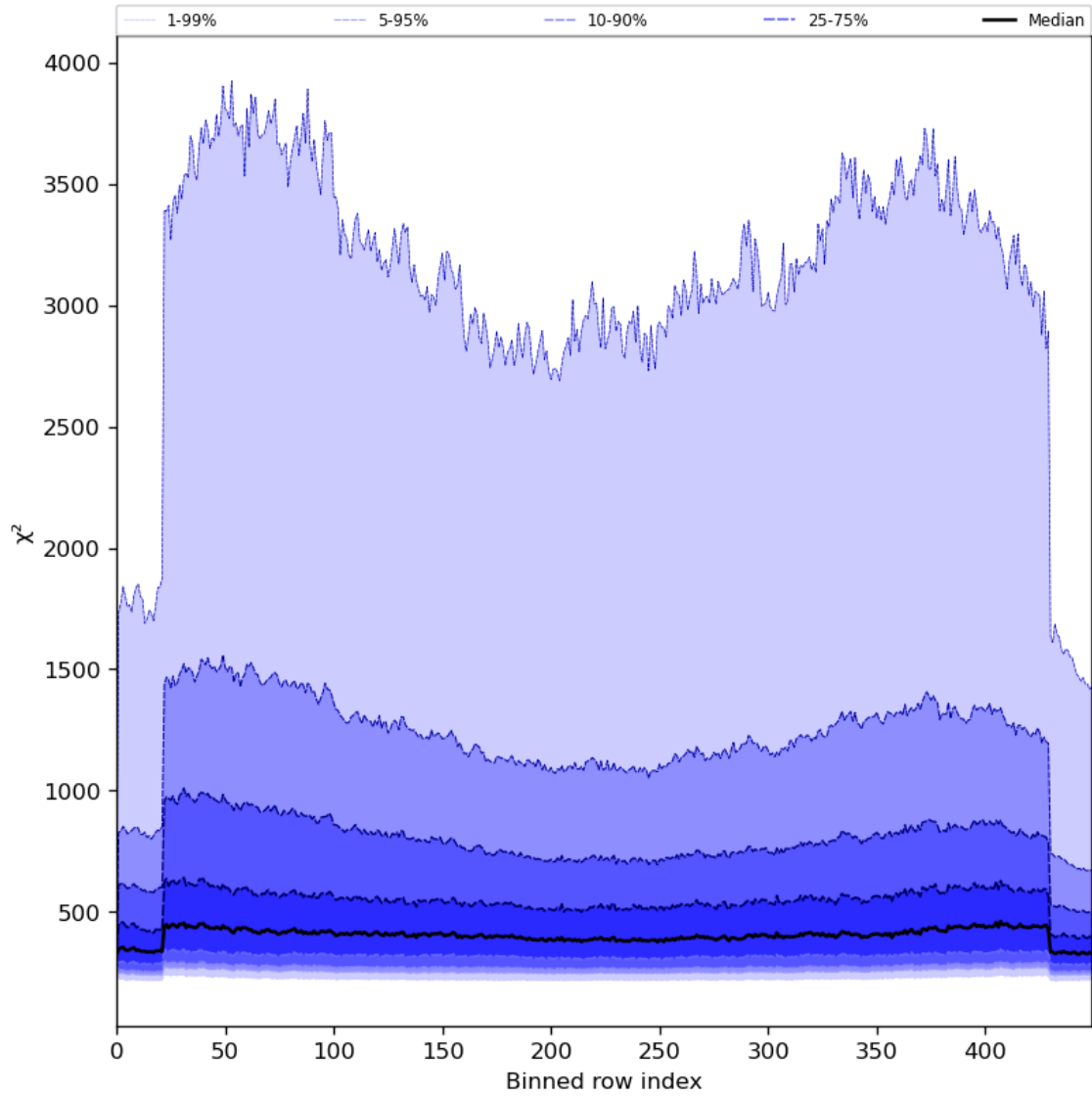
Figure 59: Along track statistics of “ \chi^2 ” for 2024-05-30 to 2024-06-01
