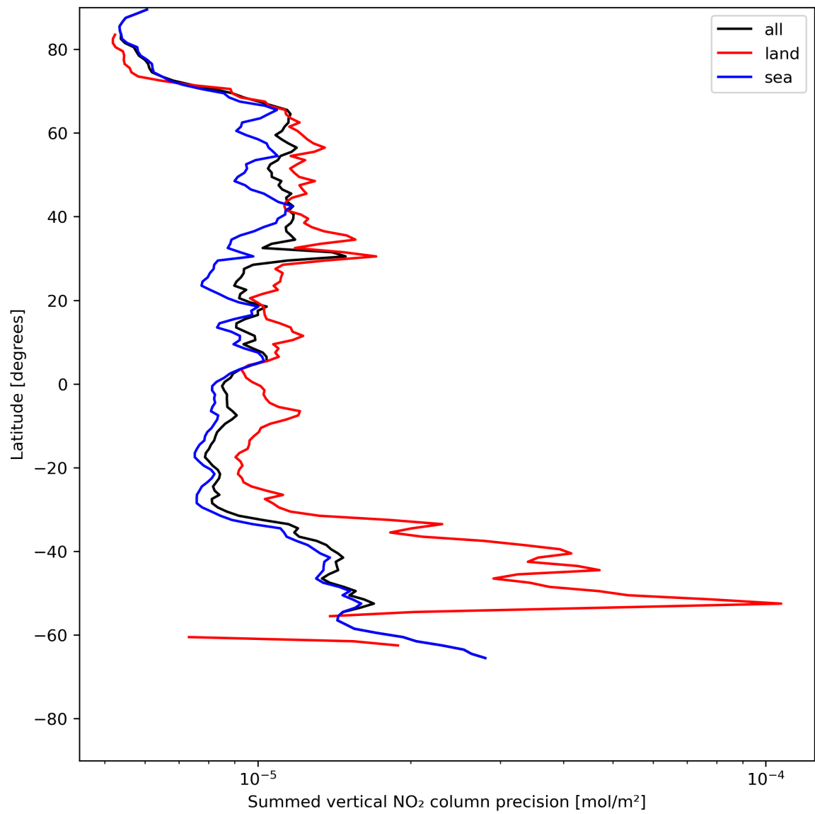
Figure 24: Zonal average of “Summed vertical NO 2 column precision” for 2024-05-30 to 2024-06-01.
