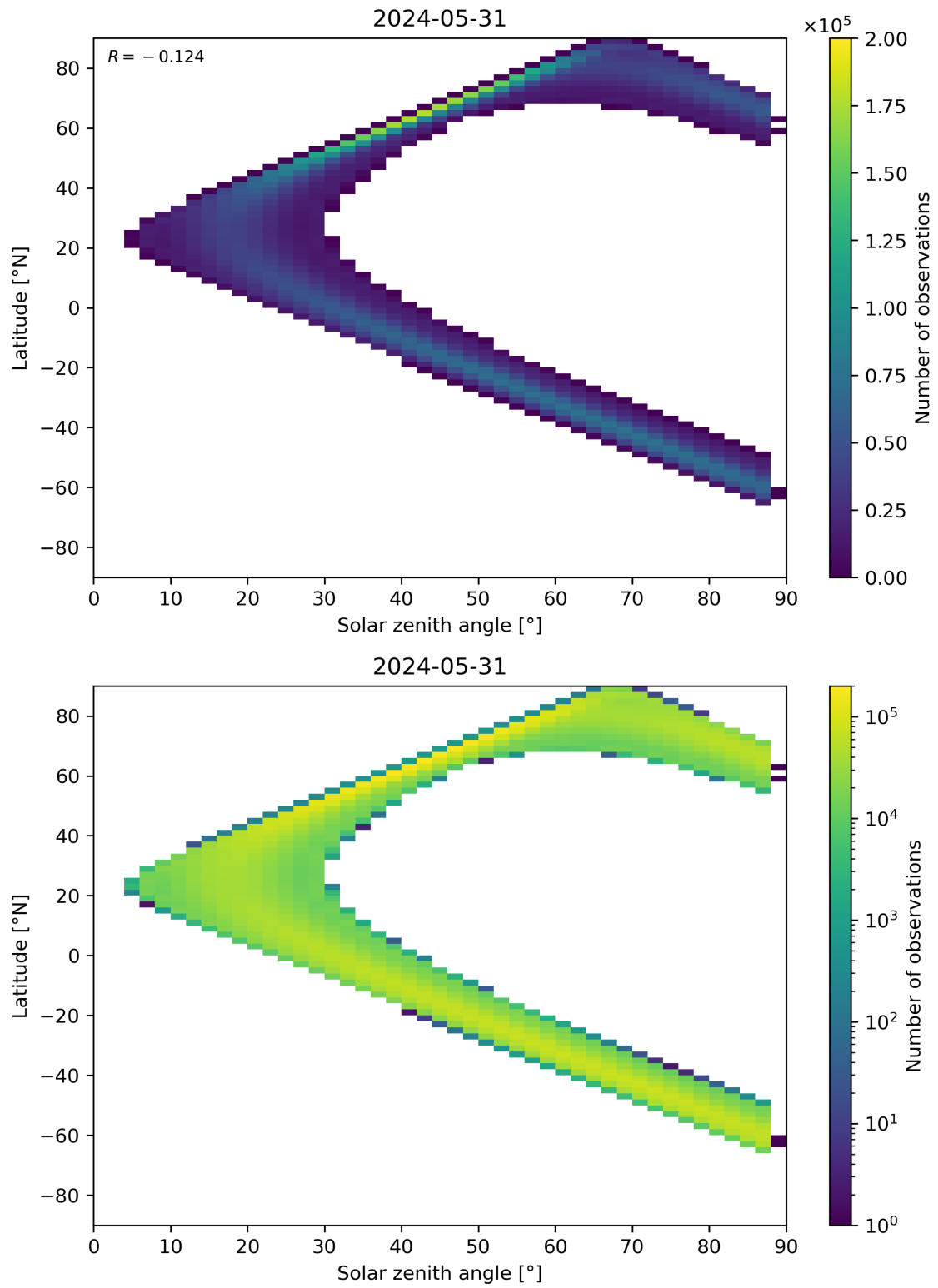
Figure 149: Scatter density plot of “Solar zenith angle” against “Latitude” for 2024-05-30 to 2024-06-01.
