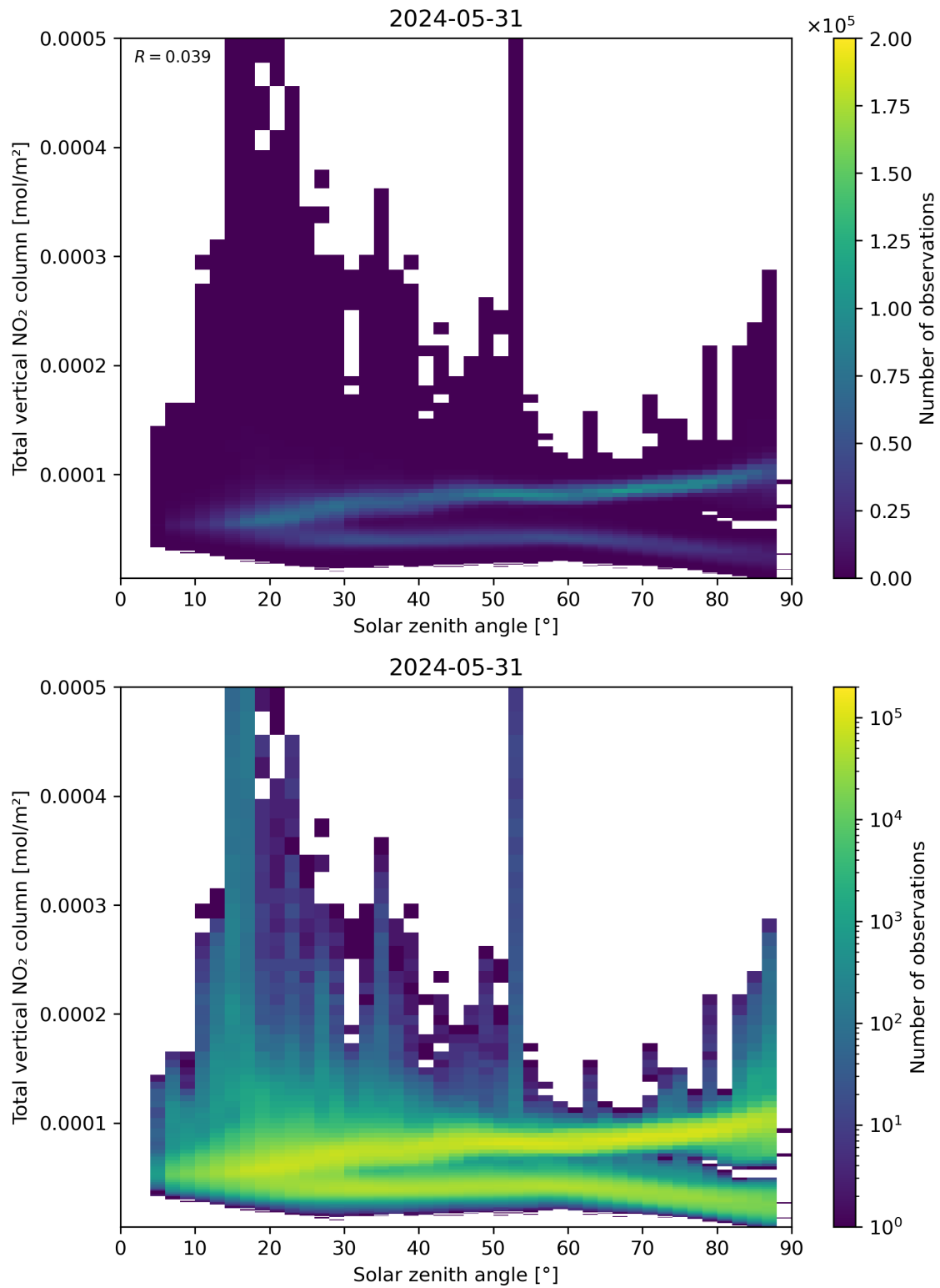
Figure 153: Scatter density plot of “Solar zenith angle” against “Total vertical NO 2 column” for 2024-05-30 to 2024-06-01.
