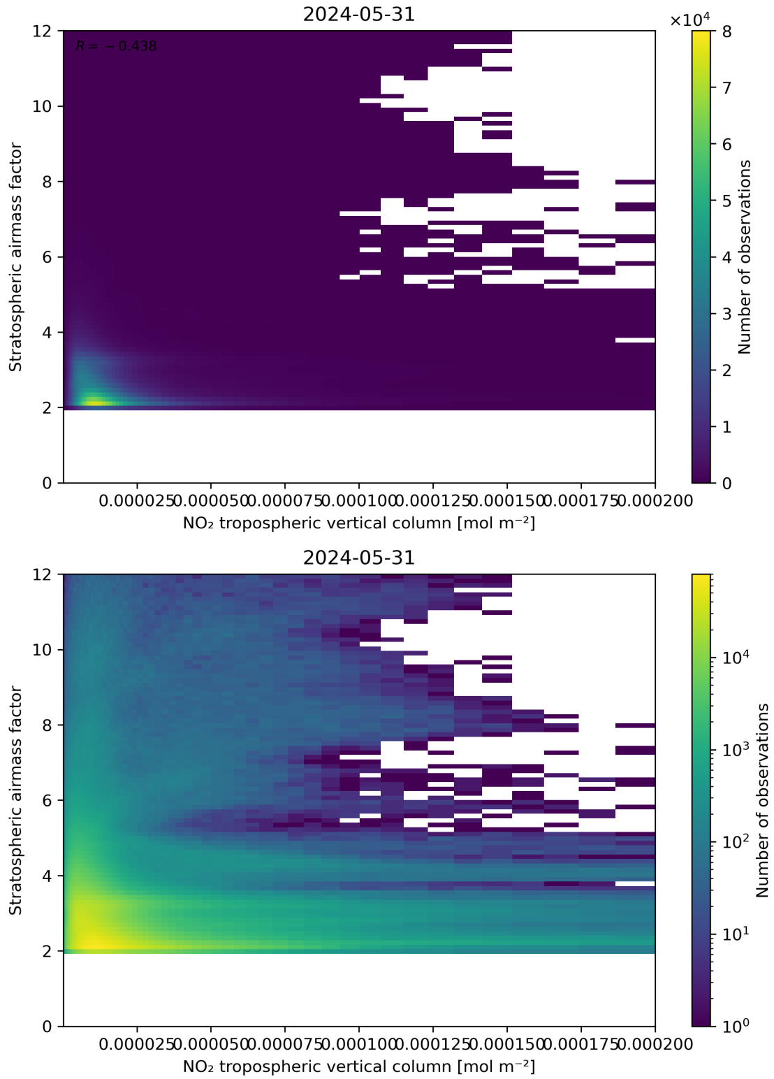
Figure 121: Scatter density plot of “NO 2 tropospheric vertical column” against “Stratospheric air mass factor” for 2024-05-30 to 2024-06-01.
