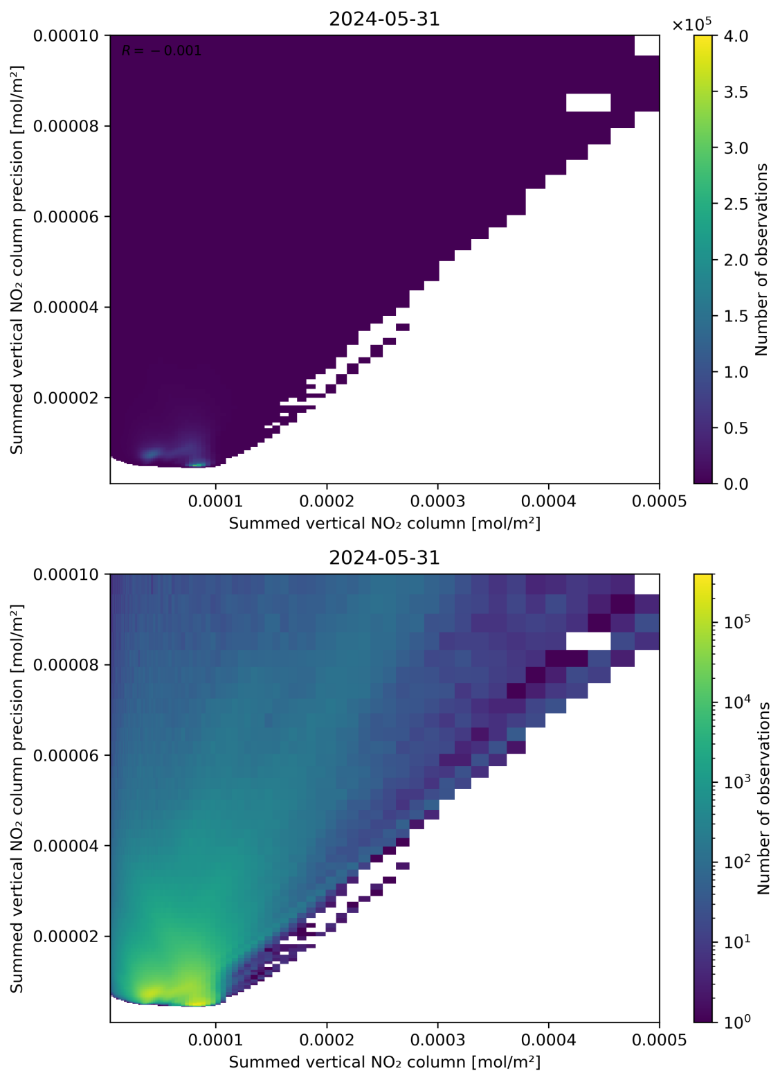
Figure 105: Scatter density plot of “Summed vertical NO 2 column” against “Summed vertical NO 2 column precision” for 2024-05-30 to 2024-06-01.
