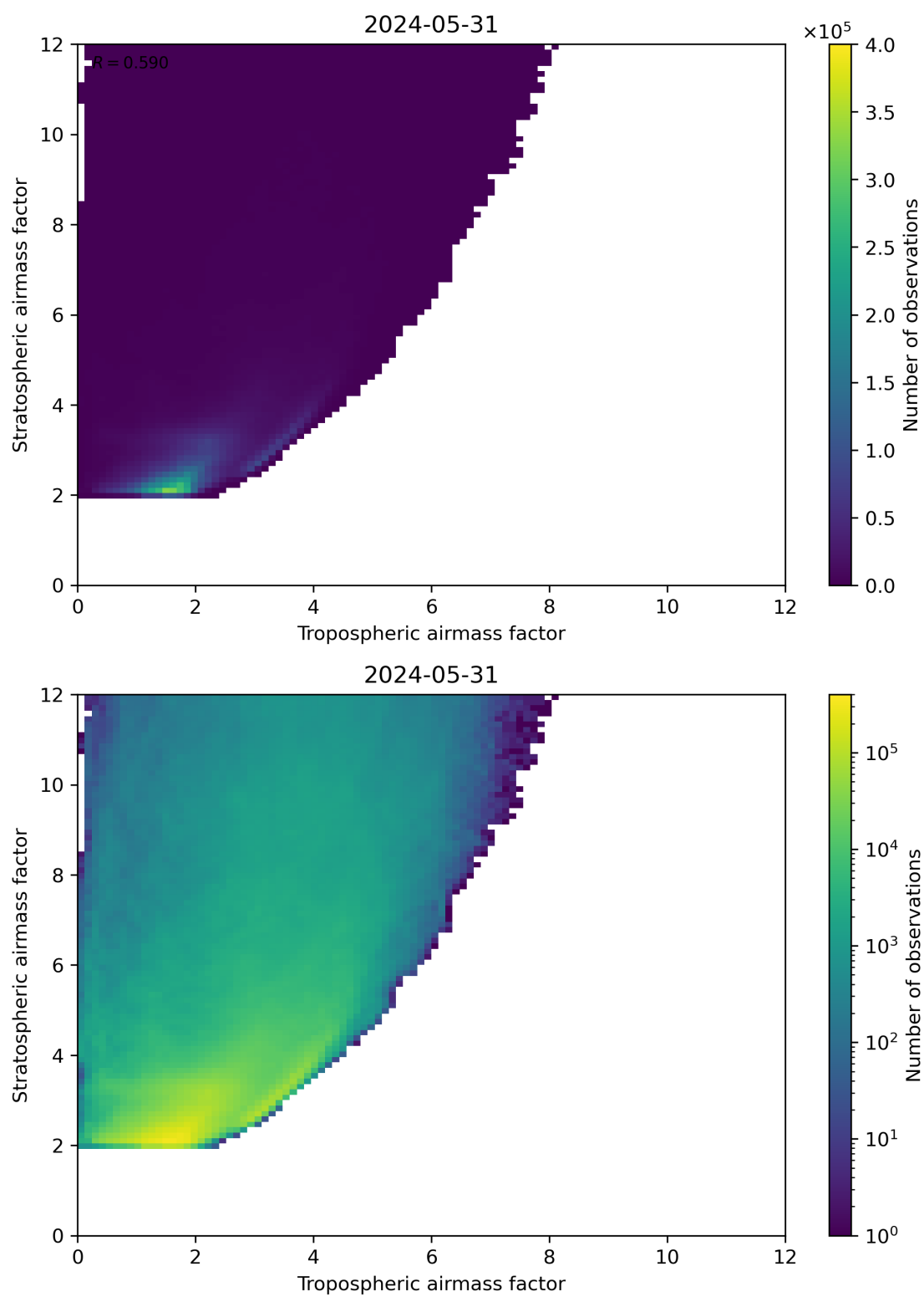
Figure 71: Scatter density plot of “Tropospheric airmass factor” against “Stratospheric airmass factor” for 2024-05-30 to 2024-06-01.
