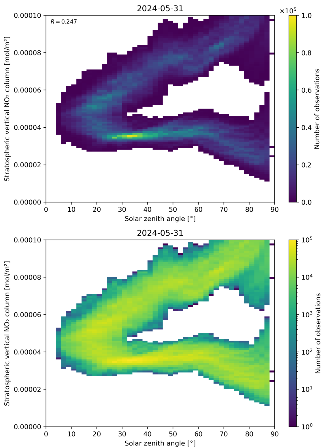
Figure 150: Scatter density plot of “Solar zenith angle” against “Stratospheric vertical NO 2 column” for 2024-05-30 to 2024-06-01.
