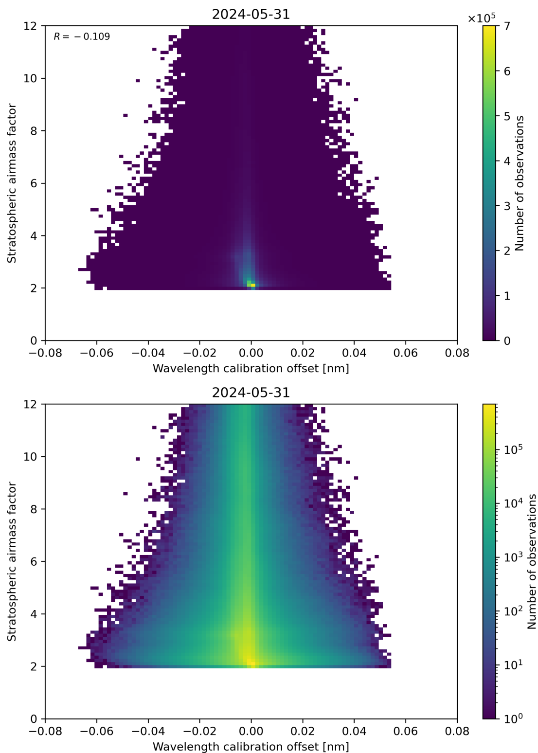
Figure 174: Scatter density plot of “Wavelength calibration offset” against “Stratospheric air mass factor” for 2024-05-30 to 2024-06-01.
