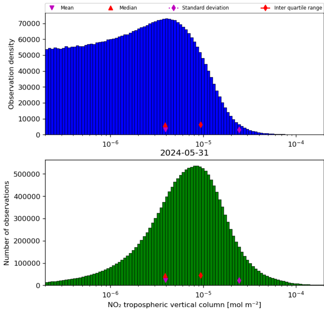
Figure 29: Histogram of “NO 2 tropospheric vertical column” for 2024-05-30 to 2024-06-01
