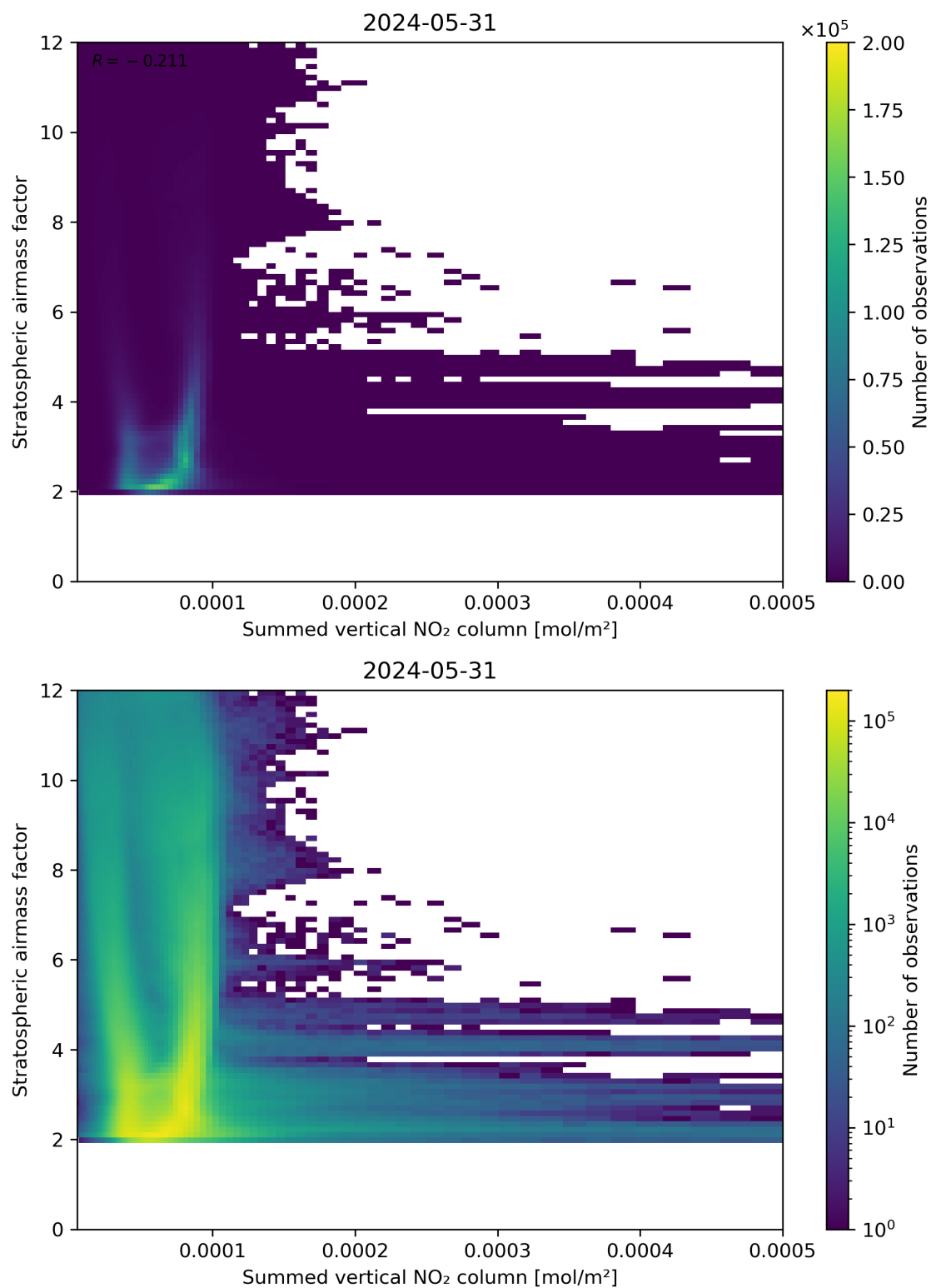
Figure 103: Scatter density plot of “Summed vertical NO 2 column” against “Stratospheric air mass factor” for 2024-05-30 to 2024-06-01.
