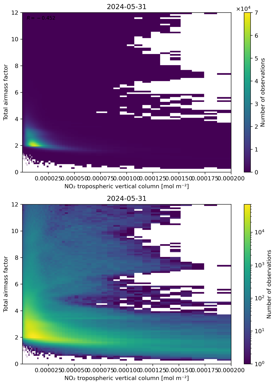
Figure 122: Scatter density plot of “NO 2 tropospheric vertical column” against “Total air mass factor” for 2024-05-30 to 2024-06-01.
