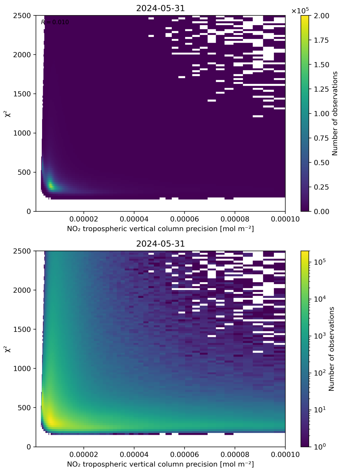
Figure 134: Scatter density plot of “NO 2 tropospheric vertical column precision” against “ \chi^2 ” for 2024-05-30 to 2024-06-01.
