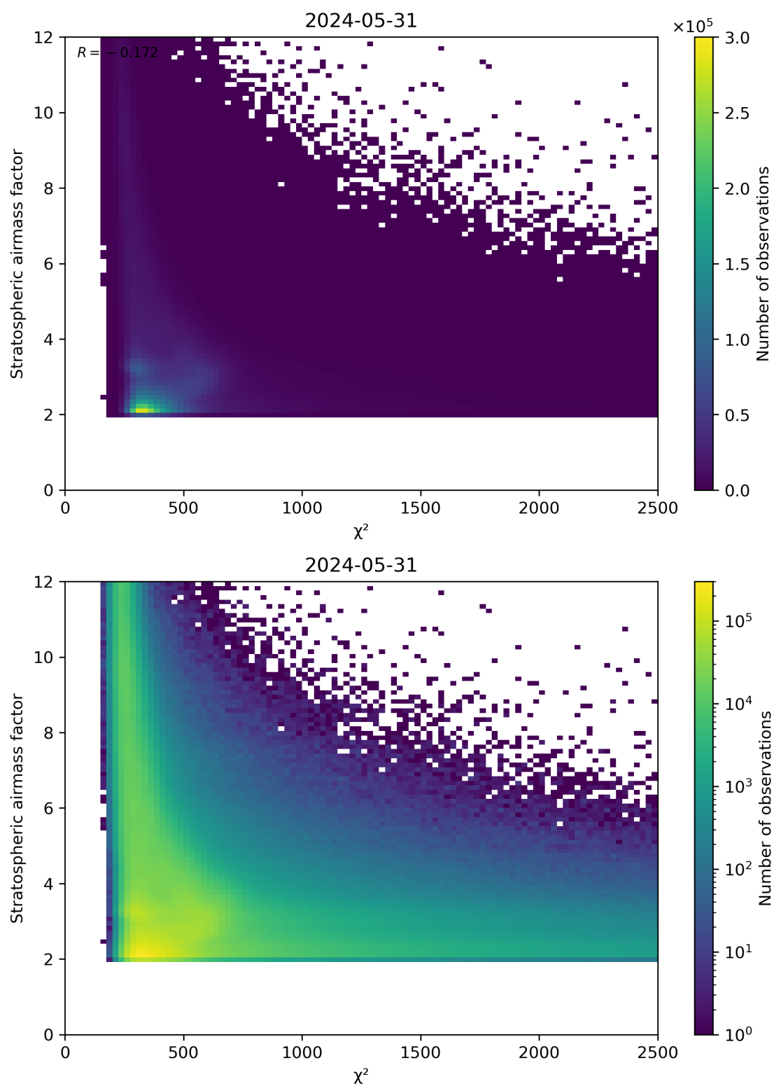
Figure 81: Scatter density plot of “ \chi^2 ” against “Stratospheric airmass factor” for 2024-05-30 to 2024-06-01.
