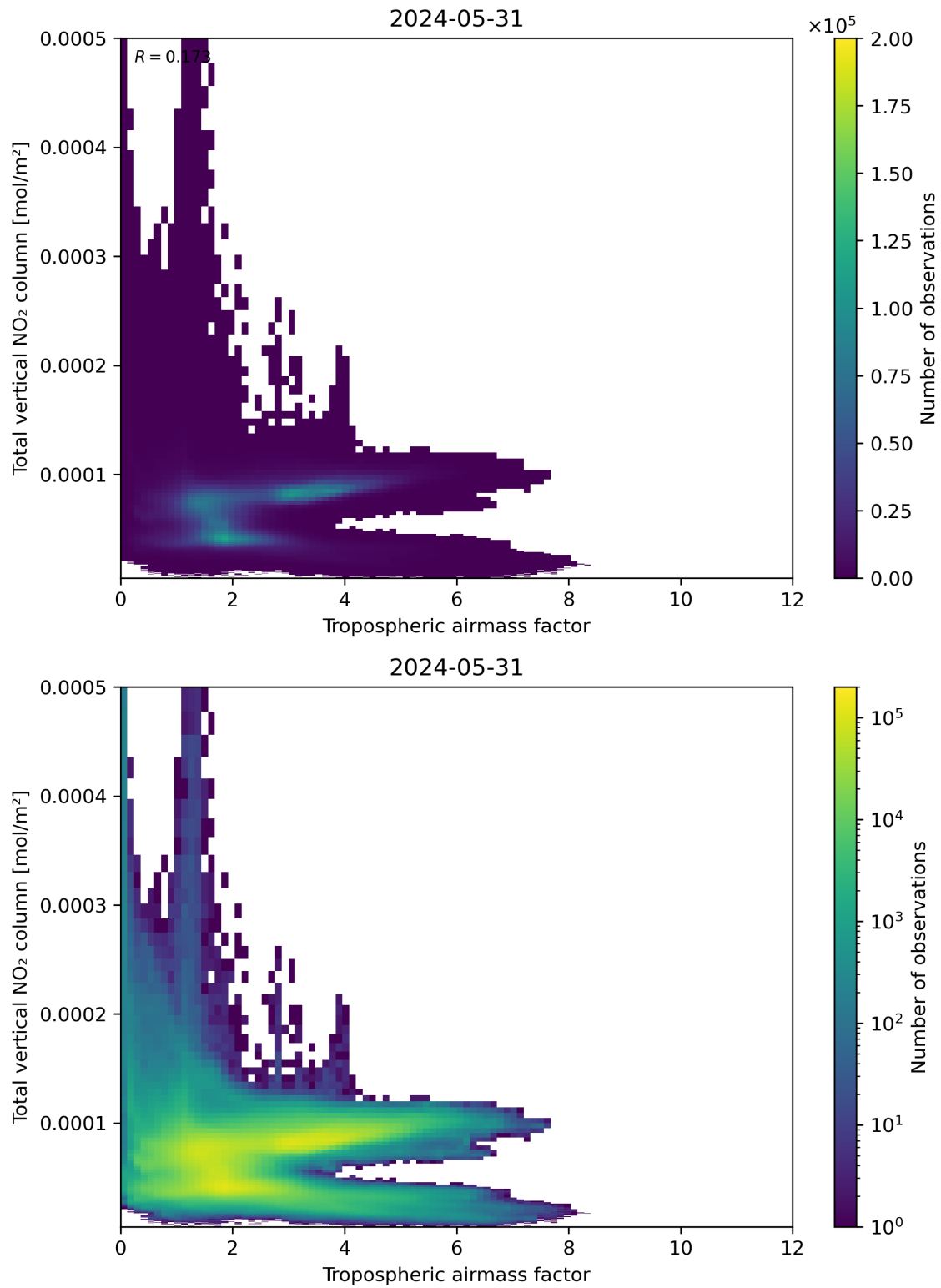
Figure 77: Scatter density plot of “Tropospheric airmass factor” against “Total vertical NO 2 column” for 2024-05-30 to 2024-06-01.
