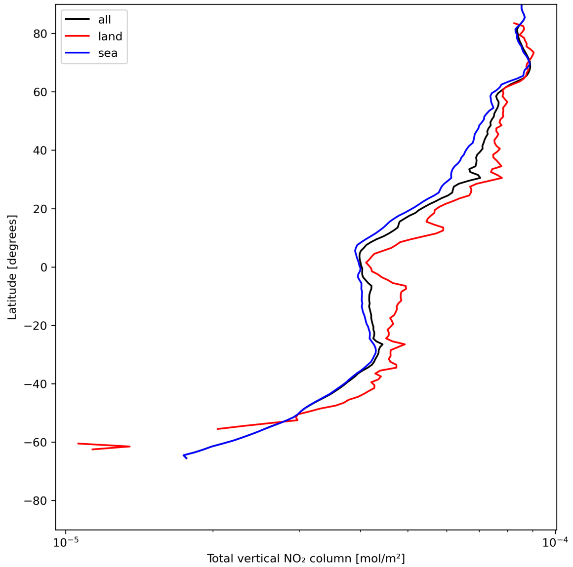
Figure 21: Zonal average of “Total vertical NO 2 column” for 2024-05-30 to 2024-06-01.
