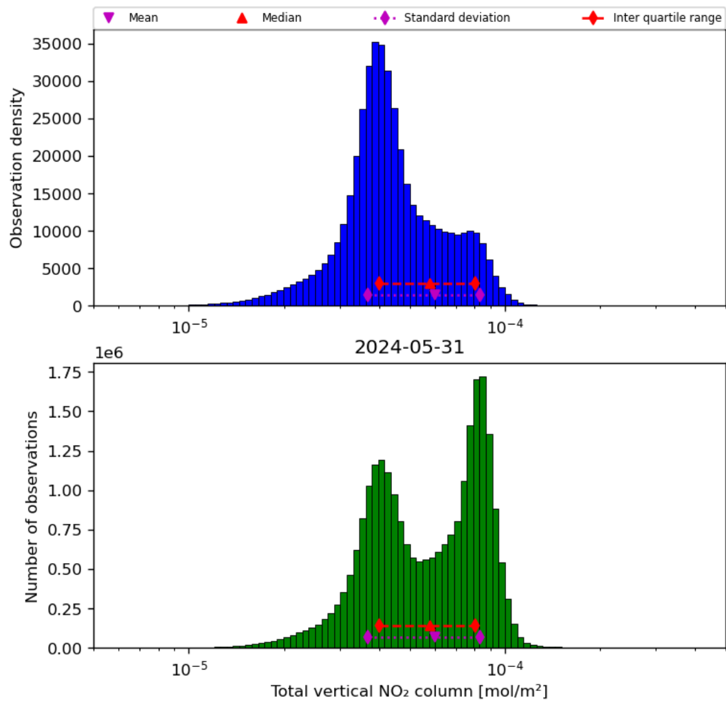
Figure 38: Histogram of “Total vertical NO 2 column” for 2024-05-30 to 2024-06-01
