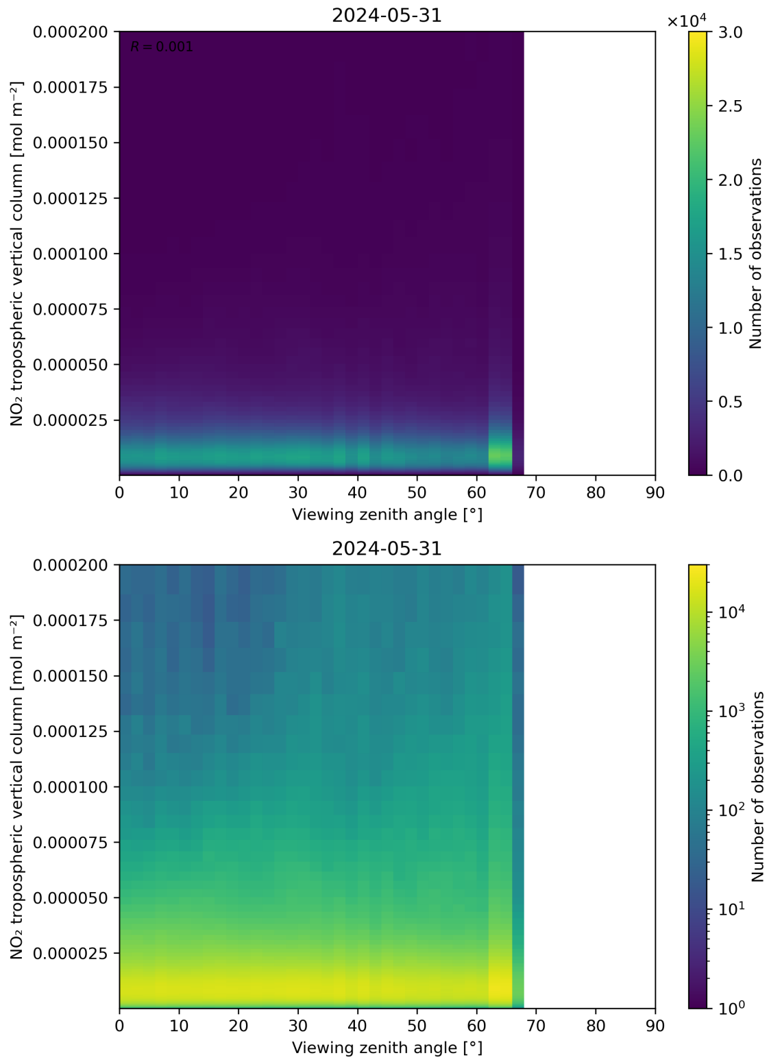
Figure 169: Scatter density plot of “Viewing zenith angle” against “NO 2 tropospheric vertical column” for 2024-05-30 to 2024-06-01.
