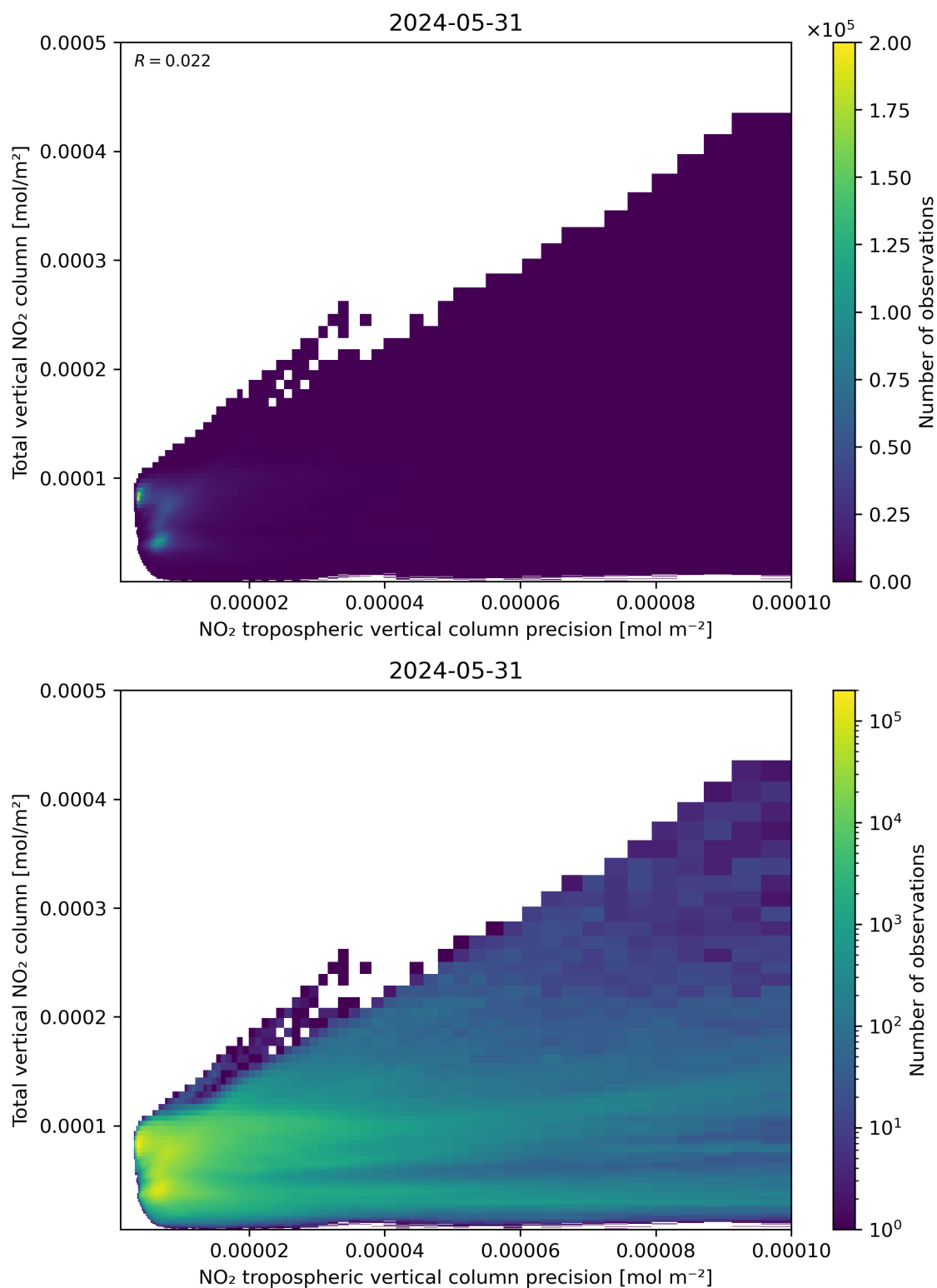
Figure 138: Scatter density plot of “NO 2 tropospheric vertical column precision” against “Total vertical NO 2 column” for 2024-05-30 to 2024-06-01.
