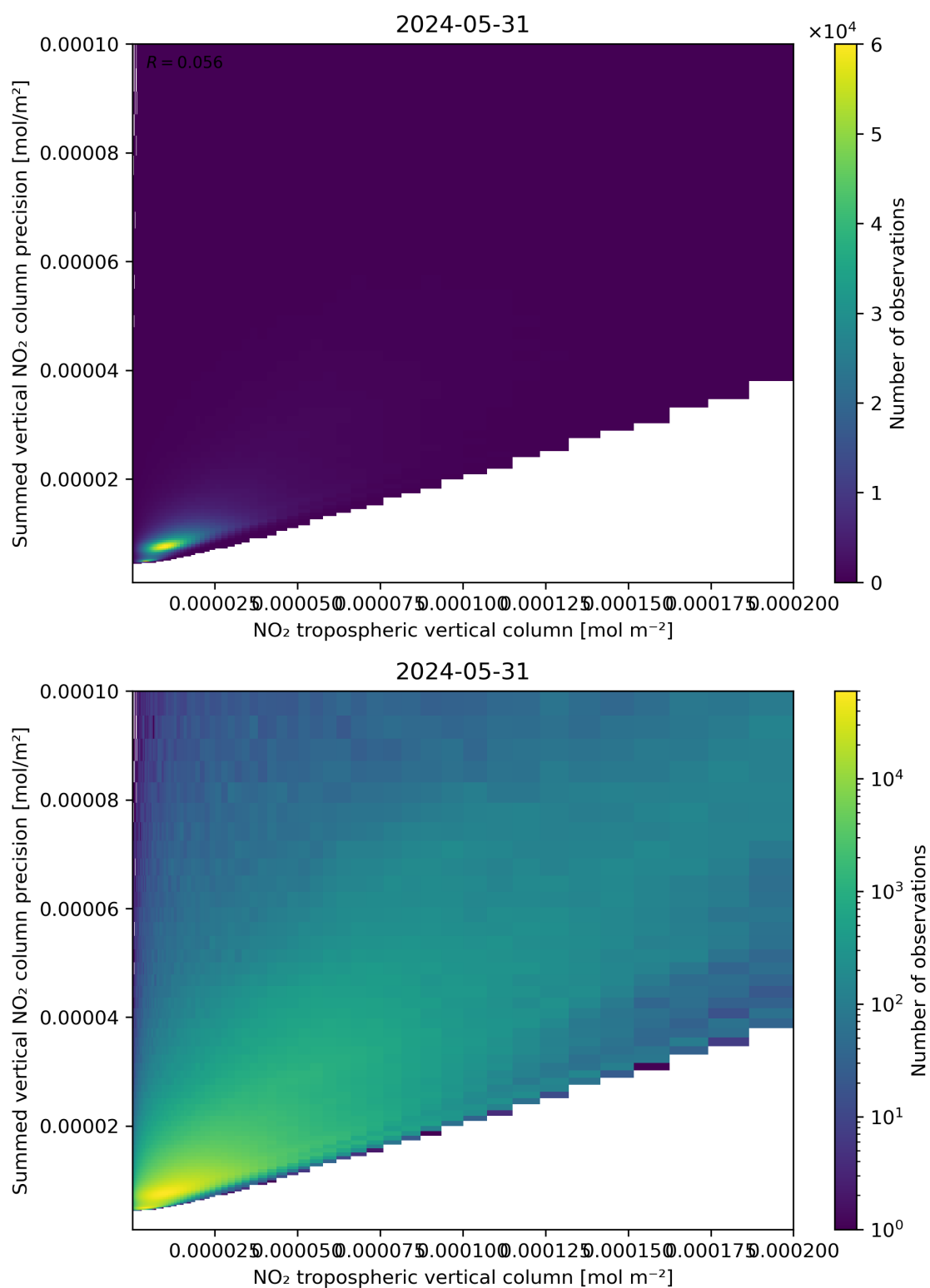
Figure 127: Scatter density plot of “NO 2 tropospheric vertical column” against “Summed vertical NO 2 column precision” for 2024-05-30 to 2024-06-01.
