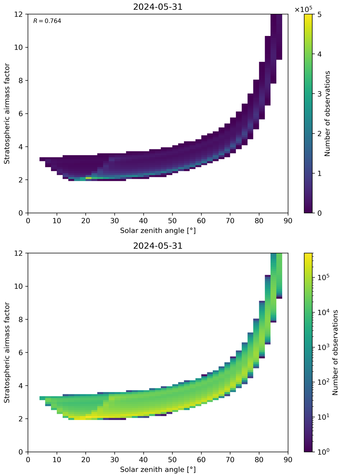
Figure 145: Scatter density plot of “Solar zenith angle” against “Stratospheric airmass factor” for 2024-05-30 to 2024-06-01.
