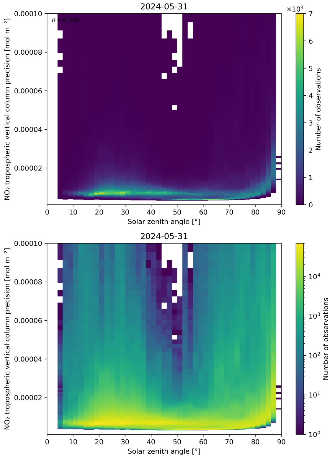
Figure 156: Scatter density plot of “Solar zenith angle” against “NO 2 tropospheric vertical column precision” for 2024-05-30 to 2024-06-01.
