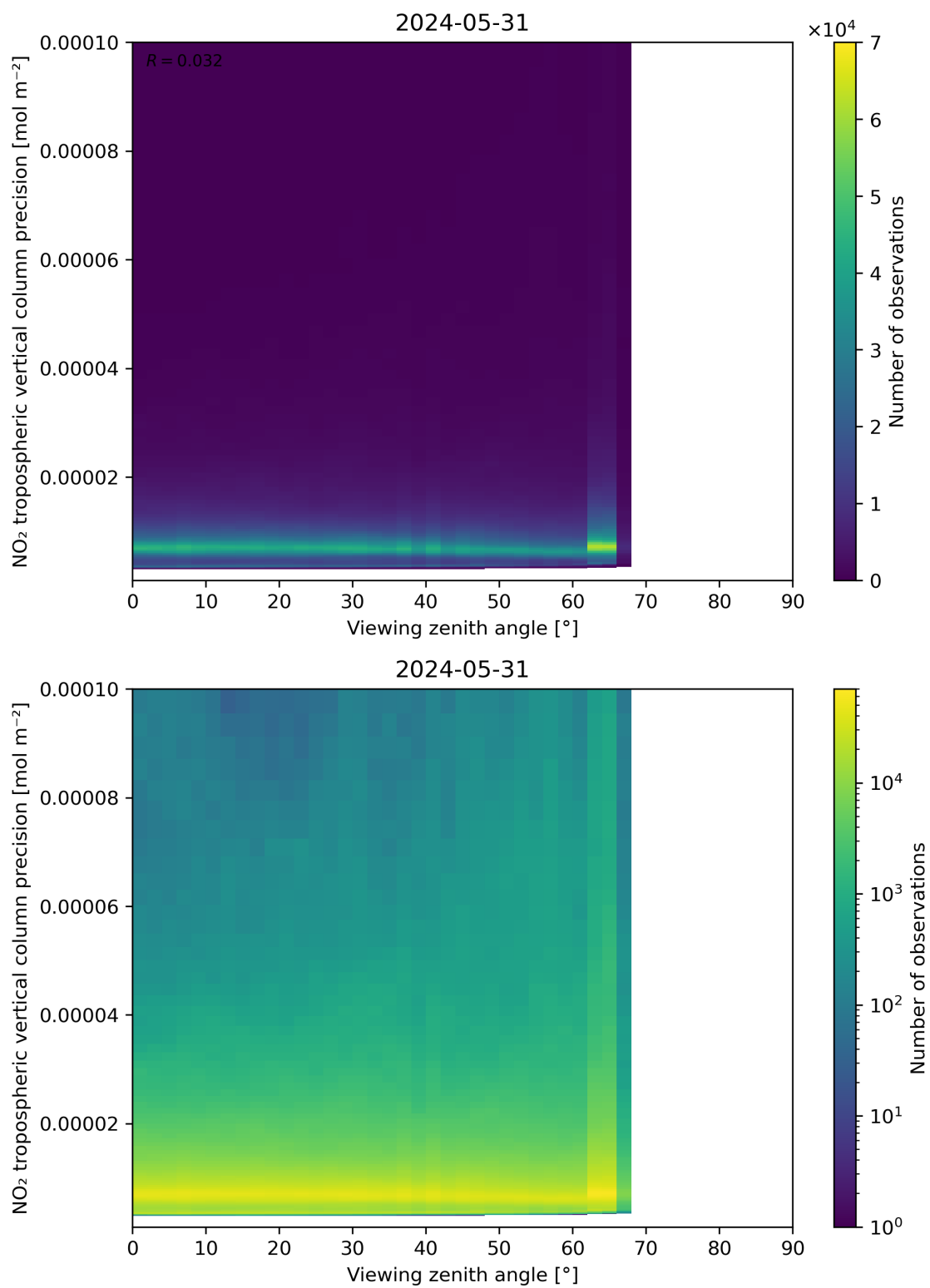
Figure 170: Scatter density plot of “Viewing zenith angle” against “NO 2 tropospheric vertical column precision” for 2024-05-30 to 2024-06-01.
