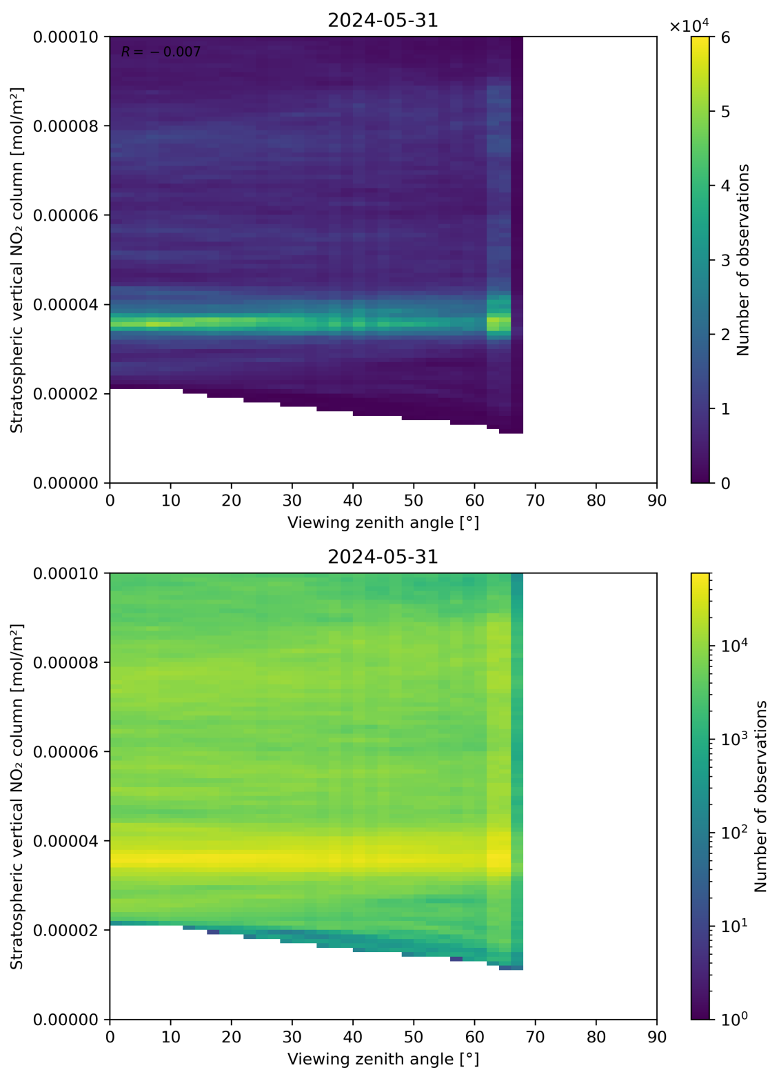
Figure 164: Scatter density plot of “Viewing zenith angle” against “Stratospheric vertical NO 2 column” for 2024-05-30 to 2024-06-01.
