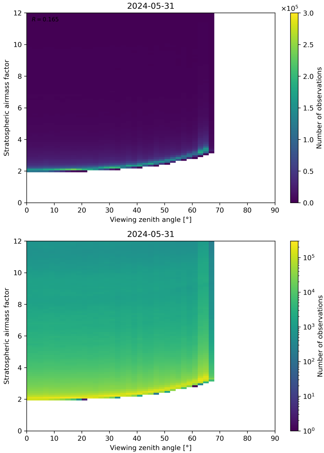
Figure 159: Scatter density plot of “Viewing zenith angle” against “Stratospheric airmass factor” for 2024-05-30 to 2024-06-01.
