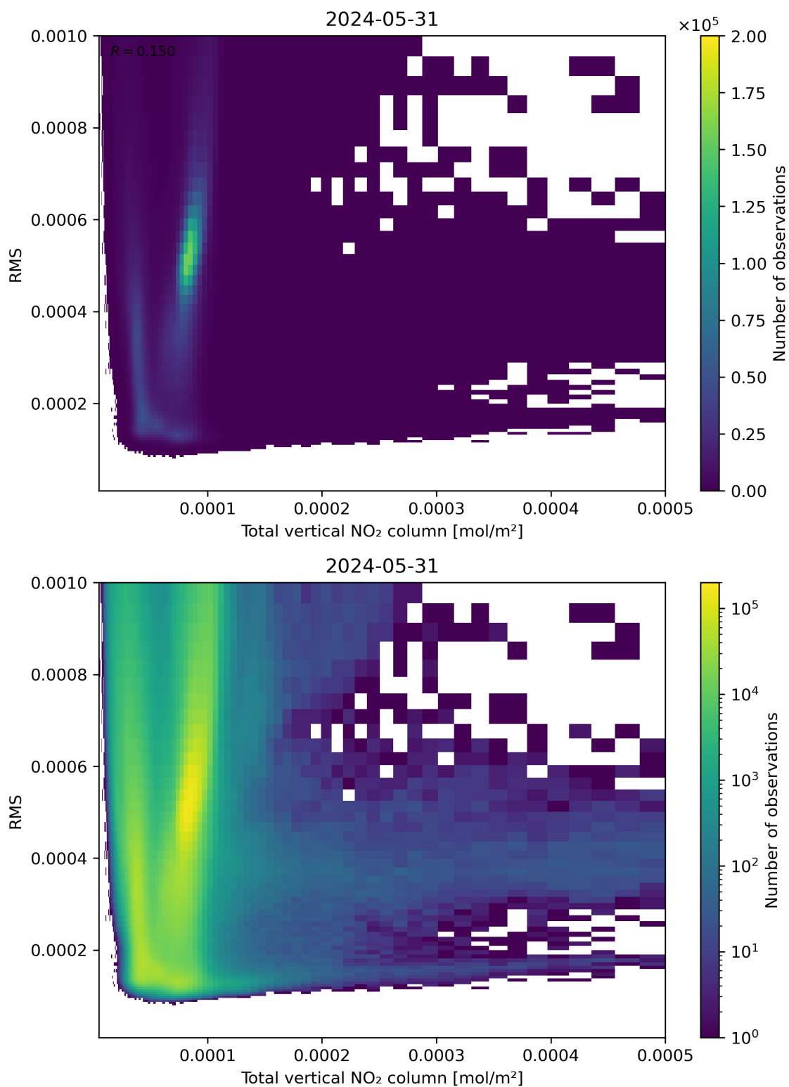
Figure 120: Scatter density plot of “Total vertical NO 2 column” against “RMS” for 2024-05-30 to 2024-06-01.
