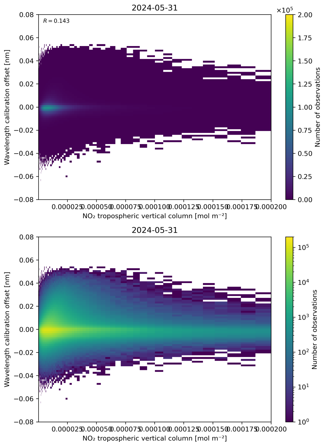
Figure 143: Scatter density plot of “NO 2 tropospheric vertical column” against “Wavelength calibration offset” for 2024-05-30 to 2024-06-01.
