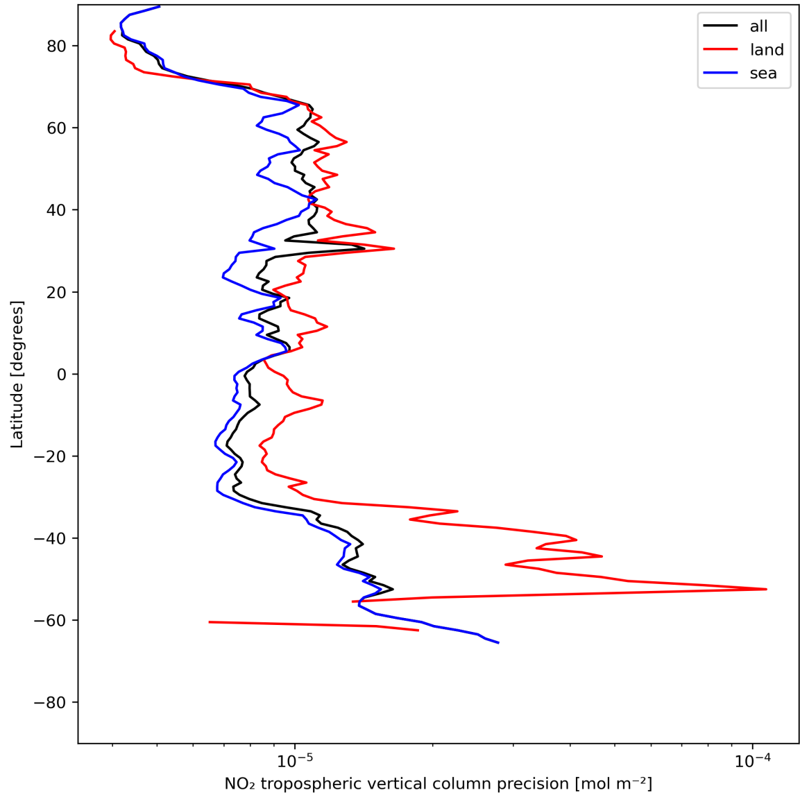
Figure 13: Zonal average of “NO 2 tropospheric vertical column precision” for 2024-05-30 to 2024-06-01.
