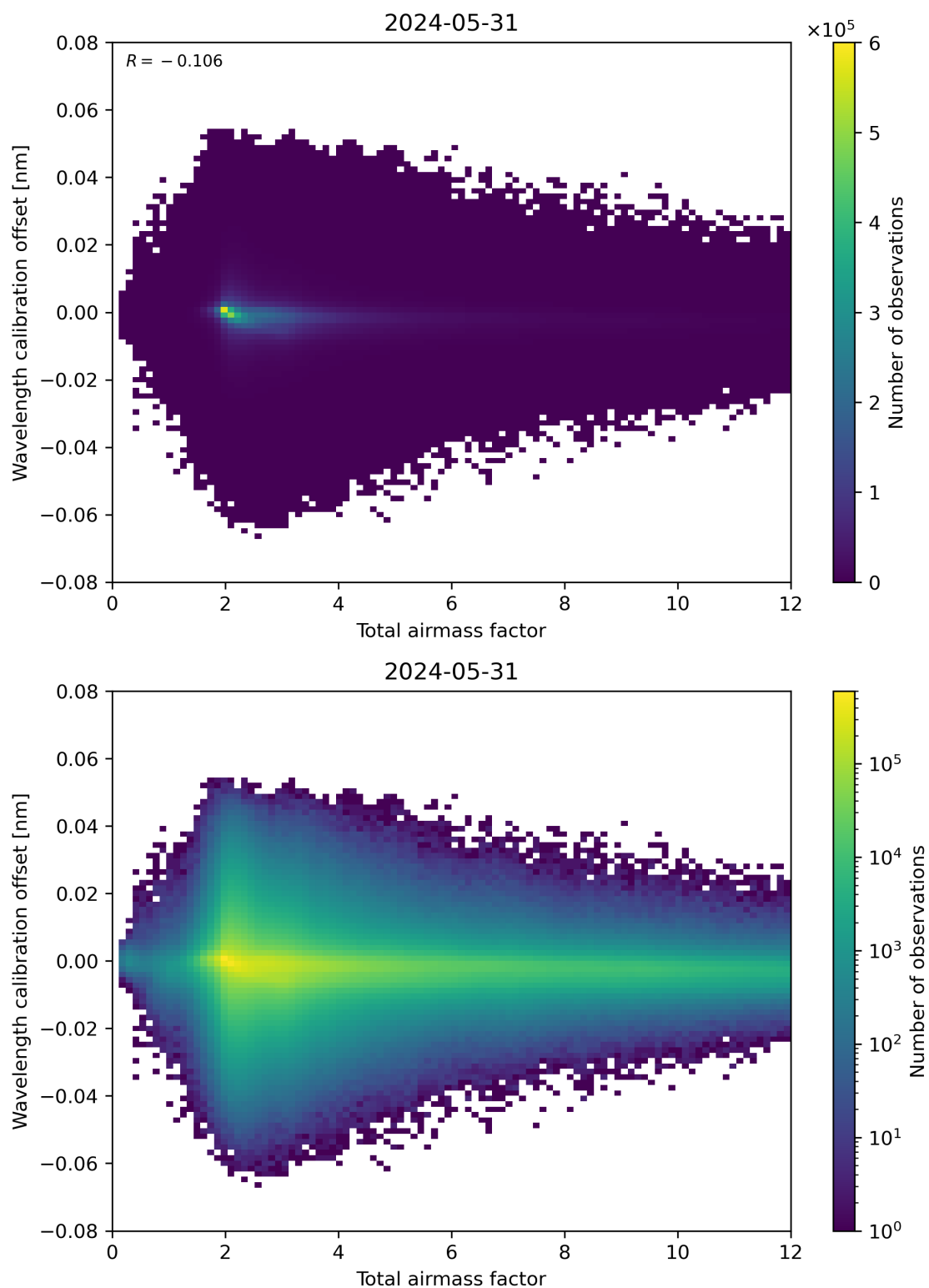
Figure 70: Scatter density plot of “Total airmass factor” against “Wavelength calibration offset” for 2024-05-30 to 2024-06-01.
