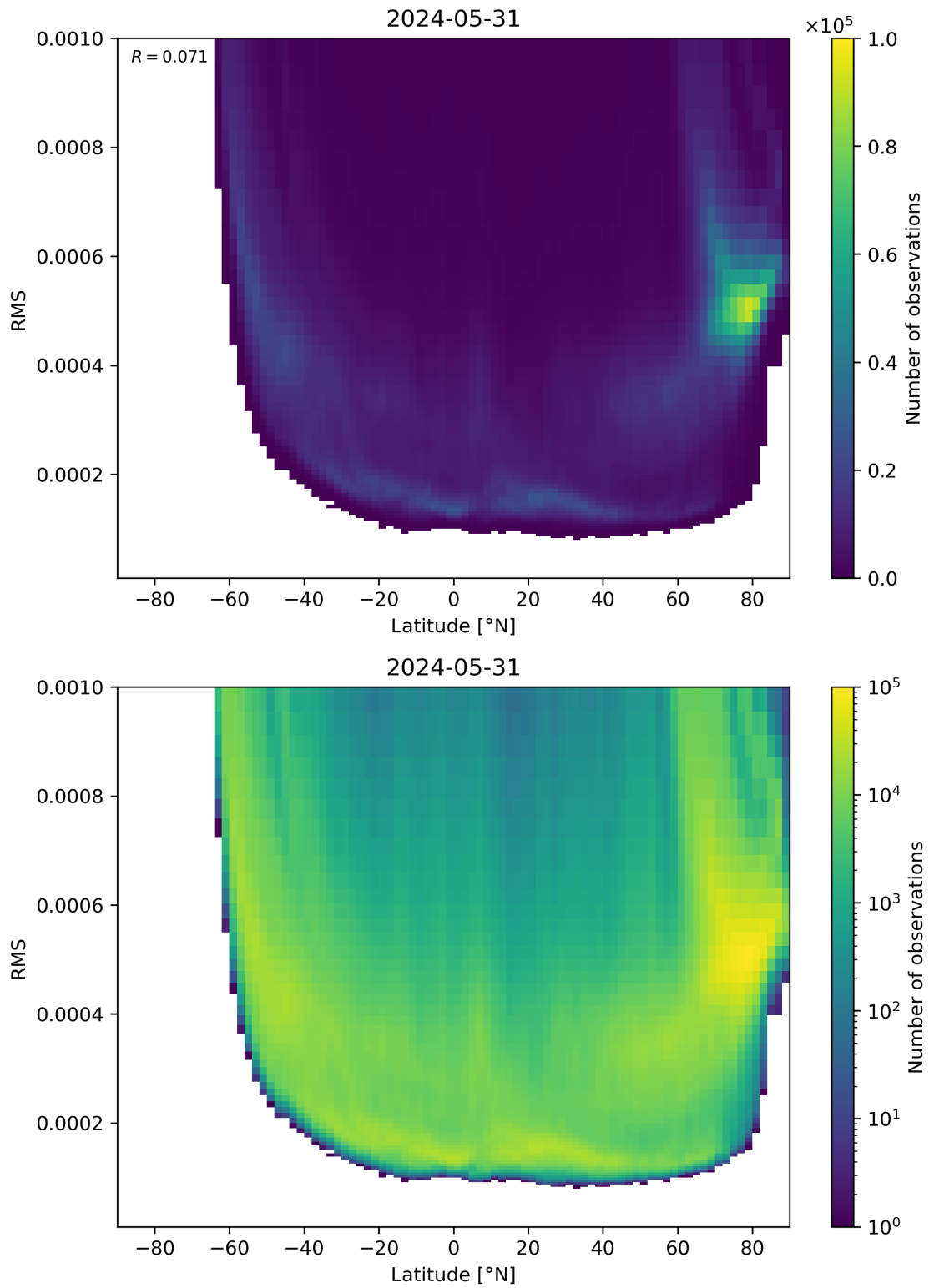
Figure 94: Scatter density plot of “Latitude” against “RMS” for 2024-05-30 to 2024-06-01.
