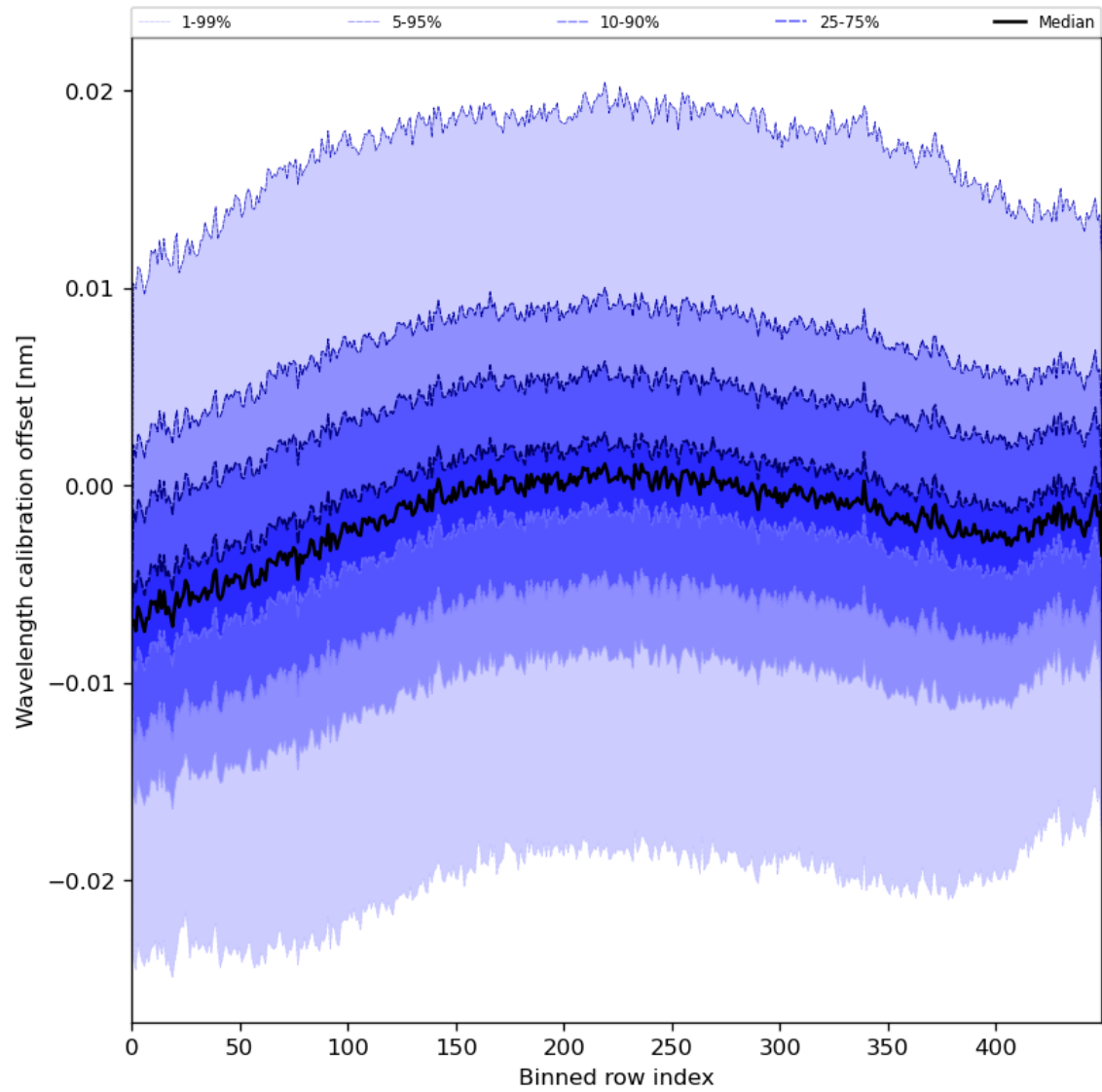
Figure 52: Along track statistics of “Wavelength calibration offset” for 2024-05-30 to 2024-06-01
