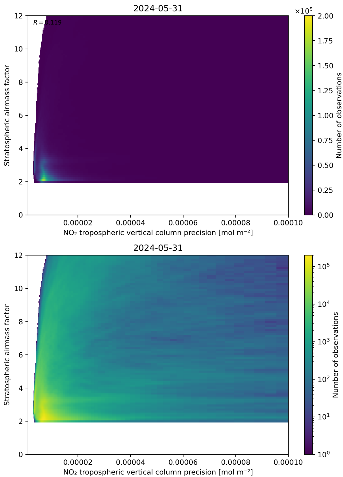
Figure 131: Scatter density plot of “NO 2 tropospheric vertical column precision” against “Stratospheric airmass factor” for 2024-05-30 to 2024-06-01.
