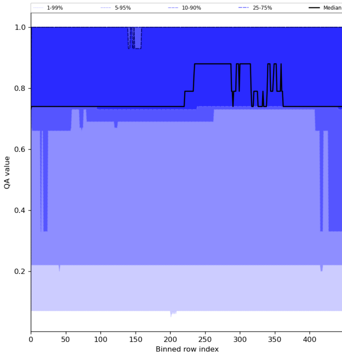
Figure 45: Along track statistics of “QA value” for 2024-05-30 to 2024-06-01
