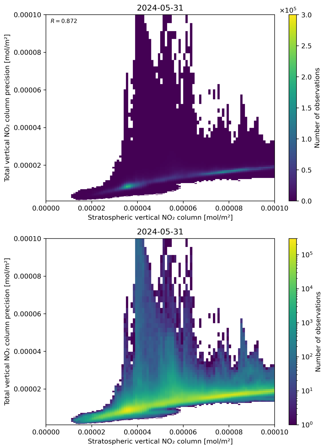
Figure 101: Scatter density plot of “Stratospheric vertical NO 2 column” against “Total vertical NO 2 column precision” for 2024-05-30 to 2024-06-01.
