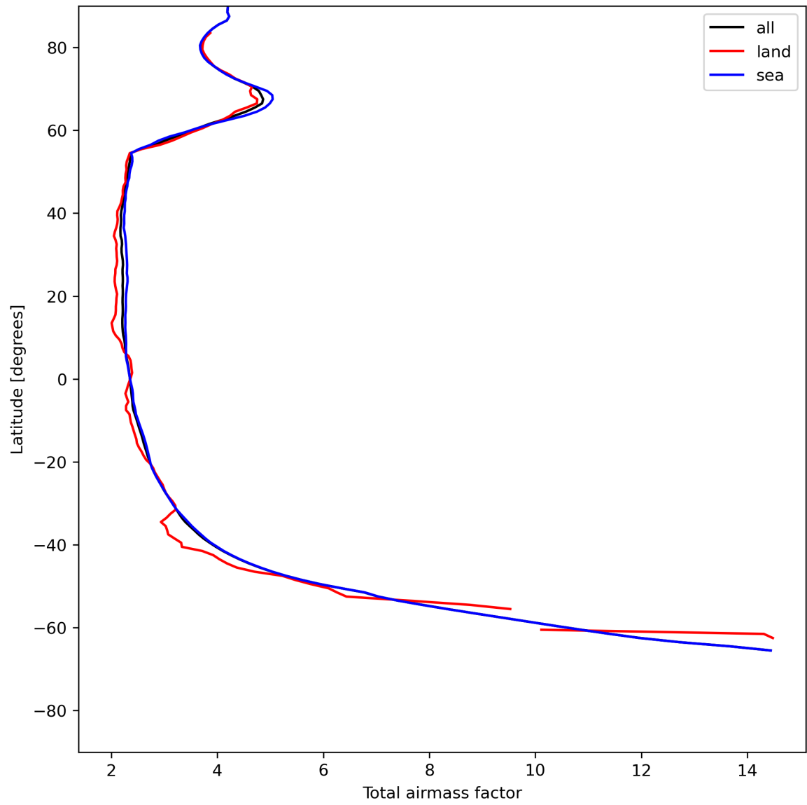
Figure 15: Zonal average of “Total airmass factor” for 2024-05-30 to 2024-06-01.
