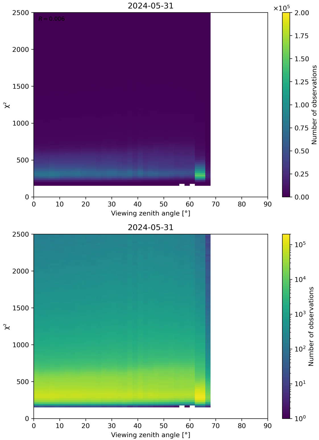
Figure 162: Scatter density plot of “Viewing zenith angle” against “ \chi^2 ” for 2024-05-30 to 2024-06-01.
