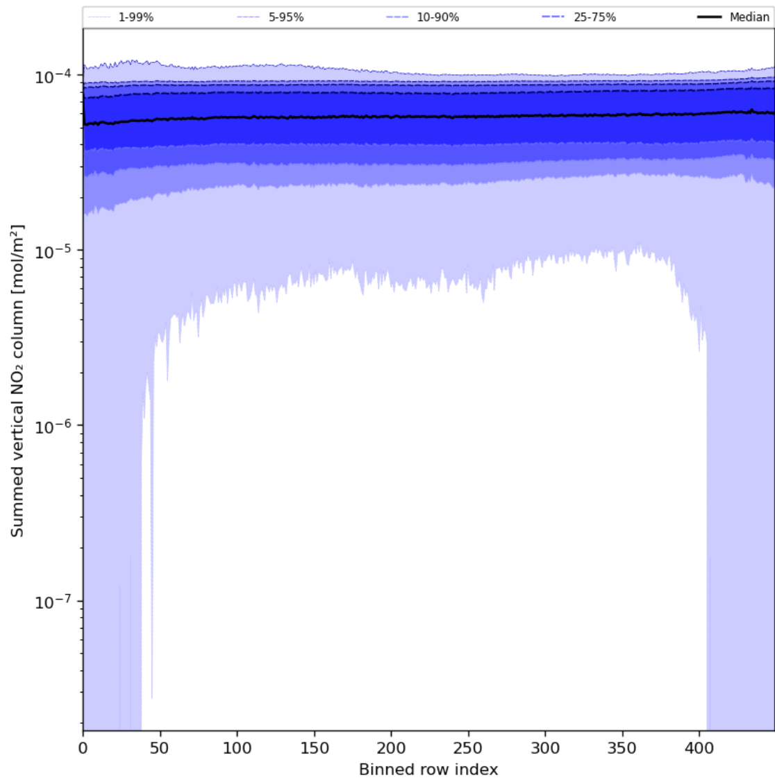
Figure 57: Along track statistics of “Summed vertical NO 2 column” for 2024-05-30 to 2024-06-01
