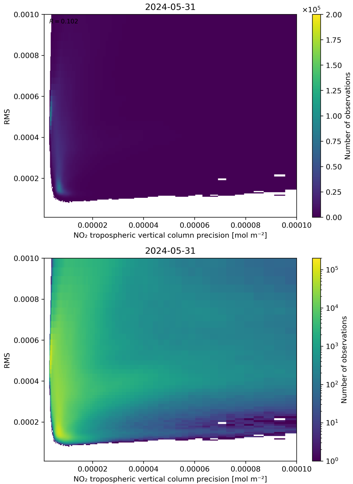
Figure 140: Scatter density plot of “NO 2 tropospheric vertical column precision” against “RMS” for 2024-05-30 to 2024-06-01.
