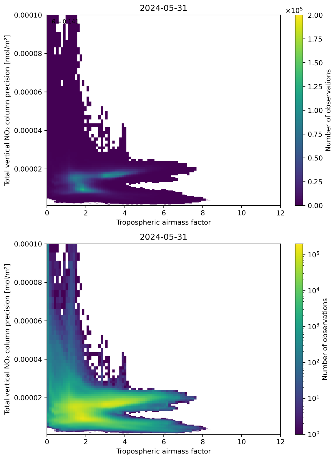
Figure 78: Scatter density plot of “Tropospheric air mass factor” against “Total vertical NO 2 column precision” for 2024-05-30 to 2024-06-01.
