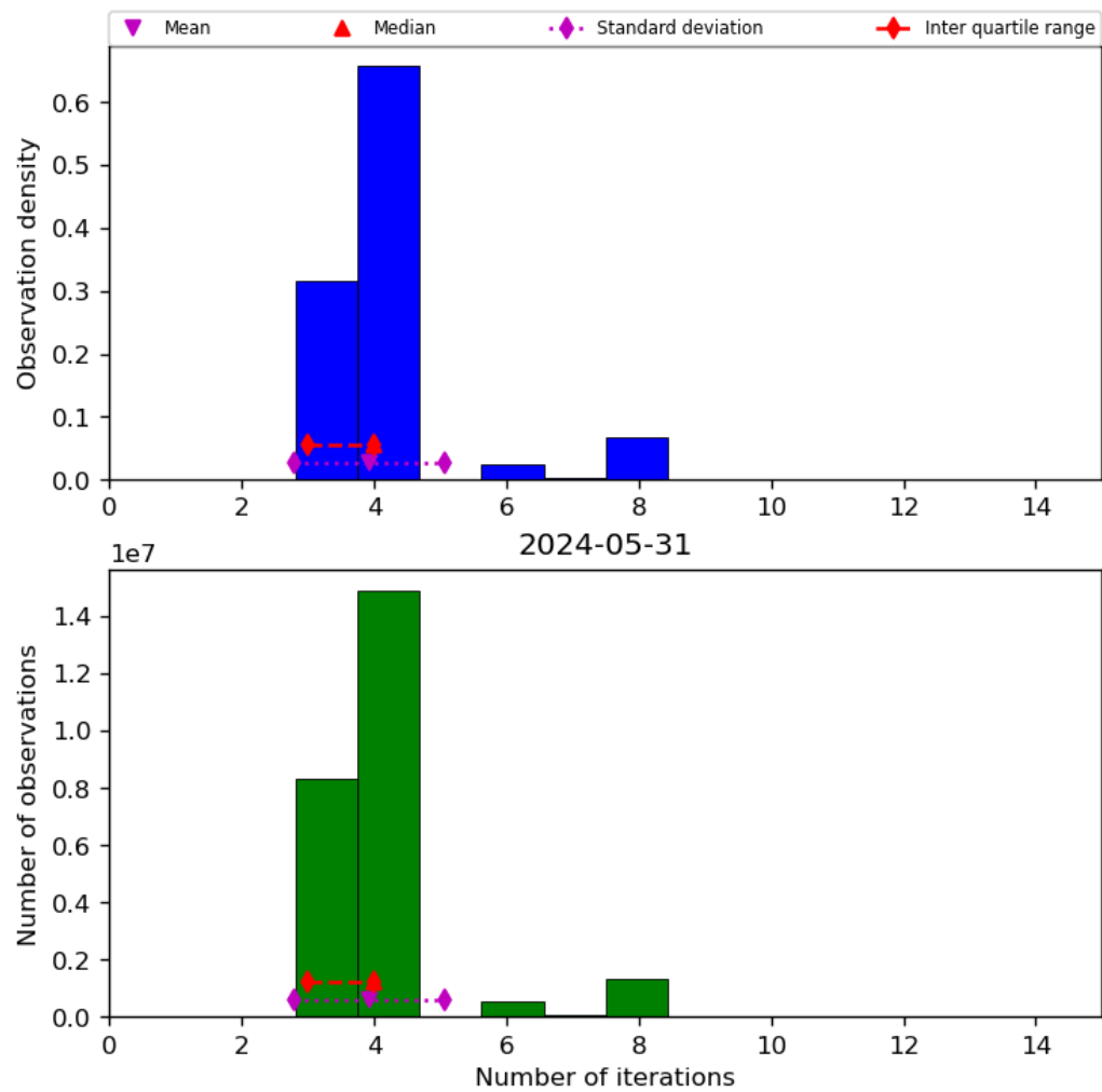
Figure 34: Histogram of "Number of iterations" for 2024-05-30 to 2024-06-01
