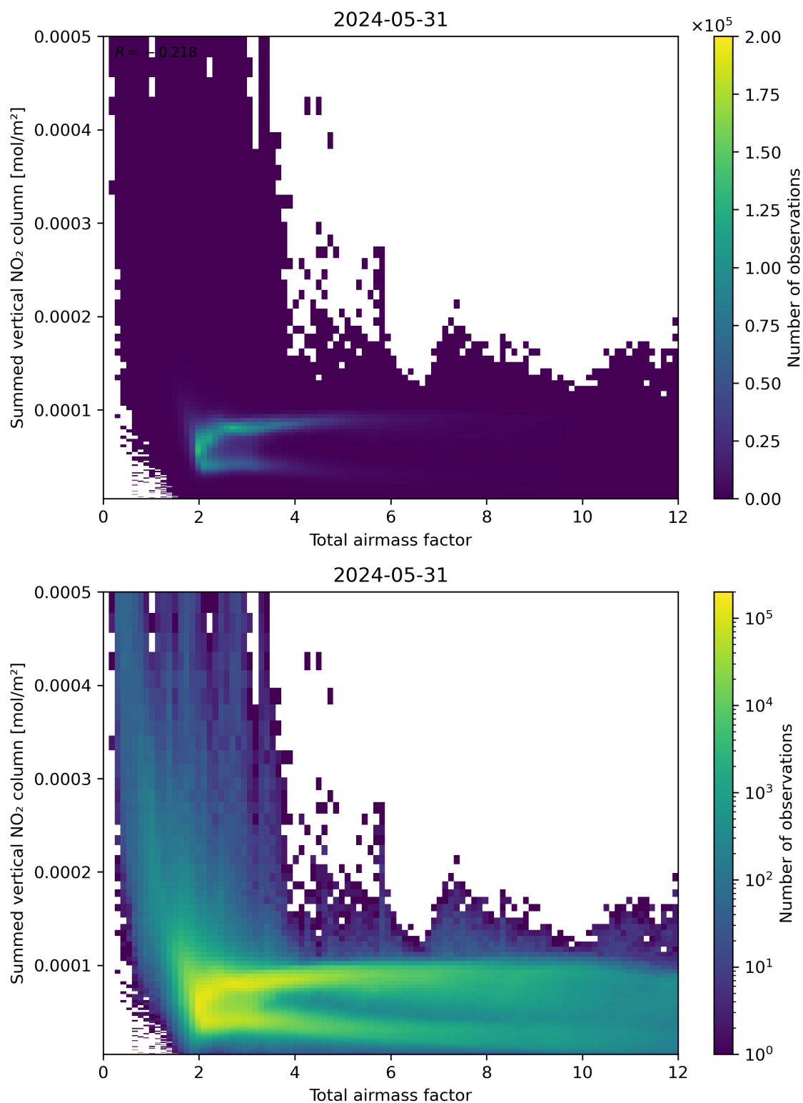
Figure 65: Scatter density plot of “Total airmass factor” against “Summed vertical NO 2 column” for 2024-05-30 to 2024-06-01.
