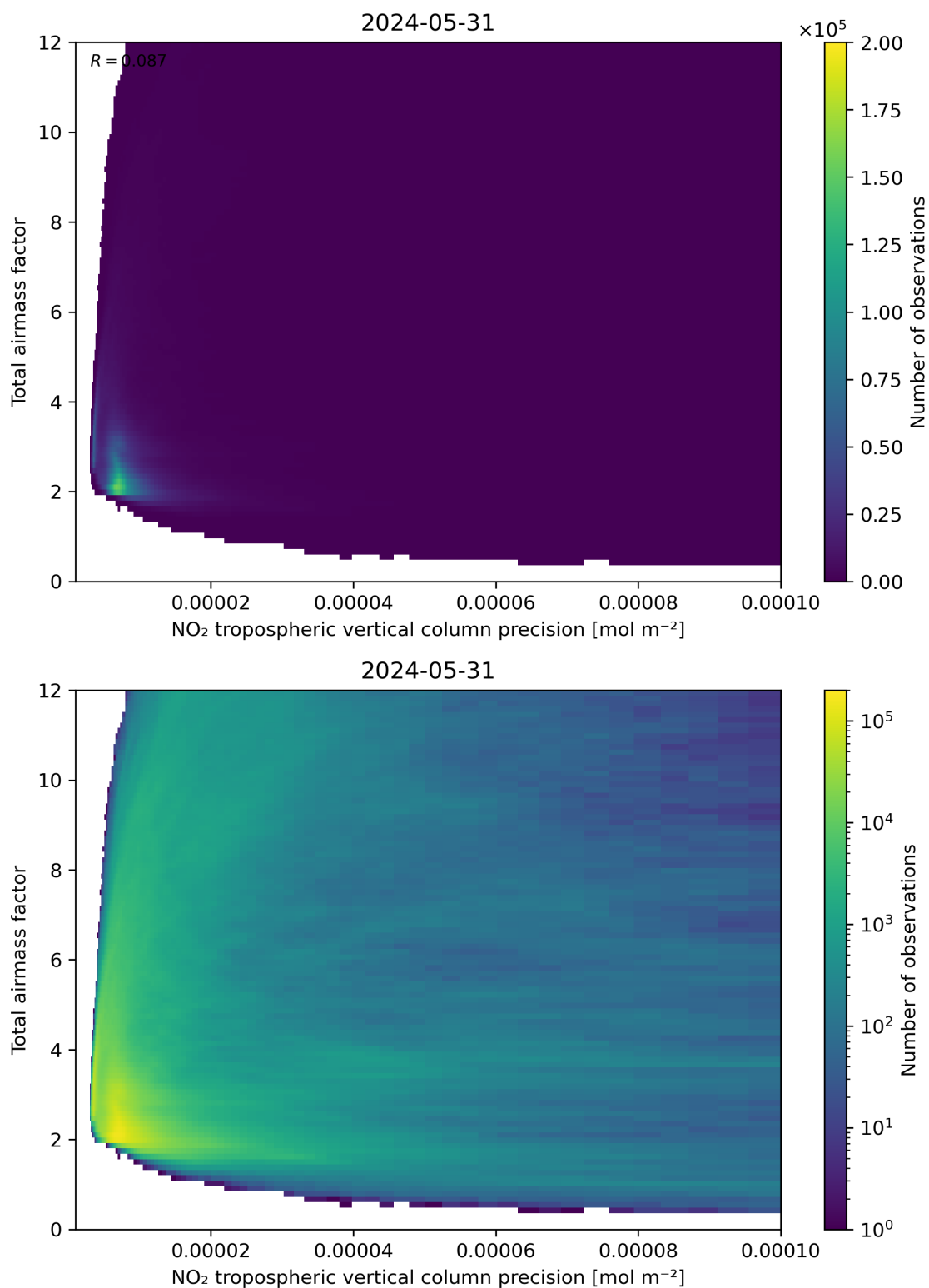
Figure 132: Scatter density plot of “NO 2 tropospheric vertical column precision” against “Total air mass factor” for 2024-05-30 to 2024-06-01.
