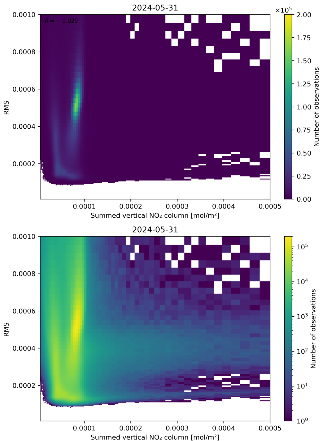
Figure 109: Scatter density plot of “Summed vertical NO 2 column” against “RMS” for 2024-05-30 to 2024-06-01.
