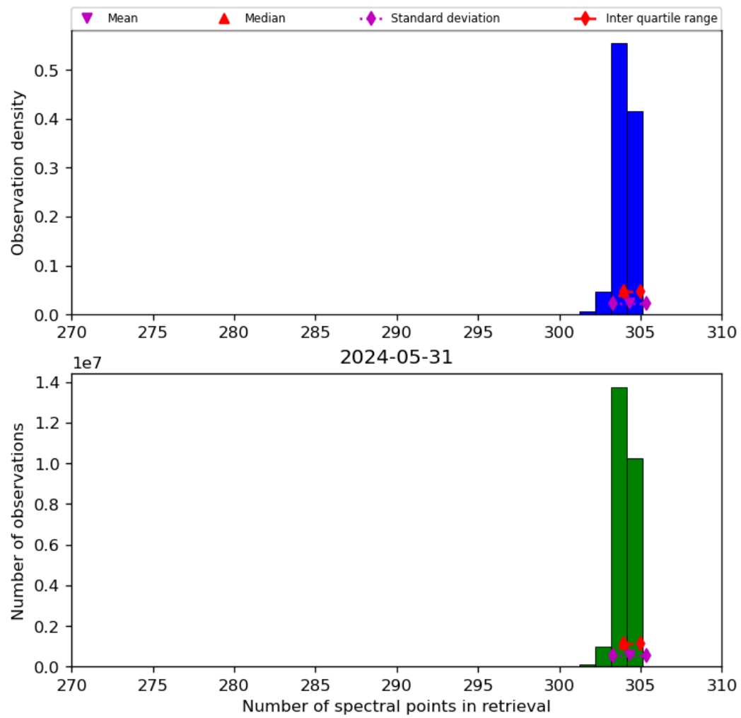
Figure 33: Histogram of “Number of spectral points in retrieval” for 2024-05-30 to 2024-06-01
