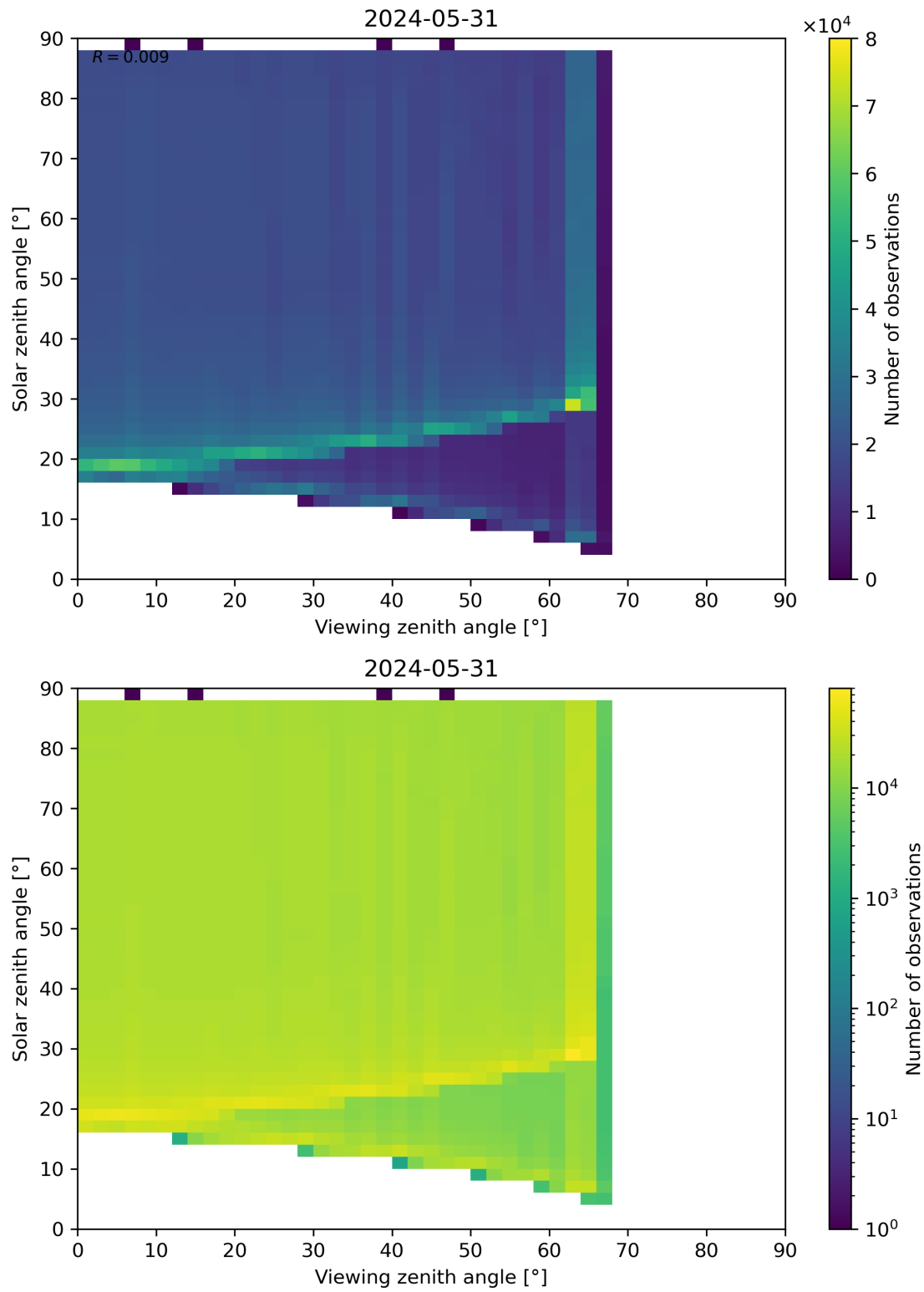
Figure 172: Scatter density plot of “Viewing zenith angle” against “Solar zenith angle” for 2024-05-30 to 2024-06-01.
