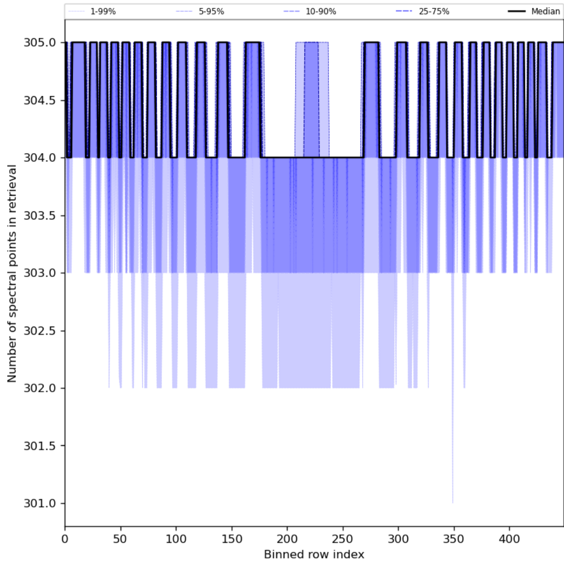
Figure 50: Along track statistics of “Number of spectral points in retrieval” for 2024-05-30 to 2024-06-01
