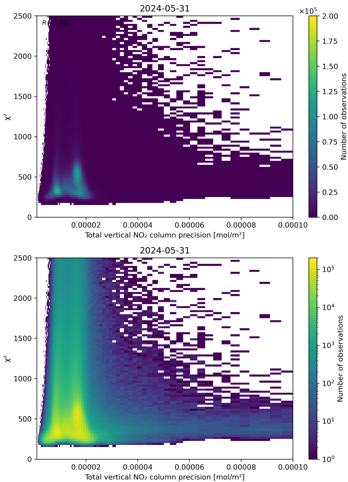
Figure 116: Scatter density plot of “Total vertical NO 2 column precision” against “ \chi^2 ” for 2024-05-30 to 2024-06-01.
