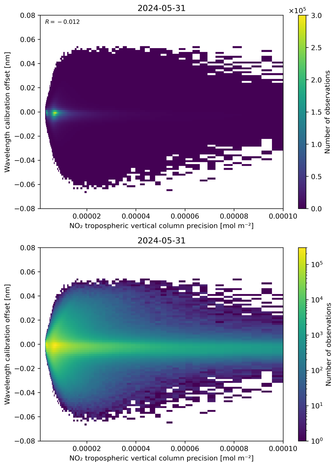
Figure 141: Scatter density plot of “NO 2 tropospheric vertical column precision” against “Wavelength calibration offset” for 2024-05-30 to 2024-06-01.
