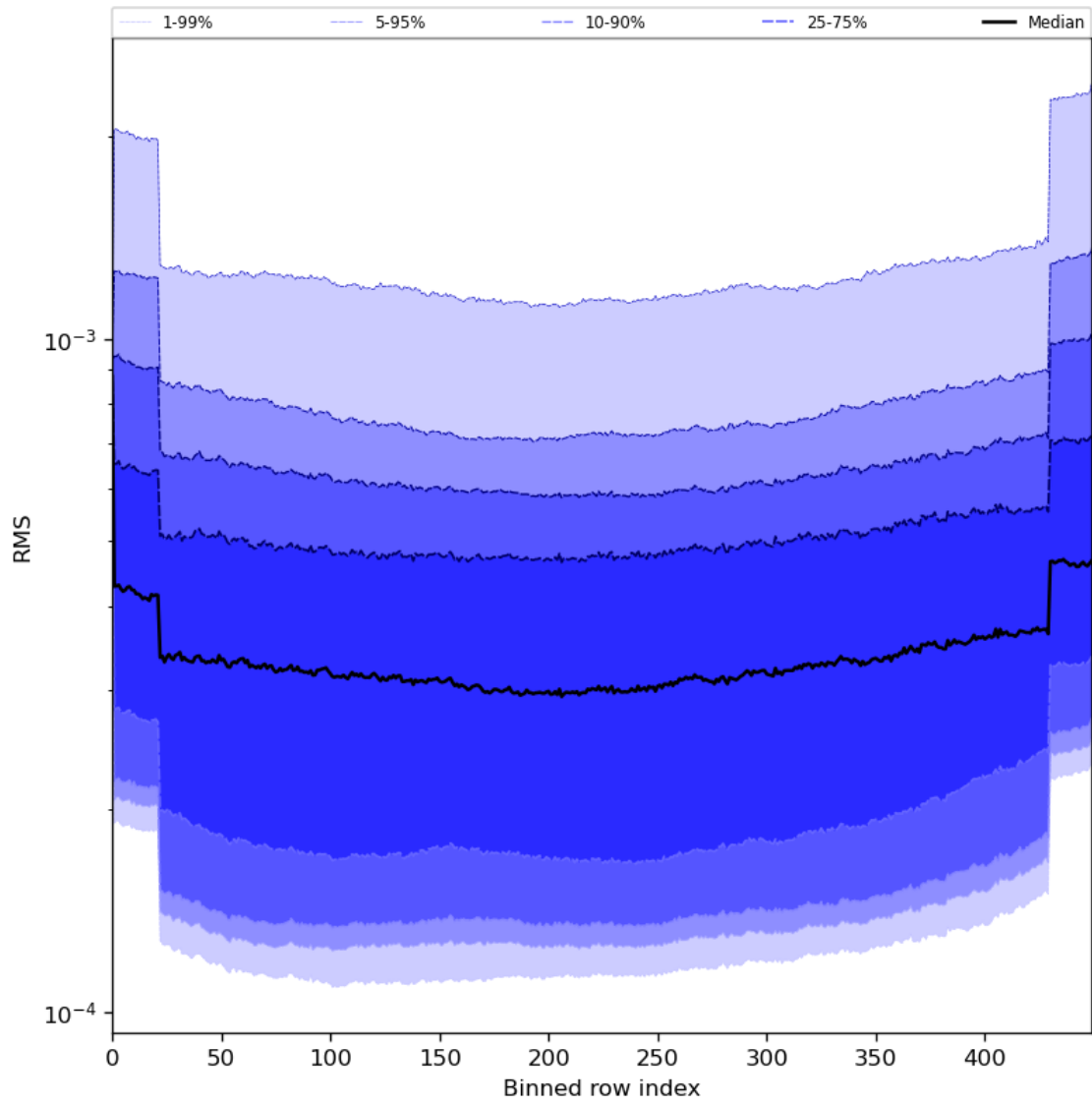
Figure 60: Along track statistics of “RMS” for 2024-05-30 to 2024-06-01
