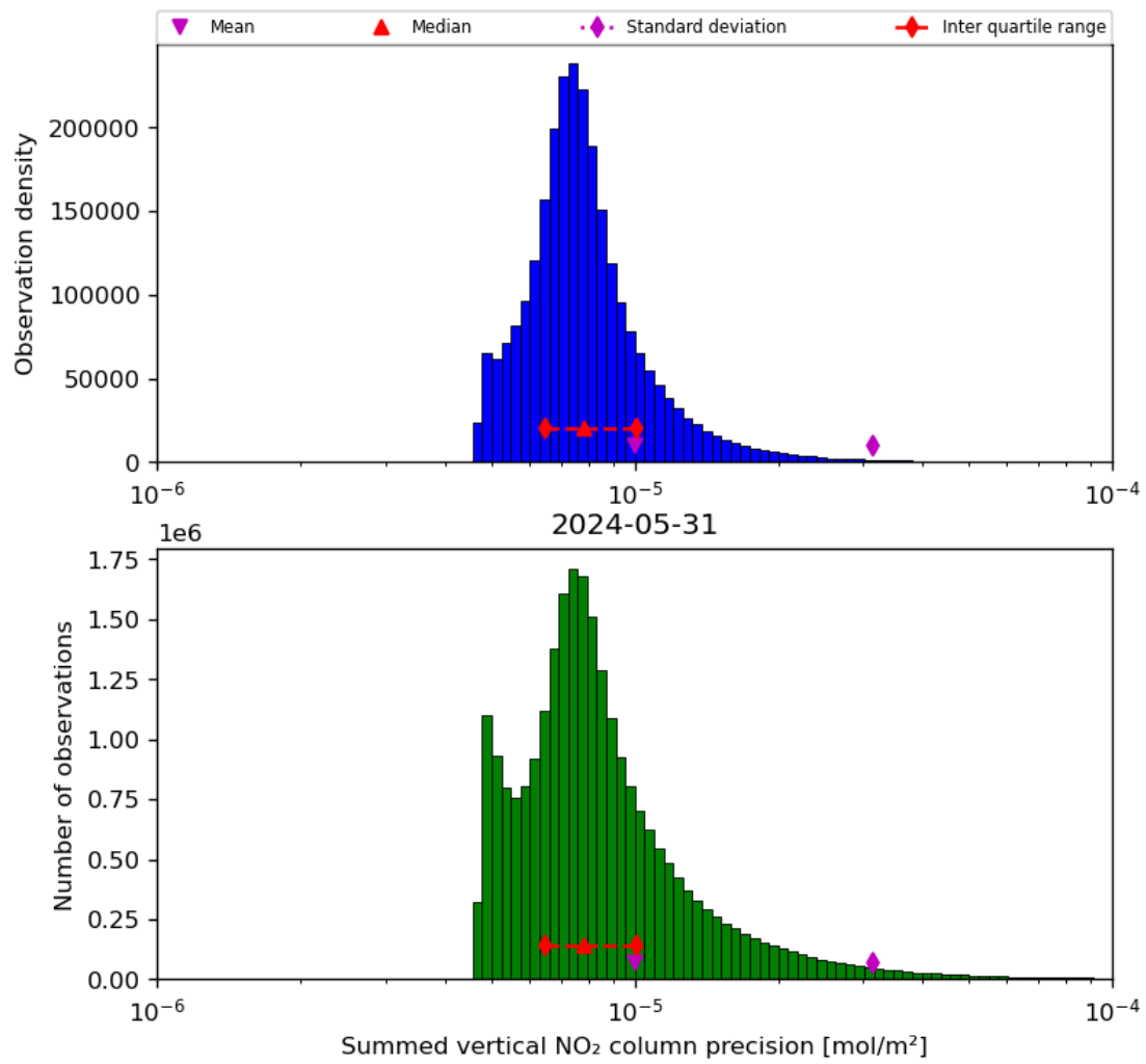
Figure 41: Histogram of "Summed vertical NO 2 column precision" for 2024-05-30 to 2024-06-01
