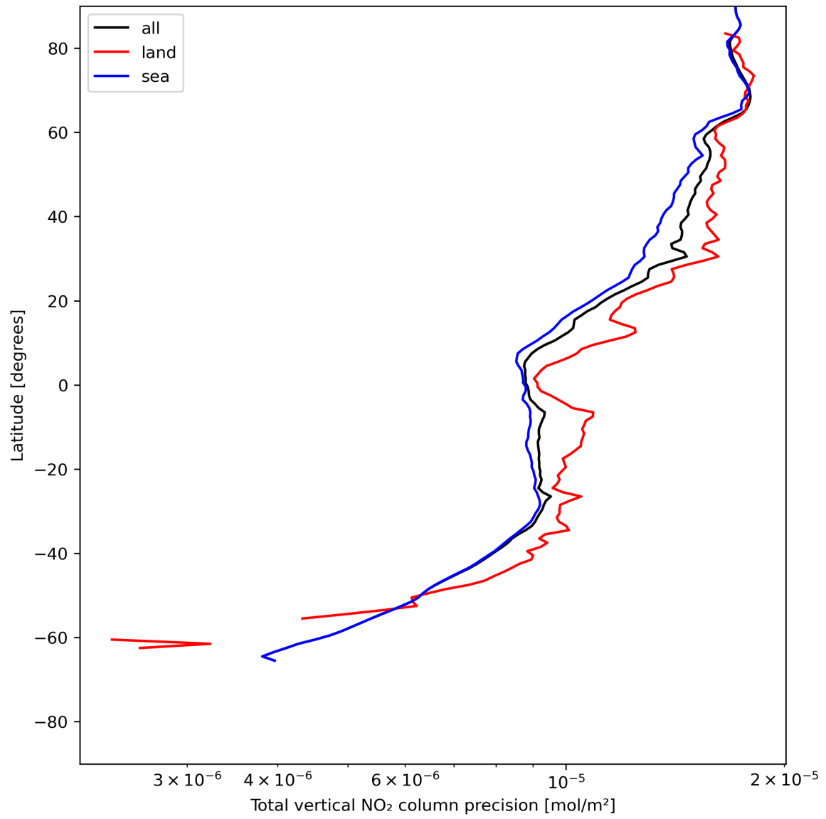
Figure 22: Zonal average of “Total vertical NO 2 column precision” for 2024-05-30 to 2024-06-01.
