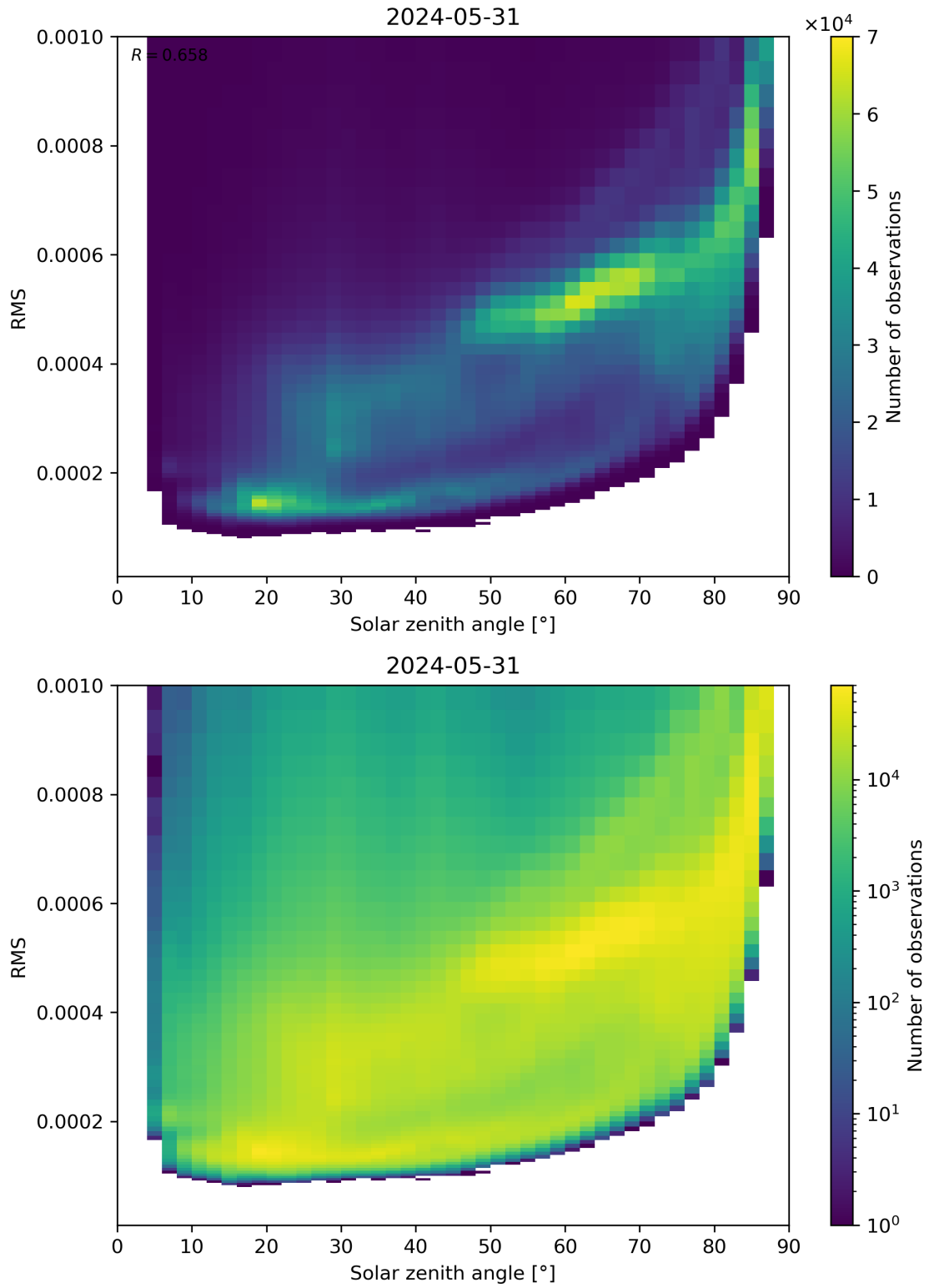
Figure 157: Scatter density plot of “Solar zenith angle” against “RMS” for 2024-05-30 to 2024-06-01.
