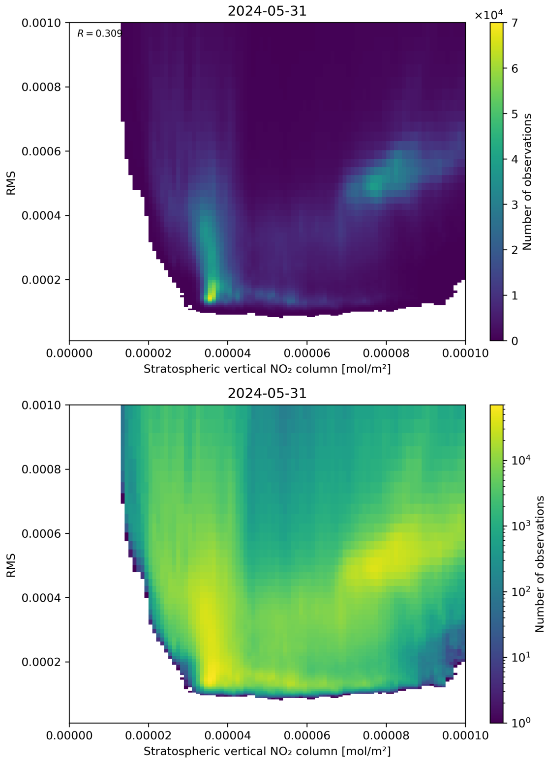
Figure 102: Scatter density plot of “Stratospheric vertical NO 2 column” against “RMS” for 2024-05-30 to 2024-06-01.
