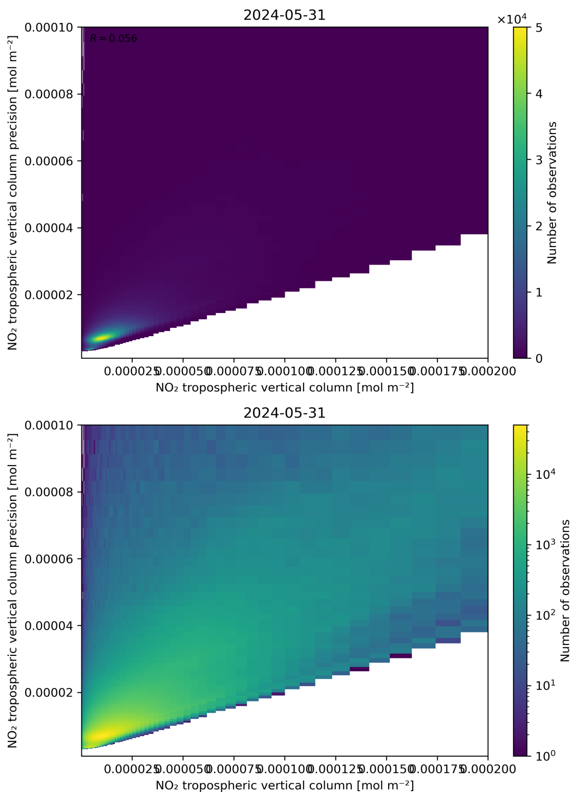
Figure 130: Scatter density plot of “NO 2 tropospheric vertical column” against “NO 2 tropospheric vertical column precision” for 2024-05-30 to 2024-06-01.
