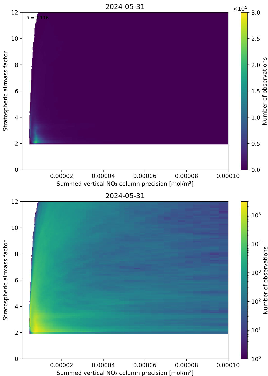
Figure 106: Scatter density plot of “Summed vertical NO 2 column precision” against “Stratospheric airmass factor” for 2024-05-30 to 2024-06-01.
