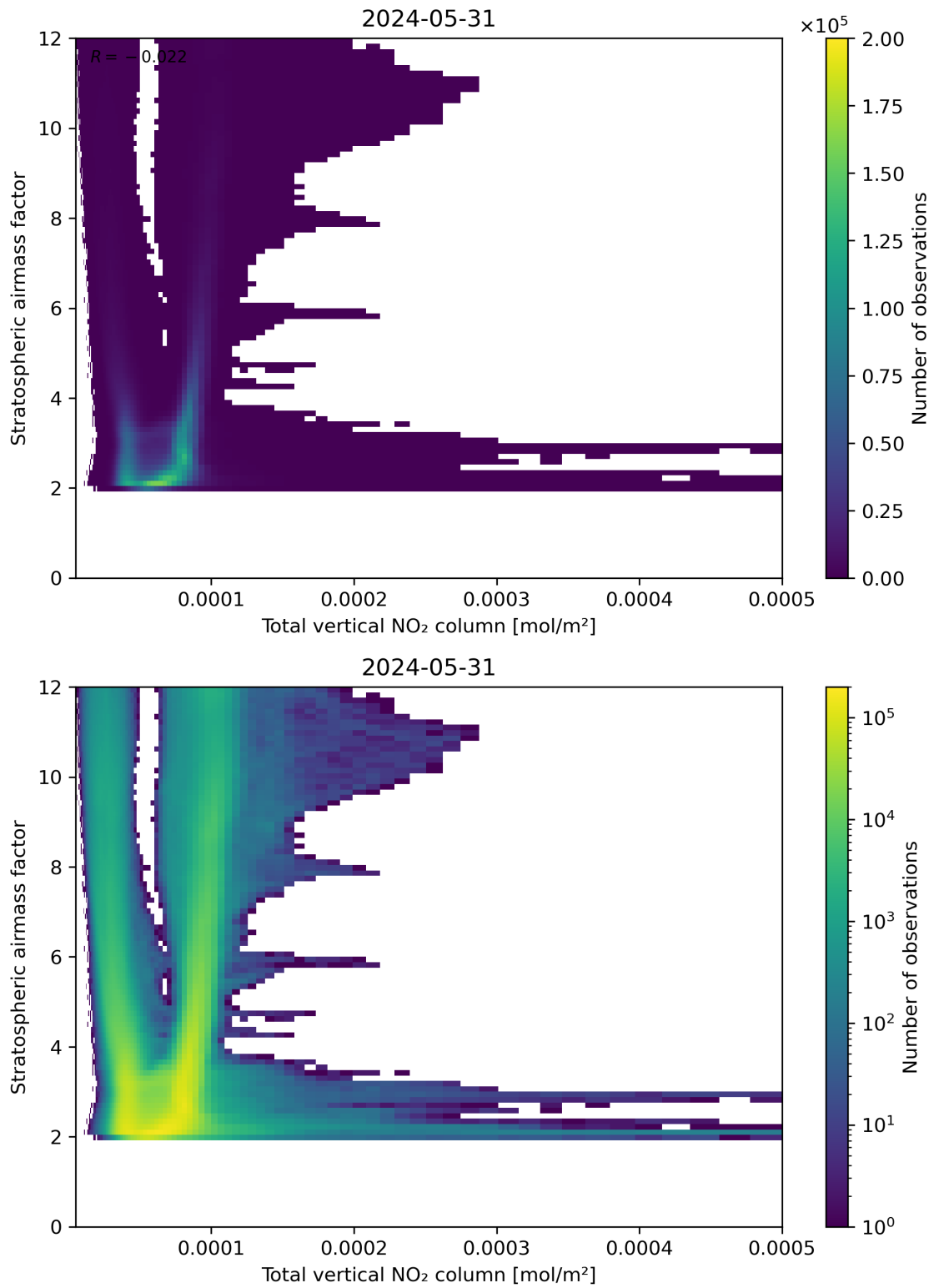
Figure 110: Scatter density plot of “Total vertical NO 2 column” against “Stratospheric airmass factor” for 2024-05-30 to 2024-06-01.
