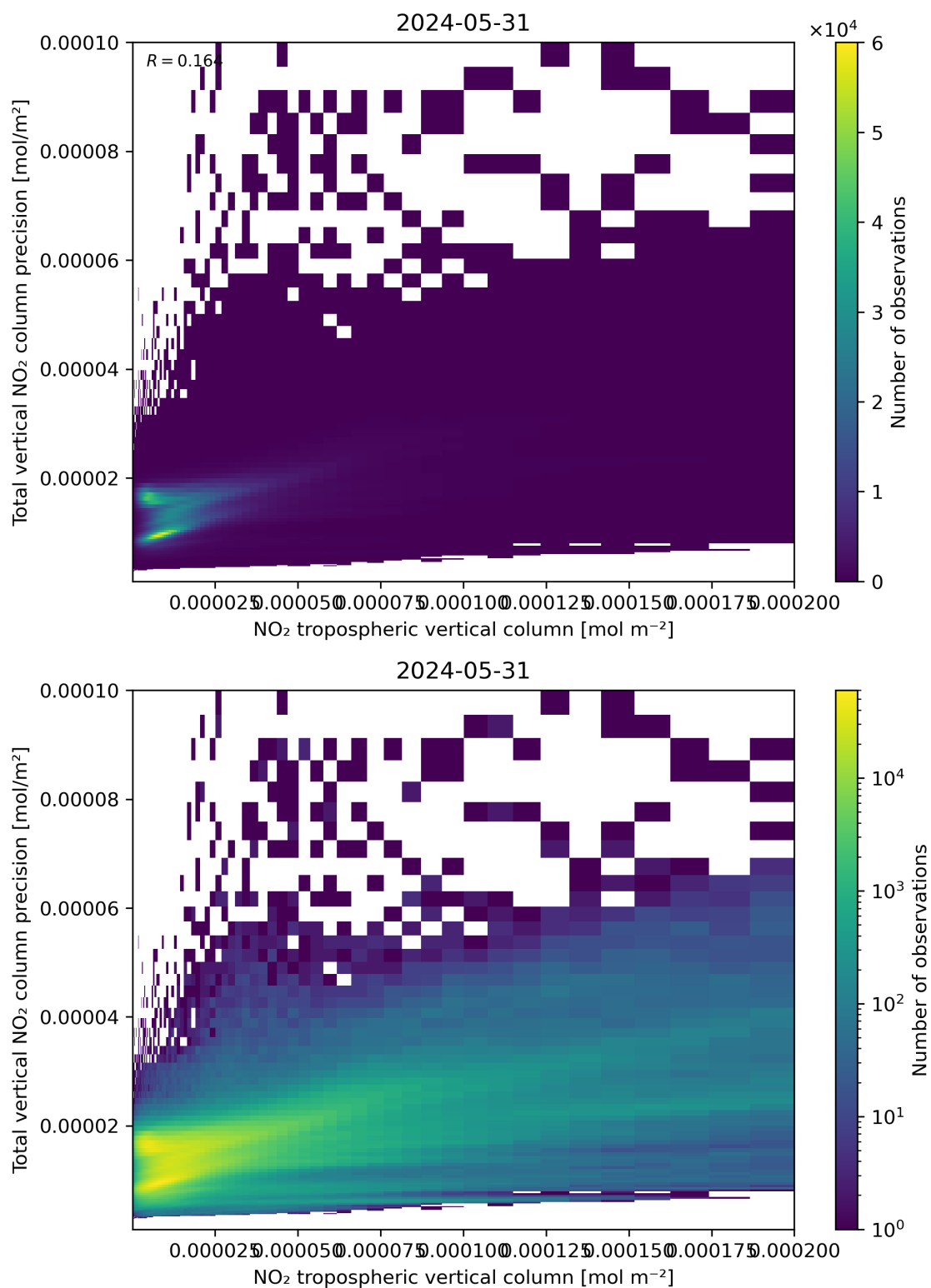
Figure 129: Scatter density plot of “NO 2 tropospheric vertical column” against “Total vertical NO 2 column precision” for 2024-05-30 to 2024-06-01.
