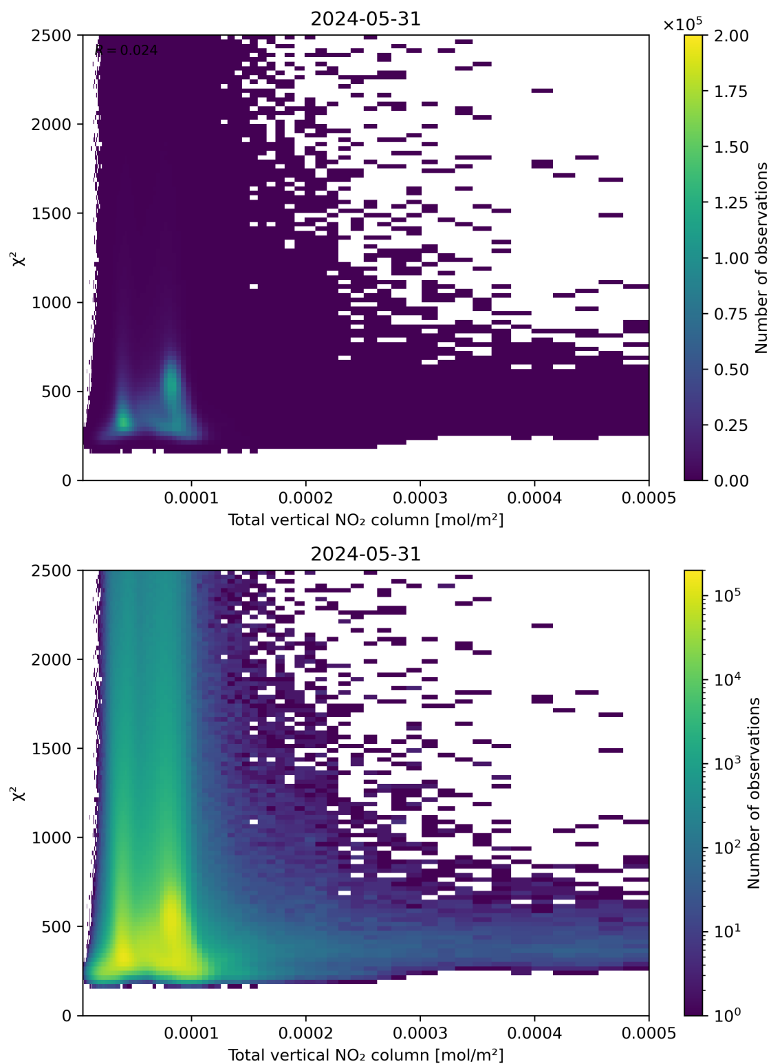
Figure 111: Scatter density plot of “Total vertical NO 2 column” against “ \chi^2 ” for 2024-05-30 to 2024-06-01.
