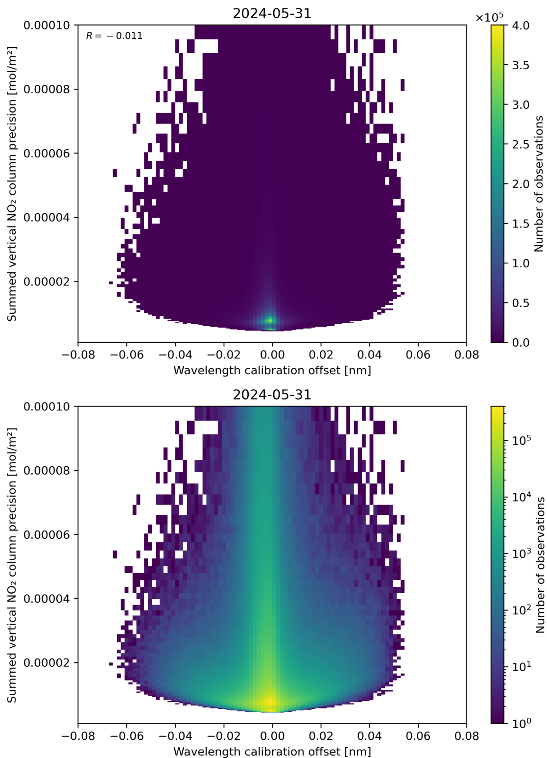
Figure 178: Scatter density plot of “Wavelength calibration offset” against “Summed vertical NO 2 column precision” for 2024-05-30 to 2024-06-01.
