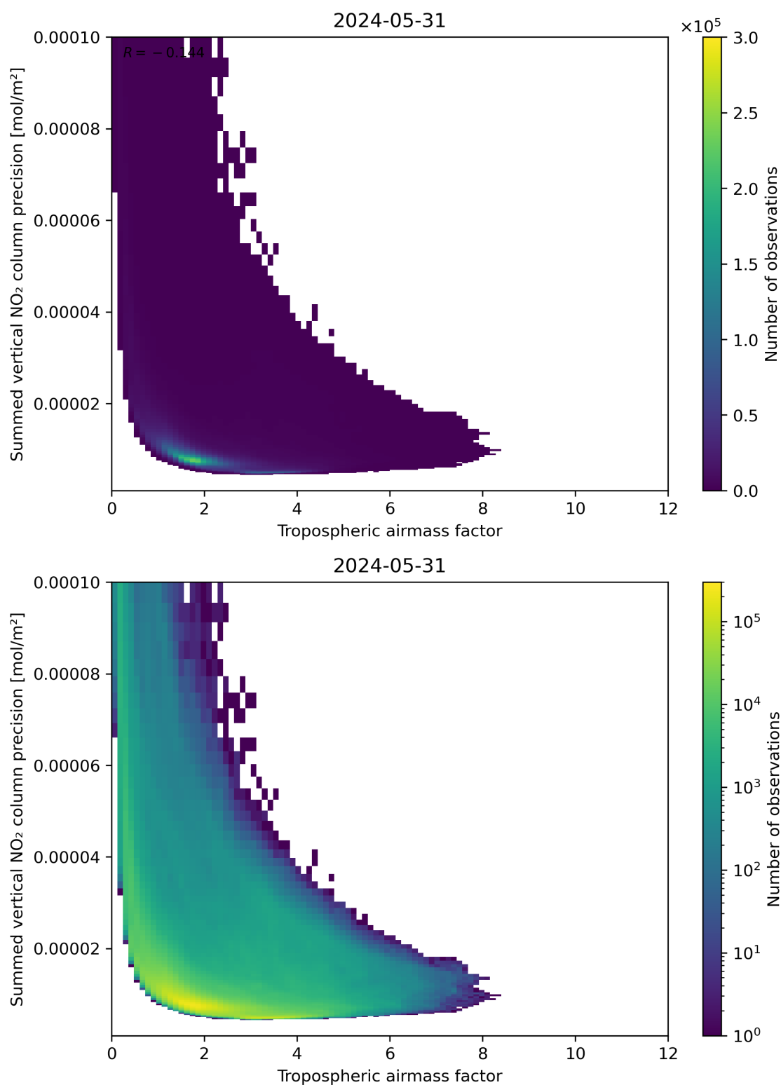
Figure 76: Scatter density plot of “Tropospheric air mass factor” against “Summed vertical NO 2 column precision” for 2024-05-30 to 2024-06-01.
