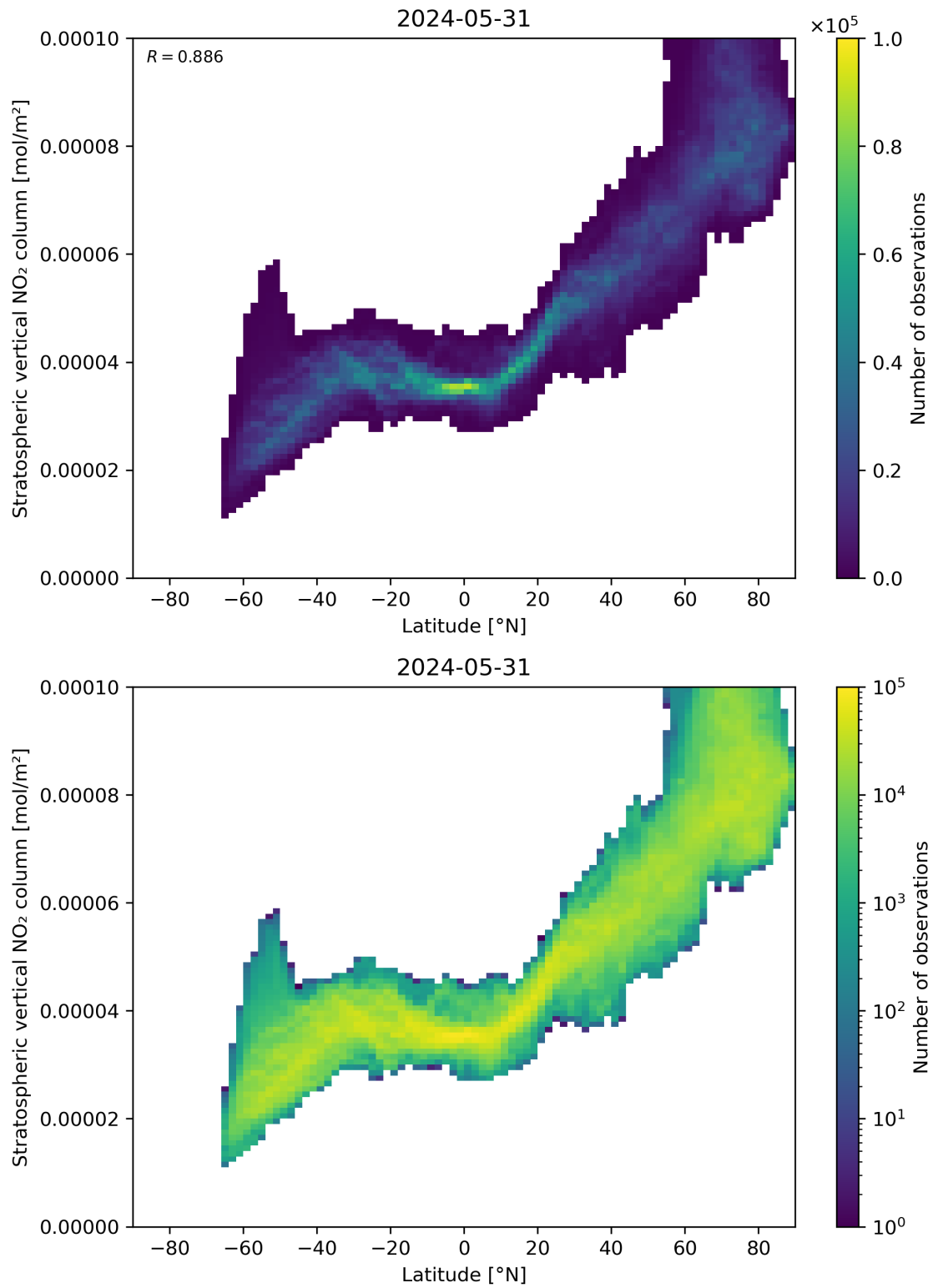
Figure 87: Scatter density plot of “Latitude” against “Stratospheric vertical NO 2 column” for 2024-05-30 to 2024-06-01.
