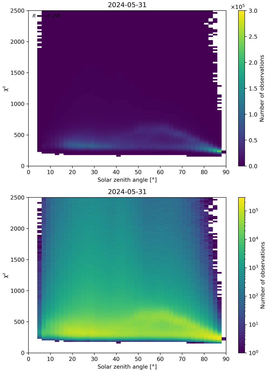
Figure 148: Scatter density plot of “Solar zenith angle” against “ \chi^2 ” for 2024-05-30 to 2024-06-01.
