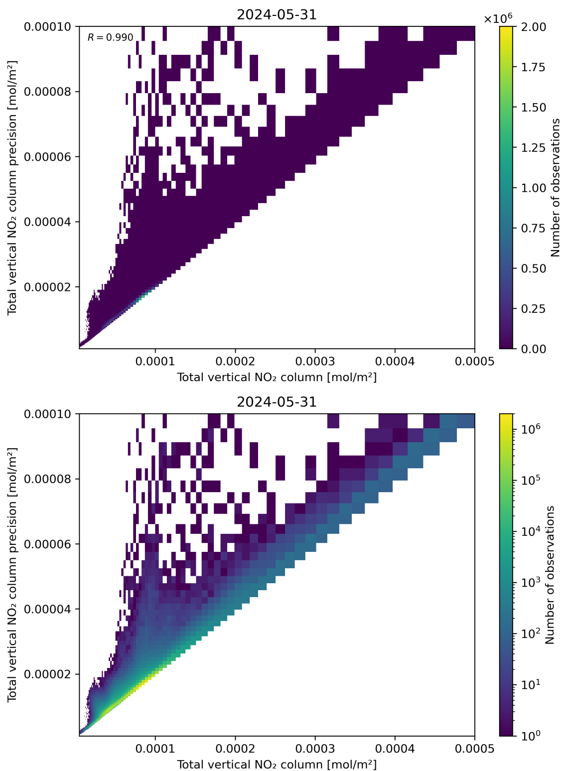
Figure 114: Scatter density plot of “Total vertical NO 2 column” against “Total vertical NO 2 column precision” for 2024-05-30 to 2024-06-01.
