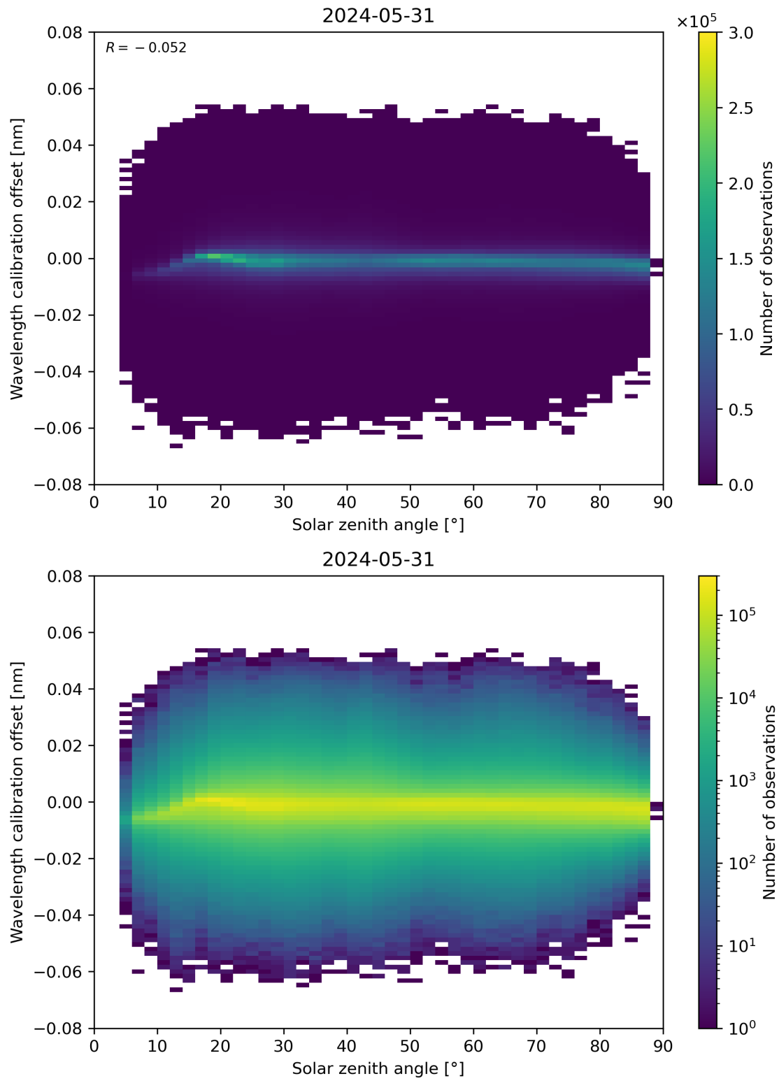
Figure 158: Scatter density plot of “Solar zenith angle” against “Wavelength calibration offset” for 2024-05-30 to 2024-06-01.
