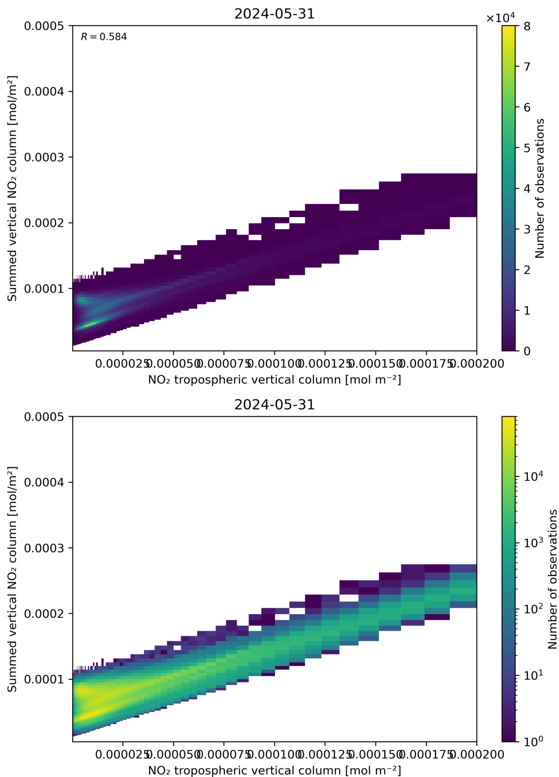
Figure 126: Scatter density plot of “NO 2 tropospheric vertical column” against “Summed vertical NO 2 column” for 2024-05-30 to 2024-06-01.
