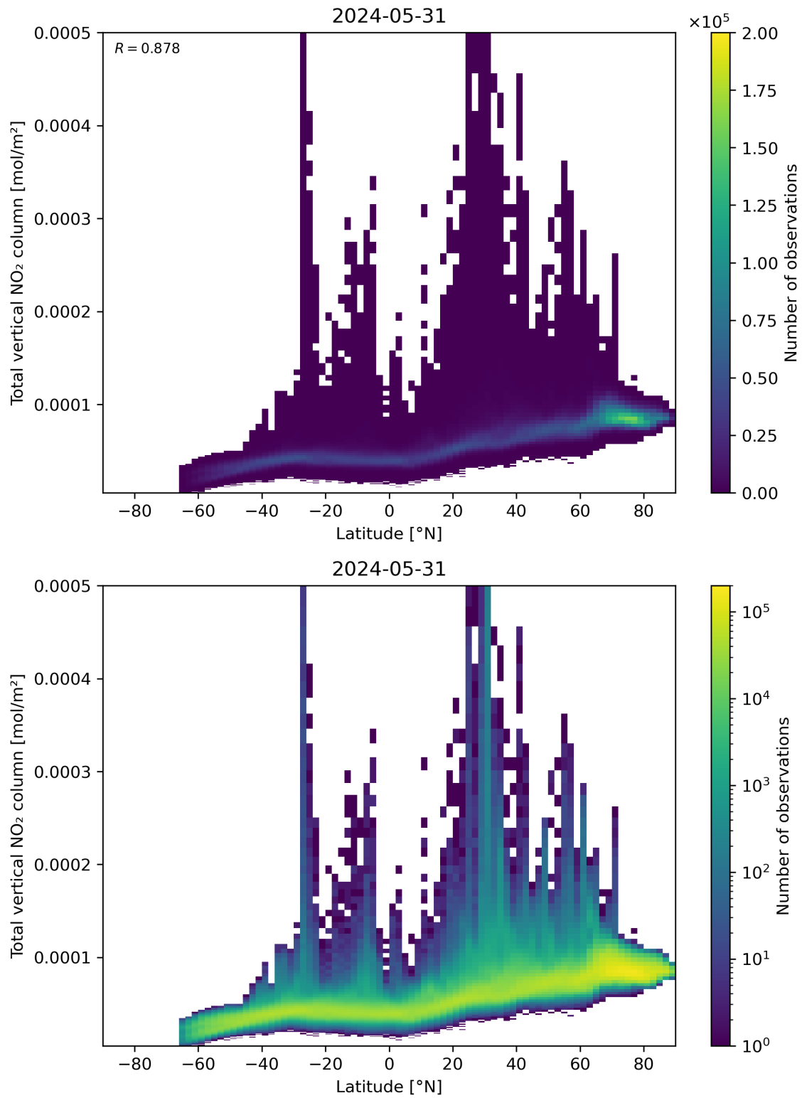
Figure 90: Scatter density plot of “Latitude” against “Total vertical NO 2 column” for 2024-05-30 to 2024-06-01.
