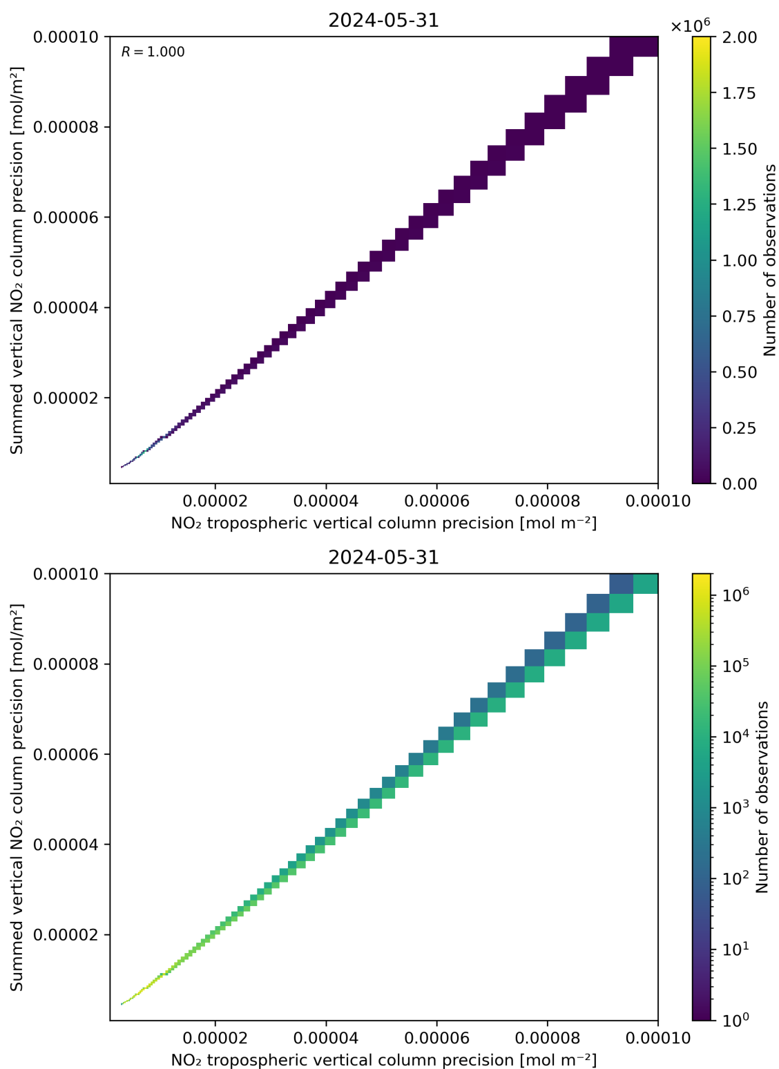
Figure 137: Scatter density plot of “NO 2 tropospheric vertical column precision” against “Summed vertical NO 2 column precision” for 2024-05-30 to 2024-06-01.
