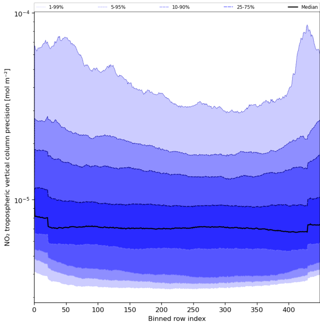
Figure 47: Along track statistics of “NO 2 tropospheric vertical column precision” for 2024-05-30 to 2024-06-01
