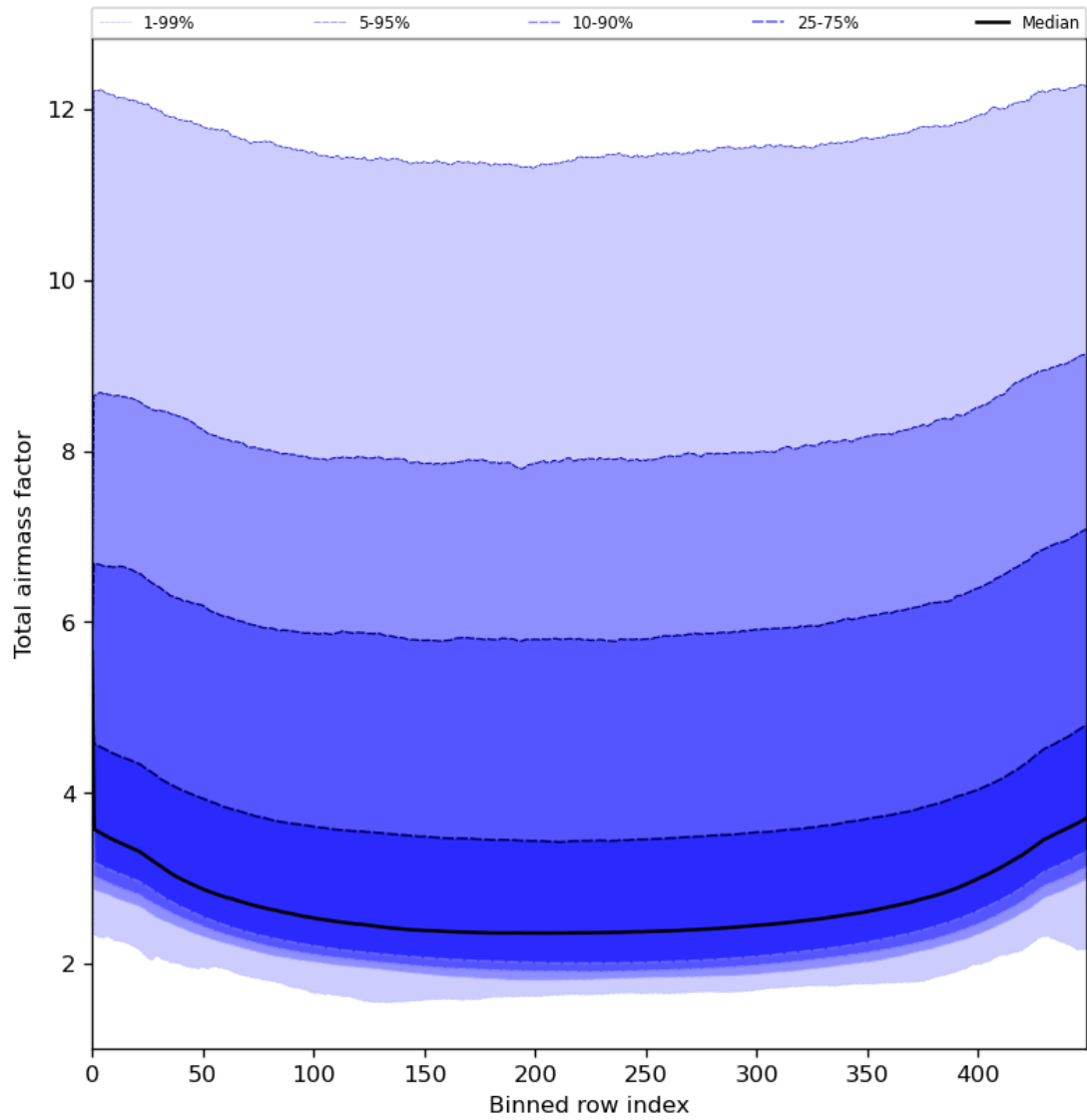
Figure 49: Along track statistics of “Total airmass factor” for 2024-05-30 to 2024-06-01
