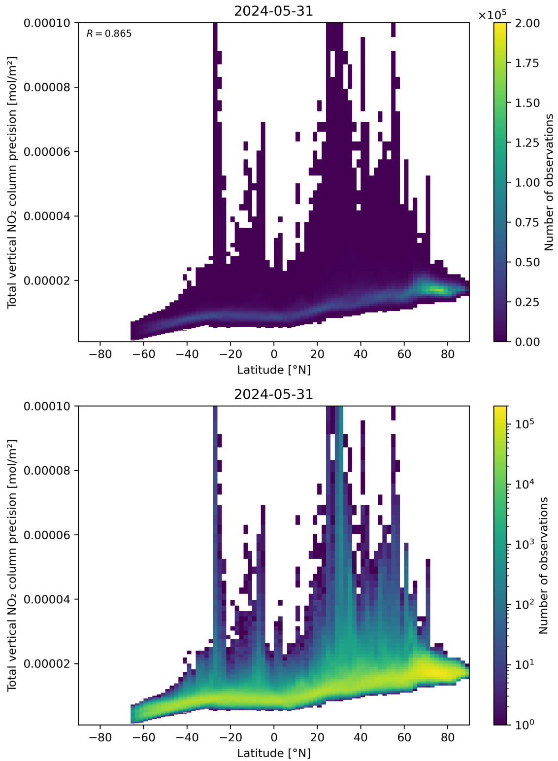
Figure 91: Scatter density plot of “Latitude” against “Total vertical NO 2 column precision” for 2024-05-30 to 2024-06-01.
