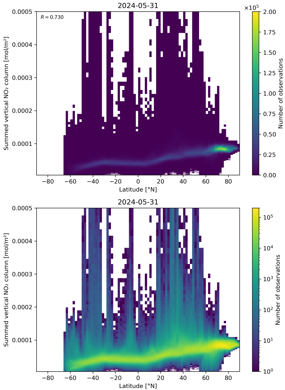
Figure 88: Scatter density plot of “Latitude” against “Summed vertical NO 2 column” for 2024-05-30 to 2024-06-01.
