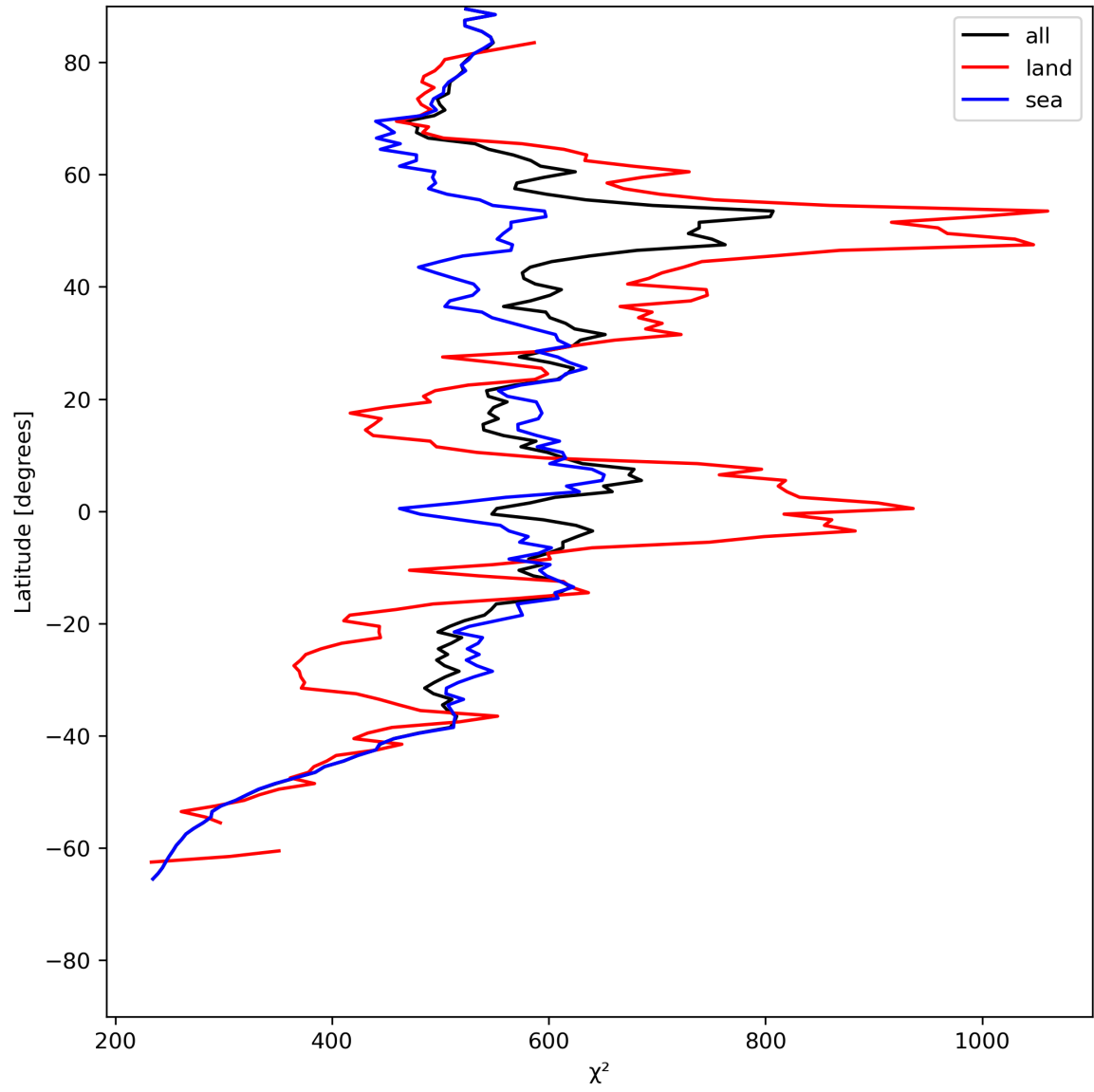
Figure 25: Zonal average of “ \chi^2 ” for 2024-05-30 to 2024-06-01.
