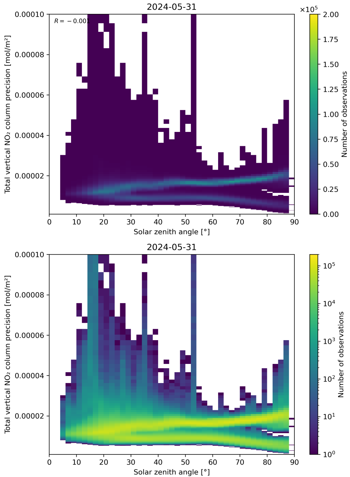
Figure 154: Scatter density plot of “Solar zenith angle” against “Total vertical NO 2 column precision” for 2024-05-30 to 2024-06-01.
