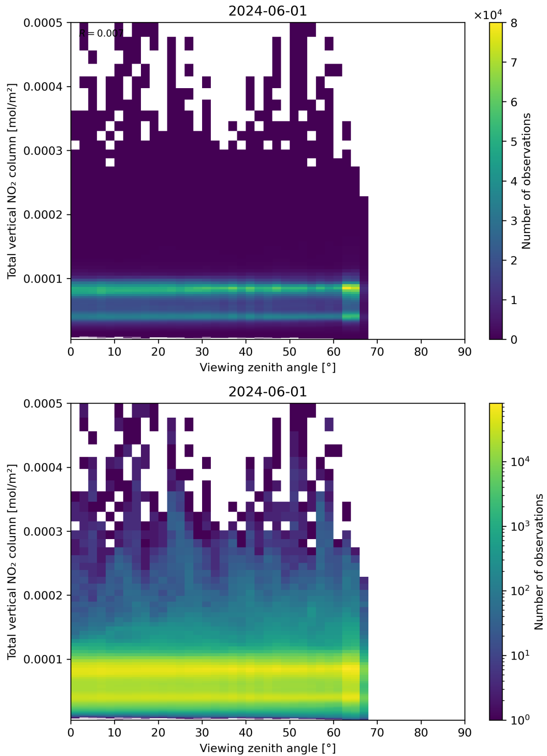
Figure 167: Scatter density plot of “Viewing zenith angle” against “Total vertical NO 2 column” for 2024-05-31 to 2024-06-02.
