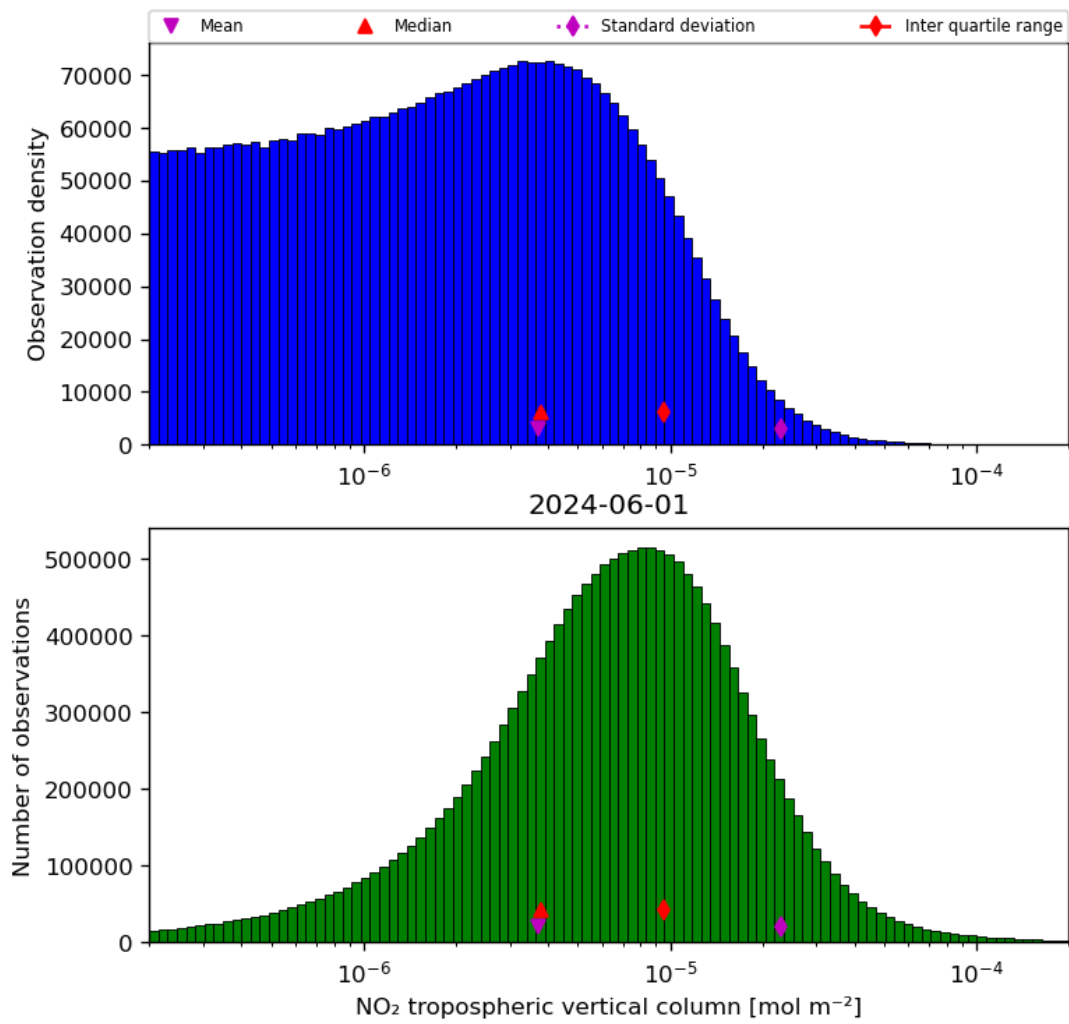
Figure 29: Histogram of “NO 2 tropospheric vertical column” for 2024-05-31 to 2024-06-02
