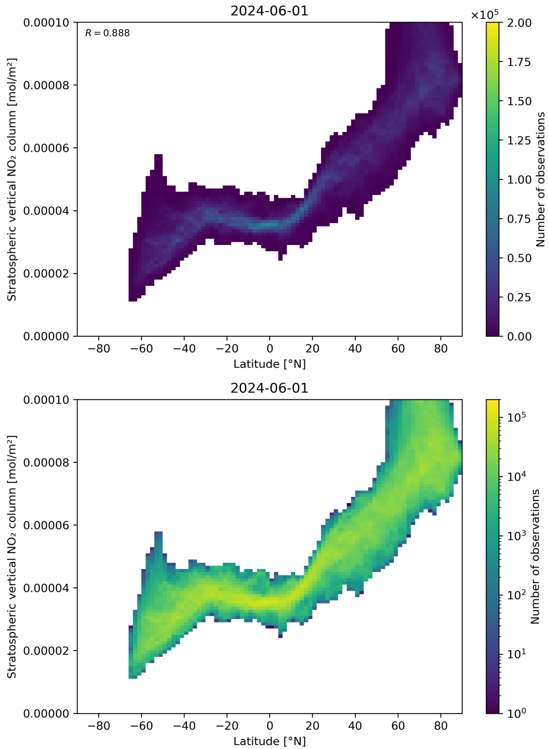
Figure 87: Scatter density plot of “Latitude” against “Stratospheric vertical NO 2 column” for 2024-05-31 to 2024-06-02.
