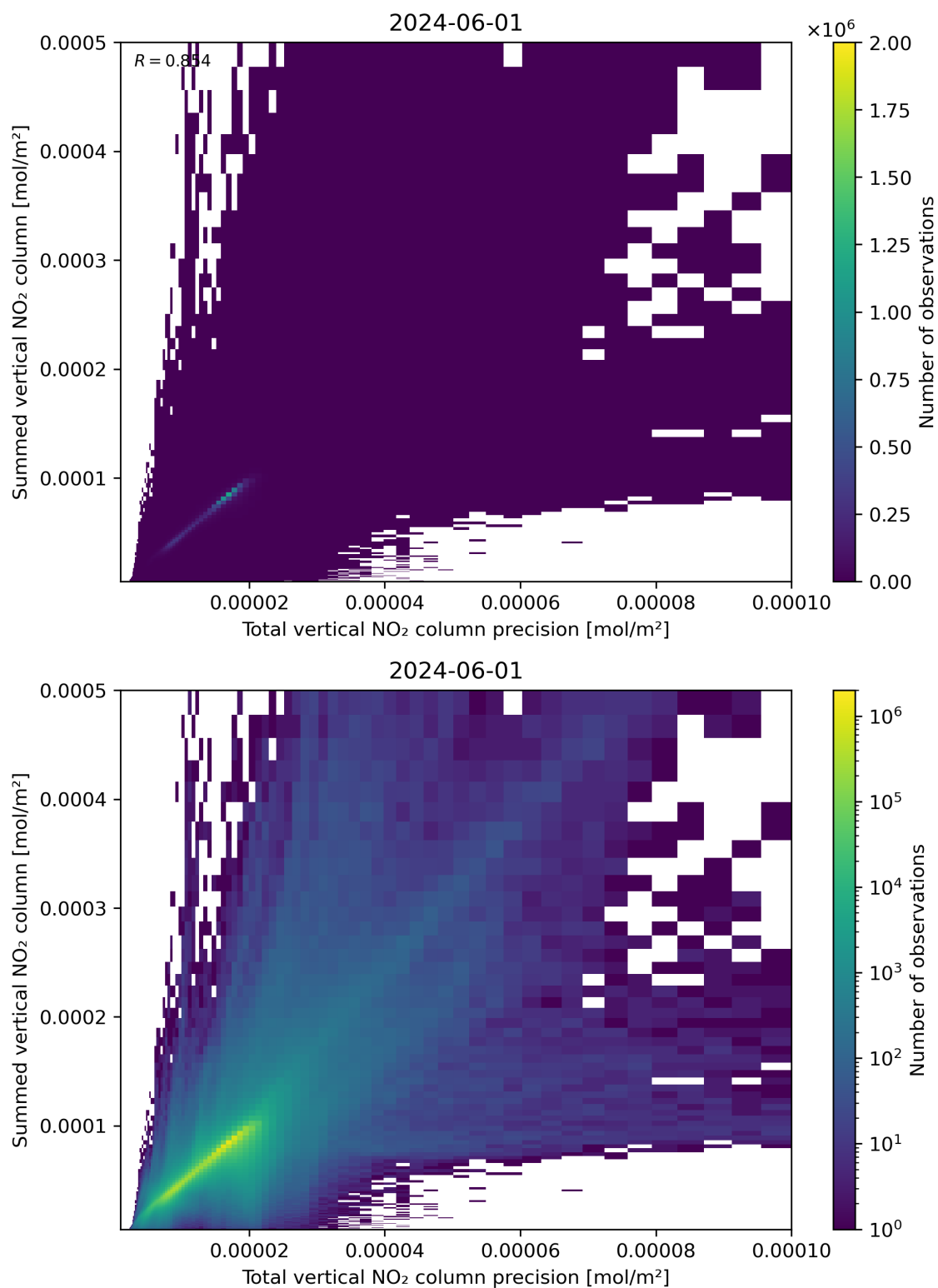
Figure 117: Scatter density plot of “Total vertical NO 2 column precision” against “Summed vertical NO 2 column” for 2024-05-31 to 2024-06-02.
