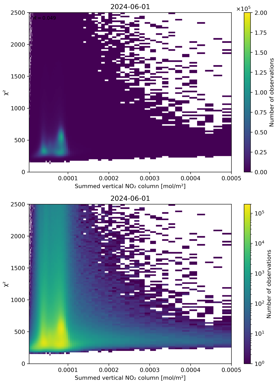
Figure 104: Scatter density plot of “Summed vertical NO 2 column” against “ \chi^2 ” for 2024-05-31 to 2024-06-02.
