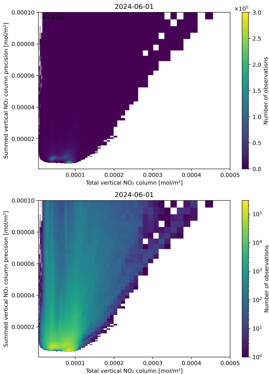
Figure 113: Scatter density plot of “Total vertical NO 2 column” against “Summed vertical NO 2 column precision” for 2024-05-31 to 2024-06-02.
