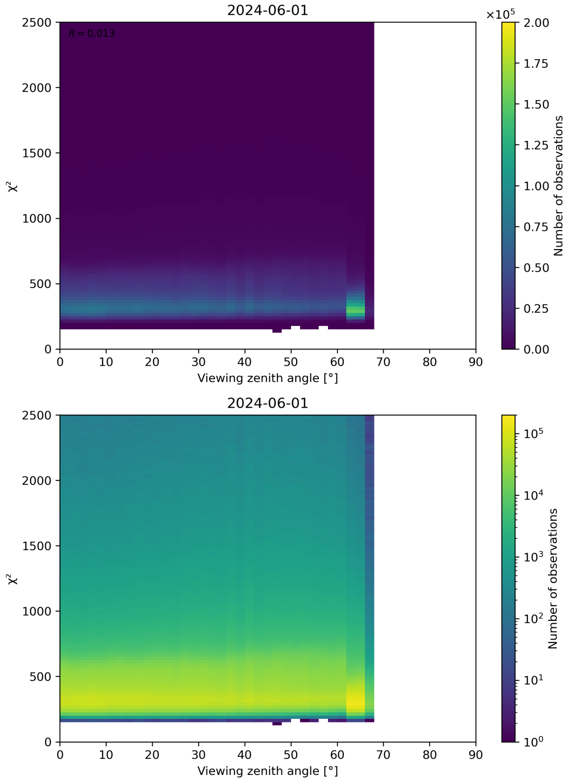
Figure 162: Scatter density plot of “Viewing zenith angle” against “ \chi^2 ” for 2024-05-31 to 2024-06-02.
