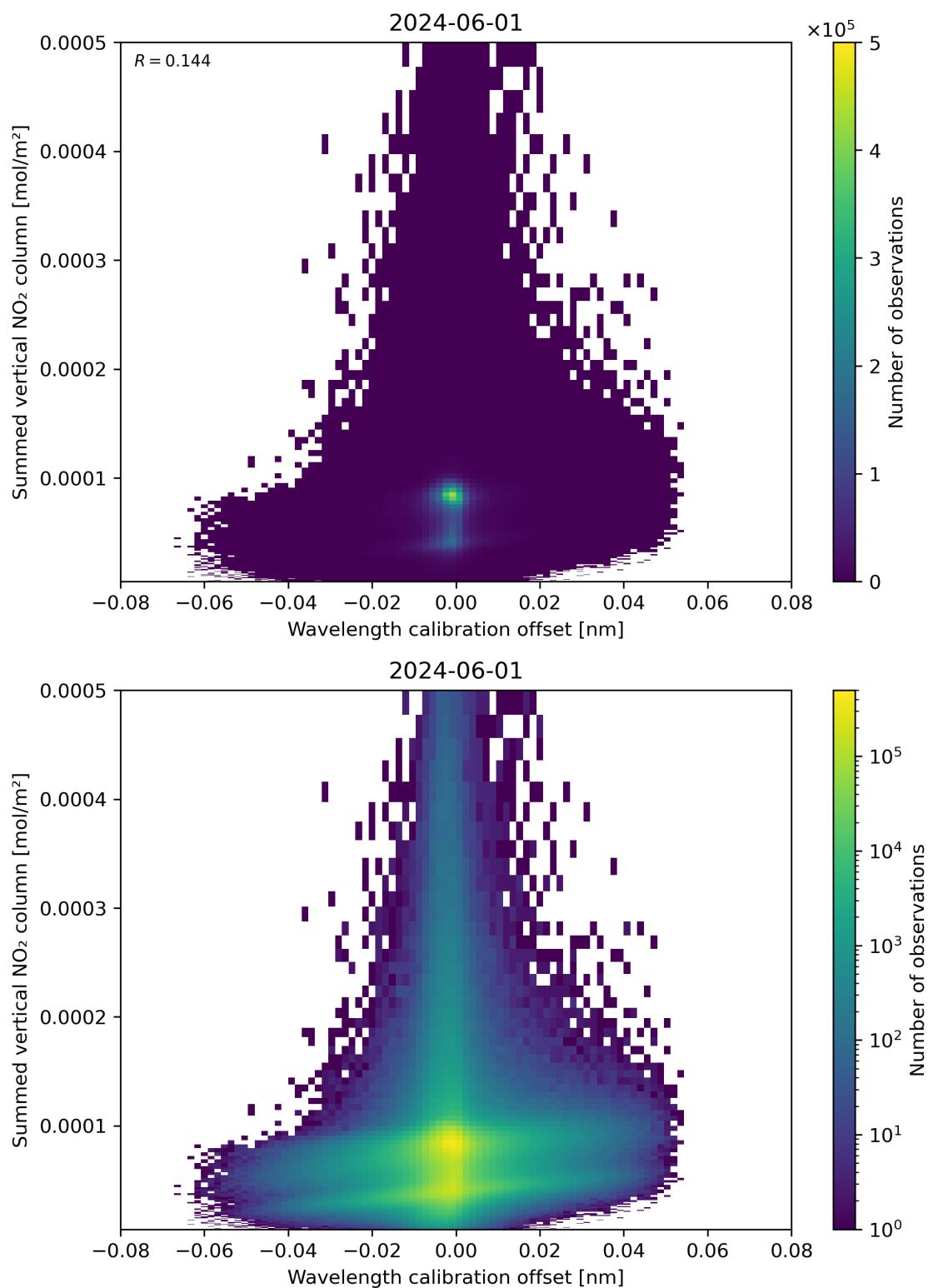
Figure 177: Scatter density plot of “Wavelength calibration offset” against “Summed vertical NO 2 column” for 2024-05-31 to 2024-06-02.
