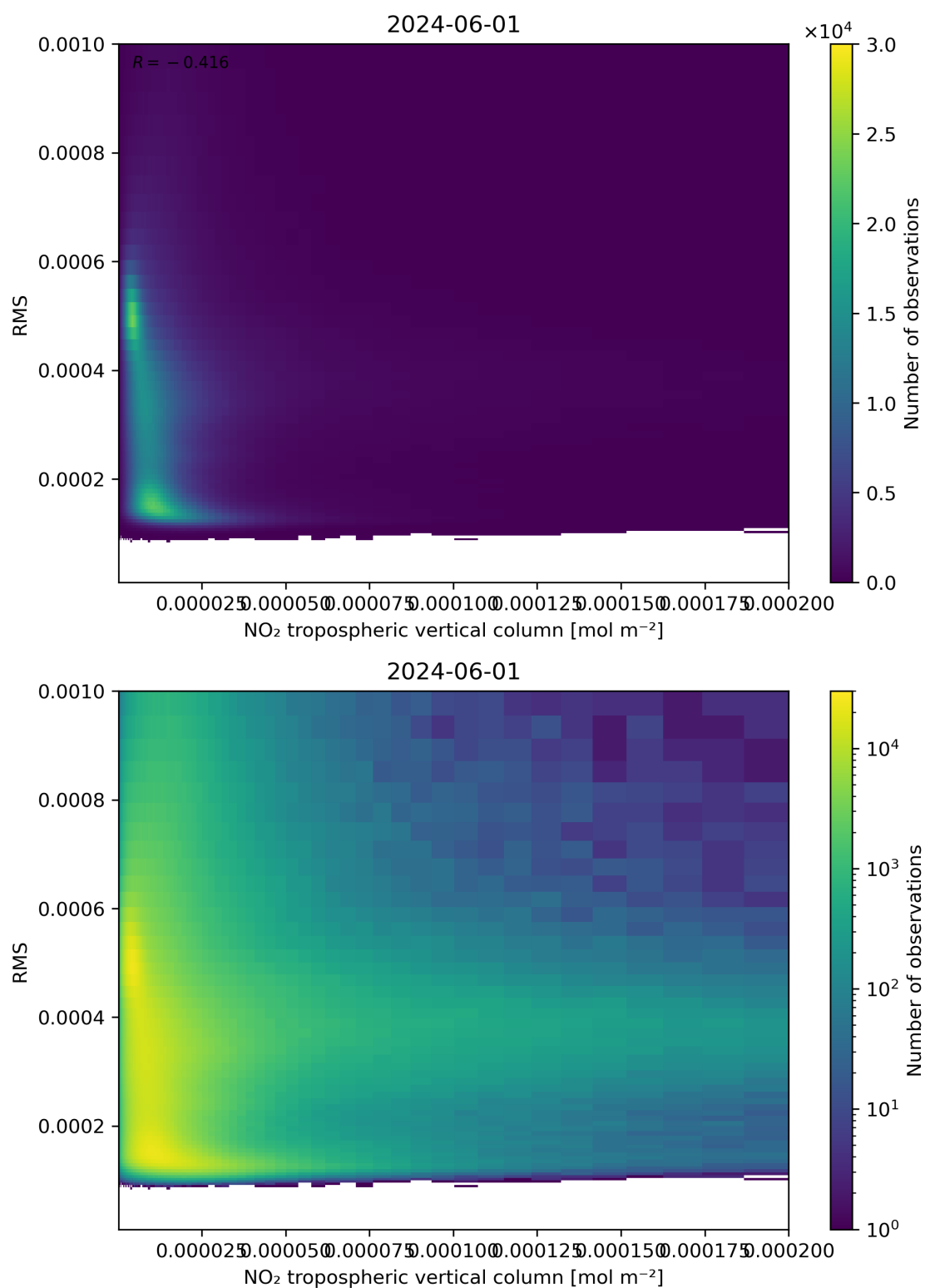
Figure 142: Scatter density plot of “NO 2 tropospheric vertical column” against “RMS” for 2024-05-31 to 2024-06-02.
