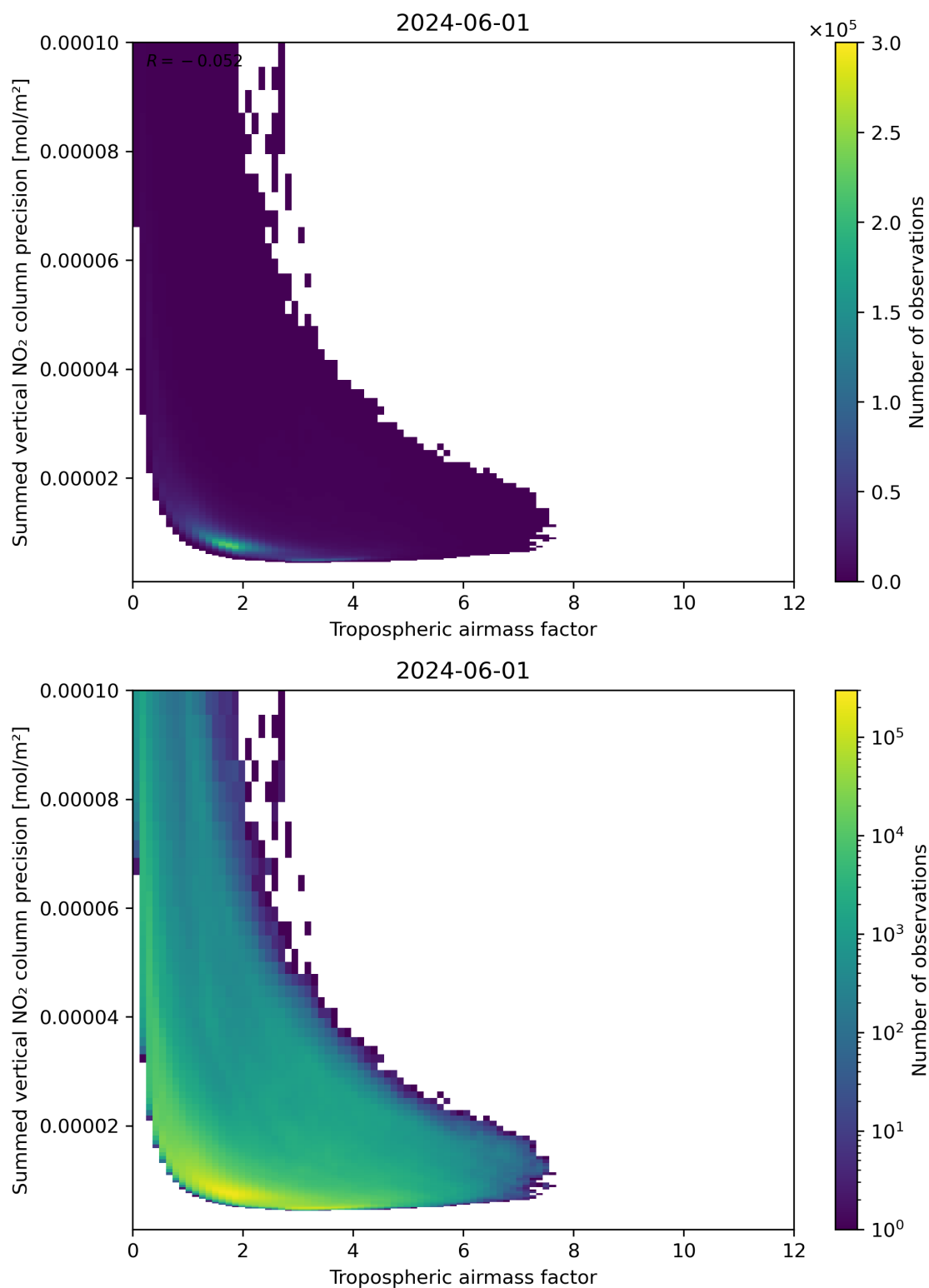
Figure 76: Scatter density plot of “Tropospheric air mass factor” against “Summed vertical NO 2 column precision” for 2024-05-31 to 2024-06-02.
