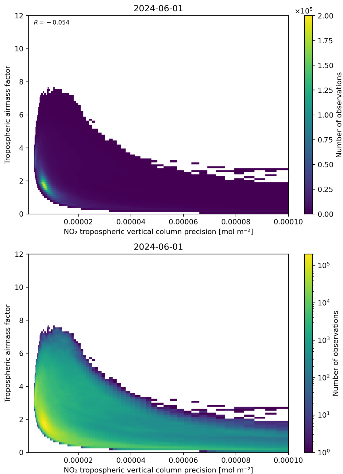
Figure 133: Scatter density plot of “NO 2 tropospheric vertical column precision” against “Tropospheric airmass factor” for 2024-05-31 to 2024-06-02.
