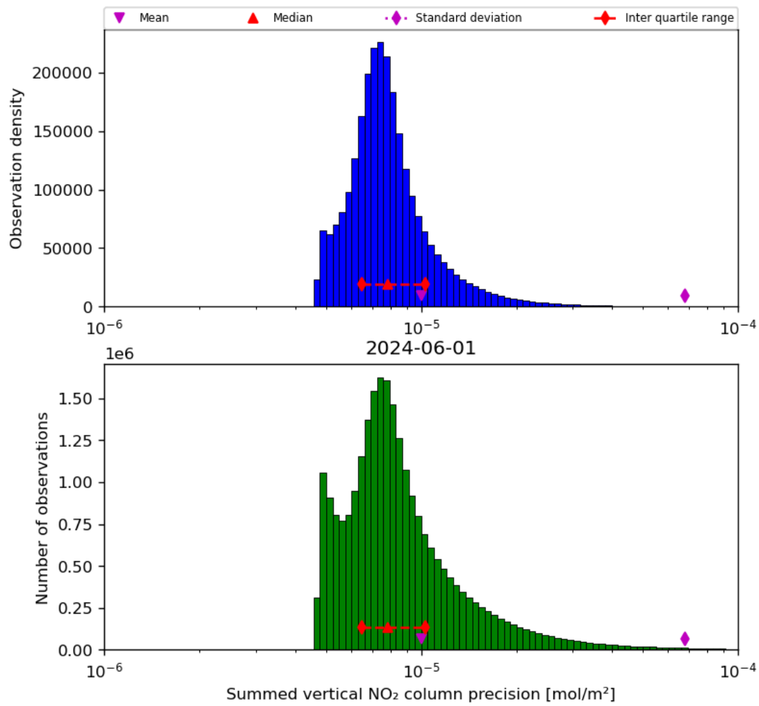
Figure 41: Histogram of "Summed vertical NO 2 column precision" for 2024-05-31 to 2024-06-02
