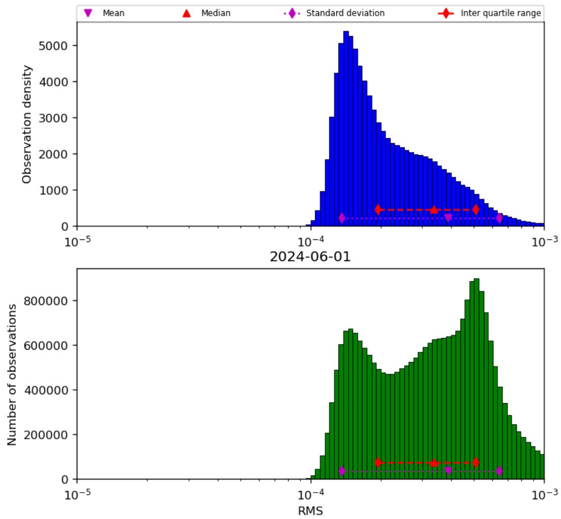
Figure 43: Histogram of “RMS” for 2024-05-31 to 2024-06-02
