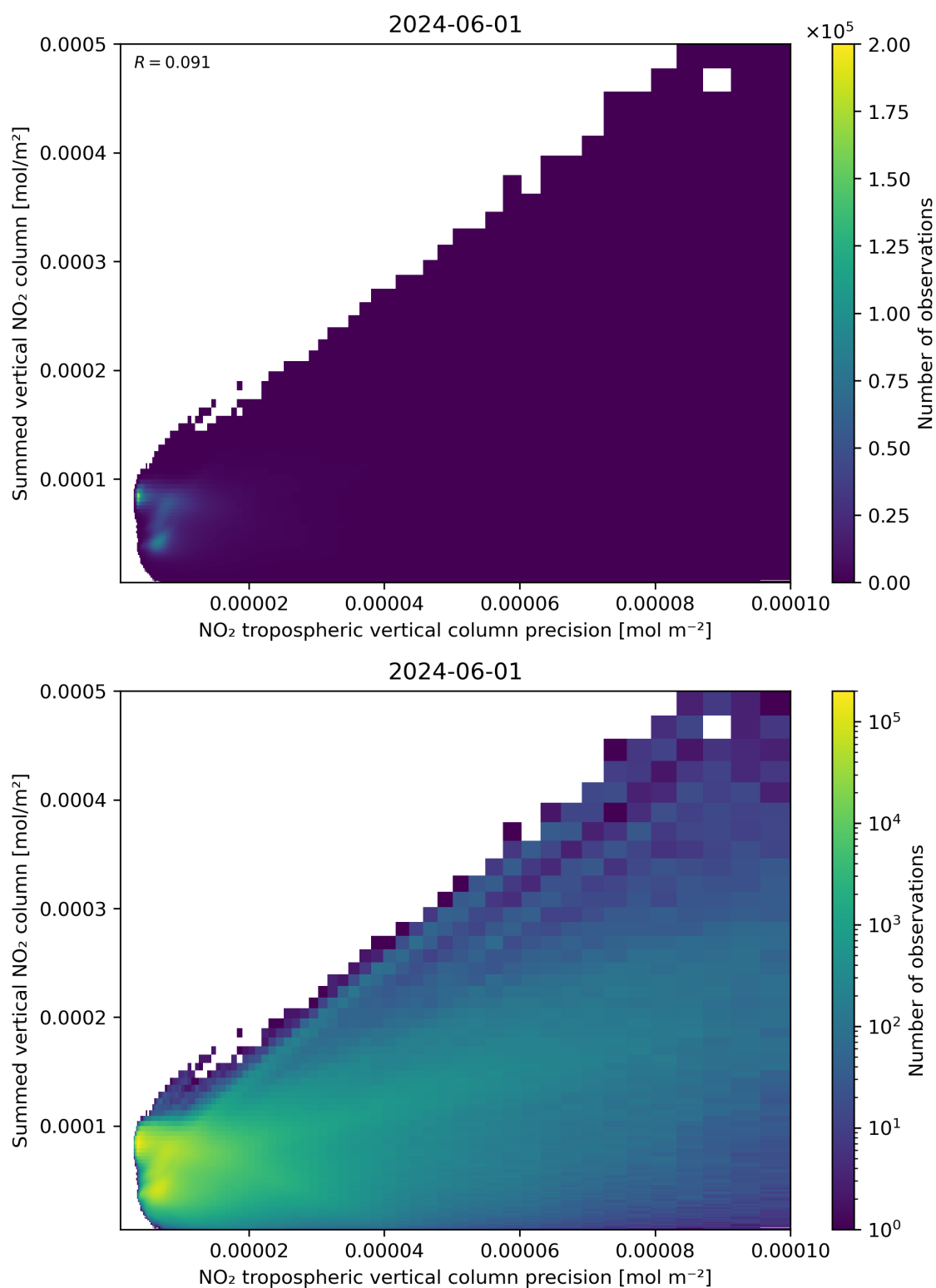
Figure 136: Scatter density plot of “NO 2 tropospheric vertical column precision” against “Summed vertical NO 2 column” for 2024-05-31 to 2024-06-02.
