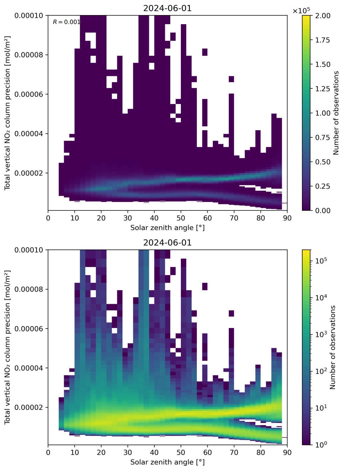
Figure 154: Scatter density plot of “Solar zenith angle” against “Total vertical NO 2 column precision” for 2024-05-31 to 2024-06-02.
