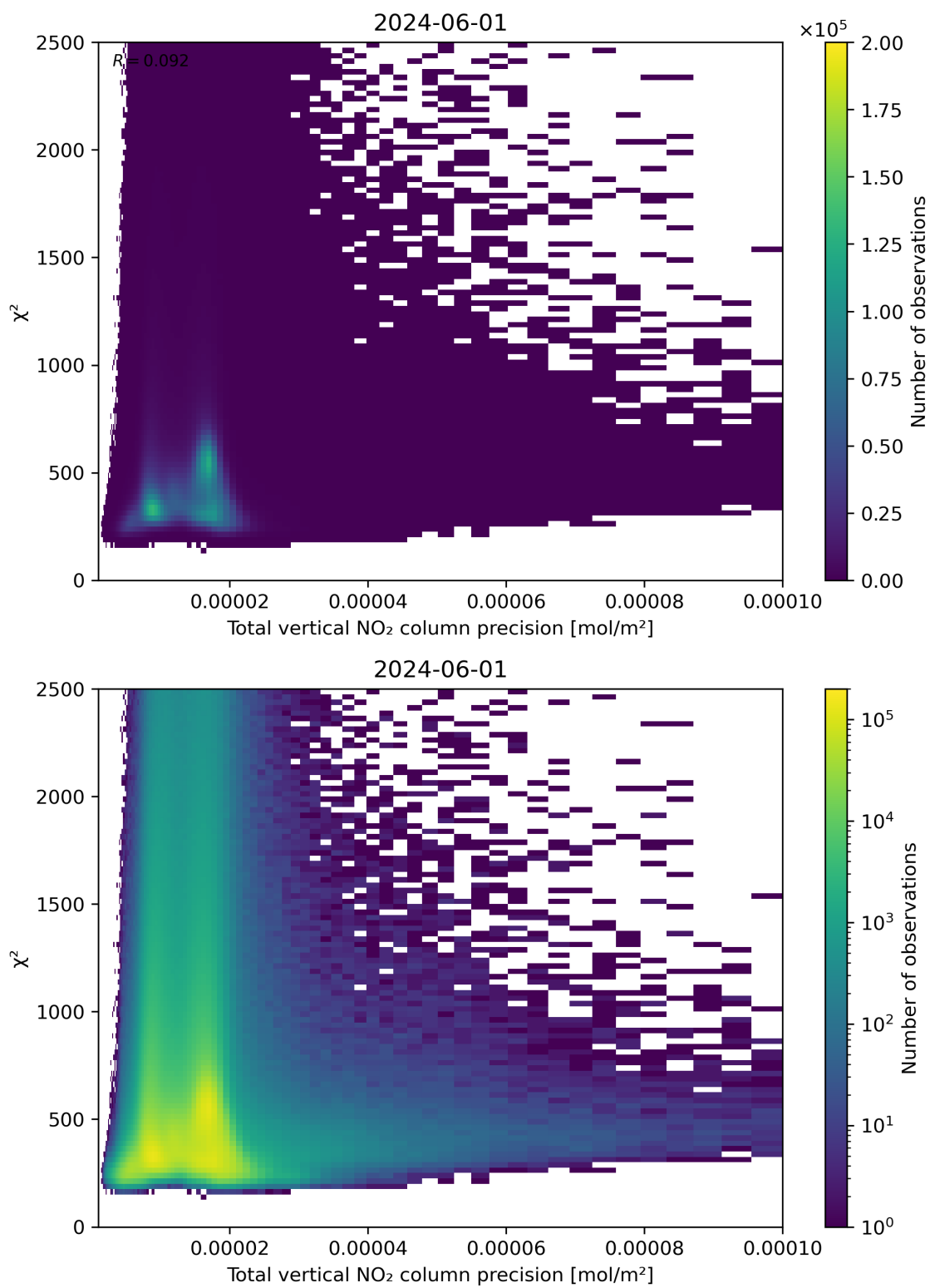
Figure 116: Scatter density plot of “Total vertical NO 2 column precision” against “ \chi^2 ” for 2024-05-31 to 2024-06-02.
