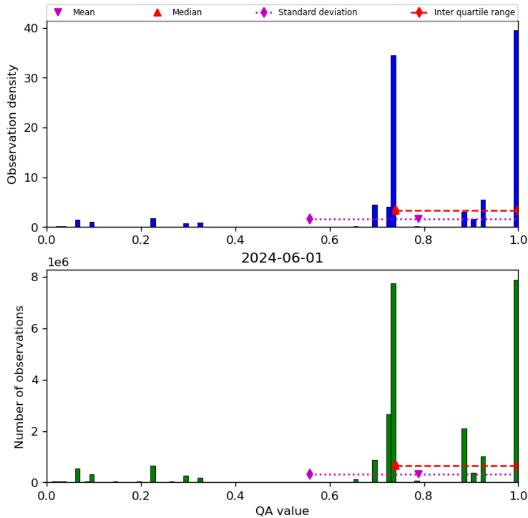
Figure 28: Histogram of “QA value” for 2024-05-31 to 2024-06-02
