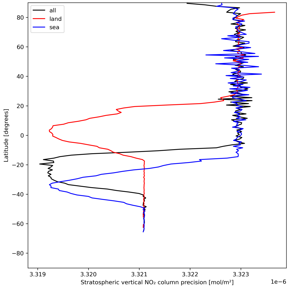
Figure 20: Zonal average of “Stratospheric vertical NO 2 column precision” for 2024-05-31 to 2024-06-02.
