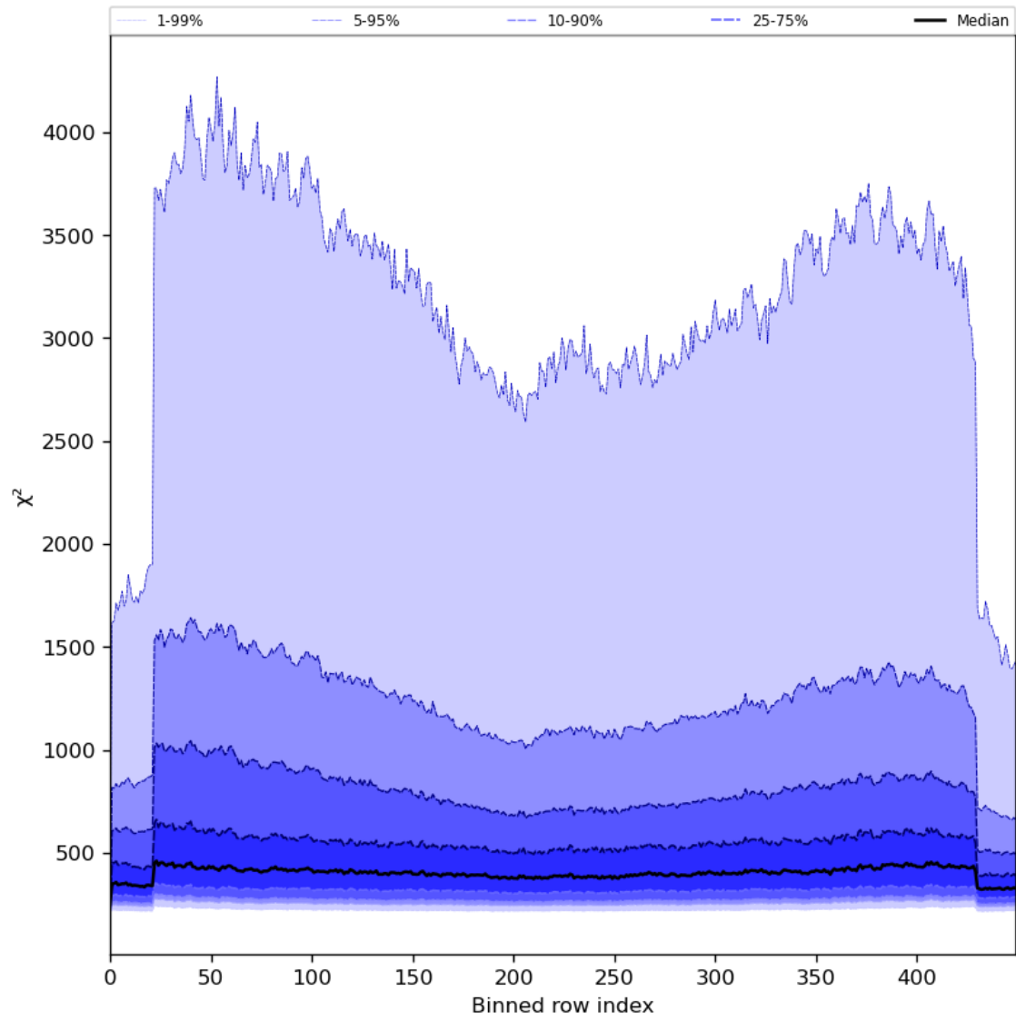
Figure 59: Along track statistics of “ \chi^2 ” for 2024-05-31 to 2024-06-02
