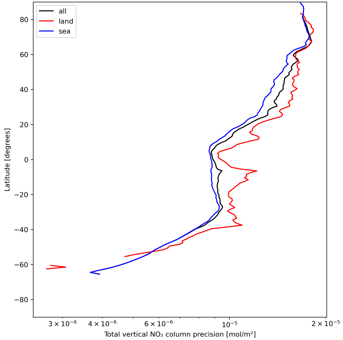
Figure 22: Zonal average of “Total vertical NO 2 column precision” for 2024-05-31 to 2024-06-02.
