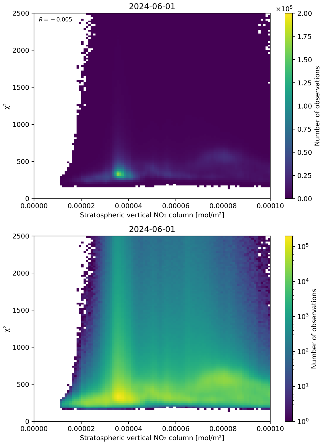
Figure 97: Scatter density plot of “Stratospheric vertical NO 2 column” against “ \chi^2 ” for 2024-05-31 to 2024-06-02.
