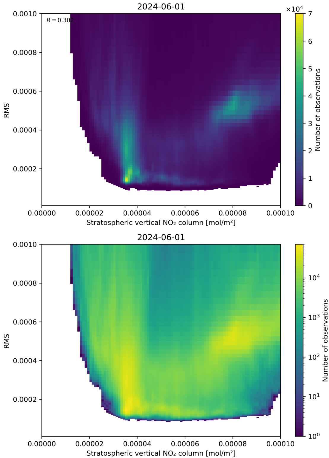
Figure 102: Scatter density plot of “Stratospheric vertical NO 2 column” against “RMS” for 2024-05-31 to 2024-06-02.
