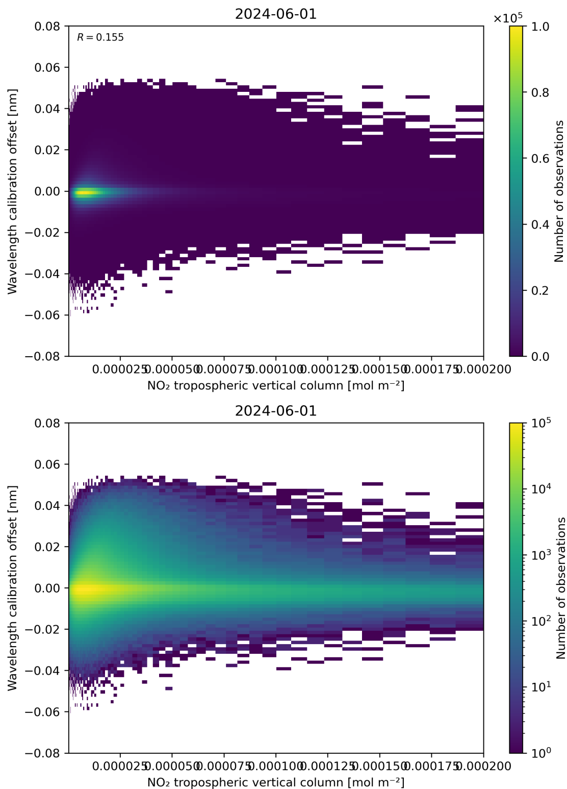
Figure 143: Scatter density plot of “NO 2 tropospheric vertical column” against “Wavelength calibration offset” for 2024-05-31 to 2024-06-02.
