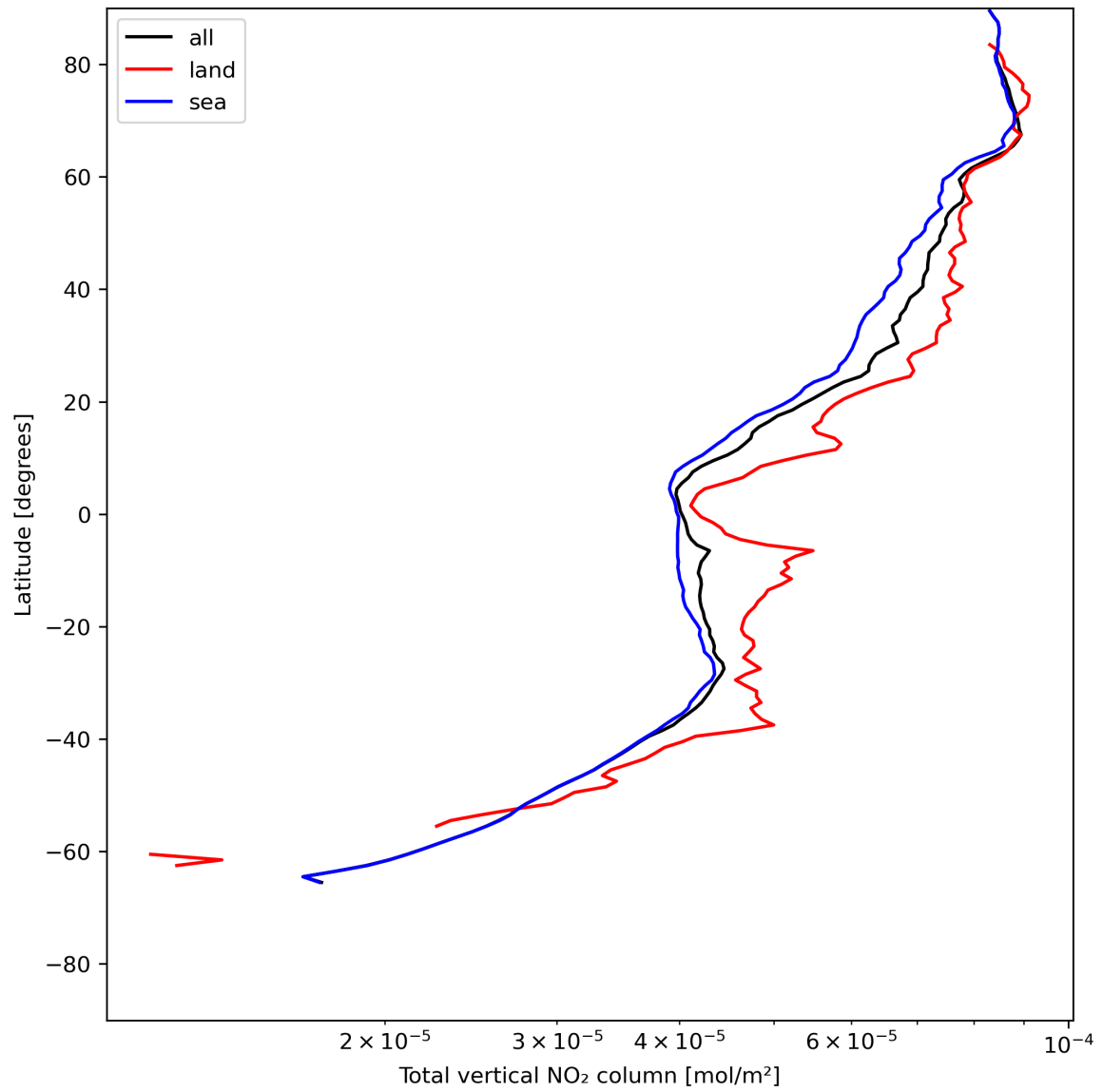
Figure 21: Zonal average of “Total vertical NO 2 column” for 2024-05-31 to 2024-06-02.
