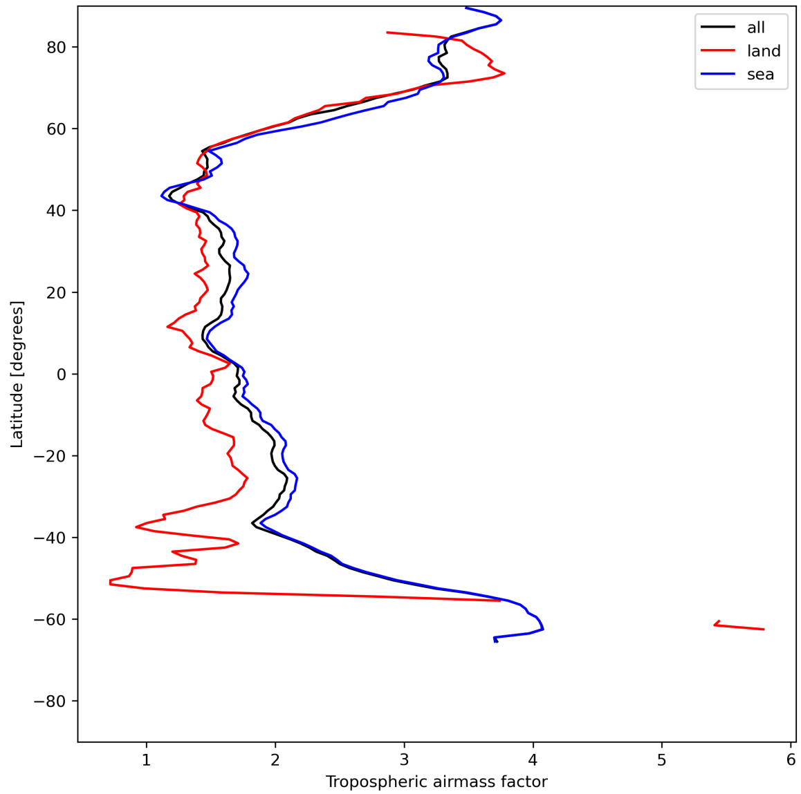
Figure 14: Zonal average of “Tropospheric air mass factor” for 2024-05-31 to 2024-06-02.
