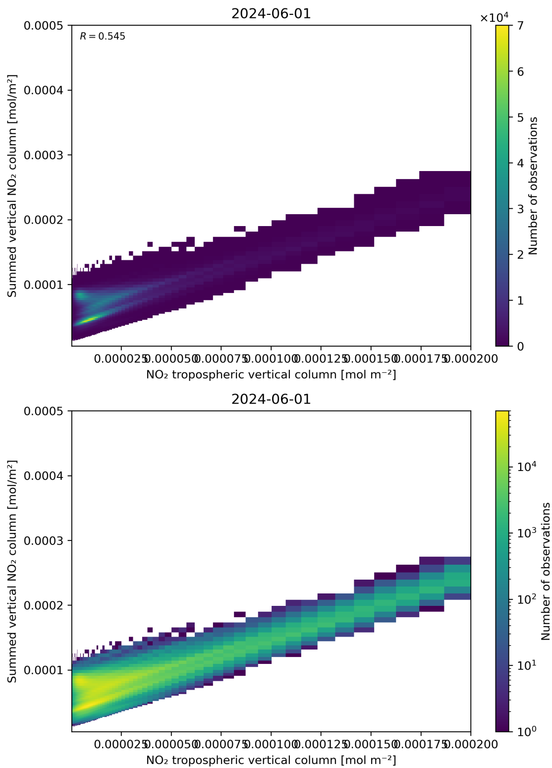
Figure 126: Scatter density plot of “NO 2 tropospheric vertical column” against “Summed vertical NO 2 column” for 2024-05-31 to 2024-06-02.
