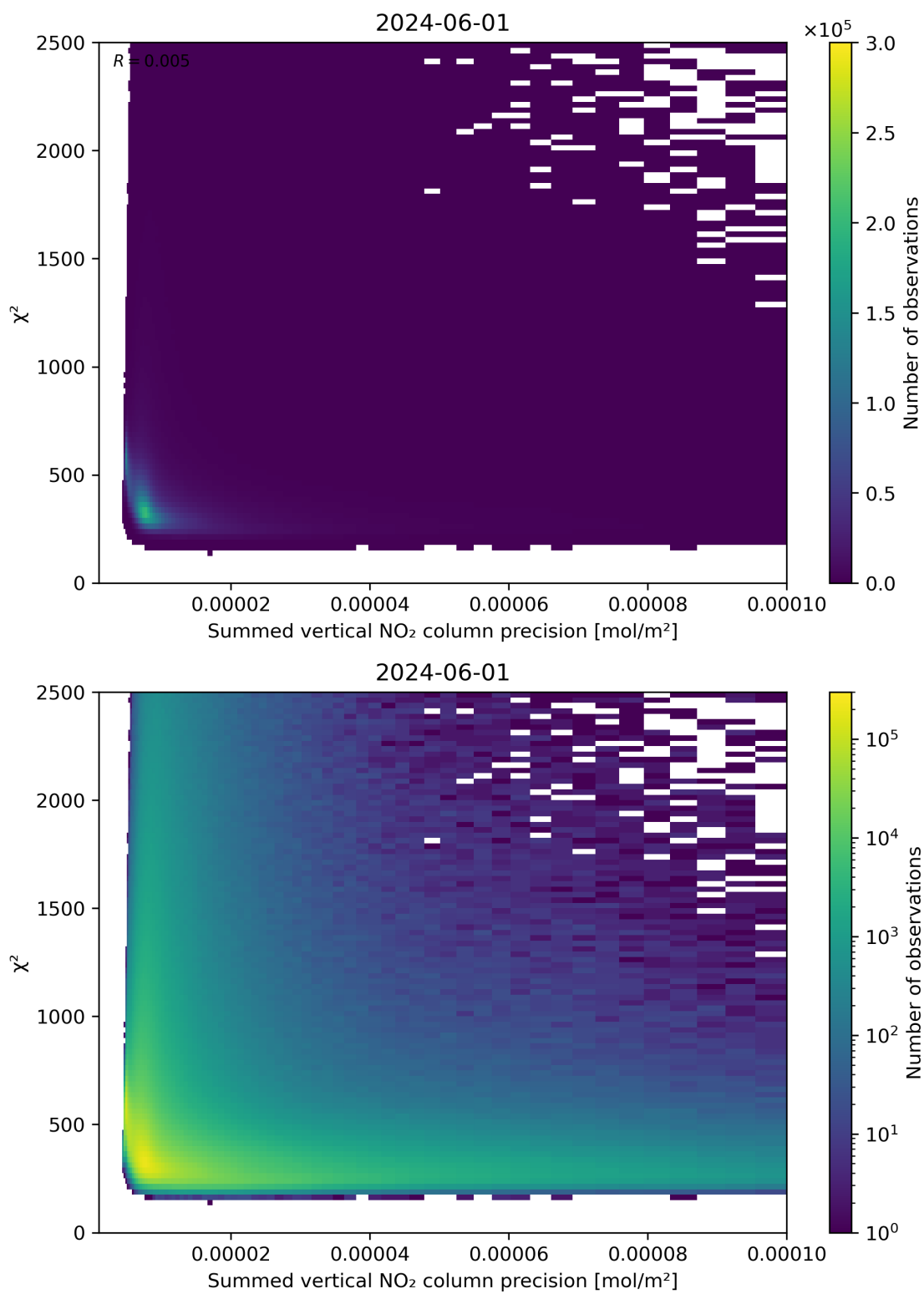
Figure 107: Scatter density plot of “Summed vertical NO 2 column precision” against “ \chi^2 ” for 2024-05-31 to 2024-06-02.
