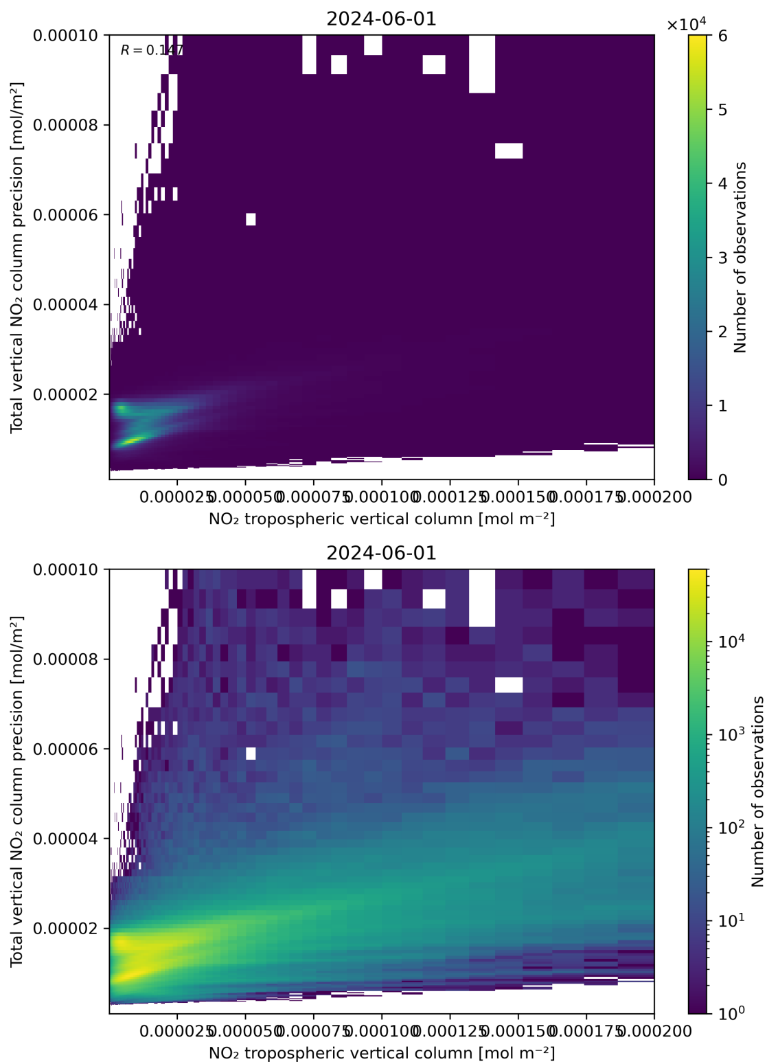
Figure 129: Scatter density plot of “NO 2 tropospheric vertical column” against “Total vertical NO 2 column precision” for 2024-05-31 to 2024-06-02.
