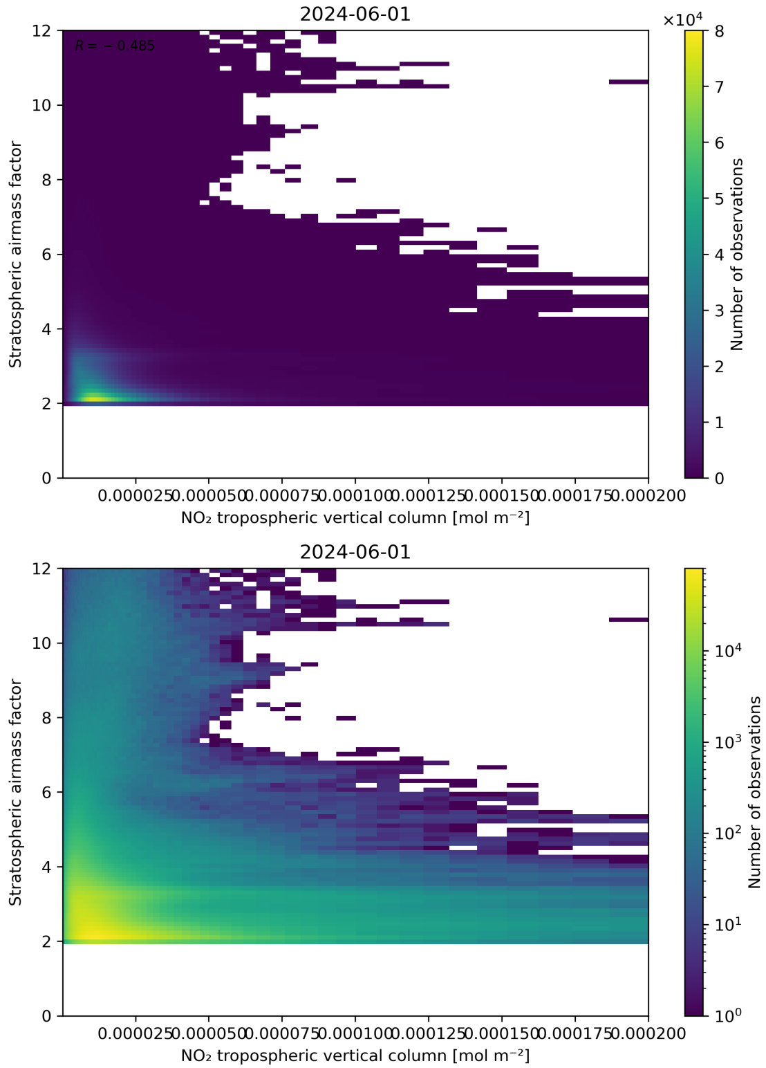
Figure 121: Scatter density plot of “NO 2 tropospheric vertical column” against “Stratospheric air mass factor” for 2024-05-31 to 2024-06-02.
