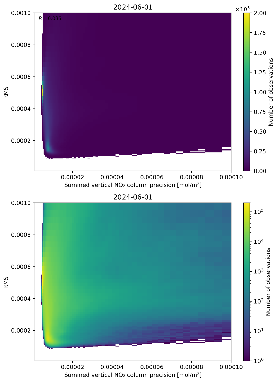
Figure 108: Scatter density plot of “Summed vertical NO 2 column precision” against “RMS” for 2024-05-31 to 2024-06-02.
