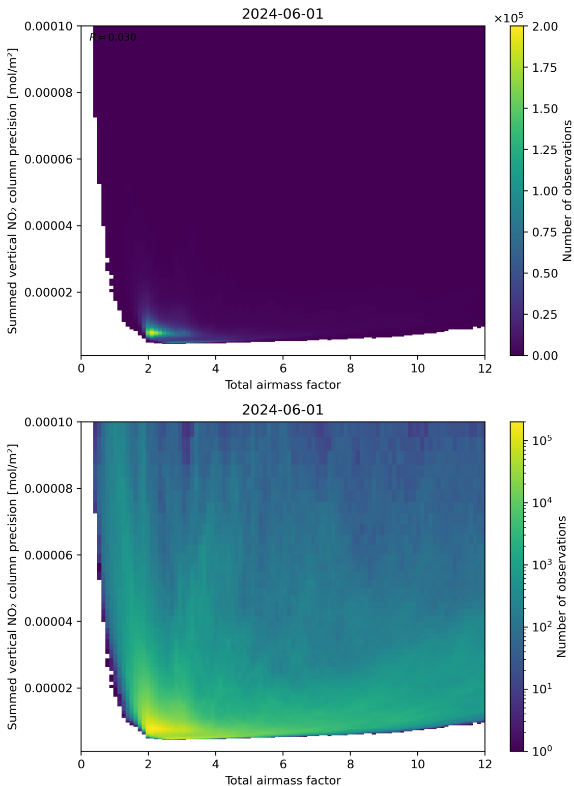
Figure 66: Scatter density plot of “Total airmass factor” against “Summed vertical NO 2 column precision” for 2024-05-31 to 2024-06-02.
