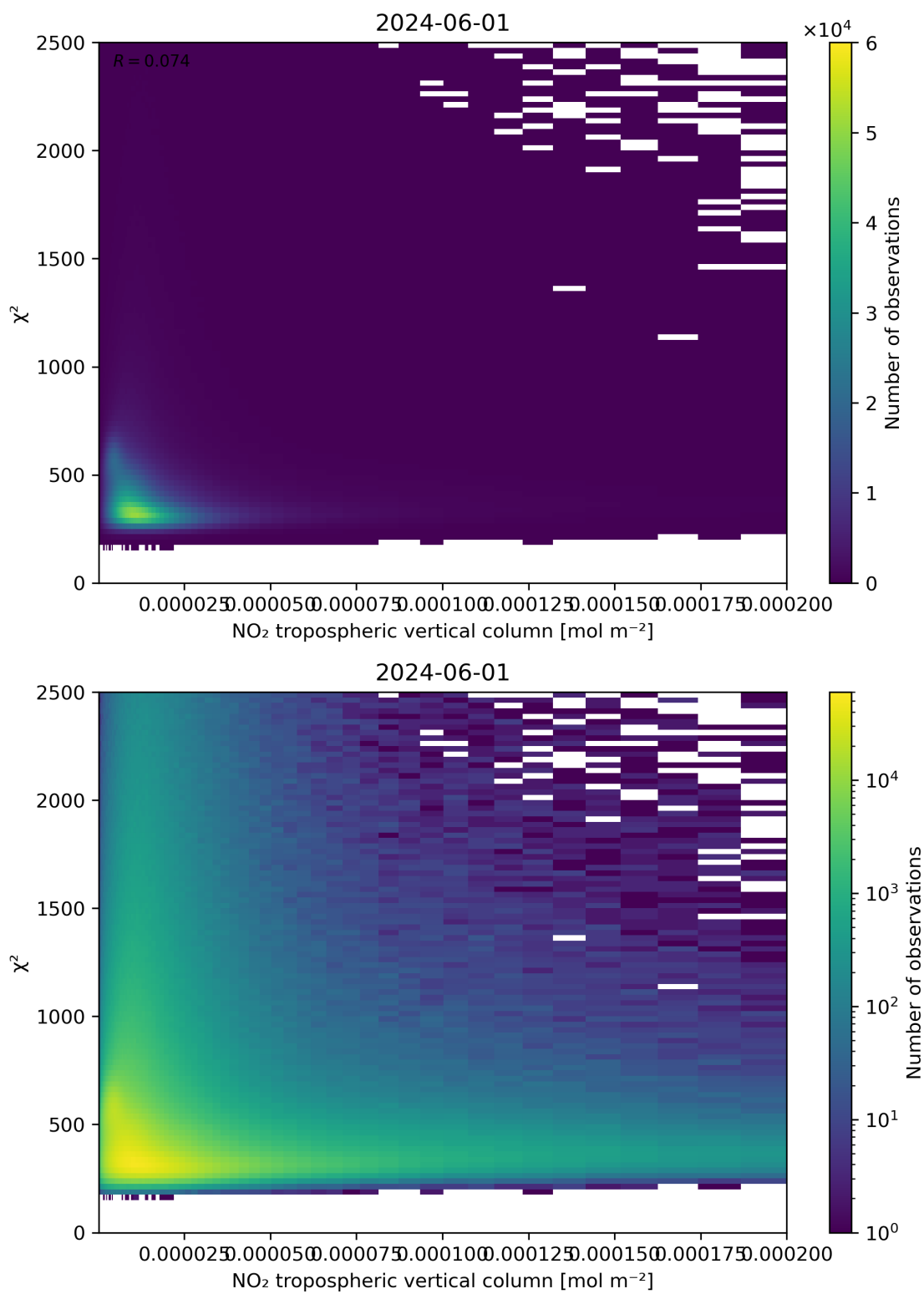
Figure 124: Scatter density plot of “NO 2 tropospheric vertical column” against “ \chi^2 ” for 2024-05-31 to 2024-06-02.
