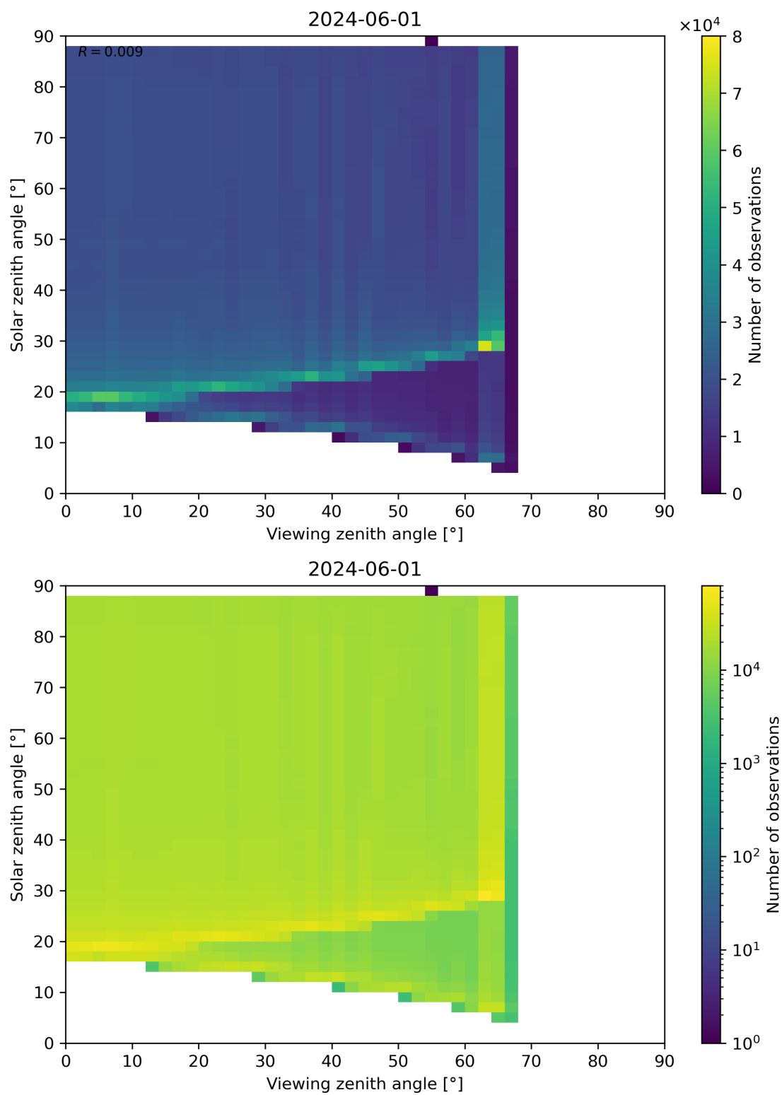
Figure 172: Scatter density plot of “Viewing zenith angle” against “Solar zenith angle” for 2024-05-31 to 2024-06-02.
