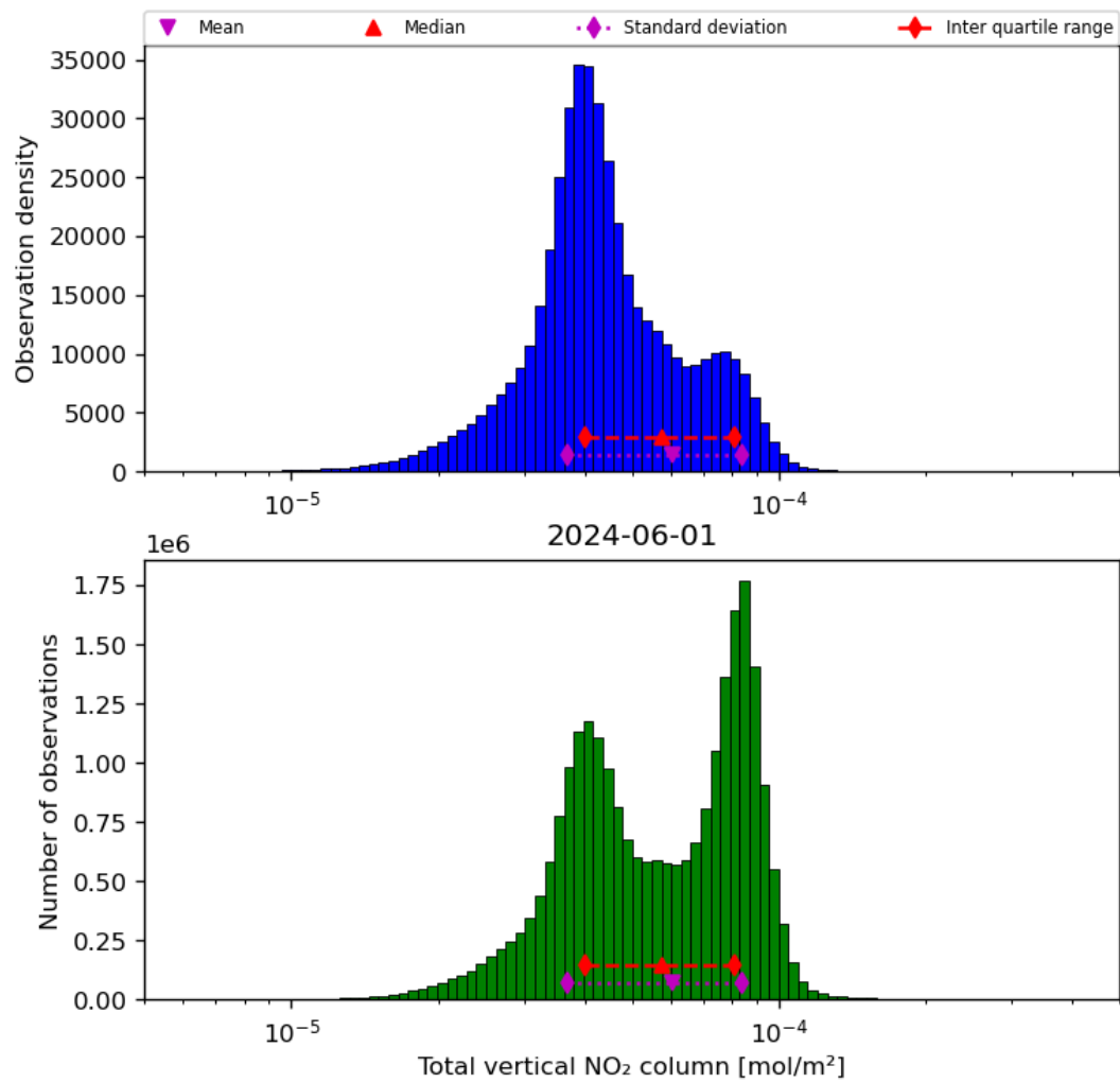
Figure 38: Histogram of “Total vertical NO 2 column” for 2024-05-31 to 2024-06-02
