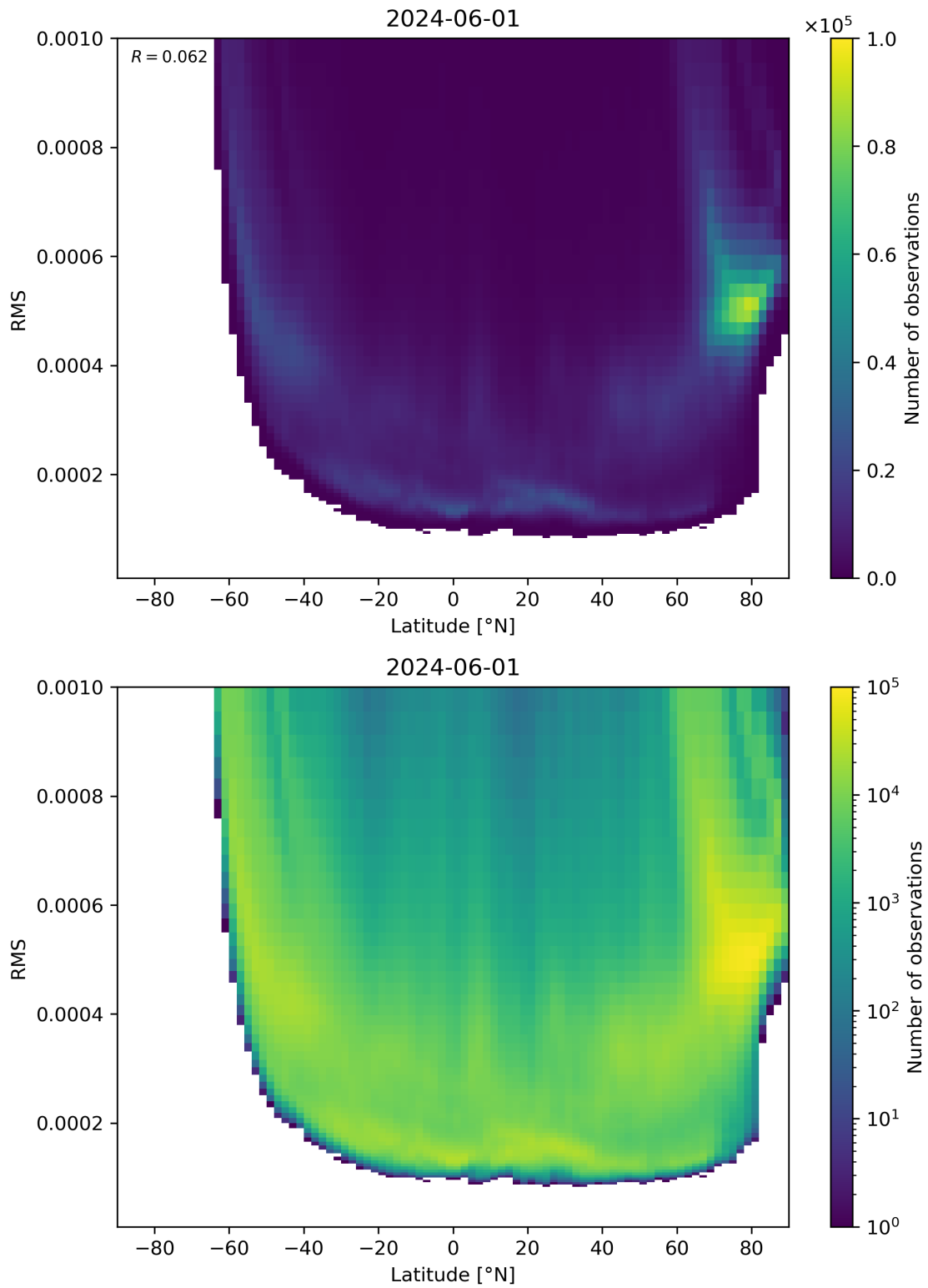
Figure 94: Scatter density plot of “Latitude” against “RMS” for 2024-05-31 to 2024-06-02.
