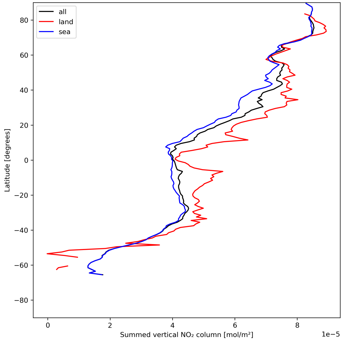
Figure 23: Zonal average of “Summed vertical NO 2 column” for 2024-05-31 to 2024-06-02.
