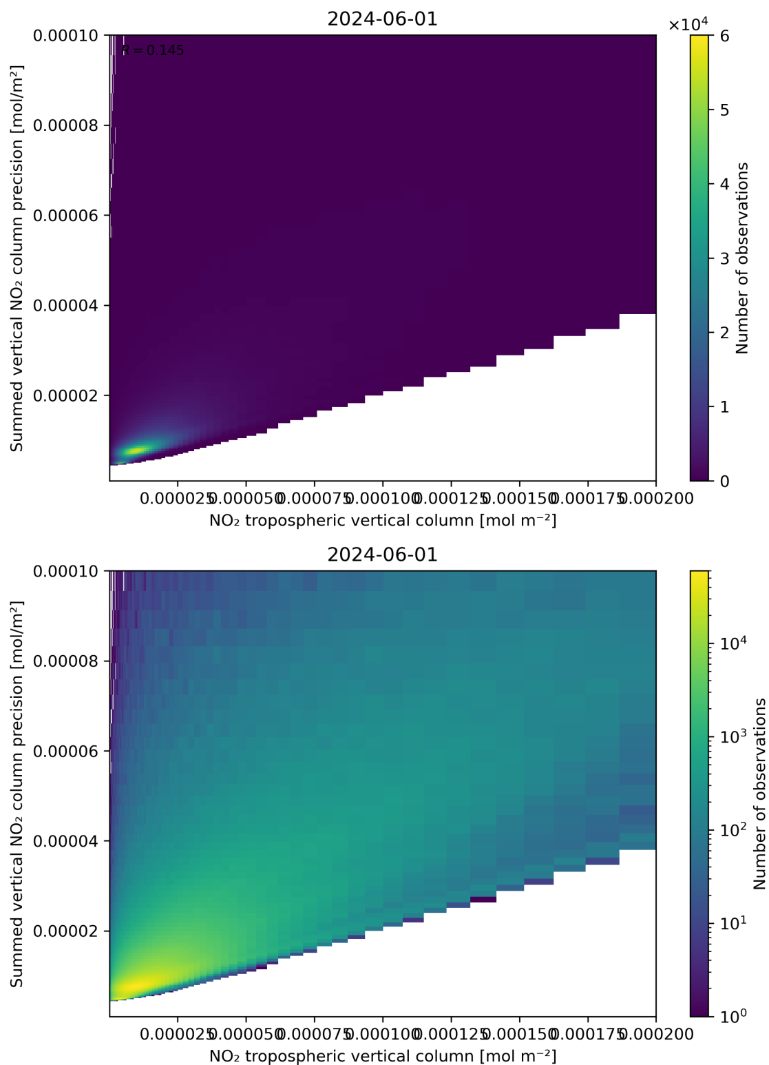
Figure 127: Scatter density plot of “NO 2 tropospheric vertical column” against “Summed vertical NO 2 column precision” for 2024-05-31 to 2024-06-02.
