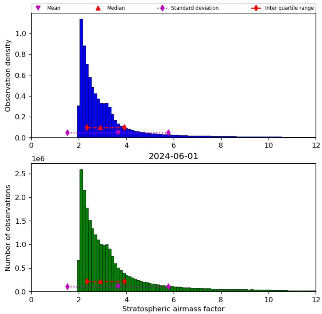
Figure 44: Histogram of “Stratospheric airmass factor” for 2024-05-31 to 2024-06-02
