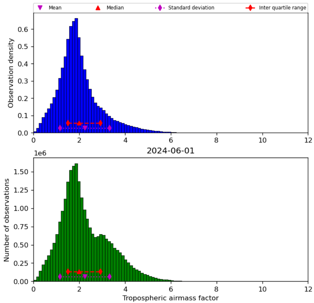
Figure 31: Histogram of “Tropospheric airmass factor” for 2024-05-31 to 2024-06-02
