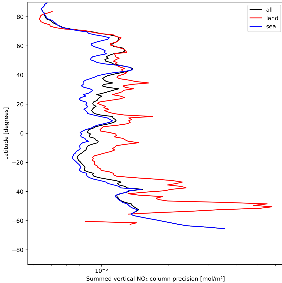
Figure 24: Zonal average of “Summed vertical NO 2 column precision” for 2024-05-31 to 2024-06-02.
