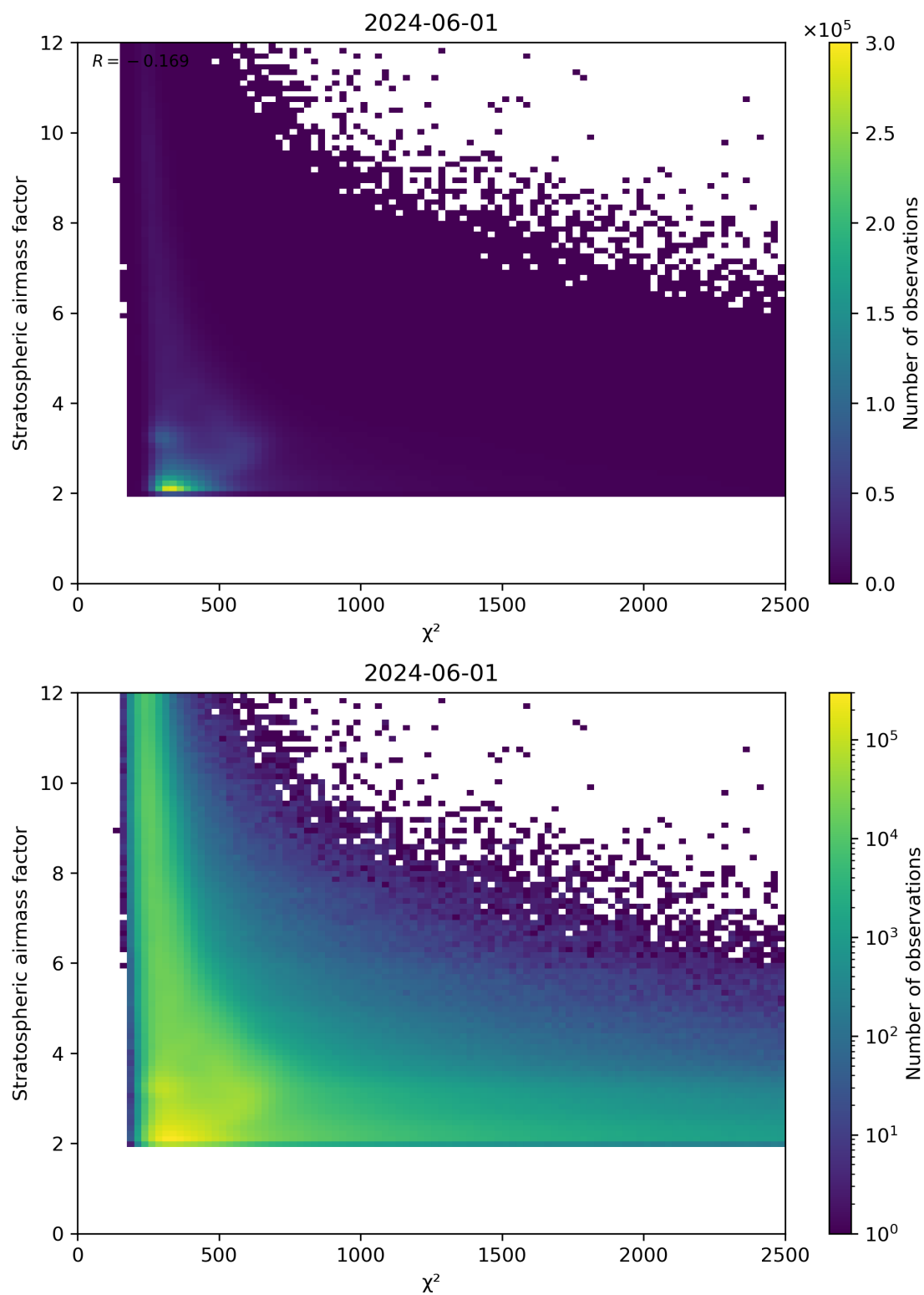
Figure 81: Scatter density plot of “ \chi^2 ” against “Stratospheric airmass factor” for 2024-05-31 to 2024-06-02.
