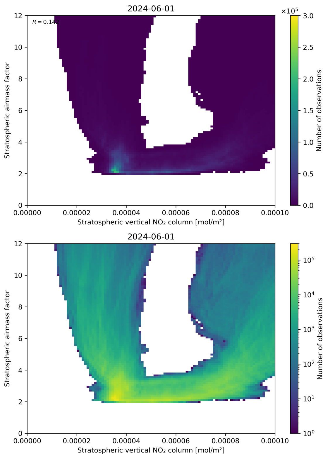
Figure 96: Scatter density plot of “Stratospheric vertical NO 2 column” against “Stratospheric airmass factor” for 2024-05-31 to 2024-06-02.
