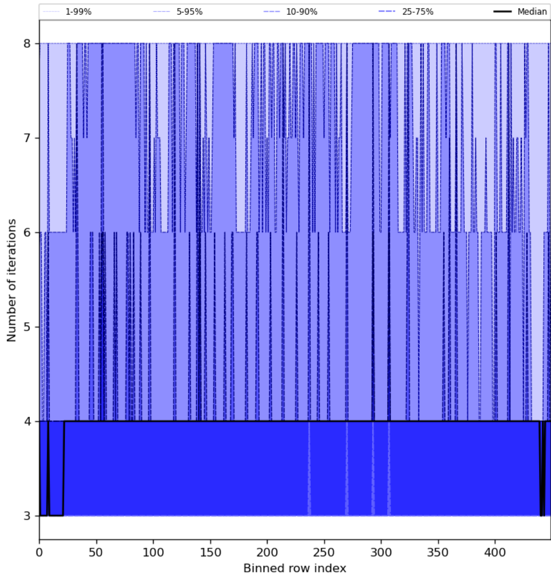
Figure 51: Along track statistics of “Number of iterations” for 2024-05-31 to 2024-06-02
