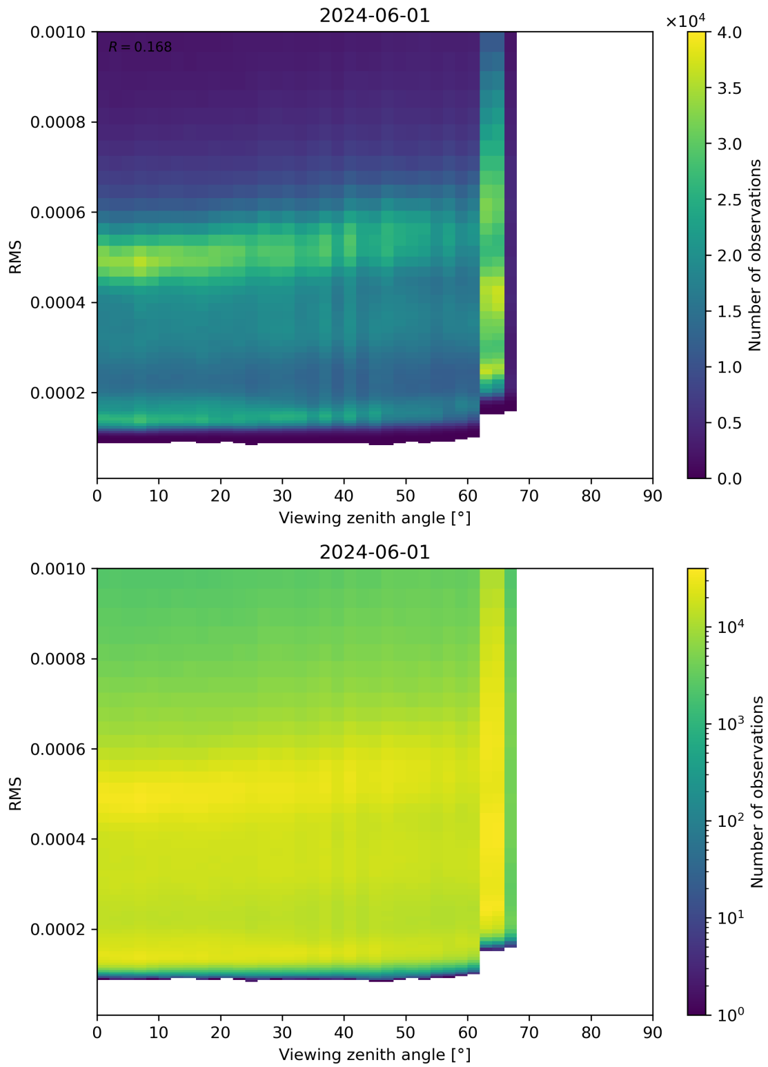
Figure 171: Scatter density plot of “Viewing zenith angle” against “RMS” for 2024-05-31 to 2024-06-02.
