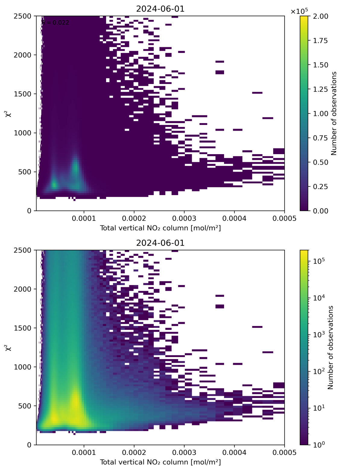
Figure 111: Scatter density plot of “Total vertical NO 2 column” against “ \chi^2 ” for 2024-05-31 to 2024-06-02.
