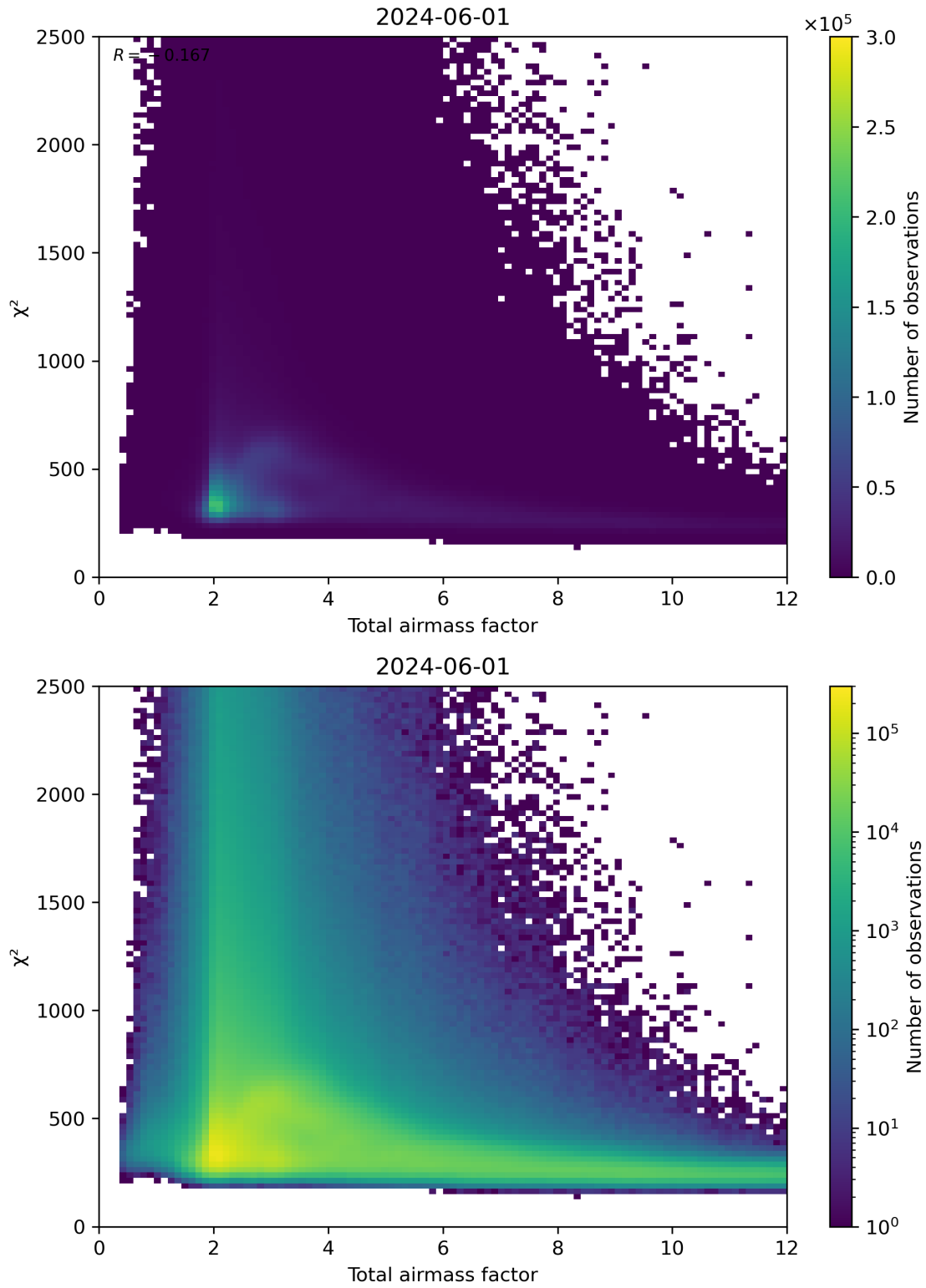
Figure 63: Scatter density plot of “Total airmass factor” against “ \chi^2 ” for 2024-05-31 to 2024-06-02.
