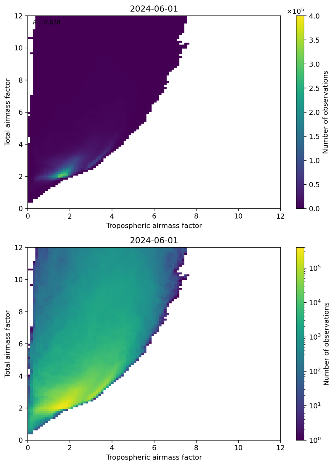
Figure 72: Scatter density plot of “Tropospheric airmass factor” against “Total airmass factor” for 2024-05-31 to 2024-06-02.
