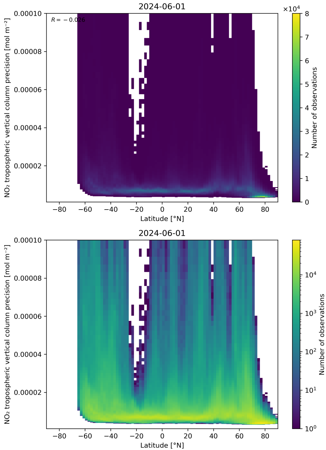
Figure 93: Scatter density plot of “Latitude” against “NO 2 tropospheric vertical column precision” for 2024-05-31 to 2024-06-02.
