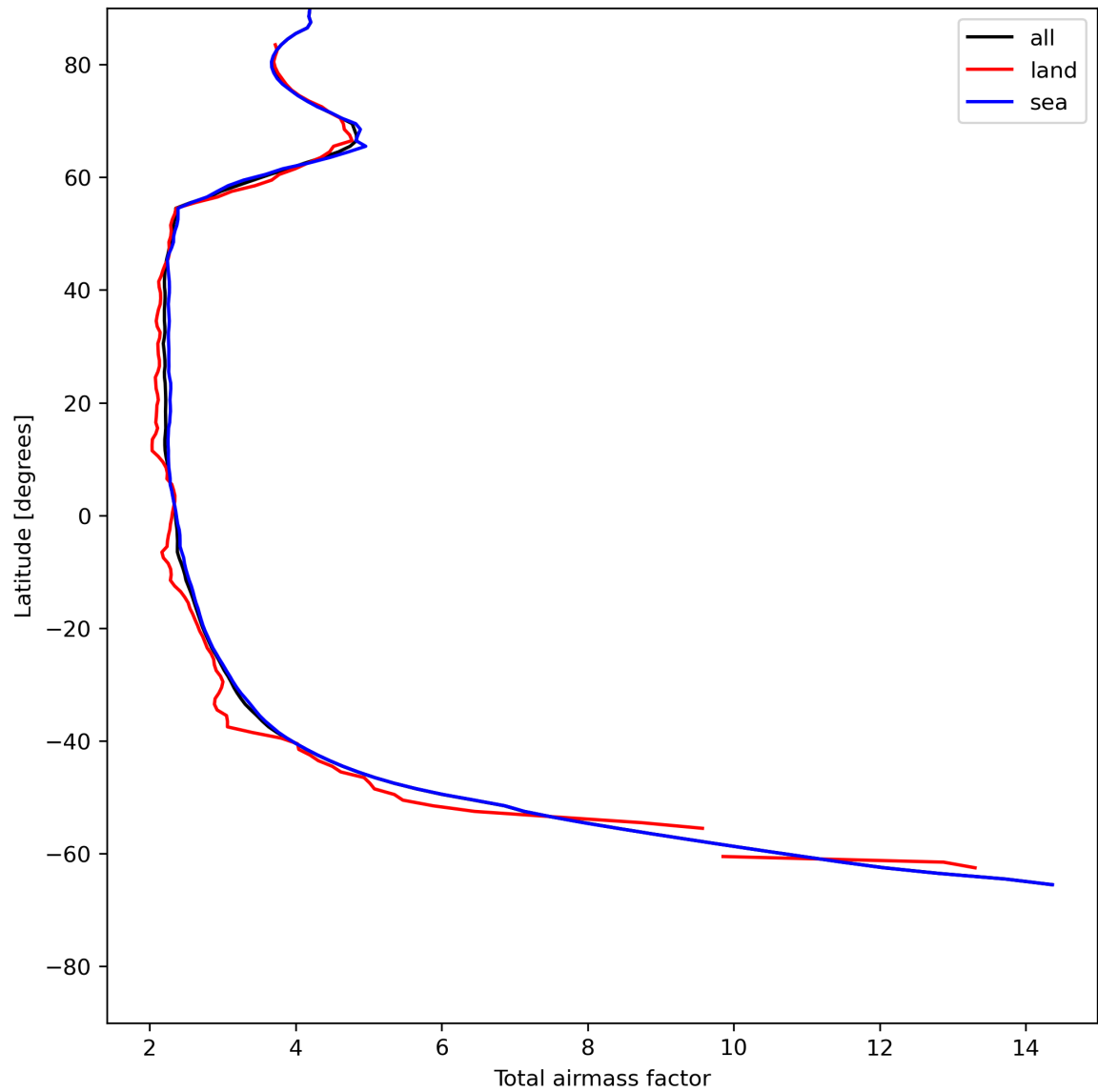
Figure 15: Zonal average of “Total airmass factor” for 2024-05-31 to 2024-06-02.
