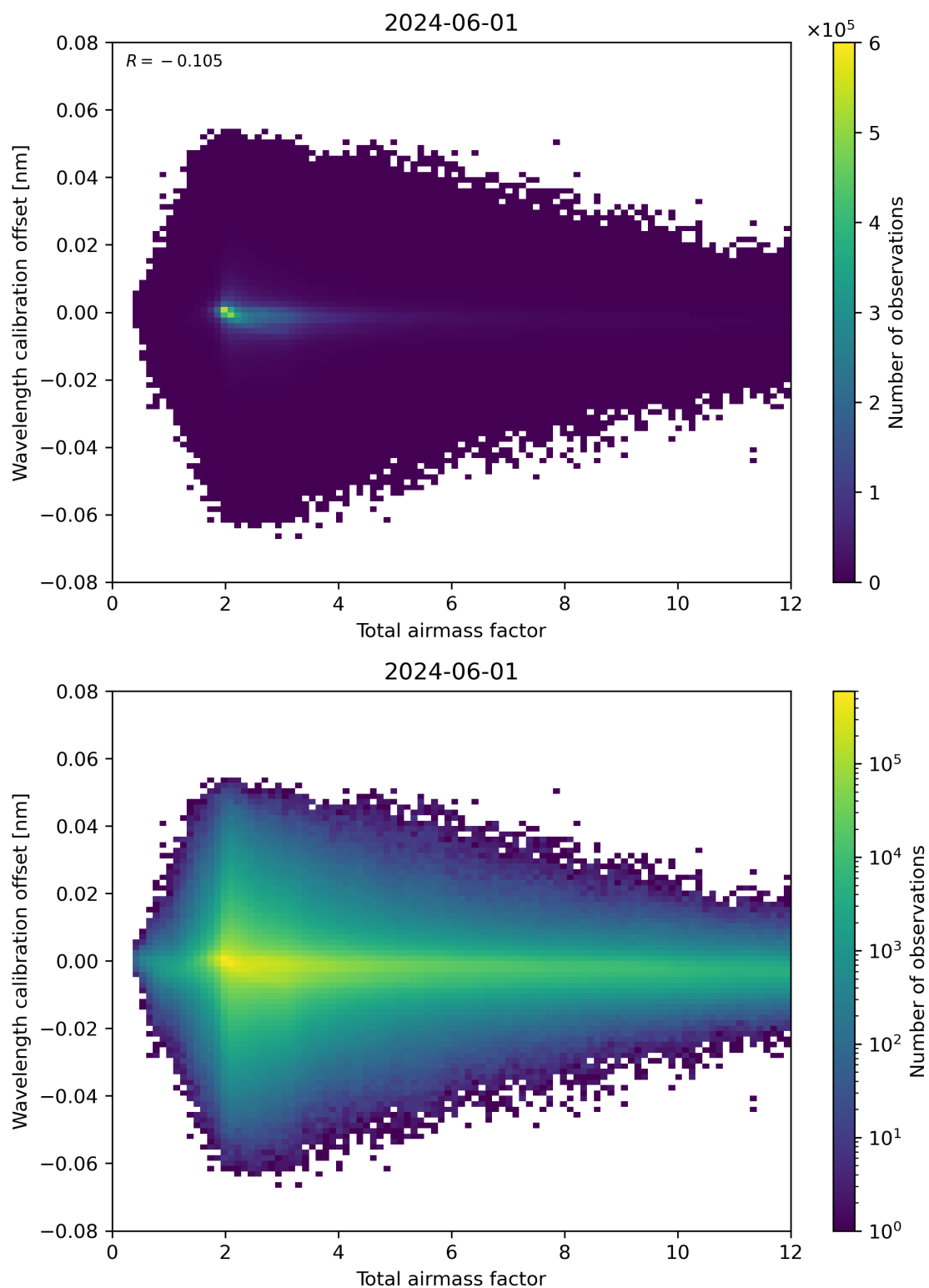
Figure 70: Scatter density plot of “Total airmass factor” against “Wavelength calibration offset” for 2024-05-31 to 2024-06-02.
