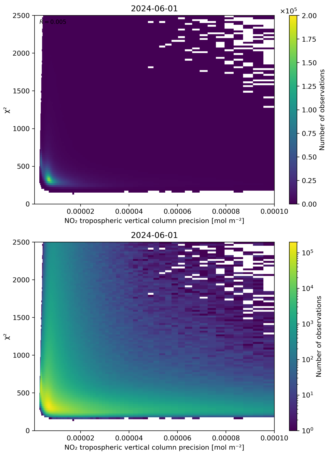
Figure 134: Scatter density plot of “NO 2 tropospheric vertical column precision” against “ \chi^2 ” for 2024-05-31 to 2024-06-02.
