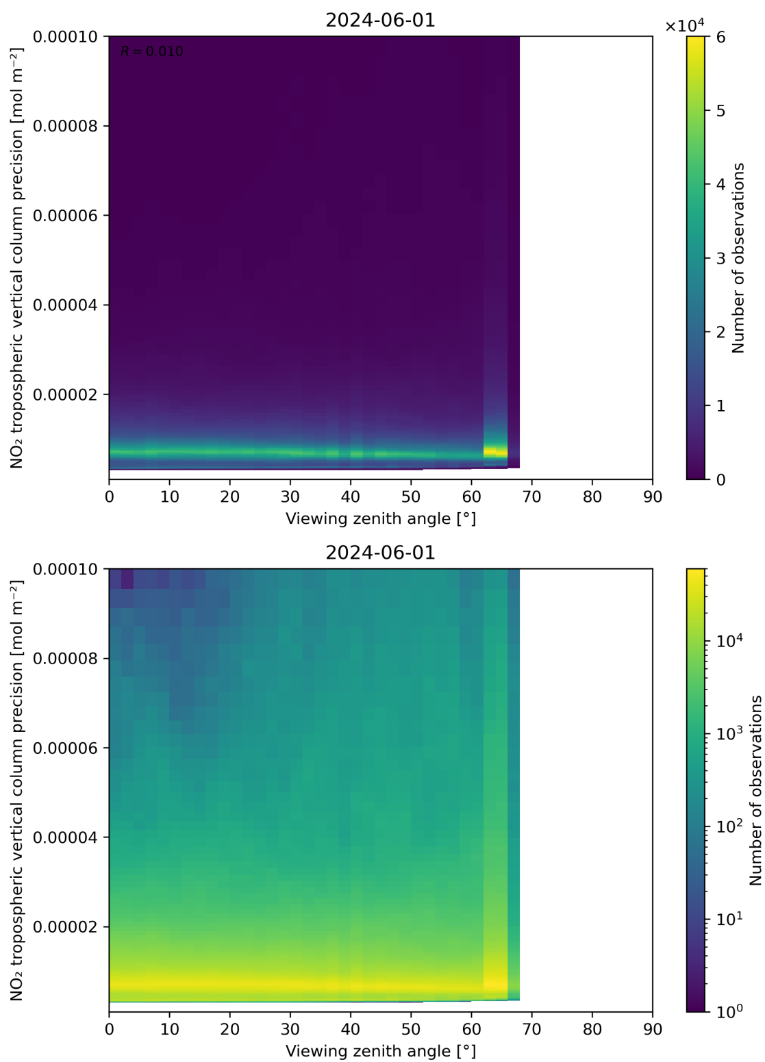
Figure 170: Scatter density plot of “Viewing zenith angle” against “NO 2 tropospheric vertical column precision” for 2024-05-31 to 2024-06-02.
