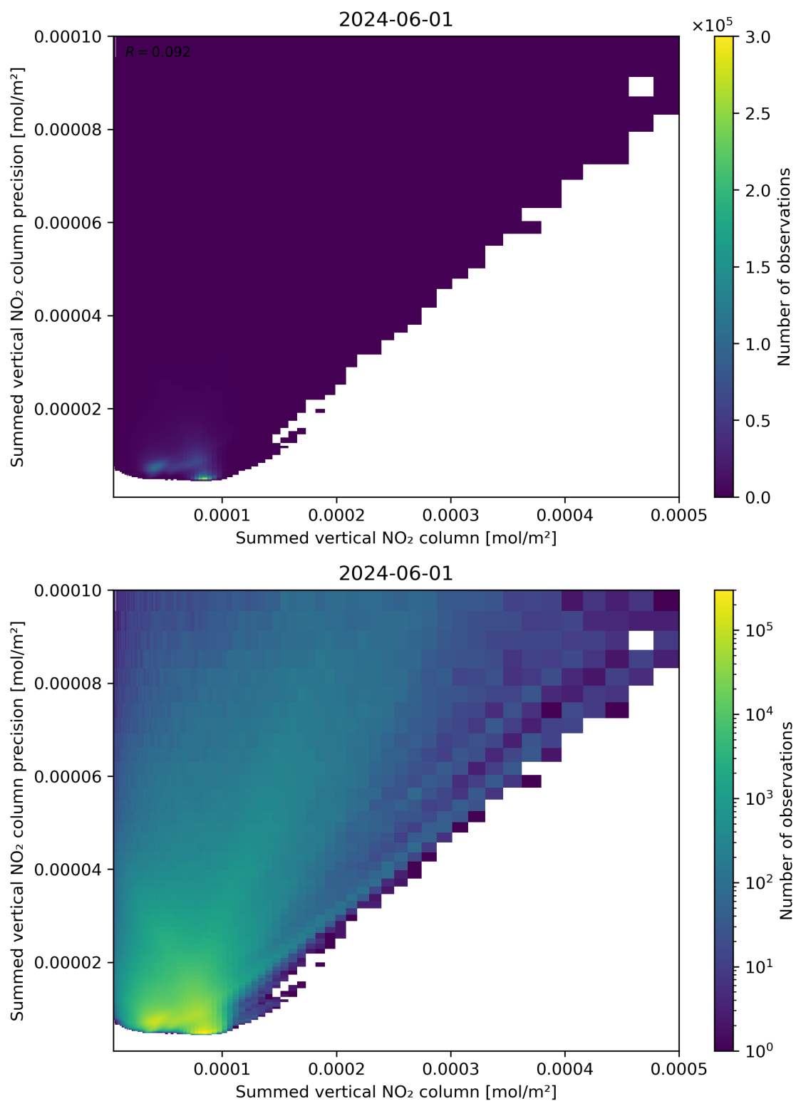
Figure 105: Scatter density plot of “Summed vertical NO 2 column” against “Summed vertical NO 2 column precision” for 2024-05-31 to 2024-06-02.
