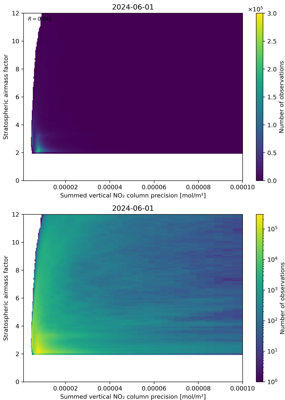
Figure 106: Scatter density plot of “Summed vertical NO 2 column precision” against “Stratospheric airmass factor” for 2024-05-31 to 2024-06-02.
