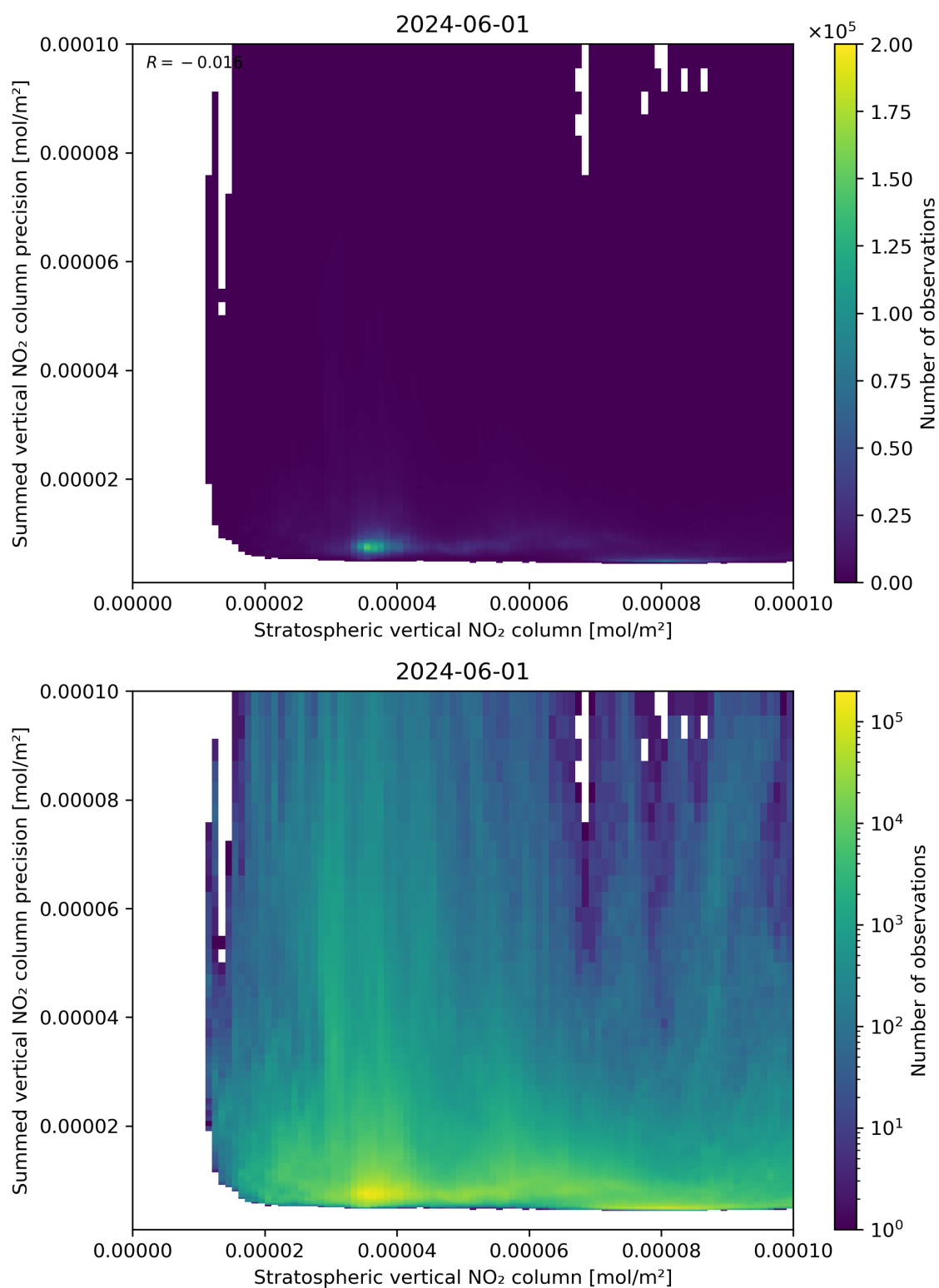
Figure 99: Scatter density plot of “Stratospheric vertical NO 2 column” against “Summed vertical NO 2 column precision” for 2024-05-31 to 2024-06-02.
