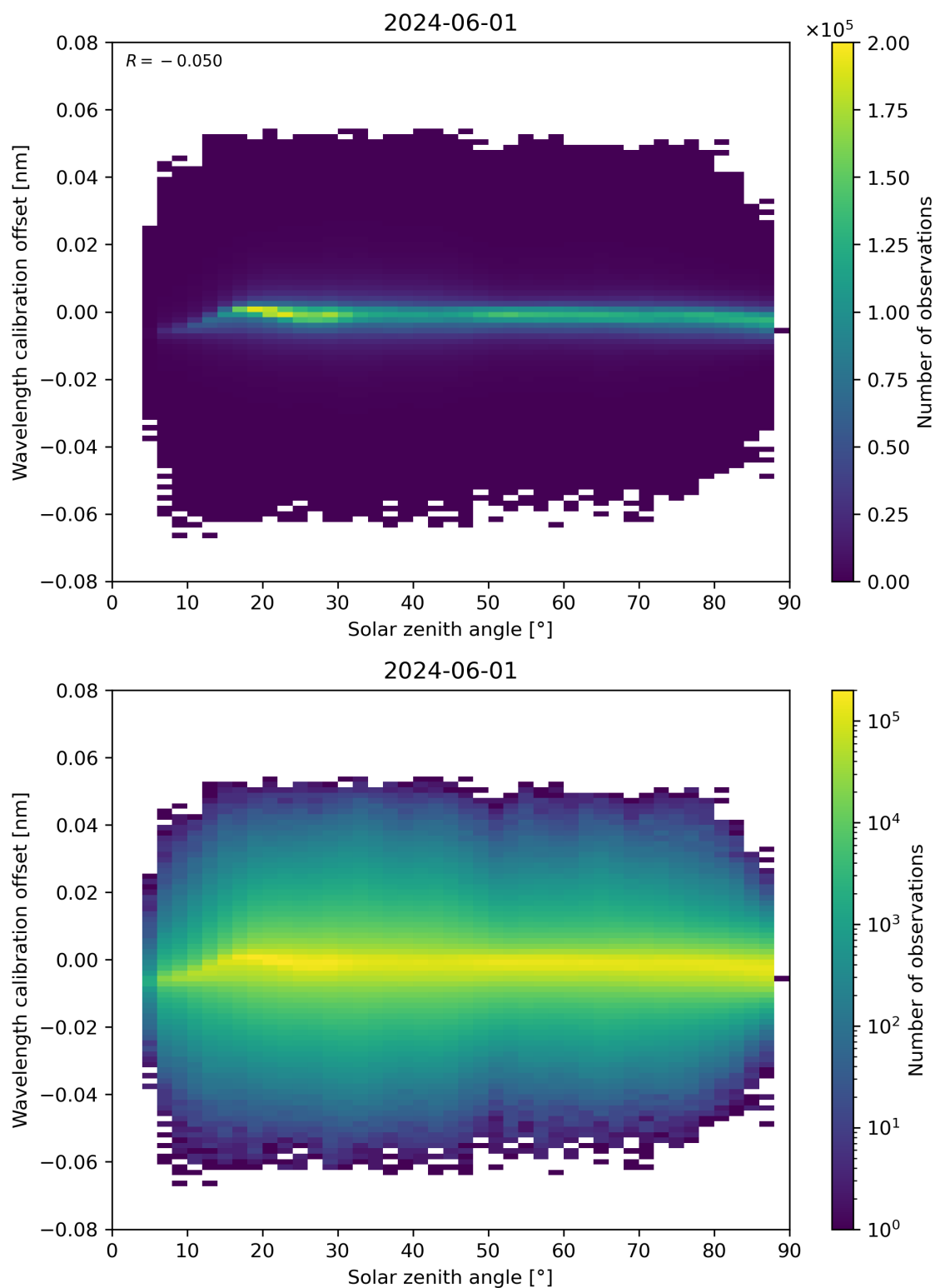
Figure 158: Scatter density plot of “Solar zenith angle” against “Wavelength calibration offset” for 2024-05-31 to 2024-06-02.
