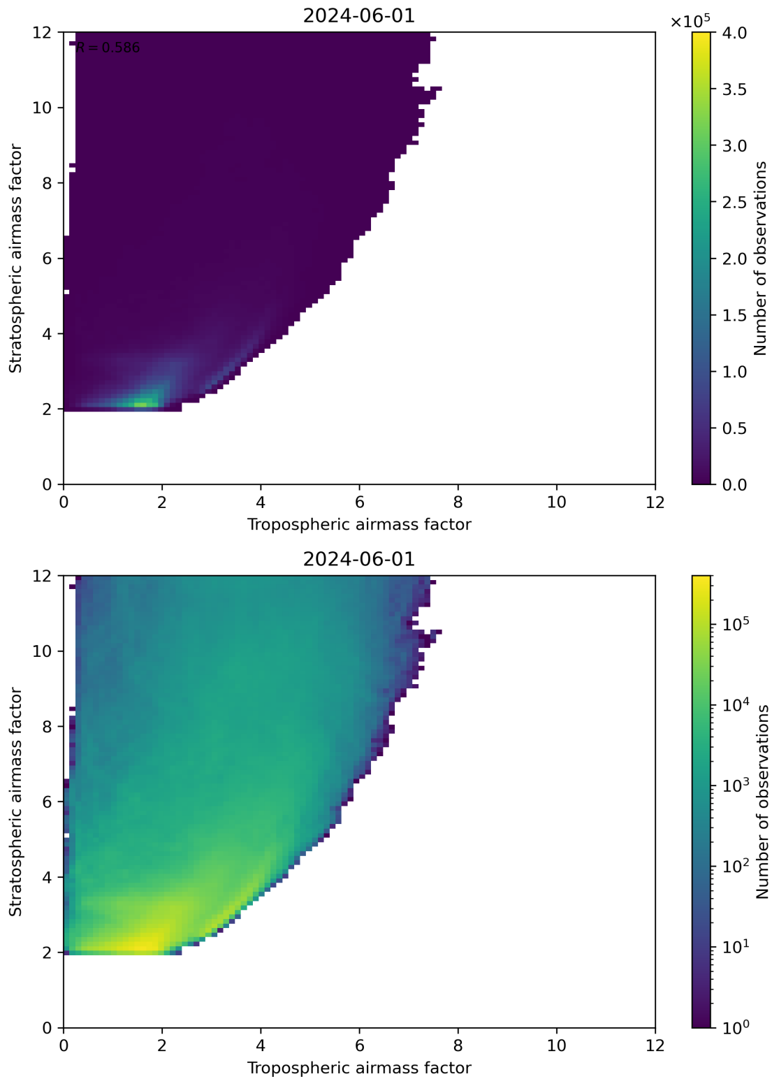
Figure 71: Scatter density plot of “Tropospheric airmass factor” against “Stratospheric airmass factor” for 2024-05-31 to 2024-06-02.
