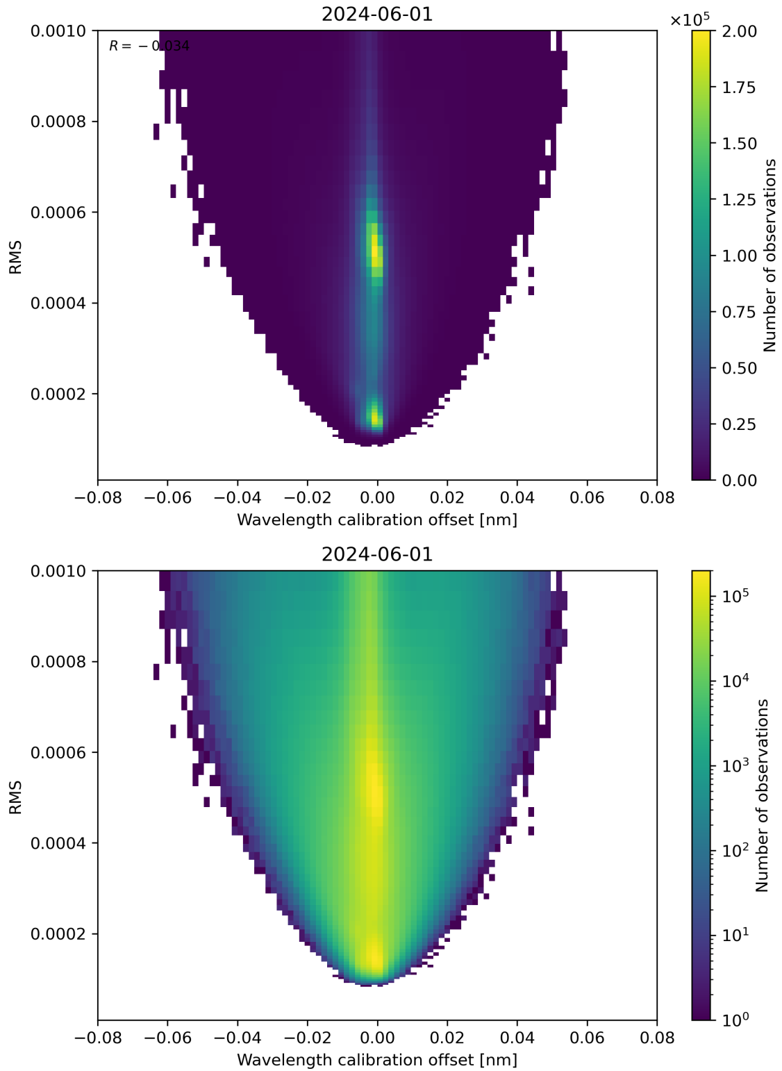
Figure 181: Scatter density plot of “Wavelength calibration offset” against “RMS” for 2024-05-31 to 2024-06-02.
