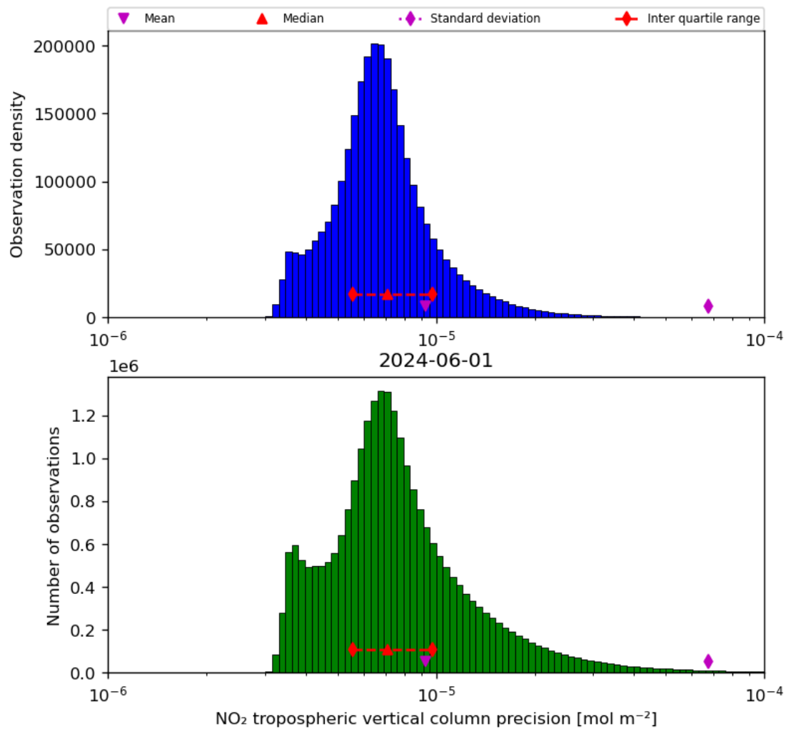
Figure 30: Histogram of “NO 2 tropospheric vertical column precision” for 2024-05-31 to 2024-06-02
