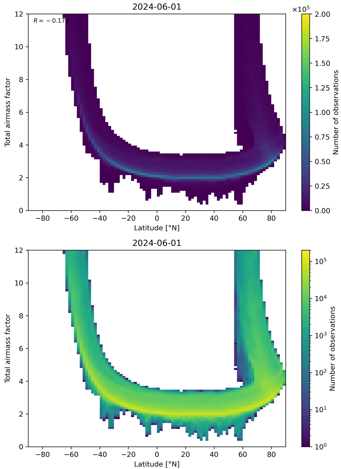
Figure 84: Scatter density plot of “Latitude” against “Total airmass factor” for 2024-05-31 to 2024-06-02.
