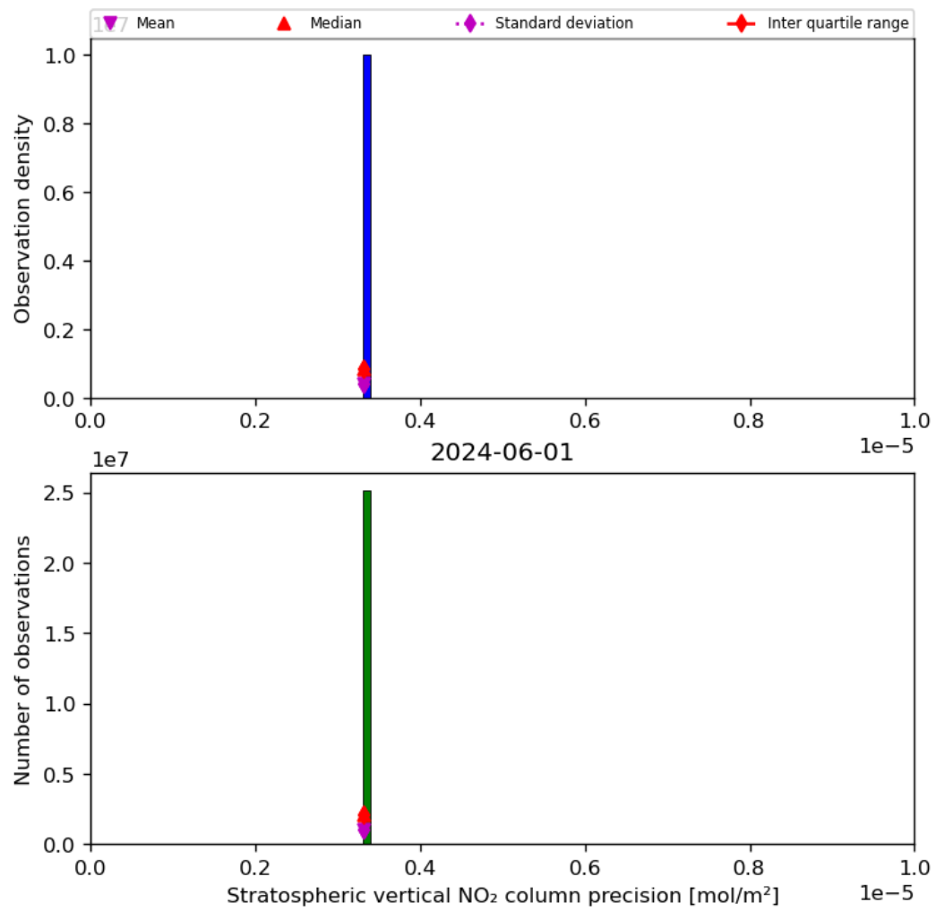
Figure 37: Histogram of “Stratospheric vertical NO 2 column precision” for 2024-05-31 to 2024-06-02
