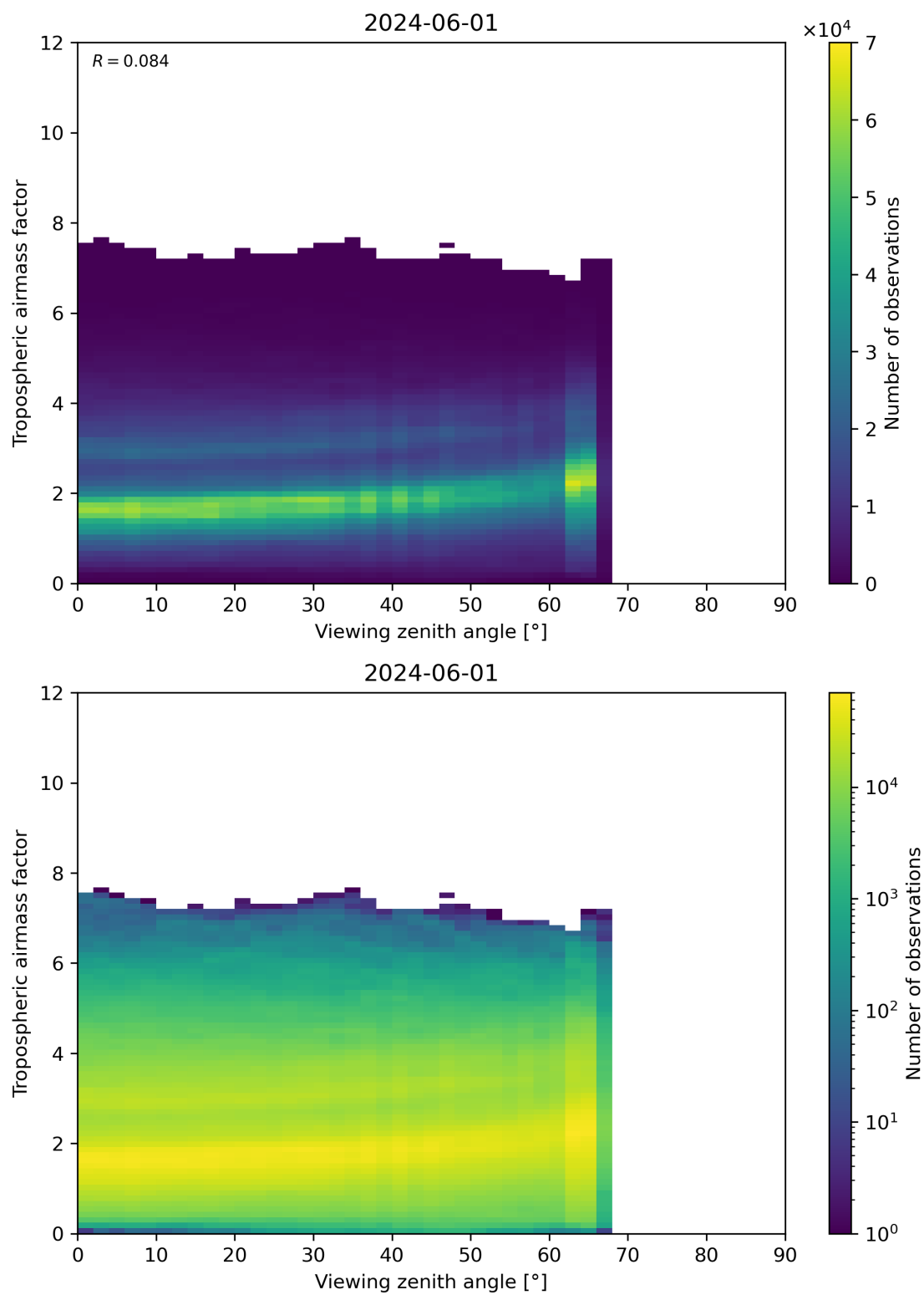
Figure 161: Scatter density plot of “Viewing zenith angle” against “Tropospheric airmass factor” for 2024-05-31 to 2024-06-02.
