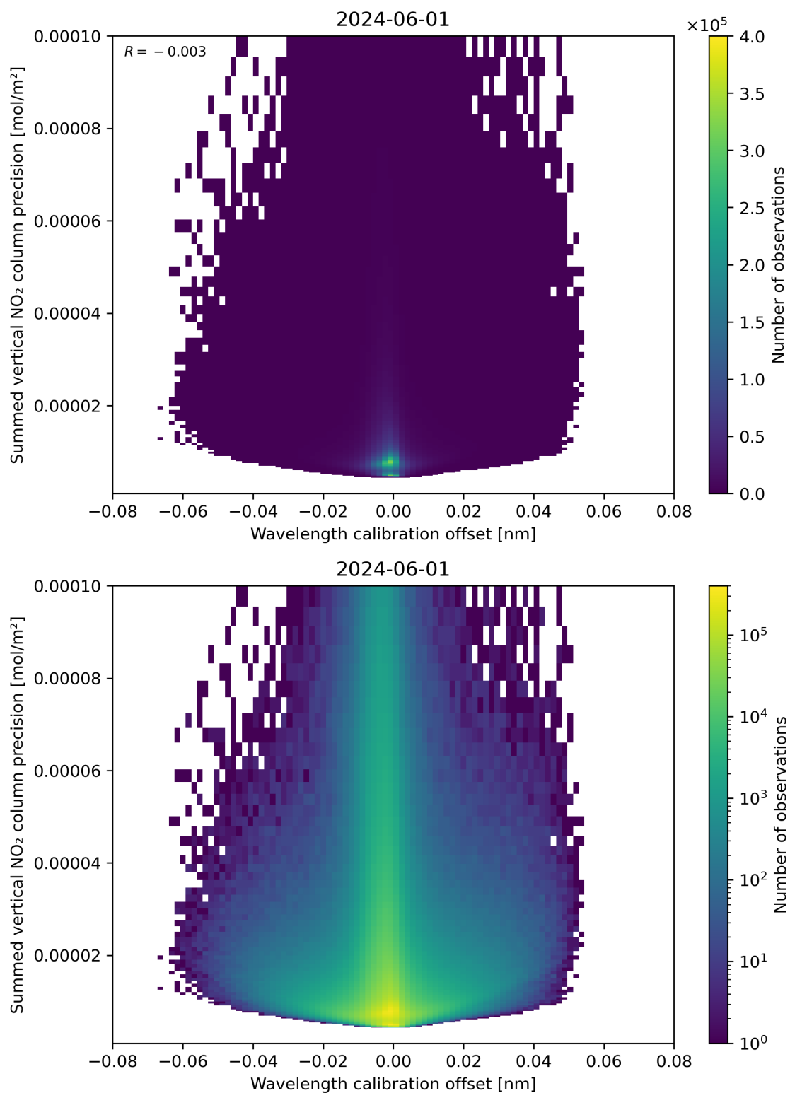
Figure 178: Scatter density plot of “Wavelength calibration offset” against “Summed vertical NO 2 column precision” for 2024-05-31 to 2024-06-02.
