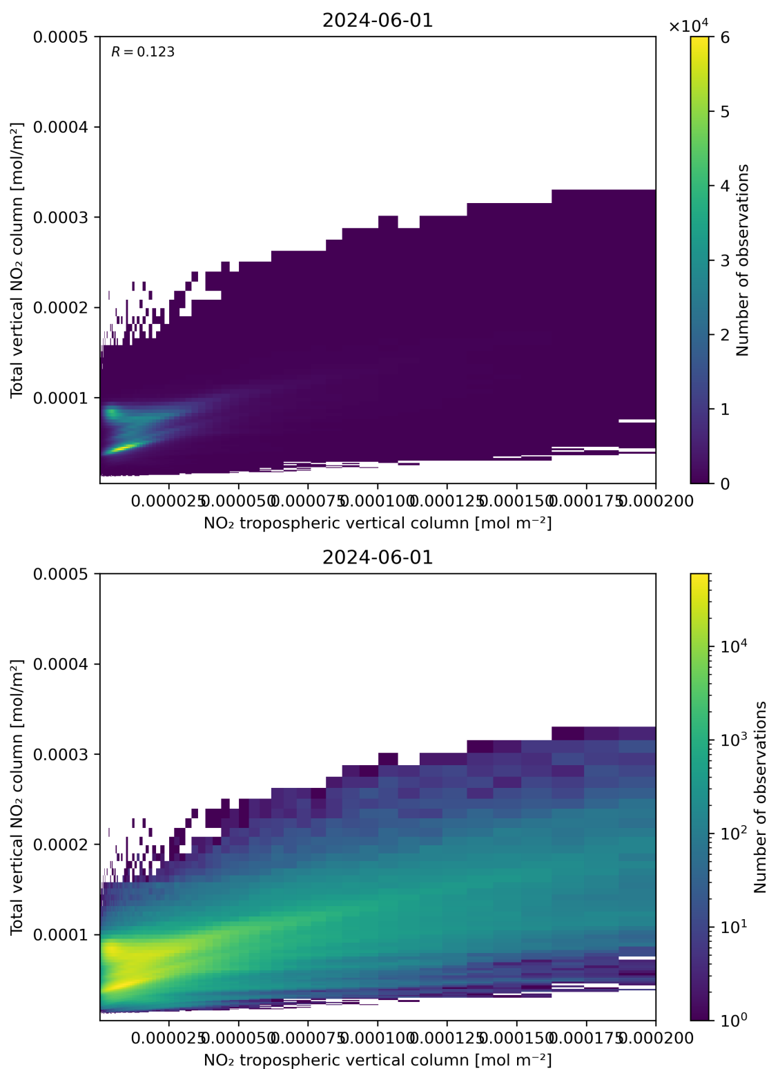
Figure 128: Scatter density plot of “NO 2 tropospheric vertical column” against “Total vertical NO 2 column” for 2024-05-31 to 2024-06-02.
