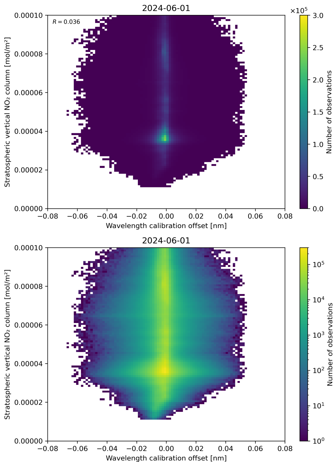
Figure 176: Scatter density plot of “Wavelength calibration offset” against “Stratospheric vertical NO 2 column” for 2024-05-31 to 2024-06-02.
