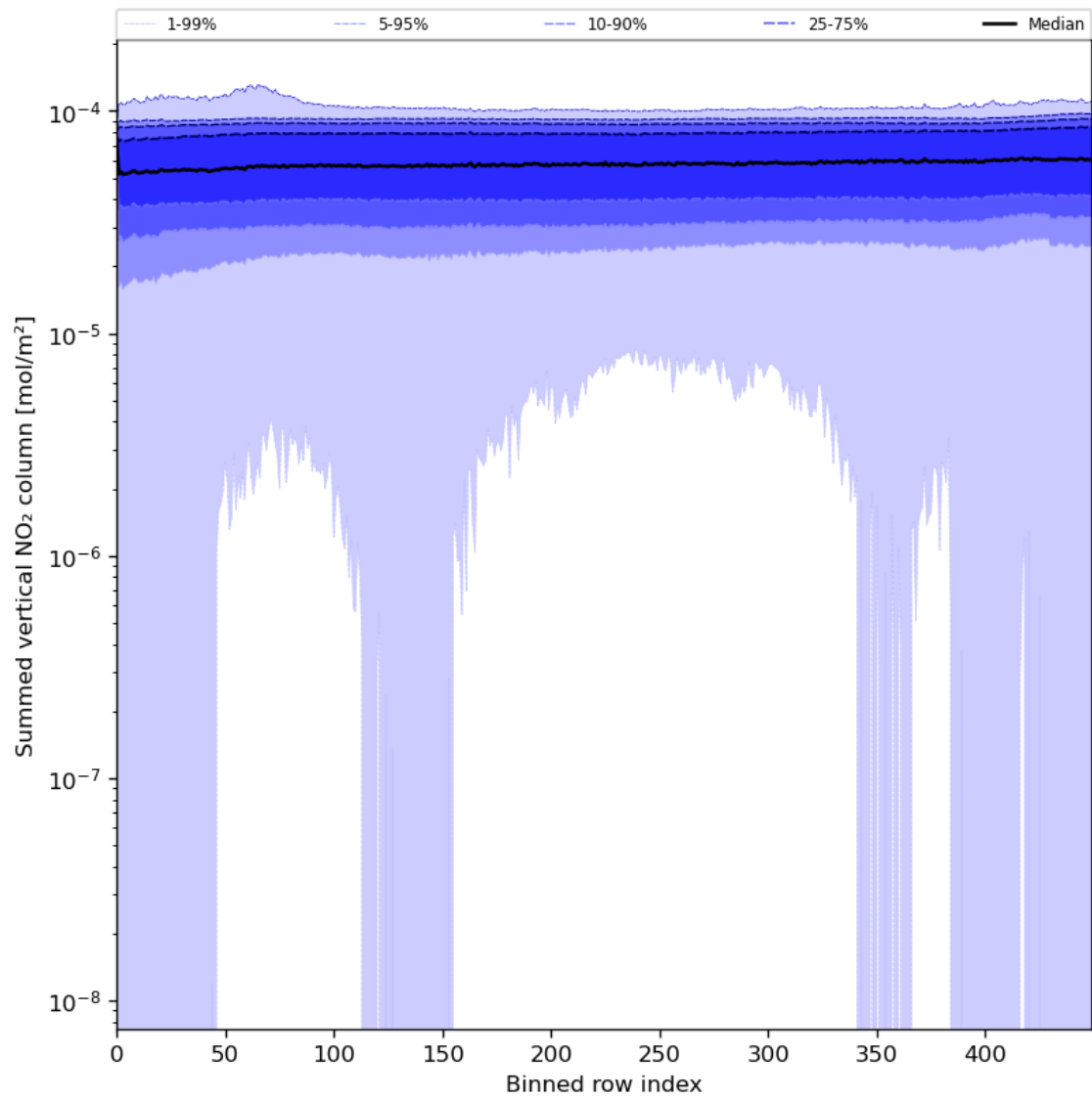
Figure 57: Along track statistics of “Summed vertical NO 2 column” for 2024-05-31 to 2024-06-02
