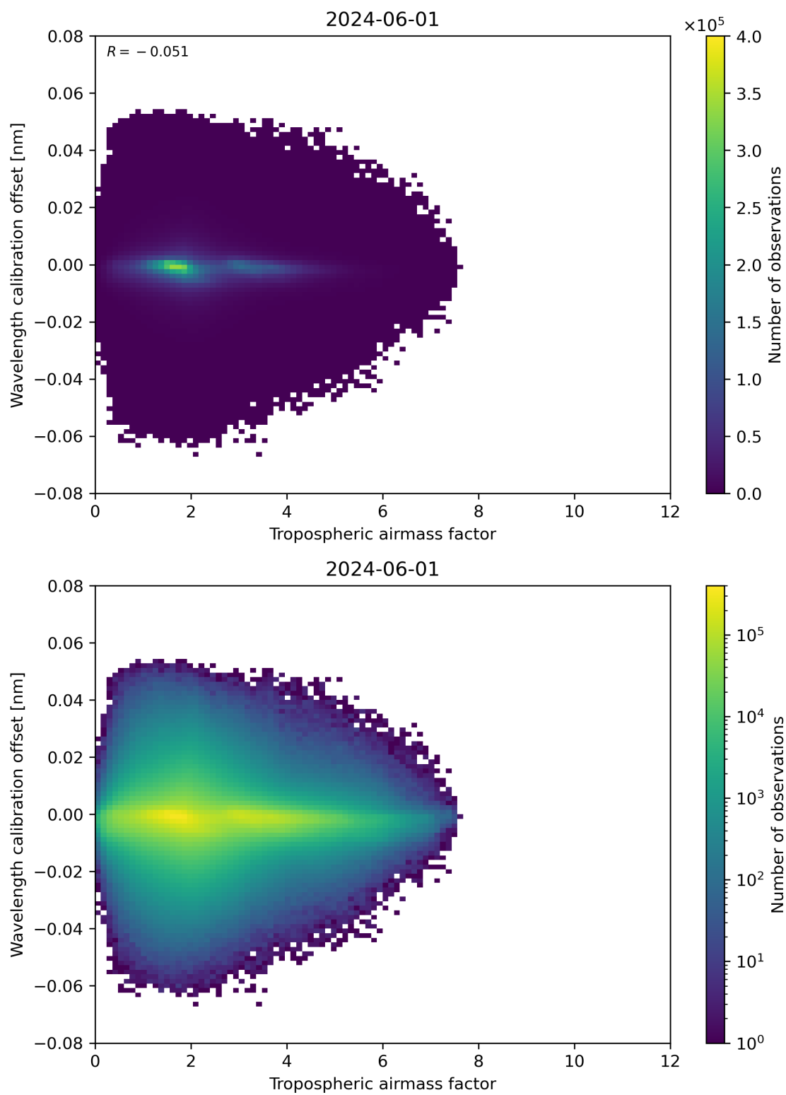
Figure 80: Scatter density plot of “Tropospheric airmass factor” against “Wavelength calibration offset” for 2024-05-31 to 2024-06-02.
