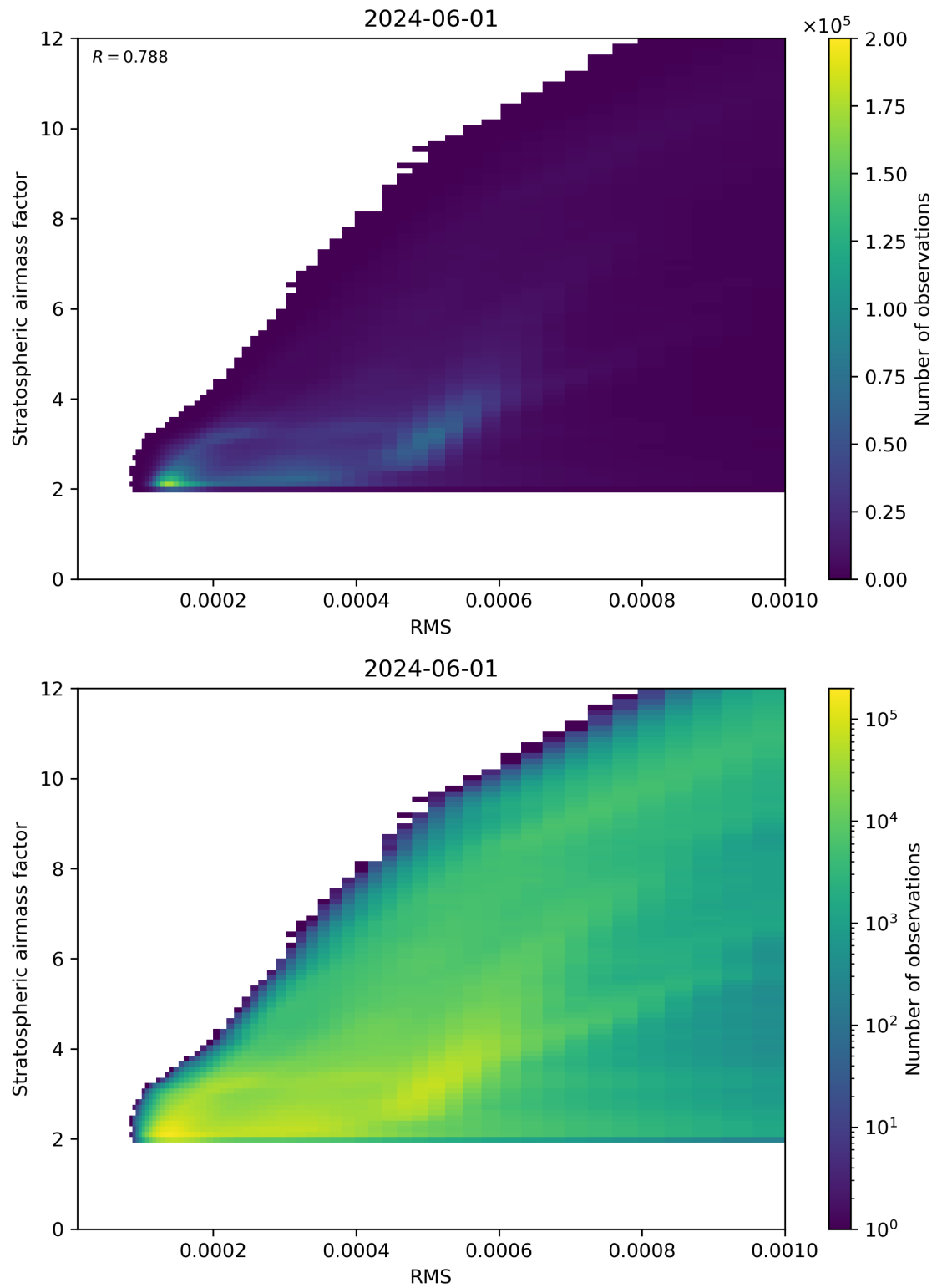
Figure 144: Scatter density plot of “RMS” against “Stratospheric airmass factor” for 2024-05-31 to 2024-06-02.
