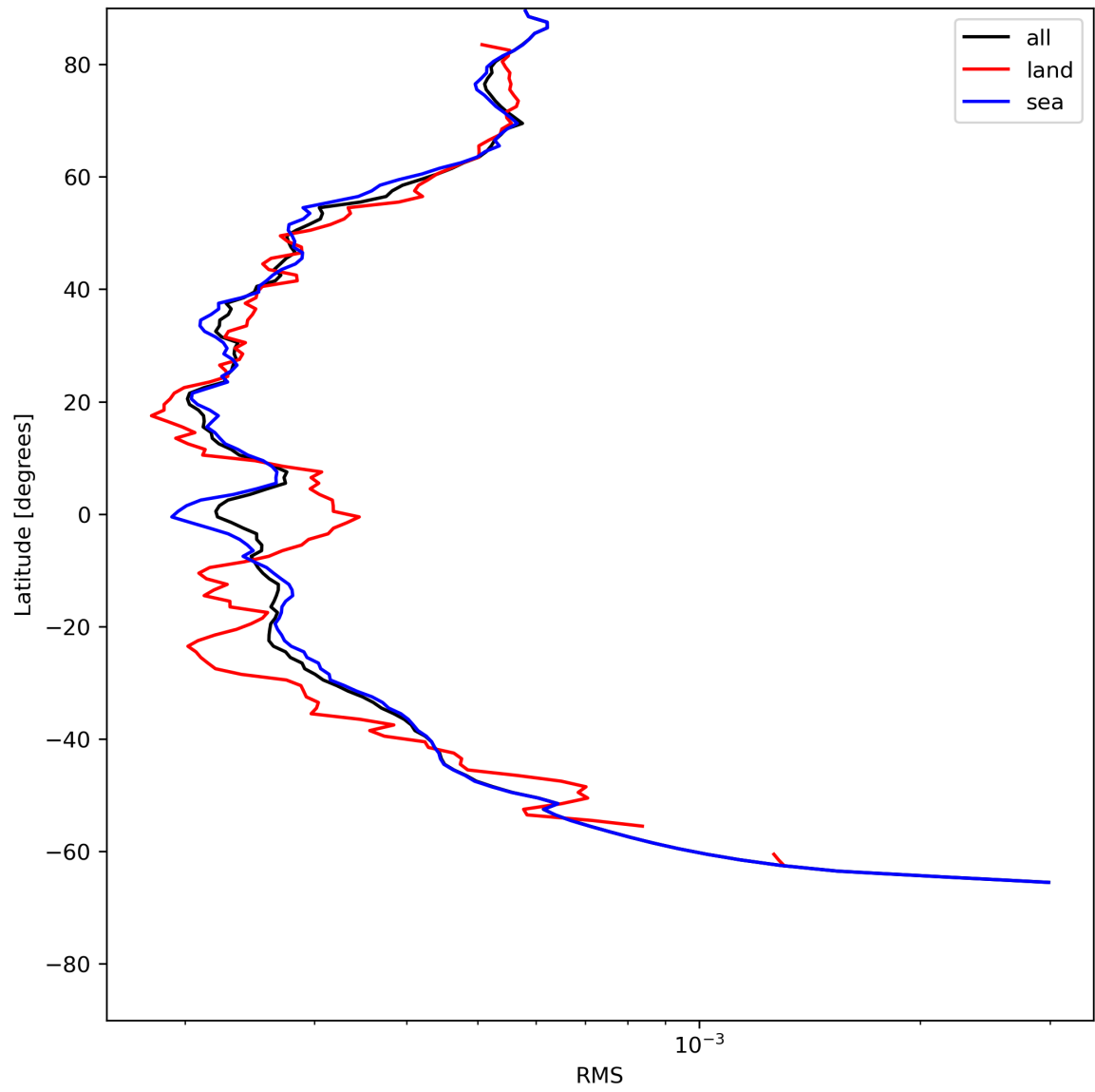
Figure 26: Zonal average of “RMS” for 2024-05-31 to 2024-06-02.
