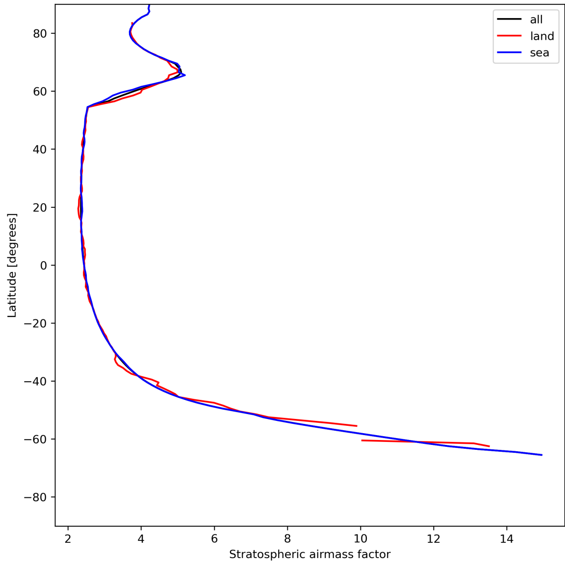
Figure 27: Zonal average of “Stratospheric airmass factor” for 2024-05-31 to 2024-06-02.
