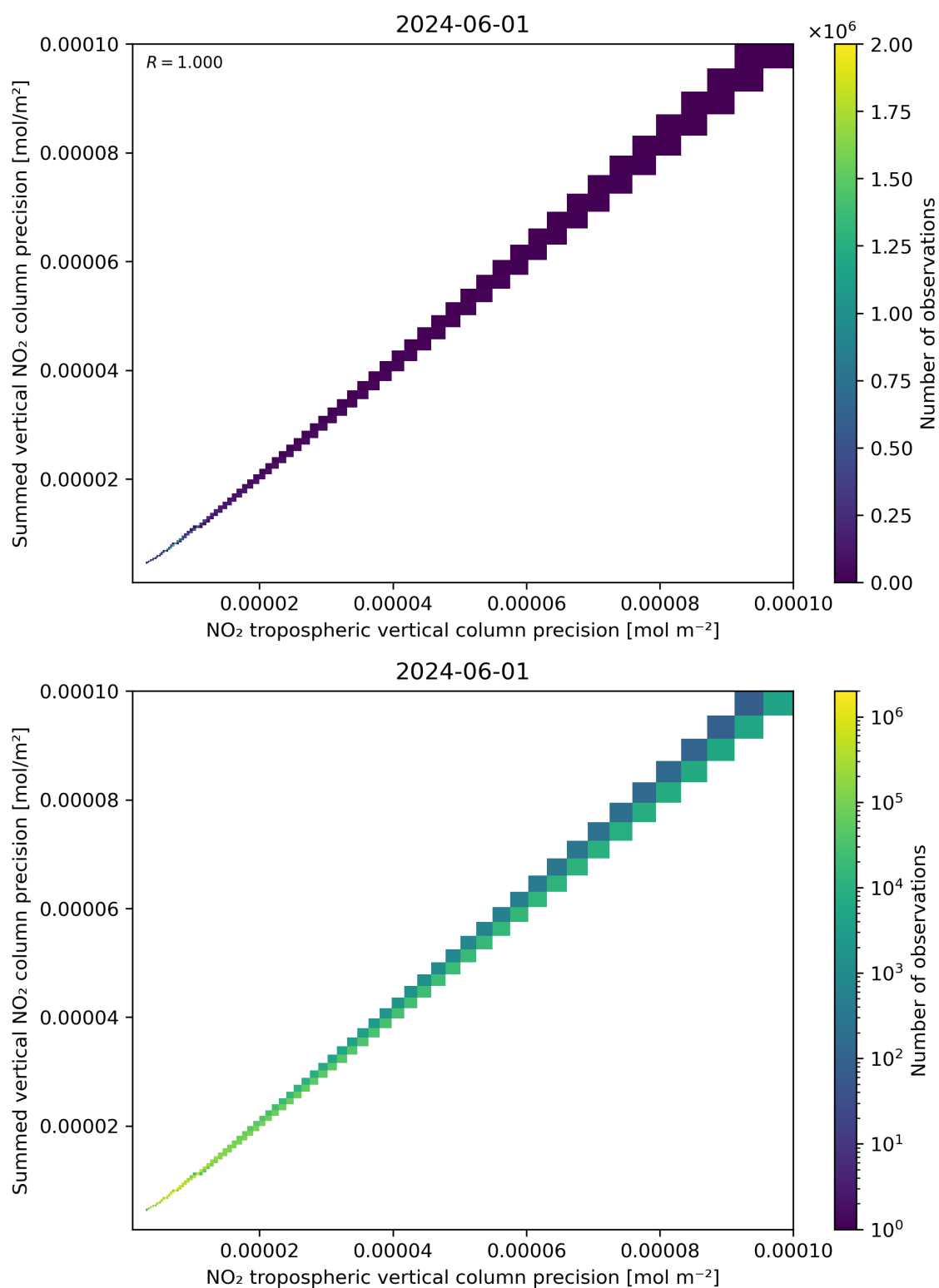
Figure 137: Scatter density plot of “NO 2 tropospheric vertical column precision” against “Summed vertical NO 2 column precision” for 2024-05-31 to 2024-06-02.
