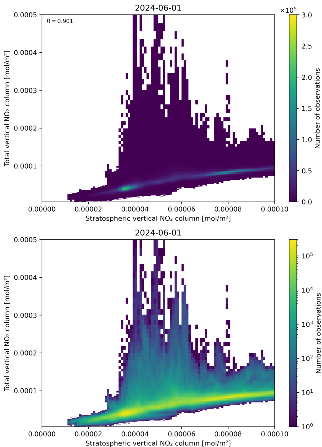
Figure 100: Scatter density plot of “Stratospheric vertical NO 2 column” against “Total vertical NO 2 column” for 2024-05-31 to 2024-06-02.
