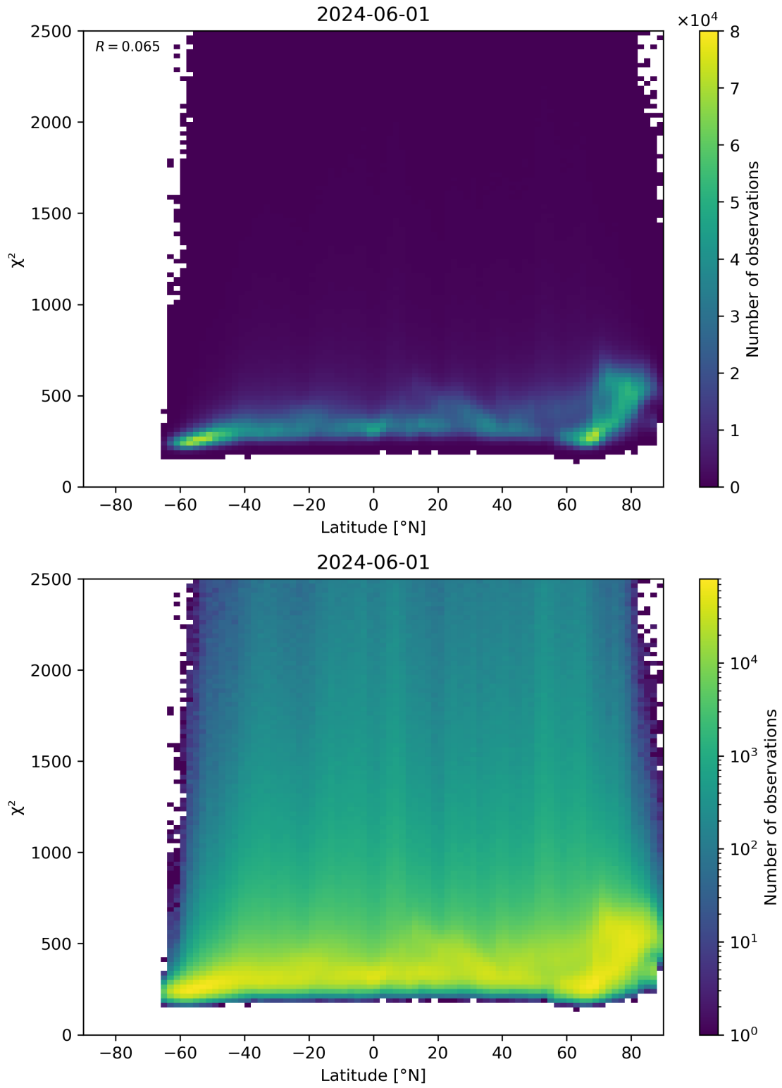
Figure 86: Scatter density plot of “Latitude” against “ \chi^2 ” for 2024-05-31 to 2024-06-02.
