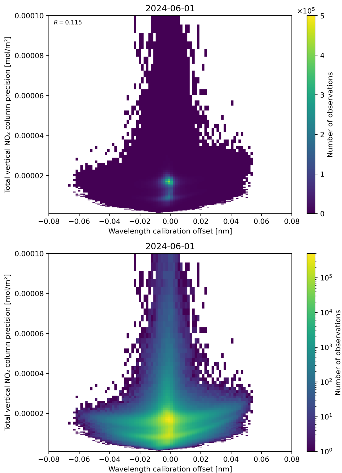
Figure 180: Scatter density plot of “Wavelength calibration offset” against “Total vertical NO 2 column precision” for 2024-05-31 to 2024-06-02.
