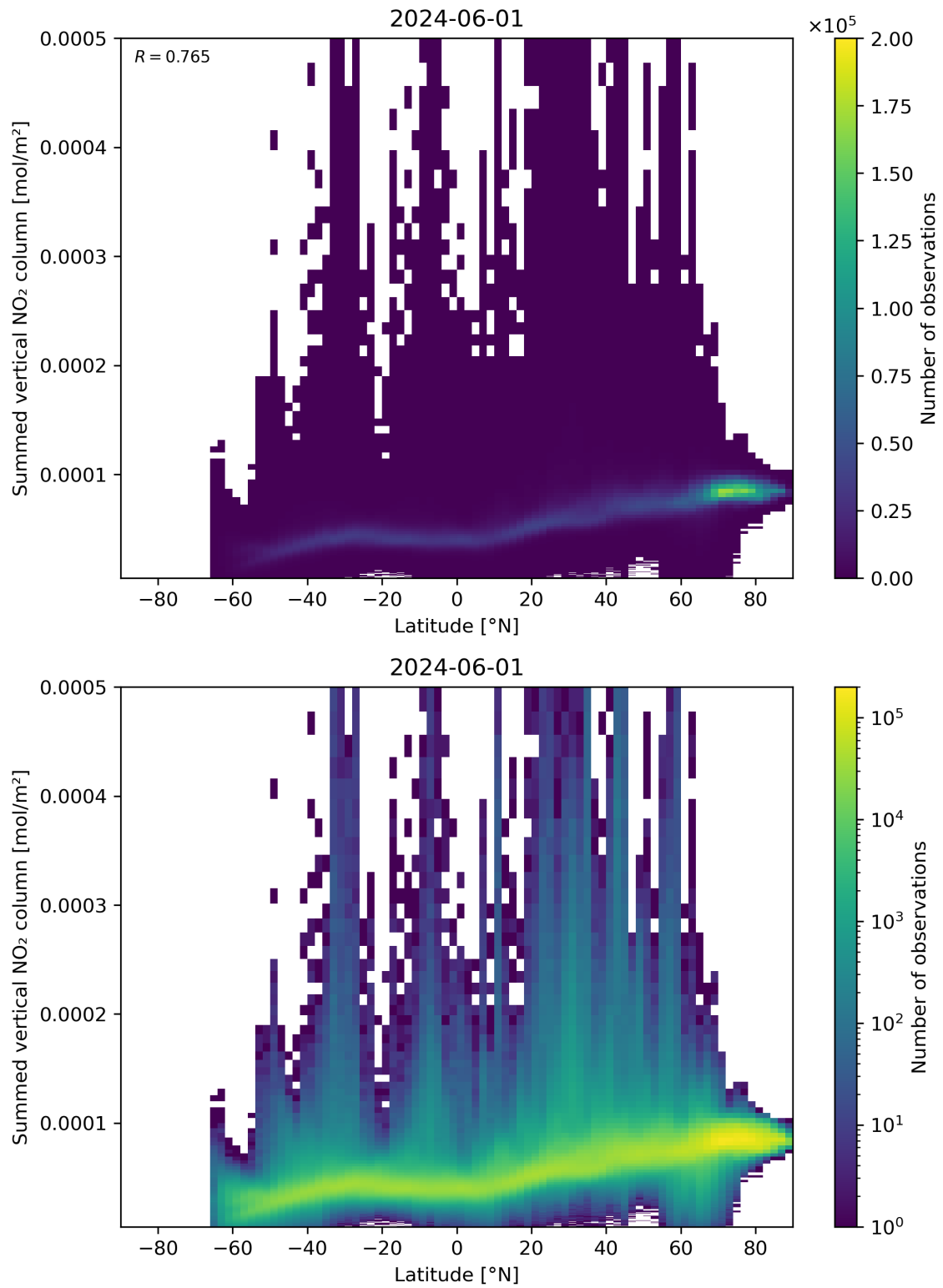
Figure 88: Scatter density plot of “Latitude” against “Summed vertical NO 2 column” for 2024-05-31 to 2024-06-02.
