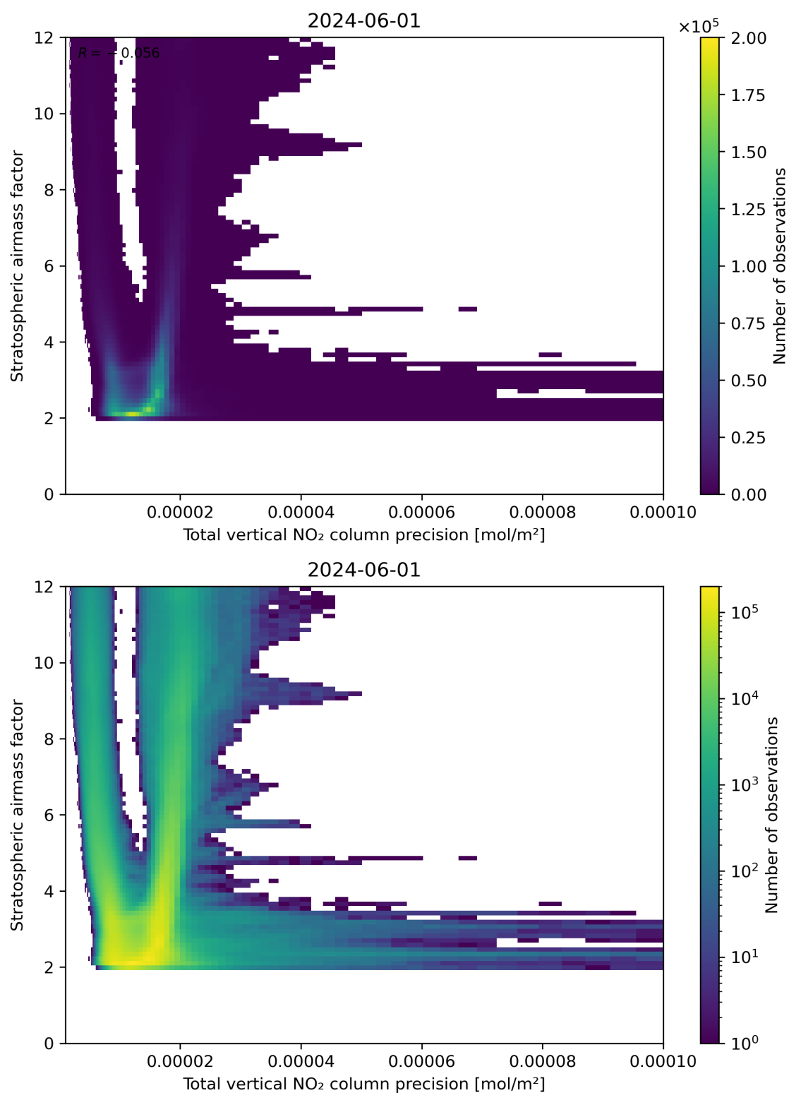
Figure 115: Scatter density plot of “Total vertical NO 2 column precision” against “Stratospheric air mass factor” for 2024-05-31 to 2024-06-02.
