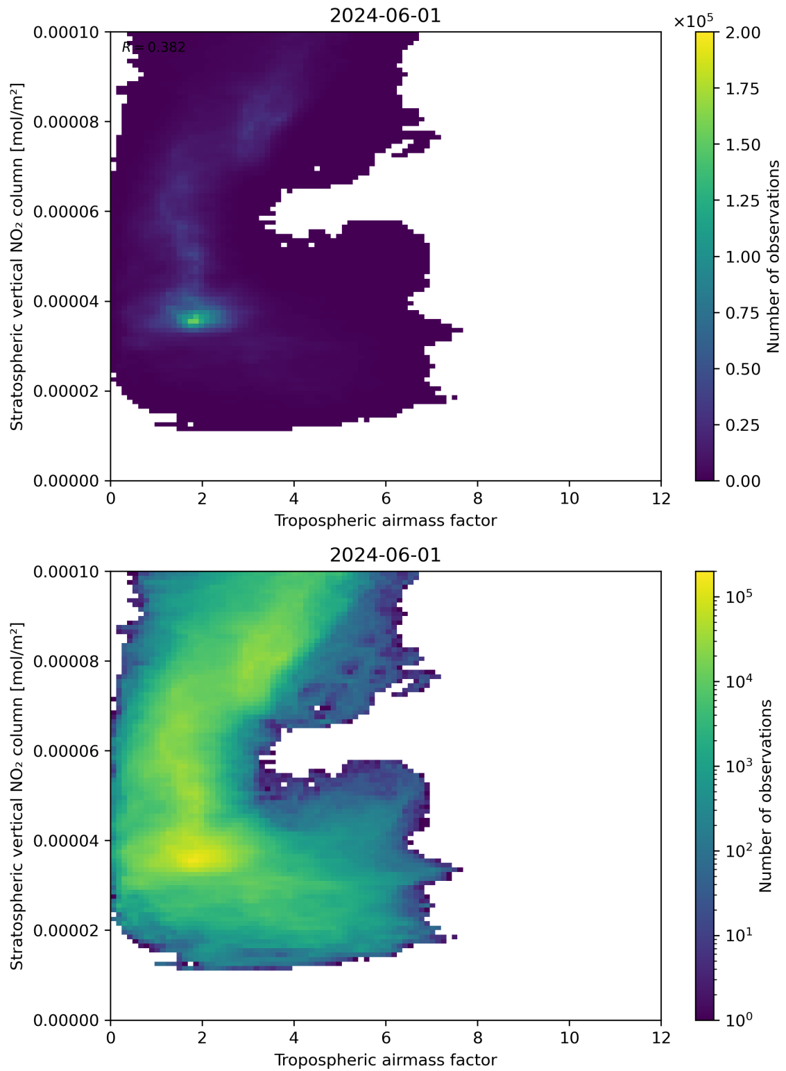
Figure 74: Scatter density plot of “Tropospheric air mass factor” against “Stratospheric vertical NO 2 column” for 2024-05-31 to 2024-06-02.
