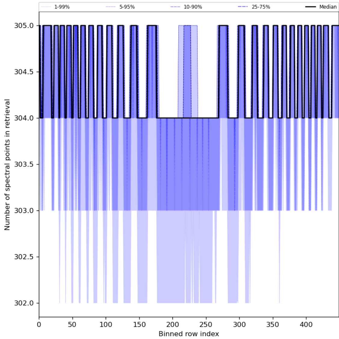
Figure 50: Along track statistics of “Number of spectral points in retrieval” for 2024-05-31 to 2024-06-02
