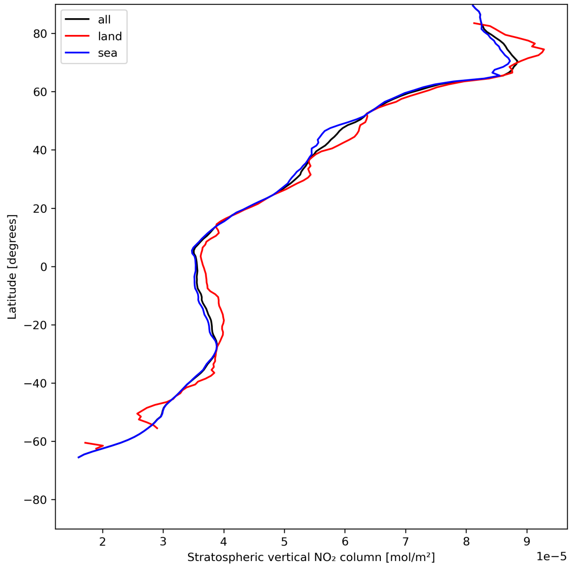
Figure 19: Zonal average of “Stratospheric vertical NO 2 column” for 2024-05-31 to 2024-06-02.
