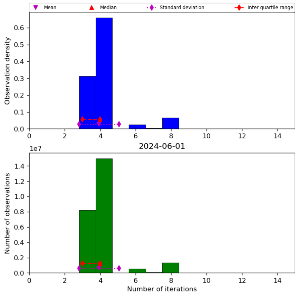
Figure 34: Histogram of “Number of iterations” for 2024-05-31 to 2024-06-02
