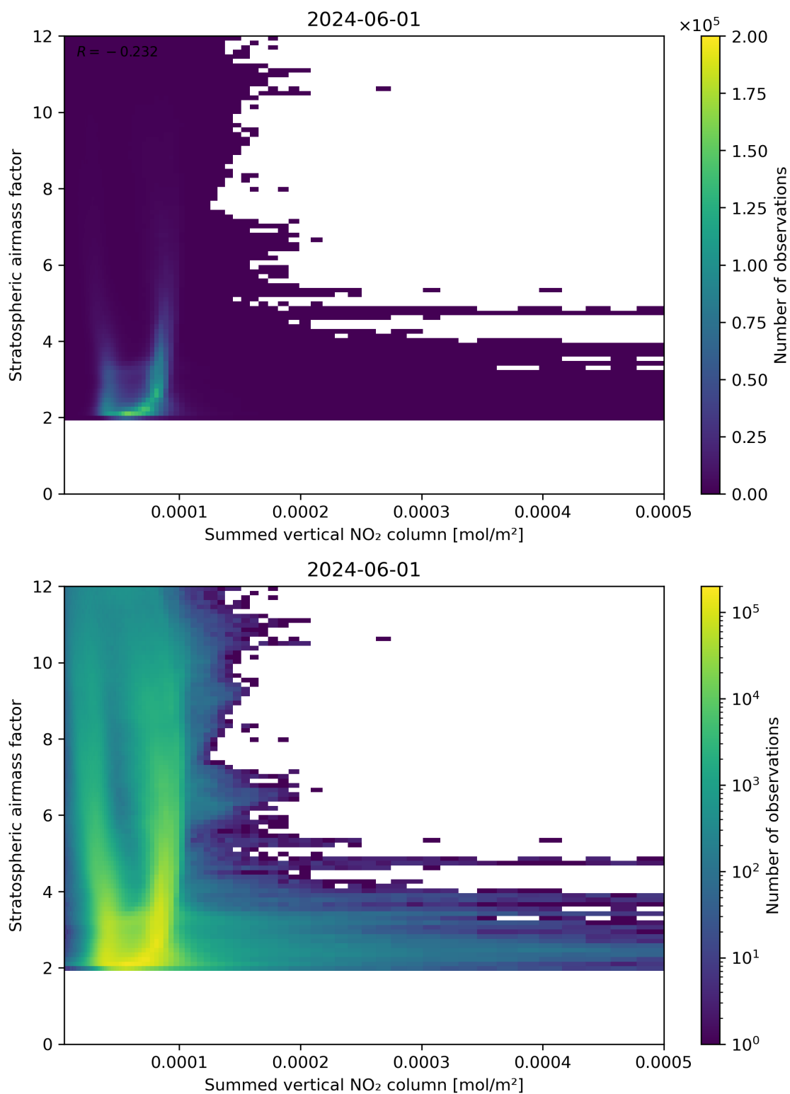
Figure 103: Scatter density plot of “Summed vertical NO 2 column” against “Stratospheric airmass factor” for 2024-05-31 to 2024-06-02.
