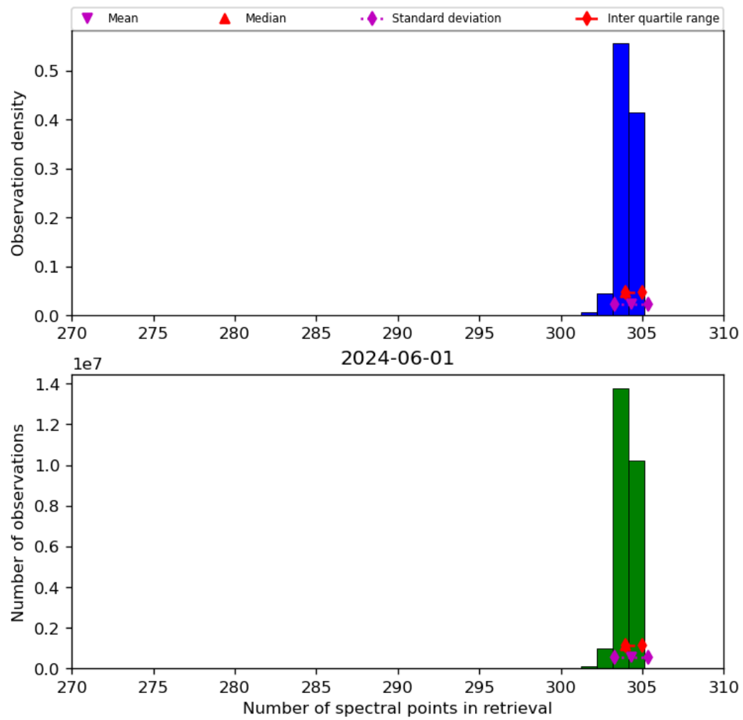
Figure 33: Histogram of “Number of spectral points in retrieval” for 2024-05-31 to 2024-06-02
