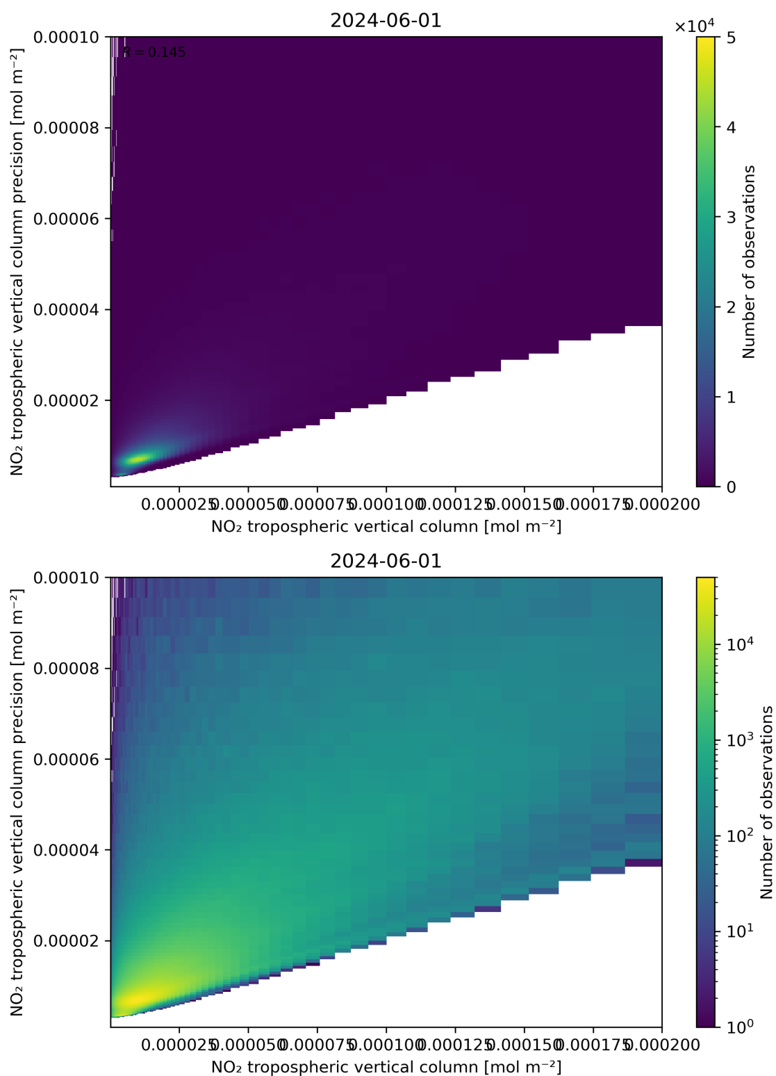
Figure 130: Scatter density plot of “NO 2 tropospheric vertical column” against “NO 2 tropospheric vertical column precision” for 2024-05-31 to 2024-06-02.
