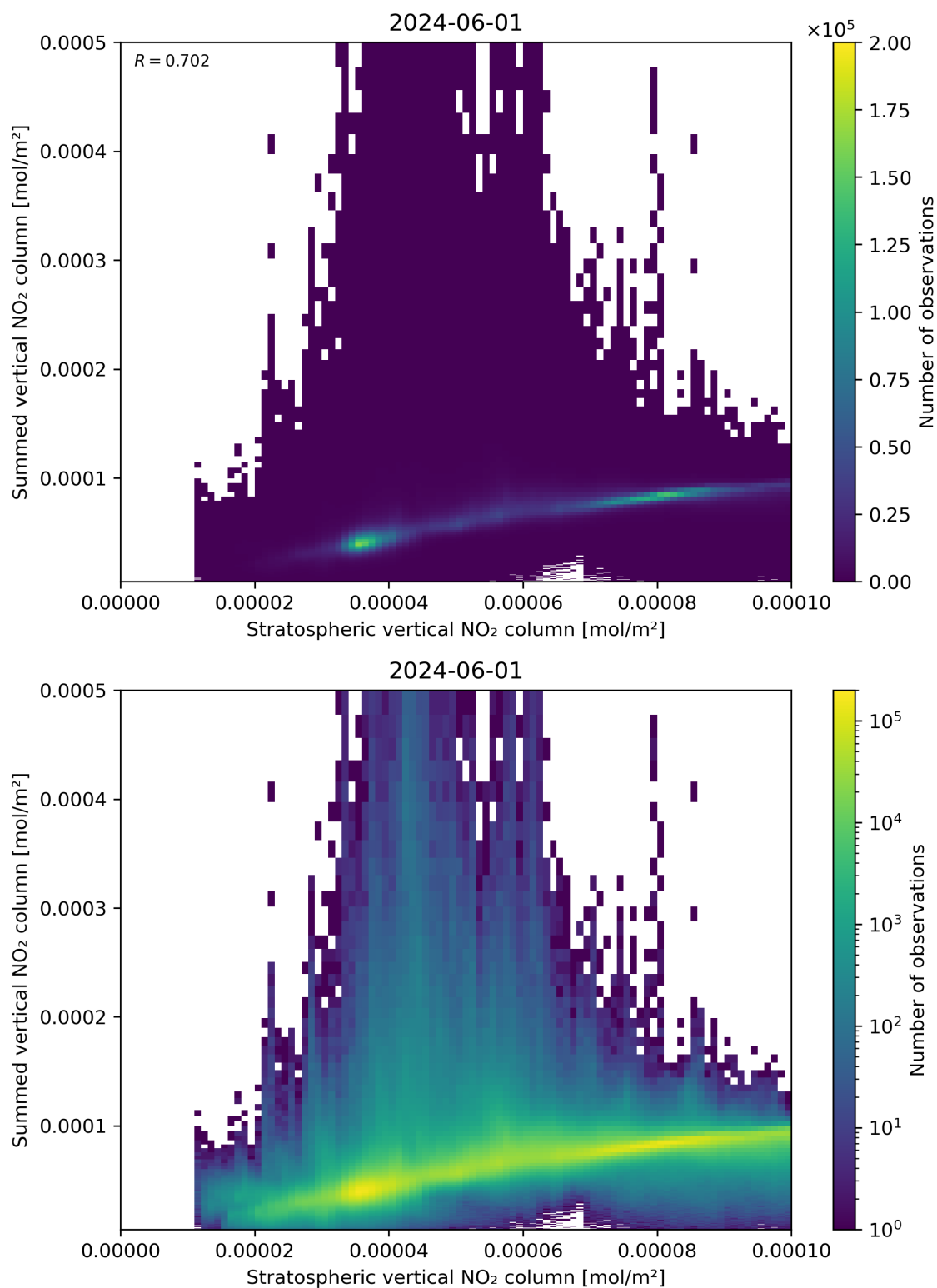
Figure 98: Scatter density plot of “Stratospheric vertical NO 2 column” against “Summed vertical NO 2 column” for 2024-05-31 to 2024-06-02.
