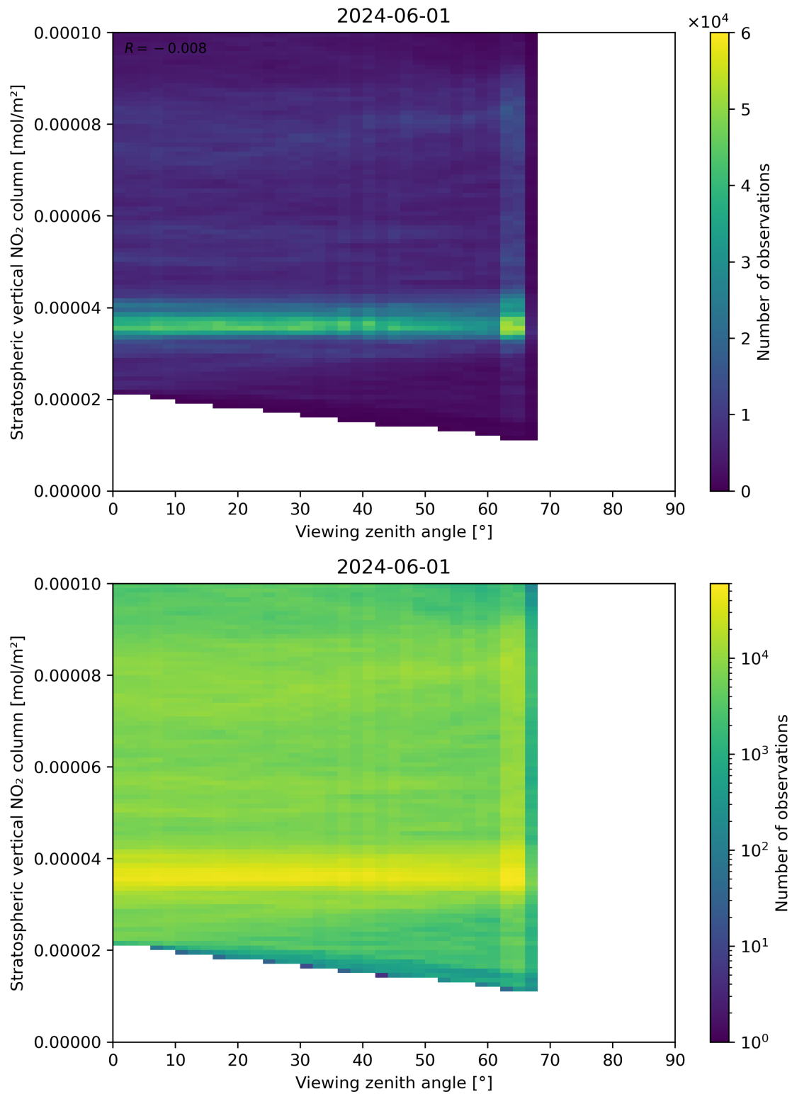
Figure 164: Scatter density plot of “Viewing zenith angle” against “Stratospheric vertical NO 2 column” for 2024-05-31 to 2024-06-02.
