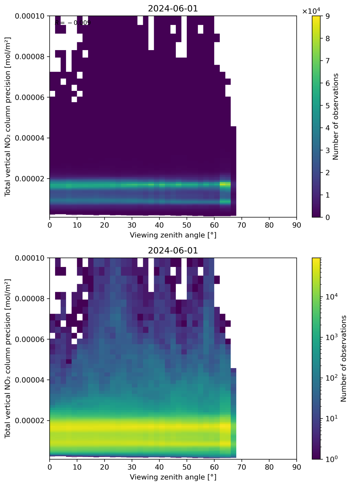
Figure 168: Scatter density plot of “Viewing zenith angle” against “Total vertical NO 2 column precision” for 2024-05-31 to 2024-06-02.
