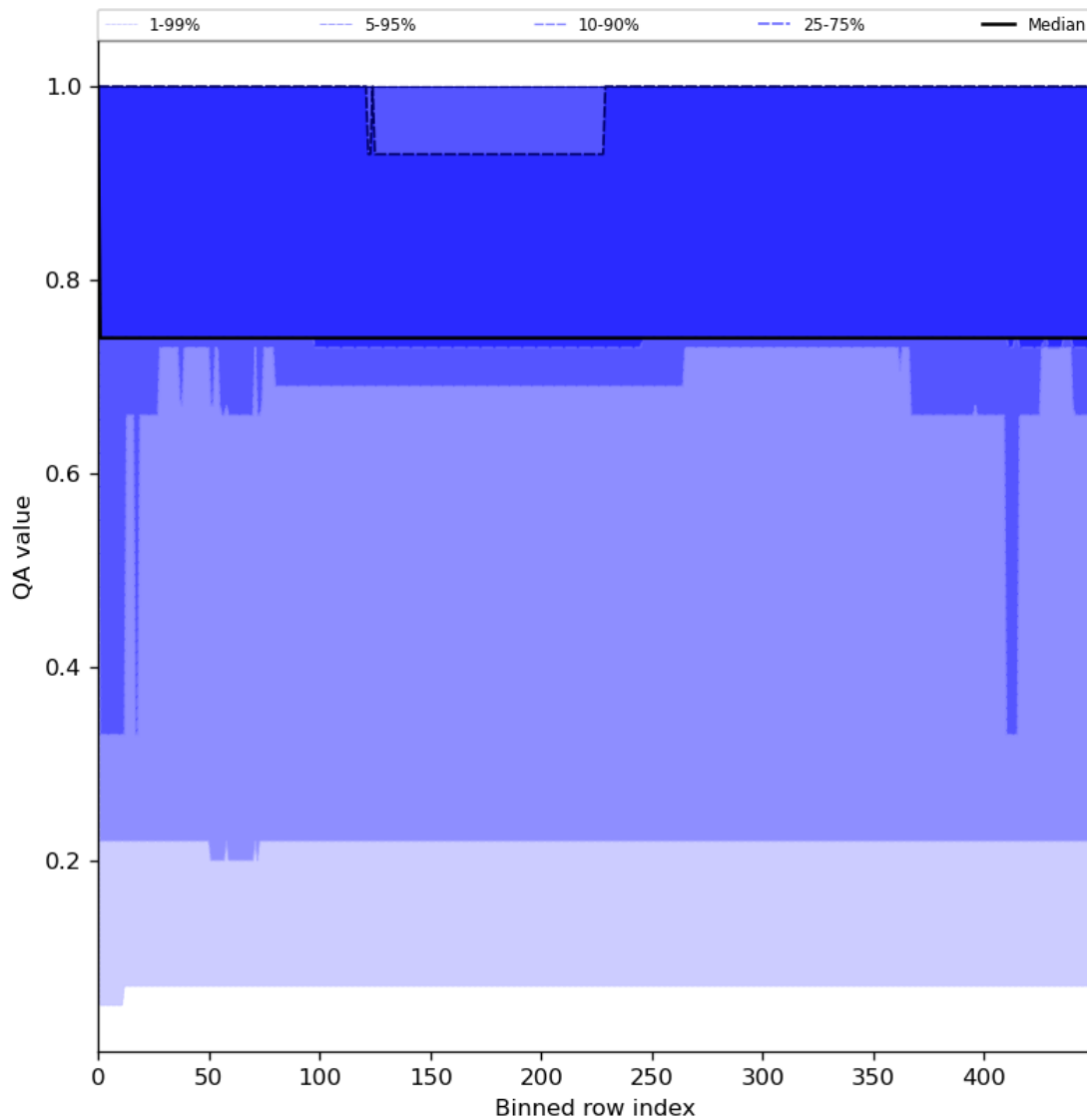
Figure 45: Along track statistics of “QA value” for 2024-05-31 to 2024-06-02
