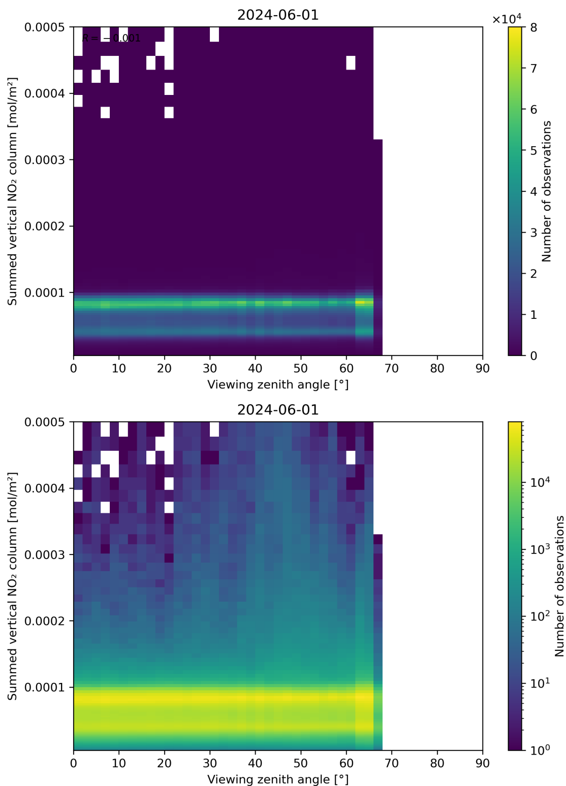
Figure 165: Scatter density plot of “Viewing zenith angle” against “Summed vertical NO 2 column” for 2024-05-31 to 2024-06-02.
