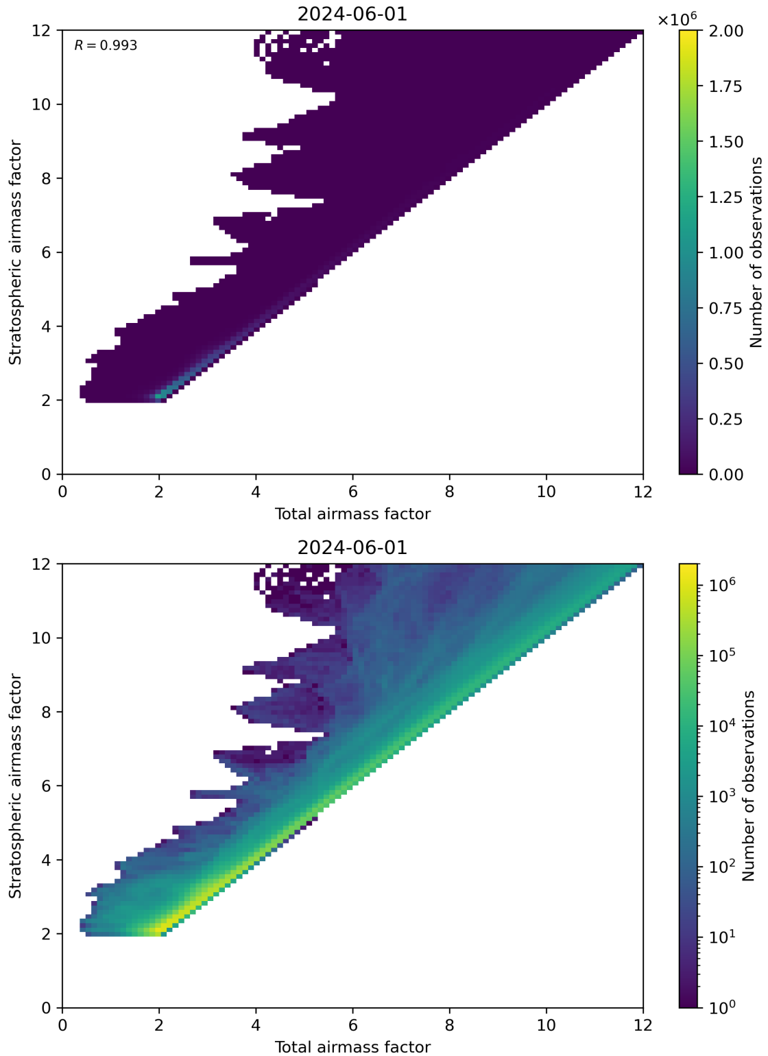
Figure 62: Scatter density plot of “Total airmass factor” against “Stratospheric airmass factor” for 2024-05-31 to 2024-06-02.
