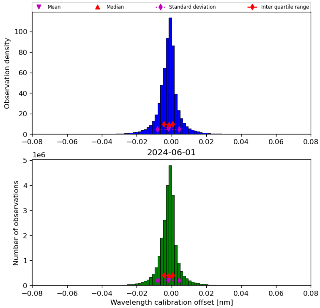
Figure 35: Histogram of “Wavelength calibration offset” for 2024-05-31 to 2024-06-02
