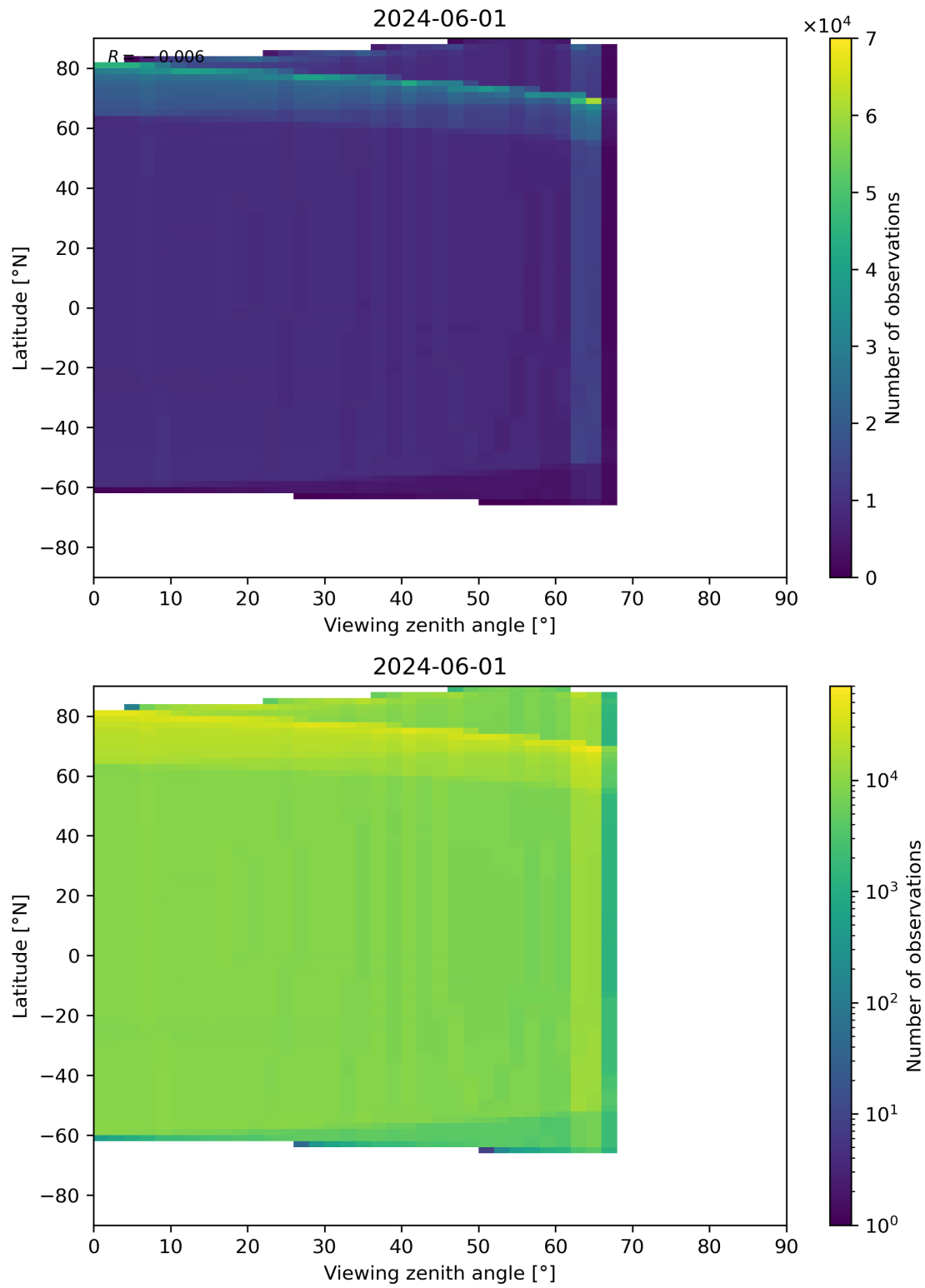
Figure 163: Scatter density plot of “Viewing zenith angle” against “Latitude” for 2024-05-31 to 2024-06-02.
