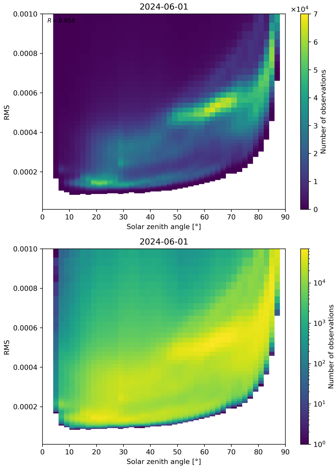
Figure 157: Scatter density plot of “Solar zenith angle” against “RMS” for 2024-05-31 to 2024-06-02.
