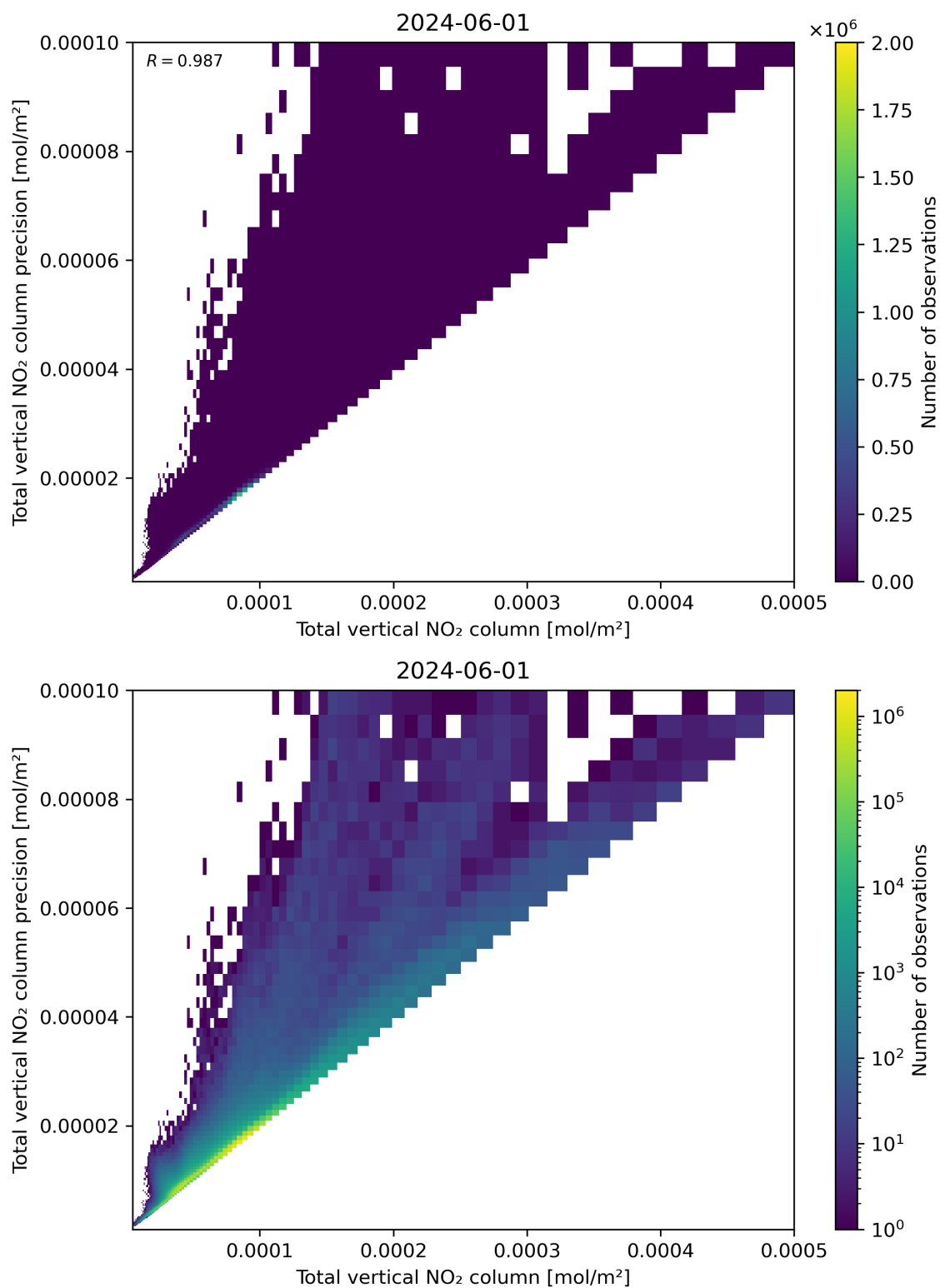
Figure 114: Scatter density plot of “Total vertical NO 2 column” against “Total vertical NO 2 column precision” for 2024-05-31 to 2024-06-02.
