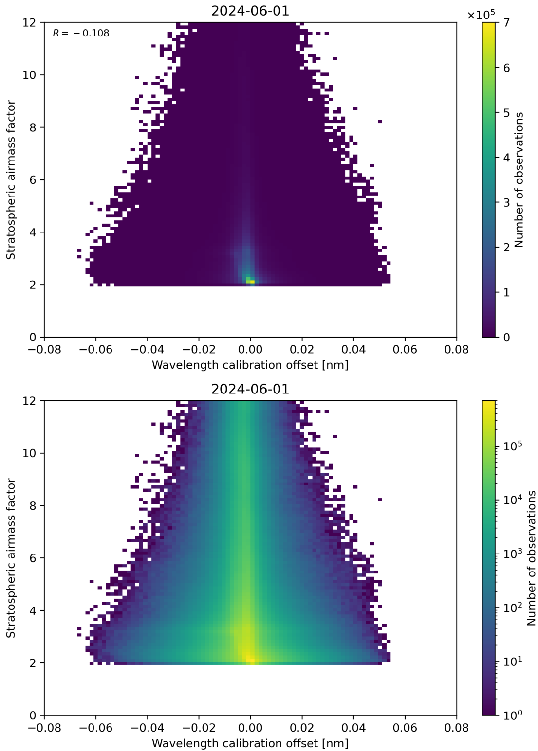
Figure 174: Scatter density plot of “Wavelength calibration offset” against “Stratospheric air mass factor” for 2024-05-31 to 2024-06-02.
