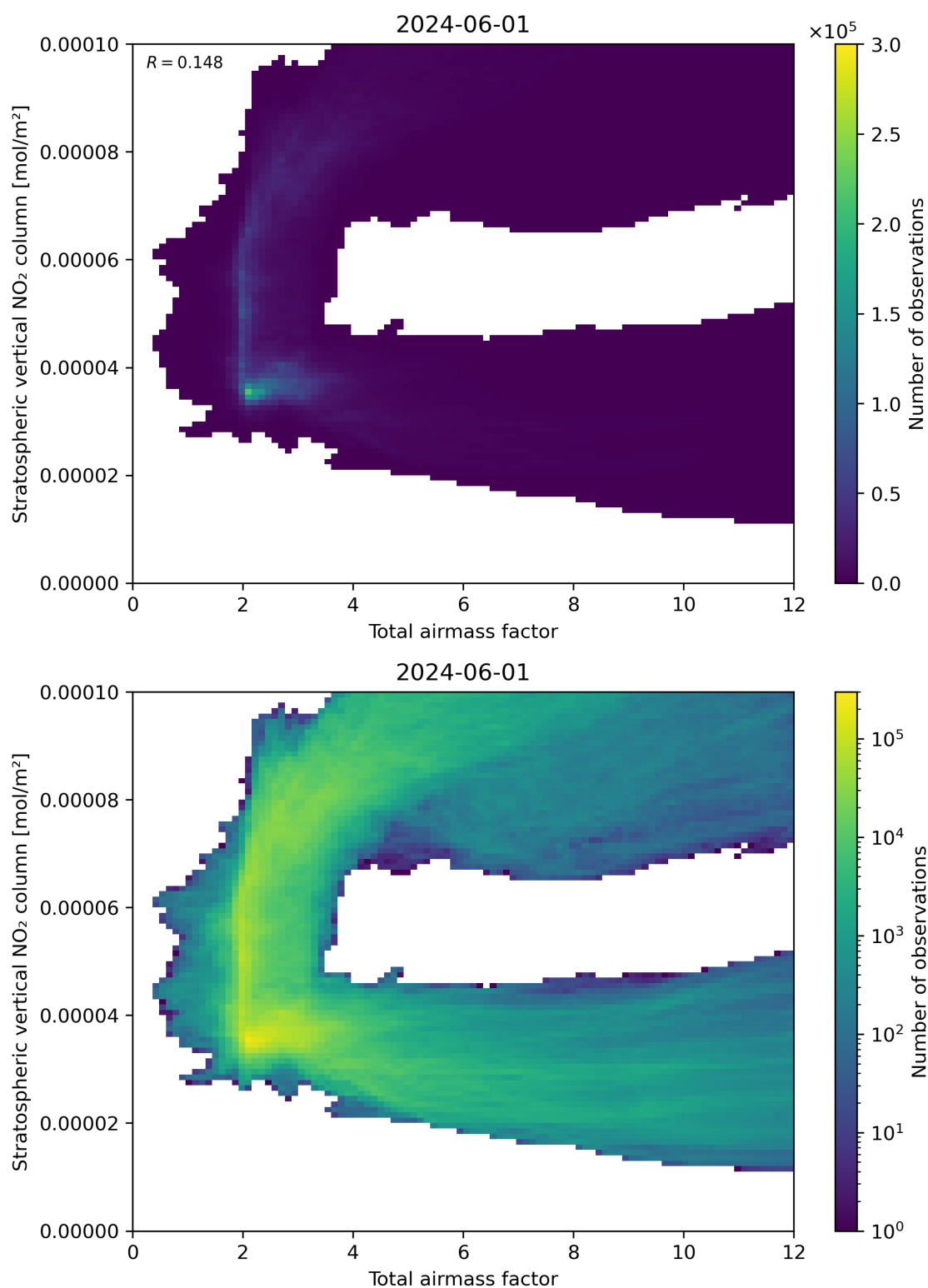
Figure 64: Scatter density plot of “Total airmass factor” against “Stratospheric vertical \text{NO}_2 column” for 2024-05-31 to 2024-06-02.
