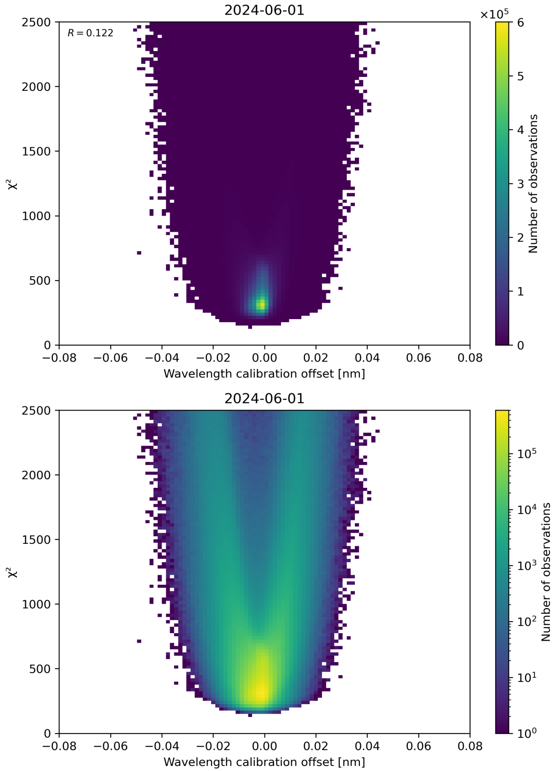
Figure 175: Scatter density plot of “Wavelength calibration offset” against “ \chi^2 ” for 2024-05-31 to 2024-06-02.
