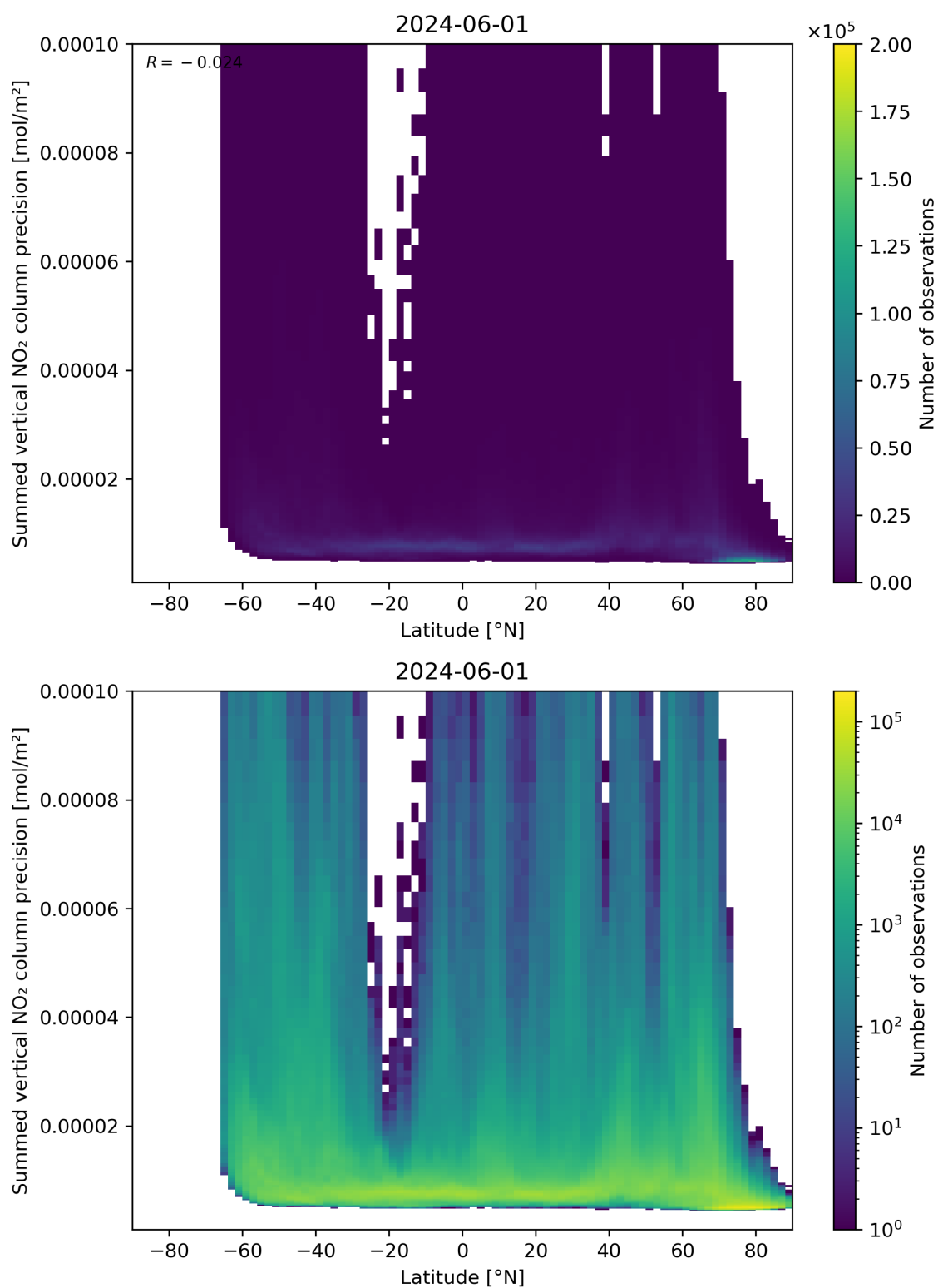
Figure 89: Scatter density plot of “Latitude” against “Summed vertical NO 2 column precision” for 2024-05-31 to 2024-06-02.
