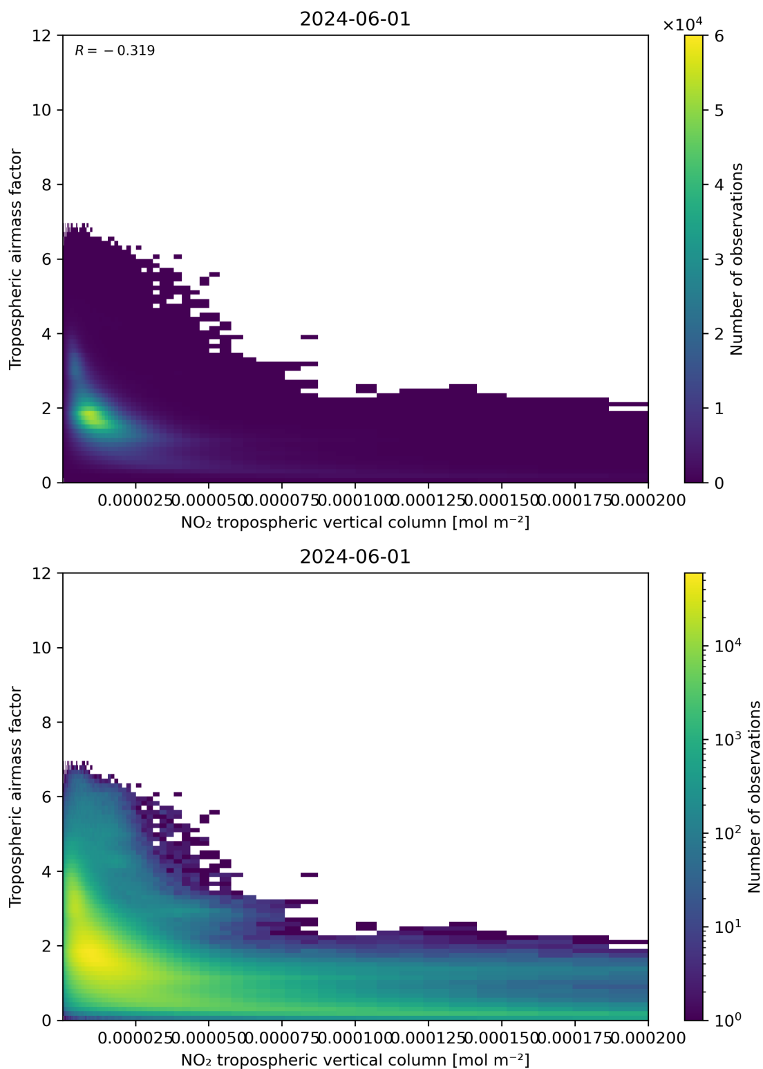
Figure 123: Scatter density plot of “NO 2 tropospheric vertical column” against “Tropospheric air mass factor” for 2024-05-31 to 2024-06-02.
