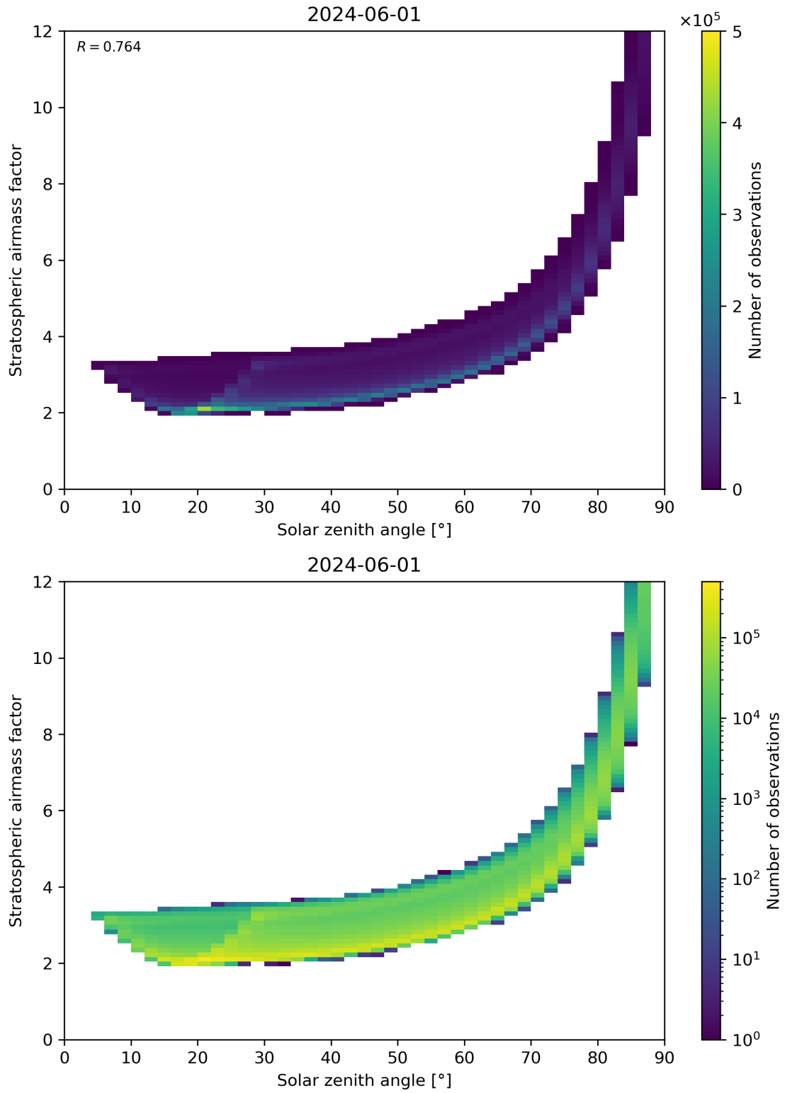
Figure 145: Scatter density plot of “Solar zenith angle” against “Stratospheric airmass factor” for 2024-05-31 to 2024-06-02.
