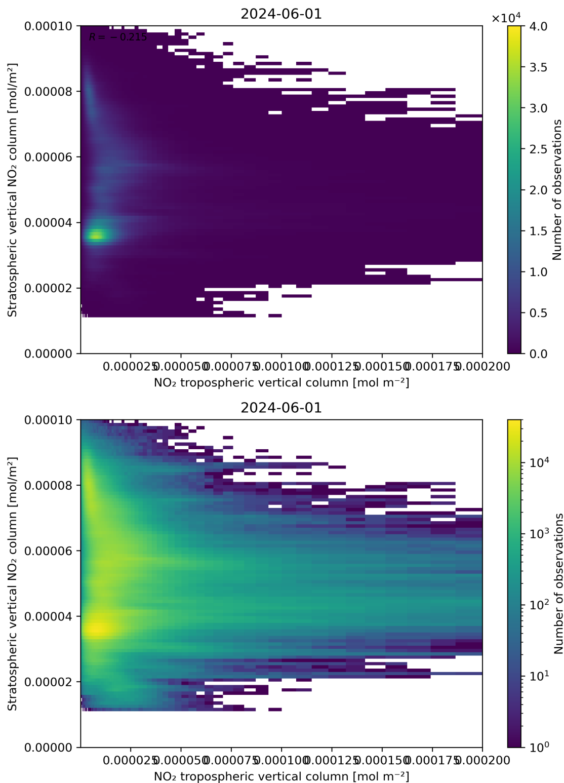
Figure 125: Scatter density plot of “NO 2 tropospheric vertical column” against “Stratospheric vertical NO 2 column” for 2024-05-31 to 2024-06-02.
