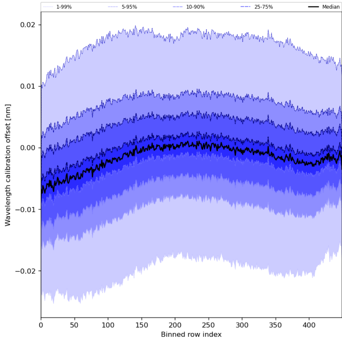
Figure 52: Along track statistics of “Wavelength calibration offset” for 2024-05-31 to 2024-06-02
