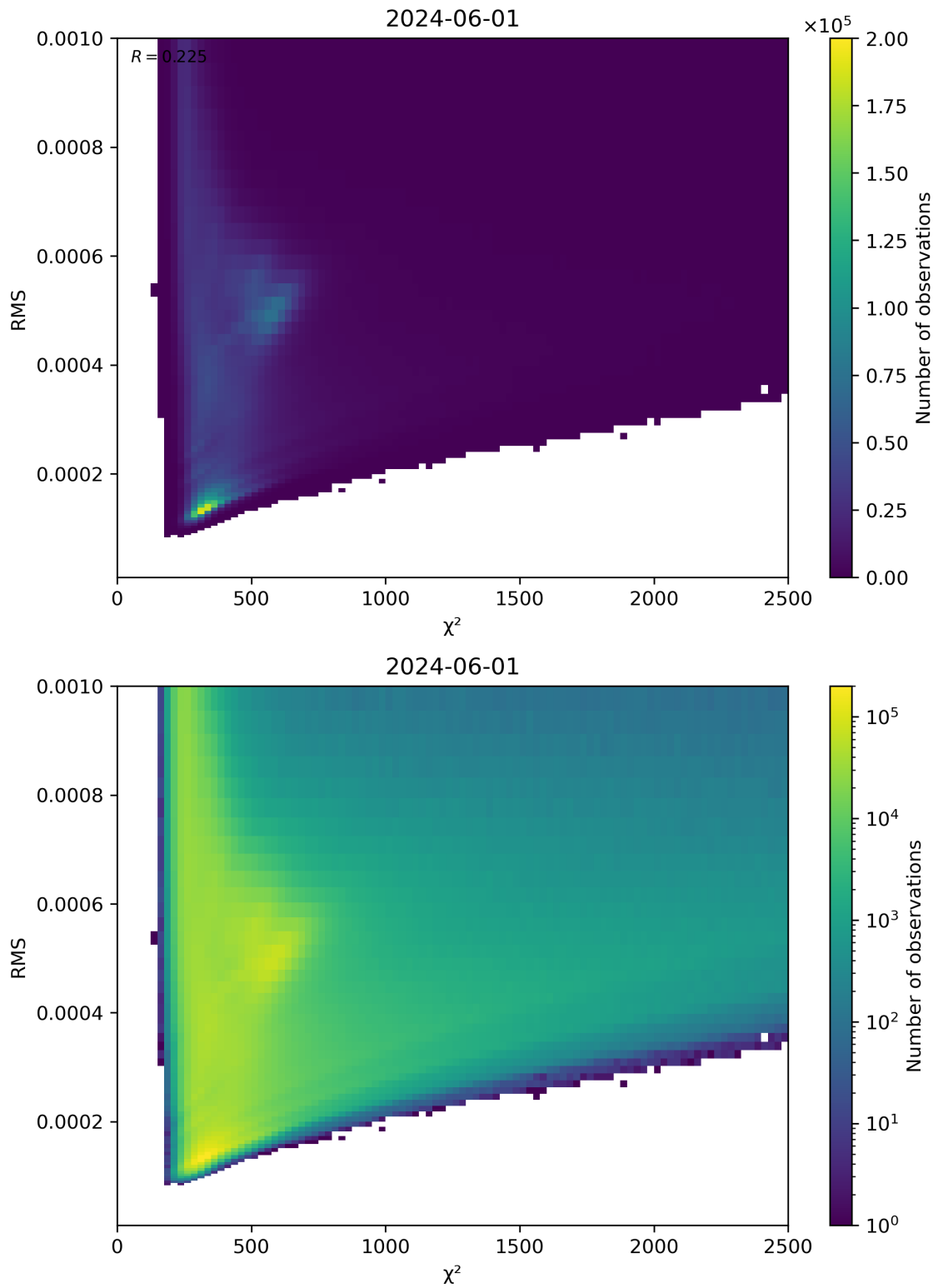
Figure 82: Scatter density plot of “ \chi^2 ” against “RMS” for 2024-05-31 to 2024-06-02.
