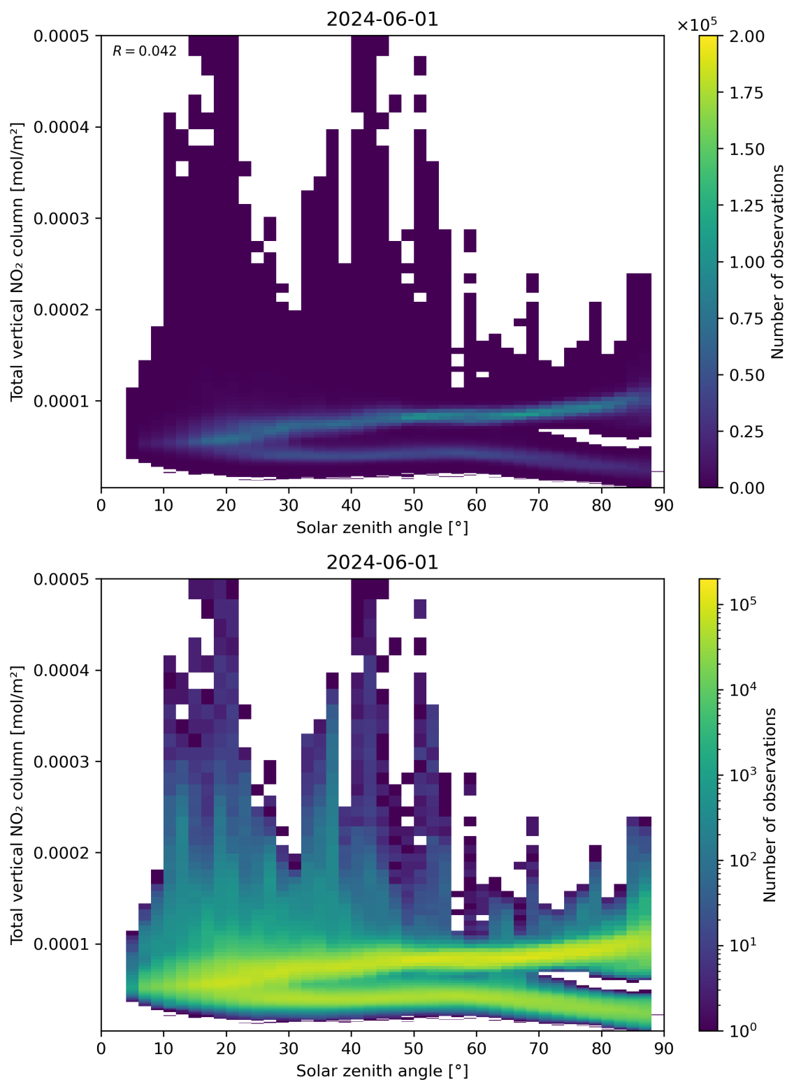
Figure 153: Scatter density plot of “Solar zenith angle” against “Total vertical NO 2 column” for 2024-05-31 to 2024-06-02.
