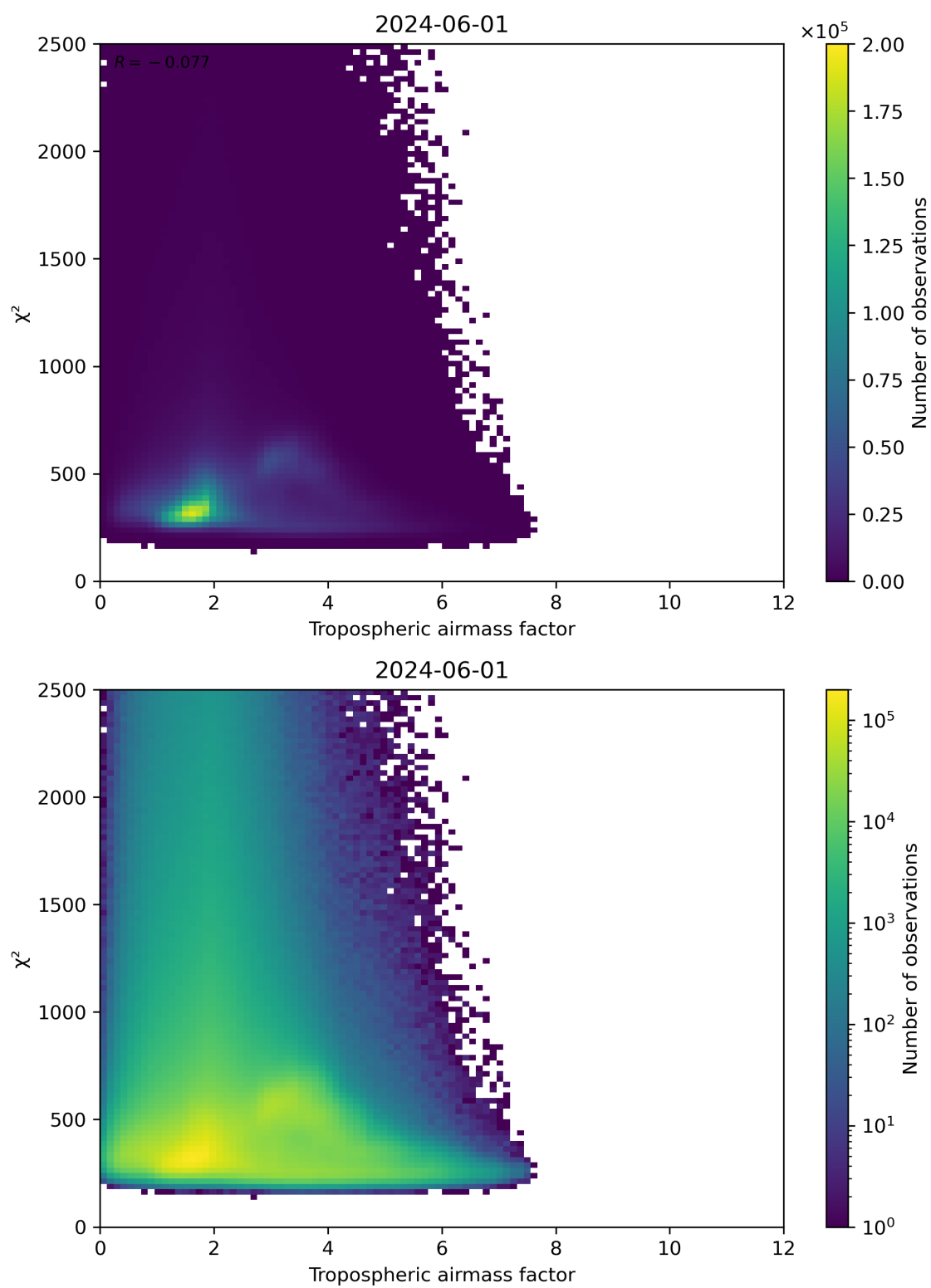
Figure 73: Scatter density plot of “Tropospheric airmass factor” against “ \chi^2 ” for 2024-05-31 to 2024-06-02.
