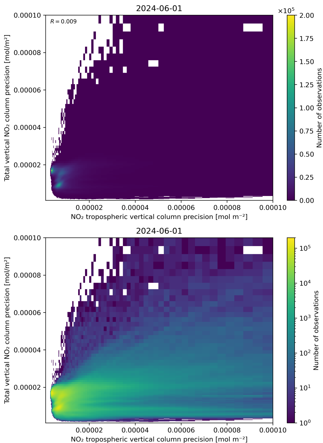
Figure 139: Scatter density plot of “NO 2 tropospheric vertical column precision” against “Total vertical NO 2 column precision” for 2024-05-31 to 2024-06-02.
