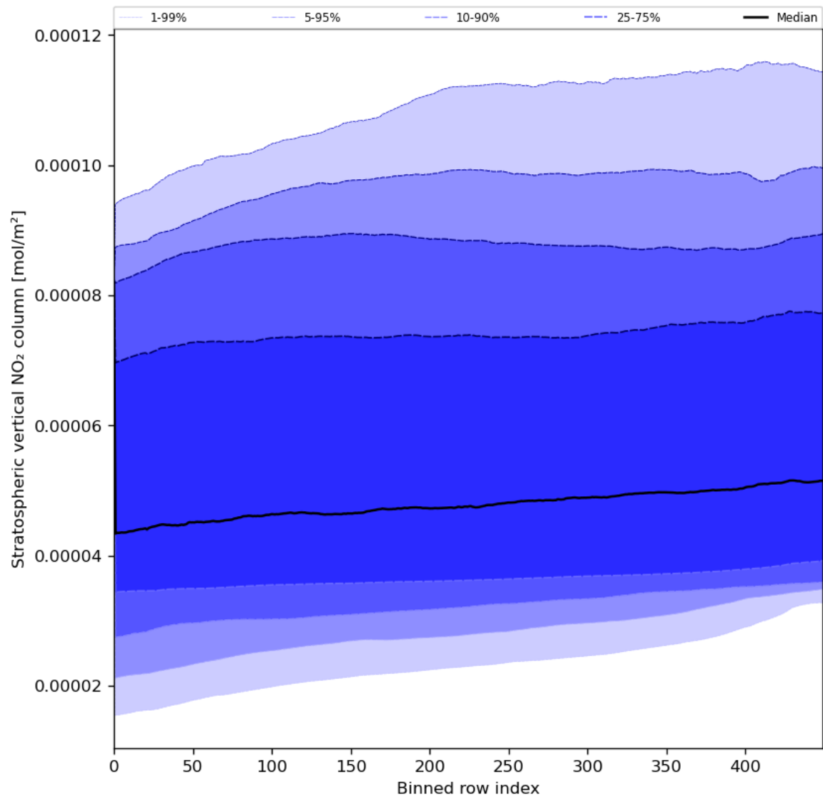
Figure 53: Along track statistics of “Stratospheric vertical NO 2 column” for 2024-05-31 to 2024-06-02
