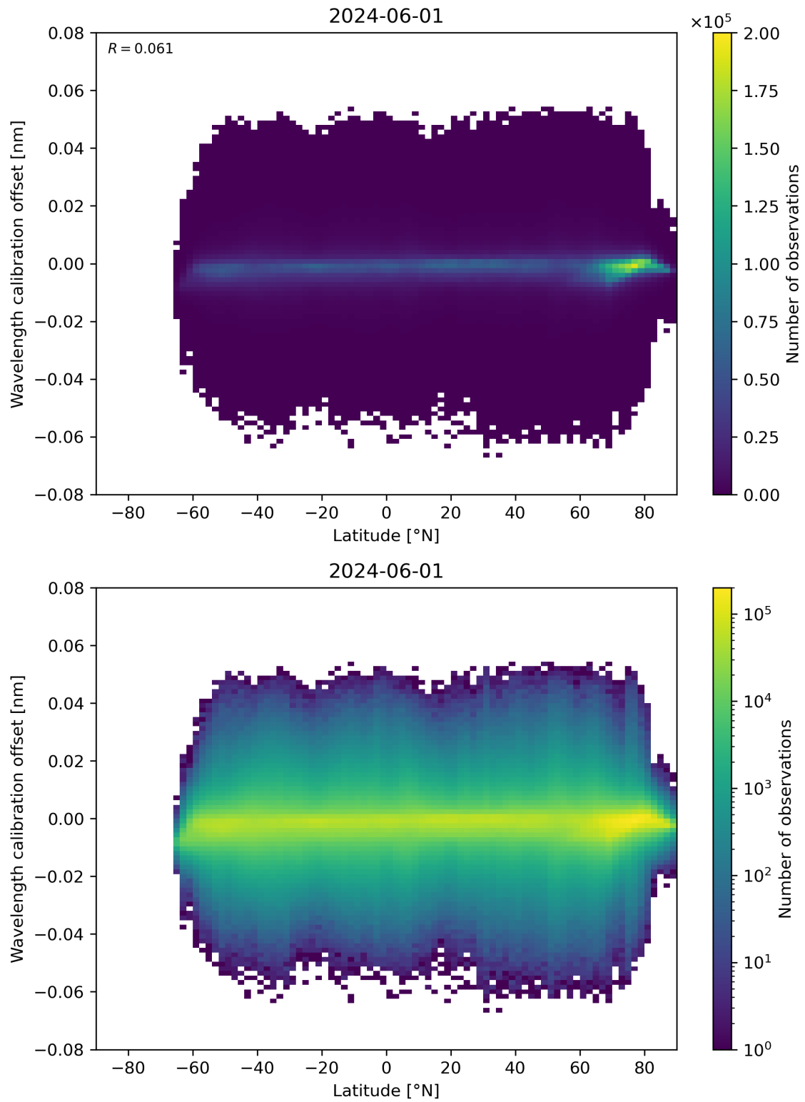
Figure 95: Scatter density plot of “Latitude” against “Wavelength calibration offset” for 2024-05-31 to 2024-06-02.
