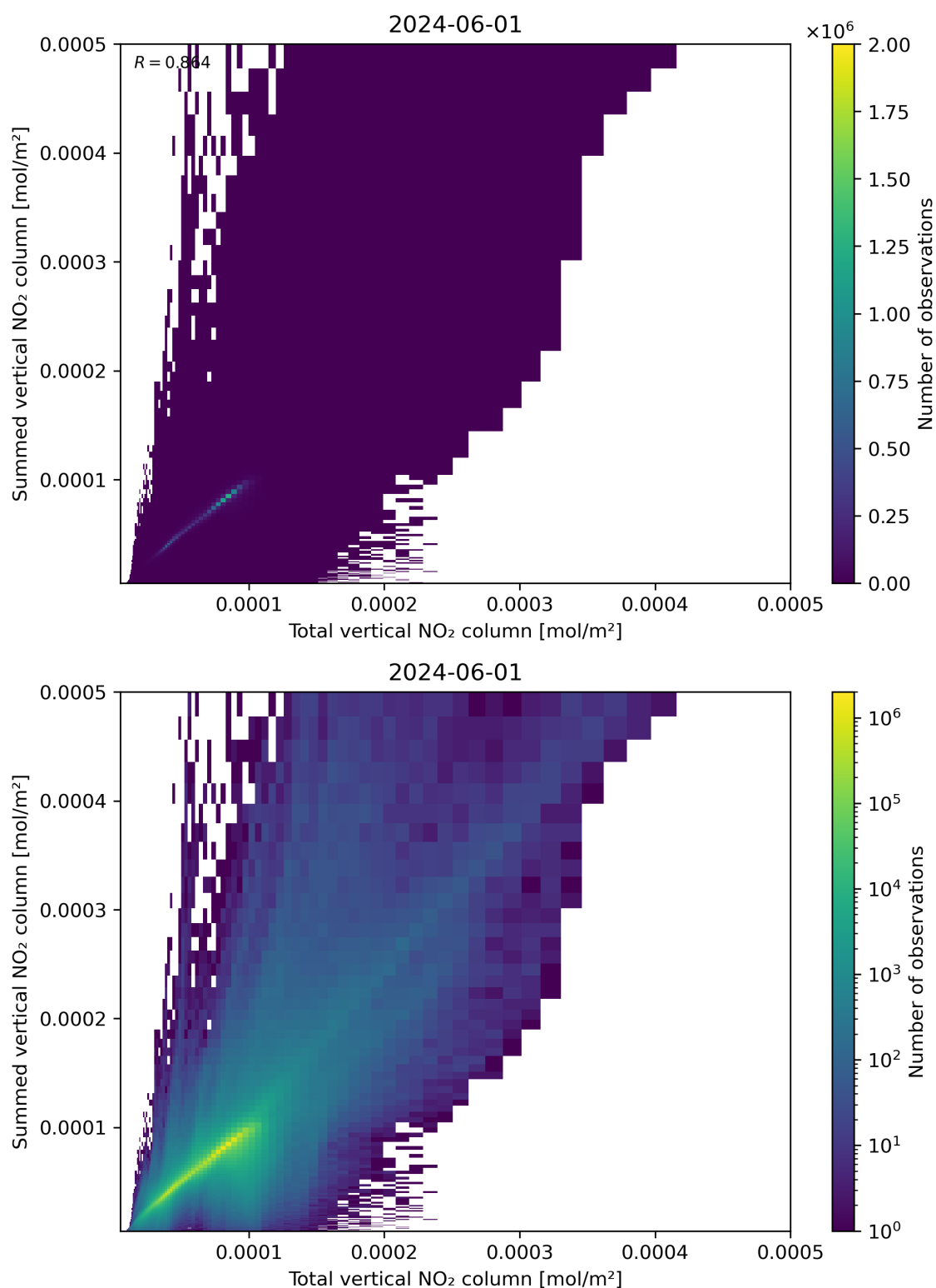
Figure 112: Scatter density plot of “Total vertical NO 2 column” against “Summed vertical NO 2 column” for 2024-05-31 to 2024-06-02.
