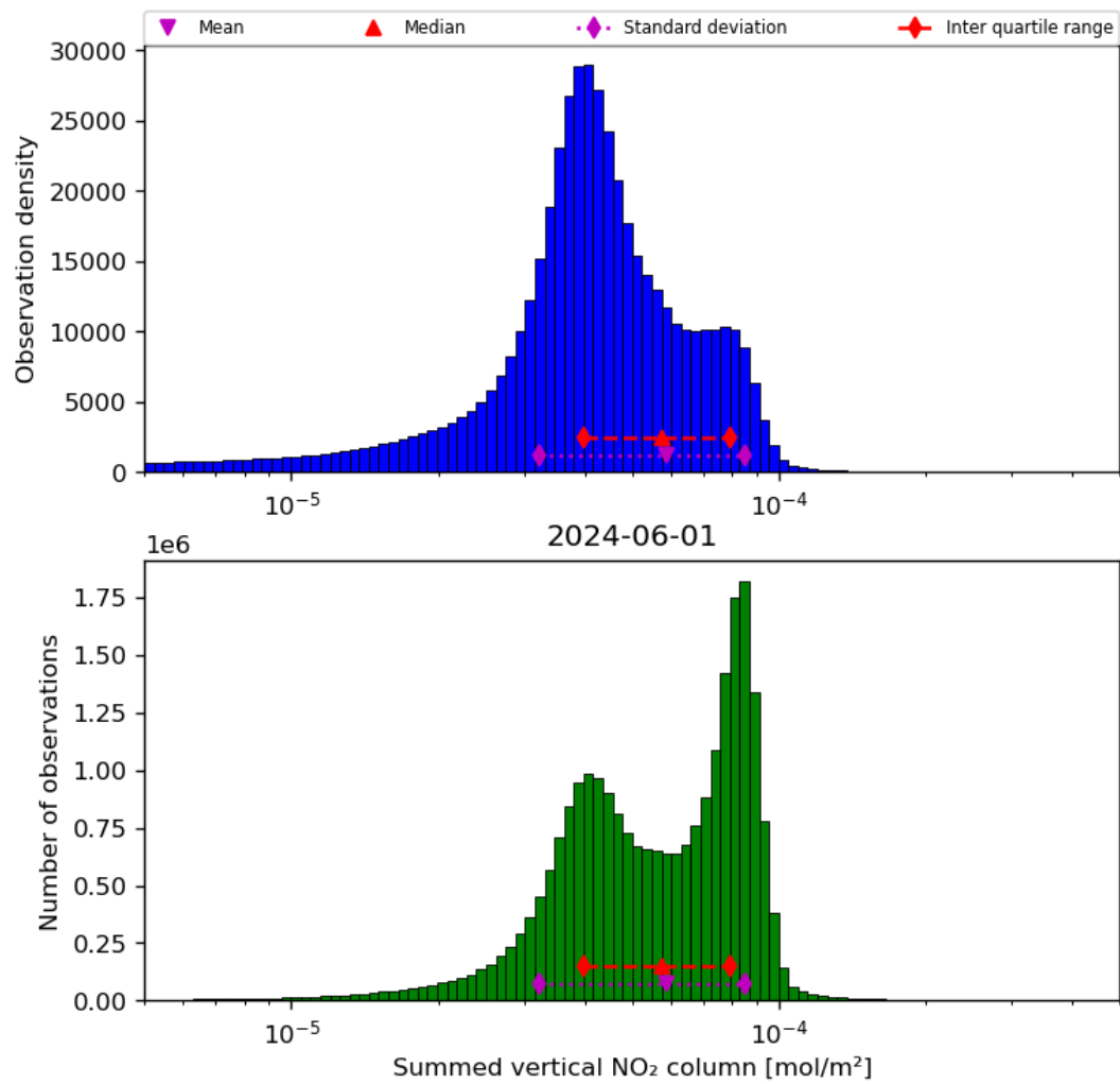
Figure 40: Histogram of “Summed vertical NO 2 column” for 2024-05-31 to 2024-06-02
