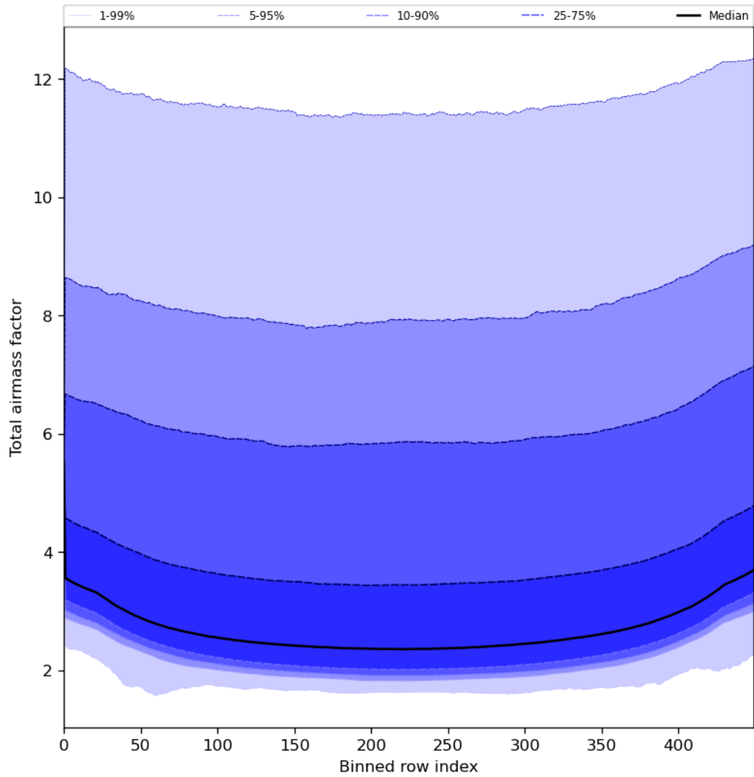
Figure 49: Along track statistics of “Total airmass factor” for 2024-05-31 to 2024-06-02
