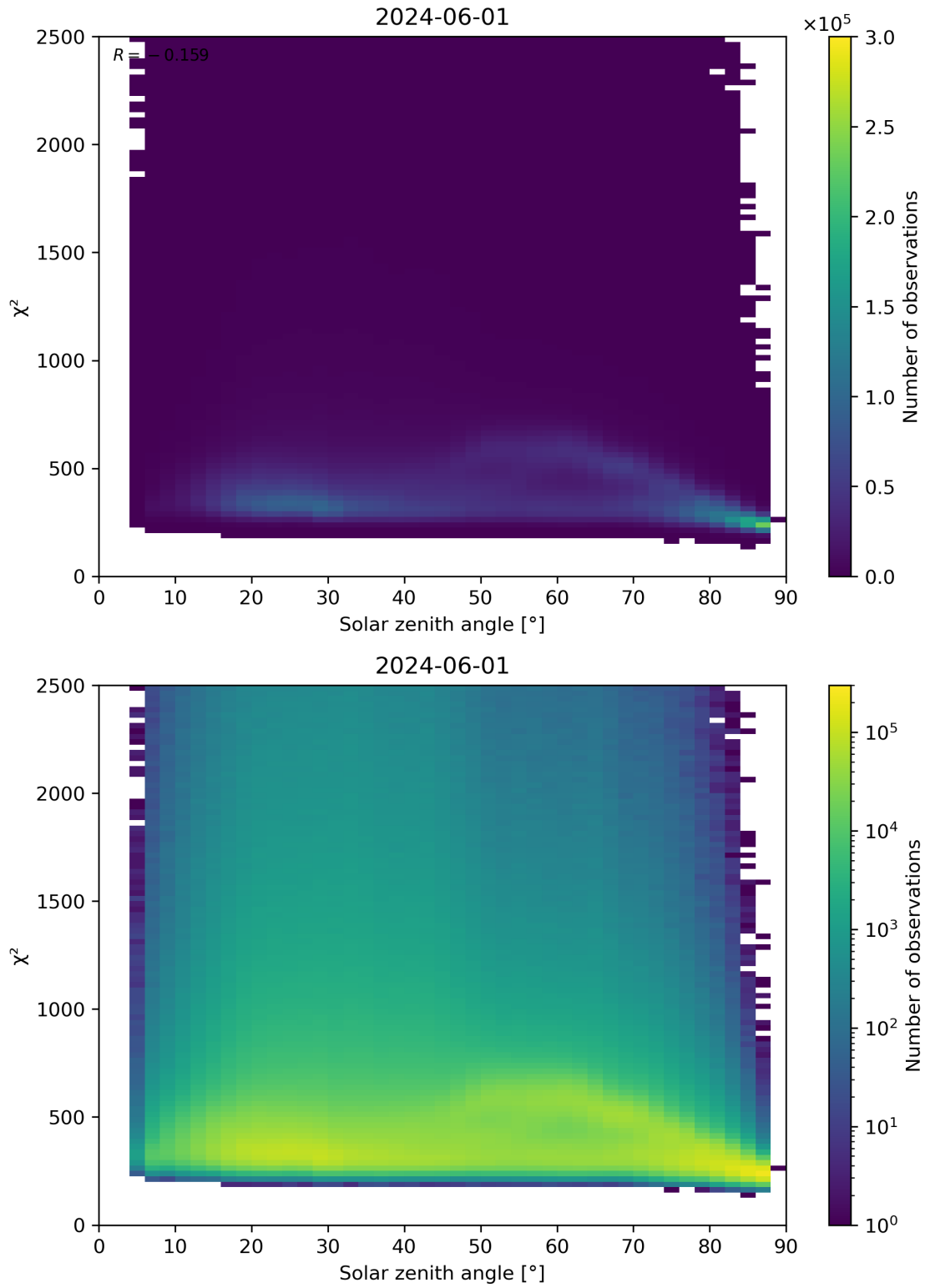
Figure 148: Scatter density plot of “Solar zenith angle” against “ \chi^2 ” for 2024-05-31 to 2024-06-02.
