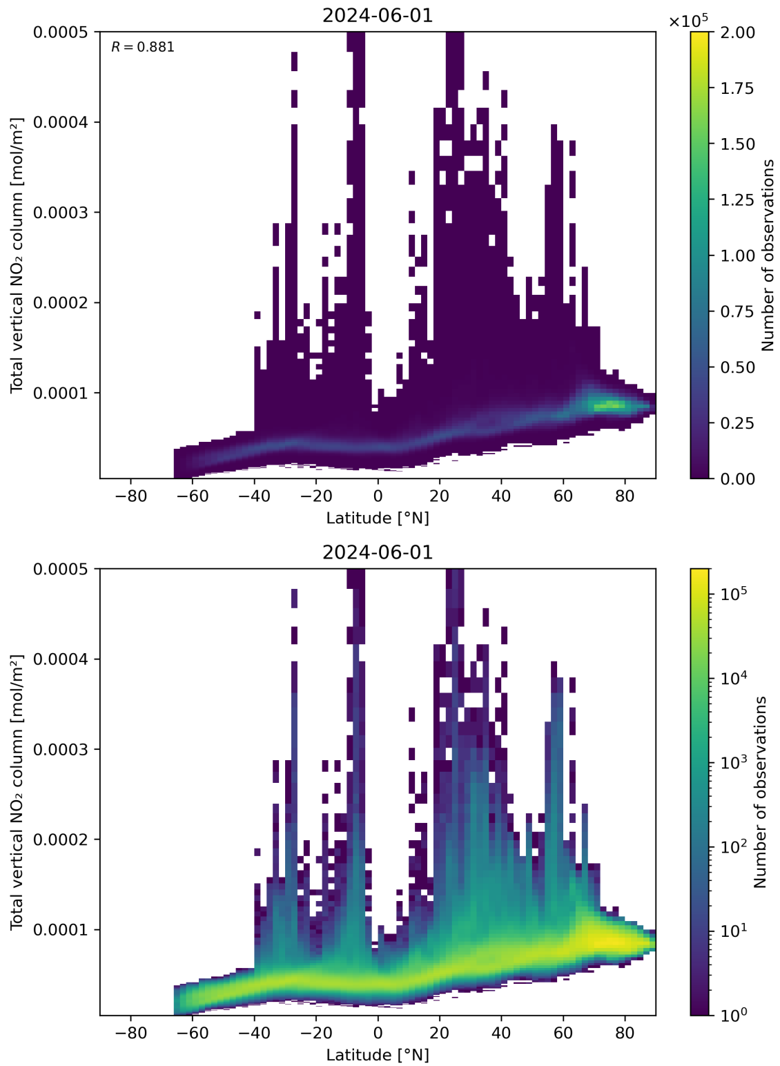
Figure 90: Scatter density plot of “Latitude” against “Total vertical NO 2 column” for 2024-05-31 to 2024-06-02.
