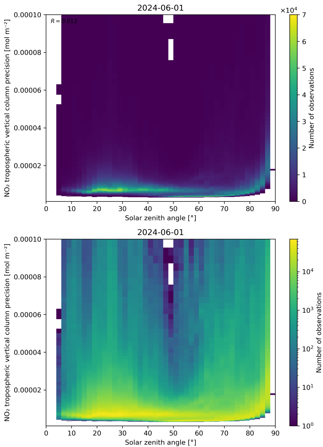
Figure 156: Scatter density plot of “Solar zenith angle” against “NO 2 tropospheric vertical column precision” for 2024-05-31 to 2024-06-02.
