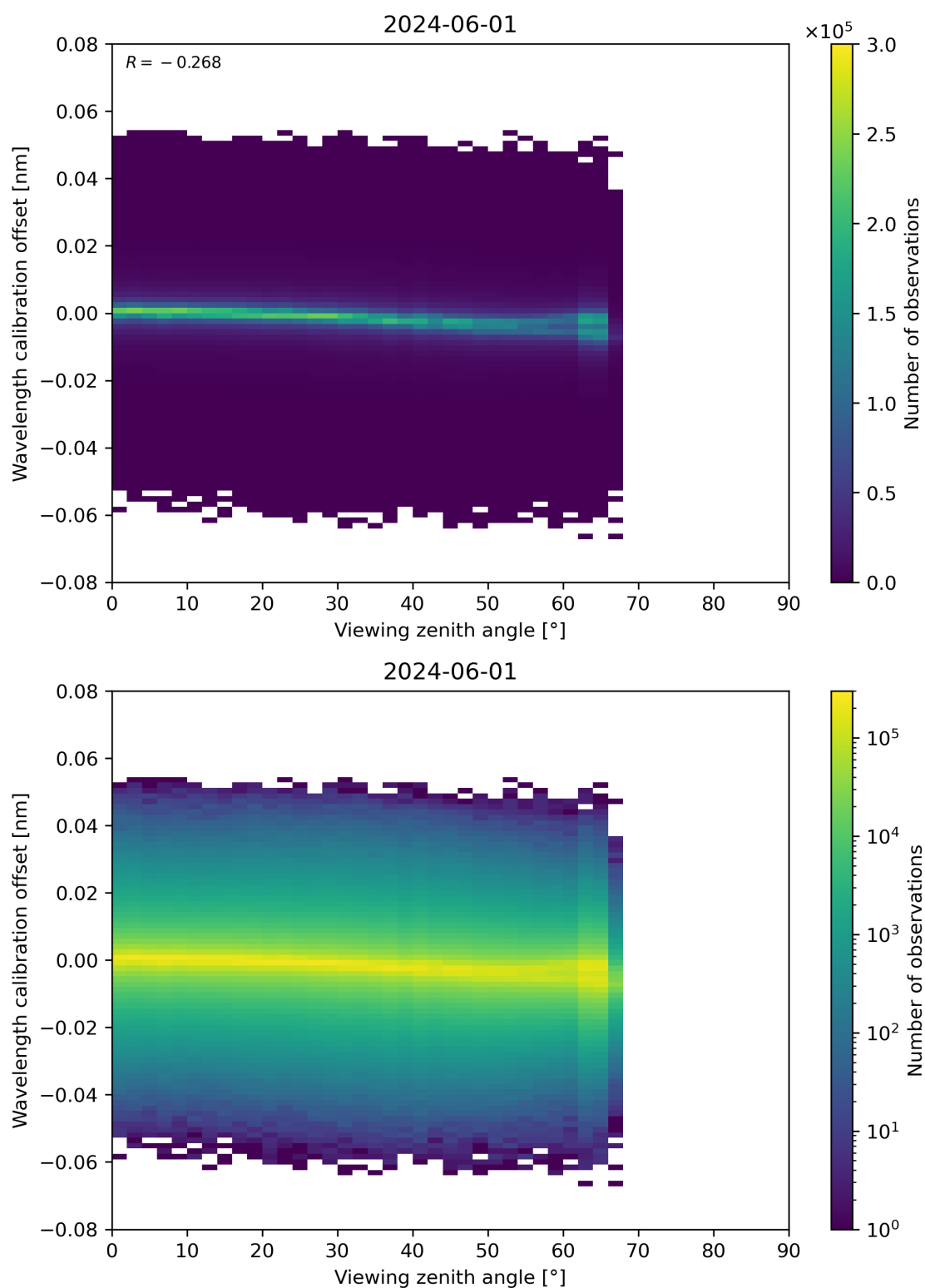
Figure 173: Scatter density plot of “Viewing zenith angle” against “Wavelength calibration offset” for 2024-05-31 to 2024-06-02.
