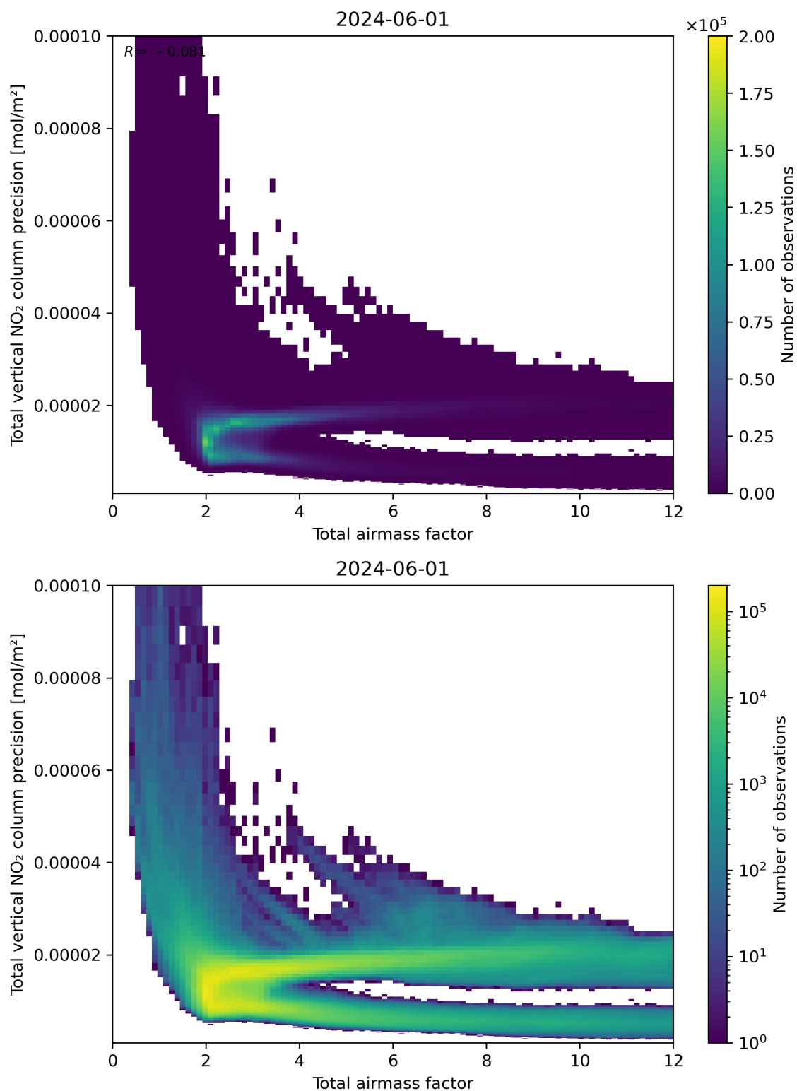
Figure 68: Scatter density plot of “Total airmass factor” against “Total vertical NO 2 column precision” for 2024-05-31 to 2024-06-02.
