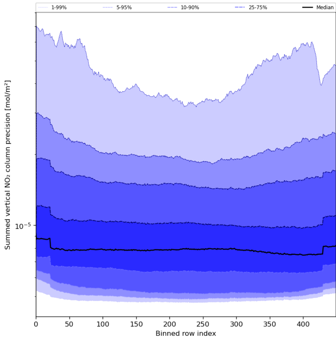
Figure 58: Along track statistics of “Summed vertical NO 2 column precision” for 2024-05-31 to 2024-06-02
