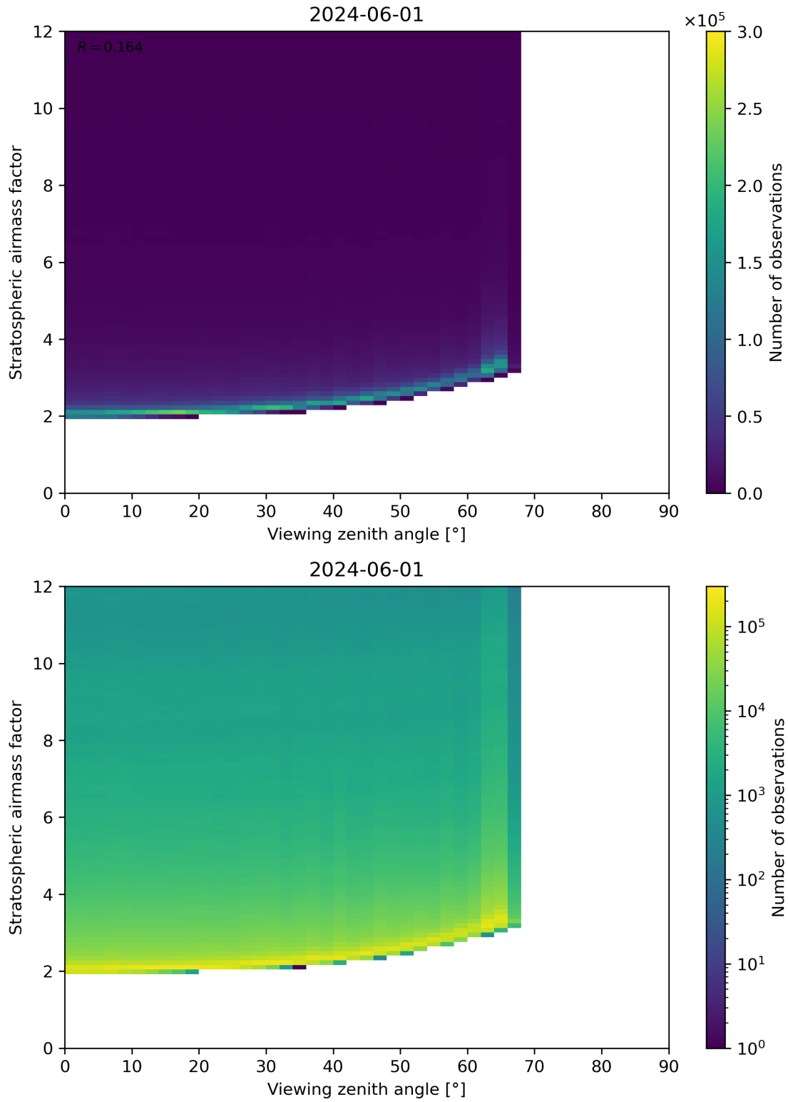
Figure 159: Scatter density plot of “Viewing zenith angle” against “Stratospheric airmass factor” for 2024-05-31 to 2024-06-02.
