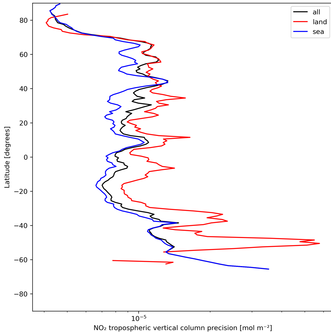
Figure 13: Zonal average of "NO 2 tropospheric vertical column precision" for 2024-05-31 to 2024-06-02.
