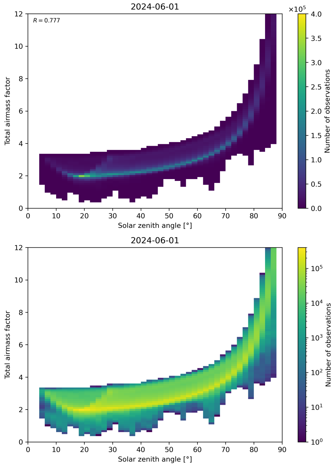
Figure 146: Scatter density plot of “Solar zenith angle” against “Total air mass factor” for 2024-05-31 to 2024-06-02.
