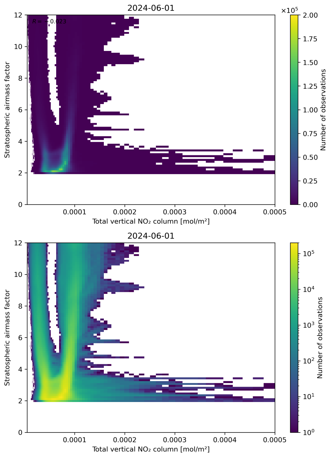
Figure 110: Scatter density plot of “Total vertical NO 2 column” against “Stratospheric airmass factor” for 2024-05-31 to 2024-06-02.
