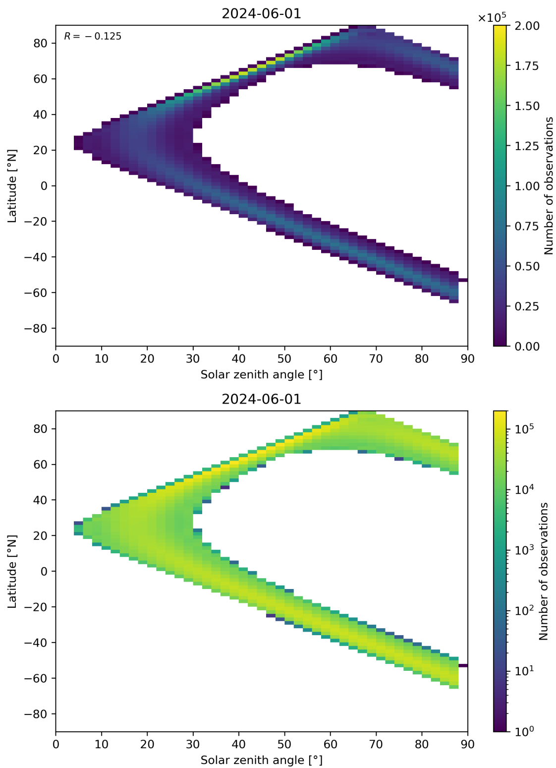
Figure 149: Scatter density plot of “Solar zenith angle” against “Latitude” for 2024-05-31 to 2024-06-02.
