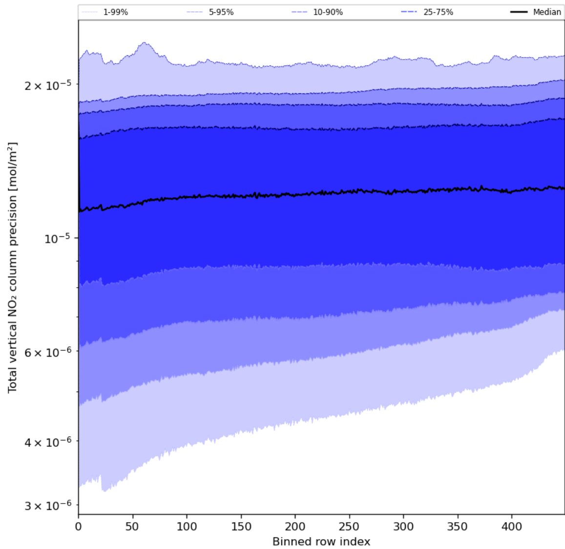
Figure 56: Along track statistics of “Total vertical NO 2 column precision” for 2024-05-31 to 2024-06-02
