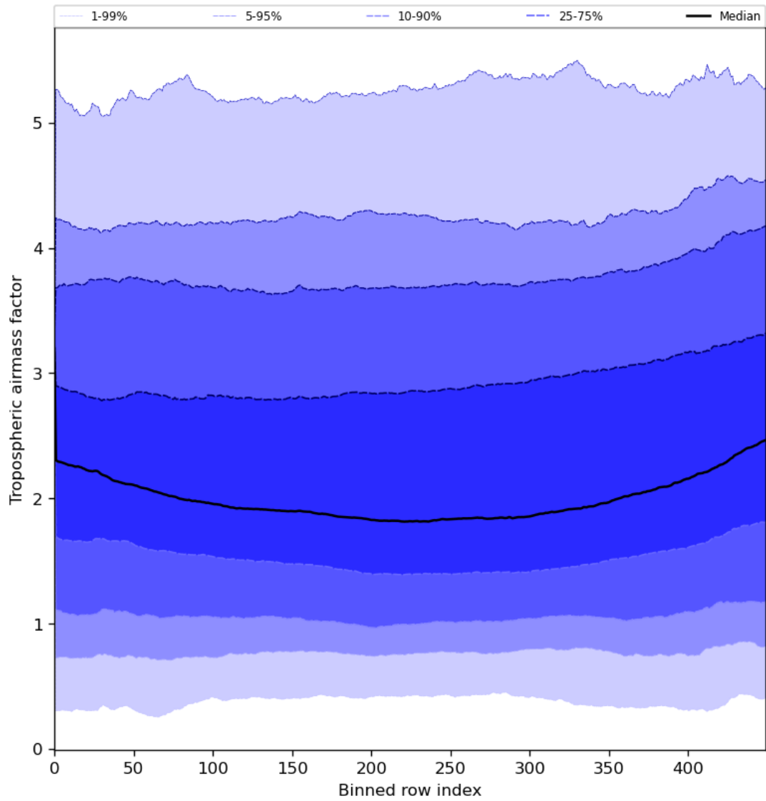
Figure 48: Along track statistics of “Tropospheric airmass factor” for 2024-05-31 to 2024-06-02
