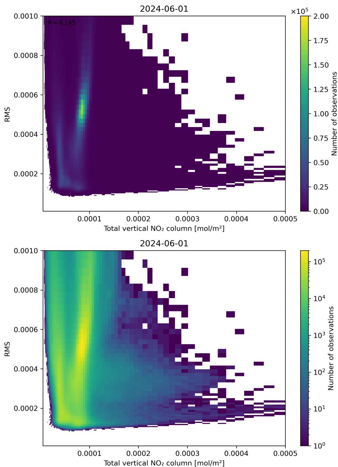
Figure 120: Scatter density plot of “Total vertical NO 2 column” against “RMS” for 2024-05-31 to 2024-06-02.
