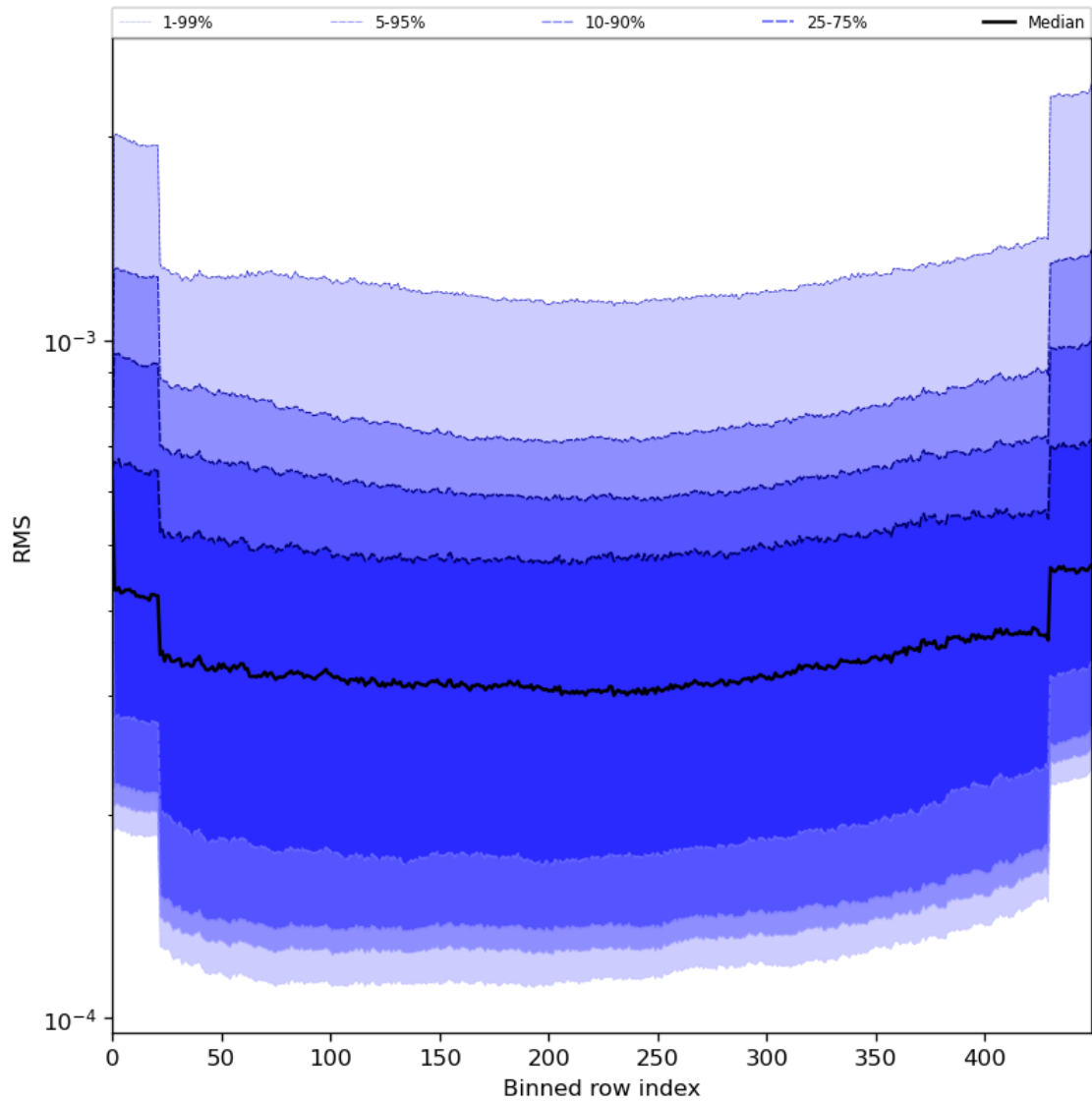
Figure 60: Along track statistics of “RMS” for 2024-05-31 to 2024-06-02
