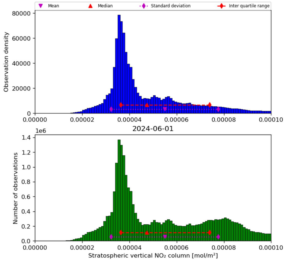
Figure 36: Histogram of “Stratospheric vertical NO 2 column” for 2024-05-31 to 2024-06-02
