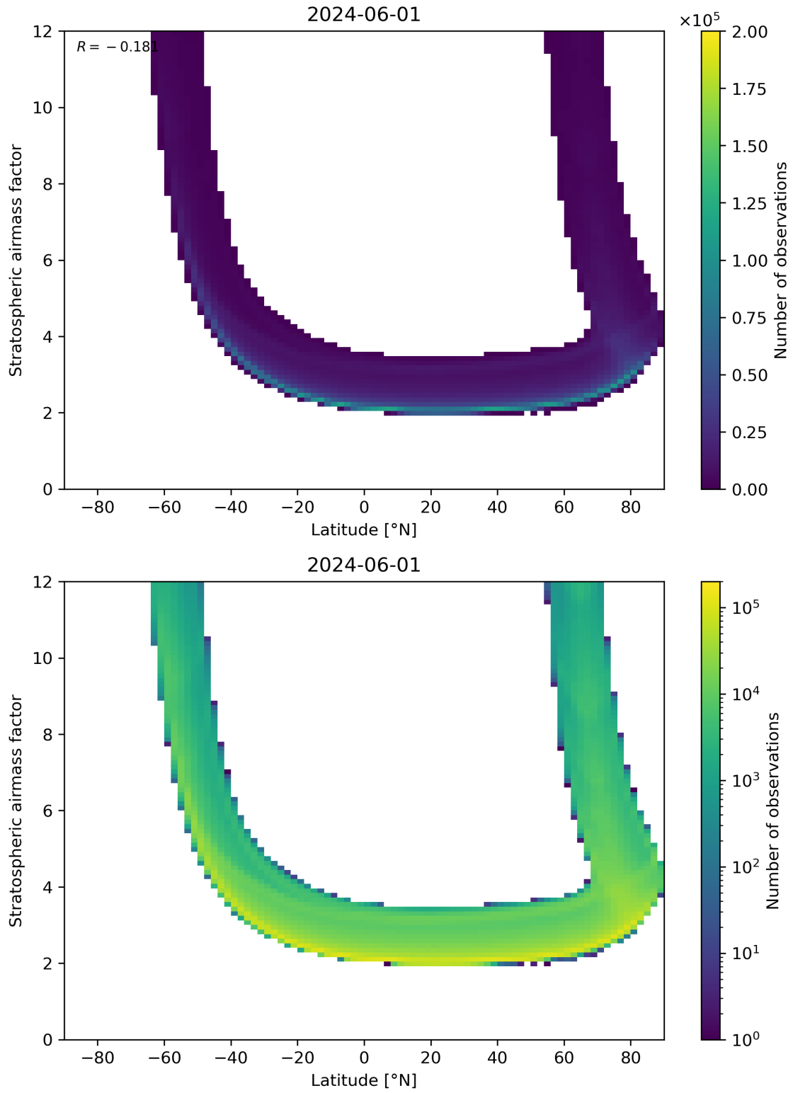
Figure 83: Scatter density plot of “Latitude” against “Stratospheric air mass factor” for 2024-05-31 to 2024-06-02.
