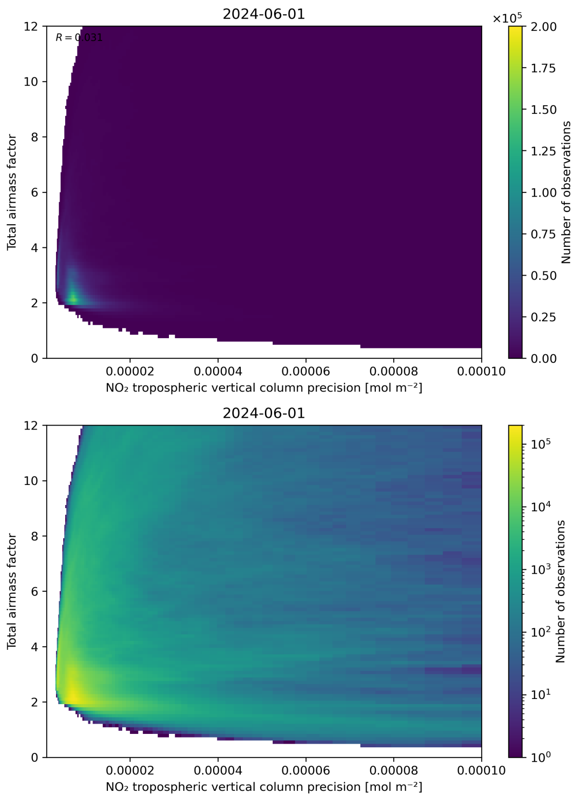
Figure 132: Scatter density plot of “NO 2 tropospheric vertical column precision” against “Total air mass factor” for 2024-05-31 to 2024-06-02.
