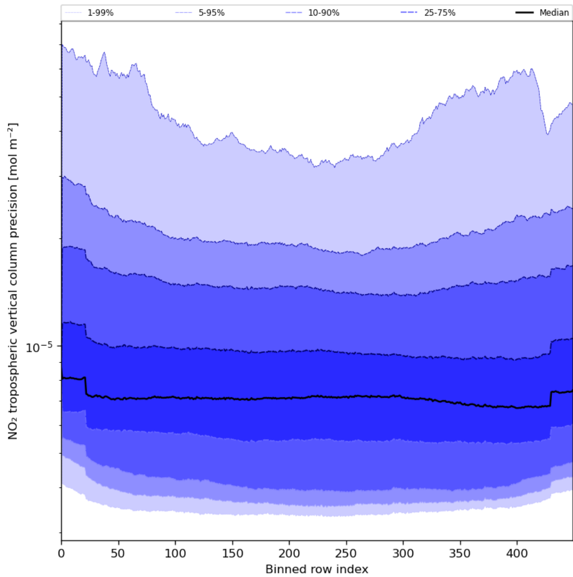
Figure 47: Along track statistics of “NO 2 tropospheric vertical column precision” for 2024-05-31 to 2024-06-02
