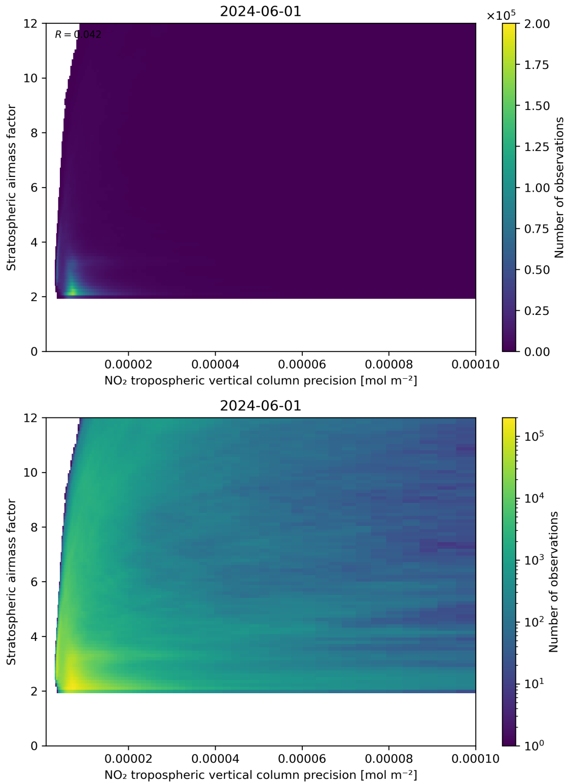
Figure 131: Scatter density plot of “NO 2 tropospheric vertical column precision” against “Stratospheric airmass factor” for 2024-05-31 to 2024-06-02.
