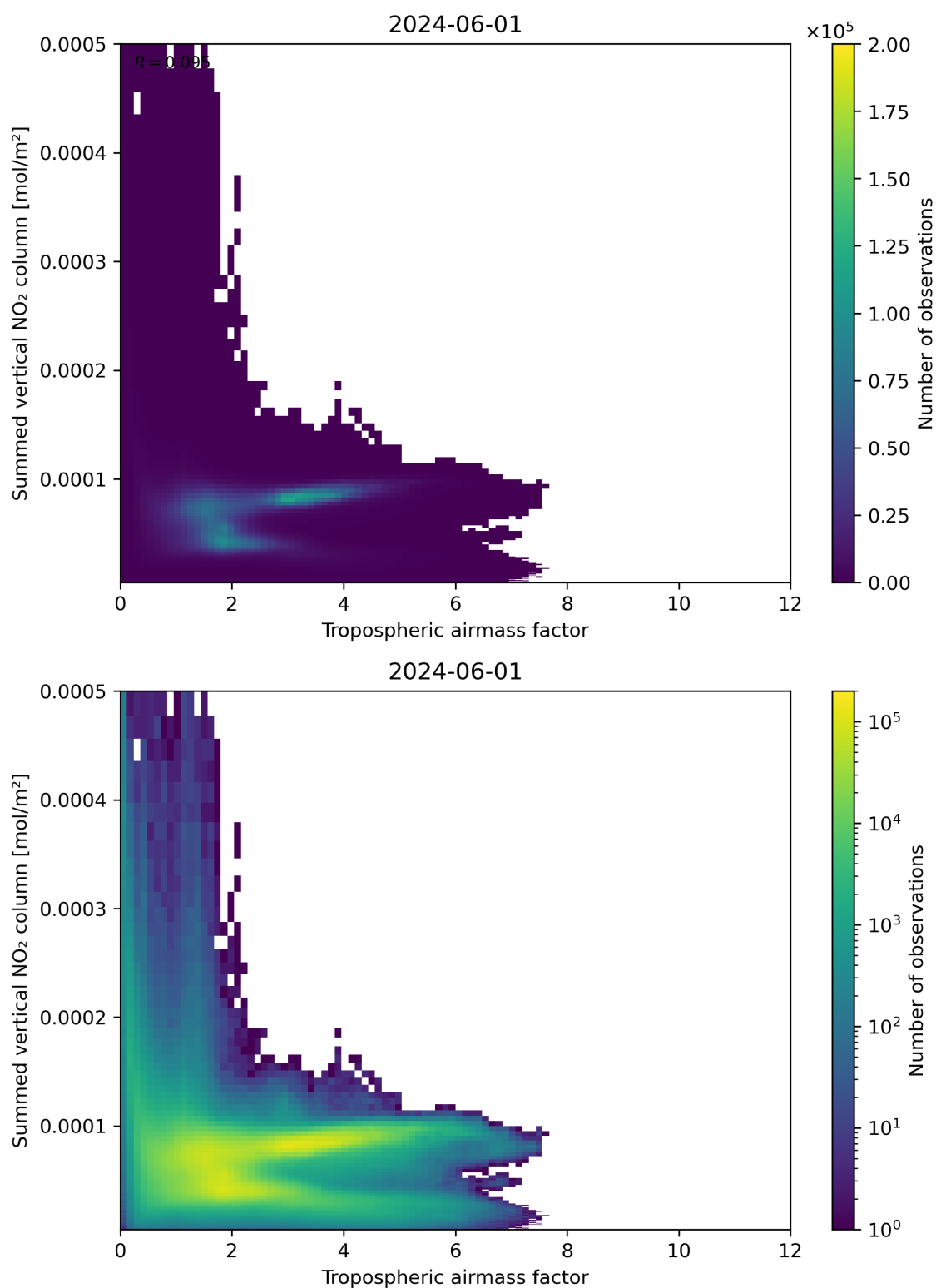
Figure 75: Scatter density plot of “Tropospheric airmass factor” against “Summed vertical NO 2 column” for 2024-05-31 to 2024-06-02.
