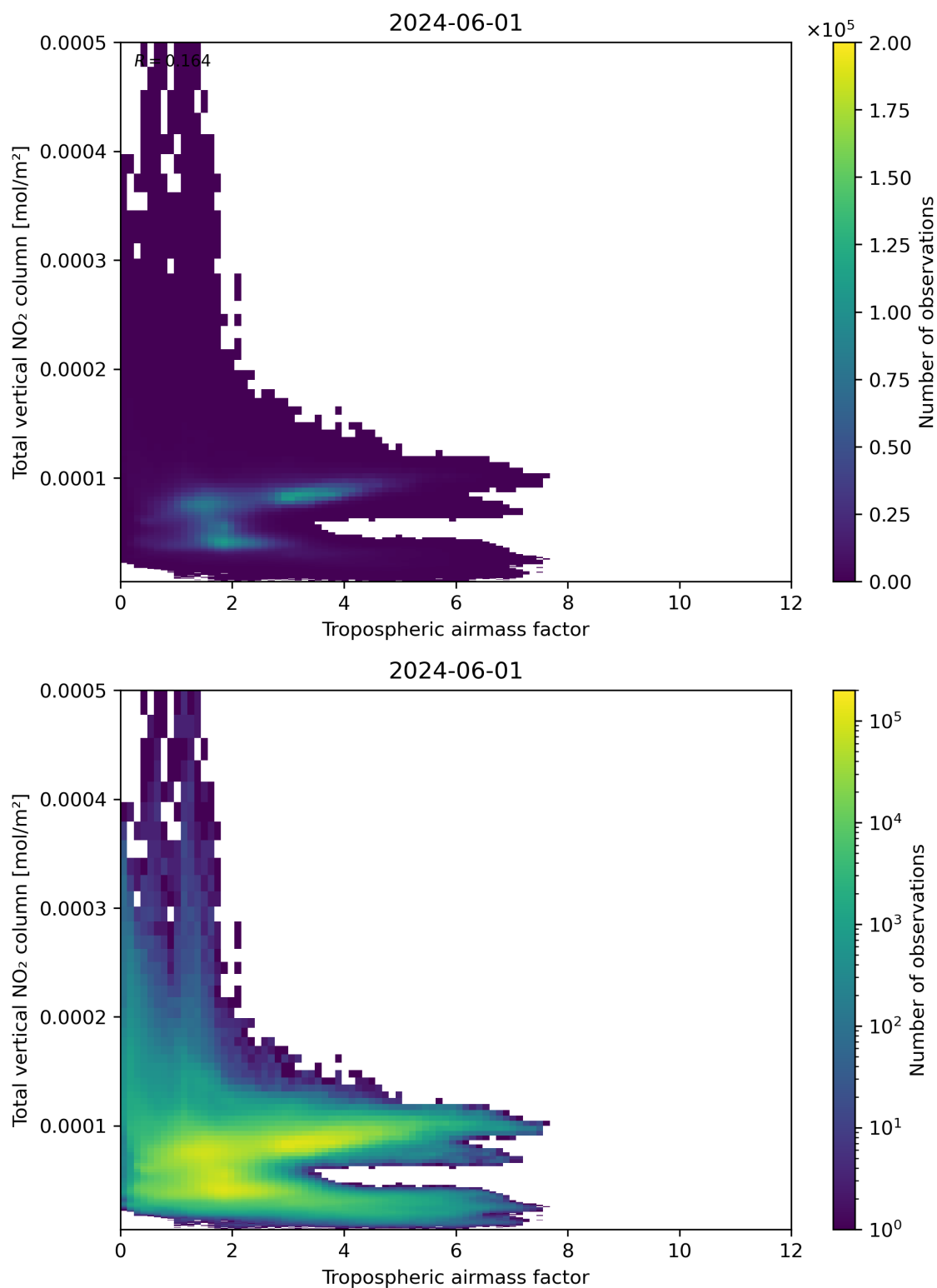
Figure 77: Scatter density plot of “Tropospheric airmass factor” against “Total vertical NO 2 column” for 2024-05-31 to 2024-06-02.
