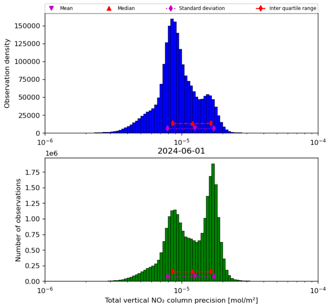
Figure 39: Histogram of "Total vertical NO 2 column precision" for 2024-05-31 to 2024-06-02
