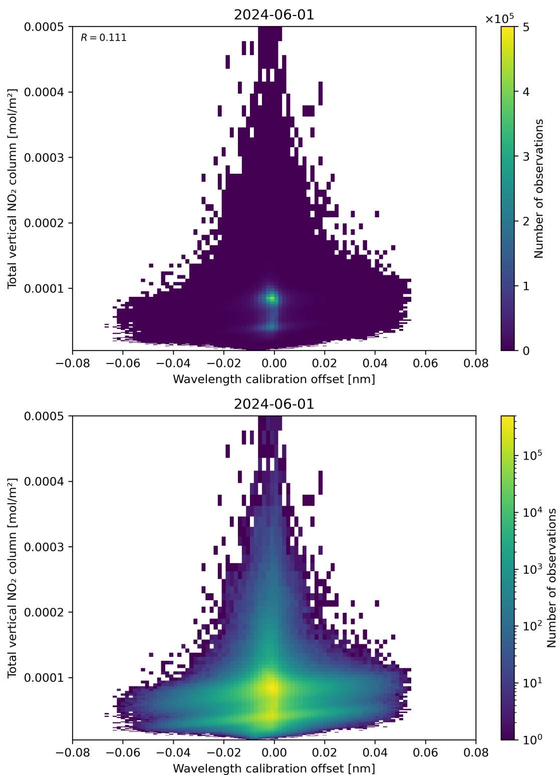
Figure 179: Scatter density plot of “Wavelength calibration offset” against “Total vertical NO 2 column” for 2024-05-31 to 2024-06-02.
