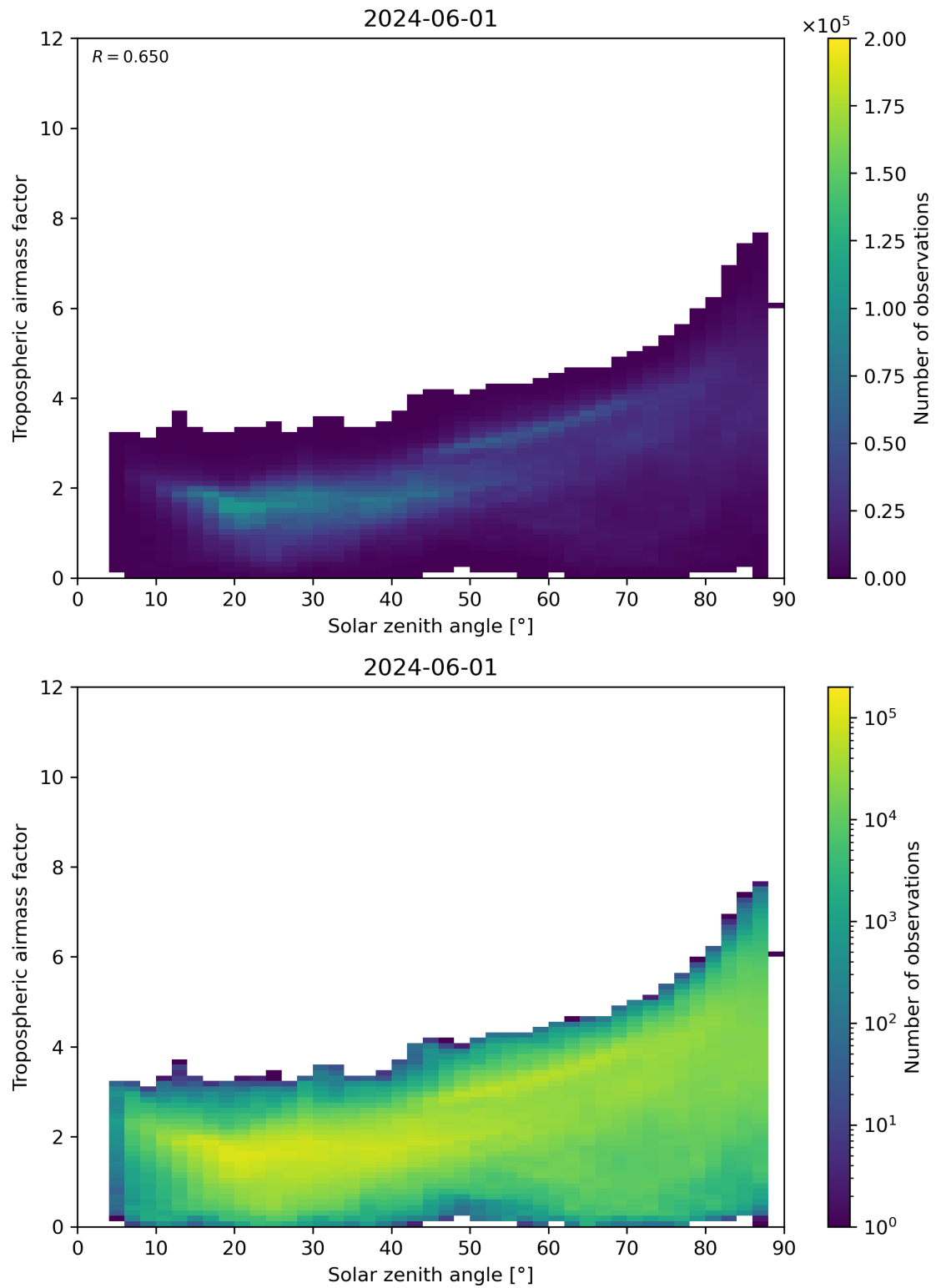
Figure 147: Scatter density plot of “Solar zenith angle” against “Tropospheric airmass factor” for 2024-05-31 to 2024-06-02.
