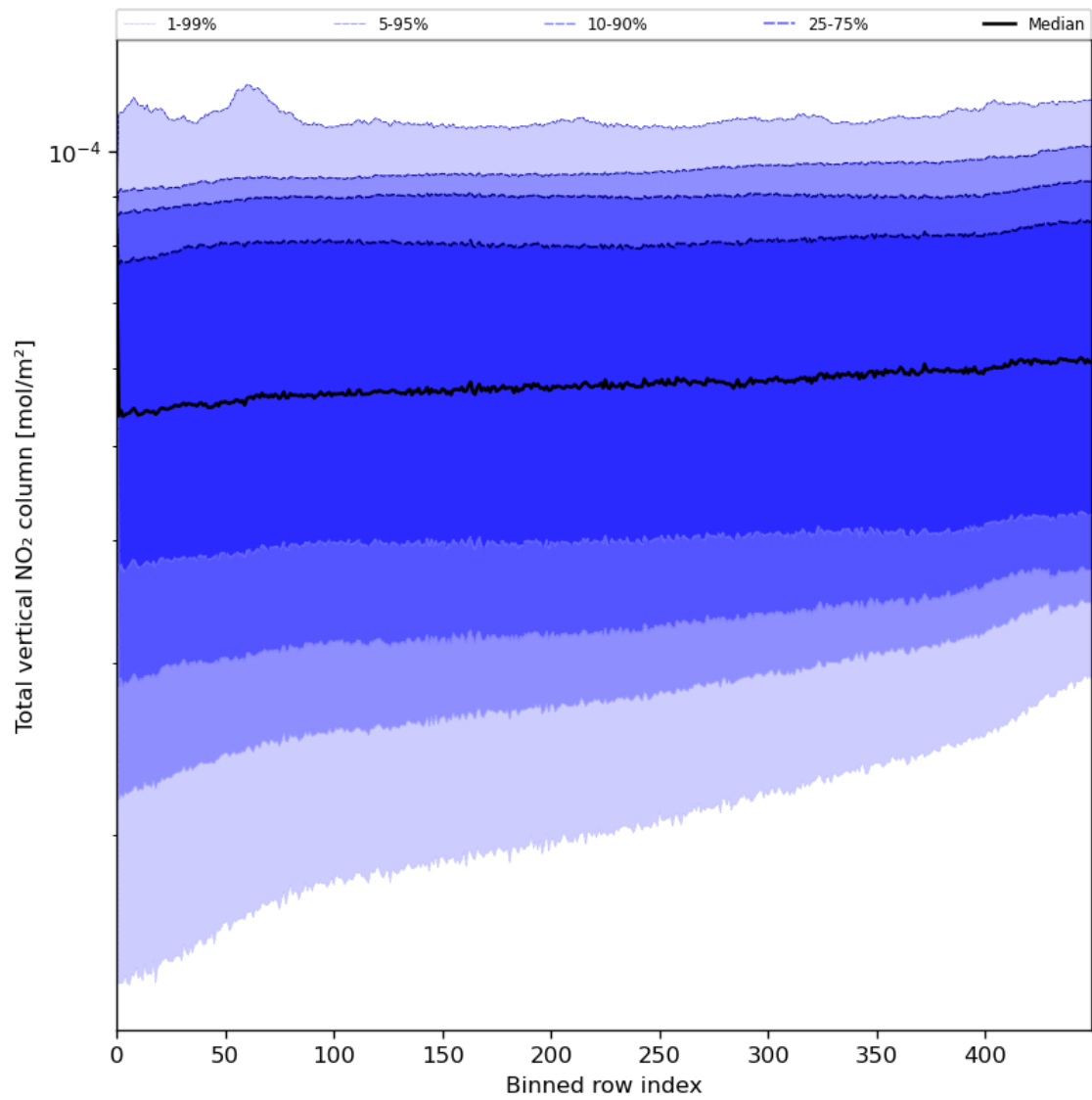
Figure 55: Along track statistics of “Total vertical NO 2 column” for 2024-05-31 to 2024-06-02
