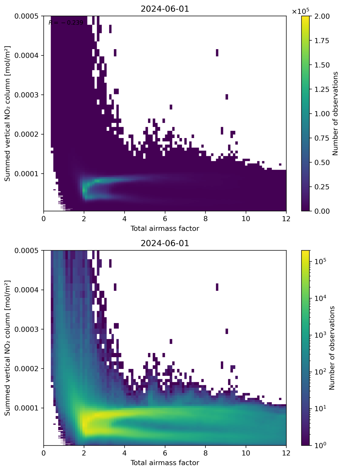
Figure 65: Scatter density plot of “Total airmass factor” against “Summed vertical NO 2 column” for 2024-05-31 to 2024-06-02.
