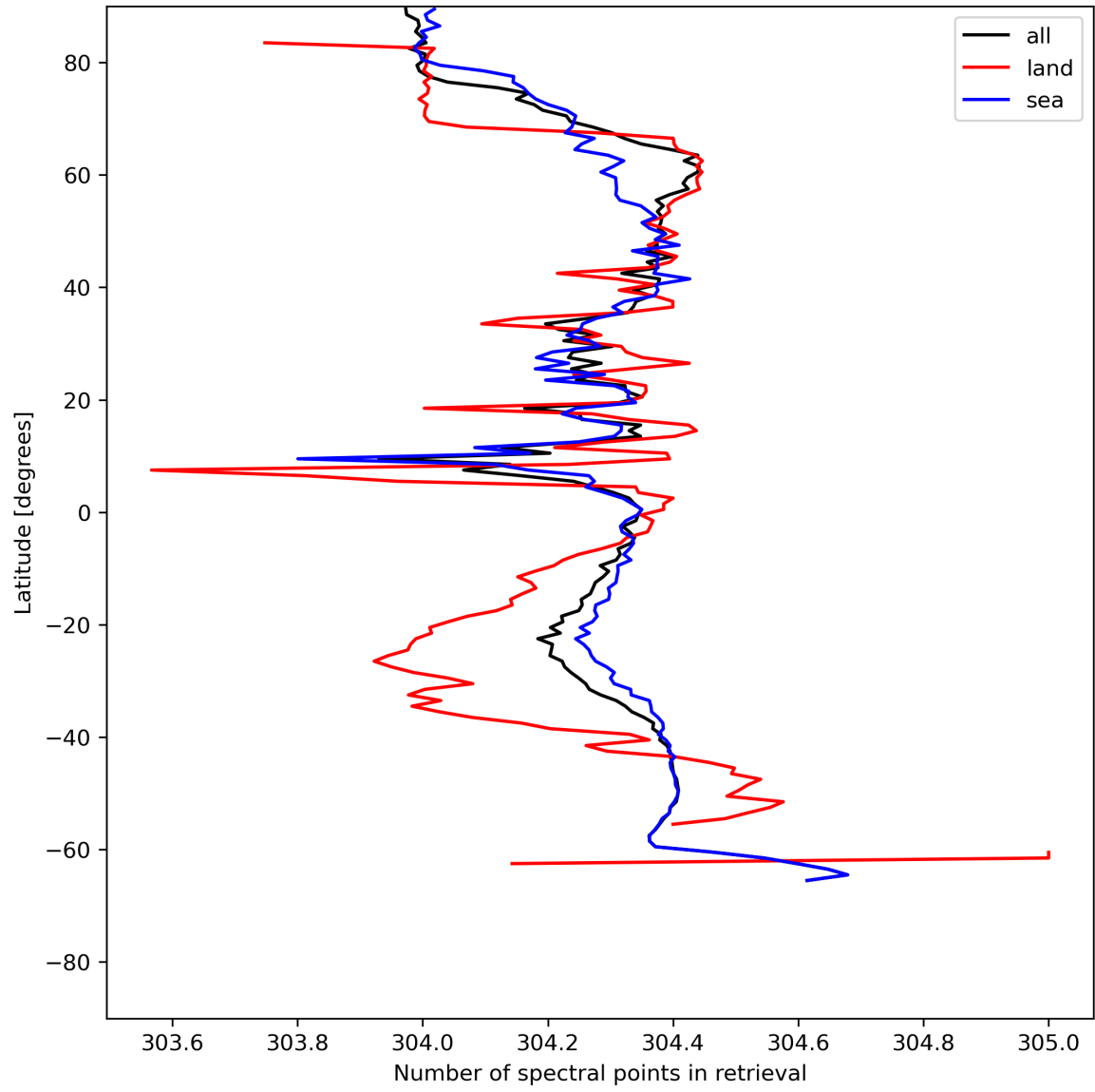
Figure 16: Zonal average of “Number of spectral points in retrieval” for 2024-05-31 to 2024-06-02.
