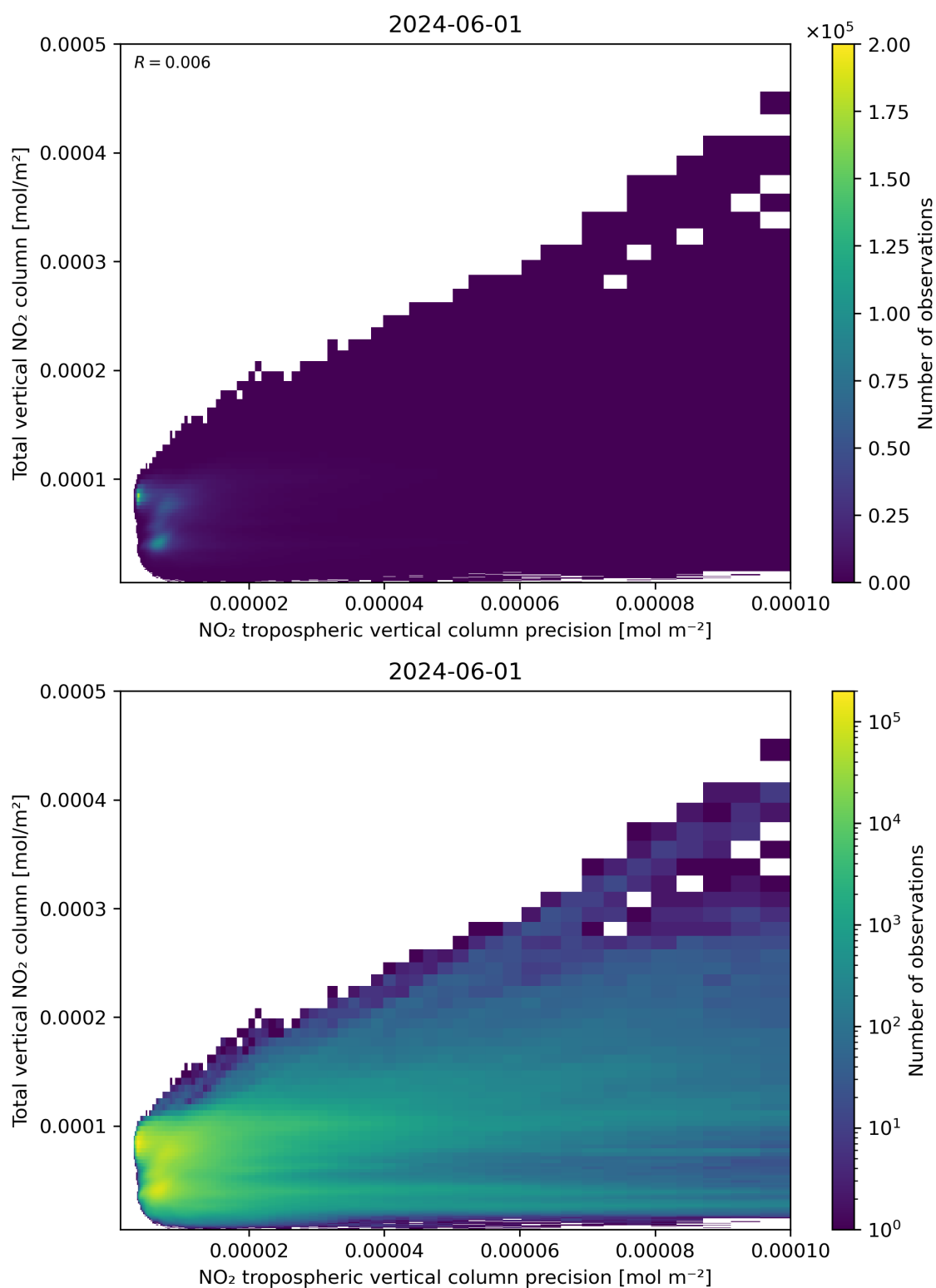
Figure 138: Scatter density plot of “NO 2 tropospheric vertical column precision” against “Total vertical NO 2 column” for 2024-05-31 to 2024-06-02.
