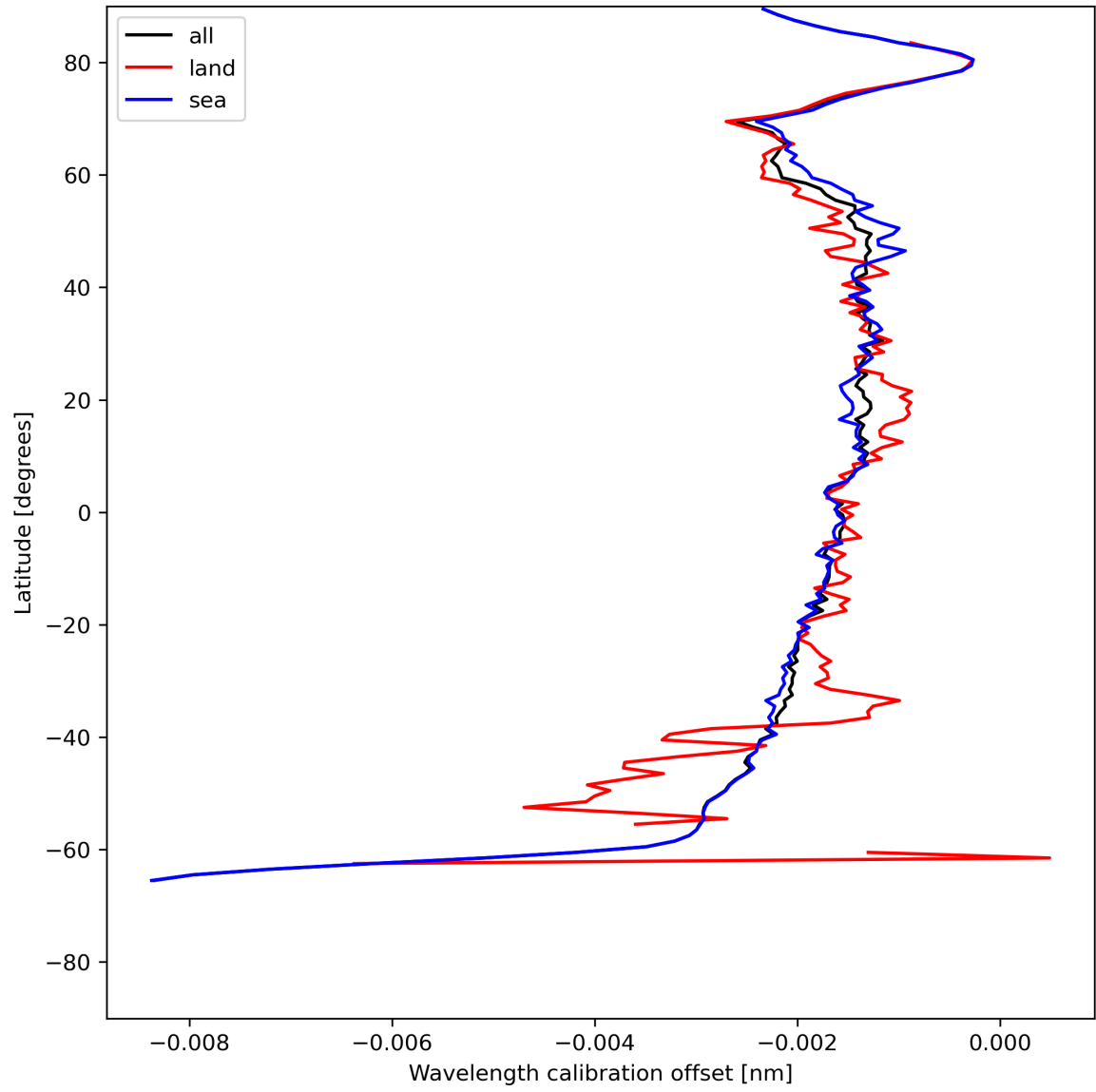
Figure 18: Zonal average of “Wavelength calibration offset” for 2024-05-31 to 2024-06-02.
