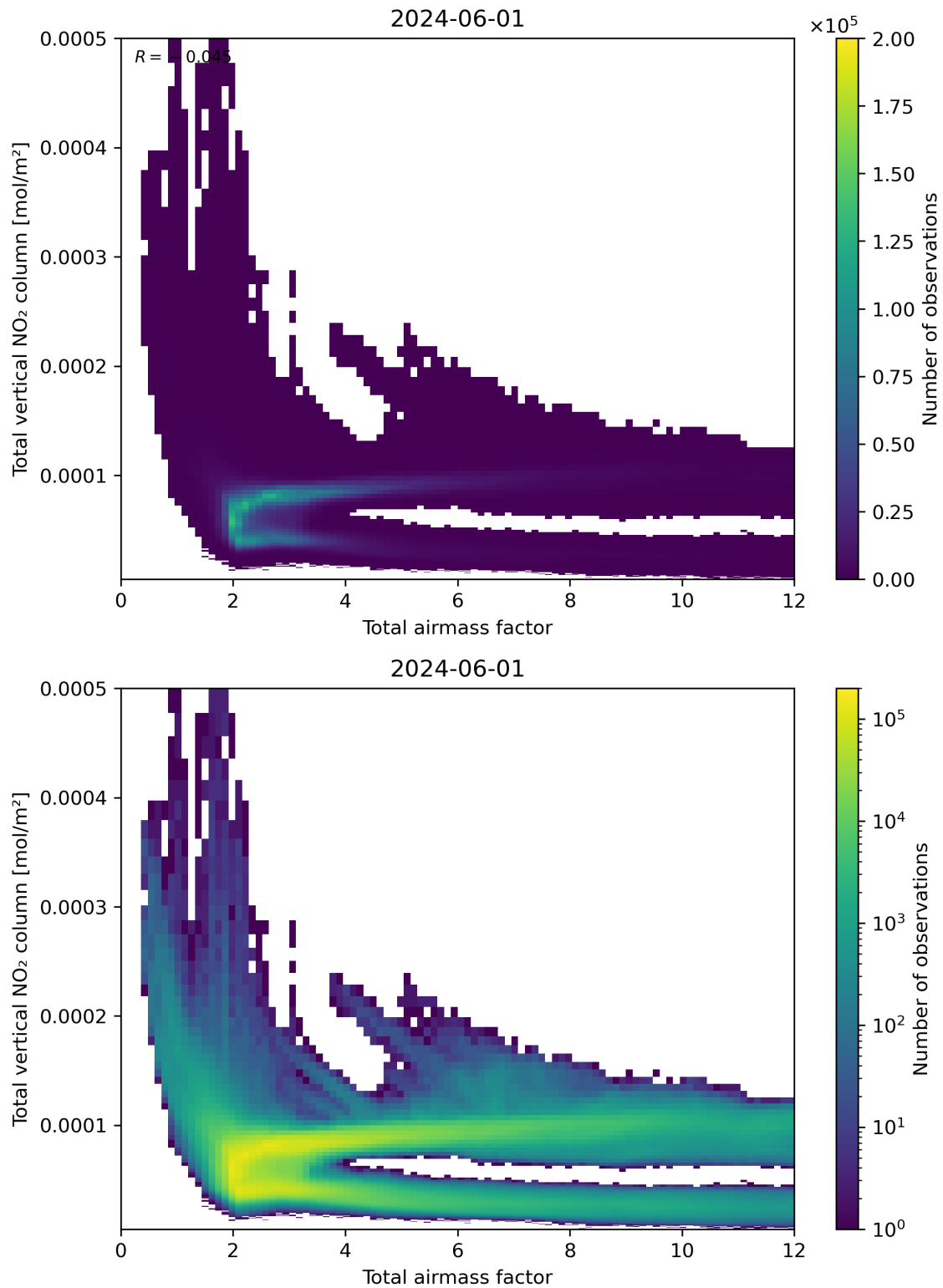
Figure 67: Scatter density plot of “Total airmass factor” against “Total vertical NO 2 column” for 2024-05-31 to 2024-06-02.
