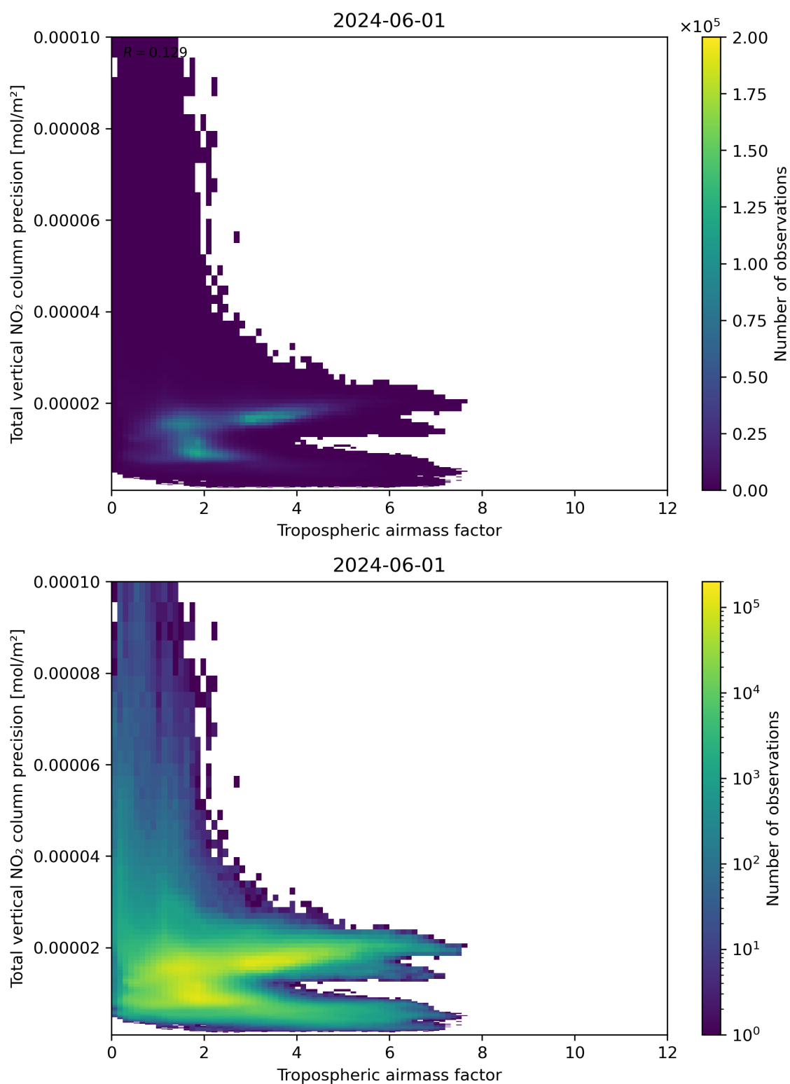
Figure 78: Scatter density plot of “Tropospheric air mass factor” against “Total vertical NO 2 column precision” for 2024-05-31 to 2024-06-02.
