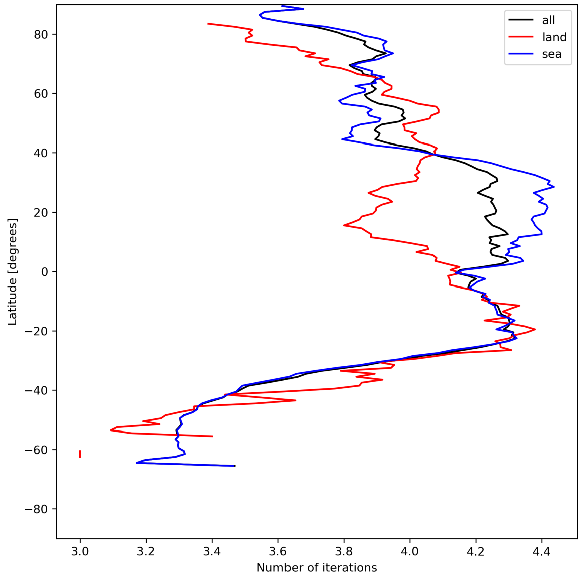
Figure 17: Zonal average of “Number of iterations” for 2024-05-31 to 2024-06-02.
