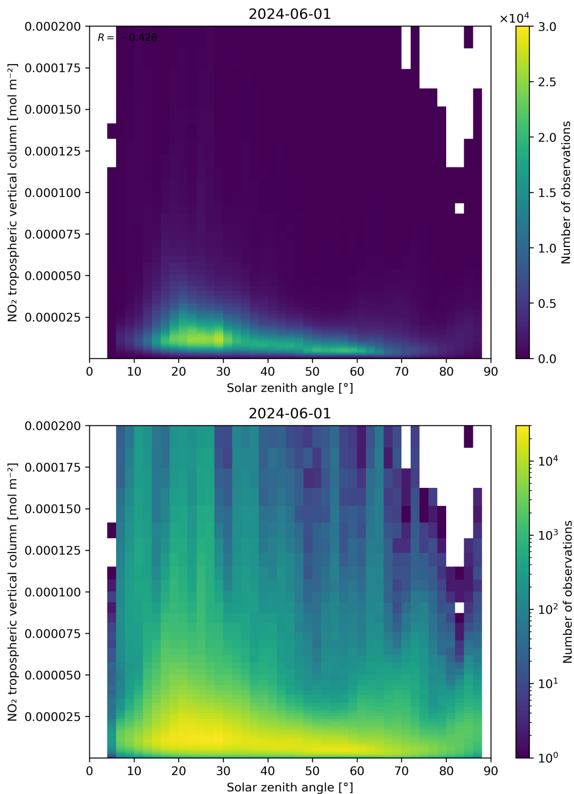
Figure 155: Scatter density plot of “Solar zenith angle” against “NO 2 tropospheric vertical column” for 2024-05-31 to 2024-06-02.
