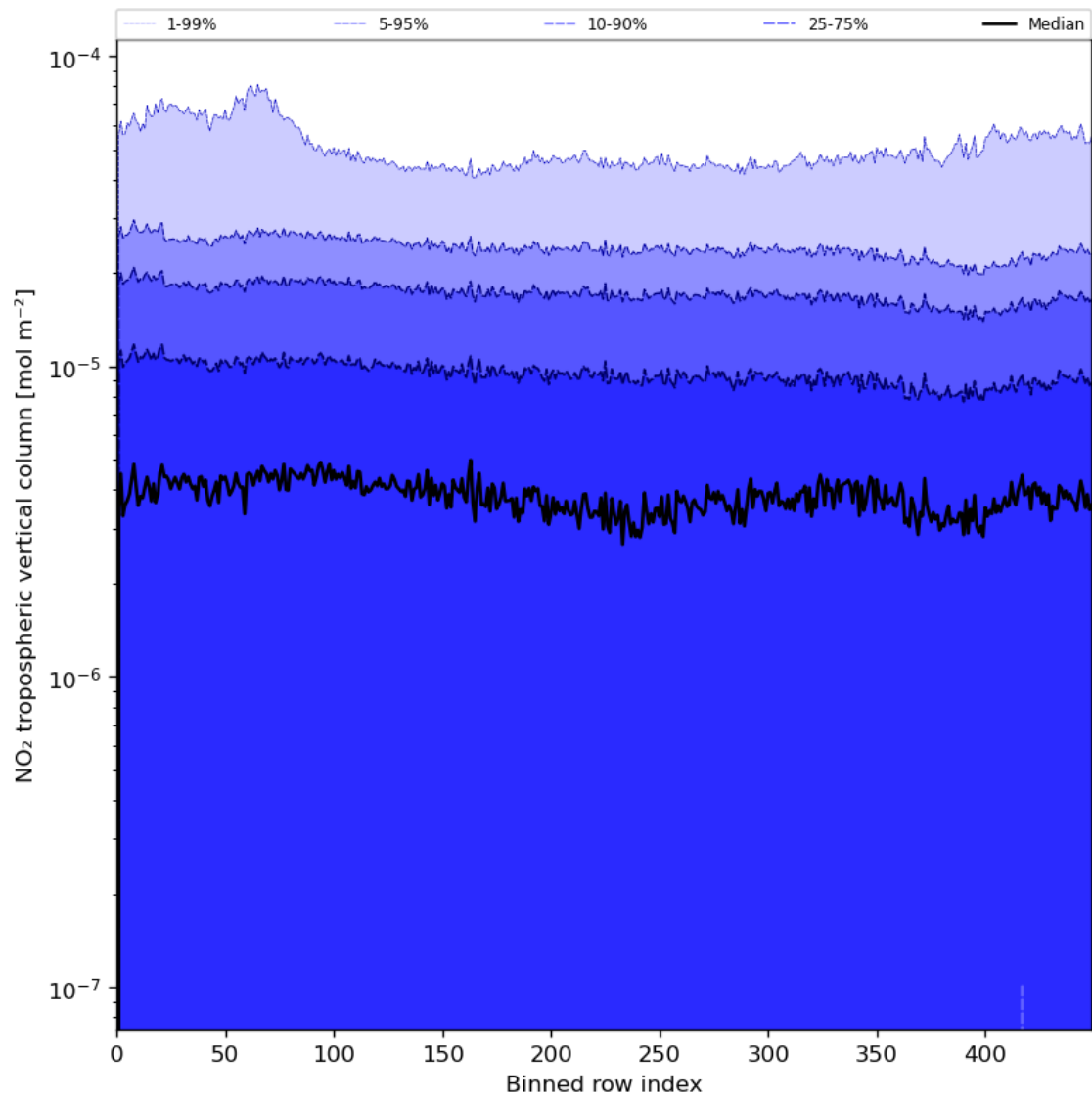
Figure 46: Along track statistics of “NO 2 tropospheric vertical column” for 2024-05-31 to 2024-06-02
