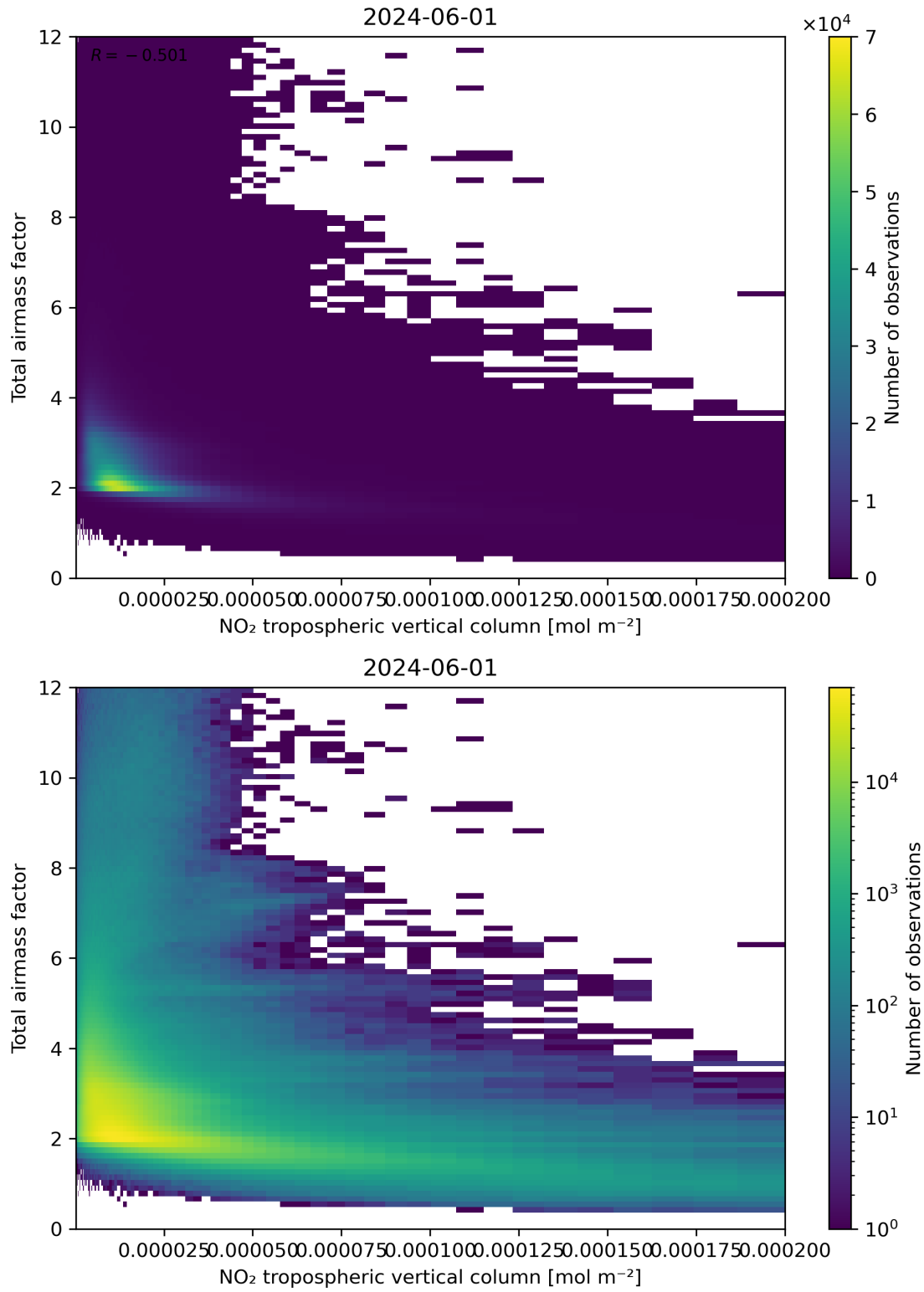
Figure 122: Scatter density plot of “NO 2 tropospheric vertical column” against “Total air mass factor” for 2024-05-31 to 2024-06-02.
