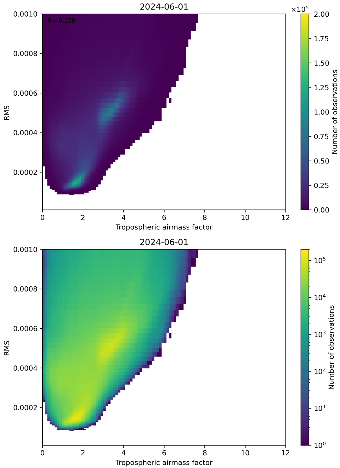
Figure 79: Scatter density plot of “Tropospheric airmass factor” against “RMS” for 2024-05-31 to 2024-06-02.
