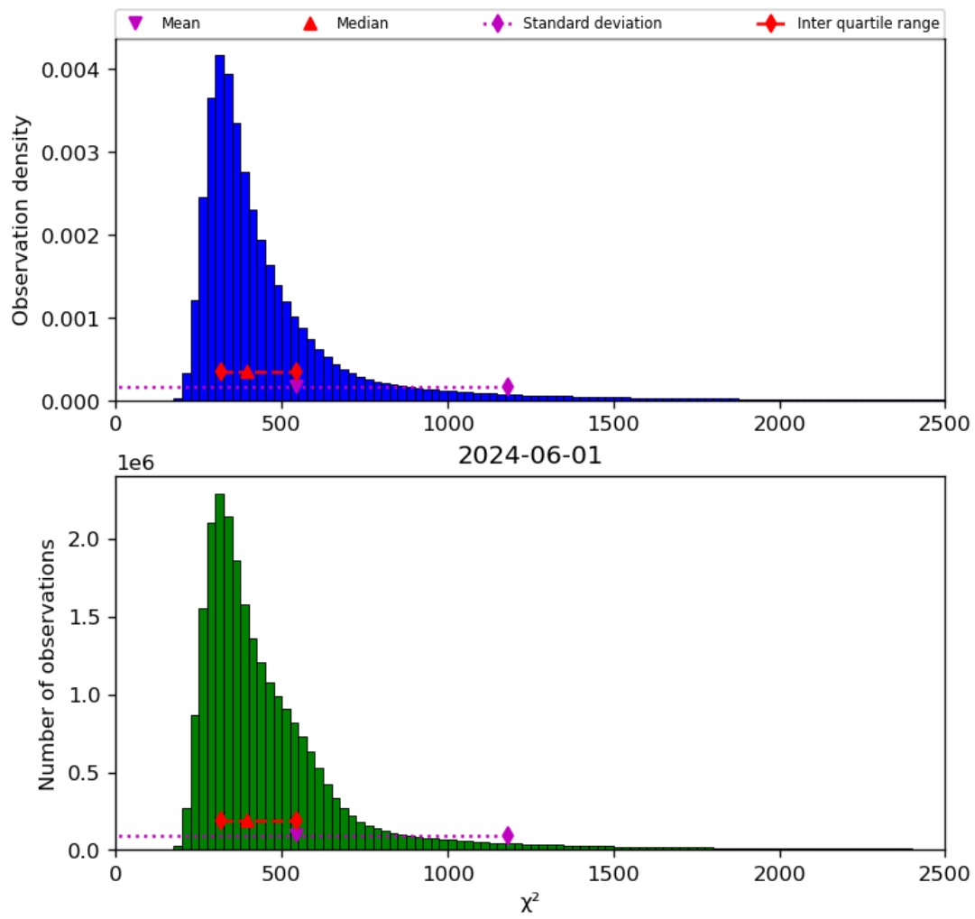
Figure 42: Histogram of “ \chi^2 ” for 2024-05-31 to 2024-06-02
