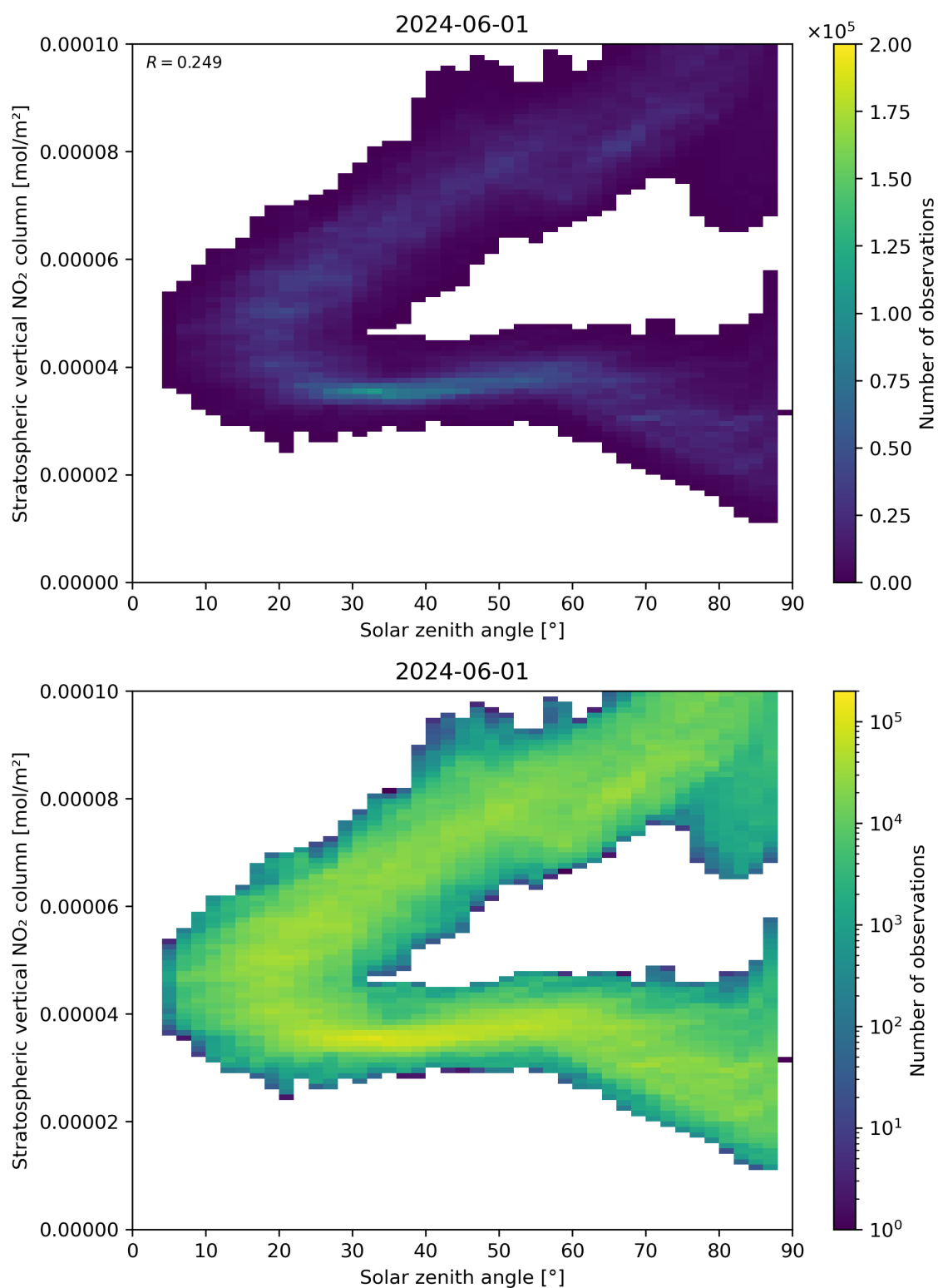
Figure 150: Scatter density plot of “Solar zenith angle” against “Stratospheric vertical NO 2 column” for 2024-05-31 to 2024-06-02.
