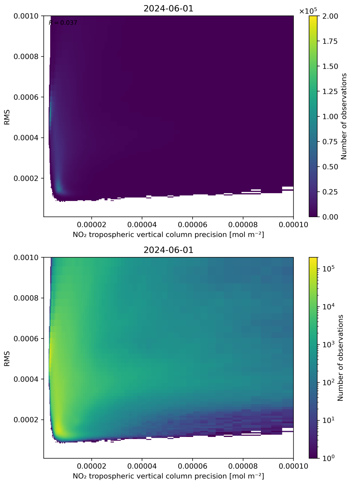
Figure 140: Scatter density plot of “NO 2 tropospheric vertical column precision” against “RMS” for 2024-05-31 to 2024-06-02.
