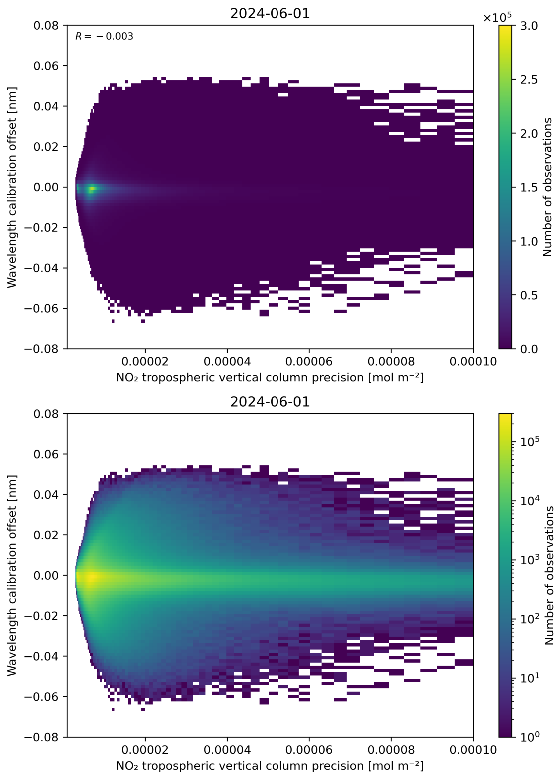
Figure 141: Scatter density plot of “NO 2 tropospheric vertical column precision” against “Wavelength calibration offset” for 2024-05-31 to 2024-06-02.
