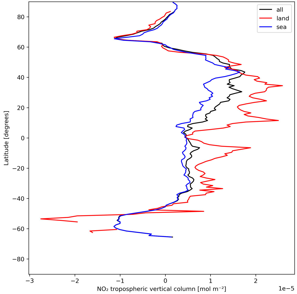
Figure 12: Zonal average of “NO 2 tropospheric vertical column” for 2024-05-31 to 2024-06-02.
