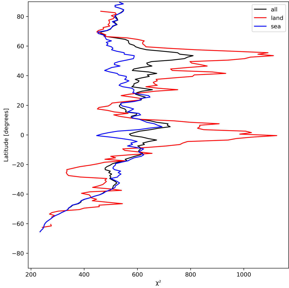
Figure 25: Zonal average of “ \chi^2 ” for 2024-05-31 to 2024-06-02.
