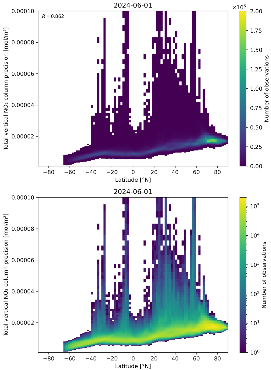
Figure 91: Scatter density plot of “Latitude” against “Total vertical NO 2 column precision” for 2024-05-31 to 2024-06-02.
