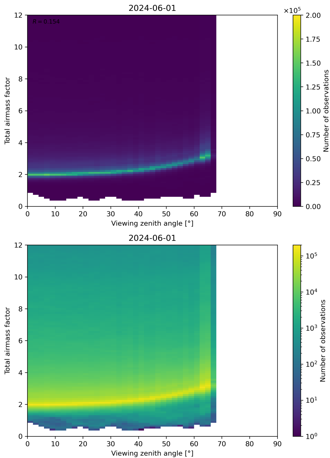
Figure 160: Scatter density plot of “Viewing zenith angle” against “Total airmass factor” for 2024-05-31 to 2024-06-02.
