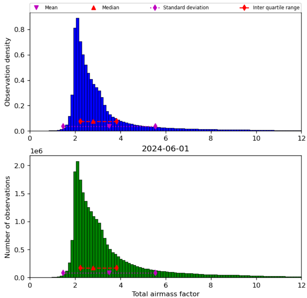
Figure 32: Histogram of “Total airmass factor” for 2024-05-31 to 2024-06-02
