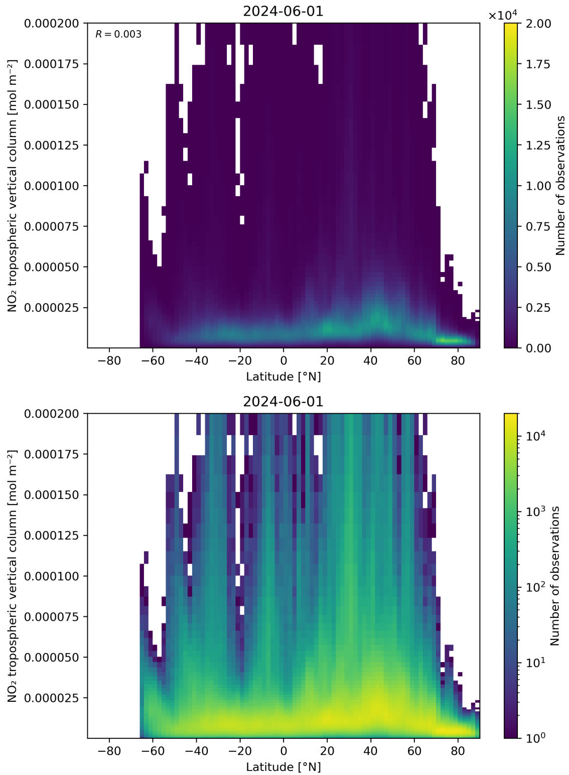
Figure 92: Scatter density plot of “Latitude” against “NO 2 tropospheric vertical column” for 2024-05-31 to 2024-06-02.
