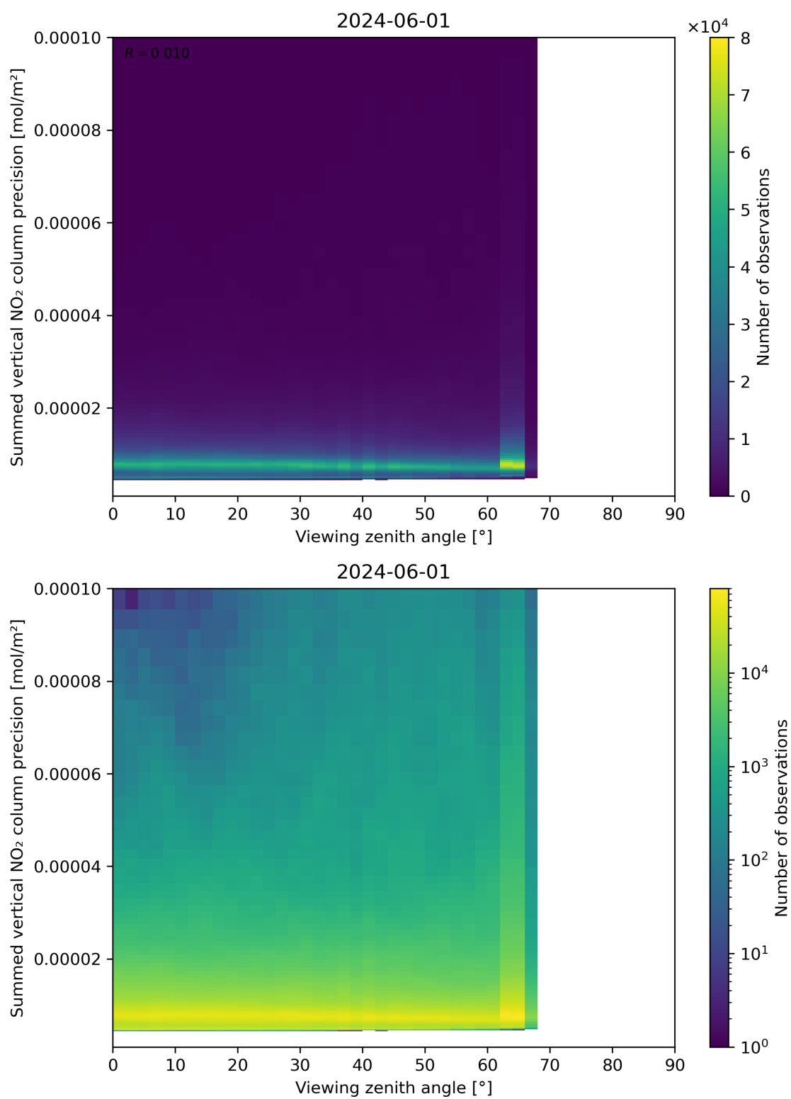
Figure 166: Scatter density plot of “Viewing zenith angle” against “Summed vertical NO 2 column precision” for 2024-05-31 to 2024-06-02.
