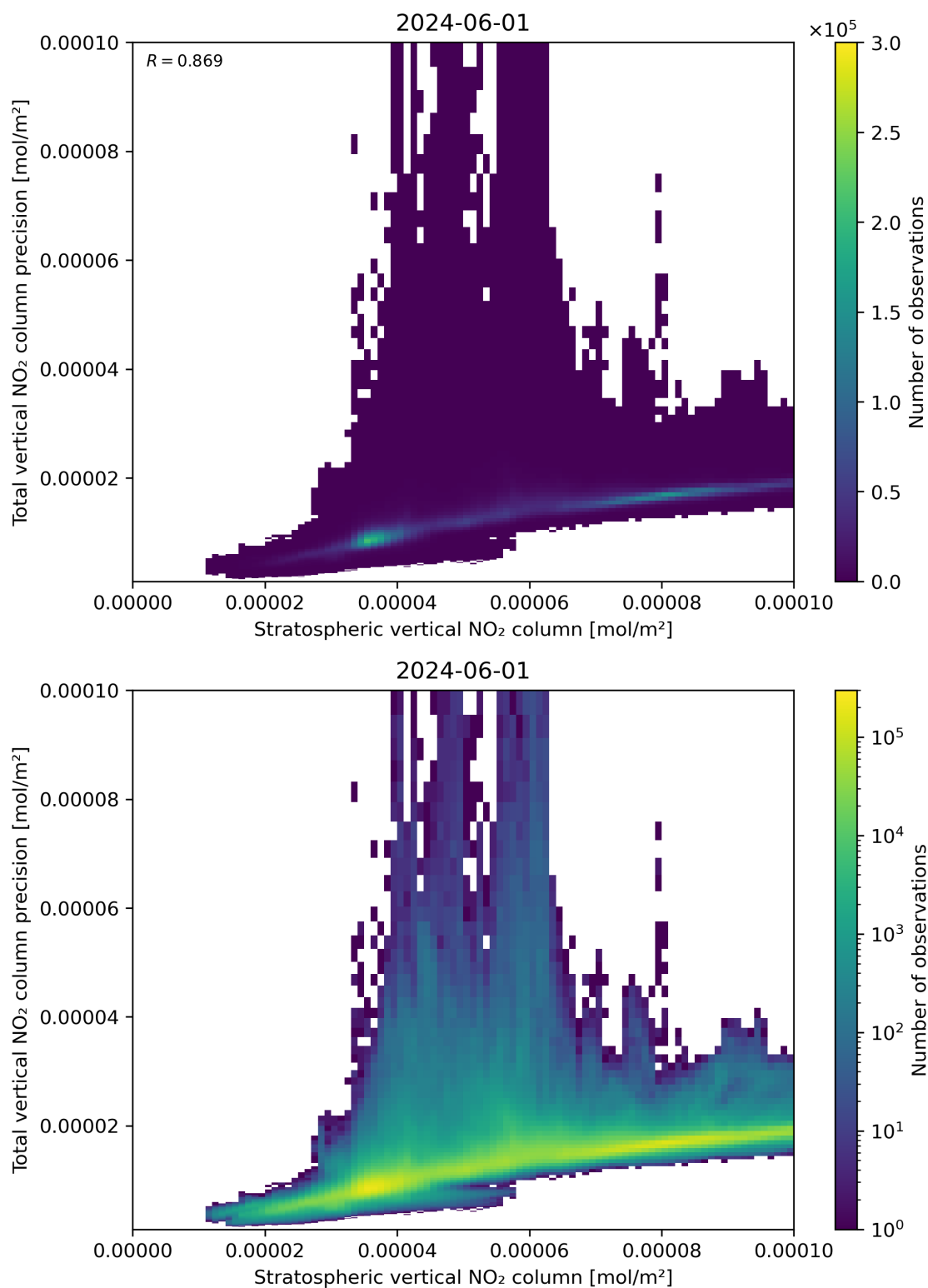
Figure 101: Scatter density plot of “Stratospheric vertical NO 2 column” against “Total vertical NO 2 column precision” for 2024-05-31 to 2024-06-02.
