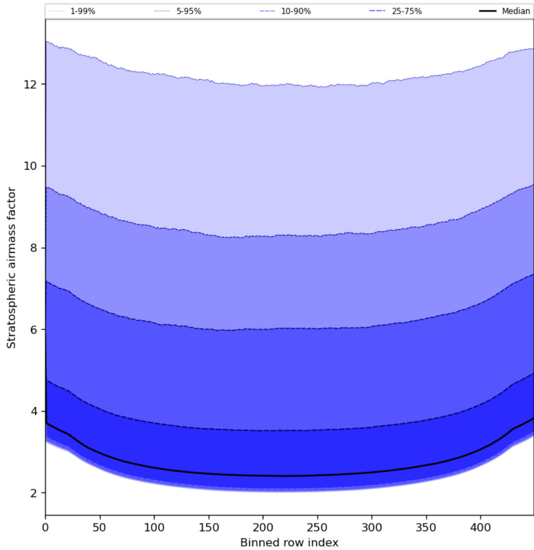
Figure 61: Along track statistics of “Stratospheric airmass factor” for 2024-05-31 to 2024-06-02
