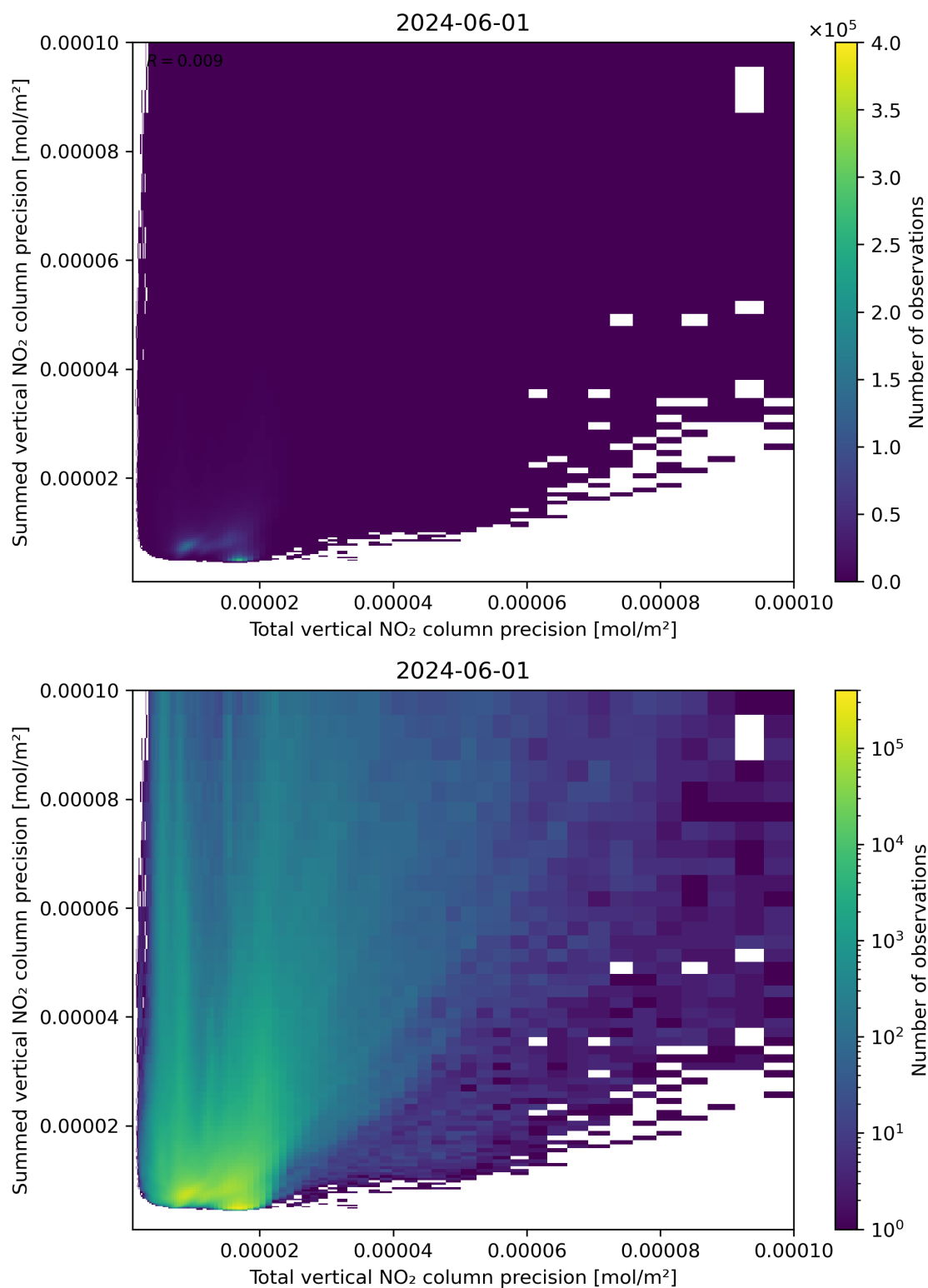
Figure 118: Scatter density plot of “Total vertical NO 2 column precision” against “Summed vertical NO 2 column precision” for 2024-05-31 to 2024-06-02.
