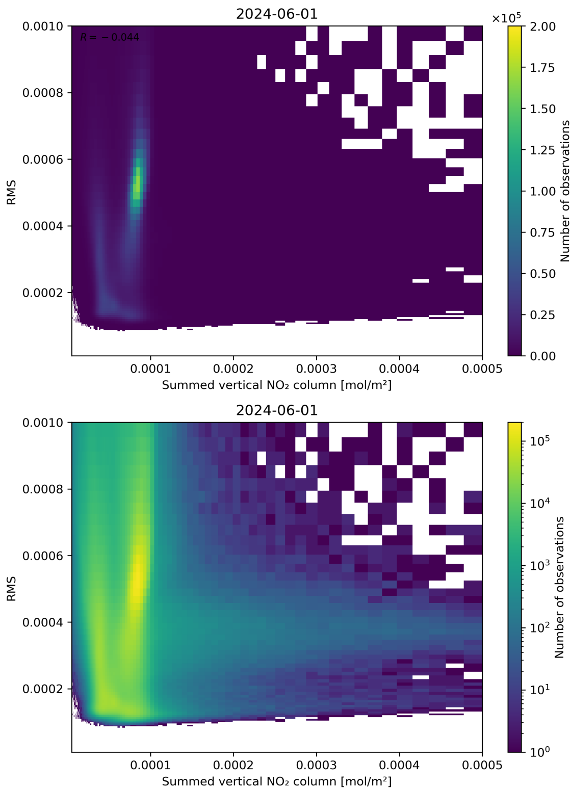
Figure 109: Scatter density plot of “Summed vertical NO 2 column” against “RMS” for 2024-05-31 to 2024-06-02.
