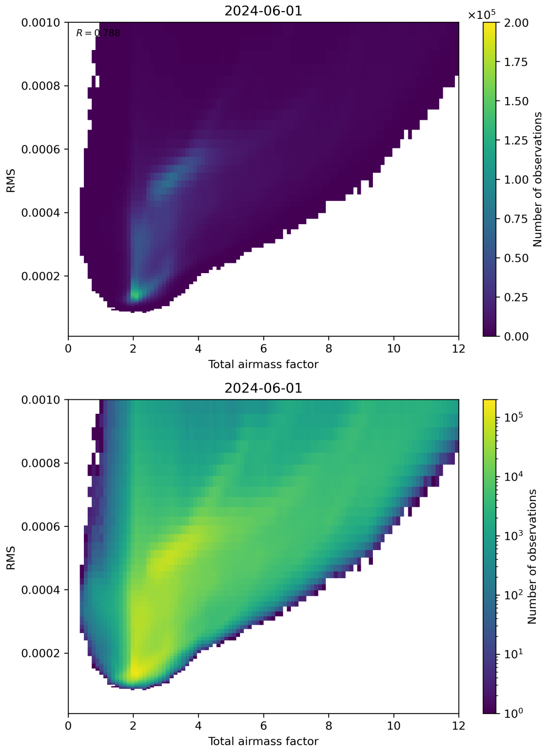
Figure 69: Scatter density plot of “Total airmass factor” against “RMS” for 2024-05-31 to 2024-06-02.
