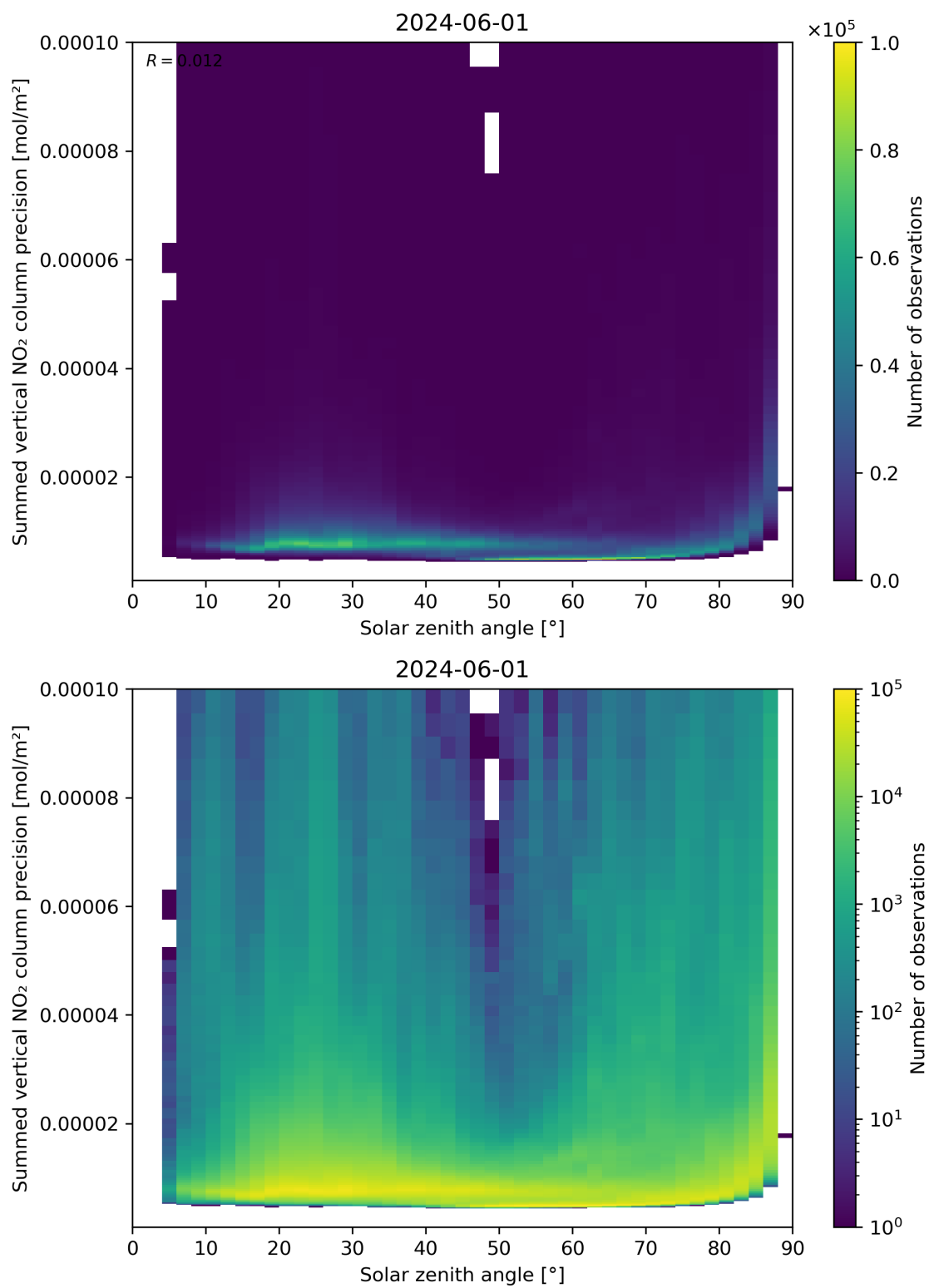
Figure 152: Scatter density plot of “Solar zenith angle” against “Summed vertical NO 2 column precision” for 2024-05-31 to 2024-06-02.
