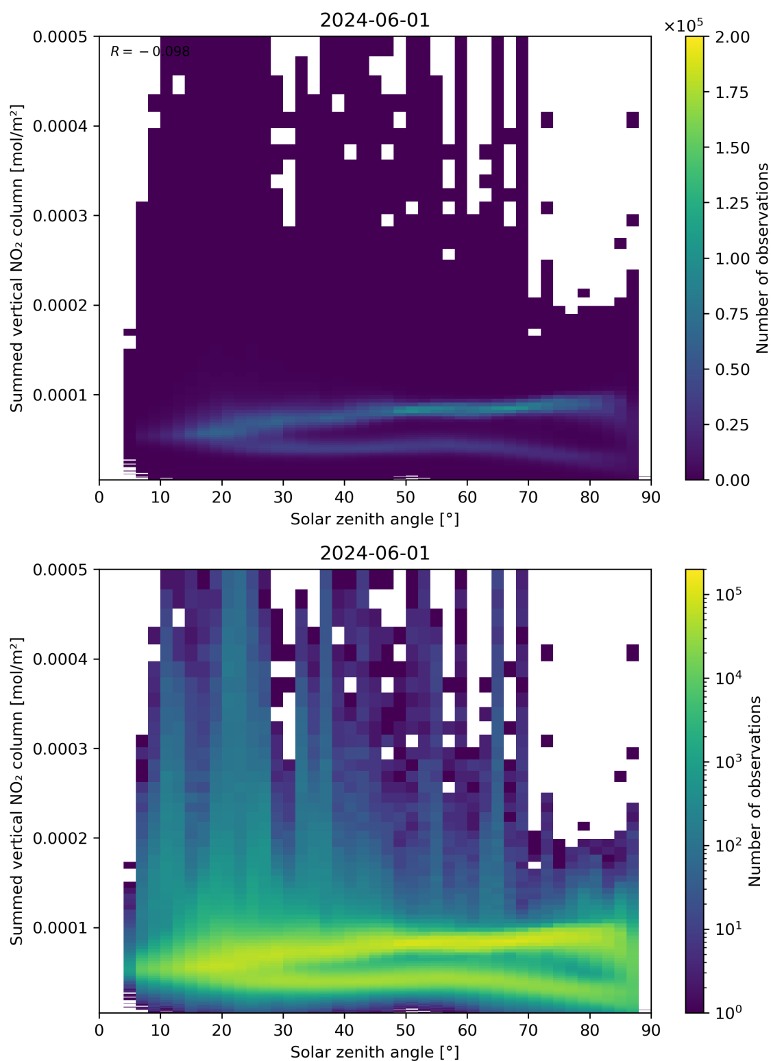
Figure 151: Scatter density plot of “Solar zenith angle” against “Summed vertical NO 2 column” for 2024-05-31 to 2024-06-02.
