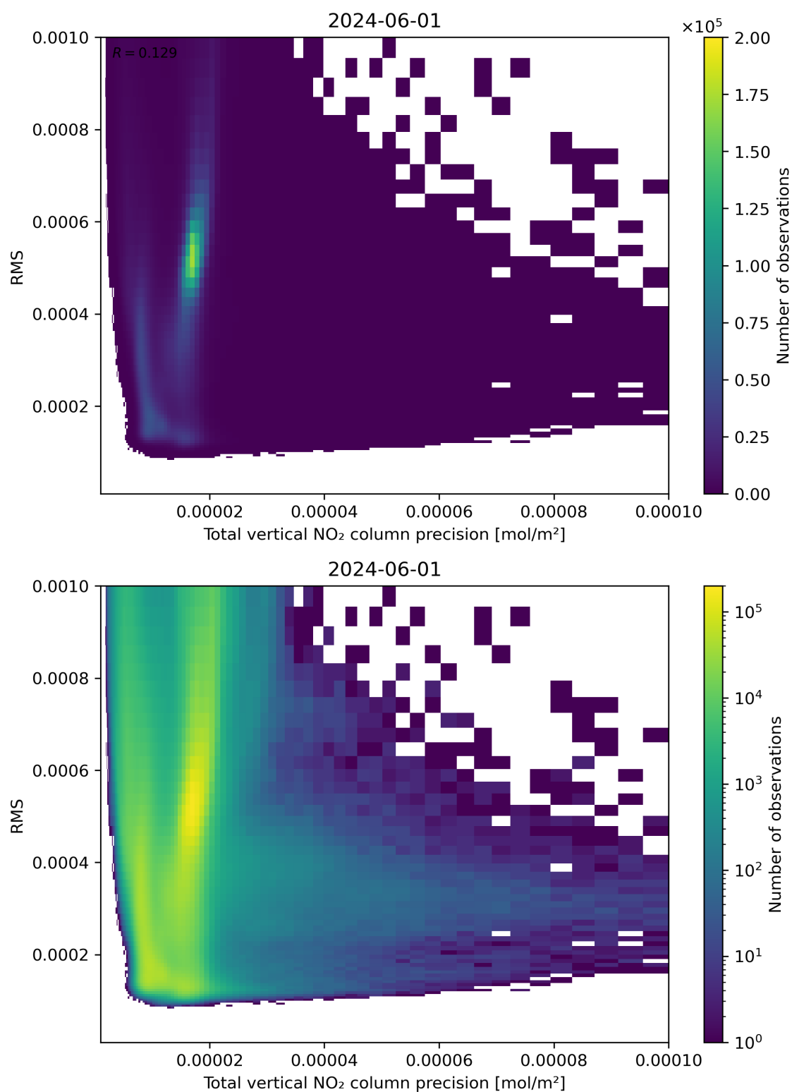
Figure 119: Scatter density plot of “Total vertical NO 2 column precision” against “RMS” for 2024-05-31 to 2024-06-02.
