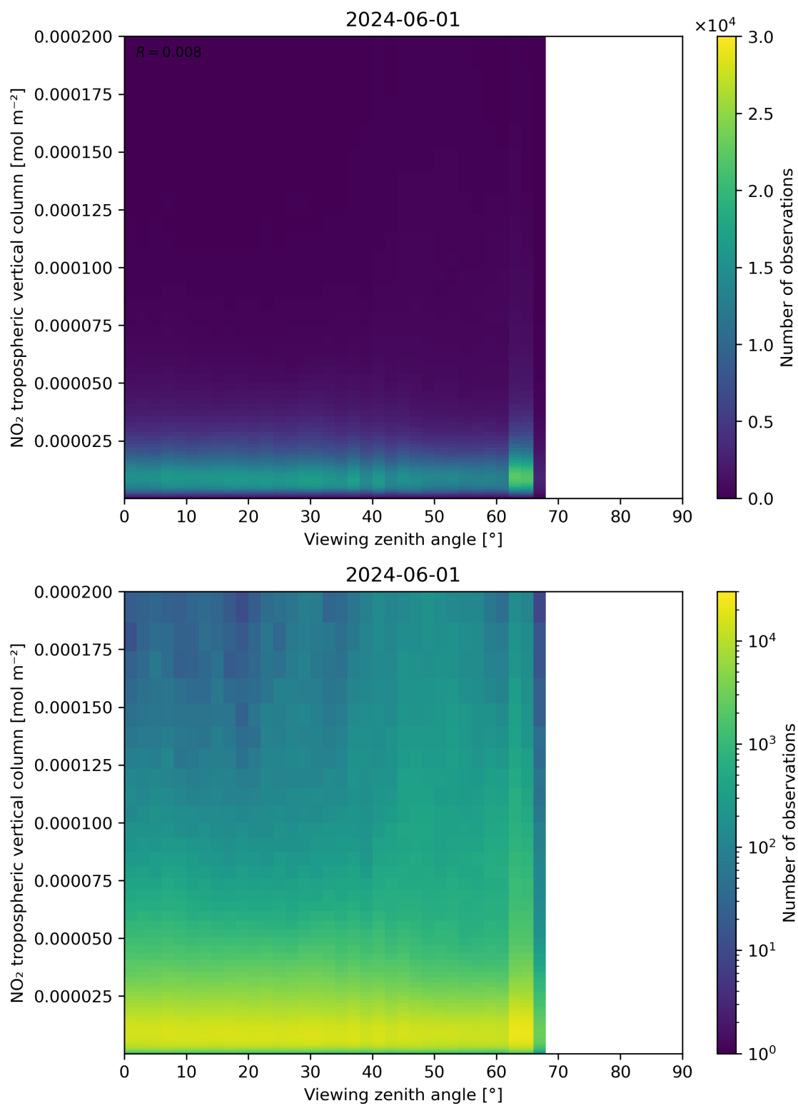
Figure 169: Scatter density plot of “Viewing zenith angle” against “NO 2 tropospheric vertical column” for 2024-05-31 to 2024-06-02.
