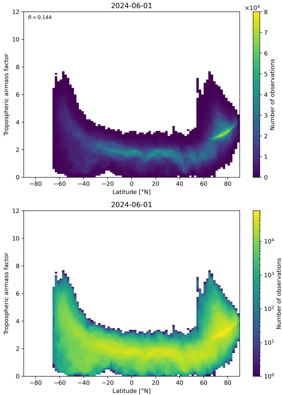
Figure 85: Scatter density plot of “Latitude” against “Tropospheric airmass factor” for 2024-05-31 to 2024-06-02.
