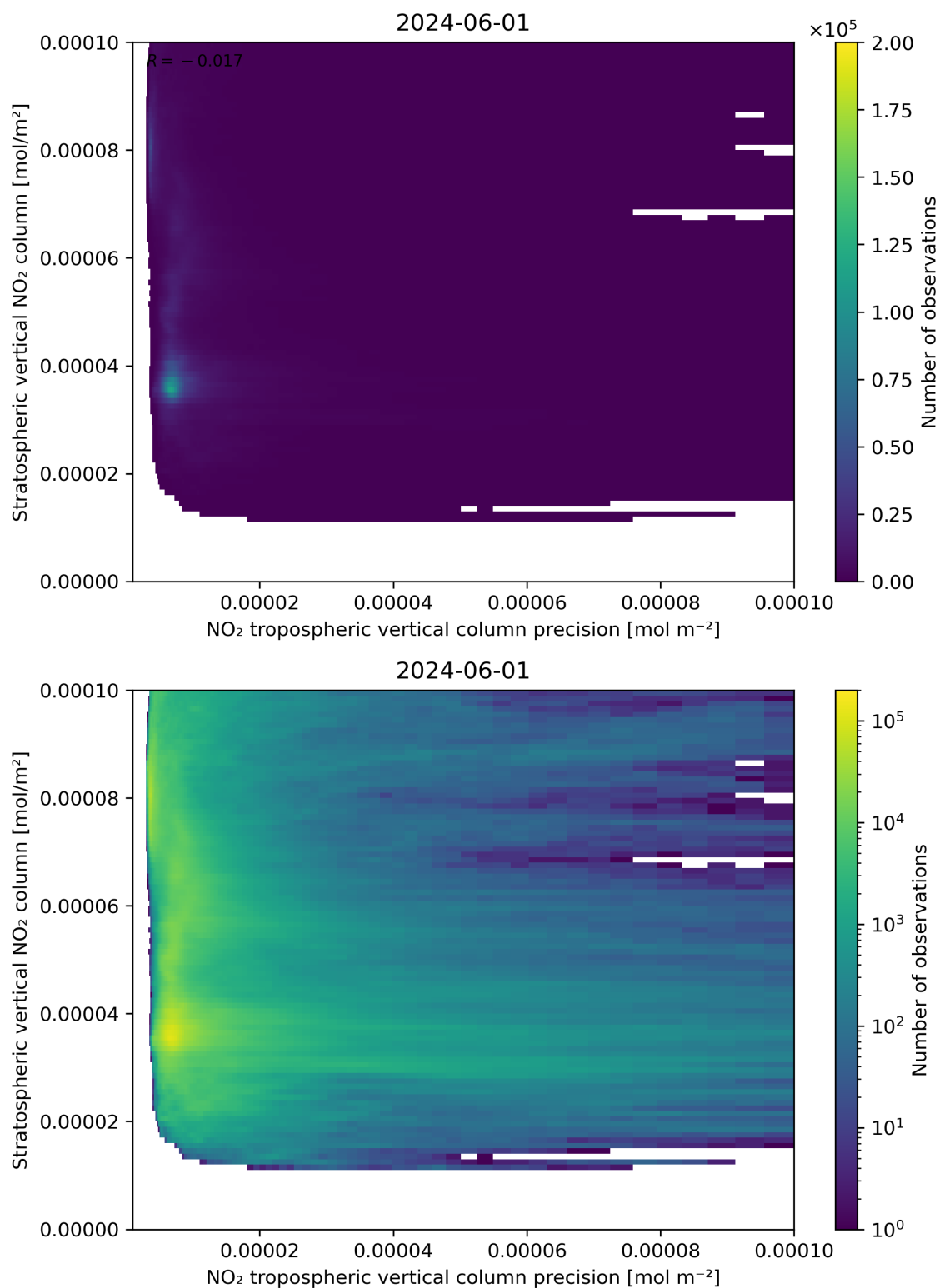
Figure 135: Scatter density plot of “NO 2 tropospheric vertical column precision” against “Stratospheric vertical NO 2 column” for 2024-05-31 to 2024-06-02.
