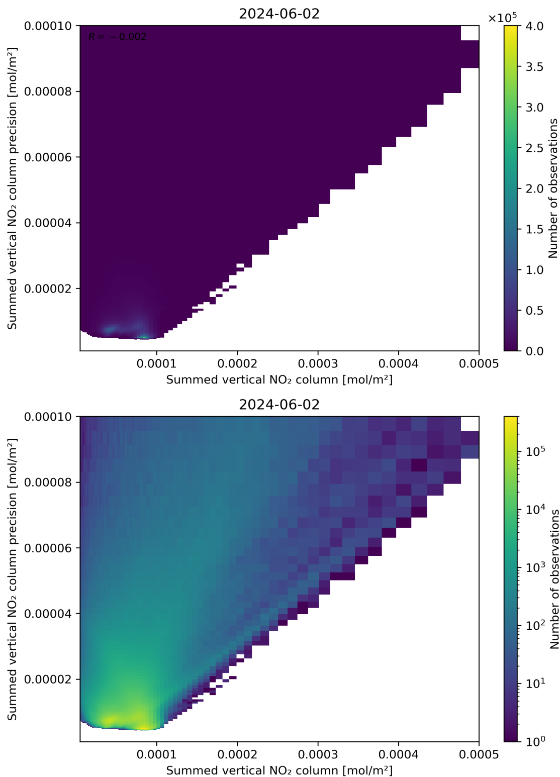
Figure 105: Scatter density plot of “Summed vertical NO 2 column” against “Summed vertical NO 2 column precision” for 2024-06-01 to 2024-06-03.
