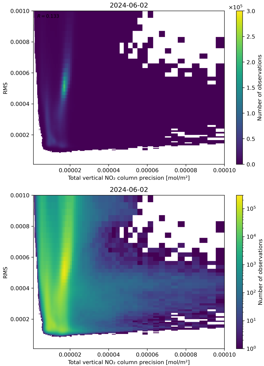
Figure 119: Scatter density plot of “Total vertical NO 2 column precision” against “RMS” for 2024-06-01 to 2024-06-03.
