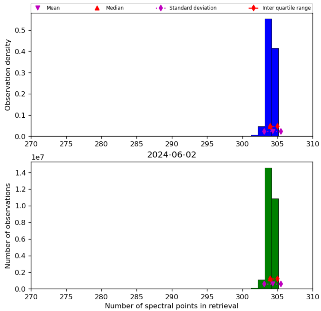
Figure 33: Histogram of “Number of spectral points in retrieval” for 2024-06-01 to 2024-06-03
