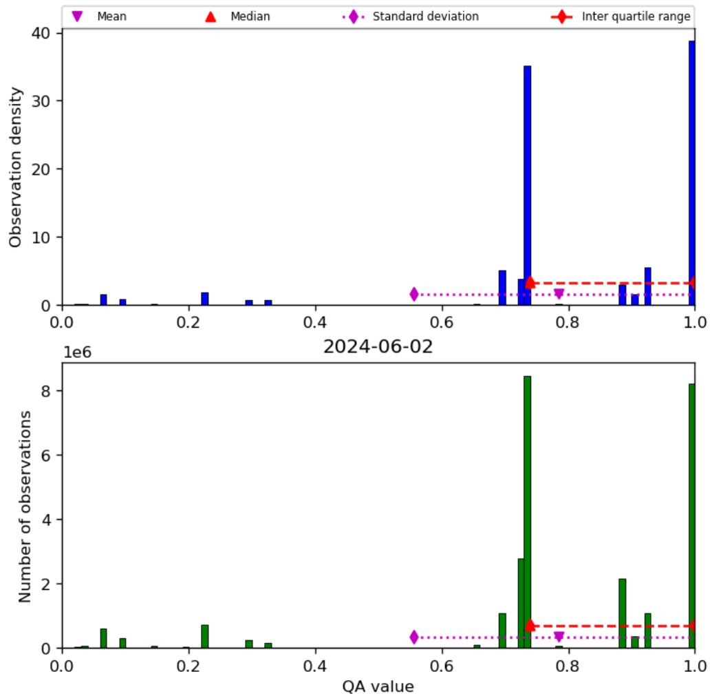
Figure 28: Histogram of “QA value” for 2024-06-01 to 2024-06-03
