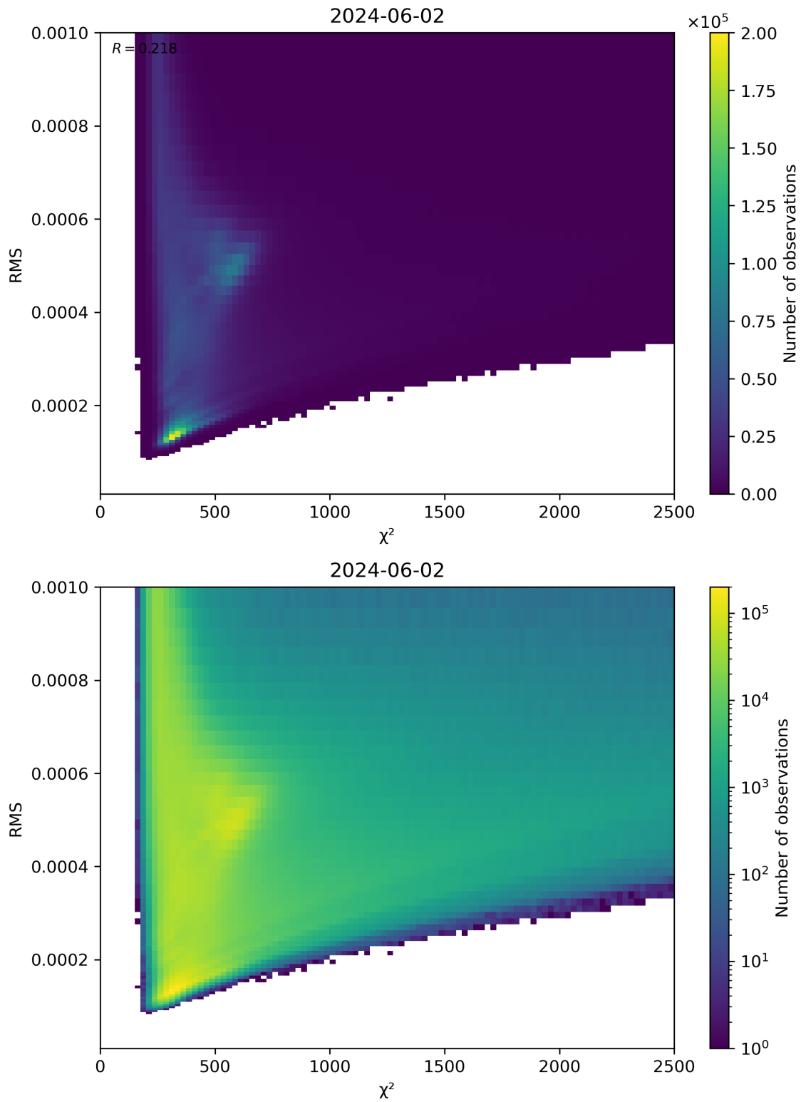
Figure 82: Scatter density plot of “ \chi^2 ” against “RMS” for 2024-06-01 to 2024-06-03.
