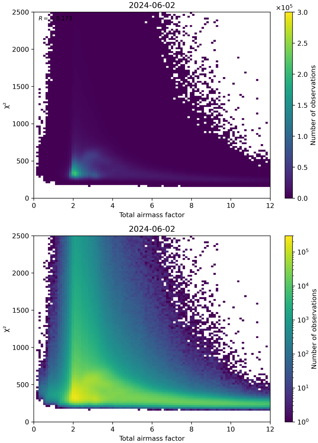
Figure 63: Scatter density plot of “Total airmass factor” against “ \chi^2 ” for 2024-06-01 to 2024-06-03.
