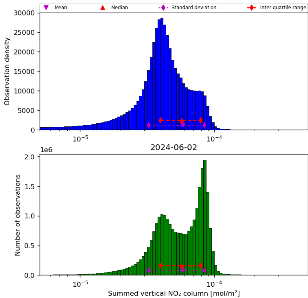
Figure 40: Histogram of “Summed vertical NO 2 column” for 2024-06-01 to 2024-06-03
