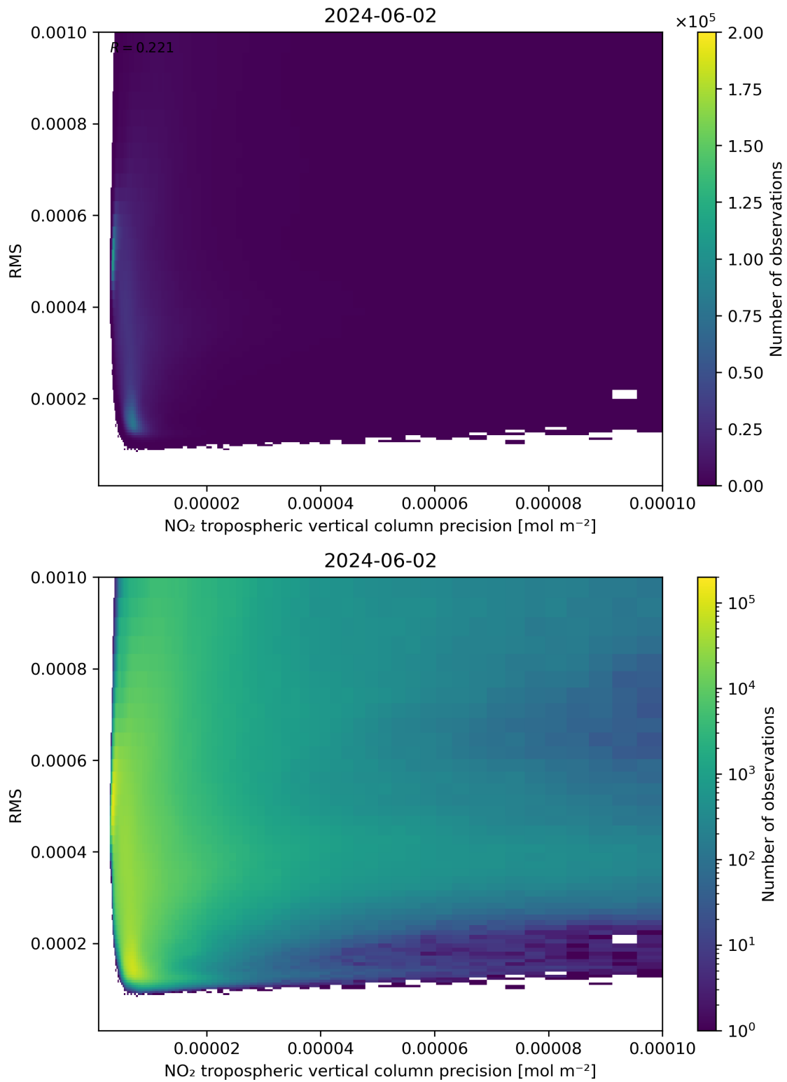
Figure 140: Scatter density plot of “NO 2 tropospheric vertical column precision” against “RMS” for 2024-06-01 to 2024-06-03.
