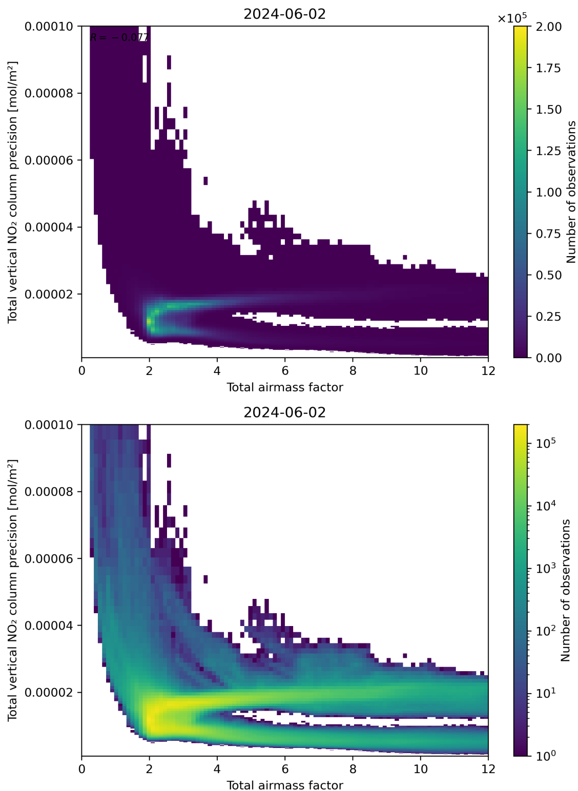
Figure 68: Scatter density plot of “Total airmass factor” against “Total vertical NO 2 column precision” for 2024-06-01 to 2024-06-03.
