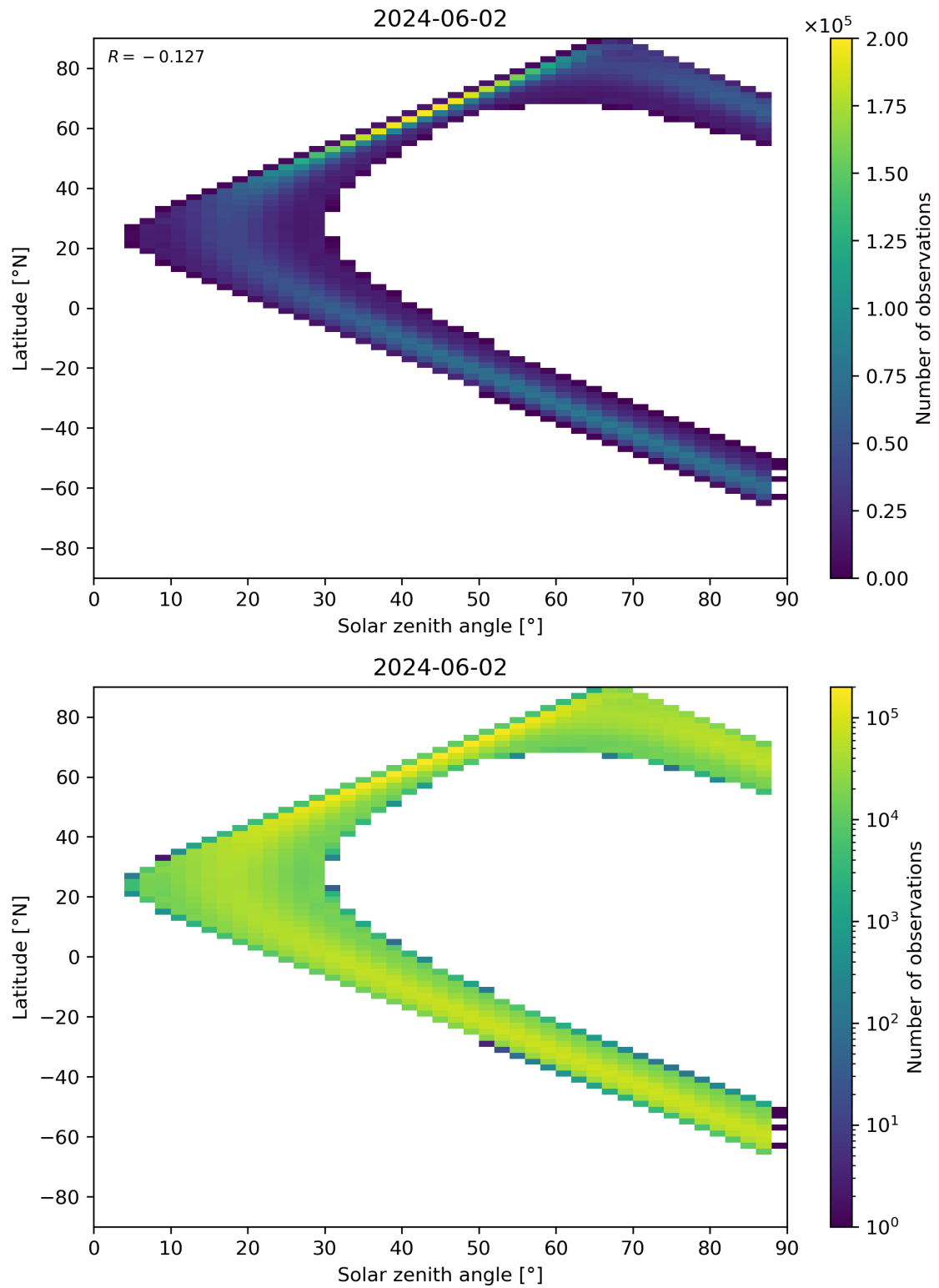
Figure 149: Scatter density plot of “Solar zenith angle” against “Latitude” for 2024-06-01 to 2024-06-03.
