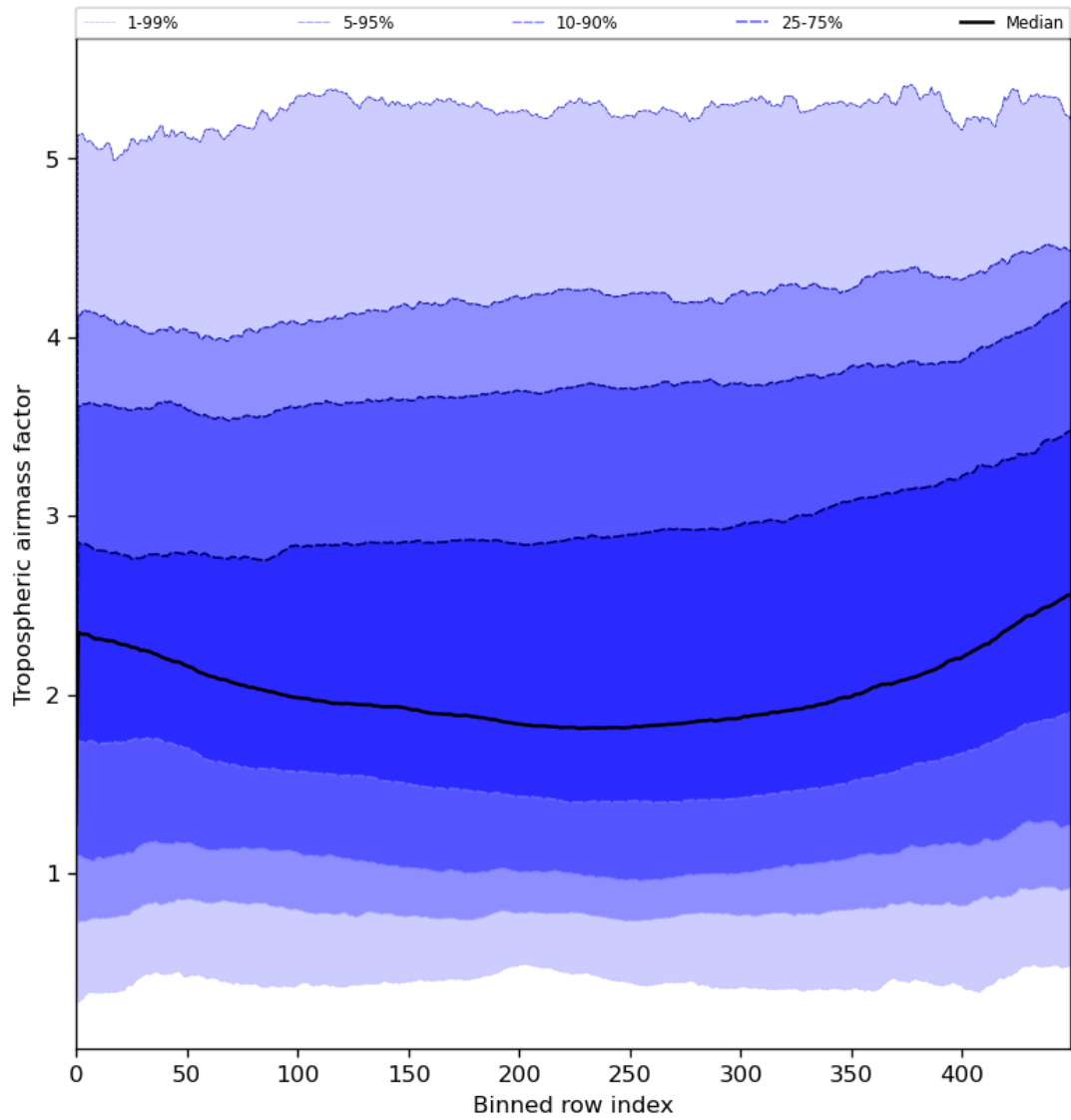
Figure 48: Along track statistics of “Tropospheric airmass factor” for 2024-06-01 to 2024-06-03
