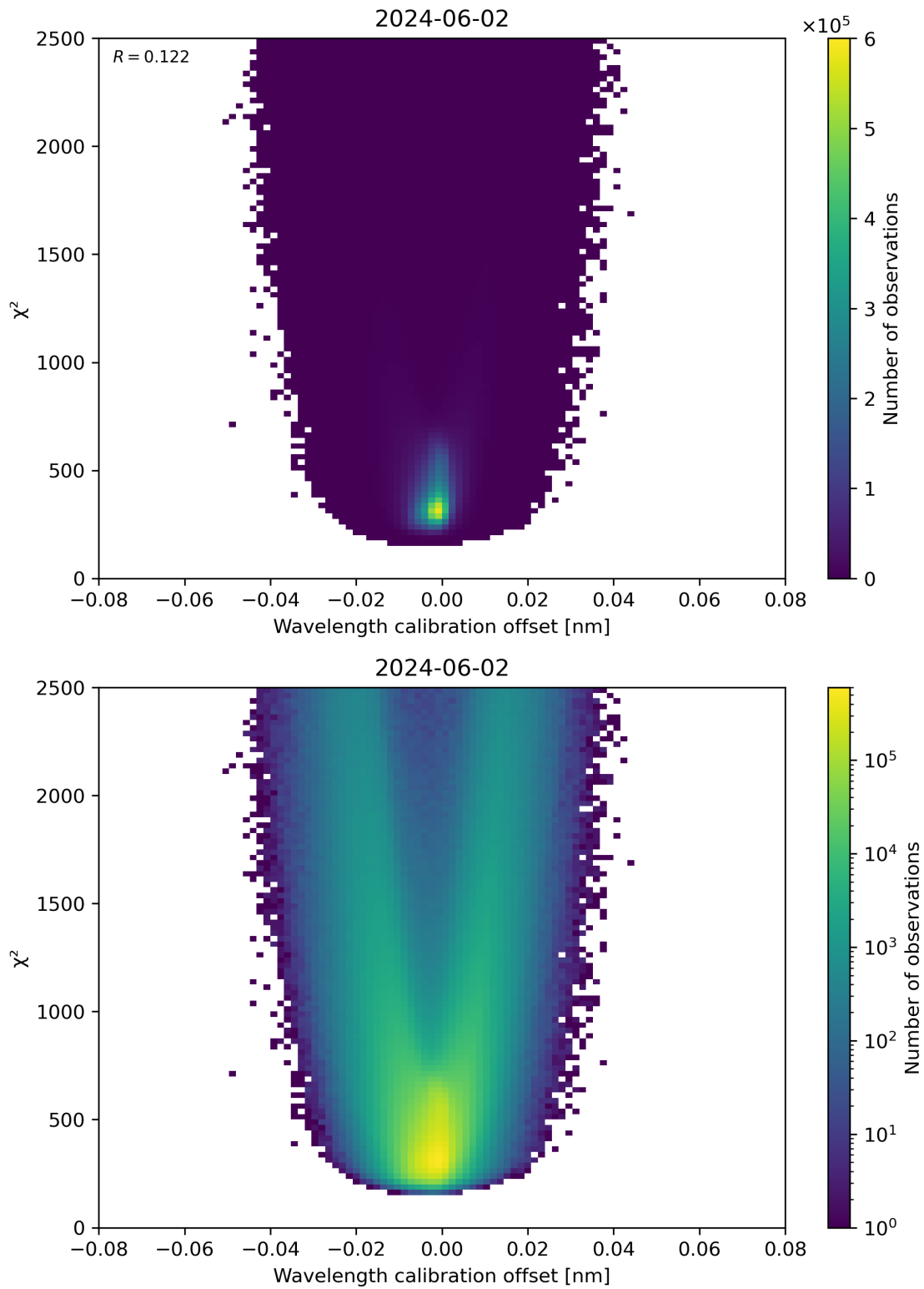
Figure 175: Scatter density plot of “Wavelength calibration offset” against “ \chi^2 ” for 2024-06-01 to 2024-06-03.
