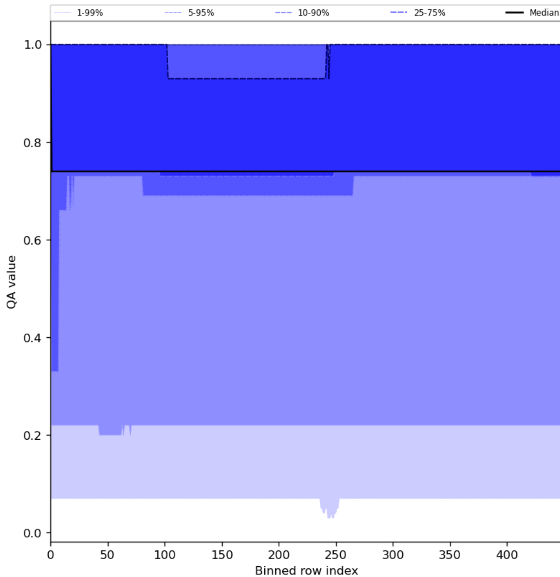
Figure 45: Along track statistics of “QA value” for 2024-06-01 to 2024-06-03
