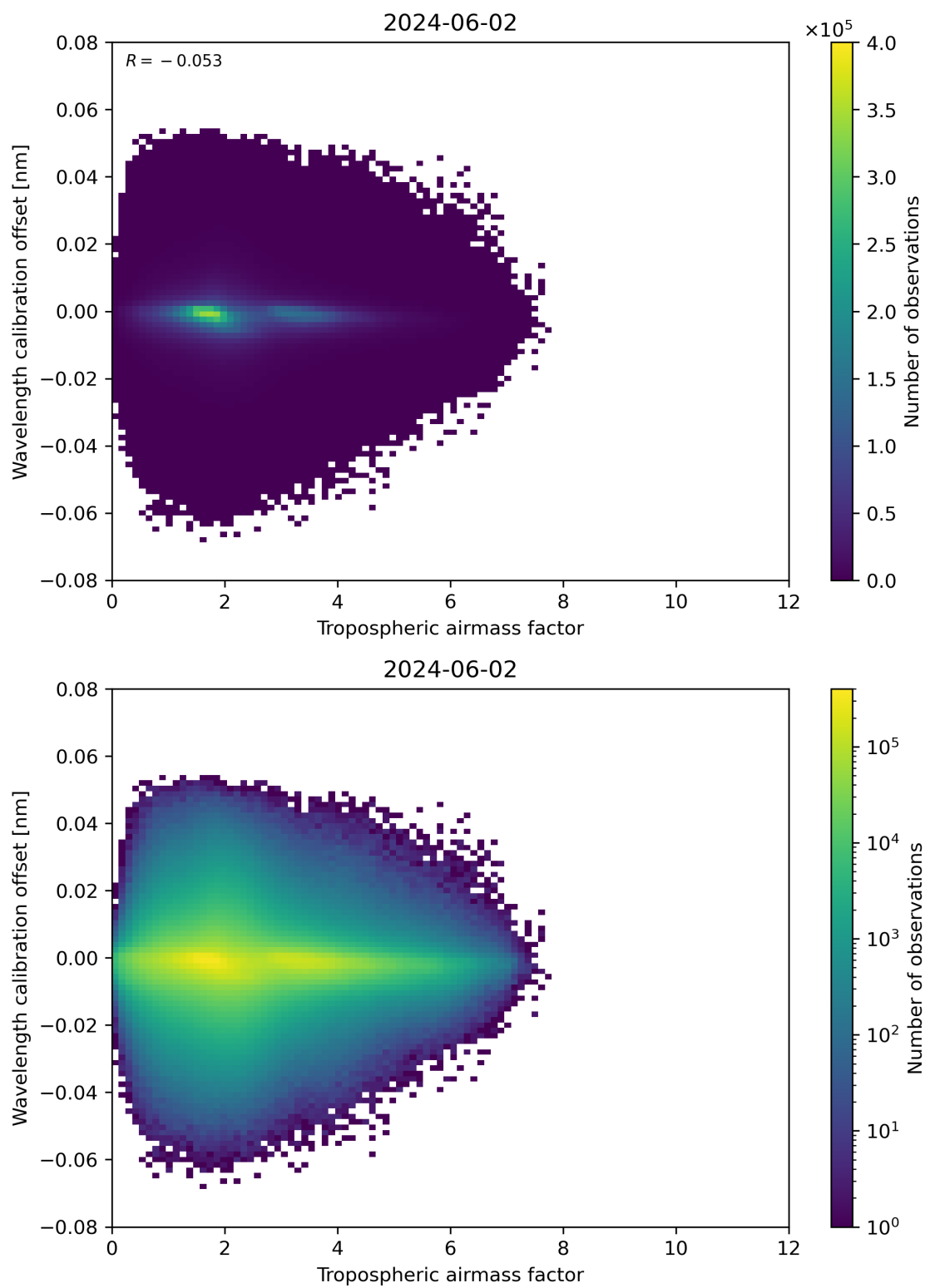
Figure 80: Scatter density plot of “Tropospheric airmass factor” against “Wavelength calibration offset” for 2024-06-01 to 2024-06-03.
