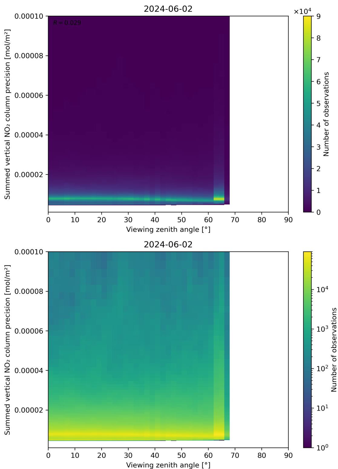
Figure 166: Scatter density plot of “Viewing zenith angle” against “Summed vertical NO 2 column precision” for 2024-06-01 to 2024-06-03.
