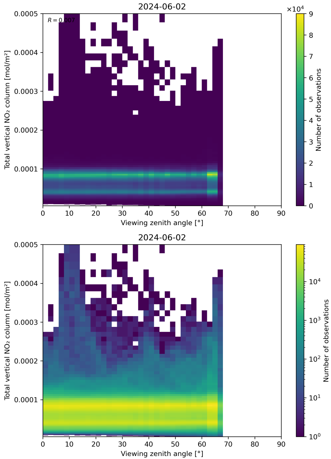
Figure 167: Scatter density plot of “Viewing zenith angle” against “Total vertical NO 2 column” for 2024-06-01 to 2024-06-03.
