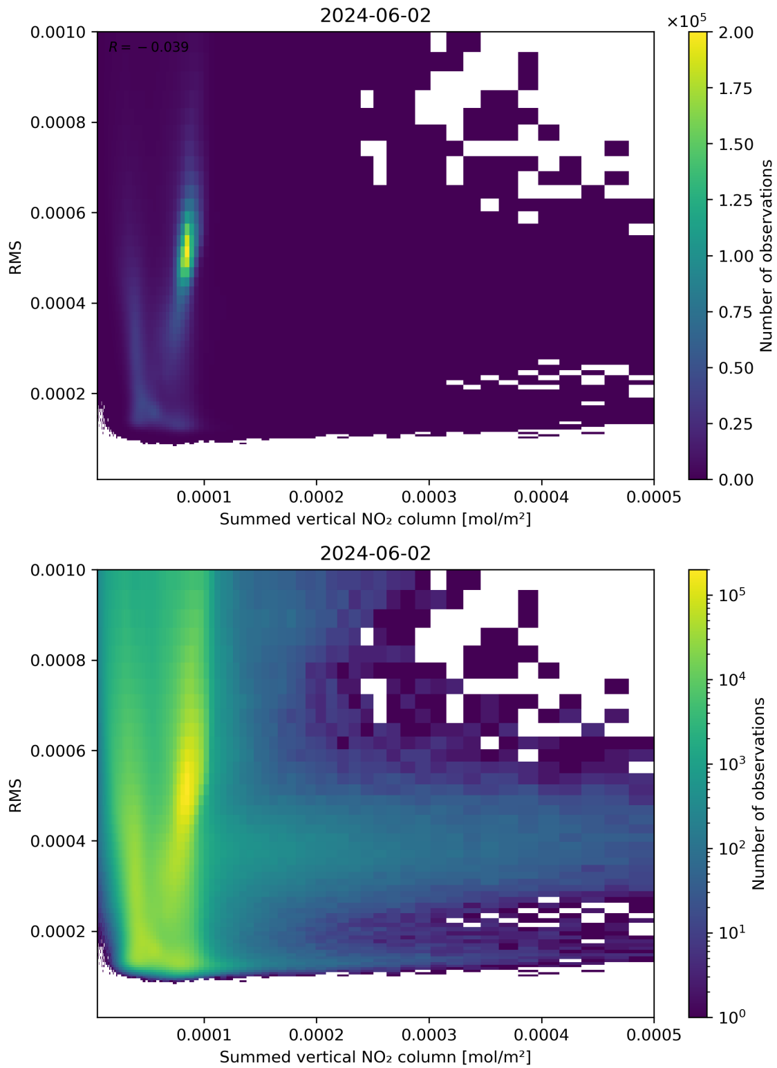
Figure 109: Scatter density plot of “Summed vertical NO 2 column” against “RMS” for 2024-06-01 to 2024-06-03.
