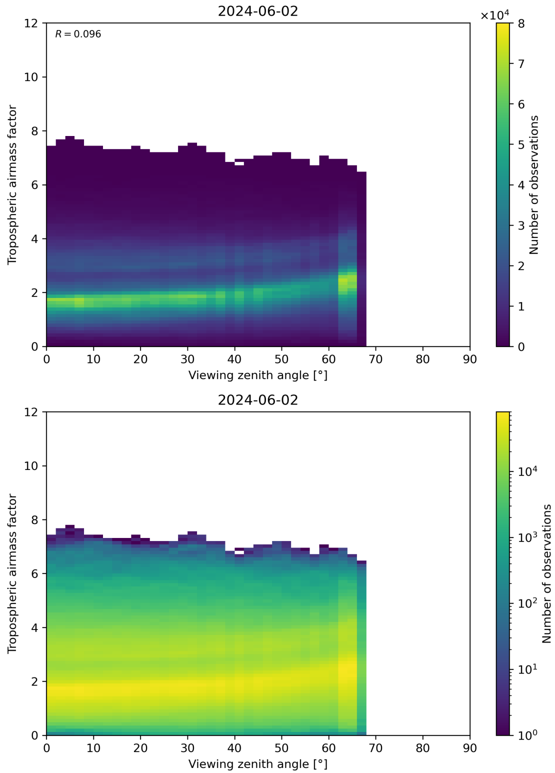
Figure 161: Scatter density plot of “Viewing zenith angle” against “Tropospheric airmass factor” for 2024-06-01 to 2024-06-03.
