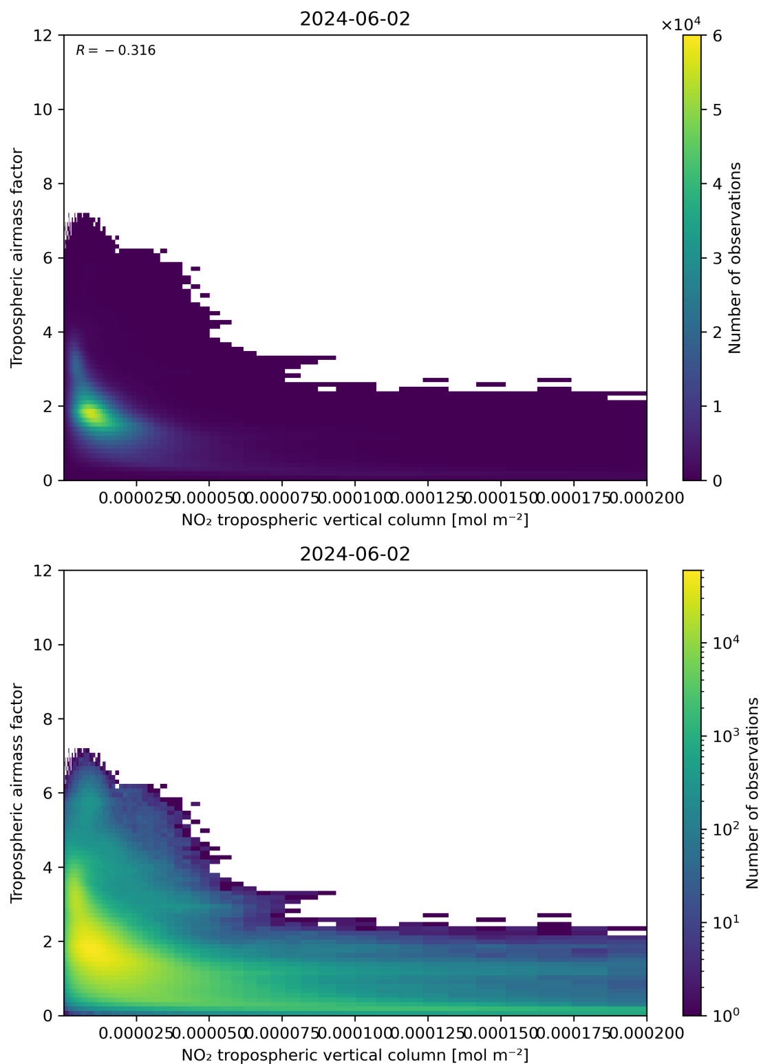
Figure 123: Scatter density plot of “NO 2 tropospheric vertical column” against “Tropospheric air mass factor” for 2024-06-01 to 2024-06-03.
