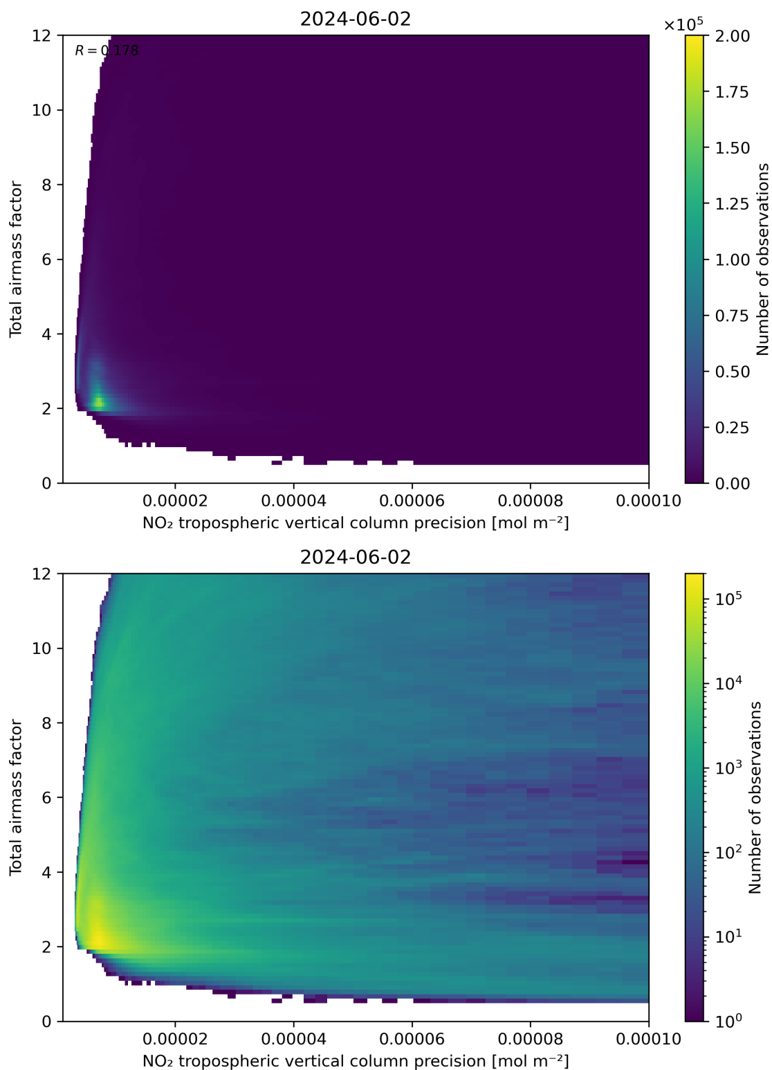
Figure 132: Scatter density plot of “NO 2 tropospheric vertical column precision” against “Total air mass factor” for 2024-06-01 to 2024-06-03.
