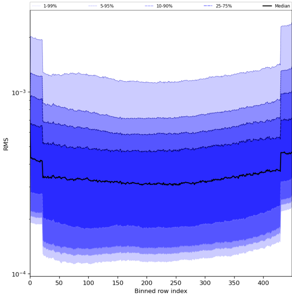
Figure 60: Along track statistics of “RMS” for 2024-06-01 to 2024-06-03
