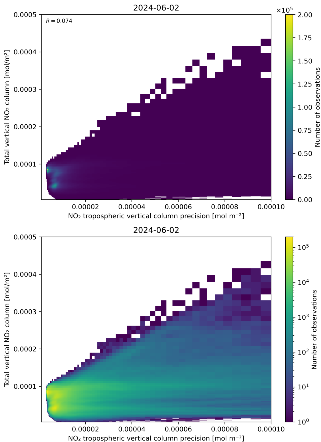
Figure 138: Scatter density plot of “NO 2 tropospheric vertical column precision” against “Total vertical NO 2 column” for 2024-06-01 to 2024-06-03.
