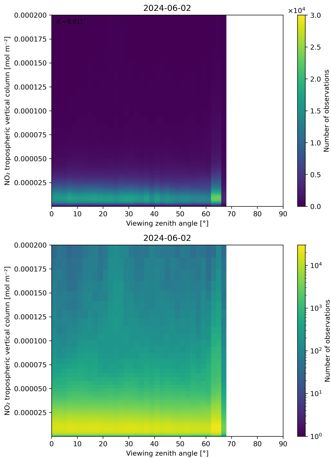
Figure 169: Scatter density plot of “Viewing zenith angle” against “NO 2 tropospheric vertical column” for 2024-06-01 to 2024-06-03.
