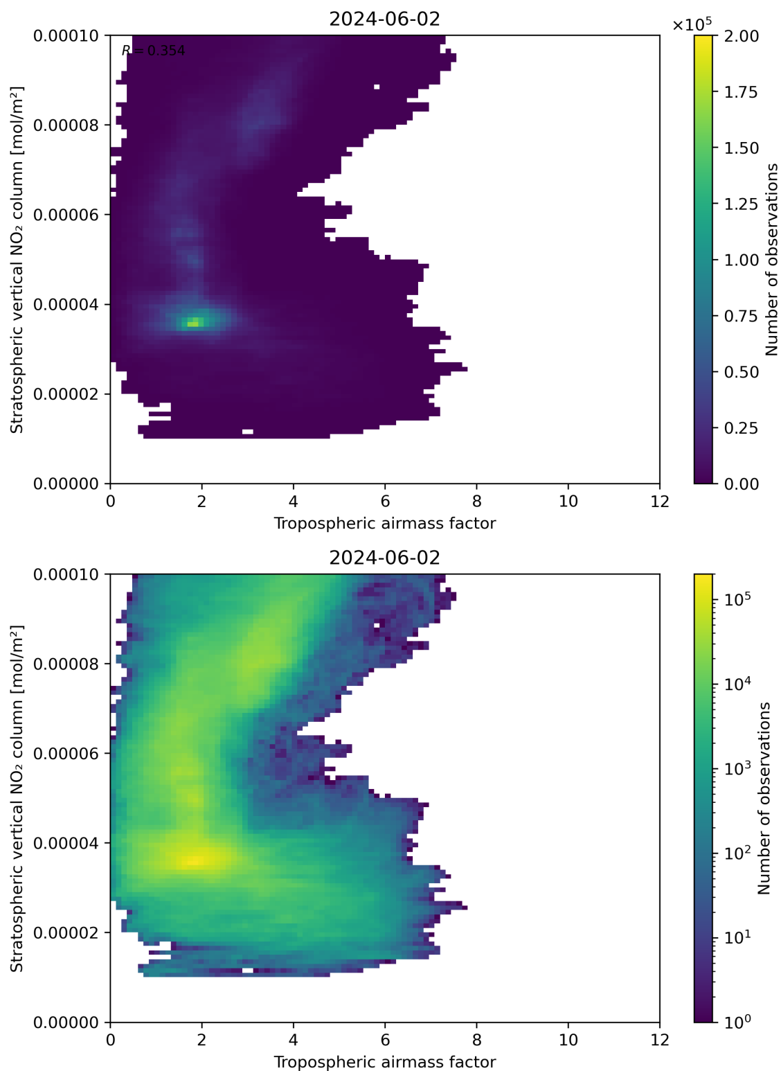
Figure 74: Scatter density plot of “Tropospheric air mass factor” against “Stratospheric vertical NO 2 column” for 2024-06-01 to 2024-06-03.
