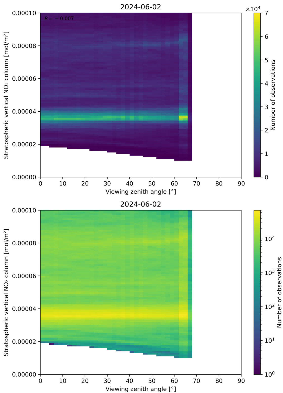
Figure 164: Scatter density plot of “Viewing zenith angle” against “Stratospheric vertical NO 2 column” for 2024-06-01 to 2024-06-03.
