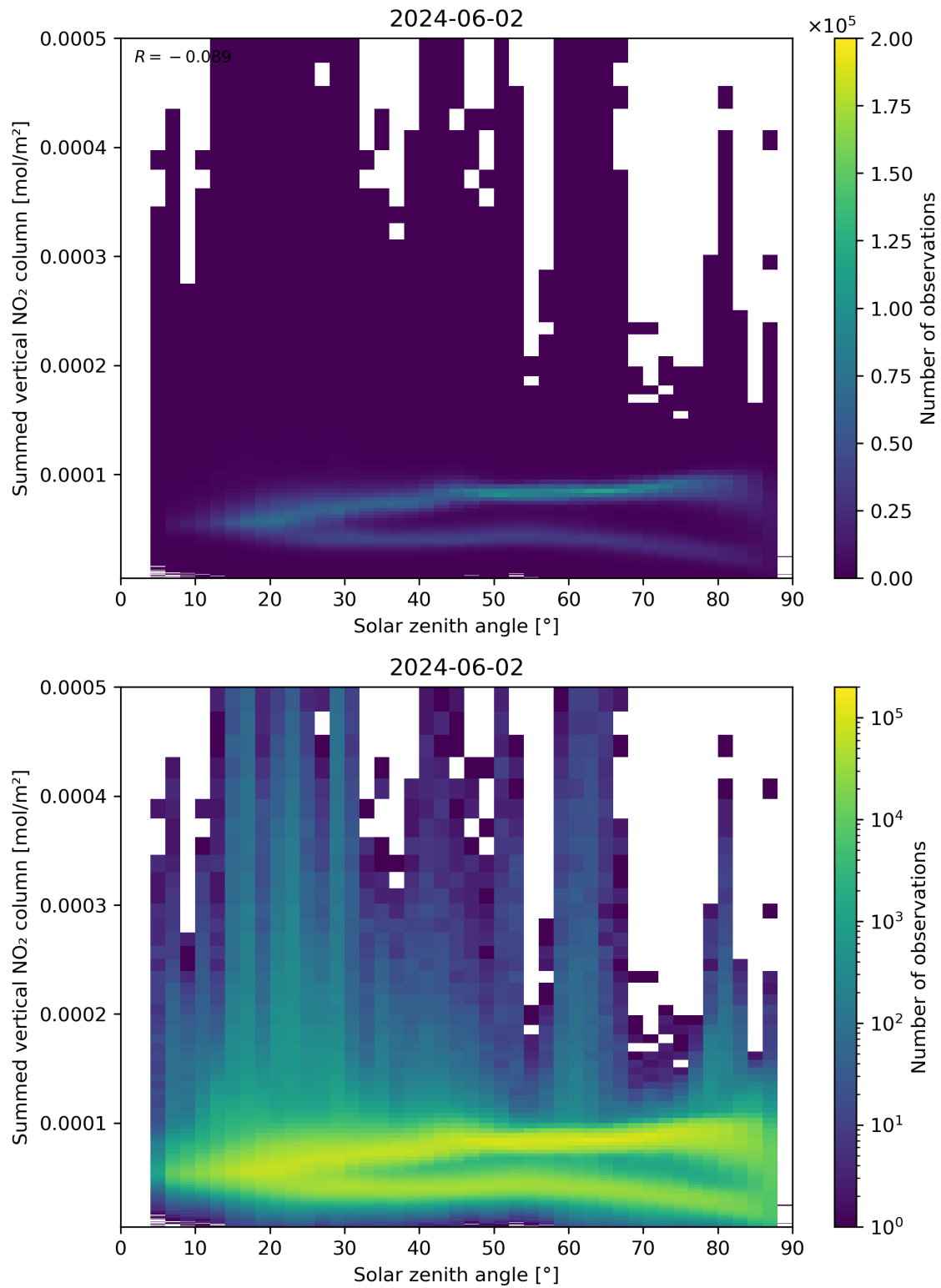
Figure 151: Scatter density plot of “Solar zenith angle” against “Summed vertical NO 2 column” for 2024-06-01 to 2024-06-03.
