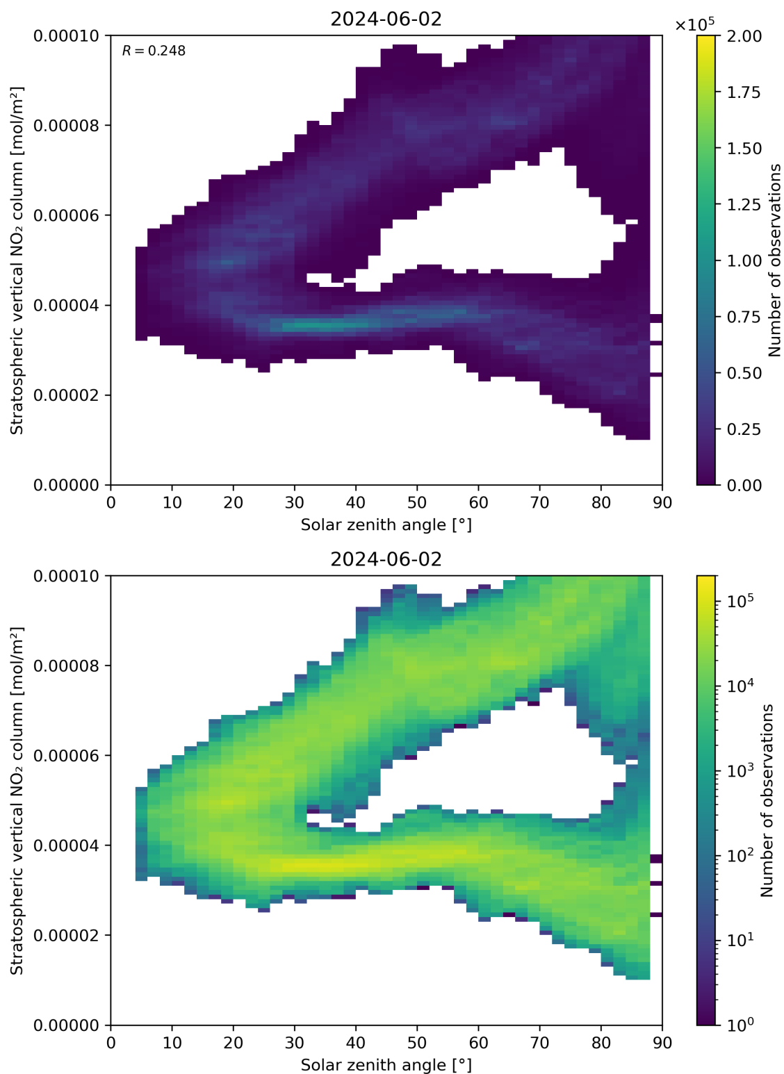
Figure 150: Scatter density plot of “Solar zenith angle” against “Stratospheric vertical NO 2 column” for 2024-06-01 to 2024-06-03.
