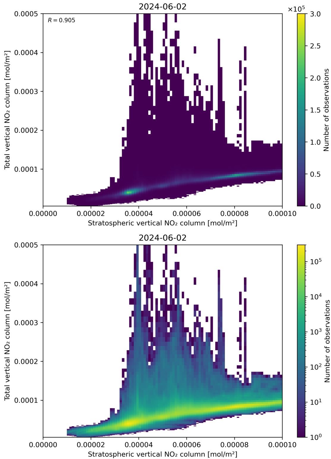
Figure 100: Scatter density plot of “Stratospheric vertical NO 2 column” against “Total vertical NO 2 column” for 2024-06-01 to 2024-06-03.
