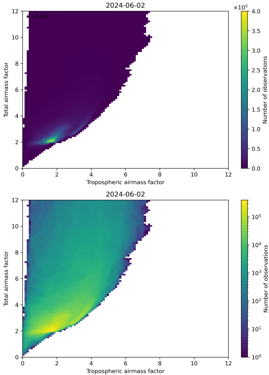
Figure 72: Scatter density plot of “Tropospheric airmass factor” against “Total airmass factor” for 2024-06-01 to 2024-06-03.
