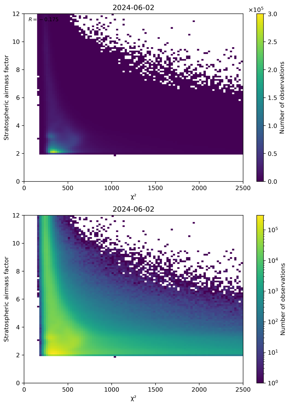
Figure 81: Scatter density plot of “ \chi^2 ” against “Stratospheric airmass factor” for 2024-06-01 to 2024-06-03.
