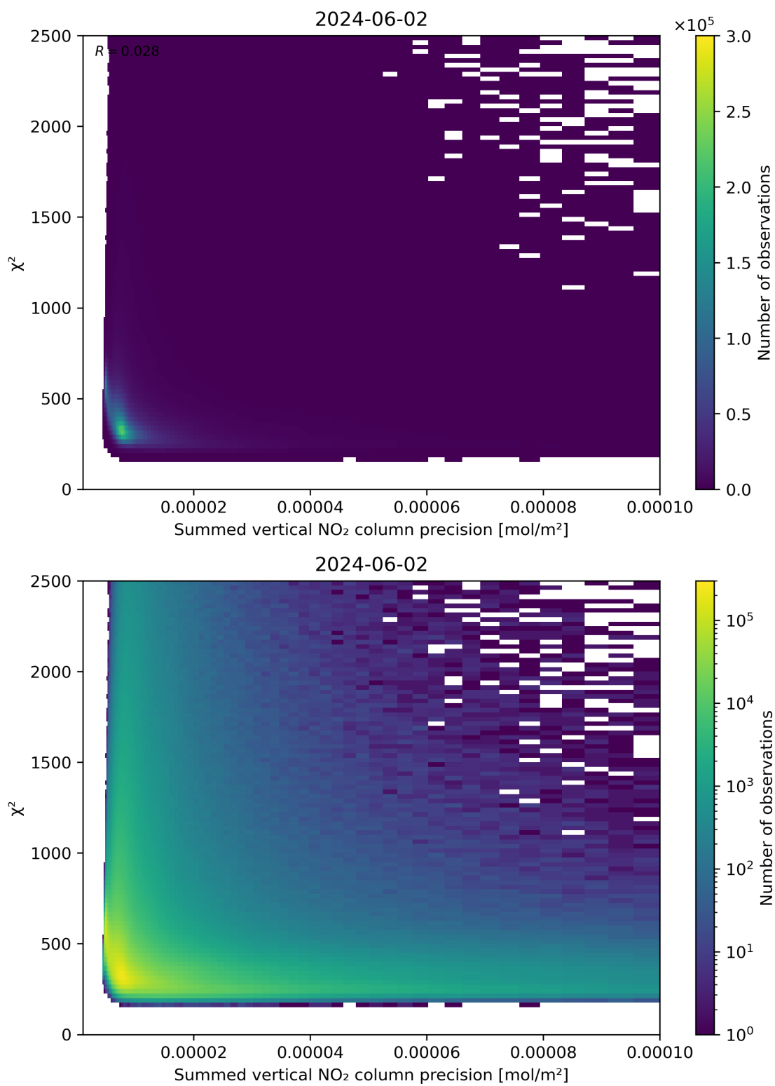
Figure 107: Scatter density plot of “Summed vertical NO 2 column precision” against “ \chi^2 ” for 2024-06-01 to 2024-06-03.
