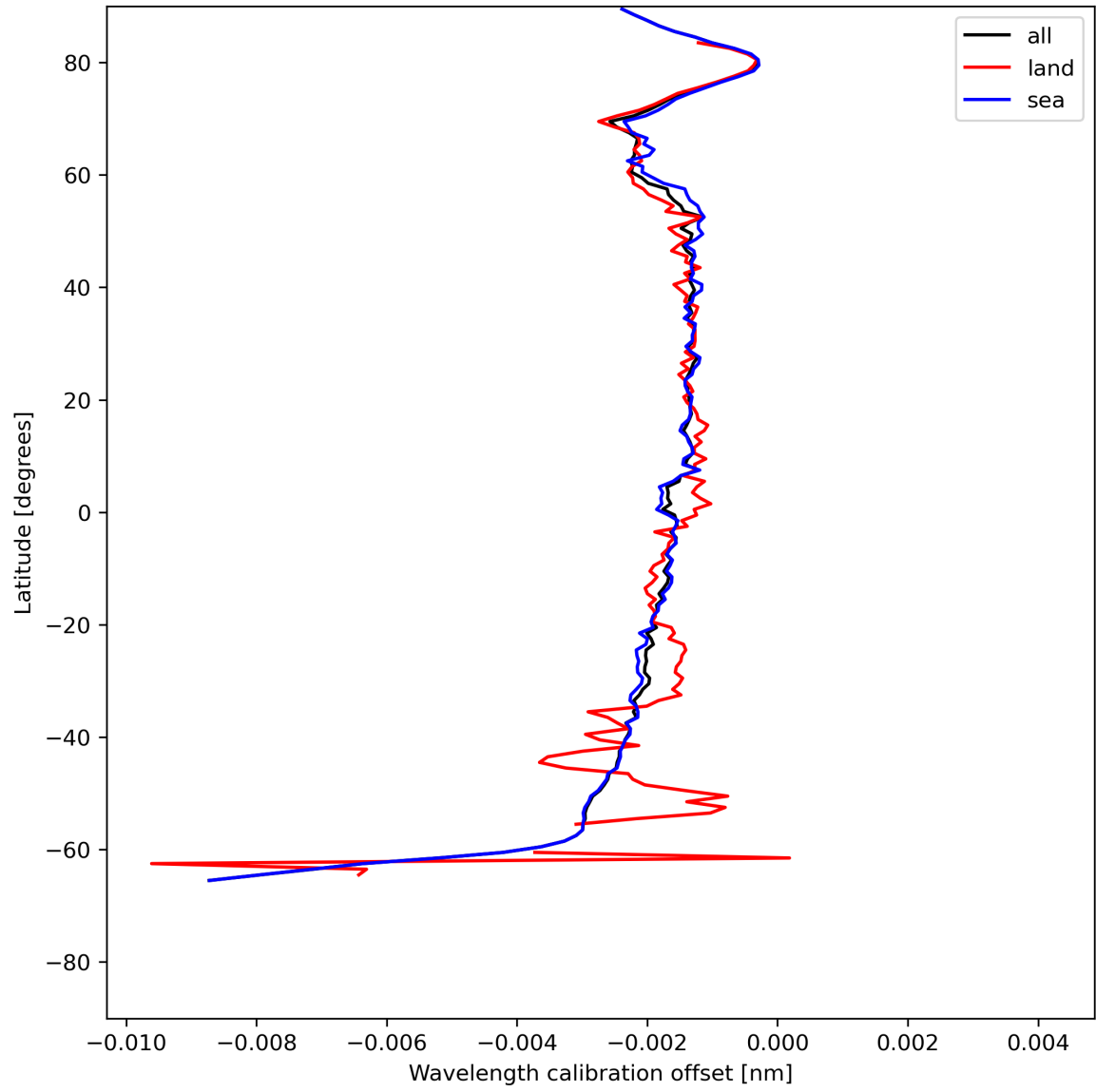
Figure 18: Zonal average of “Wavelength calibration offset” for 2024-06-01 to 2024-06-03.
