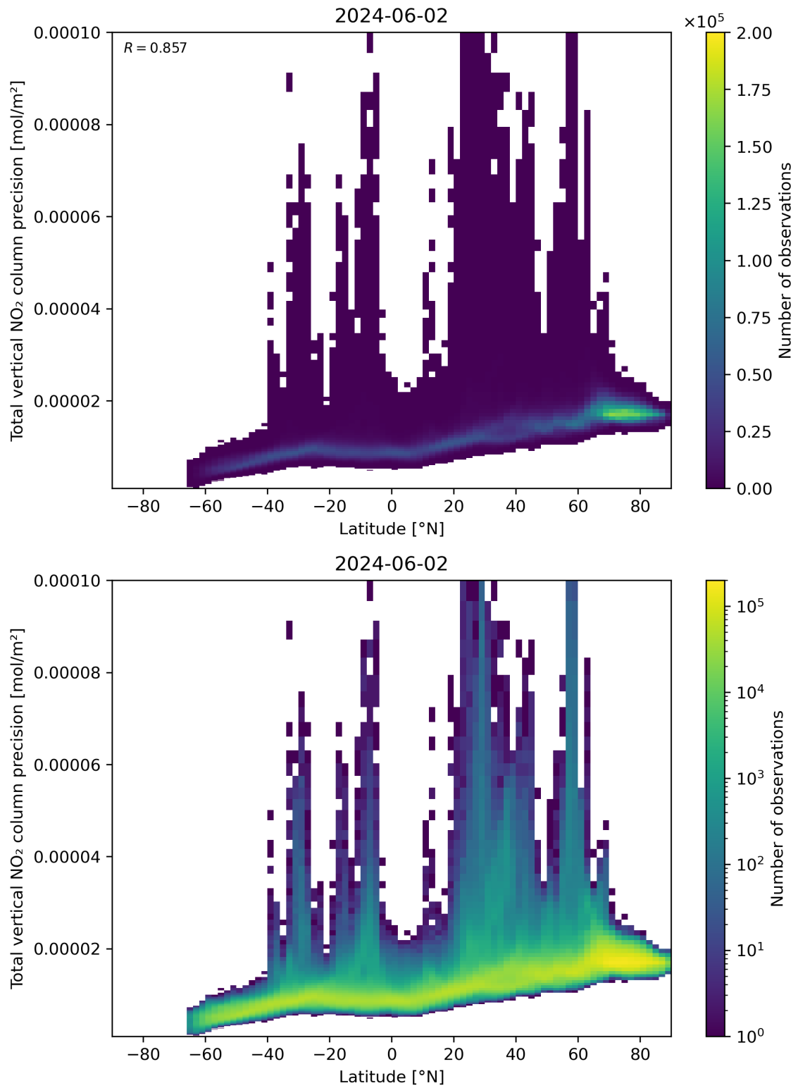
Figure 91: Scatter density plot of “Latitude” against “Total vertical NO 2 column precision” for 2024-06-01 to 2024-06-03.
