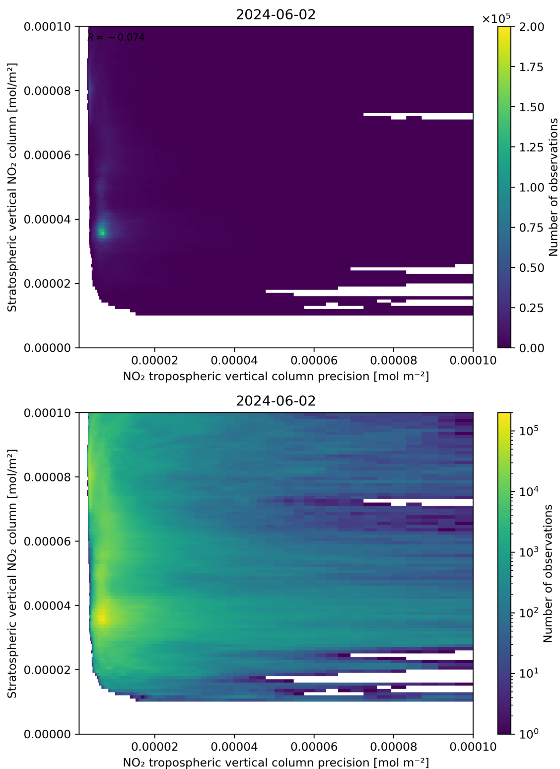
Figure 135: Scatter density plot of “NO 2 tropospheric vertical column precision” against “Stratospheric vertical NO 2 column” for 2024-06-01 to 2024-06-03.
