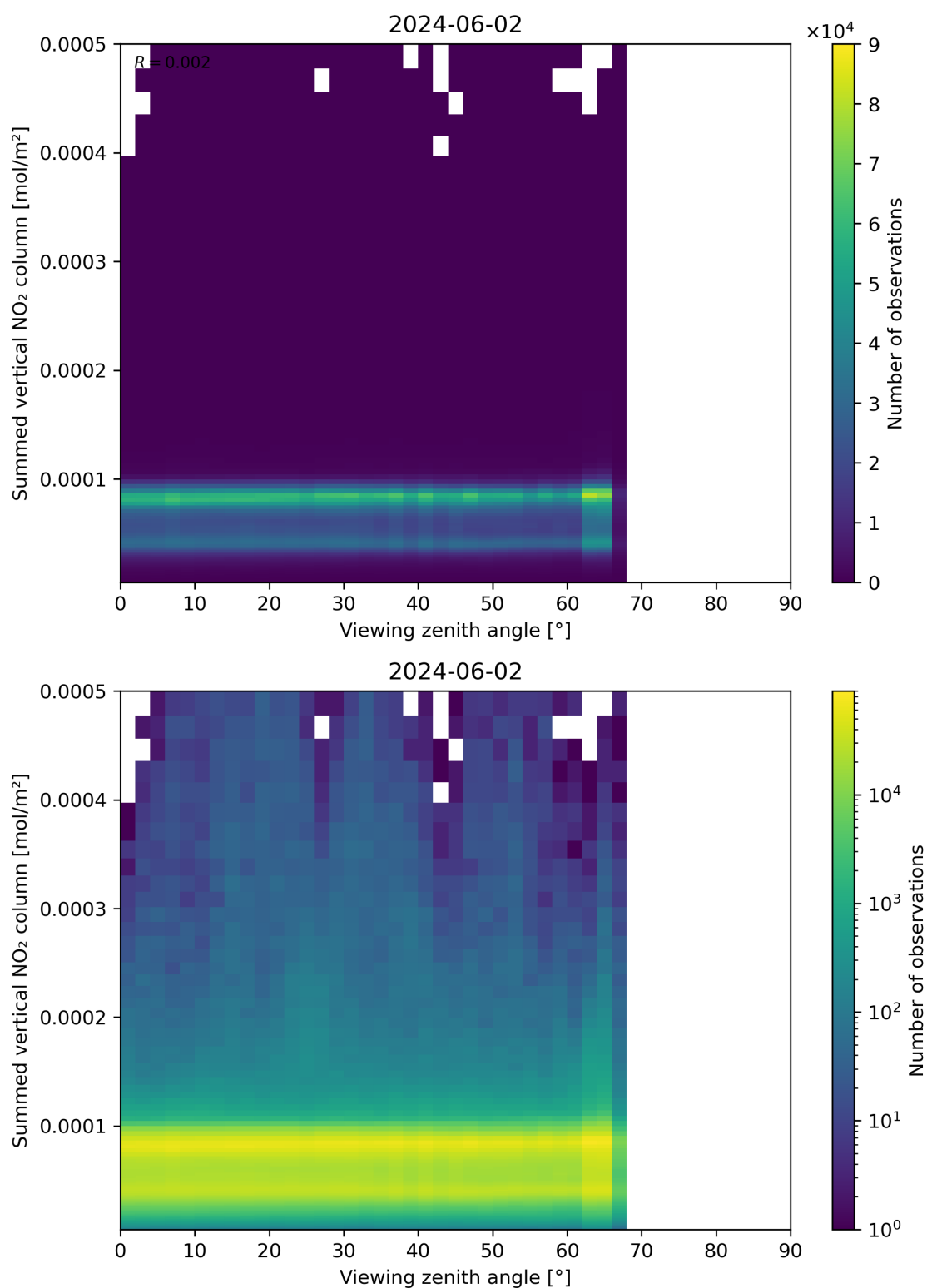
Figure 165: Scatter density plot of “Viewing zenith angle” against “Summed vertical NO 2 column” for 2024-06-01 to 2024-06-03.
