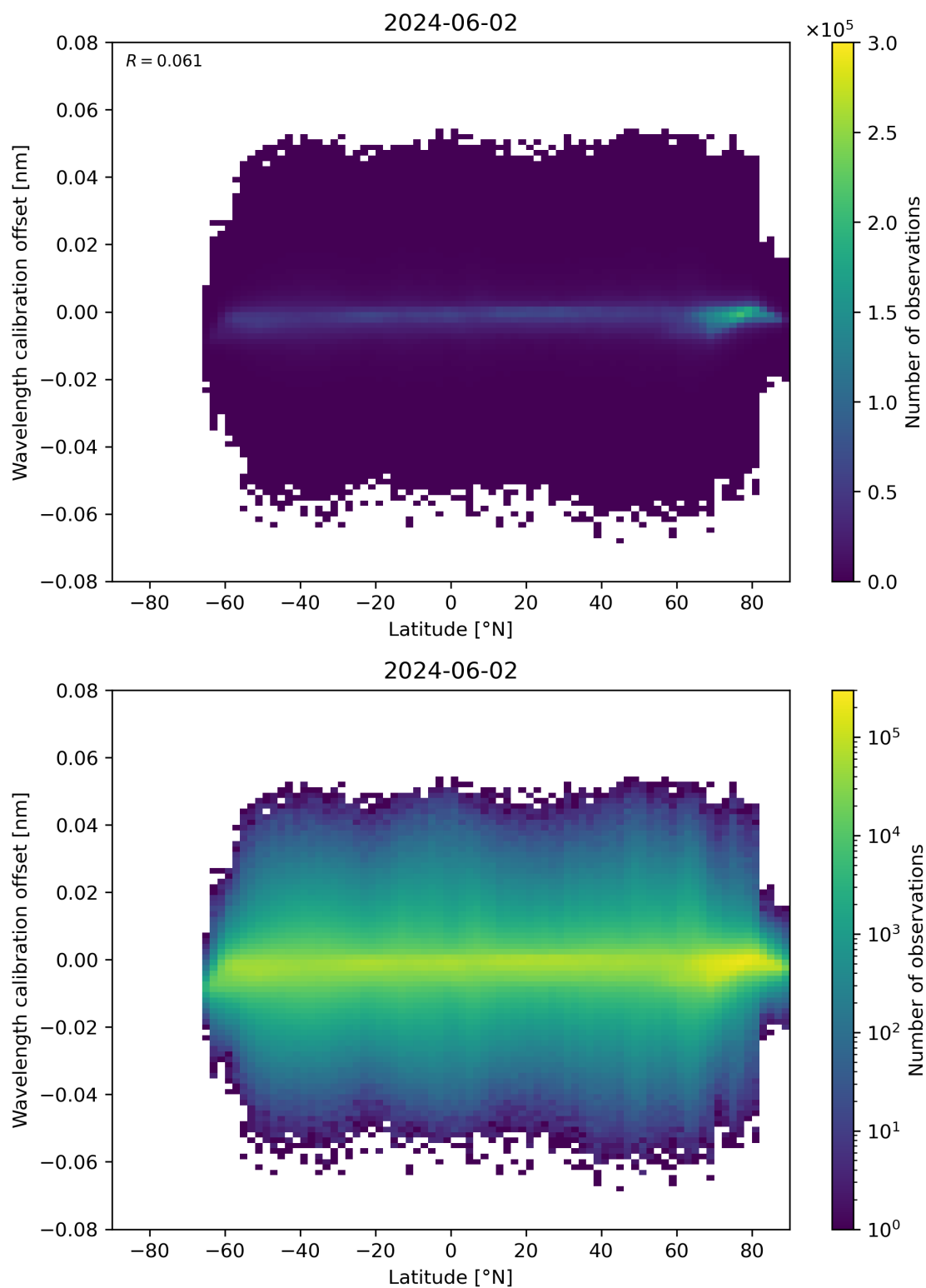
Figure 95: Scatter density plot of “Latitude” against “Wavelength calibration offset” for 2024-06-01 to 2024-06-03.
