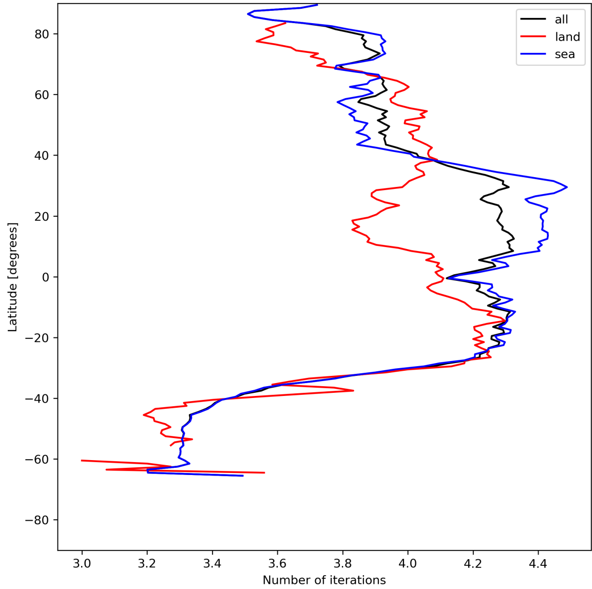
Figure 17: Zonal average of “Number of iterations” for 2024-06-01 to 2024-06-03.
