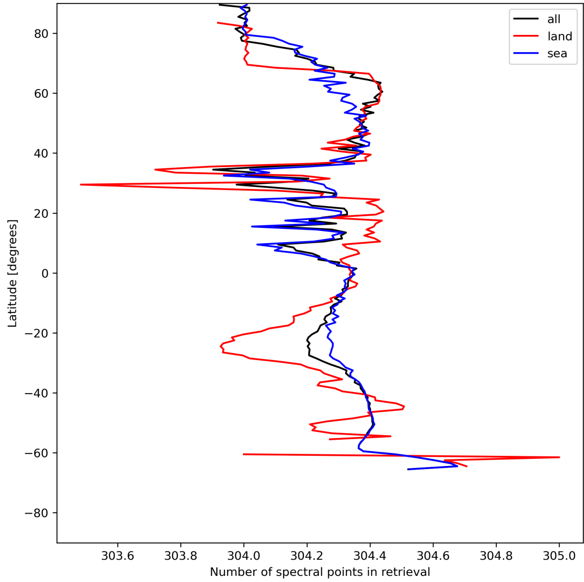
Figure 16: Zonal average of “Number of spectral points in retrieval” for 2024-06-01 to 2024-06-03.
