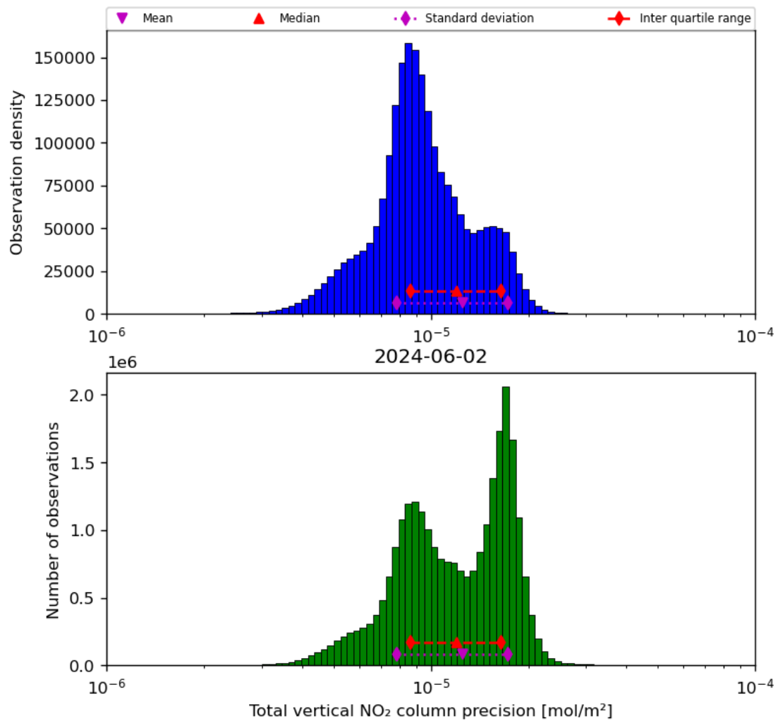
Figure 39: Histogram of “Total vertical NO 2 column precision” for 2024-06-01 to 2024-06-03
