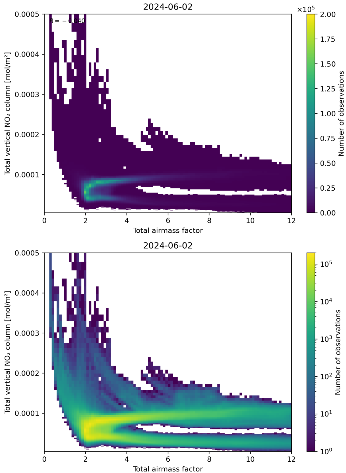
Figure 67: Scatter density plot of “Total airmass factor” against “Total vertical NO 2 column” for 2024-06-01 to 2024-06-03.
