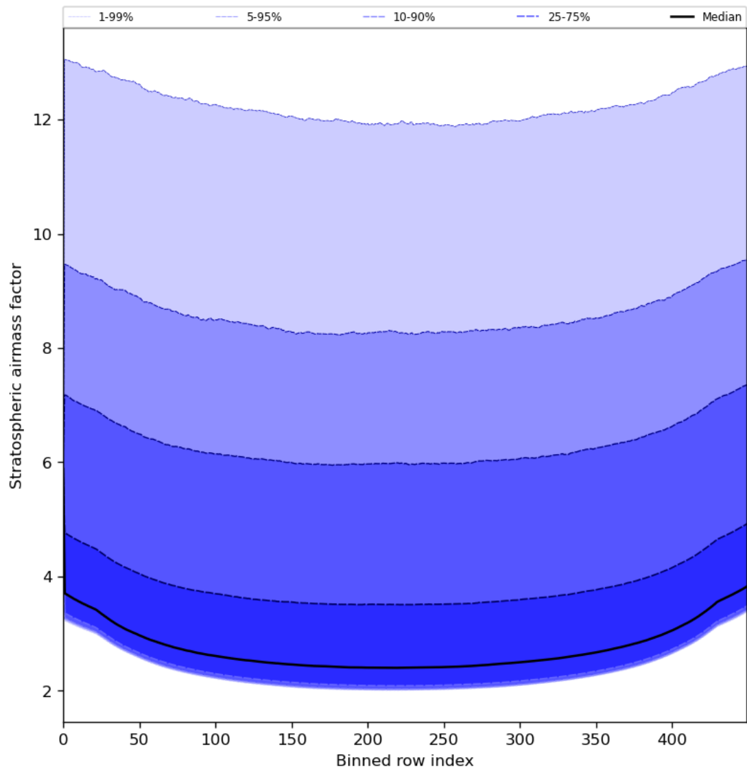
Figure 61: Along track statistics of “Stratospheric airmass factor” for 2024-06-01 to 2024-06-03
