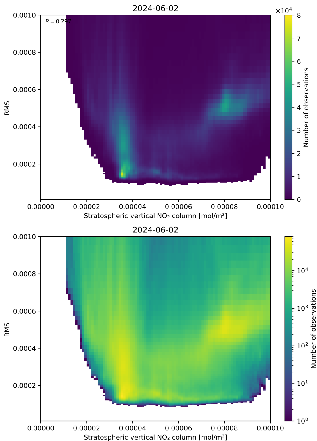
Figure 102: Scatter density plot of “Stratospheric vertical NO 2 column” against “RMS” for 2024-06-01 to 2024-06-03.
