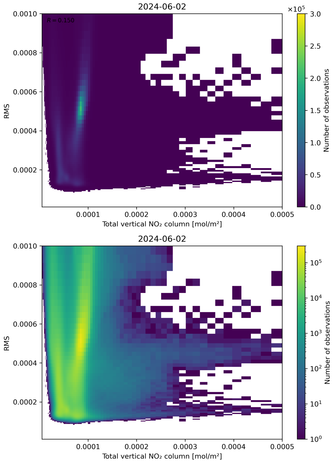
Figure 120: Scatter density plot of “Total vertical NO 2 column” against “RMS” for 2024-06-01 to 2024-06-03.
