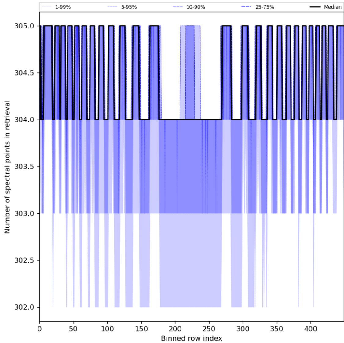
Figure 50: Along track statistics of “Number of spectral points in retrieval” for 2024-06-01 to 2024-06-03
