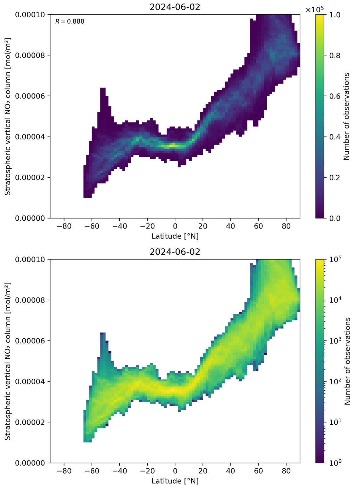
Figure 87: Scatter density plot of “Latitude” against “Stratospheric vertical NO 2 column” for 2024-06-01 to 2024-06-03.
