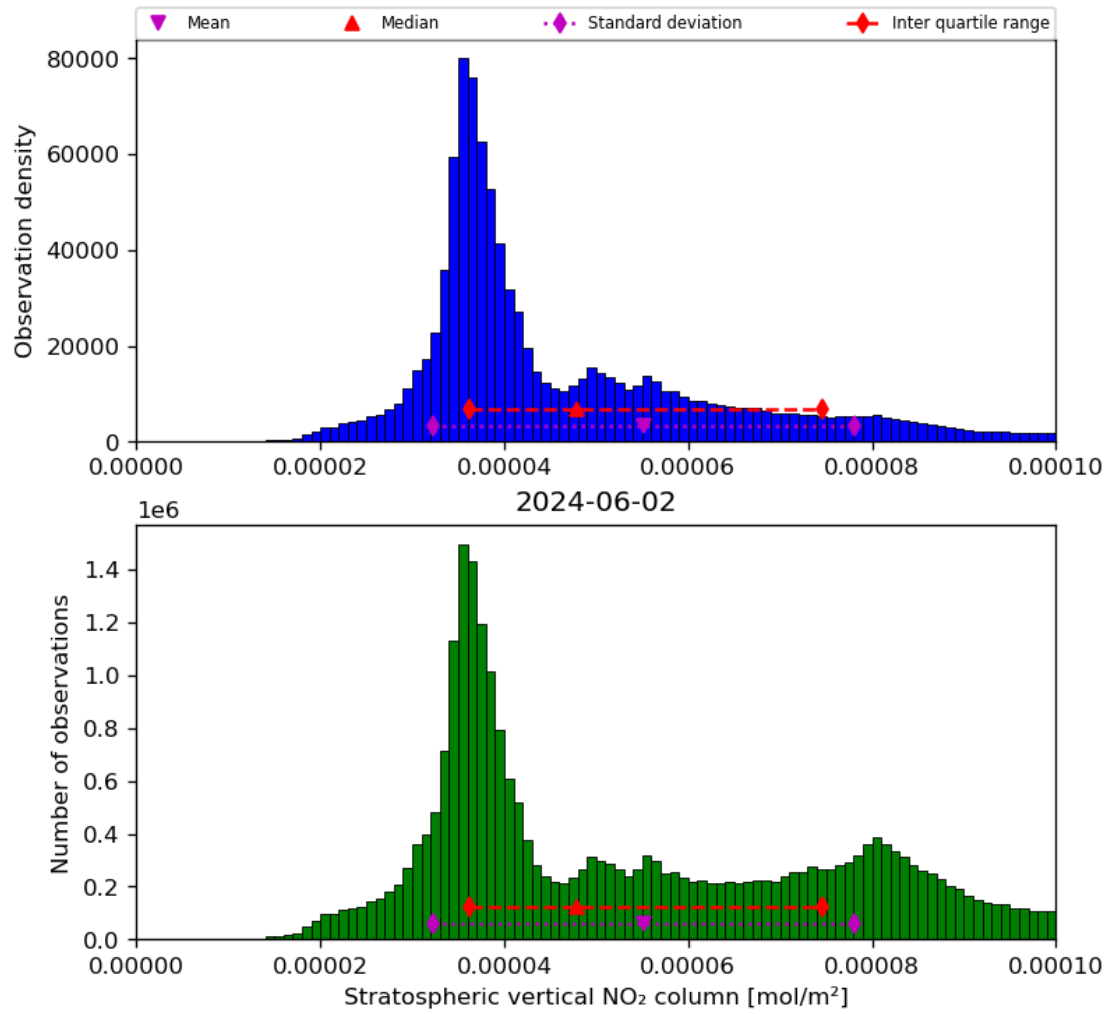
Figure 36: Histogram of “Stratospheric vertical NO 2 column” for 2024-06-01 to 2024-06-03
