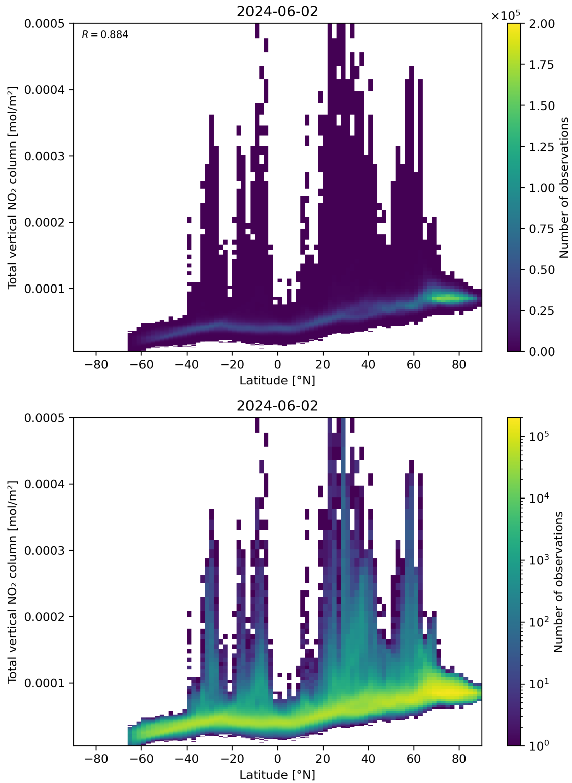
Figure 90: Scatter density plot of “Latitude” against “Total vertical NO 2 column” for 2024-06-01 to 2024-06-03.
