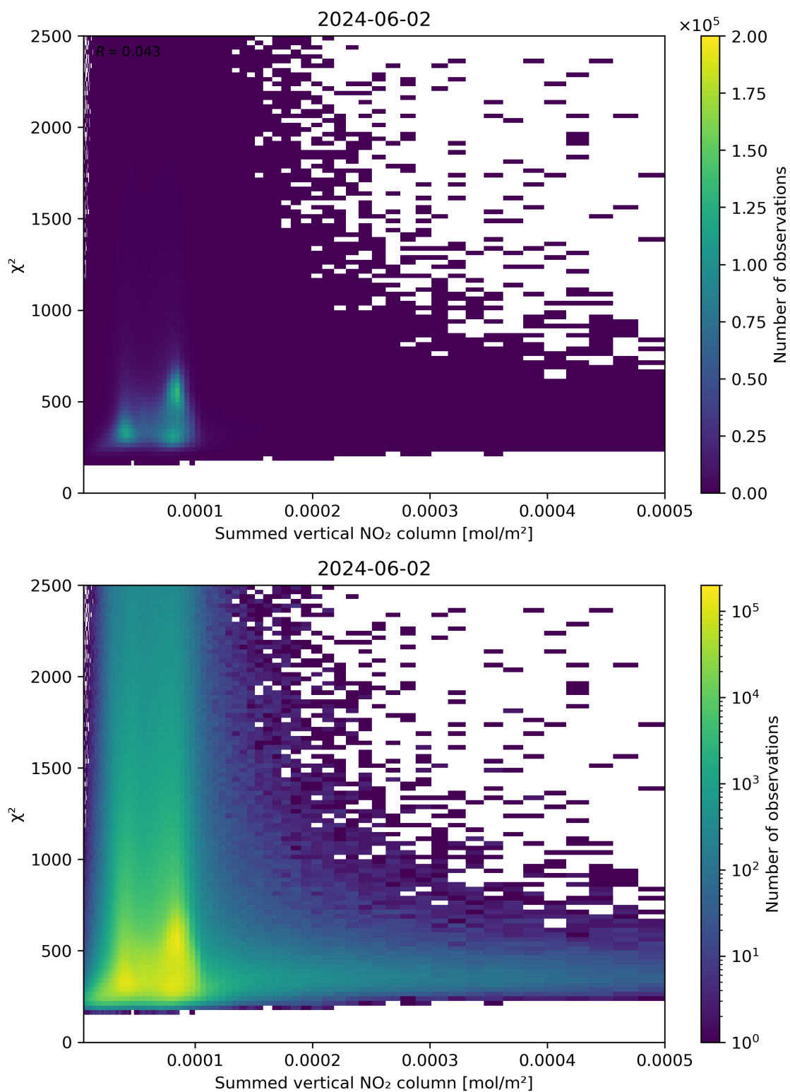
Figure 104: Scatter density plot of “Summed vertical NO 2 column” against “ \chi^2 ” for 2024-06-01 to 2024-06-03.
