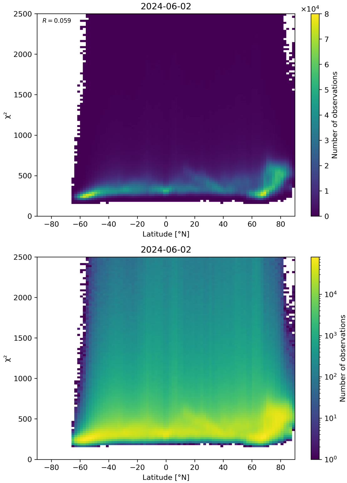
Figure 86: Scatter density plot of “Latitude” against “ \chi^2 ” for 2024-06-01 to 2024-06-03.
