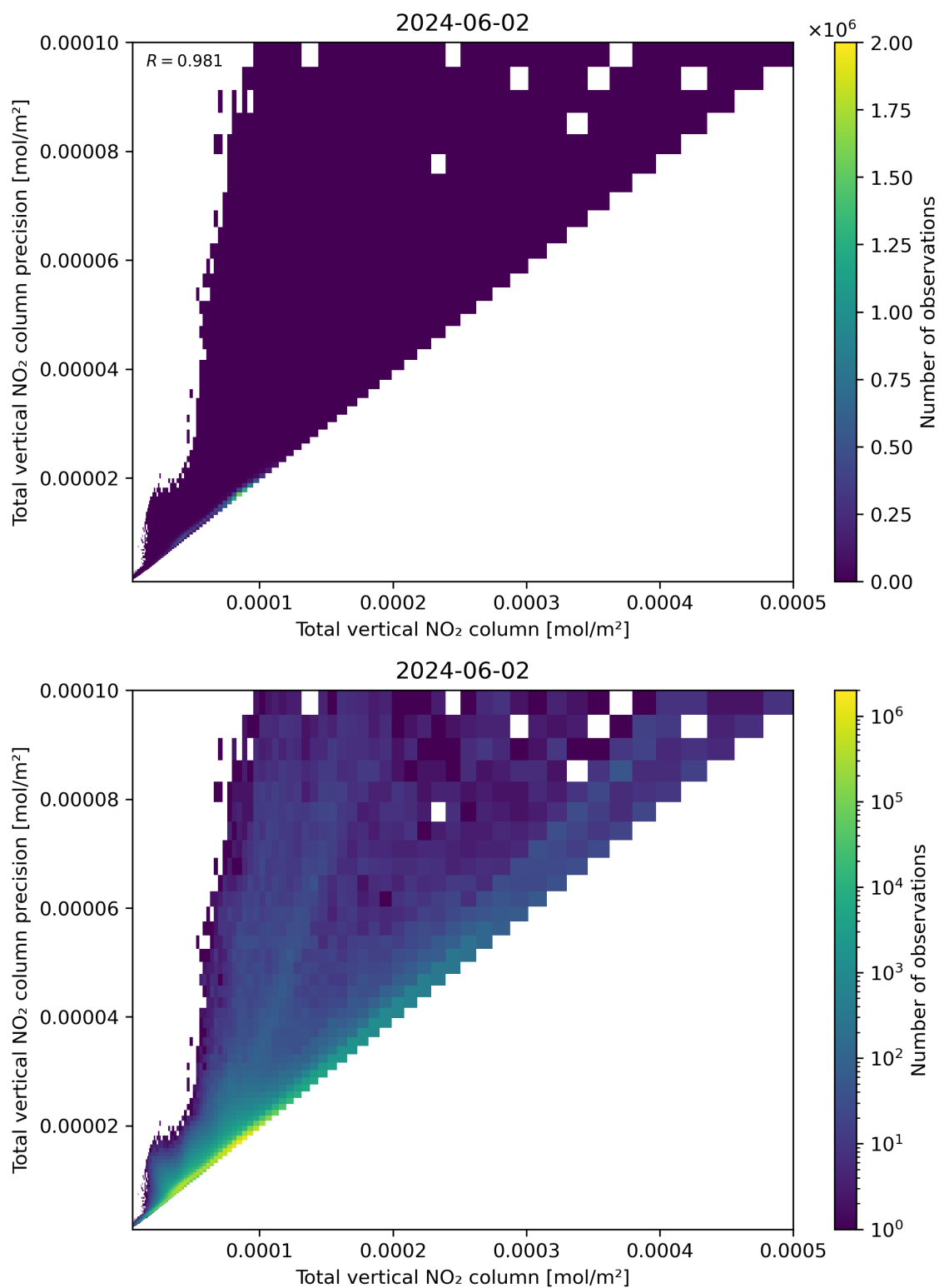
Figure 114: Scatter density plot of “Total vertical NO 2 column” against “Total vertical NO 2 column precision” for 2024-06-01 to 2024-06-03.
