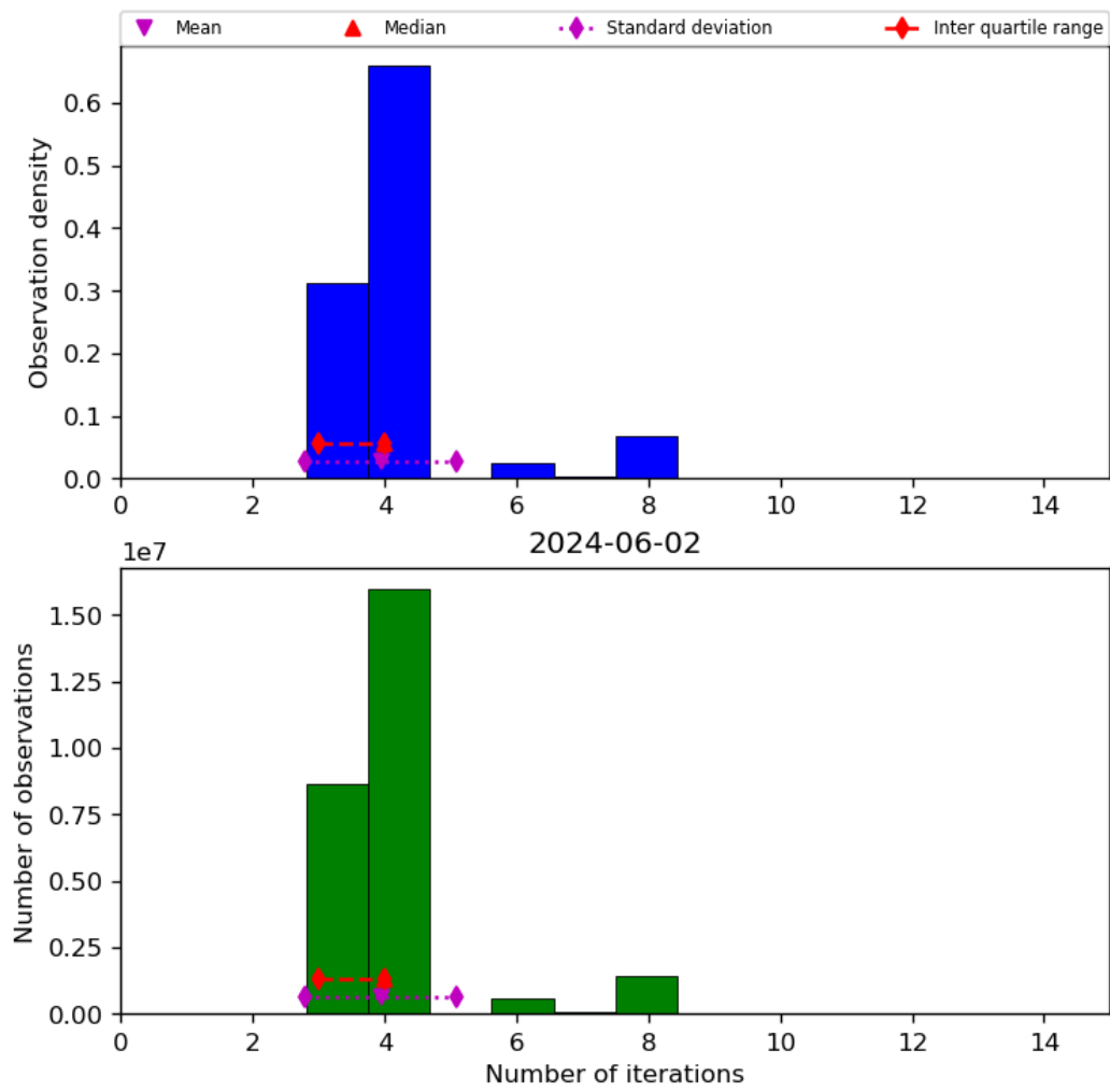
Figure 34: Histogram of “Number of iterations” for 2024-06-01 to 2024-06-03
