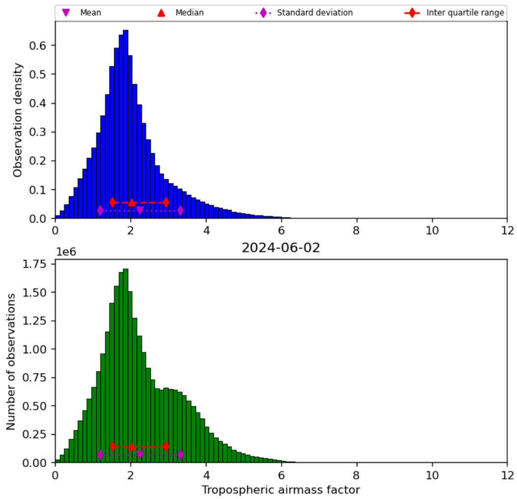
Figure 31: Histogram of “Tropospheric airmass factor” for 2024-06-01 to 2024-06-03
