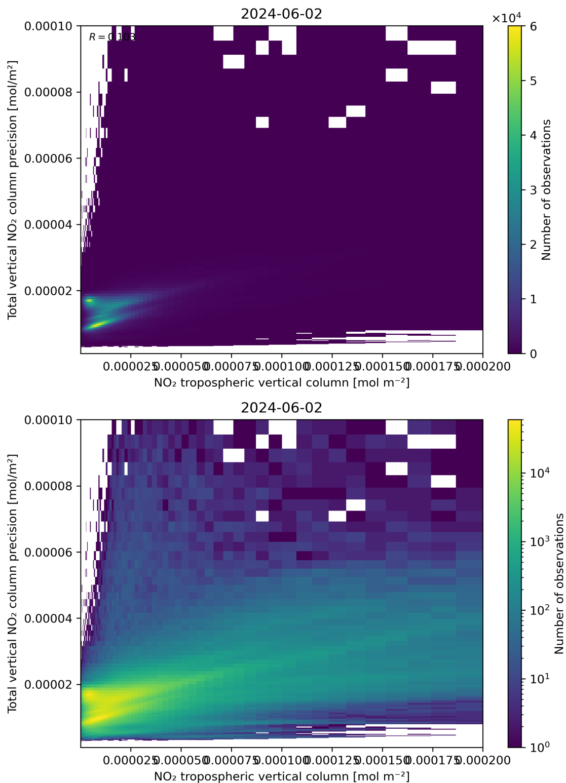
Figure 129: Scatter density plot of “NO 2 tropospheric vertical column” against “Total vertical NO 2 column precision” for 2024-06-01 to 2024-06-03.
