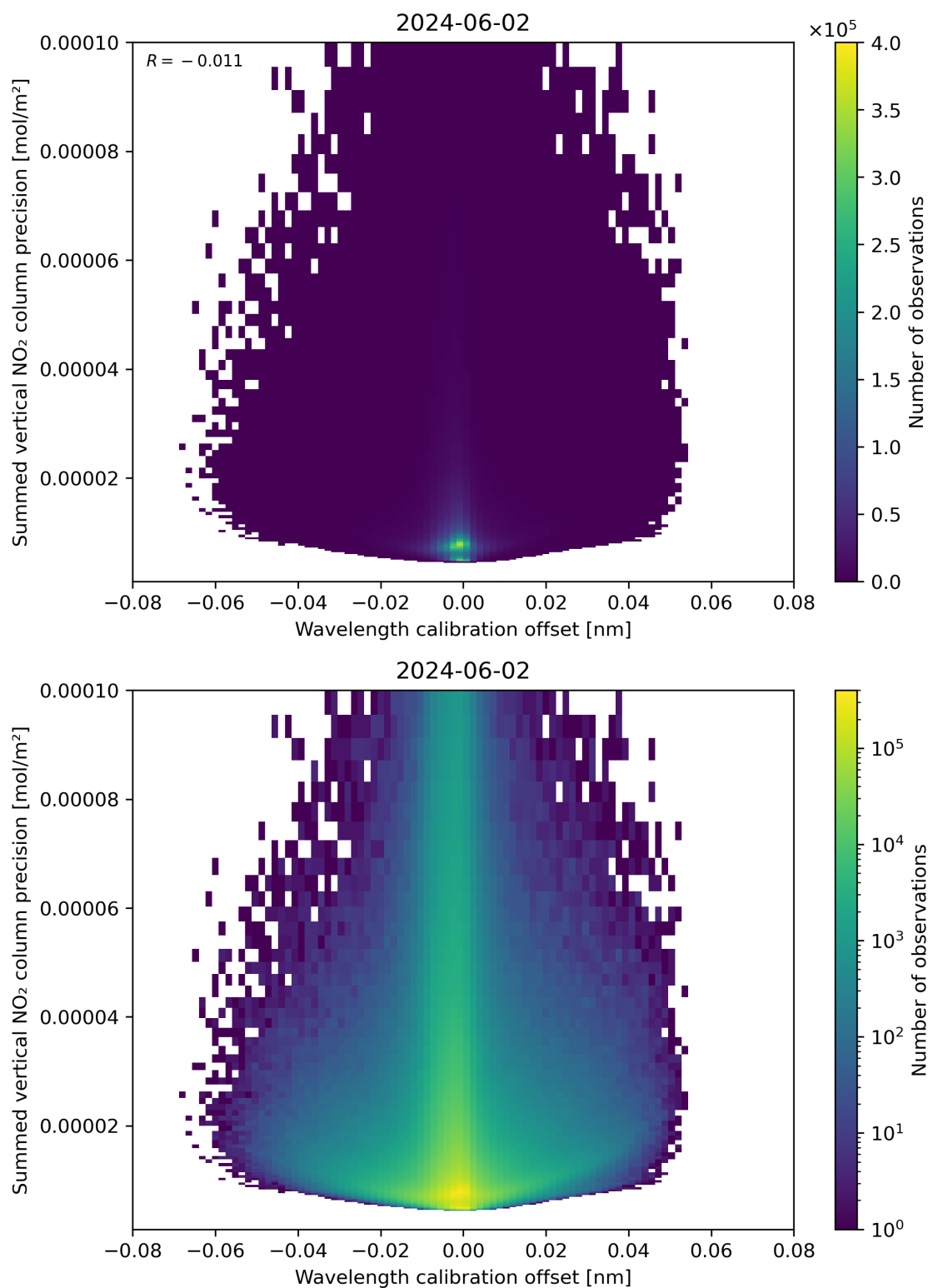
Figure 178: Scatter density plot of “Wavelength calibration offset” against “Summed vertical NO 2 column precision” for 2024-06-01 to 2024-06-03.
