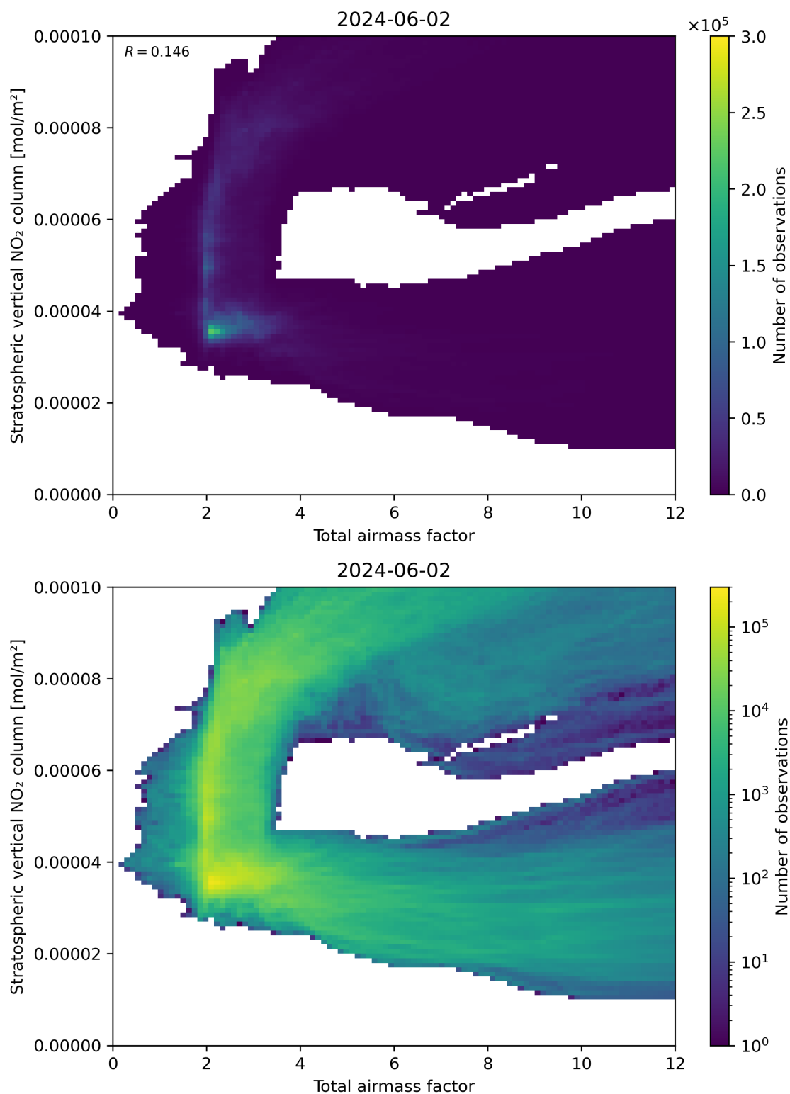
Figure 64: Scatter density plot of “Total airmass factor” against “Stratospheric vertical NO 2 column” for 2024-06-01 to 2024-06-03.
