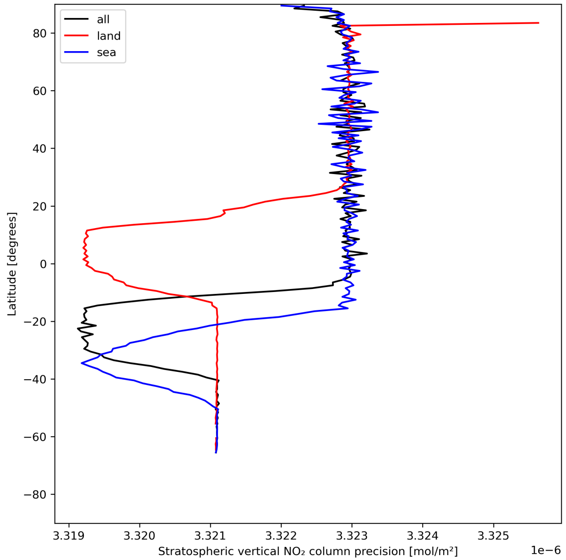
Figure 20: Zonal average of “Stratospheric vertical NO 2 column precision” for 2024-06-01 to 2024-06-03.
