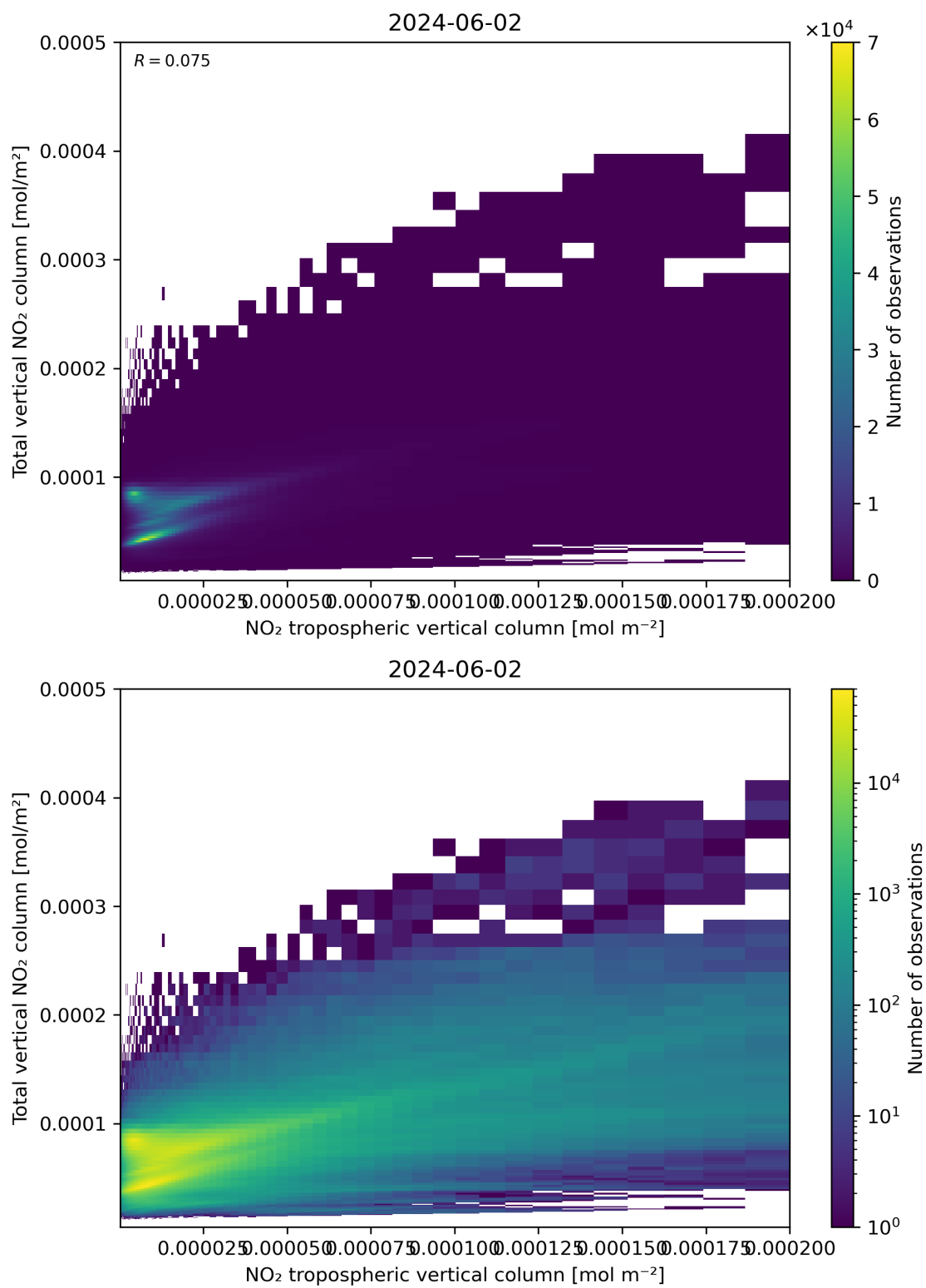
Figure 128: Scatter density plot of “NO 2 tropospheric vertical column” against “Total vertical NO 2 column” for 2024-06-01 to 2024-06-03.
