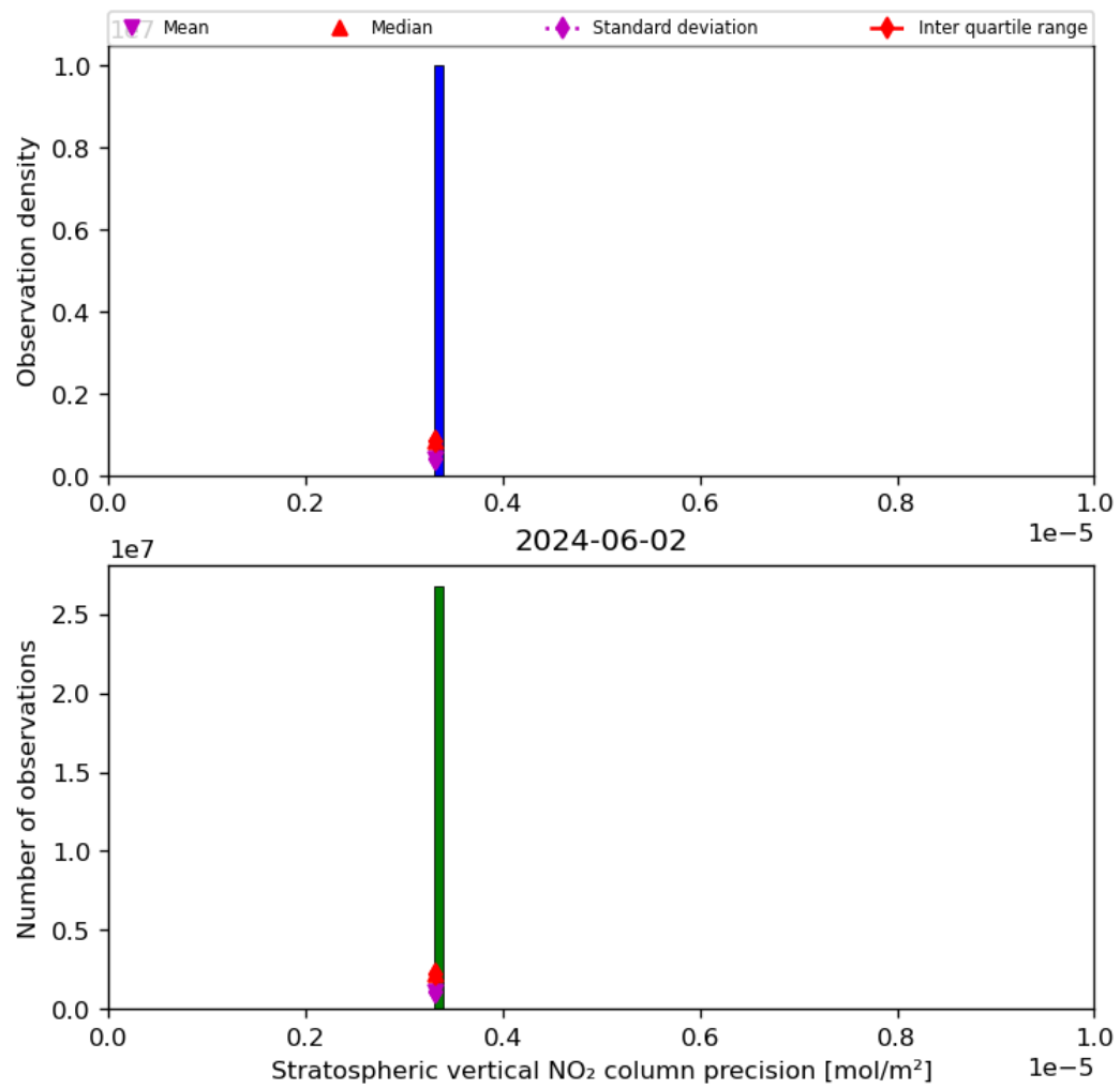
Figure 37: Histogram of “Stratospheric vertical NO 2 column precision” for 2024-06-01 to 2024-06-03
