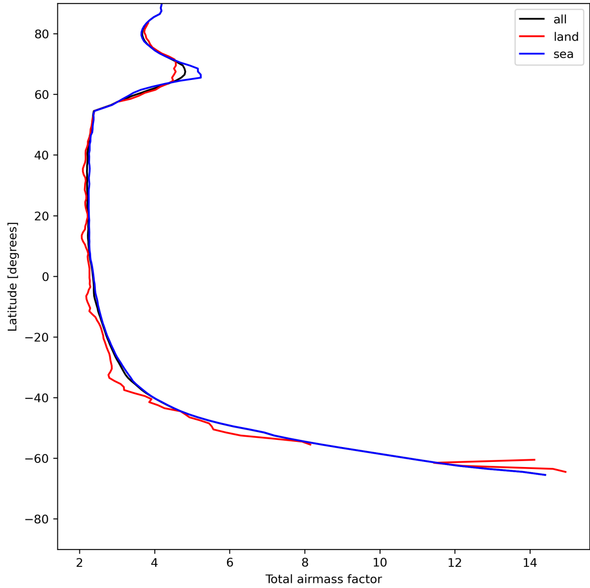
Figure 15: Zonal average of “Total airmass factor” for 2024-06-01 to 2024-06-03.
