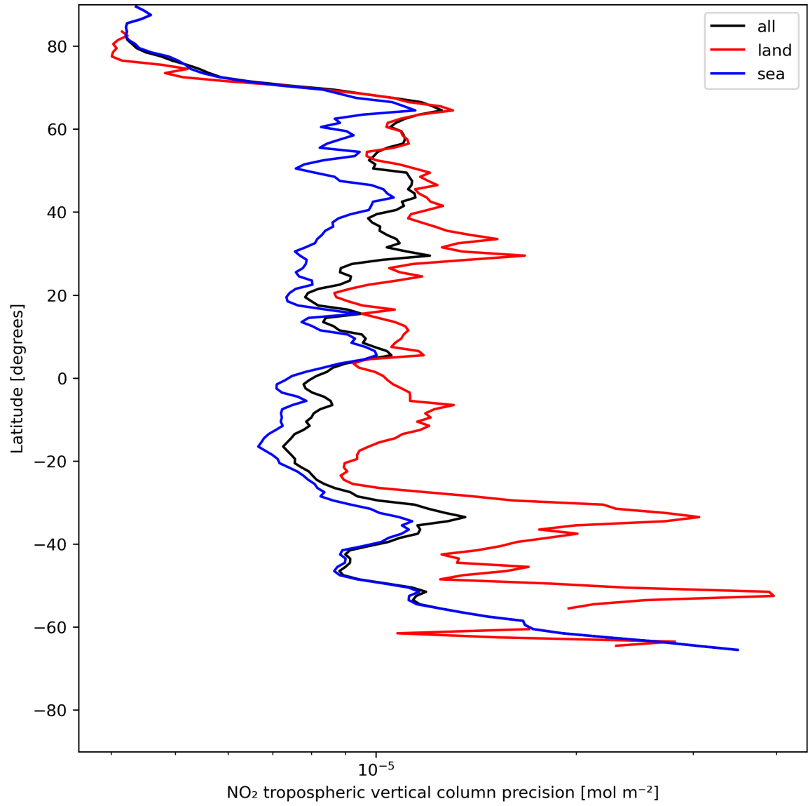
Figure 13: Zonal average of “NO 2 tropospheric vertical column precision” for 2024-06-01 to 2024-06-03.
