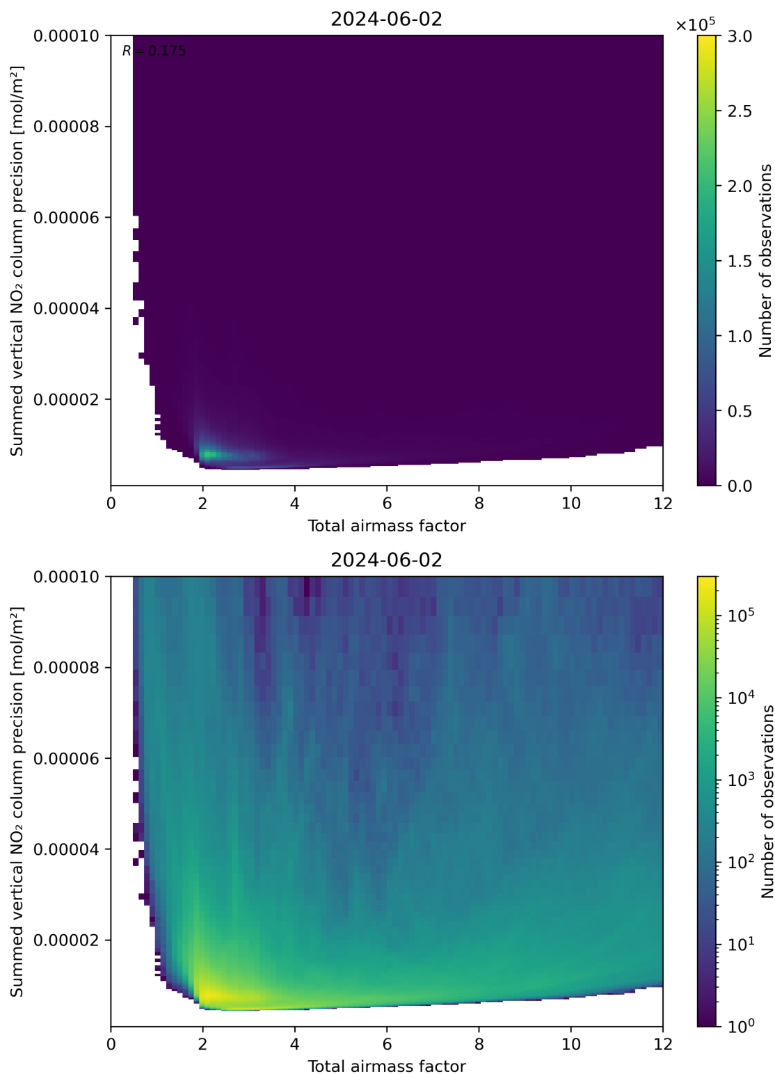
Figure 66: Scatter density plot of “Total airmass factor” against “Summed vertical NO 2 column precision” for 2024-06-01 to 2024-06-03.
