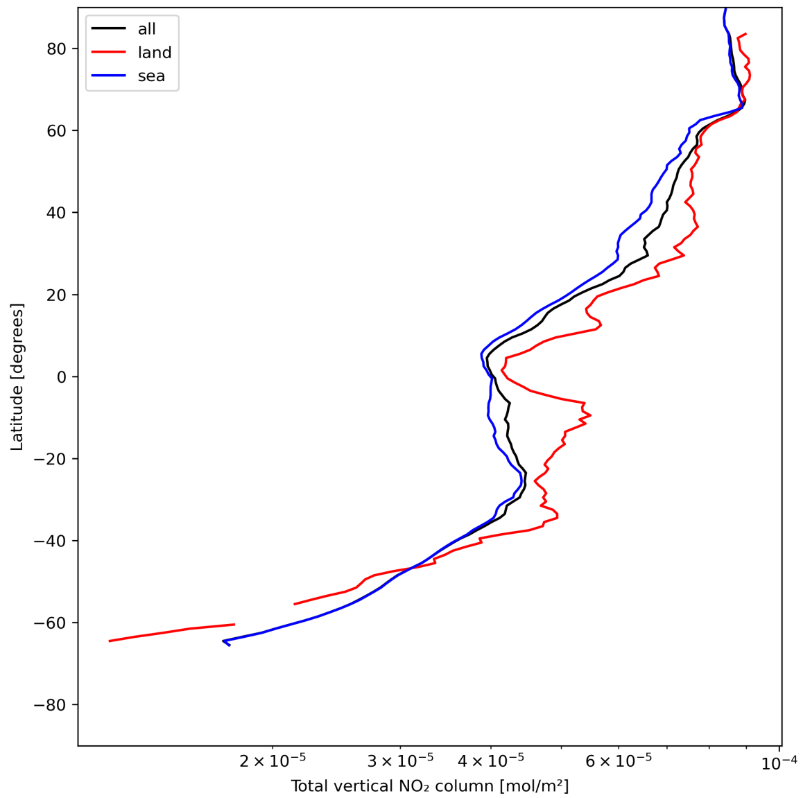
Figure 21: Zonal average of “Total vertical NO 2 column” for 2024-06-01 to 2024-06-03.
