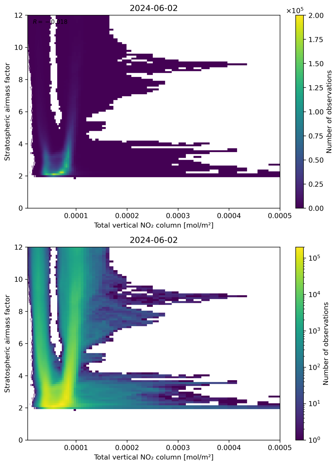
Figure 110: Scatter density plot of “Total vertical NO 2 column” against “Stratospheric airmass factor” for 2024-06-01 to 2024-06-03.
