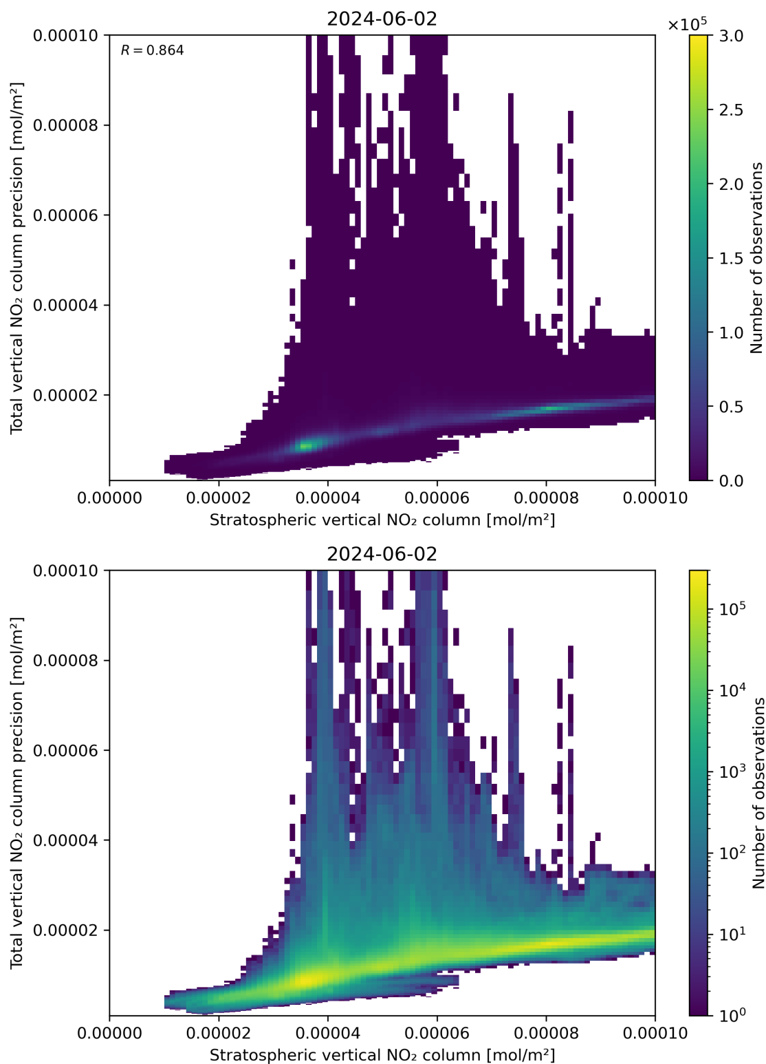
Figure 101: Scatter density plot of “Stratospheric vertical NO 2 column” against “Total vertical NO 2 column precision” for 2024-06-01 to 2024-06-03.
