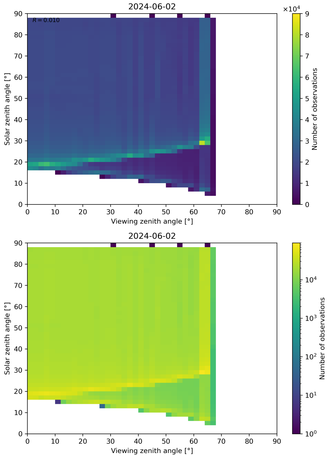
Figure 172: Scatter density plot of “Viewing zenith angle” against “Solar zenith angle” for 2024-06-01 to 2024-06-03.
