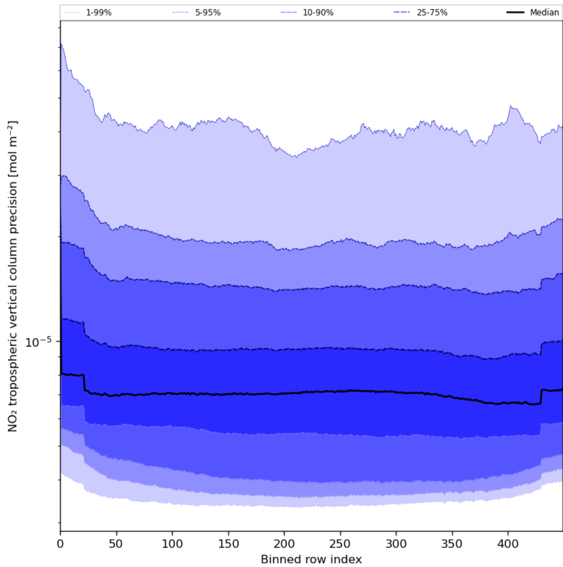
Figure 47: Along track statistics of “NO 2 tropospheric vertical column precision” for 2024-06-01 to 2024-06-03
