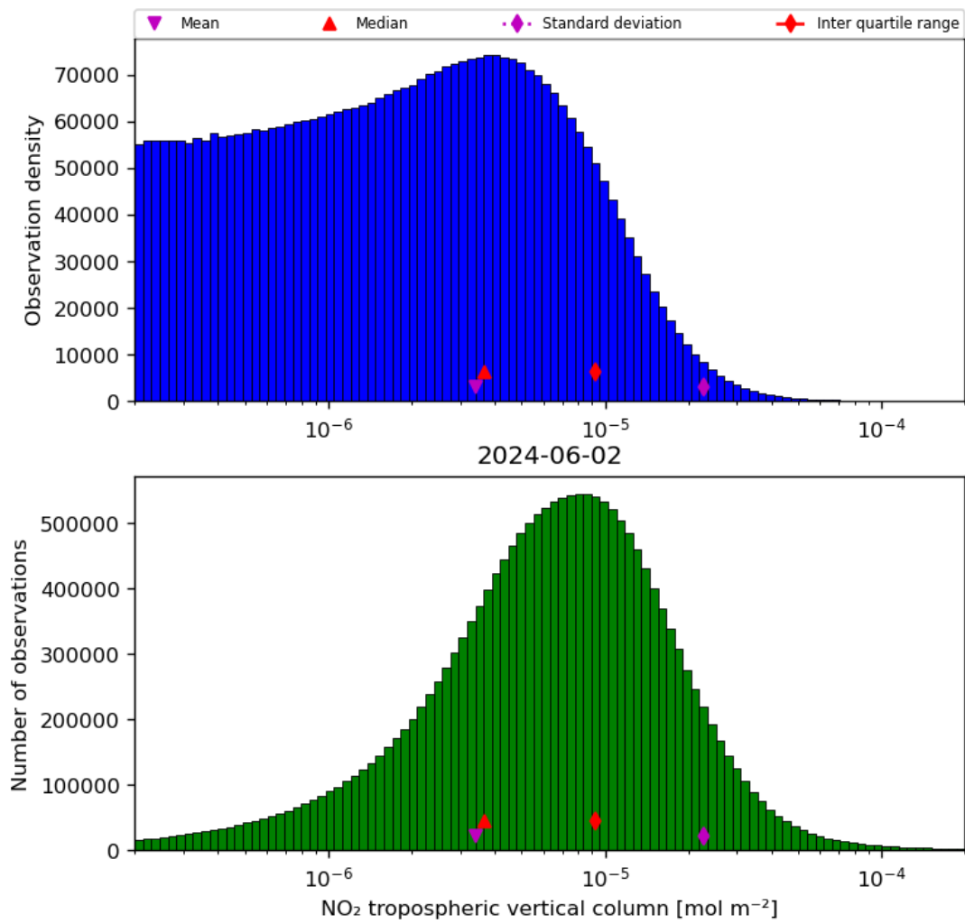
Figure 29: Histogram of “NO 2 tropospheric vertical column” for 2024-06-01 to 2024-06-03
