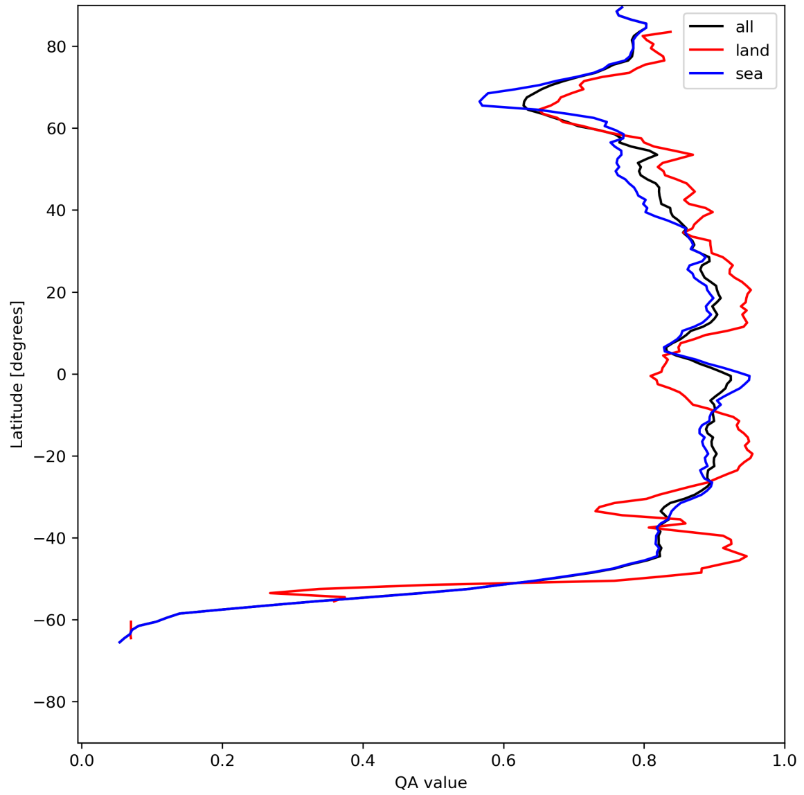
Figure 11: Zonal average of “QA value” for 2024-06-01 to 2024-06-03.
