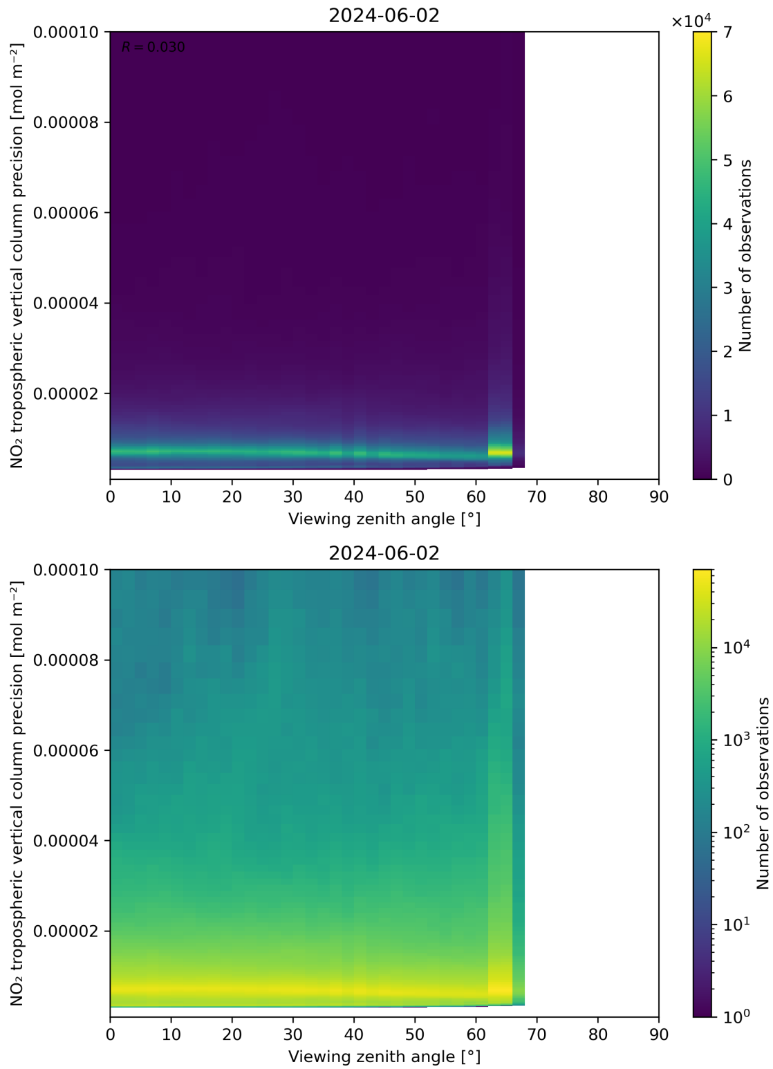
Figure 170: Scatter density plot of “Viewing zenith angle” against “NO 2 tropospheric vertical column precision” for 2024-06-01 to 2024-06-03.
