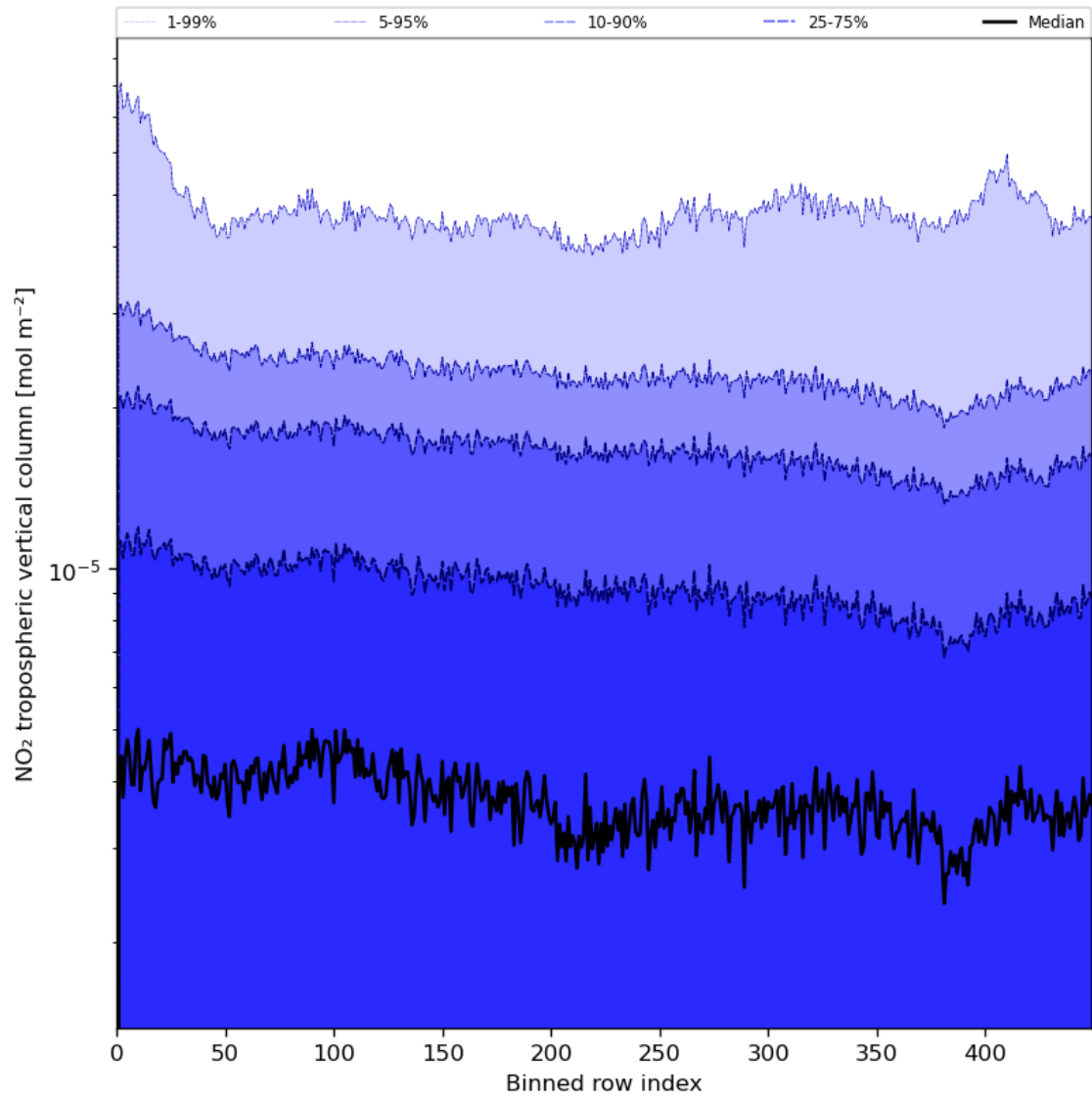
Figure 46: Along track statistics of “NO 2 tropospheric vertical column” for 2024-06-01 to 2024-06-03
