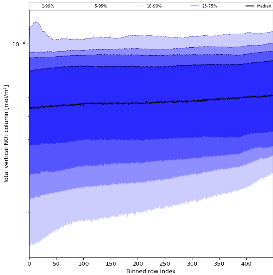
Figure 55: Along track statistics of “Total vertical NO 2 column” for 2024-06-01 to 2024-06-03
