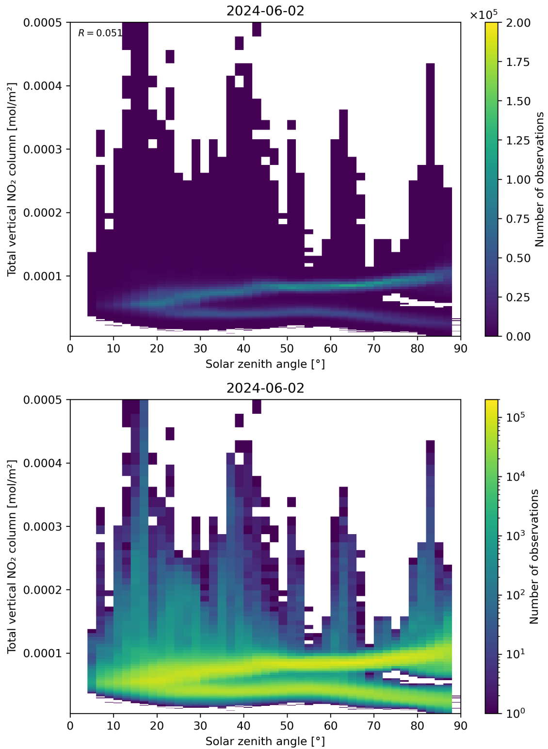
Figure 153: Scatter density plot of “Solar zenith angle” against “Total vertical NO 2 column” for 2024-06-01 to 2024-06-03.
