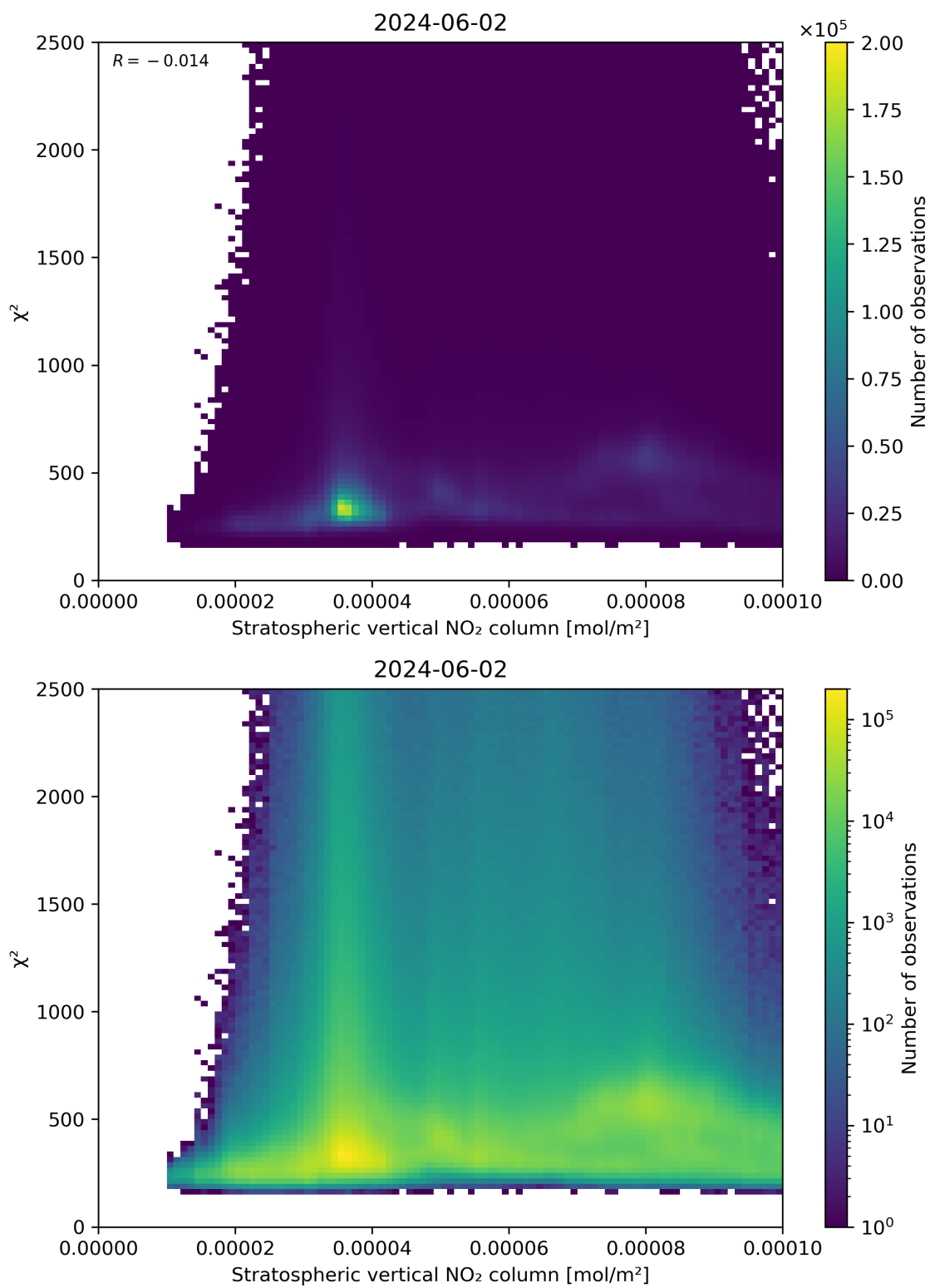
Figure 97: Scatter density plot of “Stratospheric vertical NO 2 column” against “ \chi^2 ” for 2024-06-01 to 2024-06-03.
