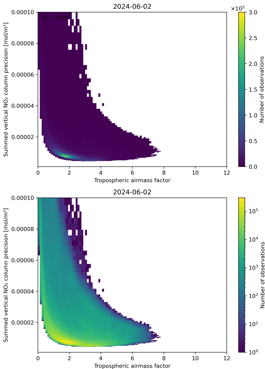
Figure 76: Scatter density plot of “Tropospheric air mass factor” against “Summed vertical NO 2 column precision” for 2024-06-01 to 2024-06-03.
