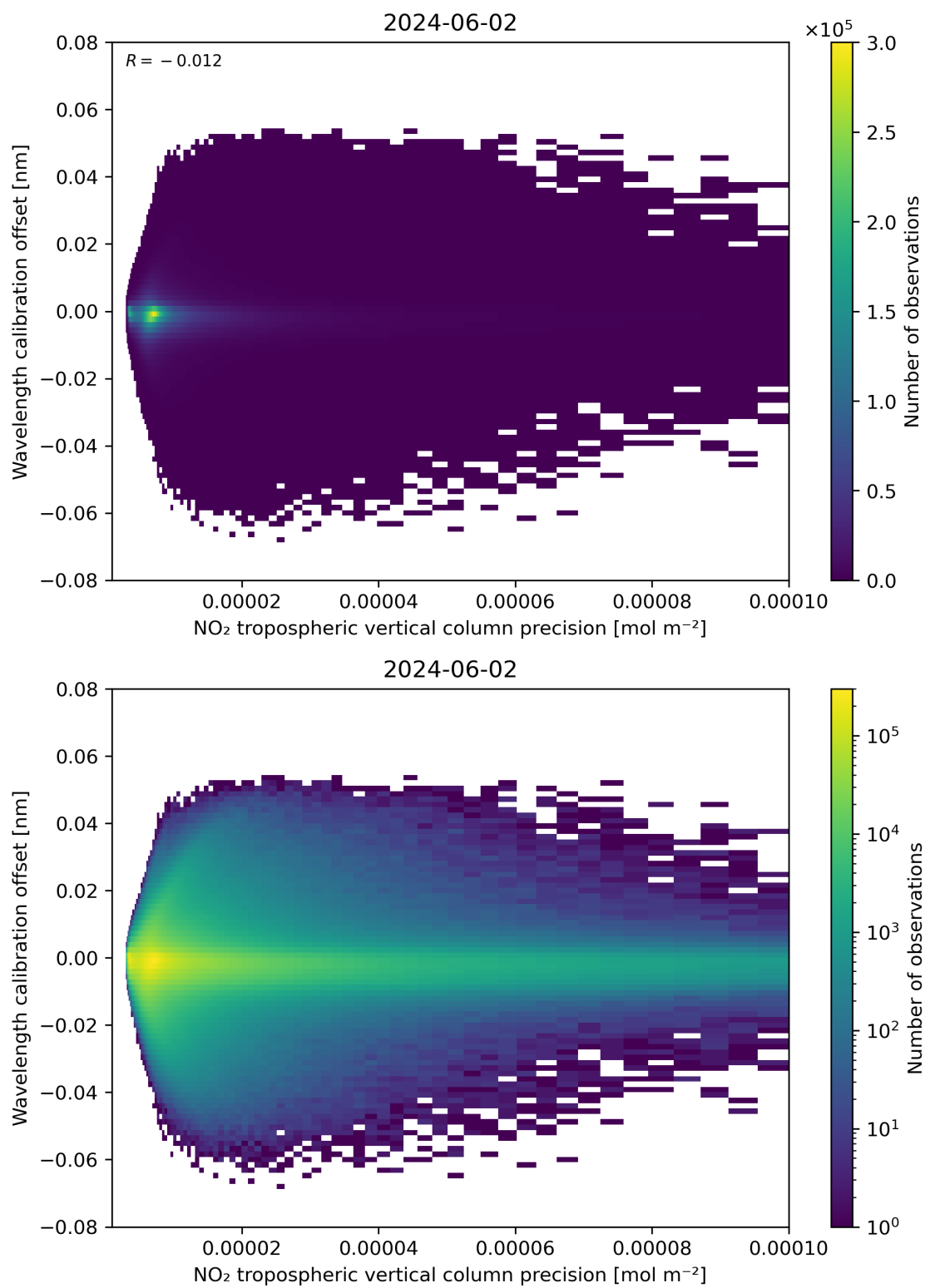
Figure 141: Scatter density plot of “NO 2 tropospheric vertical column precision” against “Wavelength calibration offset” for 2024-06-01 to 2024-06-03.
