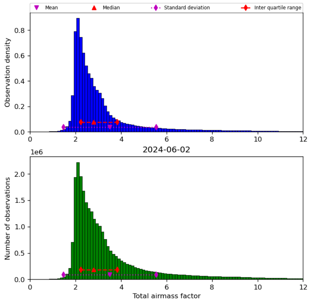
Figure 32: Histogram of “Total airmass factor” for 2024-06-01 to 2024-06-03
