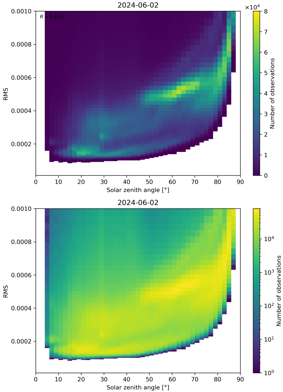
Figure 157: Scatter density plot of “Solar zenith angle” against “RMS” for 2024-06-01 to 2024-06-03.
