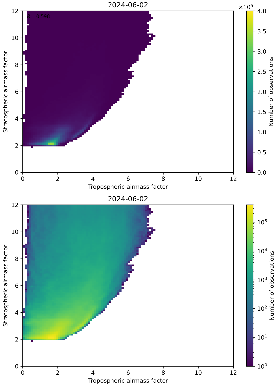
Figure 71: Scatter density plot of “Tropospheric airmass factor” against “Stratospheric airmass factor” for 2024-06-01 to 2024-06-03.
