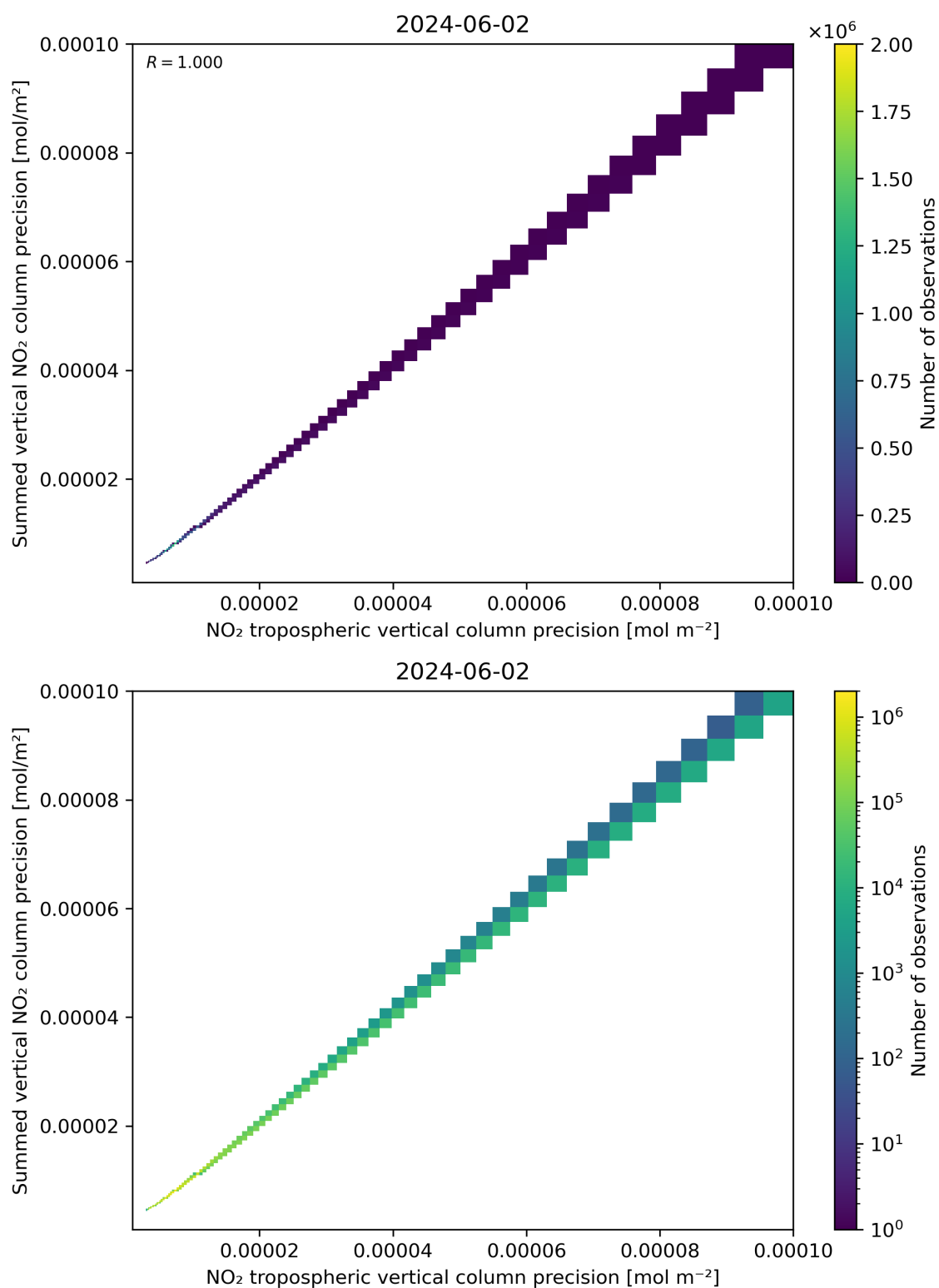
Figure 137: Scatter density plot of “NO 2 tropospheric vertical column precision” against “Summed vertical NO 2 column precision” for 2024-06-01 to 2024-06-03.
