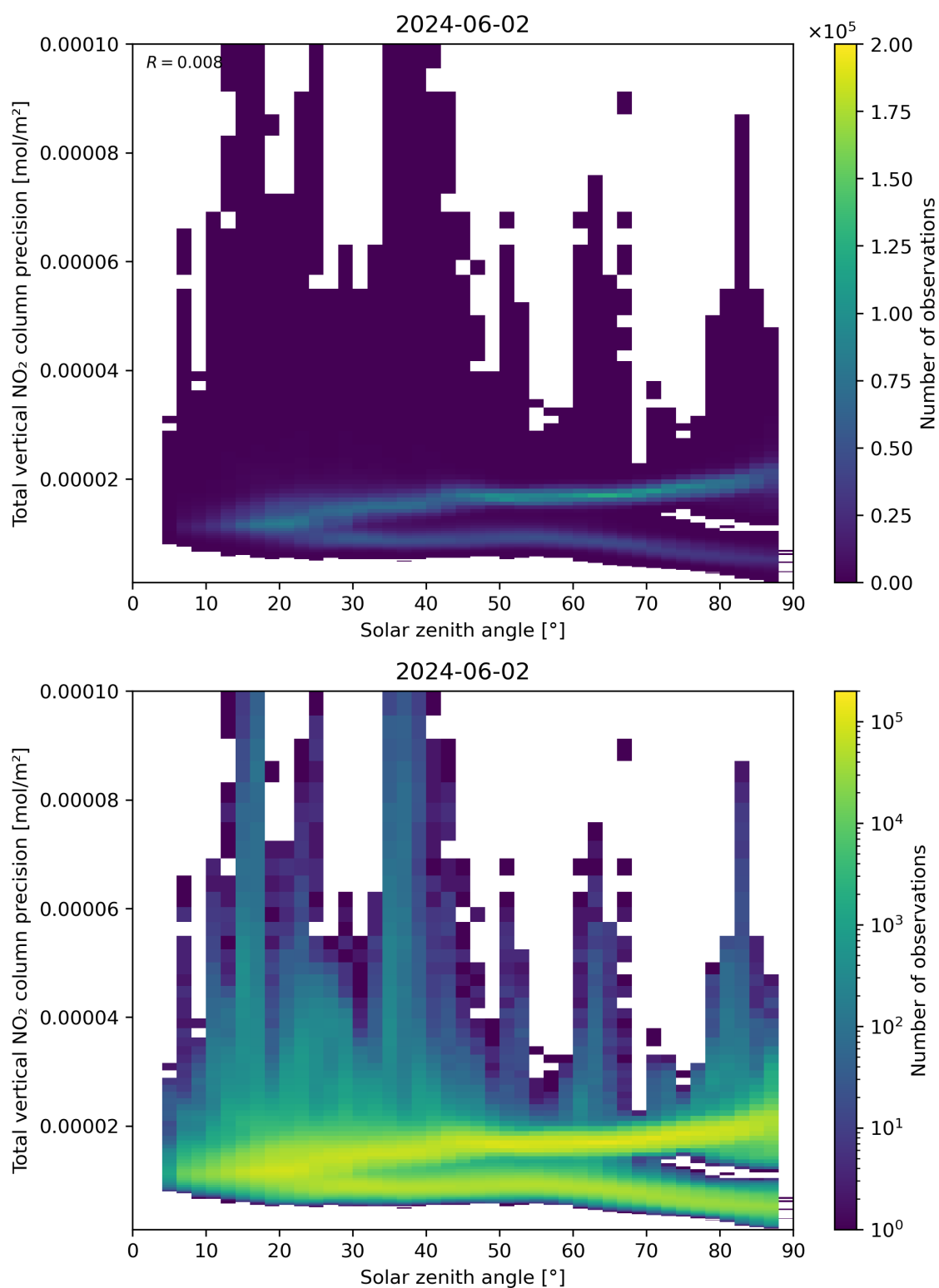
Figure 154: Scatter density plot of “Solar zenith angle” against “Total vertical NO 2 column precision” for 2024-06-01 to 2024-06-03.
