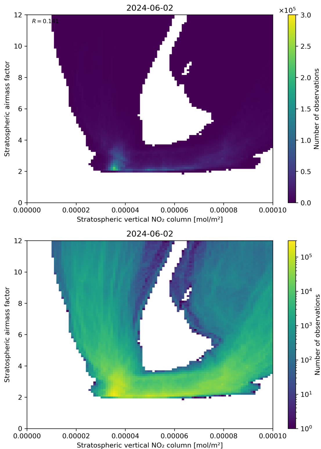
Figure 96: Scatter density plot of “Stratospheric vertical NO 2 column” against “Stratospheric airmass factor” for 2024-06-01 to 2024-06-03.
