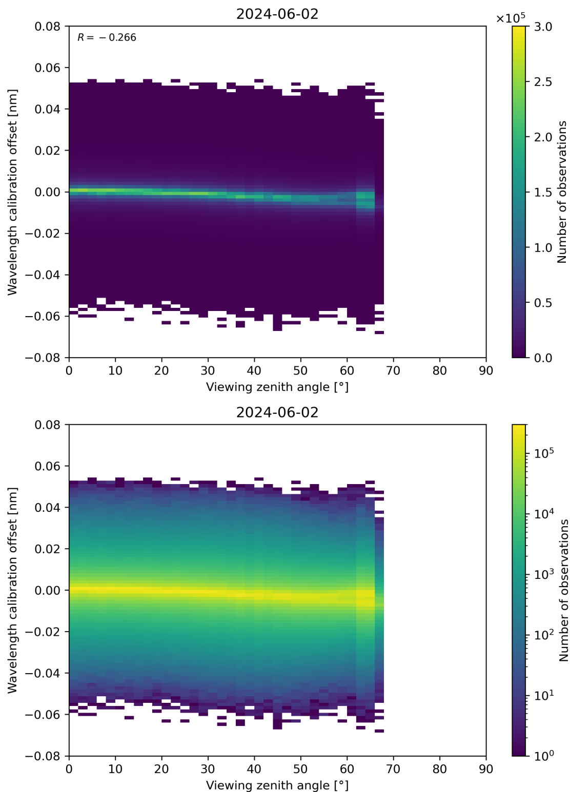
Figure 173: Scatter density plot of “Viewing zenith angle” against “Wavelength calibration offset” for 2024-06-01 to 2024-06-03.
