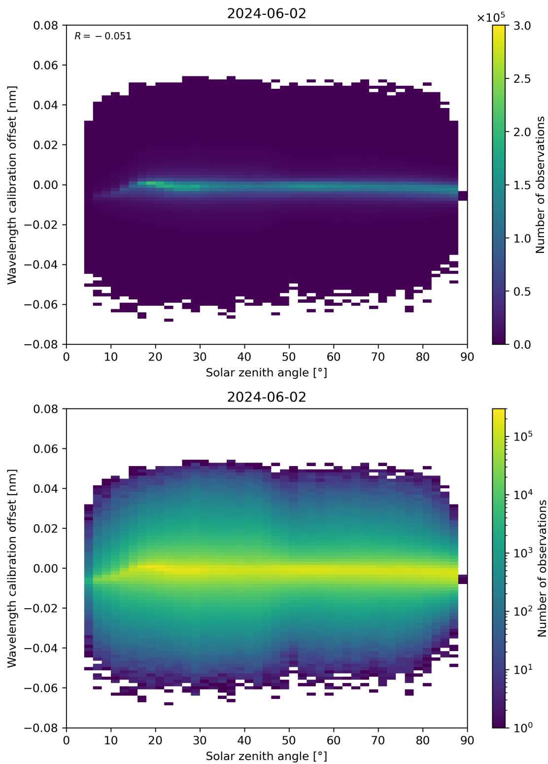
Figure 158: Scatter density plot of “Solar zenith angle” against “Wavelength calibration offset” for 2024-06-01 to 2024-06-03.
