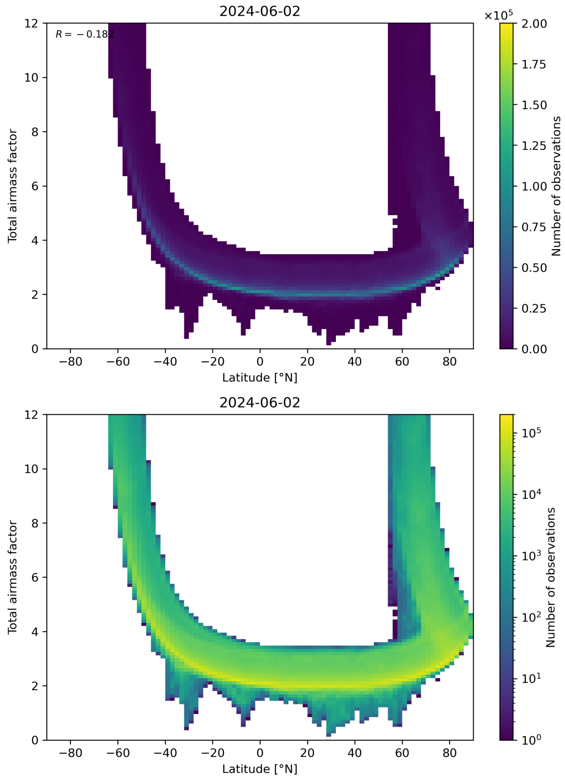
Figure 84: Scatter density plot of “Latitude” against “Total airmass factor” for 2024-06-01 to 2024-06-03.
