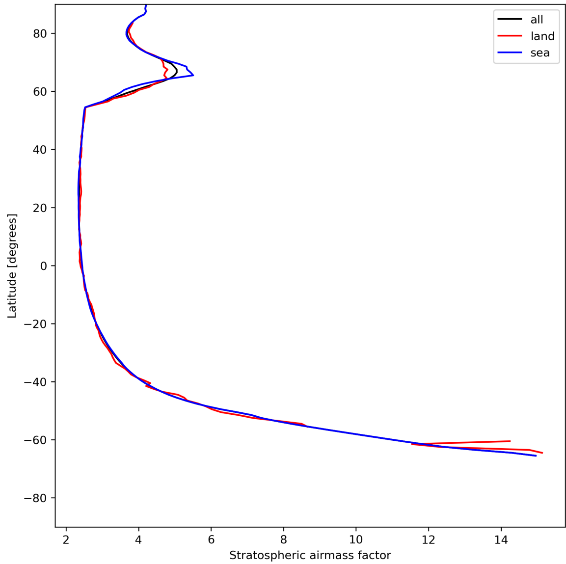
Figure 27: Zonal average of “Stratospheric air mass factor” for 2024-06-01 to 2024-06-03.
