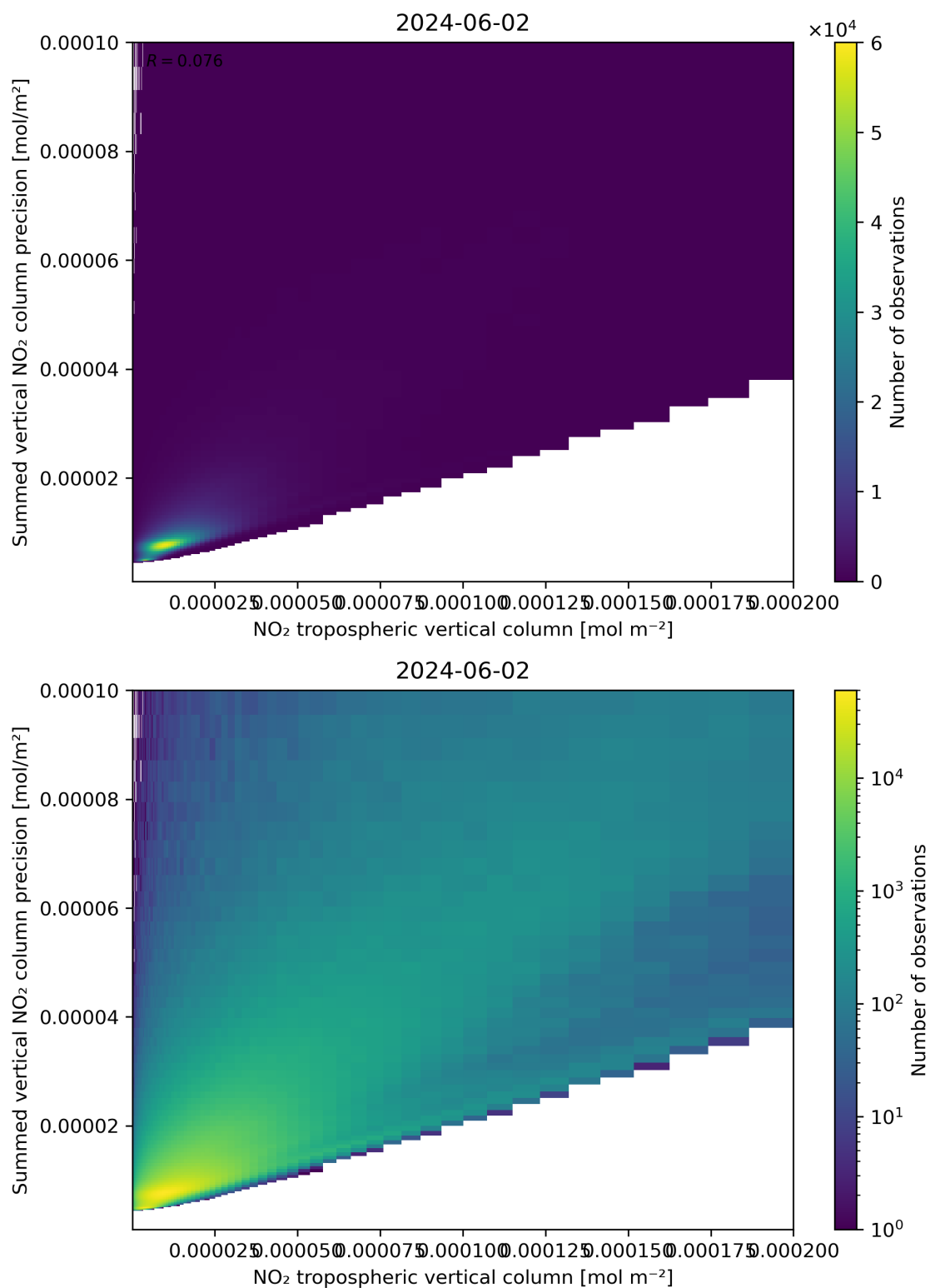
Figure 127: Scatter density plot of “NO 2 tropospheric vertical column” against “Summed vertical NO 2 column precision” for 2024-06-01 to 2024-06-03.
