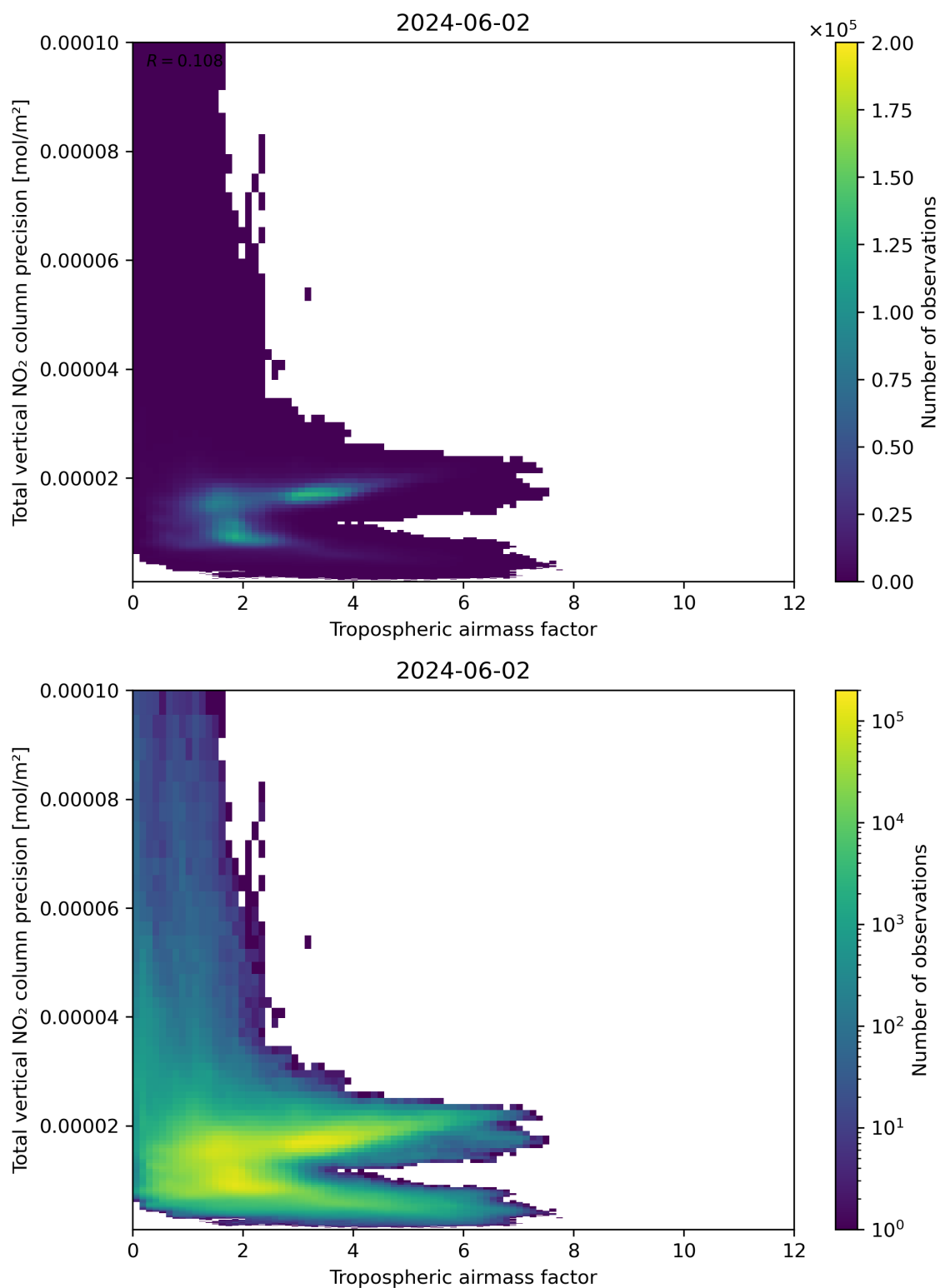
Figure 78: Scatter density plot of “Tropospheric air mass factor” against “Total vertical NO 2 column precision” for 2024-06-01 to 2024-06-03.
