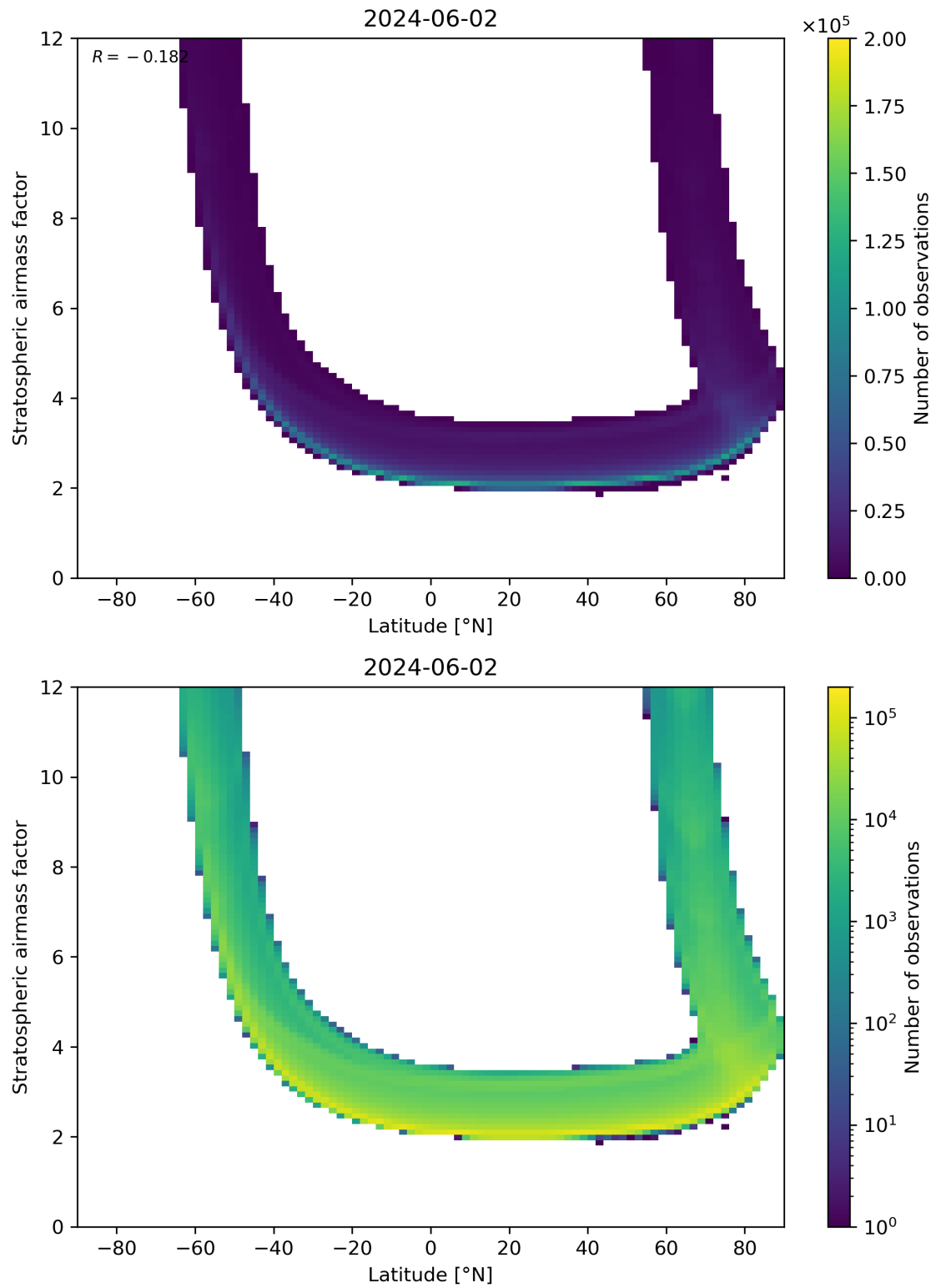
Figure 83: Scatter density plot of “Latitude” against “Stratospheric air mass factor” for 2024-06-01 to 2024-06-03.
