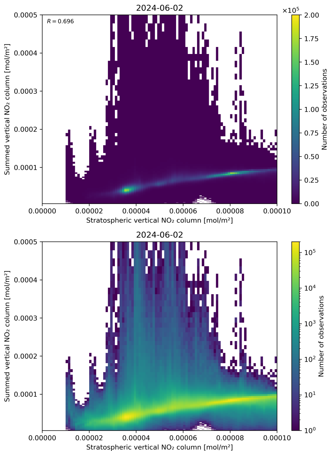
Figure 98: Scatter density plot of “Stratospheric vertical NO 2 column” against “Summed vertical NO 2 column” for 2024-06-01 to 2024-06-03.
