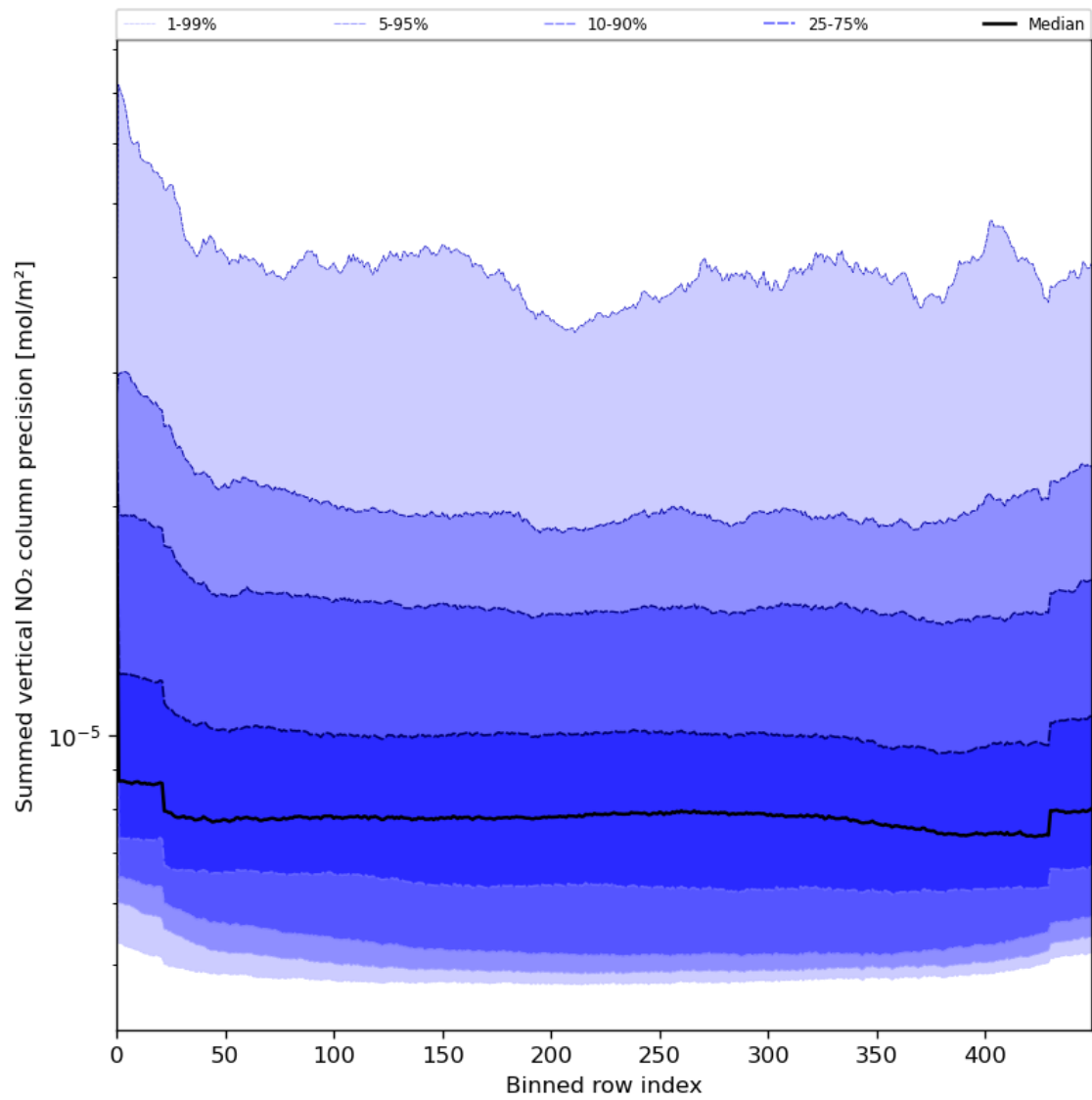
Figure 58: Along track statistics of “Summed vertical NO 2 column precision” for 2024-06-01 to 2024-06-03
