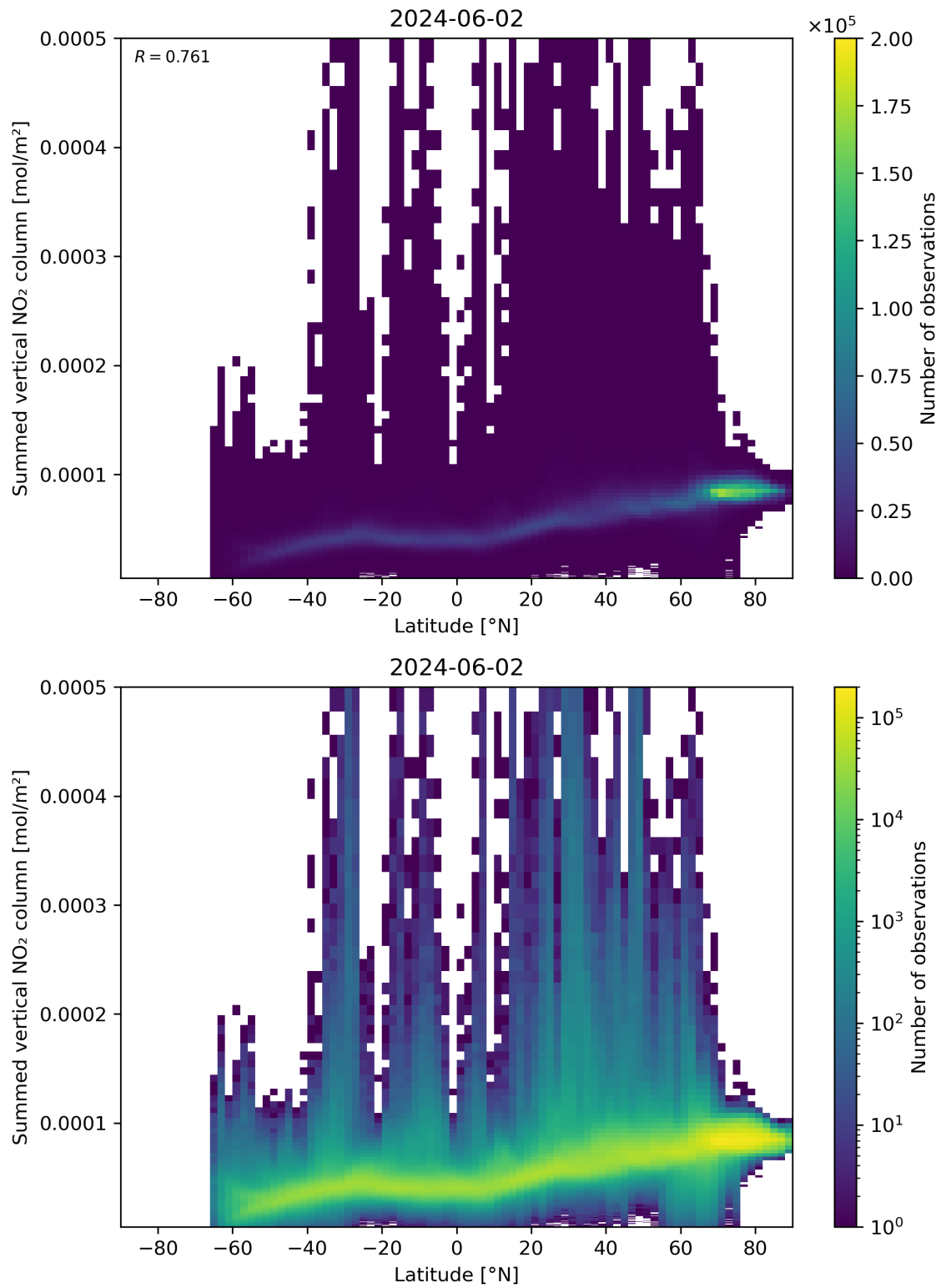
Figure 88: Scatter density plot of “Latitude” against “Summed vertical NO 2 column” for 2024-06-01 to 2024-06-03.
