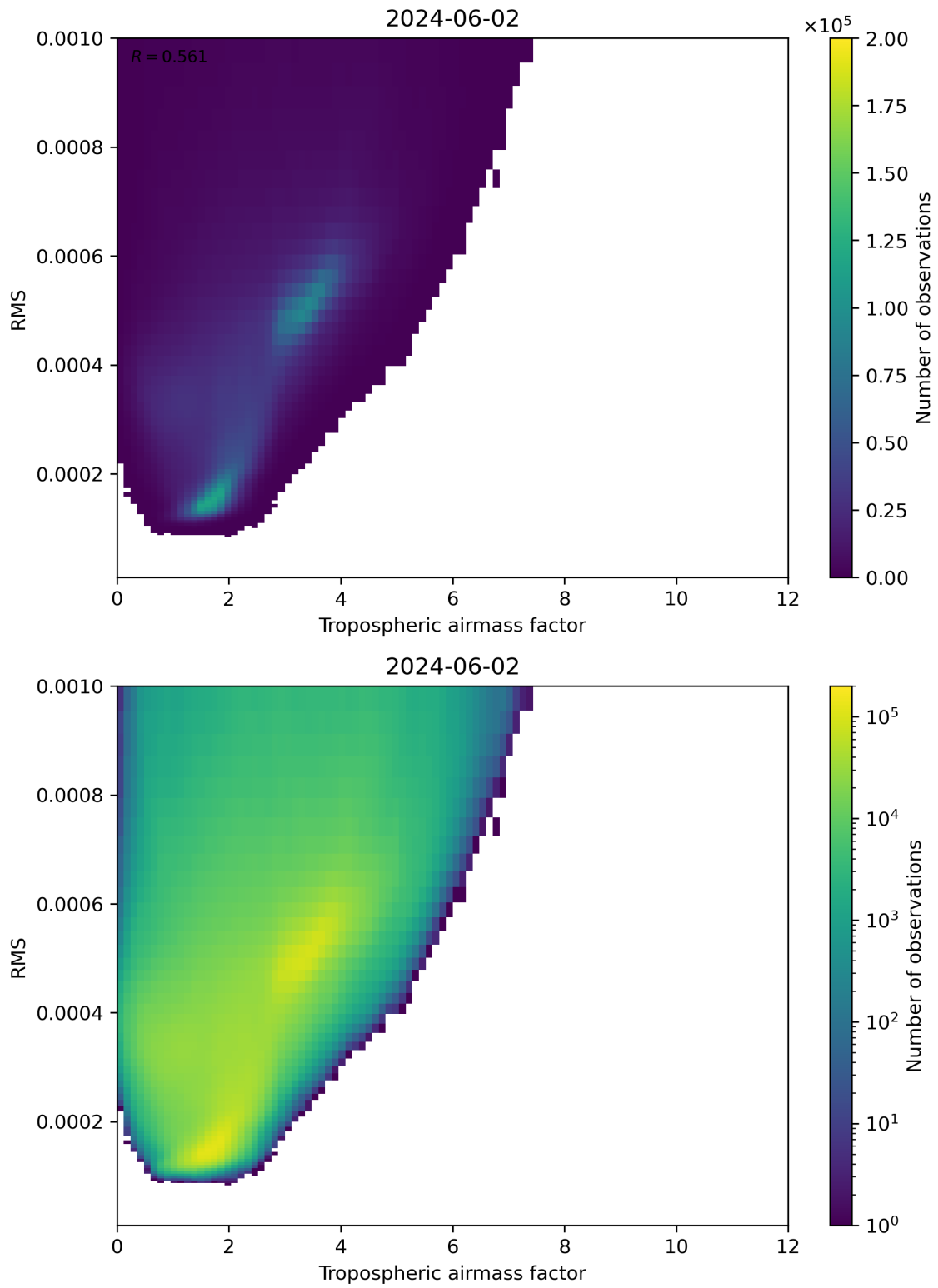
Figure 79: Scatter density plot of “Tropospheric airmass factor” against “RMS” for 2024-06-01 to 2024-06-03.
