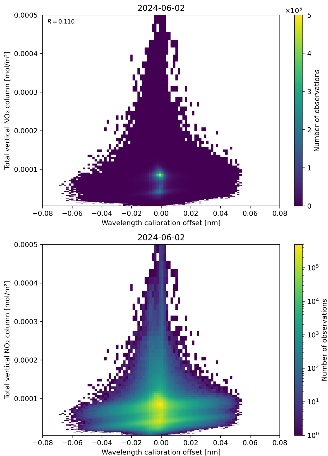
Figure 179: Scatter density plot of “Wavelength calibration offset” against “Total vertical NO 2 column” for 2024-06-01 to 2024-06-03.
