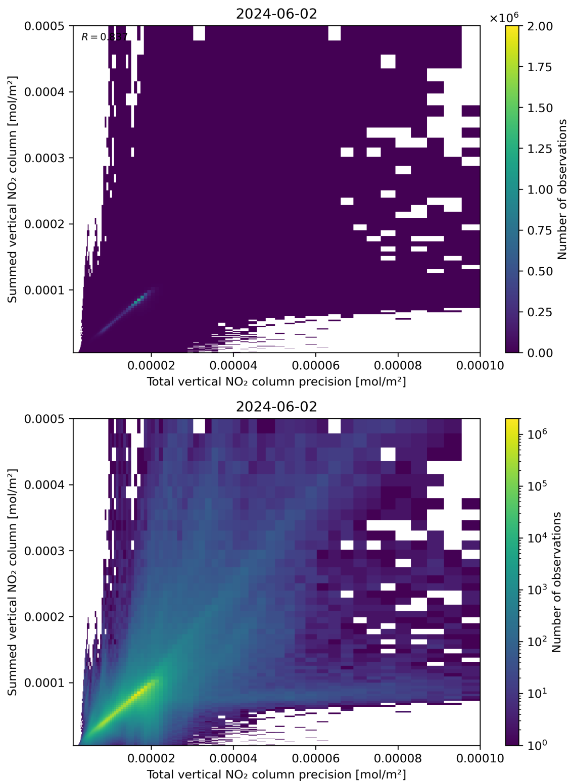
Figure 117: Scatter density plot of “Total vertical NO 2 column precision” against “Summed vertical NO 2 column” for 2024-06-01 to 2024-06-03.
