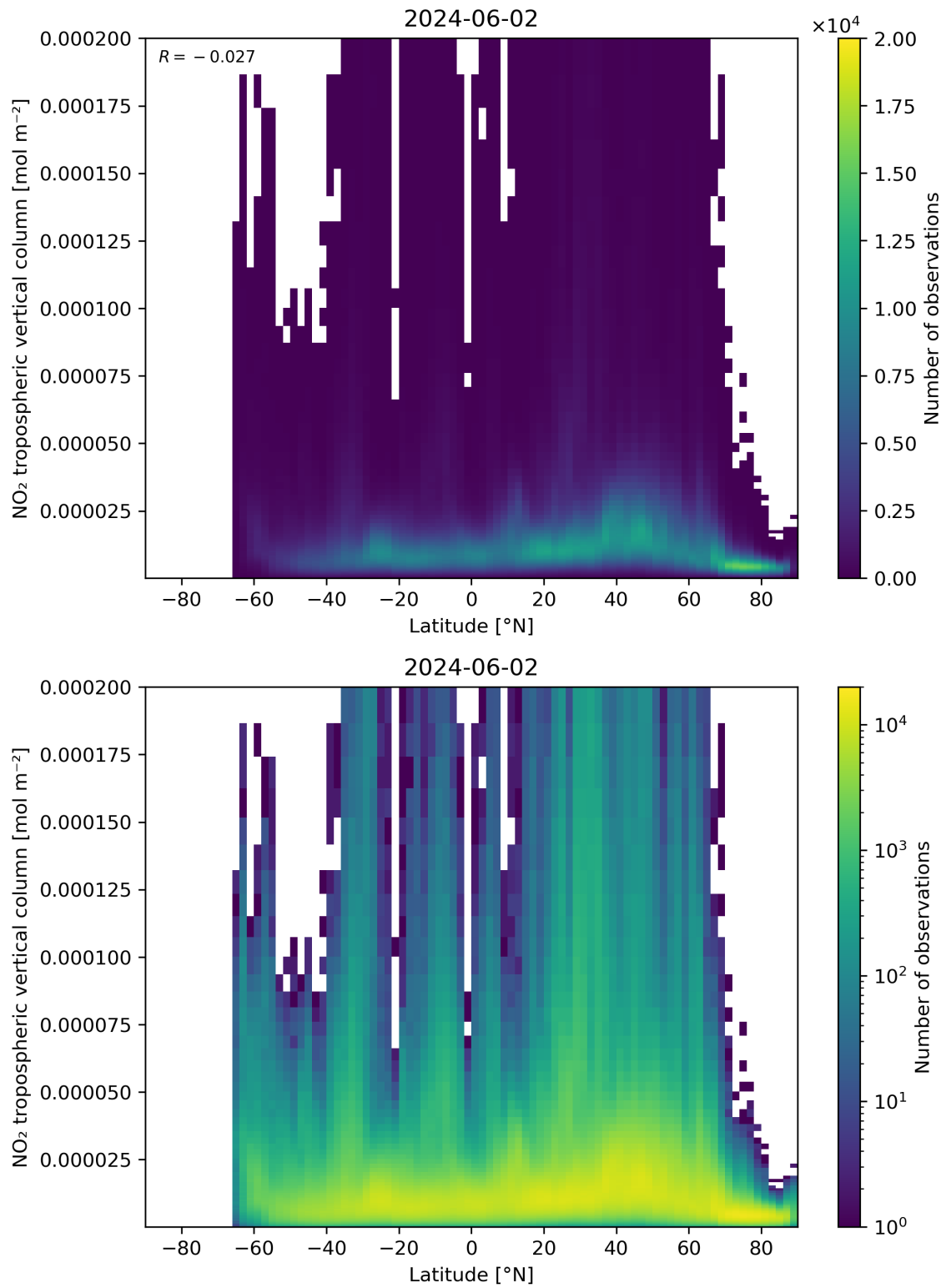
Figure 92: Scatter density plot of “Latitude” against “NO 2 tropospheric vertical column” for 2024-06-01 to 2024-06-03.
