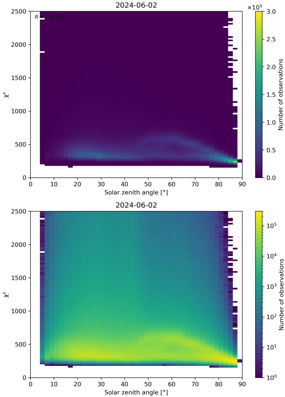
Figure 148: Scatter density plot of “Solar zenith angle” against “ \chi^2 ” for 2024-06-01 to 2024-06-03.
