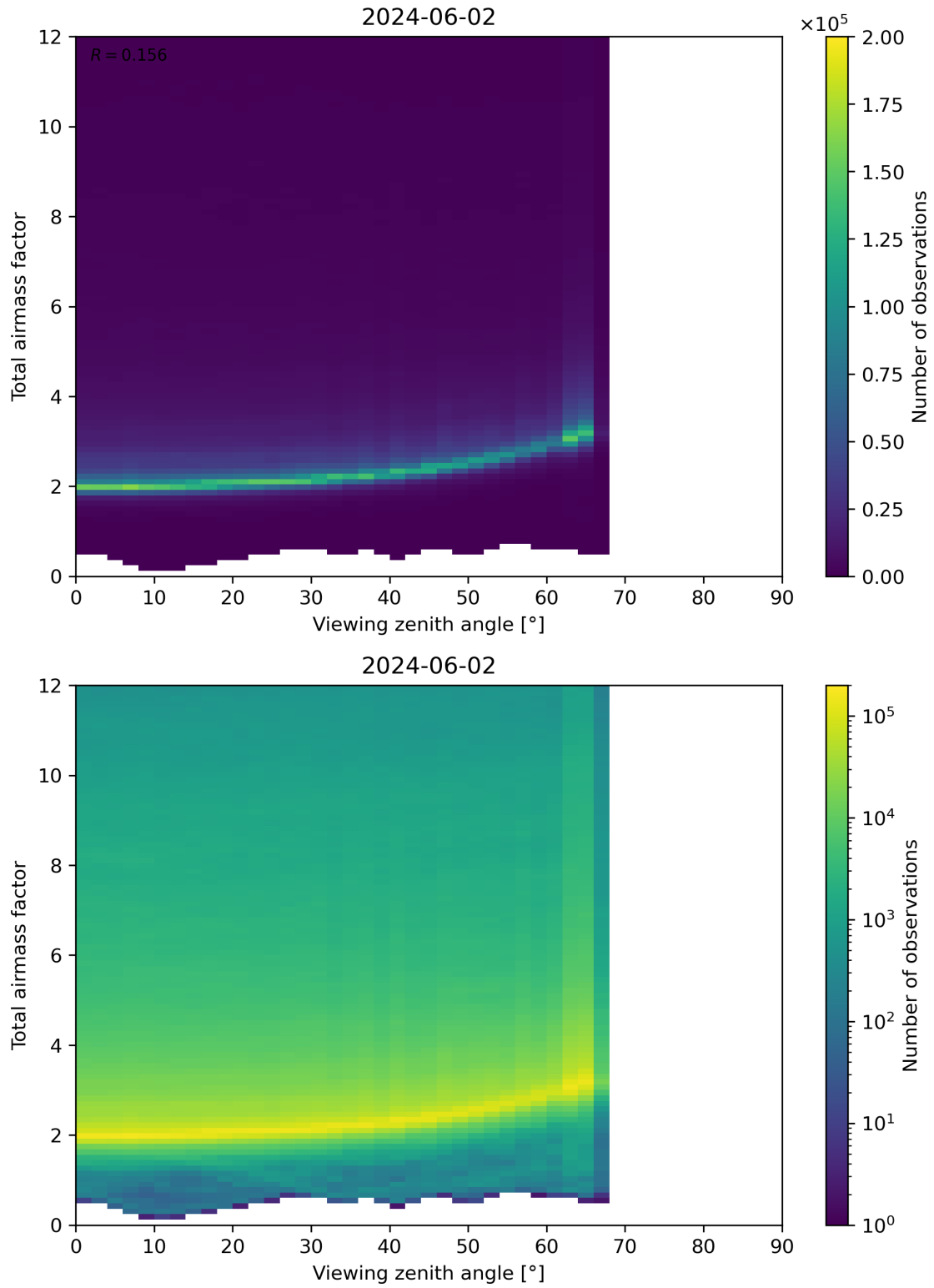
Figure 160: Scatter density plot of “Viewing zenith angle” against “Total airmass factor” for 2024-06-01 to 2024-06-03.
