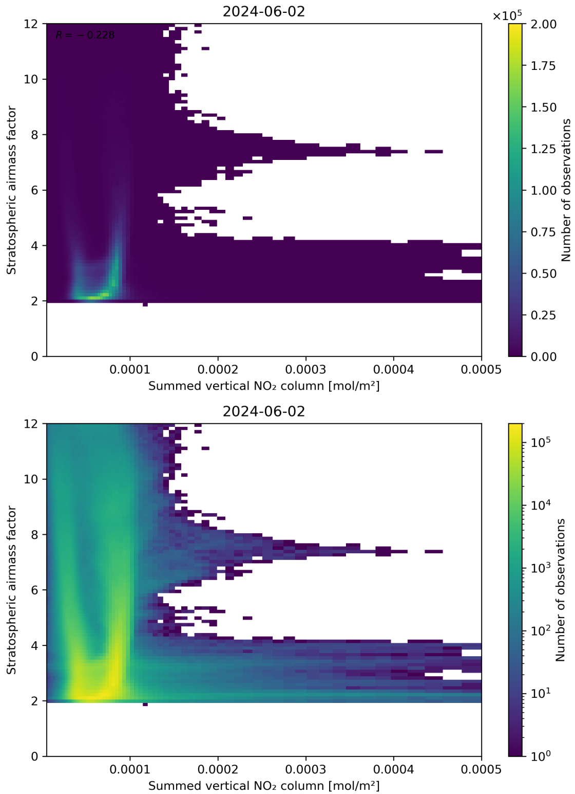
Figure 103: Scatter density plot of “Summed vertical NO 2 column” against “Stratospheric air mass factor” for 2024-06-01 to 2024-06-03.
