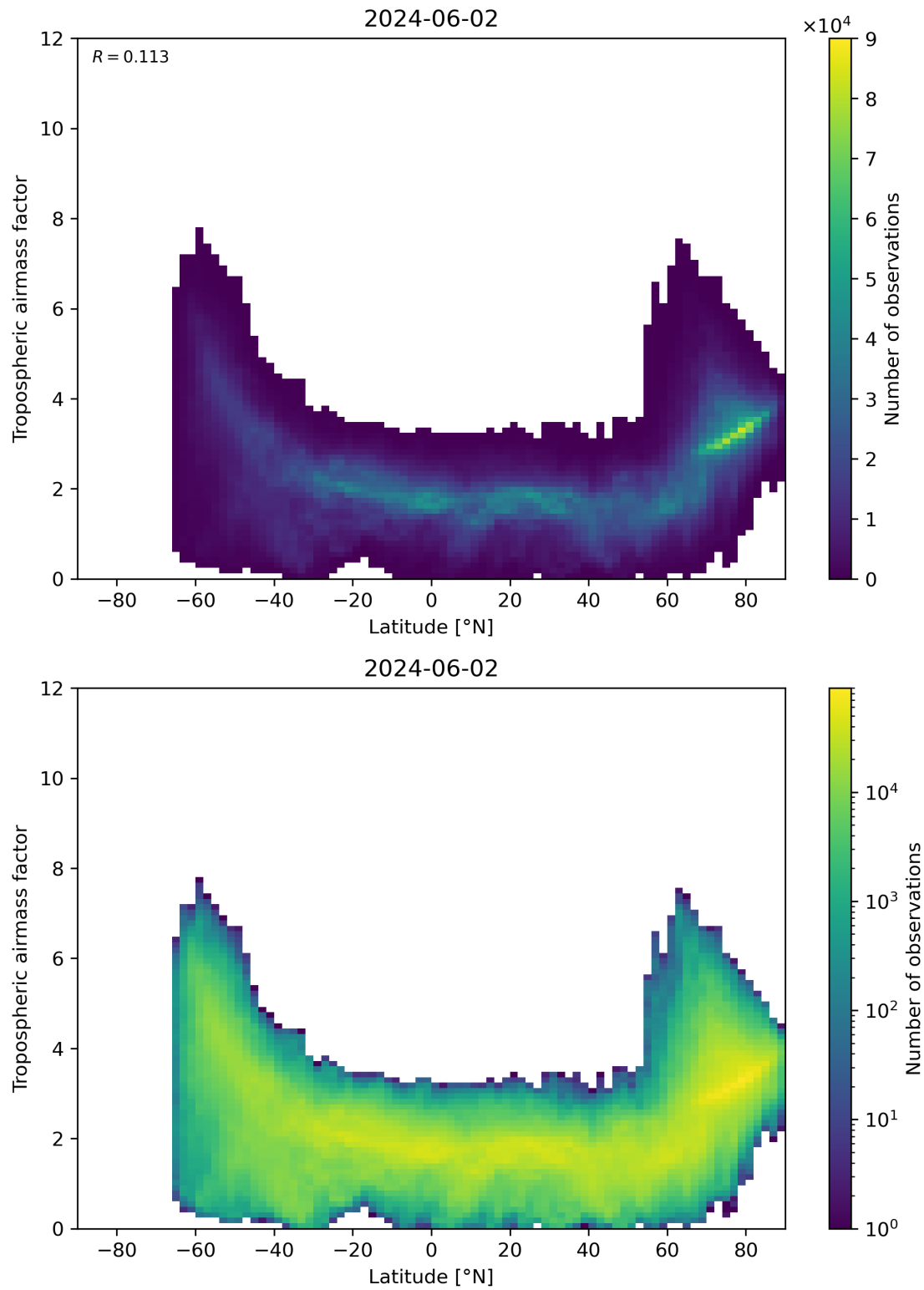
Figure 85: Scatter density plot of “Latitude” against “Tropospheric air mass factor” for 2024-06-01 to 2024-06-03.
