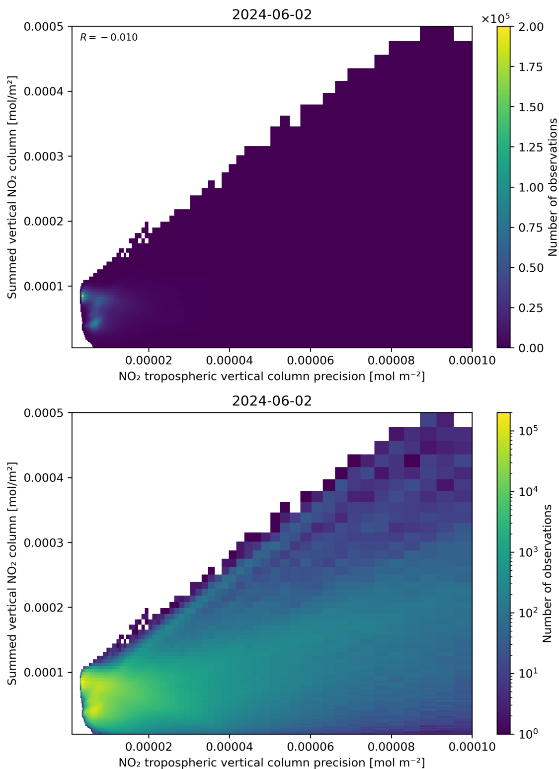
Figure 136: Scatter density plot of “NO 2 tropospheric vertical column precision” against “Summed vertical NO 2 column” for 2024-06-01 to 2024-06-03.
