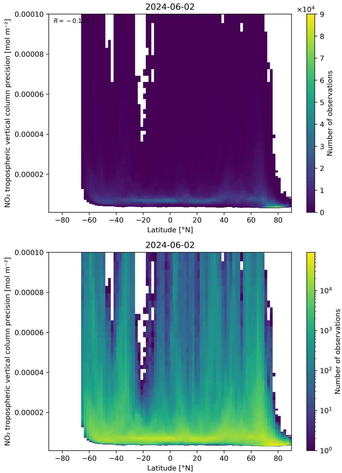
Figure 93: Scatter density plot of “Latitude” against “NO 2 tropospheric vertical column precision” for 2024-06-01 to 2024-06-03.
