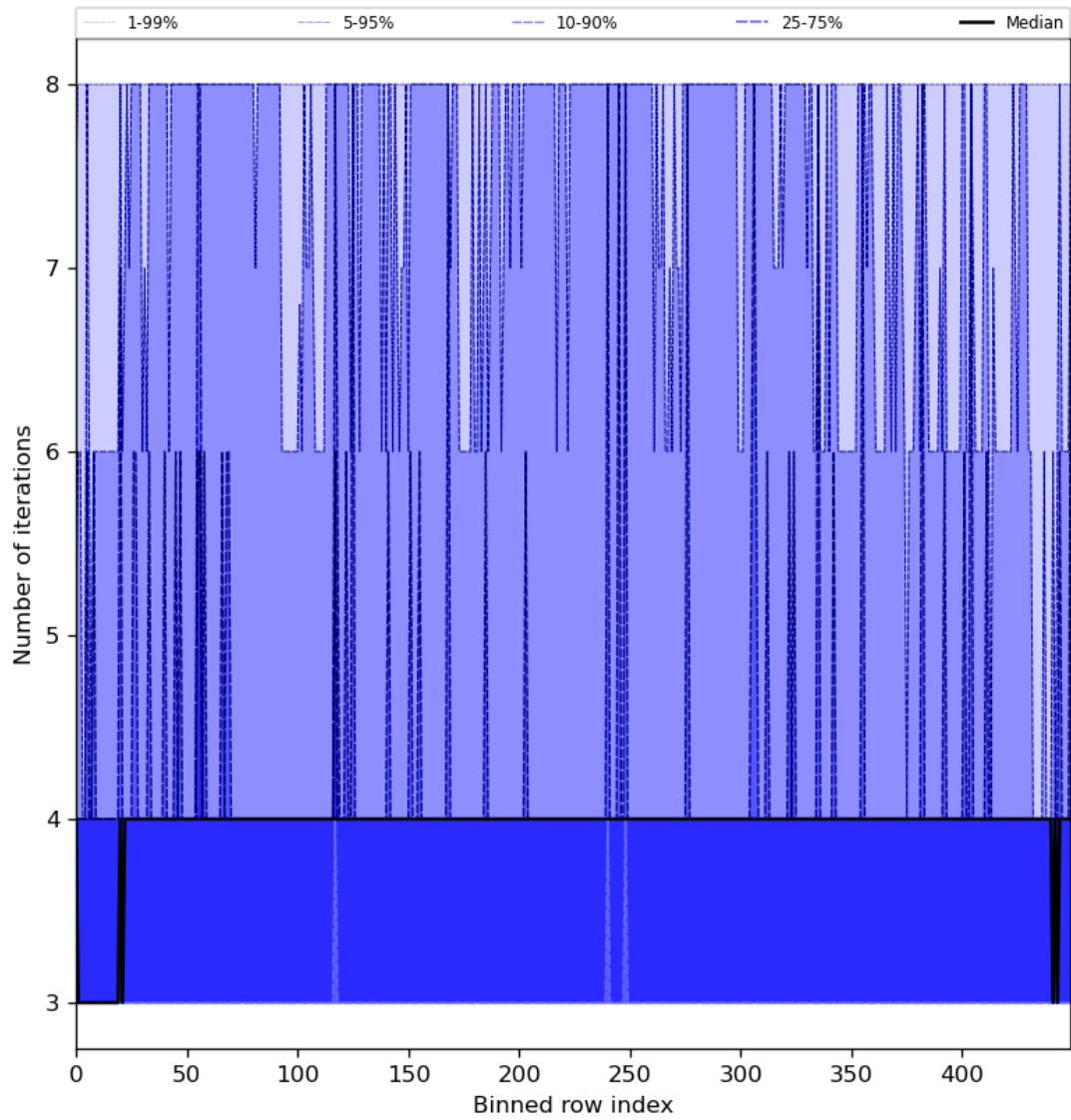
Figure 51: Along track statistics of “Number of iterations” for 2024-06-01 to 2024-06-03
