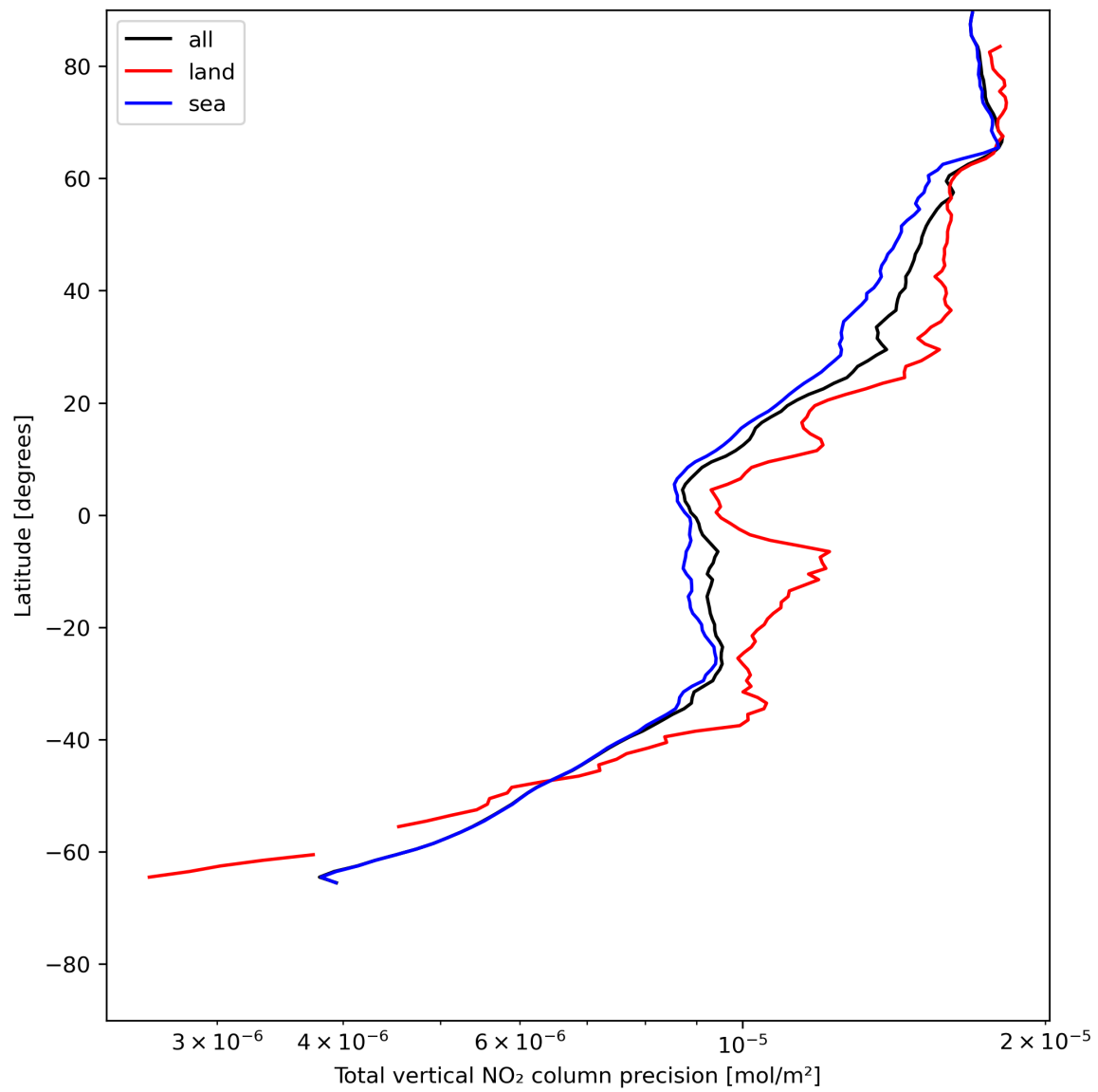
Figure 22: Zonal average of “Total vertical NO 2 column precision” for 2024-06-01 to 2024-06-03.
