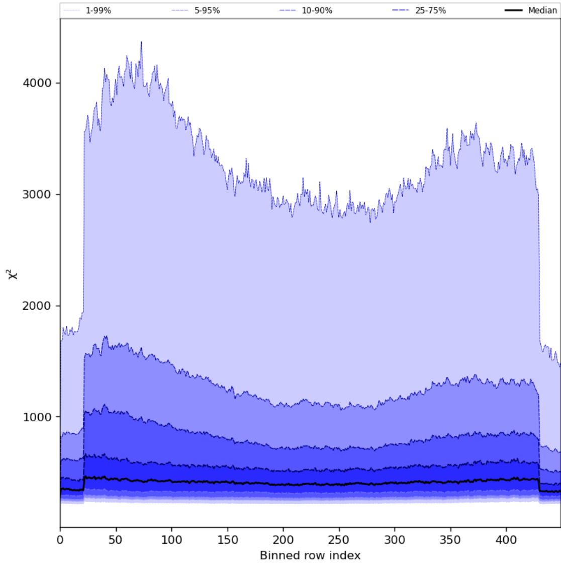
Figure 59: Along track statistics of “ \chi^2 ” for 2024-06-01 to 2024-06-03
