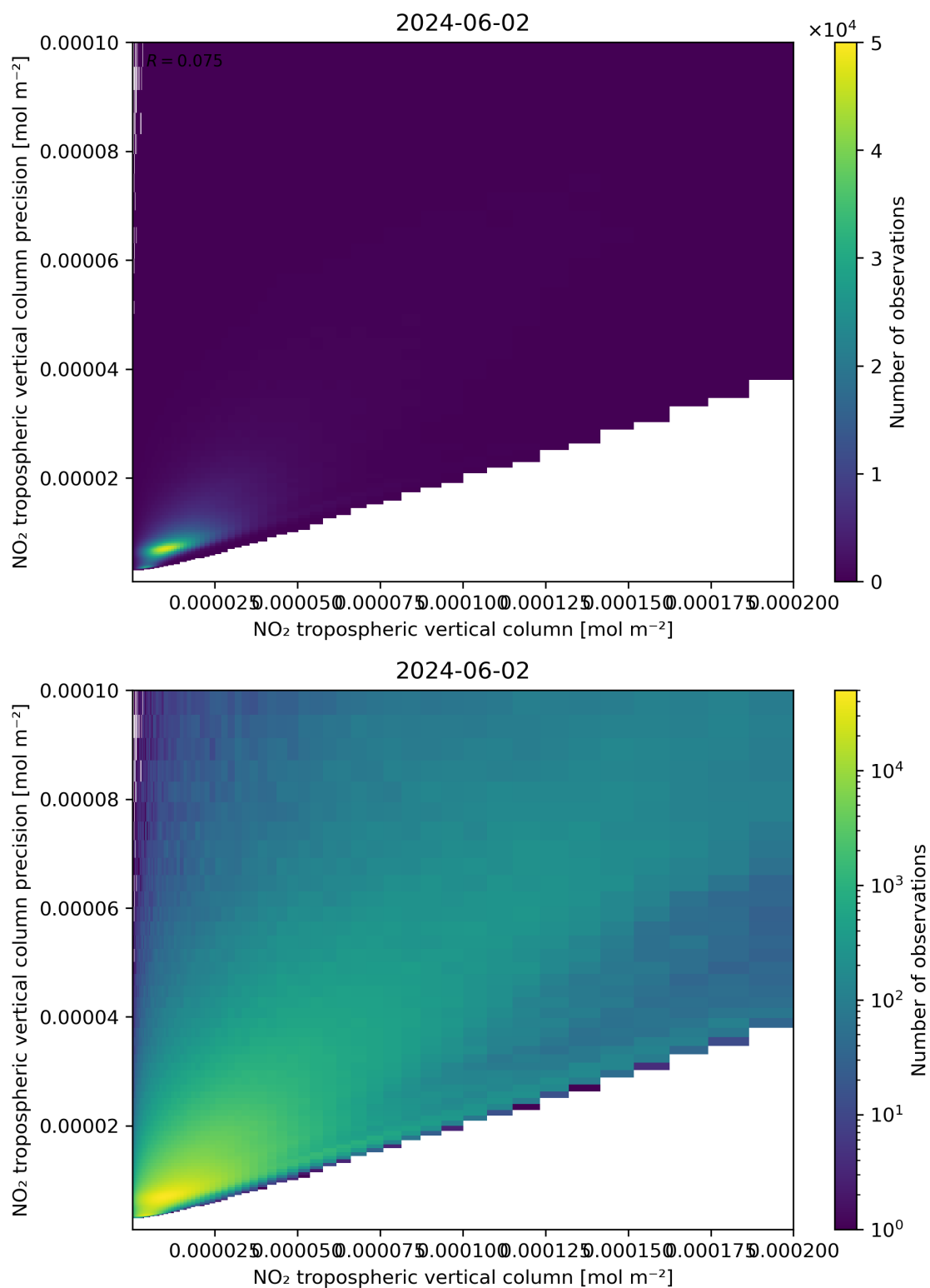
Figure 130: Scatter density plot of “NO 2 tropospheric vertical column” against “NO 2 tropospheric vertical column precision” for 2024-06-01 to 2024-06-03.
