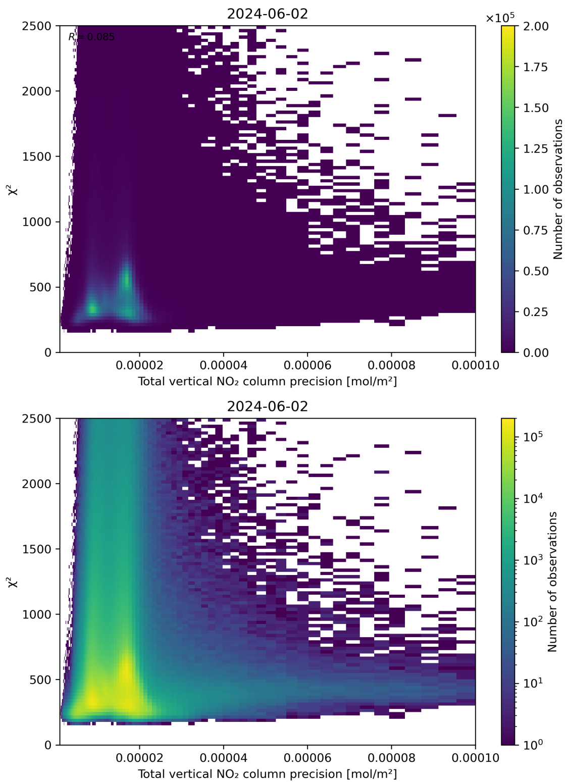
Figure 116: Scatter density plot of “Total vertical NO 2 column precision” against “ \chi^2 ” for 2024-06-01 to 2024-06-03.
