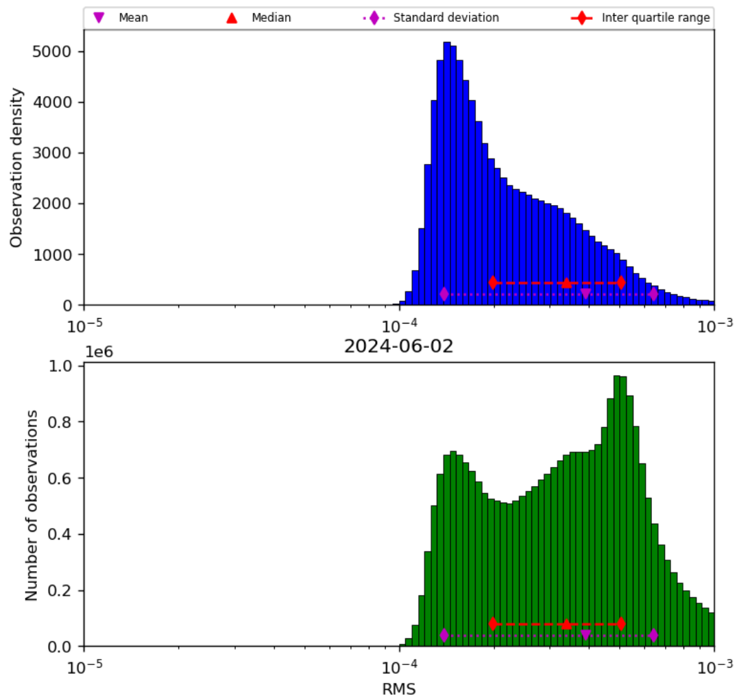
Figure 43: Histogram of “RMS” for 2024-06-01 to 2024-06-03
