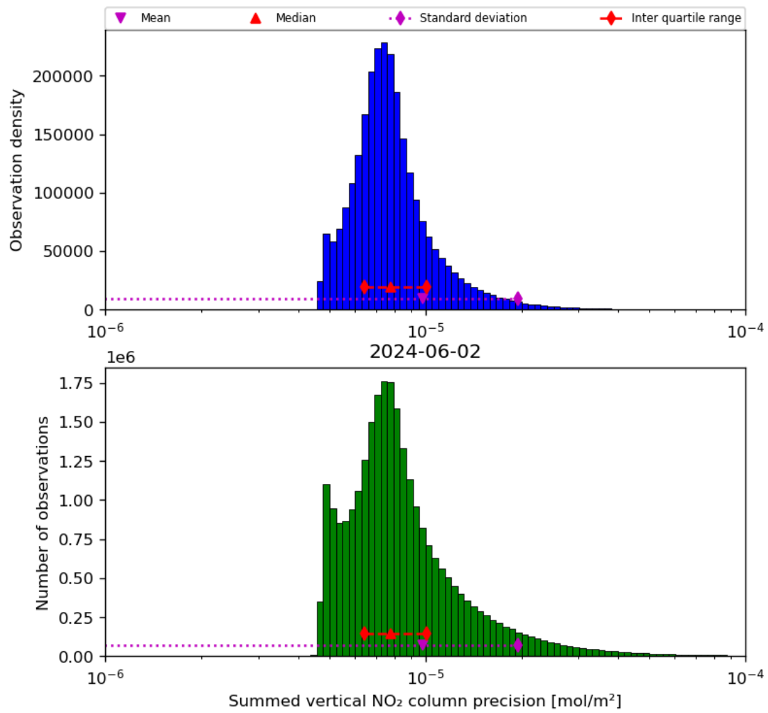
Figure 41: Histogram of "Summed vertical NO 2 column precision" for 2024-06-01 to 2024-06-03
