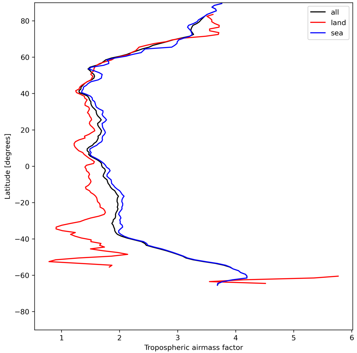
Figure 14: Zonal average of “Tropospheric airmass factor” for 2024-06-01 to 2024-06-03.
