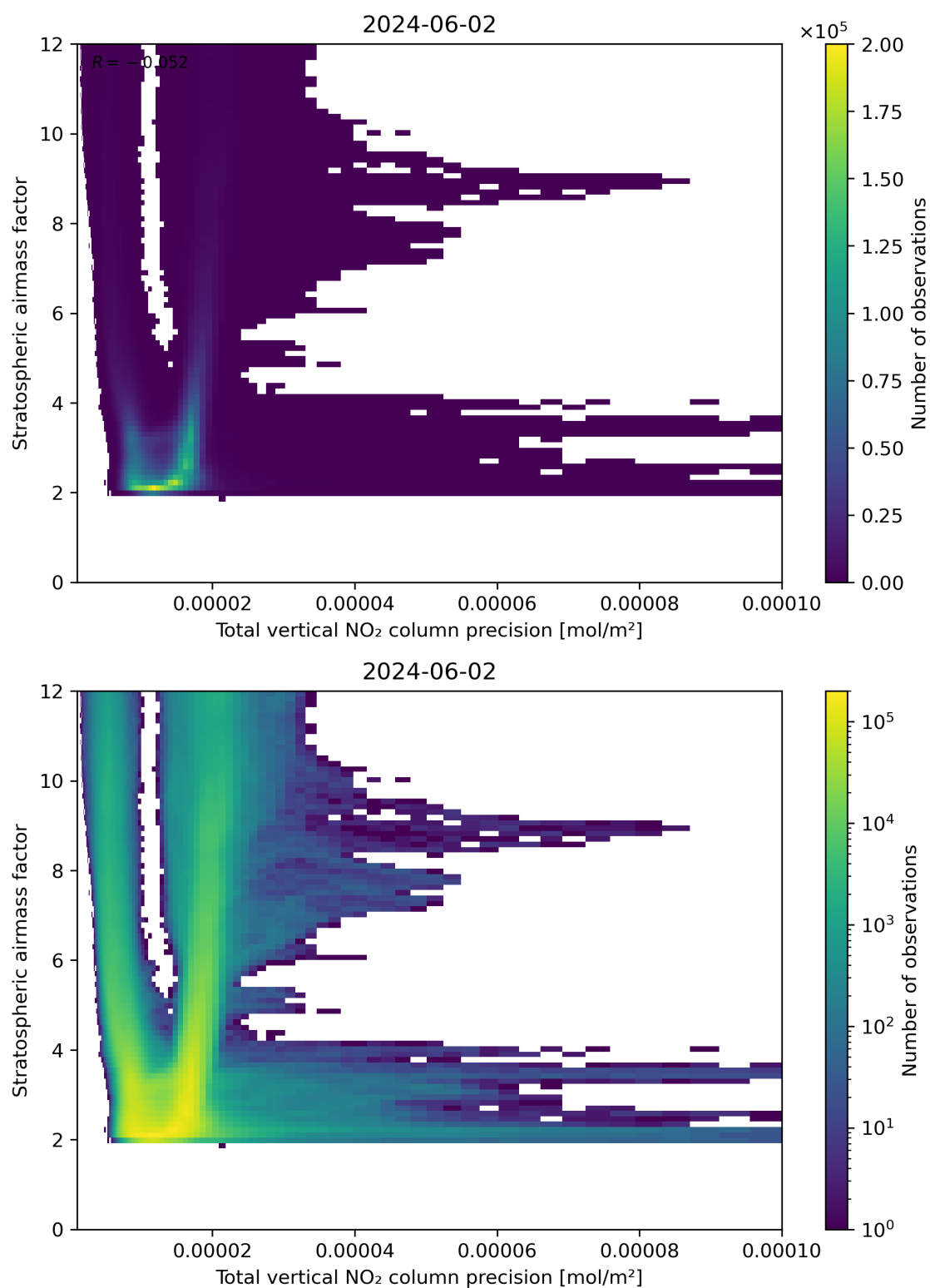
Figure 115: Scatter density plot of “Total vertical NO 2 column precision” against “Stratospheric air mass factor” for 2024-06-01 to 2024-06-03.
