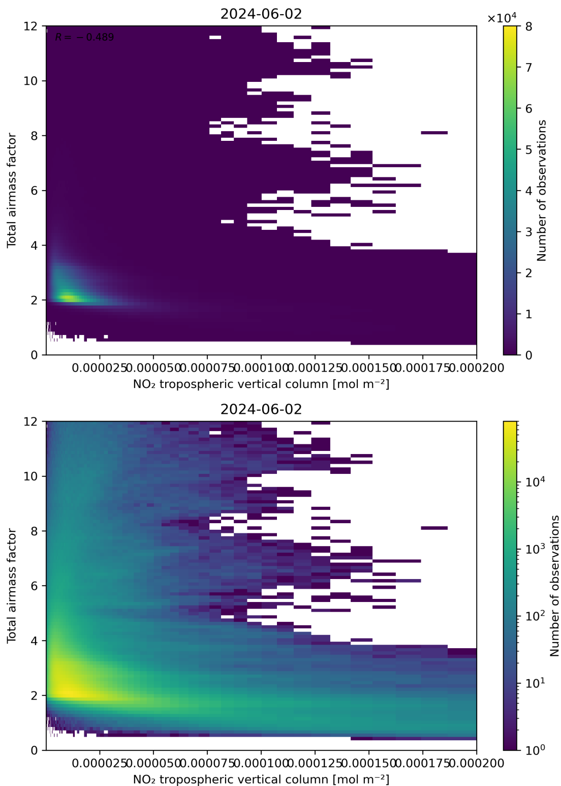
Figure 122: Scatter density plot of “NO 2 tropospheric vertical column” against “Total air mass factor” for 2024-06-01 to 2024-06-03.
