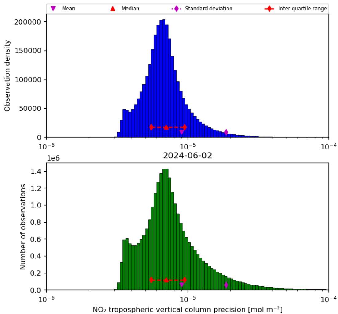
Figure 30: Histogram of “NO 2 tropospheric vertical column precision” for 2024-06-01 to 2024-06-03
