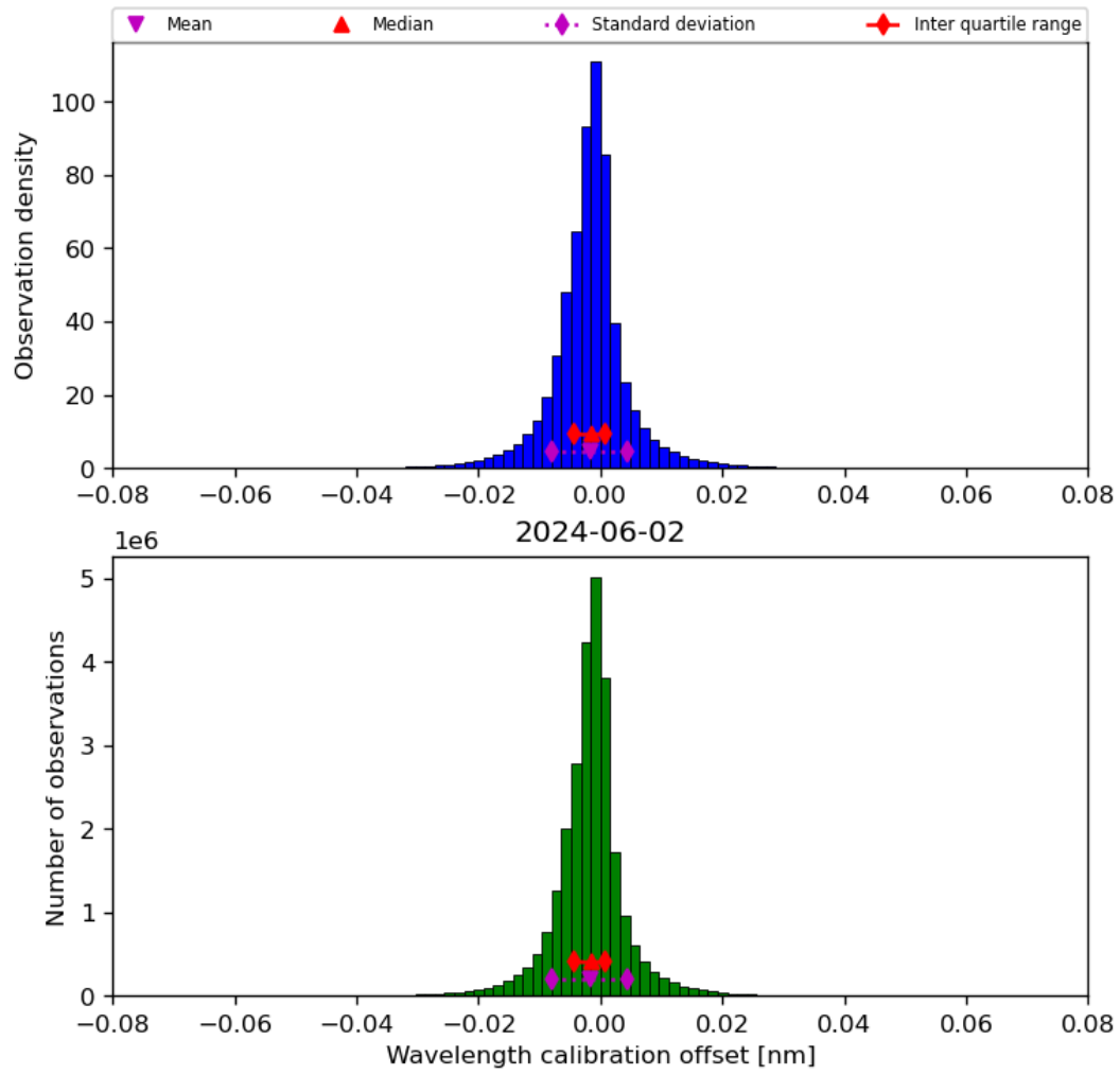
Figure 35: Histogram of “Wavelength calibration offset” for 2024-06-01 to 2024-06-03
