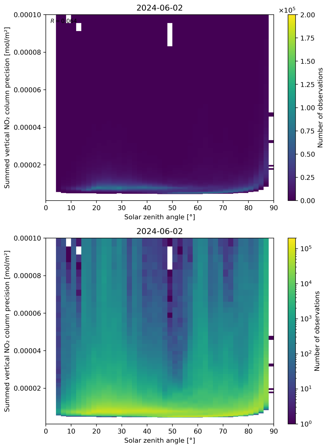
Figure 152: Scatter density plot of “Solar zenith angle” against “Summed vertical NO 2 column precision” for 2024-06-01 to 2024-06-03.
