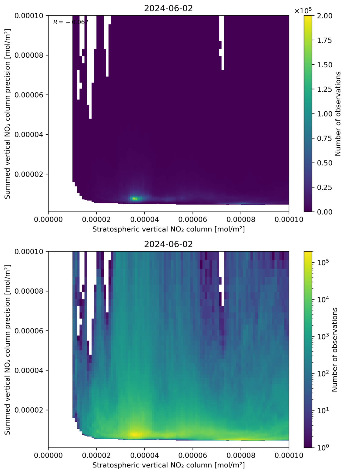
Figure 99: Scatter density plot of “Stratospheric vertical NO 2 column” against “Summed vertical NO 2 column precision” for 2024-06-01 to 2024-06-03.
