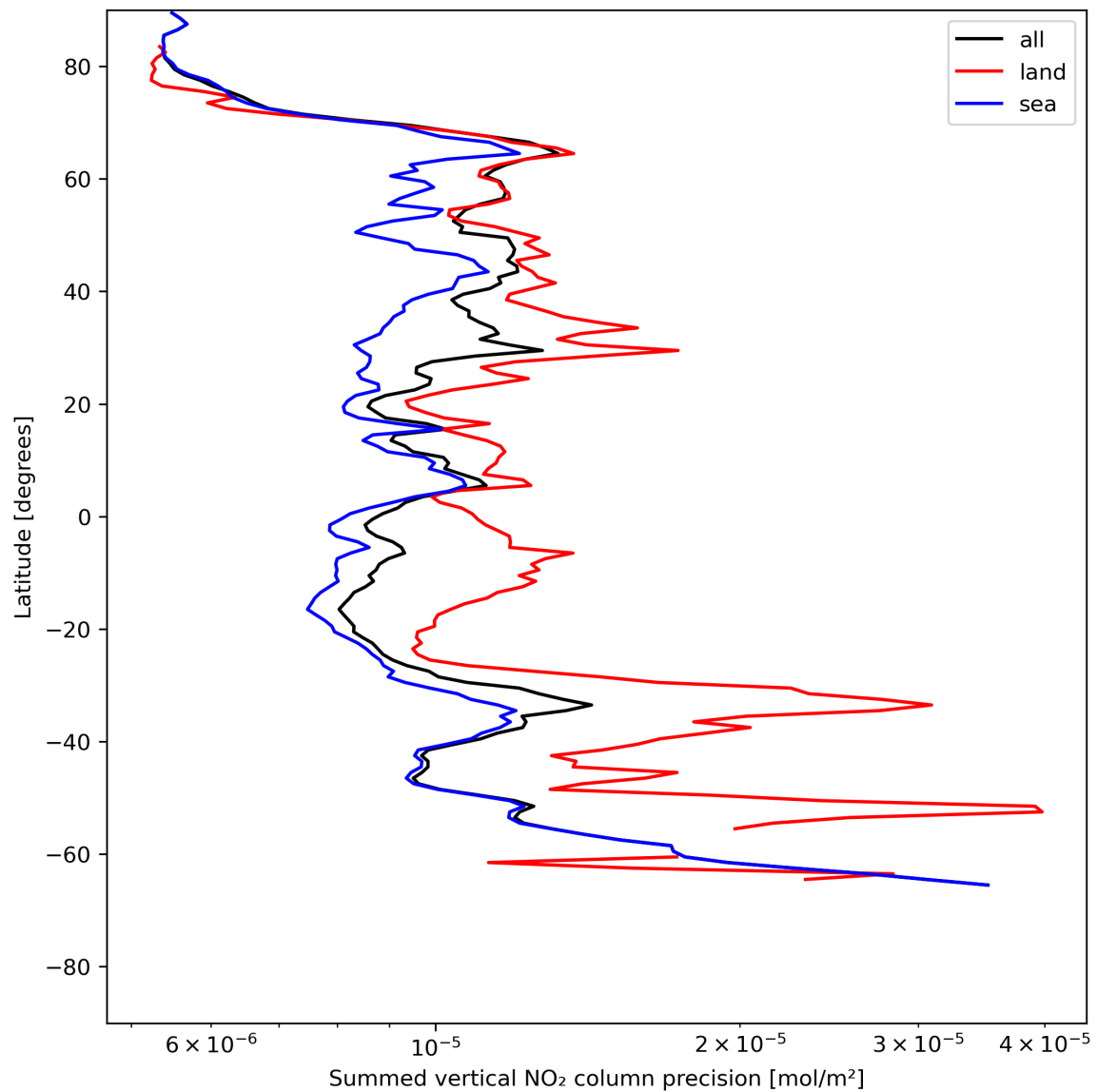
Figure 24: Zonal average of “Summed vertical NO 2 column precision” for 2024-06-01 to 2024-06-03.
