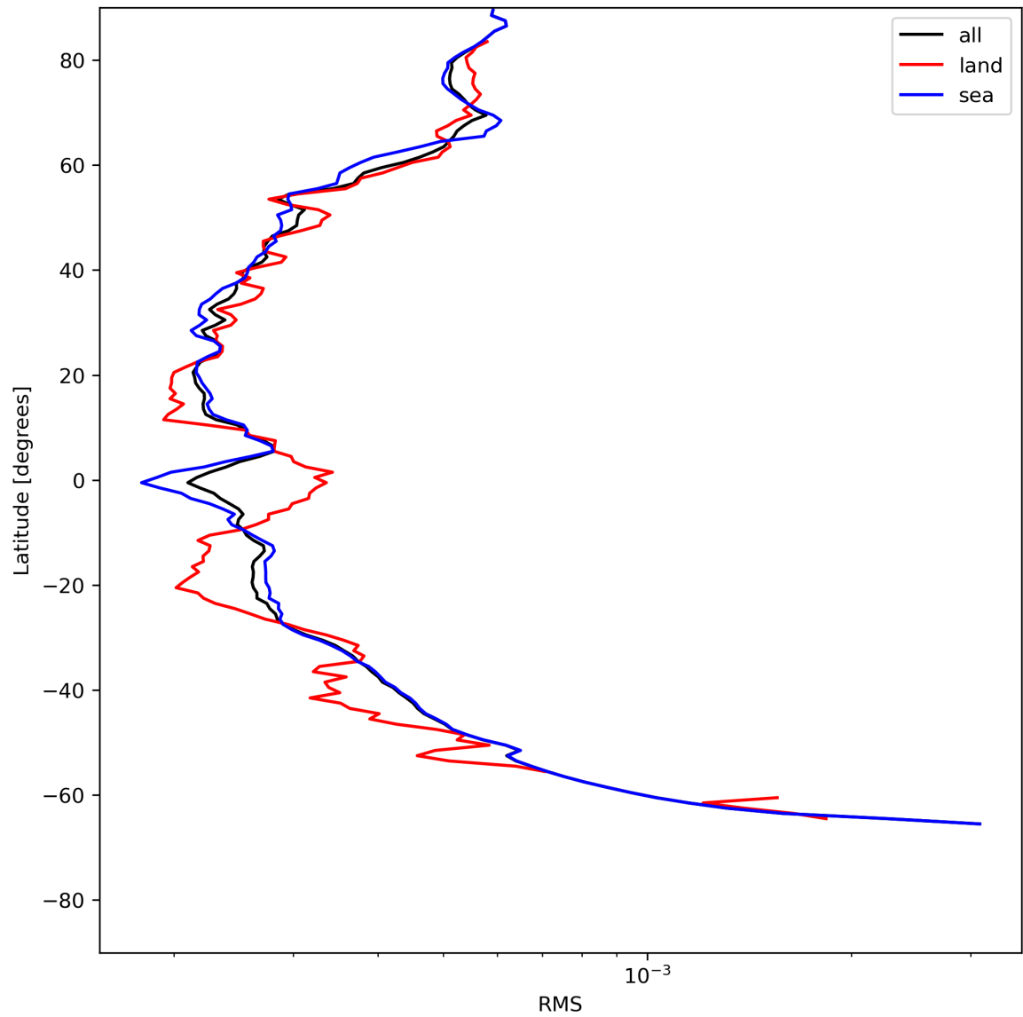
Figure 26: Zonal average of “RMS” for 2024-06-01 to 2024-06-03.
