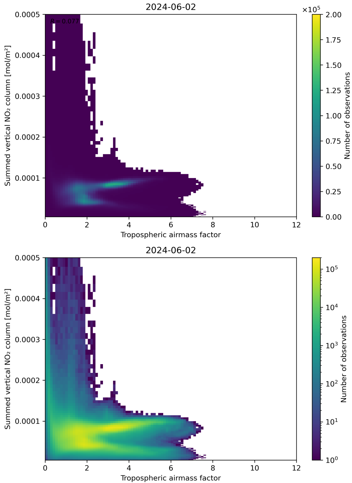
Figure 75: Scatter density plot of “Tropospheric airmass factor” against “Summed vertical NO 2 column” for 2024-06-01 to 2024-06-03.
