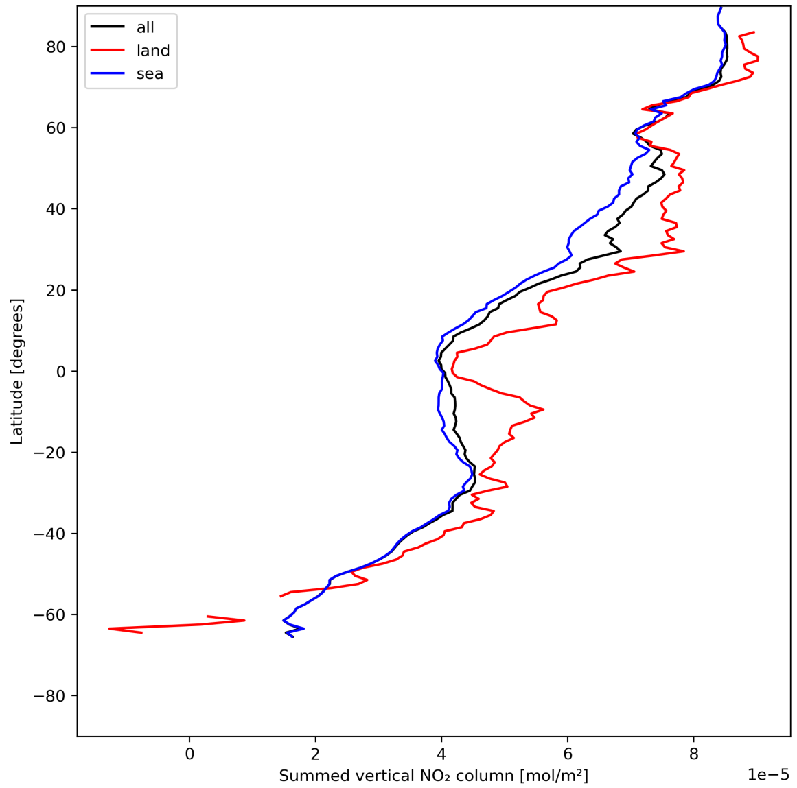
Figure 23: Zonal average of “Summed vertical NO 2 column” for 2024-06-01 to 2024-06-03.
