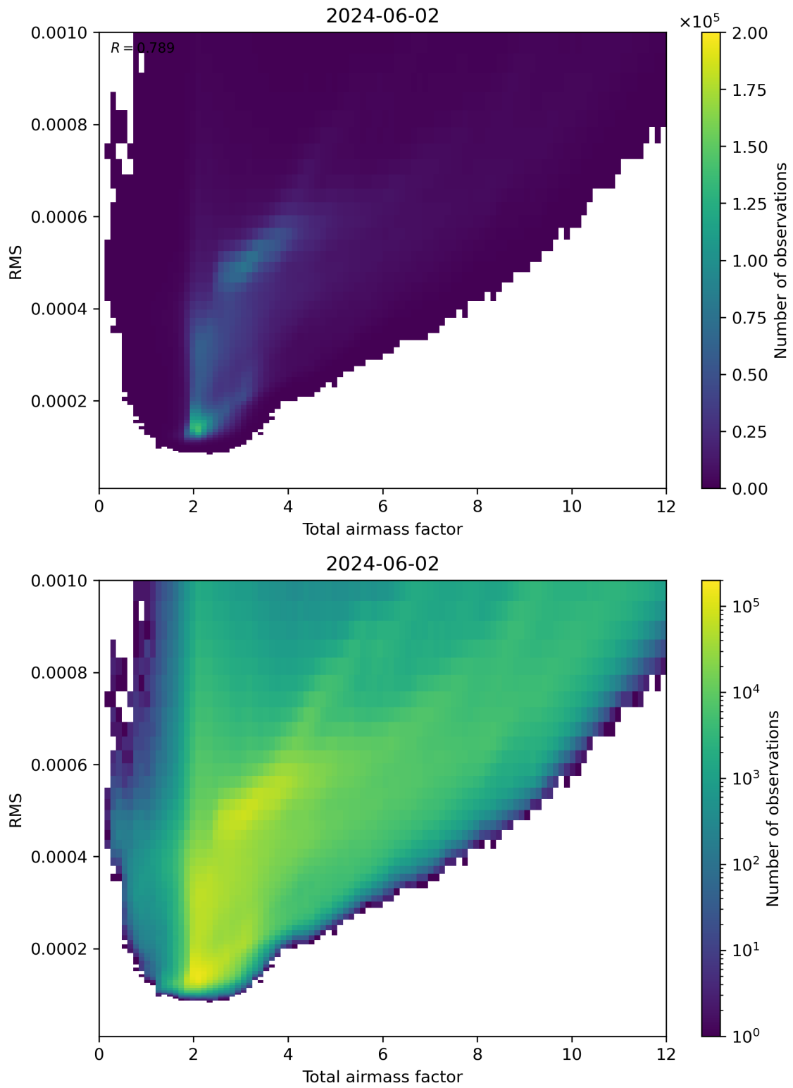
Figure 69: Scatter density plot of “Total airmass factor” against “RMS” for 2024-06-01 to 2024-06-03.
