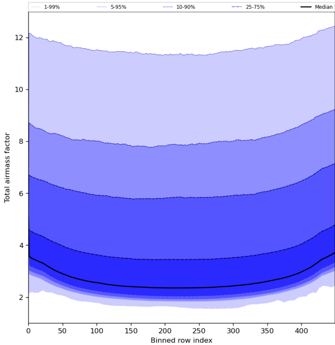
Figure 49: Along track statistics of “Total airmass factor” for 2024-06-01 to 2024-06-03
