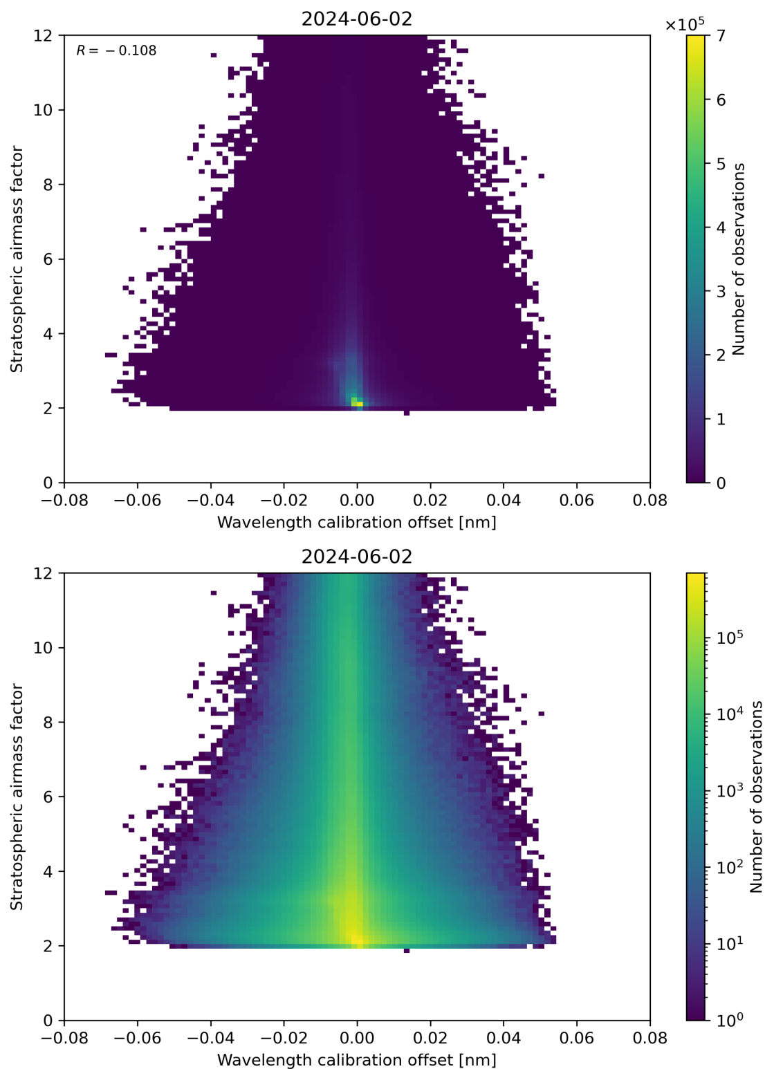
Figure 174: Scatter density plot of “Wavelength calibration offset” against “Stratospheric airmass factor” for 2024-06-01 to 2024-06-03.
