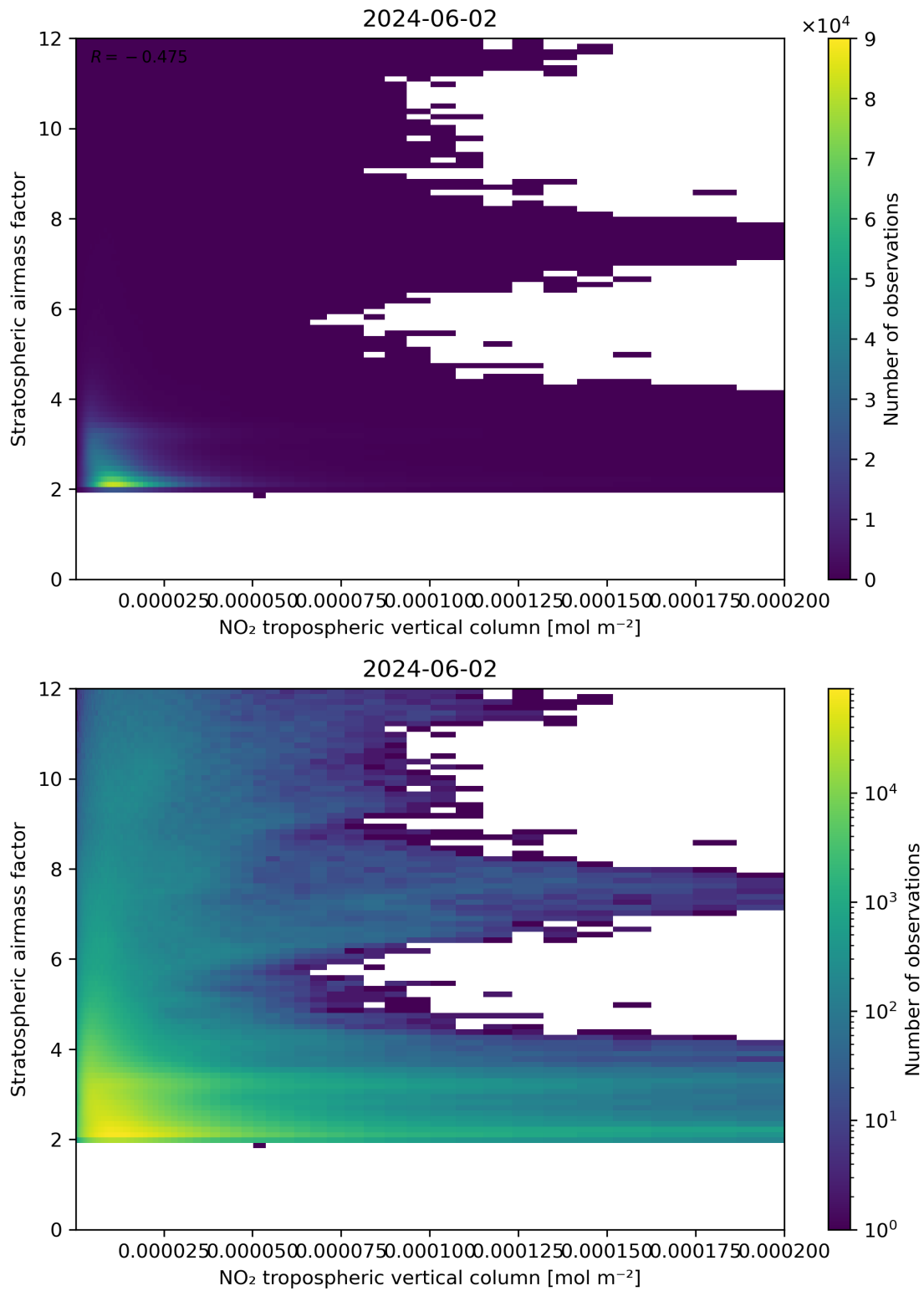
Figure 121: Scatter density plot of “NO 2 tropospheric vertical column” against “Stratospheric air mass factor” for 2024-06-01 to 2024-06-03.
