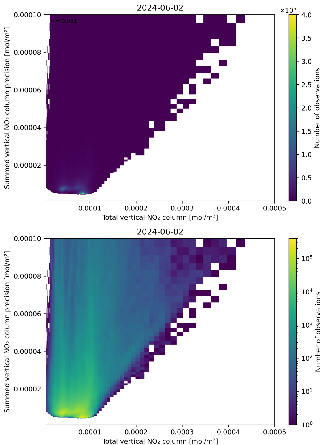
Figure 113: Scatter density plot of “Total vertical NO 2 column” against “Summed vertical NO 2 column precision” for 2024-06-01 to 2024-06-03.
