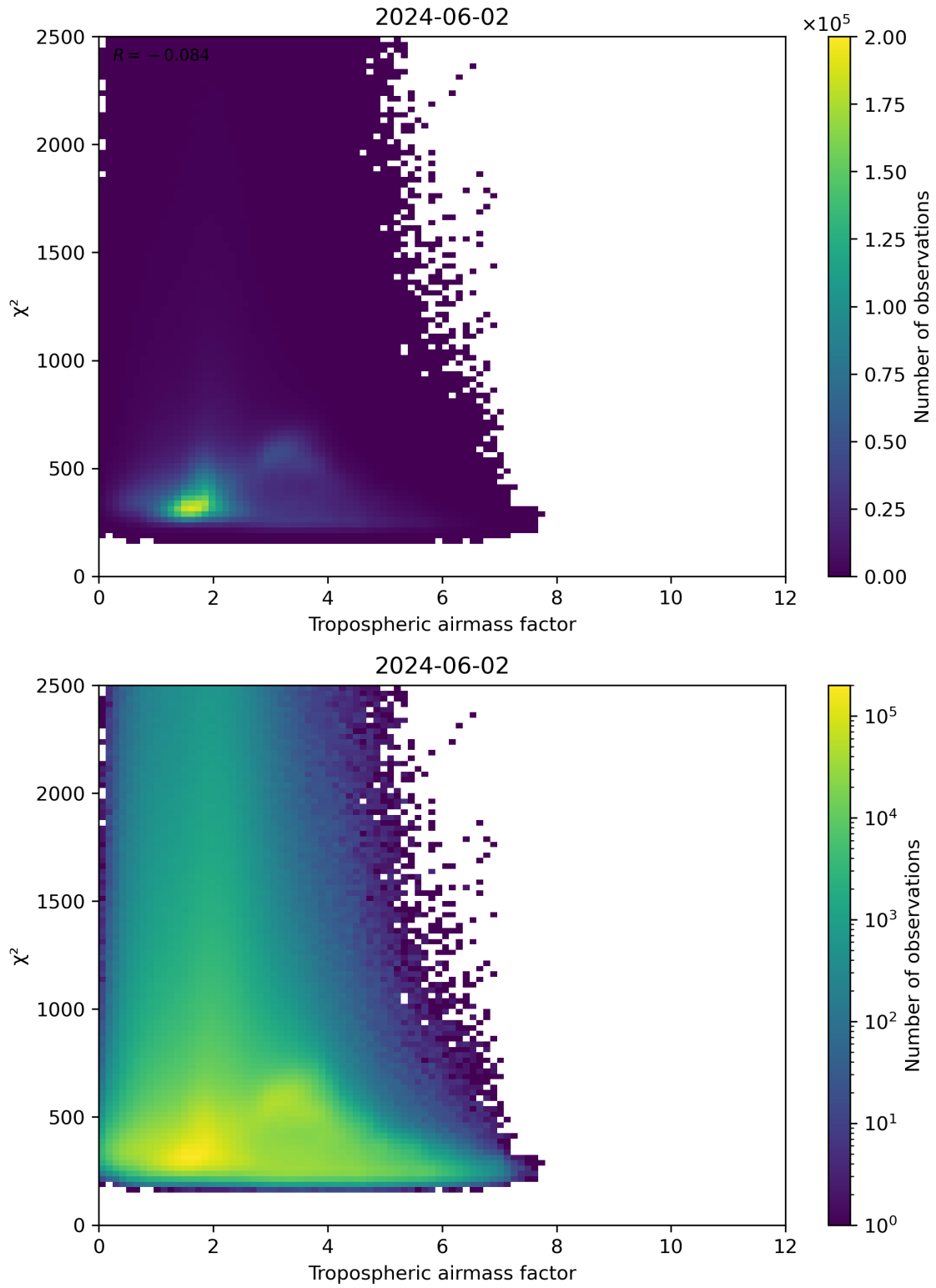
Figure 73: Scatter density plot of “Tropospheric airmass factor” against “ \chi^2 ” for 2024-06-01 to 2024-06-03.
