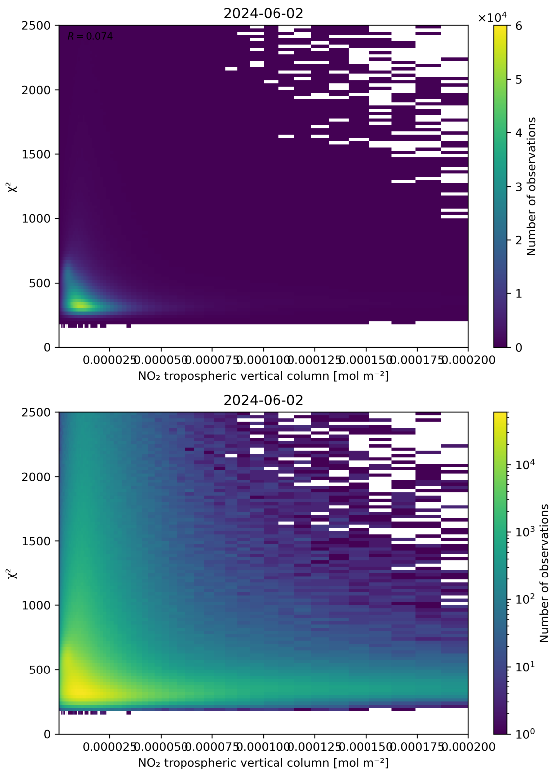
Figure 124: Scatter density plot of “NO 2 tropospheric vertical column” against “ \chi^2 ” for 2024-06-01 to 2024-06-03.
