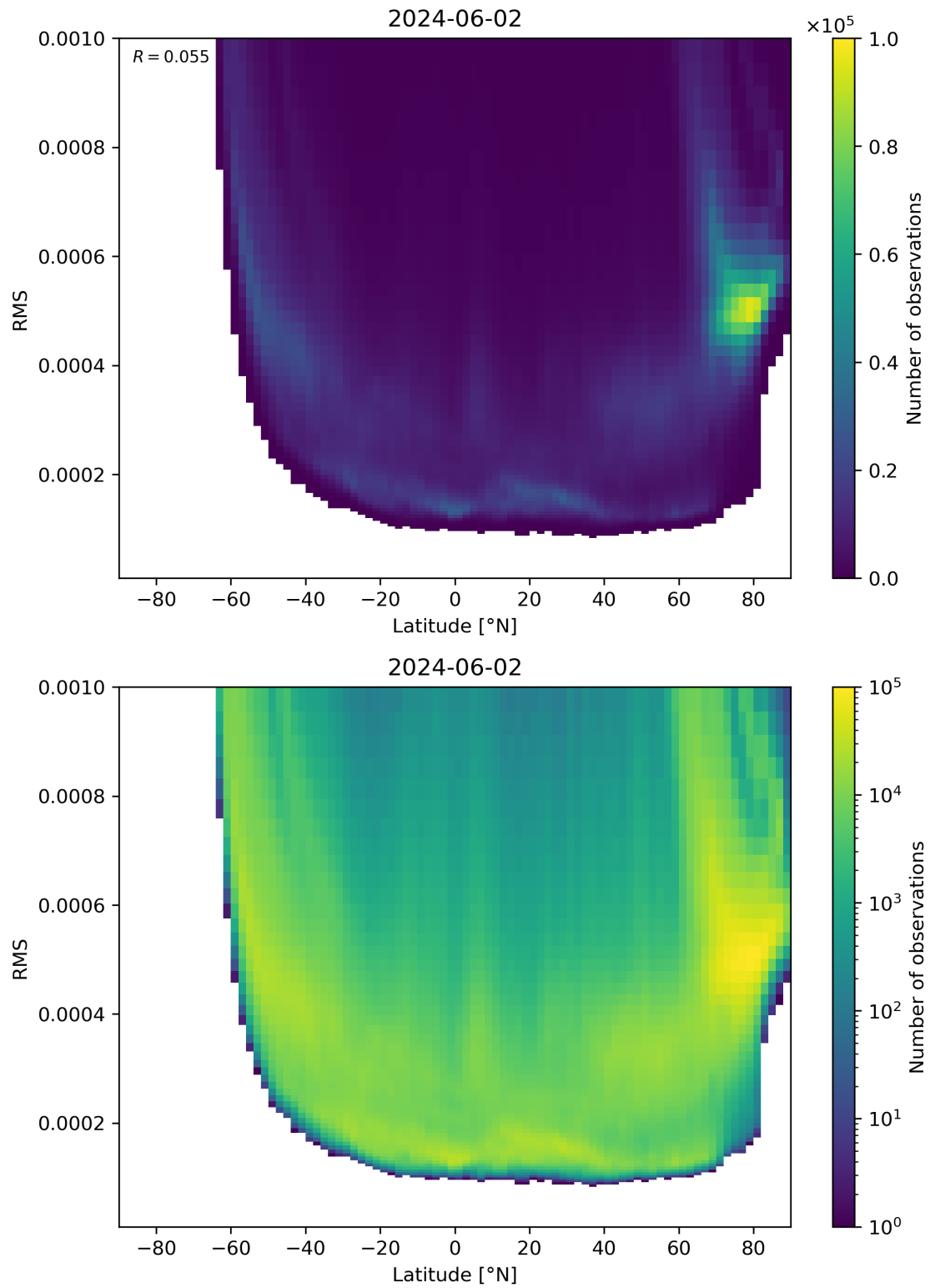
Figure 94: Scatter density plot of “Latitude” against “RMS” for 2024-06-01 to 2024-06-03.
