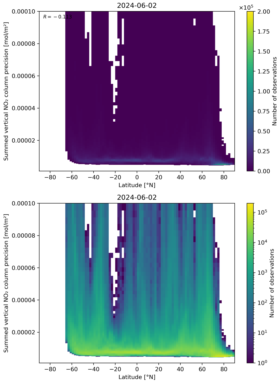
Figure 89: Scatter density plot of “Latitude” against “Summed vertical NO 2 column precision” for 2024-06-01 to 2024-06-03.
