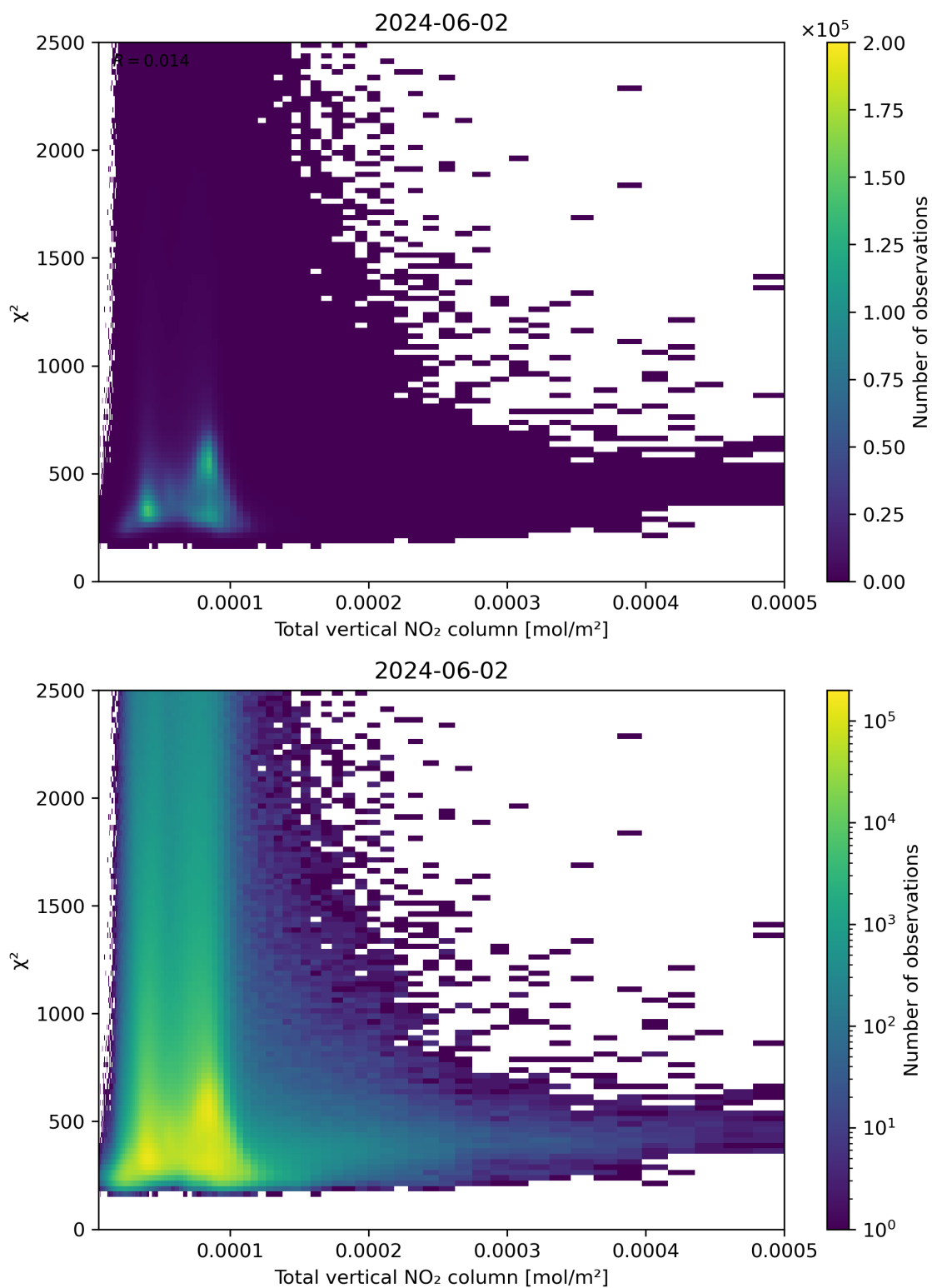
Figure 111: Scatter density plot of “Total vertical NO 2 column” against “ \chi^2 ” for 2024-06-01 to 2024-06-03.
