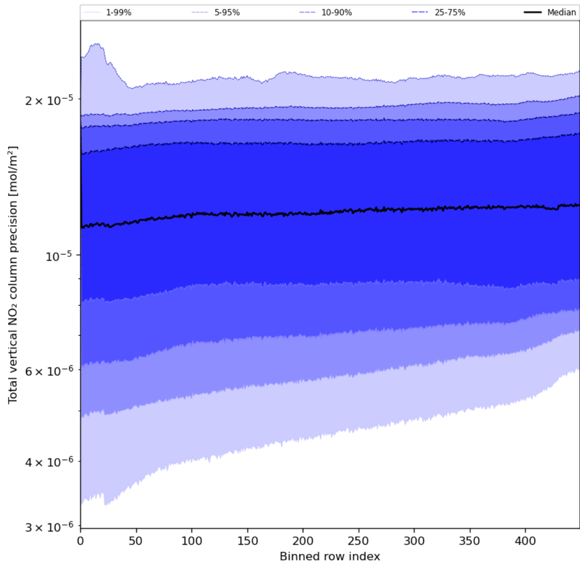
Figure 56: Along track statistics of “Total vertical NO 2 column precision” for 2024-06-01 to 2024-06-03
