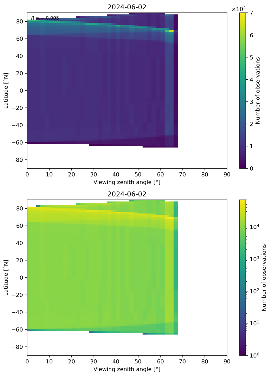
Figure 163: Scatter density plot of “Viewing zenith angle” against “Latitude” for 2024-06-01 to 2024-06-03.
