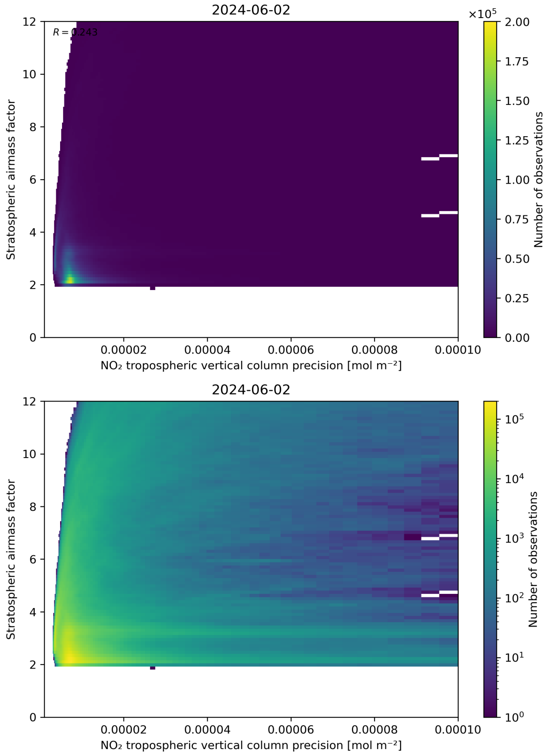
Figure 131: Scatter density plot of “NO 2 tropospheric vertical column precision” against “Stratospheric airmass factor” for 2024-06-01 to 2024-06-03.
