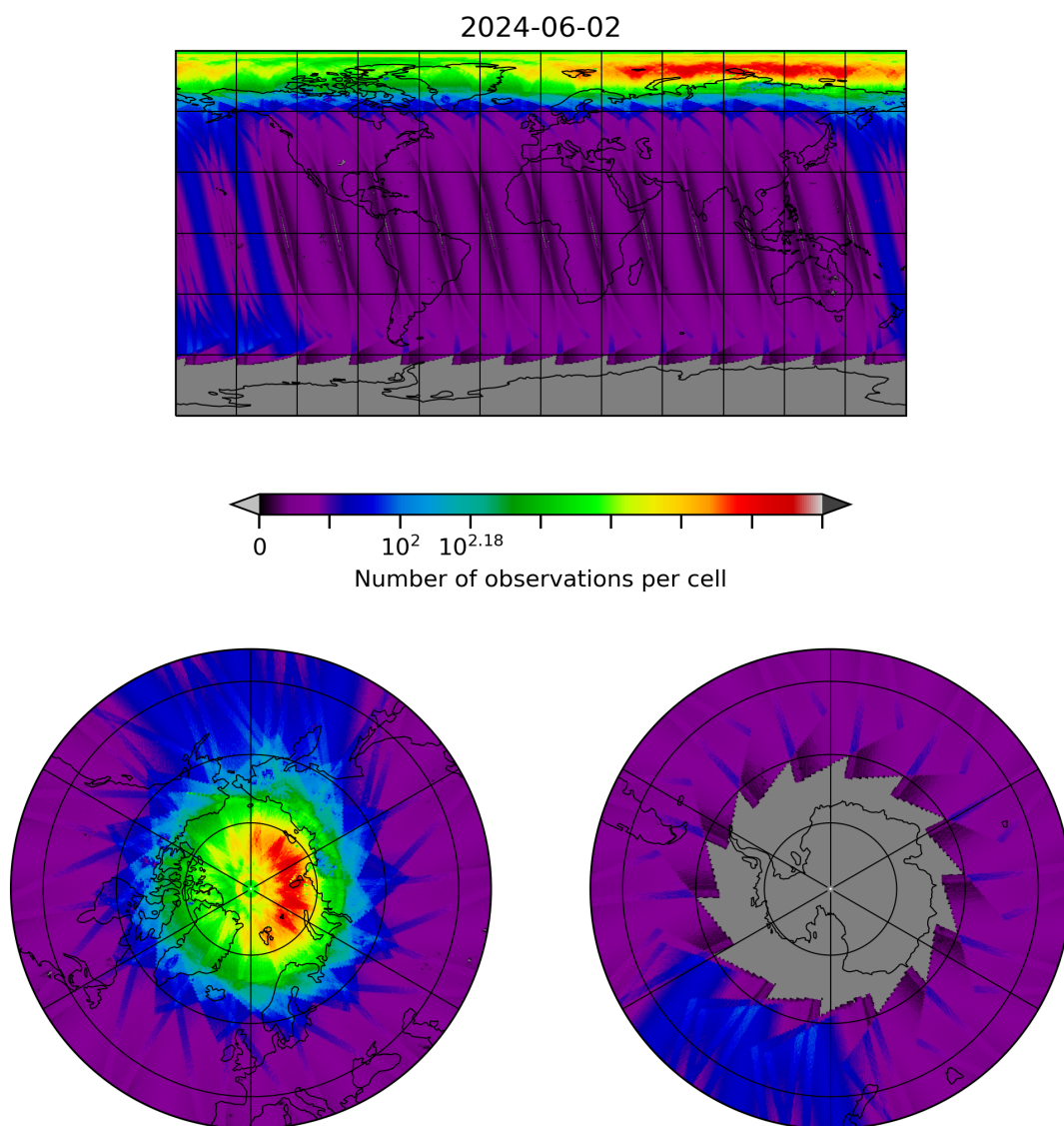
Figure 10: Map of the number of observations for 2024-06-01 to 2024-06-03
