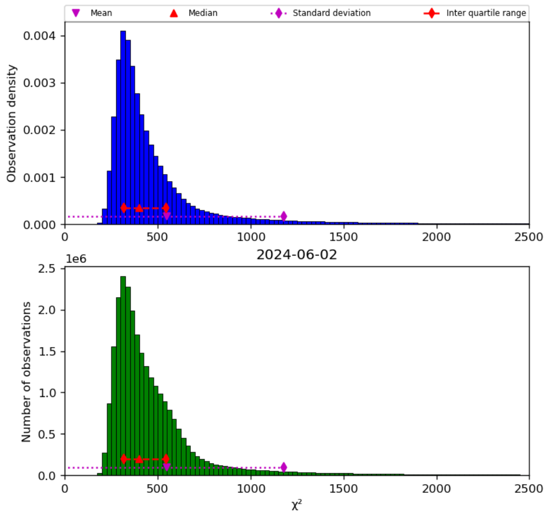
Figure 42: Histogram of “ \chi^2 ” for 2024-06-01 to 2024-06-03
