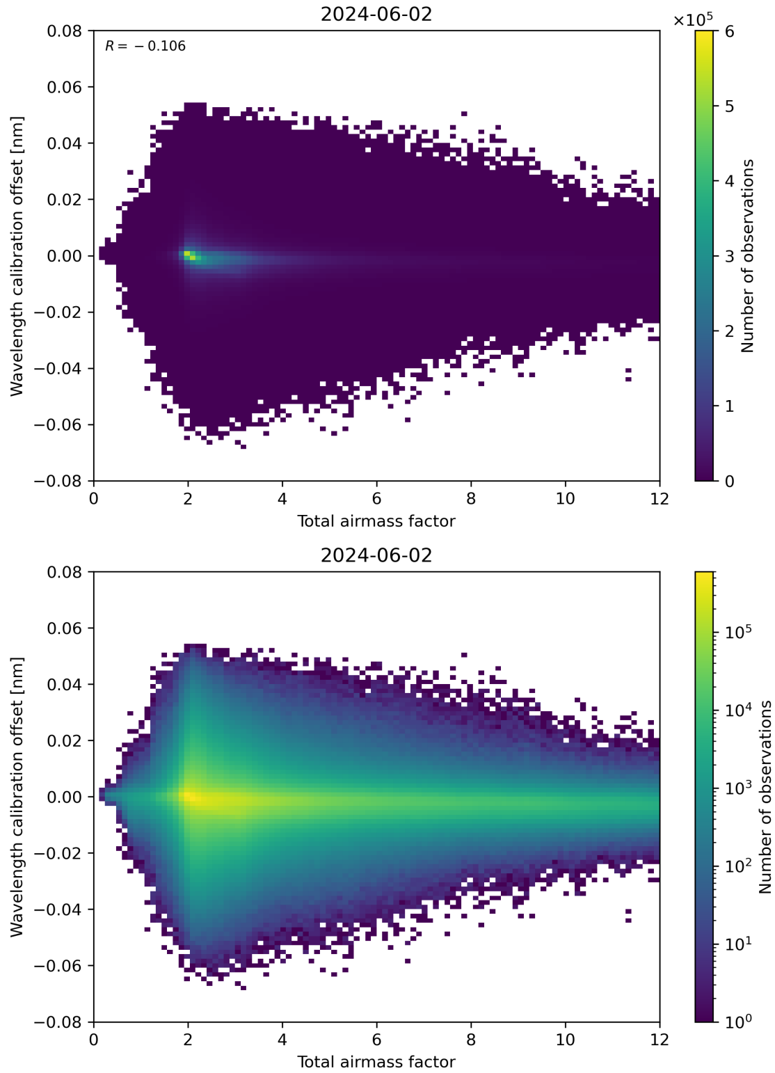
Figure 70: Scatter density plot of “Total airmass factor” against “Wavelength calibration offset” for 2024-06-01 to 2024-06-03.
