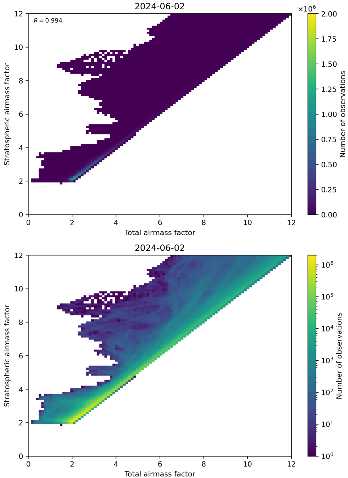
Figure 62: Scatter density plot of “Total airmass factor” against “Stratospheric airmass factor” for 2024-06-01 to 2024-06-03.
