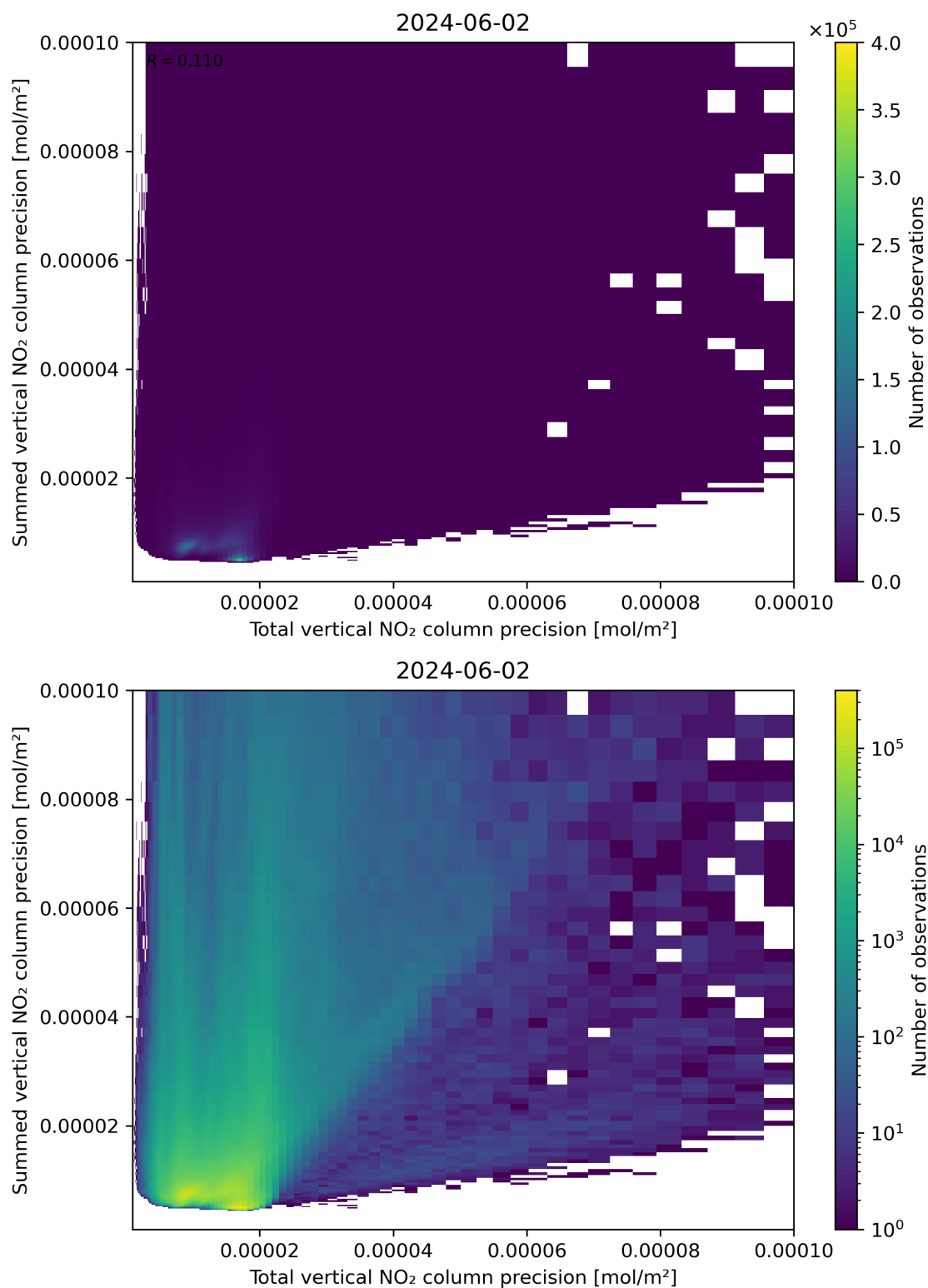
Figure 118: Scatter density plot of “Total vertical NO 2 column precision” against “Summed vertical NO 2 column precision” for 2024-06-01 to 2024-06-03.
