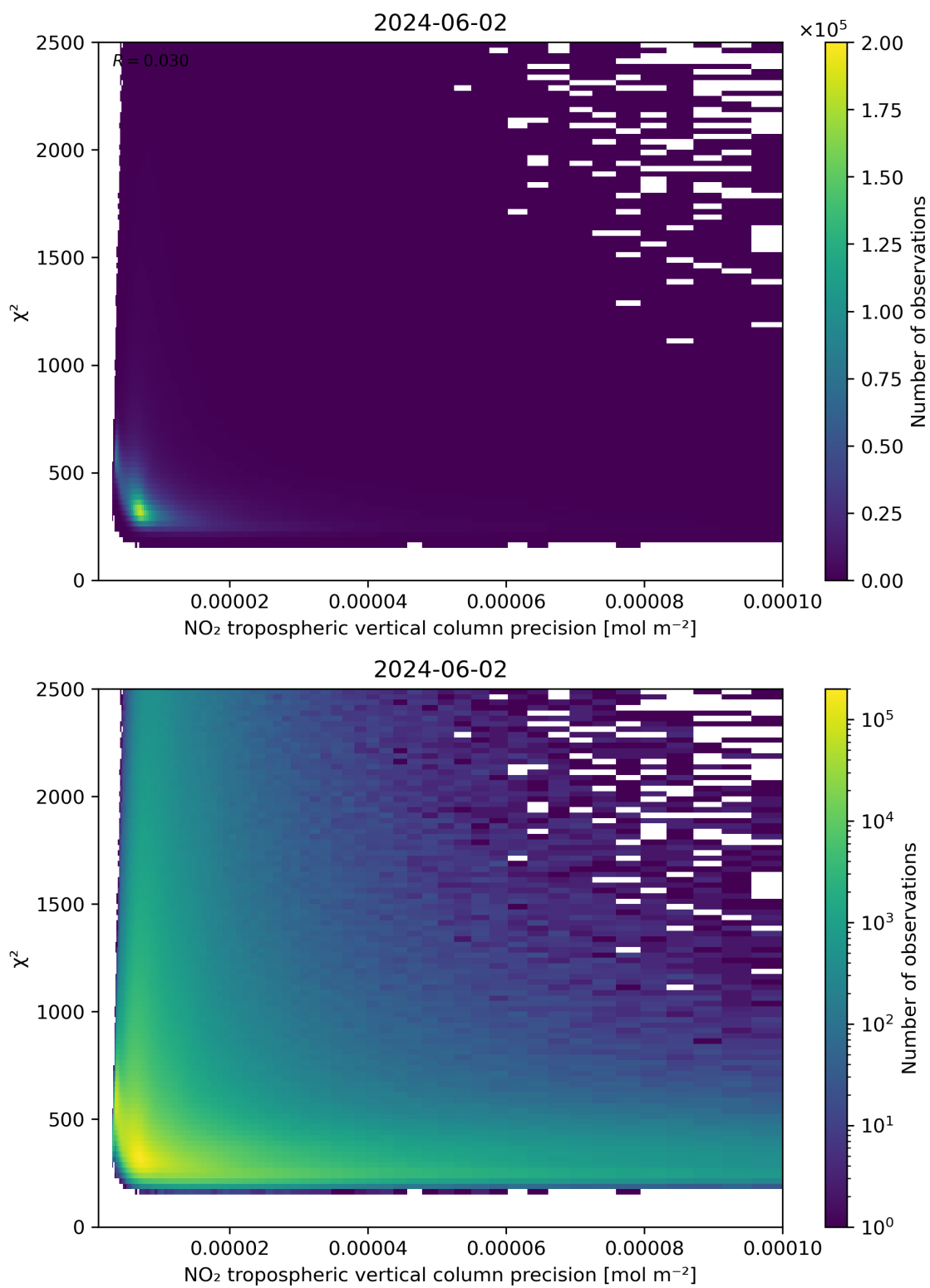
Figure 134: Scatter density plot of “NO 2 tropospheric vertical column precision” against “ \chi^2 ” for 2024-06-01 to 2024-06-03.
