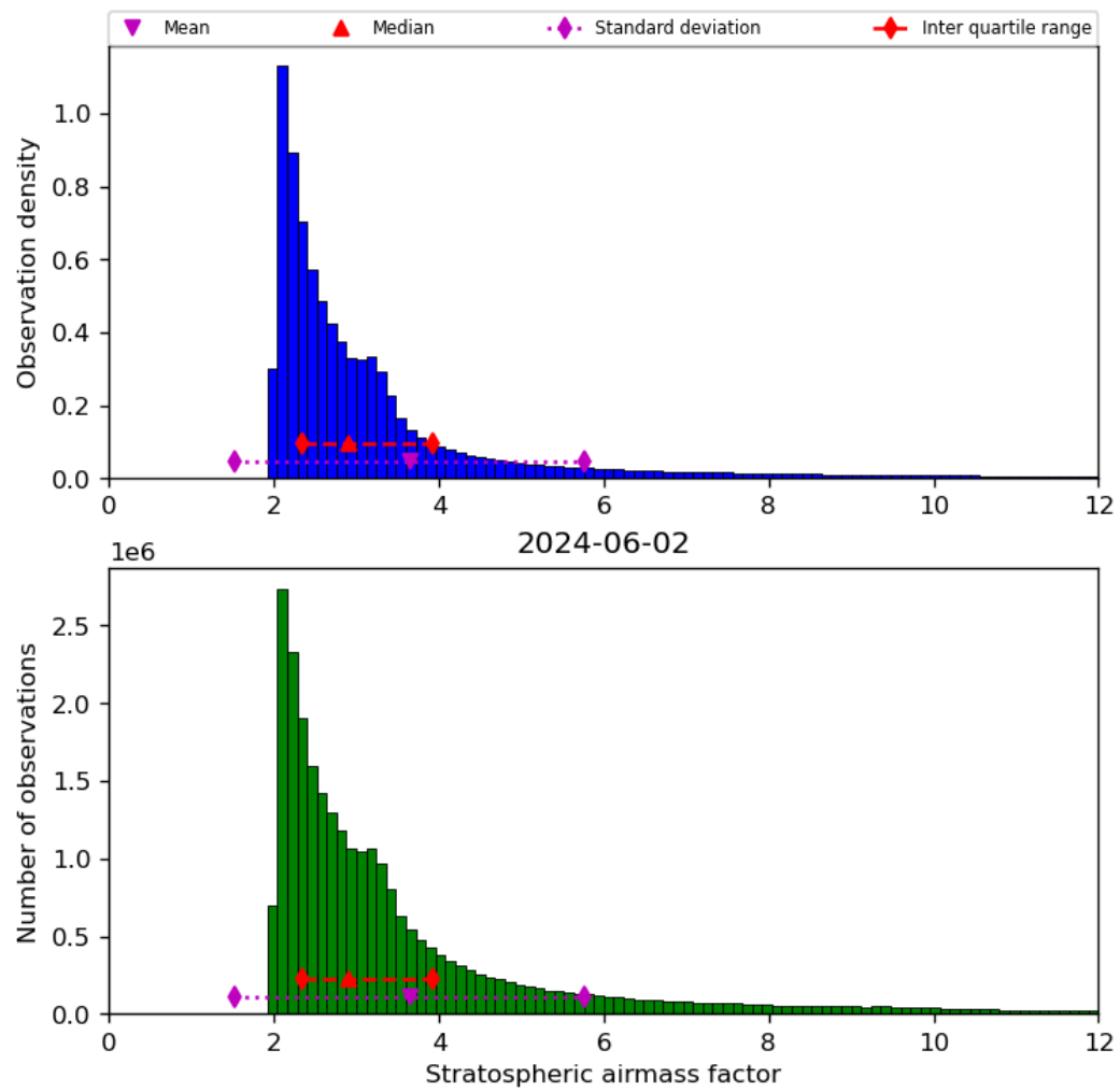
Figure 44: Histogram of “Stratospheric airmass factor” for 2024-06-01 to 2024-06-03
