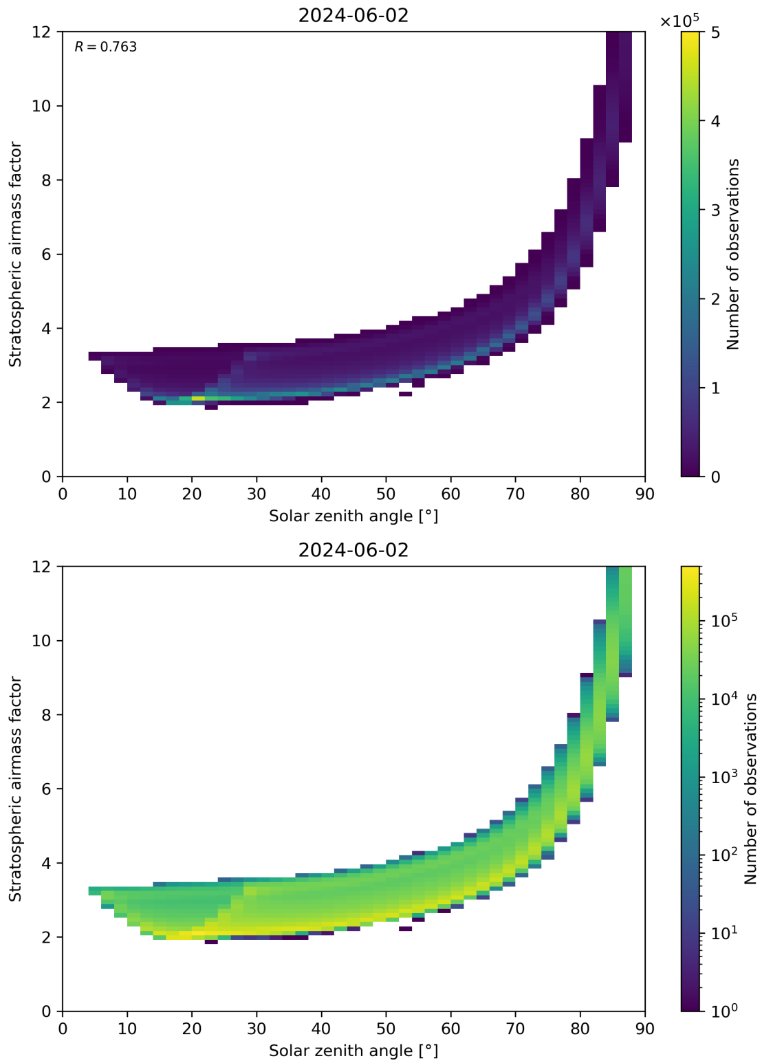
Figure 145: Scatter density plot of “Solar zenith angle” against “Stratospheric airmass factor” for 2024-06-01 to 2024-06-03.
