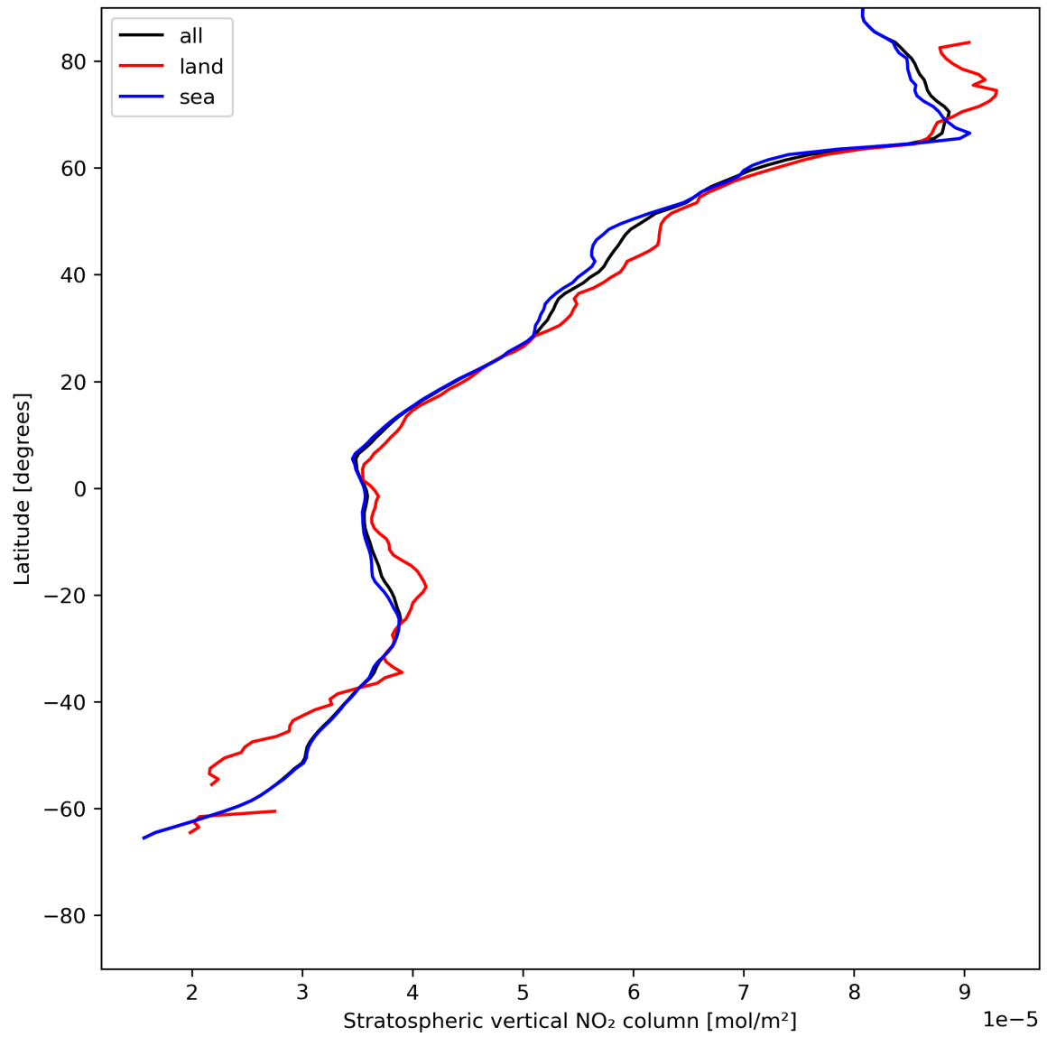
Figure 19: Zonal average of “Stratospheric vertical NO 2 column” for 2024-06-01 to 2024-06-03.
