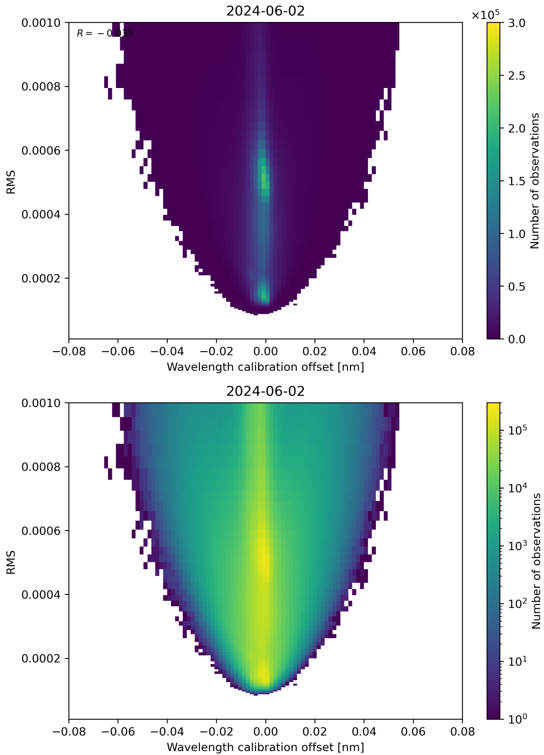
Figure 181: Scatter density plot of “Wavelength calibration offset” against “RMS” for 2024-06-01 to 2024-06-03.
