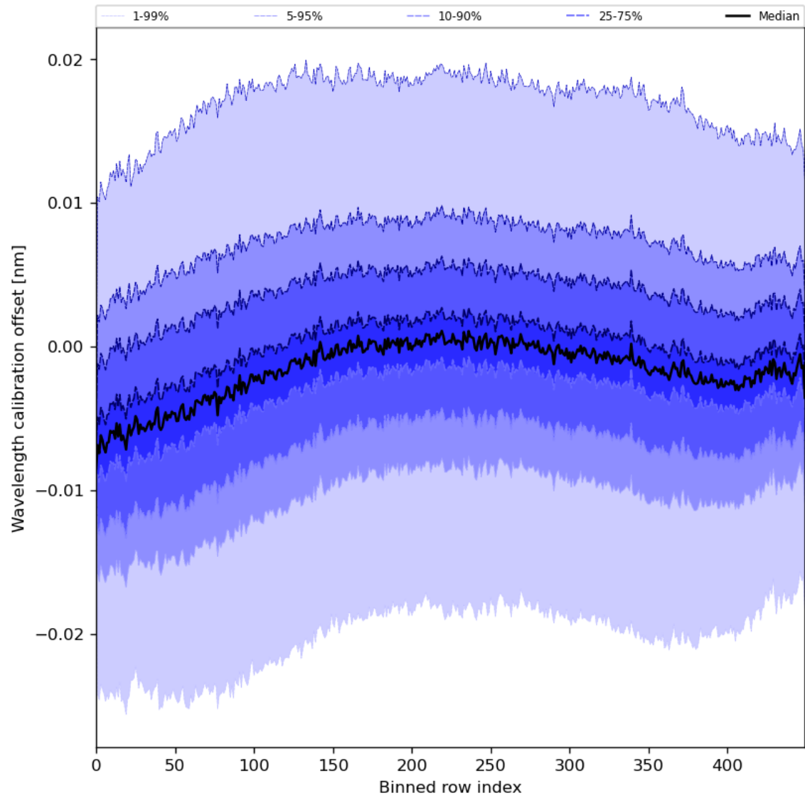
Figure 52: Along track statistics of “Wavelength calibration offset” for 2024-06-01 to 2024-06-03
