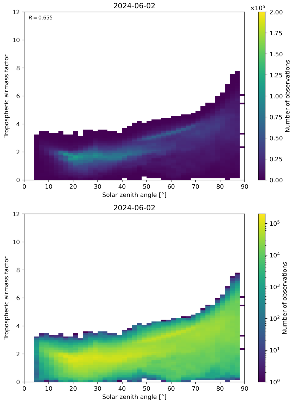
Figure 147: Scatter density plot of “Solar zenith angle” against “Tropospheric airmass factor” for 2024-06-01 to 2024-06-03.
