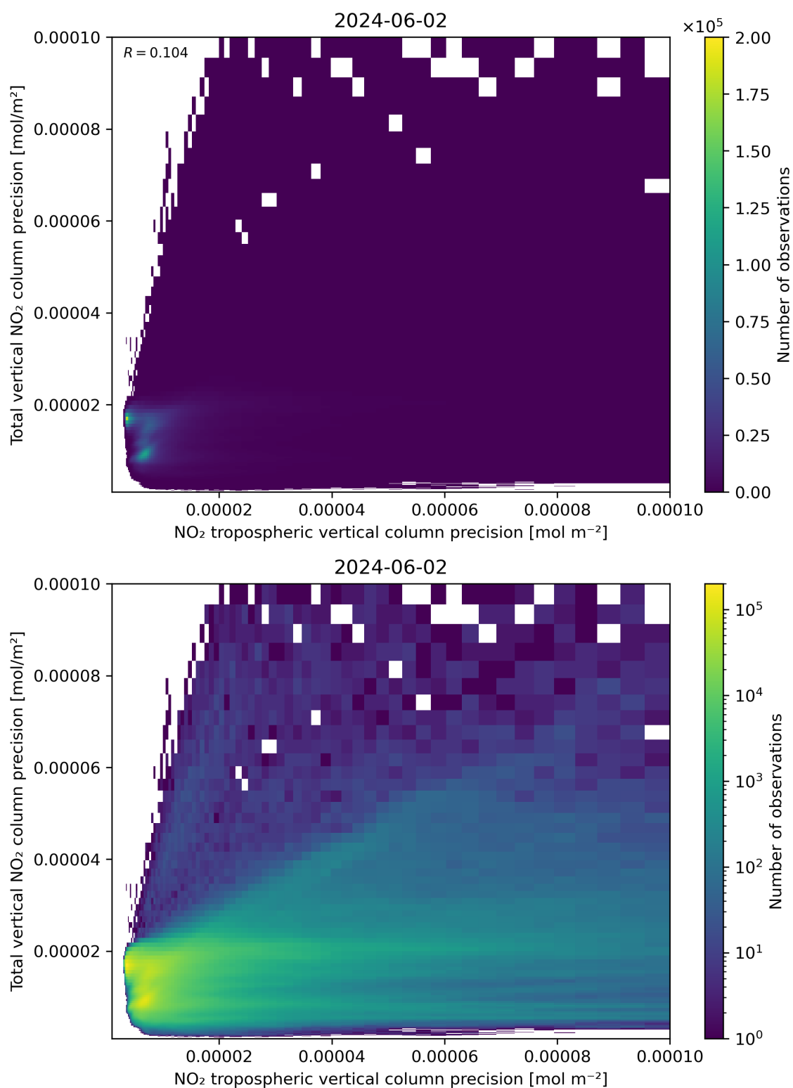
Figure 139: Scatter density plot of “NO 2 tropospheric vertical column precision” against “Total vertical NO 2 column precision” for 2024-06-01 to 2024-06-03.
