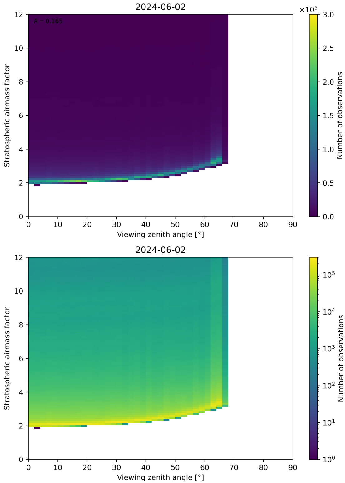
Figure 159: Scatter density plot of “Viewing zenith angle” against “Stratospheric airmass factor” for 2024-06-01 to 2024-06-03.
