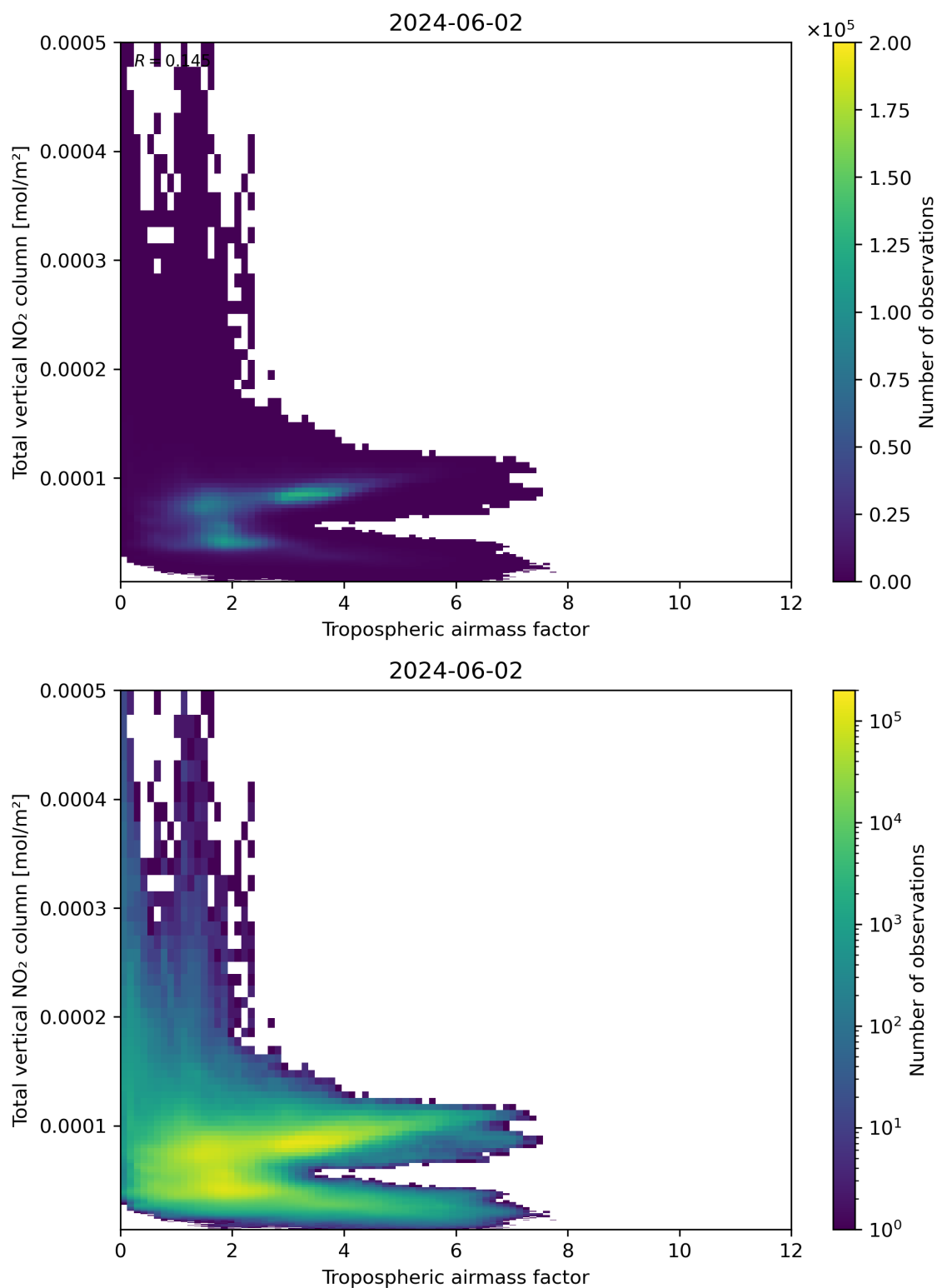
Figure 77: Scatter density plot of “Tropospheric airmass factor” against “Total vertical NO 2 column” for 2024-06-01 to 2024-06-03.
