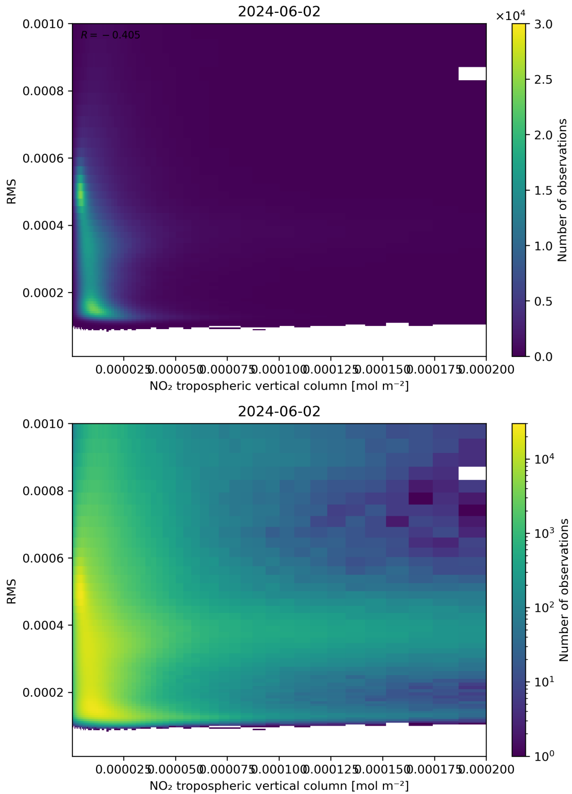
Figure 142: Scatter density plot of “NO 2 tropospheric vertical column” against “RMS” for 2024-06-01 to 2024-06-03.
