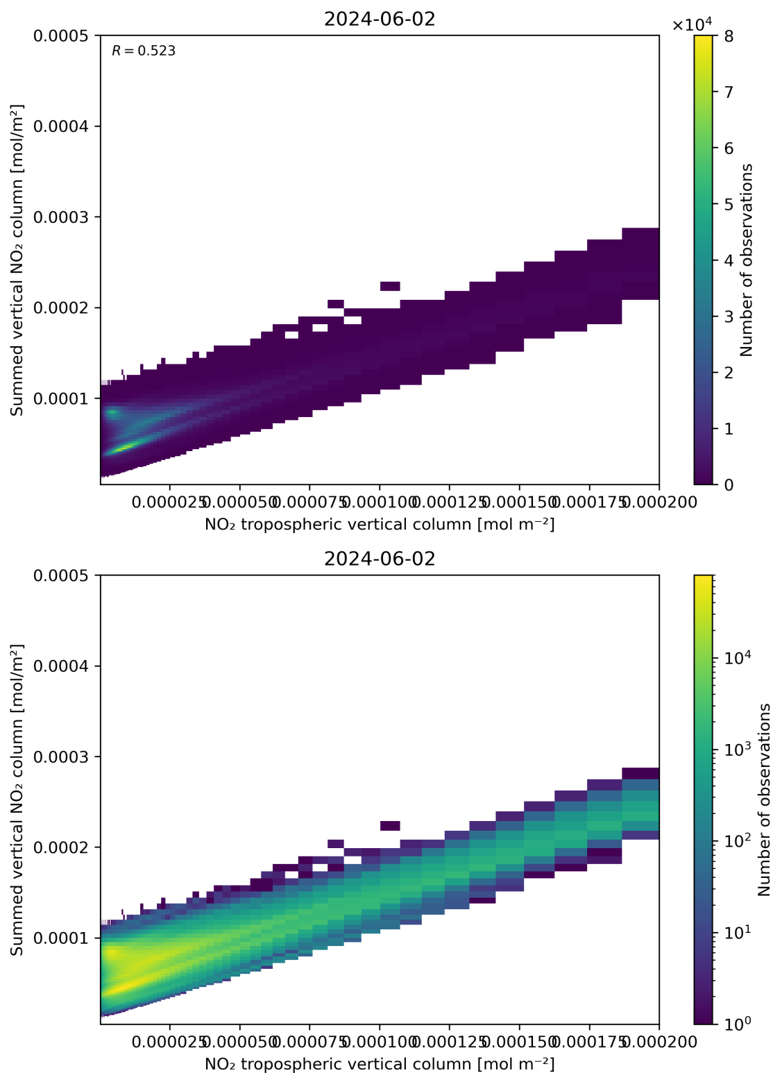
Figure 126: Scatter density plot of “NO 2 tropospheric vertical column” against “Summed vertical NO 2 column” for 2024-06-01 to 2024-06-03.
