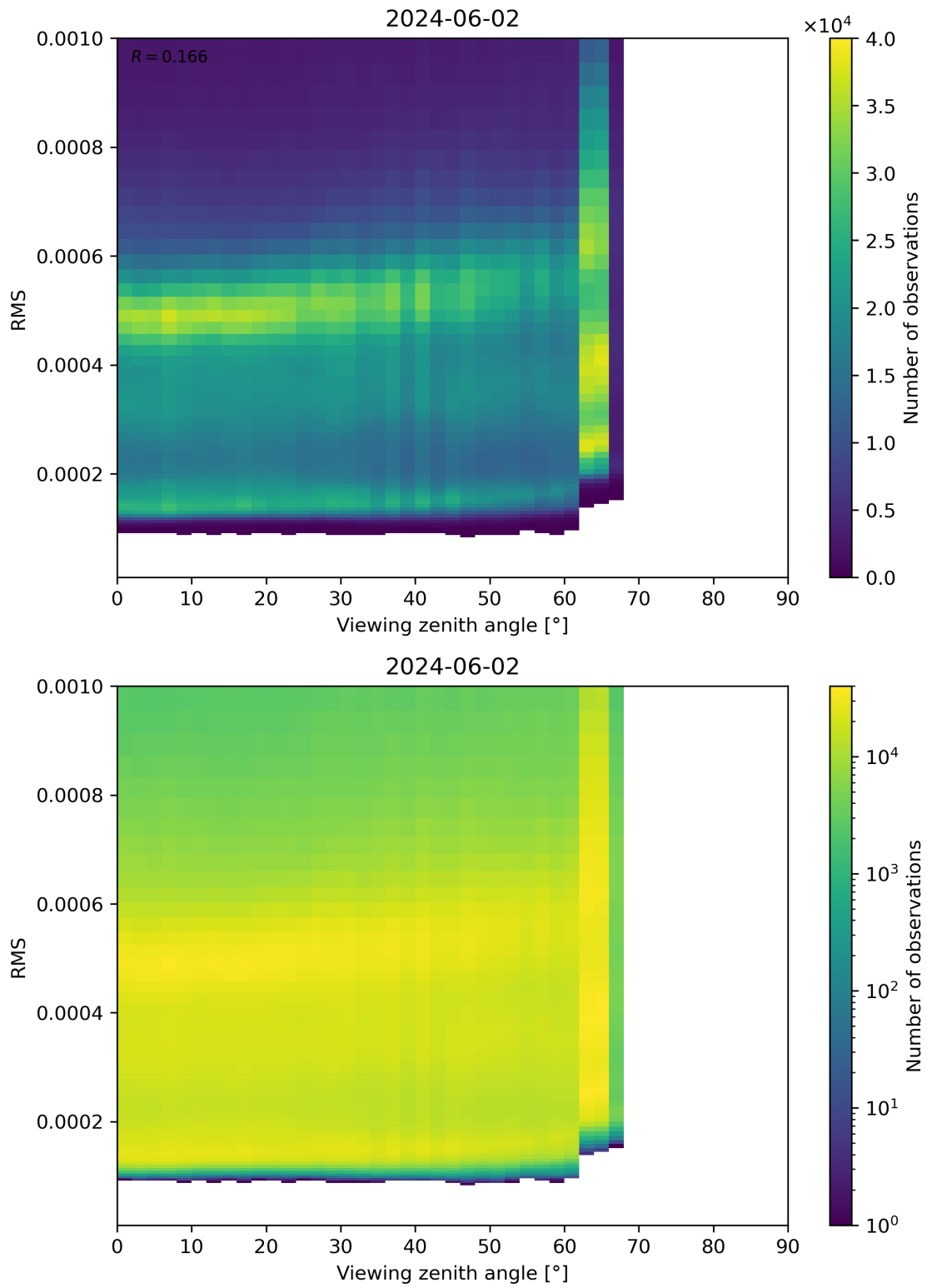
Figure 171: Scatter density plot of “Viewing zenith angle” against “RMS” for 2024-06-01 to 2024-06-03.
