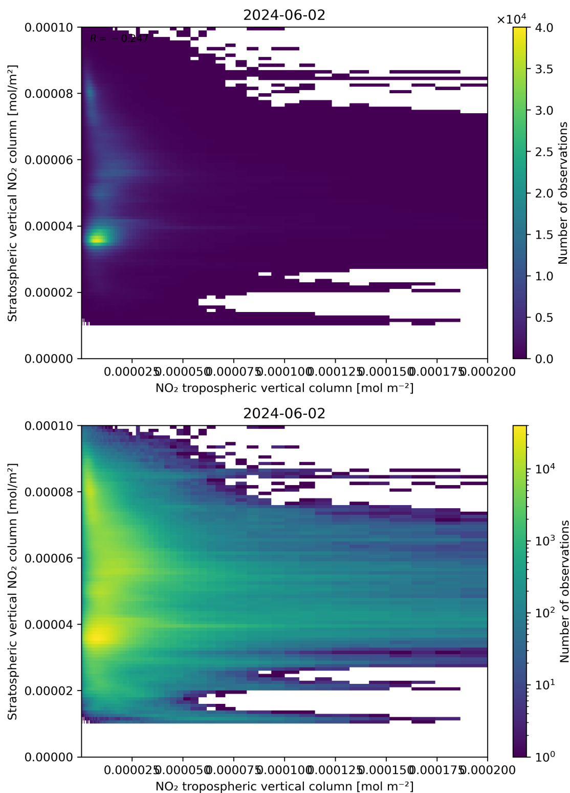
Figure 125: Scatter density plot of “NO 2 tropospheric vertical column” against “Stratospheric vertical NO 2 column” for 2024-06-01 to 2024-06-03.
