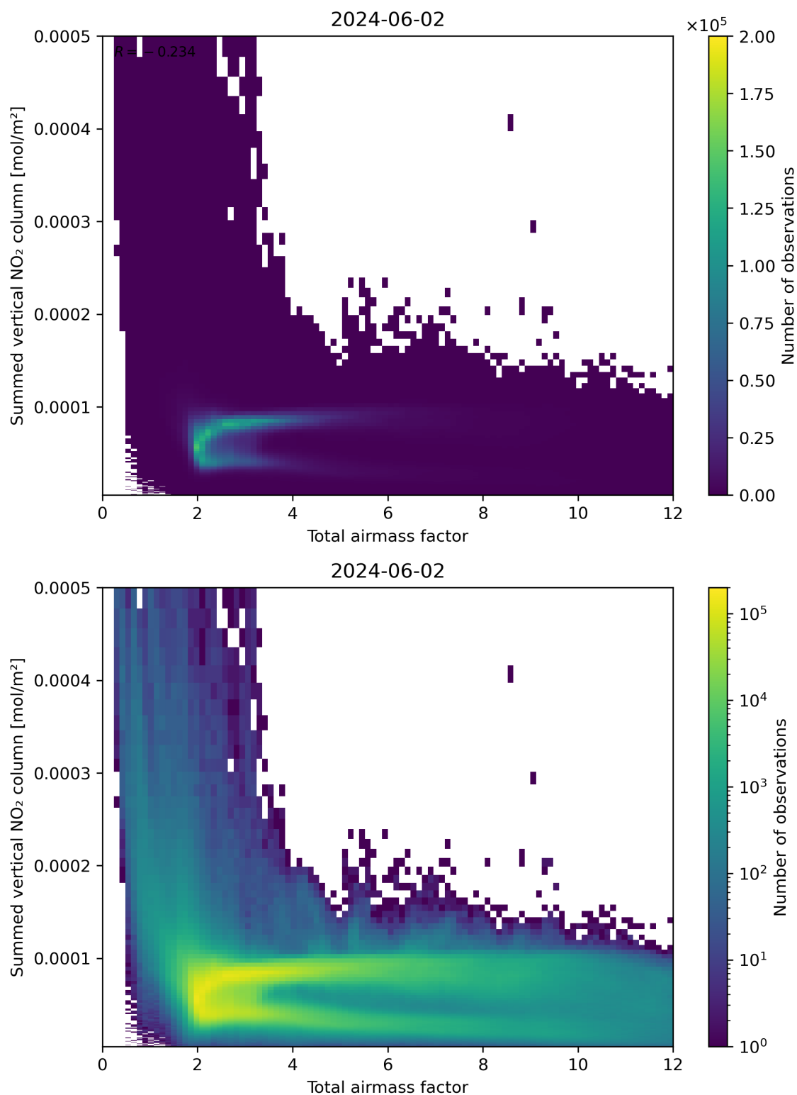
Figure 65: Scatter density plot of “Total airmass factor” against “Summed vertical NO 2 column” for 2024-06-01 to 2024-06-03.
