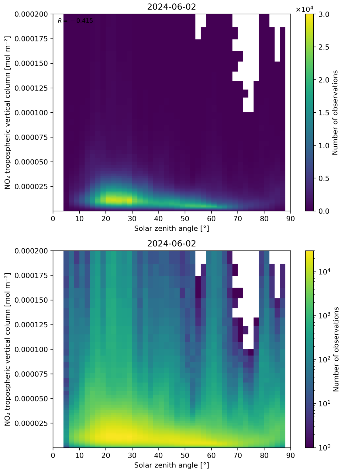
Figure 155: Scatter density plot of “Solar zenith angle” against “NO 2 tropospheric vertical column” for 2024-06-01 to 2024-06-03.
