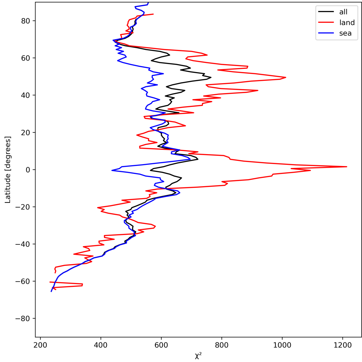
Figure 25: Zonal average of “ \chi^2 ” for 2024-06-01 to 2024-06-03.
