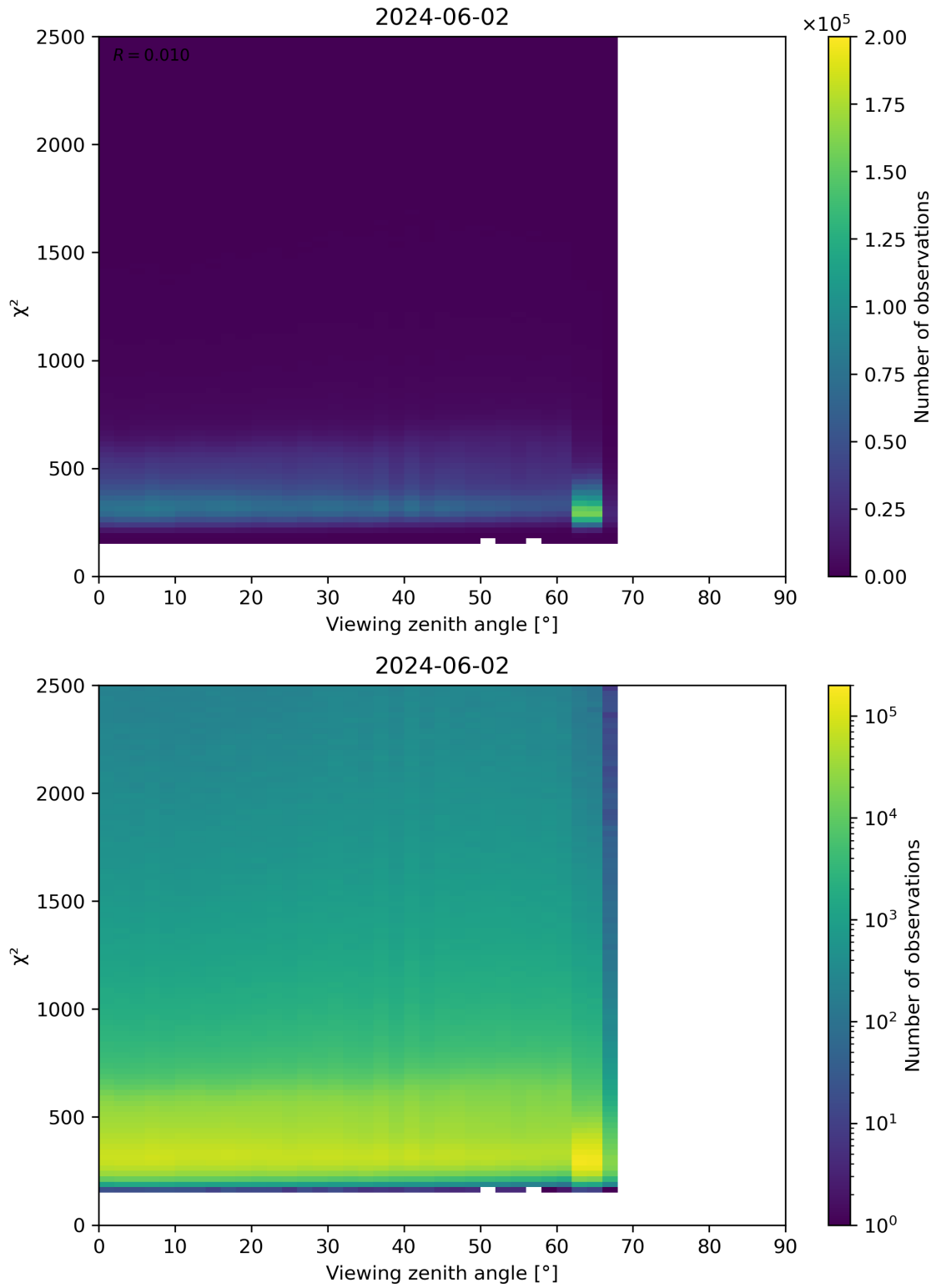
Figure 162: Scatter density plot of “Viewing zenith angle” against “ \chi^2 ” for 2024-06-01 to 2024-06-03.
