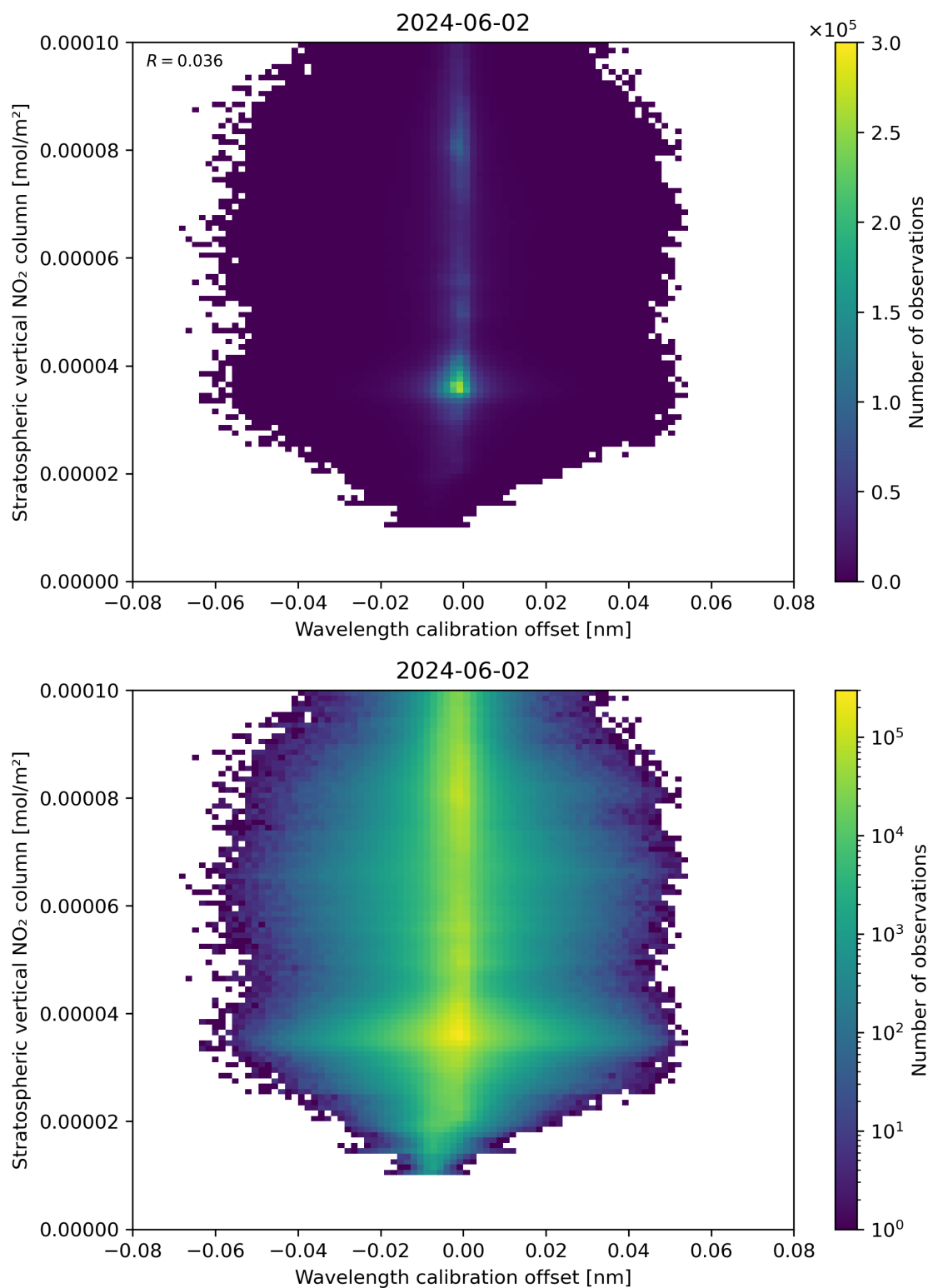
Figure 176: Scatter density plot of “Wavelength calibration offset” against “Stratospheric vertical NO 2 column” for 2024-06-01 to 2024-06-03.
