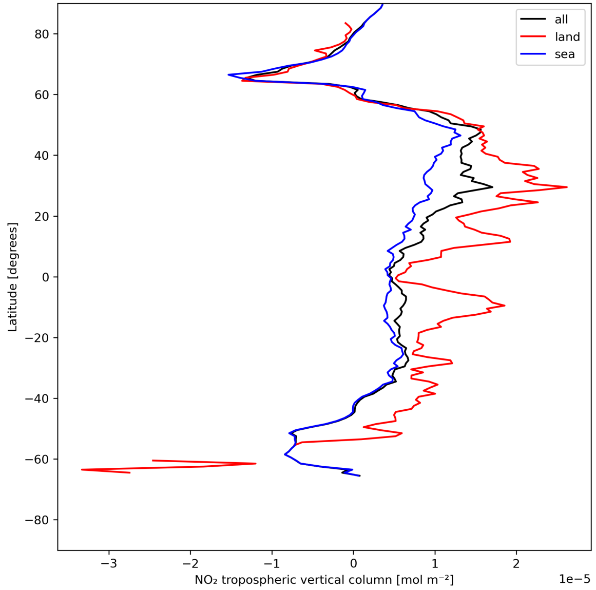
Figure 12: Zonal average of “NO 2 tropospheric vertical column” for 2024-06-01 to 2024-06-03.
