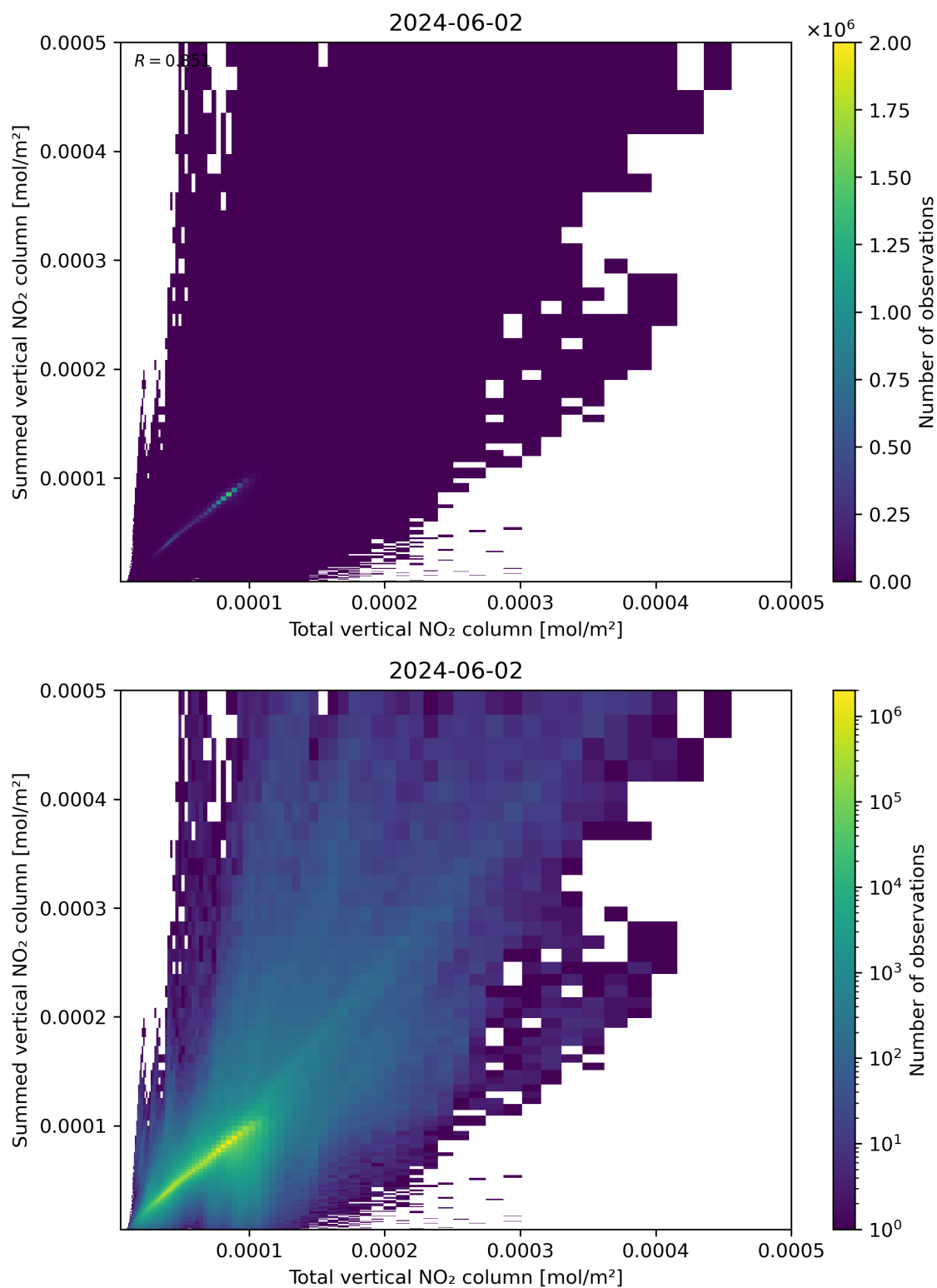
Figure 112: Scatter density plot of “Total vertical NO 2 column” against “Summed vertical NO 2 column” for 2024-06-01 to 2024-06-03.
