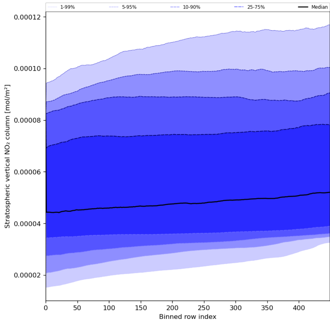
Figure 53: Along track statistics of “Stratospheric vertical NO 2 column” for 2024-06-01 to 2024-06-03
