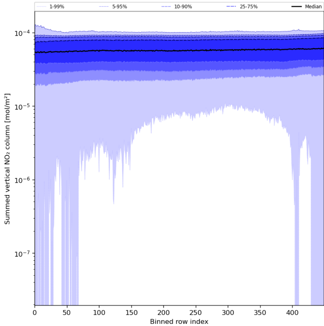
Figure 57: Along track statistics of “Summed vertical NO 2 column” for 2024-06-01 to 2024-06-03
