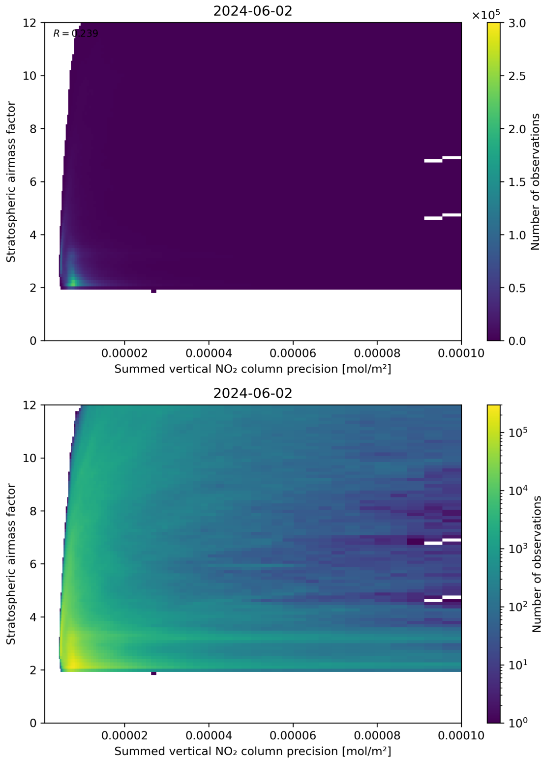
Figure 106: Scatter density plot of “Summed vertical NO 2 column precision” against “Stratospheric airmass factor” for 2024-06-01 to 2024-06-03.
