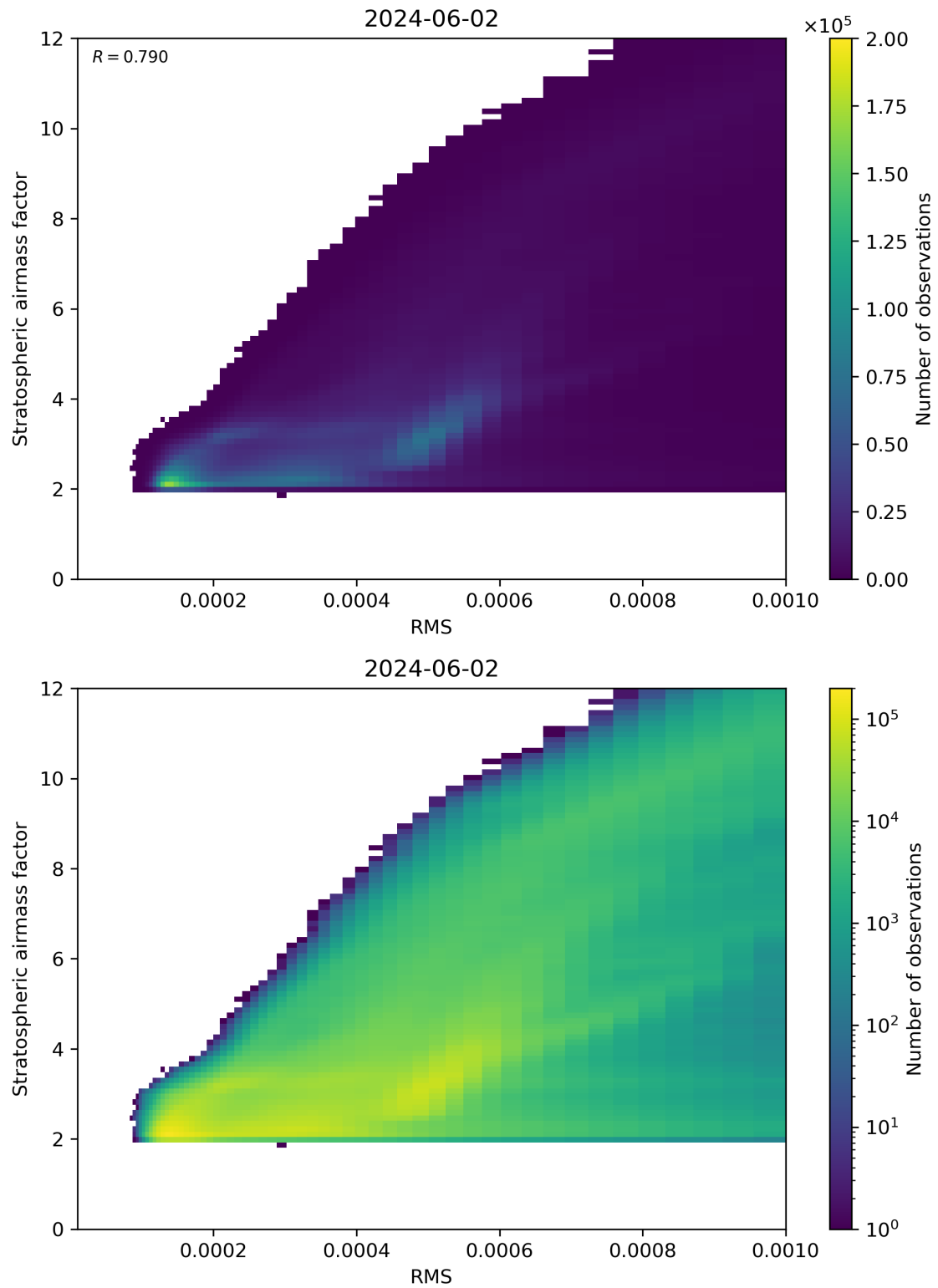
Figure 144: Scatter density plot of “RMS” against “Stratospheric airmass factor” for 2024-06-01 to 2024-06-03.
