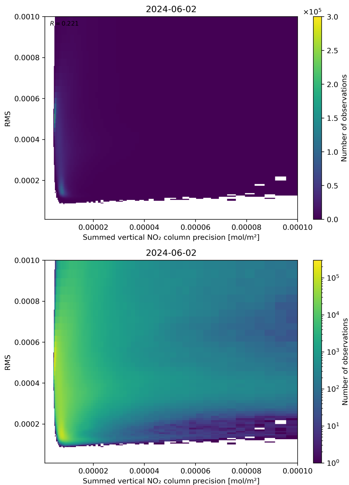
Figure 108: Scatter density plot of “Summed vertical NO 2 column precision” against “RMS” for 2024-06-01 to 2024-06-03.
