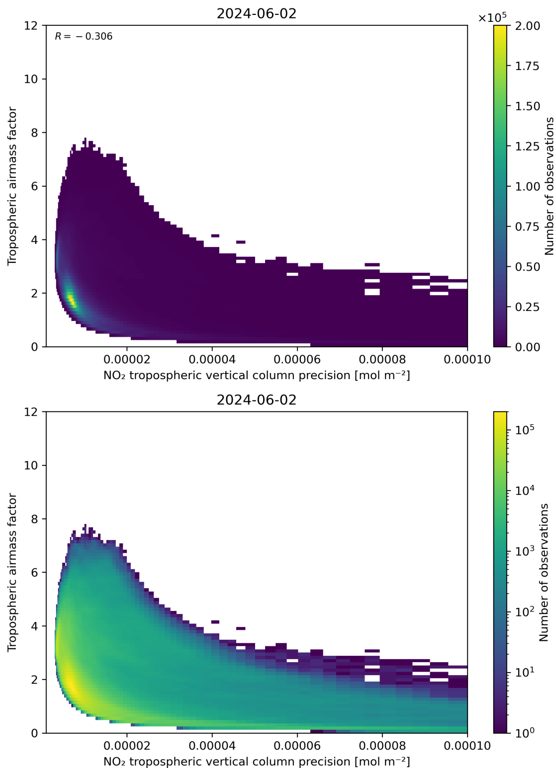
Figure 133: Scatter density plot of “NO 2 tropospheric vertical column precision” against “Tropospheric airmass factor” for 2024-06-01 to 2024-06-03.
