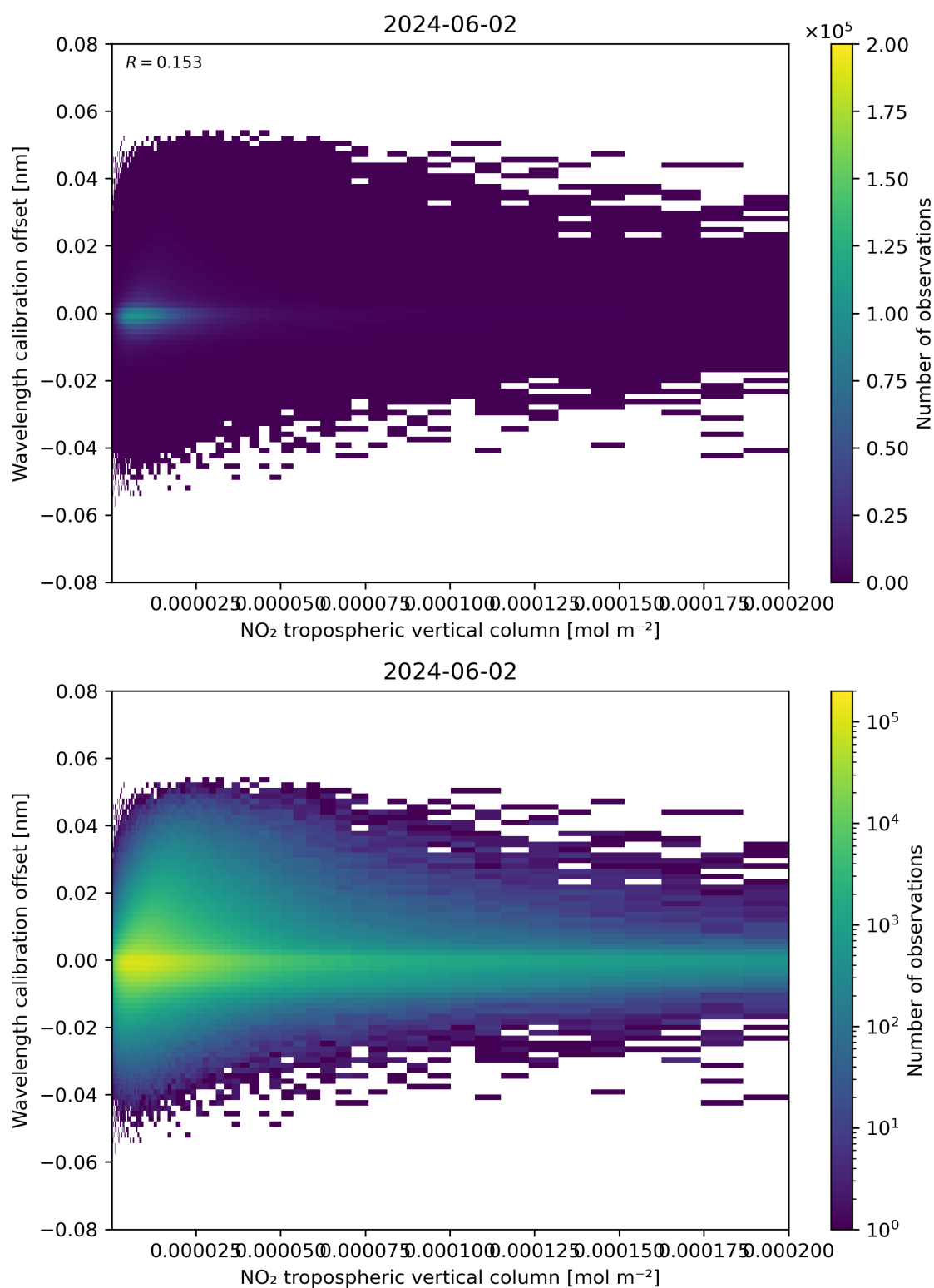
Figure 143: Scatter density plot of “NO 2 tropospheric vertical column” against “Wavelength calibration offset” for 2024-06-01 to 2024-06-03.
