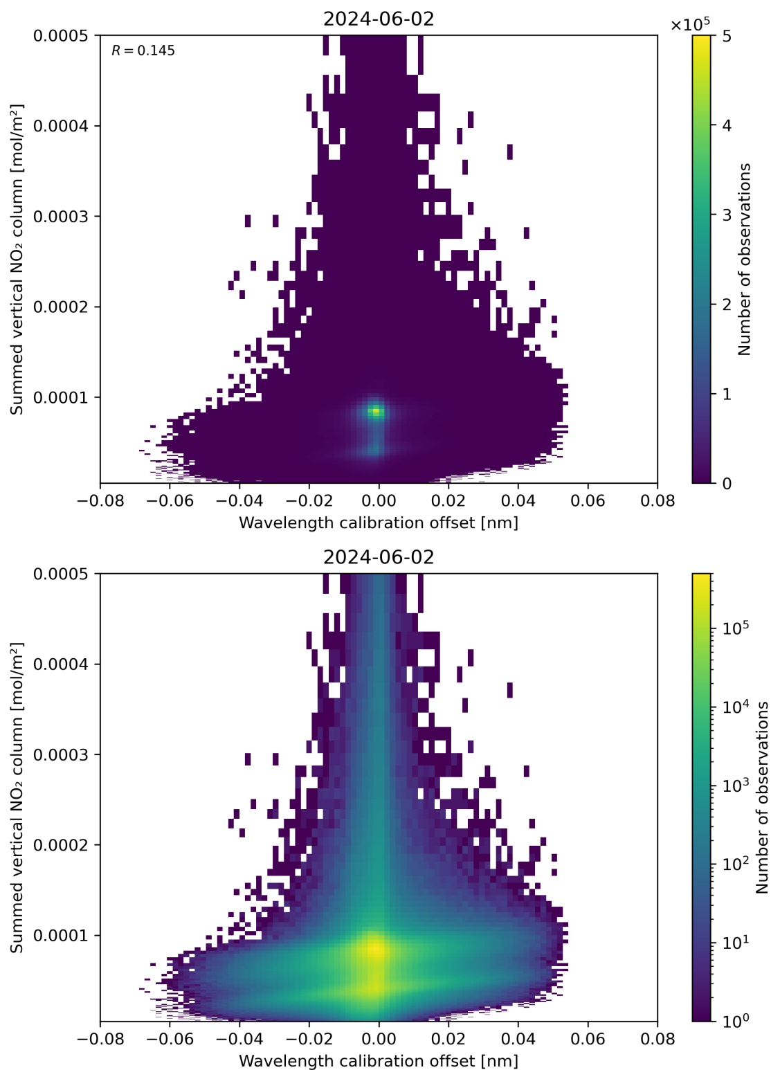
Figure 177: Scatter density plot of “Wavelength calibration offset” against “Summed vertical NO 2 column” for 2024-06-01 to 2024-06-03.
