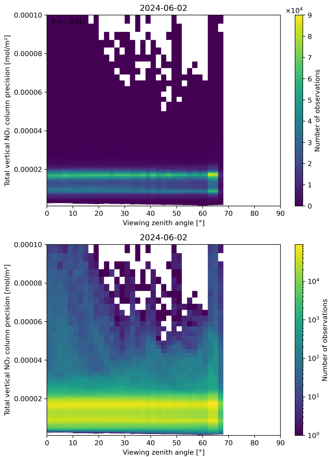
Figure 168: Scatter density plot of “Viewing zenith angle” against “Total vertical NO 2 column precision” for 2024-06-01 to 2024-06-03.
