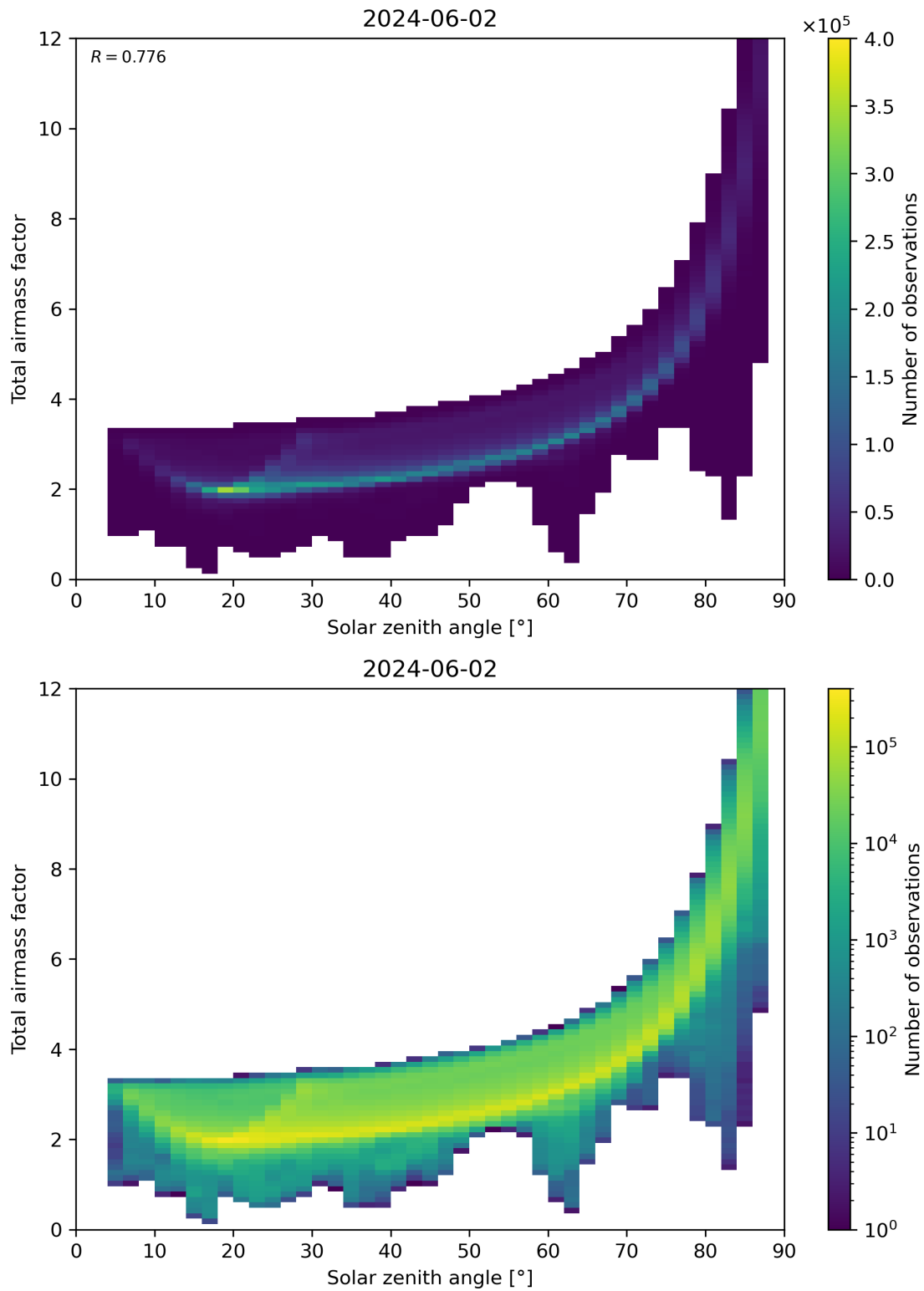
Figure 146: Scatter density plot of “Solar zenith angle” against “Total air mass factor” for 2024-06-01 to 2024-06-03.
