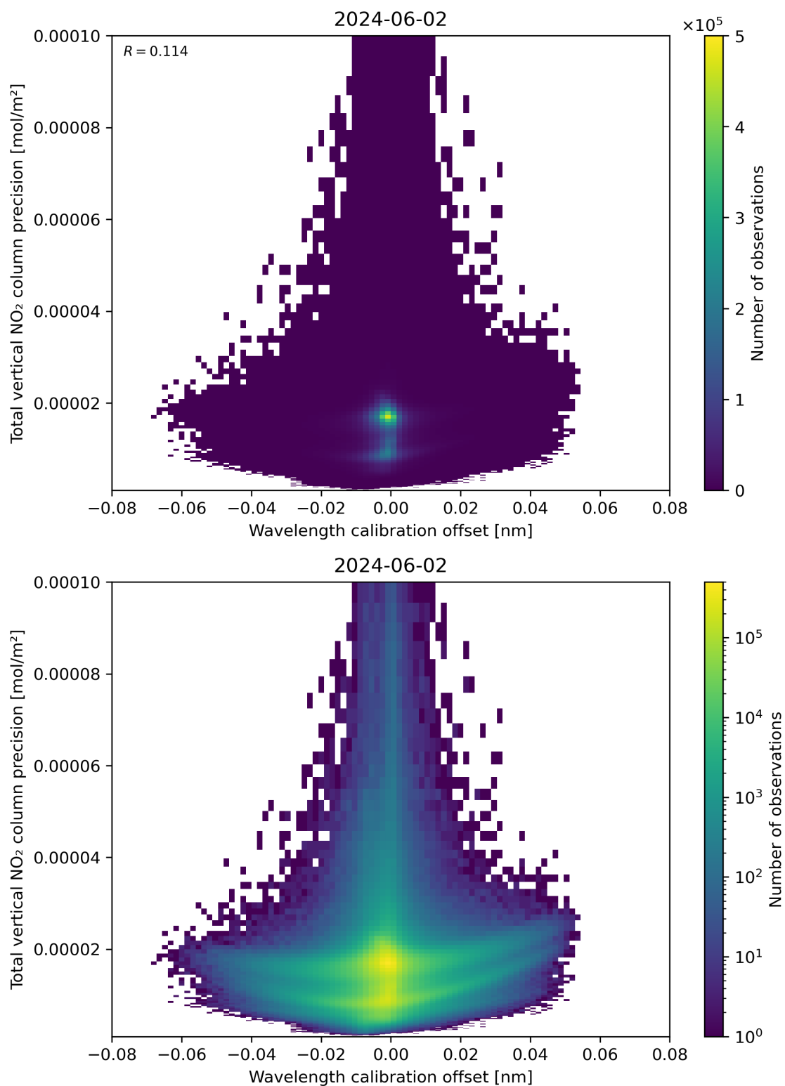
Figure 180: Scatter density plot of “Wavelength calibration offset” against “Total vertical NO 2 column precision” for 2024-06-01 to 2024-06-03.
