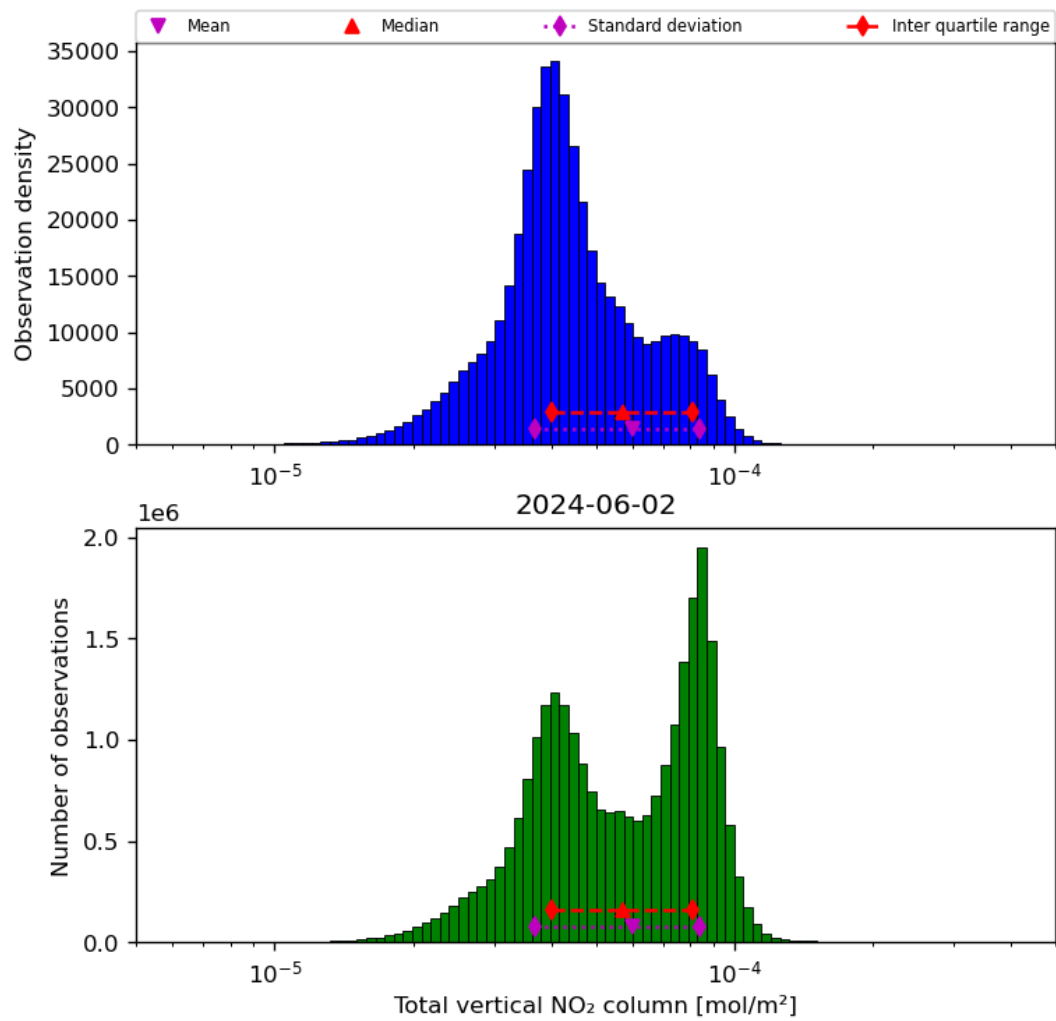
Figure 38: Histogram of “Total vertical NO 2 column” for 2024-06-01 to 2024-06-03
