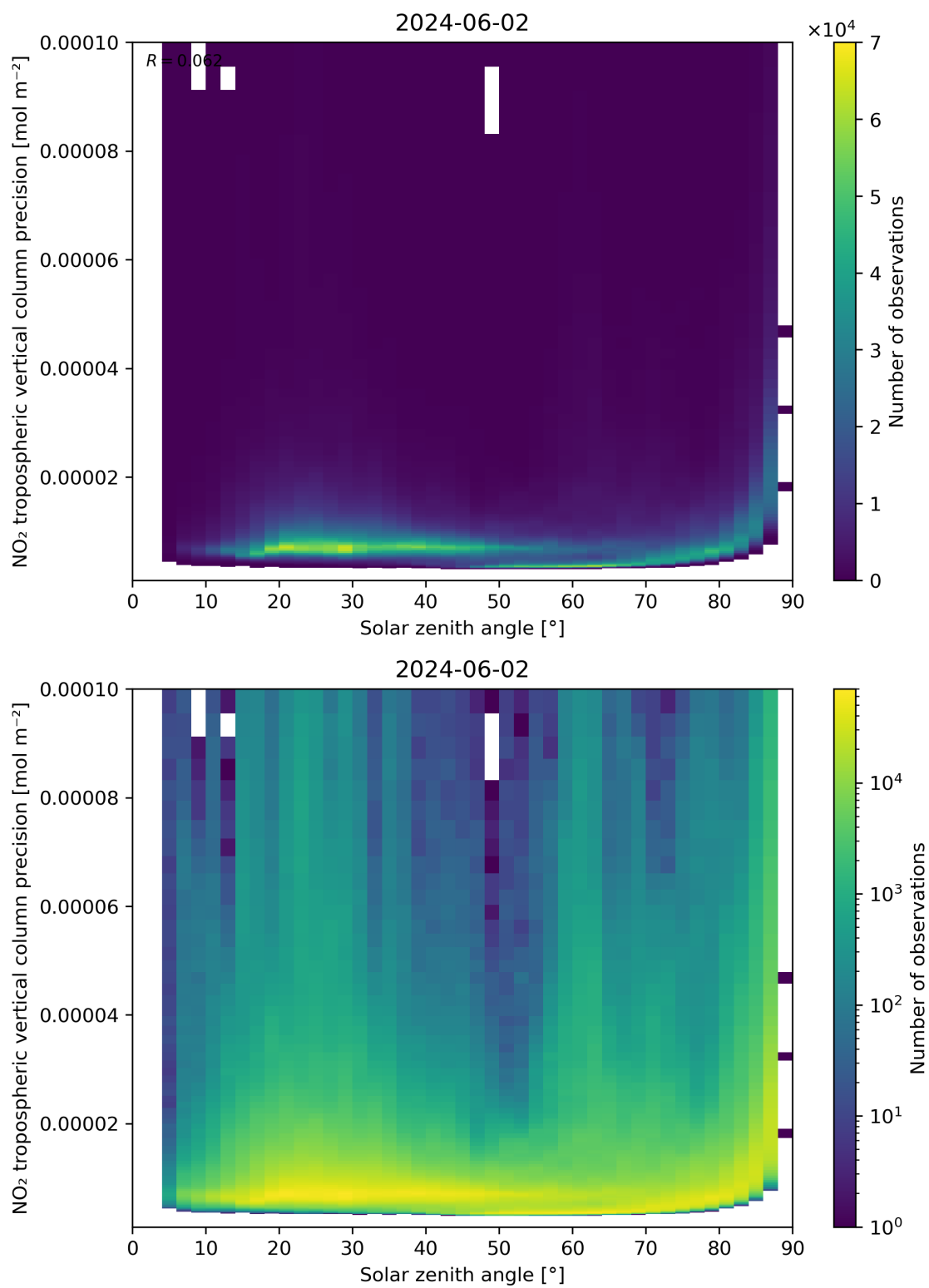
Figure 156: Scatter density plot of “Solar zenith angle” against “NO 2 tropospheric vertical column precision” for 2024-06-01 to 2024-06-03.
