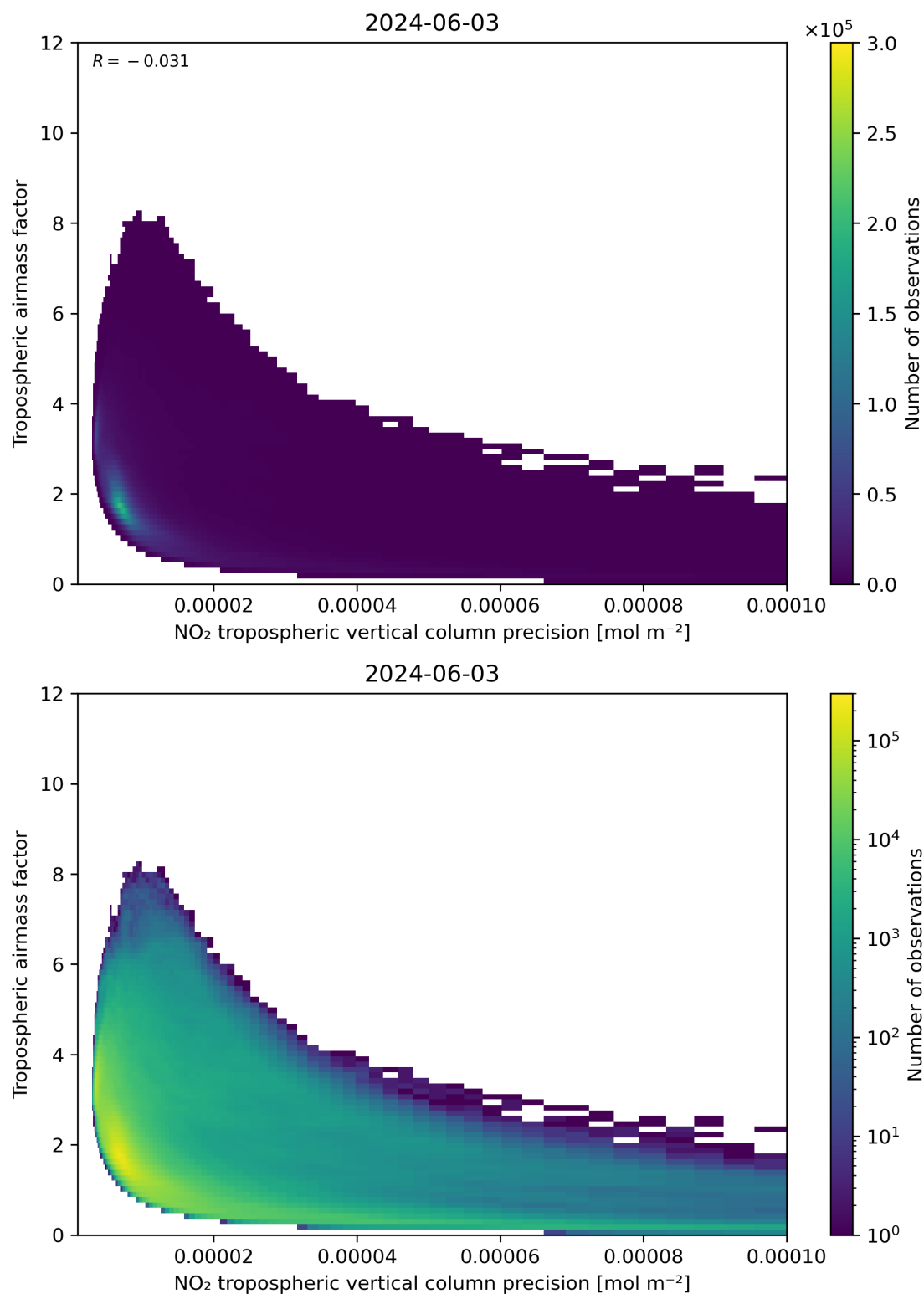
Figure 133: Scatter density plot of “NO 2 tropospheric vertical column precision” against “Tropospheric airmass factor” for 2024-06-03 to 2024-06-04.
