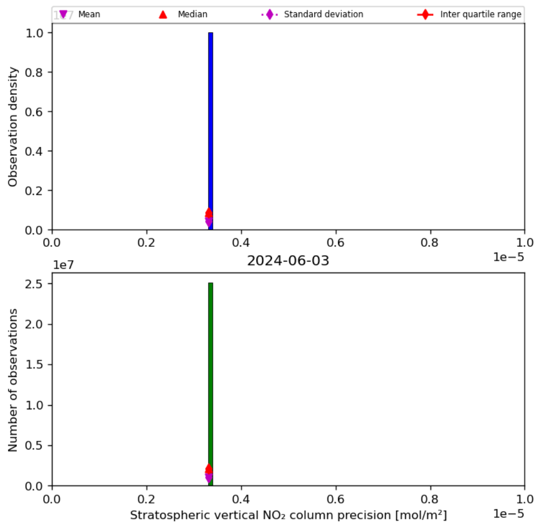
Figure 37: Histogram of “Stratospheric vertical NO 2 column precision” for 2024-06-03 to 2024-06-04
