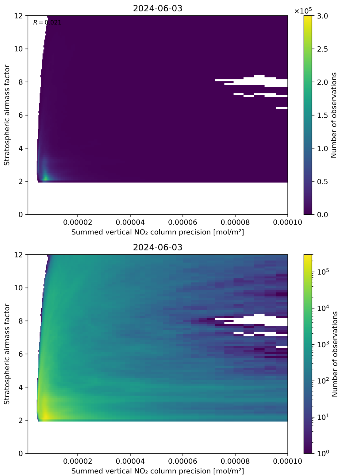
Figure 106: Scatter density plot of “Summed vertical NO 2 column precision” against “Stratospheric airmass factor” for 2024-06-03 to 2024-06-04.
