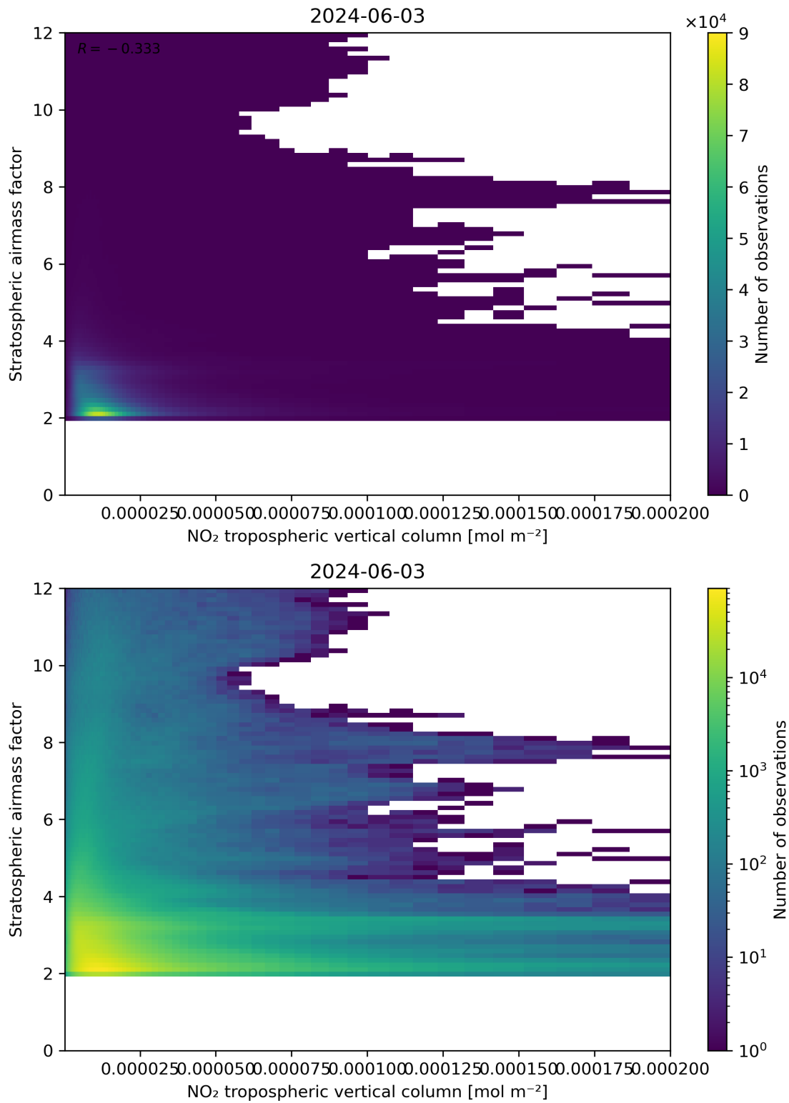
Figure 121: Scatter density plot of “NO 2 tropospheric vertical column” against “Stratospheric air mass factor” for 2024-06-03 to 2024-06-04.
