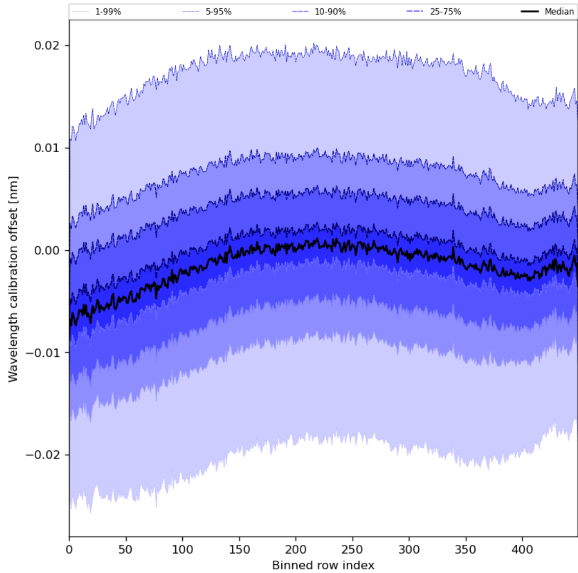
Figure 52: Along track statistics of “Wavelength calibration offset” for 2024-06-03 to 2024-06-04
