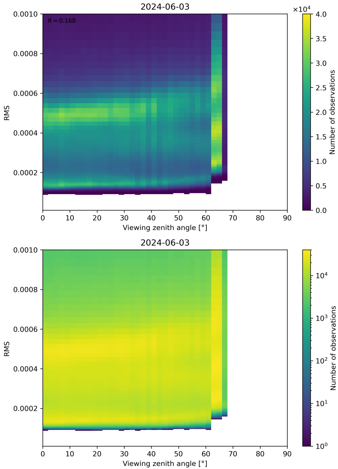
Figure 171: Scatter density plot of “Viewing zenith angle” against “RMS” for 2024-06-03 to 2024-06-04.
