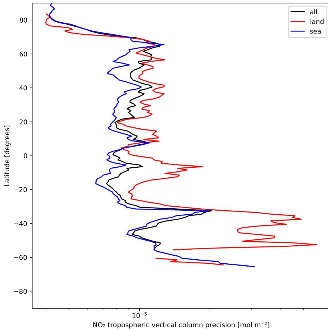
Figure 13: Zonal average of “NO 2 tropospheric vertical column precision” for 2024-06-03 to 2024-06-04.
