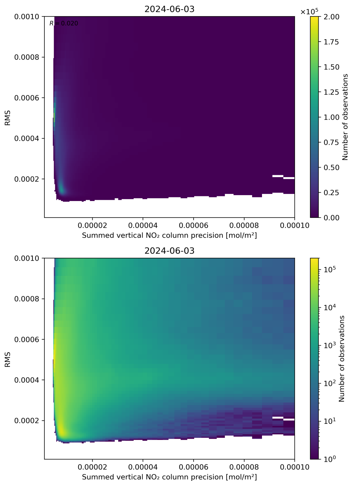
Figure 108: Scatter density plot of “Summed vertical NO 2 column precision” against “RMS” for 2024-06-03 to 2024-06-04.
