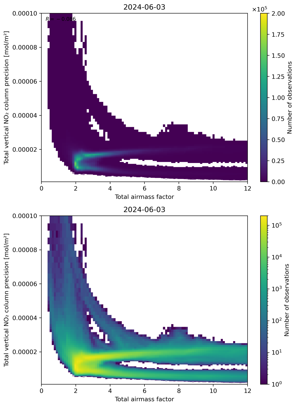
Figure 68: Scatter density plot of “Total airmass factor” against “Total vertical NO 2 column precision” for 2024-06-03 to 2024-06-04.
