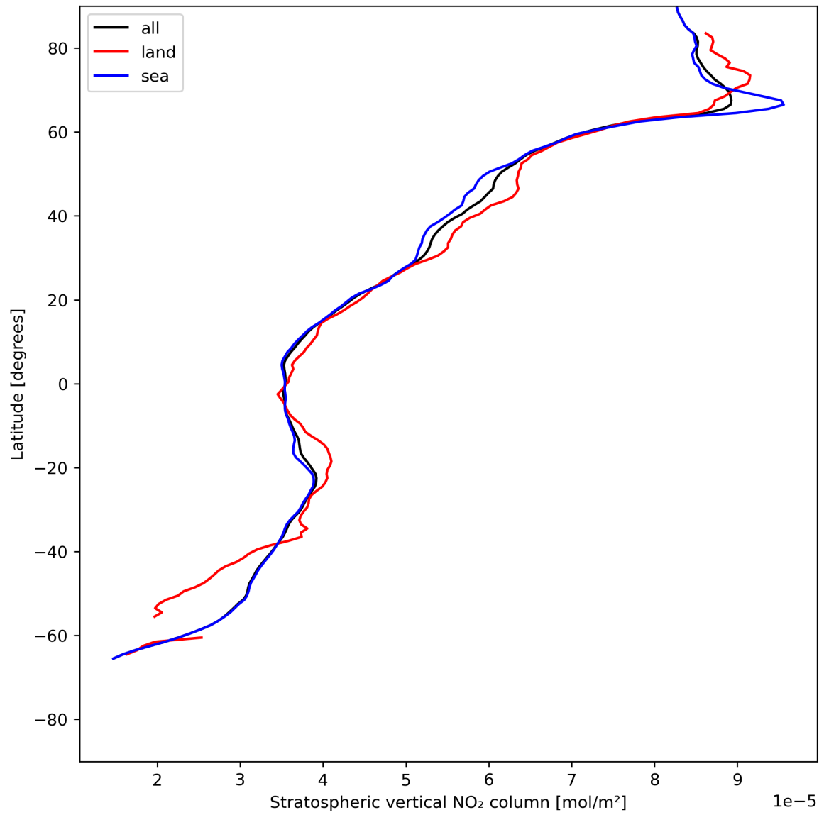
Figure 19: Zonal average of “Stratospheric vertical NO 2 column” for 2024-06-03 to 2024-06-04.
