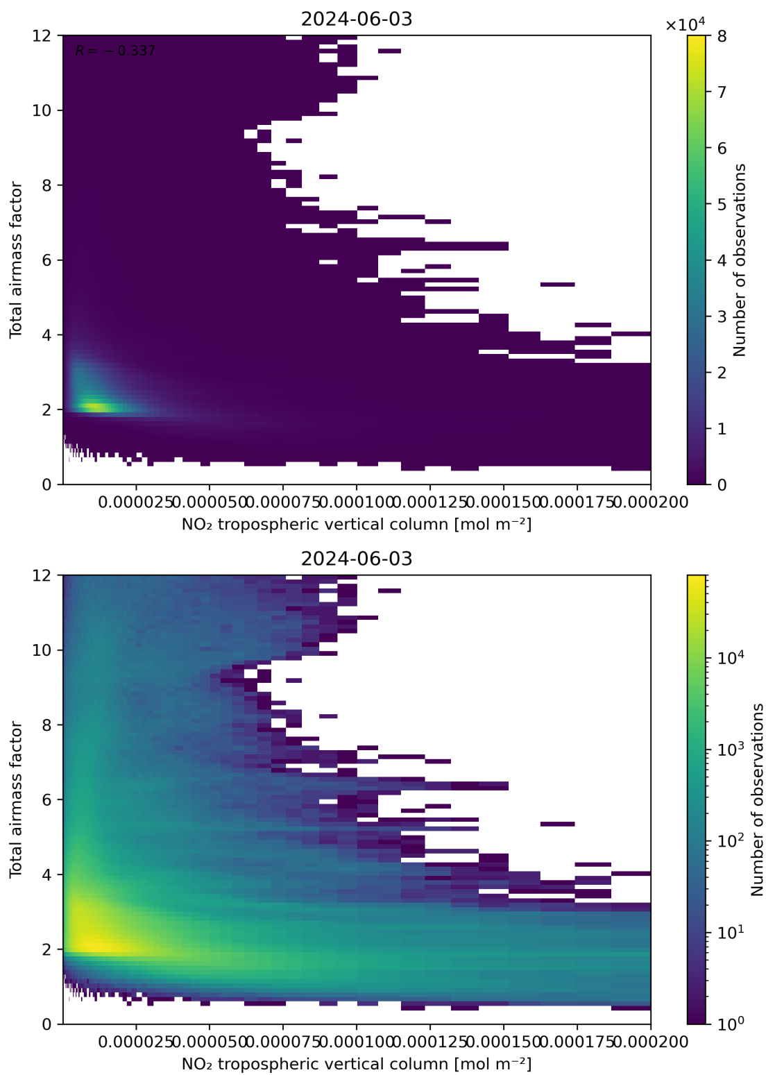
Figure 122: Scatter density plot of “NO 2 tropospheric vertical column” against “Total air mass factor” for 2024-06-03 to 2024-06-04.
