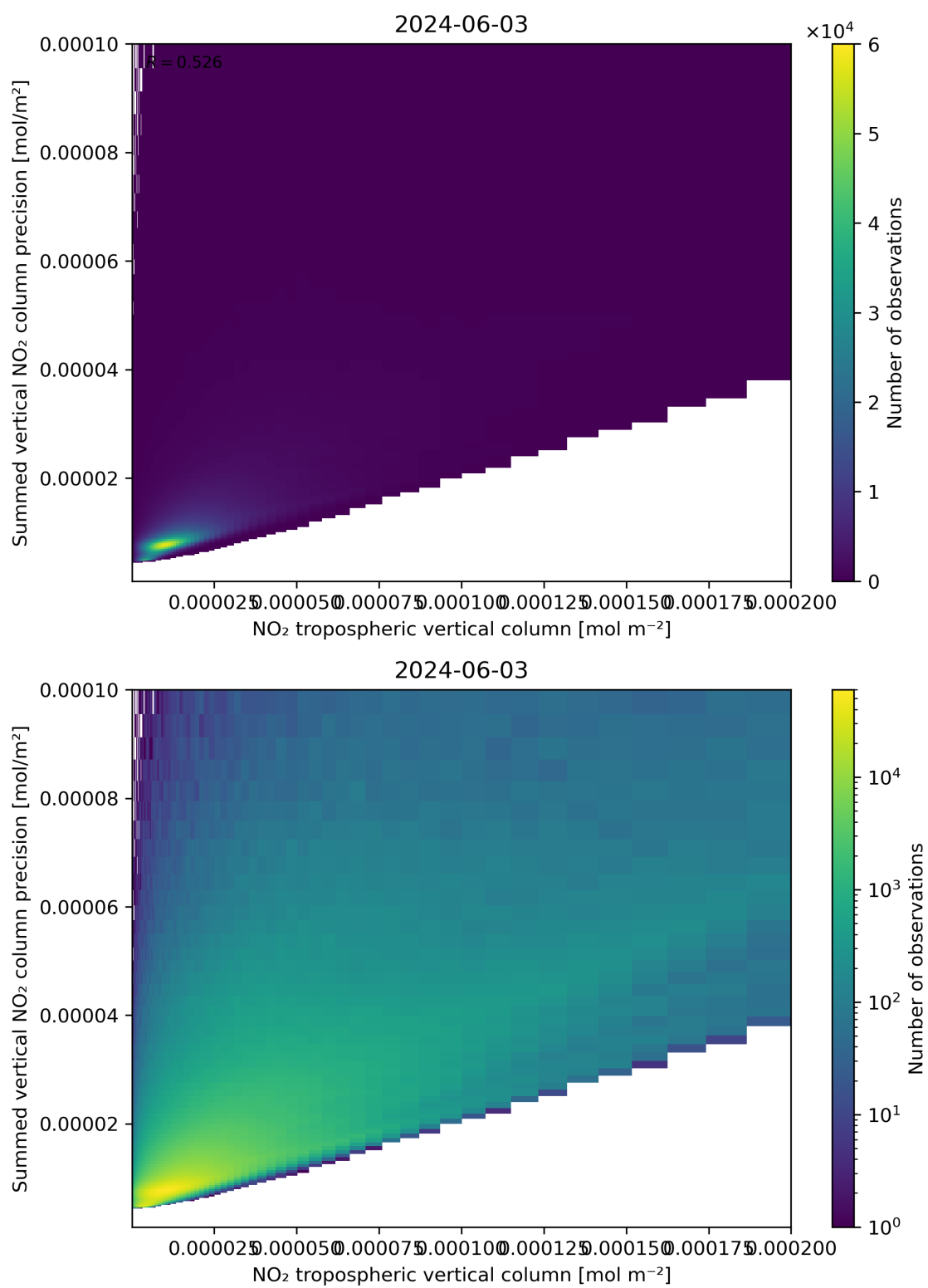
Figure 127: Scatter density plot of “NO 2 tropospheric vertical column” against “Summed vertical NO 2 column precision” for 2024-06-03 to 2024-06-04.
