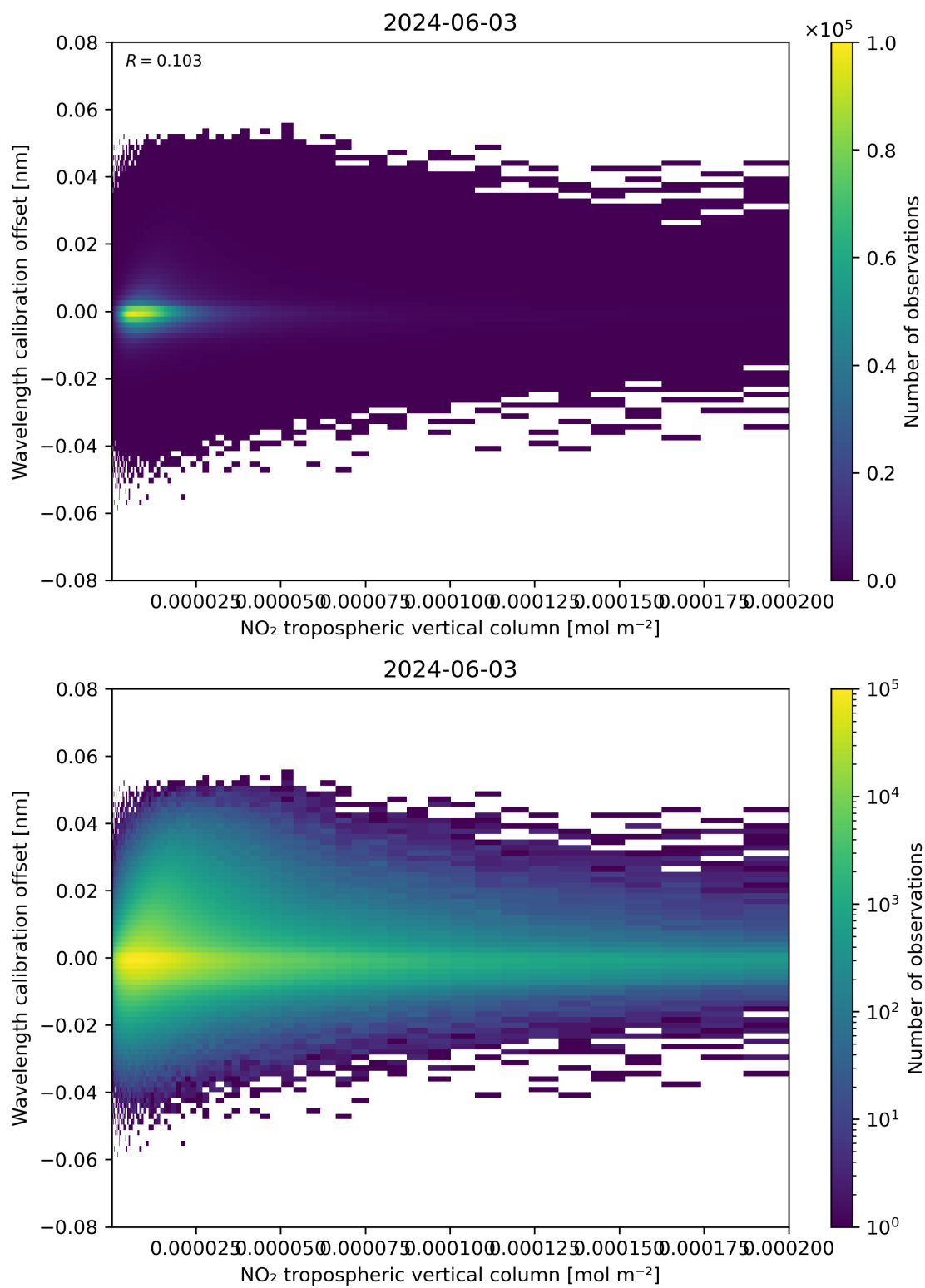
Figure 143: Scatter density plot of “NO 2 tropospheric vertical column” against “Wavelength calibration offset” for 2024-06-03 to 2024-06-04.
