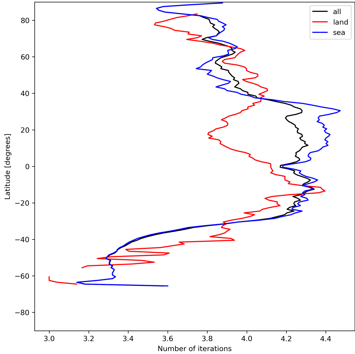
Figure 17: Zonal average of “Number of iterations” for 2024-06-03 to 2024-06-04.
