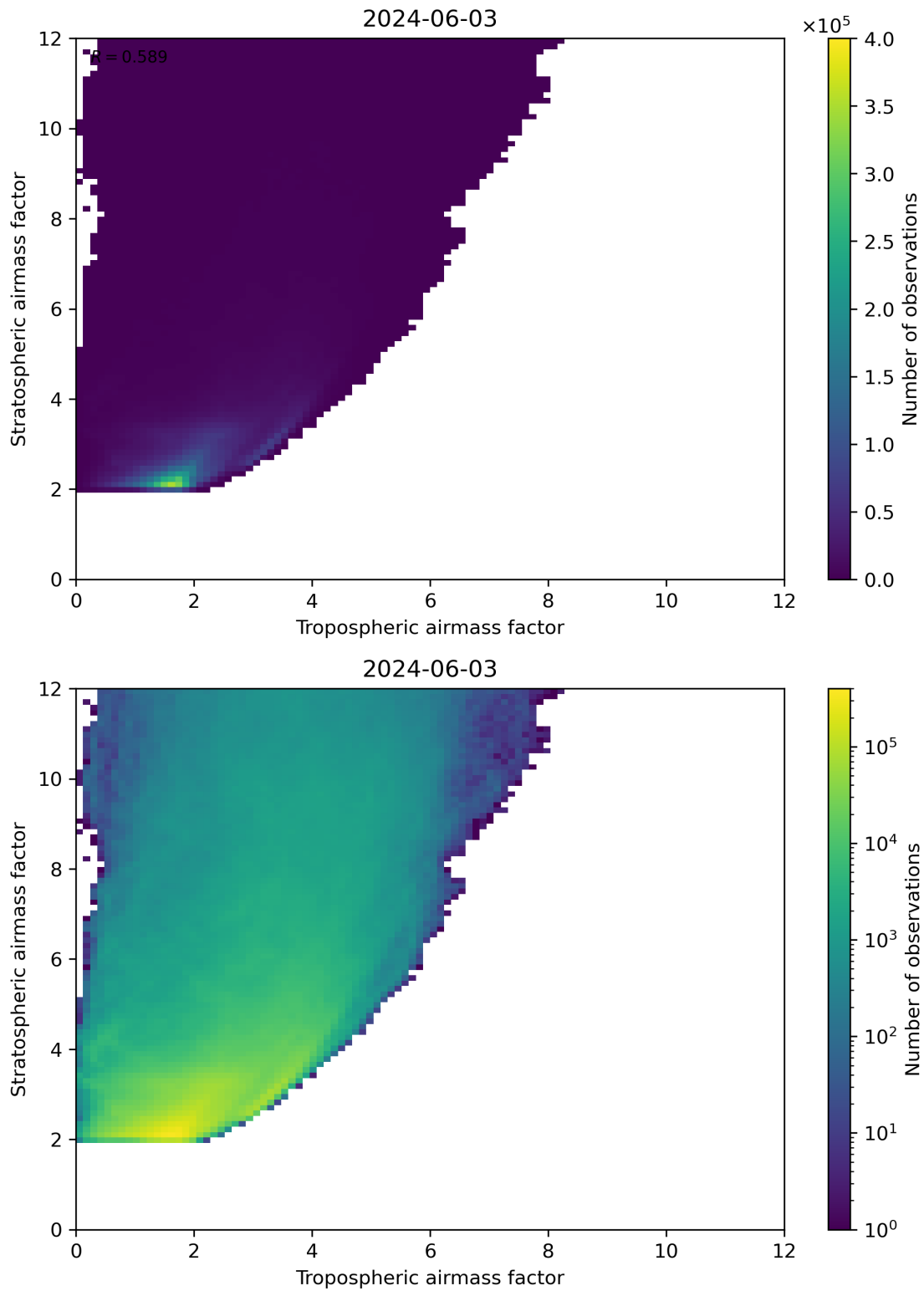
Figure 71: Scatter density plot of “Tropospheric airmass factor” against “Stratospheric airmass factor” for 2024-06-03 to 2024-06-04.
