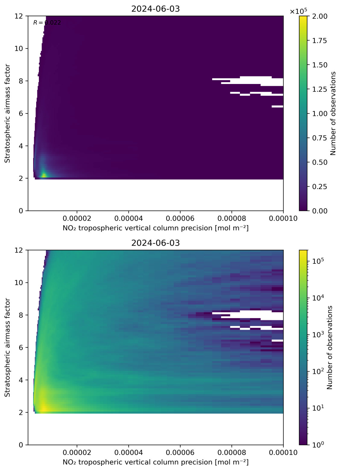
Figure 131: Scatter density plot of “NO 2 tropospheric vertical column precision” against “Stratospheric airmass factor” for 2024-06-03 to 2024-06-04.
