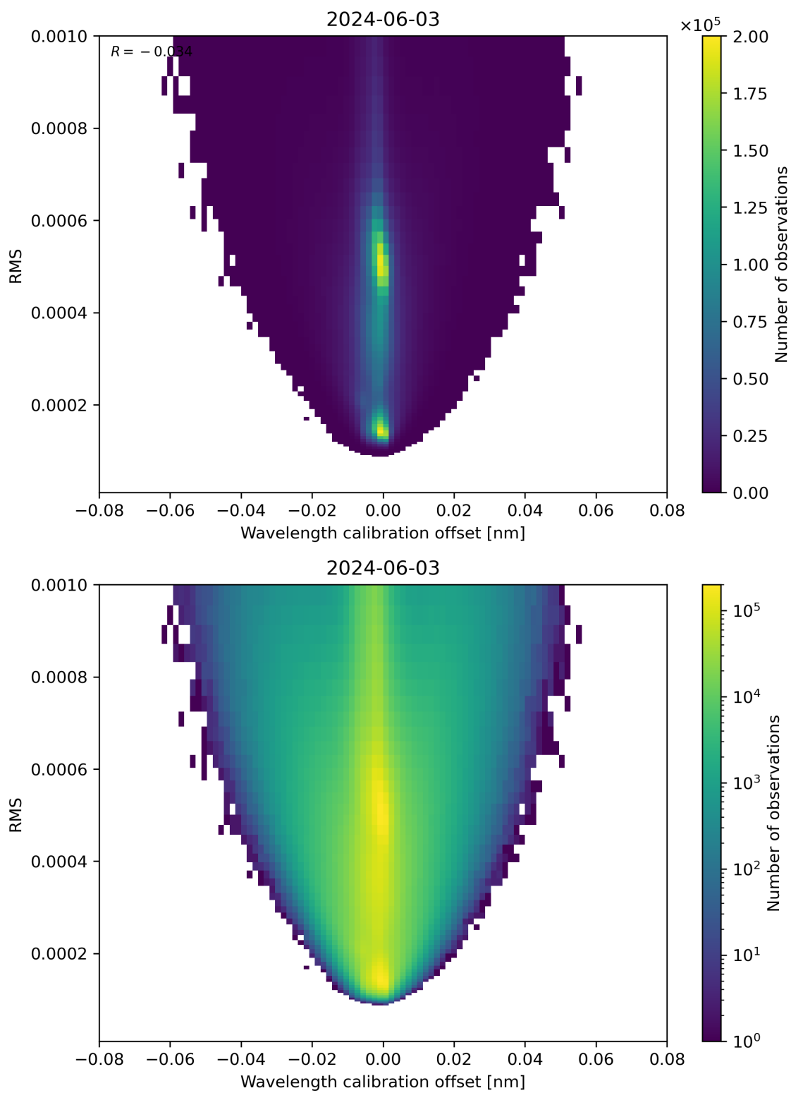
Figure 181: Scatter density plot of “Wavelength calibration offset” against “RMS” for 2024-06-03 to 2024-06-04.
