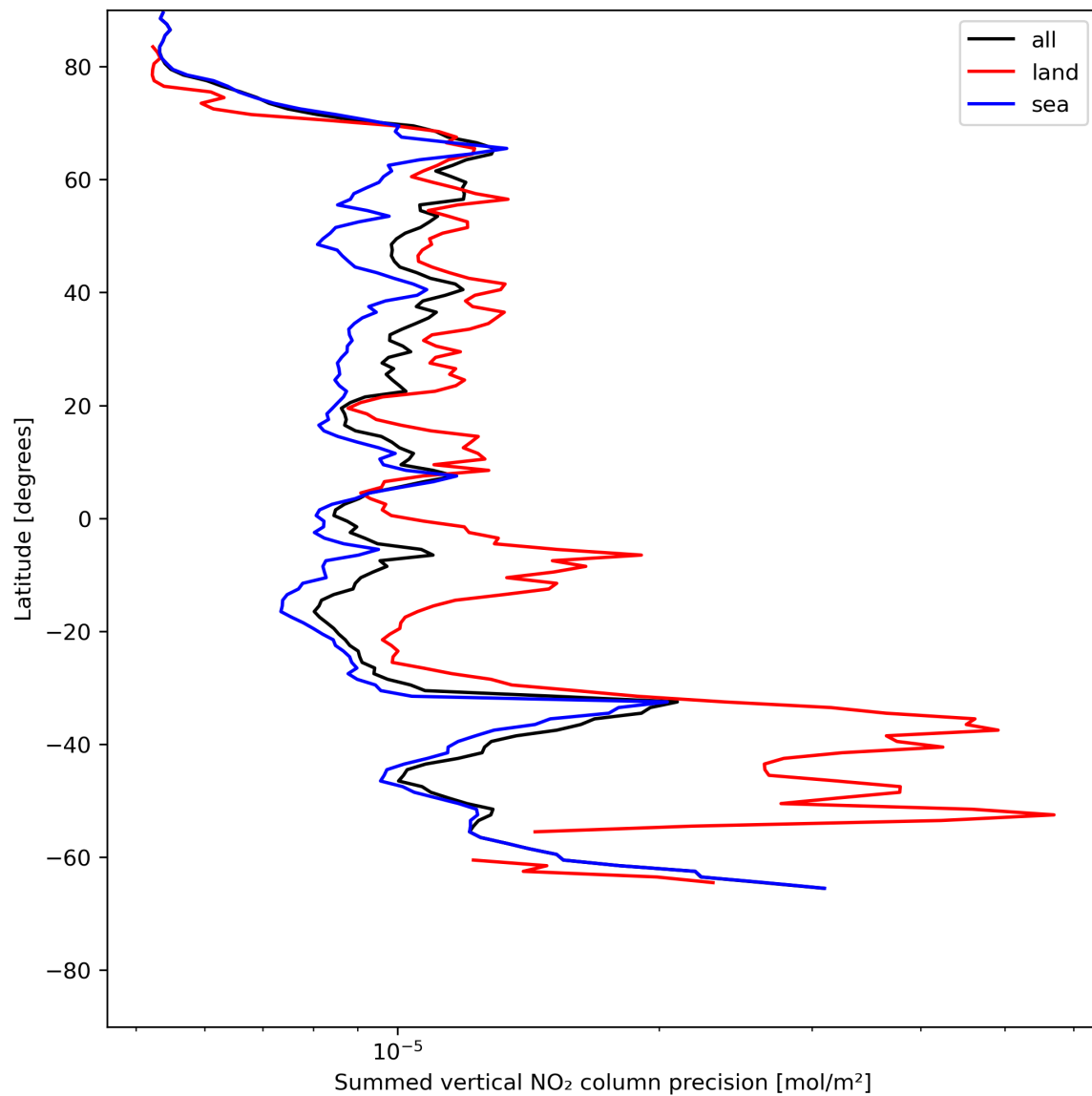
Figure 24: Zonal average of “Summed vertical NO 2 column precision” for 2024-06-03 to 2024-06-04.
