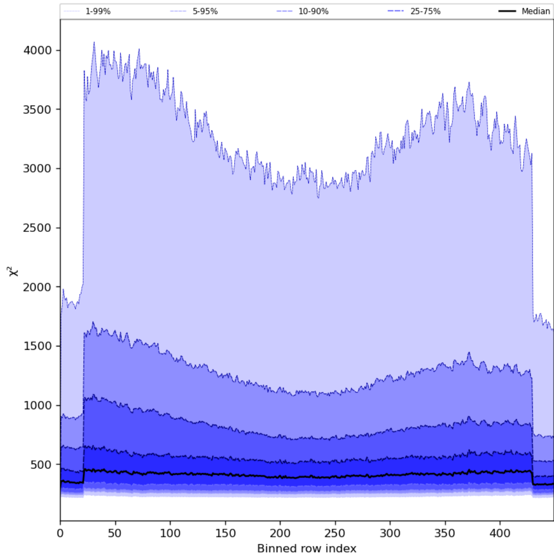
Figure 59: Along track statistics of “ \chi^2 ” for 2024-06-03 to 2024-06-04
