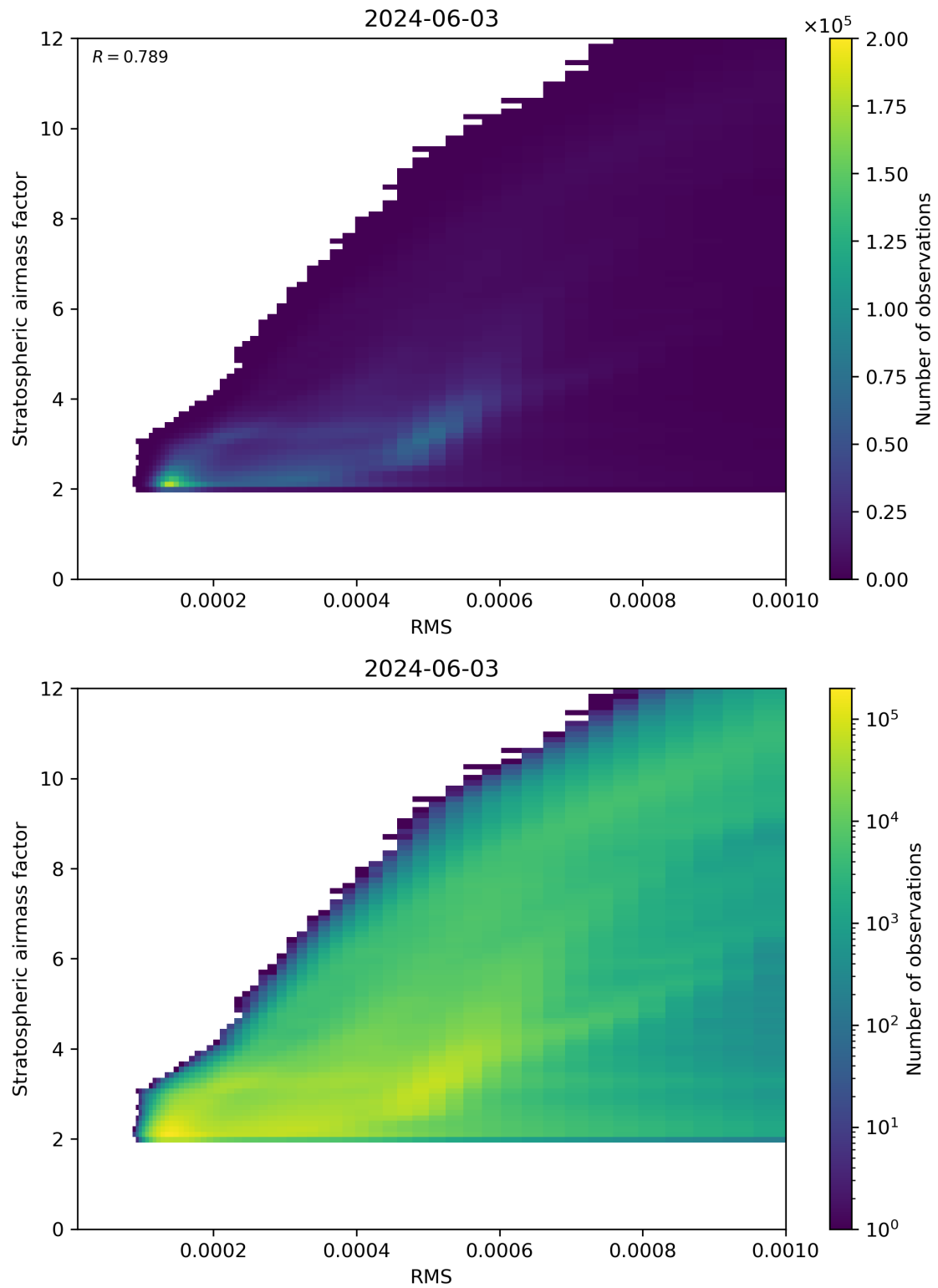
Figure 144: Scatter density plot of “RMS” against “Stratospheric airmass factor” for 2024-06-03 to 2024-06-04.
