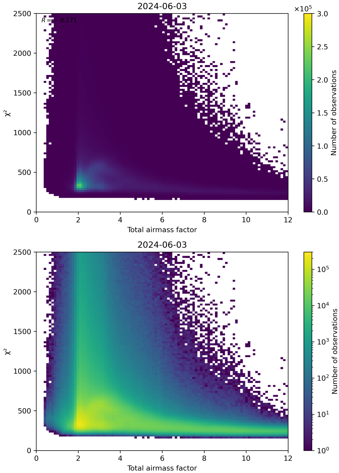
Figure 63: Scatter density plot of “Total airmass factor” against “ \chi^2 ” for 2024-06-03 to 2024-06-04.
