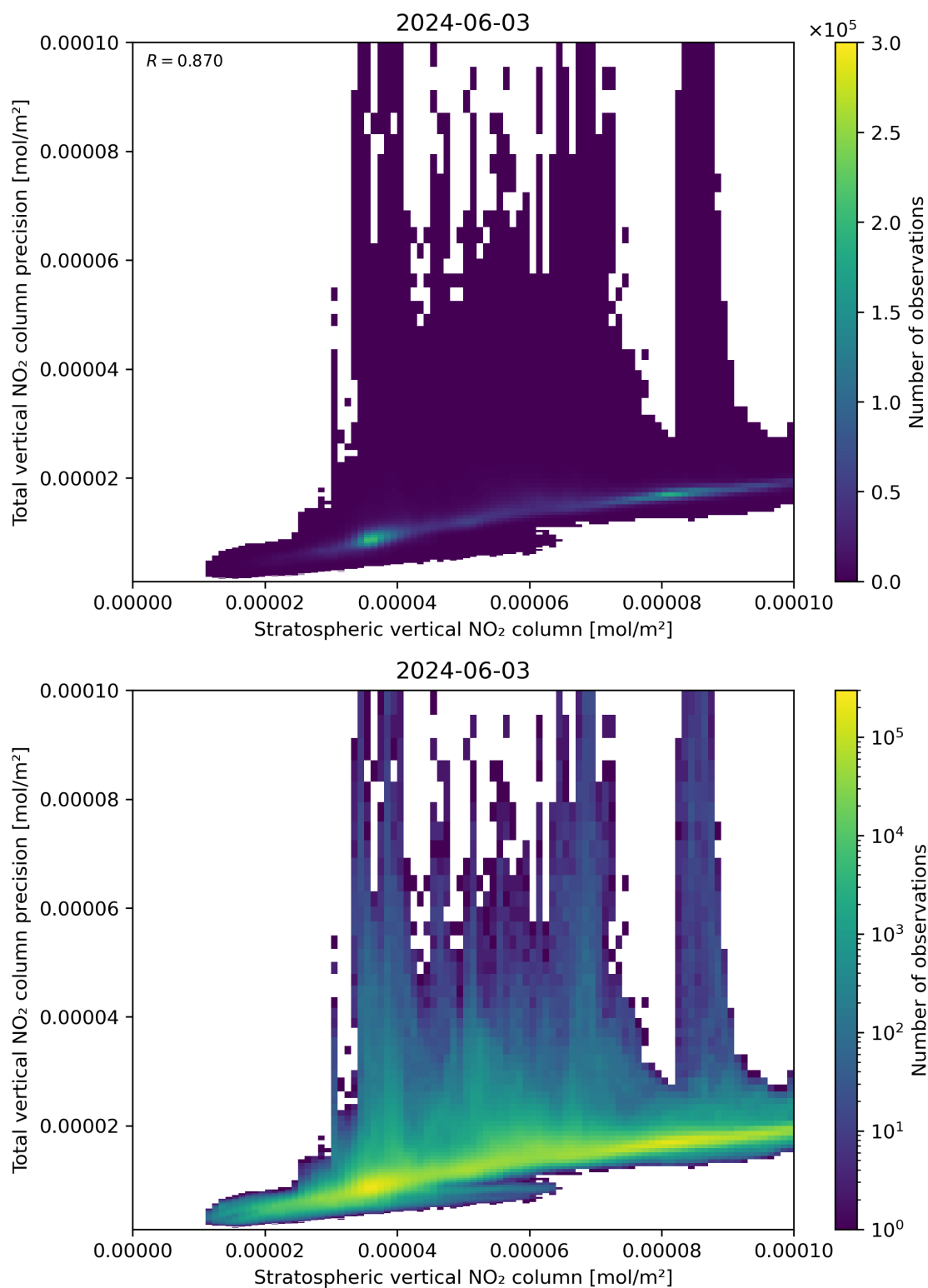
Figure 101: Scatter density plot of “Stratospheric vertical NO 2 column” against “Total vertical NO 2 column precision” for 2024-06-03 to 2024-06-04.
