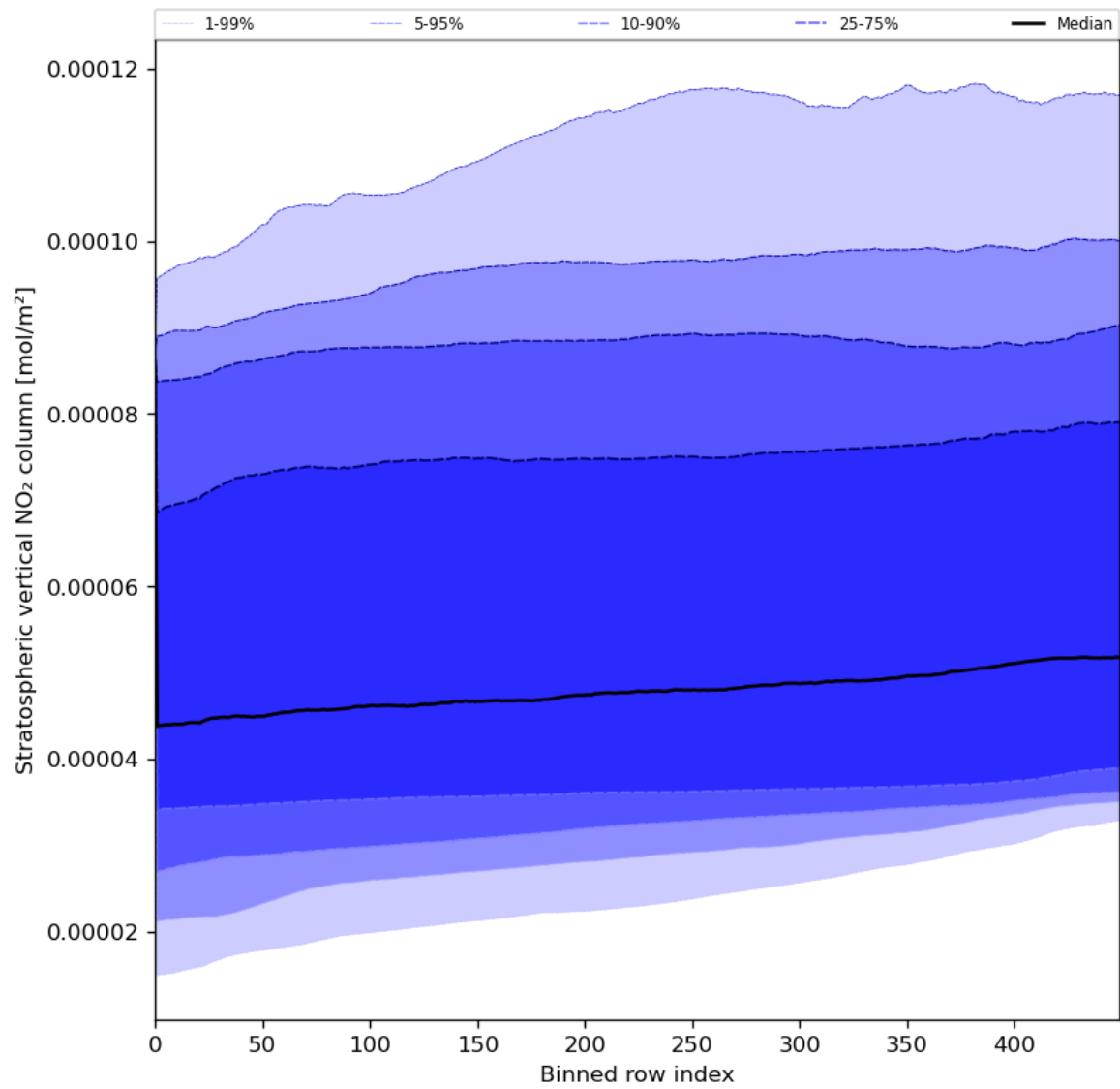
Figure 53: Along track statistics of “Stratospheric vertical NO 2 column” for 2024-06-03 to 2024-06-04
