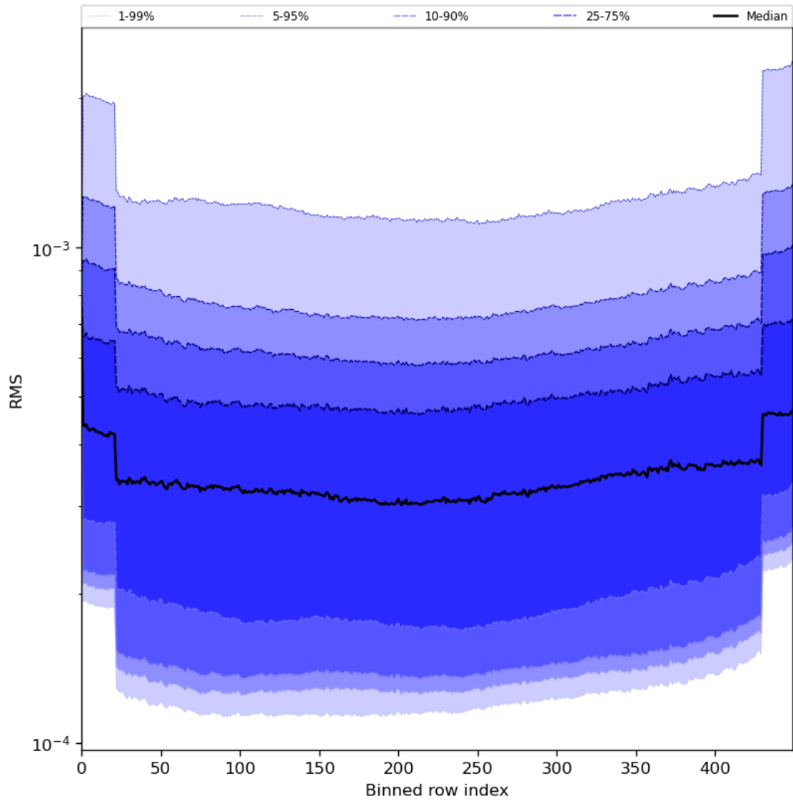
Figure 60: Along track statistics of “RMS” for 2024-06-03 to 2024-06-04
