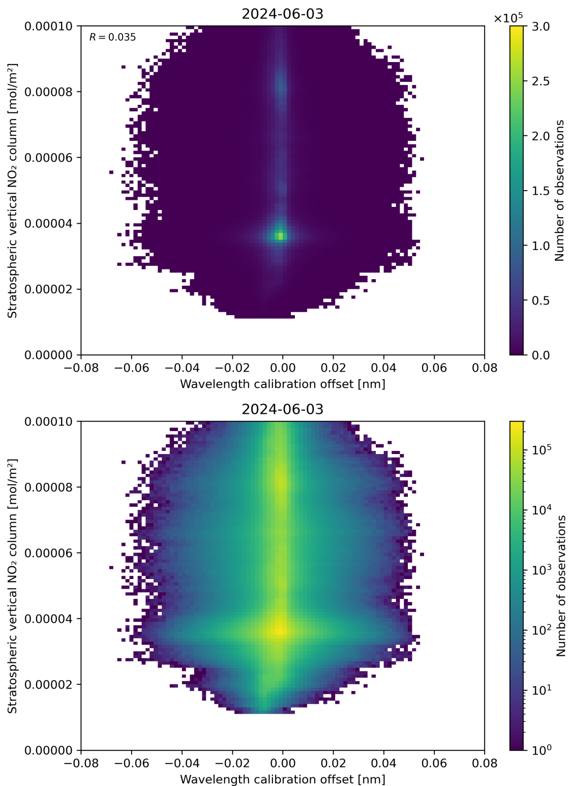
Figure 176: Scatter density plot of “Wavelength calibration offset” against “Stratospheric vertical NO 2 column” for 2024-06-03 to 2024-06-04.
