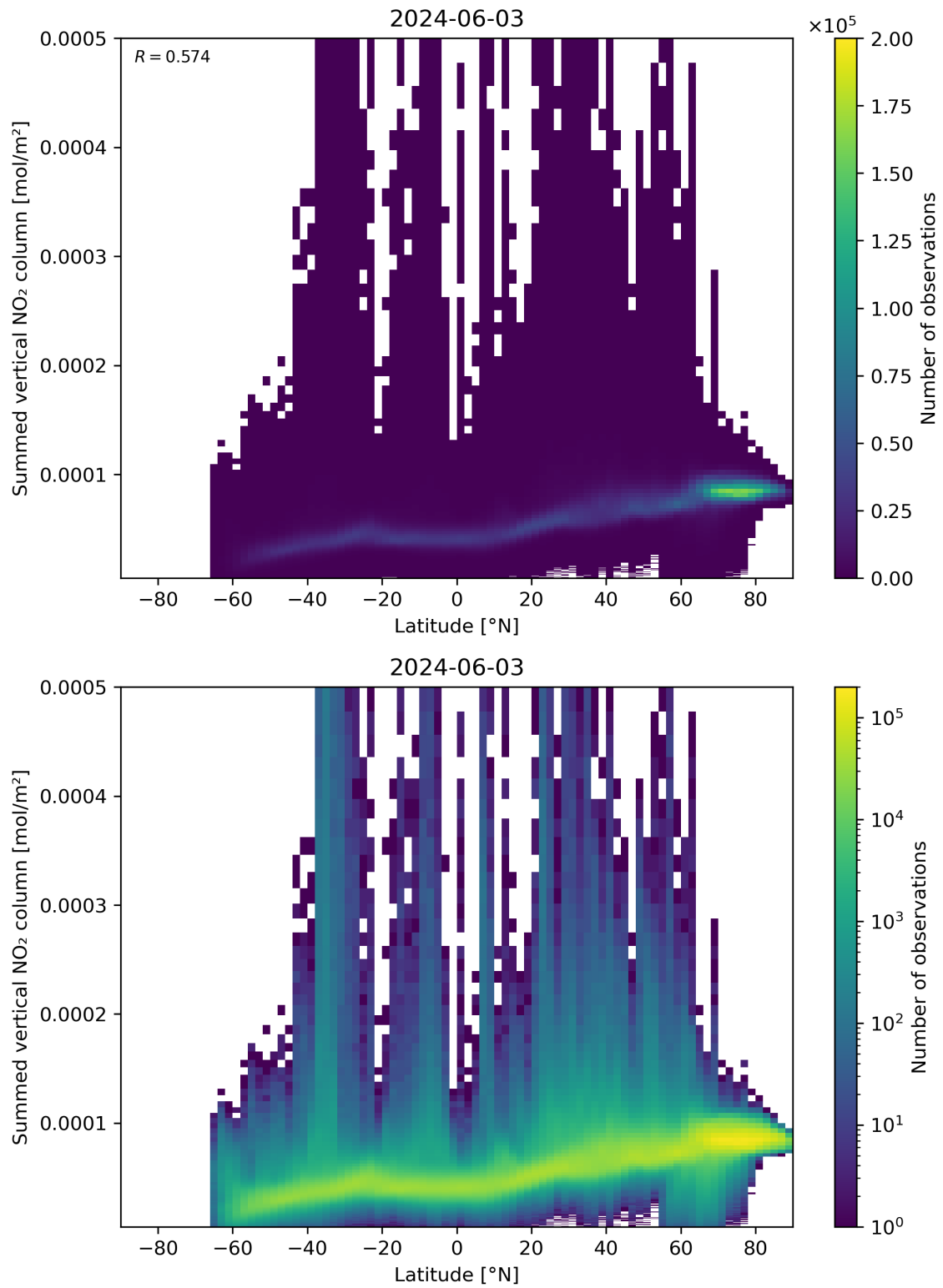
Figure 88: Scatter density plot of “Latitude” against “Summed vertical NO 2 column” for 2024-06-03 to 2024-06-04.
