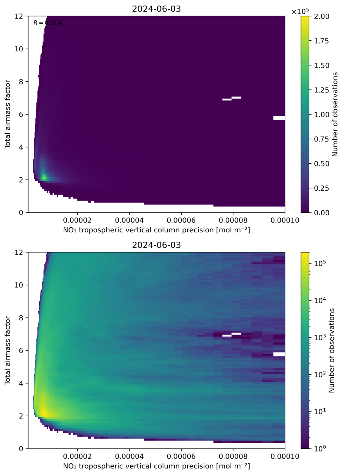
Figure 132: Scatter density plot of “NO 2 tropospheric vertical column precision” against “Total air mass factor” for 2024-06-03 to 2024-06-04.
