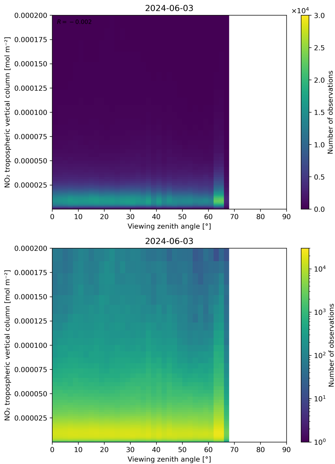
Figure 169: Scatter density plot of “Viewing zenith angle” against “NO 2 tropospheric vertical column” for 2024-06-03 to 2024-06-04.
