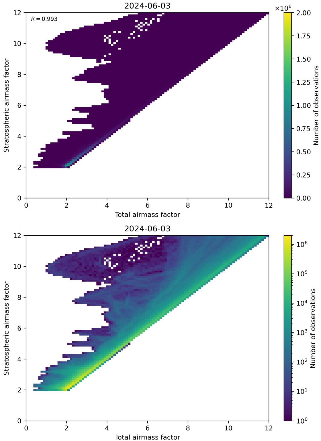
Figure 62: Scatter density plot of “Total airmass factor” against “Stratospheric airmass factor” for 2024-06-03 to 2024-06-04.
