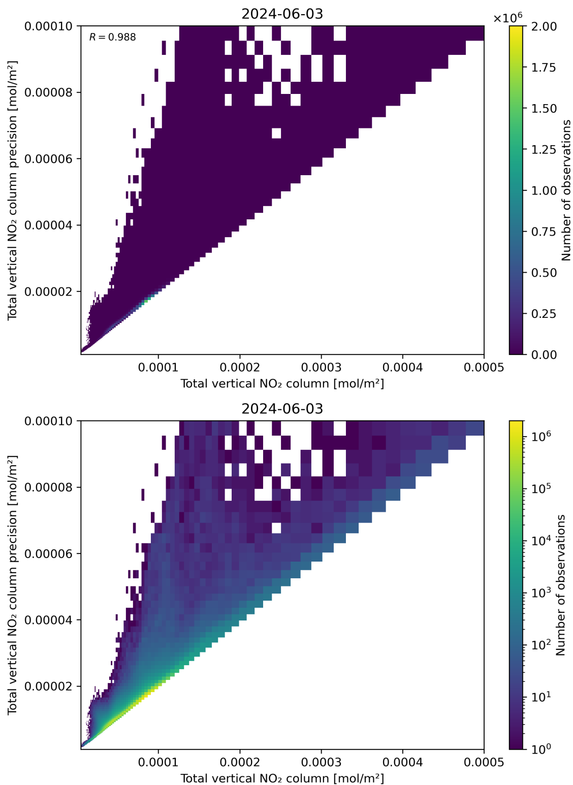
Figure 114: Scatter density plot of “Total vertical NO 2 column” against “Total vertical NO 2 column precision” for 2024-06-03 to 2024-06-04.
