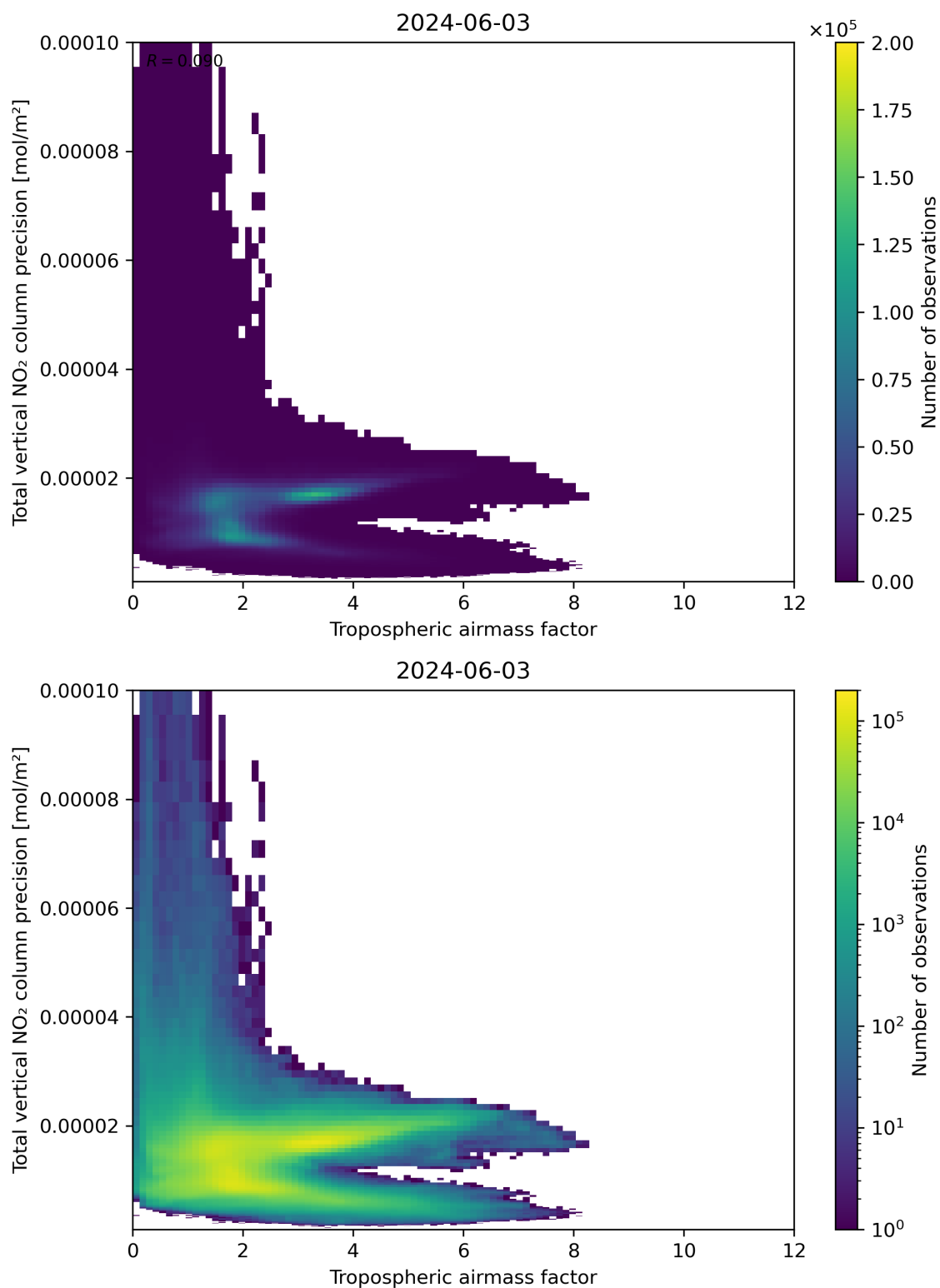
Figure 78: Scatter density plot of “Tropospheric air mass factor” against “Total vertical NO 2 column precision” for 2024-06-03 to 2024-06-04.
