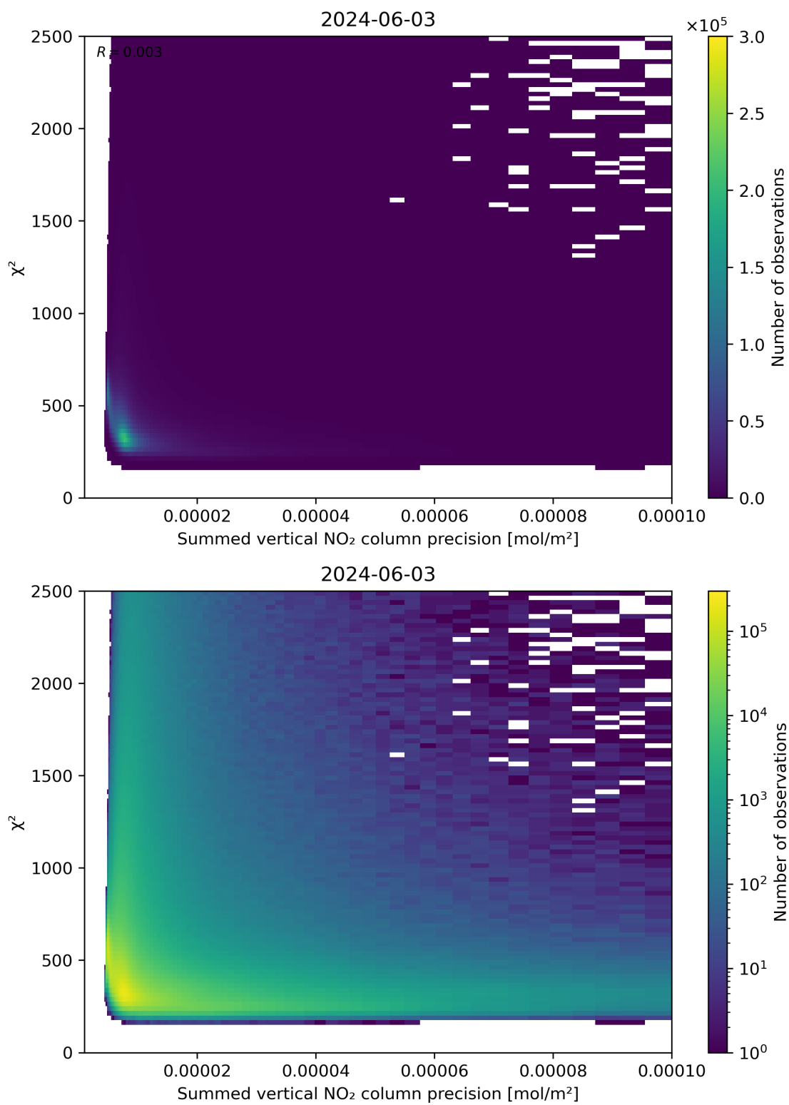
Figure 107: Scatter density plot of “Summed vertical NO 2 column precision” against “ \chi^2 ” for 2024-06-03 to 2024-06-04.
