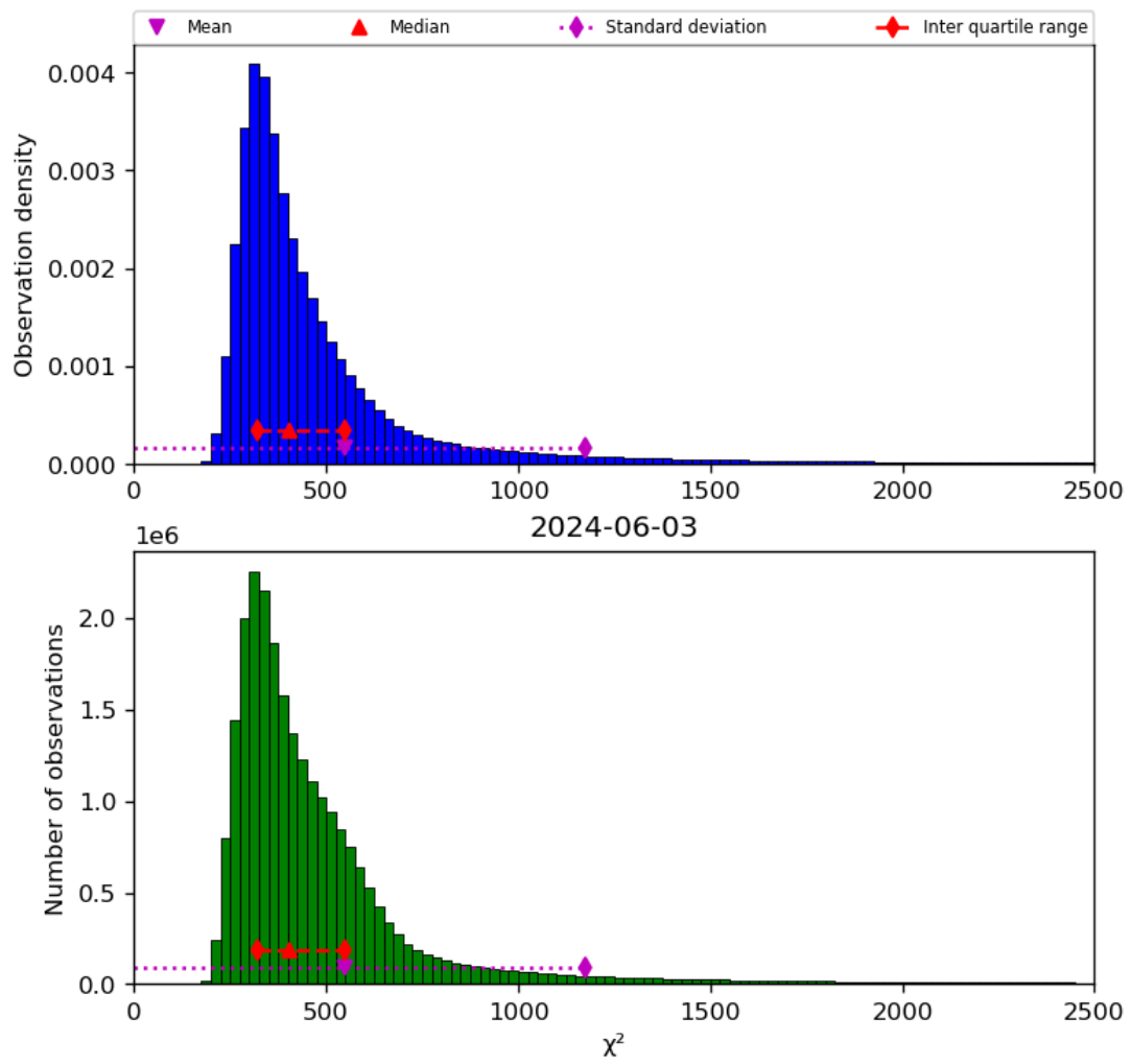
Figure 42: Histogram of “ \chi^2 ” for 2024-06-03 to 2024-06-04
