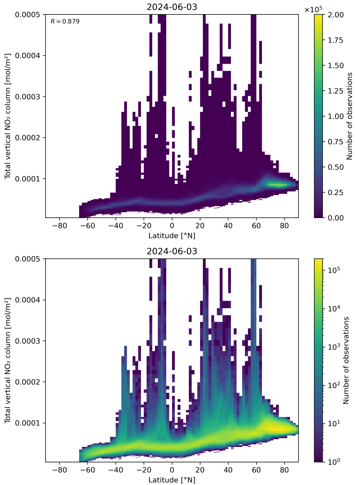
Figure 90: Scatter density plot of “Latitude” against “Total vertical NO 2 column” for 2024-06-03 to 2024-06-04.
