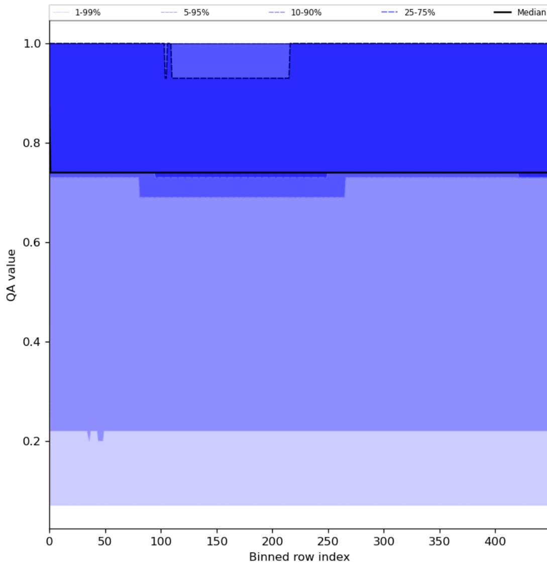
Figure 45: Along track statistics of "QA value" for 2024-06-03 to 2024-06-04
