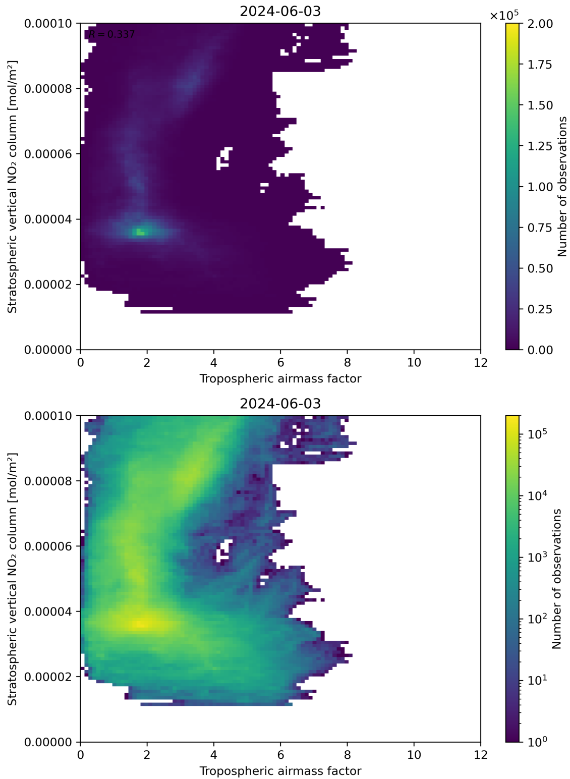
Figure 74: Scatter density plot of “Tropospheric air mass factor” against “Stratospheric vertical NO 2 column” for 2024-06-03 to 2024-06-04.
