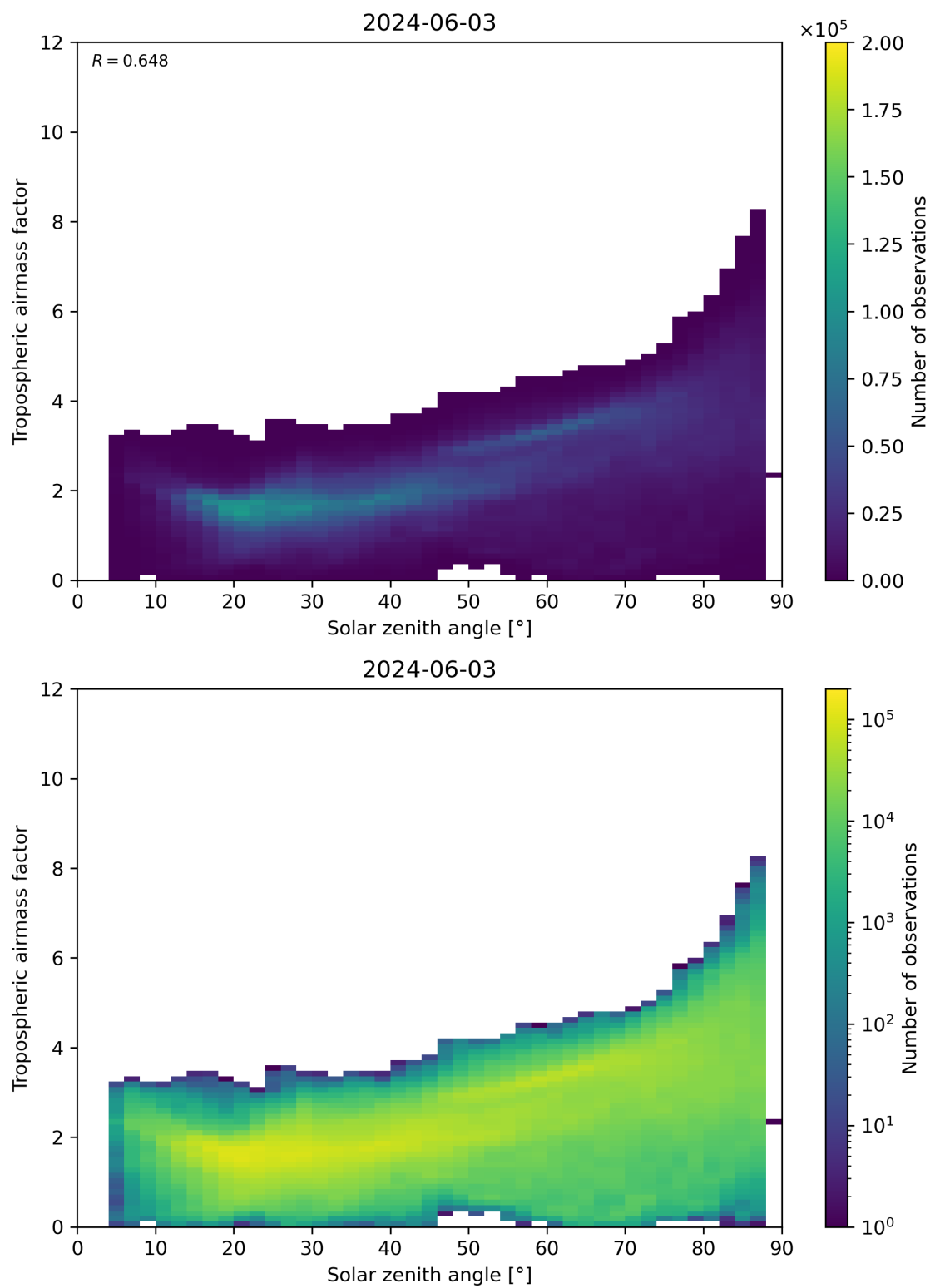
Figure 147: Scatter density plot of “Solar zenith angle” against “Tropospheric airmass factor” for 2024-06-03 to 2024-06-04.
