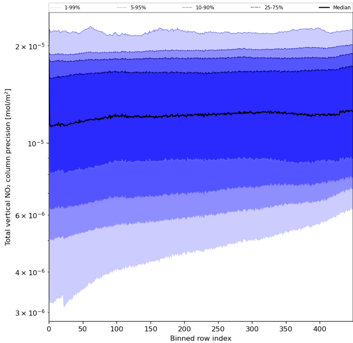
Figure 56: Along track statistics of “Total vertical NO 2 column precision” for 2024-06-03 to 2024-06-04
