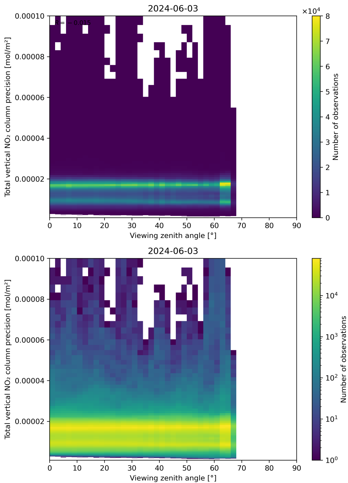
Figure 168: Scatter density plot of “Viewing zenith angle” against “Total vertical NO 2 column precision” for 2024-06-03 to 2024-06-04.
