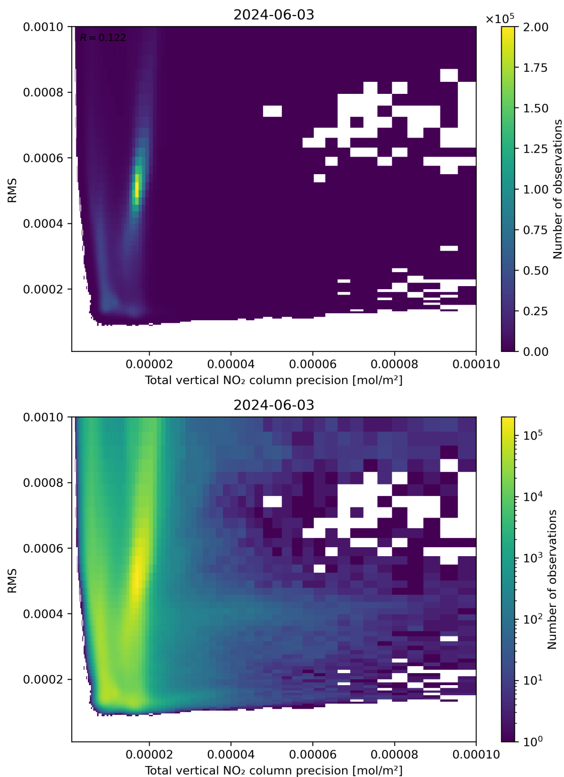
Figure 119: Scatter density plot of “Total vertical NO 2 column precision” against “RMS” for 2024-06-03 to 2024-06-04.
