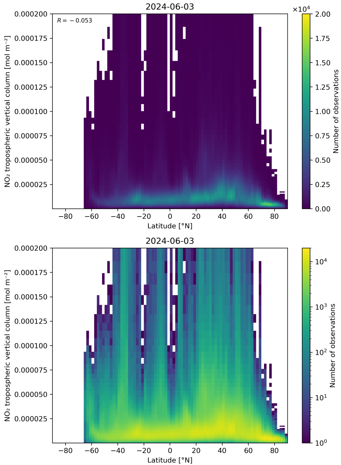
Figure 92: Scatter density plot of “Latitude” against “NO 2 tropospheric vertical column” for 2024-06-03 to 2024-06-04.
