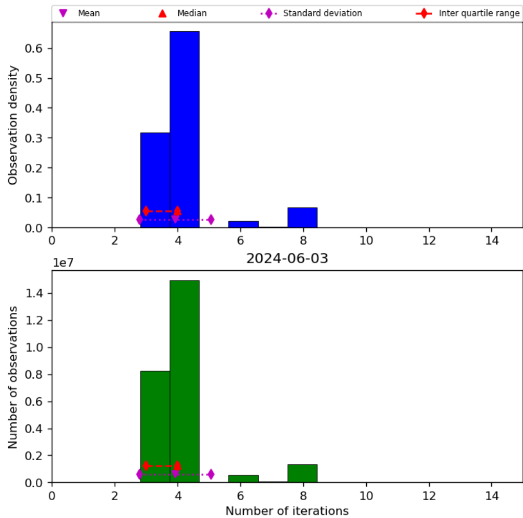
Figure 34: Histogram of “Number of iterations” for 2024-06-03 to 2024-06-04
