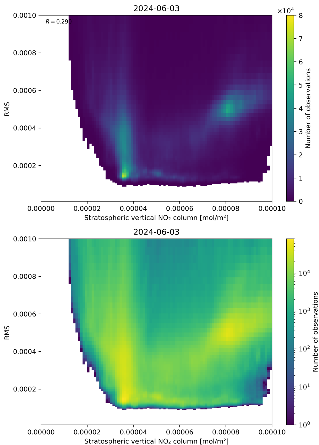
Figure 102: Scatter density plot of “Stratospheric vertical NO 2 column” against “RMS” for 2024-06-03 to 2024-06-04.
