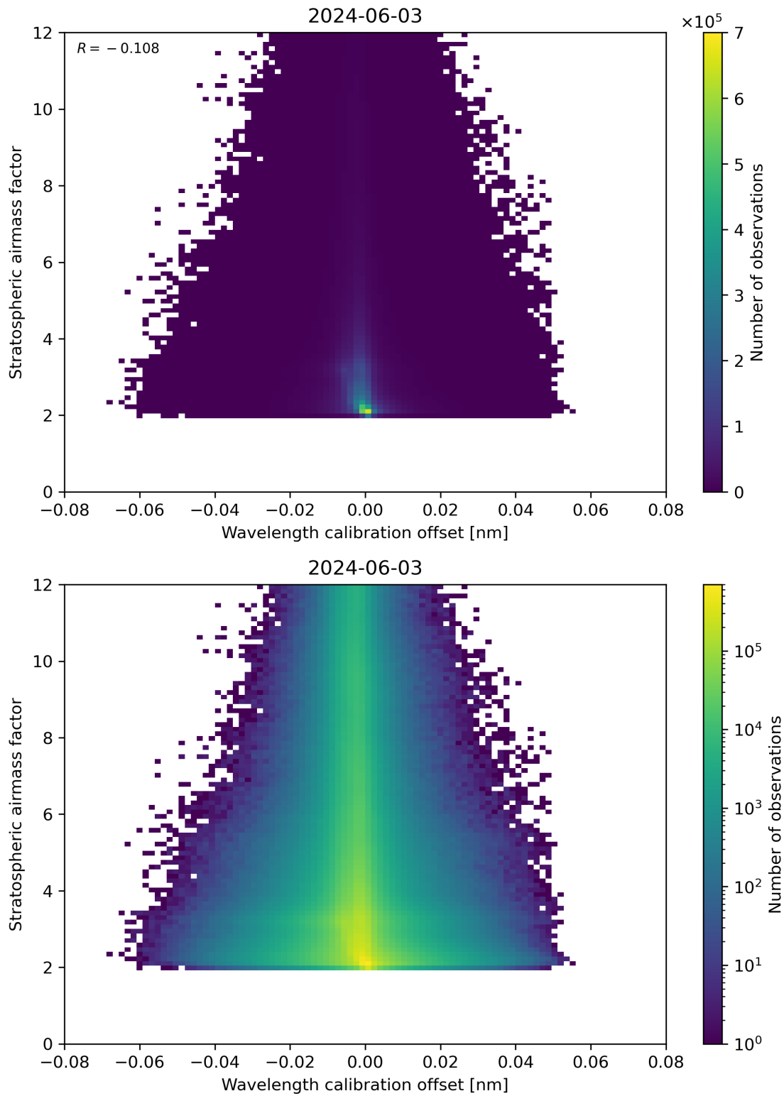
Figure 174: Scatter density plot of “Wavelength calibration offset” against “Stratospheric airmass factor” for 2024-06-03 to 2024-06-04.
