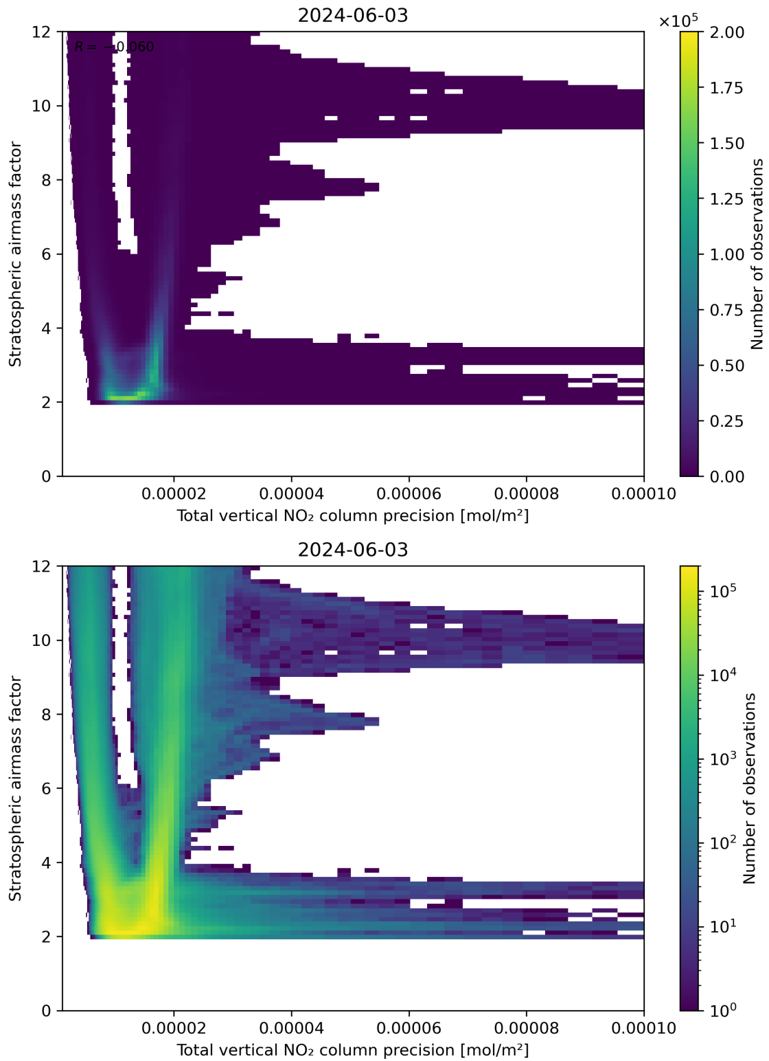
Figure 115: Scatter density plot of “Total vertical NO 2 column precision” against “Stratospheric air mass factor” for 2024-06-03 to 2024-06-04.
