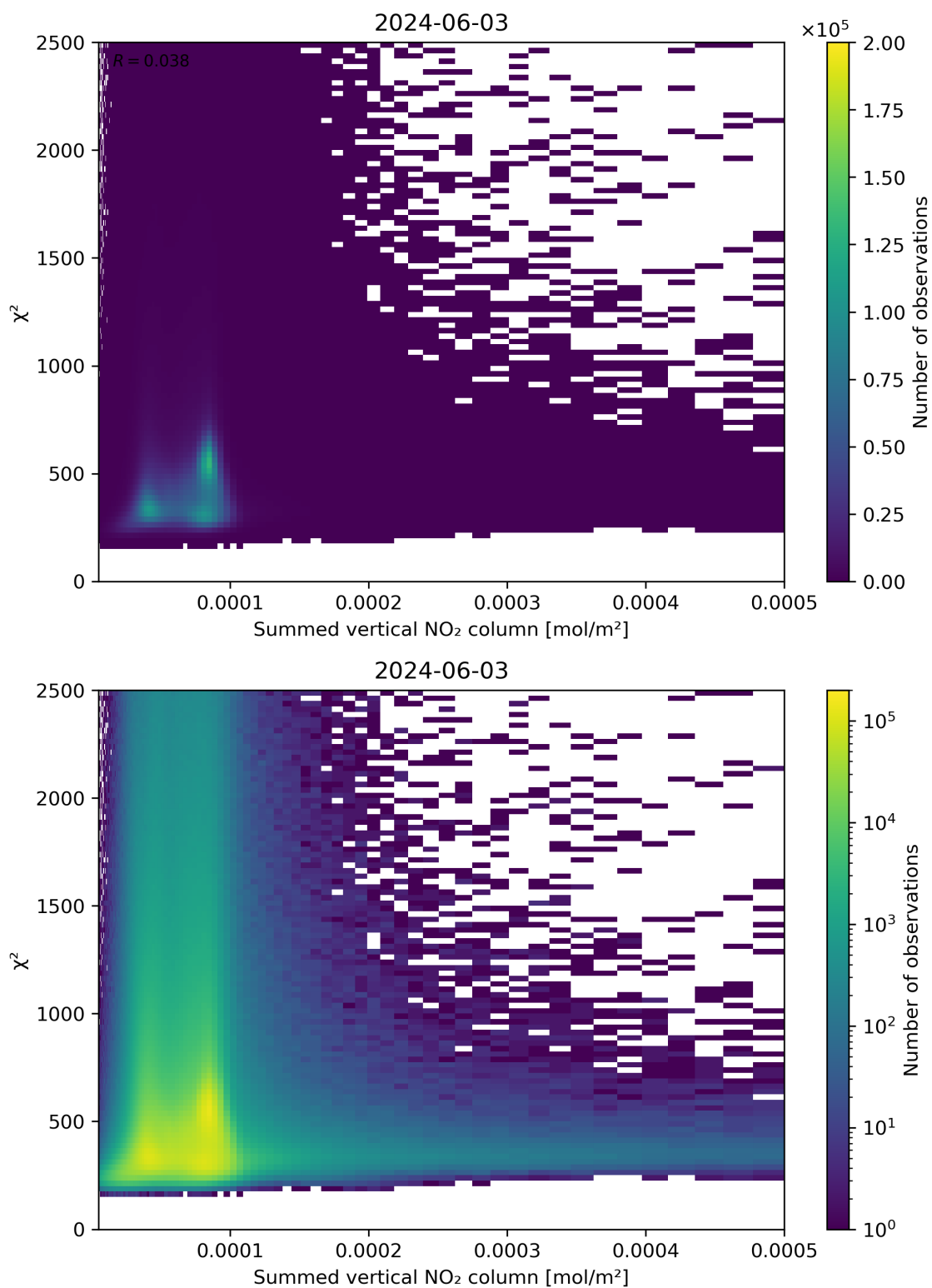
Figure 104: Scatter density plot of “Summed vertical NO 2 column” against “ \chi^2 ” for 2024-06-03 to 2024-06-04.
