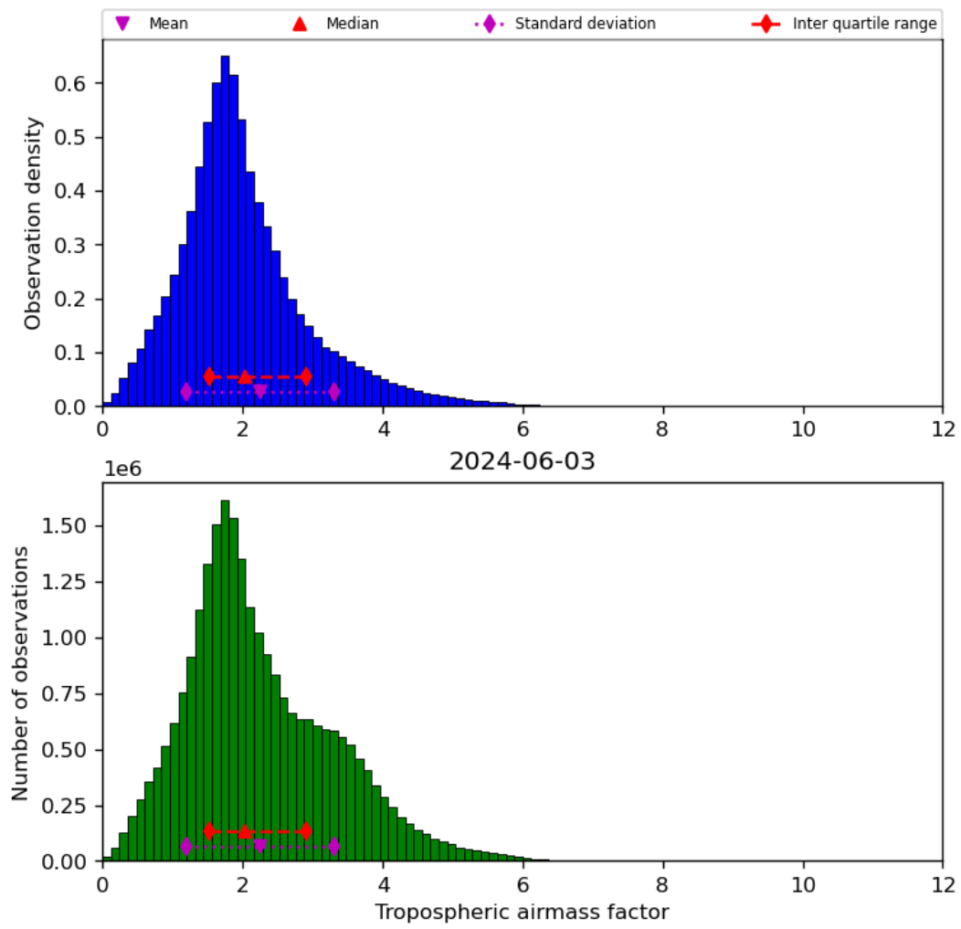
Figure 31: Histogram of “Tropospheric airmass factor” for 2024-06-03 to 2024-06-04
