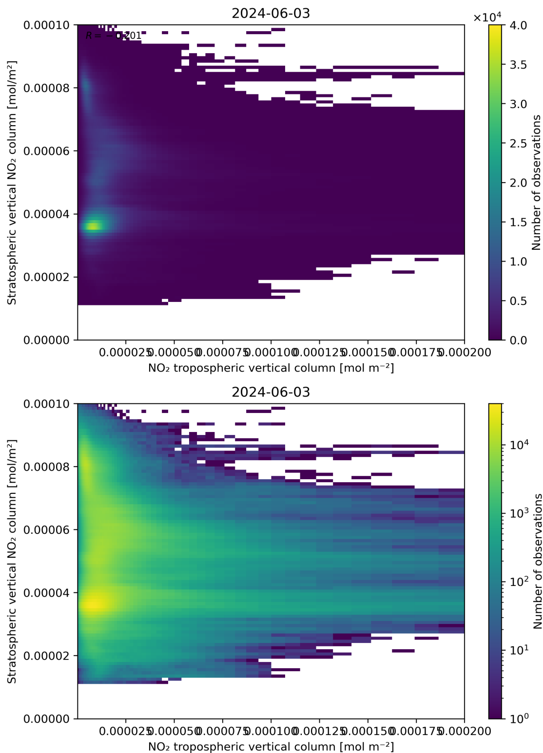
Figure 125: Scatter density plot of “NO 2 tropospheric vertical column” against “Stratospheric vertical NO 2 column” for 2024-06-03 to 2024-06-04.
