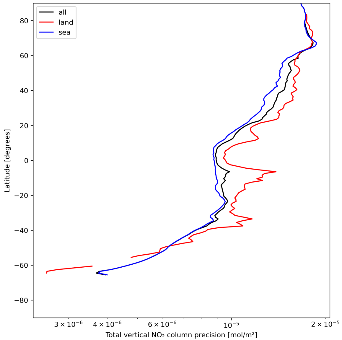
Figure 22: Zonal average of “Total vertical NO 2 column precision” for 2024-06-03 to 2024-06-04.
