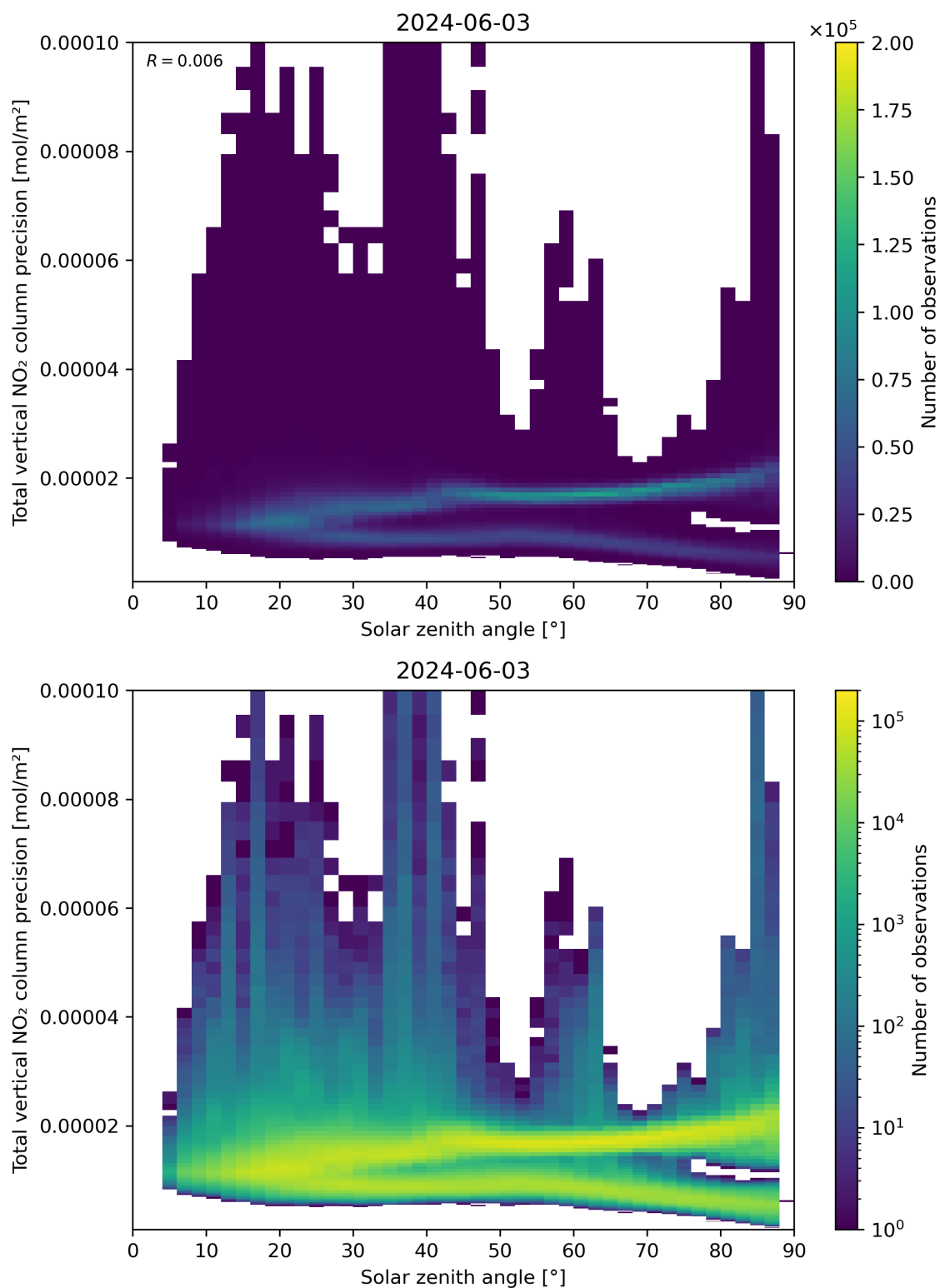
Figure 154: Scatter density plot of “Solar zenith angle” against “Total vertical NO 2 column precision” for 2024-06-03 to 2024-06-04.
