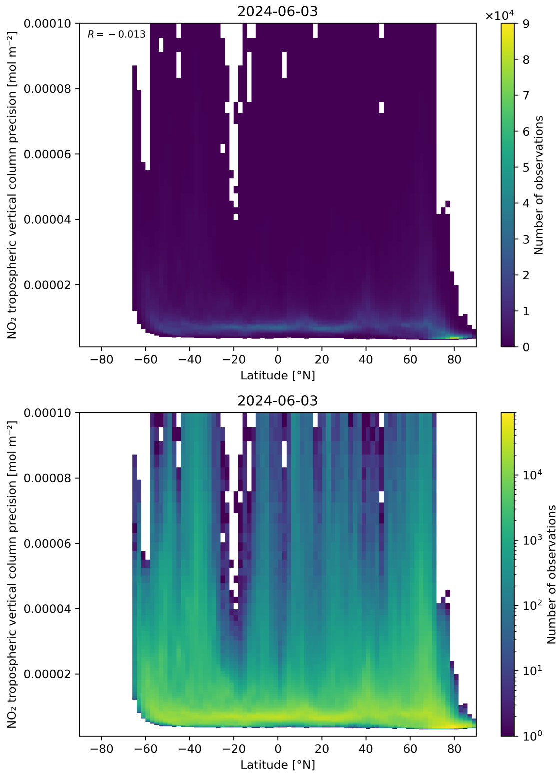
Figure 93: Scatter density plot of “Latitude” against “NO 2 tropospheric vertical column precision” for 2024-06-03 to 2024-06-04.
