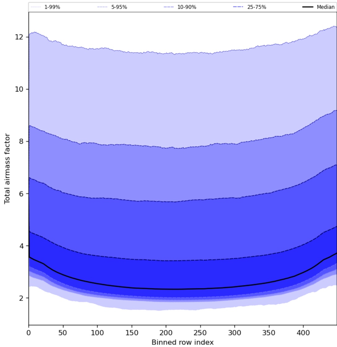
Figure 49: Along track statistics of “Total airmass factor” for 2024-06-03 to 2024-06-04
