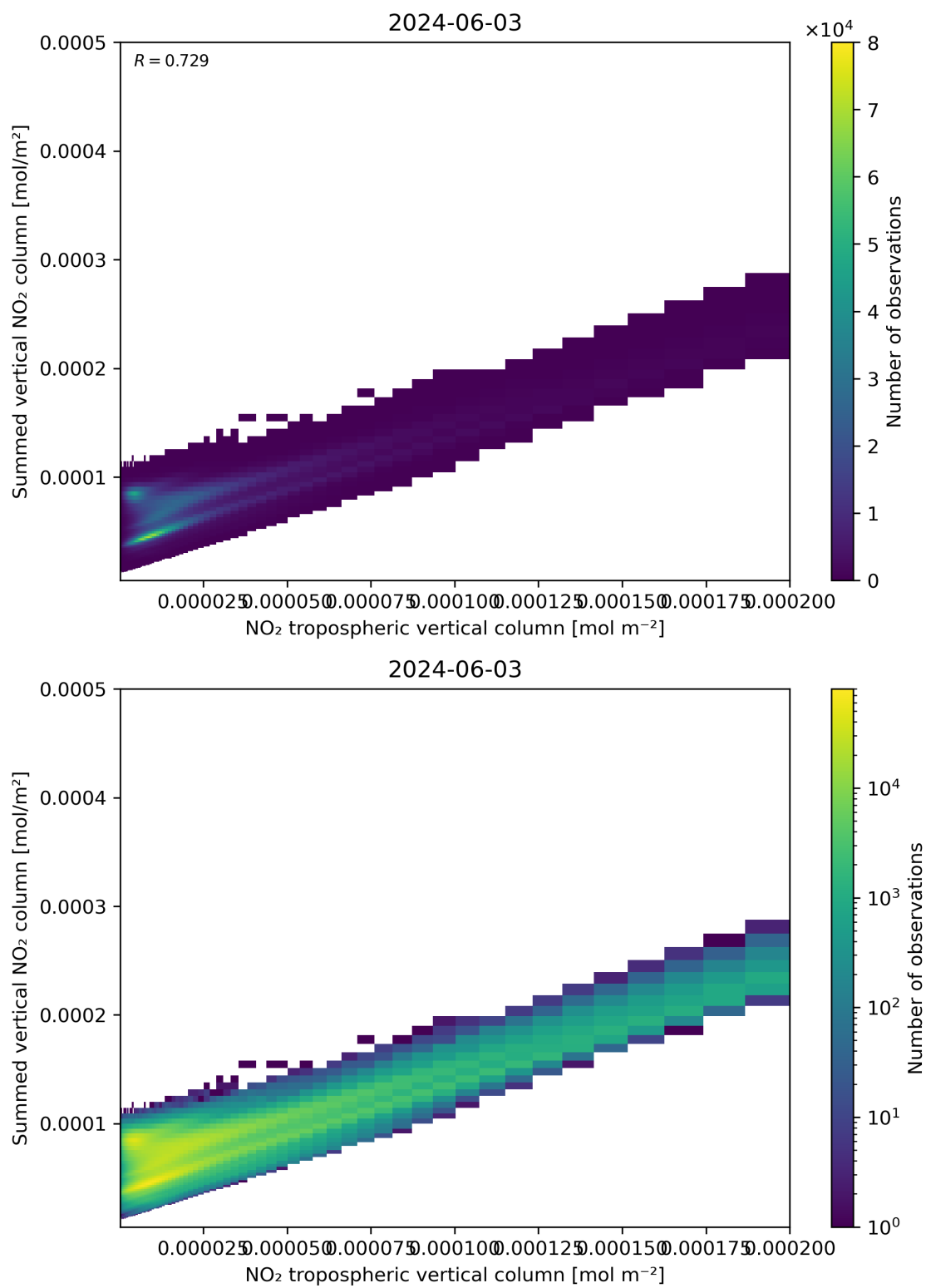
Figure 126: Scatter density plot of “NO 2 tropospheric vertical column” against “Summed vertical NO 2 column” for 2024-06-03 to 2024-06-04.
