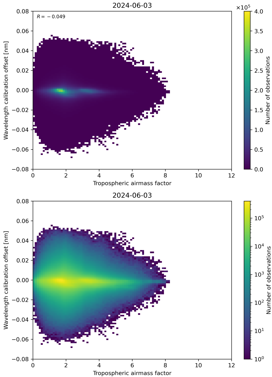
Figure 80: Scatter density plot of “Tropospheric air mass factor” against “Wavelength calibration offset” for 2024-06-03 to 2024-06-04.
