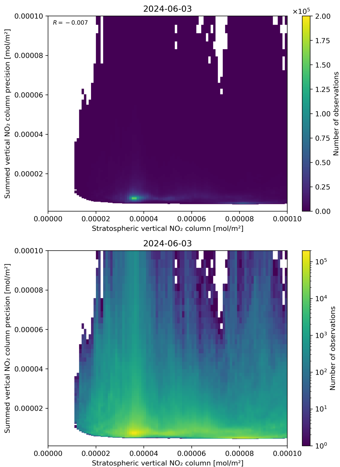
Figure 99: Scatter density plot of “Stratospheric vertical NO 2 column” against “Summed vertical NO 2 column precision” for 2024-06-03 to 2024-06-04.
