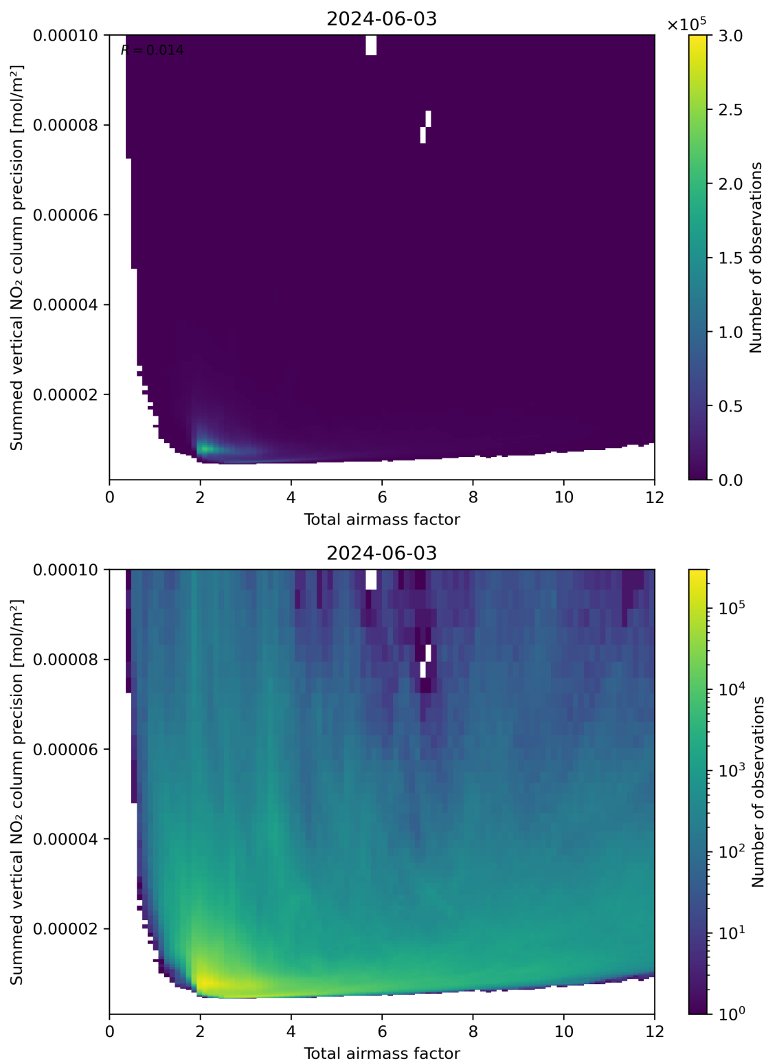
Figure 66: Scatter density plot of “Total airmass factor” against “Summed vertical NO 2 column precision” for 2024-06-03 to 2024-06-04.
