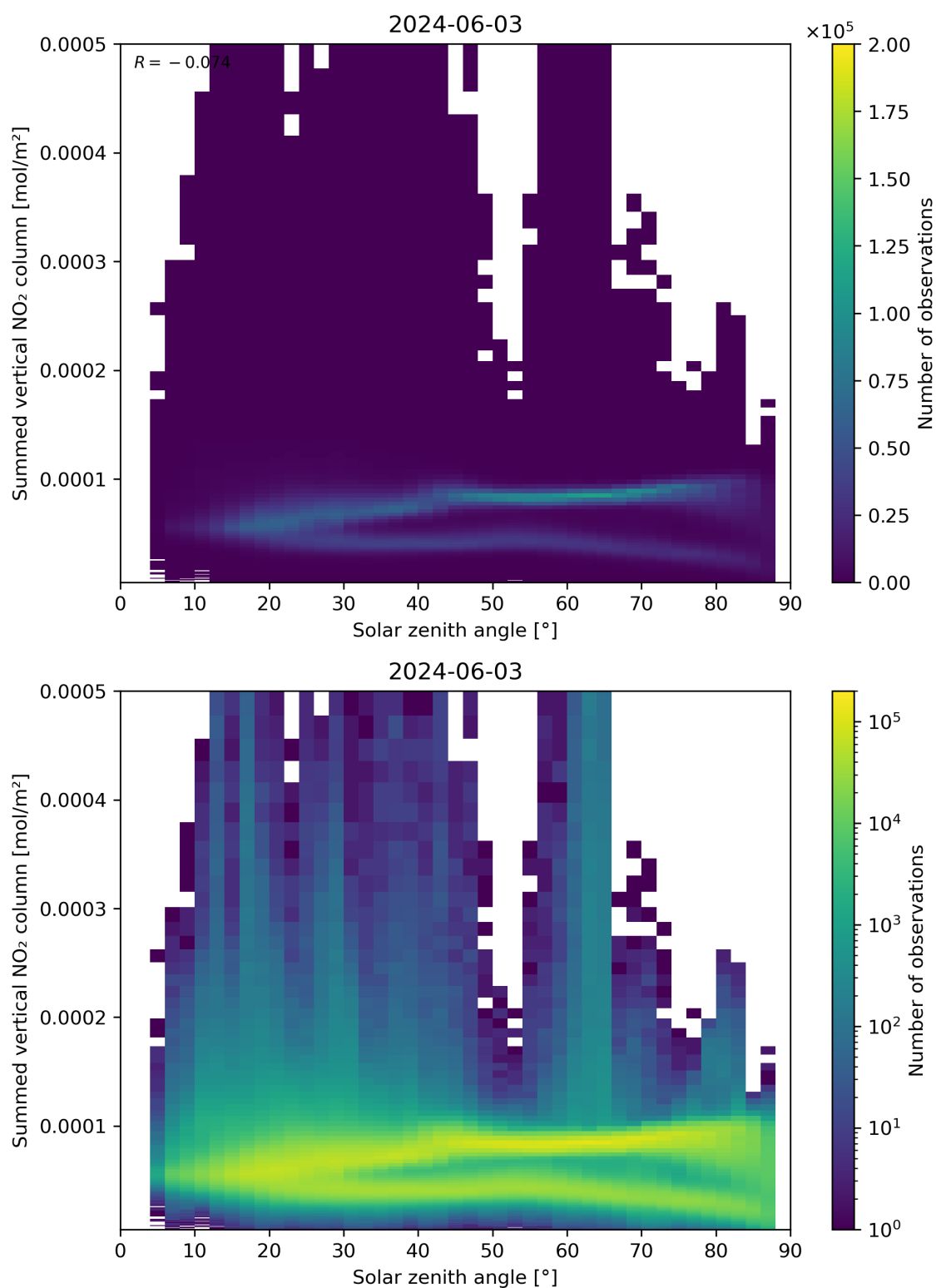
Figure 151: Scatter density plot of “Solar zenith angle” against “Summed vertical NO 2 column” for 2024-06-03 to 2024-06-04.
