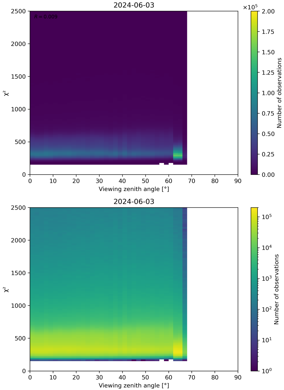
Figure 162: Scatter density plot of “Viewing zenith angle” against “ \chi^2 ” for 2024-06-03 to 2024-06-04.
