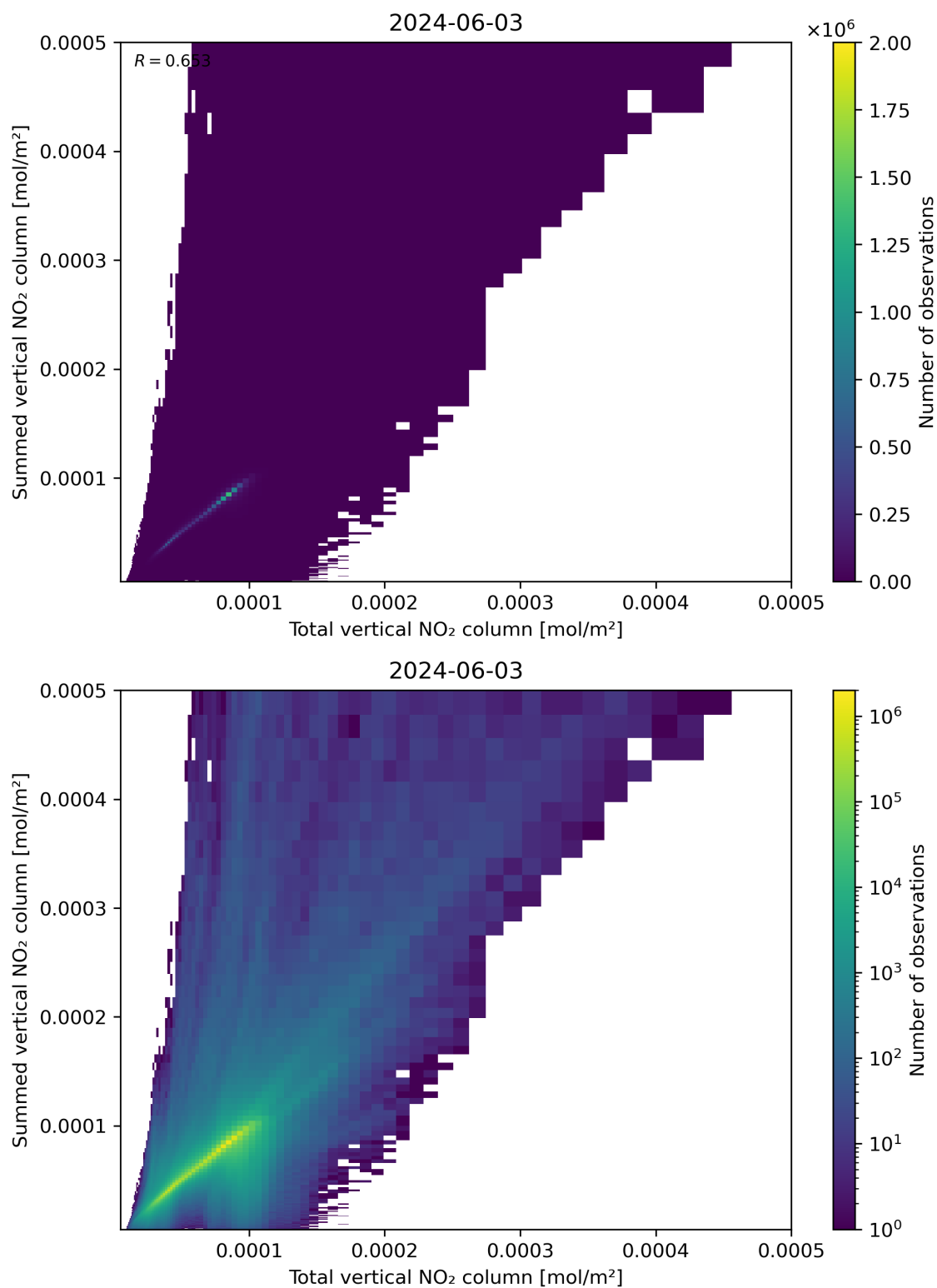
Figure 112: Scatter density plot of “Total vertical NO 2 column” against “Summed vertical NO 2 column” for 2024-06-03 to 2024-06-04.
