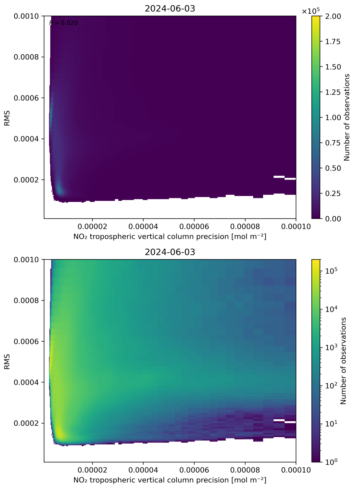
Figure 140: Scatter density plot of “NO 2 tropospheric vertical column precision” against “RMS” for 2024-06-03 to 2024-06-04.
