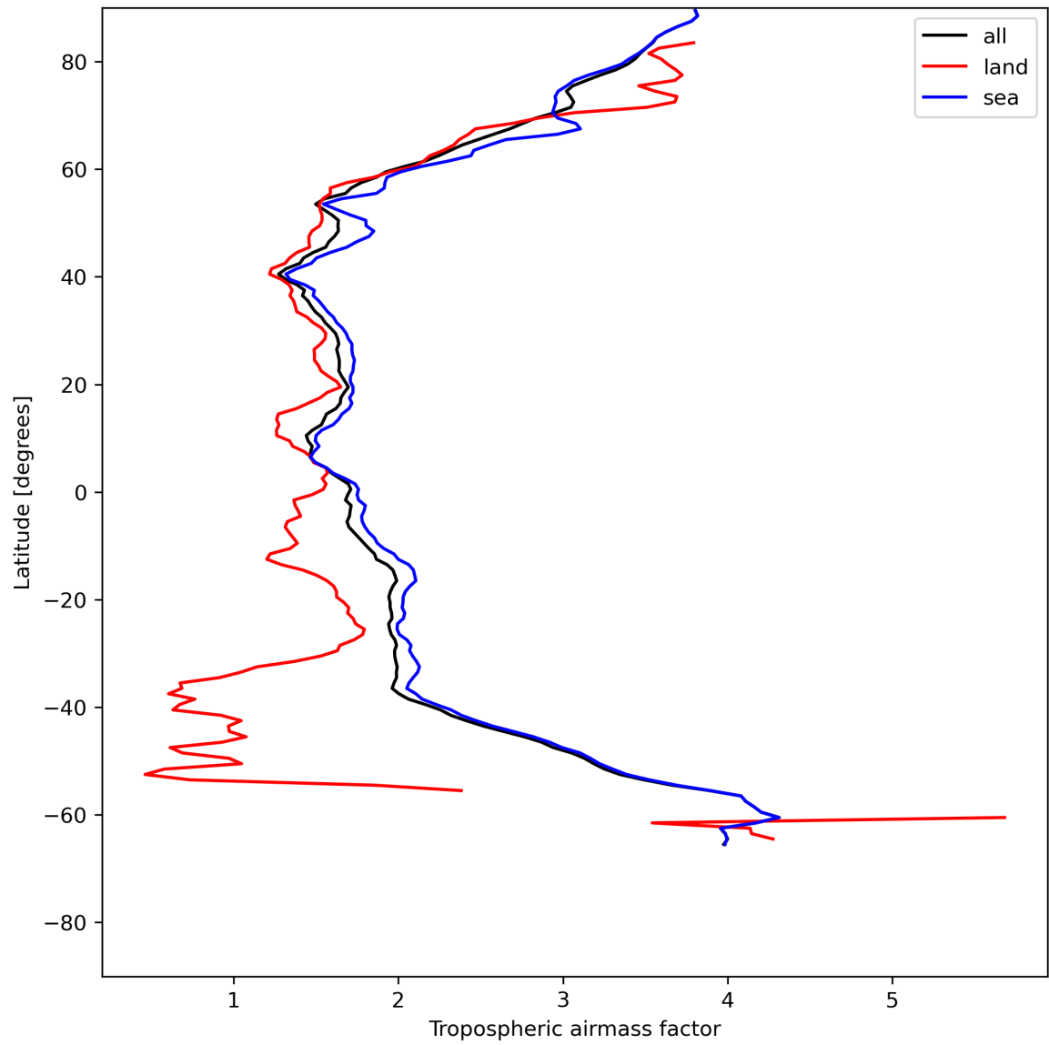
Figure 14: Zonal average of “Tropospheric airmass factor” for 2024-06-03 to 2024-06-04.
