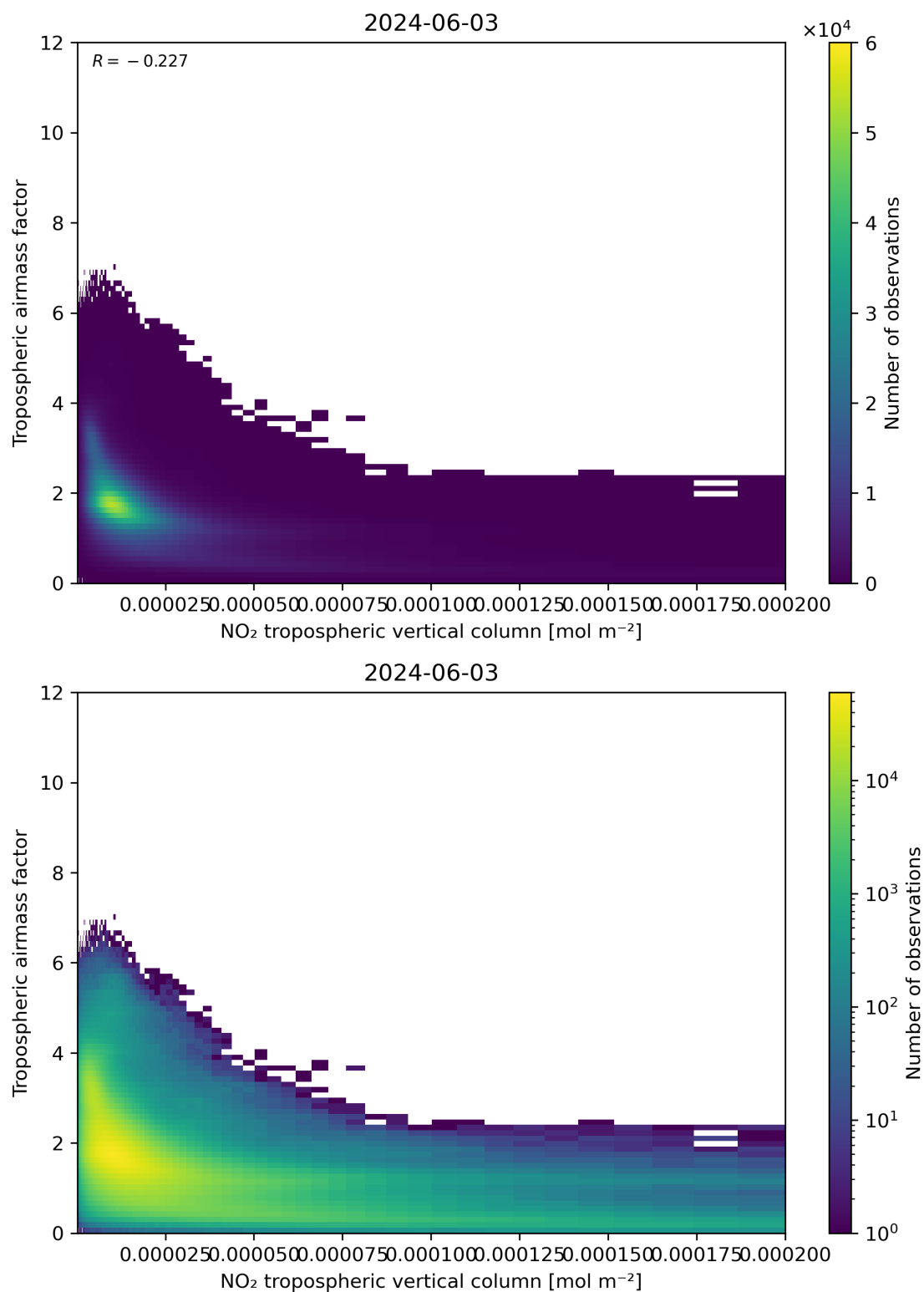
Figure 123: Scatter density plot of “NO 2 tropospheric vertical column” against “Tropospheric air mass factor” for 2024-06-03 to 2024-06-04.
