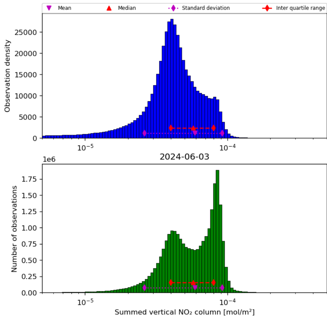
Figure 40: Histogram of “Summed vertical NO 2 column” for 2024-06-03 to 2024-06-04
