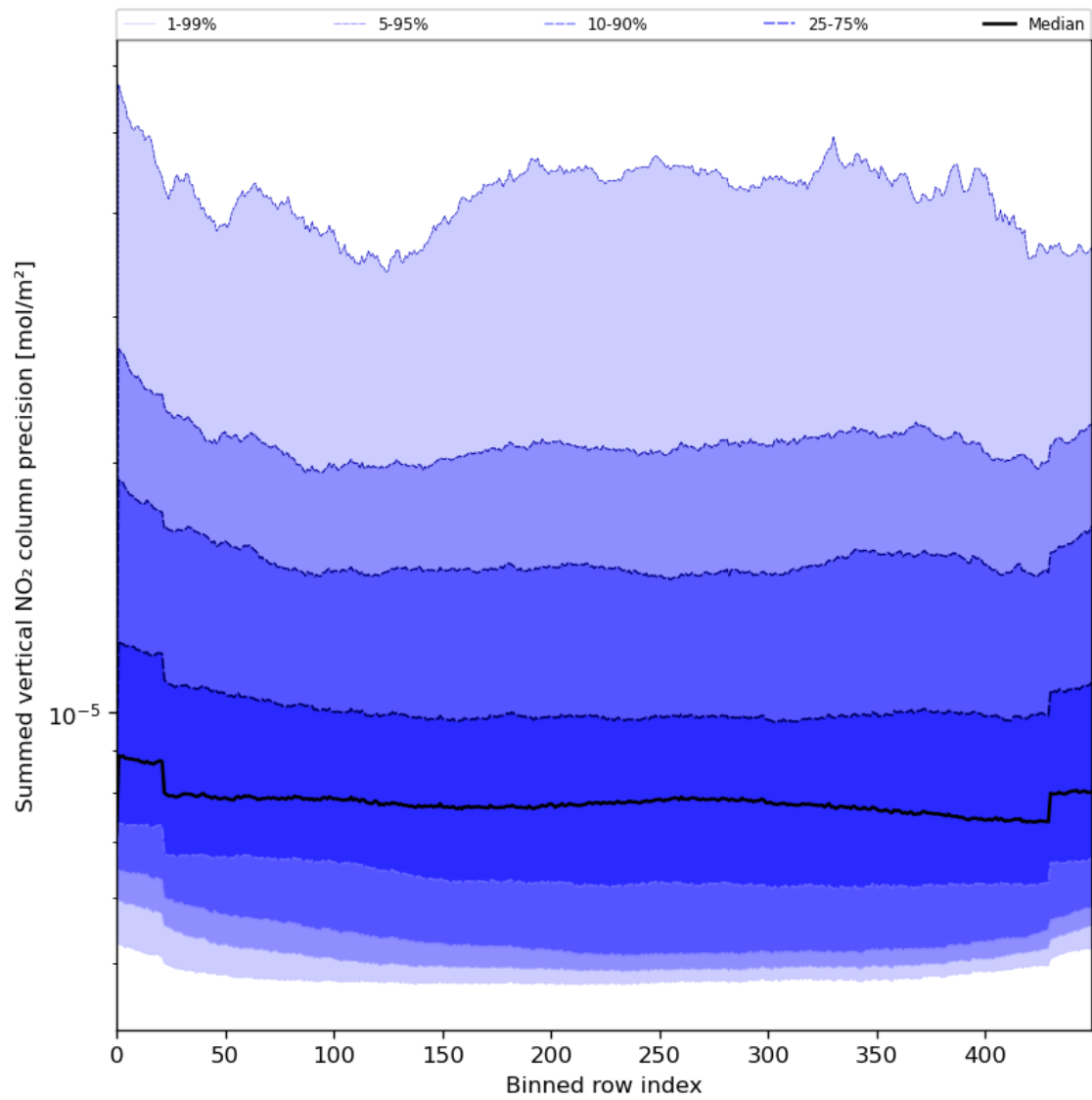
Figure 58: Along track statistics of “Summed vertical NO 2 column precision” for 2024-06-03 to 2024-06-04
