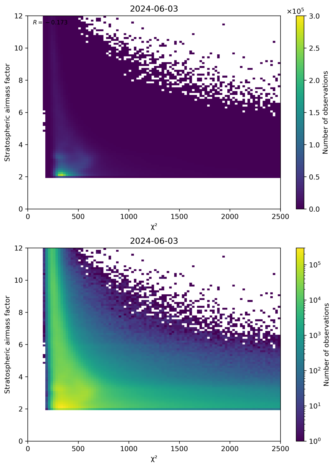
Figure 81: Scatter density plot of “ \chi^2 ” against “Stratospheric airmass factor” for 2024-06-03 to 2024-06-04.
