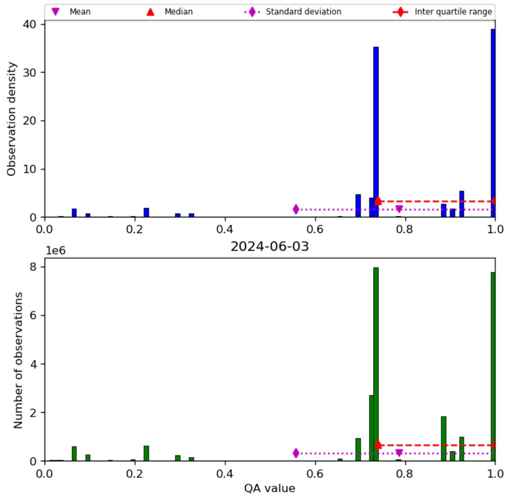
Figure 28: Histogram of “QA value” for 2024-06-03 to 2024-06-04
