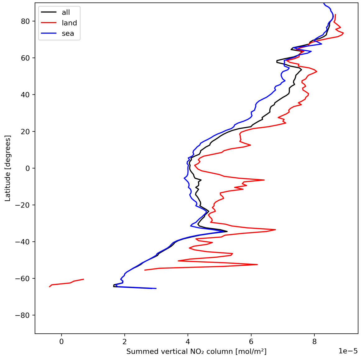
Figure 23: Zonal average of “Summed vertical NO 2 column” for 2024-06-03 to 2024-06-04.
