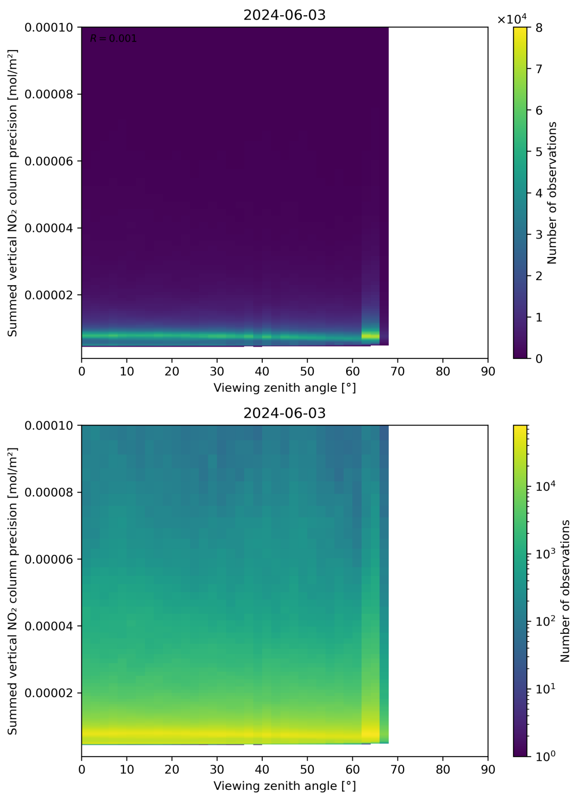
Figure 166: Scatter density plot of “Viewing zenith angle” against “Summed vertical NO 2 column precision” for 2024-06-03 to 2024-06-04.
