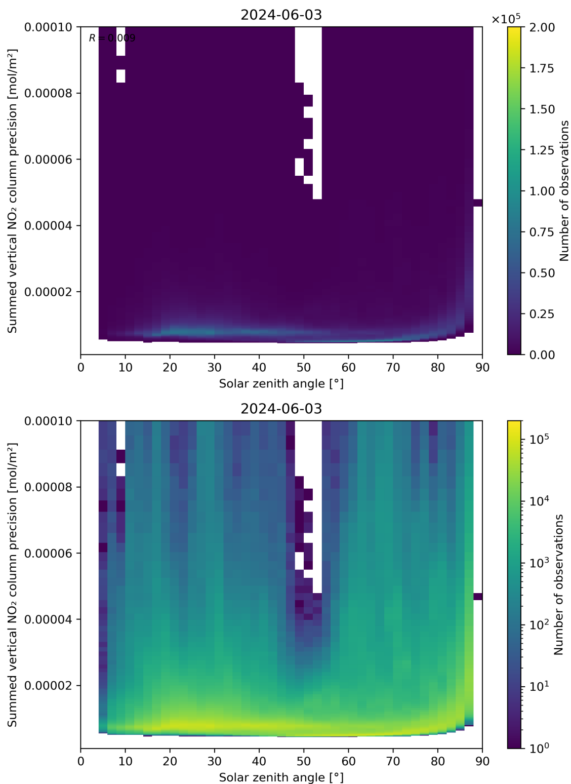
Figure 152: Scatter density plot of “Solar zenith angle” against “Summed vertical NO 2 column precision” for 2024-06-03 to 2024-06-04.
