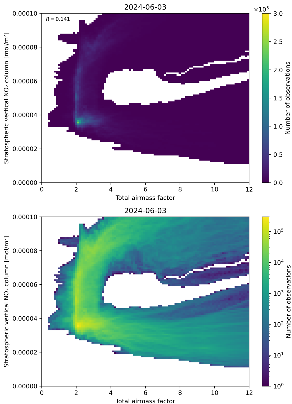
Figure 64: Scatter density plot of “Total airmass factor” against “Stratospheric vertical NO 2 column” for 2024-06-03 to 2024-06-04.
