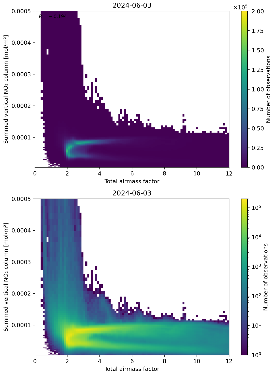
Figure 65: Scatter density plot of “Total airmass factor” against “Summed vertical NO 2 column” for 2024-06-03 to 2024-06-04.
