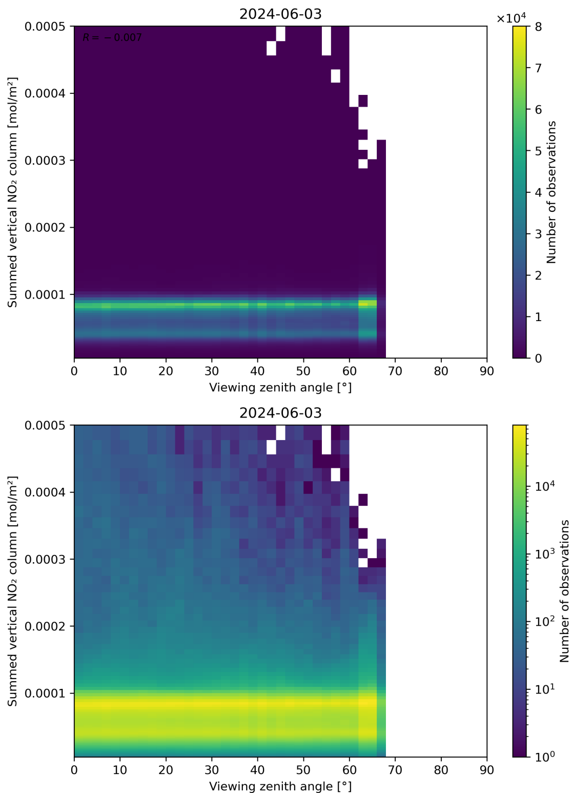
Figure 165: Scatter density plot of “Viewing zenith angle” against “Summed vertical NO 2 column” for 2024-06-03 to 2024-06-04.
