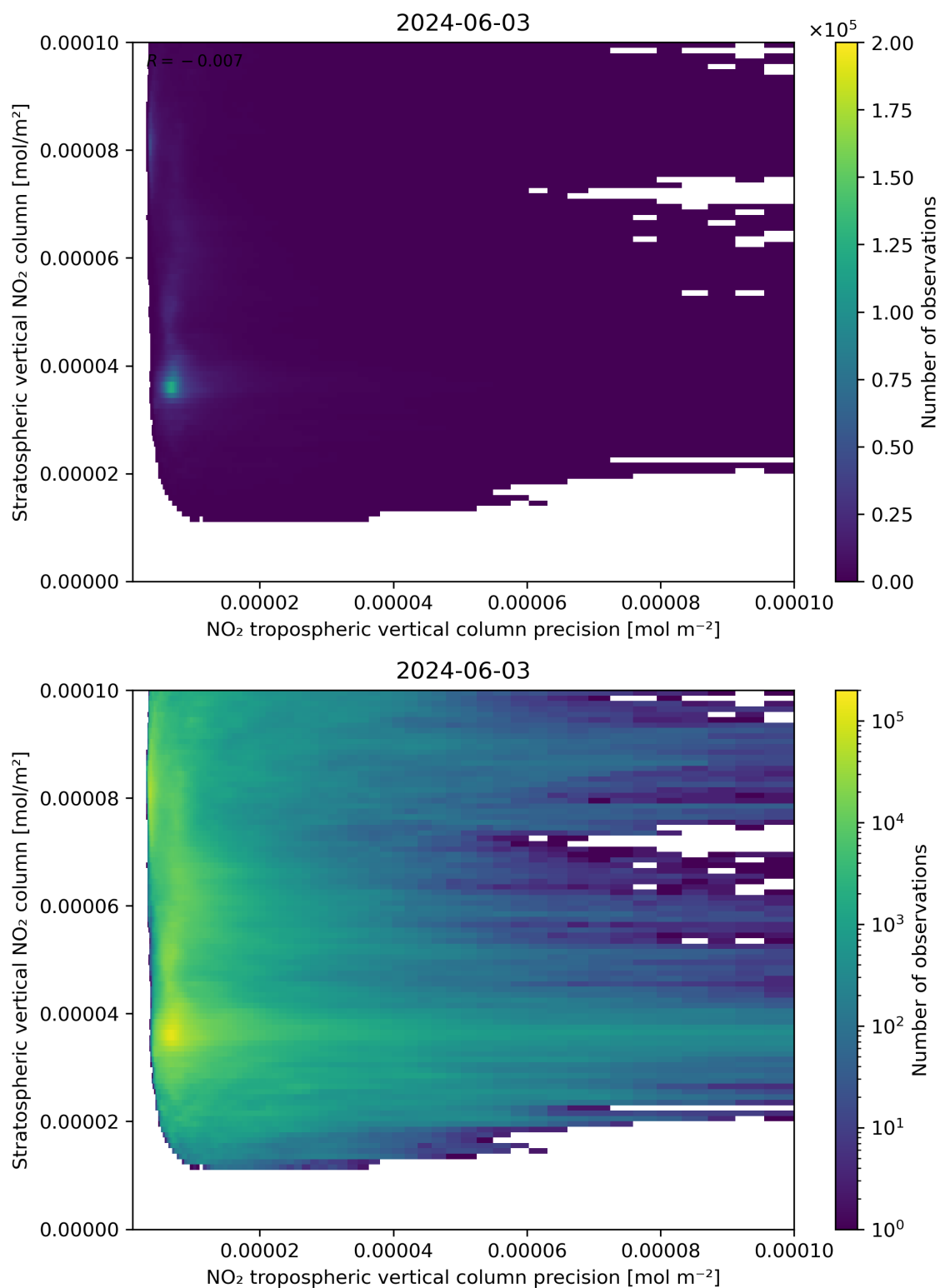
Figure 135: Scatter density plot of “NO 2 tropospheric vertical column precision” against “Stratospheric vertical NO 2 column” for 2024-06-03 to 2024-06-04.
