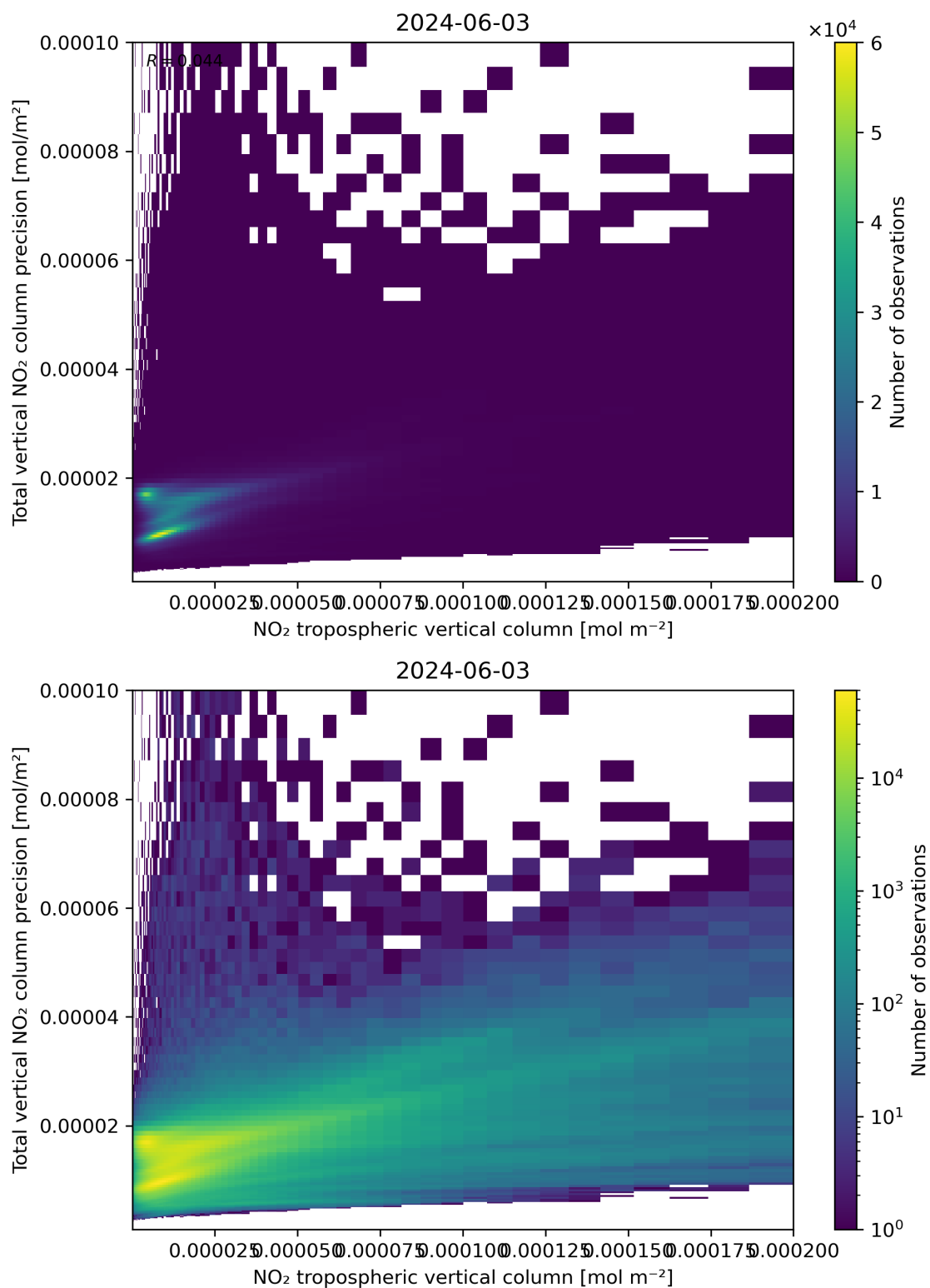
Figure 129: Scatter density plot of “NO 2 tropospheric vertical column” against “Total vertical NO 2 column precision” for 2024-06-03 to 2024-06-04.
