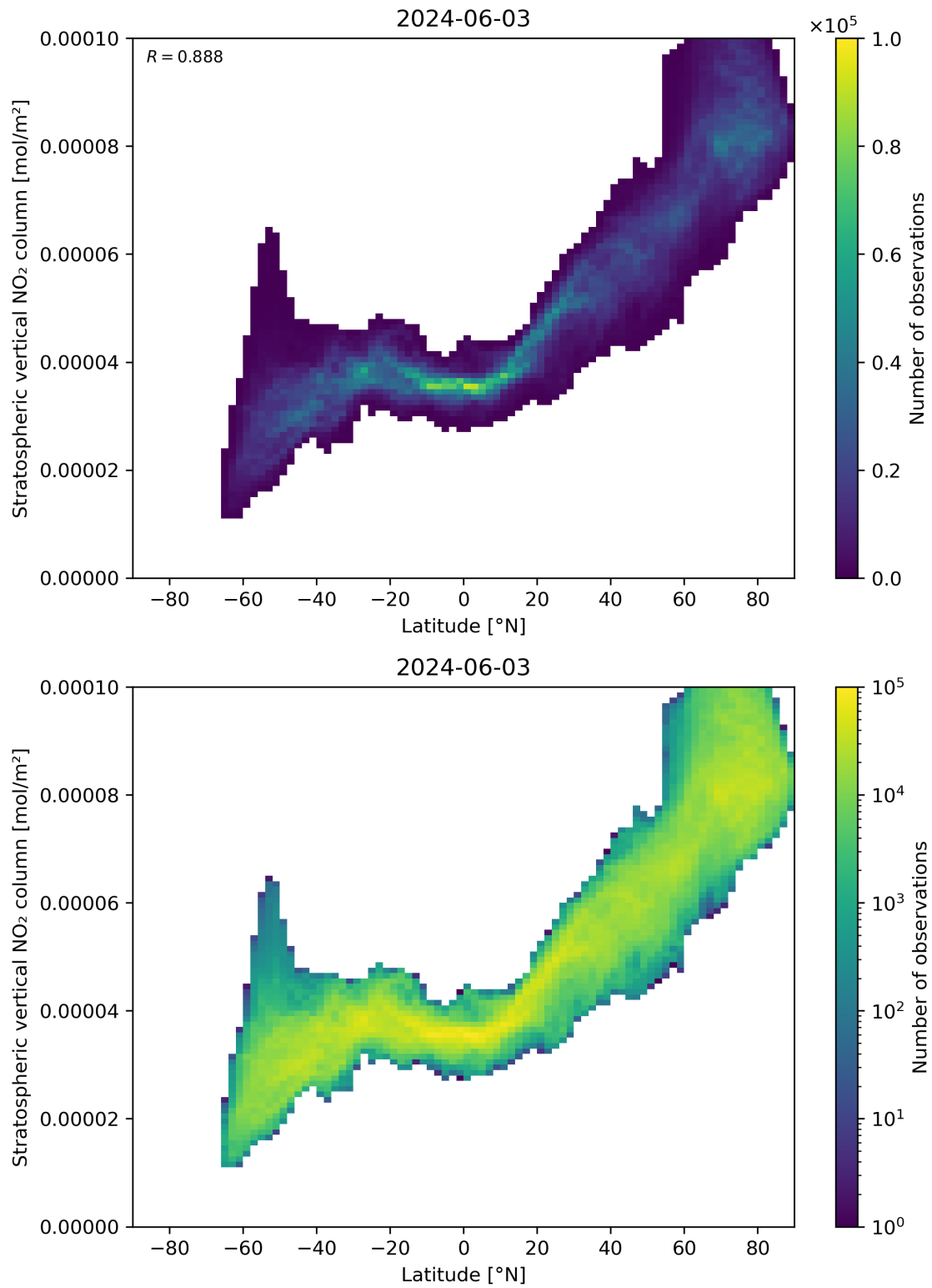
Figure 87: Scatter density plot of “Latitude” against “Stratospheric vertical NO 2 column” for 2024-06-03 to 2024-06-04.
