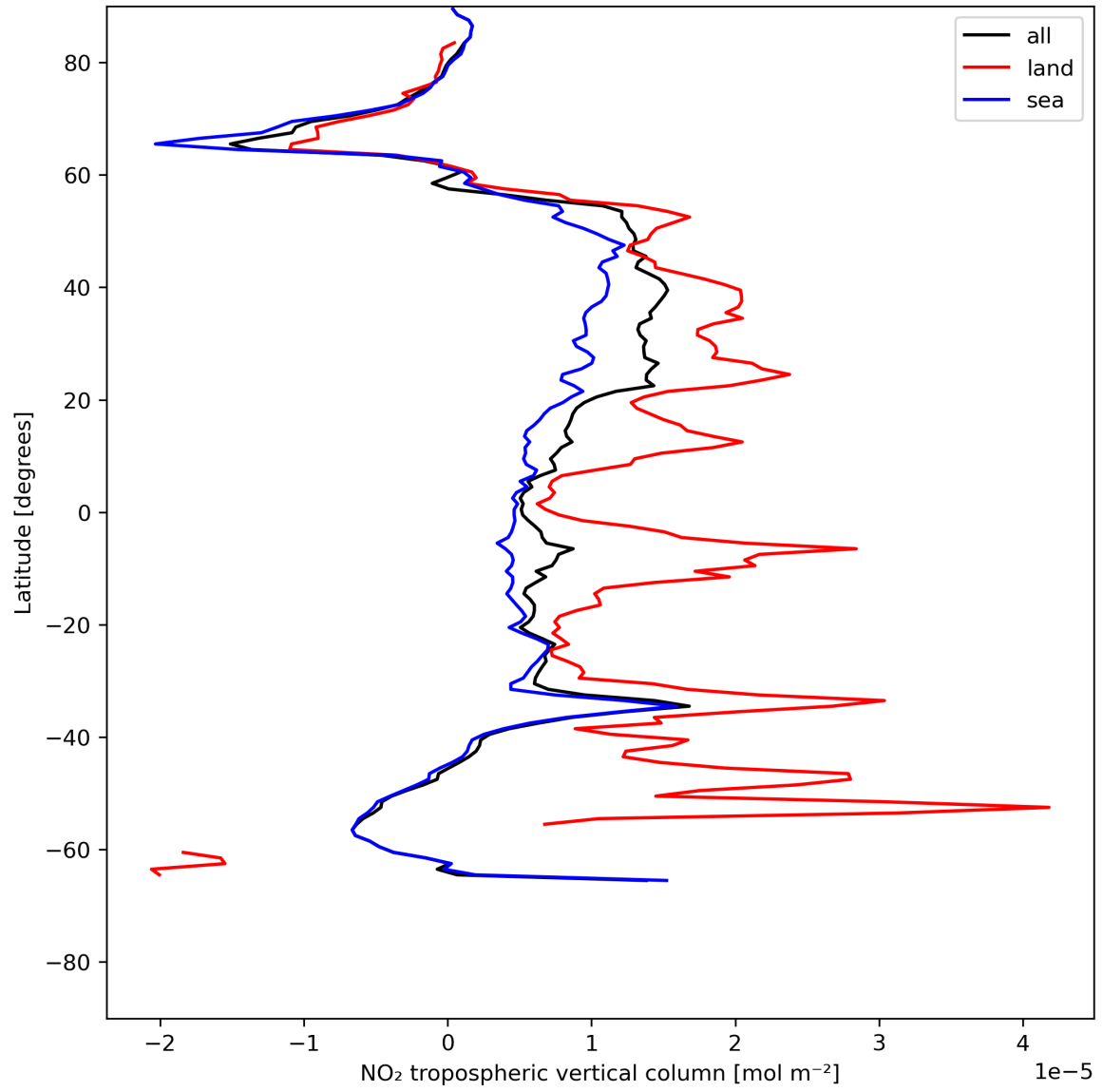
Figure 12: Zonal average of “NO 2 tropospheric vertical column” for 2024-06-03 to 2024-06-04.
