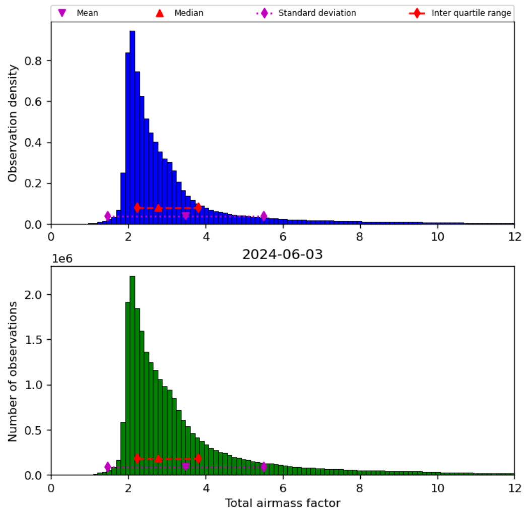
Figure 32: Histogram of “Total airmass factor” for 2024-06-03 to 2024-06-04
