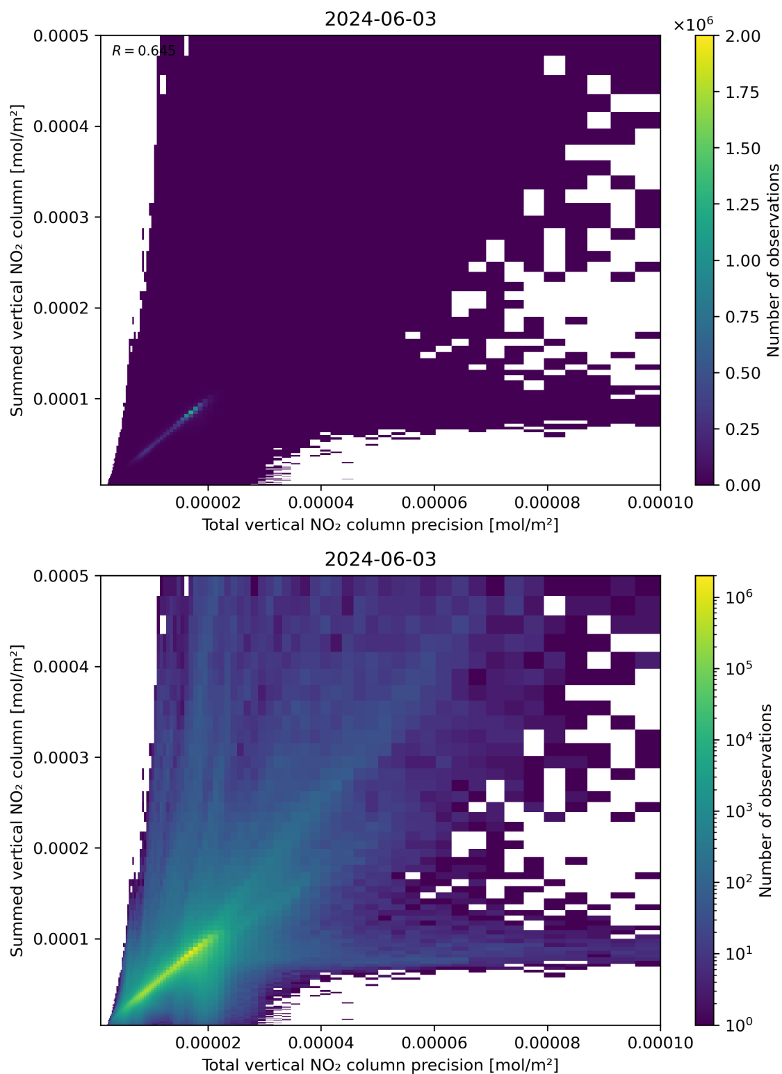
Figure 117: Scatter density plot of “Total vertical NO 2 column precision” against “Summed vertical NO 2 column” for 2024-06-03 to 2024-06-04.
