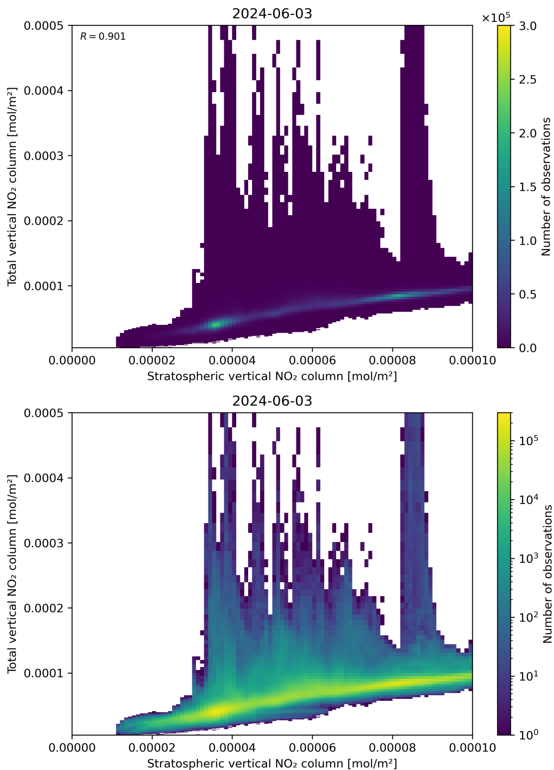
Figure 100: Scatter density plot of “Stratospheric vertical NO 2 column” against “Total vertical NO 2 column” for 2024-06-03 to 2024-06-04.
