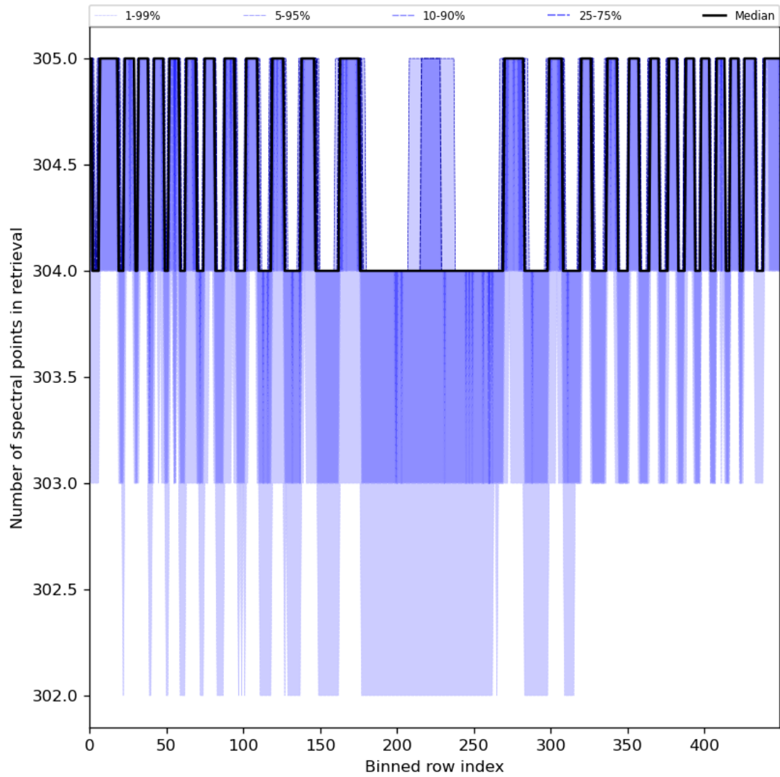
Figure 50: Along track statistics of “Number of spectral points in retrieval” for 2024-06-03 to 2024-06-04
