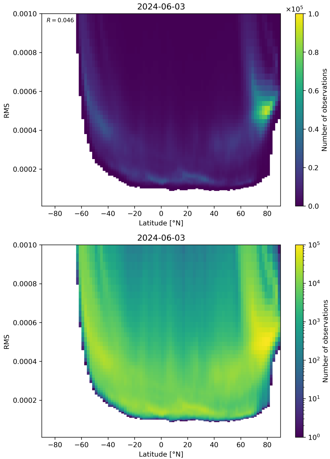
Figure 94: Scatter density plot of “Latitude” against “RMS” for 2024-06-03 to 2024-06-04.
