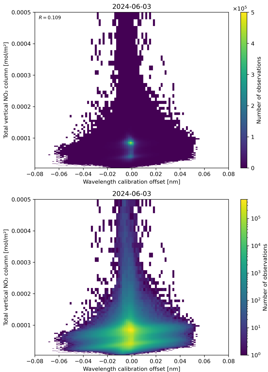
Figure 179: Scatter density plot of “Wavelength calibration offset” against “Total vertical NO 2 column” for 2024-06-03 to 2024-06-04.
