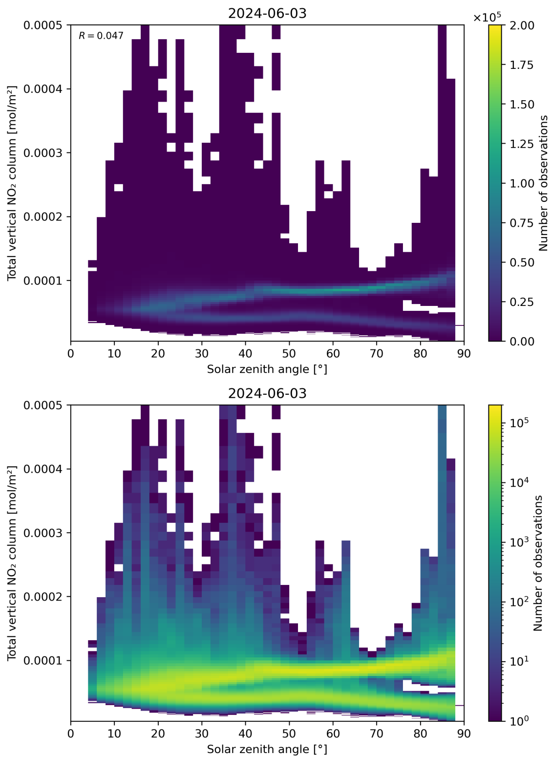
Figure 153: Scatter density plot of “Solar zenith angle” against “Total vertical NO 2 column” for 2024-06-03 to 2024-06-04.
