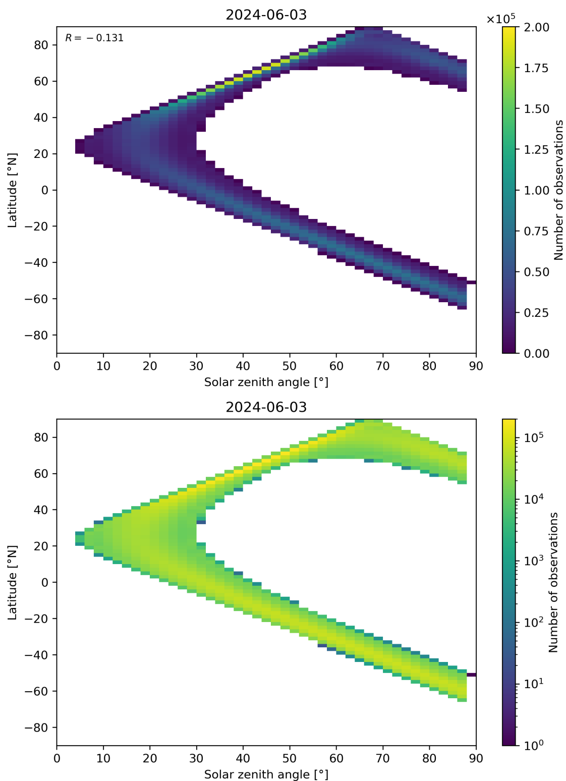
Figure 149: Scatter density plot of “Solar zenith angle” against “Latitude” for 2024-06-03 to 2024-06-04.
