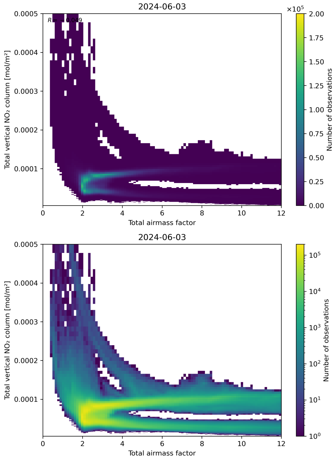
Figure 67: Scatter density plot of “Total airmass factor” against “Total vertical NO 2 column” for 2024-06-03 to 2024-06-04.
