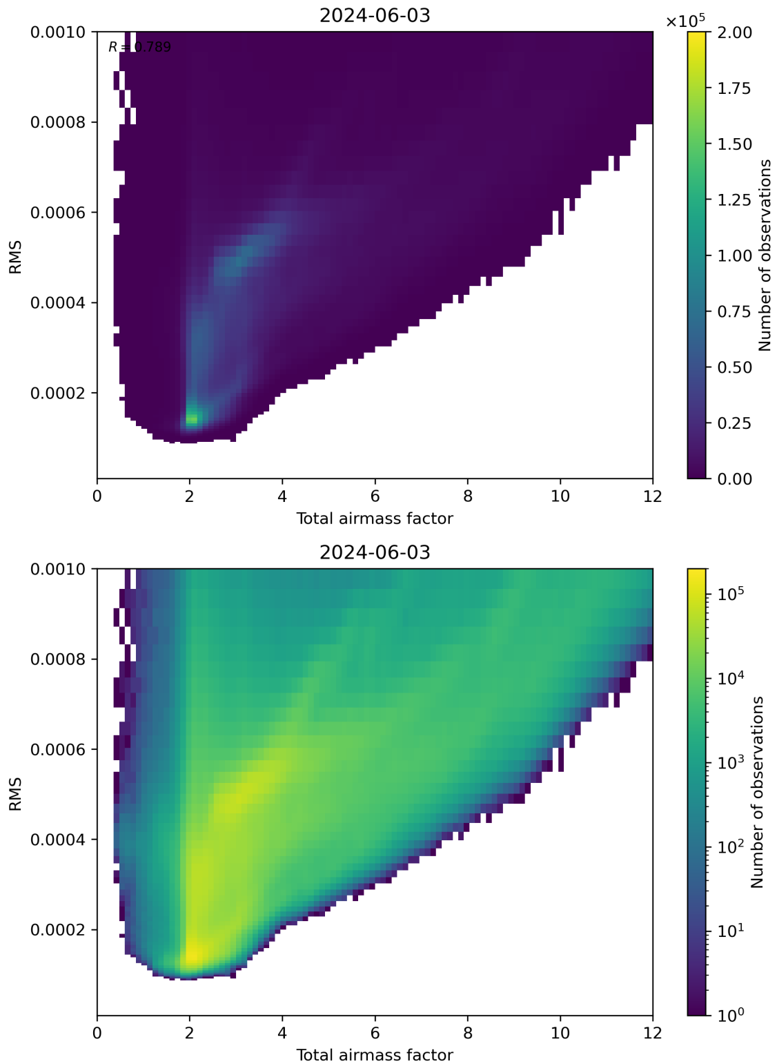
Figure 69: Scatter density plot of “Total airmass factor” against “RMS” for 2024-06-03 to 2024-06-04.
