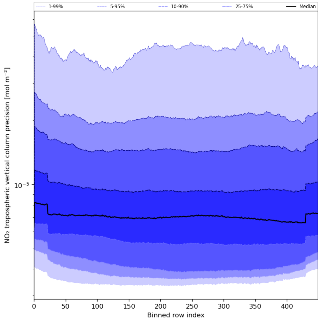
Figure 47: Along track statistics of “NO 2 tropospheric vertical column precision” for 2024-06-03 to 2024-06-04
