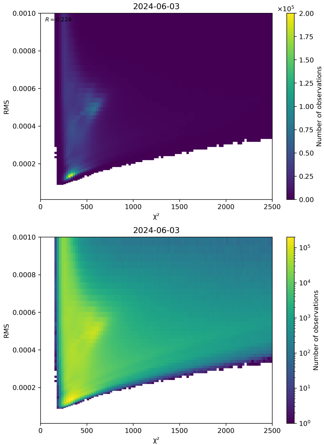
Figure 82: Scatter density plot of “ \chi^2 ” against “RMS” for 2024-06-03 to 2024-06-04.
