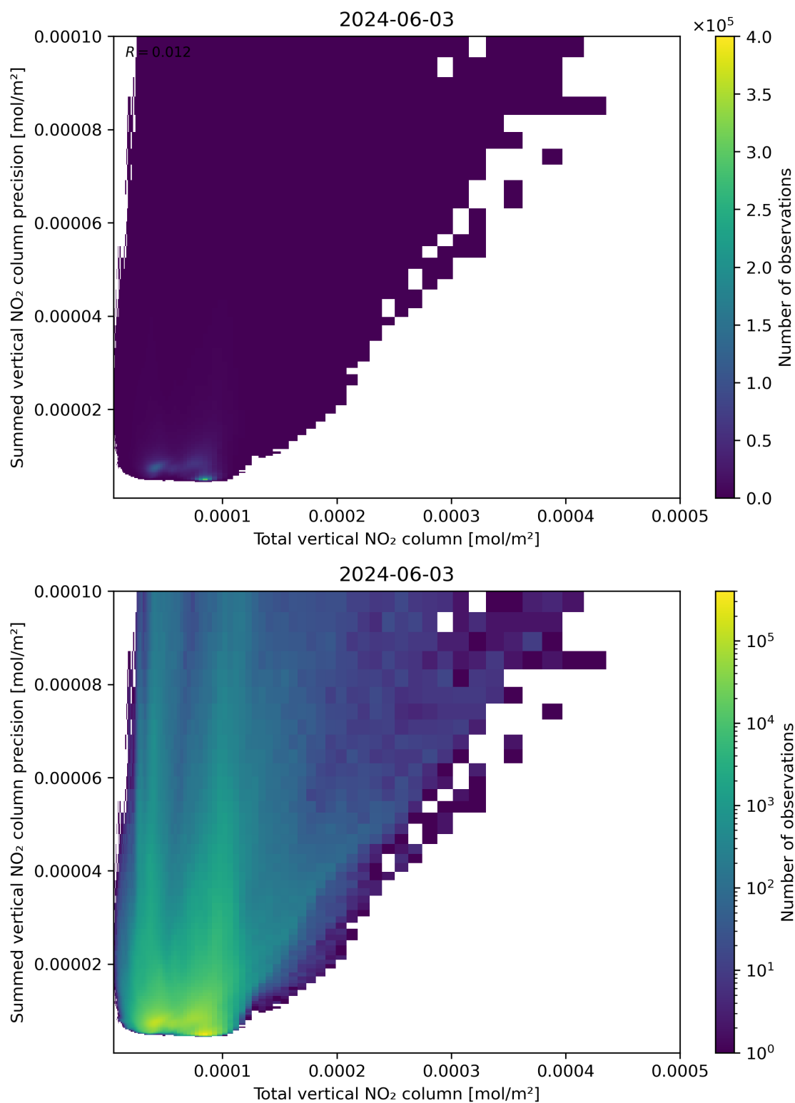
Figure 113: Scatter density plot of “Total vertical NO 2 column” against “Summed vertical NO 2 column precision” for 2024-06-03 to 2024-06-04.
