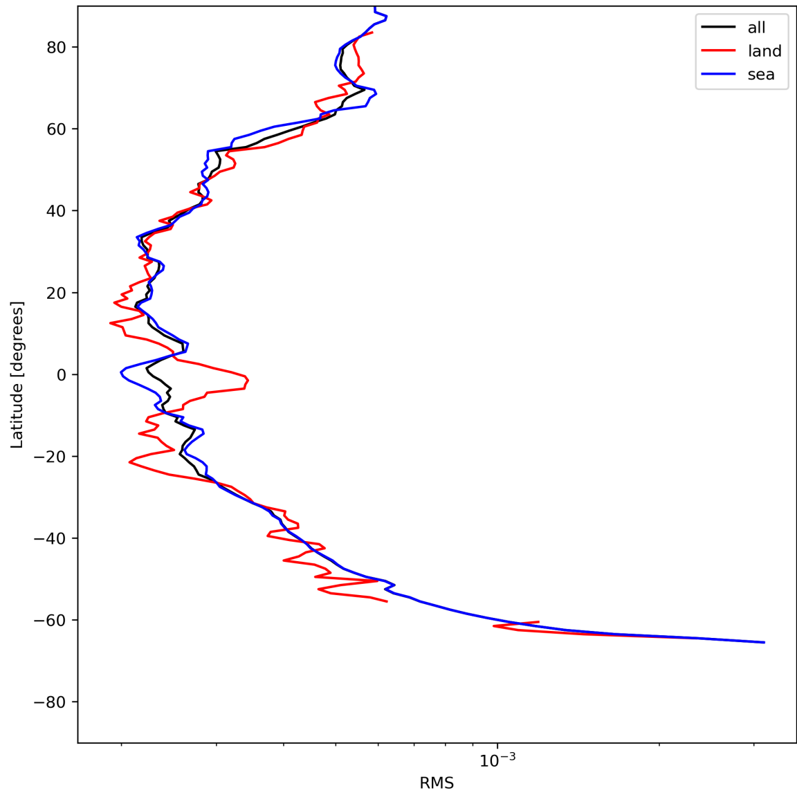
Figure 26: Zonal average of “RMS” for 2024-06-03 to 2024-06-04.
