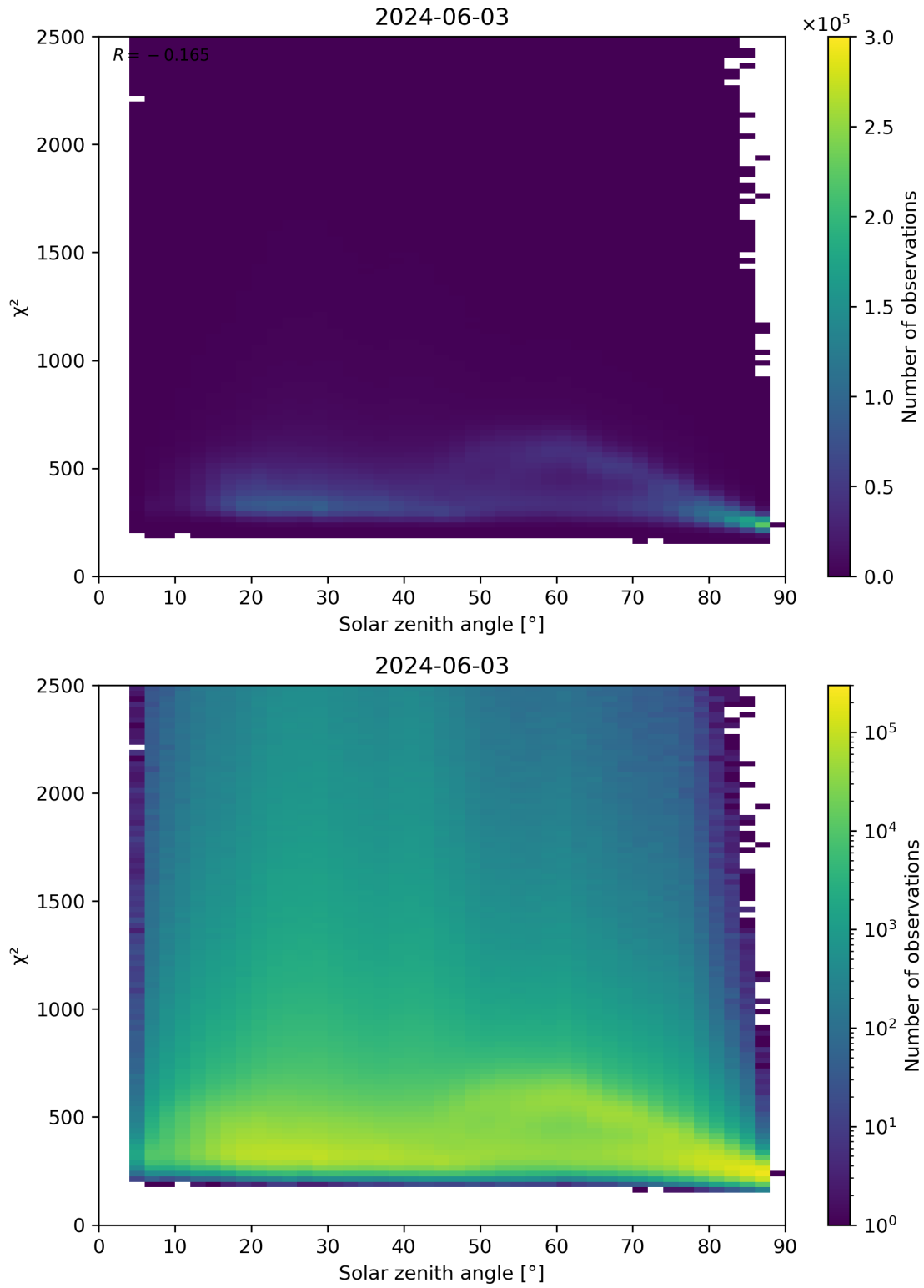
Figure 148: Scatter density plot of “Solar zenith angle” against “ \chi^2 ” for 2024-06-03 to 2024-06-04.
