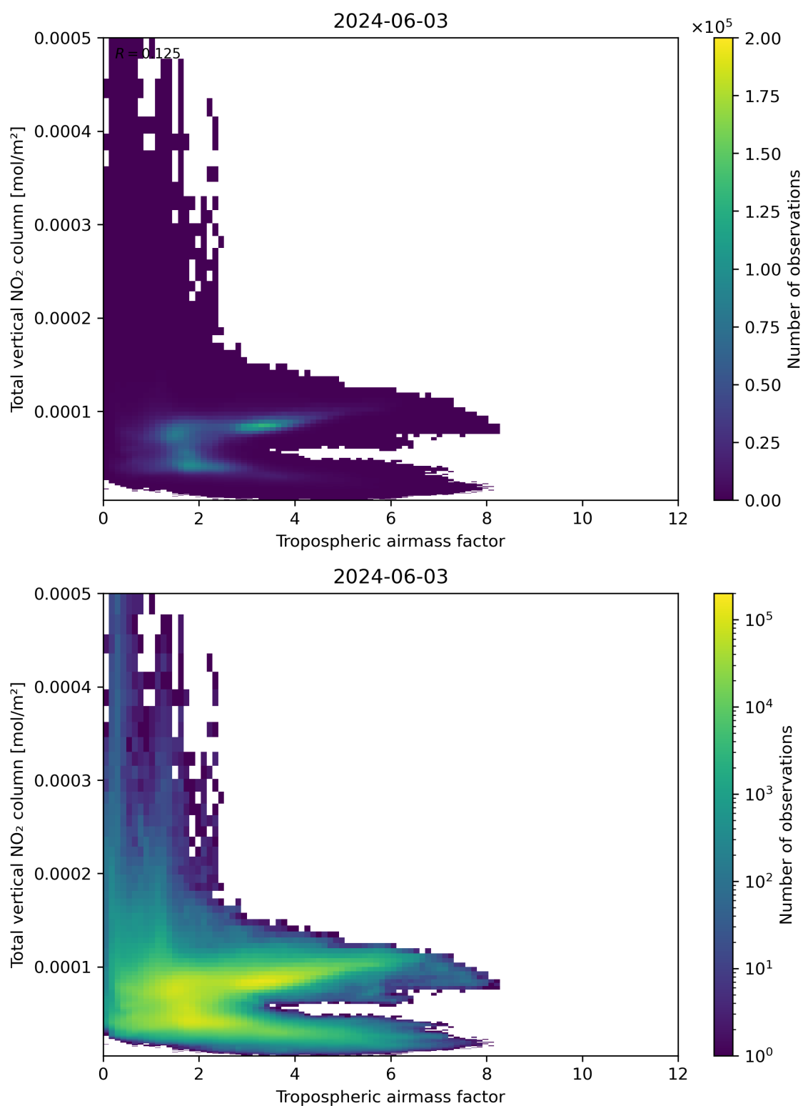
Figure 77: Scatter density plot of “Tropospheric airmass factor” against “Total vertical NO 2 column” for 2024-06-03 to 2024-06-04.
