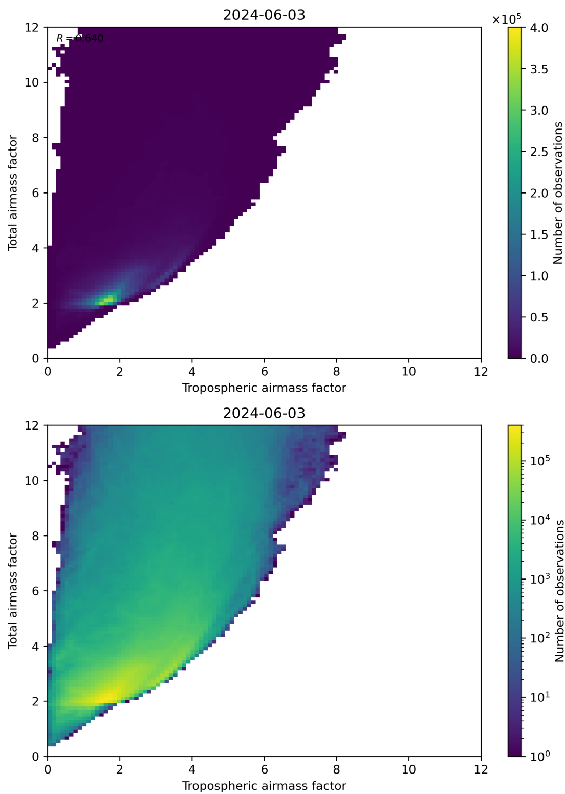
Figure 72: Scatter density plot of “Tropospheric airmass factor” against “Total airmass factor” for 2024-06-03 to 2024-06-04.
