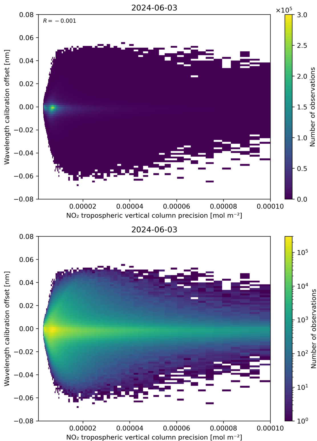
Figure 141: Scatter density plot of “NO 2 tropospheric vertical column precision” against “Wavelength calibration offset” for 2024-06-03 to 2024-06-04.
