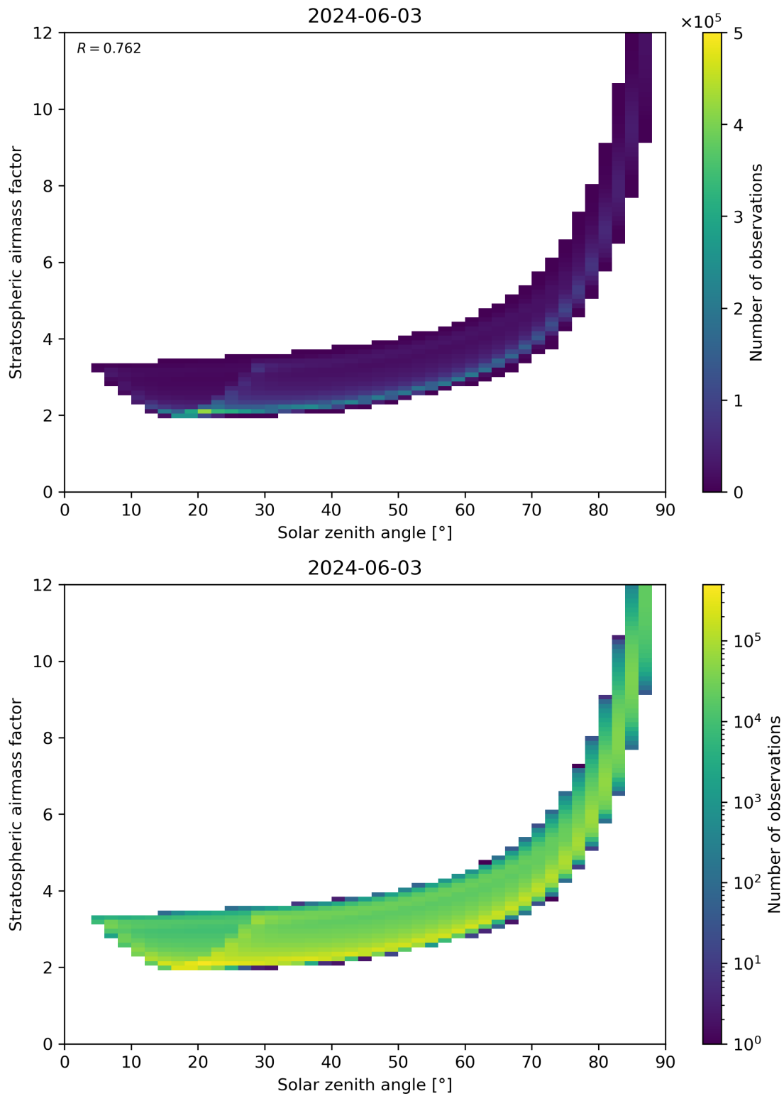
Figure 145: Scatter density plot of “Solar zenith angle” against “Stratospheric airmass factor” for 2024-06-03 to 2024-06-04.
