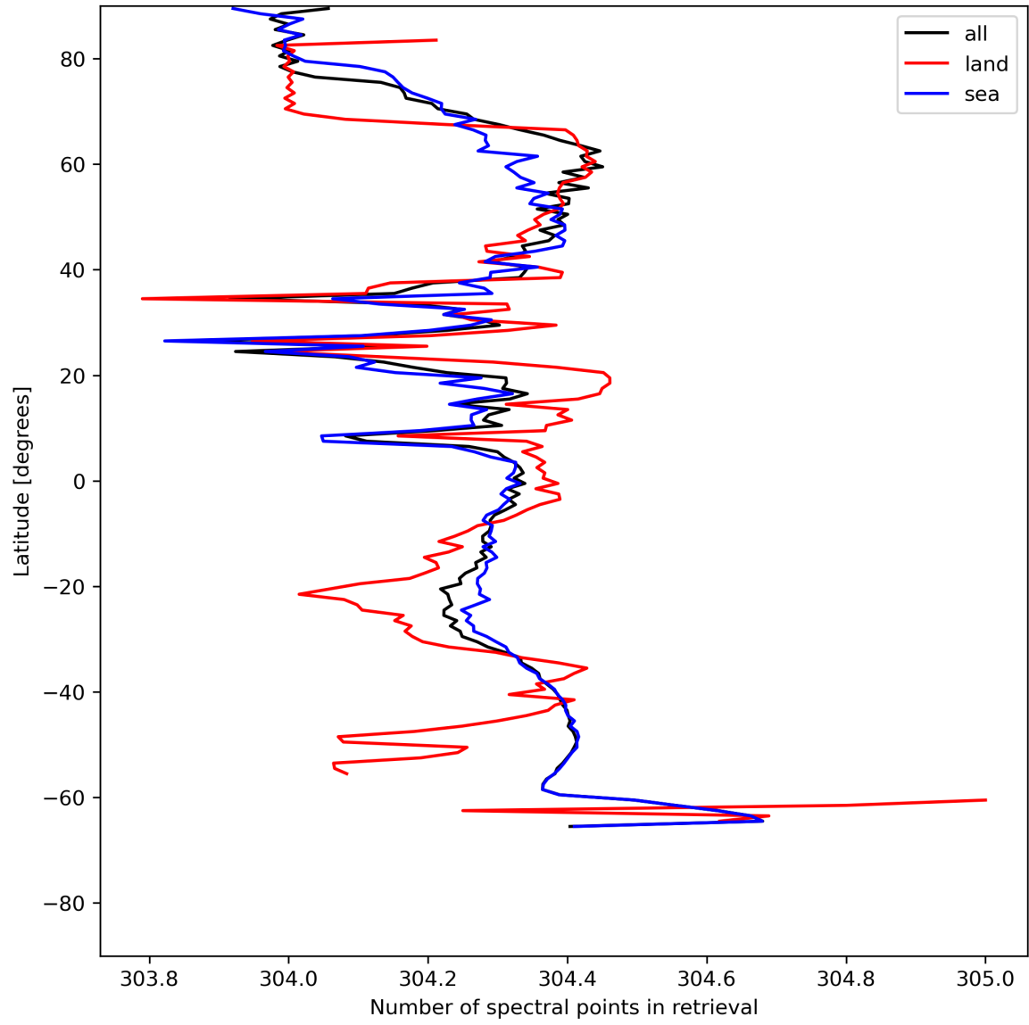
Figure 16: Zonal average of “Number of spectral points in retrieval” for 2024-06-03 to 2024-06-04.
