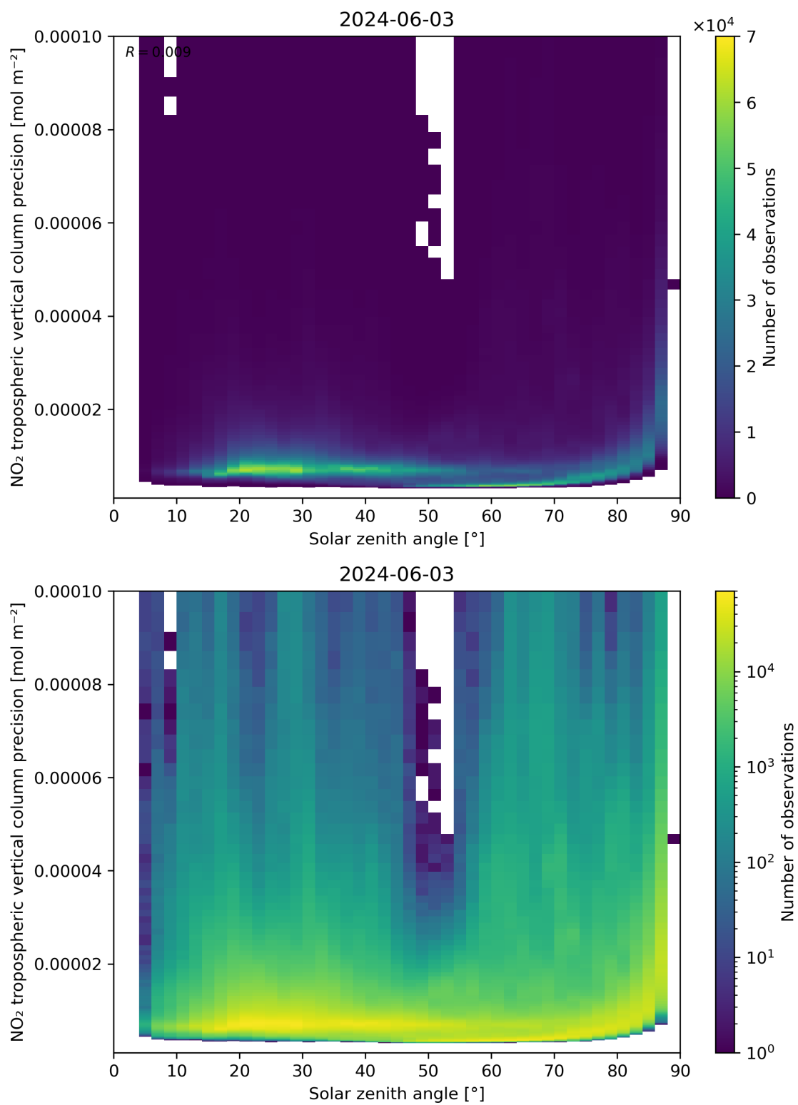
Figure 156: Scatter density plot of “Solar zenith angle” against “NO 2 tropospheric vertical column precision” for 2024-06-03 to 2024-06-04.
