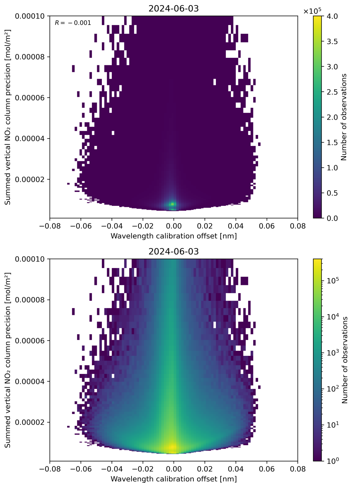
Figure 178: Scatter density plot of “Wavelength calibration offset” against “Summed vertical NO 2 column precision” for 2024-06-03 to 2024-06-04.
