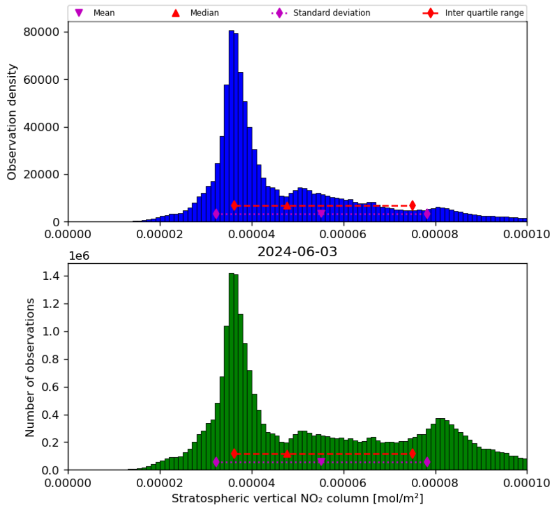
Figure 36: Histogram of “Stratospheric vertical NO 2 column” for 2024-06-03 to 2024-06-04
