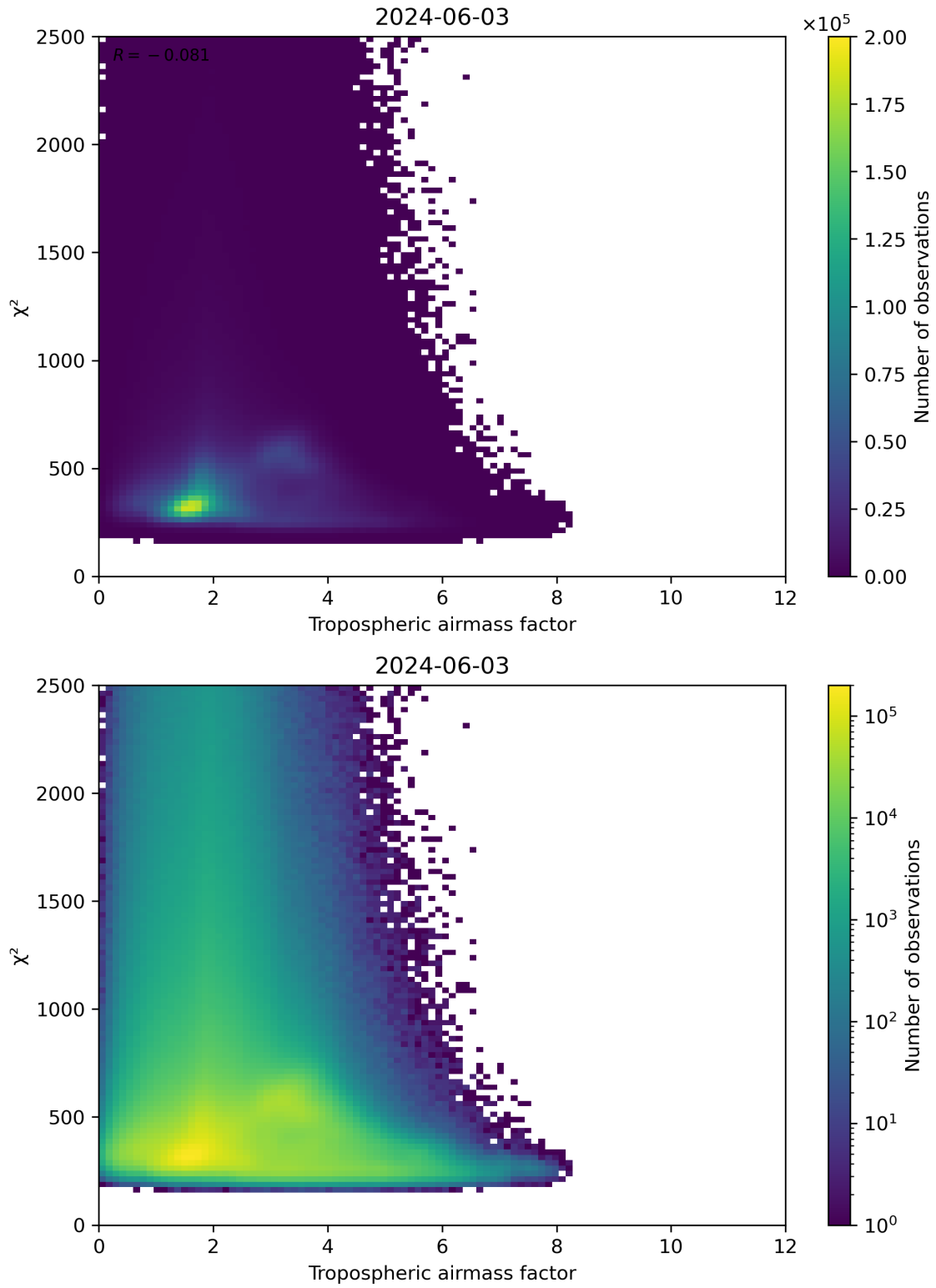
Figure 73: Scatter density plot of “Tropospheric airmass factor” against “ \chi^2 ” for 2024-06-03 to 2024-06-04.
