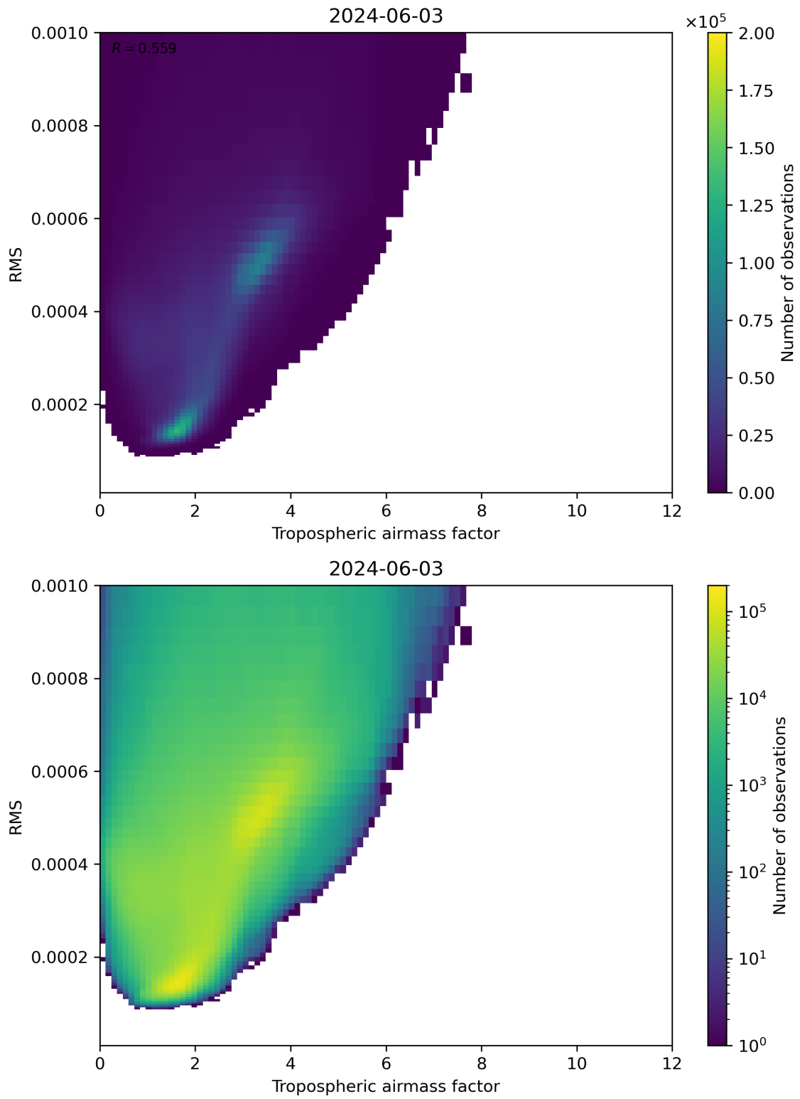
Figure 79: Scatter density plot of “Tropospheric airmass factor” against “RMS” for 2024-06-03 to 2024-06-04.
