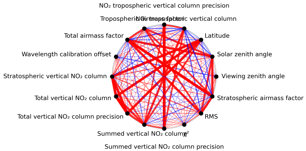
Figure 1: Map of correlation graph for 2024-06-03 to 2024-06-04.
