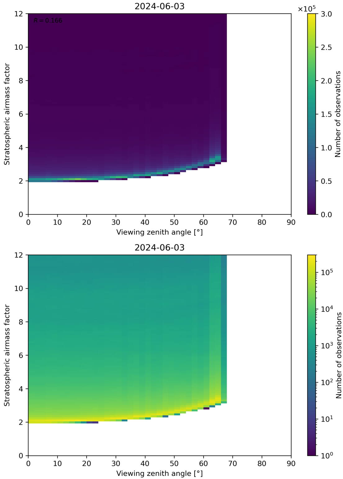
Figure 159: Scatter density plot of “Viewing zenith angle” against “Stratospheric airmass factor” for 2024-06-03 to 2024-06-04.
