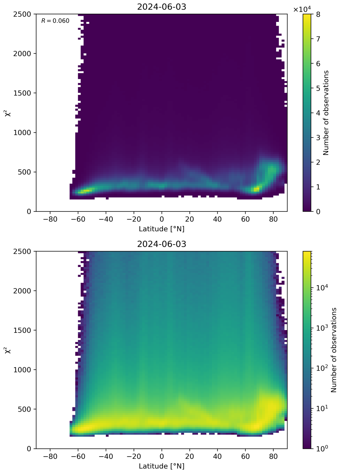
Figure 86: Scatter density plot of “Latitude” against “ \chi^2 ” for 2024-06-03 to 2024-06-04.
