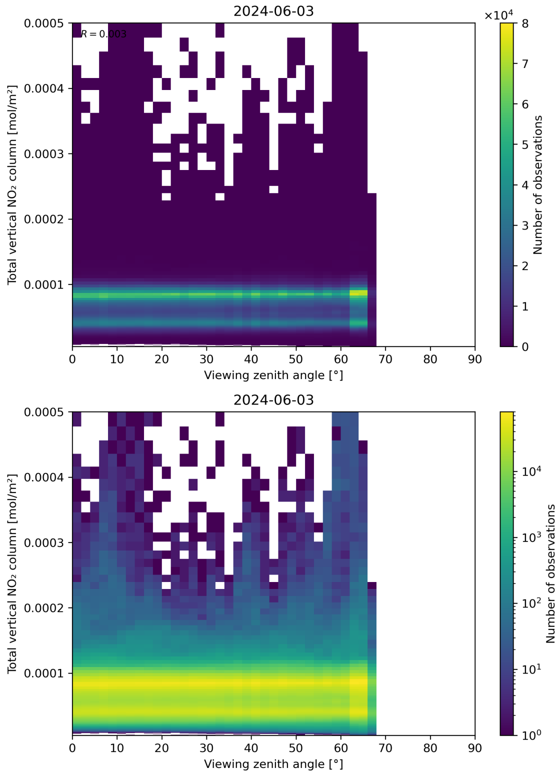
Figure 167: Scatter density plot of “Viewing zenith angle” against “Total vertical NO 2 column” for 2024-06-03 to 2024-06-04.
