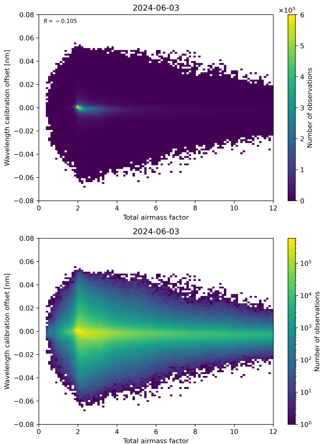
Figure 70: Scatter density plot of “Total airmass factor” against “Wavelength calibration offset” for 2024-06-03 to 2024-06-04.
