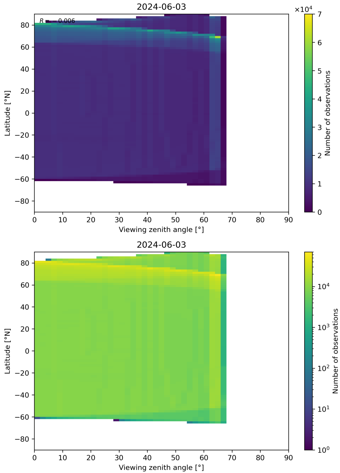
Figure 163: Scatter density plot of “Viewing zenith angle” against “Latitude” for 2024-06-03 to 2024-06-04.
