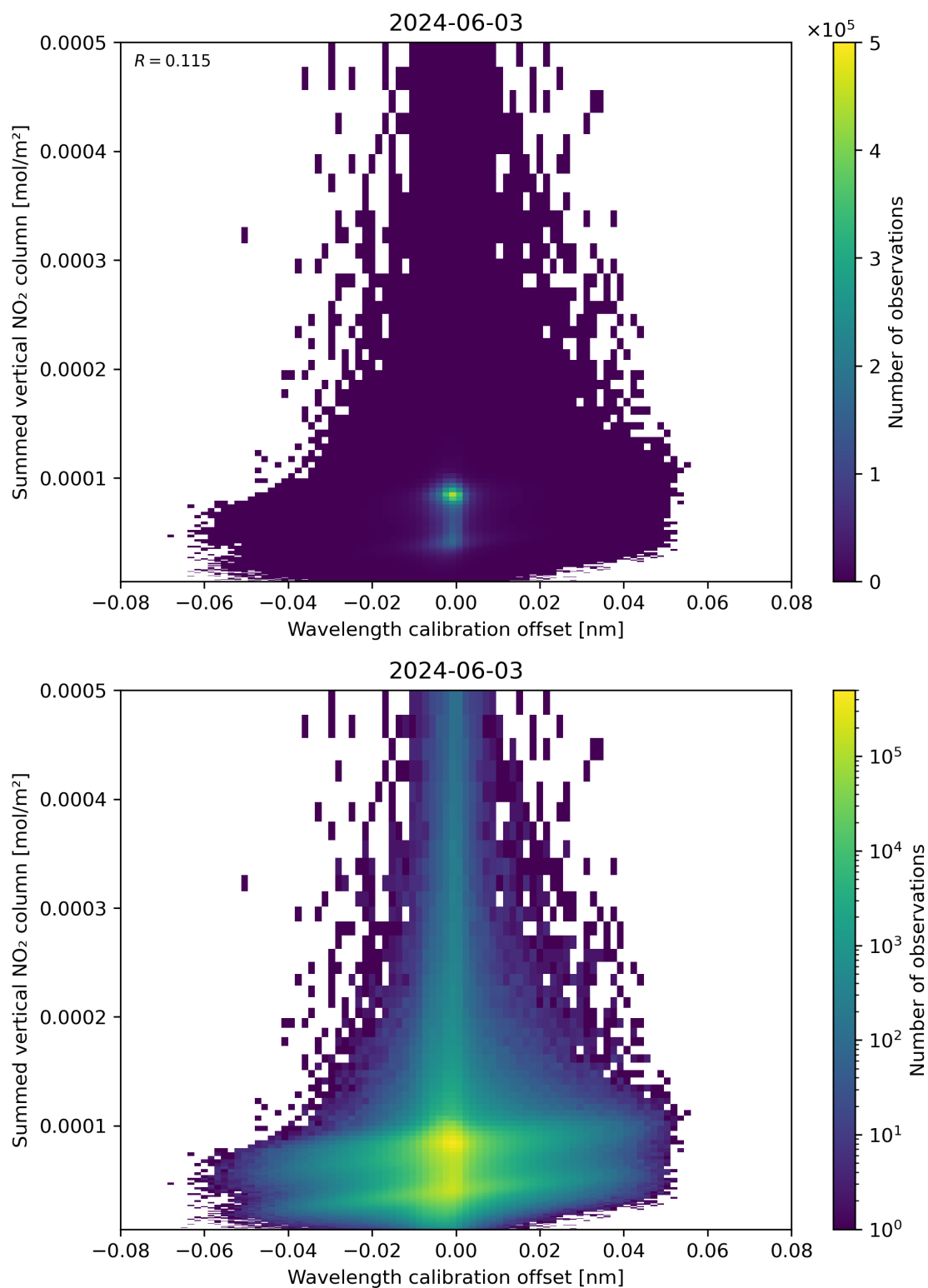
Figure 177: Scatter density plot of “Wavelength calibration offset” against “Summed vertical NO 2 column” for 2024-06-03 to 2024-06-04.
