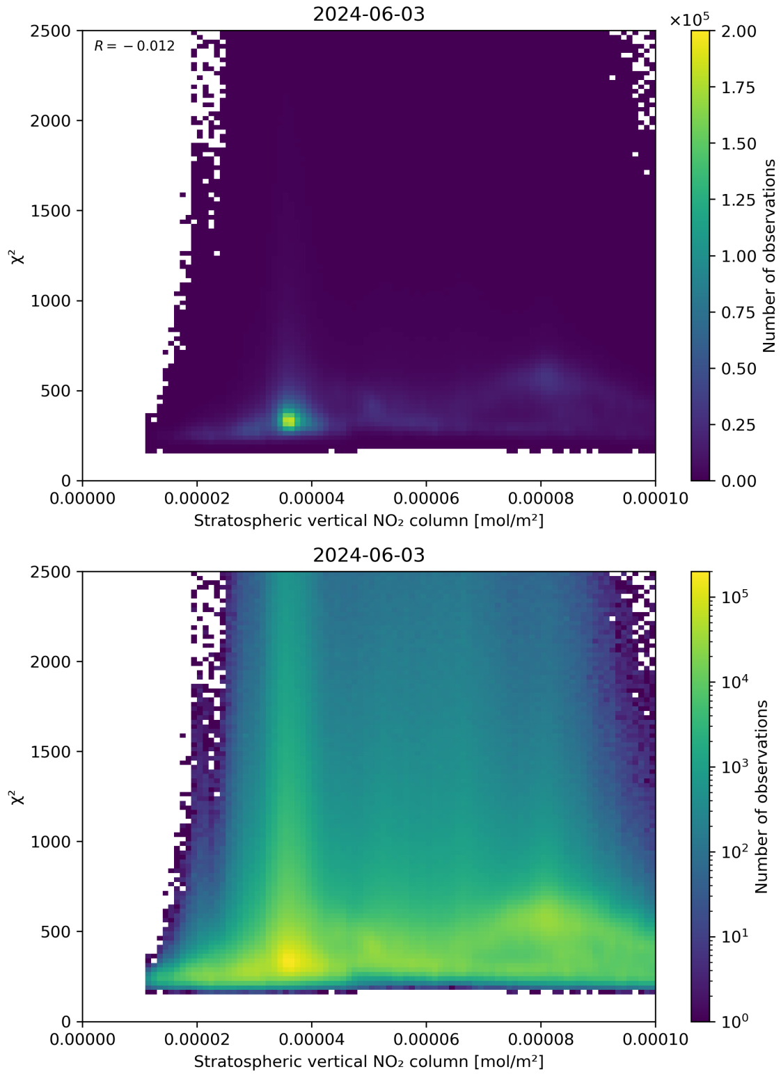
Figure 97: Scatter density plot of “Stratospheric vertical NO 2 column” against “ \chi^2 ” for 2024-06-03 to 2024-06-04.
