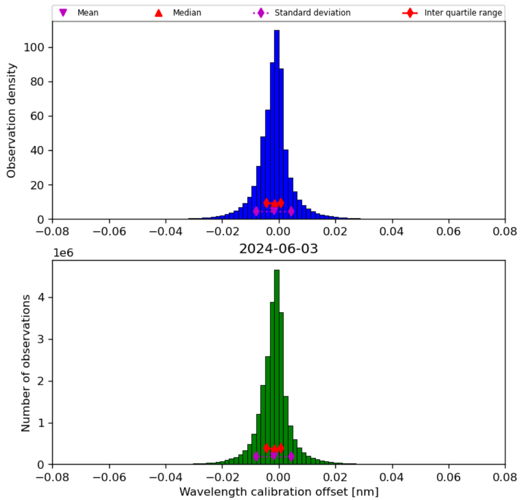
Figure 35: Histogram of “Wavelength calibration offset” for 2024-06-03 to 2024-06-04
