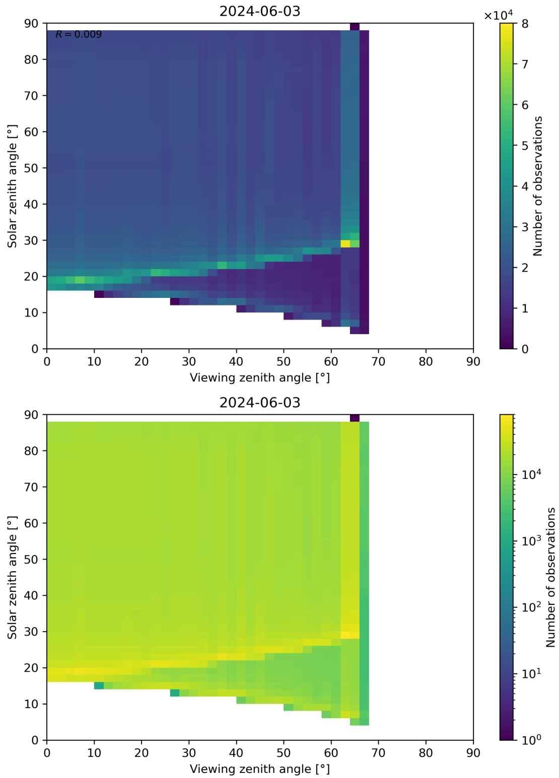
Figure 172: Scatter density plot of “Viewing zenith angle” against “Solar zenith angle” for 2024-06-03 to 2024-06-04.
