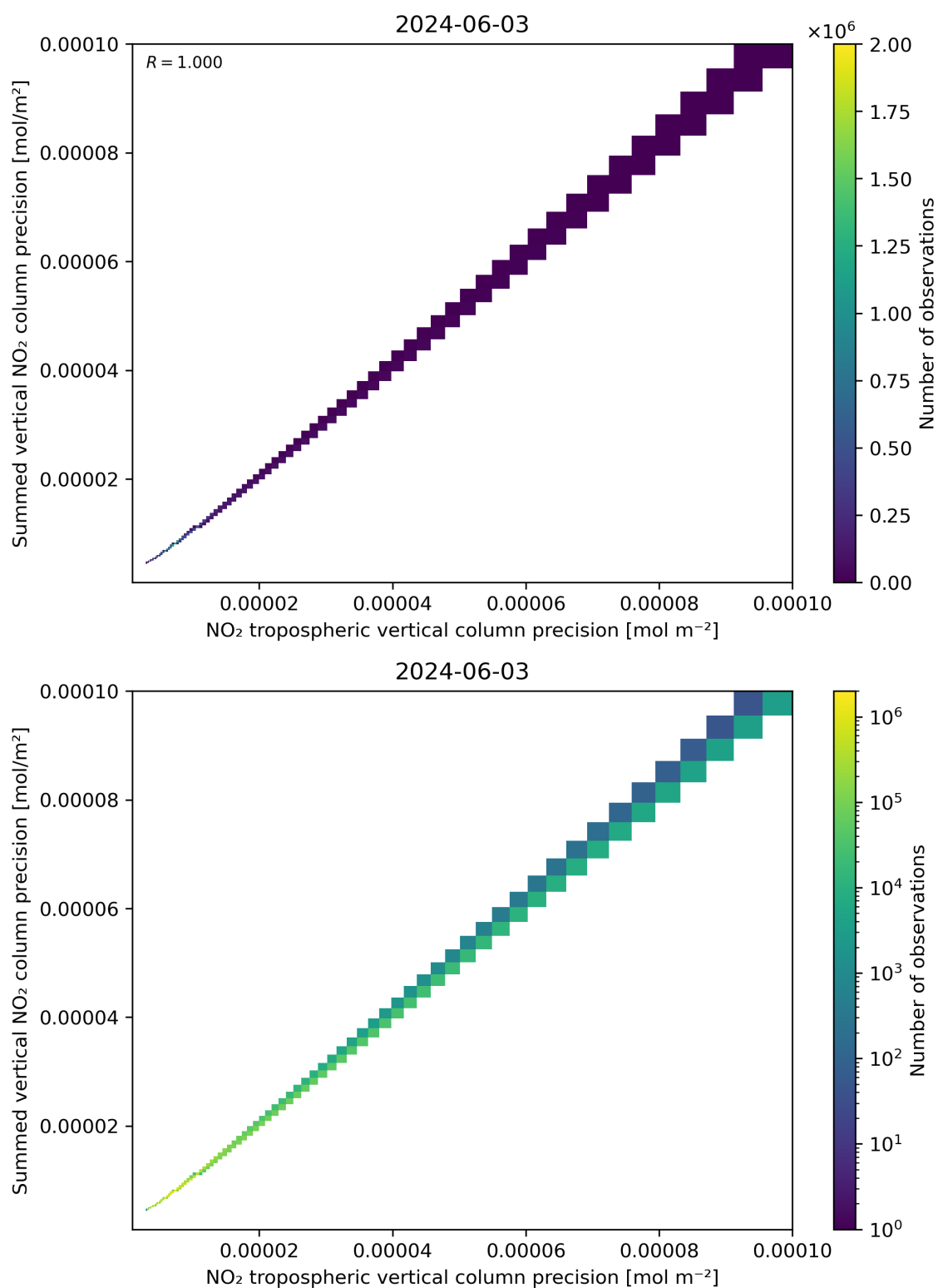
Figure 137: Scatter density plot of “NO 2 tropospheric vertical column precision” against “Summed vertical NO 2 column precision” for 2024-06-03 to 2024-06-04.
