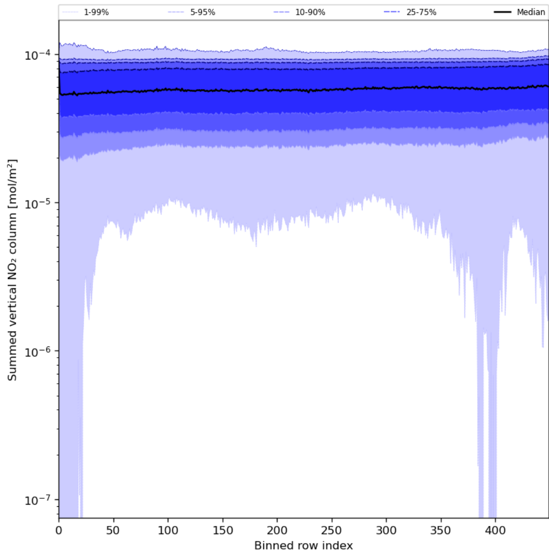
Figure 57: Along track statistics of “Summed vertical NO 2 column” for 2024-06-03 to 2024-06-04
