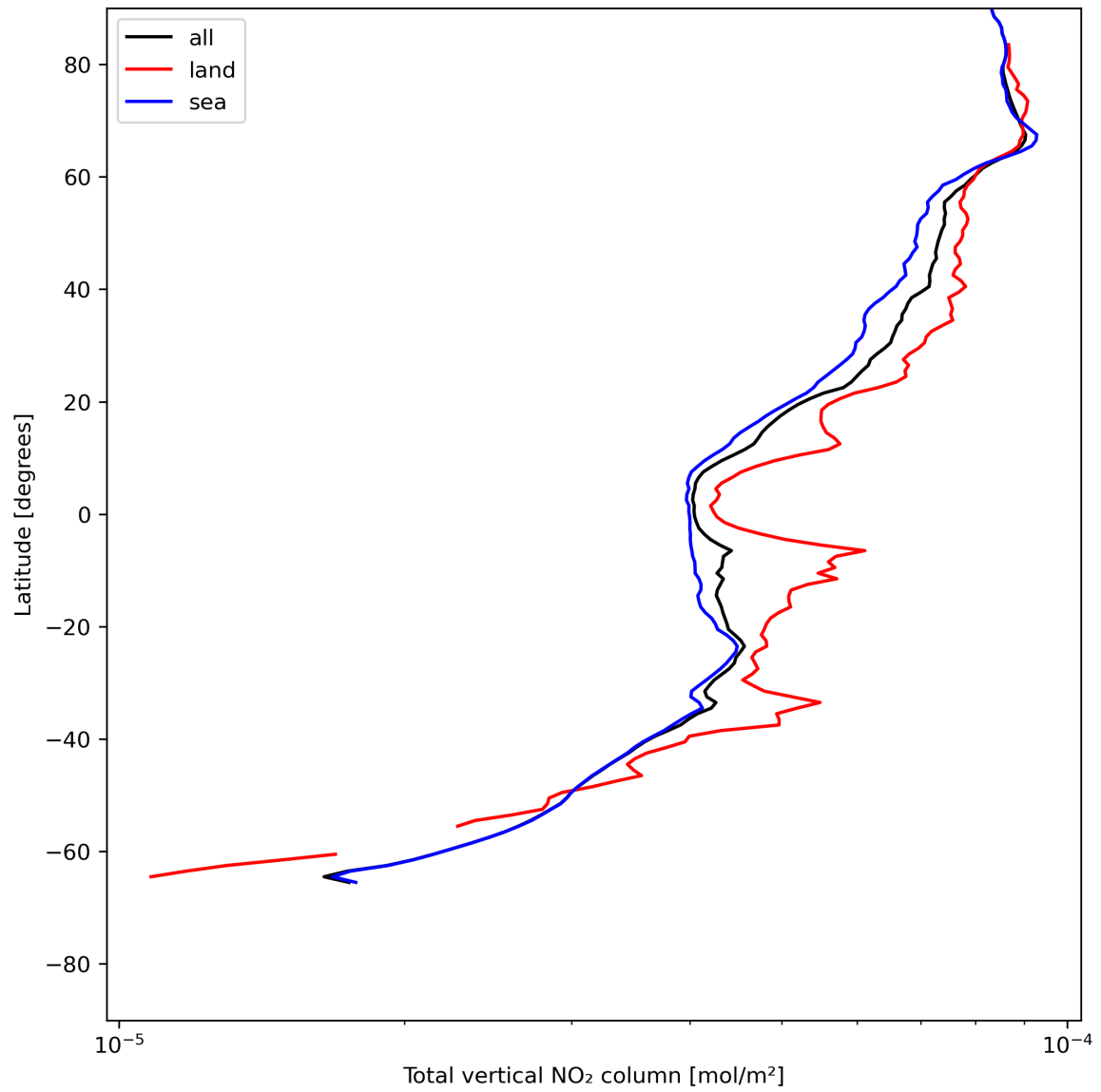
Figure 21: Zonal average of “Total vertical NO 2 column” for 2024-06-03 to 2024-06-04.
