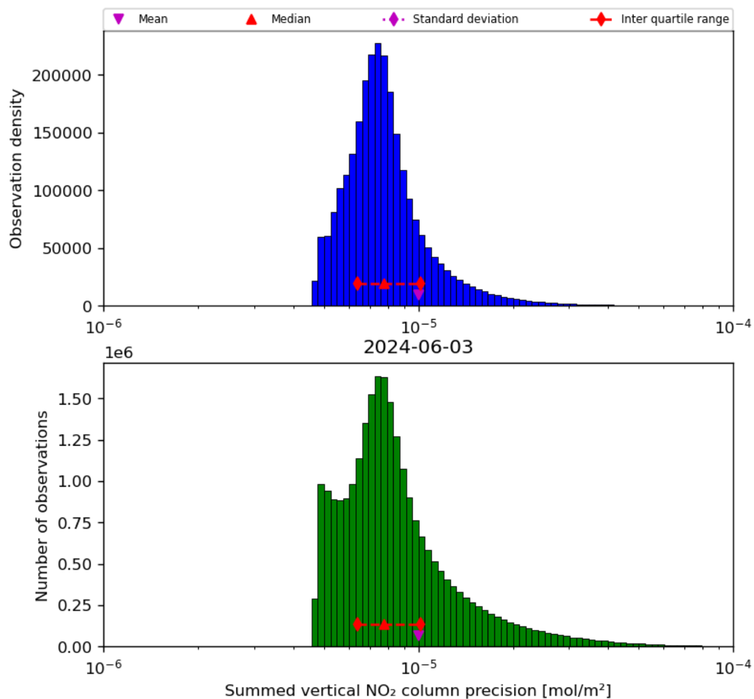
Figure 41: Histogram of “Summed vertical NO 2 column precision” for 2024-06-03 to 2024-06-04
