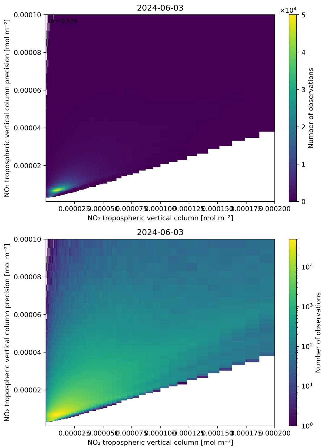
Figure 130: Scatter density plot of “NO 2 tropospheric vertical column” against “NO 2 tropospheric vertical column precision” for 2024-06-03 to 2024-06-04.
