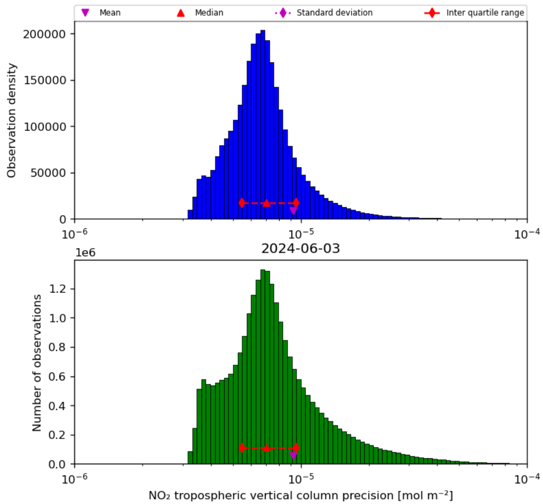
Figure 30: Histogram of “NO 2 tropospheric vertical column precision” for 2024-06-03 to 2024-06-04
