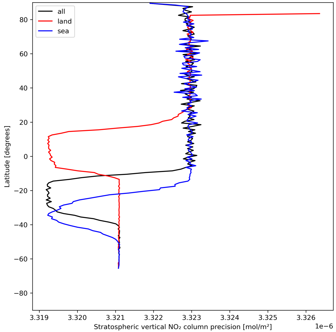
Figure 20: Zonal average of “Stratospheric vertical NO 2 column precision” for 2024-06-03 to 2024-06-04.
