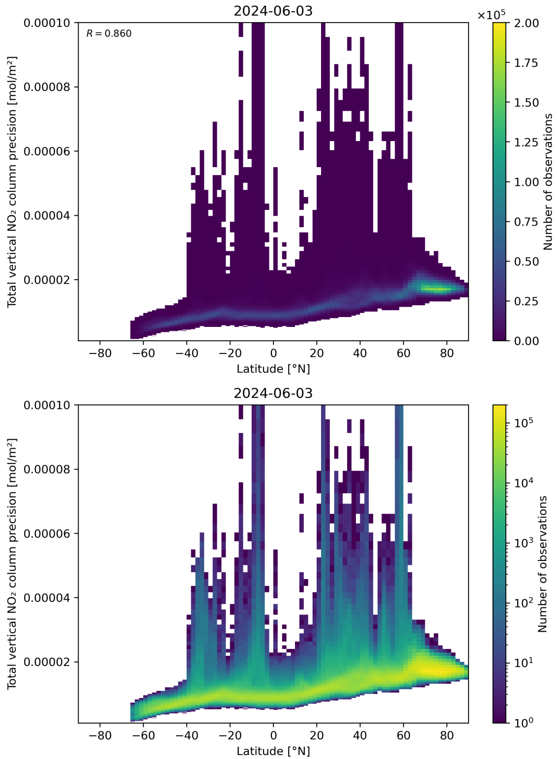
Figure 91: Scatter density plot of “Latitude” against “Total vertical NO 2 column precision” for 2024-06-03 to 2024-06-04.
