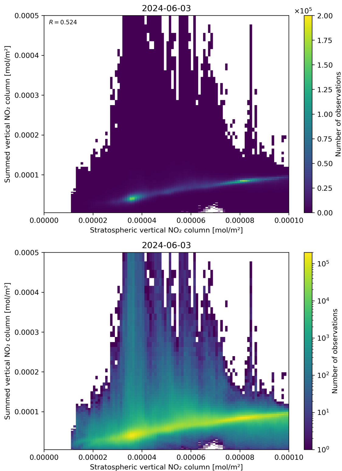
Figure 98: Scatter density plot of “Stratospheric vertical NO 2 column” against “Summed vertical NO 2 column” for 2024-06-03 to 2024-06-04.
