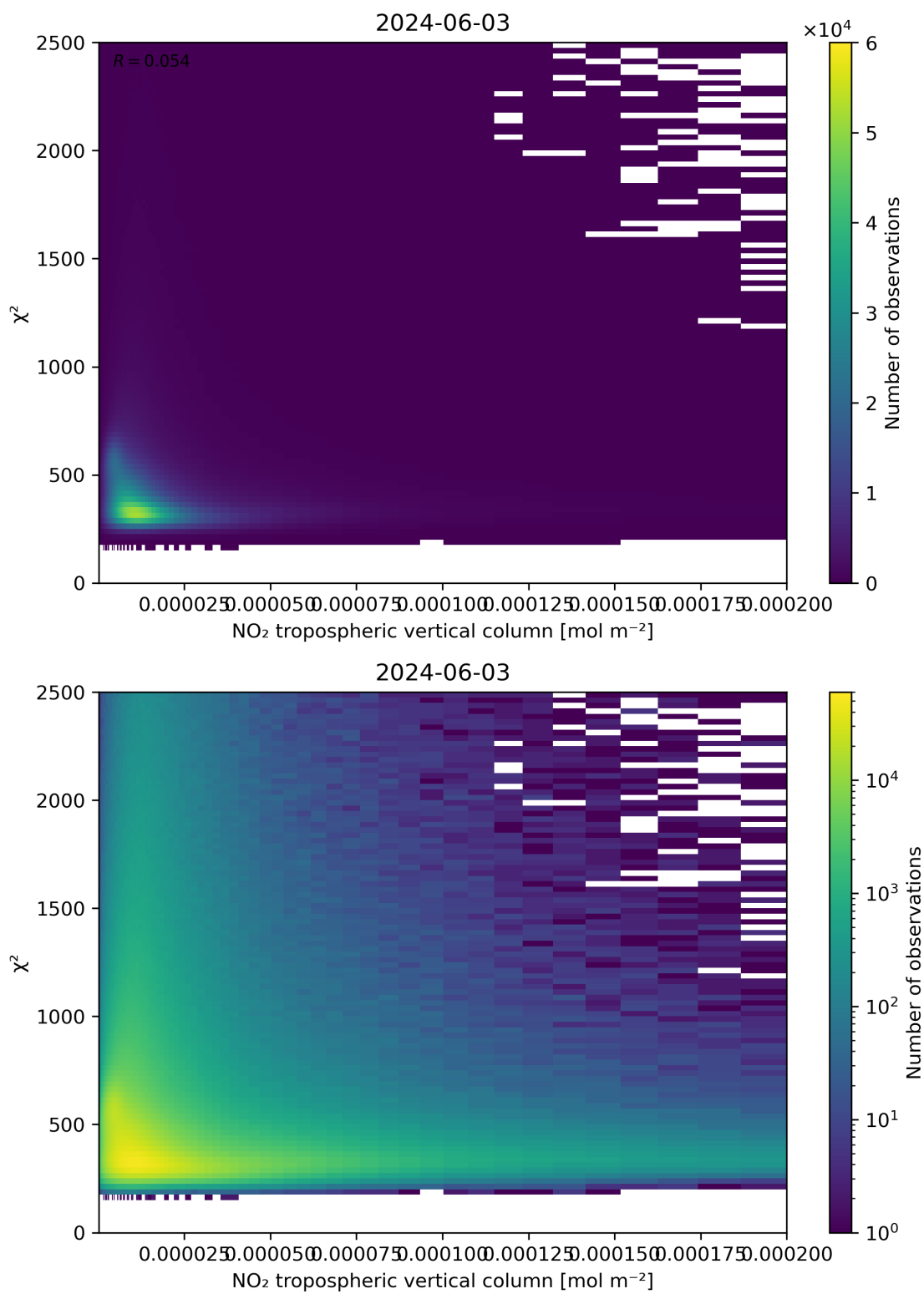
Figure 124: Scatter density plot of “NO 2 tropospheric vertical column” against “ \chi^2 ” for 2024-06-03 to 2024-06-04.
