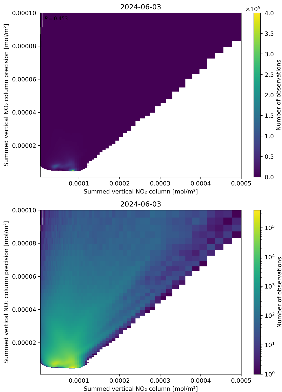
Figure 105: Scatter density plot of “Summed vertical NO 2 column” against “Summed vertical NO 2 column precision” for 2024-06-03 to 2024-06-04.
