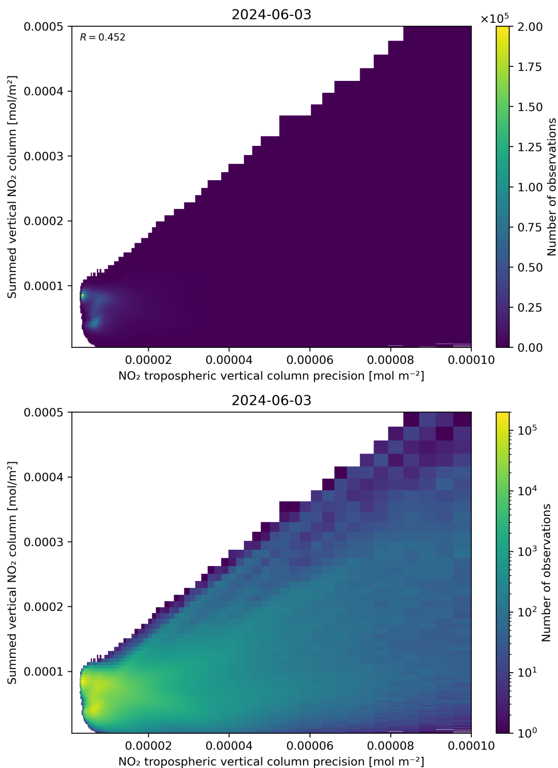
Figure 136: Scatter density plot of “NO 2 tropospheric vertical column precision” against “Summed vertical NO 2 column” for 2024-06-03 to 2024-06-04.
