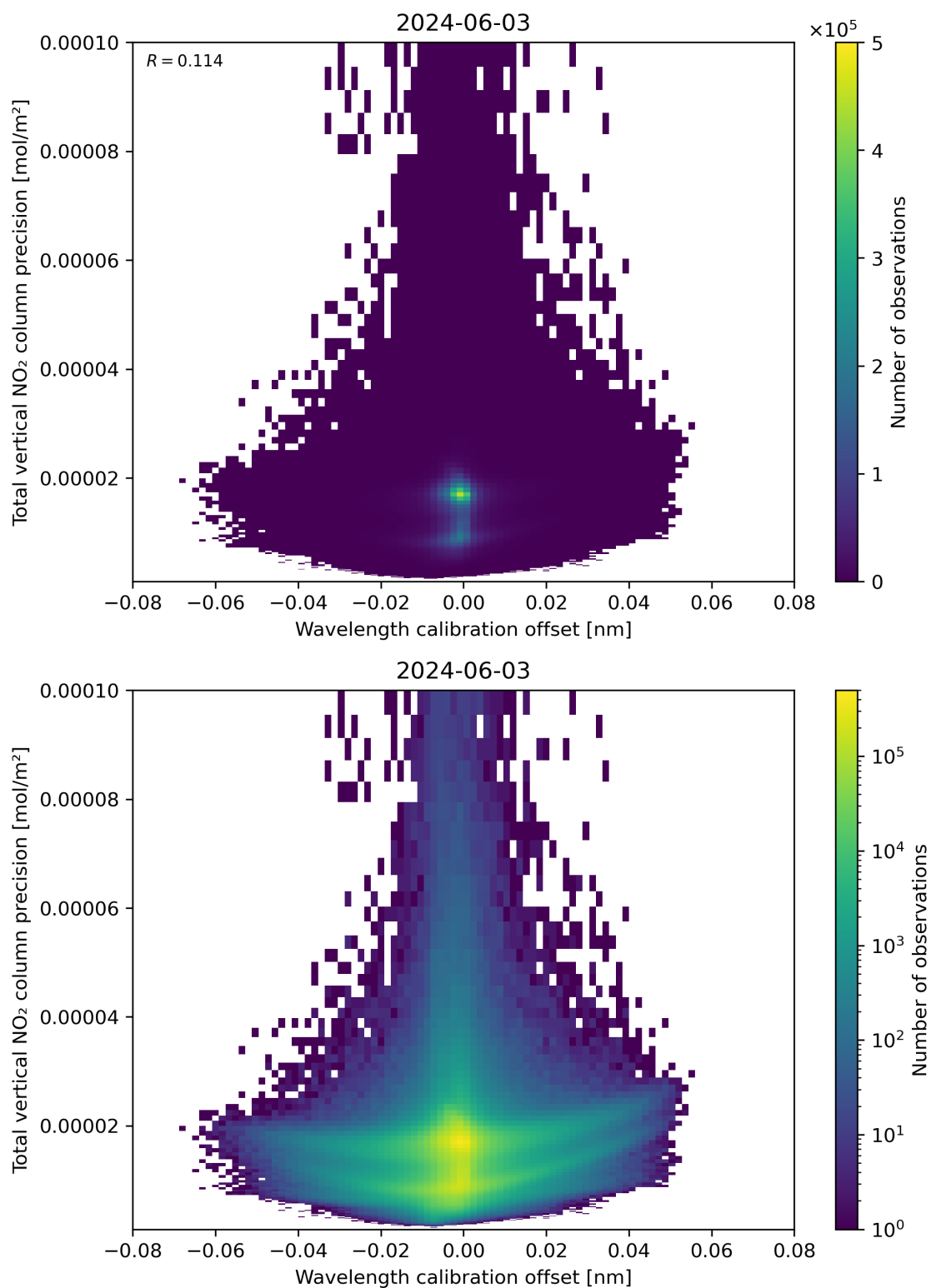
Figure 180: Scatter density plot of “Wavelength calibration offset” against “Total vertical NO 2 column precision” for 2024-06-03 to 2024-06-04.
