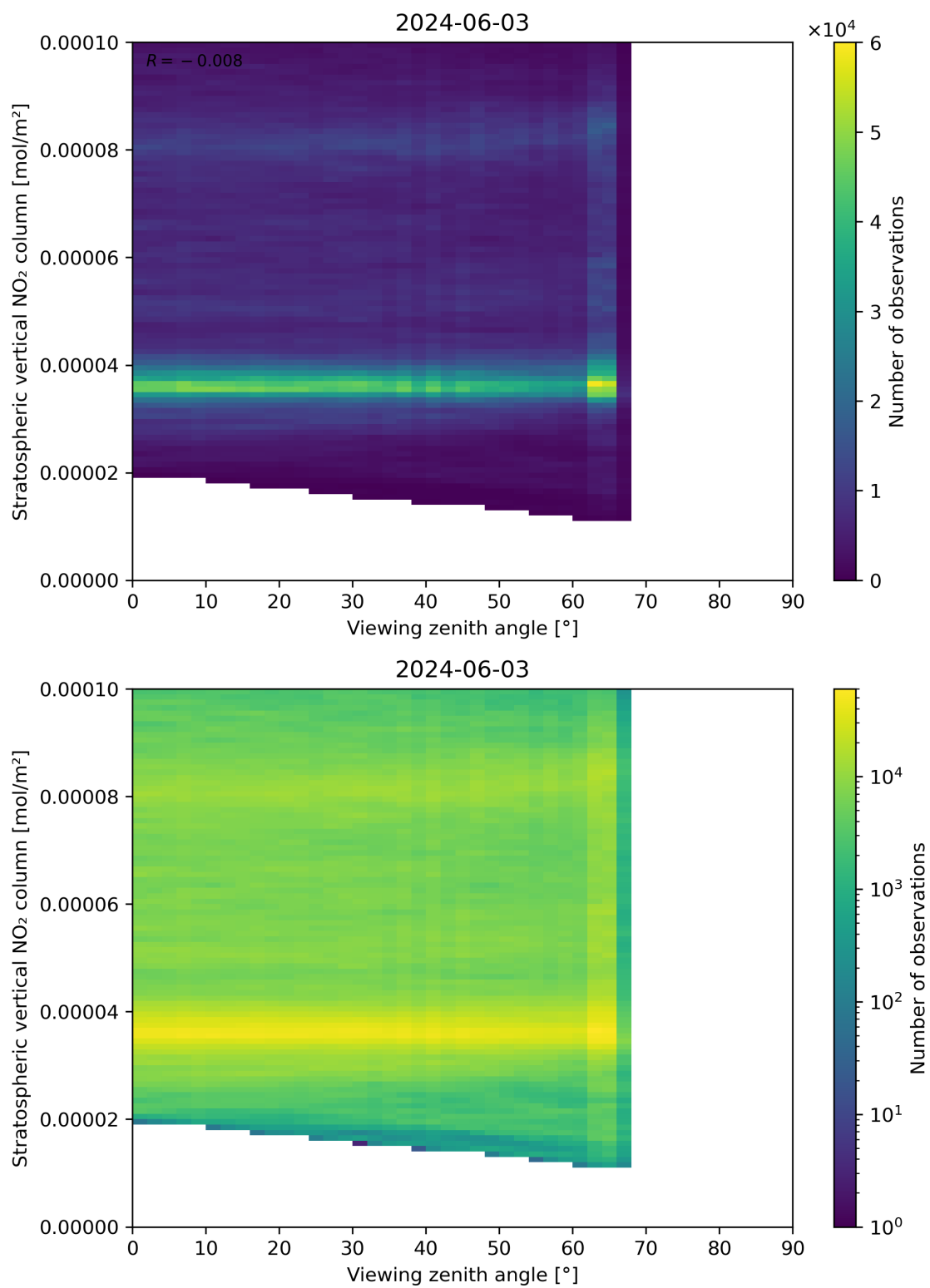
Figure 164: Scatter density plot of “Viewing zenith angle” against “Stratospheric vertical NO 2 column” for 2024-06-03 to 2024-06-04.
