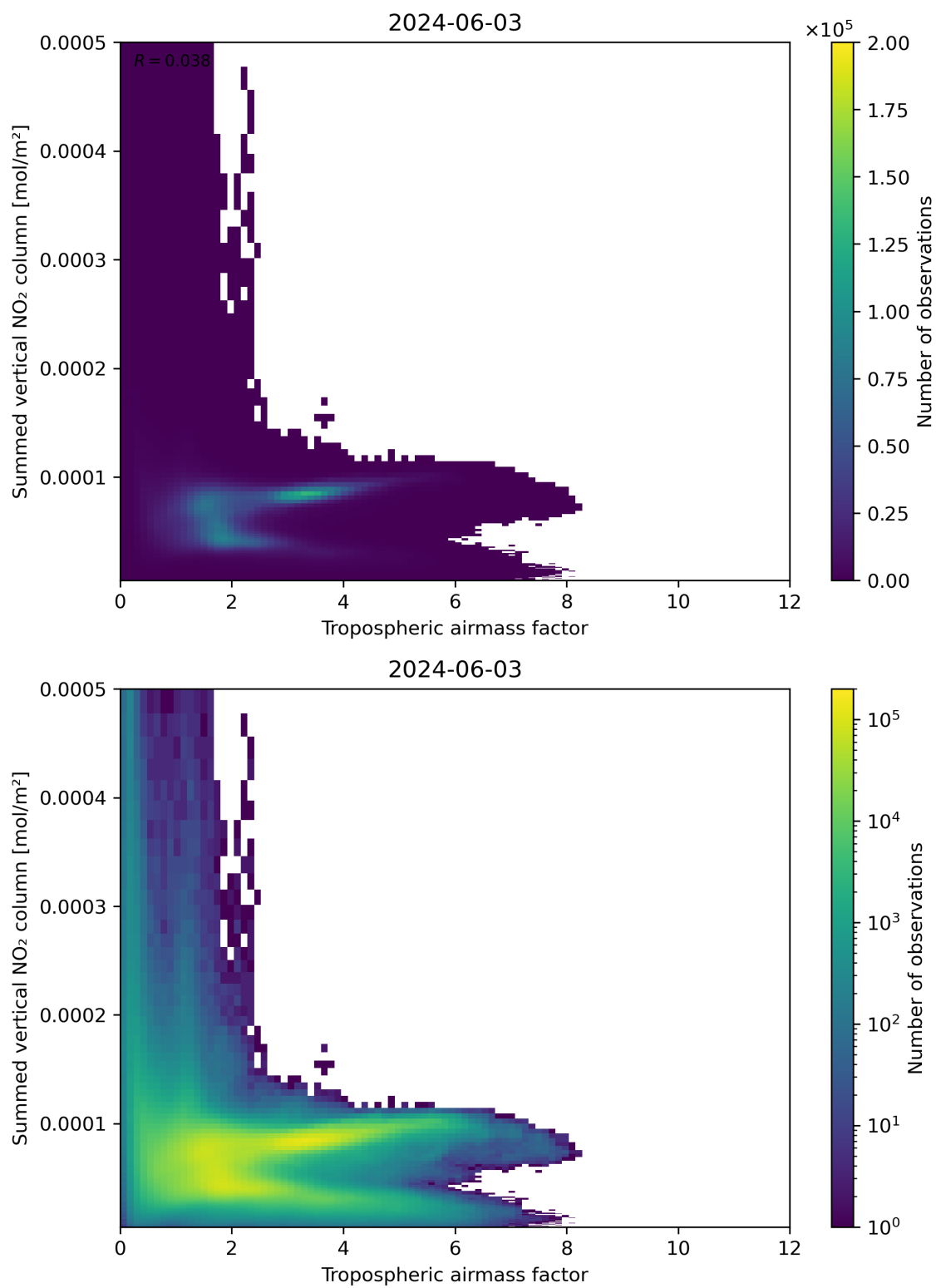
Figure 75: Scatter density plot of “Tropospheric air mass factor” against “Summed vertical NO 2 column” for 2024-06-03 to 2024-06-04.
