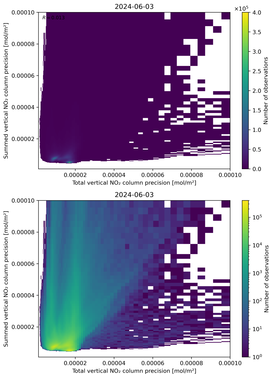
Figure 118: Scatter density plot of “Total vertical NO 2 column precision” against “Summed vertical NO 2 column precision” for 2024-06-03 to 2024-06-04.
