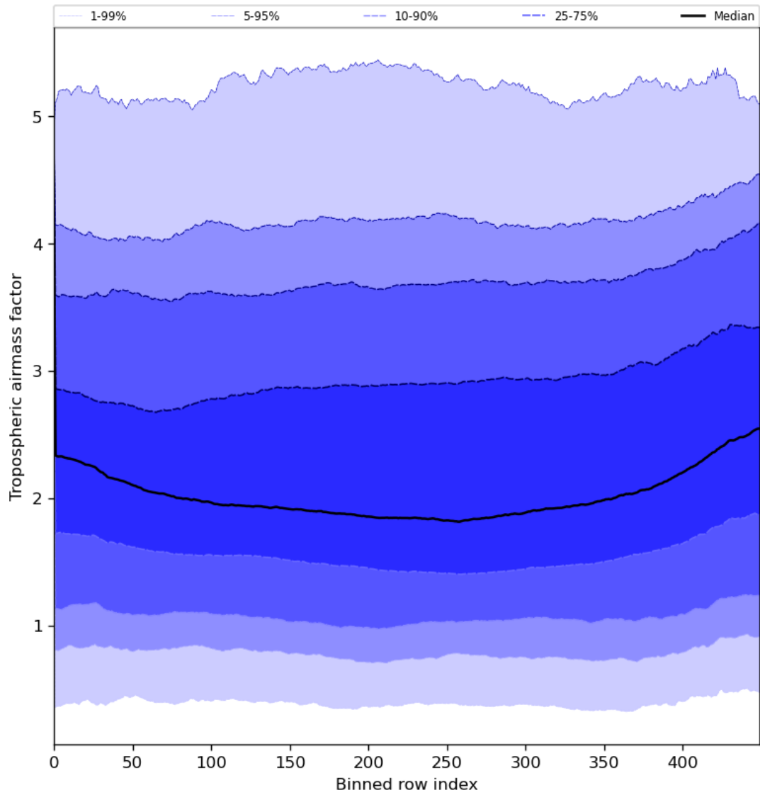
Figure 48: Along track statistics of “Tropospheric air mass factor” for 2024-06-03 to 2024-06-04
