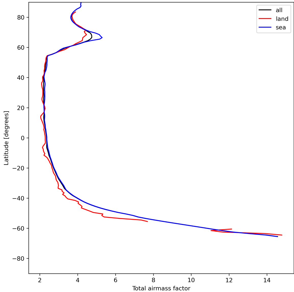
Figure 15: Zonal average of “Total airmass factor” for 2024-06-03 to 2024-06-04.
