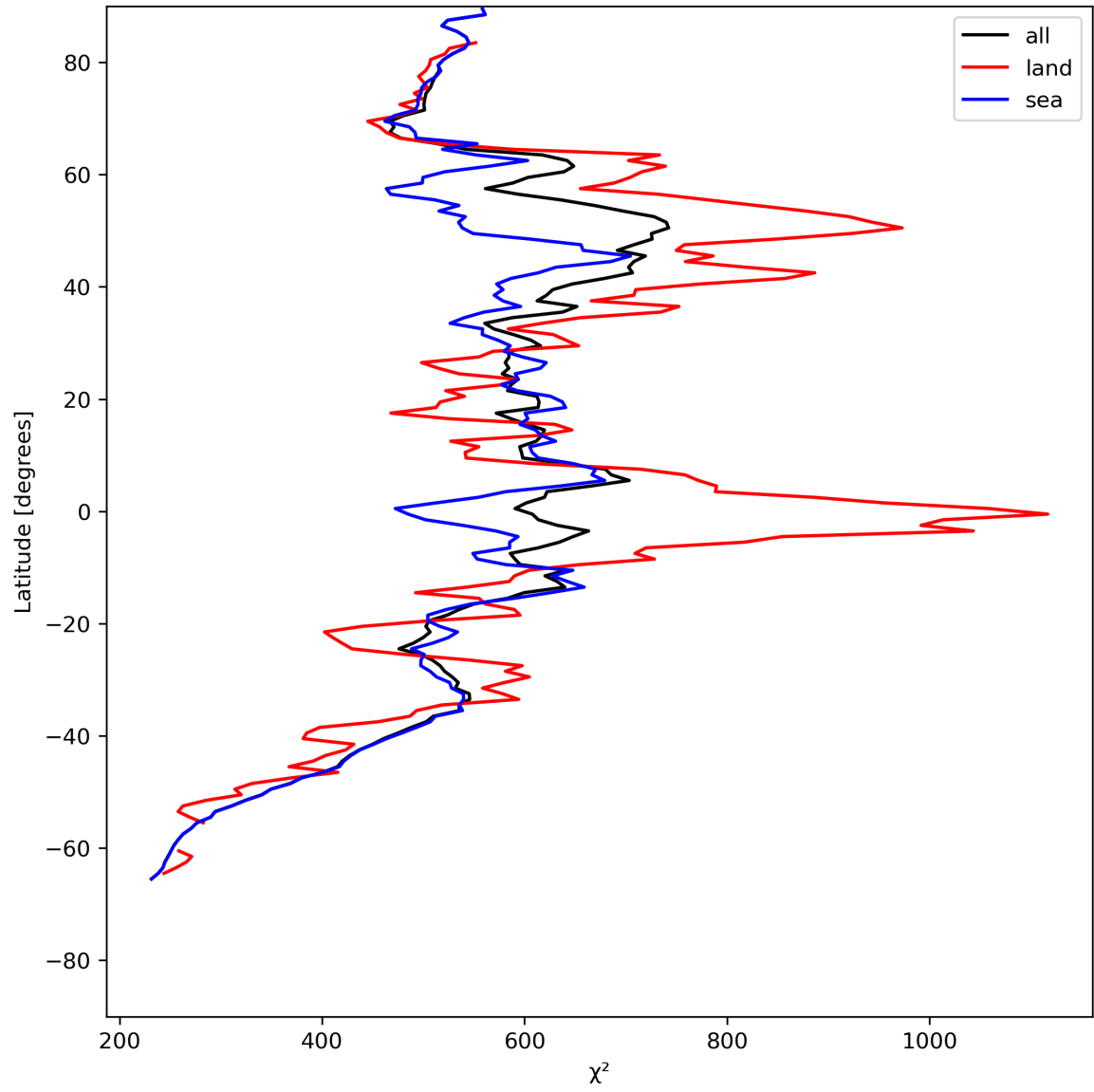
Figure 25: Zonal average of “ \chi^2 ” for 2024-06-03 to 2024-06-04.
