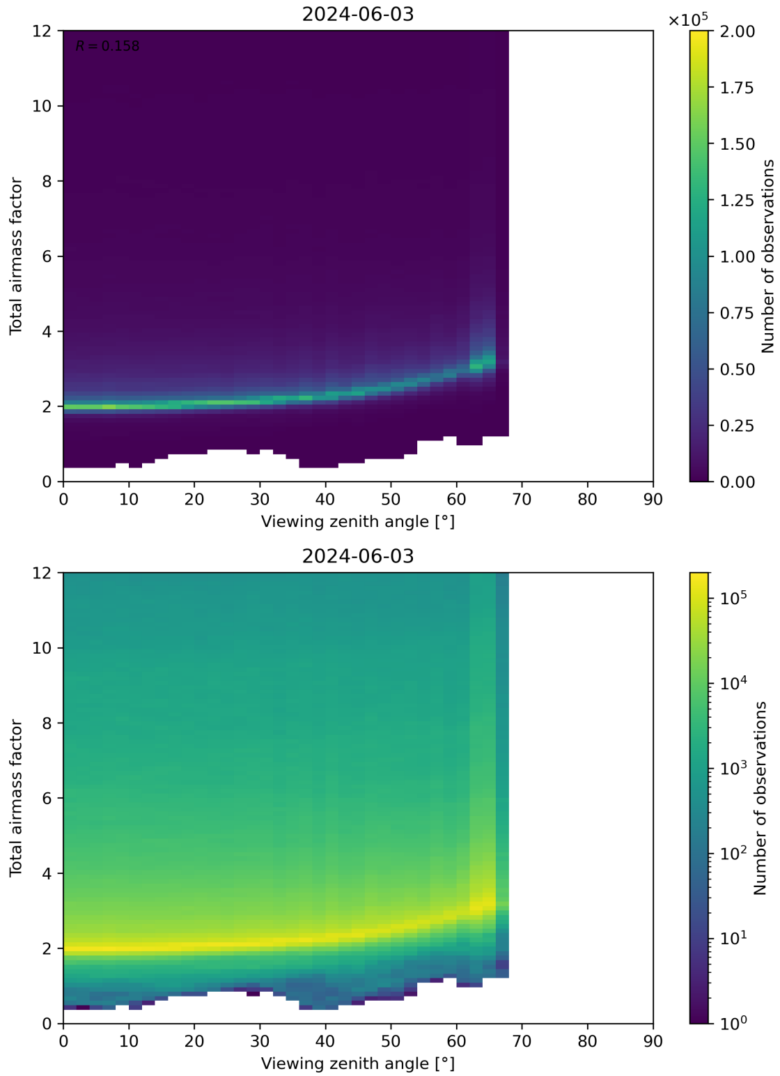
Figure 160: Scatter density plot of “Viewing zenith angle” against “Total airmass factor” for 2024-06-03 to 2024-06-04.
