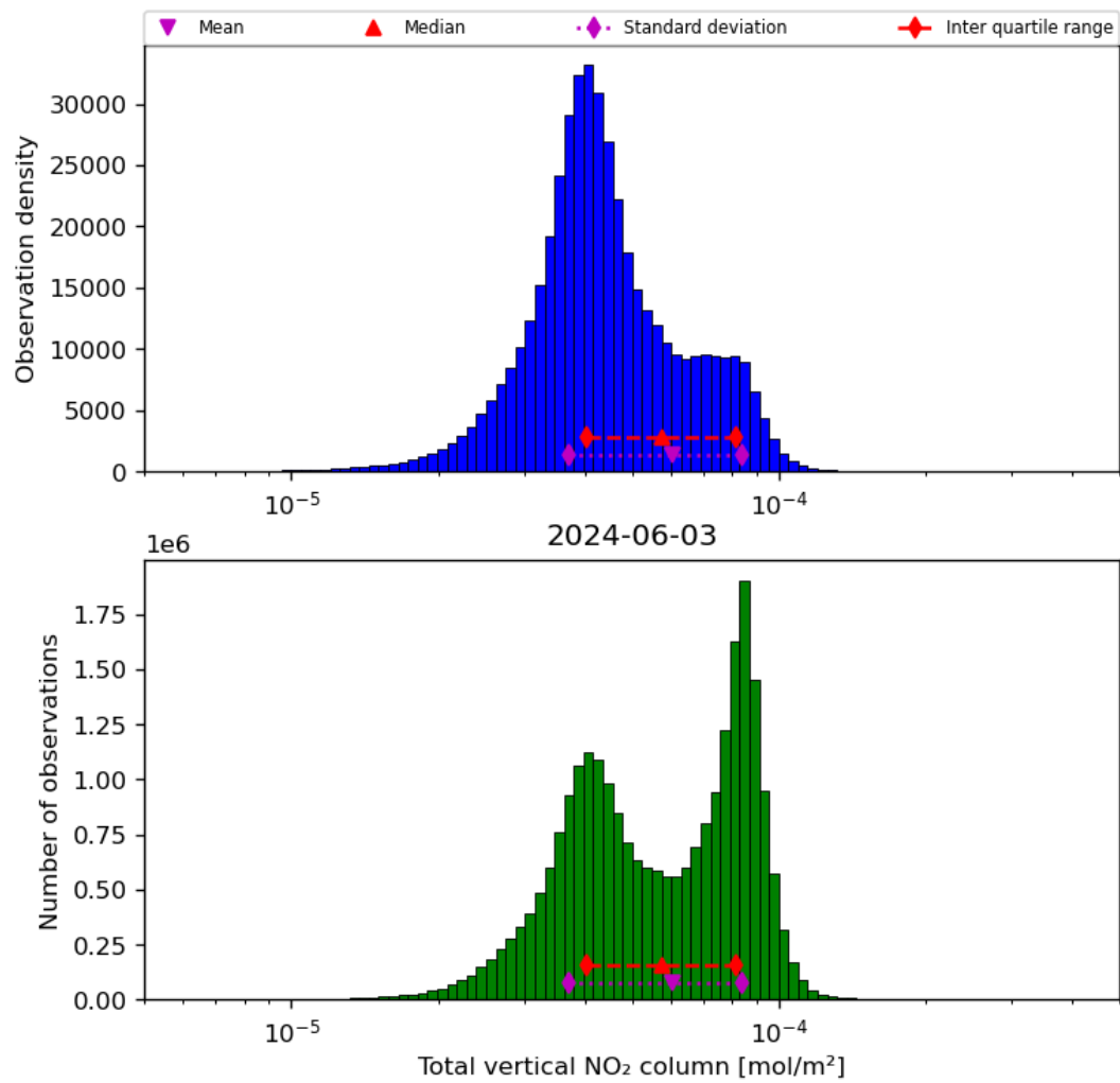
Figure 38: Histogram of “Total vertical NO 2 column” for 2024-06-03 to 2024-06-04
