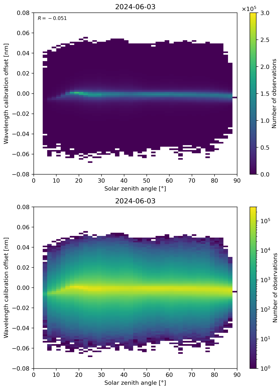
Figure 158: Scatter density plot of “Solar zenith angle” against “Wavelength calibration offset” for 2024-06-03 to 2024-06-04.
