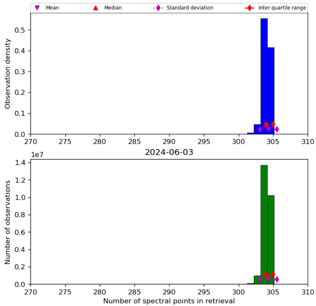
Figure 33: Histogram of “Number of spectral points in retrieval” for 2024-06-03 to 2024-06-04
