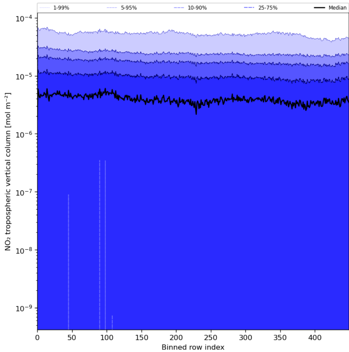
Figure 46: Along track statistics of “NO 2 tropospheric vertical column” for 2024-06-03 to 2024-06-04
