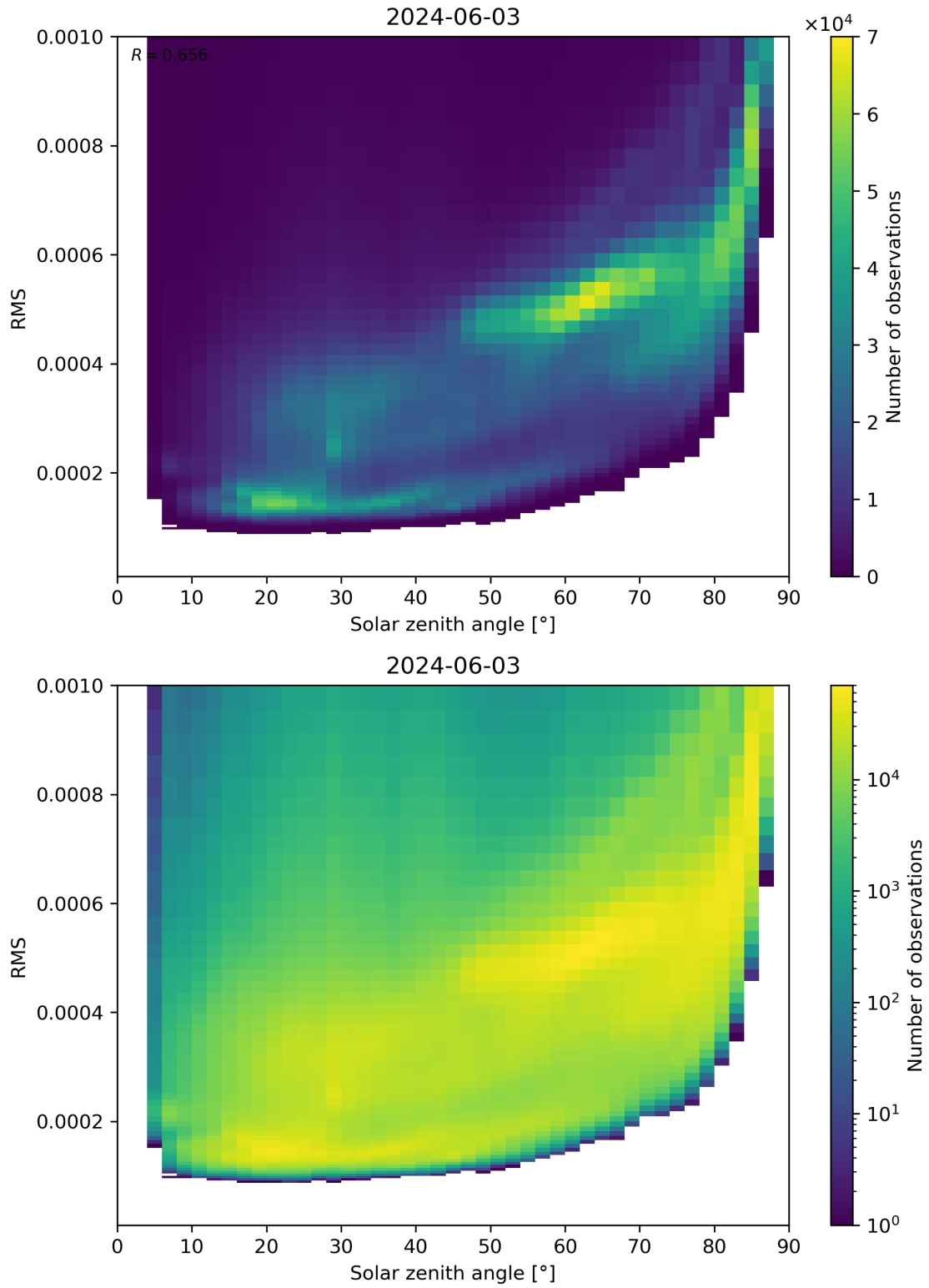
Figure 157: Scatter density plot of “Solar zenith angle” against “RMS” for 2024-06-03 to 2024-06-04.
