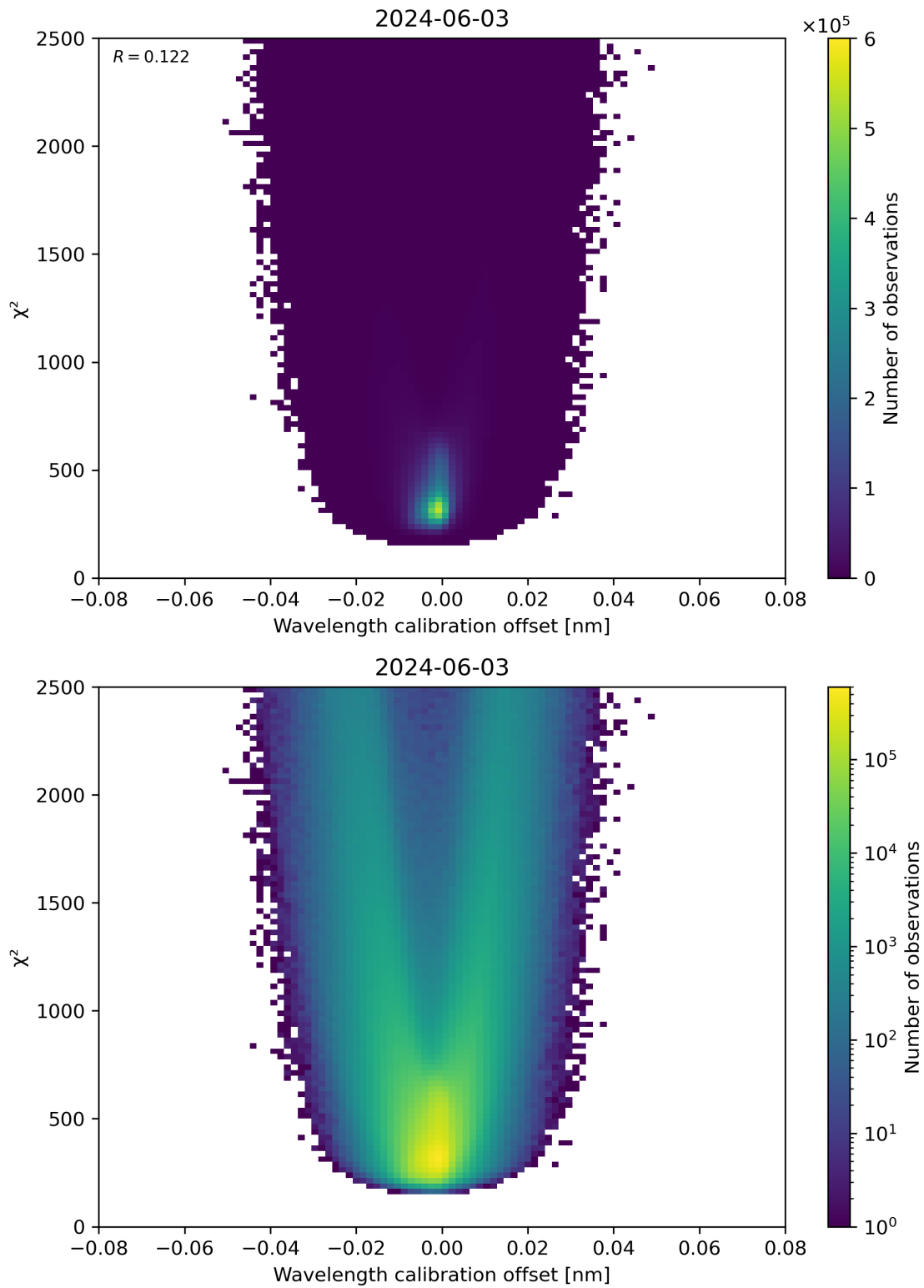
Figure 175: Scatter density plot of “Wavelength calibration offset” against “ \chi^2 ” for 2024-06-03 to 2024-06-04.
