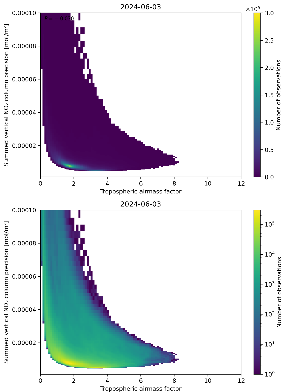
Figure 76: Scatter density plot of “Tropospheric air mass factor” against “Summed vertical NO 2 column precision” for 2024-06-03 to 2024-06-04.
