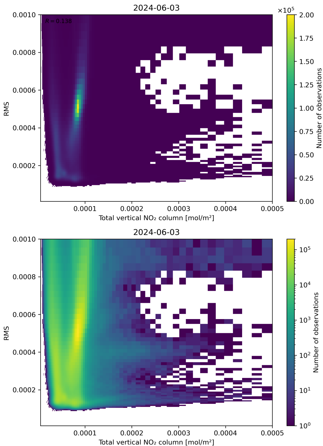
Figure 120: Scatter density plot of “Total vertical NO 2 column” against “RMS” for 2024-06-03 to 2024-06-04.
