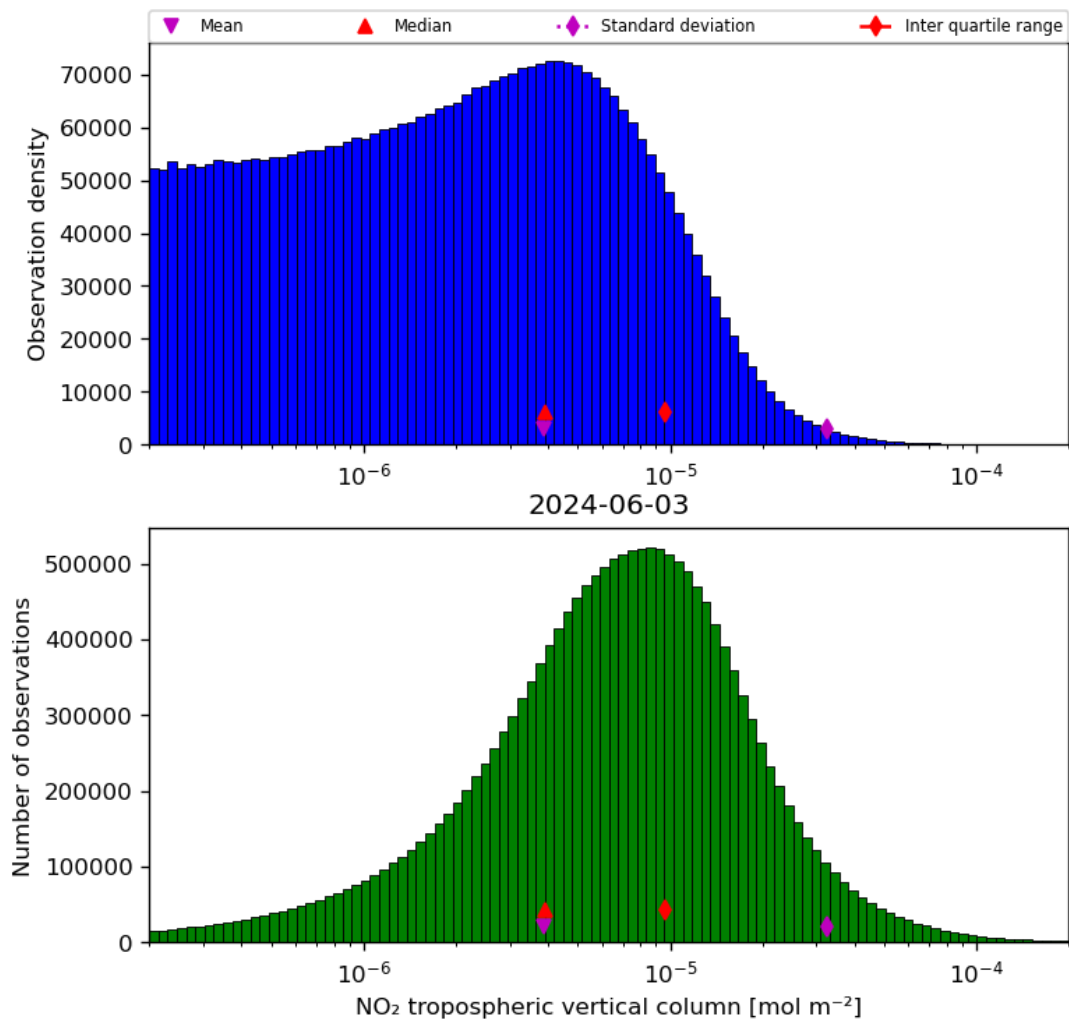
Figure 29: Histogram of “NO 2 tropospheric vertical column” for 2024-06-03 to 2024-06-04
