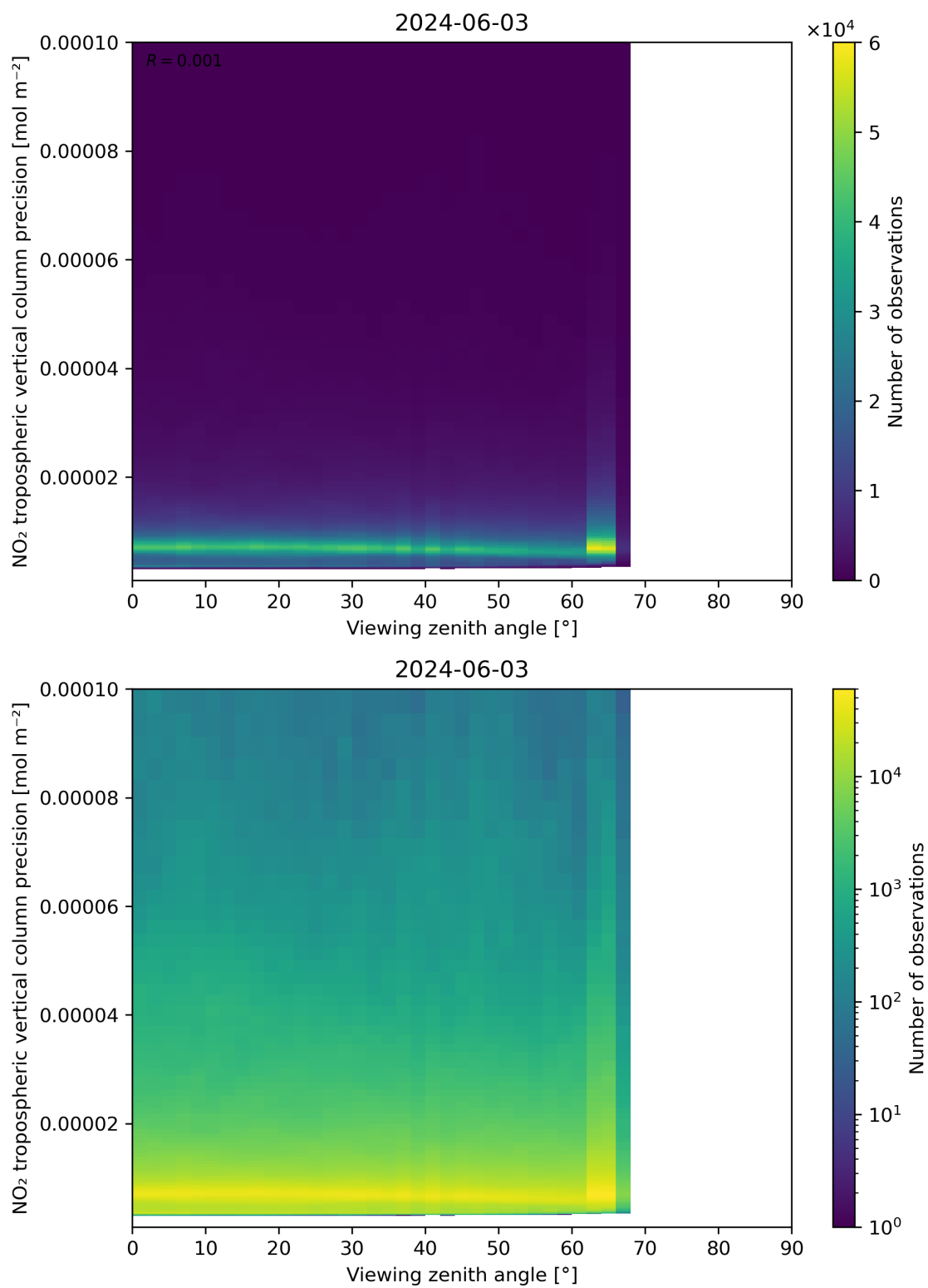
Figure 170: Scatter density plot of “Viewing zenith angle” against “NO 2 tropospheric vertical column precision” for 2024-06-03 to 2024-06-04.
