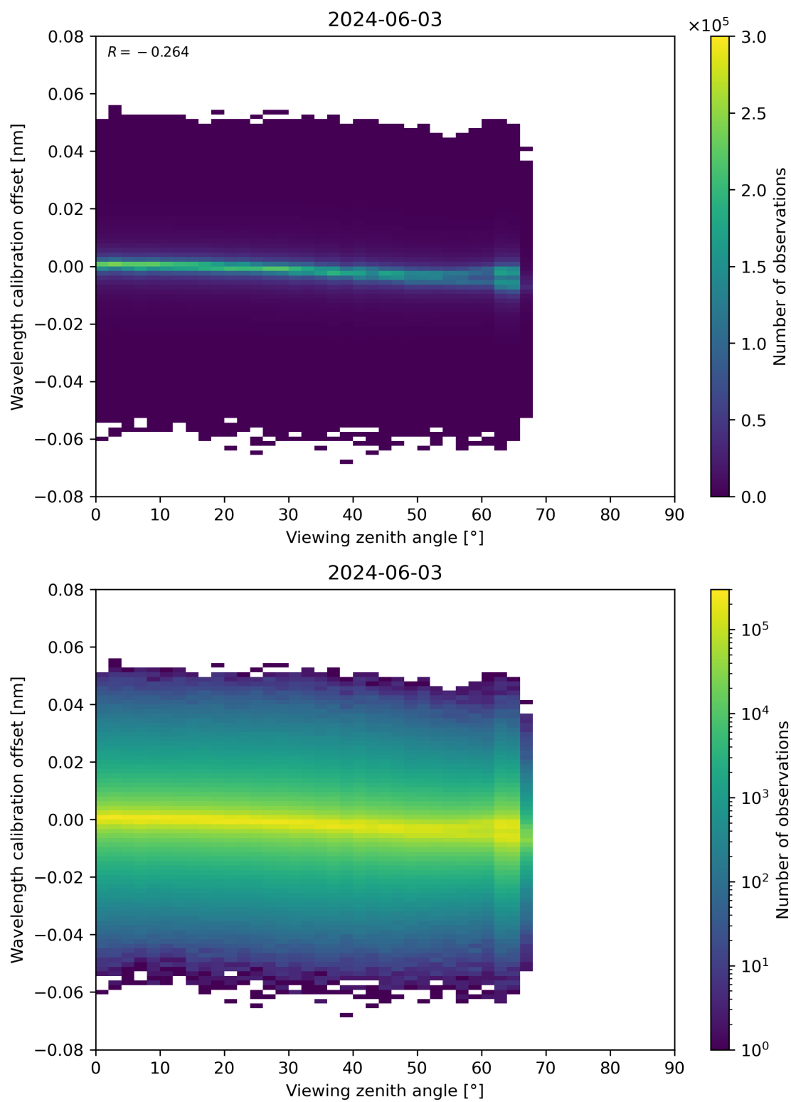
Figure 173: Scatter density plot of “Viewing zenith angle” against “Wavelength calibration offset” for 2024-06-03 to 2024-06-04.
