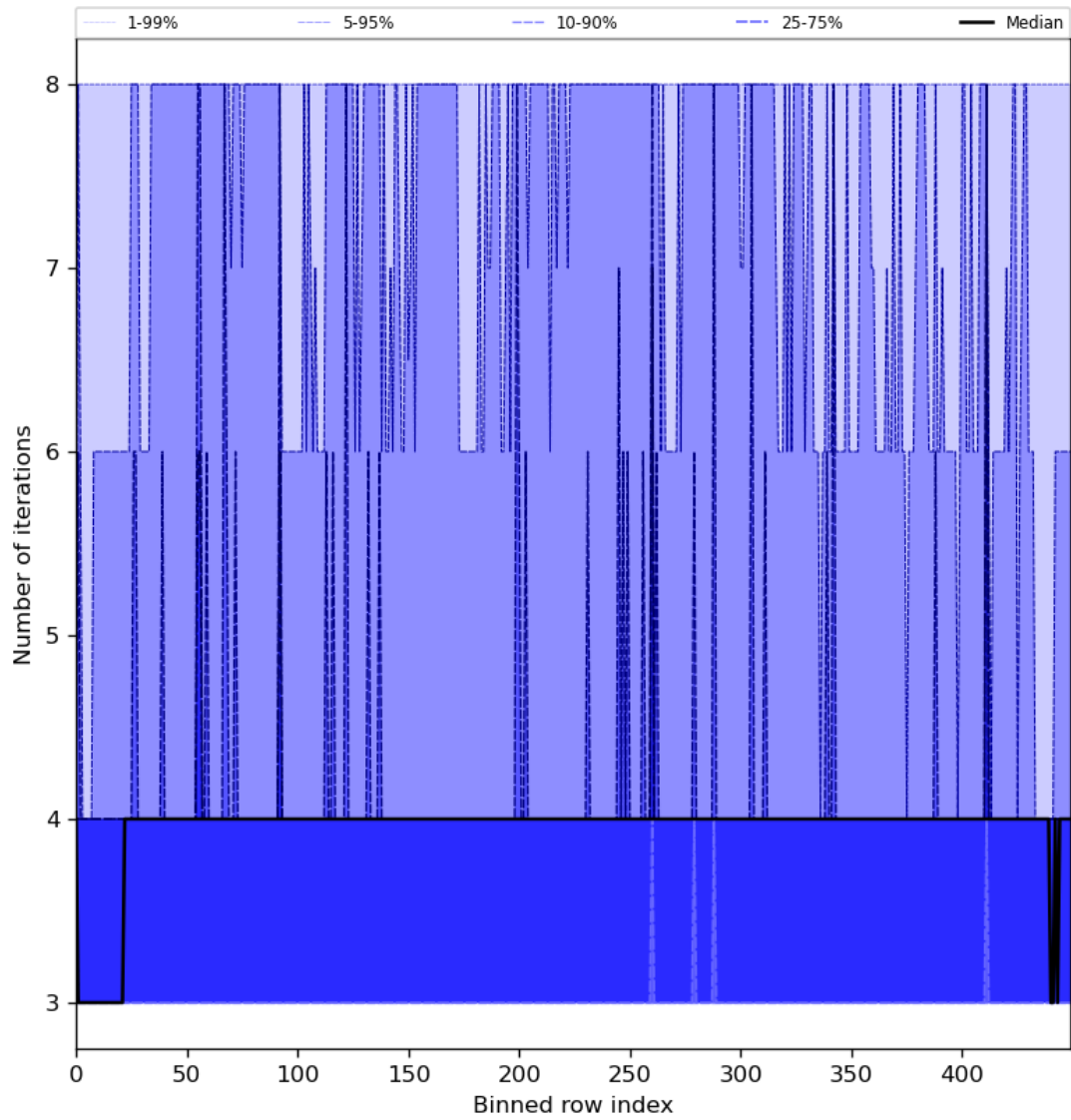
Figure 51: Along track statistics of “Number of iterations” for 2024-06-03 to 2024-06-04
