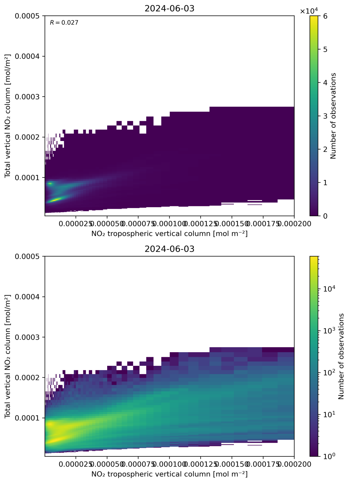
Figure 128: Scatter density plot of “NO 2 tropospheric vertical column” against “Total vertical NO 2 column” for 2024-06-03 to 2024-06-04.
