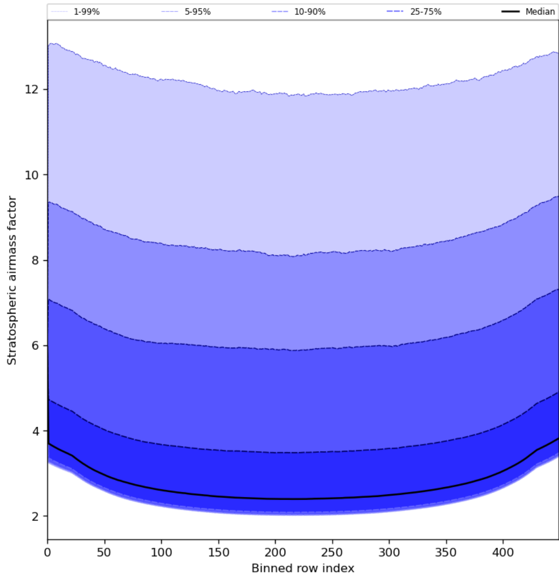
Figure 61: Along track statistics of “Stratospheric airmass factor” for 2024-06-03 to 2024-06-04
