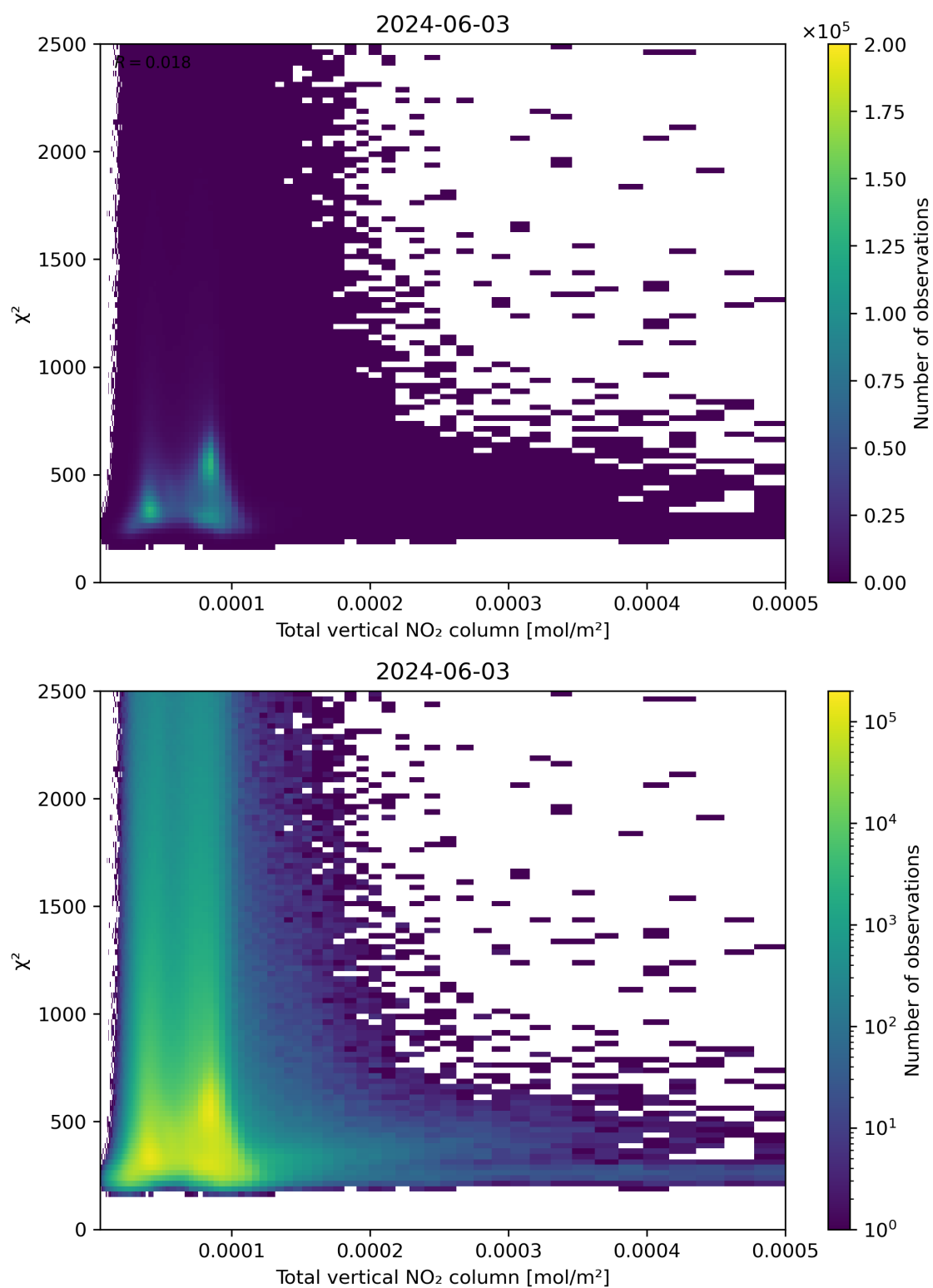
Figure 111: Scatter density plot of “Total vertical NO 2 column” against “ \chi^2 ” for 2024-06-03 to 2024-06-04.
