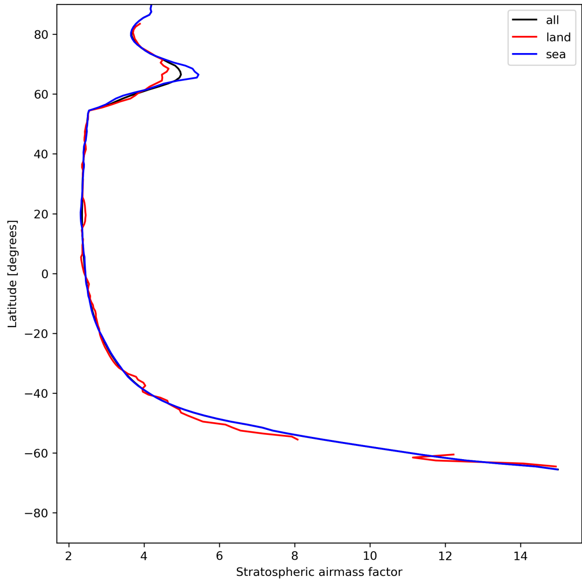
Figure 27: Zonal average of “Stratospheric air mass factor” for 2024-06-03 to 2024-06-04.
