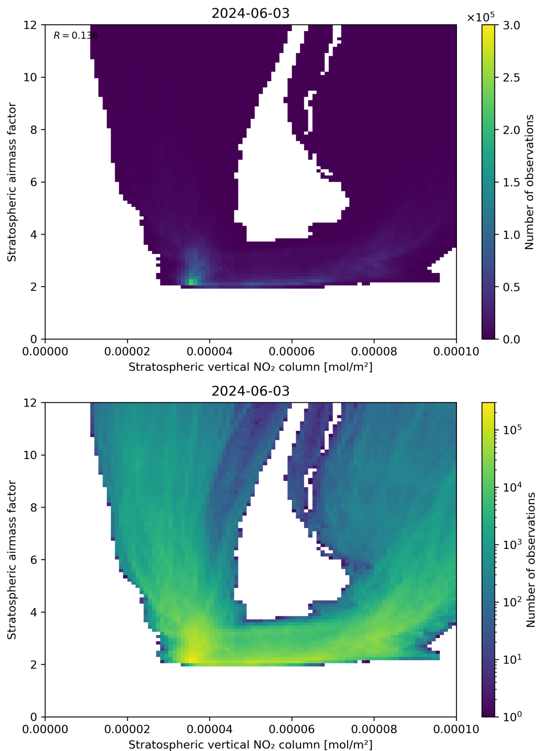
Figure 96: Scatter density plot of “Stratospheric vertical NO 2 column” against “Stratospheric airmass factor” for 2024-06-03 to 2024-06-04.
