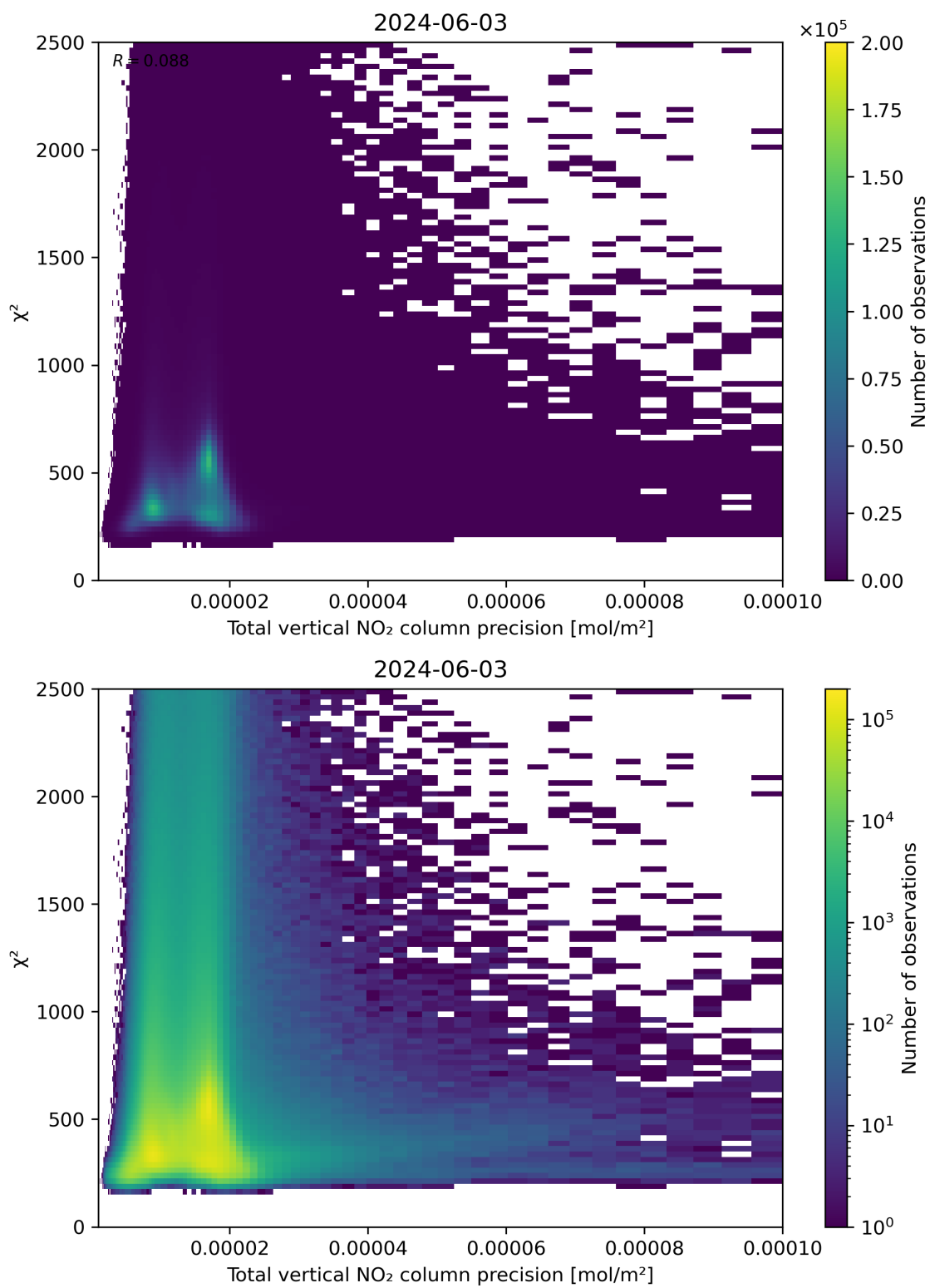
Figure 116: Scatter density plot of “Total vertical NO 2 column precision” against “ \chi^2 ” for 2024-06-03 to 2024-06-04.
