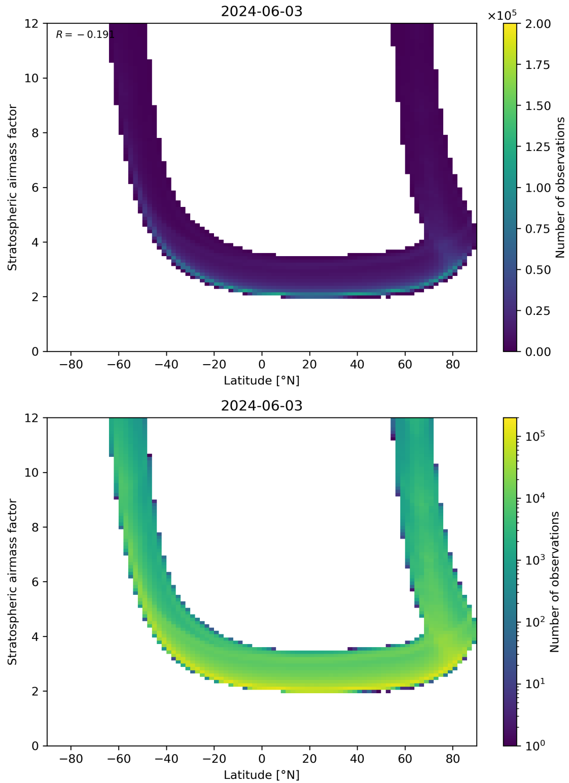
Figure 83: Scatter density plot of “Latitude” against “Stratospheric air mass factor” for 2024-06-03 to 2024-06-04.
