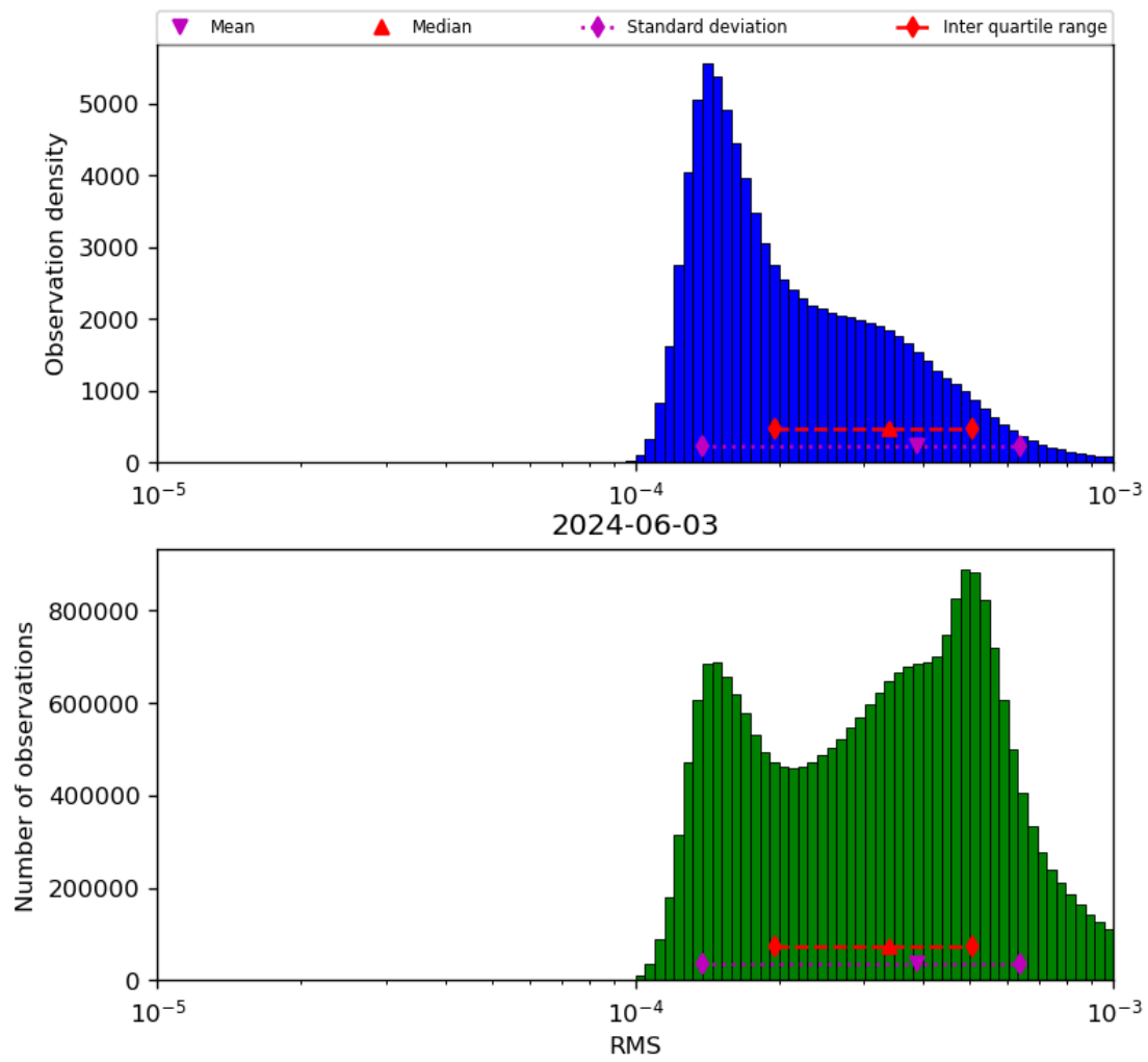
Figure 43: Histogram of “RMS” for 2024-06-03 to 2024-06-04
