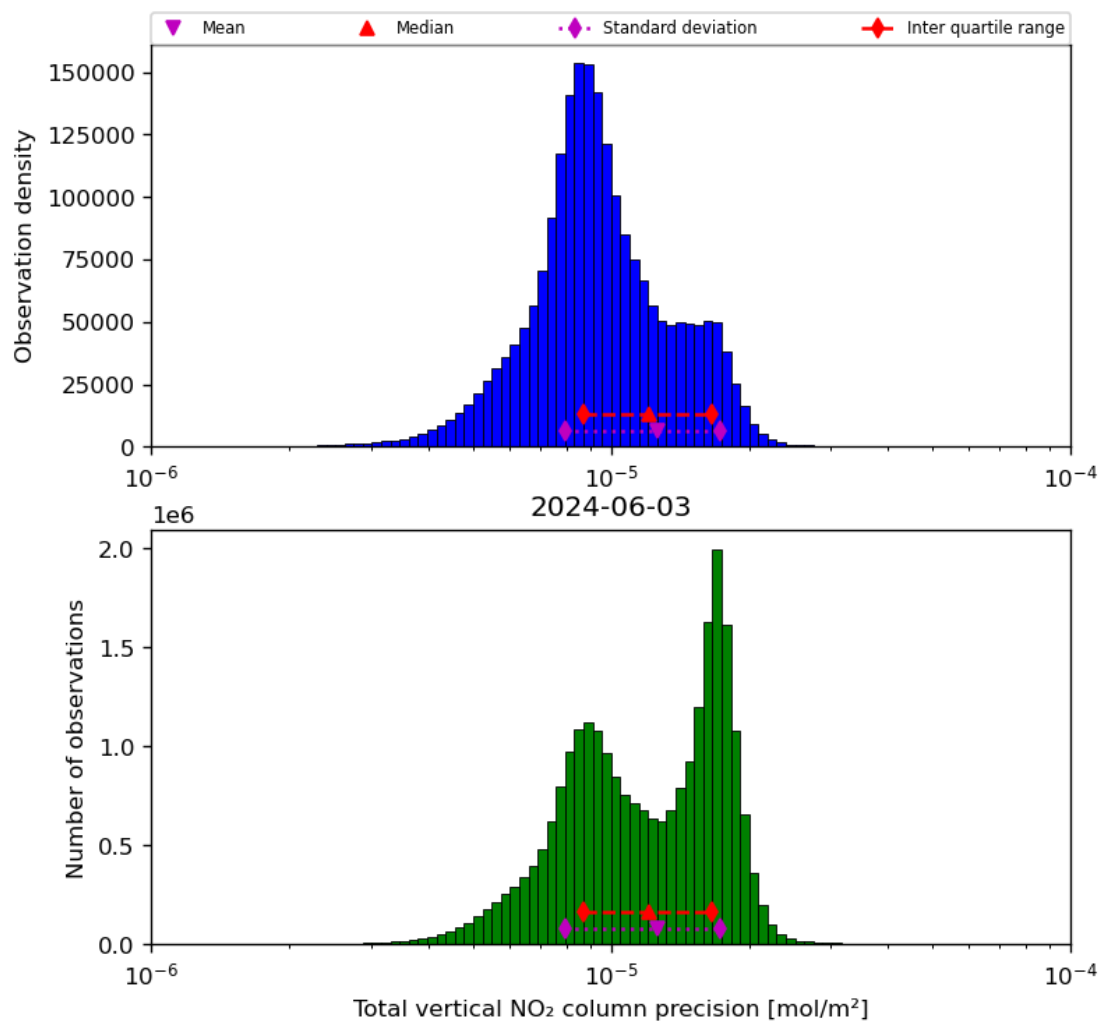
Figure 39: Histogram of “Total vertical NO 2 column precision” for 2024-06-03 to 2024-06-04
