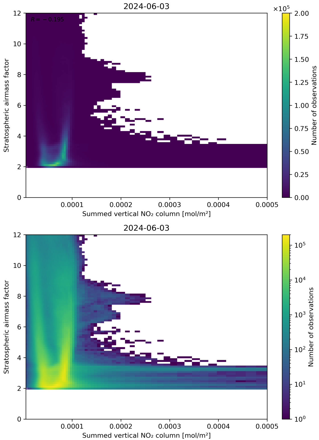
Figure 103: Scatter density plot of “Summed vertical NO 2 column” against “Stratospheric airmass factor” for 2024-06-03 to 2024-06-04.
