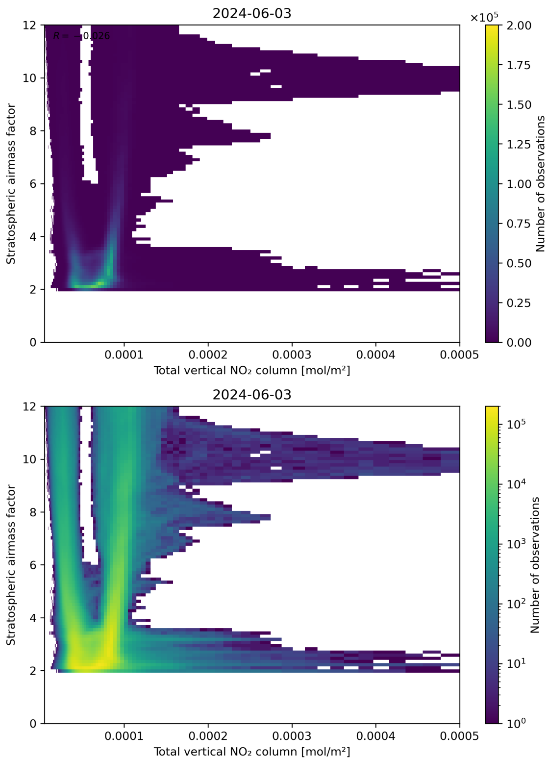
Figure 110: Scatter density plot of “Total vertical NO 2 column” against “Stratospheric airmass factor” for 2024-06-03 to 2024-06-04.
