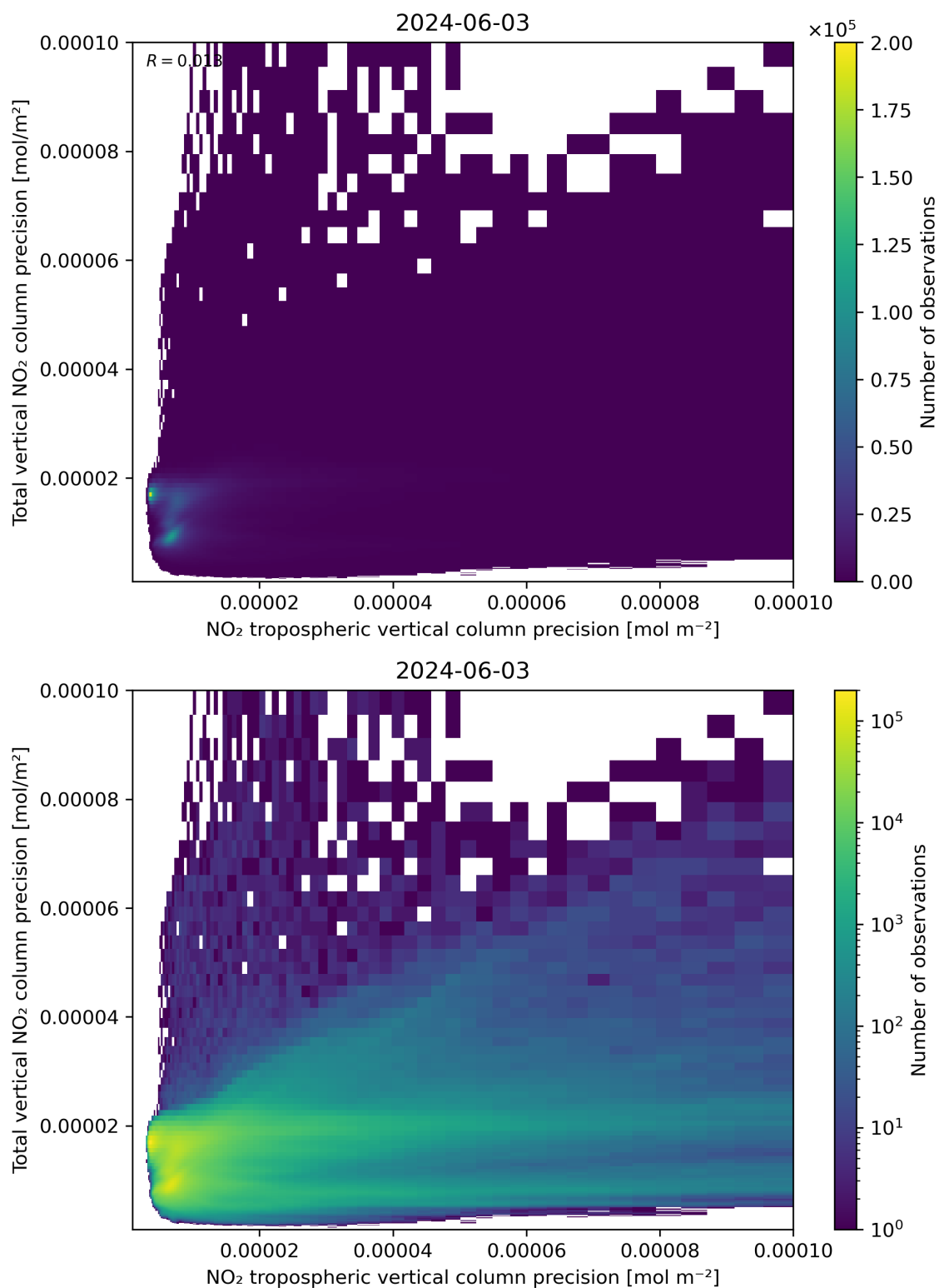
Figure 139: Scatter density plot of “NO 2 tropospheric vertical column precision” against “Total vertical NO 2 column precision” for 2024-06-03 to 2024-06-04.
