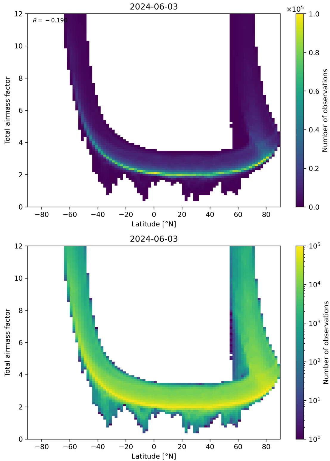
Figure 84: Scatter density plot of “Latitude” against “Total airmass factor” for 2024-06-03 to 2024-06-04.
