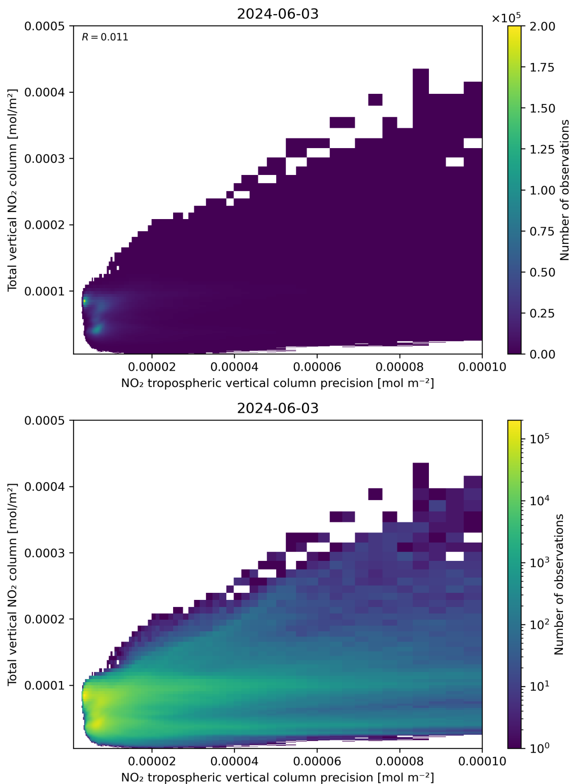
Figure 138: Scatter density plot of “NO 2 tropospheric vertical column precision” against “Total vertical NO 2 column” for 2024-06-03 to 2024-06-04.
