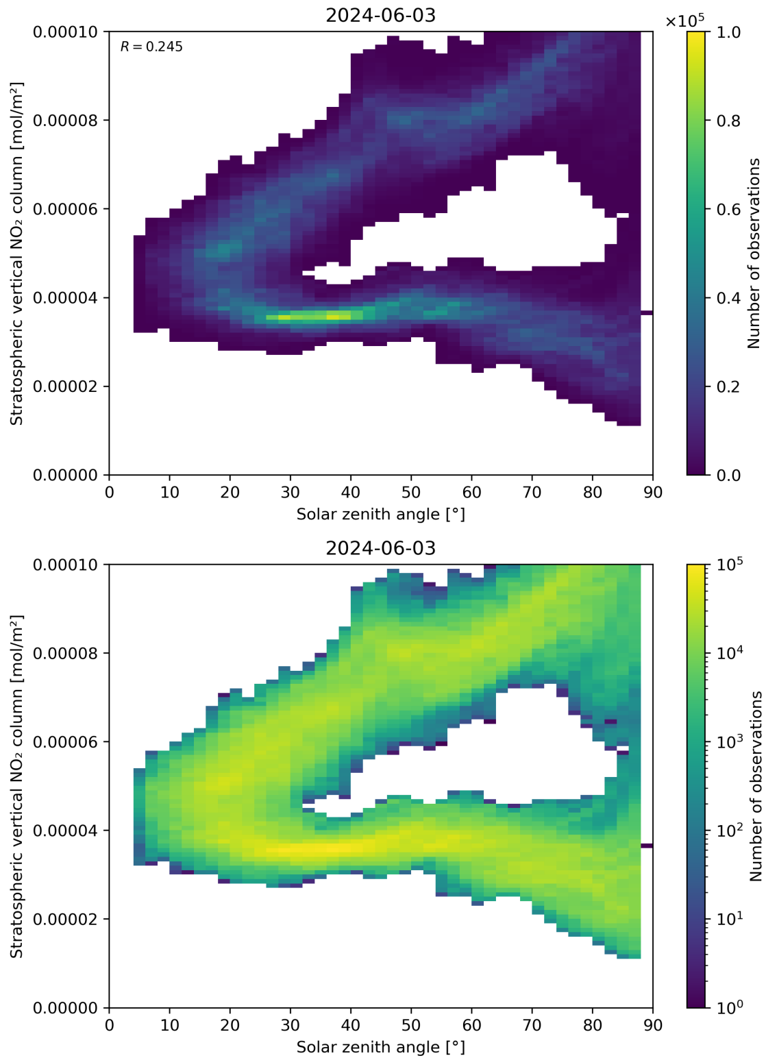
Figure 150: Scatter density plot of “Solar zenith angle” against “Stratospheric vertical NO 2 column” for 2024-06-03 to 2024-06-04.
