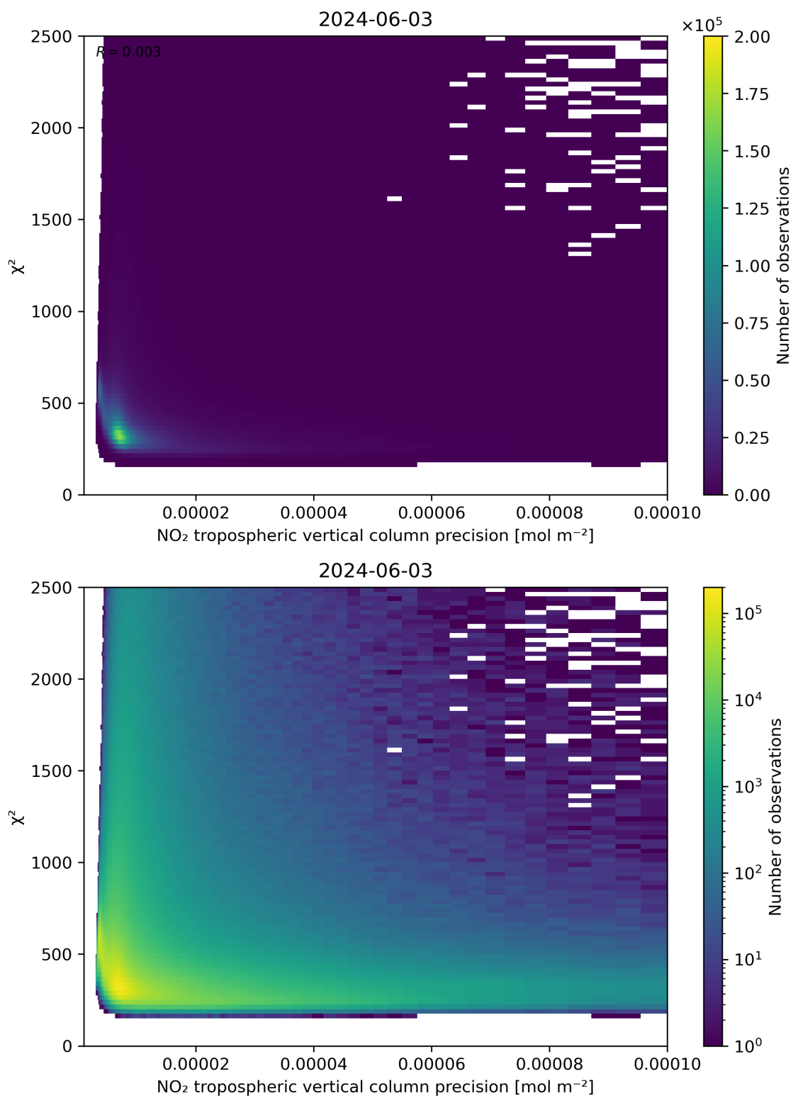
Figure 134: Scatter density plot of “NO 2 tropospheric vertical column precision” against “ \chi^2 ” for 2024-06-03 to 2024-06-04.
