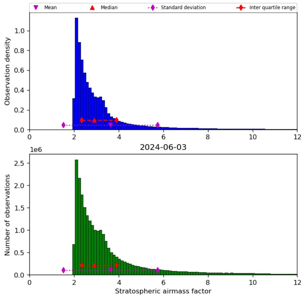
Figure 44: Histogram of “Stratospheric airmass factor” for 2024-06-03 to 2024-06-04
