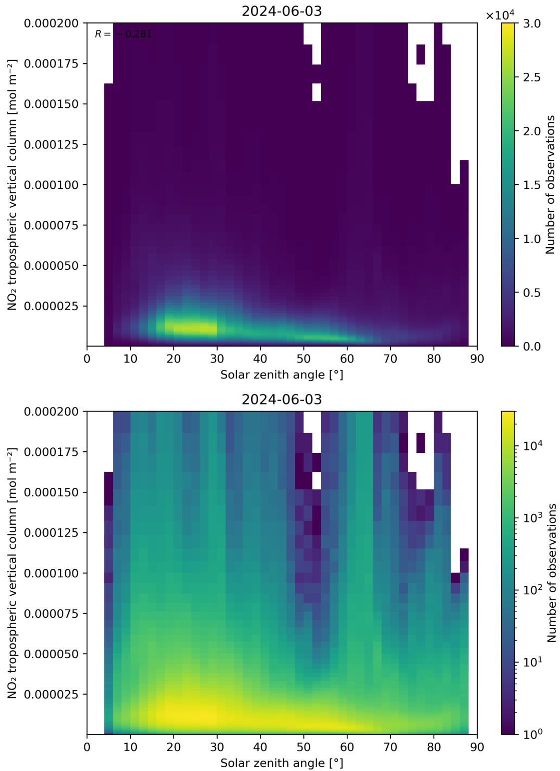
Figure 155: Scatter density plot of “Solar zenith angle” against “NO 2 tropospheric vertical column” for 2024-06-03 to 2024-06-04.
