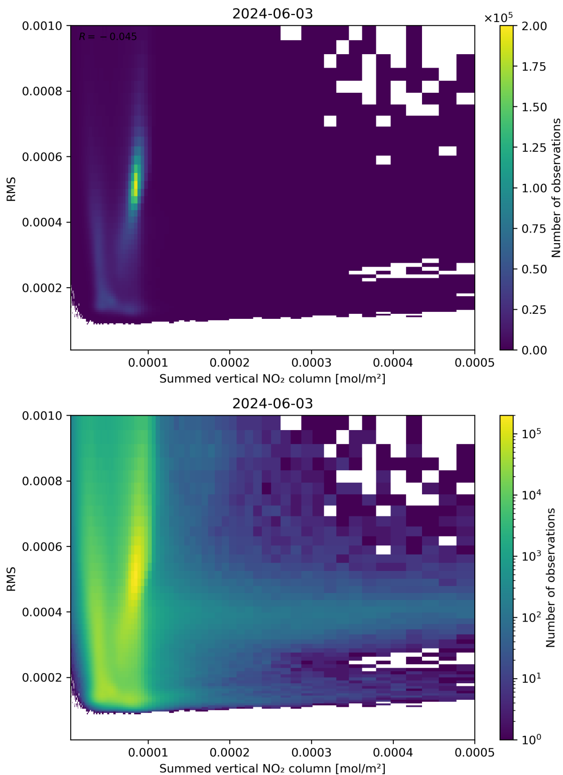
Figure 109: Scatter density plot of “Summed vertical NO 2 column” against “RMS” for 2024-06-03 to 2024-06-04.
