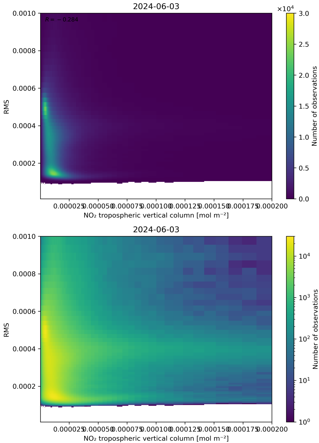
Figure 142: Scatter density plot of “NO 2 tropospheric vertical column” against “RMS” for 2024-06-03 to 2024-06-04.
