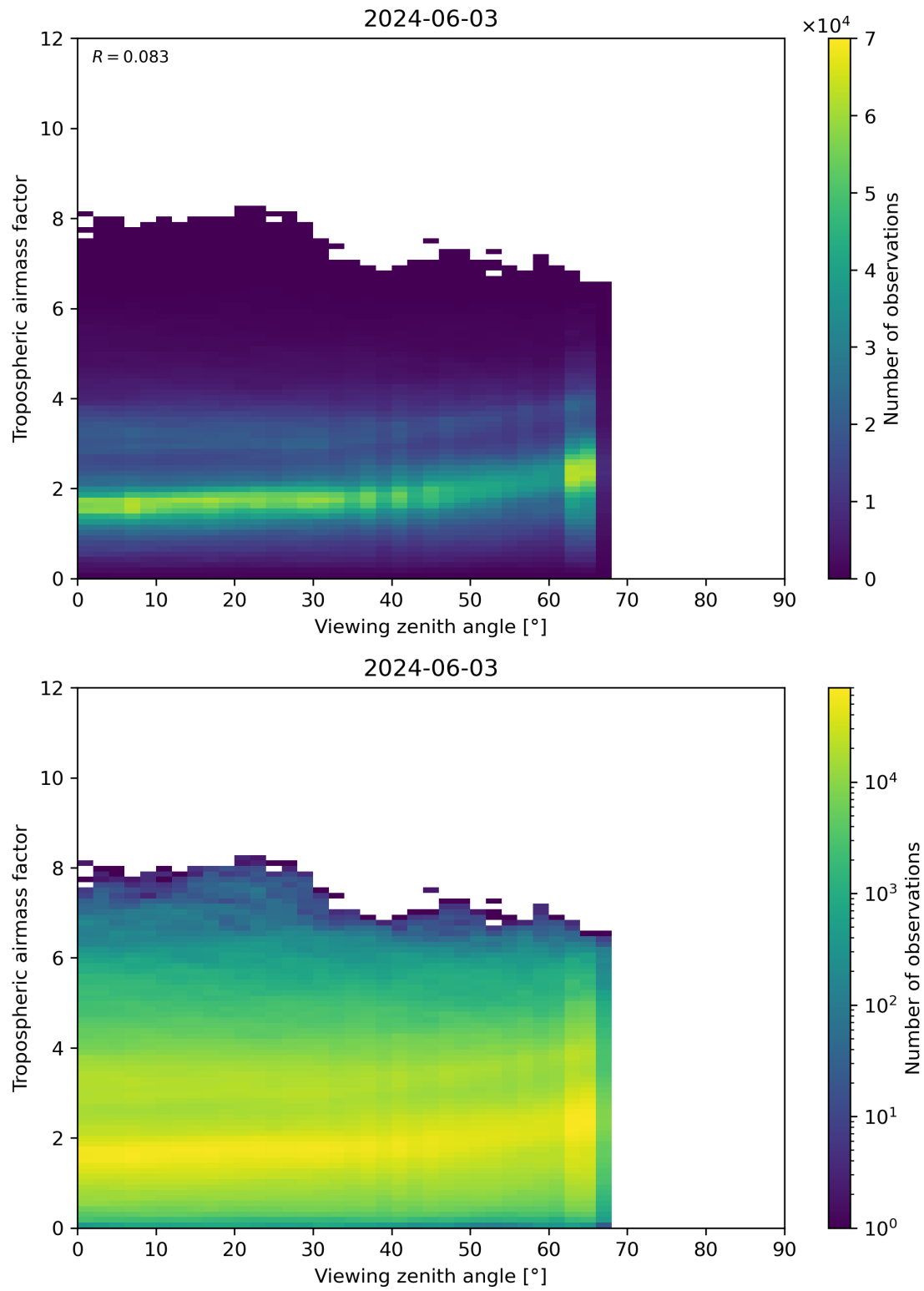
Figure 161: Scatter density plot of “Viewing zenith angle” against “Tropospheric airmass factor” for 2024-06-03 to 2024-06-04.
