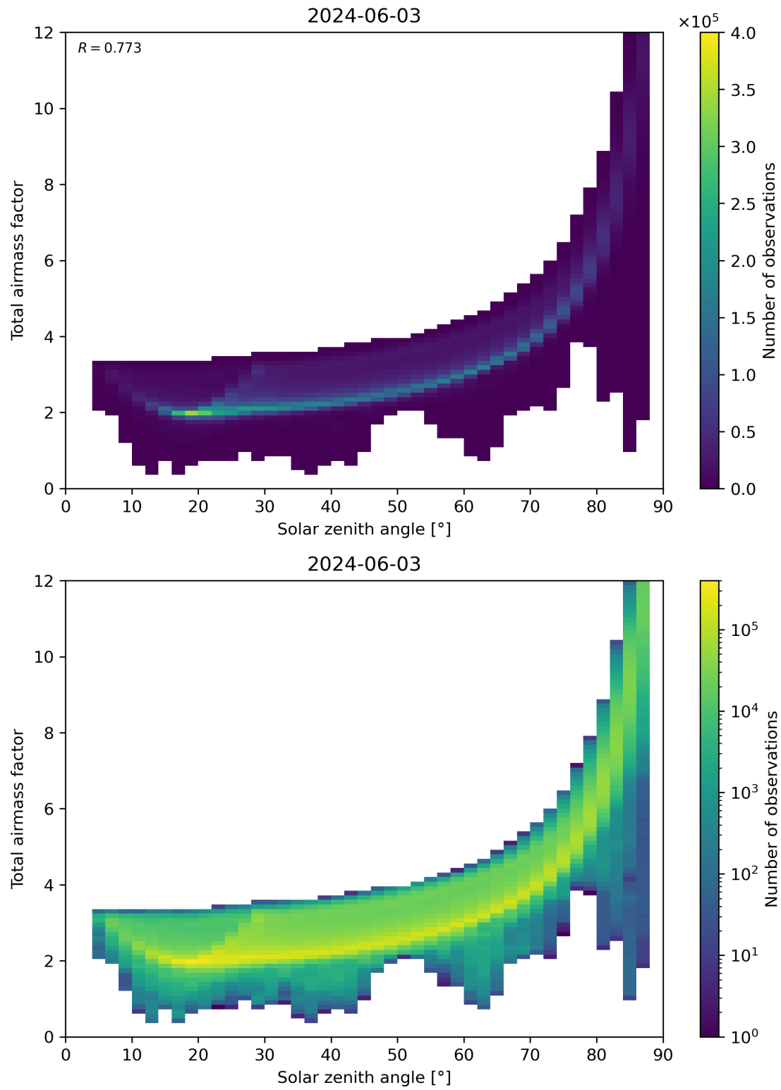
Figure 146: Scatter density plot of “Solar zenith angle” against “Total air mass factor” for 2024-06-03 to 2024-06-04.
