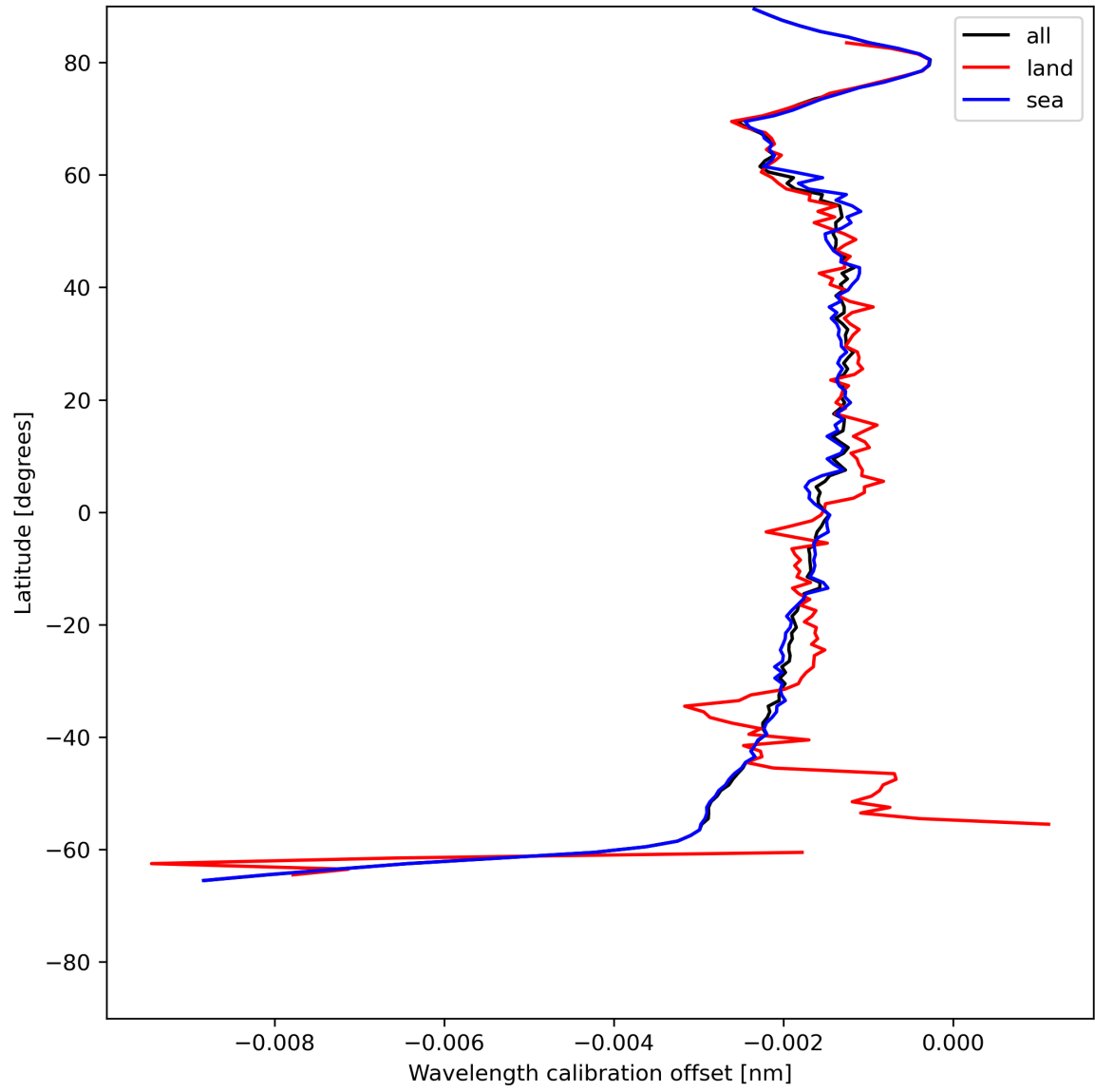
Figure 18: Zonal average of “Wavelength calibration offset” for 2024-06-03 to 2024-06-04.
