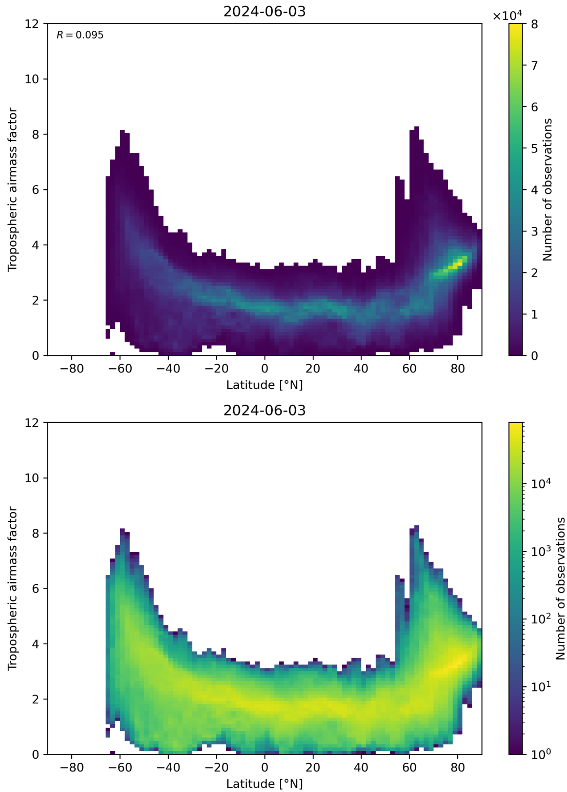
Figure 85: Scatter density plot of “Latitude” against “Tropospheric airmass factor” for 2024-06-03 to 2024-06-04.
