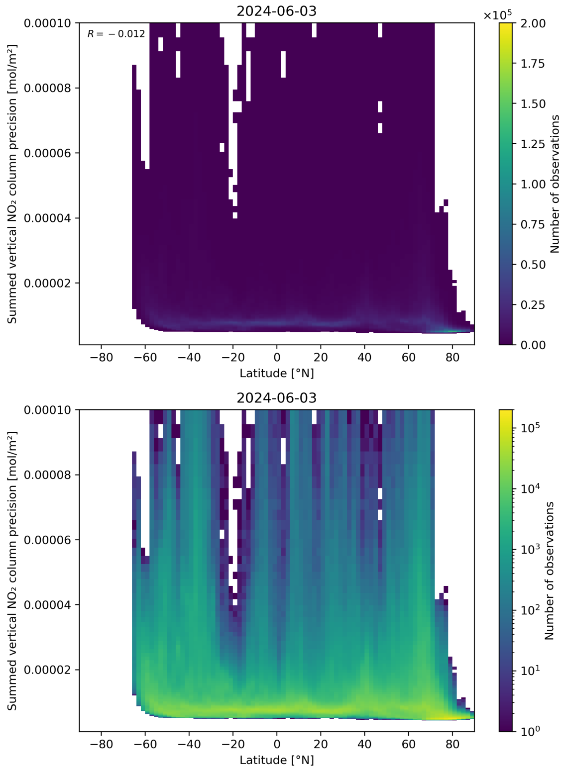
Figure 89: Scatter density plot of “Latitude” against “Summed vertical NO 2 column precision” for 2024-06-03 to 2024-06-04.
