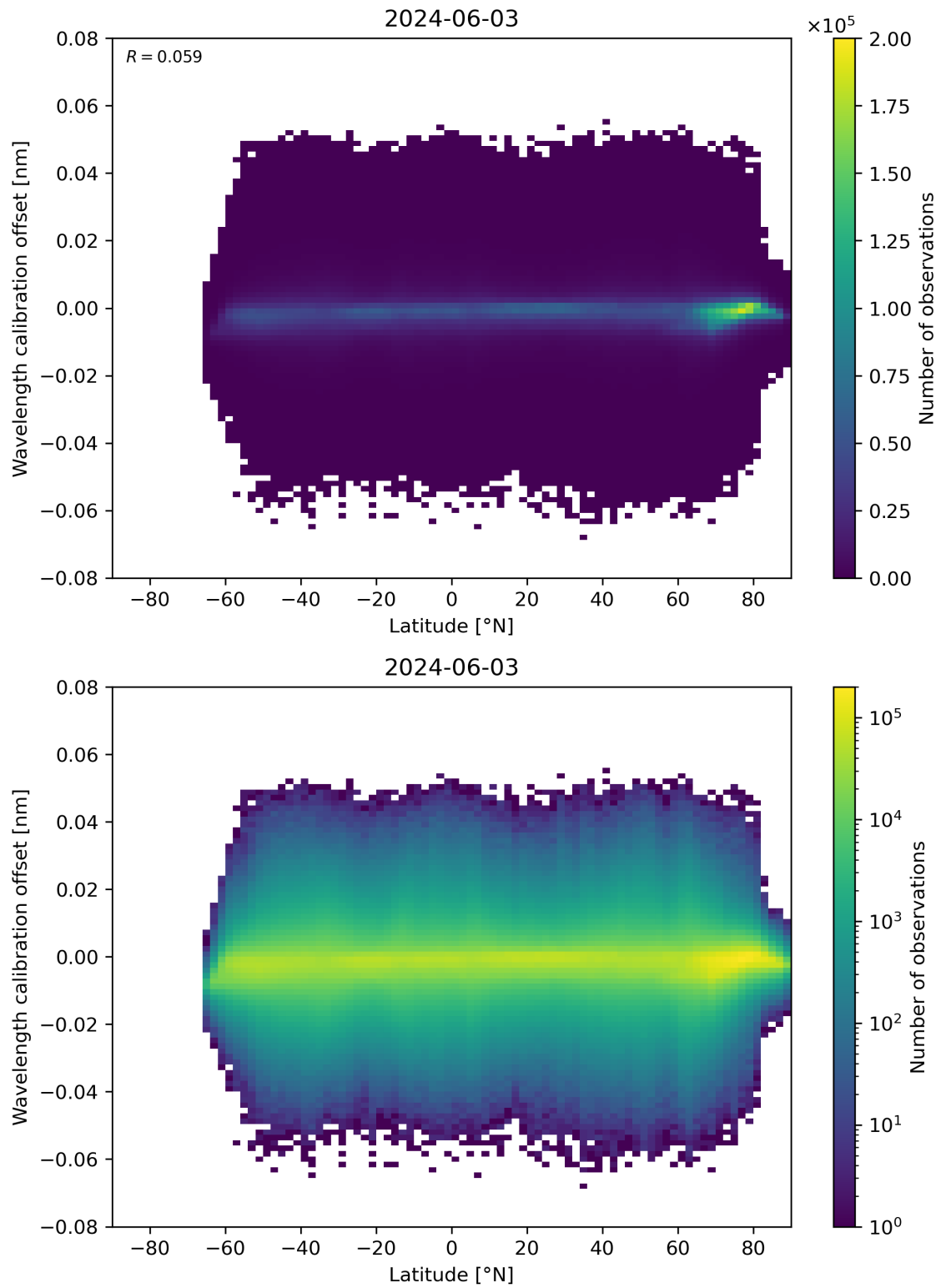
Figure 95: Scatter density plot of “Latitude” against “Wavelength calibration offset” for 2024-06-03 to 2024-06-04.
