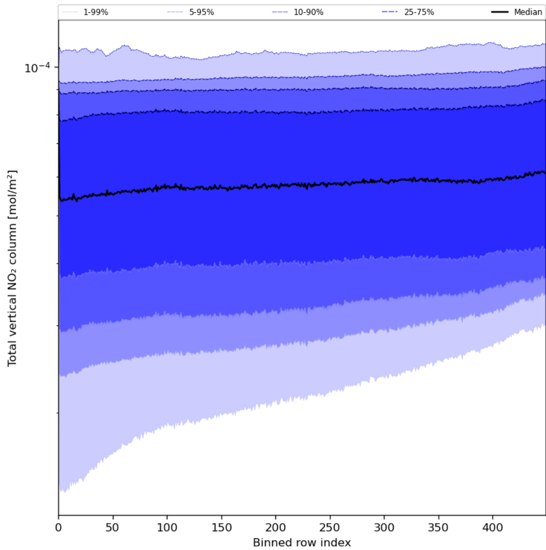
Figure 55: Along track statistics of “Total vertical NO 2 column” for 2024-06-03 to 2024-06-04
