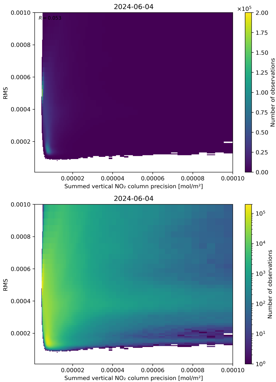
Figure 108: Scatter density plot of “Summed vertical NO 2 column precision” against “RMS” for 2024-06-03 to 2024-06-05.
