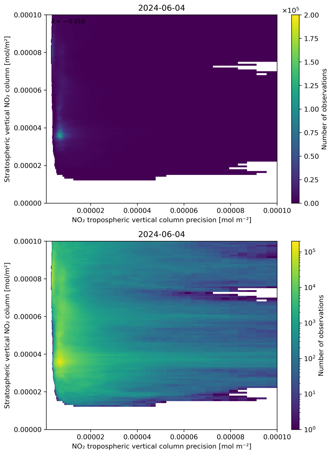
Figure 135: Scatter density plot of “NO 2 tropospheric vertical column precision” against “Stratospheric vertical NO 2 column” for 2024-06-03 to 2024-06-05.
