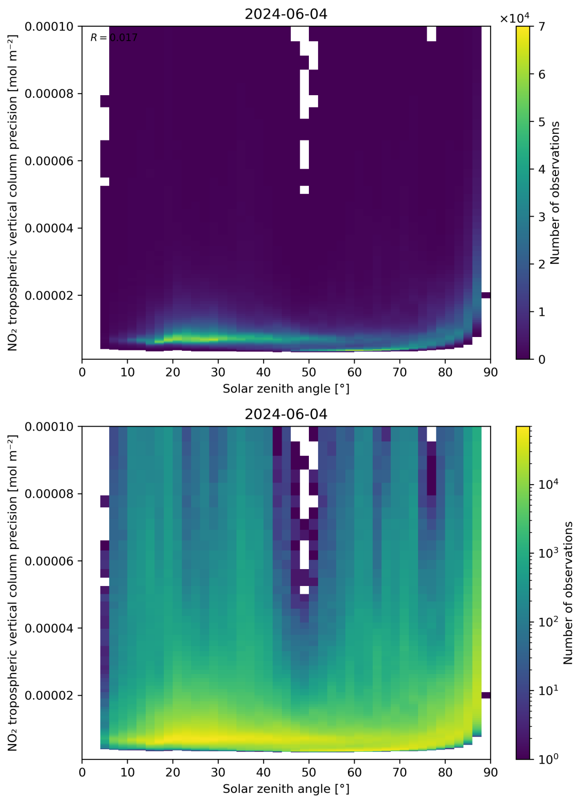
Figure 156: Scatter density plot of “Solar zenith angle” against “NO 2 tropospheric vertical column precision” for 2024-06-03 to 2024-06-05.
