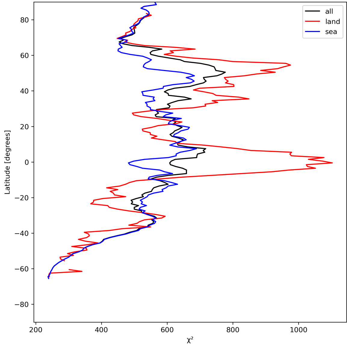
Figure 25: Zonal average of “ \chi^2 ” for 2024-06-03 to 2024-06-05.
