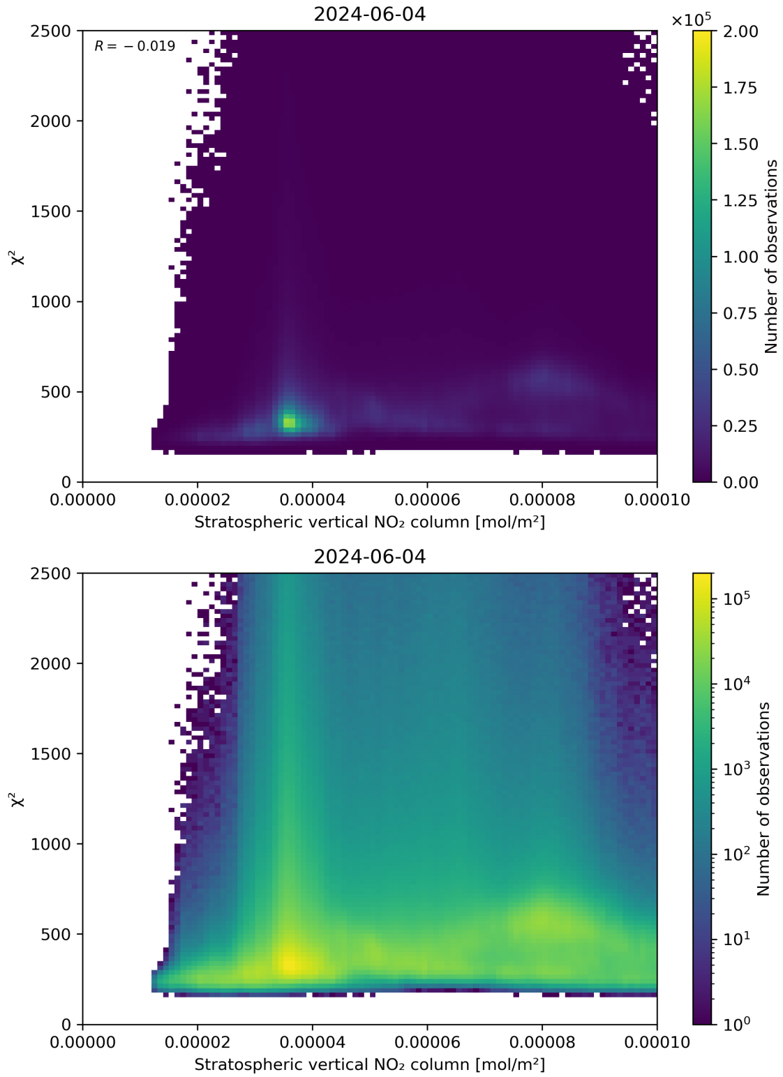
Figure 97: Scatter density plot of “Stratospheric vertical NO 2 column” against “ \chi^2 ” for 2024-06-03 to 2024-06-05.
