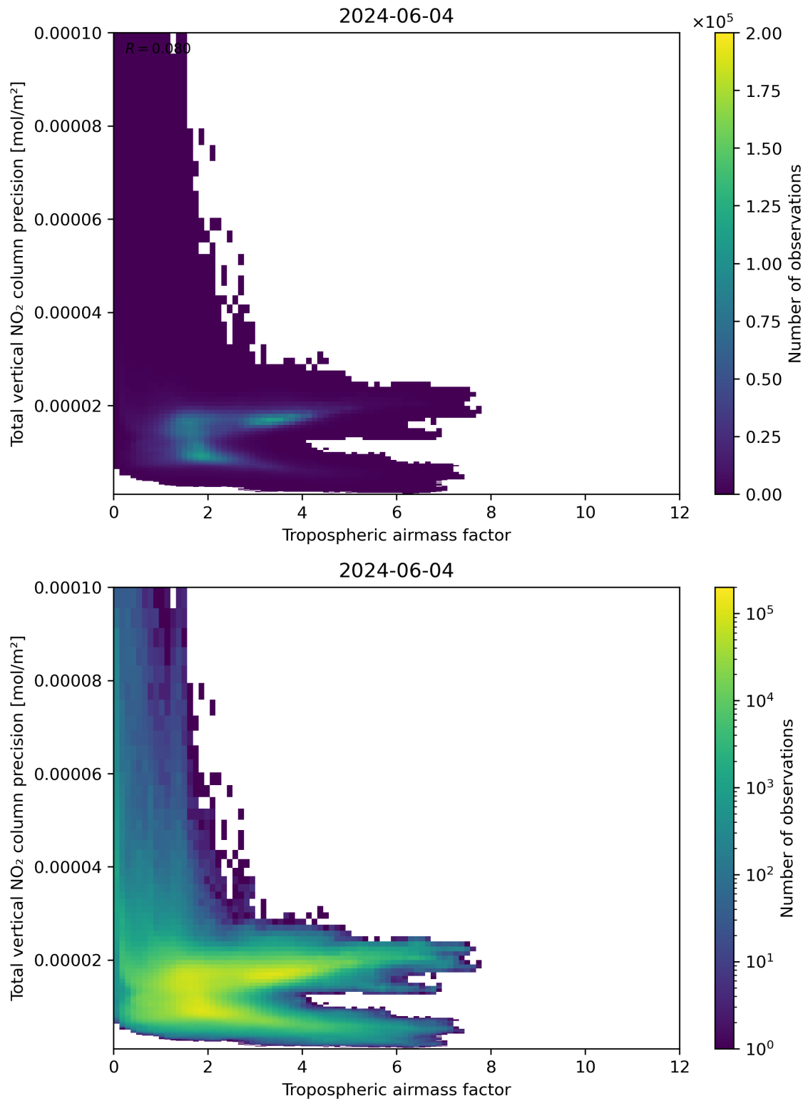
Figure 78: Scatter density plot of “Tropospheric air mass factor” against “Total vertical NO 2 column precision” for 2024-06-03 to 2024-06-05.
