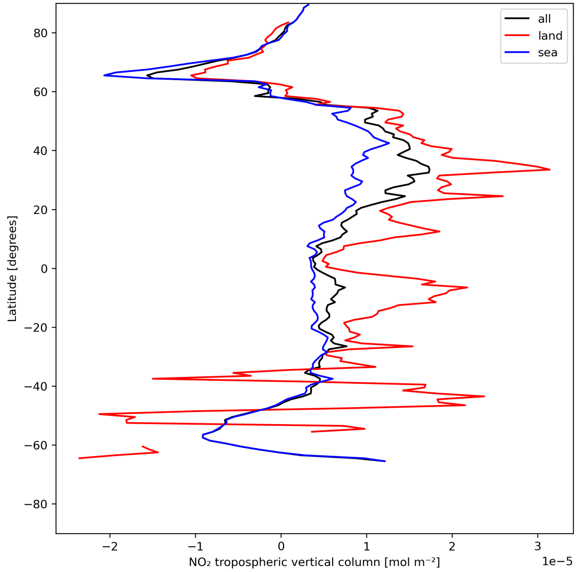
Figure 12: Zonal average of “NO 2 tropospheric vertical column” for 2024-06-03 to 2024-06-05.
