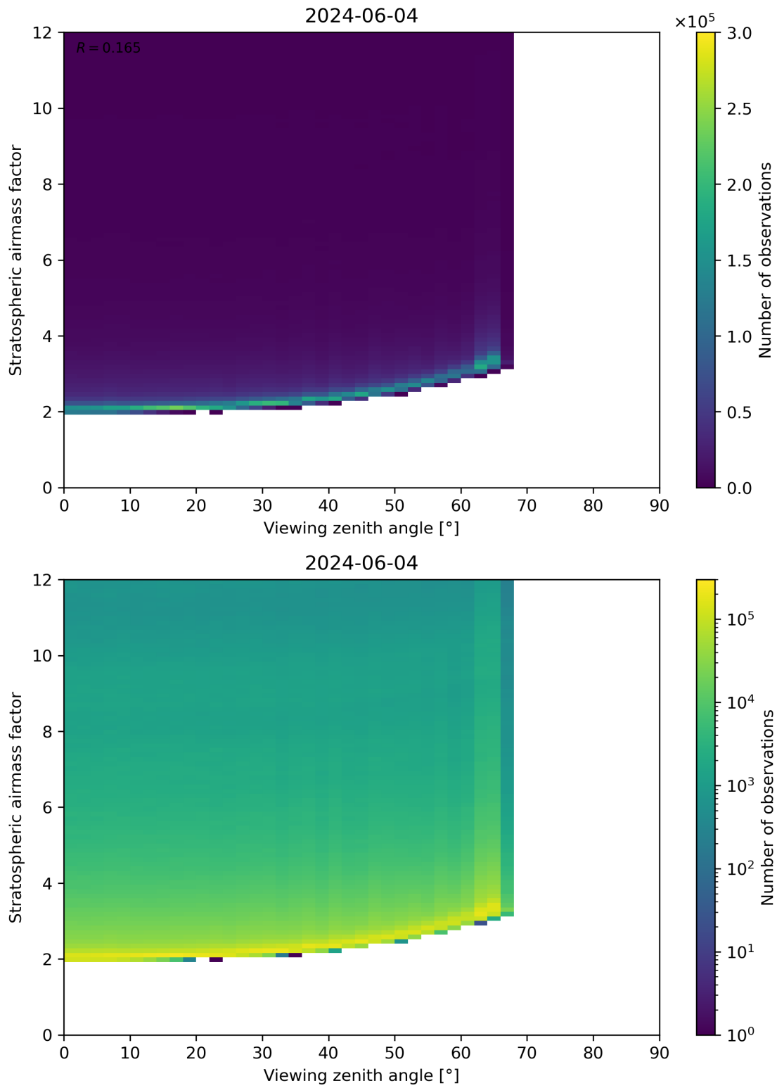
Figure 159: Scatter density plot of “Viewing zenith angle” against “Stratospheric airmass factor” for 2024-06-03 to 2024-06-05.
