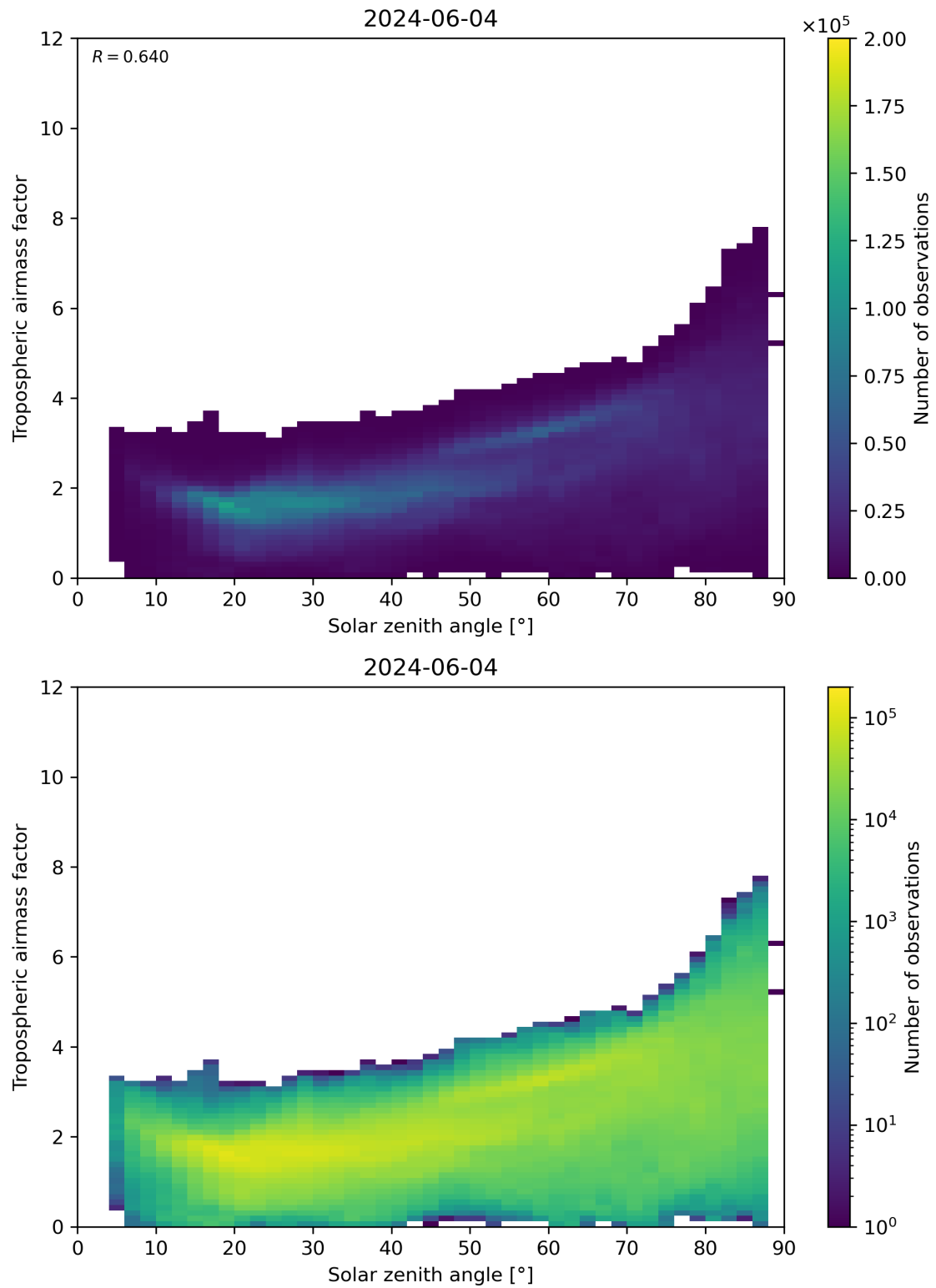
Figure 147: Scatter density plot of “Solar zenith angle” against “Tropospheric airmass factor” for 2024-06-03 to 2024-06-05.
