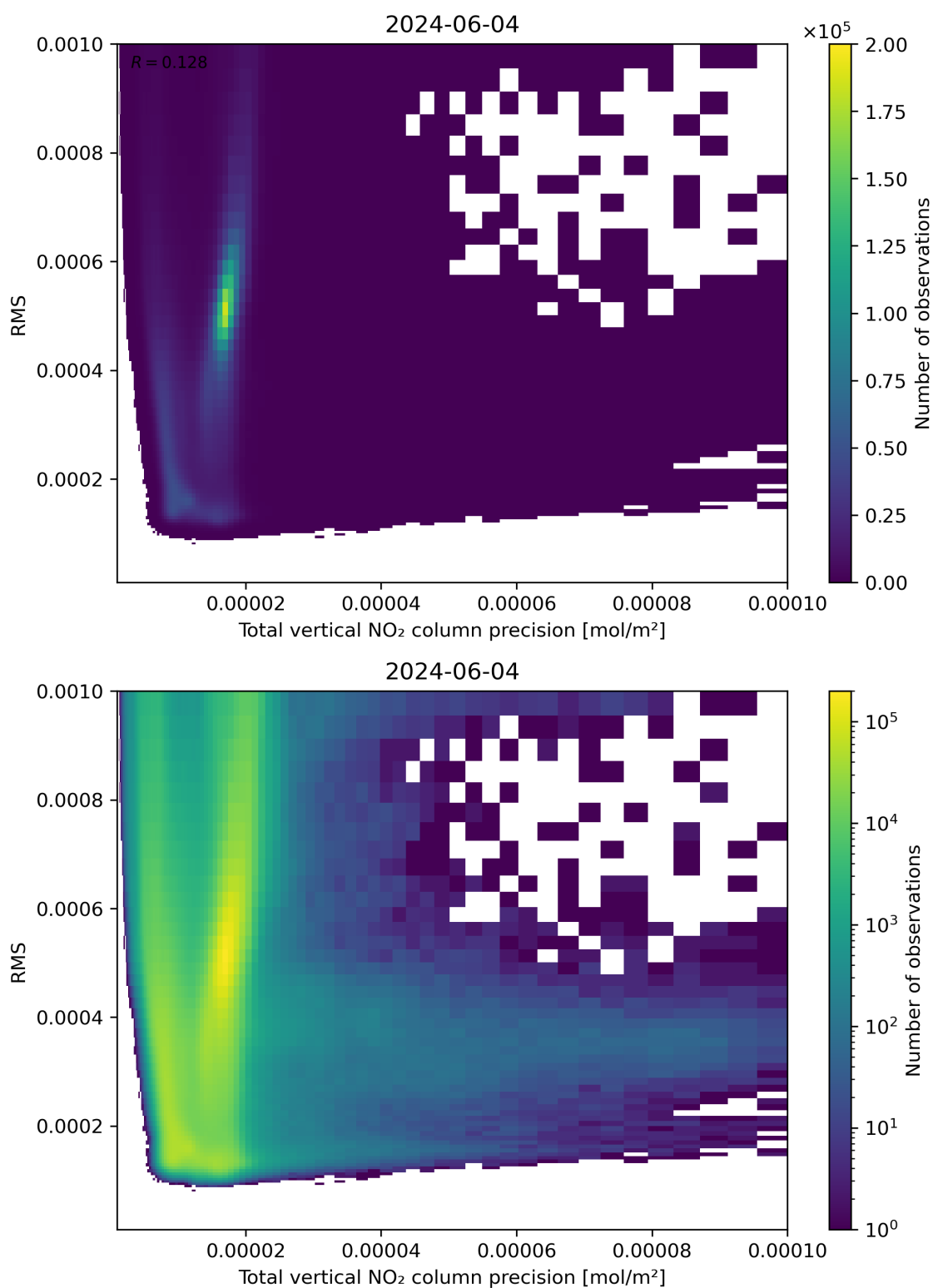
Figure 119: Scatter density plot of “Total vertical NO 2 column precision” against “RMS” for 2024-06-03 to 2024-06-05.
