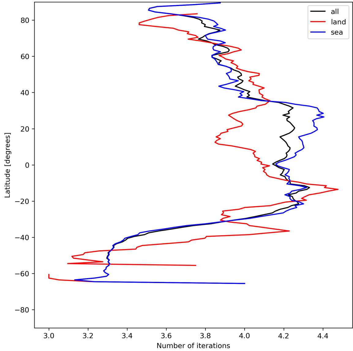
Figure 17: Zonal average of “Number of iterations” for 2024-06-03 to 2024-06-05.
