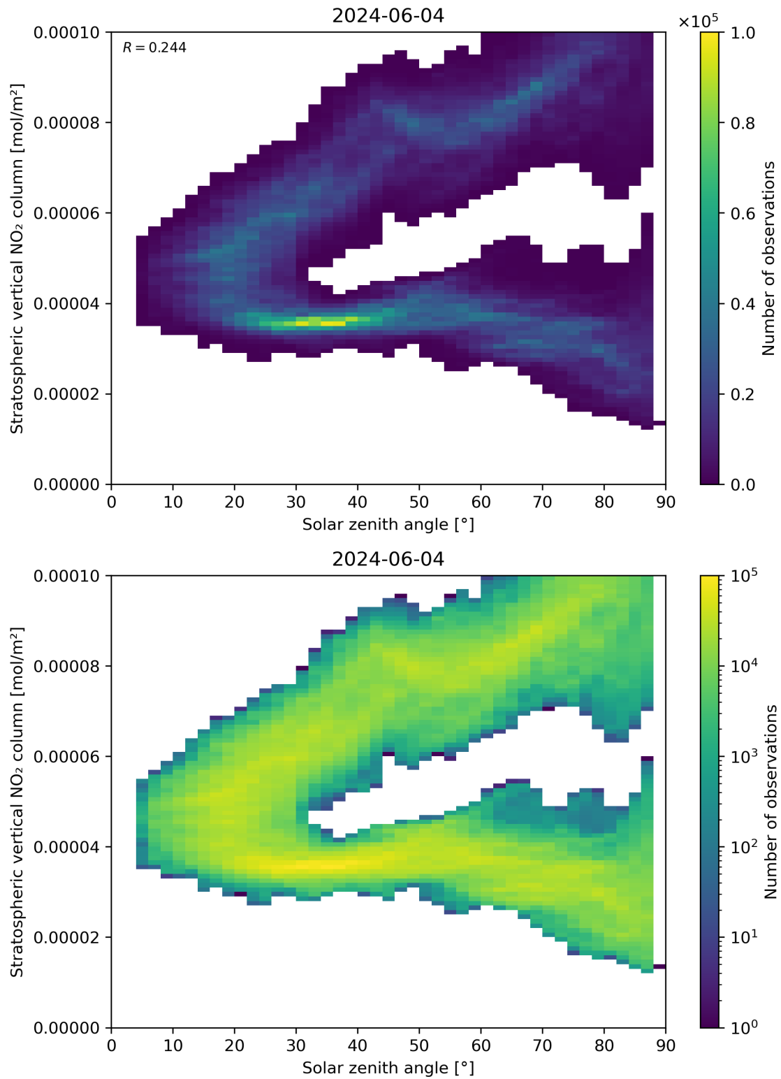
Figure 150: Scatter density plot of “Solar zenith angle” against “Stratospheric vertical NO 2 column” for 2024-06-03 to 2024-06-05.
