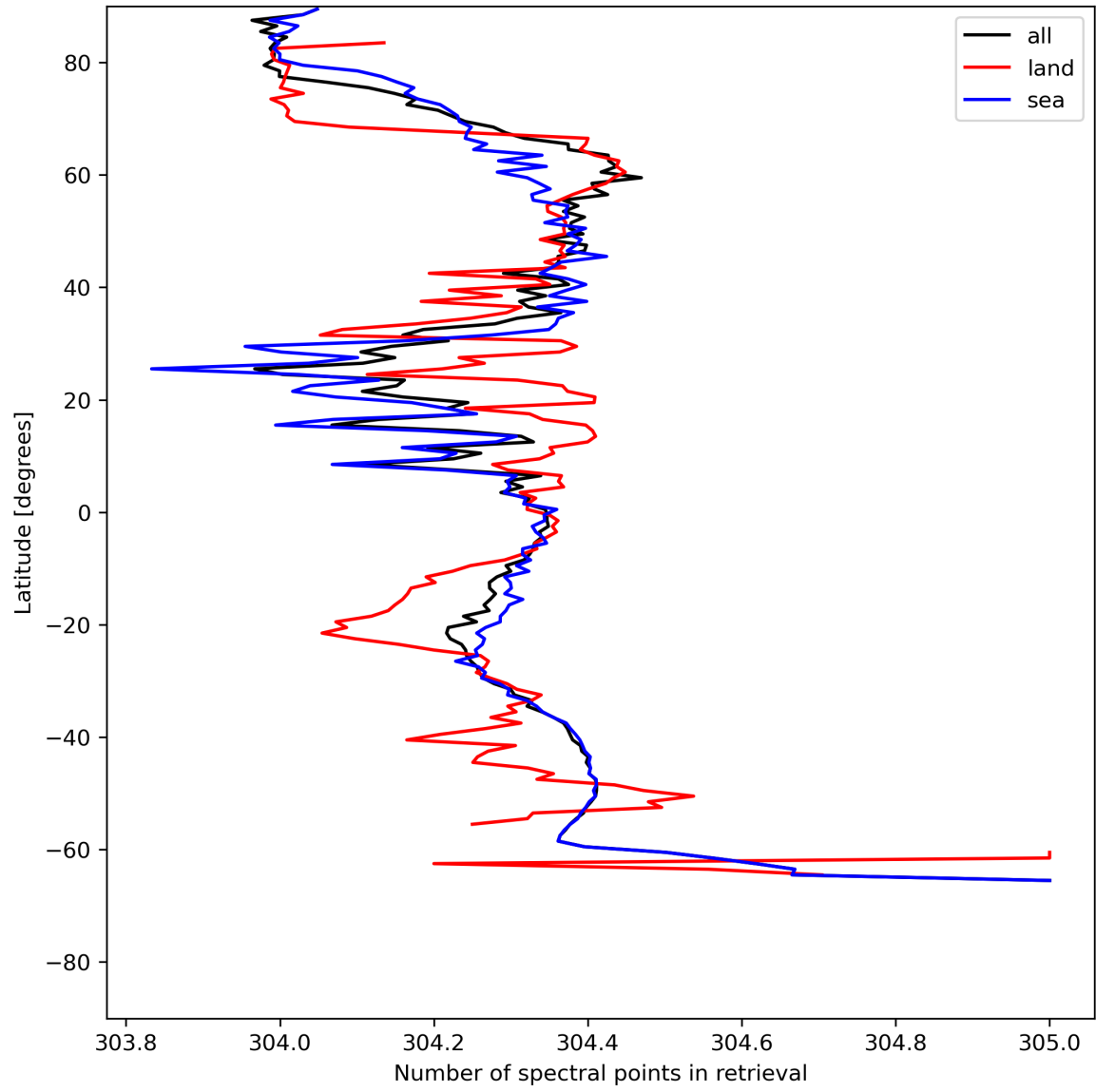
Figure 16: Zonal average of “Number of spectral points in retrieval” for 2024-06-03 to 2024-06-05.
