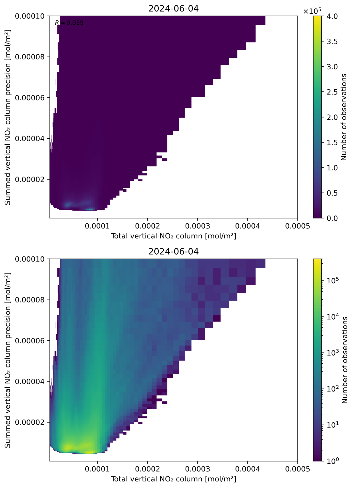
Figure 113: Scatter density plot of “Total vertical NO 2 column” against “Summed vertical NO 2 column precision” for 2024-06-03 to 2024-06-05.
