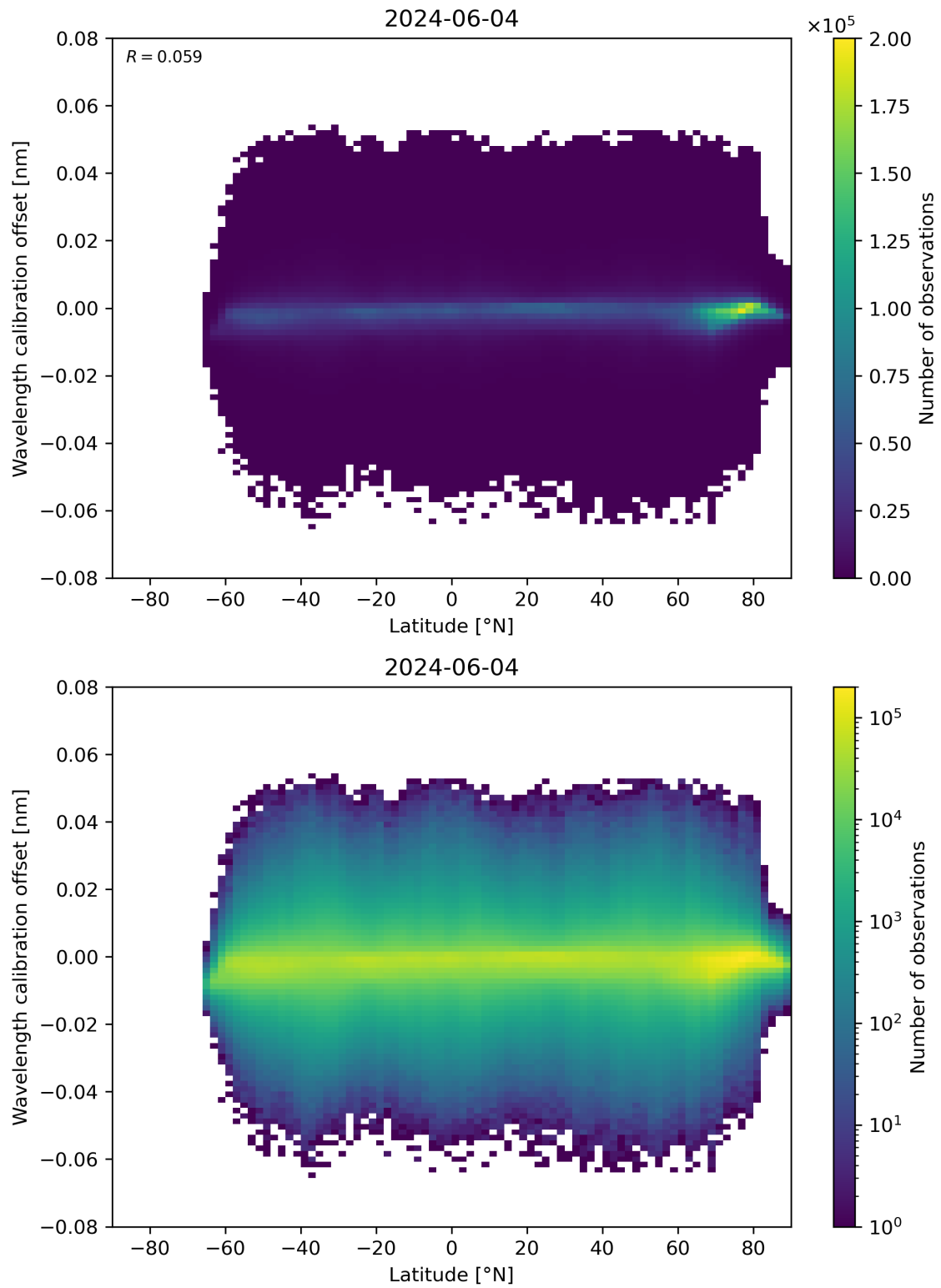
Figure 95: Scatter density plot of “Latitude” against “Wavelength calibration offset” for 2024-06-03 to 2024-06-05.
