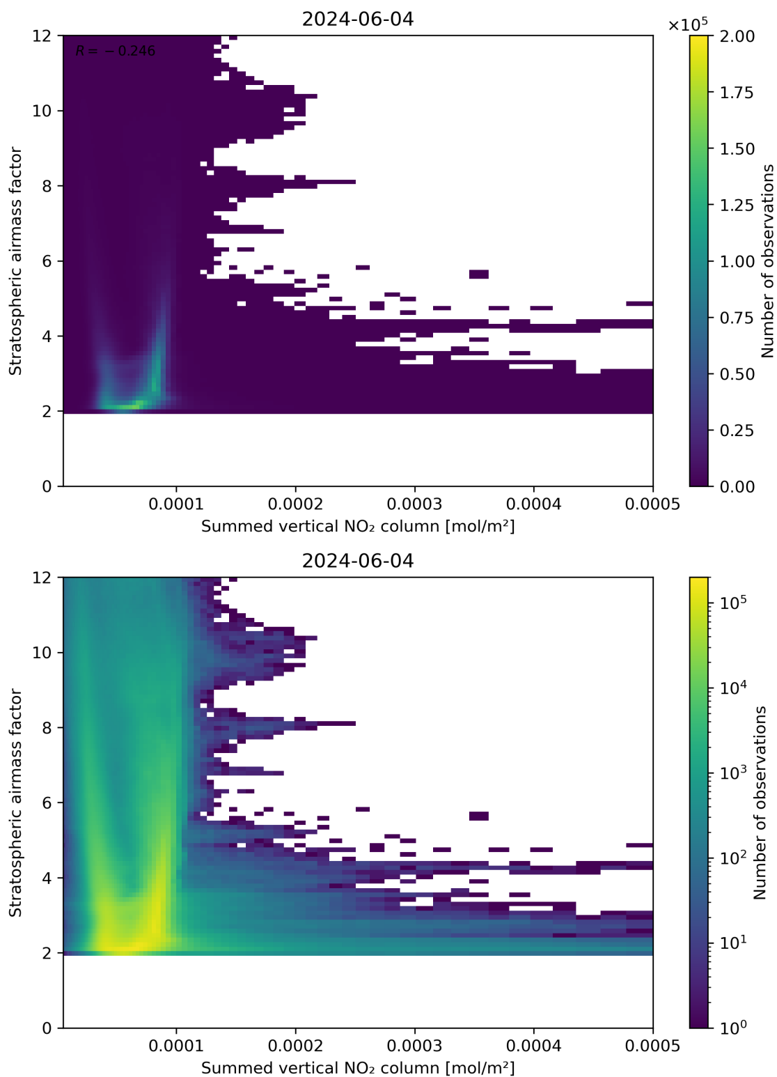
Figure 103: Scatter density plot of “Summed vertical NO 2 column” against “Stratospheric air mass factor” for 2024-06-03 to 2024-06-05.
