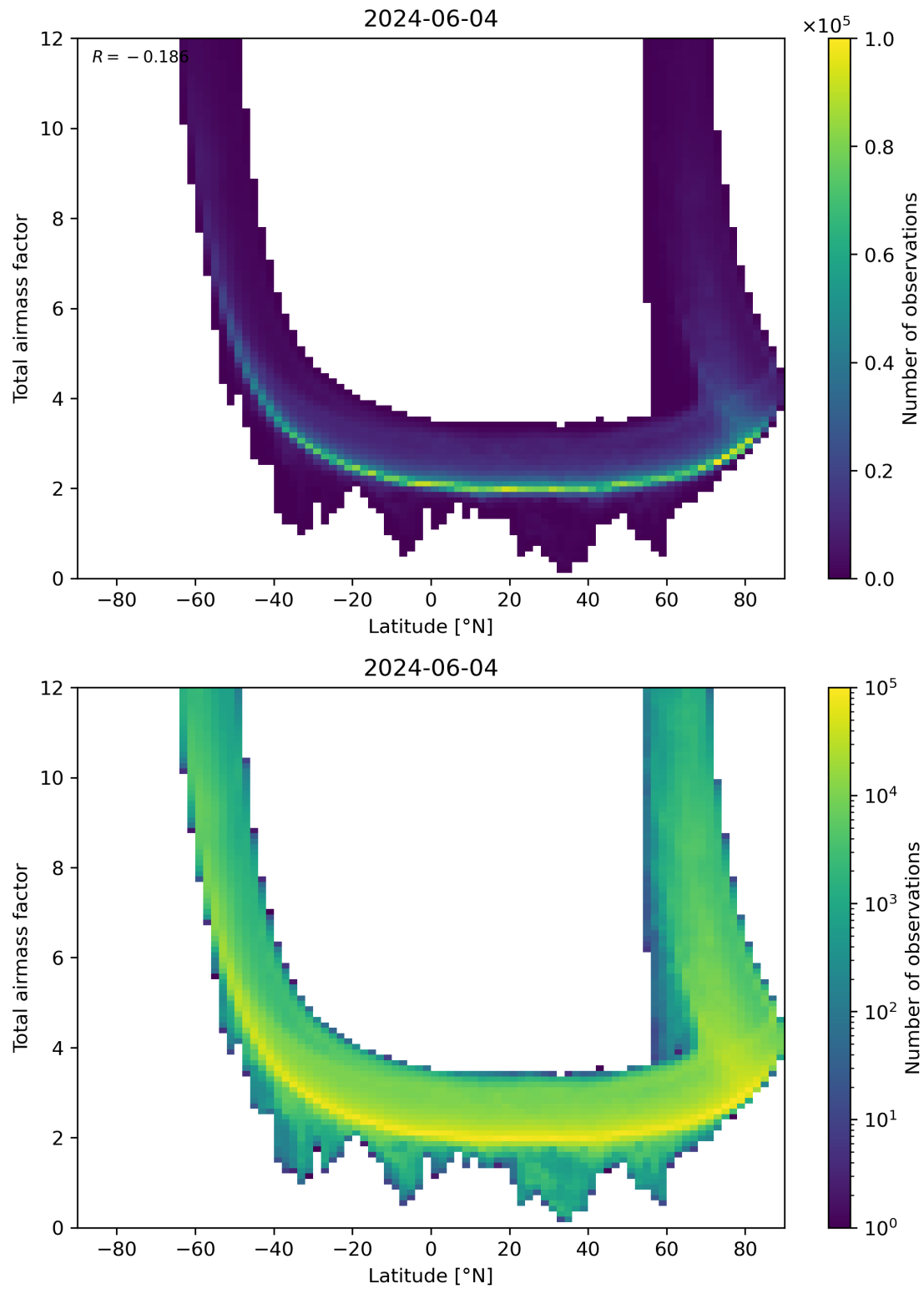
Figure 84: Scatter density plot of “Latitude” against “Total airmass factor” for 2024-06-03 to 2024-06-05.
