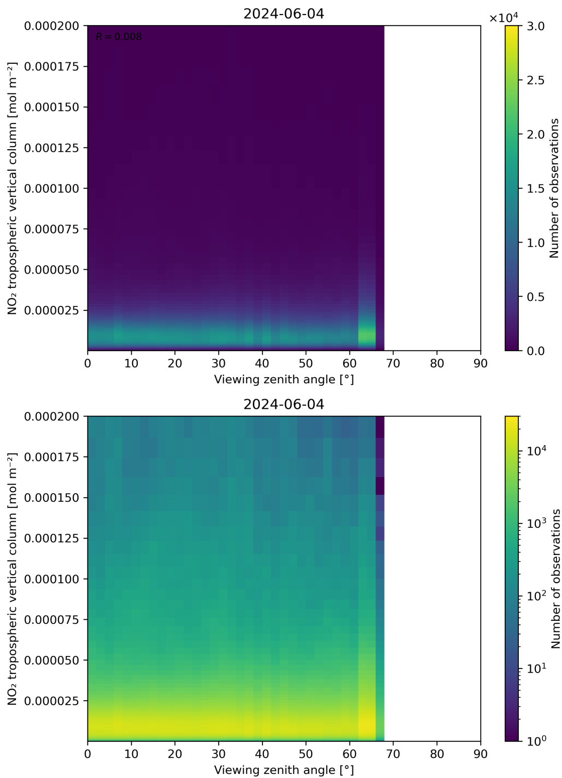
Figure 169: Scatter density plot of “Viewing zenith angle” against “NO 2 tropospheric vertical column” for 2024-06-03 to 2024-06-05.
