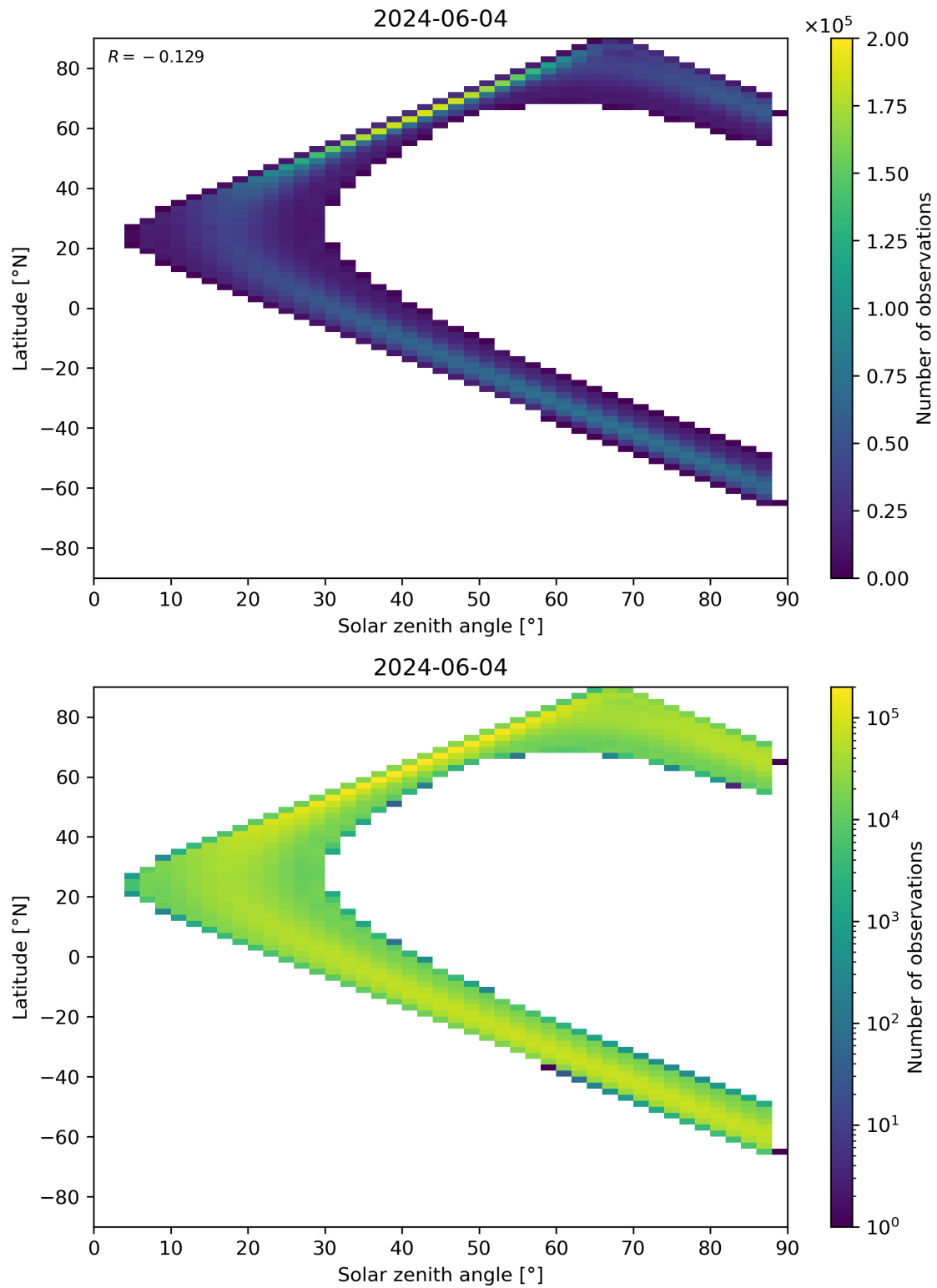
Figure 149: Scatter density plot of “Solar zenith angle” against “Latitude” for 2024-06-03 to 2024-06-05.
