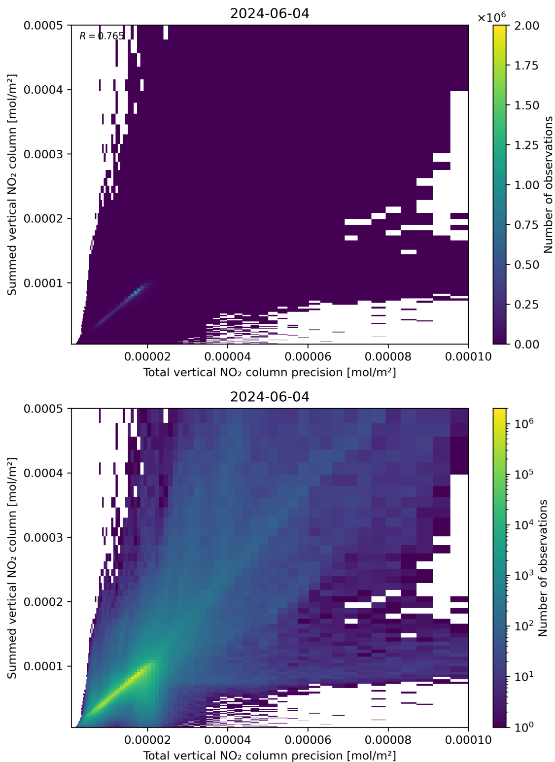
Figure 117: Scatter density plot of “Total vertical NO 2 column precision” against “Summed vertical NO 2 column” for 2024-06-03 to 2024-06-05.
