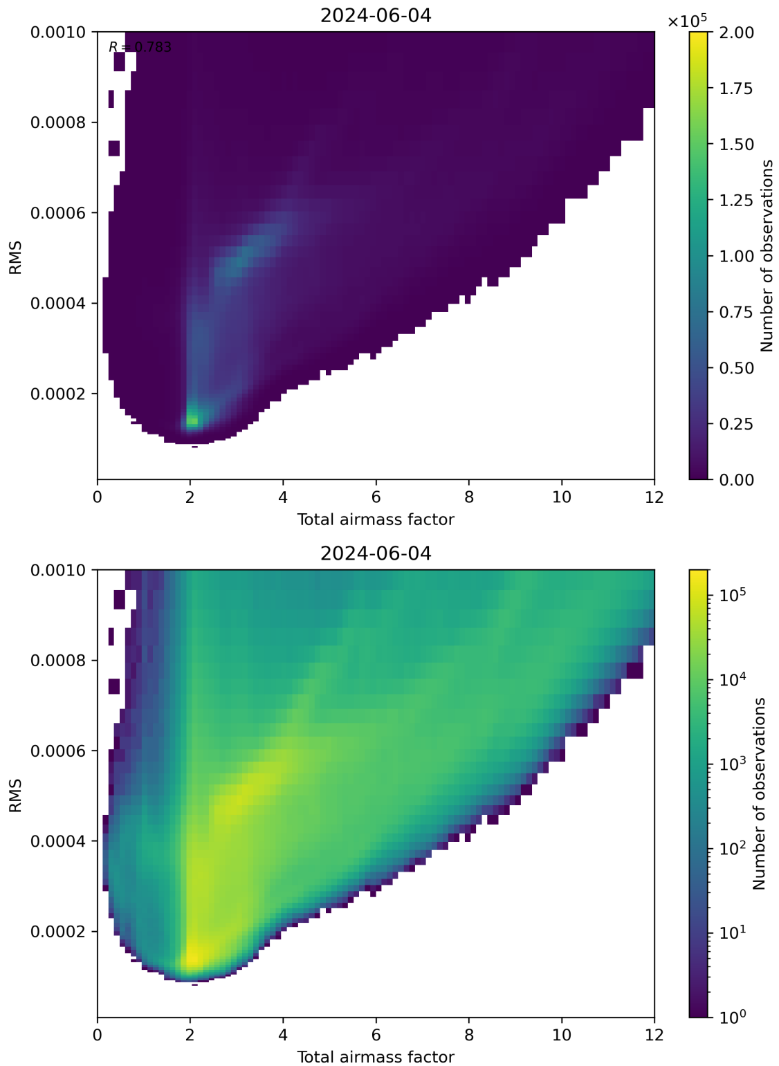
Figure 69: Scatter density plot of “Total airmass factor” against “RMS” for 2024-06-03 to 2024-06-05.
