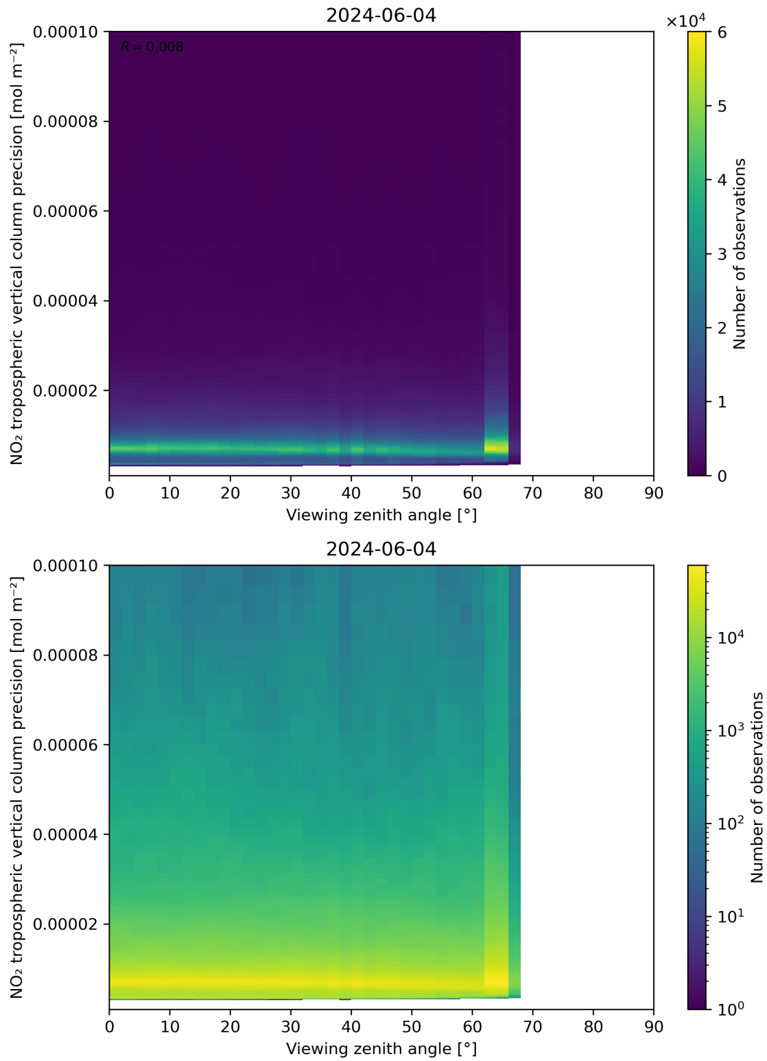
Figure 170: Scatter density plot of “Viewing zenith angle” against “NO 2 tropospheric vertical column precision” for 2024-06-03 to 2024-06-05.
