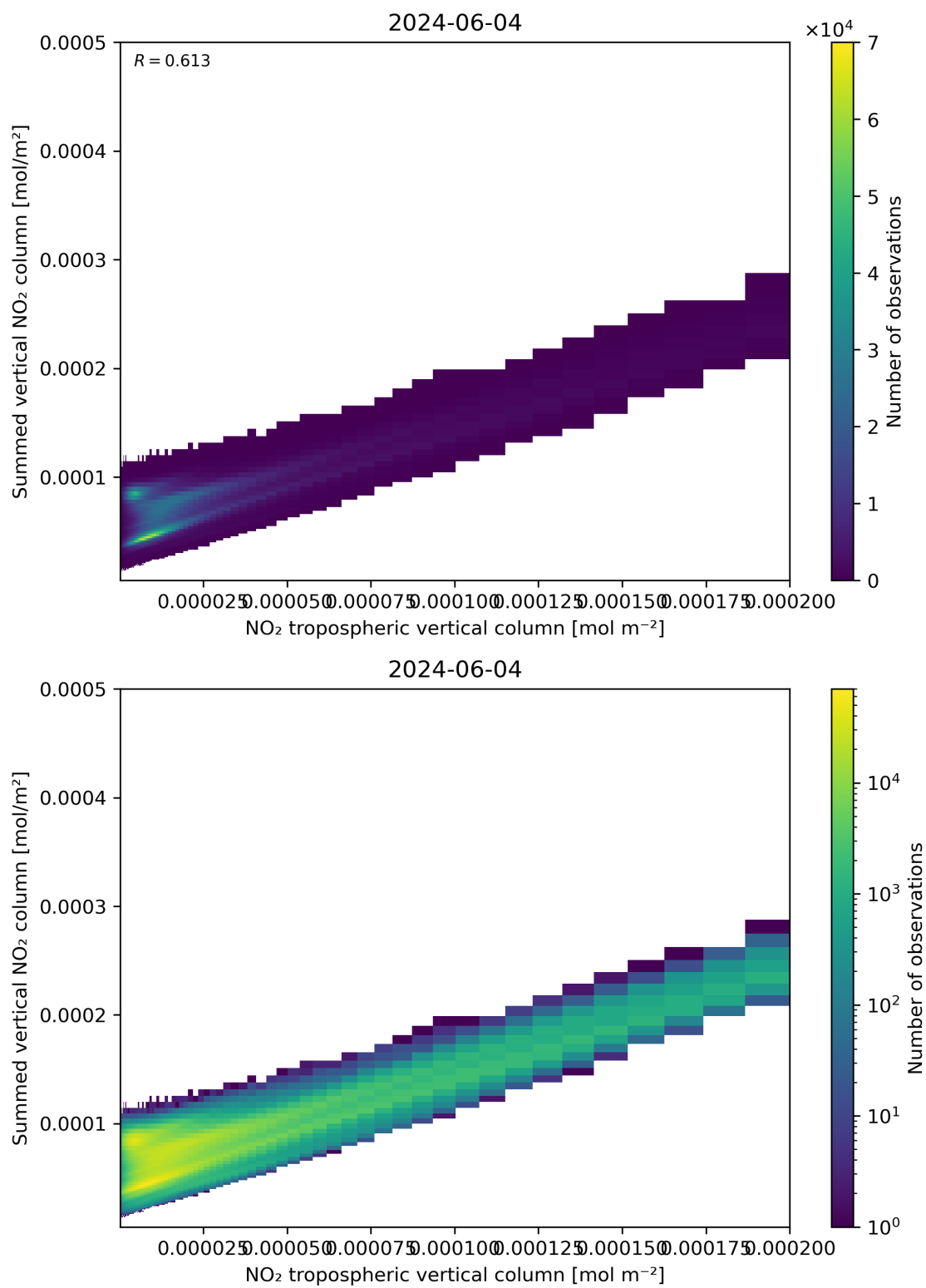
Figure 126: Scatter density plot of “NO 2 tropospheric vertical column” against “Summed vertical NO 2 column” for 2024-06-03 to 2024-06-05.
