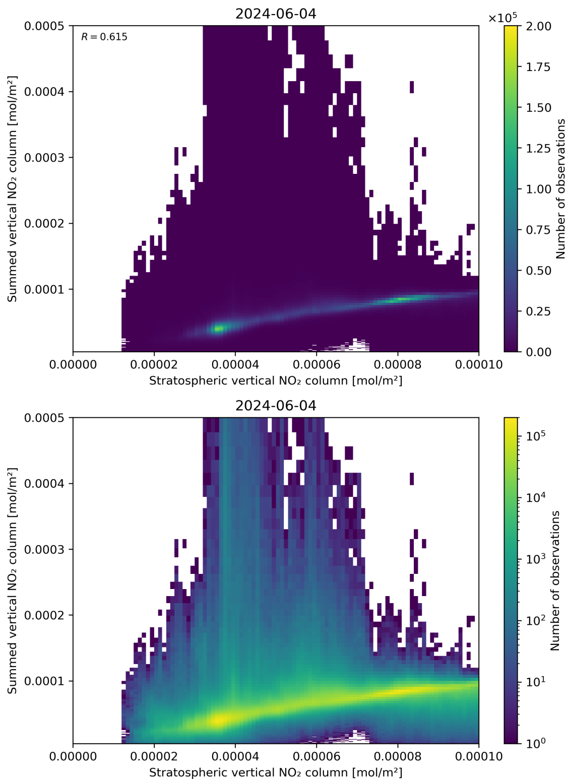
Figure 98: Scatter density plot of “Stratospheric vertical NO 2 column” against “Summed vertical NO 2 column” for 2024-06-03 to 2024-06-05.
