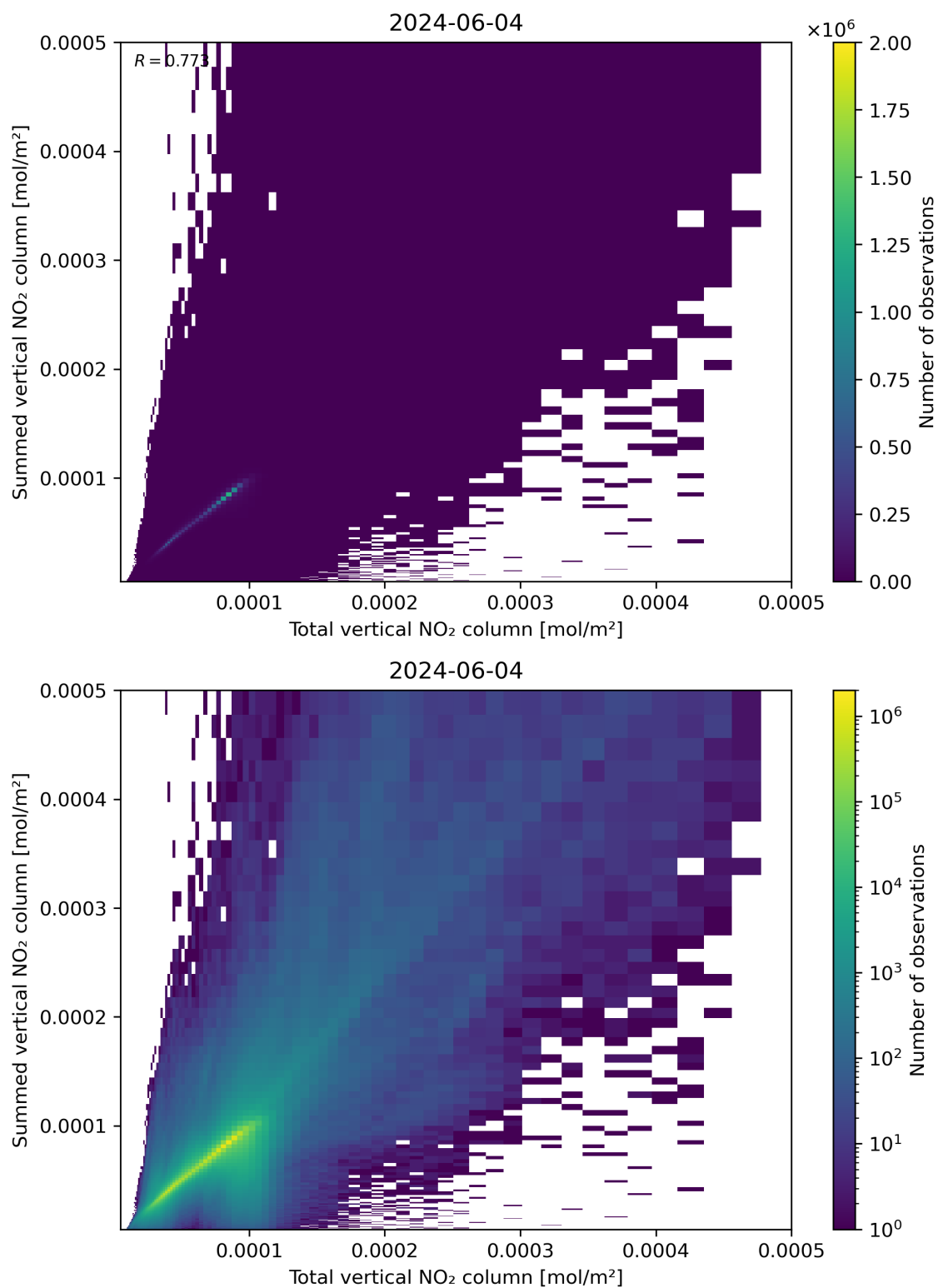
Figure 112: Scatter density plot of “Total vertical NO 2 column” against “Summed vertical NO 2 column” for 2024-06-03 to 2024-06-05.
