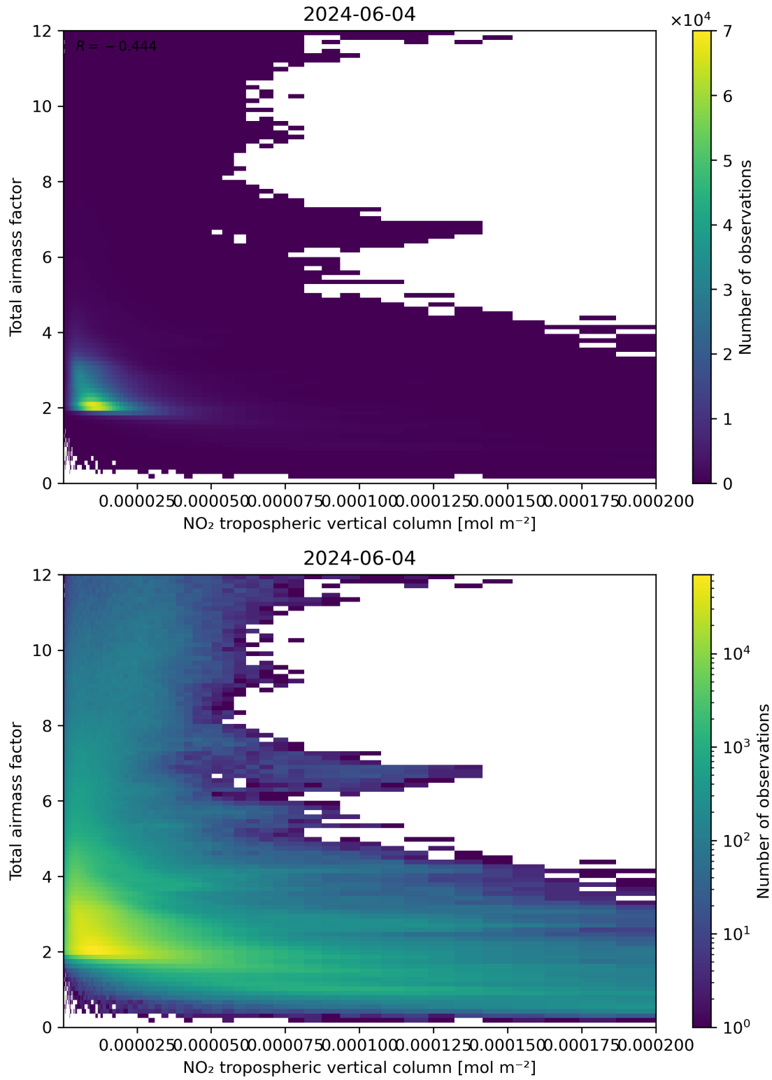
Figure 122: Scatter density plot of “NO 2 tropospheric vertical column” against “Total air mass factor” for 2024-06-03 to 2024-06-05.
