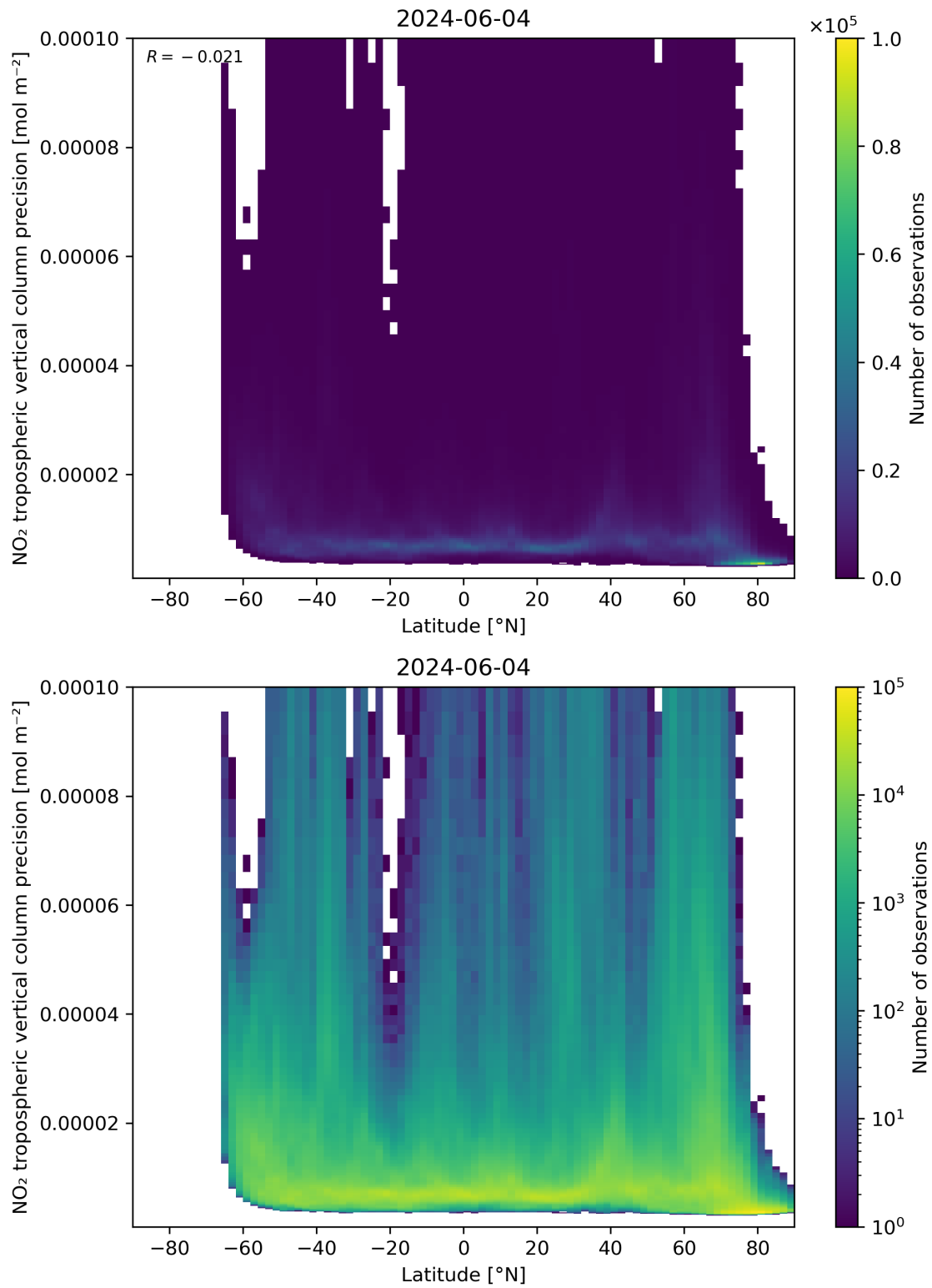
Figure 93: Scatter density plot of “Latitude” against “NO 2 tropospheric vertical column precision” for 2024-06-03 to 2024-06-05.
