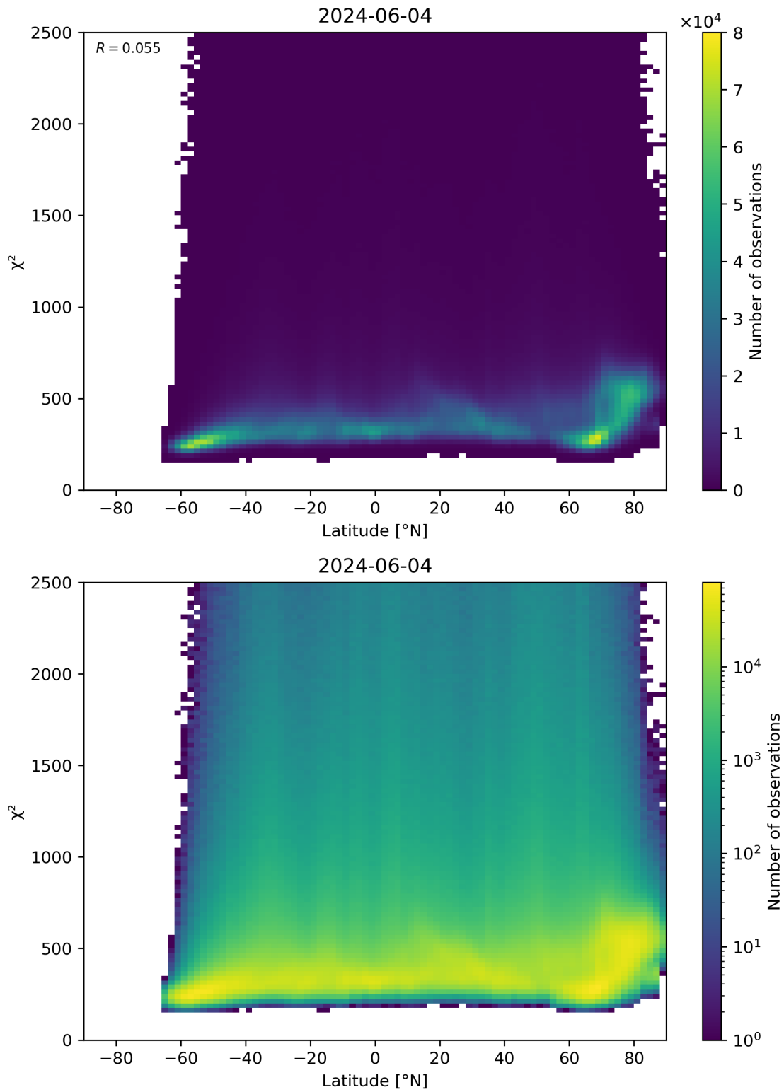
Figure 86: Scatter density plot of “Latitude” against “ \chi^2 ” for 2024-06-03 to 2024-06-05.
