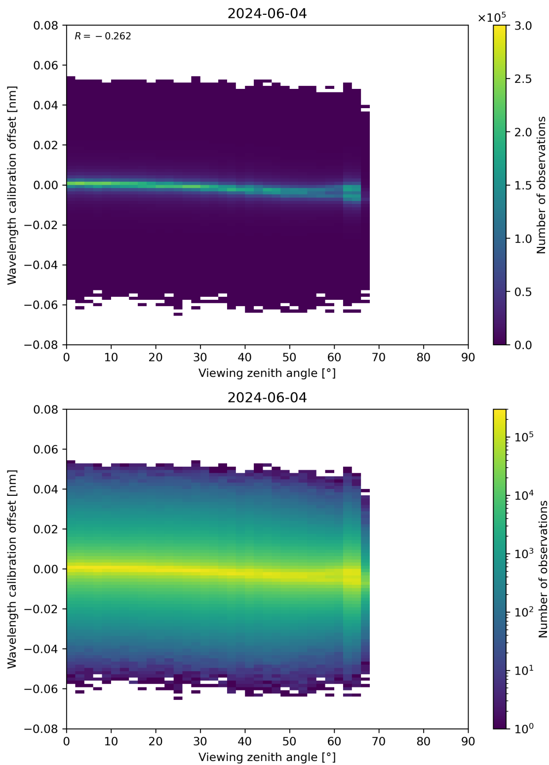
Figure 173: Scatter density plot of “Viewing zenith angle” against “Wavelength calibration offset” for 2024-06-03 to 2024-06-05.
