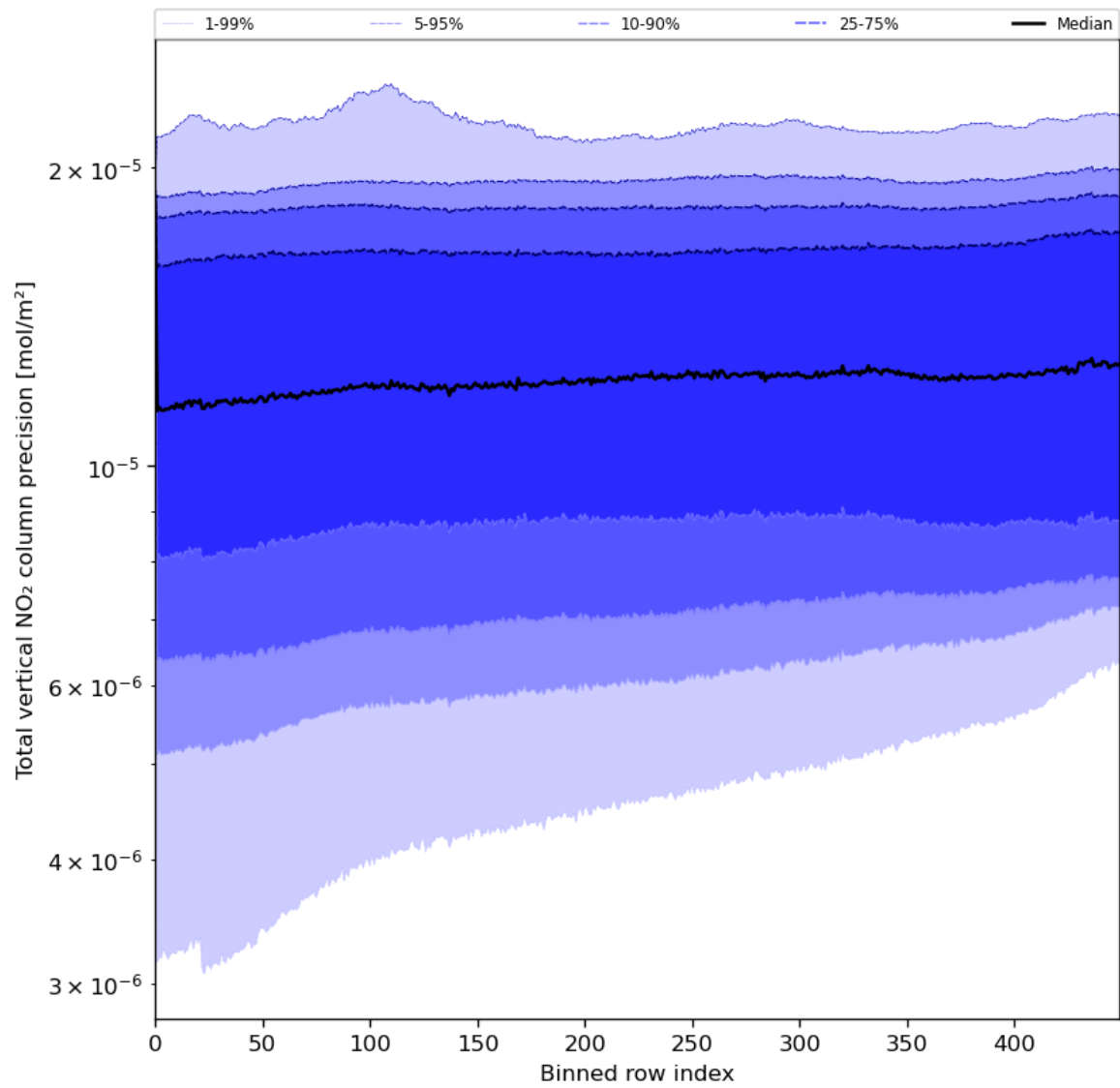
Figure 56: Along track statistics of “Total vertical NO 2 column precision” for 2024-06-03 to 2024-06-05
