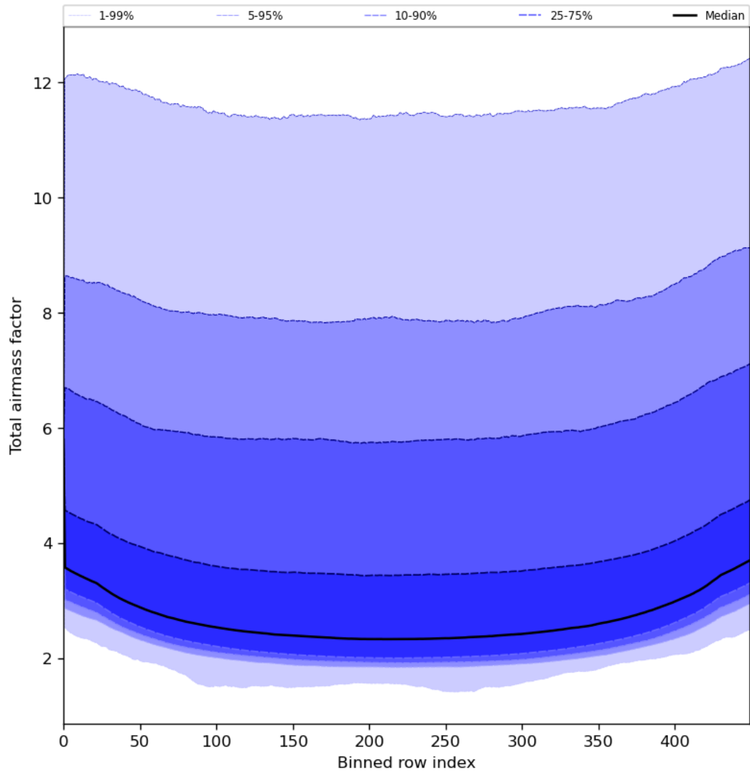
Figure 49: Along track statistics of “Total airmass factor” for 2024-06-03 to 2024-06-05
