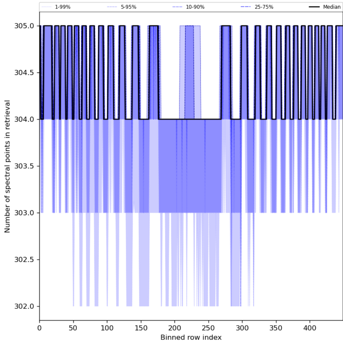
Figure 50: Along track statistics of “Number of spectral points in retrieval” for 2024-06-03 to 2024-06-05
