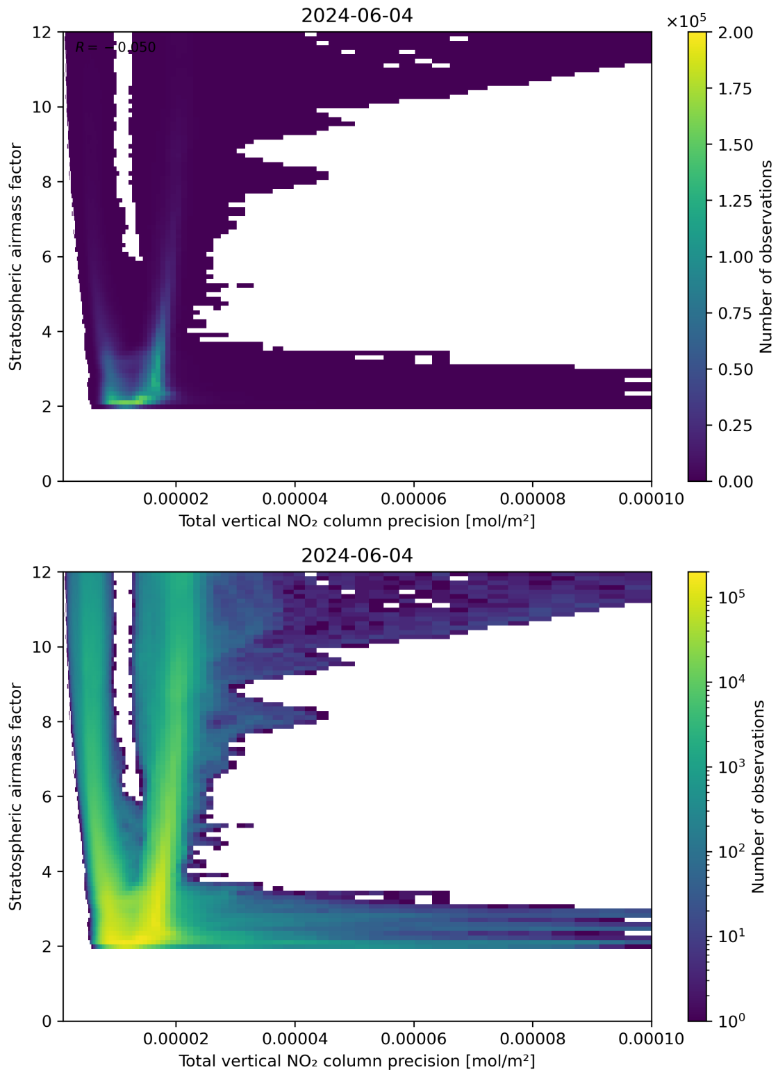
Figure 115: Scatter density plot of “Total vertical NO 2 column precision” against “Stratospheric air mass factor” for 2024-06-03 to 2024-06-05.
