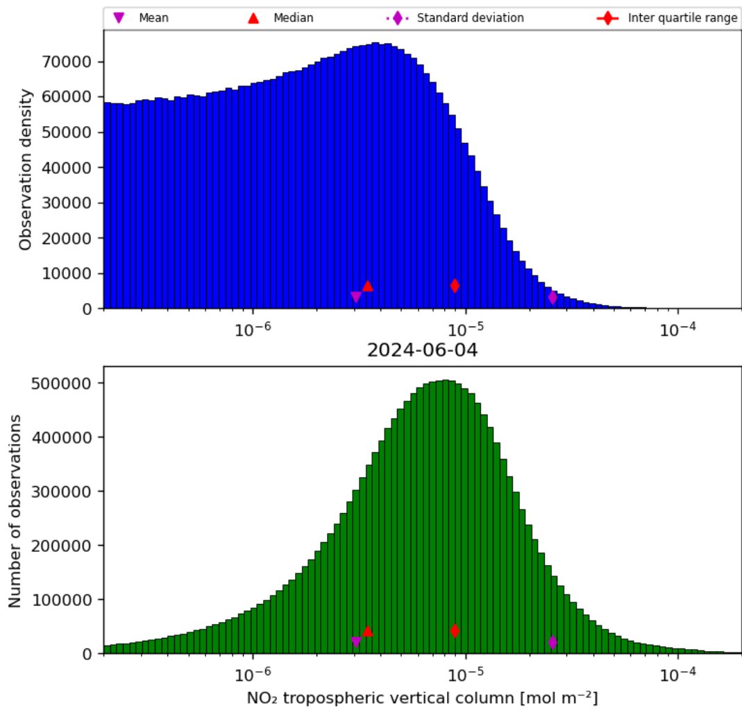
Figure 29: Histogram of “NO 2 tropospheric vertical column” for 2024-06-03 to 2024-06-05
