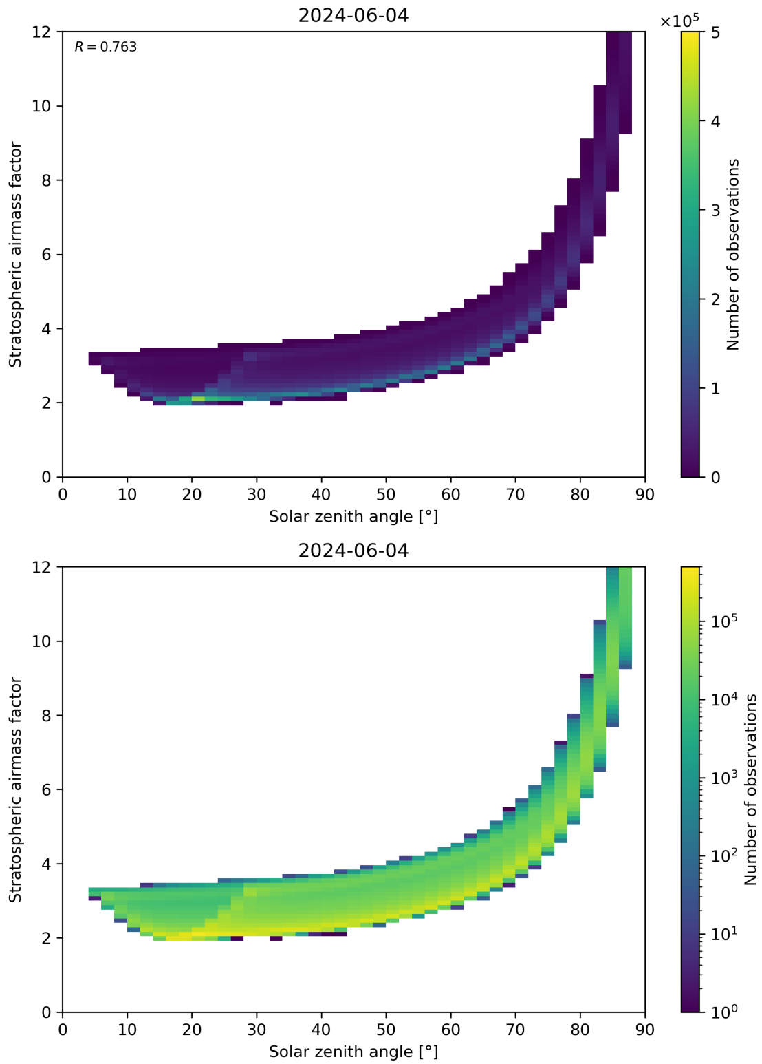
Figure 145: Scatter density plot of “Solar zenith angle” against “Stratospheric airmass factor” for 2024-06-03 to 2024-06-05.
