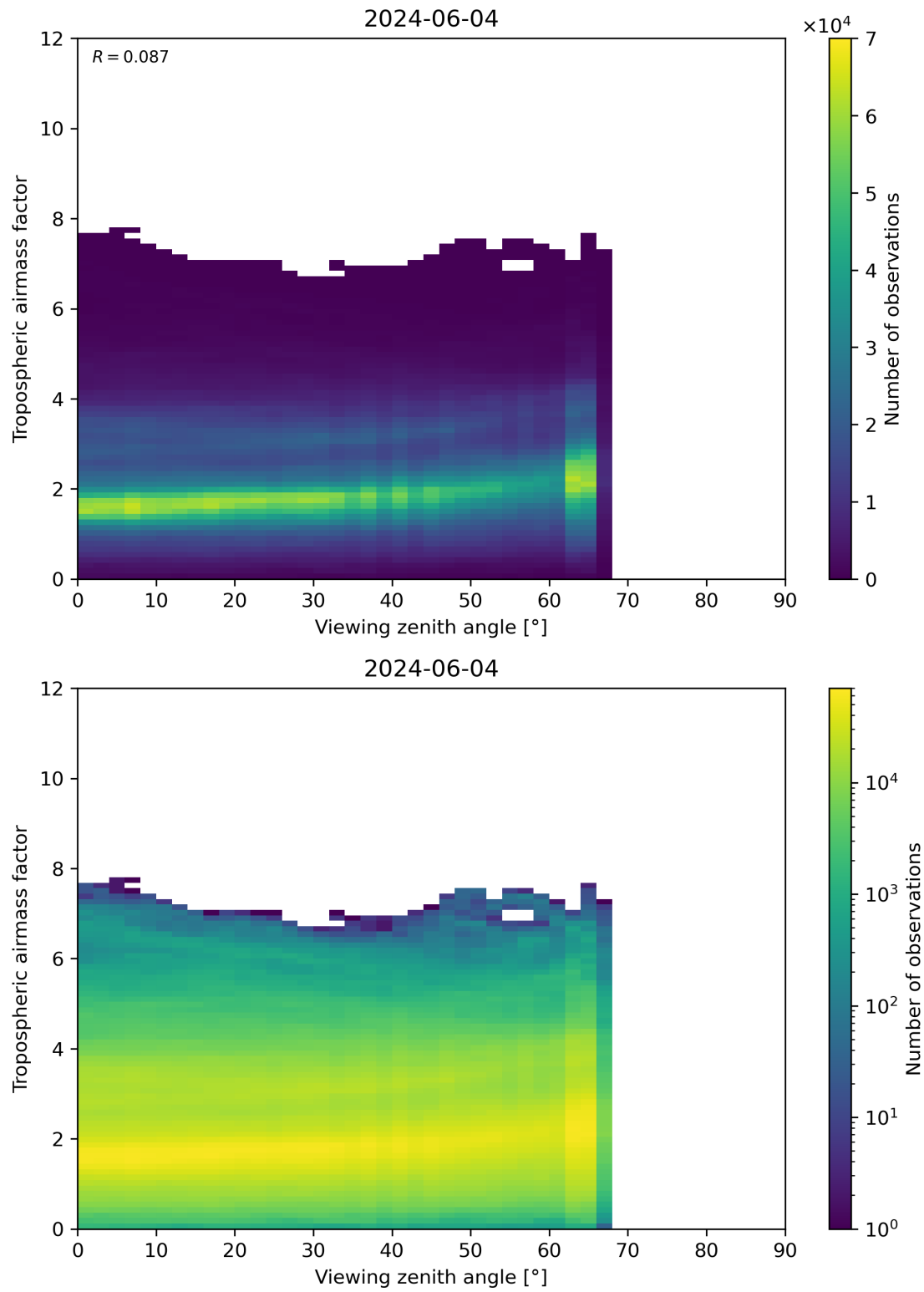
Figure 161: Scatter density plot of “Viewing zenith angle” against “Tropospheric airmass factor” for 2024-06-03 to 2024-06-05.
