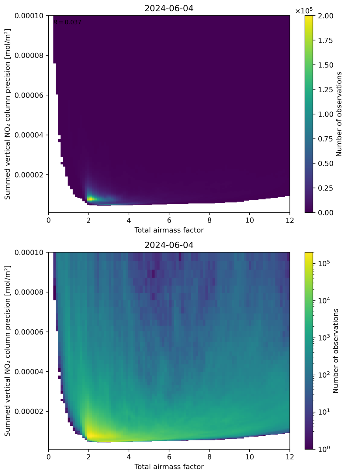
Figure 66: Scatter density plot of “Total airmass factor” against “Summed vertical NO 2 column precision” for 2024-06-03 to 2024-06-05.
