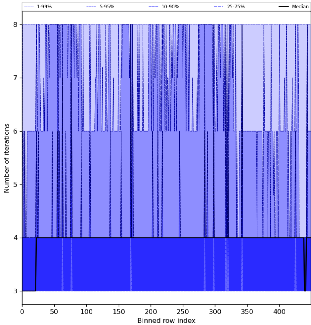
Figure 51: Along track statistics of “Number of iterations” for 2024-06-03 to 2024-06-05
