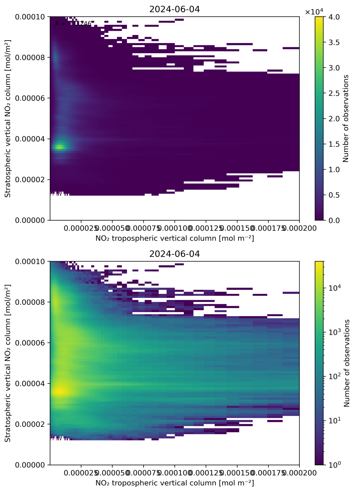
Figure 125: Scatter density plot of “NO 2 tropospheric vertical column” against “Stratospheric vertical NO 2 column” for 2024-06-03 to 2024-06-05.
