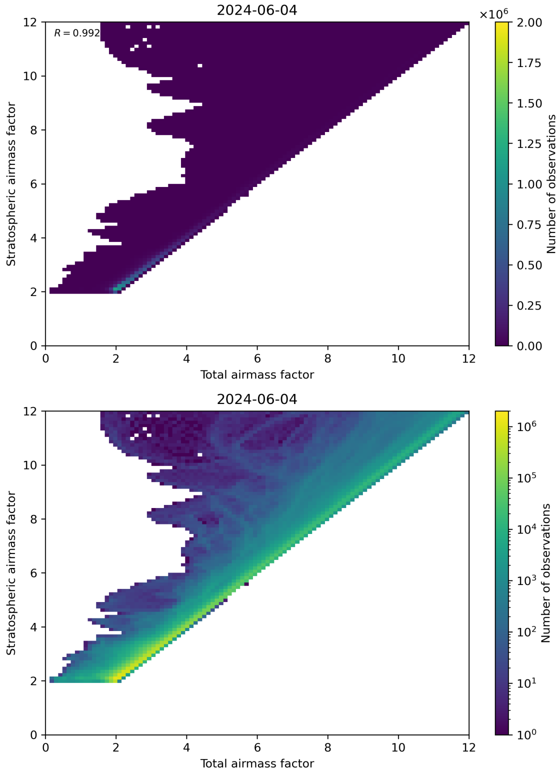
Figure 62: Scatter density plot of “Total airmass factor” against “Stratospheric airmass factor” for 2024-06-03 to 2024-06-05.
