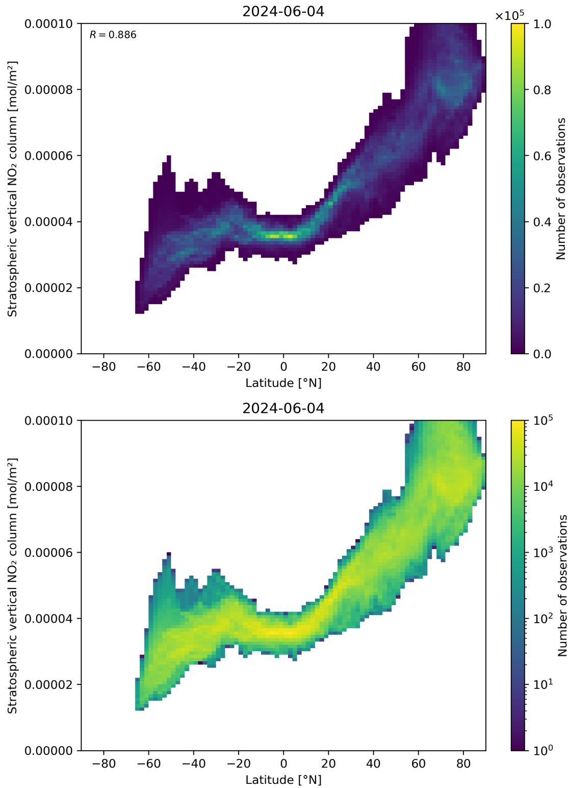
Figure 87: Scatter density plot of “Latitude” against “Stratospheric vertical NO 2 column” for 2024-06-03 to 2024-06-05.
