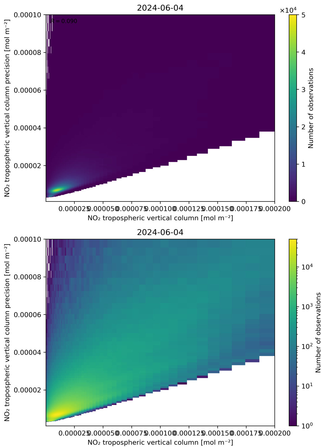
Figure 130: Scatter density plot of “NO 2 tropospheric vertical column” against “NO 2 tropospheric vertical column precision” for 2024-06-03 to 2024-06-05.
