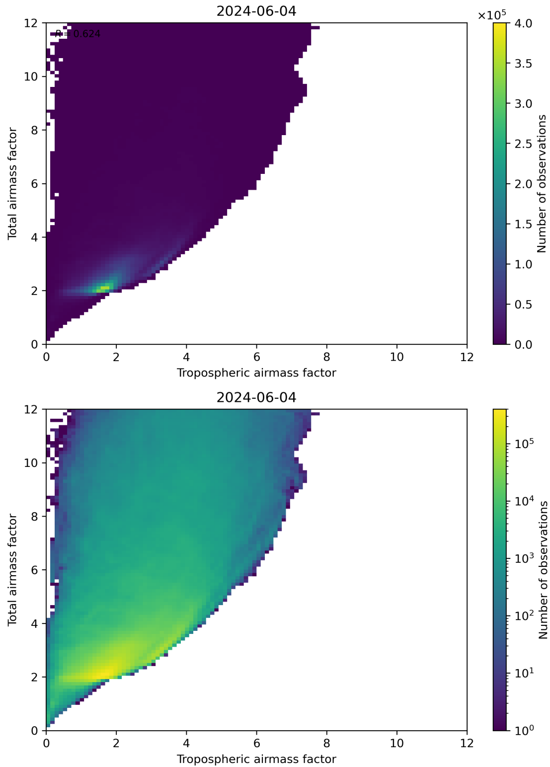
Figure 72: Scatter density plot of “Tropospheric airmass factor” against “Total airmass factor” for 2024-06-03 to 2024-06-05.
