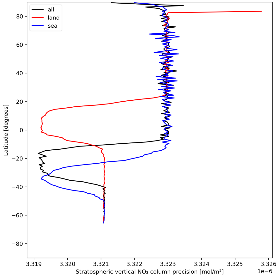
Figure 20: Zonal average of “Stratospheric vertical NO 2 column precision” for 2024-06-03 to 2024-06-05.
