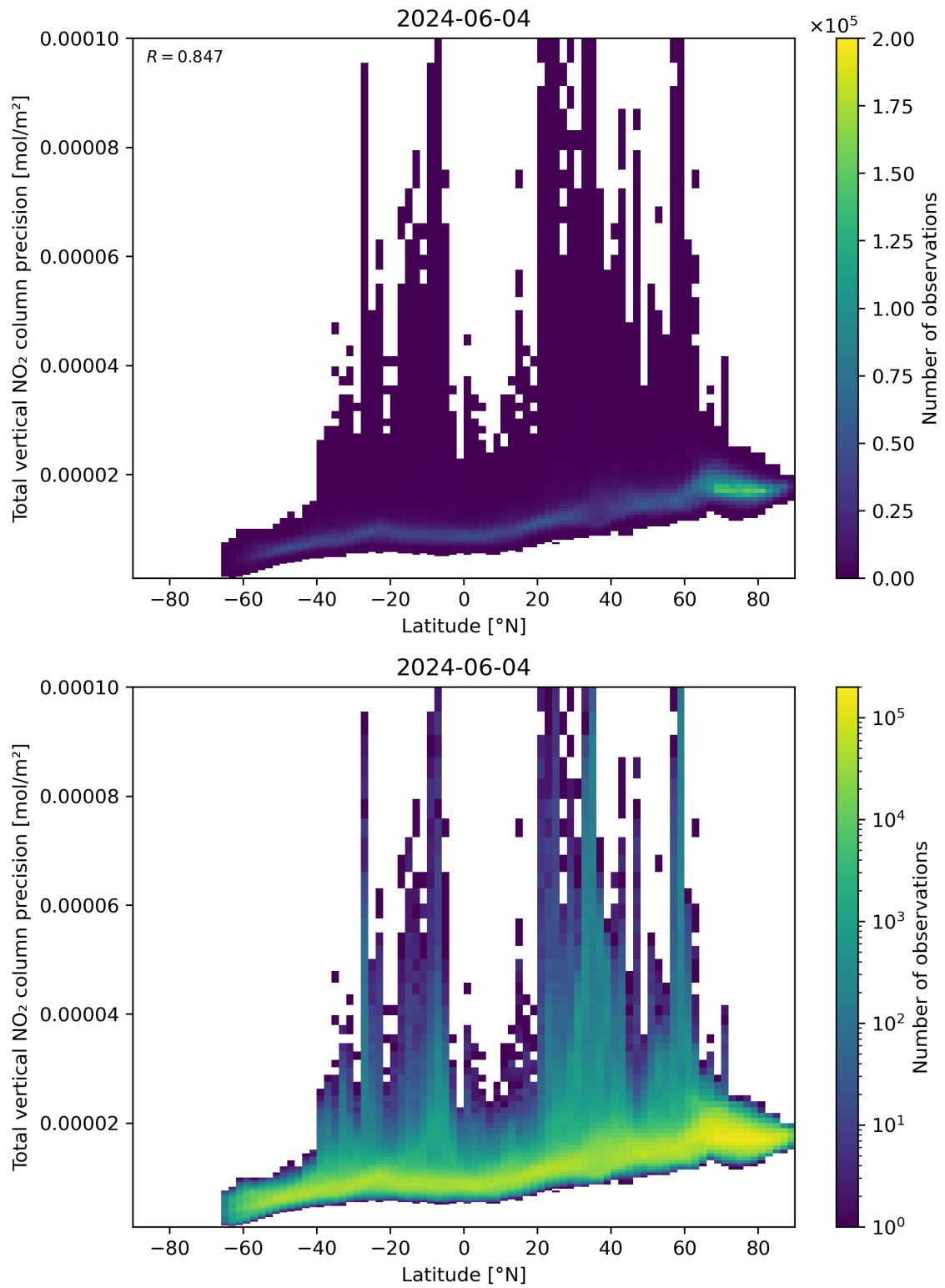
Figure 91: Scatter density plot of “Latitude” against “Total vertical NO 2 column precision” for 2024-06-03 to 2024-06-05.
