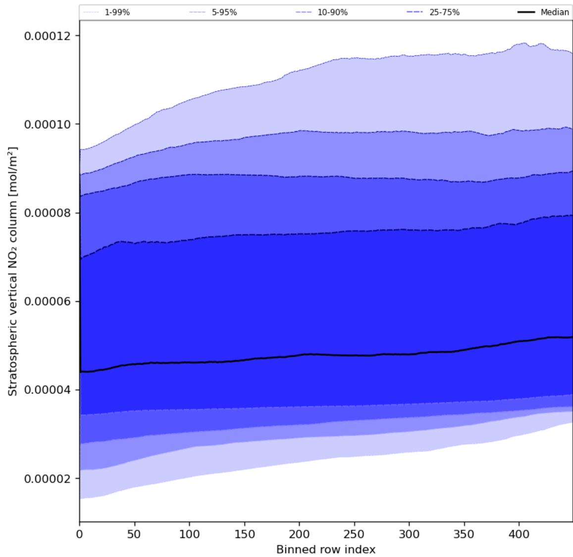
Figure 53: Along track statistics of “Stratospheric vertical NO 2 column” for 2024-06-03 to 2024-06-05
