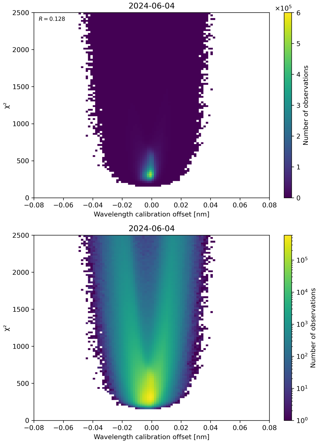
Figure 175: Scatter density plot of “Wavelength calibration offset” against “ \chi^2 ” for 2024-06-03 to 2024-06-05.
