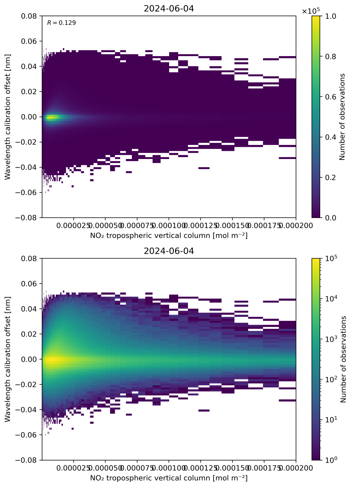
Figure 143: Scatter density plot of “NO 2 tropospheric vertical column” against “Wavelength calibration offset” for 2024-06-03 to 2024-06-05.
