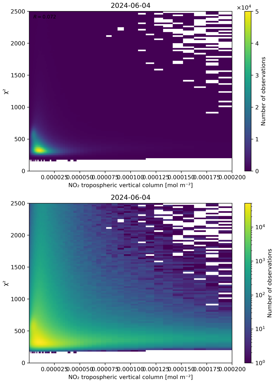
Figure 124: Scatter density plot of “NO 2 tropospheric vertical column” against “ \chi^2 ” for 2024-06-03 to 2024-06-05.
