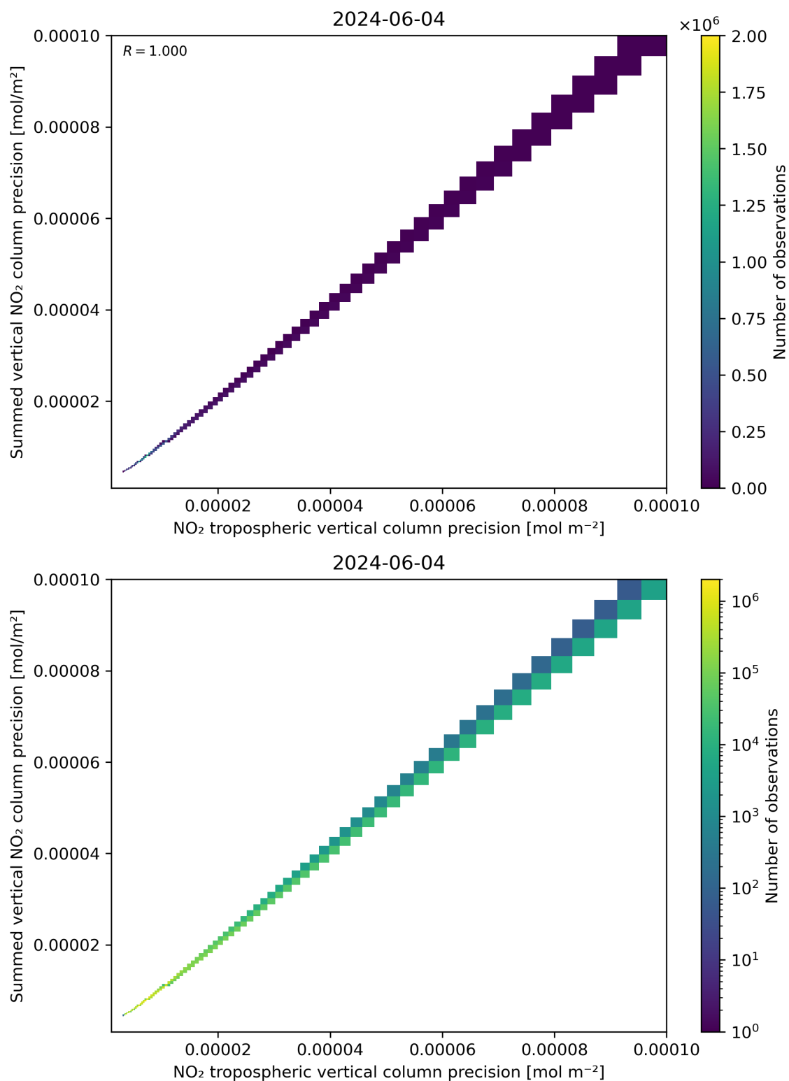
Figure 137: Scatter density plot of “NO 2 tropospheric vertical column precision” against “Summed vertical NO 2 column precision” for 2024-06-03 to 2024-06-05.
