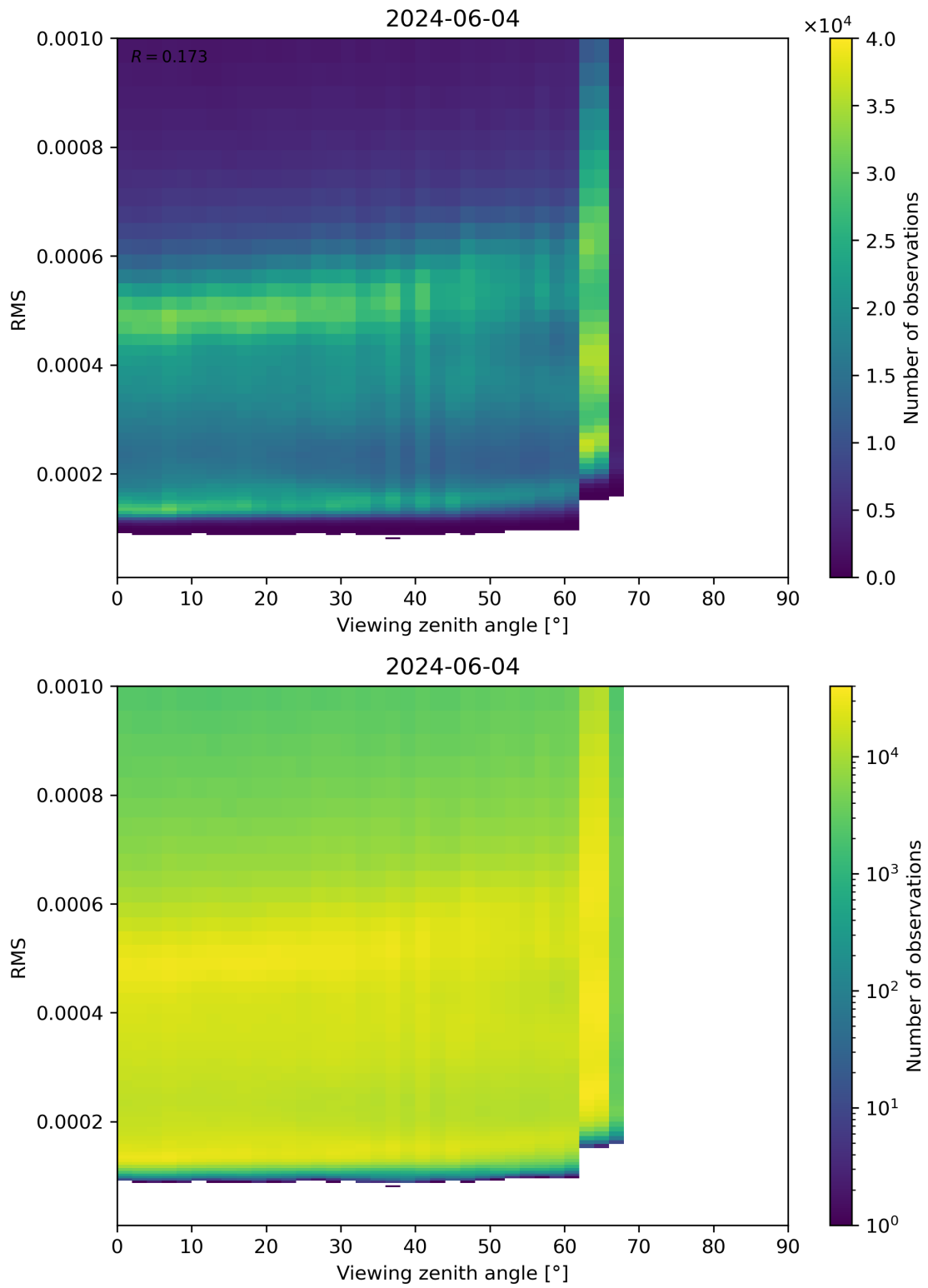
Figure 171: Scatter density plot of “Viewing zenith angle” against “RMS” for 2024-06-03 to 2024-06-05.
