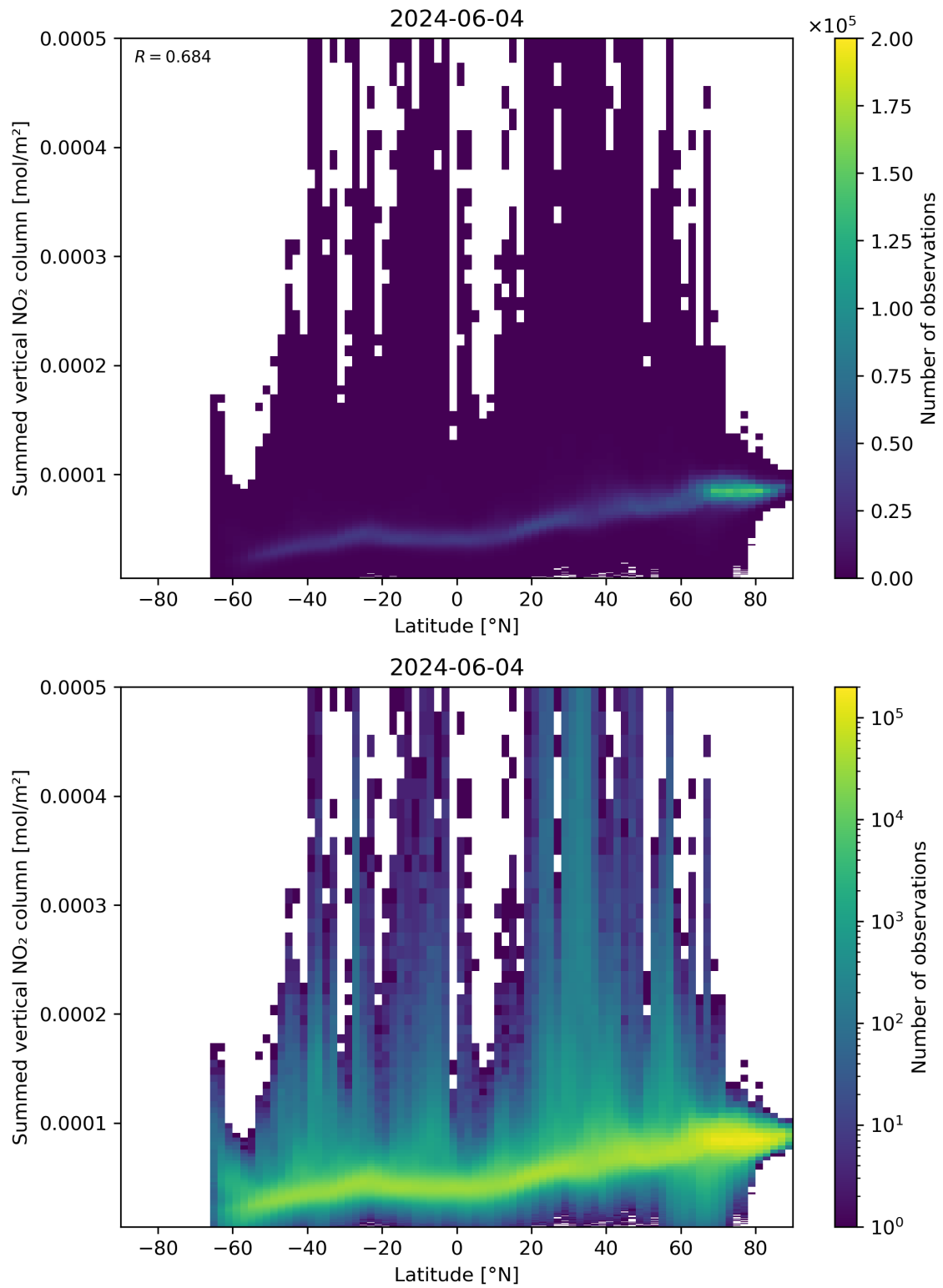
Figure 88: Scatter density plot of “Latitude” against “Summed vertical NO 2 column” for 2024-06-03 to 2024-06-05.
