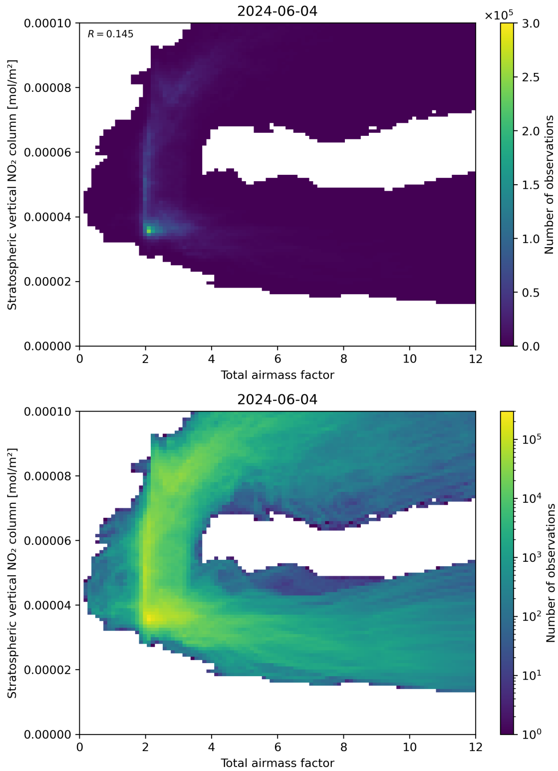
Figure 64: Scatter density plot of “Total airmass factor” against “Stratospheric vertical NO 2 column” for 2024-06-03 to 2024-06-05.
