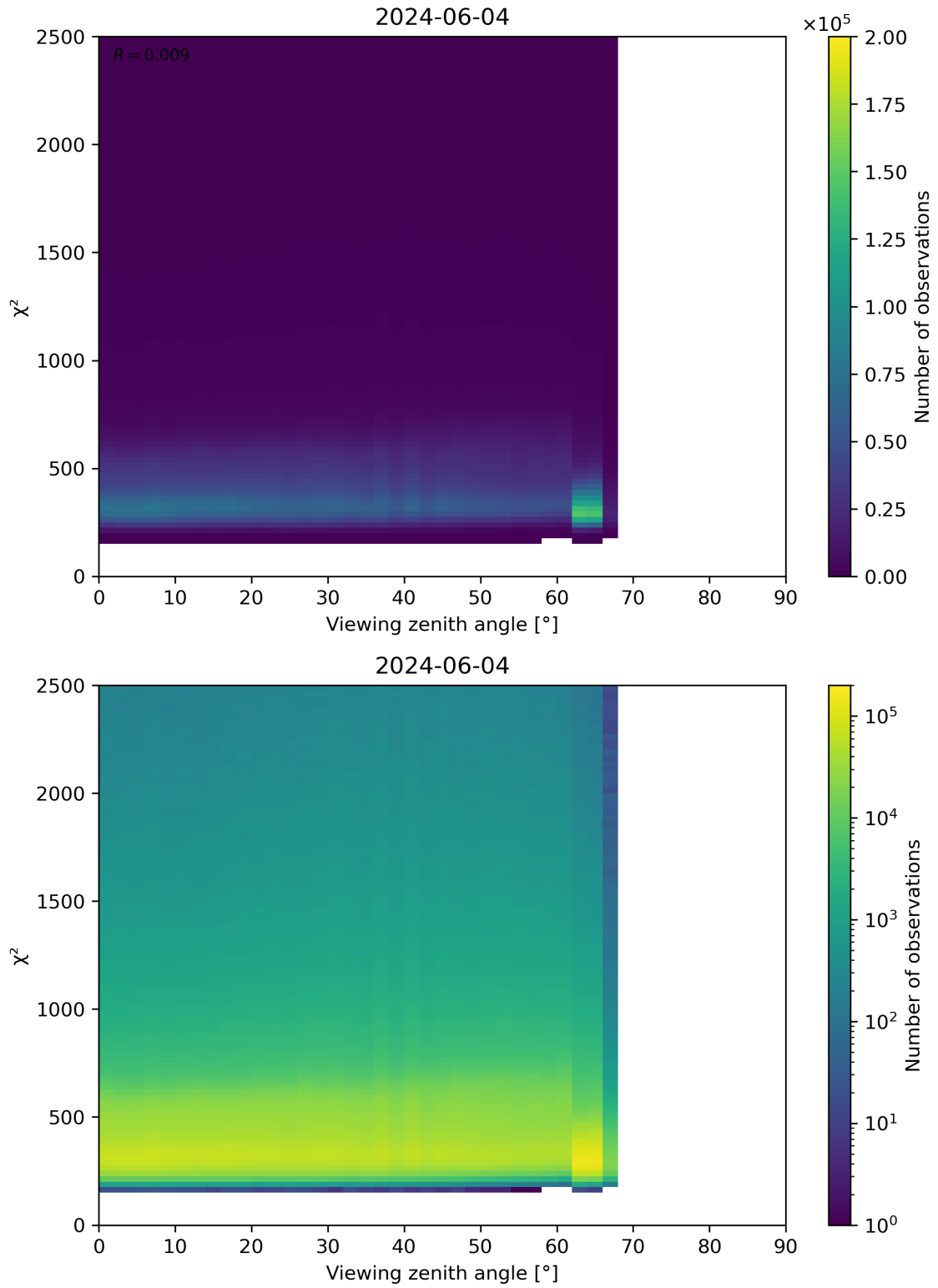
Figure 162: Scatter density plot of “Viewing zenith angle” against “ \chi^2 ” for 2024-06-03 to 2024-06-05.
