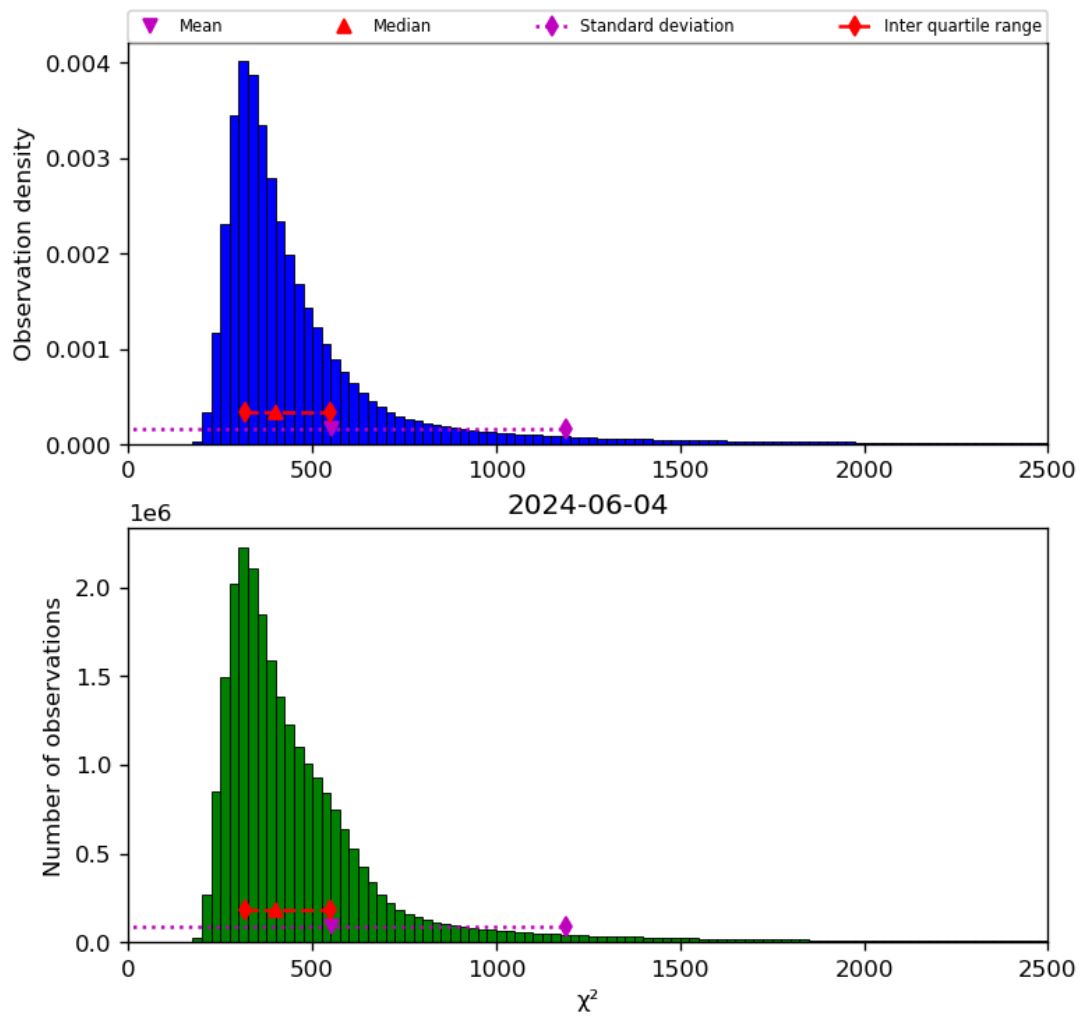
Figure 42: Histogram of “ \chi^2 ” for 2024-06-03 to 2024-06-05
