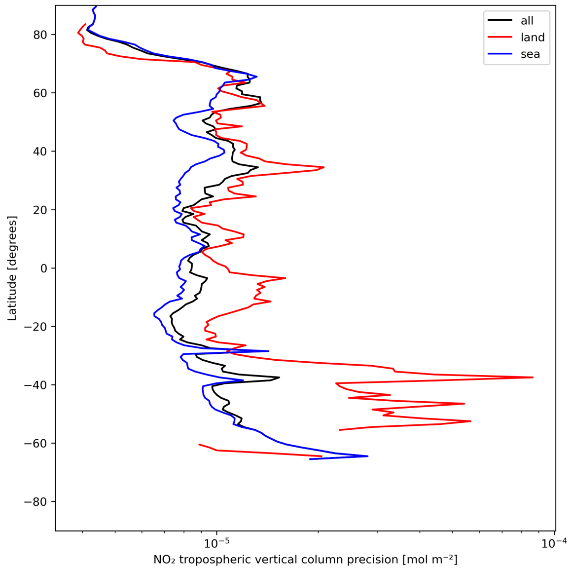
Figure 13: Zonal average of “NO 2 tropospheric vertical column precision” for 2024-06-03 to 2024-06-05.
