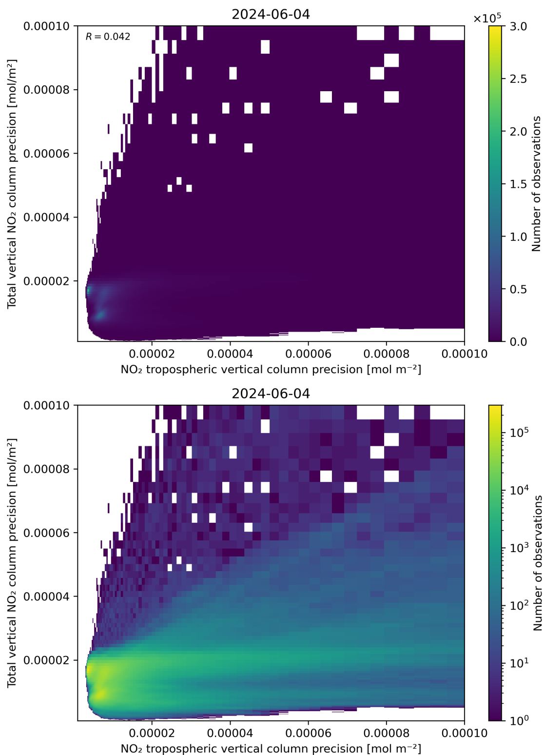
Figure 139: Scatter density plot of “NO 2 tropospheric vertical column precision” against “Total vertical NO 2 column precision” for 2024-06-03 to 2024-06-05.
