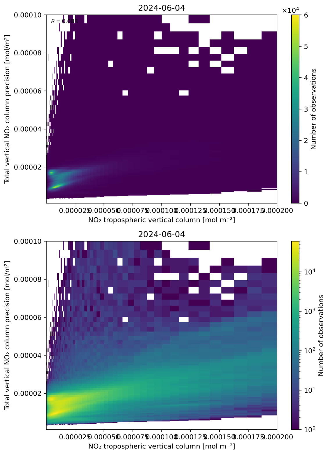
Figure 129: Scatter density plot of “NO 2 tropospheric vertical column” against “Total vertical NO 2 column precision” for 2024-06-03 to 2024-06-05.
