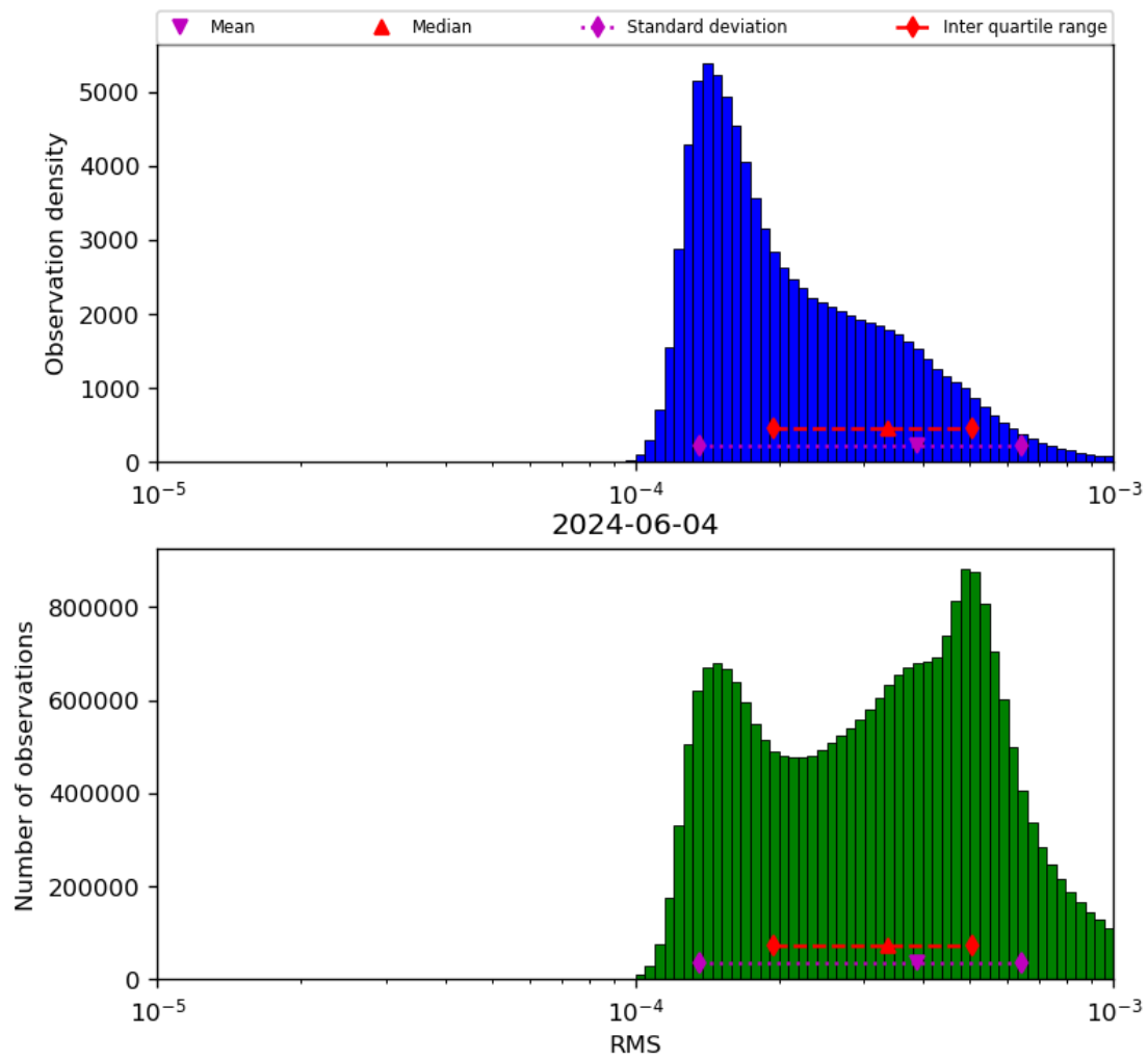
Figure 43: Histogram of “RMS” for 2024-06-03 to 2024-06-05
