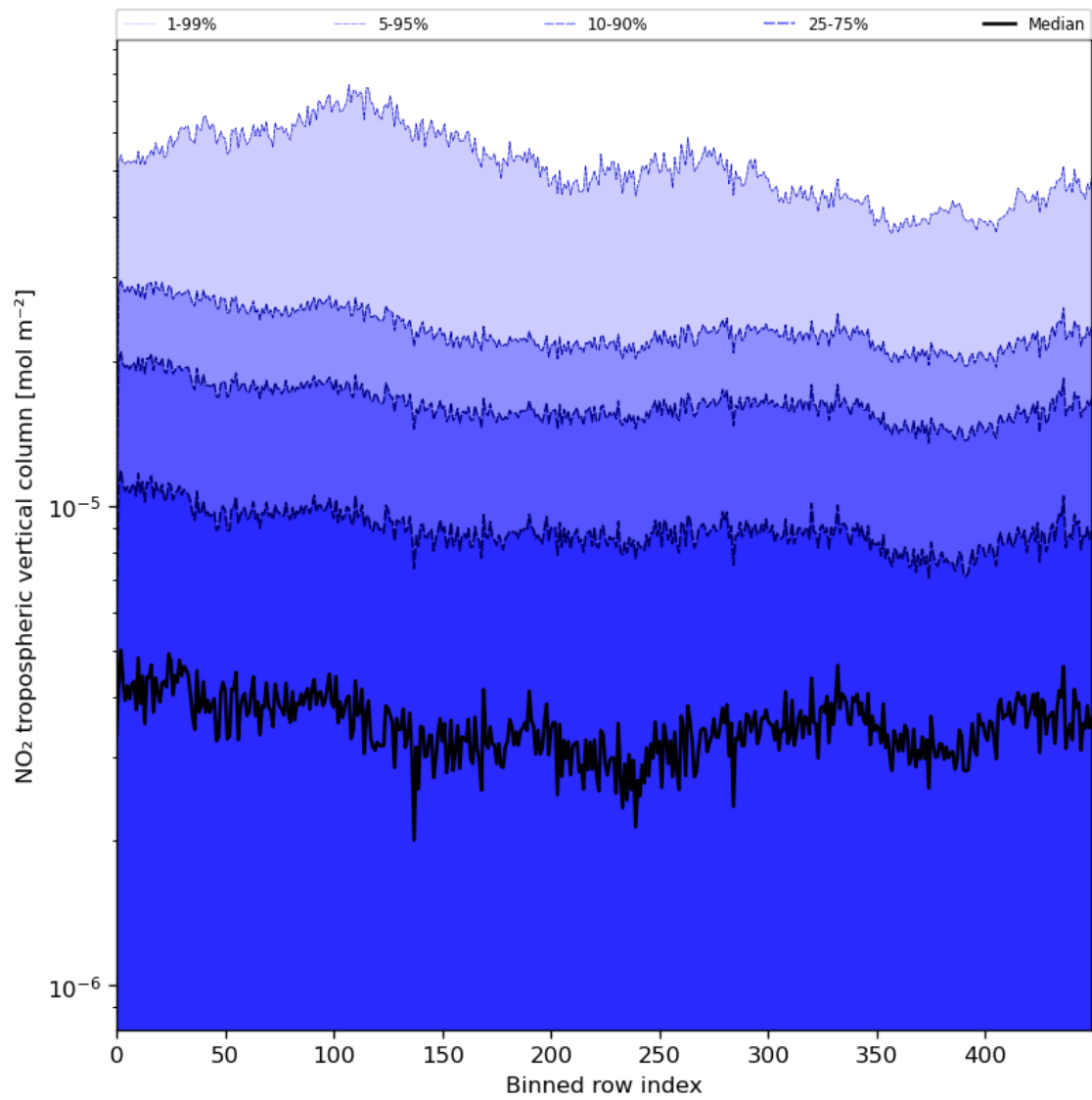
Figure 46: Along track statistics of “NO 2 tropospheric vertical column” for 2024-06-03 to 2024-06-05
