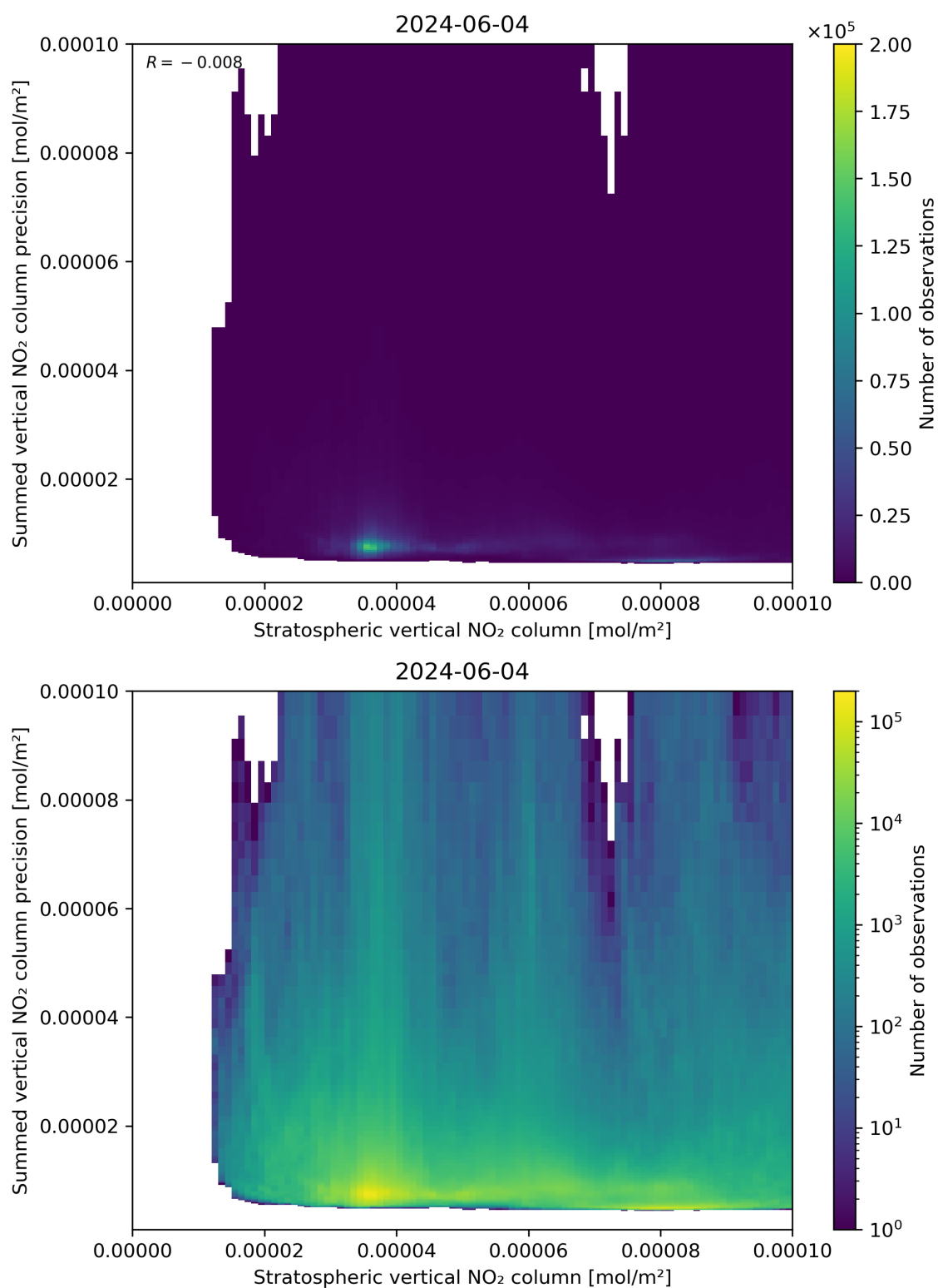
Figure 99: Scatter density plot of “Stratospheric vertical NO 2 column” against “Summed vertical NO 2 column precision” for 2024-06-03 to 2024-06-05.
