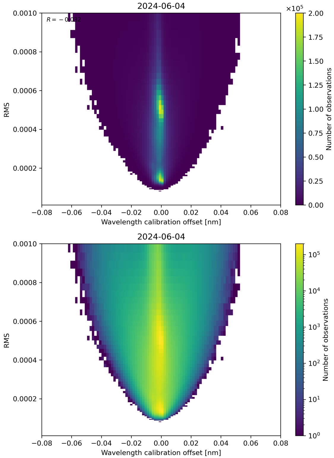
Figure 181: Scatter density plot of “Wavelength calibration offset” against “RMS” for 2024-06-03 to 2024-06-05.
