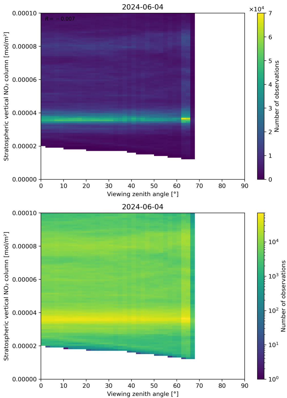
Figure 164: Scatter density plot of “Viewing zenith angle” against “Stratospheric vertical NO 2 column” for 2024-06-03 to 2024-06-05.
