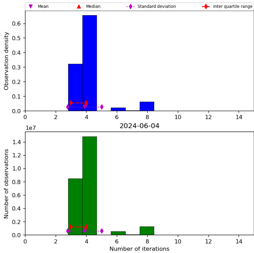
Figure 34: Histogram of “Number of iterations” for 2024-06-03 to 2024-06-05
