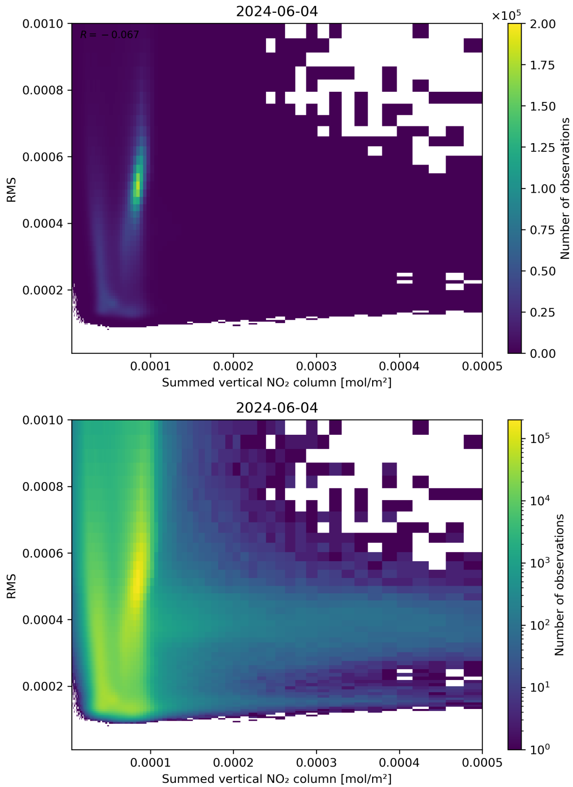
Figure 109: Scatter density plot of “Summed vertical NO 2 column” against “RMS” for 2024-06-03 to 2024-06-05.
