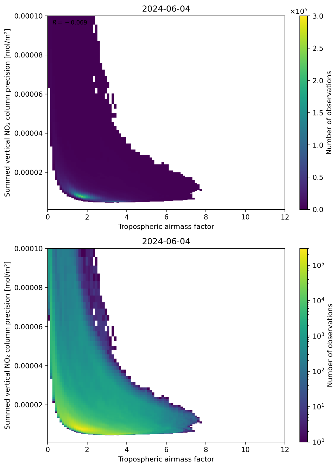
Figure 76: Scatter density plot of “Tropospheric air mass factor” against “Summed vertical NO 2 column precision” for 2024-06-03 to 2024-06-05.
