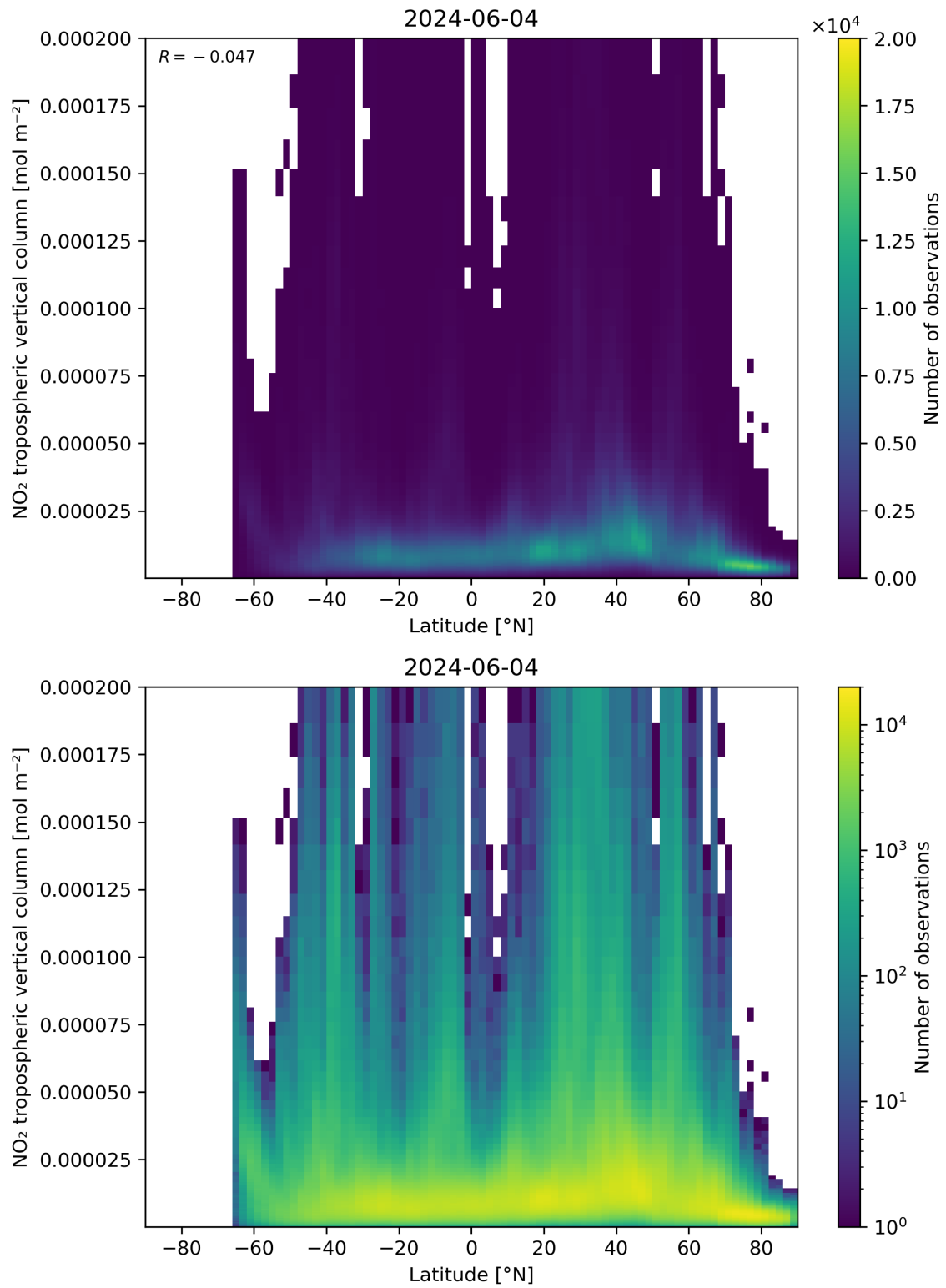
Figure 92: Scatter density plot of “Latitude” against “NO 2 tropospheric vertical column” for 2024-06-03 to 2024-06-05.
