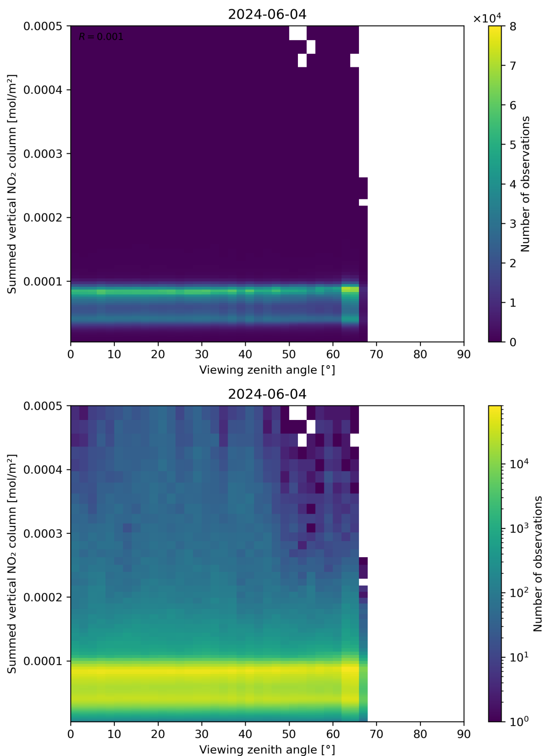
Figure 165: Scatter density plot of “Viewing zenith angle” against “Summed vertical NO 2 column” for 2024-06-03 to 2024-06-05.
