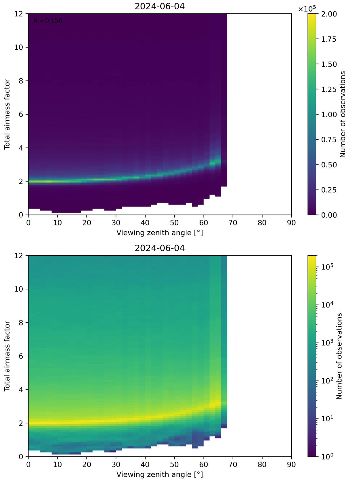
Figure 160: Scatter density plot of “Viewing zenith angle” against “Total airmass factor” for 2024-06-03 to 2024-06-05.
