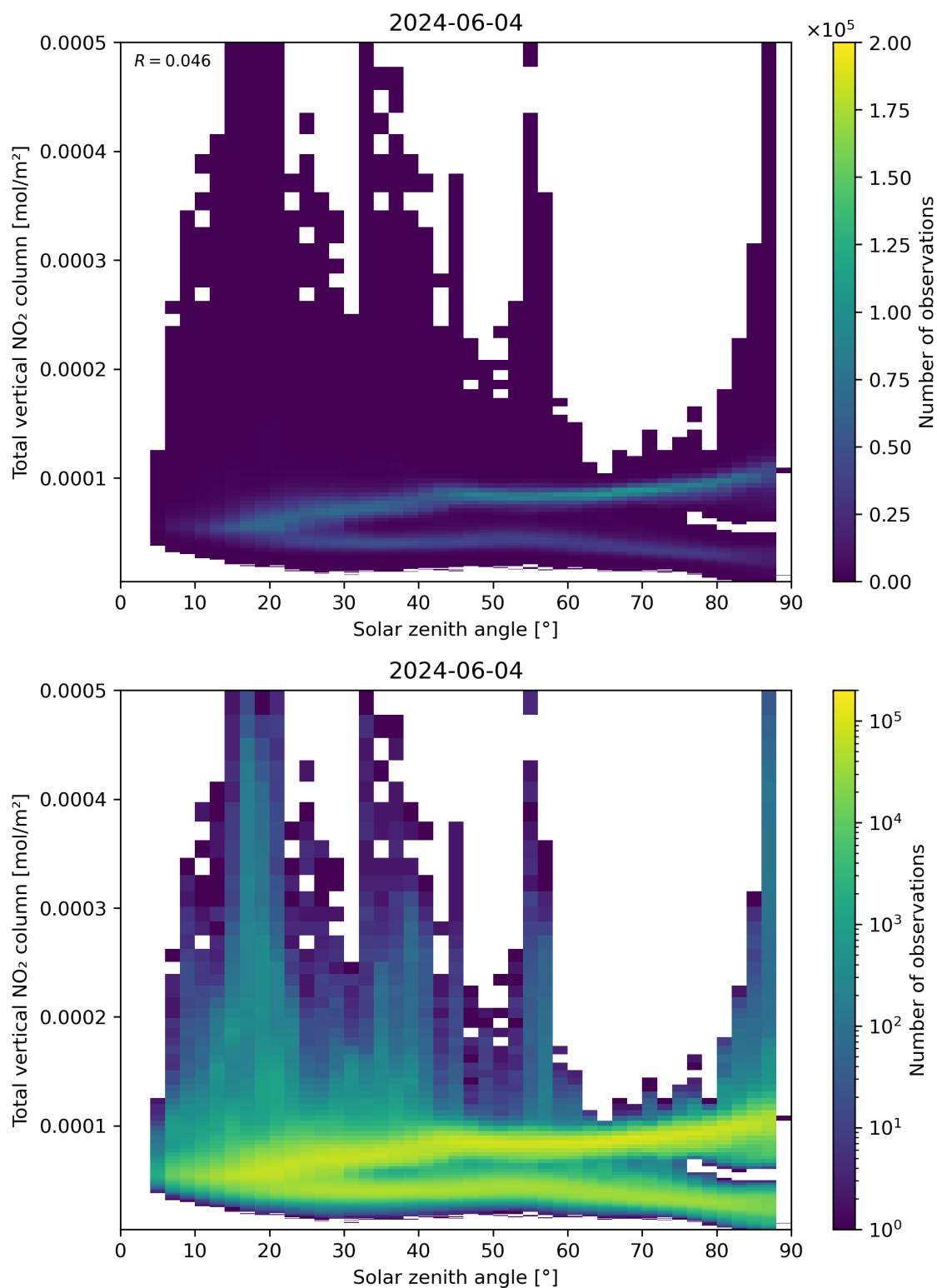
Figure 153: Scatter density plot of “Solar zenith angle” against “Total vertical NO 2 column” for 2024-06-03 to 2024-06-05.
