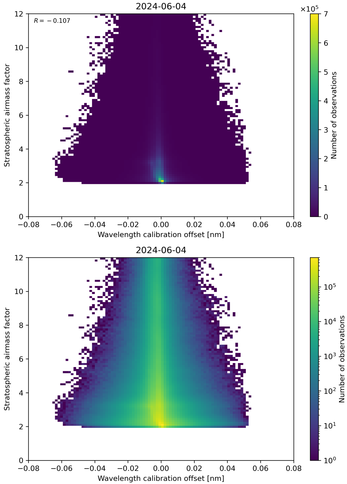
Figure 174: Scatter density plot of “Wavelength calibration offset” against “Stratospheric air mass factor” for 2024-06-03 to 2024-06-05.
