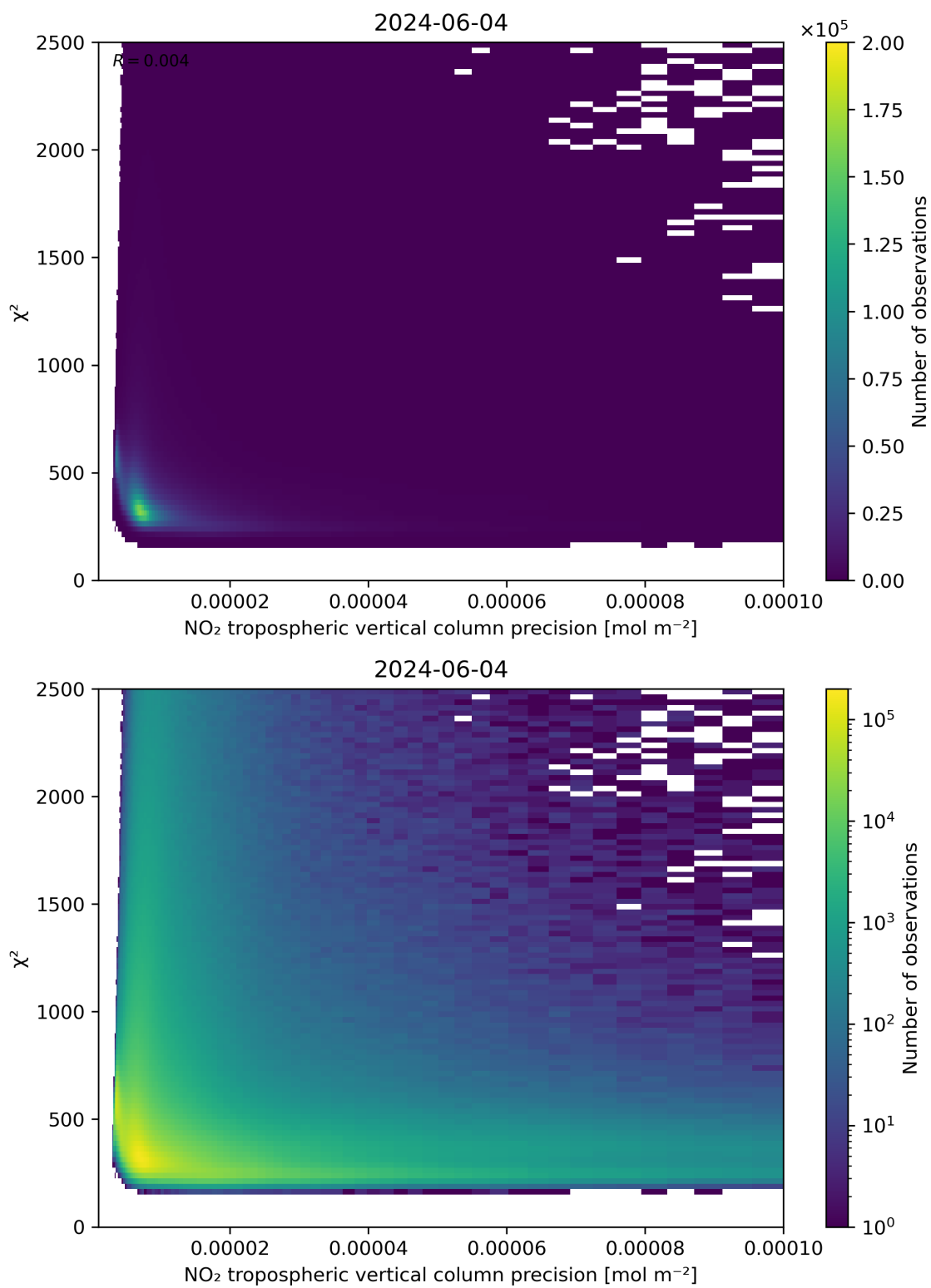
Figure 134: Scatter density plot of “NO 2 tropospheric vertical column precision” against “ \chi^2 ” for 2024-06-03 to 2024-06-05.
