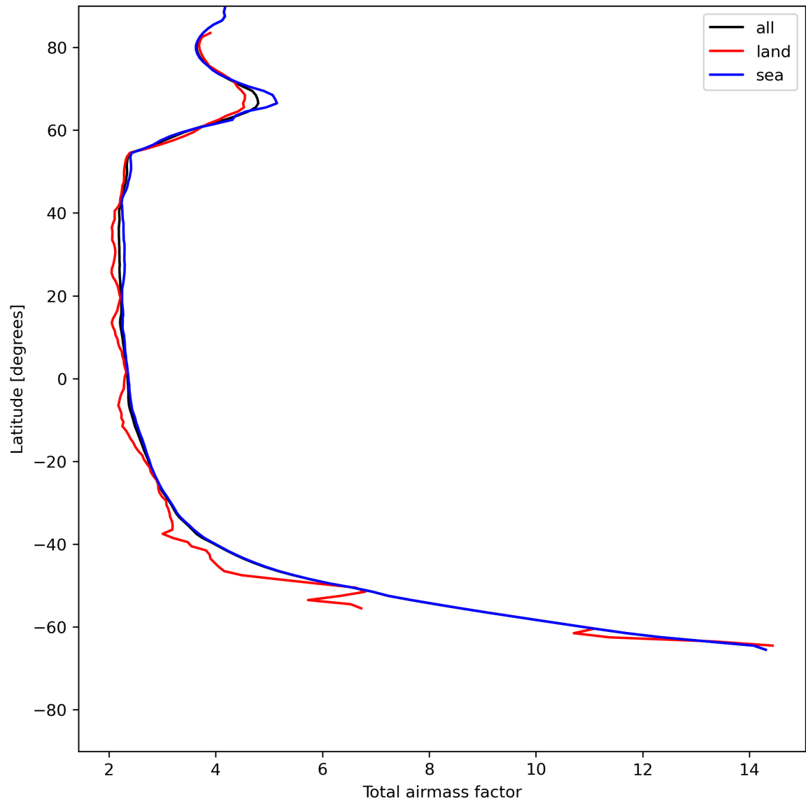
Figure 15: Zonal average of “Total airmass factor” for 2024-06-03 to 2024-06-05.
