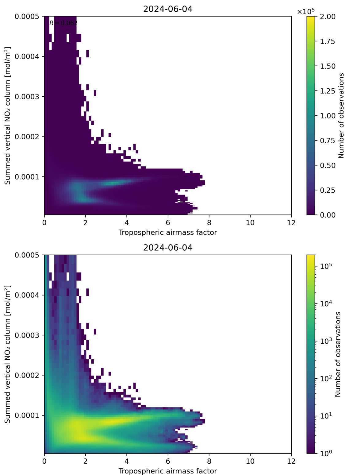
Figure 75: Scatter density plot of “Tropospheric airmass factor” against “Summed vertical NO 2 column” for 2024-06-03 to 2024-06-05.
