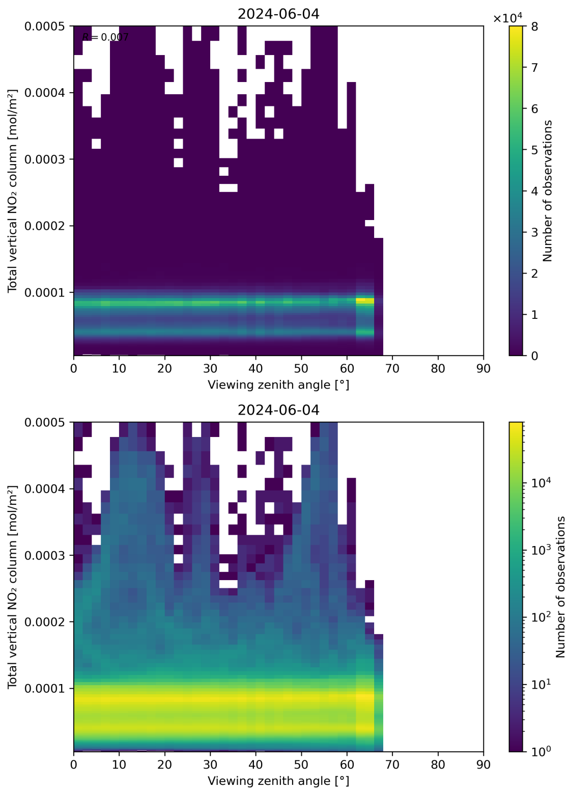
Figure 167: Scatter density plot of “Viewing zenith angle” against “Total vertical NO 2 column” for 2024-06-03 to 2024-06-05.
