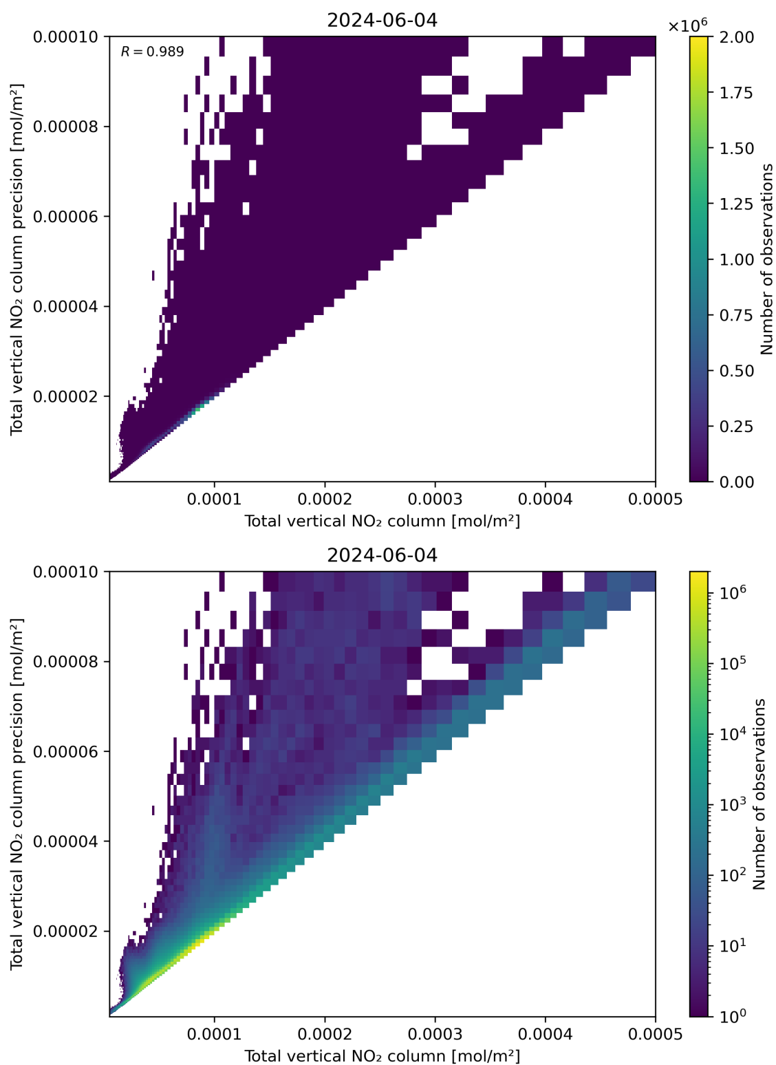
Figure 114: Scatter density plot of “Total vertical NO 2 column” against “Total vertical NO 2 column precision” for 2024-06-03 to 2024-06-05.
