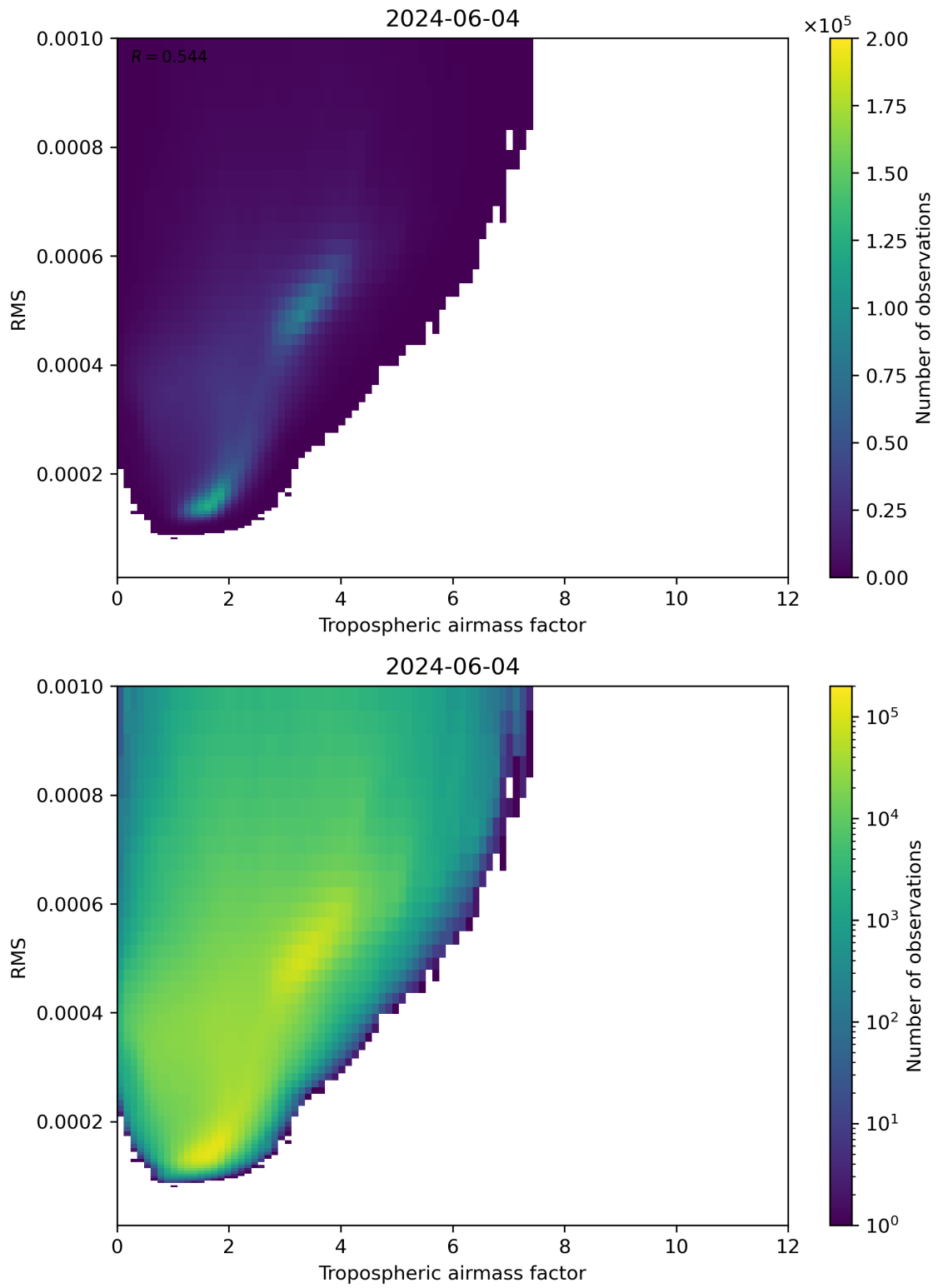
Figure 79: Scatter density plot of “Tropospheric airmass factor” against “RMS” for 2024-06-03 to 2024-06-05.
