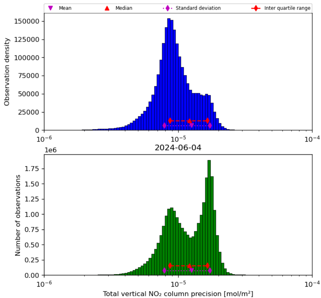
Figure 39: Histogram of “Total vertical NO 2 column precision” for 2024-06-03 to 2024-06-05
