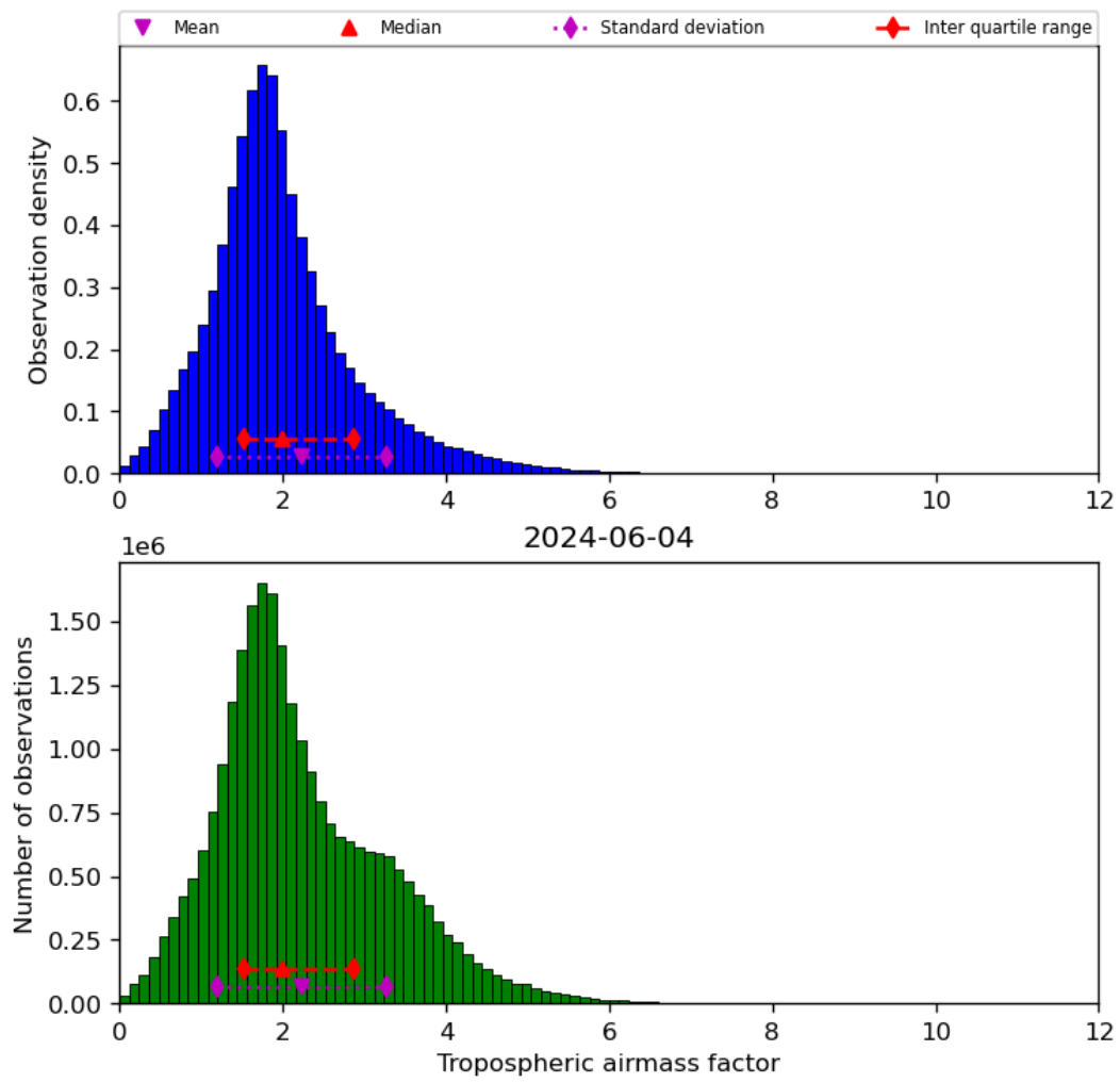
Figure 31: Histogram of “Tropospheric airmass factor” for 2024-06-03 to 2024-06-05
