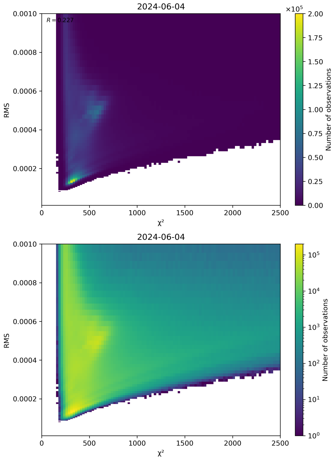
Figure 82: Scatter density plot of “ \chi^2 ” against “RMS” for 2024-06-03 to 2024-06-05.
