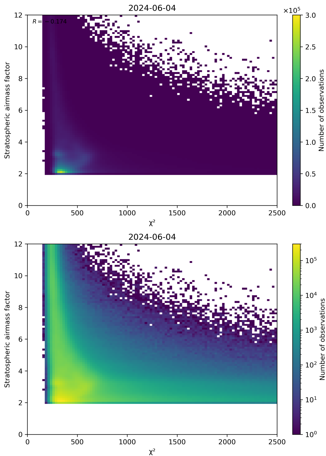
Figure 81: Scatter density plot of “ \chi^2 ” against “Stratospheric airmass factor” for 2024-06-03 to 2024-06-05.
