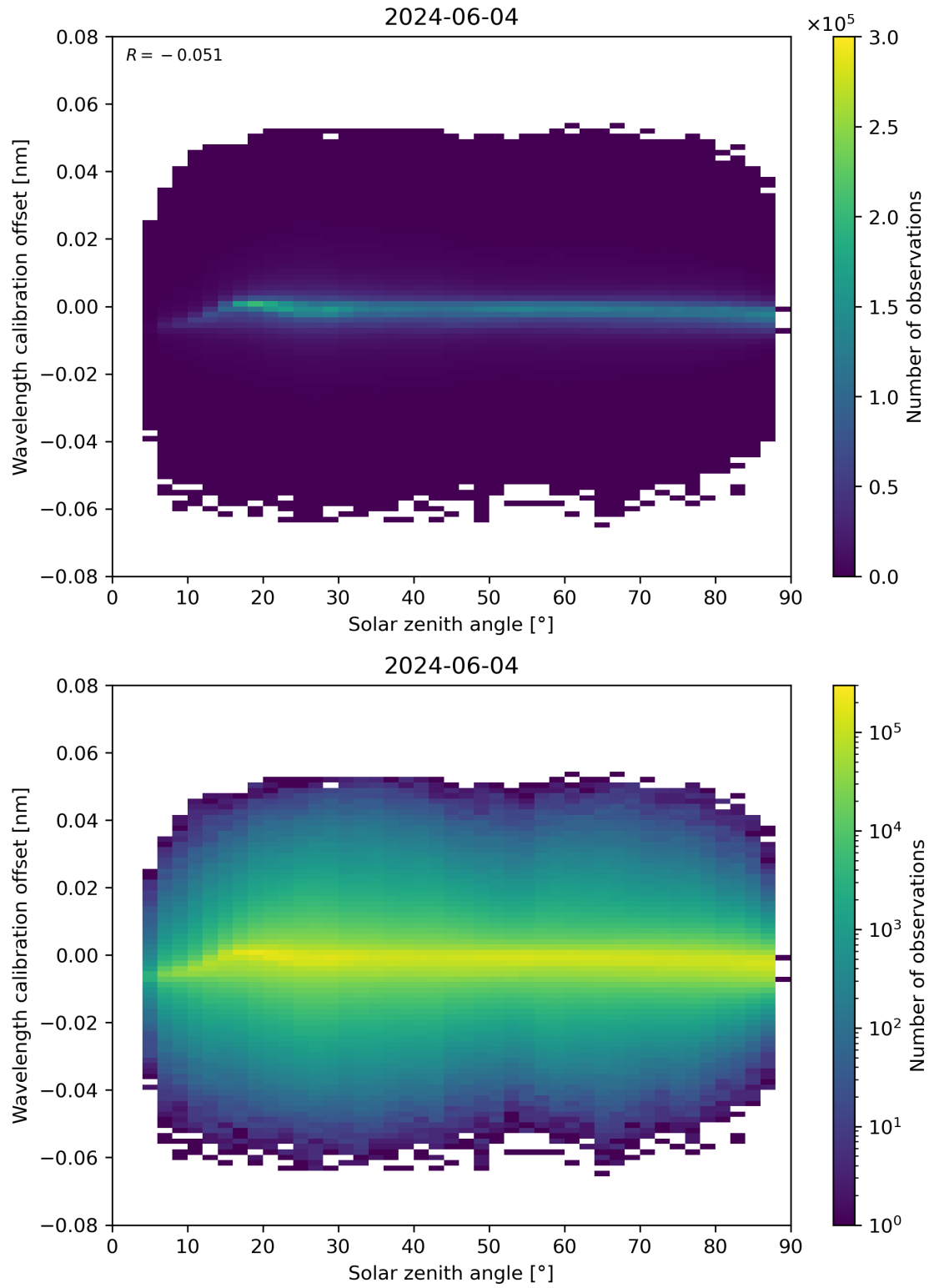
Figure 158: Scatter density plot of “Solar zenith angle” against “Wavelength calibration offset” for 2024-06-03 to 2024-06-05.
