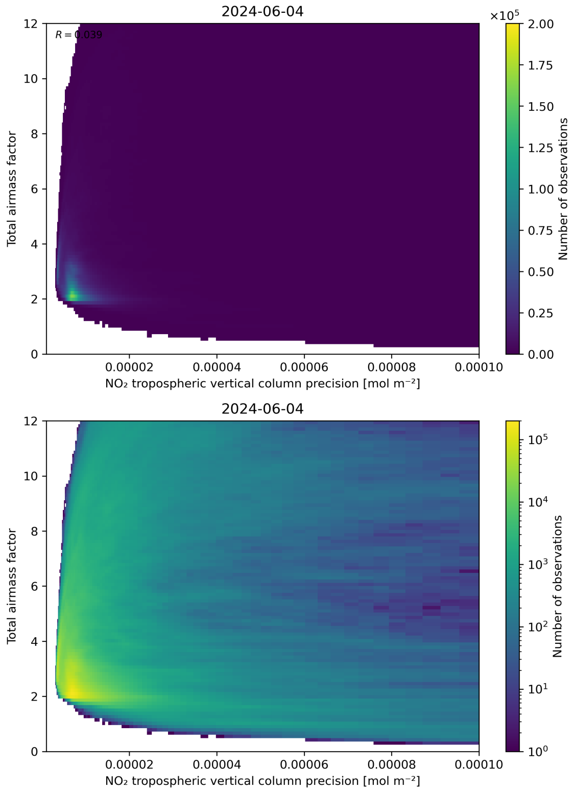
Figure 132: Scatter density plot of “NO 2 tropospheric vertical column precision” against “Total air mass factor” for 2024-06-03 to 2024-06-05.
