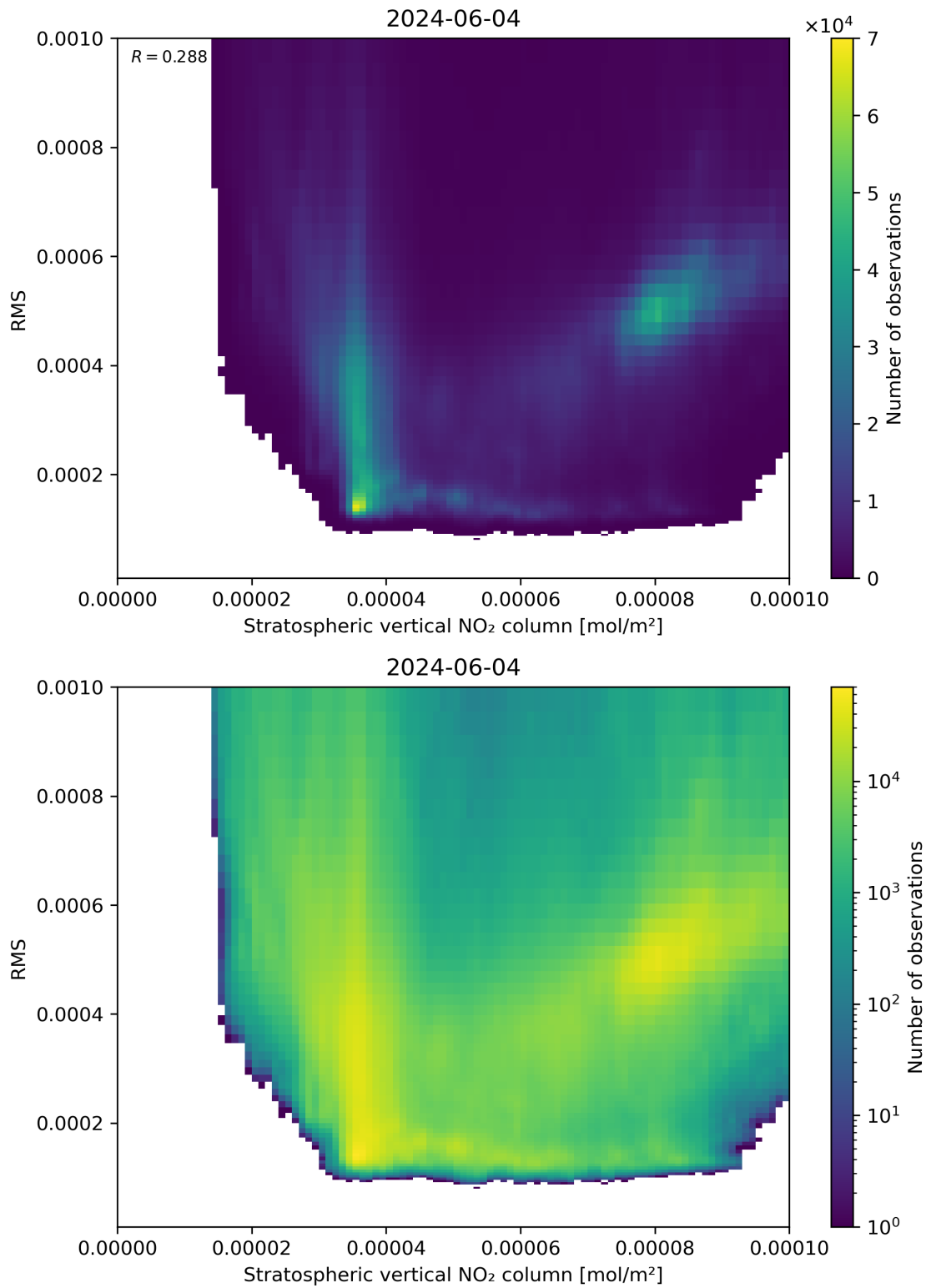
Figure 102: Scatter density plot of “Stratospheric vertical NO 2 column” against “RMS” for 2024-06-03 to 2024-06-05.
