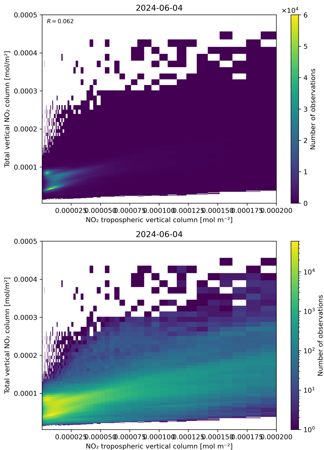
Figure 128: Scatter density plot of “NO 2 tropospheric vertical column” against “Total vertical NO 2 column” for 2024-06-03 to 2024-06-05.
