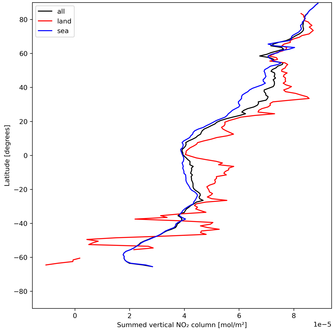
Figure 23: Zonal average of “Summed vertical NO 2 column” for 2024-06-03 to 2024-06-05.
