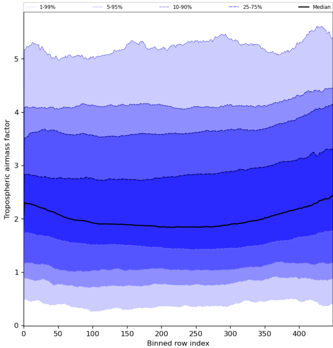
Figure 48: Along track statistics of “Tropospheric airmass factor” for 2024-06-03 to 2024-06-05
