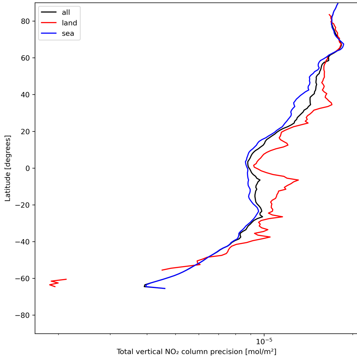
Figure 22: Zonal average of “Total vertical NO 2 column precision” for 2024-06-03 to 2024-06-05.
