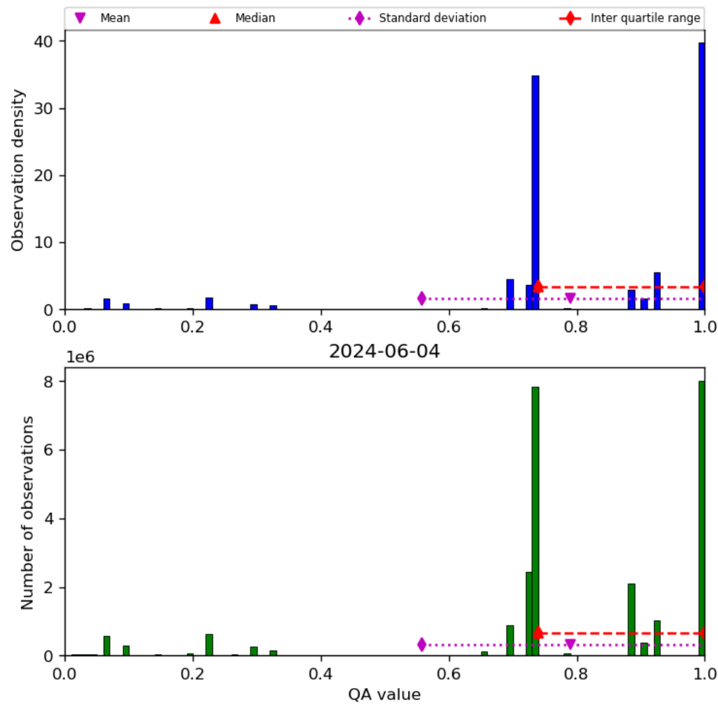
Figure 28: Histogram of “QA value” for 2024-06-03 to 2024-06-05
