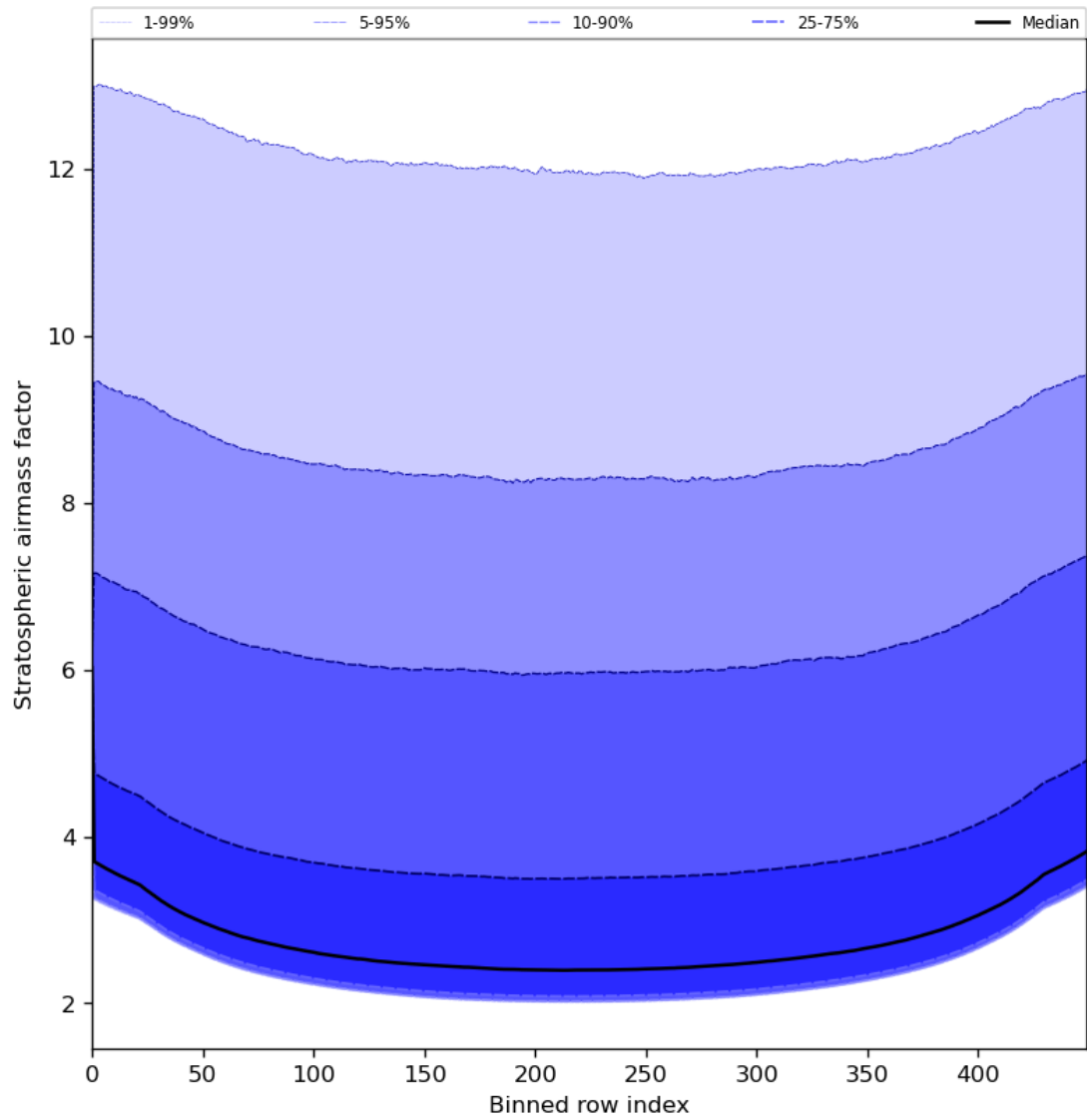
Figure 61: Along track statistics of “Stratospheric air mass factor” for 2024-06-03 to 2024-06-05
