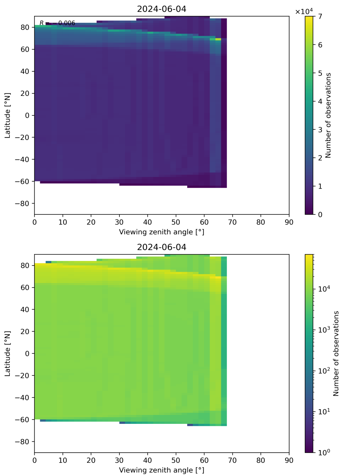
Figure 163: Scatter density plot of “Viewing zenith angle” against “Latitude” for 2024-06-03 to 2024-06-05.
