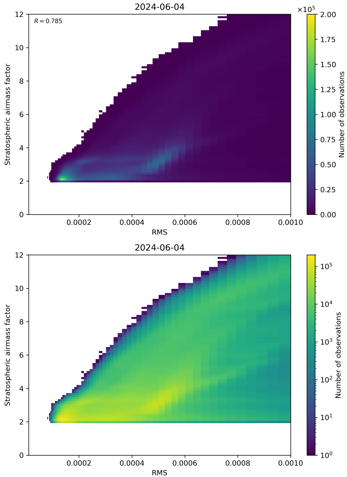
Figure 144: Scatter density plot of “RMS” against “Stratospheric airmass factor” for 2024-06-03 to 2024-06-05.
