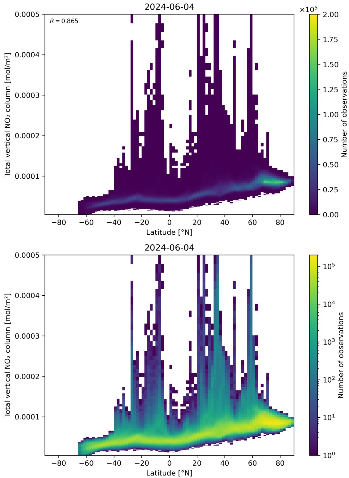
Figure 90: Scatter density plot of “Latitude” against “Total vertical NO 2 column” for 2024-06-03 to 2024-06-05.
