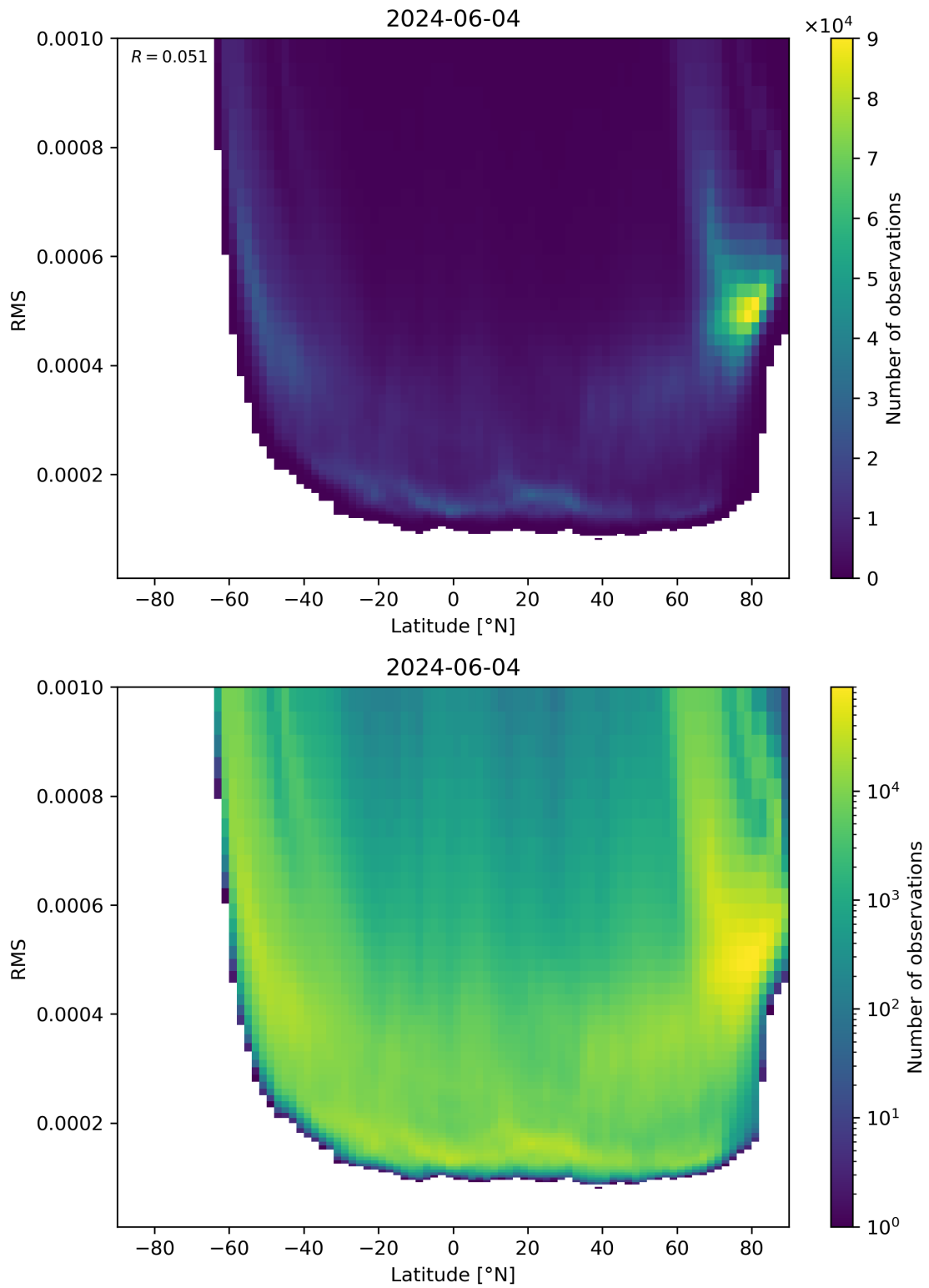
Figure 94: Scatter density plot of “Latitude” against “RMS” for 2024-06-03 to 2024-06-05.
