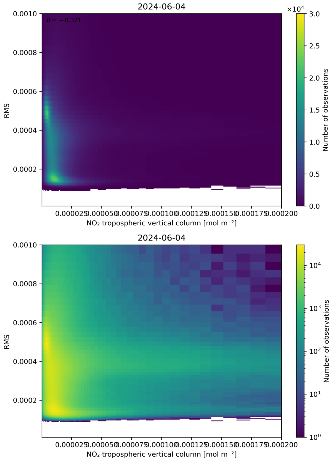
Figure 142: Scatter density plot of “NO 2 tropospheric vertical column” against “RMS” for 2024-06-03 to 2024-06-05.
