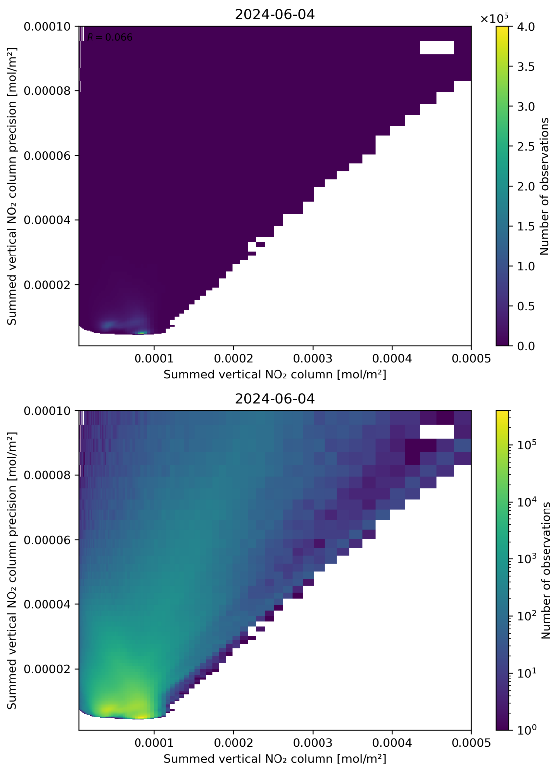
Figure 105: Scatter density plot of “Summed vertical NO 2 column” against “Summed vertical NO 2 column precision” for 2024-06-03 to 2024-06-05.
