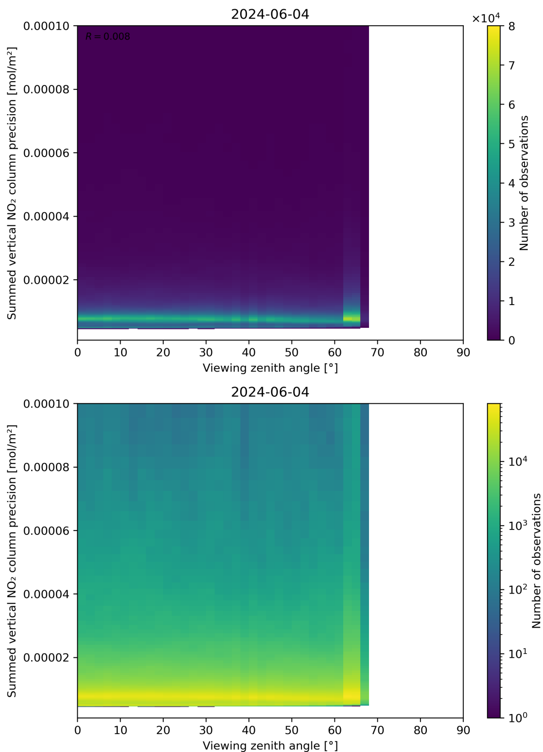
Figure 166: Scatter density plot of “Viewing zenith angle” against “Summed vertical NO 2 column precision” for 2024-06-03 to 2024-06-05.
