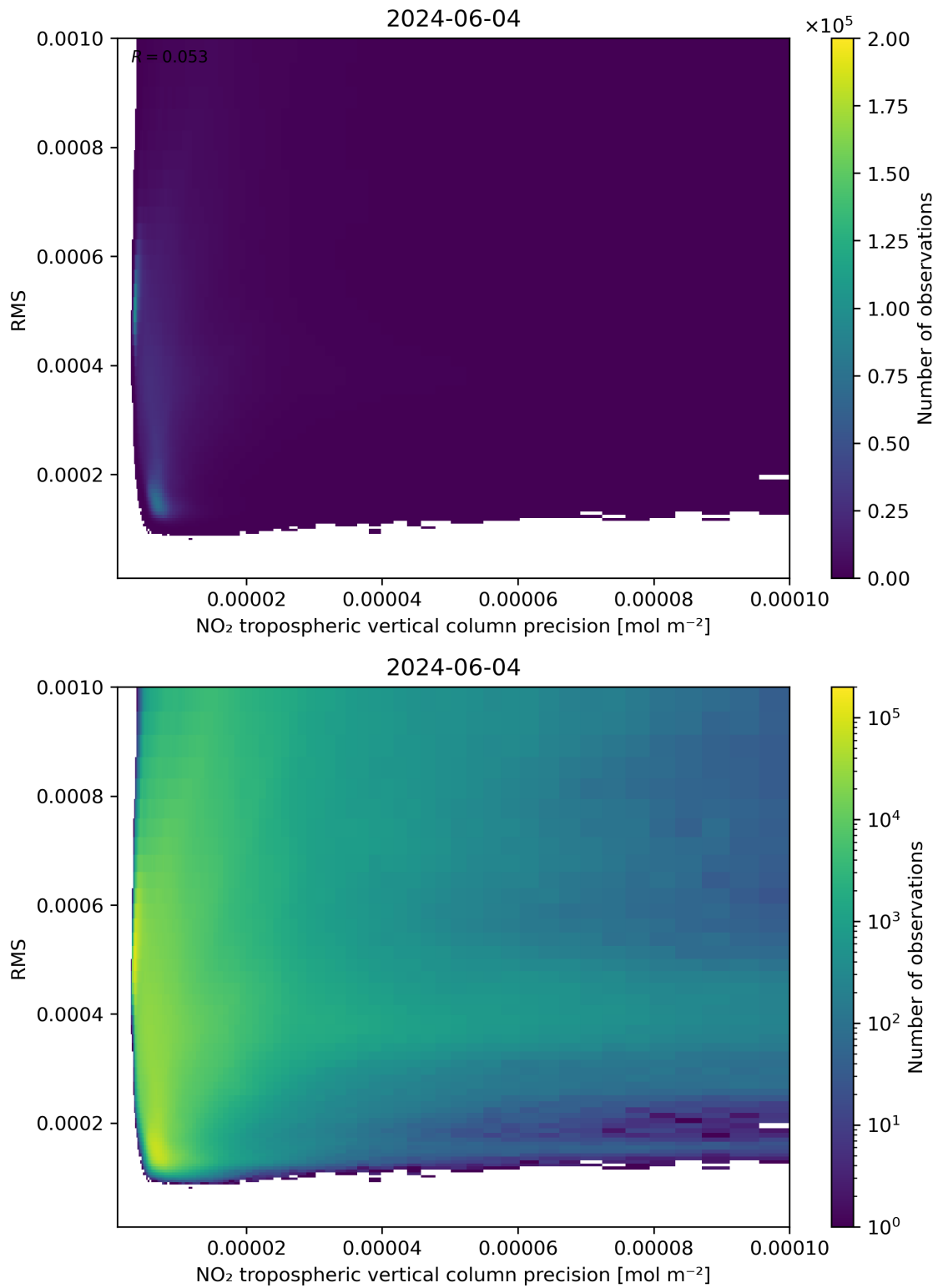
Figure 140: Scatter density plot of “NO 2 tropospheric vertical column precision” against “RMS” for 2024-06-03 to 2024-06-05.
