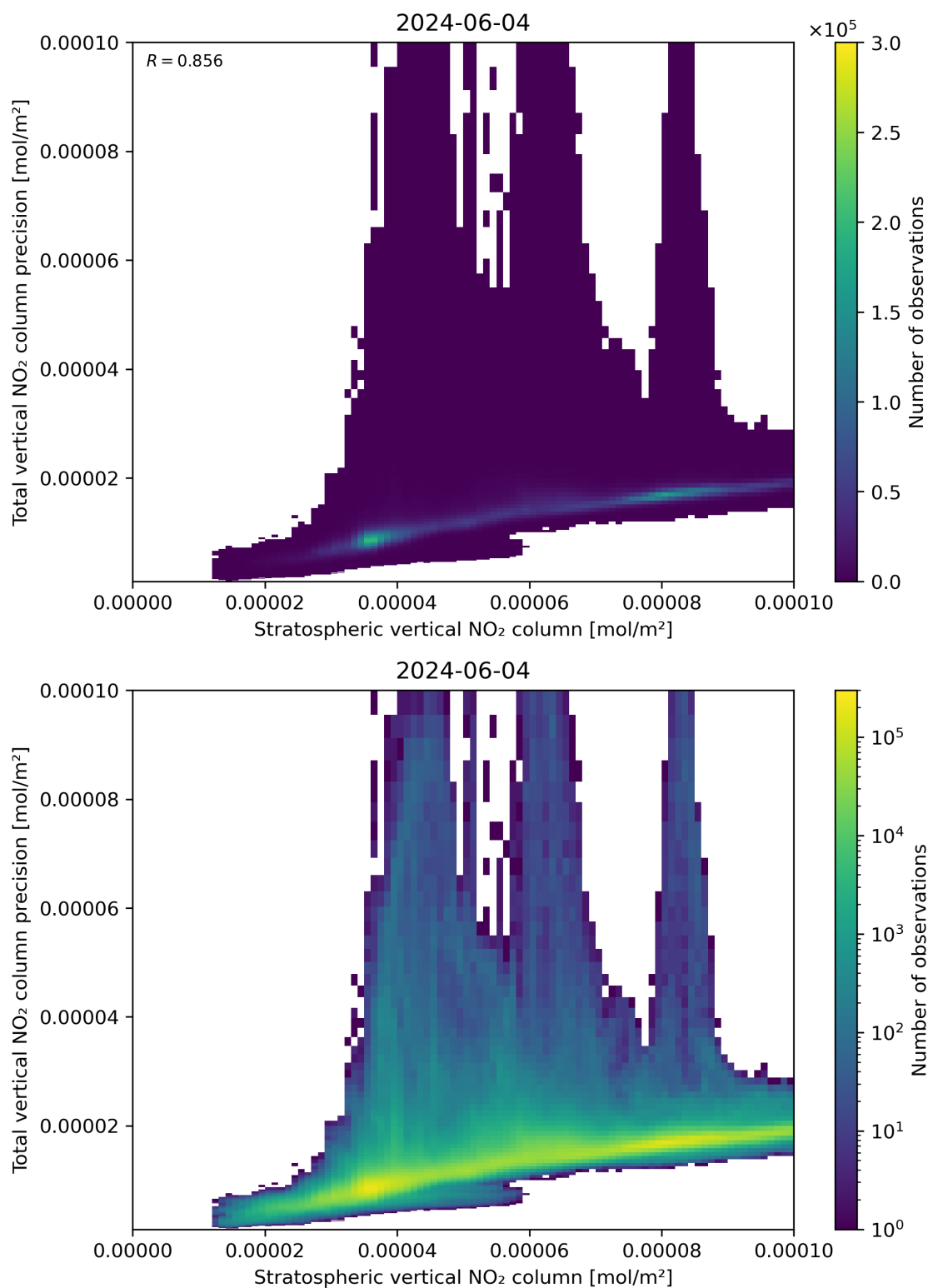
Figure 101: Scatter density plot of “Stratospheric vertical NO 2 column” against “Total vertical NO 2 column precision” for 2024-06-03 to 2024-06-05.
