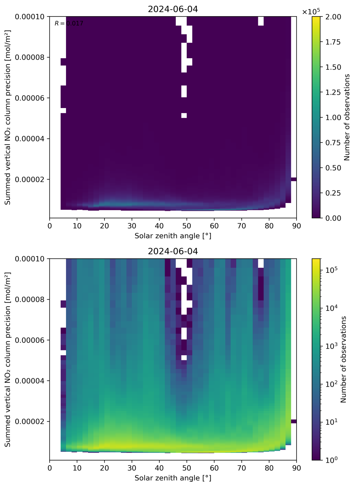
Figure 152: Scatter density plot of “Solar zenith angle” against “Summed vertical NO 2 column precision” for 2024-06-03 to 2024-06-05.
