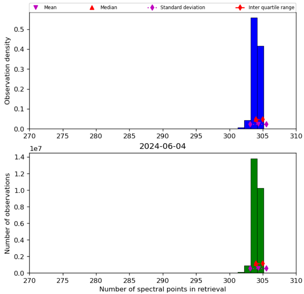
Figure 33: Histogram of “Number of spectral points in retrieval” for 2024-06-03 to 2024-06-05
