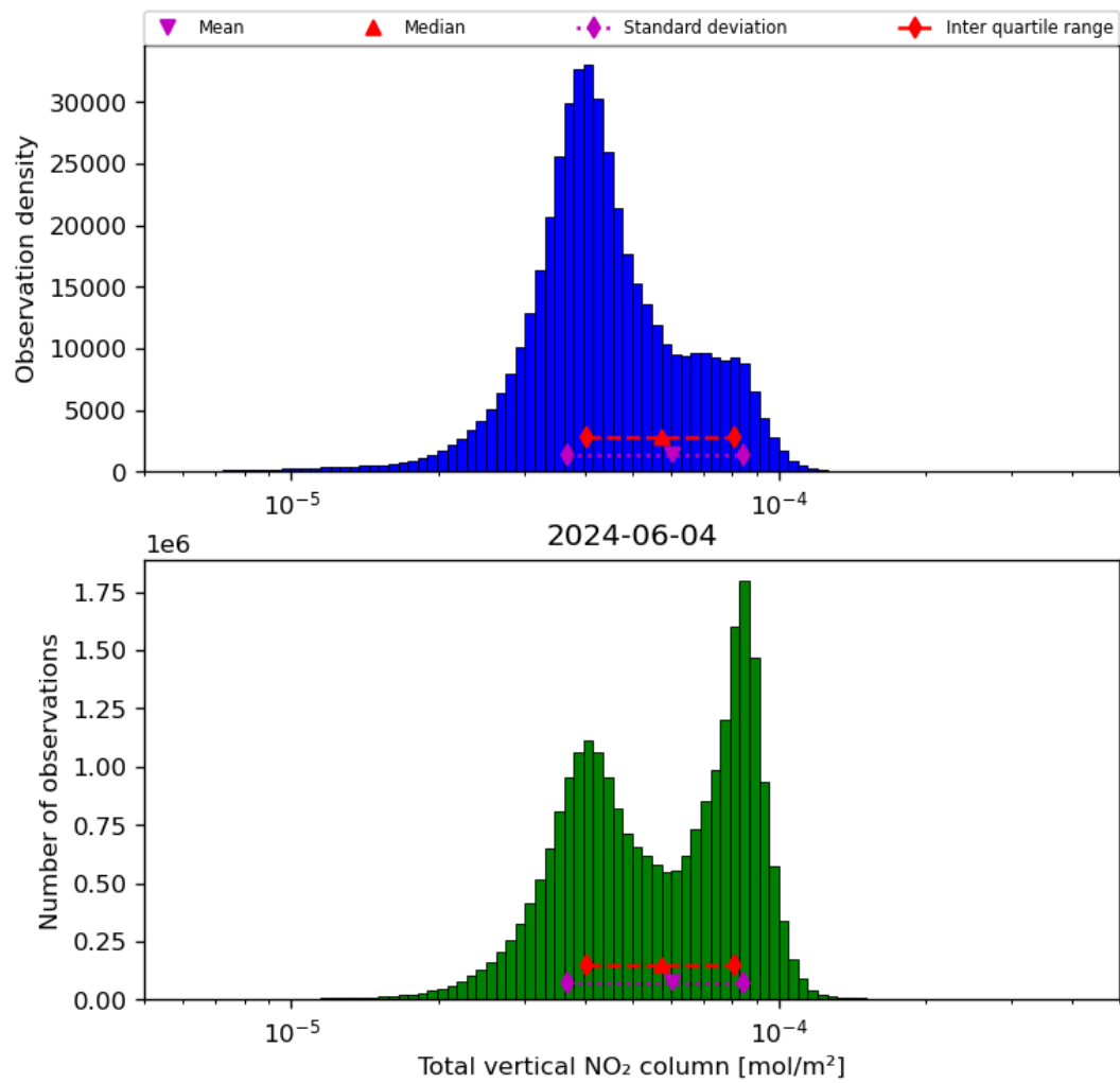
Figure 38: Histogram of “Total vertical NO 2 column” for 2024-06-03 to 2024-06-05
