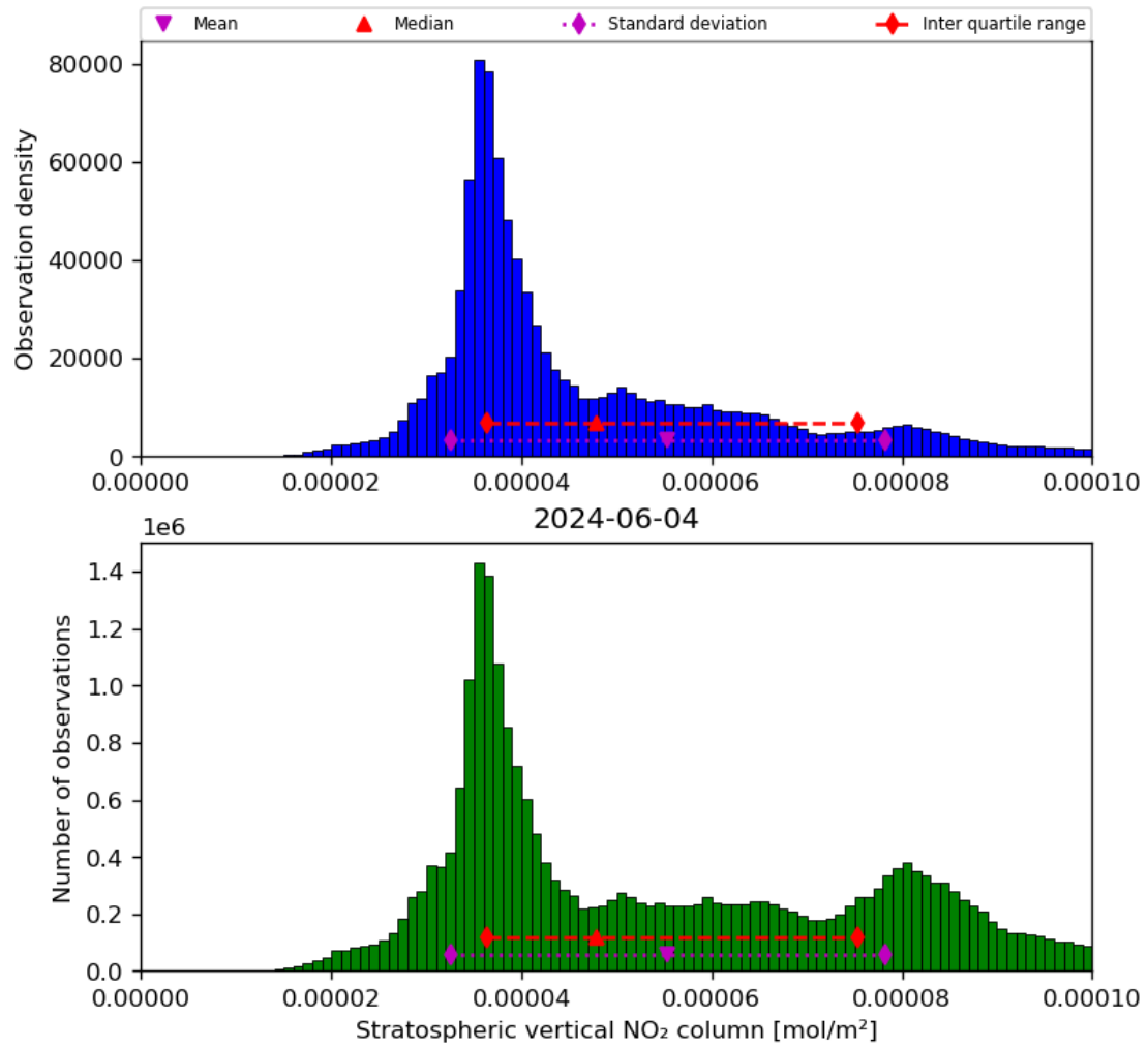
Figure 36: Histogram of “Stratospheric vertical NO 2 column” for 2024-06-03 to 2024-06-05
