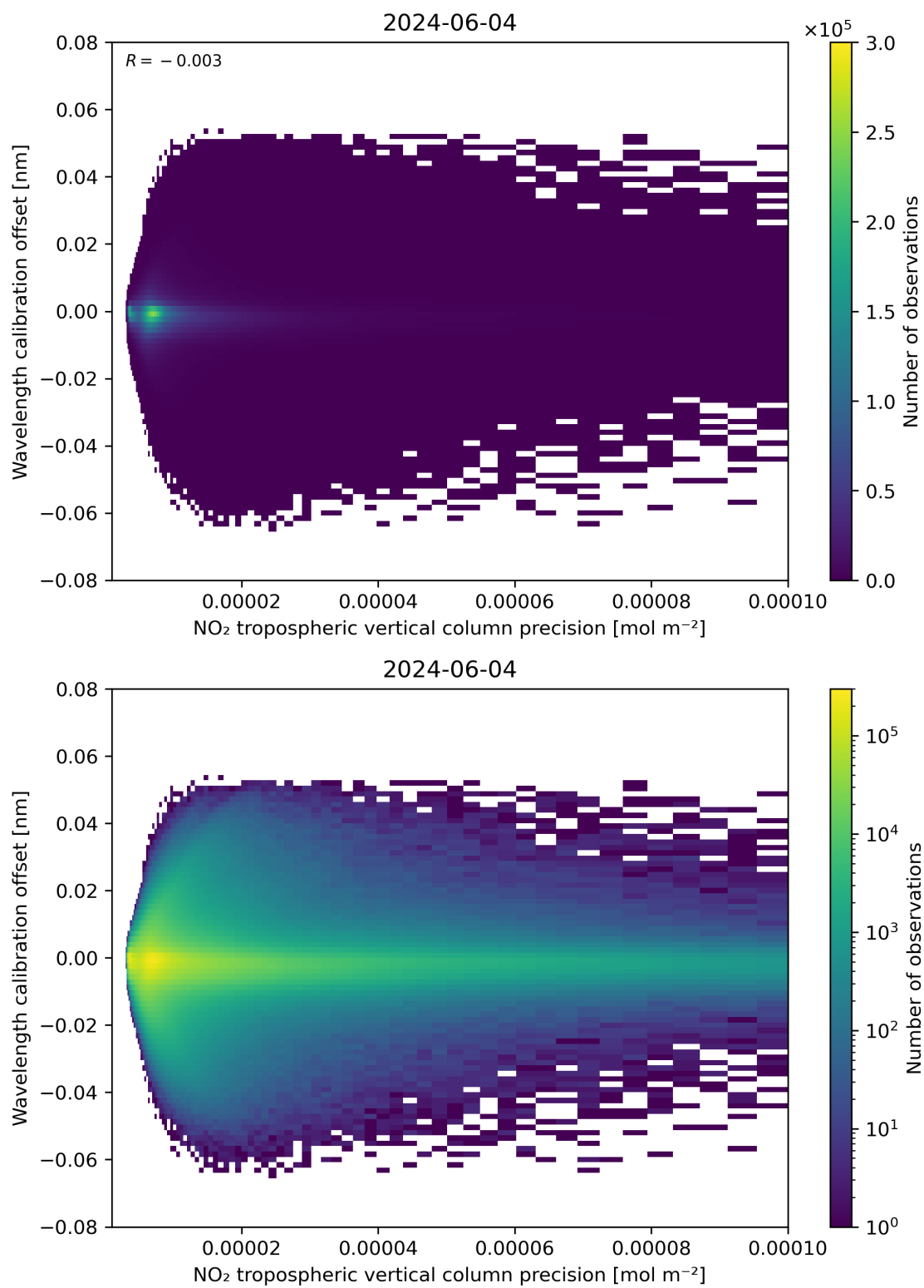
Figure 141: Scatter density plot of “NO 2 tropospheric vertical column precision” against “Wavelength calibration offset” for 2024-06-03 to 2024-06-05.
