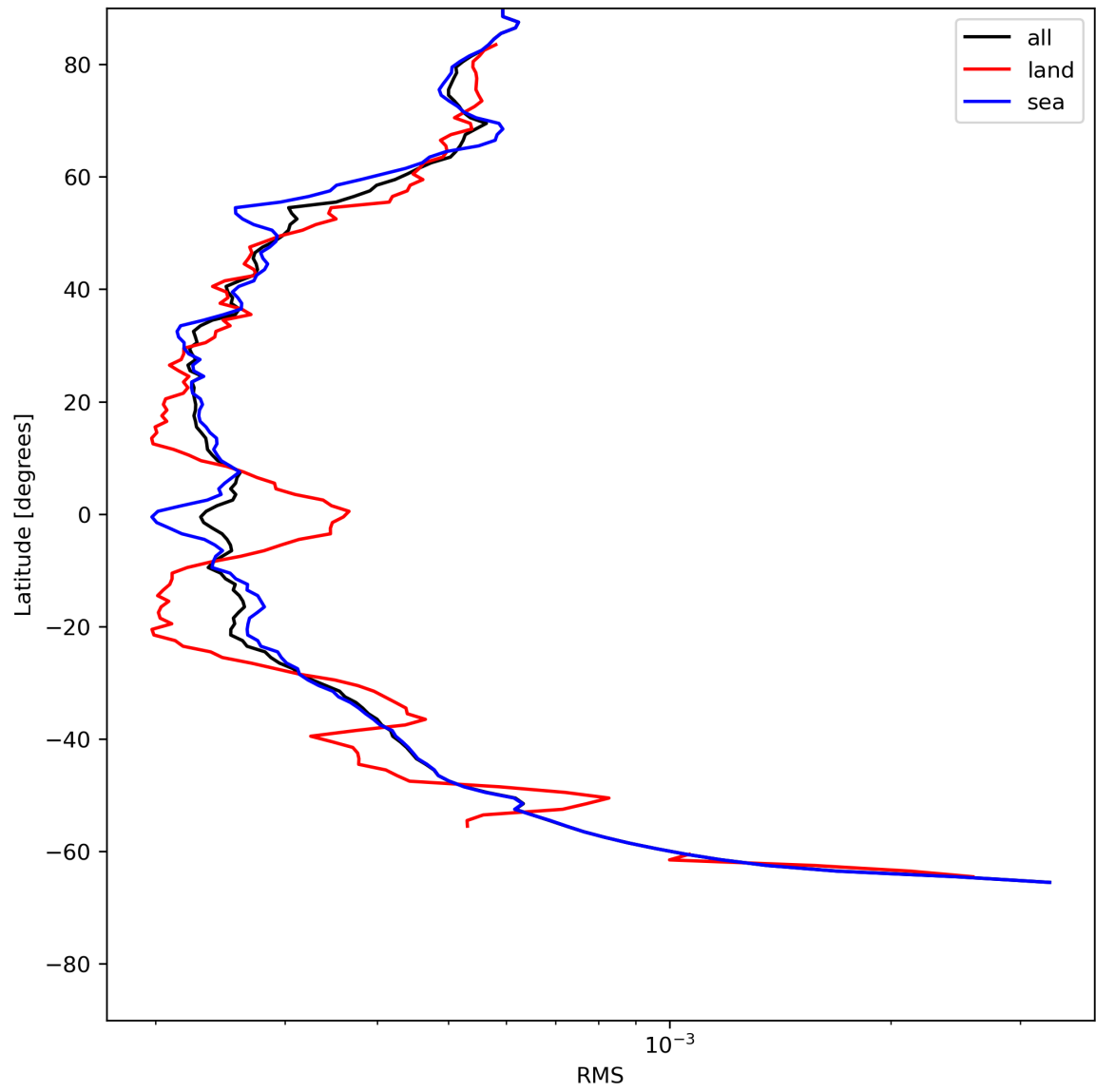
Figure 26: Zonal average of “RMS” for 2024-06-03 to 2024-06-05.
