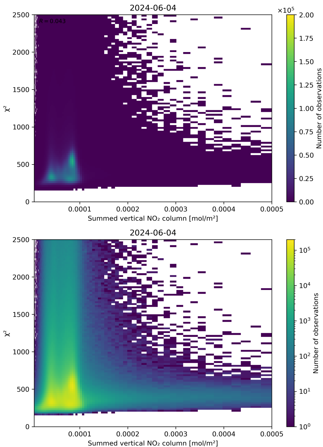
Figure 104: Scatter density plot of “Summed vertical NO 2 column” against “ \chi^2 ” for 2024-06-03 to 2024-06-05.
