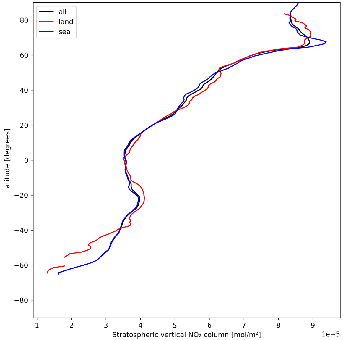
Figure 19: Zonal average of “Stratospheric vertical NO 2 column” for 2024-06-03 to 2024-06-05.
