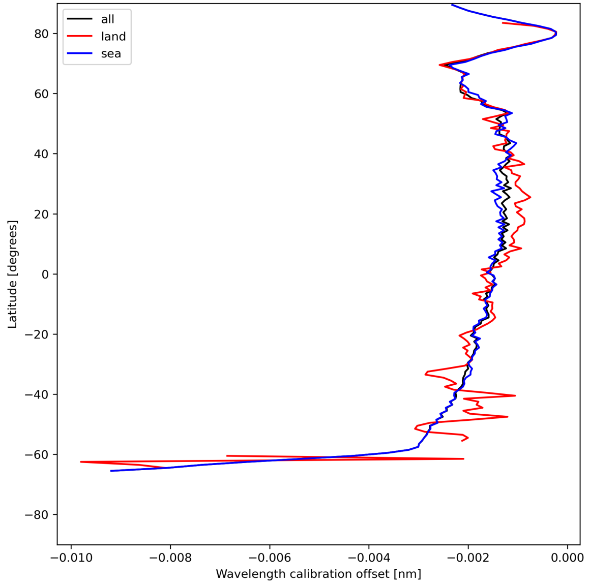
Figure 18: Zonal average of “Wavelength calibration offset” for 2024-06-03 to 2024-06-05.
