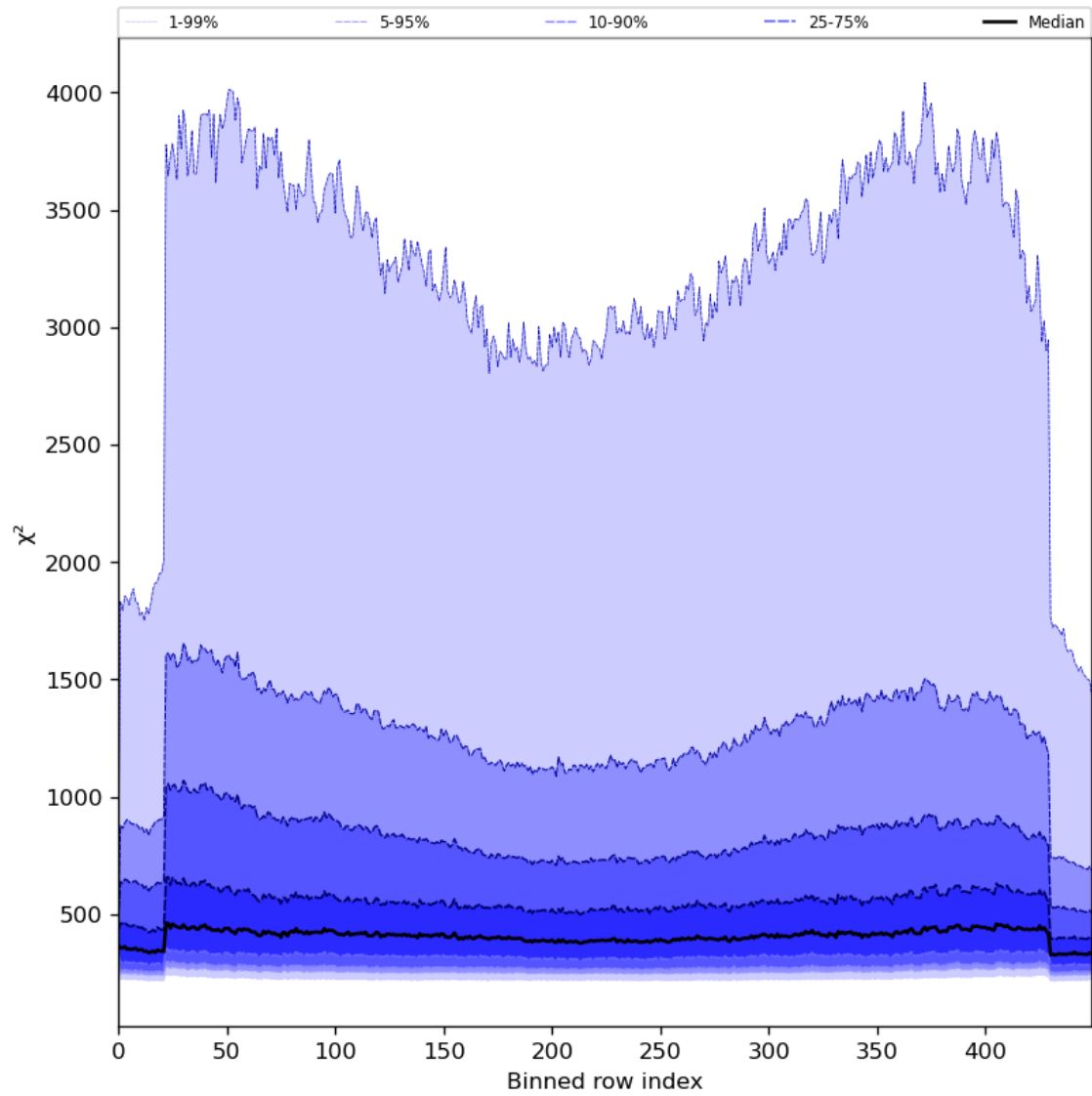
Figure 59: Along track statistics of “ \chi^2 ” for 2024-06-03 to 2024-06-05
