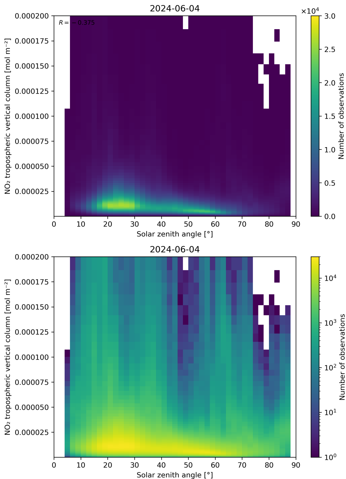
Figure 155: Scatter density plot of “Solar zenith angle” against “NO 2 tropospheric vertical column” for 2024-06-03 to 2024-06-05.
