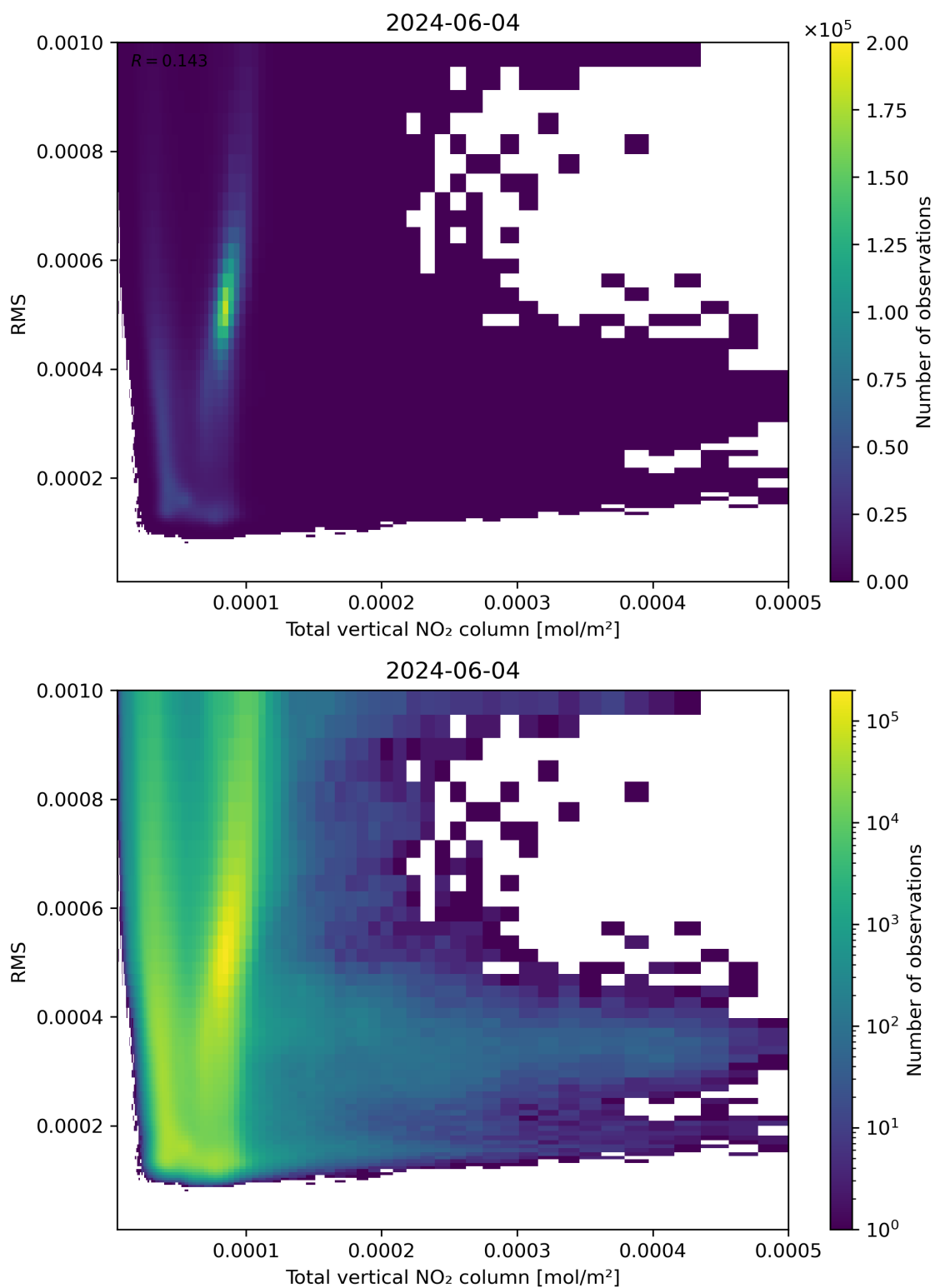
Figure 120: Scatter density plot of “Total vertical NO 2 column” against “RMS” for 2024-06-03 to 2024-06-05.
