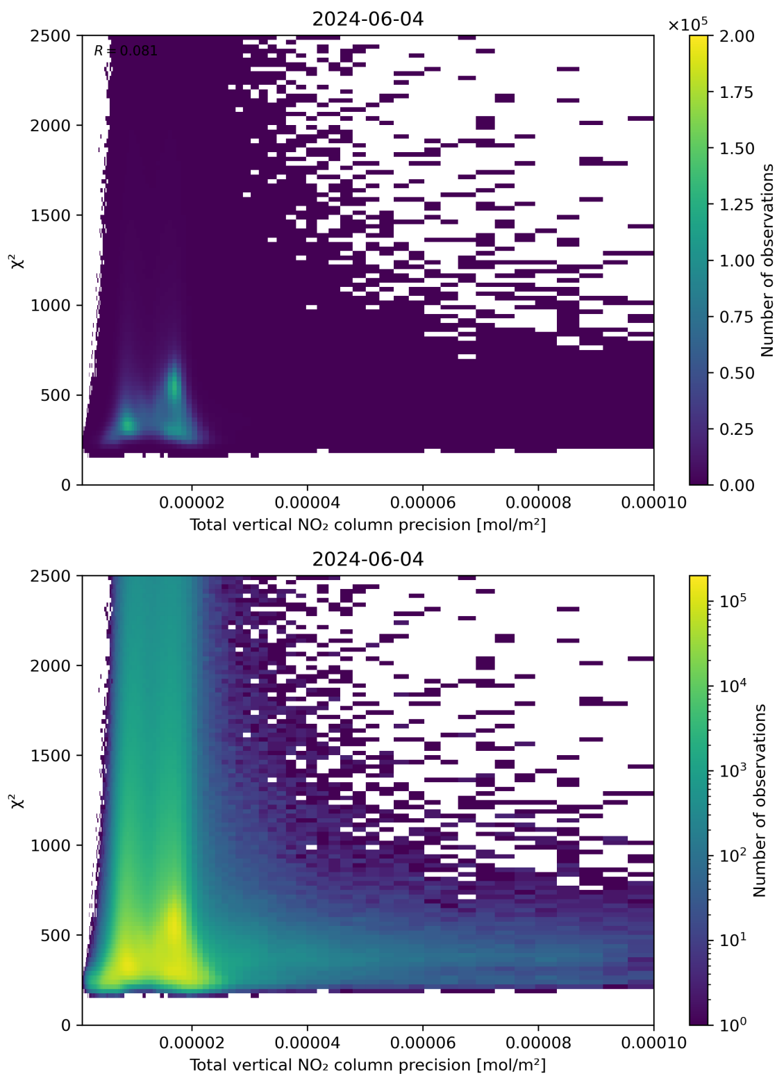
Figure 116: Scatter density plot of “Total vertical NO 2 column precision” against “ \chi^2 ” for 2024-06-03 to 2024-06-05.
