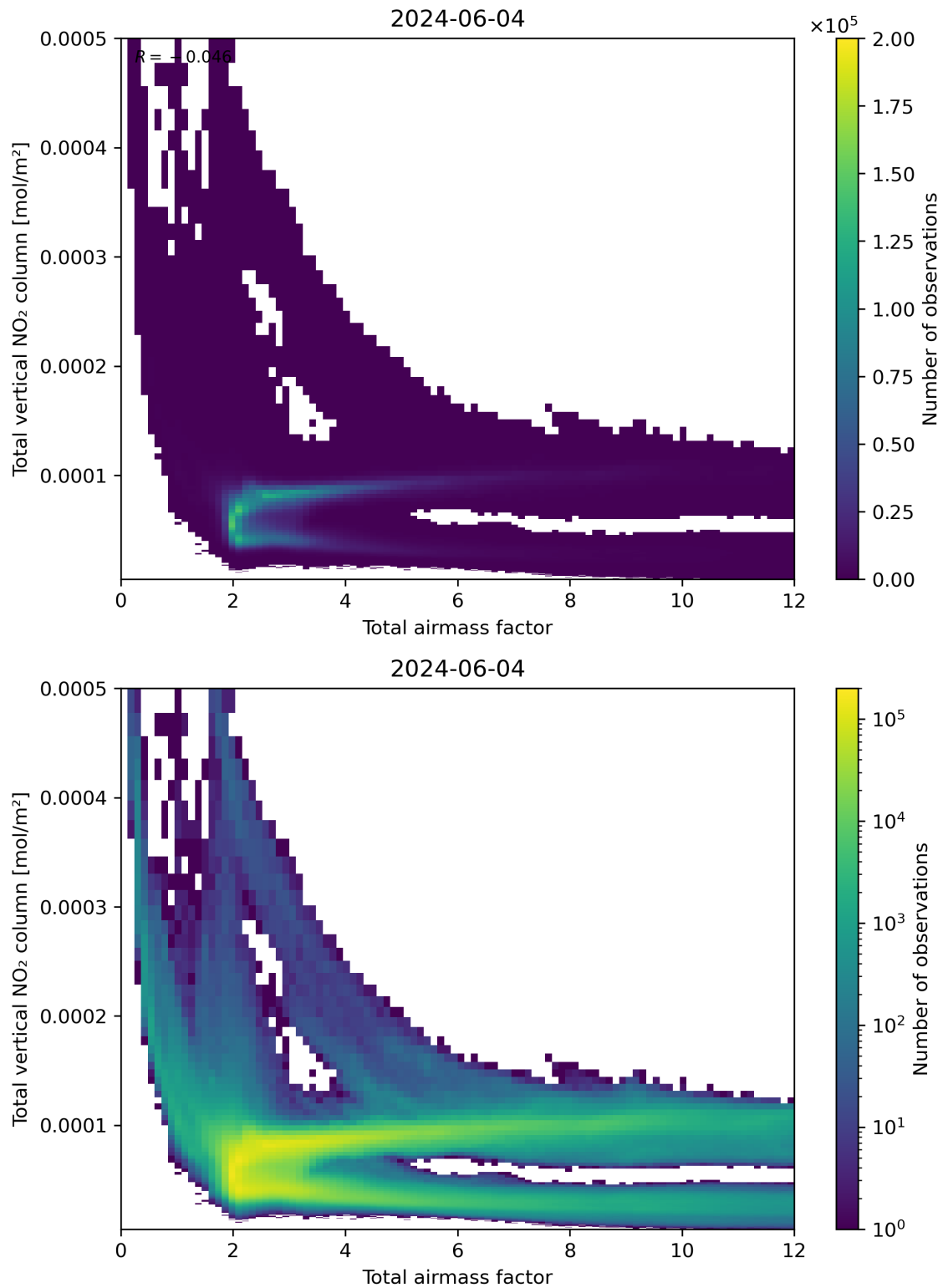
Figure 67: Scatter density plot of “Total airmass factor” against “Total vertical NO 2 column” for 2024-06-03 to 2024-06-05.
