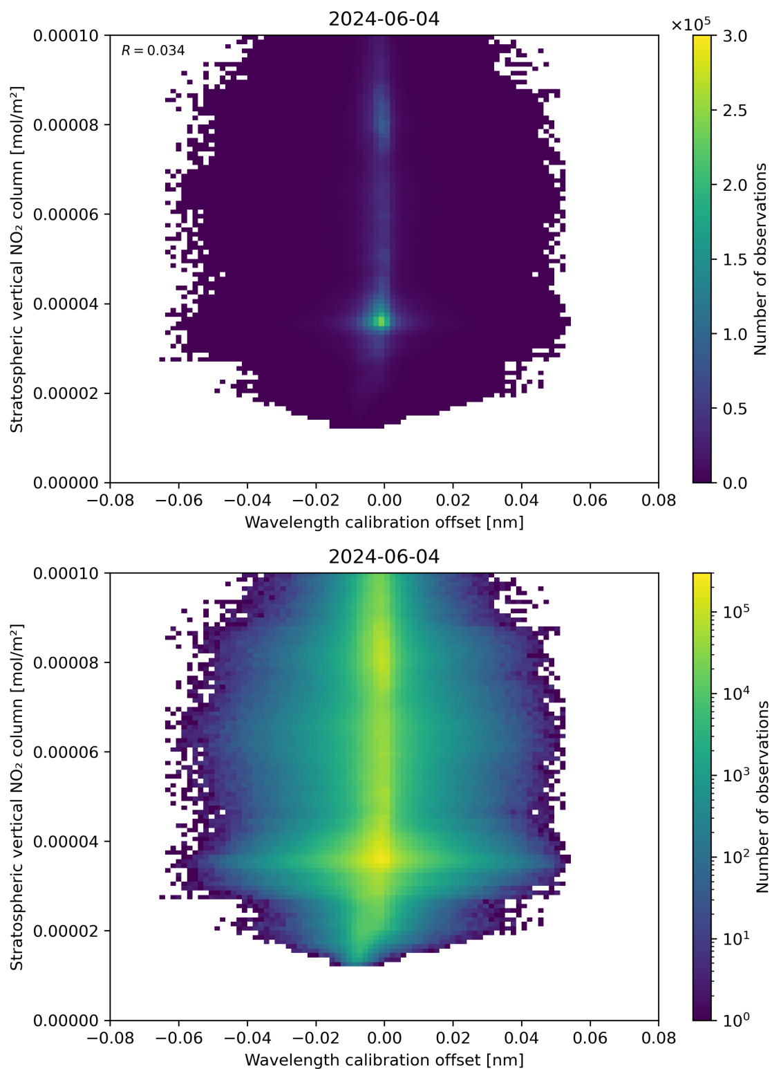
Figure 176: Scatter density plot of “Wavelength calibration offset” against “Stratospheric vertical NO 2 column” for 2024-06-03 to 2024-06-05.
