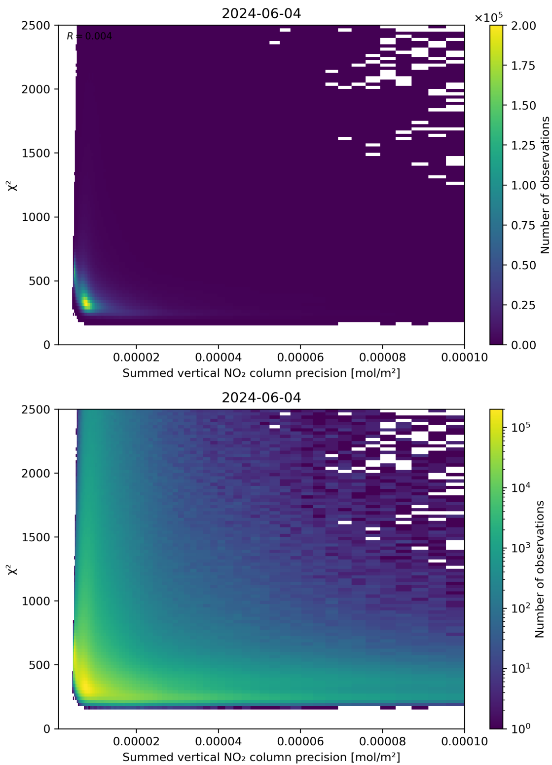
Figure 107: Scatter density plot of “Summed vertical NO 2 column precision” against “ \chi^2 ” for 2024-06-03 to 2024-06-05.
