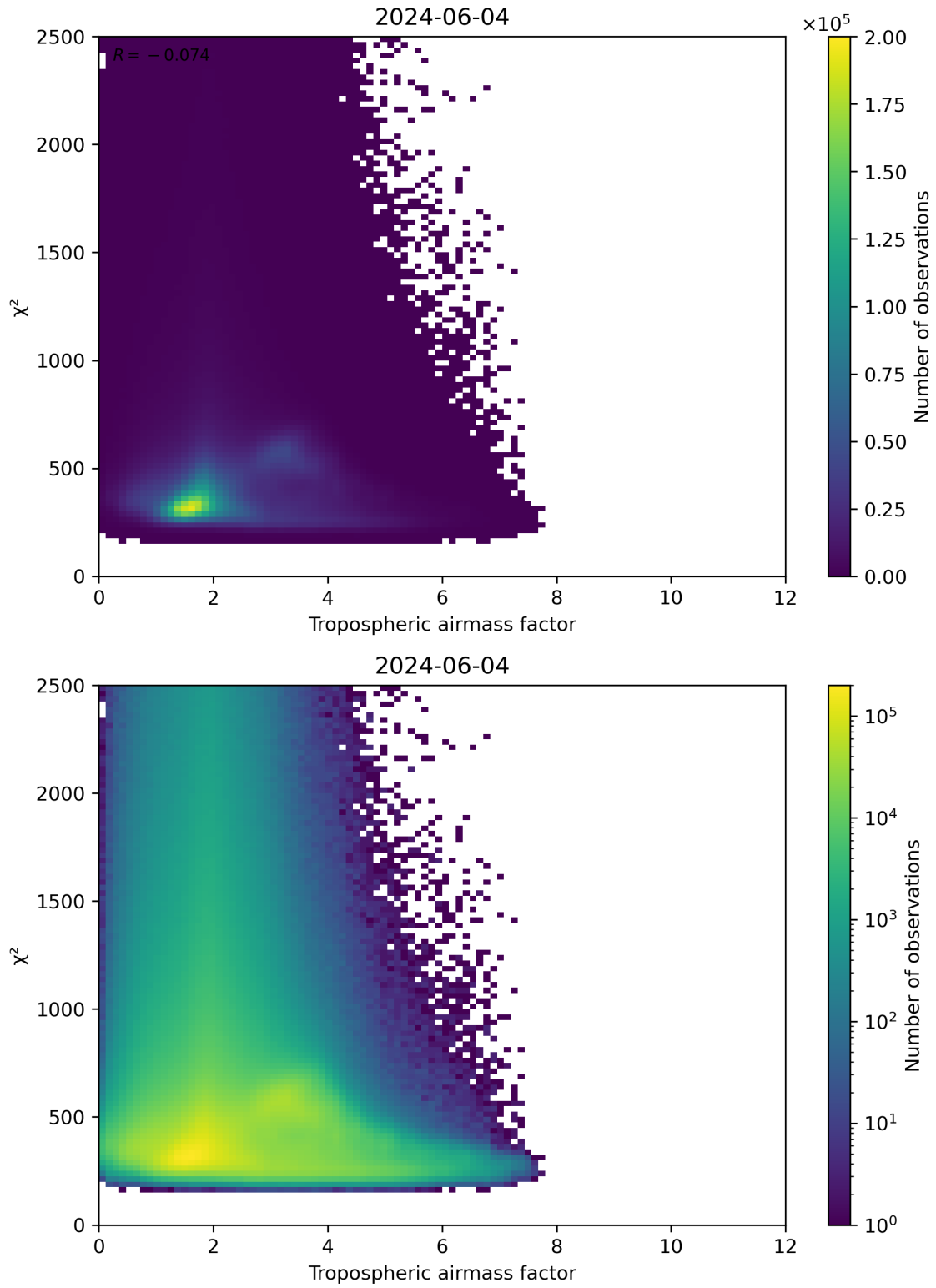
Figure 73: Scatter density plot of “Tropospheric airmass factor” against “ \chi^2 ” for 2024-06-03 to 2024-06-05.
