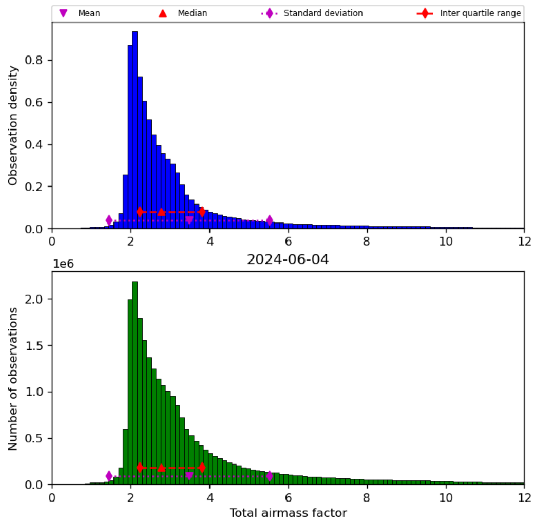
Figure 32: Histogram of “Total airmass factor” for 2024-06-03 to 2024-06-05
