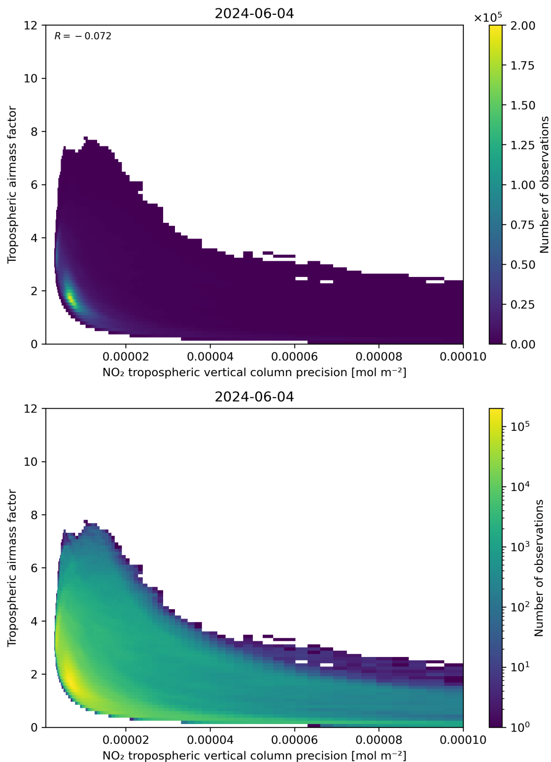
Figure 133: Scatter density plot of “NO 2 tropospheric vertical column precision” against “Tropospheric airmass factor” for 2024-06-03 to 2024-06-05.
