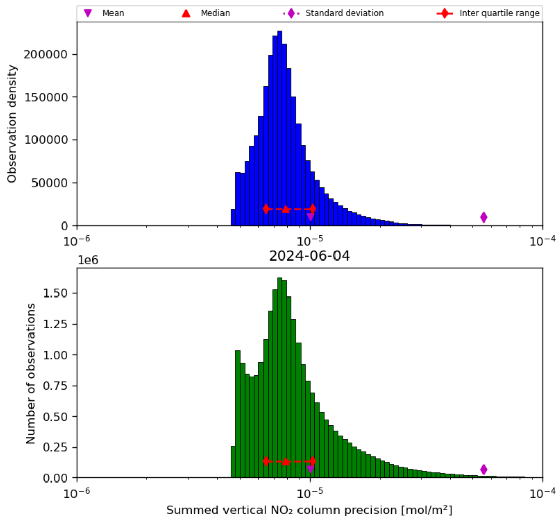
Figure 41: Histogram of "Summed vertical NO 2 column precision" for 2024-06-03 to 2024-06-05
