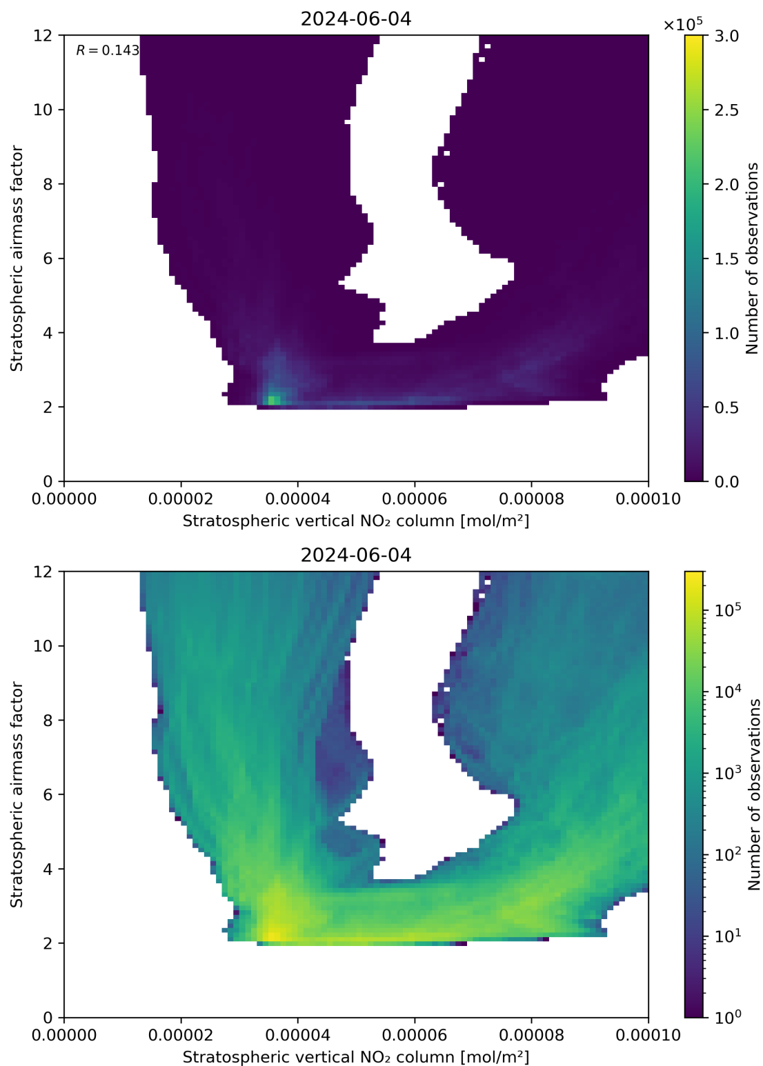
Figure 96: Scatter density plot of “Stratospheric vertical NO 2 column” against “Stratospheric airmass factor” for 2024-06-03 to 2024-06-05.
