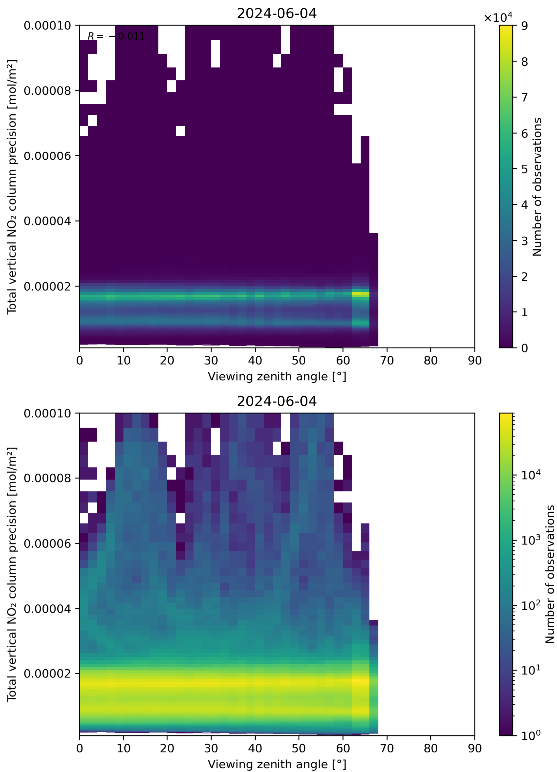
Figure 168: Scatter density plot of “Viewing zenith angle” against “Total vertical NO 2 column precision” for 2024-06-03 to 2024-06-05.
