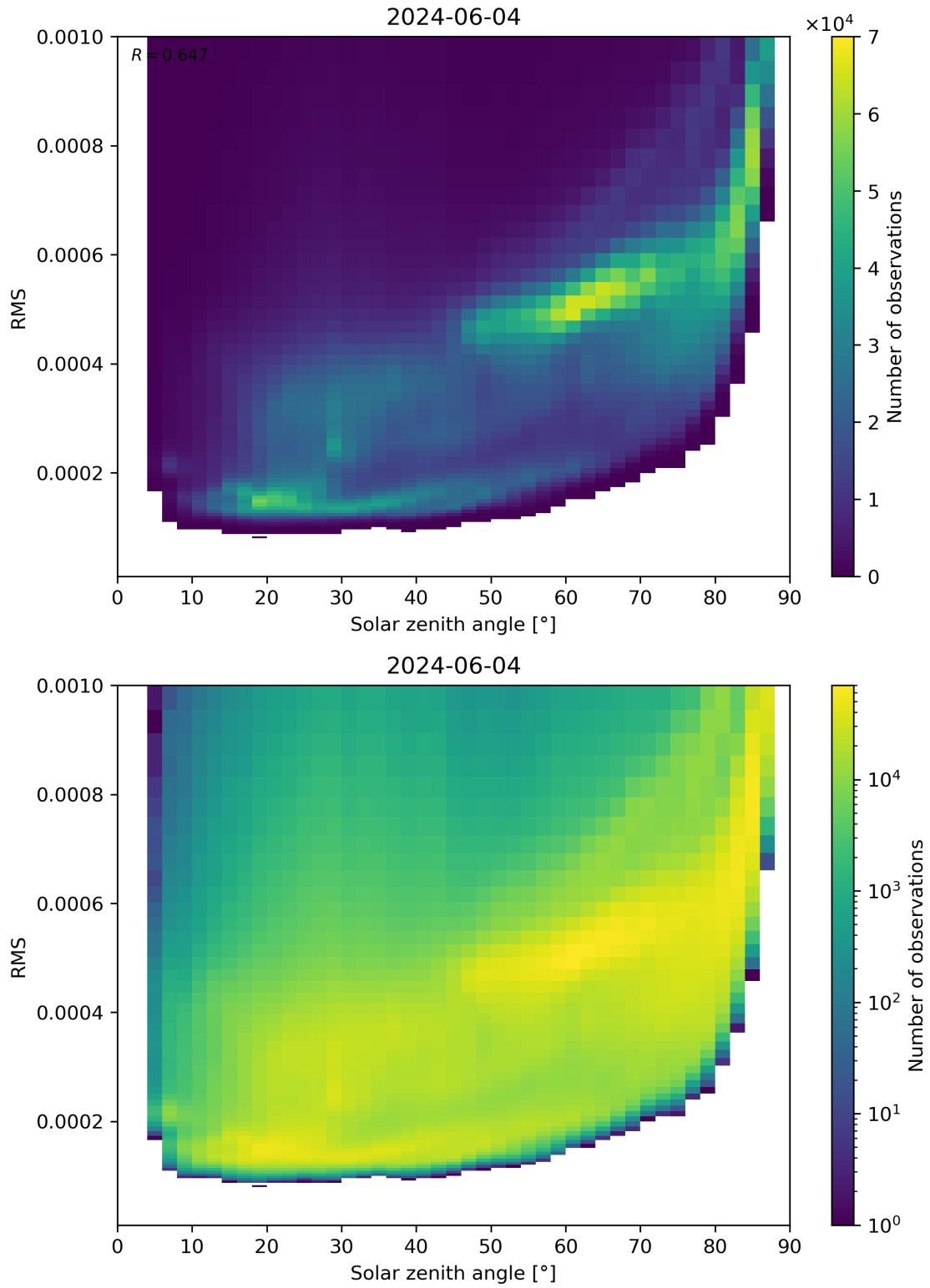
Figure 157: Scatter density plot of “Solar zenith angle” against “RMS” for 2024-06-03 to 2024-06-05.
