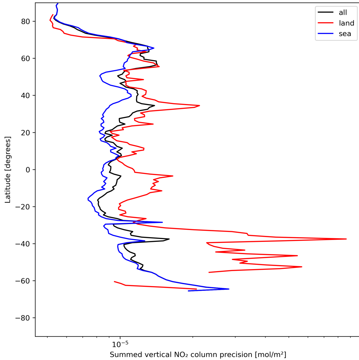
Figure 24: Zonal average of “Summed vertical NO 2 column precision” for 2024-06-03 to 2024-06-05.
