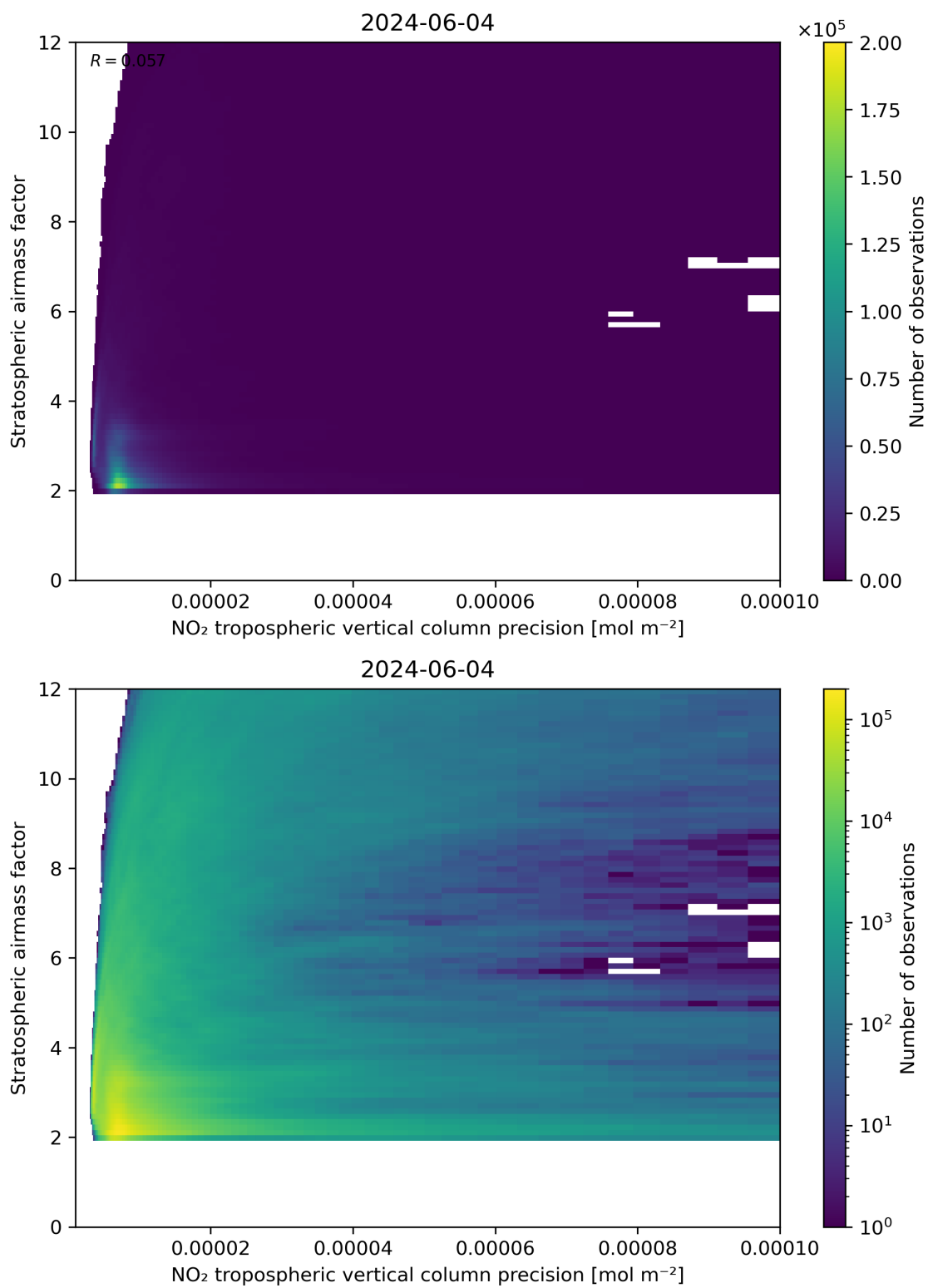
Figure 131: Scatter density plot of “NO 2 tropospheric vertical column precision” against “Stratospheric airmass factor” for 2024-06-03 to 2024-06-05.
