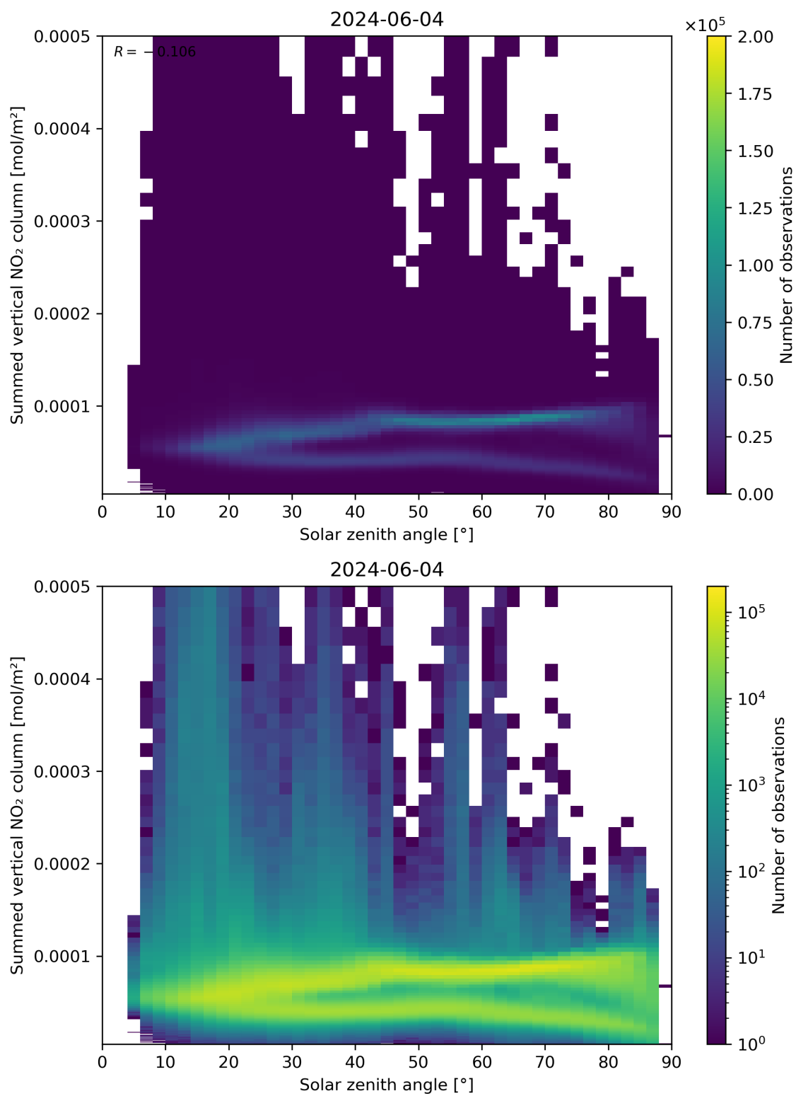
Figure 151: Scatter density plot of “Solar zenith angle” against “Summed vertical NO 2 column” for 2024-06-03 to 2024-06-05.
