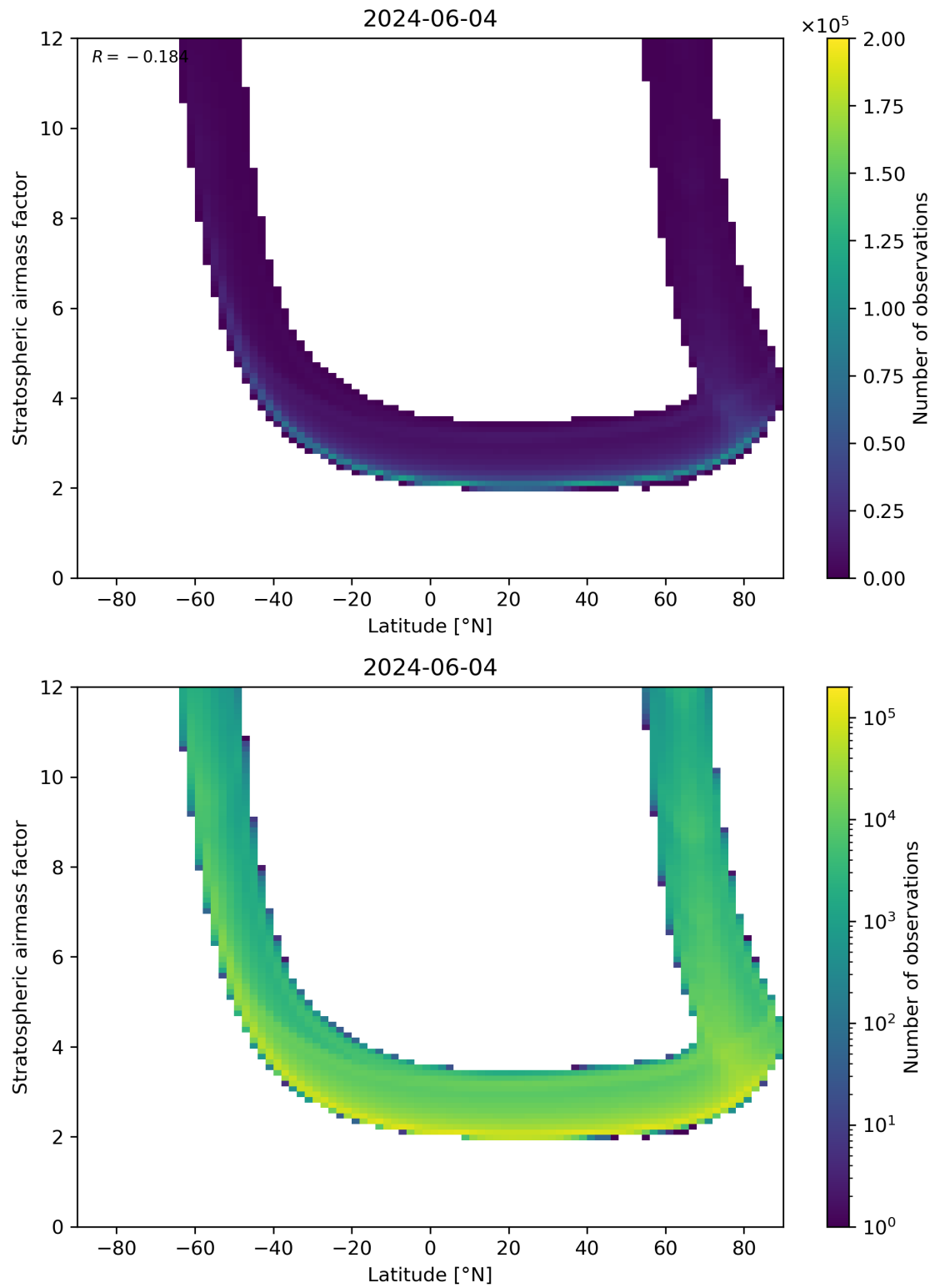
Figure 83: Scatter density plot of “Latitude” against “Stratospheric air mass factor” for 2024-06-03 to 2024-06-05.
