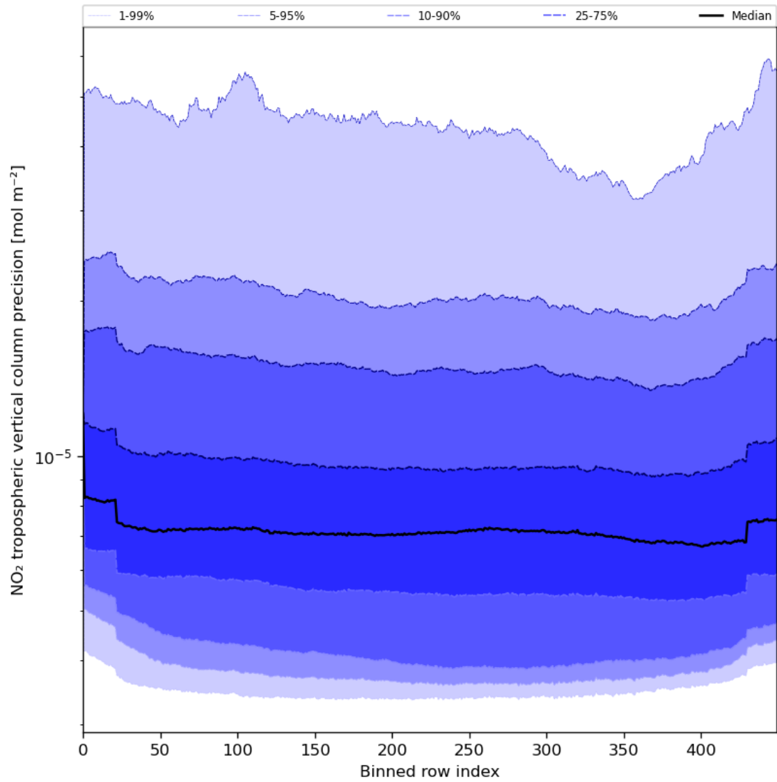
Figure 47: Along track statistics of “NO 2 tropospheric vertical column precision” for 2024-06-03 to 2024-06-05
