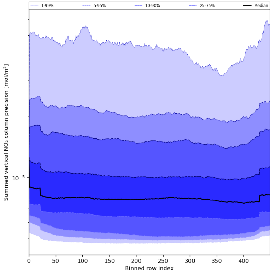
Figure 58: Along track statistics of “Summed vertical NO 2 column precision” for 2024-06-03 to 2024-06-05
