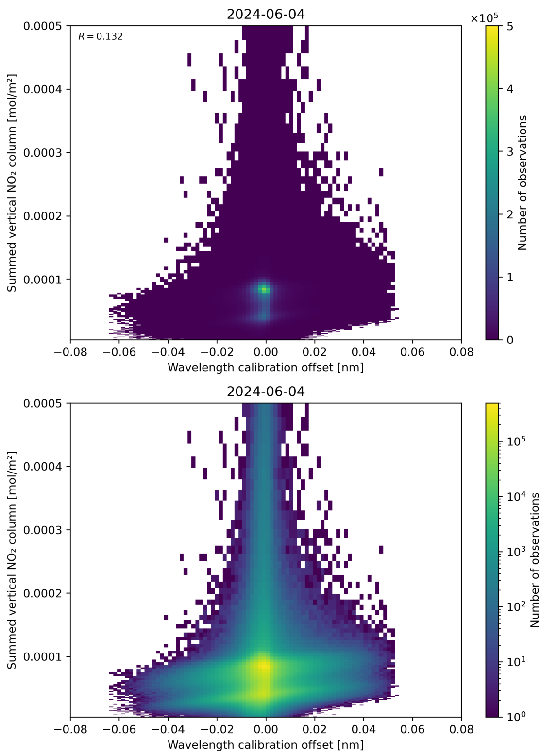
Figure 177: Scatter density plot of “Wavelength calibration offset” against “Summed vertical NO 2 column” for 2024-06-03 to 2024-06-05.
