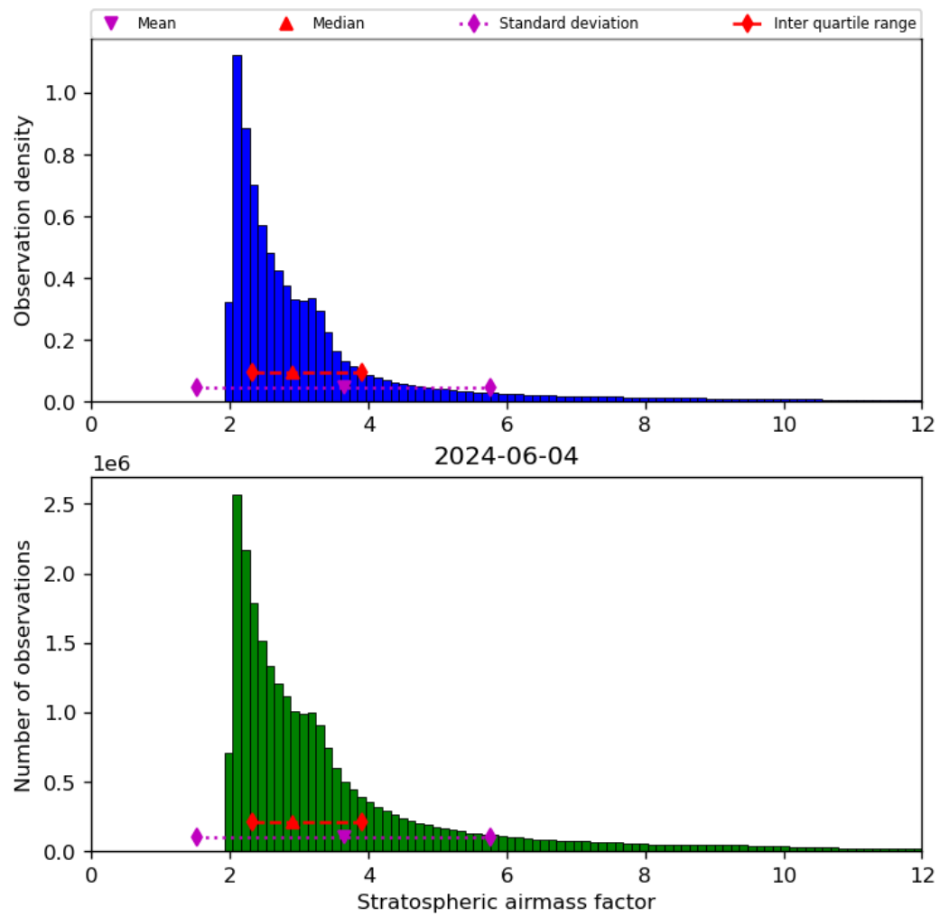
Figure 44: Histogram of “Stratospheric airmass factor” for 2024-06-03 to 2024-06-05
