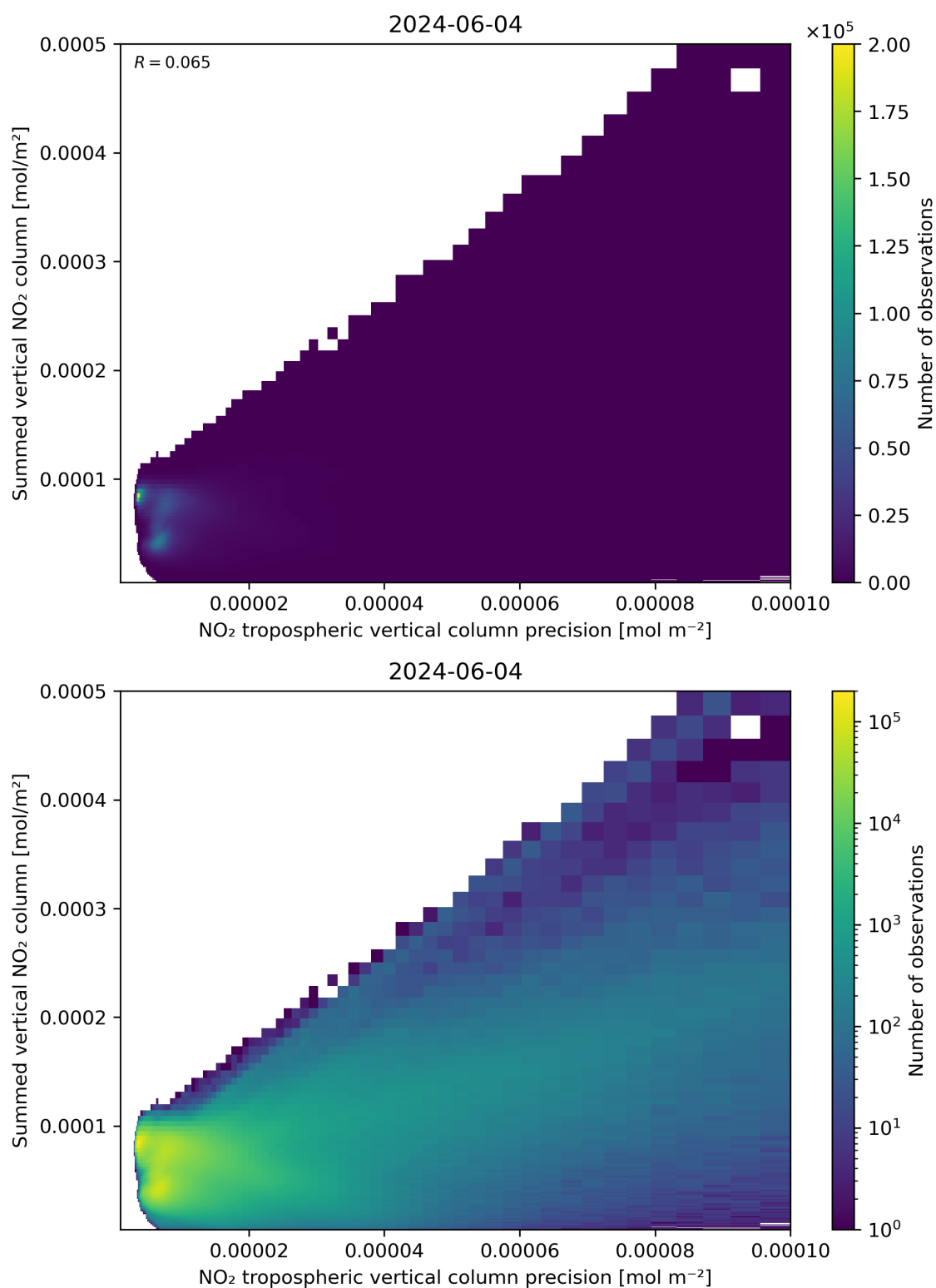
Figure 136: Scatter density plot of “NO 2 tropospheric vertical column precision” against “Summed vertical NO 2 column” for 2024-06-03 to 2024-06-05.
