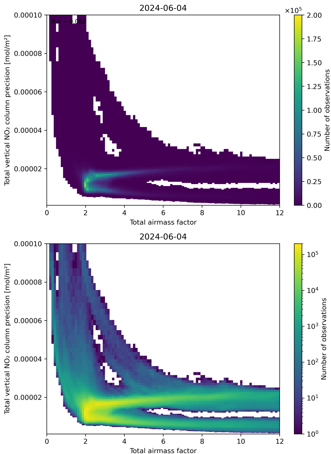
Figure 68: Scatter density plot of “Total airmass factor” against “Total vertical NO 2 column precision” for 2024-06-03 to 2024-06-05.
