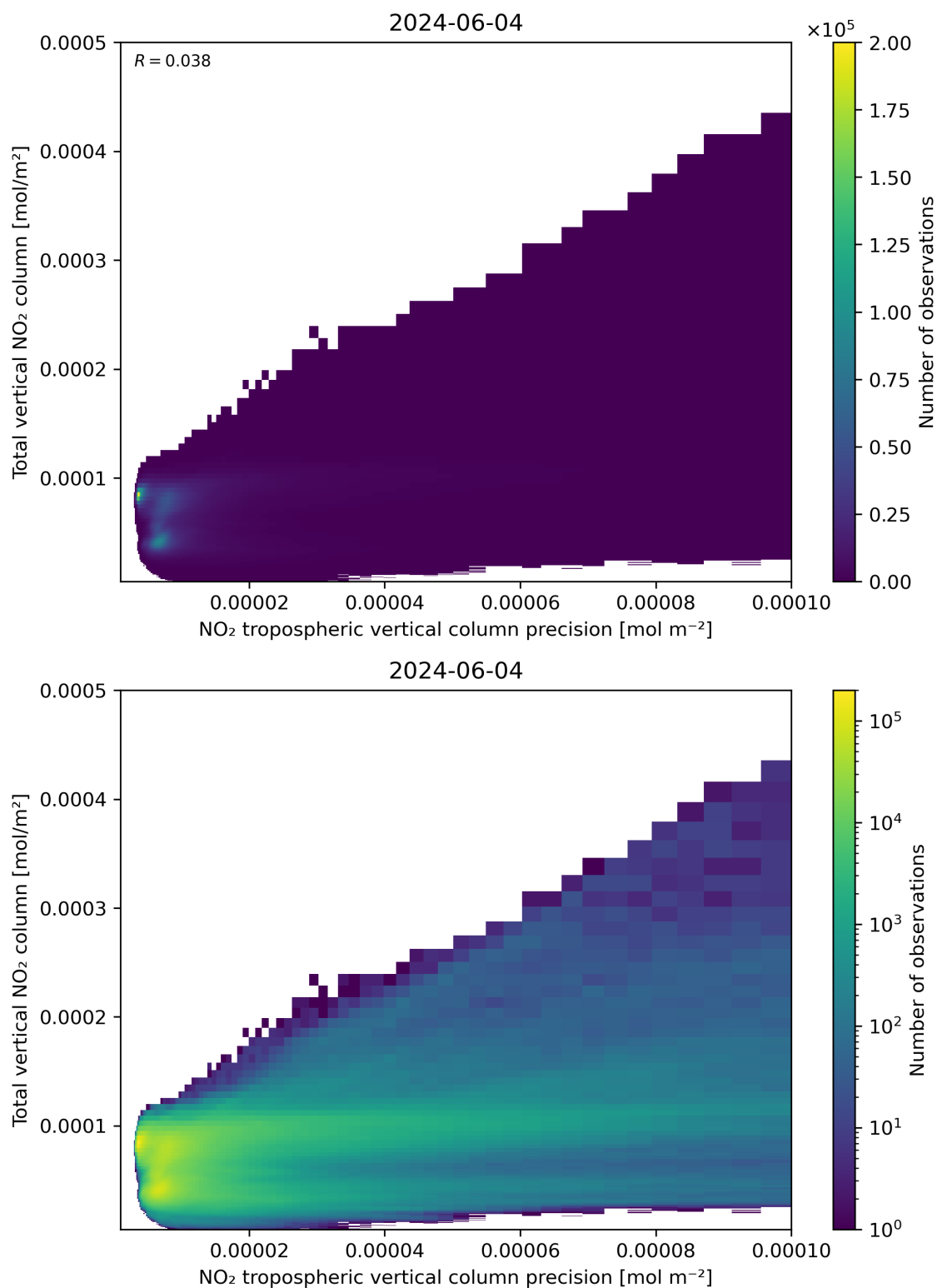
Figure 138: Scatter density plot of “NO 2 tropospheric vertical column precision” against “Total vertical NO 2 column” for 2024-06-03 to 2024-06-05.
