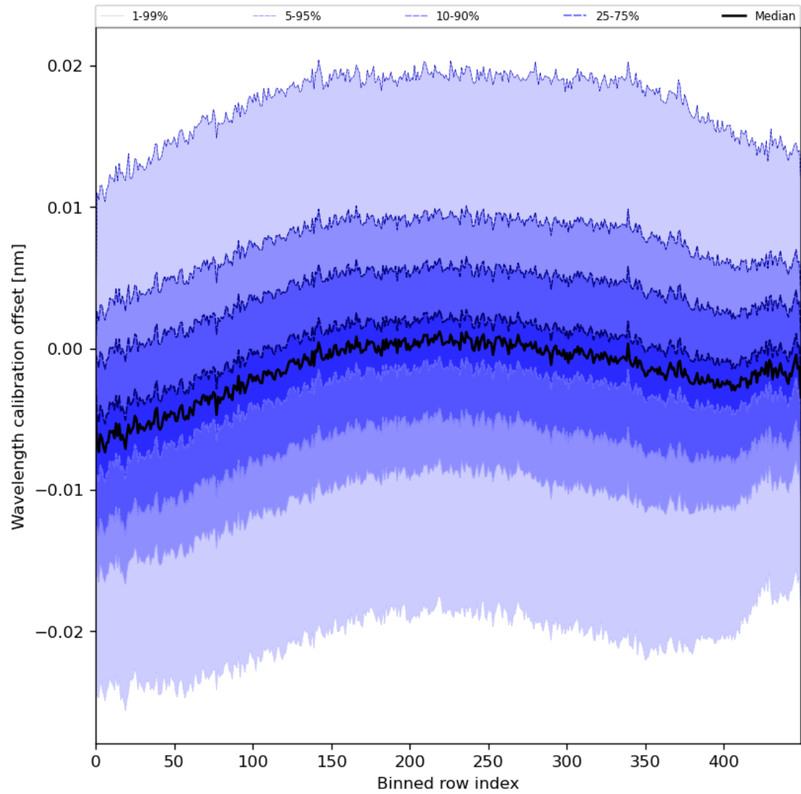
Figure 52: Along track statistics of “Wavelength calibration offset” for 2024-06-03 to 2024-06-05
