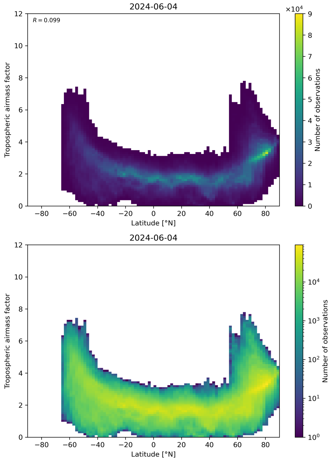
Figure 85: Scatter density plot of “Latitude” against “Tropospheric air mass factor” for 2024-06-03 to 2024-06-05.
