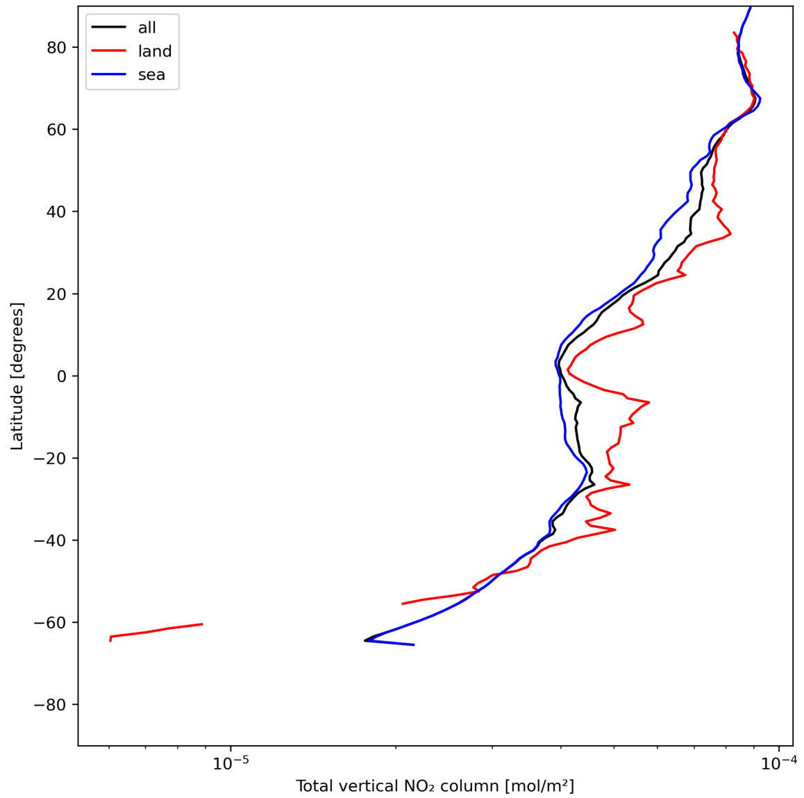
Figure 21: Zonal average of “Total vertical NO 2 column” for 2024-06-03 to 2024-06-05.
