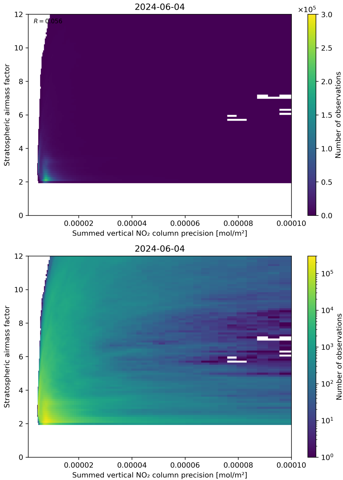
Figure 106: Scatter density plot of “Summed vertical NO 2 column precision” against “Stratospheric airmass factor” for 2024-06-03 to 2024-06-05.
