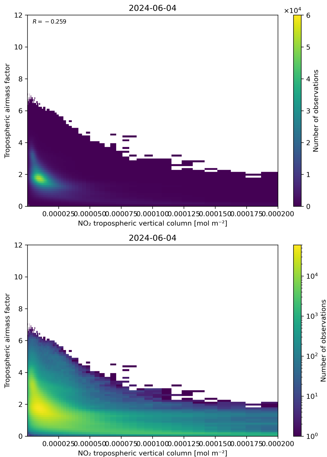
Figure 123: Scatter density plot of “NO 2 tropospheric vertical column” against “Tropospheric air mass factor” for 2024-06-03 to 2024-06-05.
