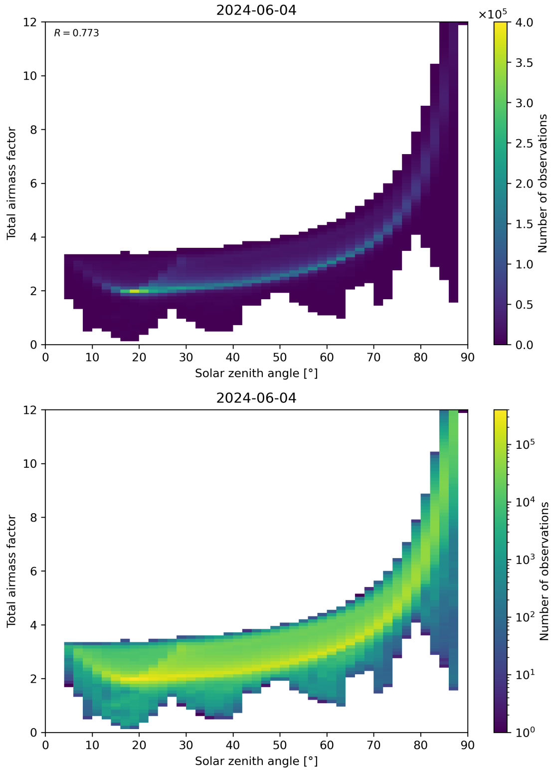
Figure 146: Scatter density plot of “Solar zenith angle” against “Total air mass factor” for 2024-06-03 to 2024-06-05.
