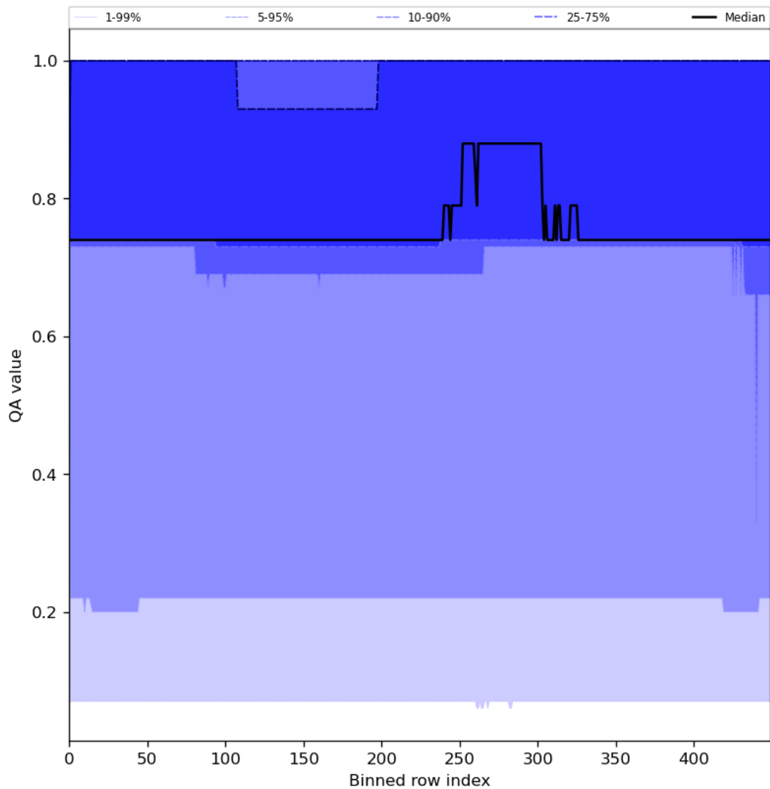
Figure 45: Along track statistics of “QA value” for 2024-06-03 to 2024-06-05
