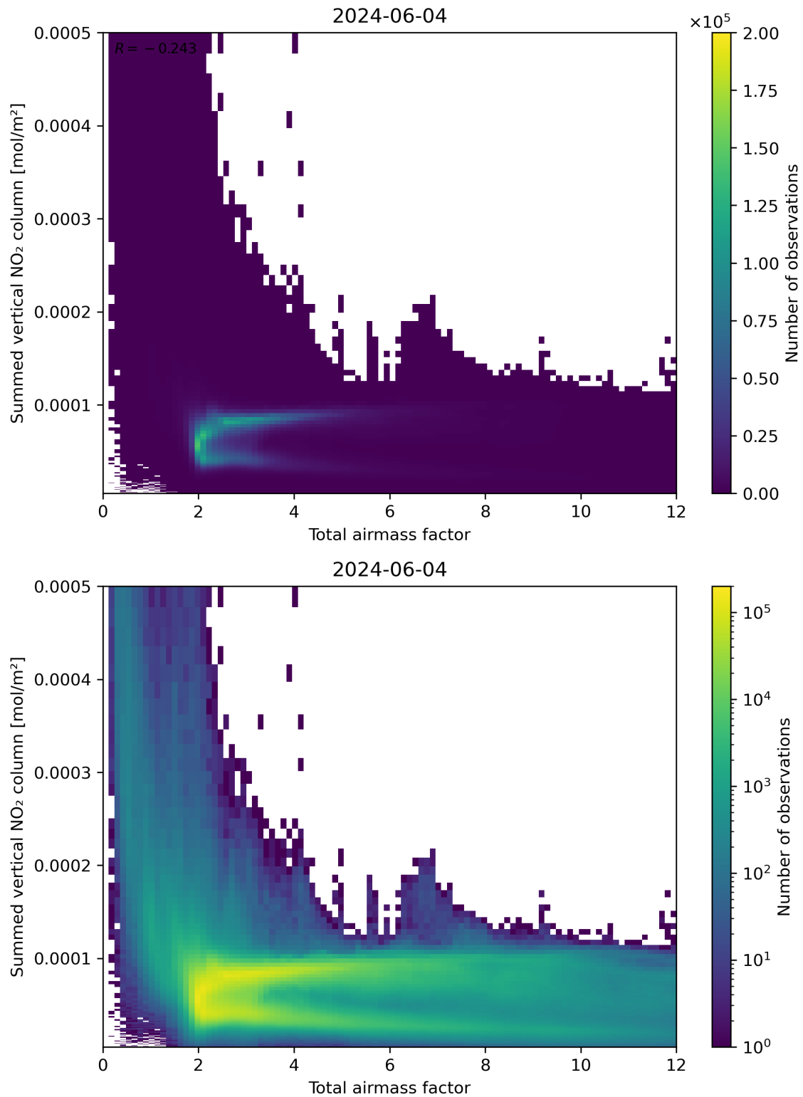
Figure 65: Scatter density plot of “Total airmass factor” against “Summed vertical NO 2 column” for 2024-06-03 to 2024-06-05.
