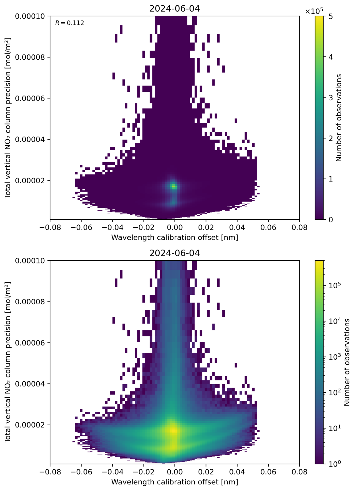
Figure 180: Scatter density plot of “Wavelength calibration offset” against “Total vertical NO 2 column precision” for 2024-06-03 to 2024-06-05.
