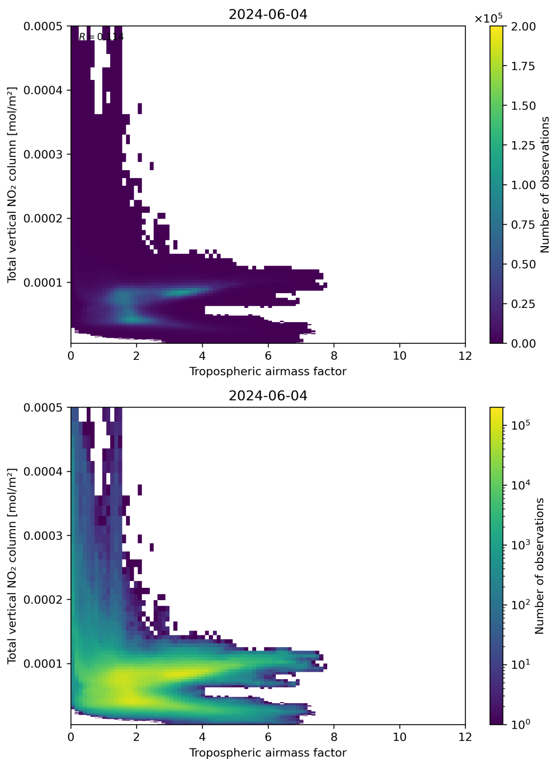
Figure 77: Scatter density plot of “Tropospheric airmass factor” against “Total vertical NO 2 column” for 2024-06-03 to 2024-06-05.
