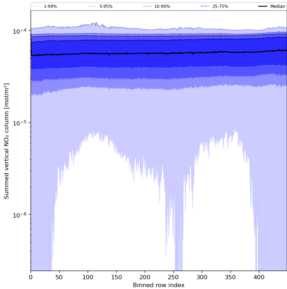
Figure 57: Along track statistics of “Summed vertical NO 2 column” for 2024-06-03 to 2024-06-05
