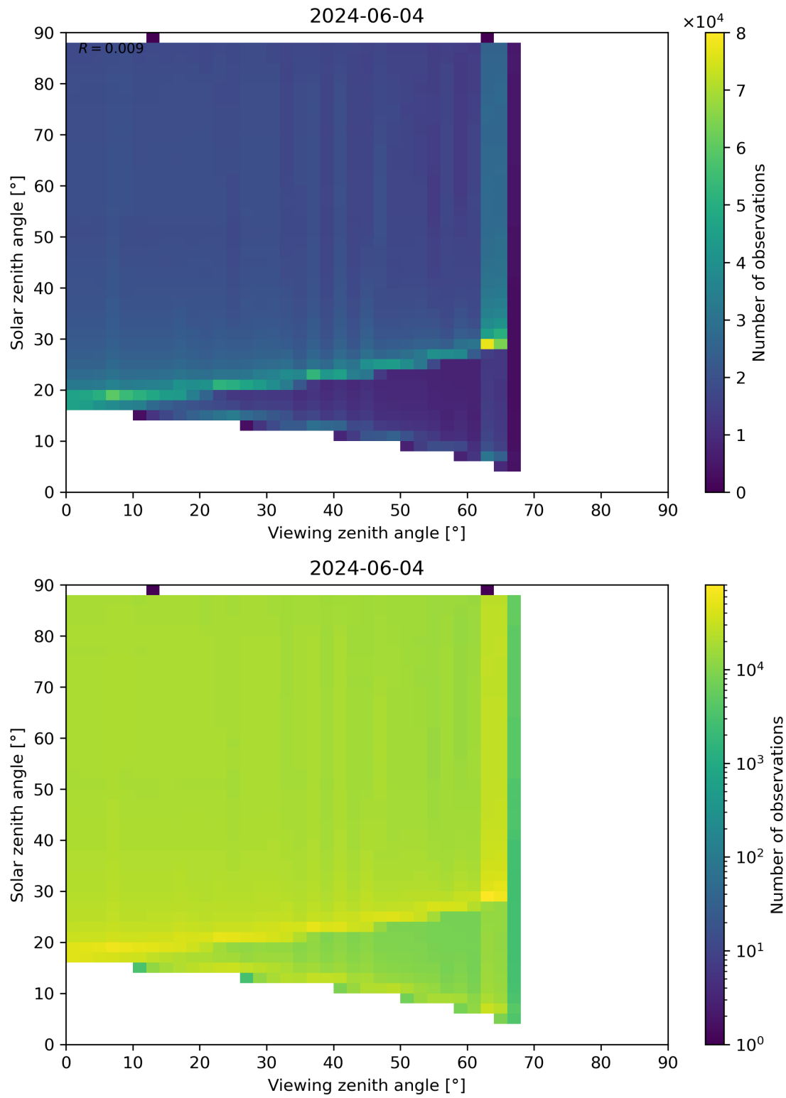
Figure 172: Scatter density plot of “Viewing zenith angle” against “Solar zenith angle” for 2024-06-03 to 2024-06-05.
