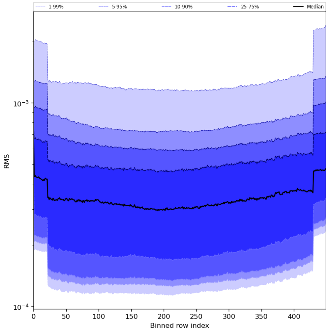
Figure 60: Along track statistics of “RMS” for 2024-06-03 to 2024-06-05
