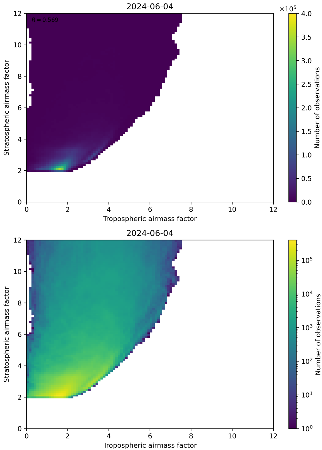
Figure 71: Scatter density plot of “Tropospheric airmass factor” against “Stratospheric airmass factor” for 2024-06-03 to 2024-06-05.
