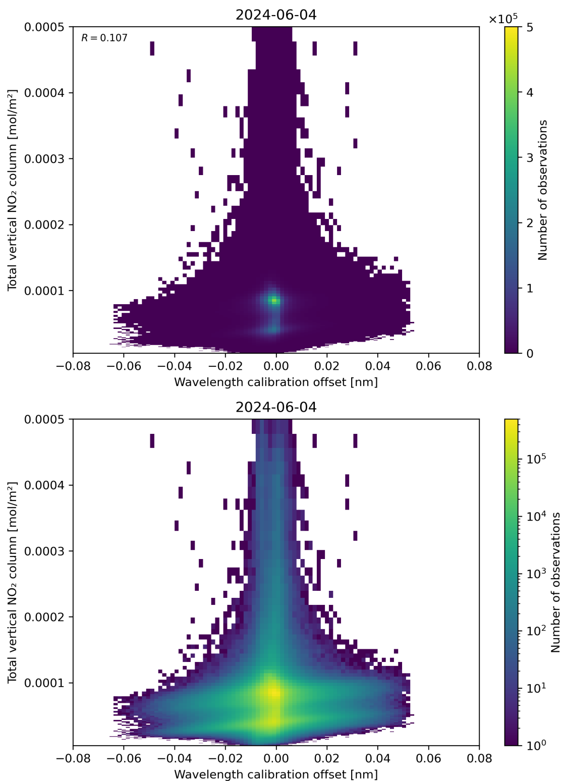
Figure 179: Scatter density plot of “Wavelength calibration offset” against “Total vertical NO 2 column” for 2024-06-03 to 2024-06-05.
