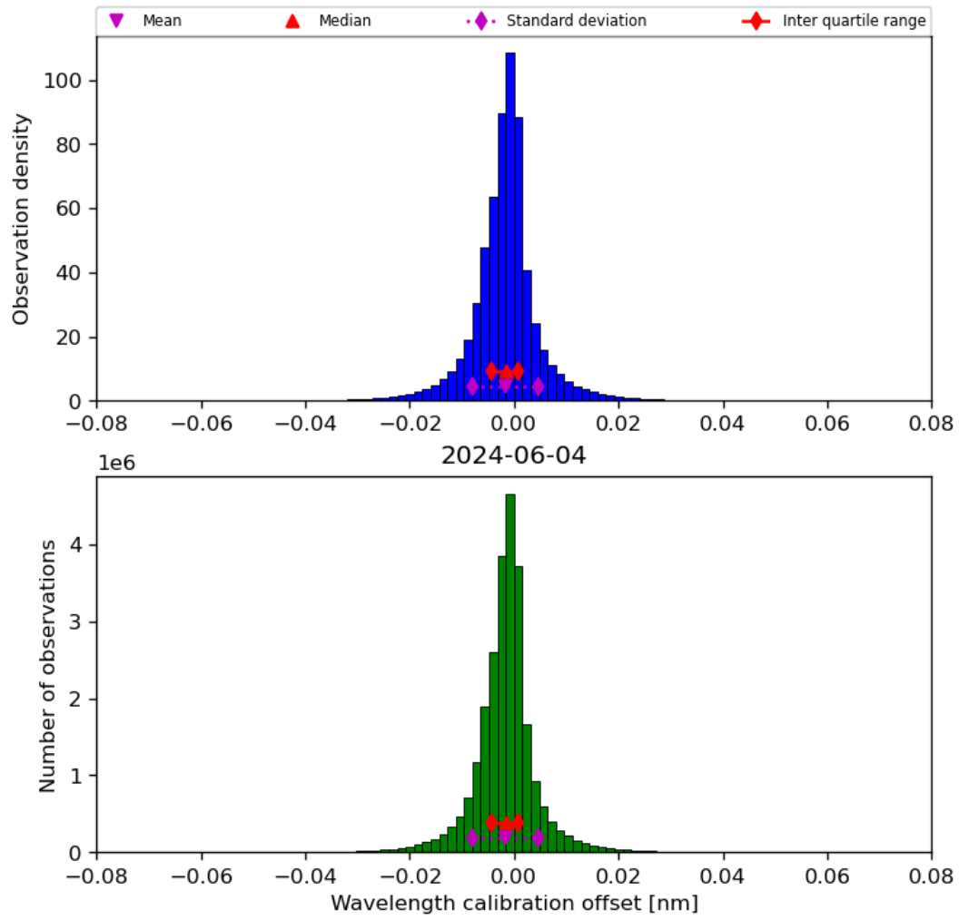
Figure 35: Histogram of “Wavelength calibration offset” for 2024-06-03 to 2024-06-05
