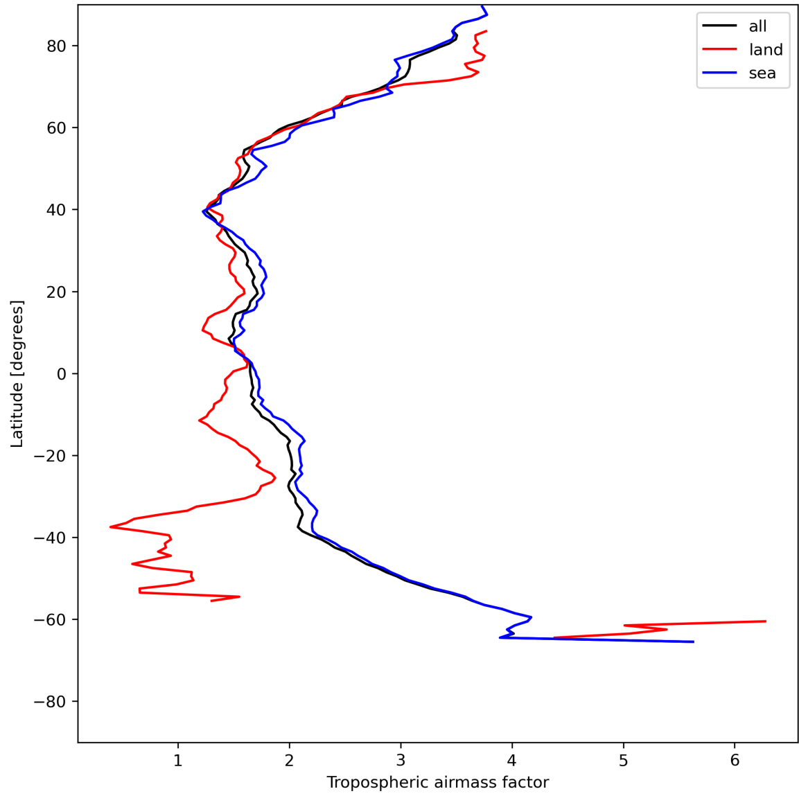
Figure 14: Zonal average of “Tropospheric airmass factor” for 2024-06-03 to 2024-06-05.
