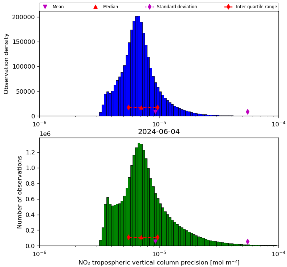
Figure 30: Histogram of “NO 2 tropospheric vertical column precision” for 2024-06-03 to 2024-06-05
