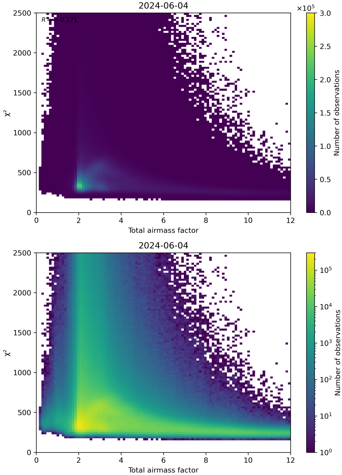
Figure 63: Scatter density plot of “Total airmass factor” against “ \chi^2 ” for 2024-06-03 to 2024-06-05.
