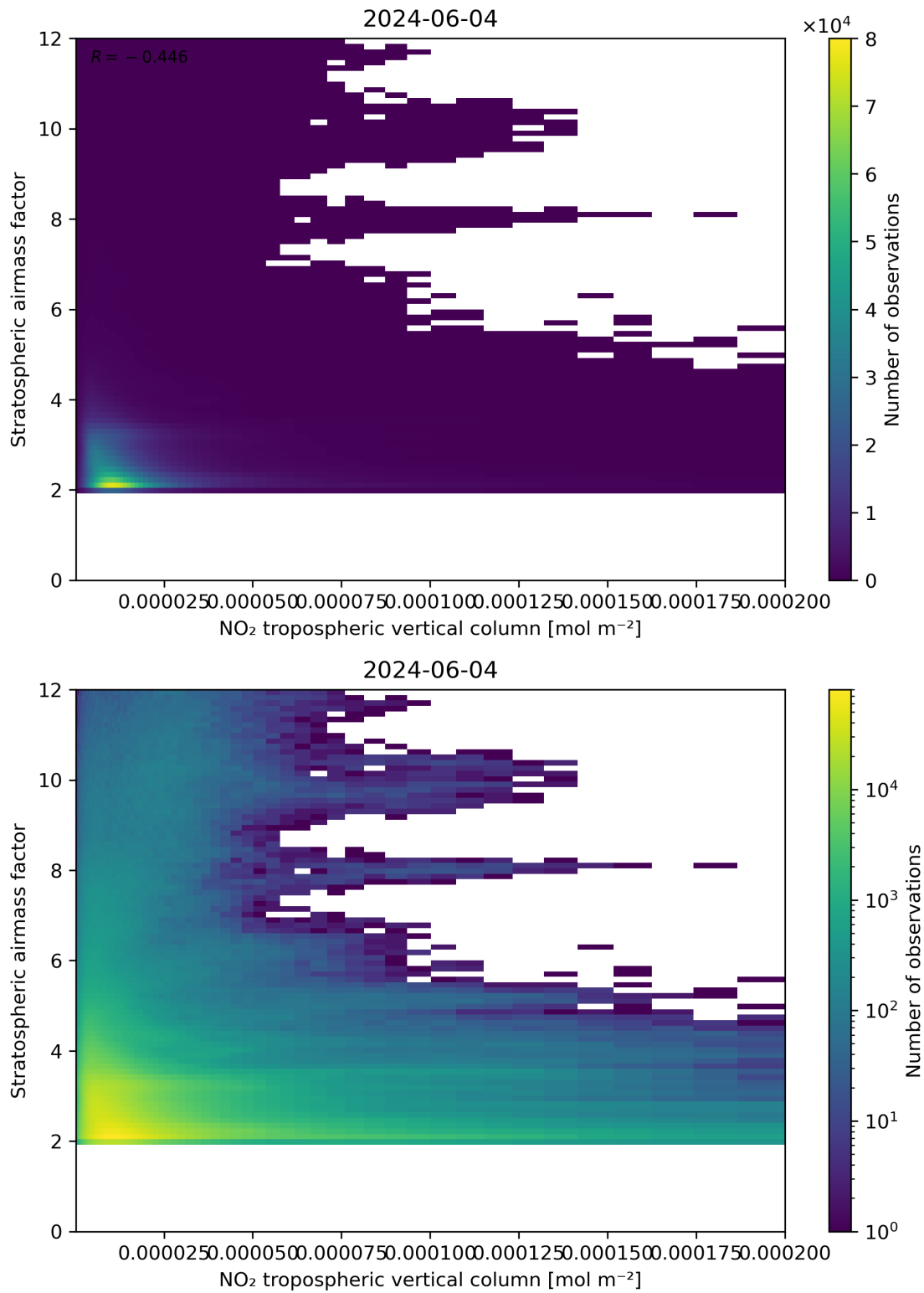
Figure 121: Scatter density plot of “NO 2 tropospheric vertical column” against “Stratospheric air mass factor” for 2024-06-03 to 2024-06-05.
