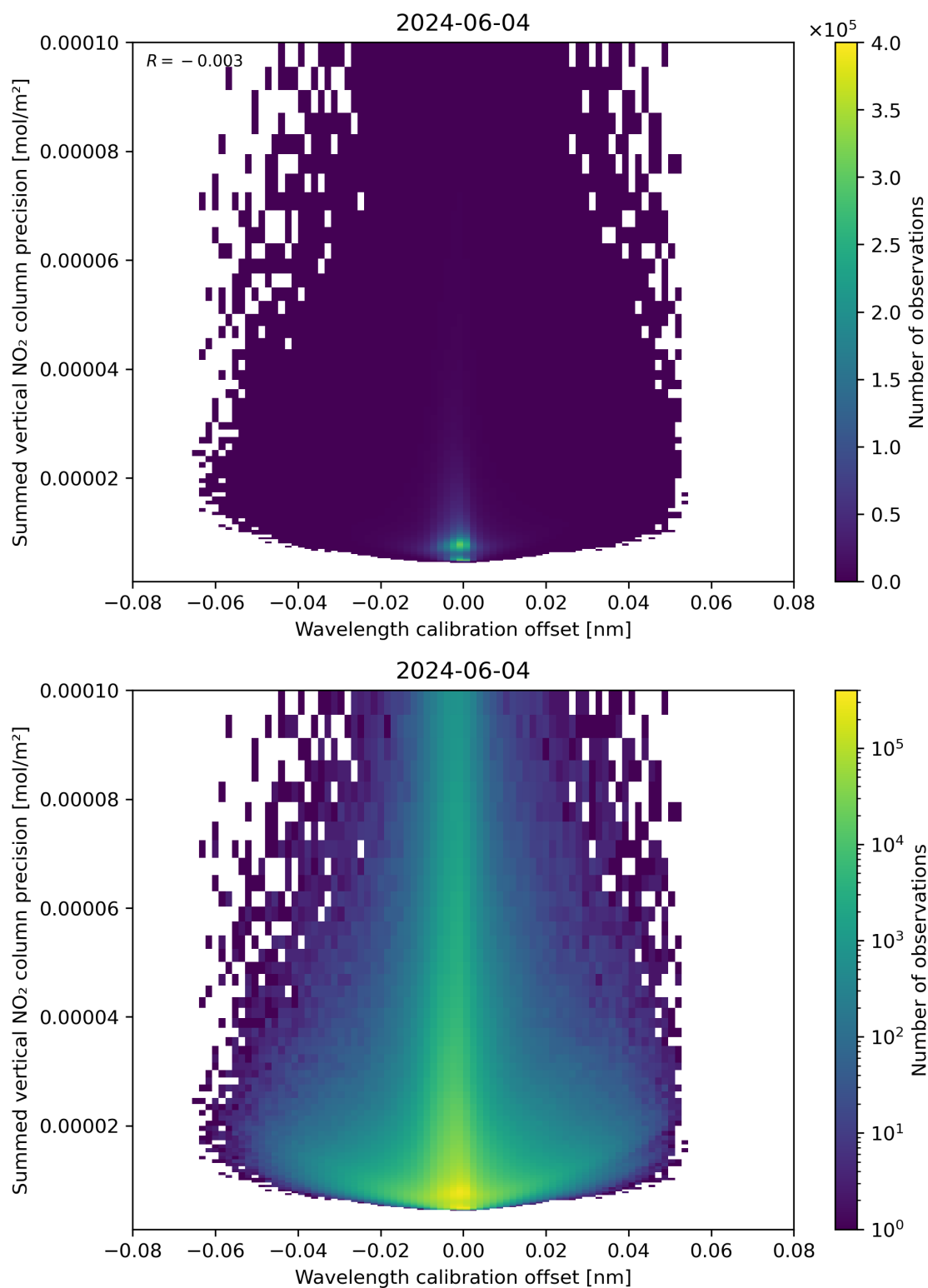
Figure 178: Scatter density plot of “Wavelength calibration offset” against “Summed vertical NO 2 column precision” for 2024-06-03 to 2024-06-05.
