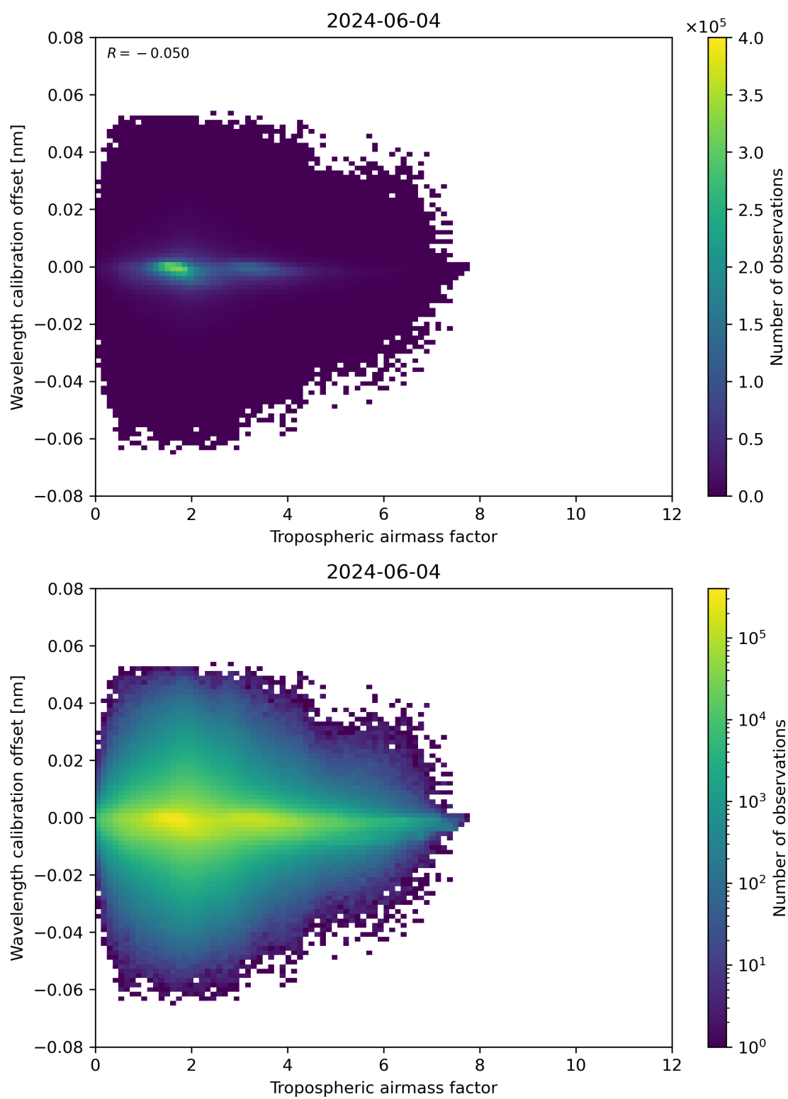
Figure 80: Scatter density plot of “Tropospheric airmass factor” against “Wavelength calibration offset” for 2024-06-03 to 2024-06-05.
