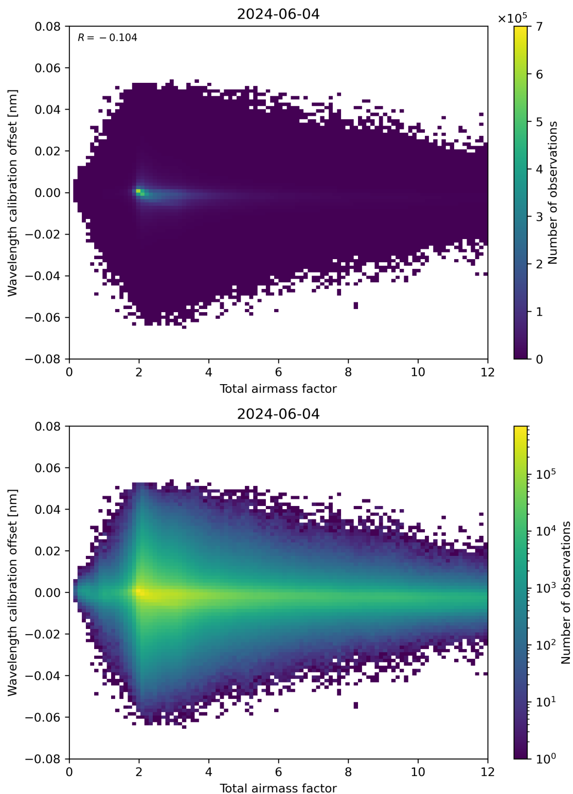
Figure 70: Scatter density plot of “Total airmass factor” against “Wavelength calibration offset” for 2024-06-03 to 2024-06-05.
