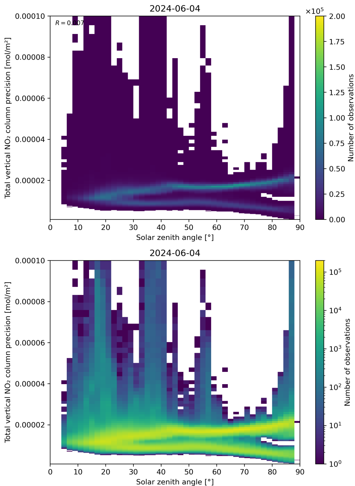
Figure 154: Scatter density plot of “Solar zenith angle” against “Total vertical NO 2 column precision” for 2024-06-03 to 2024-06-05.
