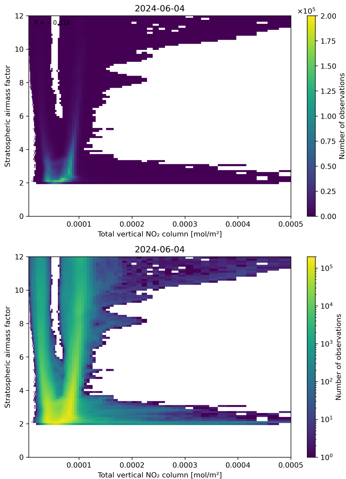
Figure 110: Scatter density plot of “Total vertical NO 2 column” against “Stratospheric air mass factor” for 2024-06-03 to 2024-06-05.
