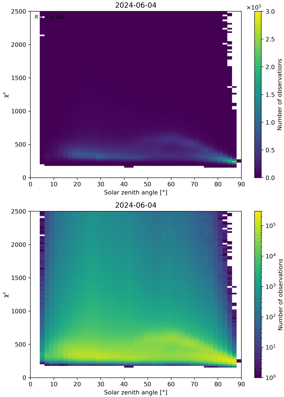
Figure 148: Scatter density plot of “Solar zenith angle” against “ \chi^2 ” for 2024-06-03 to 2024-06-05.
