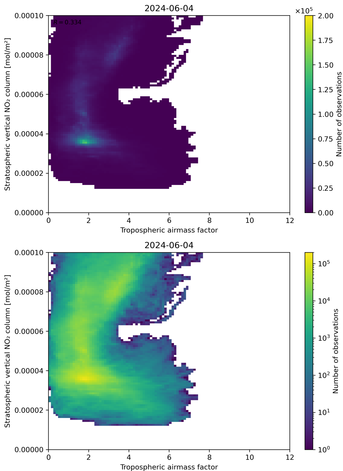
Figure 74: Scatter density plot of “Tropospheric air mass factor” against “Stratospheric vertical NO 2 column” for 2024-06-03 to 2024-06-05.
