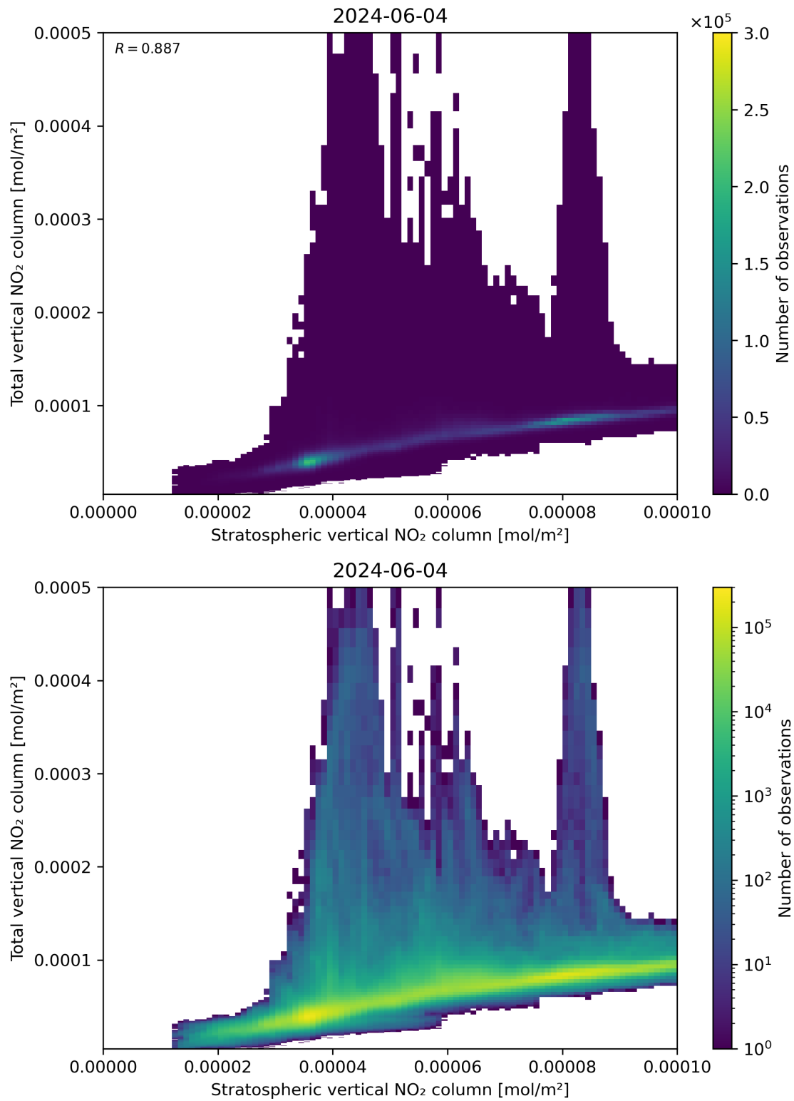
Figure 100: Scatter density plot of “Stratospheric vertical NO 2 column” against “Total vertical NO 2 column” for 2024-06-03 to 2024-06-05.
