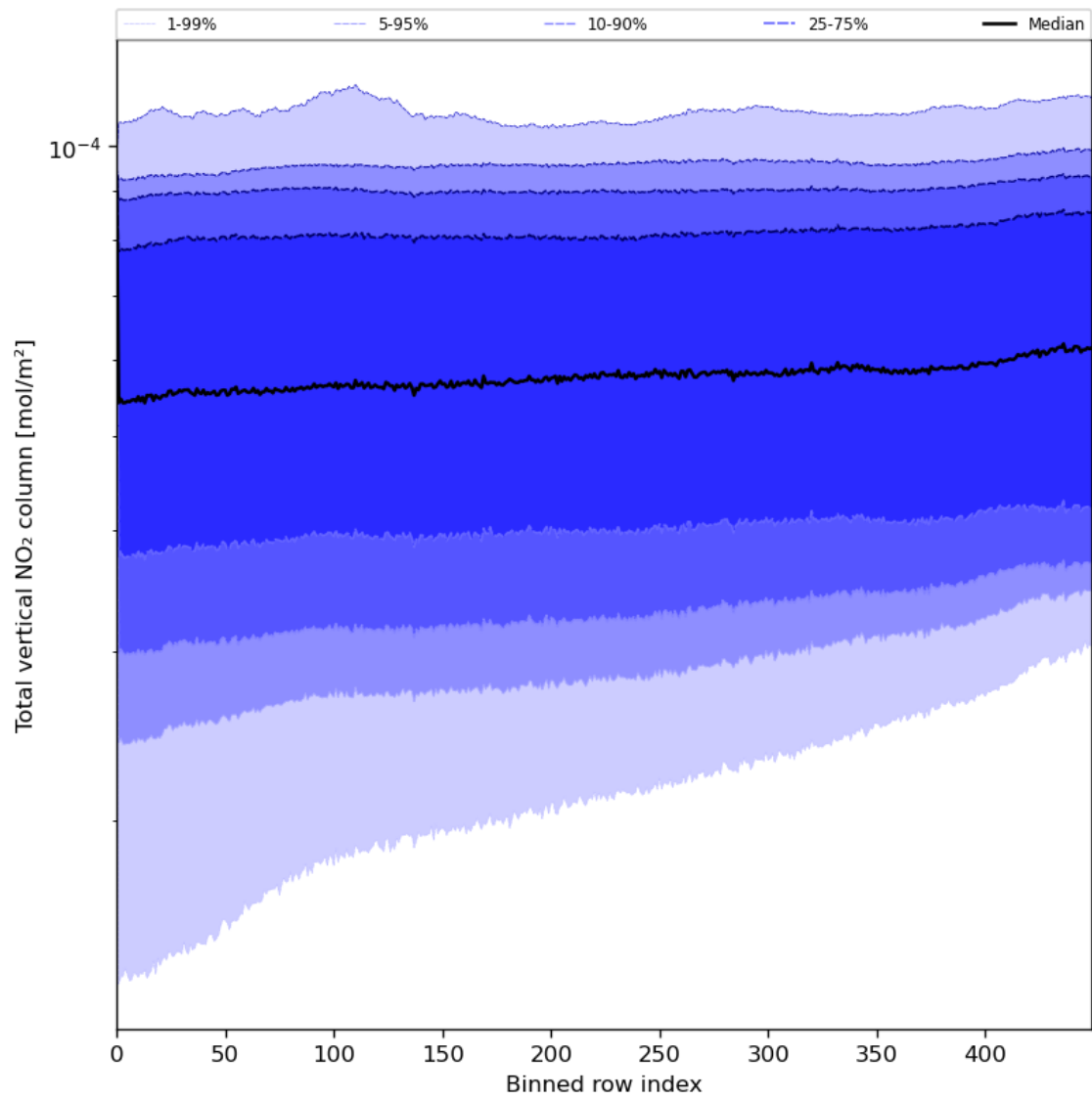
Figure 55: Along track statistics of “Total vertical NO 2 column” for 2024-06-03 to 2024-06-05
