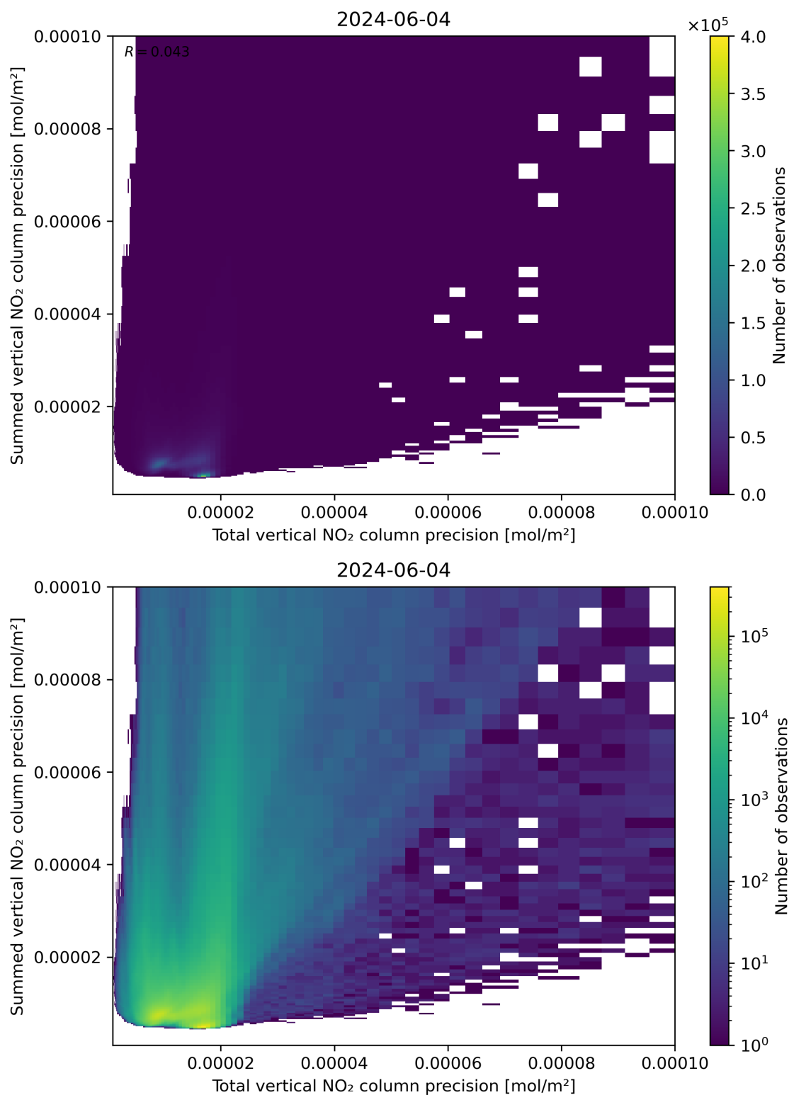
Figure 118: Scatter density plot of “Total vertical NO 2 column precision” against “Summed vertical NO 2 column precision” for 2024-06-03 to 2024-06-05.
