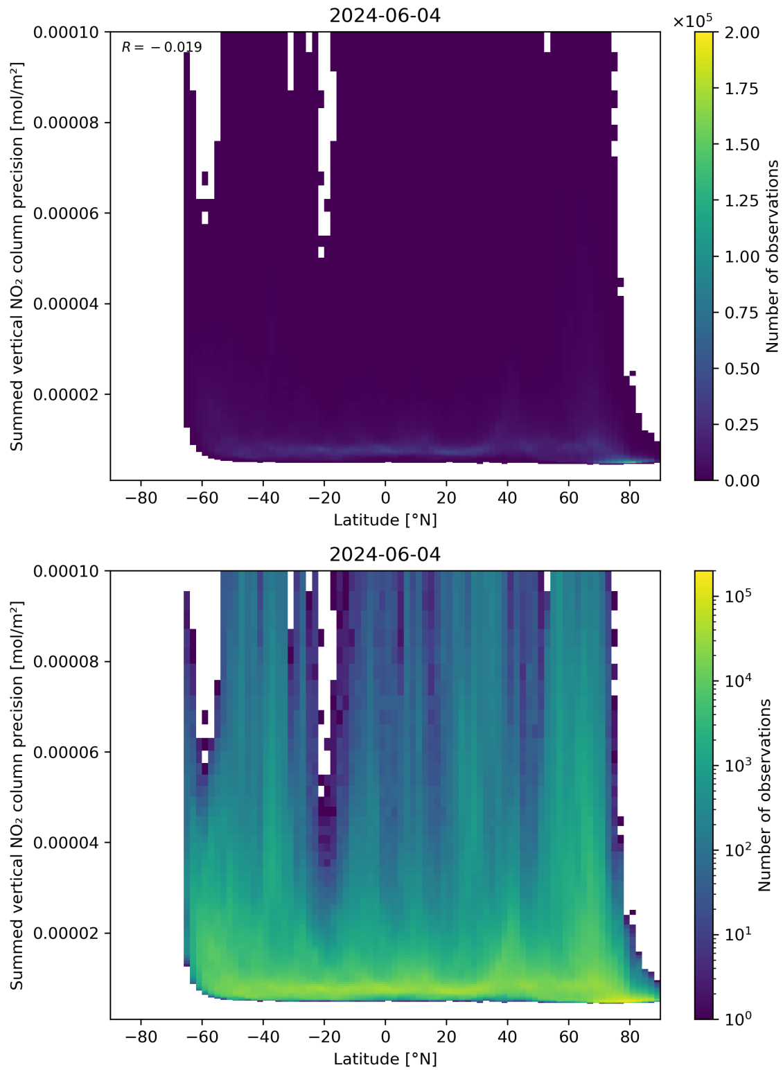
Figure 89: Scatter density plot of “Latitude” against “Summed vertical NO 2 column precision” for 2024-06-03 to 2024-06-05.
