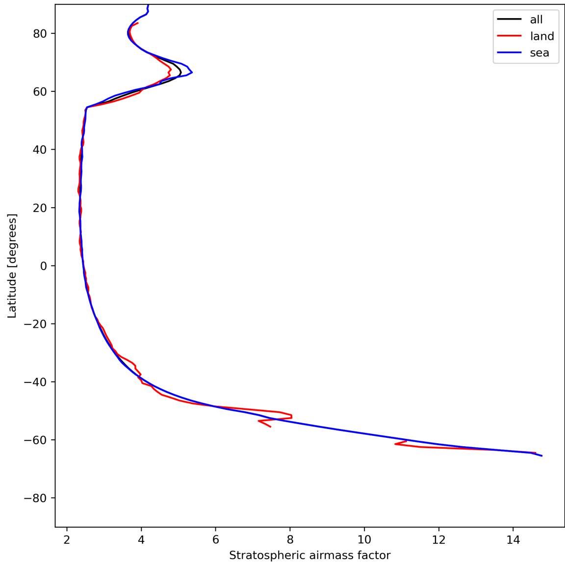
Figure 27: Zonal average of “Stratospheric airmass factor” for 2024-06-03 to 2024-06-05.
