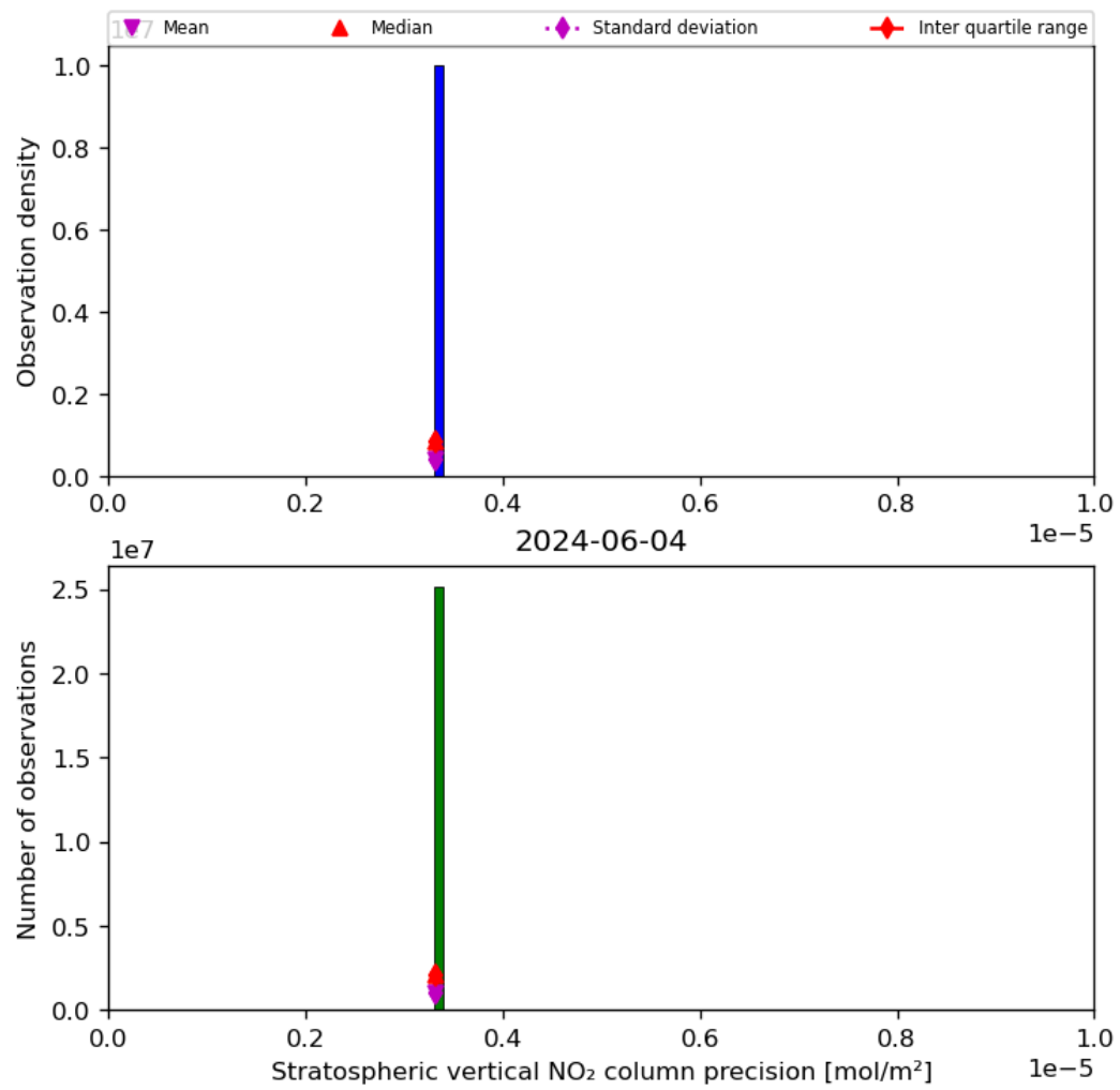
Figure 37: Histogram of “Stratospheric vertical NO 2 column precision” for 2024-06-03 to 2024-06-05
