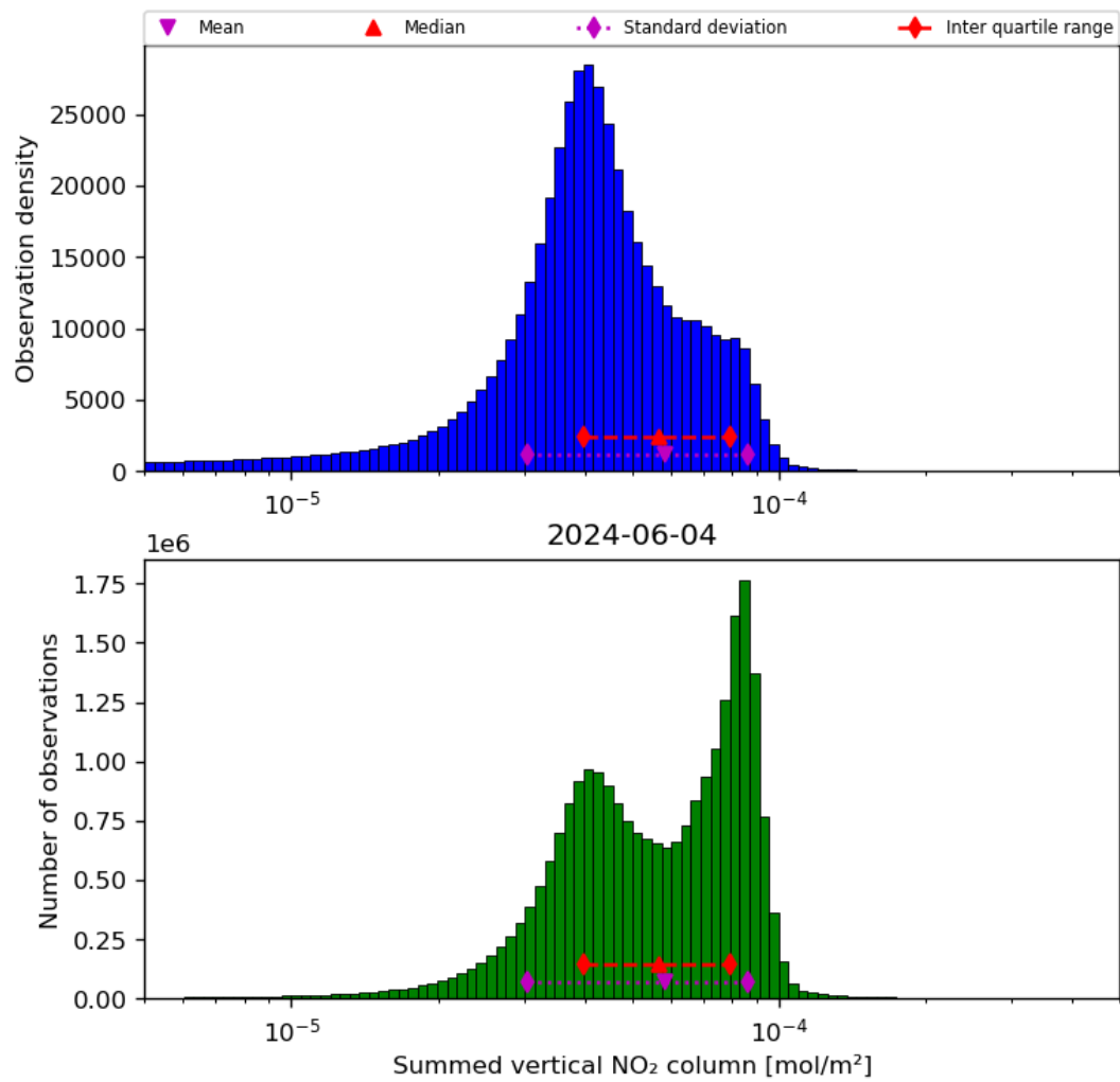
Figure 40: Histogram of “Summed vertical NO 2 column” for 2024-06-03 to 2024-06-05
