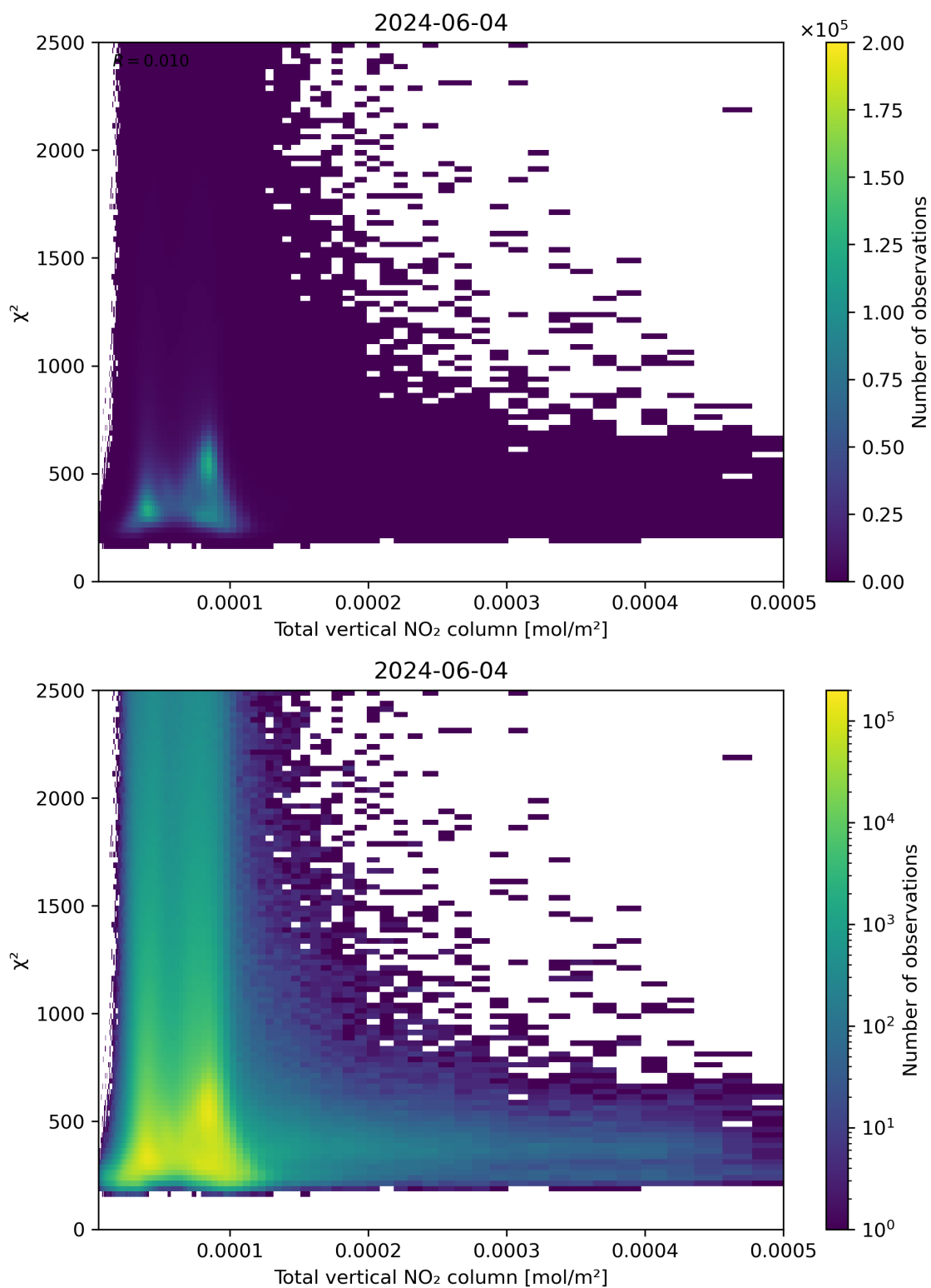
Figure 111: Scatter density plot of “Total vertical NO 2 column” against “ \chi^2 ” for 2024-06-03 to 2024-06-05.
