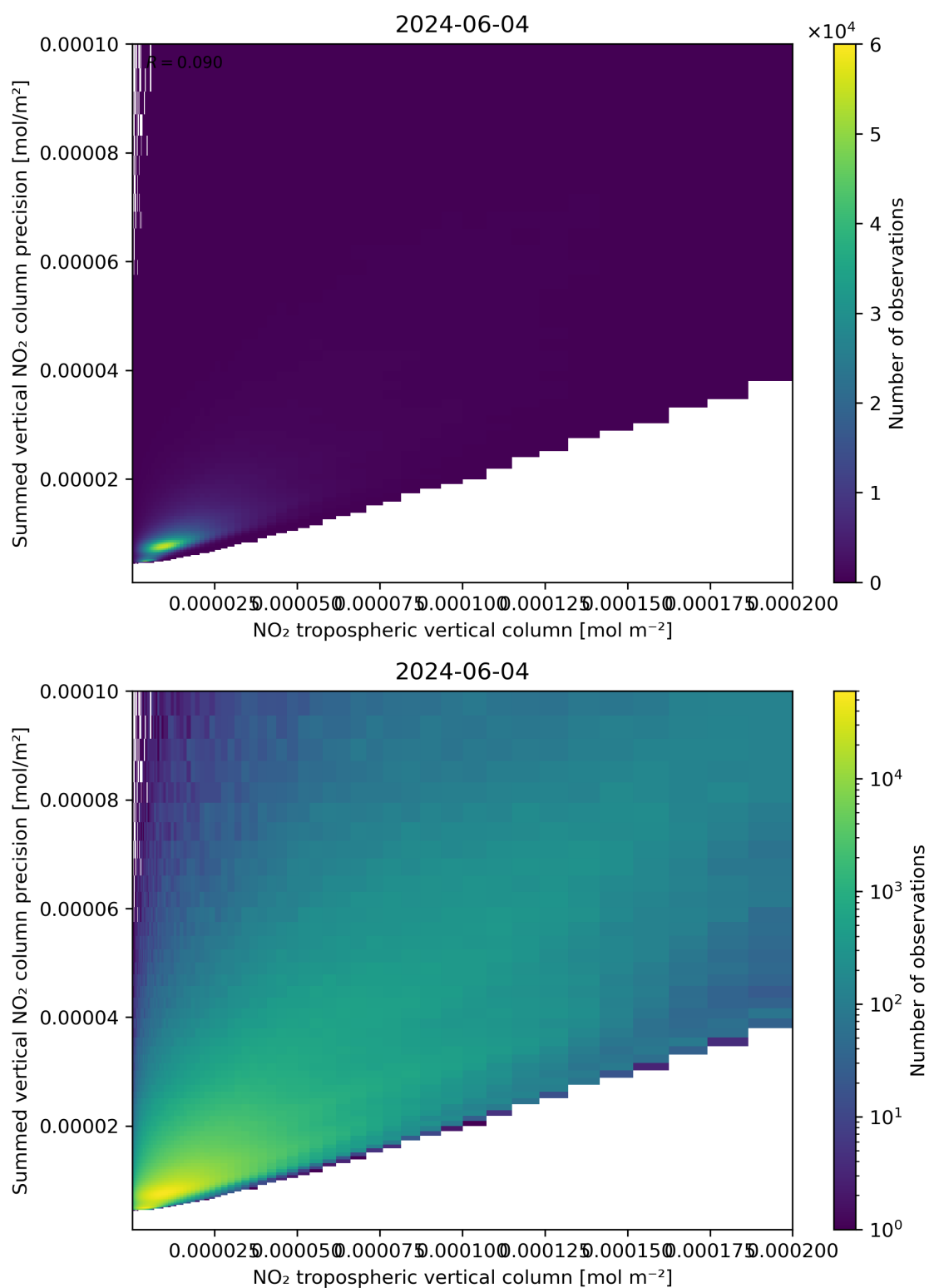
Figure 127: Scatter density plot of “NO 2 tropospheric vertical column” against “Summed vertical NO 2 column precision” for 2024-06-03 to 2024-06-05.
