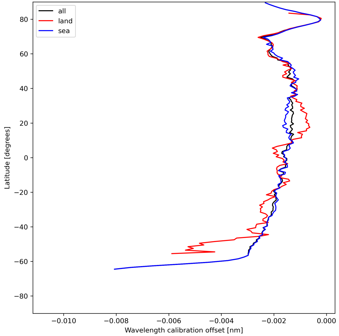
Figure 18: Zonal average of “Wavelength calibration offset” for 2024-06-04 to 2024-06-06.
