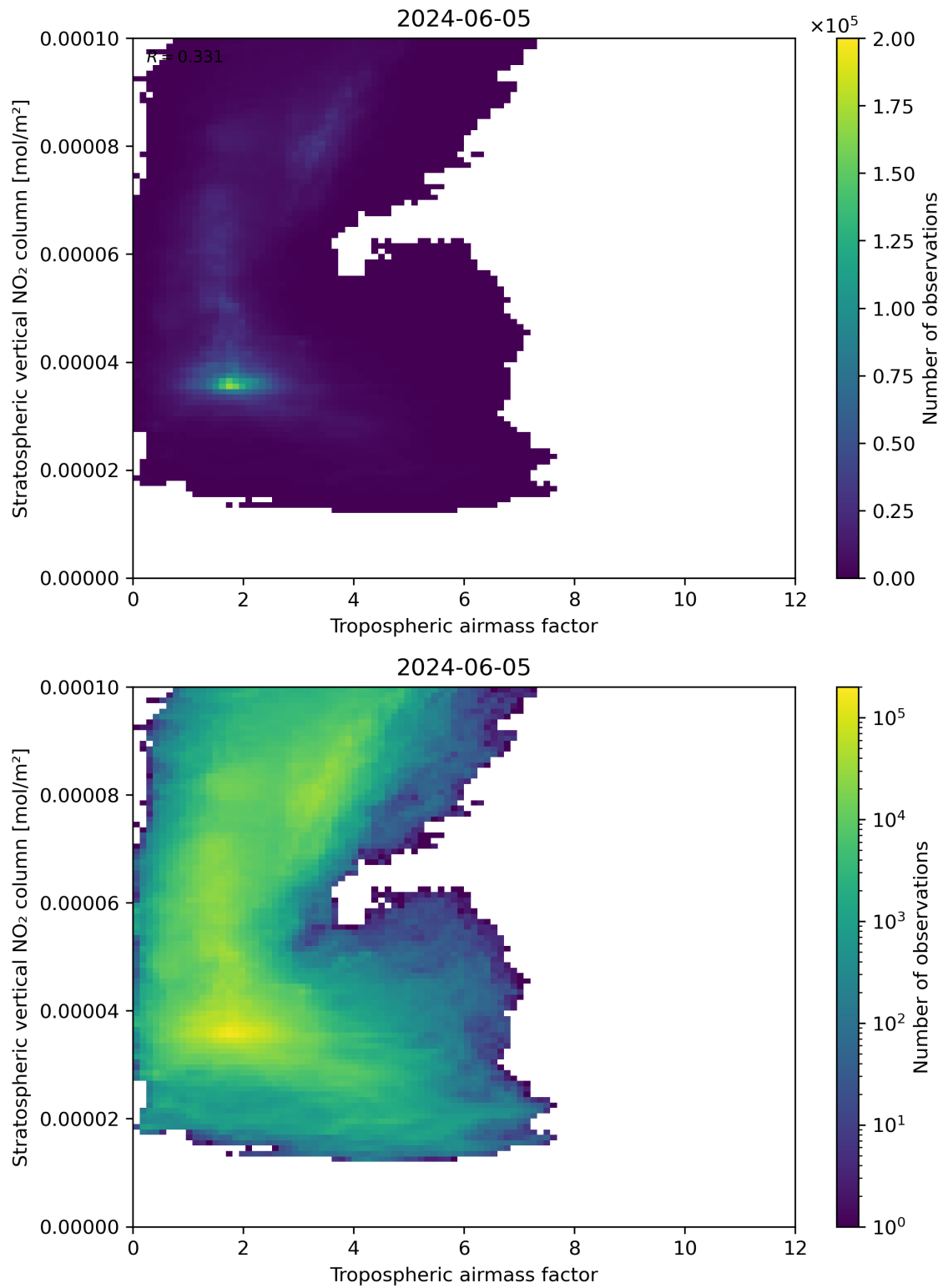
Figure 74: Scatter density plot of “Tropospheric airmass factor” against “Stratospheric vertical NO 2 column” for 2024-06-04 to 2024-06-06.
