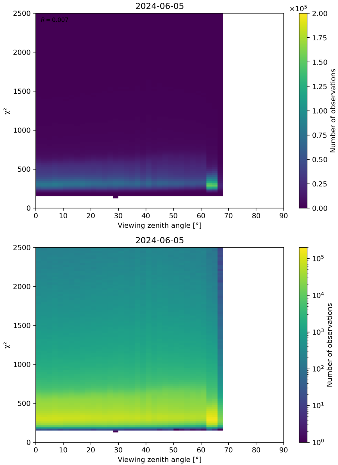
Figure 162: Scatter density plot of “Viewing zenith angle” against “ \chi^2 ” for 2024-06-04 to 2024-06-06.
