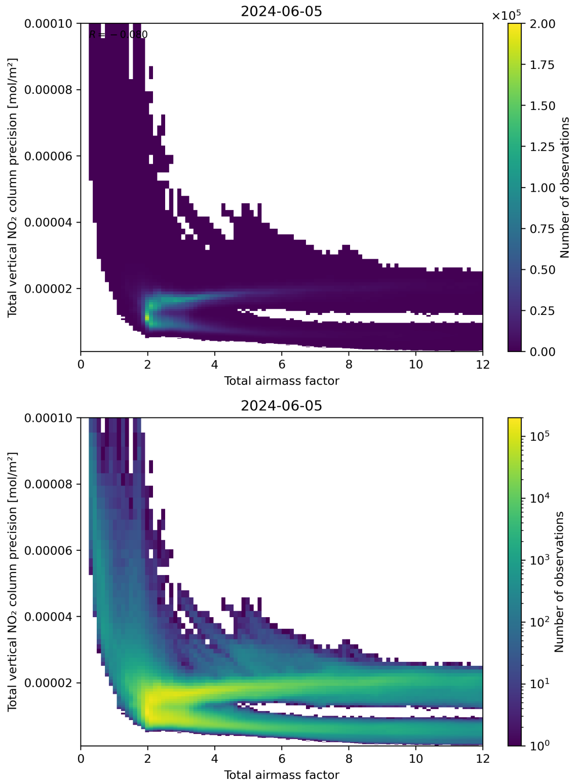
Figure 68: Scatter density plot of “Total airmass factor” against “Total vertical NO 2 column precision” for 2024-06-04 to 2024-06-06.
