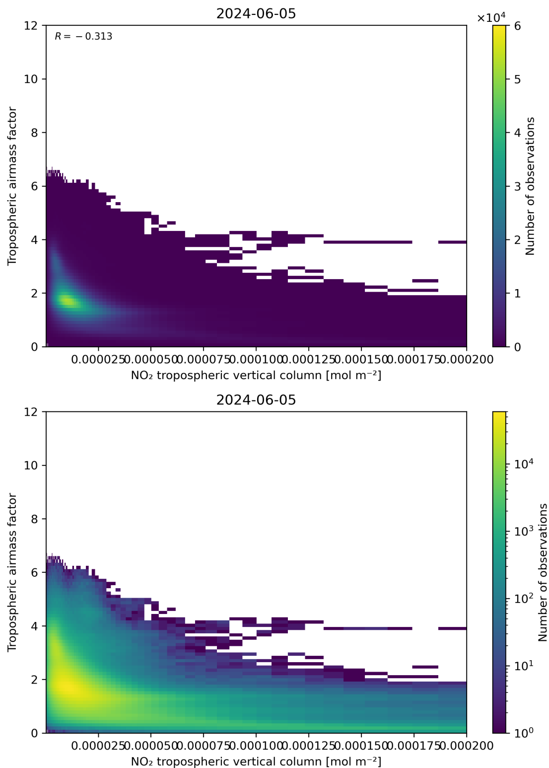
Figure 123: Scatter density plot of “NO 2 tropospheric vertical column” against “Tropospheric air mass factor” for 2024-06-04 to 2024-06-06.
