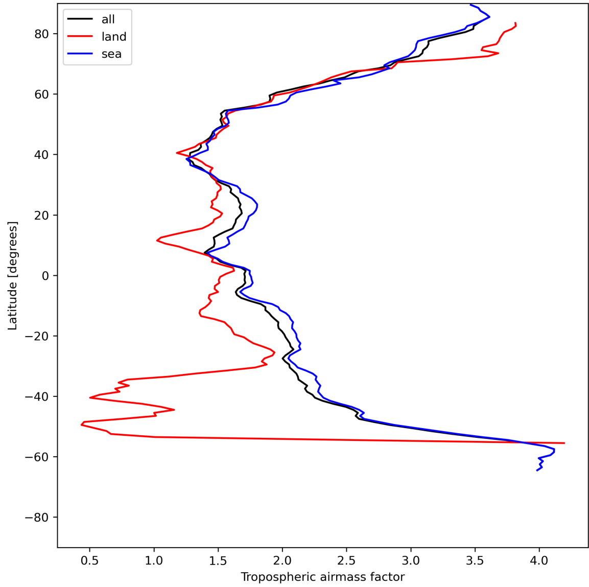
Figure 14: Zonal average of “Tropospheric airmass factor” for 2024-06-04 to 2024-06-06.
