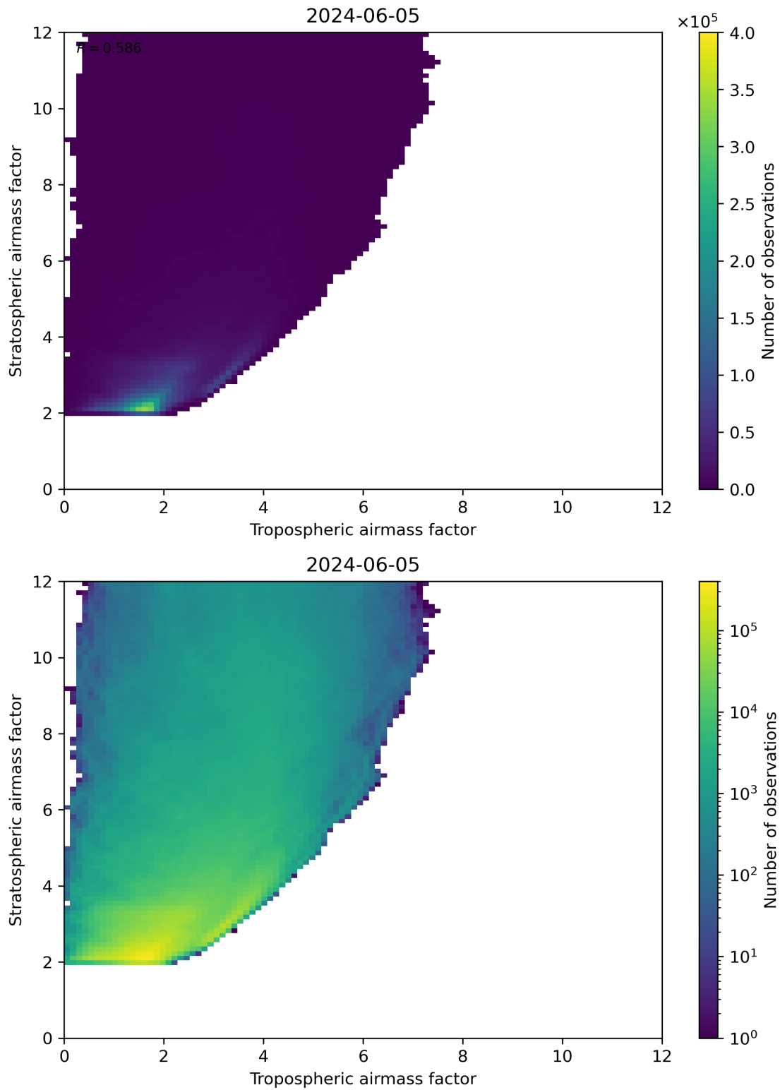
Figure 71: Scatter density plot of “Tropospheric airmass factor” against “Stratospheric airmass factor” for 2024-06-04 to 2024-06-06.
