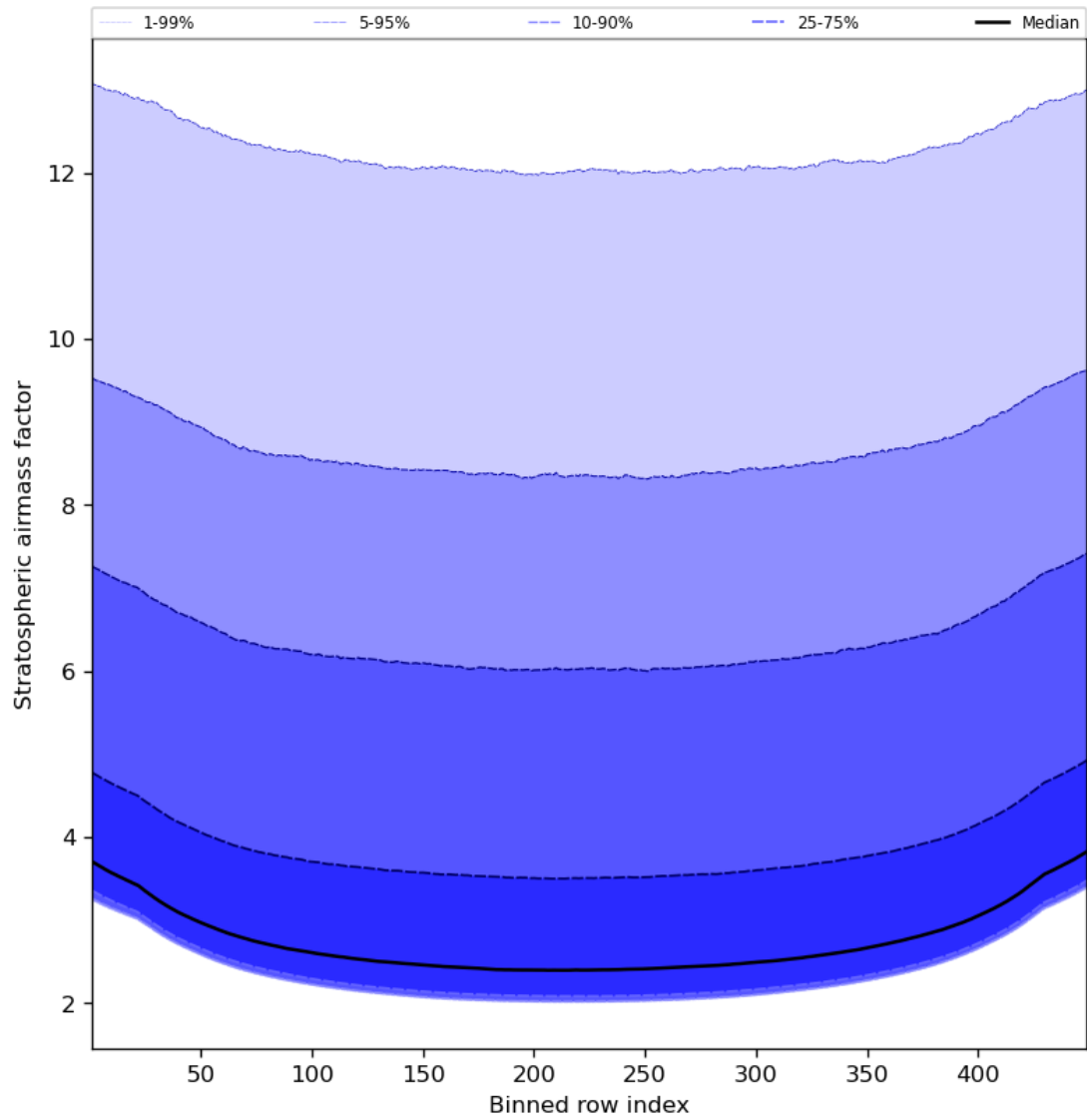
Figure 61: Along track statistics of “Stratospheric airmass factor” for 2024-06-04 to 2024-06-06
