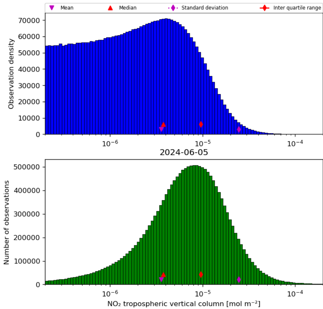
Figure 29: Histogram of “NO 2 tropospheric vertical column” for 2024-06-04 to 2024-06-06
