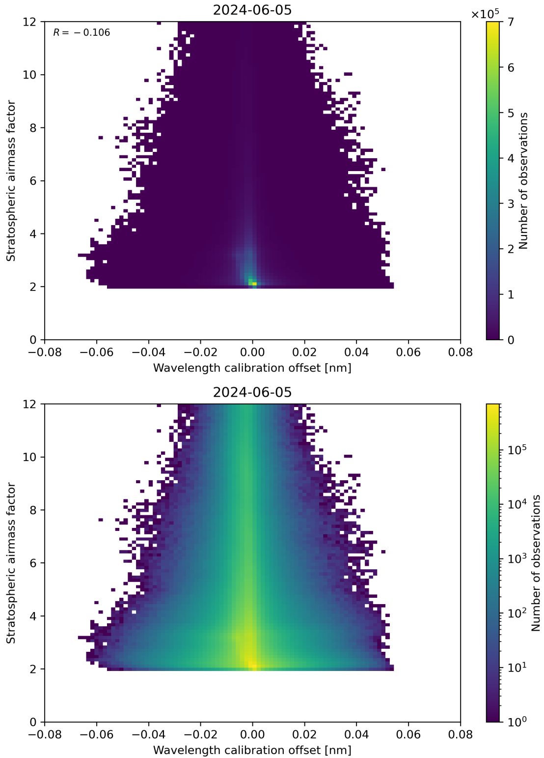
Figure 174: Scatter density plot of “Wavelength calibration offset” against “Stratospheric air mass factor” for 2024-06-04 to 2024-06-06.
