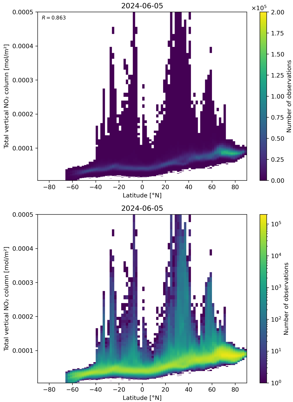
Figure 90: Scatter density plot of “Latitude” against “Total vertical NO 2 column” for 2024-06-04 to 2024-06-06.
