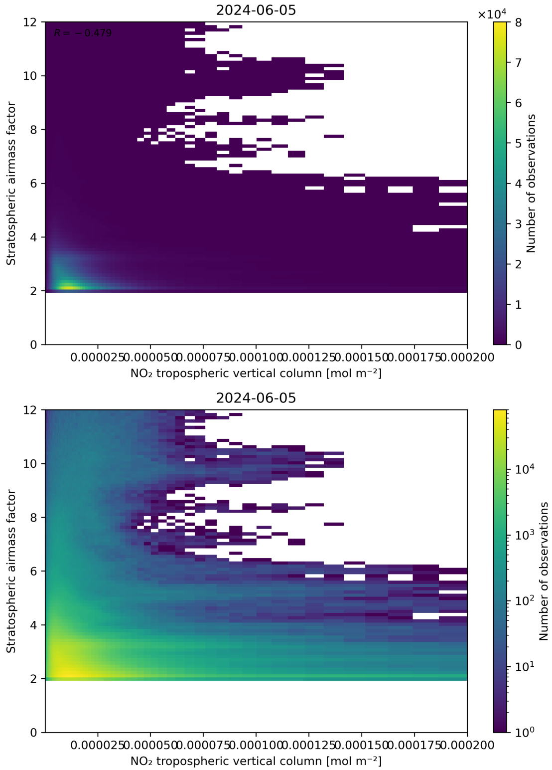
Figure 121: Scatter density plot of “NO 2 tropospheric vertical column” against “Stratospheric air mass factor” for 2024-06-04 to 2024-06-06.
