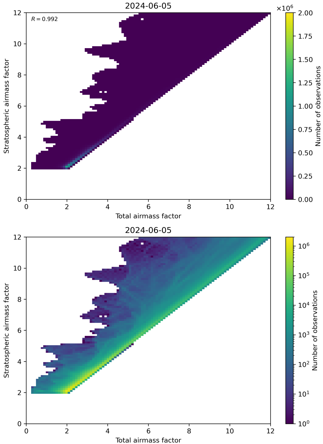
Figure 62: Scatter density plot of “Total airmass factor” against “Stratospheric airmass factor” for 2024-06-04 to 2024-06-06.
