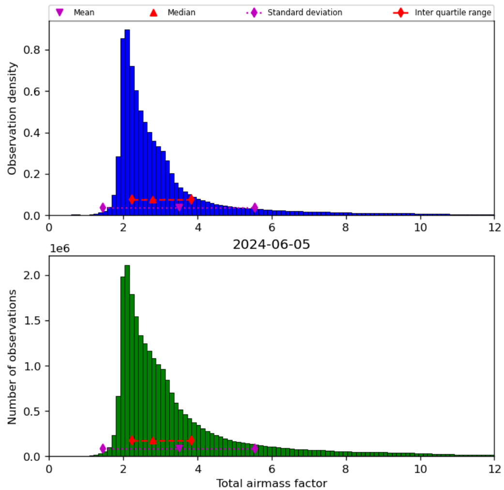
Figure 32: Histogram of “Total airmass factor” for 2024-06-04 to 2024-06-06
