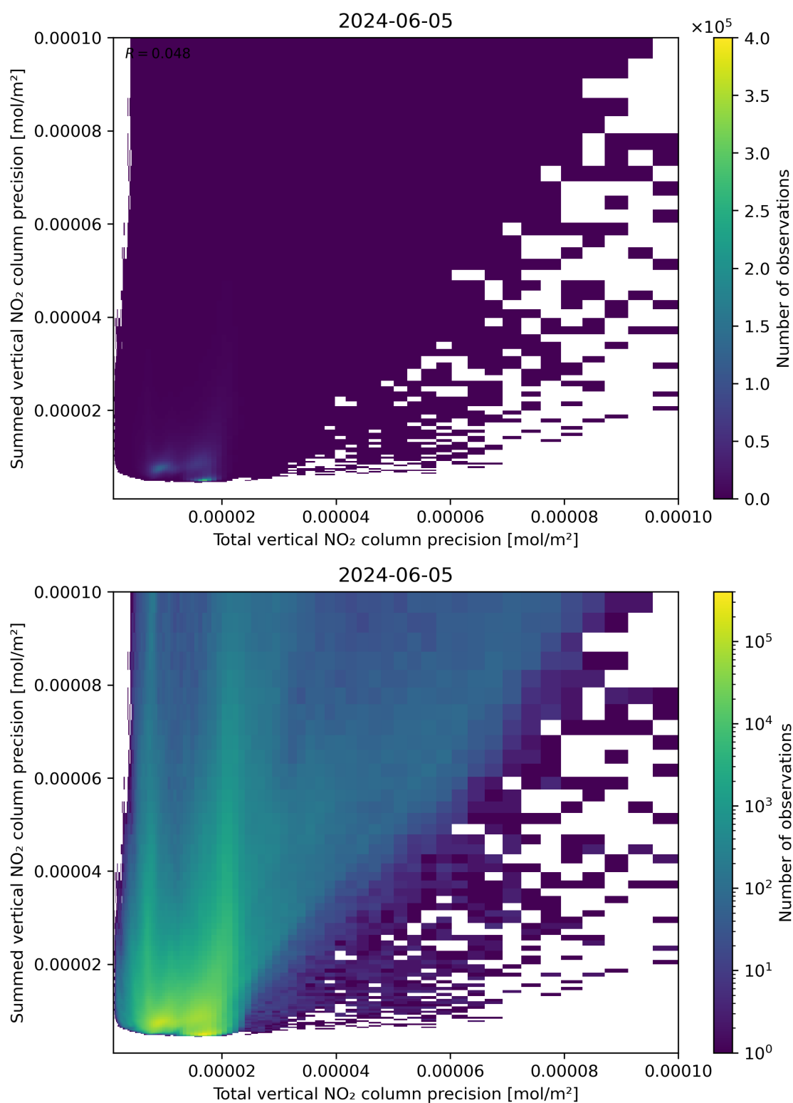
Figure 118: Scatter density plot of “Total vertical NO 2 column precision” against “Summed vertical NO 2 column precision” for 2024-06-04 to 2024-06-06.
