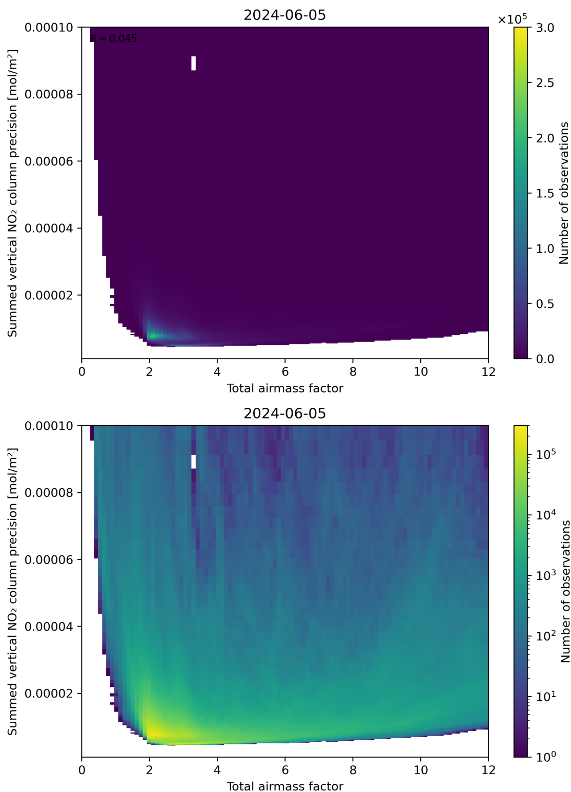
Figure 66: Scatter density plot of “Total airmass factor” against “Summed vertical NO 2 column precision” for 2024-06-04 to 2024-06-06.
