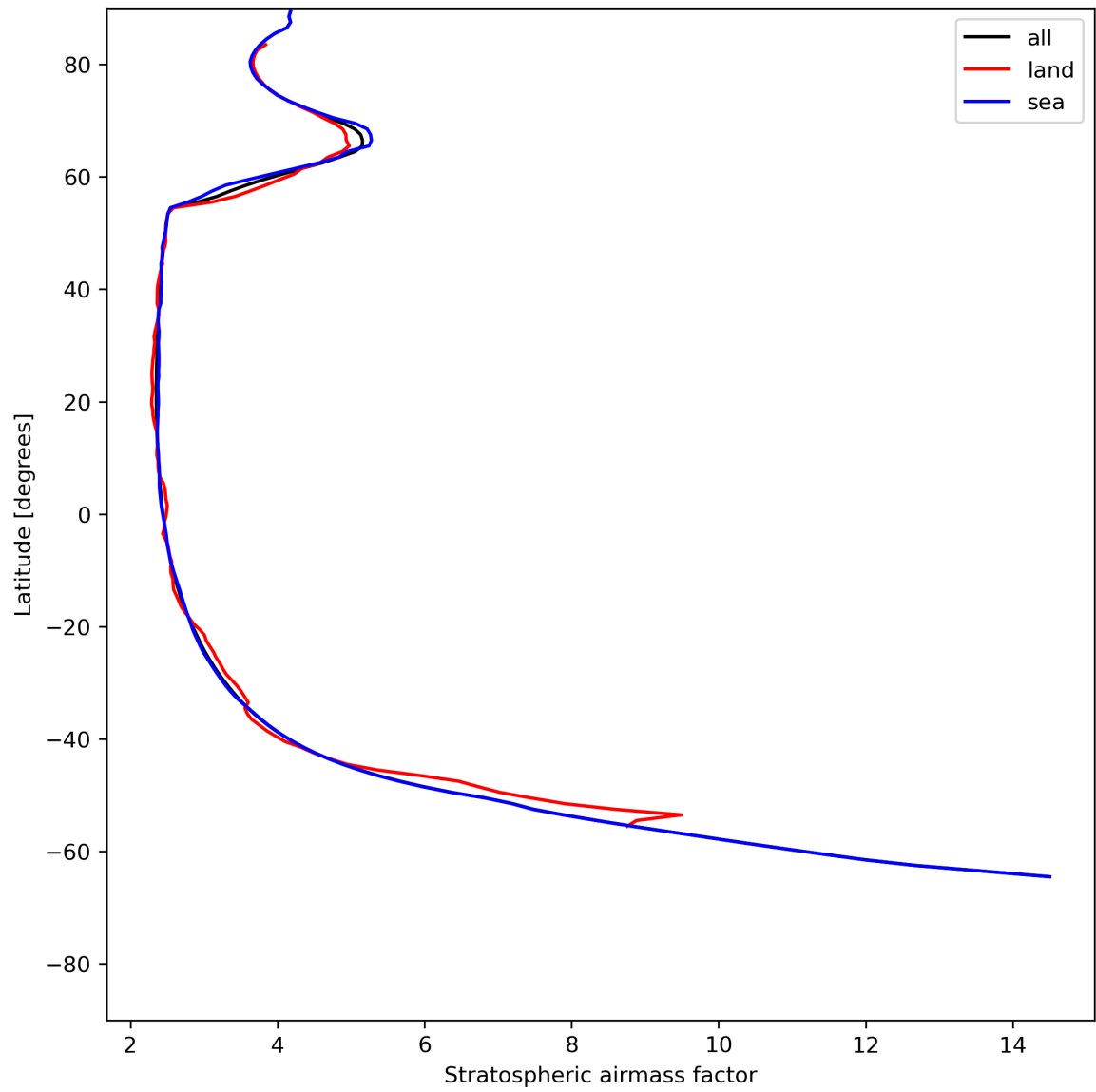
Figure 27: Zonal average of “Stratospheric air mass factor” for 2024-06-04 to 2024-06-06.
