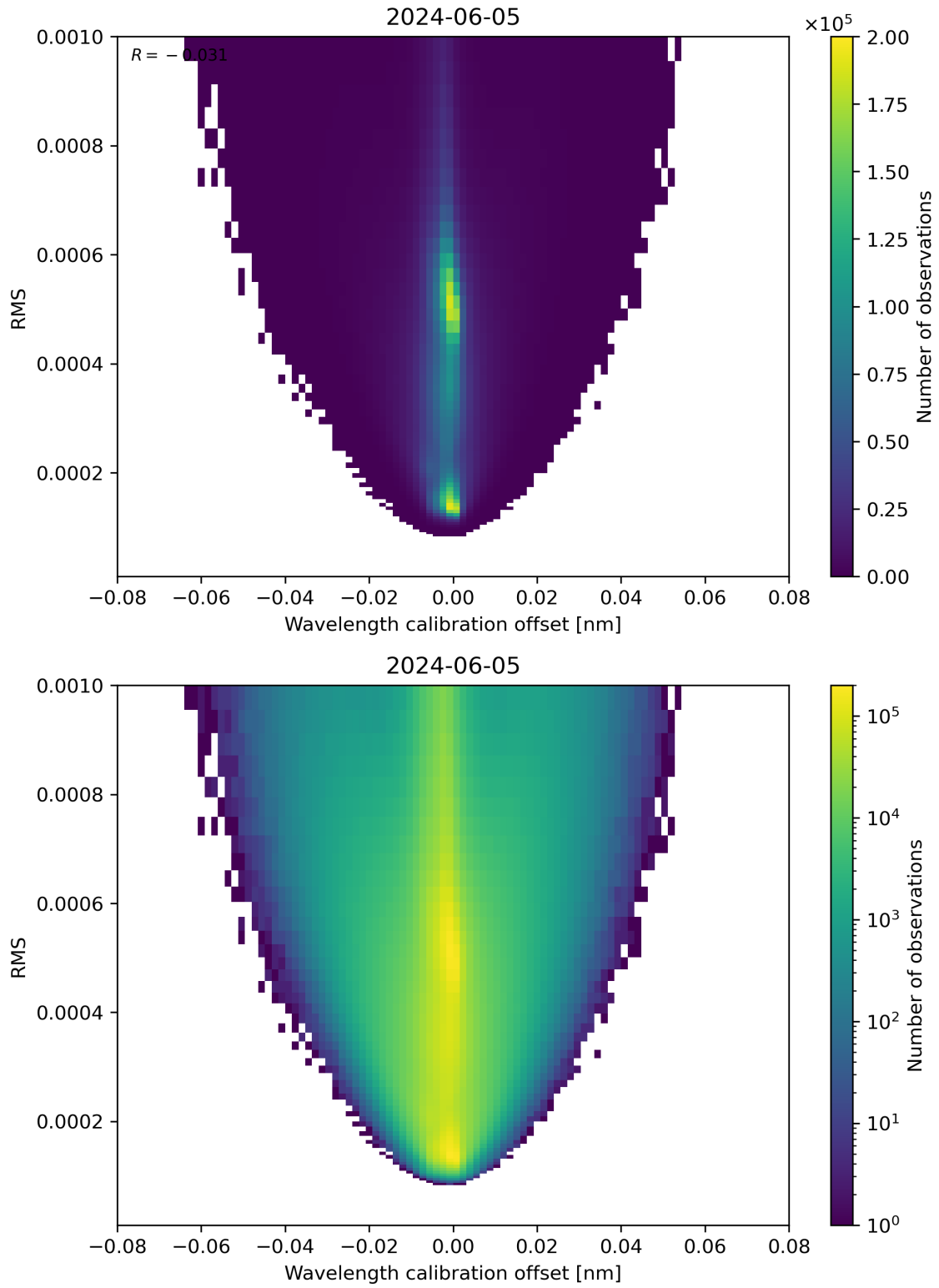
Figure 181: Scatter density plot of “Wavelength calibration offset” against “RMS” for 2024-06-04 to 2024-06-06.
