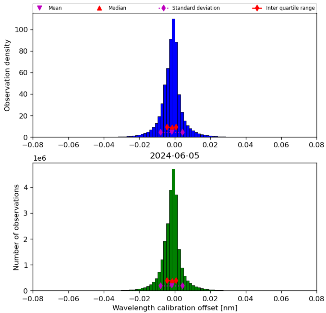
Figure 35: Histogram of “Wavelength calibration offset” for 2024-06-04 to 2024-06-06
