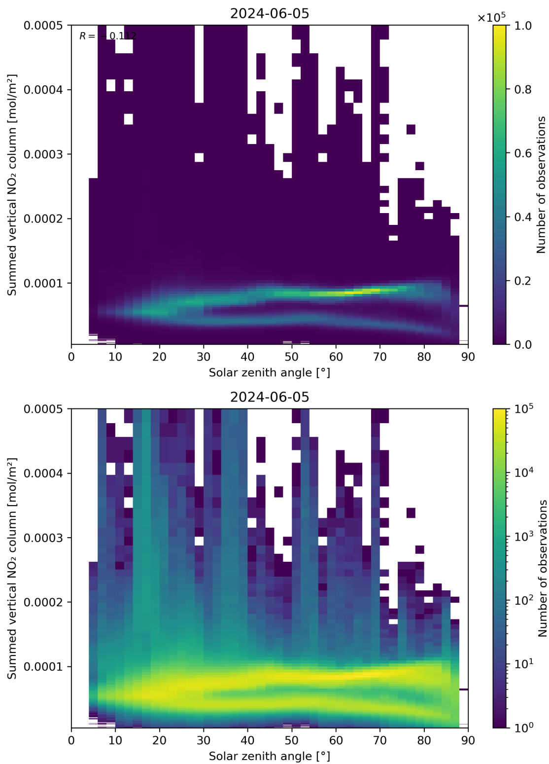
Figure 151: Scatter density plot of “Solar zenith angle” against “Summed vertical NO 2 column” for 2024-06-04 to 2024-06-06.
