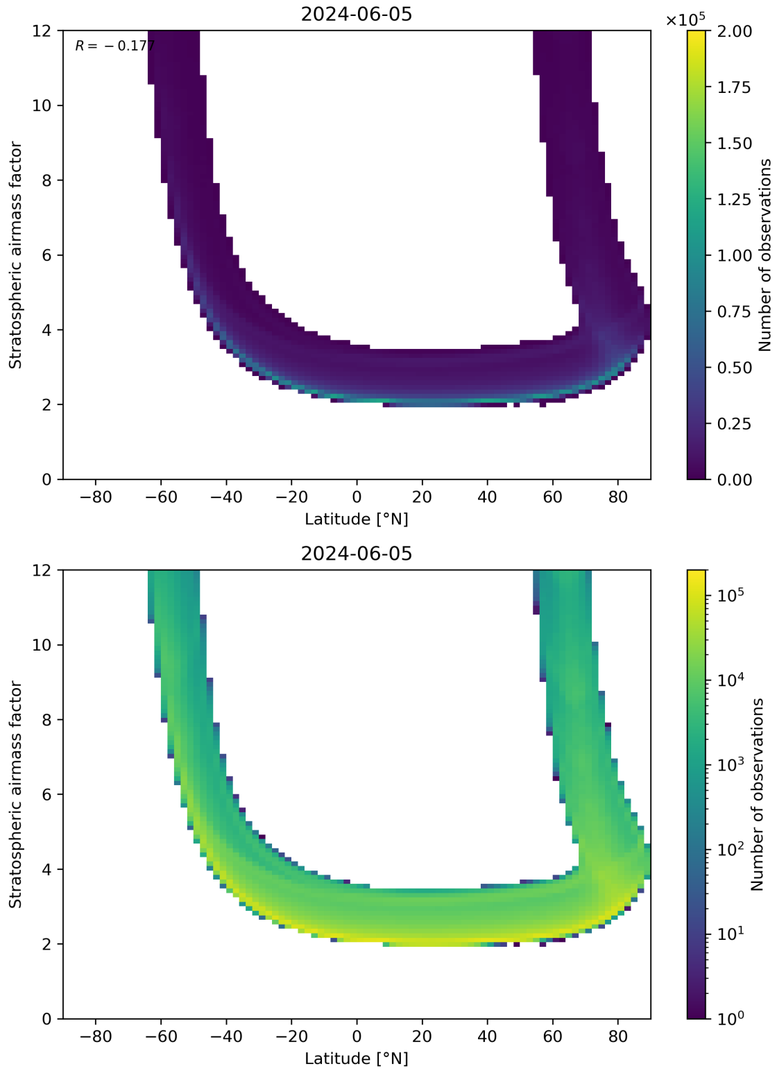
Figure 83: Scatter density plot of “Latitude” against “Stratospheric air mass factor” for 2024-06-04 to 2024-06-06.
