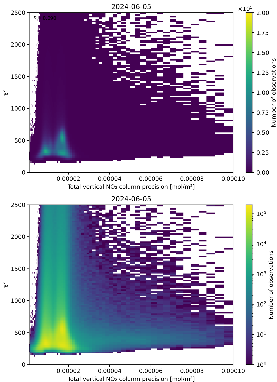
Figure 116: Scatter density plot of “Total vertical NO 2 column precision” against “ \chi^2 ” for 2024-06-04 to 2024-06-06.
