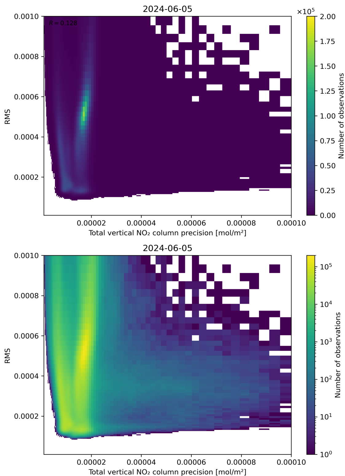
Figure 119: Scatter density plot of “Total vertical NO 2 column precision” against “RMS” for 2024-06-04 to 2024-06-06.
