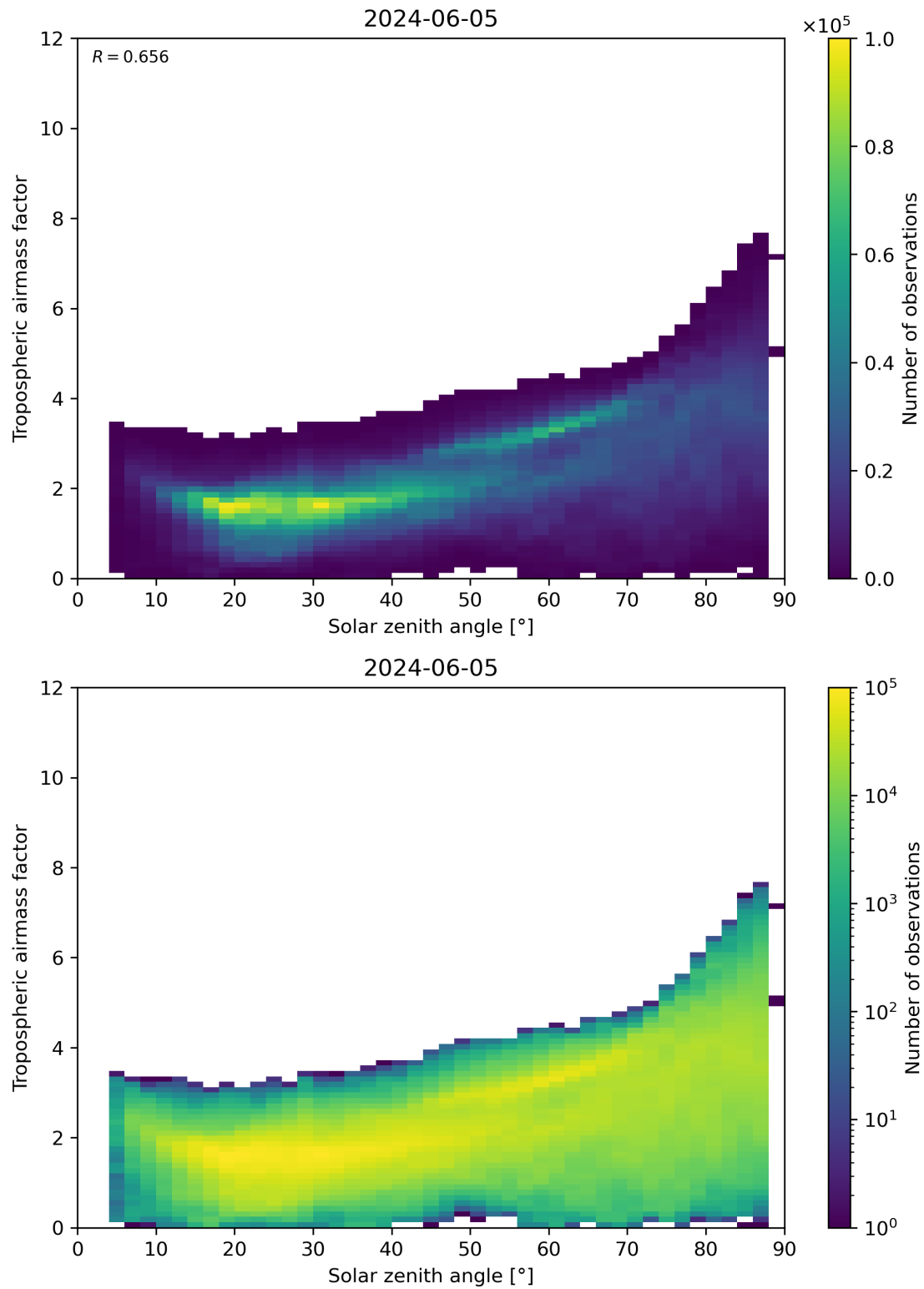
Figure 147: Scatter density plot of “Solar zenith angle” against “Tropospheric airmass factor” for 2024-06-04 to 2024-06-06.
