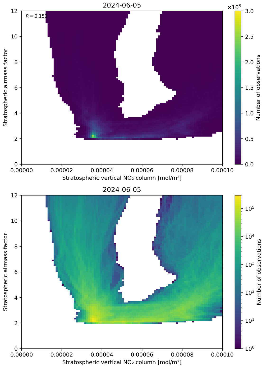
Figure 96: Scatter density plot of “Stratospheric vertical NO 2 column” against “Stratospheric airmass factor” for 2024-06-04 to 2024-06-06.
