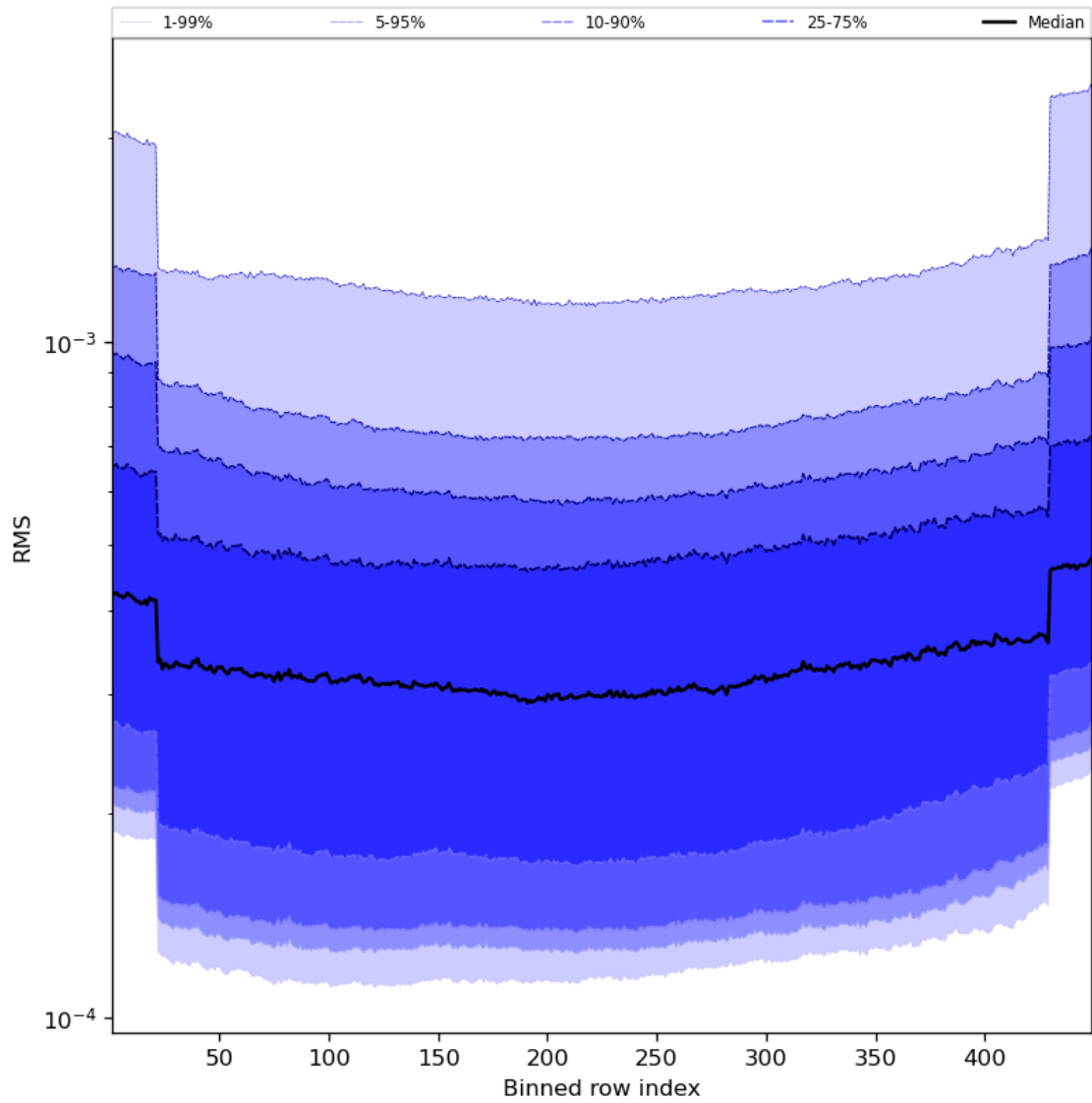
Figure 60: Along track statistics of “RMS” for 2024-06-04 to 2024-06-06
