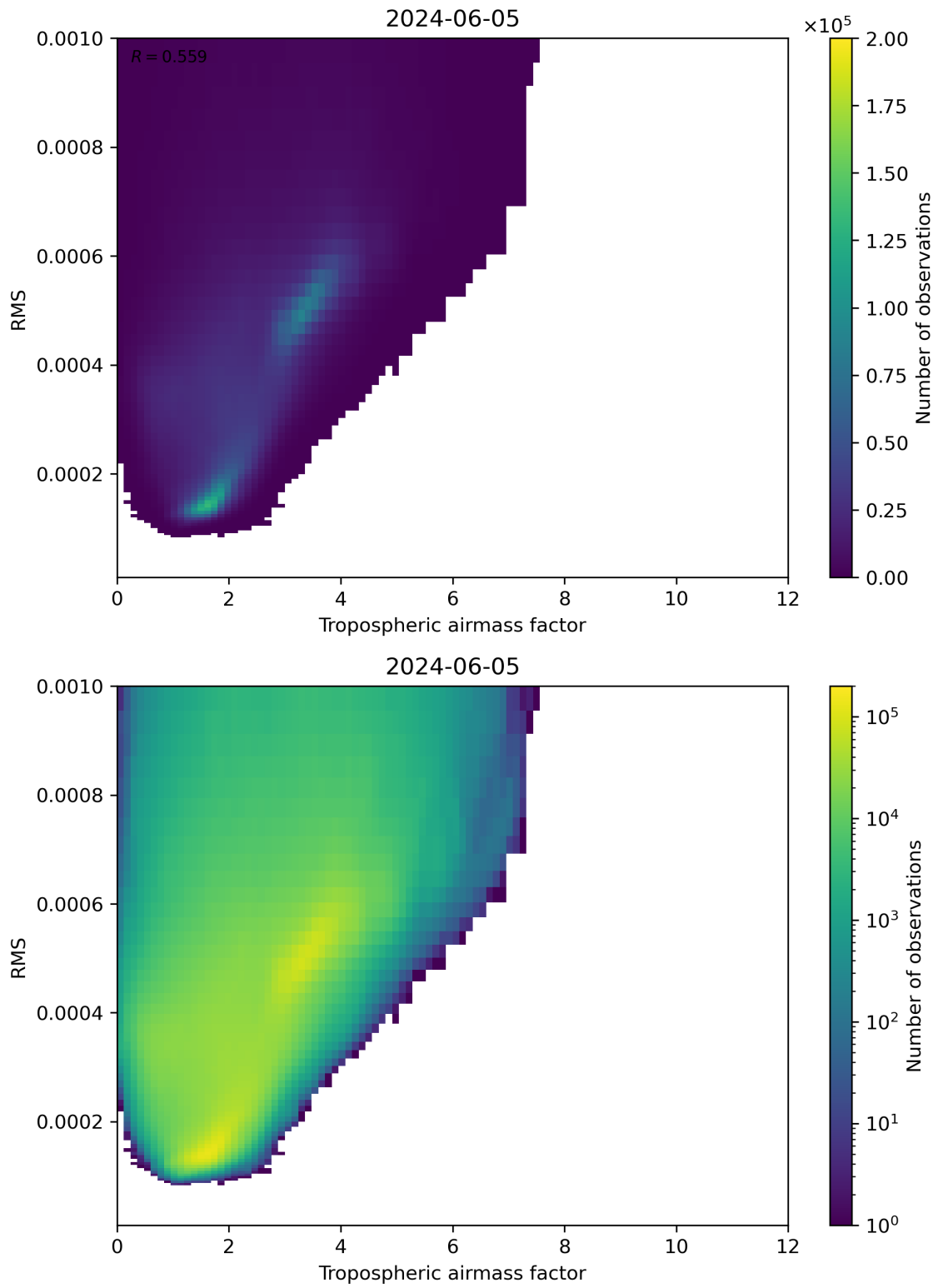
Figure 79: Scatter density plot of “Tropospheric airmass factor” against “RMS” for 2024-06-04 to 2024-06-06.
