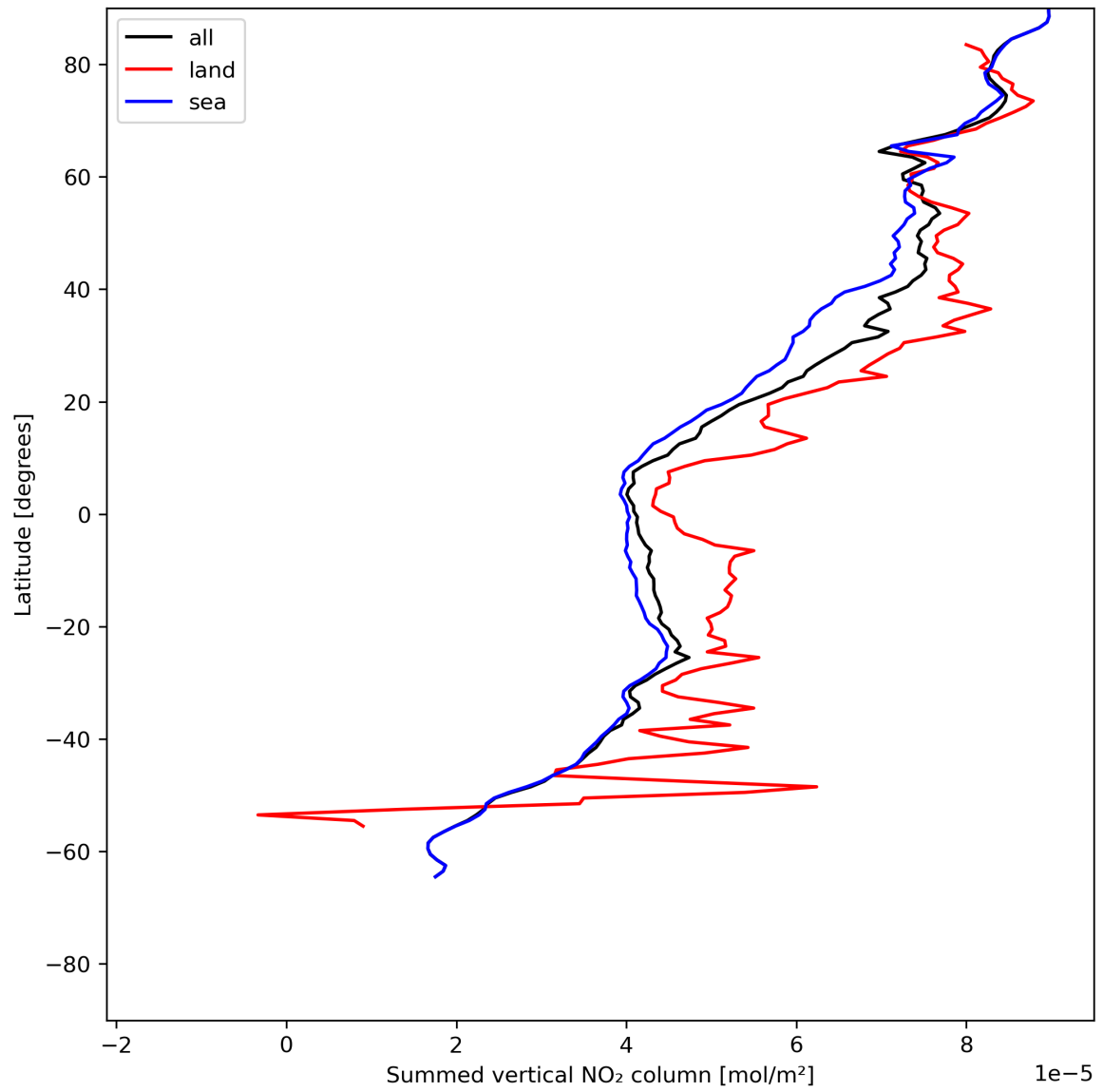
Figure 23: Zonal average of “Summed vertical NO 2 column” for 2024-06-04 to 2024-06-06.
