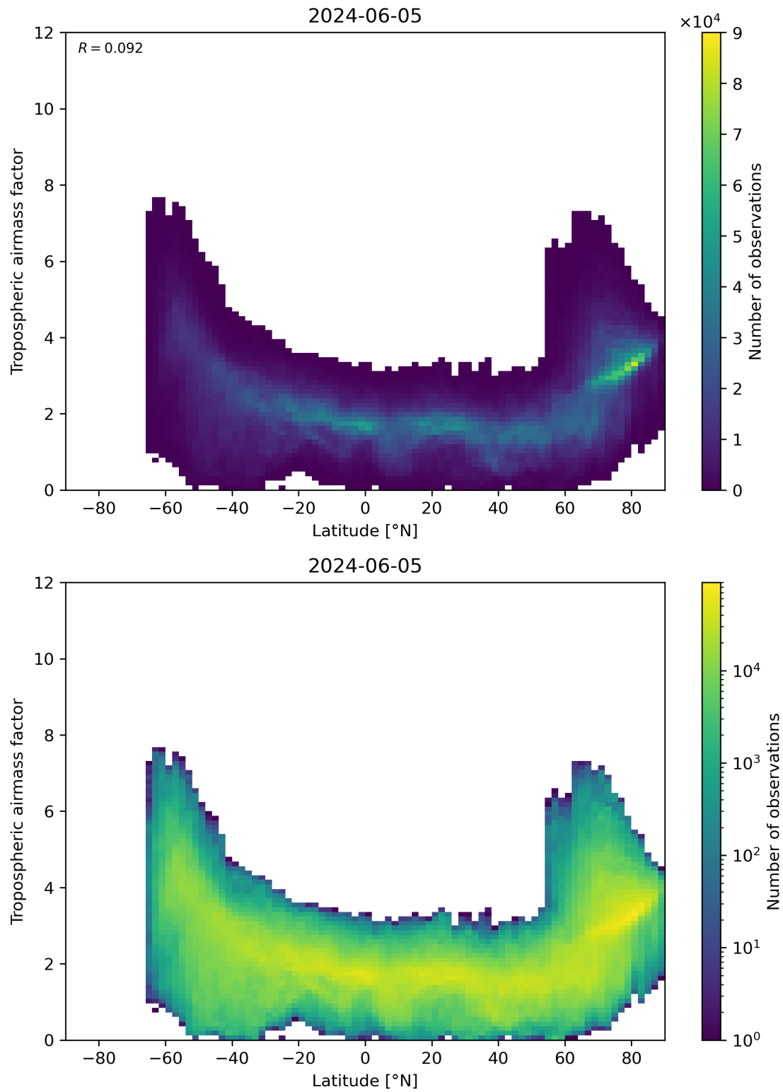
Figure 85: Scatter density plot of “Latitude” against “Tropospheric air mass factor” for 2024-06-04 to 2024-06-06.
