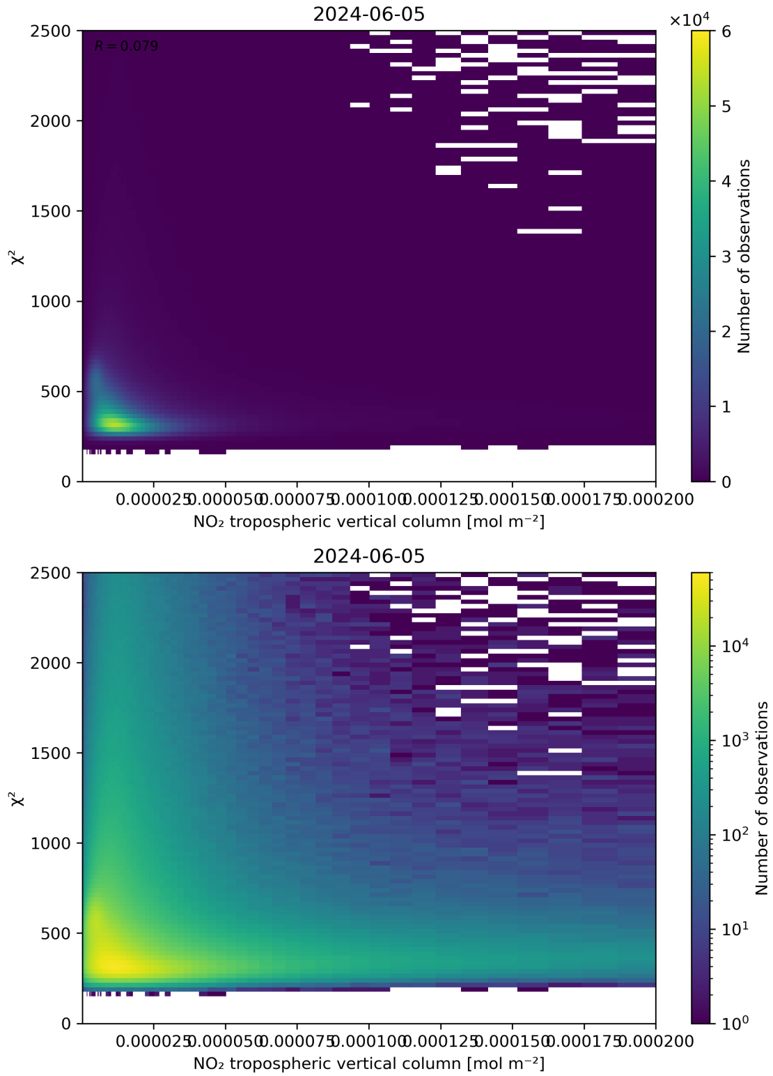
Figure 124: Scatter density plot of “NO 2 tropospheric vertical column” against “ \chi^2 ” for 2024-06-04 to 2024-06-06.
