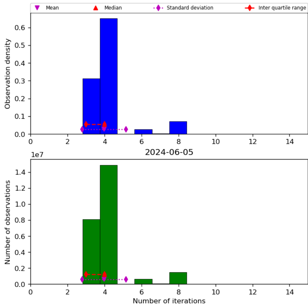
Figure 34: Histogram of “Number of iterations” for 2024-06-04 to 2024-06-06
