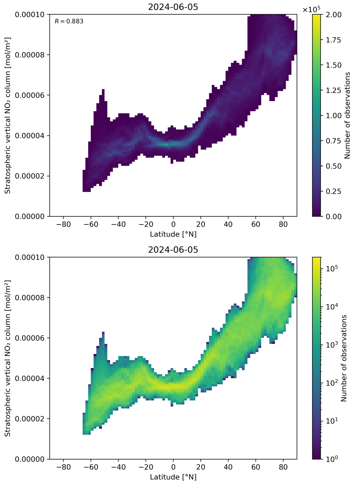
Figure 87: Scatter density plot of “Latitude” against “Stratospheric vertical NO 2 column” for 2024-06-04 to 2024-06-06.
