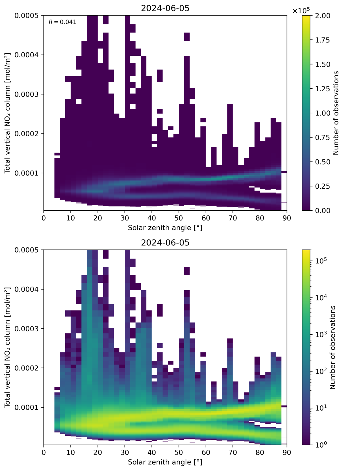
Figure 153: Scatter density plot of “Solar zenith angle” against “Total vertical NO 2 column” for 2024-06-04 to 2024-06-06.
