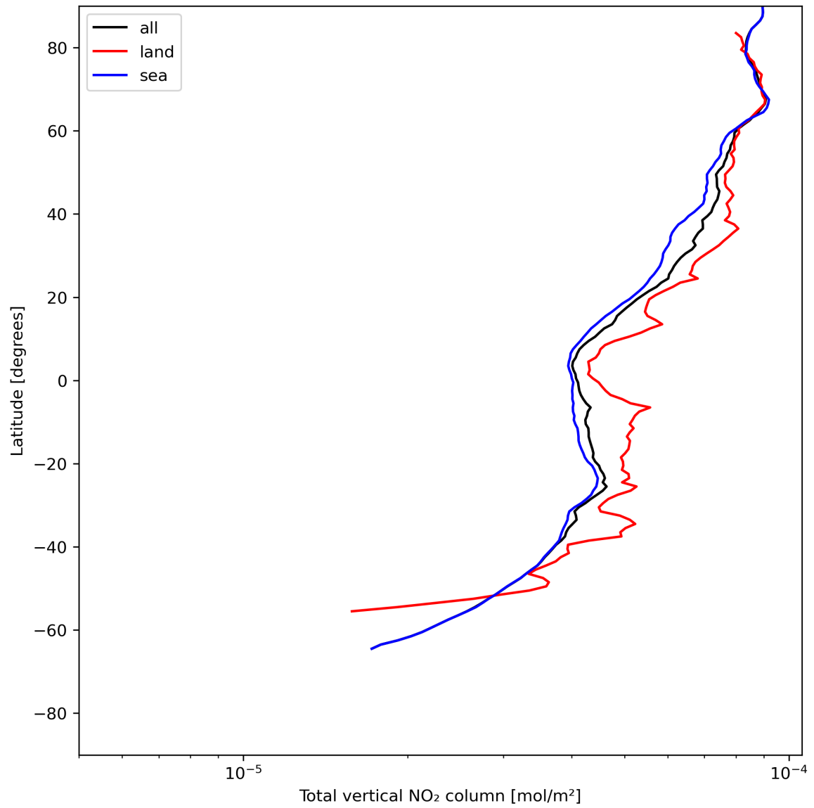
Figure 21: Zonal average of “Total vertical NO 2 column” for 2024-06-04 to 2024-06-06.
