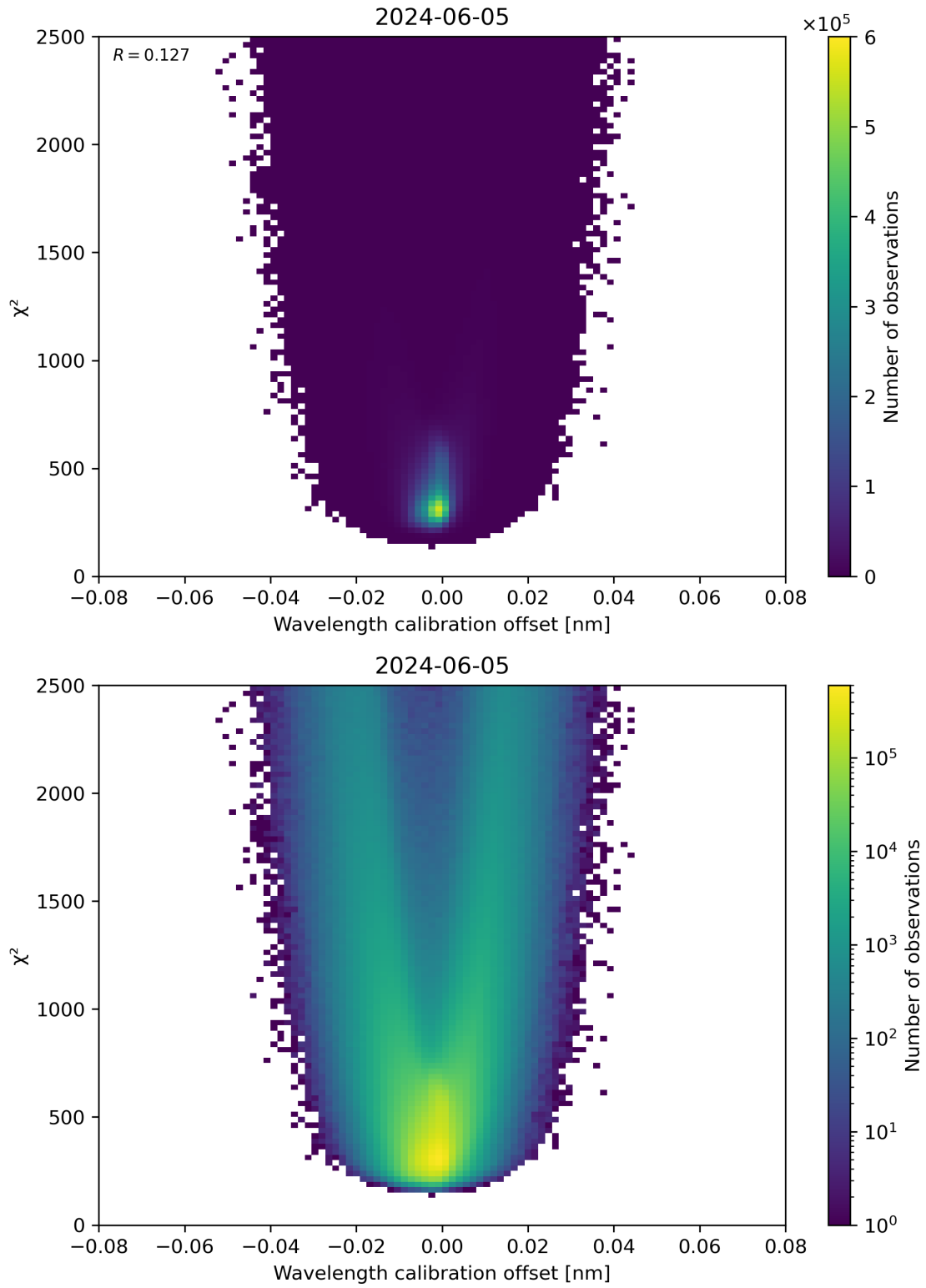
Figure 175: Scatter density plot of “Wavelength calibration offset” against “ \chi^2 ” for 2024-06-04 to 2024-06-06.
