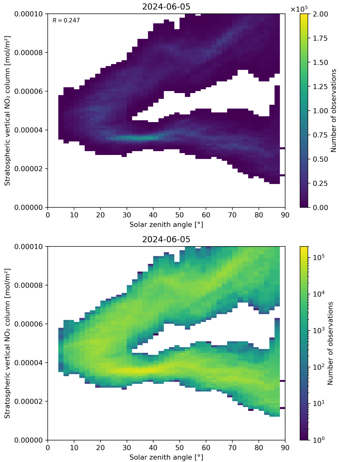
Figure 150: Scatter density plot of “Solar zenith angle” against “Stratospheric vertical NO 2 column” for 2024-06-04 to 2024-06-06.
