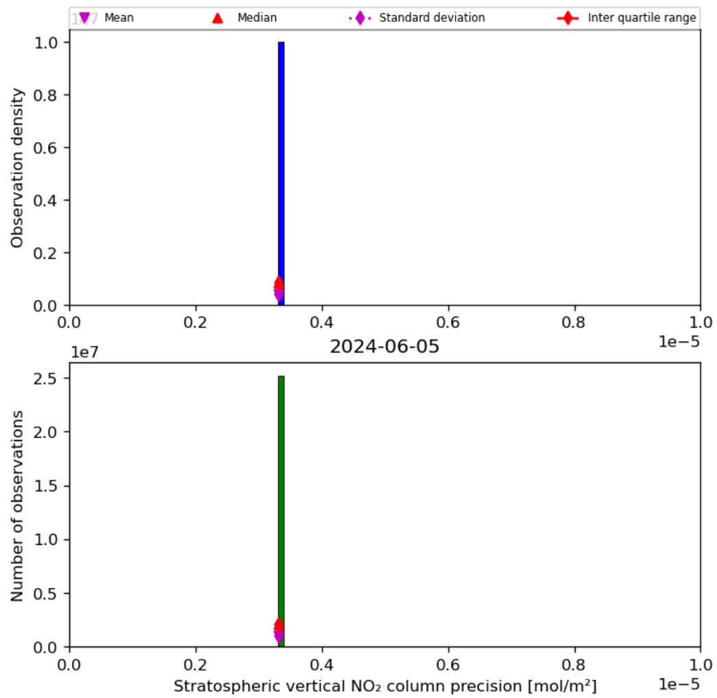
Figure 37: Histogram of “Stratospheric vertical NO 2 column precision” for 2024-06-04 to 2024-06-06
