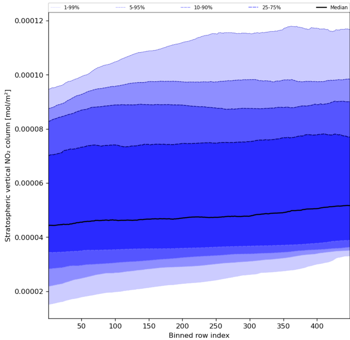
Figure 53: Along track statistics of “Stratospheric vertical NO 2 column” for 2024-06-04 to 2024-06-06
