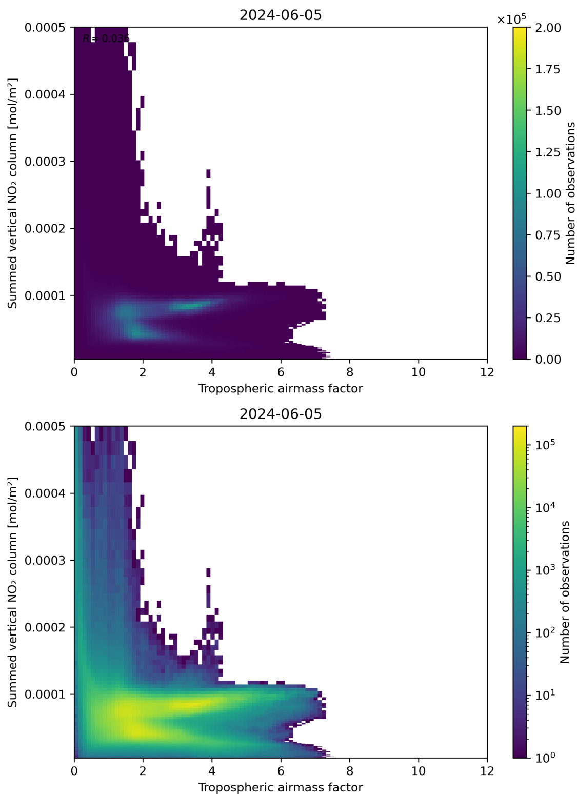
Figure 75: Scatter density plot of “Tropospheric air mass factor” against “Summed vertical NO 2 column” for 2024-06-04 to 2024-06-06.
