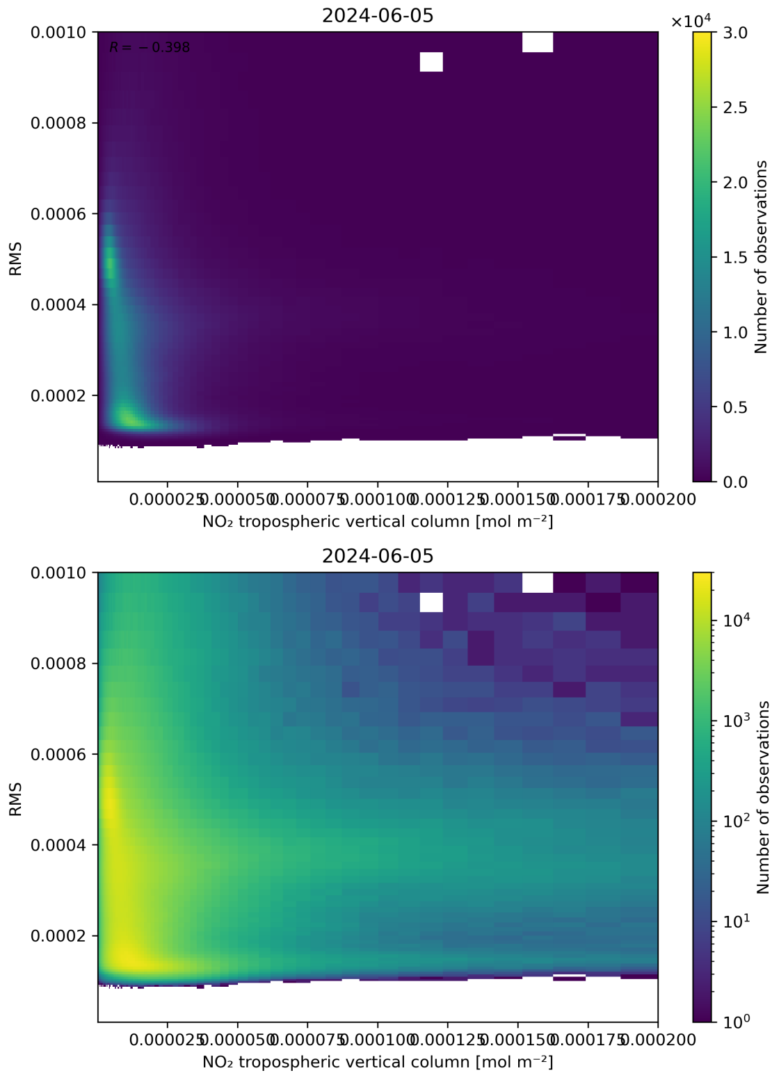
Figure 142: Scatter density plot of “NO 2 tropospheric vertical column” against “RMS” for 2024-06-04 to 2024-06-06.
