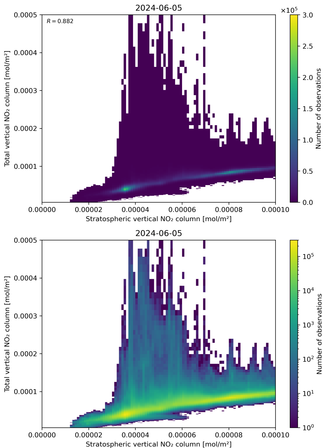
Figure 100: Scatter density plot of “Stratospheric vertical NO 2 column” against “Total vertical NO 2 column” for 2024-06-04 to 2024-06-06.
