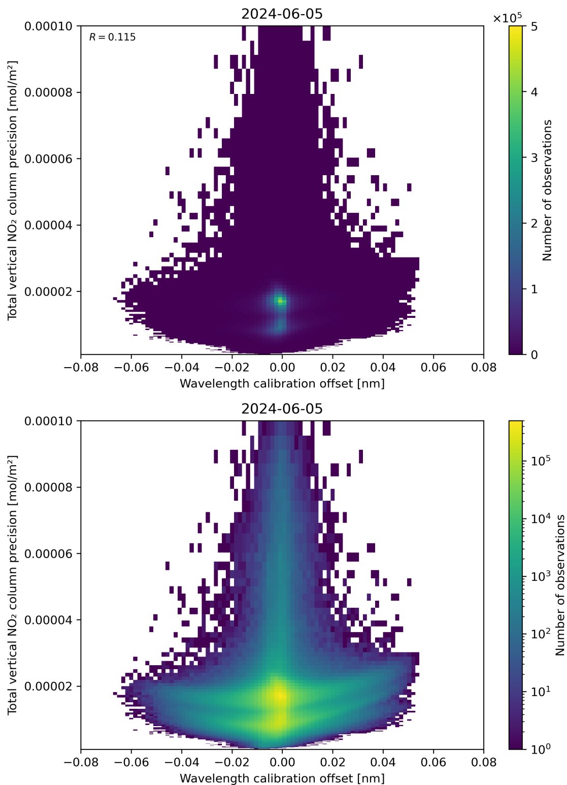
Figure 180: Scatter density plot of “Wavelength calibration offset” against “Total vertical NO 2 column precision” for 2024-06-04 to 2024-06-06.
