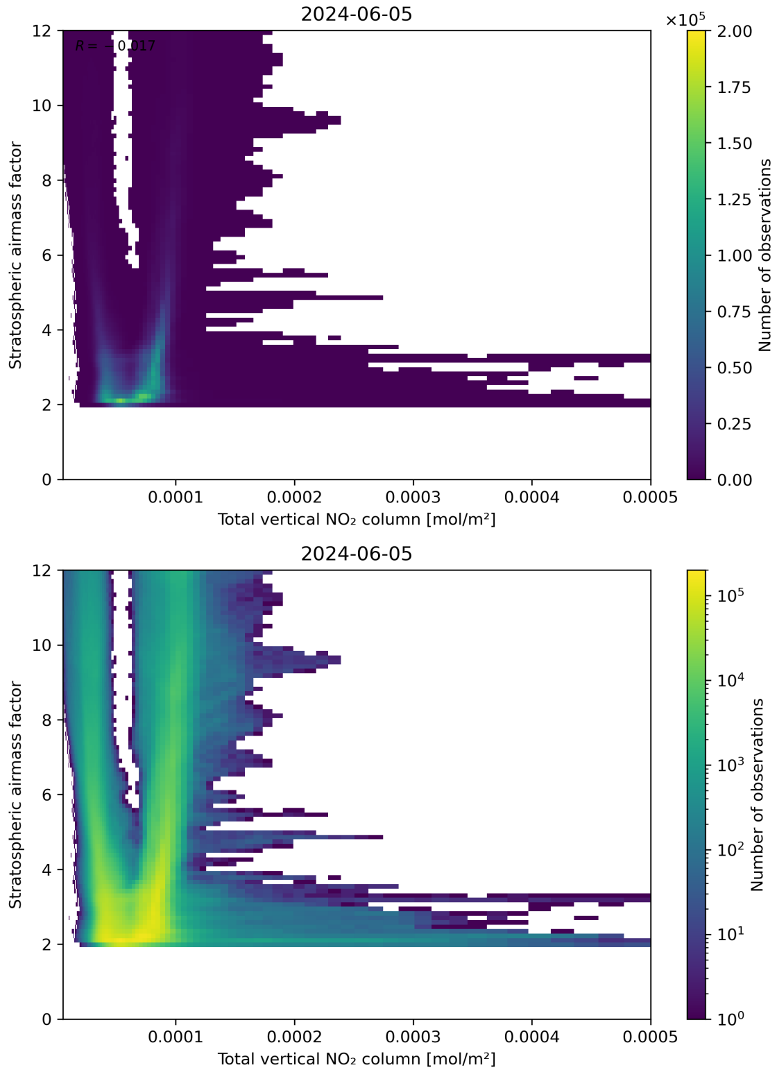
Figure 110: Scatter density plot of “Total vertical NO 2 column” against “Stratospheric airmass factor” for 2024-06-04 to 2024-06-06.
