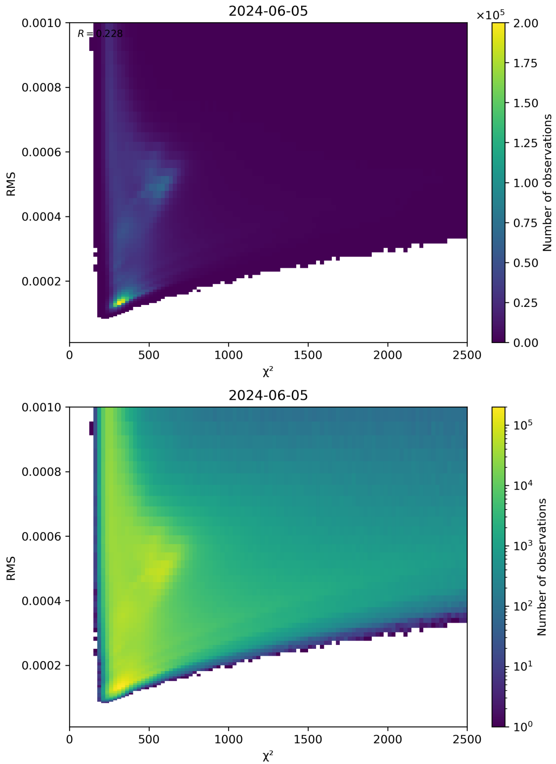
Figure 82: Scatter density plot of “ \chi^2 ” against “RMS” for 2024-06-04 to 2024-06-06.
