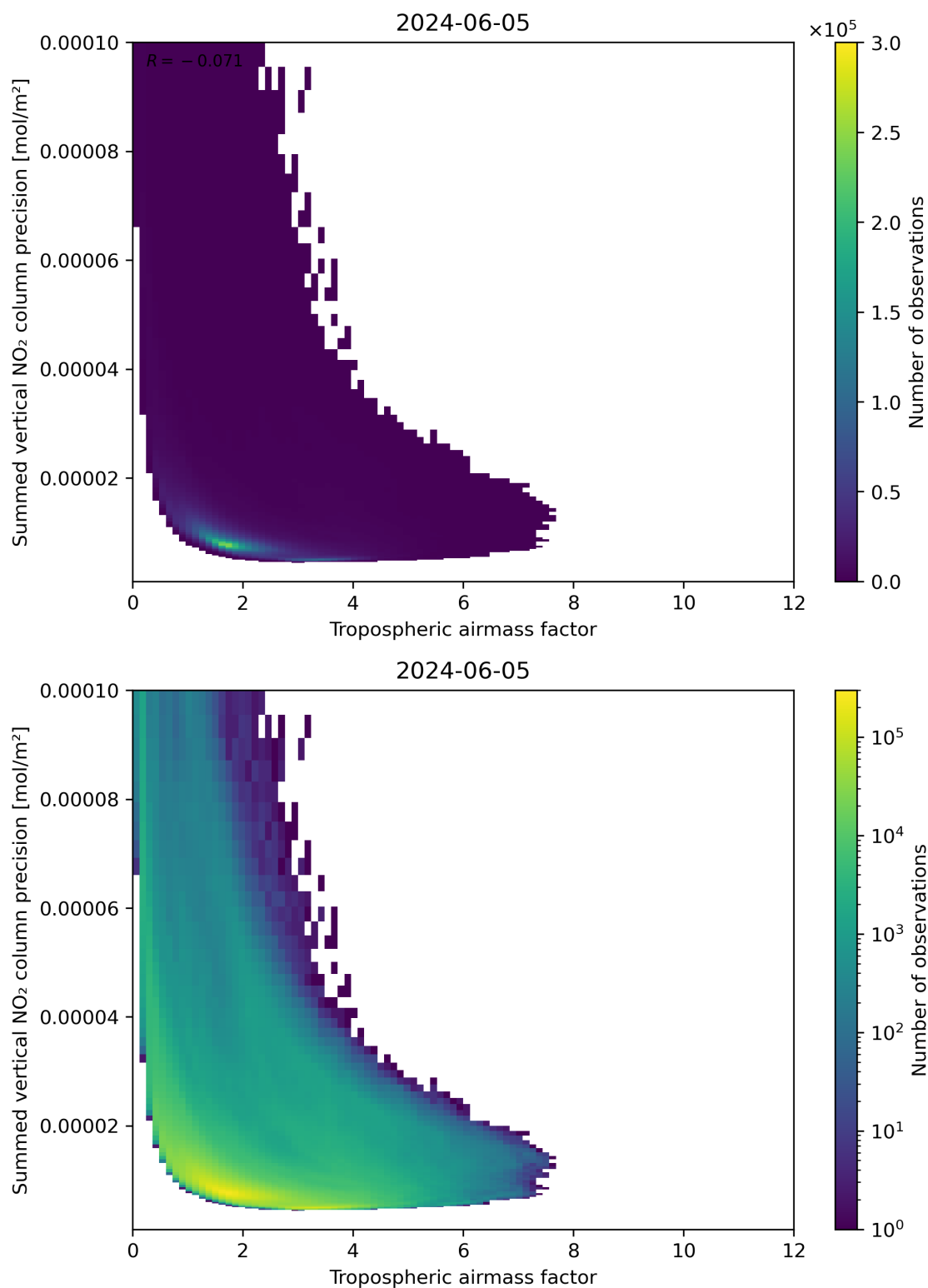
Figure 76: Scatter density plot of “Tropospheric air mass factor” against “Summed vertical NO 2 column precision” for 2024-06-04 to 2024-06-06.
