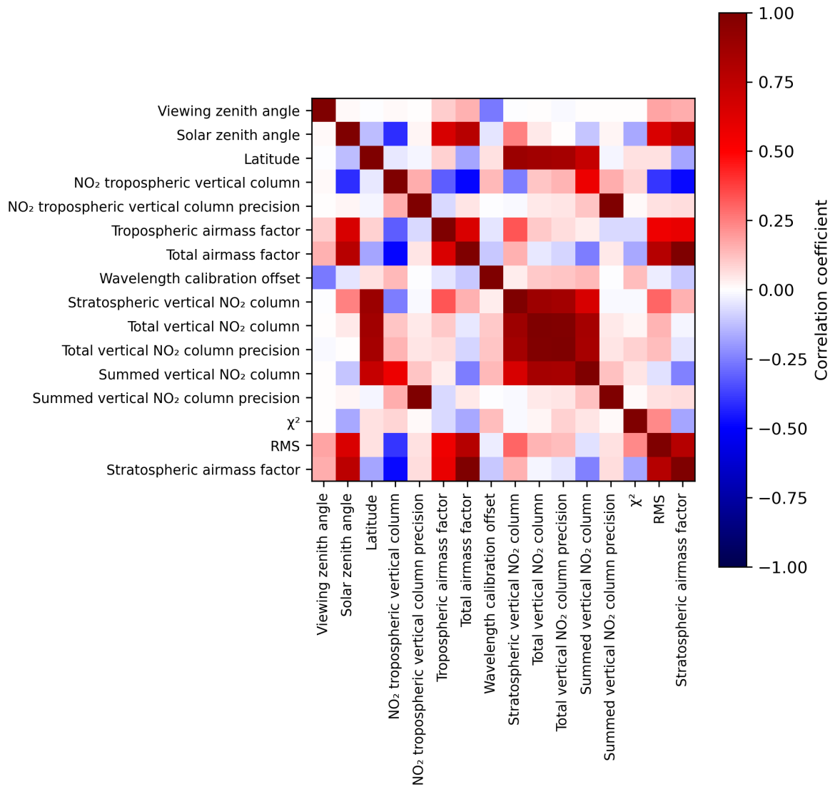
Figure 2: Map of correlation matrix for 2024-06-04 to 2024-06-06.
