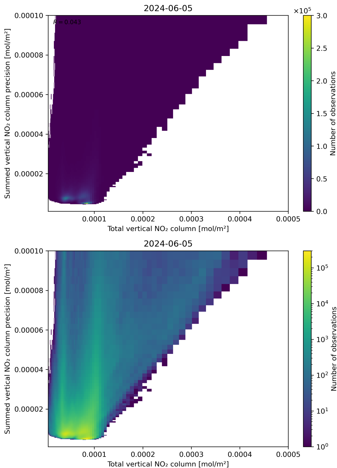
Figure 113: Scatter density plot of “Total vertical NO 2 column” against “Summed vertical NO 2 column precision” for 2024-06-04 to 2024-06-06.
