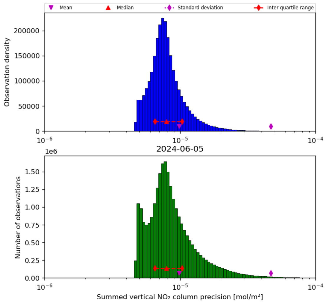
Figure 41: Histogram of "Summed vertical NO 2 column precision" for 2024-06-04 to 2024-06-06
