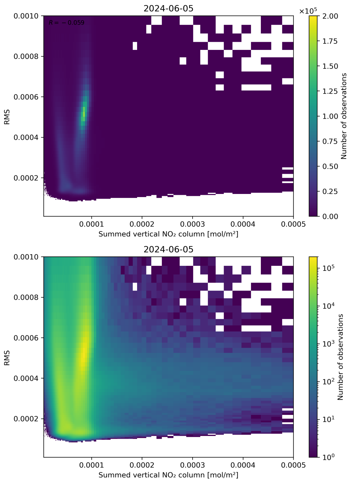
Figure 109: Scatter density plot of “Summed vertical NO 2 column” against “RMS” for 2024-06-04 to 2024-06-06.
