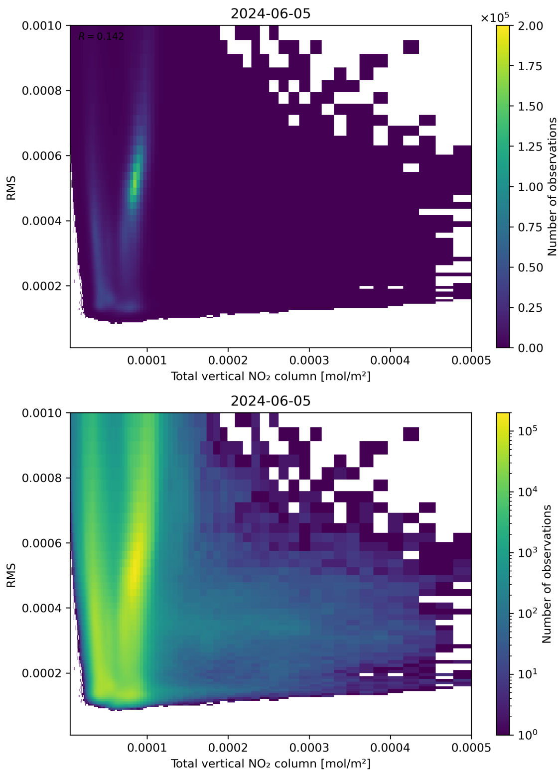
Figure 120: Scatter density plot of “Total vertical NO 2 column” against “RMS” for 2024-06-04 to 2024-06-06.
