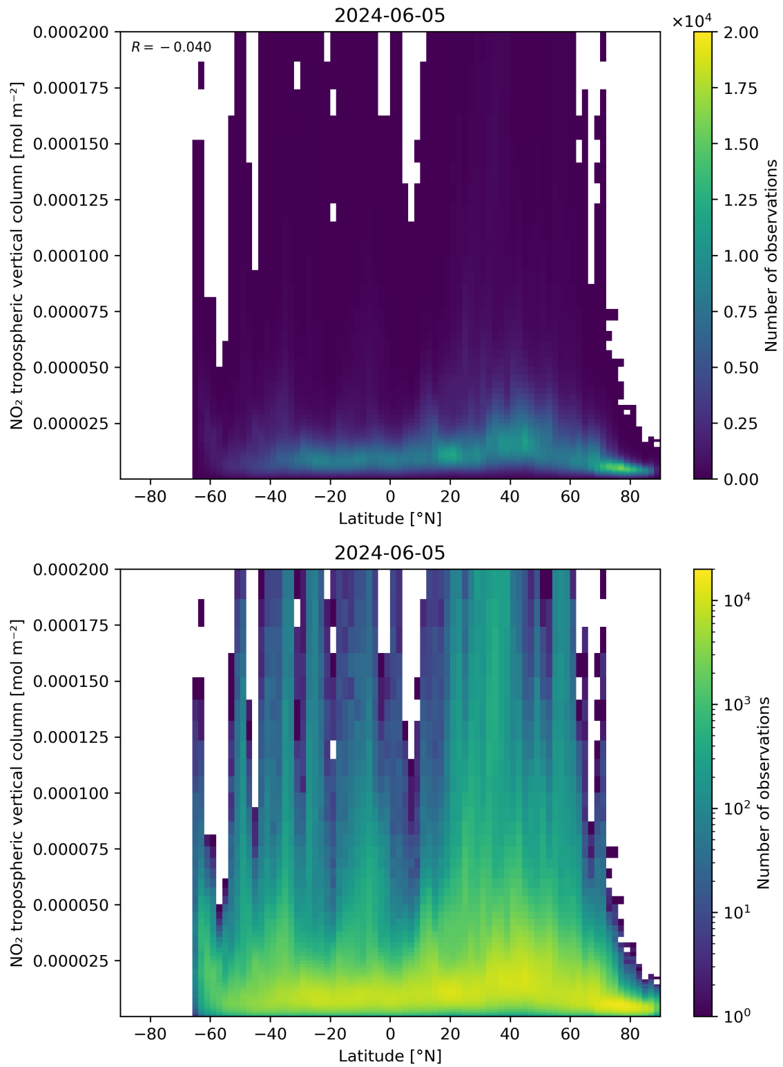
Figure 92: Scatter density plot of “Latitude” against “NO 2 tropospheric vertical column” for 2024-06-04 to 2024-06-06.
