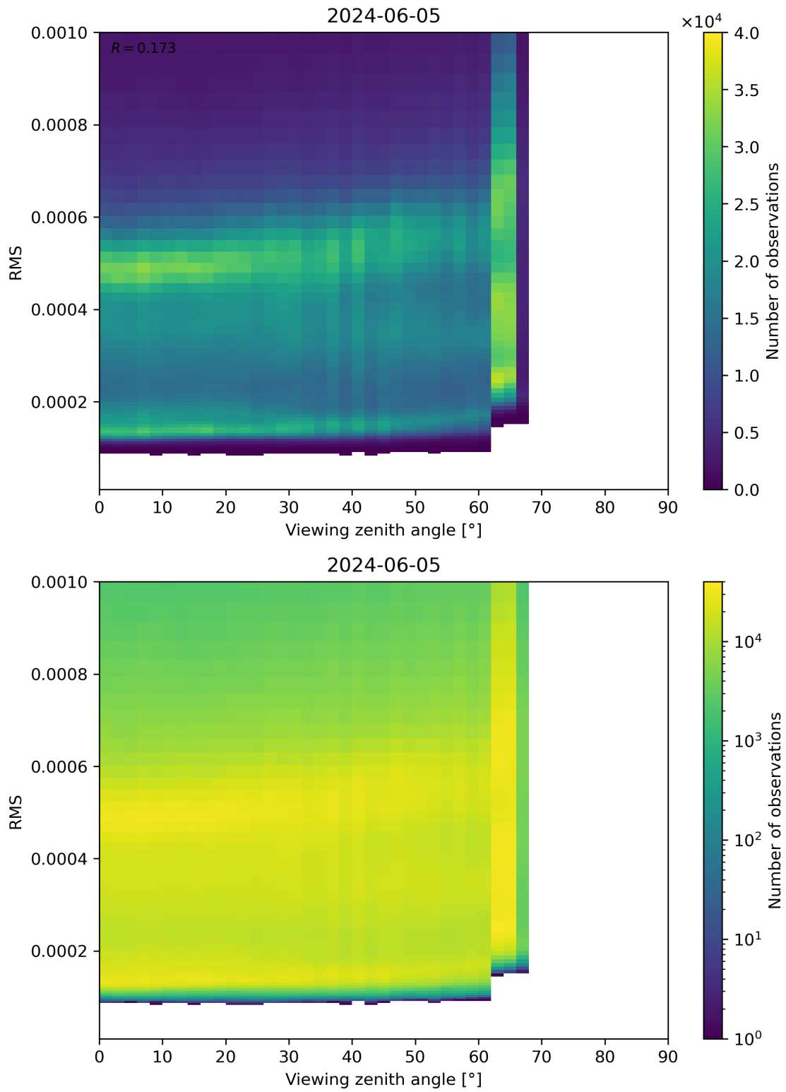
Figure 171: Scatter density plot of “Viewing zenith angle” against “RMS” for 2024-06-04 to 2024-06-06.
