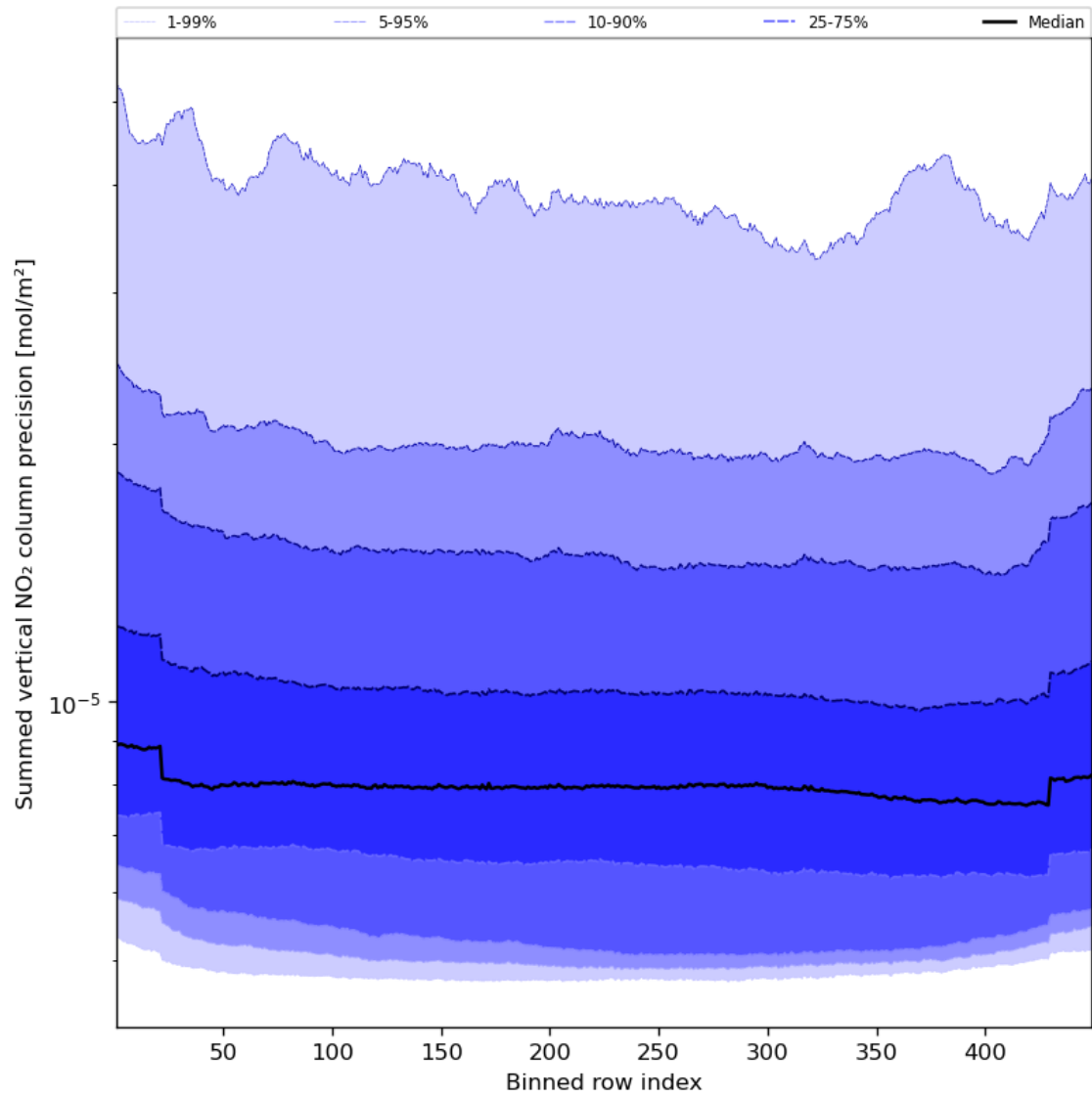
Figure 58: Along track statistics of “Summed vertical NO 2 column precision” for 2024-06-04 to 2024-06-06
