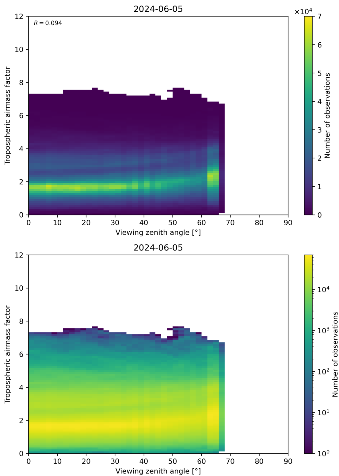
Figure 161: Scatter density plot of “Viewing zenith angle” against “Tropospheric airmass factor” for 2024-06-04 to 2024-06-06.
