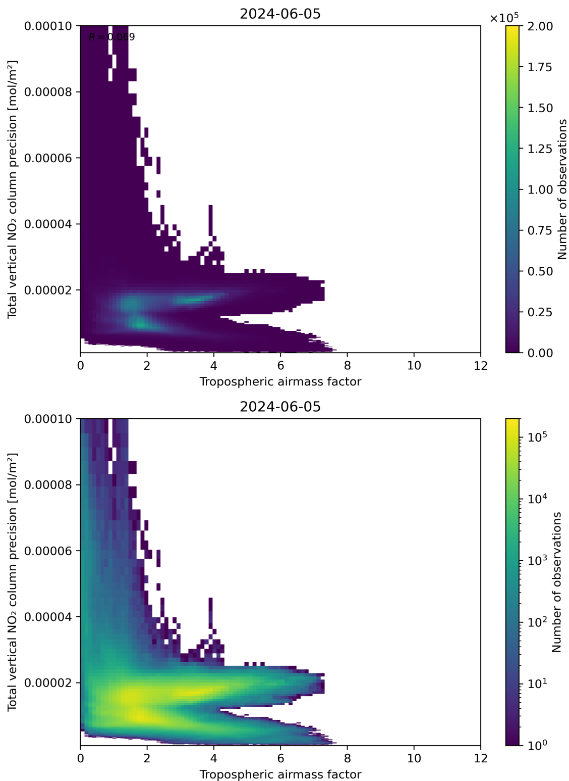
Figure 78: Scatter density plot of “Tropospheric air mass factor” against “Total vertical NO 2 column precision” for 2024-06-04 to 2024-06-06.
