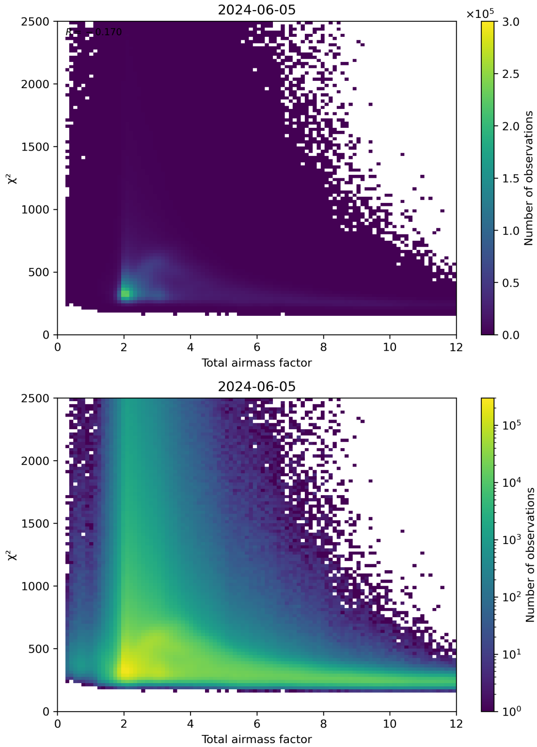
Figure 63: Scatter density plot of “Total airmass factor” against “ \chi^2 ” for 2024-06-04 to 2024-06-06.
