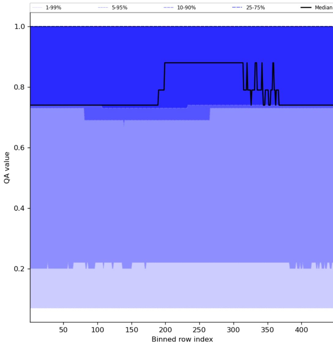
Figure 45: Along track statistics of “QA value” for 2024-06-04 to 2024-06-06
