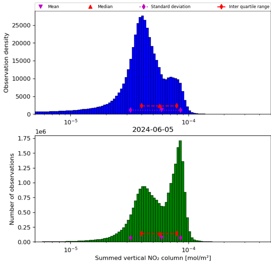
Figure 40: Histogram of “Summed vertical NO 2 column” for 2024-06-04 to 2024-06-06
