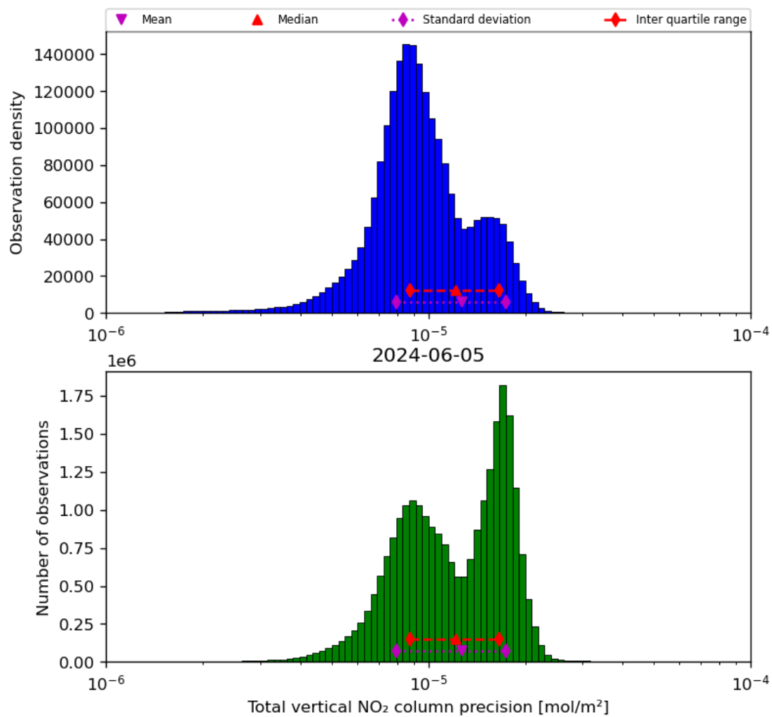
Figure 39: Histogram of “Total vertical NO 2 column precision” for 2024-06-04 to 2024-06-06
