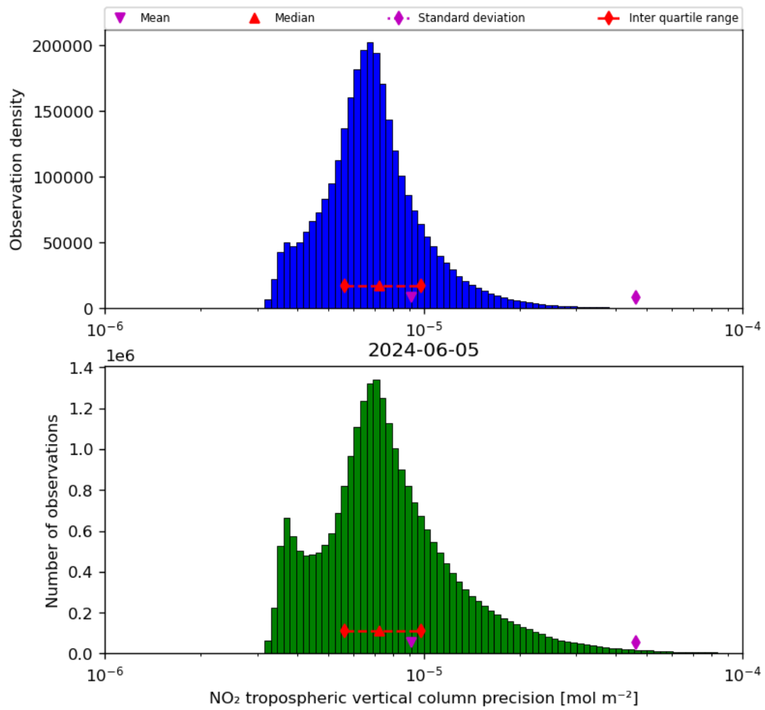
Figure 30: Histogram of “NO 2 tropospheric vertical column precision” for 2024-06-04 to 2024-06-06
