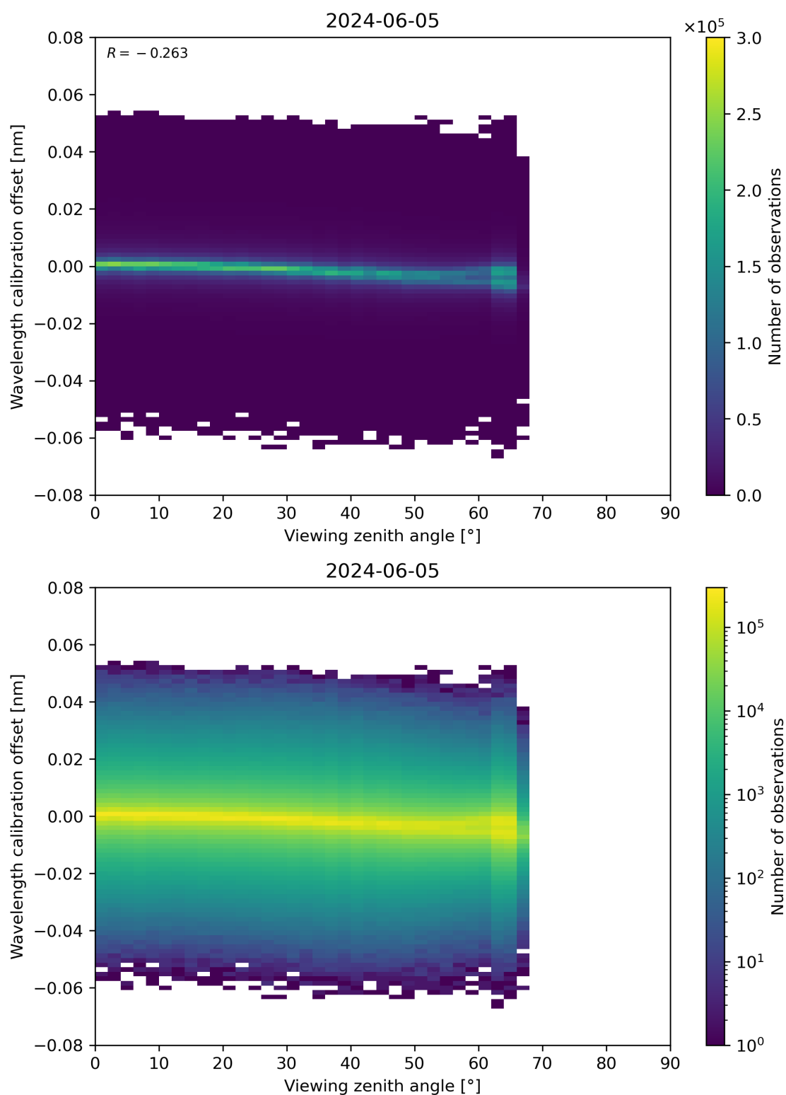
Figure 173: Scatter density plot of “Viewing zenith angle” against “Wavelength calibration offset” for 2024-06-04 to 2024-06-06.
