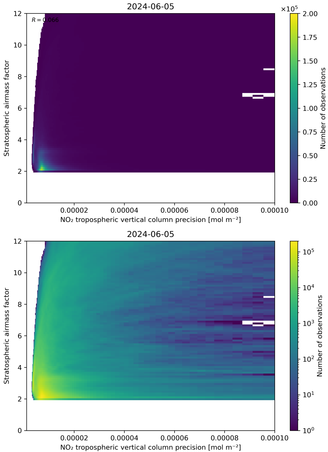
Figure 131: Scatter density plot of “NO 2 tropospheric vertical column precision” against “Stratospheric airmass factor” for 2024-06-04 to 2024-06-06.
