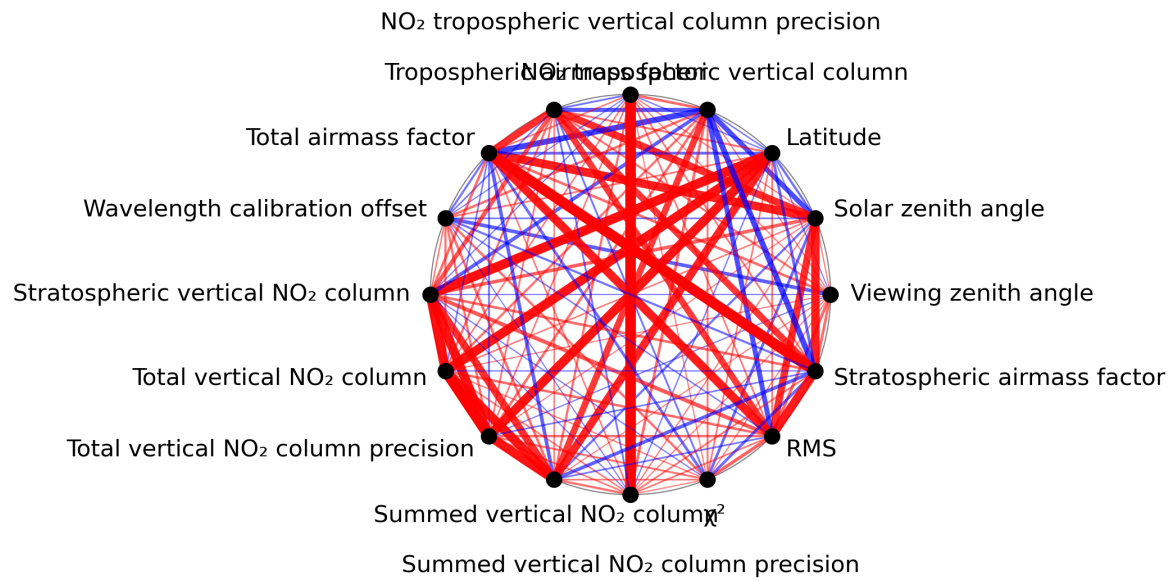
Figure 1: Map of correlation graph for 2024-06-04 to 2024-06-06.
