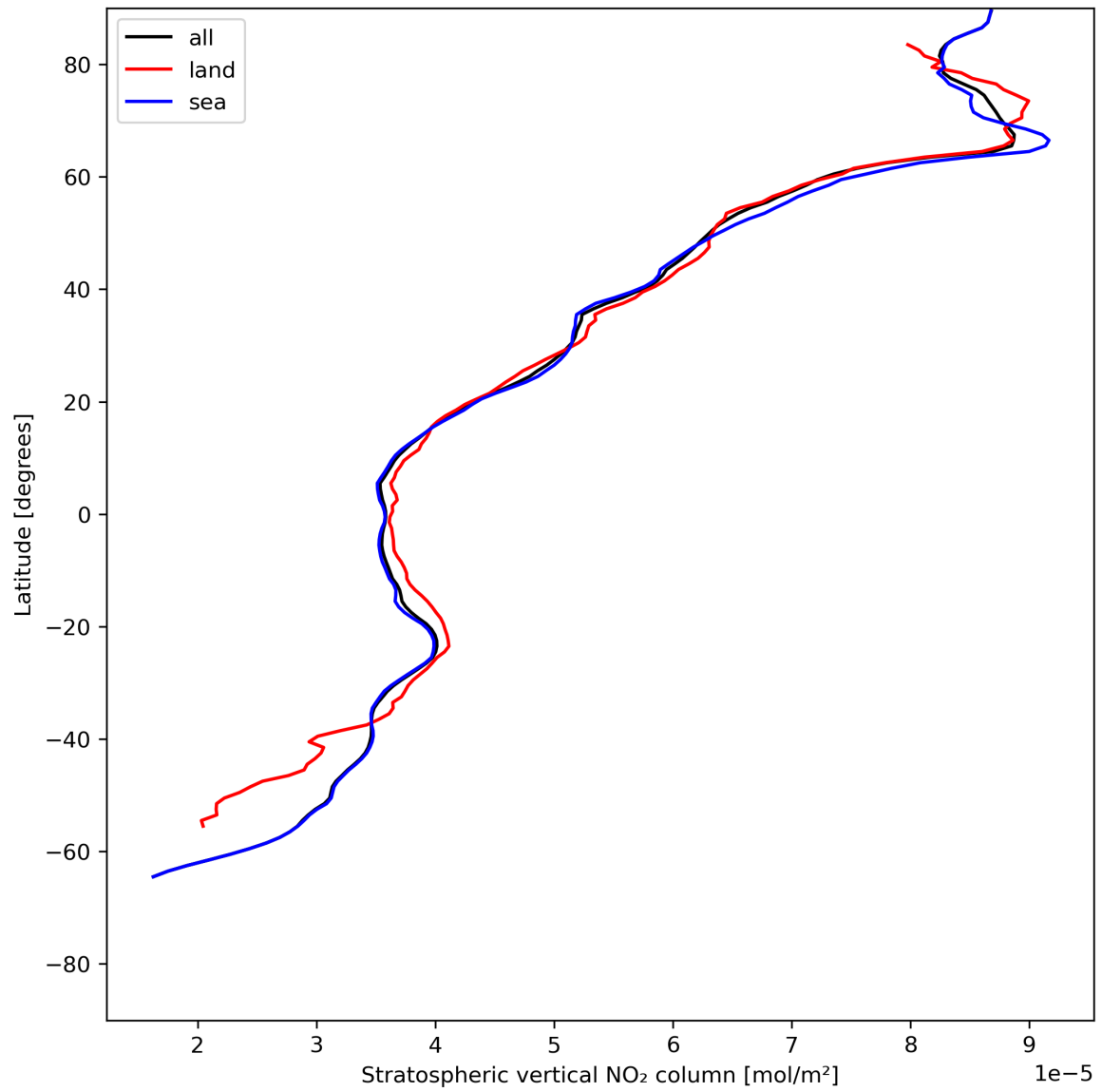
Figure 19: Zonal average of “Stratospheric vertical NO 2 column” for 2024-06-04 to 2024-06-06.
