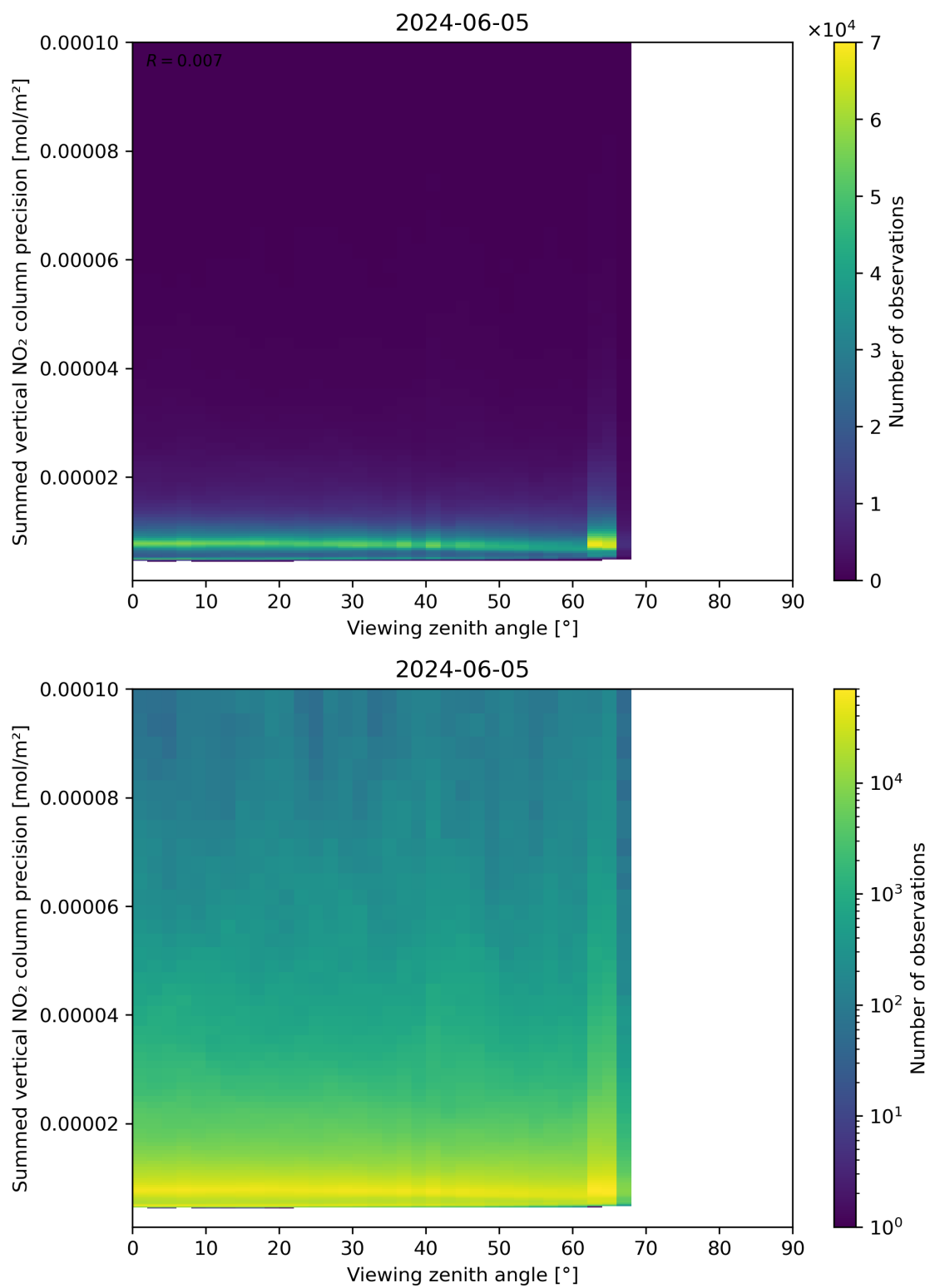
Figure 166: Scatter density plot of “Viewing zenith angle” against “Summed vertical NO 2 column precision” for 2024-06-04 to 2024-06-06.
