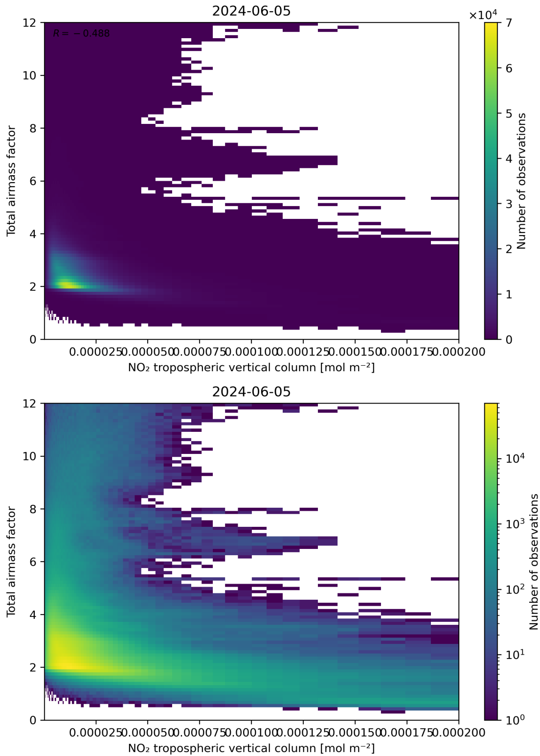
Figure 122: Scatter density plot of “NO 2 tropospheric vertical column” against “Total air mass factor” for 2024-06-04 to 2024-06-06.
