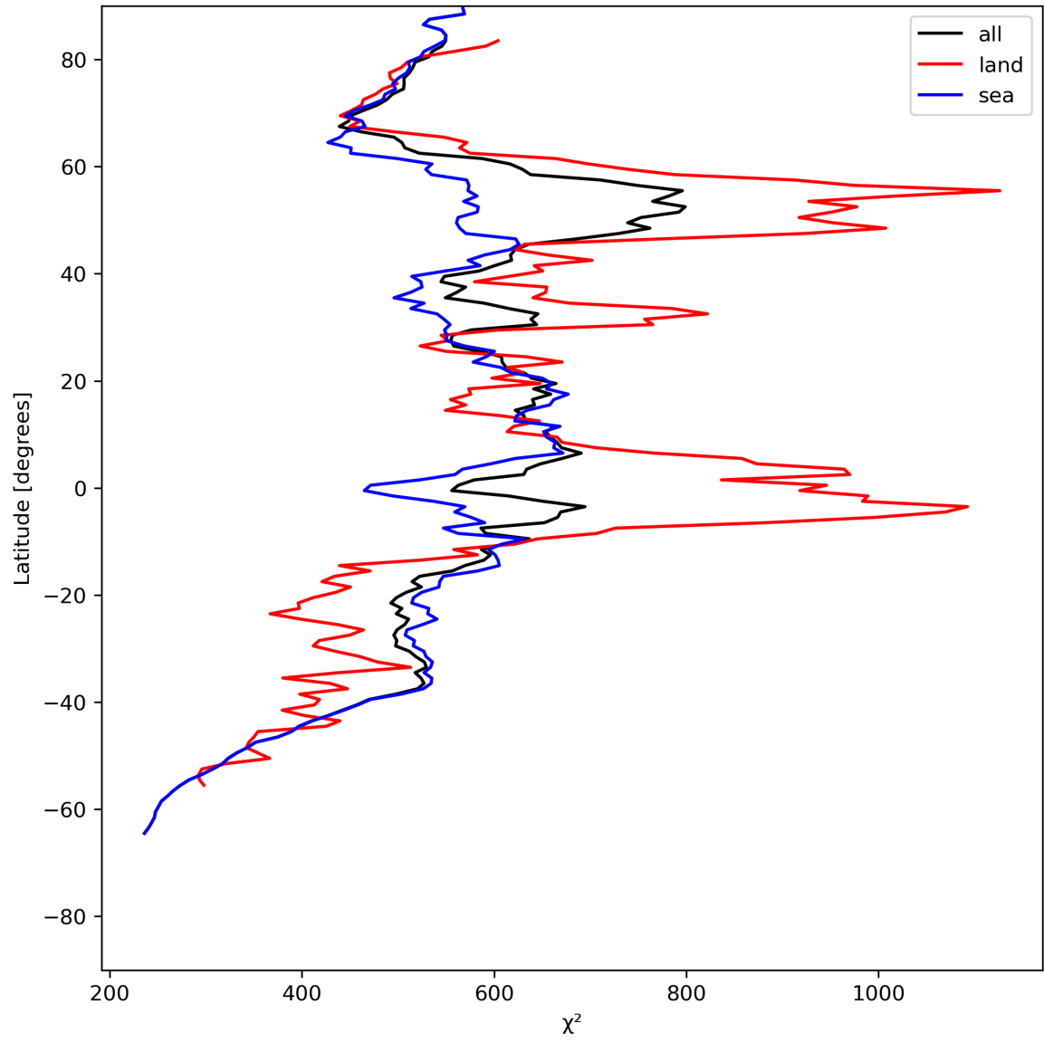
Figure 25: Zonal average of “ \chi^2 ” for 2024-06-04 to 2024-06-06.
