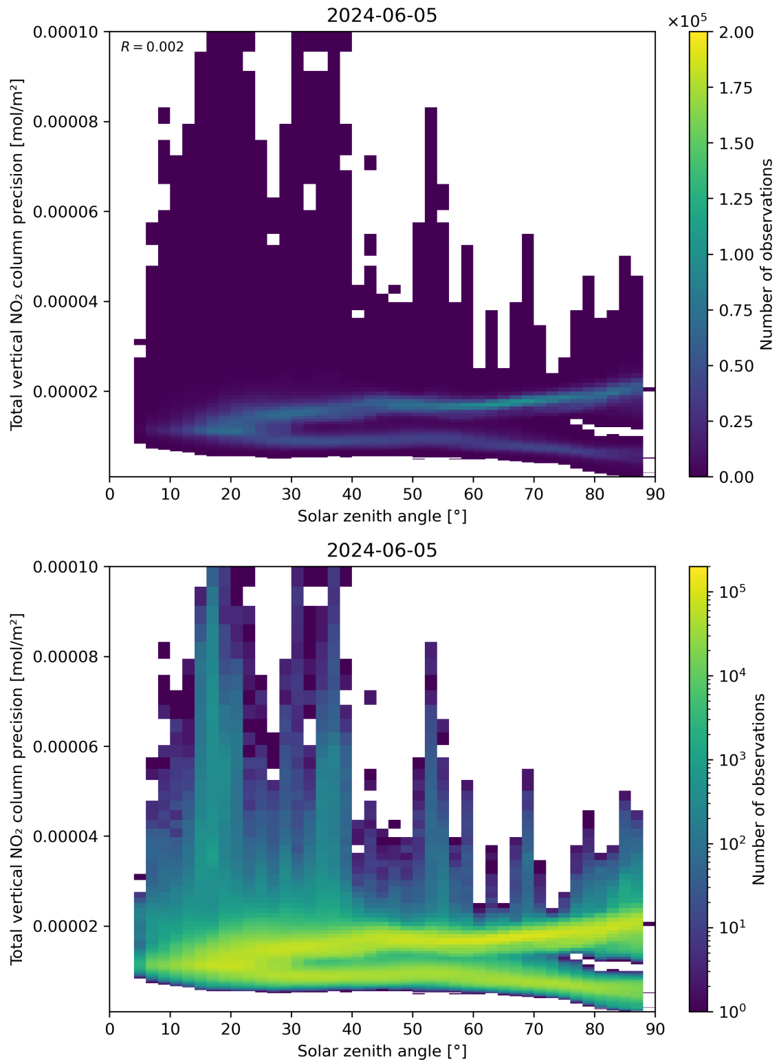
Figure 154: Scatter density plot of “Solar zenith angle” against “Total vertical NO 2 column precision” for 2024-06-04 to 2024-06-06.
