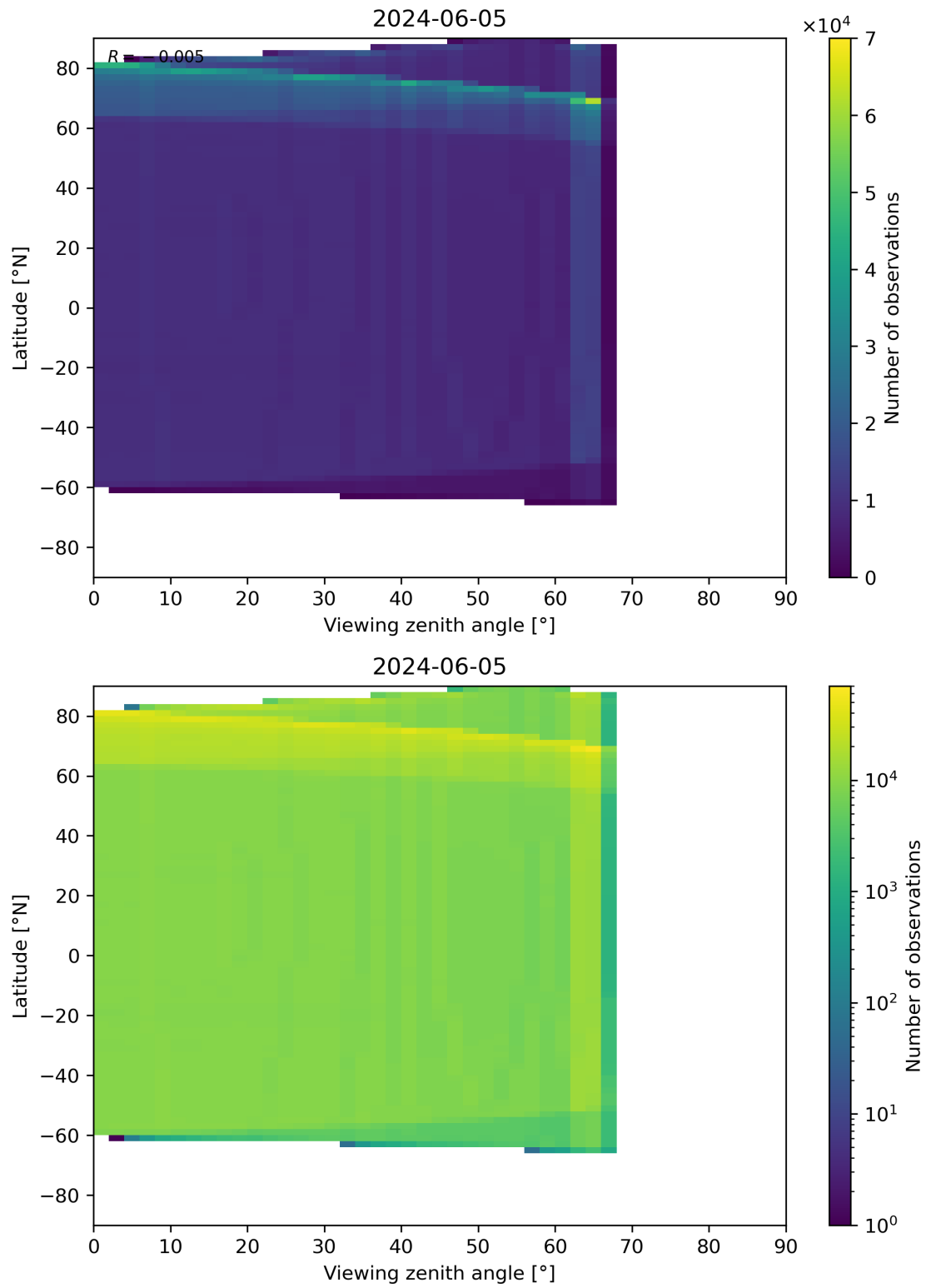
Figure 163: Scatter density plot of “Viewing zenith angle” against “Latitude” for 2024-06-04 to 2024-06-06.
