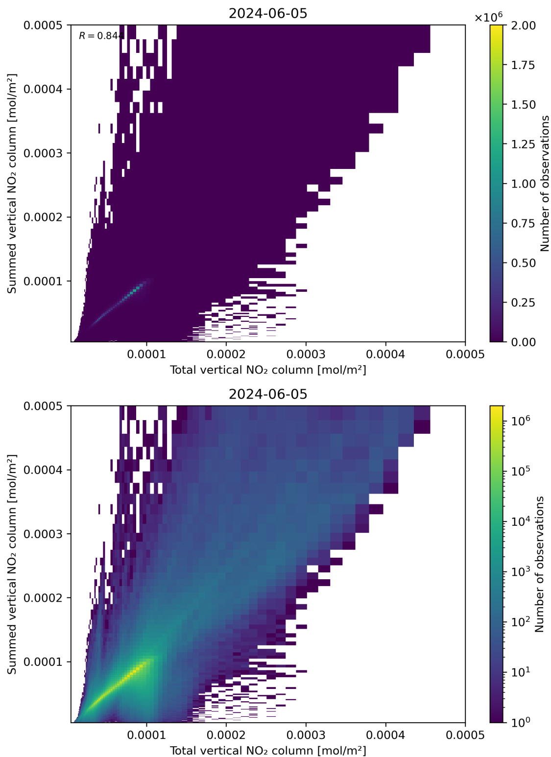
Figure 112: Scatter density plot of “Total vertical NO 2 column” against “Summed vertical NO 2 column” for 2024-06-04 to 2024-06-06.
