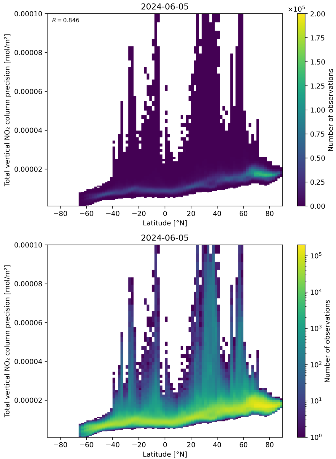
Figure 91: Scatter density plot of “Latitude” against “Total vertical NO 2 column precision” for 2024-06-04 to 2024-06-06.
