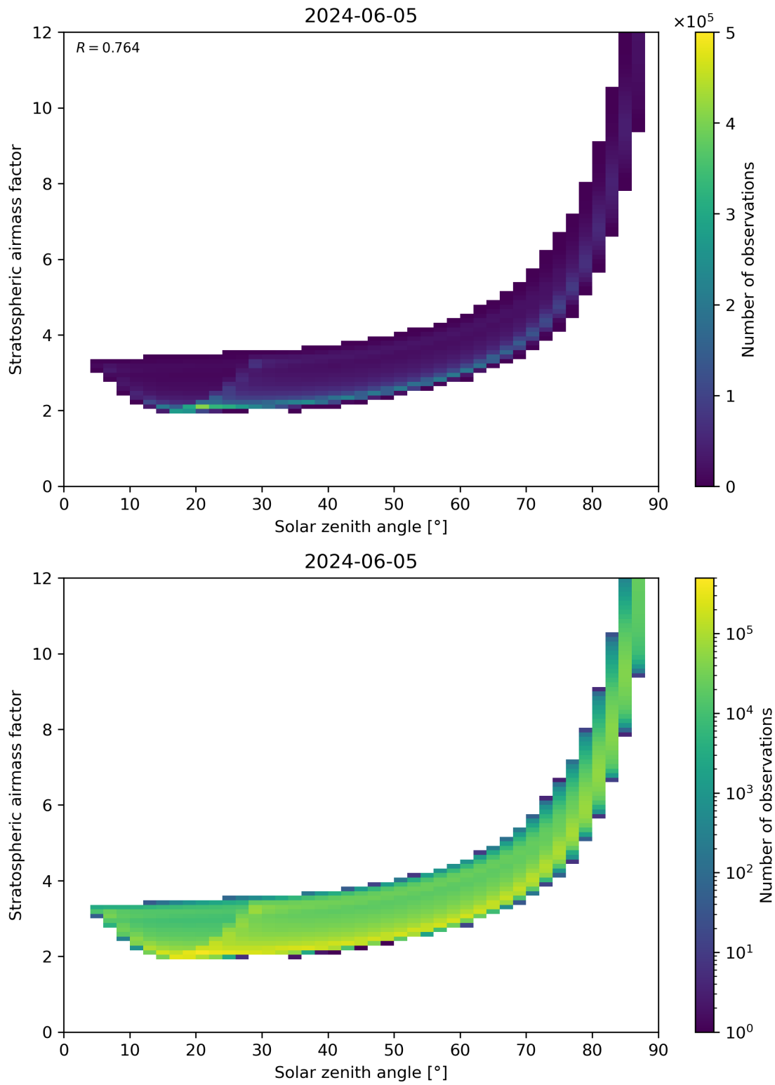
Figure 145: Scatter density plot of “Solar zenith angle” against “Stratospheric airmass factor” for 2024-06-04 to 2024-06-06.
