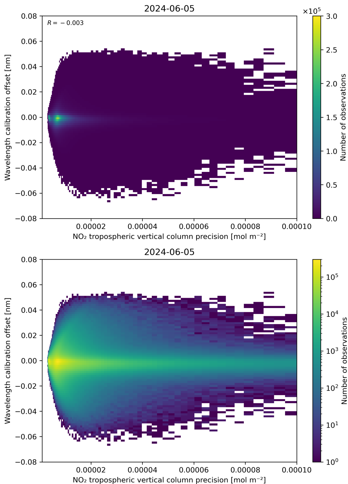
Figure 141: Scatter density plot of “NO 2 tropospheric vertical column precision” against “Wavelength calibration offset” for 2024-06-04 to 2024-06-06.
