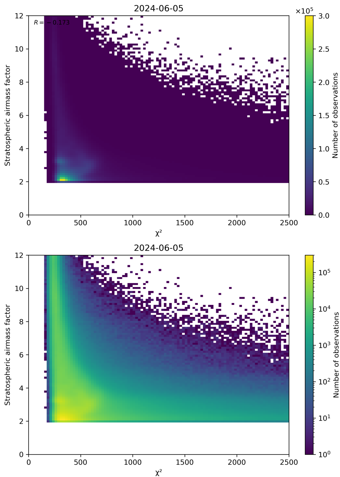
Figure 81: Scatter density plot of “ \chi^2 ” against “Stratospheric airmass factor” for 2024-06-04 to 2024-06-06.
