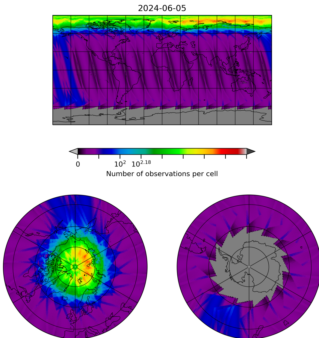
Figure 10: Map of the number of observations for 2024-06-04 to 2024-06-06
