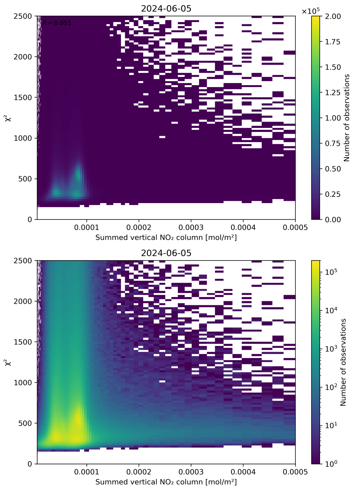
Figure 104: Scatter density plot of “Summed vertical NO 2 column” against “ \chi^2 ” for 2024-06-04 to 2024-06-06.
