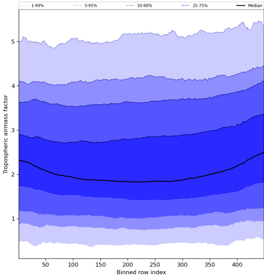
Figure 48: Along track statistics of “Tropospheric airmass factor” for 2024-06-04 to 2024-06-06
