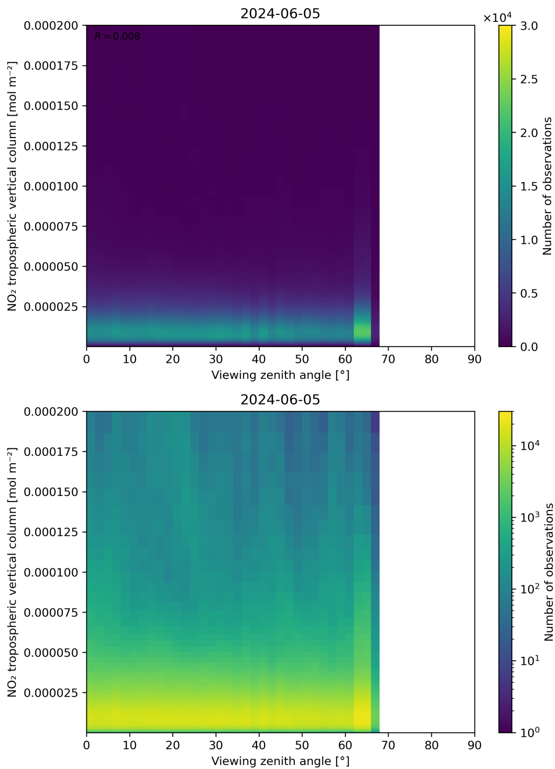
Figure 169: Scatter density plot of “Viewing zenith angle” against “NO 2 tropospheric vertical column” for 2024-06-04 to 2024-06-06.
