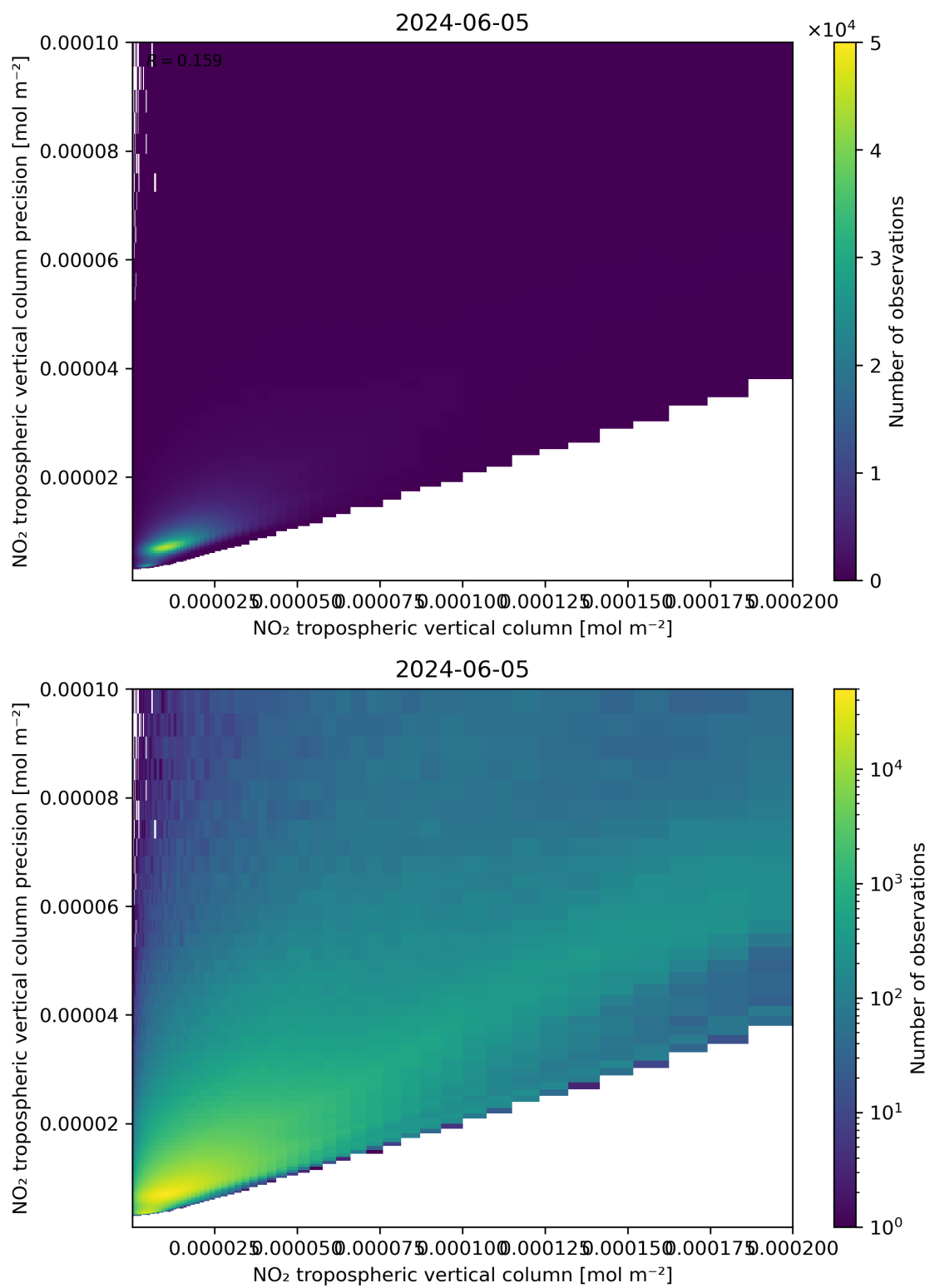
Figure 130: Scatter density plot of “NO 2 tropospheric vertical column” against “NO 2 tropospheric vertical column precision” for 2024-06-04 to 2024-06-06.
