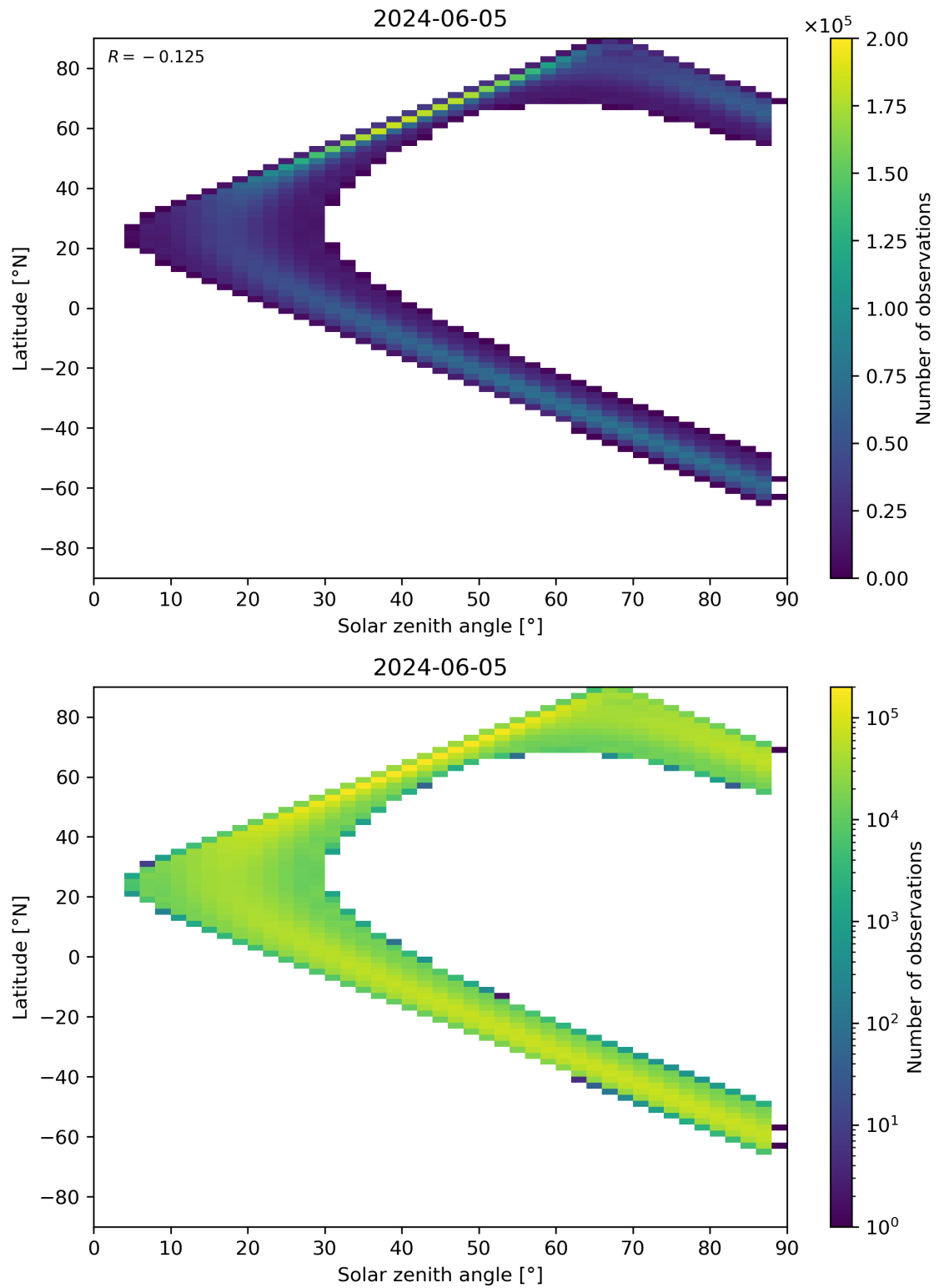
Figure 149: Scatter density plot of “Solar zenith angle” against “Latitude” for 2024-06-04 to 2024-06-06.
