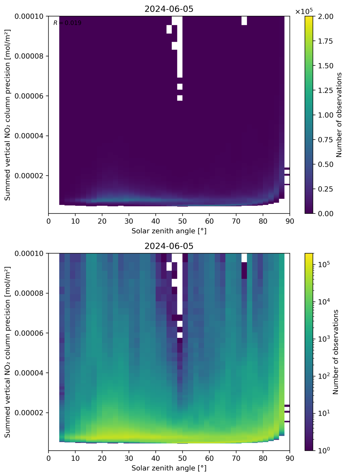
Figure 152: Scatter density plot of “Solar zenith angle” against “Summed vertical NO 2 column precision” for 2024-06-04 to 2024-06-06.
