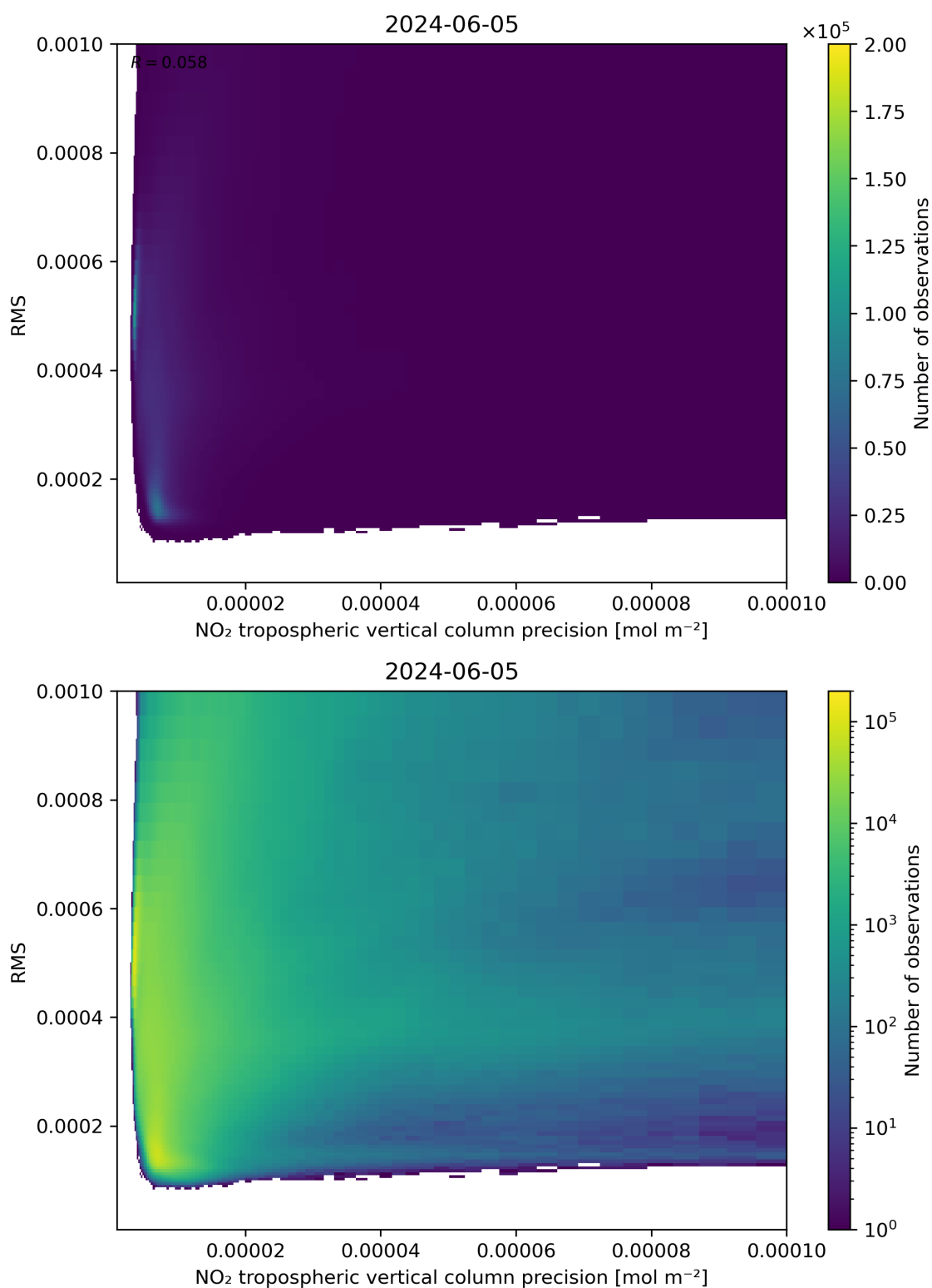
Figure 140: Scatter density plot of “NO 2 tropospheric vertical column precision” against “RMS” for 2024-06-04 to 2024-06-06.
