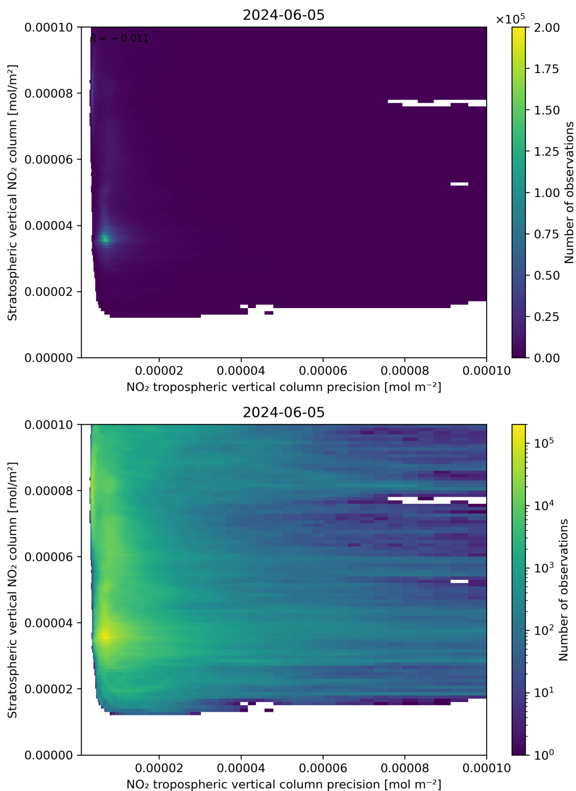
Figure 135: Scatter density plot of “NO 2 tropospheric vertical column precision” against “Stratospheric vertical NO 2 column” for 2024-06-04 to 2024-06-06.
