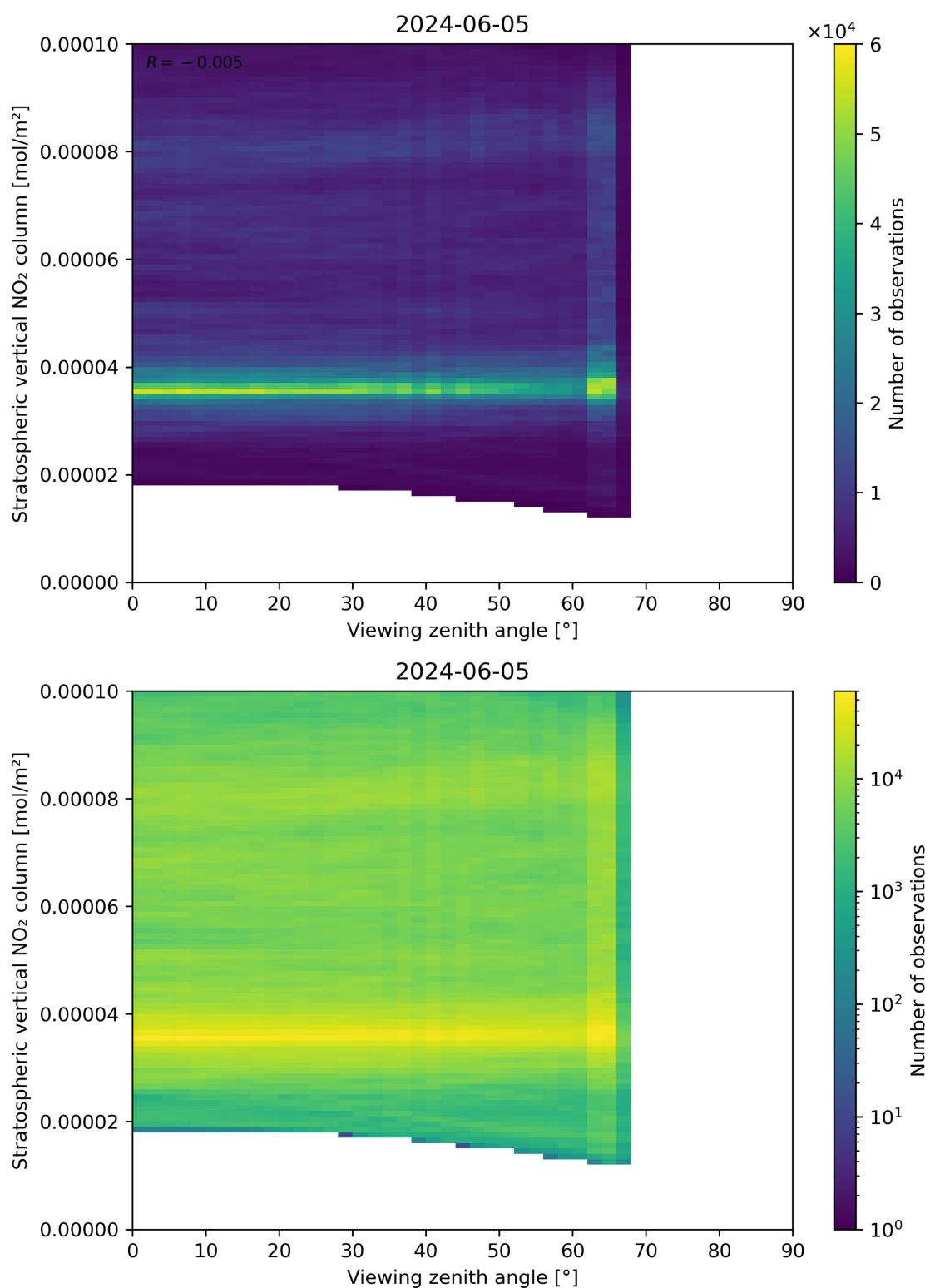
Figure 164: Scatter density plot of “Viewing zenith angle” against “Stratospheric vertical NO 2 column” for 2024-06-04 to 2024-06-06.
