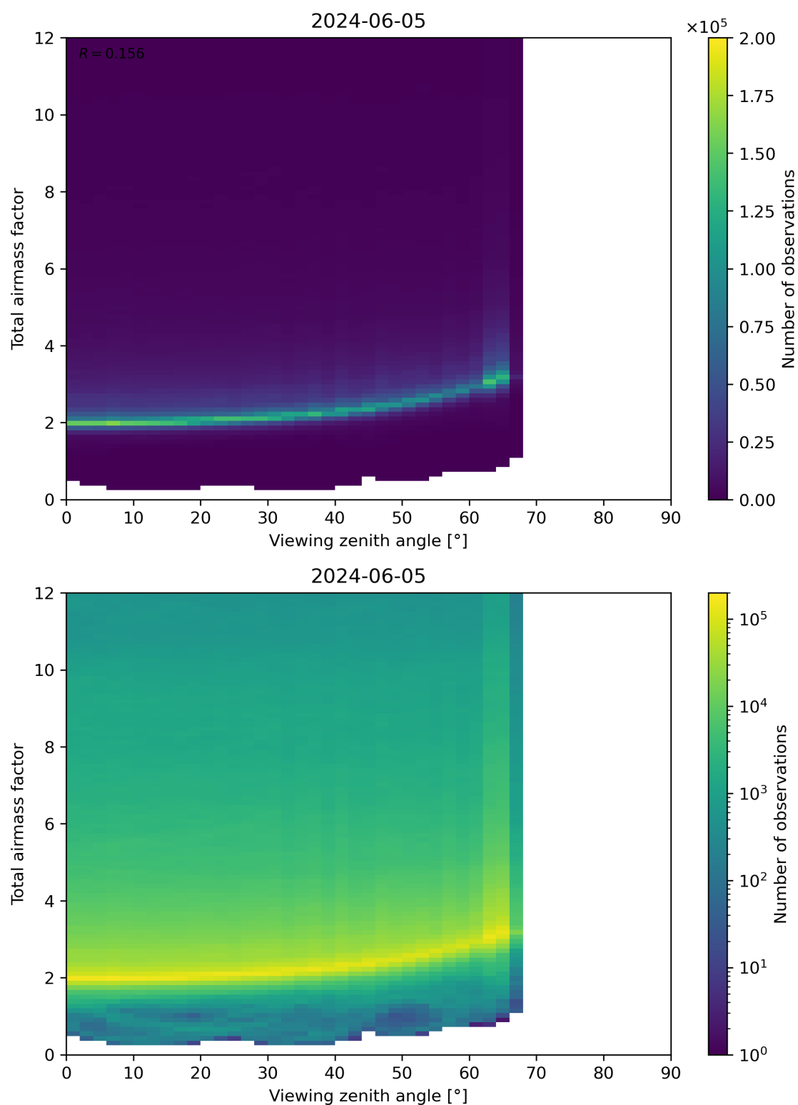
Figure 160: Scatter density plot of “Viewing zenith angle” against “Total airmass factor” for 2024-06-04 to 2024-06-06.
