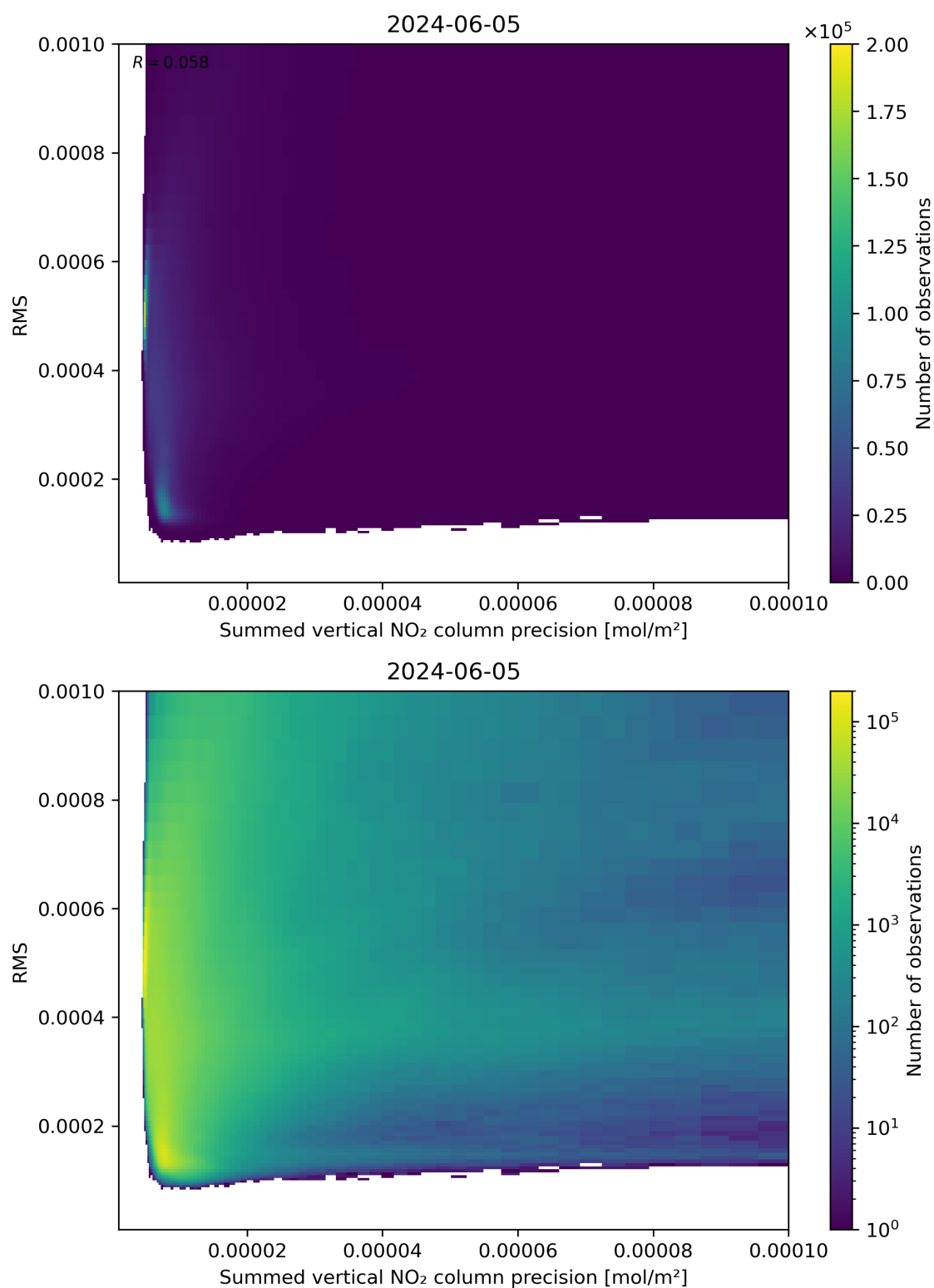
Figure 108: Scatter density plot of “Summed vertical NO 2 column precision” against “RMS” for 2024-06-04 to 2024-06-06.
