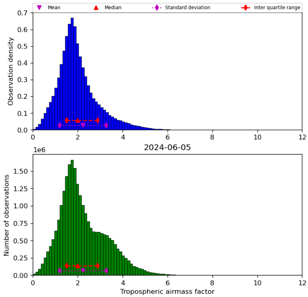
Figure 31: Histogram of “Tropospheric airmass factor” for 2024-06-04 to 2024-06-06
