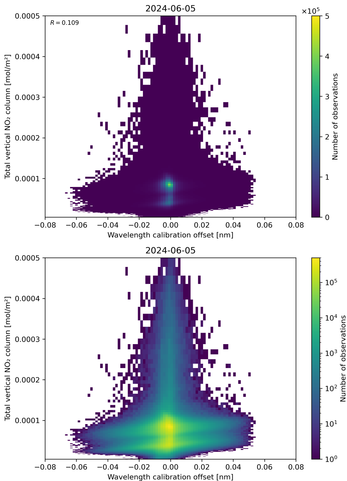
Figure 179: Scatter density plot of “Wavelength calibration offset” against “Total vertical NO 2 column” for 2024-06-04 to 2024-06-06.
