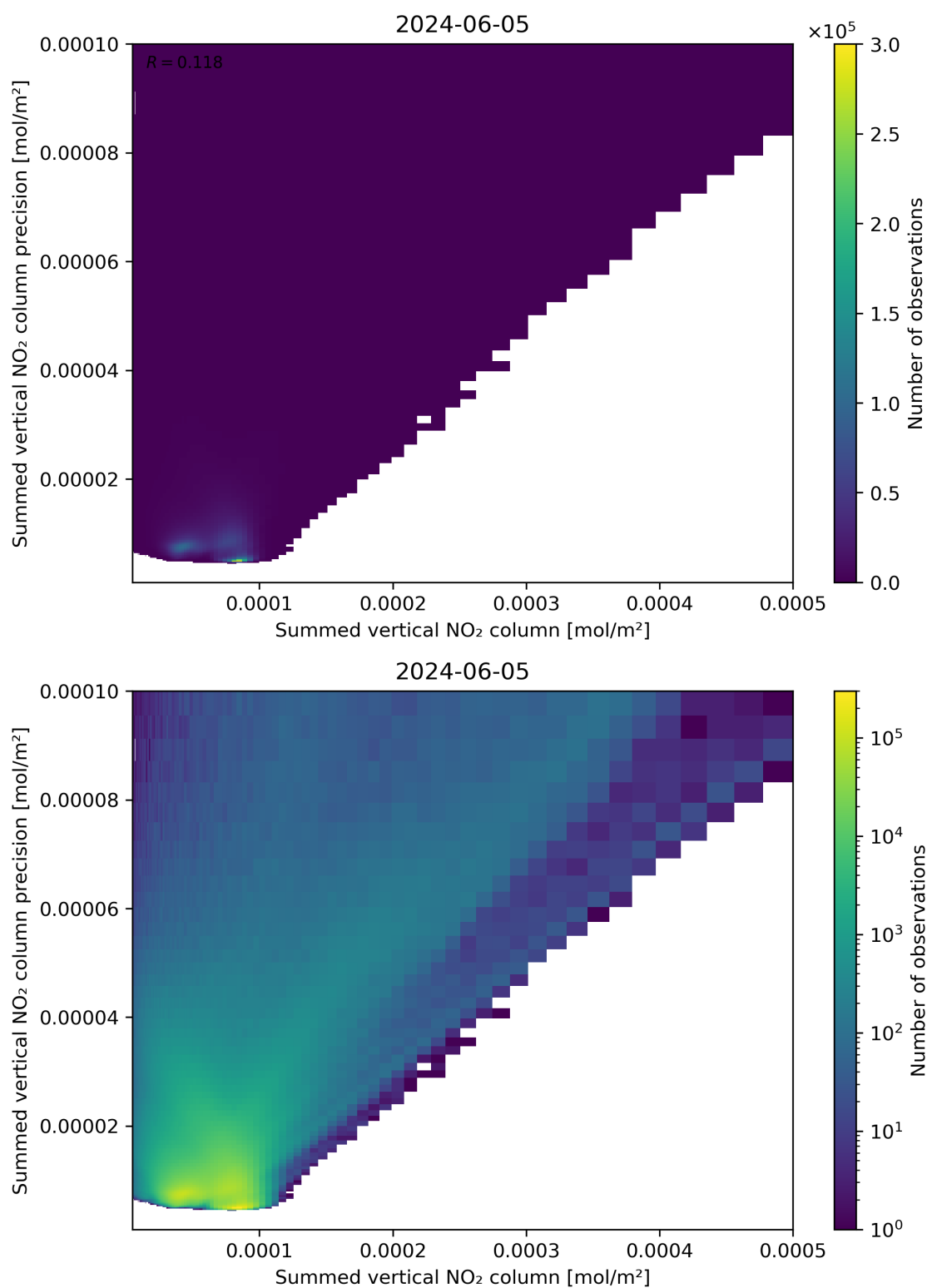
Figure 105: Scatter density plot of “Summed vertical NO 2 column” against “Summed vertical NO 2 column precision” for 2024-06-04 to 2024-06-06.
