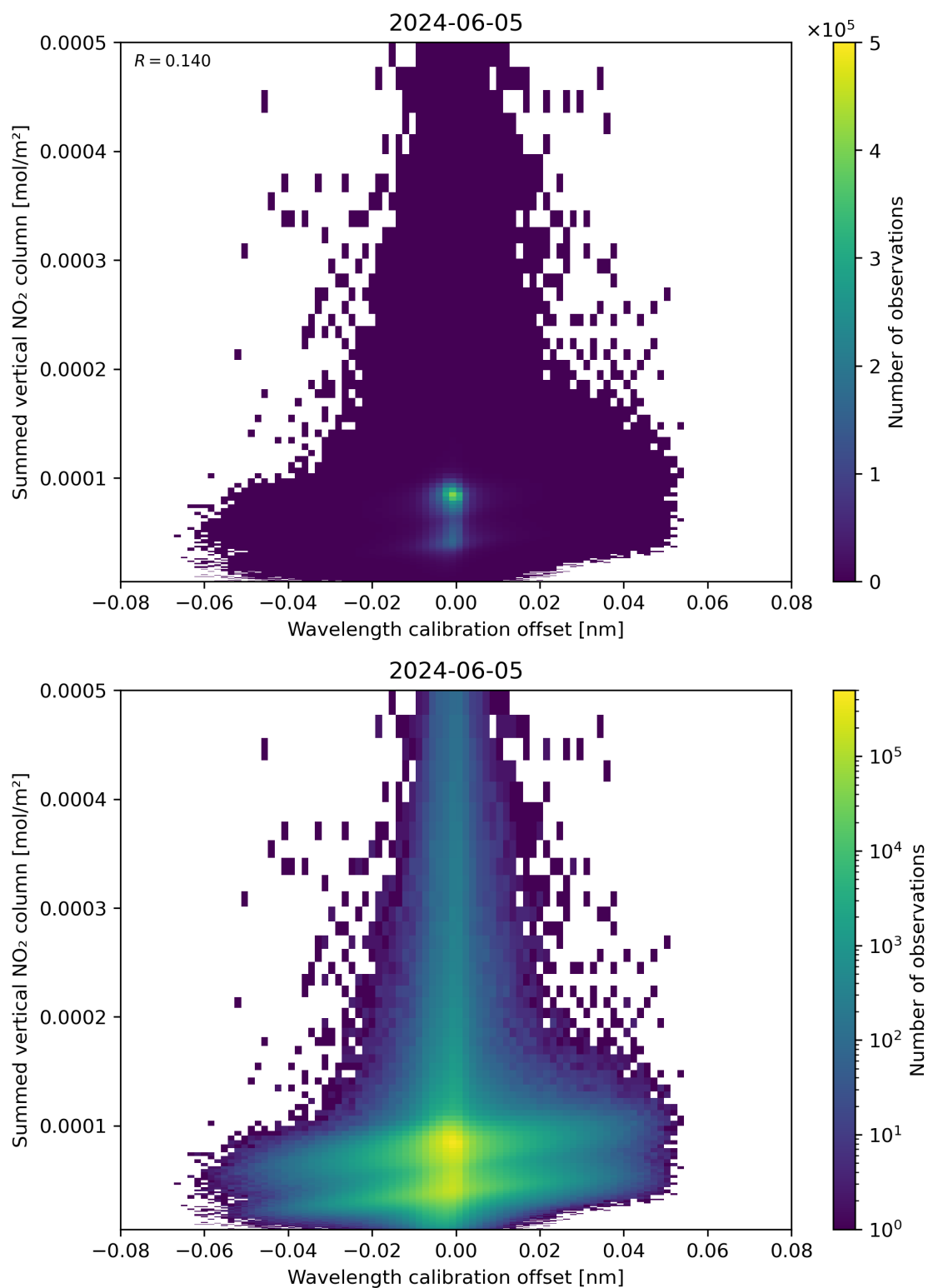
Figure 177: Scatter density plot of “Wavelength calibration offset” against “Summed vertical NO 2 column” for 2024-06-04 to 2024-06-06.
