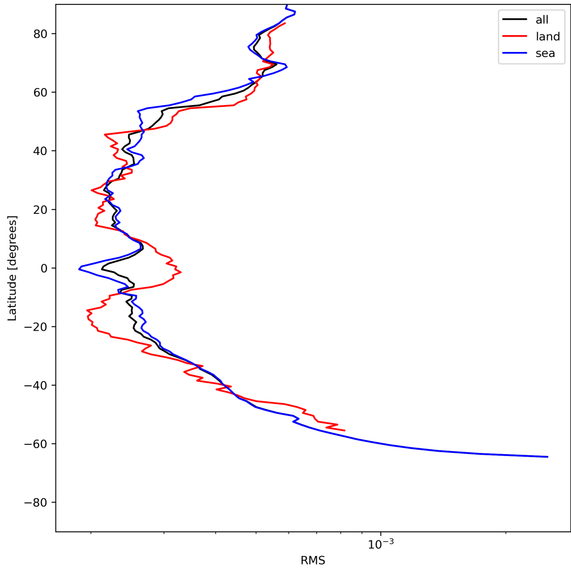
Figure 26: Zonal average of “RMS” for 2024-06-04 to 2024-06-06.
