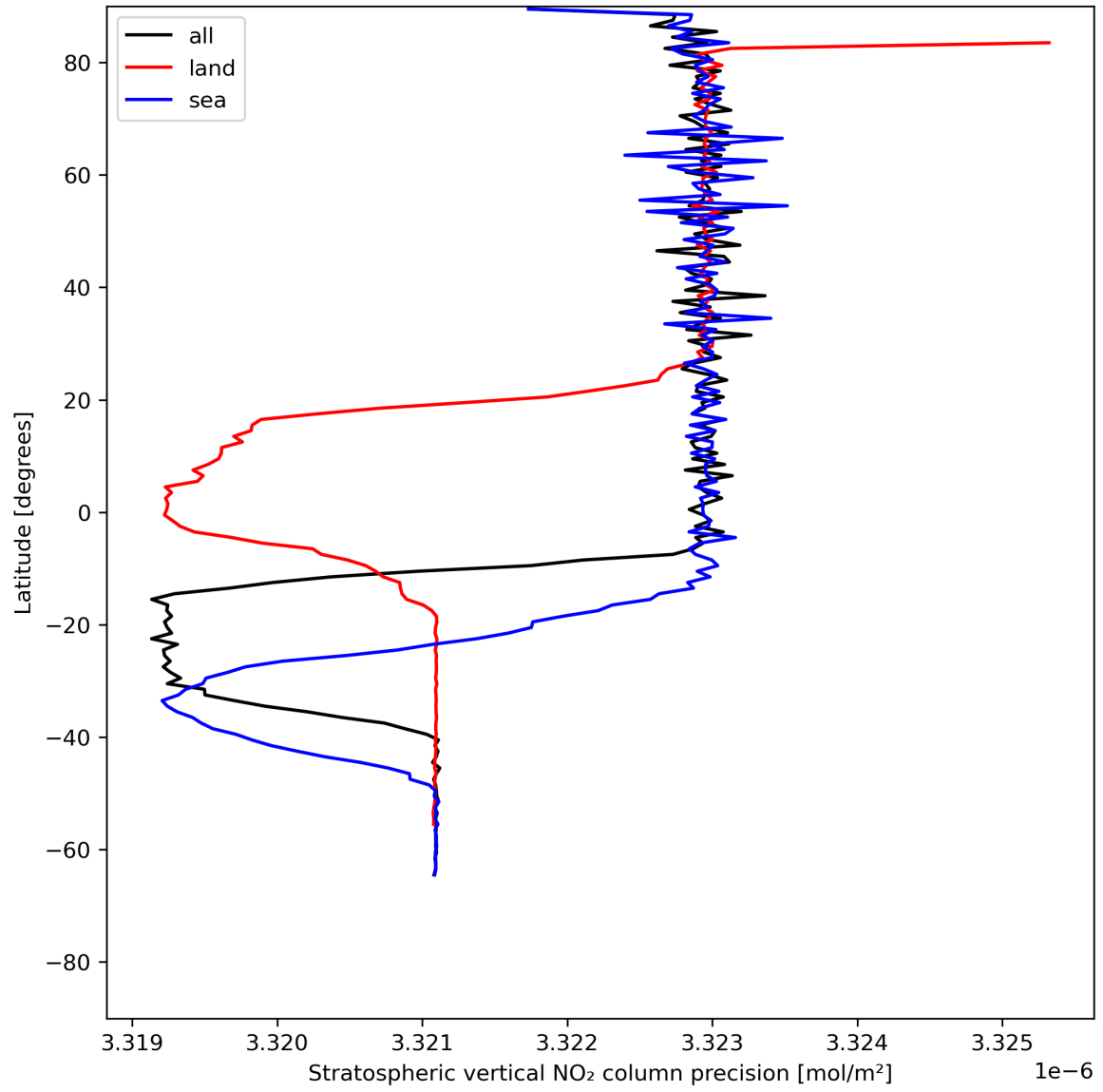
Figure 20: Zonal average of “Stratospheric vertical NO 2 column precision” for 2024-06-04 to 2024-06-06.
