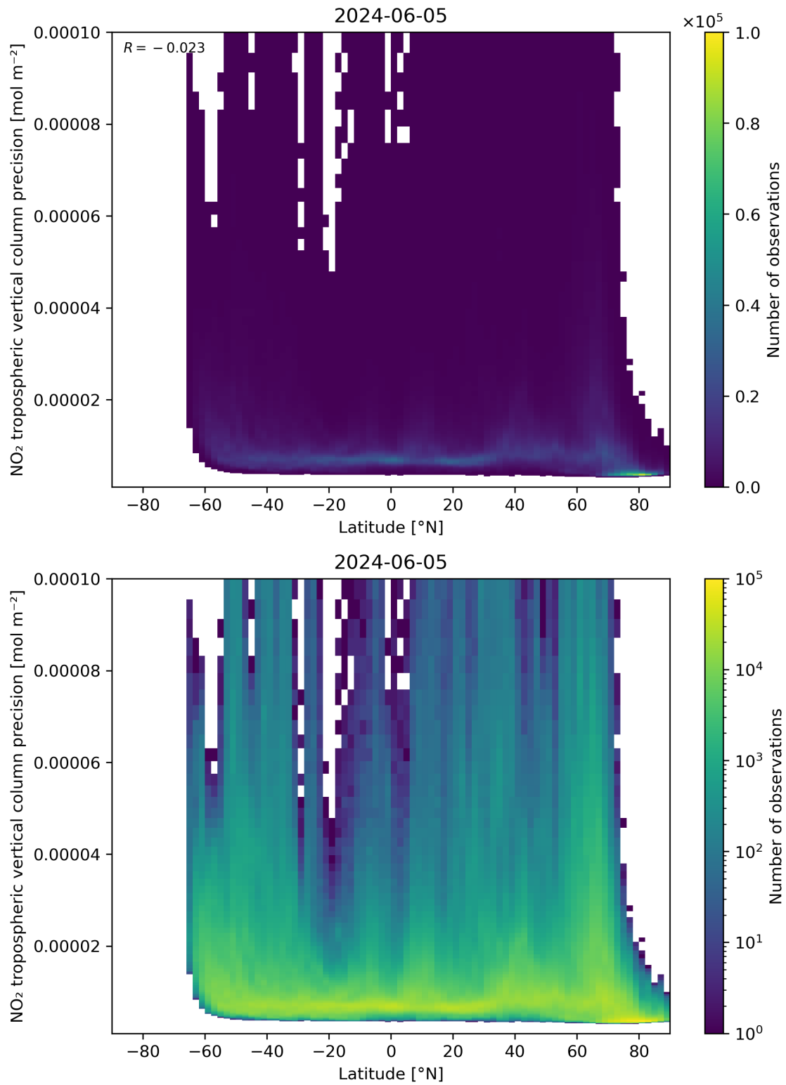
Figure 93: Scatter density plot of “Latitude” against “NO 2 tropospheric vertical column precision” for 2024-06-04 to 2024-06-06.
