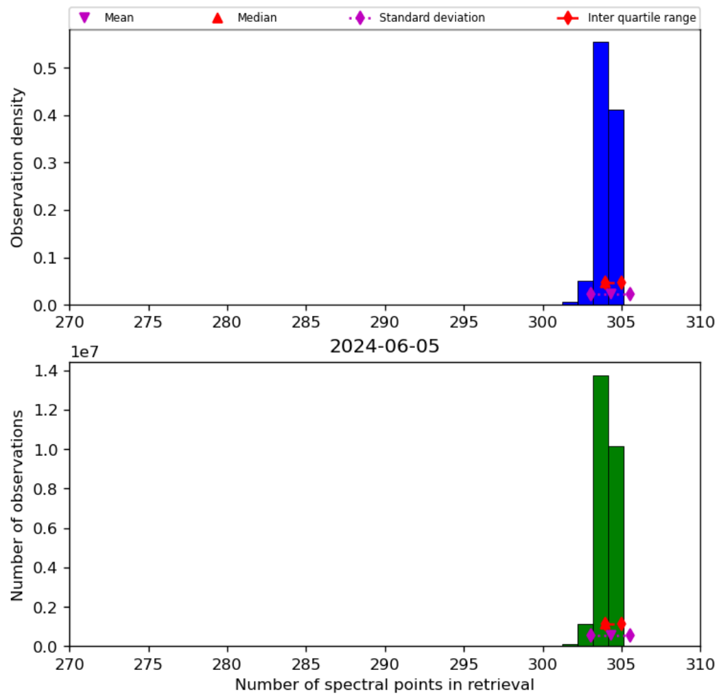
Figure 33: Histogram of “Number of spectral points in retrieval” for 2024-06-04 to 2024-06-06
