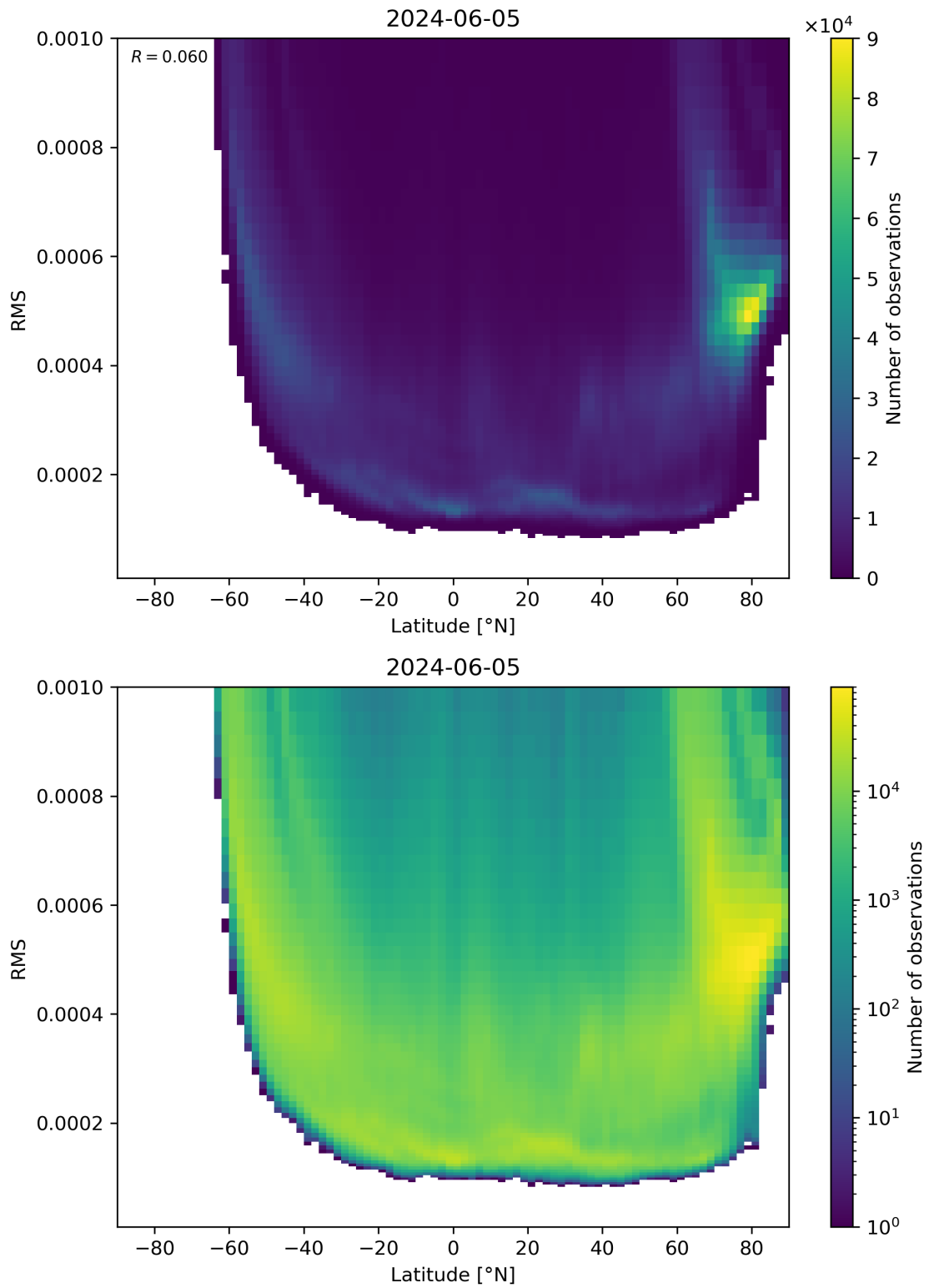
Figure 94: Scatter density plot of “Latitude” against “RMS” for 2024-06-04 to 2024-06-06.
