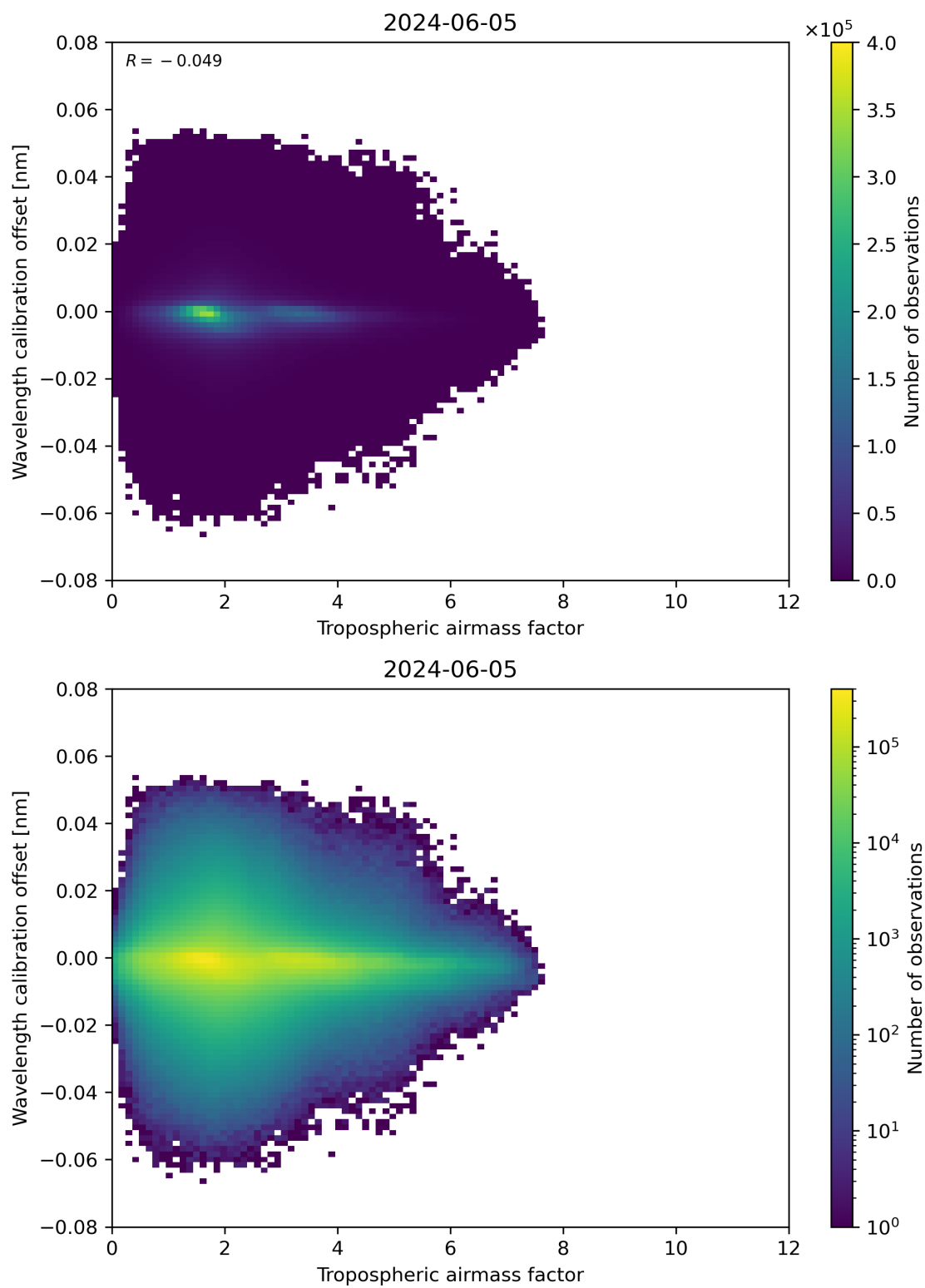
Figure 80: Scatter density plot of “Tropospheric airmass factor” against “Wavelength calibration offset” for 2024-06-04 to 2024-06-06.
