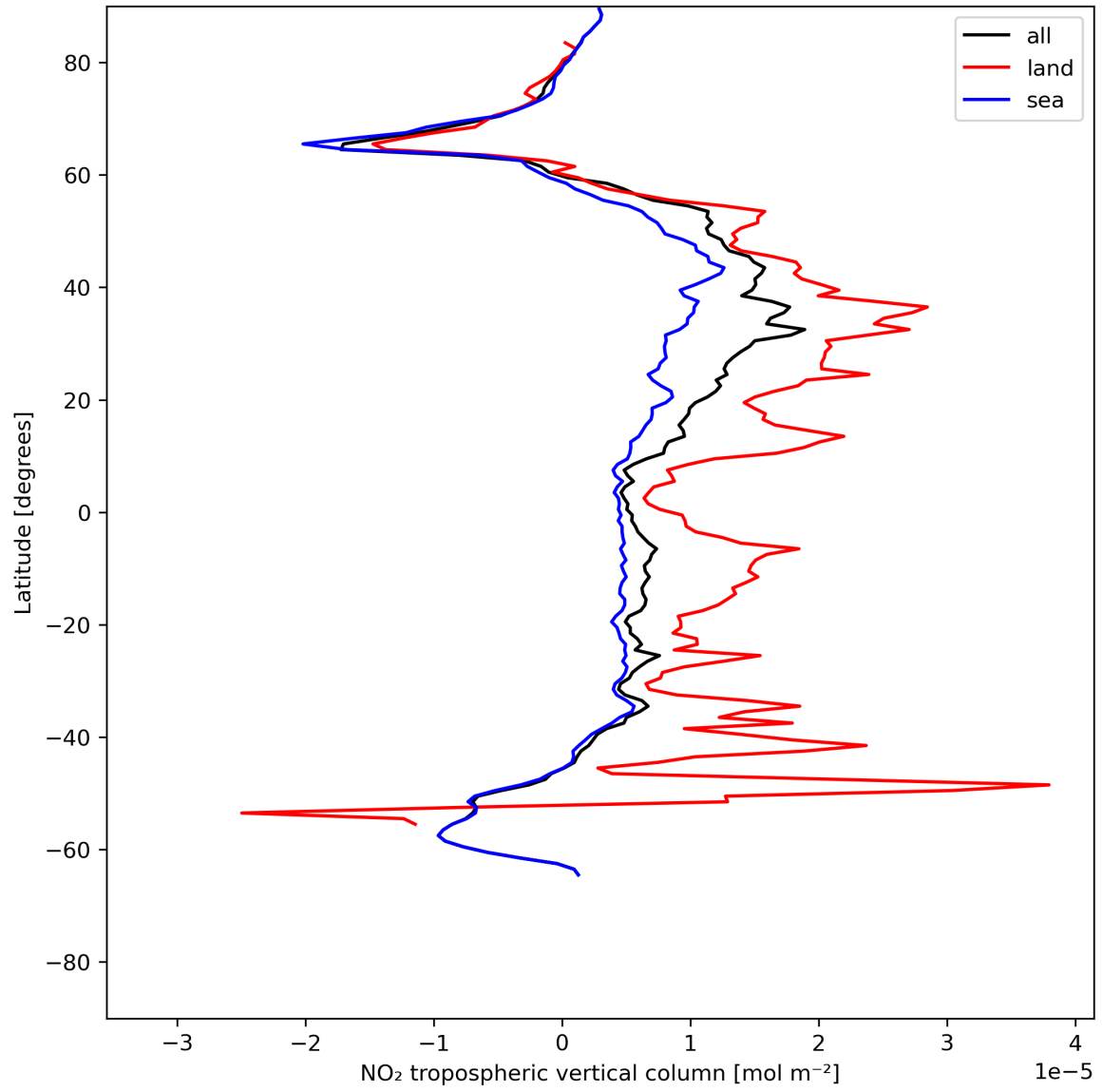
Figure 12: Zonal average of “NO 2 tropospheric vertical column” for 2024-06-04 to 2024-06-06.
