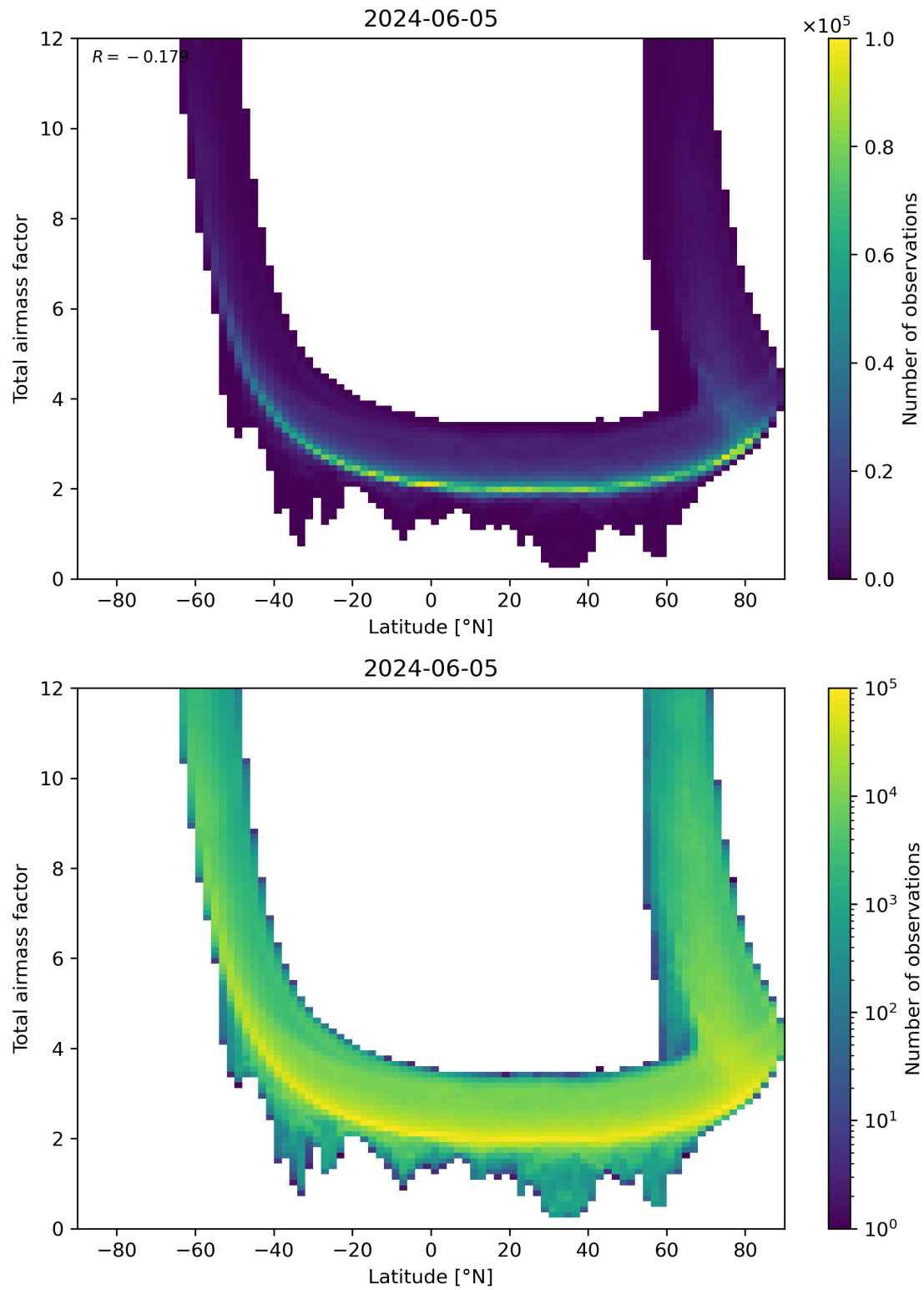
Figure 84: Scatter density plot of “Latitude” against “Total airmass factor” for 2024-06-04 to 2024-06-06.
