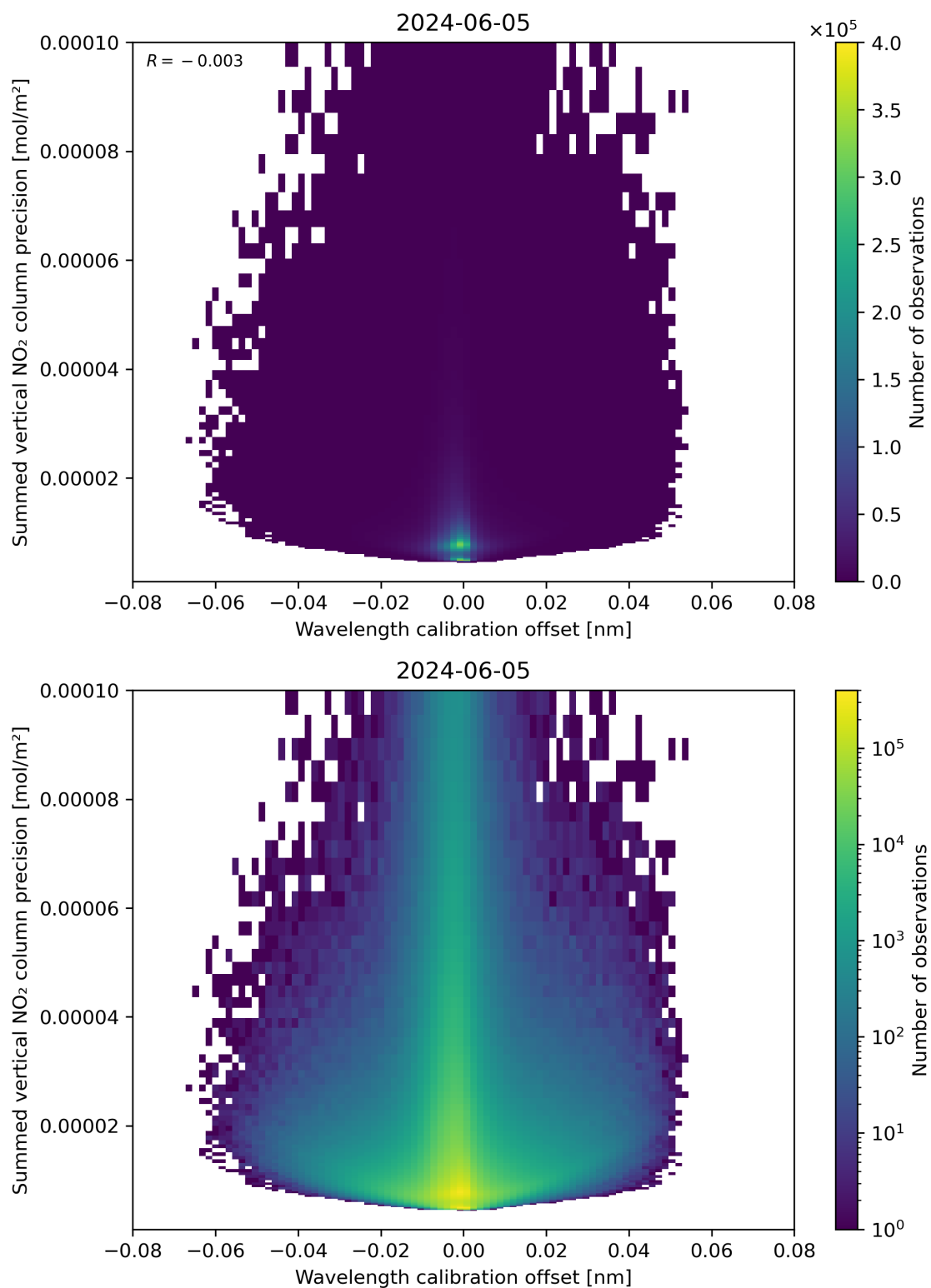
Figure 178: Scatter density plot of “Wavelength calibration offset” against “Summed vertical NO 2 column precision” for 2024-06-04 to 2024-06-06.
