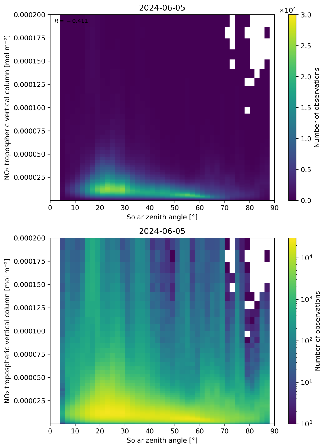
Figure 155: Scatter density plot of “Solar zenith angle” against “NO 2 tropospheric vertical column” for 2024-06-04 to 2024-06-06.
