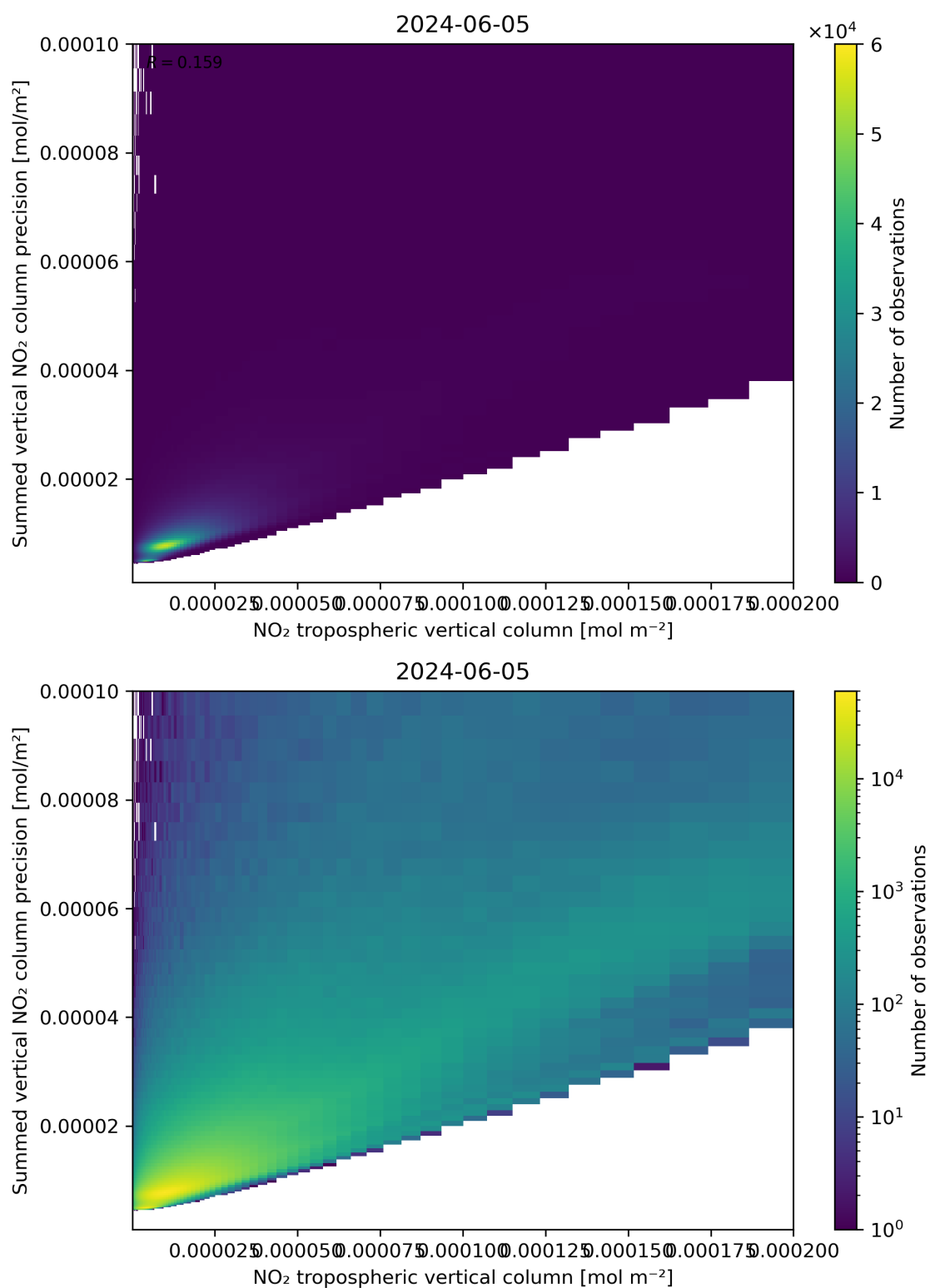
Figure 127: Scatter density plot of “NO 2 tropospheric vertical column” against “Summed vertical NO 2 column precision” for 2024-06-04 to 2024-06-06.
