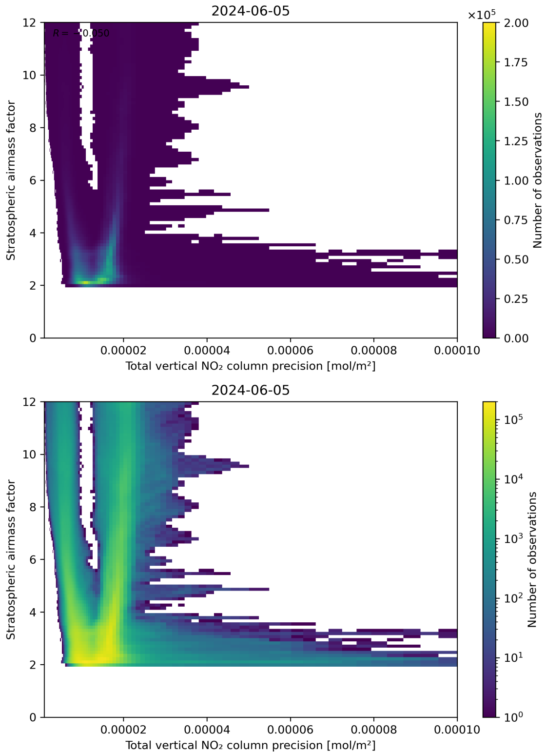
Figure 115: Scatter density plot of “Total vertical NO 2 column precision” against “Stratospheric air mass factor” for 2024-06-04 to 2024-06-06.
