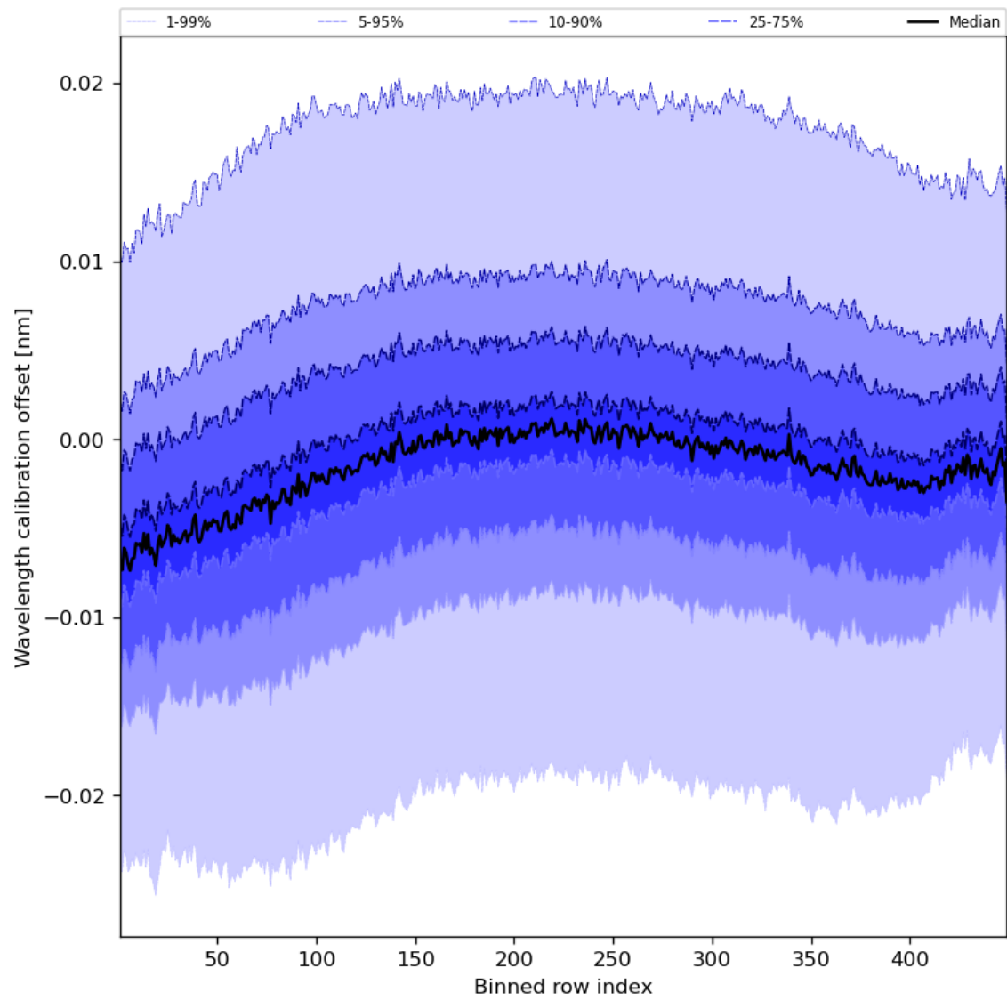
Figure 52: Along track statistics of “Wavelength calibration offset” for 2024-06-04 to 2024-06-06
