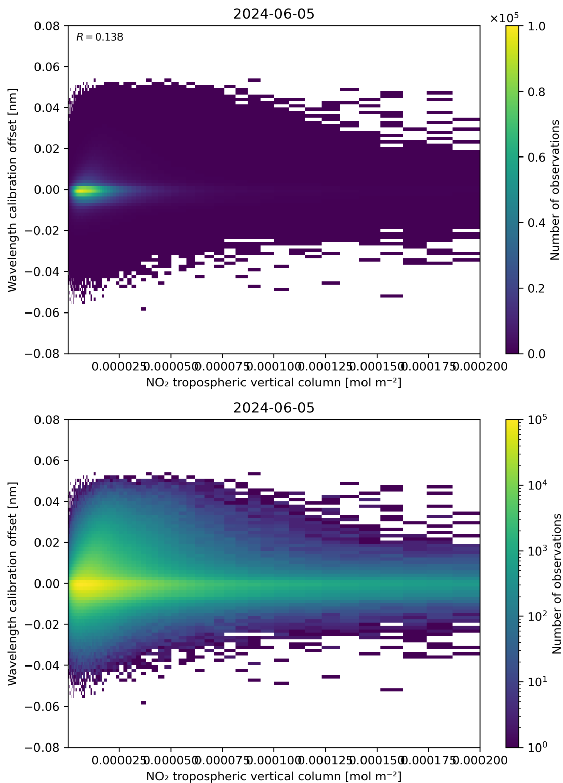
Figure 143: Scatter density plot of “NO 2 tropospheric vertical column” against “Wavelength calibration offset” for 2024-06-04 to 2024-06-06.
