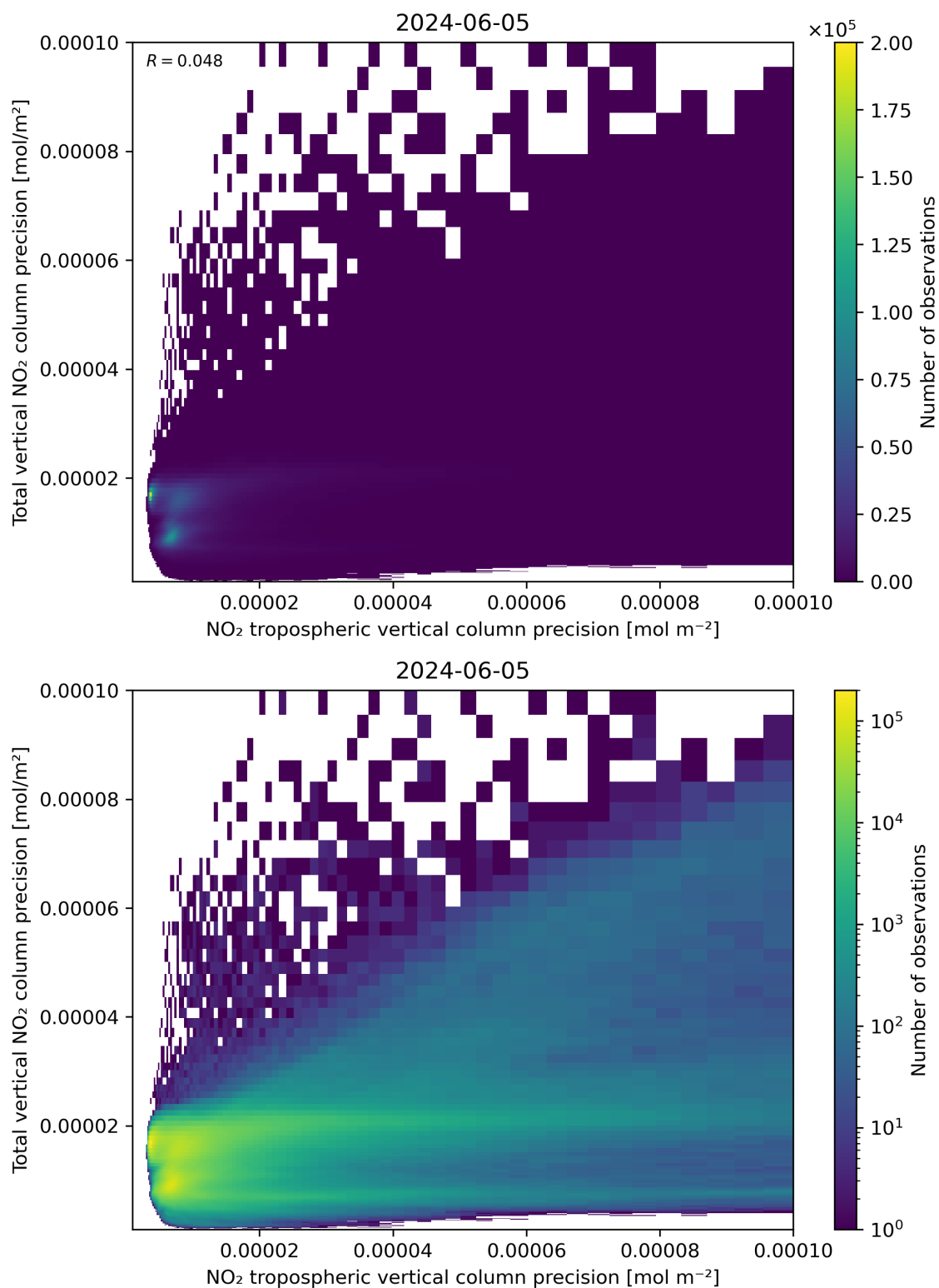
Figure 139: Scatter density plot of “NO 2 tropospheric vertical column precision” against “Total vertical NO 2 column precision” for 2024-06-04 to 2024-06-06.
