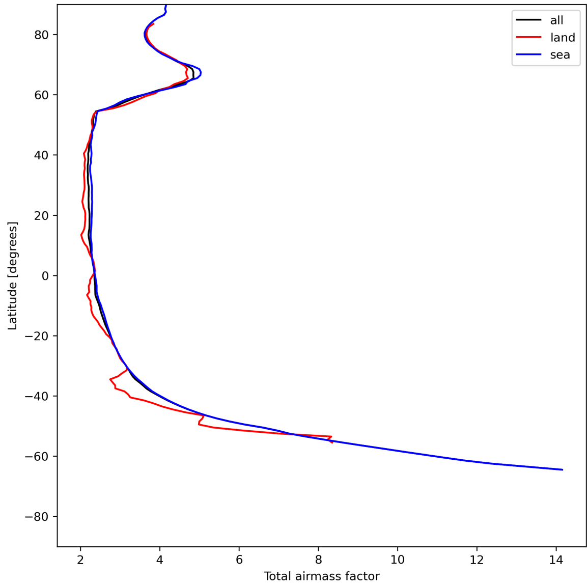
Figure 15: Zonal average of “Total airmass factor” for 2024-06-04 to 2024-06-06.
