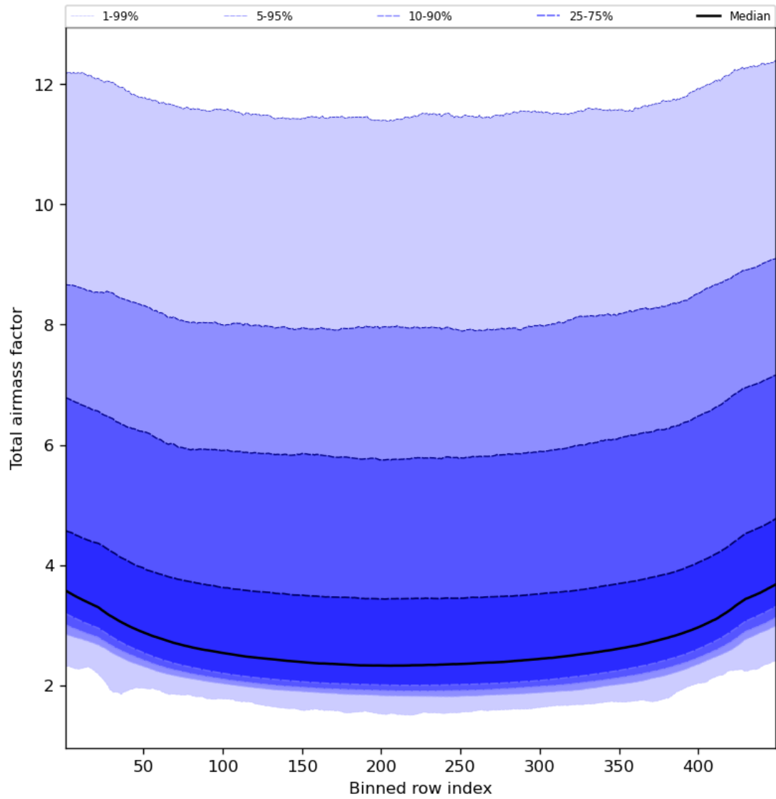
Figure 49: Along track statistics of “Total airmass factor” for 2024-06-04 to 2024-06-06
