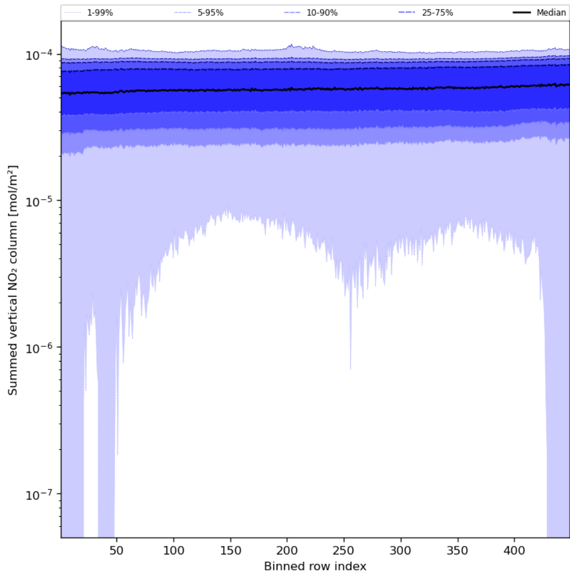
Figure 57: Along track statistics of “Summed vertical NO 2 column” for 2024-06-04 to 2024-06-06
