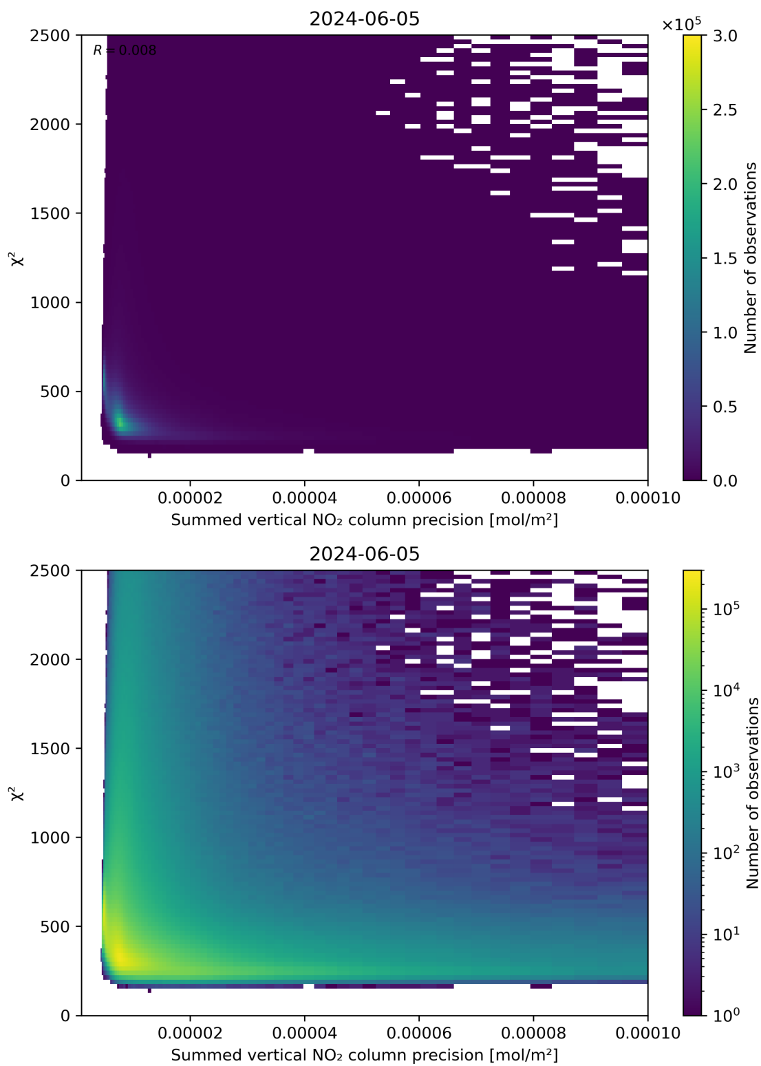
Figure 107: Scatter density plot of “Summed vertical NO 2 column precision” against “ \chi^2 ” for 2024-06-04 to 2024-06-06.
