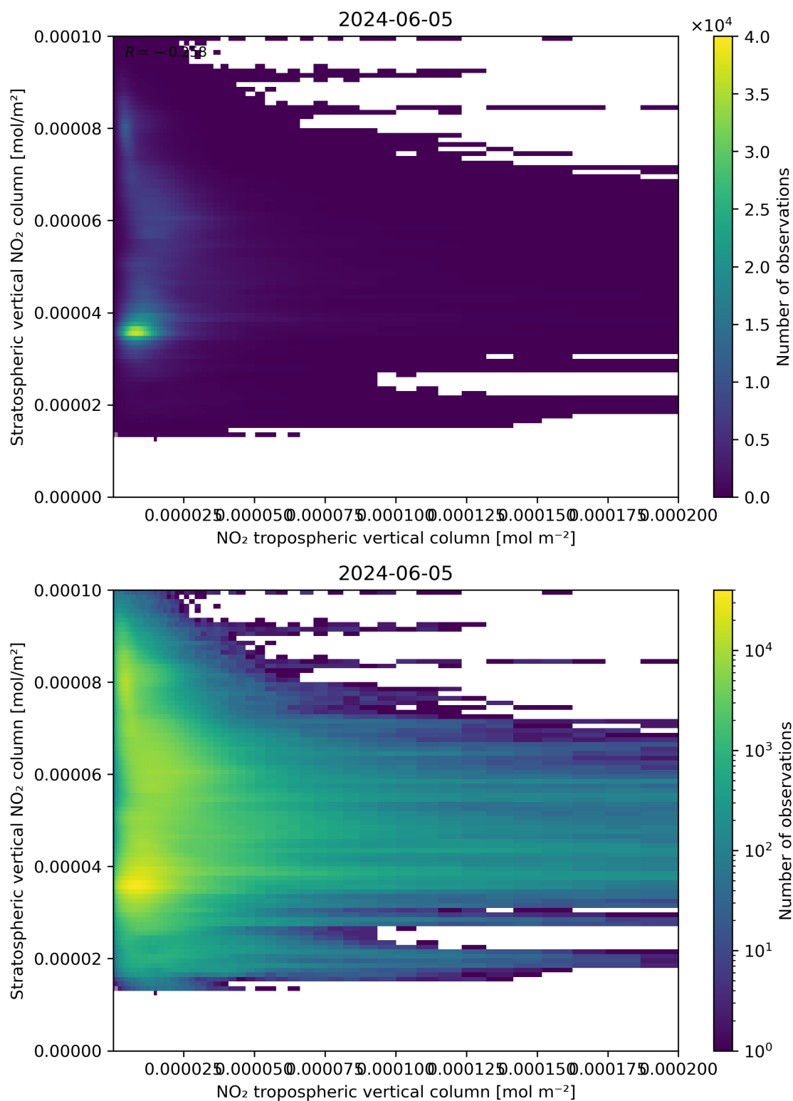
Figure 125: Scatter density plot of “NO 2 tropospheric vertical column” against “Stratospheric vertical NO 2 column” for 2024-06-04 to 2024-06-06.
