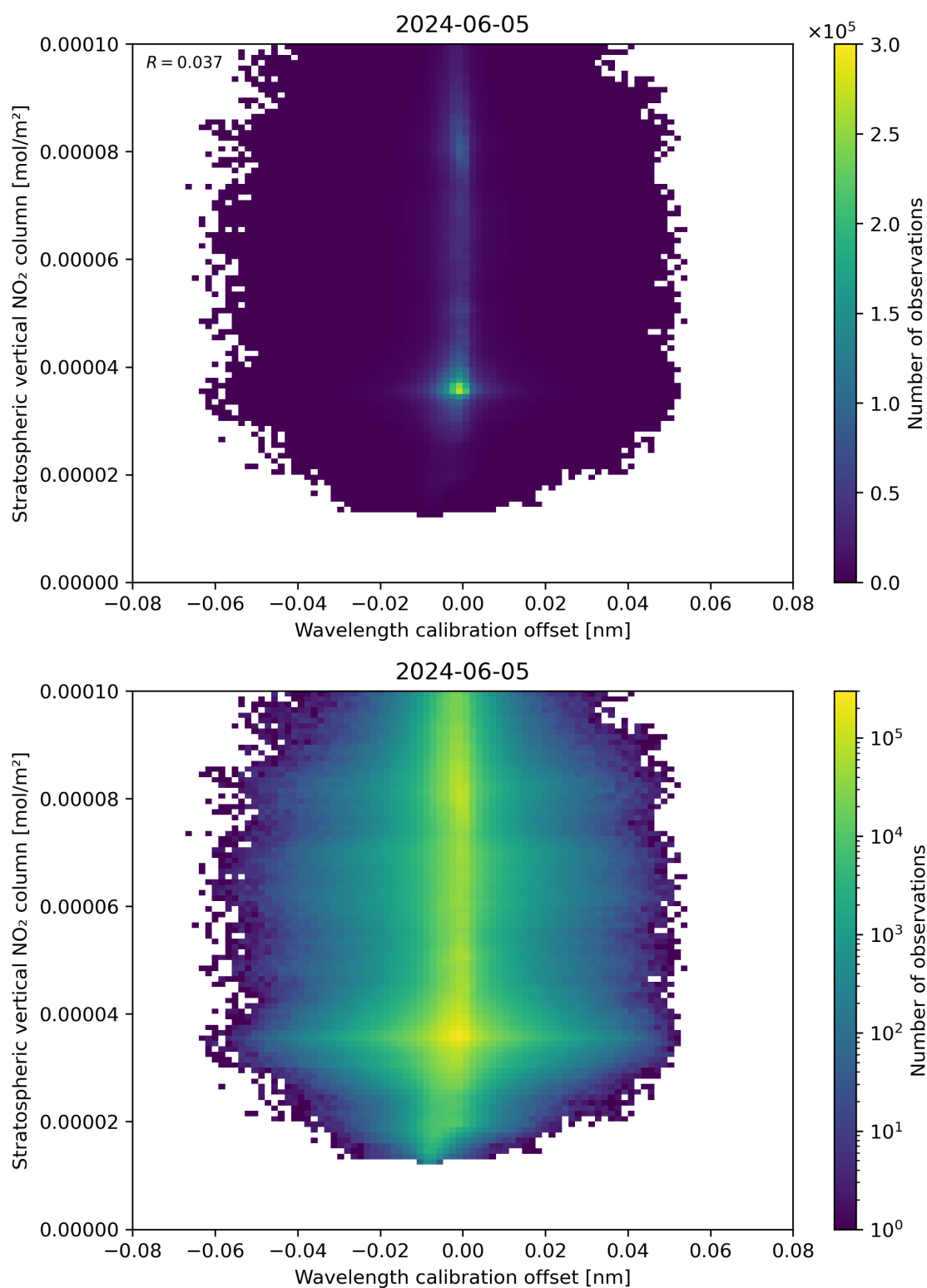
Figure 176: Scatter density plot of “Wavelength calibration offset” against “Stratospheric vertical NO 2 column” for 2024-06-04 to 2024-06-06.
