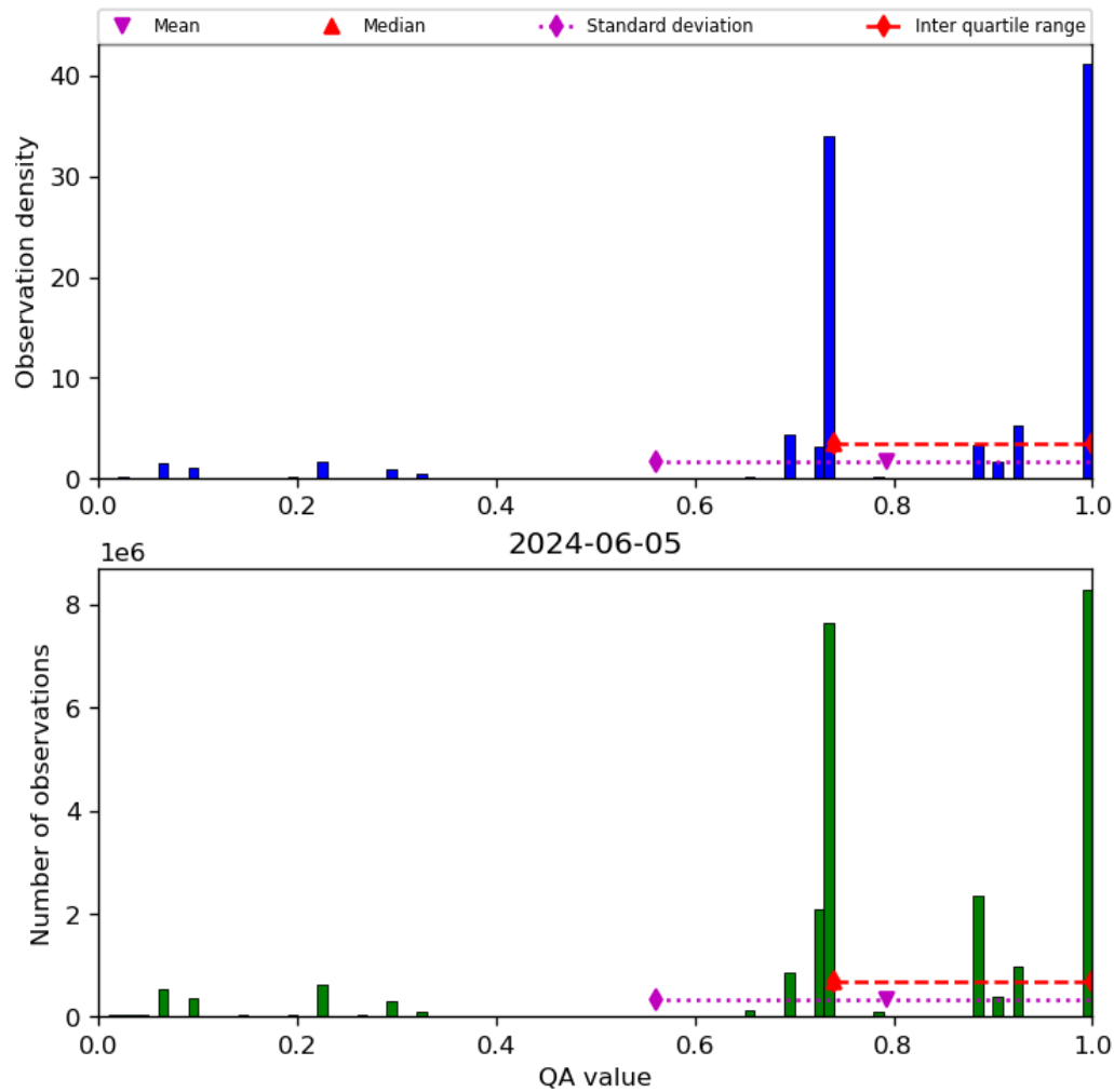
Figure 28: Histogram of “QA value” for 2024-06-04 to 2024-06-06
