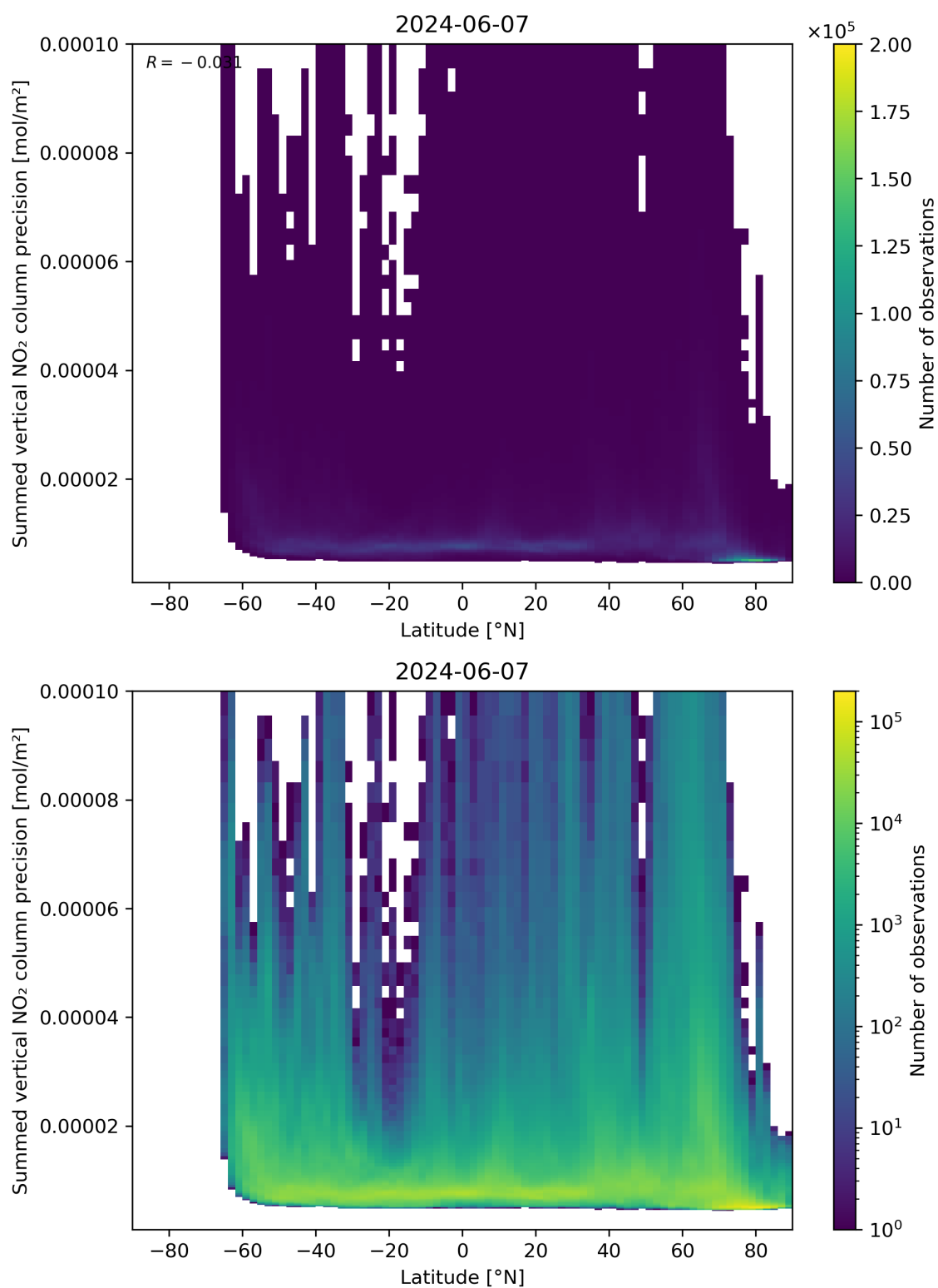
Figure 89: Scatter density plot of “Latitude” against “Summed vertical NO 2 column precision” for 2024-06-06 to 2024-06-08.
