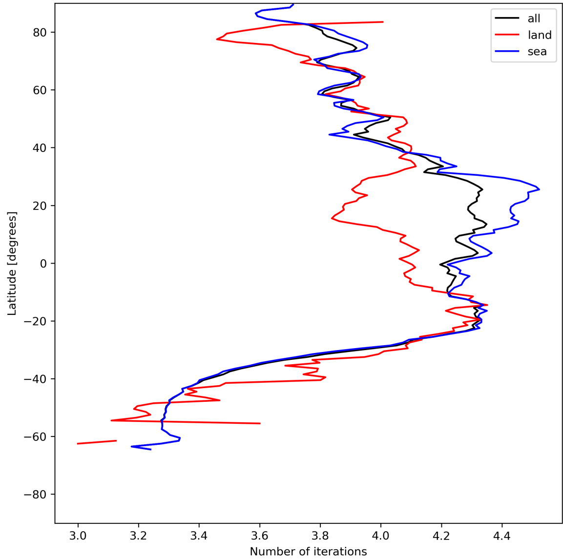
Figure 17: Zonal average of “Number of iterations” for 2024-06-06 to 2024-06-08.
