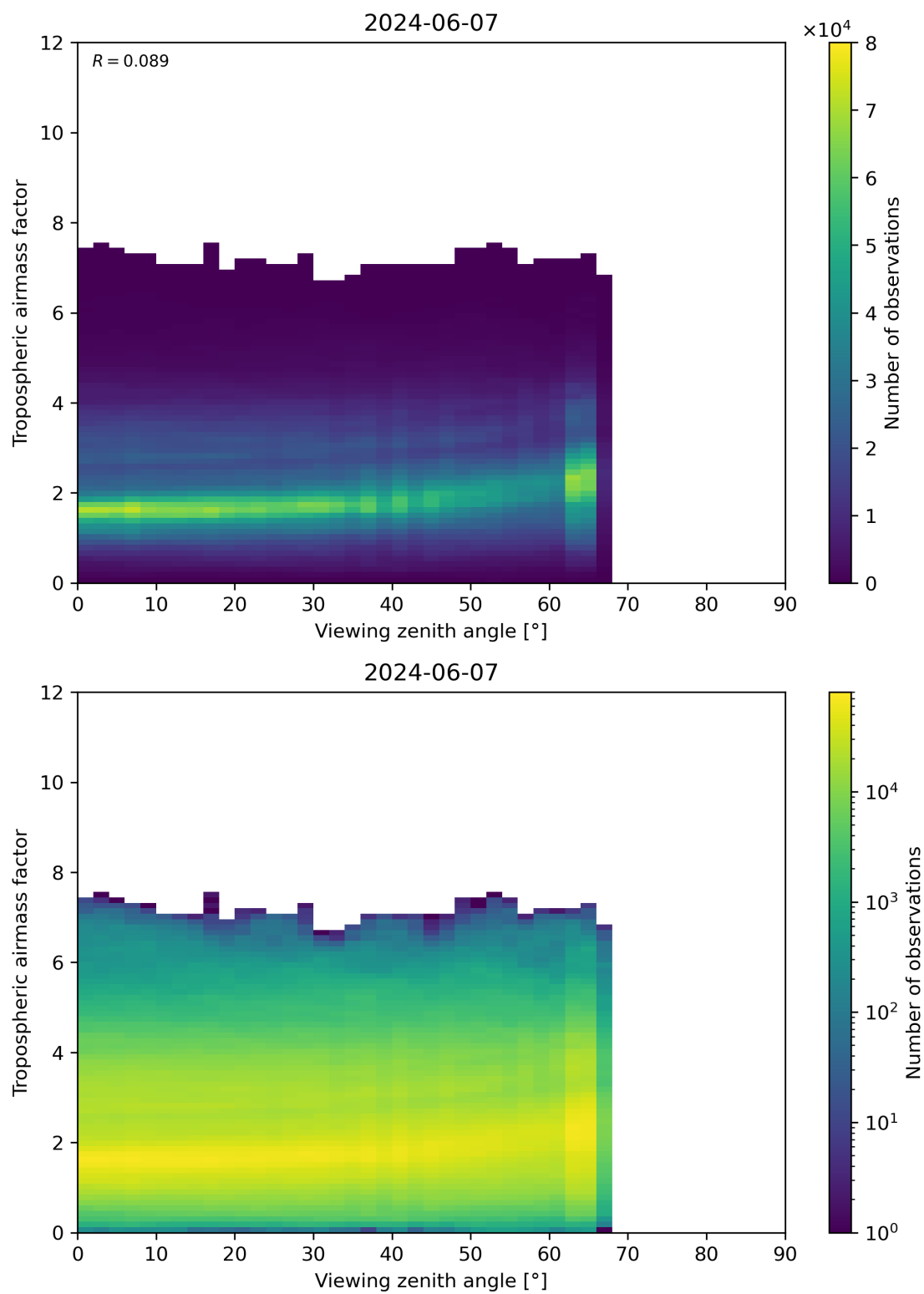
Figure 161: Scatter density plot of “Viewing zenith angle” against “Tropospheric airmass factor” for 2024-06-06 to 2024-06-08.
