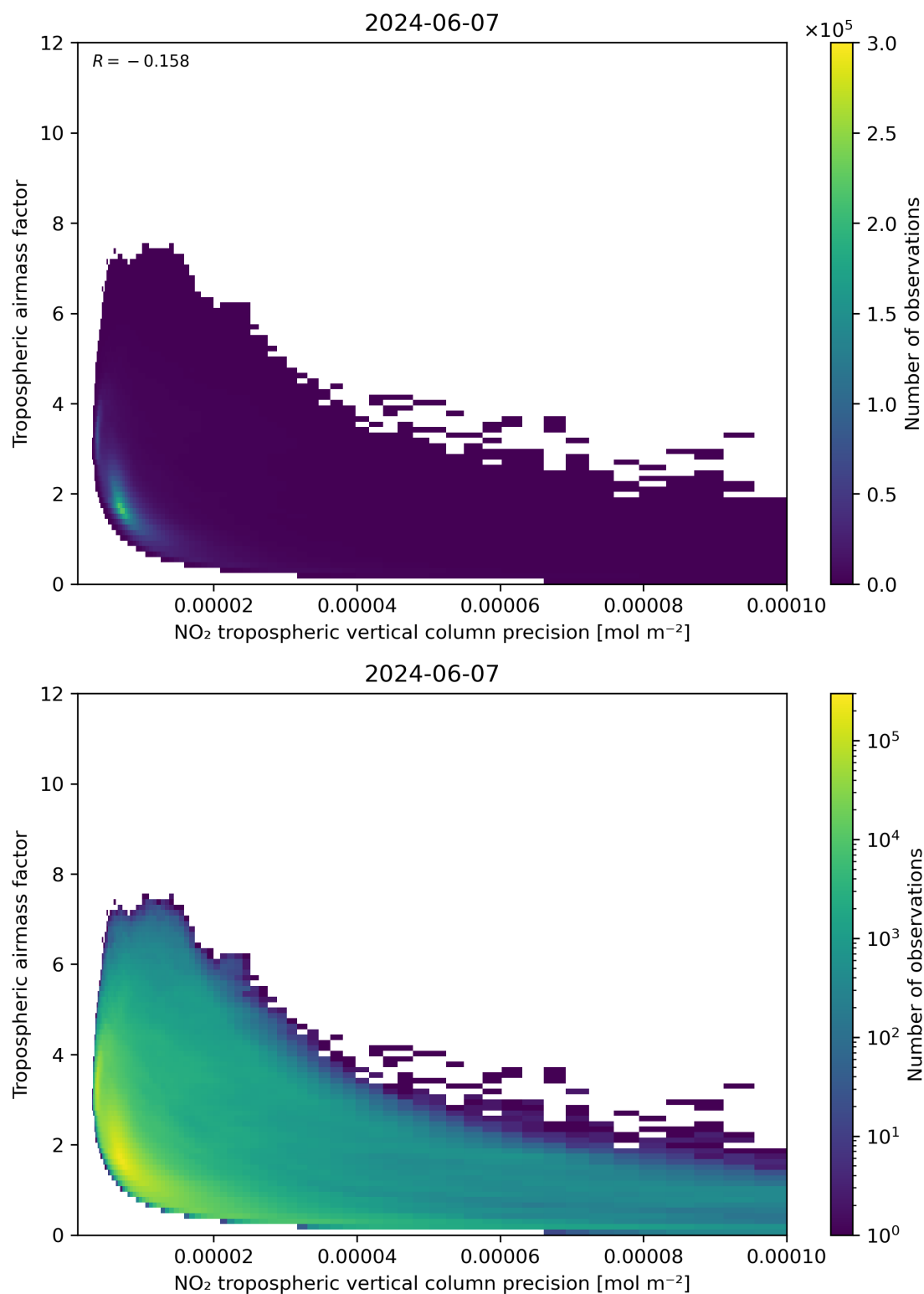
Figure 133: Scatter density plot of “NO 2 tropospheric vertical column precision” against “Tropospheric airmass factor” for 2024-06-06 to 2024-06-08.
