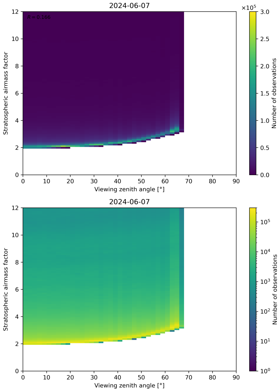
Figure 159: Scatter density plot of “Viewing zenith angle” against “Stratospheric airmass factor” for 2024-06-06 to 2024-06-08.
