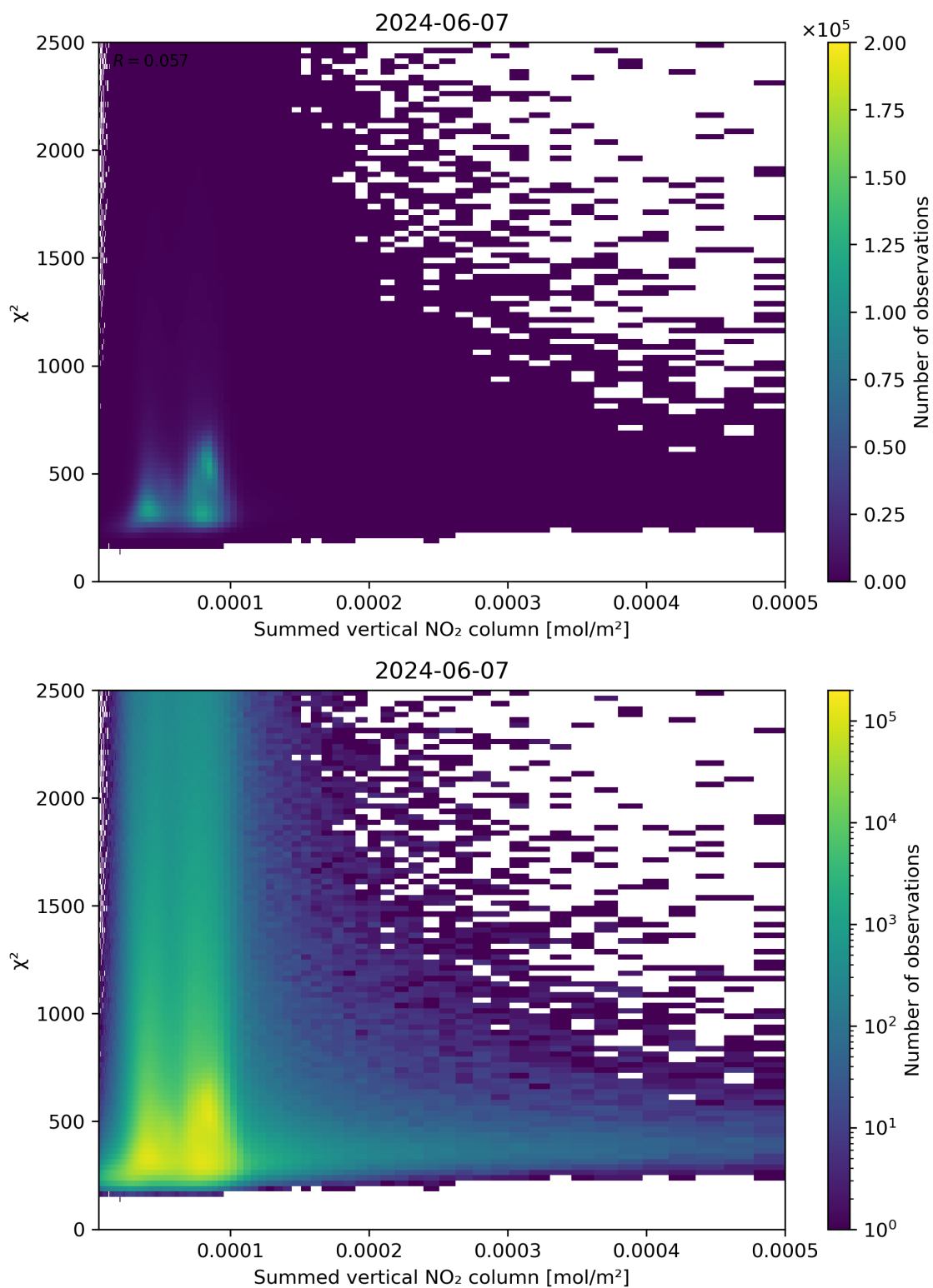
Figure 104: Scatter density plot of “Summed vertical NO 2 column” against “ \chi^2 ” for 2024-06-06 to 2024-06-08.
