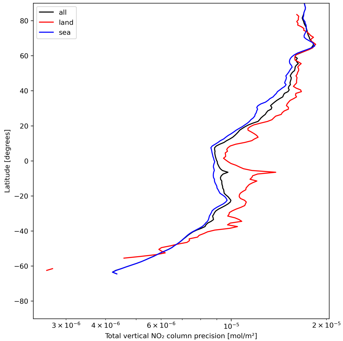
Figure 22: Zonal average of “Total vertical NO 2 column precision” for 2024-06-06 to 2024-06-08.
