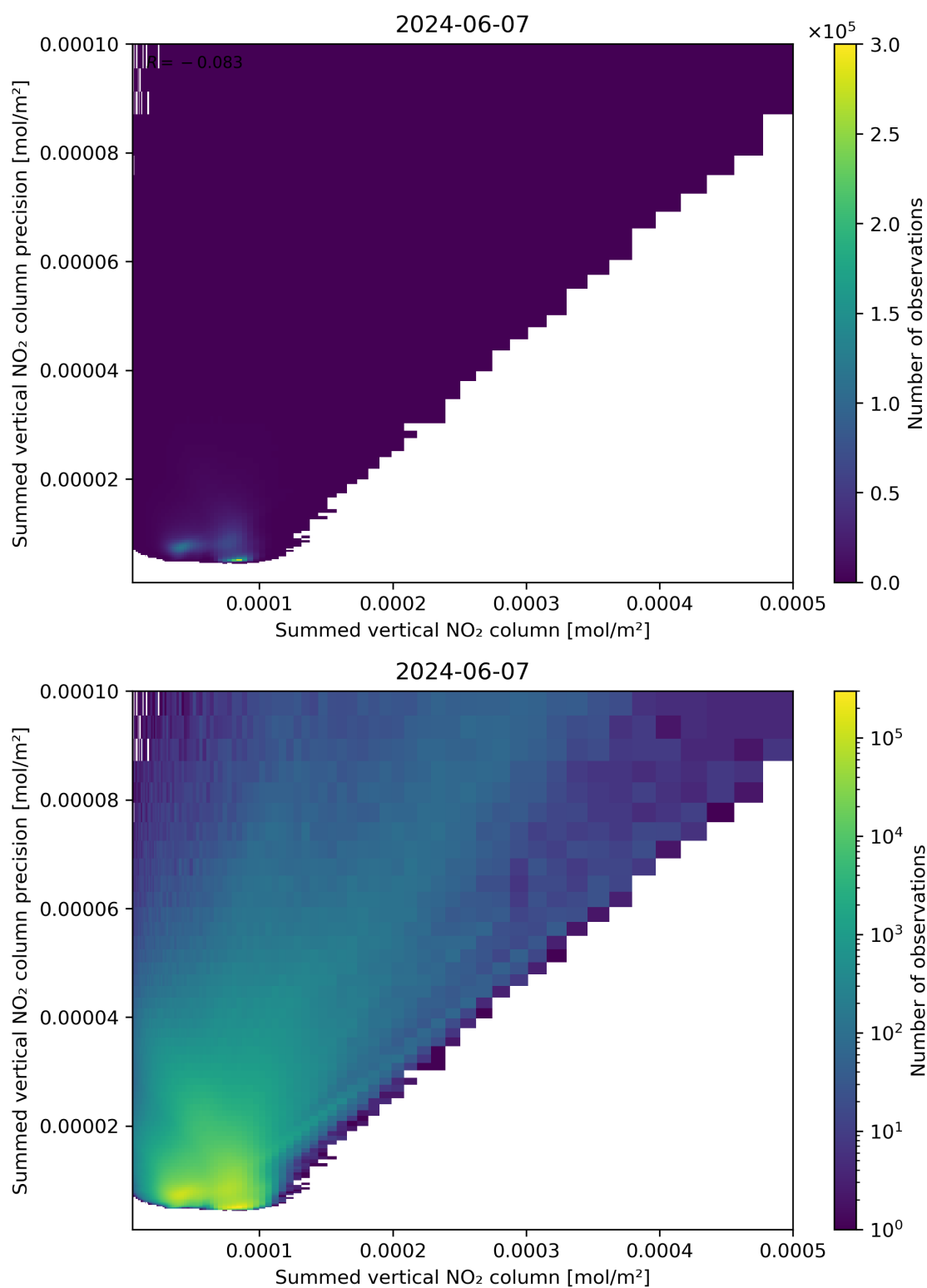
Figure 105: Scatter density plot of “Summed vertical NO 2 column” against “Summed vertical NO 2 column precision” for 2024-06-06 to 2024-06-08.
