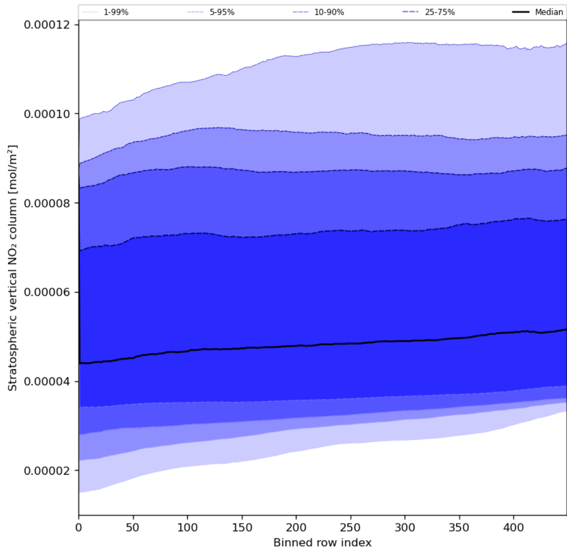
Figure 53: Along track statistics of “Stratospheric vertical NO 2 column” for 2024-06-06 to 2024-06-08
