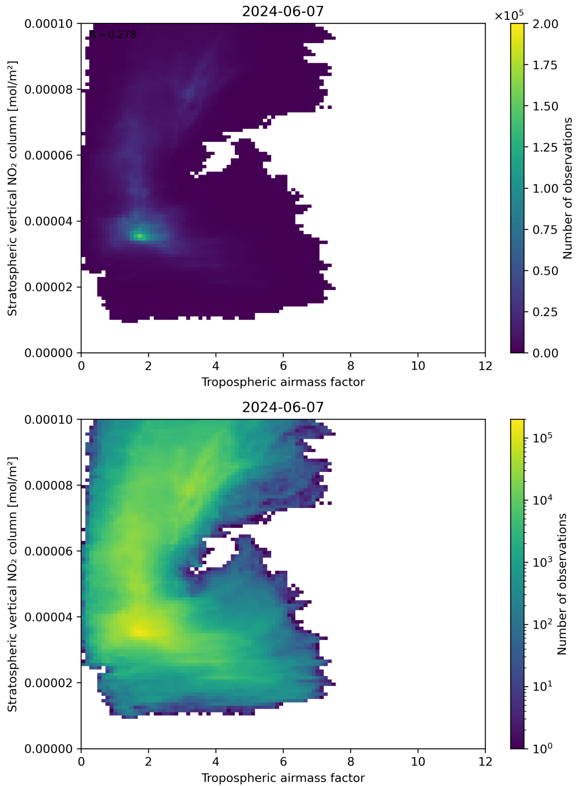
Figure 74: Scatter density plot of “Tropospheric air mass factor” against “Stratospheric vertical NO 2 column” for 2024-06-06 to 2024-06-08.
