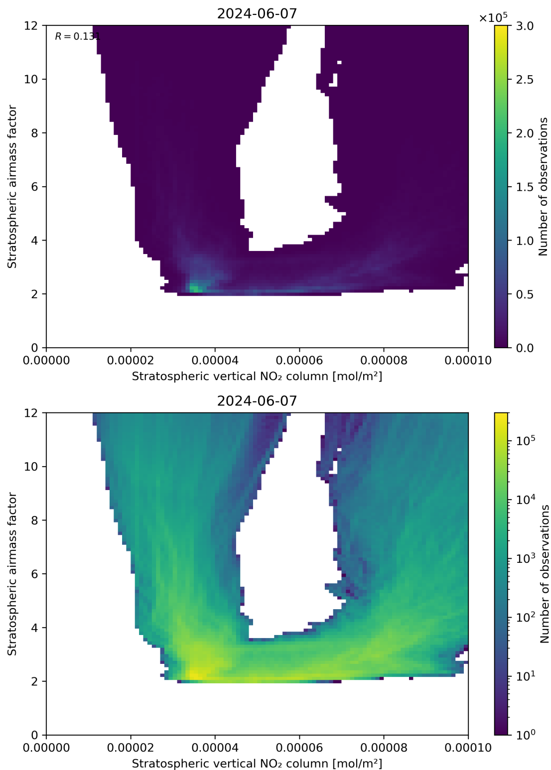
Figure 96: Scatter density plot of “Stratospheric vertical NO 2 column” against “Stratospheric airmass factor” for 2024-06-06 to 2024-06-08.
