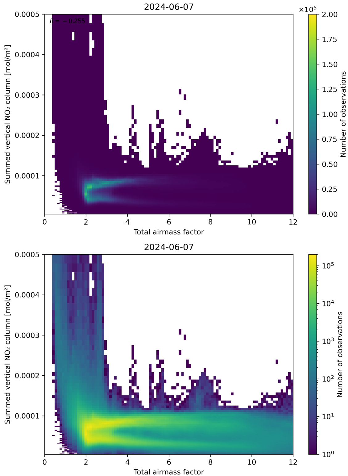
Figure 65: Scatter density plot of “Total airmass factor” against “Summed vertical NO 2 column” for 2024-06-06 to 2024-06-08.
