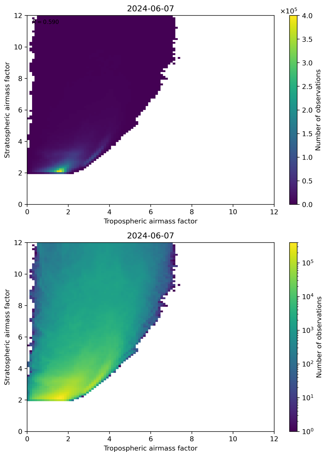
Figure 71: Scatter density plot of “Tropospheric airmass factor” against “Stratospheric airmass factor” for 2024-06-06 to 2024-06-08.
