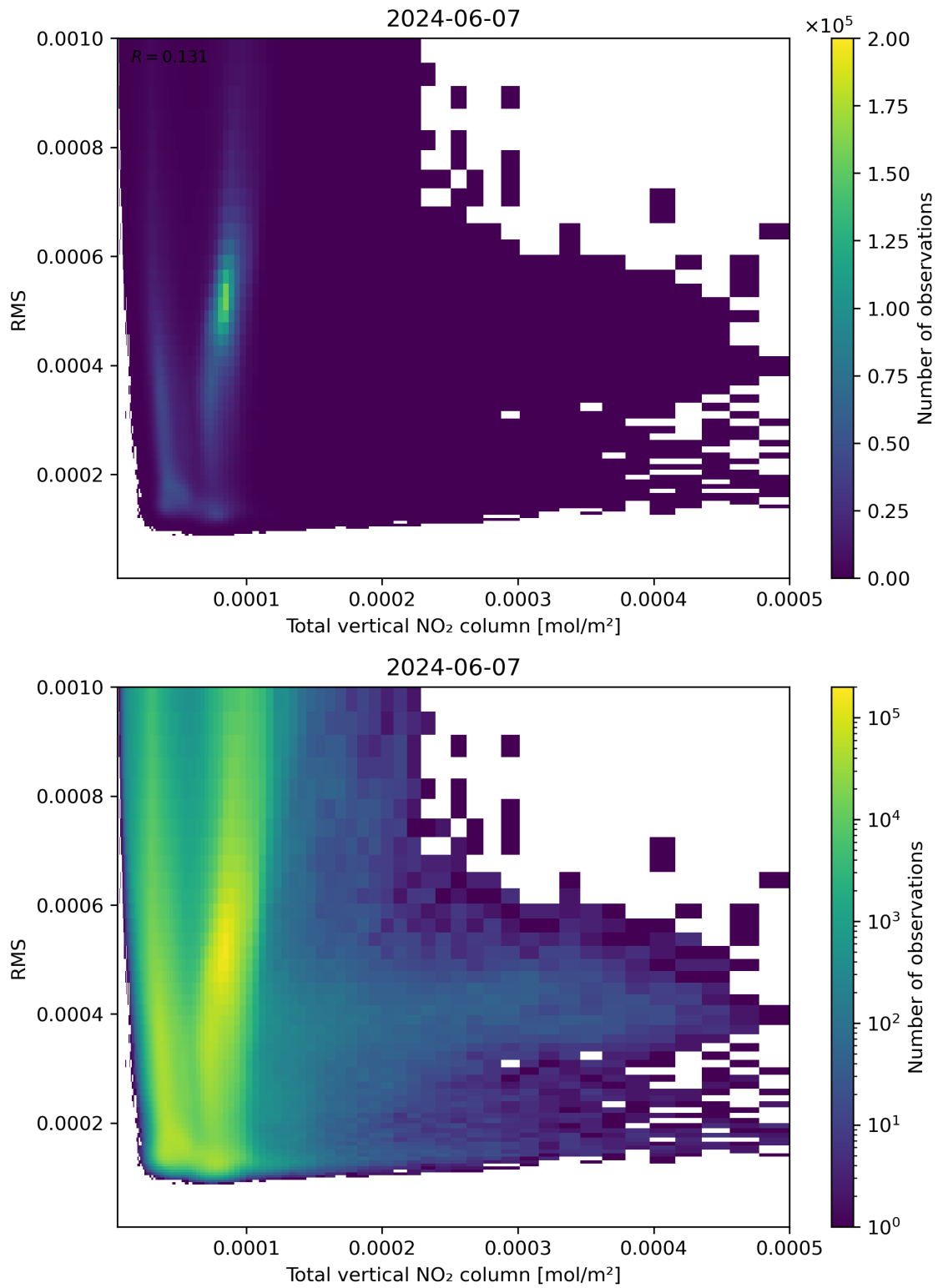
Figure 120: Scatter density plot of “Total vertical NO 2 column” against “RMS” for 2024-06-06 to 2024-06-08.
