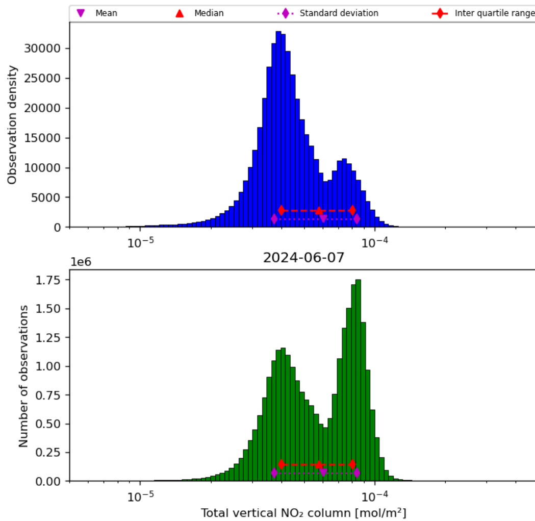
Figure 38: Histogram of “Total vertical NO 2 column” for 2024-06-06 to 2024-06-08
