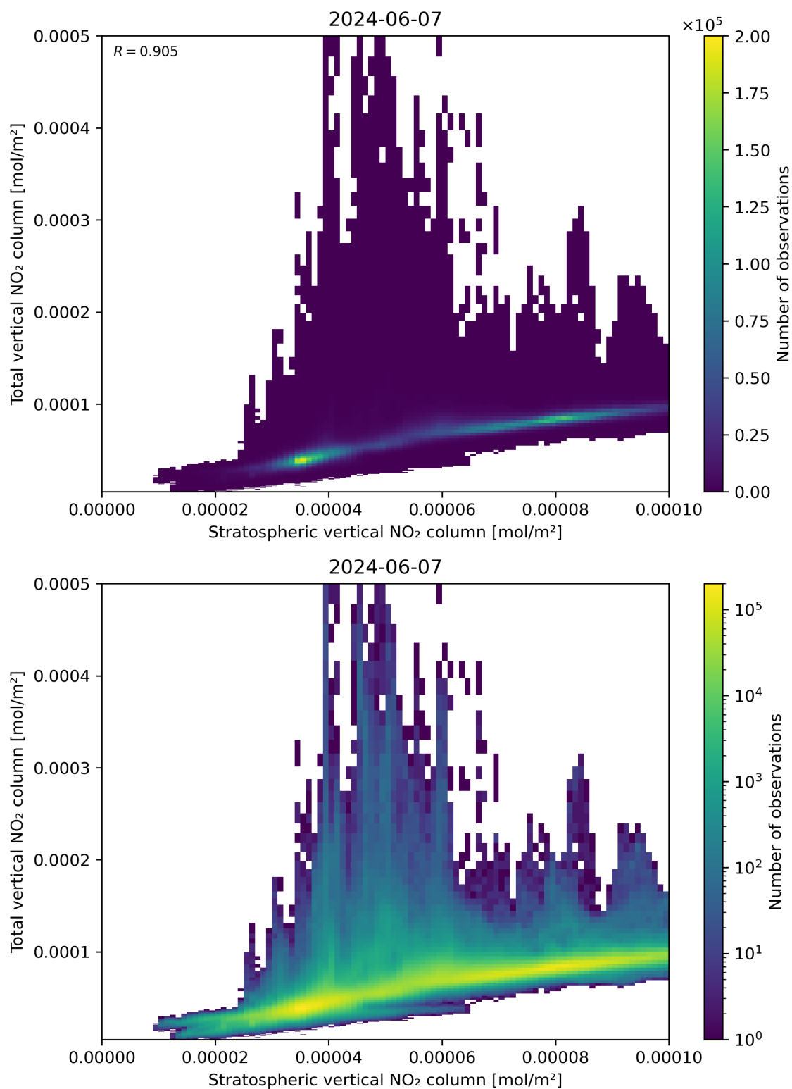
Figure 100: Scatter density plot of “Stratospheric vertical NO 2 column” against “Total vertical NO 2 column” for 2024-06-06 to 2024-06-08.
