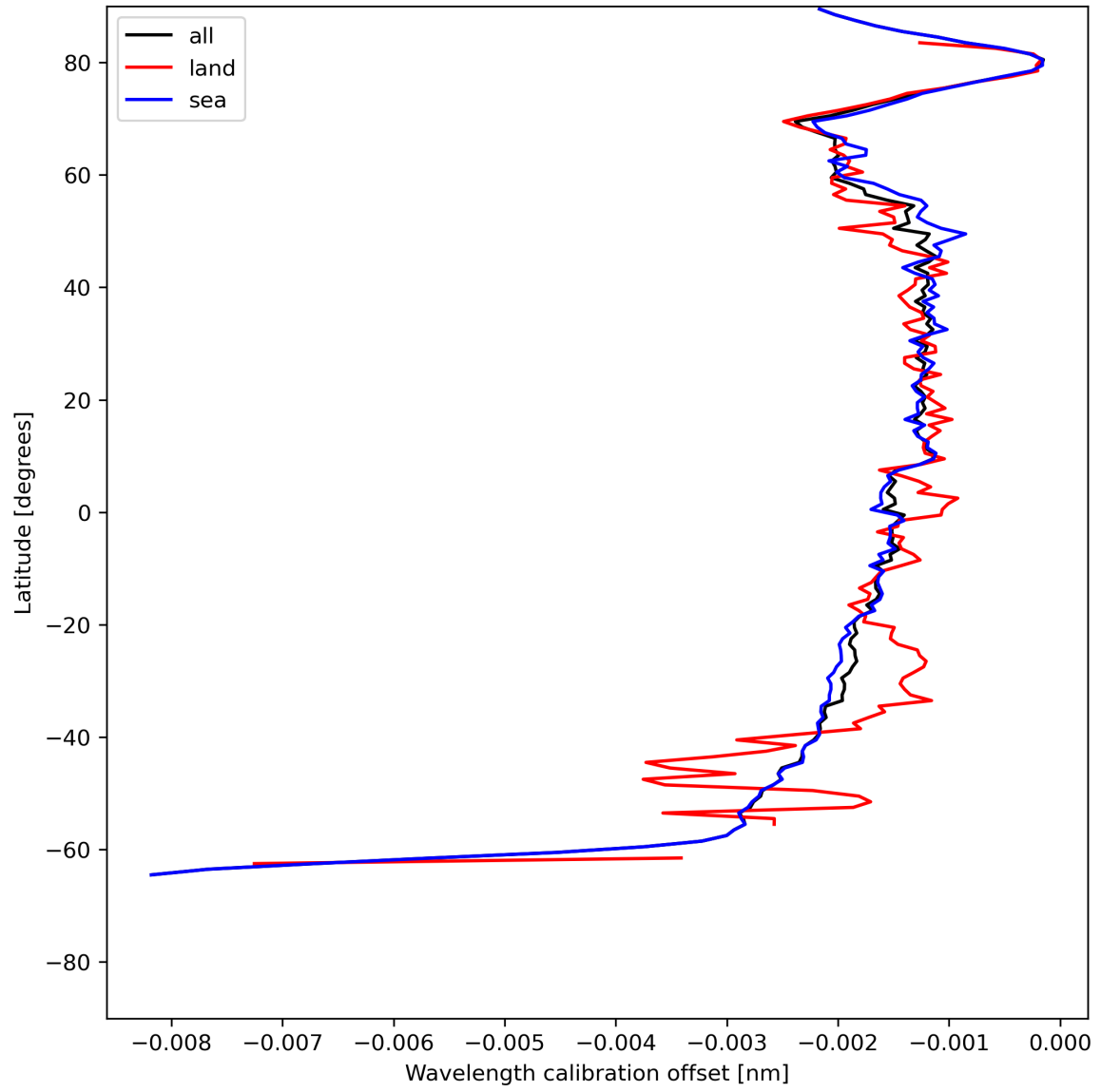
Figure 18: Zonal average of “Wavelength calibration offset” for 2024-06-06 to 2024-06-08.
