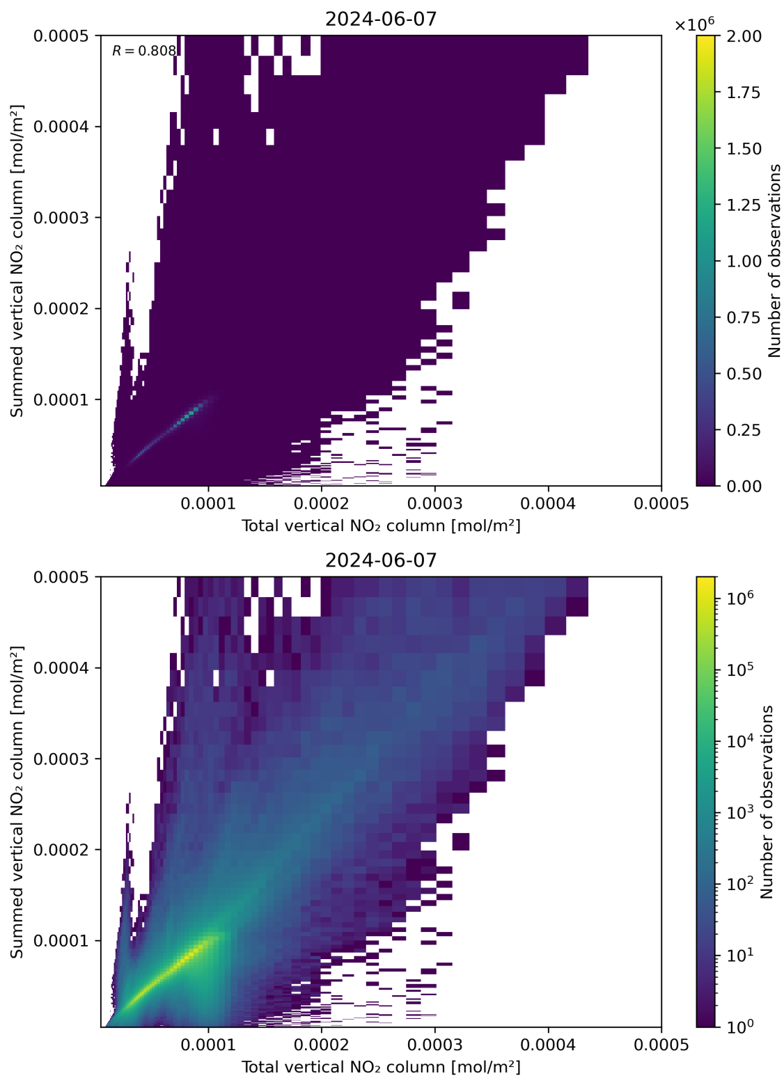
Figure 112: Scatter density plot of “Total vertical NO 2 column” against “Summed vertical NO 2 column” for 2024-06-06 to 2024-06-08.
