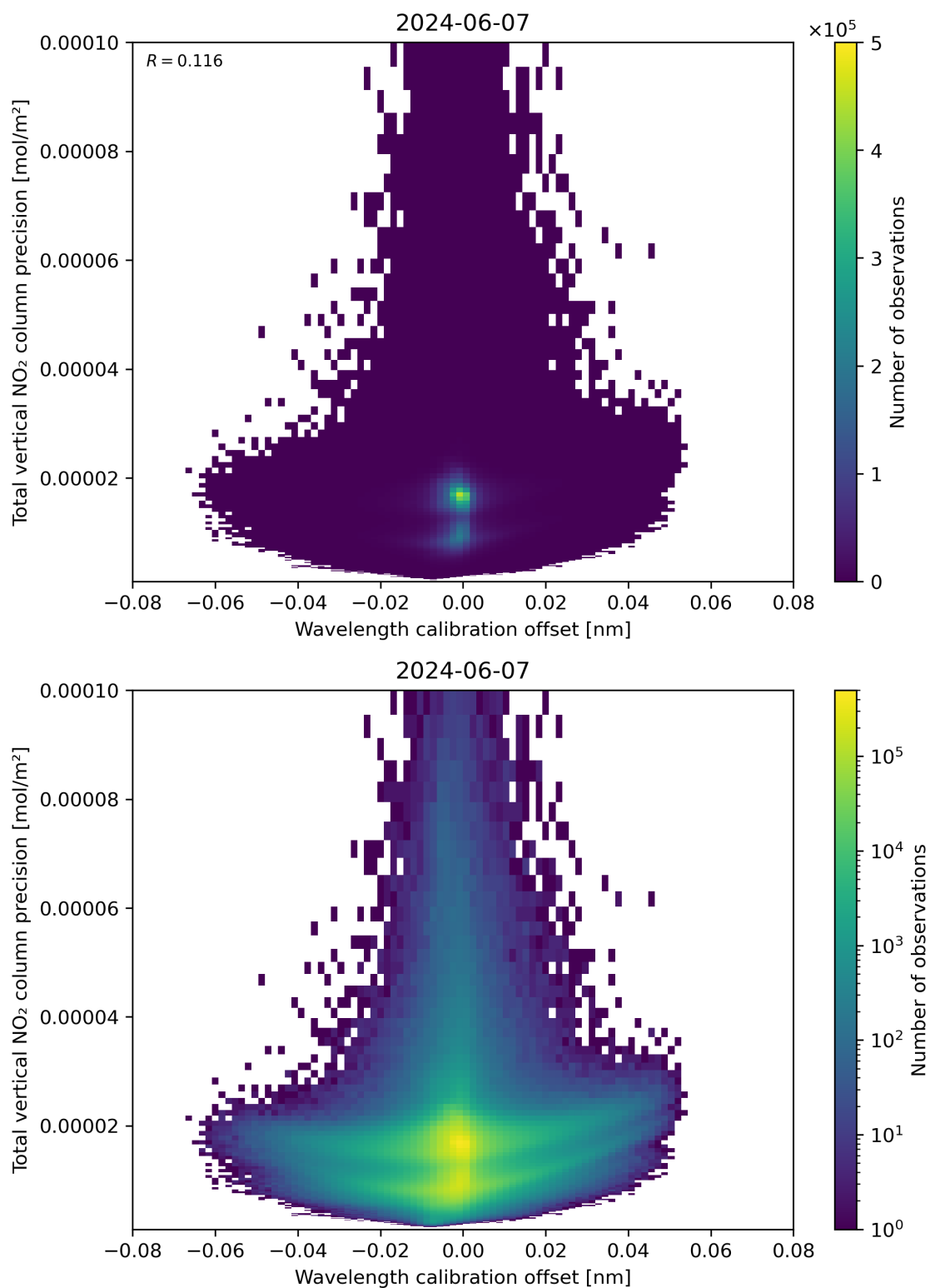
Figure 180: Scatter density plot of “Wavelength calibration offset” against “Total vertical NO 2 column precision” for 2024-06-06 to 2024-06-08.
