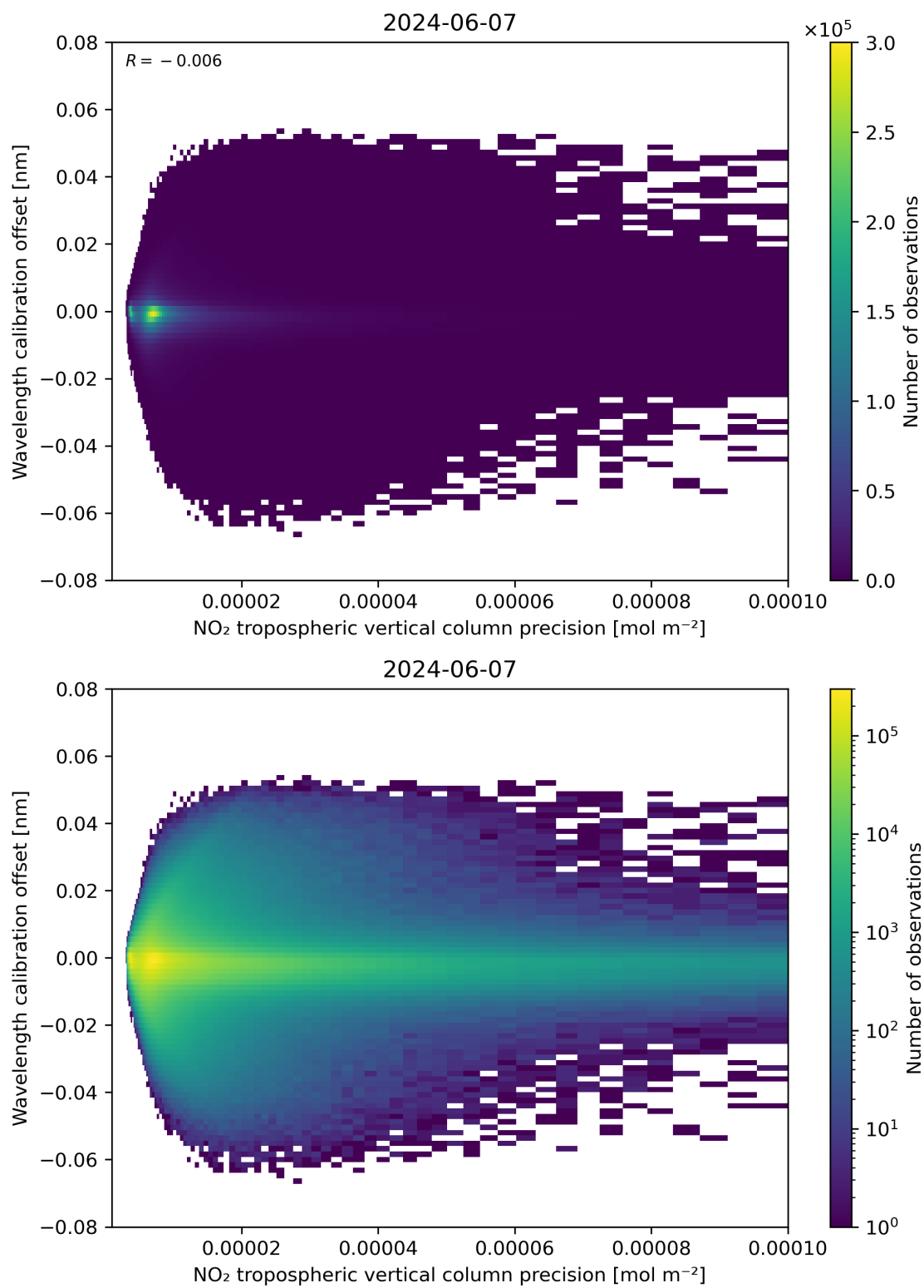
Figure 141: Scatter density plot of “NO 2 tropospheric vertical column precision” against “Wavelength calibration offset” for 2024-06-06 to 2024-06-08.
