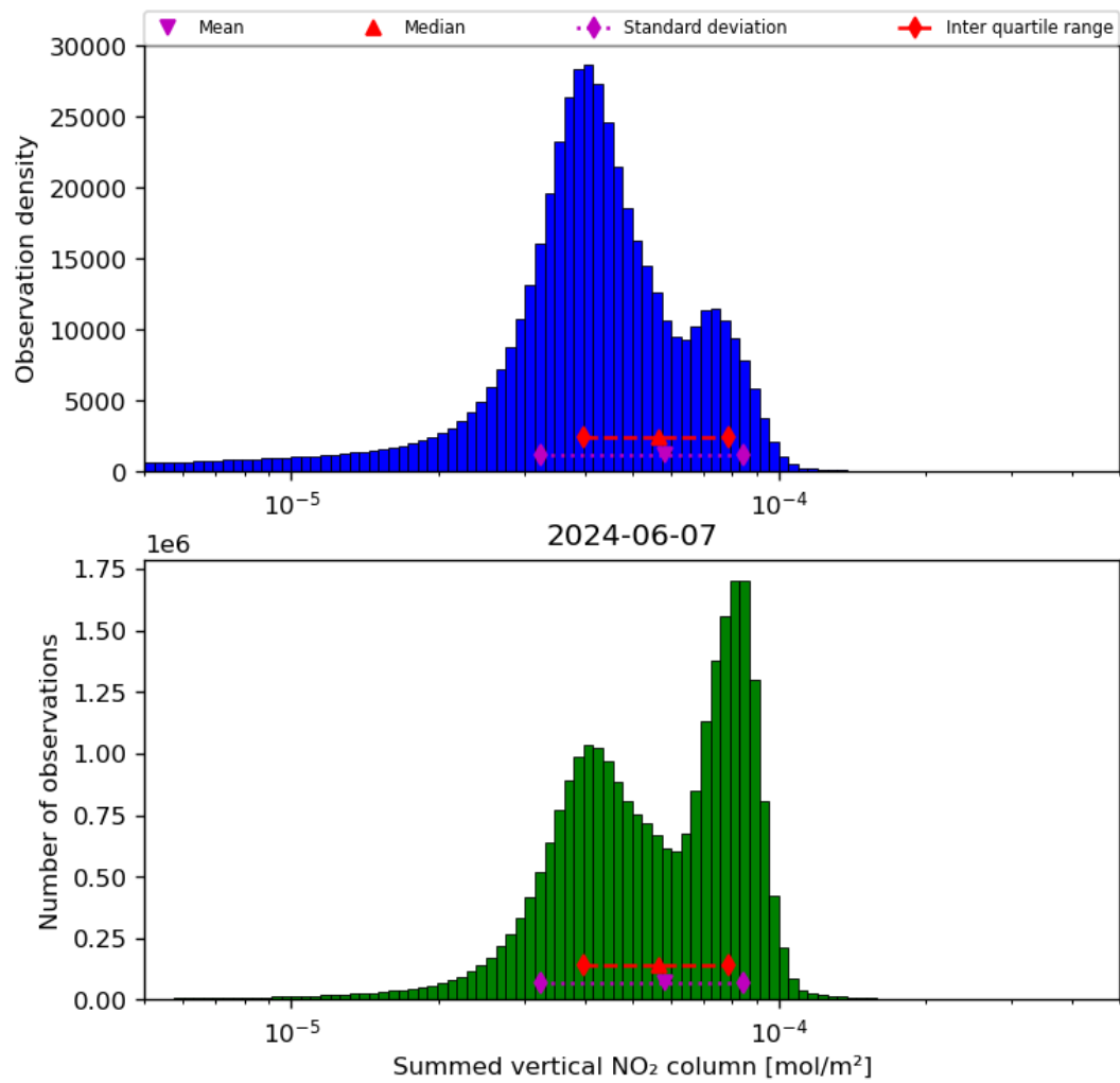
Figure 40: Histogram of “Summed vertical NO 2 column” for 2024-06-06 to 2024-06-08
