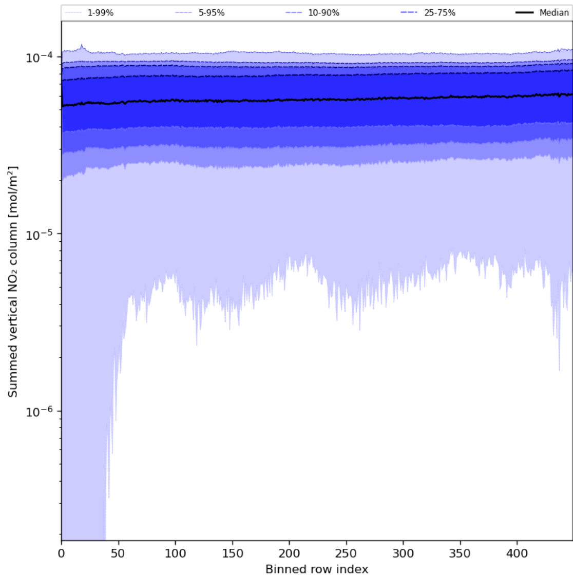
Figure 57: Along track statistics of “Summed vertical NO 2 column” for 2024-06-06 to 2024-06-08
