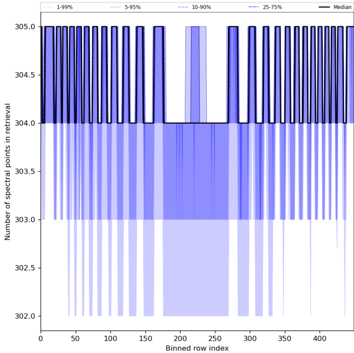
Figure 50: Along track statistics of “Number of spectral points in retrieval” for 2024-06-06 to 2024-06-08
