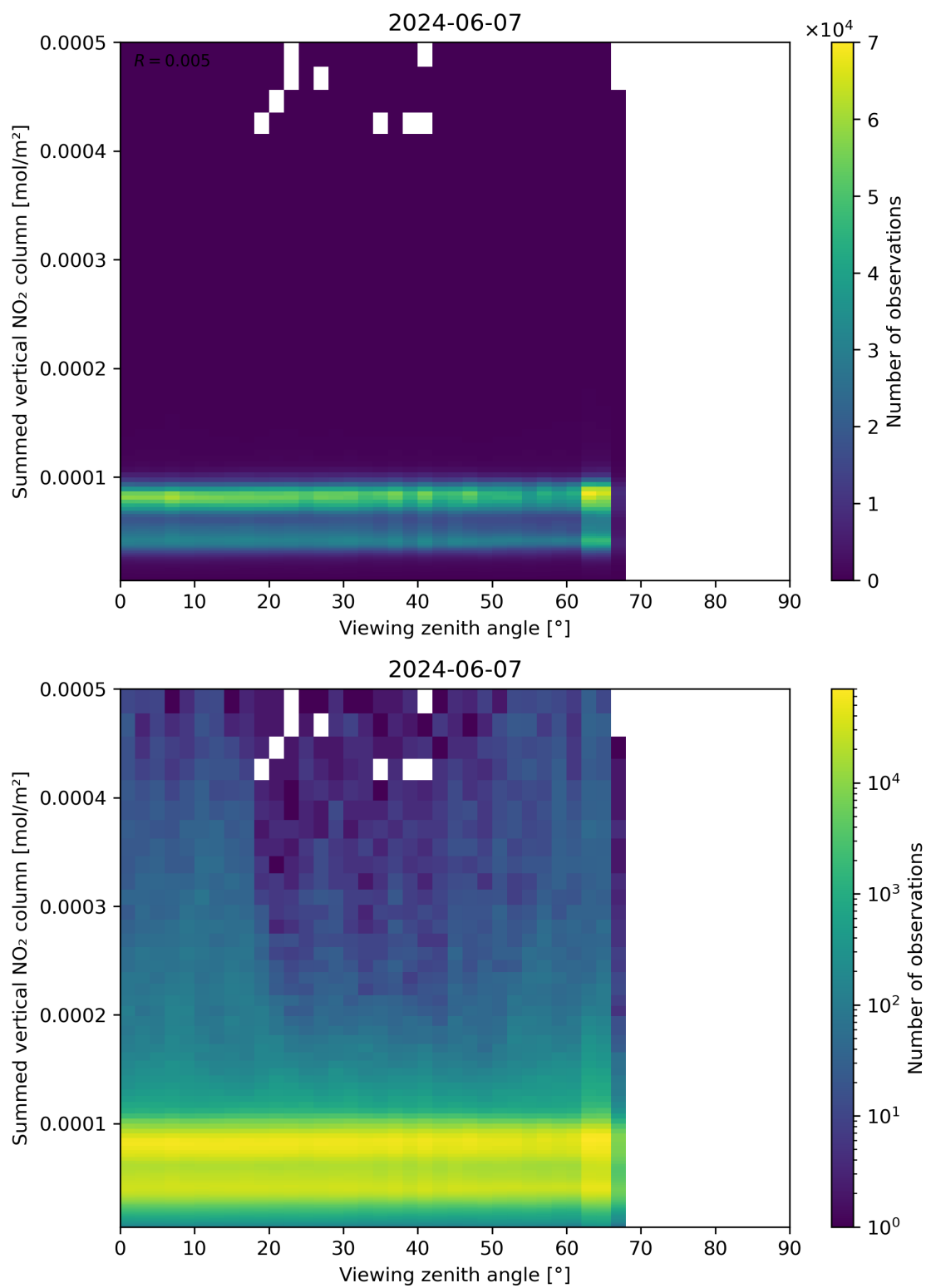
Figure 165: Scatter density plot of “Viewing zenith angle” against “Summed vertical NO 2 column” for 2024-06-06 to 2024-06-08.
