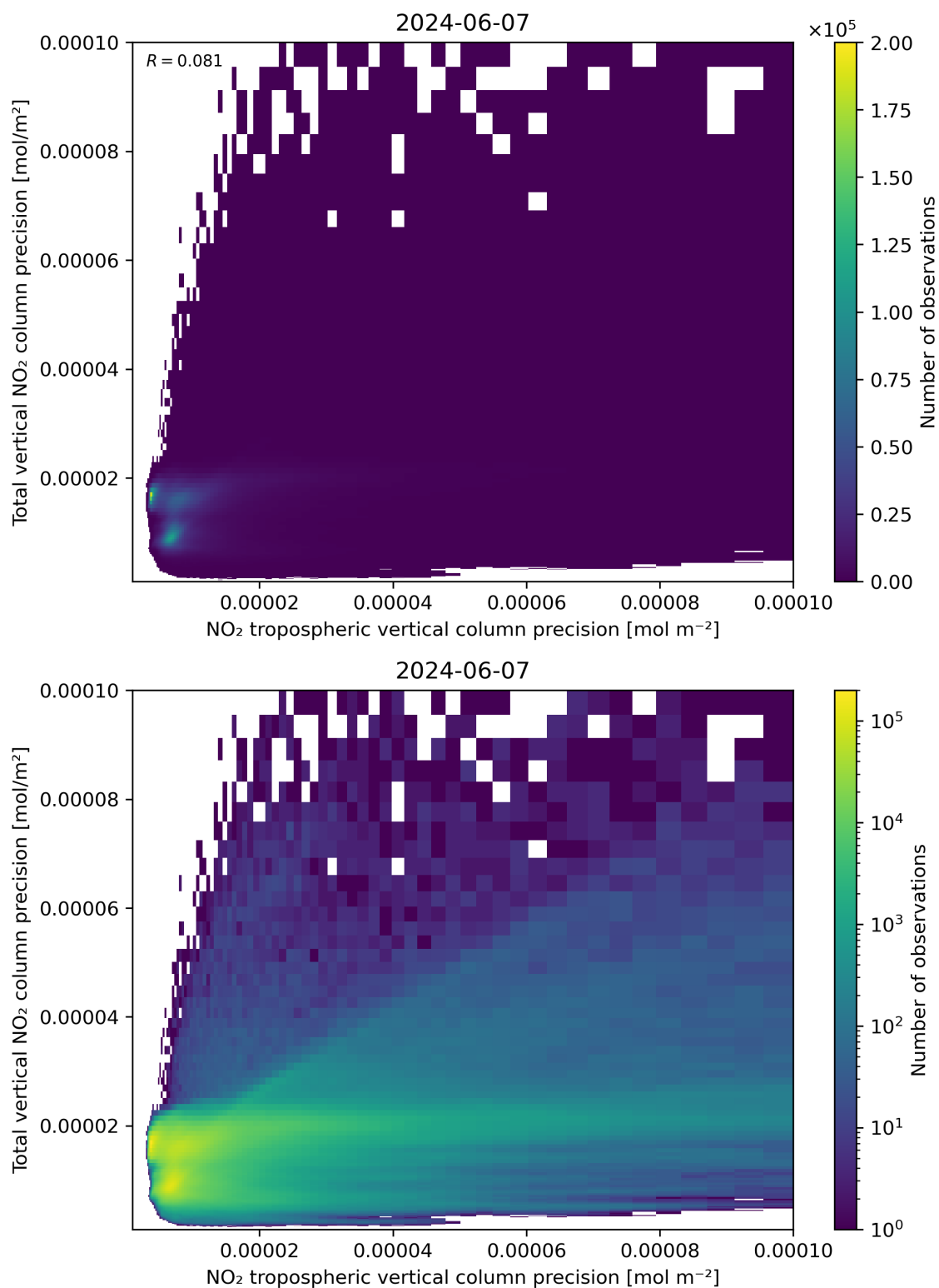
Figure 139: Scatter density plot of “NO 2 tropospheric vertical column precision” against “Total vertical NO 2 column precision” for 2024-06-06 to 2024-06-08.
