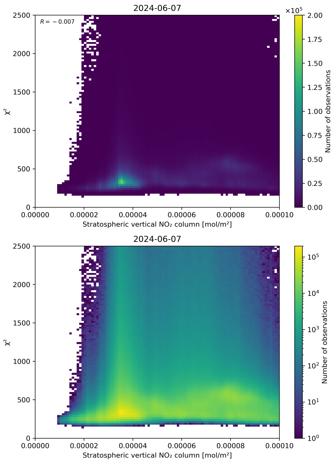
Figure 97: Scatter density plot of “Stratospheric vertical NO 2 column” against “ \chi^2 ” for 2024-06-06 to 2024-06-08.
