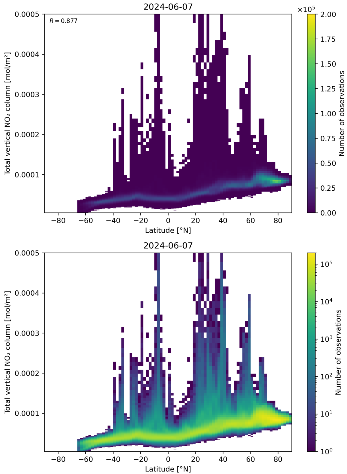
Figure 90: Scatter density plot of “Latitude” against “Total vertical NO 2 column” for 2024-06-06 to 2024-06-08.
