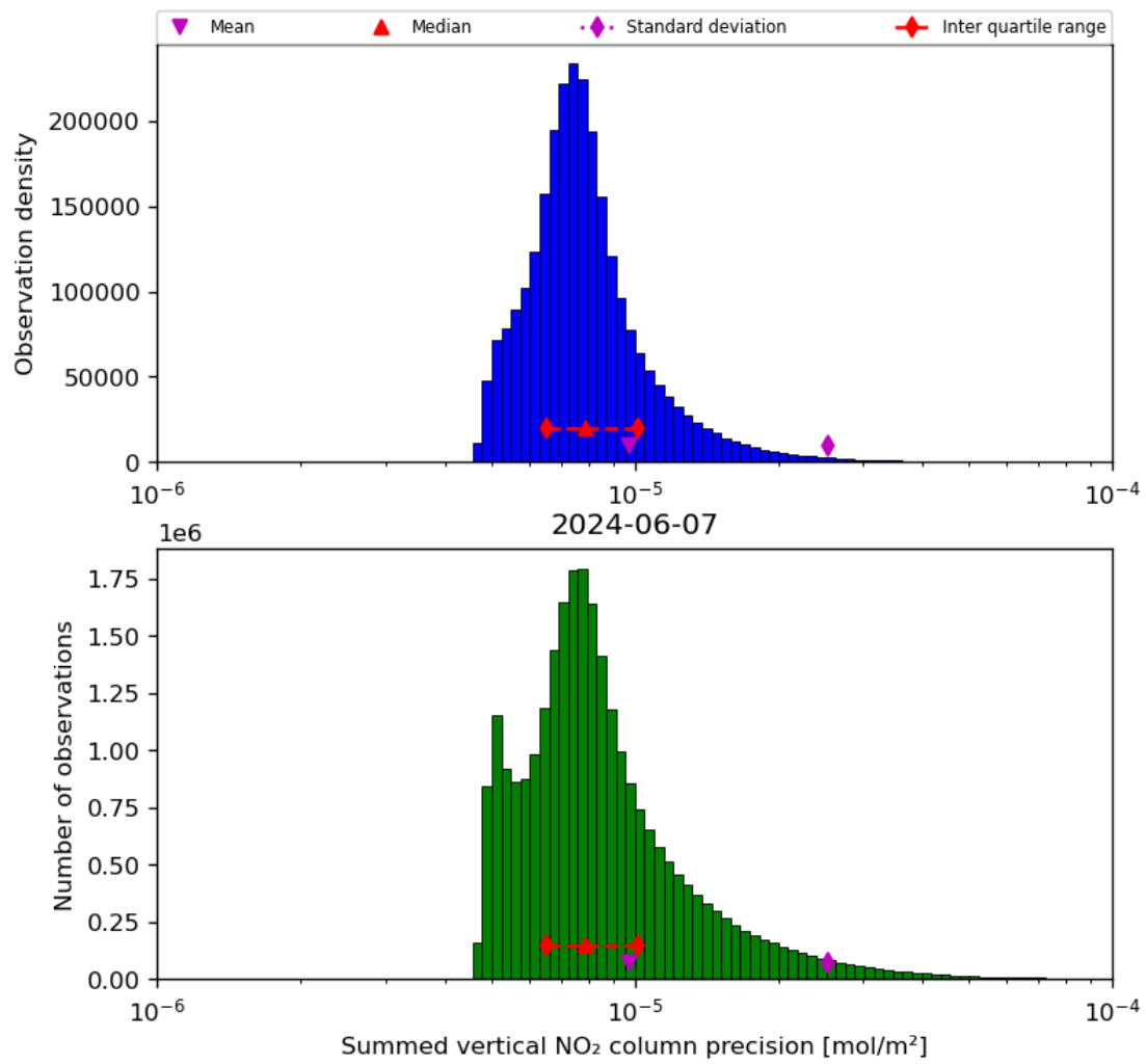
Figure 41: Histogram of “Summed vertical NO 2 column precision” for 2024-06-06 to 2024-06-08
