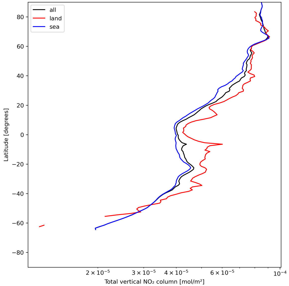
Figure 21: Zonal average of “Total vertical NO 2 column” for 2024-06-06 to 2024-06-08.
