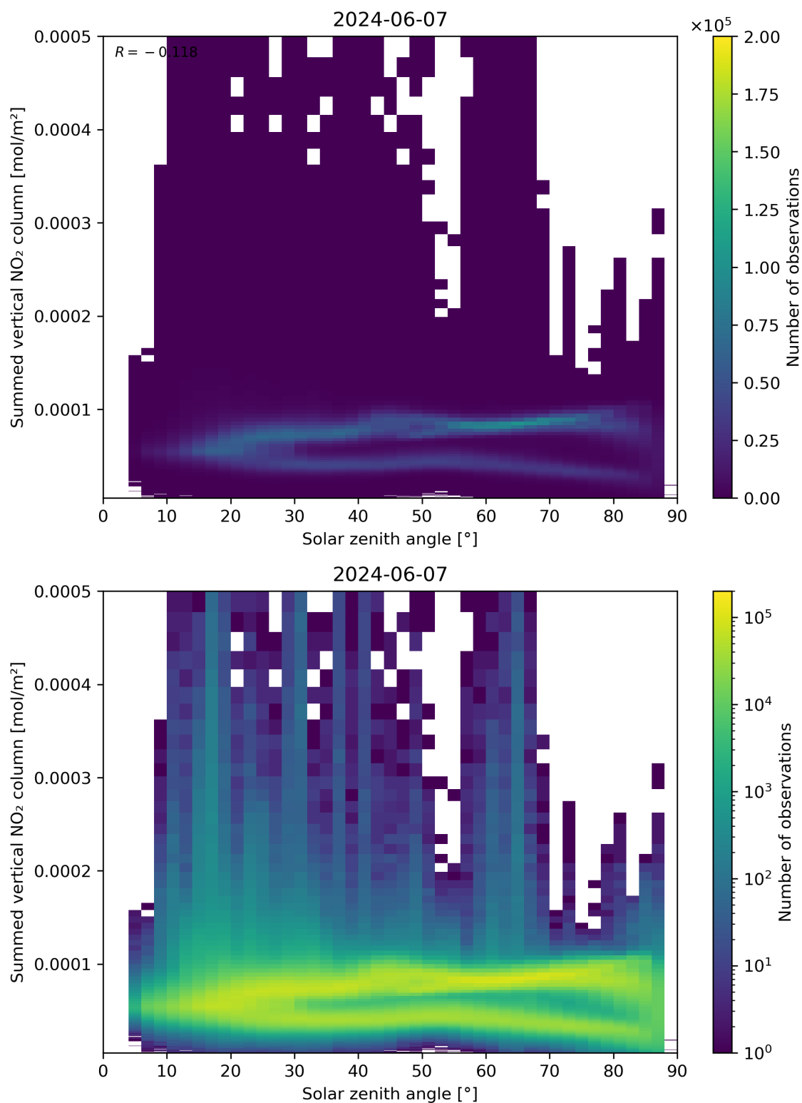
Figure 151: Scatter density plot of “Solar zenith angle” against “Summed vertical NO 2 column” for 2024-06-06 to 2024-06-08.
