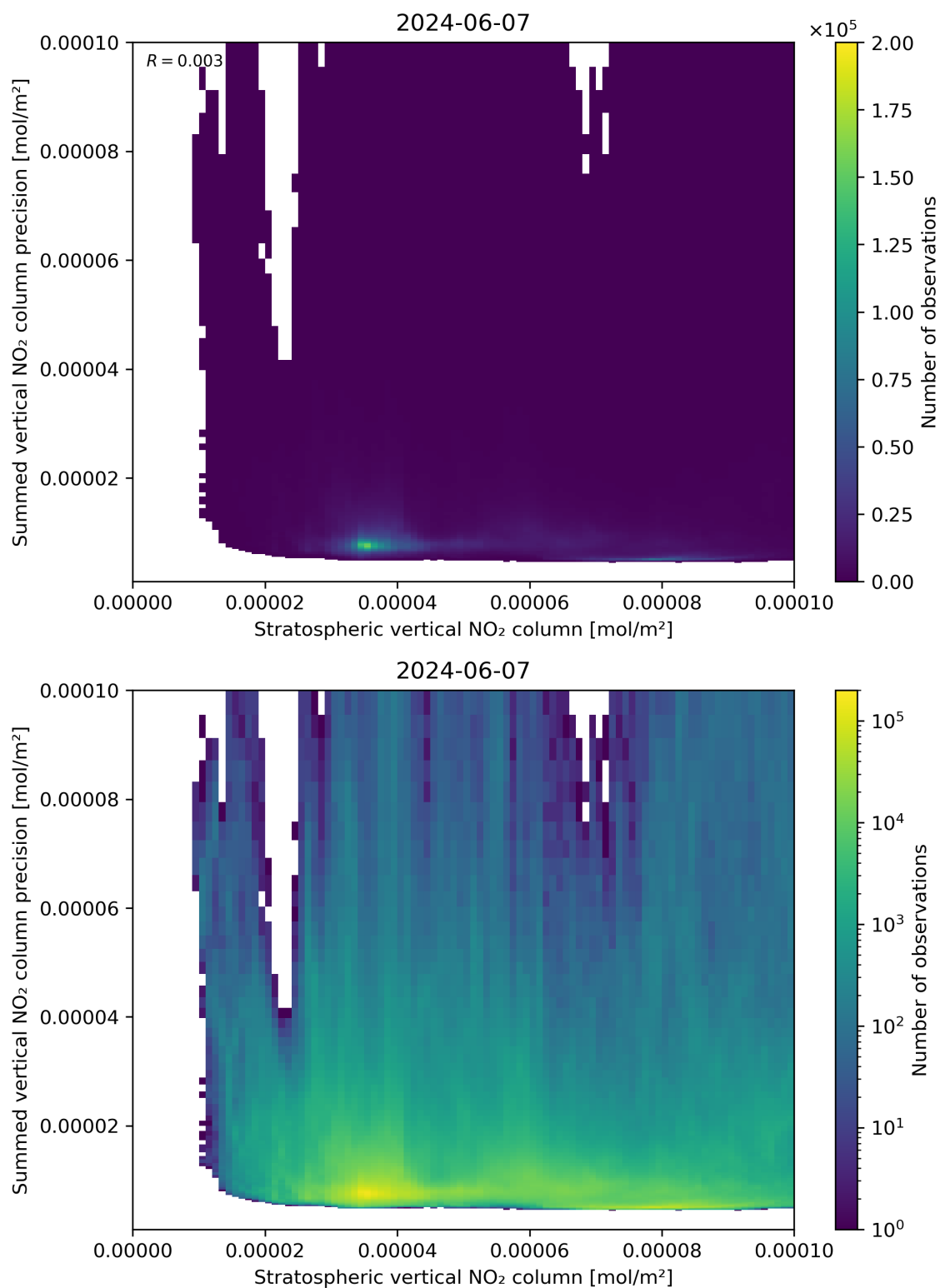
Figure 99: Scatter density plot of “Stratospheric vertical NO 2 column” against “Summed vertical NO 2 column precision” for 2024-06-06 to 2024-06-08.
