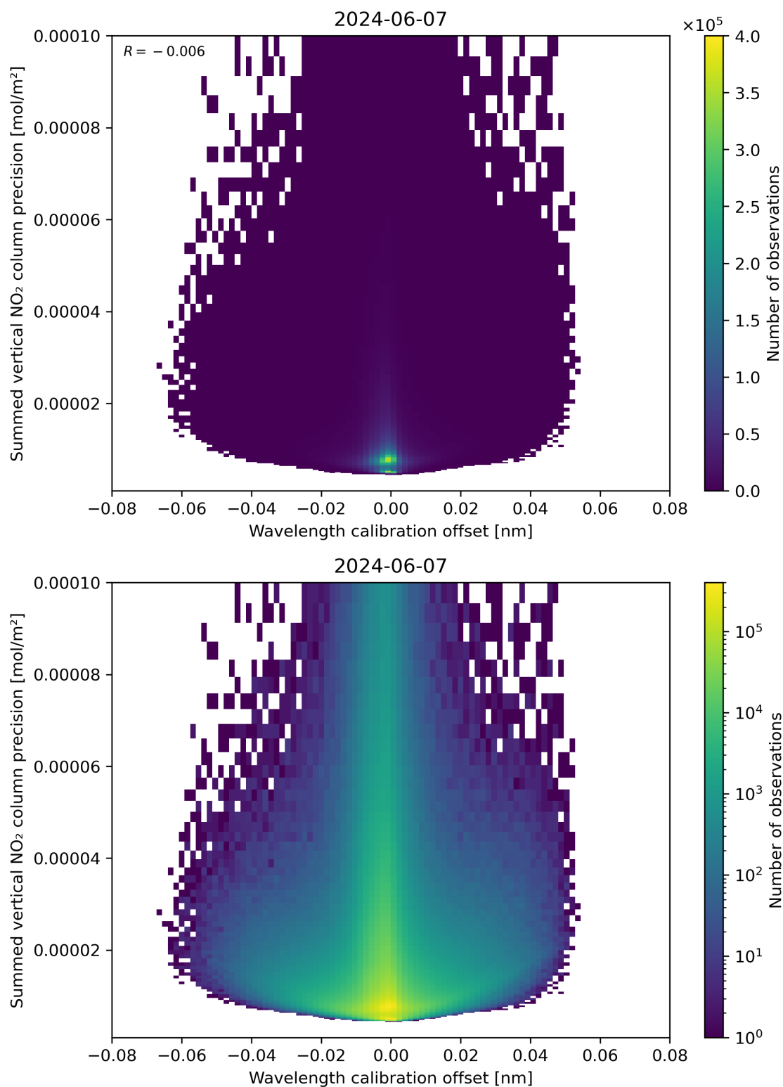
Figure 178: Scatter density plot of “Wavelength calibration offset” against “Summed vertical NO 2 column precision” for 2024-06-06 to 2024-06-08.
