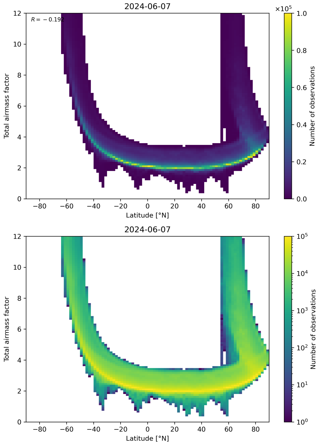
Figure 84: Scatter density plot of “Latitude” against “Total airmass factor” for 2024-06-06 to 2024-06-08.
