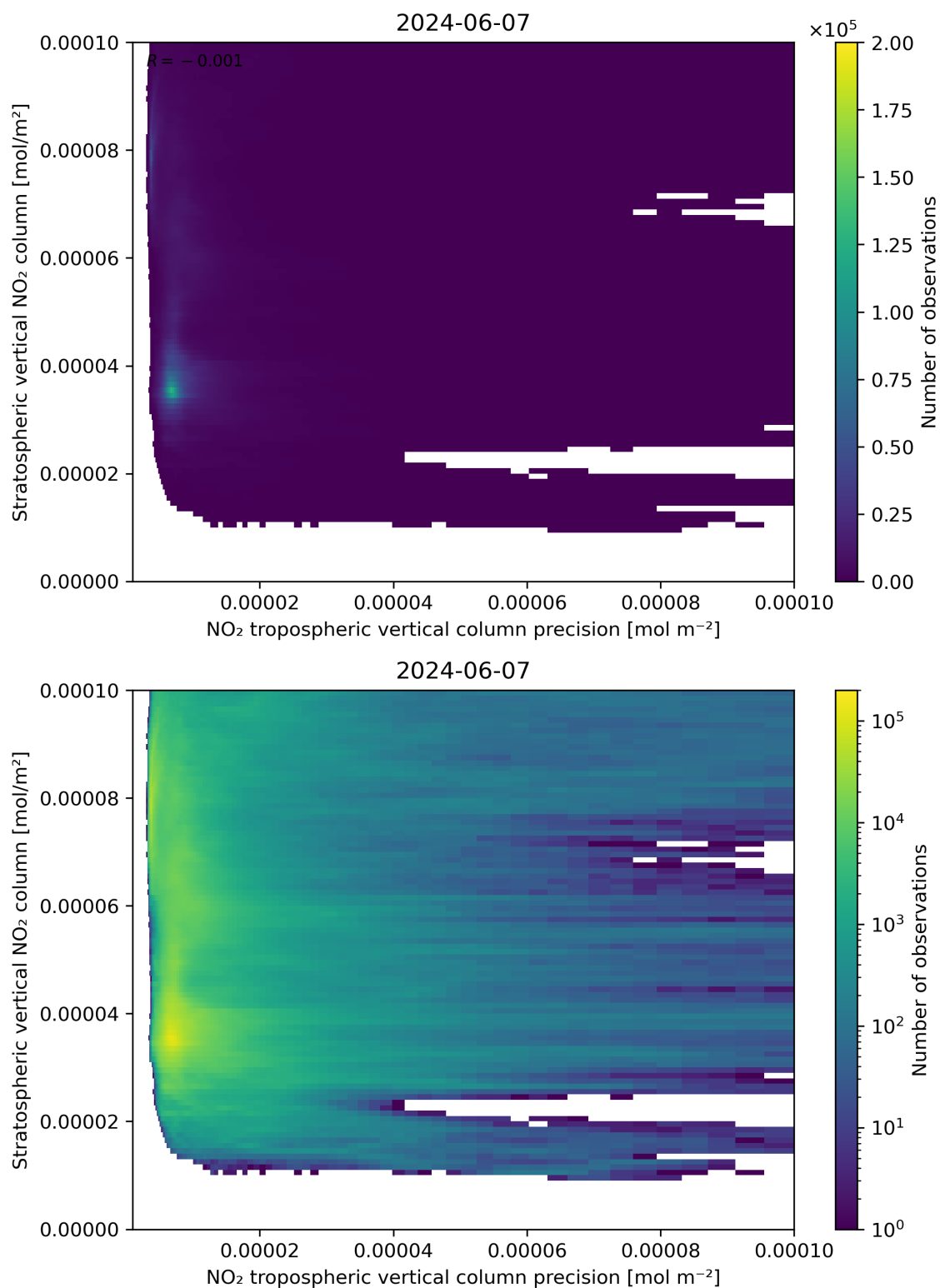
Figure 135: Scatter density plot of “NO 2 tropospheric vertical column precision” against “Stratospheric vertical NO 2 column” for 2024-06-06 to 2024-06-08.
