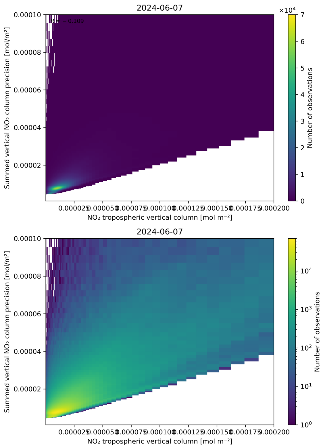
Figure 127: Scatter density plot of “NO 2 tropospheric vertical column” against “Summed vertical NO 2 column precision” for 2024-06-06 to 2024-06-08.
