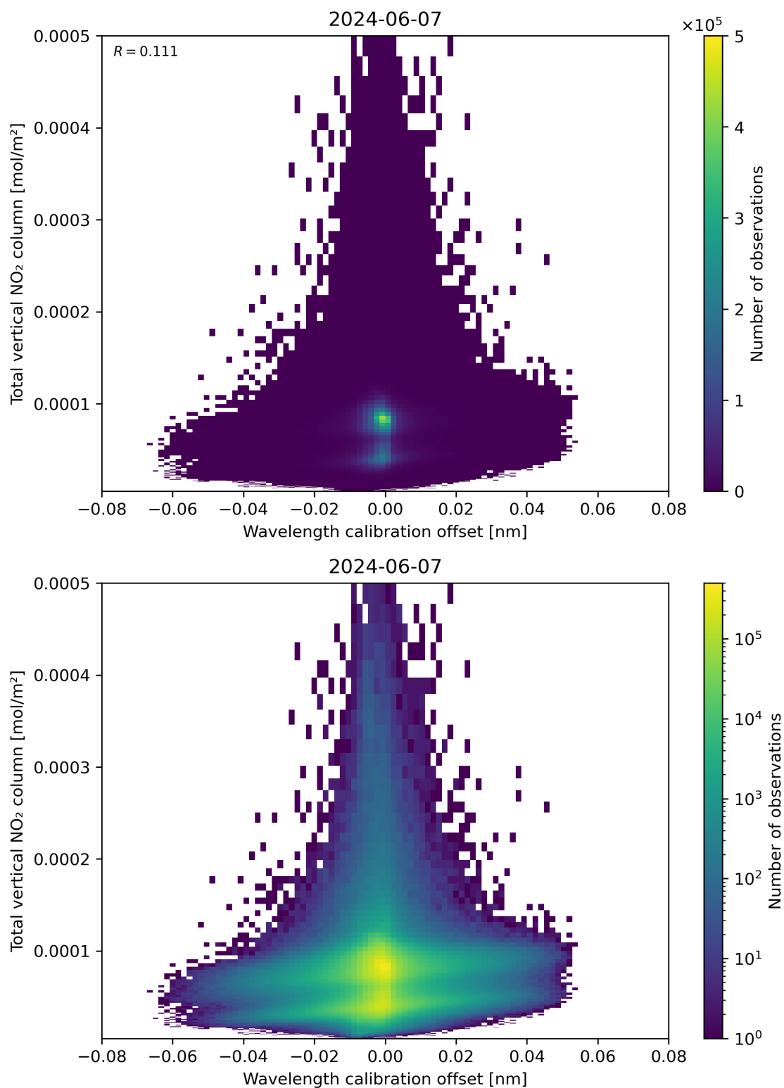
Figure 179: Scatter density plot of “Wavelength calibration offset” against “Total vertical NO 2 column” for 2024-06-06 to 2024-06-08.
