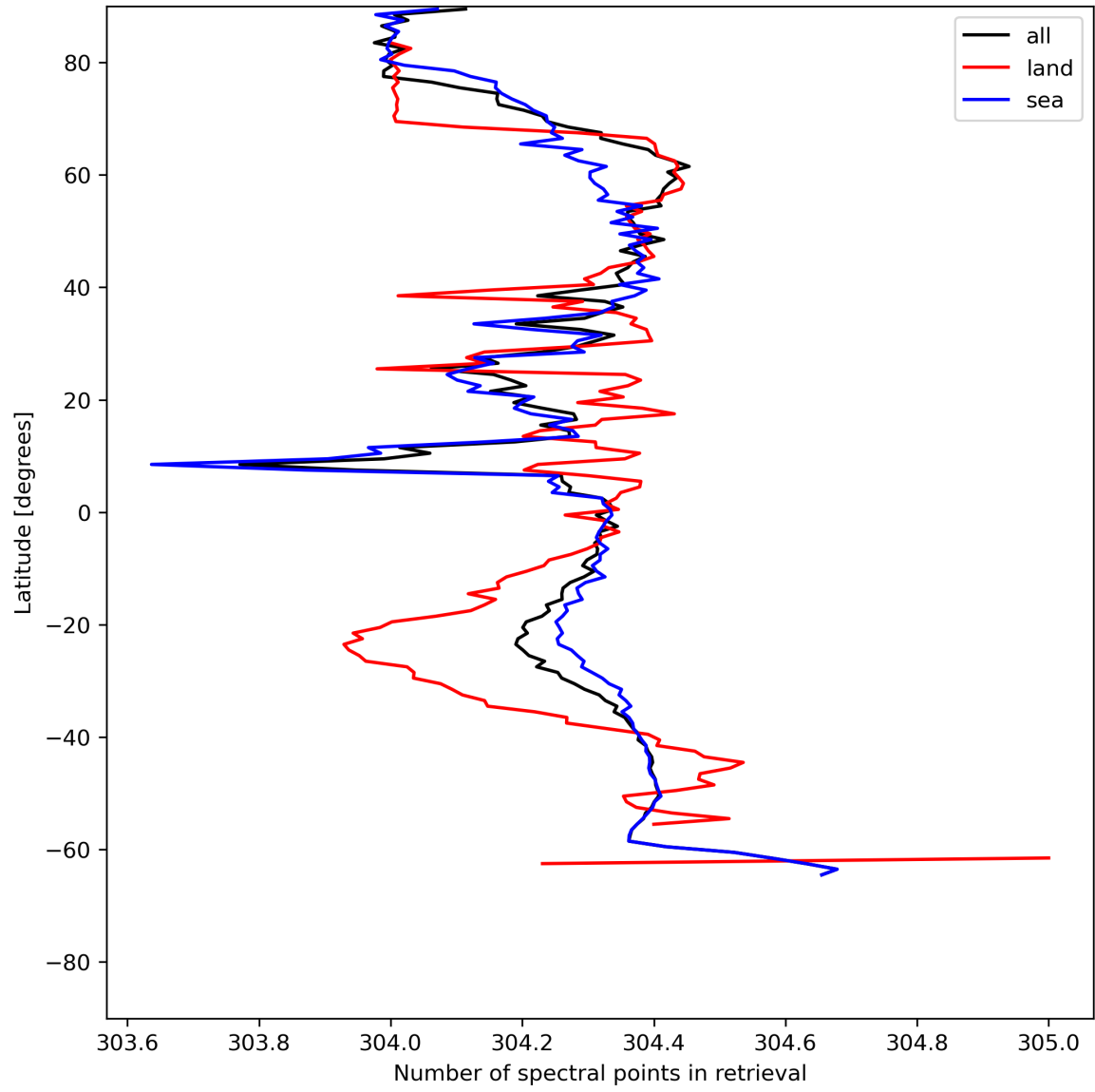
Figure 16: Zonal average of “Number of spectral points in retrieval” for 2024-06-06 to 2024-06-08.
