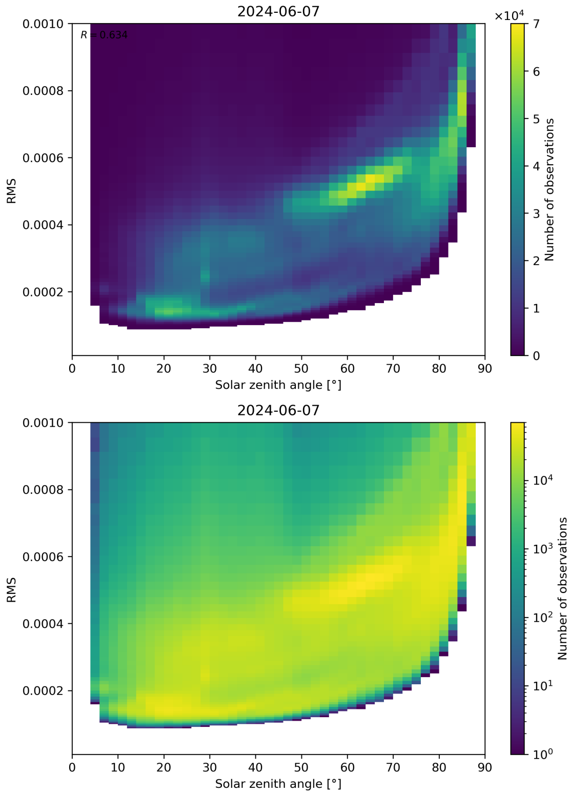
Figure 157: Scatter density plot of “Solar zenith angle” against “RMS” for 2024-06-06 to 2024-06-08.
