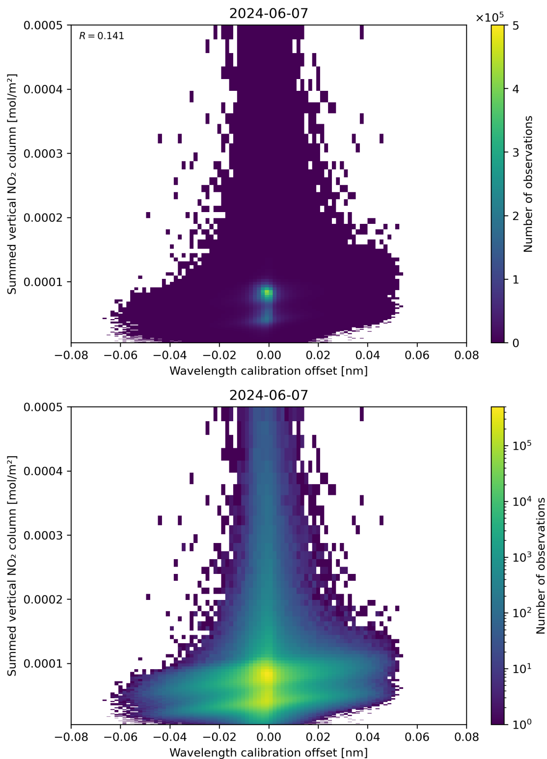
Figure 177: Scatter density plot of “Wavelength calibration offset” against “Summed vertical NO 2 column” for 2024-06-06 to 2024-06-08.
