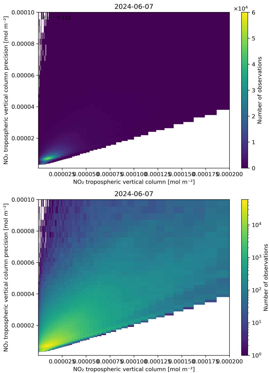
Figure 130: Scatter density plot of “NO 2 tropospheric vertical column” against “NO 2 tropospheric vertical column precision” for 2024-06-06 to 2024-06-08.
