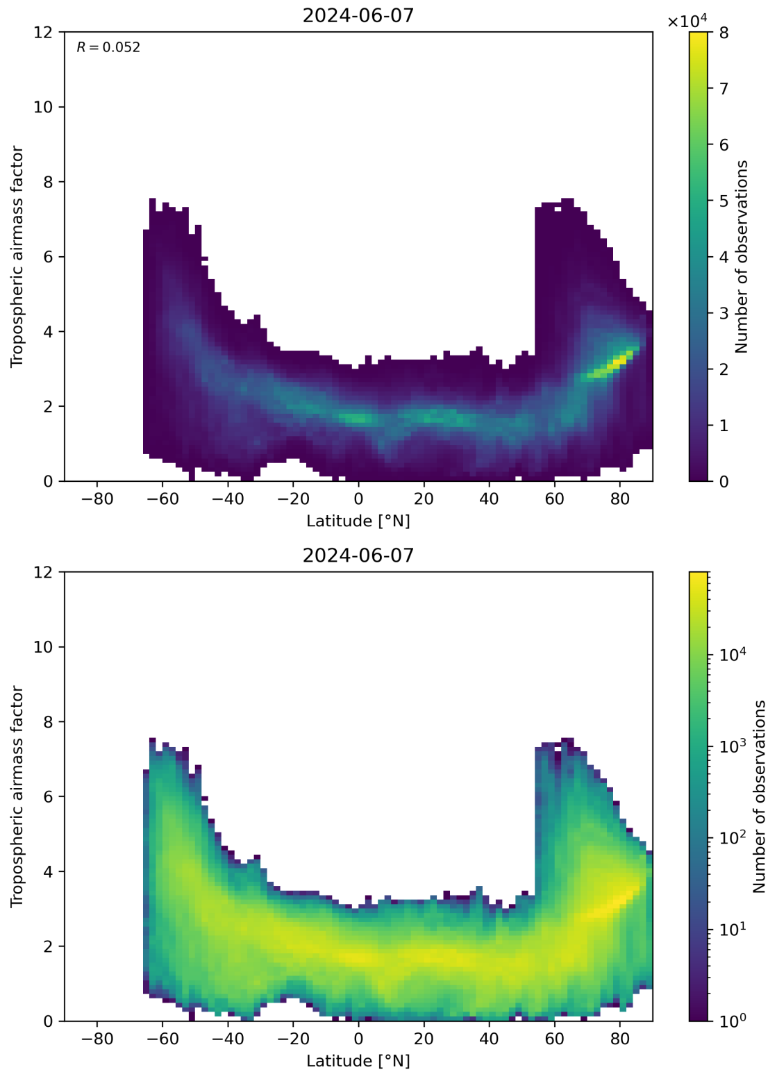
Figure 85: Scatter density plot of “Latitude” against “Tropospheric air mass factor” for 2024-06-06 to 2024-06-08.
