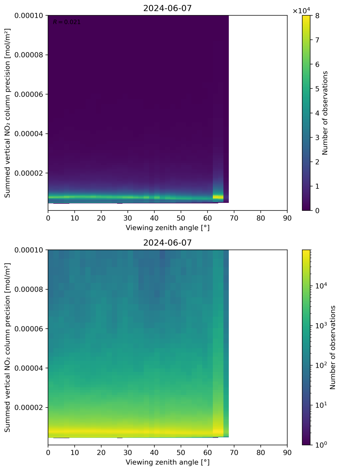
Figure 166: Scatter density plot of “Viewing zenith angle” against “Summed vertical NO 2 column precision” for 2024-06-06 to 2024-06-08.
