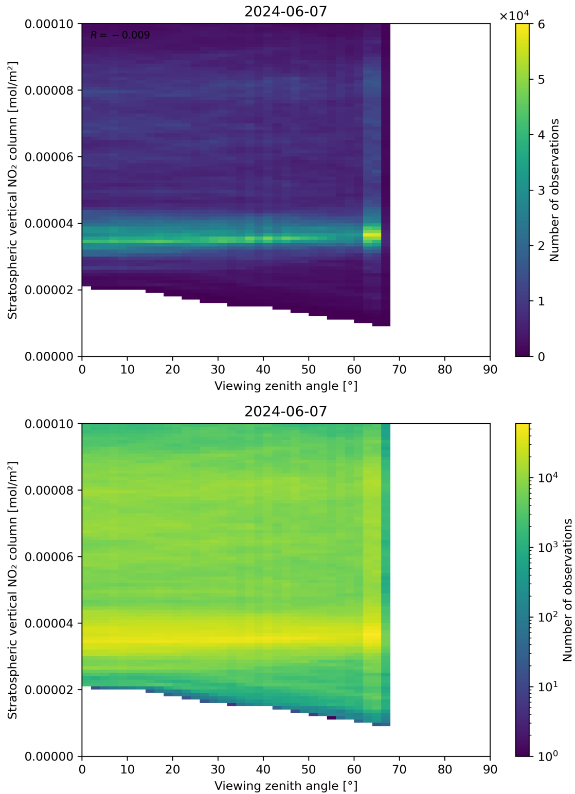
Figure 164: Scatter density plot of “Viewing zenith angle” against “Stratospheric vertical NO 2 column” for 2024-06-06 to 2024-06-08.
