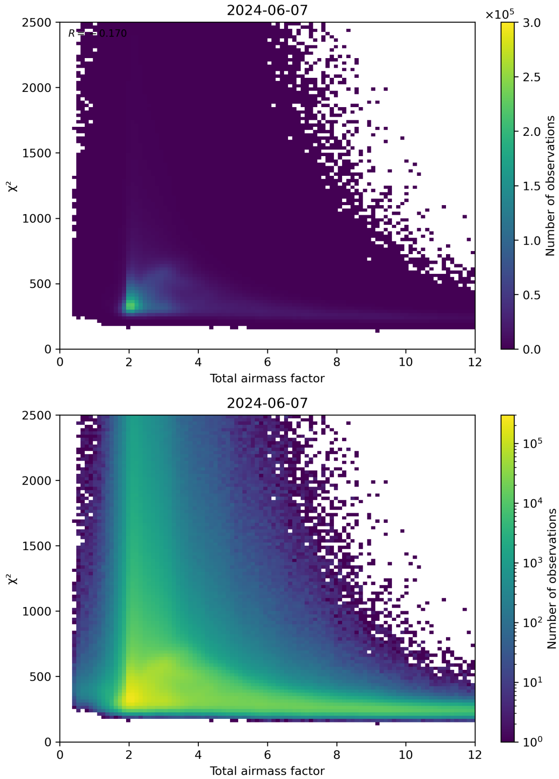
Figure 63: Scatter density plot of “Total airmass factor” against “ \chi^2 ” for 2024-06-06 to 2024-06-08.
