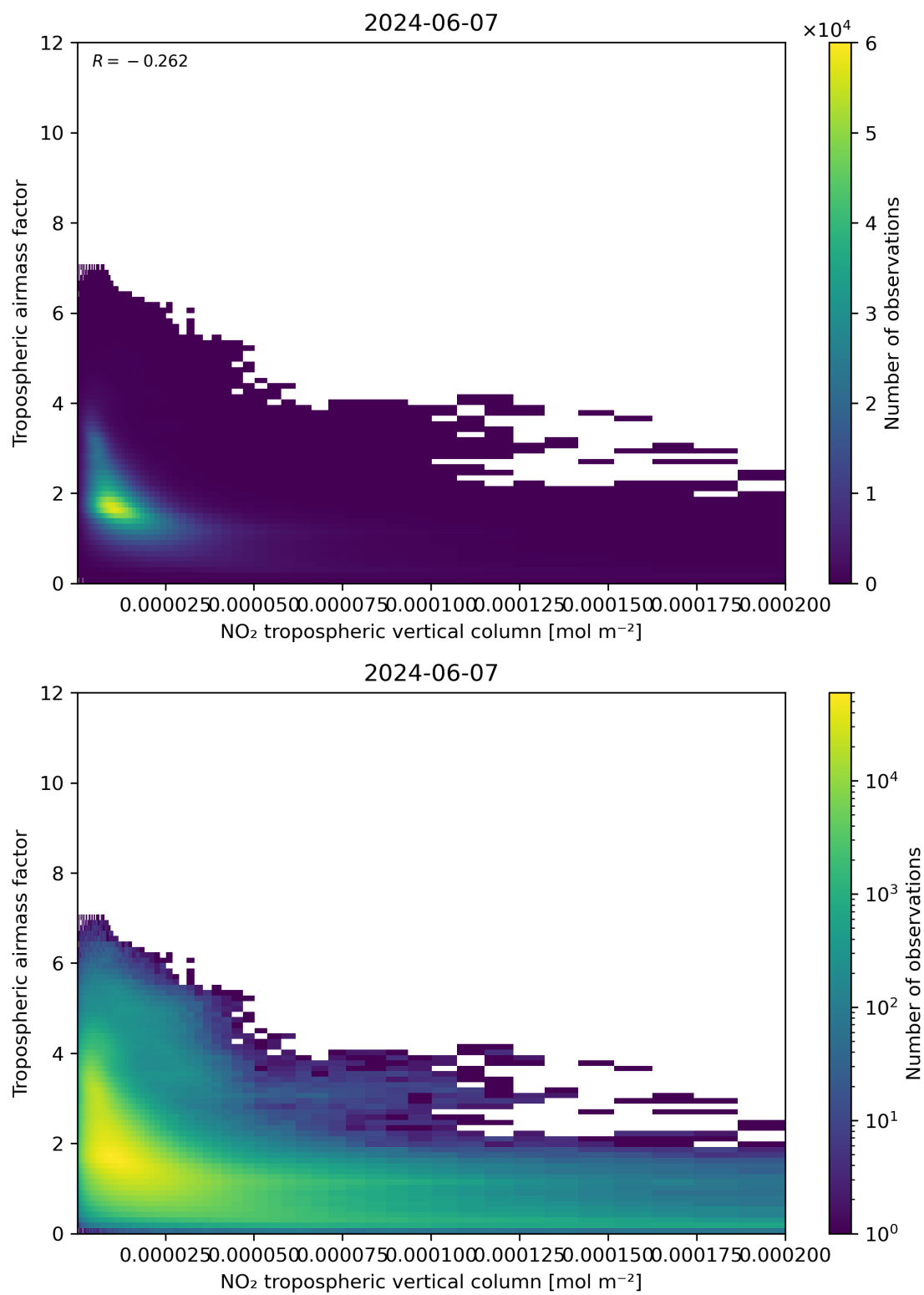
Figure 123: Scatter density plot of “NO 2 tropospheric vertical column” against “Tropospheric airmass factor” for 2024-06-06 to 2024-06-08.
