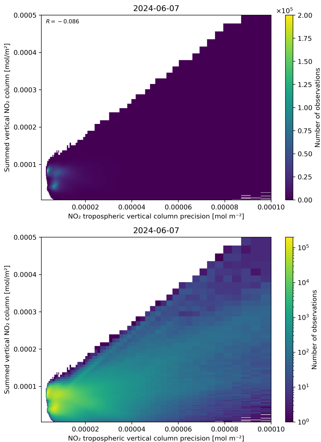
Figure 136: Scatter density plot of “NO 2 tropospheric vertical column precision” against “Summed vertical NO 2 column” for 2024-06-06 to 2024-06-08.
