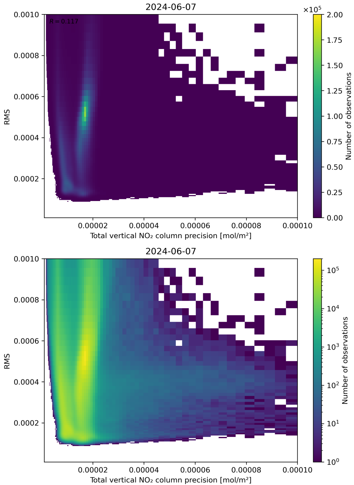
Figure 119: Scatter density plot of “Total vertical NO 2 column precision” against “RMS” for 2024-06-06 to 2024-06-08.
