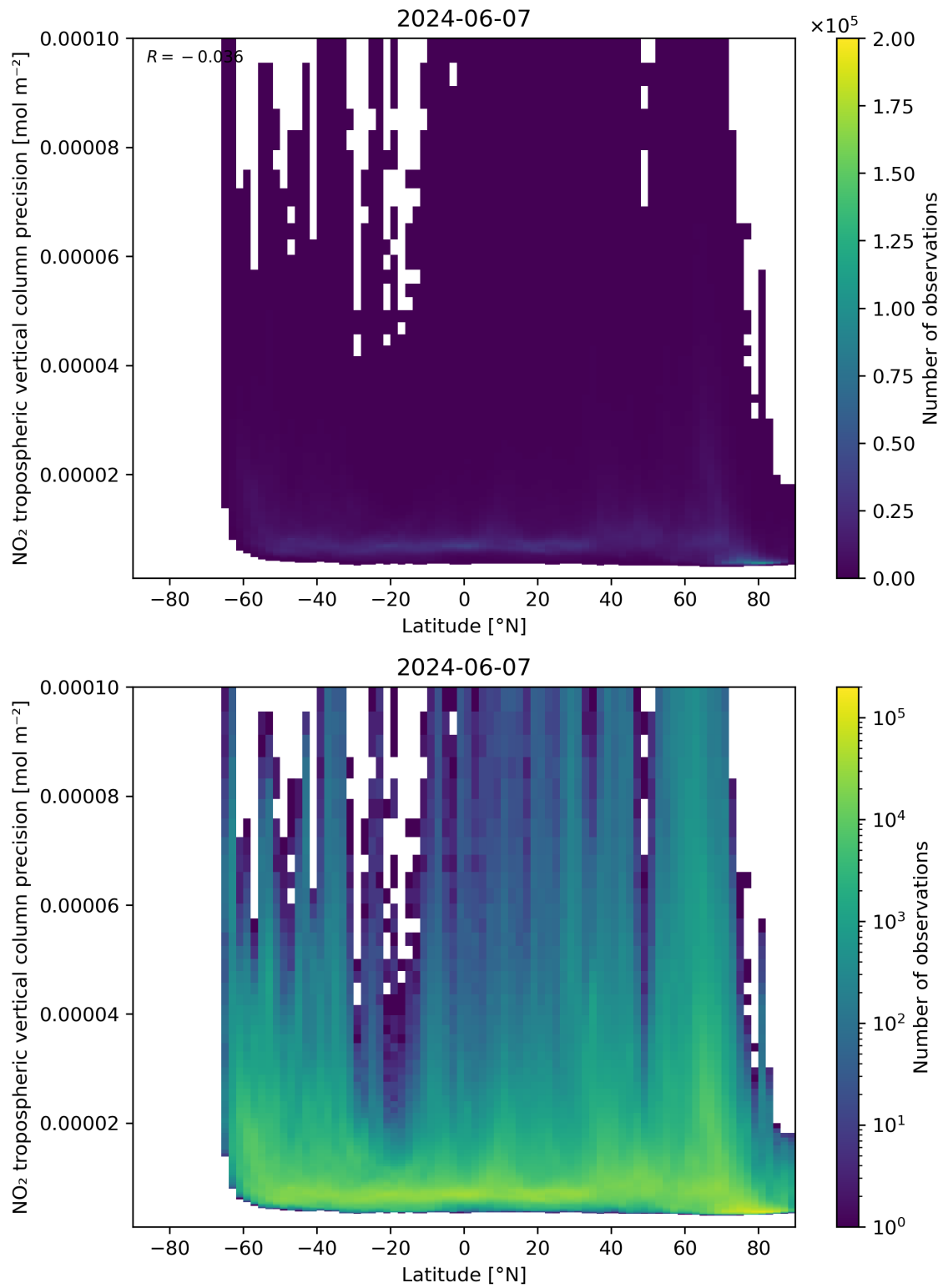
Figure 93: Scatter density plot of “Latitude” against “NO 2 tropospheric vertical column precision” for 2024-06-06 to 2024-06-08.
