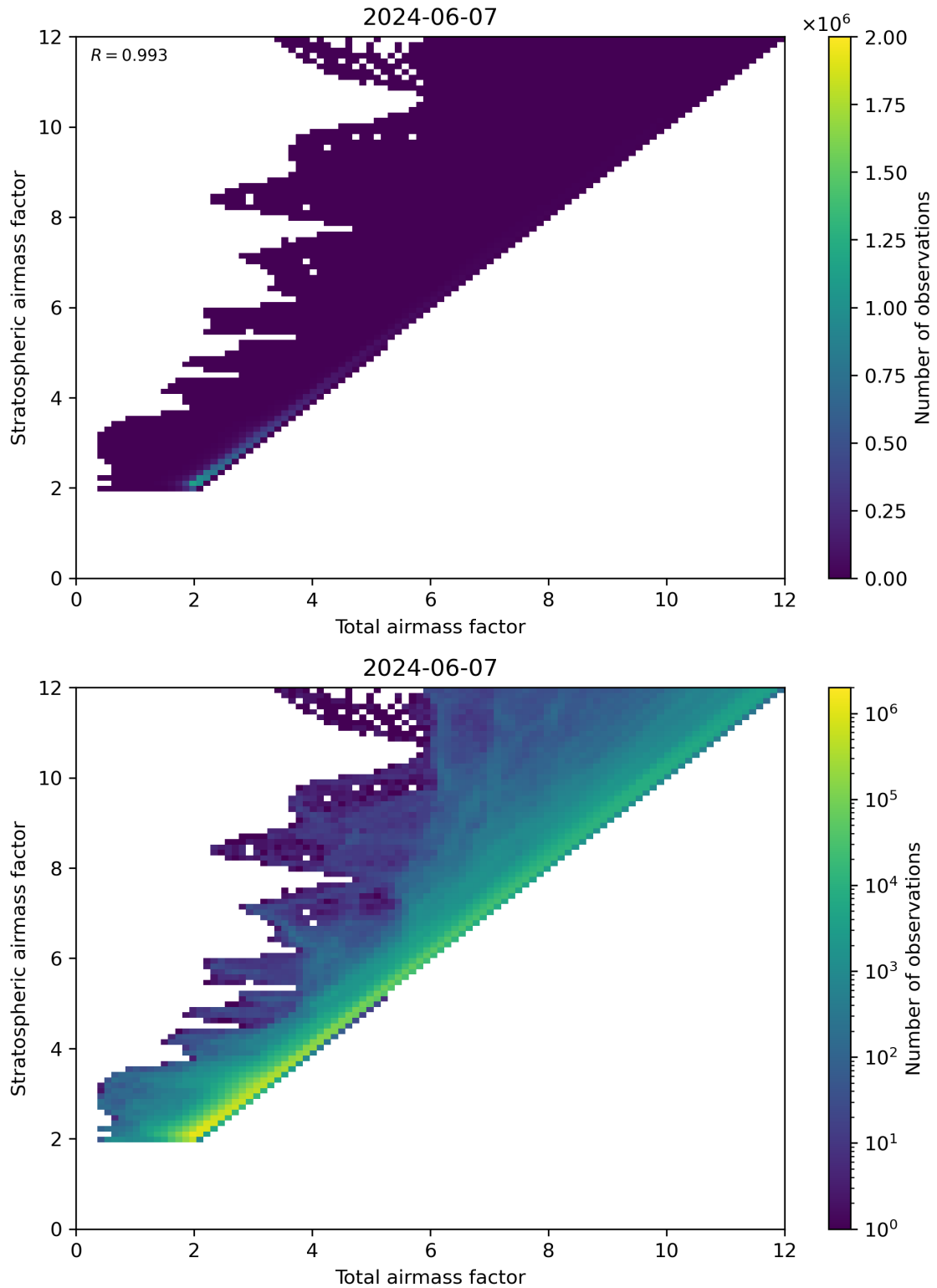
Figure 62: Scatter density plot of “Total airmass factor” against “Stratospheric airmass factor” for 2024-06-06 to 2024-06-08.
