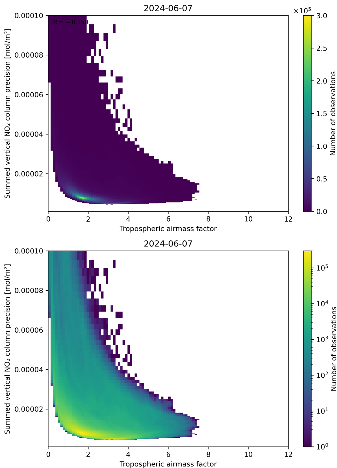
Figure 76: Scatter density plot of “Tropospheric air mass factor” against “Summed vertical NO 2 column precision” for 2024-06-06 to 2024-06-08.
