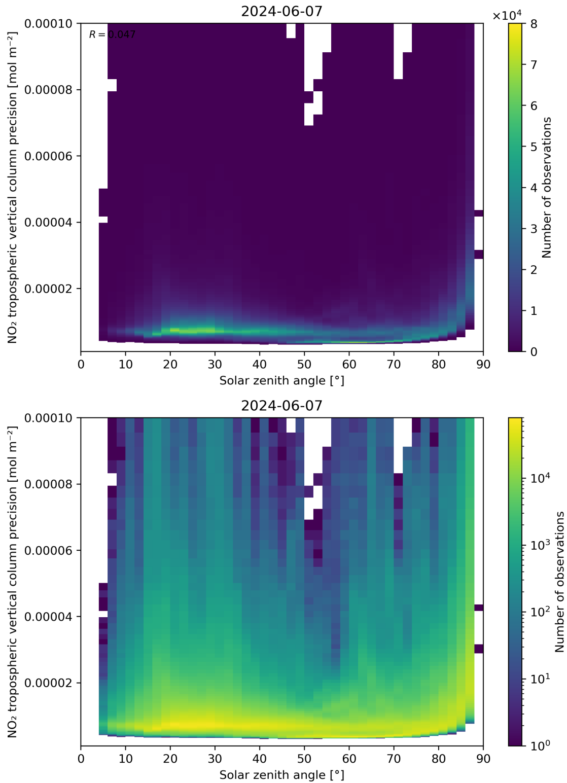
Figure 156: Scatter density plot of “Solar zenith angle” against “NO 2 tropospheric vertical column precision” for 2024-06-06 to 2024-06-08.
