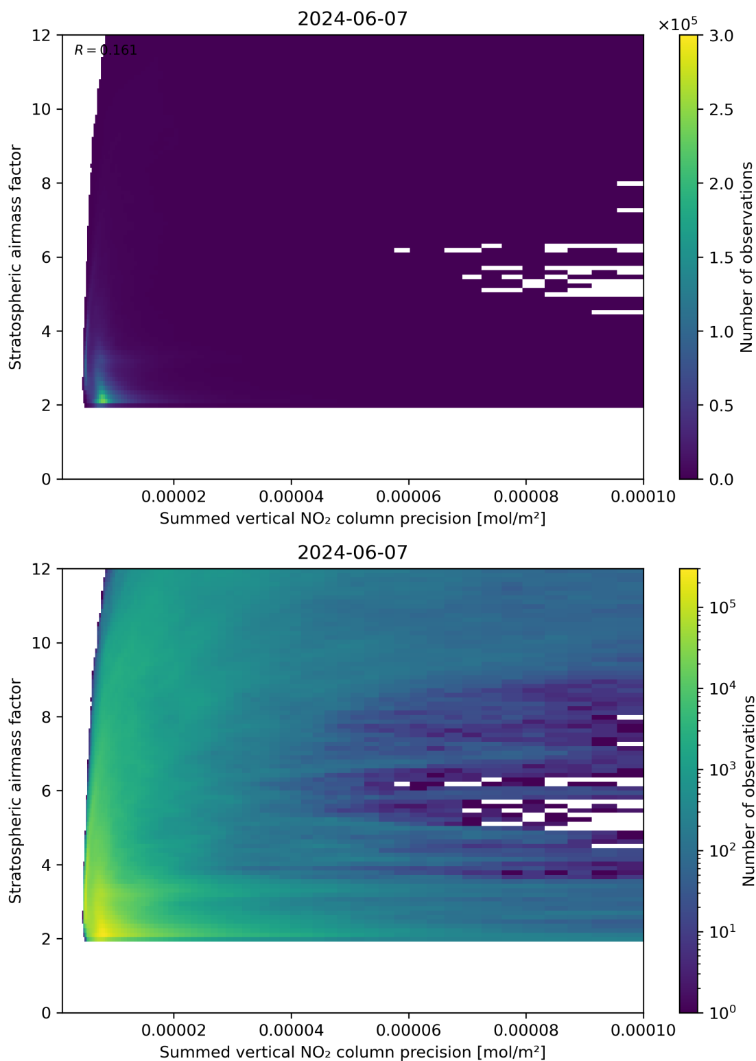
Figure 106: Scatter density plot of “Summed vertical NO 2 column precision” against “Stratospheric airmass factor” for 2024-06-06 to 2024-06-08.
