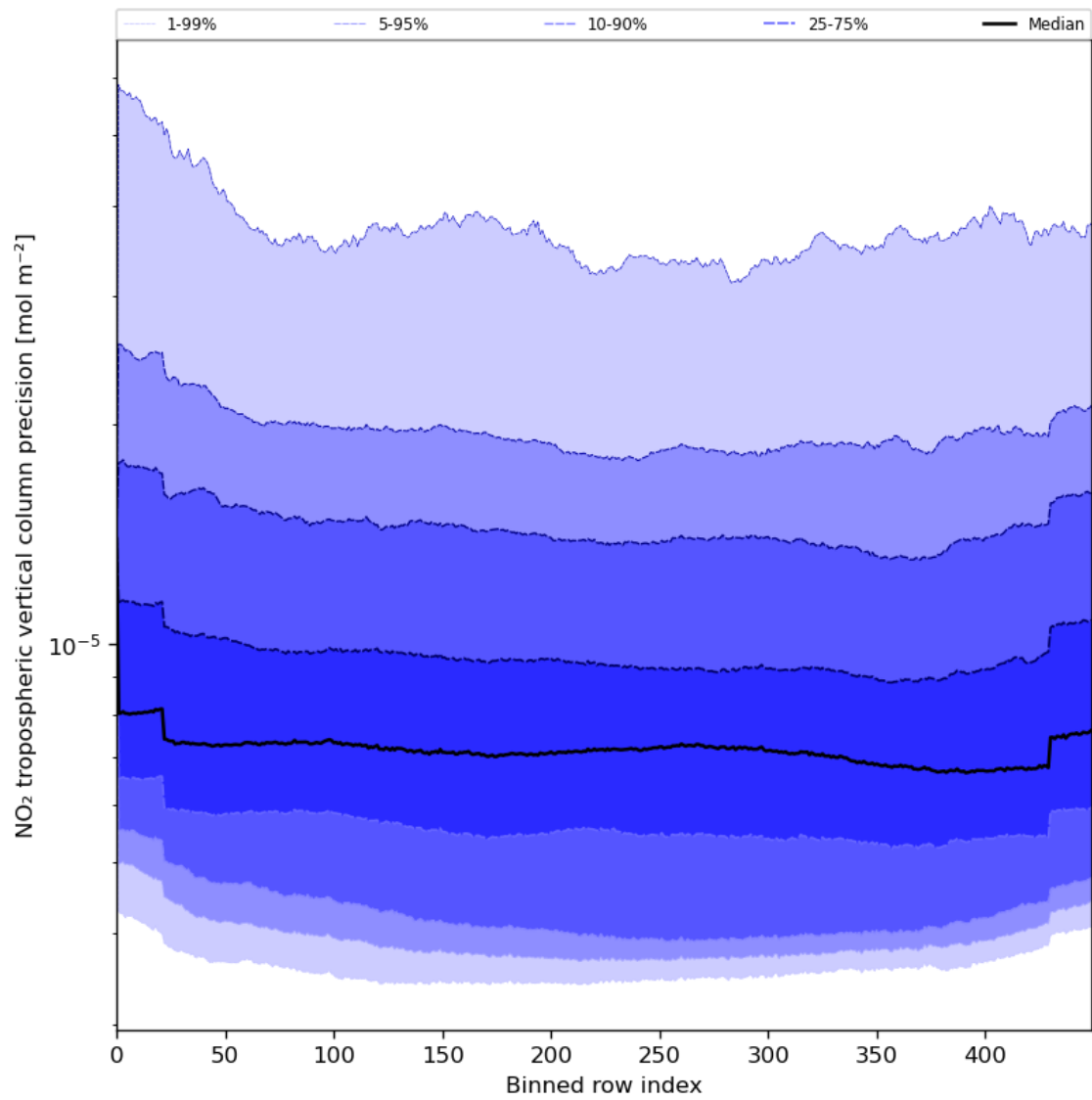
Figure 47: Along track statistics of “NO 2 tropospheric vertical column precision” for 2024-06-06 to 2024-06-08
