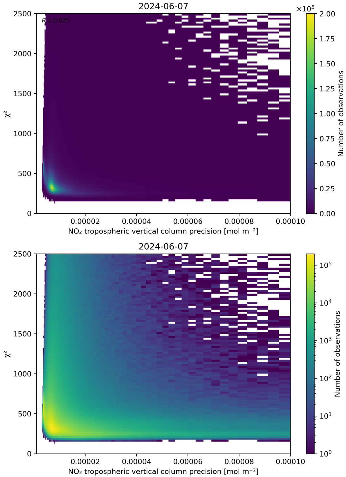
Figure 134: Scatter density plot of “NO 2 tropospheric vertical column precision” against “ \chi^2 ” for 2024-06-06 to 2024-06-08.
