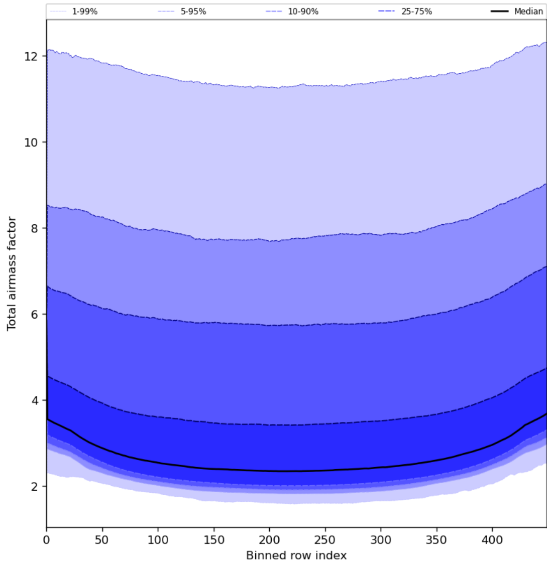
Figure 49: Along track statistics of “Total airmass factor” for 2024-06-06 to 2024-06-08
