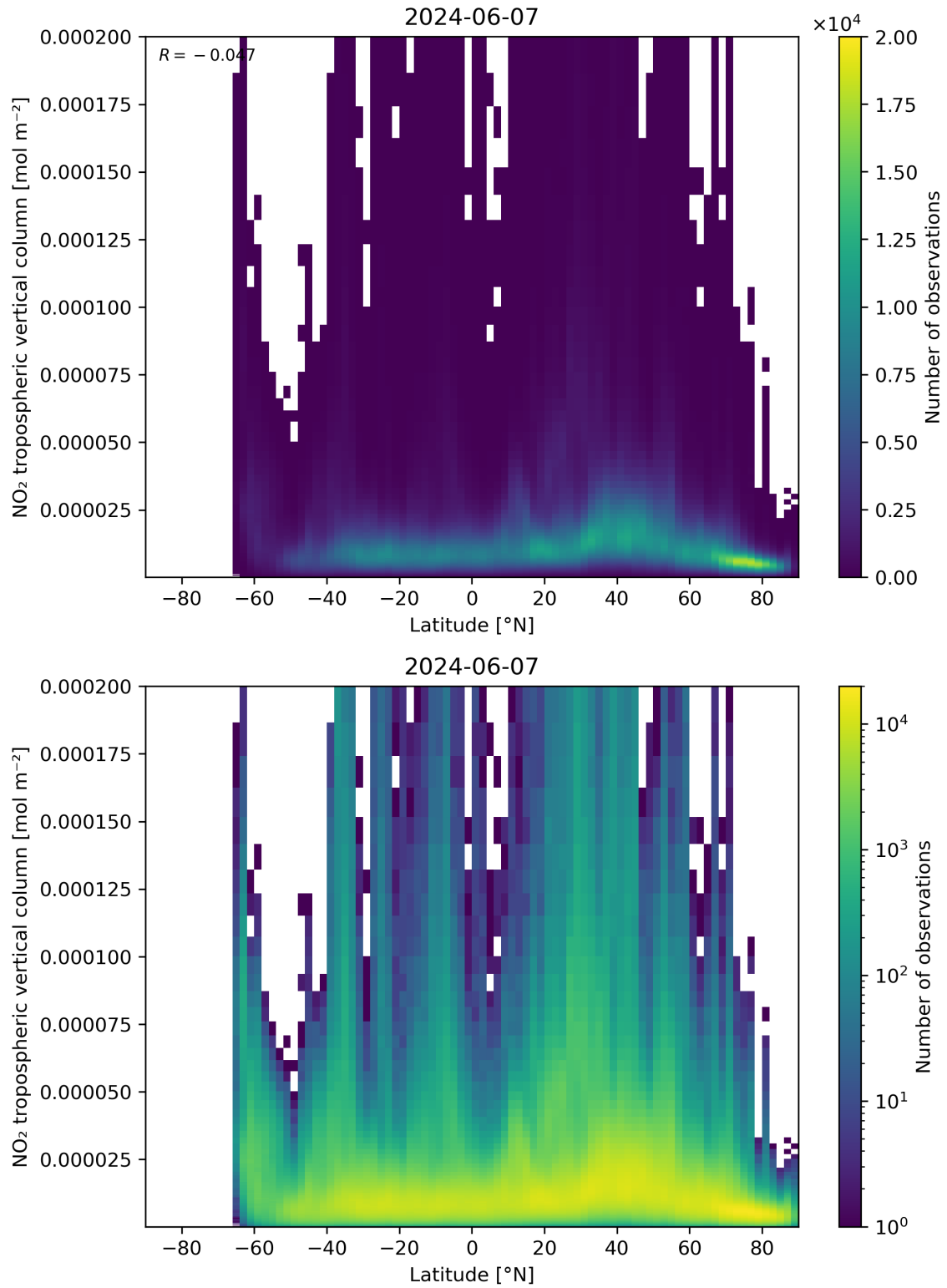
Figure 92: Scatter density plot of “Latitude” against “NO 2 tropospheric vertical column” for 2024-06-06 to 2024-06-08.
