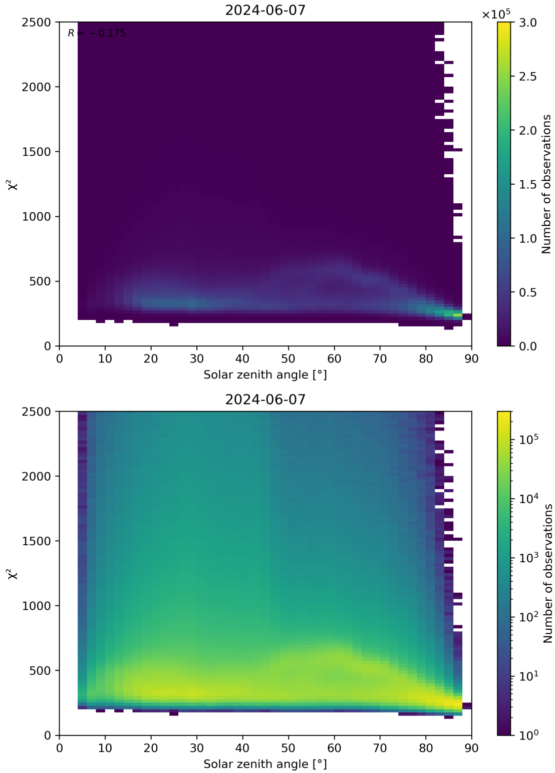
Figure 148: Scatter density plot of “Solar zenith angle” against “ \chi^2 ” for 2024-06-06 to 2024-06-08.
