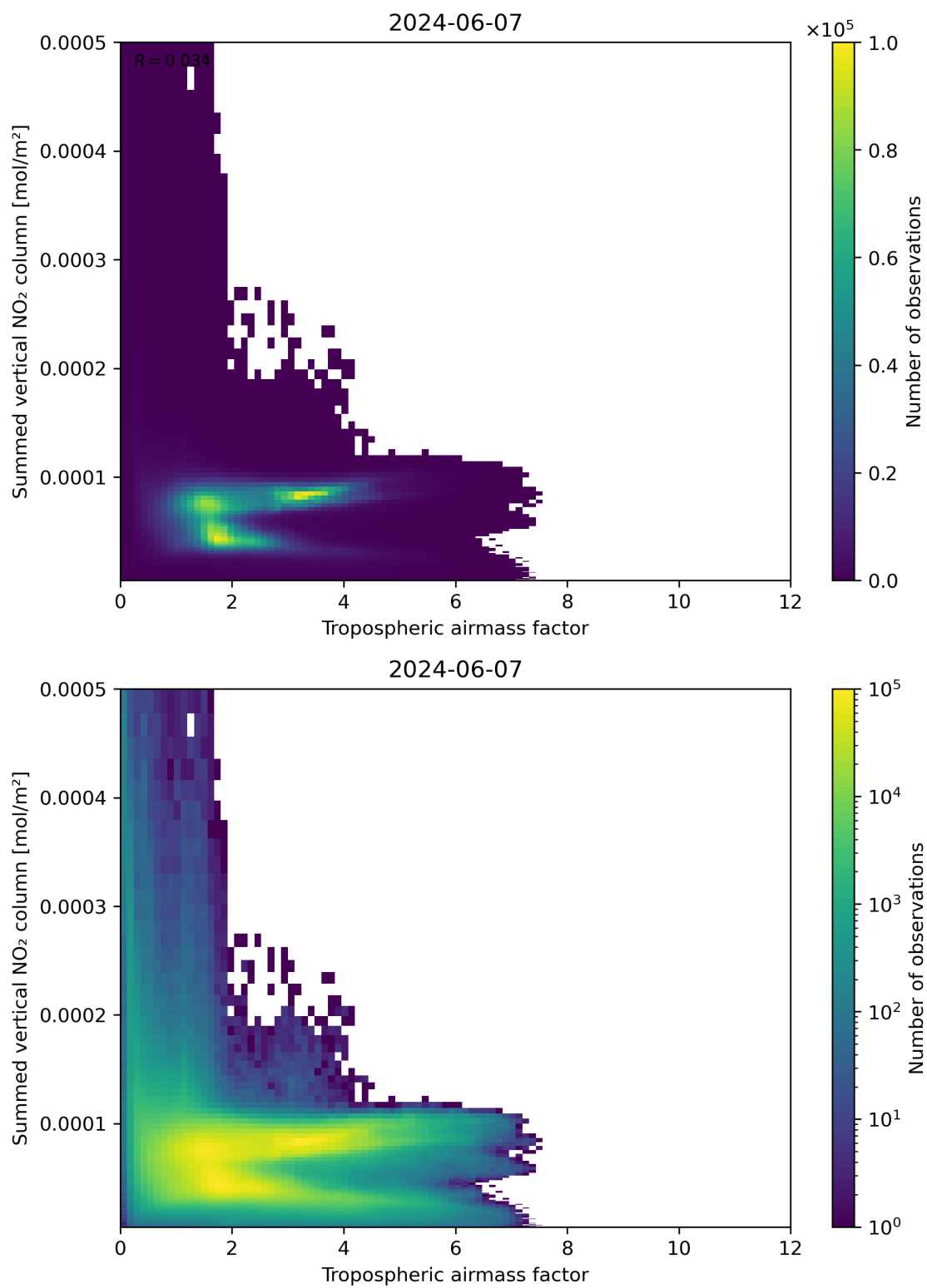
Figure 75: Scatter density plot of “Tropospheric airmass factor” against “Summed vertical NO 2 column” for 2024-06-06 to 2024-06-08.
