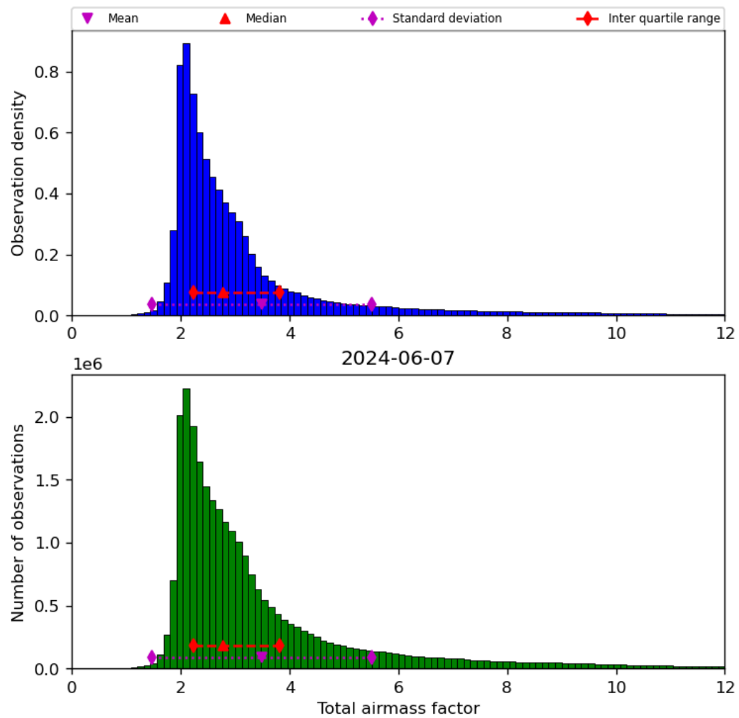
Figure 32: Histogram of “Total airmass factor” for 2024-06-06 to 2024-06-08
