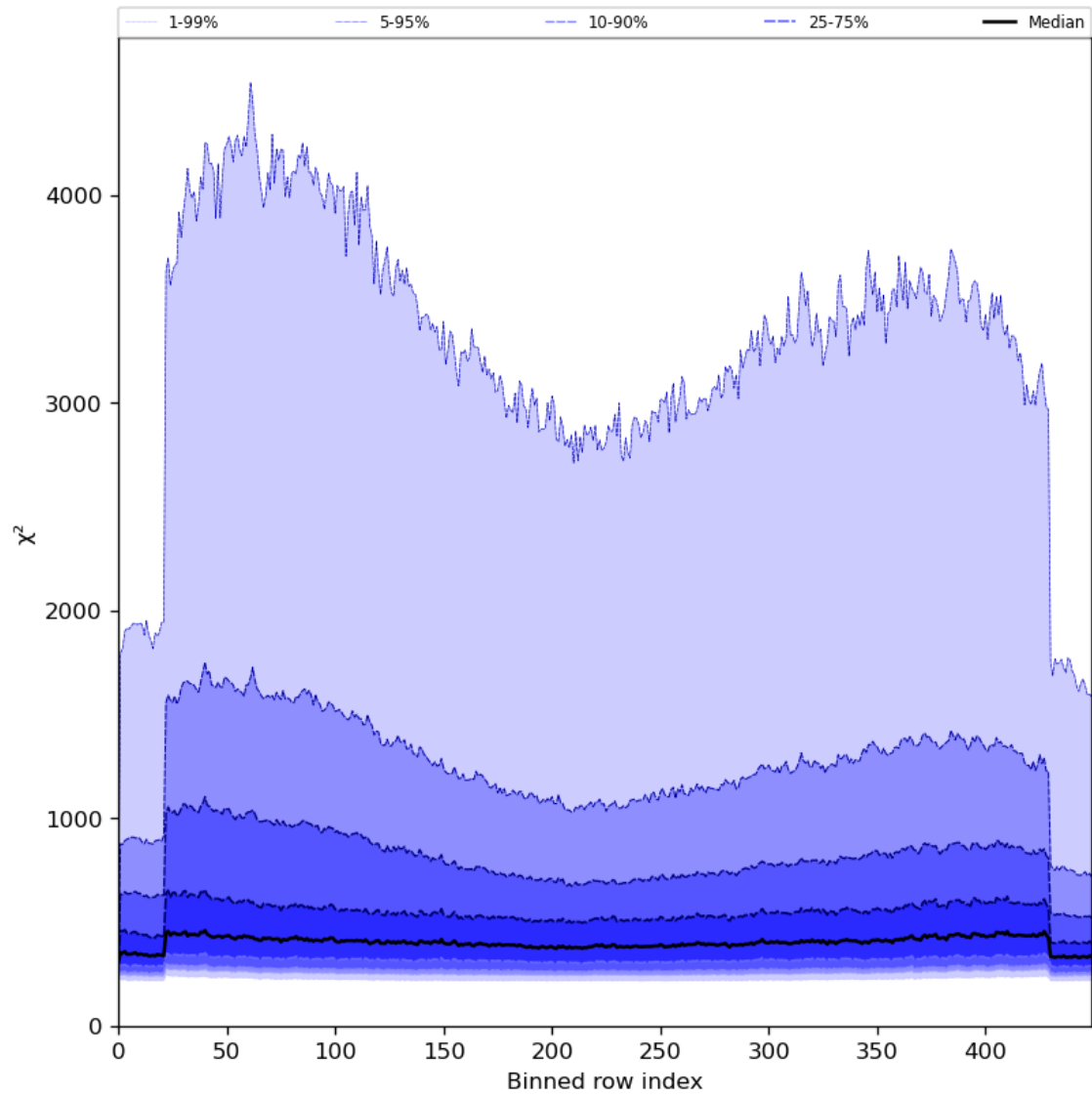
Figure 59: Along track statistics of “ \chi^2 ” for 2024-06-06 to 2024-06-08
