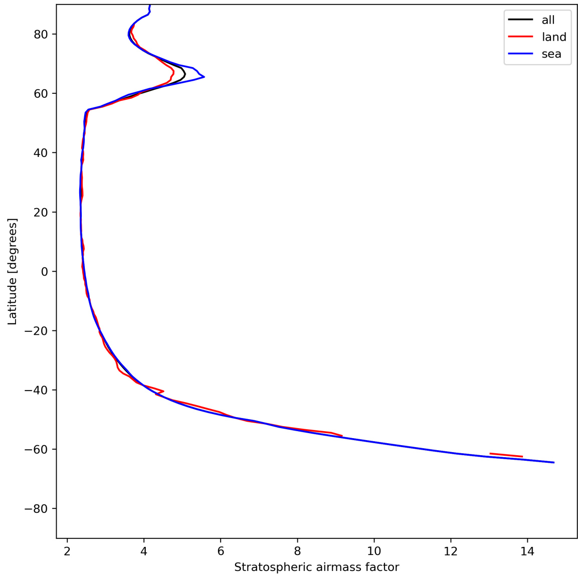
Figure 27: Zonal average of “Stratospheric air mass factor” for 2024-06-06 to 2024-06-08.
