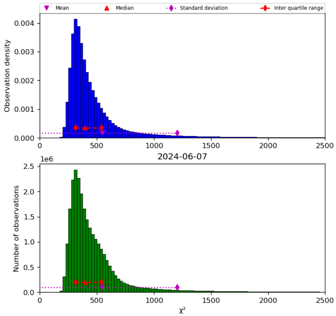
Figure 42: Histogram of “ \chi^2 ” for 2024-06-06 to 2024-06-08
