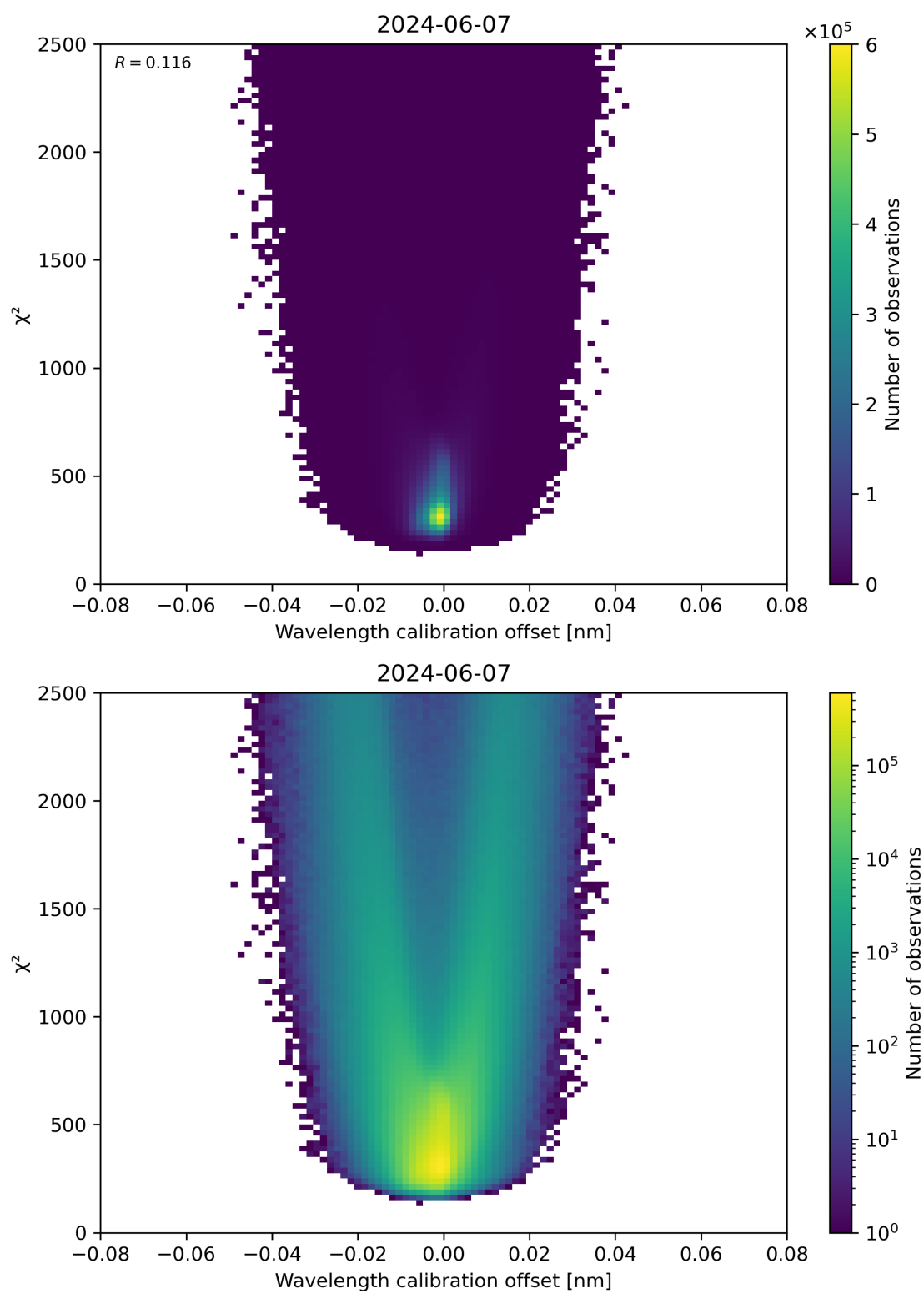
Figure 175: Scatter density plot of “Wavelength calibration offset” against “ \chi^2 ” for 2024-06-06 to 2024-06-08.
