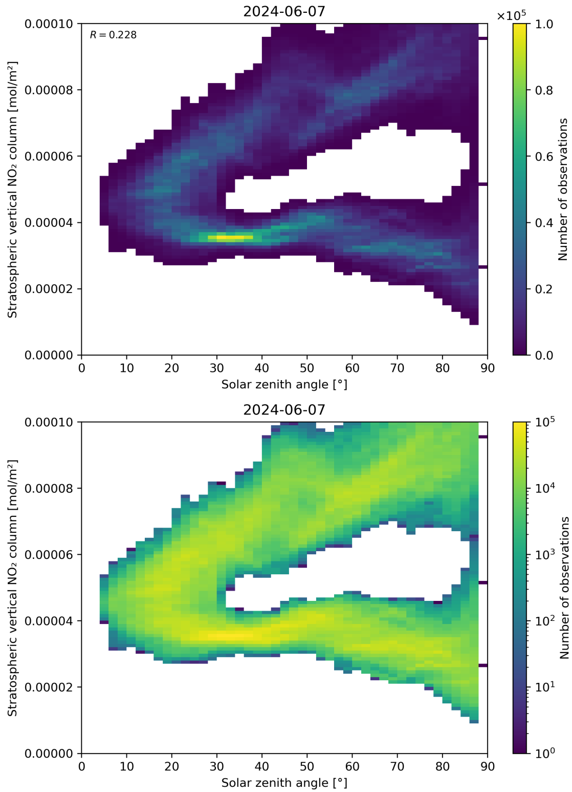
Figure 150: Scatter density plot of “Solar zenith angle” against “Stratospheric vertical NO 2 column” for 2024-06-06 to 2024-06-08.
