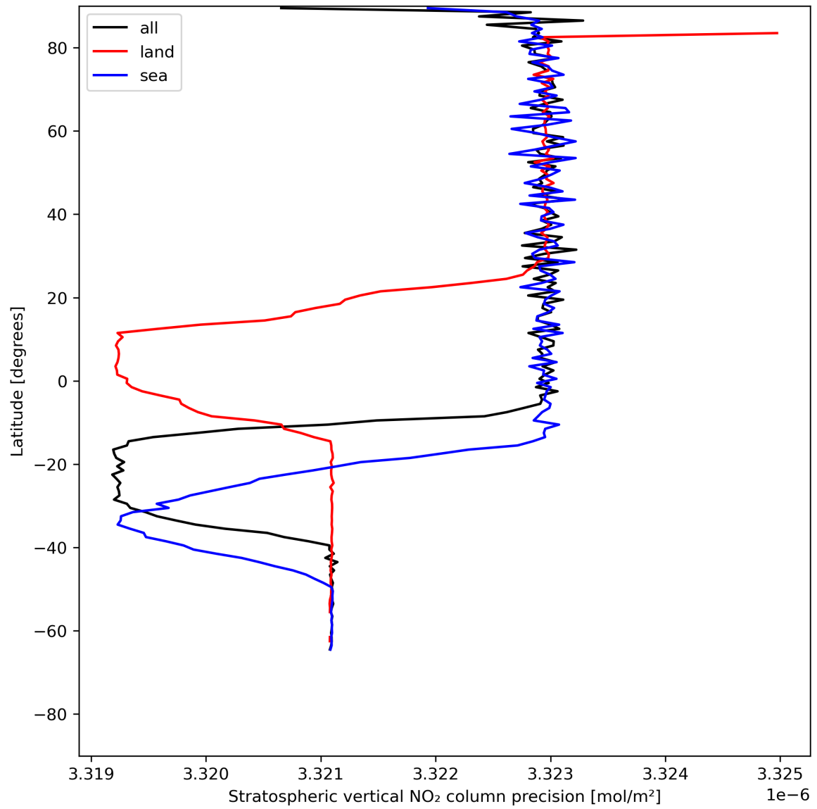
Figure 20: Zonal average of “Stratospheric vertical NO 2 column precision” for 2024-06-06 to 2024-06-08.
