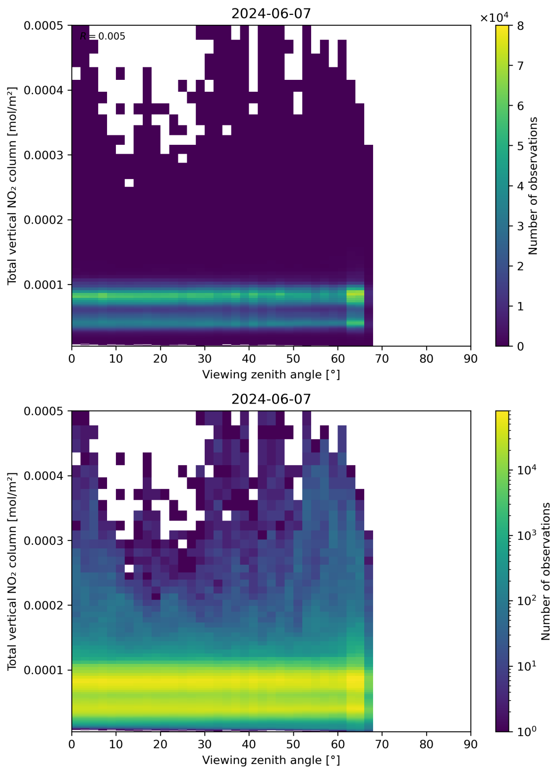
Figure 167: Scatter density plot of “Viewing zenith angle” against “Total vertical NO 2 column” for 2024-06-06 to 2024-06-08.
