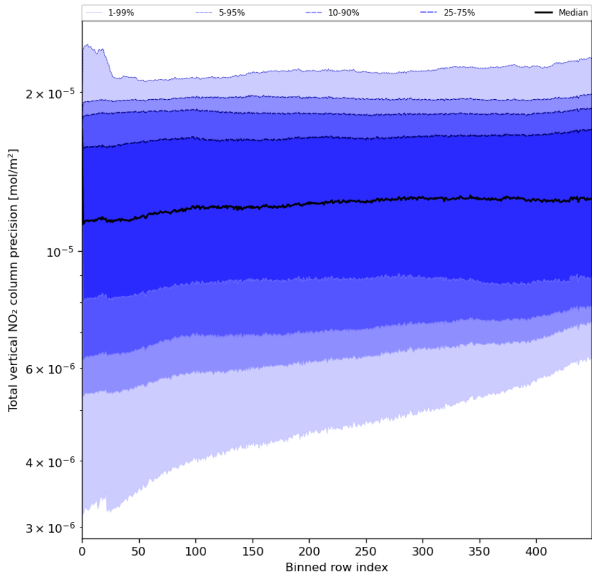
Figure 56: Along track statistics of “Total vertical NO 2 column precision” for 2024-06-06 to 2024-06-08
