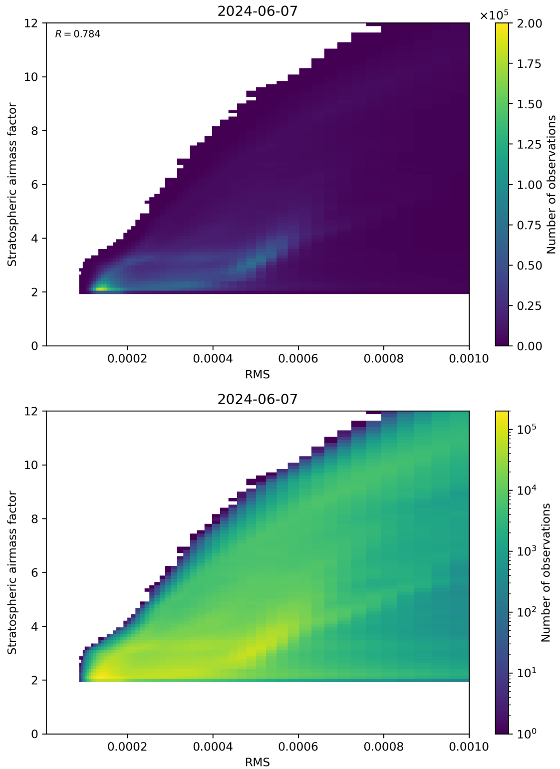
Figure 144: Scatter density plot of “RMS” against “Stratospheric airmass factor” for 2024-06-06 to 2024-06-08.
