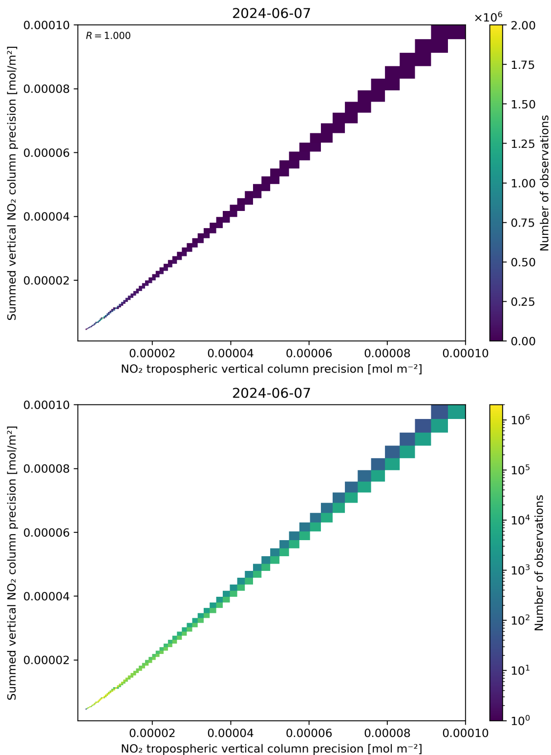
Figure 137: Scatter density plot of “NO 2 tropospheric vertical column precision” against “Summed vertical NO 2 column precision” for 2024-06-06 to 2024-06-08.
