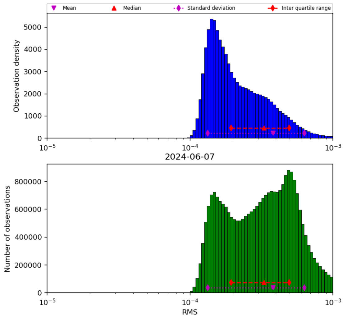
Figure 43: Histogram of “RMS” for 2024-06-06 to 2024-06-08
