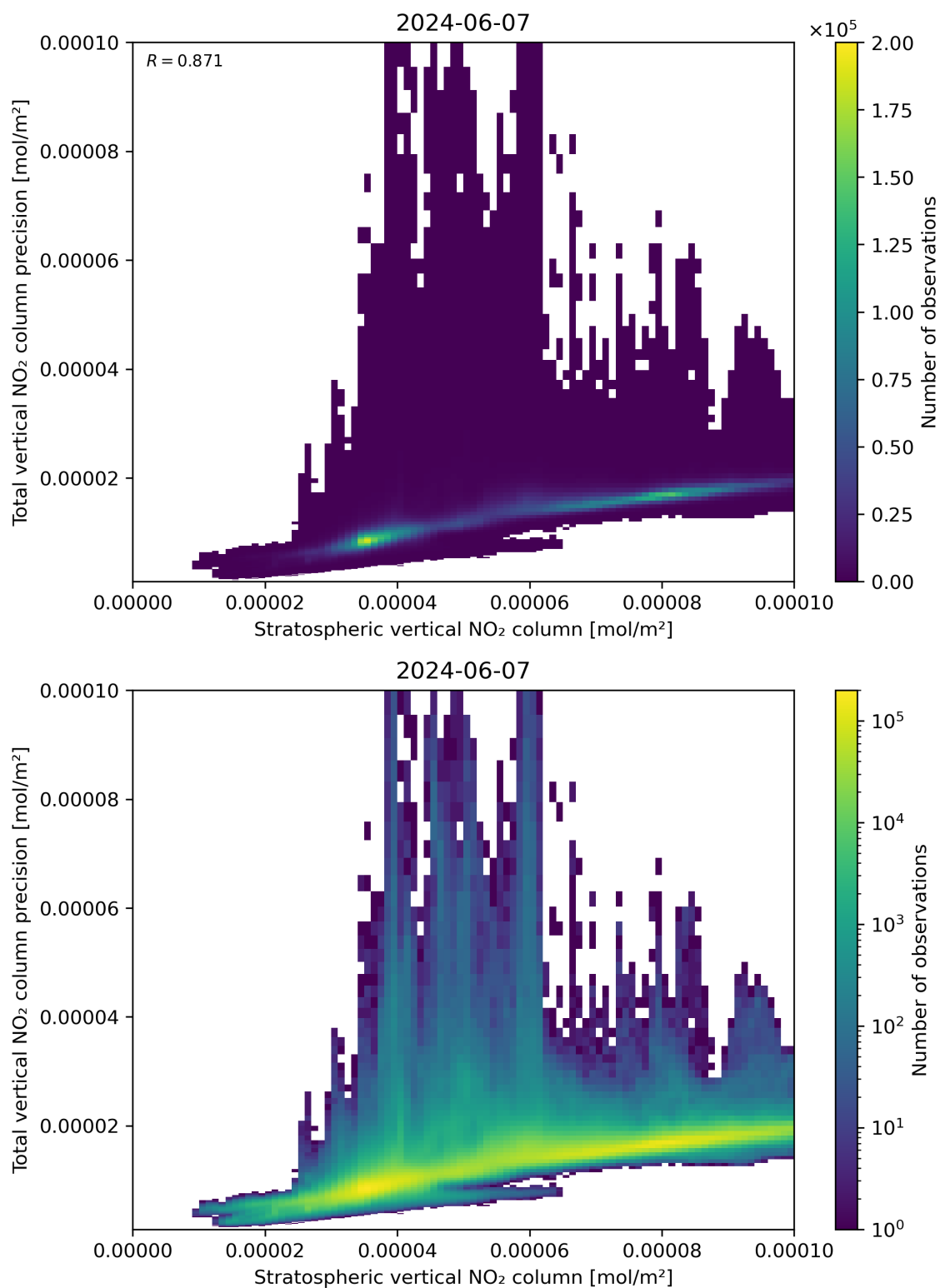
Figure 101: Scatter density plot of “Stratospheric vertical NO 2 column” against “Total vertical NO 2 column precision” for 2024-06-06 to 2024-06-08.
