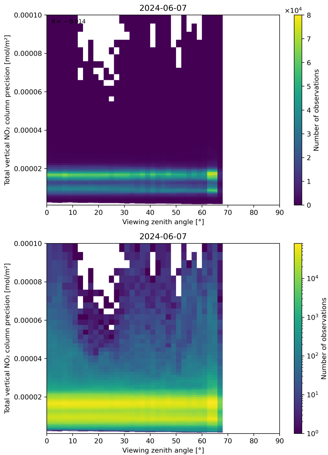
Figure 168: Scatter density plot of “Viewing zenith angle” against “Total vertical NO 2 column precision” for 2024-06-06 to 2024-06-08.
