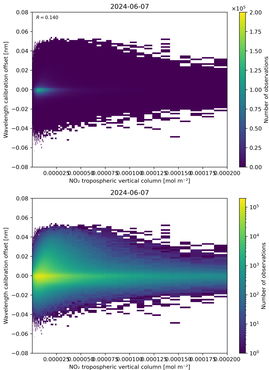
Figure 143: Scatter density plot of “NO 2 tropospheric vertical column” against “Wavelength calibration offset” for 2024-06-06 to 2024-06-08.
