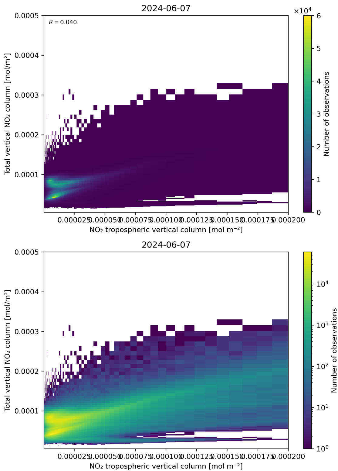
Figure 128: Scatter density plot of “NO 2 tropospheric vertical column” against “Total vertical NO 2 column” for 2024-06-06 to 2024-06-08.
