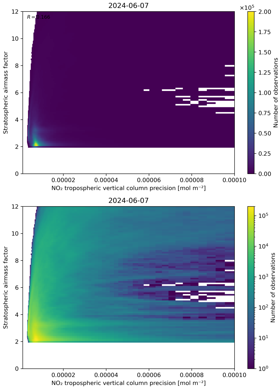
Figure 131: Scatter density plot of “NO 2 tropospheric vertical column precision” against “Stratospheric airmass factor” for 2024-06-06 to 2024-06-08.
