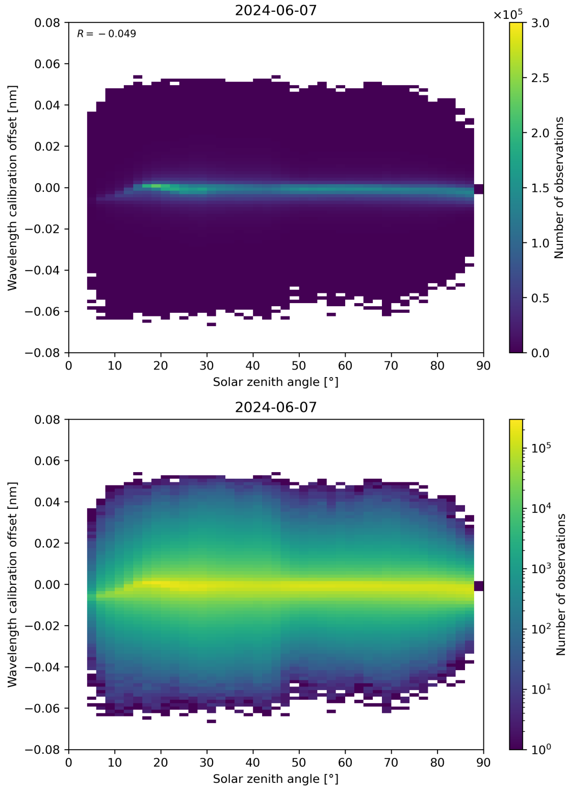
Figure 158: Scatter density plot of “Solar zenith angle” against “Wavelength calibration offset” for 2024-06-06 to 2024-06-08.
