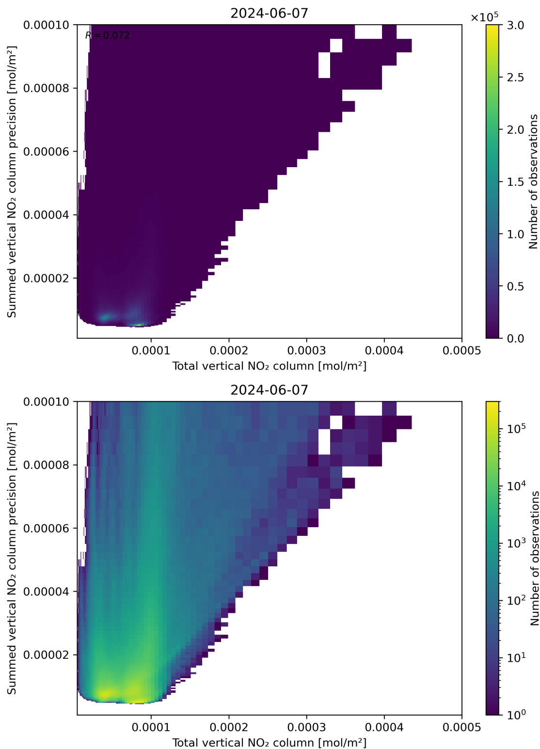
Figure 113: Scatter density plot of “Total vertical NO 2 column” against “Summed vertical NO 2 column precision” for 2024-06-06 to 2024-06-08.
