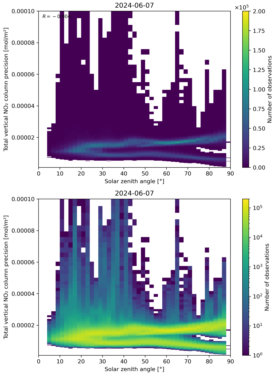
Figure 154: Scatter density plot of “Solar zenith angle” against “Total vertical NO 2 column precision” for 2024-06-06 to 2024-06-08.
