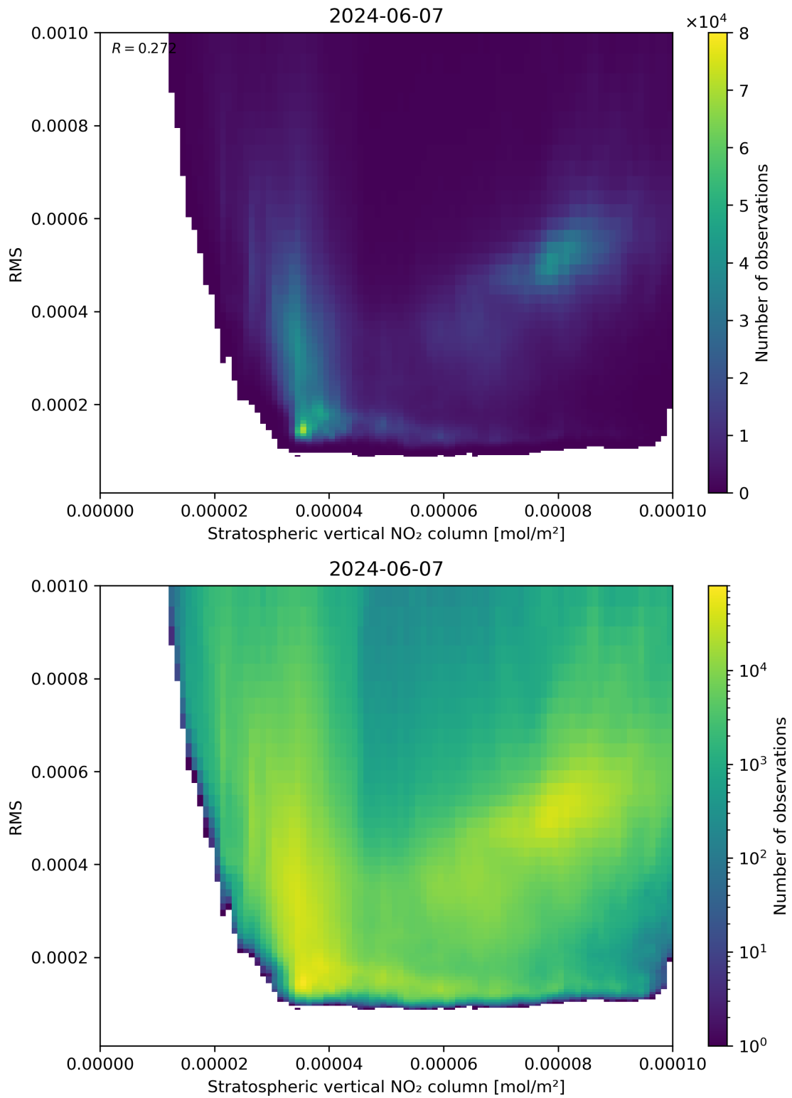
Figure 102: Scatter density plot of “Stratospheric vertical NO 2 column” against “RMS” for 2024-06-06 to 2024-06-08.
