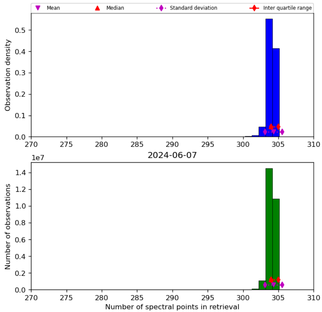
Figure 33: Histogram of “Number of spectral points in retrieval” for 2024-06-06 to 2024-06-08
