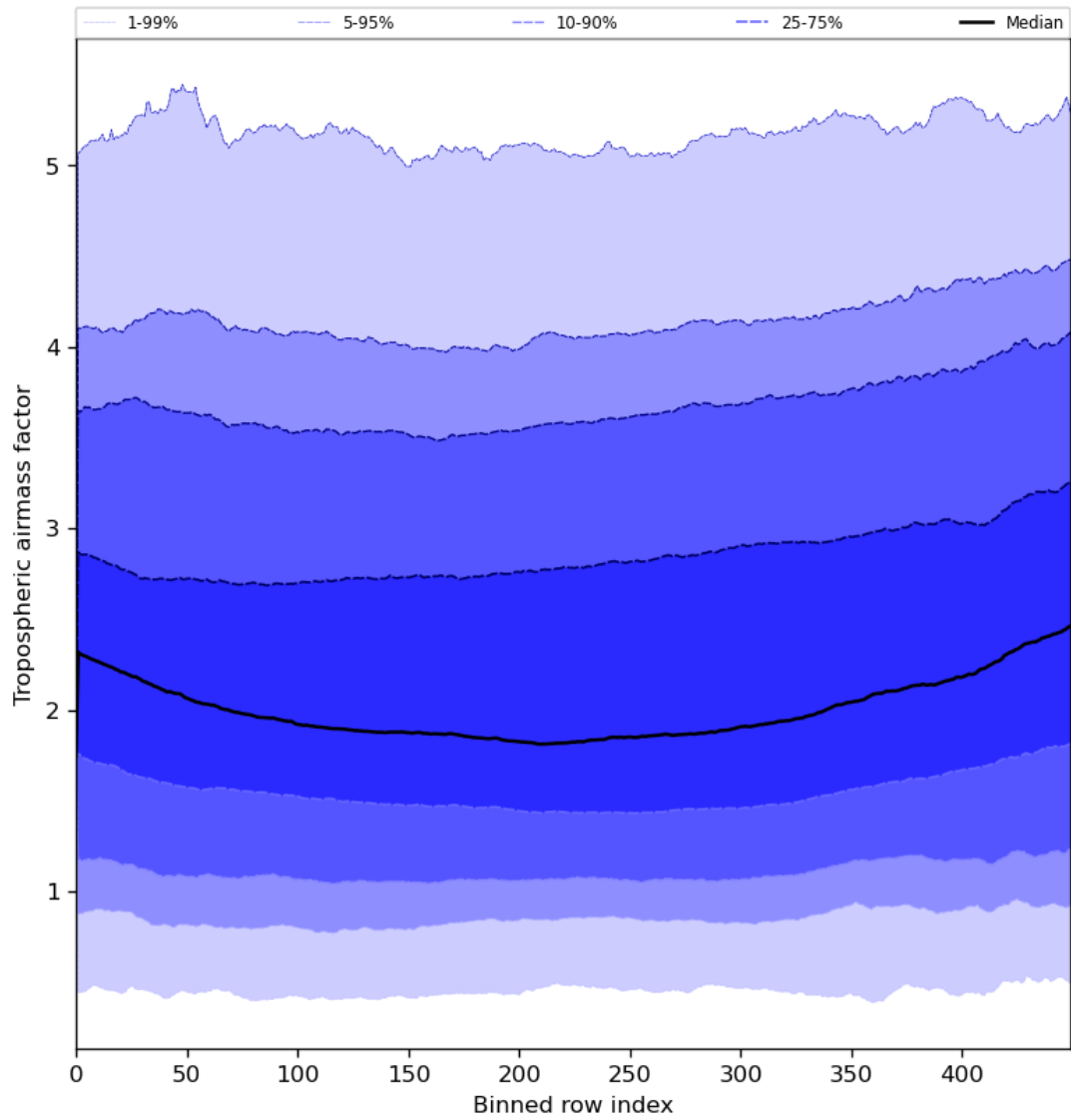
Figure 48: Along track statistics of “Tropospheric airmass factor” for 2024-06-06 to 2024-06-08
