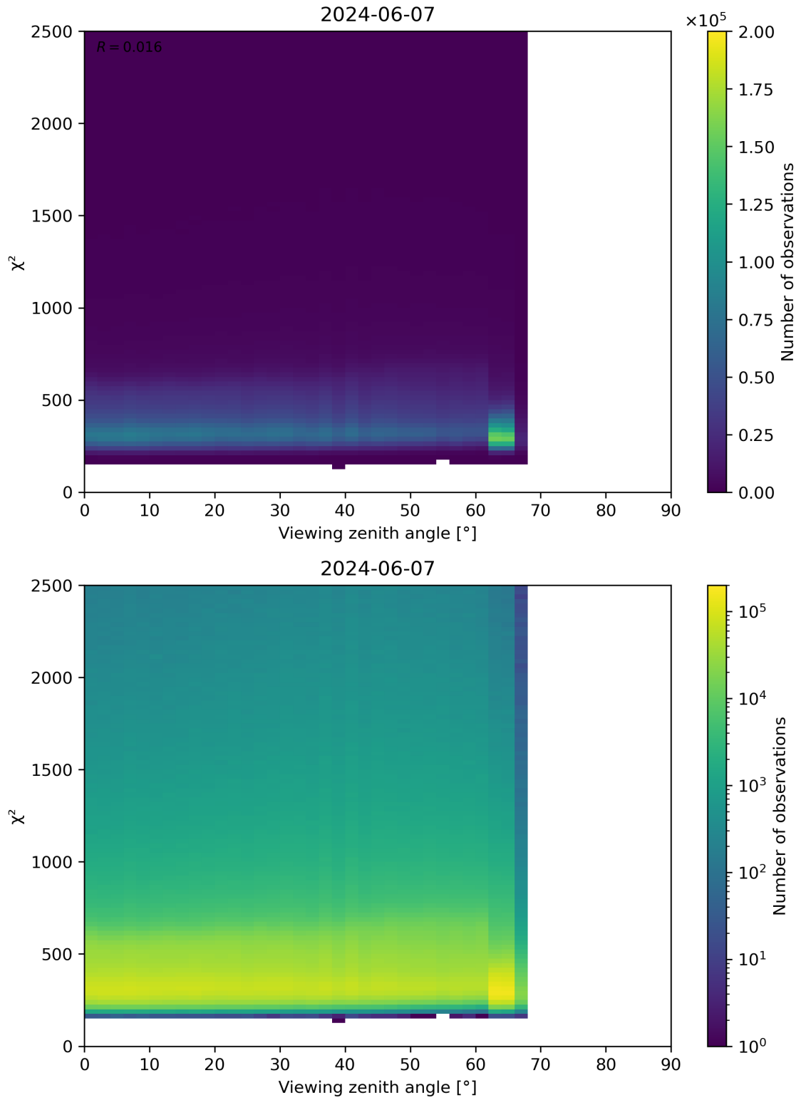
Figure 162: Scatter density plot of “Viewing zenith angle” against “ \chi^2 ” for 2024-06-06 to 2024-06-08.
