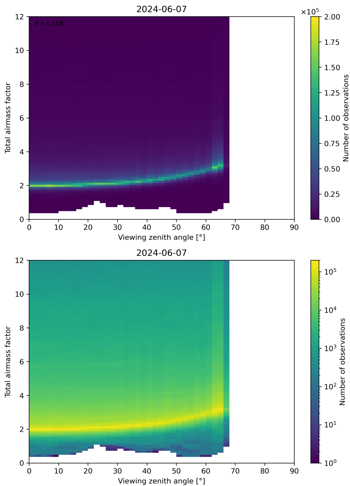
Figure 160: Scatter density plot of “Viewing zenith angle” against “Total airmass factor” for 2024-06-06 to 2024-06-08.
