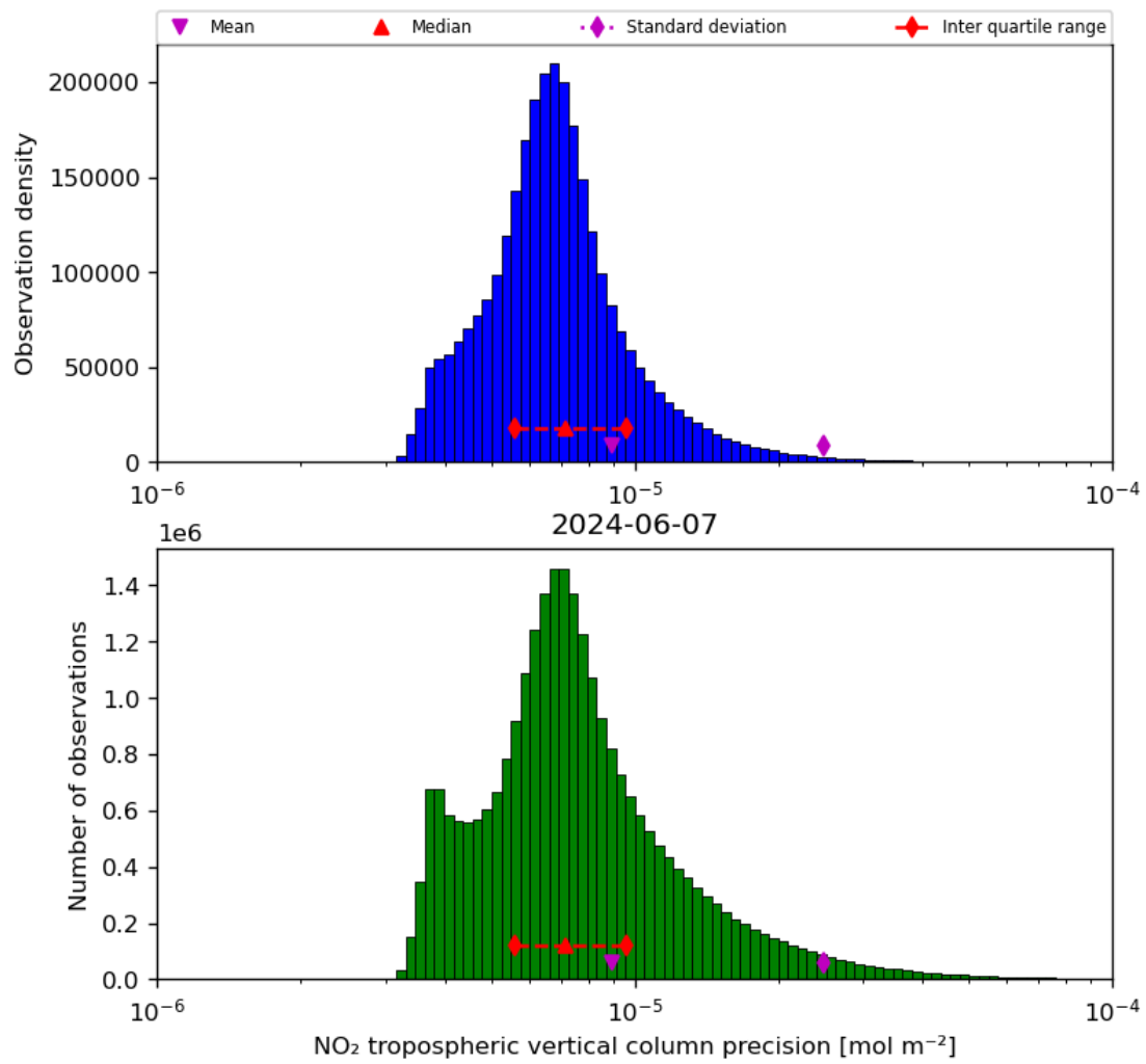
Figure 30: Histogram of “NO 2 tropospheric vertical column precision” for 2024-06-06 to 2024-06-08
