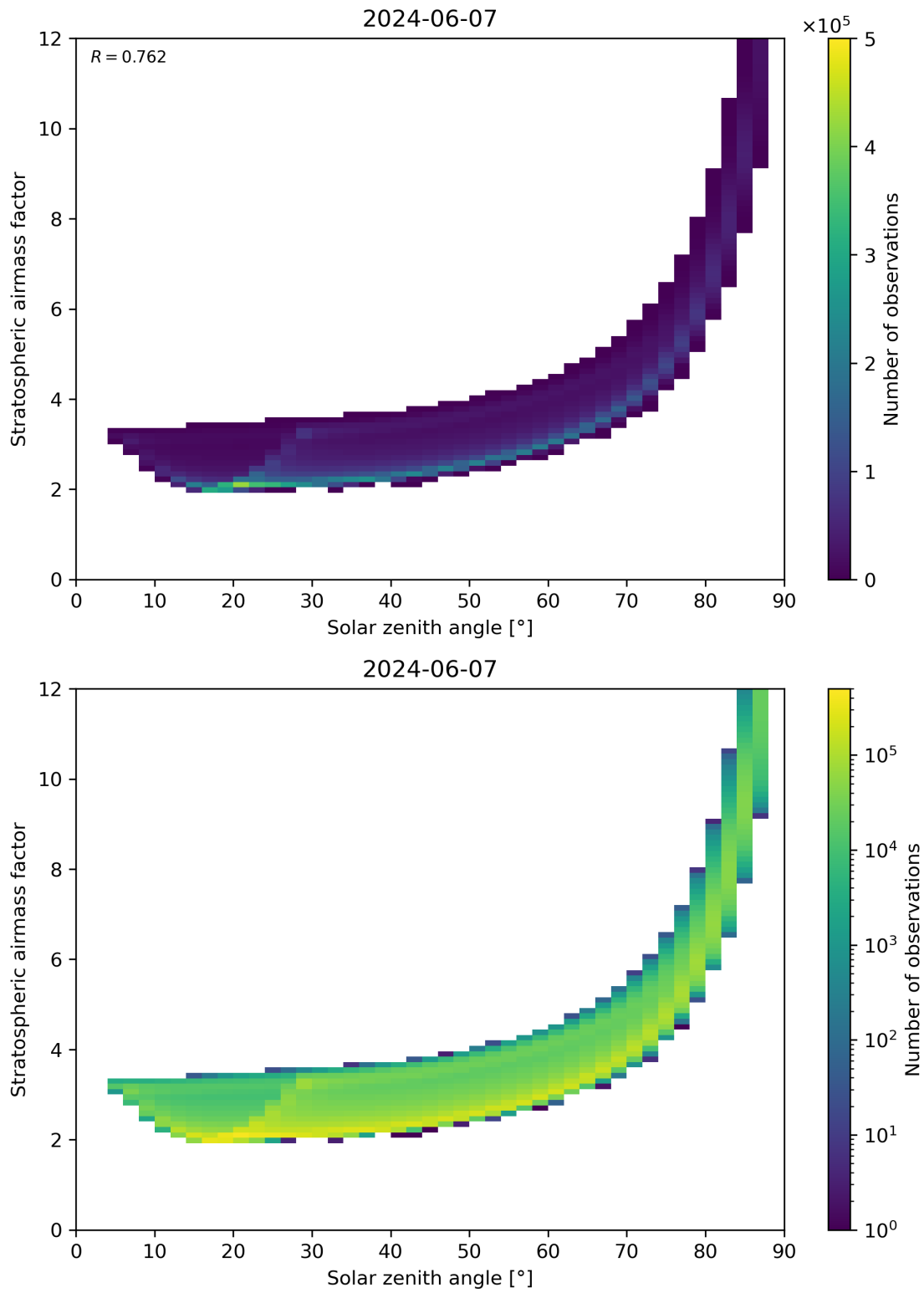
Figure 145: Scatter density plot of “Solar zenith angle” against “Stratospheric airmass factor” for 2024-06-06 to 2024-06-08.
