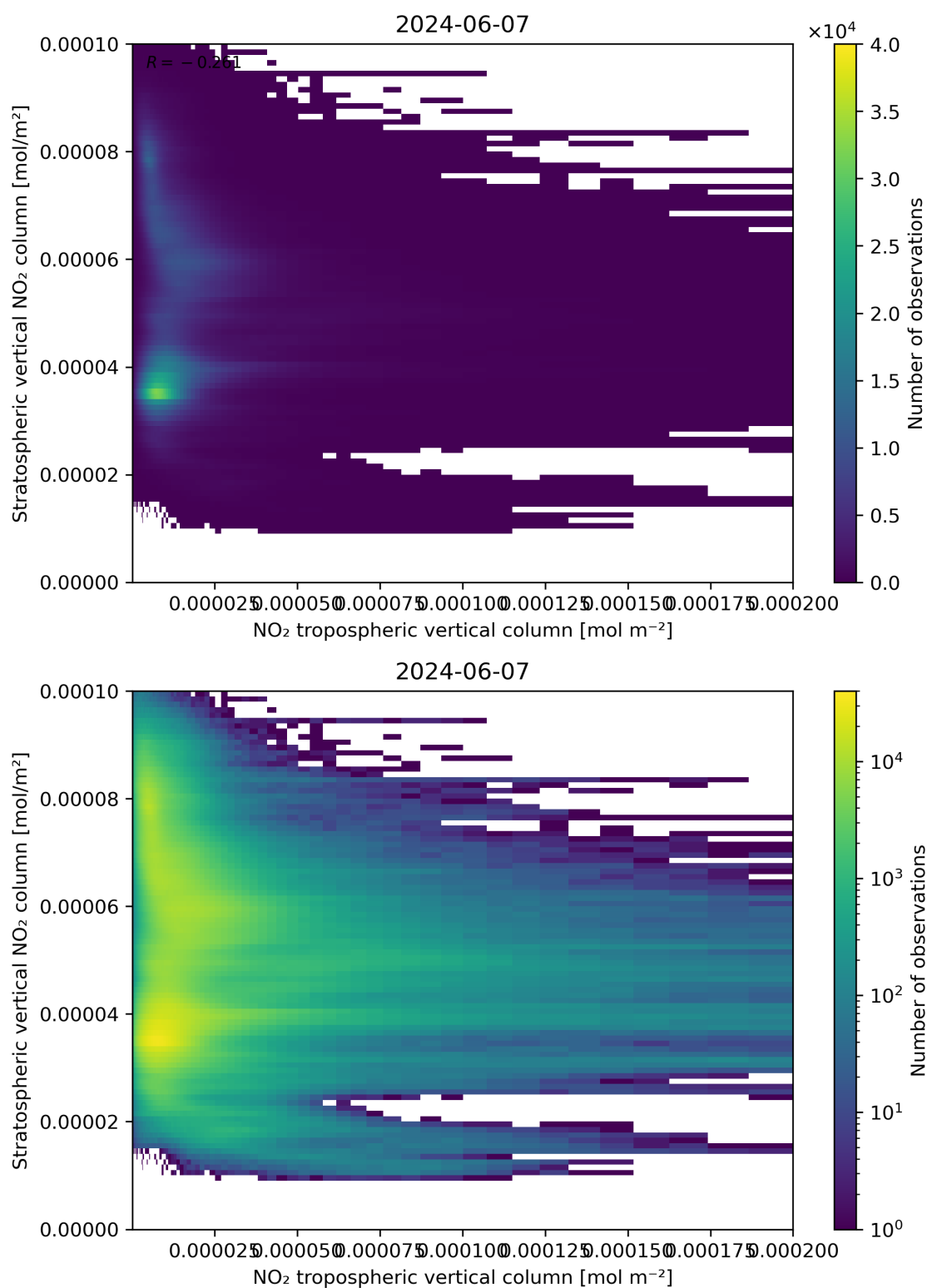
Figure 125: Scatter density plot of “NO 2 tropospheric vertical column” against “Stratospheric vertical NO 2 column” for 2024-06-06 to 2024-06-08.
