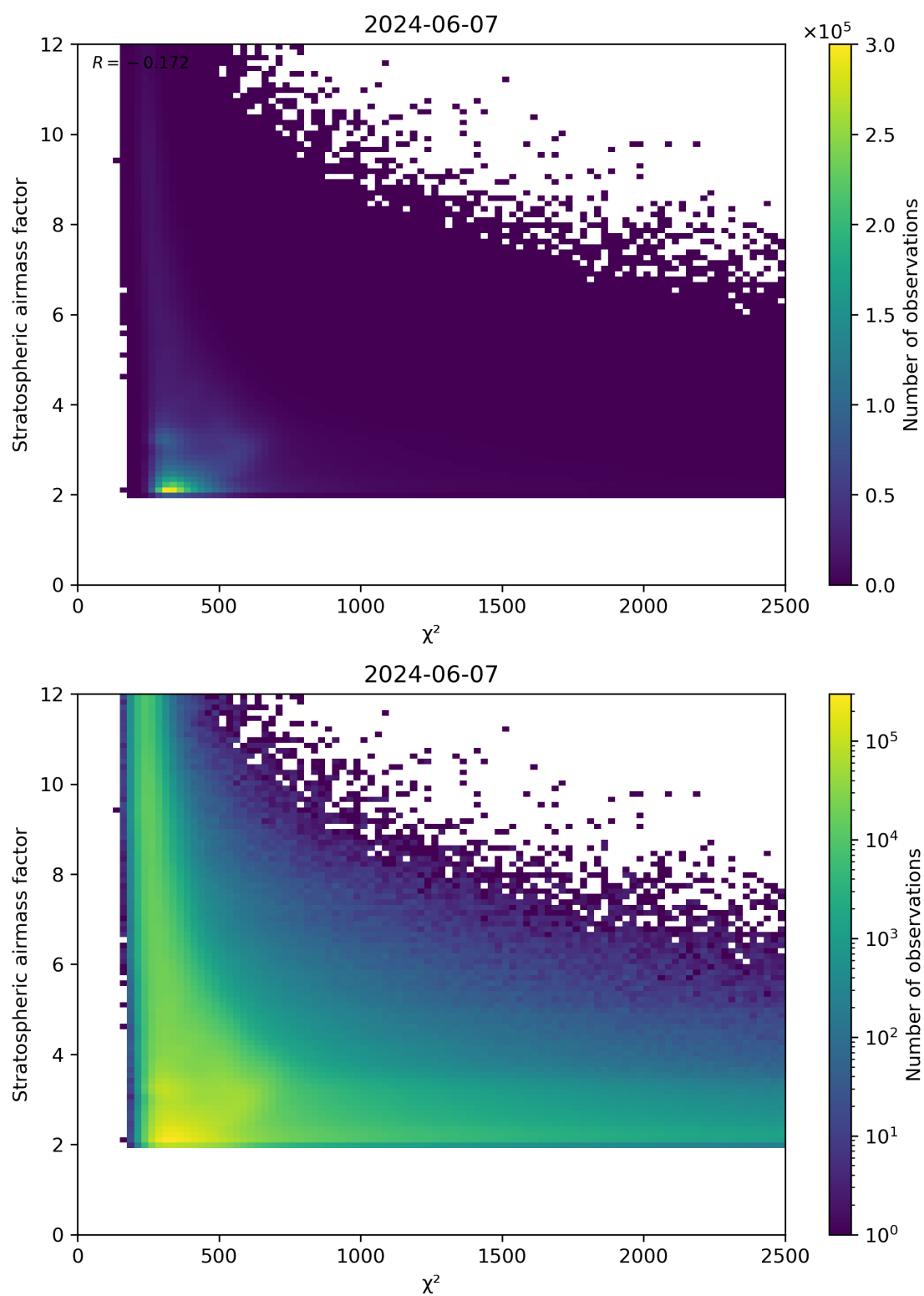
Figure 81: Scatter density plot of “ \chi^2 ” against “Stratospheric airmass factor” for 2024-06-06 to 2024-06-08.
