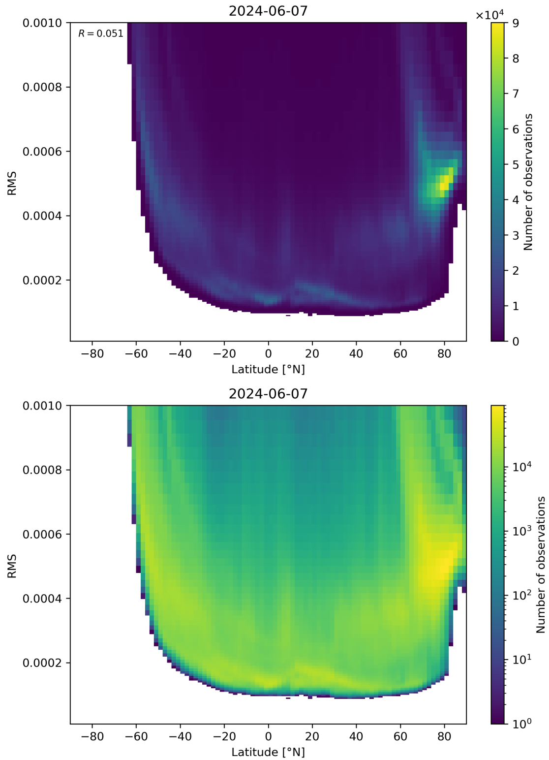
Figure 94: Scatter density plot of “Latitude” against “RMS” for 2024-06-06 to 2024-06-08.
