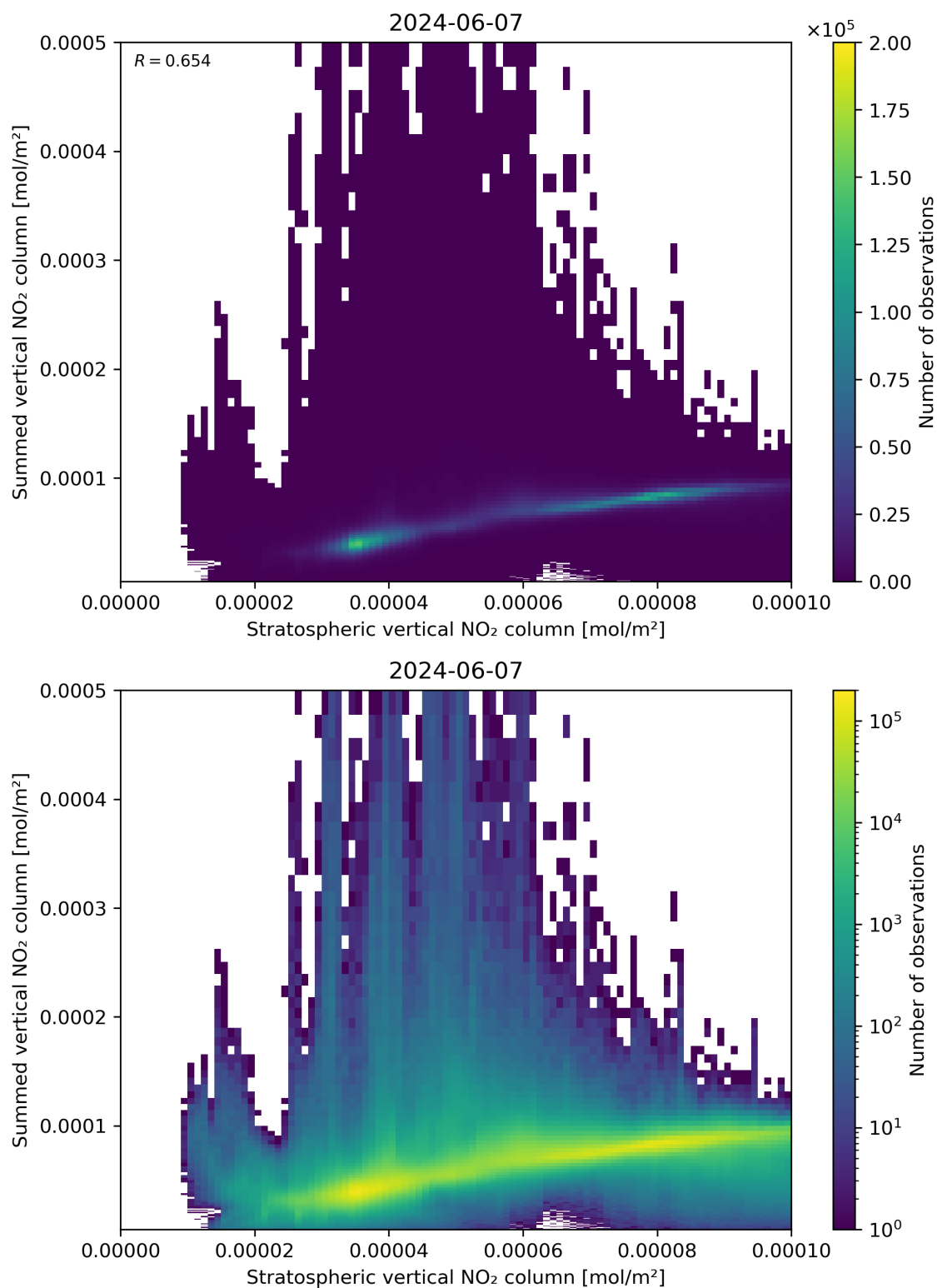
Figure 98: Scatter density plot of “Stratospheric vertical NO 2 column” against “Summed vertical NO 2 column” for 2024-06-06 to 2024-06-08.
