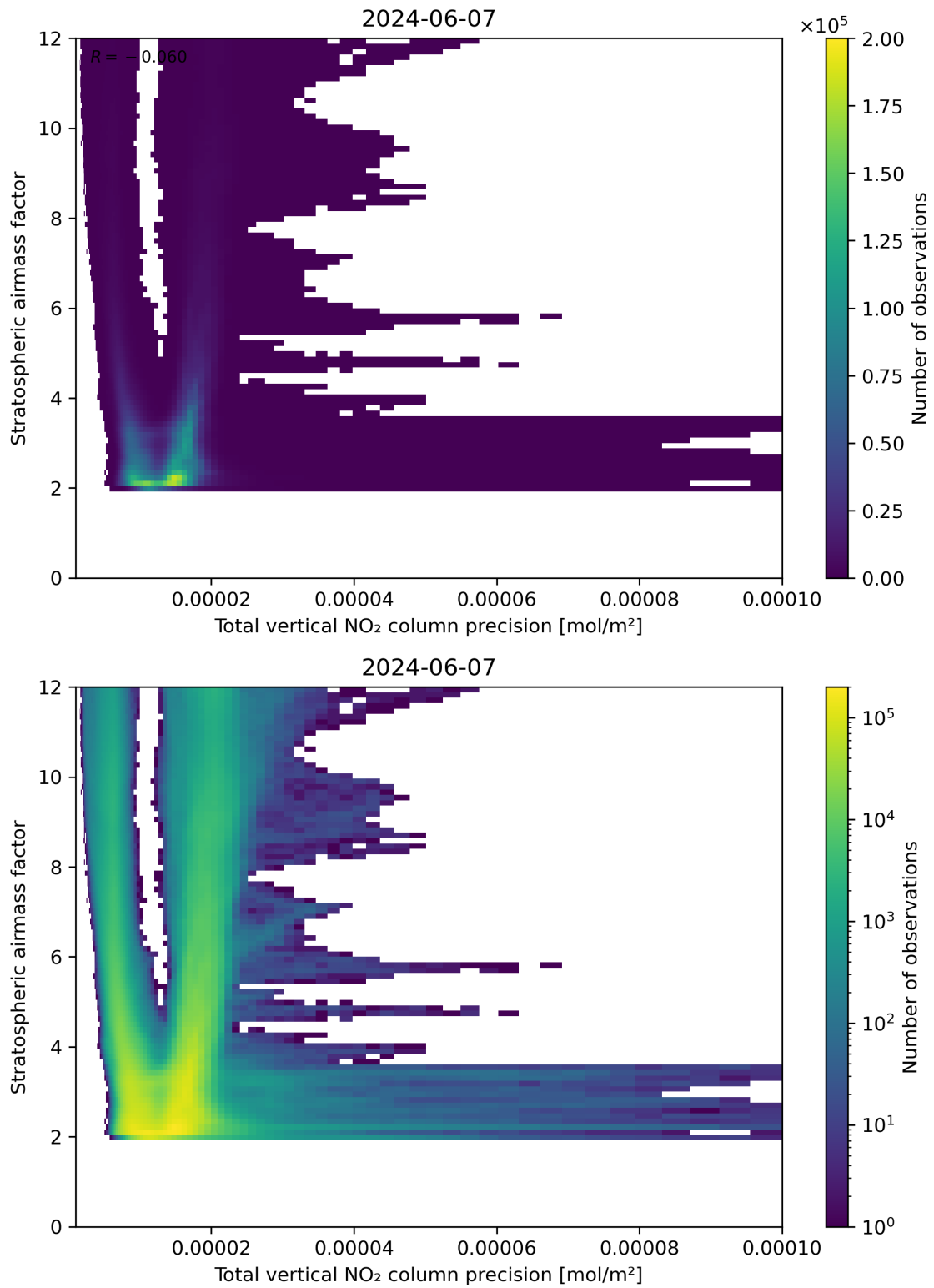
Figure 115: Scatter density plot of “Total vertical NO 2 column precision” against “Stratospheric air mass factor” for 2024-06-06 to 2024-06-08.
