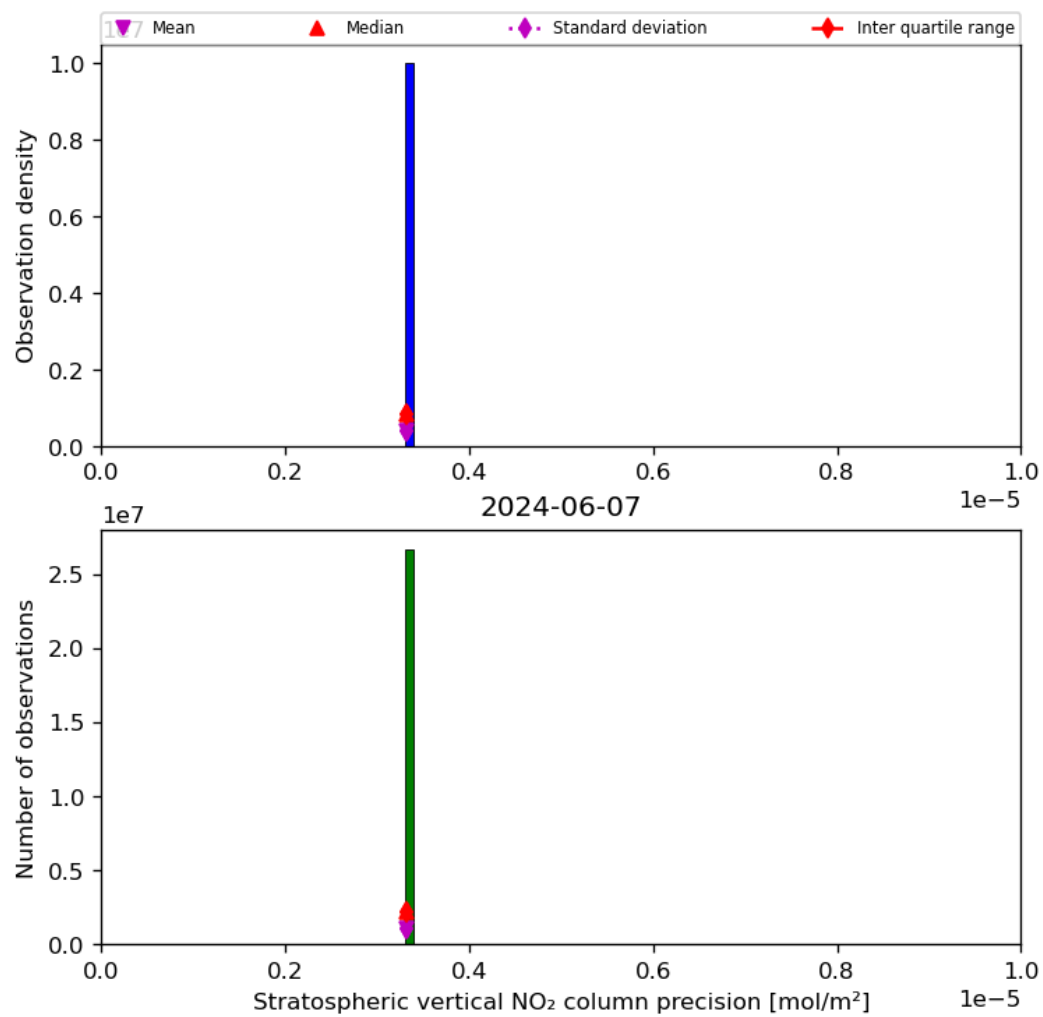
Figure 37: Histogram of “Stratospheric vertical NO 2 column precision” for 2024-06-06 to 2024-06-08
