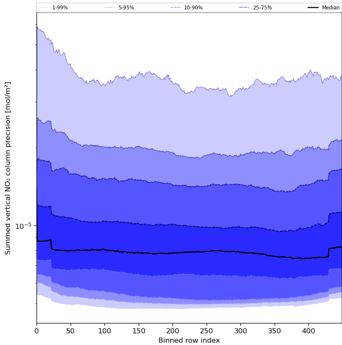
Figure 58: Along track statistics of “Summed vertical NO 2 column precision” for 2024-06-06 to 2024-06-08
