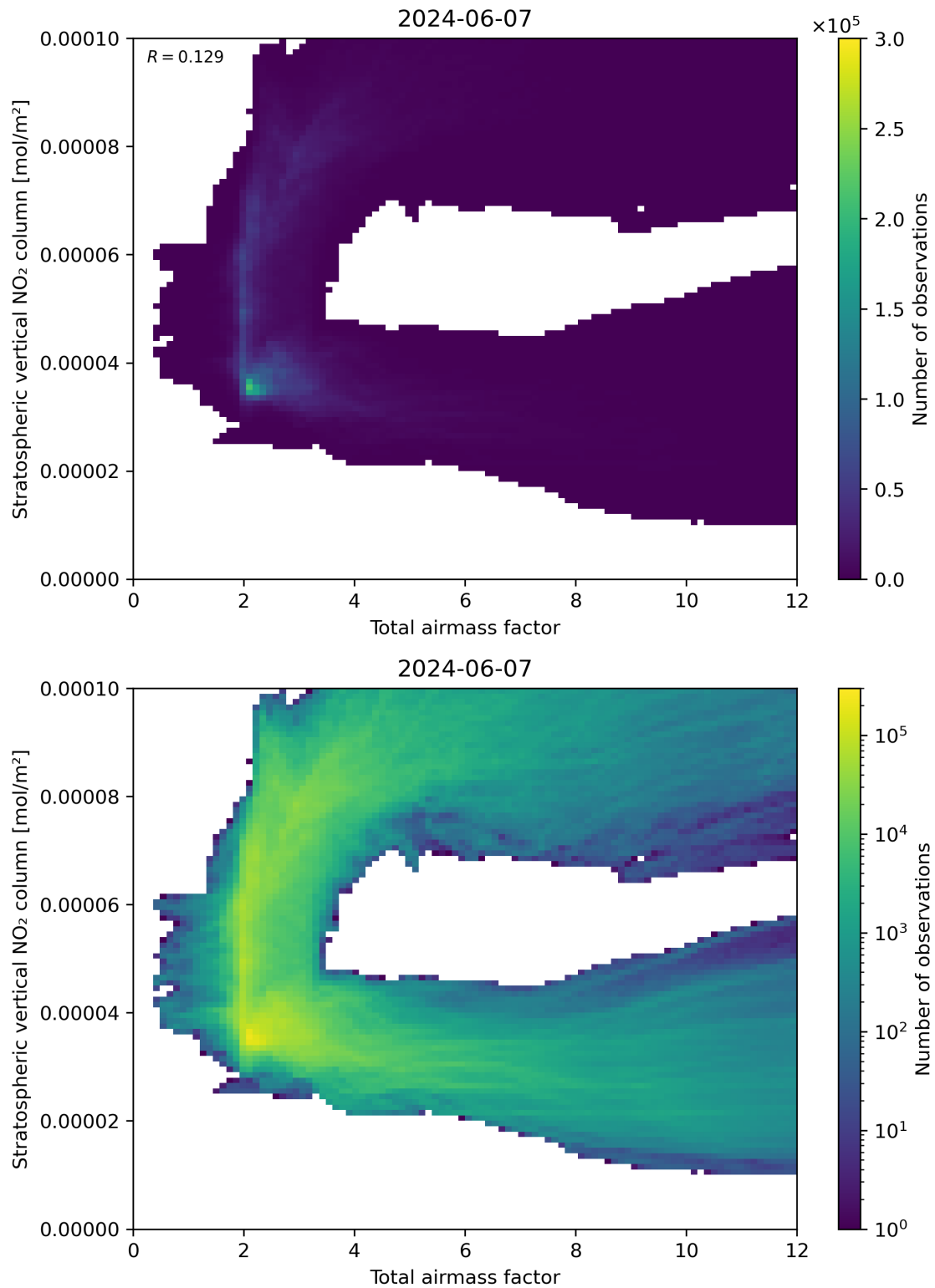
Figure 64: Scatter density plot of “Total airmass factor” against “Stratospheric vertical NO 2 column” for 2024-06-06 to 2024-06-08.
