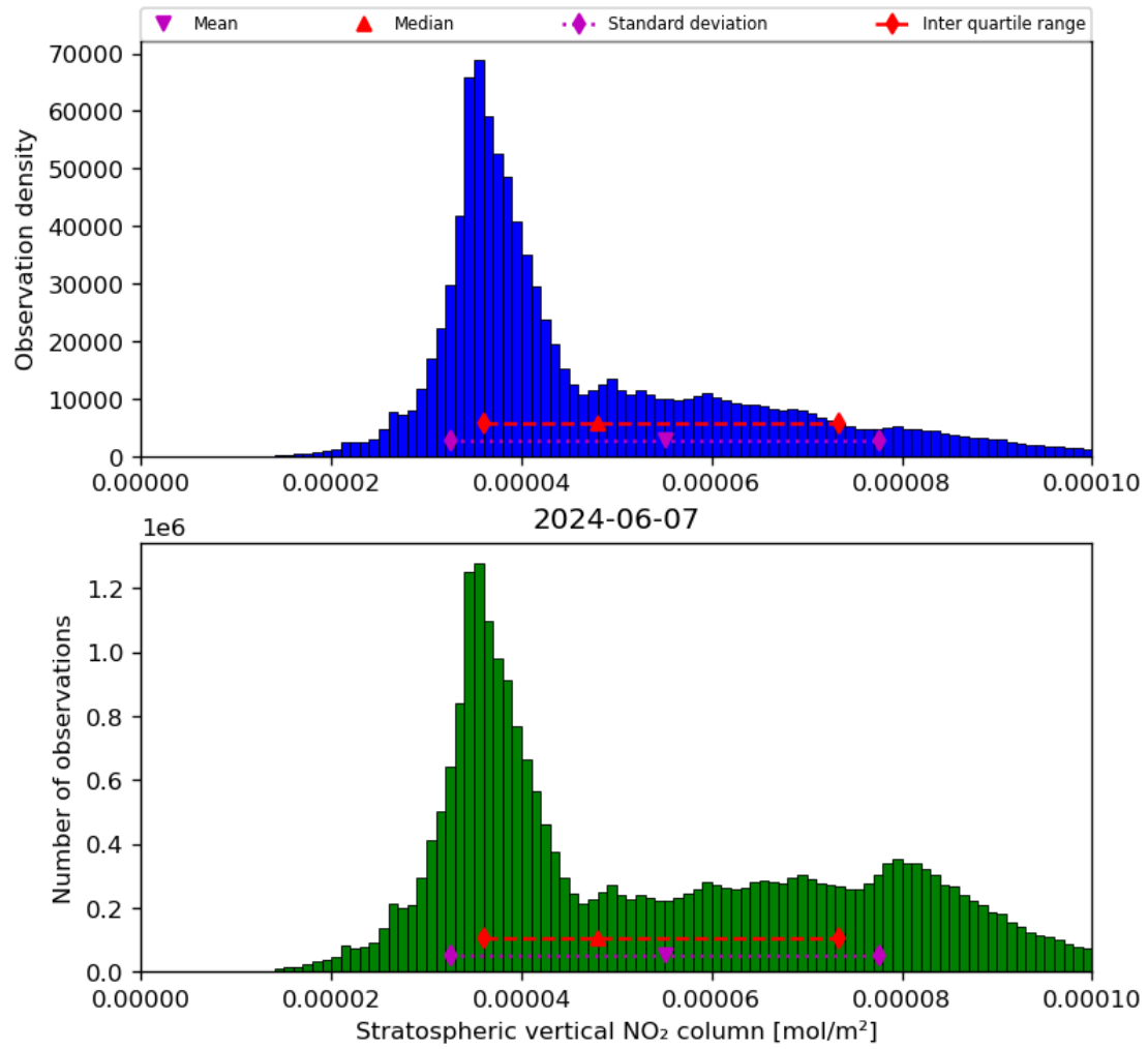
Figure 36: Histogram of “Stratospheric vertical NO 2 column” for 2024-06-06 to 2024-06-08
