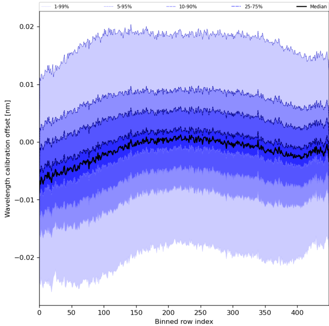
Figure 52: Along track statistics of “Wavelength calibration offset” for 2024-06-06 to 2024-06-08
