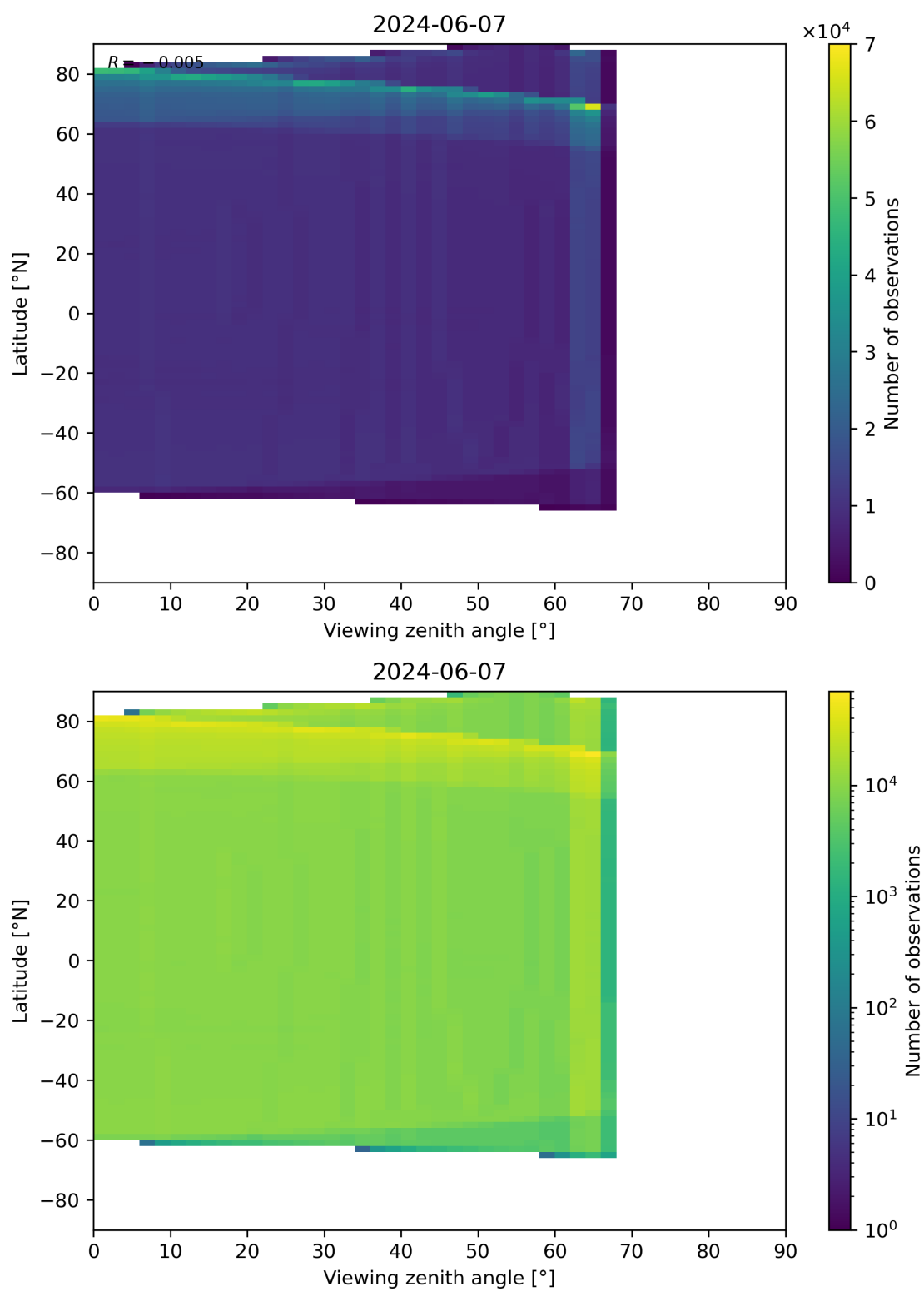
Figure 163: Scatter density plot of “Viewing zenith angle” against “Latitude” for 2024-06-06 to 2024-06-08.
