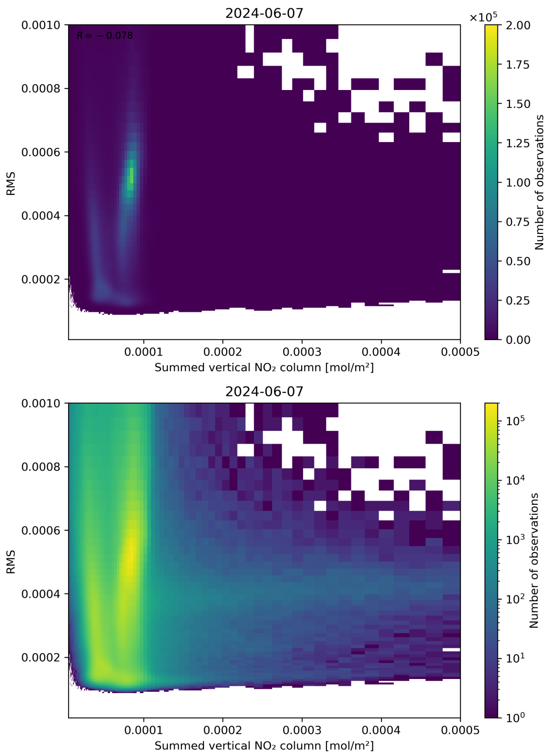
Figure 109: Scatter density plot of “Summed vertical NO 2 column” against “RMS” for 2024-06-06 to 2024-06-08.
