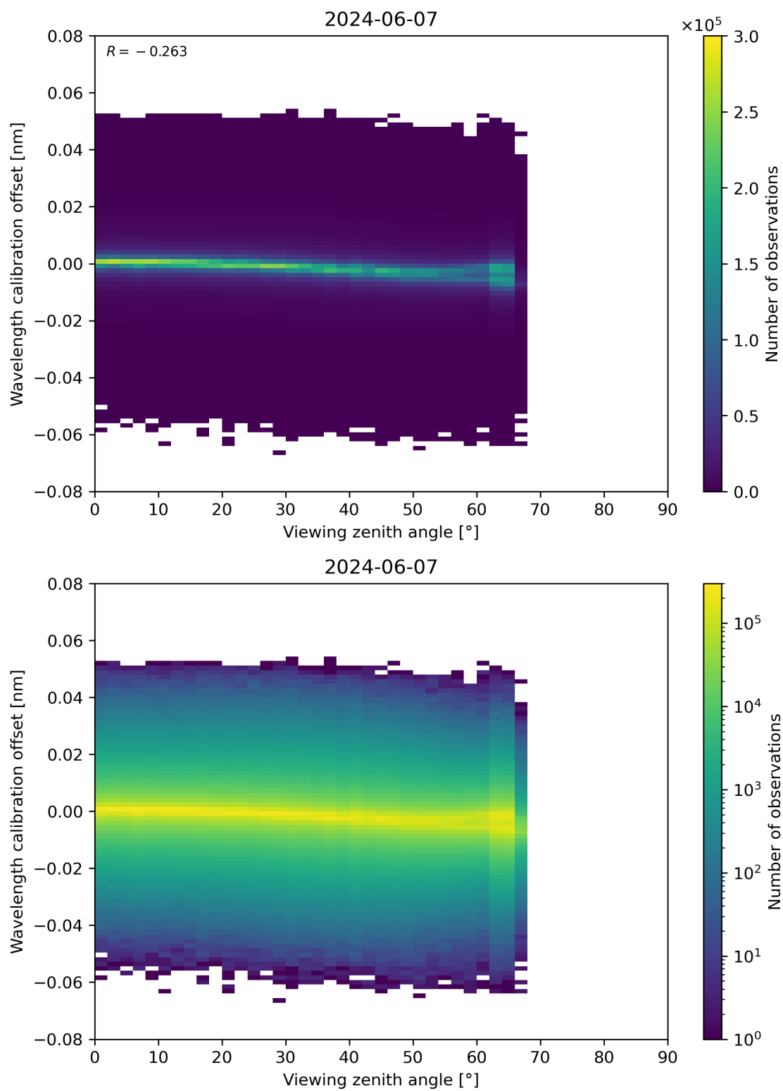
Figure 173: Scatter density plot of “Viewing zenith angle” against “Wavelength calibration offset” for 2024-06-06 to 2024-06-08.
