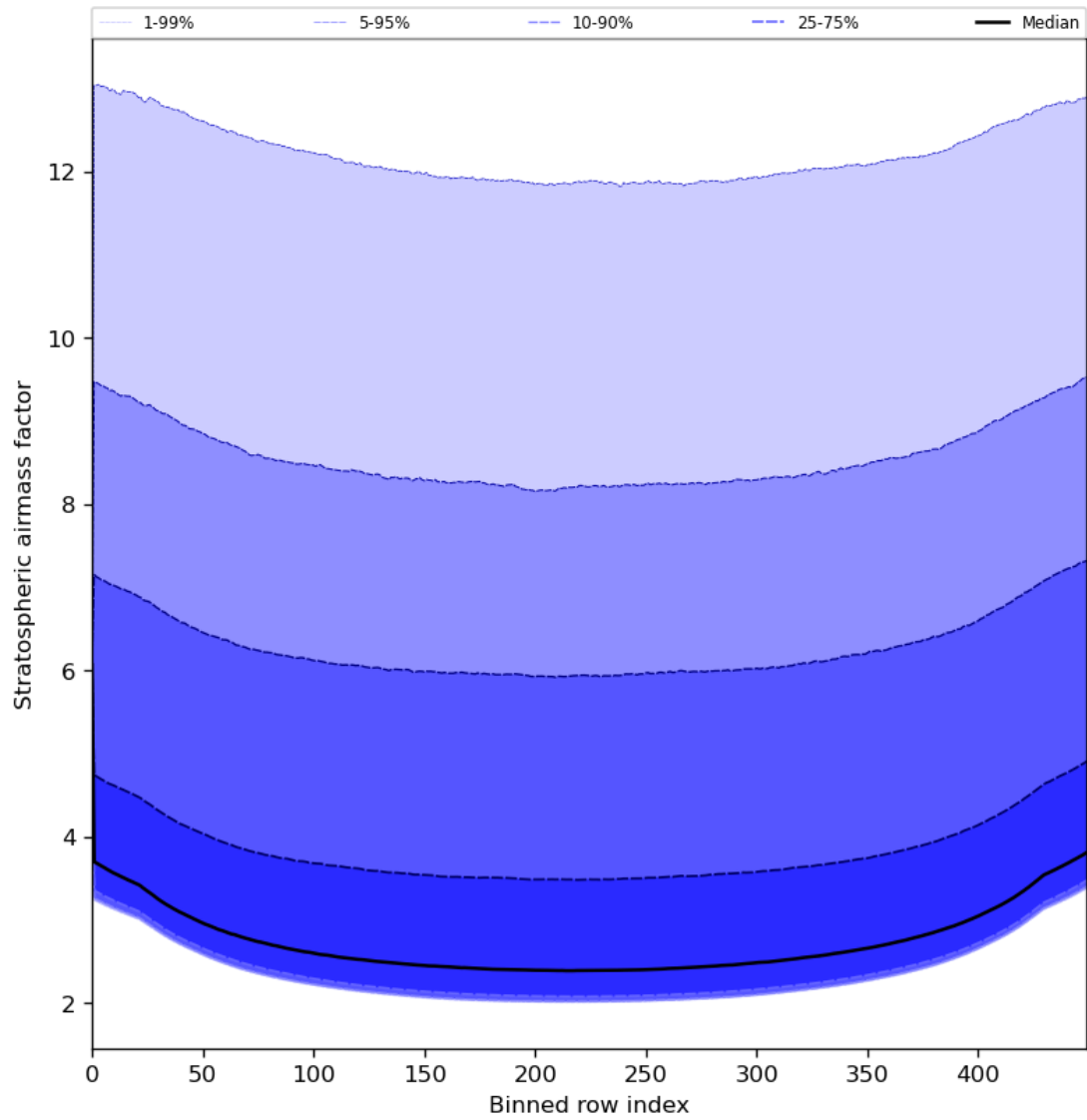
Figure 61: Along track statistics of “Stratospheric airmass factor” for 2024-06-06 to 2024-06-08
