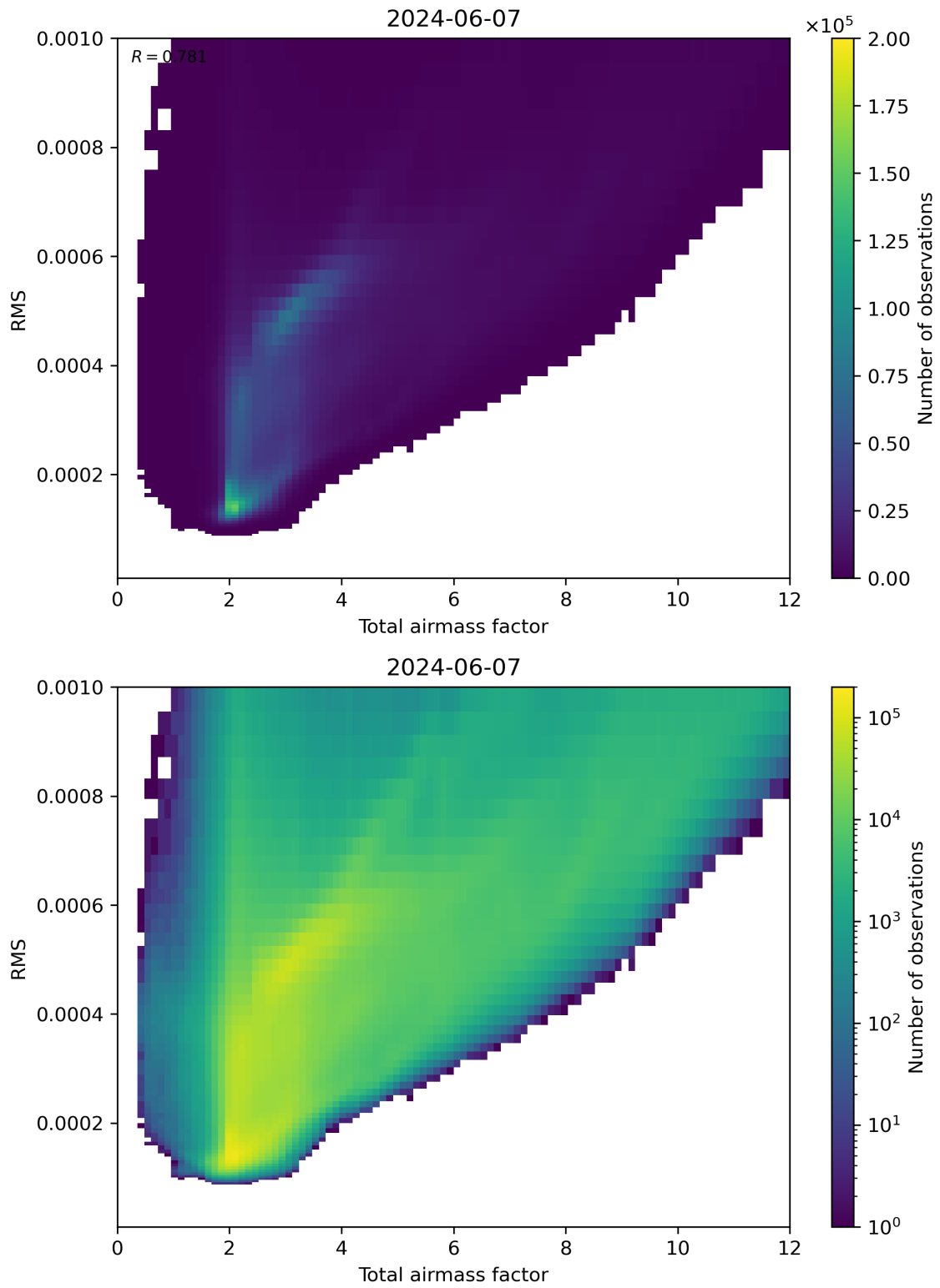
Figure 69: Scatter density plot of “Total airmass factor” against “RMS” for 2024-06-06 to 2024-06-08.
