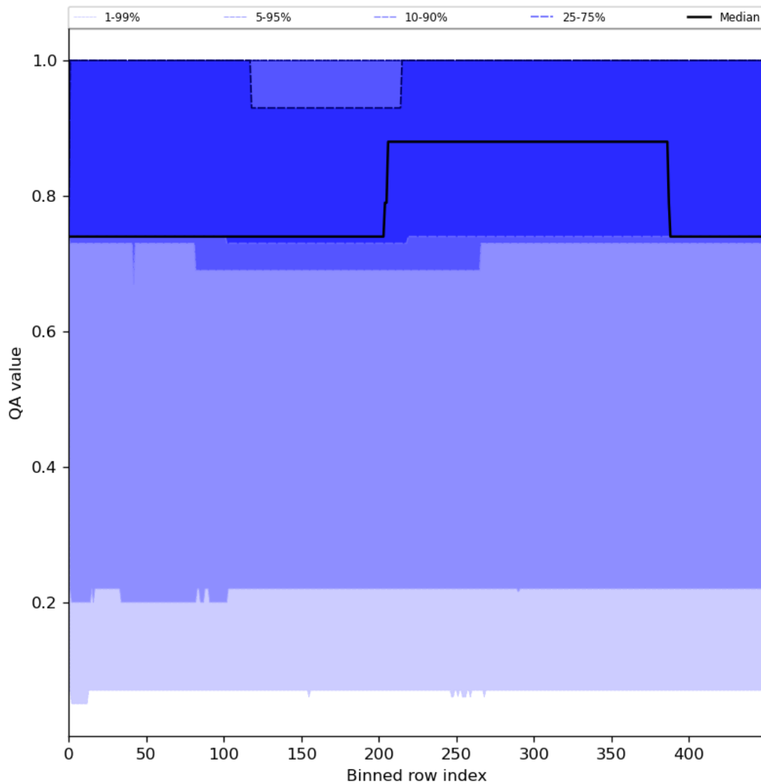
Figure 45: Along track statistics of “QA value” for 2024-06-06 to 2024-06-08
