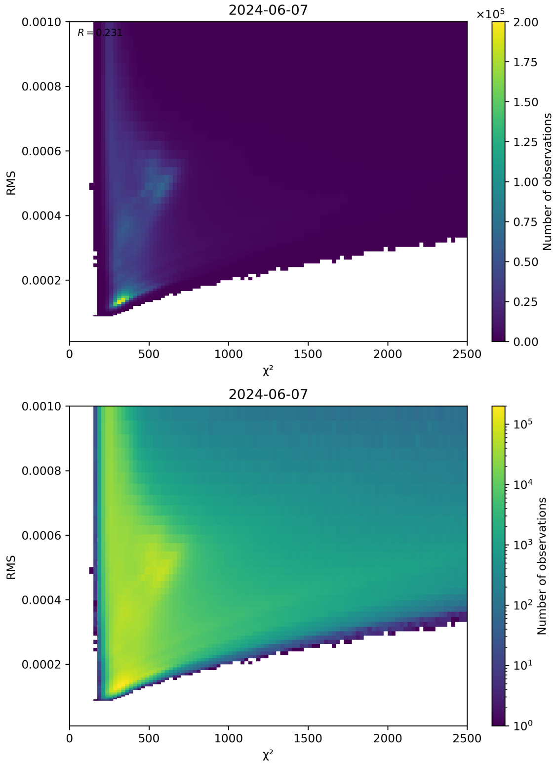
Figure 82: Scatter density plot of “ \chi^2 ” against “RMS” for 2024-06-06 to 2024-06-08.
