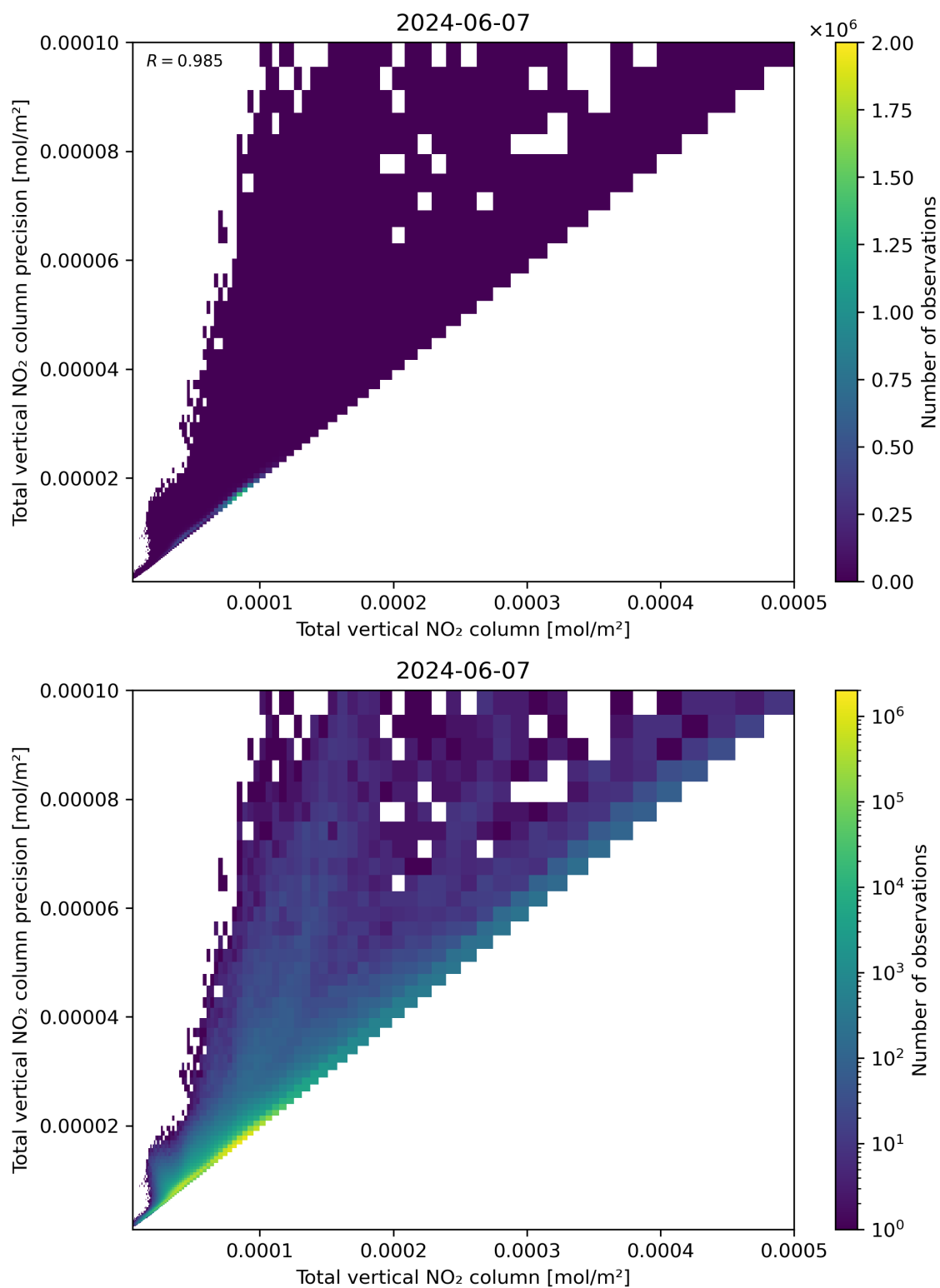
Figure 114: Scatter density plot of “Total vertical NO 2 column” against “Total vertical NO 2 column precision” for 2024-06-06 to 2024-06-08.
