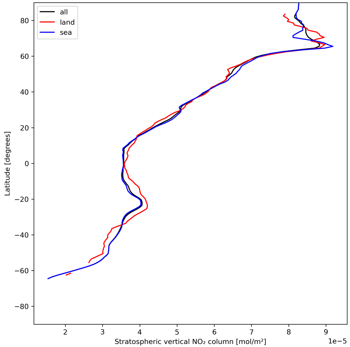
Figure 19: Zonal average of “Stratospheric vertical NO 2 column” for 2024-06-06 to 2024-06-08.
