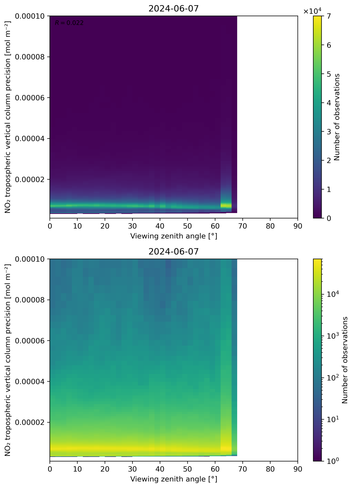
Figure 170: Scatter density plot of “Viewing zenith angle” against “NO 2 tropospheric vertical column precision” for 2024-06-06 to 2024-06-08.
