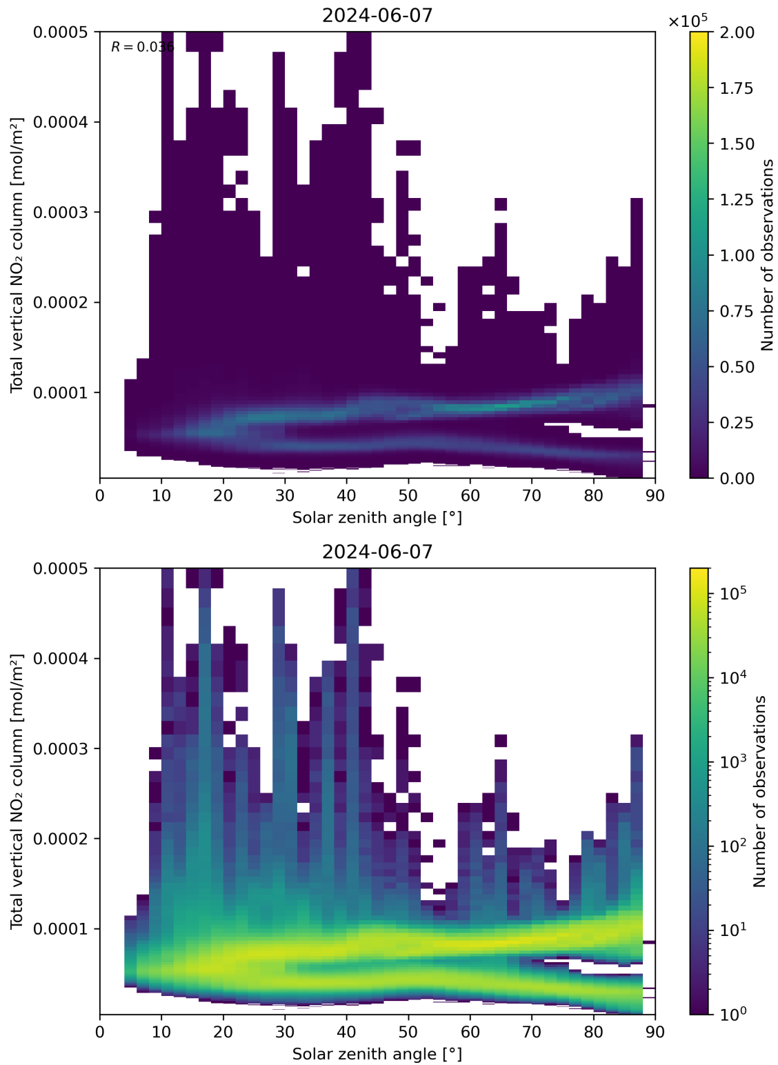
Figure 153: Scatter density plot of “Solar zenith angle” against “Total vertical NO 2 column” for 2024-06-06 to 2024-06-08.
