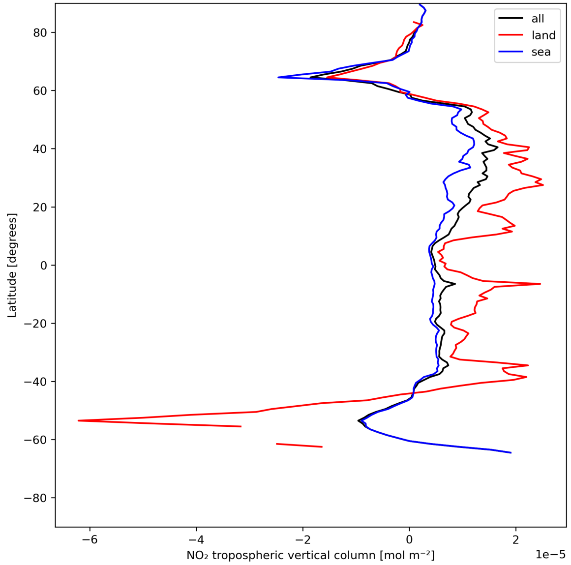
Figure 12: Zonal average of “NO 2 tropospheric vertical column” for 2024-06-06 to 2024-06-08.
