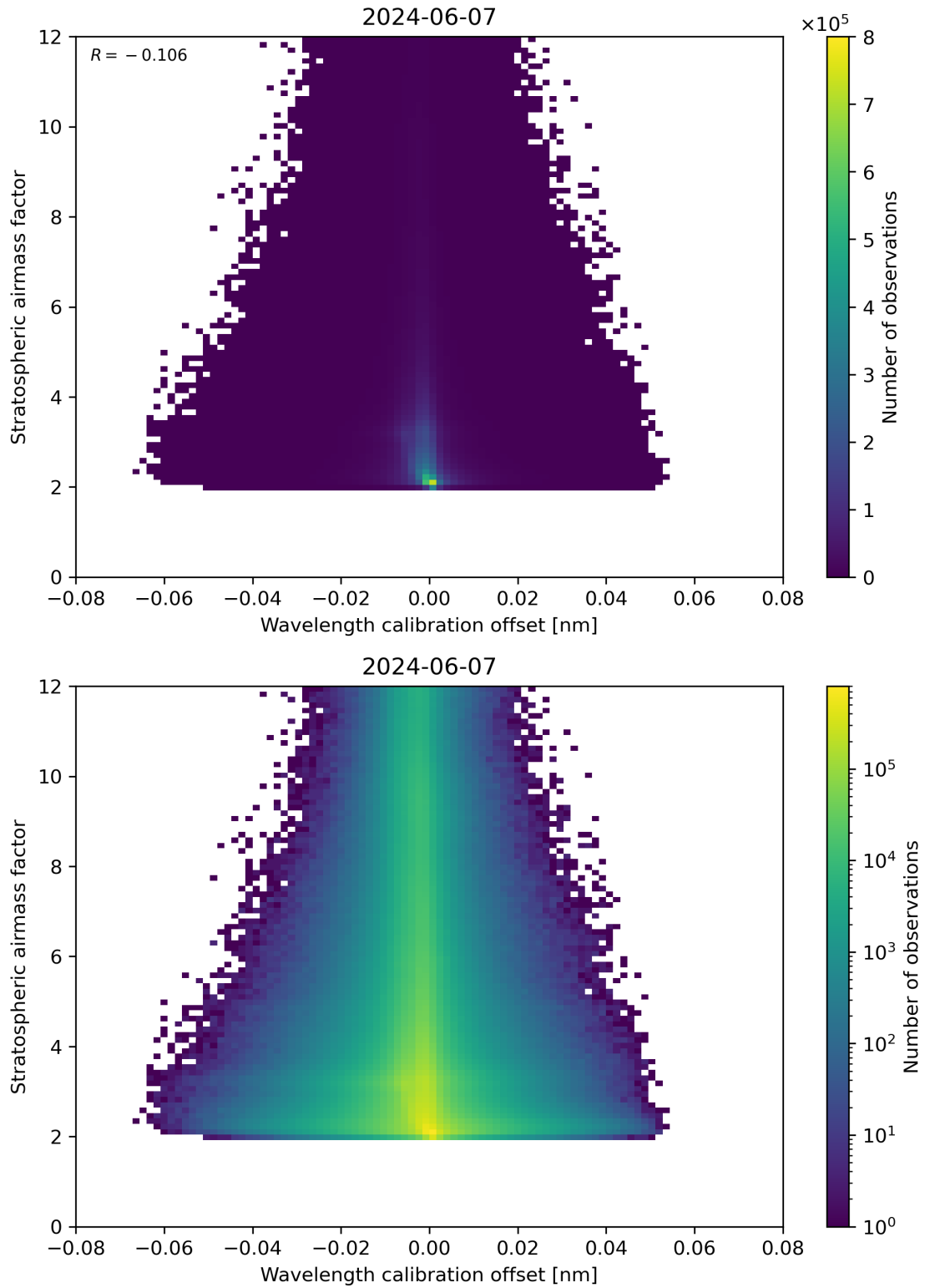
Figure 174: Scatter density plot of “Wavelength calibration offset” against “Stratospheric airmass factor” for 2024-06-06 to 2024-06-08.
