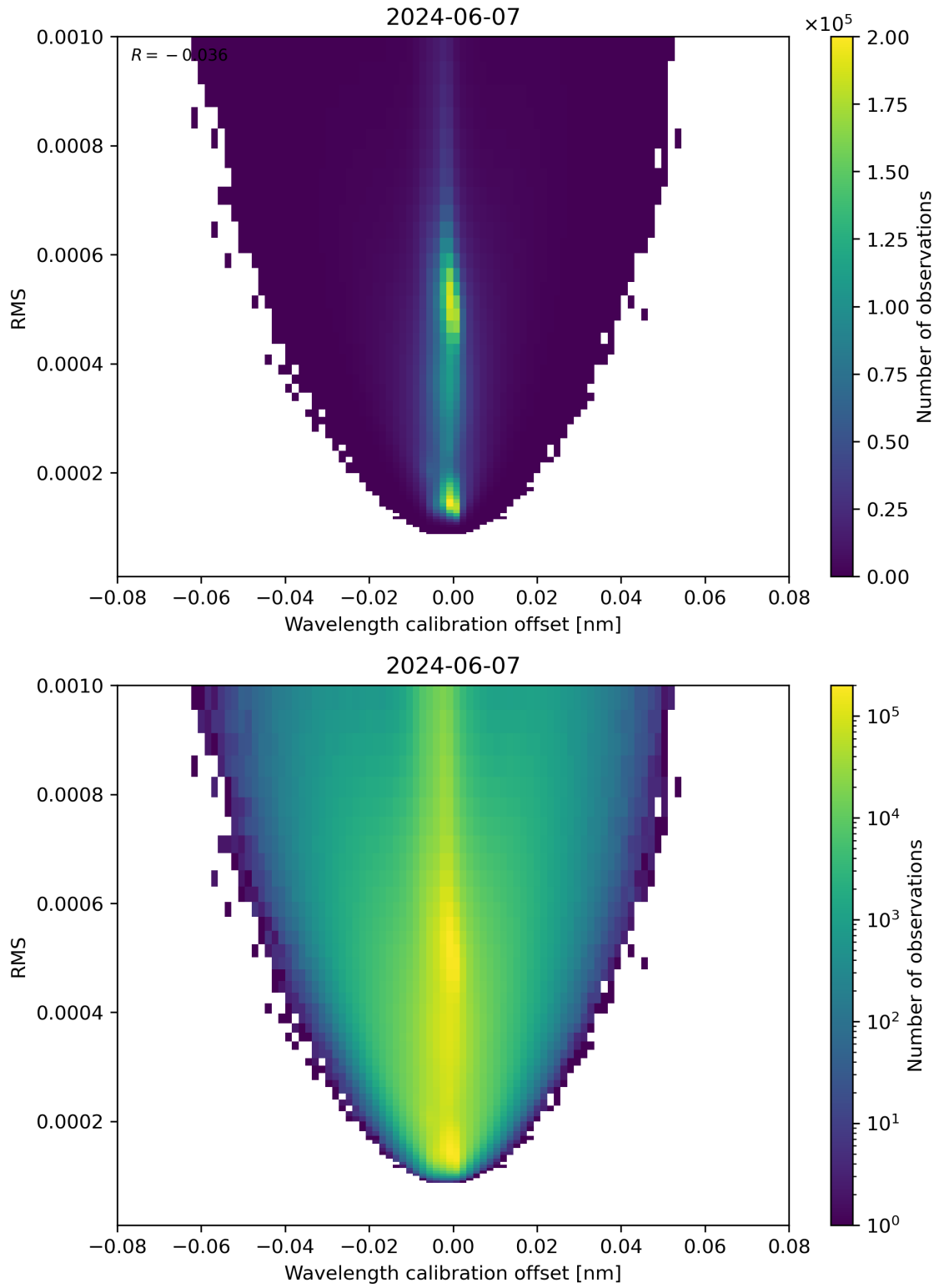
Figure 181: Scatter density plot of “Wavelength calibration offset” against “RMS” for 2024-06-06 to 2024-06-08.
