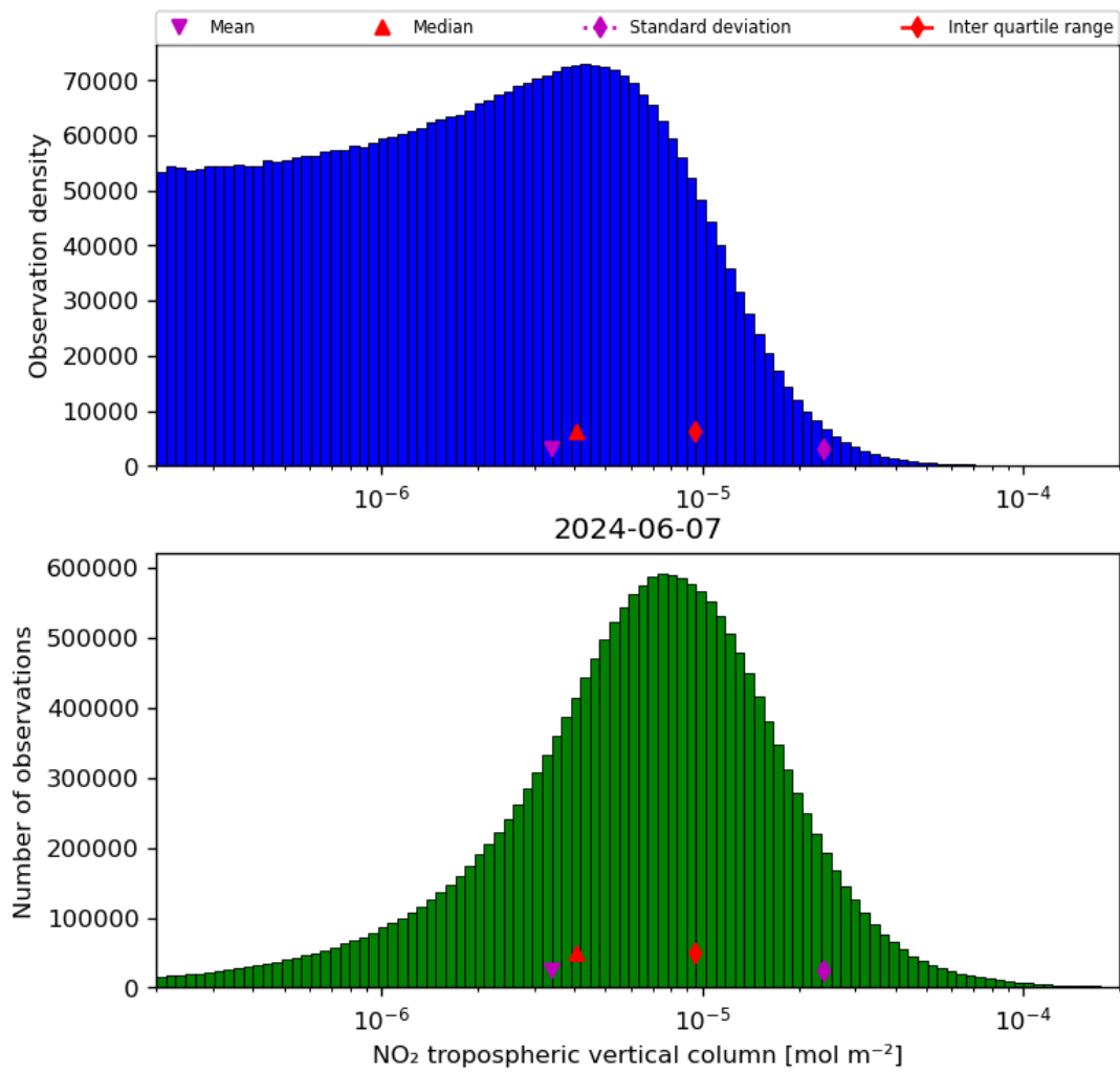
Figure 29: Histogram of “NO 2 tropospheric vertical column” for 2024-06-06 to 2024-06-08
