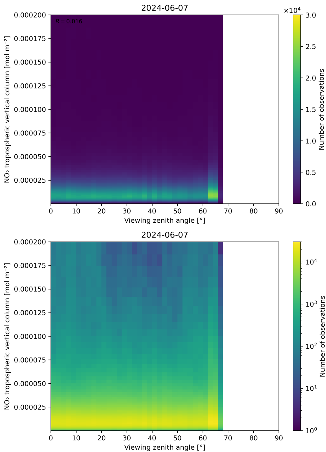
Figure 169: Scatter density plot of “Viewing zenith angle” against “NO 2 tropospheric vertical column” for 2024-06-06 to 2024-06-08.
