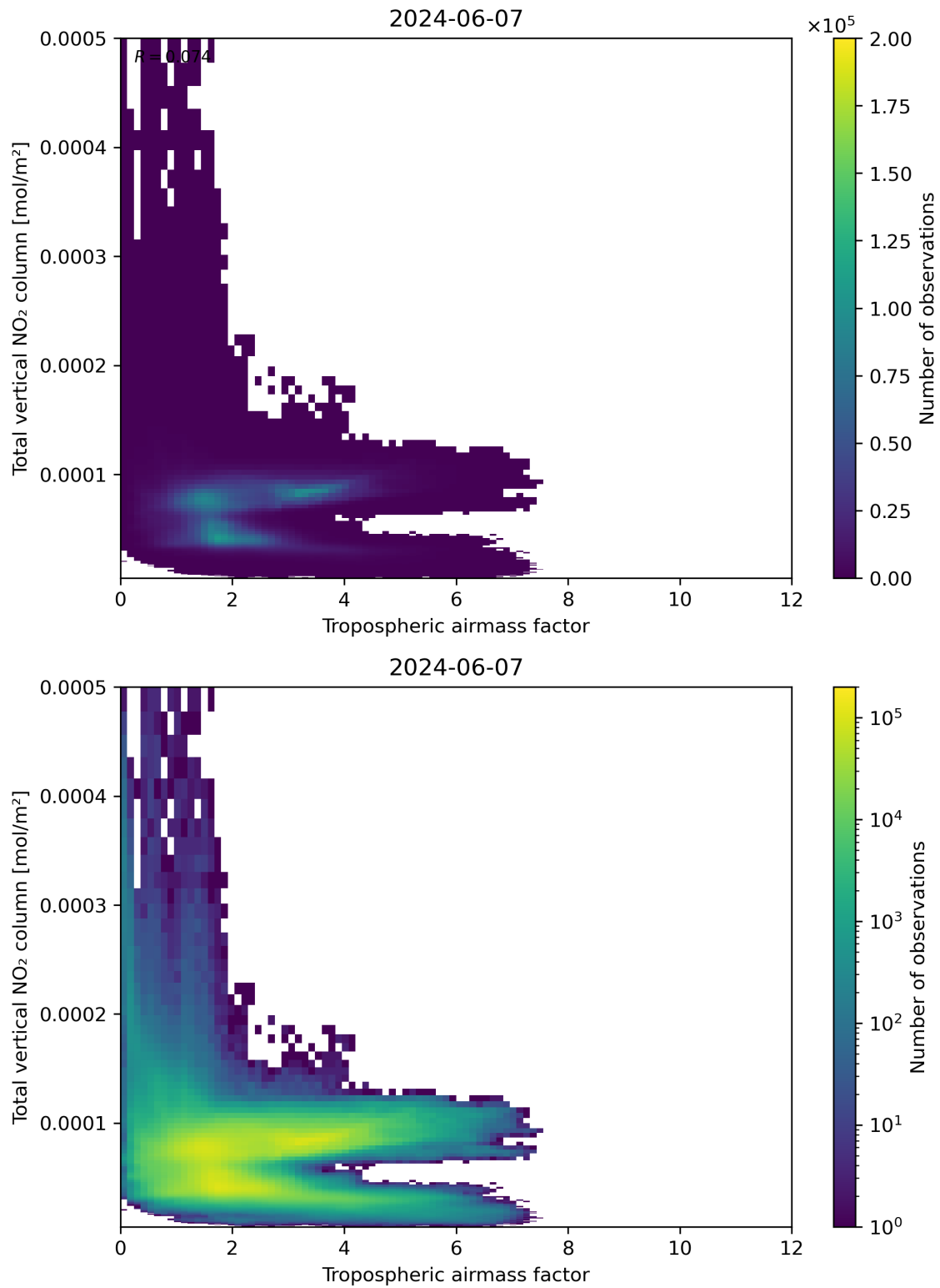
Figure 77: Scatter density plot of “Tropospheric airmass factor” against “Total vertical NO 2 column” for 2024-06-06 to 2024-06-08.
