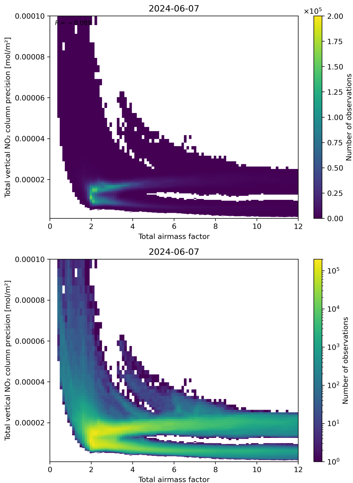
Figure 68: Scatter density plot of “Total airmass factor” against “Total vertical NO 2 column precision” for 2024-06-06 to 2024-06-08.
