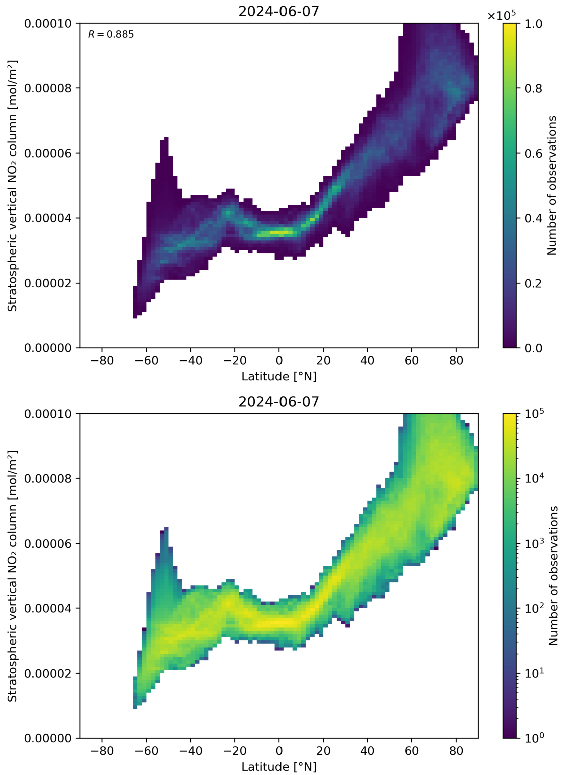
Figure 87: Scatter density plot of “Latitude” against “Stratospheric vertical NO 2 column” for 2024-06-06 to 2024-06-08.
