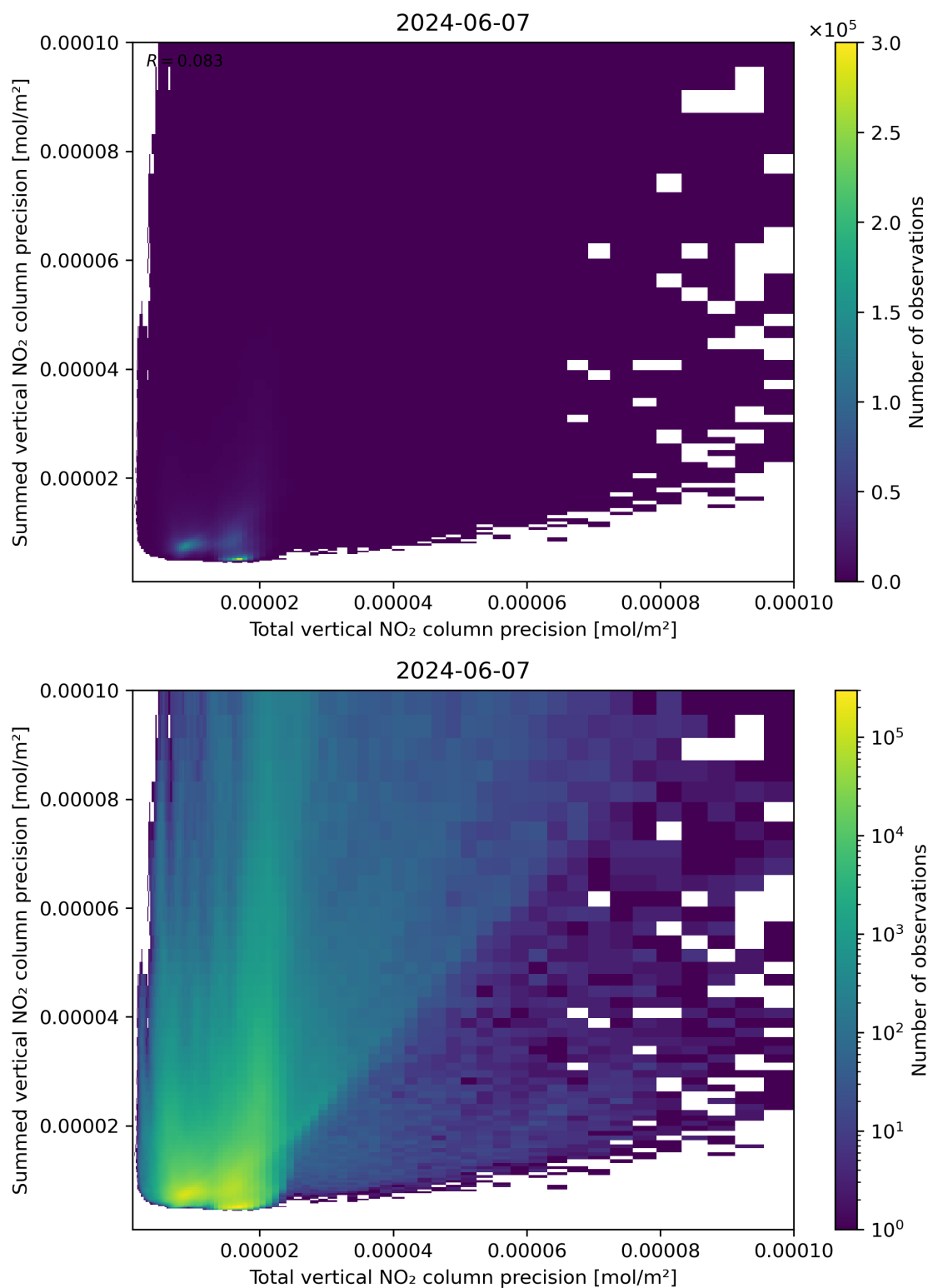
Figure 118: Scatter density plot of “Total vertical NO 2 column precision” against “Summed vertical NO 2 column precision” for 2024-06-06 to 2024-06-08.
