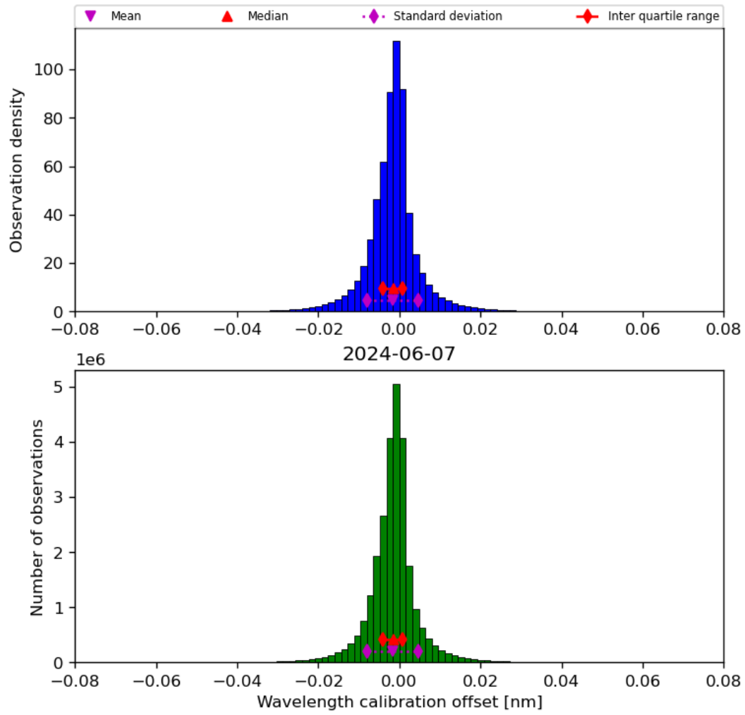
Figure 35: Histogram of “Wavelength calibration offset” for 2024-06-06 to 2024-06-08
