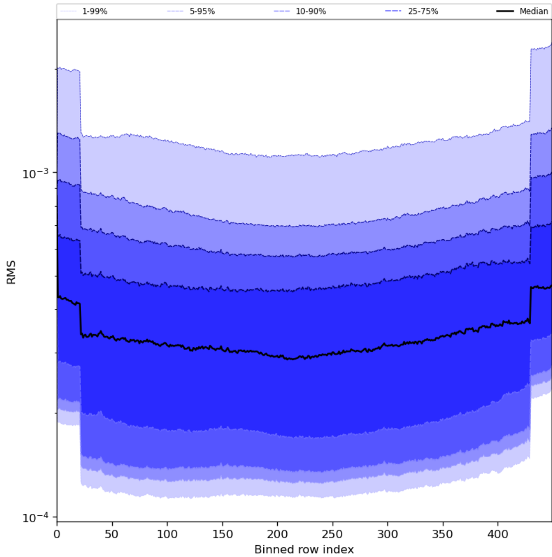
Figure 60: Along track statistics of “RMS” for 2024-06-06 to 2024-06-08
