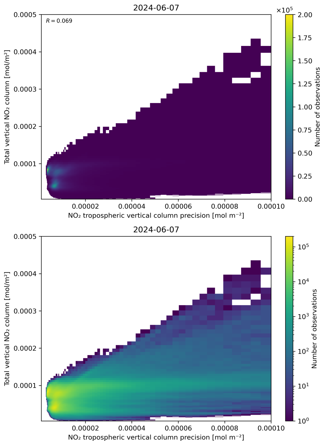
Figure 138: Scatter density plot of “NO 2 tropospheric vertical column precision” against “Total vertical NO 2 column” for 2024-06-06 to 2024-06-08.
