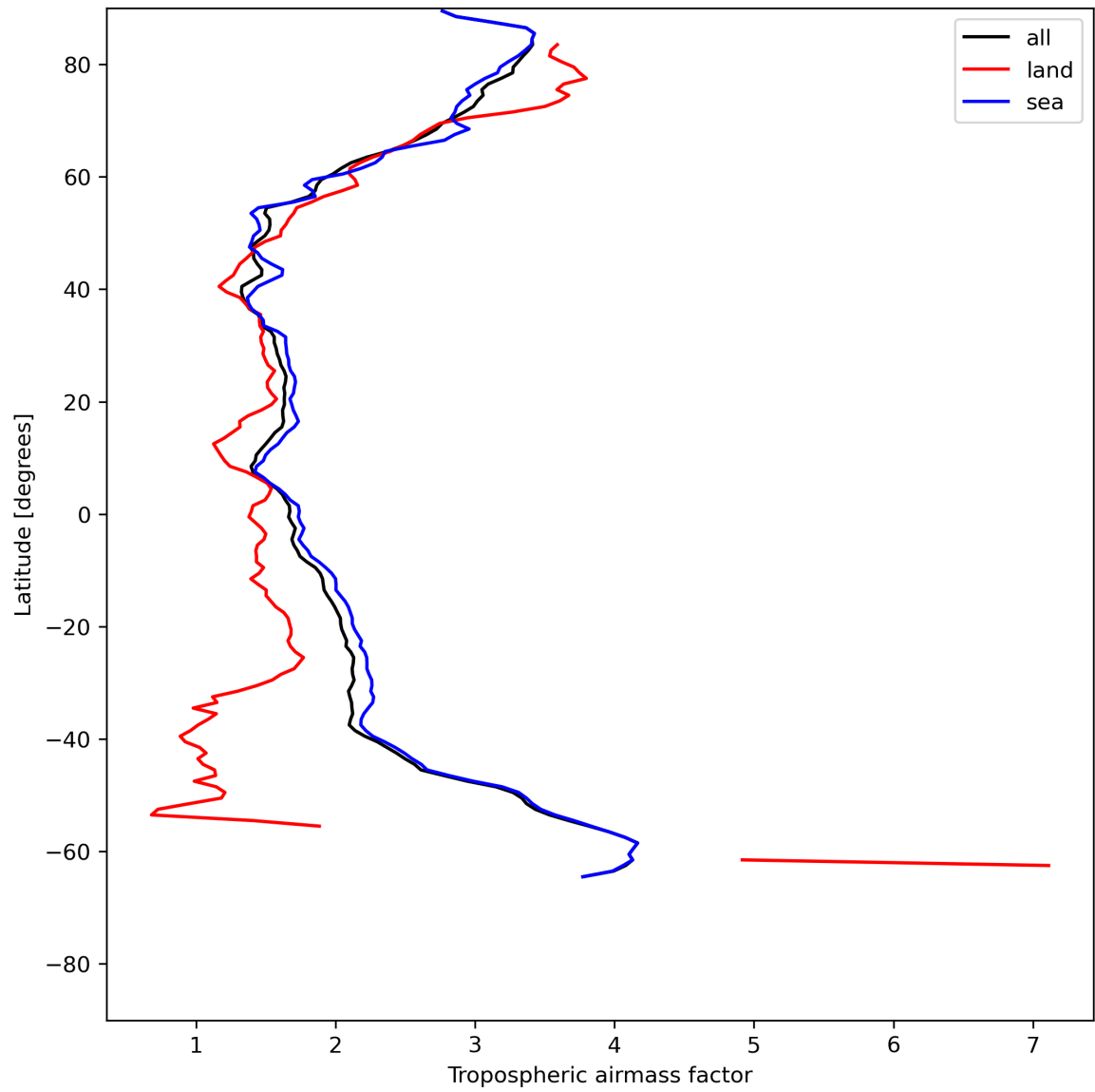
Figure 14: Zonal average of “Tropospheric airmass factor” for 2024-06-06 to 2024-06-08.
