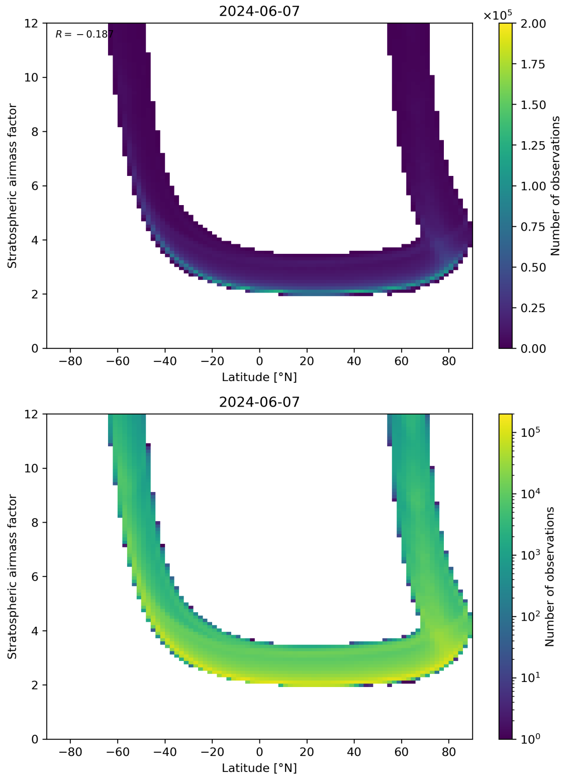
Figure 83: Scatter density plot of “Latitude” against “Stratospheric air mass factor” for 2024-06-06 to 2024-06-08.
