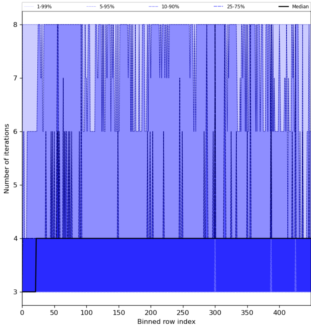
Figure 51: Along track statistics of “Number of iterations” for 2024-06-06 to 2024-06-08
