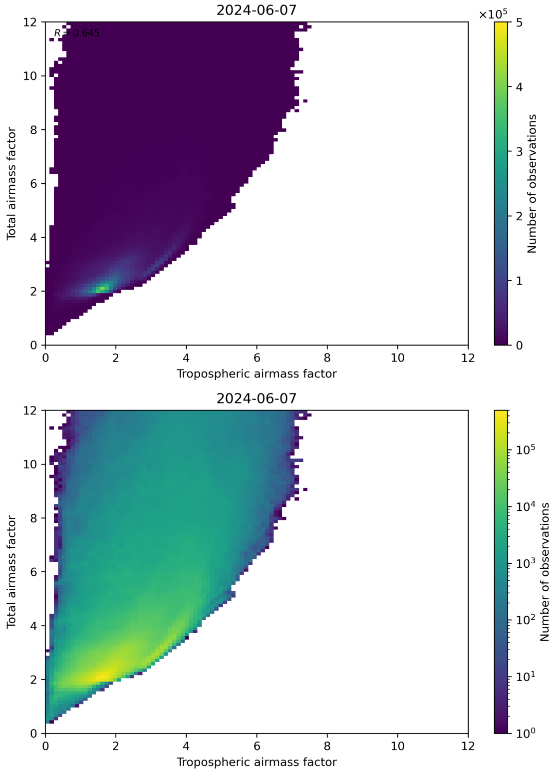
Figure 72: Scatter density plot of “Tropospheric airmass factor” against “Total airmass factor” for 2024-06-06 to 2024-06-08.
