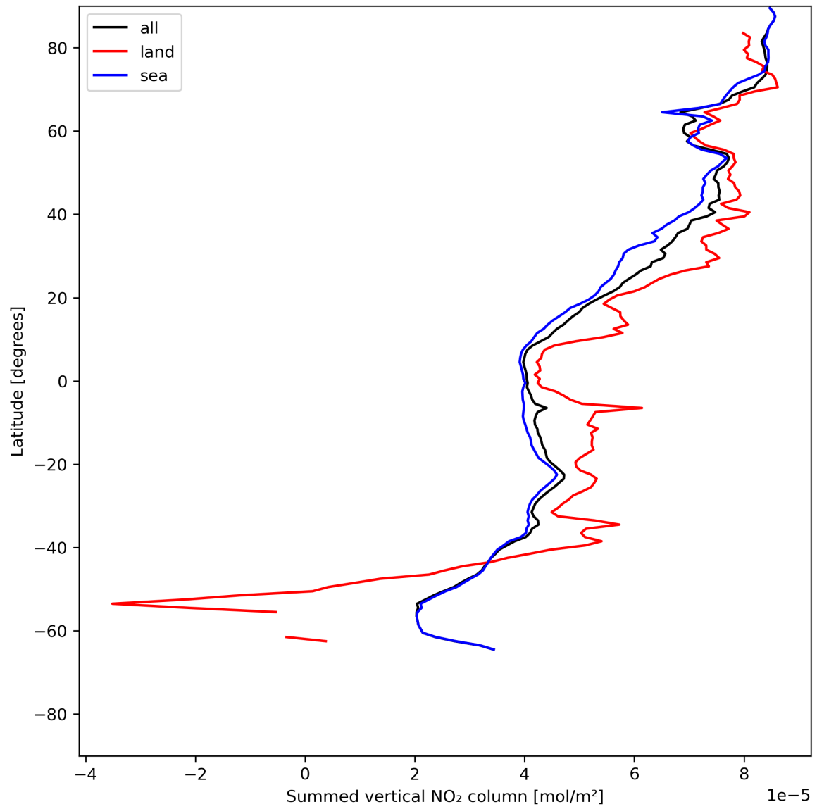
Figure 23: Zonal average of “Summed vertical NO 2 column” for 2024-06-06 to 2024-06-08.
