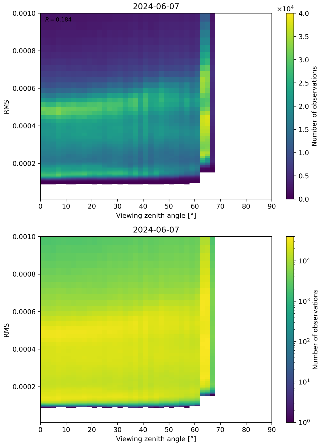
Figure 171: Scatter density plot of “Viewing zenith angle” against “RMS” for 2024-06-06 to 2024-06-08.
