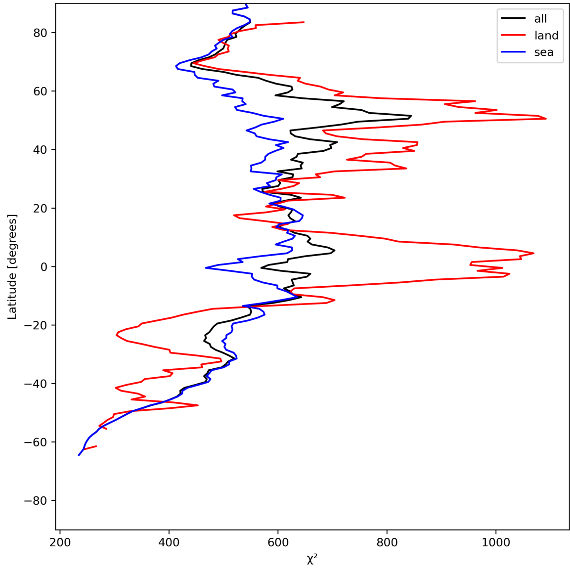
Figure 25: Zonal average of “ \chi^2 ” for 2024-06-06 to 2024-06-08.
