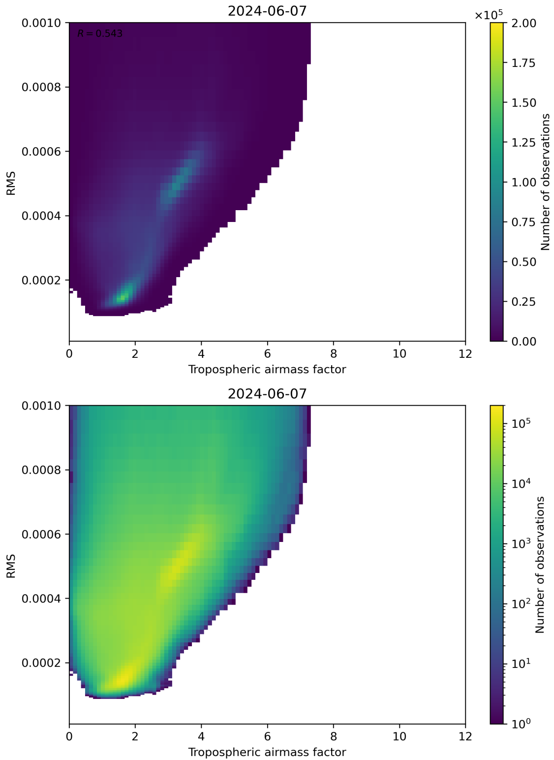
Figure 79: Scatter density plot of “Tropospheric airmass factor” against “RMS” for 2024-06-06 to 2024-06-08.
