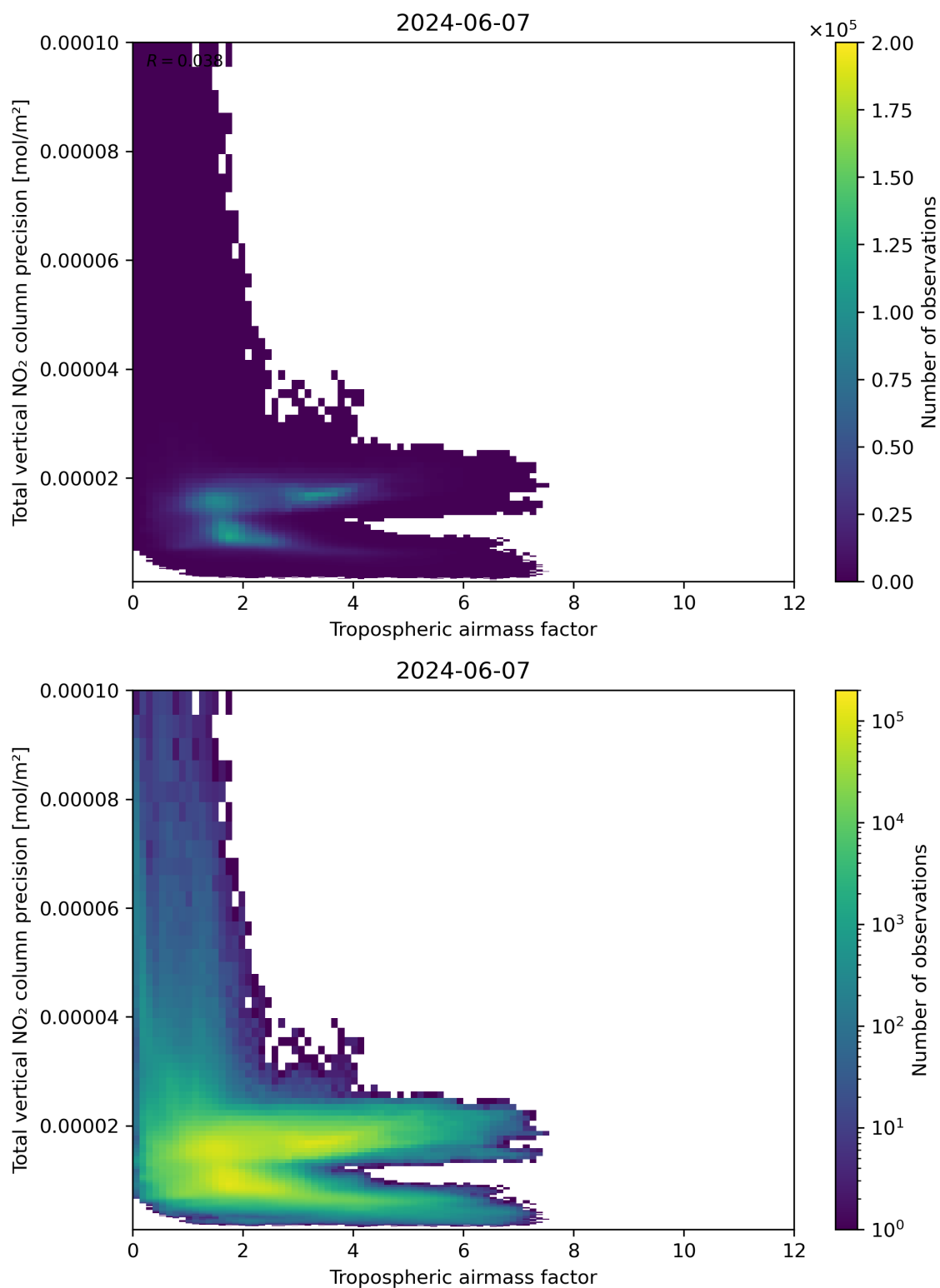
Figure 78: Scatter density plot of “Tropospheric air mass factor” against “Total vertical NO 2 column precision” for 2024-06-06 to 2024-06-08.
