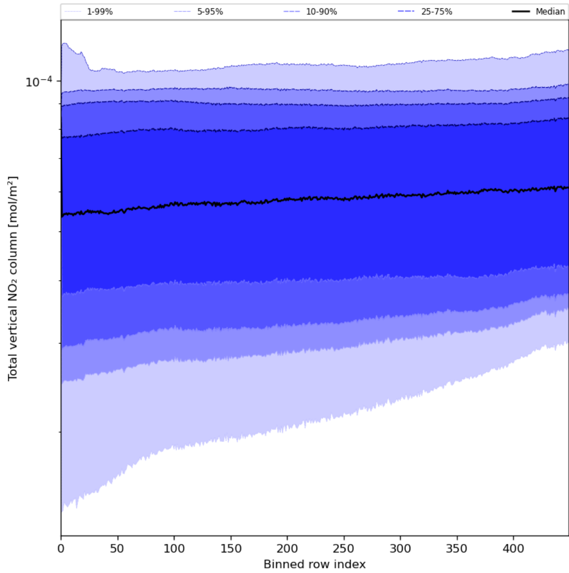
Figure 55: Along track statistics of “Total vertical NO 2 column” for 2024-06-06 to 2024-06-08
