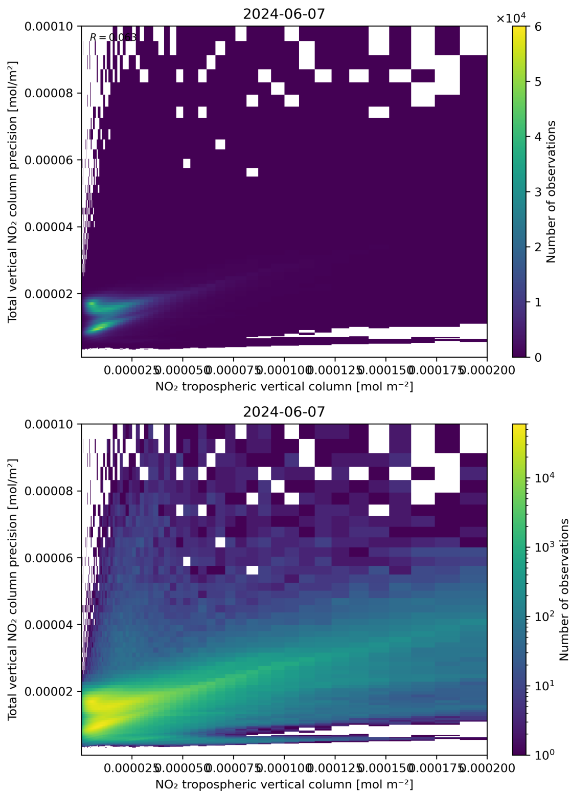
Figure 129: Scatter density plot of “NO 2 tropospheric vertical column” against “Total vertical NO 2 column precision” for 2024-06-06 to 2024-06-08.
