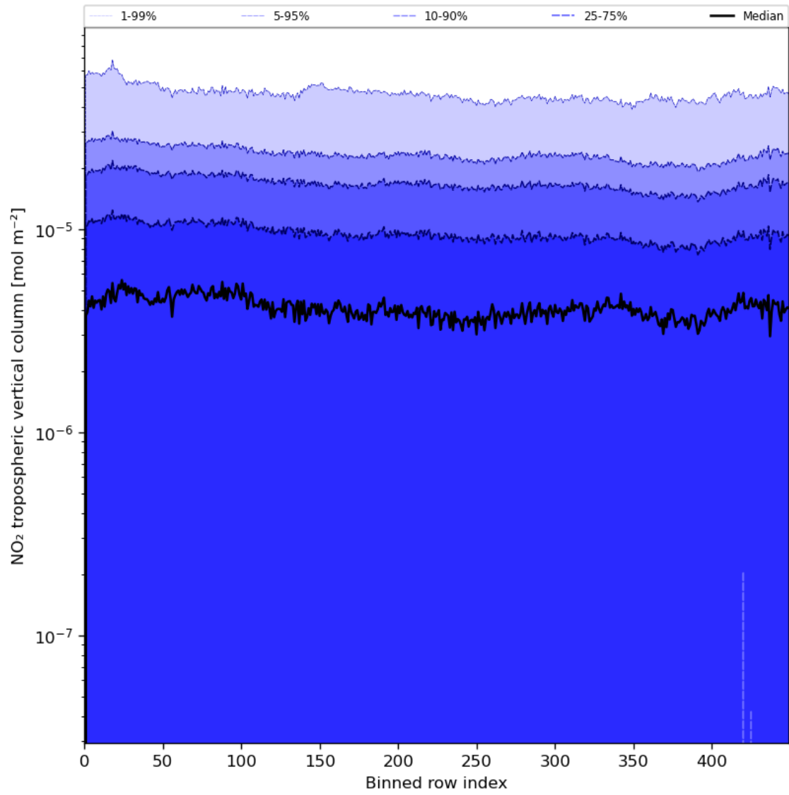
Figure 46: Along track statistics of “NO 2 tropospheric vertical column” for 2024-06-06 to 2024-06-08
