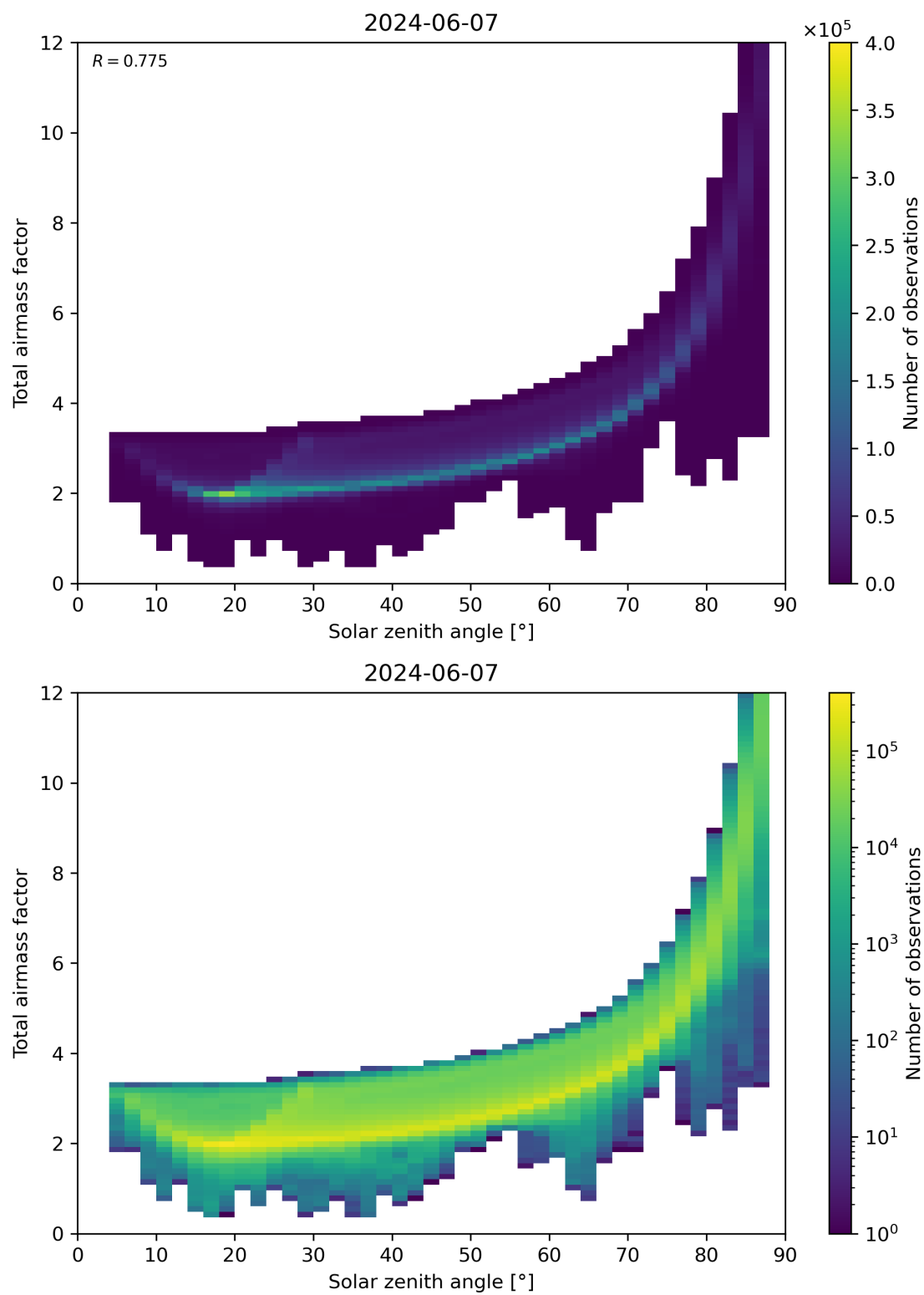
Figure 146: Scatter density plot of “Solar zenith angle” against “Total air mass factor” for 2024-06-06 to 2024-06-08.
