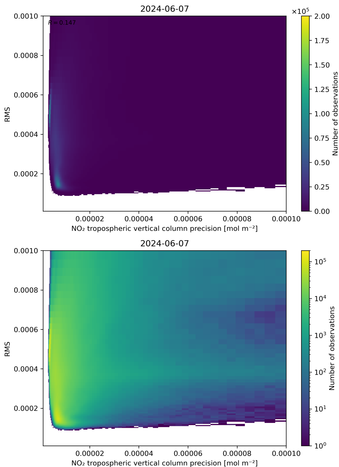
Figure 140: Scatter density plot of “NO 2 tropospheric vertical column precision” against “RMS” for 2024-06-06 to 2024-06-08.
