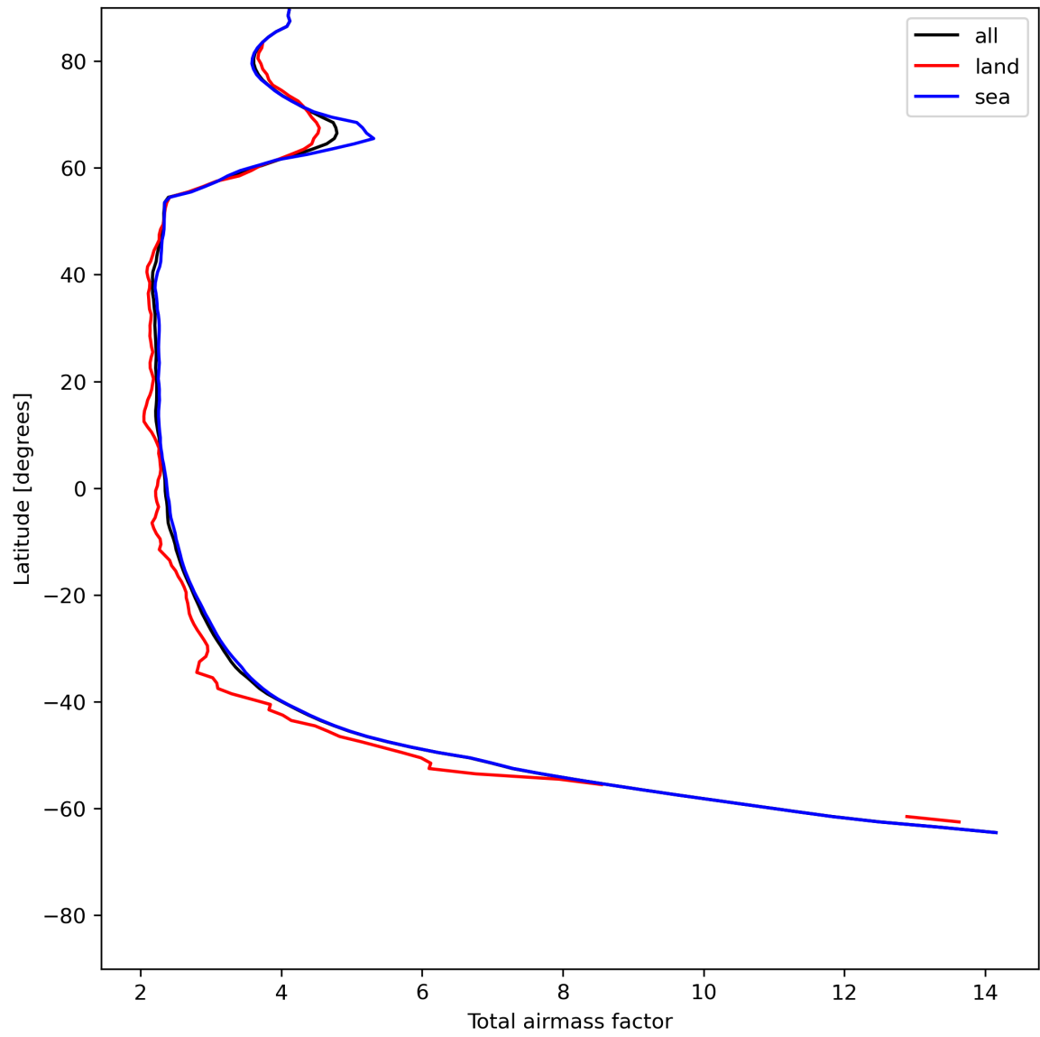
Figure 15: Zonal average of “Total airmass factor” for 2024-06-06 to 2024-06-08.
