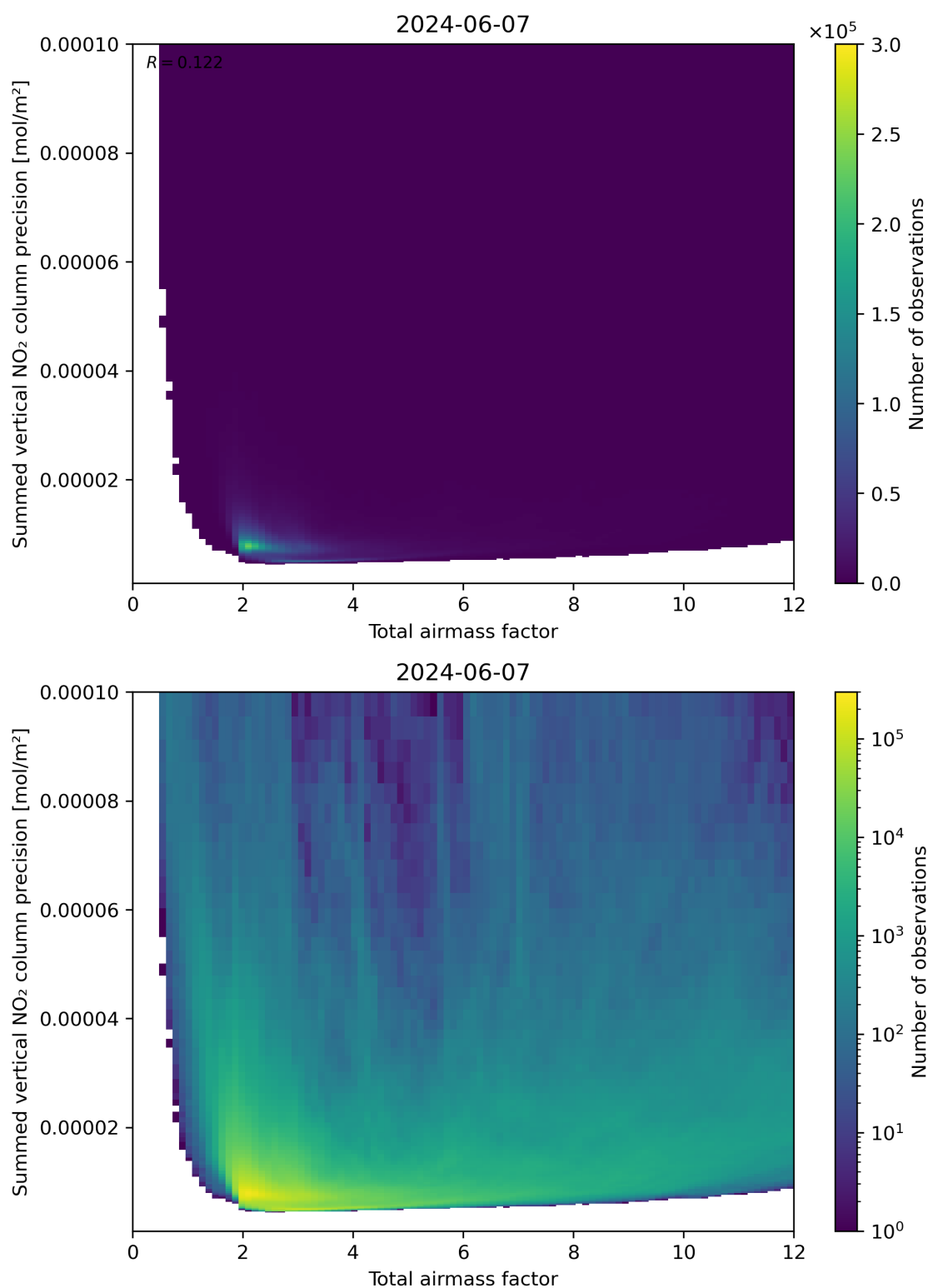
Figure 66: Scatter density plot of “Total airmass factor” against “Summed vertical NO 2 column precision” for 2024-06-06 to 2024-06-08.
