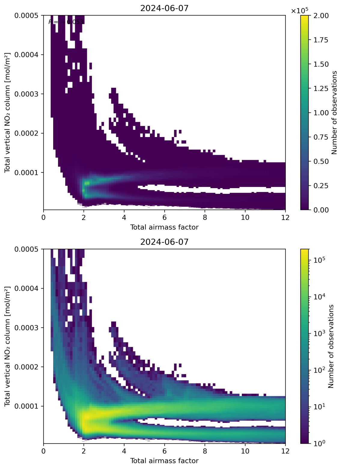
Figure 67: Scatter density plot of “Total airmass factor” against “Total vertical NO 2 column” for 2024-06-06 to 2024-06-08.
