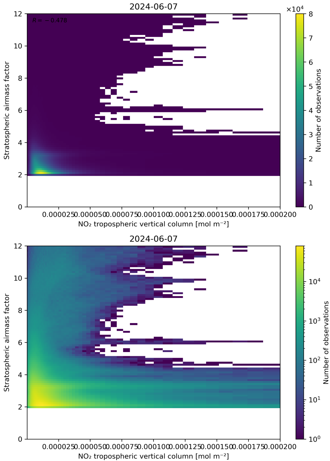
Figure 121: Scatter density plot of “NO 2 tropospheric vertical column” against “Stratospheric air mass factor” for 2024-06-06 to 2024-06-08.
