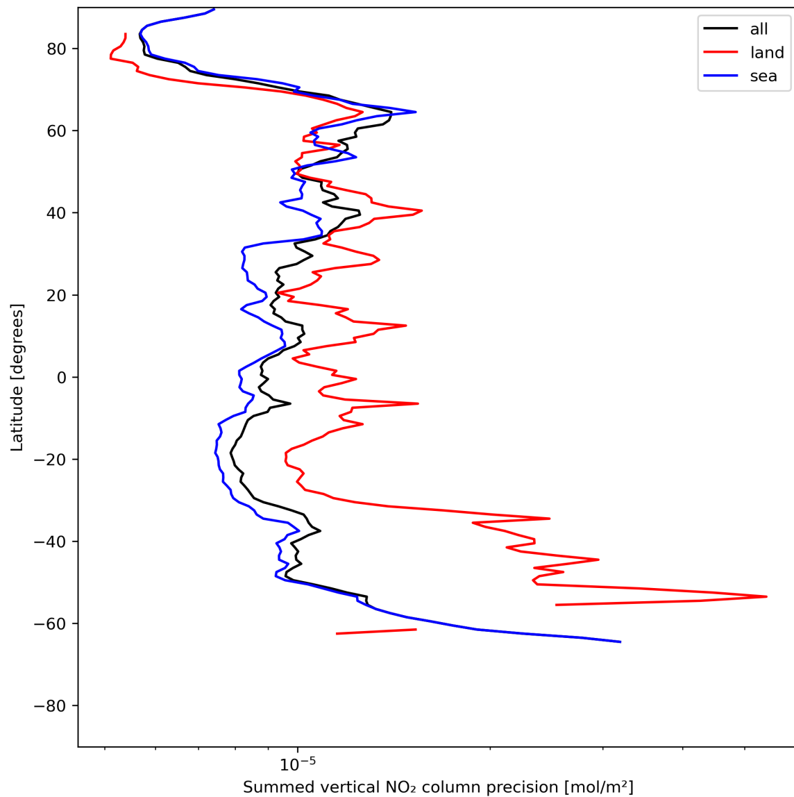
Figure 24: Zonal average of “Summed vertical NO 2 column precision” for 2024-06-06 to 2024-06-08.
