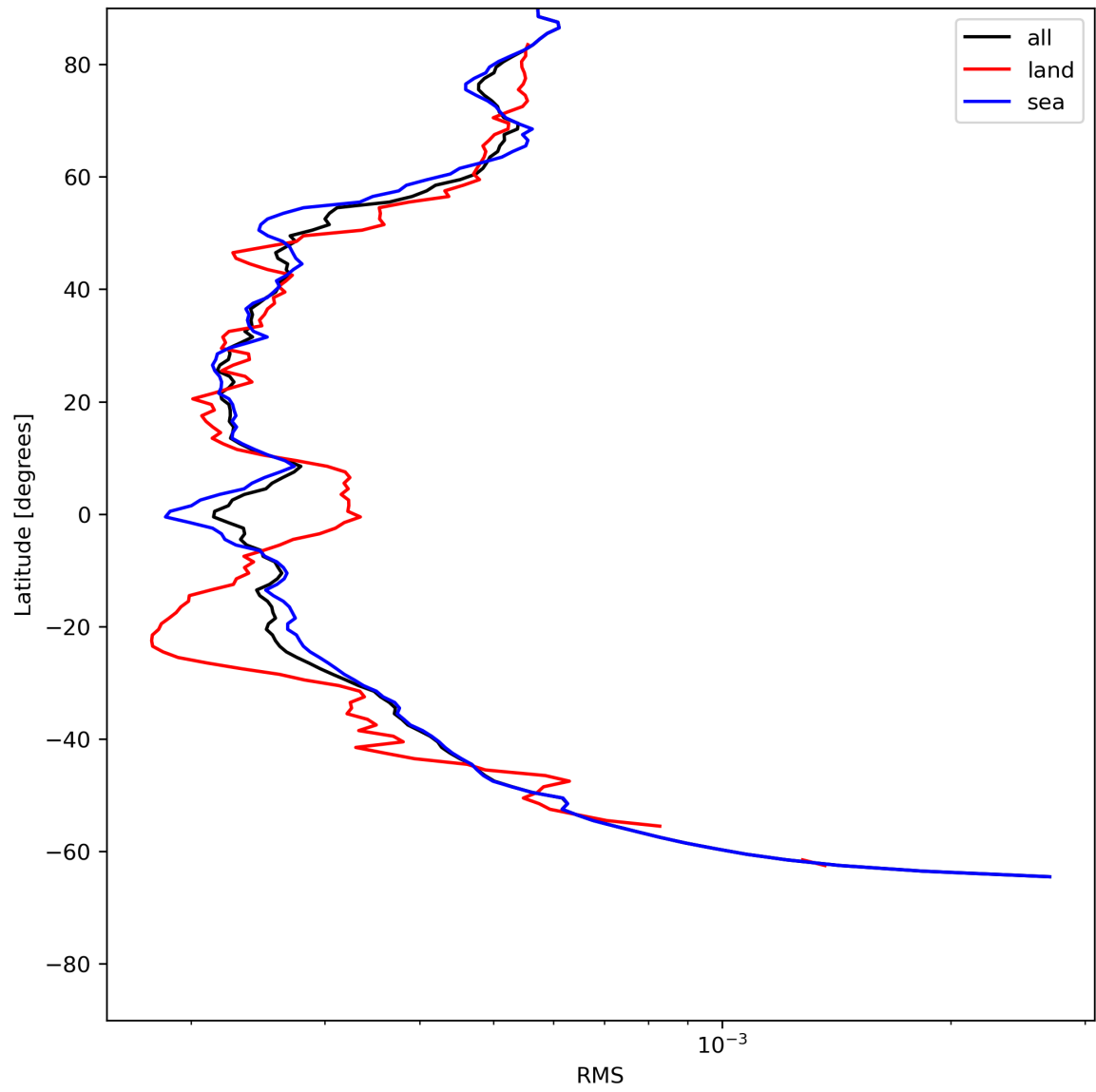
Figure 26: Zonal average of “RMS” for 2024-06-06 to 2024-06-08.
