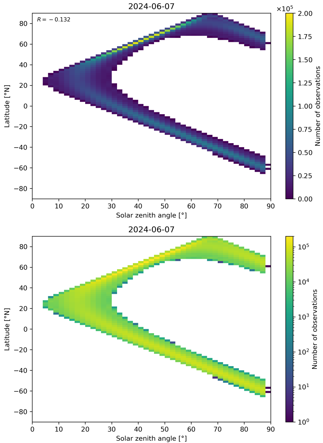
Figure 149: Scatter density plot of “Solar zenith angle” against “Latitude” for 2024-06-06 to 2024-06-08.
