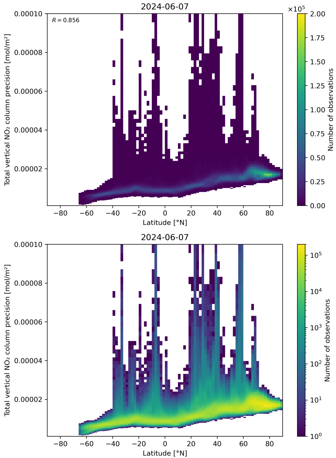
Figure 91: Scatter density plot of “Latitude” against “Total vertical NO 2 column precision” for 2024-06-06 to 2024-06-08.
