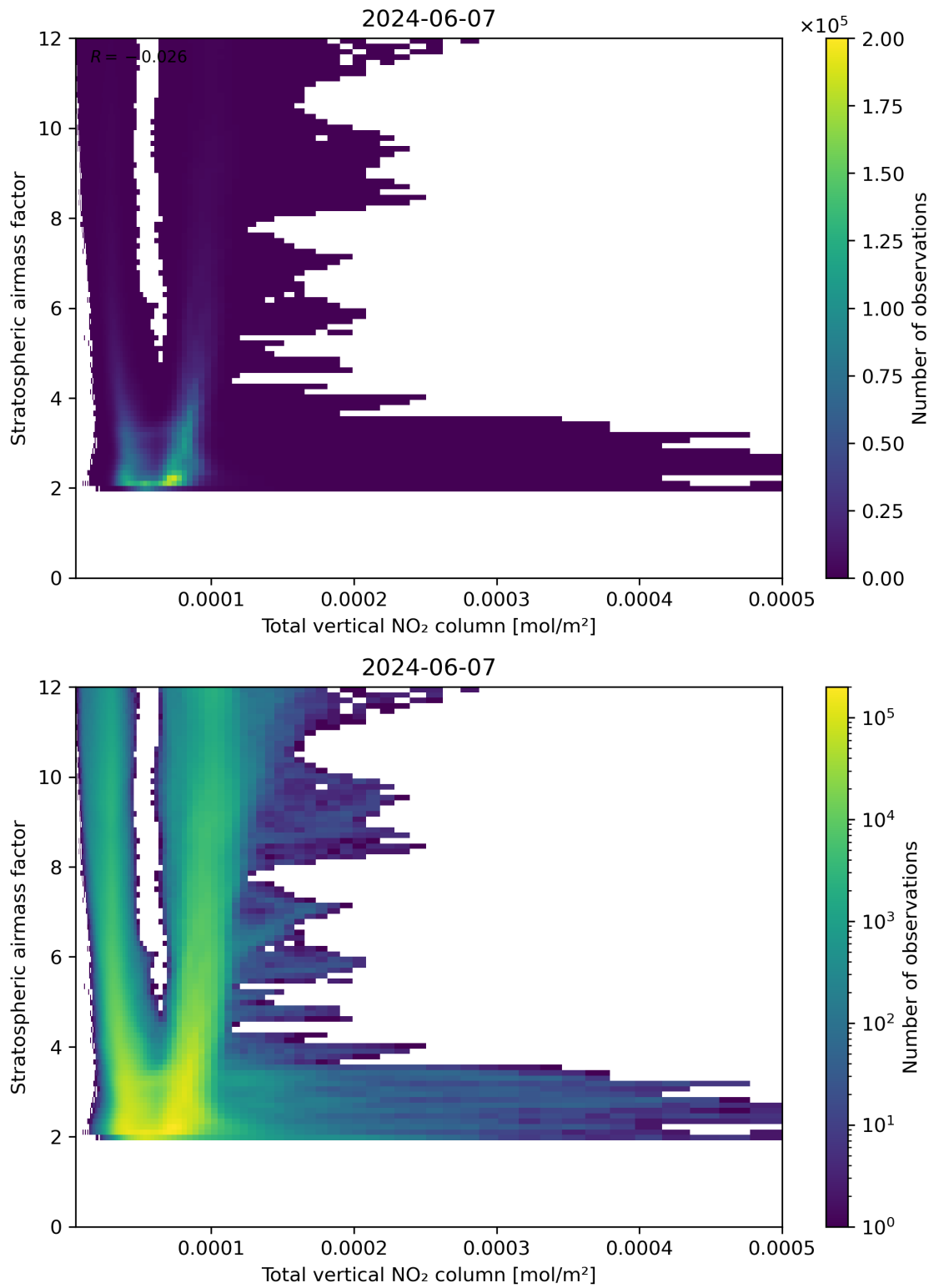
Figure 110: Scatter density plot of “Total vertical NO 2 column” against “Stratospheric airmass factor” for 2024-06-06 to 2024-06-08.
