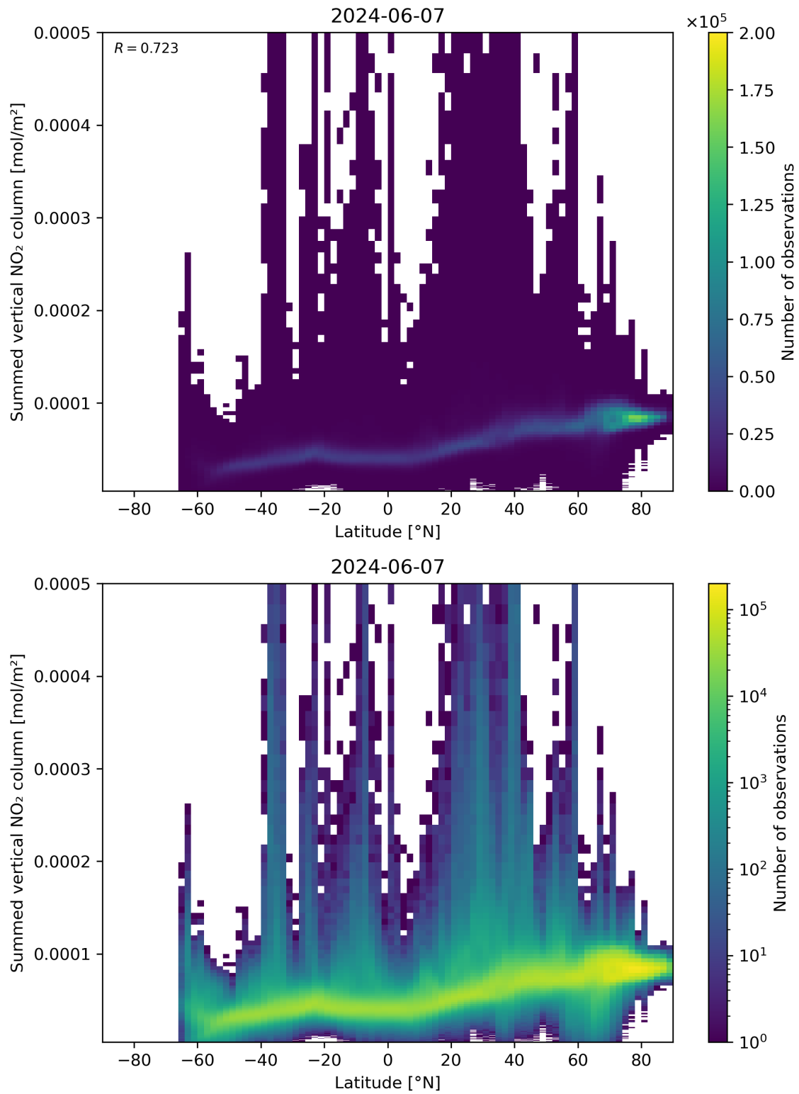
Figure 88: Scatter density plot of “Latitude” against “Summed vertical NO 2 column” for 2024-06-06 to 2024-06-08.
