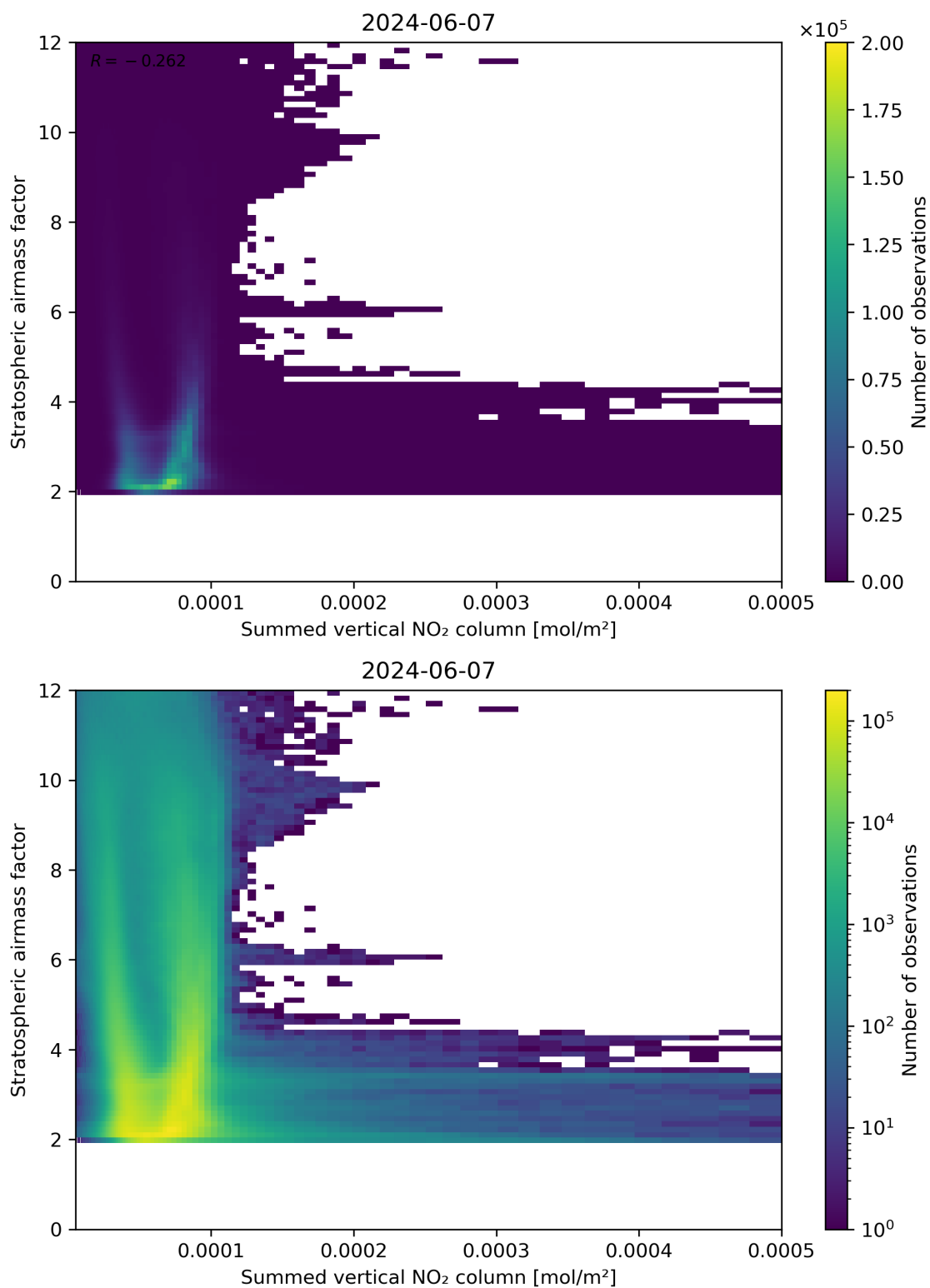
Figure 103: Scatter density plot of “Summed vertical NO 2 column” against “Stratospheric airmass factor” for 2024-06-06 to 2024-06-08.
