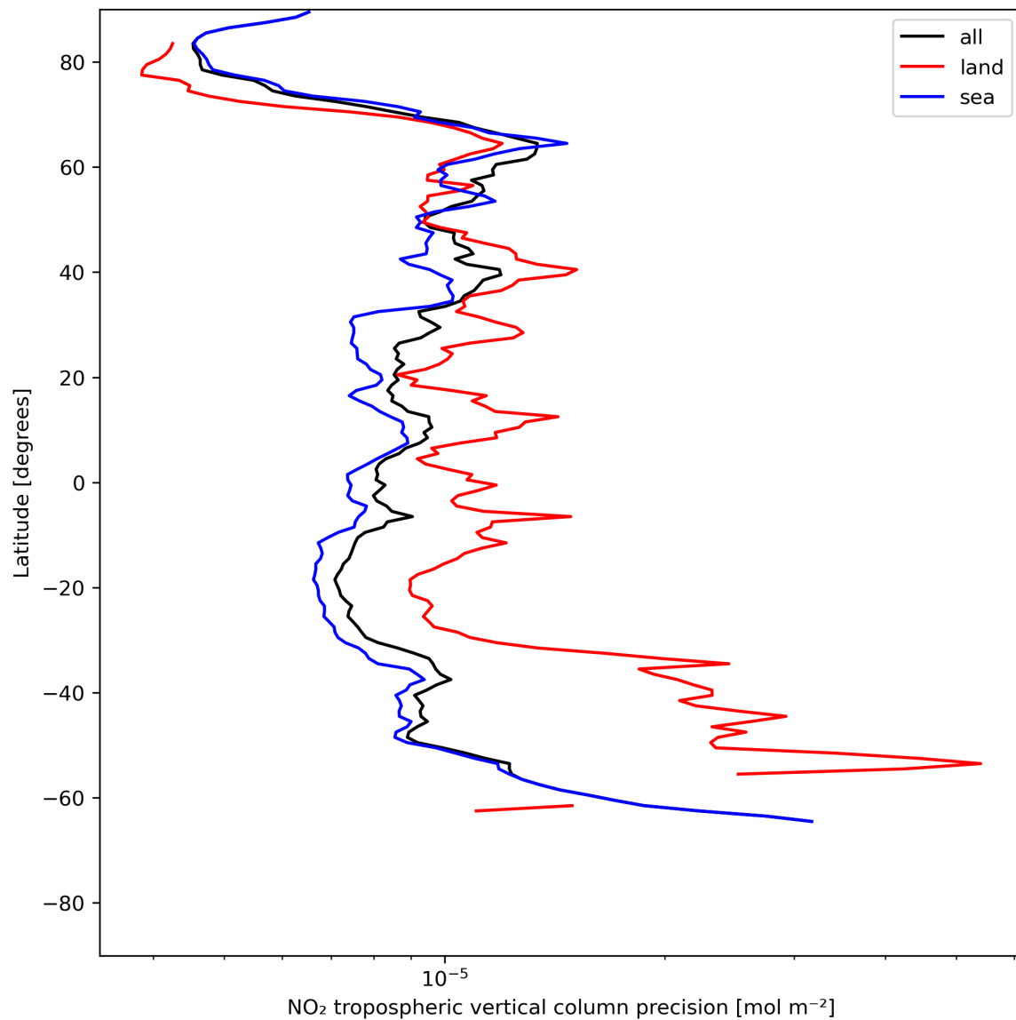
Figure 13: Zonal average of “NO 2 tropospheric vertical column precision” for 2024-06-06 to 2024-06-08.
