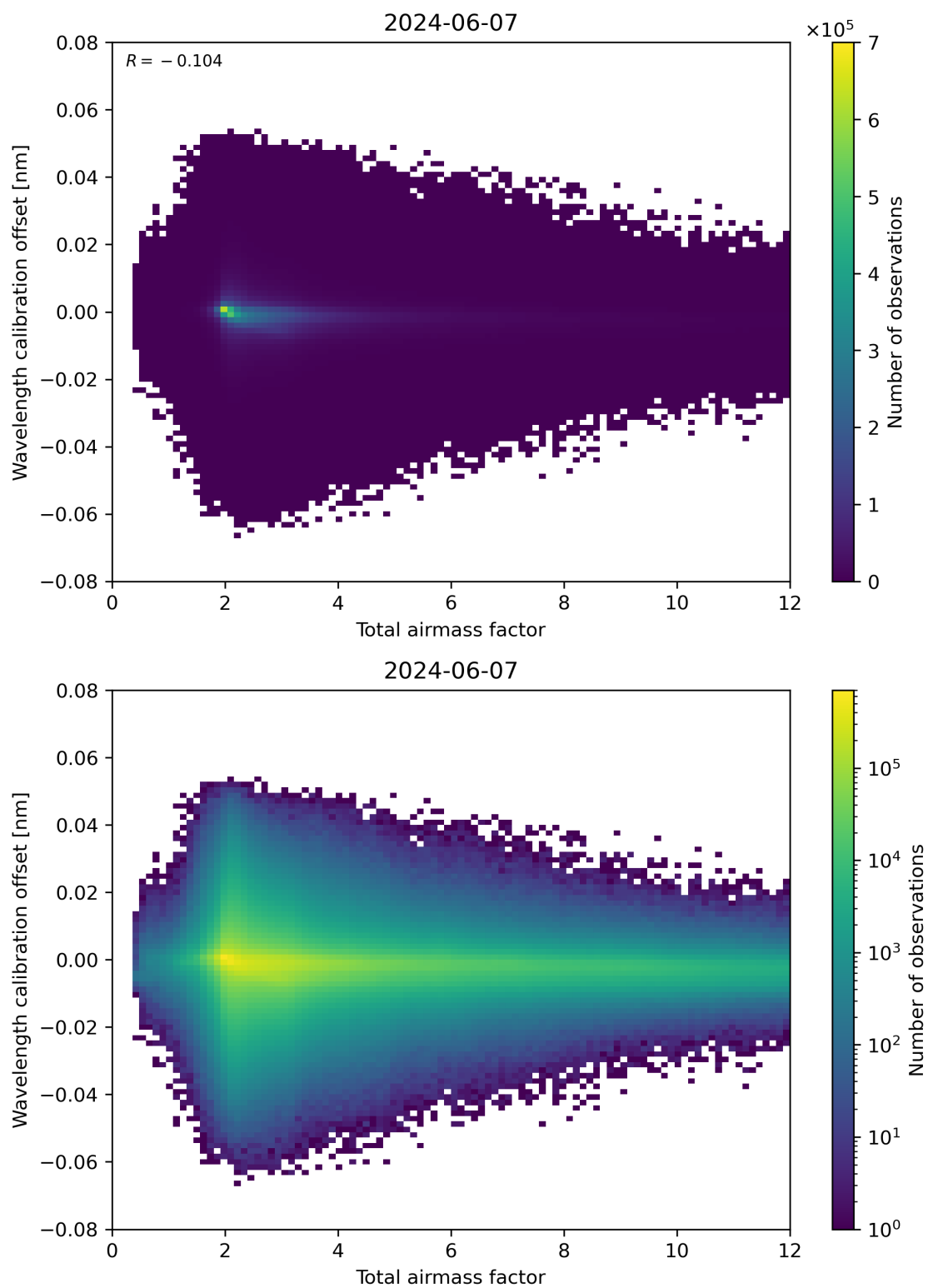
Figure 70: Scatter density plot of “Total airmass factor” against “Wavelength calibration offset” for 2024-06-06 to 2024-06-08.
