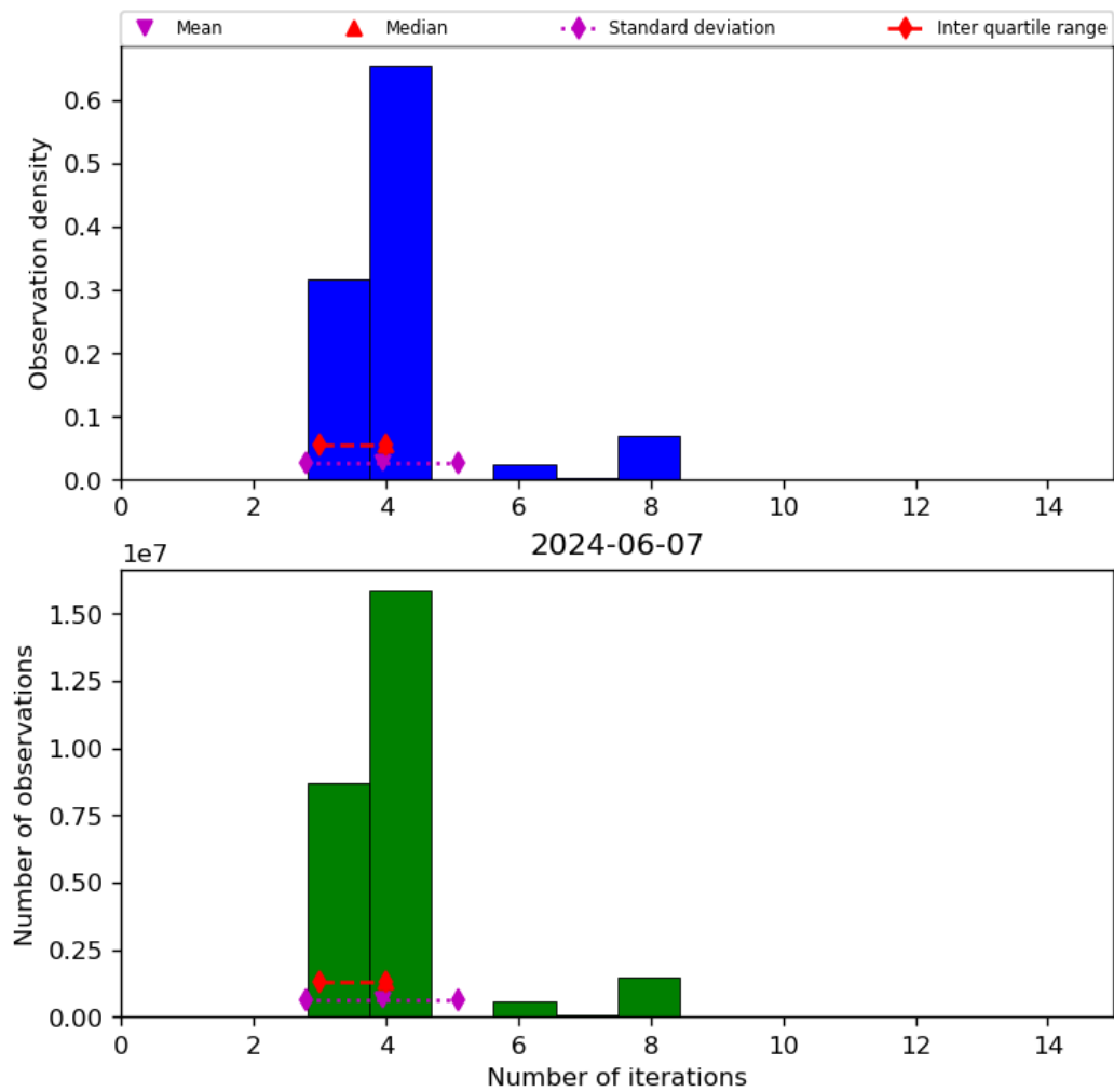
Figure 34: Histogram of “Number of iterations” for 2024-06-06 to 2024-06-08
