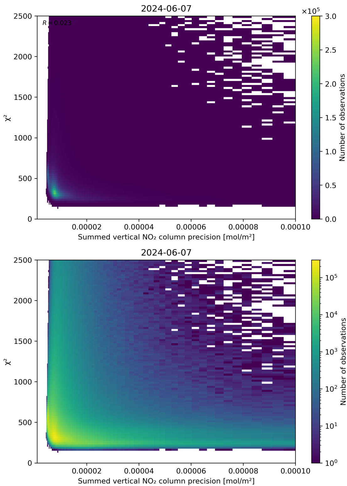
Figure 107: Scatter density plot of “Summed vertical NO 2 column precision” against “ \chi^2 ” for 2024-06-06 to 2024-06-08.
