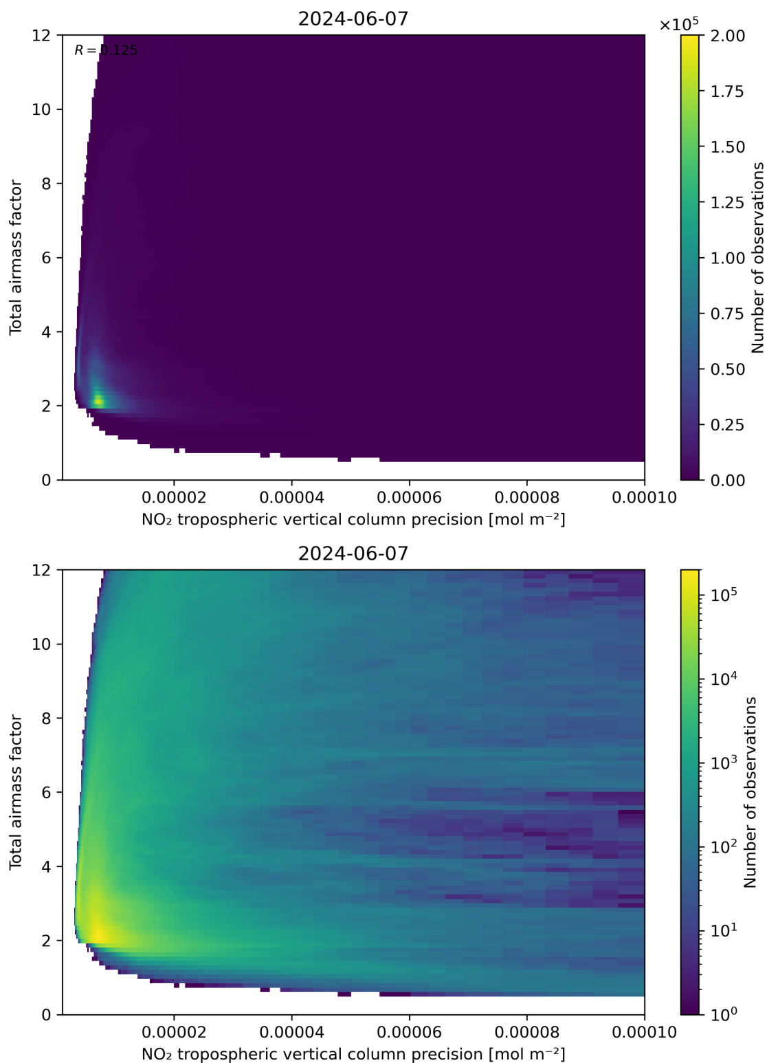
Figure 132: Scatter density plot of “NO 2 tropospheric vertical column precision” against “Total airmass factor” for 2024-06-06 to 2024-06-08.
