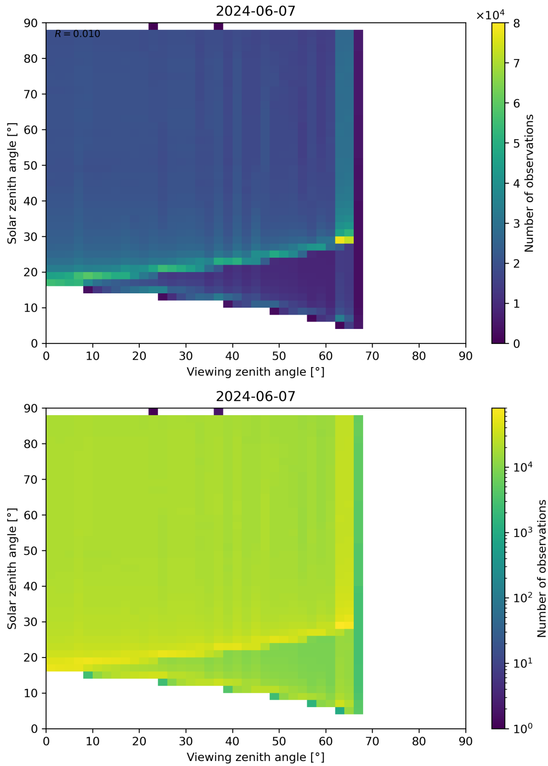
Figure 172: Scatter density plot of “Viewing zenith angle” against “Solar zenith angle” for 2024-06-06 to 2024-06-08.
