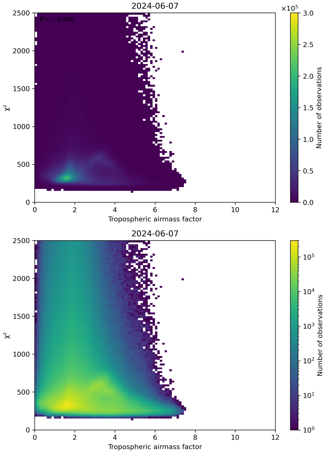
Figure 73: Scatter density plot of “Tropospheric airmass factor” against “ \chi^2 ” for 2024-06-06 to 2024-06-08.
