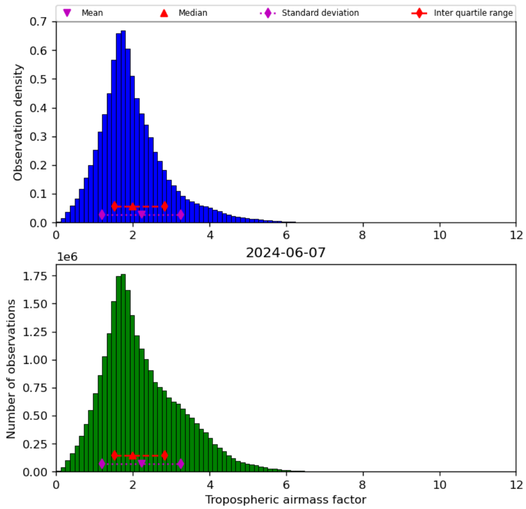
Figure 31: Histogram of “Tropospheric airmass factor” for 2024-06-06 to 2024-06-08
