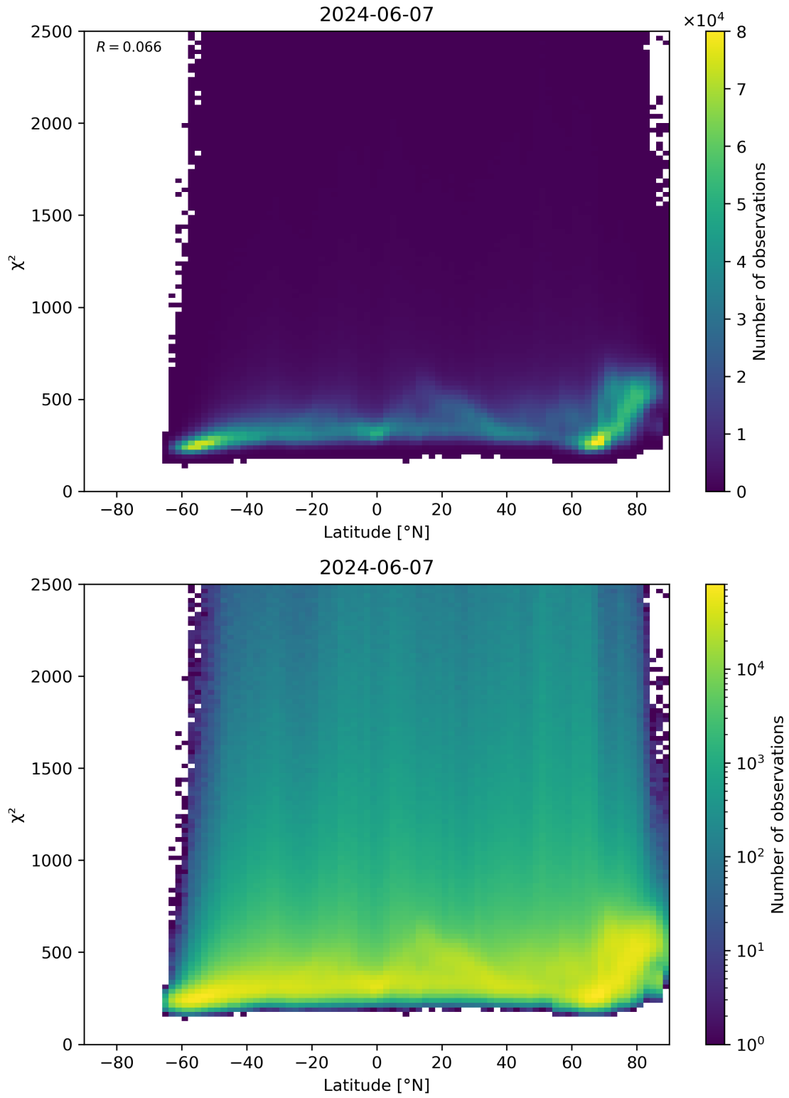
Figure 86: Scatter density plot of “Latitude” against “ \chi^2 ” for 2024-06-06 to 2024-06-08.
