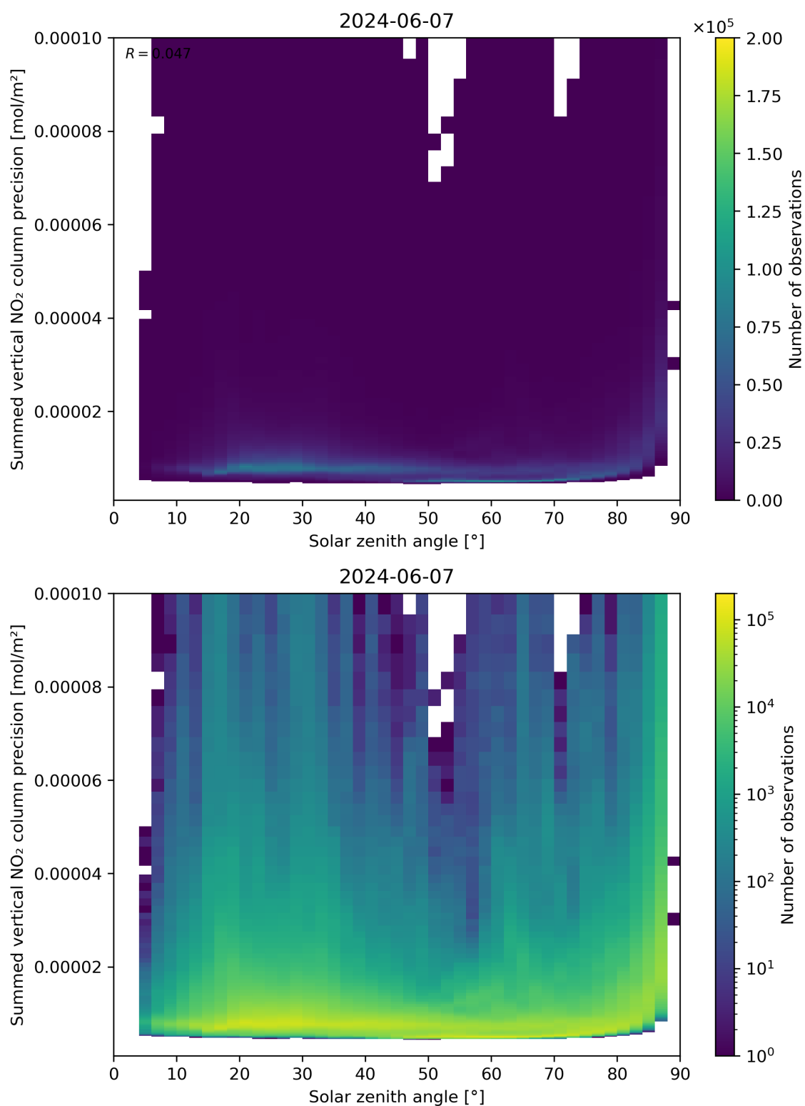
Figure 152: Scatter density plot of “Solar zenith angle” against “Summed vertical NO 2 column precision” for 2024-06-06 to 2024-06-08.
