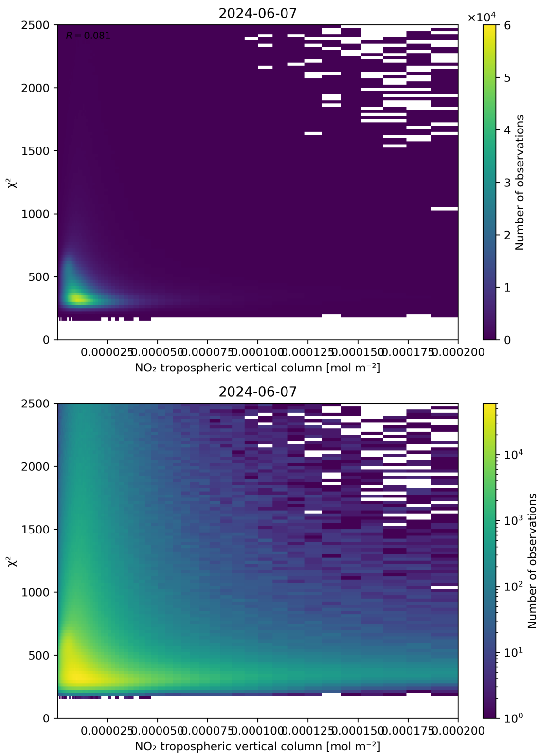
Figure 124: Scatter density plot of “NO 2 tropospheric vertical column” against “ \chi^2 ” for 2024-06-06 to 2024-06-08.
