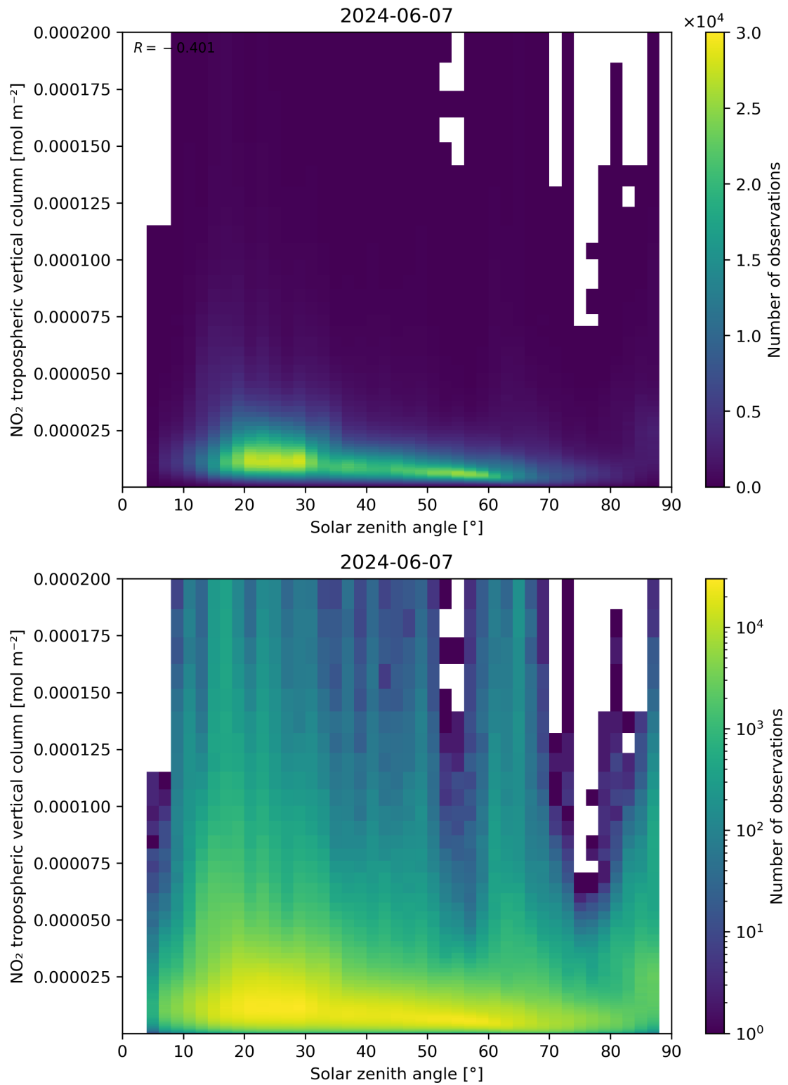
Figure 155: Scatter density plot of “Solar zenith angle” against “NO 2 tropospheric vertical column” for 2024-06-06 to 2024-06-08.
