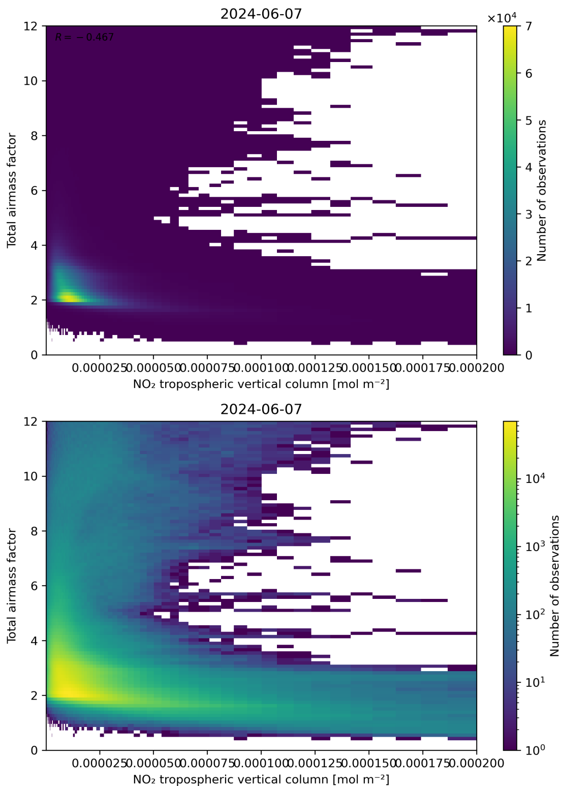
Figure 122: Scatter density plot of “NO 2 tropospheric vertical column” against “Total air mass factor” for 2024-06-06 to 2024-06-08.
