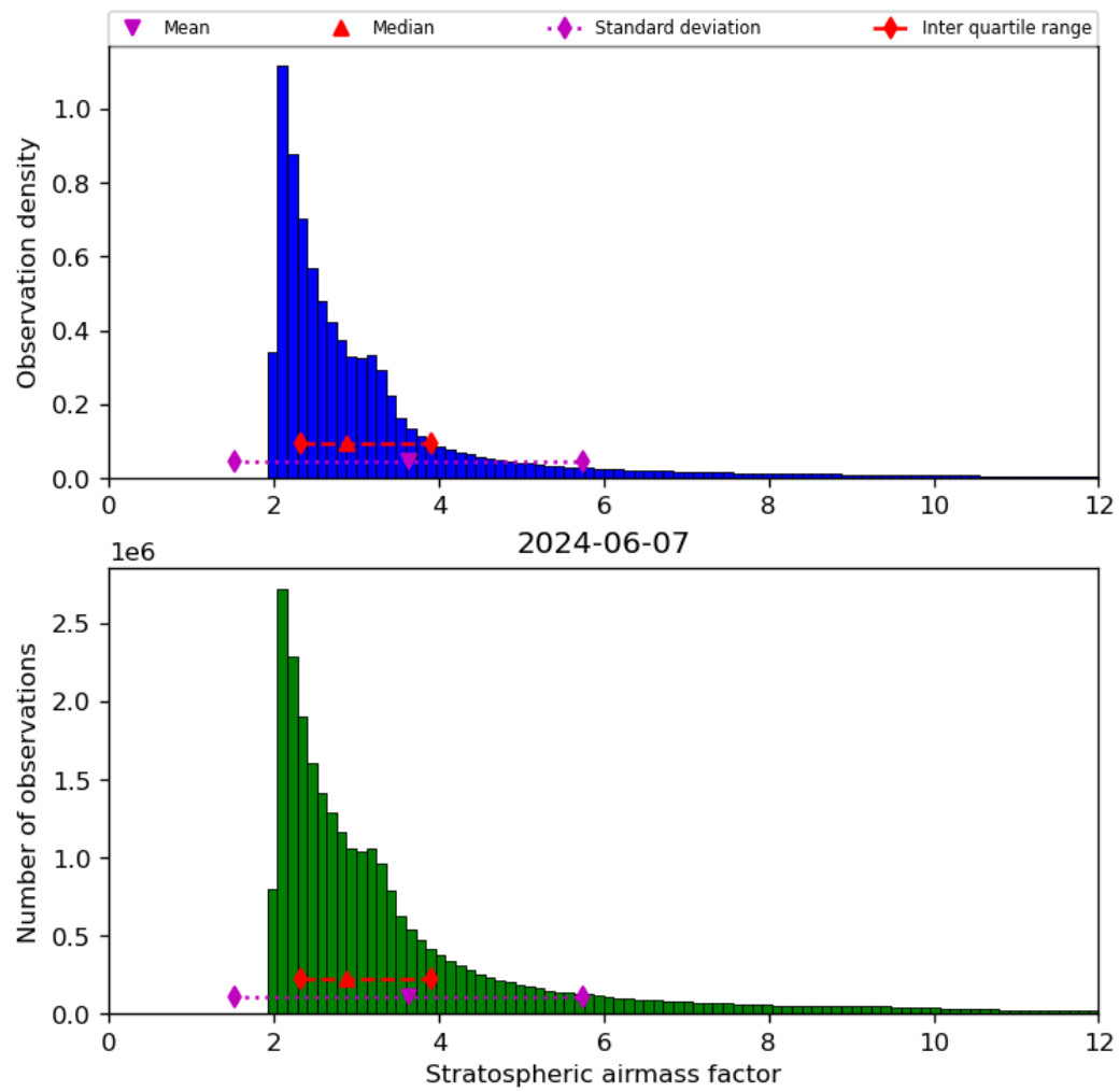
Figure 44: Histogram of “Stratospheric airmass factor” for 2024-06-06 to 2024-06-08
