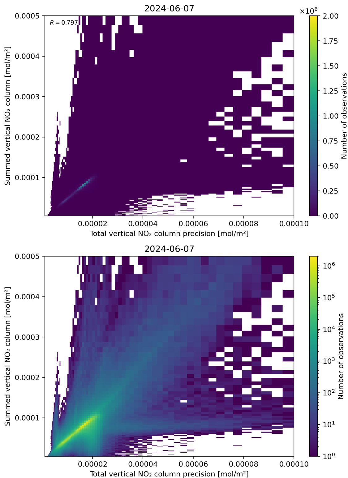
Figure 117: Scatter density plot of “Total vertical NO 2 column precision” against “Summed vertical NO 2 column” for 2024-06-06 to 2024-06-08.
