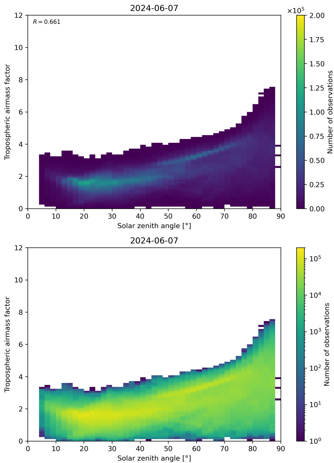
Figure 147: Scatter density plot of “Solar zenith angle” against “Tropospheric airmass factor” for 2024-06-06 to 2024-06-08.
