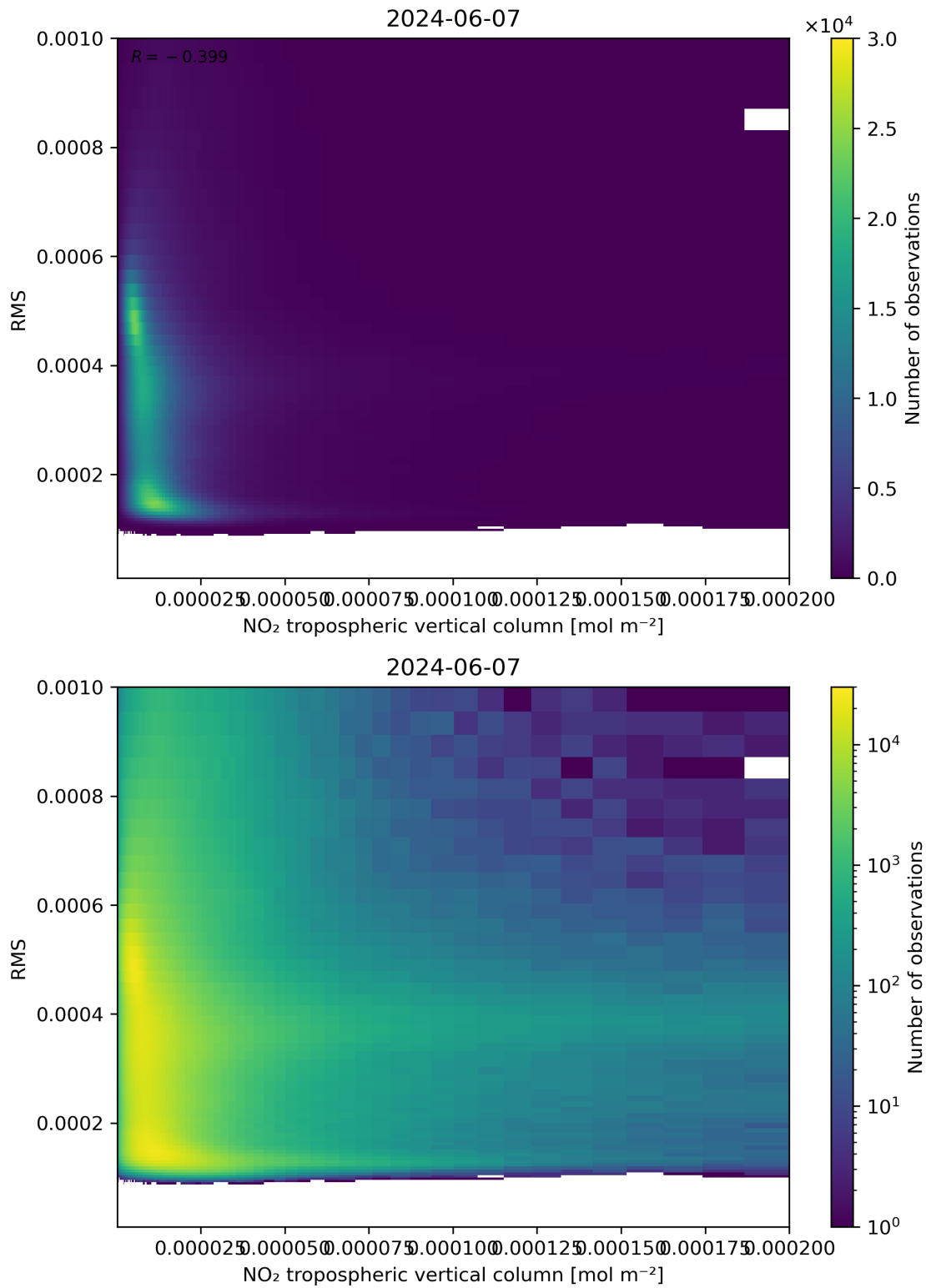
Figure 142: Scatter density plot of “NO 2 tropospheric vertical column” against “RMS” for 2024-06-06 to 2024-06-08.
