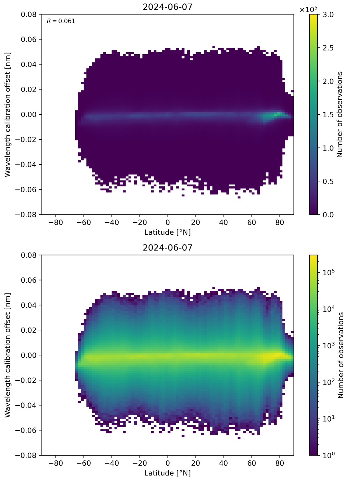
Figure 95: Scatter density plot of “Latitude” against “Wavelength calibration offset” for 2024-06-06 to 2024-06-08.
