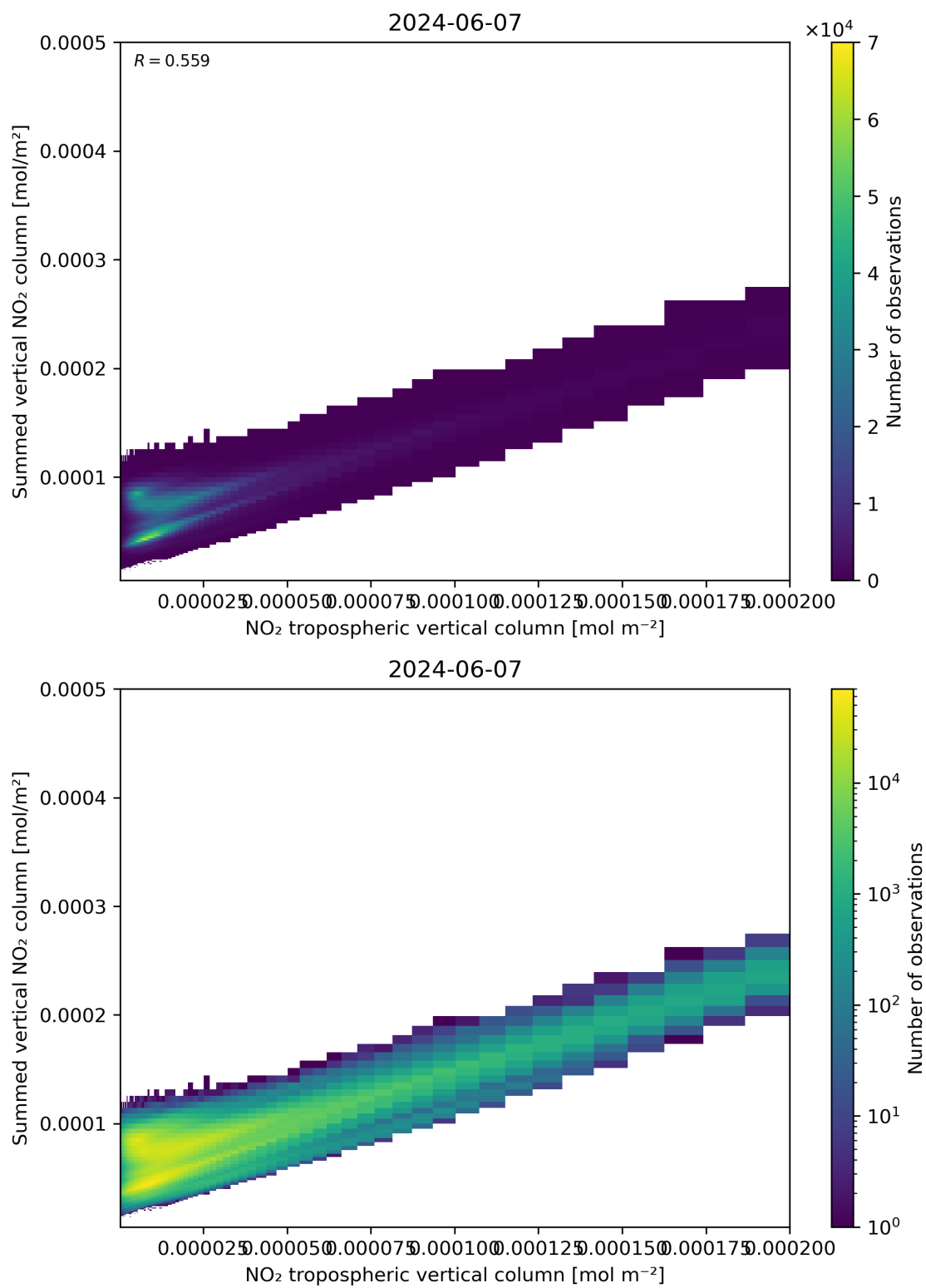
Figure 126: Scatter density plot of “NO 2 tropospheric vertical column” against “Summed vertical NO 2 column” for 2024-06-06 to 2024-06-08.
