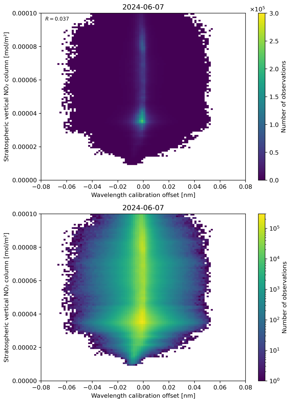
Figure 176: Scatter density plot of “Wavelength calibration offset” against “Stratospheric vertical NO 2 column” for 2024-06-06 to 2024-06-08.
