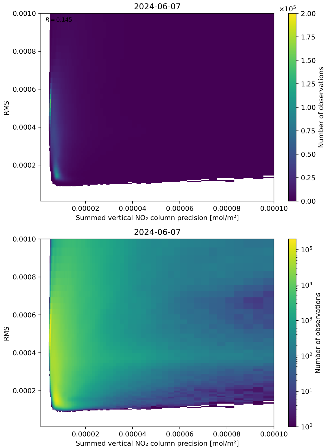
Figure 108: Scatter density plot of “Summed vertical NO 2 column precision” against “RMS” for 2024-06-06 to 2024-06-08.
