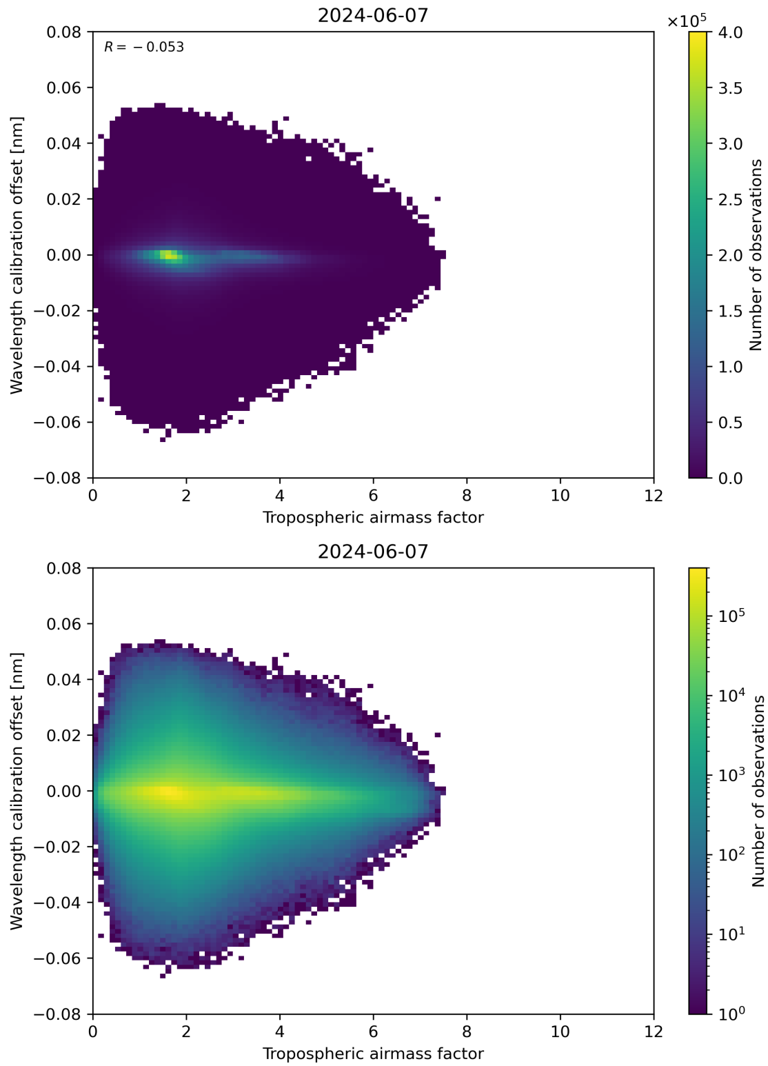
Figure 80: Scatter density plot of “Tropospheric airmass factor” against “Wavelength calibration offset” for 2024-06-06 to 2024-06-08.
