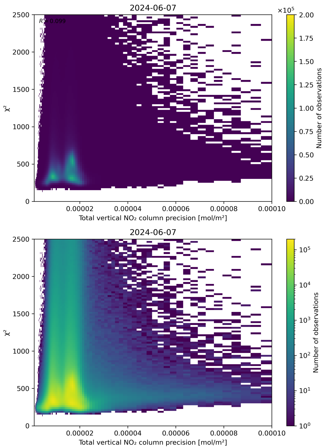
Figure 116: Scatter density plot of “Total vertical NO 2 column precision” against “ \chi^2 ” for 2024-06-06 to 2024-06-08.
