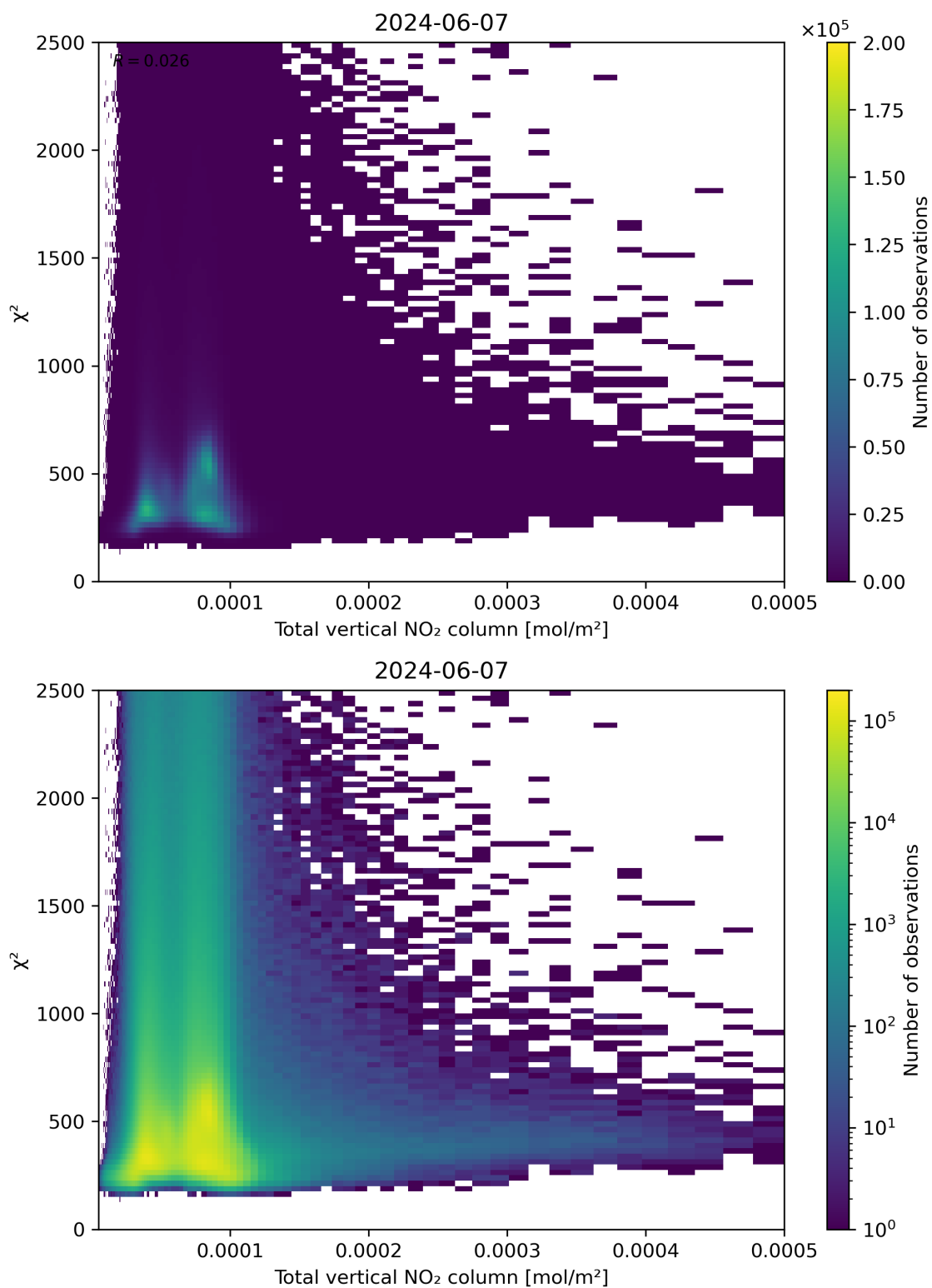
Figure 111: Scatter density plot of “Total vertical NO 2 column” against “ \chi^2 ” for 2024-06-06 to 2024-06-08.
