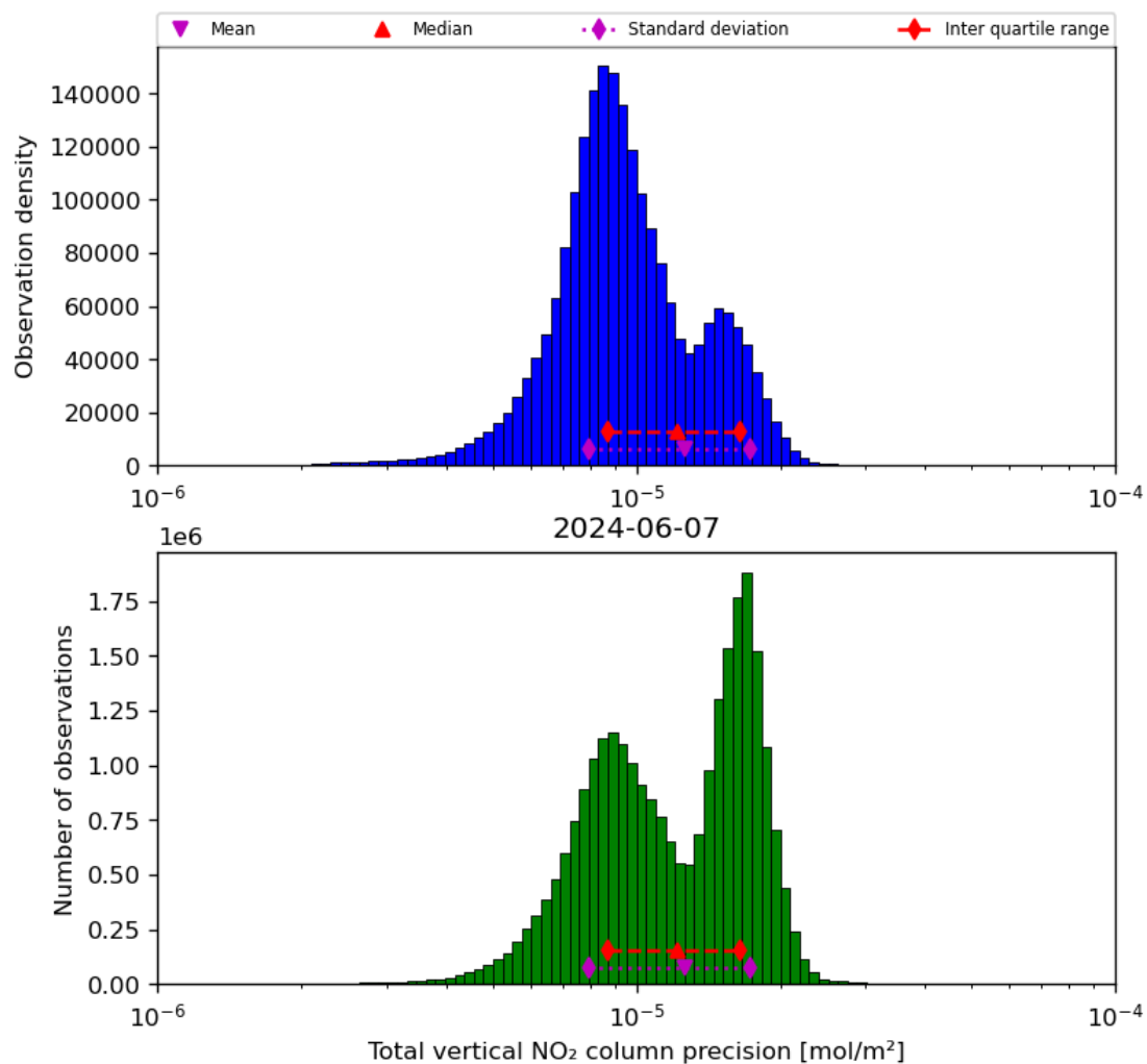
Figure 39: Histogram of “Total vertical NO 2 column precision” for 2024-06-06 to 2024-06-08
