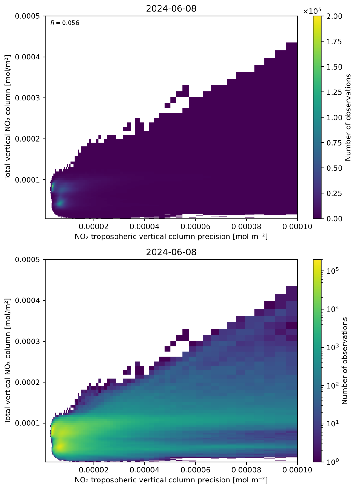
Figure 138: Scatter density plot of “NO 2 tropospheric vertical column precision” against “Total vertical NO 2 column” for 2024-06-08 to 2024-06-09.
