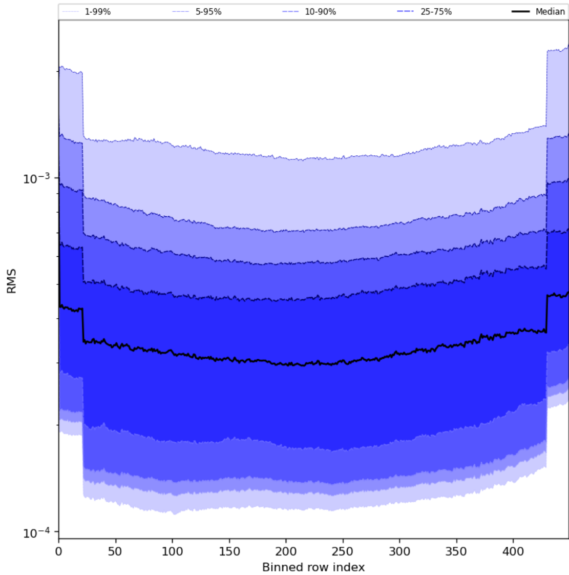
Figure 60: Along track statistics of “RMS” for 2024-06-08 to 2024-06-09
