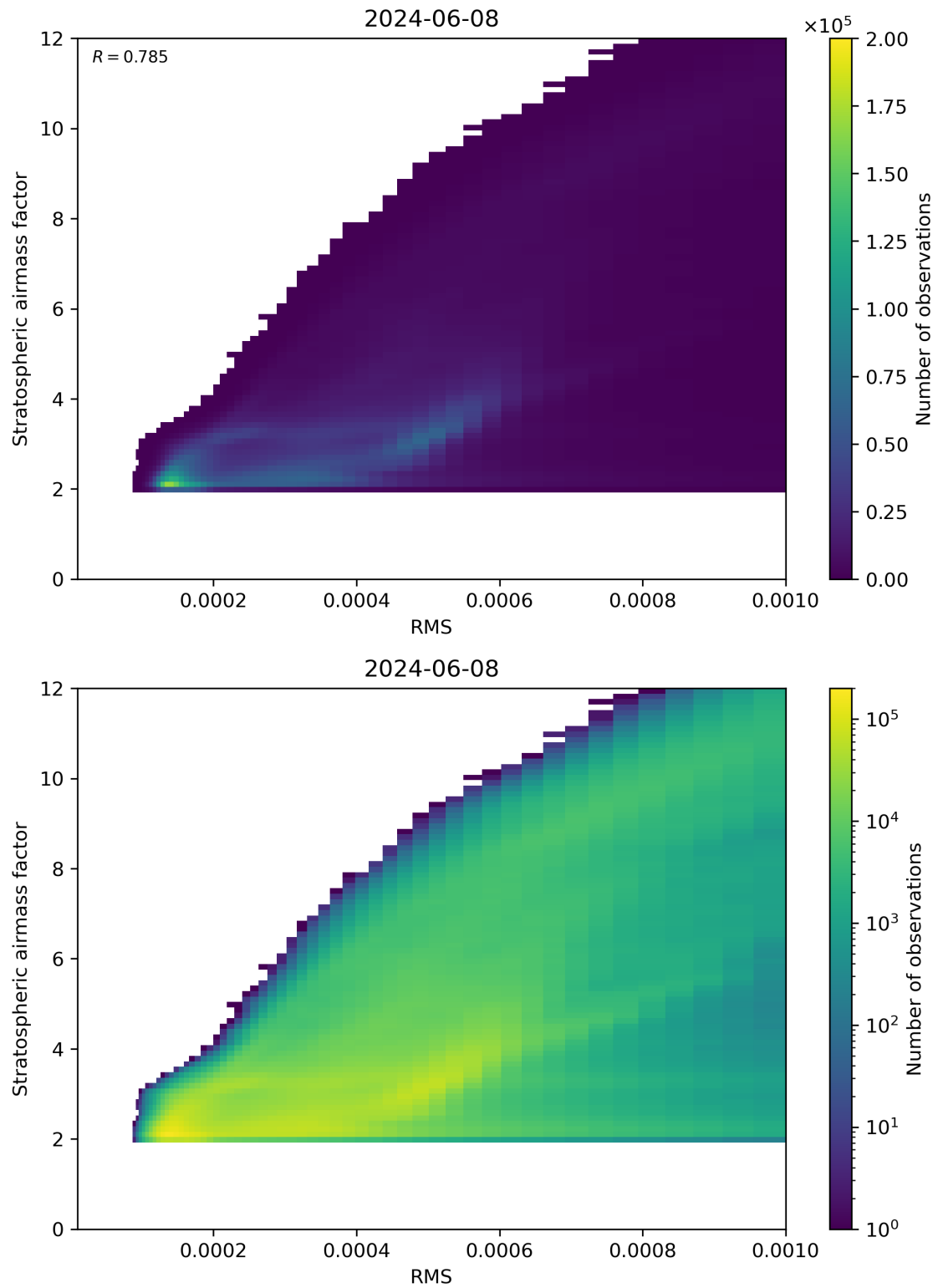
Figure 144: Scatter density plot of “RMS” against “Stratospheric airmass factor” for 2024-06-08 to 2024-06-09.
