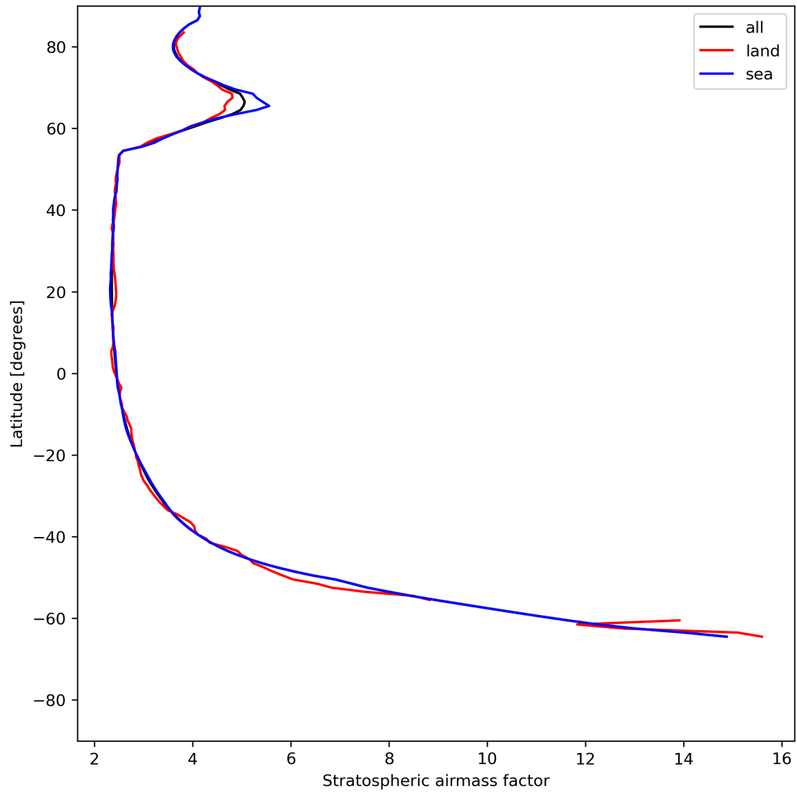
Figure 27: Zonal average of “Stratospheric airmass factor” for 2024-06-08 to 2024-06-09.
