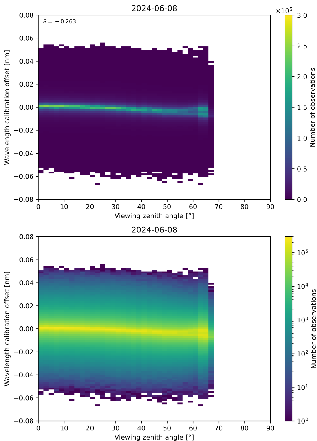
Figure 173: Scatter density plot of “Viewing zenith angle” against “Wavelength calibration offset” for 2024-06-08 to 2024-06-09.
