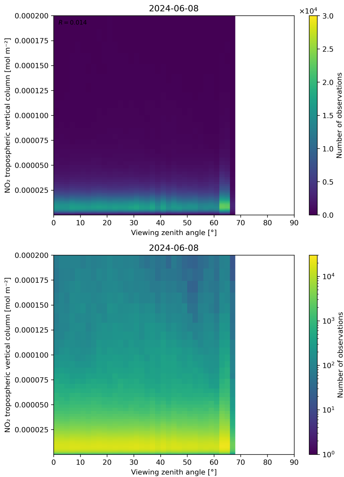
Figure 169: Scatter density plot of “Viewing zenith angle” against “NO 2 tropospheric vertical column” for 2024-06-08 to 2024-06-09.
