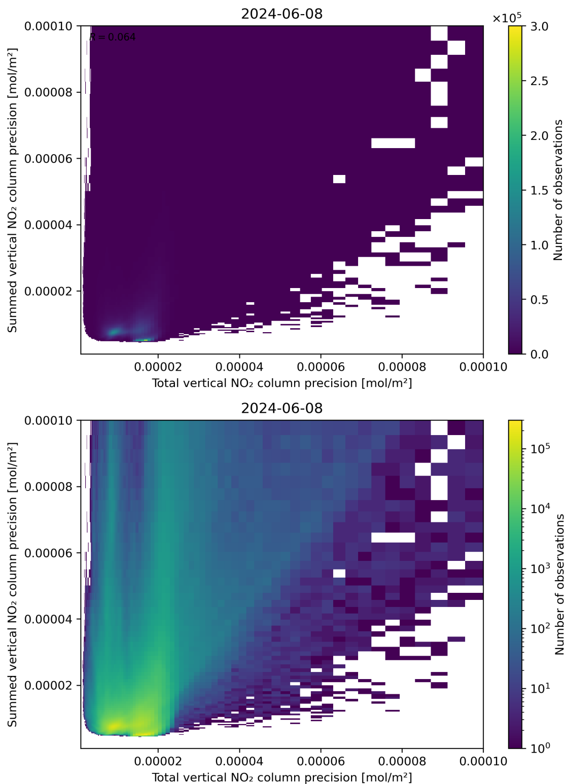
Figure 118: Scatter density plot of “Total vertical NO 2 column precision” against “Summed vertical NO 2 column precision” for 2024-06-08 to 2024-06-09.
