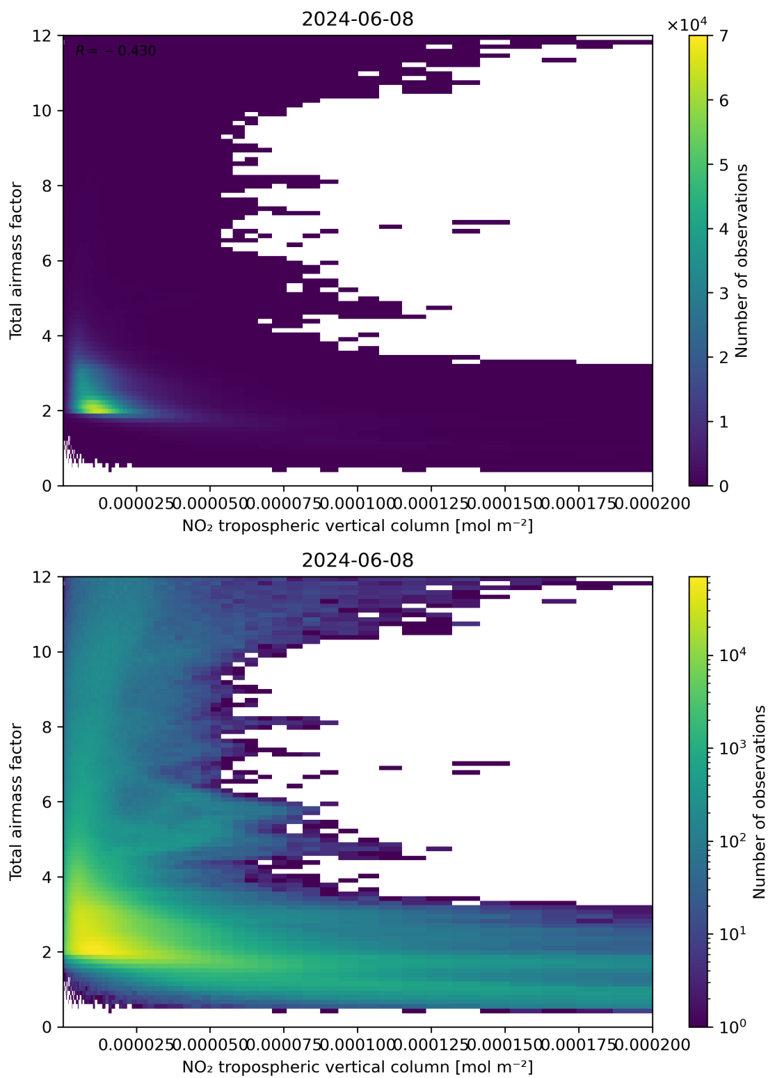
Figure 122: Scatter density plot of “NO 2 tropospheric vertical column” against “Total air mass factor” for 2024-06-08 to 2024-06-09.
