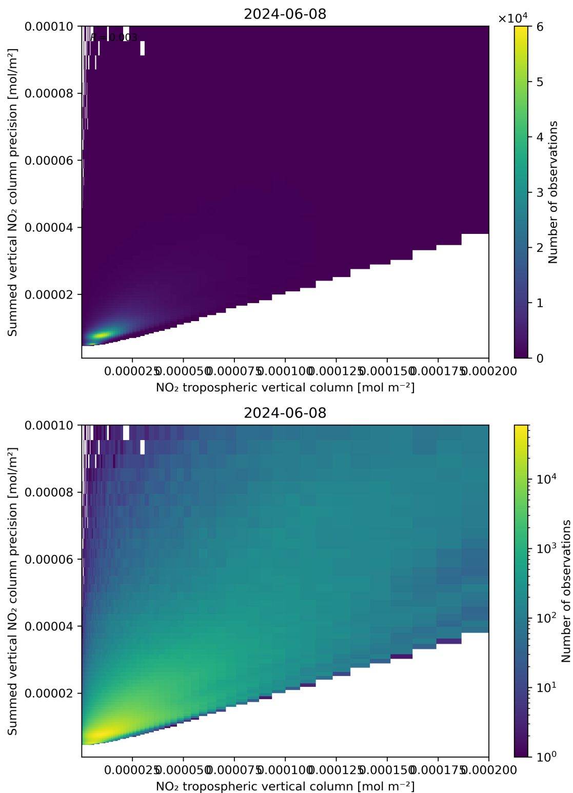
Figure 127: Scatter density plot of “NO 2 tropospheric vertical column” against “Summed vertical NO 2 column precision” for 2024-06-08 to 2024-06-09.
