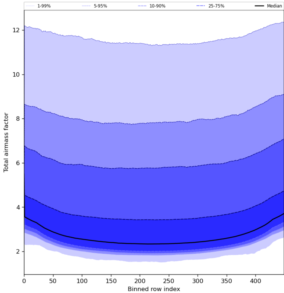
Figure 49: Along track statistics of “Total airmass factor” for 2024-06-08 to 2024-06-09
