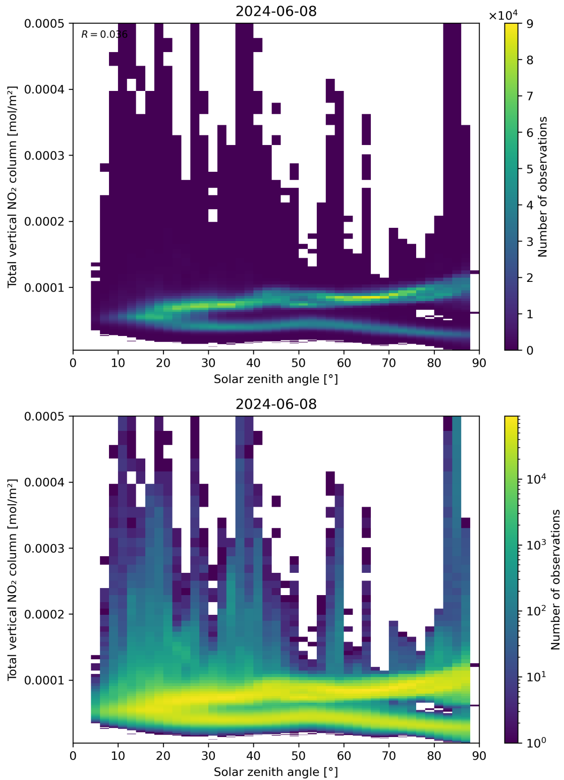
Figure 153: Scatter density plot of “Solar zenith angle” against “Total vertical NO 2 column” for 2024-06-08 to 2024-06-09.
