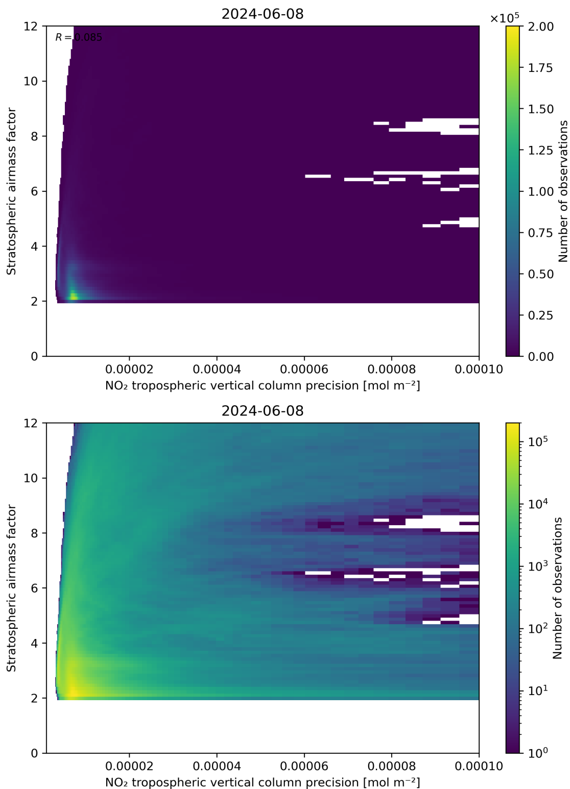
Figure 131: Scatter density plot of “NO 2 tropospheric vertical column precision” against “Stratospheric airmass factor” for 2024-06-08 to 2024-06-09.
