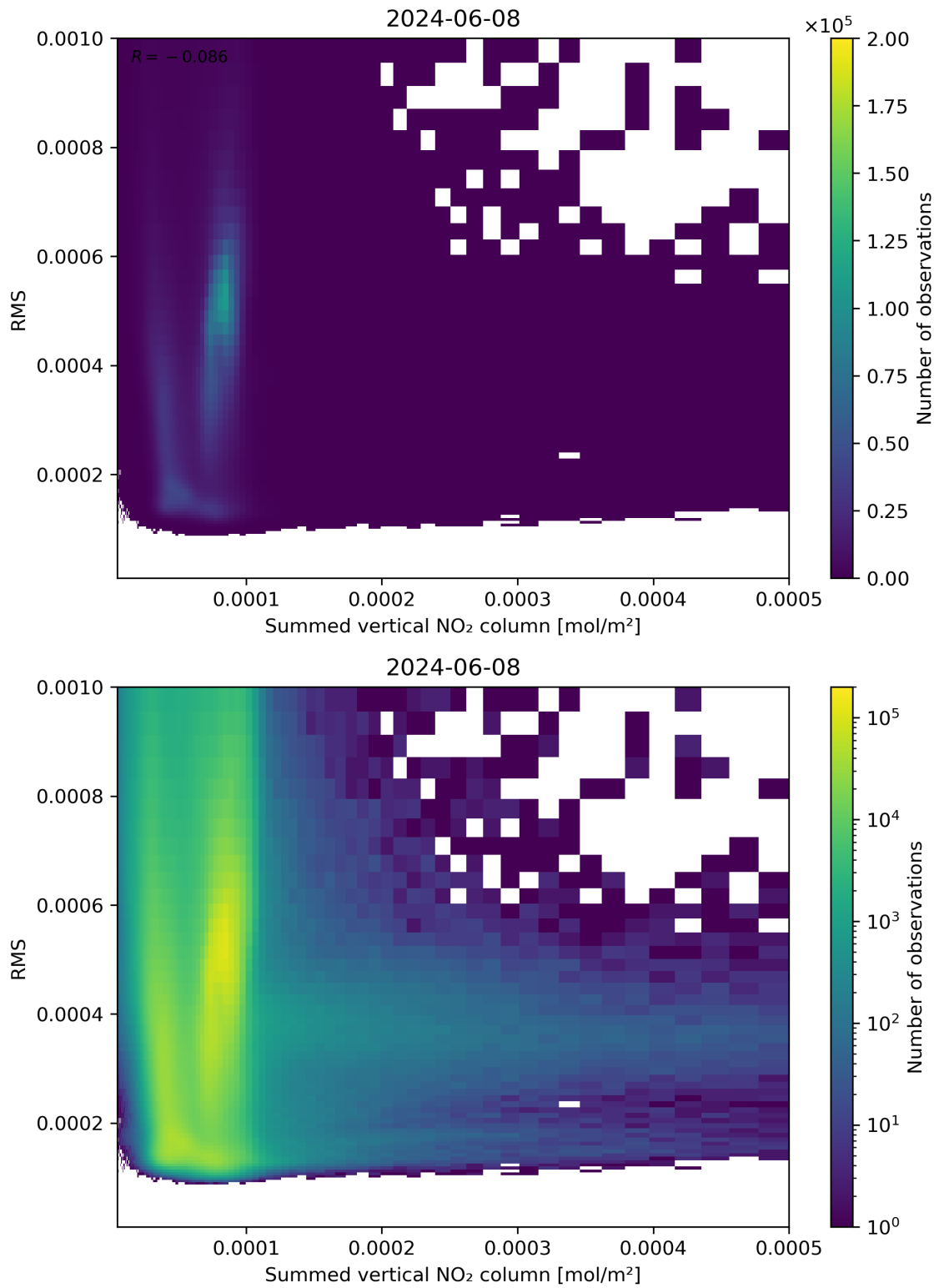
Figure 109: Scatter density plot of “Summed vertical NO 2 column” against “RMS” for 2024-06-08 to 2024-06-09.
