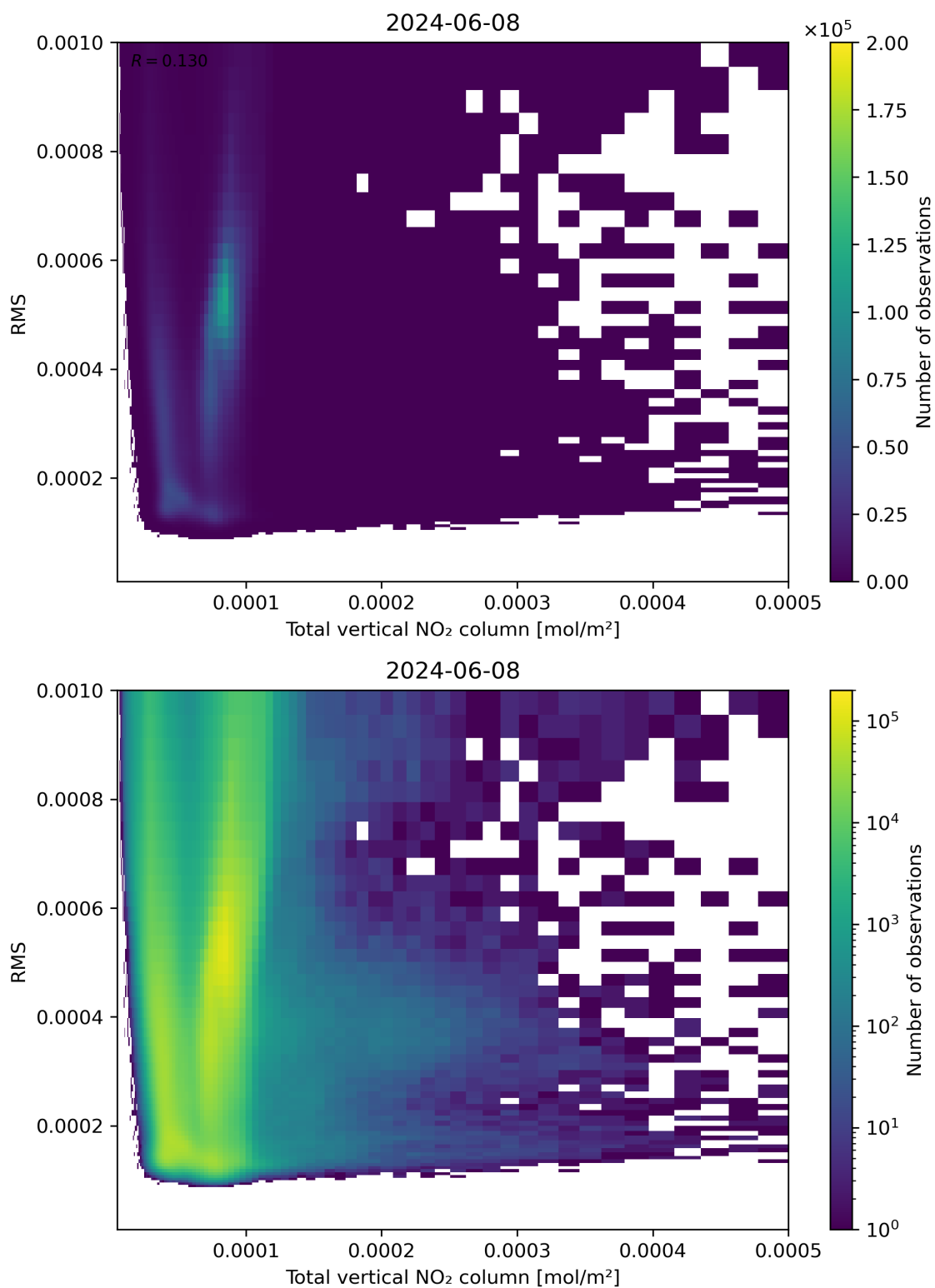
Figure 120: Scatter density plot of “Total vertical NO 2 column” against “RMS” for 2024-06-08 to 2024-06-09.
