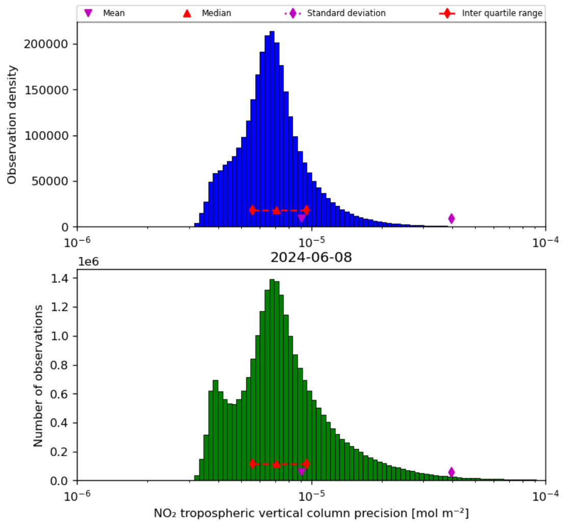
Figure 30: Histogram of “NO 2 tropospheric vertical column precision” for 2024-06-08 to 2024-06-09
