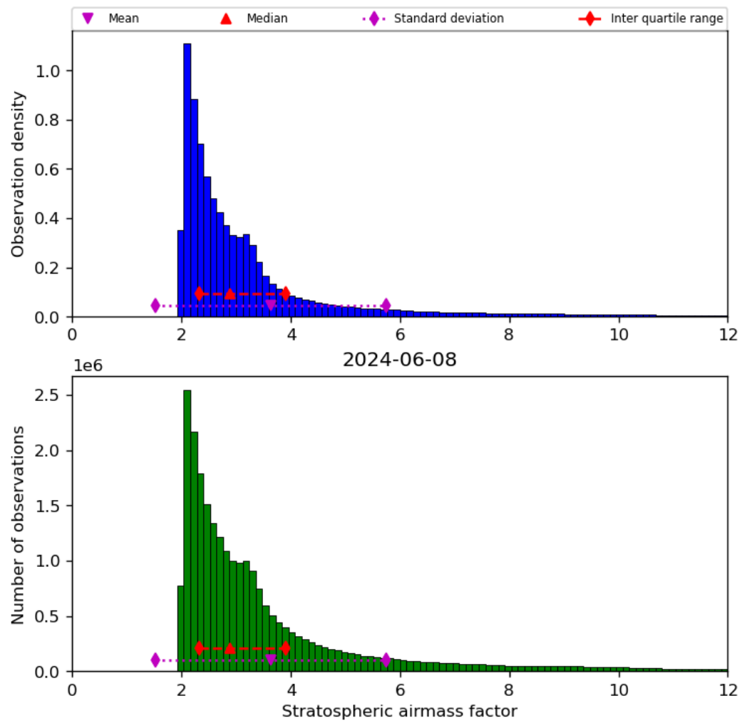
Figure 44: Histogram of “Stratospheric airmass factor” for 2024-06-08 to 2024-06-09
