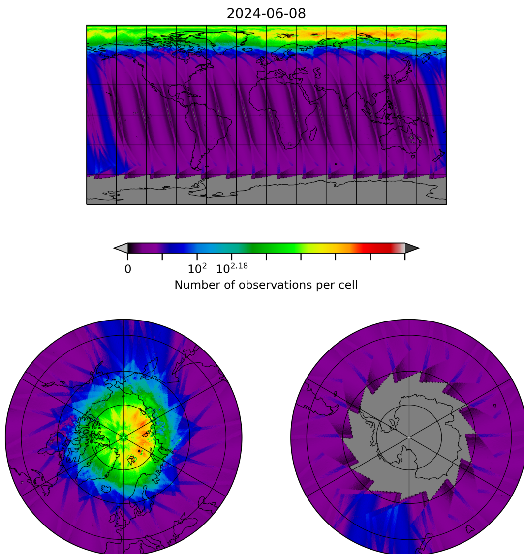
Figure 10: Map of the number of observations for 2024-06-08 to 2024-06-09
