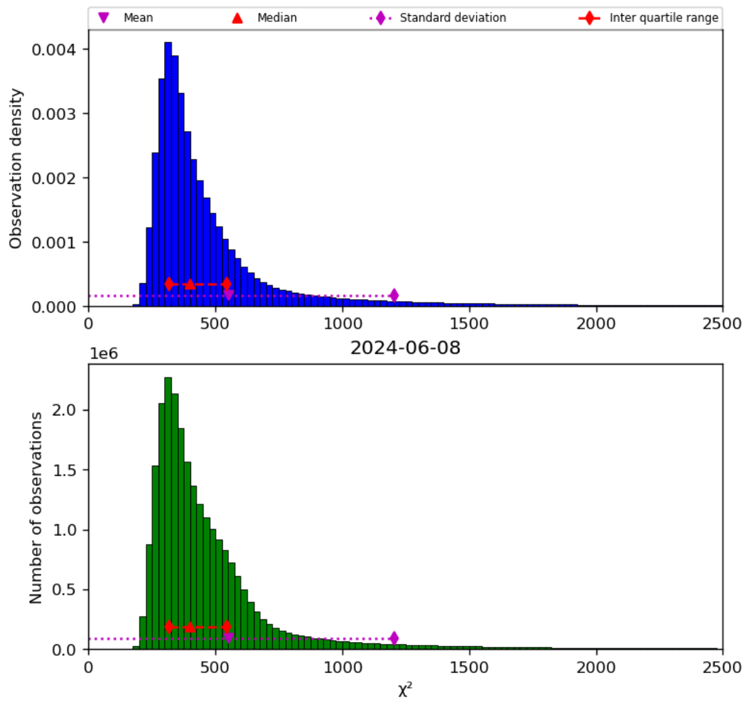
Figure 42: Histogram of “ \chi^2 ” for 2024-06-08 to 2024-06-09
