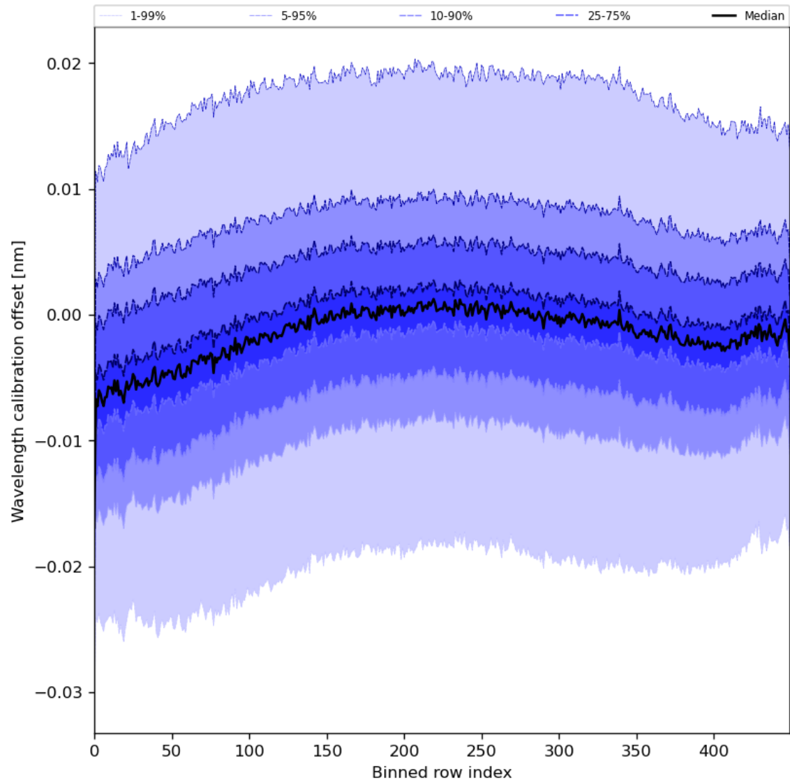
Figure 52: Along track statistics of “Wavelength calibration offset” for 2024-06-08 to 2024-06-09
