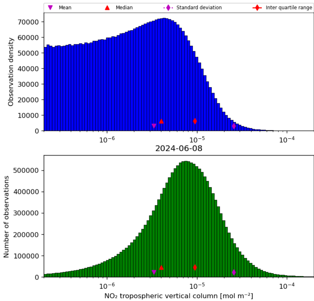
Figure 29: Histogram of “NO 2 tropospheric vertical column” for 2024-06-08 to 2024-06-09
