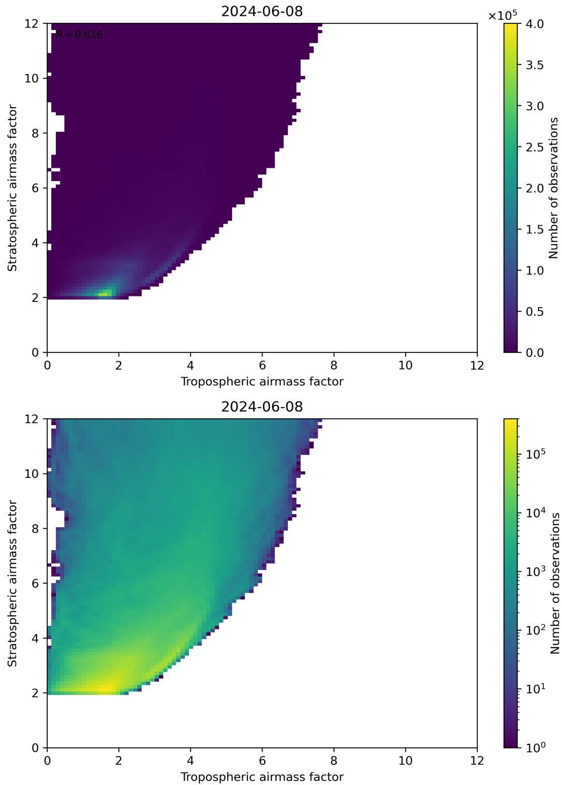
Figure 71: Scatter density plot of “Tropospheric airmass factor” against “Stratospheric airmass factor” for 2024-06-08 to 2024-06-09.
