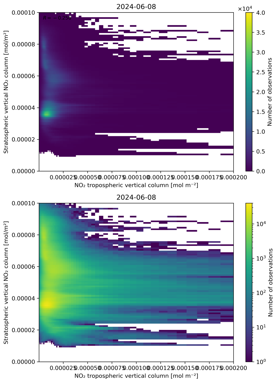
Figure 125: Scatter density plot of “NO 2 tropospheric vertical column” against “Stratospheric vertical NO 2 column” for 2024-06-08 to 2024-06-09.
