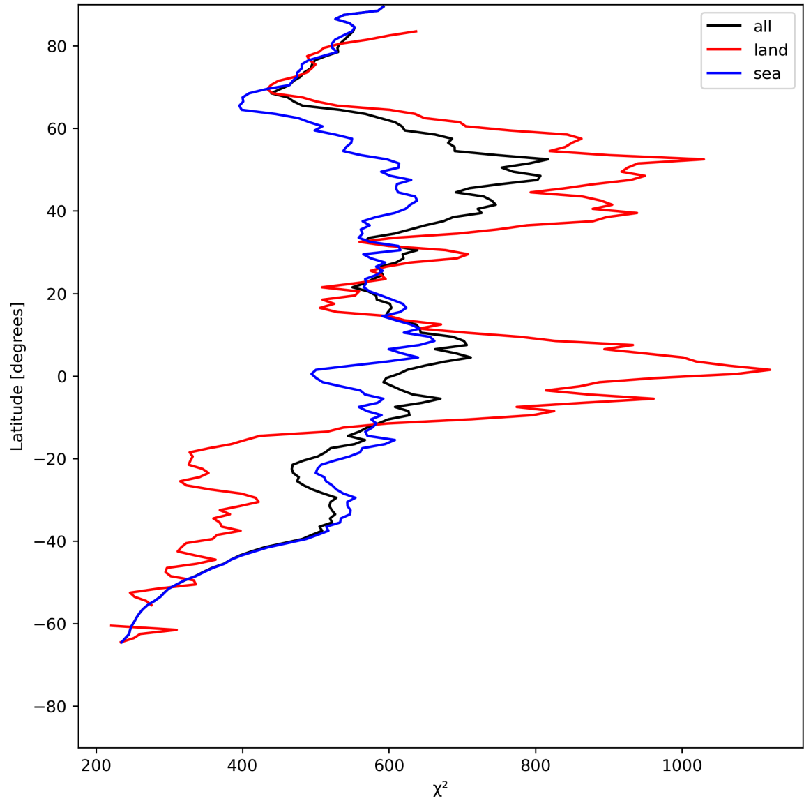
Figure 25: Zonal average of “ \chi^2 ” for 2024-06-08 to 2024-06-09.
