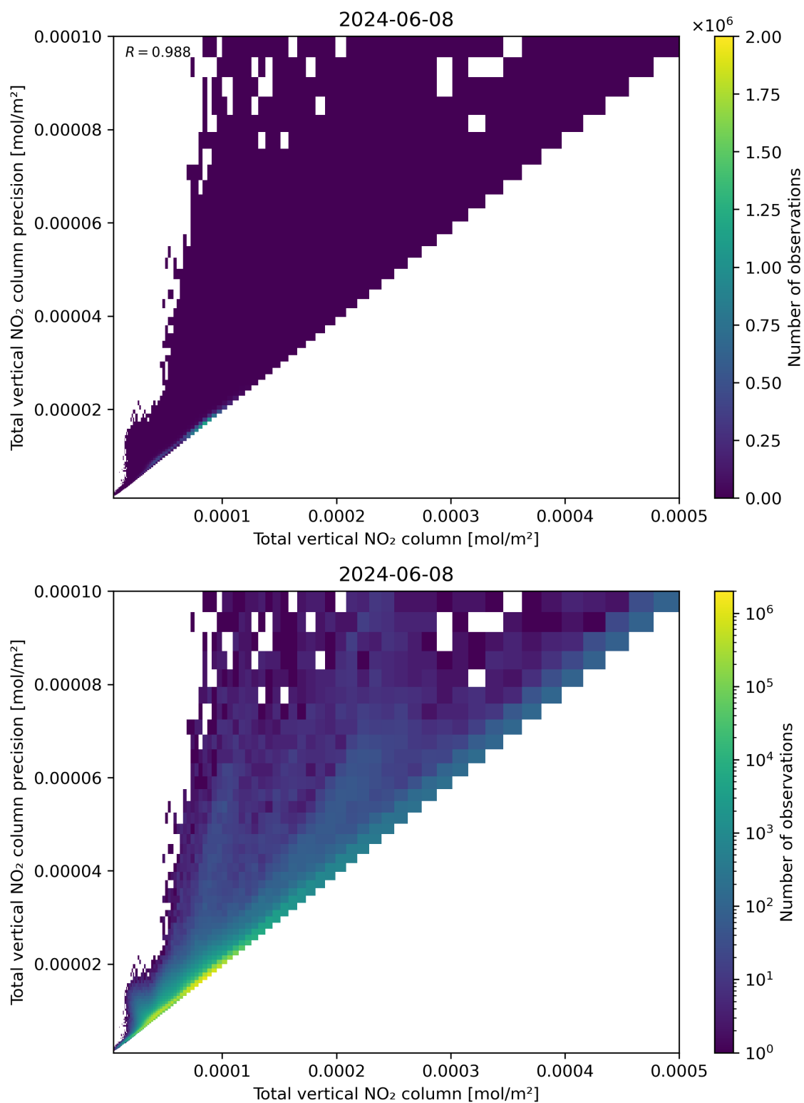
Figure 114: Scatter density plot of “Total vertical NO 2 column” against “Total vertical NO 2 column precision” for 2024-06-08 to 2024-06-09.
