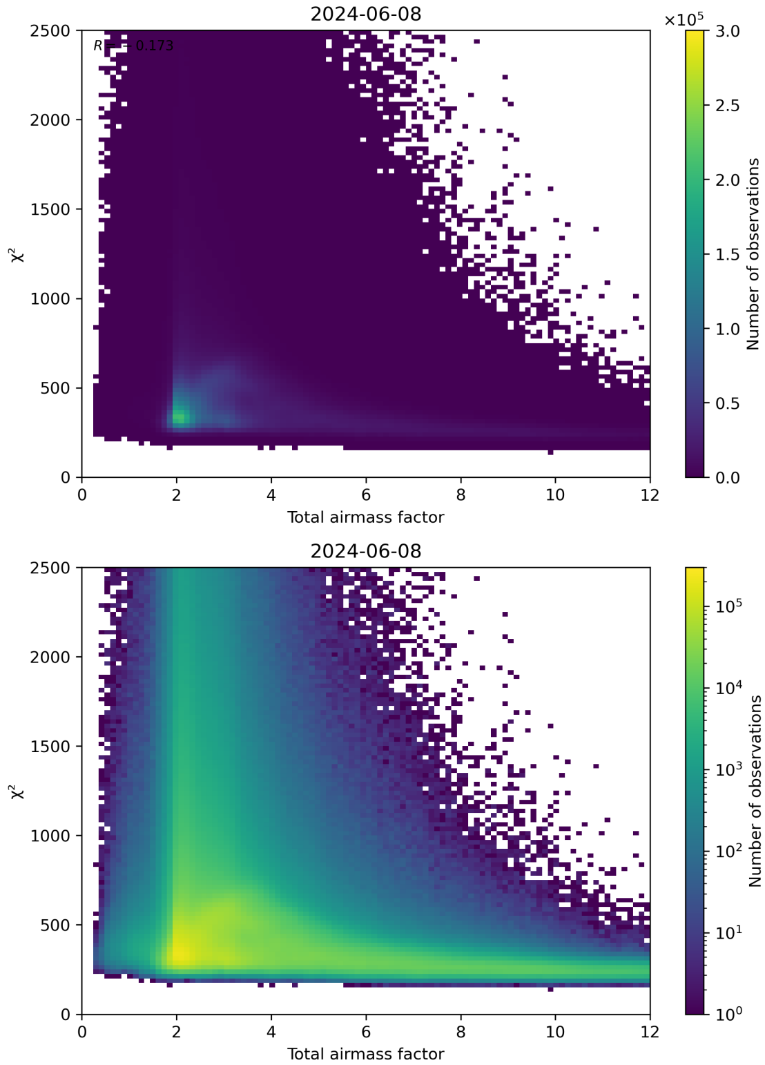
Figure 63: Scatter density plot of “Total airmass factor” against “ \chi^2 ” for 2024-06-08 to 2024-06-09.
