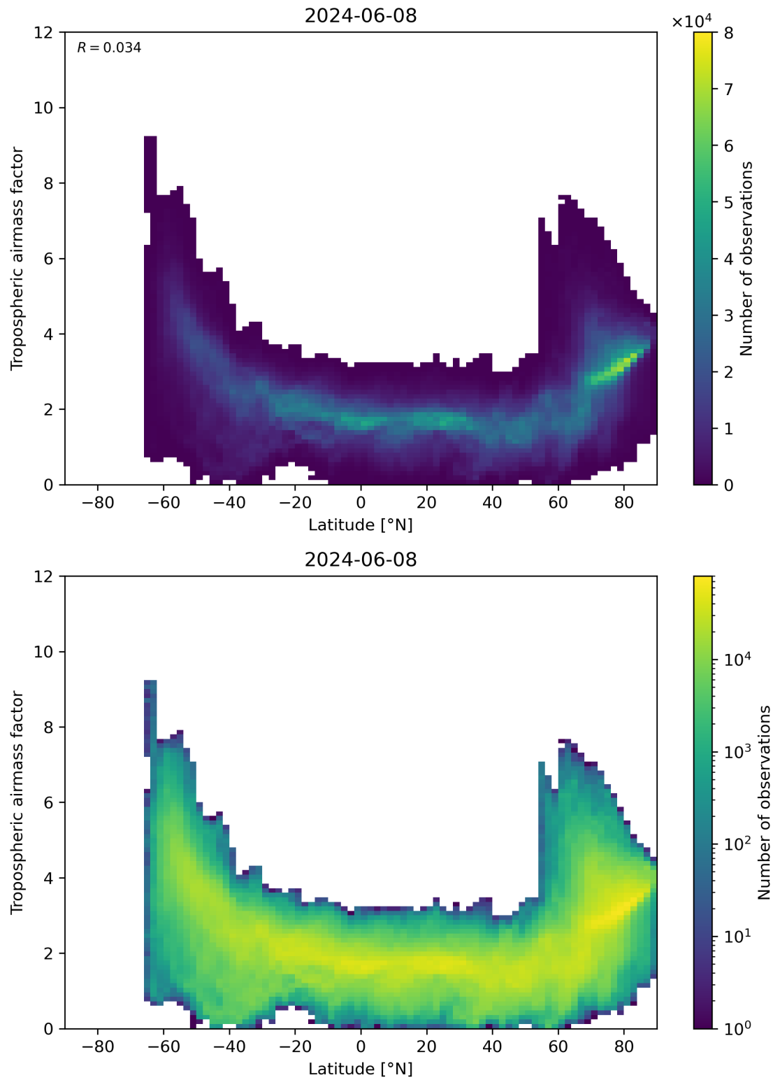
Figure 85: Scatter density plot of “Latitude” against “Tropospheric airmass factor” for 2024-06-08 to 2024-06-09.
