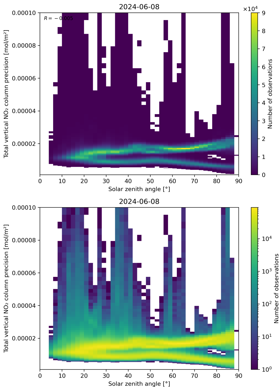
Figure 154: Scatter density plot of “Solar zenith angle” against “Total vertical NO 2 column precision” for 2024-06-08 to 2024-06-09.
