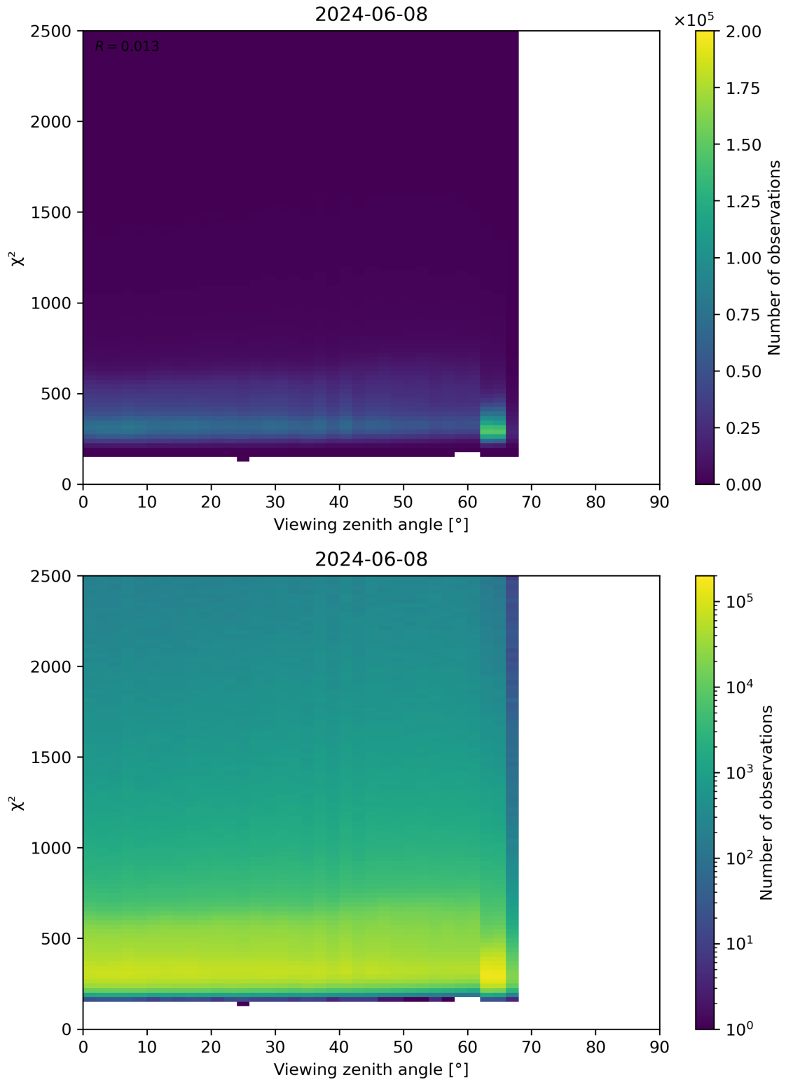
Figure 162: Scatter density plot of “Viewing zenith angle” against “ \chi^2 ” for 2024-06-08 to 2024-06-09.
