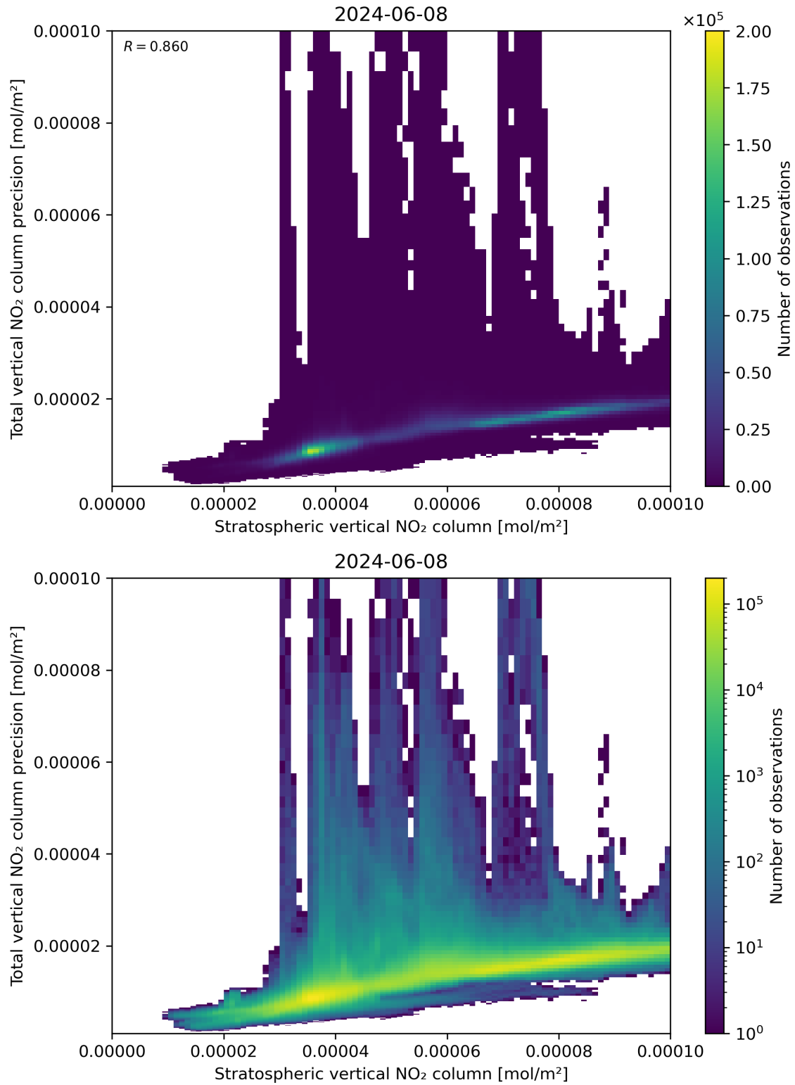
Figure 101: Scatter density plot of “Stratospheric vertical NO 2 column” against “Total vertical NO 2 column precision” for 2024-06-08 to 2024-06-09.
