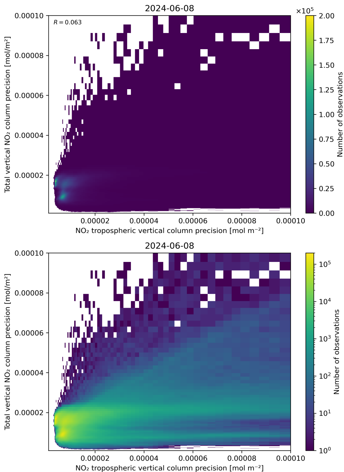
Figure 139: Scatter density plot of “NO 2 tropospheric vertical column precision” against “Total vertical NO 2 column precision” for 2024-06-08 to 2024-06-09.
