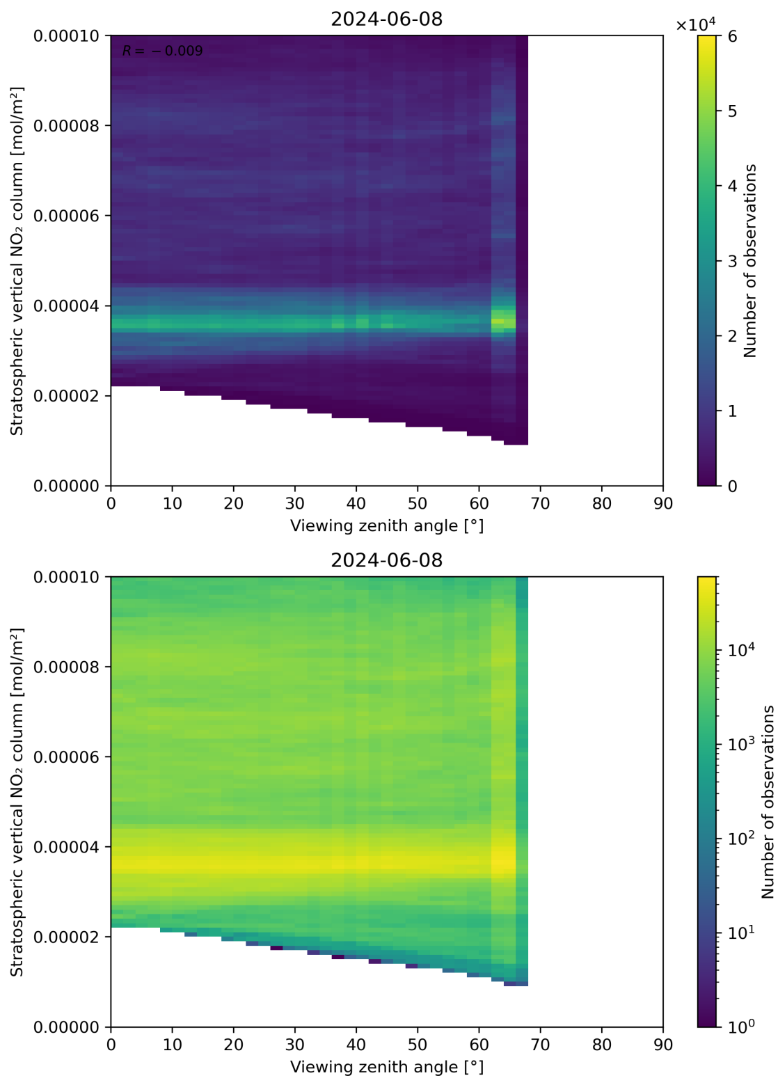
Figure 164: Scatter density plot of “Viewing zenith angle” against “Stratospheric vertical NO 2 column” for 2024-06-08 to 2024-06-09.
