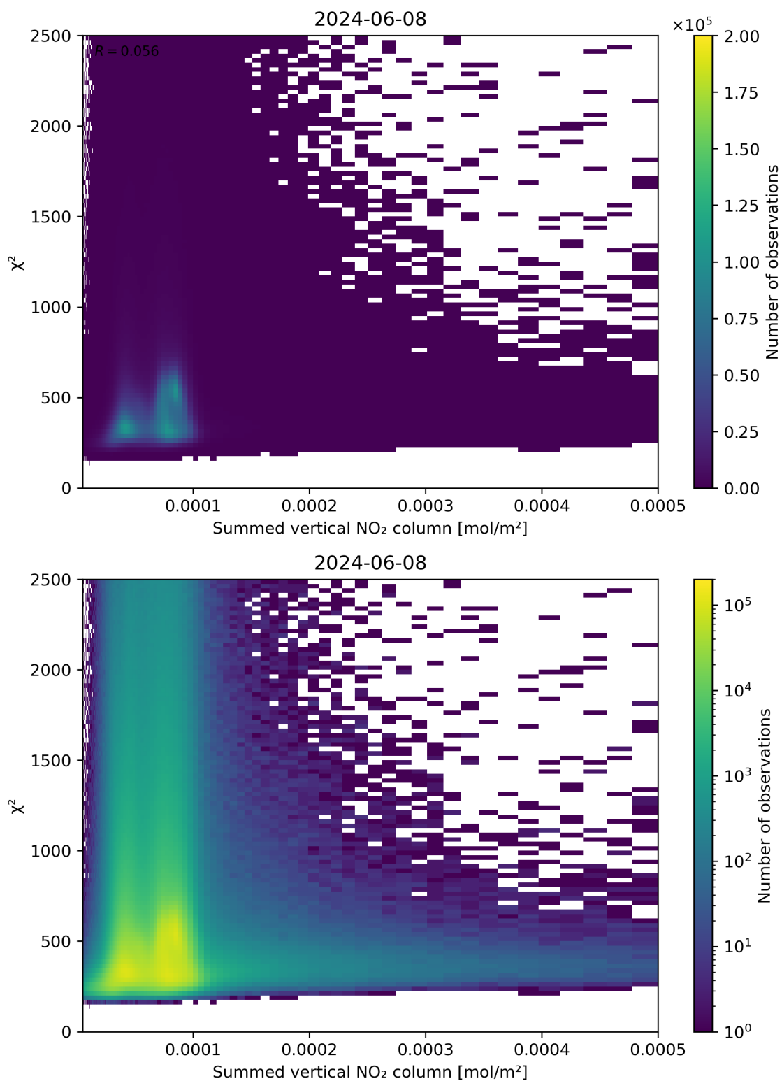
Figure 104: Scatter density plot of “Summed vertical NO 2 column” against “ \chi^2 ” for 2024-06-08 to 2024-06-09.
