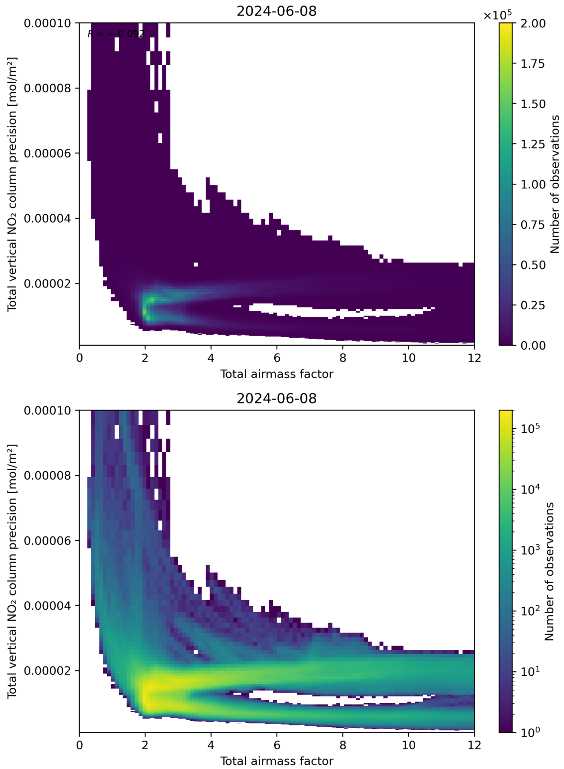
Figure 68: Scatter density plot of “Total airmass factor” against “Total vertical NO 2 column precision” for 2024-06-08 to 2024-06-09.
