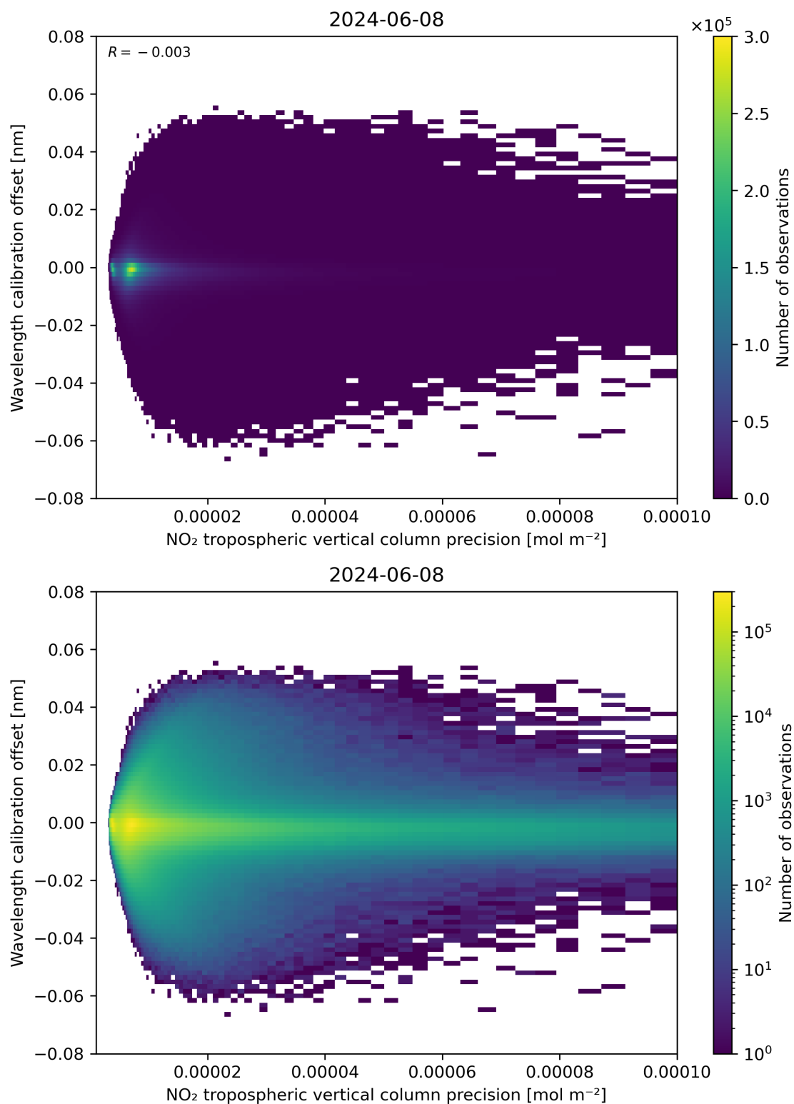
Figure 141: Scatter density plot of “NO 2 tropospheric vertical column precision” against “Wavelength calibration offset” for 2024-06-08 to 2024-06-09.
