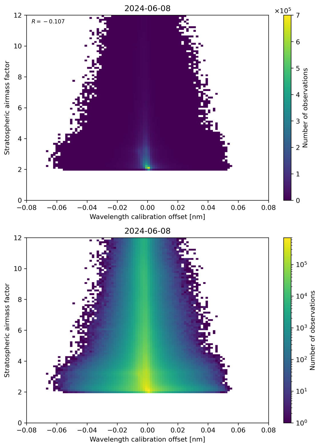
Figure 174: Scatter density plot of “Wavelength calibration offset” against “Stratospheric airmass factor” for 2024-06-08 to 2024-06-09.
