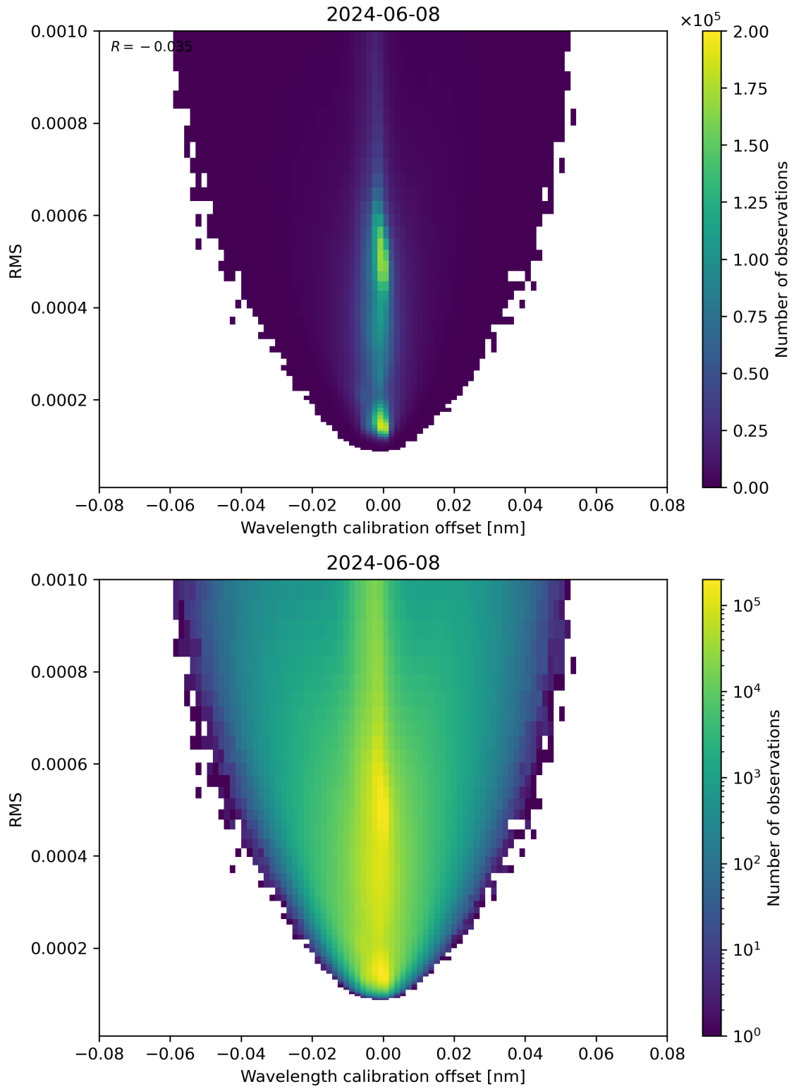
Figure 181: Scatter density plot of “Wavelength calibration offset” against “RMS” for 2024-06-08 to 2024-06-09.
