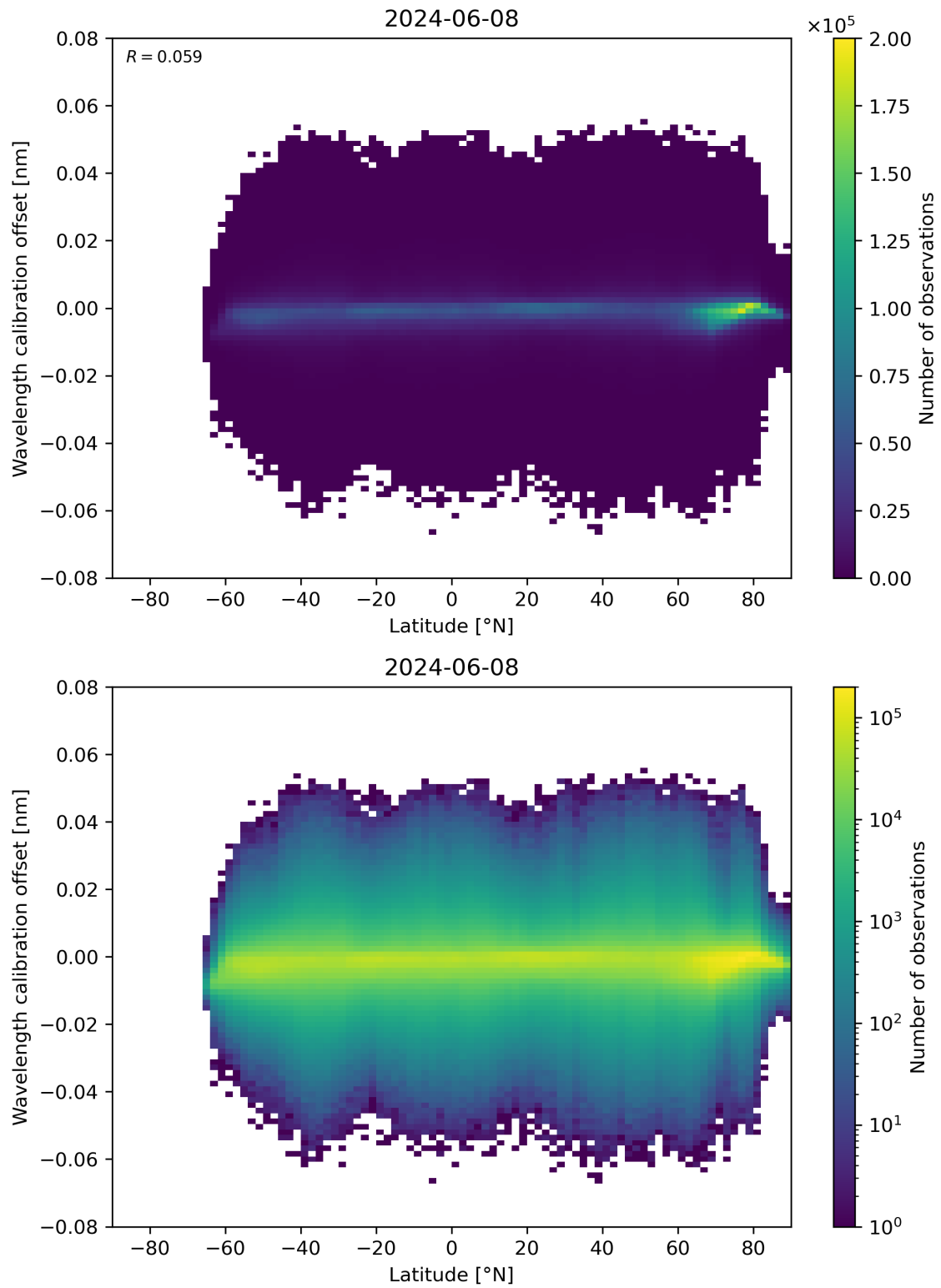
Figure 95: Scatter density plot of “Latitude” against “Wavelength calibration offset” for 2024-06-08 to 2024-06-09.
