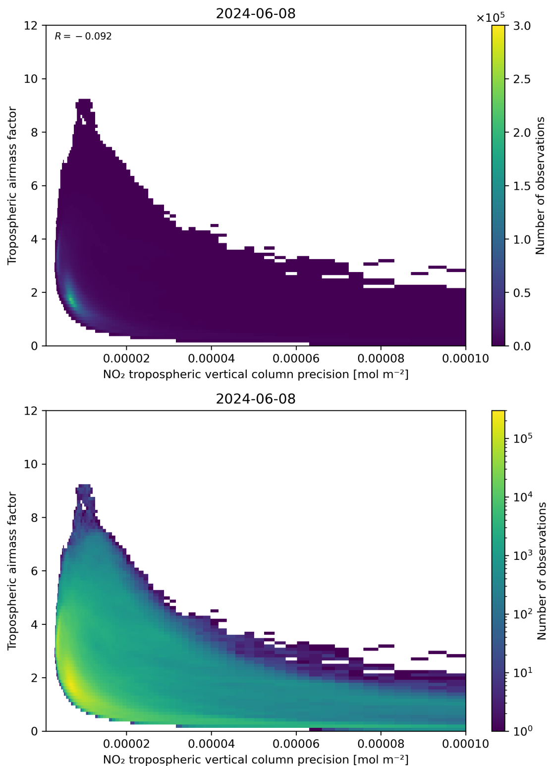
Figure 133: Scatter density plot of “NO 2 tropospheric vertical column precision” against “Tropospheric airmass factor” for 2024-06-08 to 2024-06-09.
