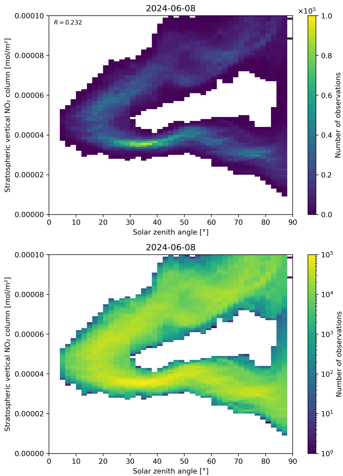
Figure 150: Scatter density plot of “Solar zenith angle” against “Stratospheric vertical NO 2 column” for 2024-06-08 to 2024-06-09.
