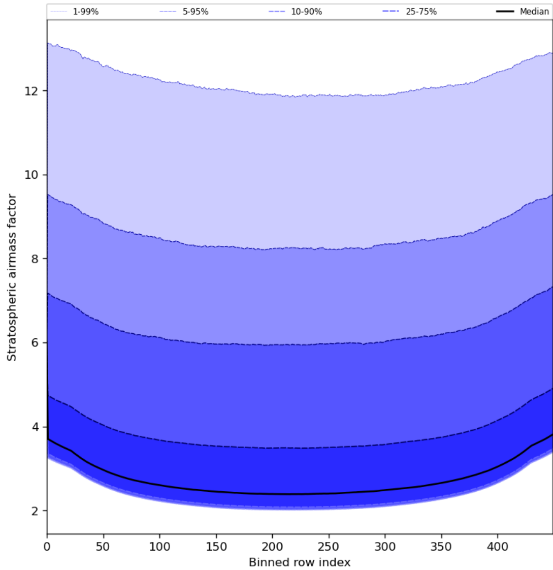
Figure 61: Along track statistics of “Stratospheric airmass factor” for 2024-06-08 to 2024-06-09
