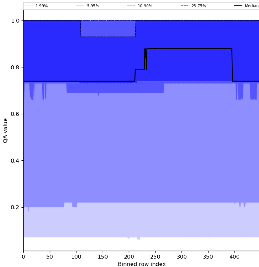
Figure 45: Along track statistics of “QA value” for 2024-06-08 to 2024-06-09
