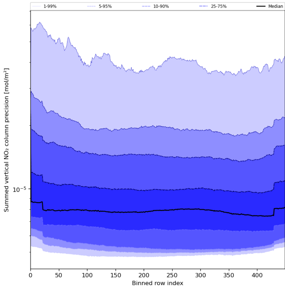
Figure 58: Along track statistics of “Summed vertical NO 2 column precision” for 2024-06-08 to 2024-06-09
