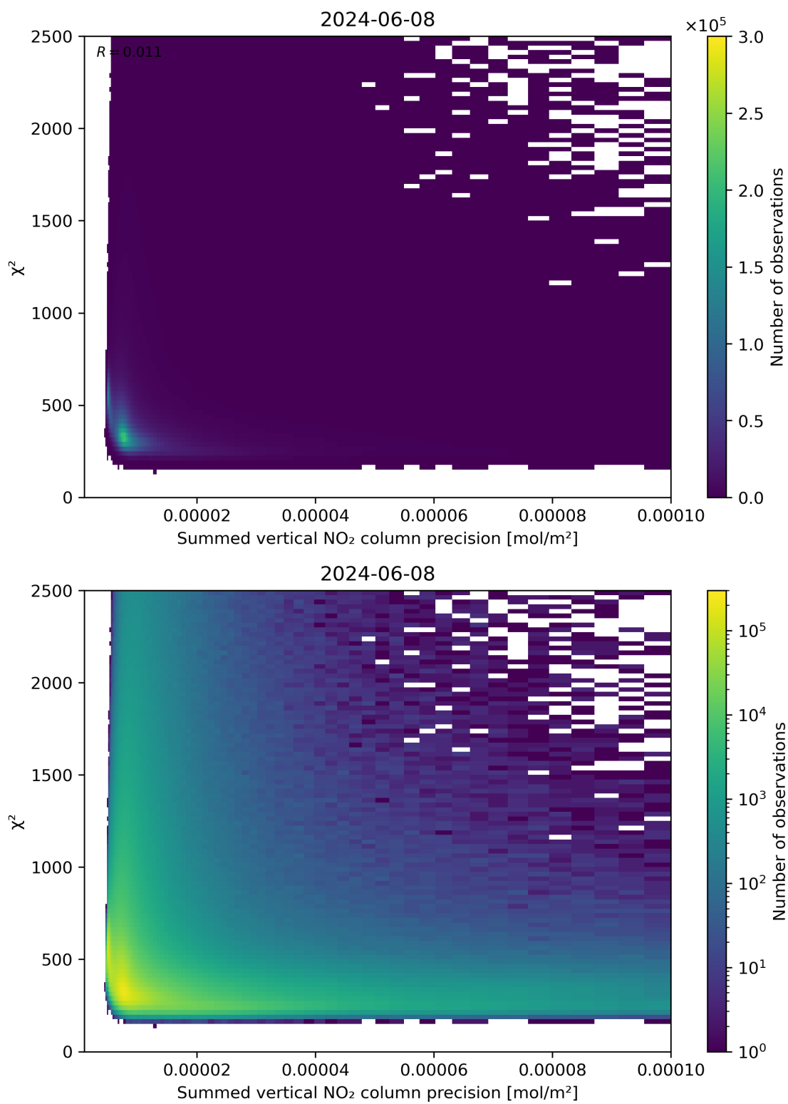
Figure 107: Scatter density plot of “Summed vertical NO 2 column precision” against “ \chi^2 ” for 2024-06-08 to 2024-06-09.
