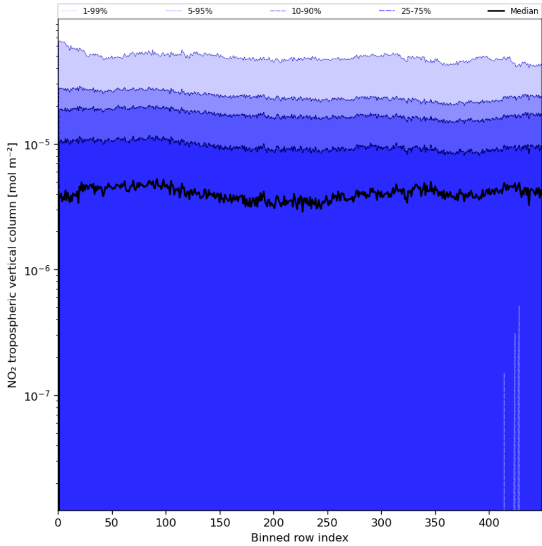
Figure 46: Along track statistics of “NO 2 tropospheric vertical column” for 2024-06-08 to 2024-06-09
