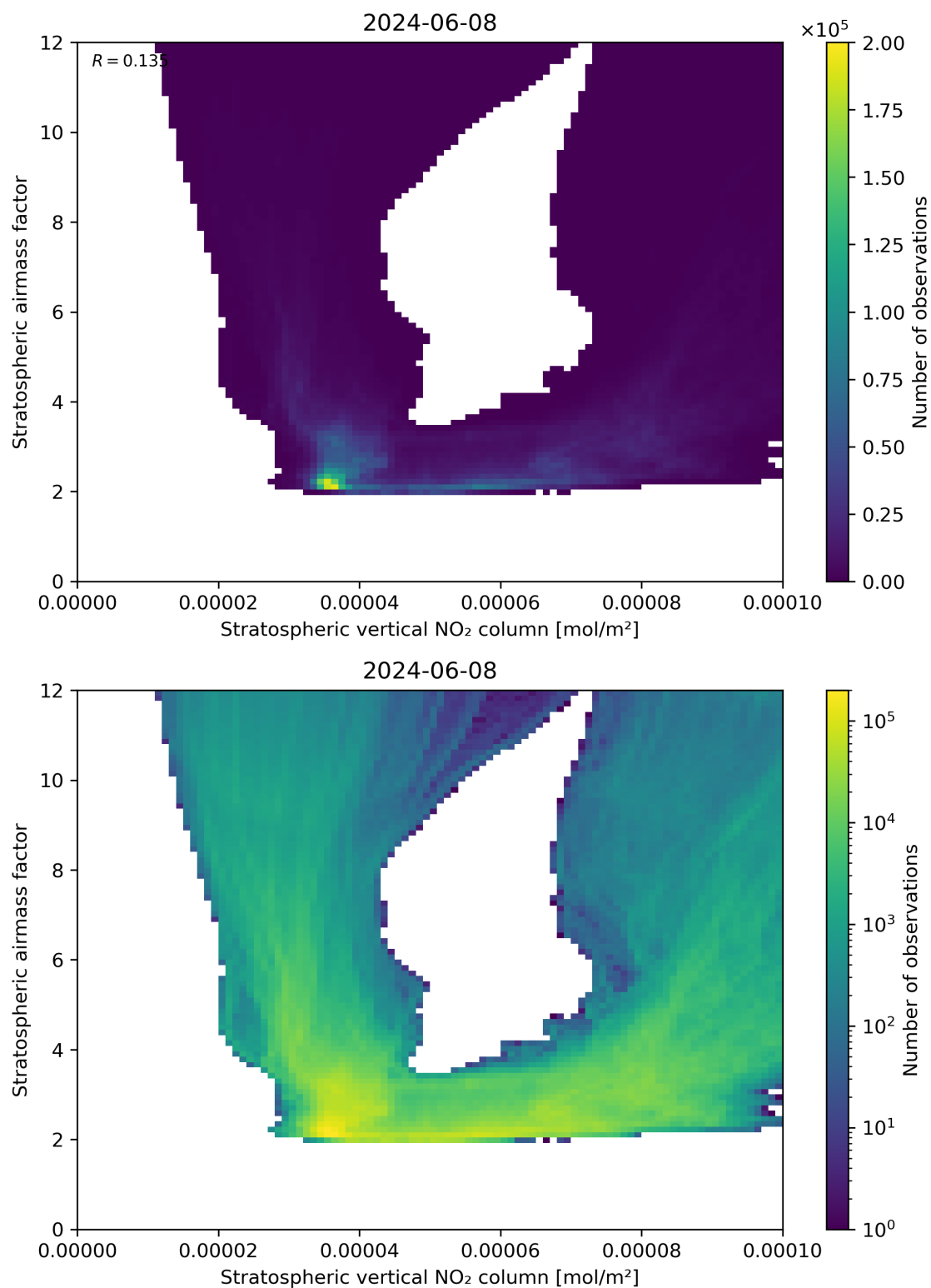
Figure 96: Scatter density plot of “Stratospheric vertical NO 2 column” against “Stratospheric airmass factor” for 2024-06-08 to 2024-06-09.
