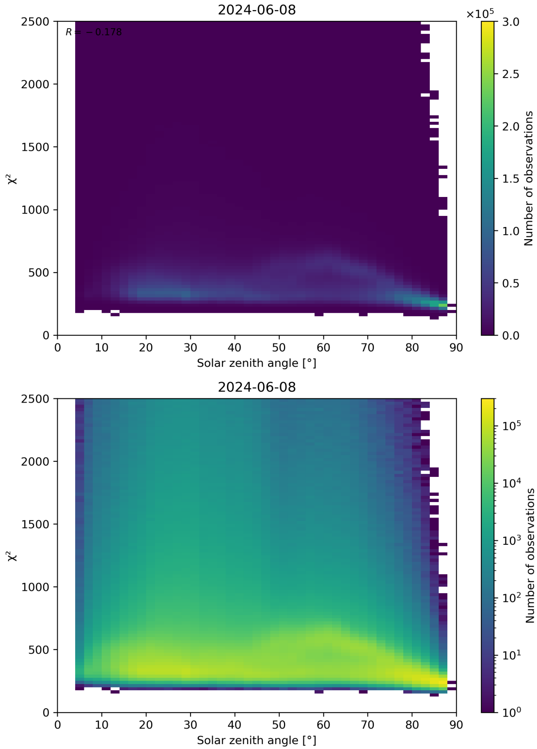
Figure 148: Scatter density plot of “Solar zenith angle” against “ \chi^2 ” for 2024-06-08 to 2024-06-09.
