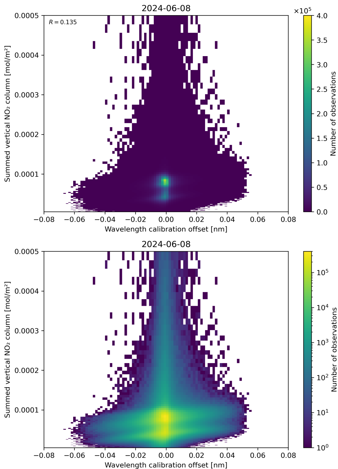
Figure 177: Scatter density plot of “Wavelength calibration offset” against “Summed vertical NO 2 column” for 2024-06-08 to 2024-06-09.
