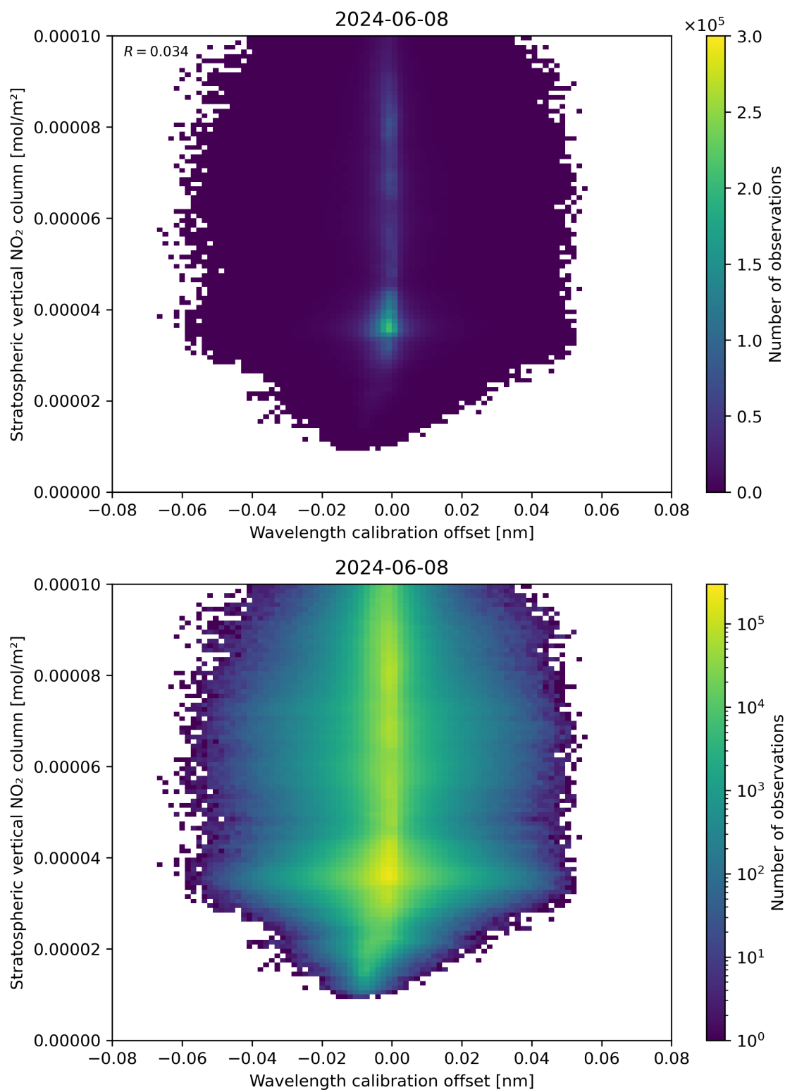
Figure 176: Scatter density plot of “Wavelength calibration offset” against “Stratospheric vertical NO 2 column” for 2024-06-08 to 2024-06-09.
