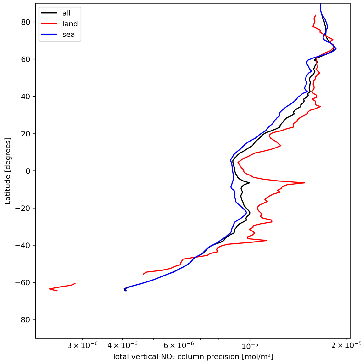
Figure 22: Zonal average of “Total vertical NO 2 column precision” for 2024-06-08 to 2024-06-09.
