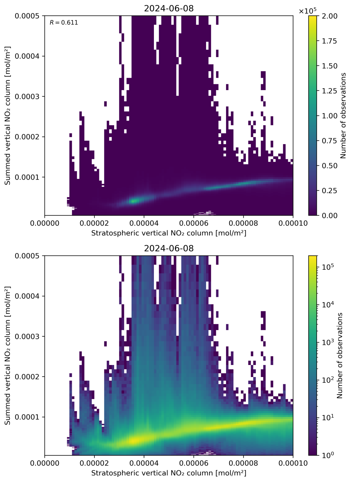
Figure 98: Scatter density plot of “Stratospheric vertical NO 2 column” against “Summed vertical NO 2 column” for 2024-06-08 to 2024-06-09.
