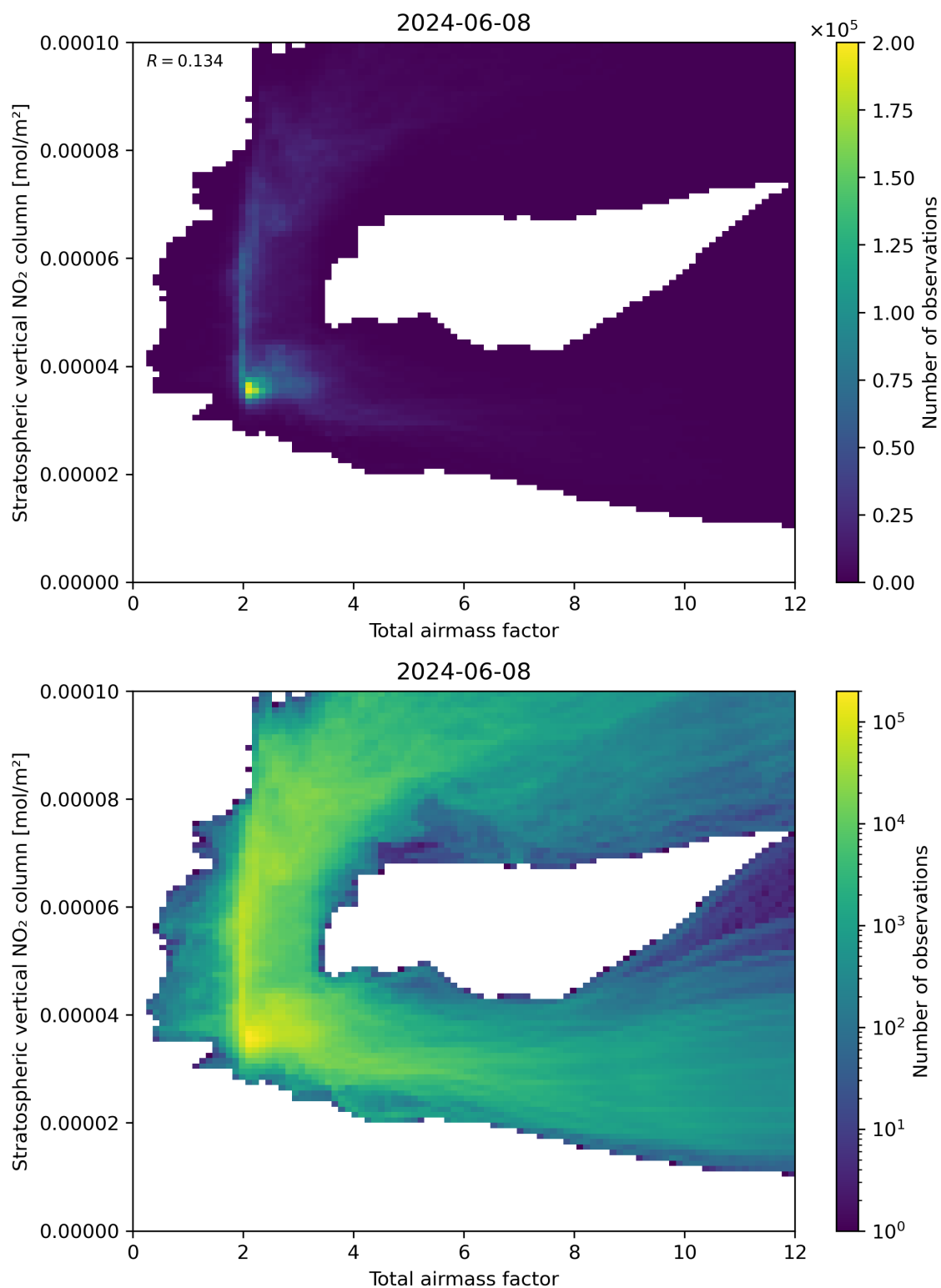
Figure 64: Scatter density plot of “Total airmass factor” against “Stratospheric vertical \text{NO}_2 column” for 2024-06-08 to 2024-06-09.
