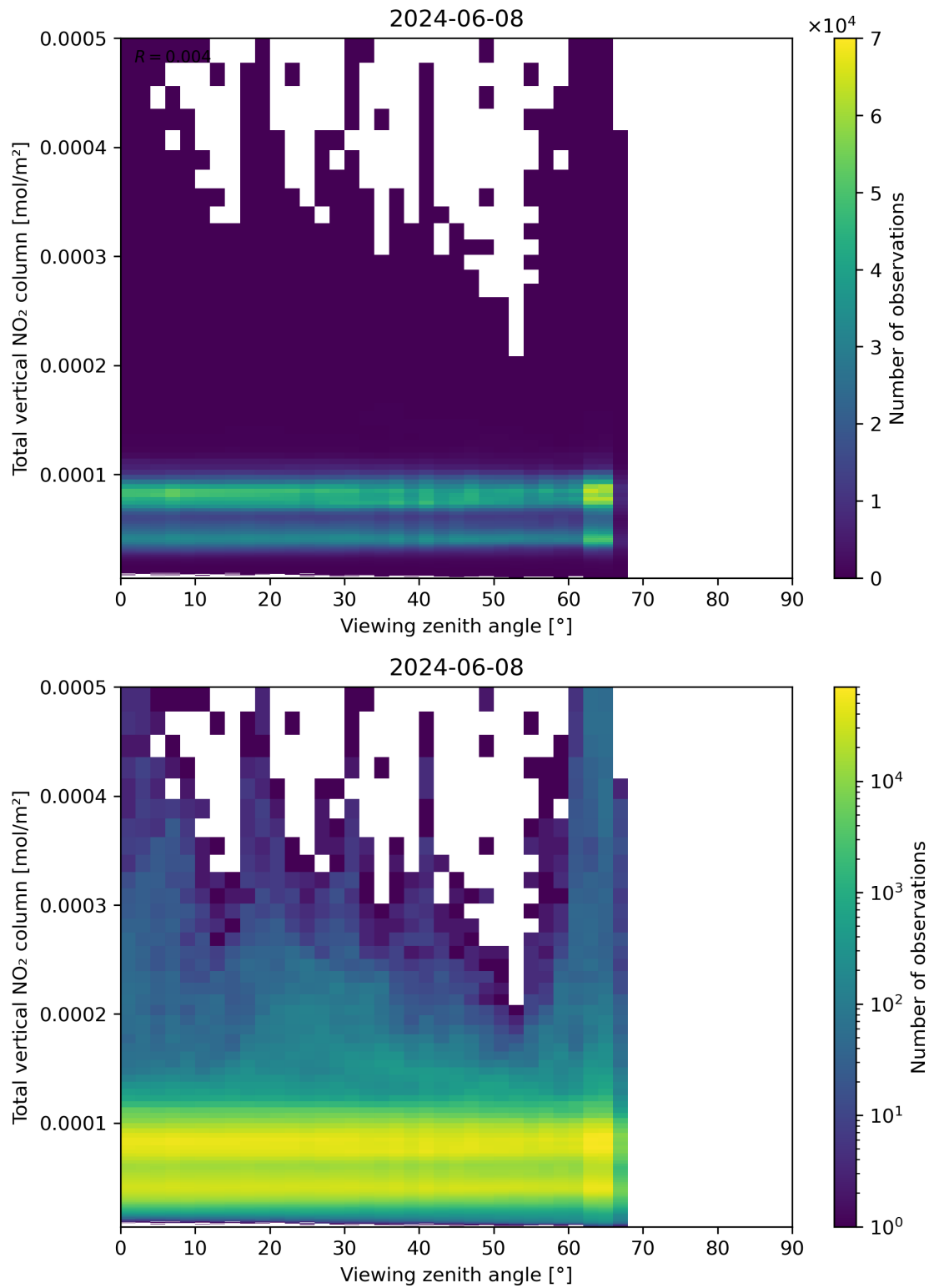
Figure 167: Scatter density plot of “Viewing zenith angle” against “Total vertical NO 2 column” for 2024-06-08 to 2024-06-09.
