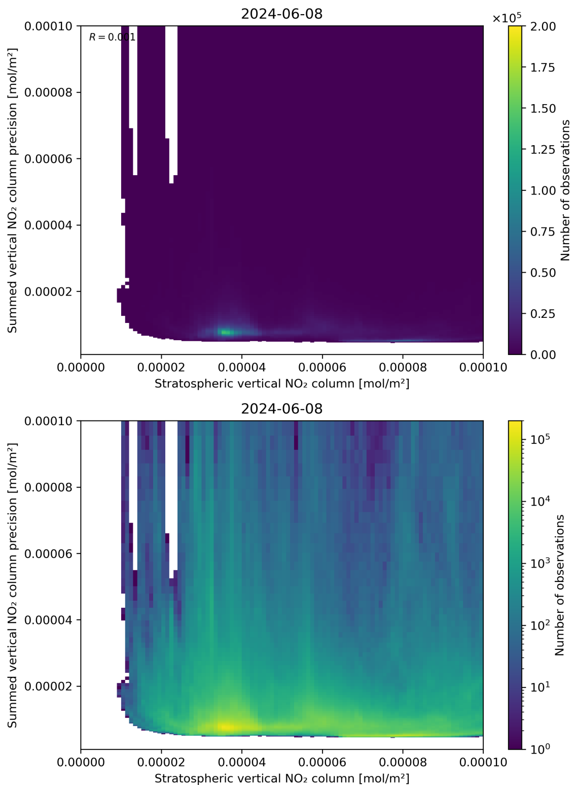
Figure 99: Scatter density plot of “Stratospheric vertical NO 2 column” against “Summed vertical NO 2 column precision” for 2024-06-08 to 2024-06-09.
