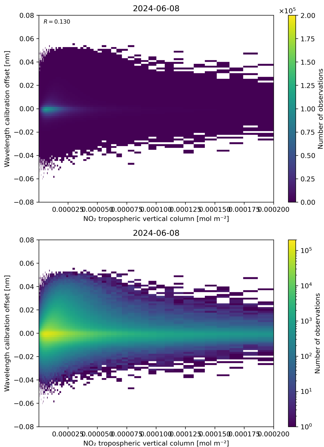
Figure 143: Scatter density plot of “NO 2 tropospheric vertical column” against “Wavelength calibration offset” for 2024-06-08 to 2024-06-09.
