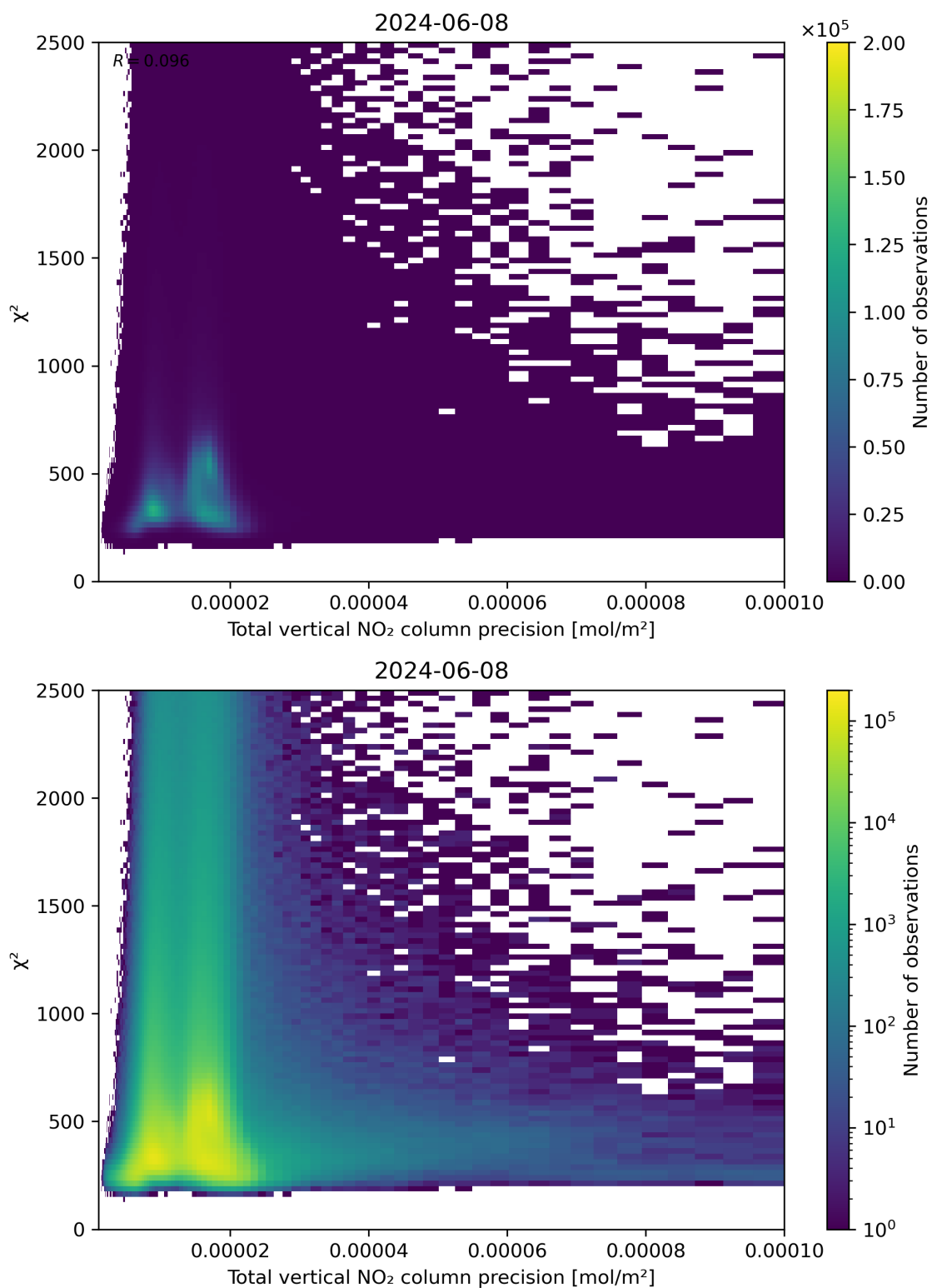
Figure 116: Scatter density plot of “Total vertical NO 2 column precision” against “ \chi^2 ” for 2024-06-08 to 2024-06-09.
