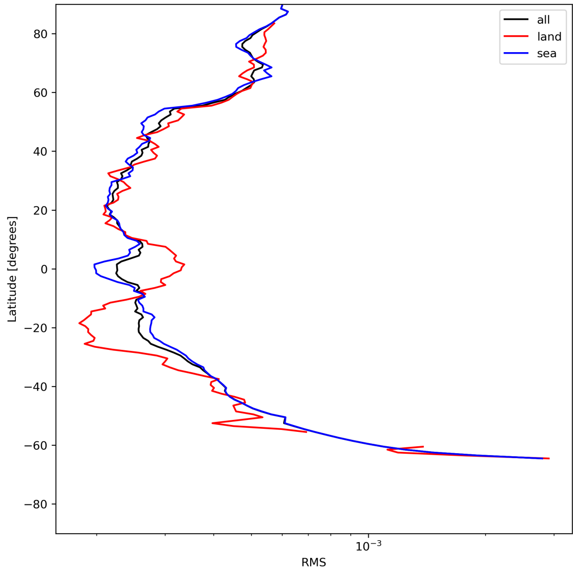
Figure 26: Zonal average of “RMS” for 2024-06-08 to 2024-06-09.
