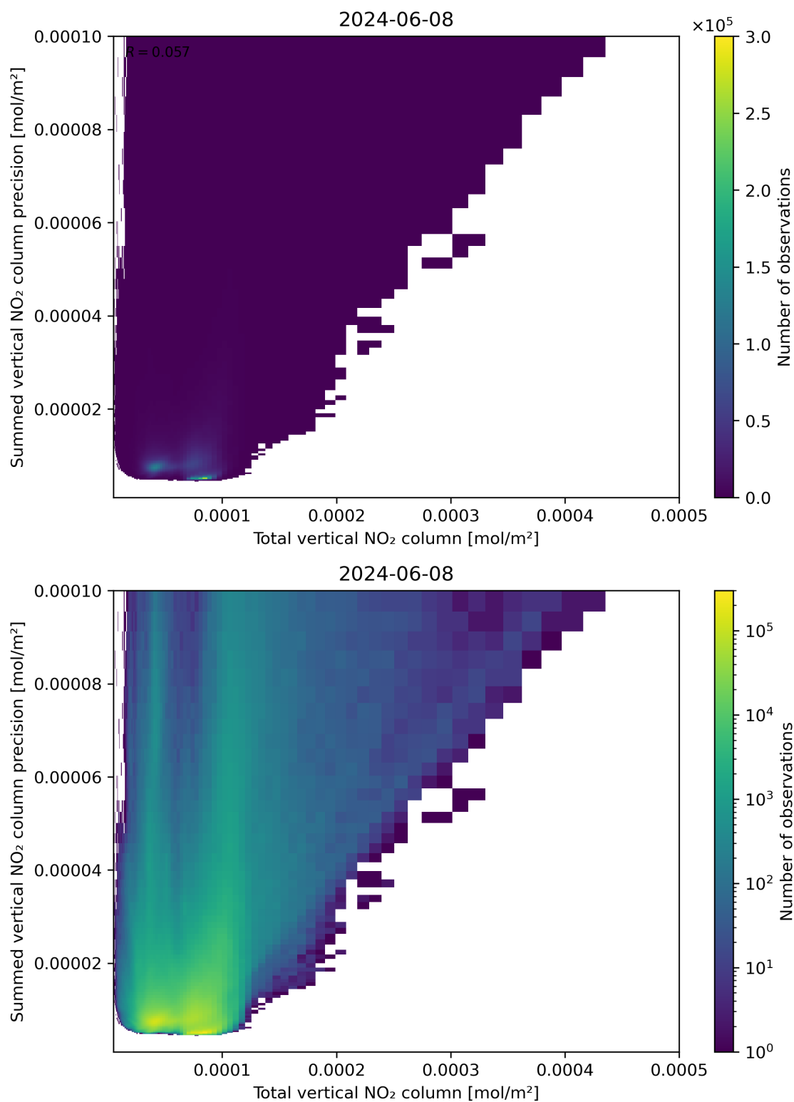
Figure 113: Scatter density plot of “Total vertical NO 2 column” against “Summed vertical NO 2 column precision” for 2024-06-08 to 2024-06-09.
