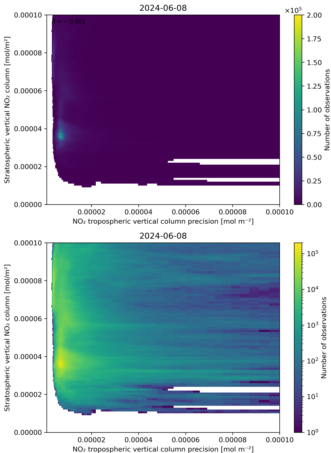
Figure 135: Scatter density plot of “NO 2 tropospheric vertical column precision” against “Stratospheric vertical NO 2 column” for 2024-06-08 to 2024-06-09.
