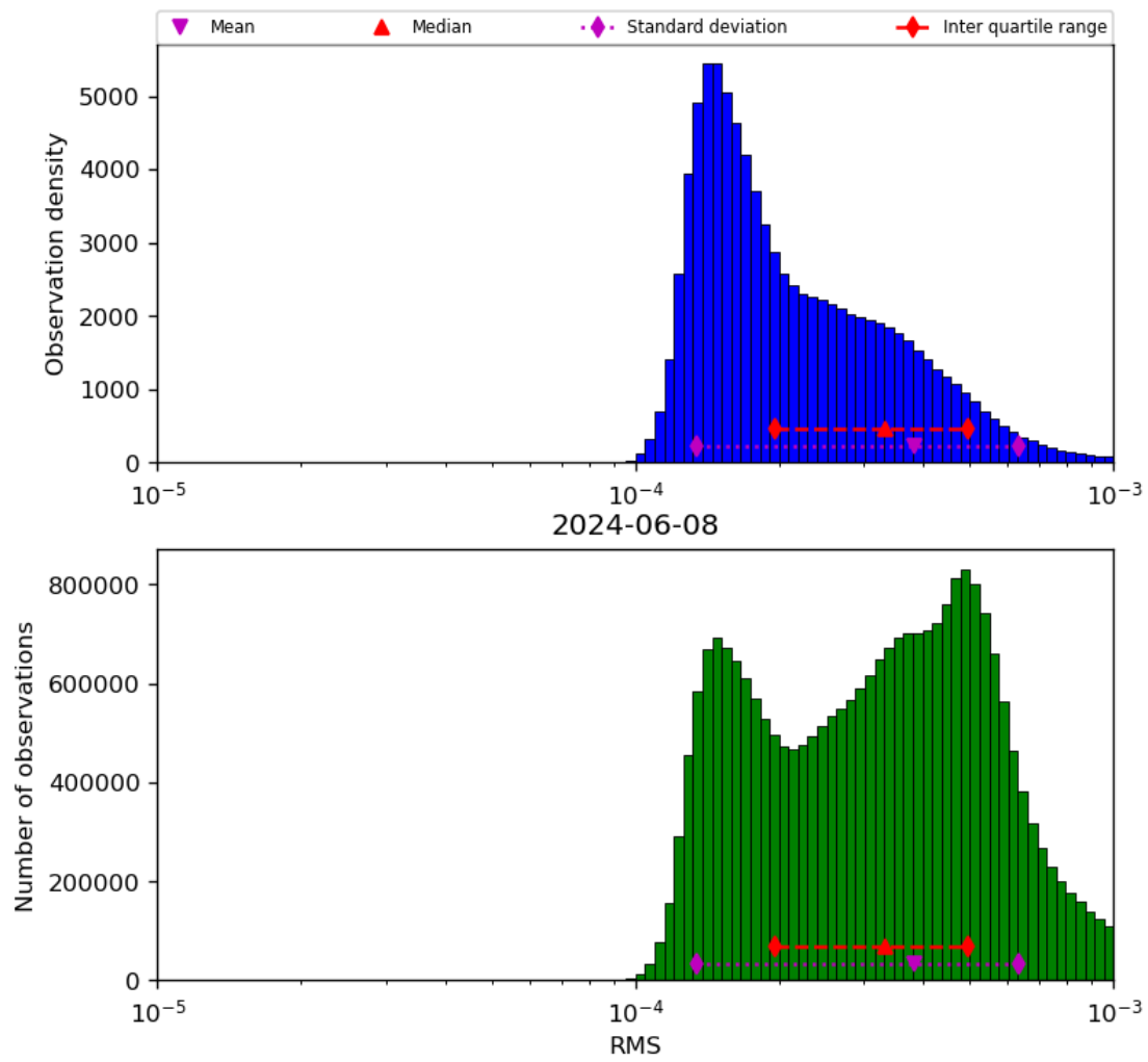
Figure 43: Histogram of “RMS” for 2024-06-08 to 2024-06-09
