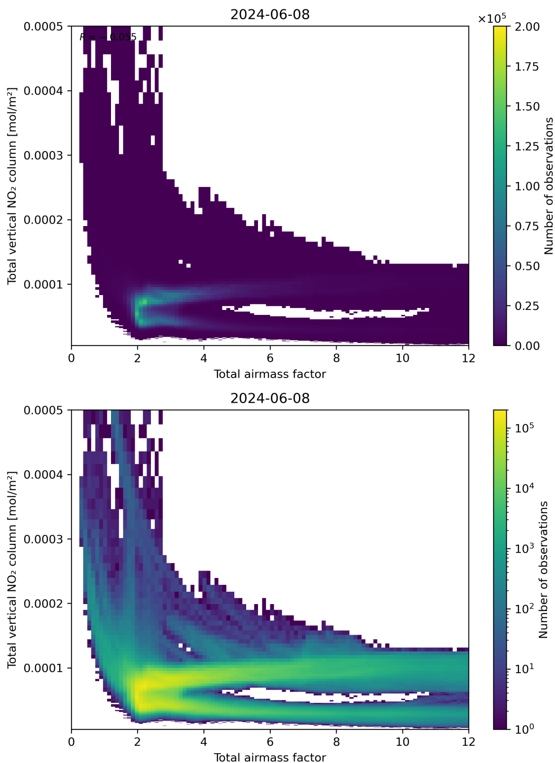
Figure 67: Scatter density plot of “Total airmass factor” against “Total vertical NO 2 column” for 2024-06-08 to 2024-06-09.
