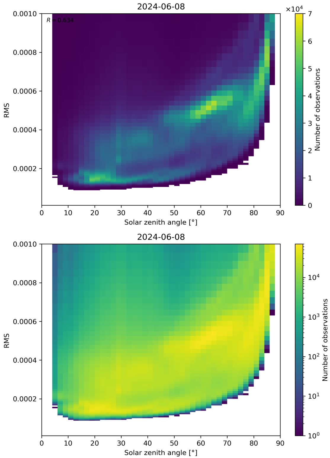
Figure 157: Scatter density plot of “Solar zenith angle” against “RMS” for 2024-06-08 to 2024-06-09.
