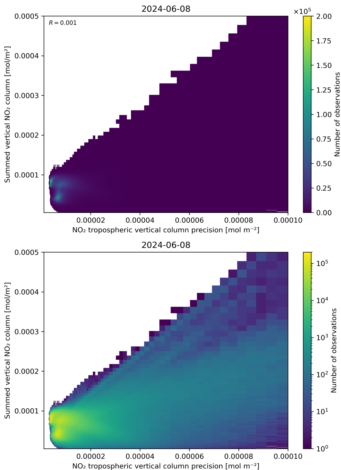
Figure 136: Scatter density plot of “NO 2 tropospheric vertical column precision” against “Summed vertical NO 2 column” for 2024-06-08 to 2024-06-09.
