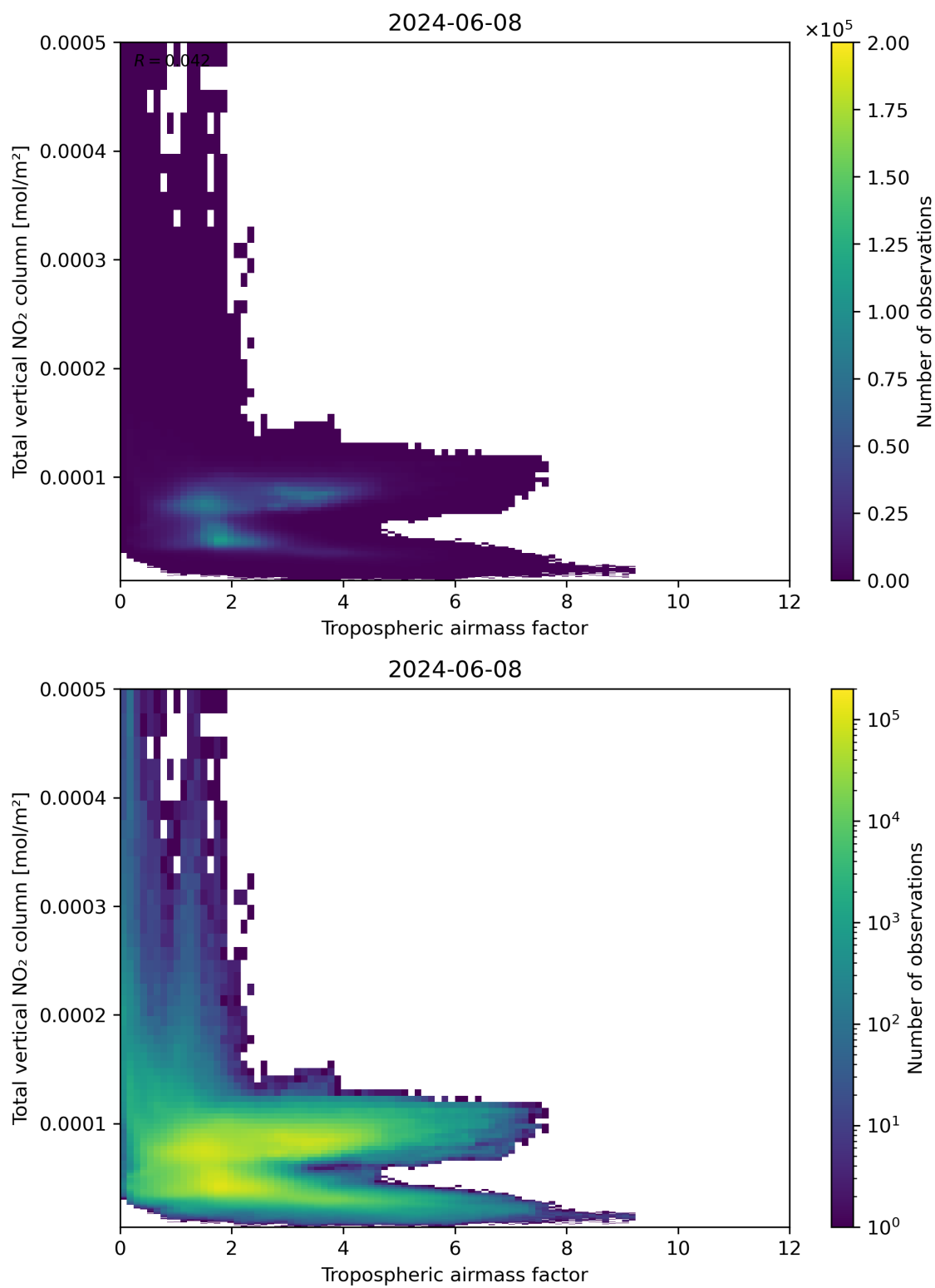
Figure 77: Scatter density plot of “Tropospheric airmass factor” against “Total vertical NO 2 column” for 2024-06-08 to 2024-06-09.
