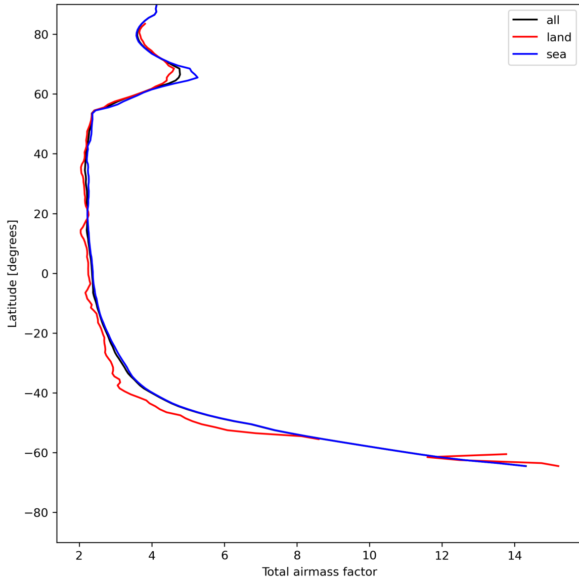
Figure 15: Zonal average of “Total airmass factor” for 2024-06-08 to 2024-06-09.
