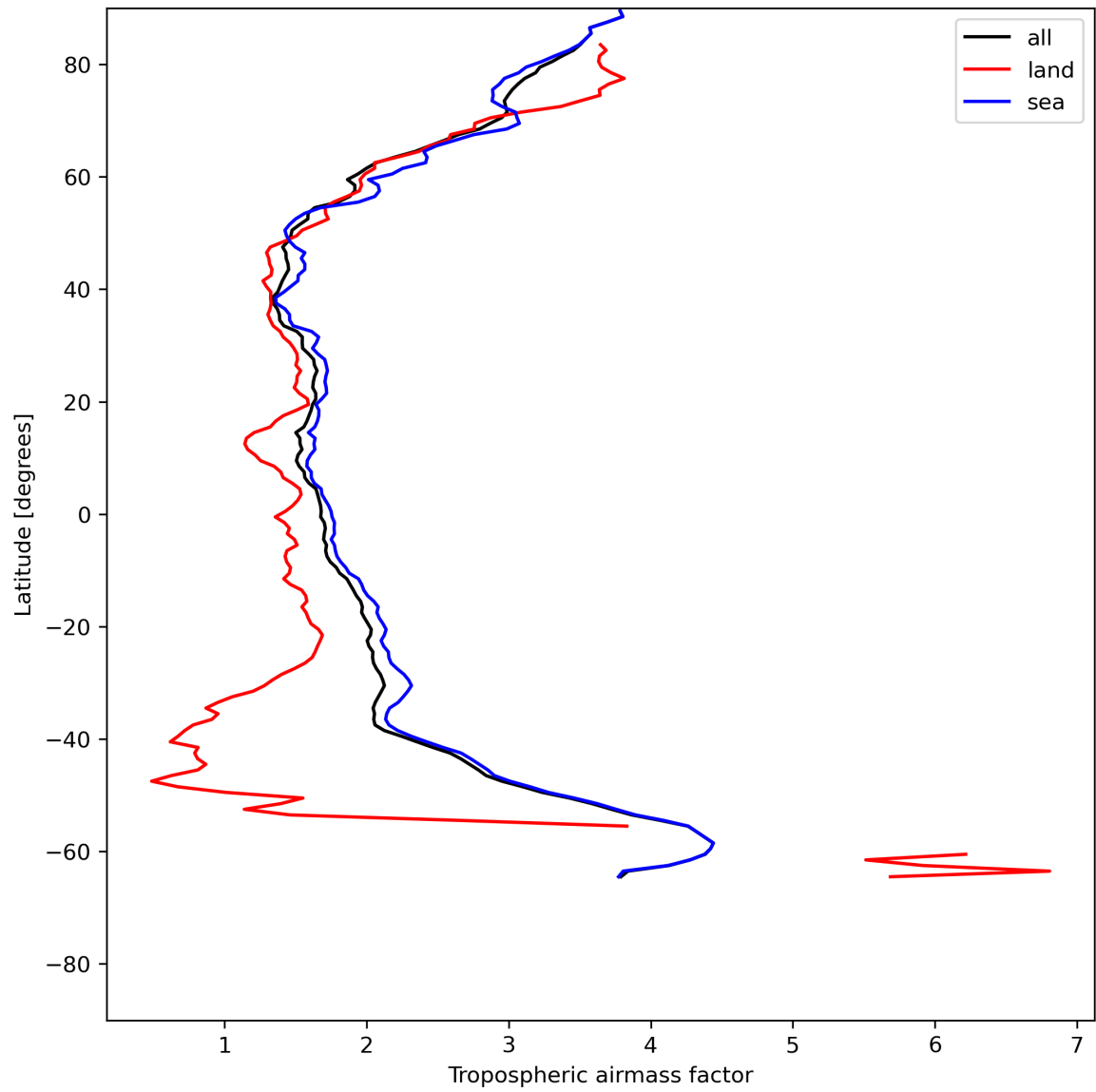
Figure 14: Zonal average of “Tropospheric airmass factor” for 2024-06-08 to 2024-06-09.
