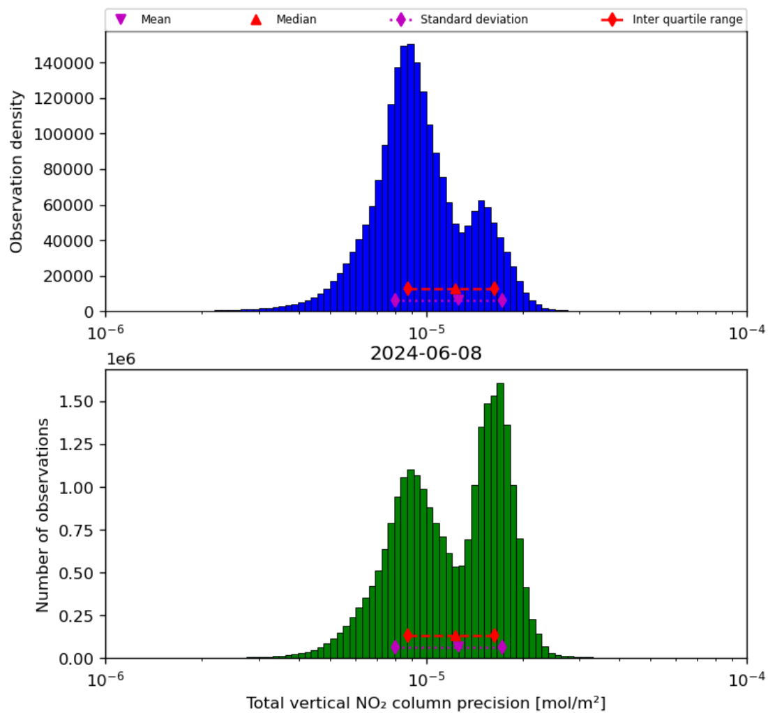
Figure 39: Histogram of “Total vertical NO 2 column precision” for 2024-06-08 to 2024-06-09
