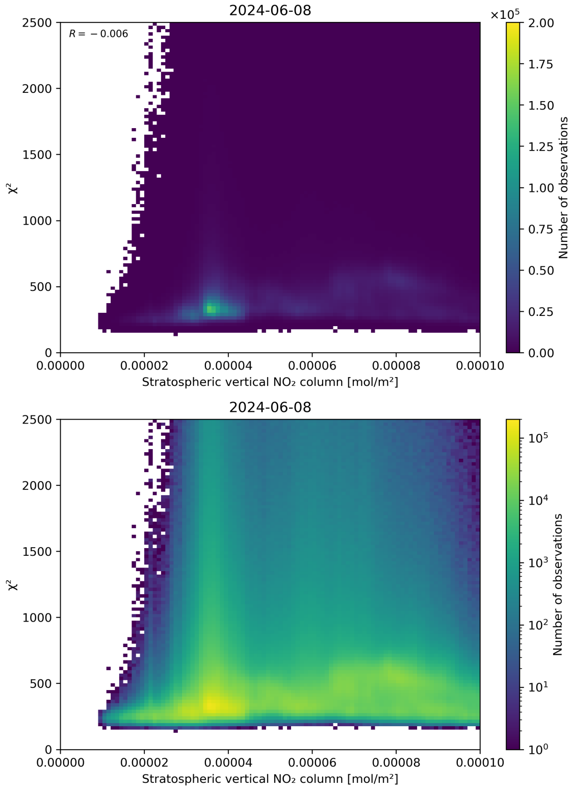
Figure 97: Scatter density plot of “Stratospheric vertical NO 2 column” against “ \chi^2 ” for 2024-06-08 to 2024-06-09.
