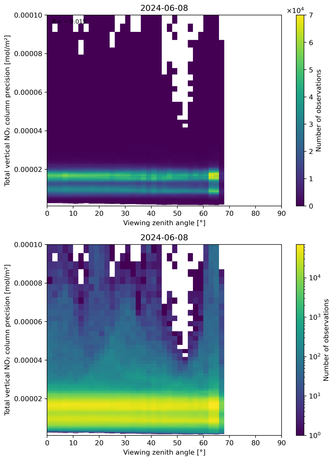
Figure 168: Scatter density plot of “Viewing zenith angle” against “Total vertical NO 2 column precision” for 2024-06-08 to 2024-06-09.
