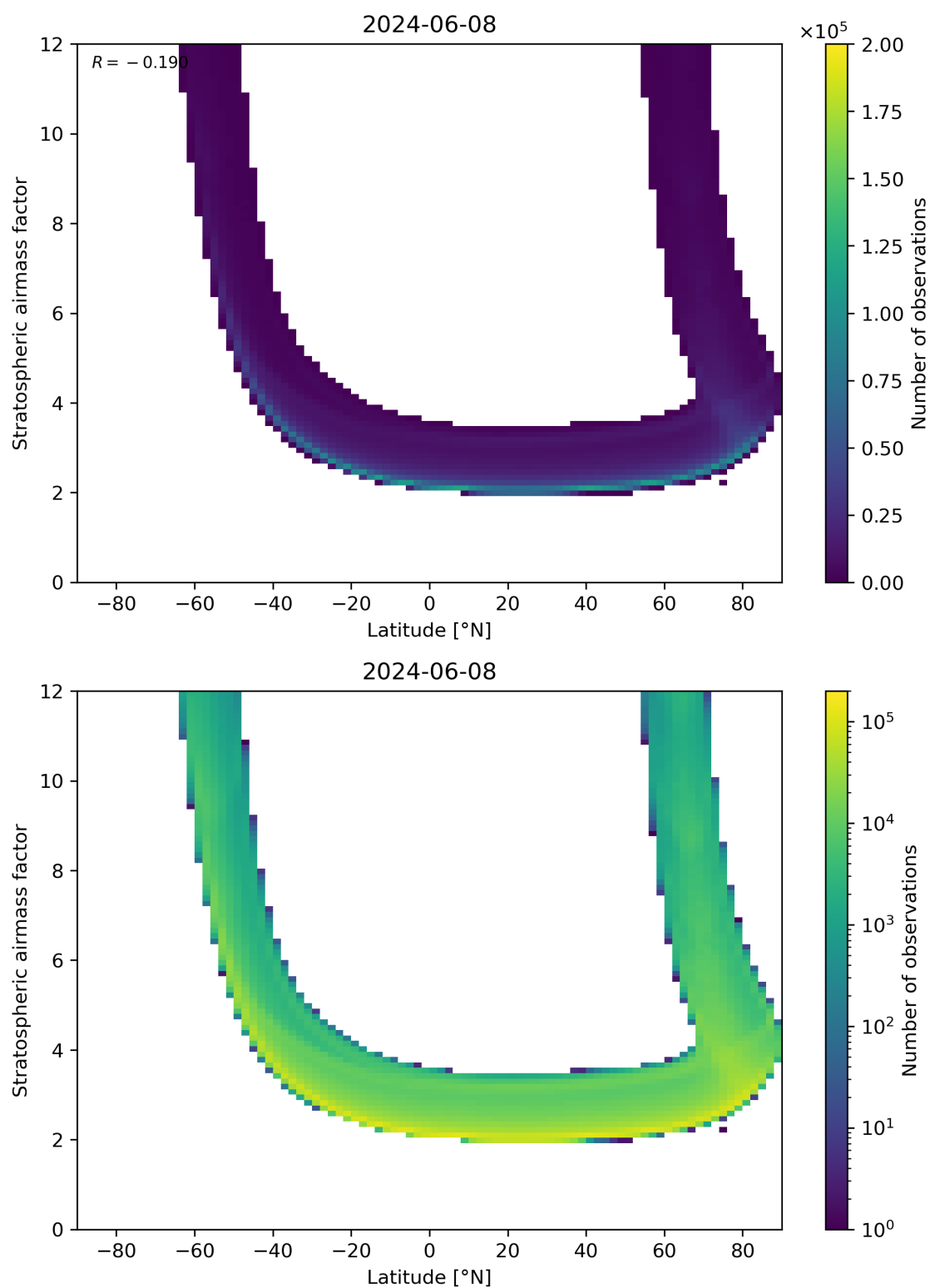
Figure 83: Scatter density plot of “Latitude” against “Stratospheric air mass factor” for 2024-06-08 to 2024-06-09.
