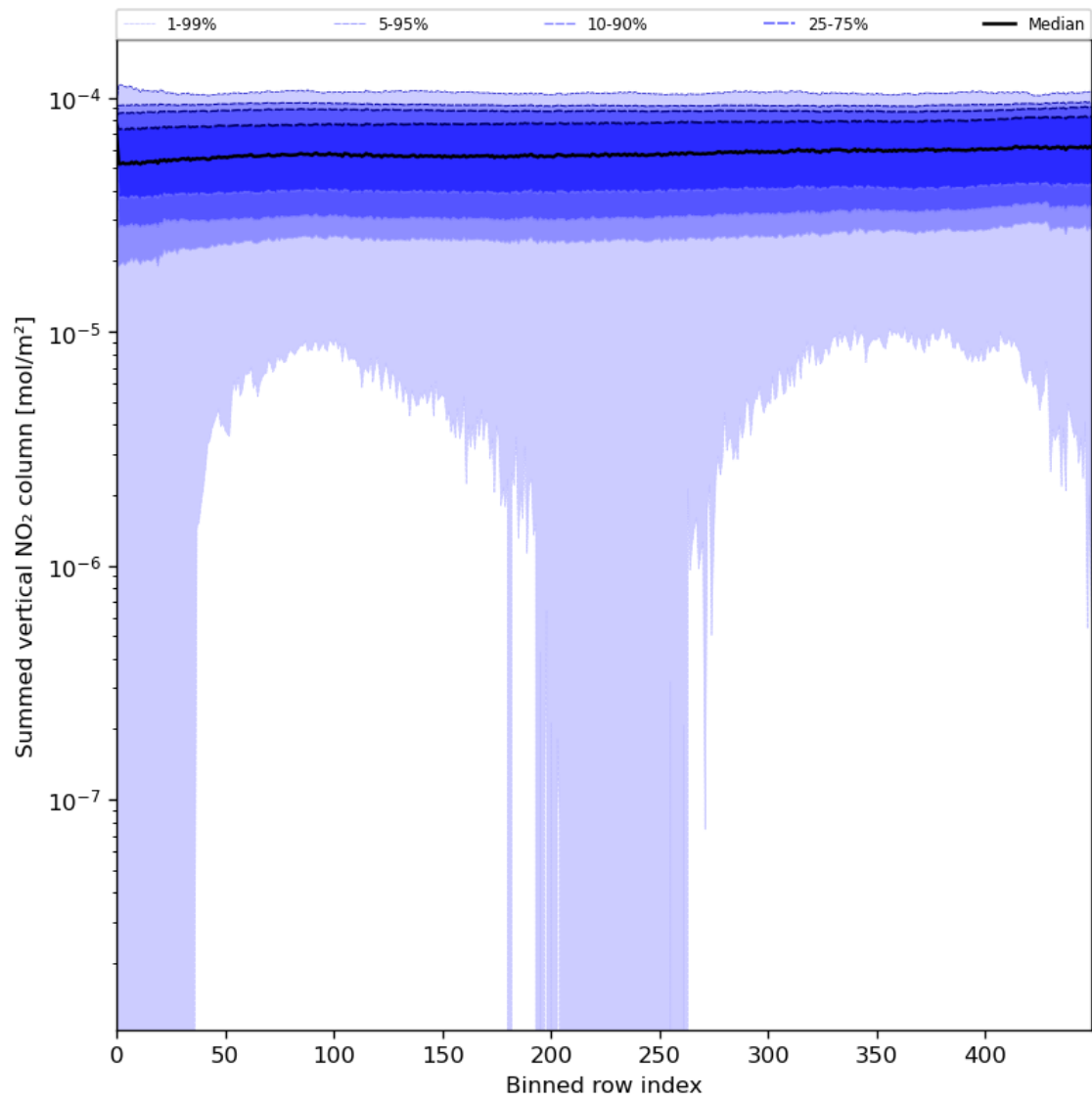
Figure 57: Along track statistics of “Summed vertical NO 2 column” for 2024-06-08 to 2024-06-09
