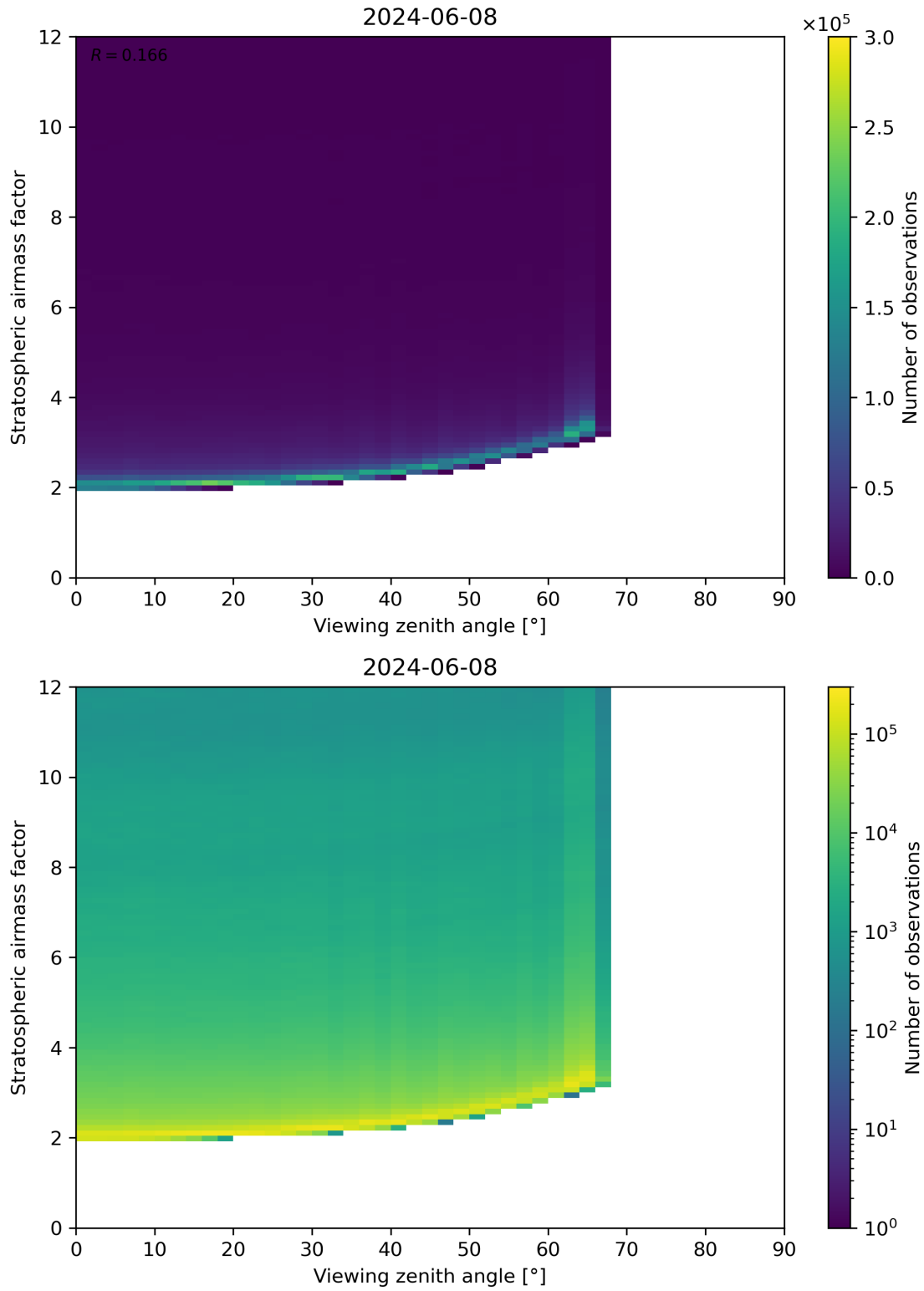
Figure 159: Scatter density plot of “Viewing zenith angle” against “Stratospheric airmass factor” for 2024-06-08 to 2024-06-09.
