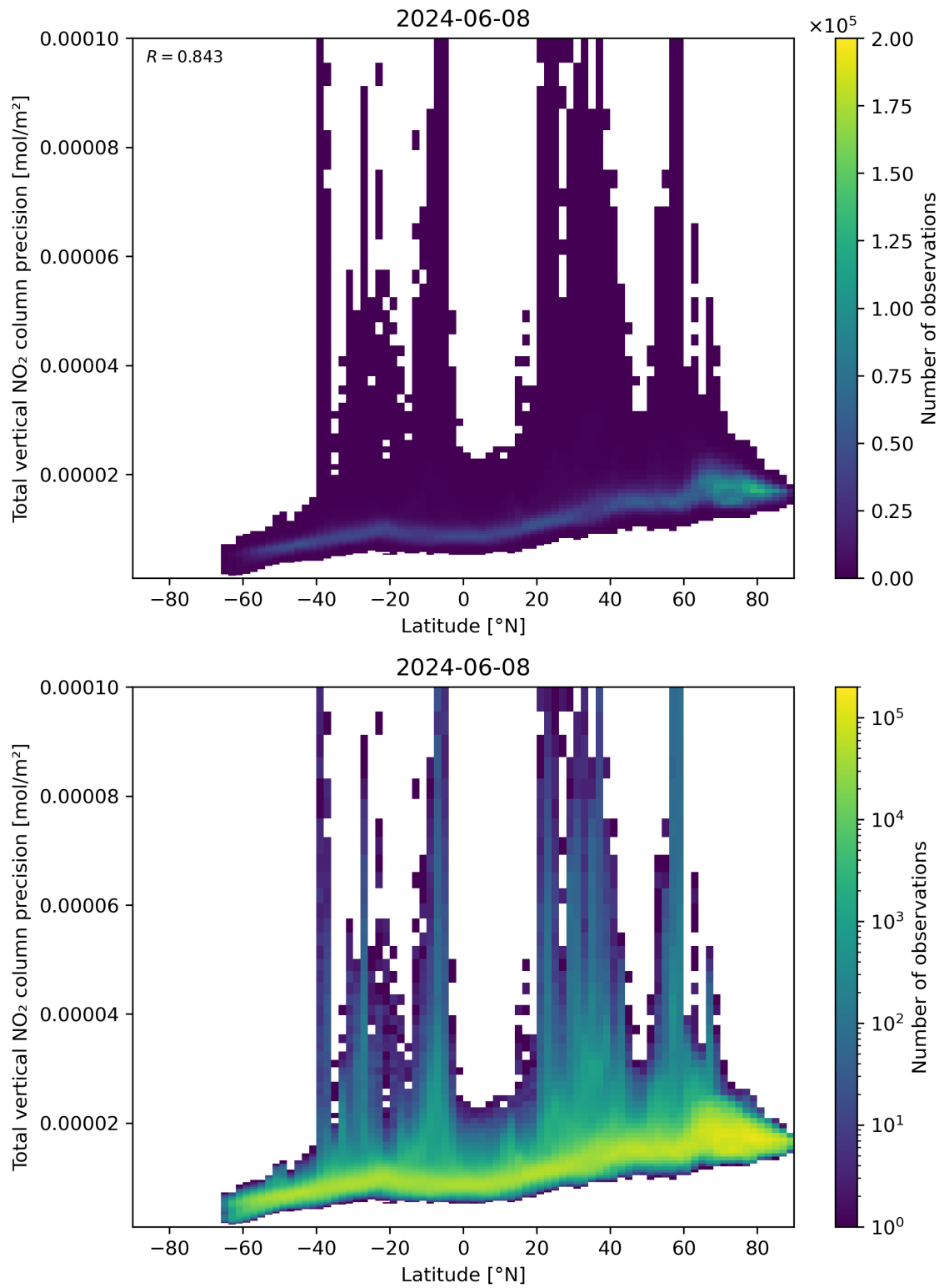
Figure 91: Scatter density plot of “Latitude” against “Total vertical NO 2 column precision” for 2024-06-08 to 2024-06-09.
