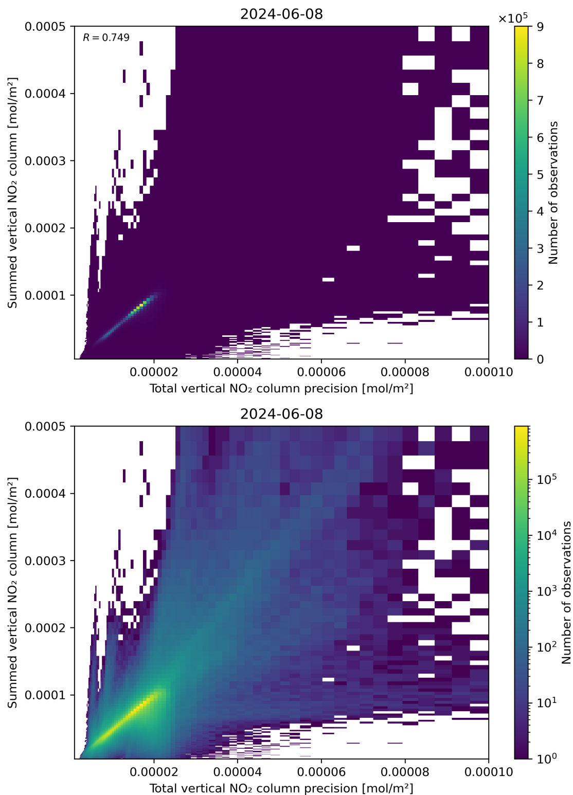
Figure 117: Scatter density plot of “Total vertical NO 2 column precision” against “Summed vertical NO 2 column” for 2024-06-08 to 2024-06-09.
