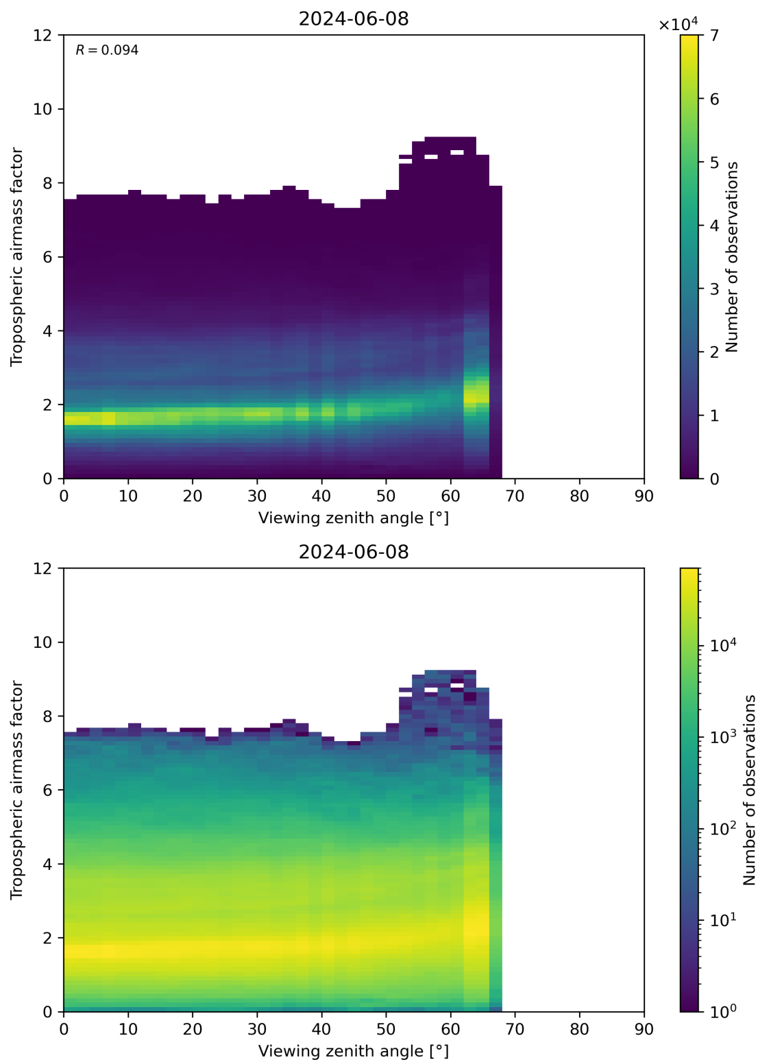
Figure 161: Scatter density plot of “Viewing zenith angle” against “Tropospheric airmass factor” for 2024-06-08 to 2024-06-09.
