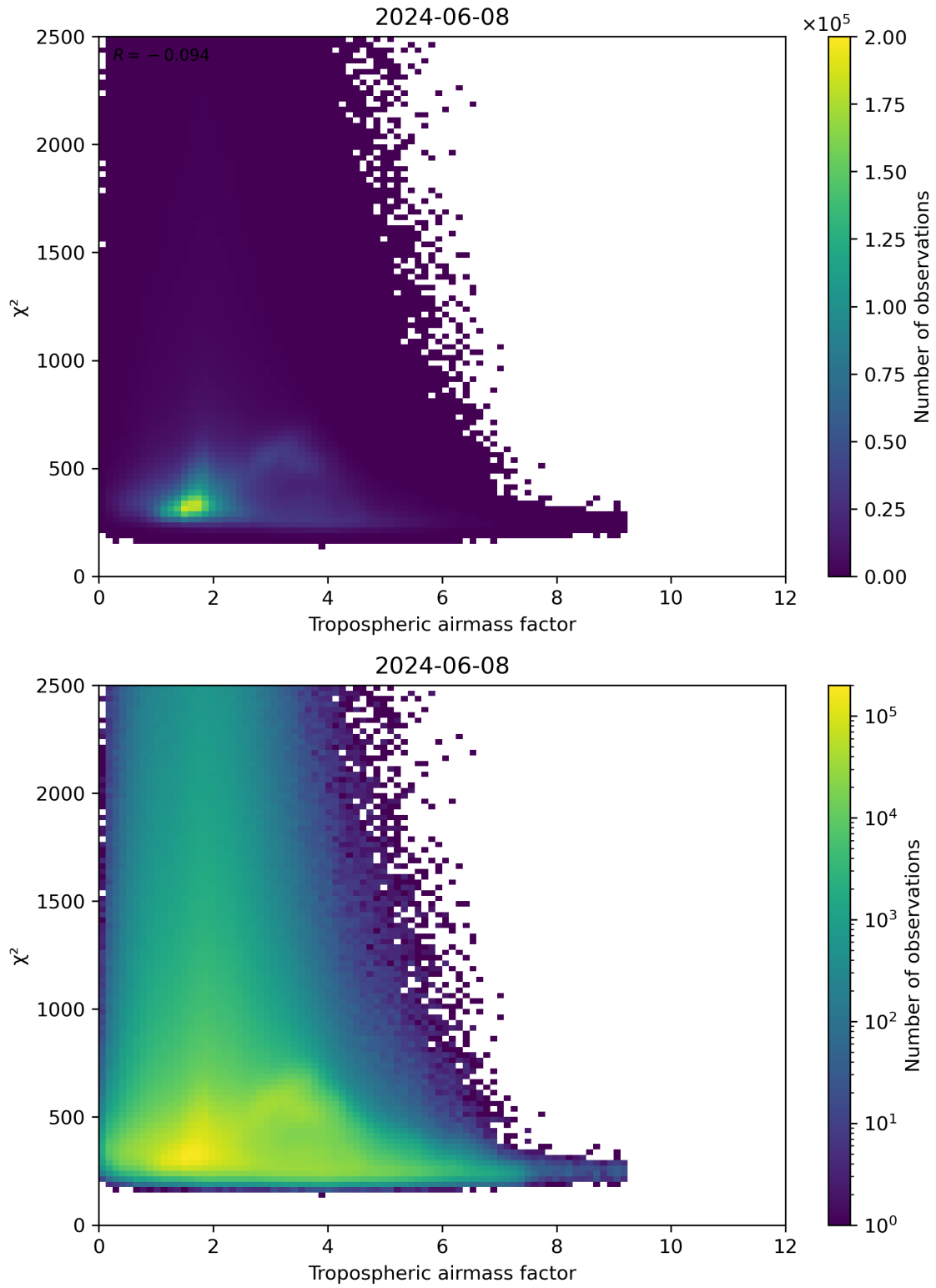
Figure 73: Scatter density plot of “Tropospheric airmass factor” against “ \chi^2 ” for 2024-06-08 to 2024-06-09.
