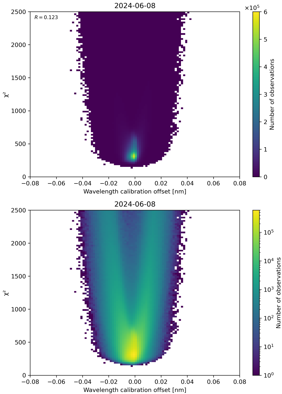
Figure 175: Scatter density plot of “Wavelength calibration offset” against “ \chi^2 ” for 2024-06-08 to 2024-06-09.
