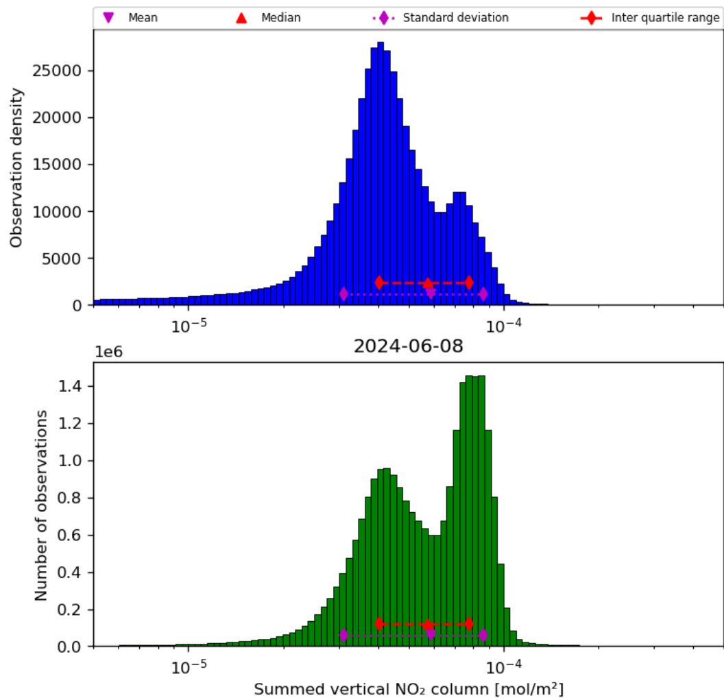
Figure 40: Histogram of “Summed vertical NO 2 column” for 2024-06-08 to 2024-06-09
