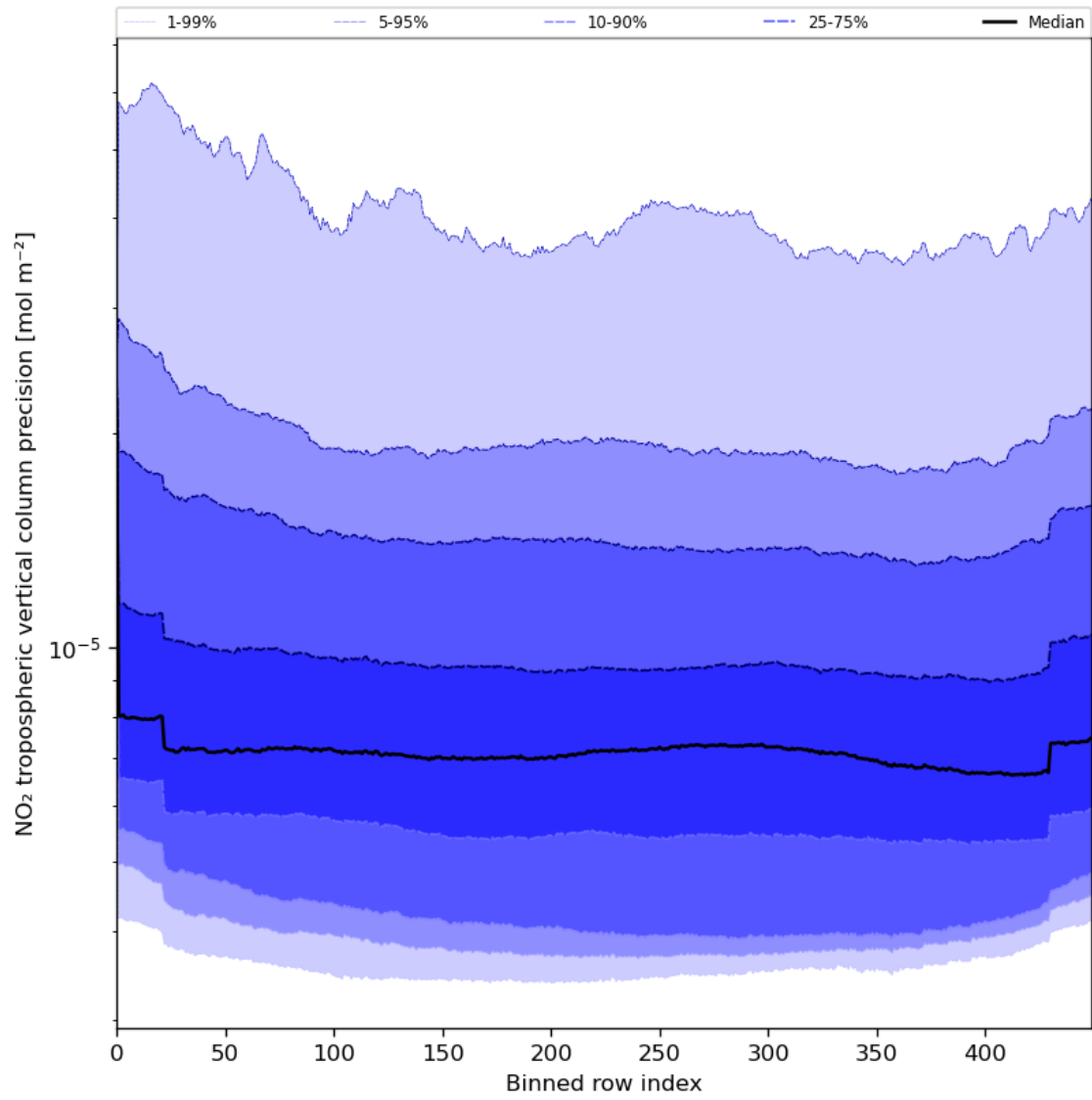
Figure 47: Along track statistics of “NO 2 tropospheric vertical column precision” for 2024-06-08 to 2024-06-09
