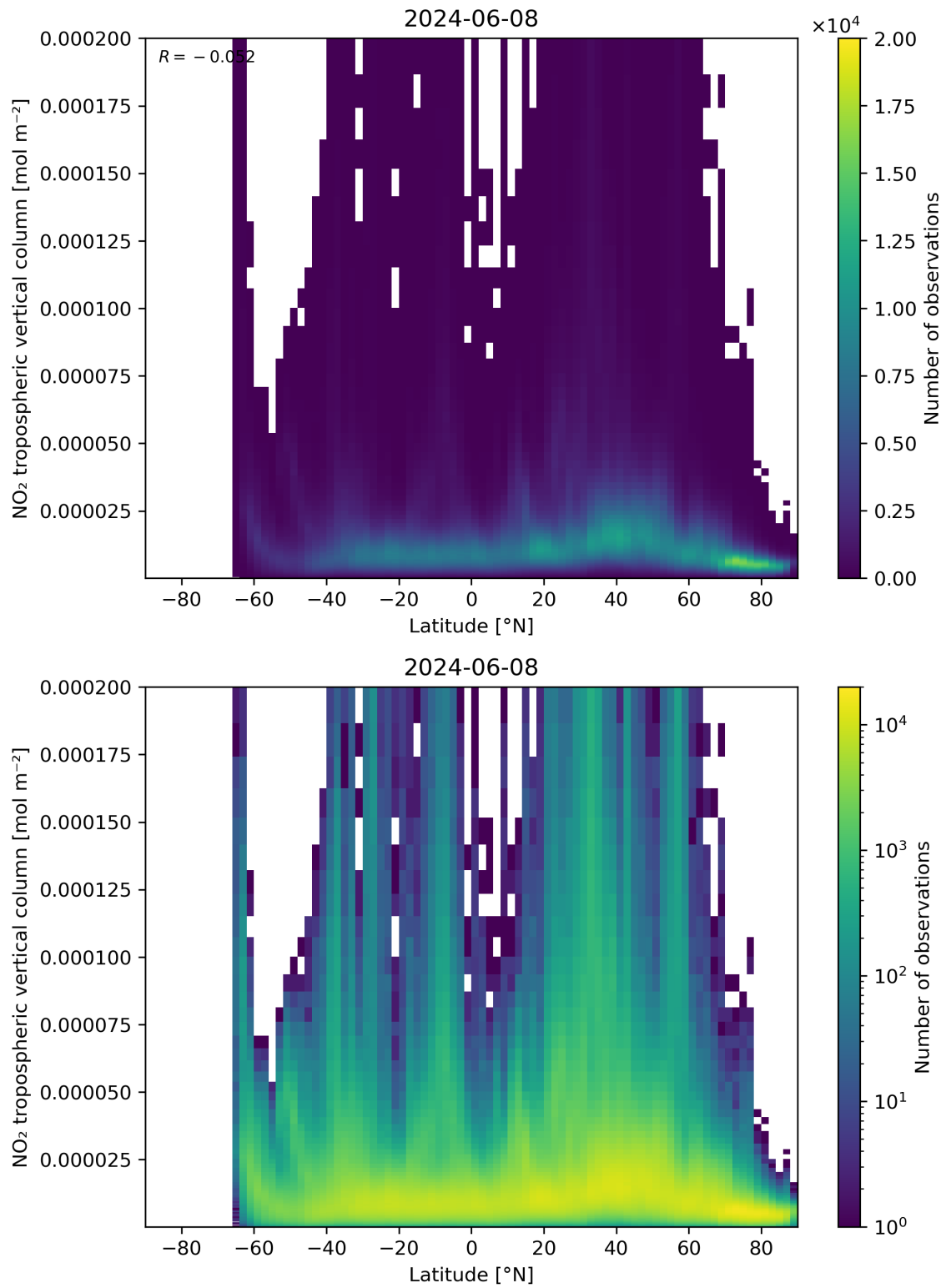
Figure 92: Scatter density plot of “Latitude” against “NO 2 tropospheric vertical column” for 2024-06-08 to 2024-06-09.
