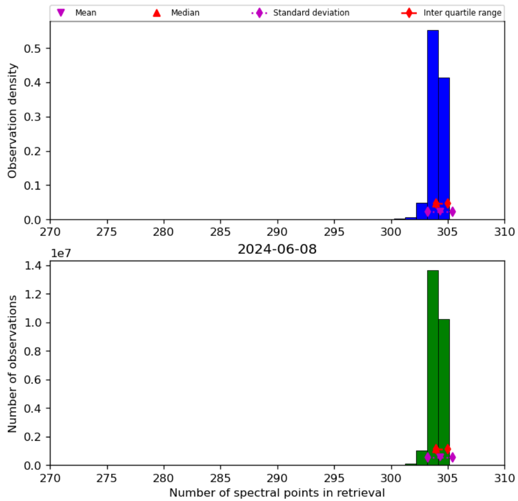
Figure 33: Histogram of “Number of spectral points in retrieval” for 2024-06-08 to 2024-06-09
