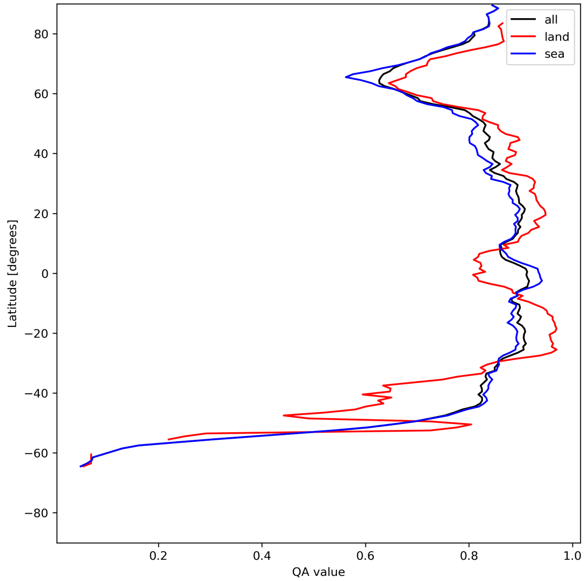
Figure 11: Zonal average of “QA value” for 2024-06-08 to 2024-06-09.
