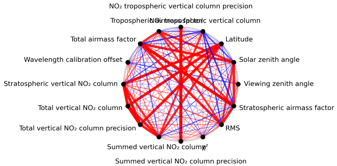
Figure 1: Map of correlation graph for 2024-06-08 to 2024-06-09.
