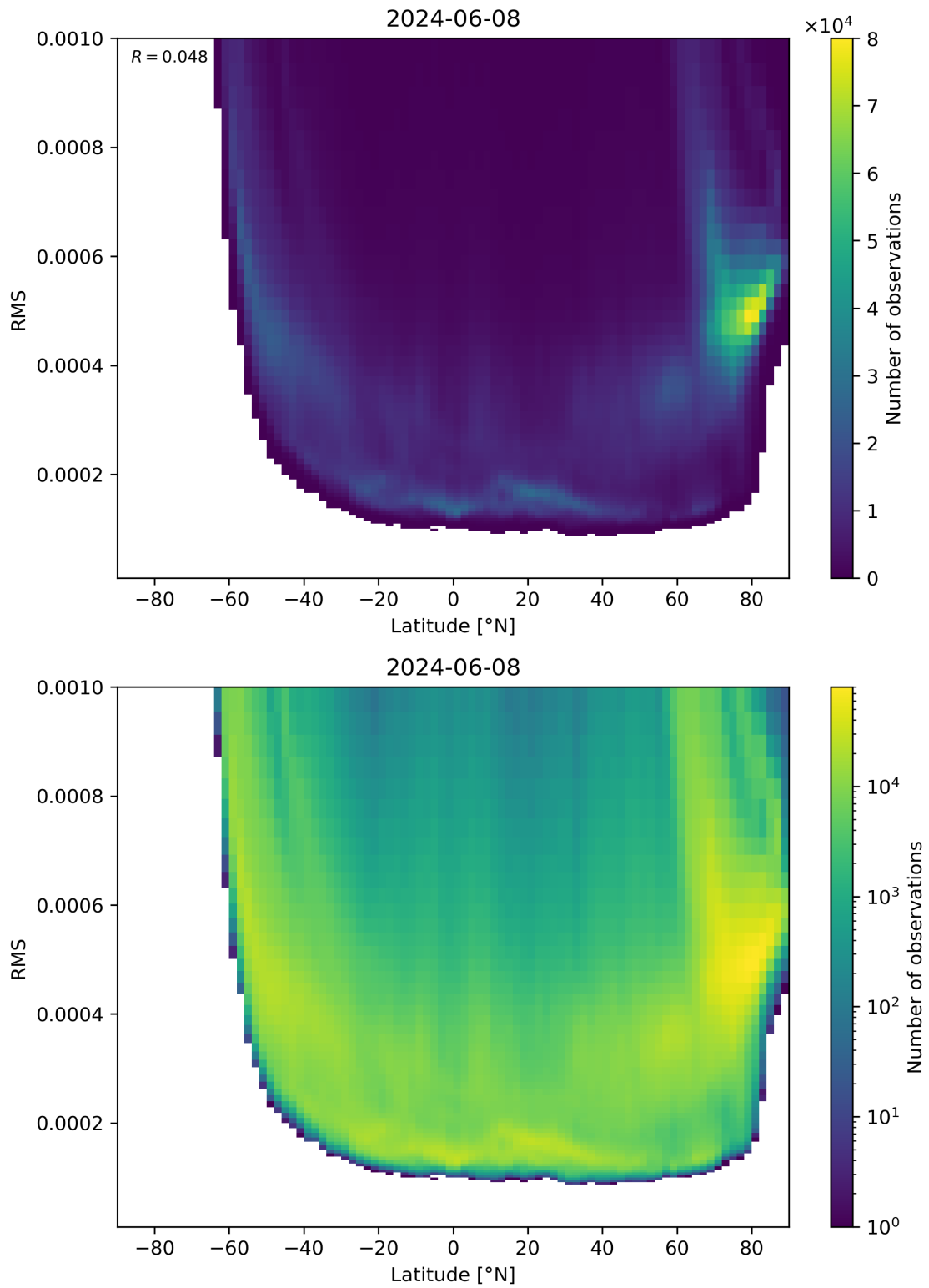
Figure 94: Scatter density plot of “Latitude” against “RMS” for 2024-06-08 to 2024-06-09.
