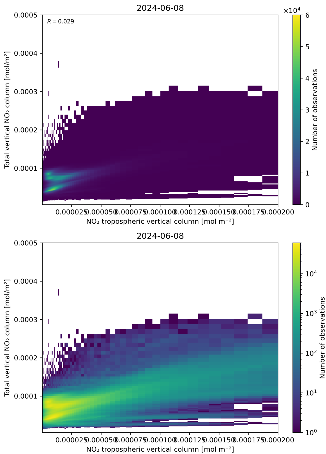
Figure 128: Scatter density plot of “NO 2 tropospheric vertical column” against “Total vertical NO 2 column” for 2024-06-08 to 2024-06-09.
