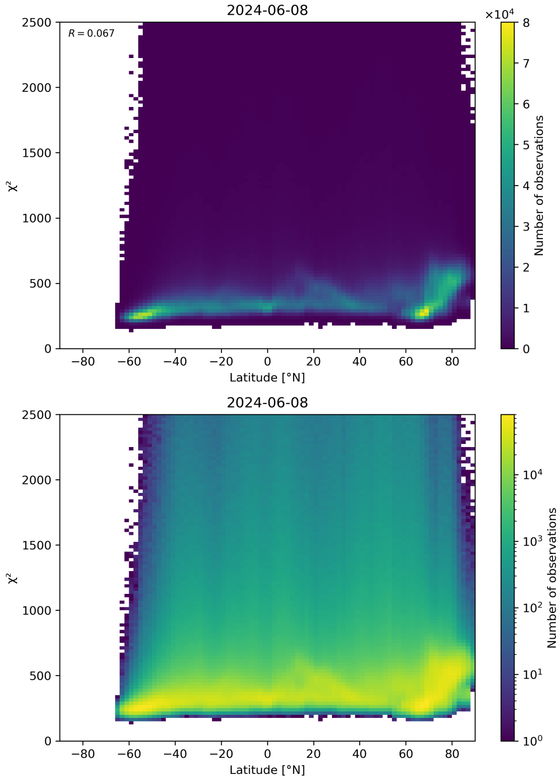
Figure 86: Scatter density plot of “Latitude” against “ \chi^2 ” for 2024-06-08 to 2024-06-09.
