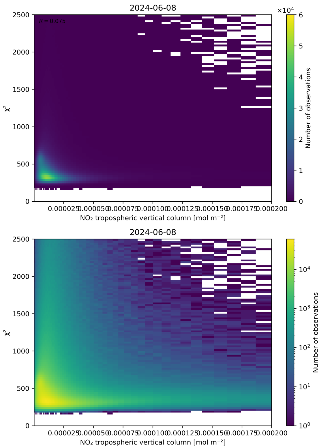
Figure 124: Scatter density plot of “NO 2 tropospheric vertical column” against “ \chi^2 ” for 2024-06-08 to 2024-06-09.
