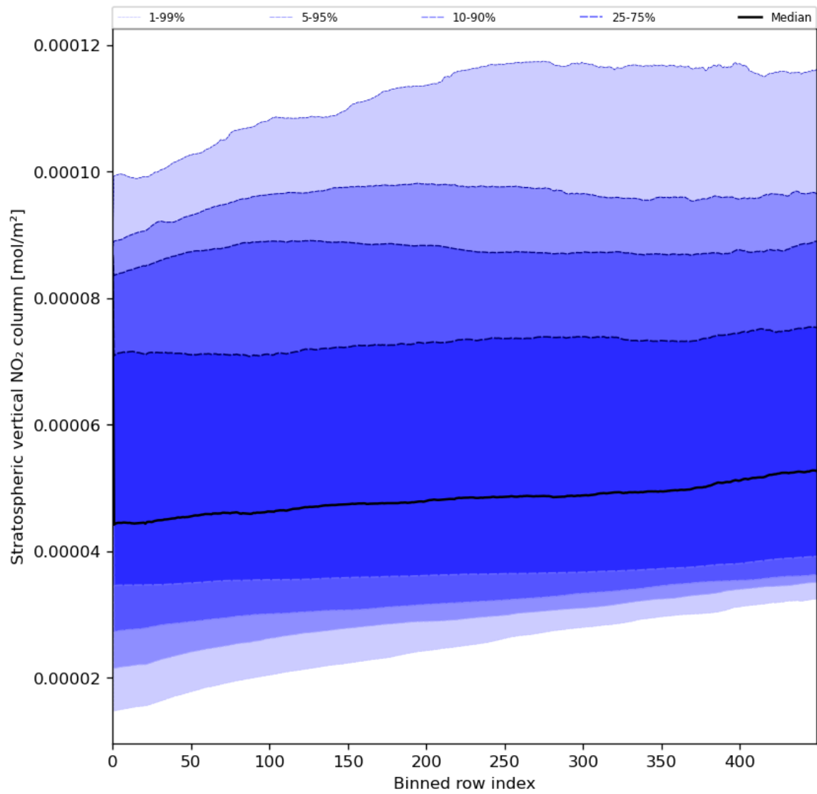
Figure 53: Along track statistics of “Stratospheric vertical NO 2 column” for 2024-06-08 to 2024-06-09
