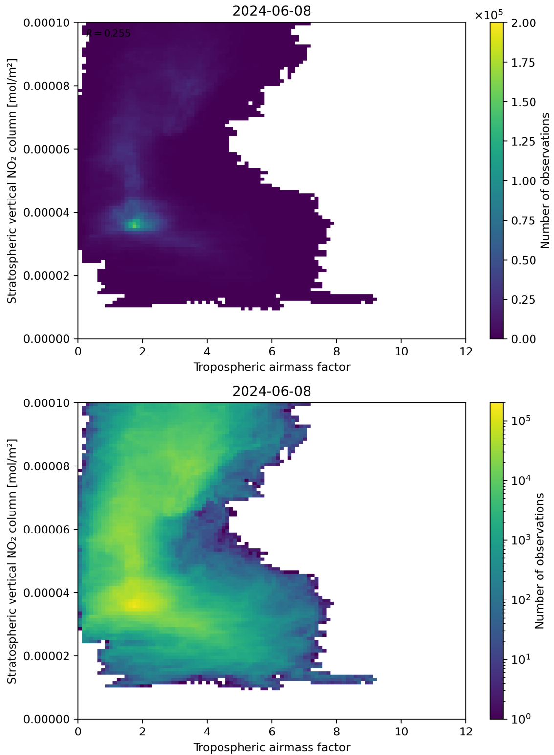
Figure 74: Scatter density plot of “Tropospheric air mass factor” against “Stratospheric vertical NO 2 column” for 2024-06-08 to 2024-06-09.
