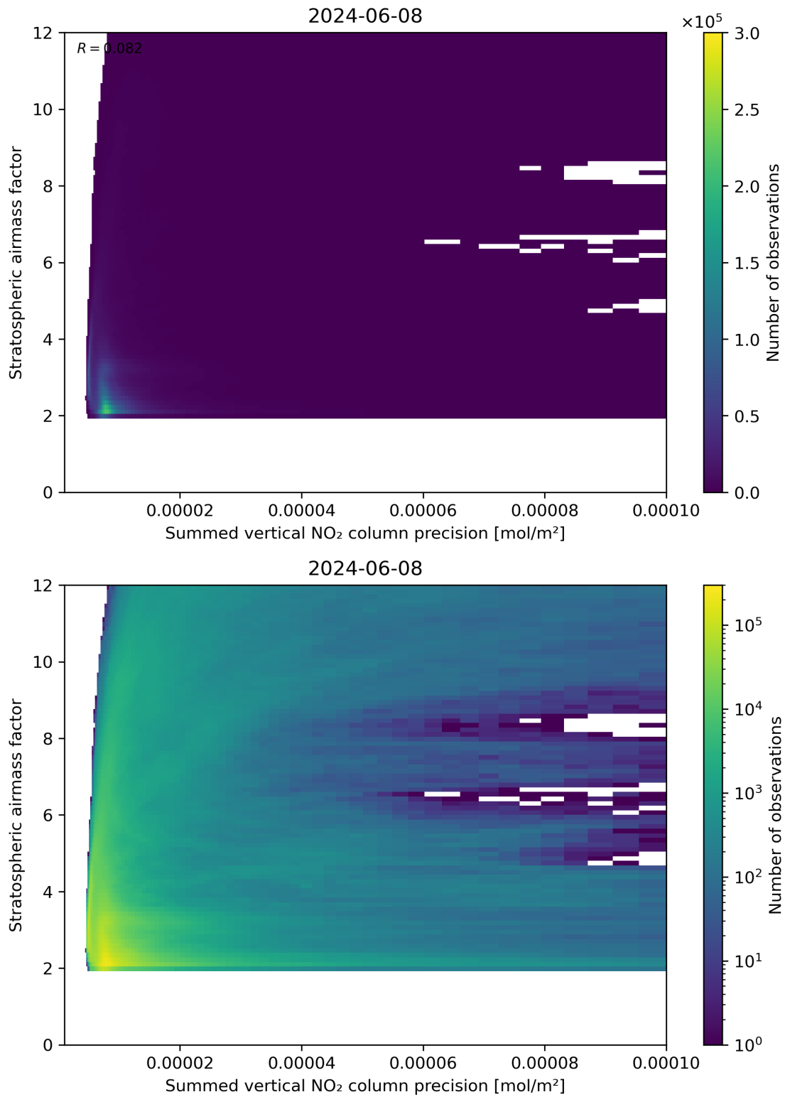
Figure 106: Scatter density plot of “Summed vertical NO 2 column precision” against “Stratospheric airmass factor” for 2024-06-08 to 2024-06-09.
