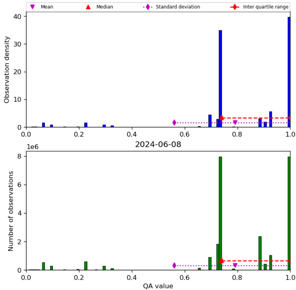
Figure 28: Histogram of “QA value” for 2024-06-08 to 2024-06-09
