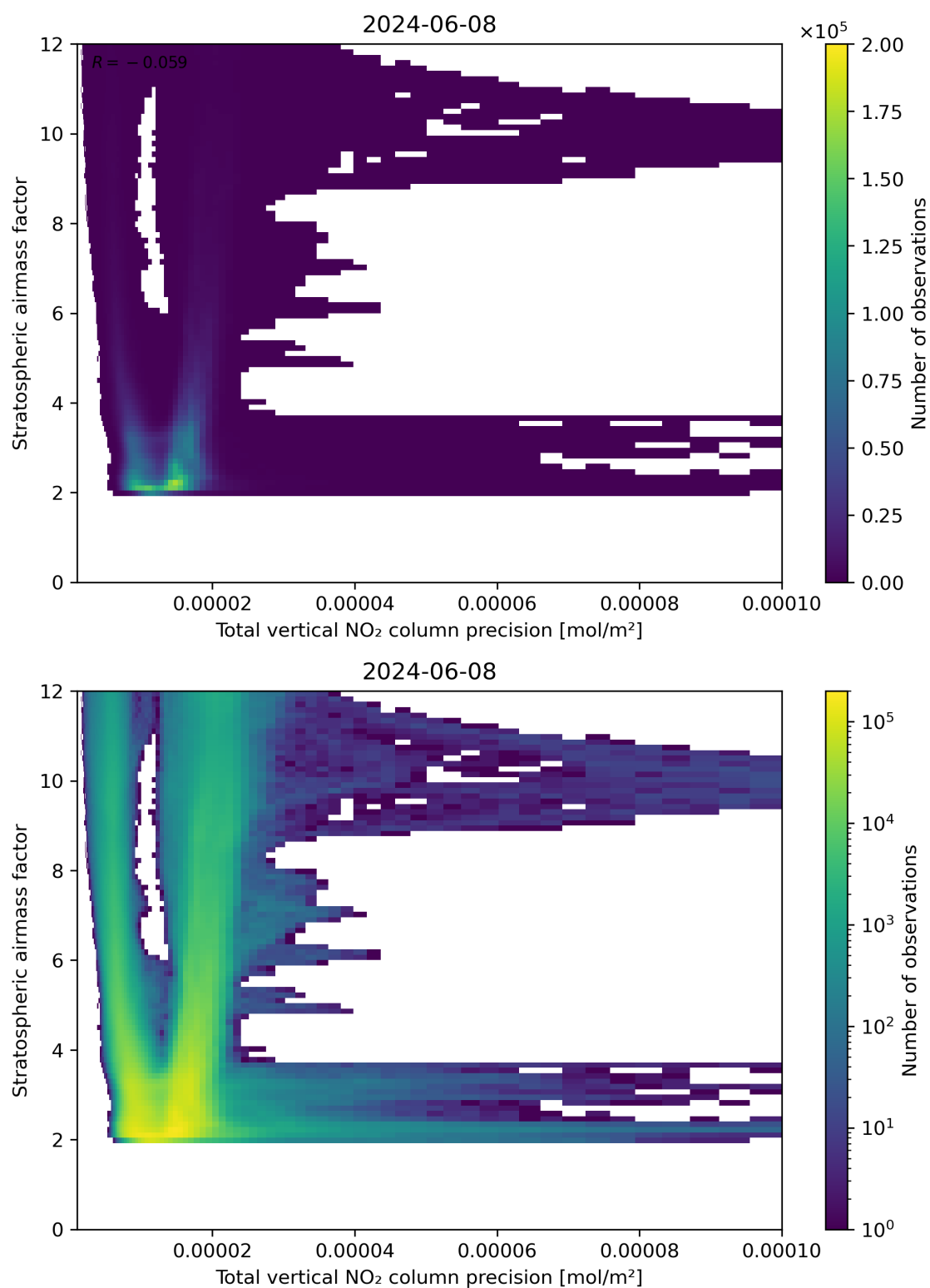
Figure 115: Scatter density plot of “Total vertical NO 2 column precision” against “Stratospheric air mass factor” for 2024-06-08 to 2024-06-09.
