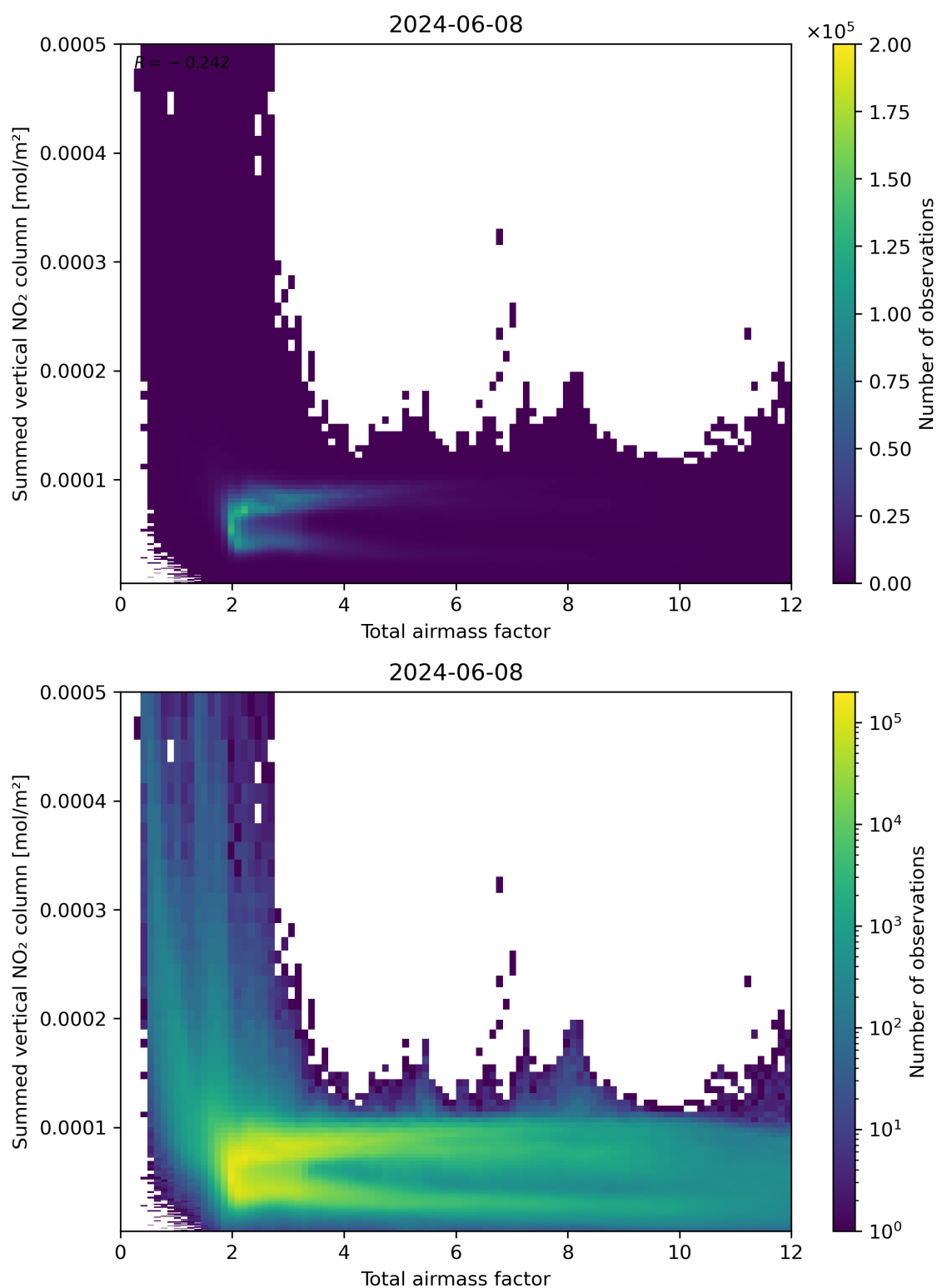
Figure 65: Scatter density plot of “Total airmass factor” against “Summed vertical NO 2 column” for 2024-06-08 to 2024-06-09.
