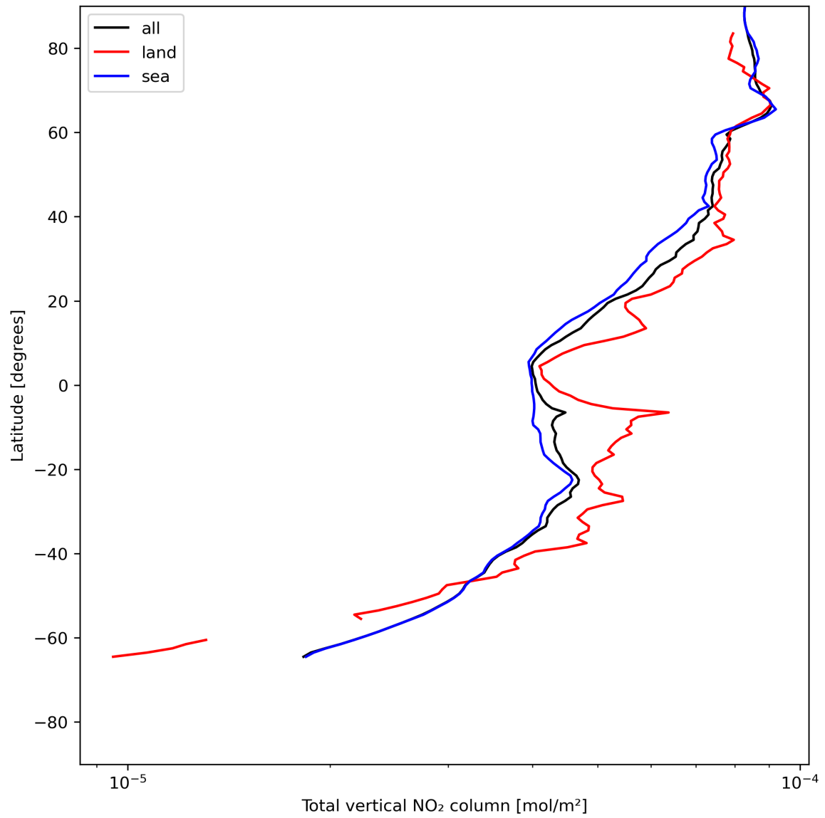
Figure 21: Zonal average of “Total vertical NO 2 column” for 2024-06-08 to 2024-06-09.
