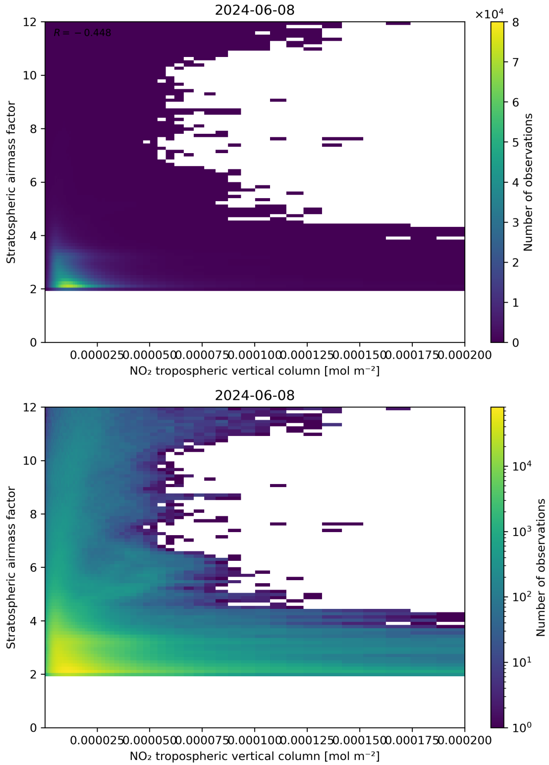
Figure 121: Scatter density plot of “NO 2 tropospheric vertical column” against “Stratospheric air mass factor” for 2024-06-08 to 2024-06-09.
