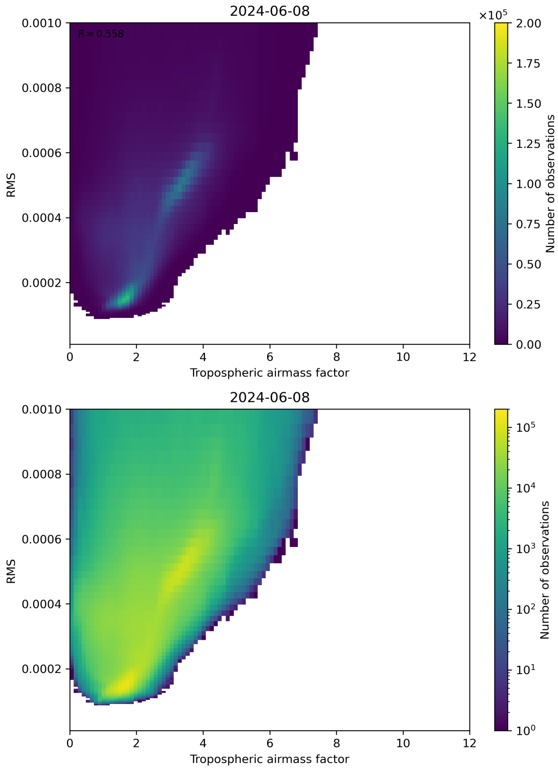
Figure 79: Scatter density plot of “Tropospheric airmass factor” against “RMS” for 2024-06-08 to 2024-06-09.
