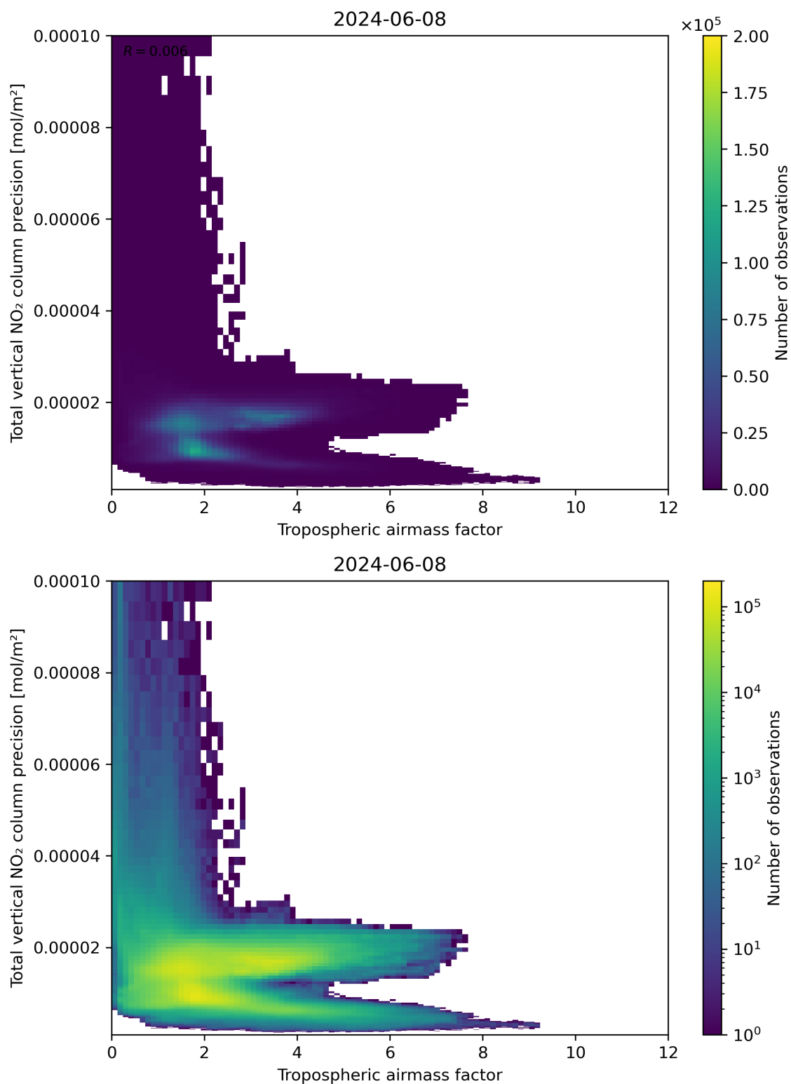
Figure 78: Scatter density plot of “Tropospheric air mass factor” against “Total vertical NO 2 column precision” for 2024-06-08 to 2024-06-09.
