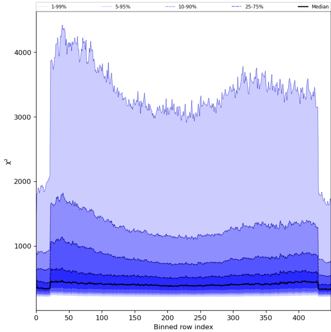
Figure 59: Along track statistics of “ \chi^2 ” for 2024-06-08 to 2024-06-09
