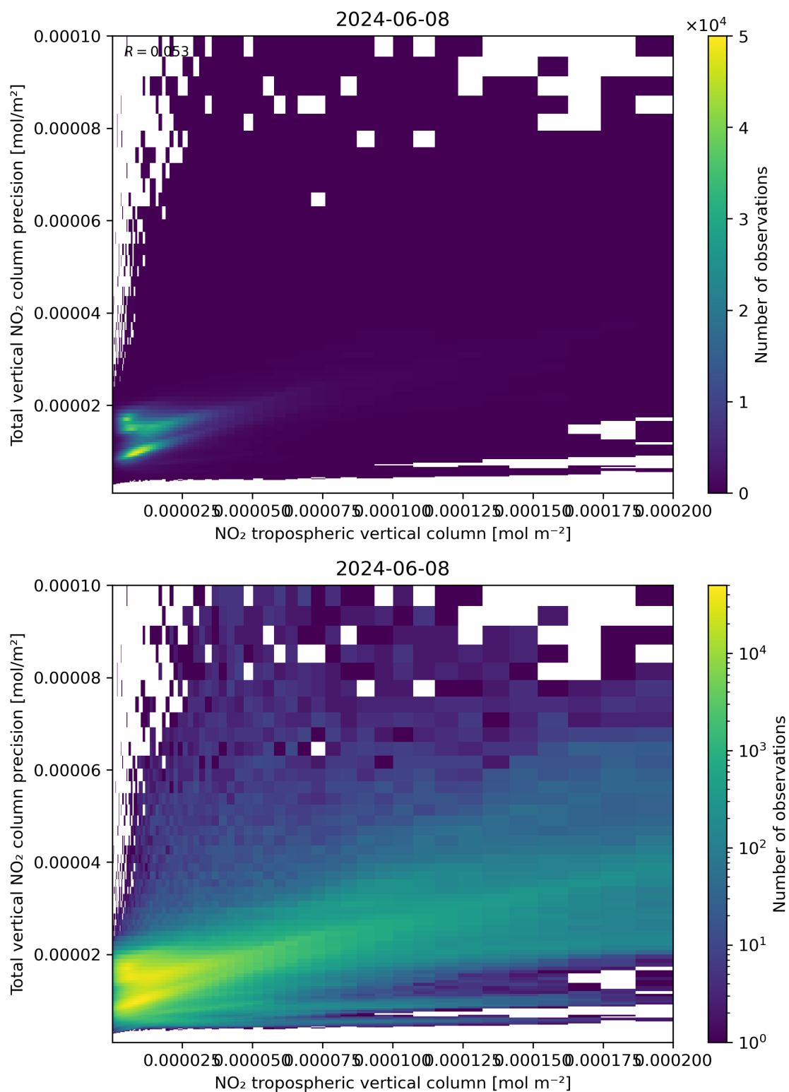
Figure 129: Scatter density plot of “NO 2 tropospheric vertical column” against “Total vertical NO 2 column precision” for 2024-06-08 to 2024-06-09.
