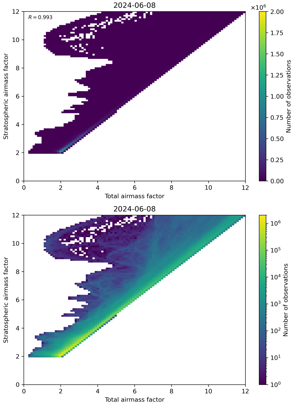
Figure 62: Scatter density plot of “Total airmass factor” against “Stratospheric airmass factor” for 2024-06-08 to 2024-06-09.
