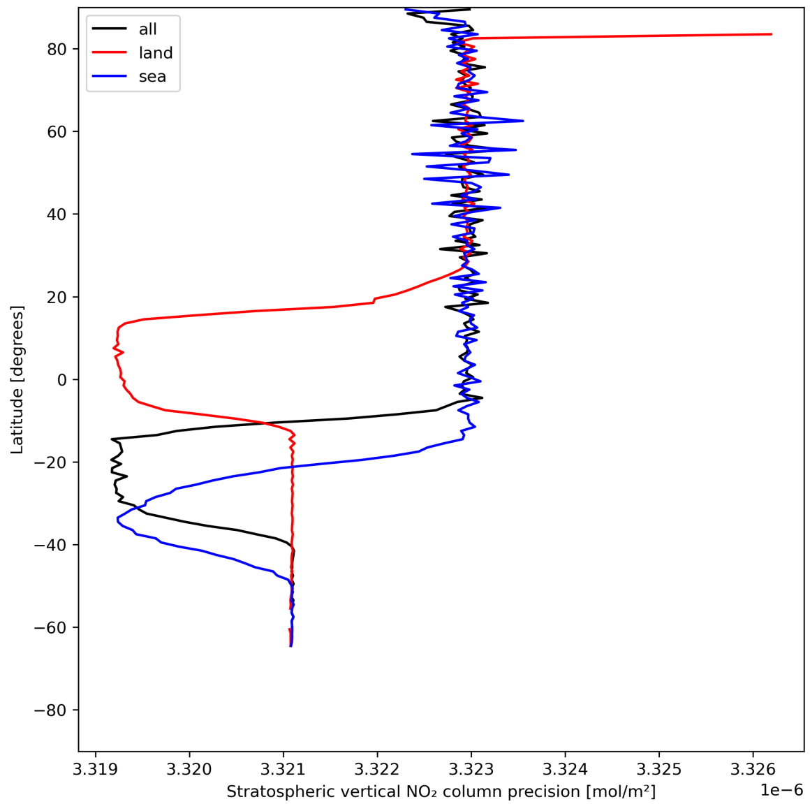
Figure 20: Zonal average of “Stratospheric vertical NO 2 column precision” for 2024-06-08 to 2024-06-09.
