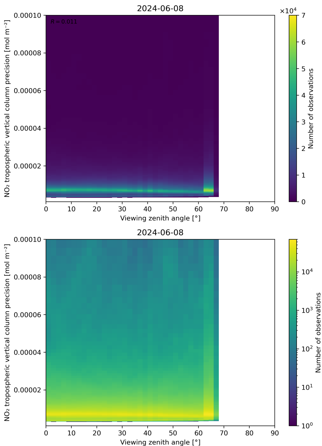
Figure 170: Scatter density plot of “Viewing zenith angle” against “NO 2 tropospheric vertical column precision” for 2024-06-08 to 2024-06-09.
