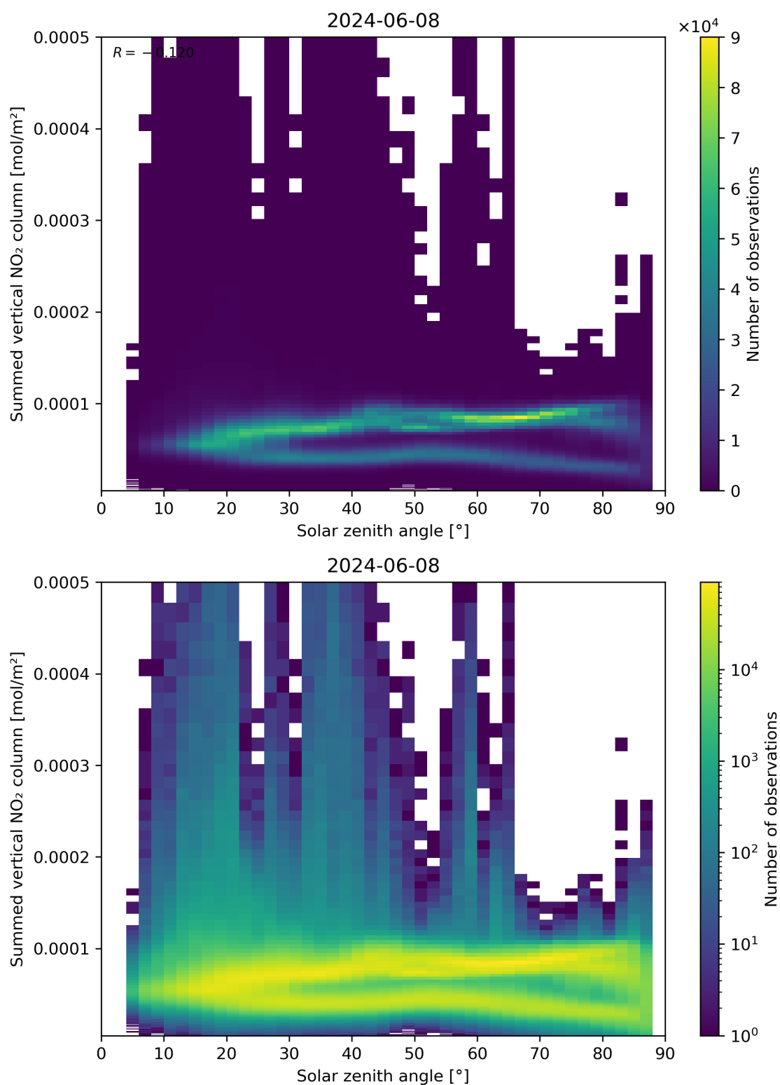
Figure 151: Scatter density plot of “Solar zenith angle” against “Summed vertical NO 2 column” for 2024-06-08 to 2024-06-09.
