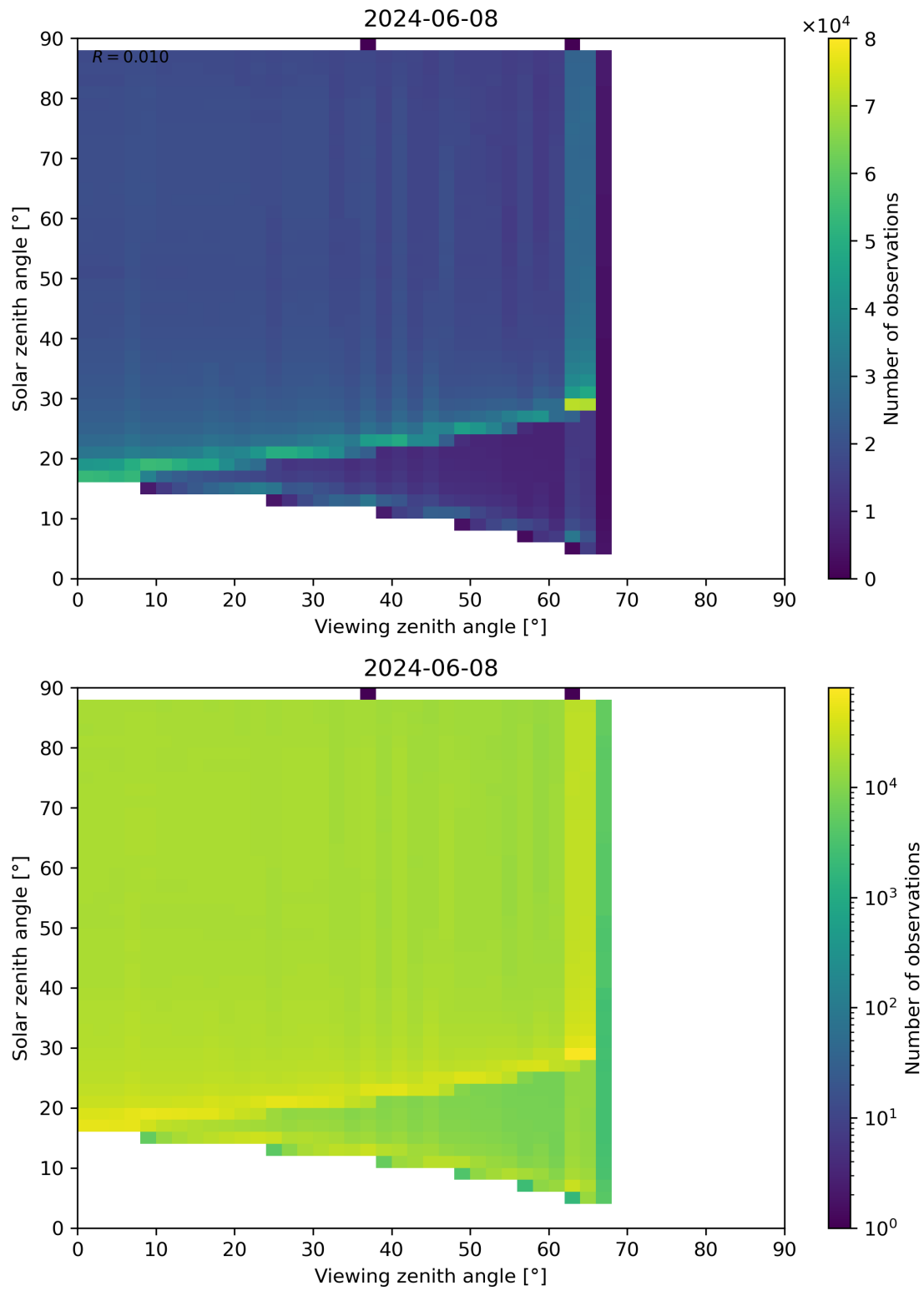
Figure 172: Scatter density plot of “Viewing zenith angle” against “Solar zenith angle” for 2024-06-08 to 2024-06-09.
