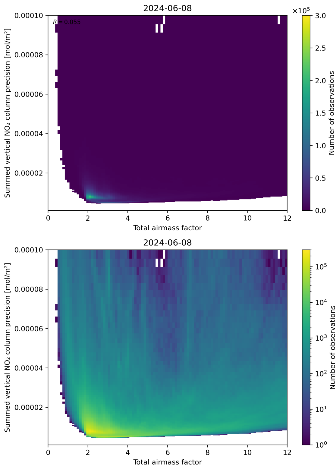
Figure 66: Scatter density plot of “Total airmass factor” against “Summed vertical NO 2 column precision” for 2024-06-08 to 2024-06-09.
