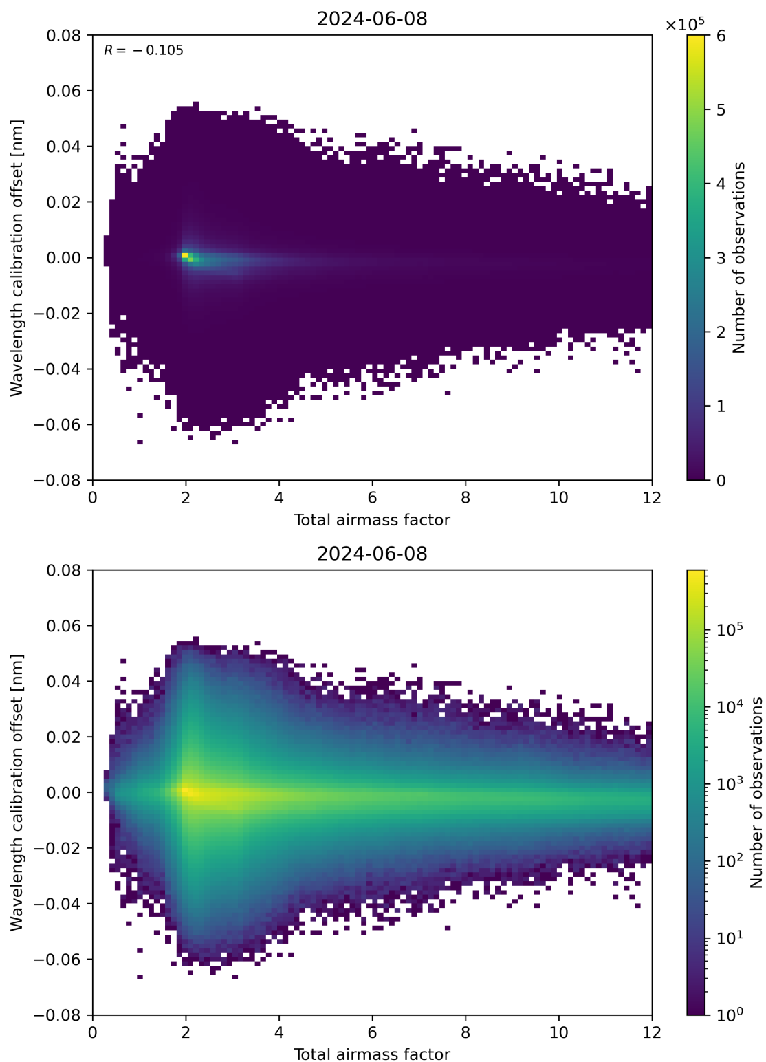
Figure 70: Scatter density plot of “Total airmass factor” against “Wavelength calibration offset” for 2024-06-08 to 2024-06-09.
