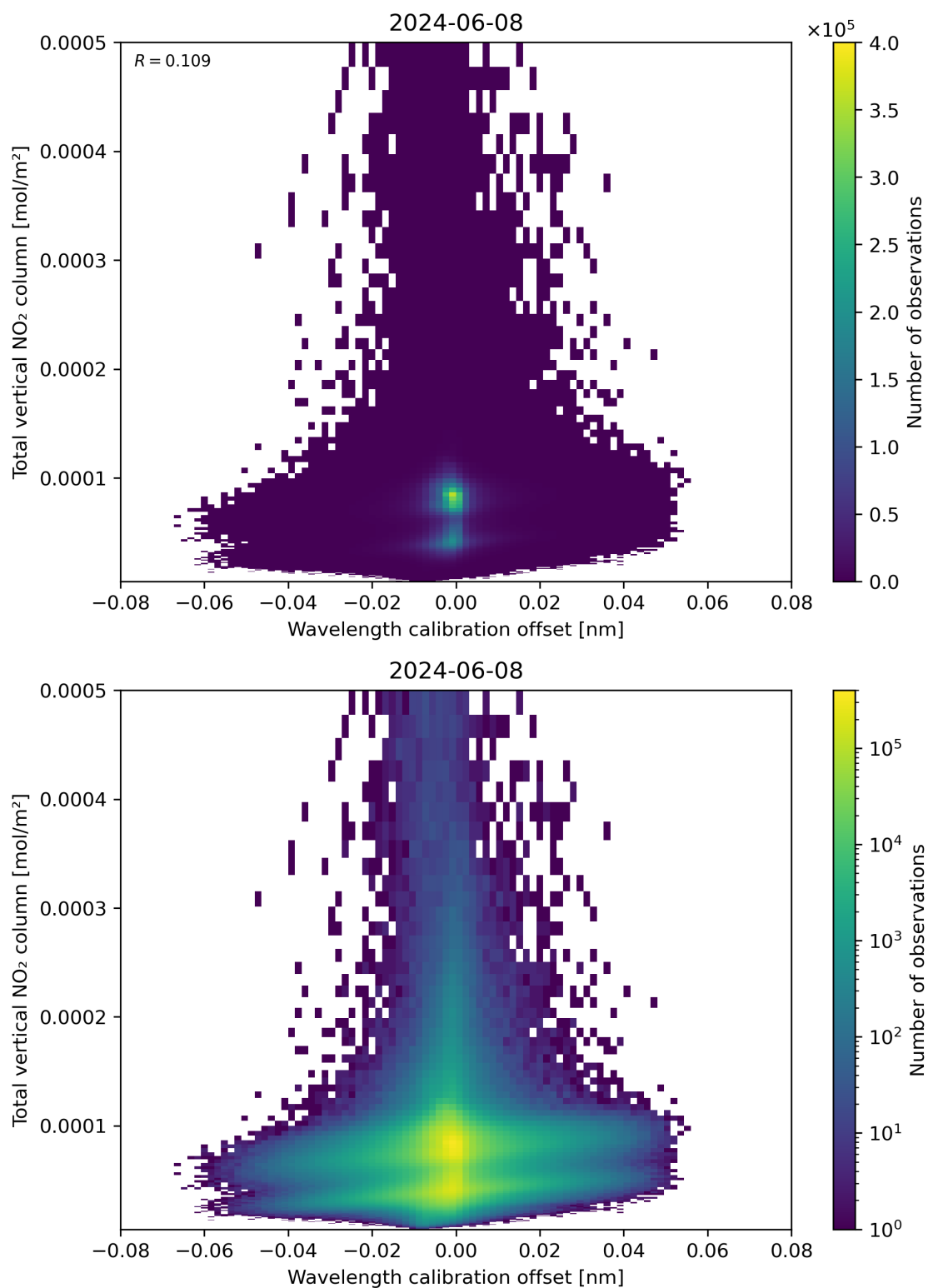
Figure 179: Scatter density plot of “Wavelength calibration offset” against “Total vertical NO 2 column” for 2024-06-08 to 2024-06-09.
