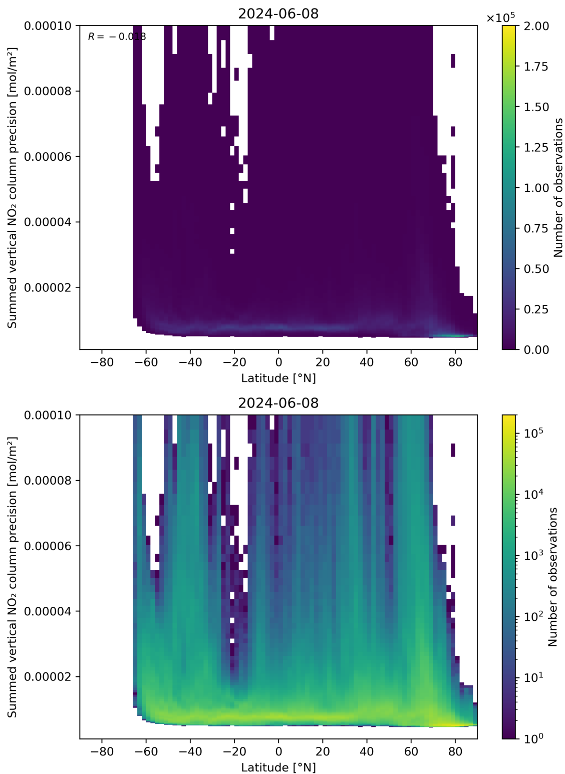
Figure 89: Scatter density plot of “Latitude” against “Summed vertical NO 2 column precision” for 2024-06-08 to 2024-06-09.
