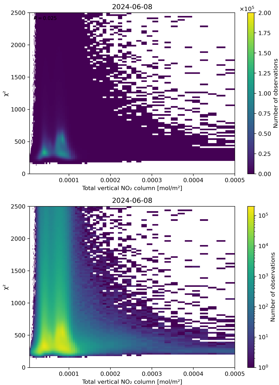
Figure 111: Scatter density plot of “Total vertical NO 2 column” against “ \chi^2 ” for 2024-06-08 to 2024-06-09.
