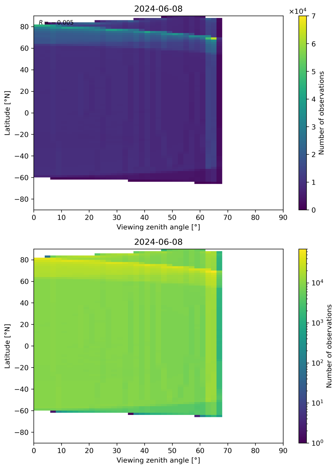
Figure 163: Scatter density plot of “Viewing zenith angle” against “Latitude” for 2024-06-08 to 2024-06-09.
