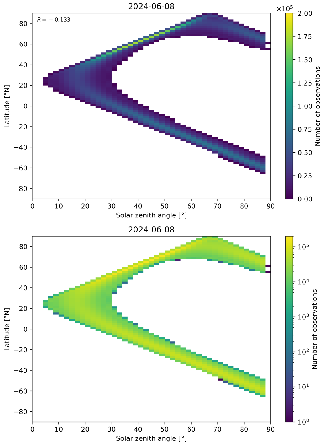
Figure 149: Scatter density plot of “Solar zenith angle” against “Latitude” for 2024-06-08 to 2024-06-09.
