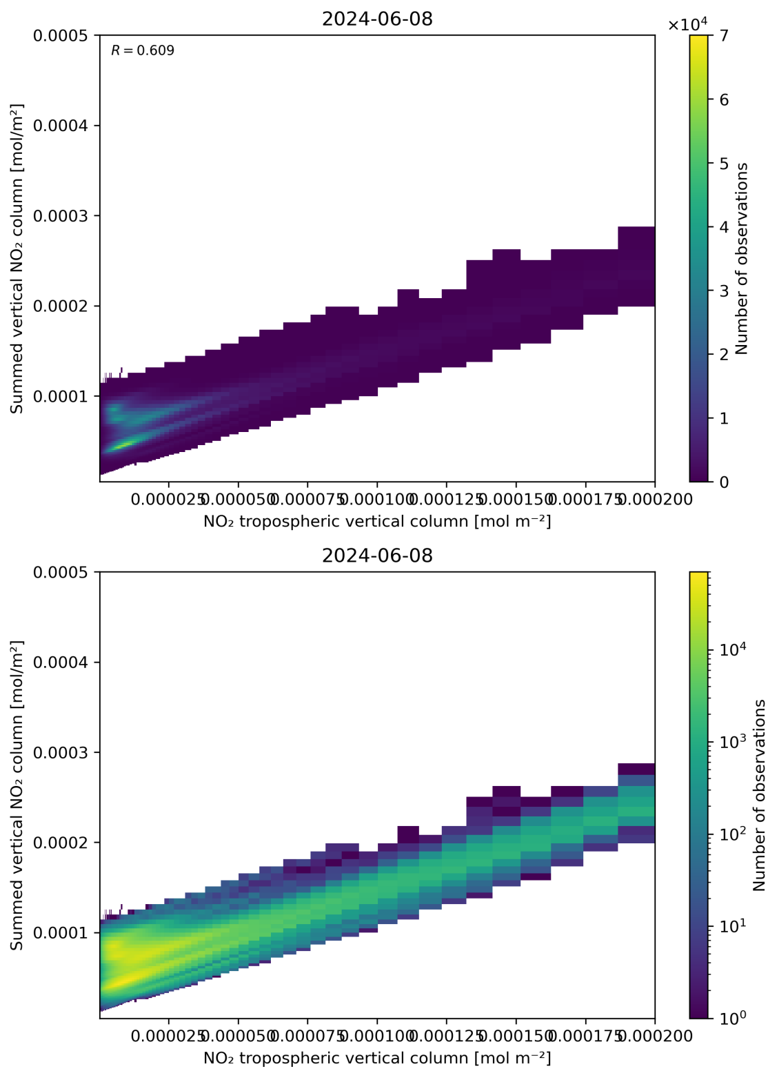
Figure 126: Scatter density plot of “NO 2 tropospheric vertical column” against “Summed vertical NO 2 column” for 2024-06-08 to 2024-06-09.
