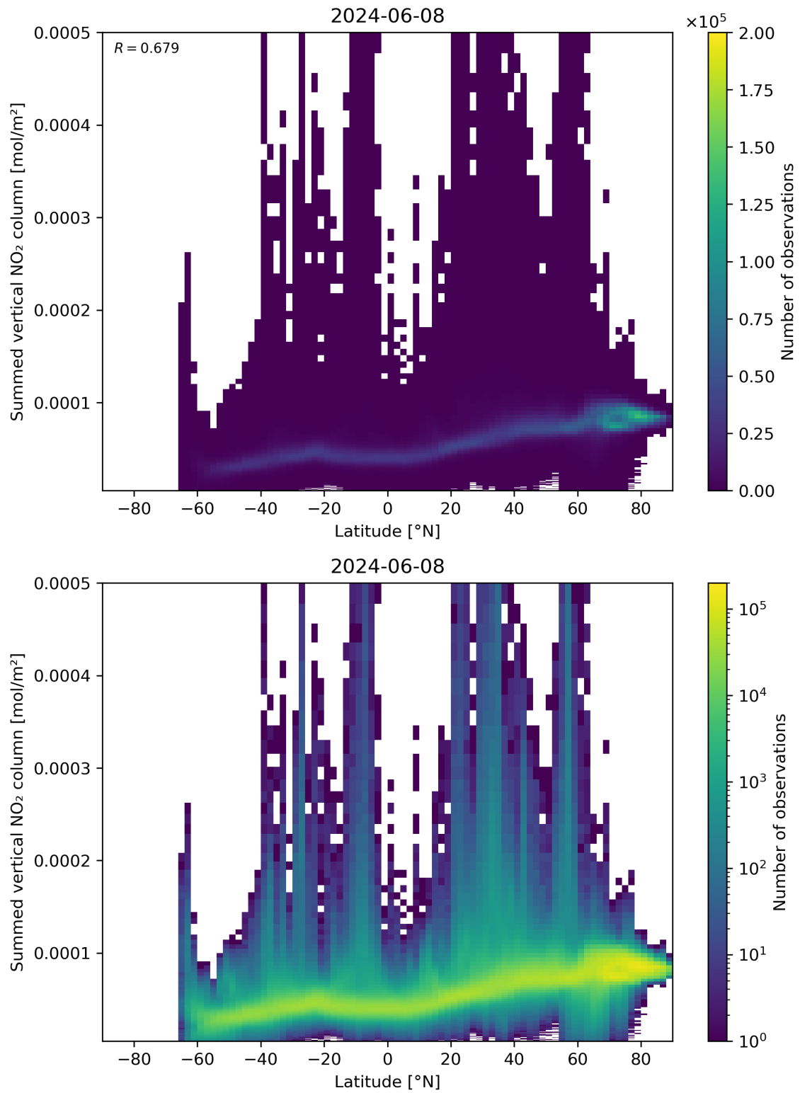
Figure 88: Scatter density plot of “Latitude” against “Summed vertical NO 2 column” for 2024-06-08 to 2024-06-09.
