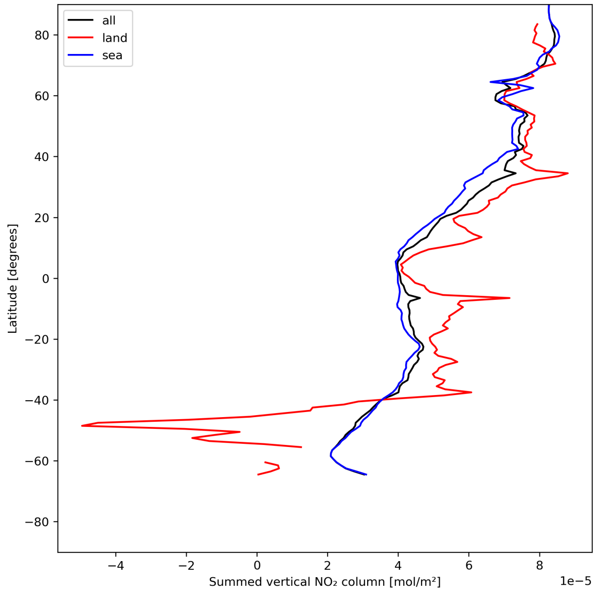
Figure 23: Zonal average of “Summed vertical NO 2 column” for 2024-06-08 to 2024-06-09.
