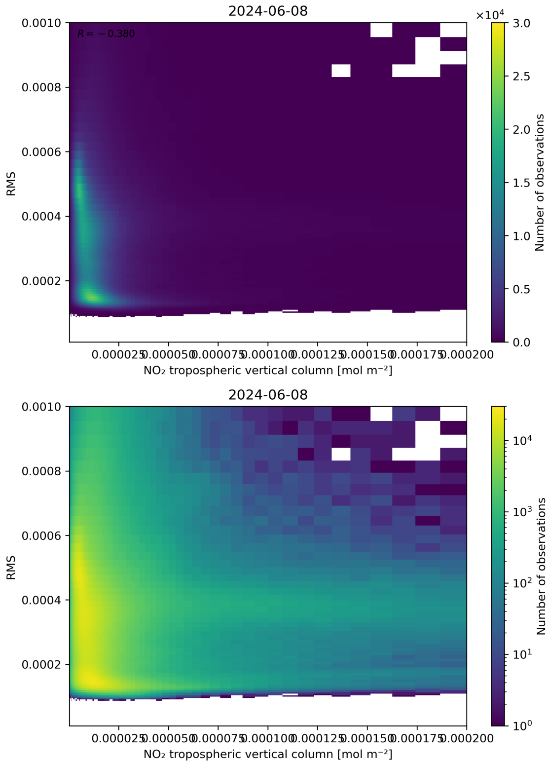
Figure 142: Scatter density plot of “NO 2 tropospheric vertical column” against “RMS” for 2024-06-08 to 2024-06-09.
