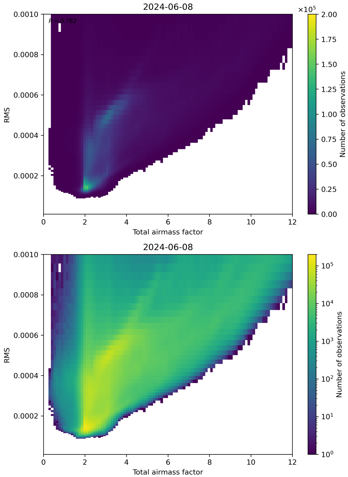
Figure 69: Scatter density plot of “Total airmass factor” against “RMS” for 2024-06-08 to 2024-06-09.
