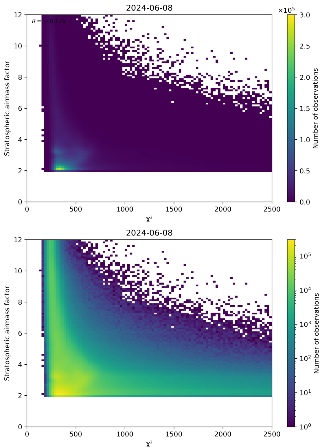
Figure 81: Scatter density plot of “ \chi^2 ” against “Stratospheric airmass factor” for 2024-06-08 to 2024-06-09.
