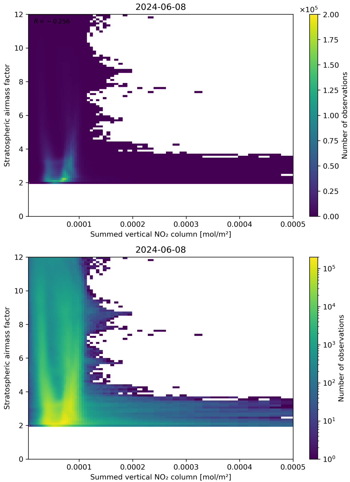
Figure 103: Scatter density plot of “Summed vertical NO 2 column” against “Stratospheric air mass factor” for 2024-06-08 to 2024-06-09.
