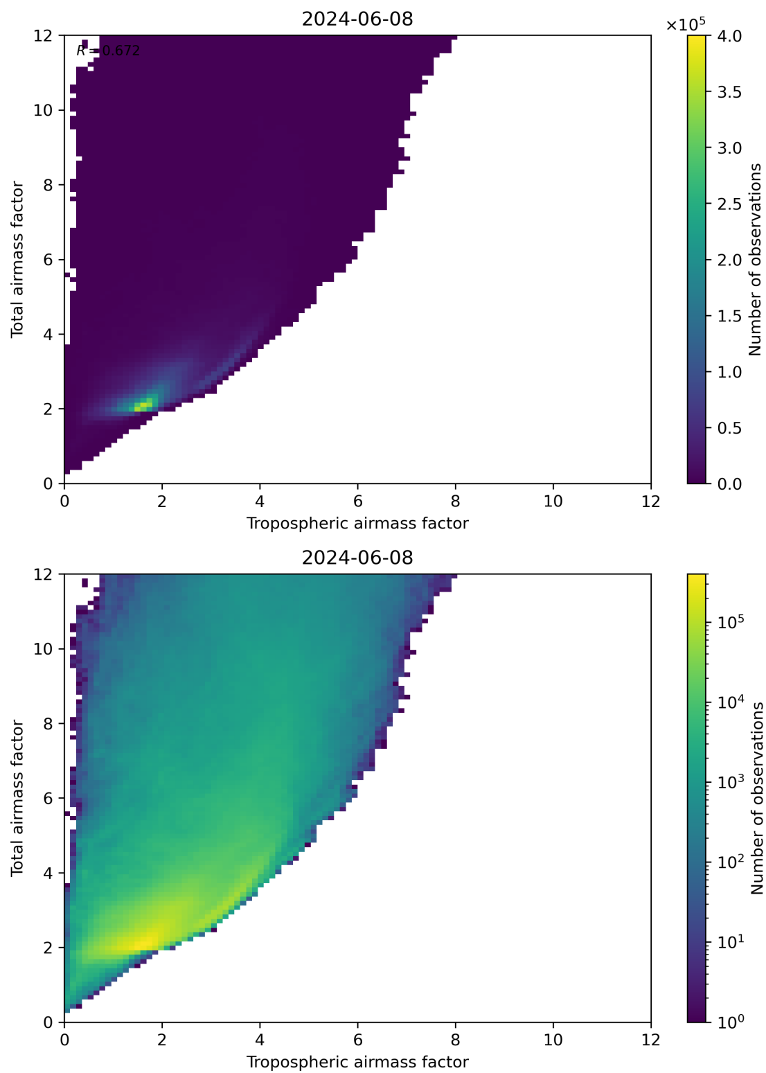
Figure 72: Scatter density plot of “Tropospheric airmass factor” against “Total airmass factor” for 2024-06-08 to 2024-06-09.
