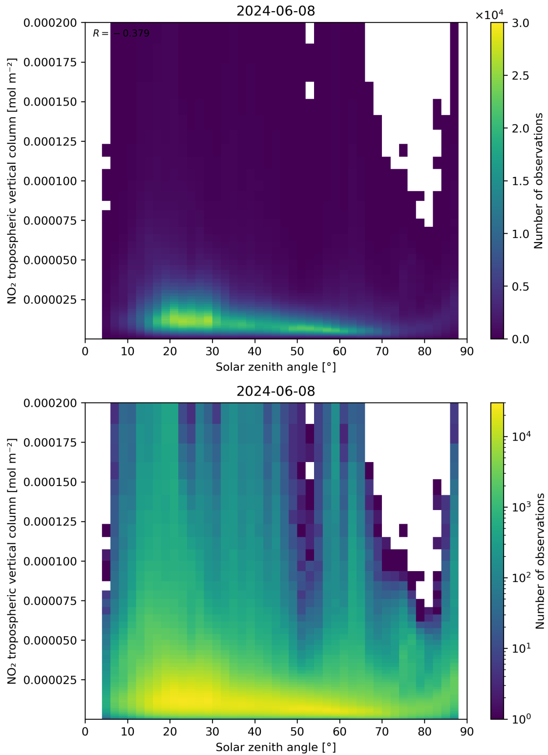
Figure 155: Scatter density plot of “Solar zenith angle” against “NO 2 tropospheric vertical column” for 2024-06-08 to 2024-06-09.
