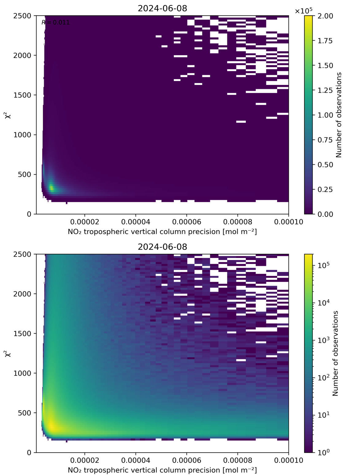
Figure 134: Scatter density plot of “NO 2 tropospheric vertical column precision” against “ \chi^2 ” for 2024-06-08 to 2024-06-09.
