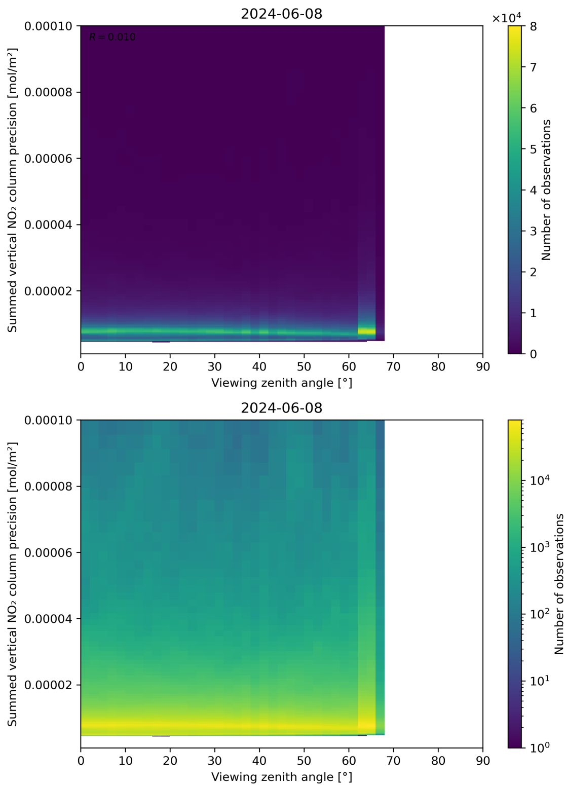
Figure 166: Scatter density plot of “Viewing zenith angle” against “Summed vertical NO 2 column precision” for 2024-06-08 to 2024-06-09.
