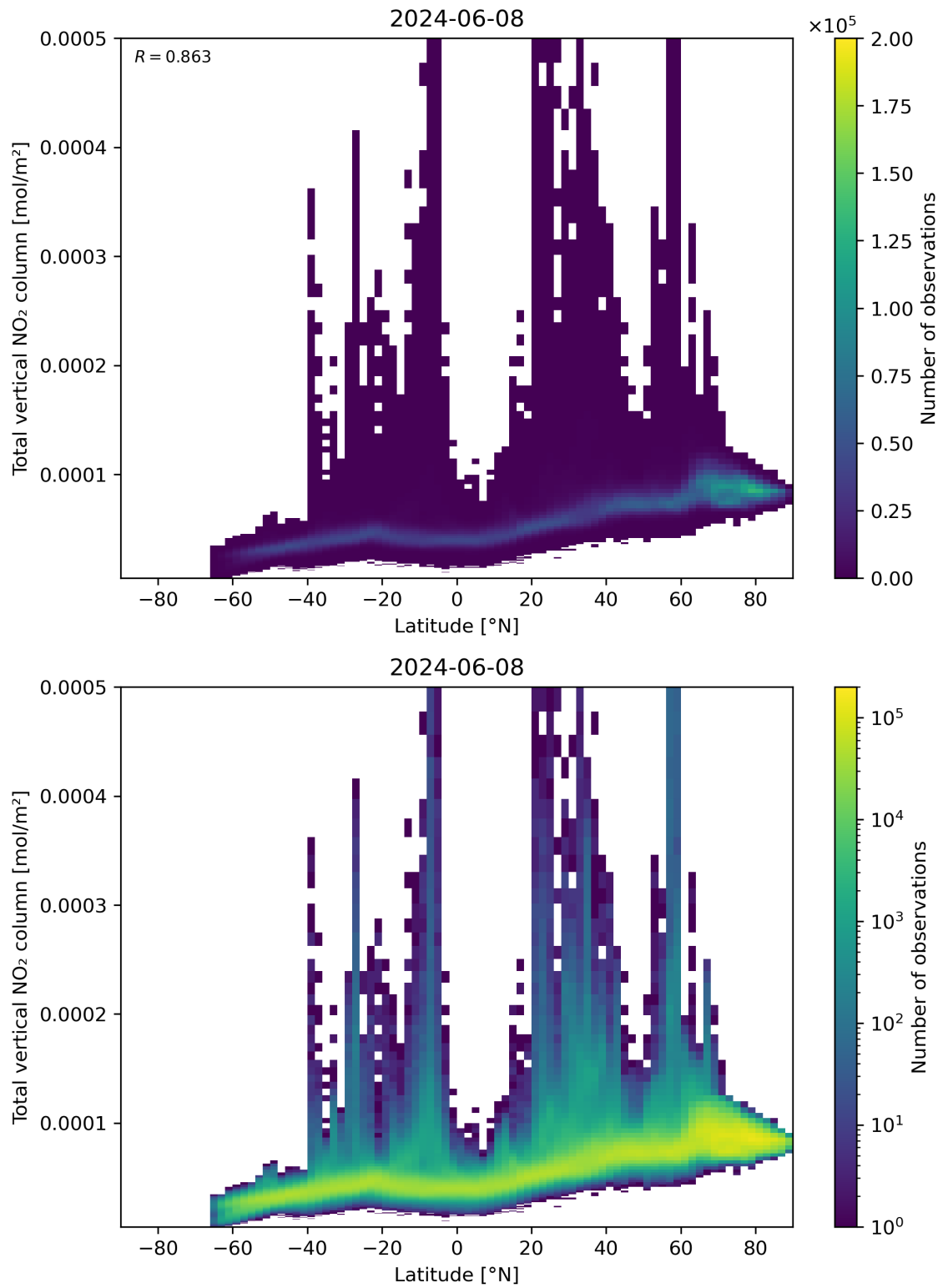
Figure 90: Scatter density plot of “Latitude” against “Total vertical NO 2 column” for 2024-06-08 to 2024-06-09.
