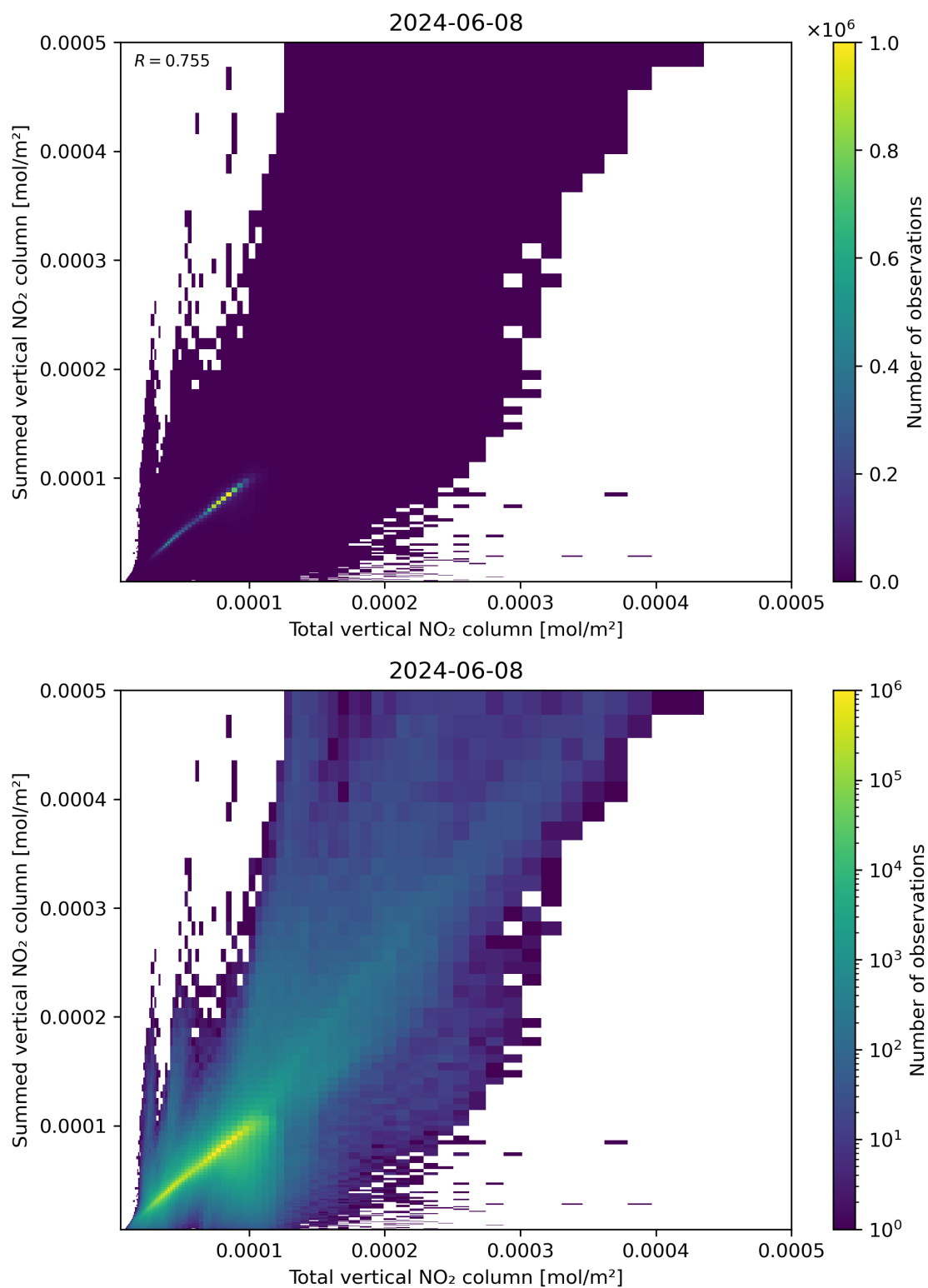
Figure 112: Scatter density plot of “Total vertical NO 2 column” against “Summed vertical NO 2 column” for 2024-06-08 to 2024-06-09.
