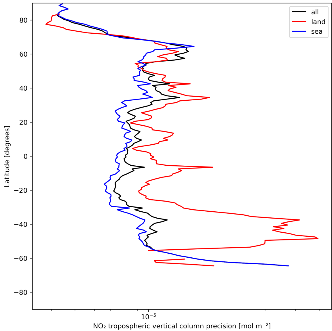
Figure 13: Zonal average of “NO 2 tropospheric vertical column precision” for 2024-06-08 to 2024-06-09.
