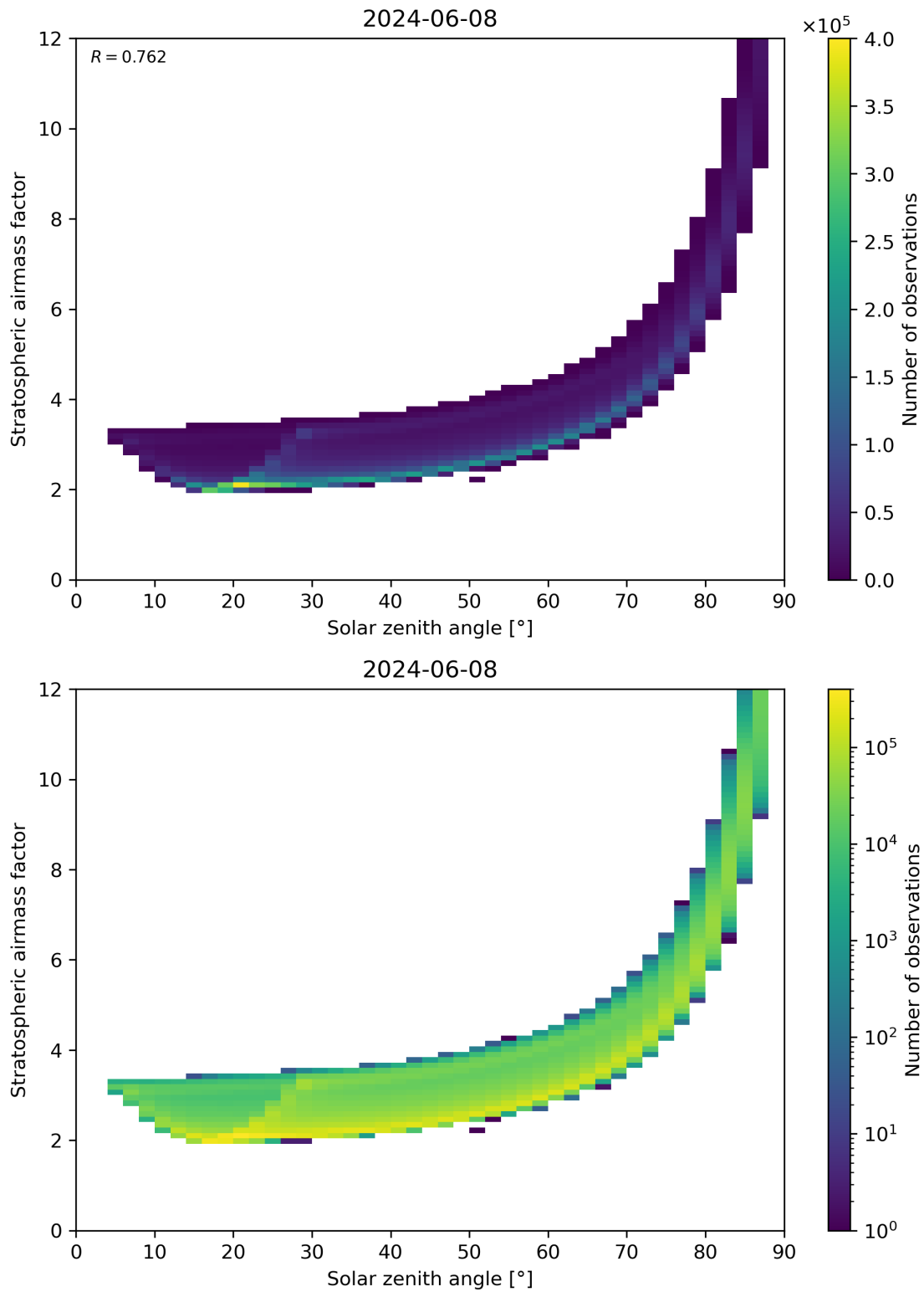
Figure 145: Scatter density plot of “Solar zenith angle” against “Stratospheric airmass factor” for 2024-06-08 to 2024-06-09.
