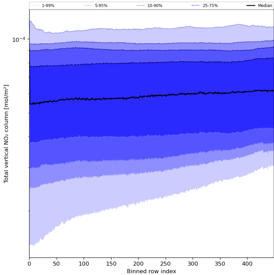
Figure 55: Along track statistics of “Total vertical NO 2 column” for 2024-06-08 to 2024-06-09
