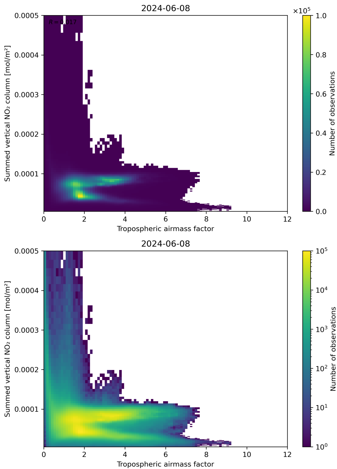
Figure 75: Scatter density plot of “Tropospheric airmass factor” against “Summed vertical NO 2 column” for 2024-06-08 to 2024-06-09.
