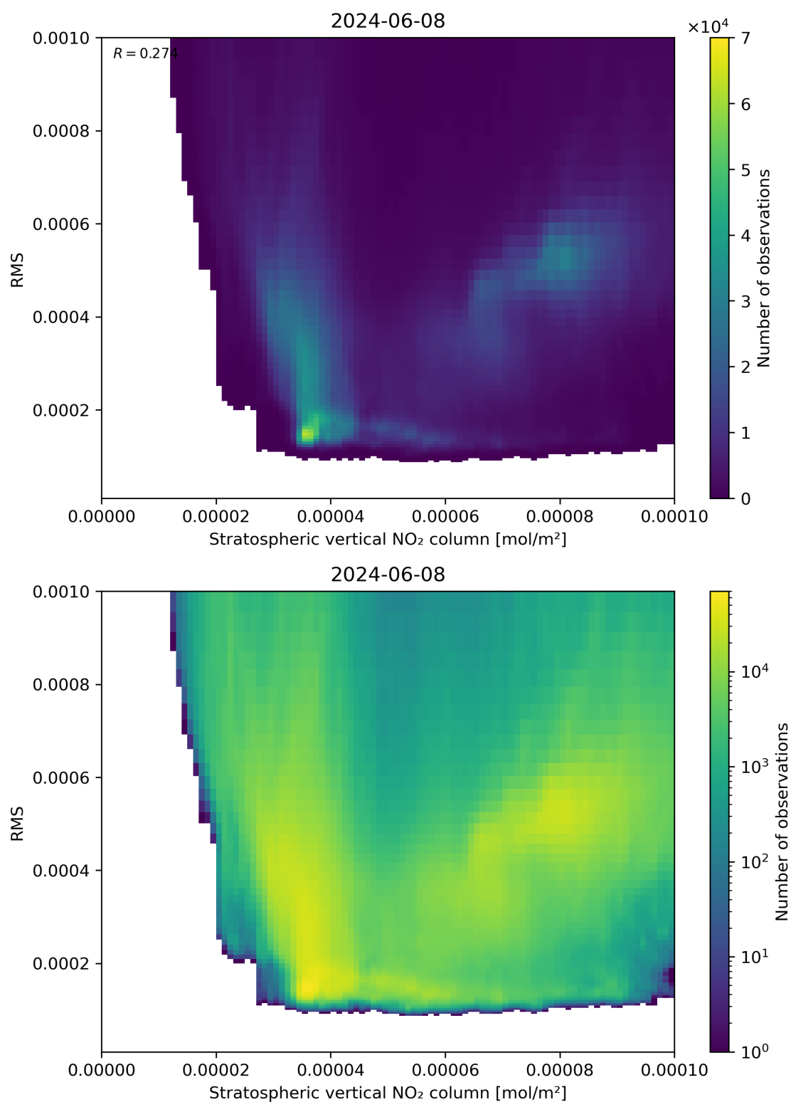
Figure 102: Scatter density plot of “Stratospheric vertical NO 2 column” against “RMS” for 2024-06-08 to 2024-06-09.
