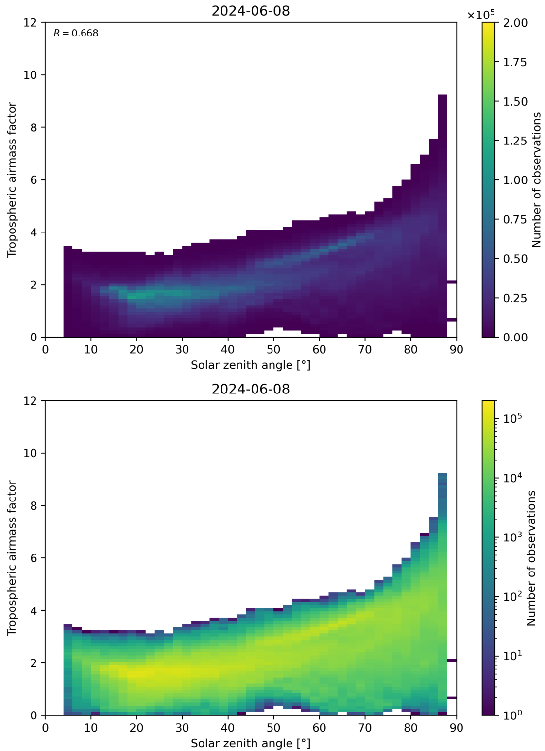
Figure 147: Scatter density plot of “Solar zenith angle” against “Tropospheric airmass factor” for 2024-06-08 to 2024-06-09.
