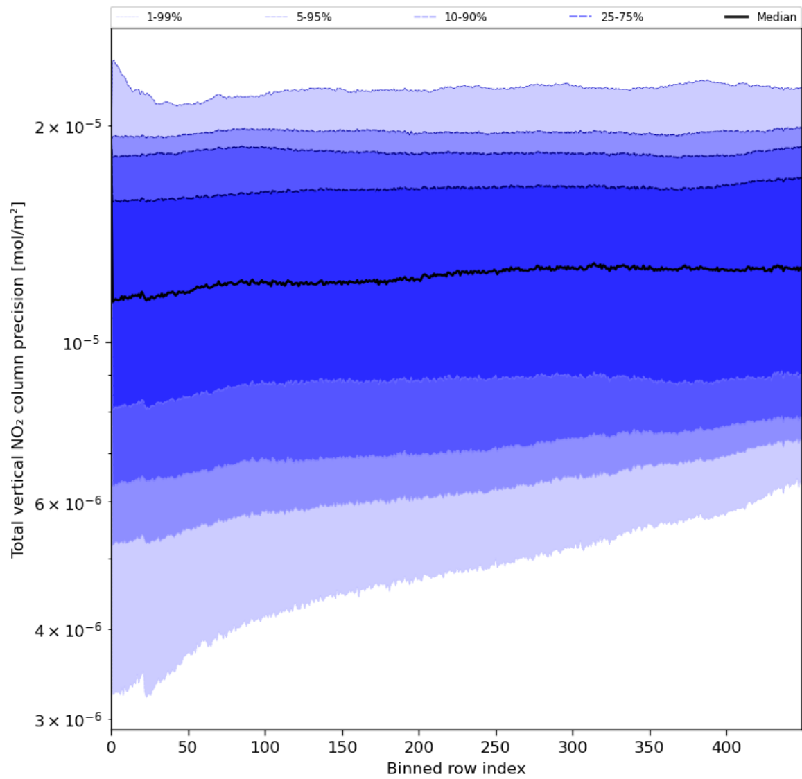
Figure 56: Along track statistics of “Total vertical NO 2 column precision” for 2024-06-08 to 2024-06-09
