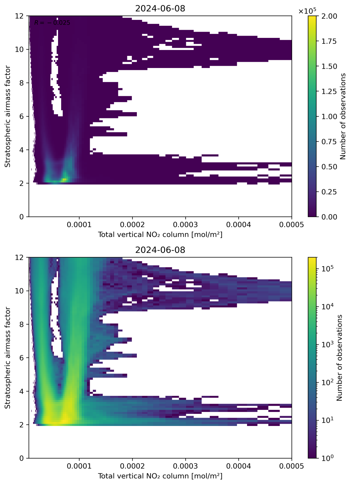
Figure 110: Scatter density plot of “Total vertical NO 2 column” against “Stratospheric airmass factor” for 2024-06-08 to 2024-06-09.
