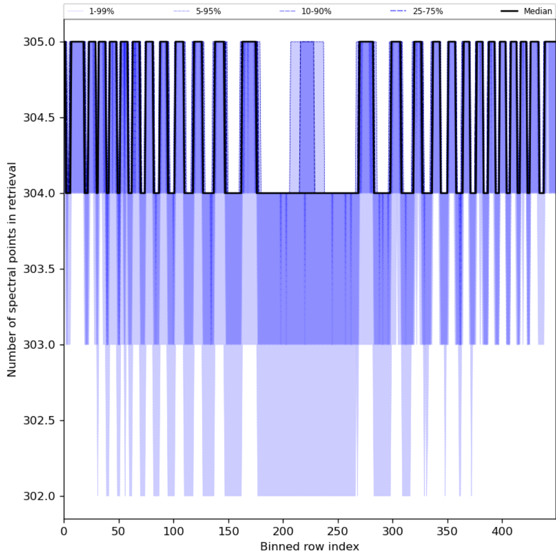
Figure 50: Along track statistics of “Number of spectral points in retrieval” for 2024-06-08 to 2024-06-09
