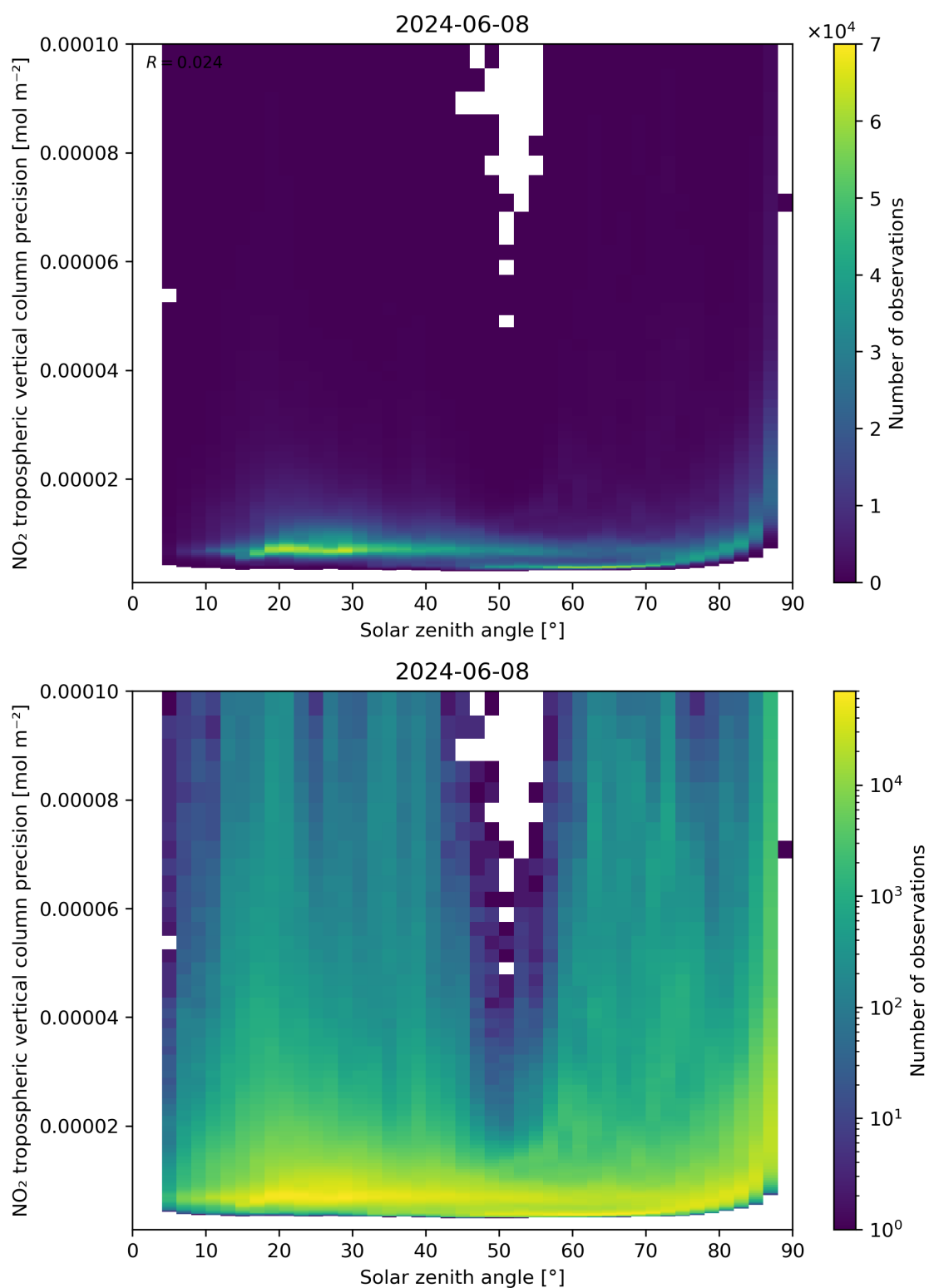
Figure 156: Scatter density plot of “Solar zenith angle” against “NO 2 tropospheric vertical column precision” for 2024-06-08 to 2024-06-09.
