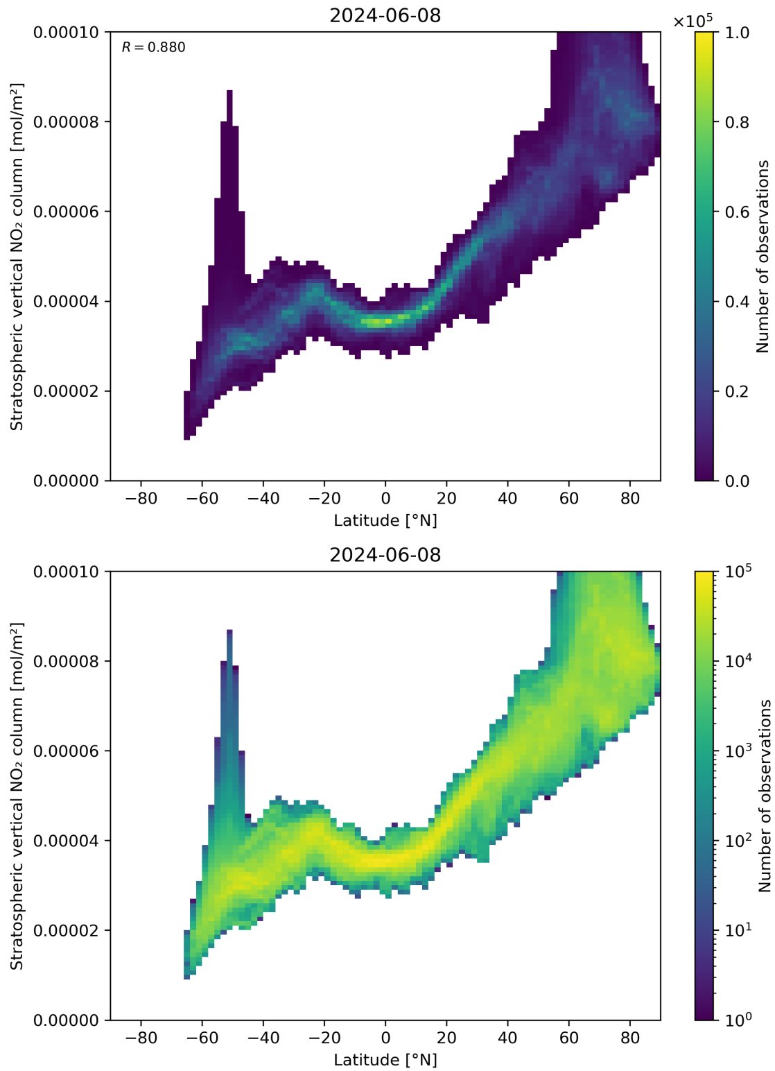
Figure 87: Scatter density plot of “Latitude” against “Stratospheric vertical NO 2 column” for 2024-06-08 to 2024-06-09.
