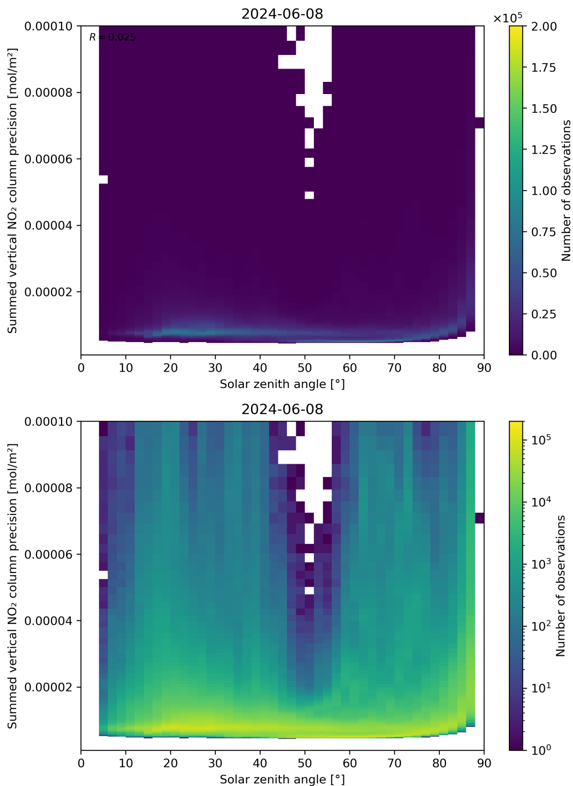
Figure 152: Scatter density plot of “Solar zenith angle” against “Summed vertical NO 2 column precision” for 2024-06-08 to 2024-06-09.
