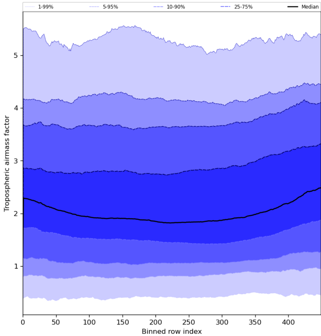
Figure 48: Along track statistics of “Tropospheric airmass factor” for 2024-06-08 to 2024-06-09
