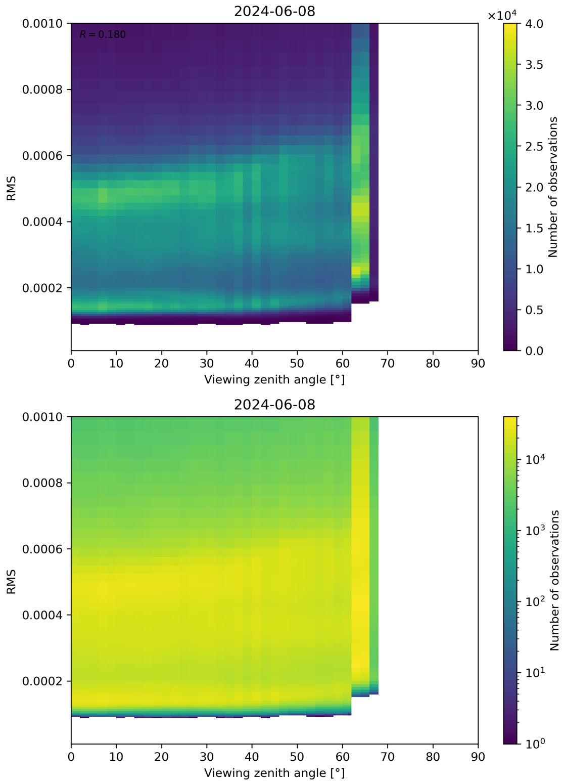
Figure 171: Scatter density plot of “Viewing zenith angle” against “RMS” for 2024-06-08 to 2024-06-09.
