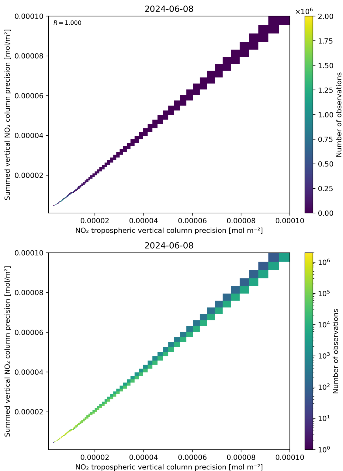
Figure 137: Scatter density plot of “NO 2 tropospheric vertical column precision” against “Summed vertical NO 2 column precision” for 2024-06-08 to 2024-06-09.
