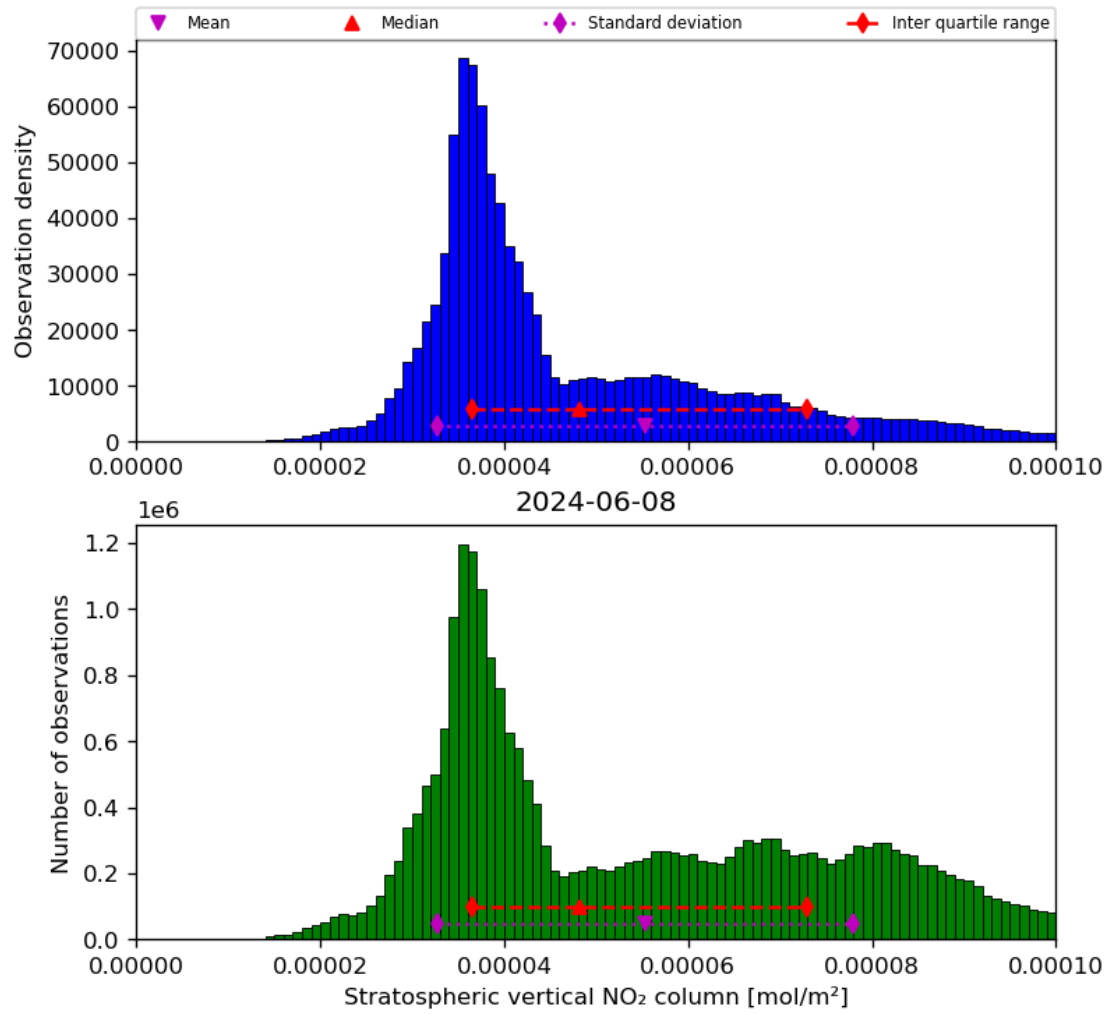
Figure 36: Histogram of “Stratospheric vertical NO 2 column” for 2024-06-08 to 2024-06-09
