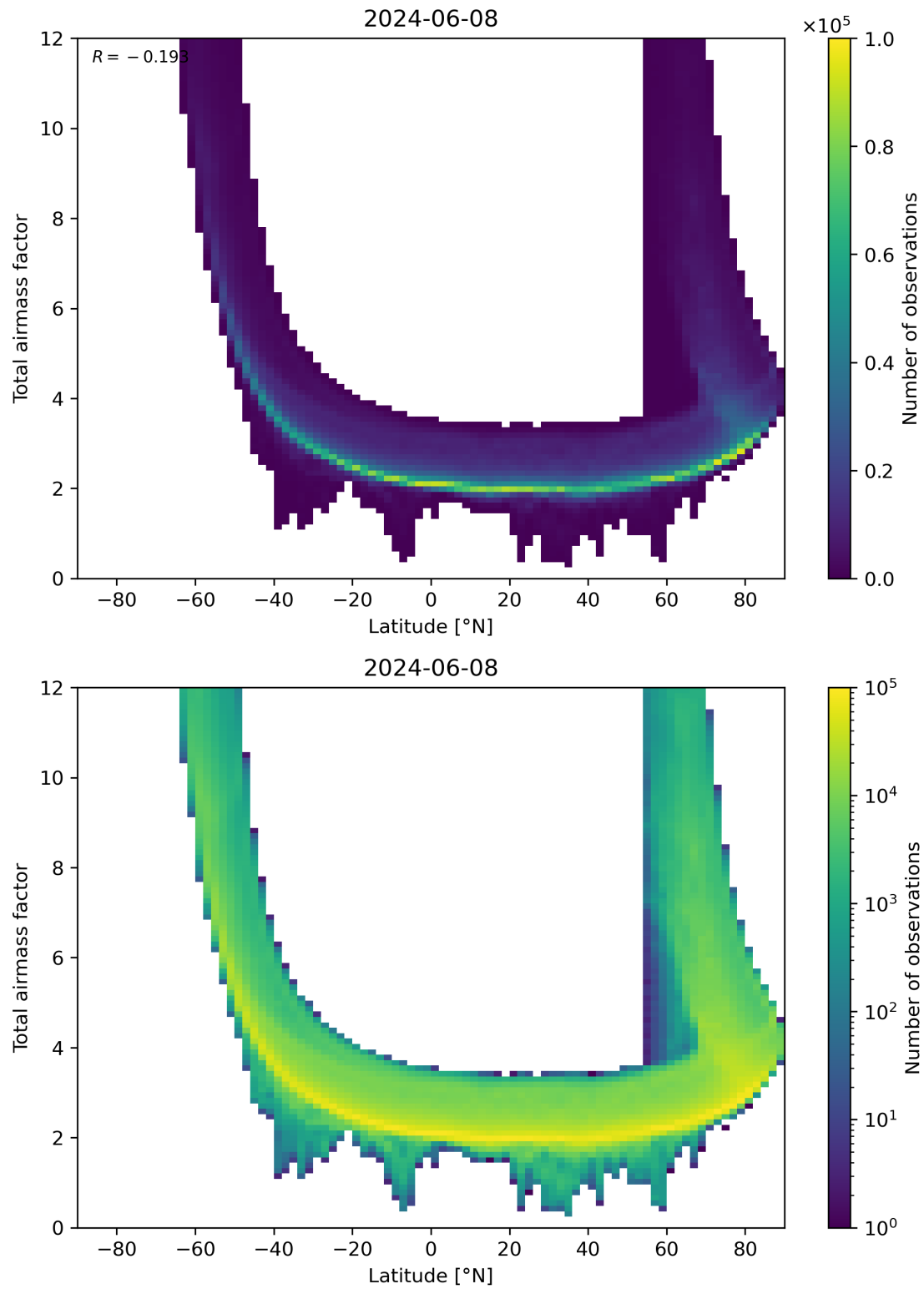
Figure 84: Scatter density plot of “Latitude” against “Total airmass factor” for 2024-06-08 to 2024-06-09.
