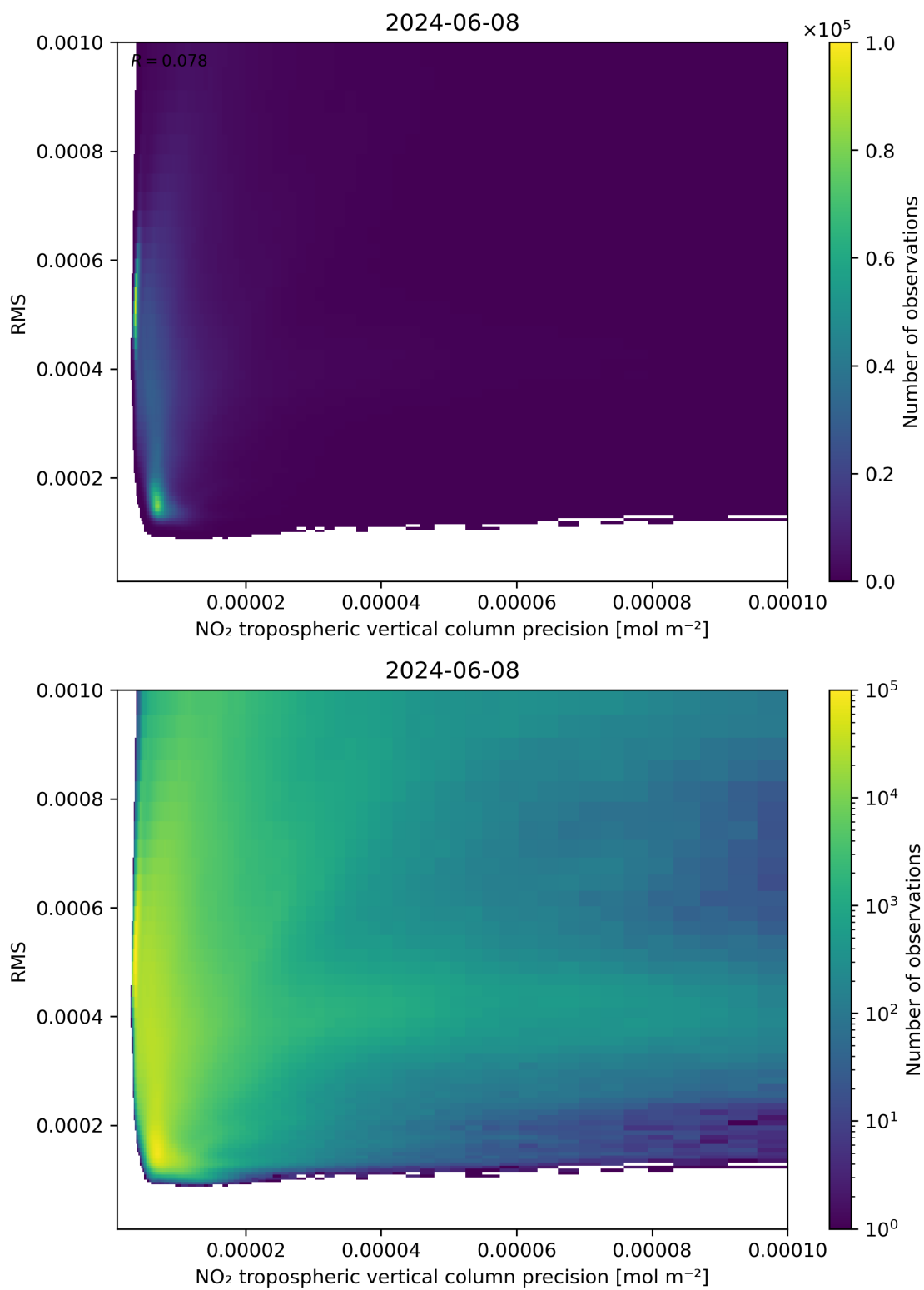
Figure 140: Scatter density plot of “NO 2 tropospheric vertical column precision” against “RMS” for 2024-06-08 to 2024-06-09.
