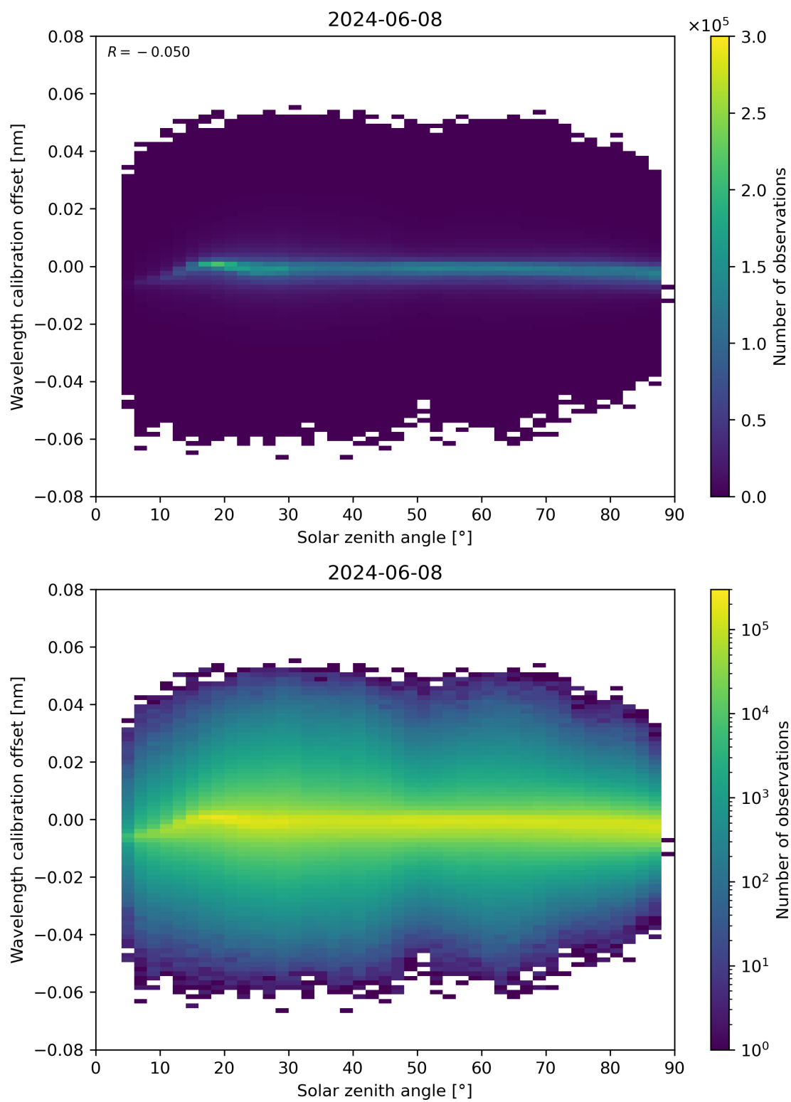
Figure 158: Scatter density plot of “Solar zenith angle” against “Wavelength calibration offset” for 2024-06-08 to 2024-06-09.
