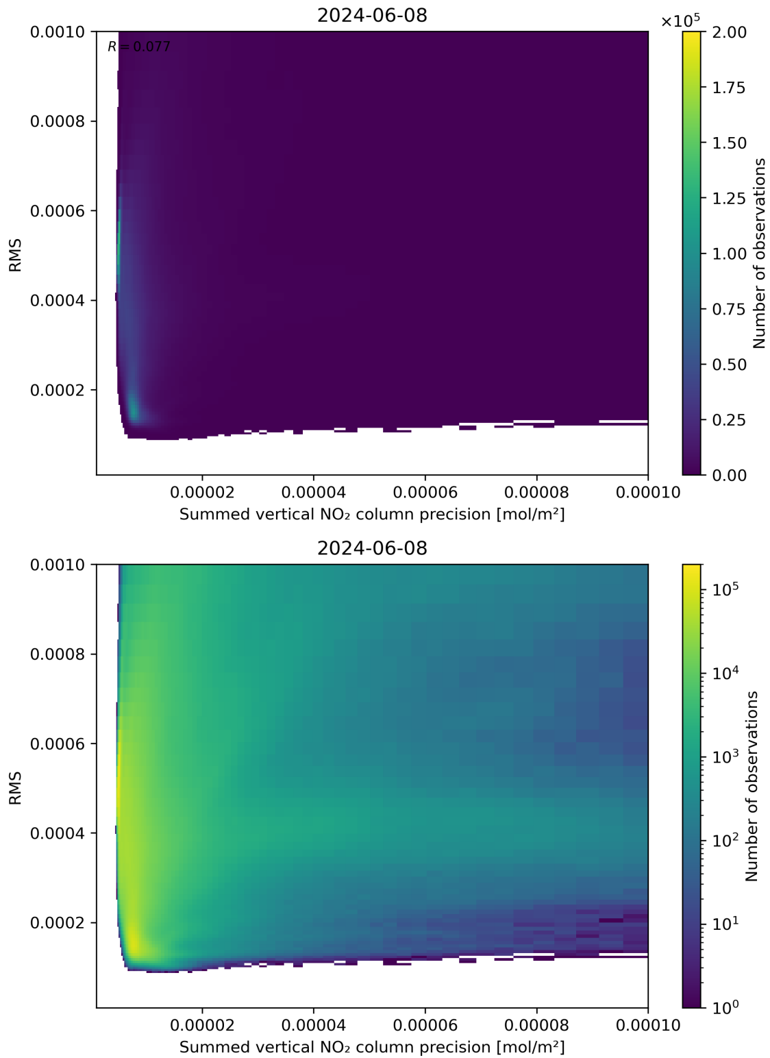
Figure 108: Scatter density plot of “Summed vertical NO 2 column precision” against “RMS” for 2024-06-08 to 2024-06-09.
