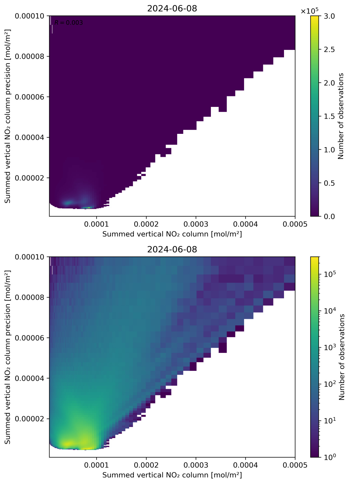
Figure 105: Scatter density plot of “Summed vertical NO 2 column” against “Summed vertical NO 2 column precision” for 2024-06-08 to 2024-06-09.
