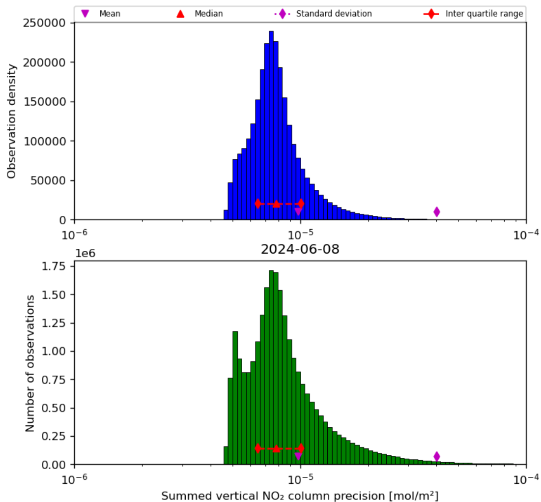
Figure 41: Histogram of “Summed vertical NO 2 column precision” for 2024-06-08 to 2024-06-09
