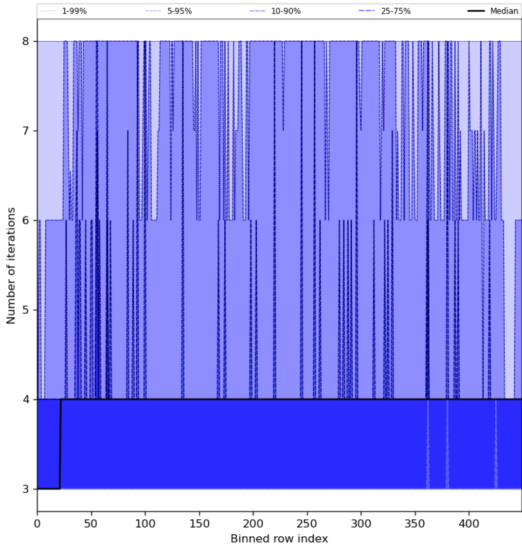
Figure 51: Along track statistics of “Number of iterations” for 2024-06-08 to 2024-06-09
