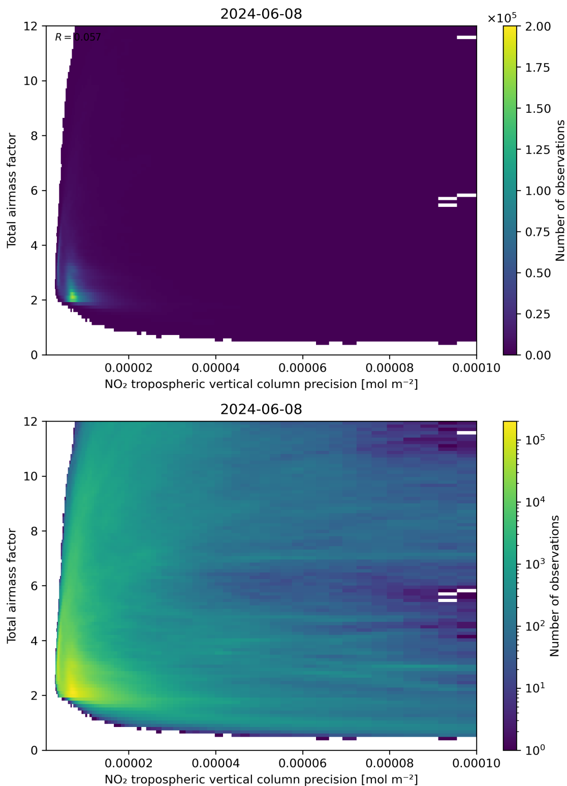
Figure 132: Scatter density plot of “NO 2 tropospheric vertical column precision” against “Total air mass factor” for 2024-06-08 to 2024-06-09.
