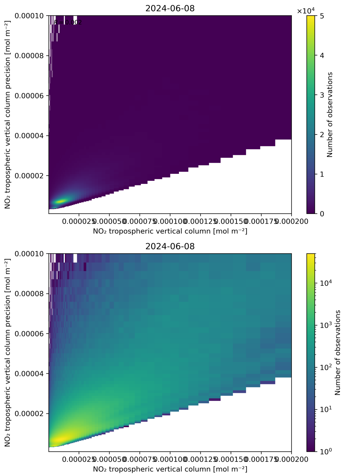
Figure 130: Scatter density plot of “NO 2 tropospheric vertical column” against “NO 2 tropospheric vertical column precision” for 2024-06-08 to 2024-06-09.
