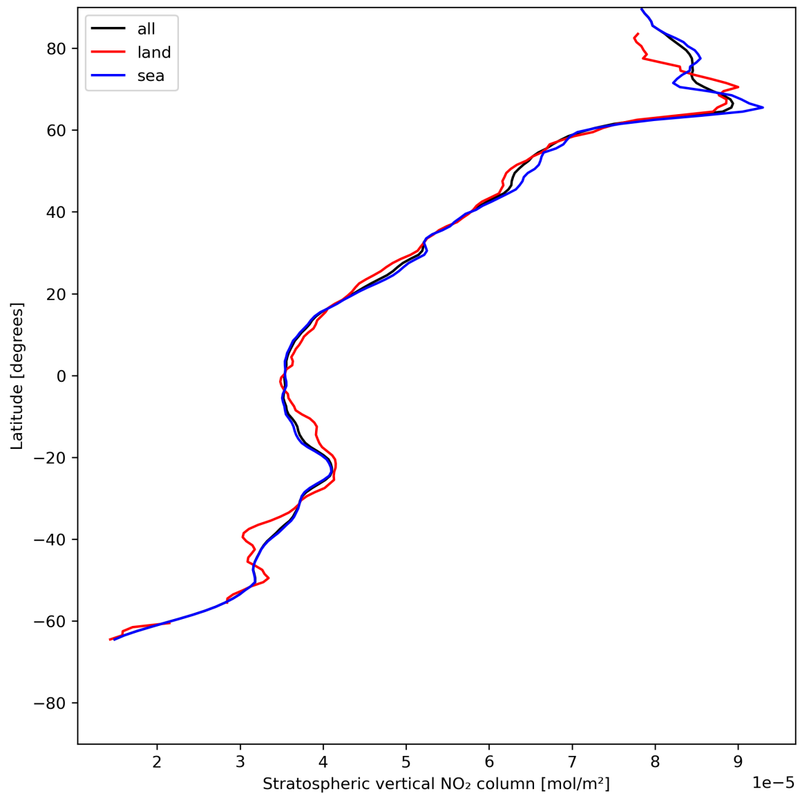
Figure 19: Zonal average of “Stratospheric vertical NO 2 column” for 2024-06-08 to 2024-06-09.
