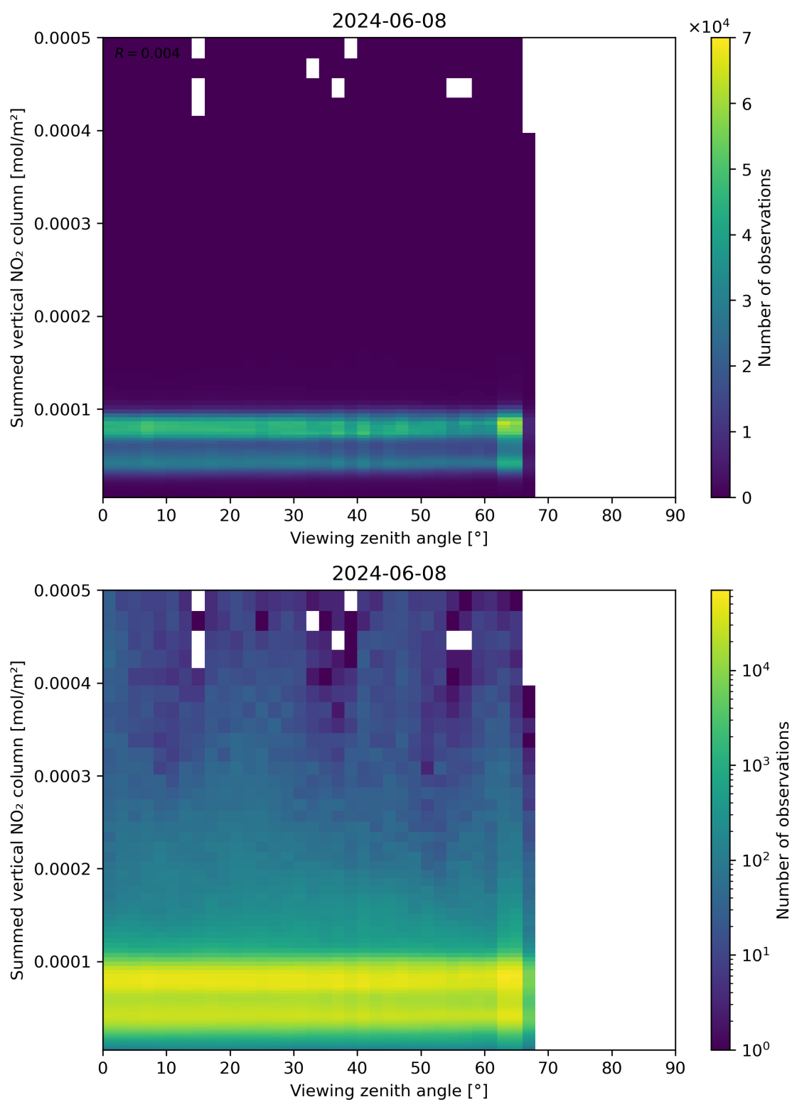
Figure 165: Scatter density plot of “Viewing zenith angle” against “Summed vertical NO 2 column” for 2024-06-08 to 2024-06-09.
