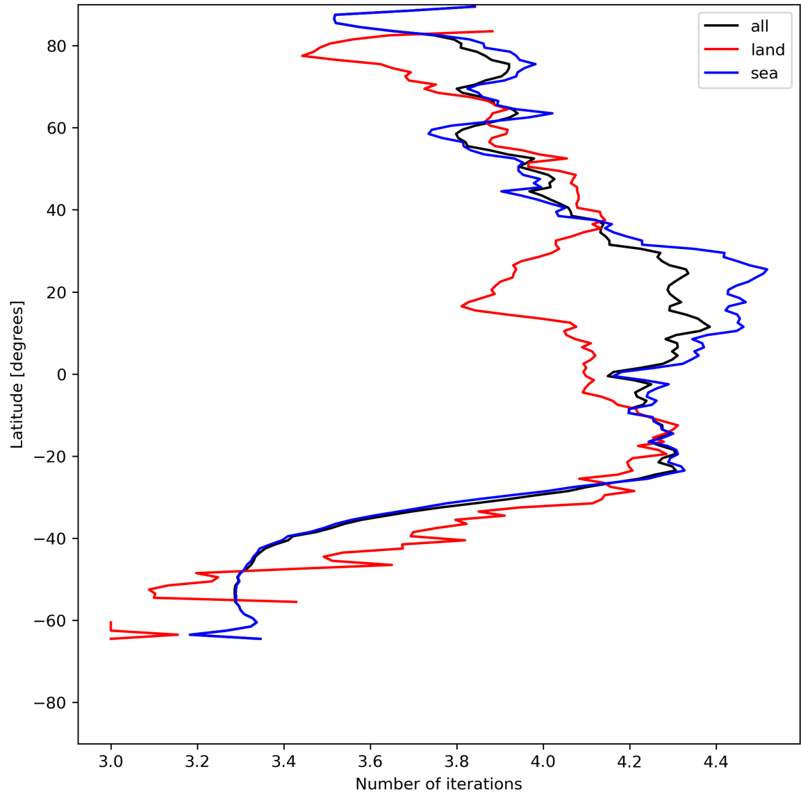
Figure 17: Zonal average of “Number of iterations” for 2024-06-08 to 2024-06-09.
