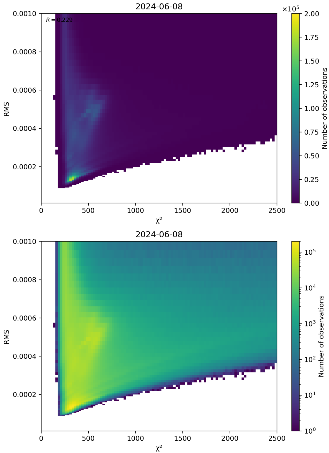
Figure 82: Scatter density plot of “ \chi^2 ” against “RMS” for 2024-06-08 to 2024-06-09.
