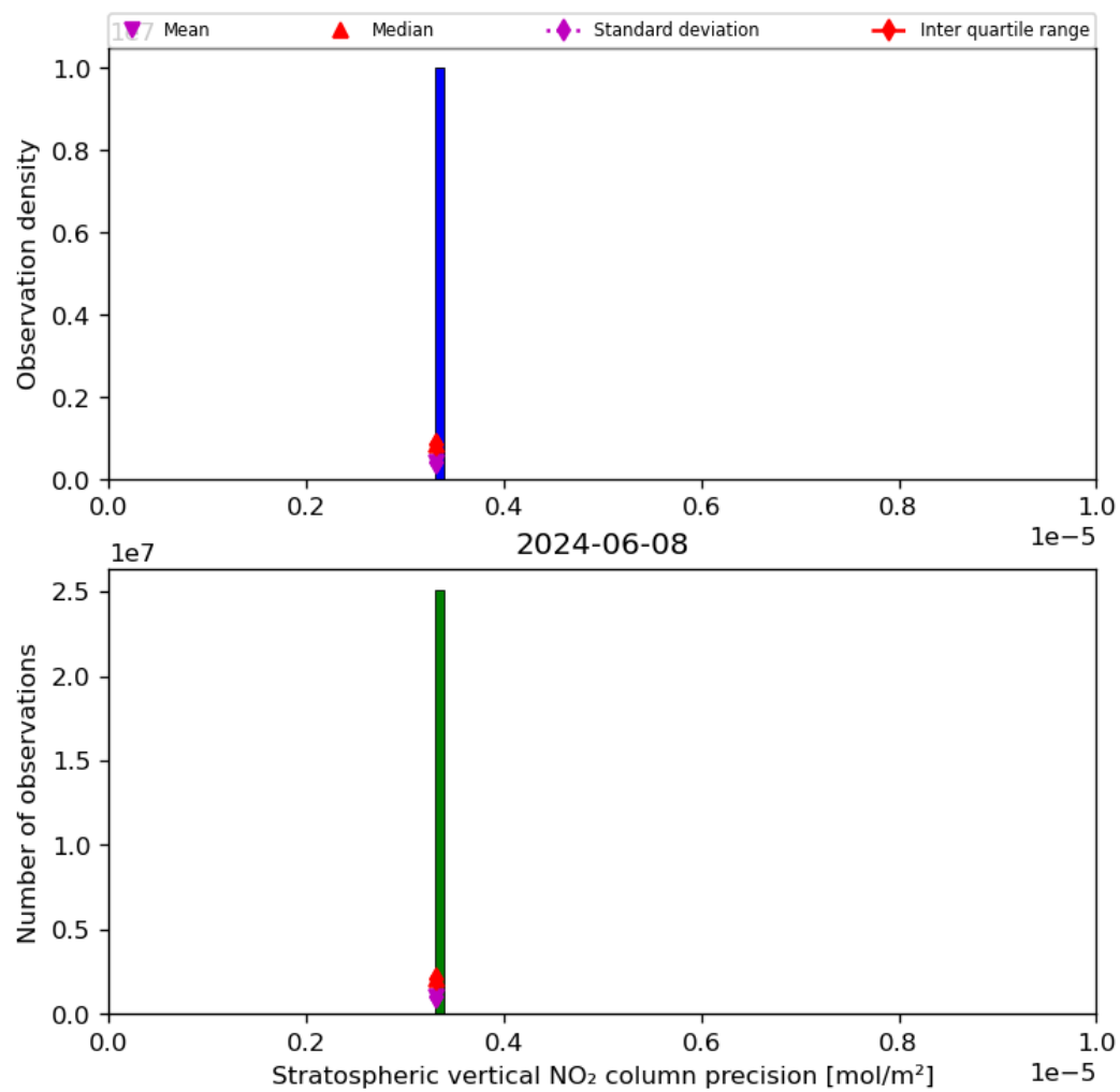
Figure 37: Histogram of “Stratospheric vertical NO 2 column precision” for 2024-06-08 to 2024-06-09
