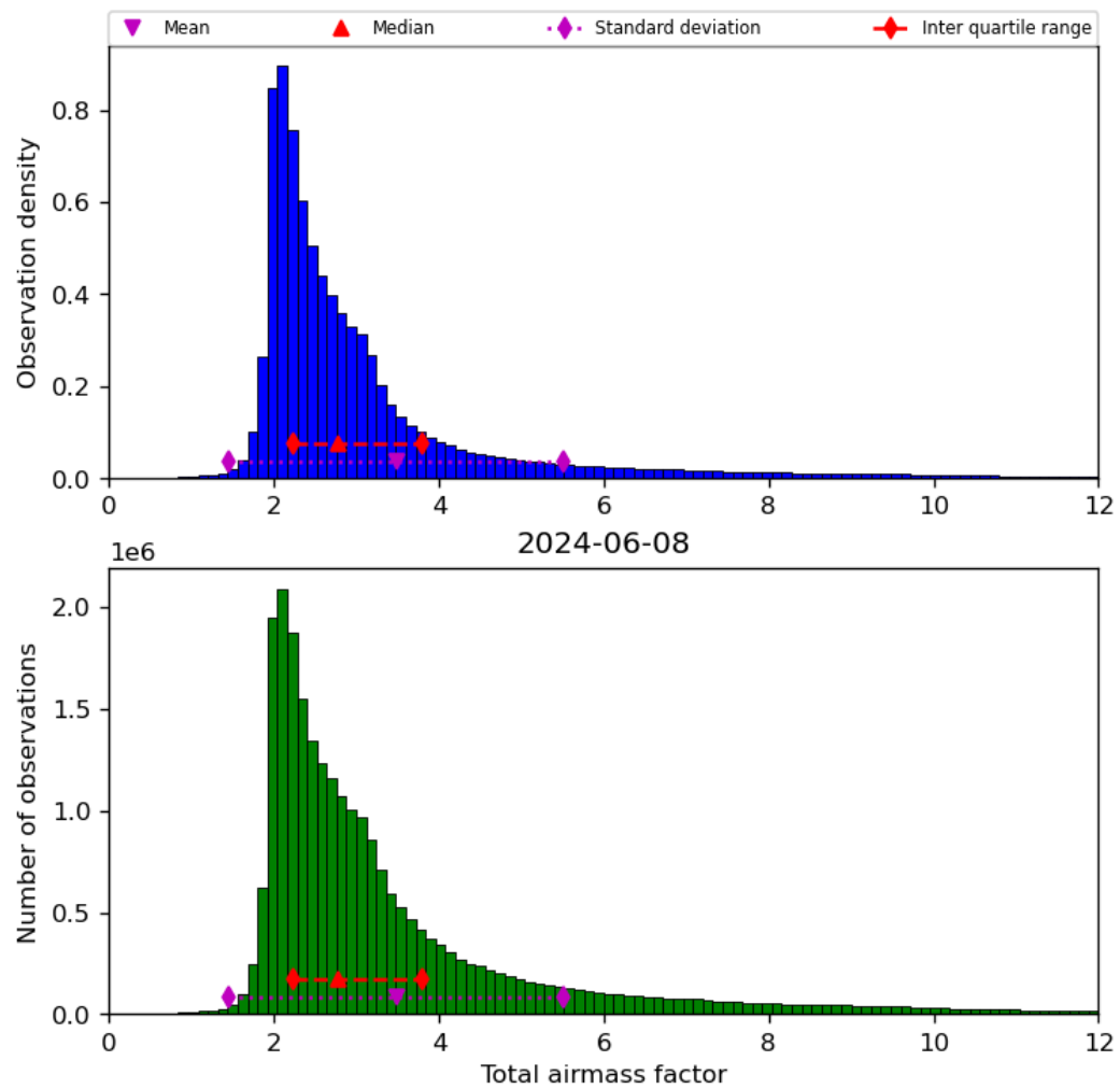
Figure 32: Histogram of “Total airmass factor” for 2024-06-08 to 2024-06-09
