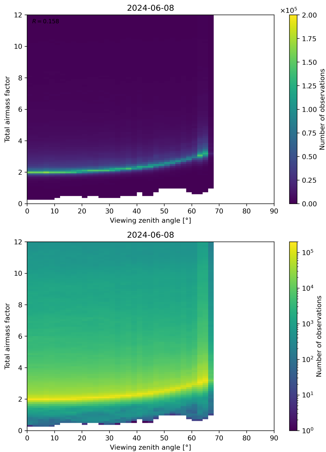
Figure 160: Scatter density plot of “Viewing zenith angle” against “Total airmass factor” for 2024-06-08 to 2024-06-09.
