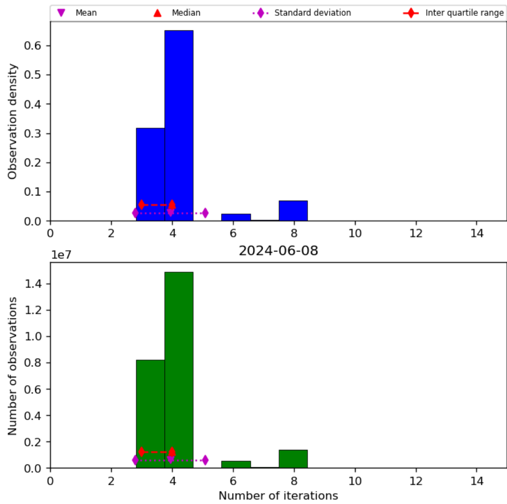
Figure 34: Histogram of “Number of iterations” for 2024-06-08 to 2024-06-09
