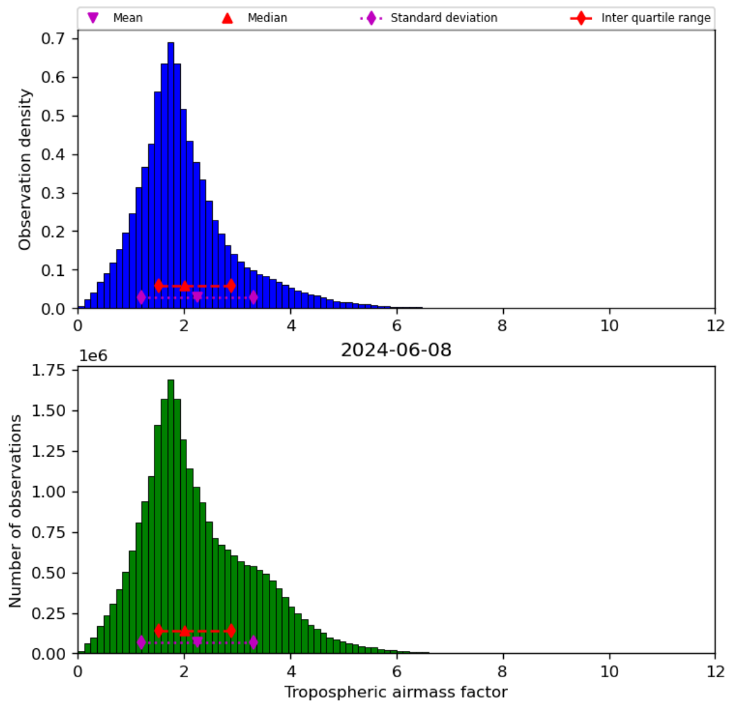
Figure 31: Histogram of “Tropospheric airmass factor” for 2024-06-08 to 2024-06-09
