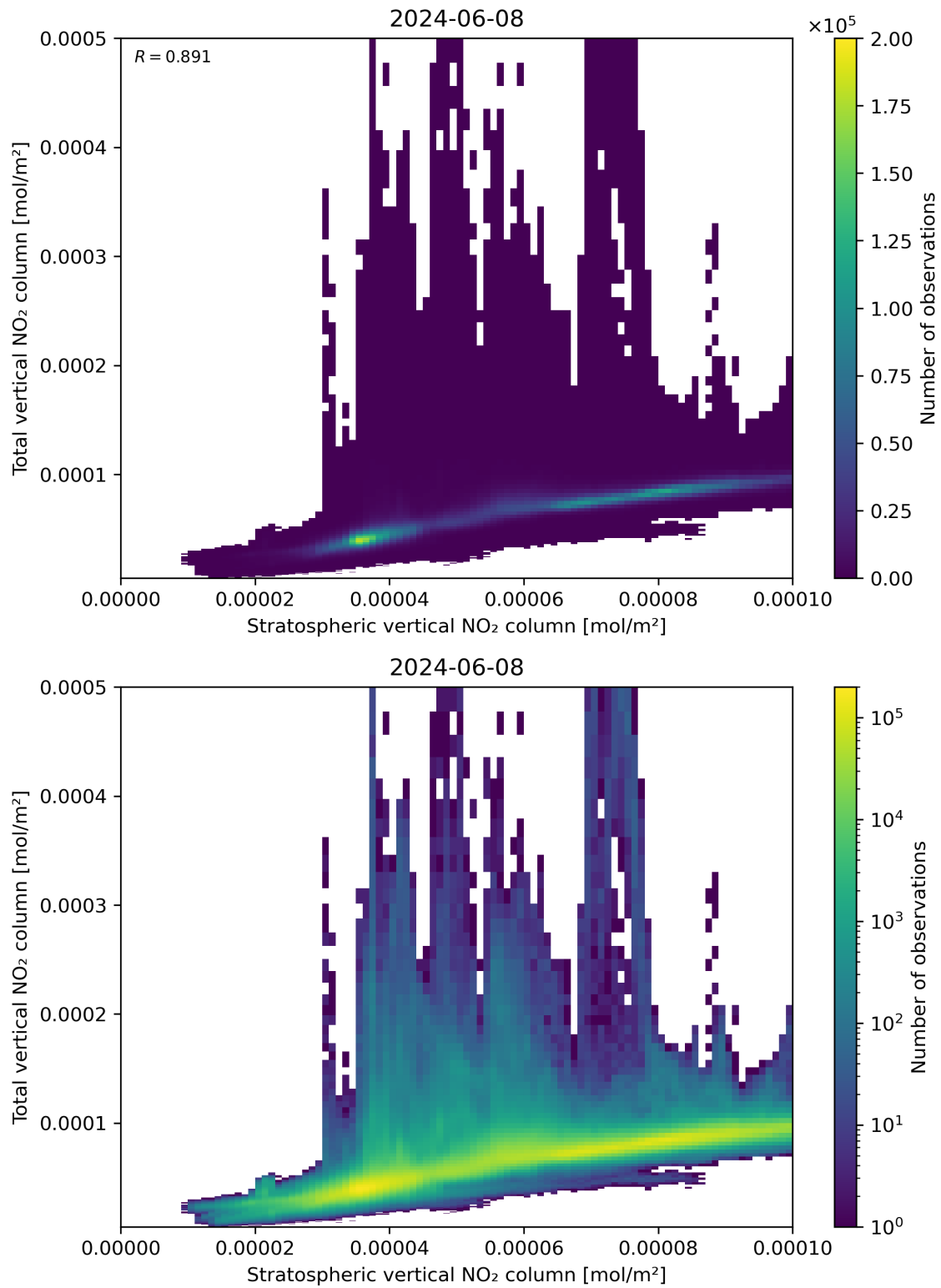
Figure 100: Scatter density plot of “Stratospheric vertical NO 2 column” against “Total vertical NO 2 column” for 2024-06-08 to 2024-06-09.
