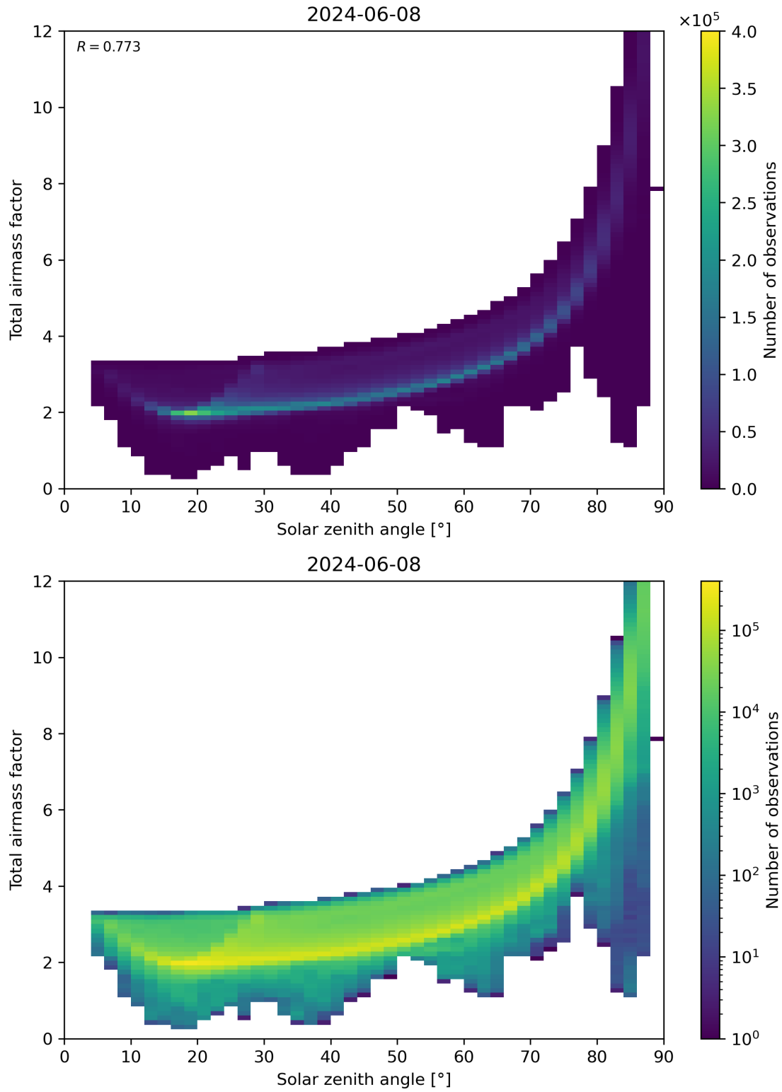
Figure 146: Scatter density plot of “Solar zenith angle” against “Total air mass factor” for 2024-06-08 to 2024-06-09.
