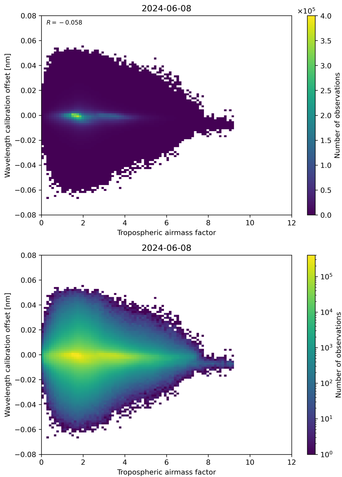
Figure 80: Scatter density plot of “Tropospheric airmass factor” against “Wavelength calibration offset” for 2024-06-08 to 2024-06-09.
