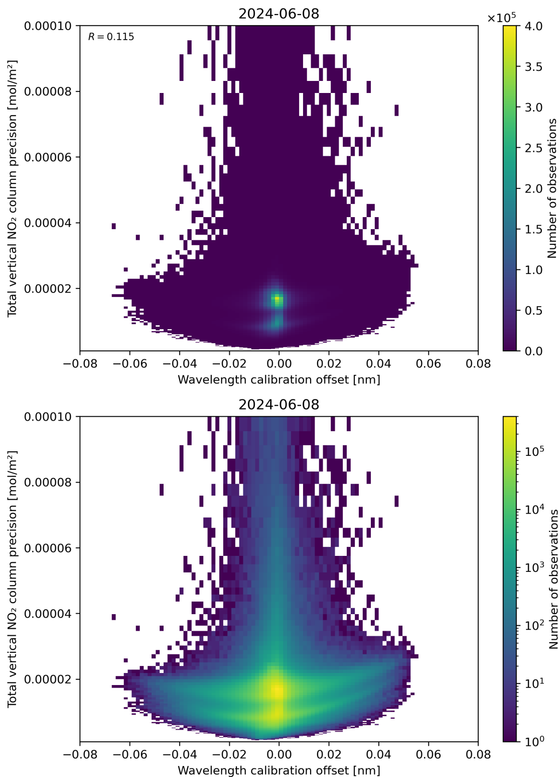
Figure 180: Scatter density plot of “Wavelength calibration offset” against “Total vertical NO 2 column precision” for 2024-06-08 to 2024-06-09.
