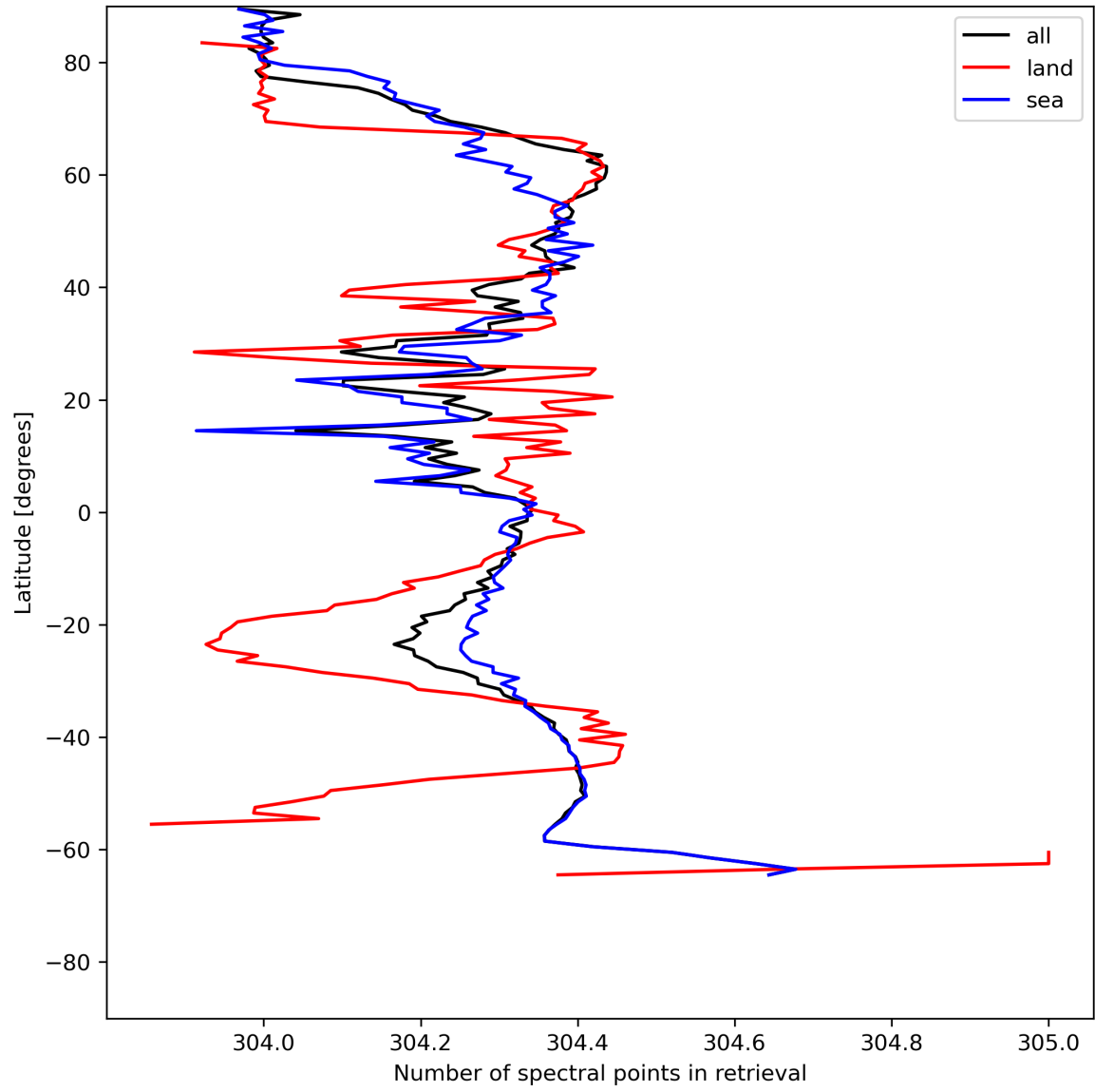
Figure 16: Zonal average of “Number of spectral points in retrieval” for 2024-06-08 to 2024-06-09.
