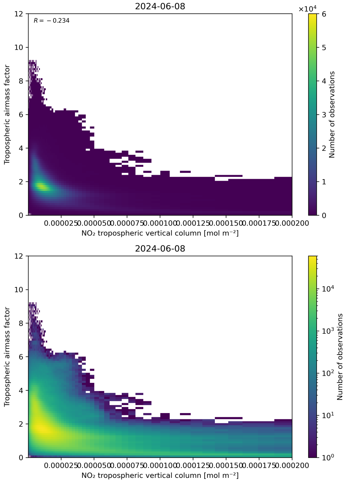
Figure 123: Scatter density plot of “NO 2 tropospheric vertical column” against “Tropospheric air mass factor” for 2024-06-08 to 2024-06-09.
