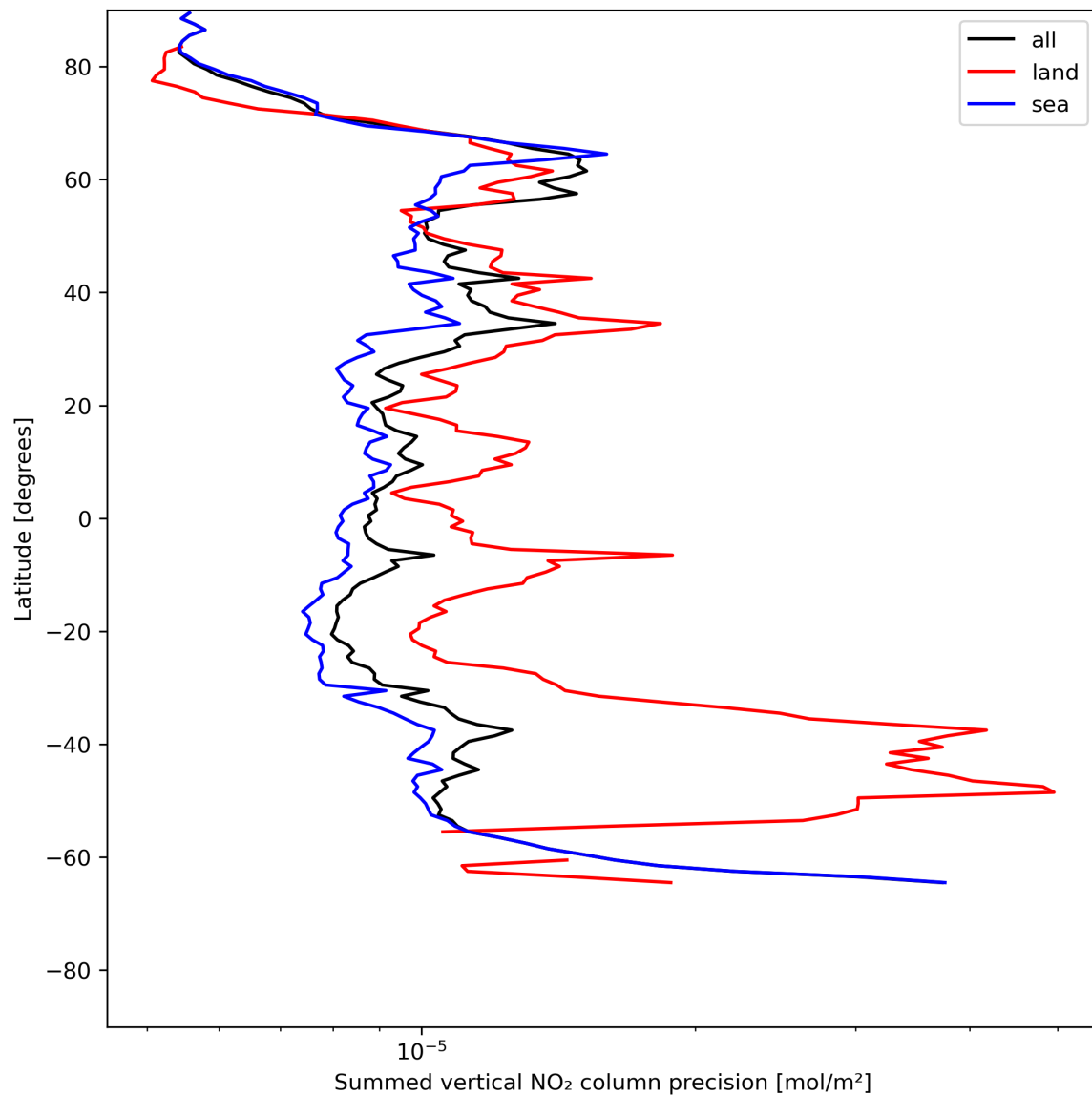
Figure 24: Zonal average of “Summed vertical NO 2 column precision” for 2024-06-08 to 2024-06-09.
