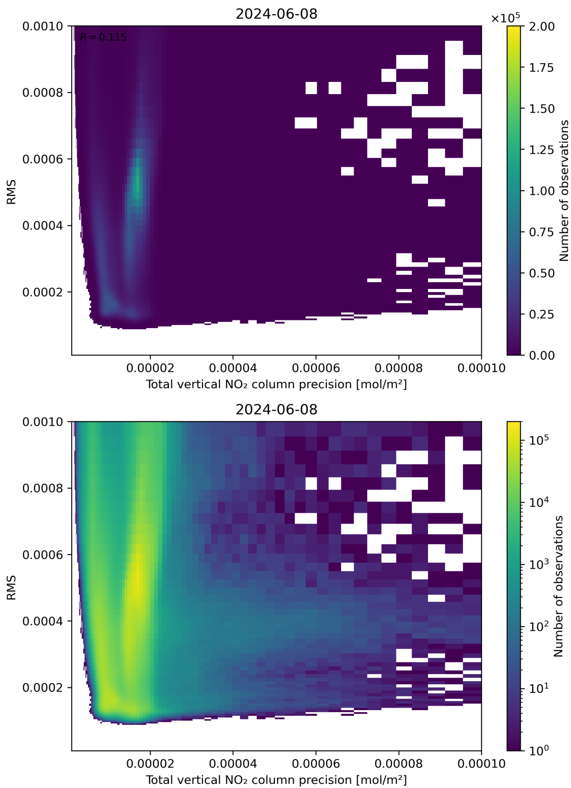
Figure 119: Scatter density plot of “Total vertical NO 2 column precision” against “RMS” for 2024-06-08 to 2024-06-09.
