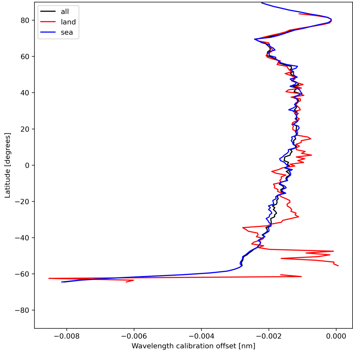
Figure 18: Zonal average of “Wavelength calibration offset” for 2024-06-08 to 2024-06-09.
