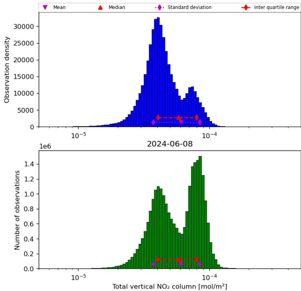
Figure 38: Histogram of “Total vertical NO 2 column” for 2024-06-08 to 2024-06-09
