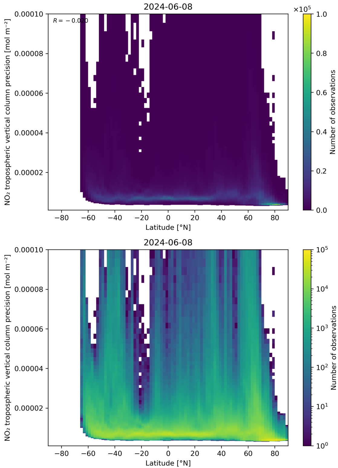
Figure 93: Scatter density plot of “Latitude” against “NO 2 tropospheric vertical column precision” for 2024-06-08 to 2024-06-09.
