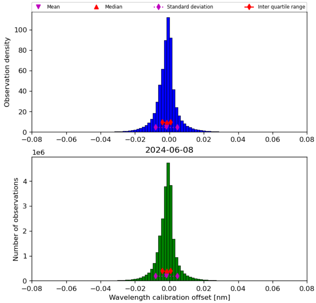
Figure 35: Histogram of “Wavelength calibration offset” for 2024-06-08 to 2024-06-09
