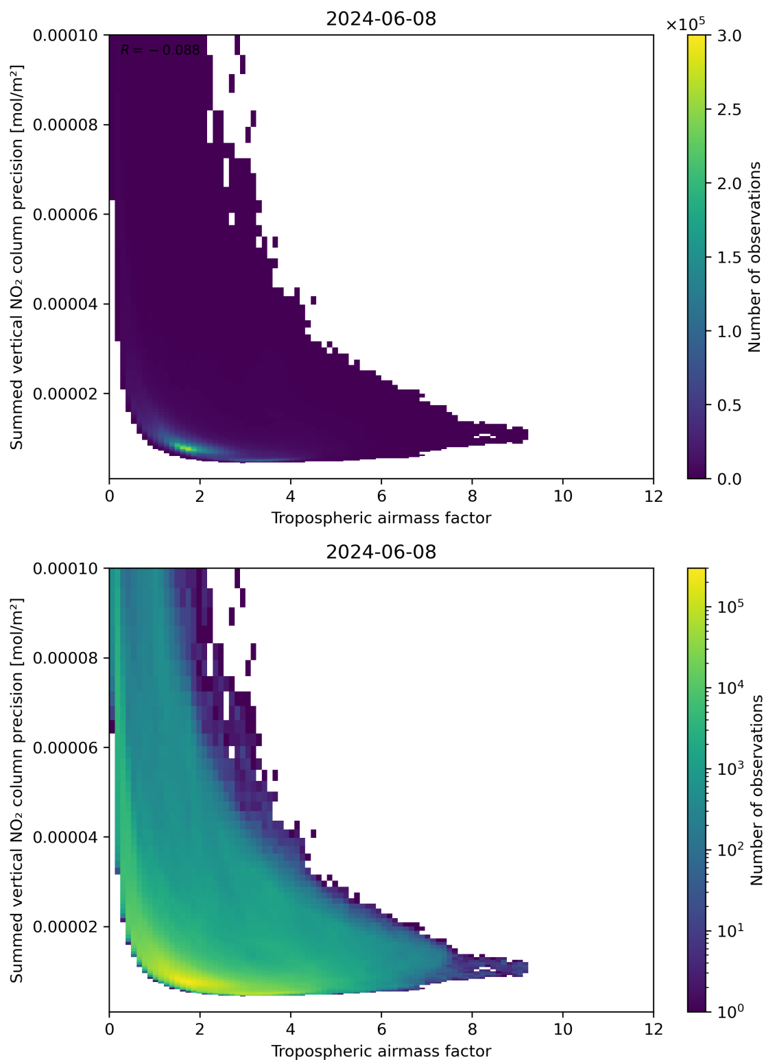
Figure 76: Scatter density plot of “Tropospheric air mass factor” against “Summed vertical NO 2 column precision” for 2024-06-08 to 2024-06-09.
