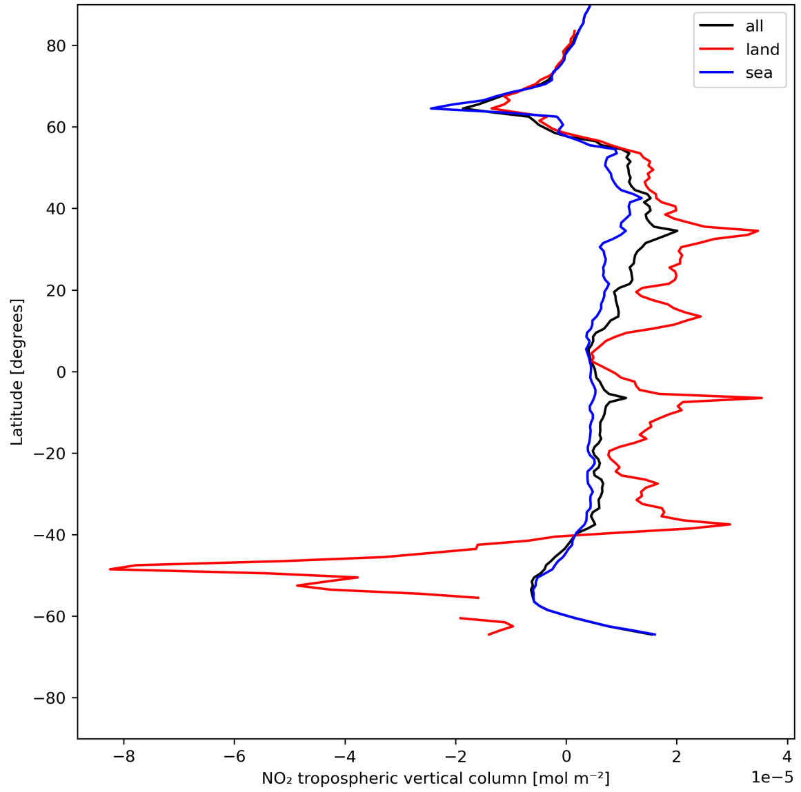
Figure 12: Zonal average of “NO 2 tropospheric vertical column” for 2024-06-08 to 2024-06-09.
