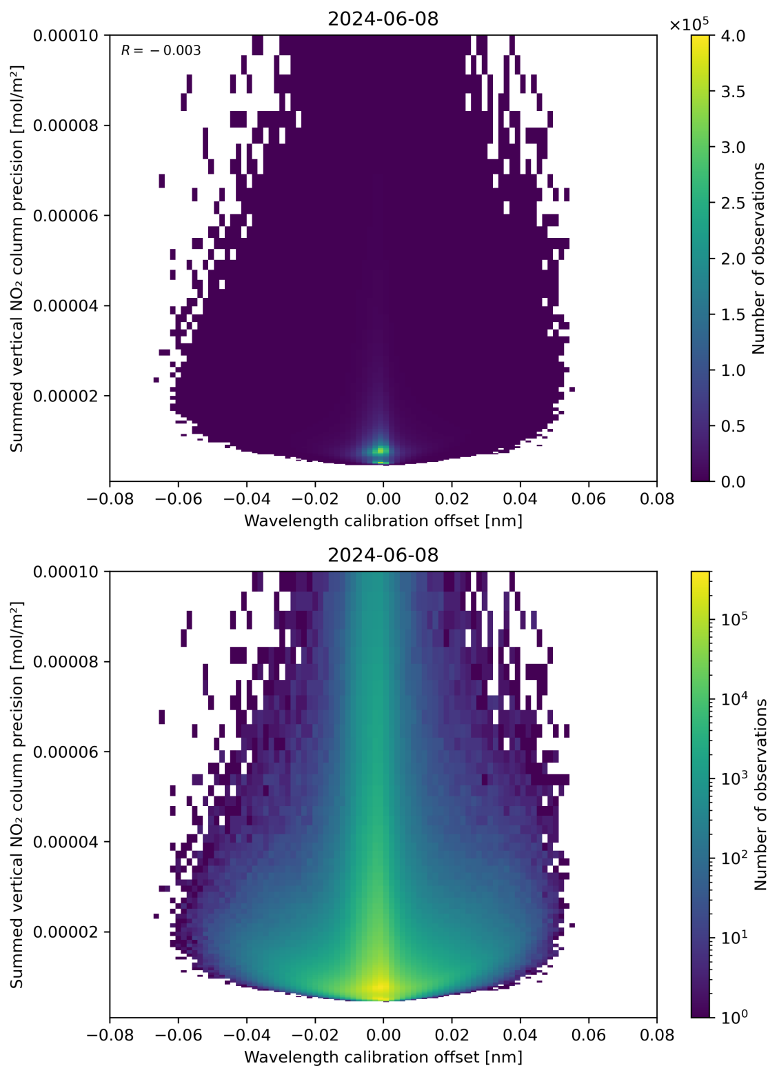
Figure 178: Scatter density plot of “Wavelength calibration offset” against “Summed vertical NO 2 column precision” for 2024-06-08 to 2024-06-09.
