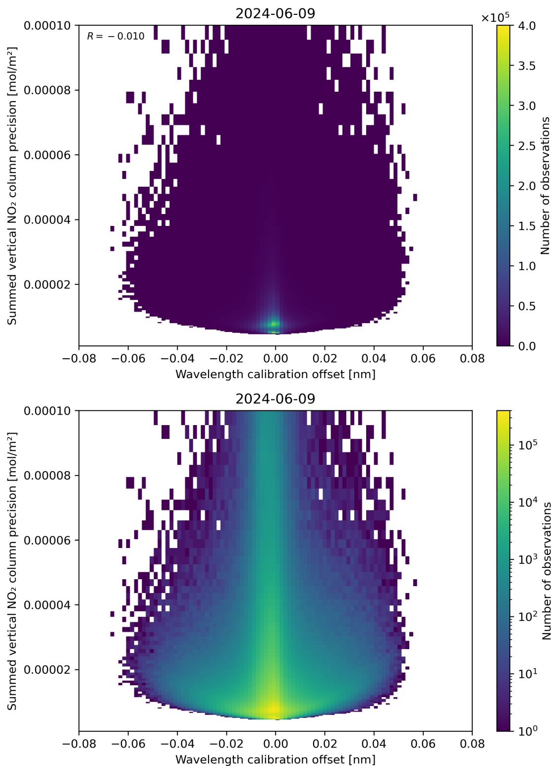
Figure 178: Scatter density plot of “Wavelength calibration offset” against “Summed vertical NO 2 column precision” for 2024-06-08 to 2024-06-10.
