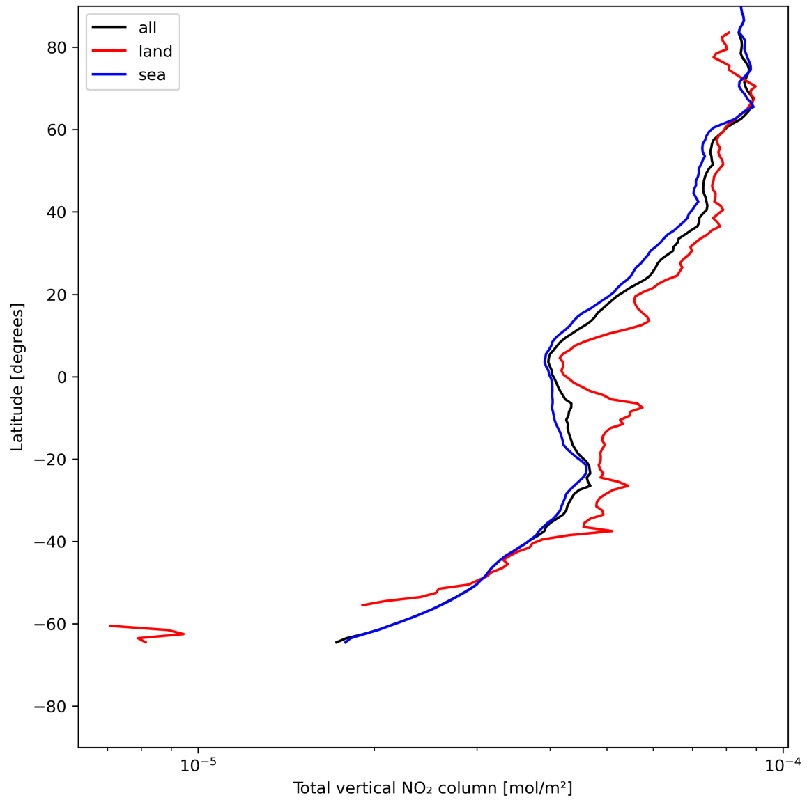
Figure 21: Zonal average of “Total vertical NO 2 column” for 2024-06-08 to 2024-06-10.
