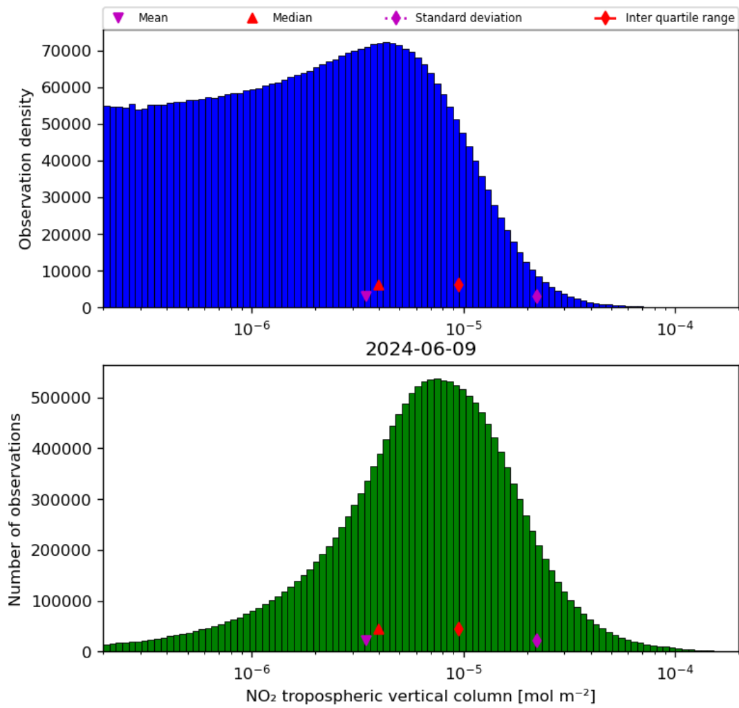
Figure 29: Histogram of “NO 2 tropospheric vertical column” for 2024-06-08 to 2024-06-10
