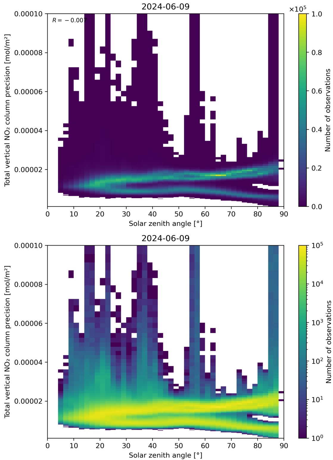
Figure 154: Scatter density plot of “Solar zenith angle” against “Total vertical NO 2 column precision” for 2024-06-08 to 2024-06-10.
