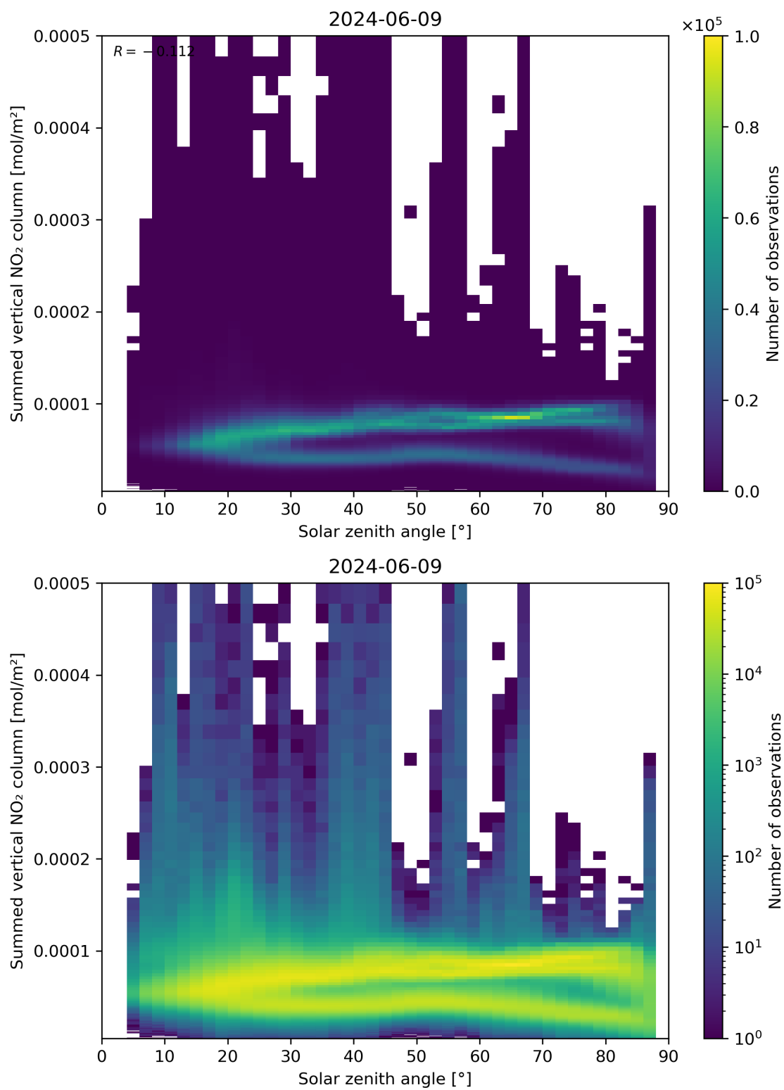
Figure 151: Scatter density plot of “Solar zenith angle” against “Summed vertical NO 2 column” for 2024-06-08 to 2024-06-10.
