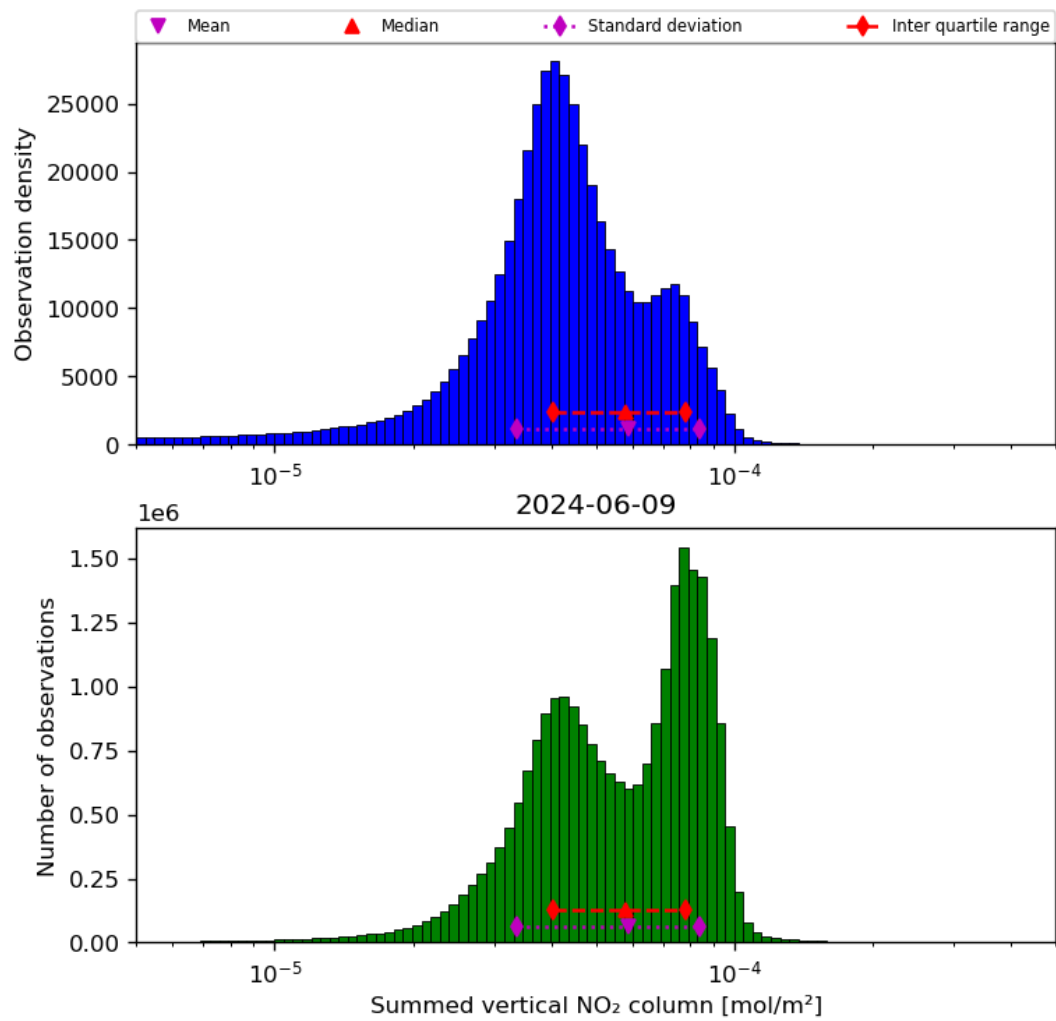
Figure 40: Histogram of “Summed vertical NO 2 column” for 2024-06-08 to 2024-06-10
