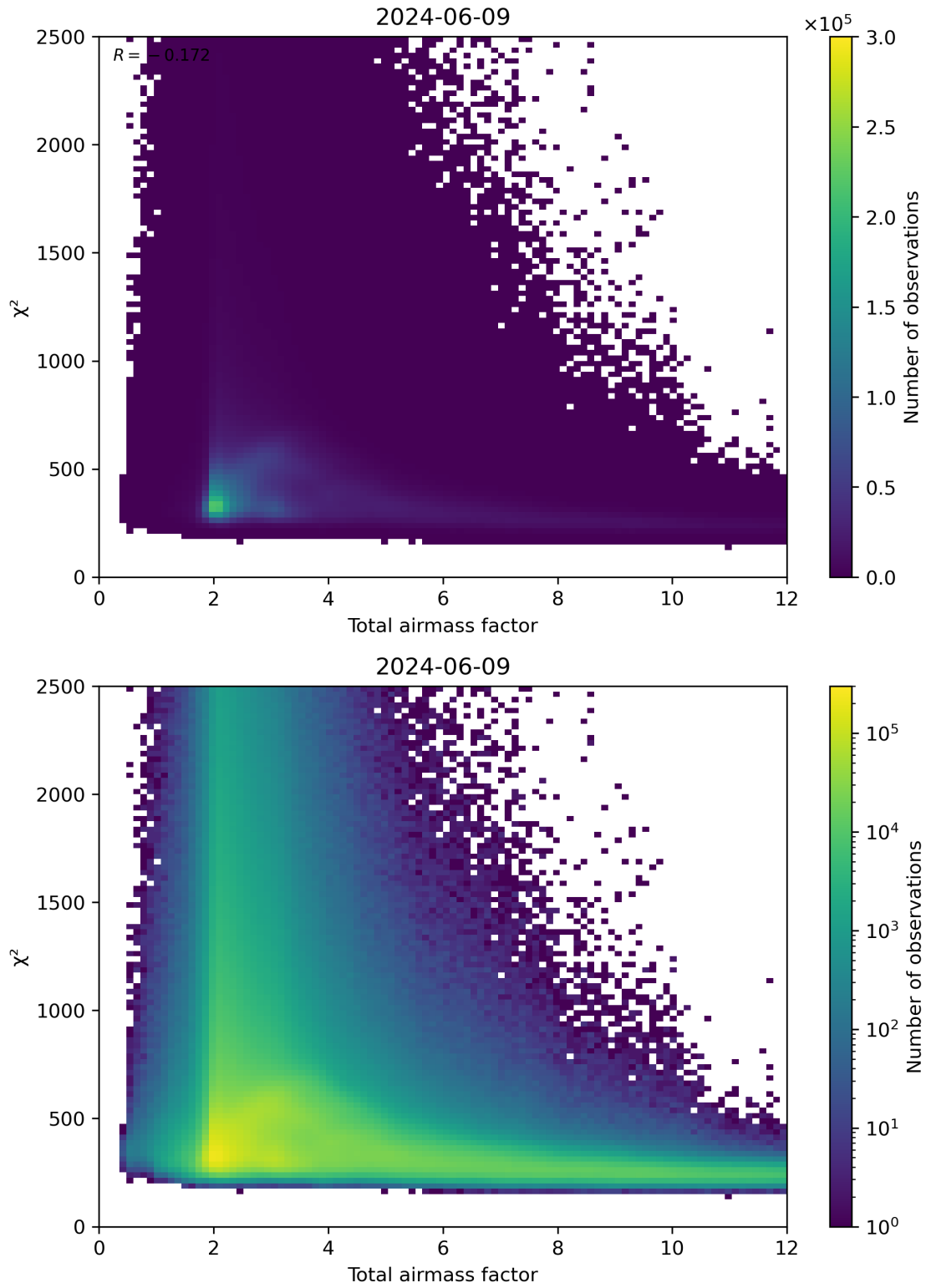
Figure 63: Scatter density plot of “Total airmass factor” against “ \chi^2 ” for 2024-06-08 to 2024-06-10.
