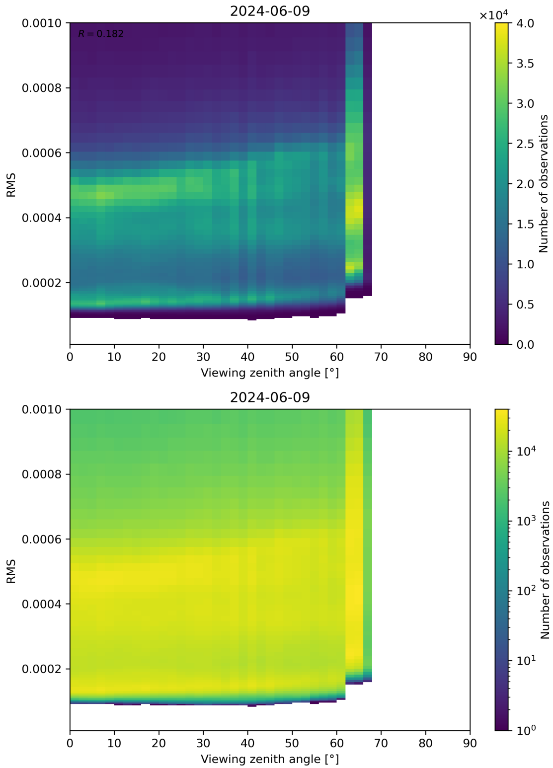
Figure 171: Scatter density plot of “Viewing zenith angle” against “RMS” for 2024-06-08 to 2024-06-10.
