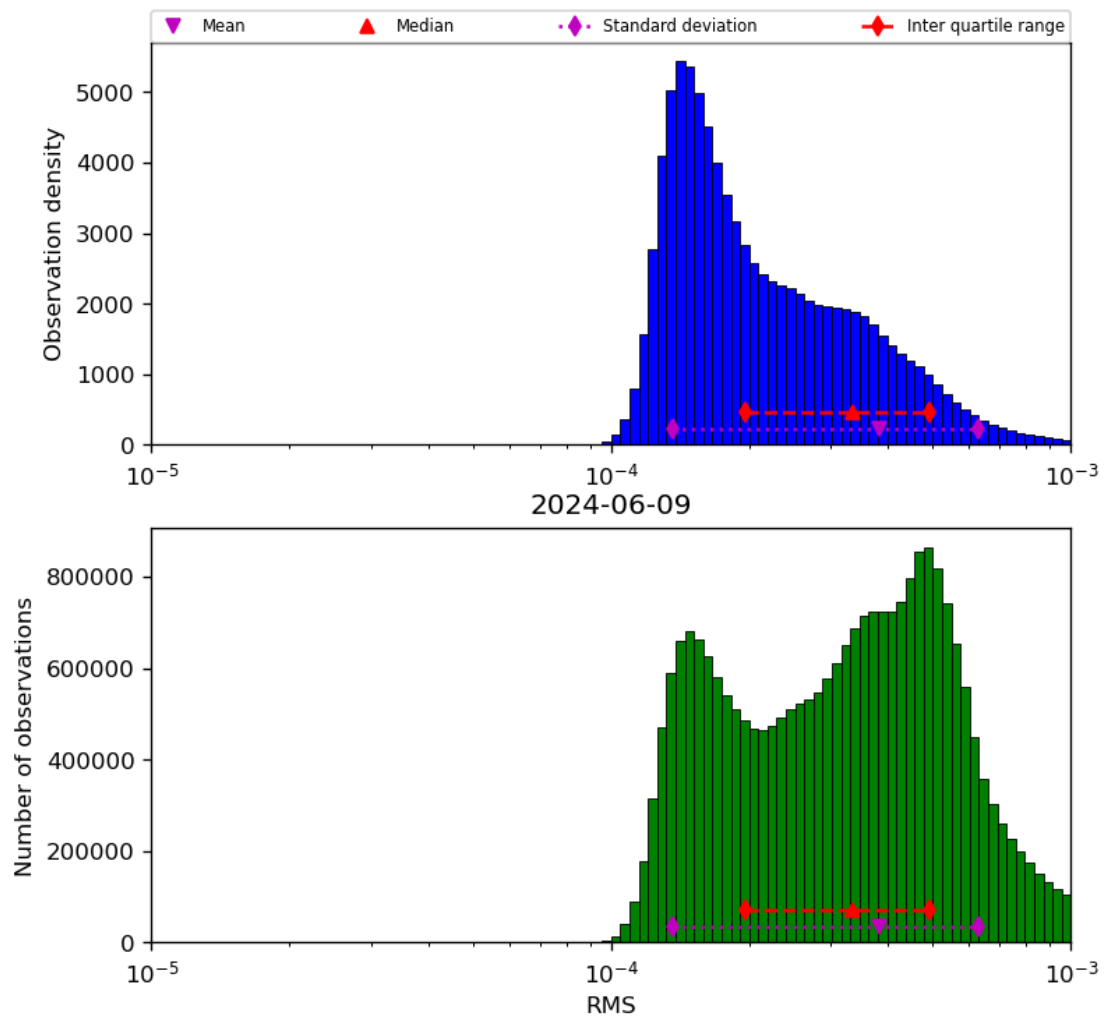
Figure 43: Histogram of “RMS” for 2024-06-08 to 2024-06-10
