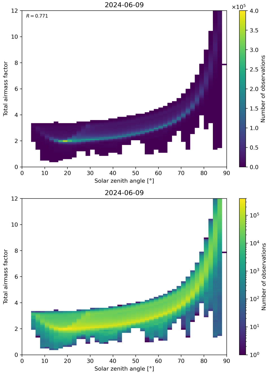
Figure 146: Scatter density plot of “Solar zenith angle” against “Total air mass factor” for 2024-06-08 to 2024-06-10.
