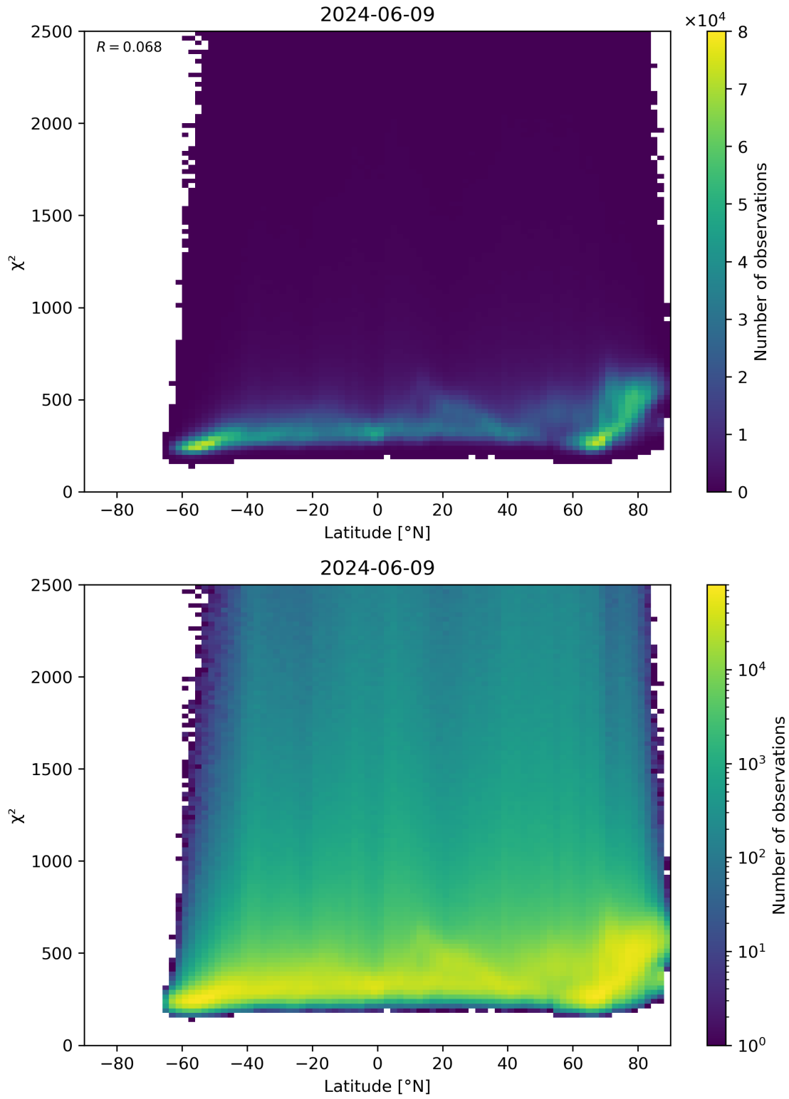
Figure 86: Scatter density plot of “Latitude” against “ \chi^2 ” for 2024-06-08 to 2024-06-10.
