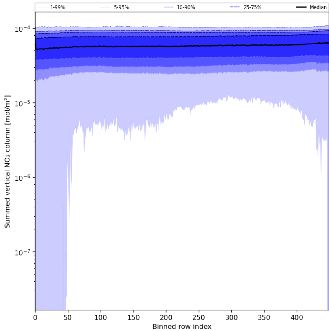
Figure 57: Along track statistics of “Summed vertical NO 2 column” for 2024-06-08 to 2024-06-10
