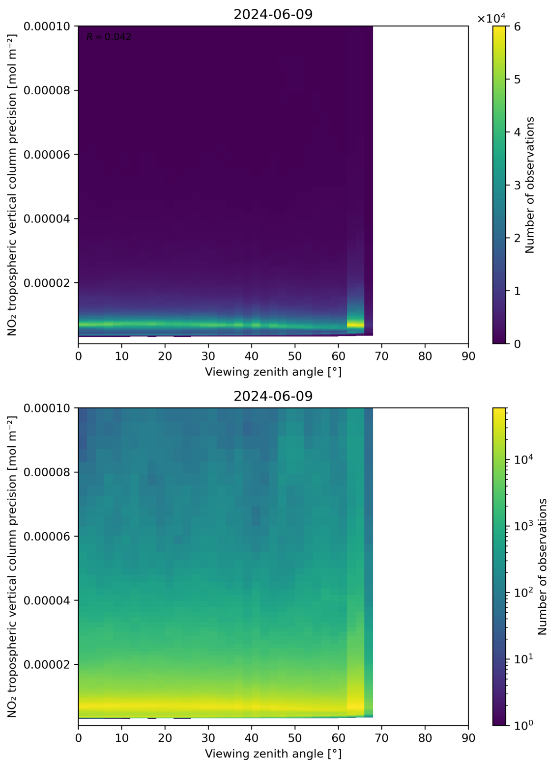
Figure 170: Scatter density plot of “Viewing zenith angle” against “NO 2 tropospheric vertical column precision” for 2024-06-08 to 2024-06-10.
