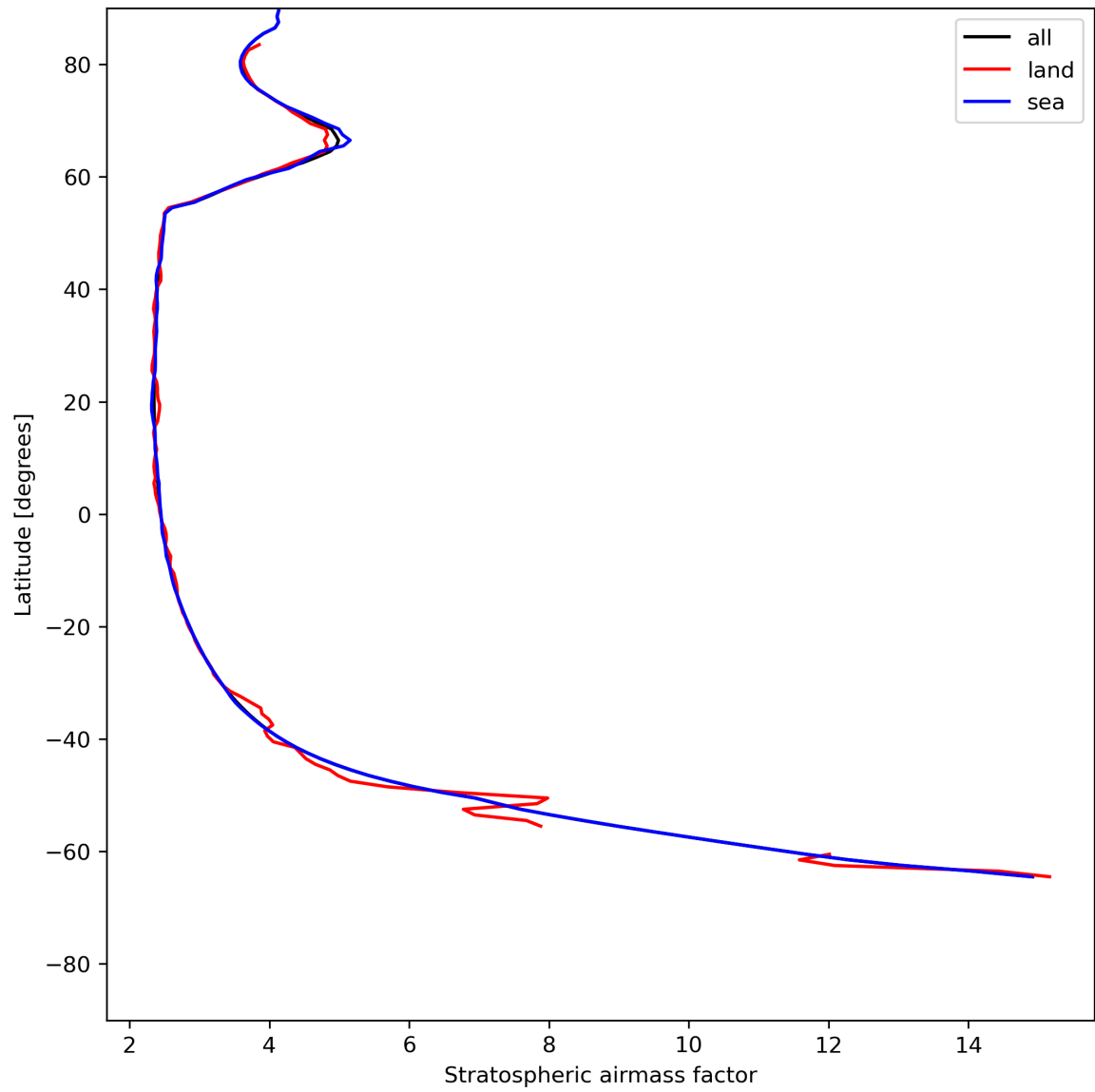
Figure 27: Zonal average of “Stratospheric air mass factor” for 2024-06-08 to 2024-06-10.
