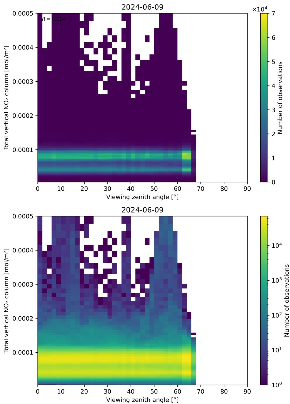
Figure 167: Scatter density plot of “Viewing zenith angle” against “Total vertical NO 2 column” for 2024-06-08 to 2024-06-10.
