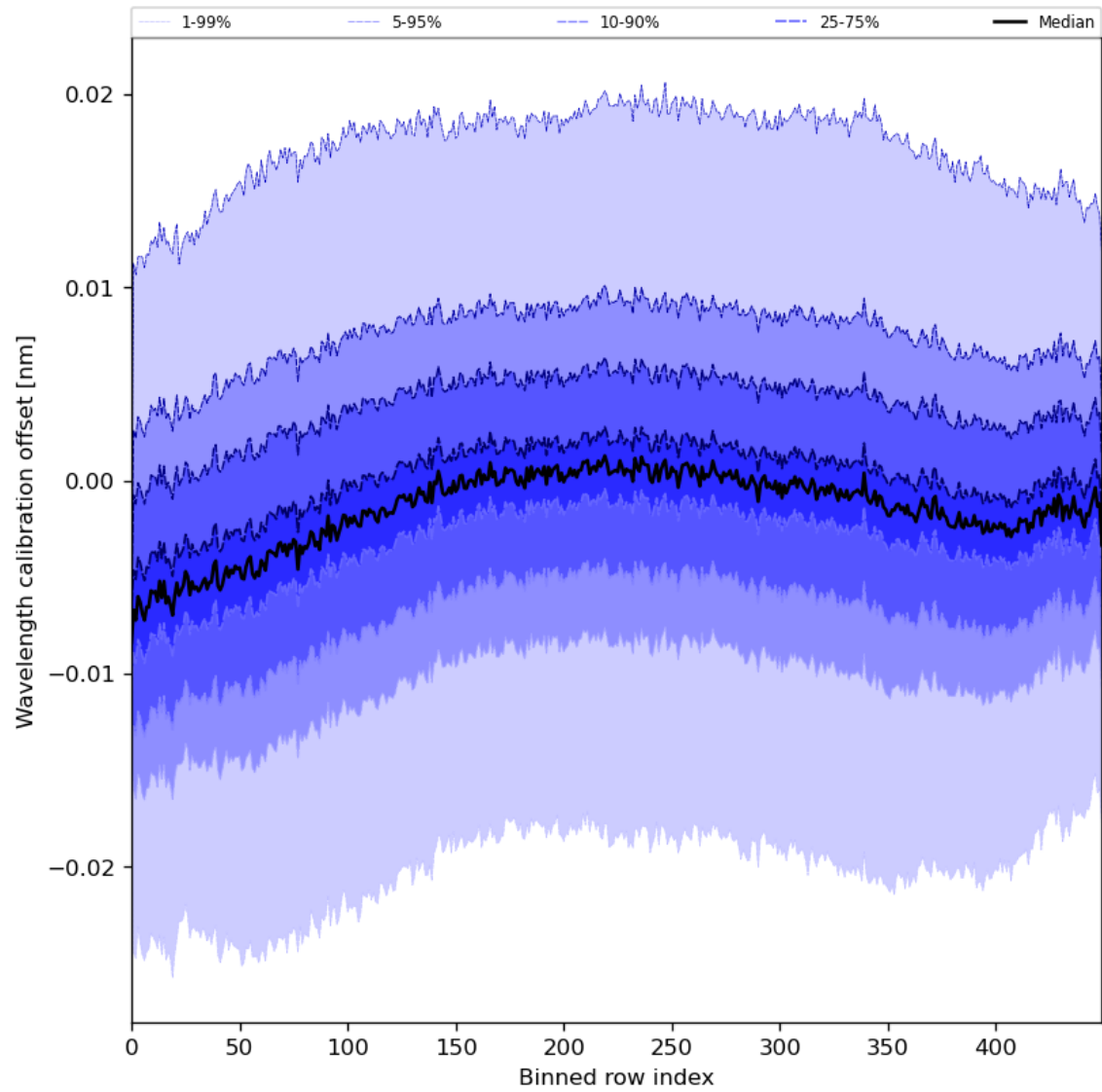
Figure 52: Along track statistics of “Wavelength calibration offset” for 2024-06-08 to 2024-06-10
