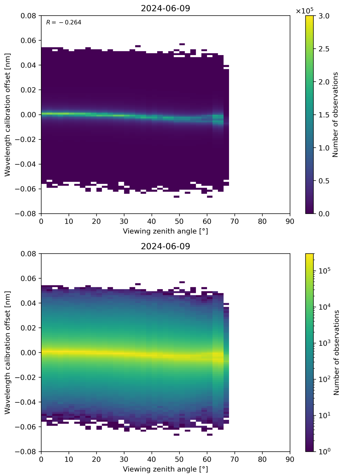
Figure 173: Scatter density plot of “Viewing zenith angle” against “Wavelength calibration offset” for 2024-06-08 to 2024-06-10.
