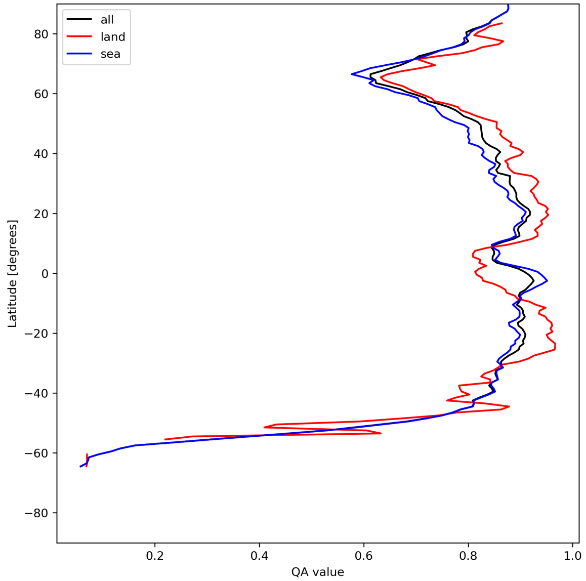
Figure 11: Zonal average of “QA value” for 2024-06-08 to 2024-06-10.
