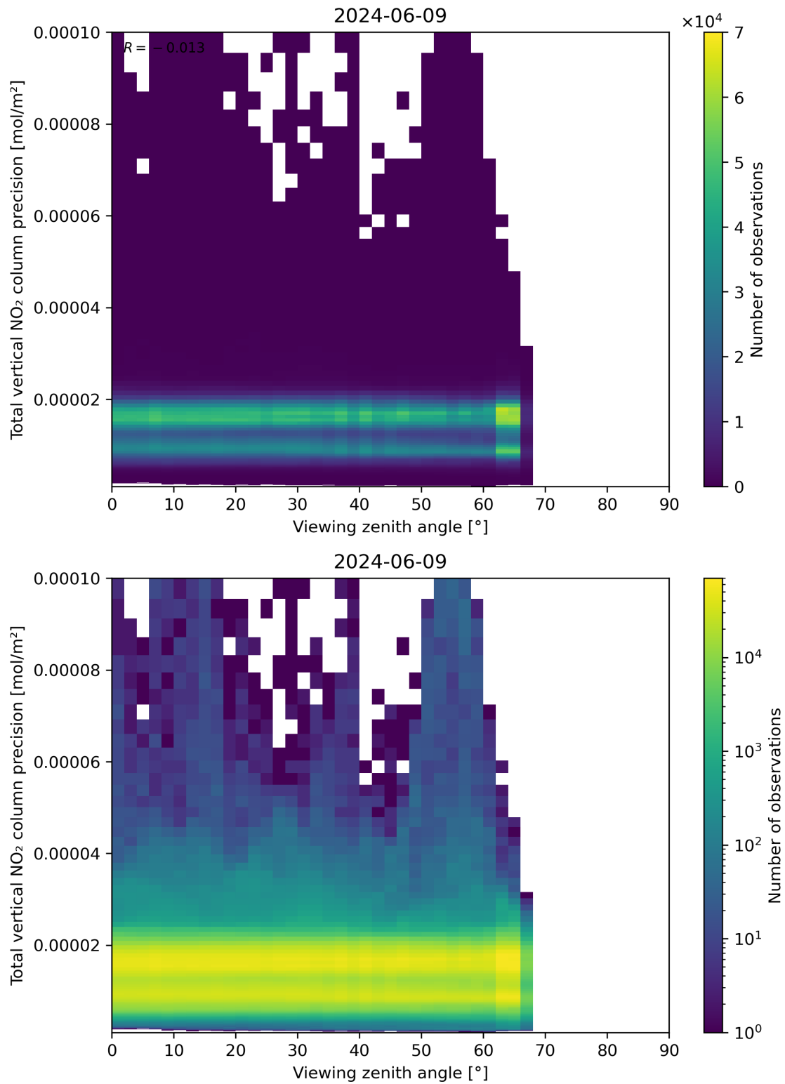
Figure 168: Scatter density plot of “Viewing zenith angle” against “Total vertical NO 2 column precision” for 2024-06-08 to 2024-06-10.
