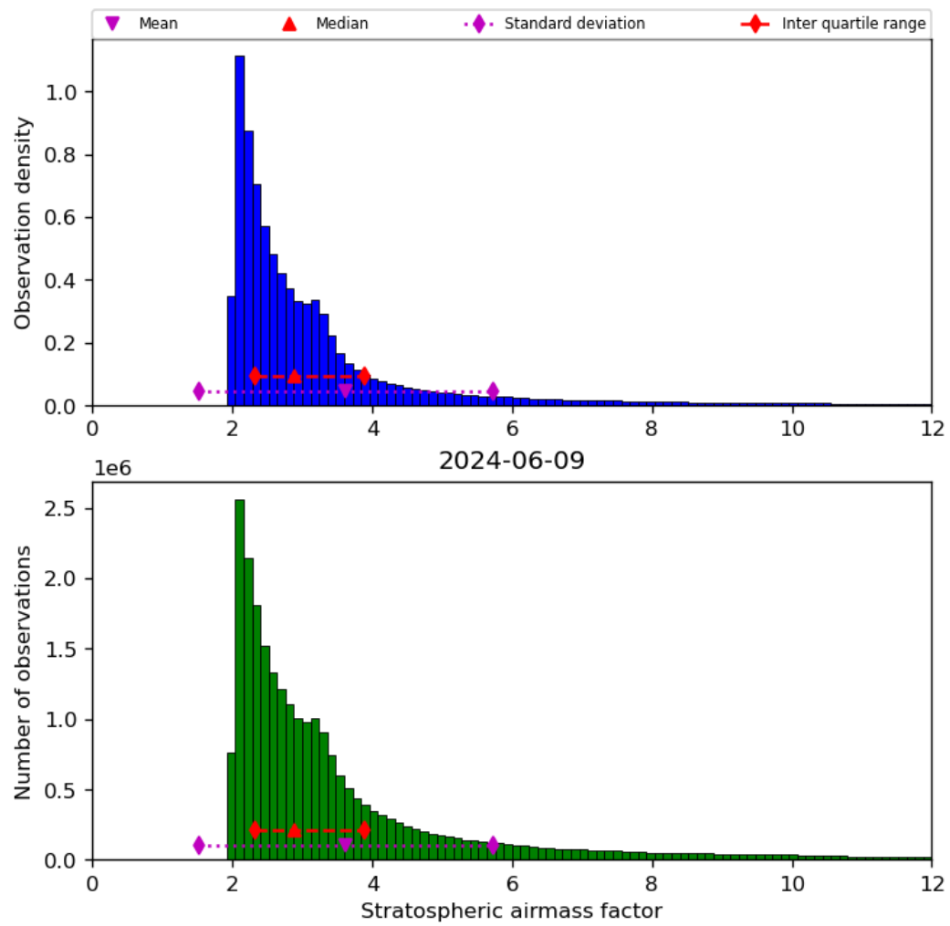
Figure 44: Histogram of “Stratospheric airmass factor” for 2024-06-08 to 2024-06-10
