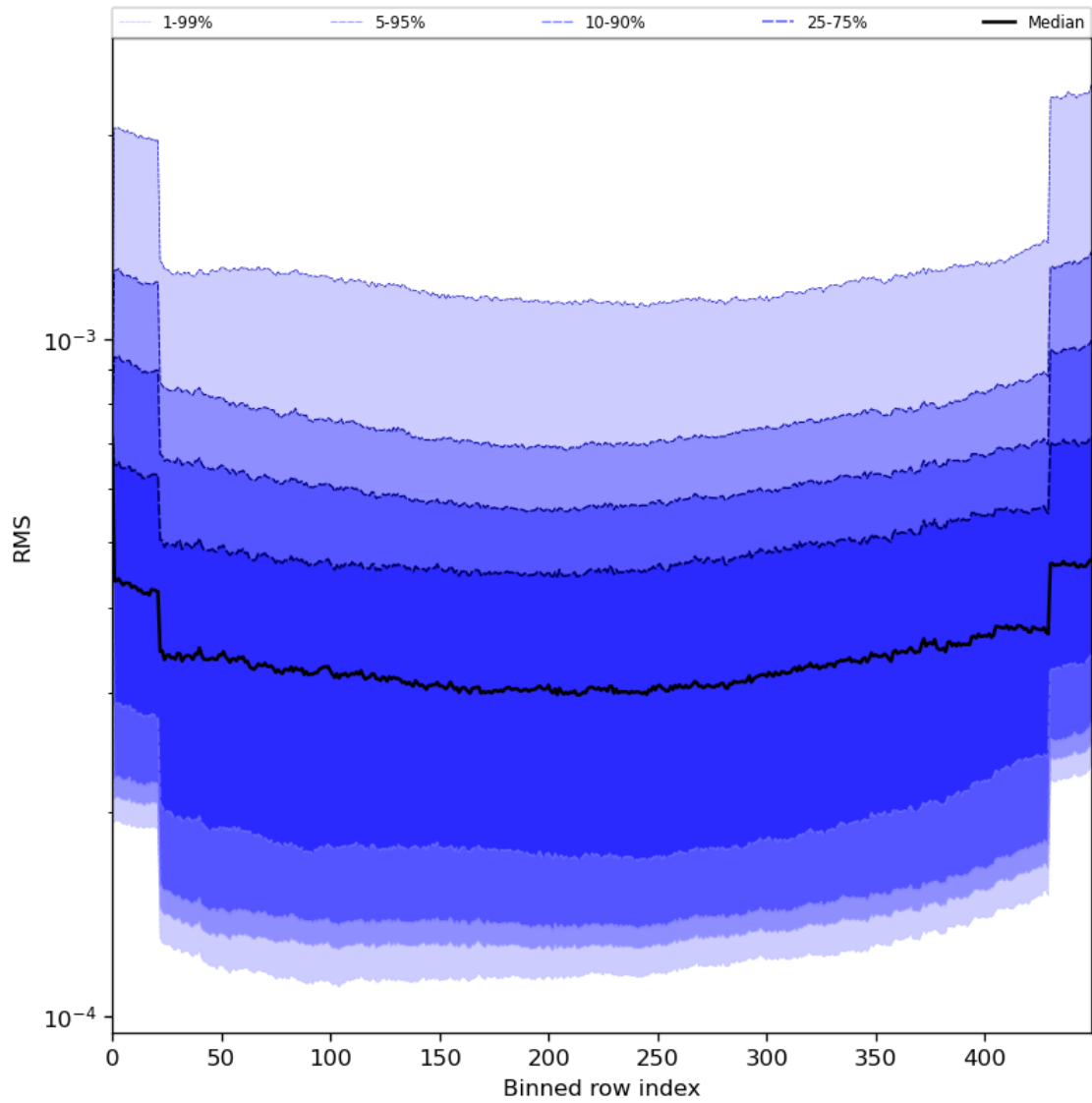
Figure 60: Along track statistics of “RMS” for 2024-06-08 to 2024-06-10
