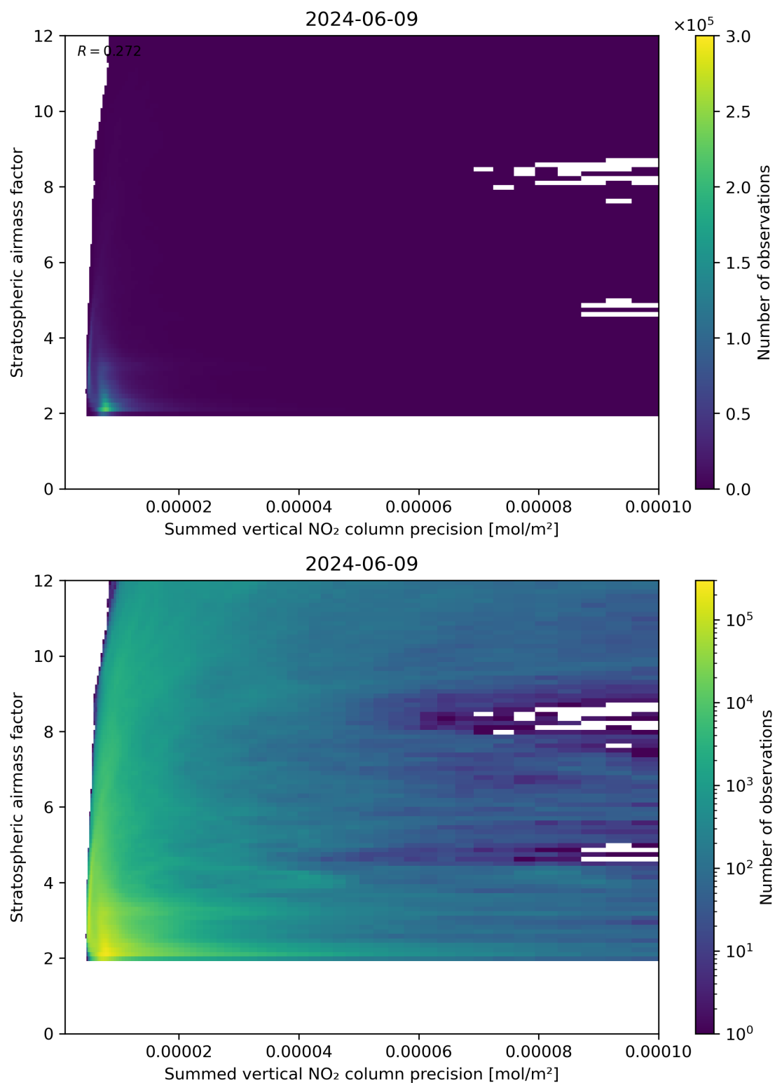
Figure 106: Scatter density plot of “Summed vertical NO 2 column precision” against “Stratospheric airmass factor” for 2024-06-08 to 2024-06-10.
