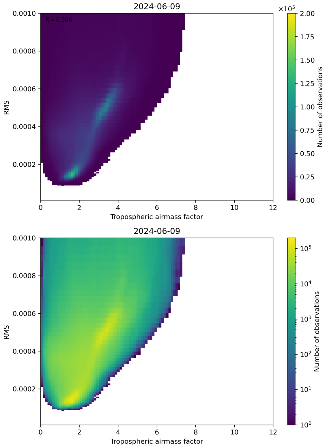
Figure 79: Scatter density plot of “Tropospheric airmass factor” against “RMS” for 2024-06-08 to 2024-06-10.
