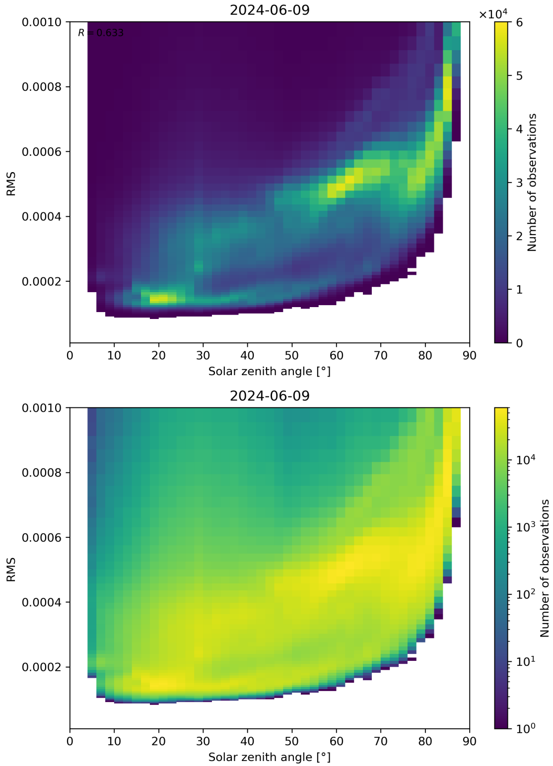
Figure 157: Scatter density plot of “Solar zenith angle” against “RMS” for 2024-06-08 to 2024-06-10.
