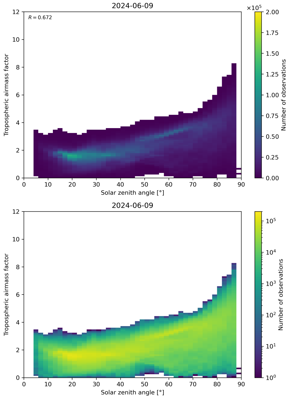
Figure 147: Scatter density plot of “Solar zenith angle” against “Tropospheric airmass factor” for 2024-06-08 to 2024-06-10.
