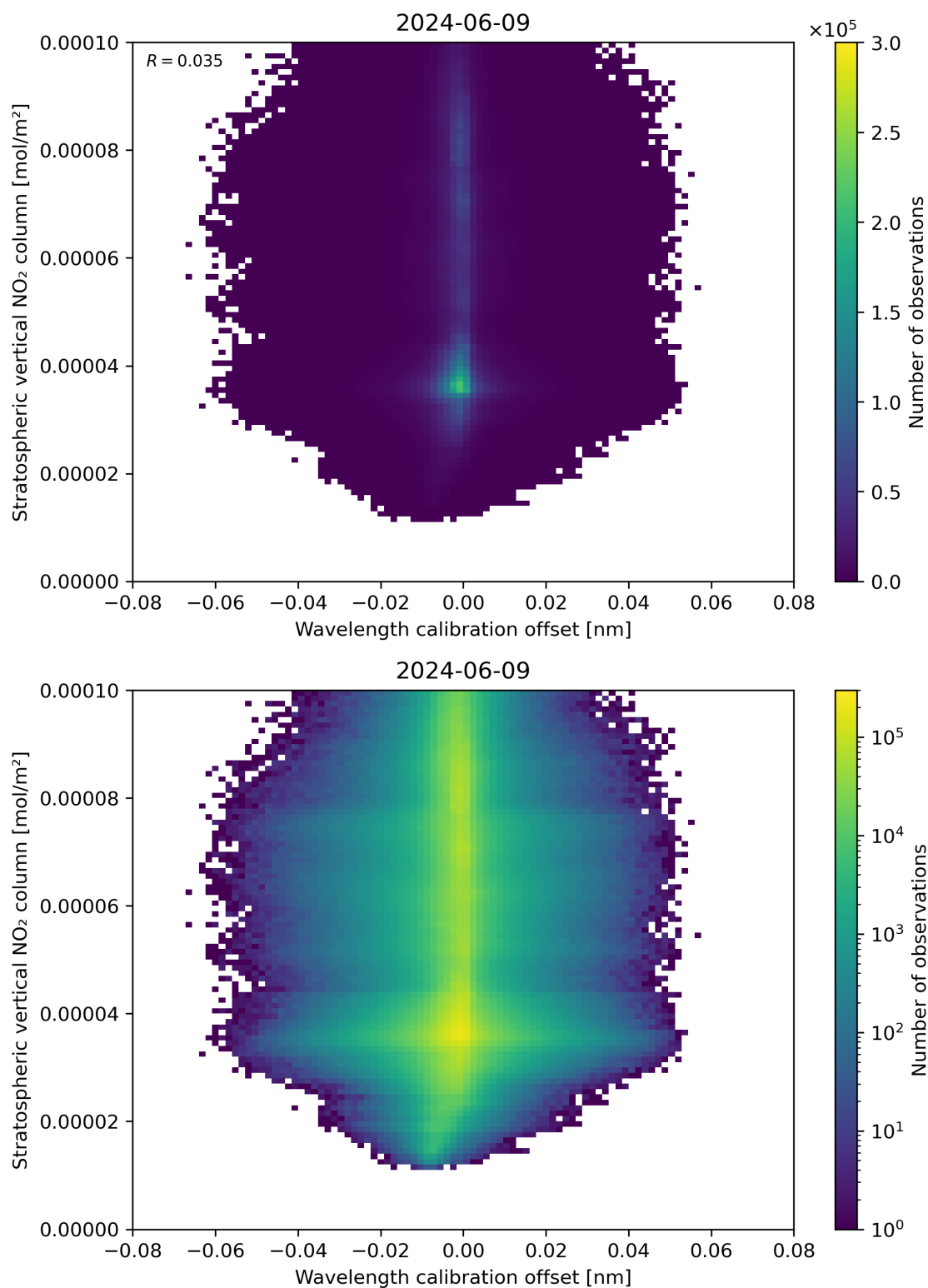
Figure 176: Scatter density plot of “Wavelength calibration offset” against “Stratospheric vertical NO 2 column” for 2024-06-08 to 2024-06-10.
