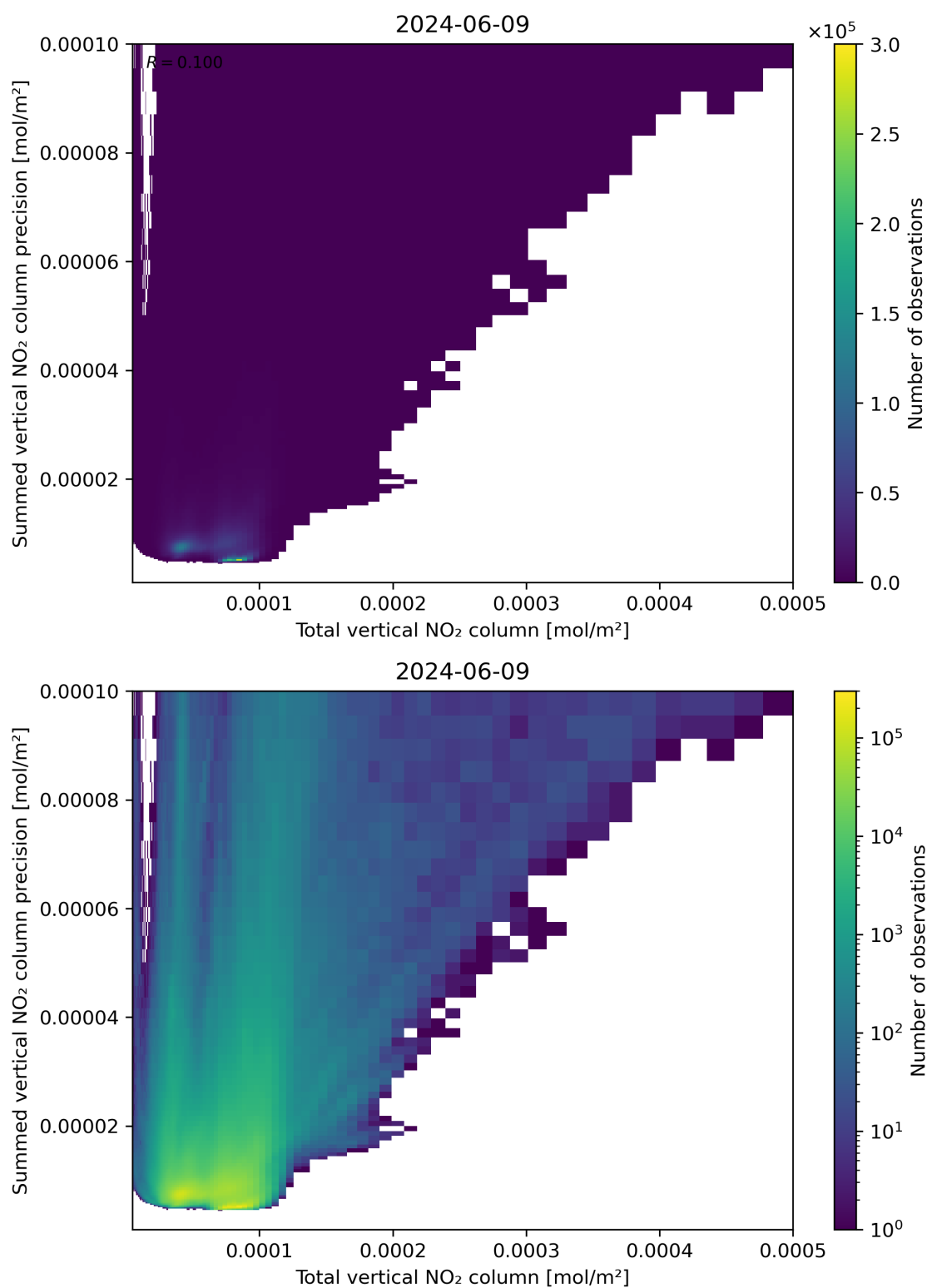
Figure 113: Scatter density plot of “Total vertical NO 2 column” against “Summed vertical NO 2 column precision” for 2024-06-08 to 2024-06-10.
