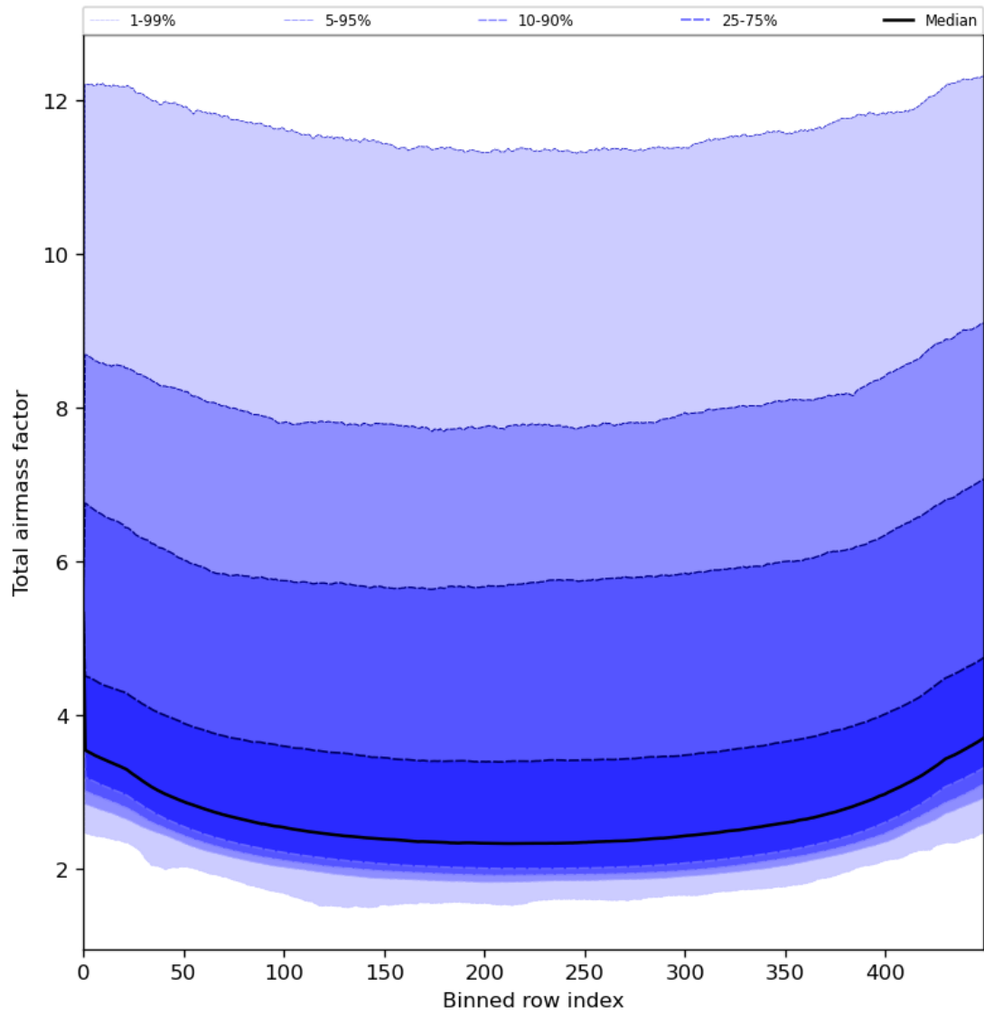
Figure 49: Along track statistics of “Total airmass factor” for 2024-06-08 to 2024-06-10
