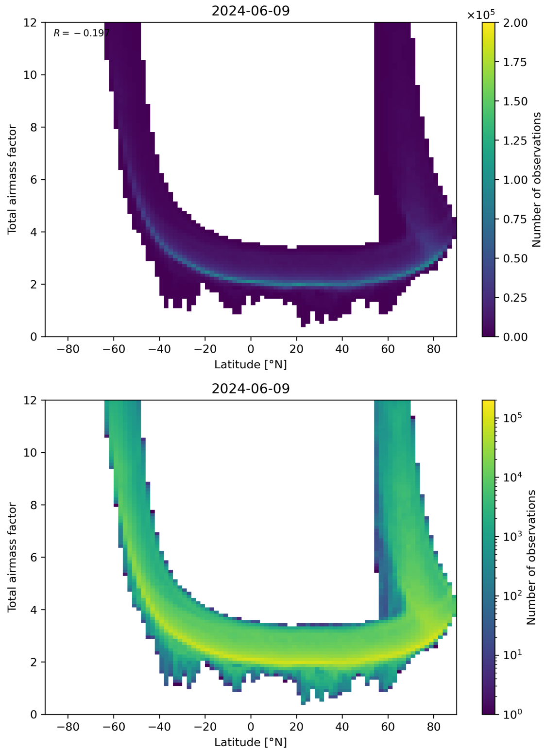
Figure 84: Scatter density plot of “Latitude” against “Total airmass factor” for 2024-06-08 to 2024-06-10.
