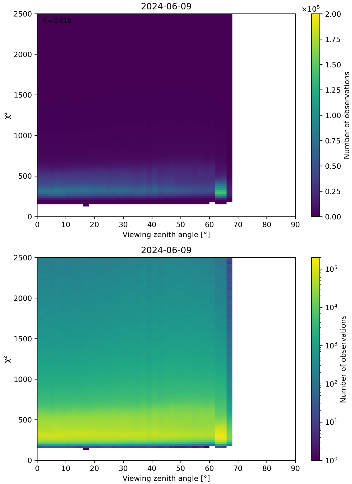
Figure 162: Scatter density plot of “Viewing zenith angle” against “ \chi^2 ” for 2024-06-08 to 2024-06-10.
