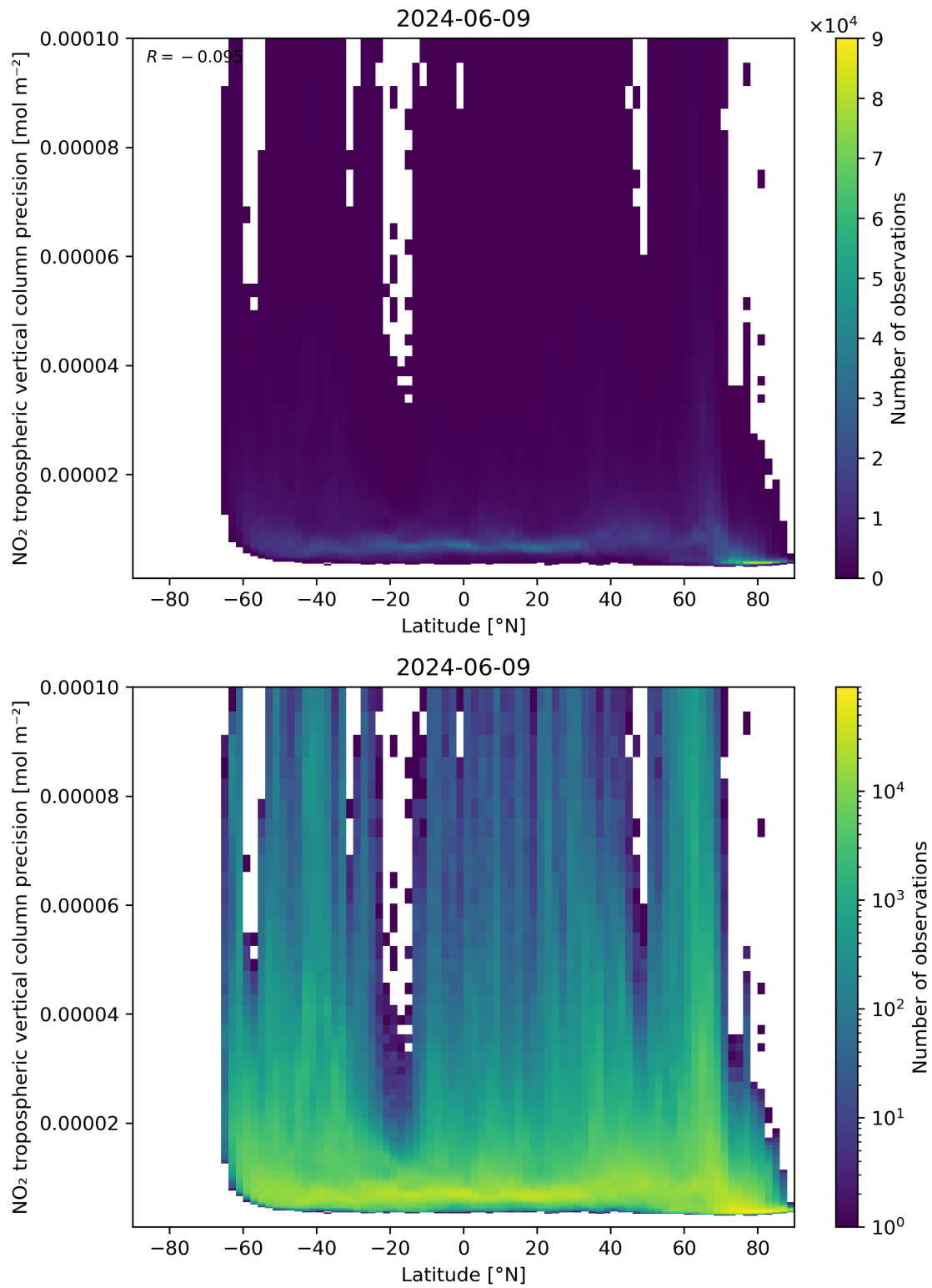
Figure 93: Scatter density plot of “Latitude” against “NO 2 tropospheric vertical column precision” for 2024-06-08 to 2024-06-10.
