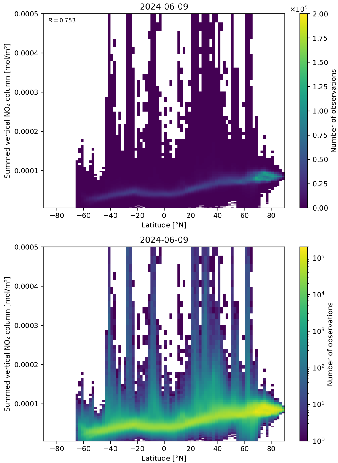
Figure 88: Scatter density plot of “Latitude” against “Summed vertical NO 2 column” for 2024-06-08 to 2024-06-10.
