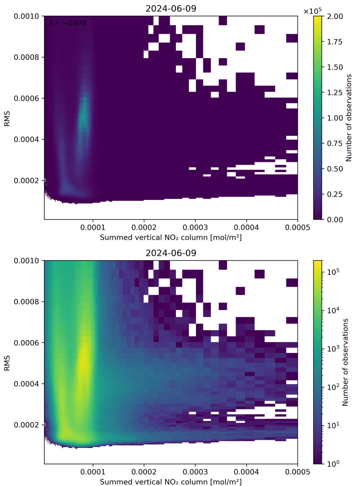
Figure 109: Scatter density plot of “Summed vertical NO 2 column” against “RMS” for 2024-06-08 to 2024-06-10.
