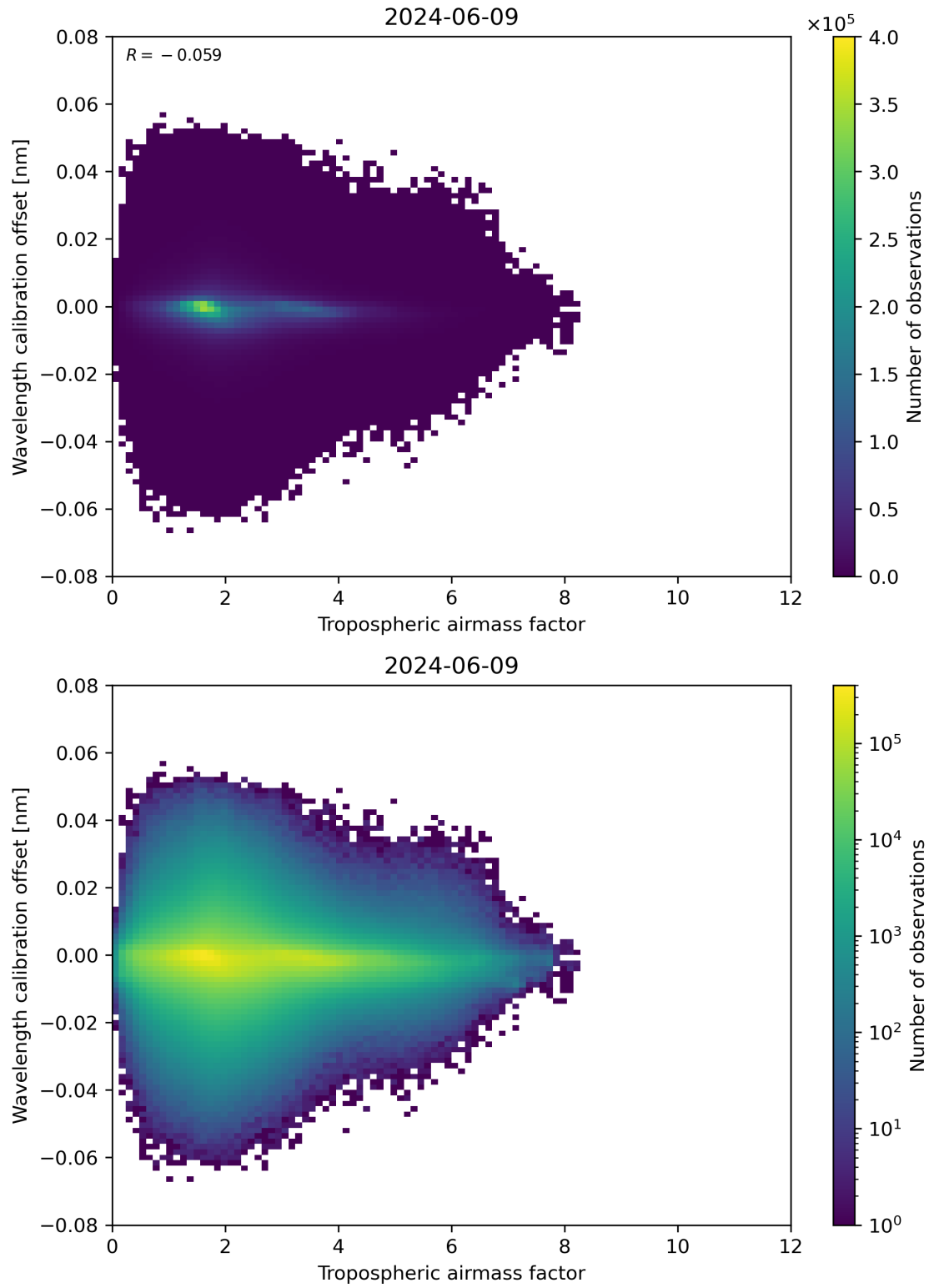
Figure 80: Scatter density plot of “Tropospheric airmass factor” against “Wavelength calibration offset” for 2024-06-08 to 2024-06-10.
