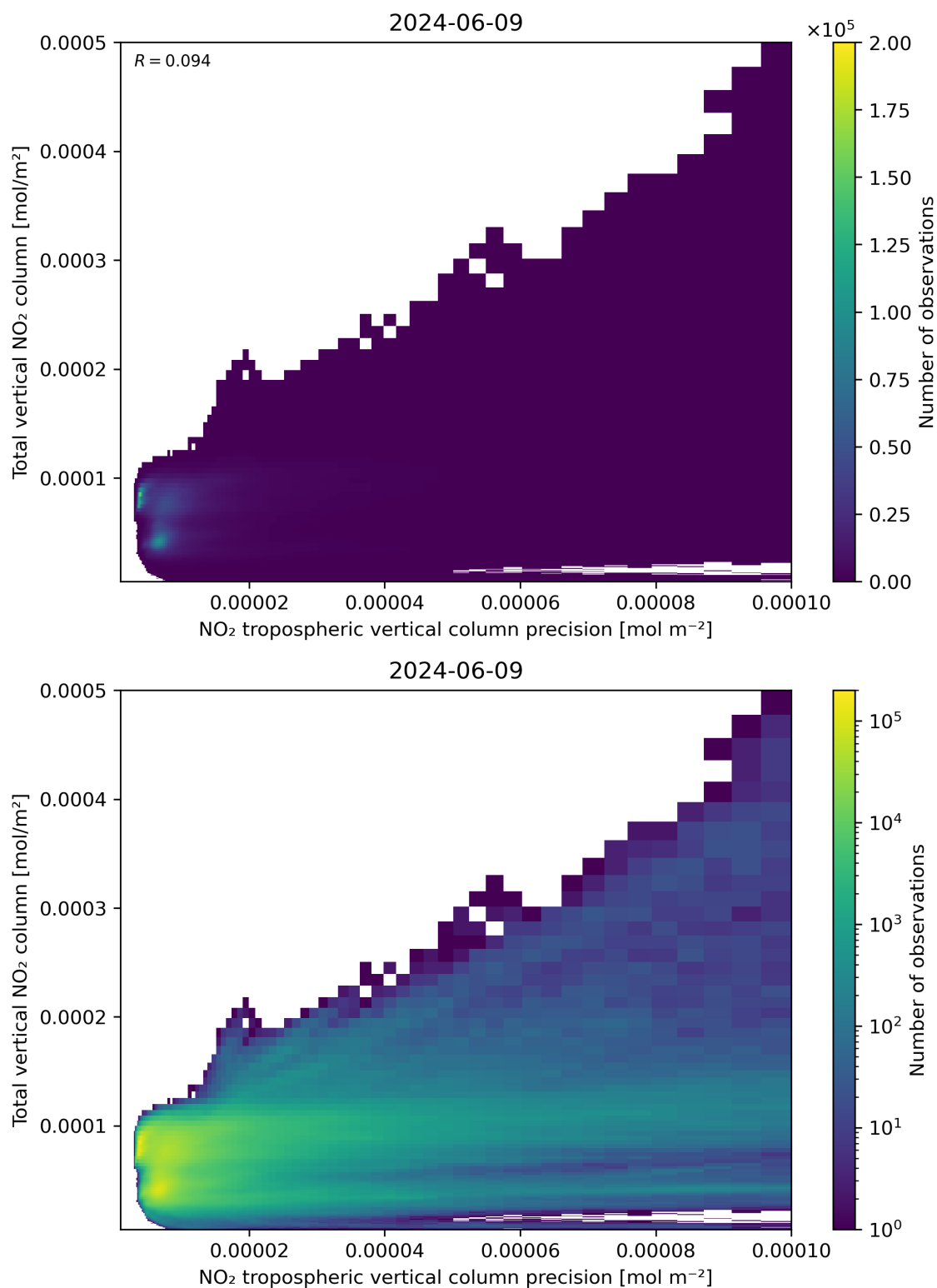
Figure 138: Scatter density plot of “NO 2 tropospheric vertical column precision” against “Total vertical NO 2 column” for 2024-06-08 to 2024-06-10.
