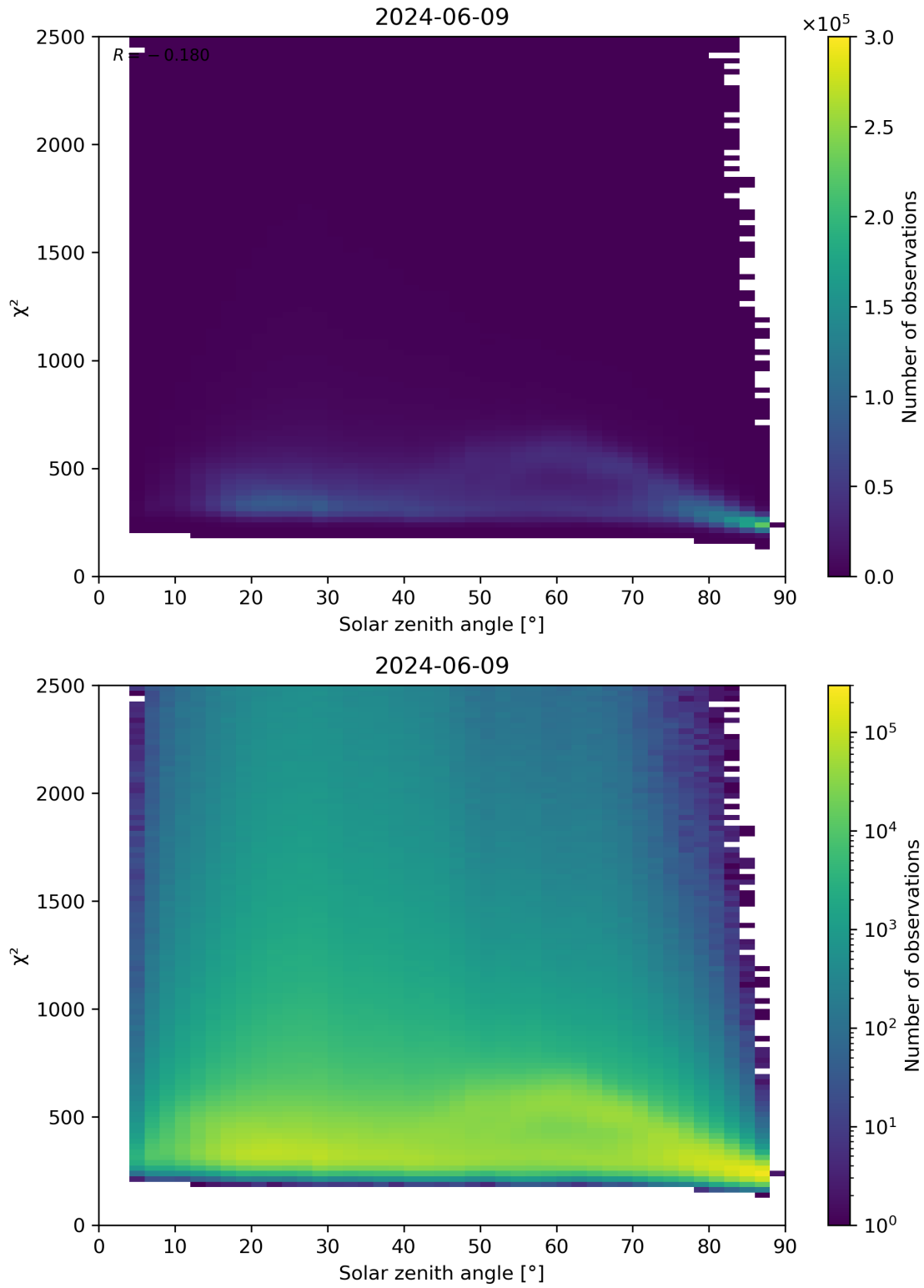
Figure 148: Scatter density plot of “Solar zenith angle” against “ \chi^2 ” for 2024-06-08 to 2024-06-10.
