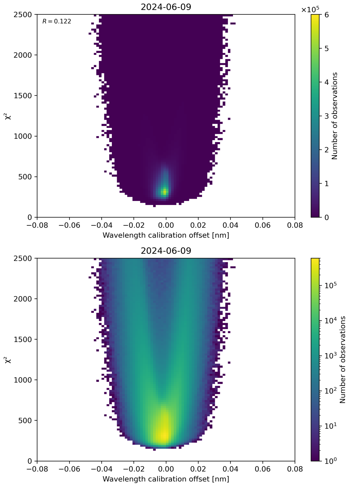
Figure 175: Scatter density plot of “Wavelength calibration offset” against “ \chi^2 ” for 2024-06-08 to 2024-06-10.
