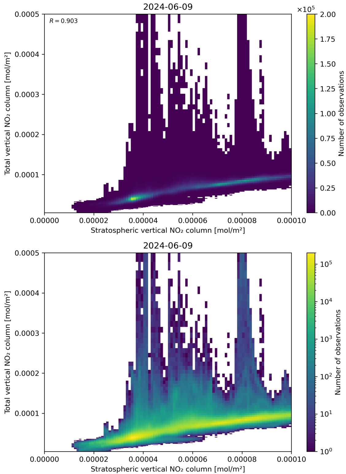
Figure 100: Scatter density plot of “Stratospheric vertical NO 2 column” against “Total vertical NO 2 column” for 2024-06-08 to 2024-06-10.
