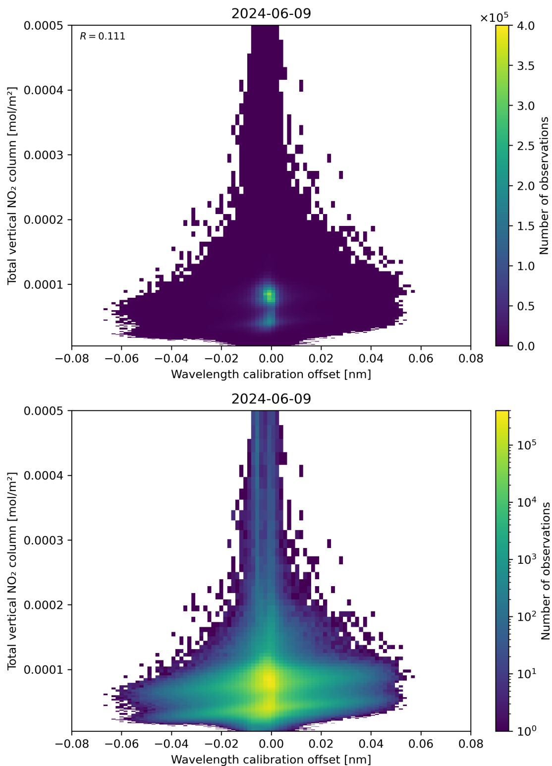
Figure 179: Scatter density plot of “Wavelength calibration offset” against “Total vertical NO 2 column” for 2024-06-08 to 2024-06-10.
