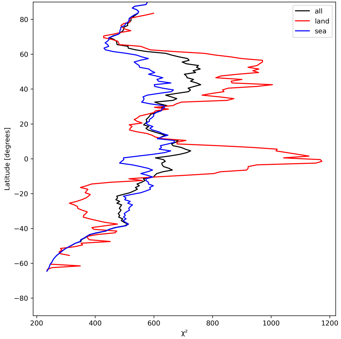
Figure 25: Zonal average of “ \chi^2 ” for 2024-06-08 to 2024-06-10.
