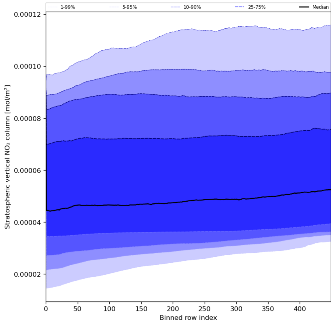
Figure 53: Along track statistics of “Stratospheric vertical NO 2 column” for 2024-06-08 to 2024-06-10
