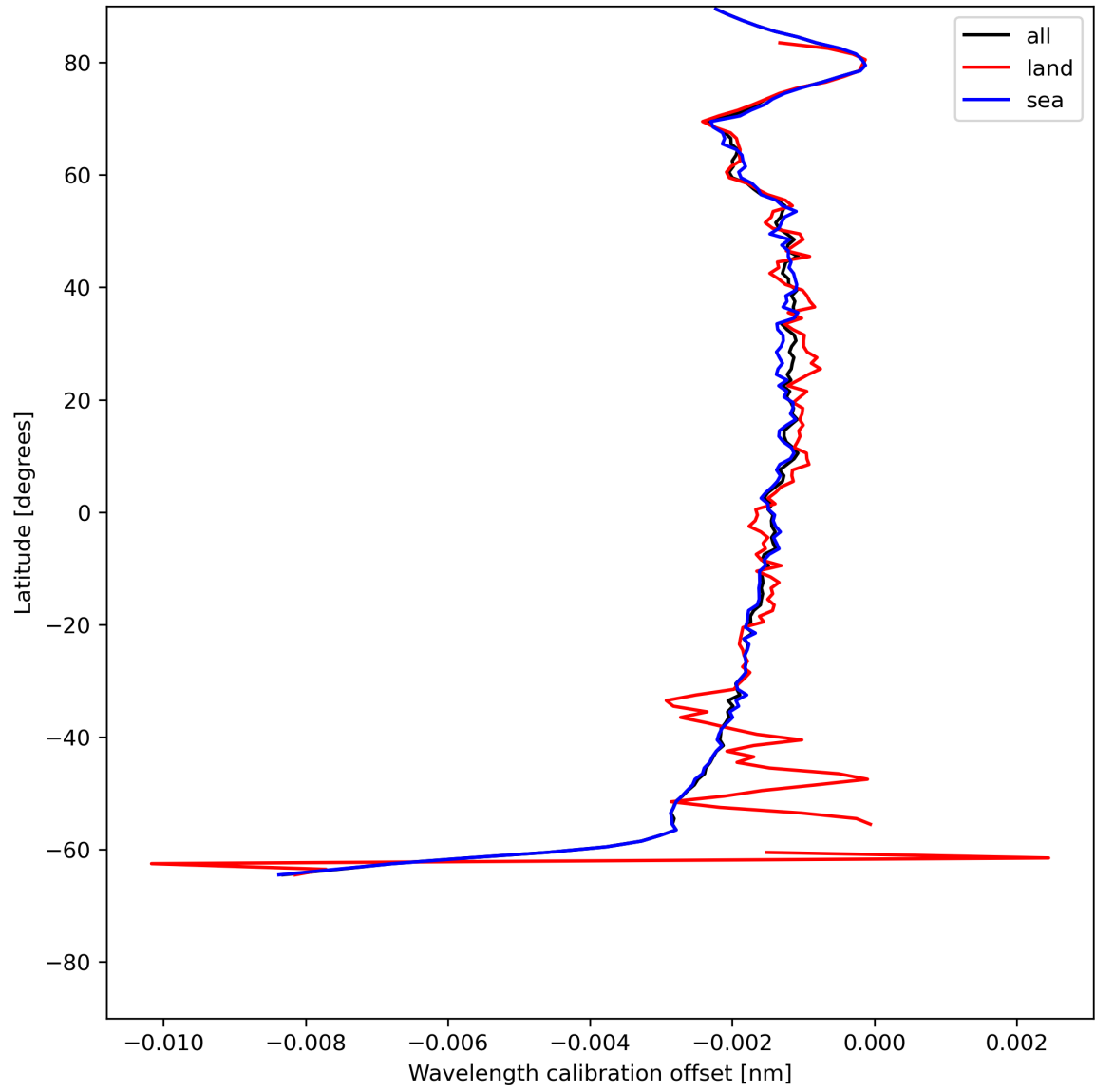
Figure 18: Zonal average of “Wavelength calibration offset” for 2024-06-08 to 2024-06-10.
