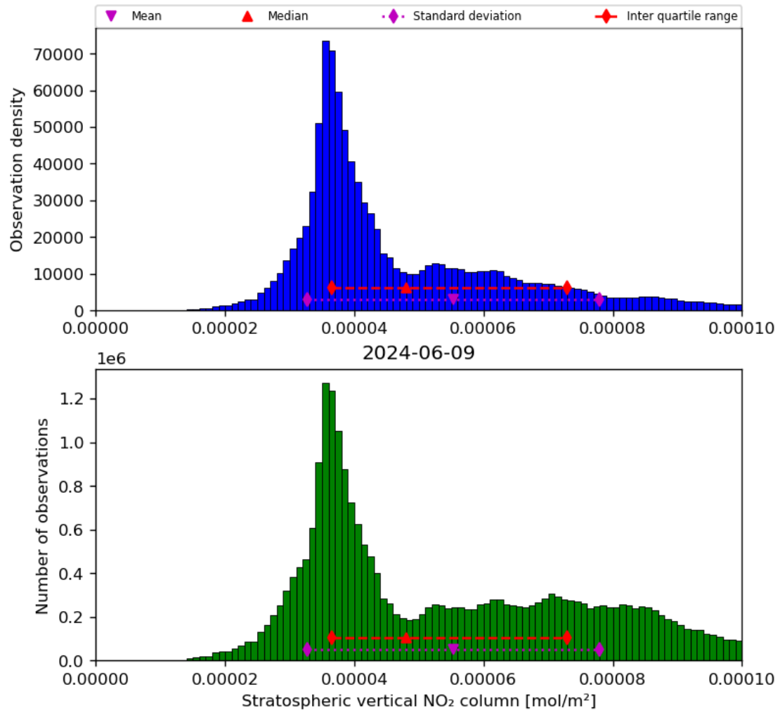
Figure 36: Histogram of “Stratospheric vertical NO 2 column” for 2024-06-08 to 2024-06-10
