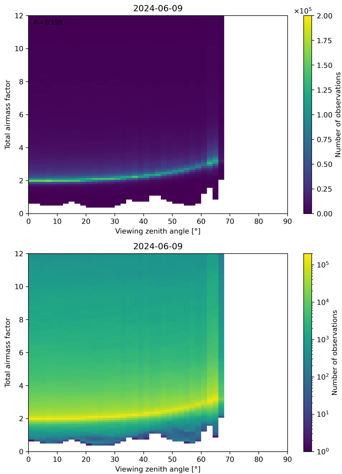
Figure 160: Scatter density plot of “Viewing zenith angle” against “Total airmass factor” for 2024-06-08 to 2024-06-10.
