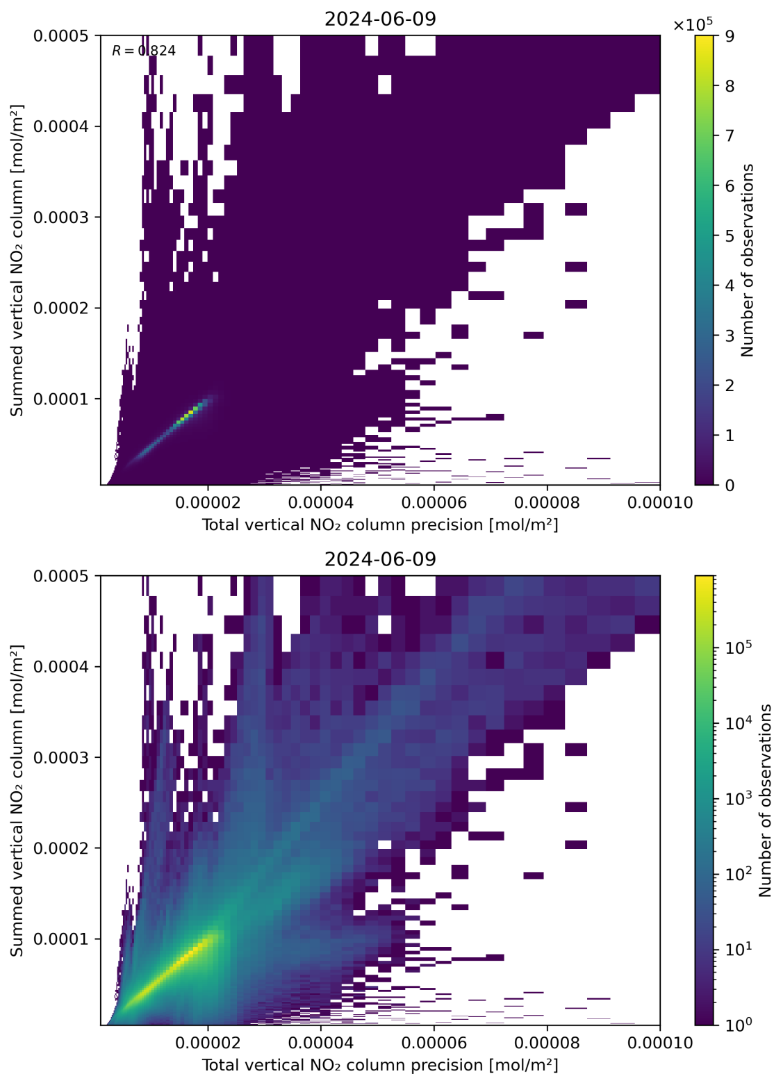
Figure 117: Scatter density plot of “Total vertical NO 2 column precision” against “Summed vertical NO 2 column” for 2024-06-08 to 2024-06-10.
