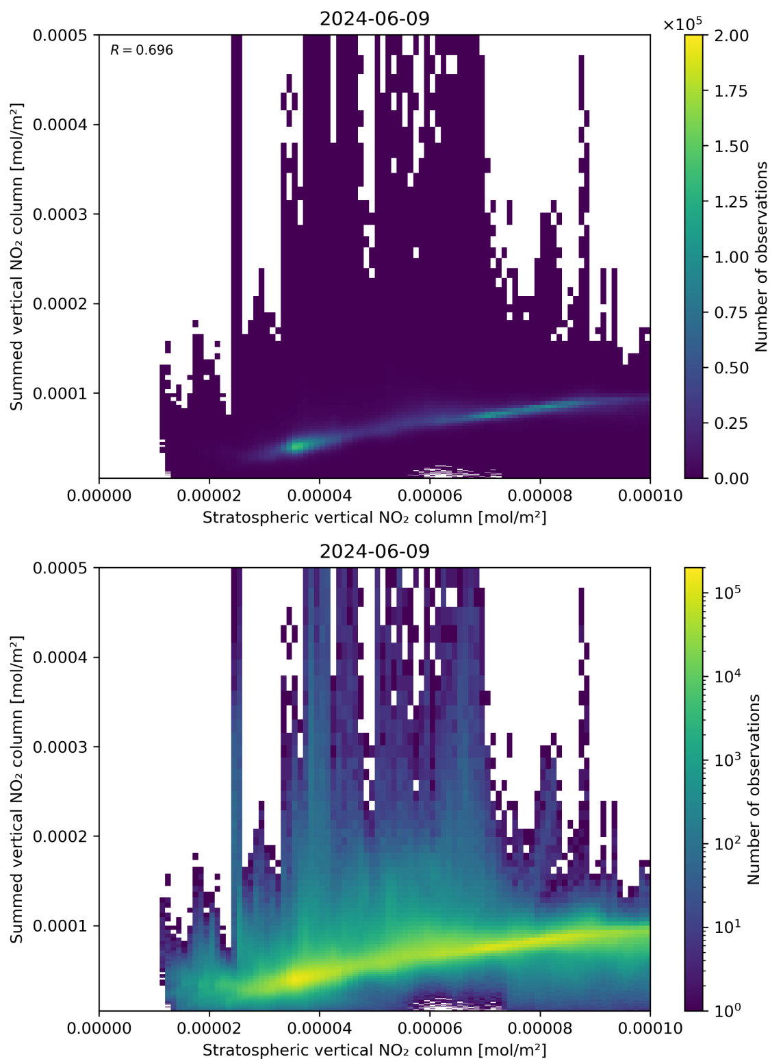
Figure 98: Scatter density plot of “Stratospheric vertical NO 2 column” against “Summed vertical NO 2 column” for 2024-06-08 to 2024-06-10.
