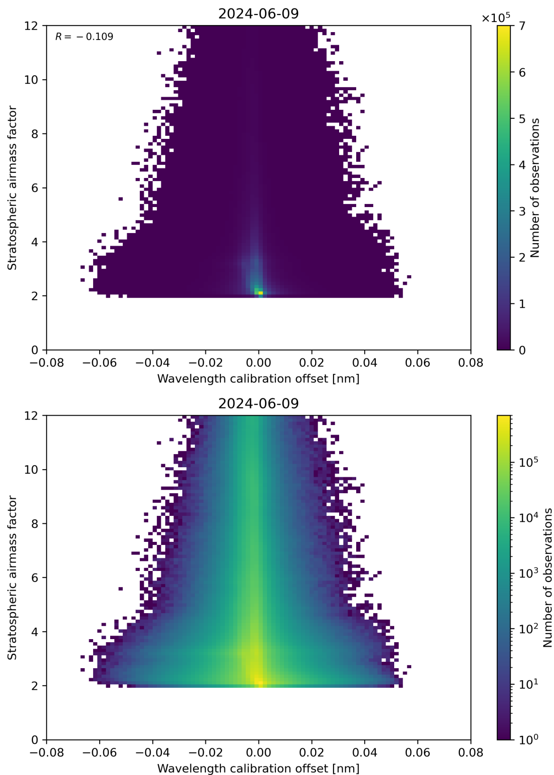
Figure 174: Scatter density plot of “Wavelength calibration offset” against “Stratospheric airmass factor” for 2024-06-08 to 2024-06-10.
