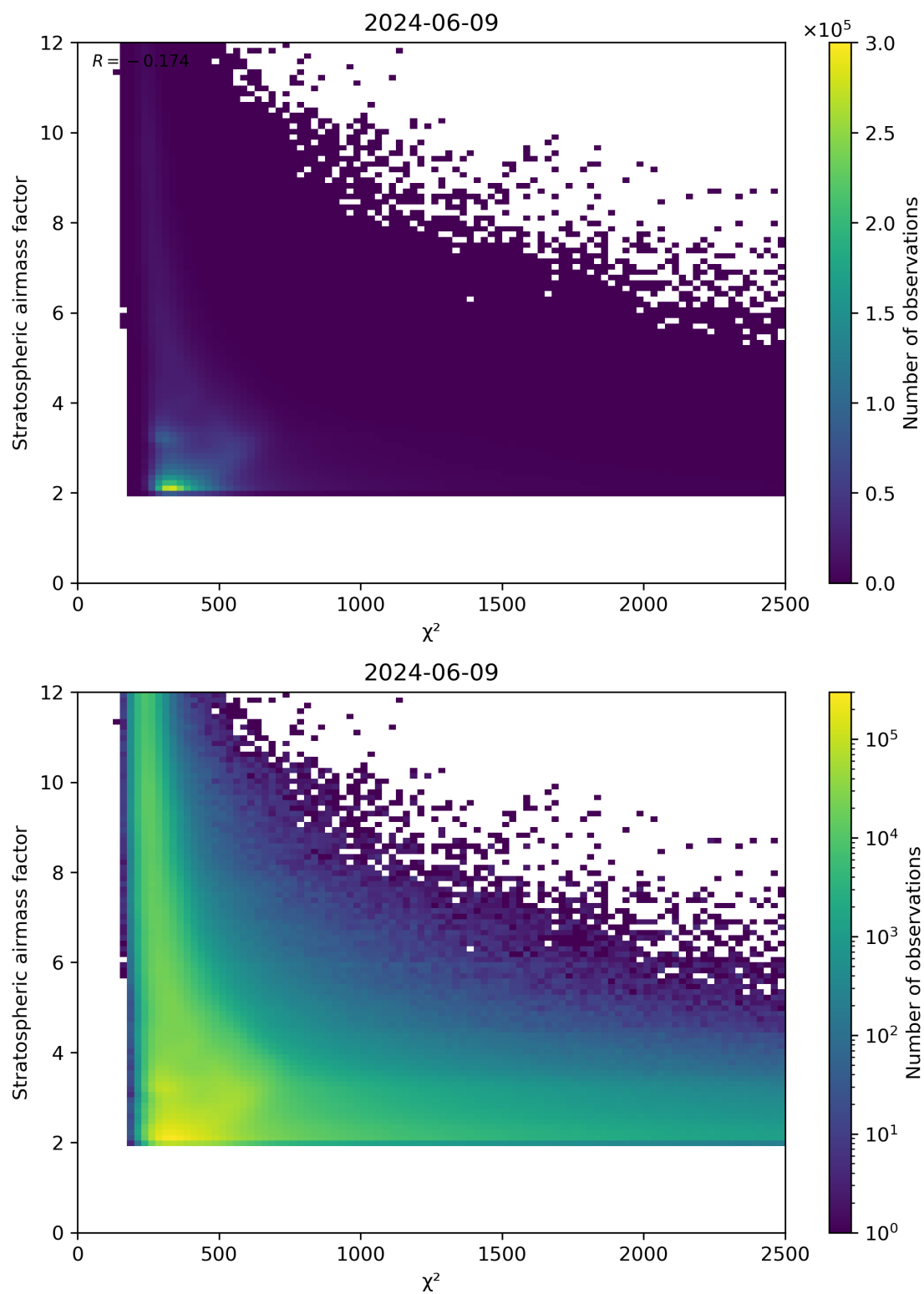
Figure 81: Scatter density plot of “ \chi^2 ” against “Stratospheric airmass factor” for 2024-06-08 to 2024-06-10.
