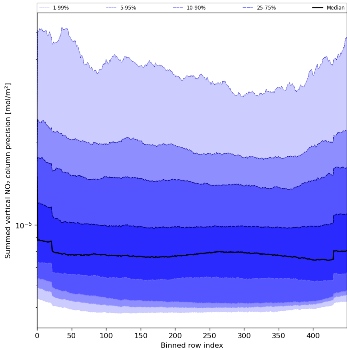
Figure 58: Along track statistics of “Summed vertical NO 2 column precision” for 2024-06-08 to 2024-06-10
