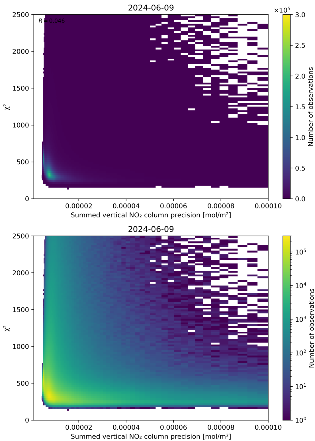
Figure 107: Scatter density plot of “Summed vertical NO 2 column precision” against “ \chi^2 ” for 2024-06-08 to 2024-06-10.
