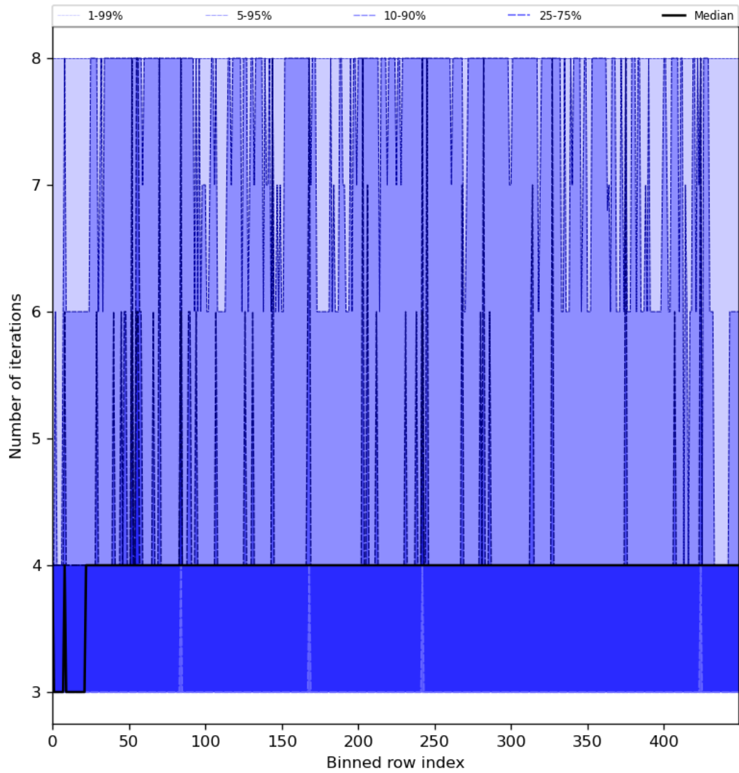
Figure 51: Along track statistics of “Number of iterations” for 2024-06-08 to 2024-06-10
