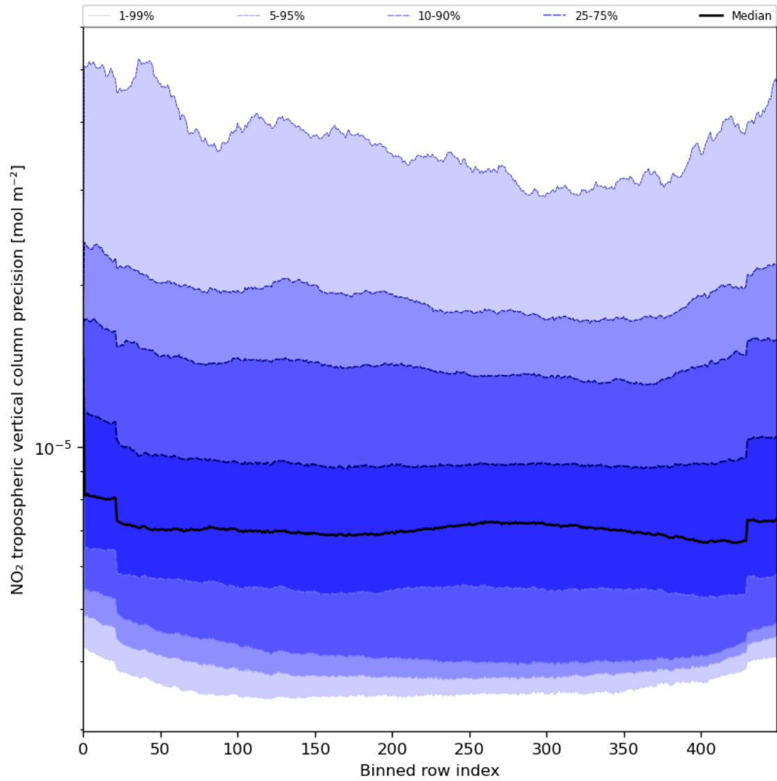
Figure 47: Along track statistics of “NO 2 tropospheric vertical column precision” for 2024-06-08 to 2024-06-10
