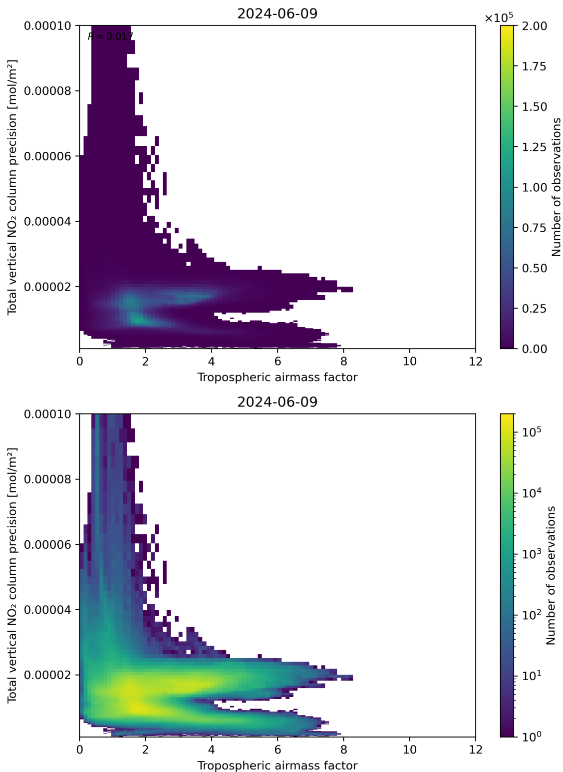
Figure 78: Scatter density plot of “Tropospheric airmass factor” against “Total vertical NO 2 column precision” for 2024-06-08 to 2024-06-10.
