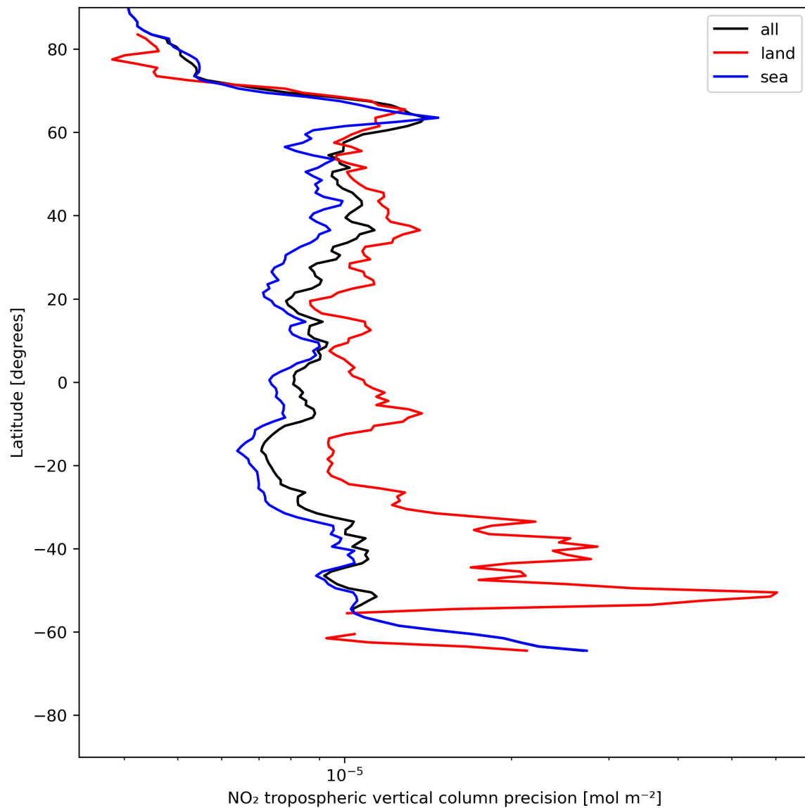
Figure 13: Zonal average of “NO 2 tropospheric vertical column precision” for 2024-06-08 to 2024-06-10.
