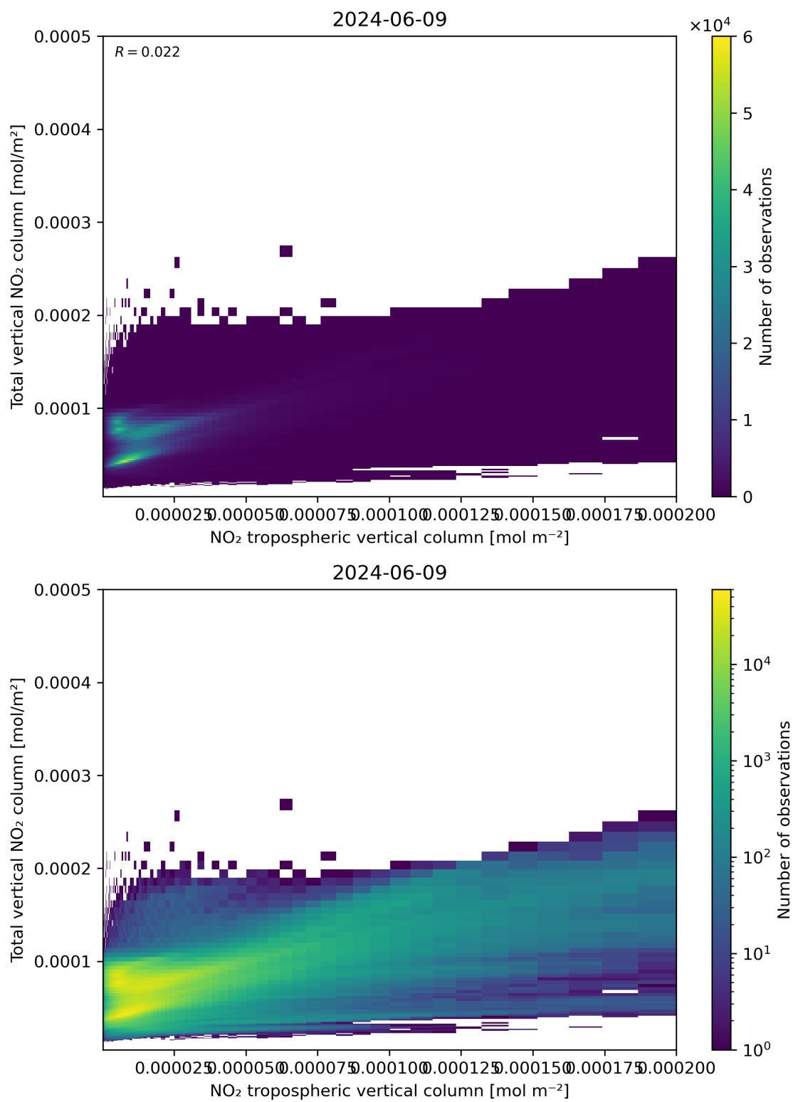
Figure 128: Scatter density plot of “NO 2 tropospheric vertical column” against “Total vertical NO 2 column” for 2024-06-08 to 2024-06-10.
