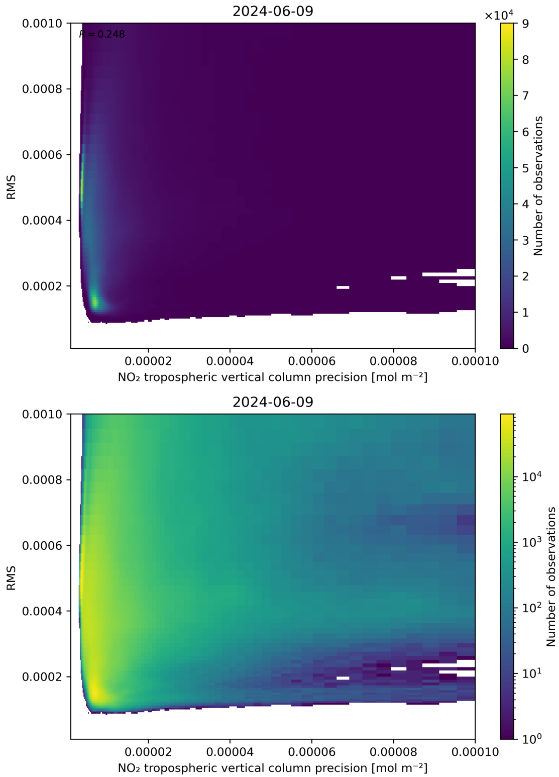
Figure 140: Scatter density plot of “NO 2 tropospheric vertical column precision” against “RMS” for 2024-06-08 to 2024-06-10.
