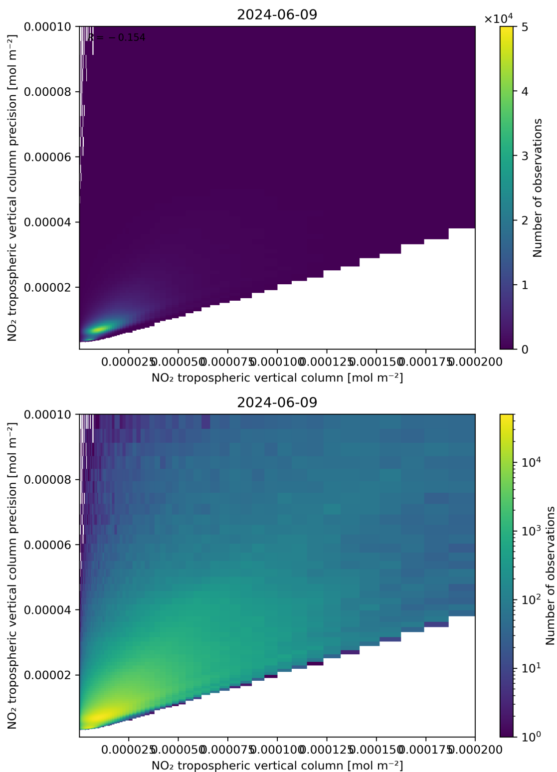
Figure 130: Scatter density plot of “NO 2 tropospheric vertical column” against “NO 2 tropospheric vertical column precision” for 2024-06-08 to 2024-06-10.
