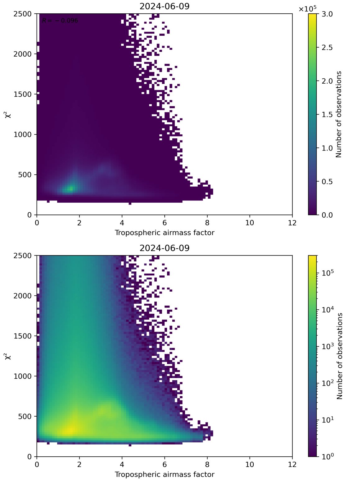
Figure 73: Scatter density plot of “Tropospheric airmass factor” against “ \chi^2 ” for 2024-06-08 to 2024-06-10.
