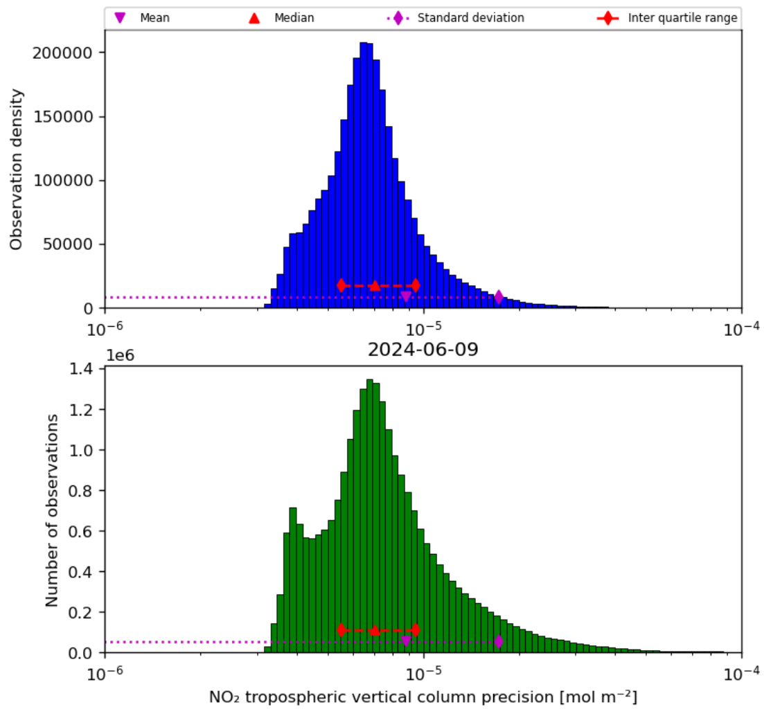
Figure 30: Histogram of “NO 2 tropospheric vertical column precision” for 2024-06-08 to 2024-06-10
