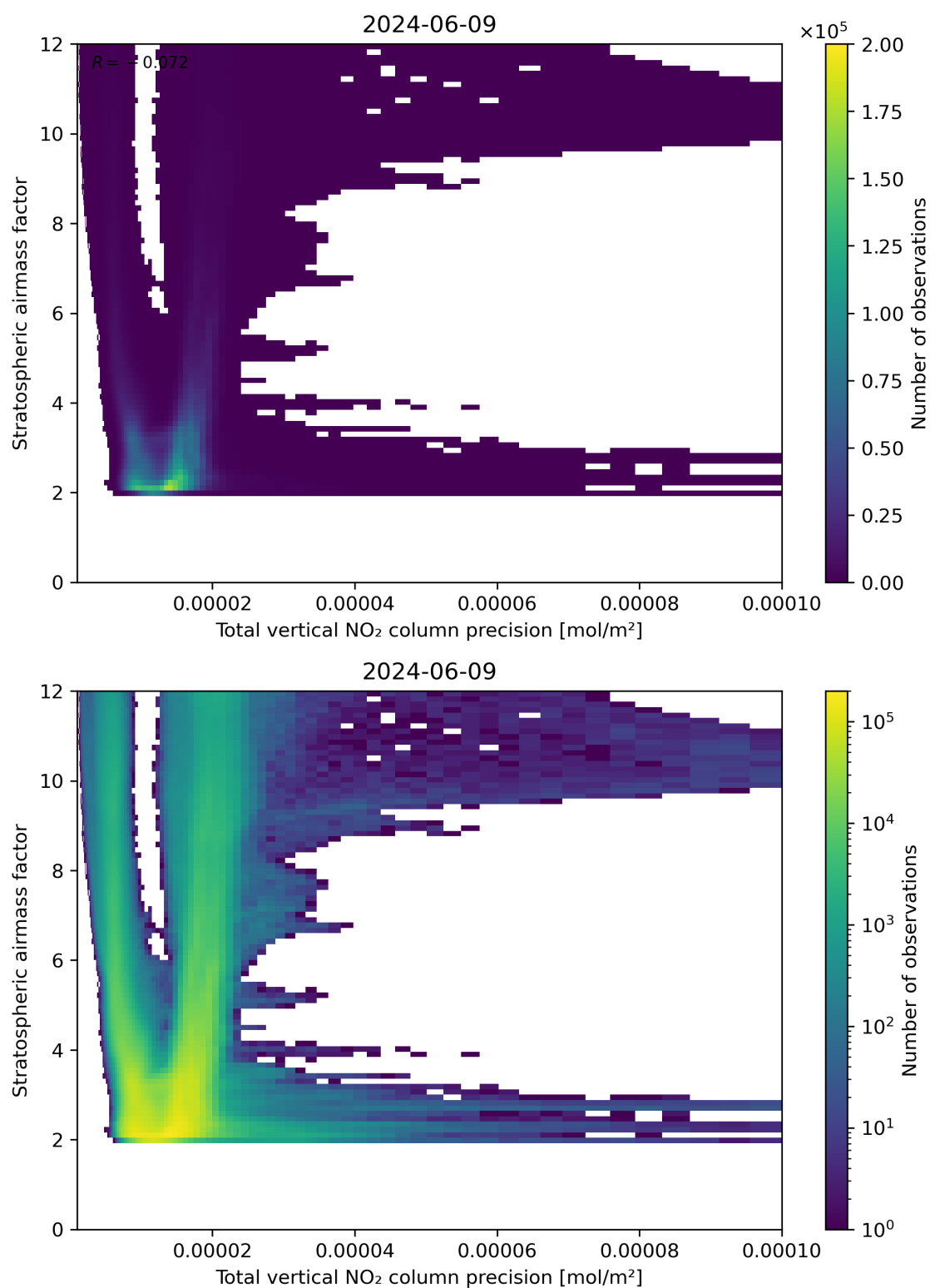
Figure 115: Scatter density plot of “Total vertical NO 2 column precision” against “Stratospheric air mass factor” for 2024-06-08 to 2024-06-10.
