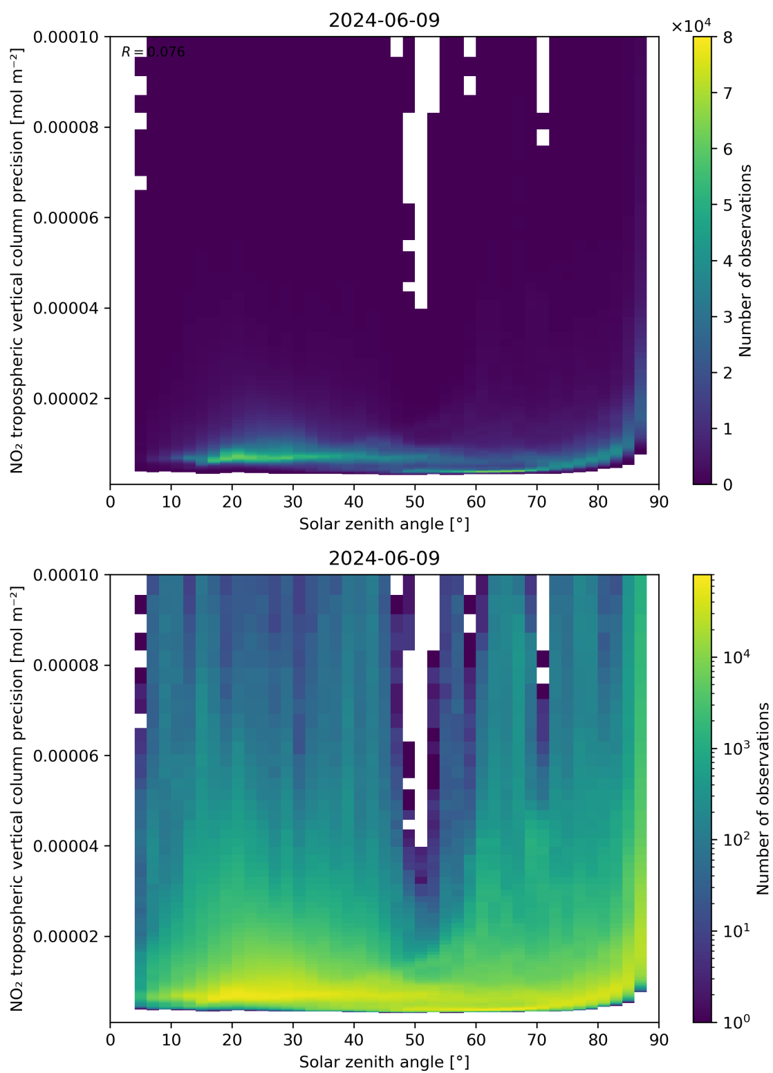
Figure 156: Scatter density plot of “Solar zenith angle” against “NO 2 tropospheric vertical column precision” for 2024-06-08 to 2024-06-10.
