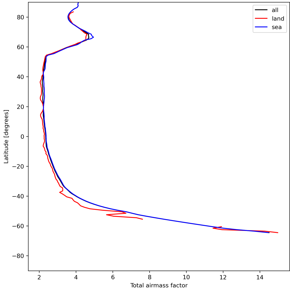
Figure 15: Zonal average of “Total airmass factor” for 2024-06-08 to 2024-06-10.
