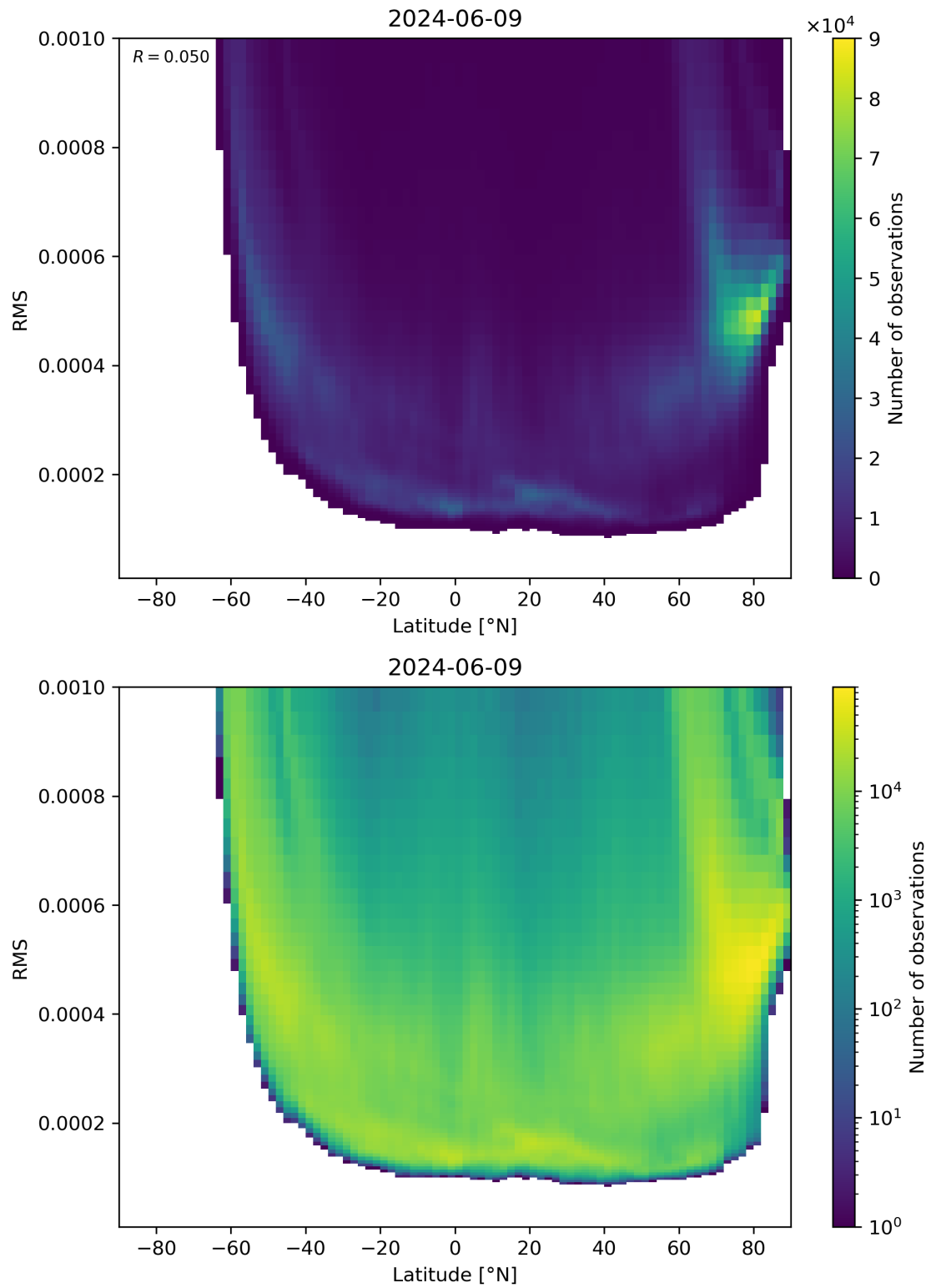
Figure 94: Scatter density plot of “Latitude” against “RMS” for 2024-06-08 to 2024-06-10.
