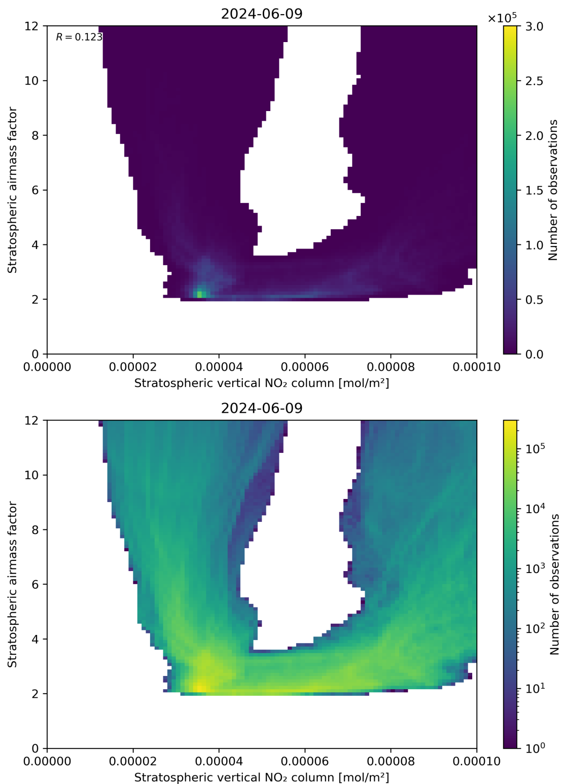
Figure 96: Scatter density plot of “Stratospheric vertical NO 2 column” against “Stratospheric airmass factor” for 2024-06-08 to 2024-06-10.
