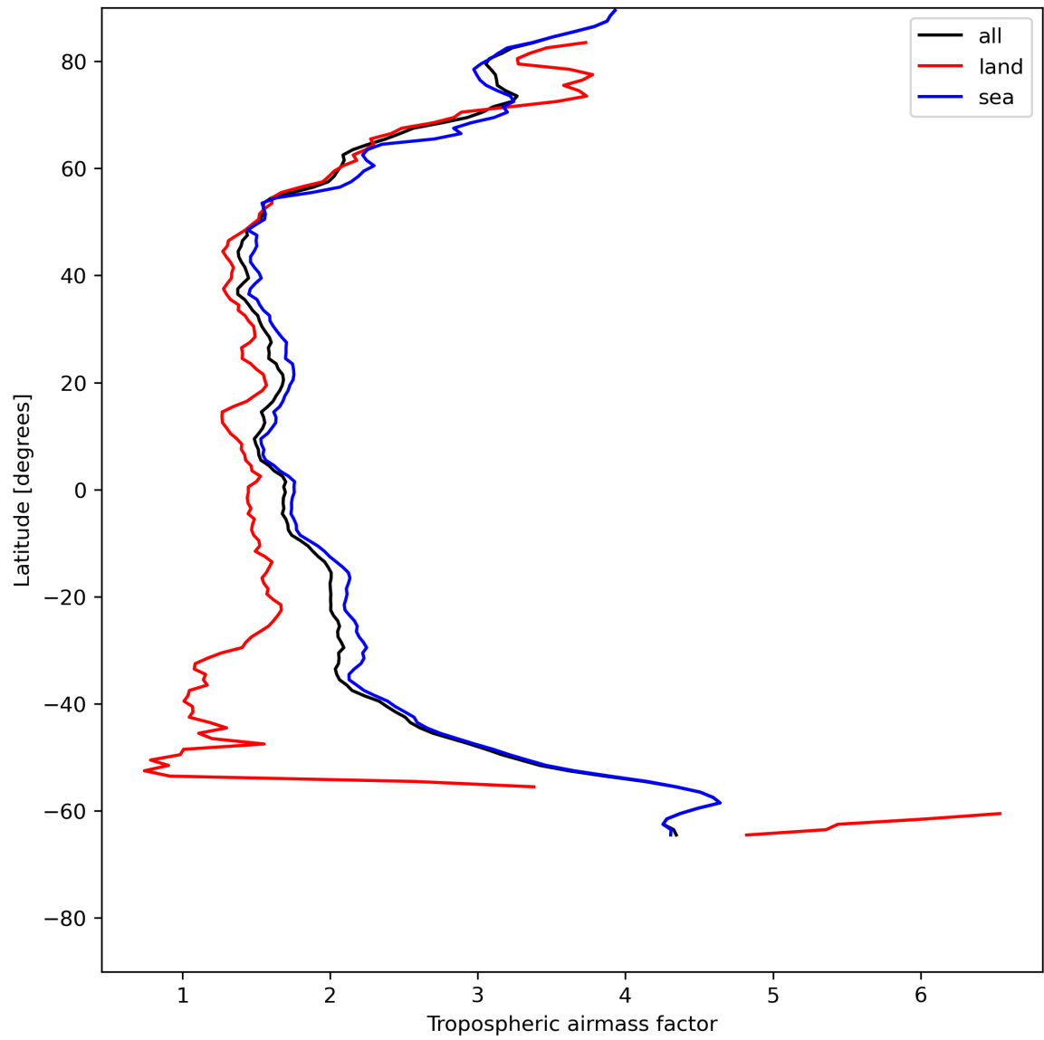
Figure 14: Zonal average of “Tropospheric airmass factor” for 2024-06-08 to 2024-06-10.
