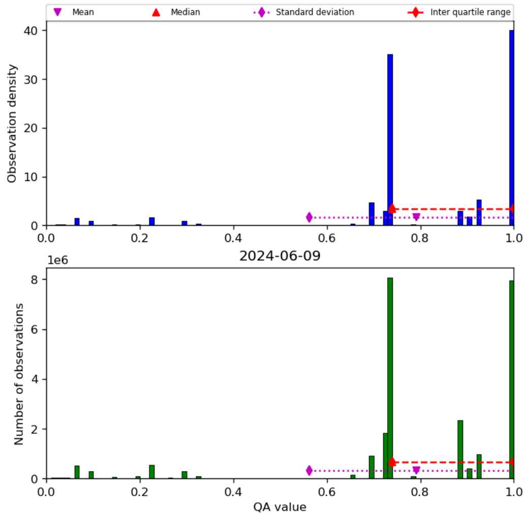
Figure 28: Histogram of “QA value” for 2024-06-08 to 2024-06-10
