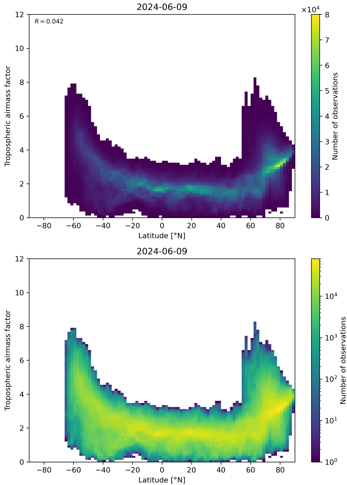
Figure 85: Scatter density plot of “Latitude” against “Tropospheric airmass factor” for 2024-06-08 to 2024-06-10.
