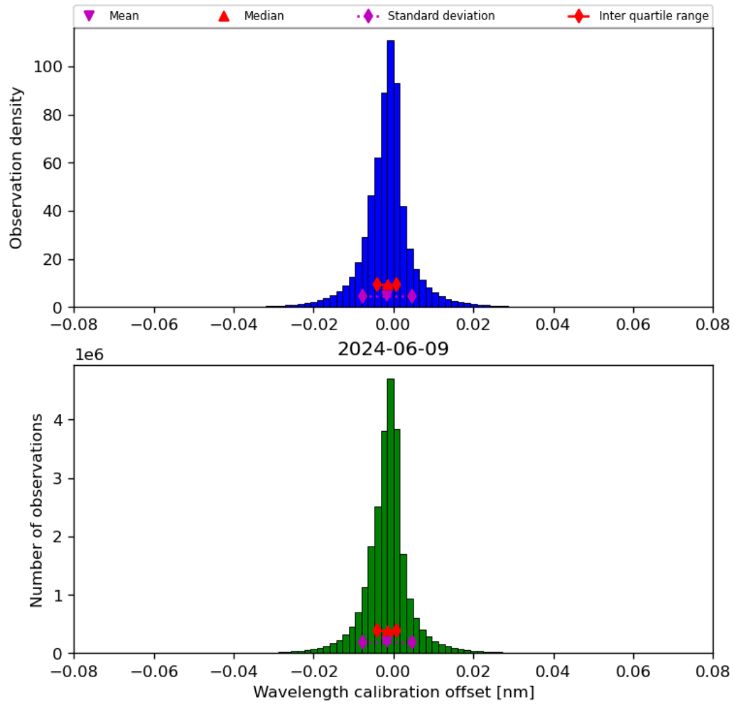
Figure 35: Histogram of “Wavelength calibration offset” for 2024-06-08 to 2024-06-10
