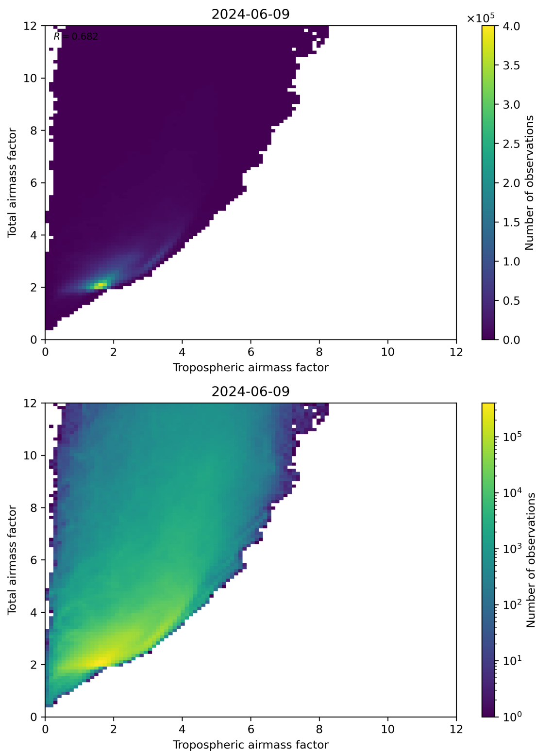
Figure 72: Scatter density plot of “Tropospheric airmass factor” against “Total airmass factor” for 2024-06-08 to 2024-06-10.
