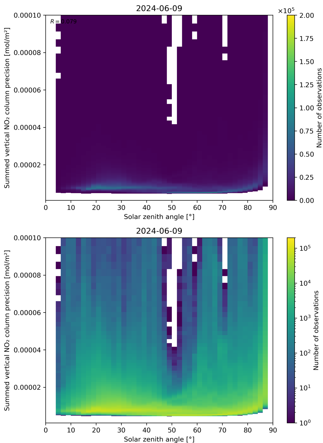
Figure 152: Scatter density plot of “Solar zenith angle” against “Summed vertical NO 2 column precision” for 2024-06-08 to 2024-06-10.
