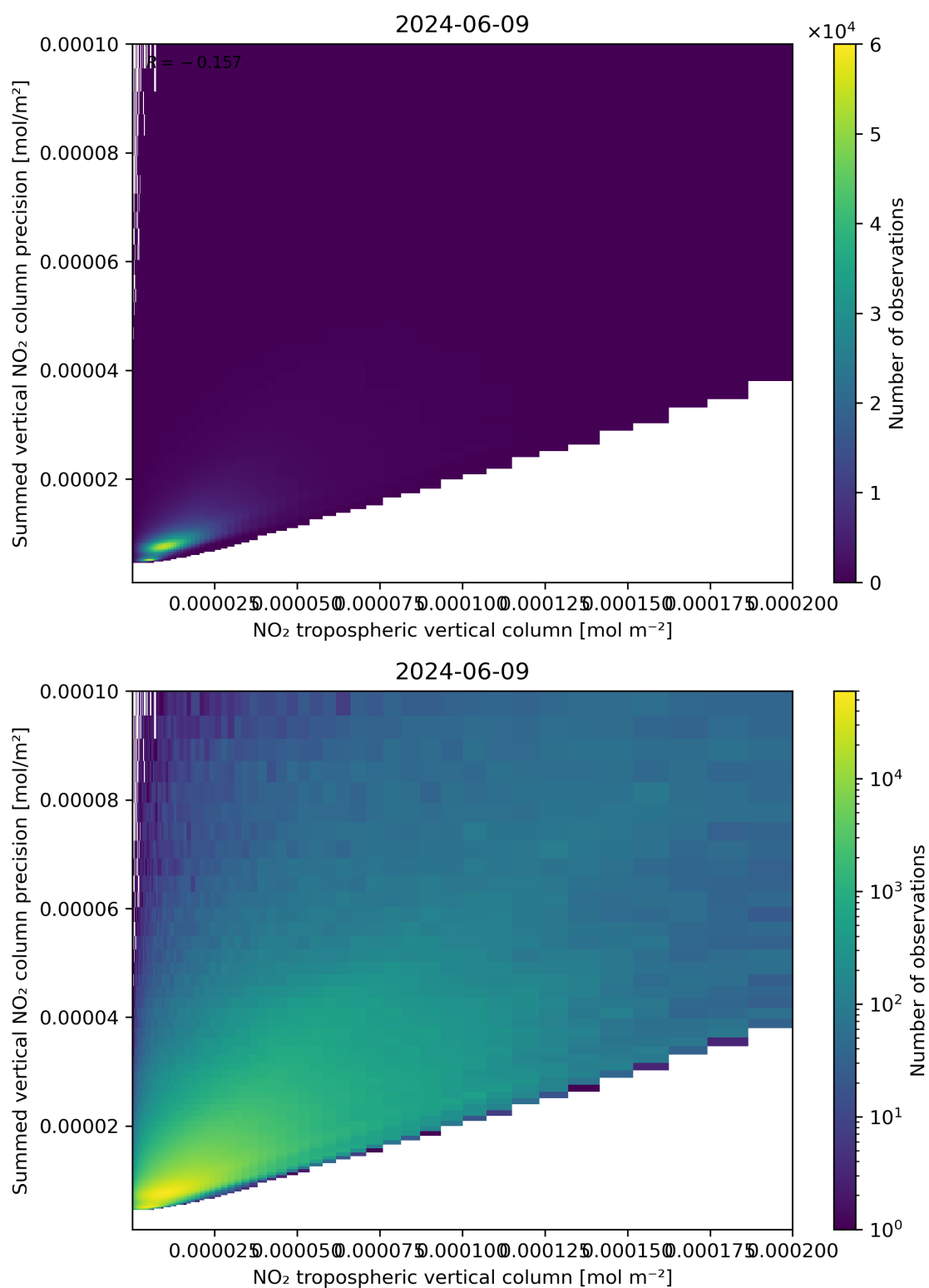
Figure 127: Scatter density plot of “NO 2 tropospheric vertical column” against “Summed vertical NO 2 column precision” for 2024-06-08 to 2024-06-10.
