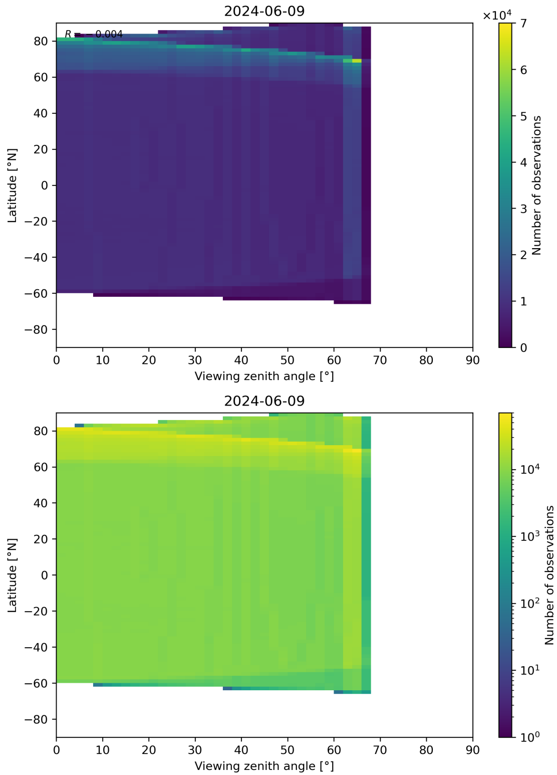
Figure 163: Scatter density plot of “Viewing zenith angle” against “Latitude” for 2024-06-08 to 2024-06-10.
