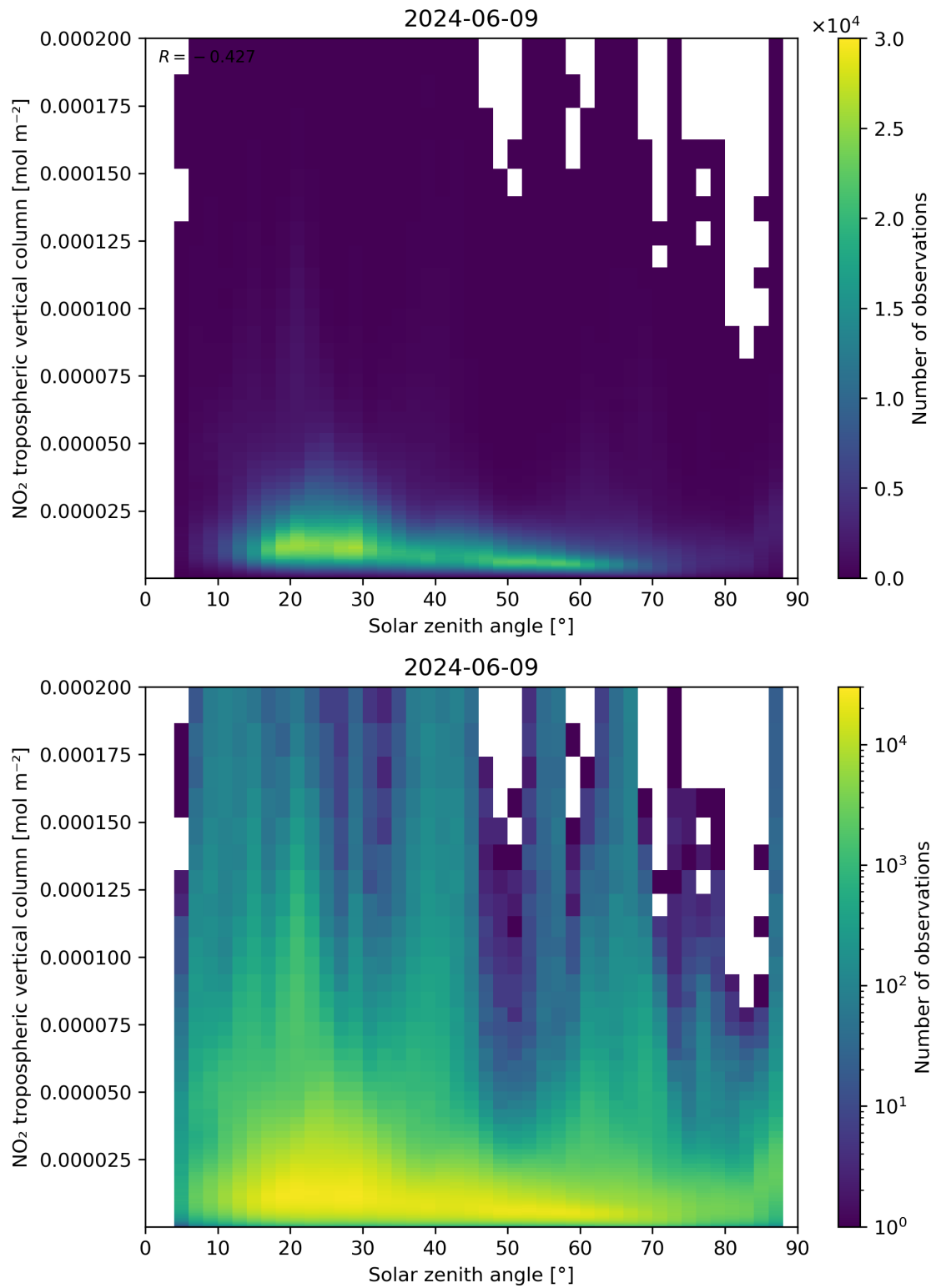
Figure 155: Scatter density plot of “Solar zenith angle” against “NO 2 tropospheric vertical column” for 2024-06-08 to 2024-06-10.
