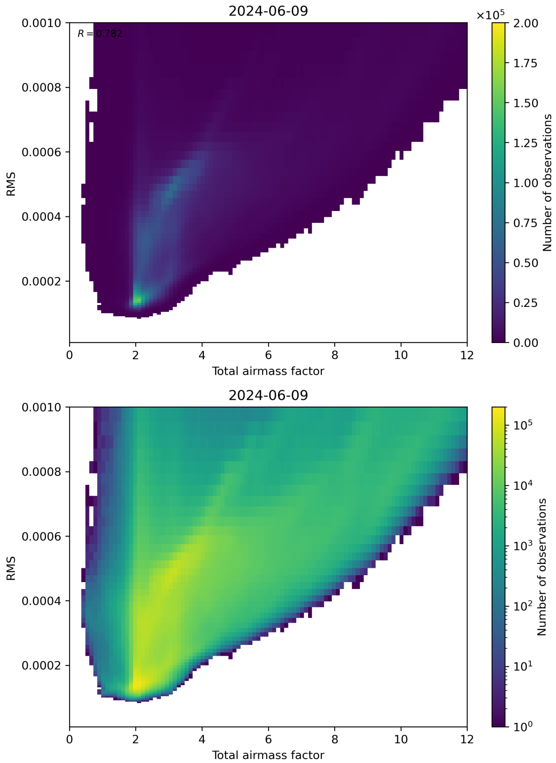
Figure 69: Scatter density plot of “Total airmass factor” against “RMS” for 2024-06-08 to 2024-06-10.
