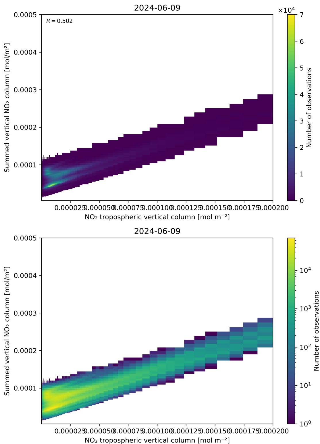
Figure 126: Scatter density plot of “NO 2 tropospheric vertical column” against “Summed vertical NO 2 column” for 2024-06-08 to 2024-06-10.
