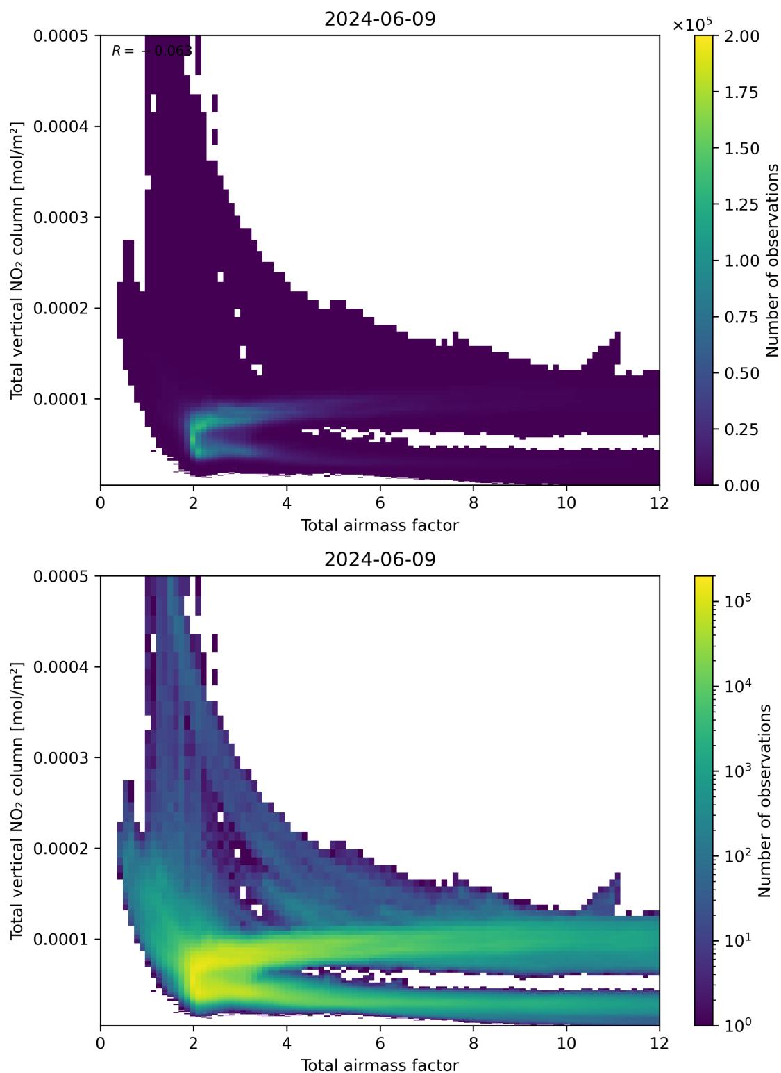
Figure 67: Scatter density plot of “Total airmass factor” against “Total vertical NO 2 column” for 2024-06-08 to 2024-06-10.
