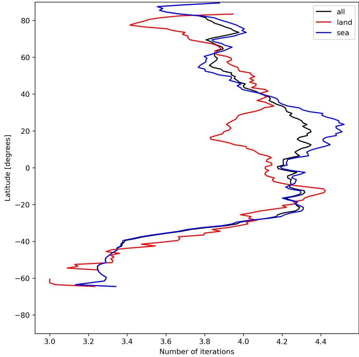
Figure 17: Zonal average of “Number of iterations” for 2024-06-08 to 2024-06-10.
