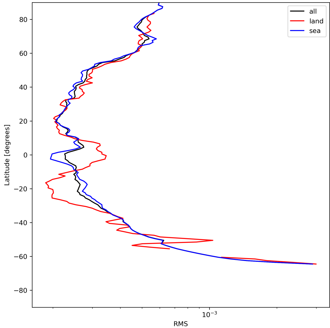
Figure 26: Zonal average of “RMS” for 2024-06-08 to 2024-06-10.
