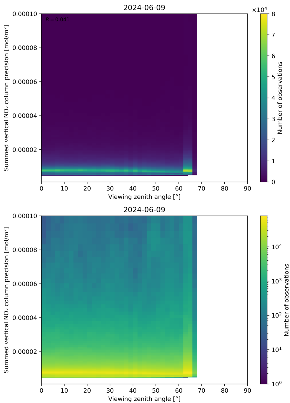
Figure 166: Scatter density plot of “Viewing zenith angle” against “Summed vertical NO 2 column precision” for 2024-06-08 to 2024-06-10.
