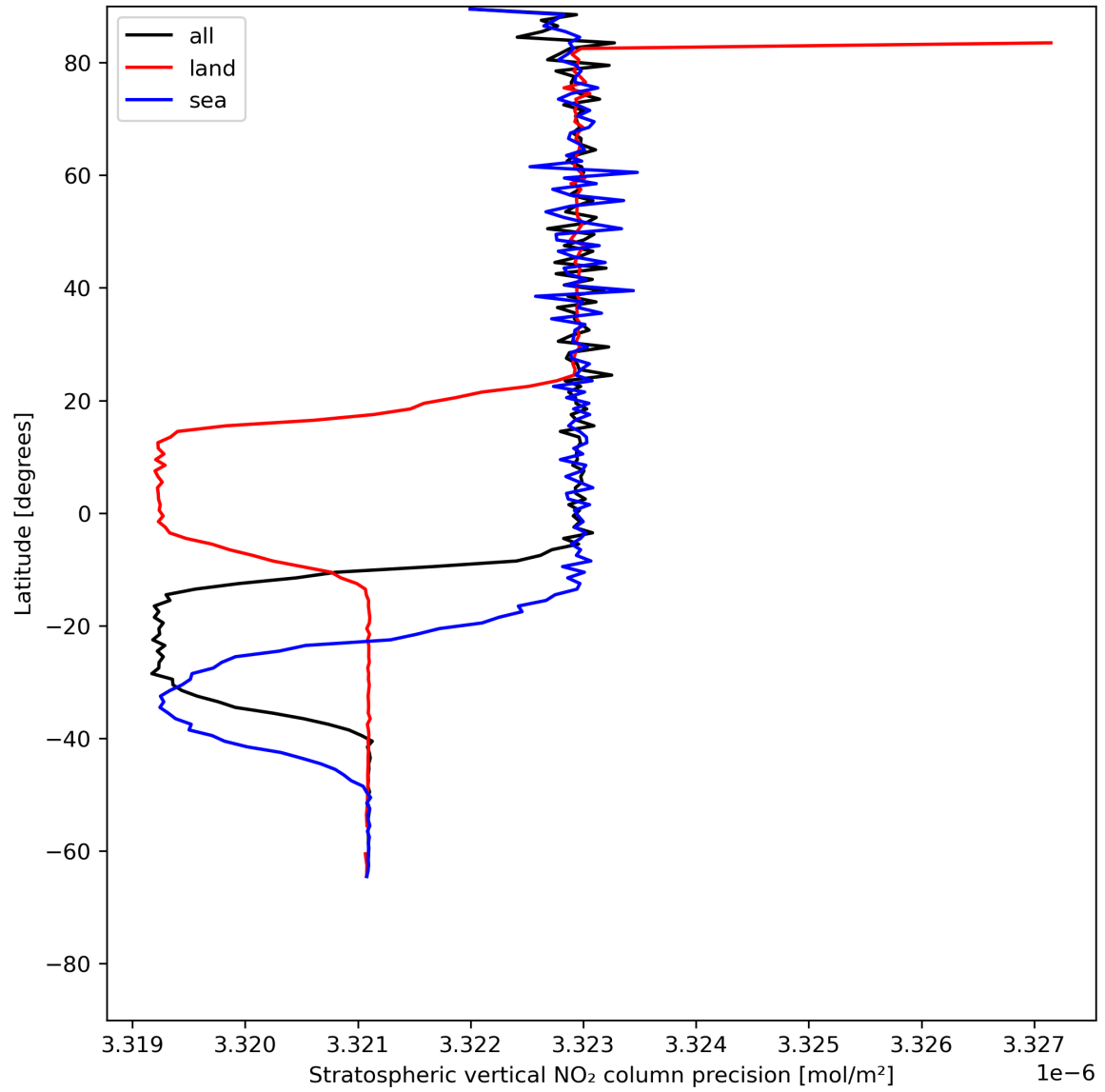
Figure 20: Zonal average of “Stratospheric vertical NO 2 column precision” for 2024-06-08 to 2024-06-10.
