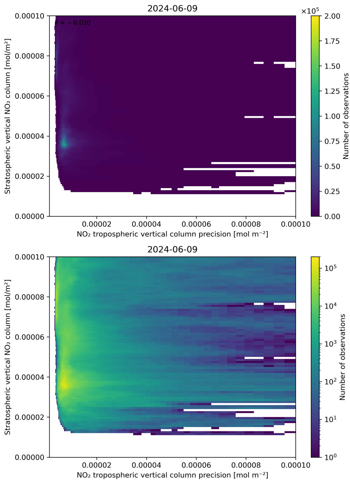
Figure 135: Scatter density plot of “NO 2 tropospheric vertical column precision” against “Stratospheric vertical NO 2 column” for 2024-06-08 to 2024-06-10.
