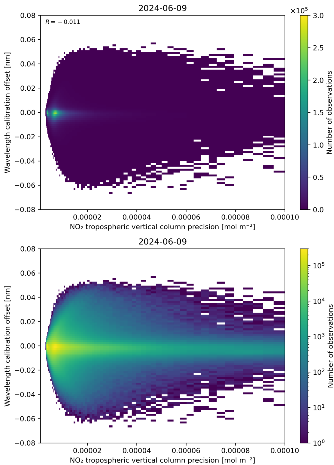
Figure 141: Scatter density plot of “NO 2 tropospheric vertical column precision” against “Wavelength calibration offset” for 2024-06-08 to 2024-06-10.
