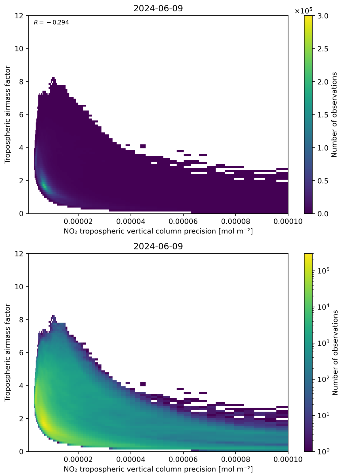
Figure 133: Scatter density plot of “NO 2 tropospheric vertical column precision” against “Tropospheric airmass factor” for 2024-06-08 to 2024-06-10.
