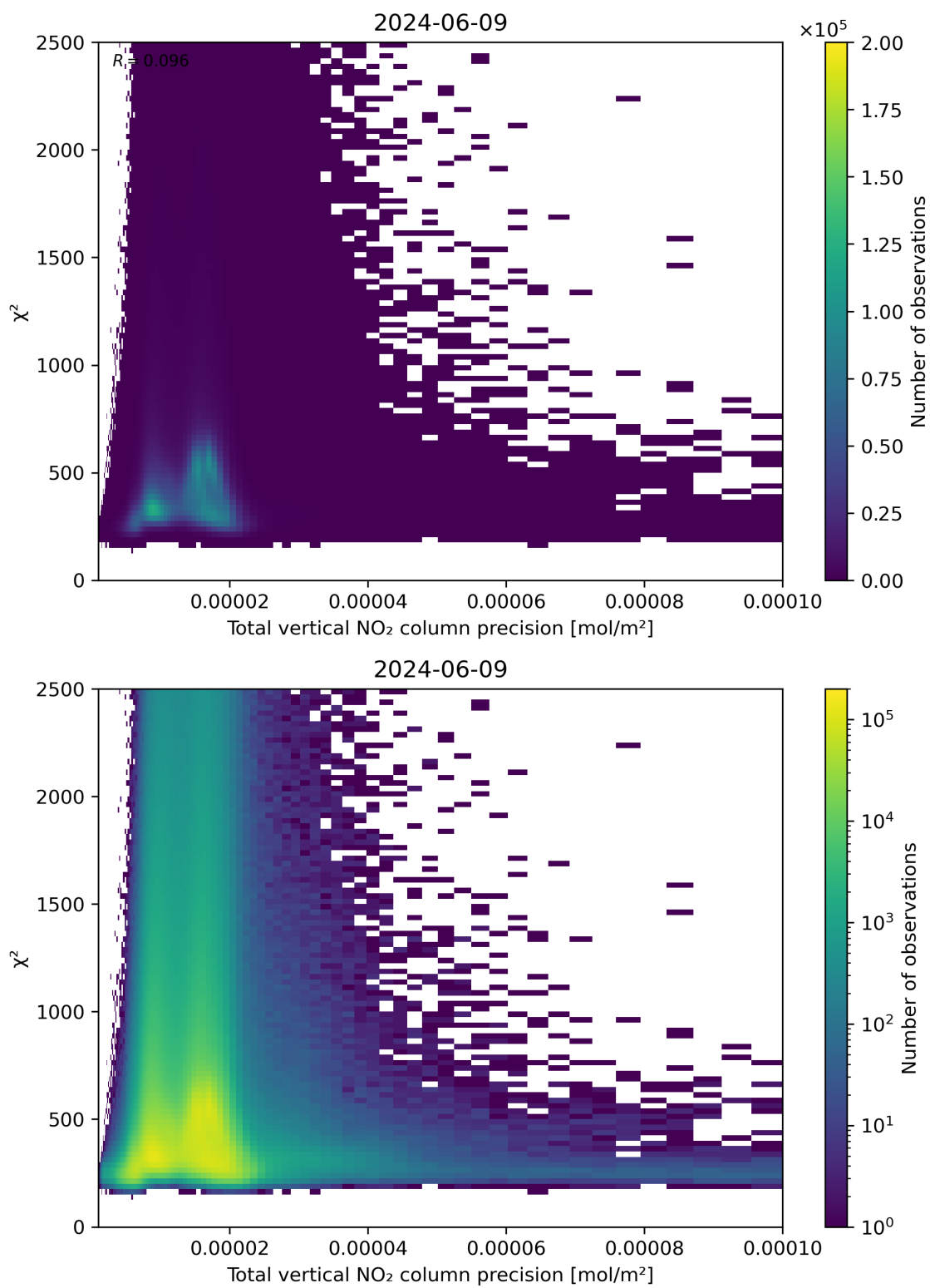
Figure 116: Scatter density plot of “Total vertical NO 2 column precision” against “ \chi^2 ” for 2024-06-08 to 2024-06-10.
