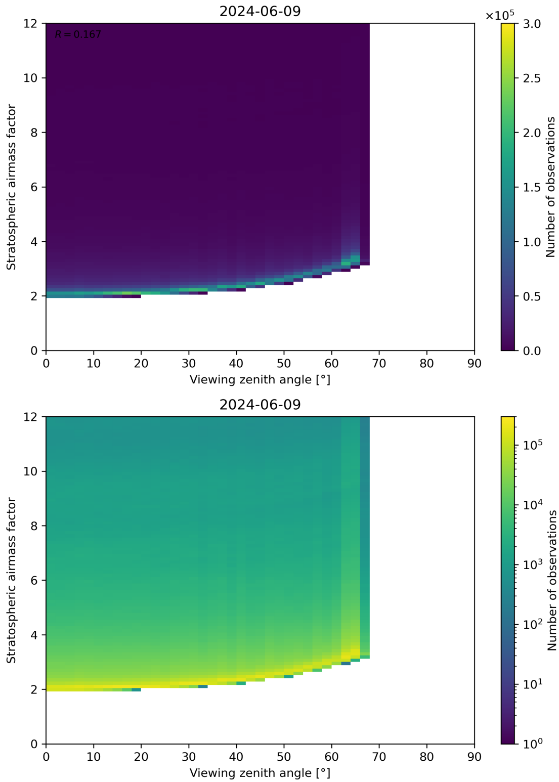
Figure 159: Scatter density plot of “Viewing zenith angle” against “Stratospheric airmass factor” for 2024-06-08 to 2024-06-10.
