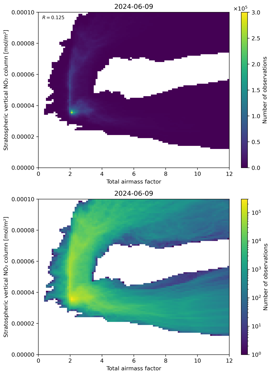
Figure 64: Scatter density plot of “Total airmass factor” against “Stratospheric vertical NO 2 column” for 2024-06-08 to 2024-06-10.
