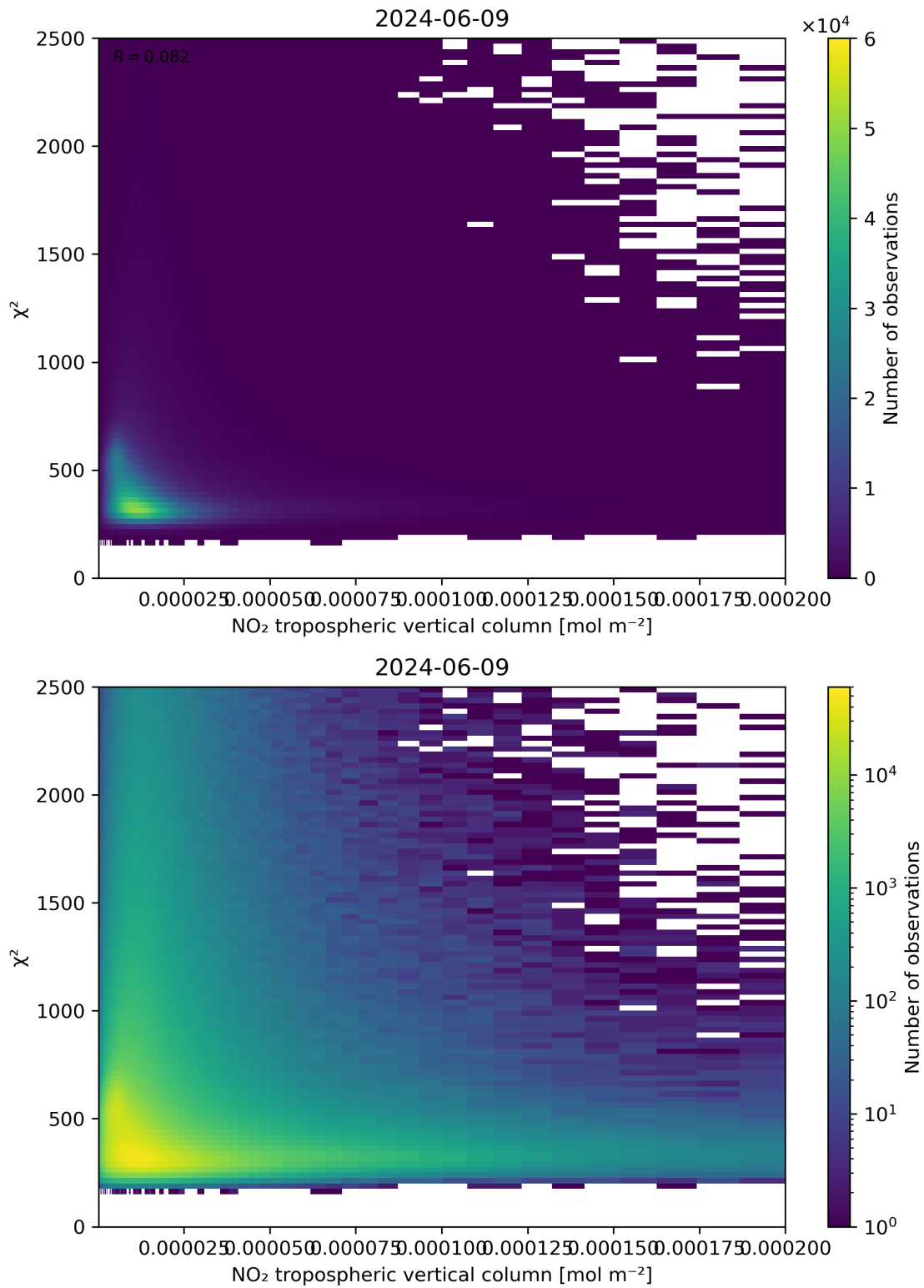
Figure 124: Scatter density plot of “NO 2 tropospheric vertical column” against “ \chi^2 ” for 2024-06-08 to 2024-06-10.
