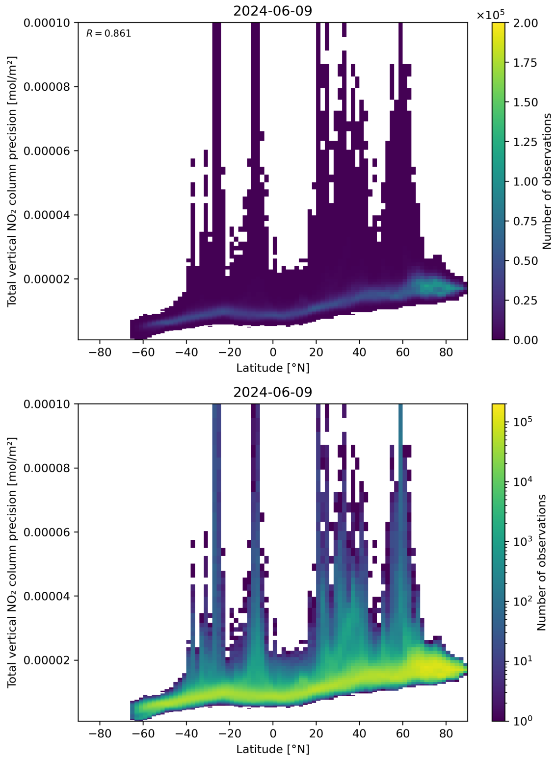
Figure 91: Scatter density plot of “Latitude” against “Total vertical NO 2 column precision” for 2024-06-08 to 2024-06-10.
