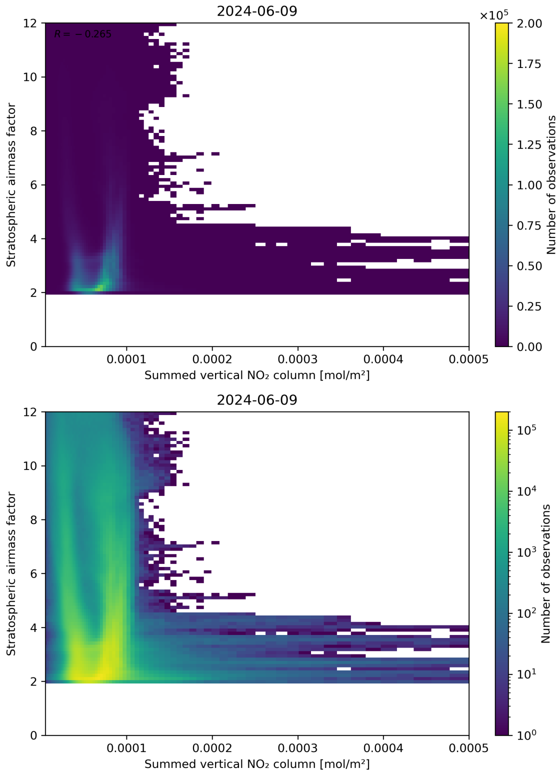
Figure 103: Scatter density plot of “Summed vertical NO 2 column” against “Stratospheric airmass factor” for 2024-06-08 to 2024-06-10.
