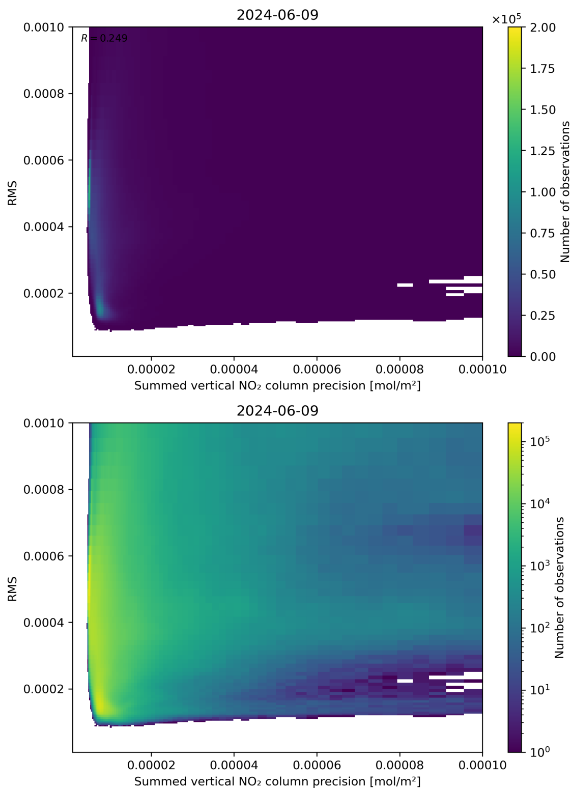
Figure 108: Scatter density plot of “Summed vertical NO 2 column precision” against “RMS” for 2024-06-08 to 2024-06-10.
