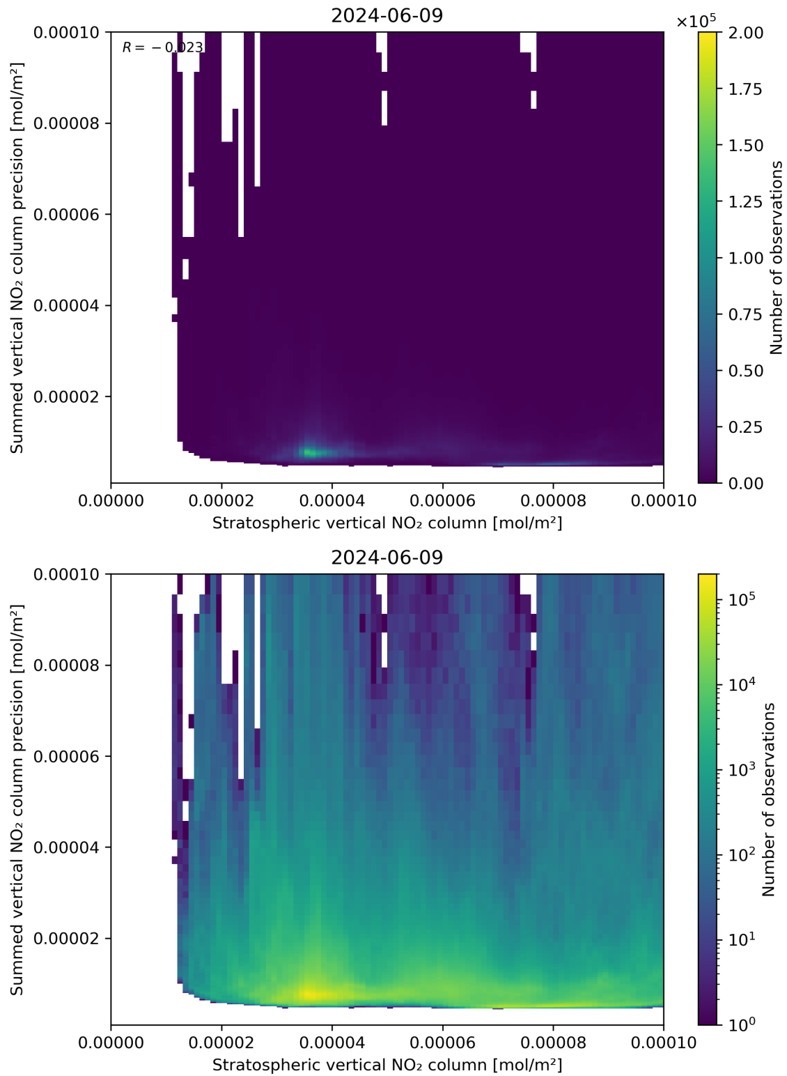
Figure 99: Scatter density plot of “Stratospheric vertical NO 2 column” against “Summed vertical NO 2 column precision” for 2024-06-08 to 2024-06-10.
