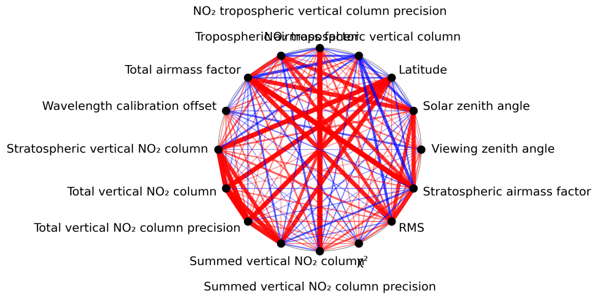
Figure 1: Map of correlation graph for 2024-06-08 to 2024-06-10.
