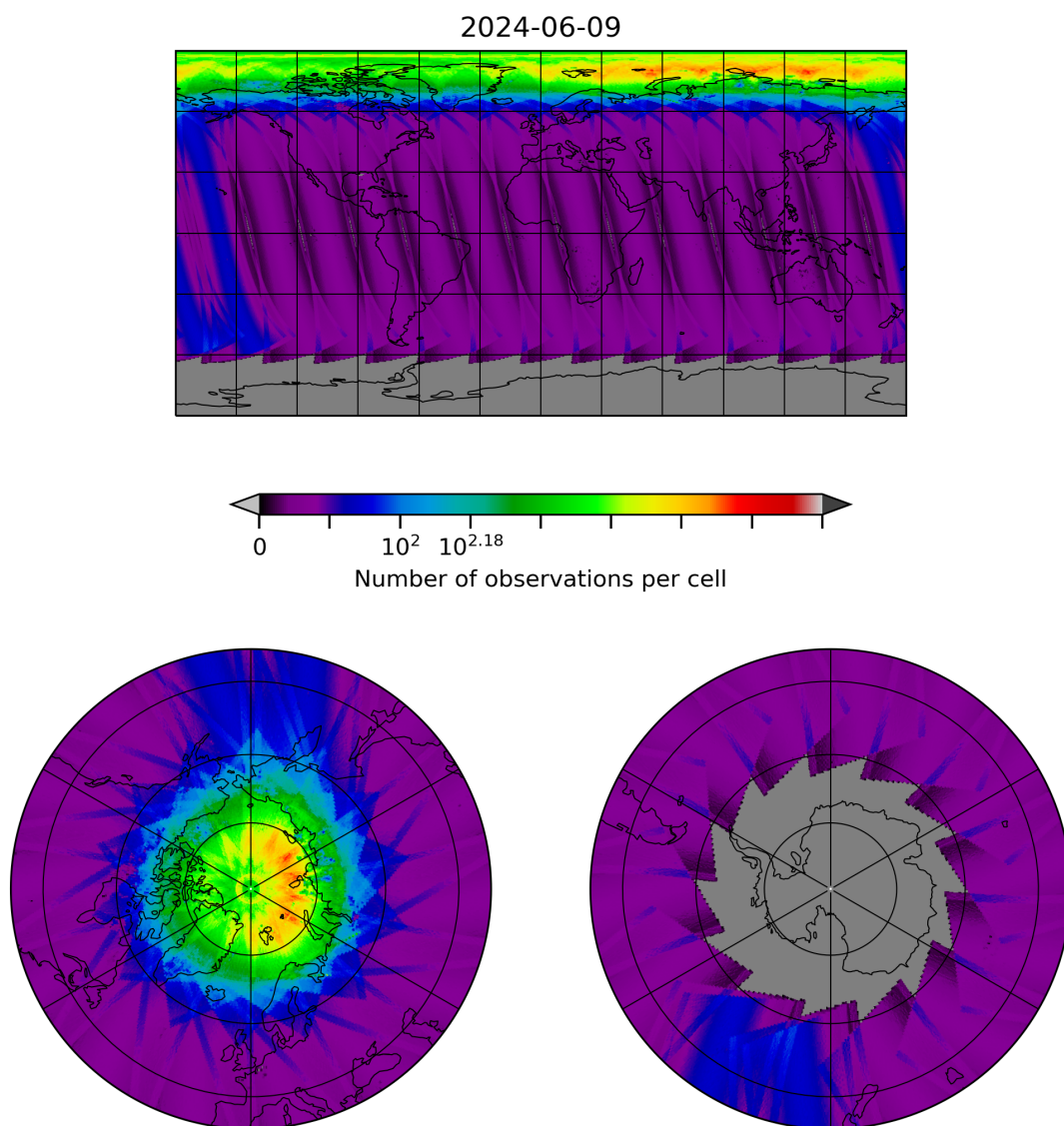
Figure 10: Map of the number of observations for 2024-06-08 to 2024-06-10
