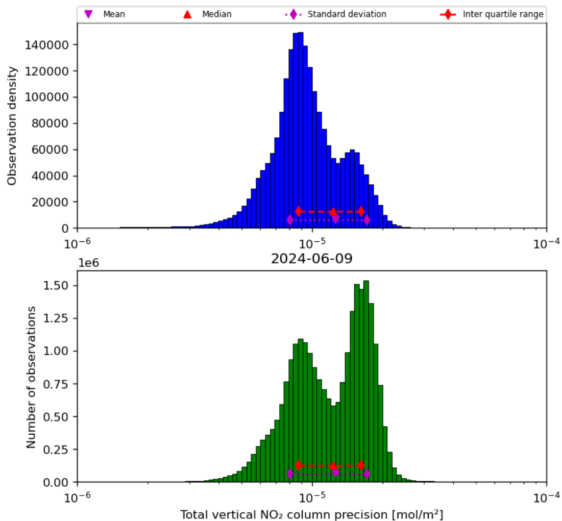
Figure 39: Histogram of “Total vertical NO 2 column precision” for 2024-06-08 to 2024-06-10
