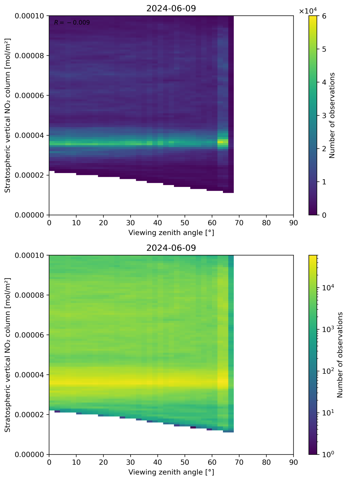
Figure 164: Scatter density plot of “Viewing zenith angle” against “Stratospheric vertical NO 2 column” for 2024-06-08 to 2024-06-10.
