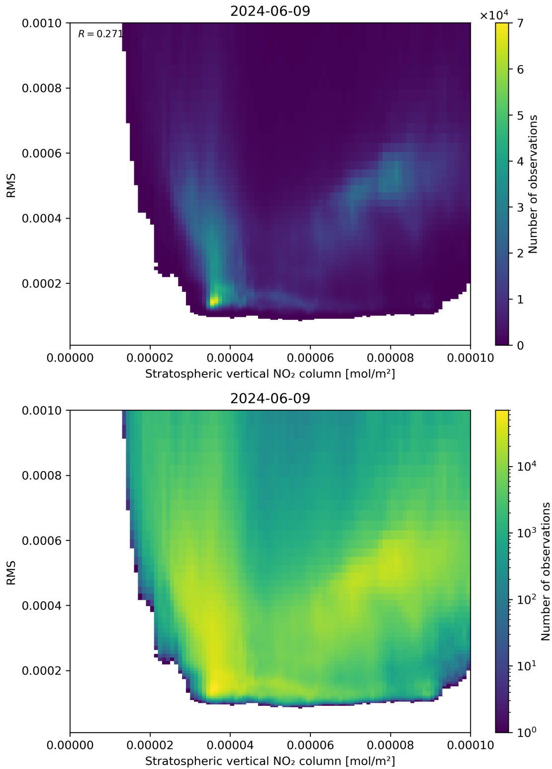
Figure 102: Scatter density plot of “Stratospheric vertical NO 2 column” against “RMS” for 2024-06-08 to 2024-06-10.
