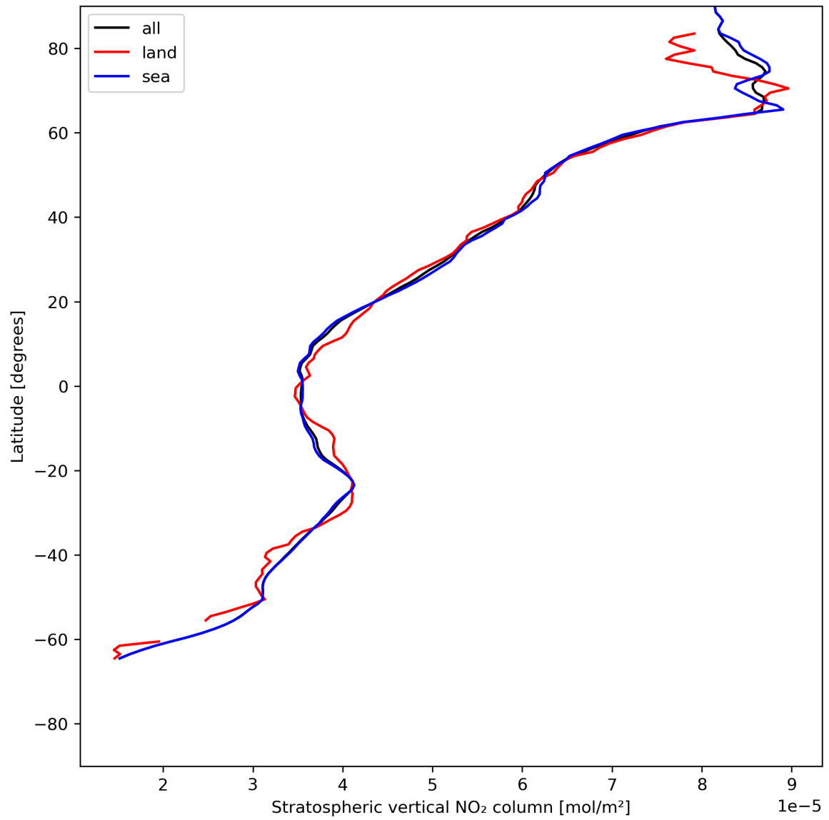
Figure 19: Zonal average of “Stratospheric vertical NO 2 column” for 2024-06-08 to 2024-06-10.
