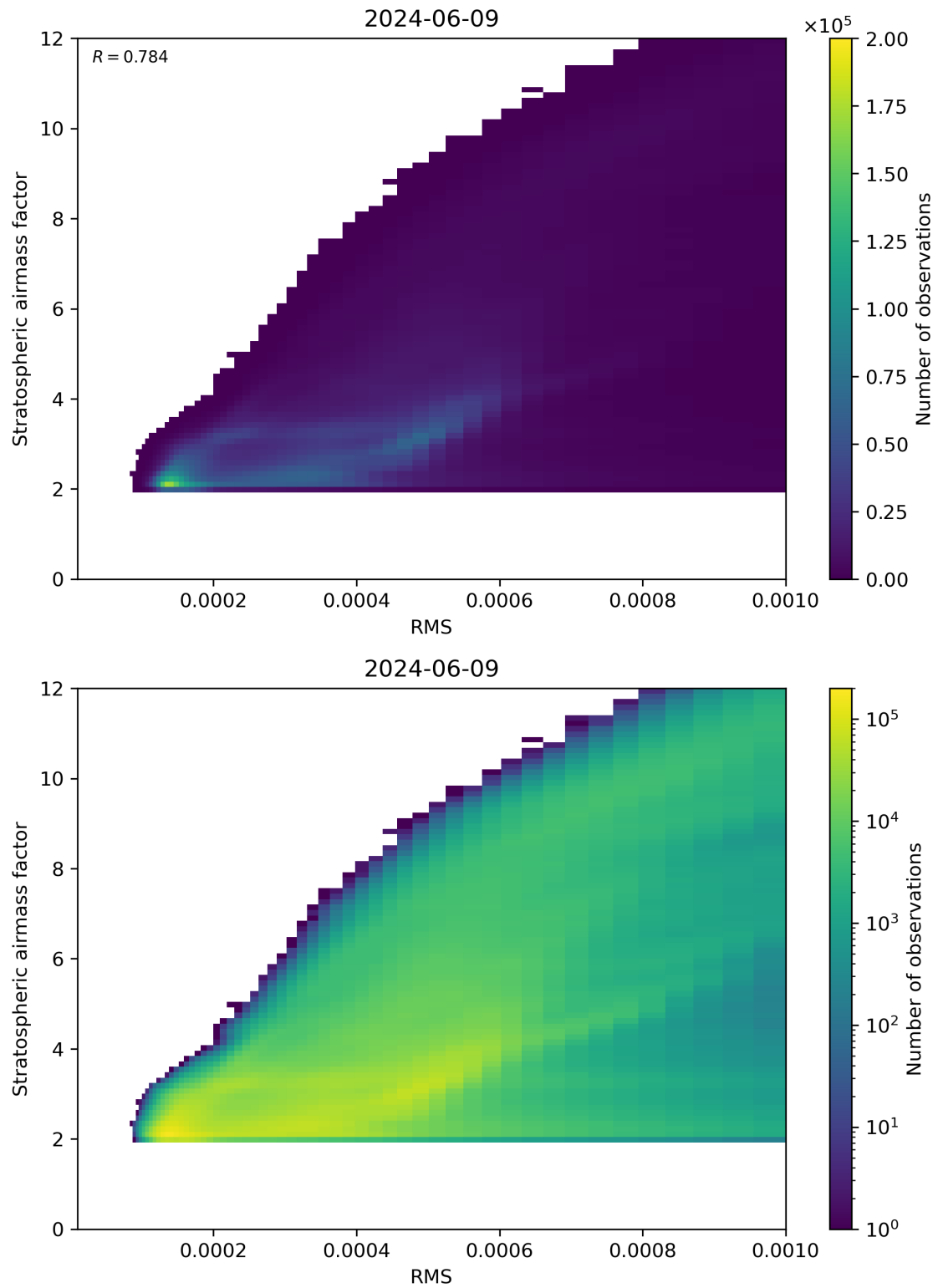
Figure 144: Scatter density plot of “RMS” against “Stratospheric airmass factor” for 2024-06-08 to 2024-06-10.
