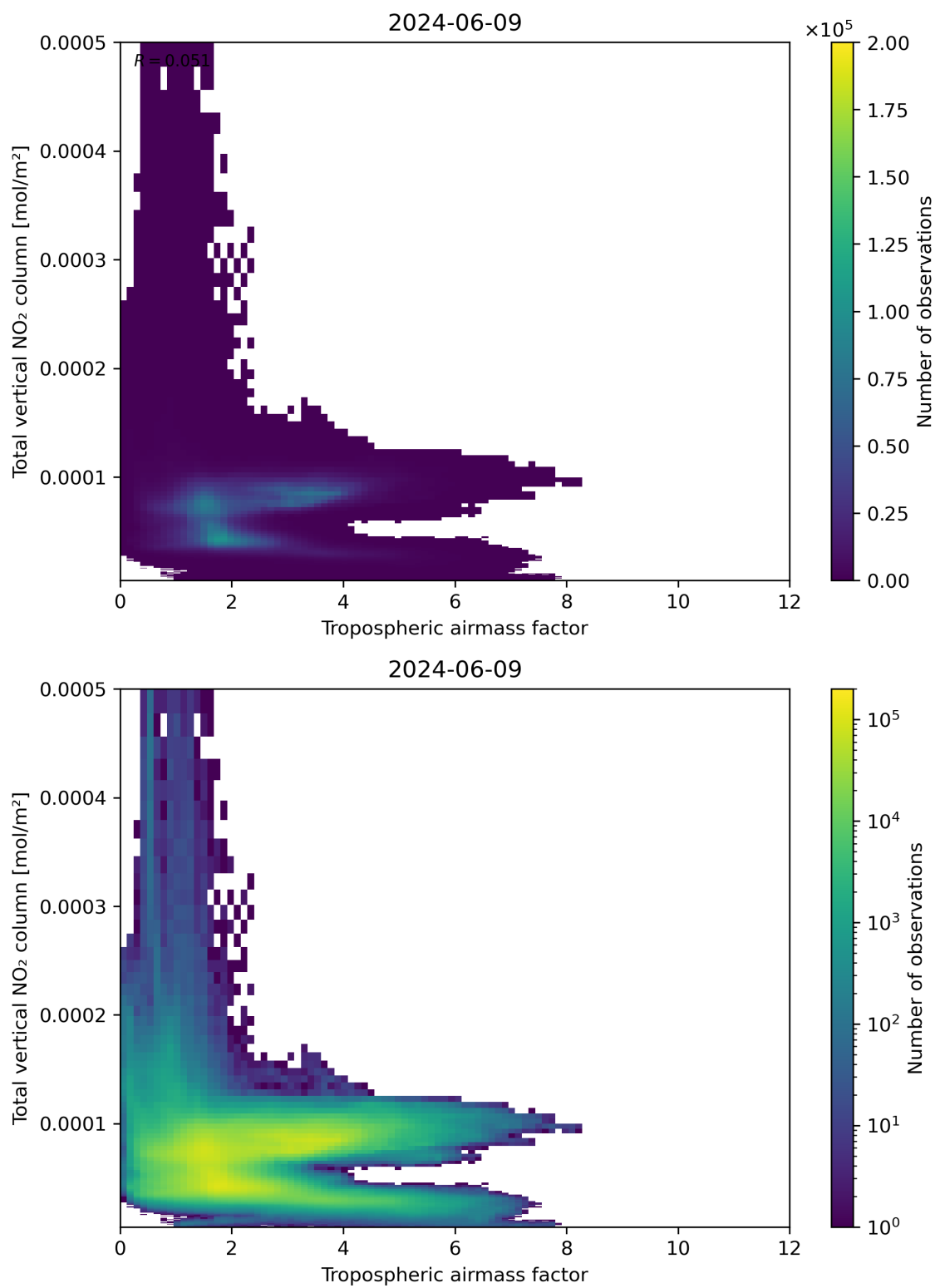
Figure 77: Scatter density plot of “Tropospheric airmass factor” against “Total vertical NO 2 column” for 2024-06-08 to 2024-06-10.
