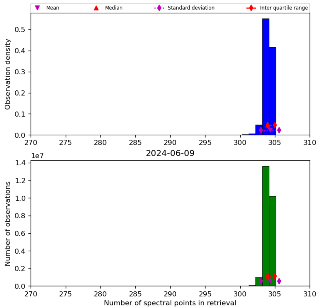
Figure 33: Histogram of “Number of spectral points in retrieval” for 2024-06-08 to 2024-06-10
