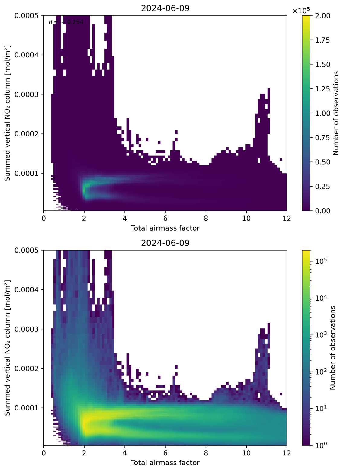
Figure 65: Scatter density plot of “Total airmass factor” against “Summed vertical NO 2 column” for 2024-06-08 to 2024-06-10.
