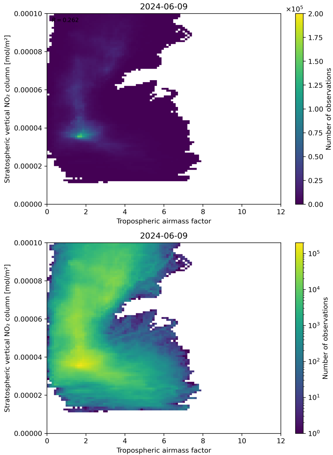
Figure 74: Scatter density plot of “Tropospheric air mass factor” against “Stratospheric vertical NO 2 column” for 2024-06-08 to 2024-06-10.
