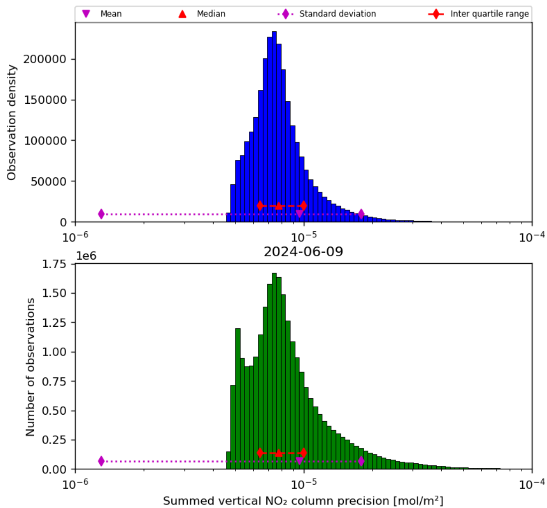
Figure 41: Histogram of "Summed vertical NO 2 column precision" for 2024-06-08 to 2024-06-10
