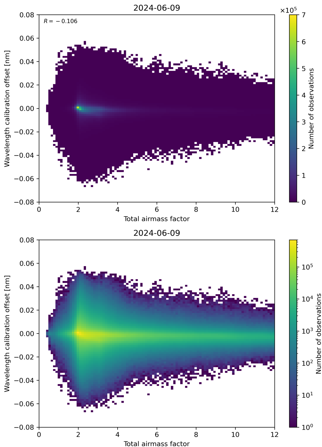
Figure 70: Scatter density plot of “Total airmass factor” against “Wavelength calibration offset” for 2024-06-08 to 2024-06-10.
