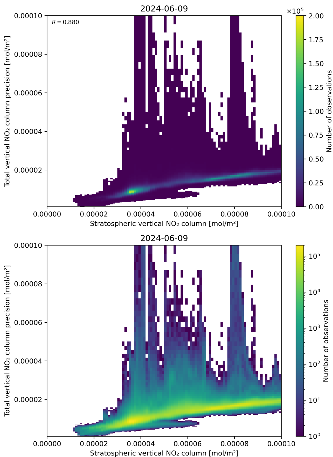
Figure 101: Scatter density plot of “Stratospheric vertical NO 2 column” against “Total vertical NO 2 column precision” for 2024-06-08 to 2024-06-10.
