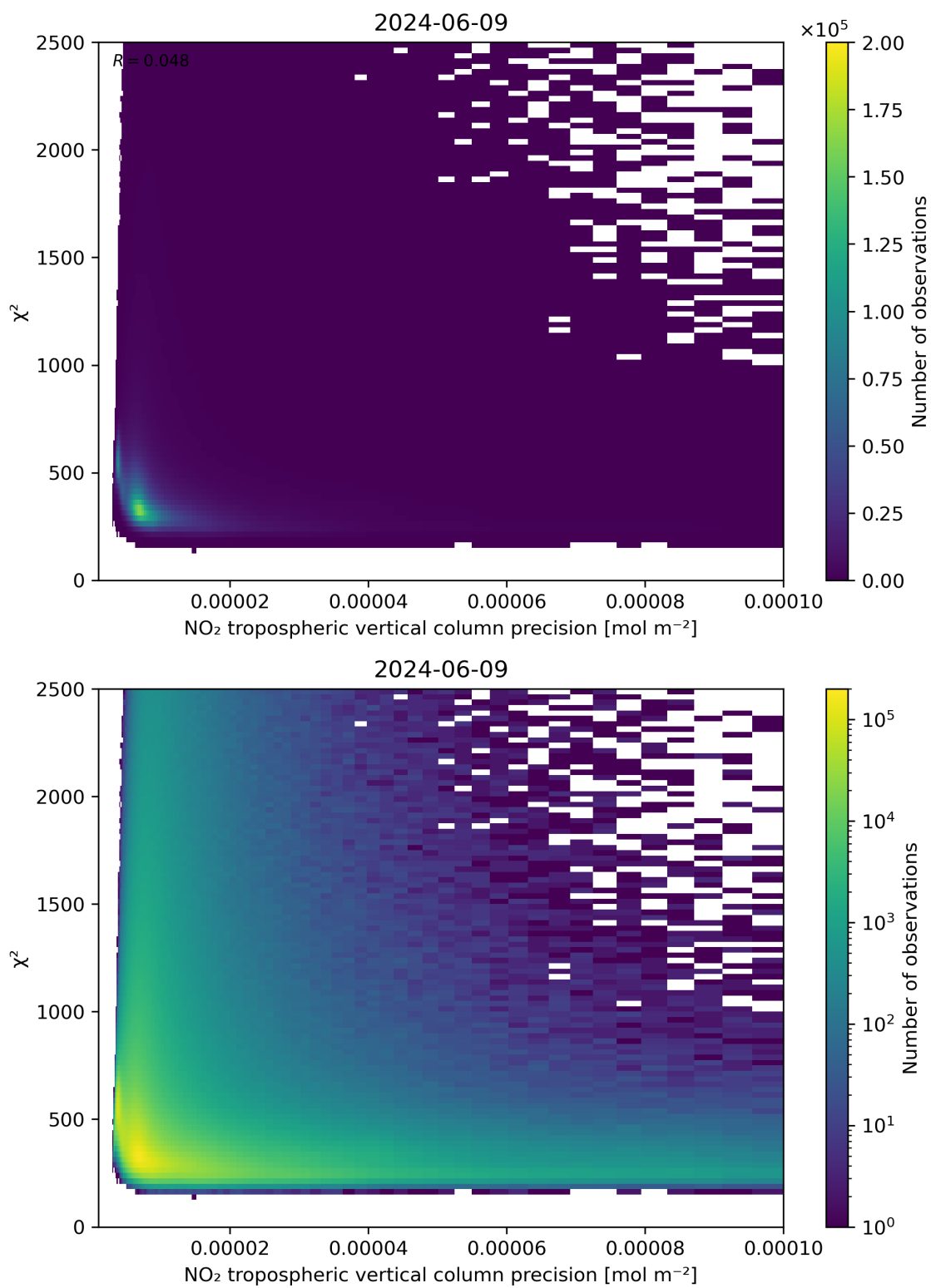
Figure 134: Scatter density plot of “NO 2 tropospheric vertical column precision” against “ \chi^2 ” for 2024-06-08 to 2024-06-10.
