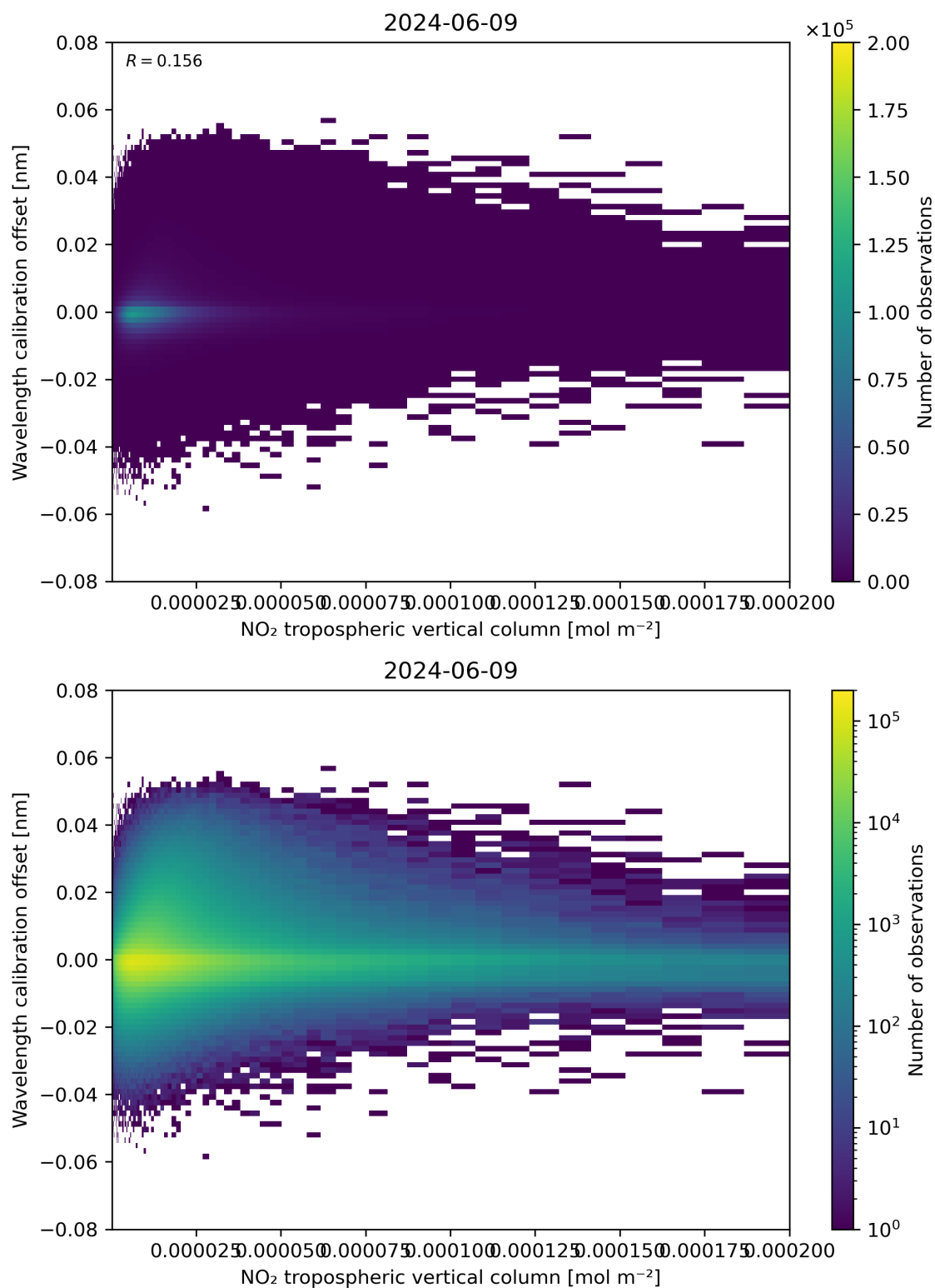
Figure 143: Scatter density plot of “NO 2 tropospheric vertical column” against “Wavelength calibration offset” for 2024-06-08 to 2024-06-10.
