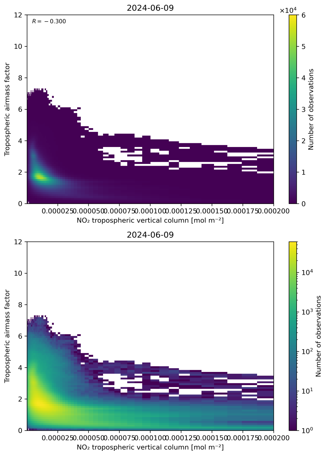
Figure 123: Scatter density plot of “NO 2 tropospheric vertical column” against “Tropospheric air mass factor” for 2024-06-08 to 2024-06-10.
