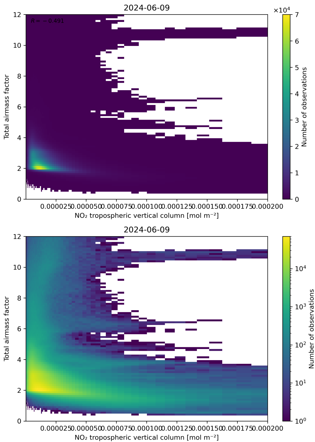
Figure 122: Scatter density plot of “NO 2 tropospheric vertical column” against “Total air mass factor” for 2024-06-08 to 2024-06-10.
