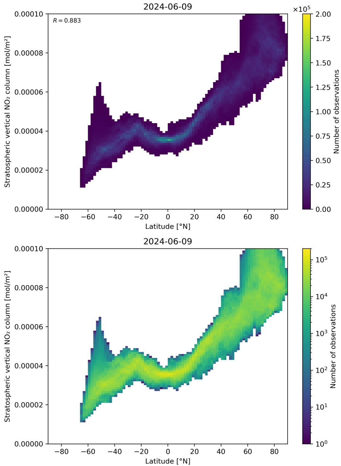
Figure 87: Scatter density plot of “Latitude” against “Stratospheric vertical \text{NO}_2 column” for 2024-06-08 to 2024-06-10.
