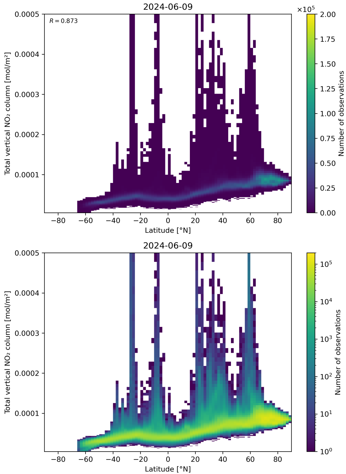
Figure 90: Scatter density plot of “Latitude” against “Total vertical NO 2 column” for 2024-06-08 to 2024-06-10.
