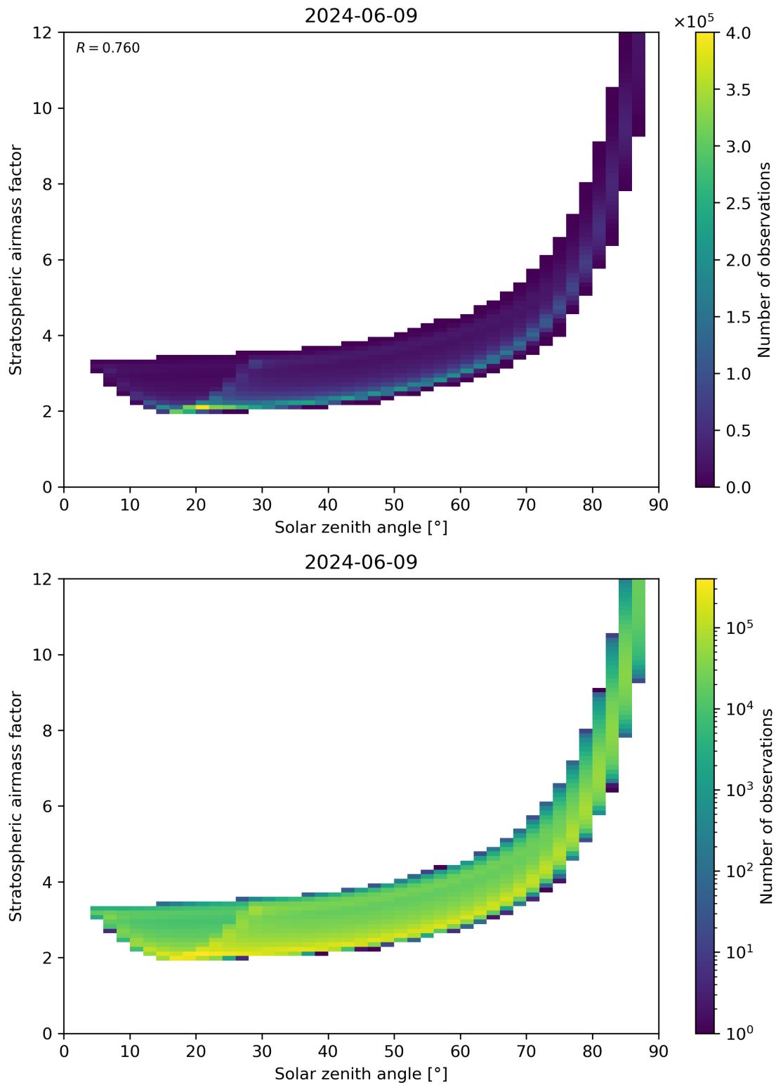
Figure 145: Scatter density plot of “Solar zenith angle” against “Stratospheric airmass factor” for 2024-06-08 to 2024-06-10.
