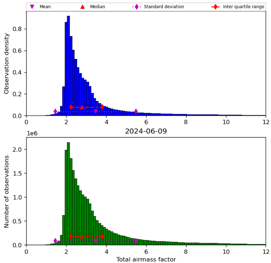
Figure 32: Histogram of “Total airmass factor” for 2024-06-08 to 2024-06-10
