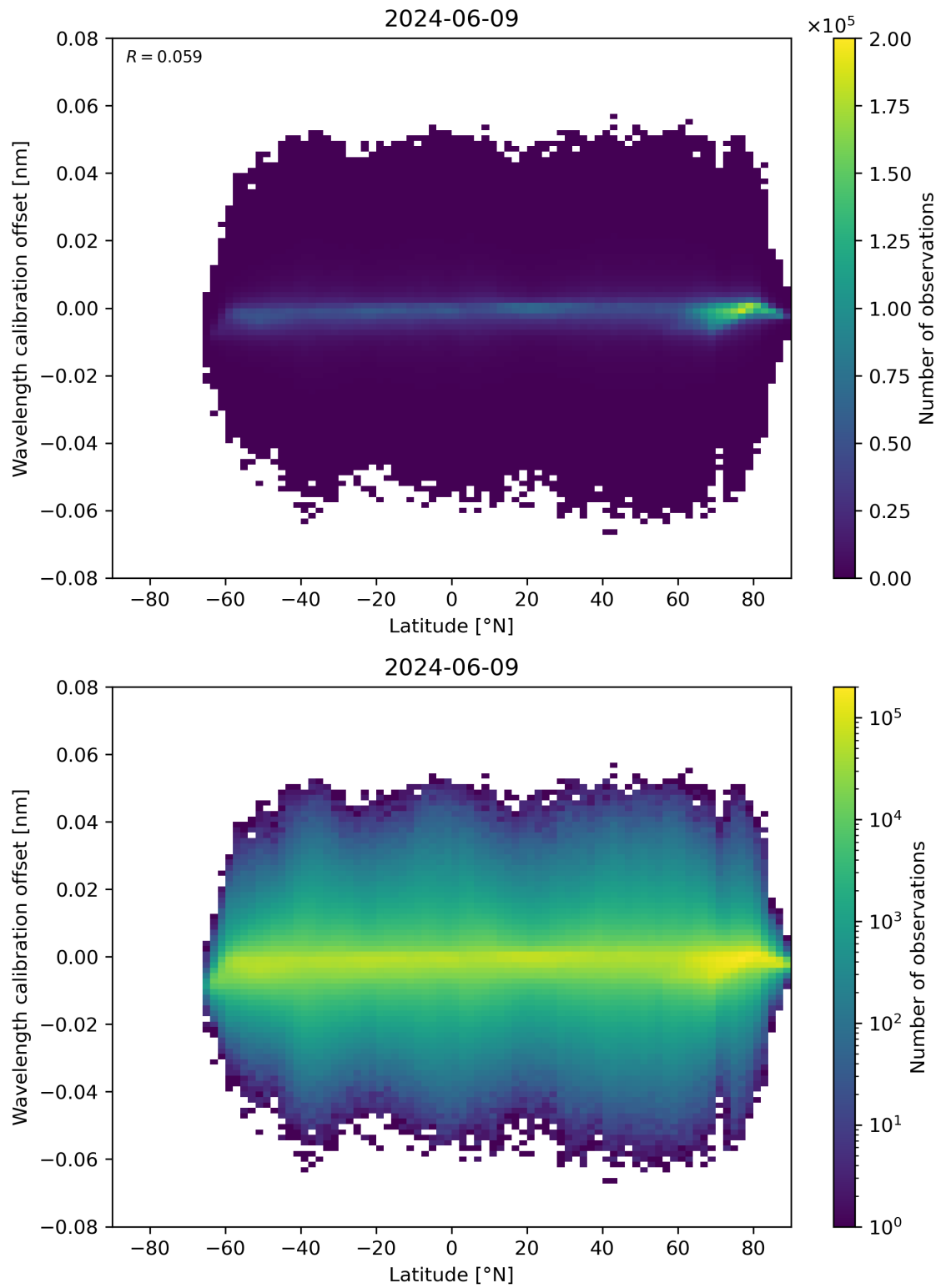
Figure 95: Scatter density plot of “Latitude” against “Wavelength calibration offset” for 2024-06-08 to 2024-06-10.
