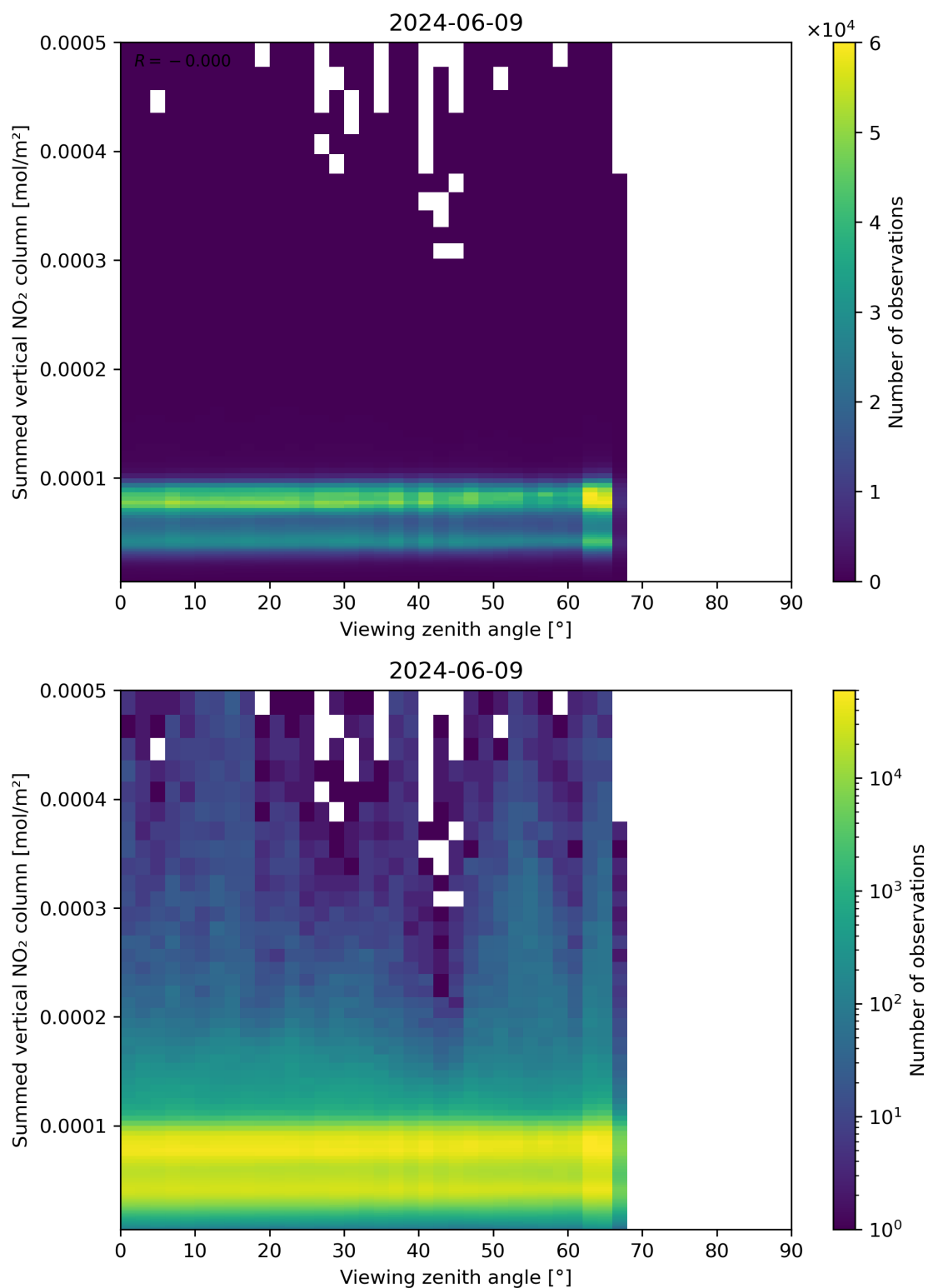
Figure 165: Scatter density plot of “Viewing zenith angle” against “Summed vertical NO 2 column” for 2024-06-08 to 2024-06-10.
