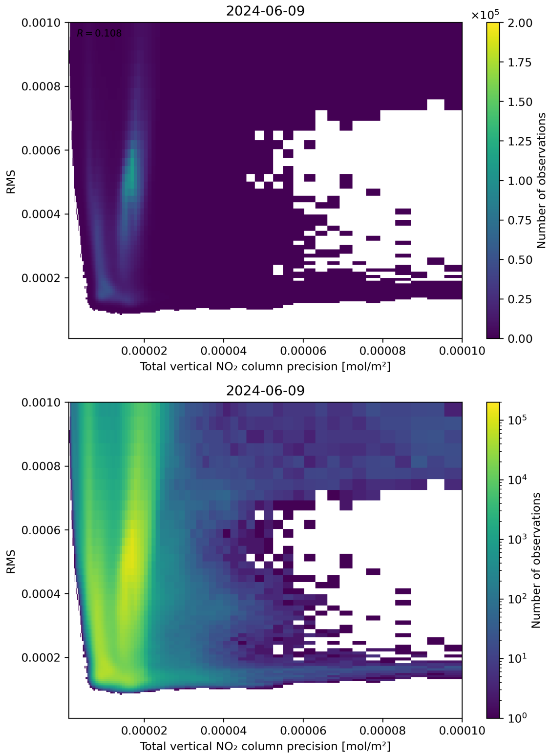
Figure 119: Scatter density plot of “Total vertical NO 2 column precision” against “RMS” for 2024-06-08 to 2024-06-10.
