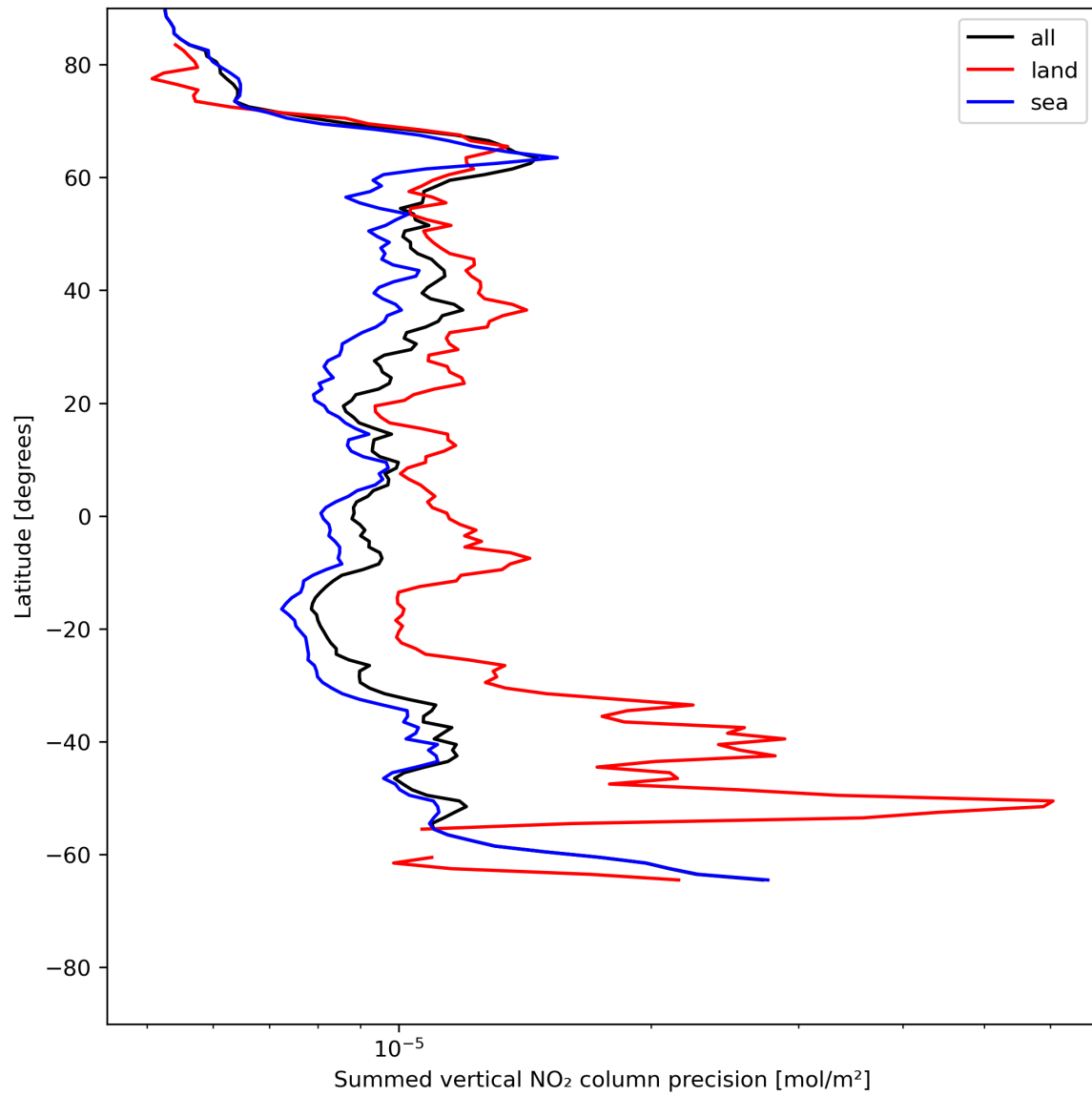
Figure 24: Zonal average of “Summed vertical NO 2 column precision” for 2024-06-08 to 2024-06-10.
