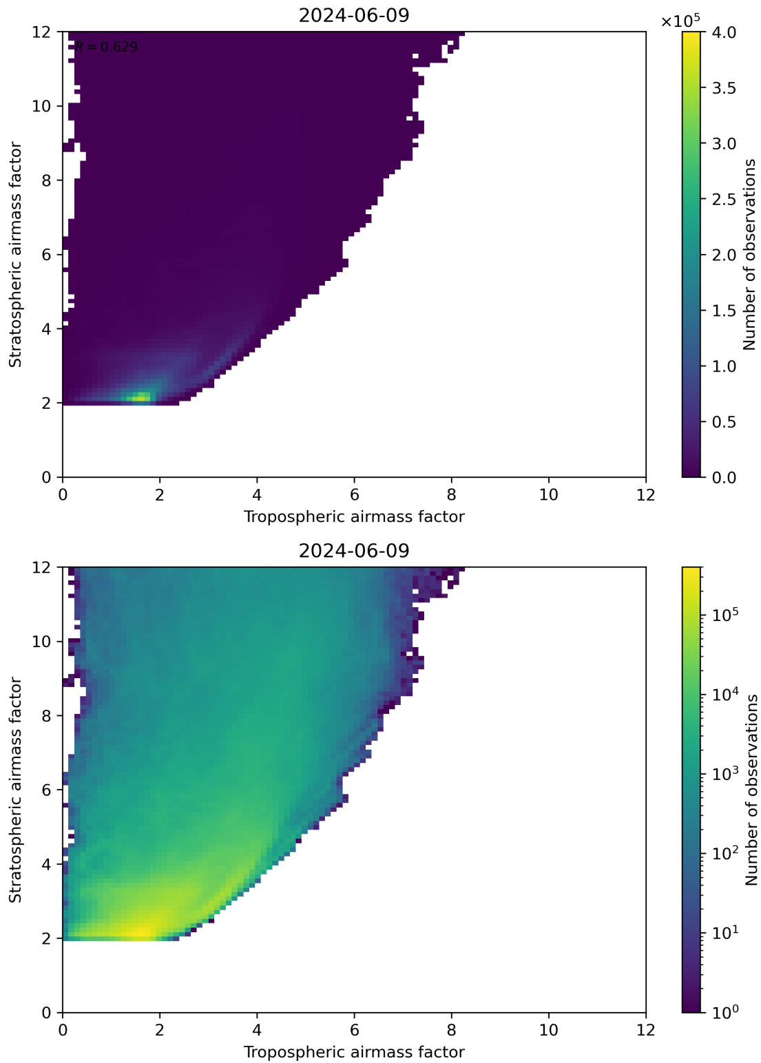
Figure 71: Scatter density plot of “Tropospheric airmass factor” against “Stratospheric airmass factor” for 2024-06-08 to 2024-06-10.
