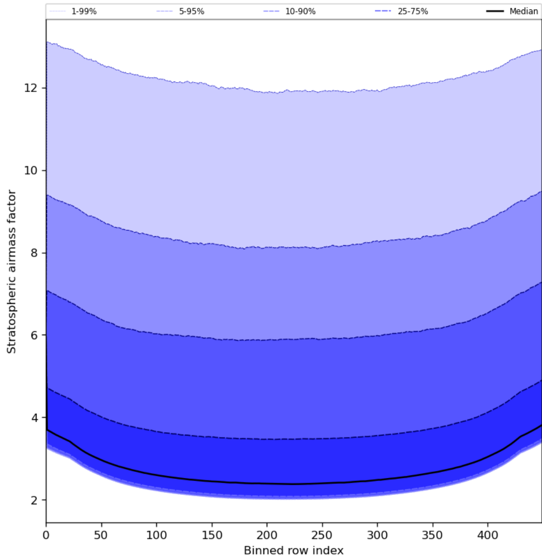
Figure 61: Along track statistics of “Stratospheric airmass factor” for 2024-06-08 to 2024-06-10
