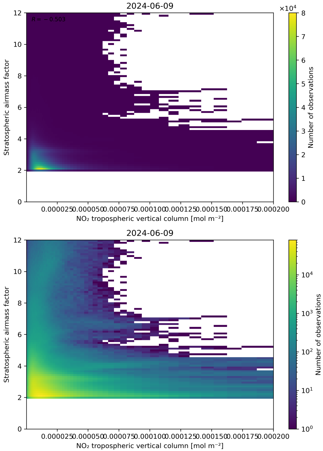
Figure 121: Scatter density plot of “NO 2 tropospheric vertical column” against “Stratospheric air mass factor” for 2024-06-08 to 2024-06-10.
