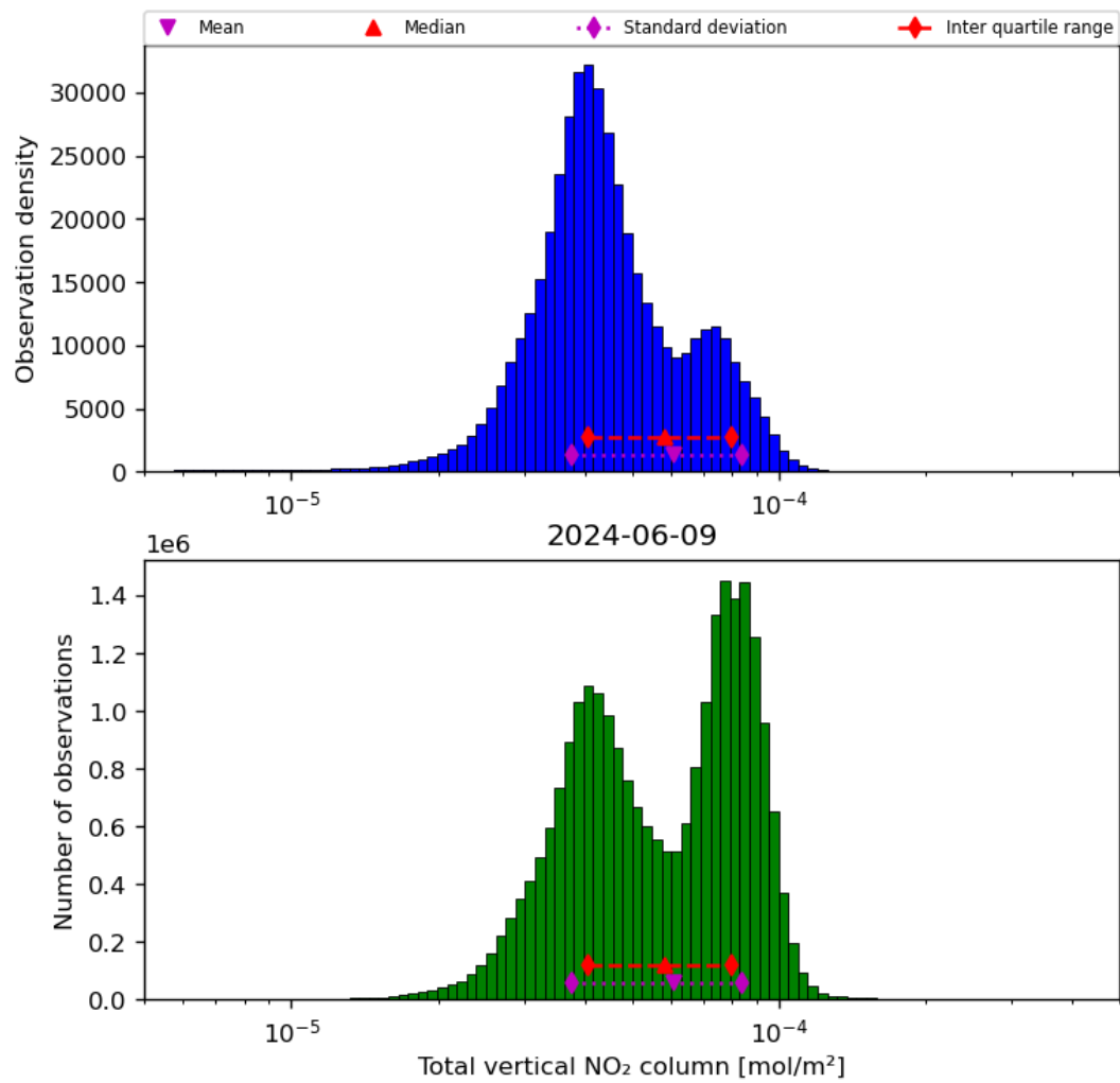
Figure 38: Histogram of "Total vertical NO 2 column" for 2024-06-08 to 2024-06-10
