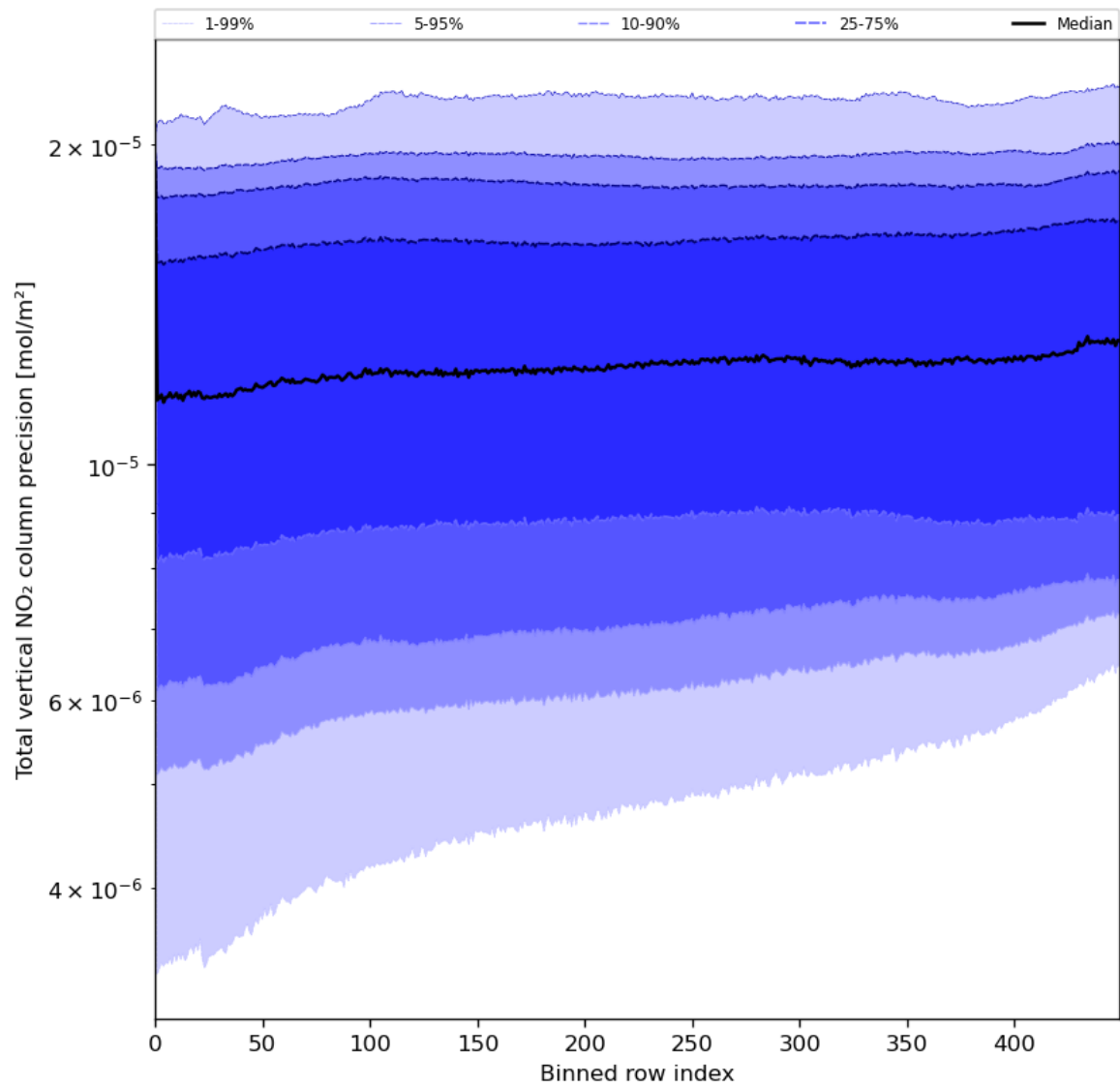
Figure 56: Along track statistics of “Total vertical NO 2 column precision” for 2024-06-08 to 2024-06-10
