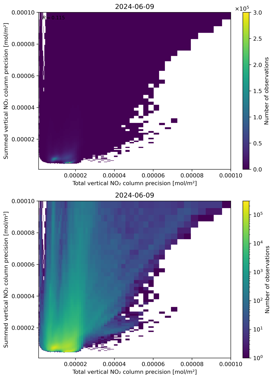
Figure 118: Scatter density plot of “Total vertical NO 2 column precision” against “Summed vertical NO 2 column precision” for 2024-06-08 to 2024-06-10.
