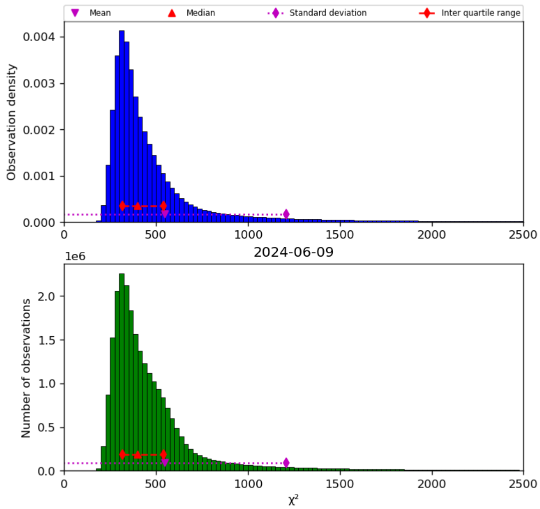
Figure 42: Histogram of “ \chi^2 ” for 2024-06-08 to 2024-06-10
