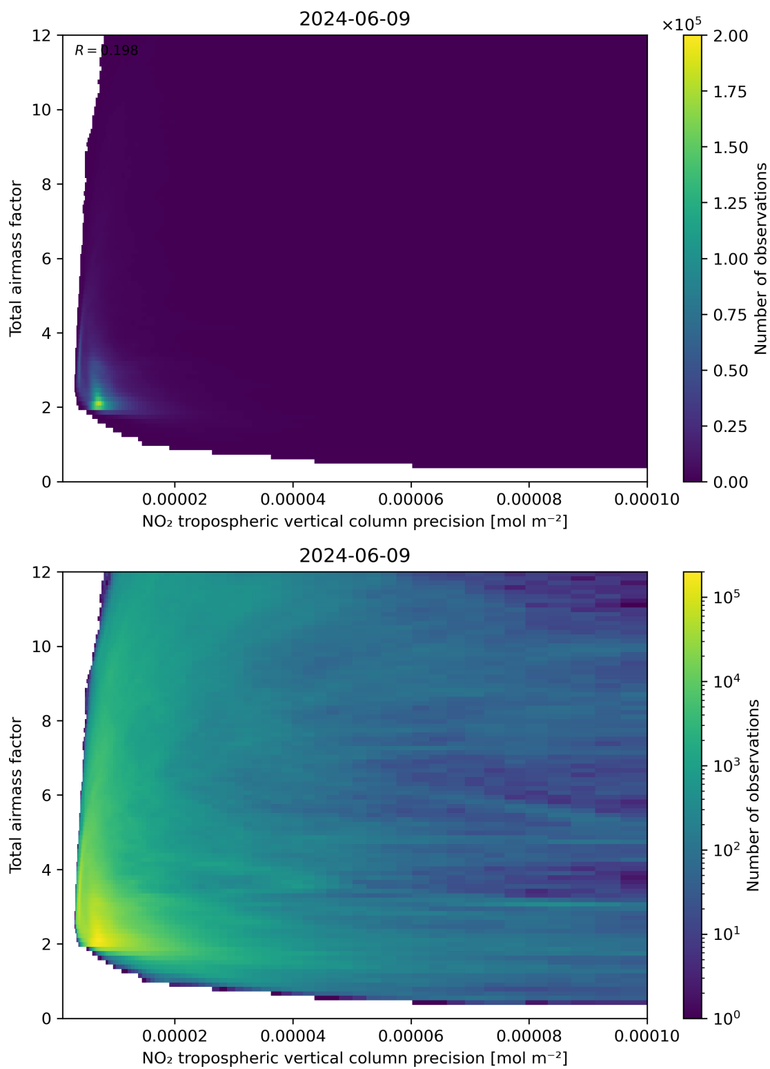
Figure 132: Scatter density plot of “NO 2 tropospheric vertical column precision” against “Total air mass factor” for 2024-06-08 to 2024-06-10.
