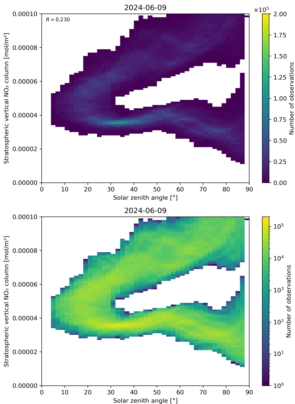
Figure 150: Scatter density plot of “Solar zenith angle” against “Stratospheric vertical NO 2 column” for 2024-06-08 to 2024-06-10.
