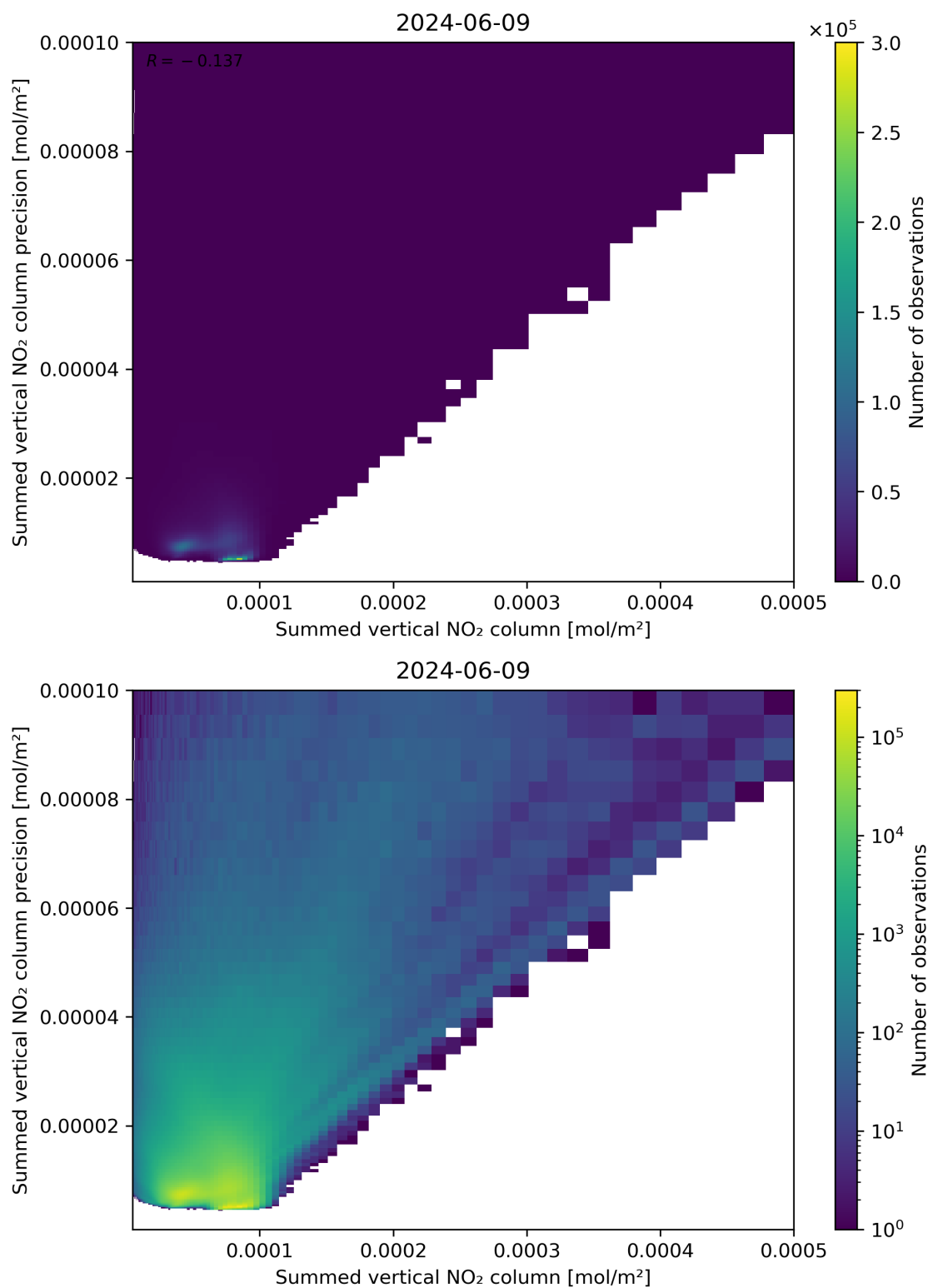
Figure 105: Scatter density plot of “Summed vertical NO 2 column” against “Summed vertical NO 2 column precision” for 2024-06-08 to 2024-06-10.
