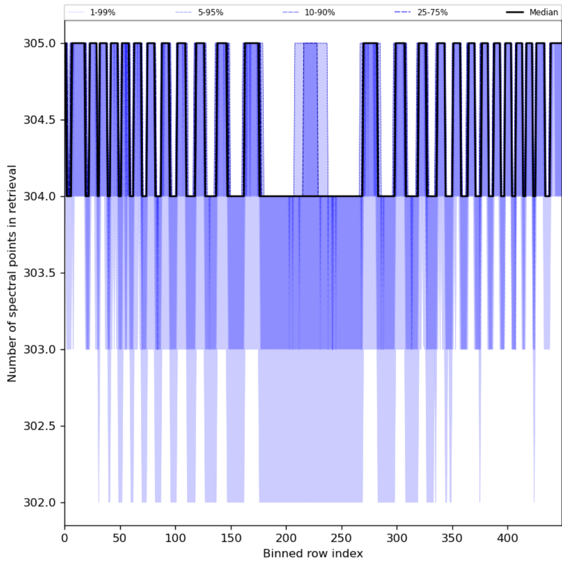
Figure 50: Along track statistics of “Number of spectral points in retrieval” for 2024-06-08 to 2024-06-10
