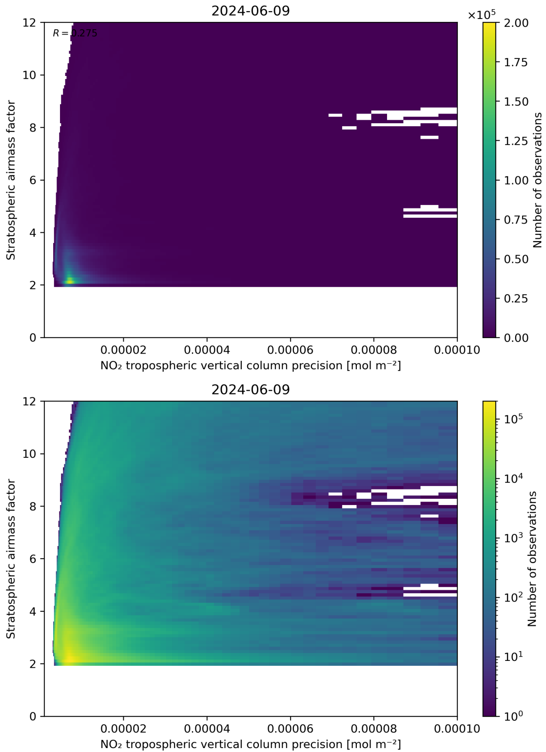
Figure 131: Scatter density plot of “NO 2 tropospheric vertical column precision” against “Stratospheric airmass factor” for 2024-06-08 to 2024-06-10.
