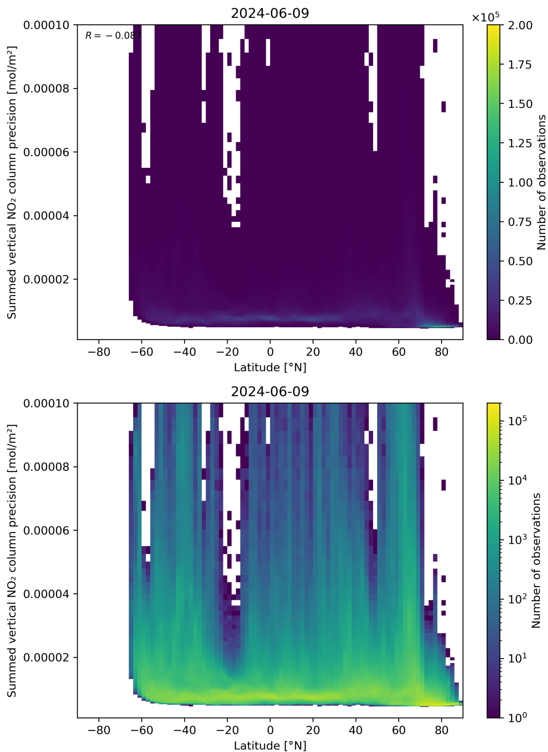
Figure 89: Scatter density plot of “Latitude” against “Summed vertical NO 2 column precision” for 2024-06-08 to 2024-06-10.
