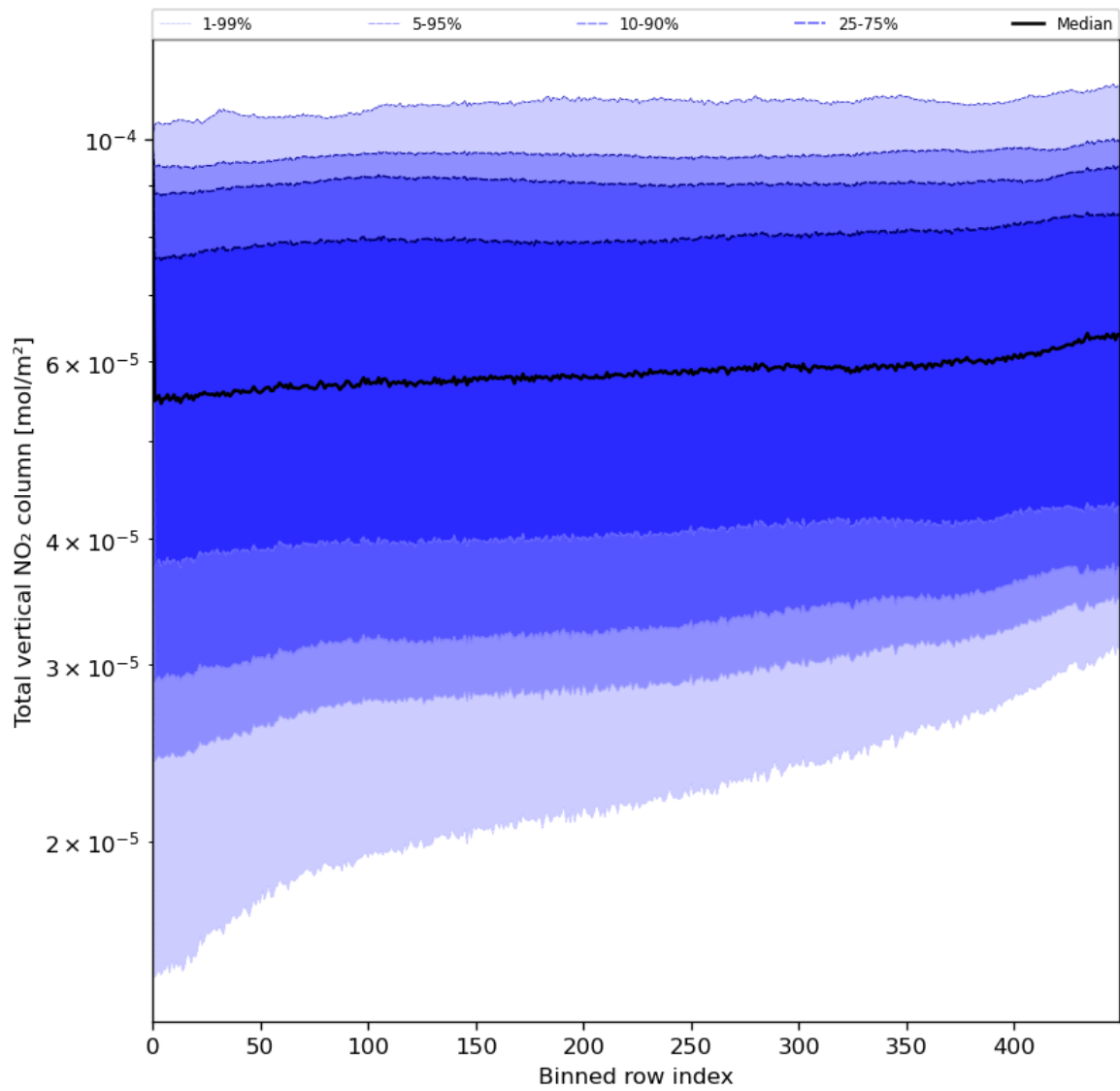
Figure 55: Along track statistics of “Total vertical NO 2 column” for 2024-06-08 to 2024-06-10
