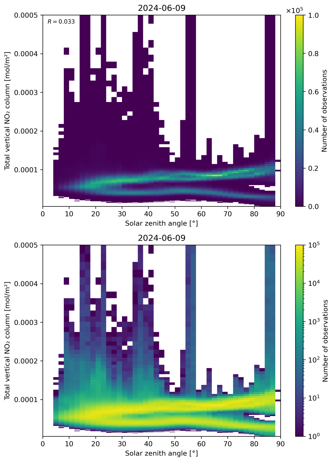
Figure 153: Scatter density plot of “Solar zenith angle” against “Total vertical NO 2 column” for 2024-06-08 to 2024-06-10.
