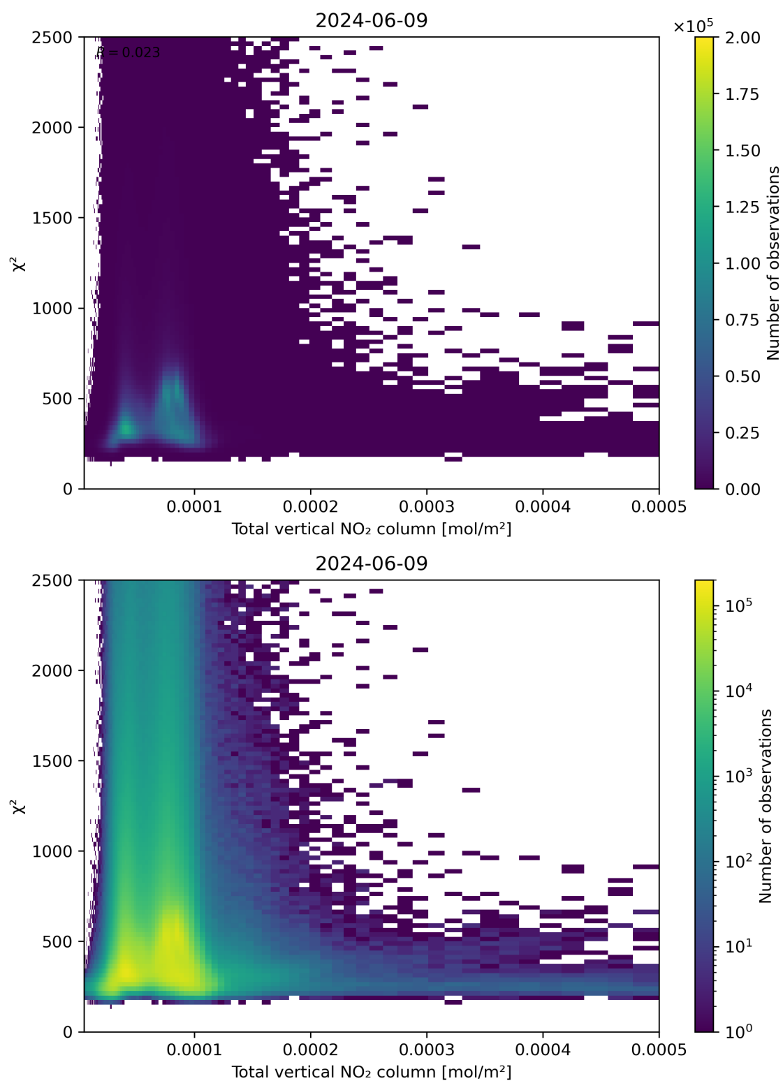
Figure 111: Scatter density plot of “Total vertical NO 2 column” against “ \chi^2 ” for 2024-06-08 to 2024-06-10.
