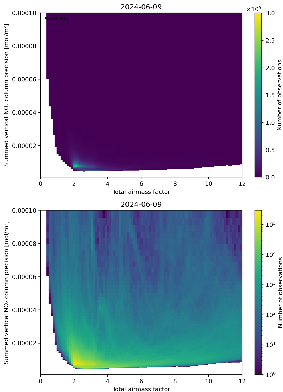
Figure 66: Scatter density plot of “Total airmass factor” against “Summed vertical NO 2 column precision” for 2024-06-08 to 2024-06-10.
