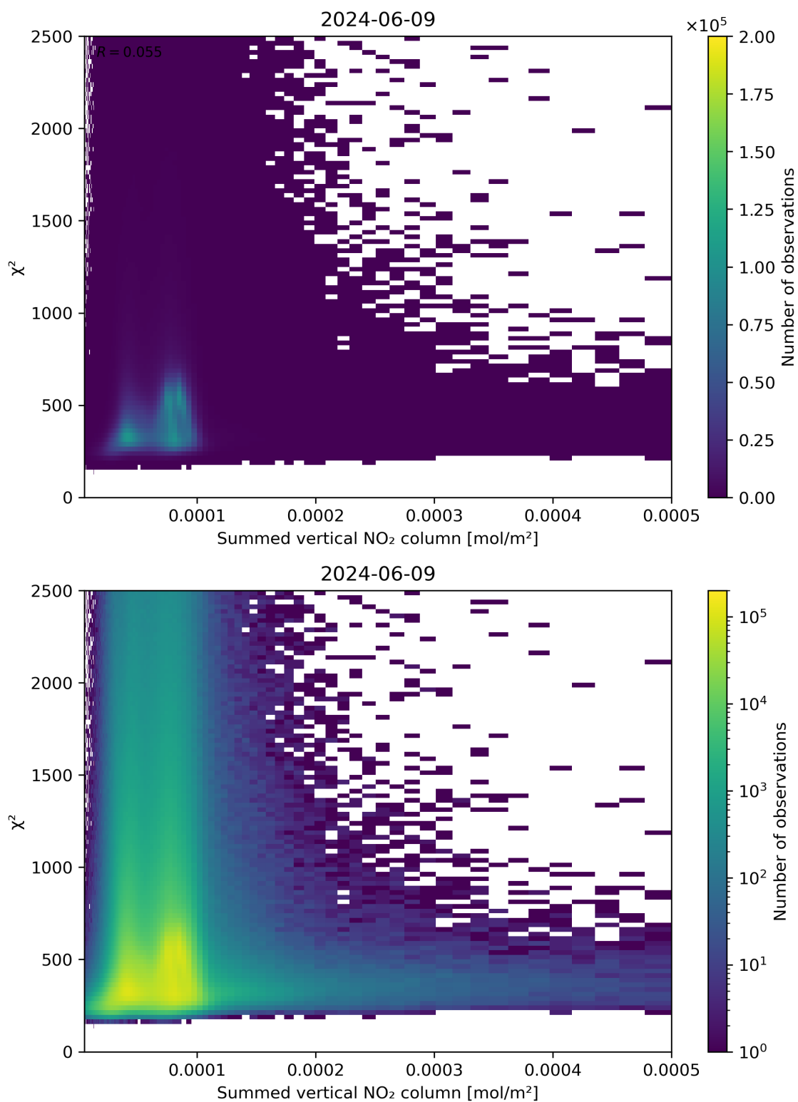
Figure 104: Scatter density plot of “Summed vertical NO 2 column” against “ \chi^2 ” for 2024-06-08 to 2024-06-10.
