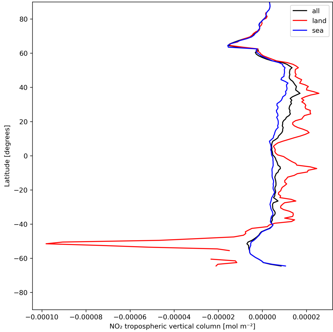
Figure 12: Zonal average of “NO 2 tropospheric vertical column” for 2024-06-08 to 2024-06-10.
