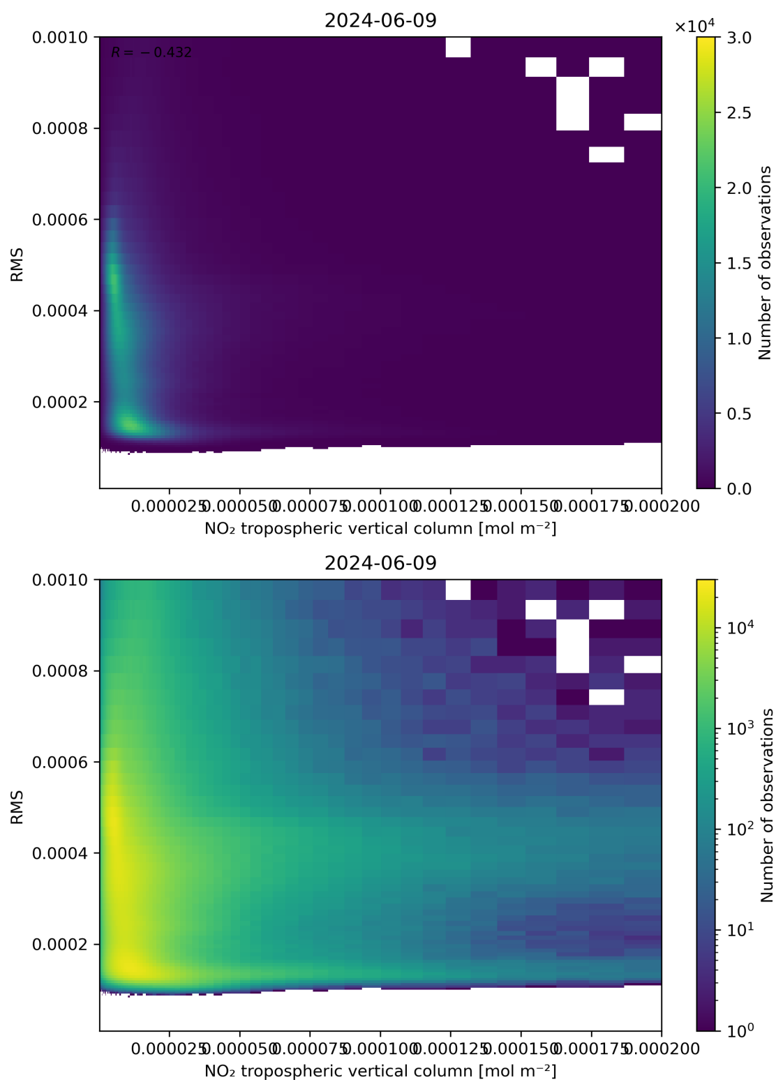
Figure 142: Scatter density plot of “NO 2 tropospheric vertical column” against “RMS” for 2024-06-08 to 2024-06-10.
