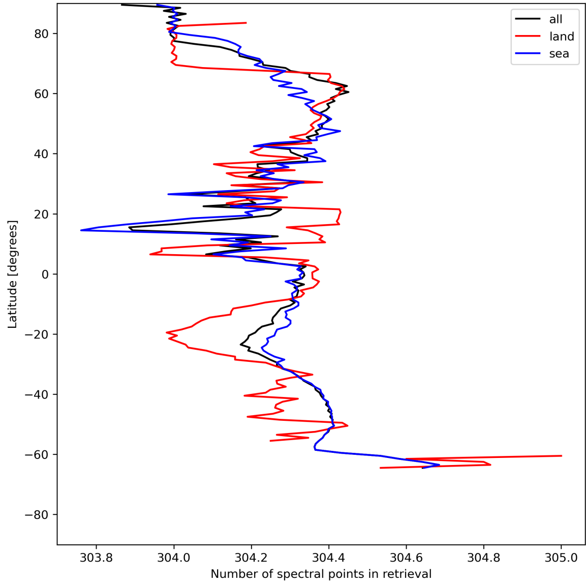
Figure 16: Zonal average of “Number of spectral points in retrieval” for 2024-06-08 to 2024-06-10.
