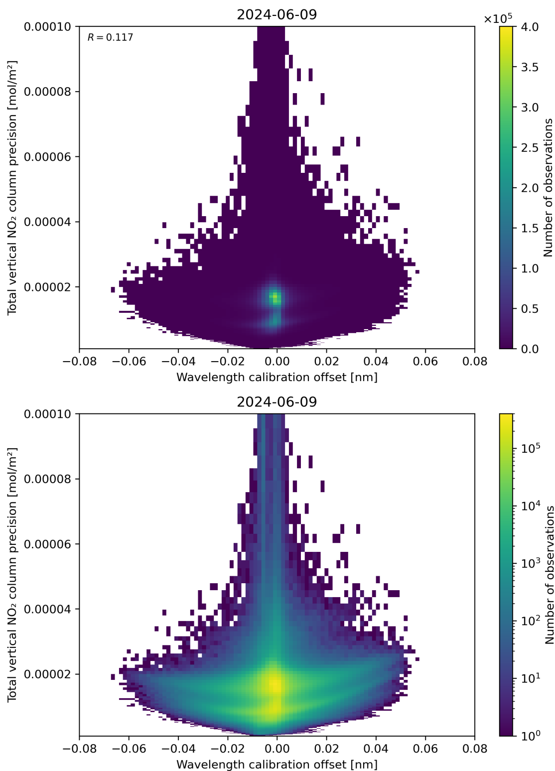
Figure 180: Scatter density plot of “Wavelength calibration offset” against “Total vertical NO 2 column precision” for 2024-06-08 to 2024-06-10.
