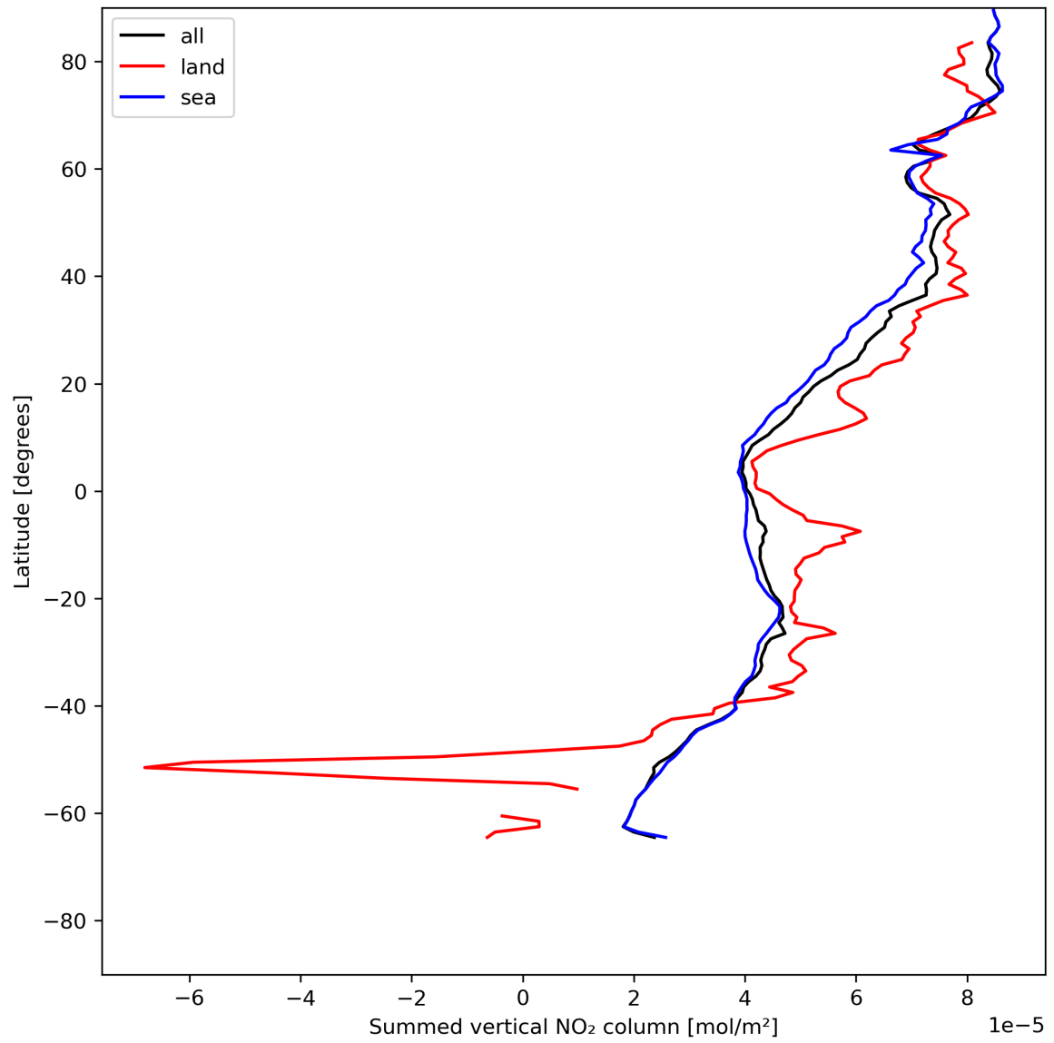
Figure 23: Zonal average of “Summed vertical NO 2 column” for 2024-06-08 to 2024-06-10.
