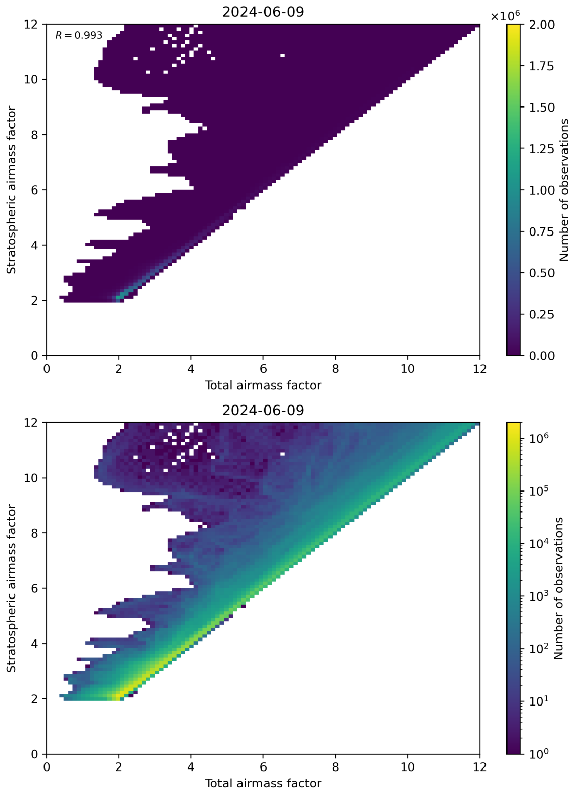
Figure 62: Scatter density plot of “Total airmass factor” against “Stratospheric airmass factor” for 2024-06-08 to 2024-06-10.
