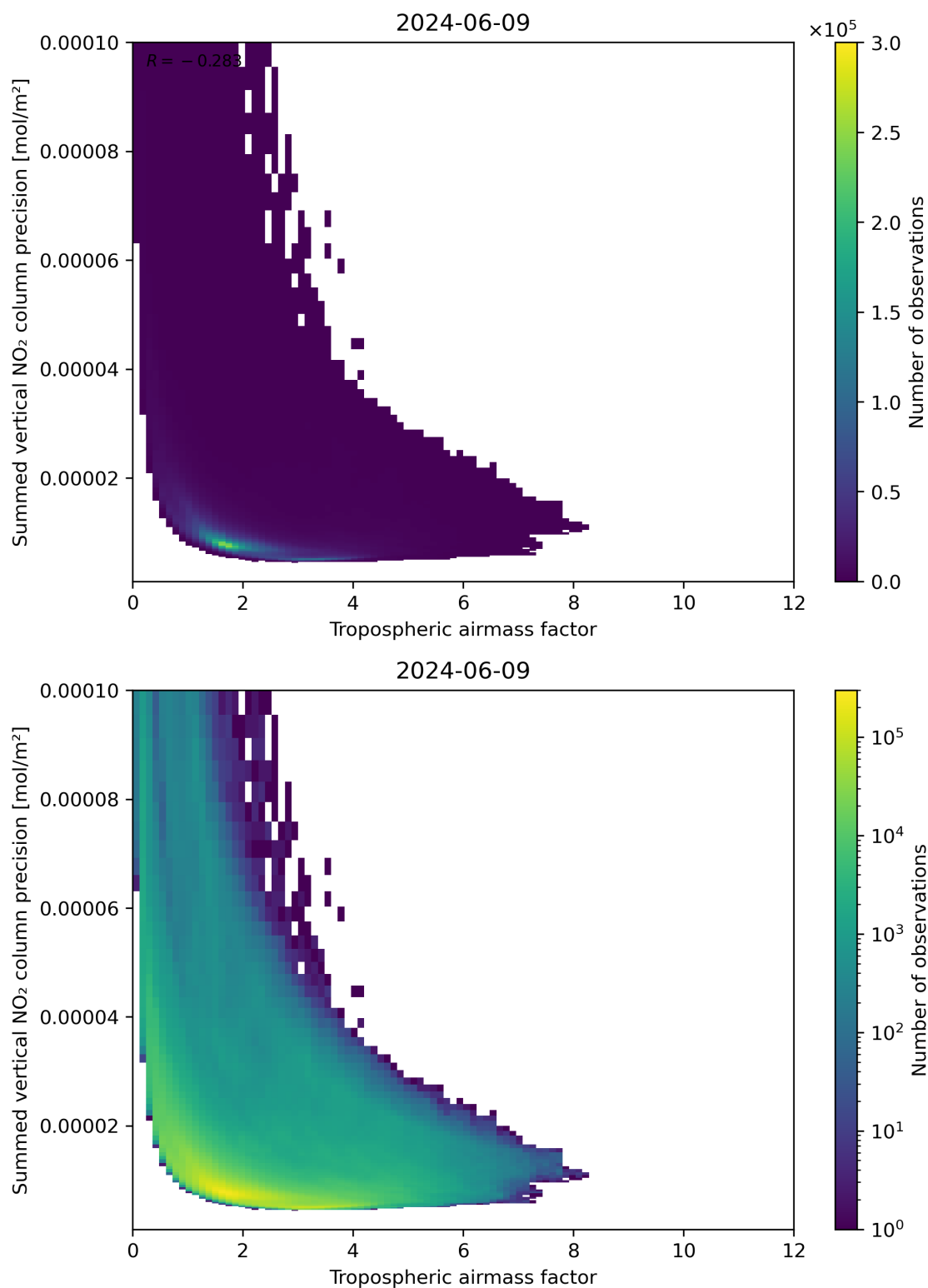
Figure 76: Scatter density plot of “Tropospheric air mass factor” against “Summed vertical NO 2 column precision” for 2024-06-08 to 2024-06-10.
