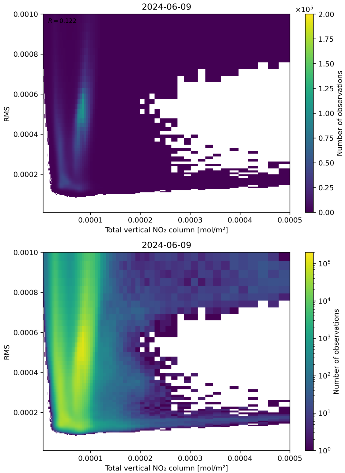
Figure 120: Scatter density plot of “Total vertical NO 2 column” against “RMS” for 2024-06-08 to 2024-06-10.
