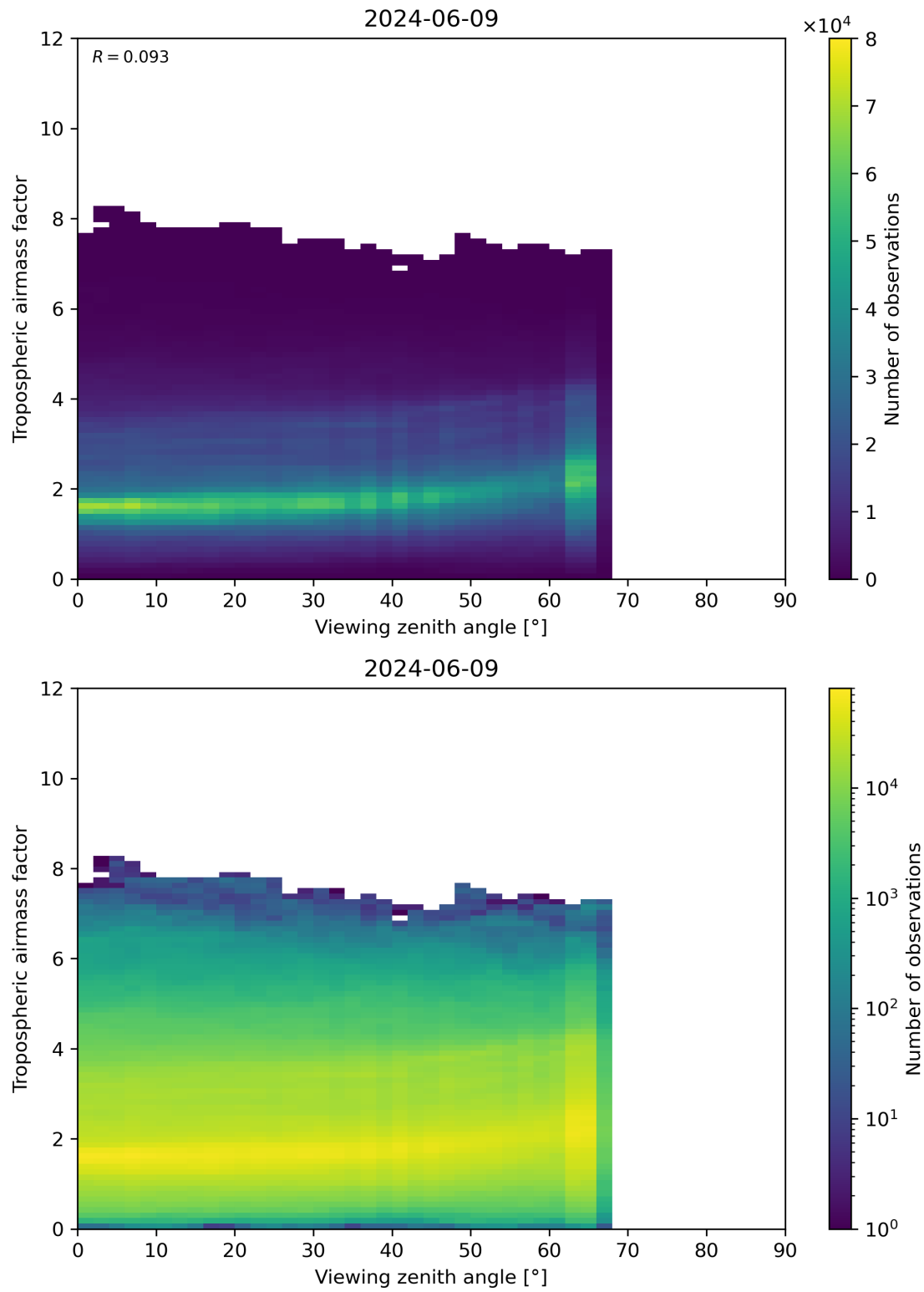
Figure 161: Scatter density plot of “Viewing zenith angle” against “Tropospheric airmass factor” for 2024-06-08 to 2024-06-10.
