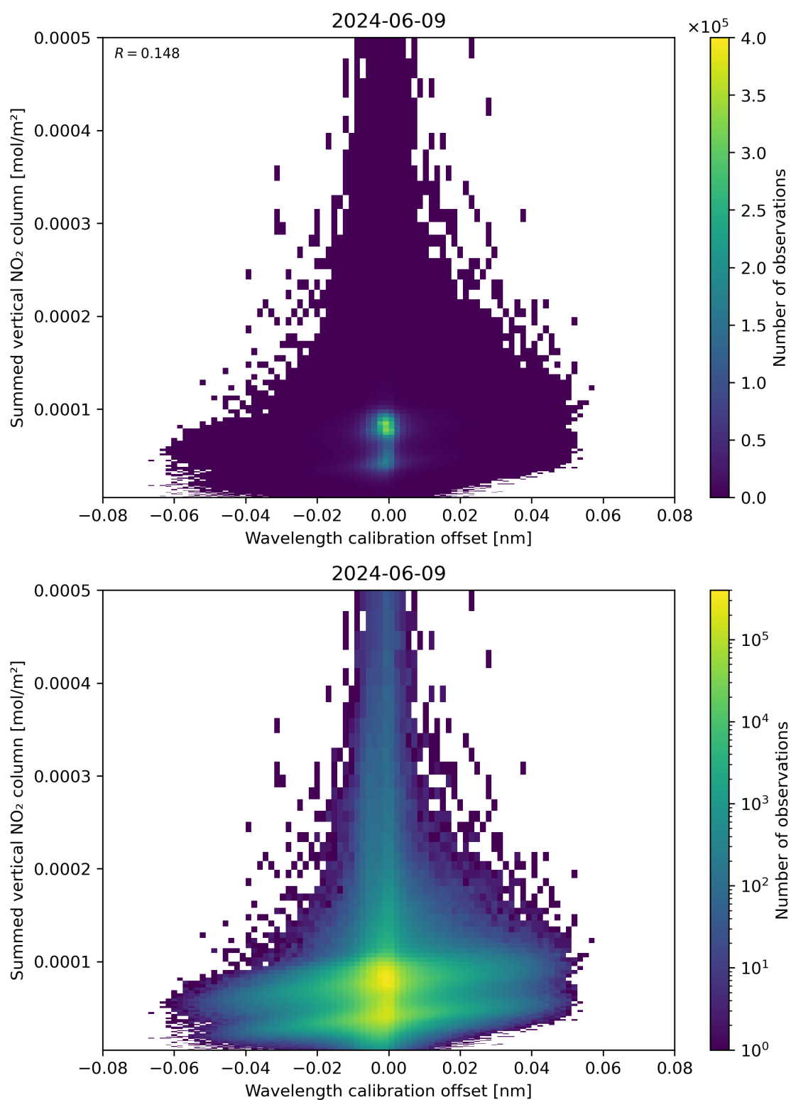
Figure 177: Scatter density plot of “Wavelength calibration offset” against “Summed vertical NO 2 column” for 2024-06-08 to 2024-06-10.
