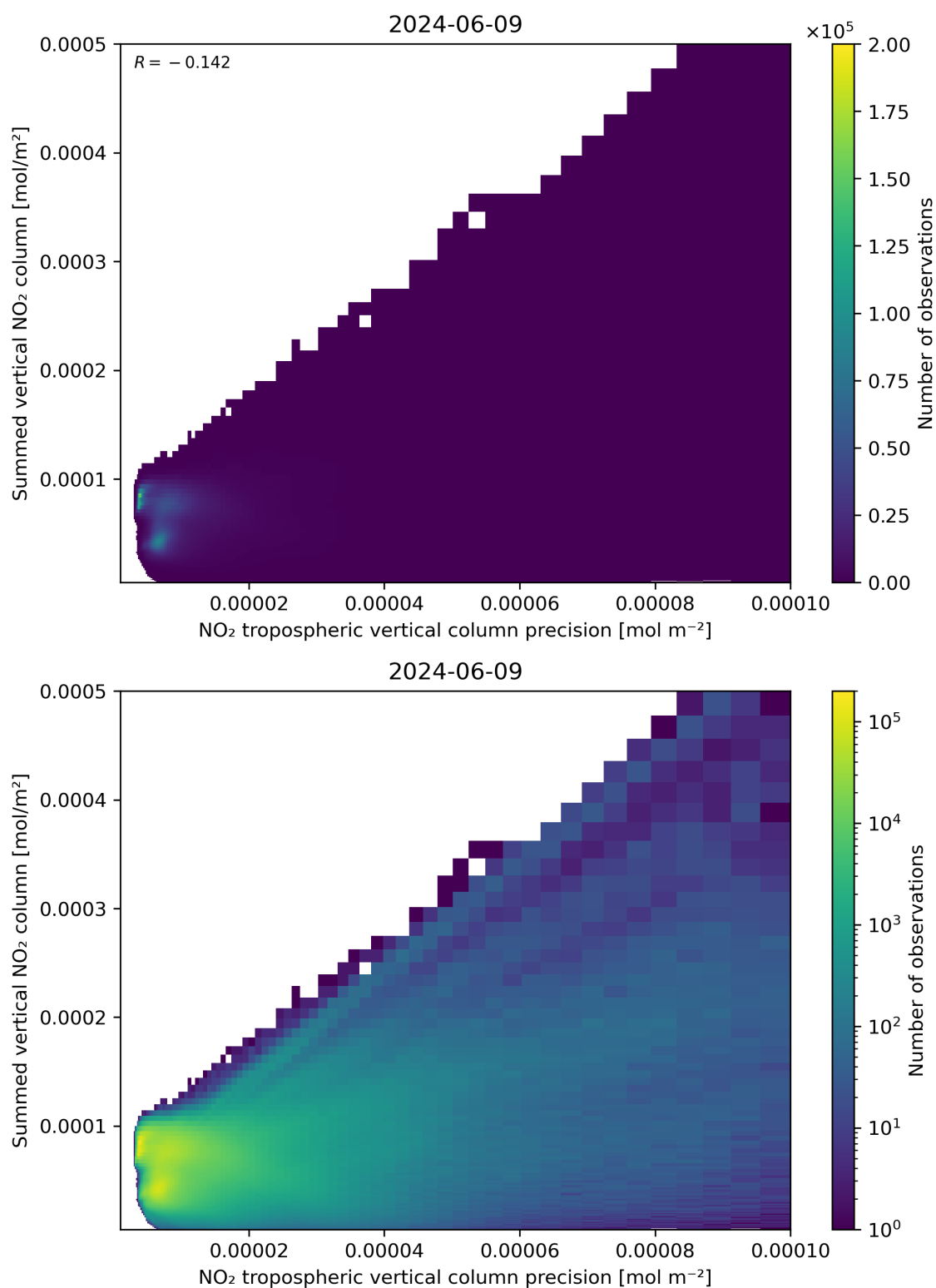
Figure 136: Scatter density plot of “NO 2 tropospheric vertical column precision” against “Summed vertical NO 2 column” for 2024-06-08 to 2024-06-10.
