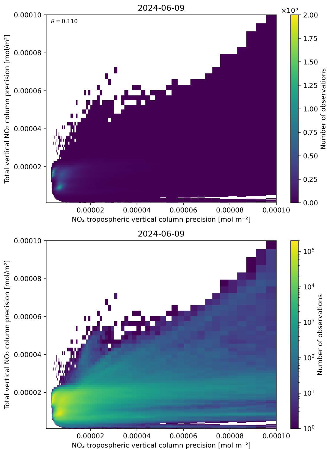
Figure 139: Scatter density plot of “NO 2 tropospheric vertical column precision” against “Total vertical NO 2 column precision” for 2024-06-08 to 2024-06-10.
