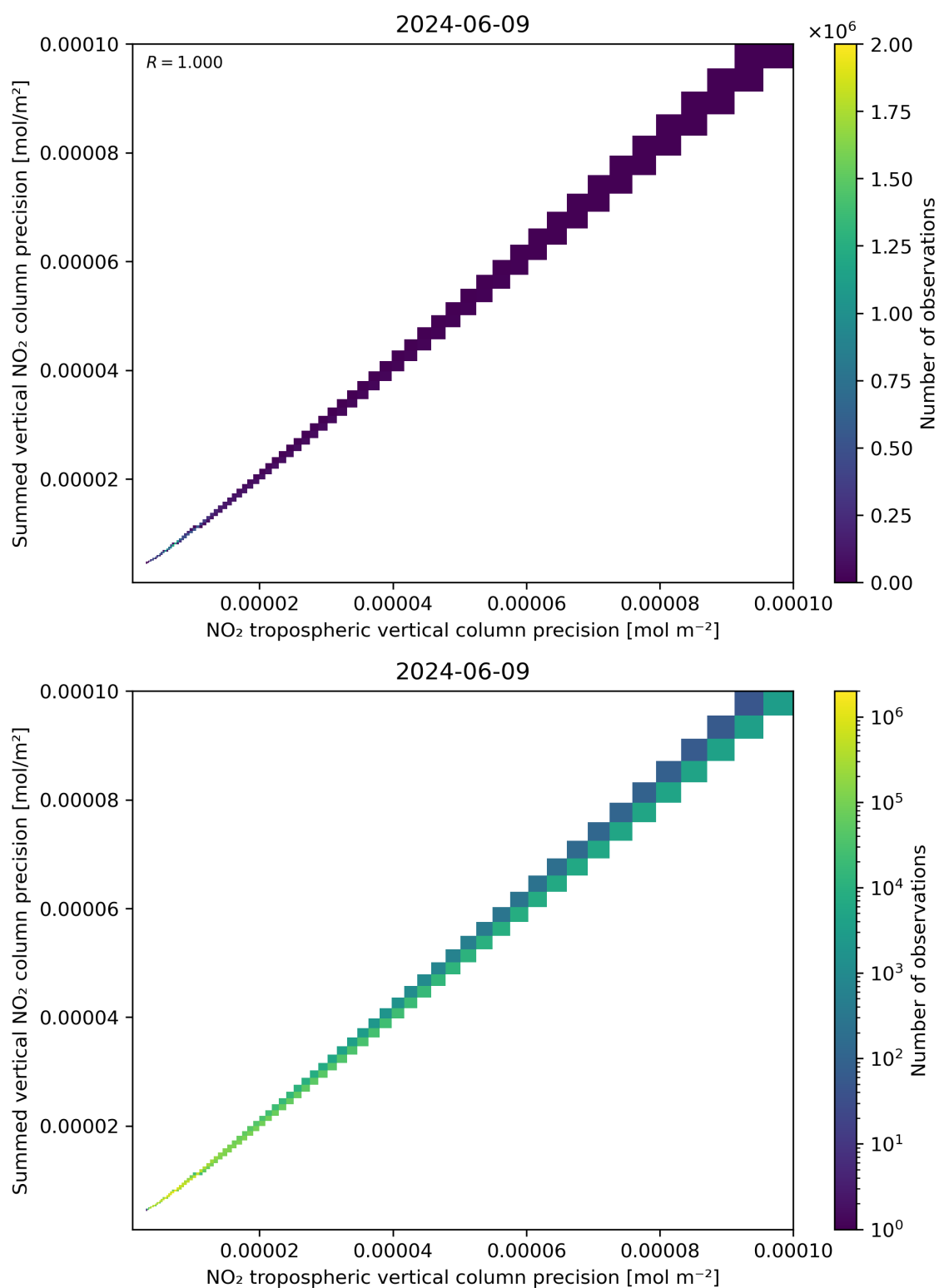
Figure 137: Scatter density plot of “NO 2 tropospheric vertical column precision” against “Summed vertical NO 2 column precision” for 2024-06-08 to 2024-06-10.
