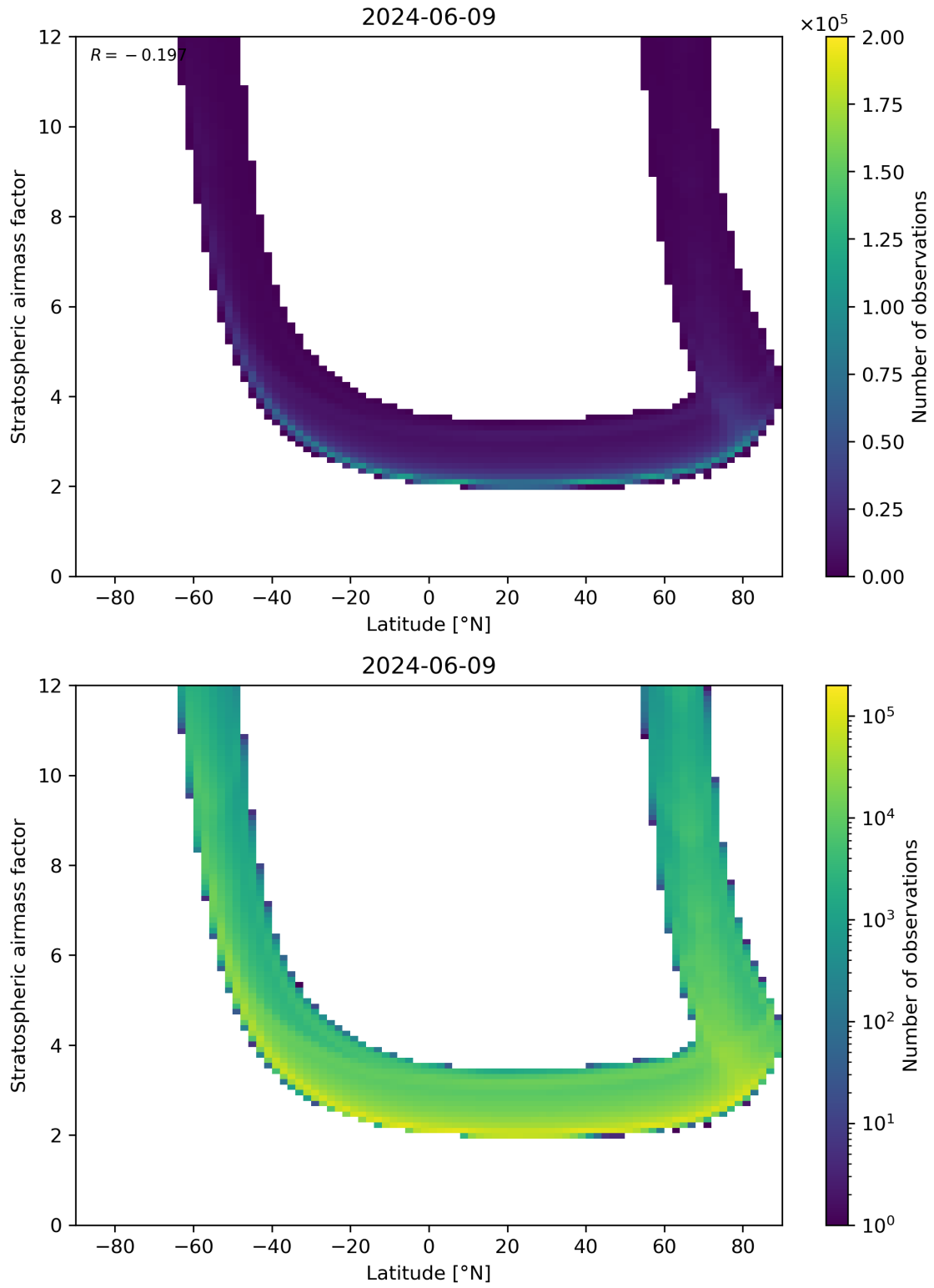
Figure 83: Scatter density plot of “Latitude” against “Stratospheric air mass factor” for 2024-06-08 to 2024-06-10.
