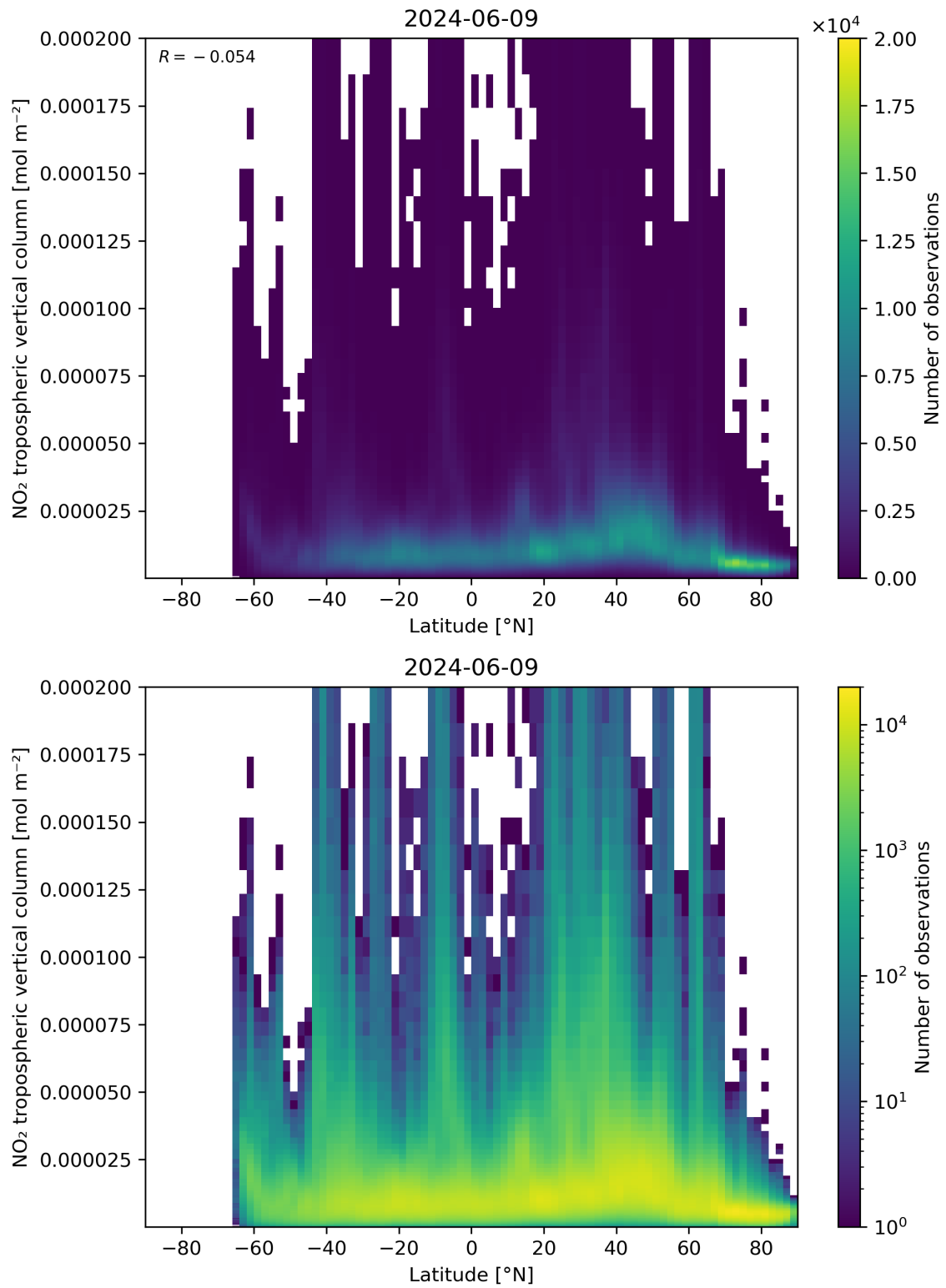
Figure 92: Scatter density plot of “Latitude” against “NO 2 tropospheric vertical column” for 2024-06-08 to 2024-06-10.
