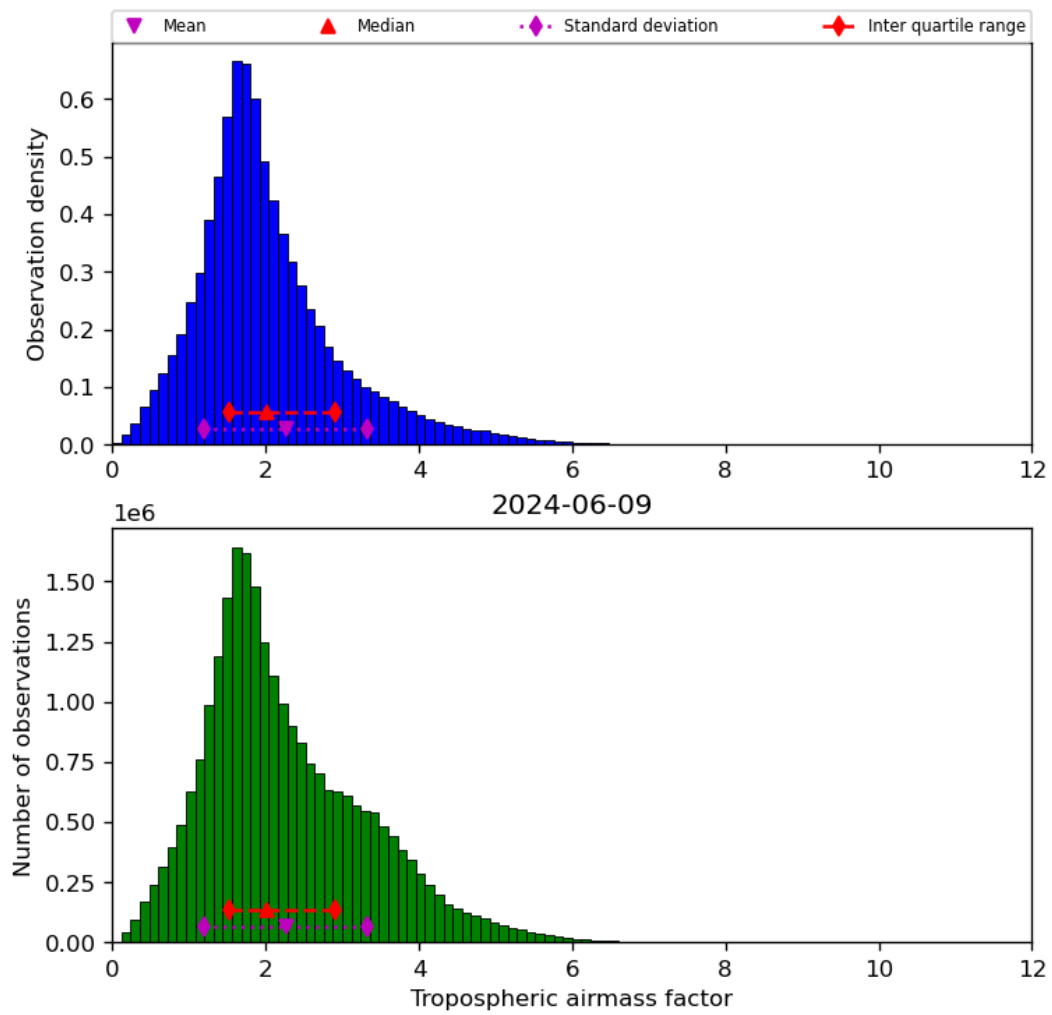
Figure 31: Histogram of “Tropospheric airmass factor” for 2024-06-08 to 2024-06-10
