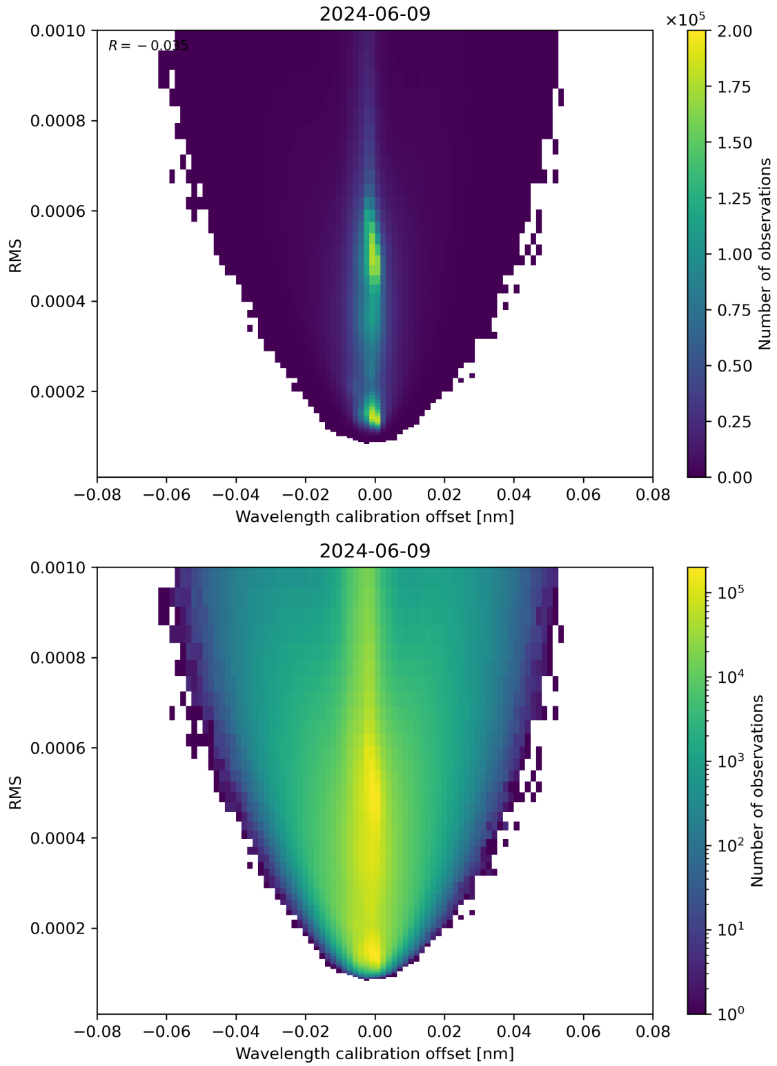
Figure 181: Scatter density plot of “Wavelength calibration offset” against “RMS” for 2024-06-08 to 2024-06-10.
