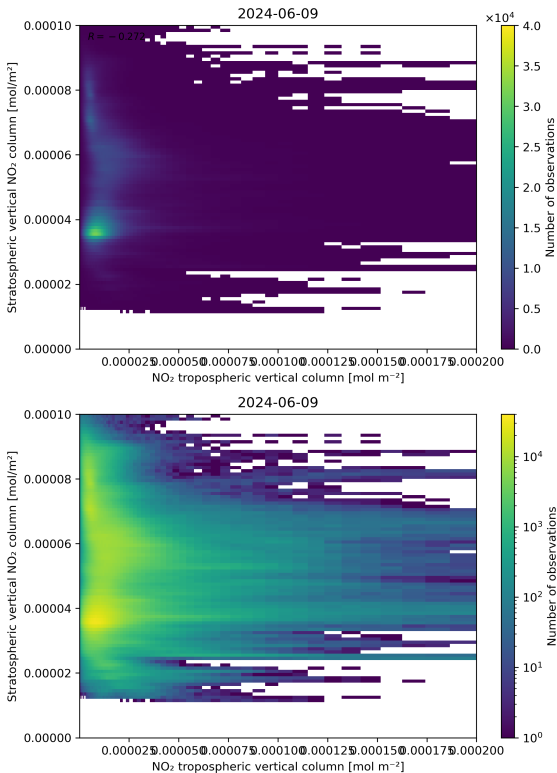
Figure 125: Scatter density plot of “NO 2 tropospheric vertical column” against “Stratospheric vertical NO 2 column” for 2024-06-08 to 2024-06-10.
