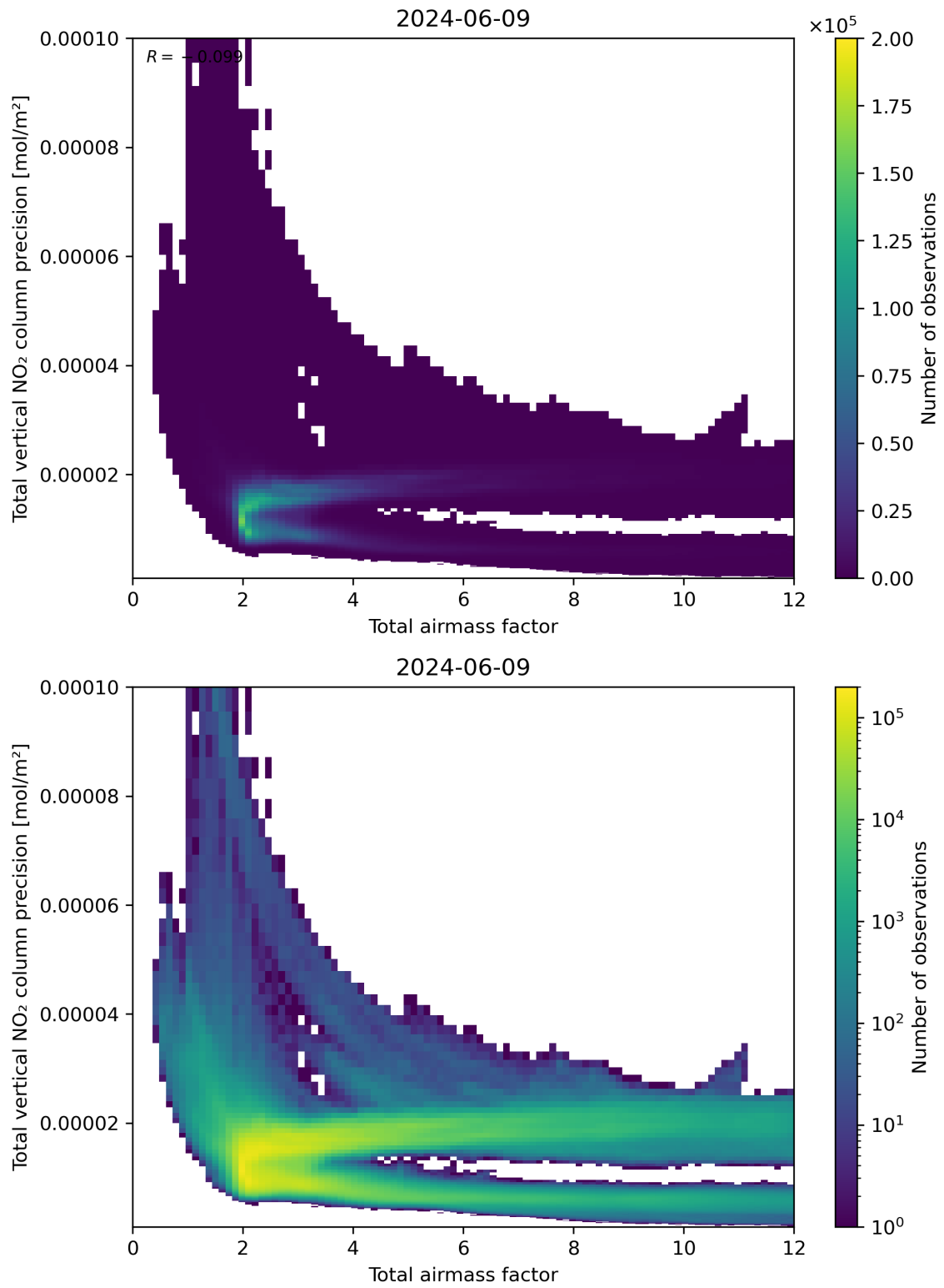
Figure 68: Scatter density plot of “Total airmass factor” against “Total vertical NO 2 column precision” for 2024-06-08 to 2024-06-10.
