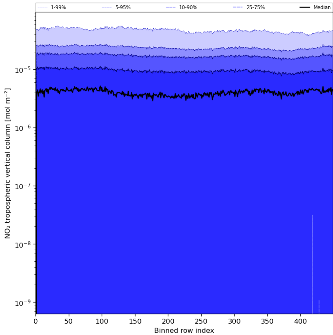
Figure 46: Along track statistics of “NO 2 tropospheric vertical column” for 2024-06-08 to 2024-06-10
