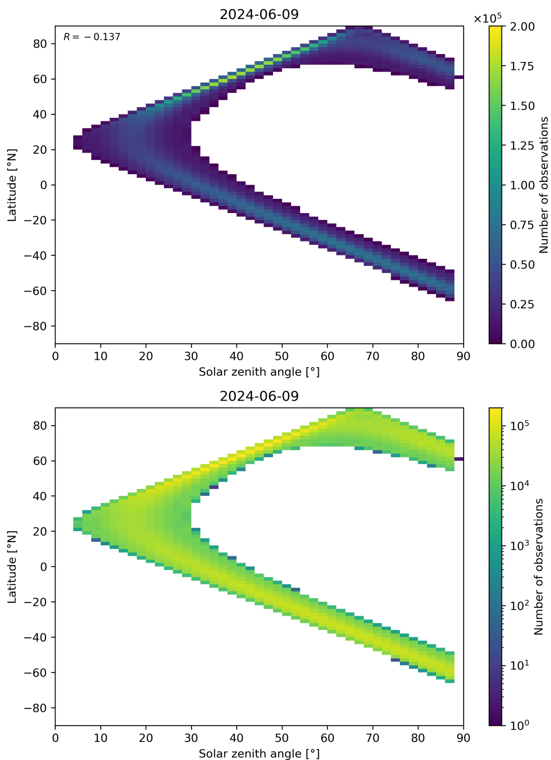
Figure 149: Scatter density plot of “Solar zenith angle” against “Latitude” for 2024-06-08 to 2024-06-10.
