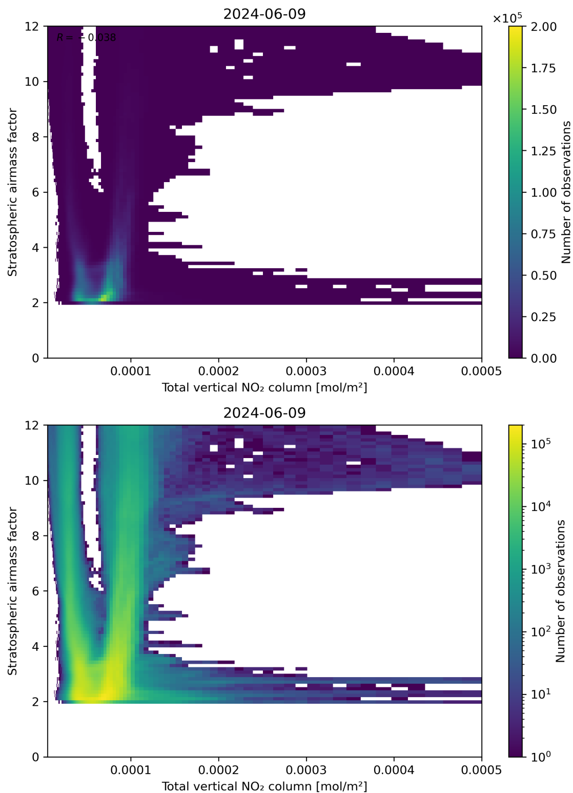
Figure 110: Scatter density plot of “Total vertical NO 2 column” against “Stratospheric airmass factor” for 2024-06-08 to 2024-06-10.
