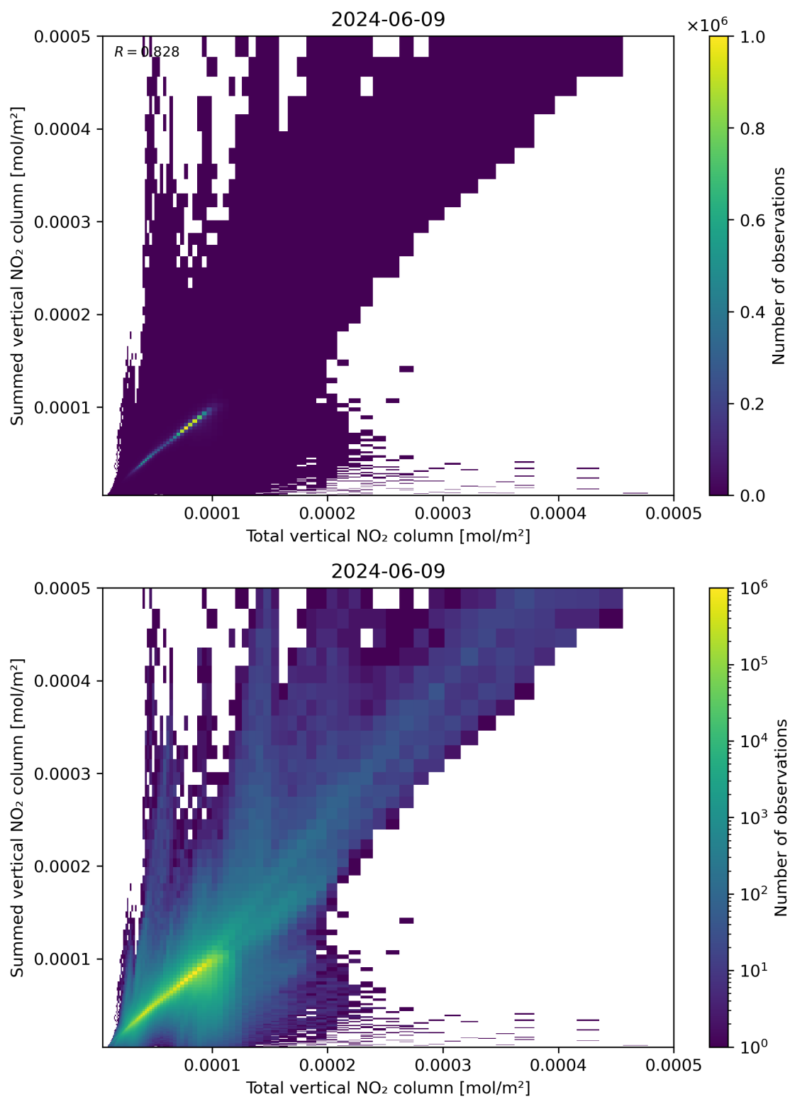
Figure 112: Scatter density plot of “Total vertical NO 2 column” against “Summed vertical NO 2 column” for 2024-06-08 to 2024-06-10.
