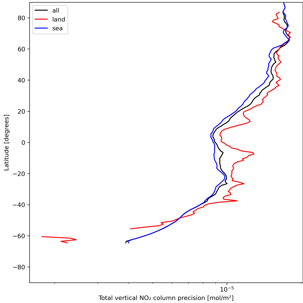
Figure 22: Zonal average of “Total vertical NO 2 column precision” for 2024-06-08 to 2024-06-10.
