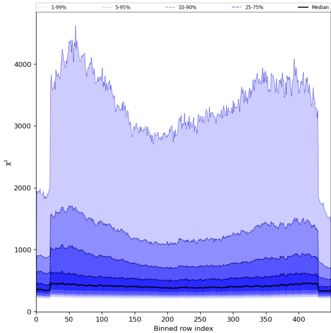
Figure 59: Along track statistics of “ \chi^2 ” for 2024-06-08 to 2024-06-10
