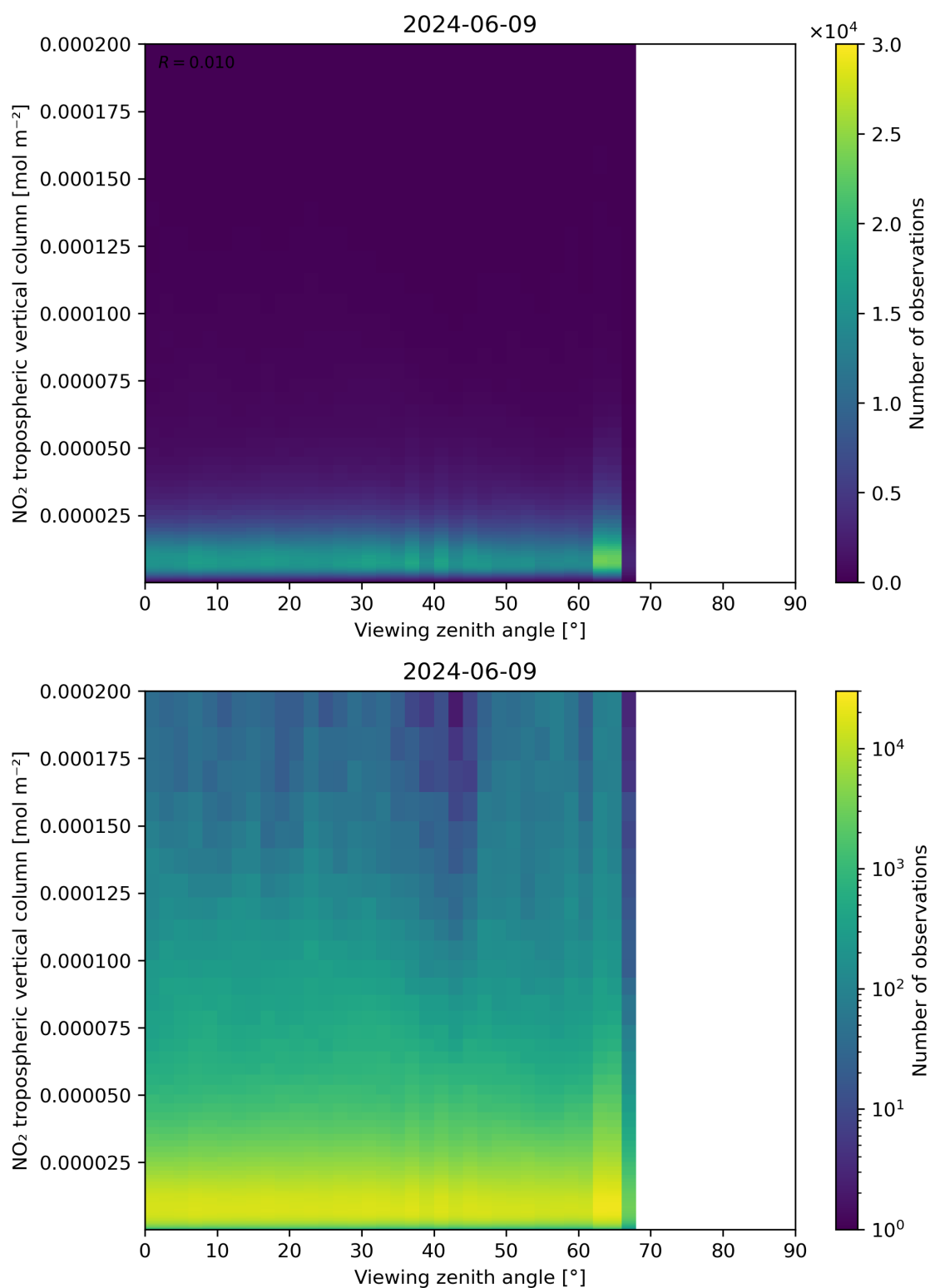
Figure 169: Scatter density plot of “Viewing zenith angle” against “NO 2 tropospheric vertical column” for 2024-06-08 to 2024-06-10.
