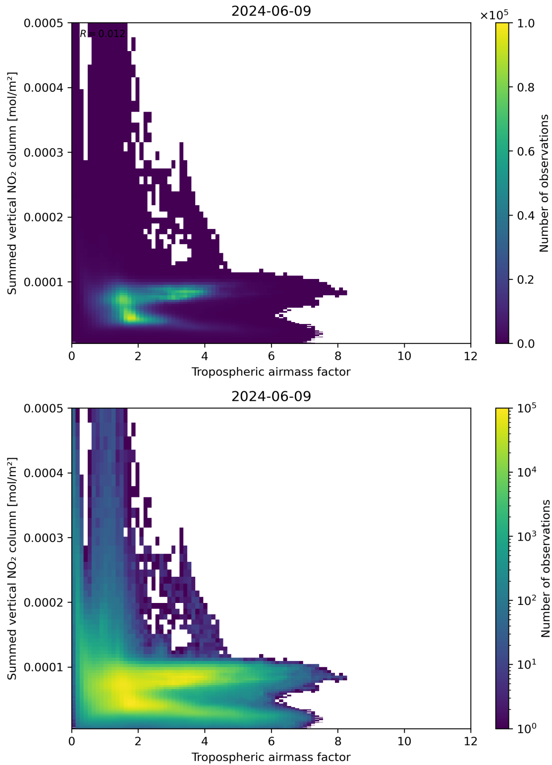
Figure 75: Scatter density plot of “Tropospheric airmass factor” against “Summed vertical NO 2 column” for 2024-06-08 to 2024-06-10.
