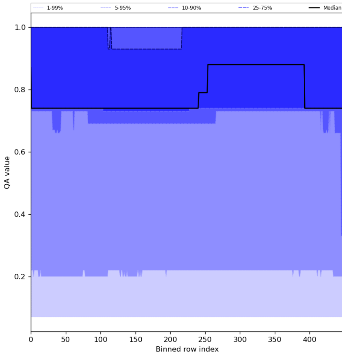
Figure 45: Along track statistics of "QA value" for 2024-06-08 to 2024-06-10
