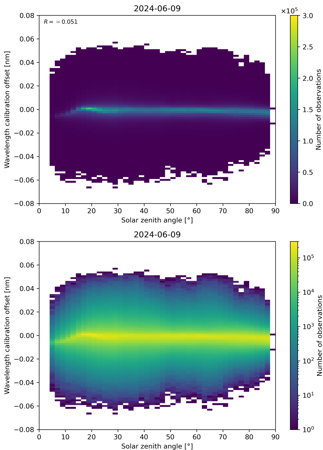
Figure 158: Scatter density plot of “Solar zenith angle” against “Wavelength calibration offset” for 2024-06-08 to 2024-06-10.
