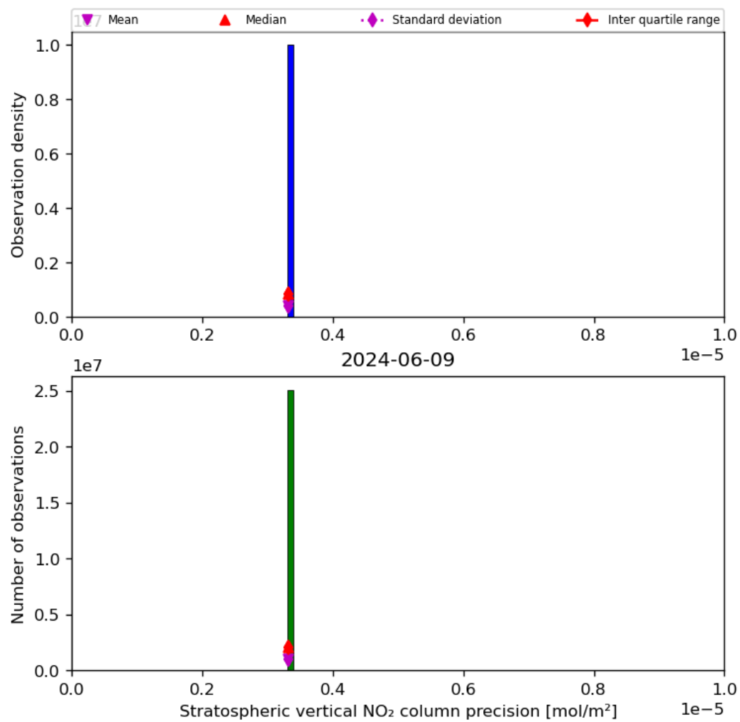
Figure 37: Histogram of “Stratospheric vertical NO 2 column precision” for 2024-06-08 to 2024-06-10
