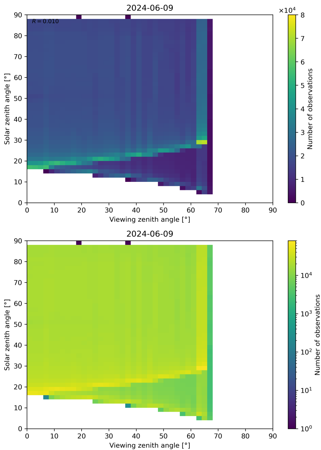
Figure 172: Scatter density plot of “Viewing zenith angle” against “Solar zenith angle” for 2024-06-08 to 2024-06-10.
