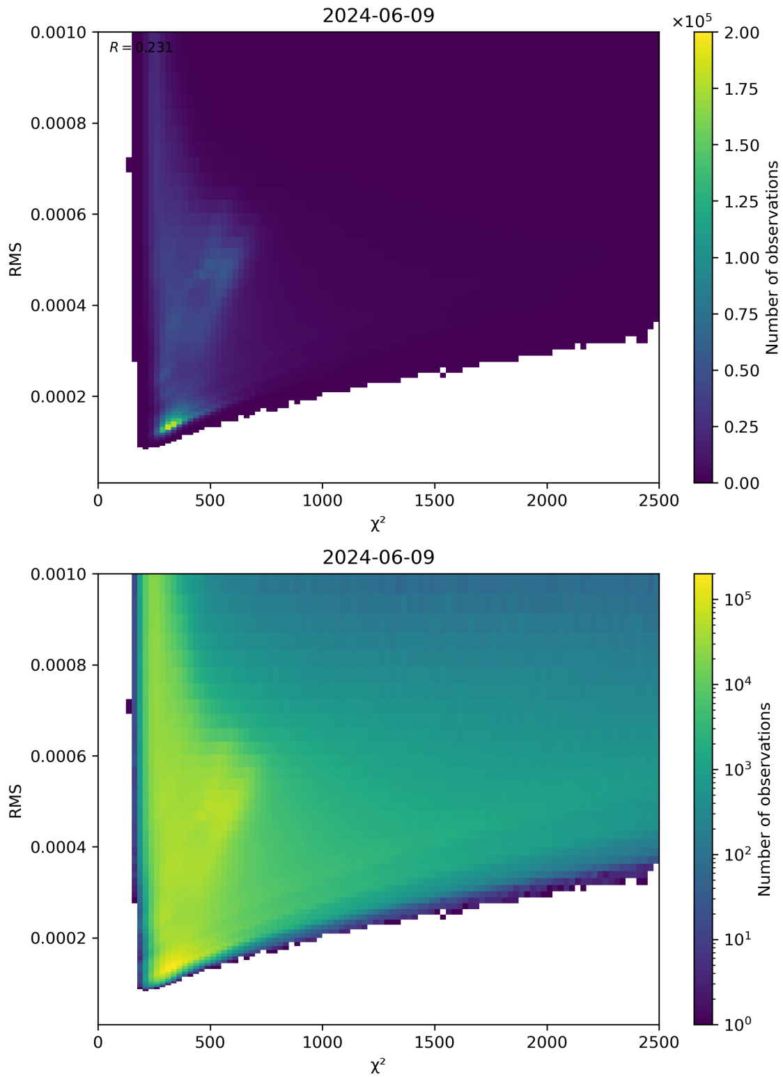
Figure 82: Scatter density plot of “ \chi^2 ” against “RMS” for 2024-06-08 to 2024-06-10.
