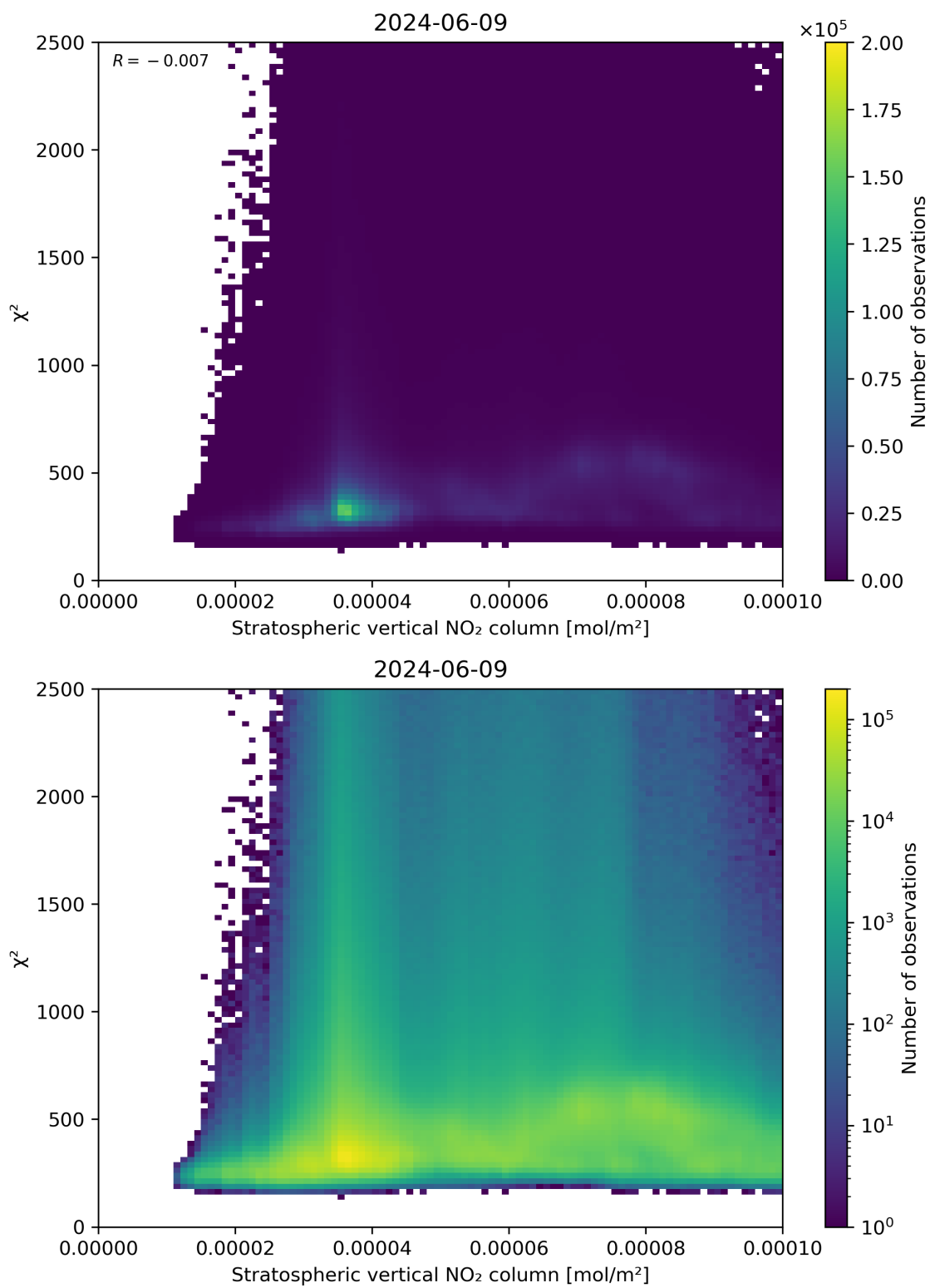
Figure 97: Scatter density plot of “Stratospheric vertical NO 2 column” against “ \chi^2 ” for 2024-06-08 to 2024-06-10.
