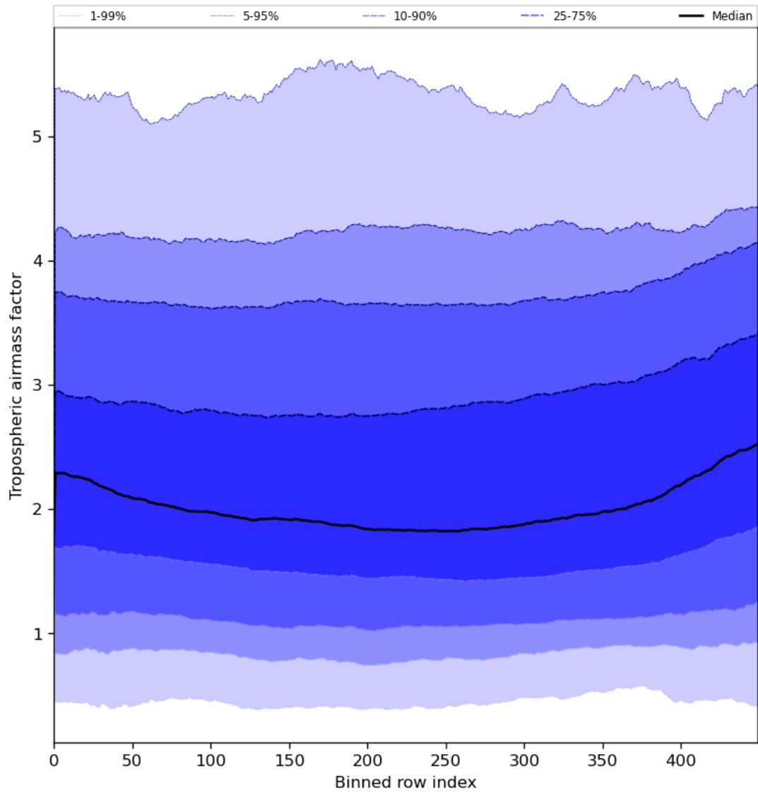
Figure 48: Along track statistics of “Tropospheric airmass factor” for 2024-06-08 to 2024-06-10
