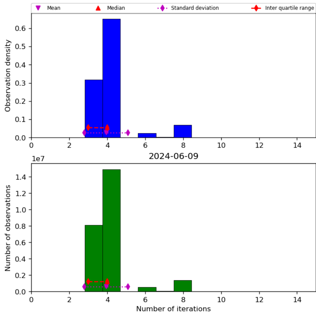
Figure 34: Histogram of “Number of iterations” for 2024-06-08 to 2024-06-10
