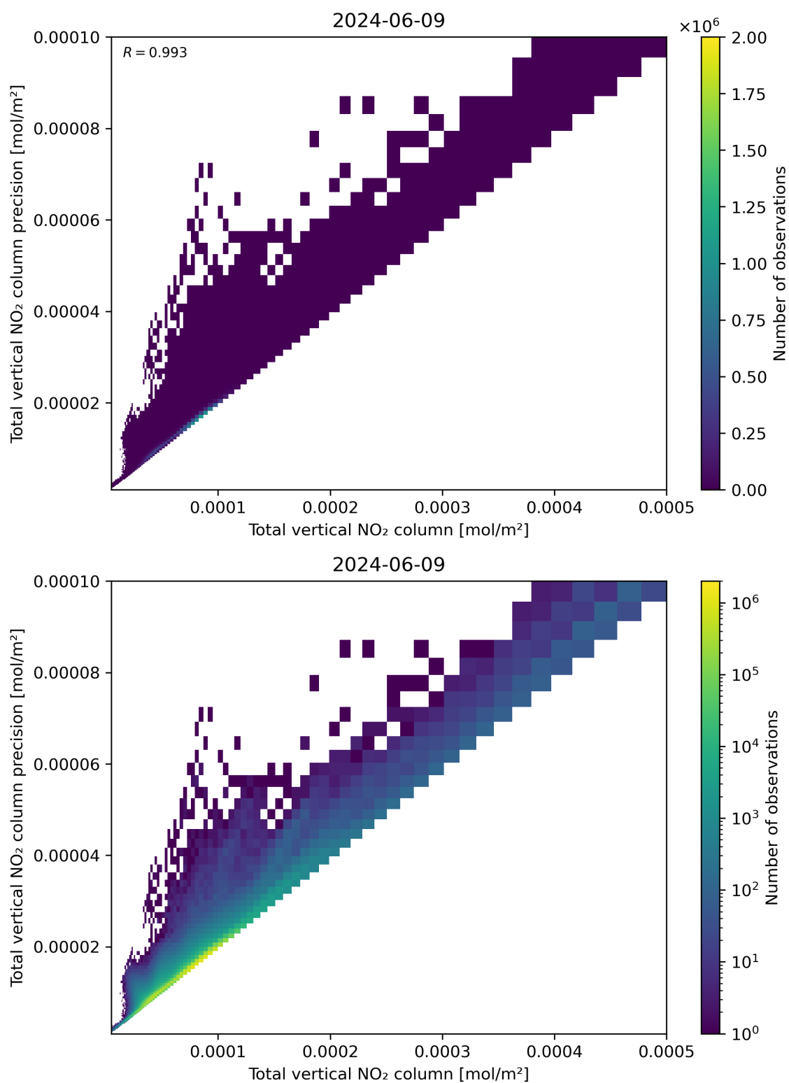
Figure 114: Scatter density plot of “Total vertical NO 2 column” against “Total vertical NO 2 column precision” for 2024-06-08 to 2024-06-10.
