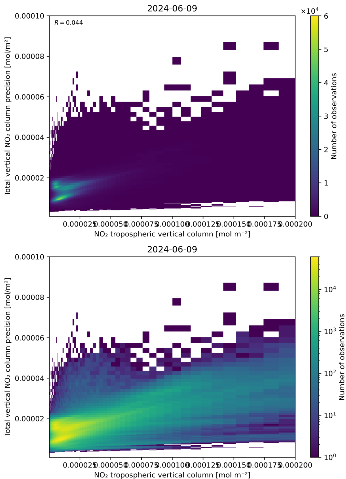
Figure 129: Scatter density plot of “NO 2 tropospheric vertical column” against “Total vertical NO 2 column precision” for 2024-06-08 to 2024-06-10.
