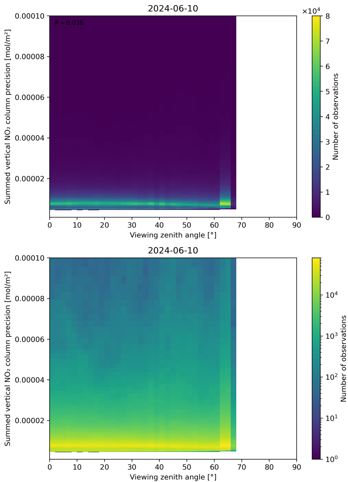
Figure 166: Scatter density plot of “Viewing zenith angle” against “Summed vertical NO 2 column precision” for 2024-06-09 to 2024-06-11.
