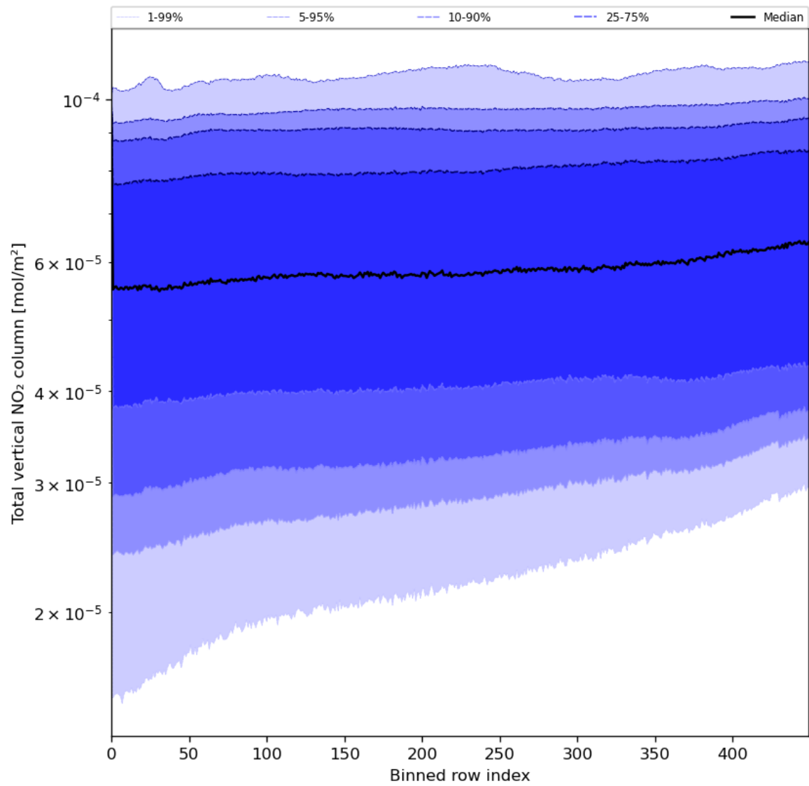
Figure 55: Along track statistics of “Total vertical NO 2 column” for 2024-06-09 to 2024-06-11
