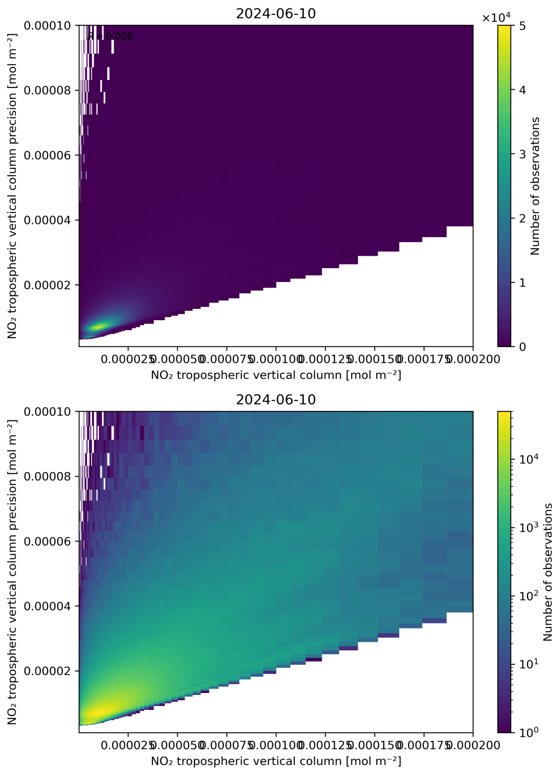
Figure 130: Scatter density plot of “NO 2 tropospheric vertical column” against “NO 2 tropospheric vertical column precision” for 2024-06-09 to 2024-06-11.
