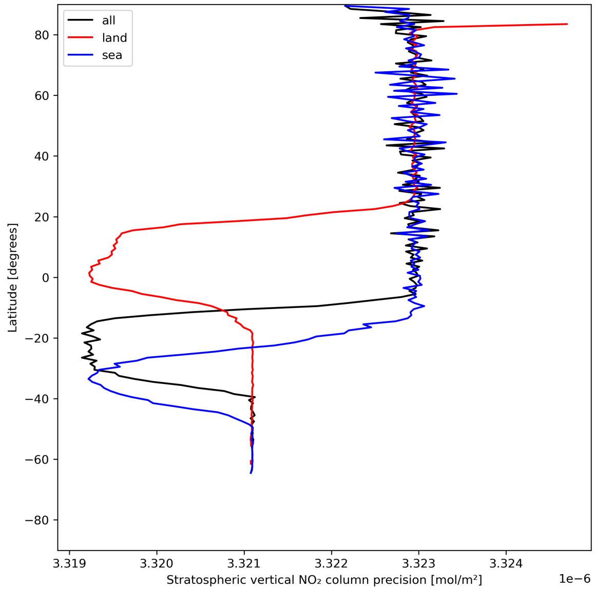
Figure 20: Zonal average of “Stratospheric vertical NO 2 column precision” for 2024-06-09 to 2024-06-11.
