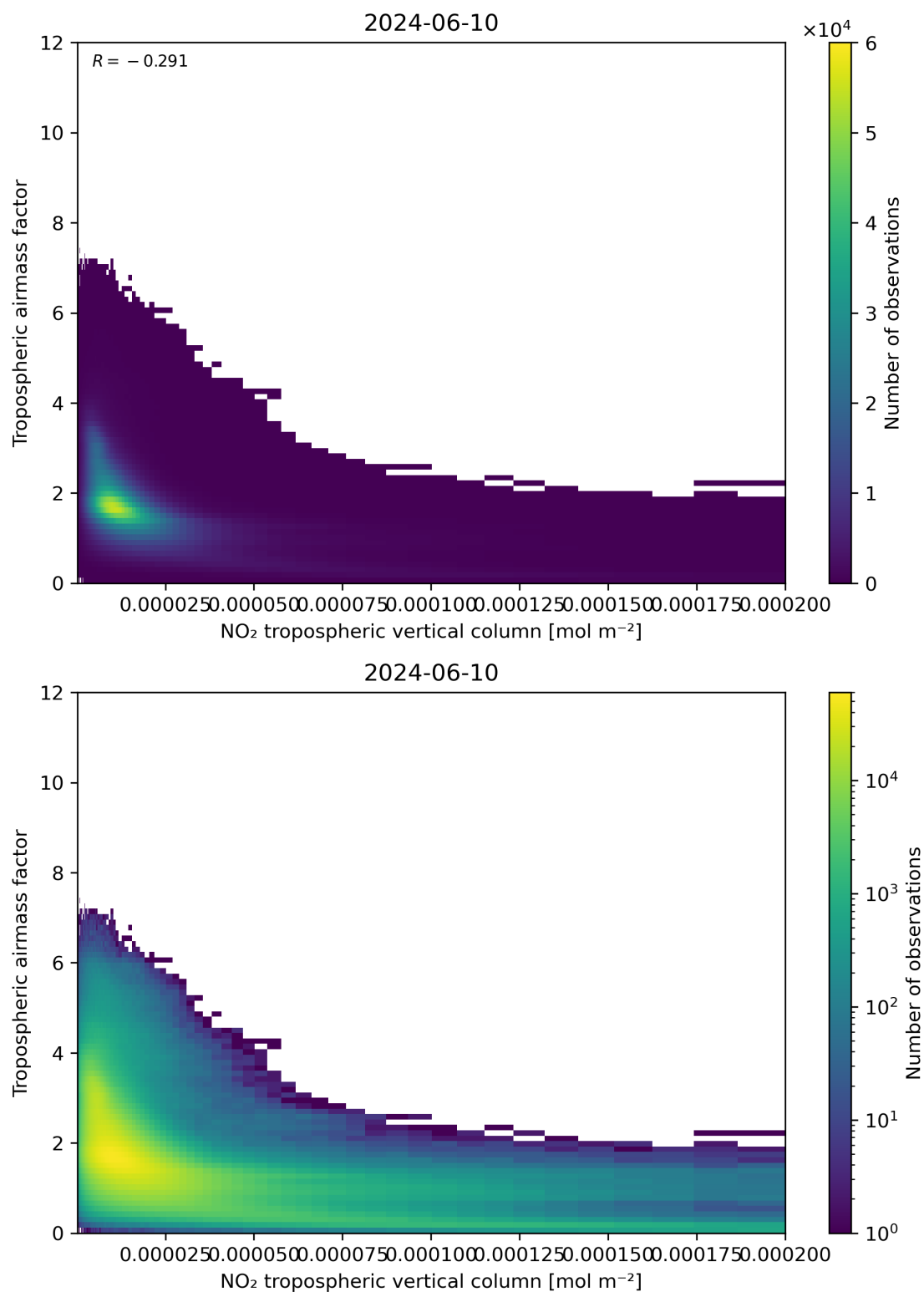
Figure 123: Scatter density plot of “NO 2 tropospheric vertical column” against “Tropospheric air mass factor” for 2024-06-09 to 2024-06-11.
