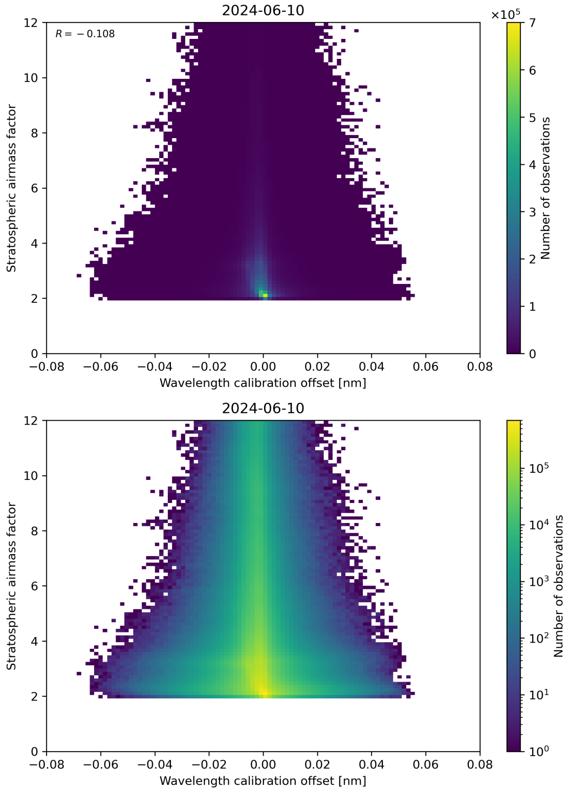
Figure 174: Scatter density plot of “Wavelength calibration offset” against “Stratospheric airmass factor” for 2024-06-09 to 2024-06-11.
