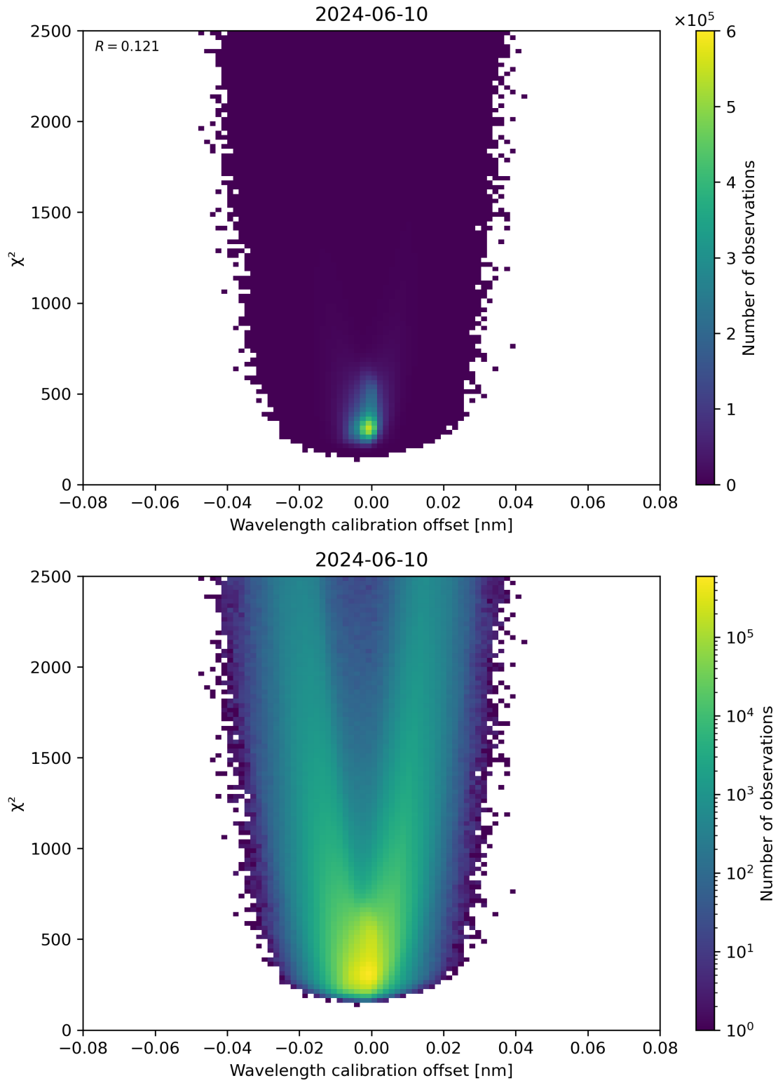
Figure 175: Scatter density plot of “Wavelength calibration offset” against “ \chi^2 ” for 2024-06-09 to 2024-06-11.
