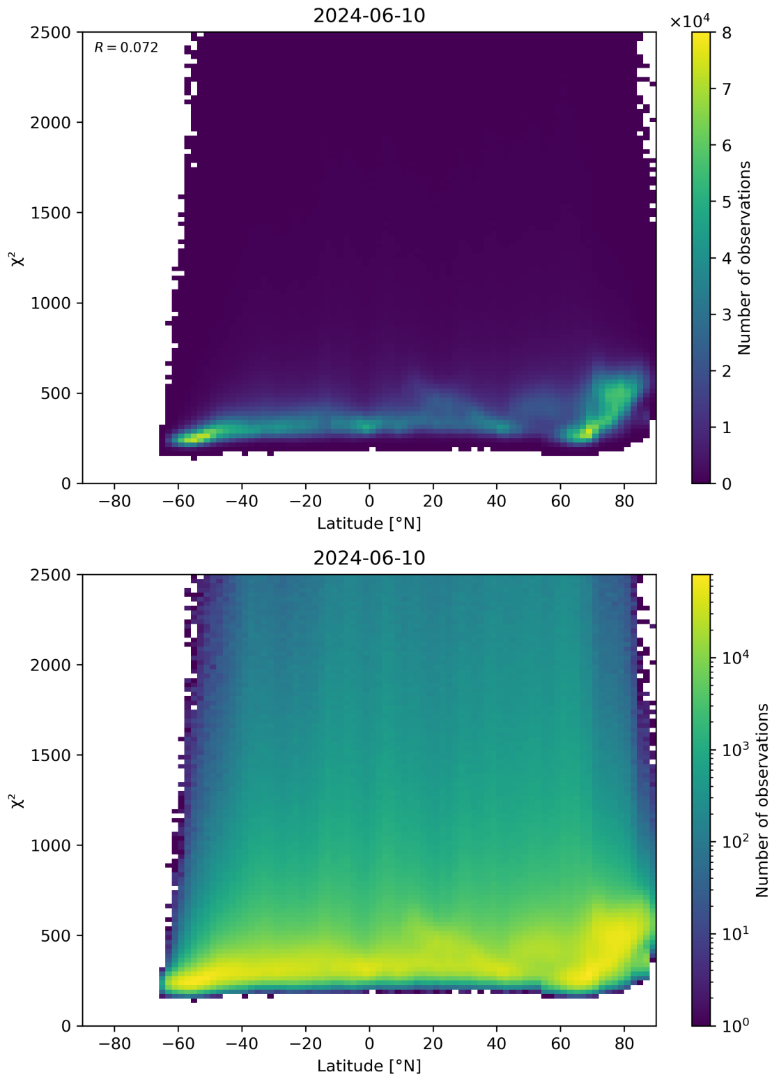
Figure 86: Scatter density plot of “Latitude” against “ \chi^2 ” for 2024-06-09 to 2024-06-11.
