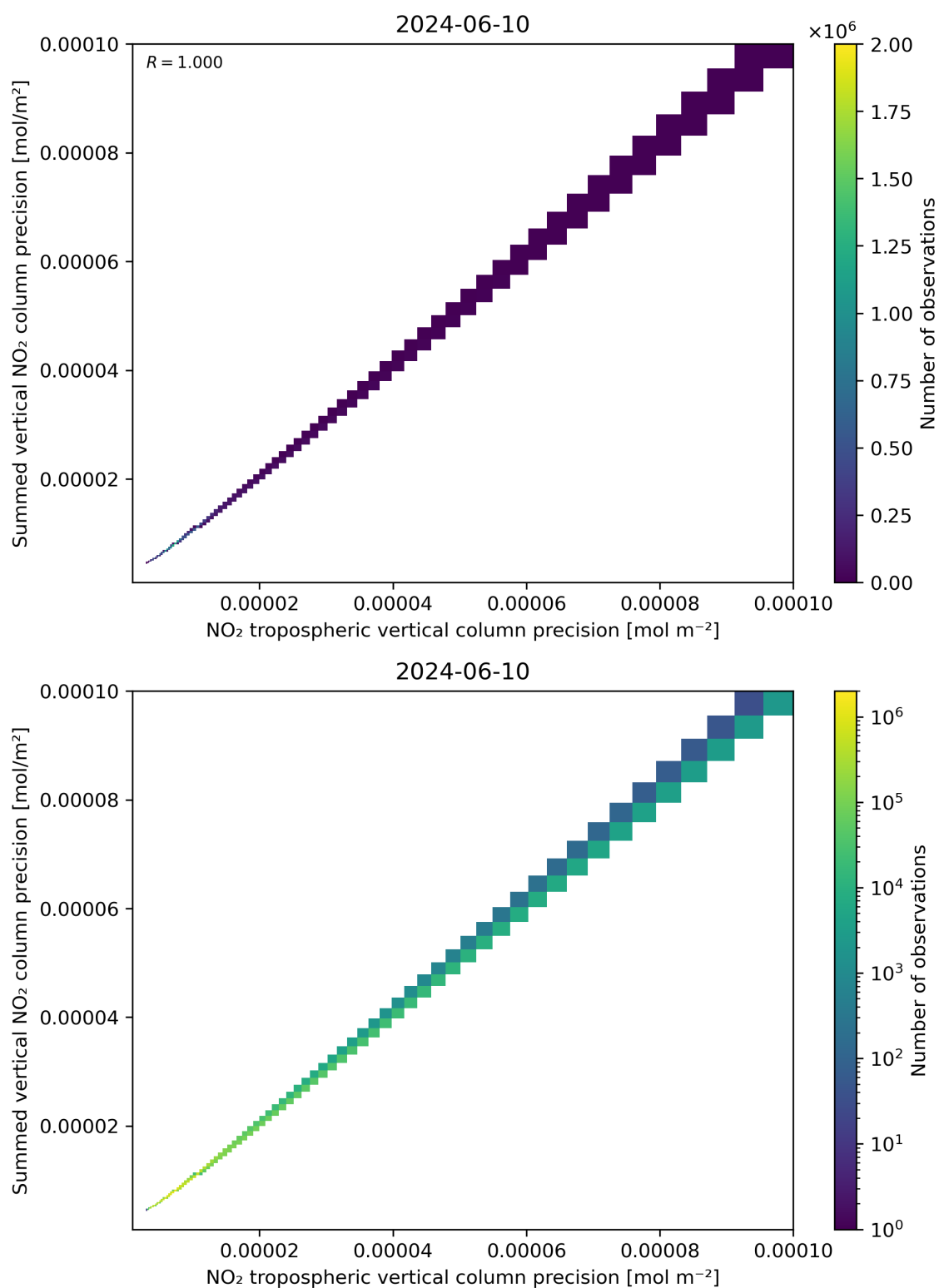
Figure 137: Scatter density plot of “NO 2 tropospheric vertical column precision” against “Summed vertical NO 2 column precision” for 2024-06-09 to 2024-06-11.
