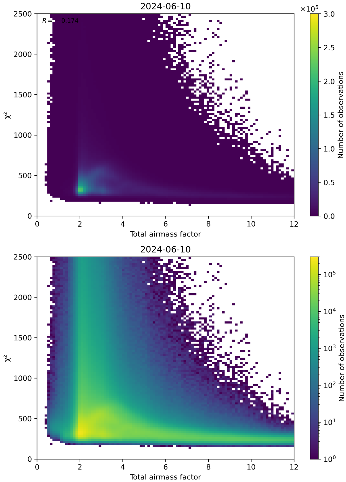
Figure 63: Scatter density plot of “Total airmass factor” against “ \chi^2 ” for 2024-06-09 to 2024-06-11.
