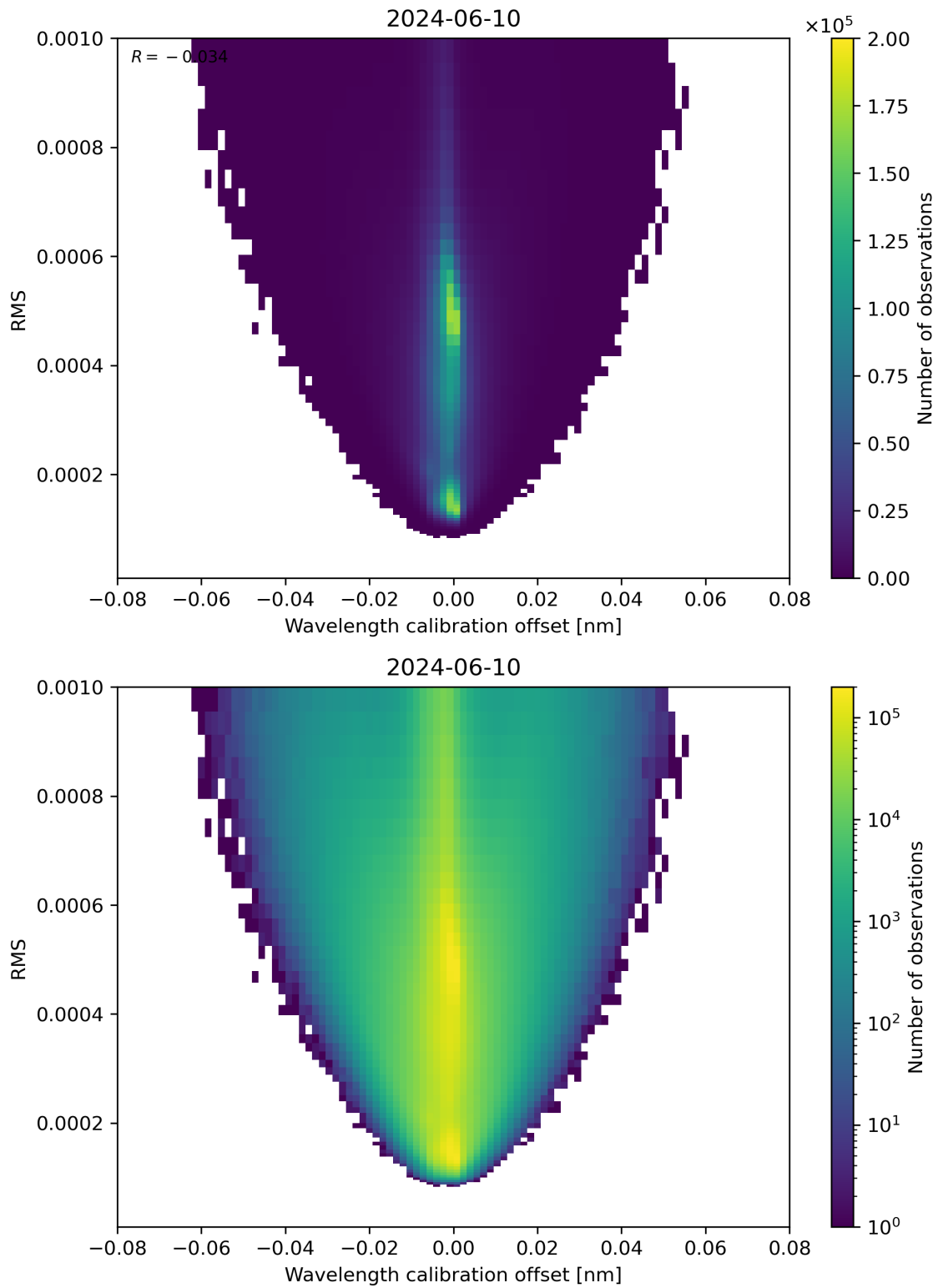
Figure 181: Scatter density plot of “Wavelength calibration offset” against “RMS” for 2024-06-09 to 2024-06-11.
