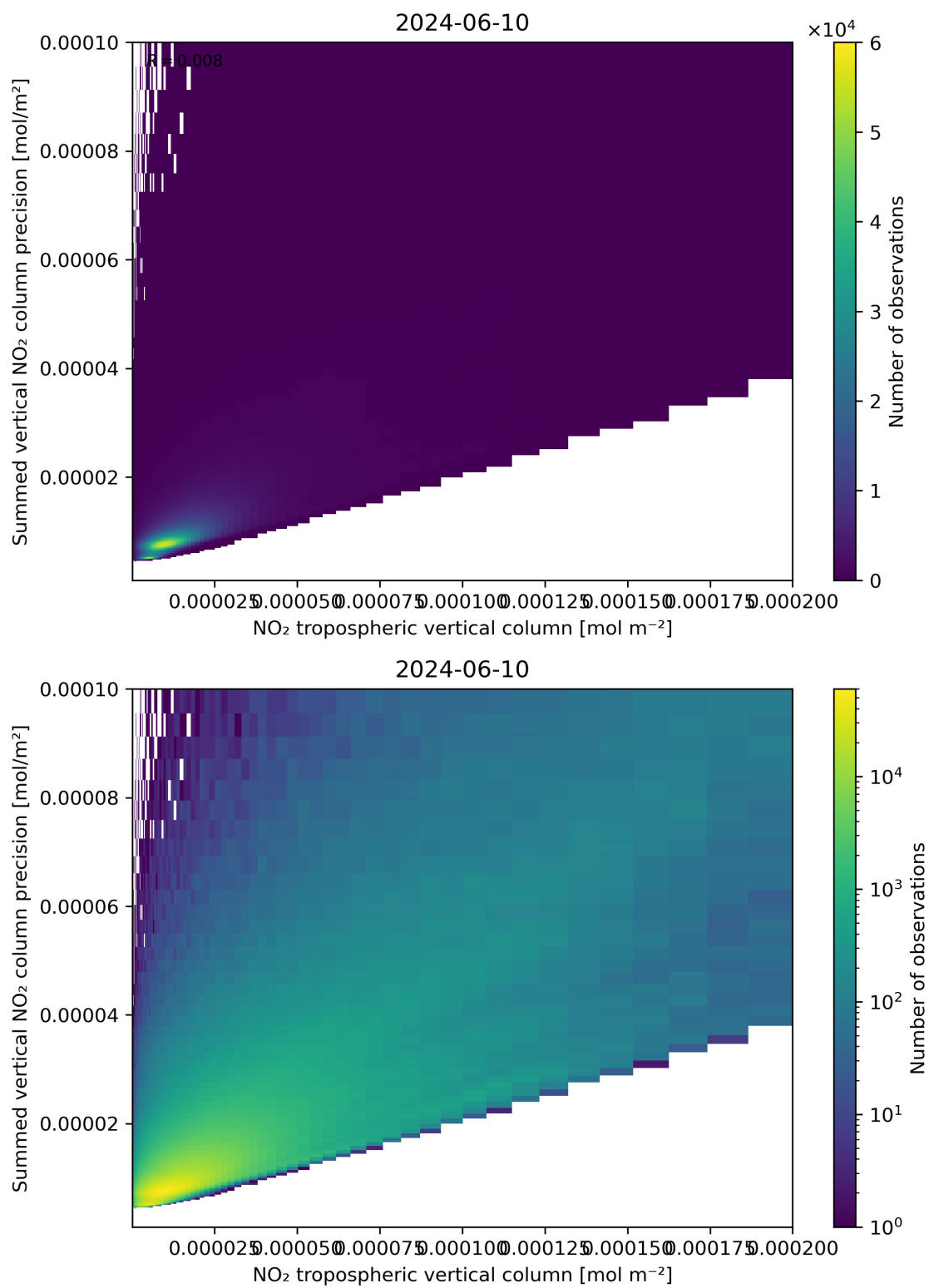
Figure 127: Scatter density plot of “NO 2 tropospheric vertical column” against “Summed vertical NO 2 column precision” for 2024-06-09 to 2024-06-11.
