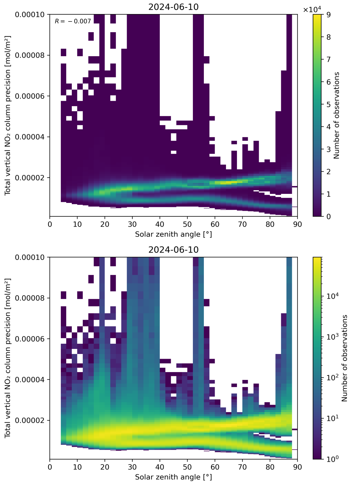
Figure 154: Scatter density plot of “Solar zenith angle” against “Total vertical NO 2 column precision” for 2024-06-09 to 2024-06-11.
