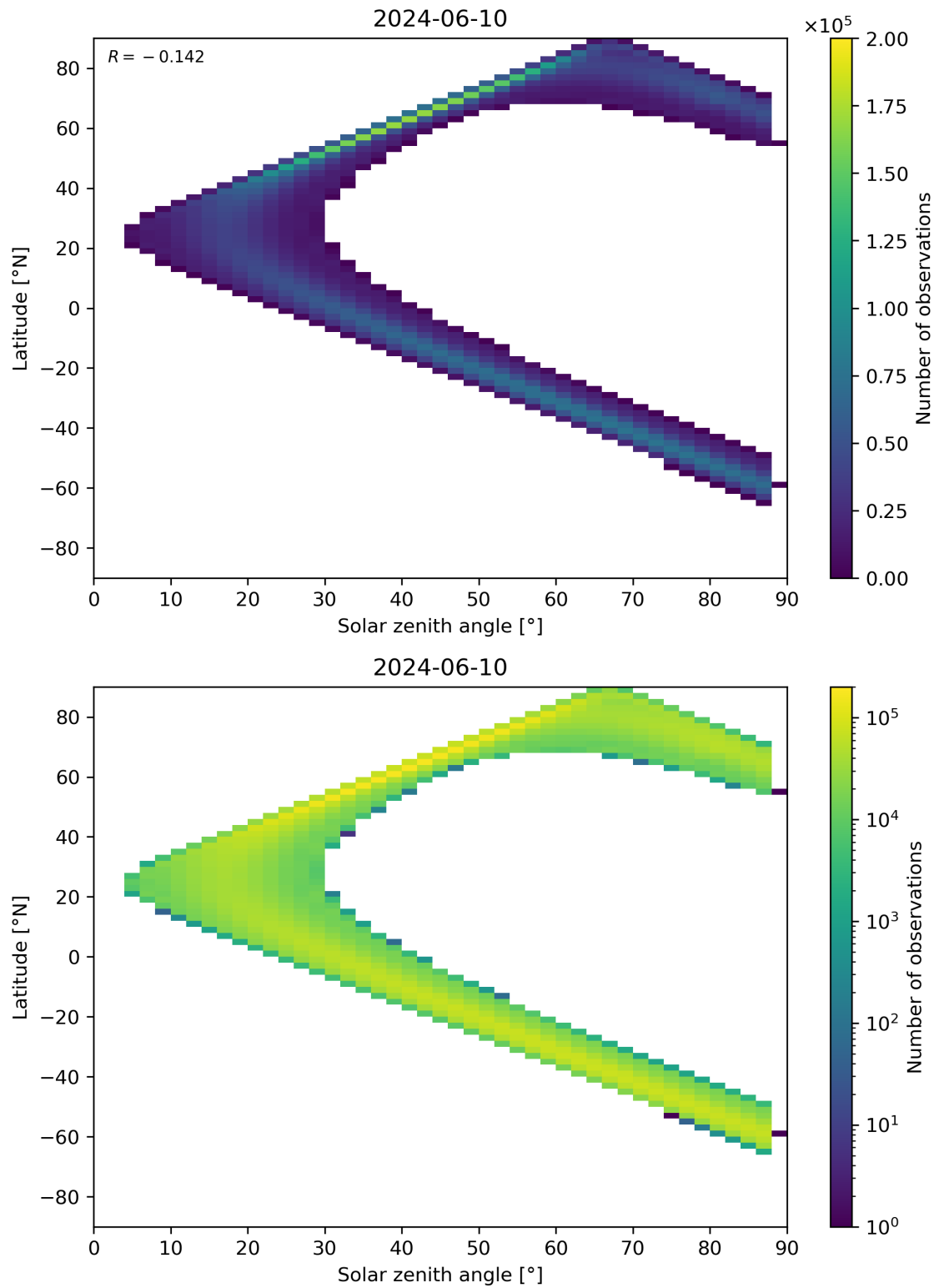
Figure 149: Scatter density plot of “Solar zenith angle” against “Latitude” for 2024-06-09 to 2024-06-11.
