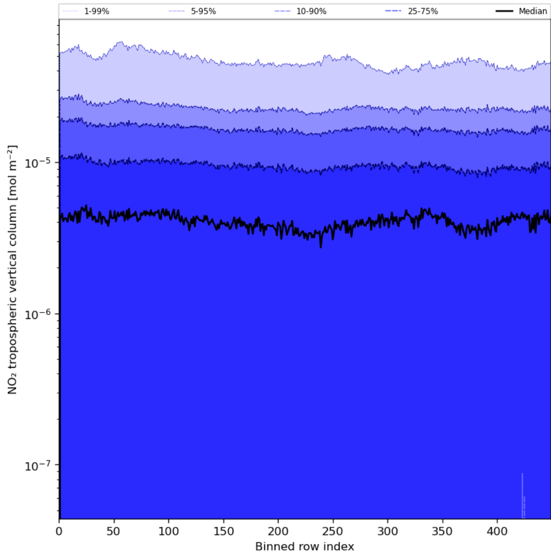
Figure 46: Along track statistics of "NO 2 tropospheric vertical column" for 2024-06-09 to 2024-06-11
