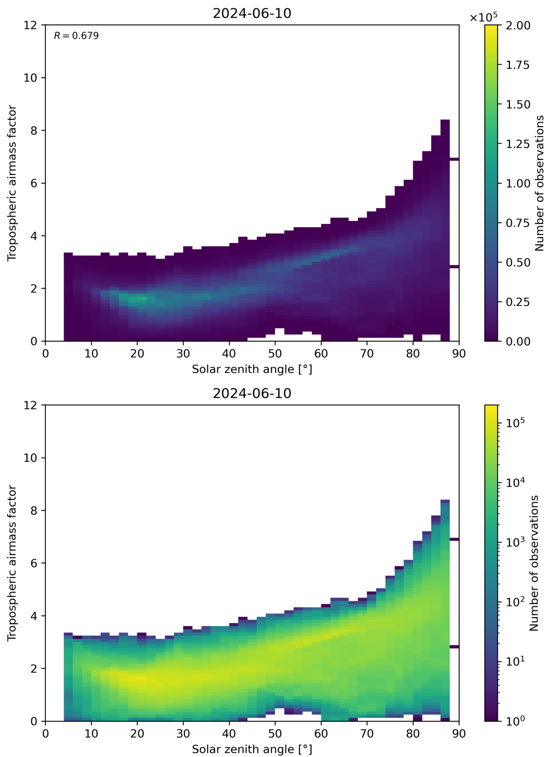
Figure 147: Scatter density plot of “Solar zenith angle” against “Tropospheric airmass factor” for 2024-06-09 to 2024-06-11.
