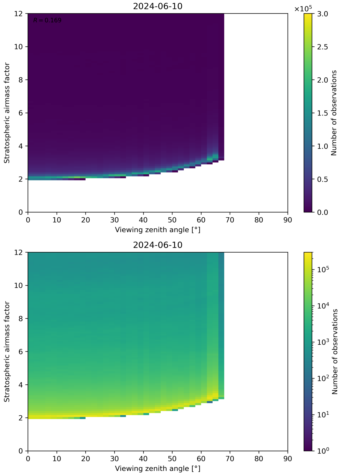
Figure 159: Scatter density plot of “Viewing zenith angle” against “Stratospheric airmass factor” for 2024-06-09 to 2024-06-11.
