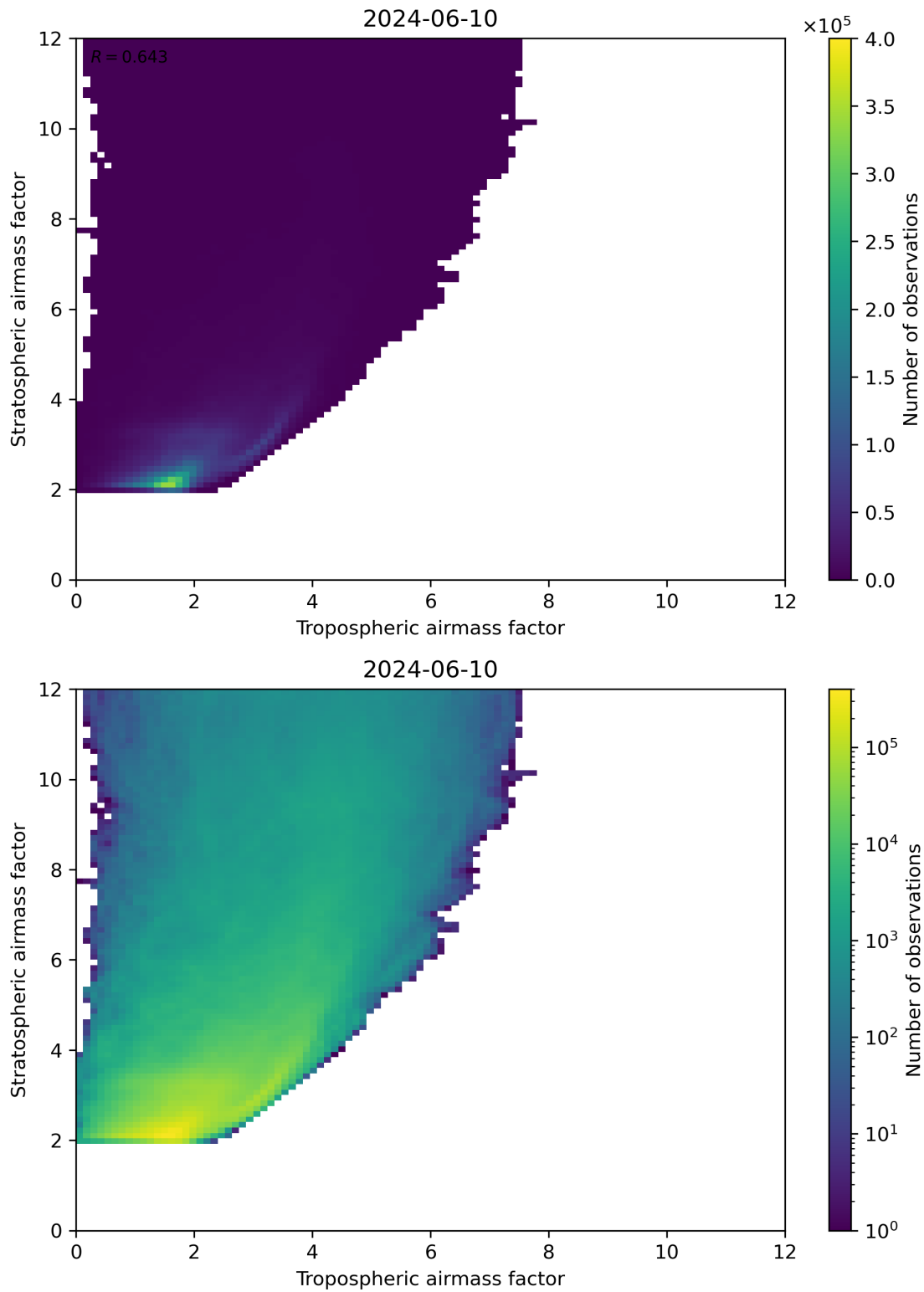
Figure 71: Scatter density plot of “Tropospheric airmass factor” against “Stratospheric airmass factor” for 2024-06-09 to 2024-06-11.
