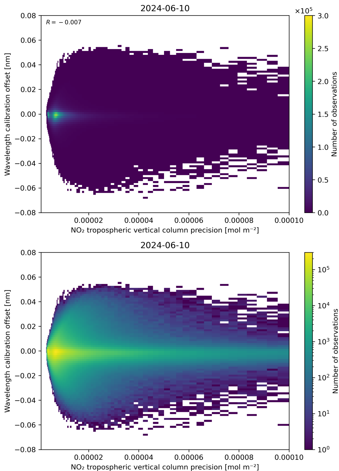
Figure 141: Scatter density plot of “NO 2 tropospheric vertical column precision” against “Wavelength calibration offset” for 2024-06-09 to 2024-06-11.
