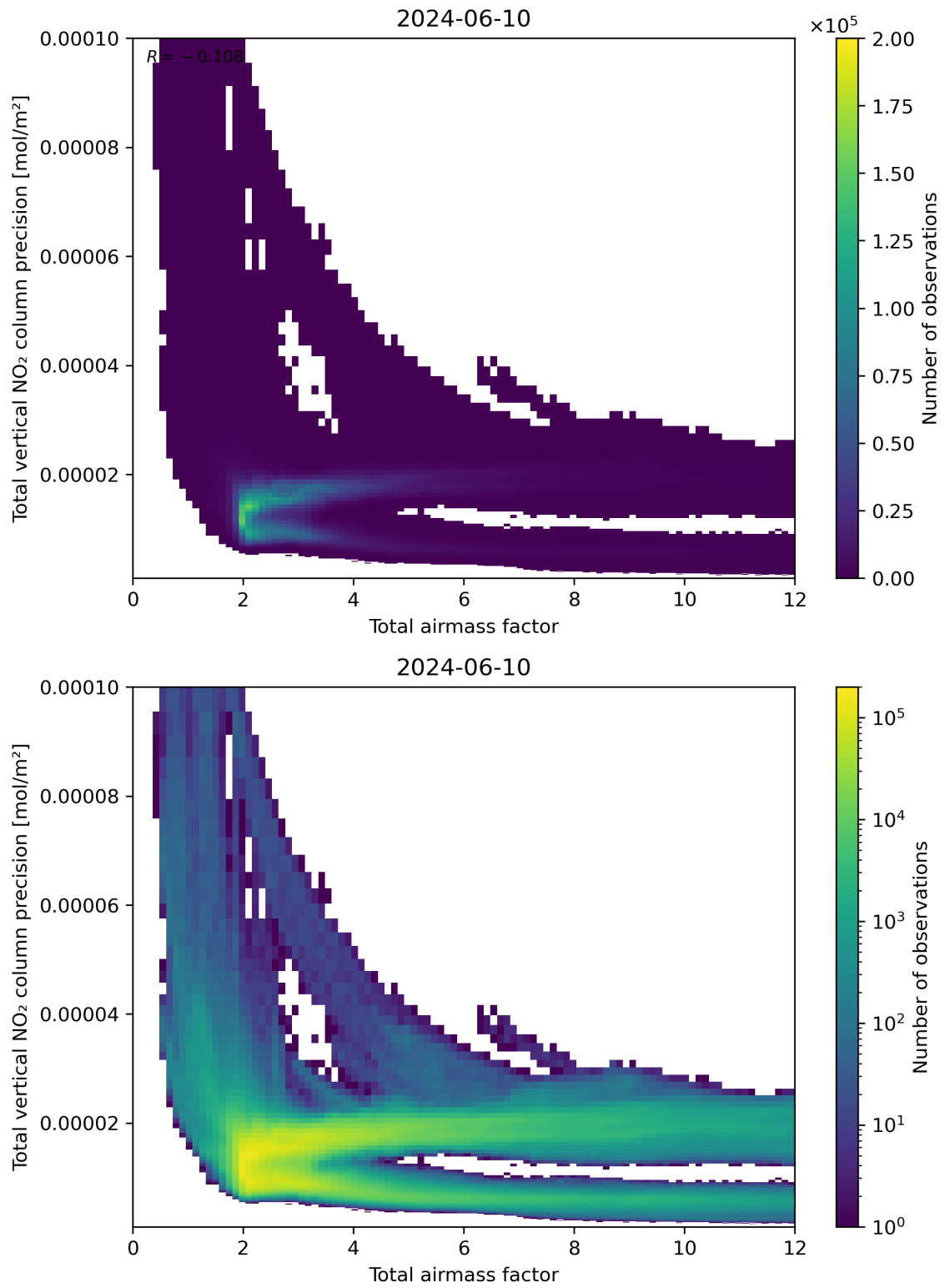
Figure 68: Scatter density plot of “Total airmass factor” against “Total vertical NO 2 column precision” for 2024-06-09 to 2024-06-11.
