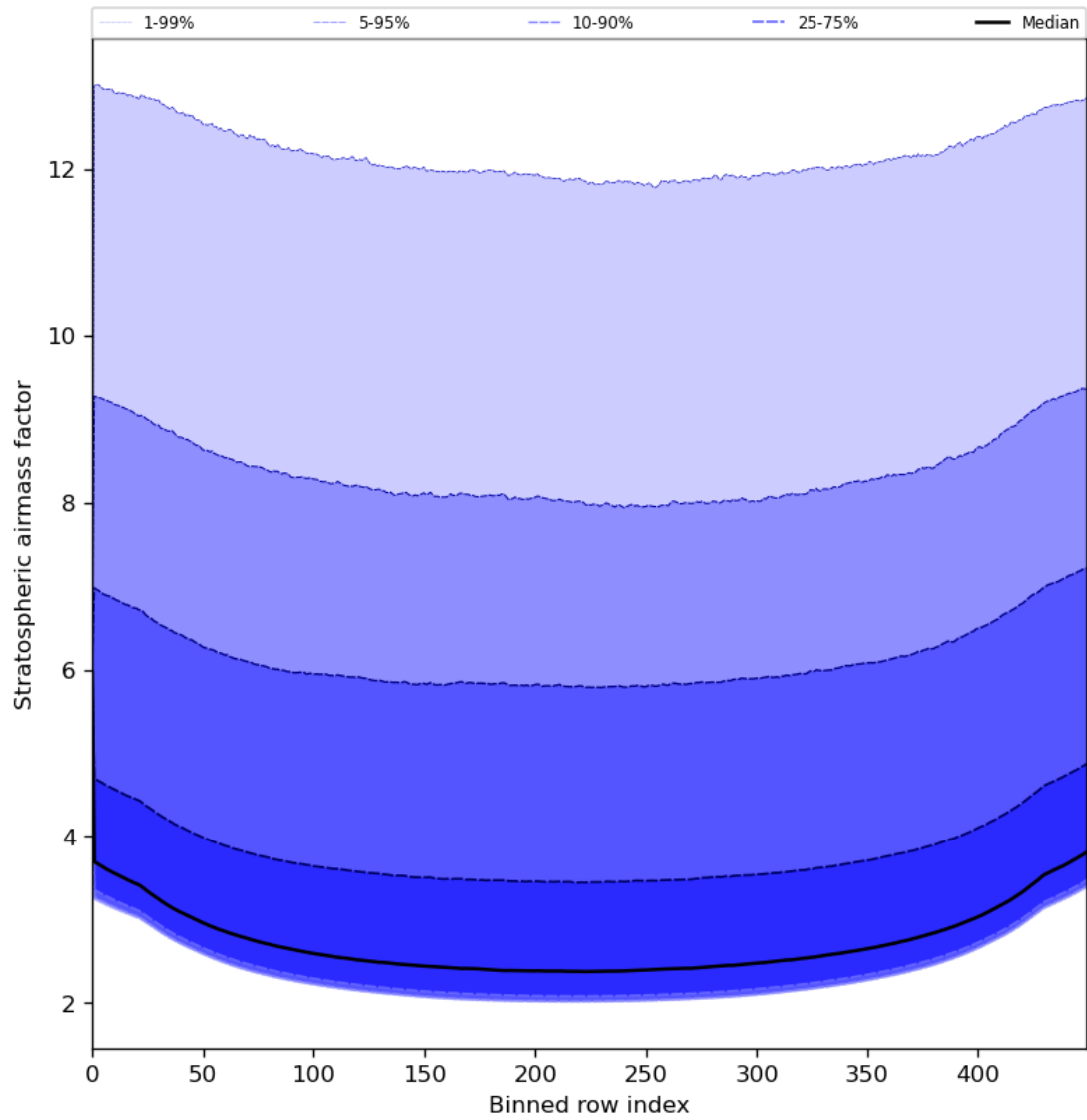
Figure 61: Along track statistics of “Stratospheric airmass factor” for 2024-06-09 to 2024-06-11
