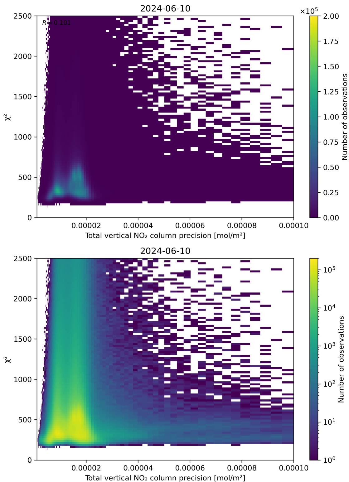
Figure 116: Scatter density plot of “Total vertical NO 2 column precision” against “ \chi^2 ” for 2024-06-09 to 2024-06-11.
