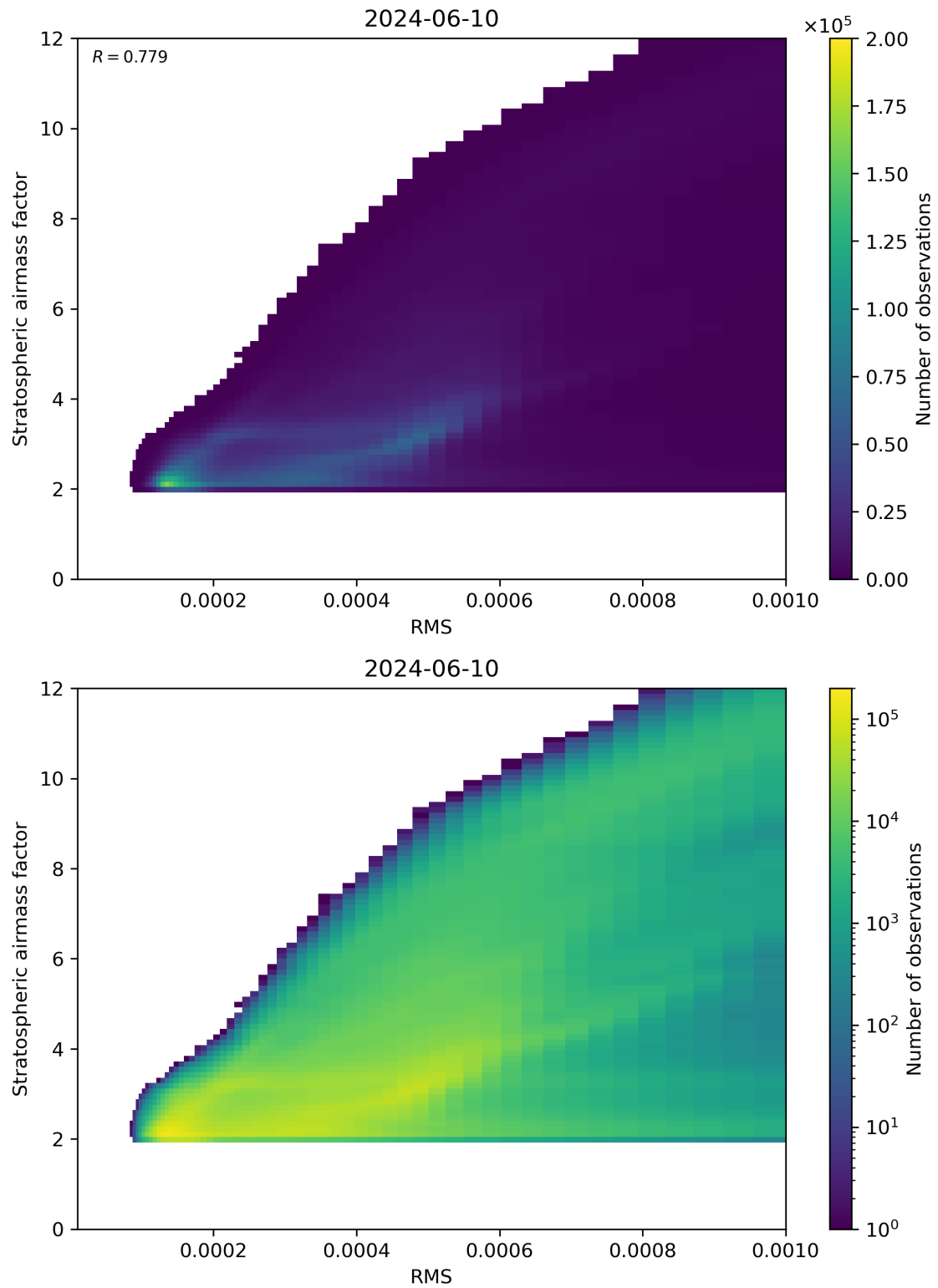
Figure 144: Scatter density plot of “RMS” against “Stratospheric airmass factor” for 2024-06-09 to 2024-06-11.
