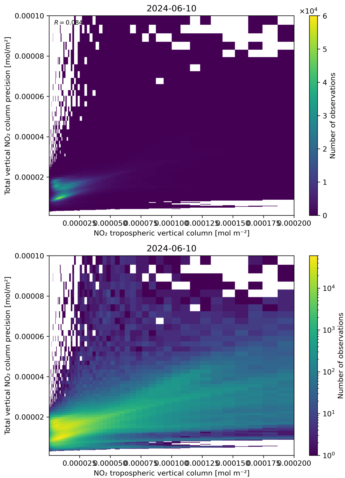
Figure 129: Scatter density plot of “NO 2 tropospheric vertical column” against “Total vertical NO 2 column precision” for 2024-06-09 to 2024-06-11.
