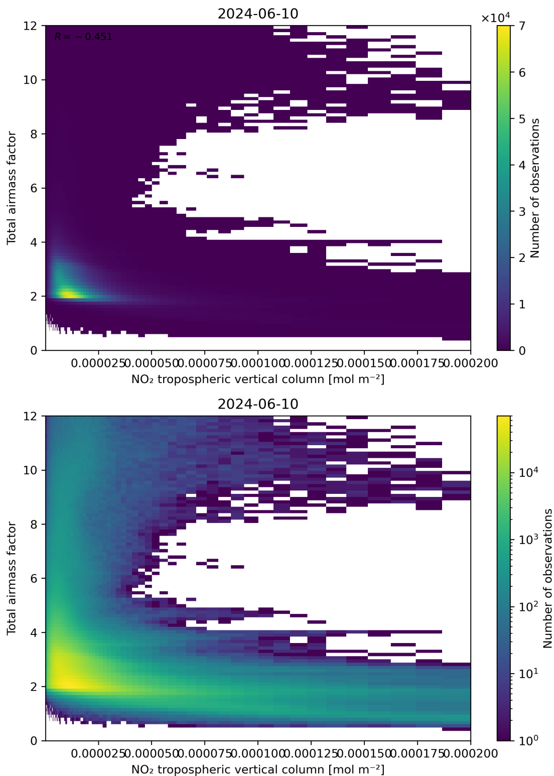
Figure 122: Scatter density plot of “NO 2 tropospheric vertical column” against “Total air mass factor” for 2024-06-09 to 2024-06-11.
