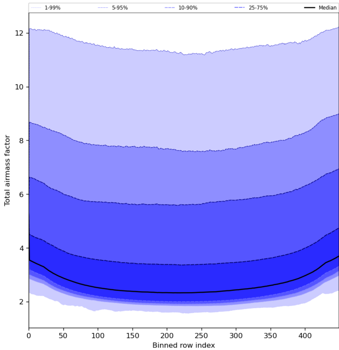
Figure 49: Along track statistics of “Total airmass factor” for 2024-06-09 to 2024-06-11
