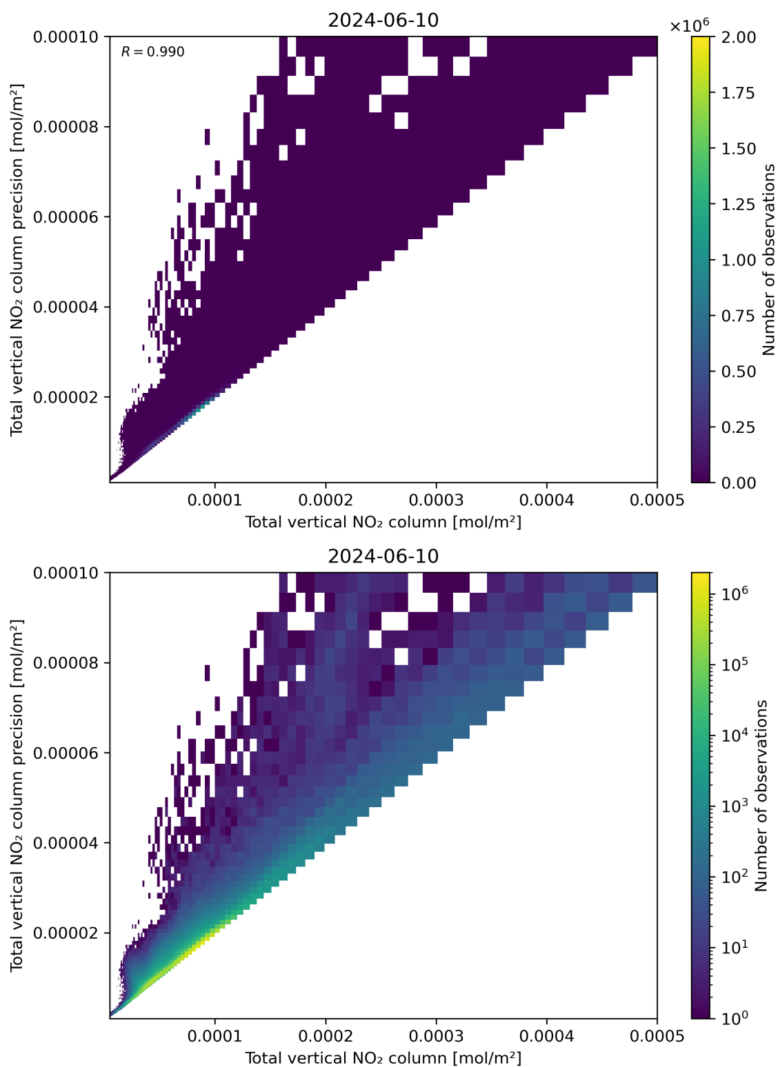
Figure 114: Scatter density plot of “Total vertical NO 2 column” against “Total vertical NO 2 column precision” for 2024-06-09 to 2024-06-11.
