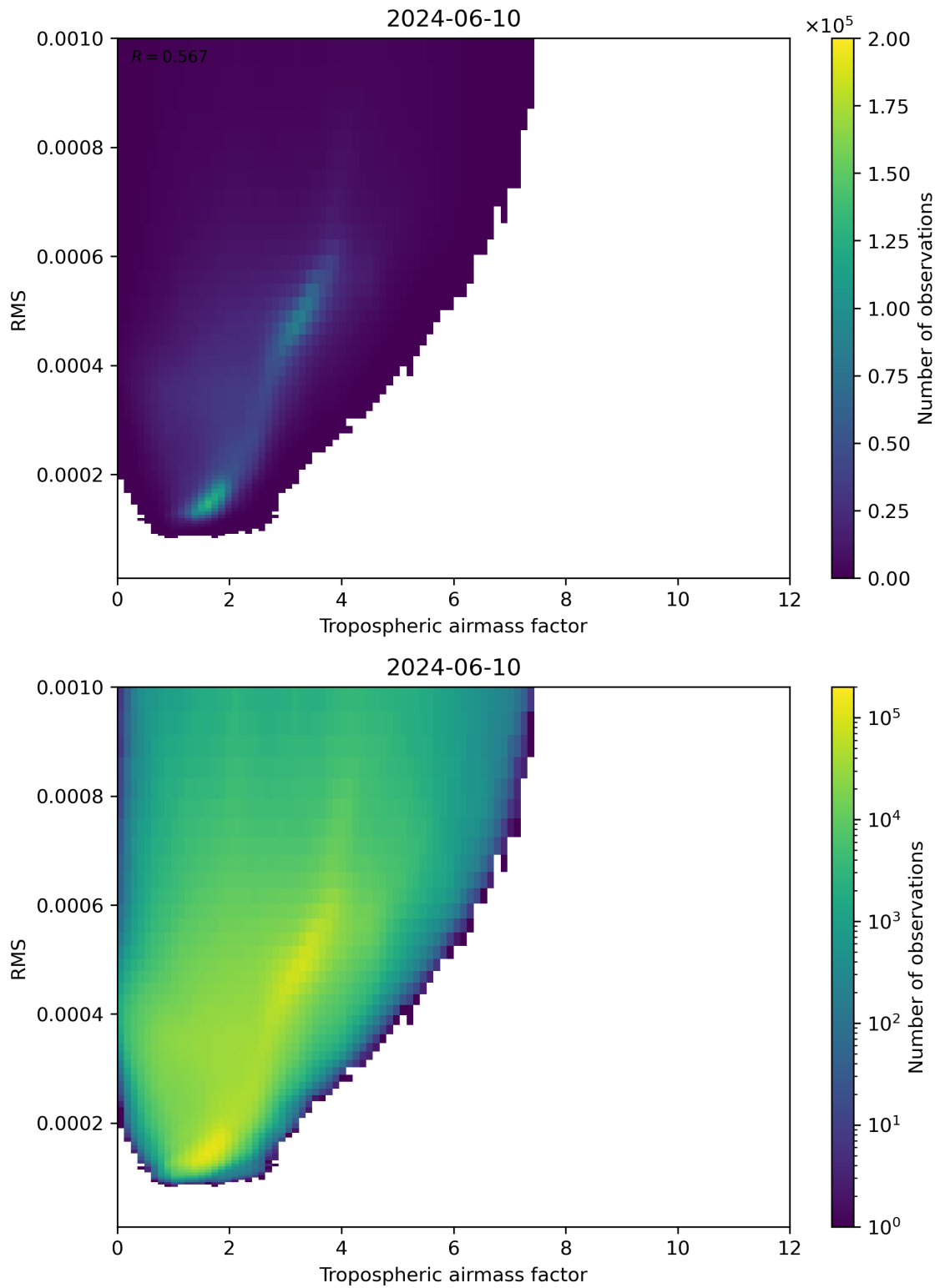
Figure 79: Scatter density plot of “Tropospheric airmass factor” against “RMS” for 2024-06-09 to 2024-06-11.
