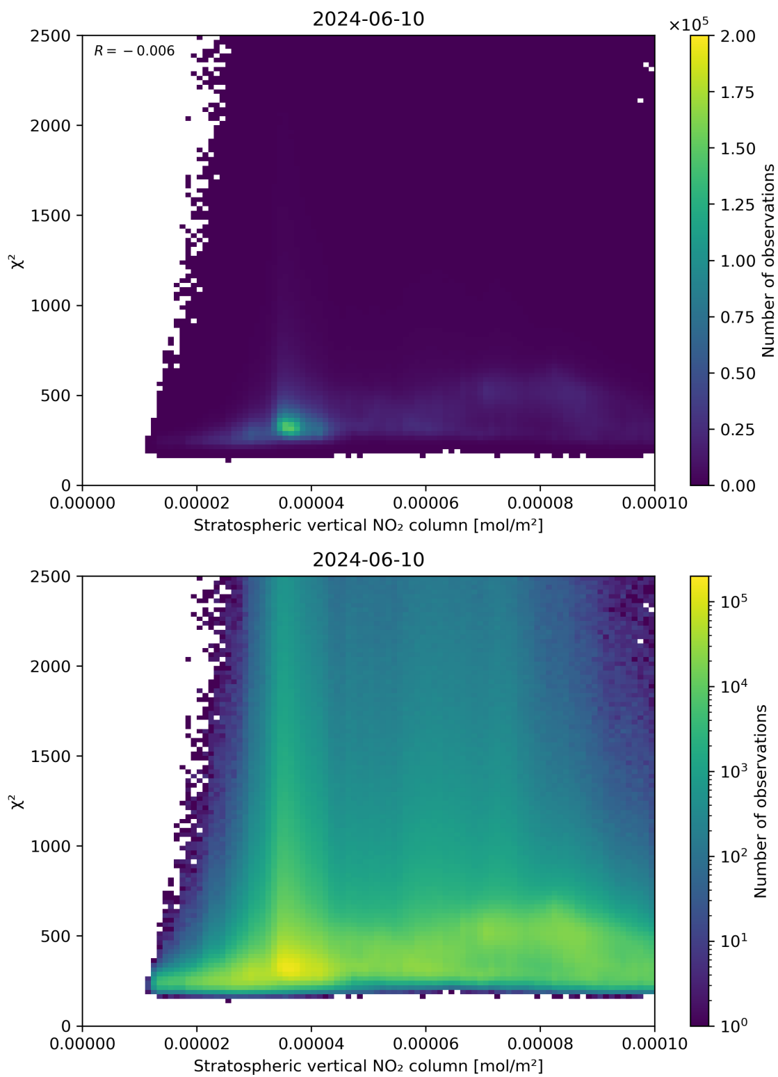
Figure 97: Scatter density plot of “Stratospheric vertical NO 2 column” against “ \chi^2 ” for 2024-06-09 to 2024-06-11.
