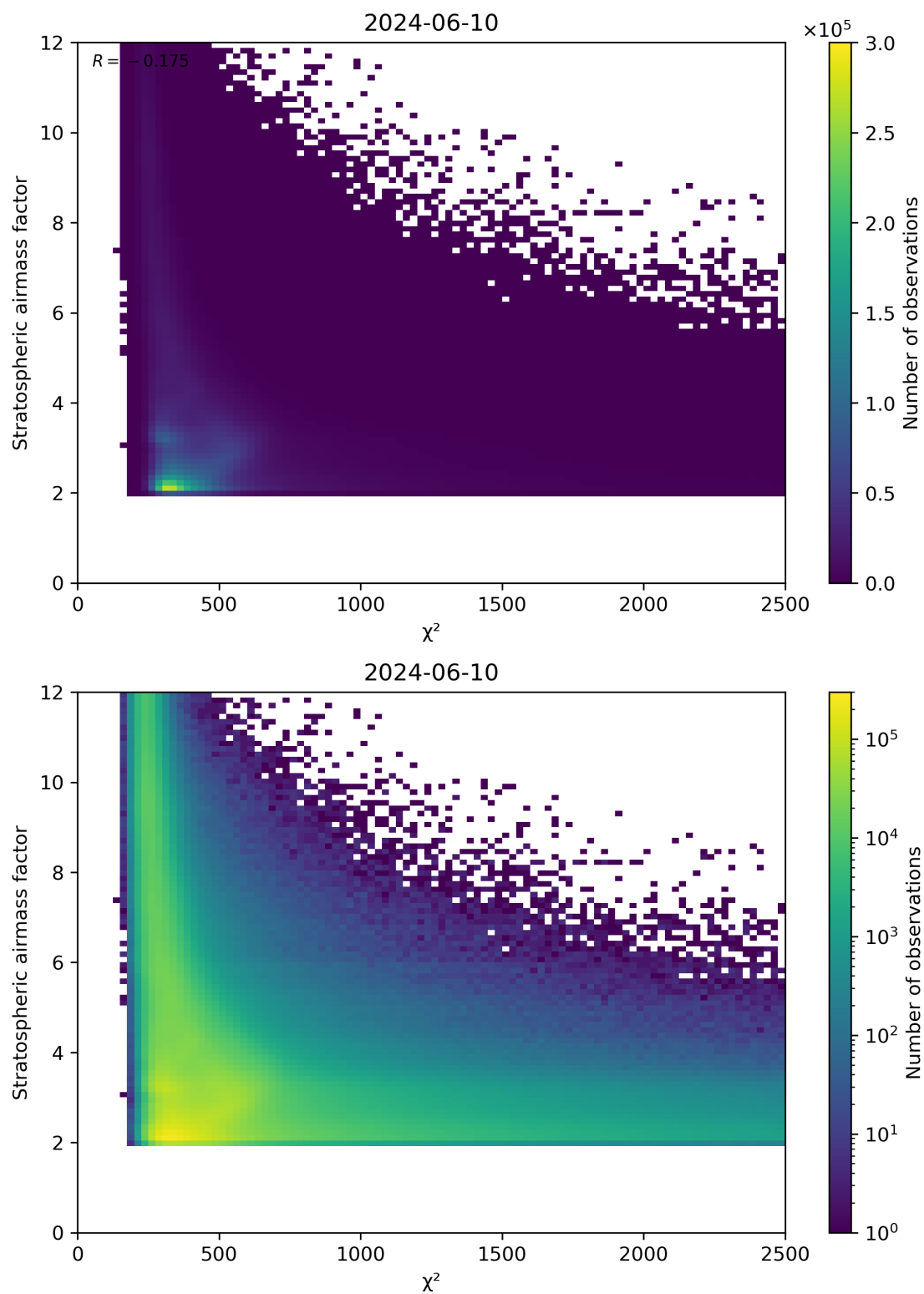
Figure 81: Scatter density plot of “ \chi^2 ” against “Stratospheric airmass factor” for 2024-06-09 to 2024-06-11.
