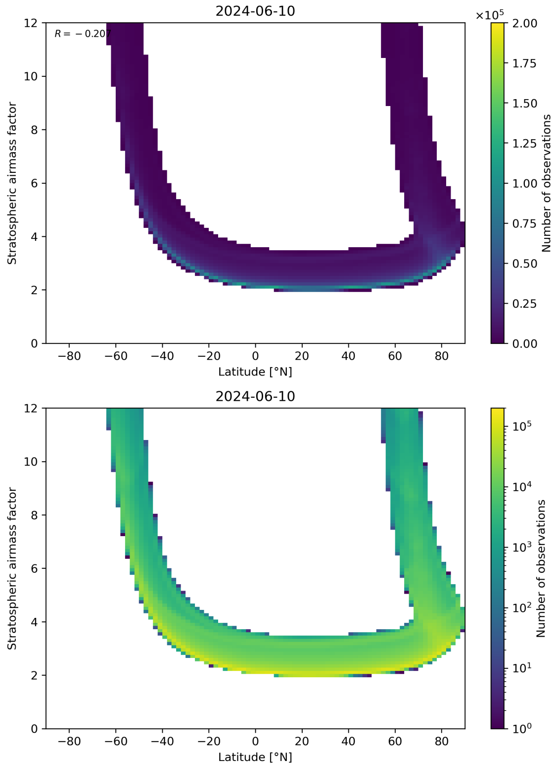
Figure 83: Scatter density plot of “Latitude” against “Stratospheric air mass factor” for 2024-06-09 to 2024-06-11.
