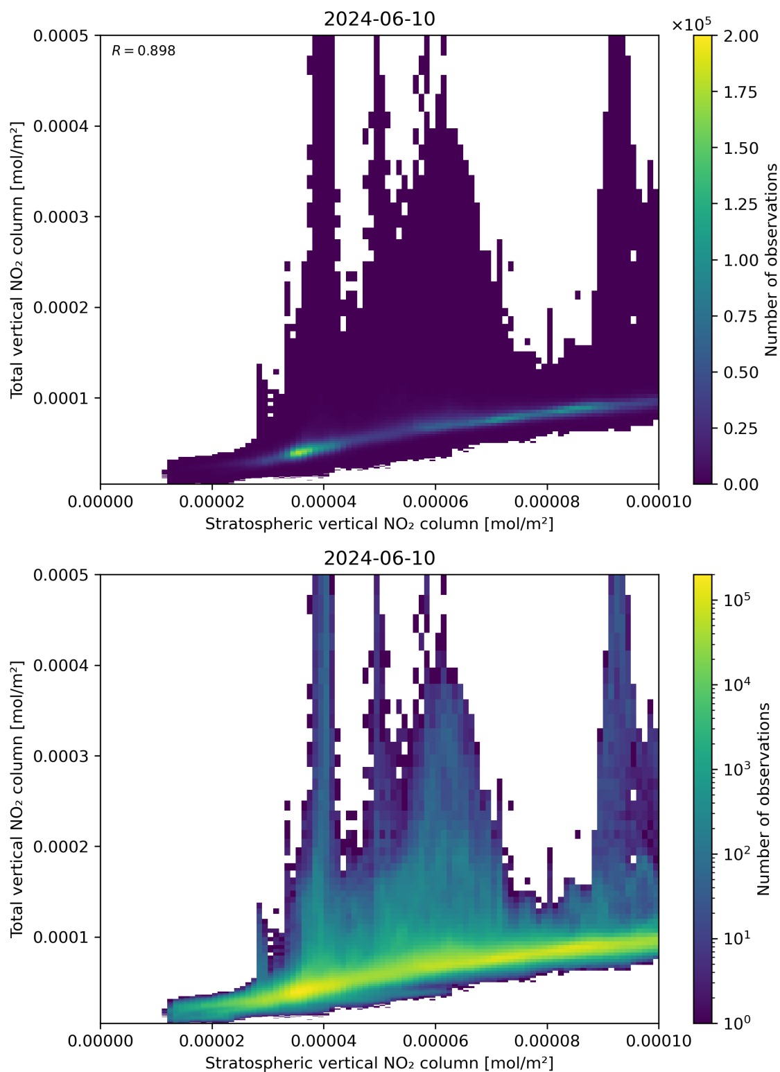
Figure 100: Scatter density plot of “Stratospheric vertical NO 2 column” against “Total vertical NO 2 column” for 2024-06-09 to 2024-06-11.
