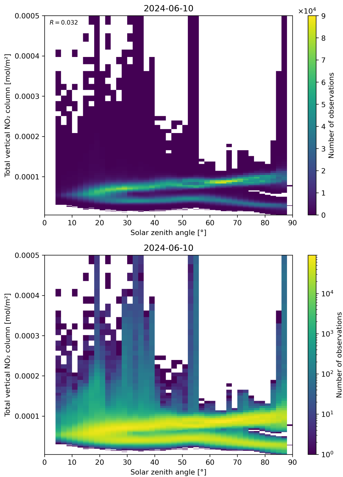
Figure 153: Scatter density plot of “Solar zenith angle” against “Total vertical NO 2 column” for 2024-06-09 to 2024-06-11.
