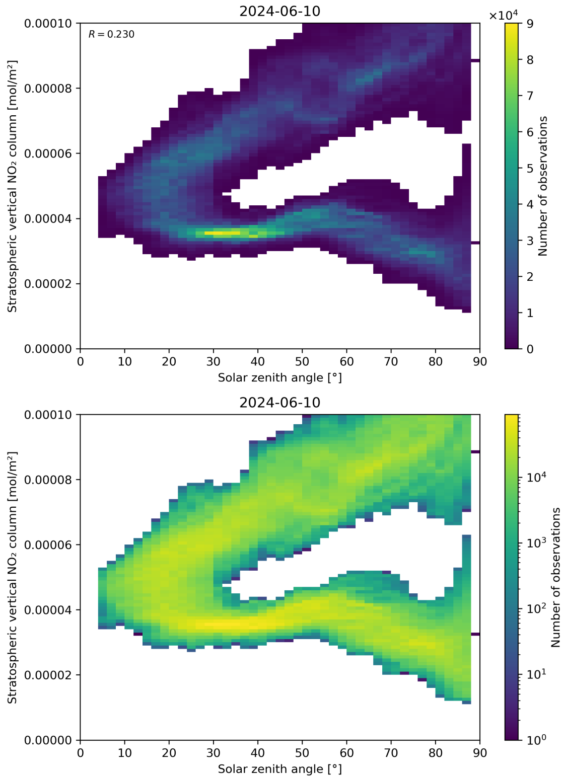
Figure 150: Scatter density plot of “Solar zenith angle” against “Stratospheric vertical NO 2 column” for 2024-06-09 to 2024-06-11.
