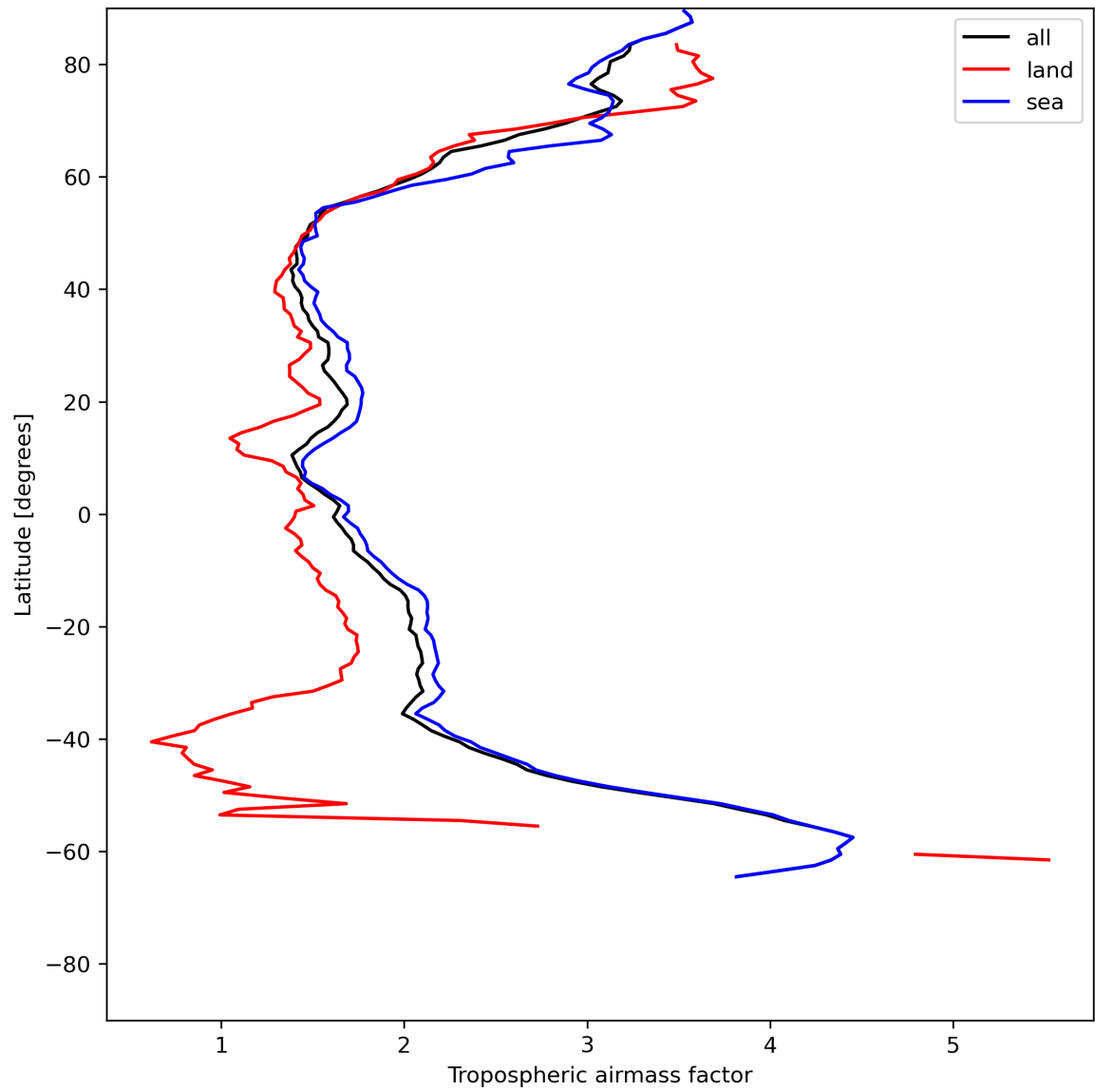
Figure 14: Zonal average of “Tropospheric airmass factor” for 2024-06-09 to 2024-06-11.
