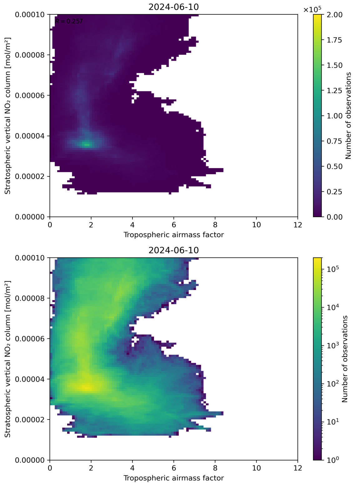
Figure 74: Scatter density plot of “Tropospheric air mass factor” against “Stratospheric vertical NO 2 column” for 2024-06-09 to 2024-06-11.
