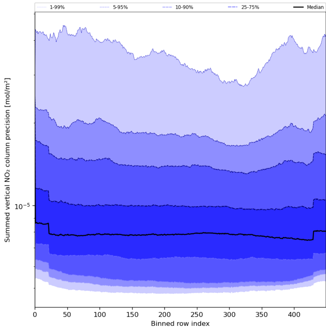
Figure 58: Along track statistics of “Summed vertical NO 2 column precision” for 2024-06-09 to 2024-06-11
