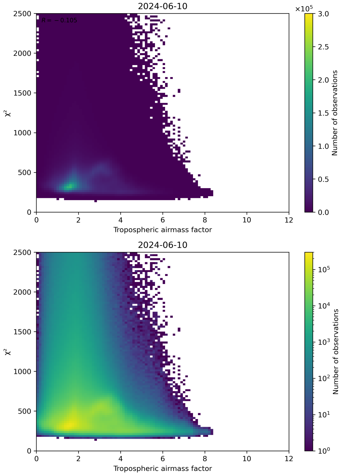
Figure 73: Scatter density plot of “Tropospheric airmass factor” against “ \chi^2 ” for 2024-06-09 to 2024-06-11.
