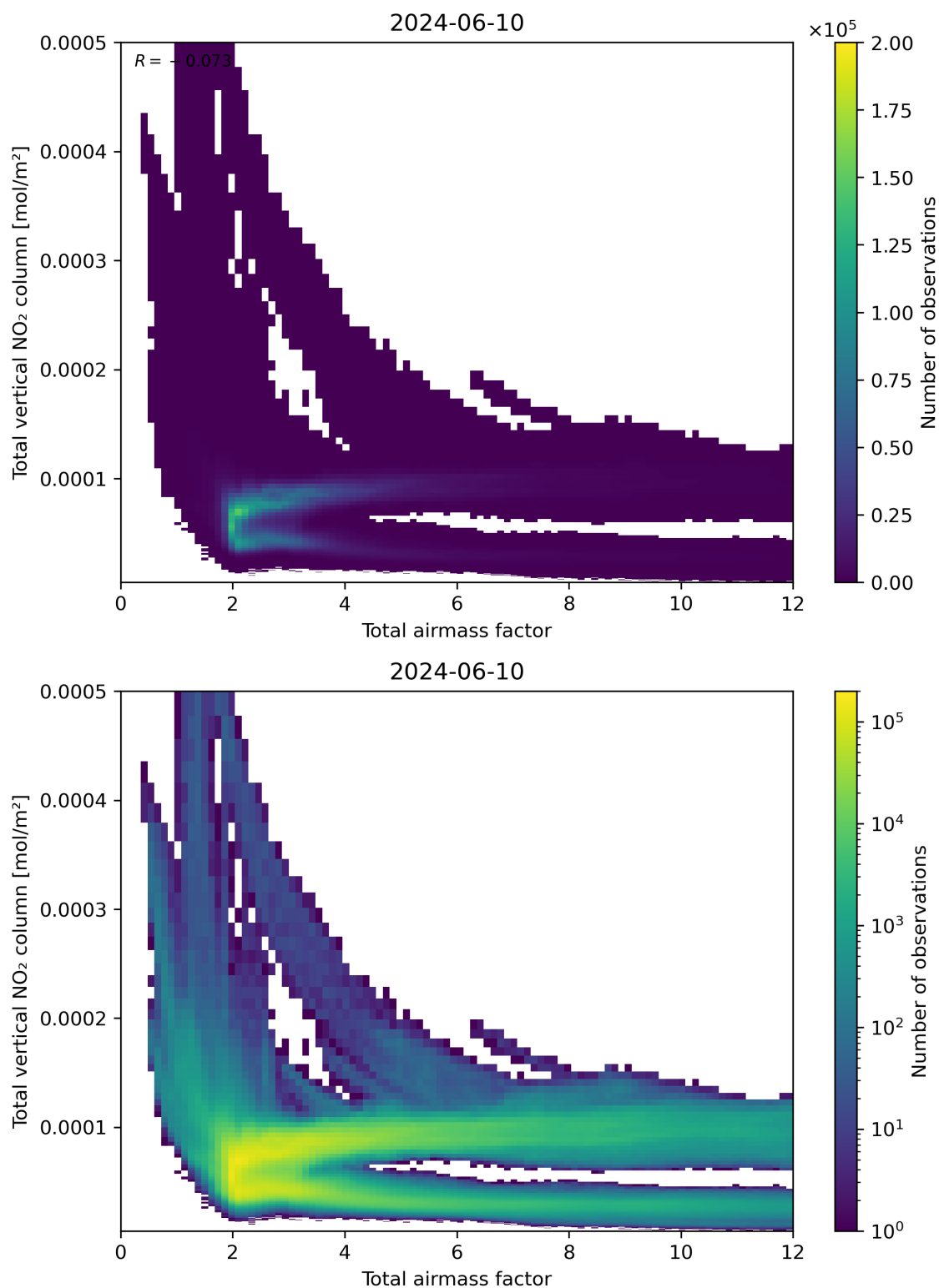
Figure 67: Scatter density plot of “Total air mass factor” against “Total vertical NO 2 column” for 2024-06-09 to 2024-06-11.
