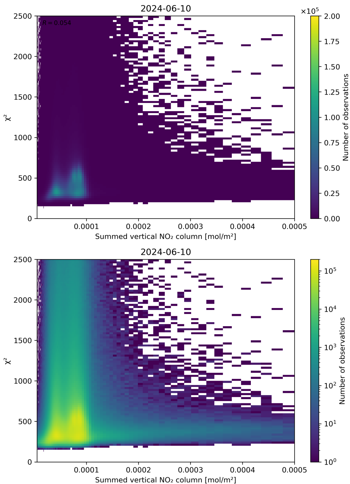
Figure 104: Scatter density plot of “Summed vertical NO 2 column” against “ \chi^2 ” for 2024-06-09 to 2024-06-11.
