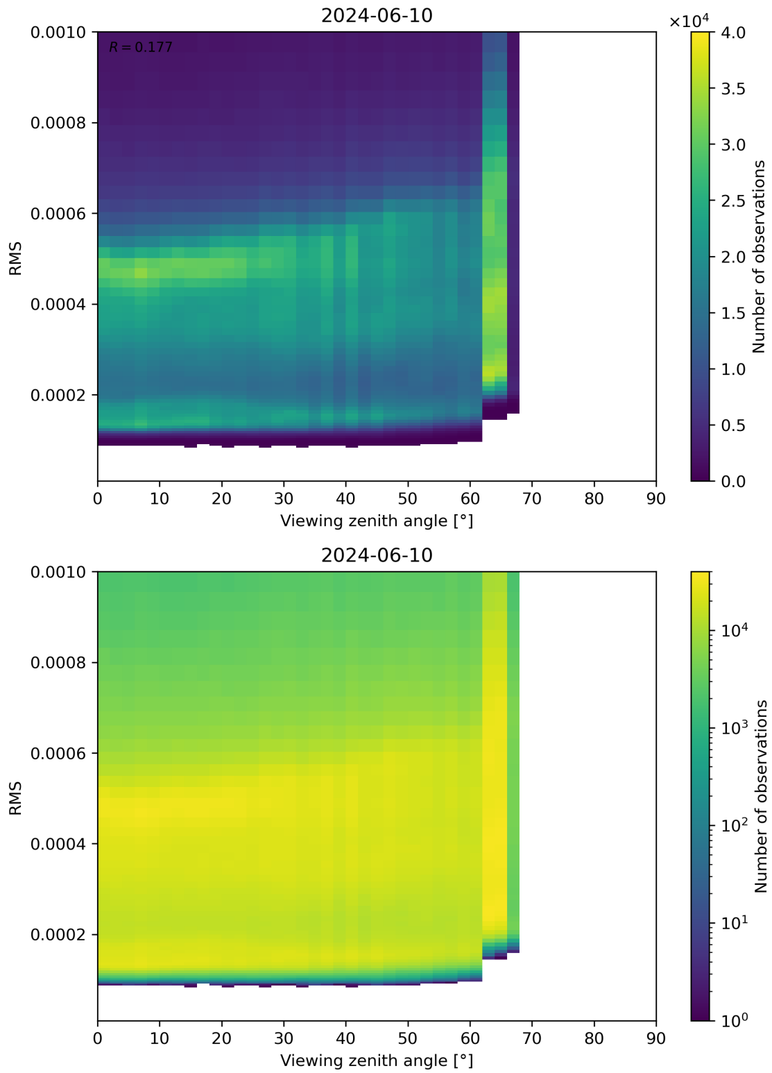
Figure 171: Scatter density plot of “Viewing zenith angle” against “RMS” for 2024-06-09 to 2024-06-11.
