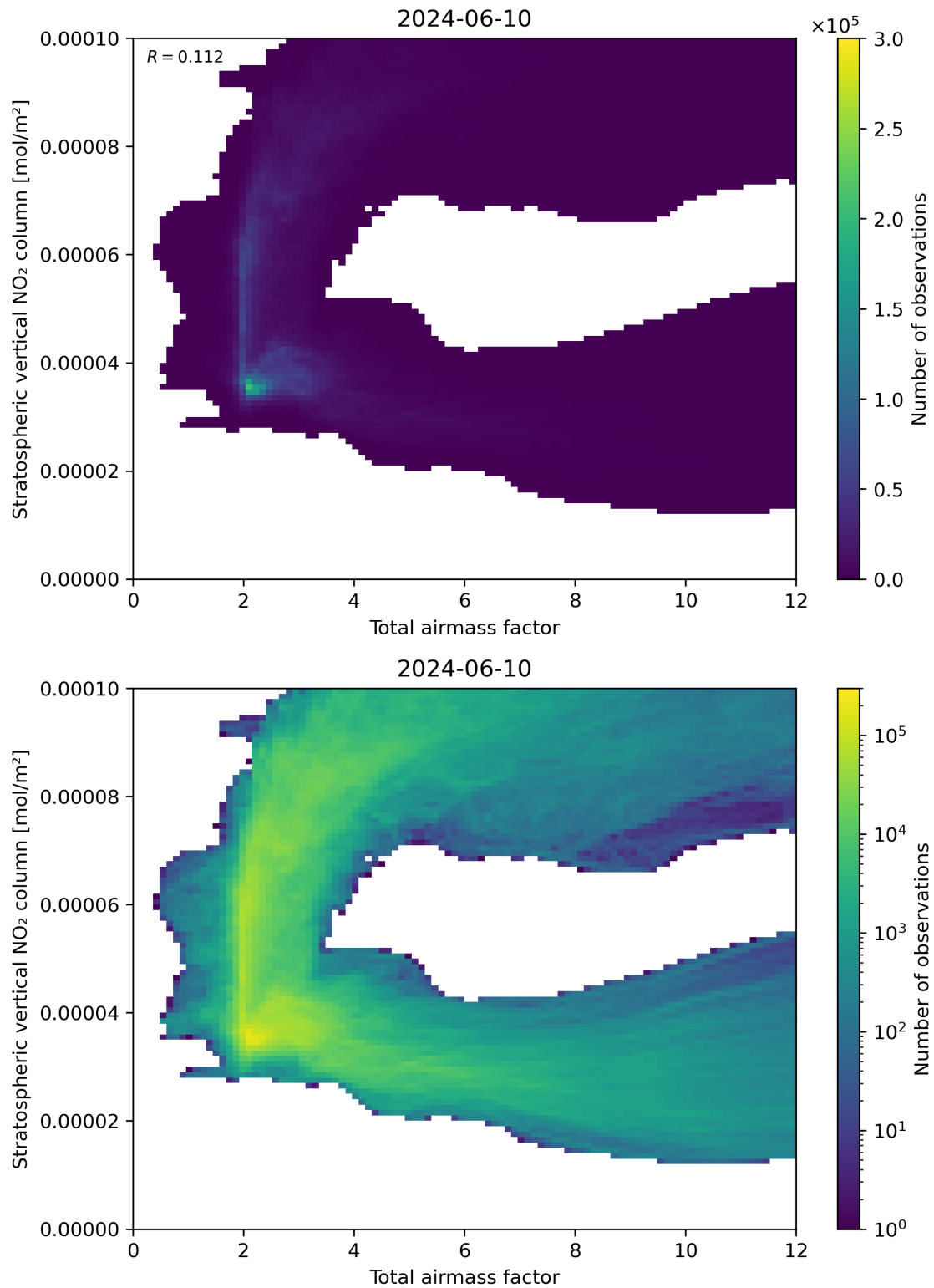
Figure 64: Scatter density plot of “Total airmass factor” against “Stratospheric vertical NO 2 column” for 2024-06-09 to 2024-06-11.
