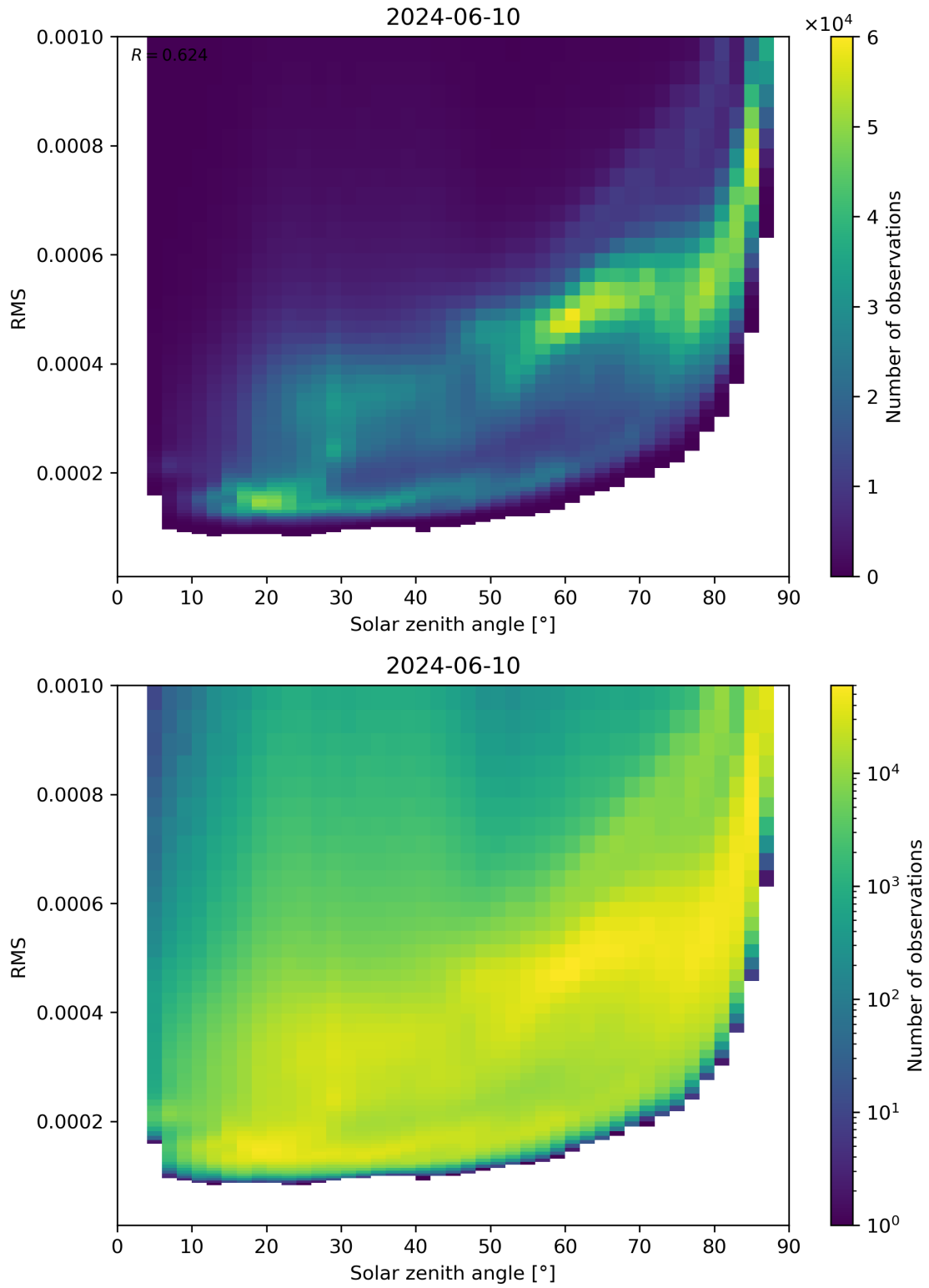
Figure 157: Scatter density plot of “Solar zenith angle” against “RMS” for 2024-06-09 to 2024-06-11.
