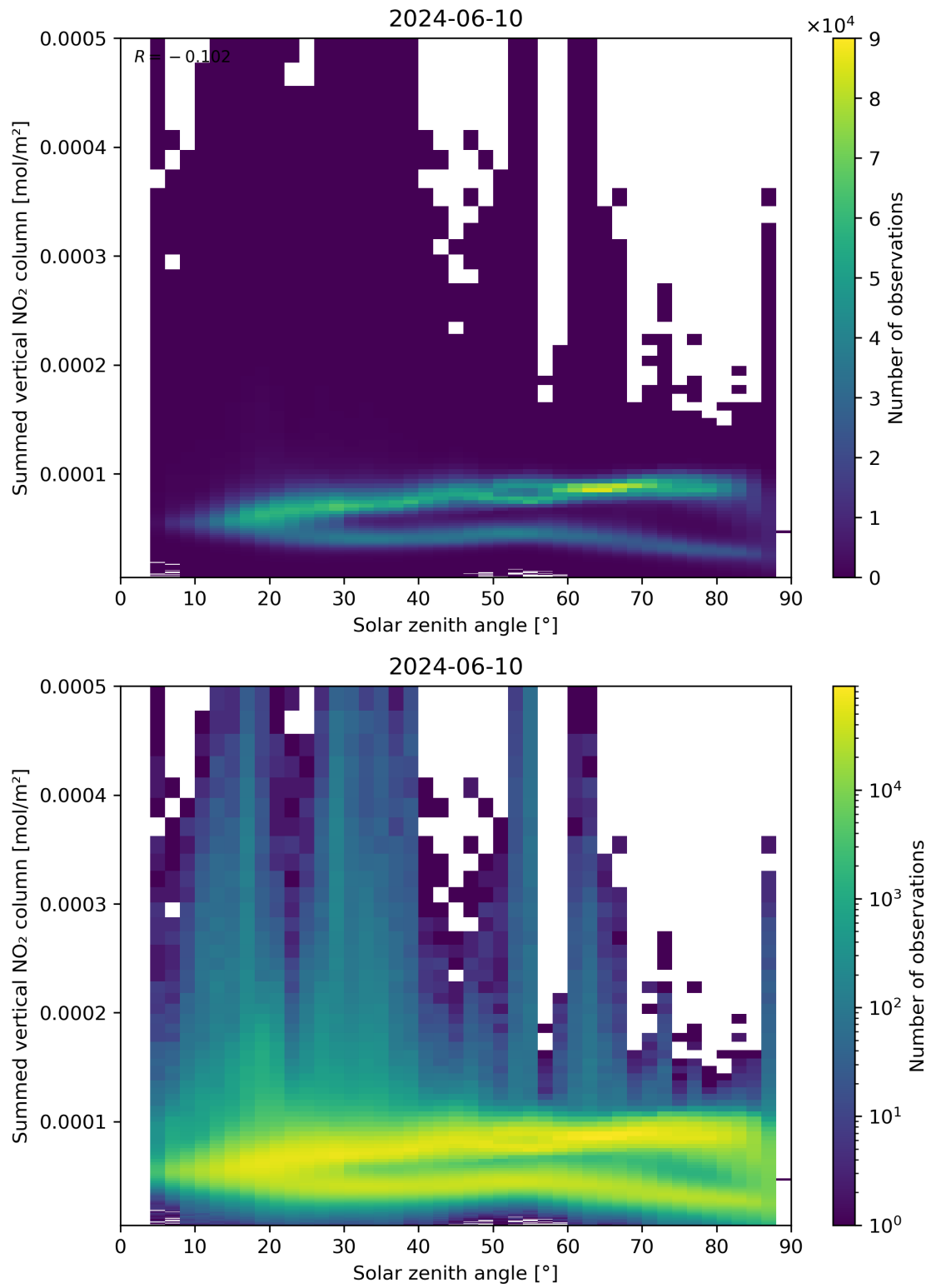
Figure 151: Scatter density plot of “Solar zenith angle” against “Summed vertical NO 2 column” for 2024-06-09 to 2024-06-11.
