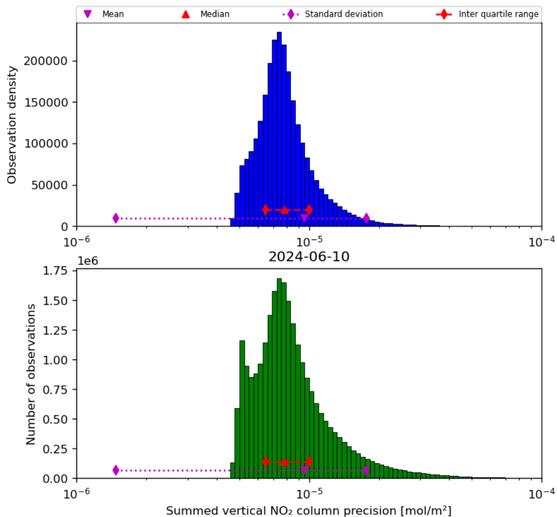
Figure 41: Histogram of "Summed vertical NO 2 column precision" for 2024-06-09 to 2024-06-11
