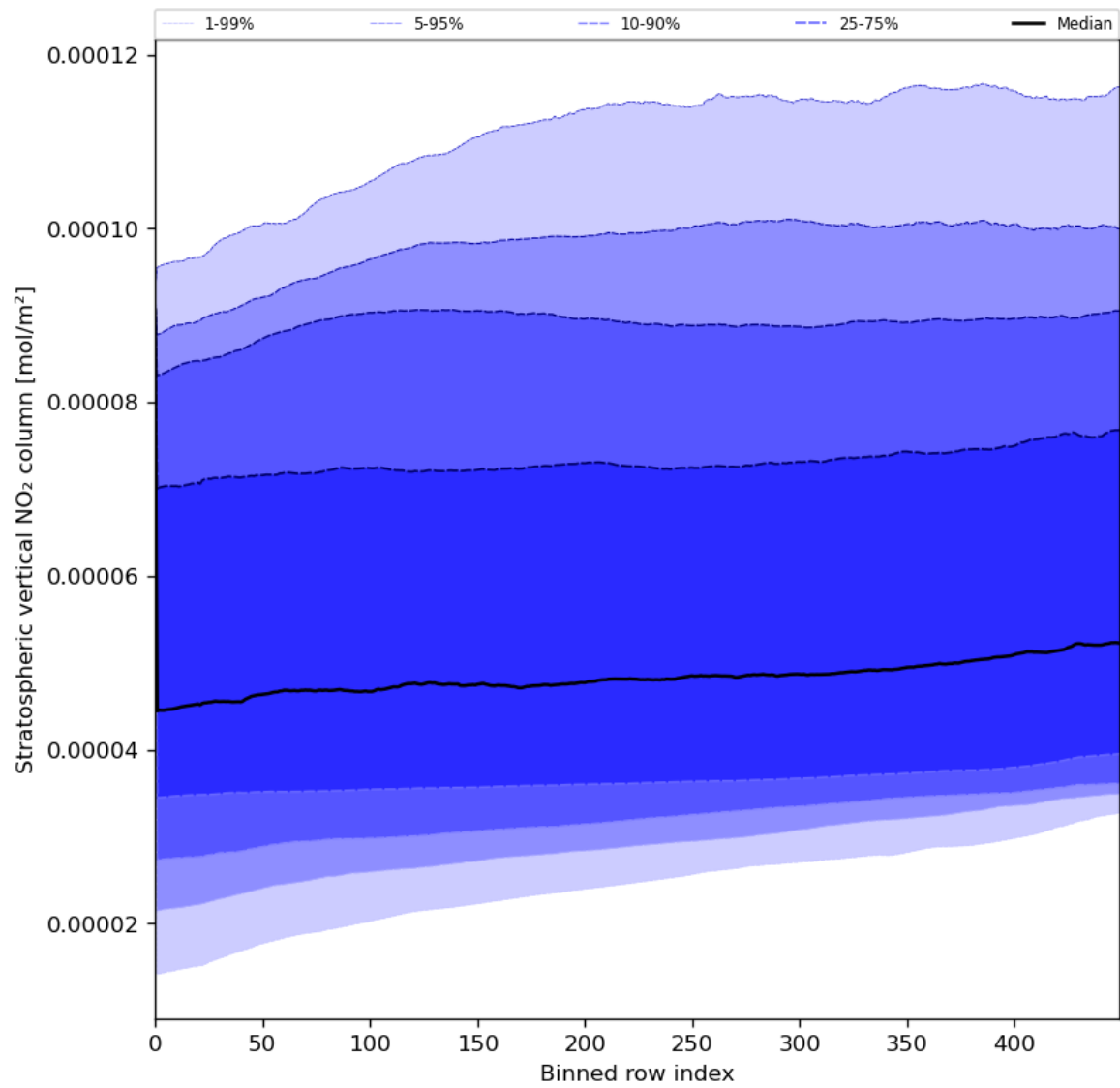
Figure 53: Along track statistics of “Stratospheric vertical NO 2 column” for 2024-06-09 to 2024-06-11
