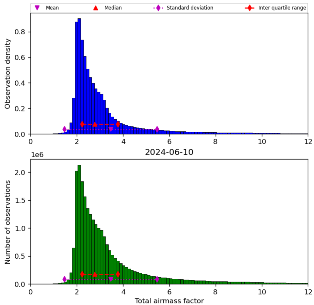
Figure 32: Histogram of “Total airmass factor” for 2024-06-09 to 2024-06-11
