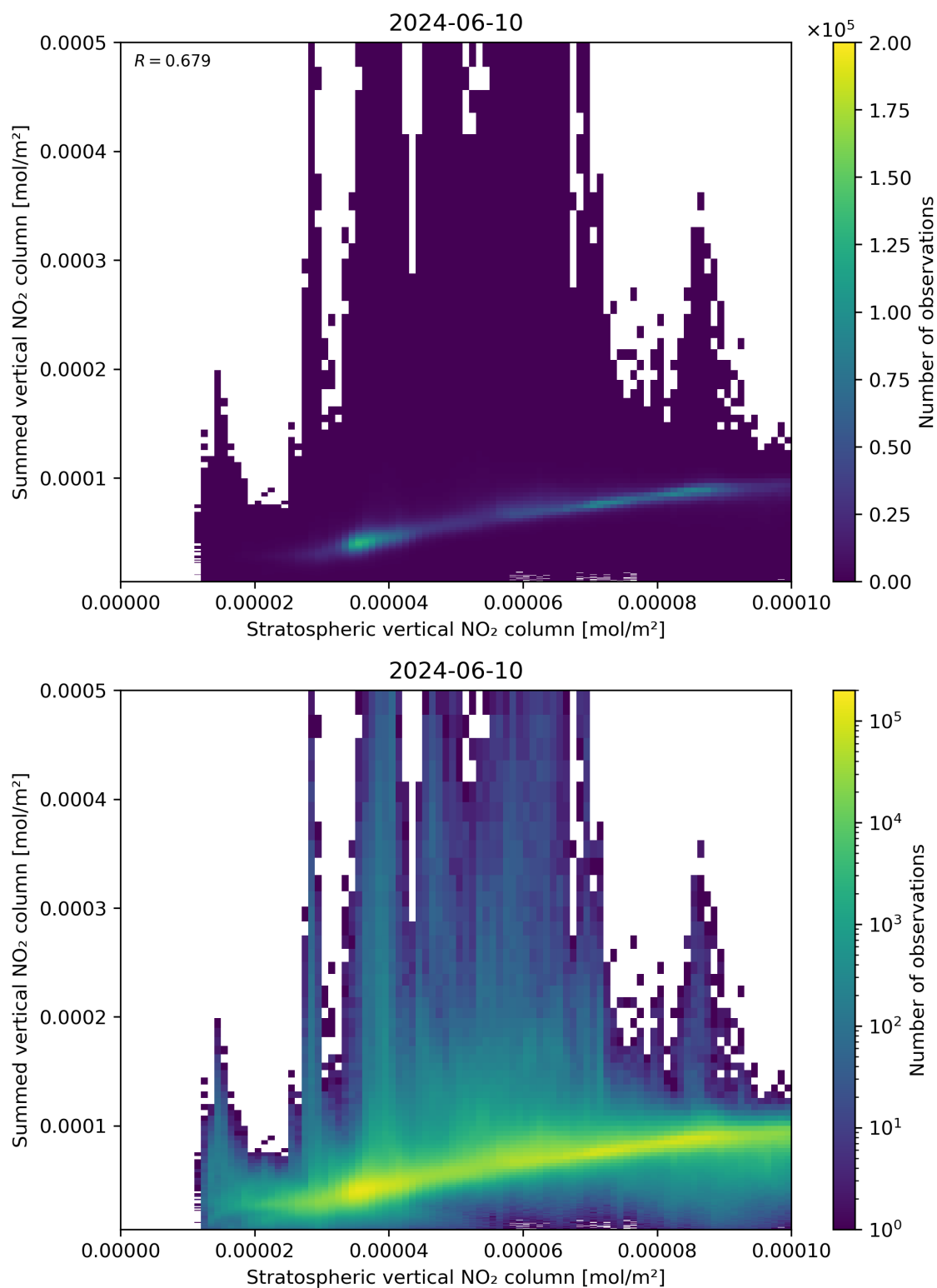
Figure 98: Scatter density plot of “Stratospheric vertical NO 2 column” against “Summed vertical NO 2 column” for 2024-06-09 to 2024-06-11.
