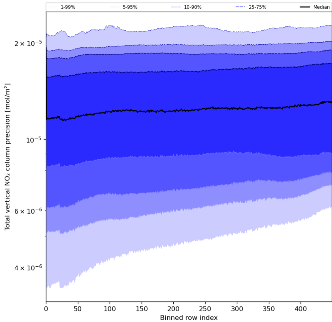
Figure 56: Along track statistics of “Total vertical NO 2 column precision” for 2024-06-09 to 2024-06-11
