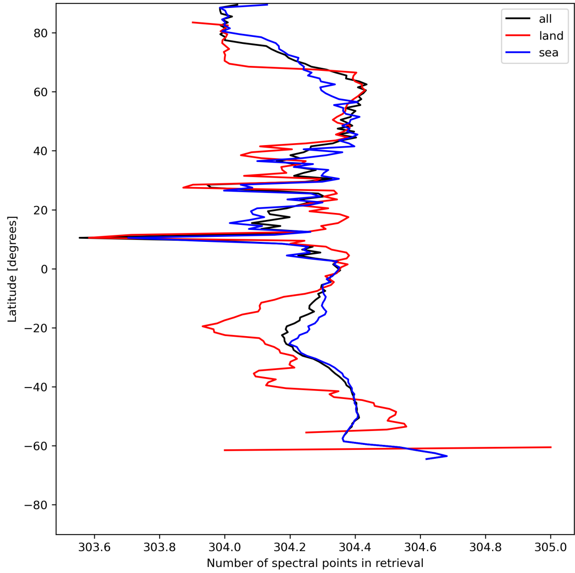
Figure 16: Zonal average of “Number of spectral points in retrieval” for 2024-06-09 to 2024-06-11.
