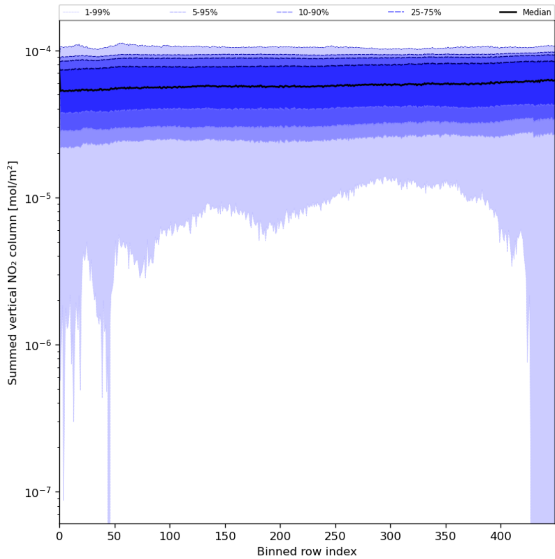
Figure 57: Along track statistics of “Summed vertical NO 2 column” for 2024-06-09 to 2024-06-11
