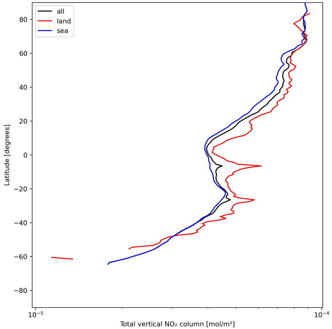
Figure 21: Zonal average of “Total vertical NO 2 column” for 2024-06-09 to 2024-06-11.
