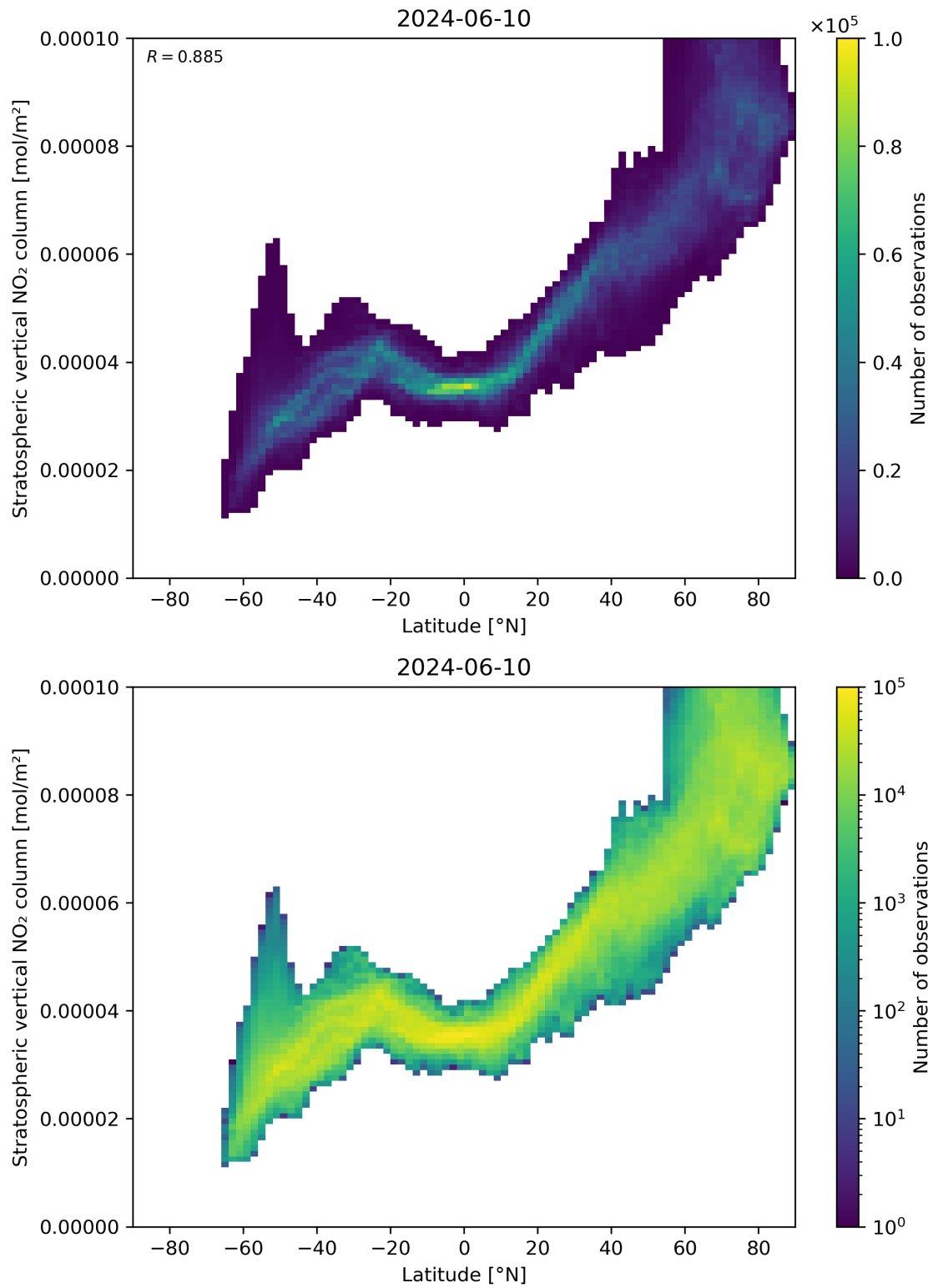
Figure 87: Scatter density plot of “Latitude” against “Stratospheric vertical NO 2 column” for 2024-06-09 to 2024-06-11.
