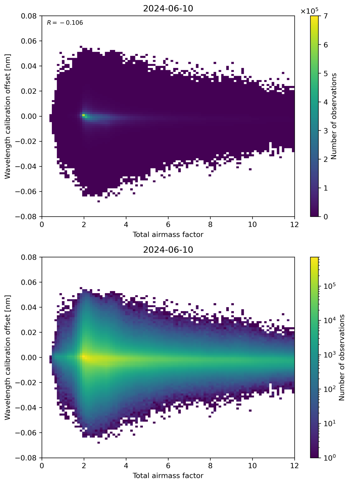
Figure 70: Scatter density plot of “Total airmass factor” against “Wavelength calibration offset” for 2024-06-09 to 2024-06-11.
