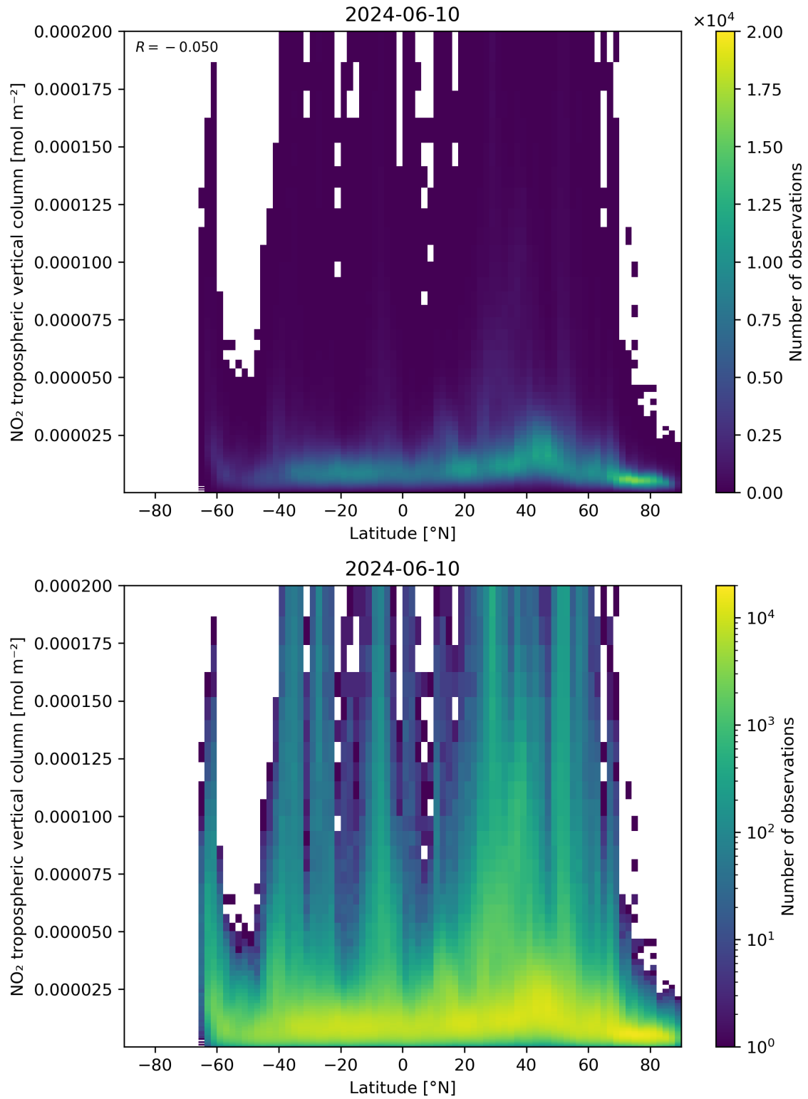
Figure 92: Scatter density plot of “Latitude” against “NO 2 tropospheric vertical column” for 2024-06-09 to 2024-06-11.
