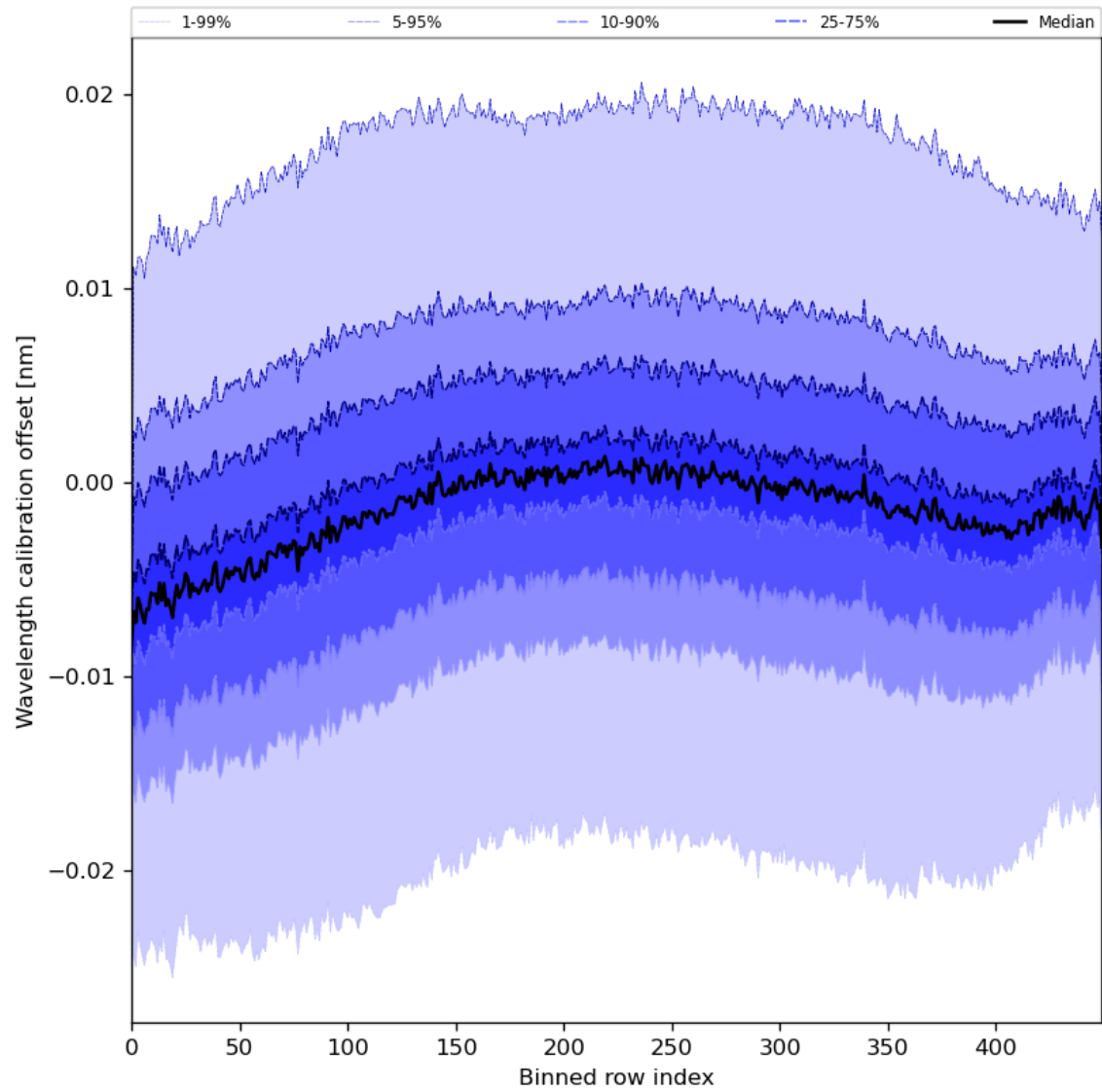
Figure 52: Along track statistics of “Wavelength calibration offset” for 2024-06-09 to 2024-06-11
