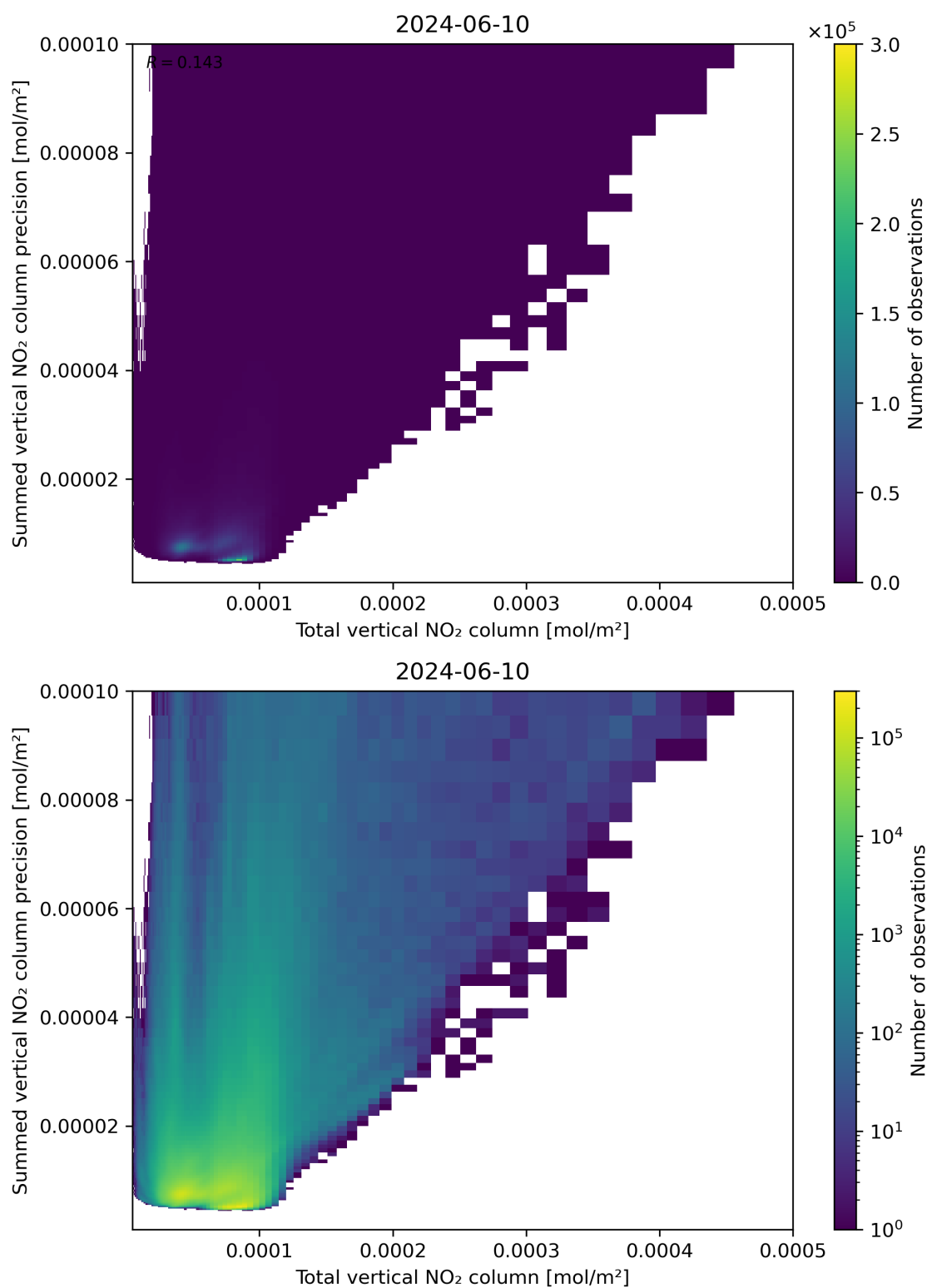
Figure 113: Scatter density plot of “Total vertical NO 2 column” against “Summed vertical NO 2 column precision” for 2024-06-09 to 2024-06-11.
