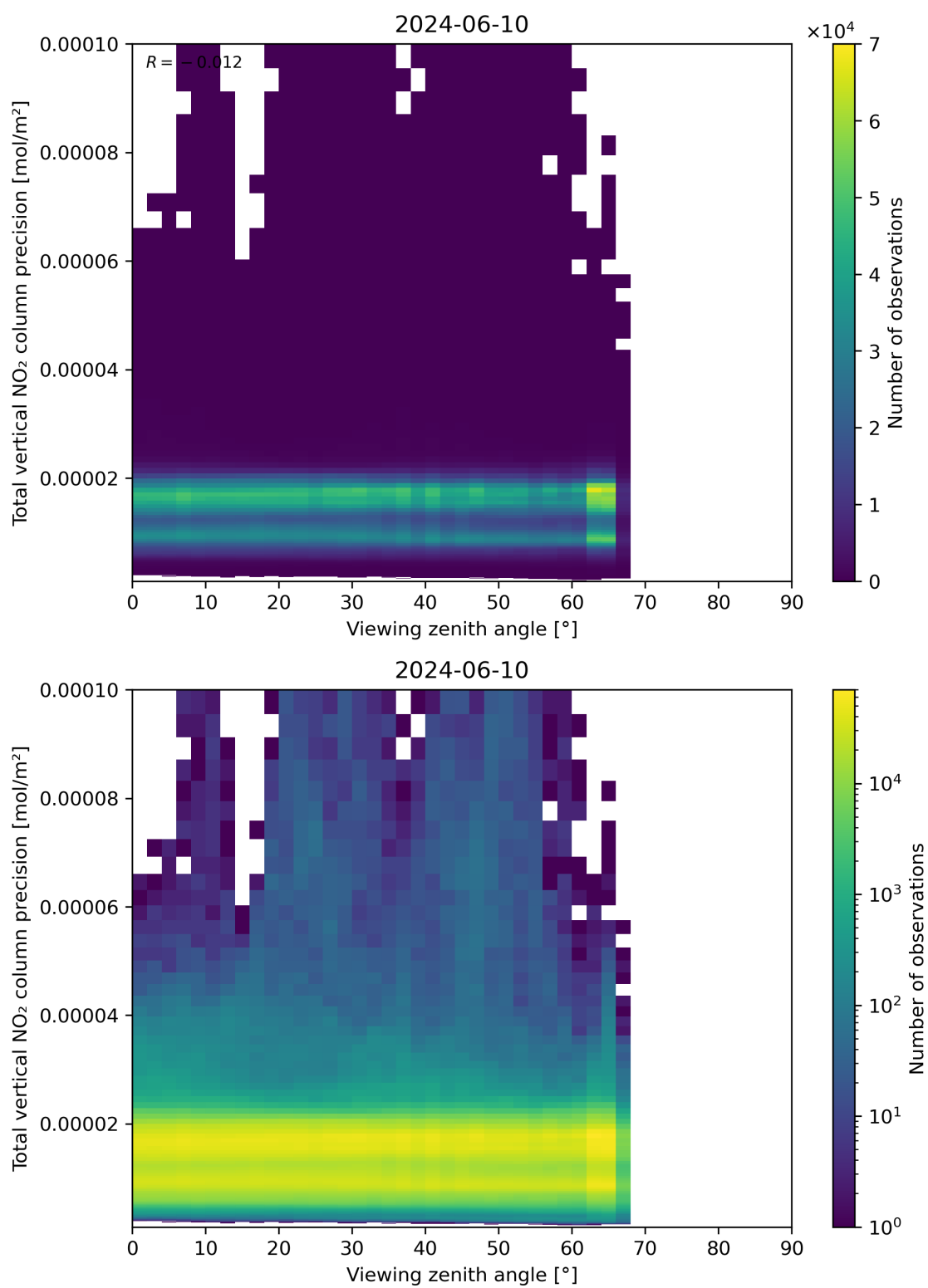
Figure 168: Scatter density plot of “Viewing zenith angle” against “Total vertical NO 2 column precision” for 2024-06-09 to 2024-06-11.
