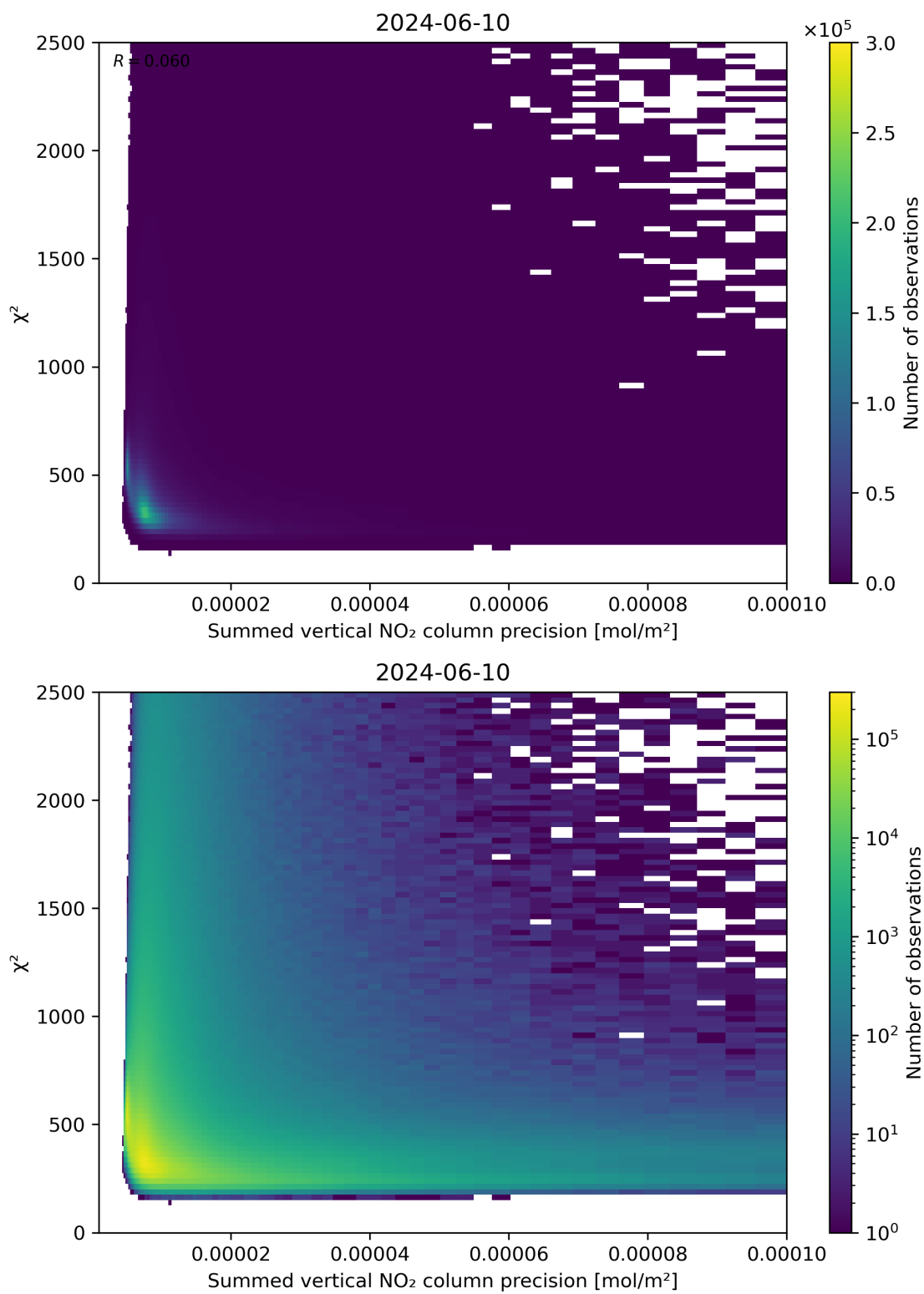
Figure 107: Scatter density plot of “Summed vertical NO 2 column precision” against “ \chi^2 ” for 2024-06-09 to 2024-06-11.
