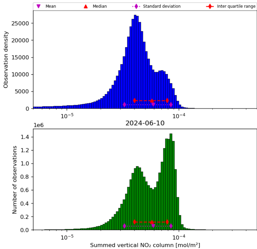
Figure 40: Histogram of “Summed vertical NO 2 column” for 2024-06-09 to 2024-06-11
