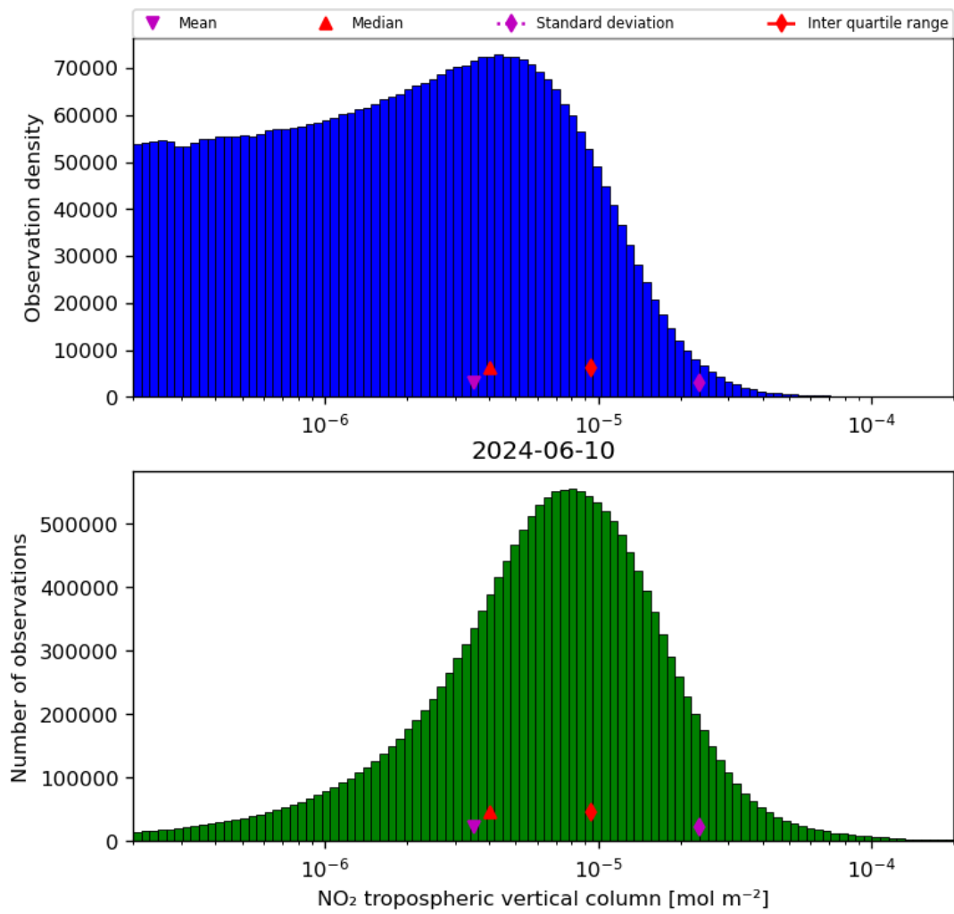
Figure 29: Histogram of “NO 2 tropospheric vertical column” for 2024-06-09 to 2024-06-11
