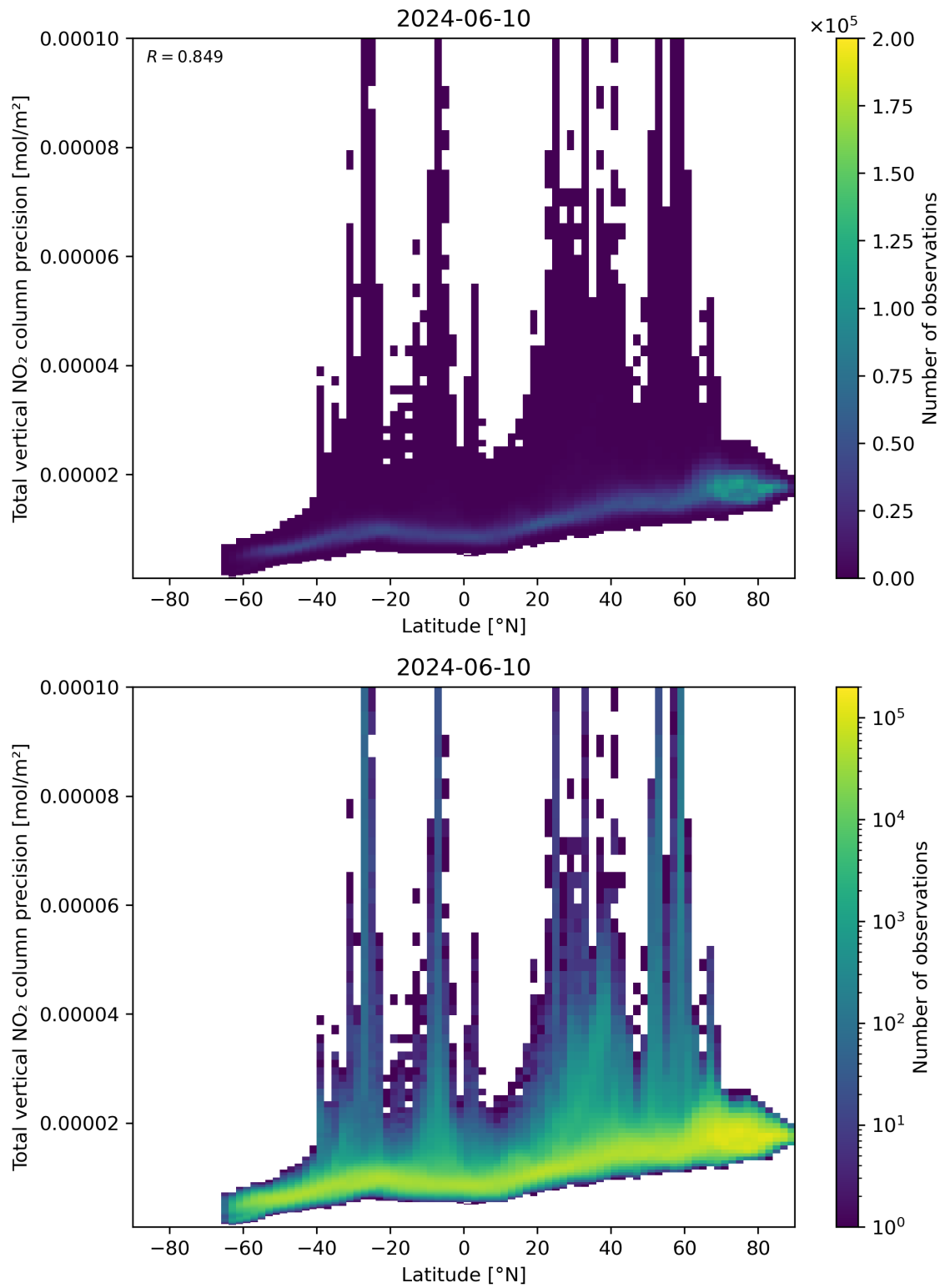
Figure 91: Scatter density plot of “Latitude” against “Total vertical NO 2 column precision” for 2024-06-09 to 2024-06-11.
