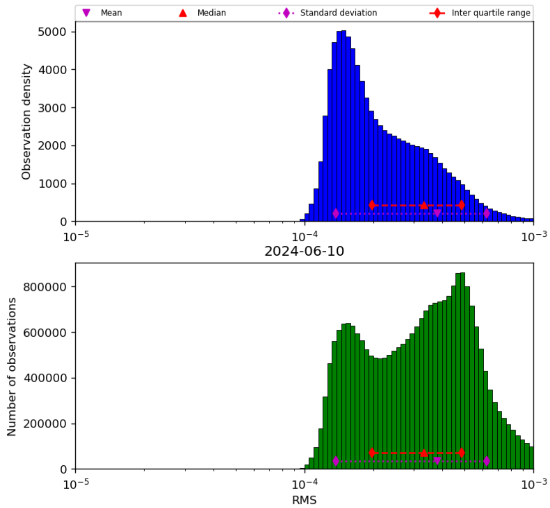
Figure 43: Histogram of “RMS” for 2024-06-09 to 2024-06-11
