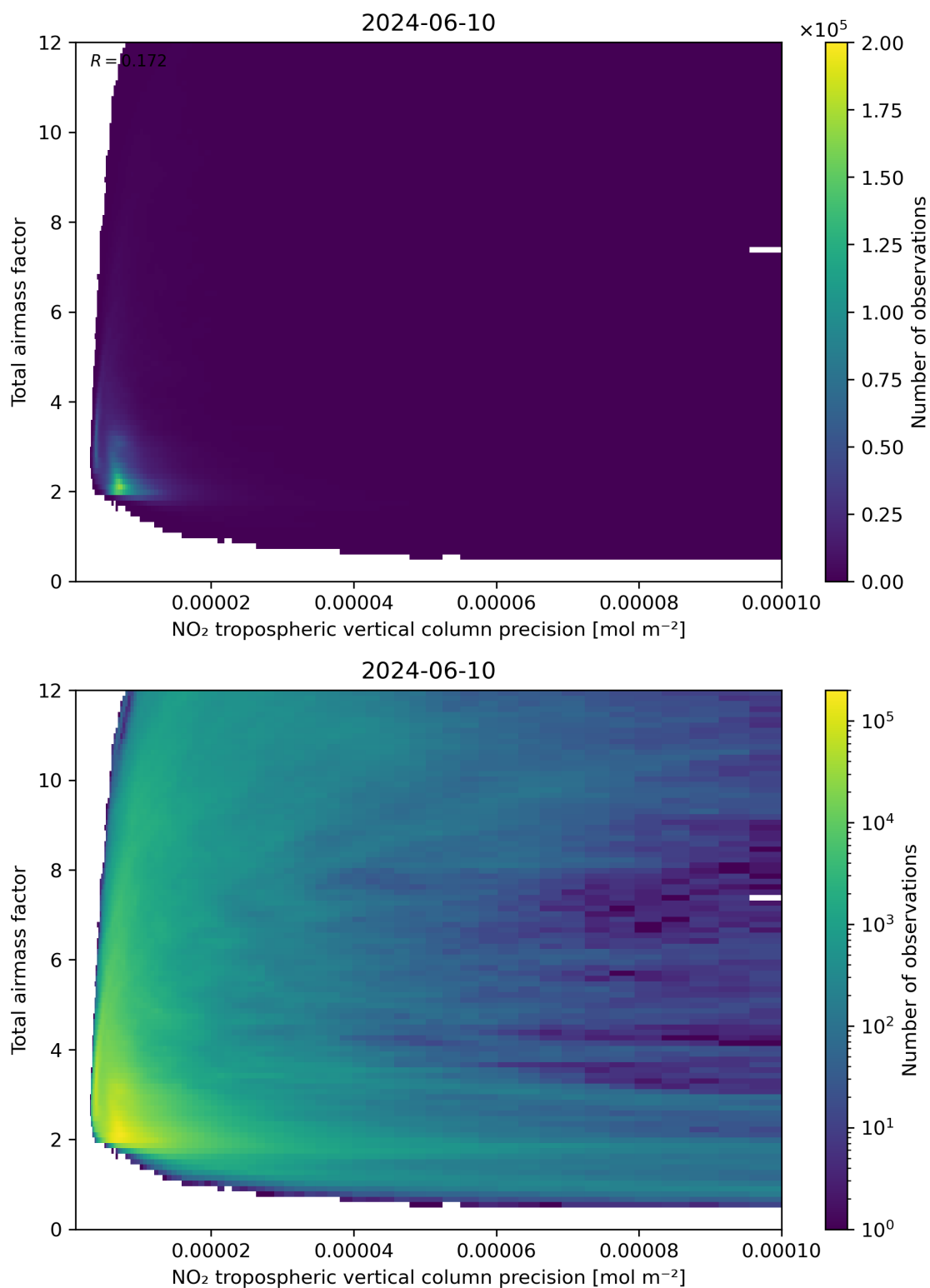
Figure 132: Scatter density plot of “NO 2 tropospheric vertical column precision” against “Total air mass factor” for 2024-06-09 to 2024-06-11.
