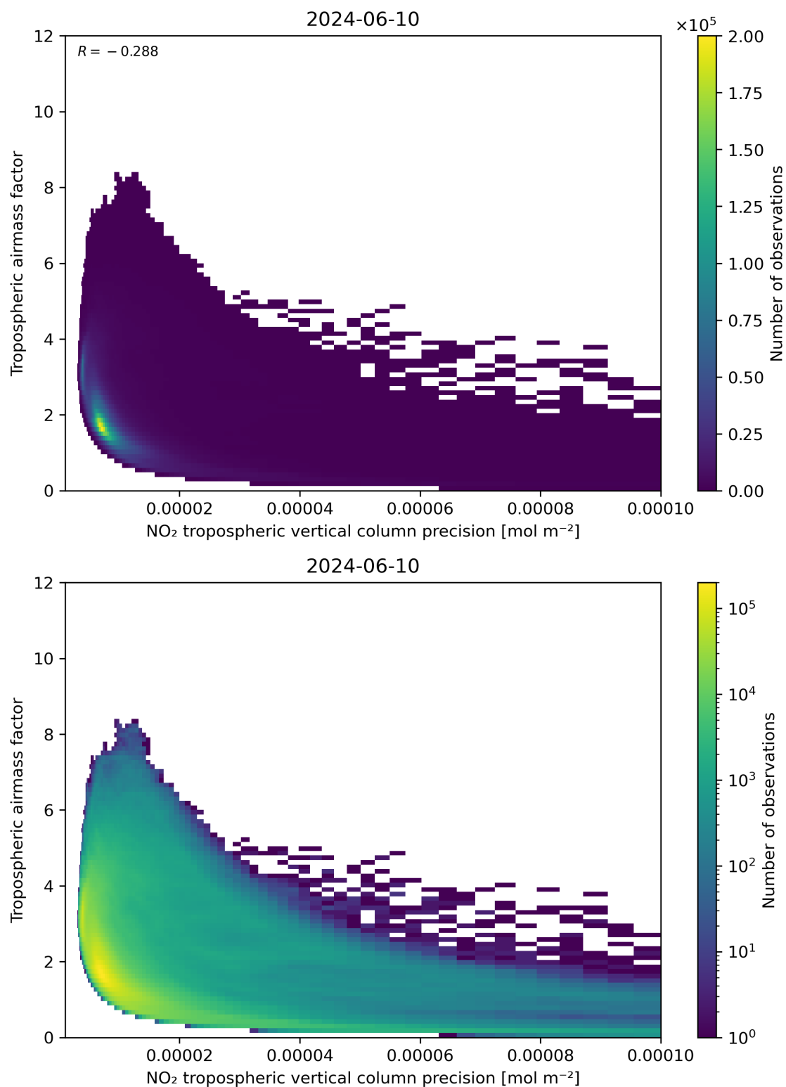
Figure 133: Scatter density plot of “NO 2 tropospheric vertical column precision” against “Tropospheric airmass factor” for 2024-06-09 to 2024-06-11.
