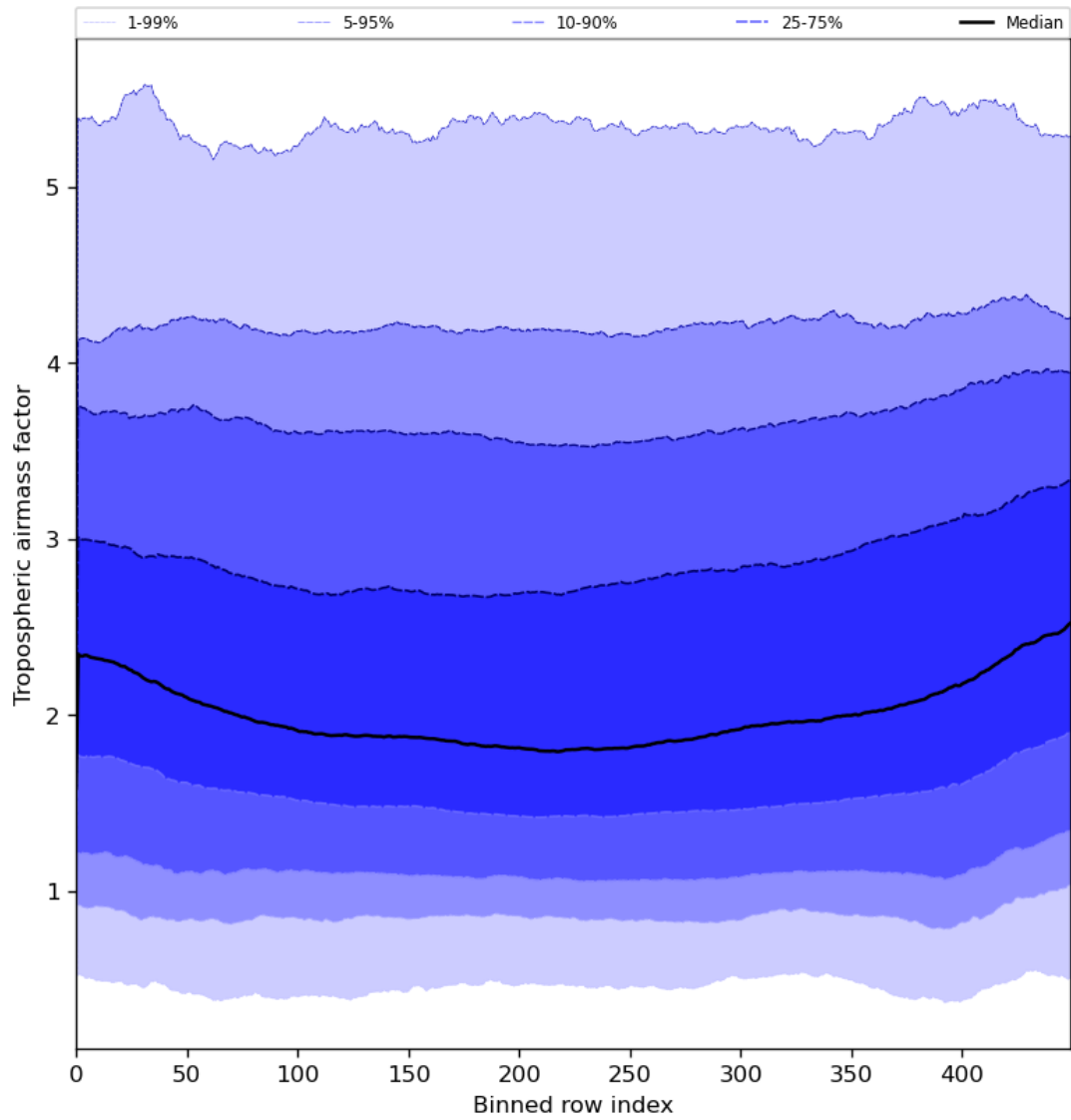
Figure 48: Along track statistics of “Tropospheric airmass factor” for 2024-06-09 to 2024-06-11
