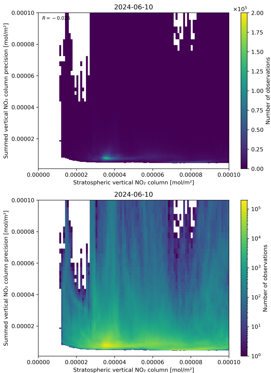
Figure 99: Scatter density plot of “Stratospheric vertical NO 2 column” against “Summed vertical NO 2 column precision” for 2024-06-09 to 2024-06-11.
