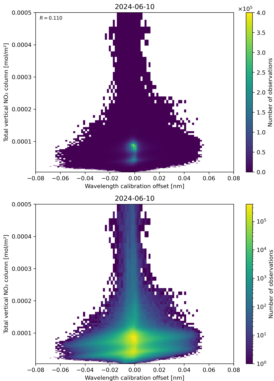
Figure 179: Scatter density plot of “Wavelength calibration offset” against “Total vertical NO 2 column” for 2024-06-09 to 2024-06-11.
