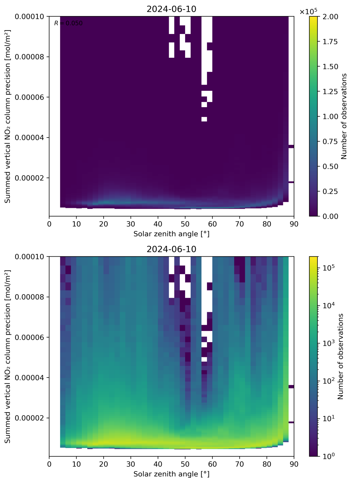
Figure 152: Scatter density plot of “Solar zenith angle” against “Summed vertical NO 2 column precision” for 2024-06-09 to 2024-06-11.
