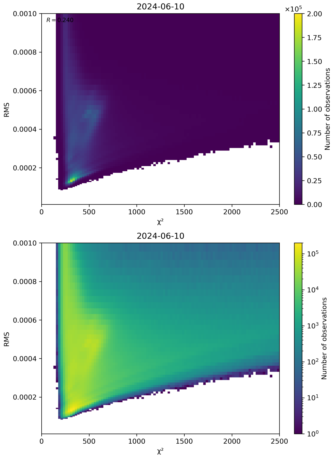
Figure 82: Scatter density plot of “ \chi^2 ” against “RMS” for 2024-06-09 to 2024-06-11.
