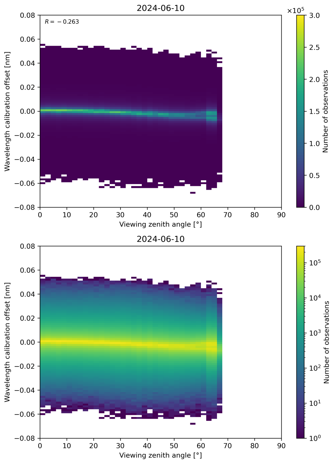
Figure 173: Scatter density plot of “Viewing zenith angle” against “Wavelength calibration offset” for 2024-06-09 to 2024-06-11.
