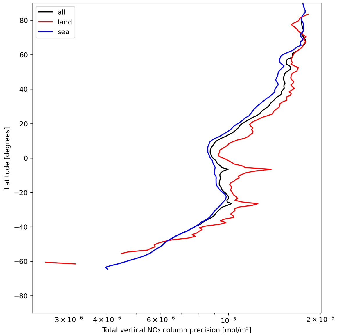
Figure 22: Zonal average of “Total vertical NO 2 column precision” for 2024-06-09 to 2024-06-11.
