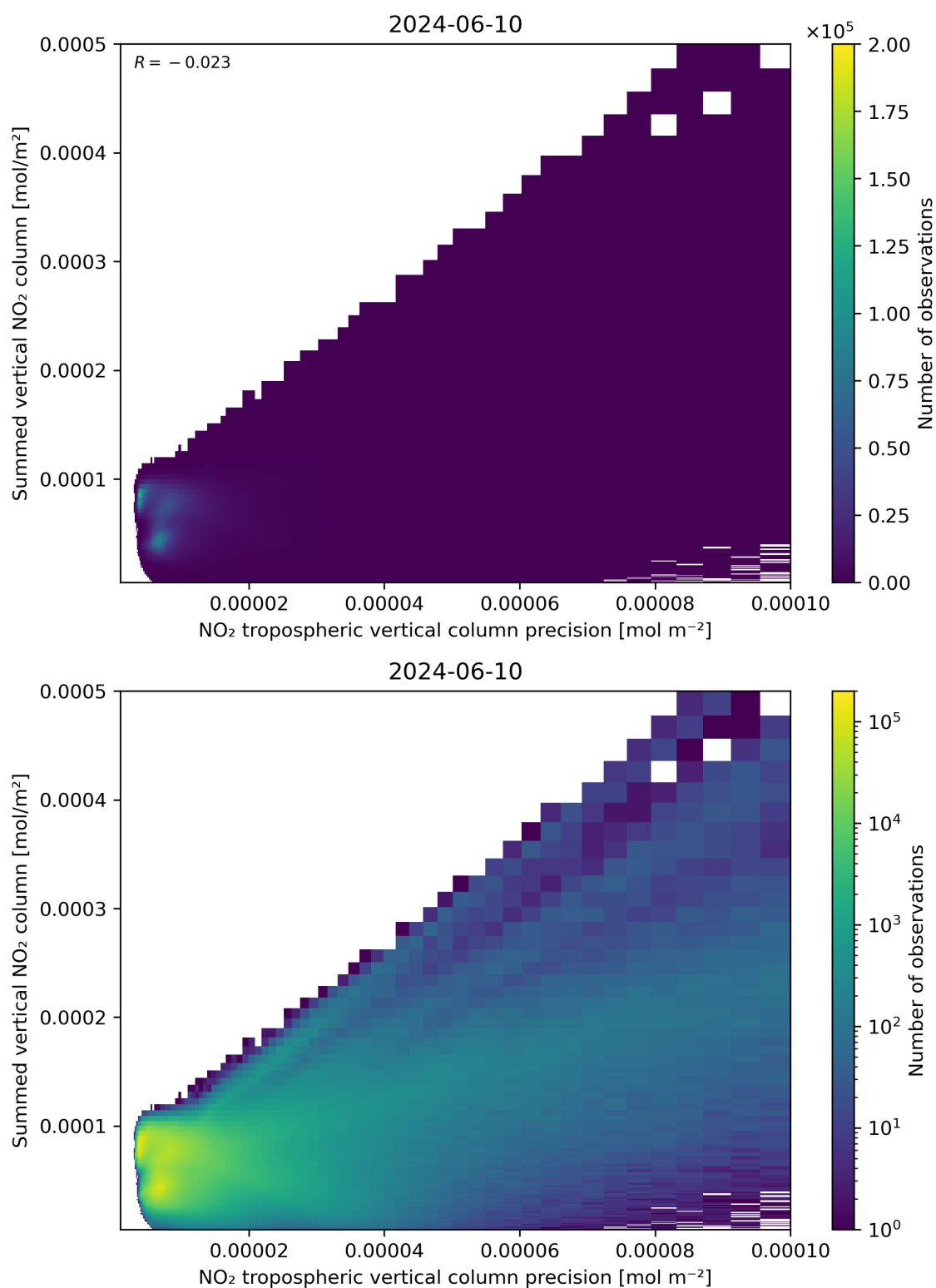
Figure 136: Scatter density plot of “NO 2 tropospheric vertical column precision” against “Summed vertical NO 2 column” for 2024-06-09 to 2024-06-11.
