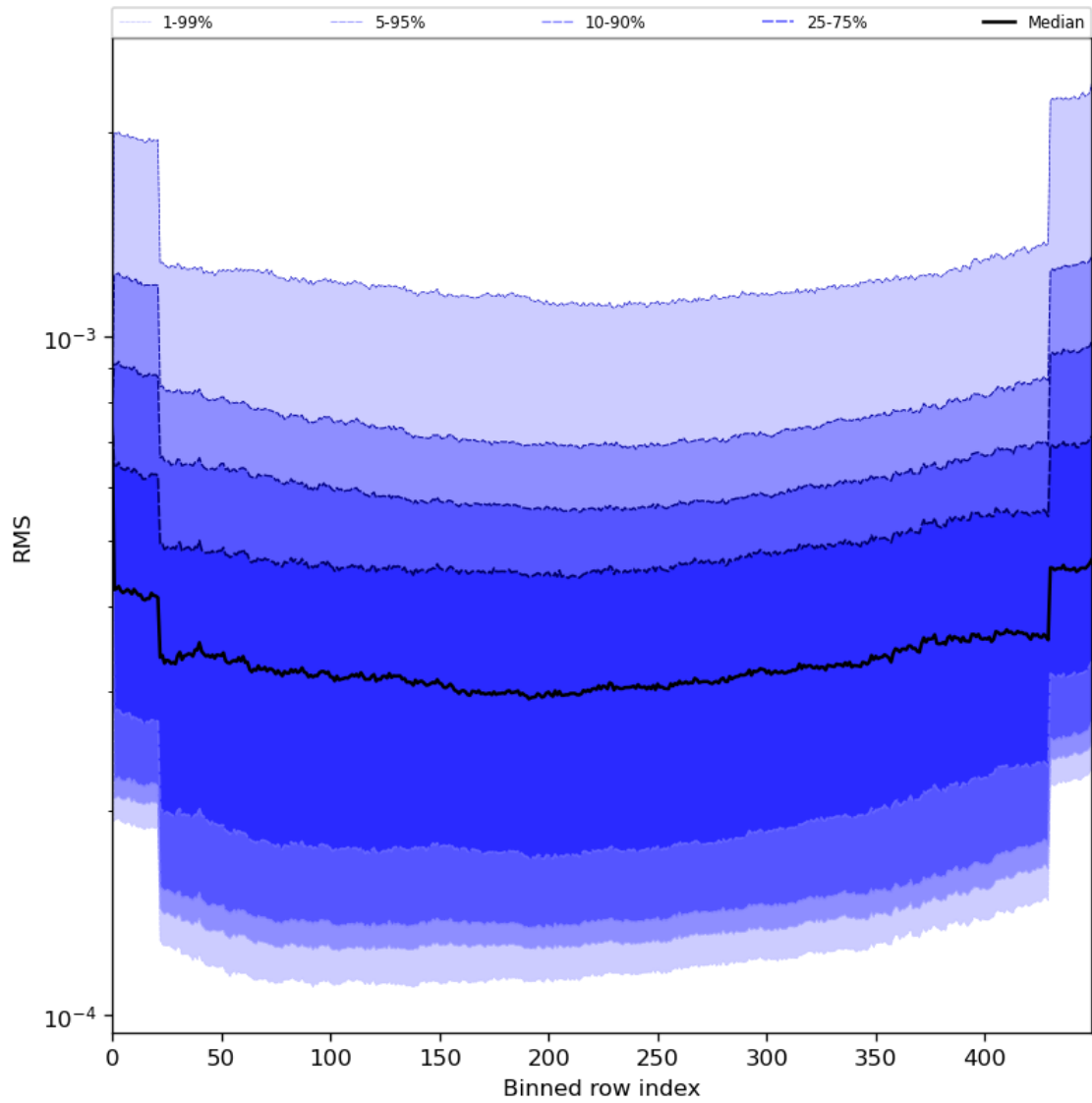
Figure 60: Along track statistics of “RMS” for 2024-06-09 to 2024-06-11
