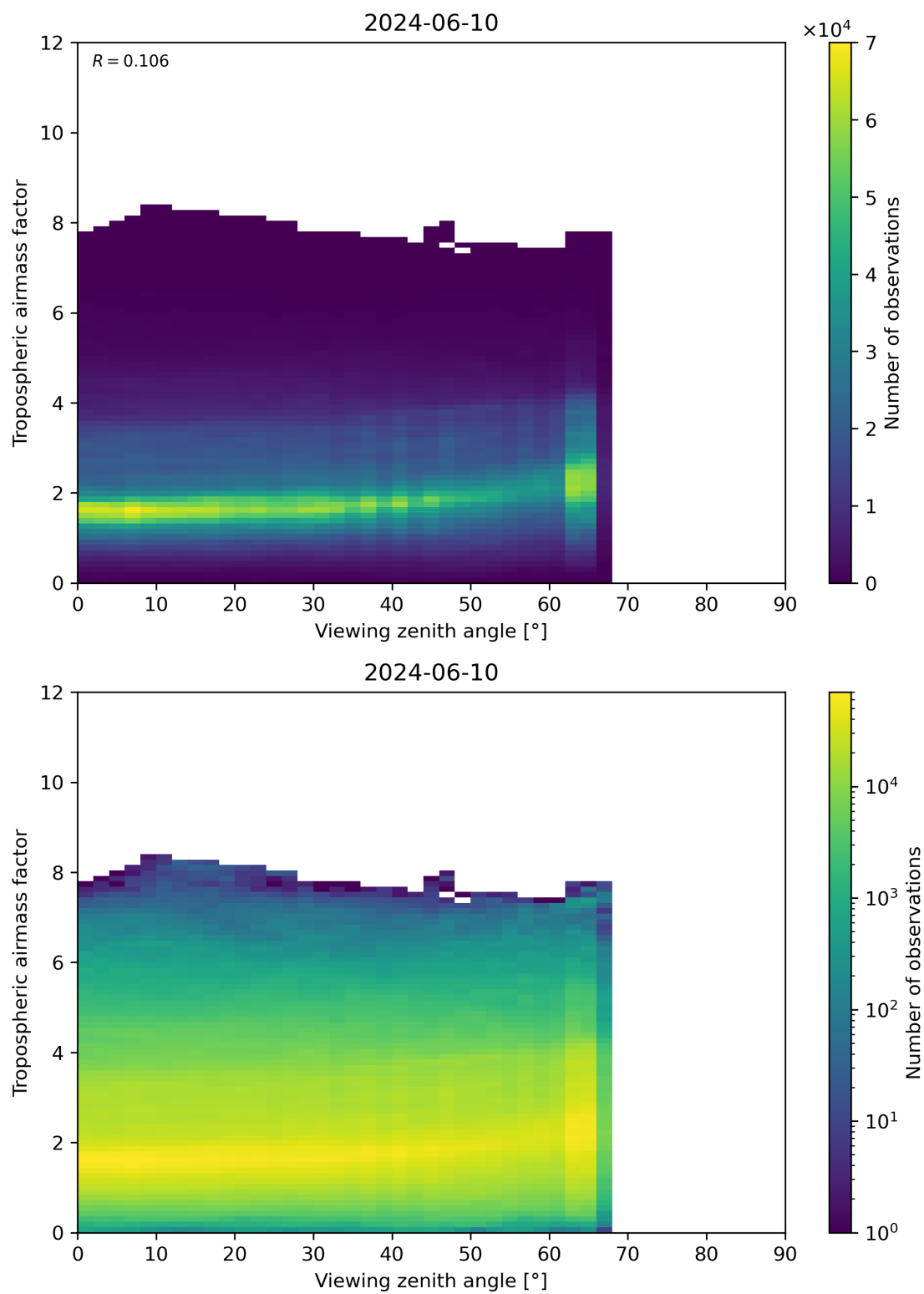
Figure 161: Scatter density plot of “Viewing zenith angle” against “Tropospheric airmass factor” for 2024-06-09 to 2024-06-11.
