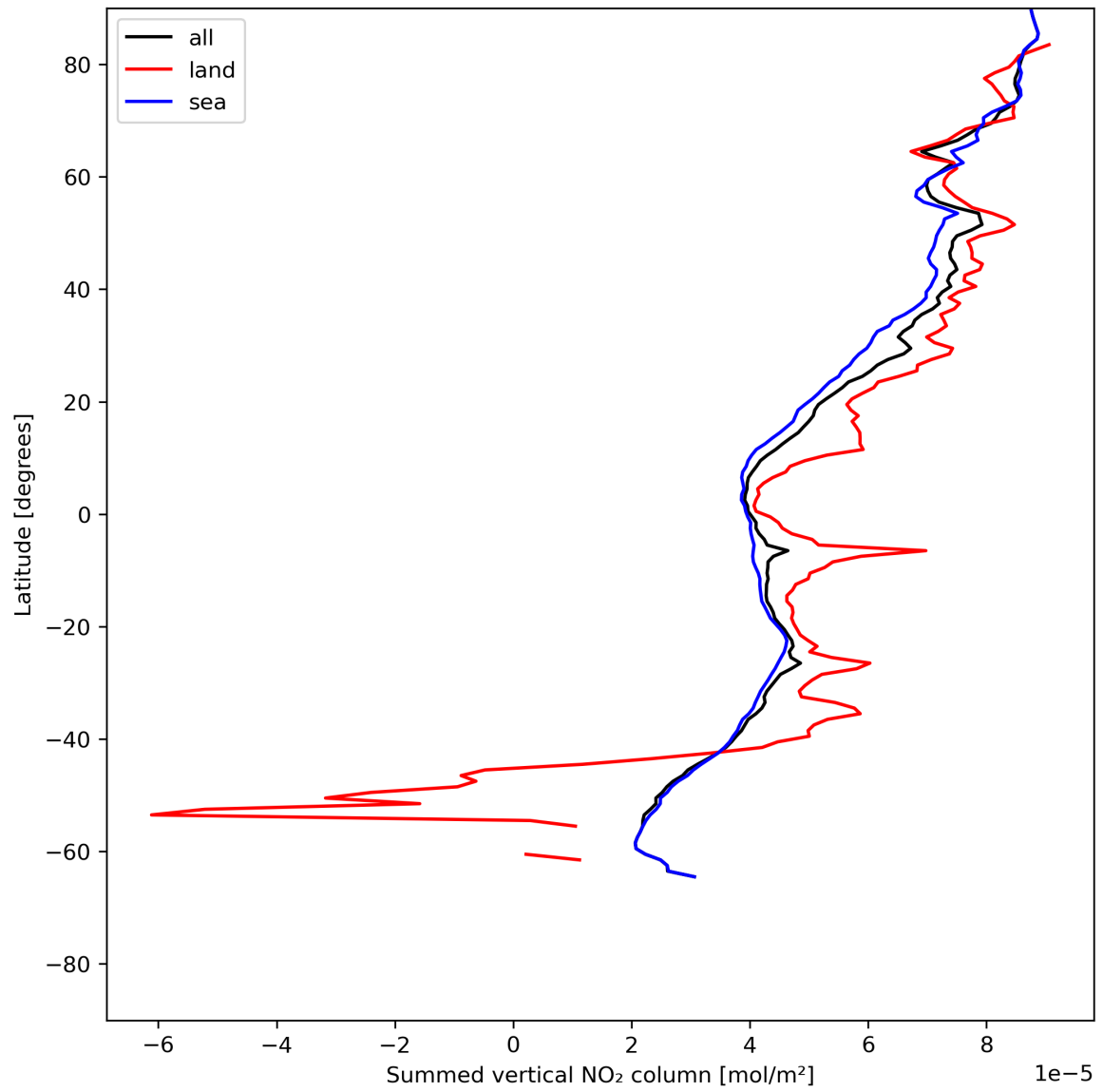
Figure 23: Zonal average of “Summed vertical NO 2 column” for 2024-06-09 to 2024-06-11.
