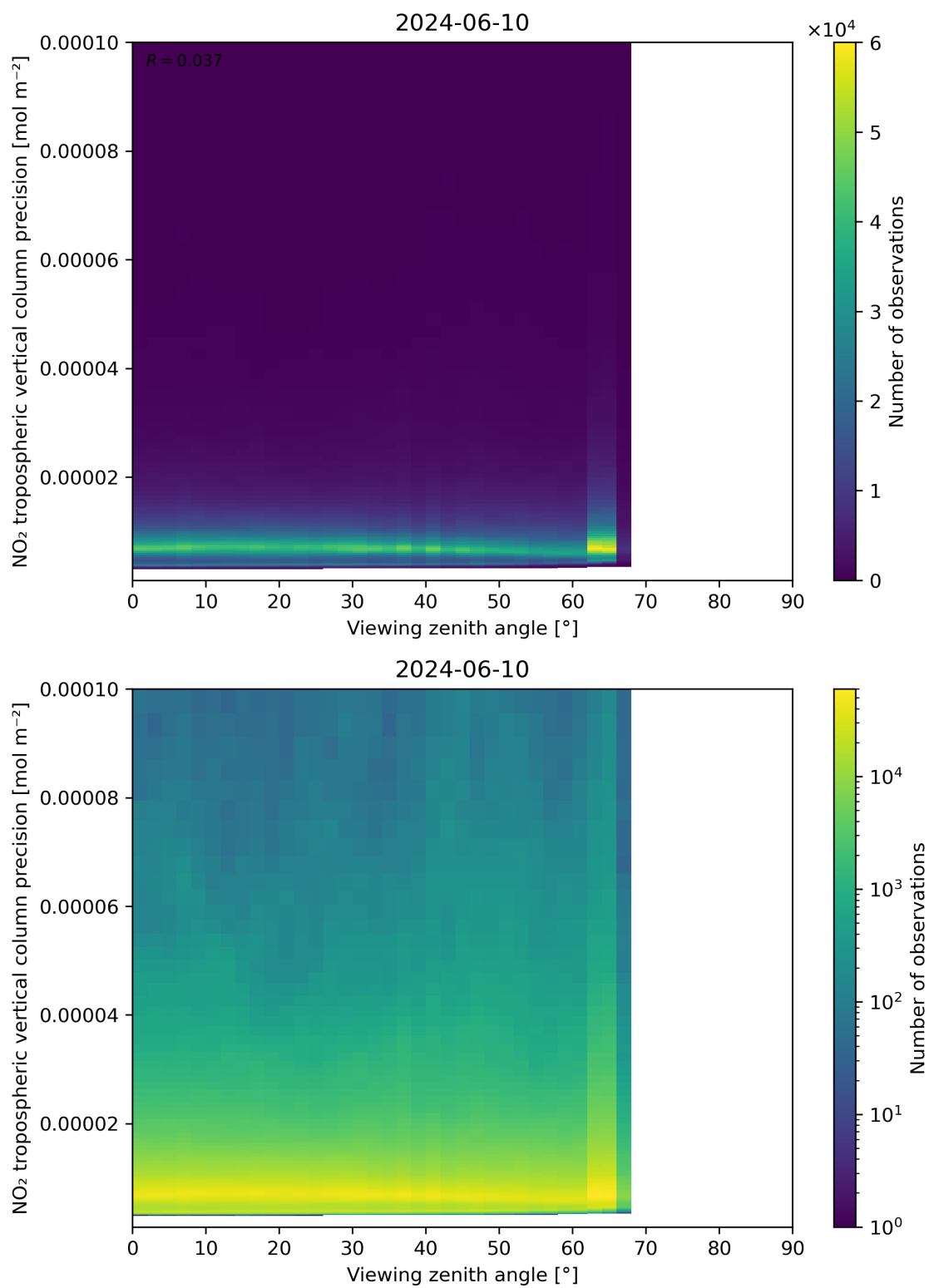
Figure 170: Scatter density plot of “Viewing zenith angle” against “NO 2 tropospheric vertical column precision” for 2024-06-09 to 2024-06-11.
