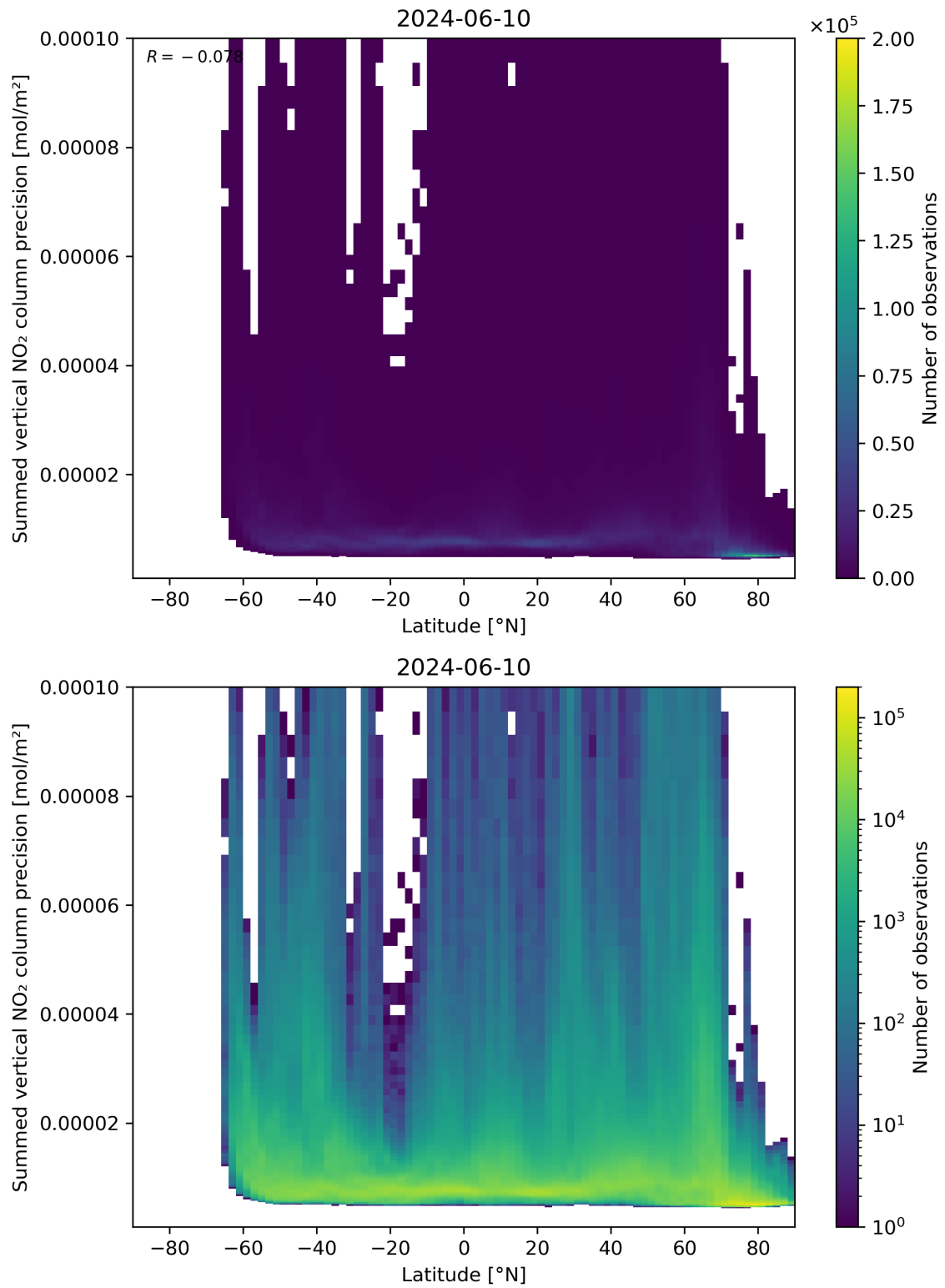
Figure 89: Scatter density plot of “Latitude” against “Summed vertical NO 2 column precision” for 2024-06-09 to 2024-06-11.
