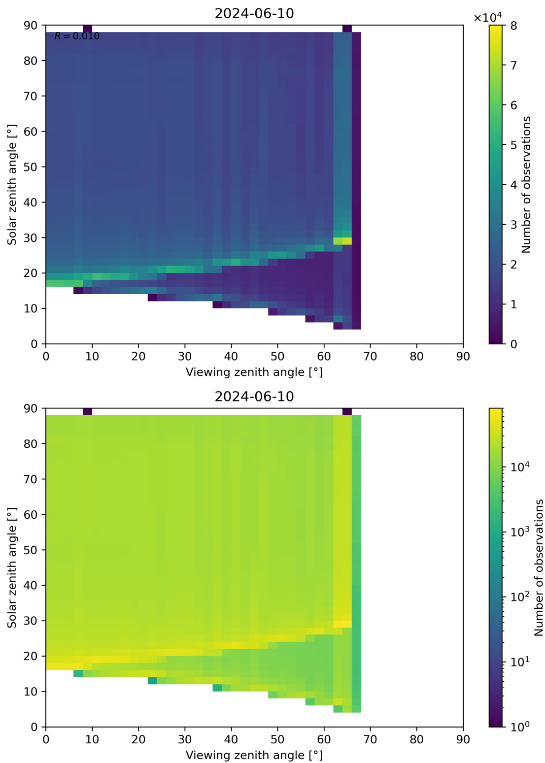
Figure 172: Scatter density plot of “Viewing zenith angle” against “Solar zenith angle” for 2024-06-09 to 2024-06-11.
