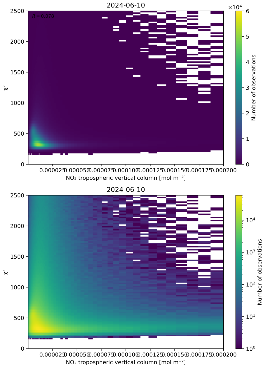
Figure 124: Scatter density plot of “NO 2 tropospheric vertical column” against “ \chi^2 ” for 2024-06-09 to 2024-06-11.
