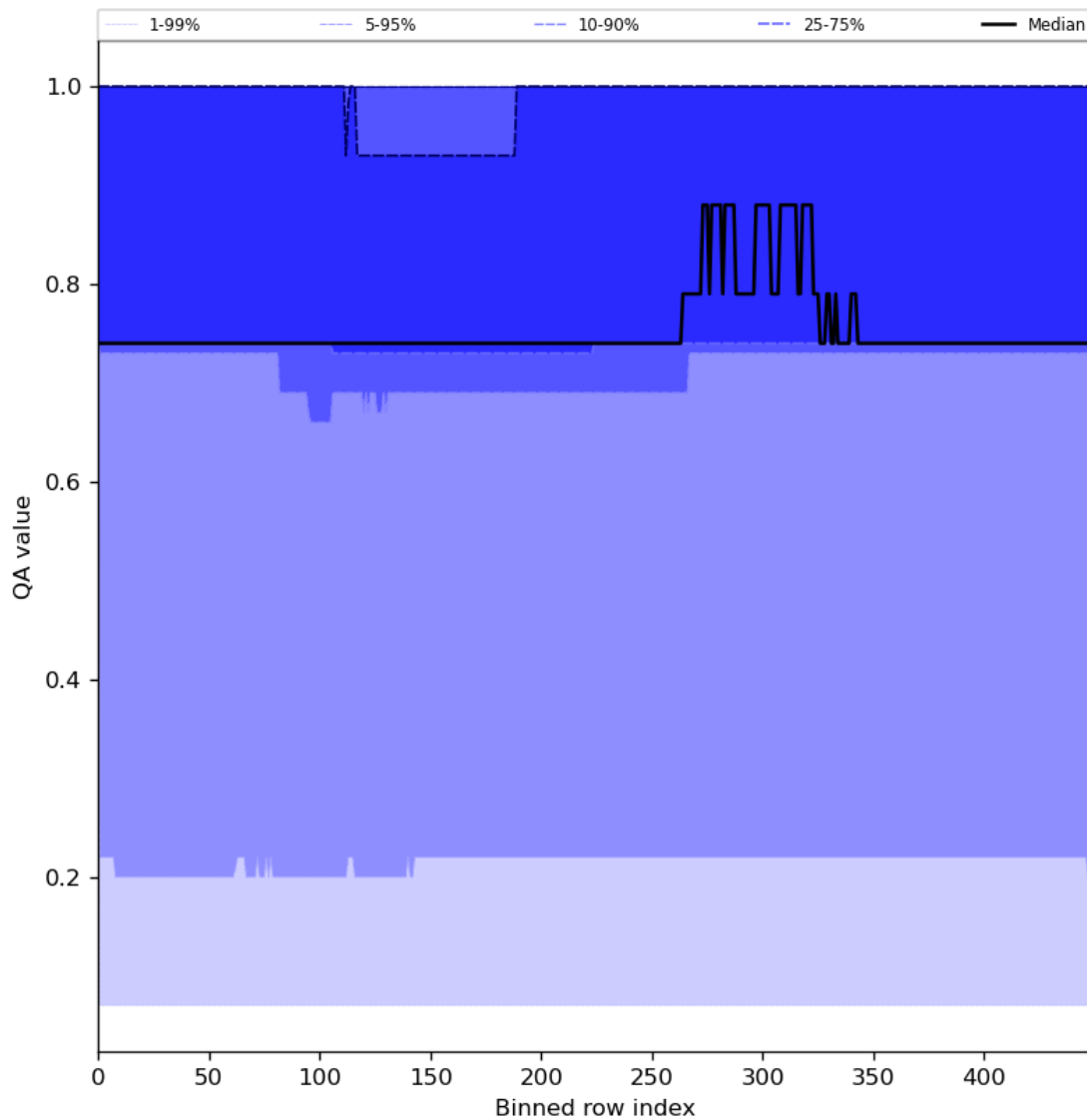
Figure 45: Along track statistics of “QA value” for 2024-06-09 to 2024-06-11
