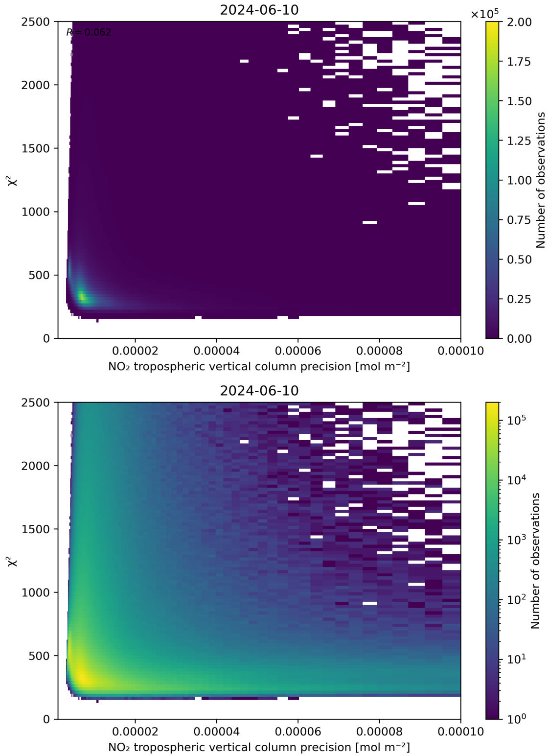
Figure 134: Scatter density plot of “NO 2 tropospheric vertical column precision” against “ \chi^2 ” for 2024-06-09 to 2024-06-11.
