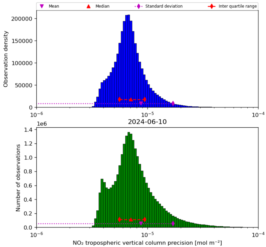
Figure 30: Histogram of “NO 2 tropospheric vertical column precision” for 2024-06-09 to 2024-06-11
