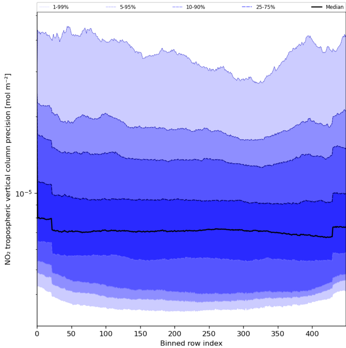
Figure 47: Along track statistics of “NO 2 tropospheric vertical column precision” for 2024-06-09 to 2024-06-11
