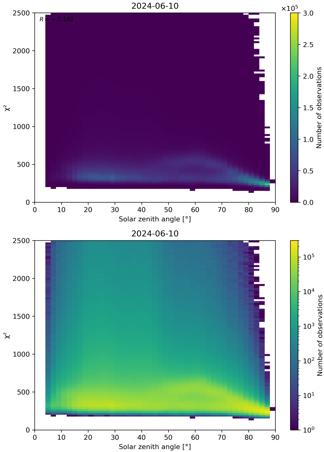
Figure 148: Scatter density plot of “Solar zenith angle” against “ \chi^2 ” for 2024-06-09 to 2024-06-11.
