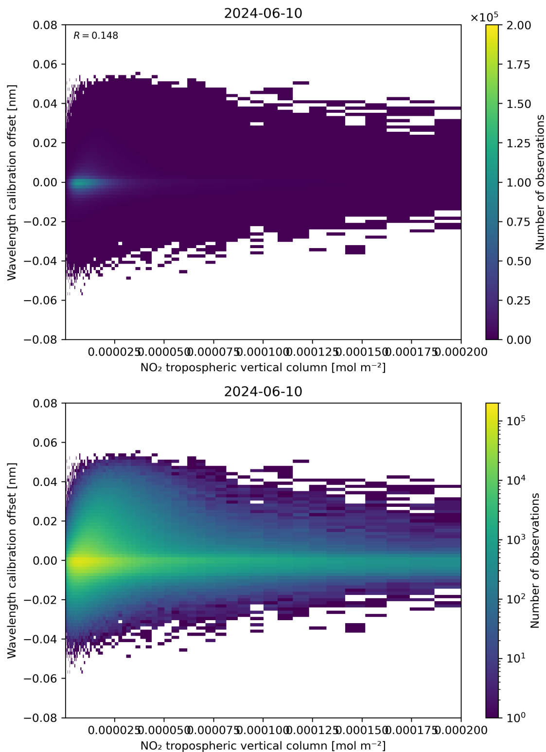
Figure 143: Scatter density plot of “NO 2 tropospheric vertical column” against “Wavelength calibration offset” for 2024-06-09 to 2024-06-11.
