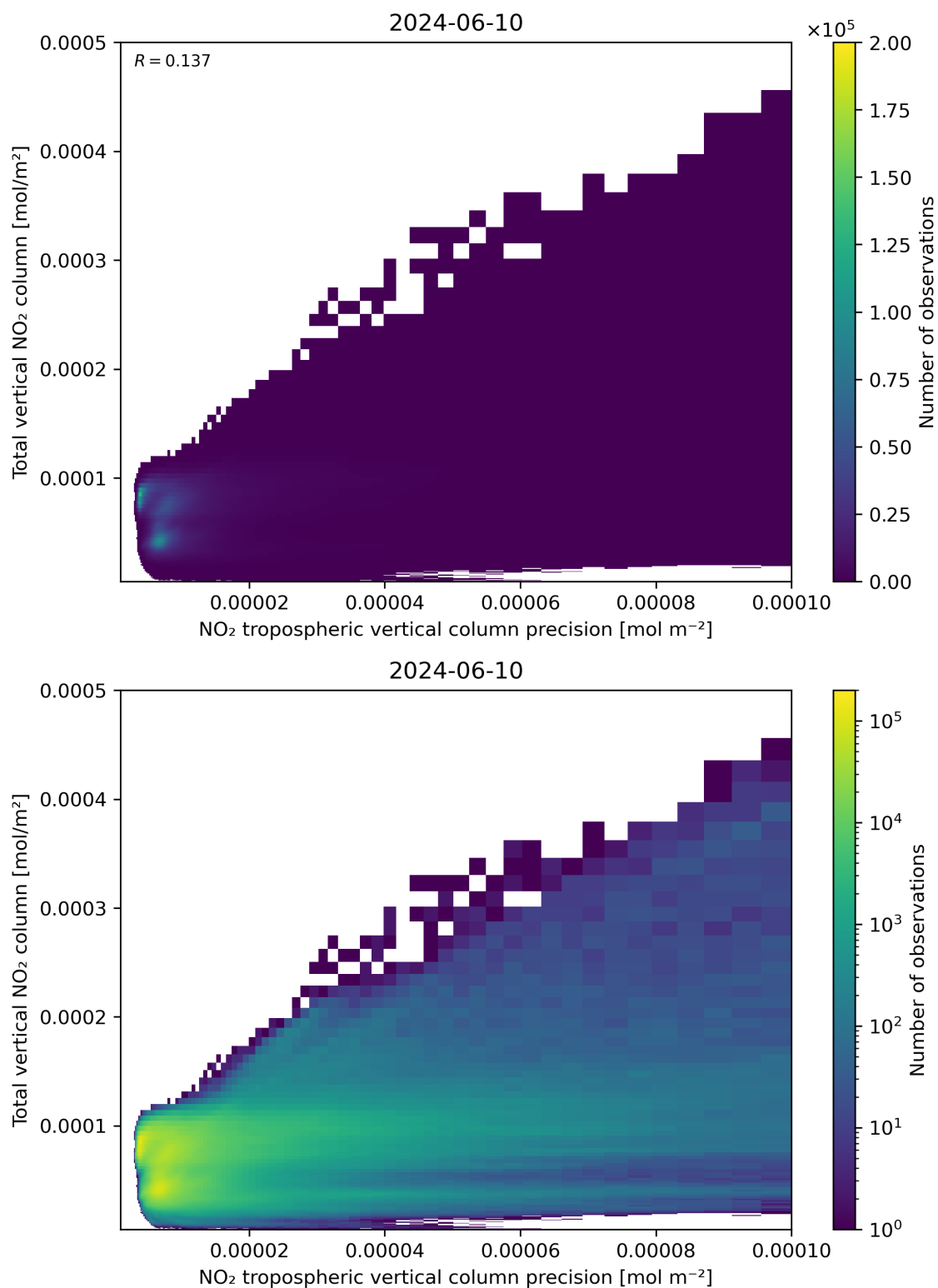
Figure 138: Scatter density plot of “NO 2 tropospheric vertical column precision” against “Total vertical NO 2 column” for 2024-06-09 to 2024-06-11.
