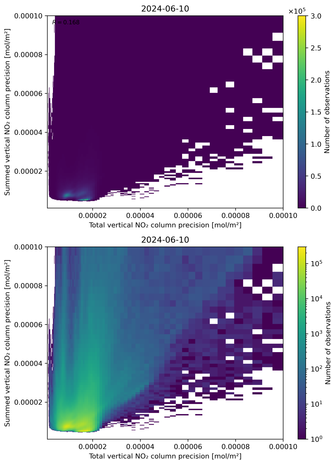
Figure 118: Scatter density plot of “Total vertical NO 2 column precision” against “Summed vertical NO 2 column precision” for 2024-06-09 to 2024-06-11.
