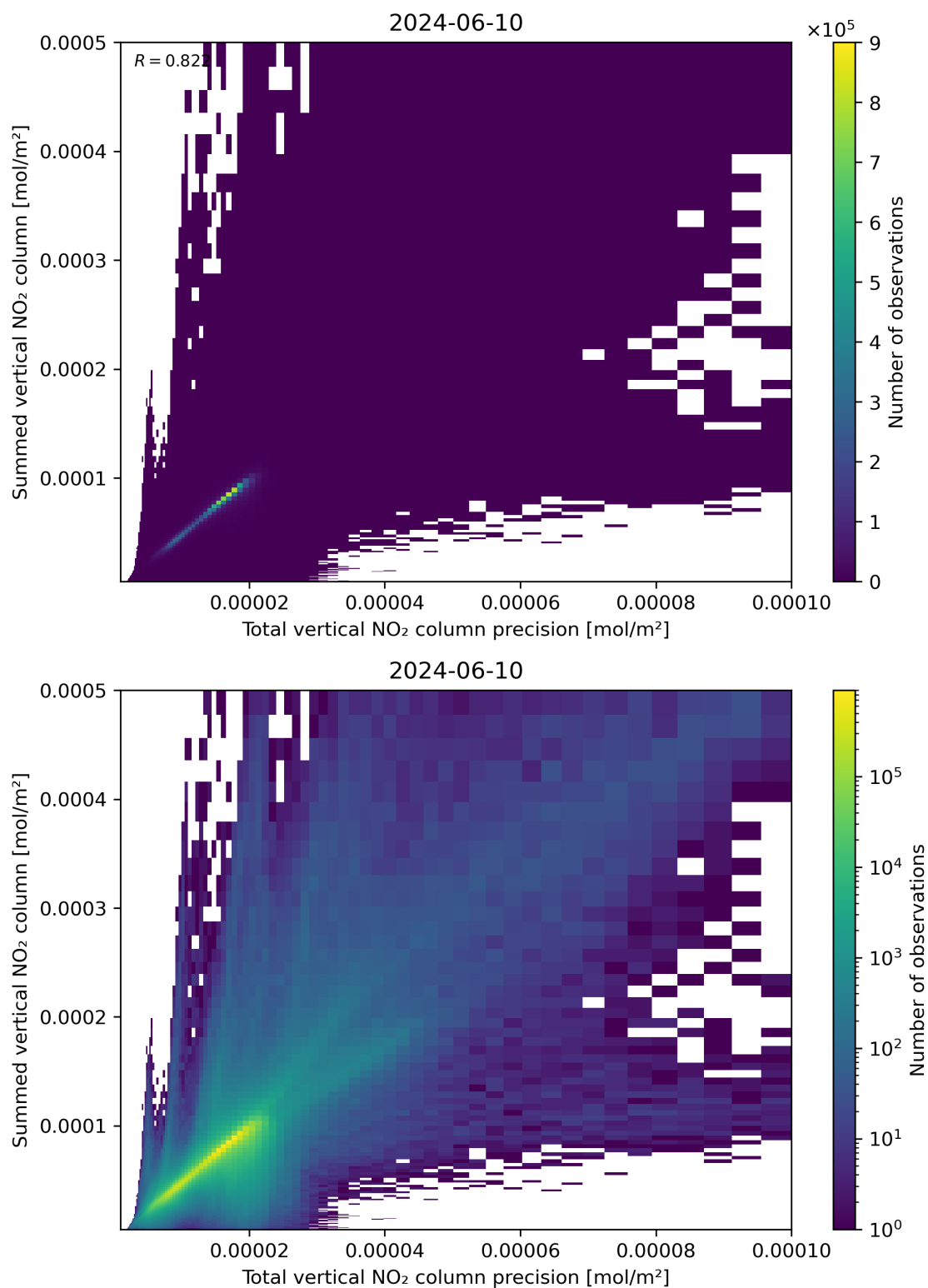
Figure 117: Scatter density plot of “Total vertical NO 2 column precision” against “Summed vertical NO 2 column” for 2024-06-09 to 2024-06-11.
