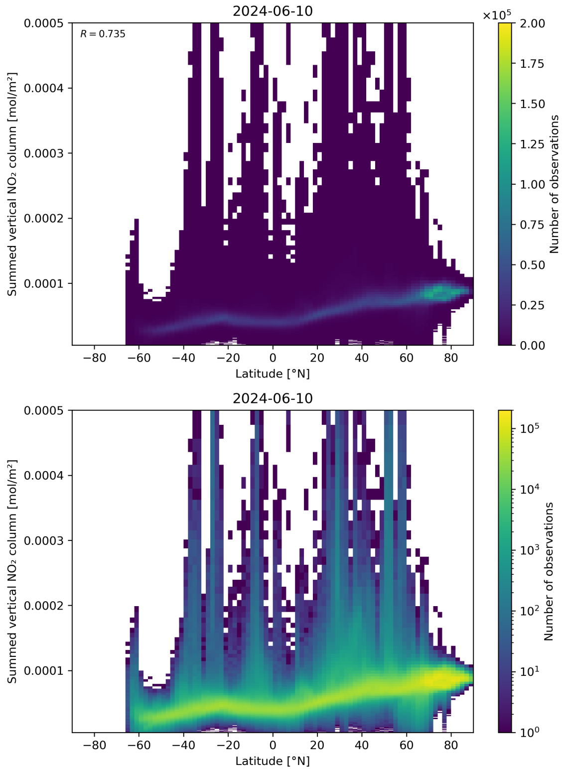
Figure 88: Scatter density plot of “Latitude” against “Summed vertical NO 2 column” for 2024-06-09 to 2024-06-11.
