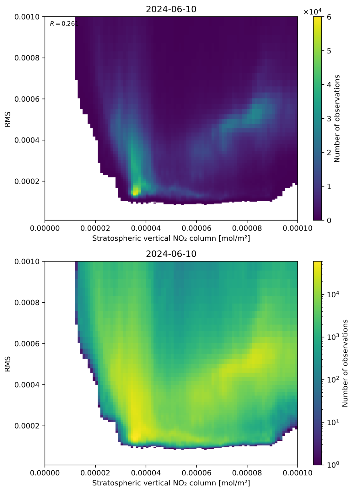
Figure 102: Scatter density plot of “Stratospheric vertical NO 2 column” against “RMS” for 2024-06-09 to 2024-06-11.
