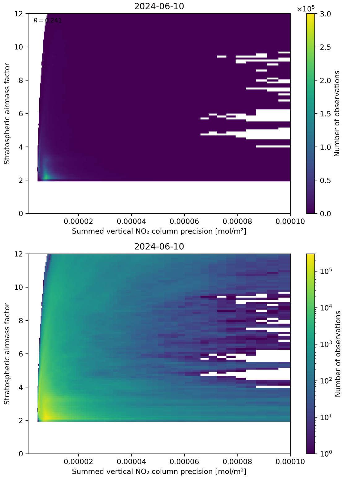
Figure 106: Scatter density plot of “Summed vertical NO 2 column precision” against “Stratospheric airmass factor” for 2024-06-09 to 2024-06-11.
