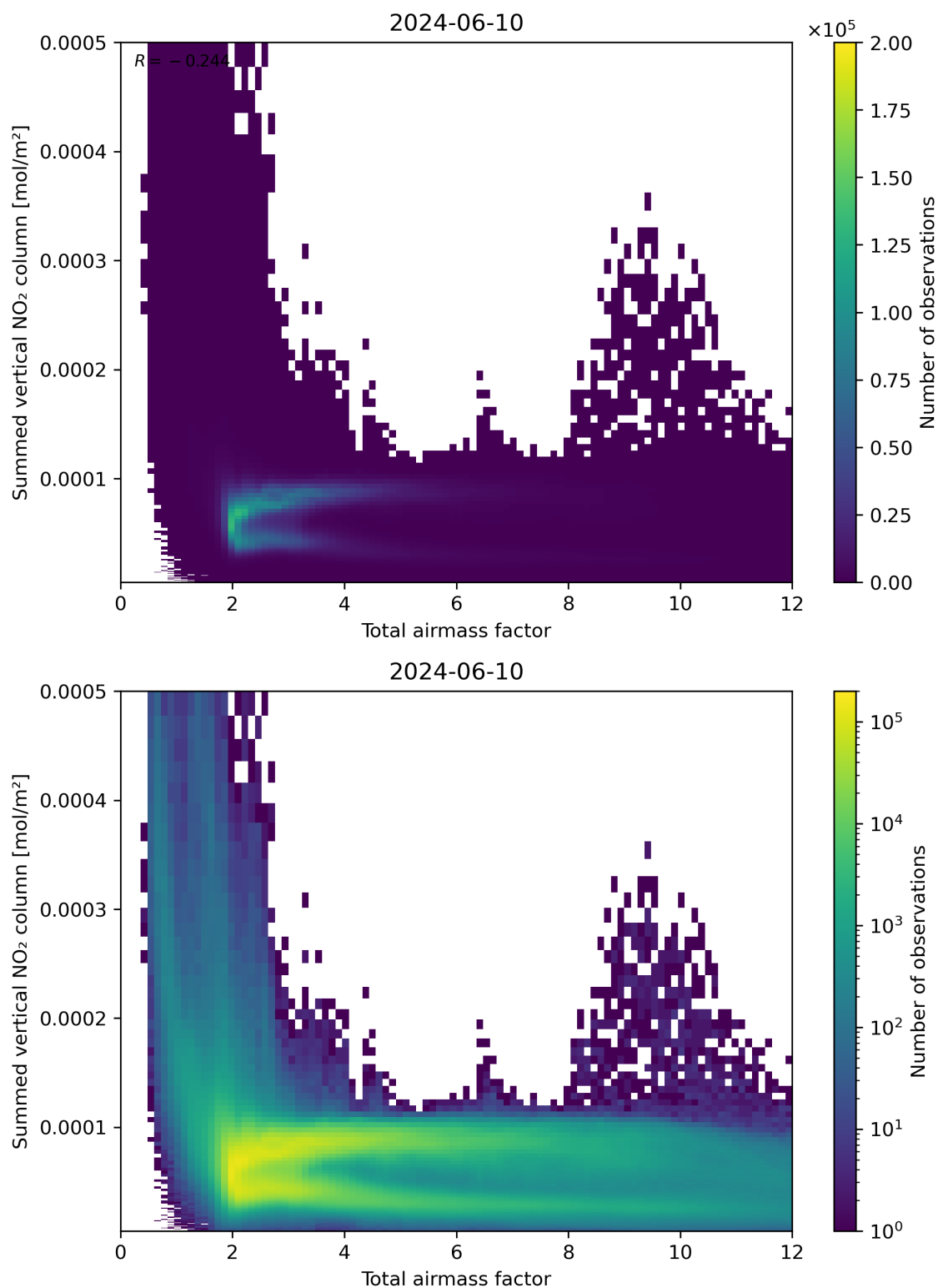
Figure 65: Scatter density plot of “Total airmass factor” against “Summed vertical NO 2 column” for 2024-06-09 to 2024-06-11.
