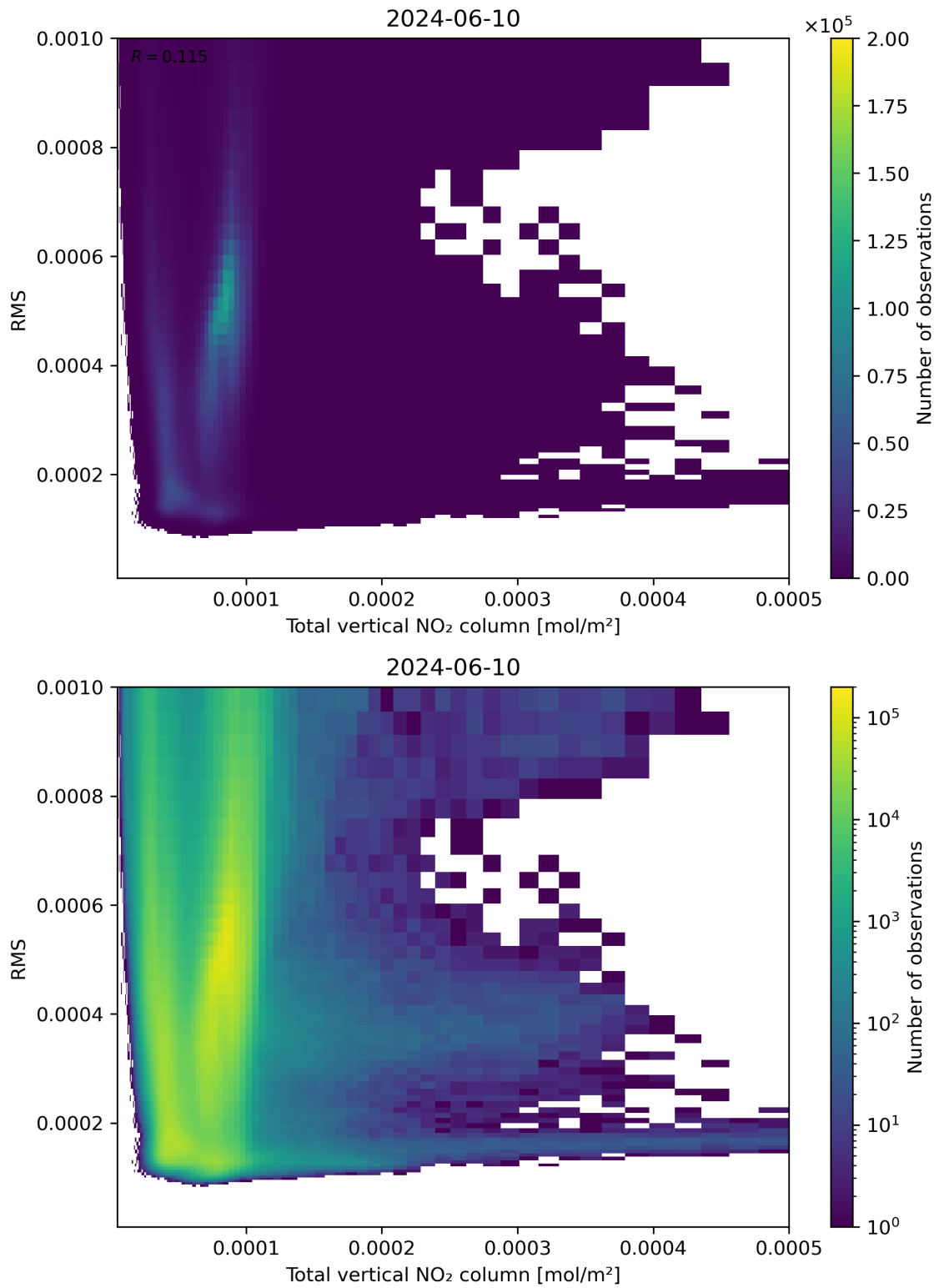
Figure 120: Scatter density plot of “Total vertical NO 2 column” against “RMS” for 2024-06-09 to 2024-06-11.
