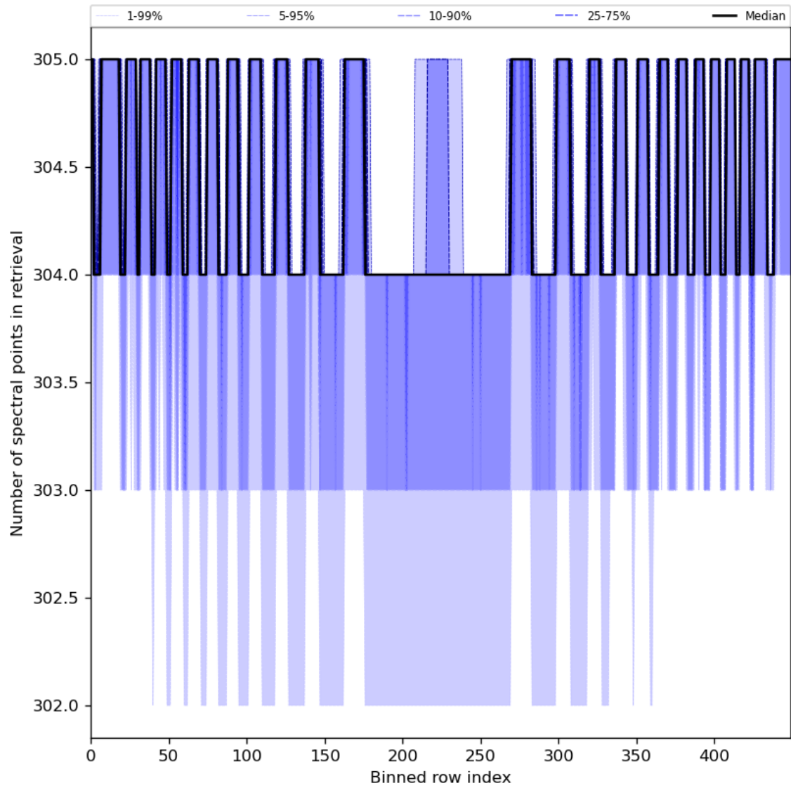
Figure 50: Along track statistics of “Number of spectral points in retrieval” for 2024-06-09 to 2024-06-11
