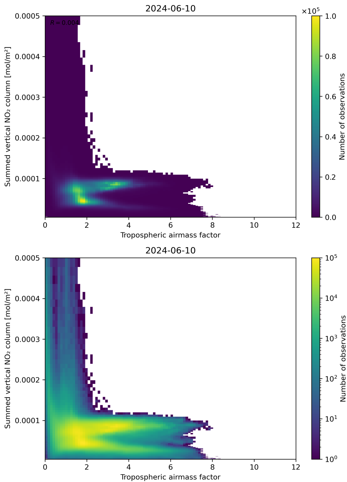
Figure 75: Scatter density plot of “Tropospheric air mass factor” against “Summed vertical NO 2 column” for 2024-06-09 to 2024-06-11.
