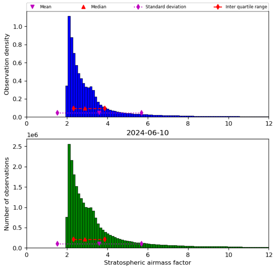
Figure 44: Histogram of “Stratospheric airmass factor” for 2024-06-09 to 2024-06-11
