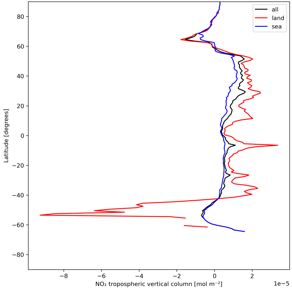
Figure 12: Zonal average of “NO 2 tropospheric vertical column” for 2024-06-09 to 2024-06-11.
