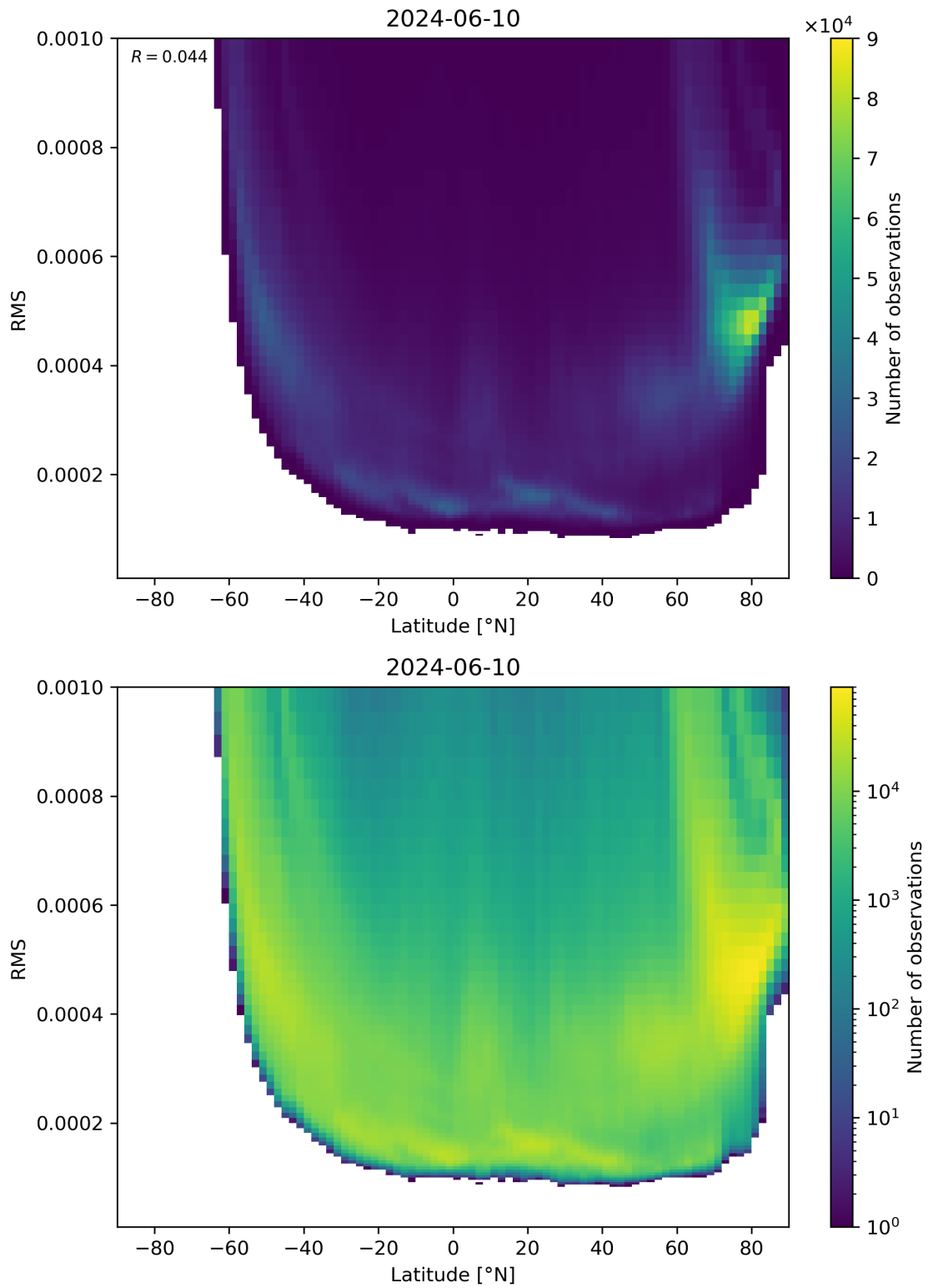
Figure 94: Scatter density plot of “Latitude” against “RMS” for 2024-06-09 to 2024-06-11.
