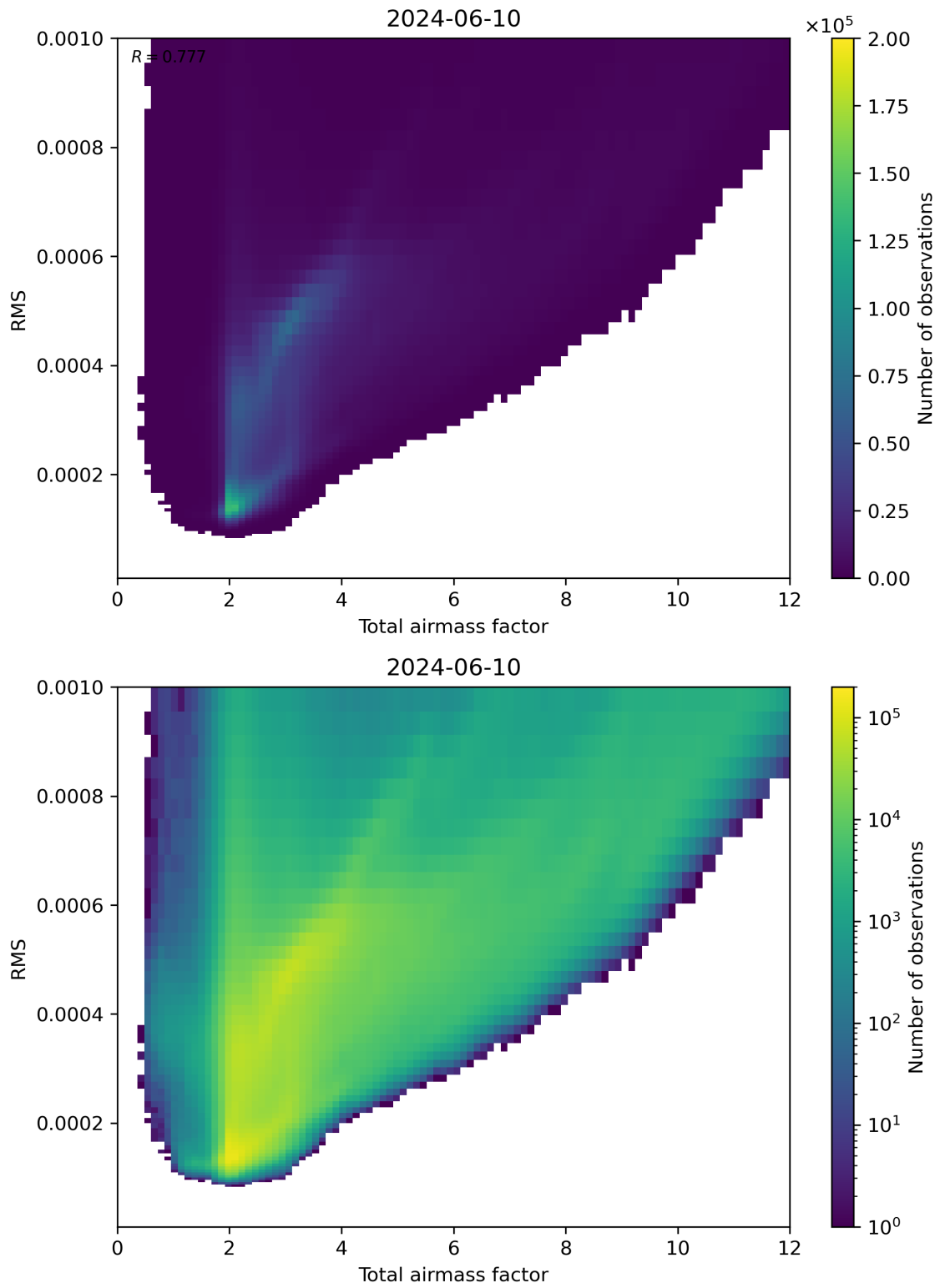
Figure 69: Scatter density plot of “Total airmass factor” against “RMS” for 2024-06-09 to 2024-06-11.
