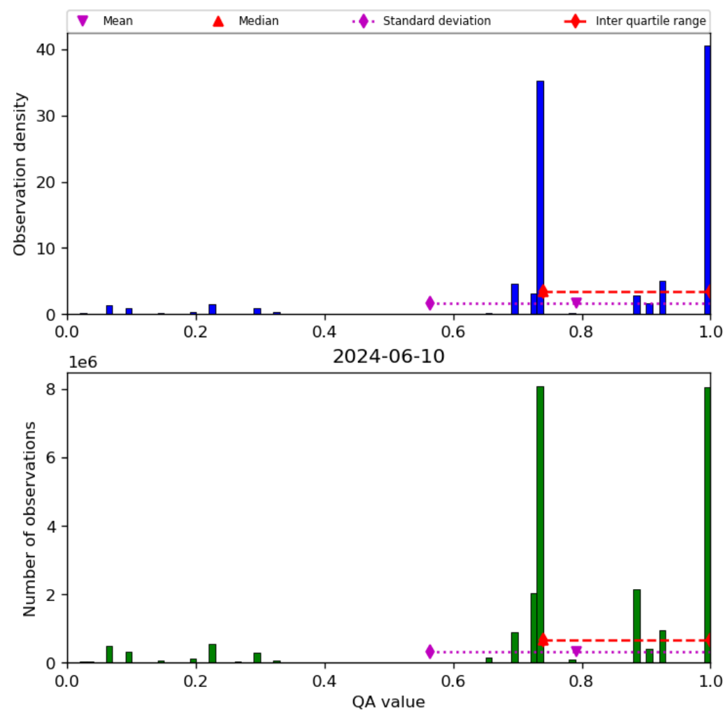
Figure 28: Histogram of “QA value” for 2024-06-09 to 2024-06-11
