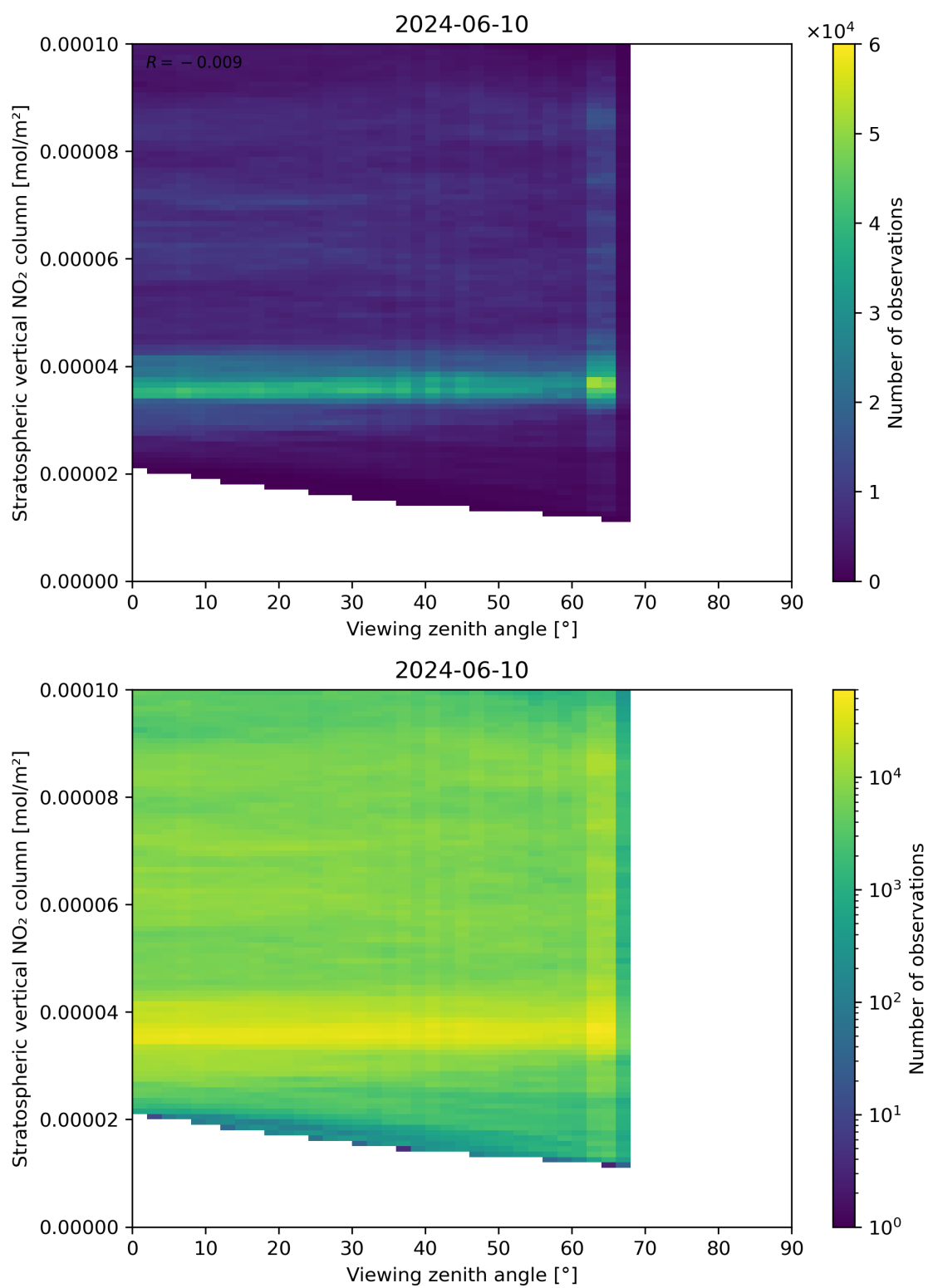
Figure 164: Scatter density plot of “Viewing zenith angle” against “Stratospheric vertical NO 2 column” for 2024-06-09 to 2024-06-11.
