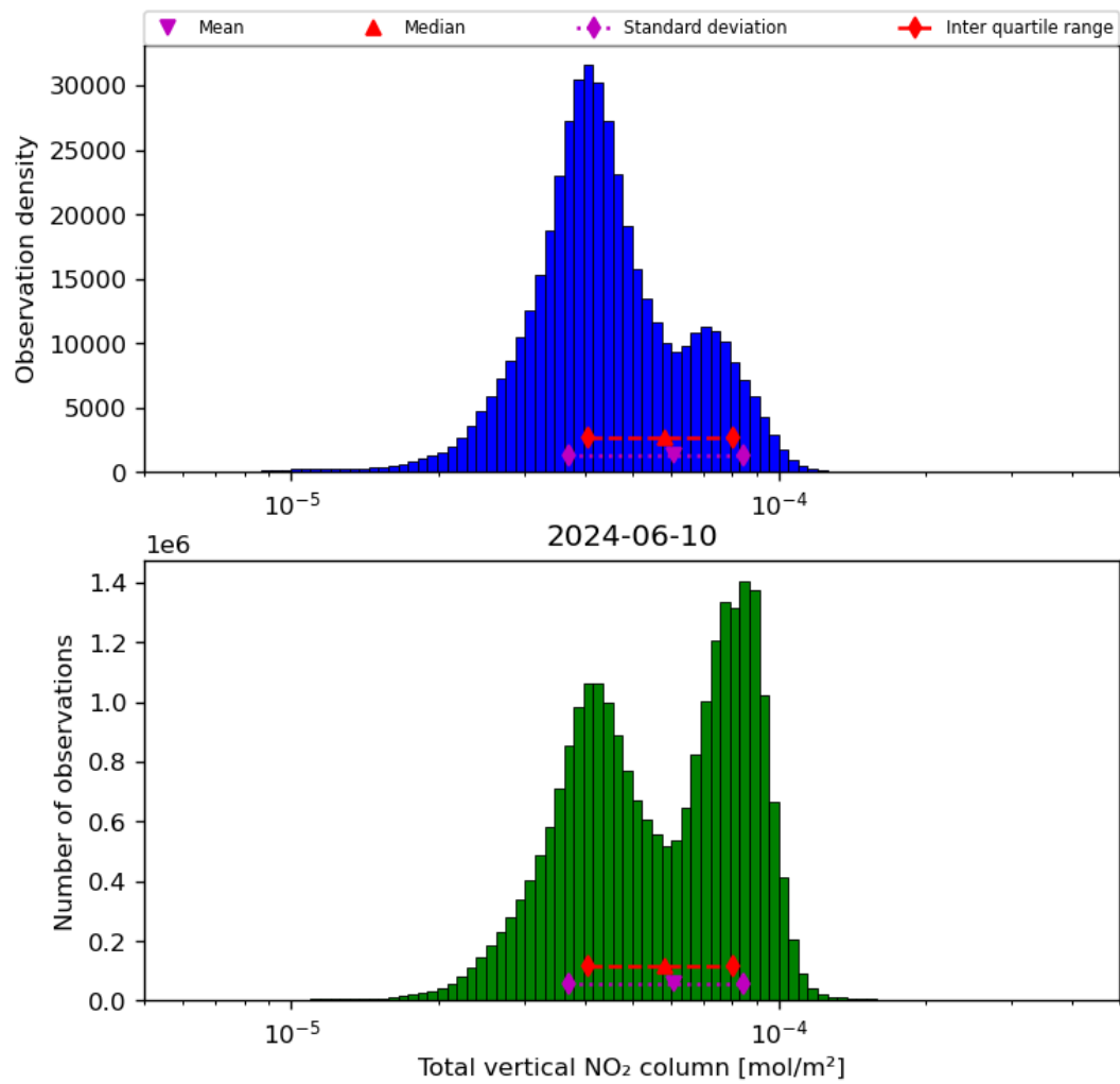
Figure 38: Histogram of “Total vertical NO 2 column” for 2024-06-09 to 2024-06-11
