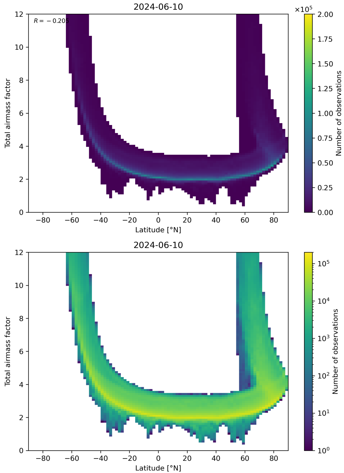
Figure 84: Scatter density plot of “Latitude” against “Total airmass factor” for 2024-06-09 to 2024-06-11.
