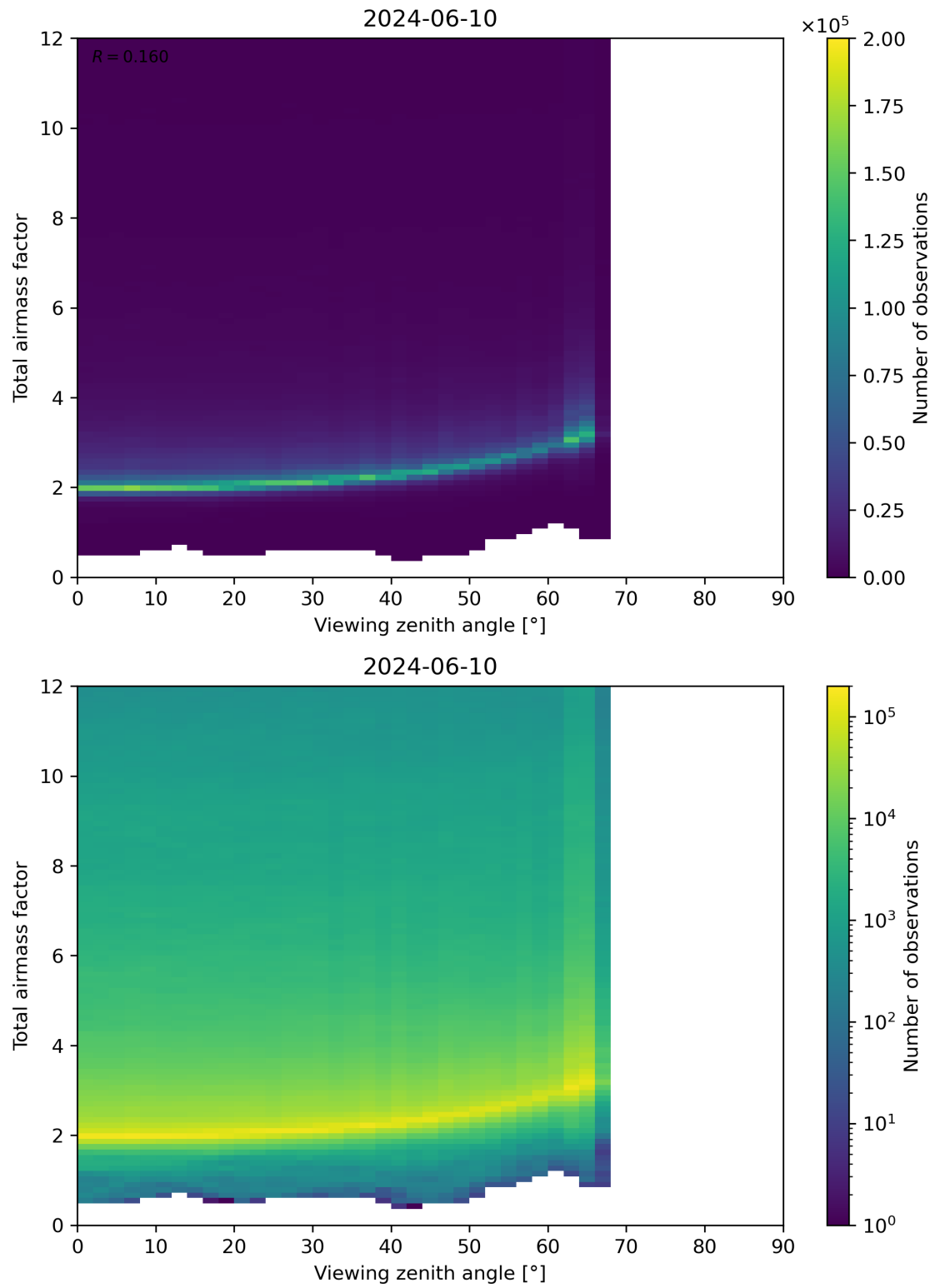
Figure 160: Scatter density plot of “Viewing zenith angle” against “Total airmass factor” for 2024-06-09 to 2024-06-11.
