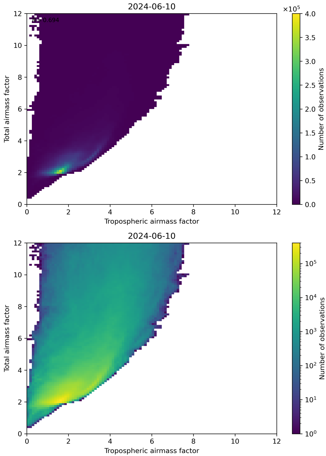
Figure 72: Scatter density plot of “Tropospheric airmass factor” against “Total airmass factor” for 2024-06-09 to 2024-06-11.
