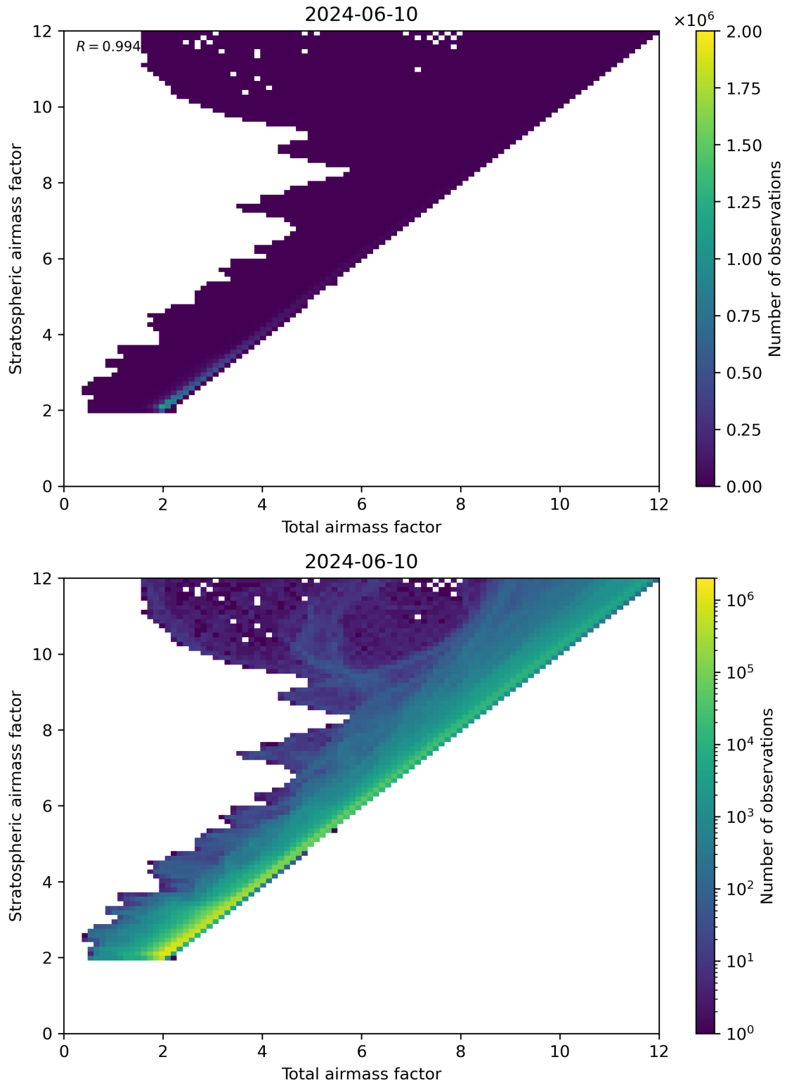
Figure 62: Scatter density plot of “Total airmass factor” against “Stratospheric airmass factor” for 2024-06-09 to 2024-06-11.
