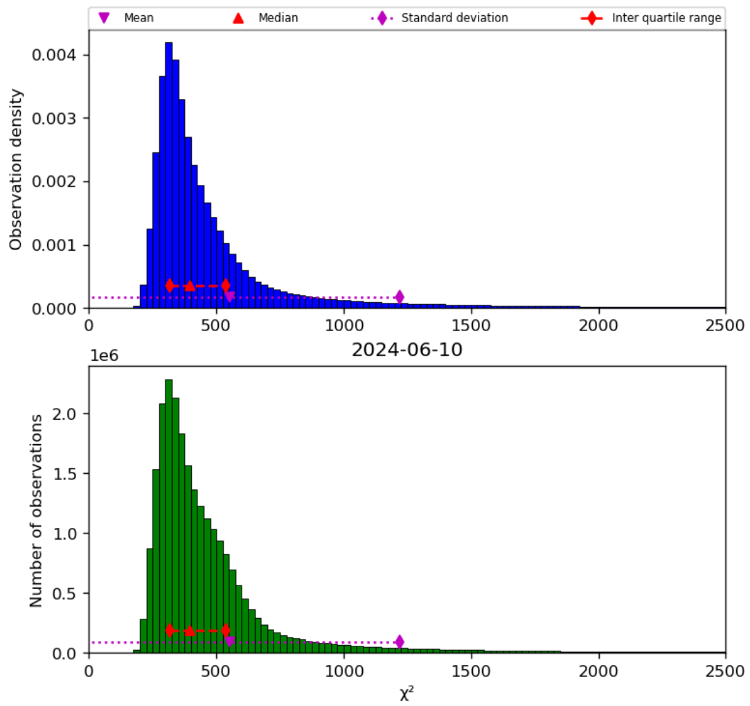
Figure 42: Histogram of “ \chi^2 ” for 2024-06-09 to 2024-06-11
