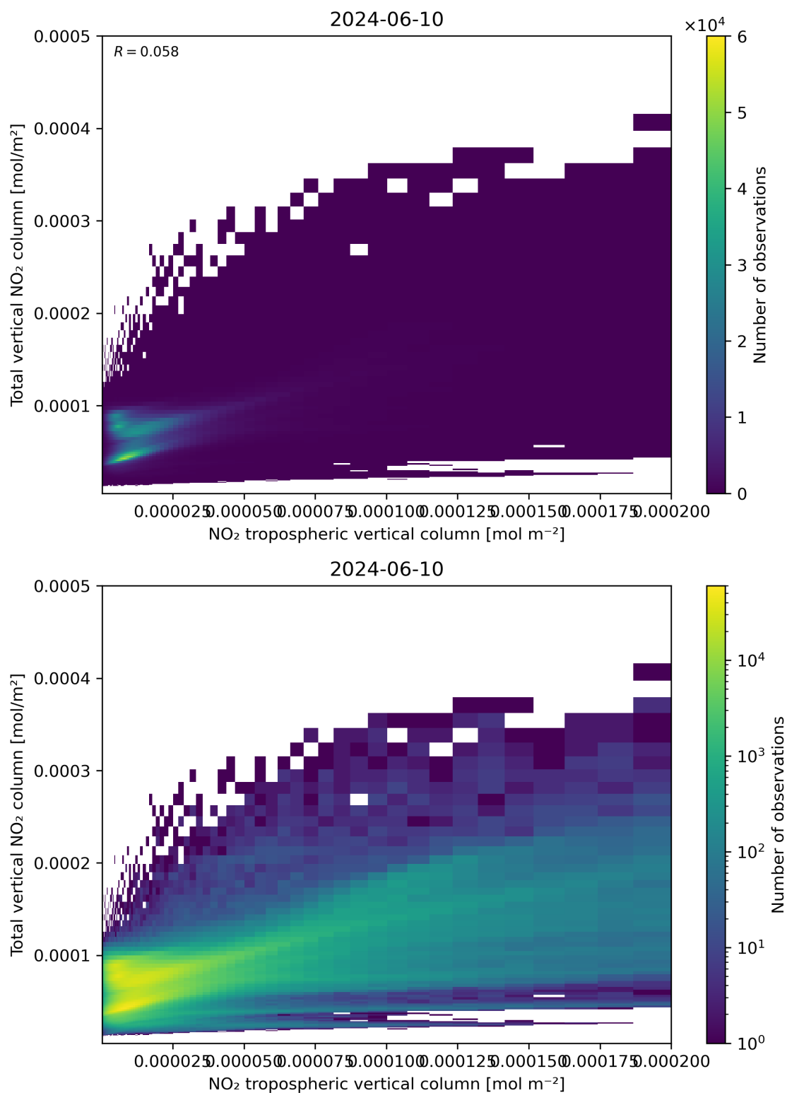
Figure 128: Scatter density plot of “NO 2 tropospheric vertical column” against “Total vertical NO 2 column” for 2024-06-09 to 2024-06-11.
