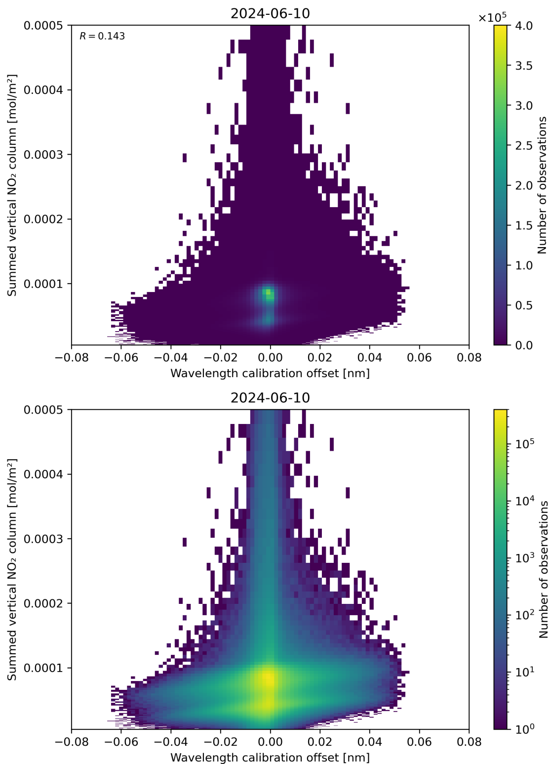
Figure 177: Scatter density plot of “Wavelength calibration offset” against “Summed vertical NO 2 column” for 2024-06-09 to 2024-06-11.
