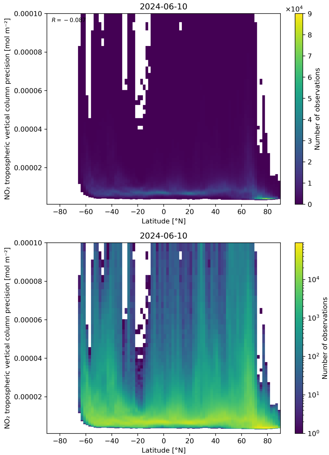
Figure 93: Scatter density plot of “Latitude” against “NO 2 tropospheric vertical column precision” for 2024-06-09 to 2024-06-11.
