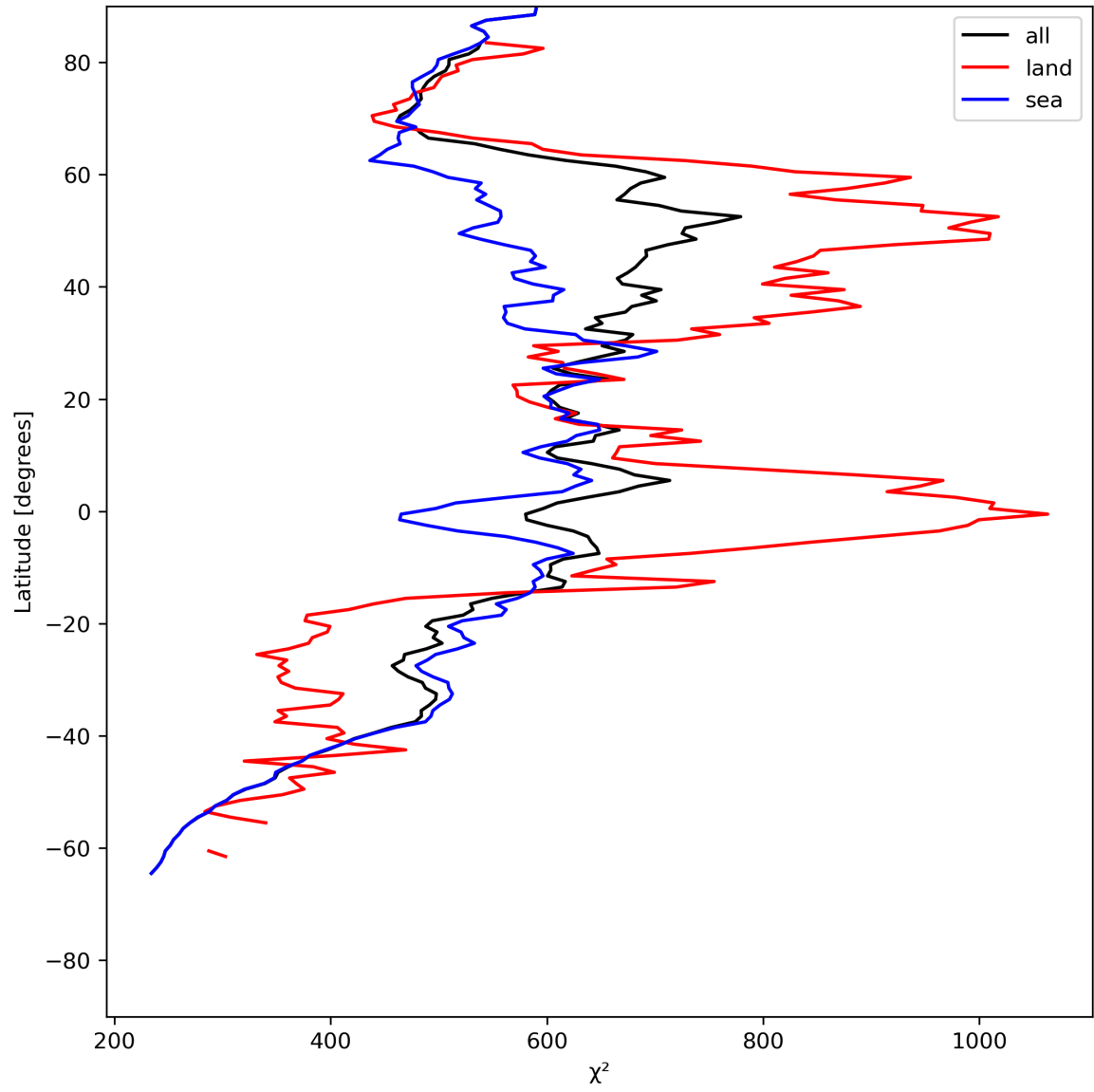
Figure 25: Zonal average of “ \chi^2 ” for 2024-06-09 to 2024-06-11.
