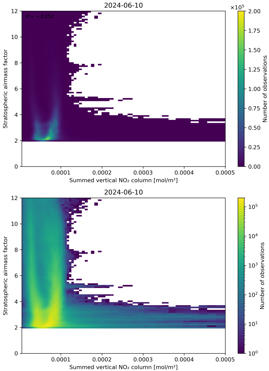
Figure 103: Scatter density plot of “Summed vertical NO 2 column” against “Stratospheric air mass factor” for 2024-06-09 to 2024-06-11.
