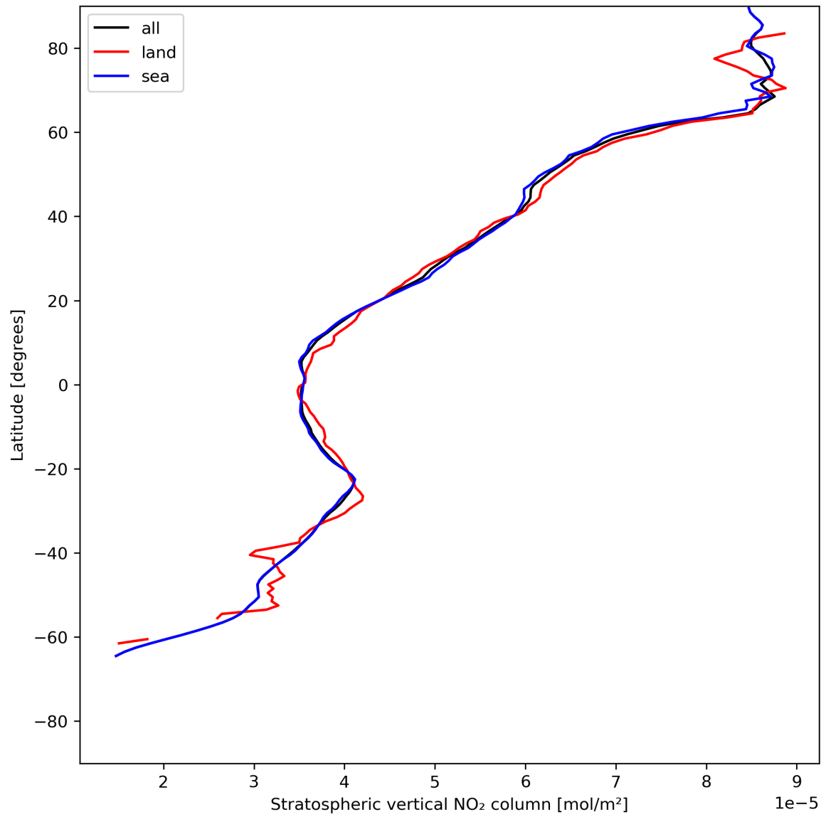
Figure 19: Zonal average of “Stratospheric vertical NO 2 column” for 2024-06-09 to 2024-06-11.
