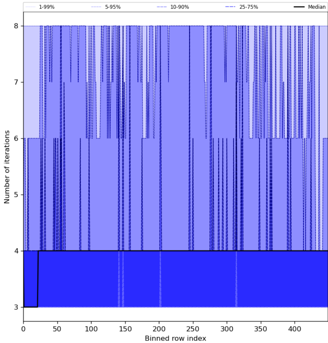
Figure 51: Along track statistics of “Number of iterations” for 2024-06-09 to 2024-06-11
