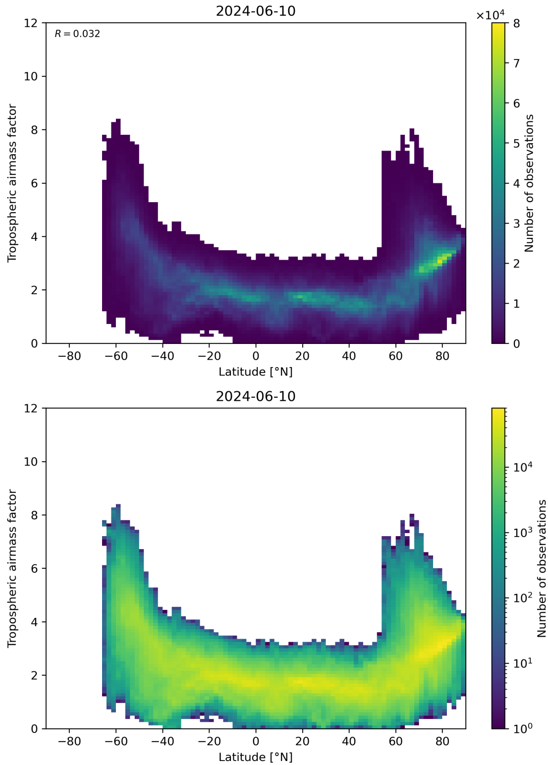
Figure 85: Scatter density plot of “Latitude” against “Tropospheric airmass factor” for 2024-06-09 to 2024-06-11.
