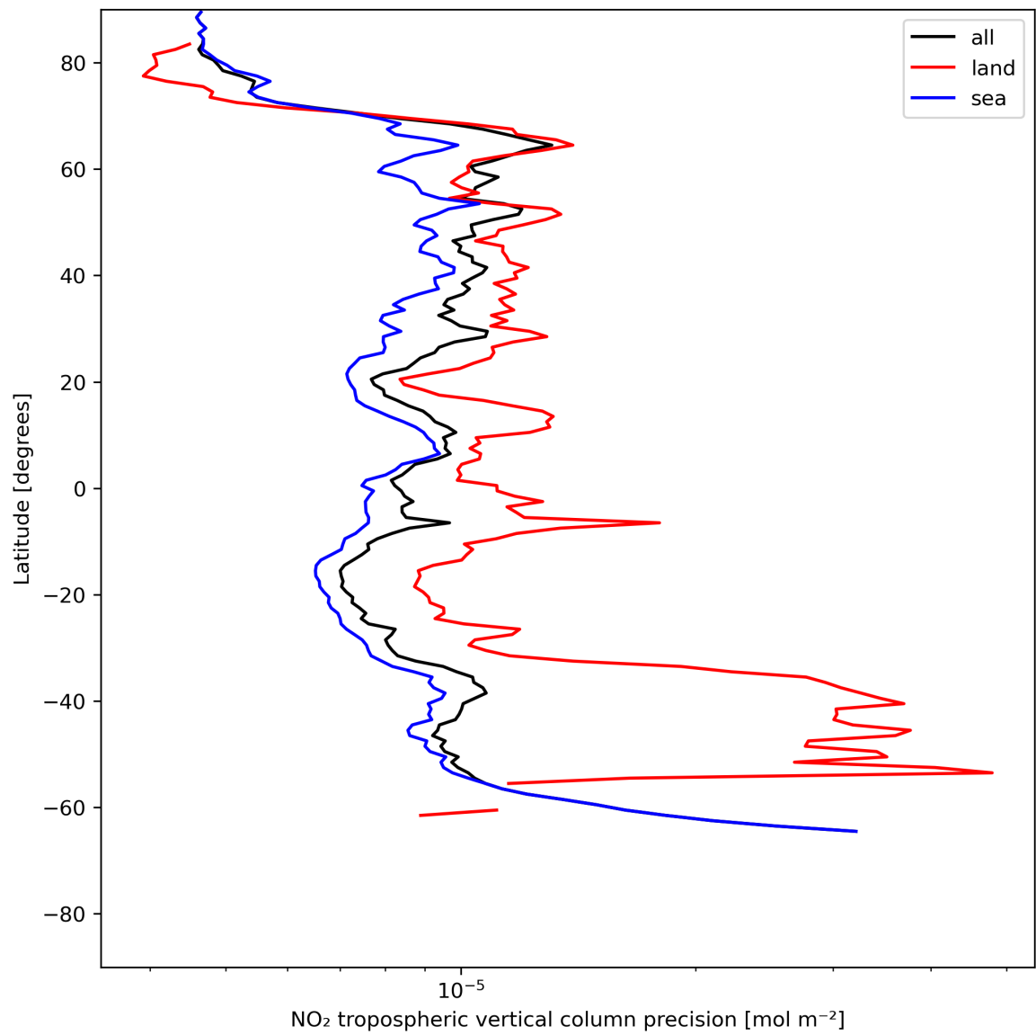
Figure 13: Zonal average of “NO 2 tropospheric vertical column precision” for 2024-06-09 to 2024-06-11.
