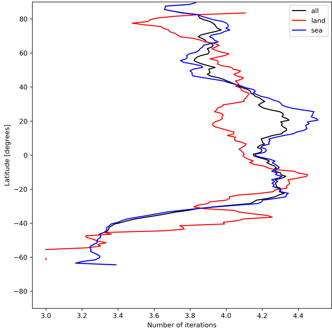
Figure 17: Zonal average of “Number of iterations” for 2024-06-09 to 2024-06-11.
