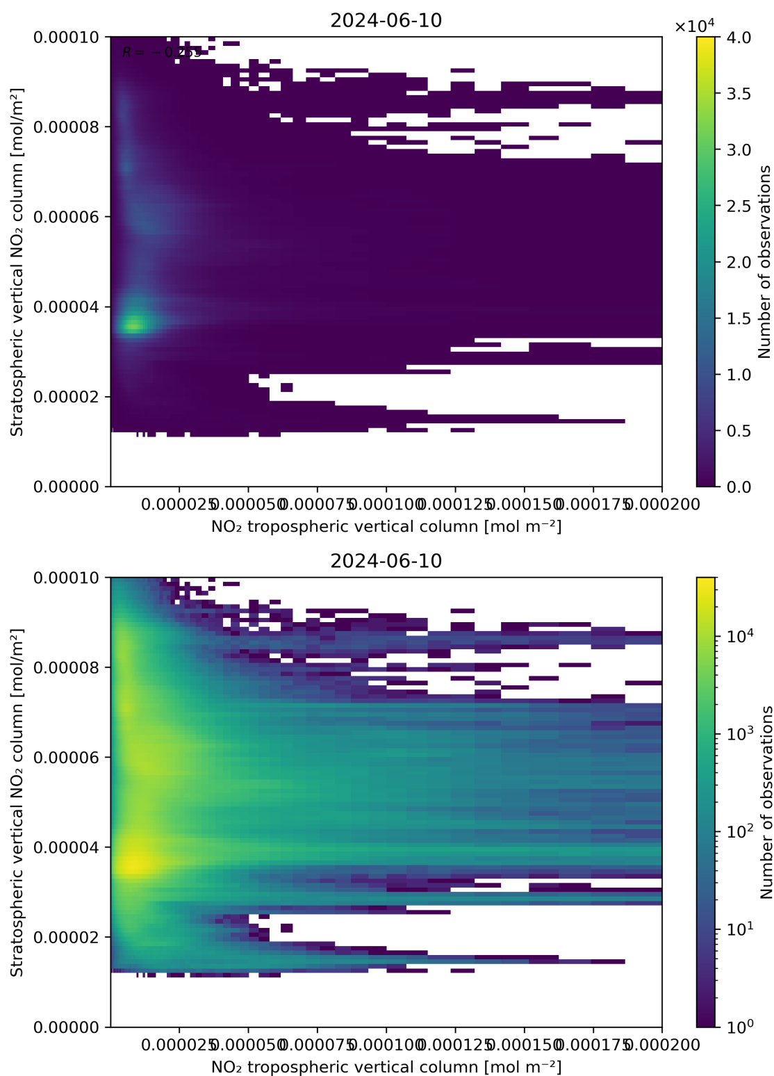
Figure 125: Scatter density plot of “NO 2 tropospheric vertical column” against “Stratospheric vertical NO 2 column” for 2024-06-09 to 2024-06-11.
