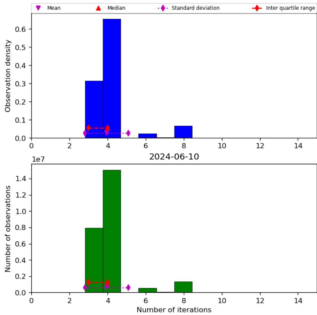
Figure 34: Histogram of “Number of iterations” for 2024-06-09 to 2024-06-11
