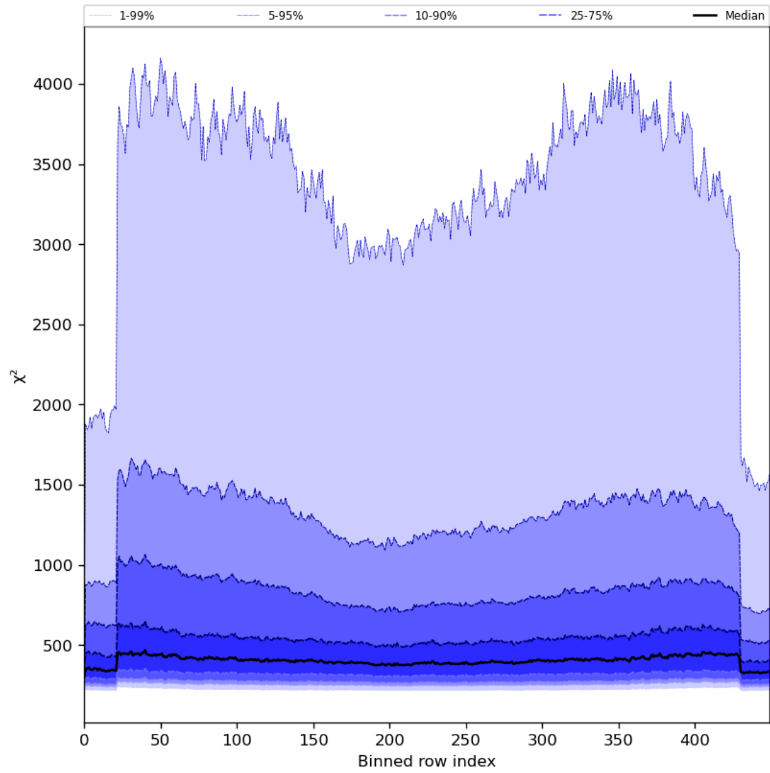
Figure 59: Along track statistics of “ \chi^2 ” for 2024-06-09 to 2024-06-11
