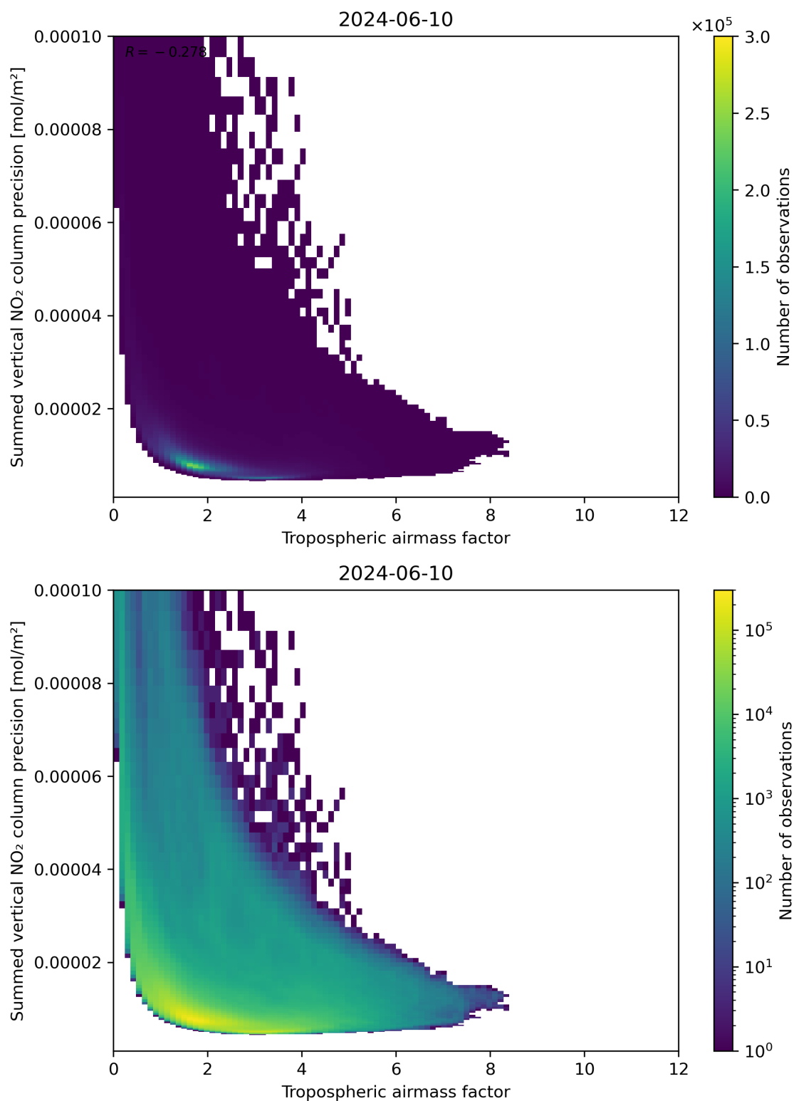
Figure 76: Scatter density plot of “Tropospheric air mass factor” against “Summed vertical NO 2 column precision” for 2024-06-09 to 2024-06-11.
