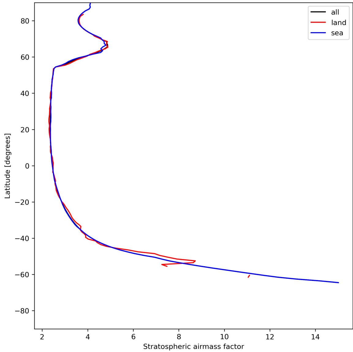
Figure 27: Zonal average of “Stratospheric airmass factor” for 2024-06-09 to 2024-06-11.
