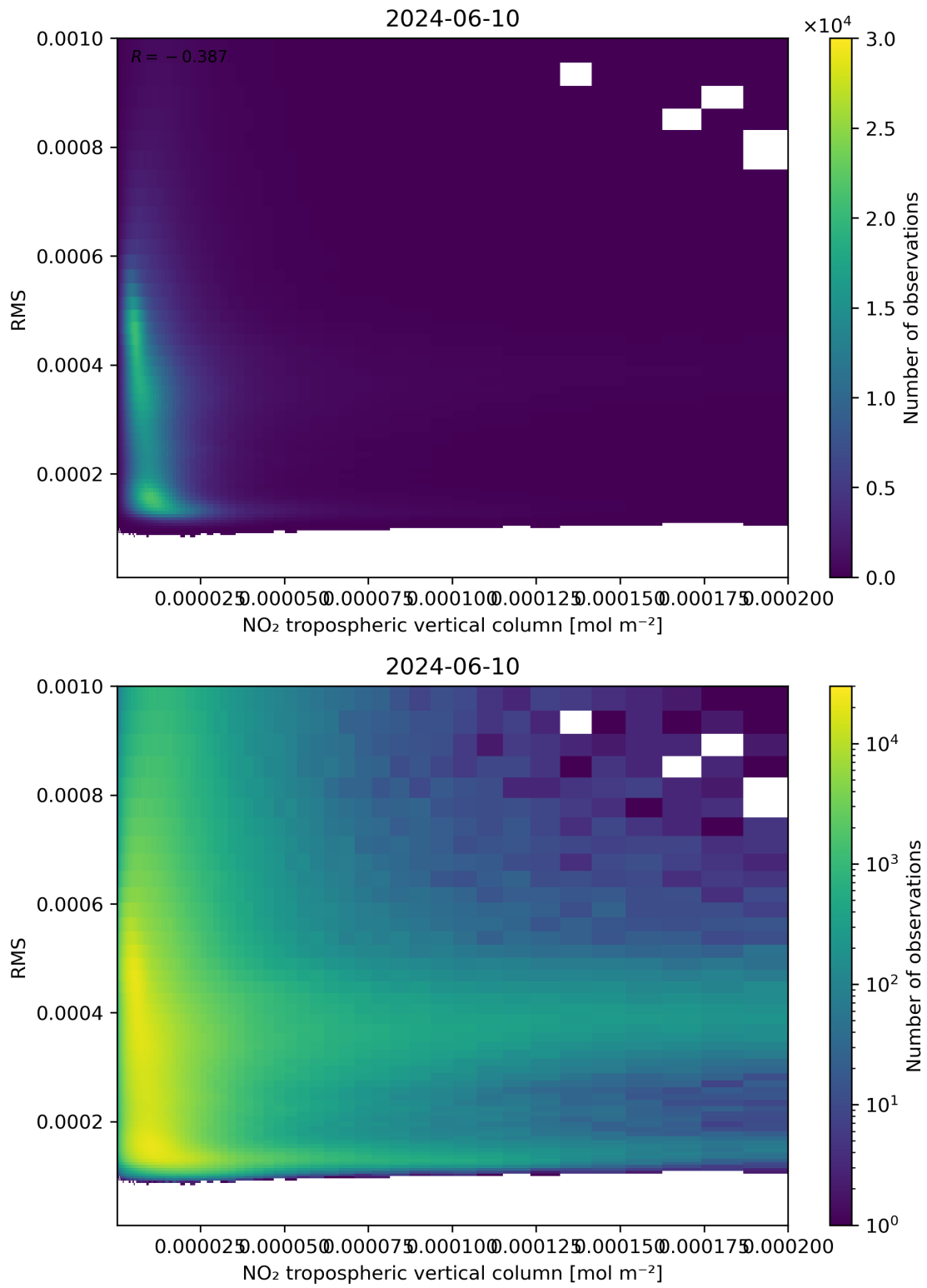
Figure 142: Scatter density plot of “NO 2 tropospheric vertical column” against “RMS” for 2024-06-09 to 2024-06-11.
