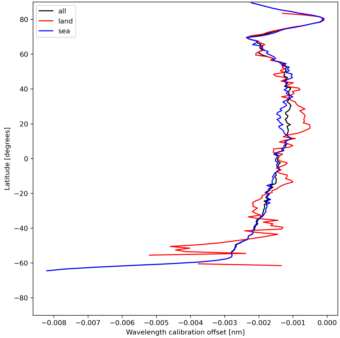
Figure 18: Zonal average of “Wavelength calibration offset” for 2024-06-09 to 2024-06-11.
