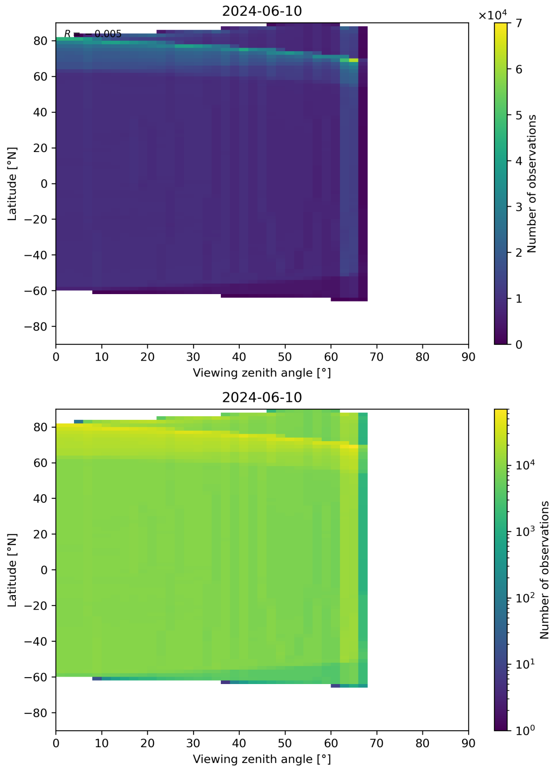
Figure 163: Scatter density plot of “Viewing zenith angle” against “Latitude” for 2024-06-09 to 2024-06-11.
