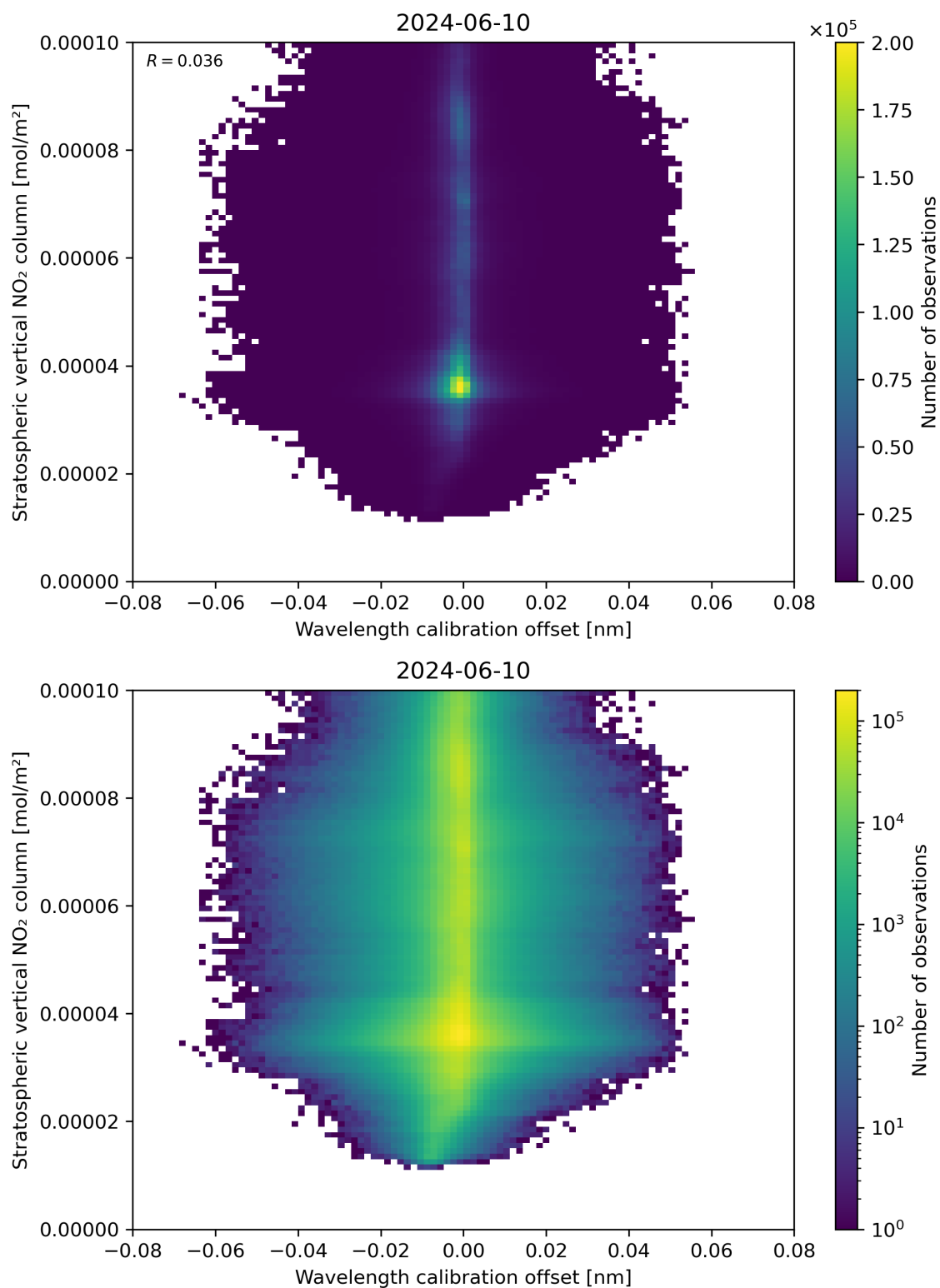
Figure 176: Scatter density plot of “Wavelength calibration offset” against “Stratospheric vertical NO 2 column” for 2024-06-09 to 2024-06-11.
