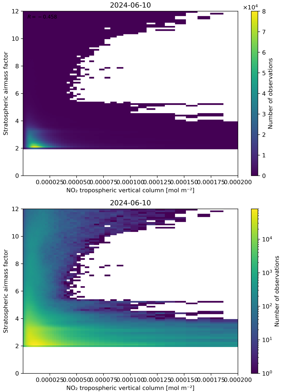
Figure 121: Scatter density plot of “NO 2 tropospheric vertical column” against “Stratospheric air mass factor” for 2024-06-09 to 2024-06-11.
