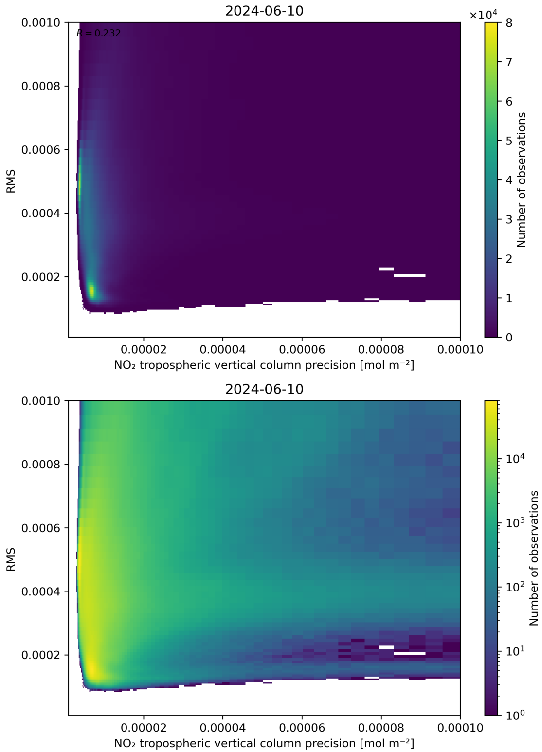
Figure 140: Scatter density plot of “NO 2 tropospheric vertical column precision” against “RMS” for 2024-06-09 to 2024-06-11.
