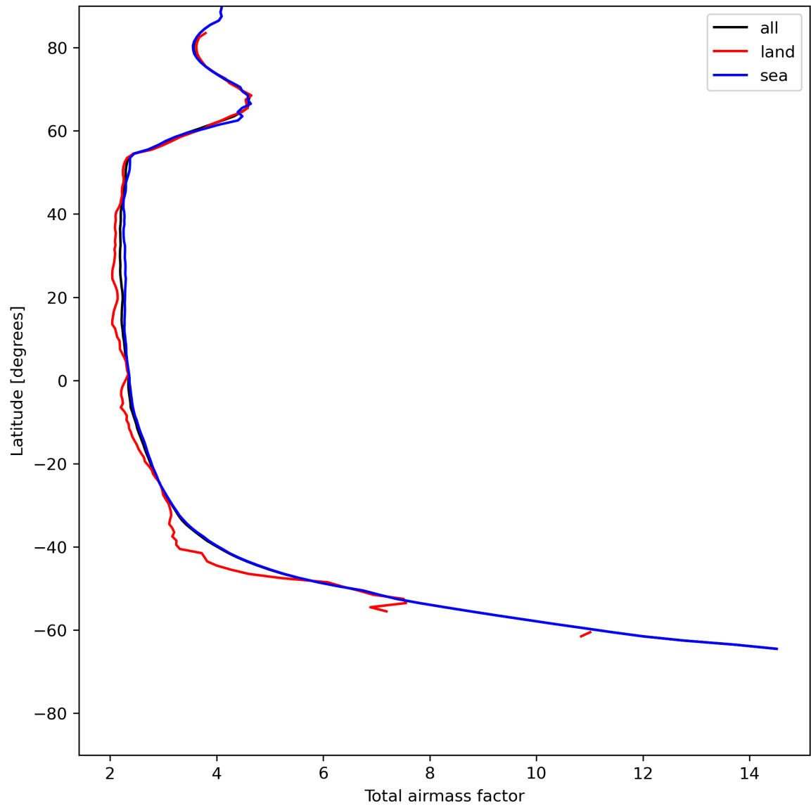
Figure 15: Zonal average of “Total airmass factor” for 2024-06-09 to 2024-06-11.
