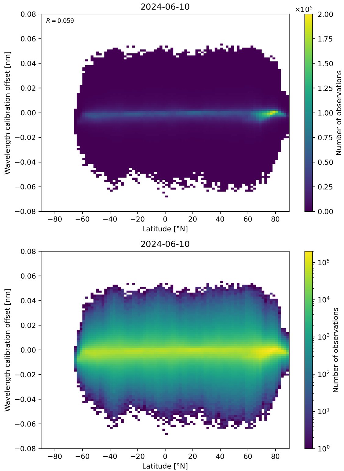
Figure 95: Scatter density plot of “Latitude” against “Wavelength calibration offset” for 2024-06-09 to 2024-06-11.
