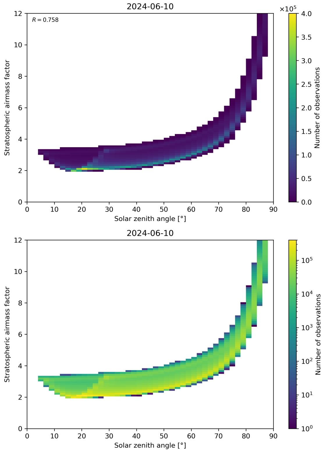
Figure 145: Scatter density plot of “Solar zenith angle” against “Stratospheric airmass factor” for 2024-06-09 to 2024-06-11.
