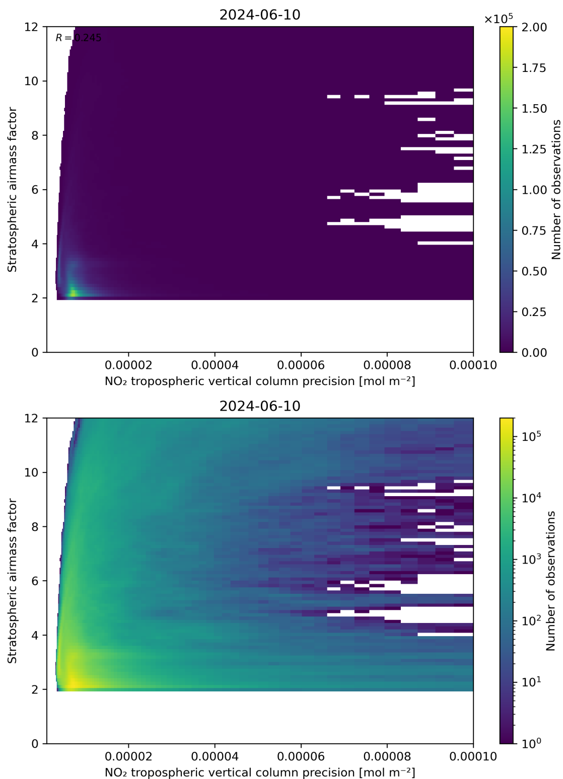
Figure 131: Scatter density plot of “NO 2 tropospheric vertical column precision” against “Stratospheric airmass factor” for 2024-06-09 to 2024-06-11.
