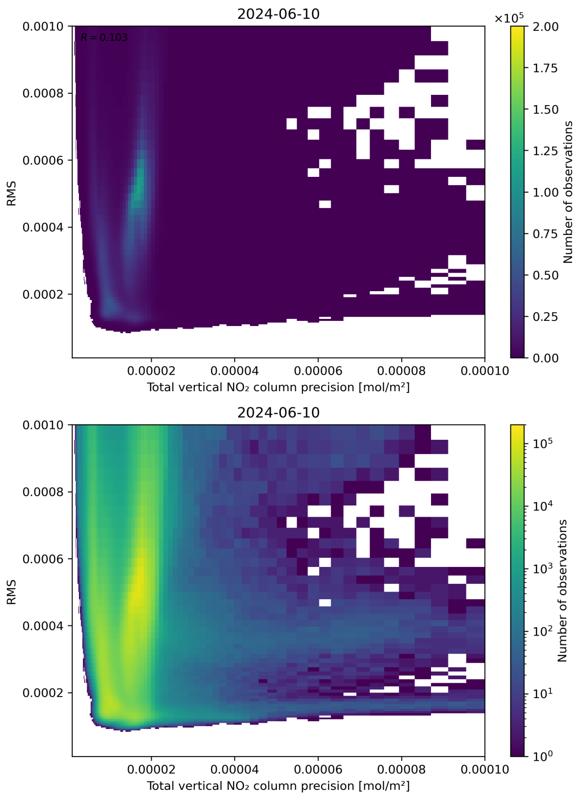
Figure 119: Scatter density plot of “Total vertical NO 2 column precision” against “RMS” for 2024-06-09 to 2024-06-11.
