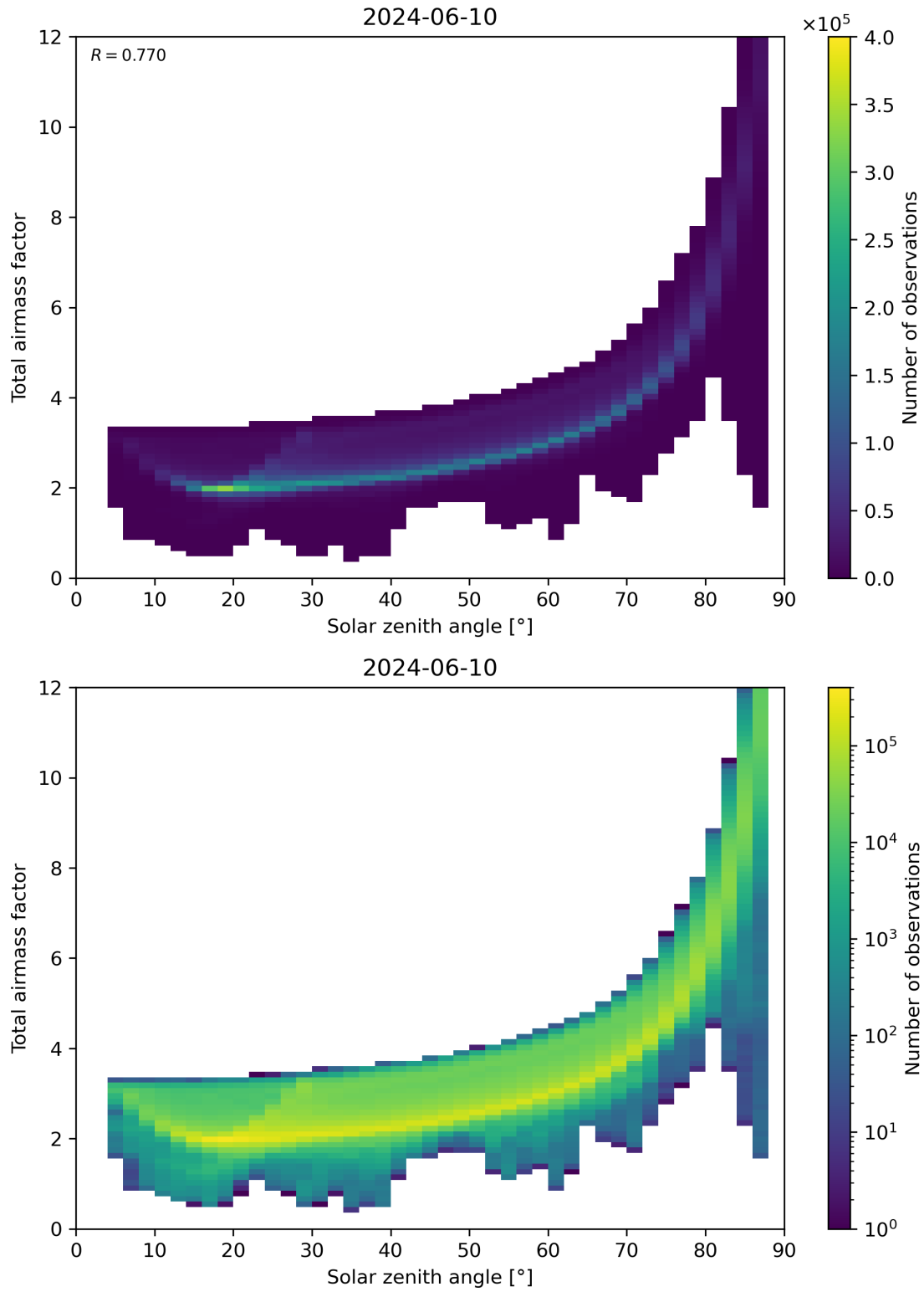
Figure 146: Scatter density plot of “Solar zenith angle” against “Total air mass factor” for 2024-06-09 to 2024-06-11.
