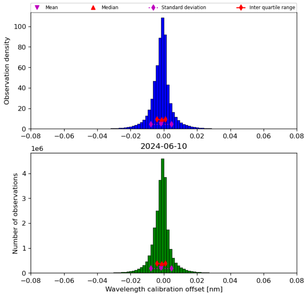
Figure 35: Histogram of “Wavelength calibration offset” for 2024-06-09 to 2024-06-11
