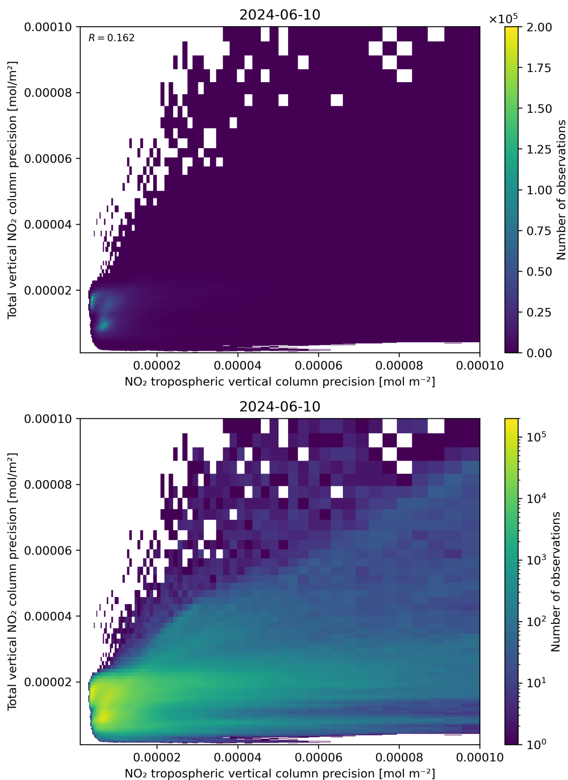
Figure 139: Scatter density plot of “NO 2 tropospheric vertical column precision” against “Total vertical NO 2 column precision” for 2024-06-09 to 2024-06-11.
