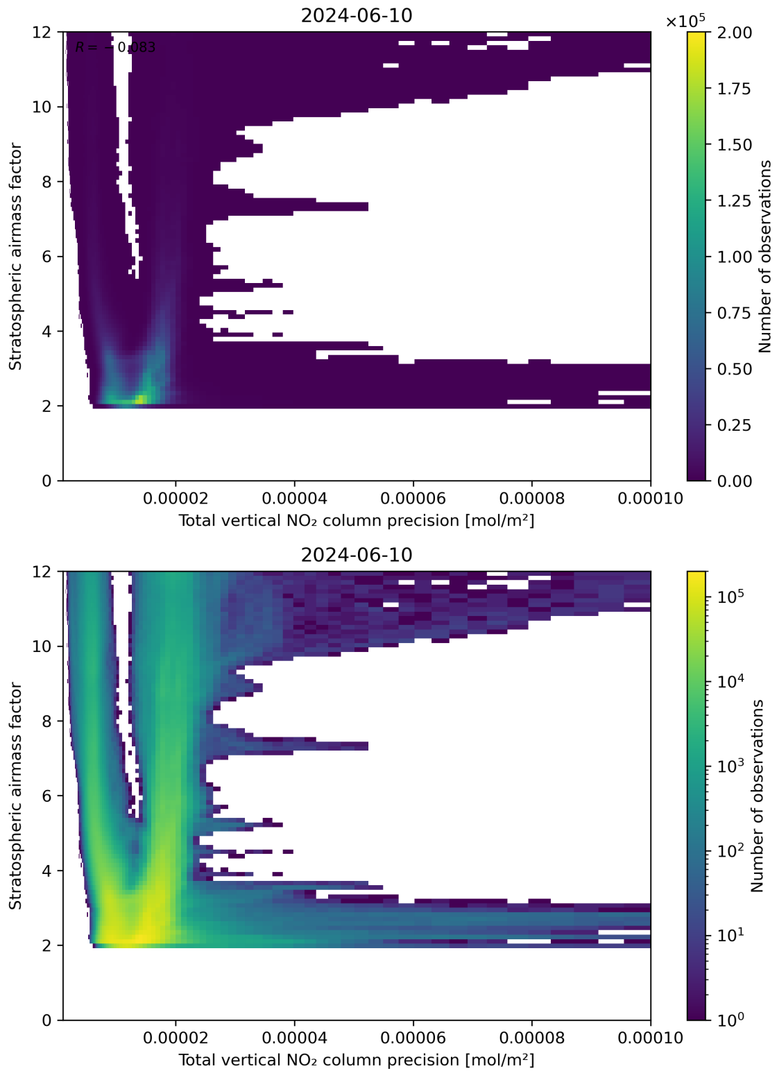
Figure 115: Scatter density plot of “Total vertical NO 2 column precision” against “Stratospheric air mass factor” for 2024-06-09 to 2024-06-11.
