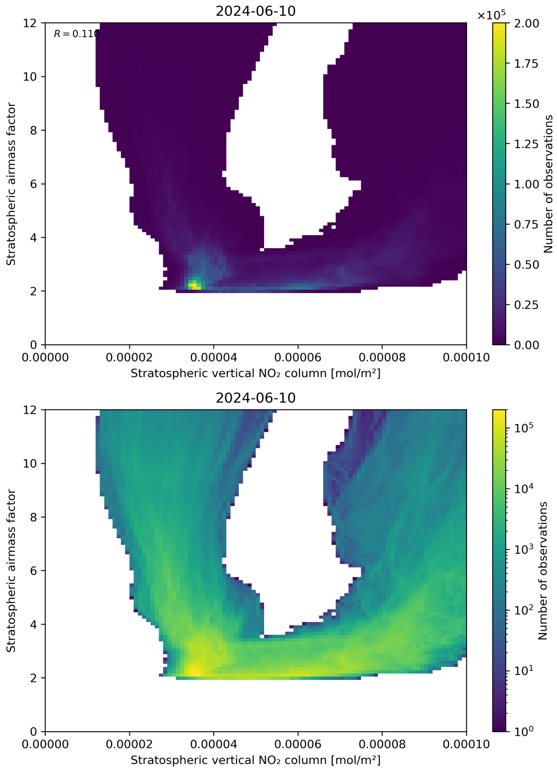
Figure 96: Scatter density plot of “Stratospheric vertical NO 2 column” against “Stratospheric airmass factor” for 2024-06-09 to 2024-06-11.
