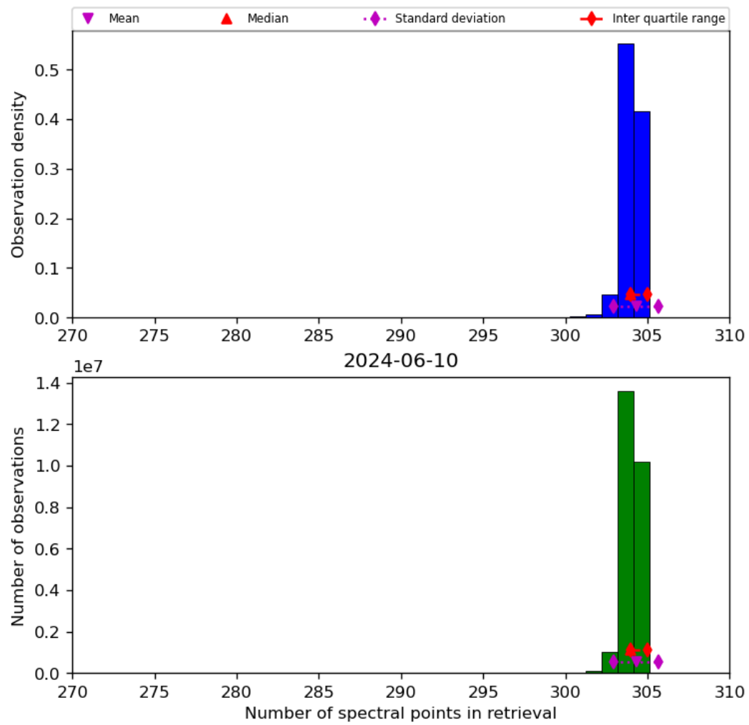
Figure 33: Histogram of “Number of spectral points in retrieval” for 2024-06-09 to 2024-06-11
