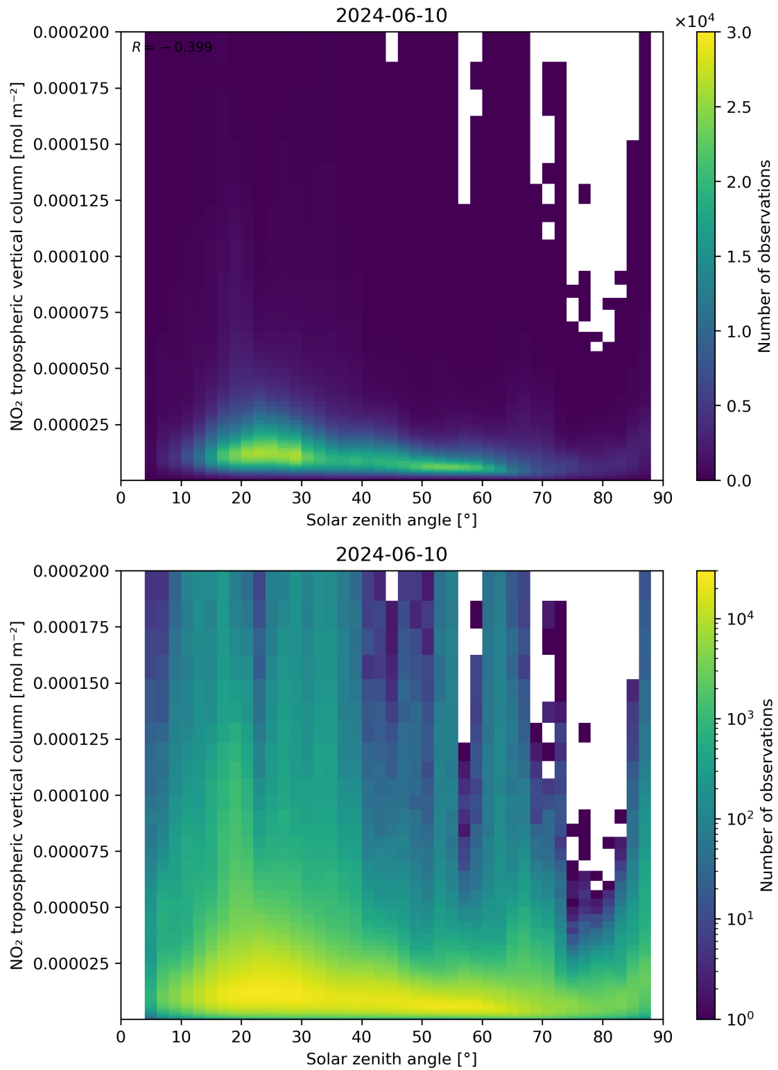
Figure 155: Scatter density plot of “Solar zenith angle” against “NO 2 tropospheric vertical column” for 2024-06-09 to 2024-06-11.
