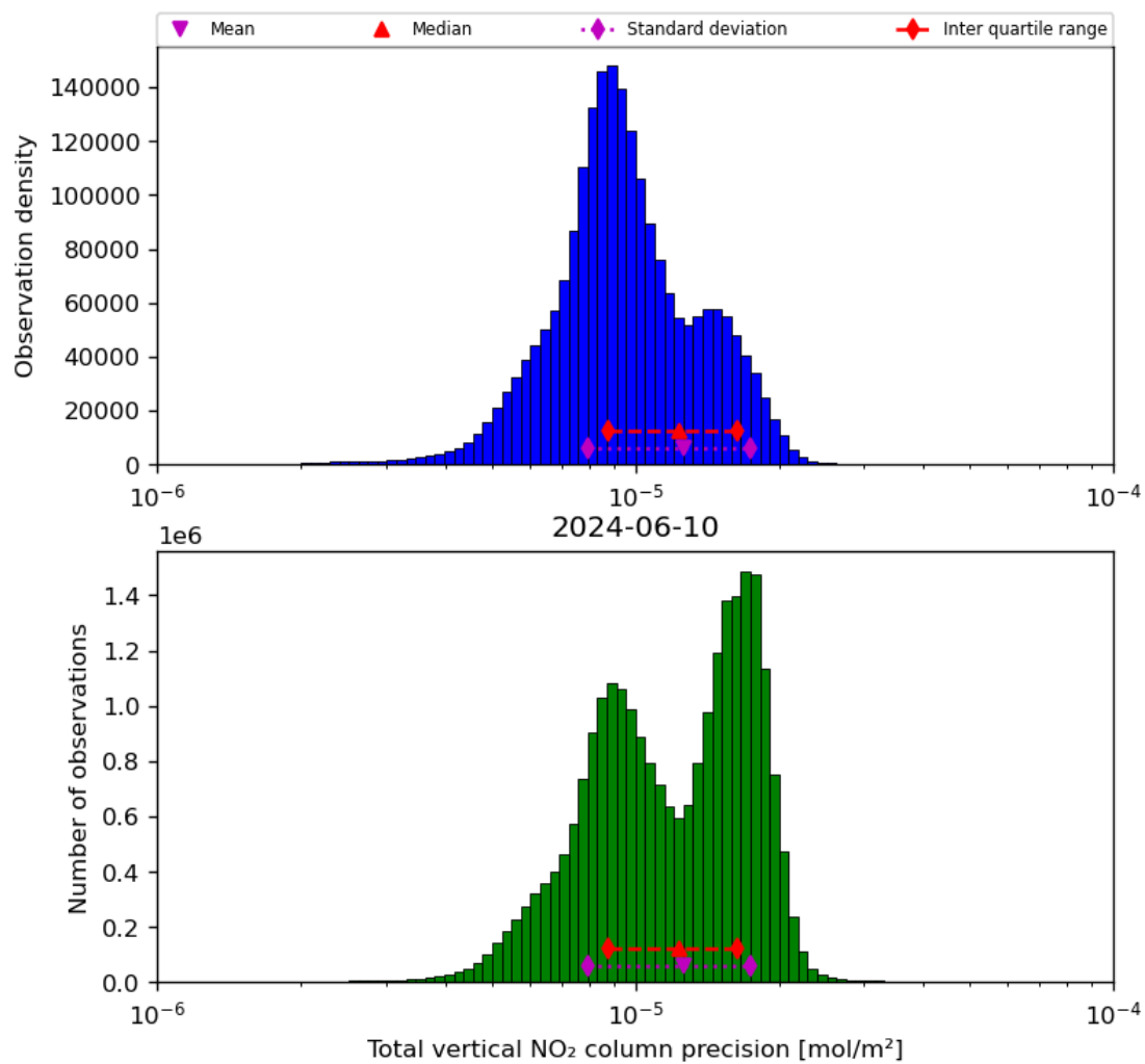
Figure 39: Histogram of “Total vertical NO 2 column precision” for 2024-06-09 to 2024-06-11
