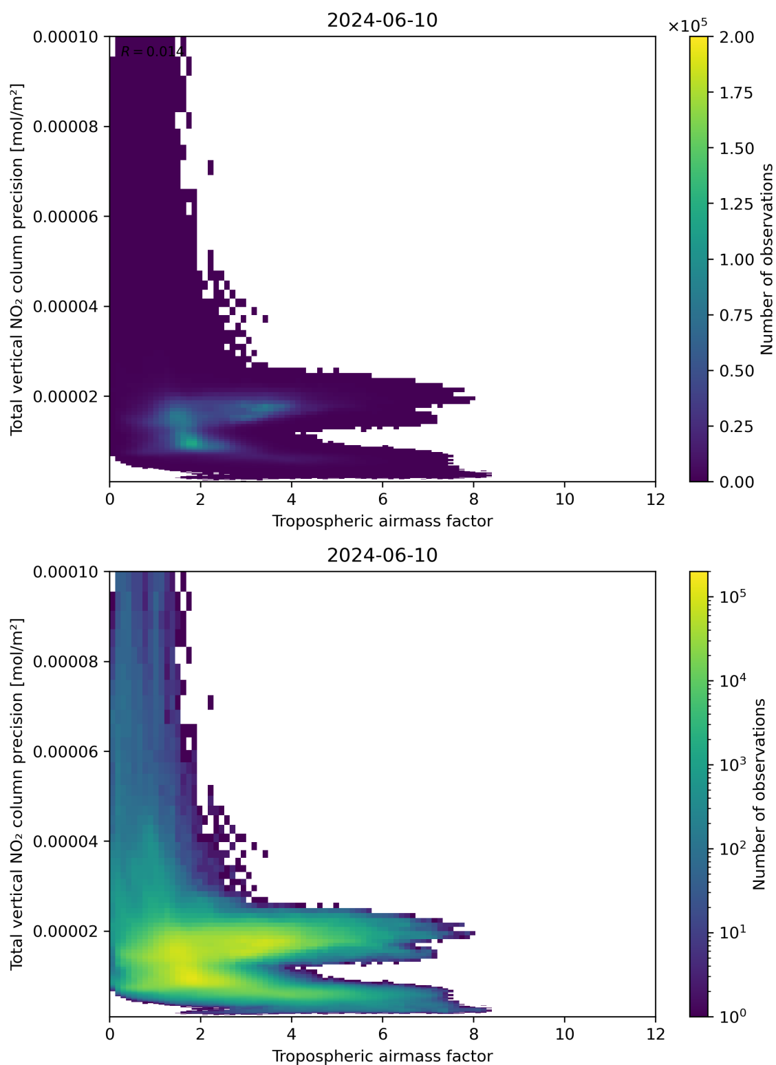
Figure 78: Scatter density plot of “Tropospheric air mass factor” against “Total vertical NO 2 column precision” for 2024-06-09 to 2024-06-11.
