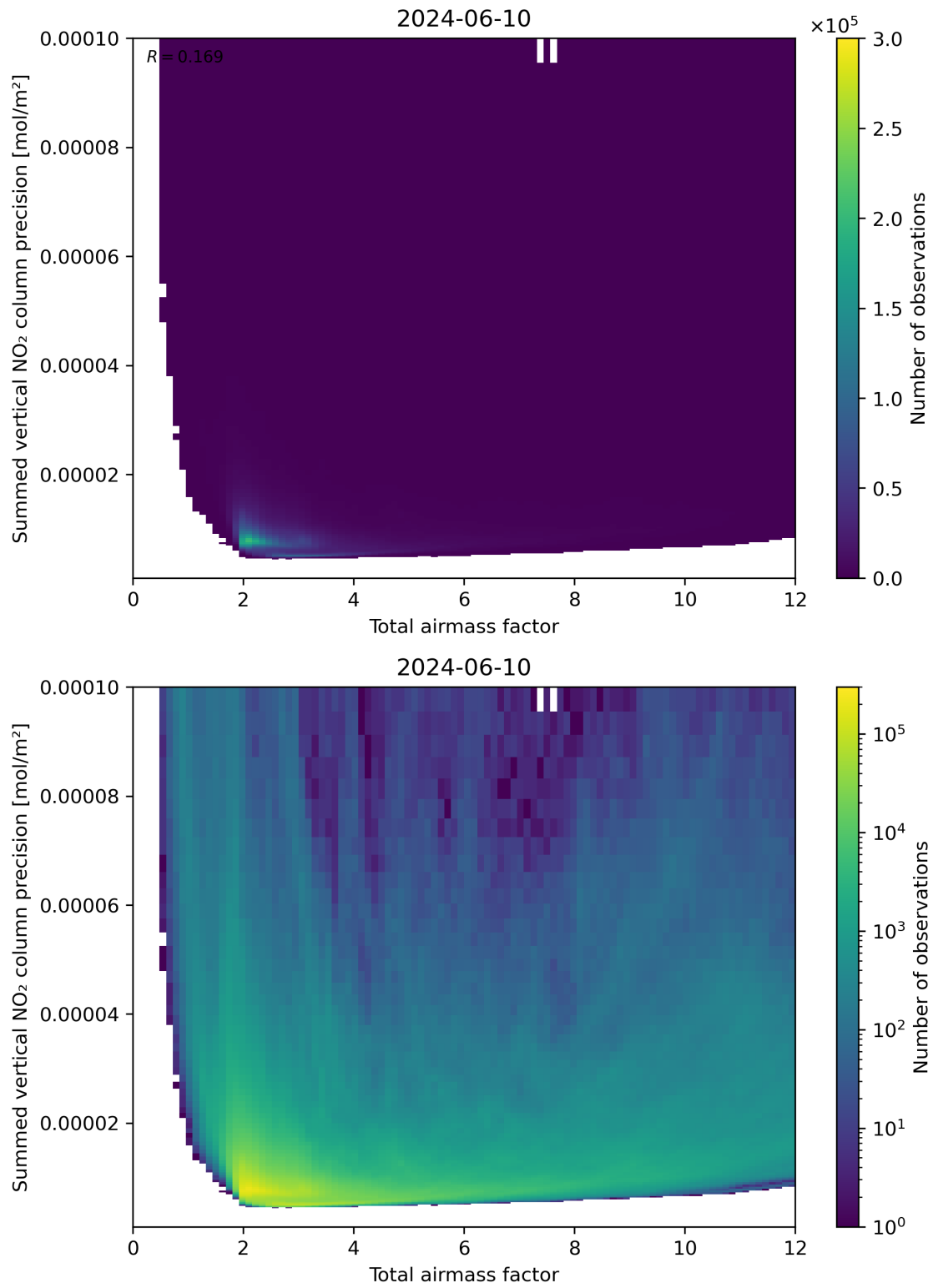
Figure 66: Scatter density plot of “Total airmass factor” against “Summed vertical NO 2 column precision” for 2024-06-09 to 2024-06-11.
