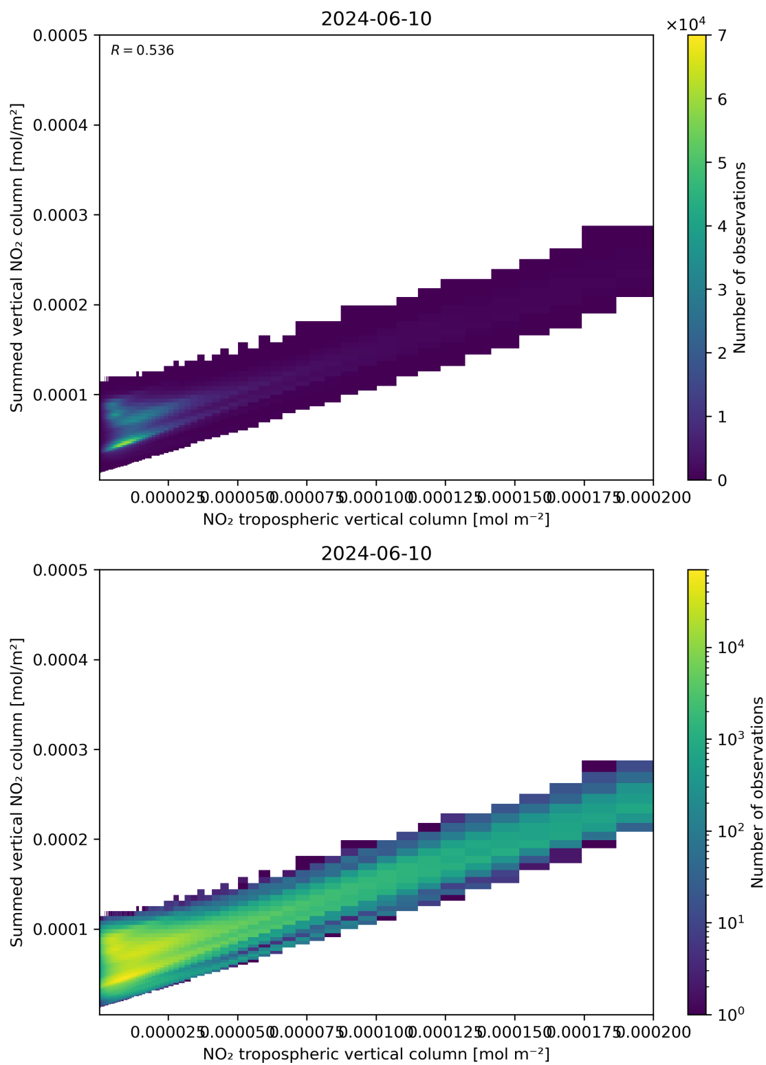
Figure 126: Scatter density plot of “NO 2 tropospheric vertical column” against “Summed vertical NO 2 column” for 2024-06-09 to 2024-06-11.
