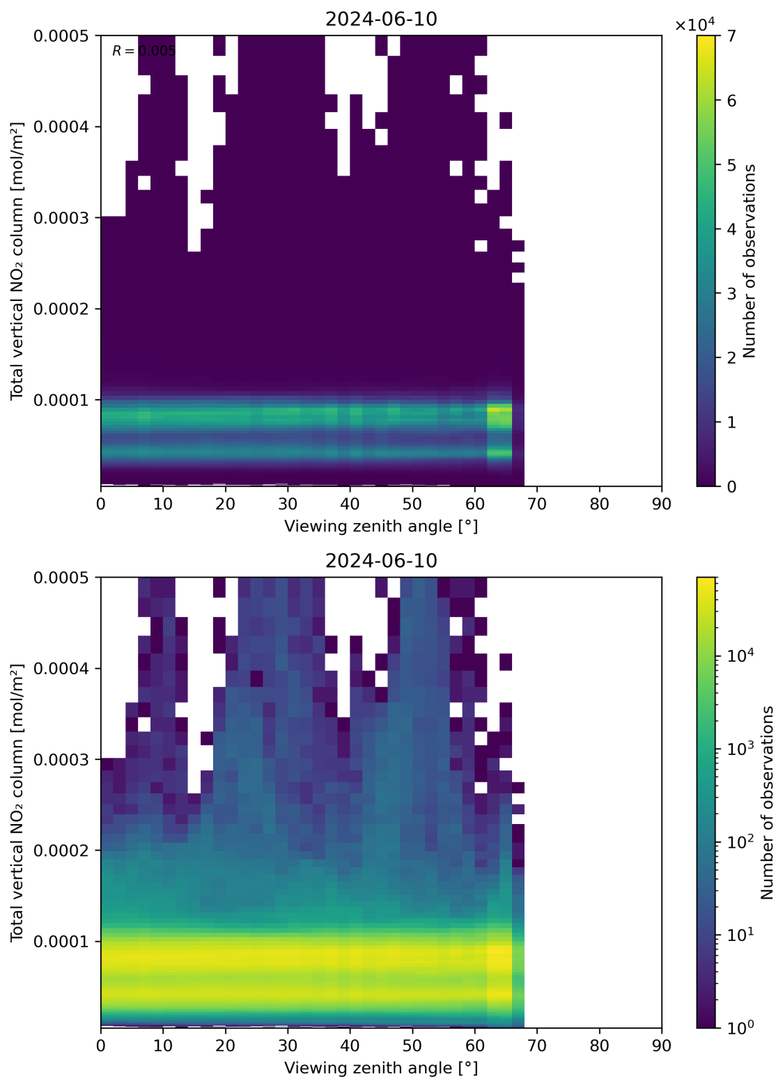
Figure 167: Scatter density plot of “Viewing zenith angle” against “Total vertical NO 2 column” for 2024-06-09 to 2024-06-11.
