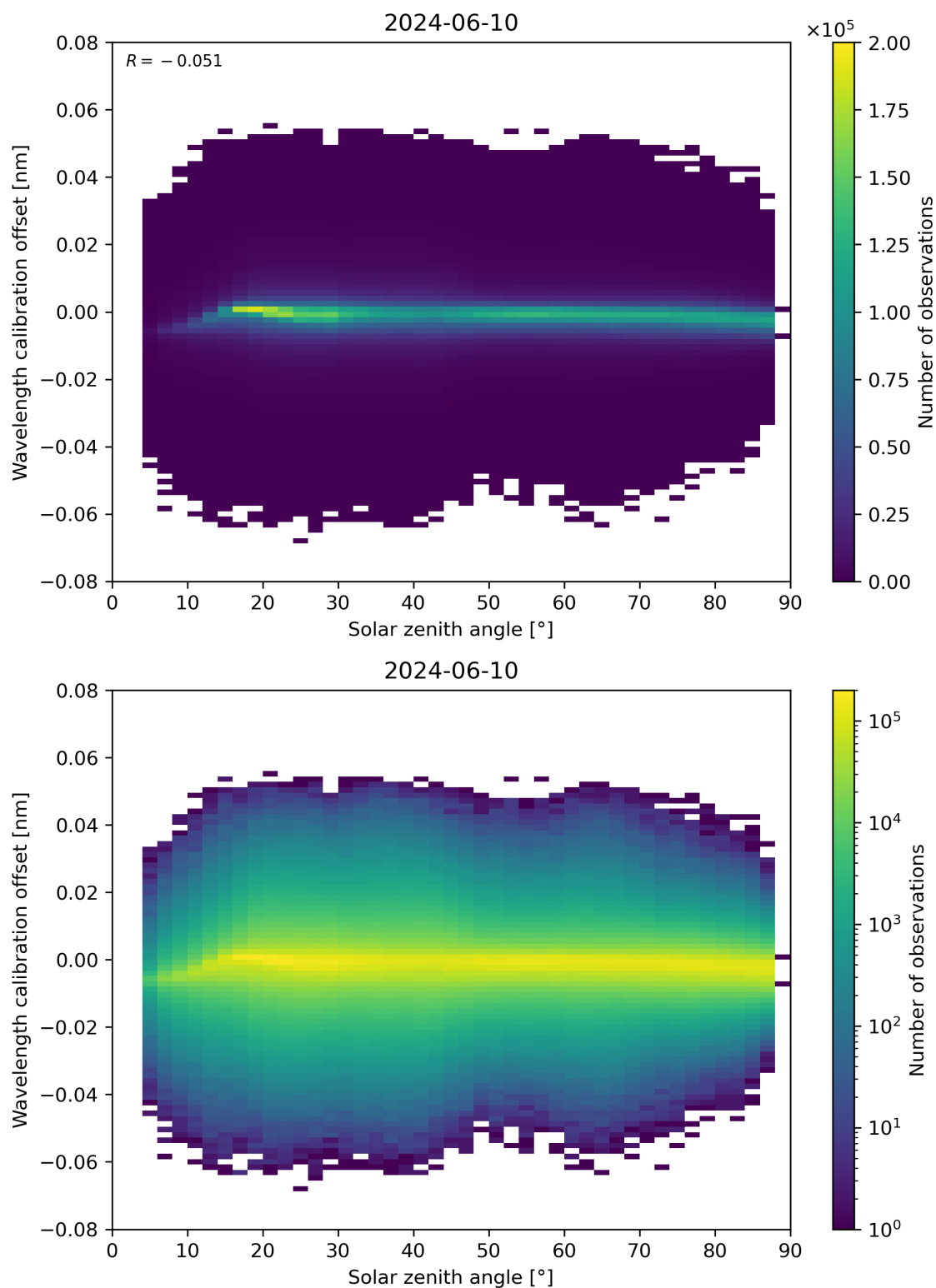
Figure 158: Scatter density plot of “Solar zenith angle” against “Wavelength calibration offset” for 2024-06-09 to 2024-06-11.
