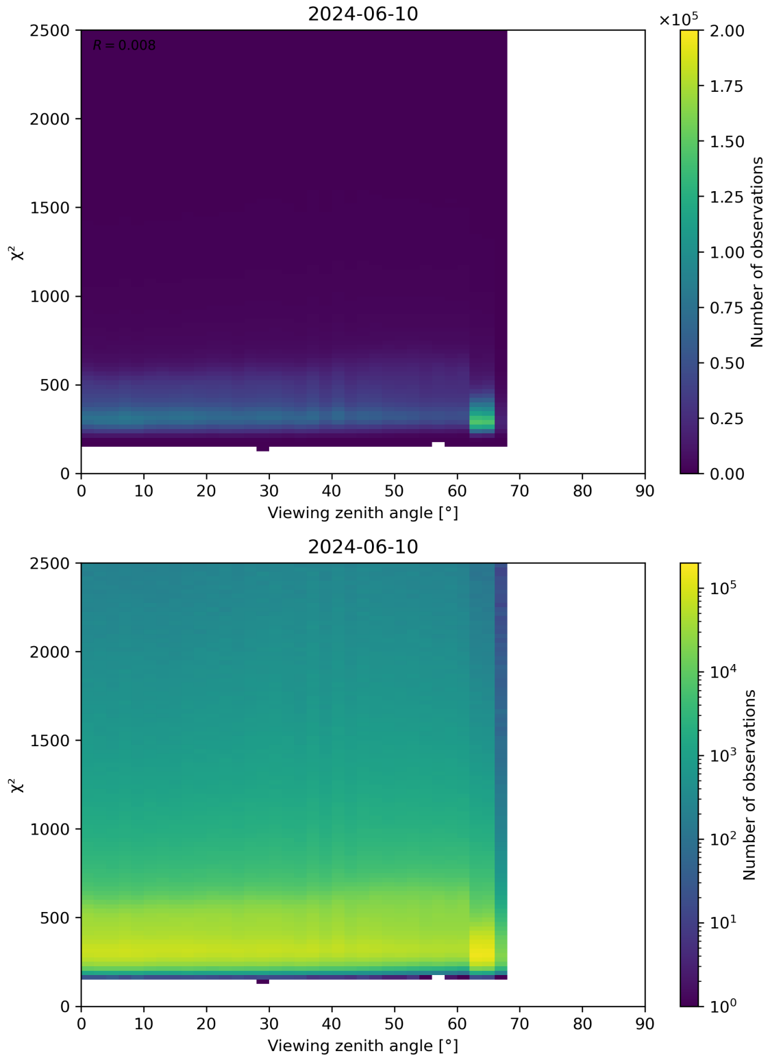
Figure 162: Scatter density plot of “Viewing zenith angle” against “ \chi^2 ” for 2024-06-09 to 2024-06-11.
