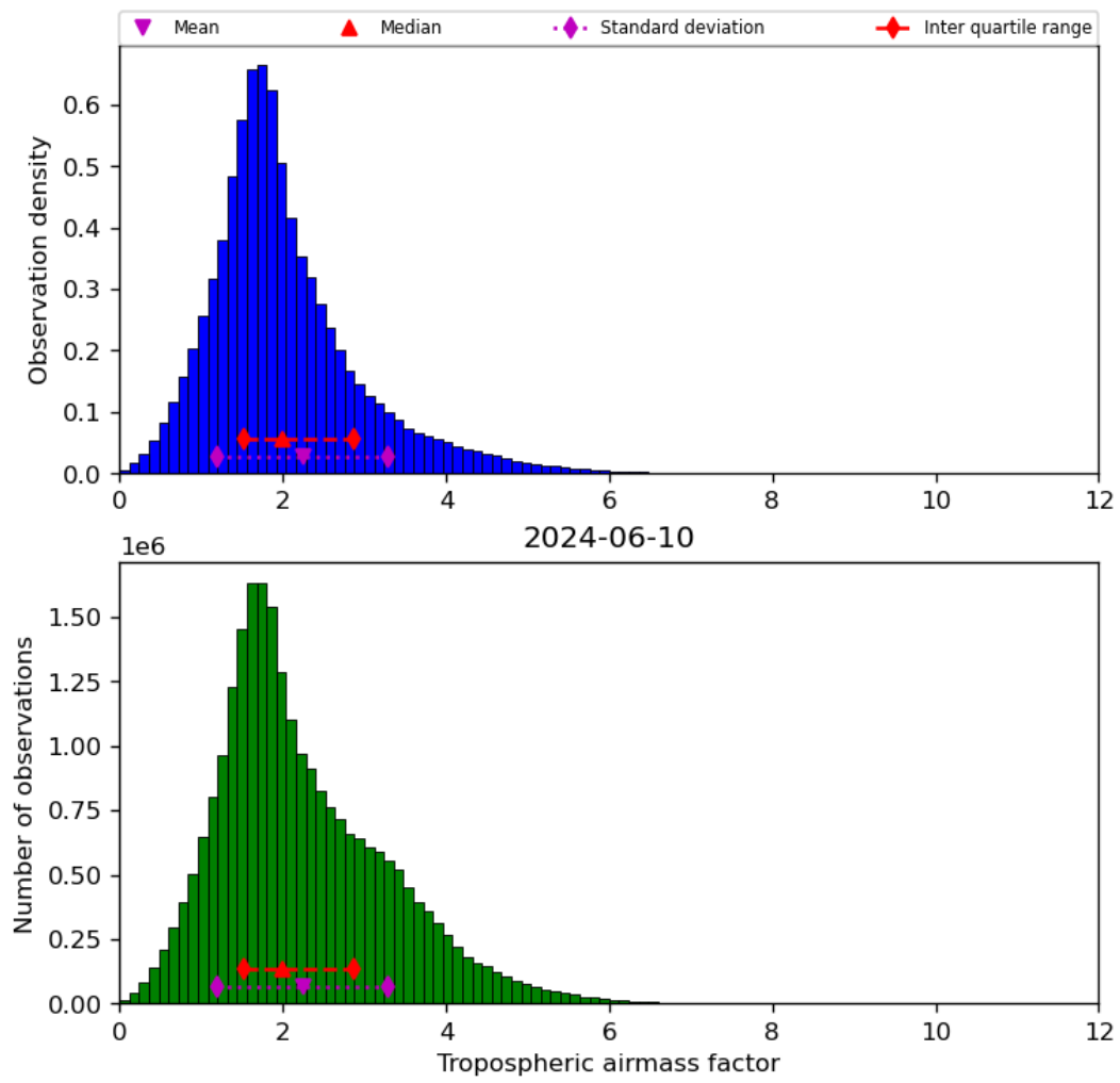
Figure 31: Histogram of “Tropospheric airmass factor” for 2024-06-09 to 2024-06-11
