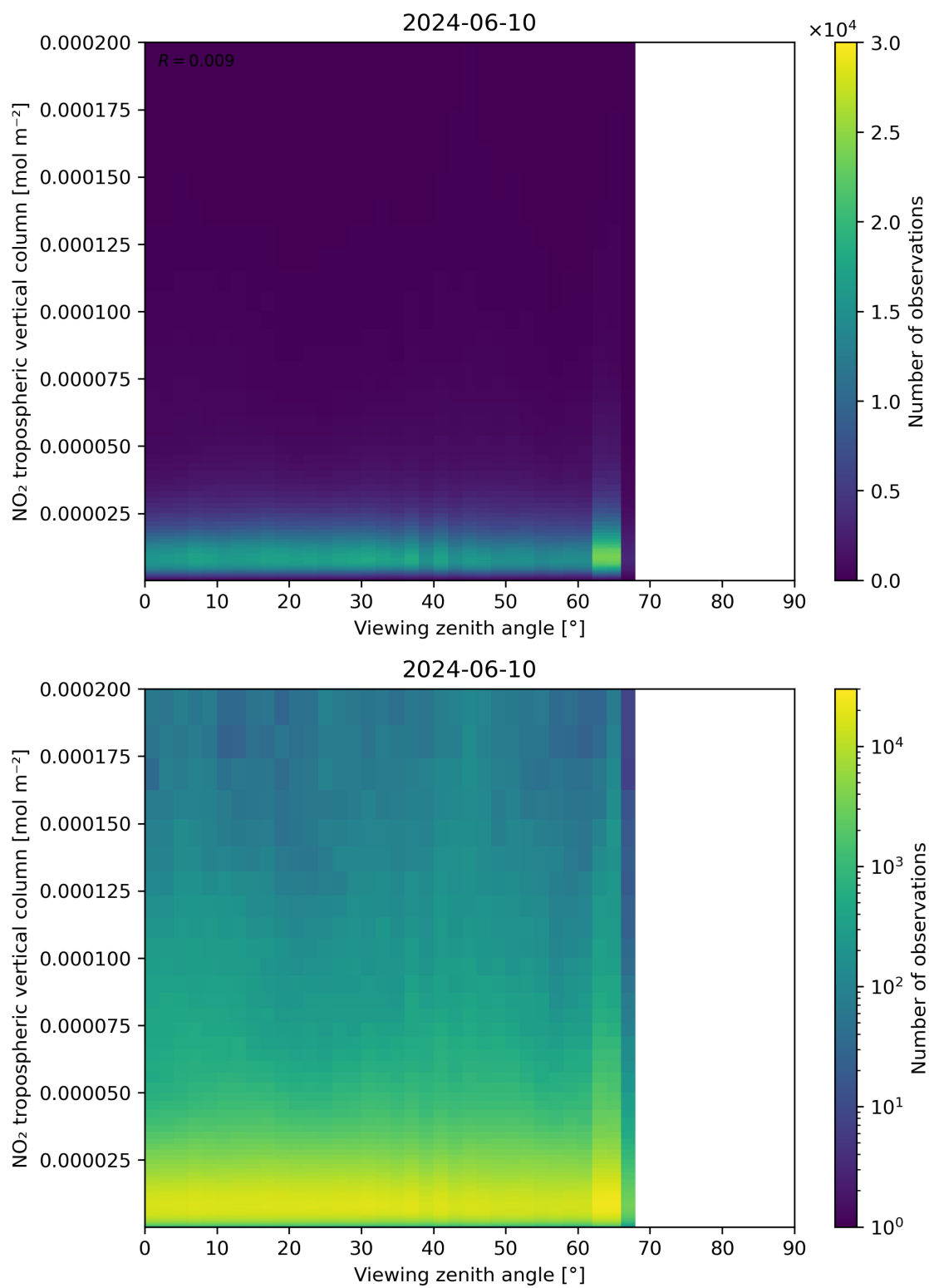
Figure 169: Scatter density plot of “Viewing zenith angle” against “NO 2 tropospheric vertical column” for 2024-06-09 to 2024-06-11.
