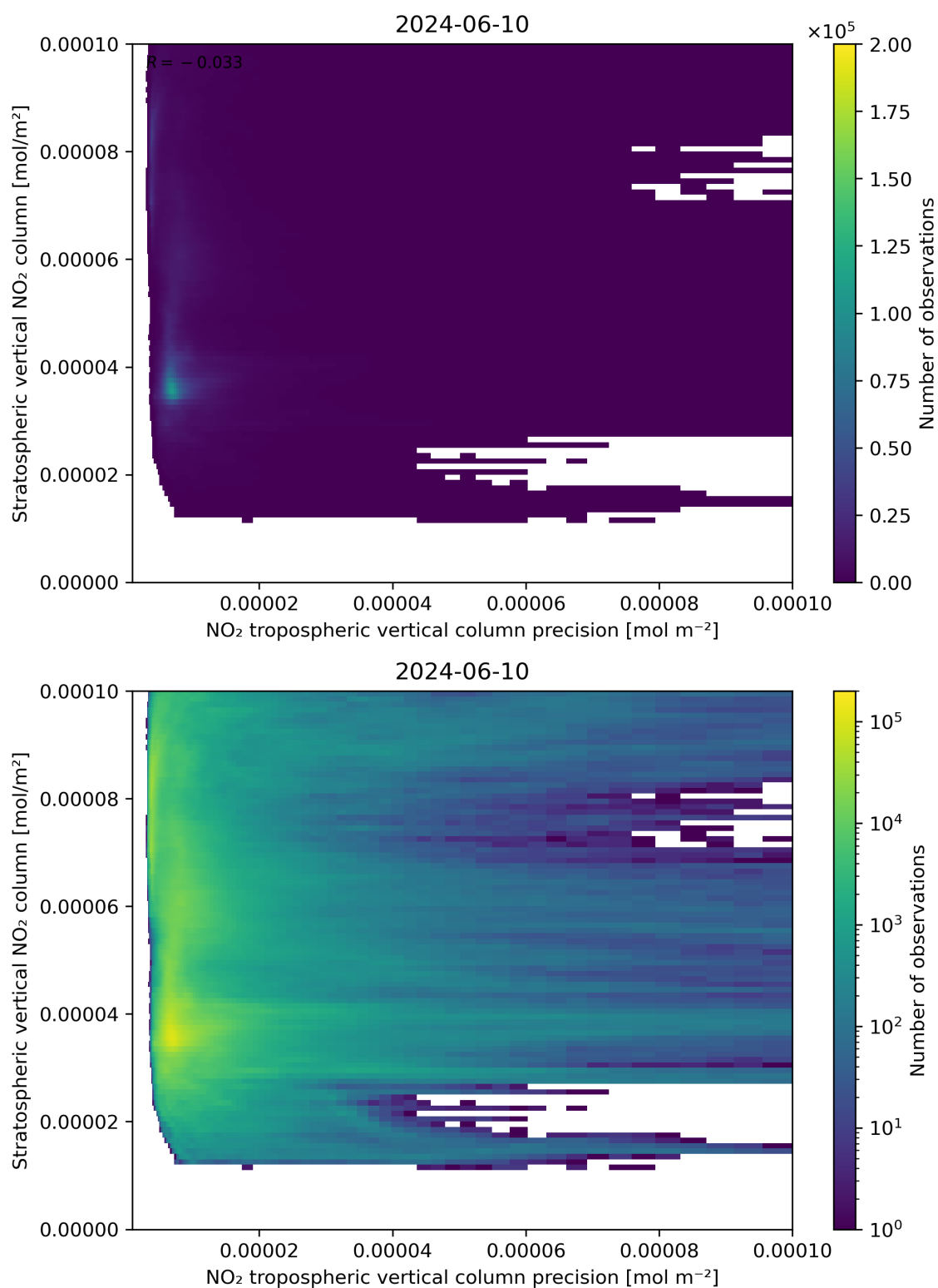
Figure 135: Scatter density plot of “NO 2 tropospheric vertical column precision” against “Stratospheric vertical NO 2 column” for 2024-06-09 to 2024-06-11.
