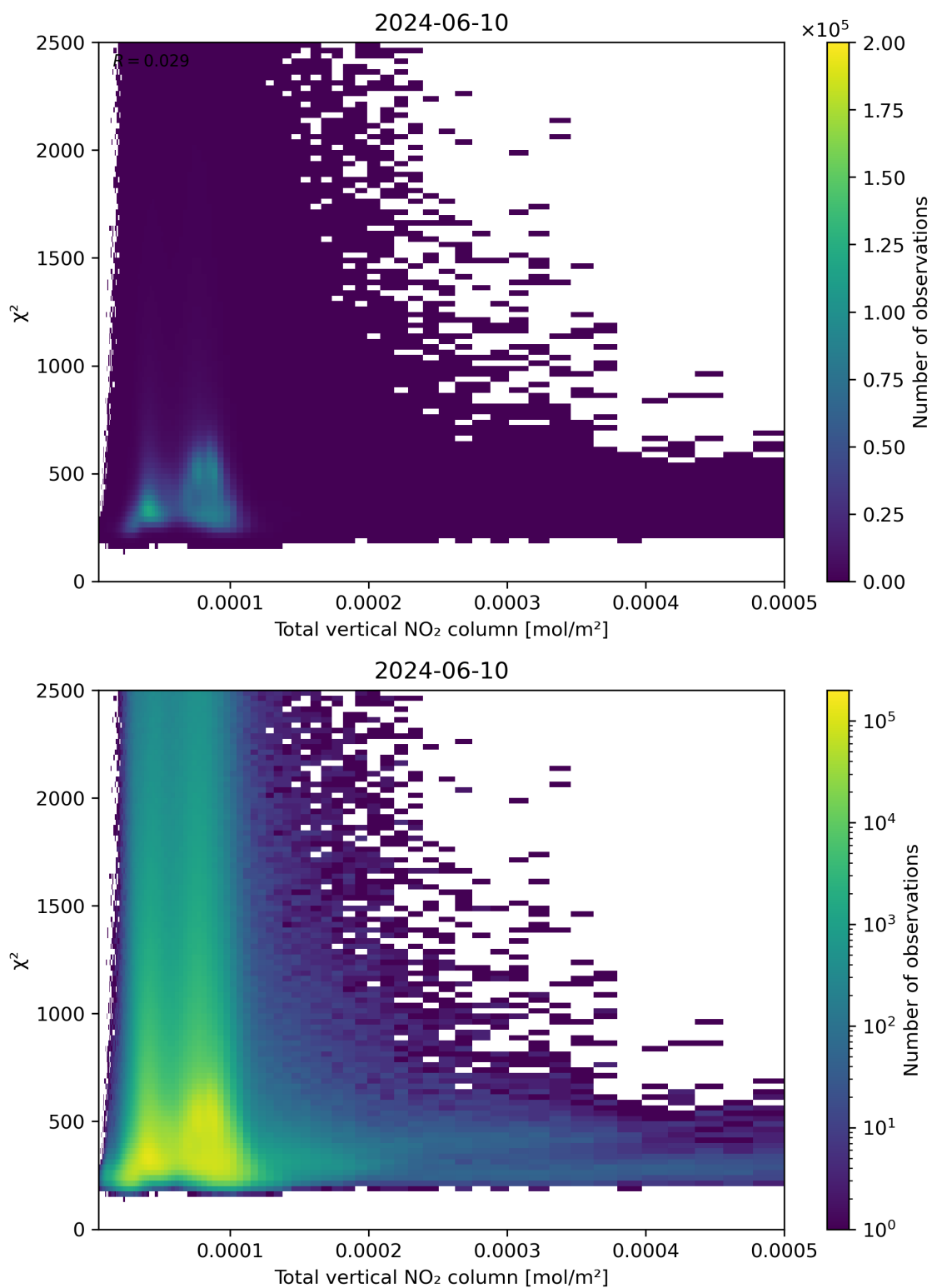
Figure 111: Scatter density plot of “Total vertical NO 2 column” against “ \chi^2 ” for 2024-06-09 to 2024-06-11.
