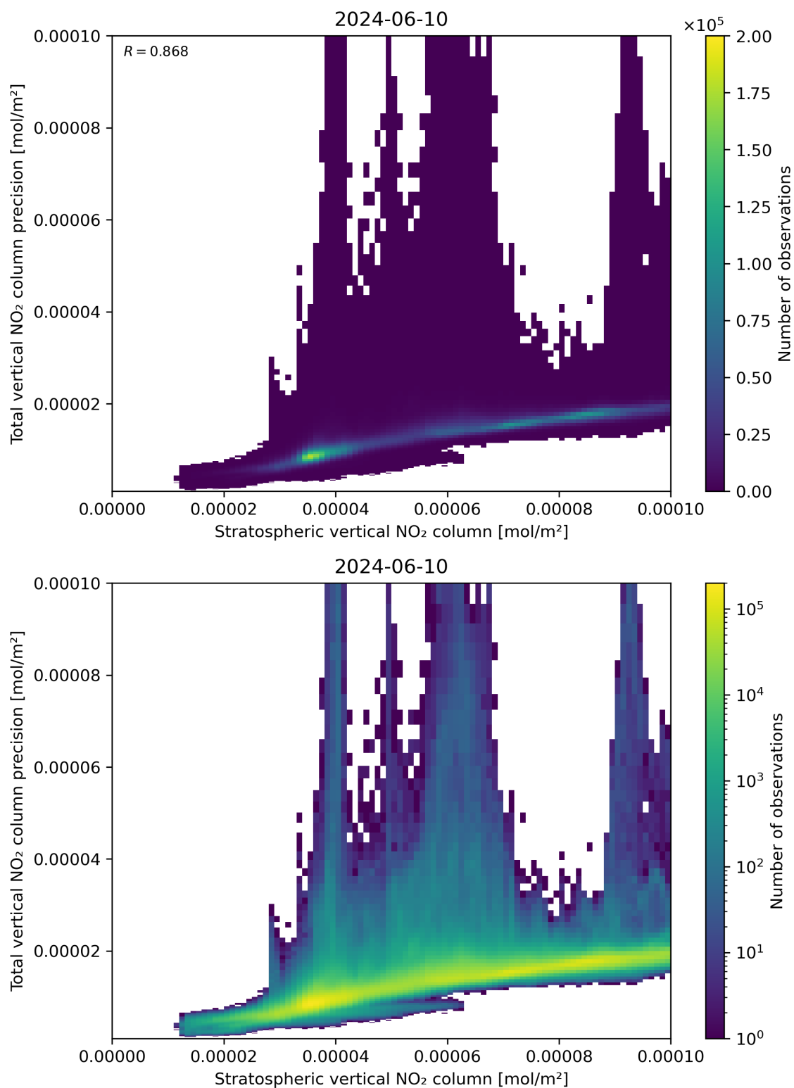
Figure 101: Scatter density plot of “Stratospheric vertical NO 2 column” against “Total vertical NO 2 column precision” for 2024-06-09 to 2024-06-11.
