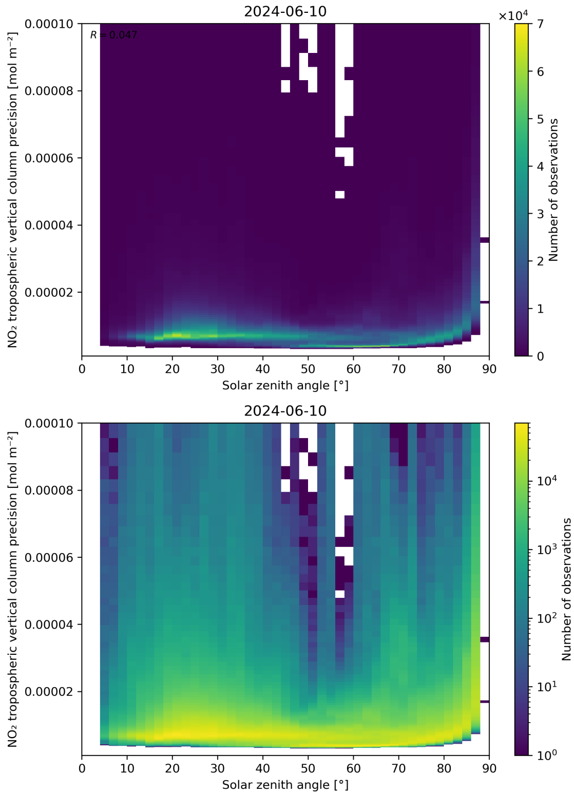
Figure 156: Scatter density plot of “Solar zenith angle” against “NO 2 tropospheric vertical column precision” for 2024-06-09 to 2024-06-11.
