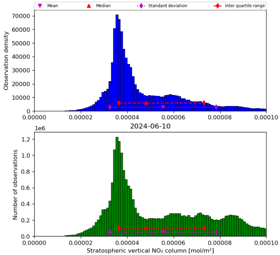
Figure 36: Histogram of “Stratospheric vertical NO 2 column” for 2024-06-09 to 2024-06-11
