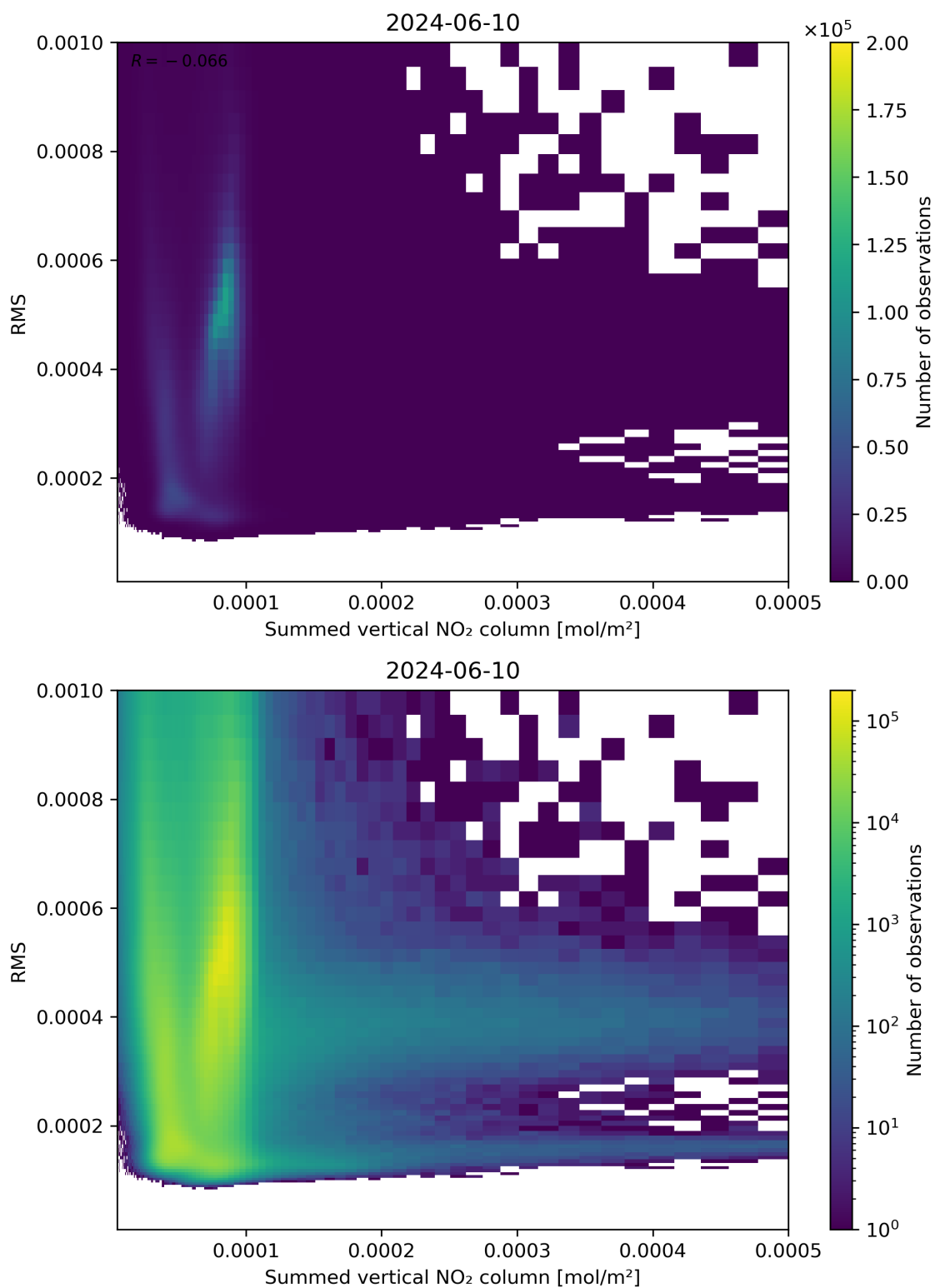
Figure 109: Scatter density plot of “Summed vertical NO 2 column” against “RMS” for 2024-06-09 to 2024-06-11.
