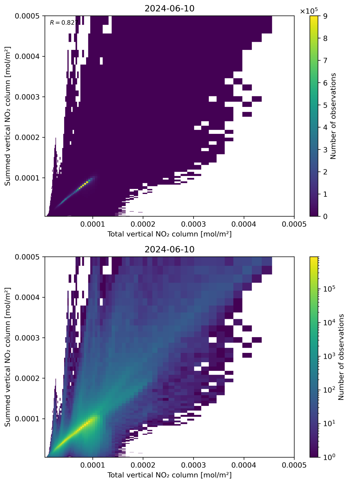
Figure 112: Scatter density plot of “Total vertical NO 2 column” against “Summed vertical NO 2 column” for 2024-06-09 to 2024-06-11.
