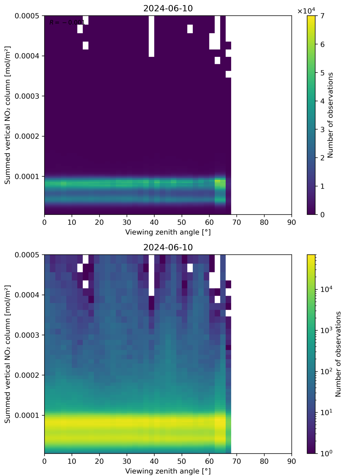
Figure 165: Scatter density plot of “Viewing zenith angle” against “Summed vertical NO 2 column” for 2024-06-09 to 2024-06-11.
