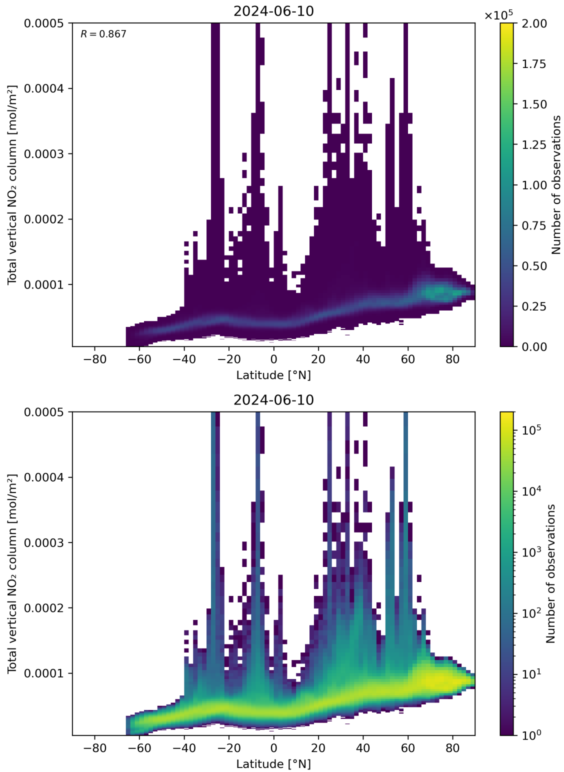
Figure 90: Scatter density plot of “Latitude” against “Total vertical NO 2 column” for 2024-06-09 to 2024-06-11.
