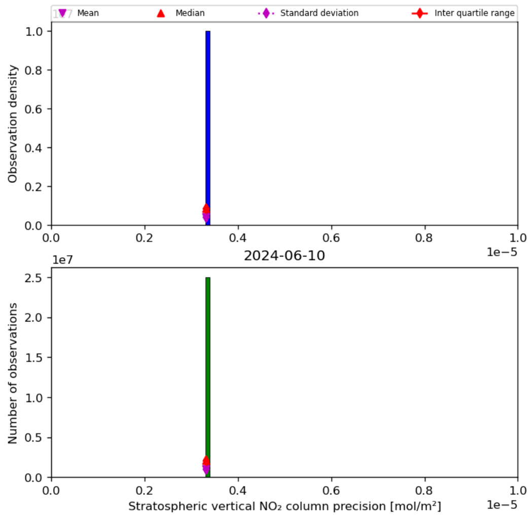
Figure 37: Histogram of “Stratospheric vertical NO 2 column precision” for 2024-06-09 to 2024-06-11
