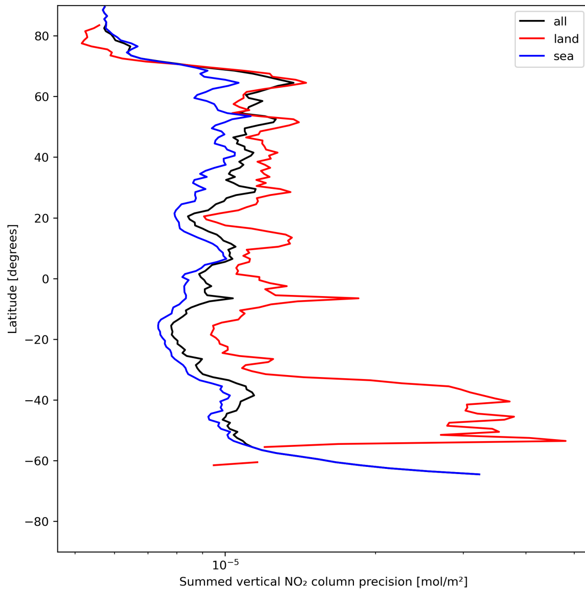
Figure 24: Zonal average of “Summed vertical NO 2 column precision” for 2024-06-09 to 2024-06-11.
