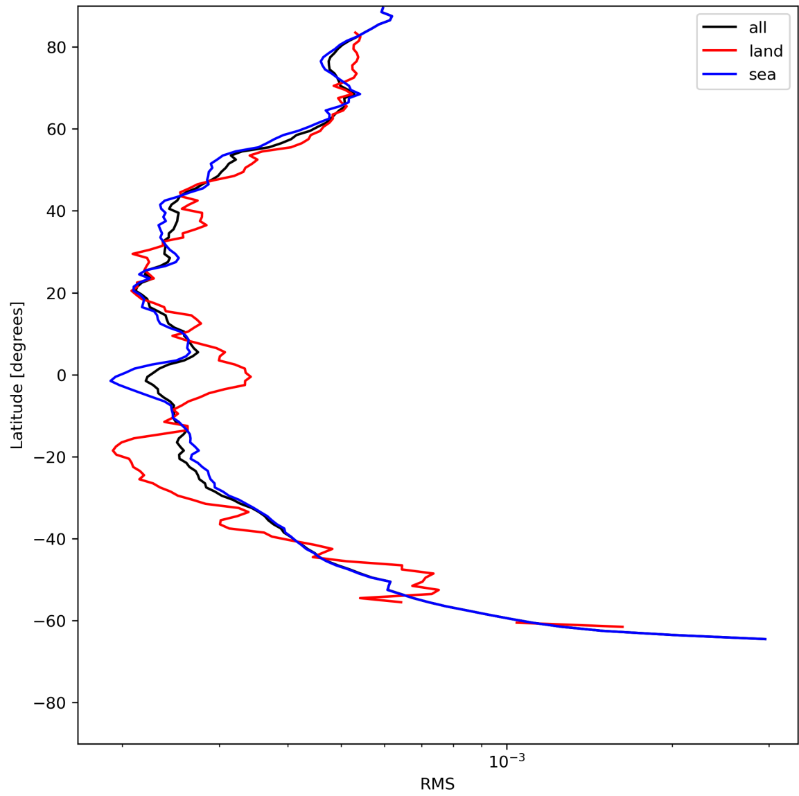
Figure 26: Zonal average of “RMS” for 2024-06-09 to 2024-06-11.
