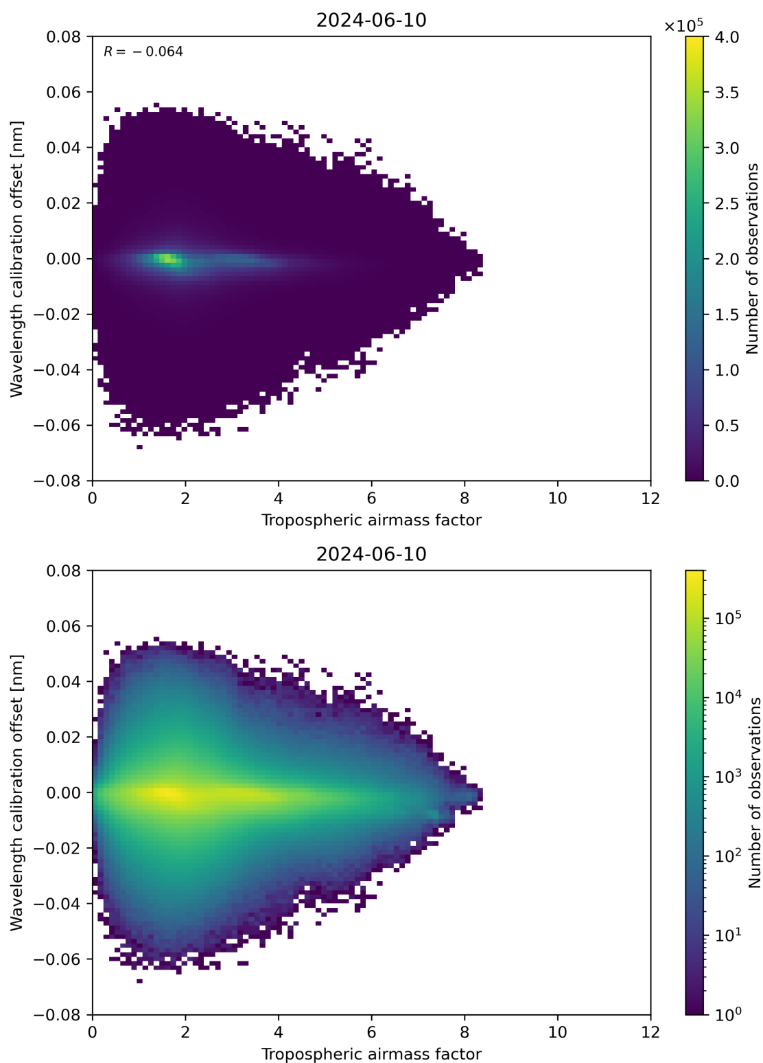
Figure 80: Scatter density plot of “Tropospheric airmass factor” against “Wavelength calibration offset” for 2024-06-09 to 2024-06-11.
