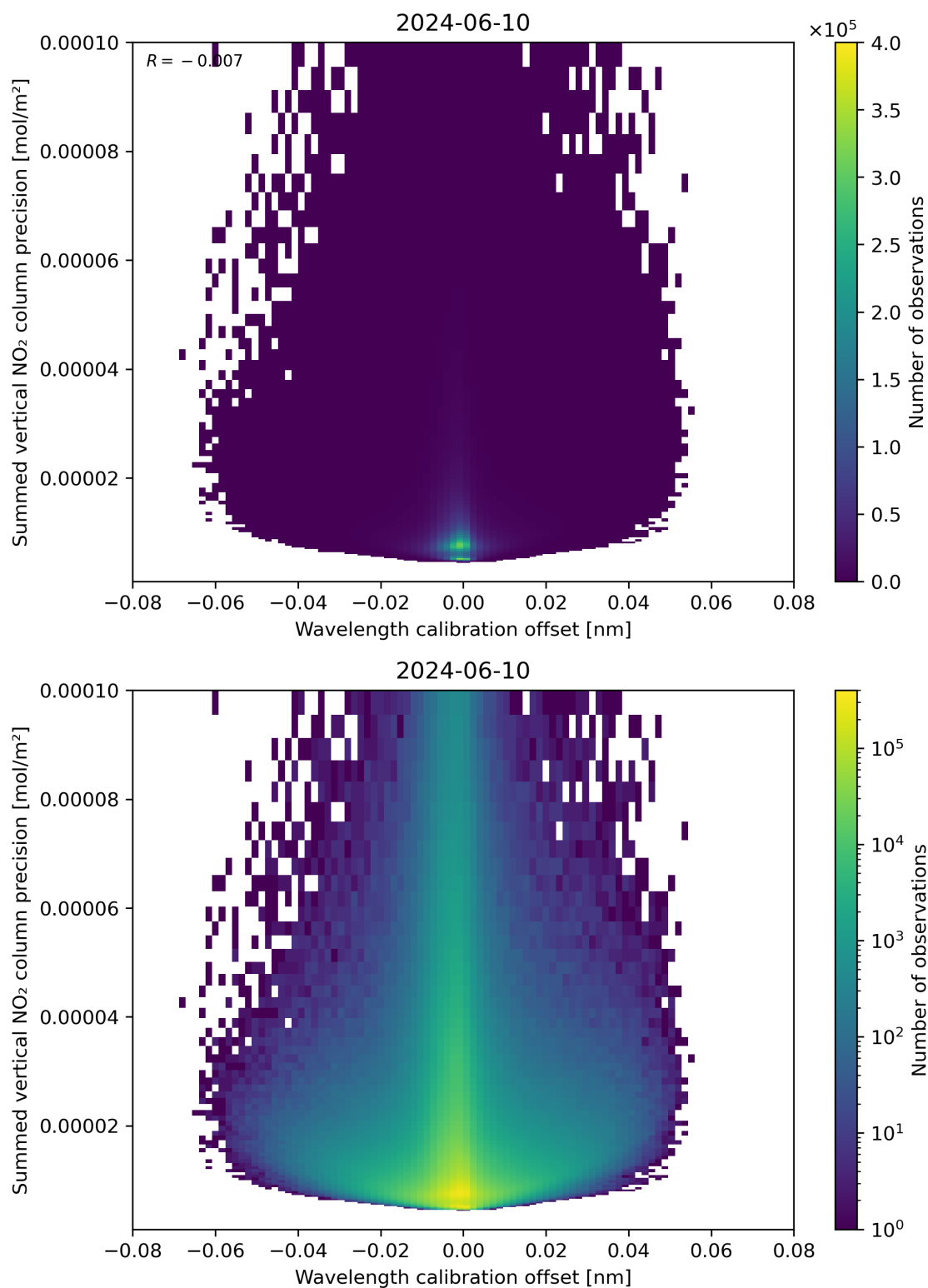
Figure 178: Scatter density plot of “Wavelength calibration offset” against “Summed vertical NO 2 column precision” for 2024-06-09 to 2024-06-11.
