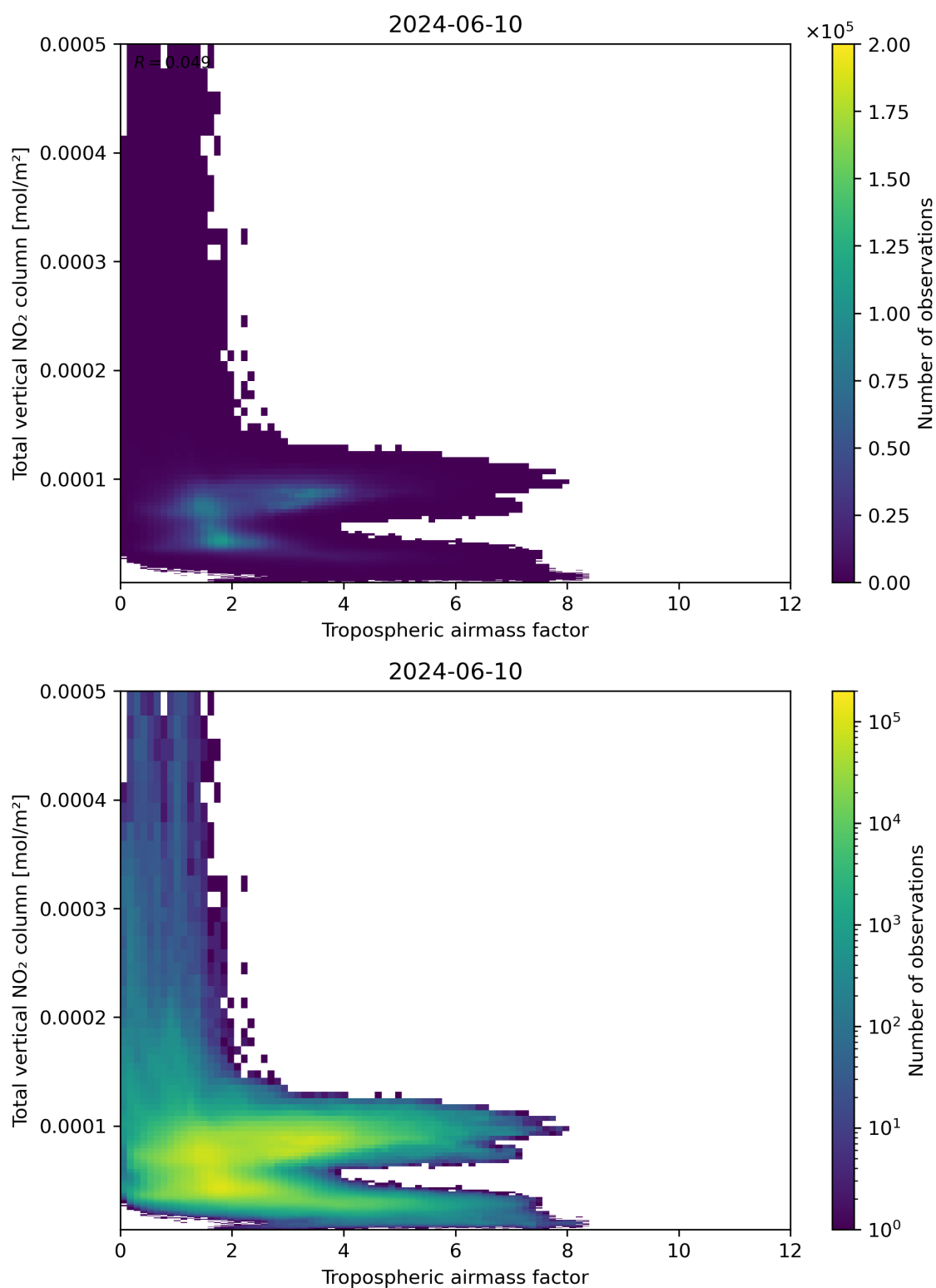
Figure 77: Scatter density plot of “Tropospheric airmass factor” against “Total vertical NO 2 column” for 2024-06-09 to 2024-06-11.
