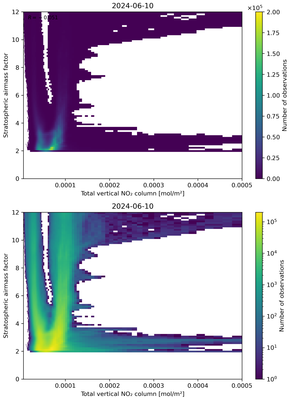
Figure 110: Scatter density plot of “Total vertical NO 2 column” against “Stratospheric airmass factor” for 2024-06-09 to 2024-06-11.
