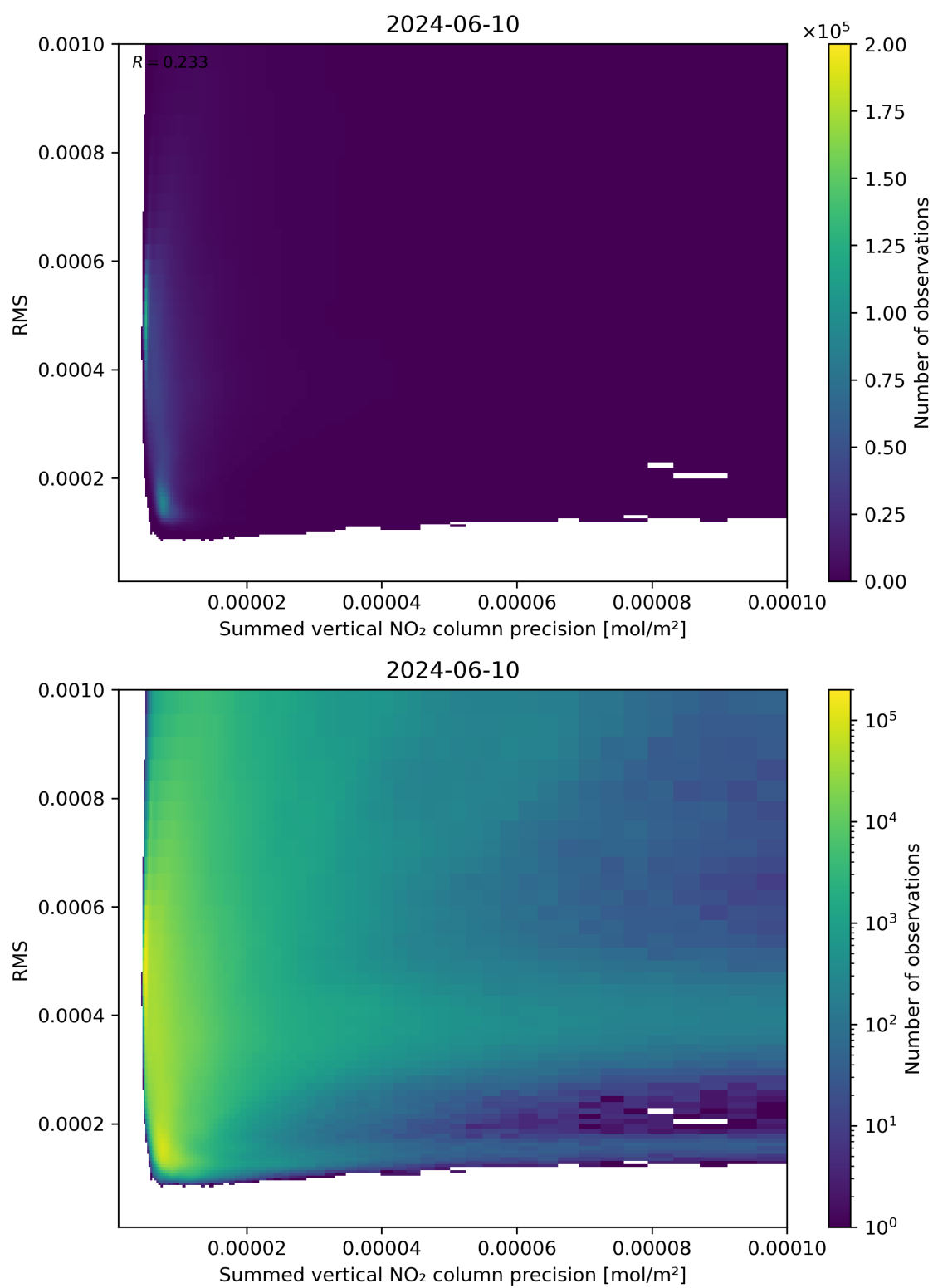
Figure 108: Scatter density plot of “Summed vertical NO 2 column precision” against “RMS” for 2024-06-09 to 2024-06-11.
