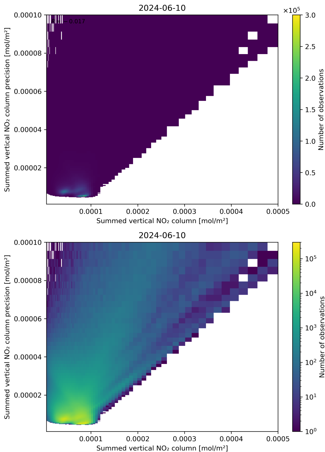
Figure 105: Scatter density plot of “Summed vertical NO 2 column” against “Summed vertical NO 2 column precision” for 2024-06-09 to 2024-06-11.
