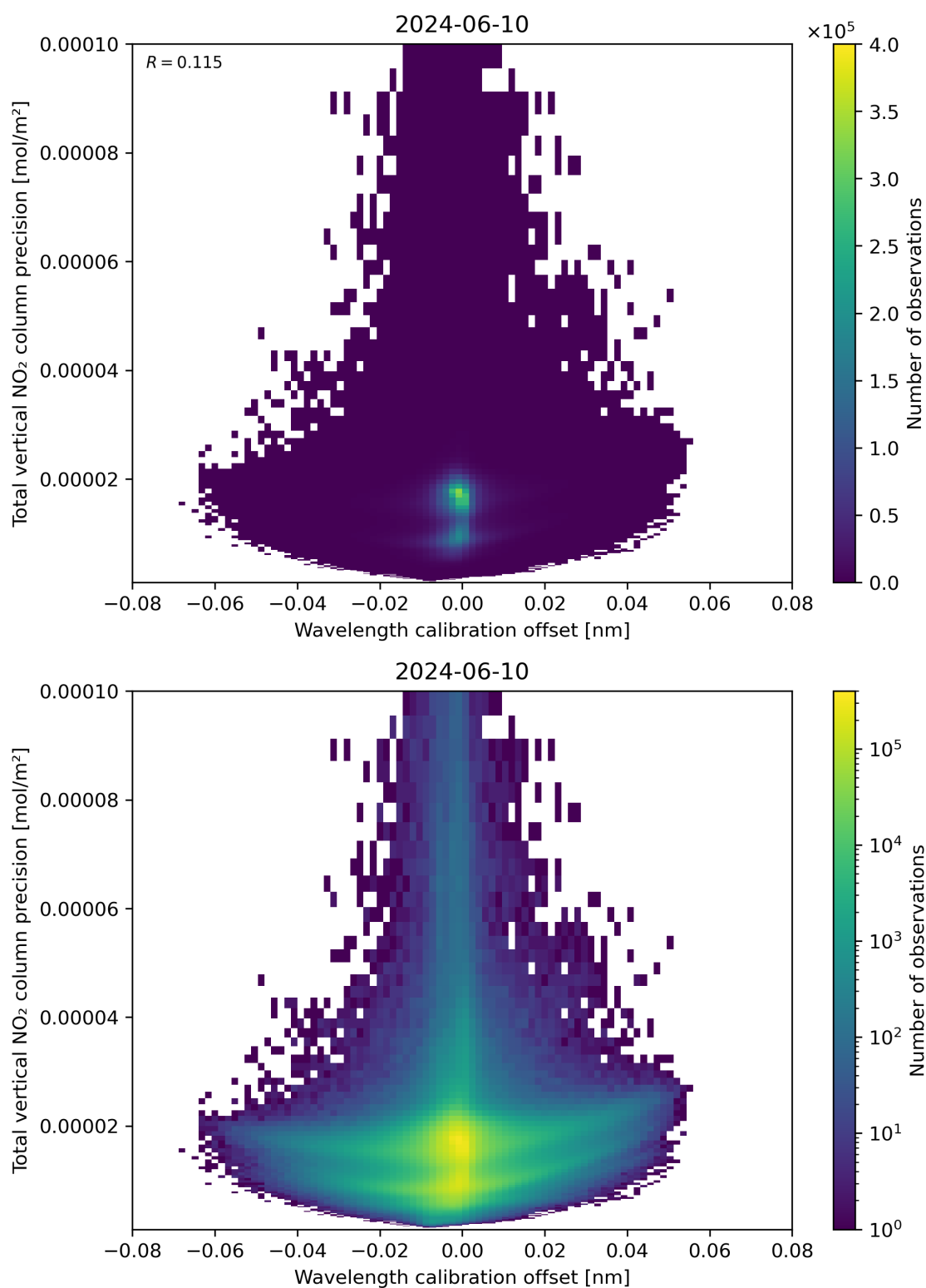
Figure 180: Scatter density plot of “Wavelength calibration offset” against “Total vertical NO 2 column precision” for 2024-06-09 to 2024-06-11.
