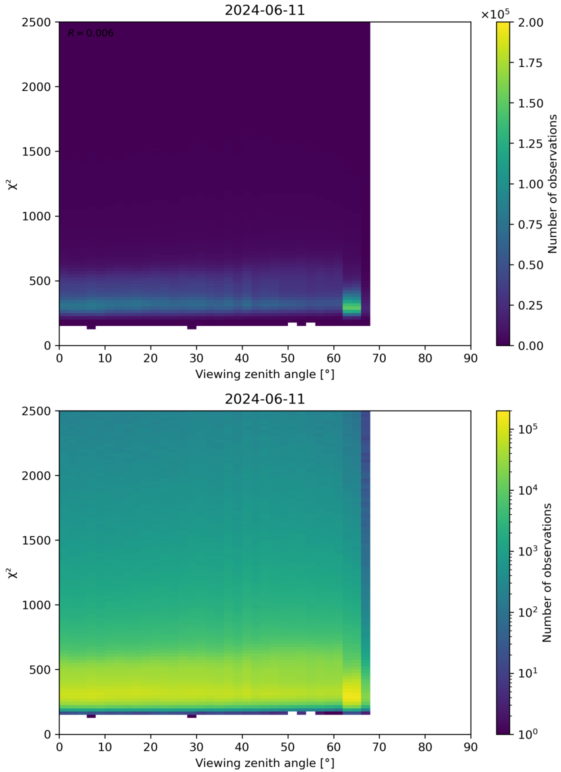
Figure 162: Scatter density plot of “Viewing zenith angle” against “ \chi^2 ” for 2024-06-10 to 2024-06-12.
