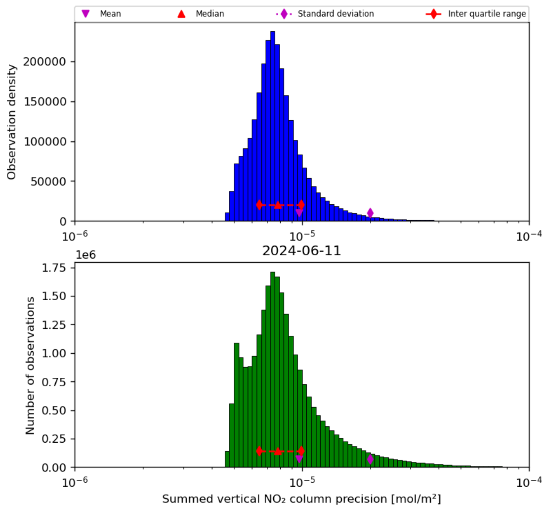
Figure 41: Histogram of "Summed vertical NO 2 column precision" for 2024-06-10 to 2024-06-12
