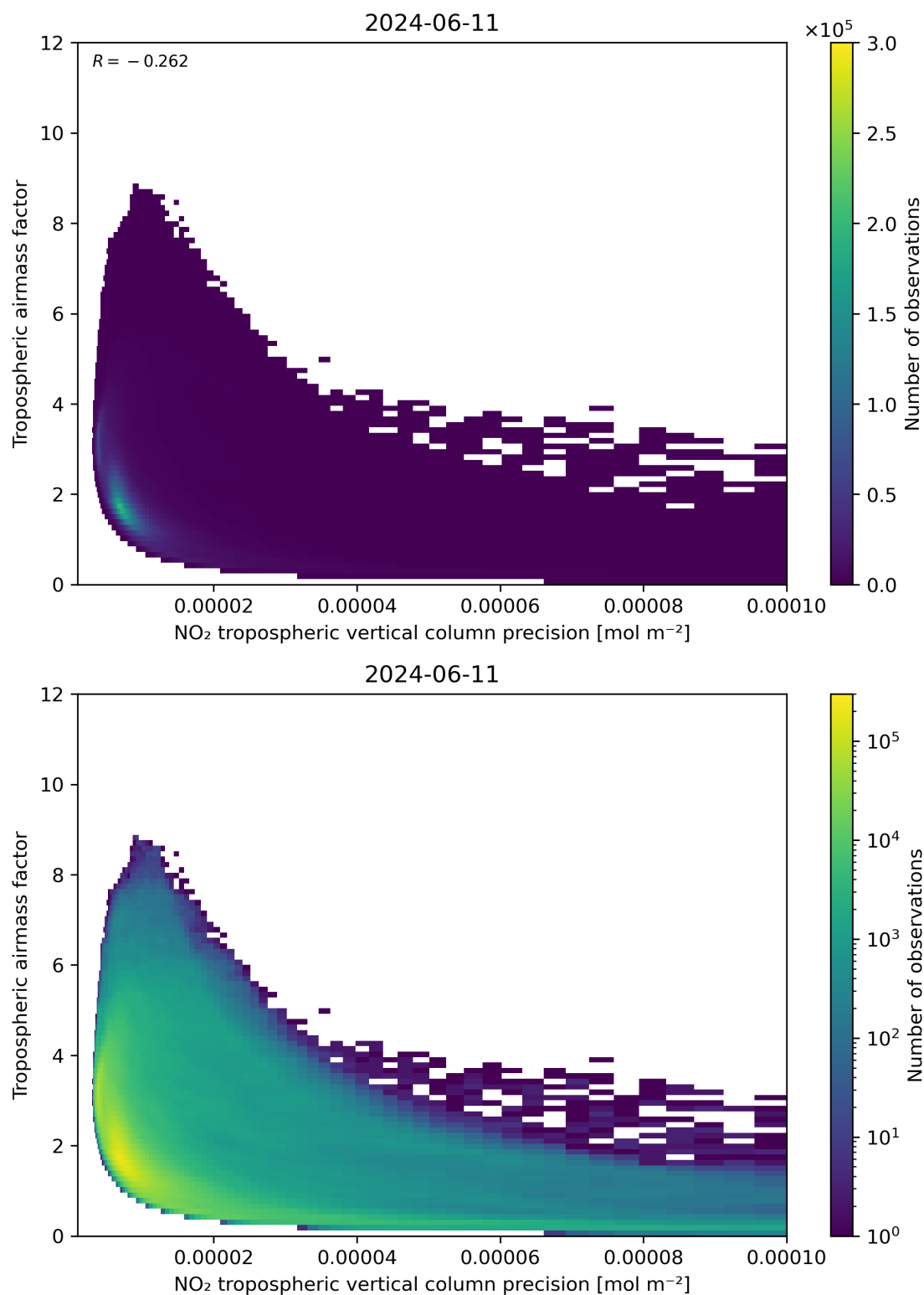
Figure 133: Scatter density plot of “NO 2 tropospheric vertical column precision” against “Tropospheric air mass factor” for 2024-06-10 to 2024-06-12.
