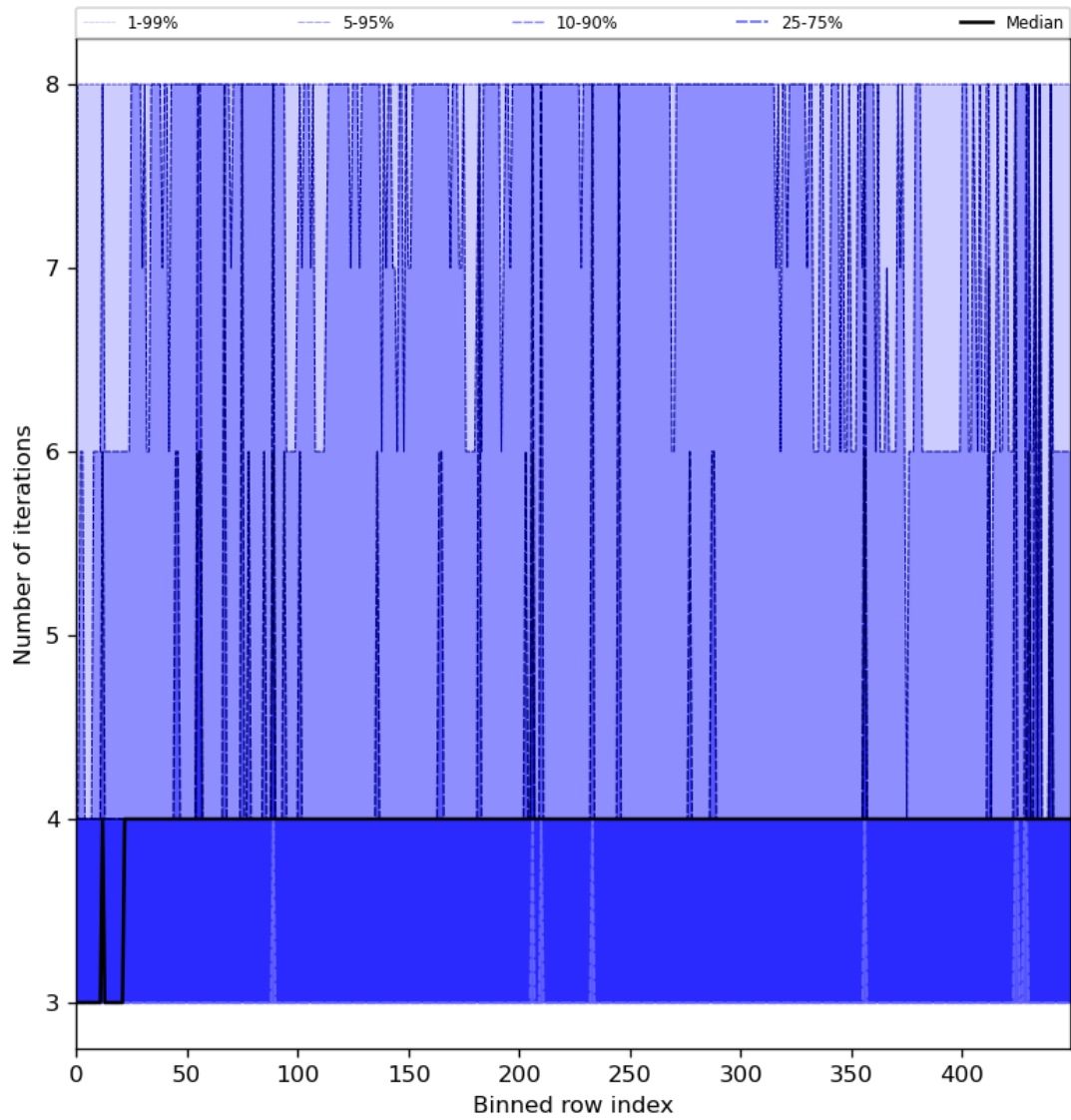
Figure 51: Along track statistics of “Number of iterations” for 2024-06-10 to 2024-06-12
