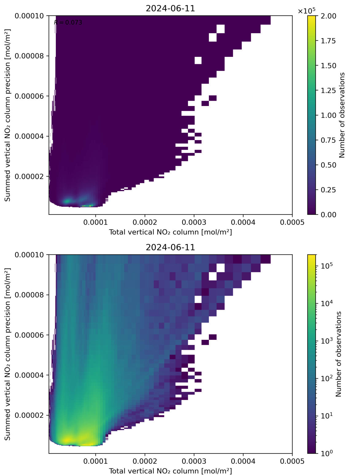
Figure 113: Scatter density plot of “Total vertical NO 2 column” against “Summed vertical NO 2 column precision” for 2024-06-10 to 2024-06-12.
