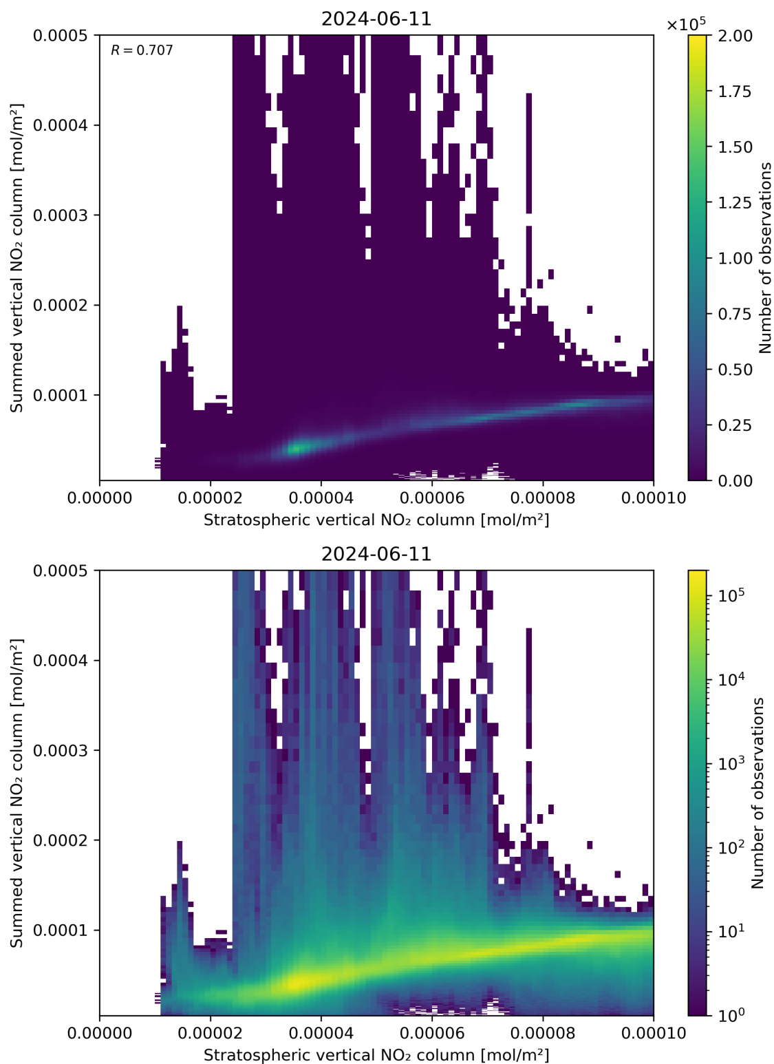
Figure 98: Scatter density plot of “Stratospheric vertical NO 2 column” against “Summed vertical NO 2 column” for 2024-06-10 to 2024-06-12.
