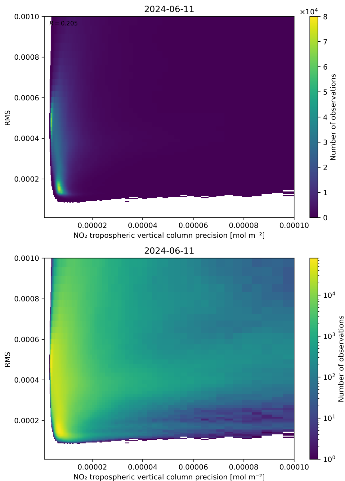
Figure 140: Scatter density plot of “NO 2 tropospheric vertical column precision” against “RMS” for 2024-06-10 to 2024-06-12.
