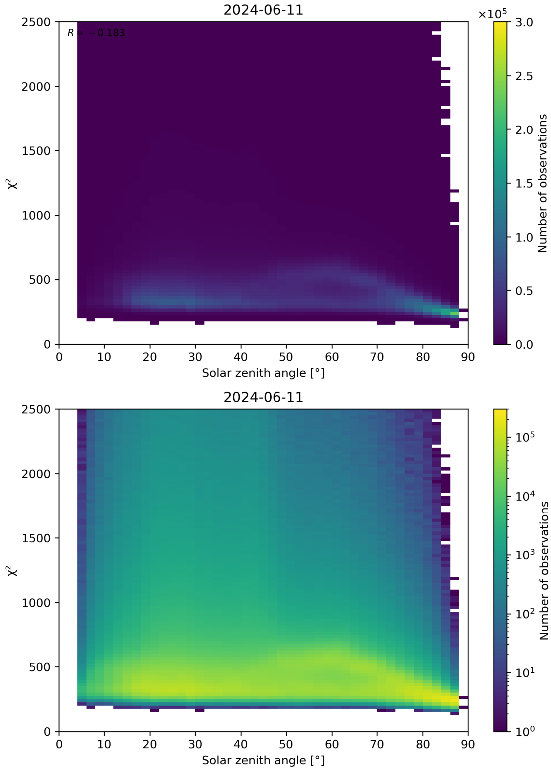
Figure 148: Scatter density plot of “Solar zenith angle” against “ \chi^2 ” for 2024-06-10 to 2024-06-12.
