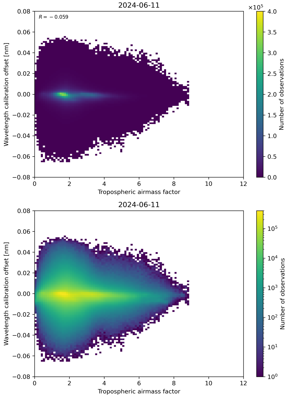
Figure 80: Scatter density plot of “Tropospheric airmass factor” against “Wavelength calibration offset” for 2024-06-10 to 2024-06-12.
