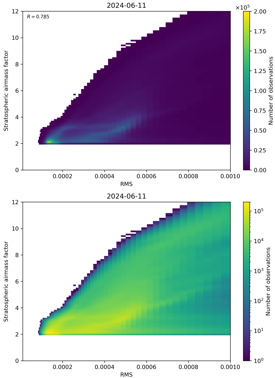
Figure 144: Scatter density plot of “RMS” against “Stratospheric airmass factor” for 2024-06-10 to 2024-06-12.
