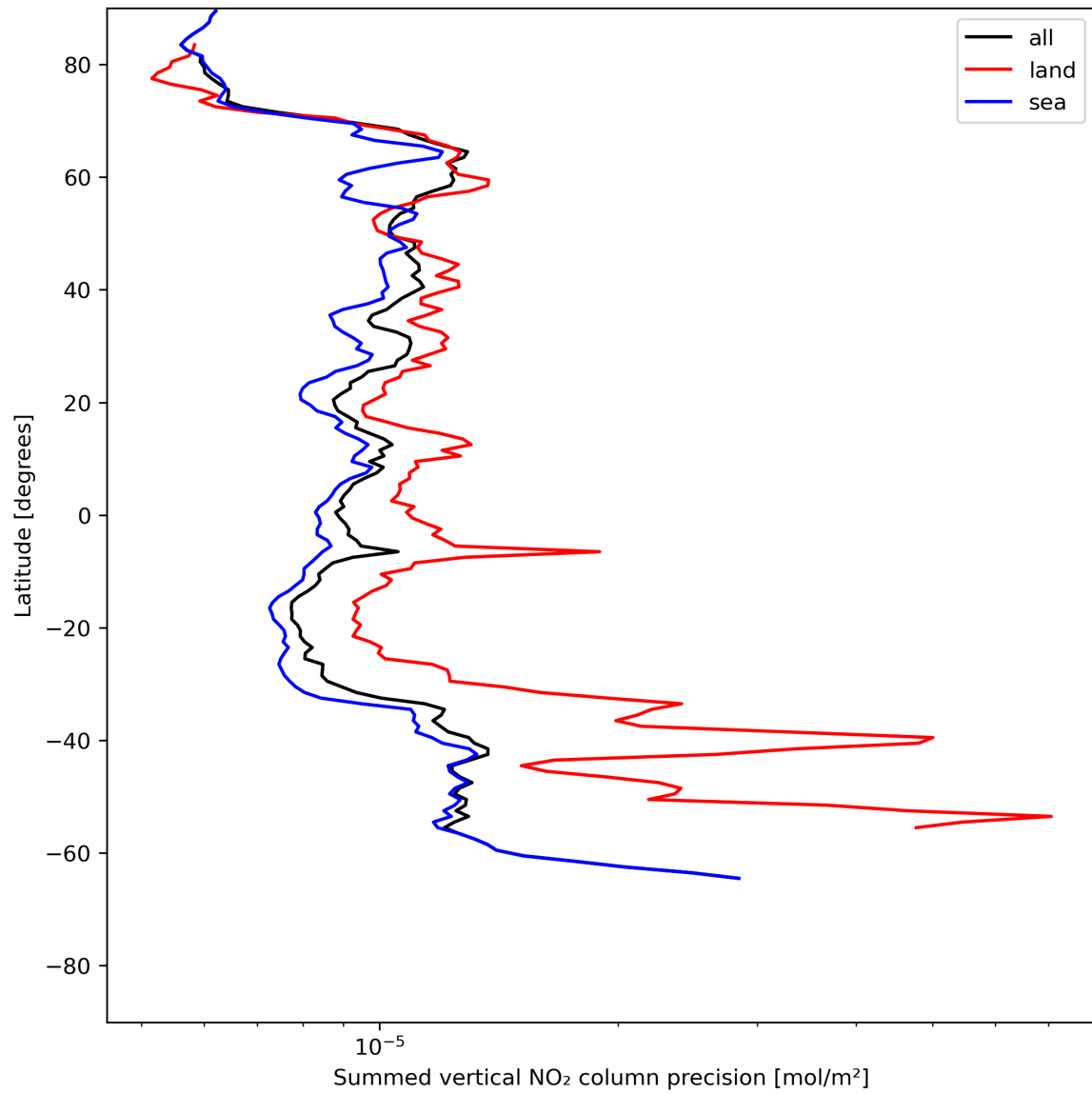
Figure 24: Zonal average of “Summed vertical NO 2 column precision” for 2024-06-10 to 2024-06-12.
