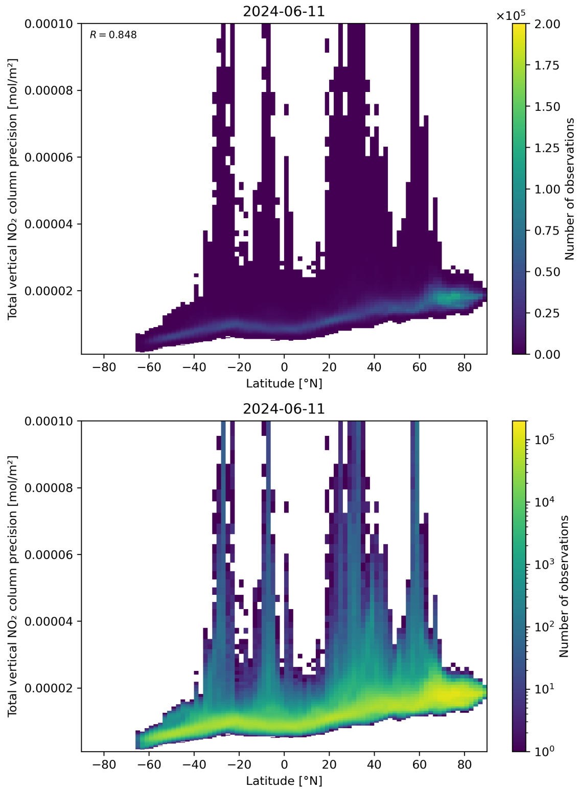
Figure 91: Scatter density plot of “Latitude” against “Total vertical NO 2 column precision” for 2024-06-10 to 2024-06-12.
