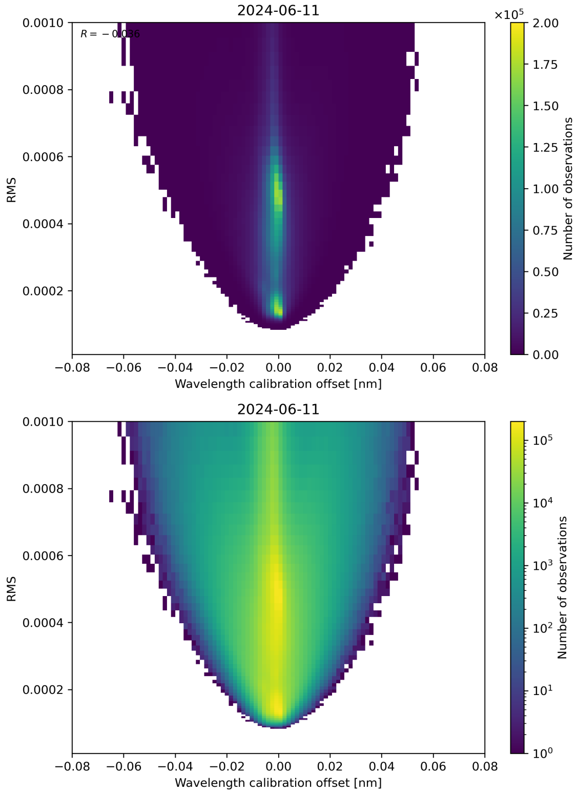
Figure 181: Scatter density plot of “Wavelength calibration offset” against “RMS” for 2024-06-10 to 2024-06-12.
