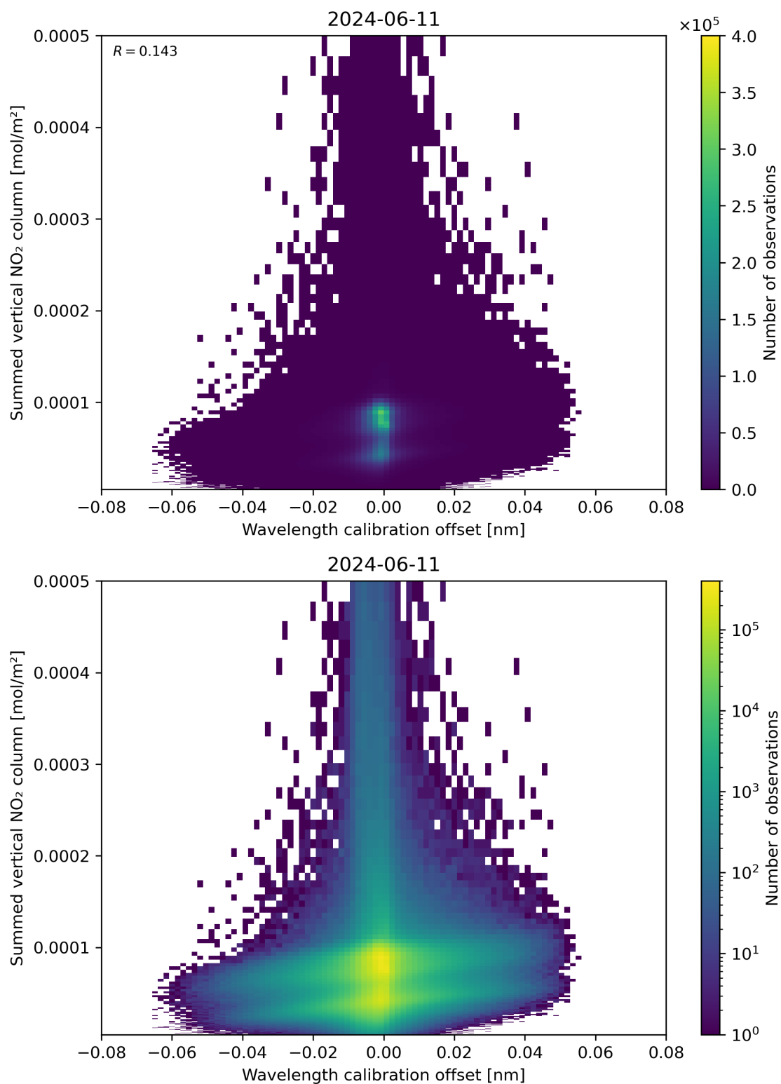
Figure 177: Scatter density plot of “Wavelength calibration offset” against “Summed vertical NO 2 column” for 2024-06-10 to 2024-06-12.
