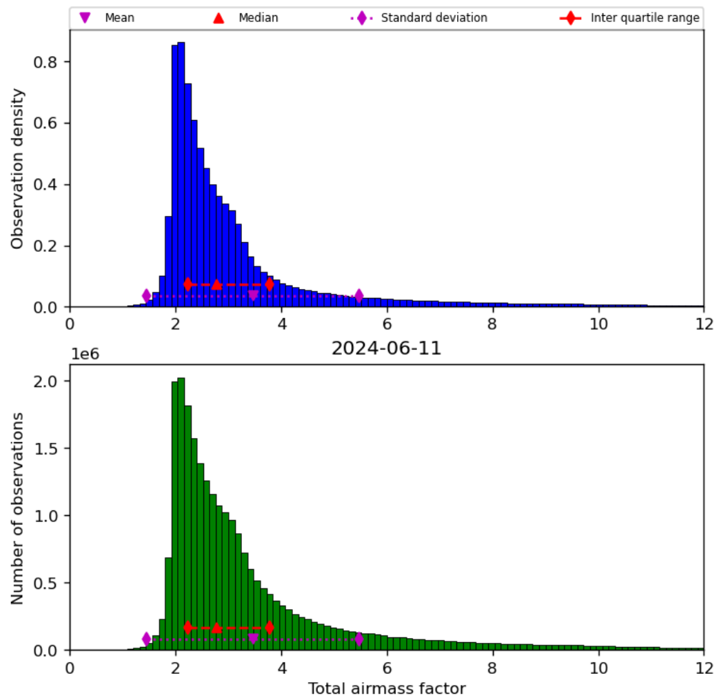
Figure 32: Histogram of “Total airmass factor” for 2024-06-10 to 2024-06-12
