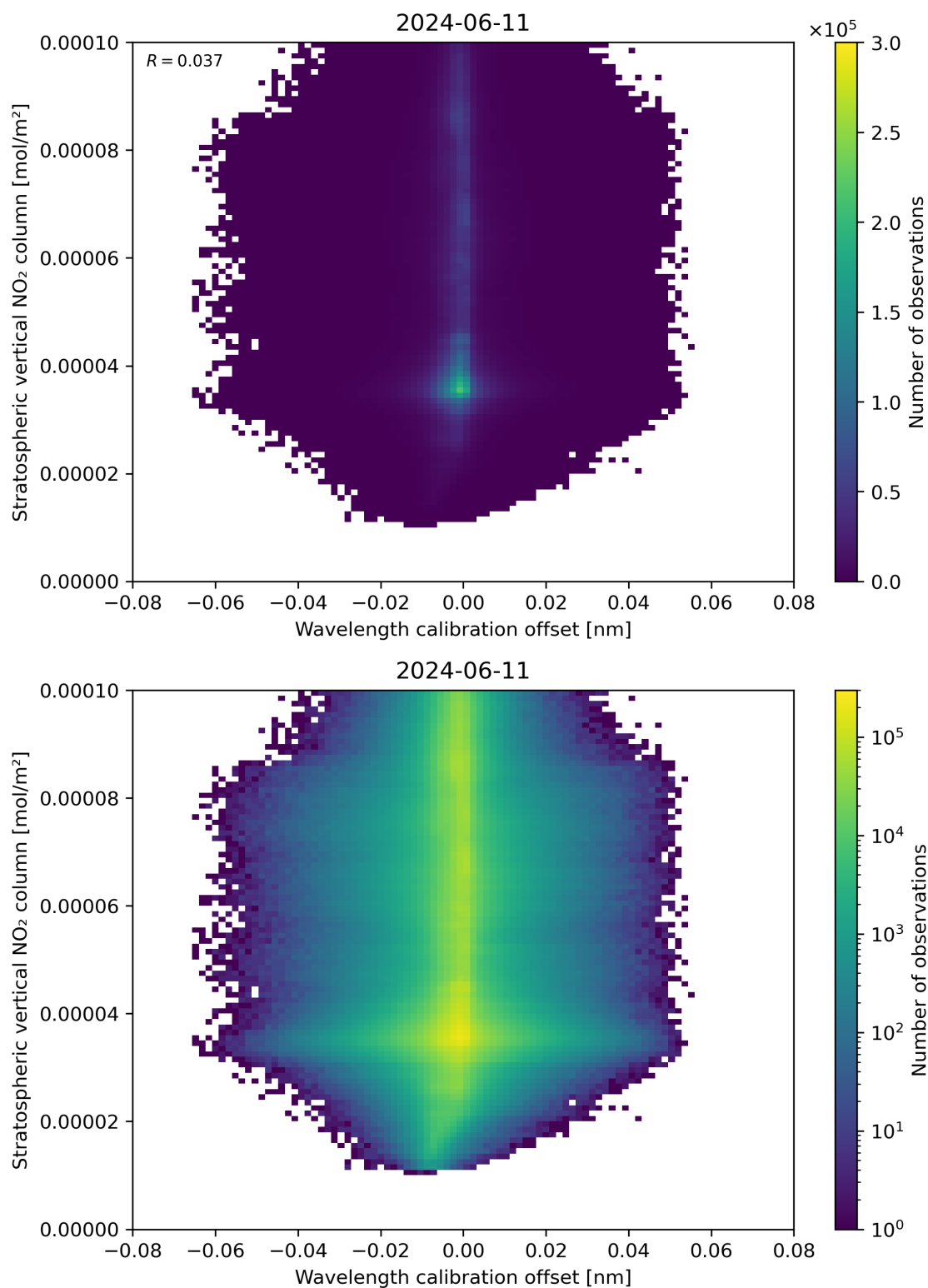
Figure 176: Scatter density plot of “Wavelength calibration offset” against “Stratospheric vertical NO 2 column” for 2024-06-10 to 2024-06-12.
