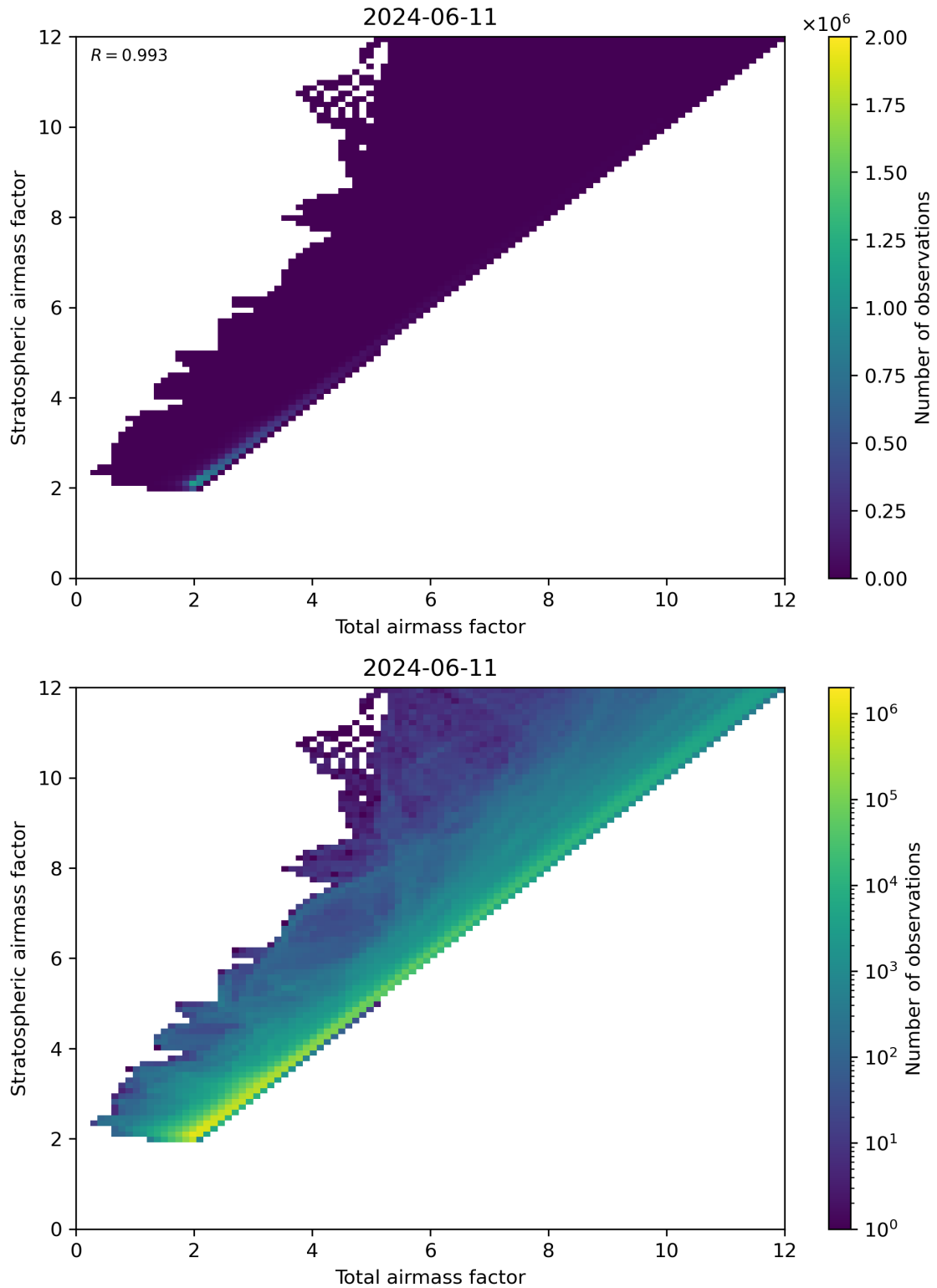
Figure 62: Scatter density plot of “Total airmass factor” against “Stratospheric airmass factor” for 2024-06-10 to 2024-06-12.
