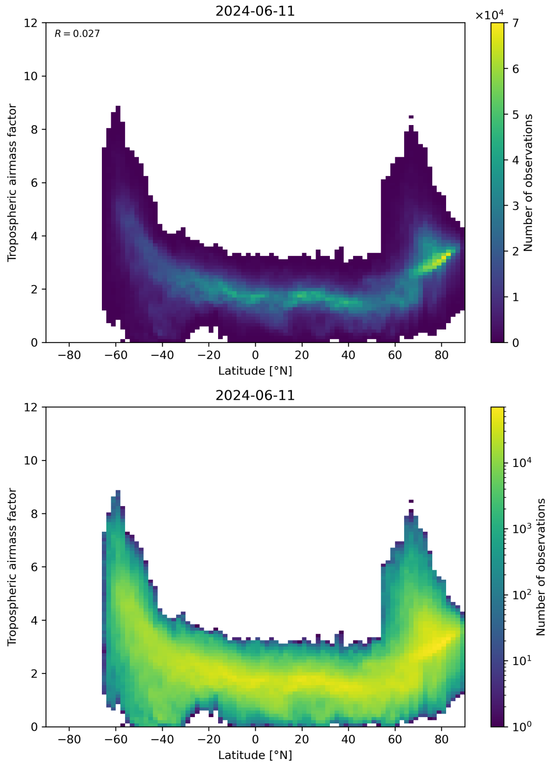
Figure 85: Scatter density plot of “Latitude” against “Tropospheric airmass factor” for 2024-06-10 to 2024-06-12.
