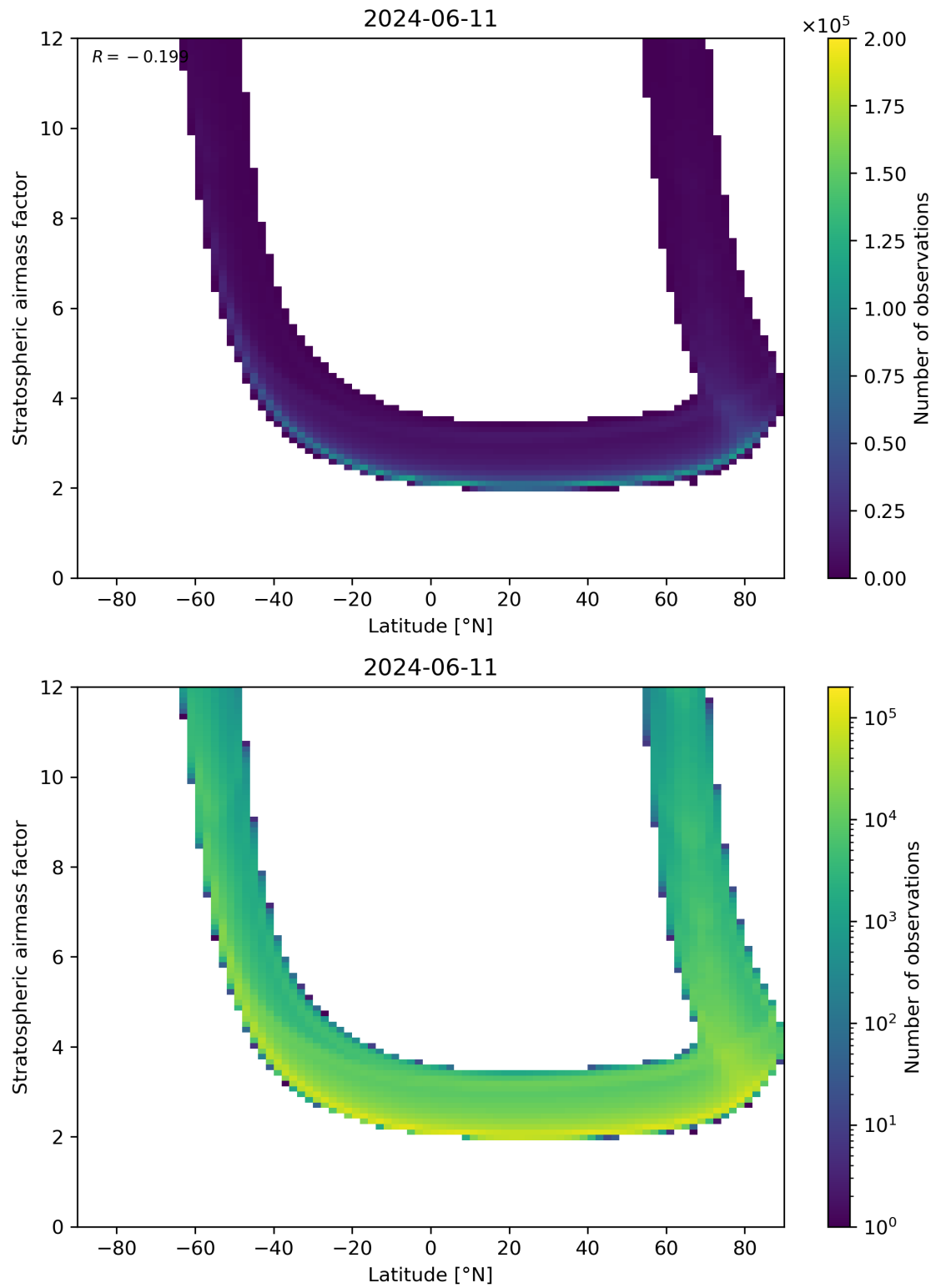
Figure 83: Scatter density plot of “Latitude” against “Stratospheric air mass factor” for 2024-06-10 to 2024-06-12.
