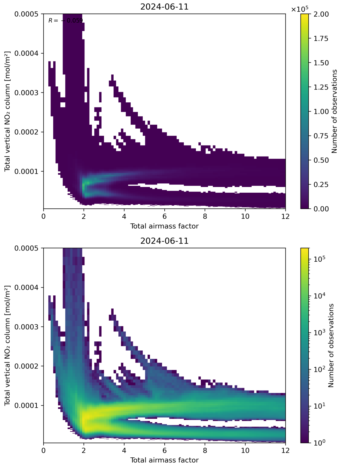
Figure 67: Scatter density plot of “Total airmass factor” against “Total vertical NO 2 column” for 2024-06-10 to 2024-06-12.
