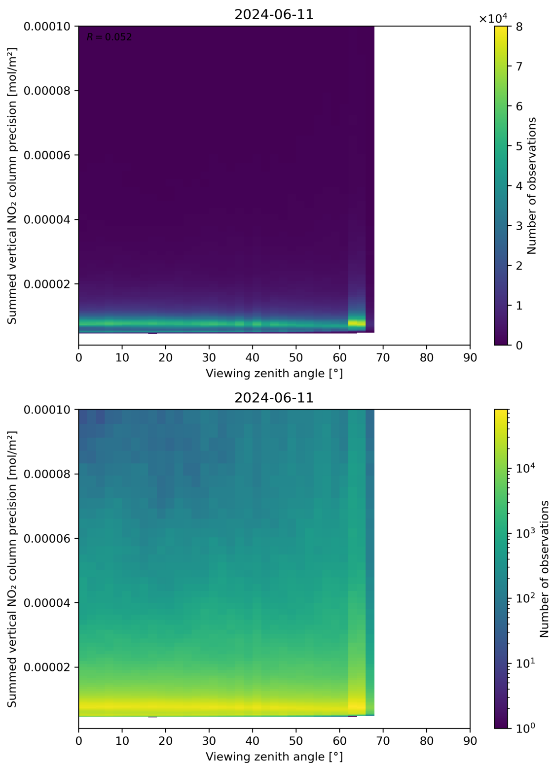
Figure 166: Scatter density plot of “Viewing zenith angle” against “Summed vertical NO 2 column precision” for 2024-06-10 to 2024-06-12.
