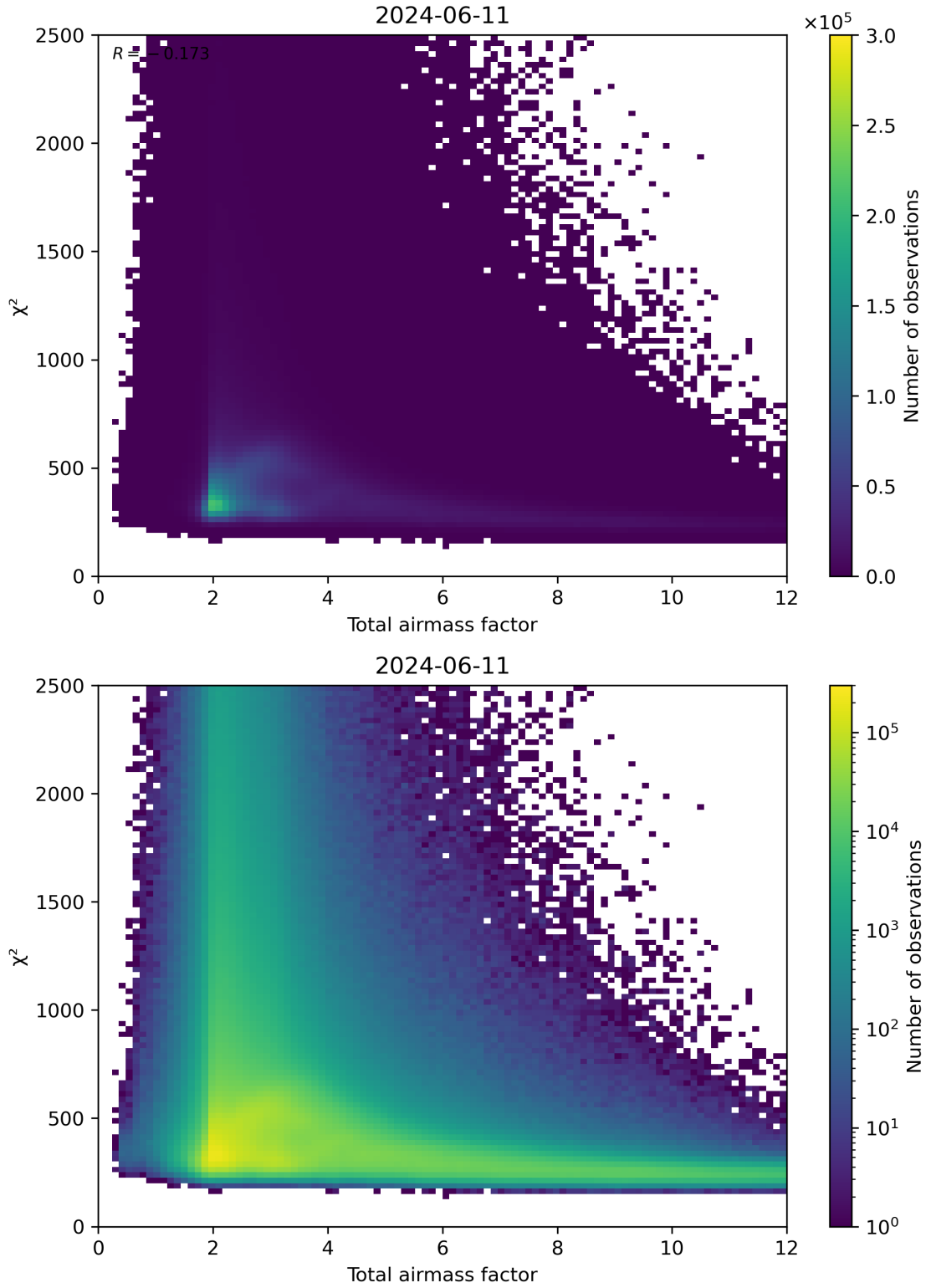
Figure 63: Scatter density plot of “Total airmass factor” against “ \chi^2 ” for 2024-06-10 to 2024-06-12.
