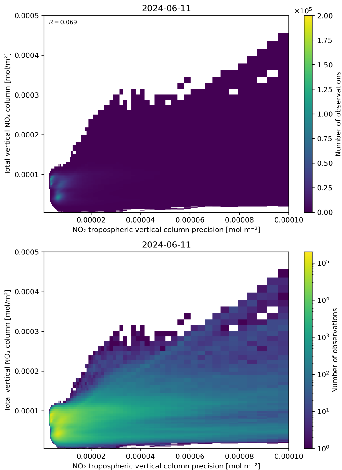
Figure 138: Scatter density plot of “NO 2 tropospheric vertical column precision” against “Total vertical NO 2 column” for 2024-06-10 to 2024-06-12.
