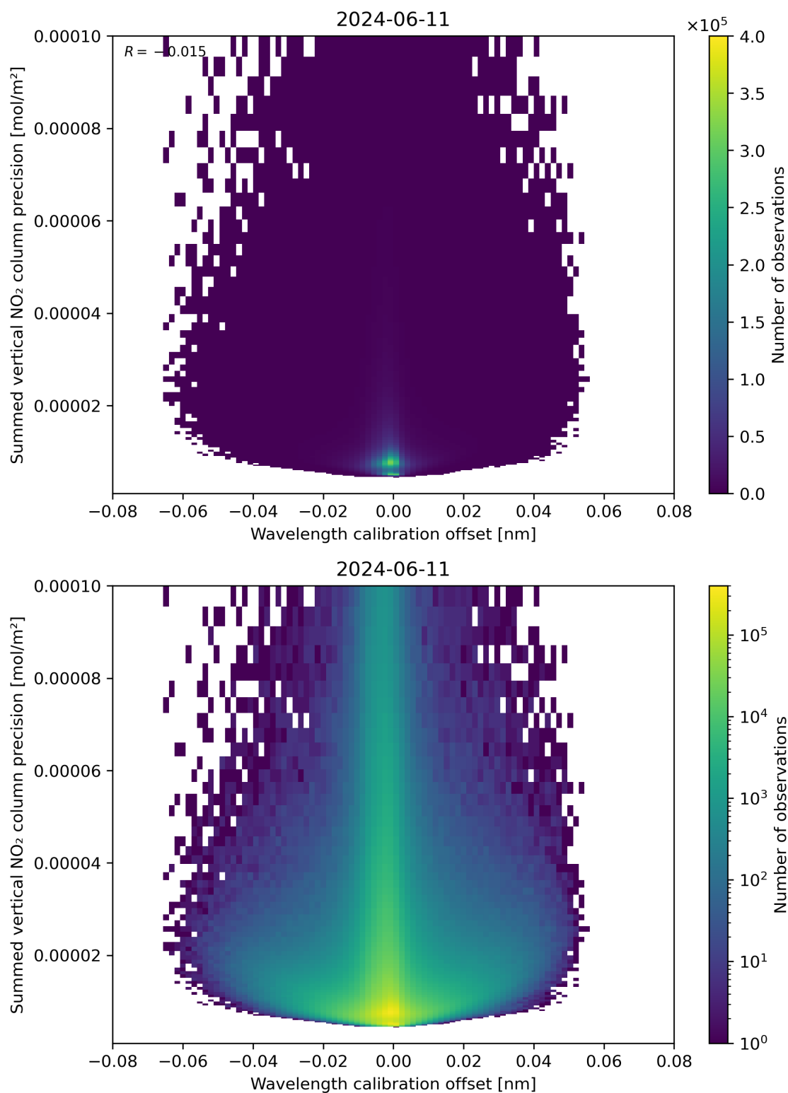
Figure 178: Scatter density plot of “Wavelength calibration offset” against “Summed vertical NO 2 column precision” for 2024-06-10 to 2024-06-12.
