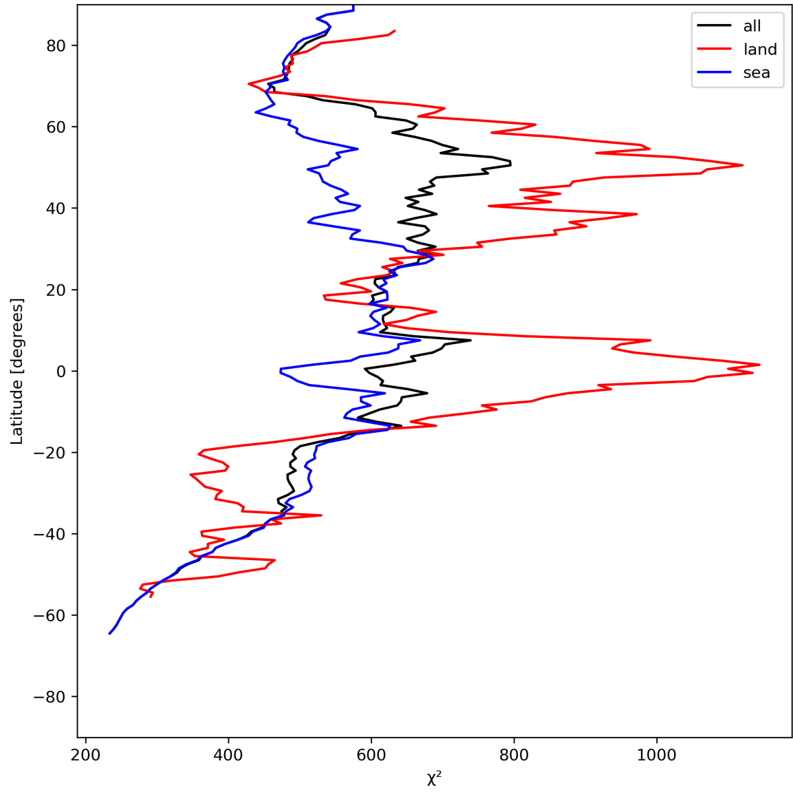
Figure 25: Zonal average of “ \chi^2 ” for 2024-06-10 to 2024-06-12.
