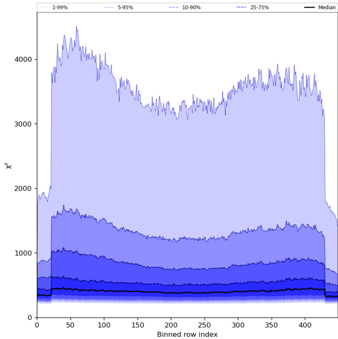
Figure 59: Along track statistics of “ \chi^2 ” for 2024-06-10 to 2024-06-12
