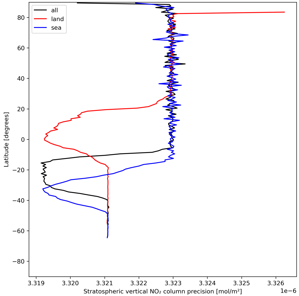
Figure 20: Zonal average of “Stratospheric vertical NO 2 column precision” for 2024-06-10 to 2024-06-12.
