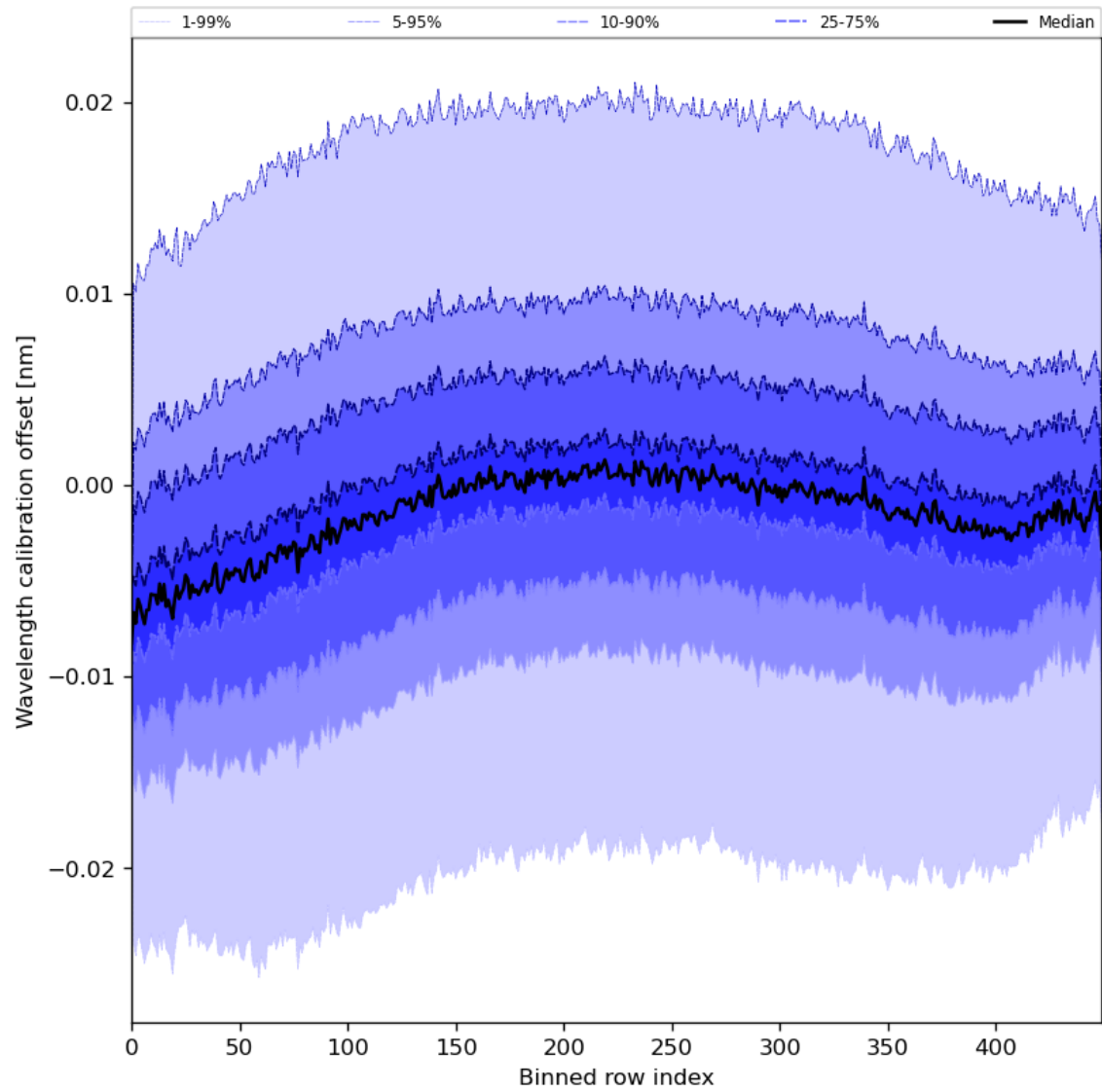
Figure 52: Along track statistics of “Wavelength calibration offset” for 2024-06-10 to 2024-06-12
