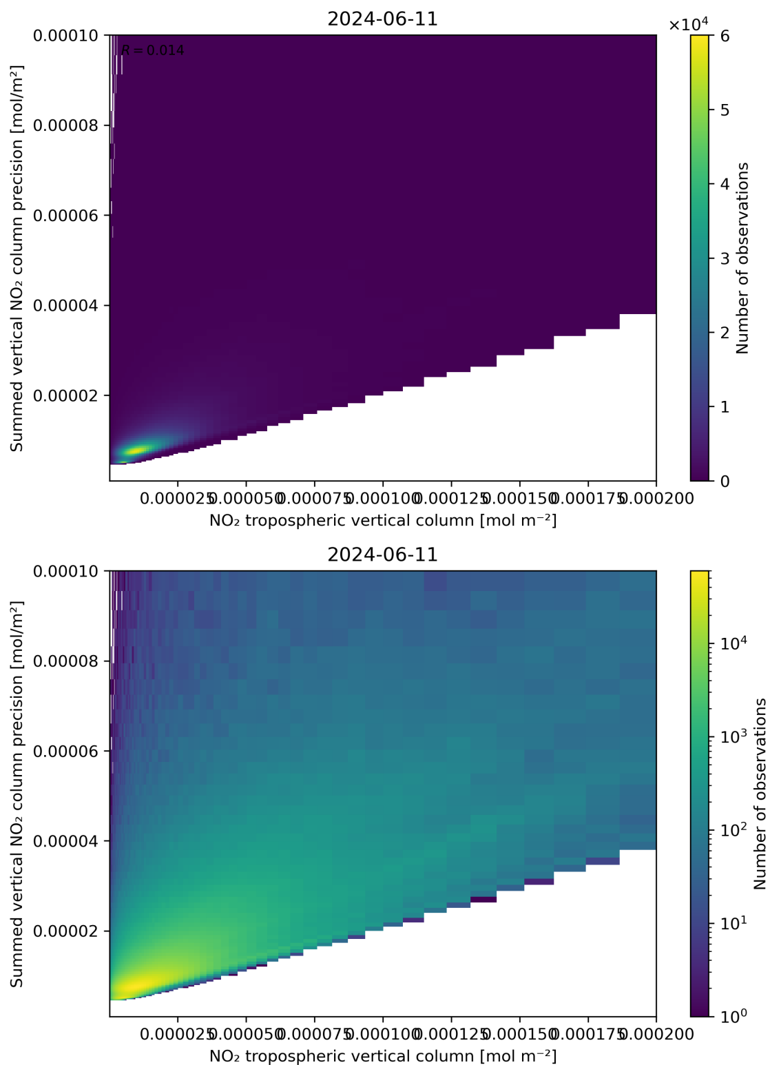
Figure 127: Scatter density plot of “NO 2 tropospheric vertical column” against “Summed vertical NO 2 column precision” for 2024-06-10 to 2024-06-12.
