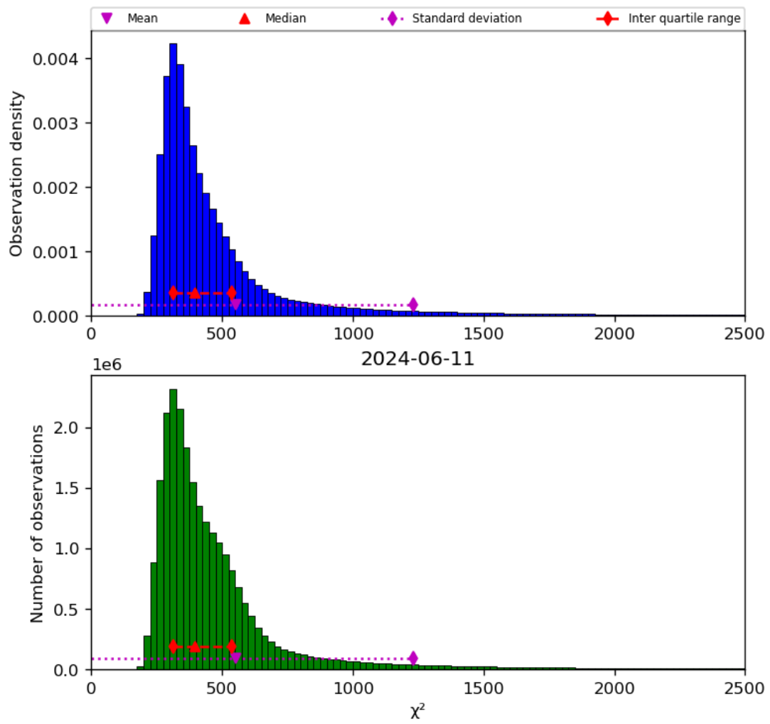
Figure 42: Histogram of “ \chi^2 ” for 2024-06-10 to 2024-06-12
