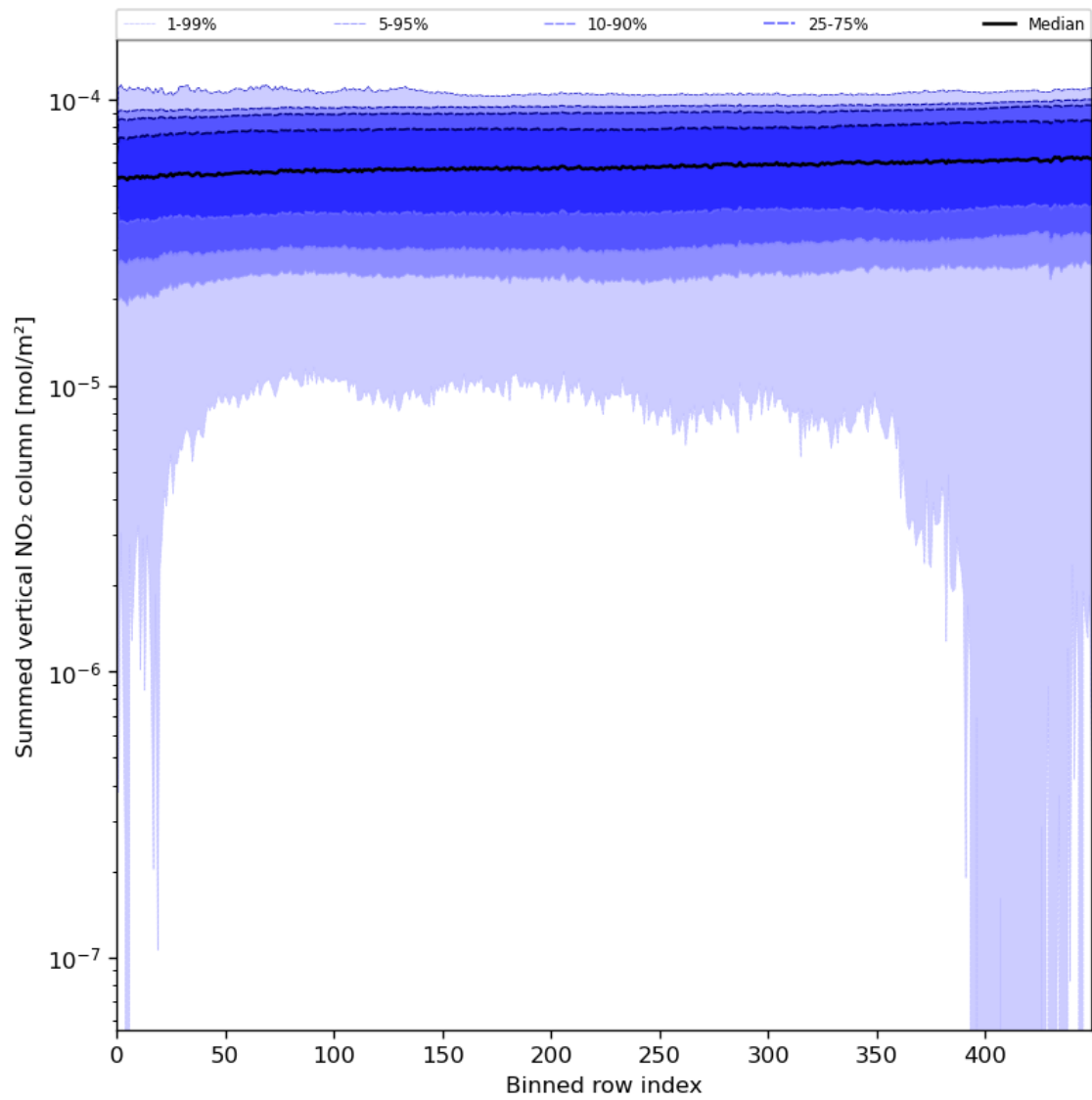
Figure 57: Along track statistics of “Summed vertical NO 2 column” for 2024-06-10 to 2024-06-12
