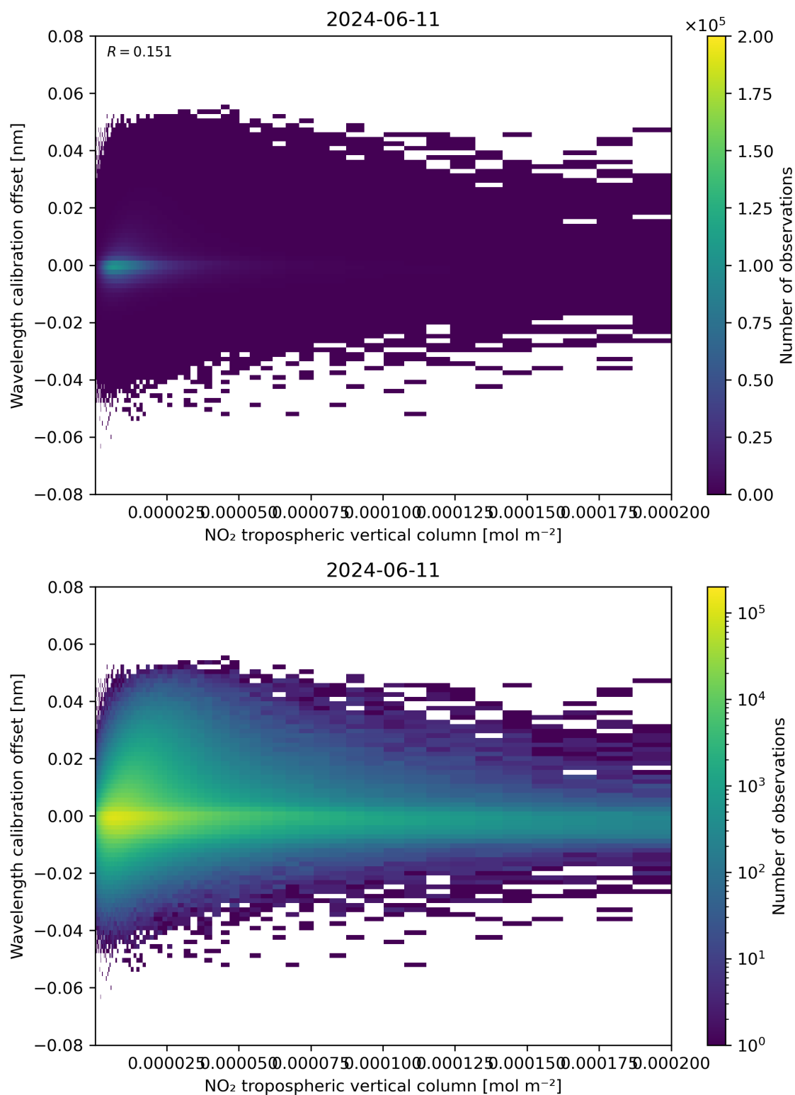
Figure 143: Scatter density plot of “NO 2 tropospheric vertical column” against “Wavelength calibration offset” for 2024-06-10 to 2024-06-12.
