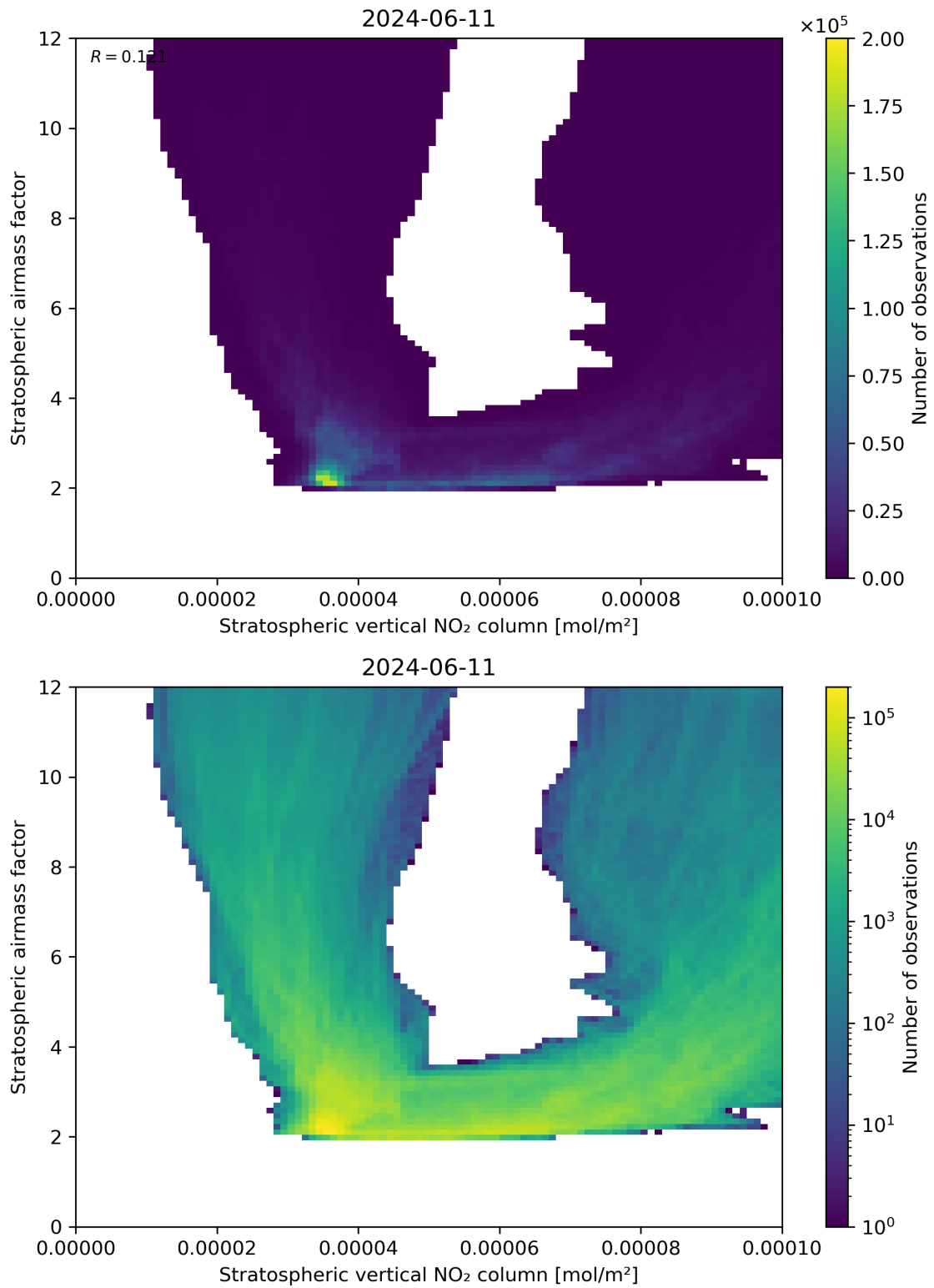
Figure 96: Scatter density plot of “Stratospheric vertical NO 2 column” against “Stratospheric airmass factor” for 2024-06-10 to 2024-06-12.
