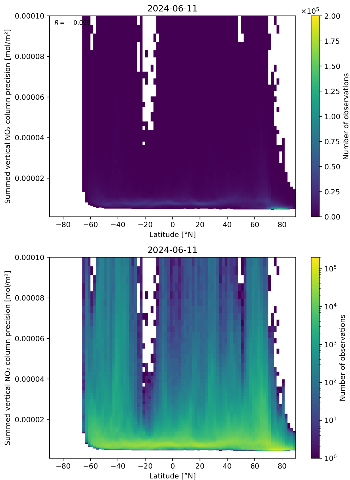
Figure 89: Scatter density plot of “Latitude” against “Summed vertical NO 2 column precision” for 2024-06-10 to 2024-06-12.
