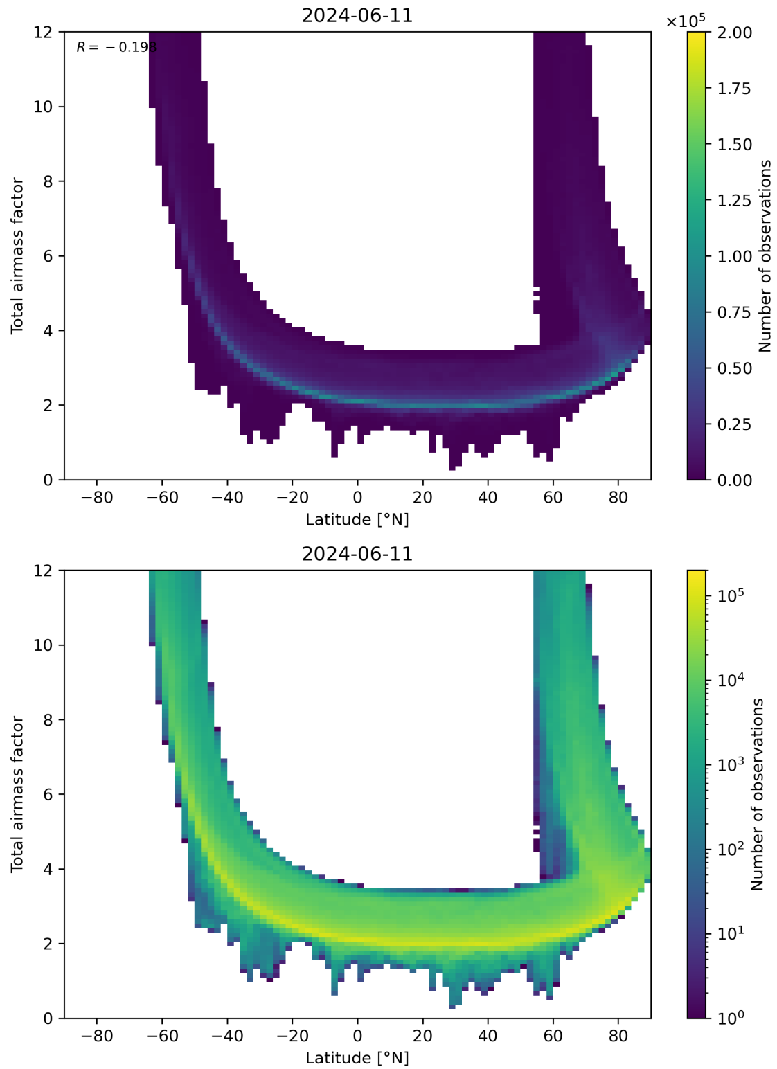
Figure 84: Scatter density plot of “Latitude” against “Total airmass factor” for 2024-06-10 to 2024-06-12.
