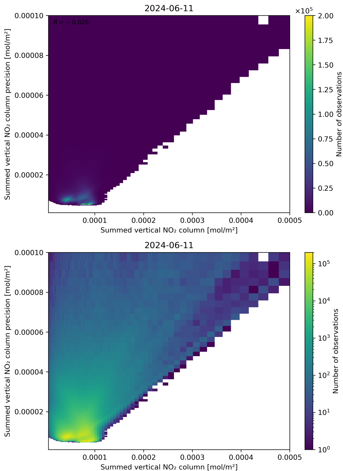
Figure 105: Scatter density plot of “Summed vertical NO 2 column” against “Summed vertical NO 2 column precision” for 2024-06-10 to 2024-06-12.
