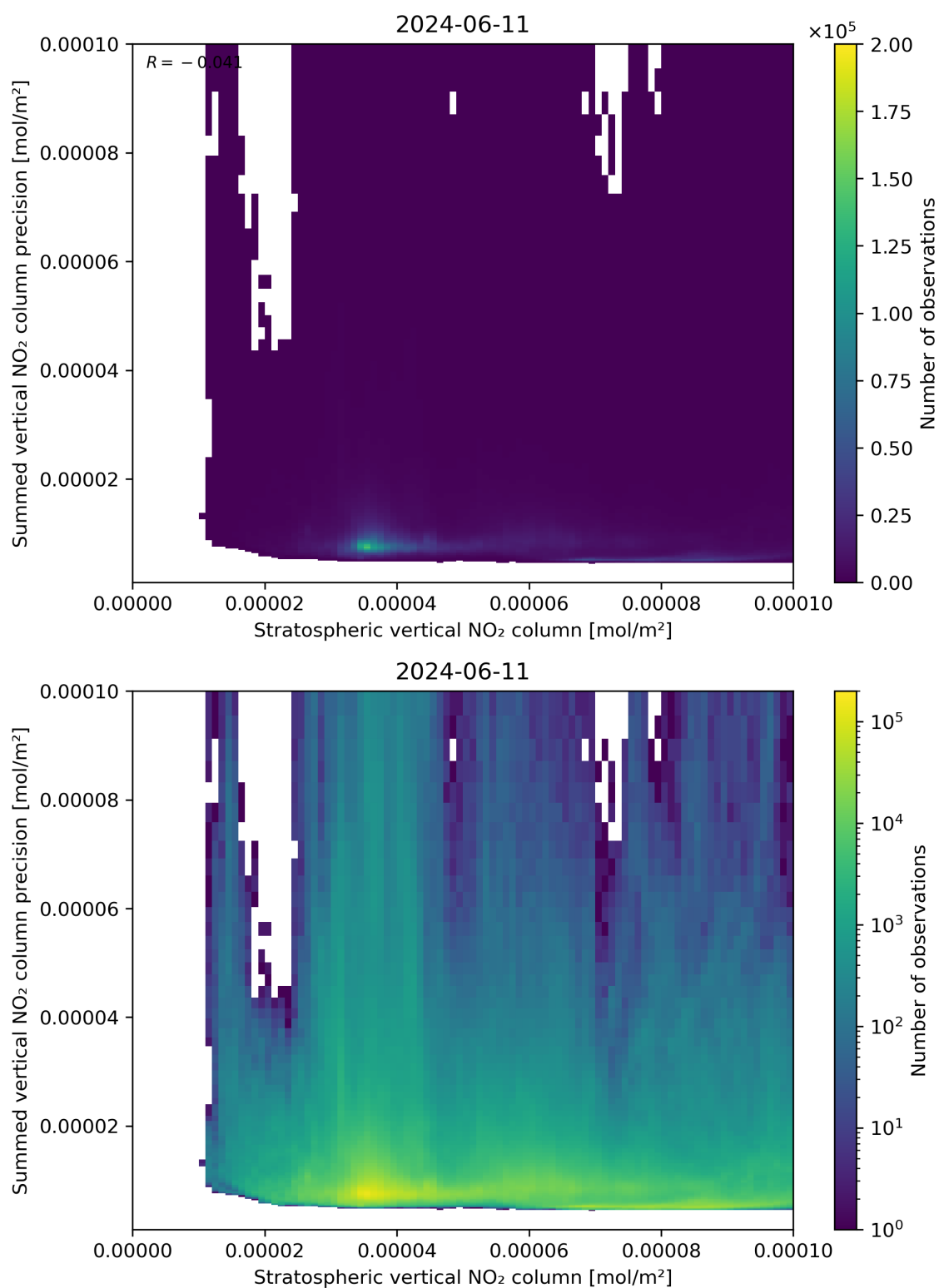
Figure 99: Scatter density plot of “Stratospheric vertical NO 2 column” against “Summed vertical NO 2 column precision” for 2024-06-10 to 2024-06-12.
