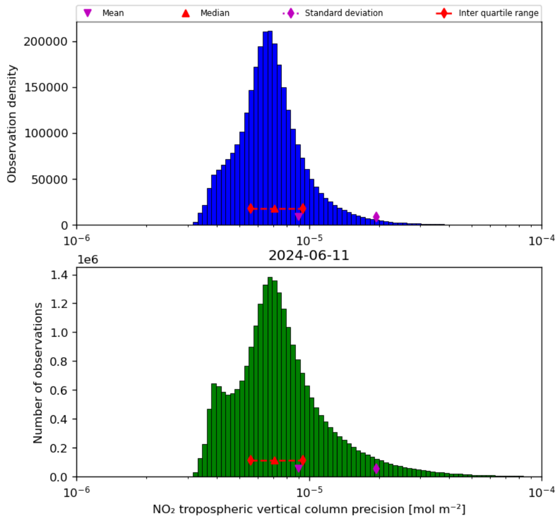
Figure 30: Histogram of “NO 2 tropospheric vertical column precision” for 2024-06-10 to 2024-06-12
