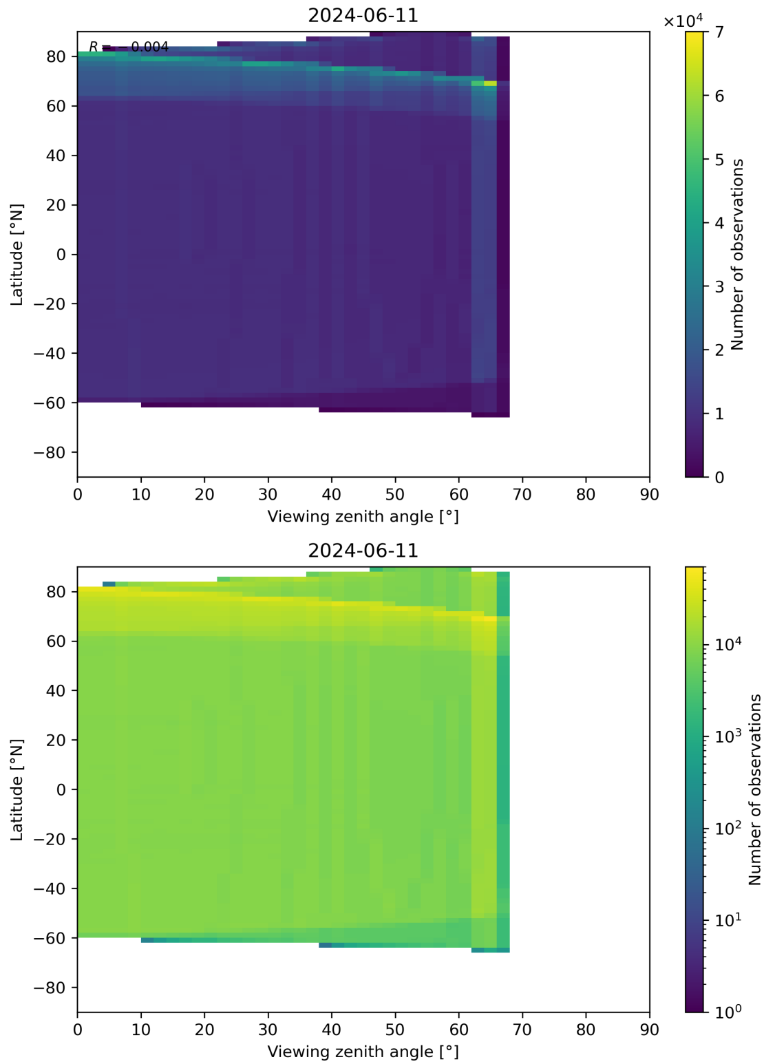
Figure 163: Scatter density plot of “Viewing zenith angle” against “Latitude” for 2024-06-10 to 2024-06-12.
