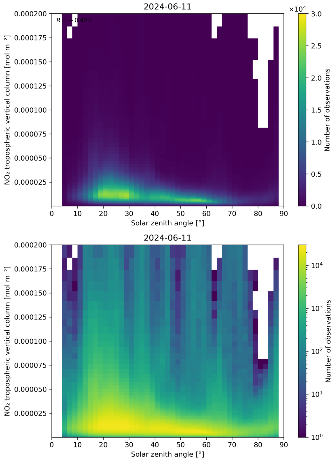
Figure 155: Scatter density plot of “Solar zenith angle” against “NO 2 tropospheric vertical column” for 2024-06-10 to 2024-06-12.
