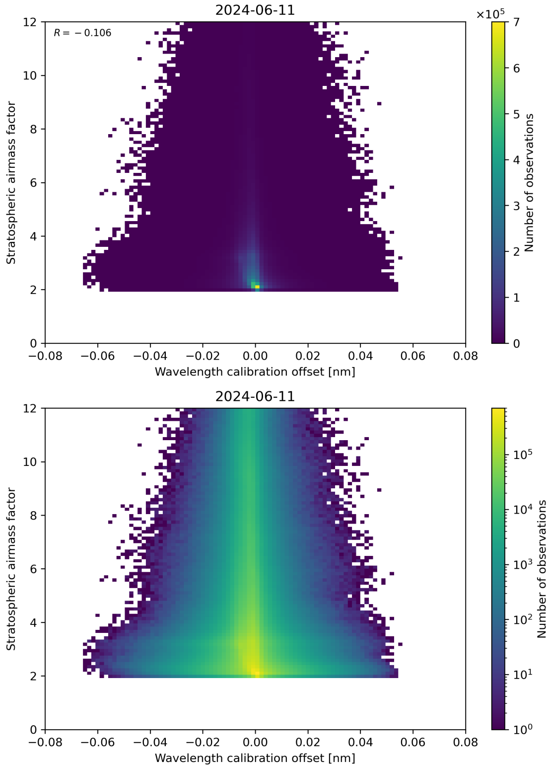
Figure 174: Scatter density plot of “Wavelength calibration offset” against “Stratospheric airmass factor” for 2024-06-10 to 2024-06-12.
