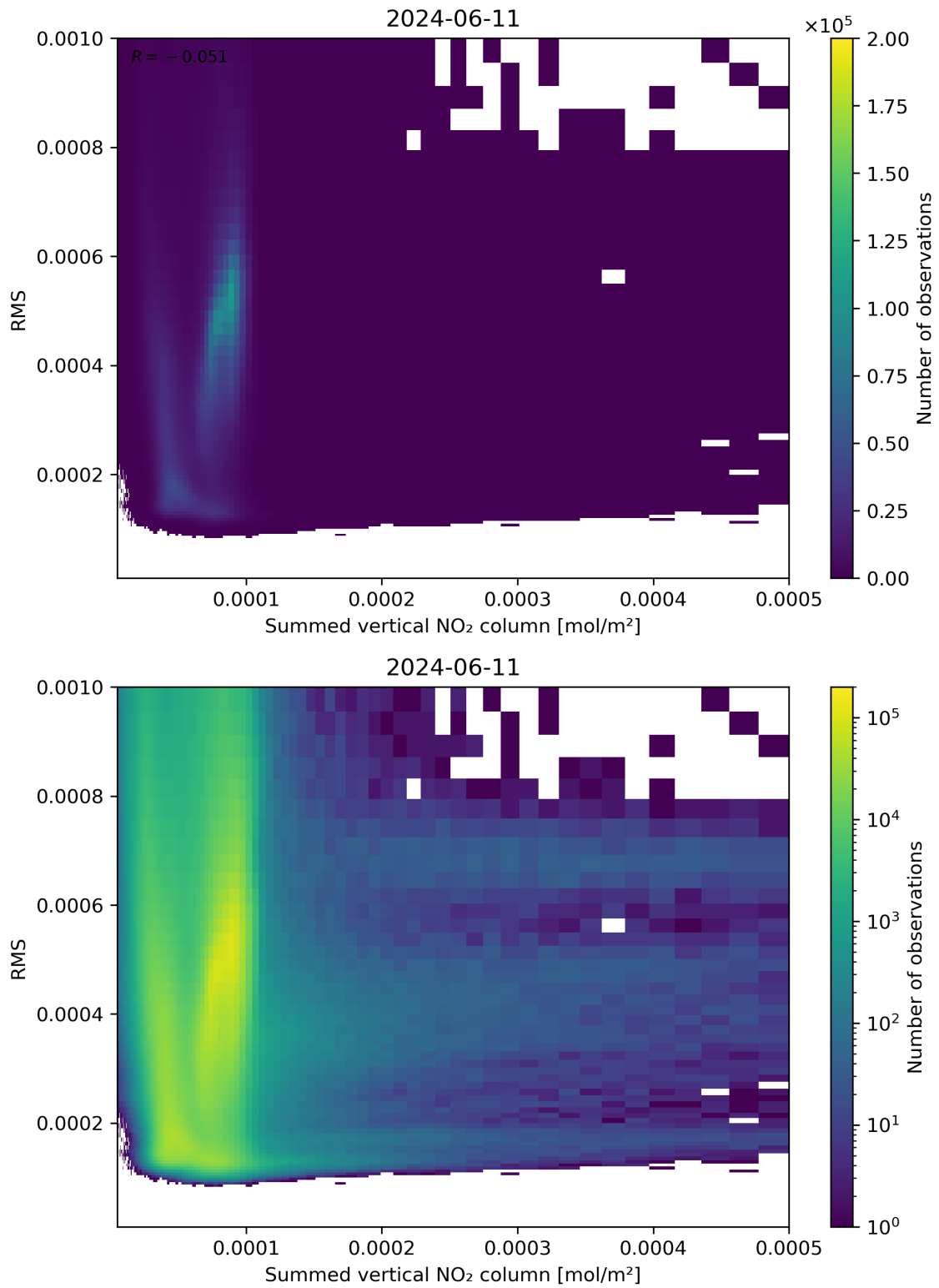
Figure 109: Scatter density plot of “Summed vertical NO 2 column” against “RMS” for 2024-06-10 to 2024-06-12.
