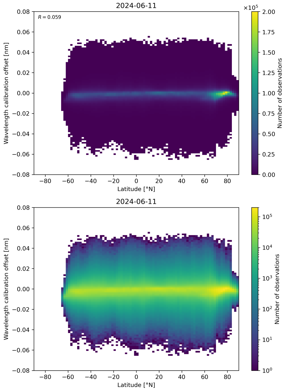
Figure 95: Scatter density plot of “Latitude” against “Wavelength calibration offset” for 2024-06-10 to 2024-06-12.
