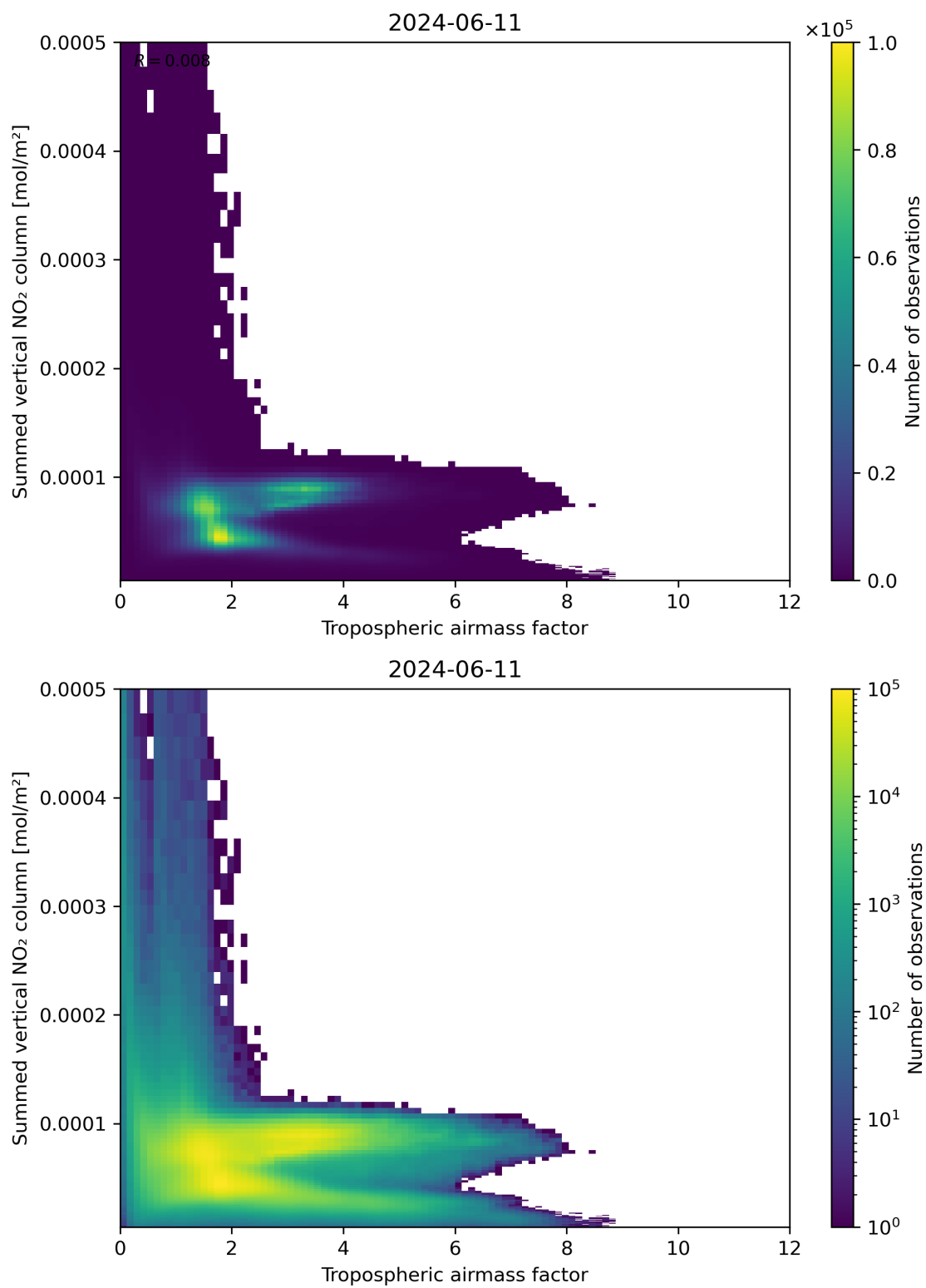
Figure 75: Scatter density plot of “Tropospheric air mass factor” against “Summed vertical NO 2 column” for 2024-06-10 to 2024-06-12.
