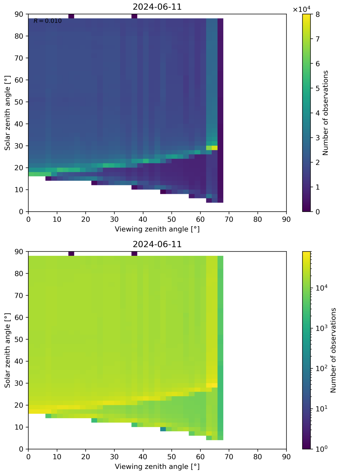
Figure 172: Scatter density plot of “Viewing zenith angle” against “Solar zenith angle” for 2024-06-10 to 2024-06-12.
