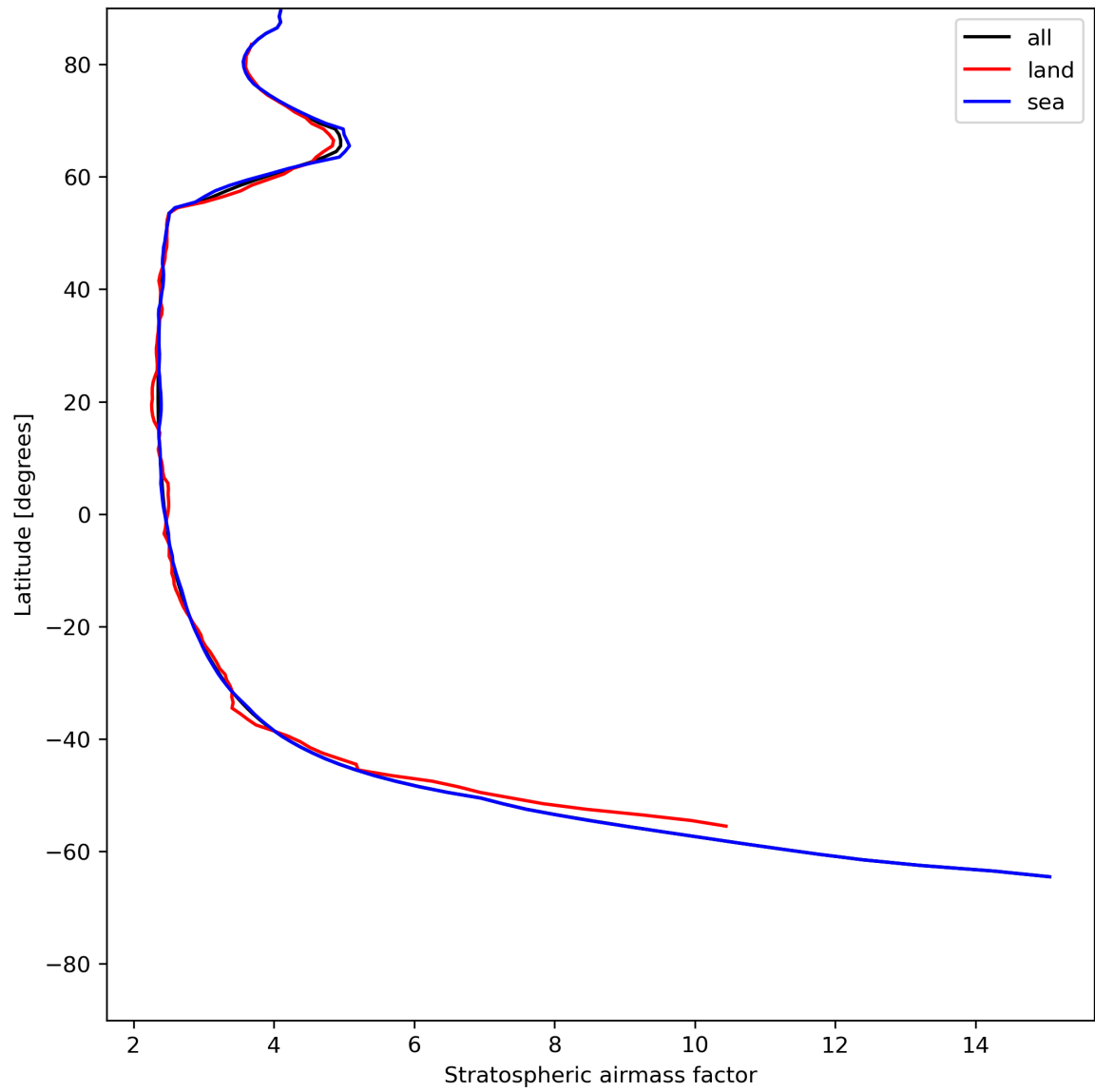
Figure 27: Zonal average of “Stratospheric air mass factor” for 2024-06-10 to 2024-06-12.
