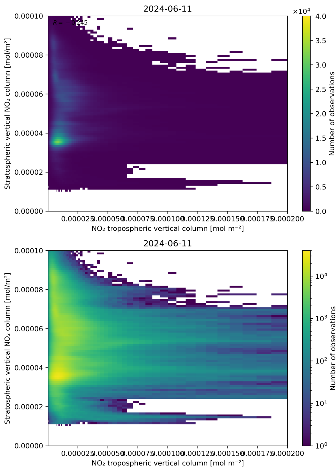
Figure 125: Scatter density plot of “NO 2 tropospheric vertical column” against “Stratospheric vertical NO 2 column” for 2024-06-10 to 2024-06-12.
