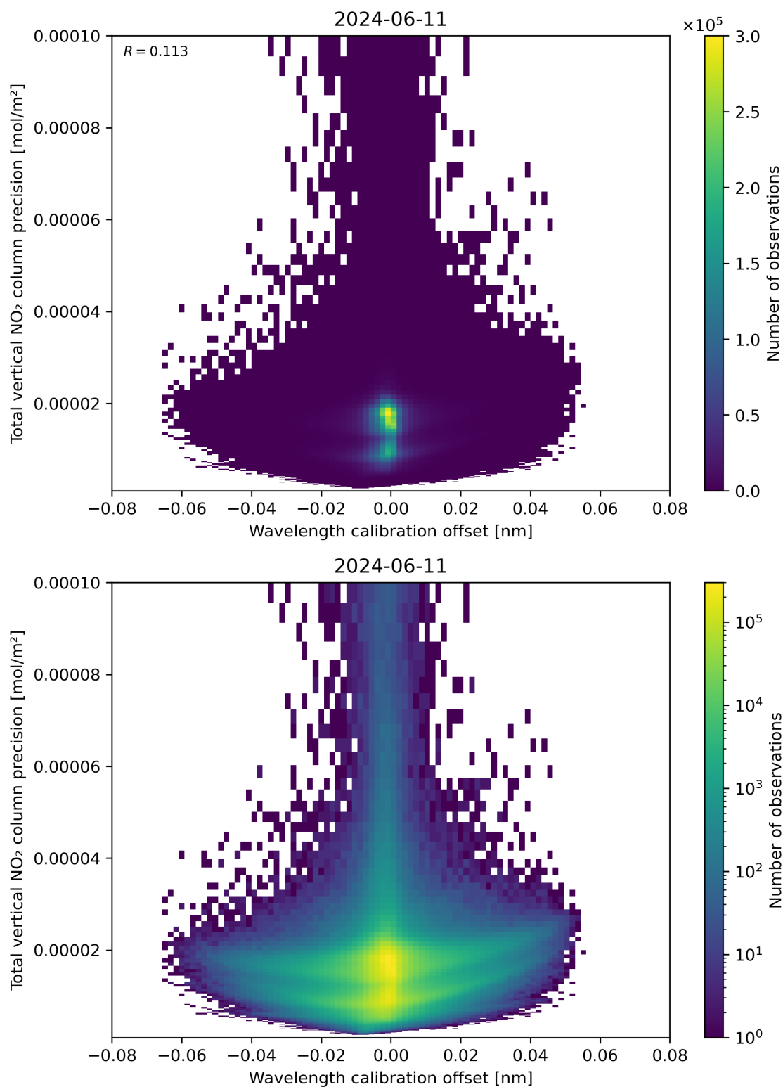
Figure 180: Scatter density plot of “Wavelength calibration offset” against “Total vertical NO 2 column precision” for 2024-06-10 to 2024-06-12.
