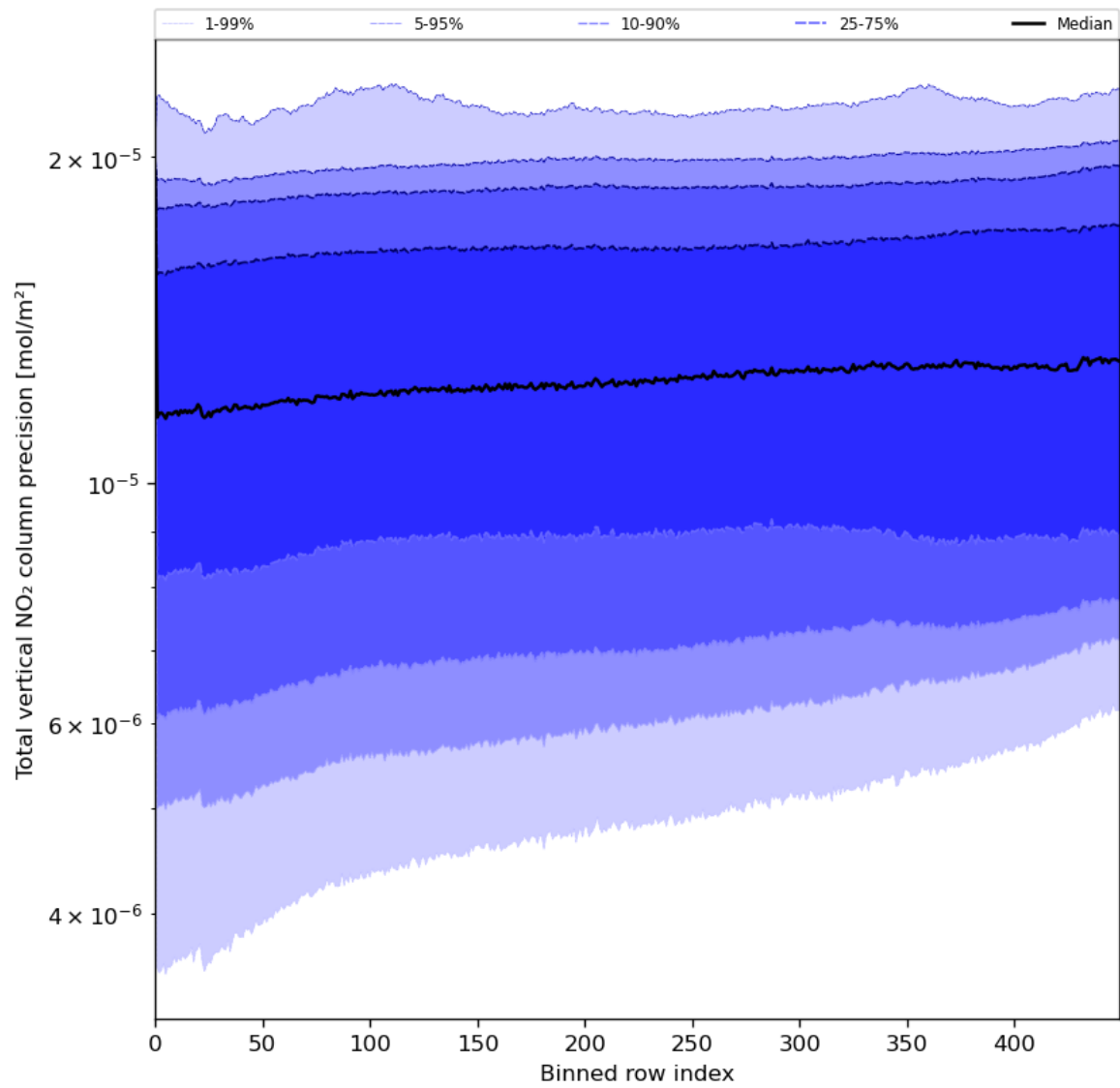
Figure 56: Along track statistics of “Total vertical NO 2 column precision” for 2024-06-10 to 2024-06-12
