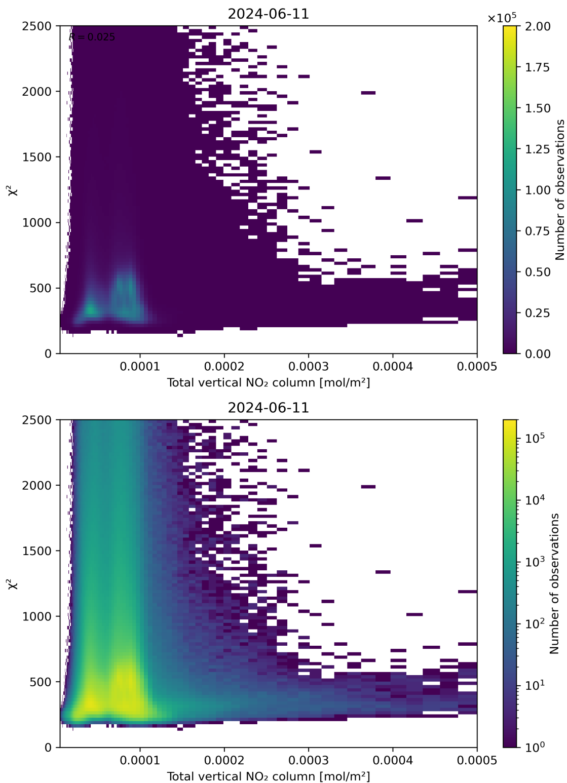
Figure 111: Scatter density plot of “Total vertical NO 2 column” against “ \chi^2 ” for 2024-06-10 to 2024-06-12.
