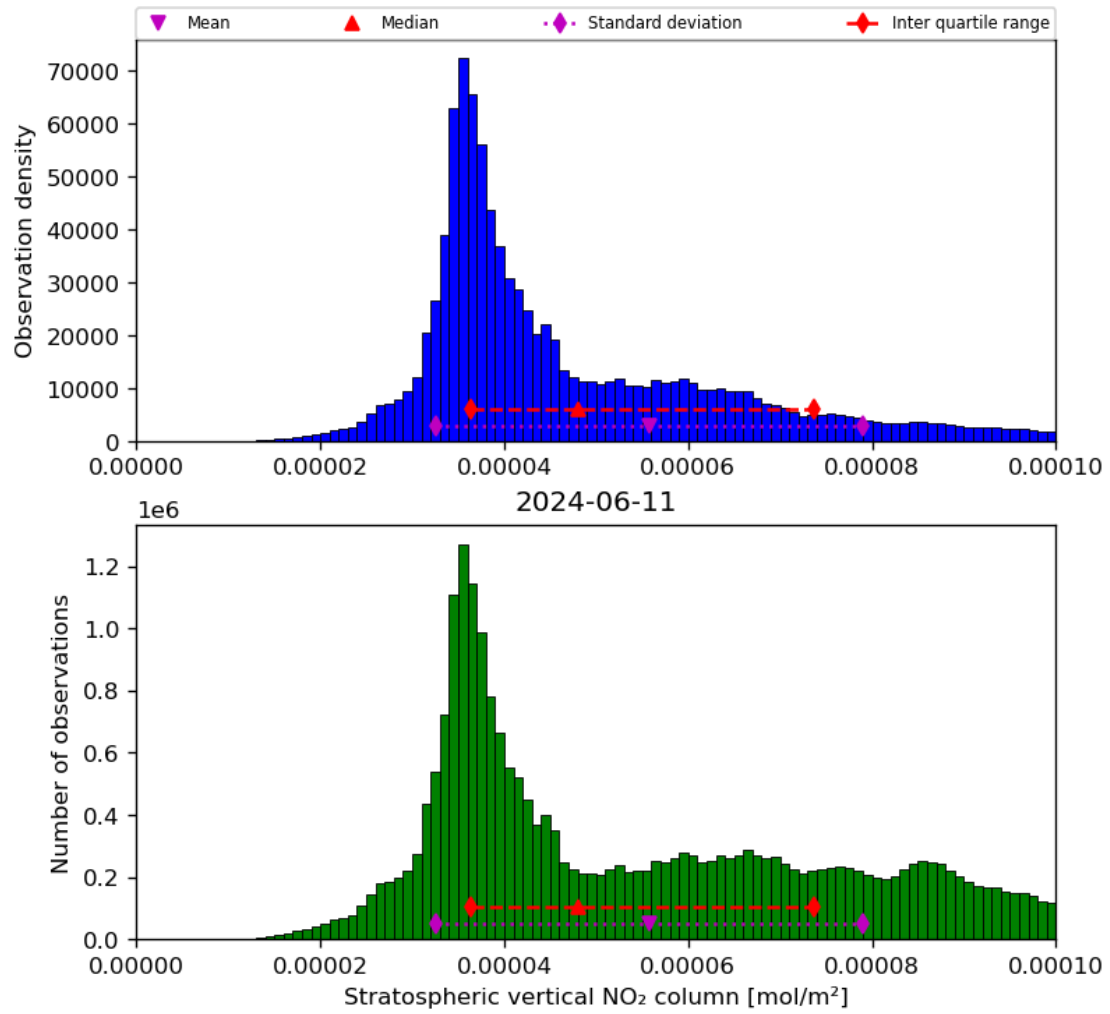
Figure 36: Histogram of “Stratospheric vertical NO 2 column” for 2024-06-10 to 2024-06-12
