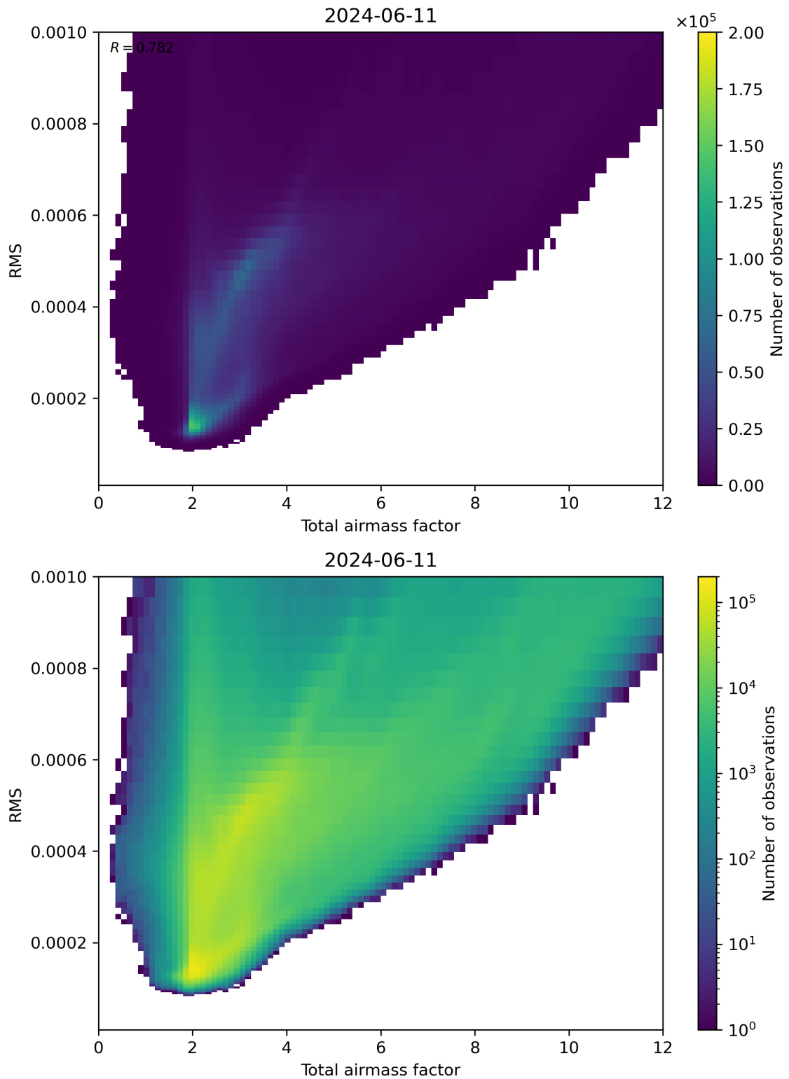
Figure 69: Scatter density plot of “Total airmass factor” against “RMS” for 2024-06-10 to 2024-06-12.
