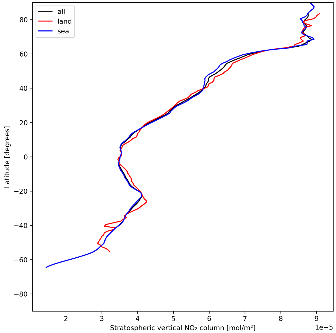
Figure 19: Zonal average of “Stratospheric vertical NO 2 column” for 2024-06-10 to 2024-06-12.
