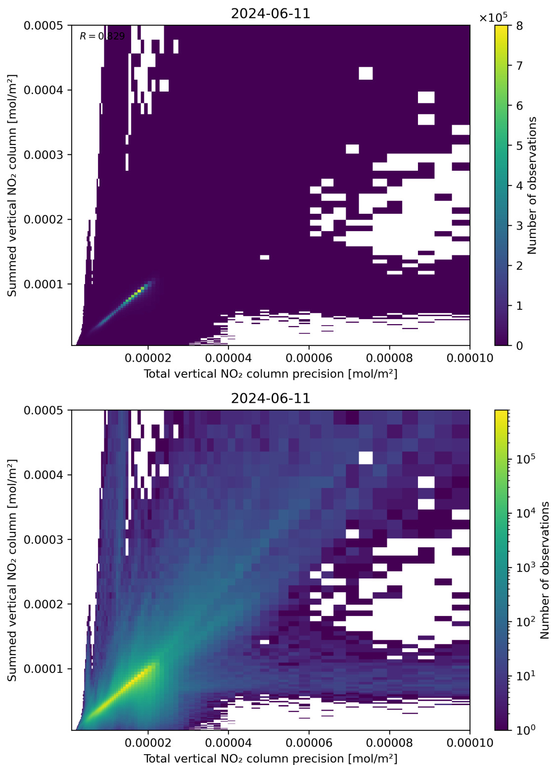
Figure 117: Scatter density plot of “Total vertical NO 2 column precision” against “Summed vertical NO 2 column” for 2024-06-10 to 2024-06-12.
