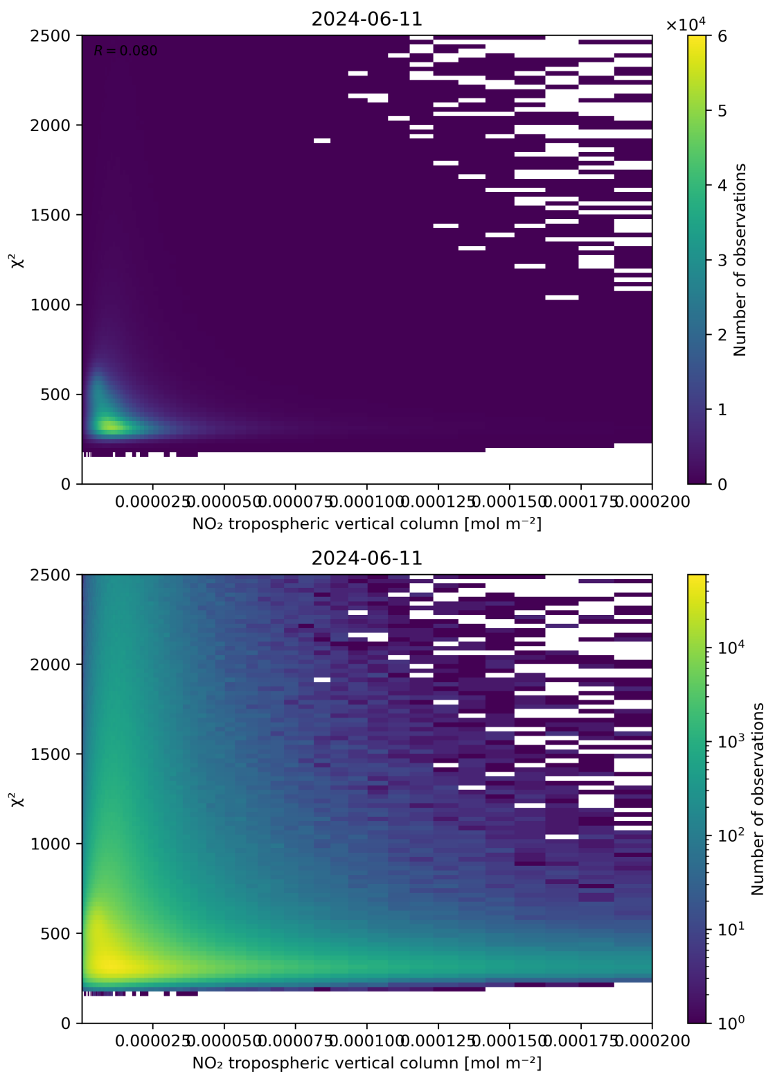
Figure 124: Scatter density plot of “NO 2 tropospheric vertical column” against “ \chi^2 ” for 2024-06-10 to 2024-06-12.
