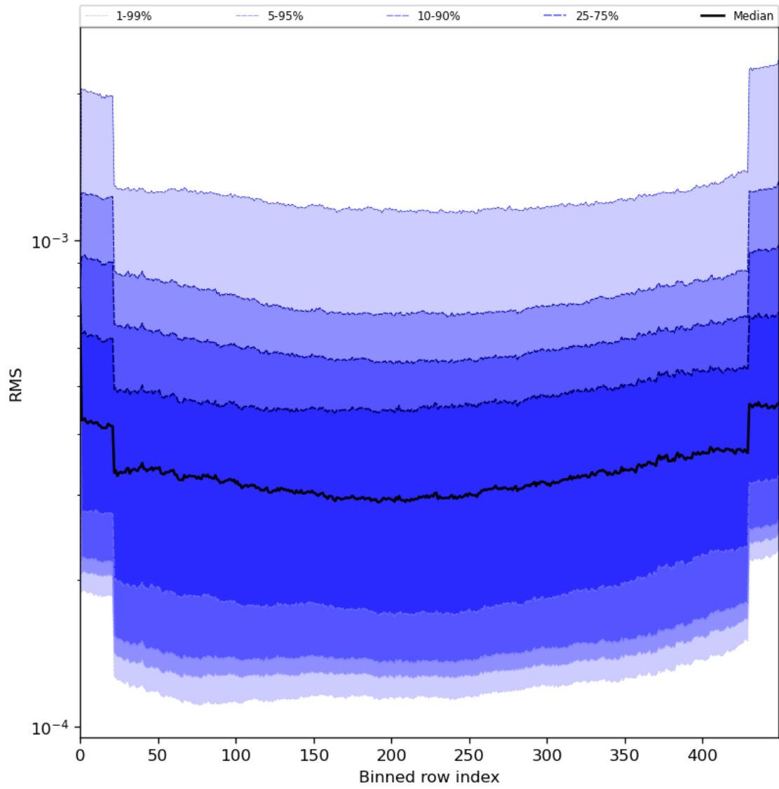
Figure 60: Along track statistics of “RMS” for 2024-06-10 to 2024-06-12
