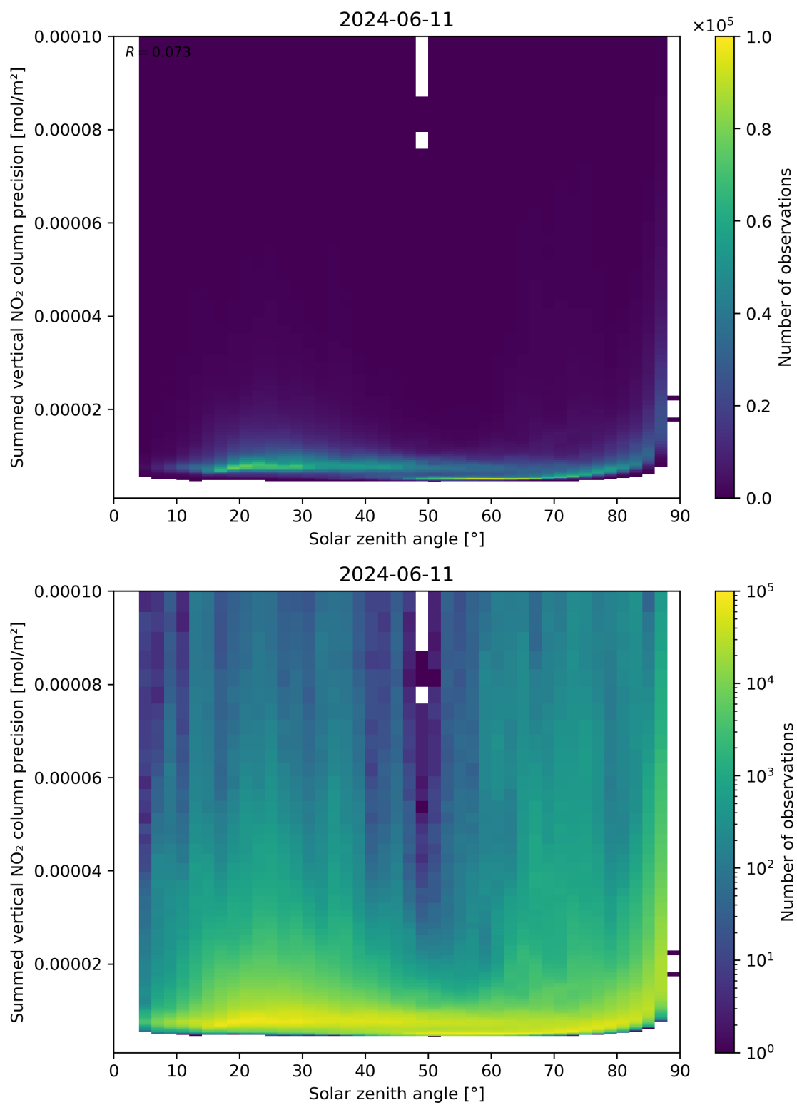
Figure 152: Scatter density plot of “Solar zenith angle” against “Summed vertical NO 2 column precision” for 2024-06-10 to 2024-06-12.
