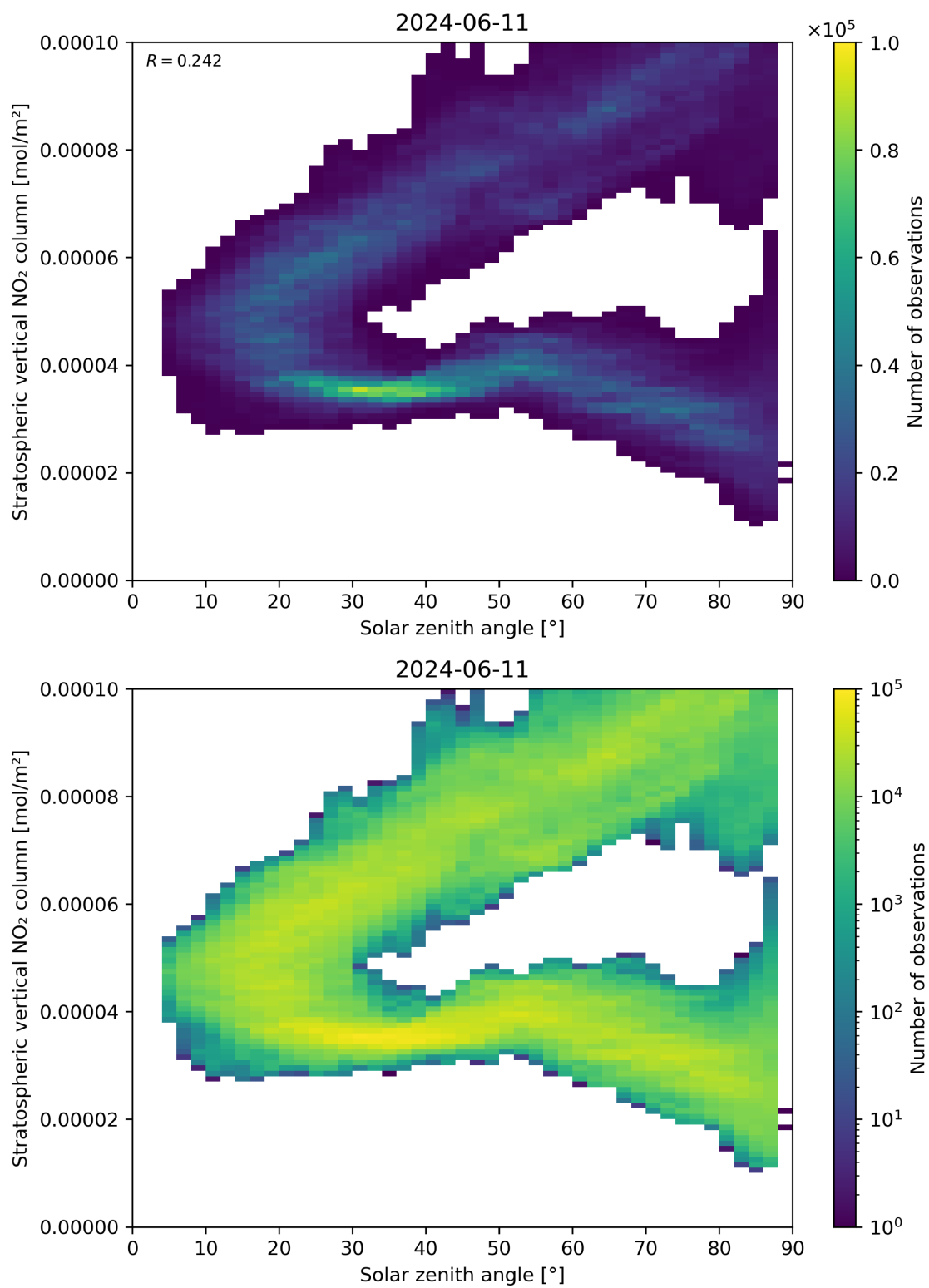
Figure 150: Scatter density plot of “Solar zenith angle” against “Stratospheric vertical NO 2 column” for 2024-06-10 to 2024-06-12.
