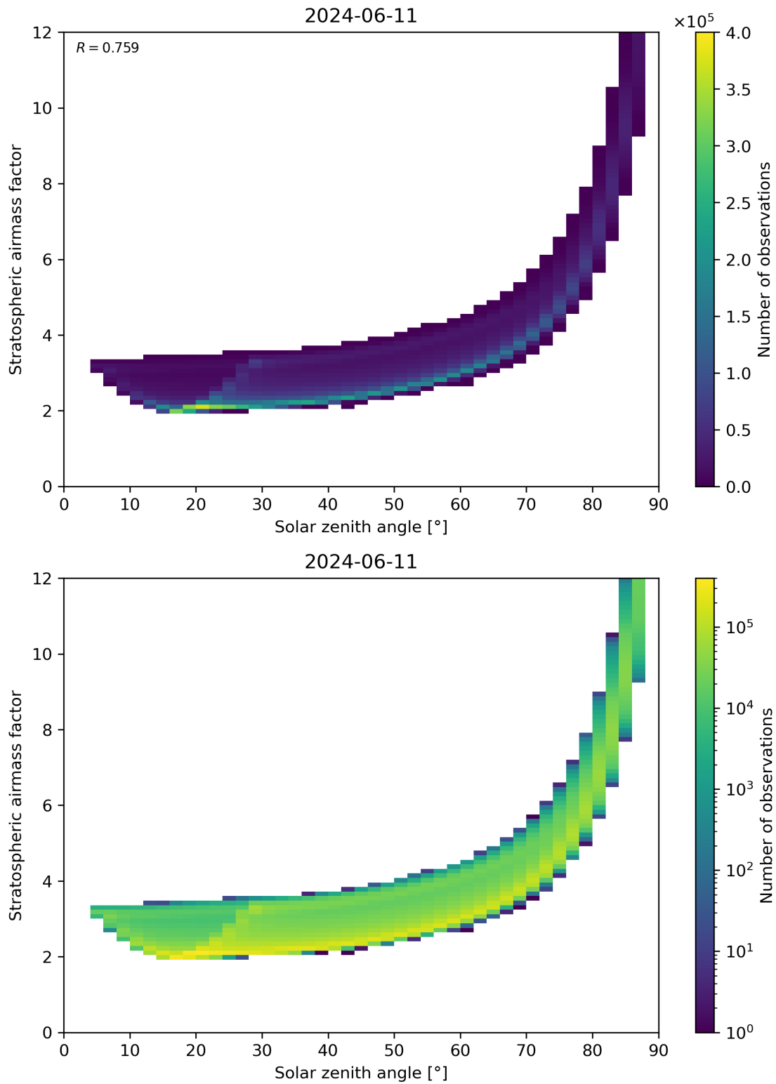
Figure 145: Scatter density plot of “Solar zenith angle” against “Stratospheric airmass factor” for 2024-06-10 to 2024-06-12.
