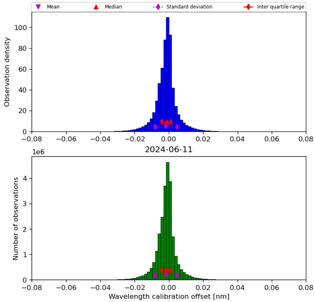
Figure 35: Histogram of “Wavelength calibration offset” for 2024-06-10 to 2024-06-12
