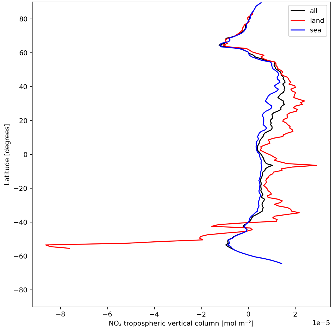
Figure 12: Zonal average of “NO 2 tropospheric vertical column” for 2024-06-10 to 2024-06-12.
