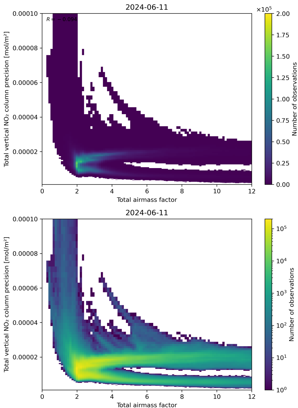
Figure 68: Scatter density plot of “Total airmass factor” against “Total vertical NO 2 column precision” for 2024-06-10 to 2024-06-12.
