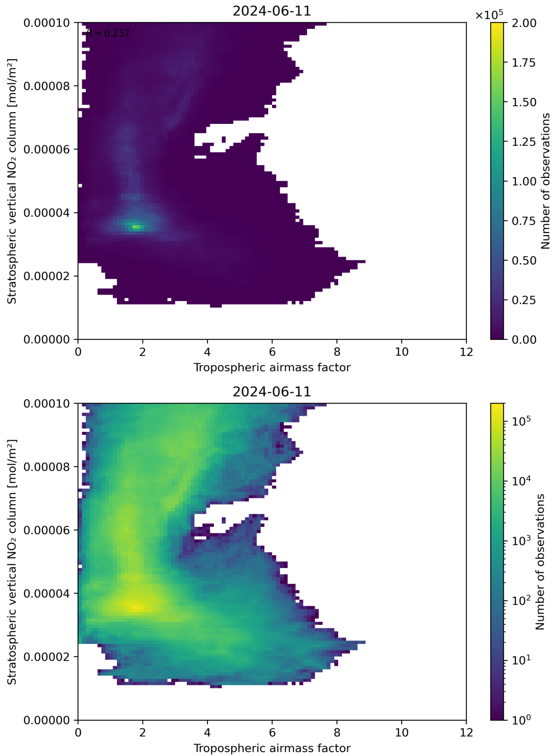
Figure 74: Scatter density plot of “Tropospheric air mass factor” against “Stratospheric vertical NO 2 column” for 2024-06-10 to 2024-06-12.
