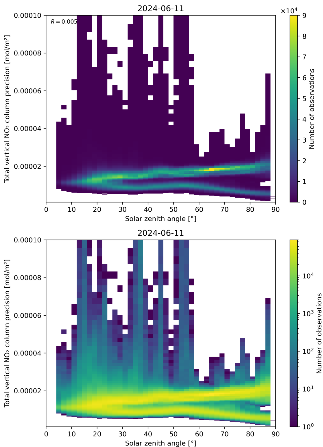
Figure 154: Scatter density plot of “Solar zenith angle” against “Total vertical NO 2 column precision” for 2024-06-10 to 2024-06-12.
