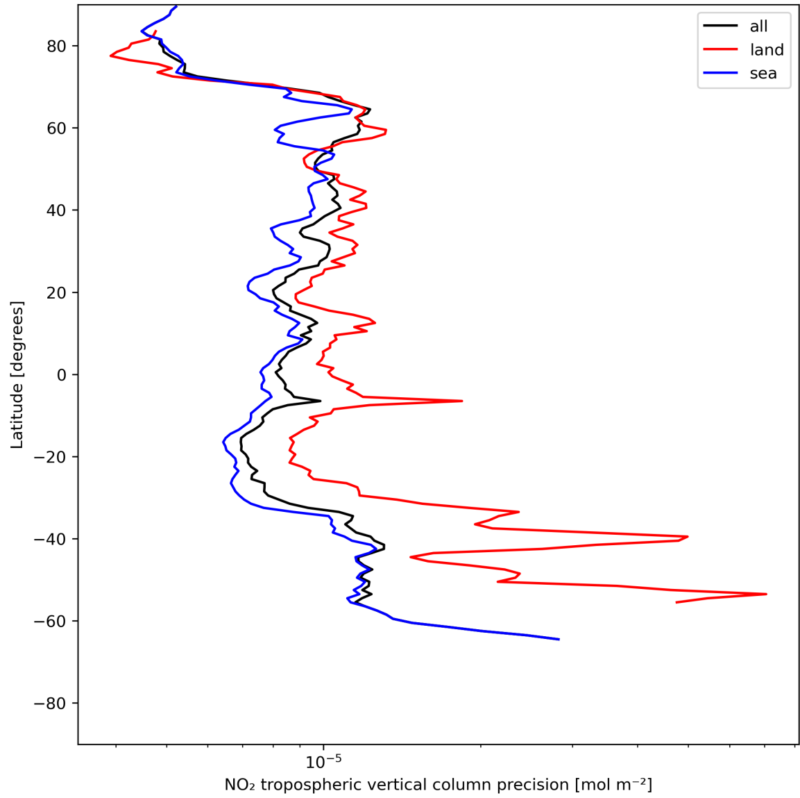
Figure 13: Zonal average of “NO 2 tropospheric vertical column precision” for 2024-06-10 to 2024-06-12.
