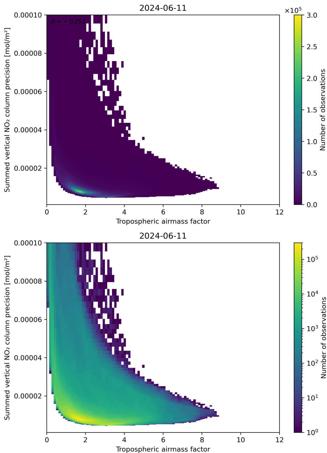
Figure 76: Scatter density plot of “Tropospheric air mass factor” against “Summed vertical NO 2 column precision” for 2024-06-10 to 2024-06-12.
