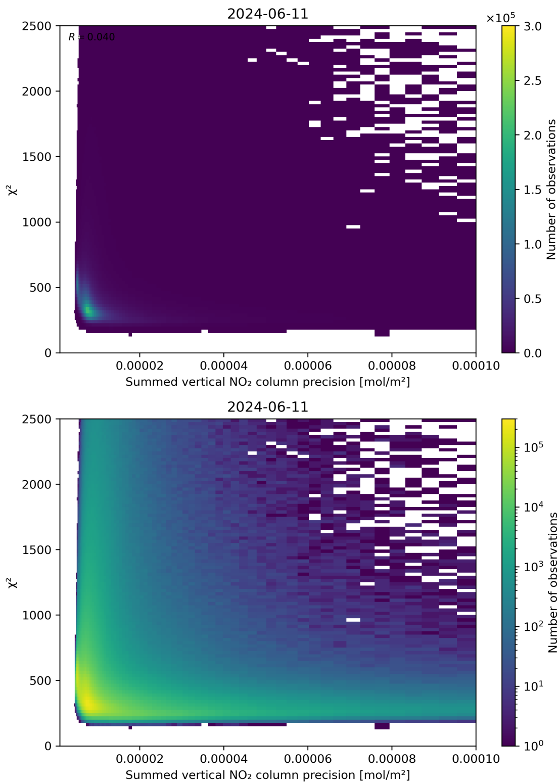
Figure 107: Scatter density plot of “Summed vertical NO 2 column precision” against “ \chi^2 ” for 2024-06-10 to 2024-06-12.
