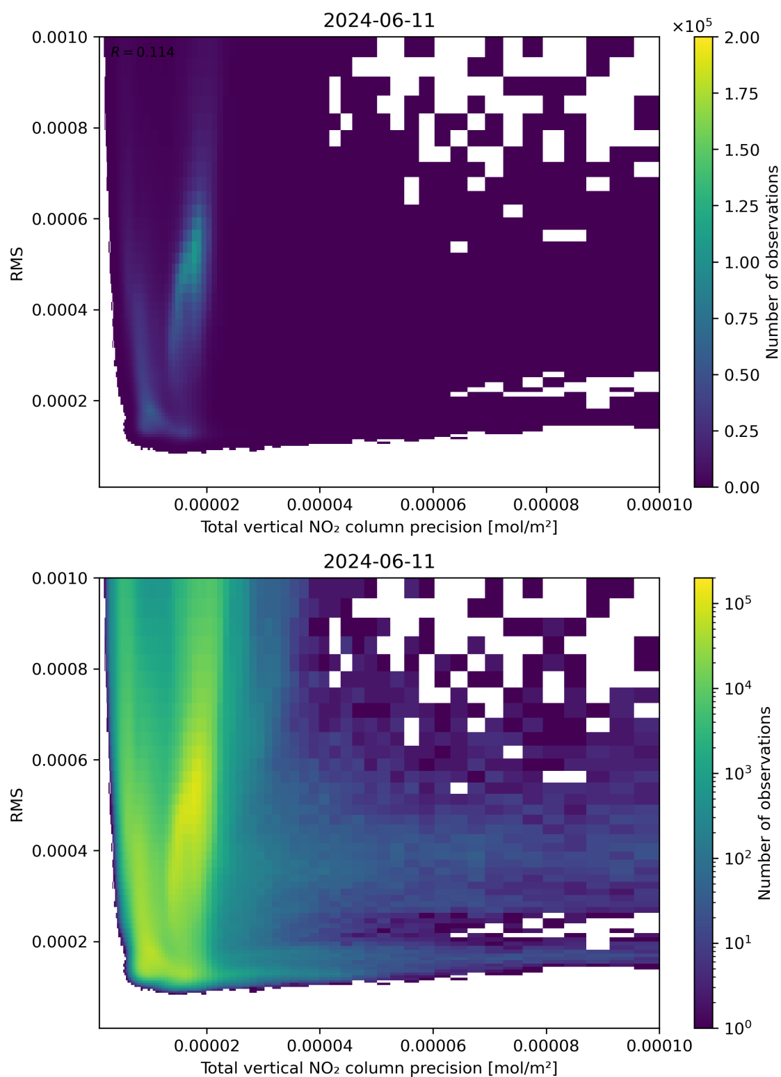
Figure 119: Scatter density plot of “Total vertical NO 2 column precision” against “RMS” for 2024-06-10 to 2024-06-12.
