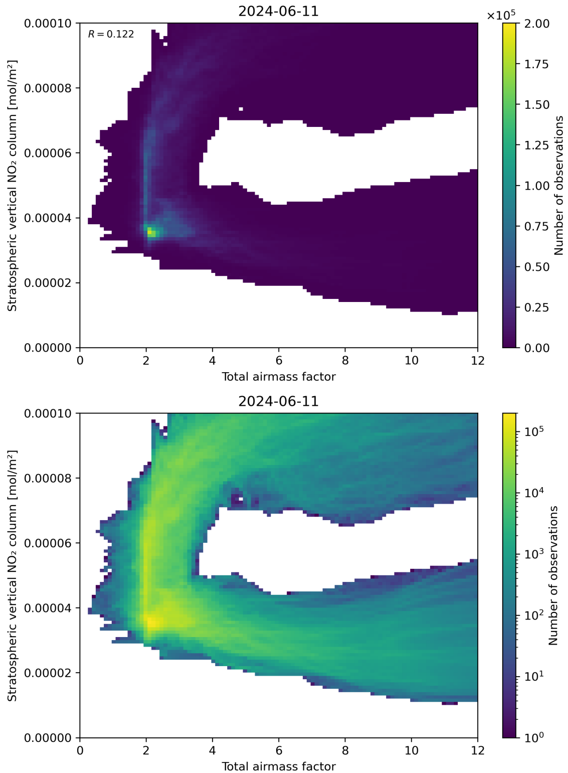
Figure 64: Scatter density plot of “Total airmass factor” against “Stratospheric vertical NO 2 column” for 2024-06-10 to 2024-06-12.
