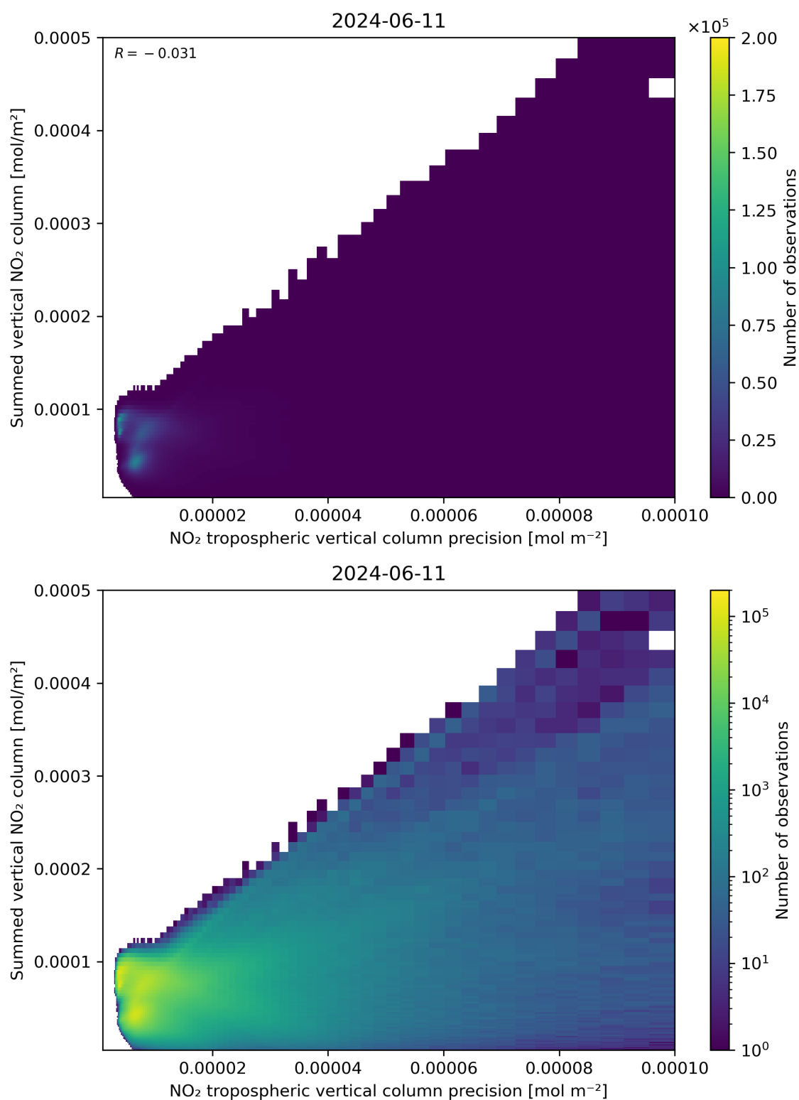
Figure 136: Scatter density plot of “NO 2 tropospheric vertical column precision” against “Summed vertical NO 2 column” for 2024-06-10 to 2024-06-12.
