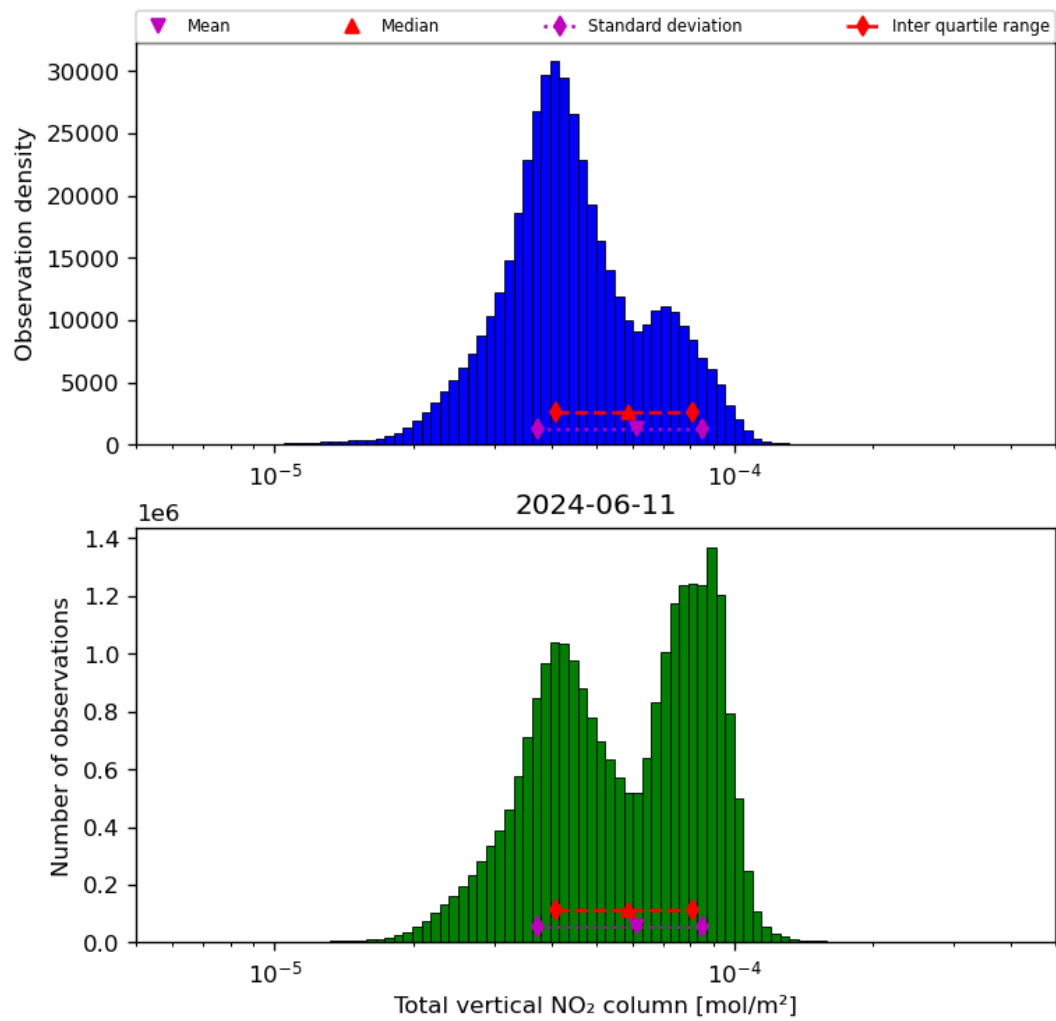
Figure 38: Histogram of “Total vertical NO 2 column” for 2024-06-10 to 2024-06-12
