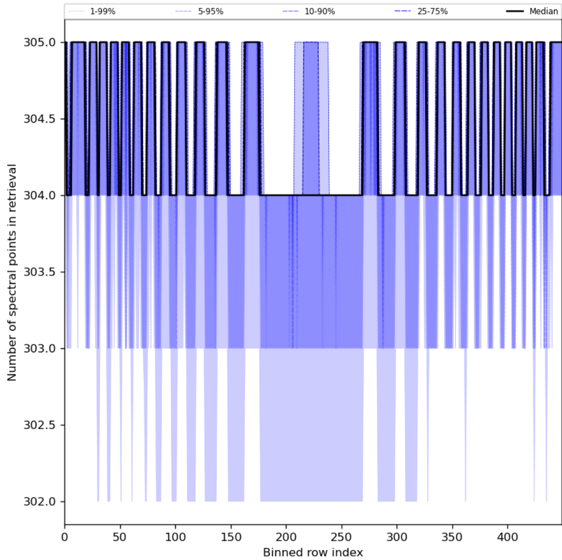
Figure 50: Along track statistics of “Number of spectral points in retrieval” for 2024-06-10 to 2024-06-12
