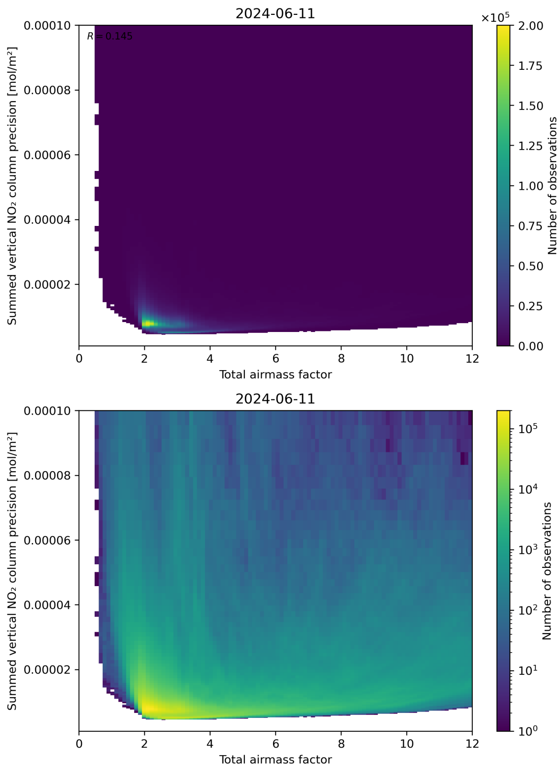
Figure 66: Scatter density plot of “Total airmass factor” against “Summed vertical NO 2 column precision” for 2024-06-10 to 2024-06-12.
