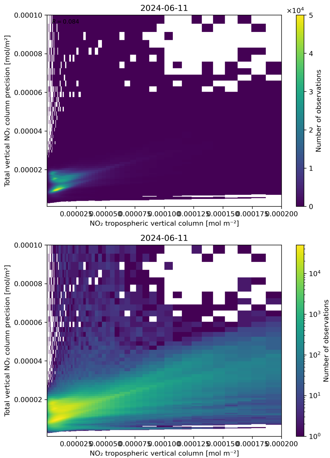
Figure 129: Scatter density plot of “NO 2 tropospheric vertical column” against “Total vertical NO 2 column precision” for 2024-06-10 to 2024-06-12.
