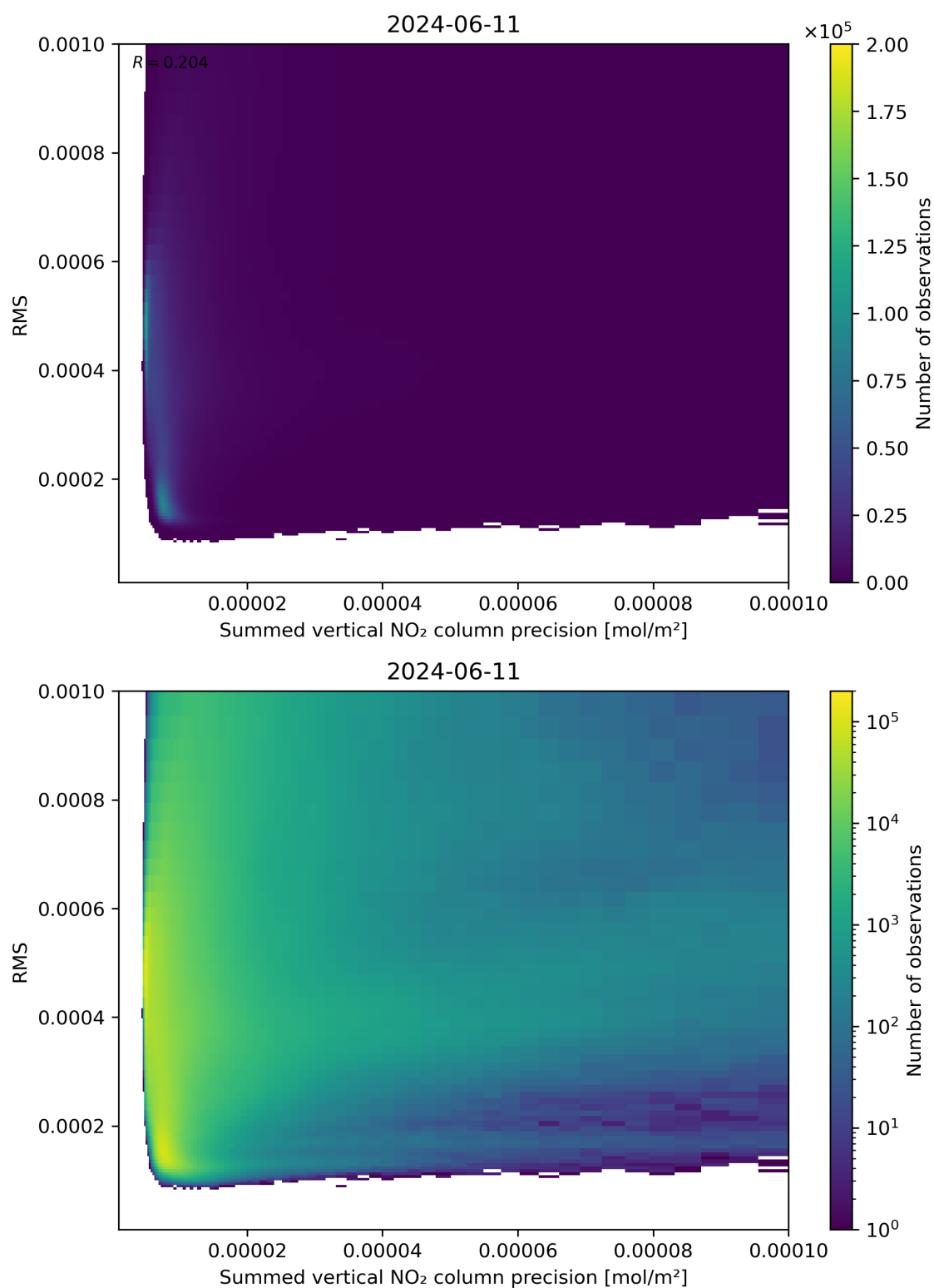
Figure 108: Scatter density plot of “Summed vertical NO 2 column precision” against “RMS” for 2024-06-10 to 2024-06-12.
