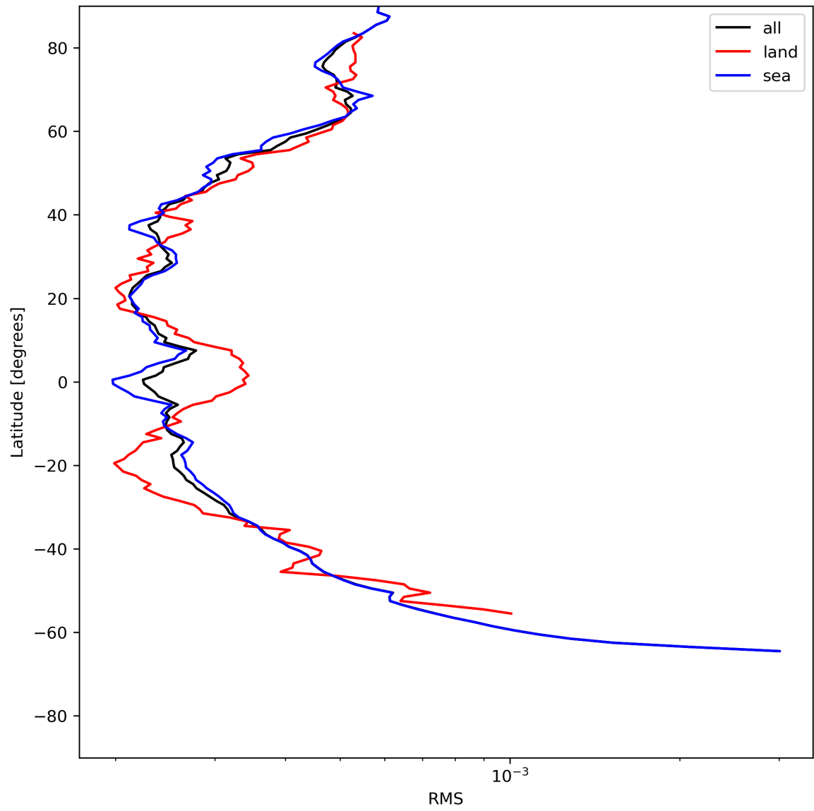
Figure 26: Zonal average of “RMS” for 2024-06-10 to 2024-06-12.
