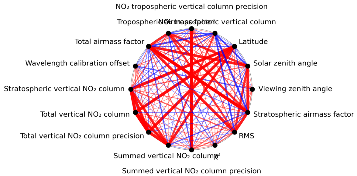
Figure 1: Map of correlation graph for 2024-06-10 to 2024-06-12.
