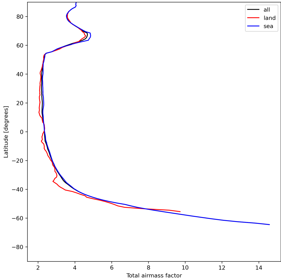
Figure 15: Zonal average of “Total airmass factor” for 2024-06-10 to 2024-06-12.
