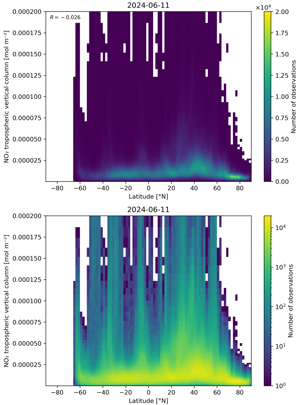
Figure 92: Scatter density plot of “Latitude” against “NO 2 tropospheric vertical column” for 2024-06-10 to 2024-06-12.
