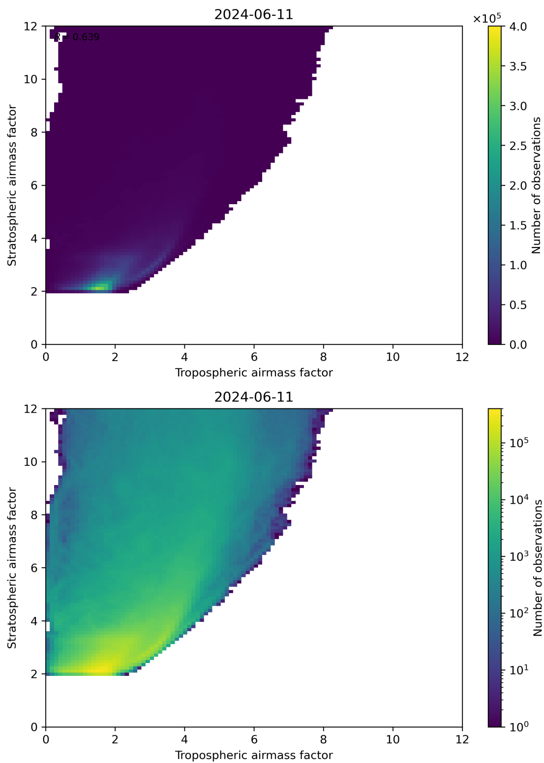
Figure 71: Scatter density plot of “Tropospheric airmass factor” against “Stratospheric airmass factor” for 2024-06-10 to 2024-06-12.
