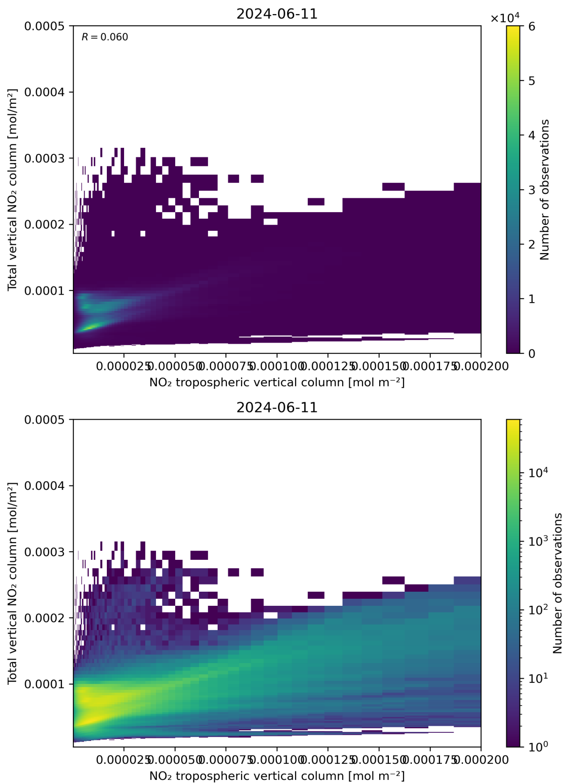
Figure 128: Scatter density plot of “NO 2 tropospheric vertical column” against “Total vertical NO 2 column” for 2024-06-10 to 2024-06-12.
