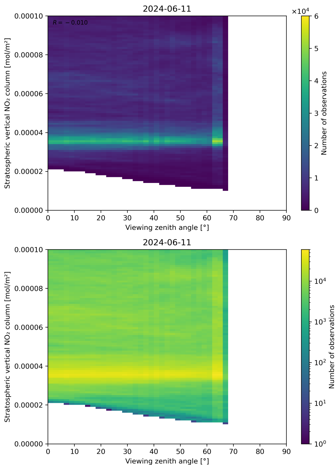
Figure 164: Scatter density plot of “Viewing zenith angle” against “Stratospheric vertical NO 2 column” for 2024-06-10 to 2024-06-12.
