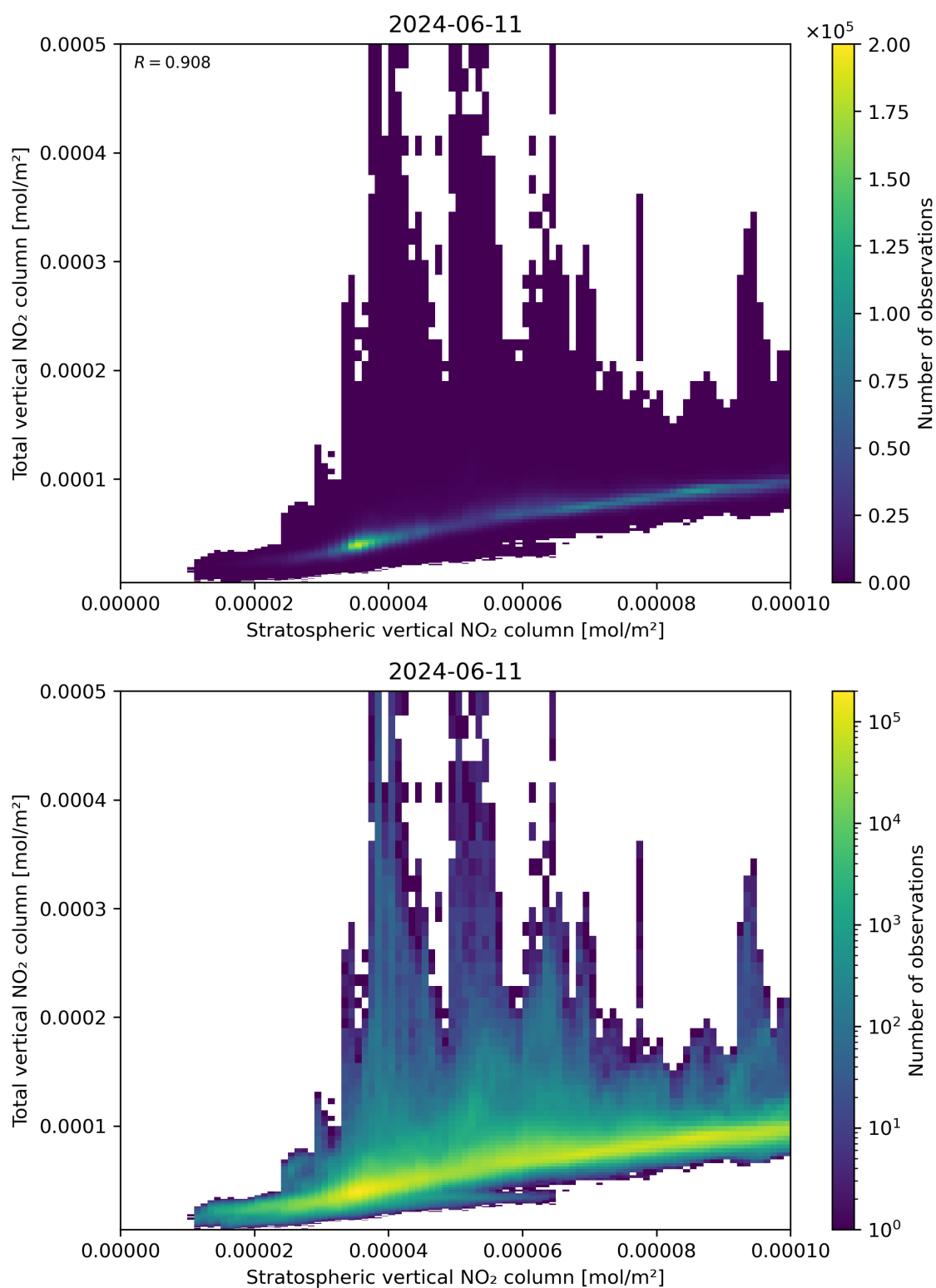
Figure 100: Scatter density plot of “Stratospheric vertical NO 2 column” against “Total vertical NO 2 column” for 2024-06-10 to 2024-06-12.
