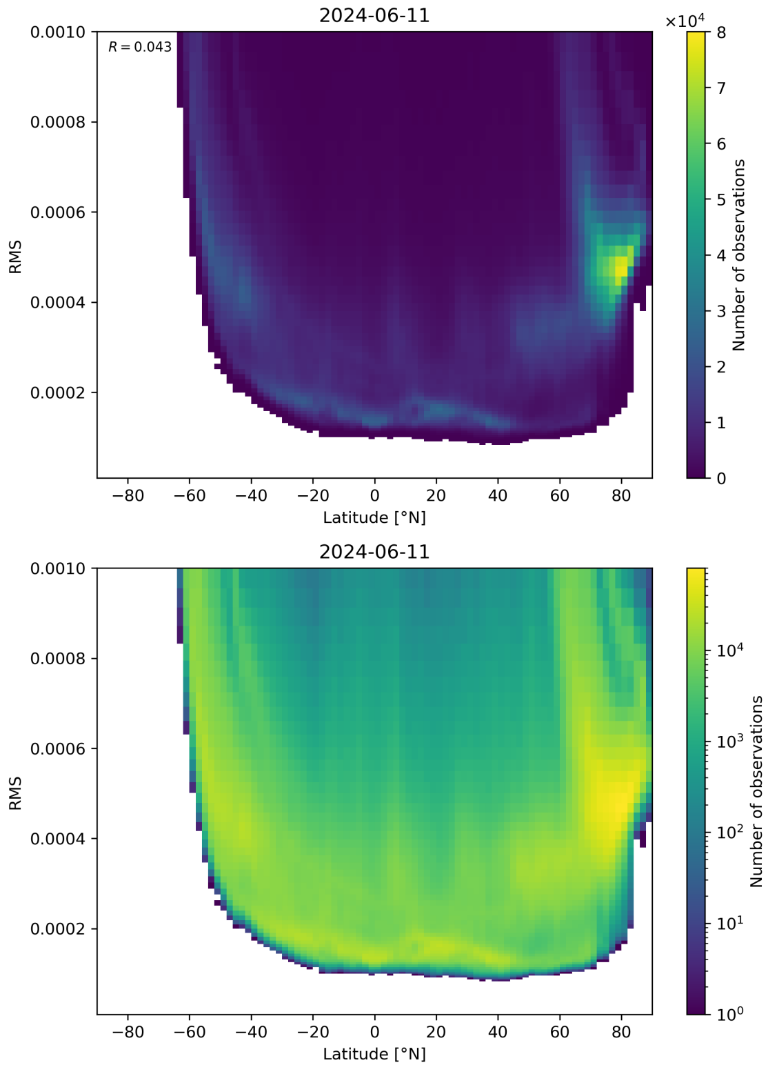
Figure 94: Scatter density plot of “Latitude” against “RMS” for 2024-06-10 to 2024-06-12.
