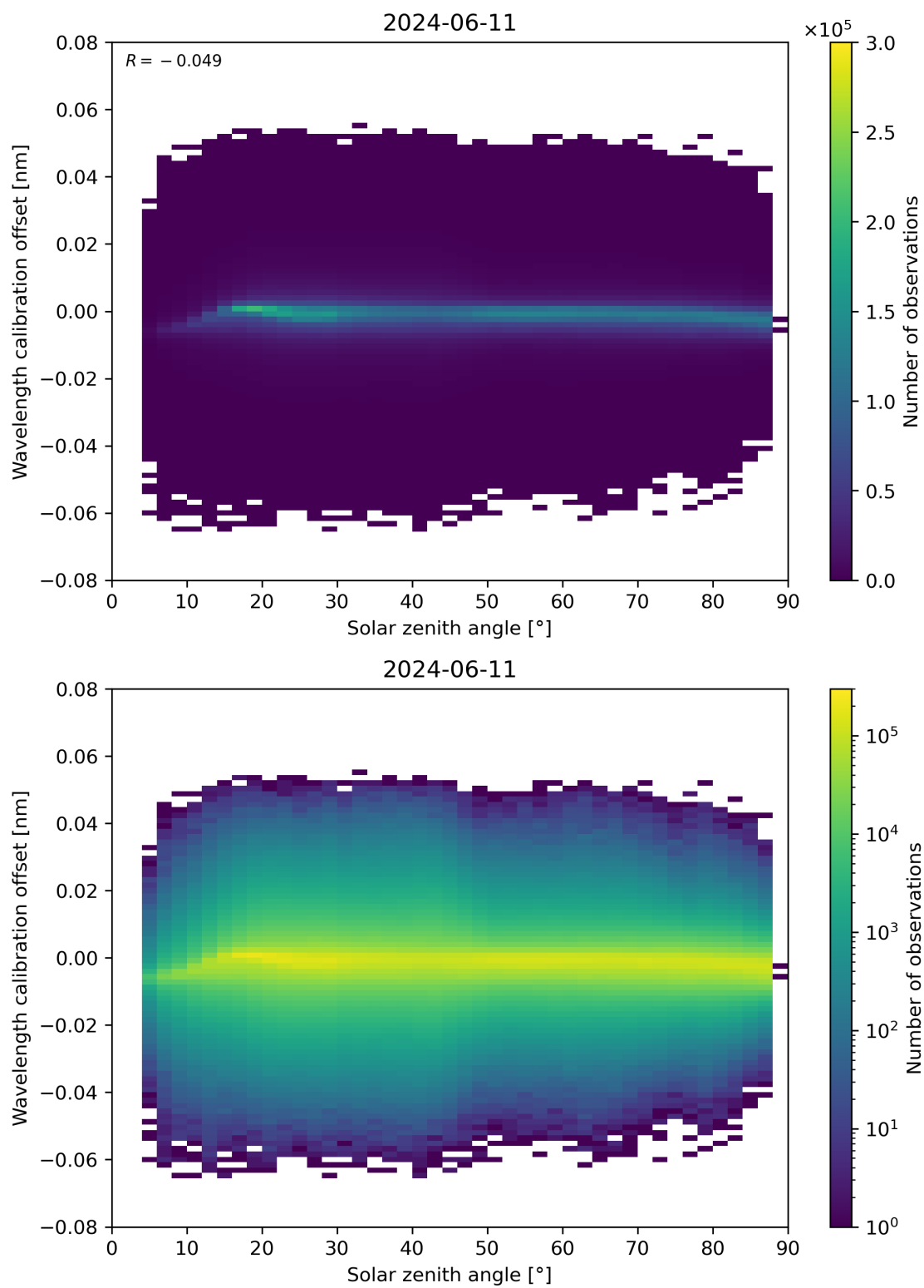
Figure 158: Scatter density plot of “Solar zenith angle” against “Wavelength calibration offset” for 2024-06-10 to 2024-06-12.
