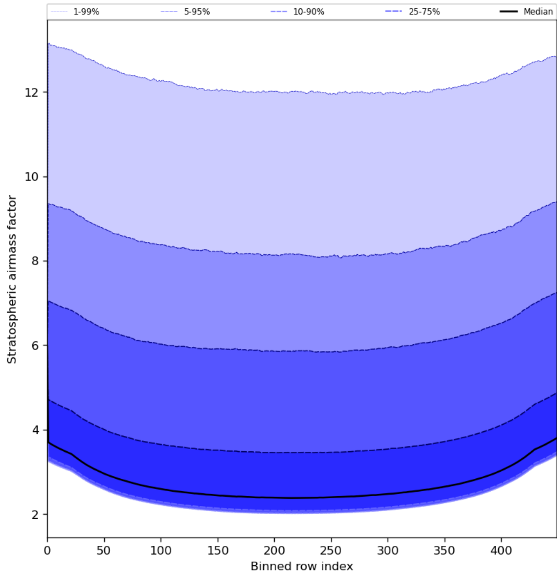
Figure 61: Along track statistics of “Stratospheric airmass factor” for 2024-06-10 to 2024-06-12
