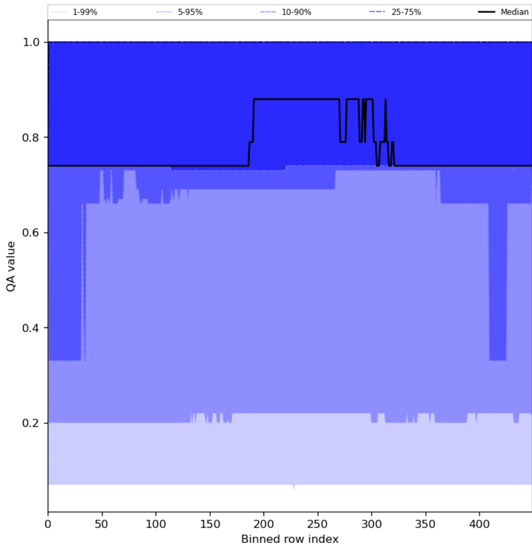
Figure 45: Along track statistics of “QA value” for 2024-06-10 to 2024-06-12
