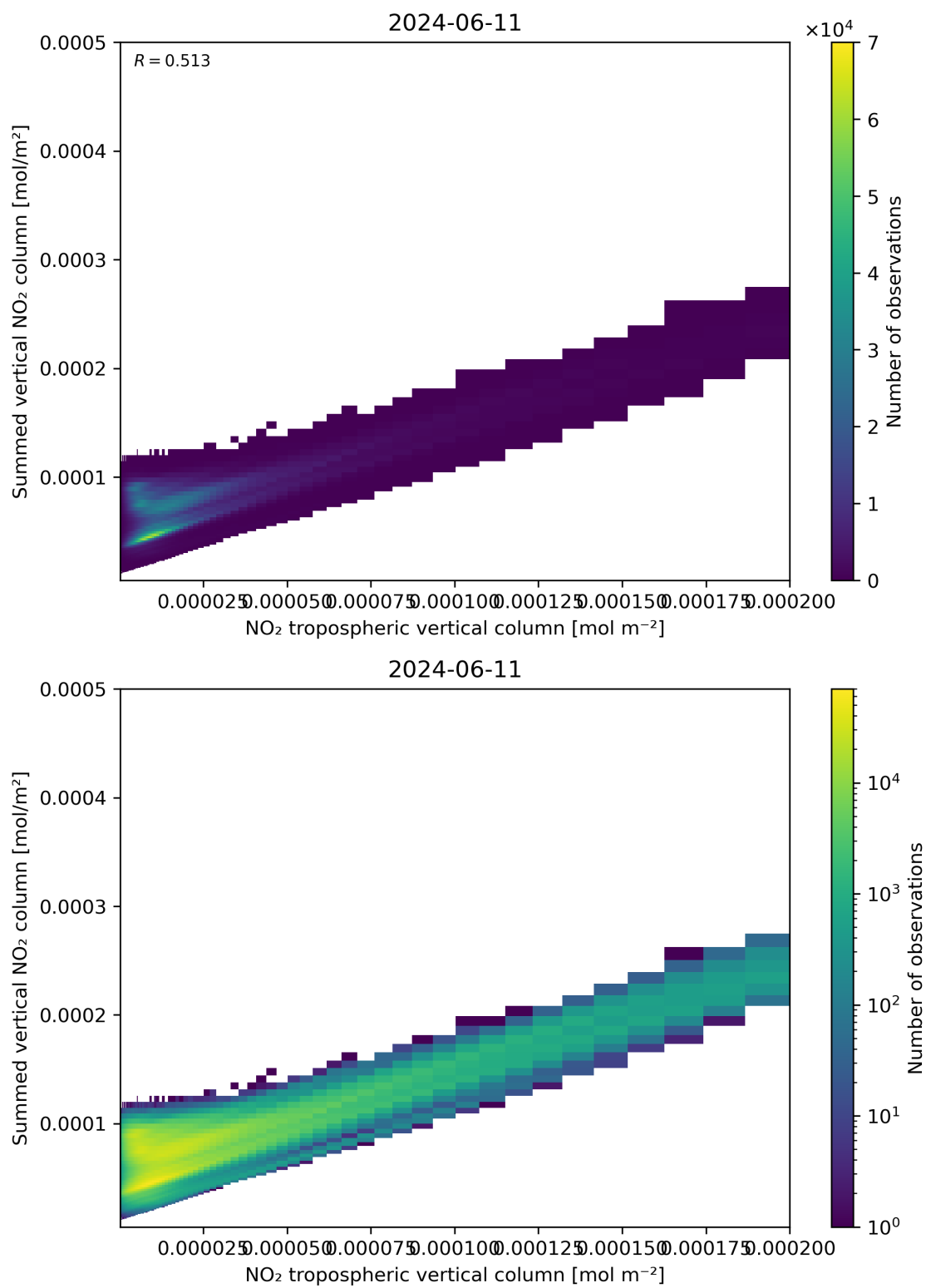
Figure 126: Scatter density plot of “NO 2 tropospheric vertical column” against “Summed vertical NO 2 column” for 2024-06-10 to 2024-06-12.
