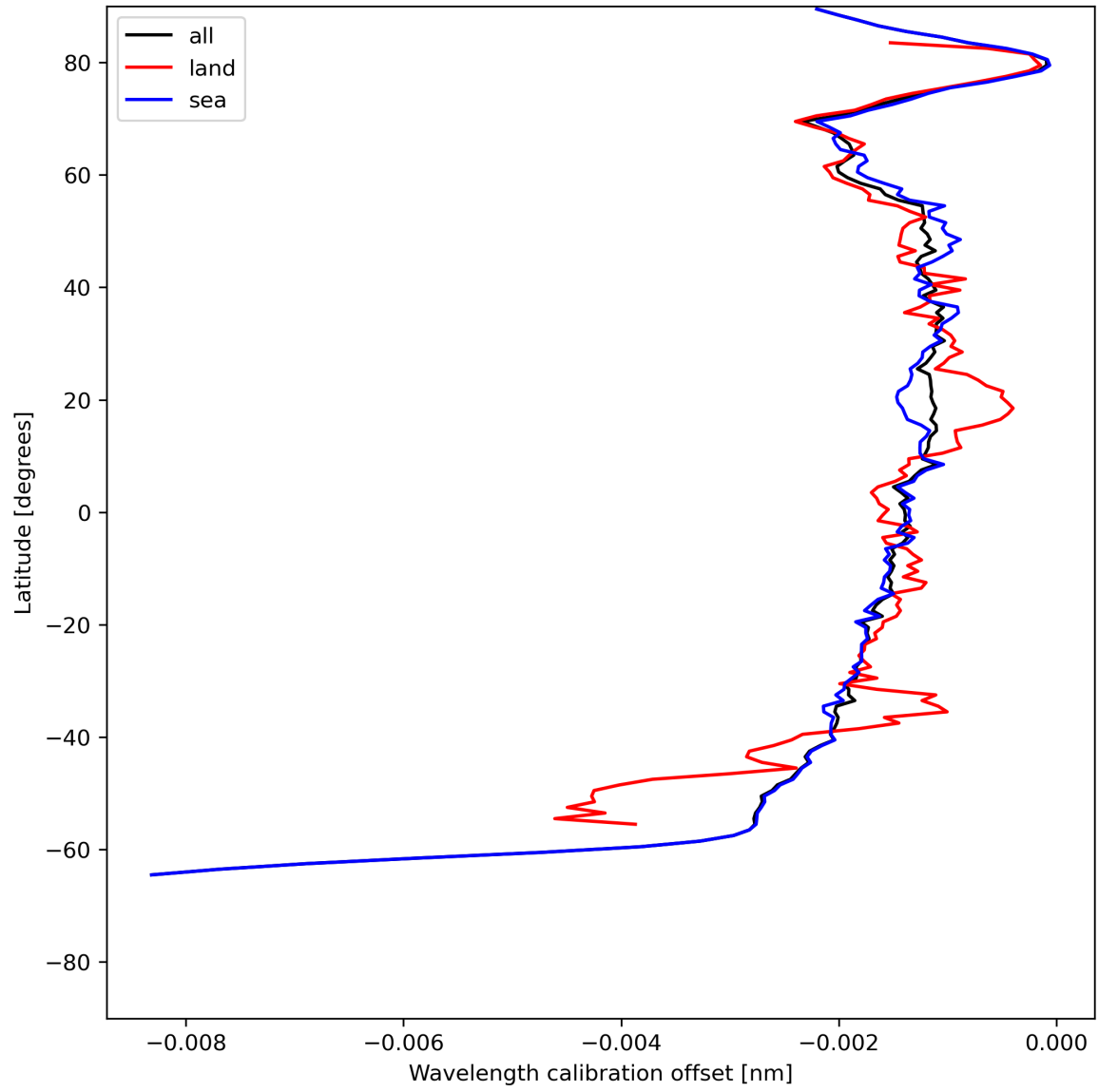
Figure 18: Zonal average of “Wavelength calibration offset” for 2024-06-10 to 2024-06-12.
