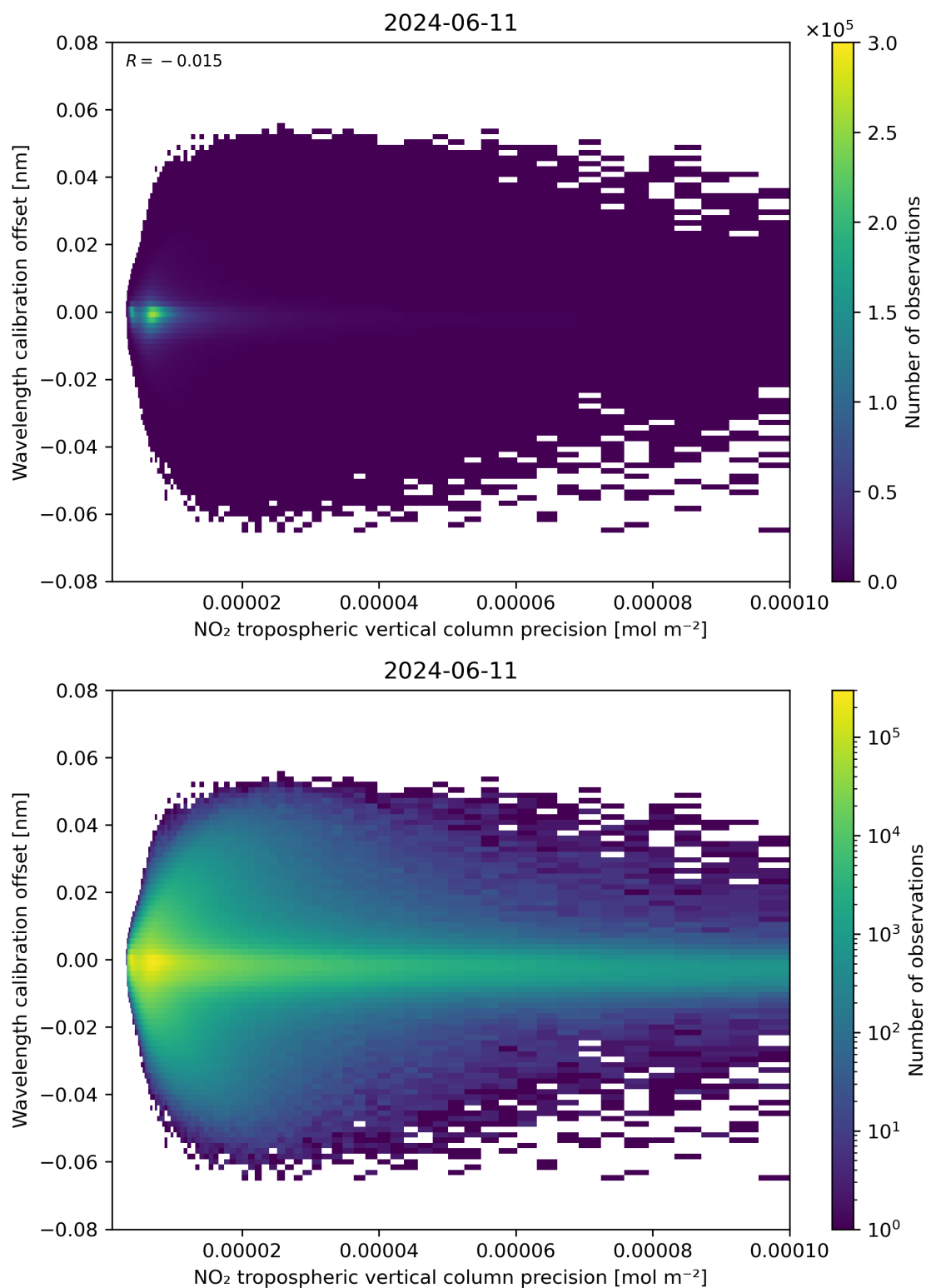
Figure 141: Scatter density plot of “NO 2 tropospheric vertical column precision” against “Wavelength calibration offset” for 2024-06-10 to 2024-06-12.
