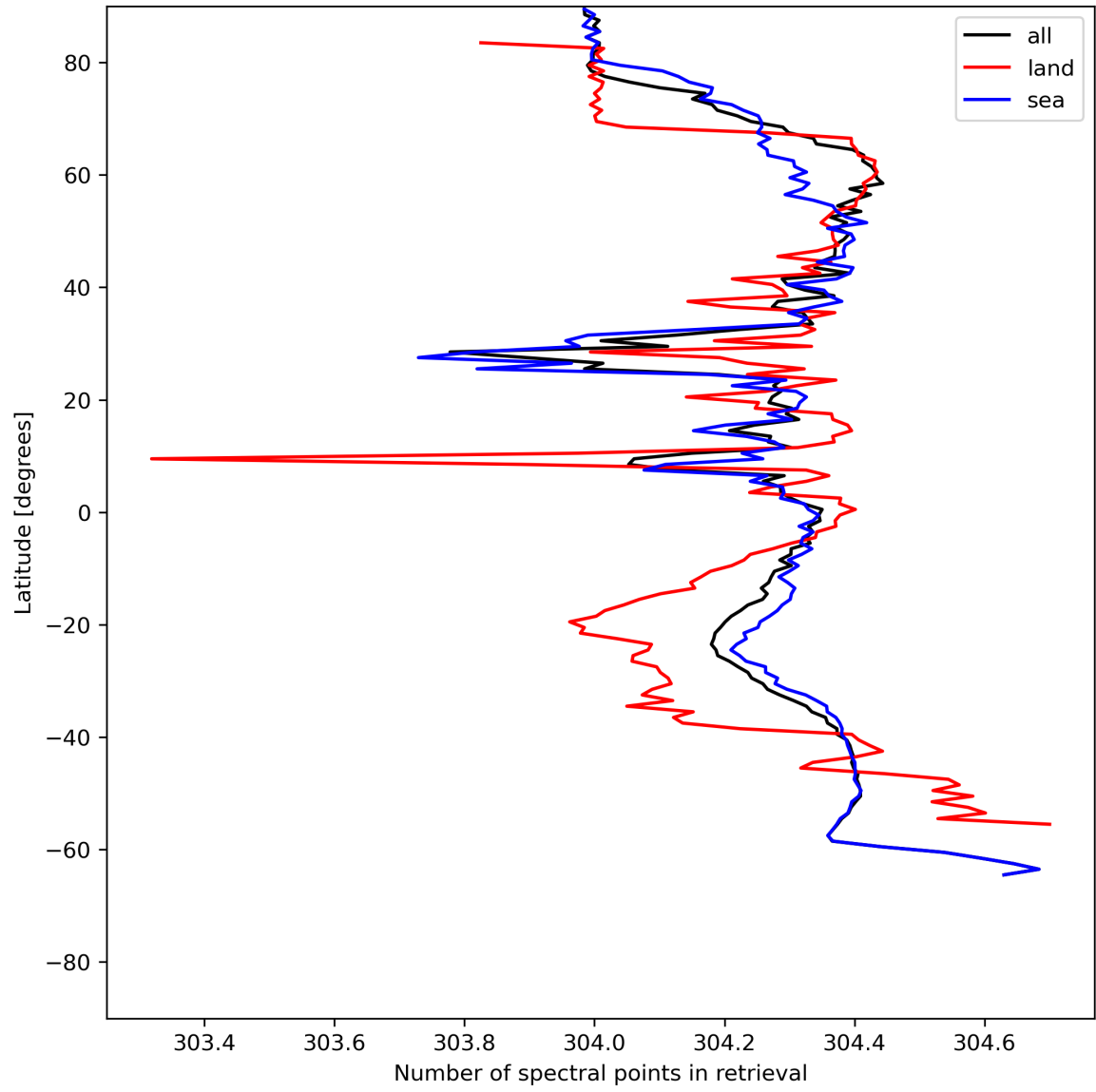
Figure 16: Zonal average of “Number of spectral points in retrieval” for 2024-06-10 to 2024-06-12.
