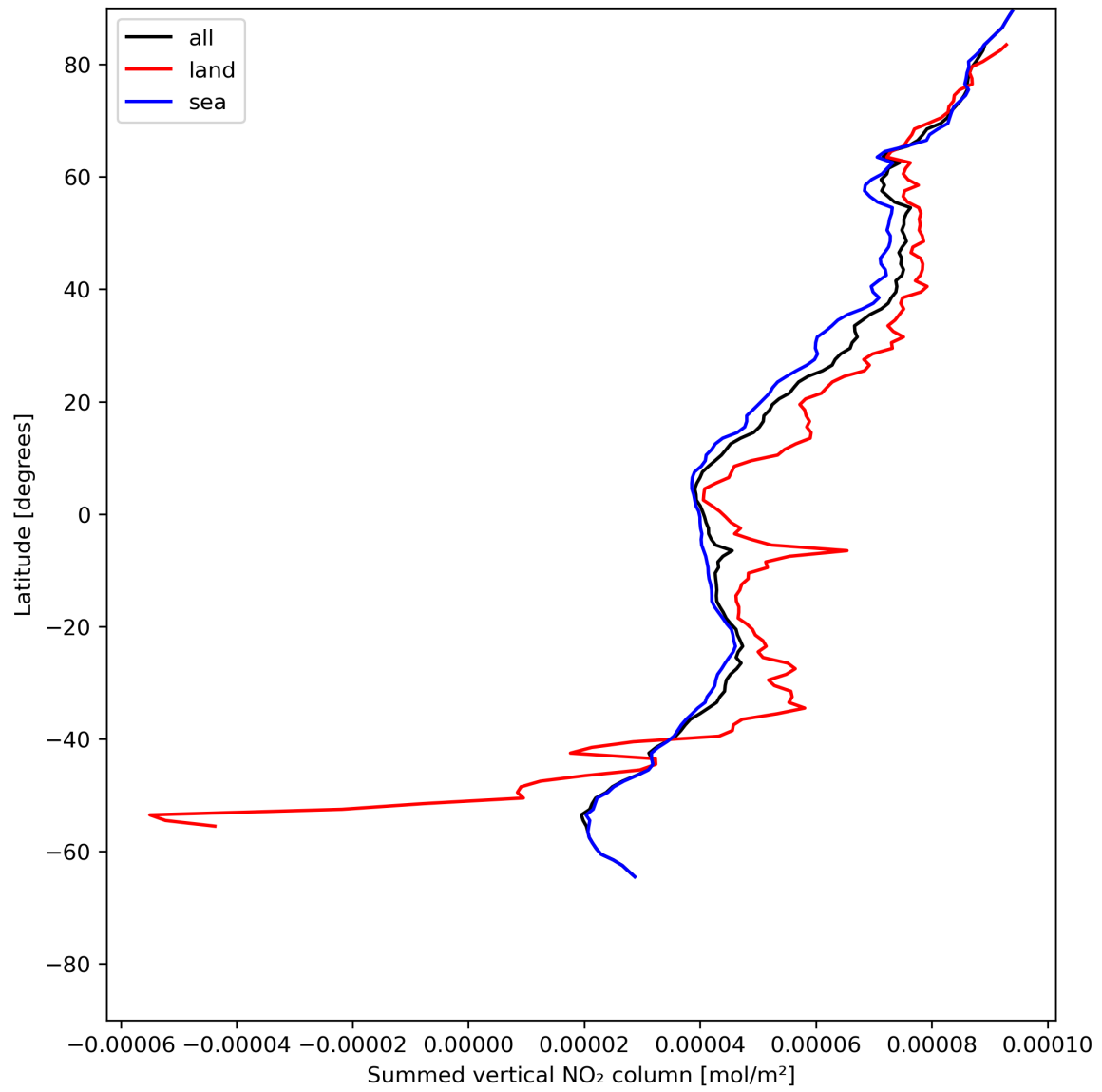
Figure 23: Zonal average of “Summed vertical NO 2 column” for 2024-06-10 to 2024-06-12.
