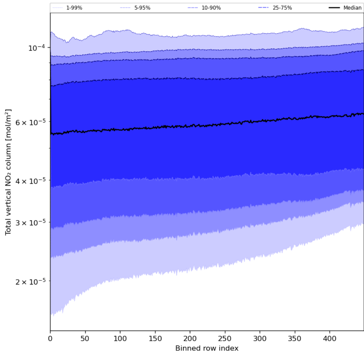
Figure 55: Along track statistics of “Total vertical NO 2 column” for 2024-06-10 to 2024-06-12
