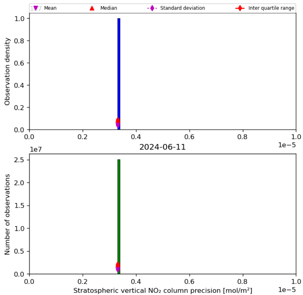
Figure 37: Histogram of “Stratospheric vertical NO 2 column precision” for 2024-06-10 to 2024-06-12
