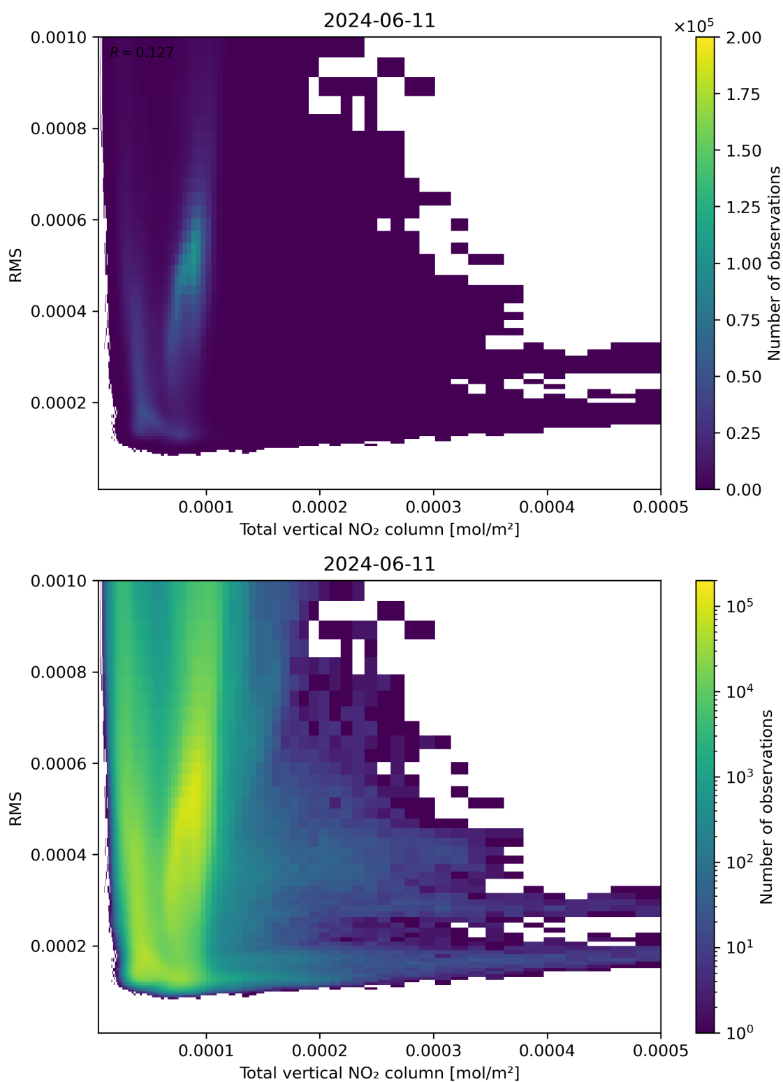
Figure 120: Scatter density plot of “Total vertical NO 2 column” against “RMS” for 2024-06-10 to 2024-06-12.
