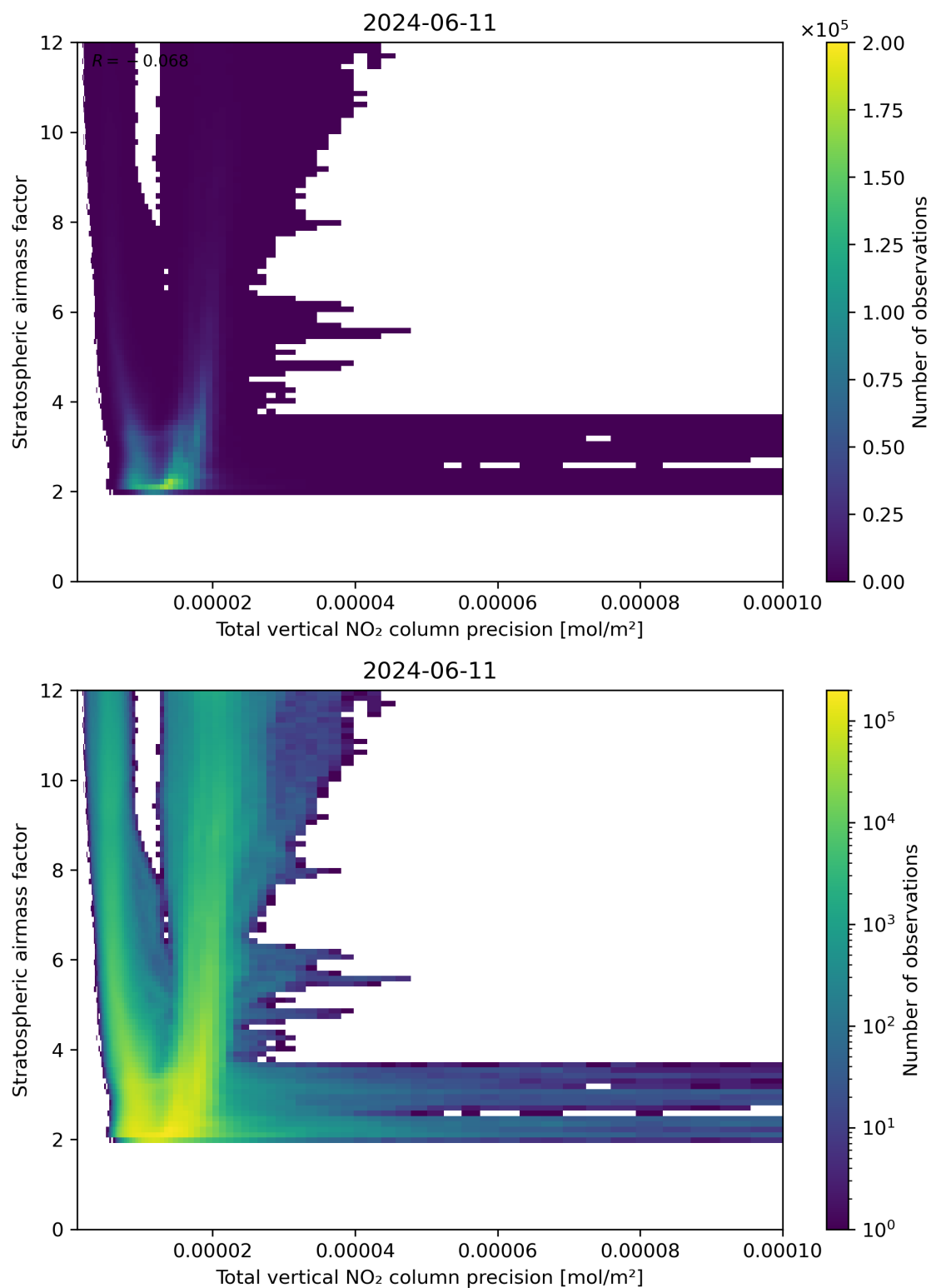
Figure 115: Scatter density plot of “Total vertical NO 2 column precision” against “Stratospheric air mass factor” for 2024-06-10 to 2024-06-12.
