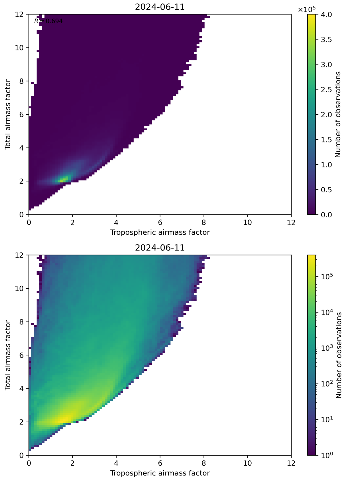
Figure 72: Scatter density plot of “Tropospheric airmass factor” against “Total airmass factor” for 2024-06-10 to 2024-06-12.
