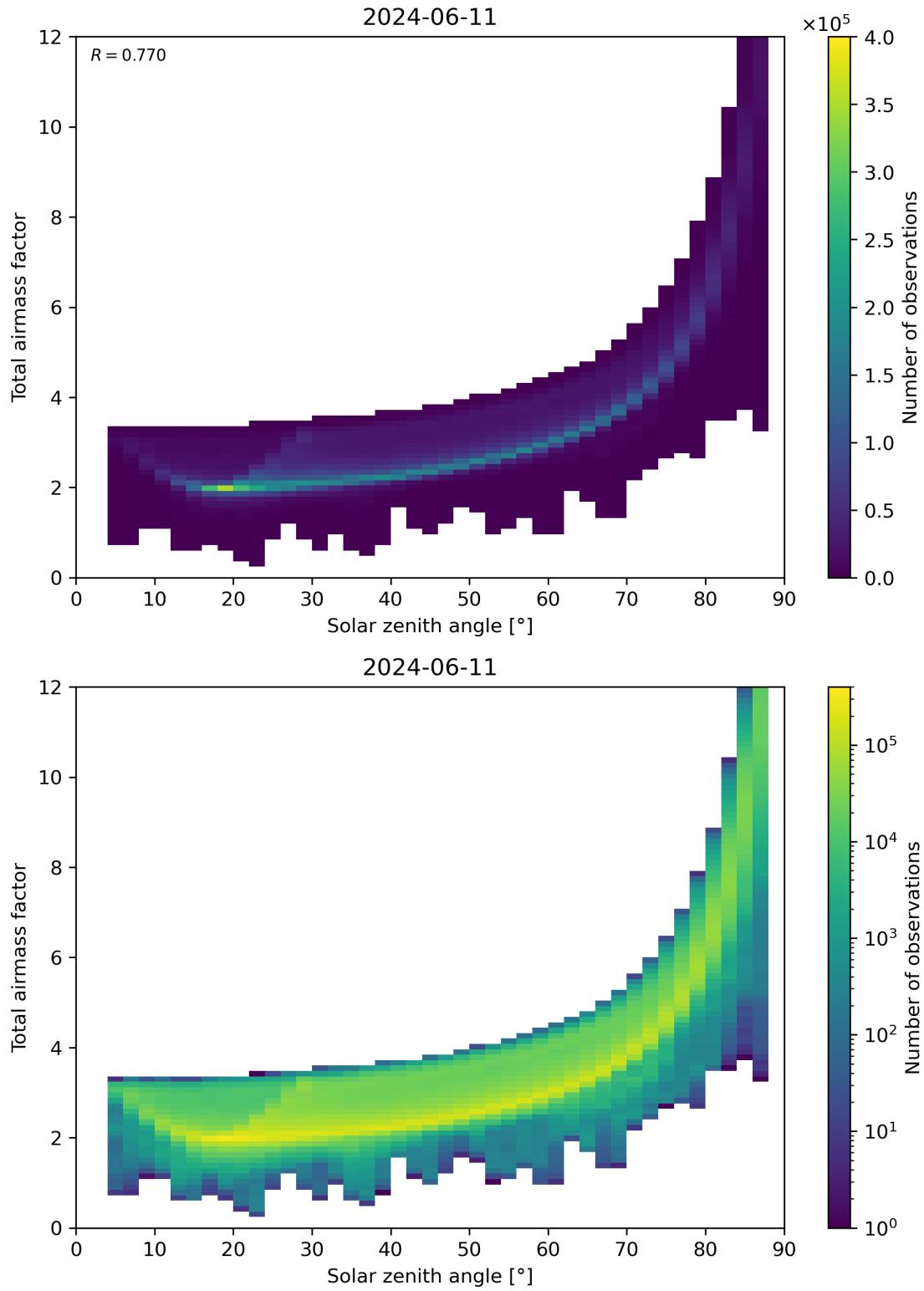
Figure 146: Scatter density plot of “Solar zenith angle” against “Total air mass factor” for 2024-06-10 to 2024-06-12.
