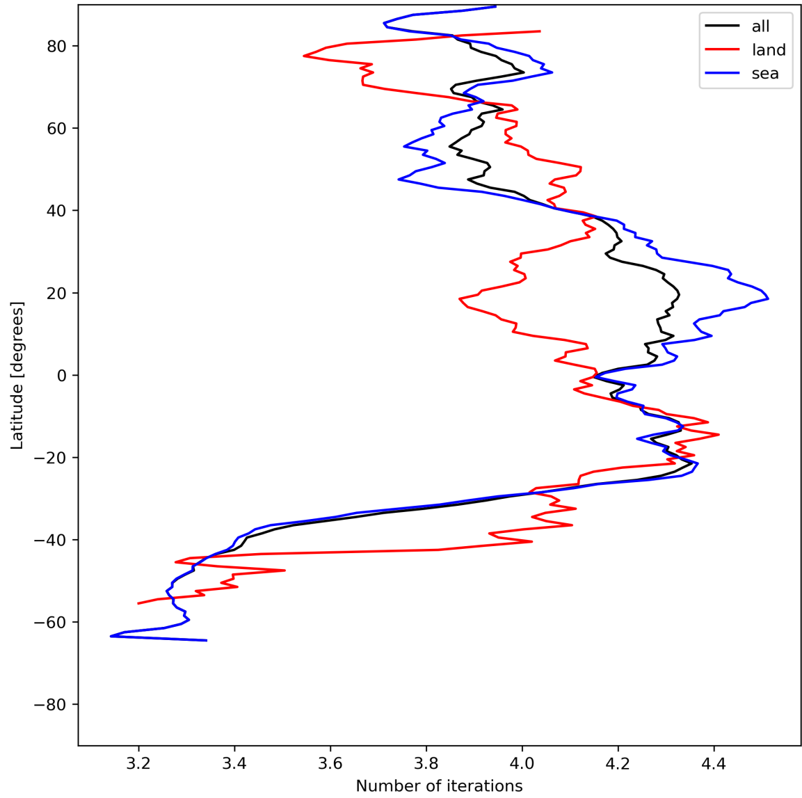
Figure 17: Zonal average of “Number of iterations” for 2024-06-10 to 2024-06-12.
