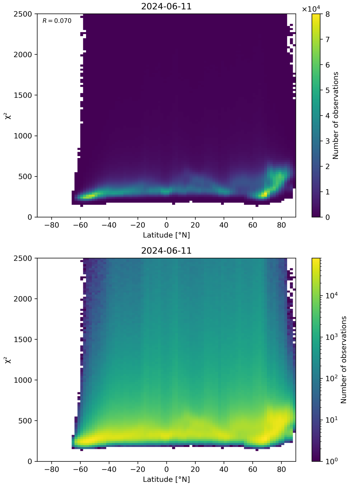
Figure 86: Scatter density plot of “Latitude” against “ \chi^2 ” for 2024-06-10 to 2024-06-12.
