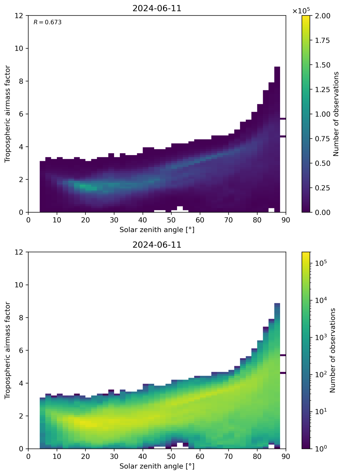
Figure 147: Scatter density plot of “Solar zenith angle” against “Tropospheric airmass factor” for 2024-06-10 to 2024-06-12.
