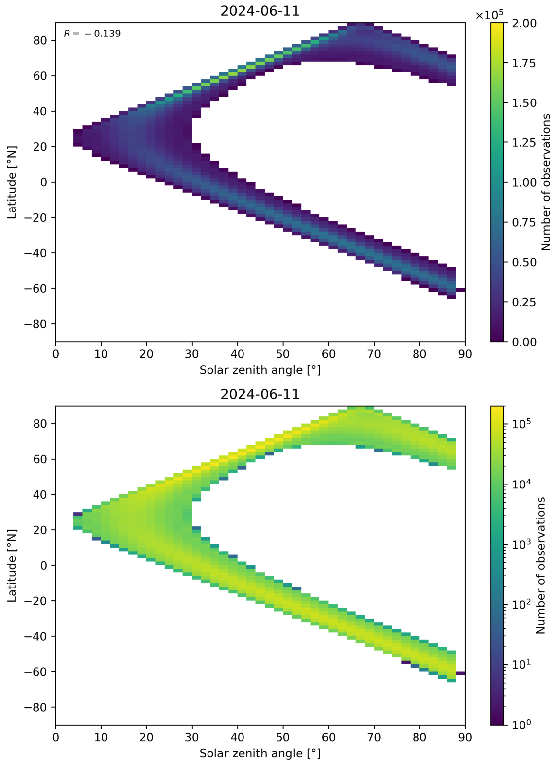
Figure 149: Scatter density plot of “Solar zenith angle” against “Latitude” for 2024-06-10 to 2024-06-12.
