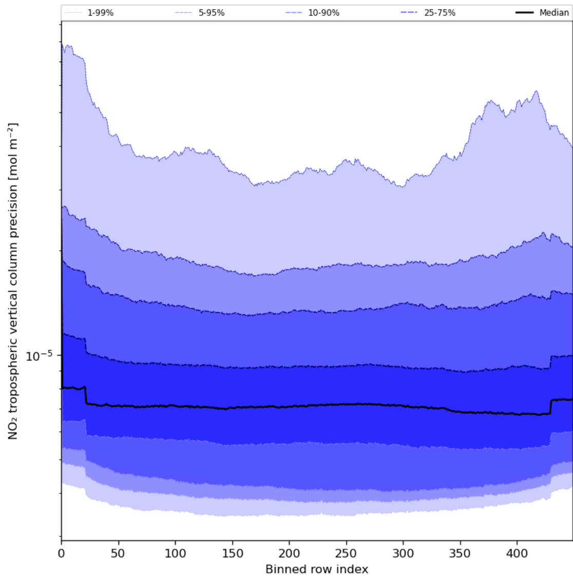
Figure 47: Along track statistics of “NO 2 tropospheric vertical column precision” for 2024-06-10 to 2024-06-12
