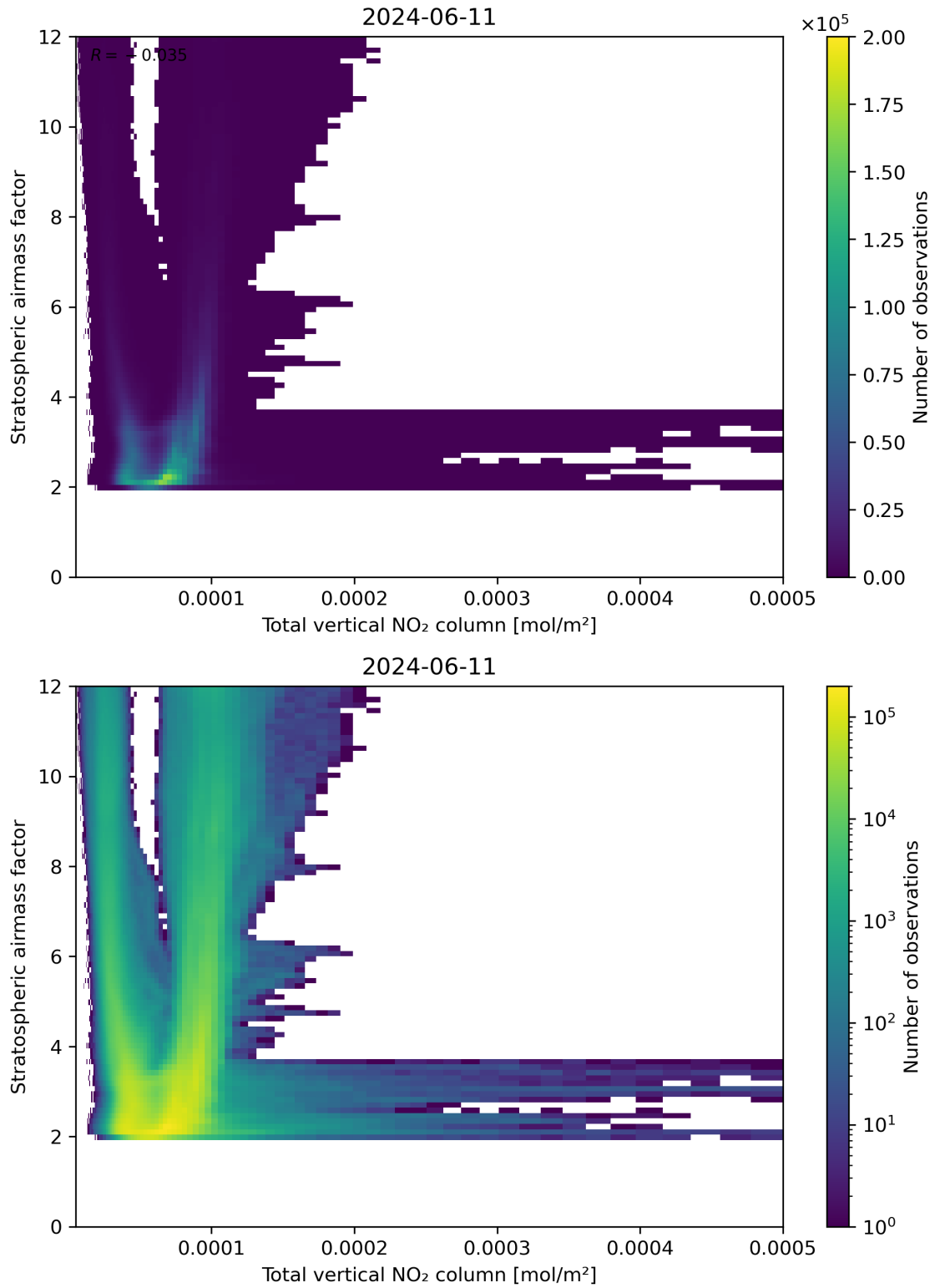
Figure 110: Scatter density plot of “Total vertical NO 2 column” against “Stratospheric airmass factor” for 2024-06-10 to 2024-06-12.
