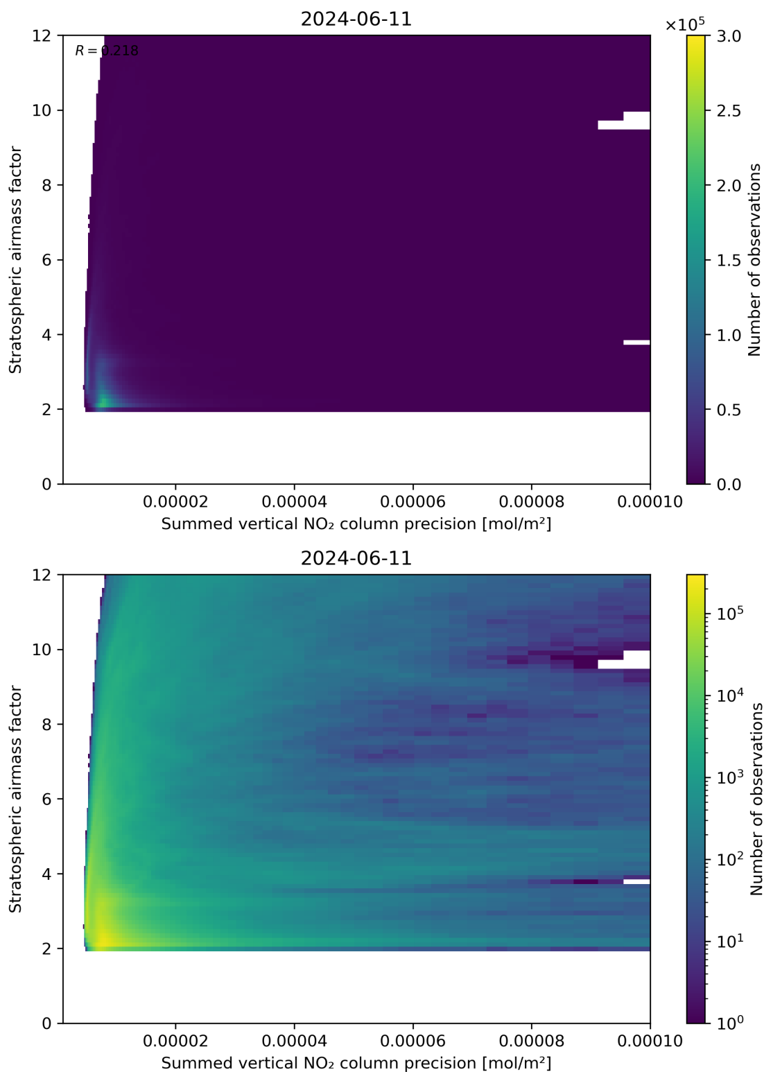
Figure 106: Scatter density plot of “Summed vertical NO 2 column precision” against “Stratospheric airmass factor” for 2024-06-10 to 2024-06-12.
