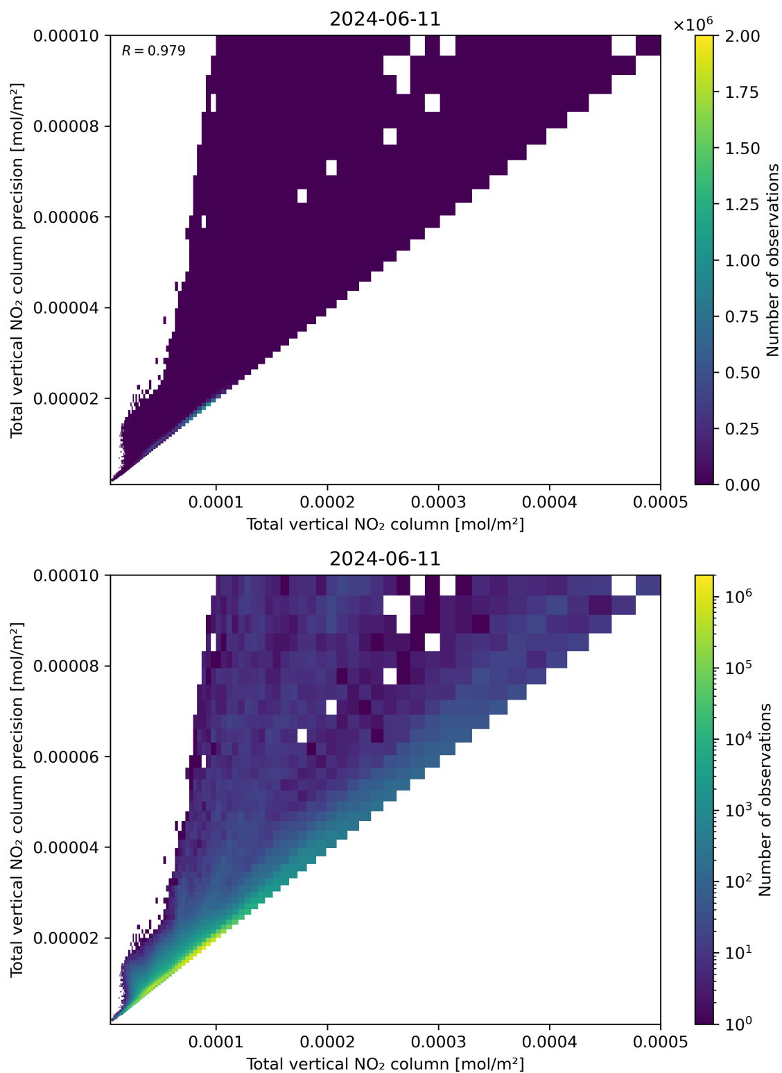
Figure 114: Scatter density plot of “Total vertical NO 2 column” against “Total vertical NO 2 column precision” for 2024-06-10 to 2024-06-12.
