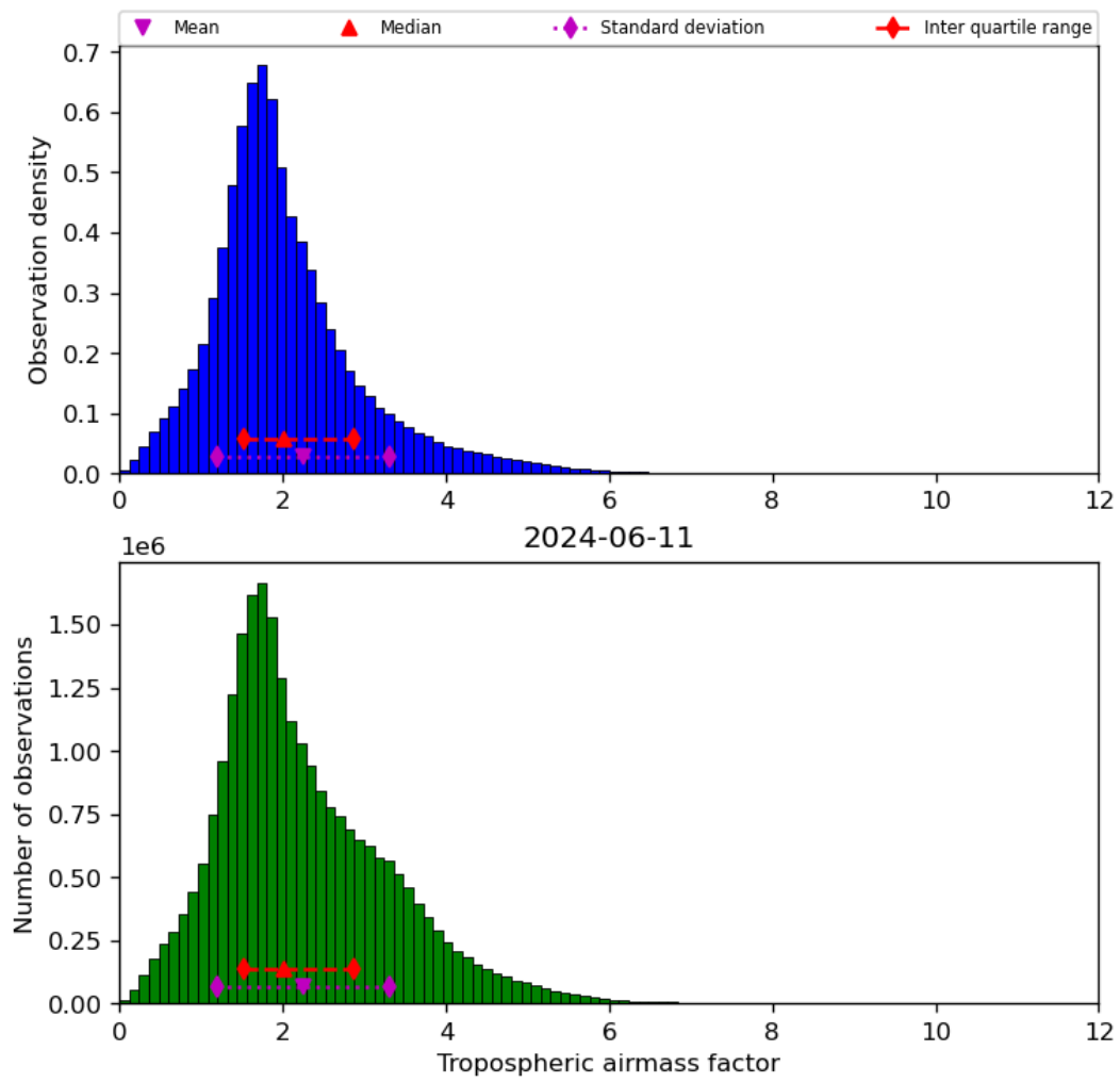
Figure 31: Histogram of “Tropospheric airmass factor” for 2024-06-10 to 2024-06-12
