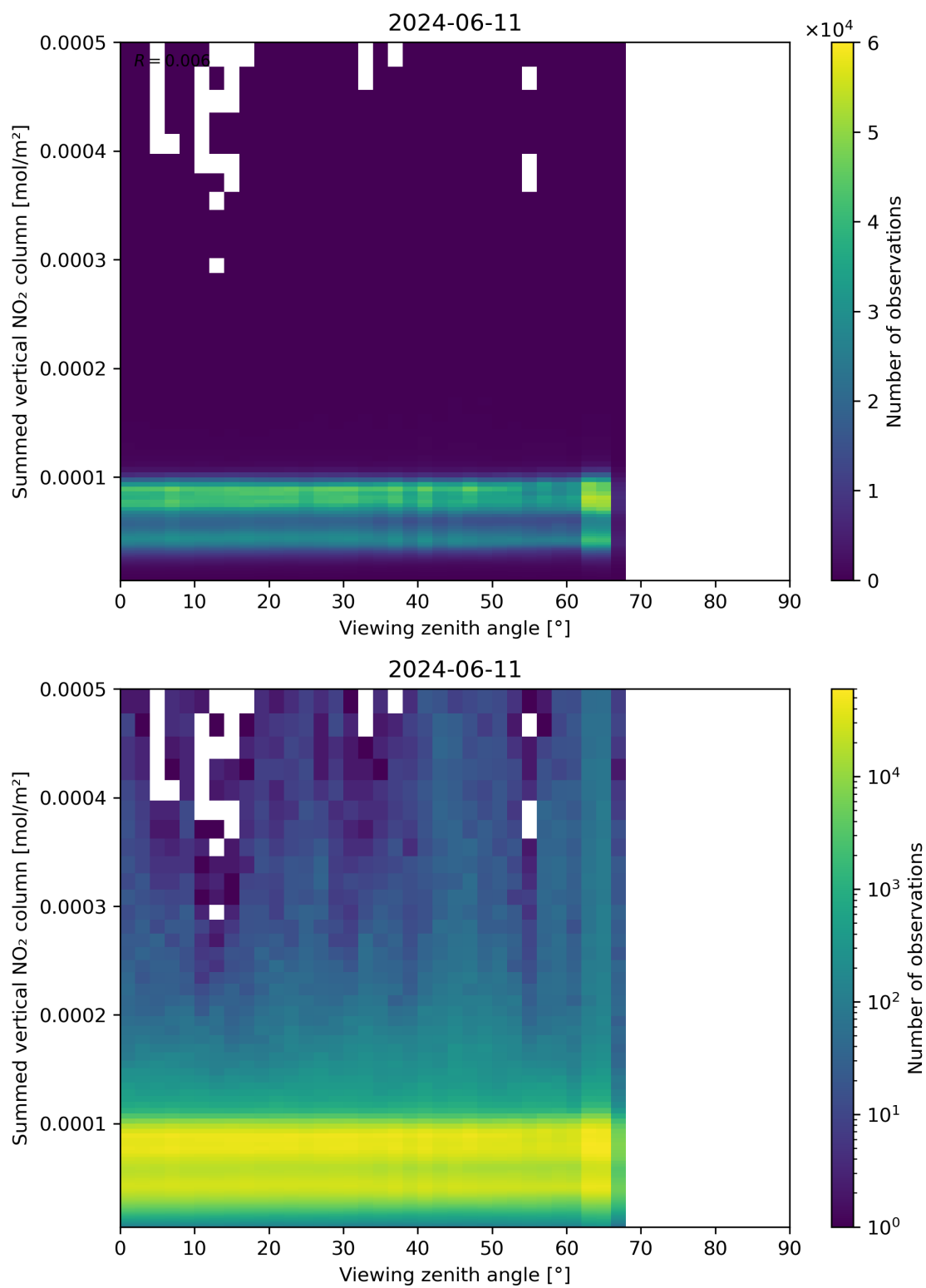
Figure 165: Scatter density plot of “Viewing zenith angle” against “Summed vertical NO 2 column” for 2024-06-10 to 2024-06-12.
