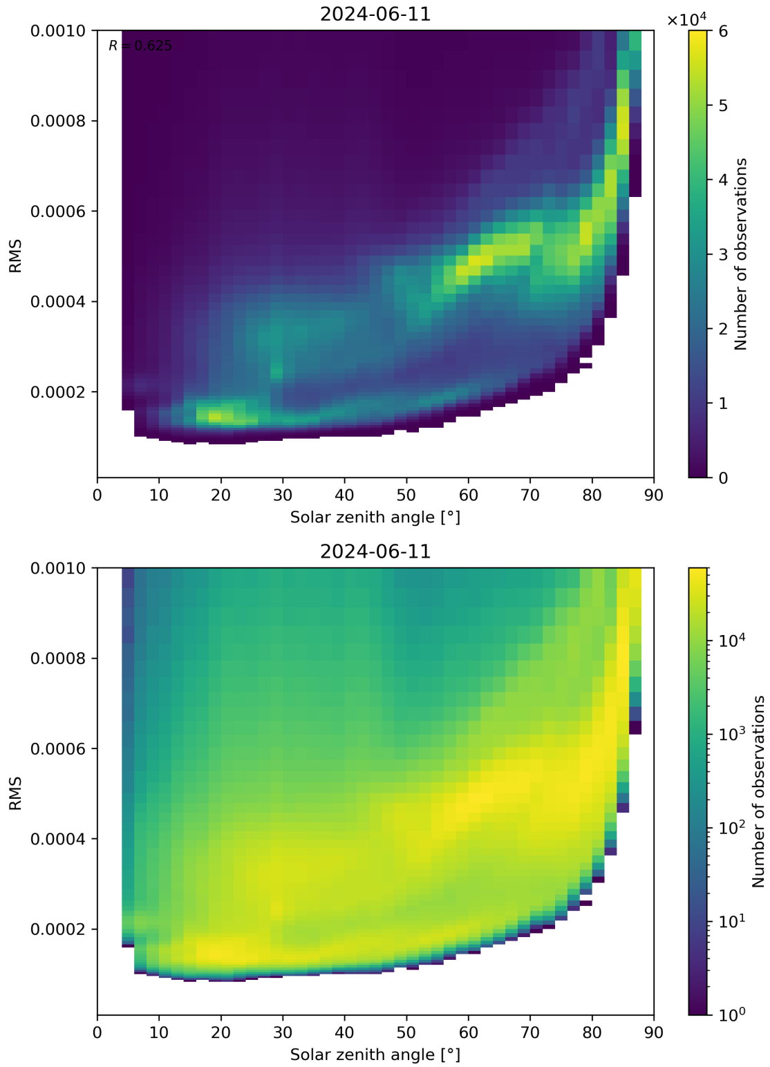
Figure 157: Scatter density plot of “Solar zenith angle” against “RMS” for 2024-06-10 to 2024-06-12.
