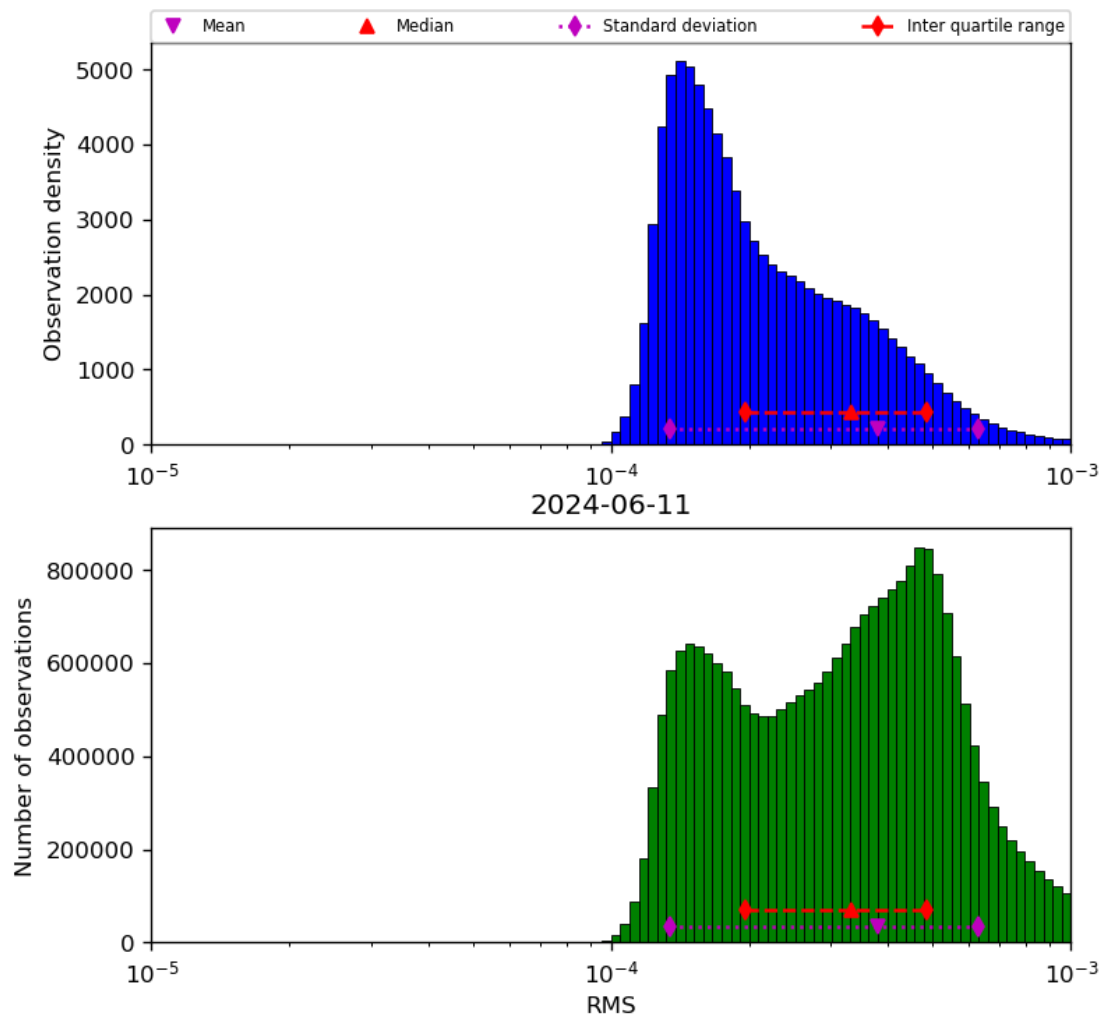
Figure 43: Histogram of “RMS” for 2024-06-10 to 2024-06-12
