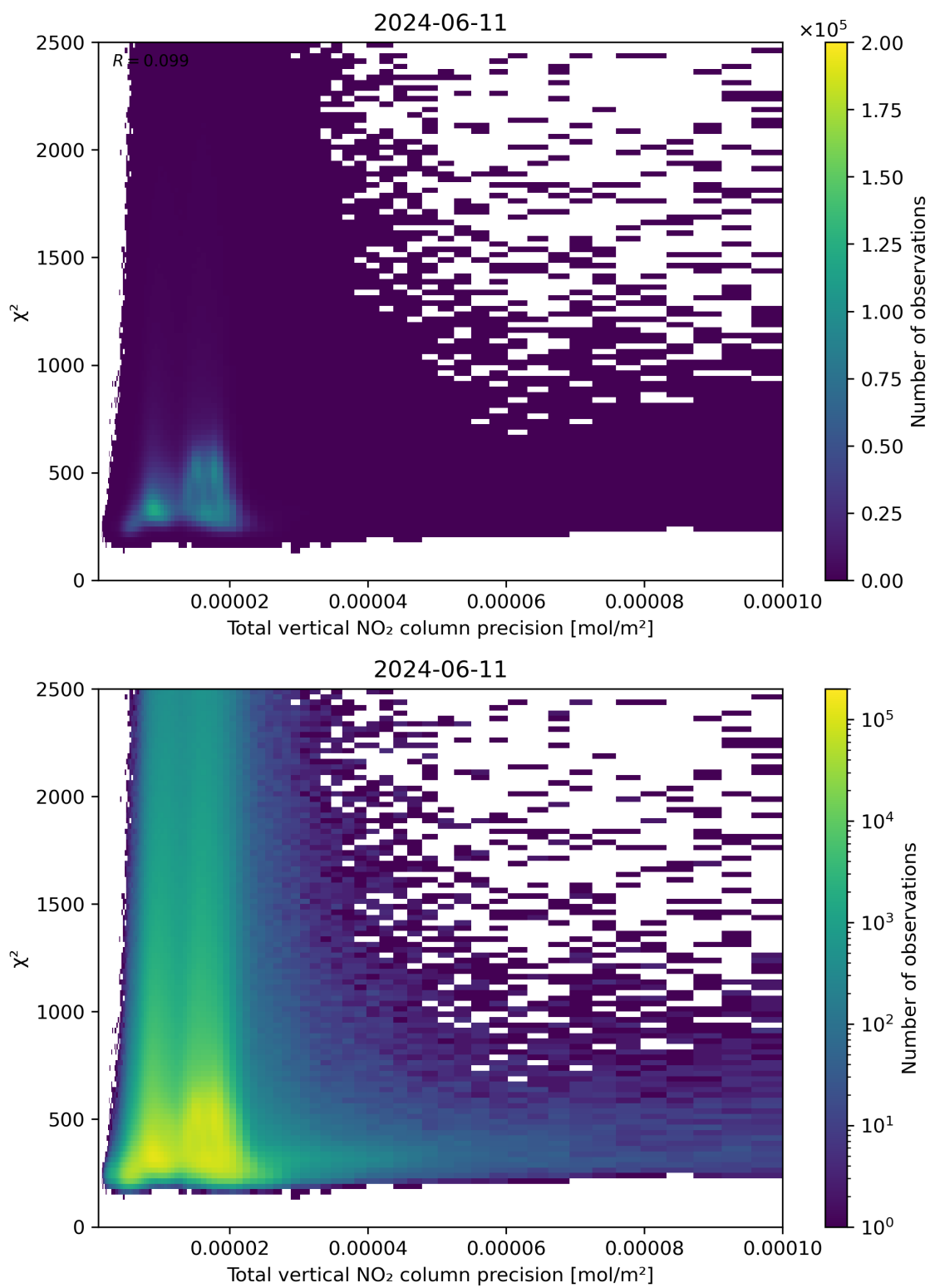
Figure 116: Scatter density plot of “Total vertical NO 2 column precision” against “ \chi^2 ” for 2024-06-10 to 2024-06-12.
