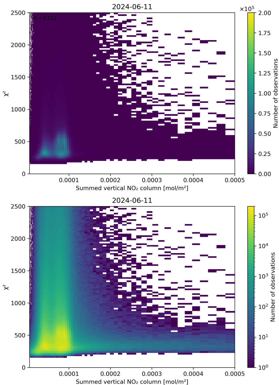
Figure 104: Scatter density plot of “Summed vertical NO 2 column” against “ \chi^2 ” for 2024-06-10 to 2024-06-12.
