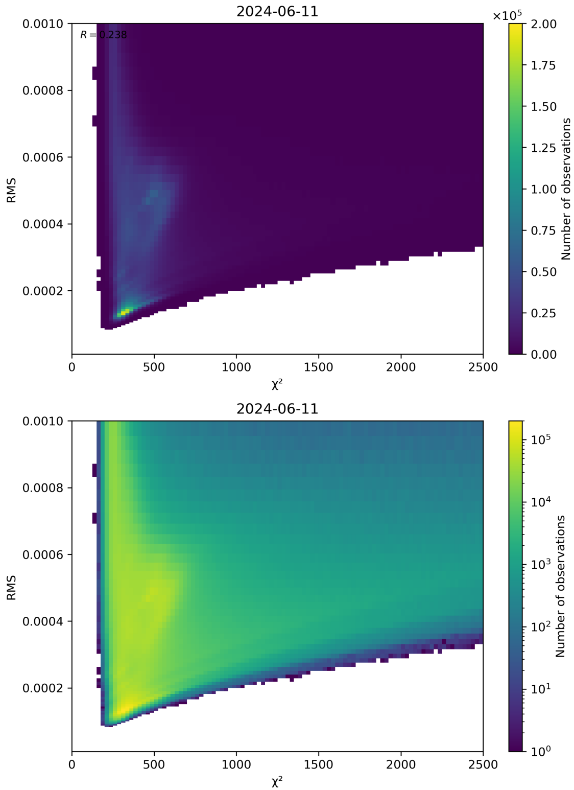
Figure 82: Scatter density plot of “ \chi^2 ” against “RMS” for 2024-06-10 to 2024-06-12.
