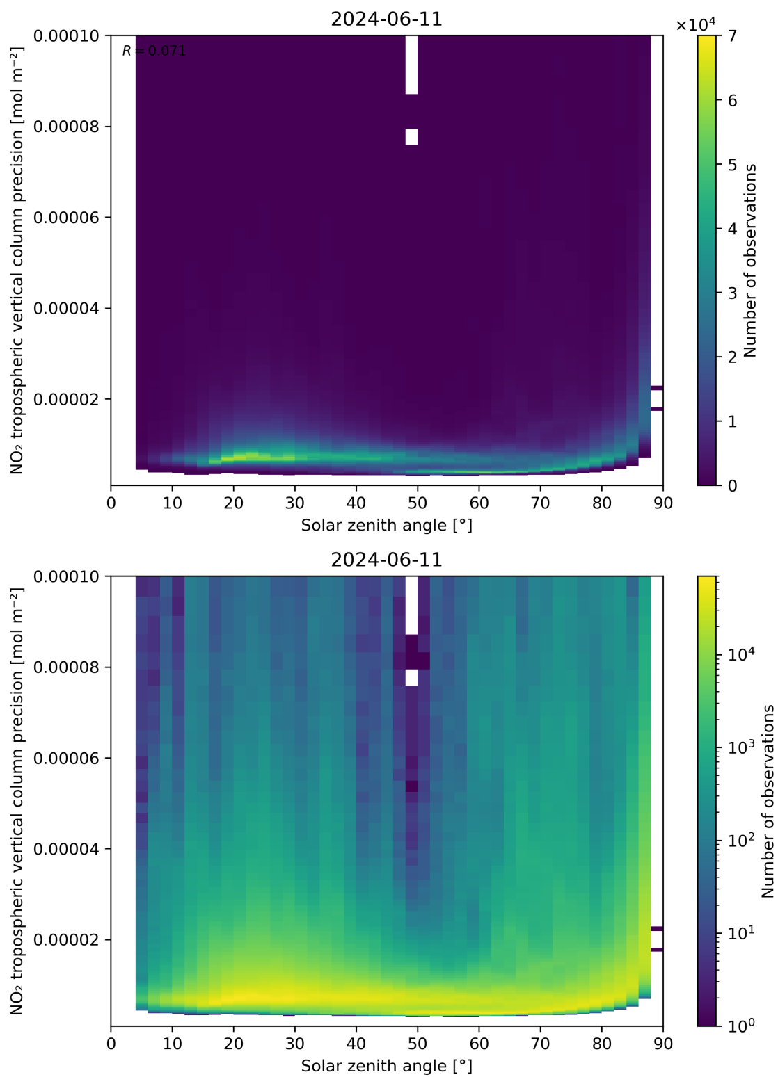
Figure 156: Scatter density plot of “Solar zenith angle” against “NO 2 tropospheric vertical column precision” for 2024-06-10 to 2024-06-12.
