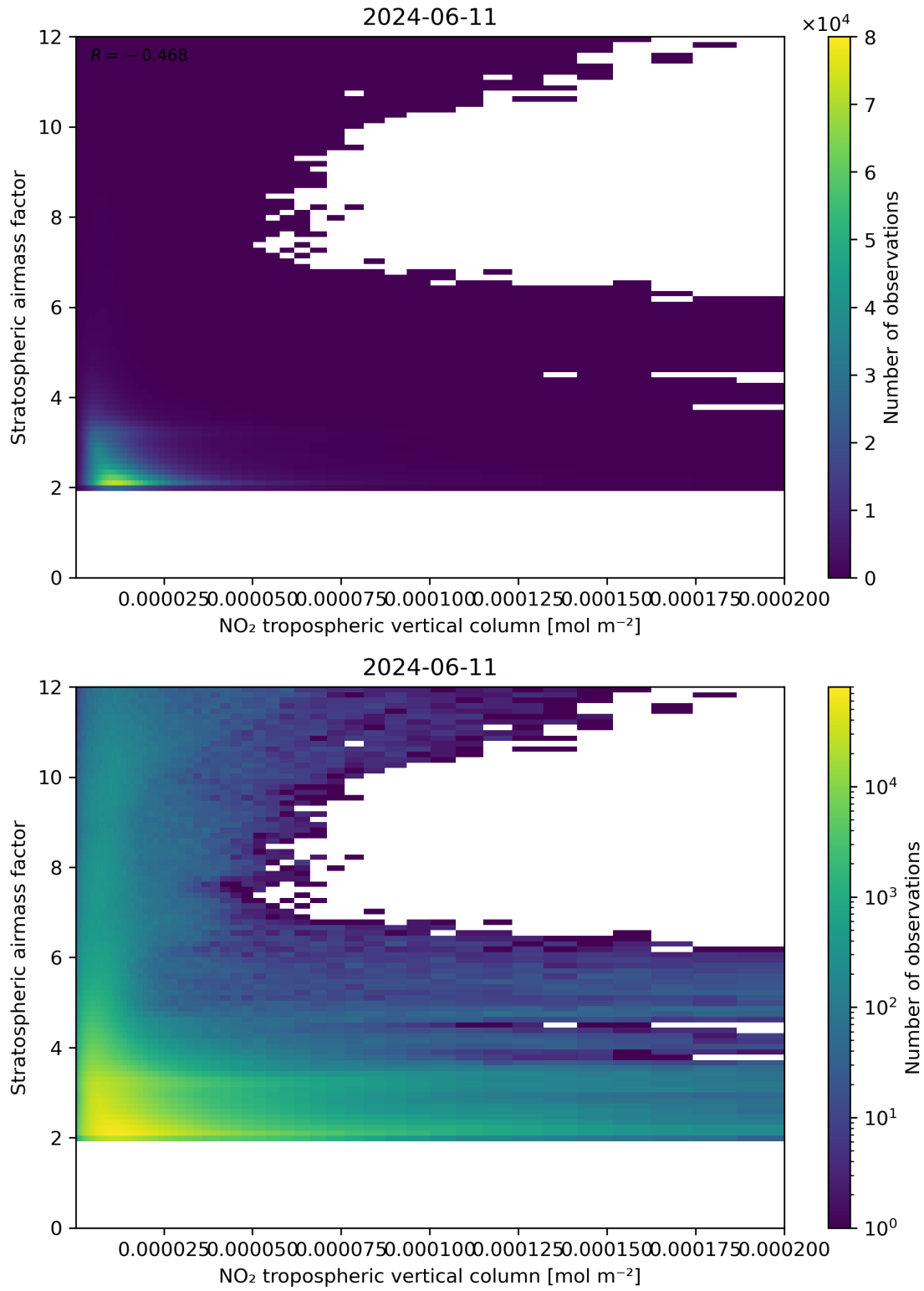
Figure 121: Scatter density plot of “NO 2 tropospheric vertical column” against “Stratospheric air mass factor” for 2024-06-10 to 2024-06-12.
