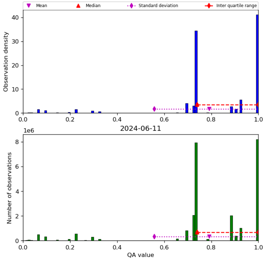
Figure 28: Histogram of “QA value” for 2024-06-10 to 2024-06-12
