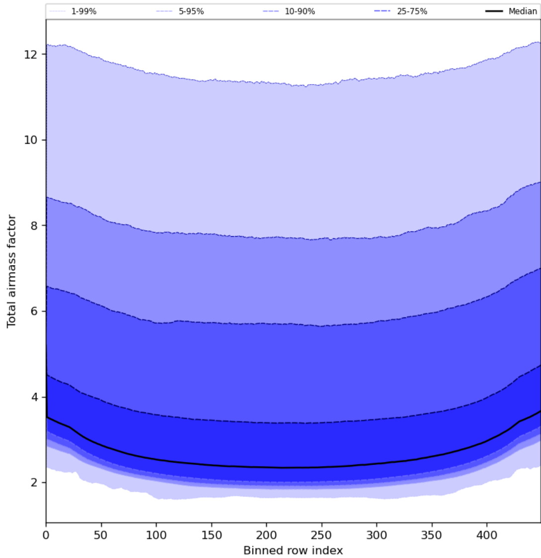
Figure 49: Along track statistics of “Total airmass factor” for 2024-06-10 to 2024-06-12
