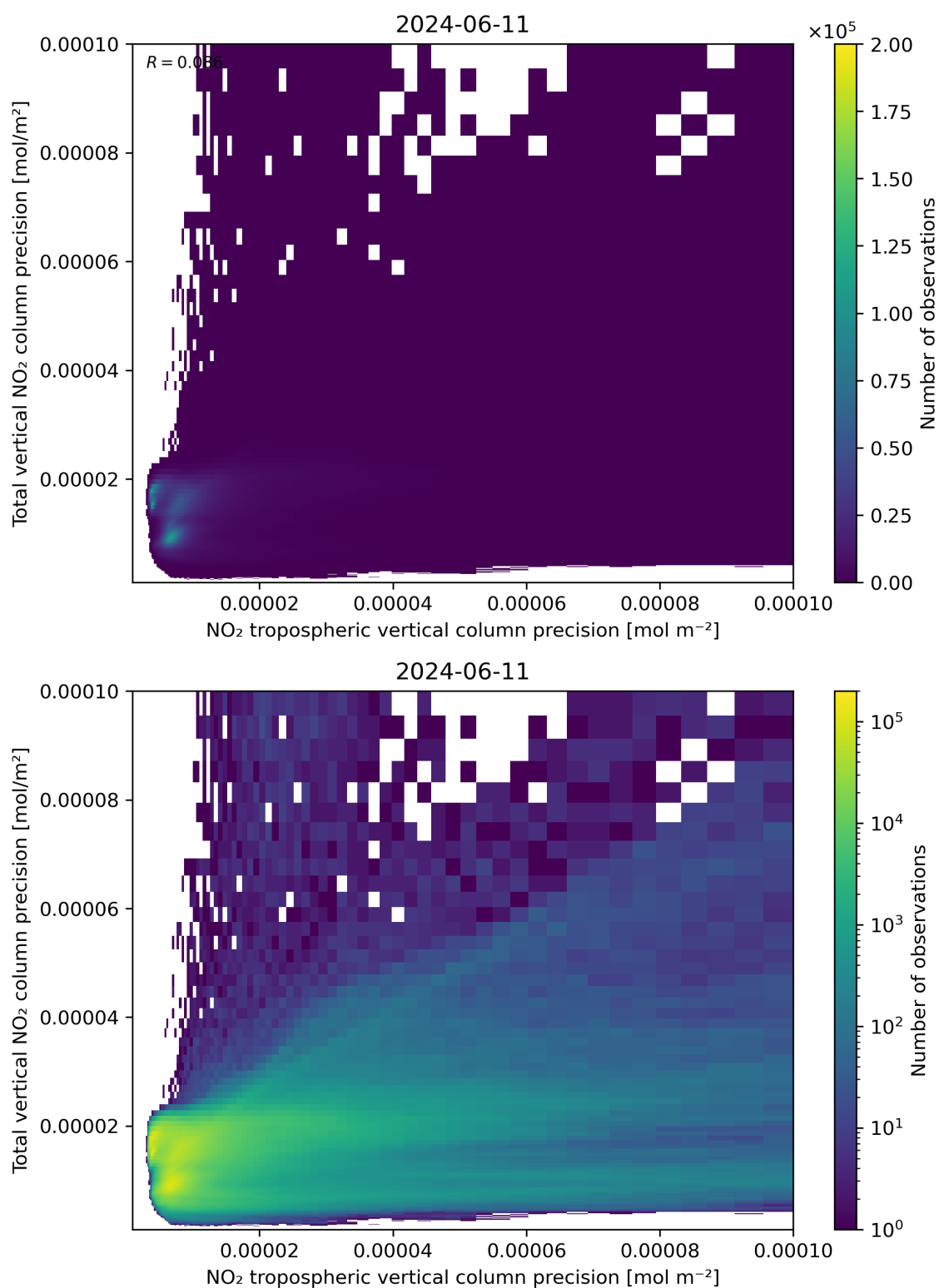
Figure 139: Scatter density plot of “NO 2 tropospheric vertical column precision” against “Total vertical NO 2 column precision” for 2024-06-10 to 2024-06-12.
