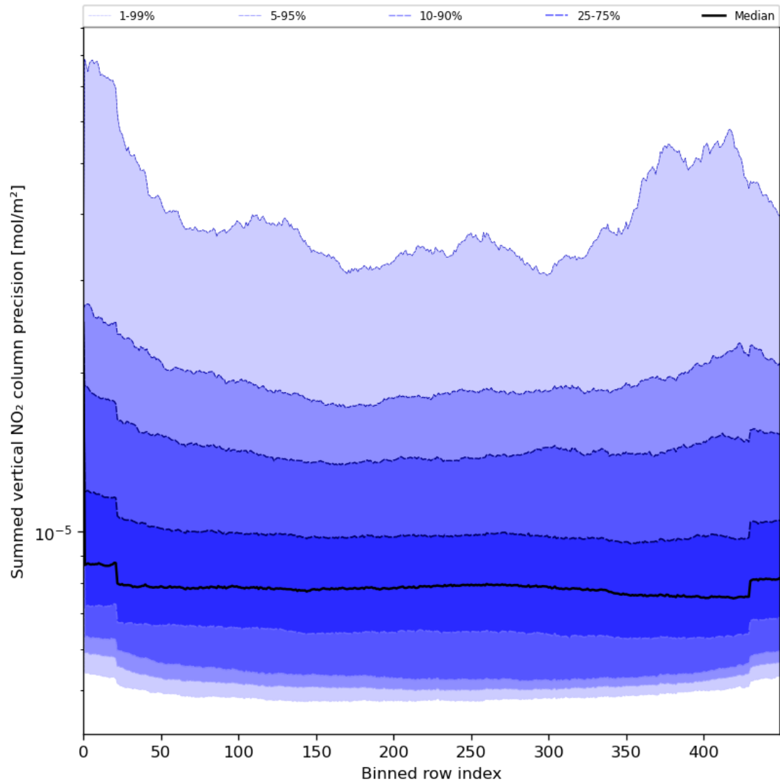
Figure 58: Along track statistics of “Summed vertical NO 2 column precision” for 2024-06-10 to 2024-06-12
