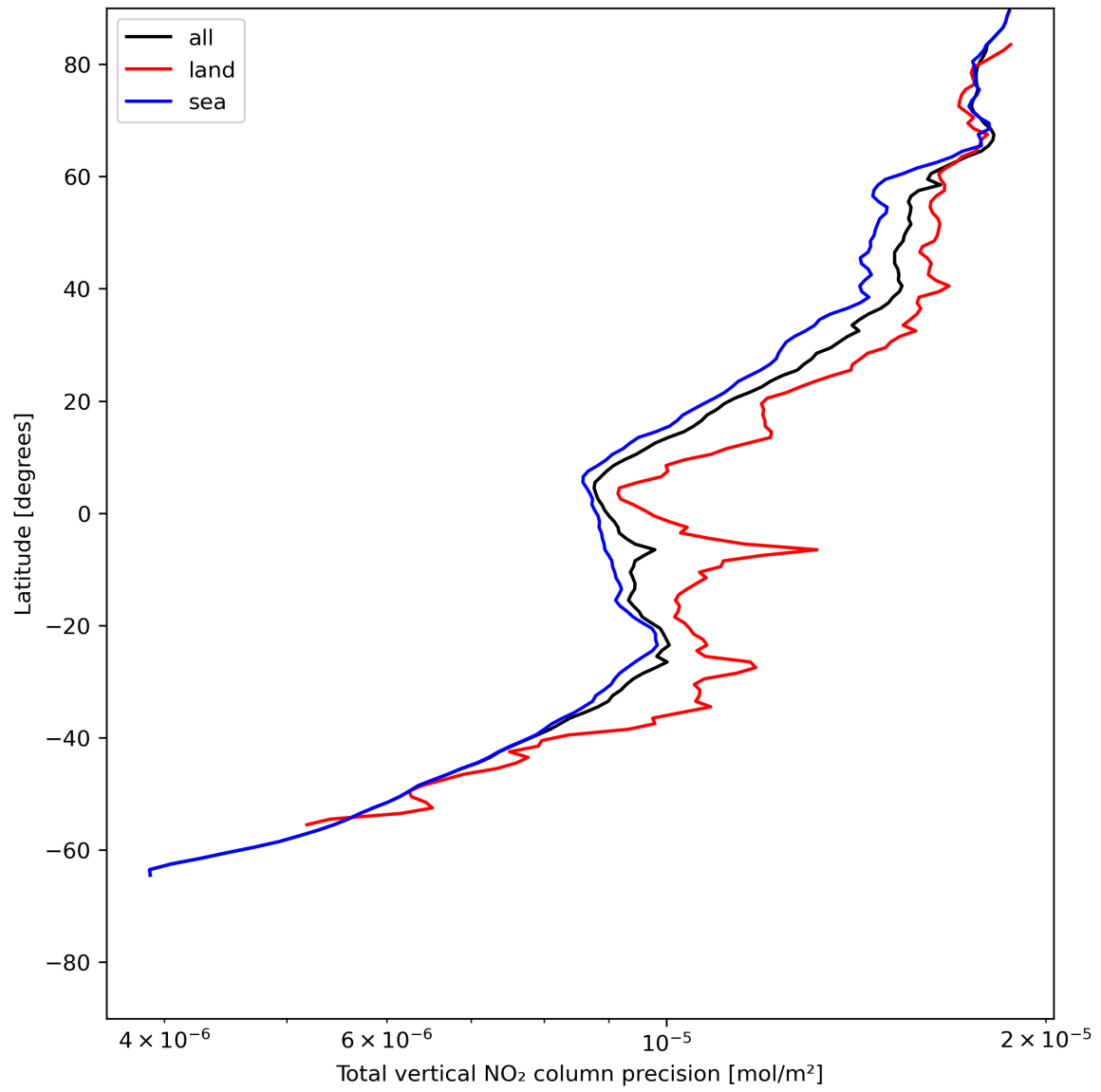
Figure 22: Zonal average of “Total vertical NO 2 column precision” for 2024-06-10 to 2024-06-12.
