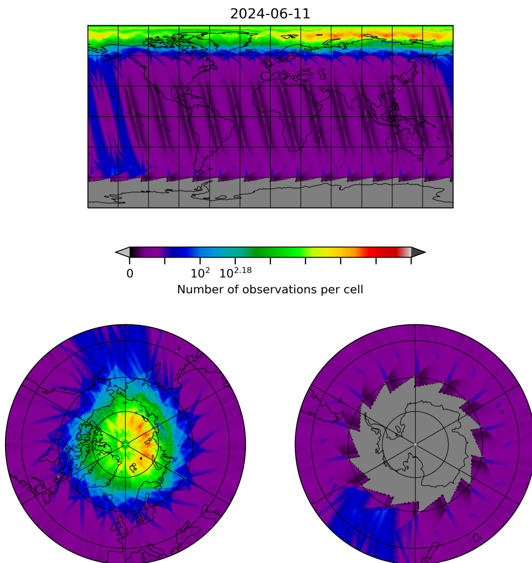
Figure 10: Map of the number of observations for 2024-06-10 to 2024-06-12
