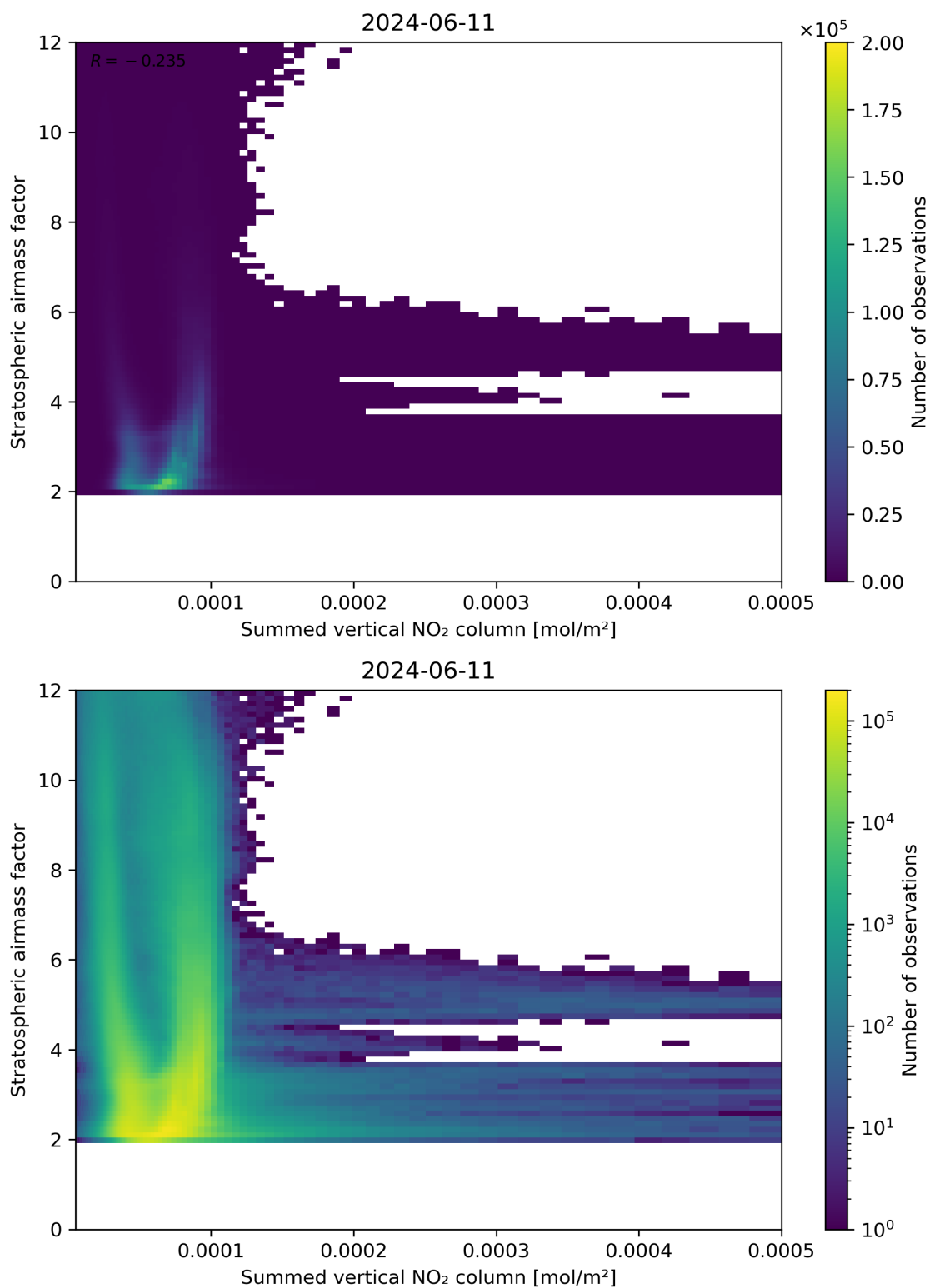
Figure 103: Scatter density plot of “Summed vertical NO 2 column” against “Stratospheric air mass factor” for 2024-06-10 to 2024-06-12.
