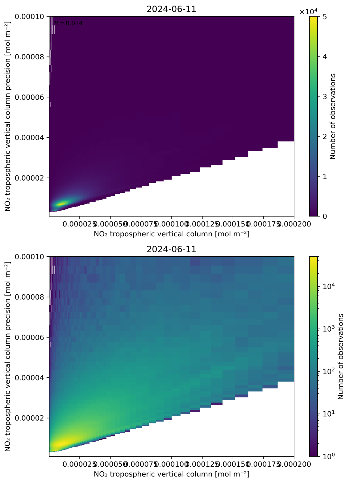
Figure 130: Scatter density plot of “NO 2 tropospheric vertical column” against “NO 2 tropospheric vertical column precision” for 2024-06-10 to 2024-06-12.
