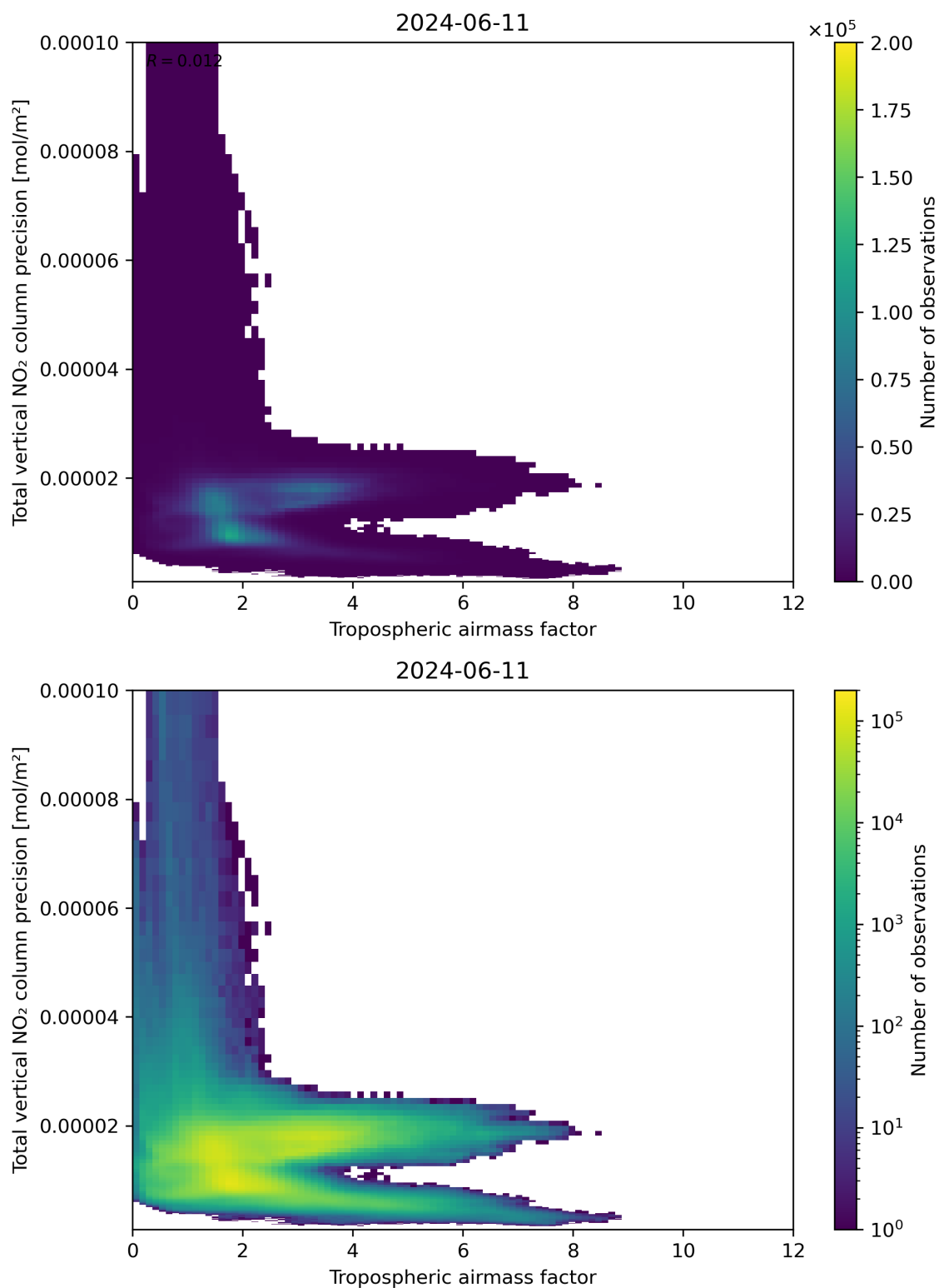
Figure 78: Scatter density plot of “Tropospheric air mass factor” against “Total vertical NO 2 column precision” for 2024-06-10 to 2024-06-12.
