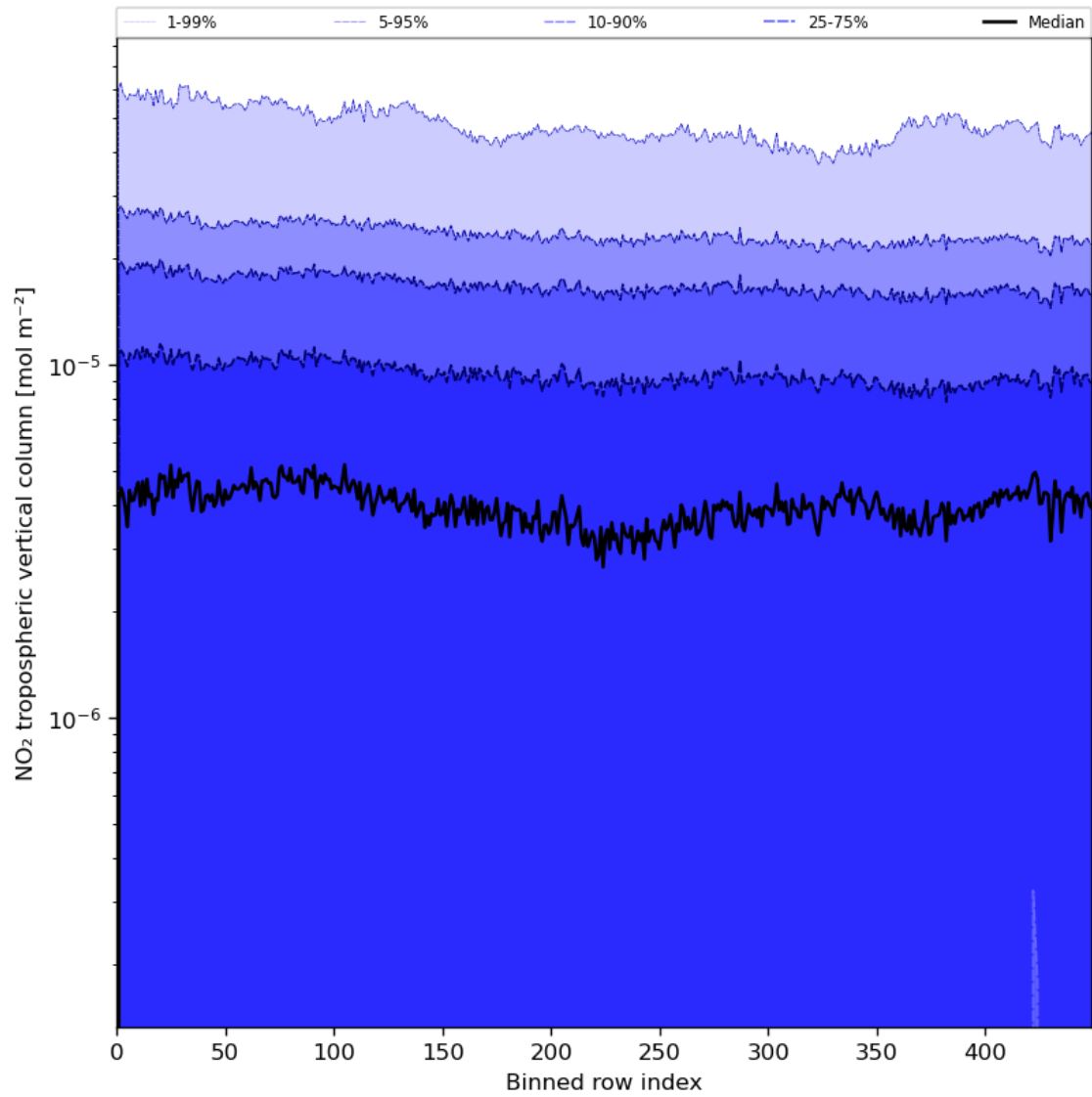
Figure 46: Along track statistics of “NO 2 tropospheric vertical column” for 2024-06-10 to 2024-06-12
