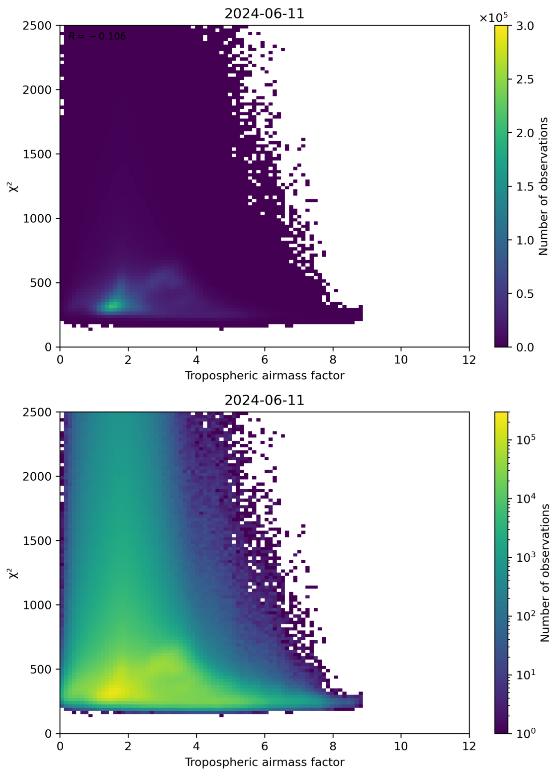
Figure 73: Scatter density plot of “Tropospheric airmass factor” against “ \chi^2 ” for 2024-06-10 to 2024-06-12.
