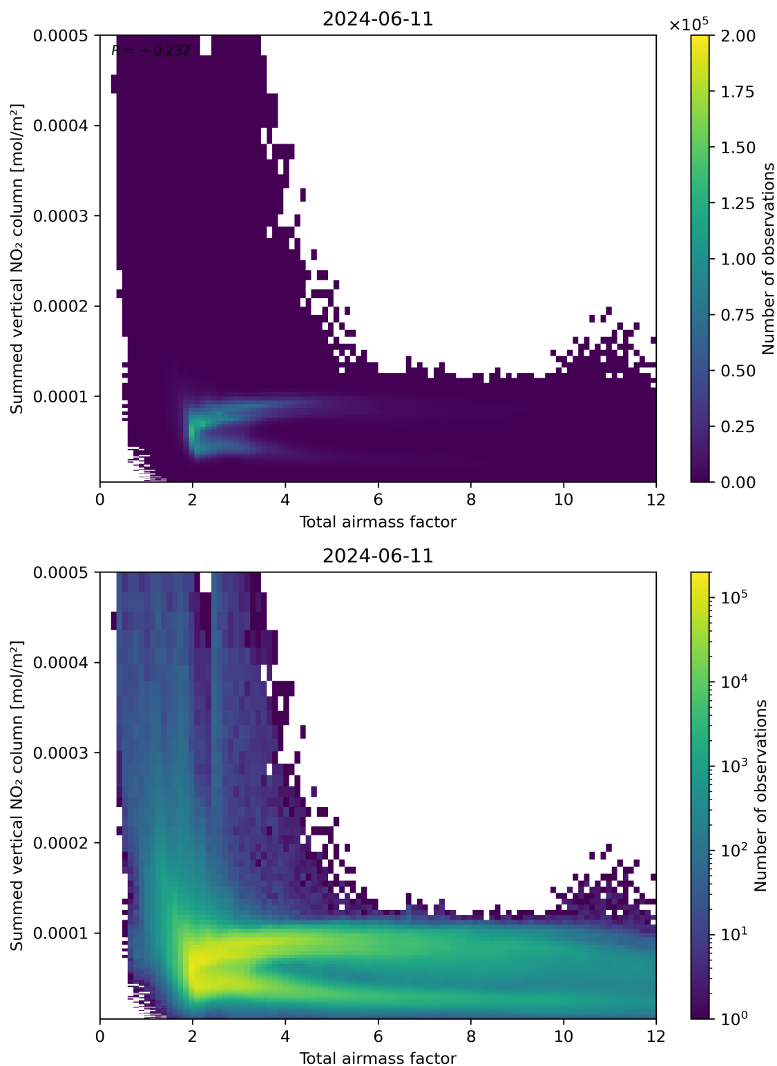
Figure 65: Scatter density plot of “Total airmass factor” against “Summed vertical NO 2 column” for 2024-06-10 to 2024-06-12.
