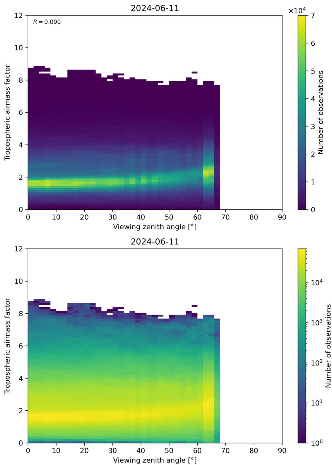
Figure 161: Scatter density plot of “Viewing zenith angle” against “Tropospheric airmass factor” for 2024-06-10 to 2024-06-12.
