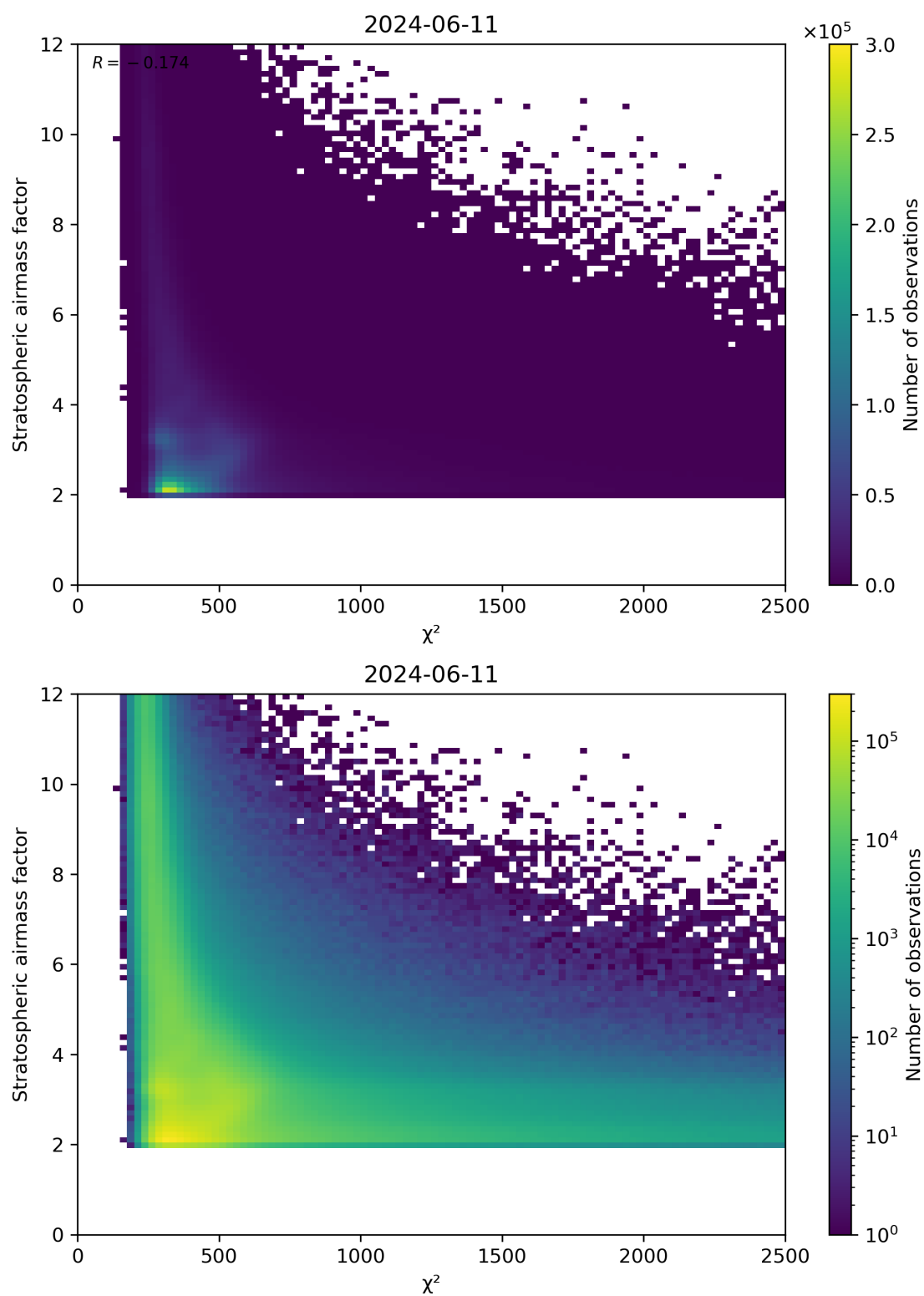
Figure 81: Scatter density plot of “ \chi^2 ” against “Stratospheric airmass factor” for 2024-06-10 to 2024-06-12.
