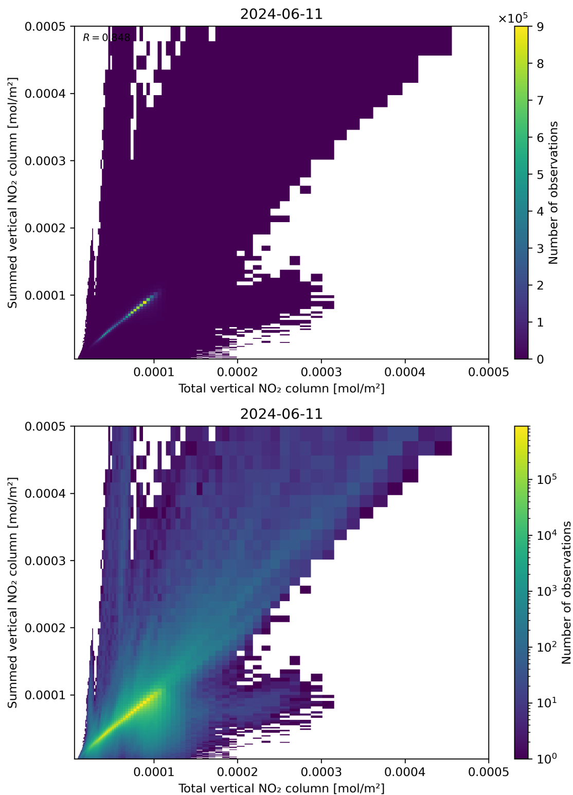
Figure 112: Scatter density plot of “Total vertical NO 2 column” against “Summed vertical NO 2 column” for 2024-06-10 to 2024-06-12.
