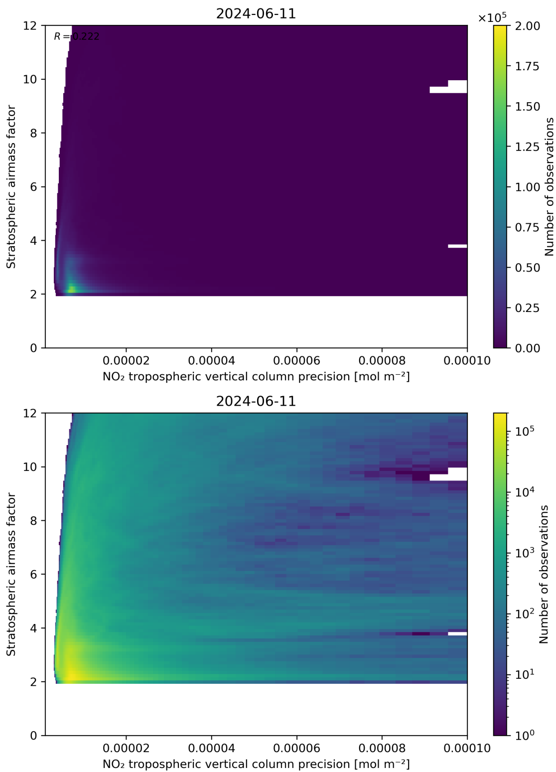
Figure 131: Scatter density plot of “NO 2 tropospheric vertical column precision” against “Stratospheric airmass factor” for 2024-06-10 to 2024-06-12.
