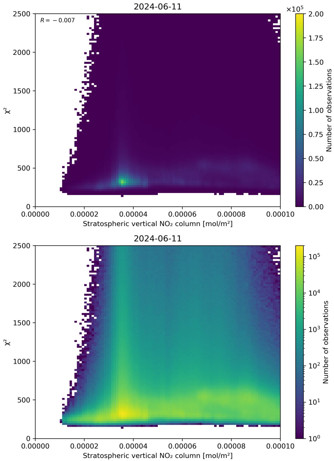
Figure 97: Scatter density plot of “Stratospheric vertical NO 2 column” against “ \chi^2 ” for 2024-06-10 to 2024-06-12.
