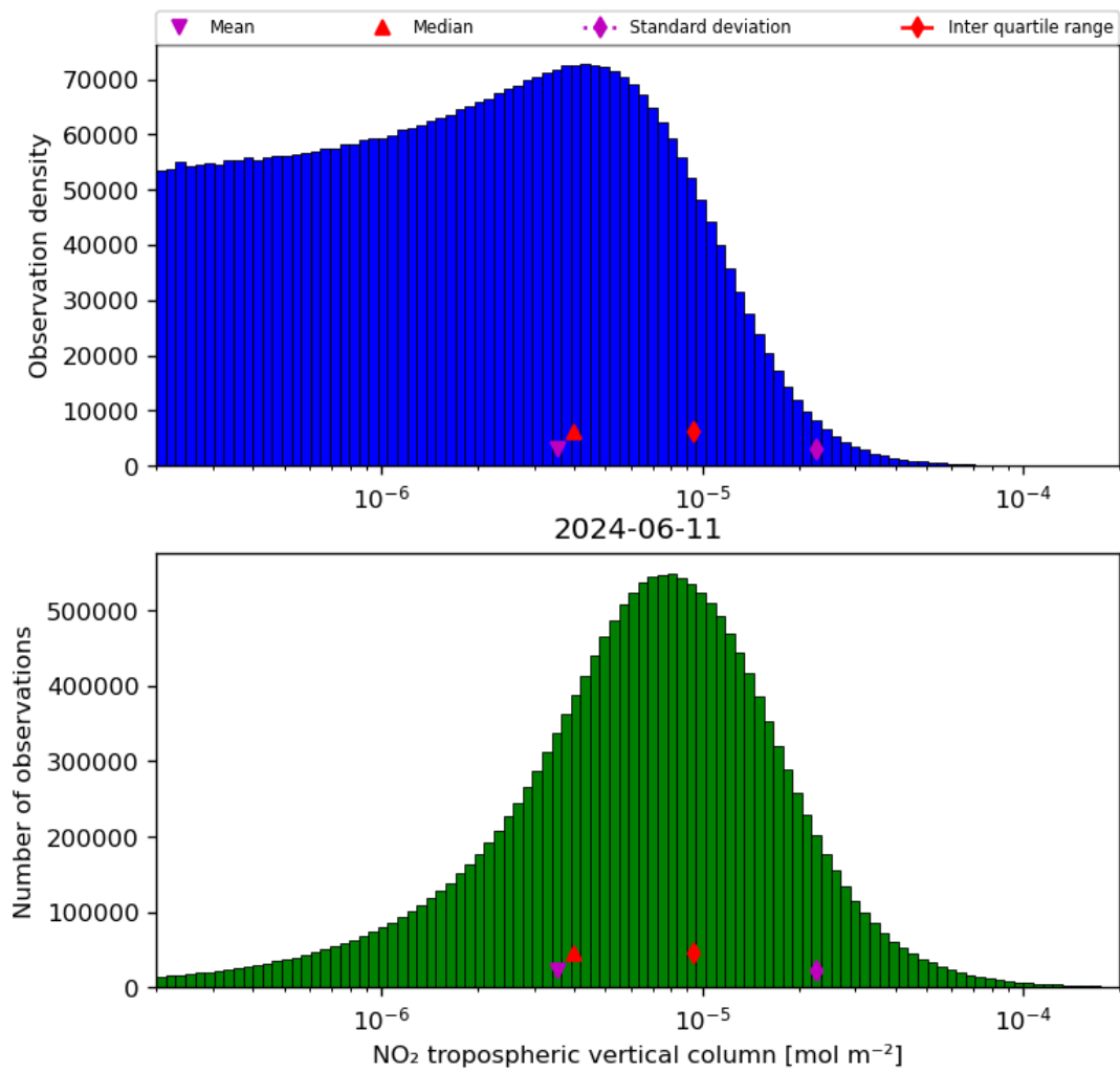
Figure 29: Histogram of “NO 2 tropospheric vertical column” for 2024-06-10 to 2024-06-12
