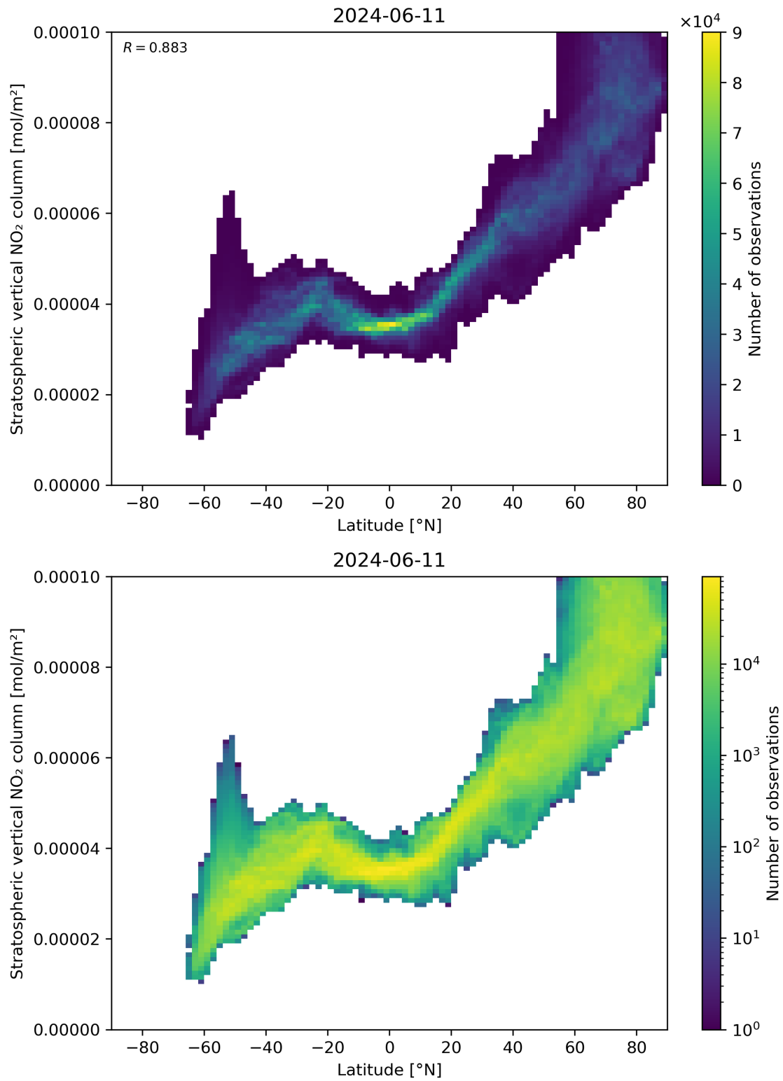
Figure 87: Scatter density plot of “Latitude” against “Stratospheric vertical NO 2 column” for 2024-06-10 to 2024-06-12.
