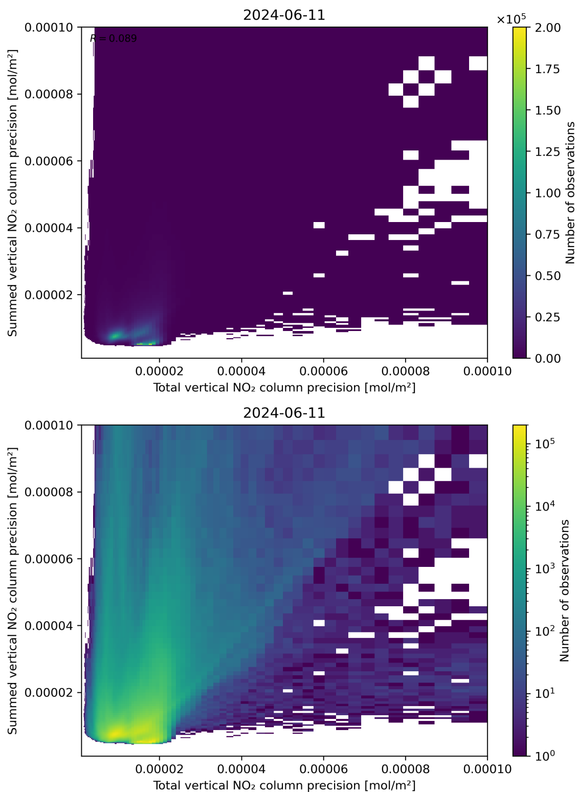
Figure 118: Scatter density plot of “Total vertical NO 2 column precision” against “Summed vertical NO 2 column precision” for 2024-06-10 to 2024-06-12.
