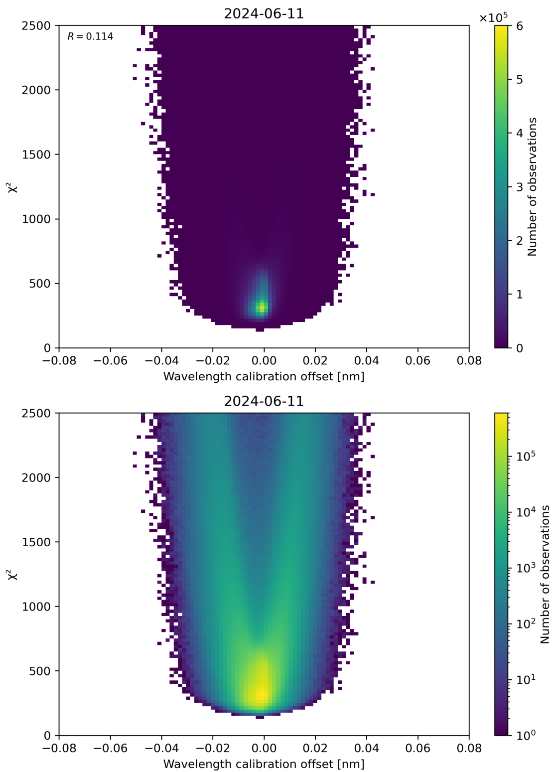
Figure 175: Scatter density plot of “Wavelength calibration offset” against “ \chi^2 ” for 2024-06-10 to 2024-06-12.
