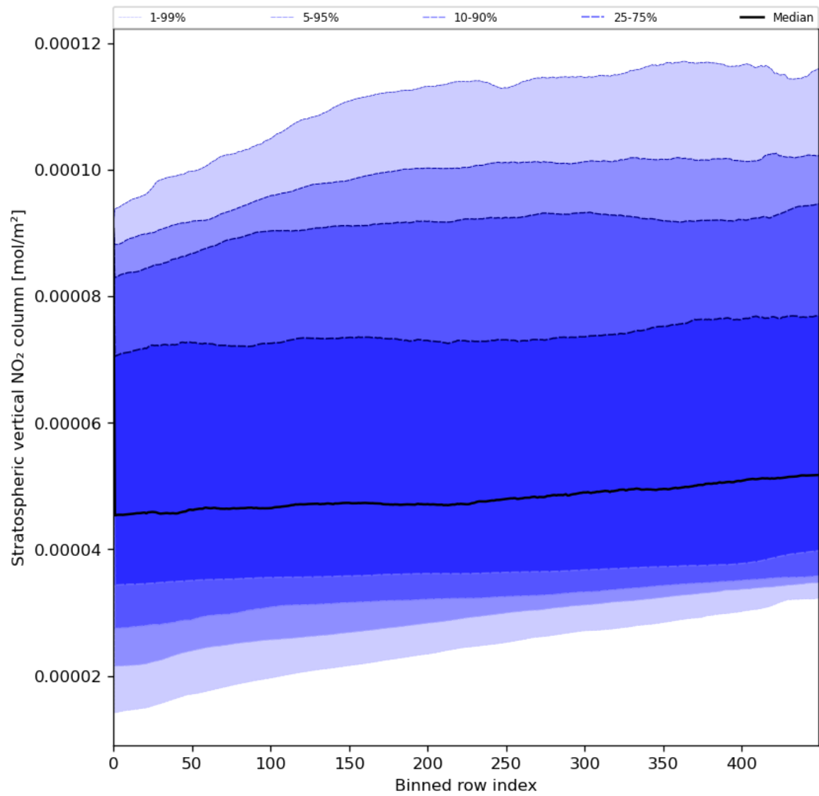
Figure 53: Along track statistics of “Stratospheric vertical NO 2 column” for 2024-06-10 to 2024-06-12
