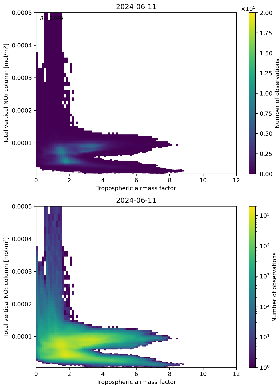
Figure 77: Scatter density plot of “Tropospheric airmass factor” against “Total vertical NO 2 column” for 2024-06-10 to 2024-06-12.
