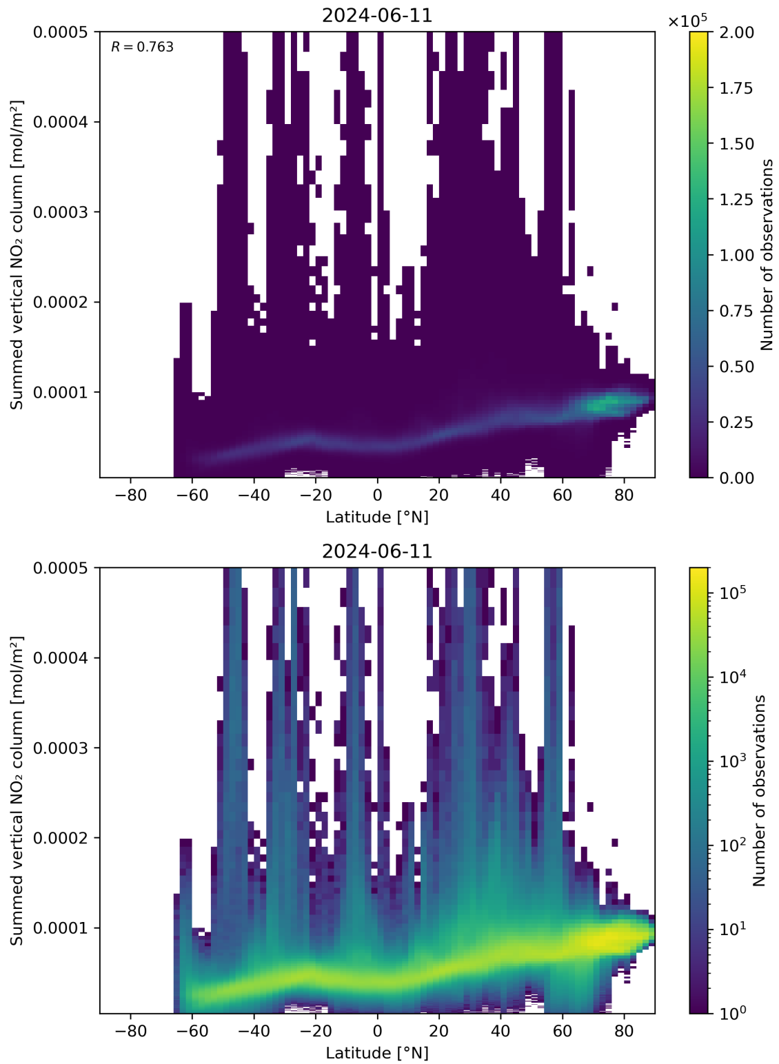
Figure 88: Scatter density plot of “Latitude” against “Summed vertical NO 2 column” for 2024-06-10 to 2024-06-12.
