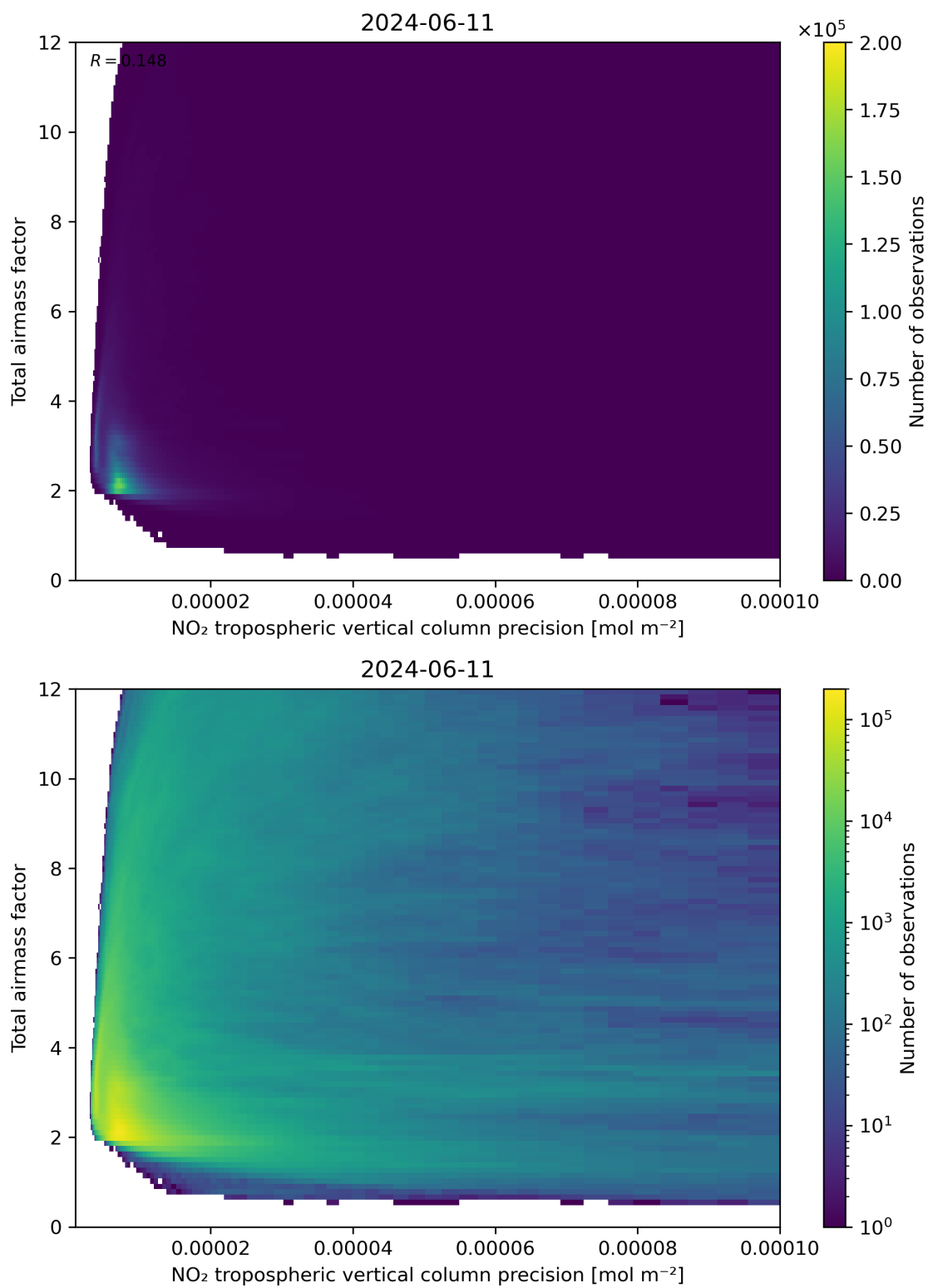
Figure 132: Scatter density plot of “NO 2 tropospheric vertical column precision” against “Total air mass factor” for 2024-06-10 to 2024-06-12.
