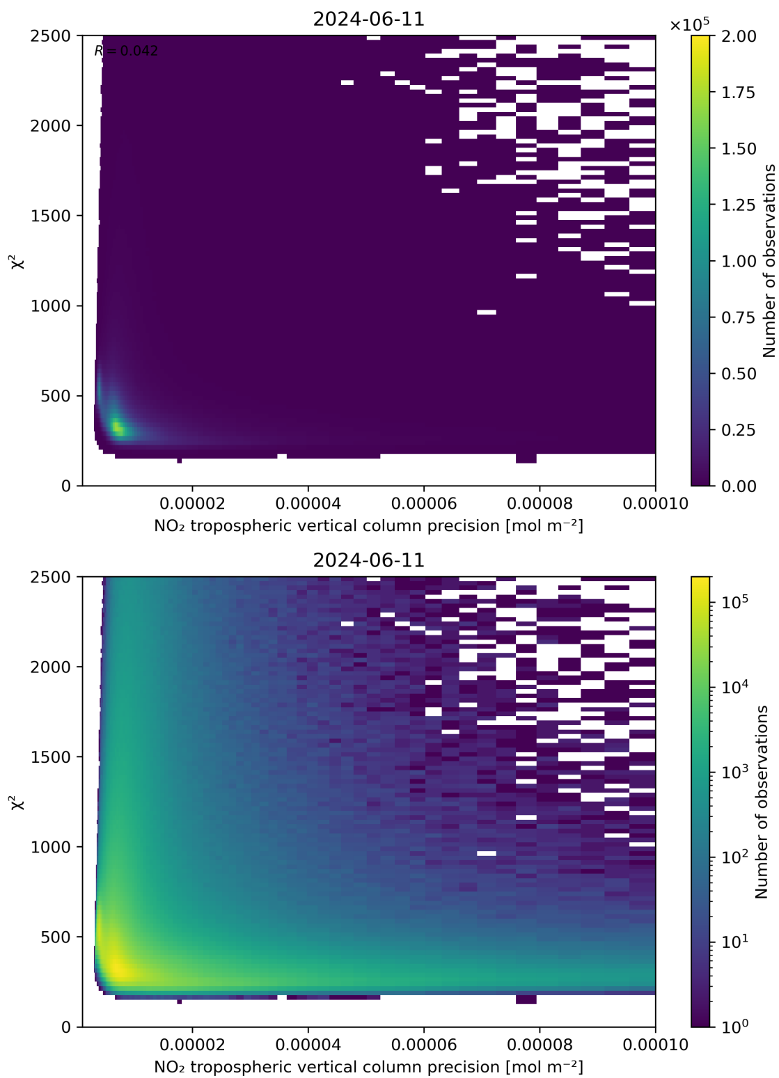
Figure 134: Scatter density plot of “NO 2 tropospheric vertical column precision” against “ \chi^2 ” for 2024-06-10 to 2024-06-12.
