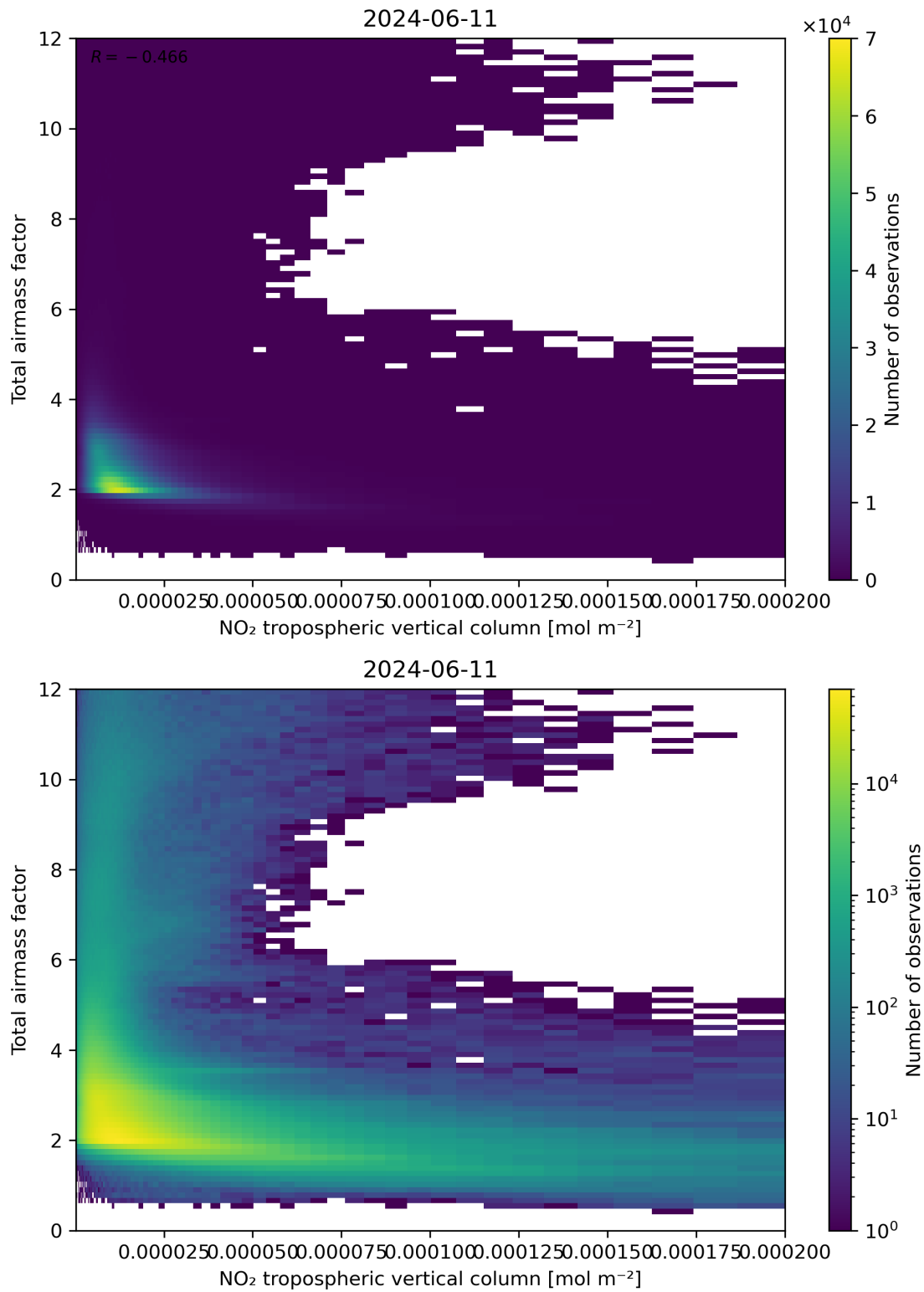
Figure 122: Scatter density plot of “NO 2 tropospheric vertical column” against “Total air mass factor” for 2024-06-10 to 2024-06-12.
