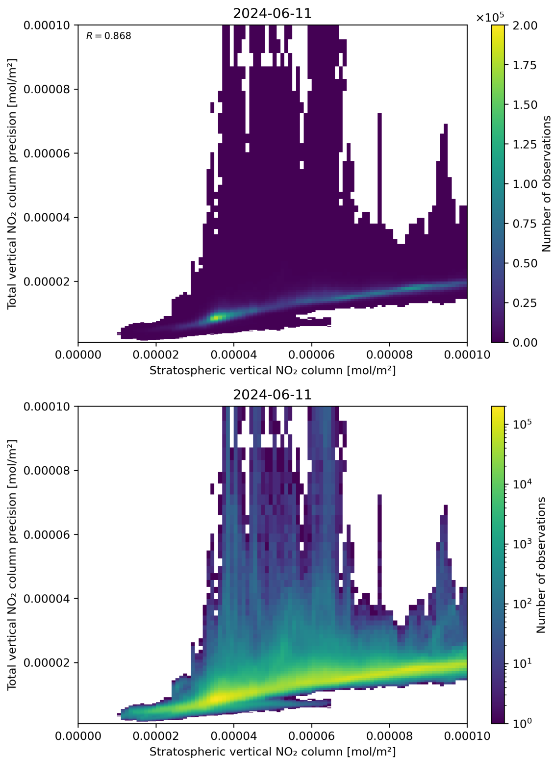
Figure 101: Scatter density plot of “Stratospheric vertical NO 2 column” against “Total vertical NO 2 column precision” for 2024-06-10 to 2024-06-12.
