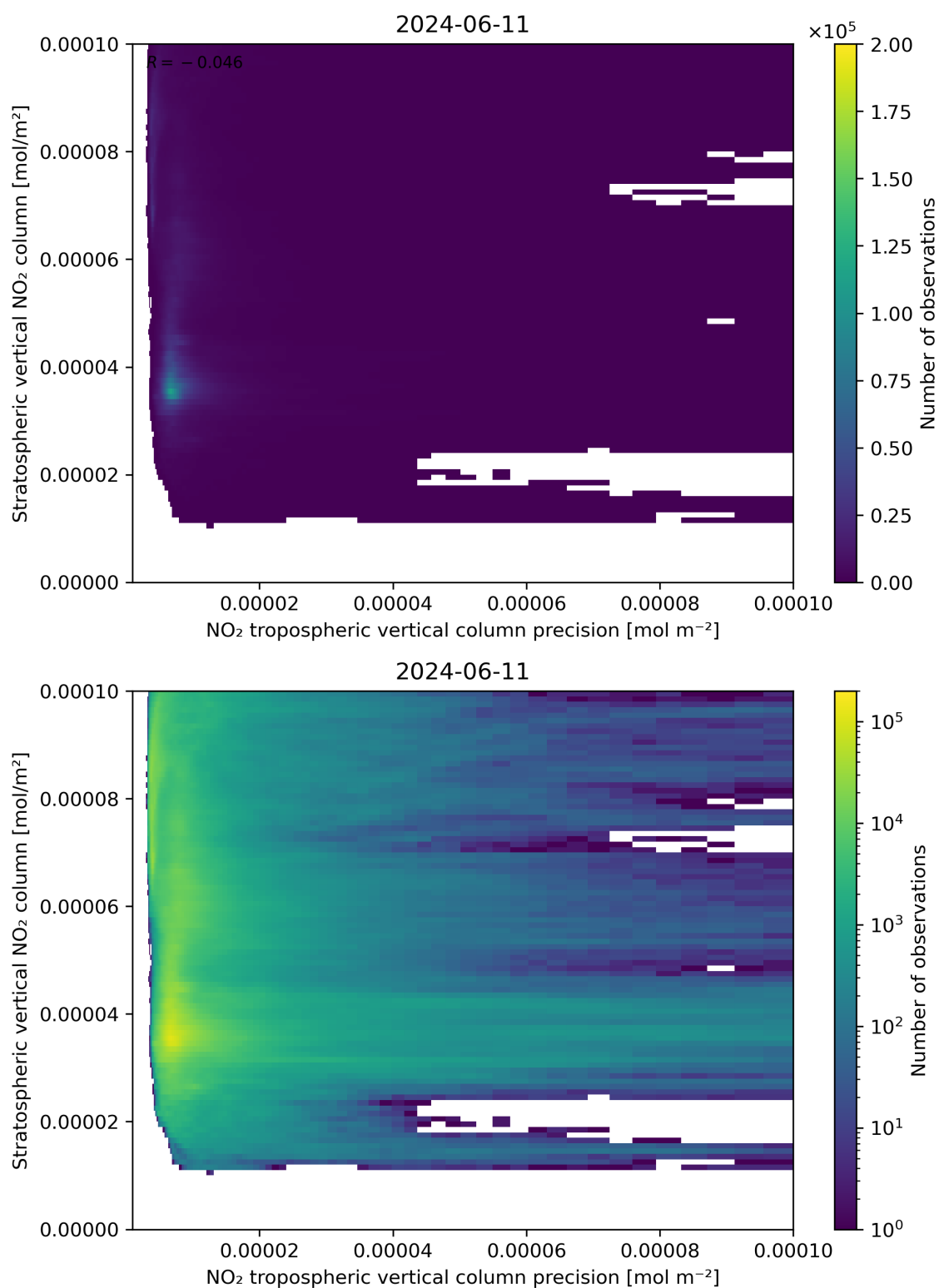
Figure 135: Scatter density plot of “NO 2 tropospheric vertical column precision” against “Stratospheric vertical NO 2 column” for 2024-06-10 to 2024-06-12.
