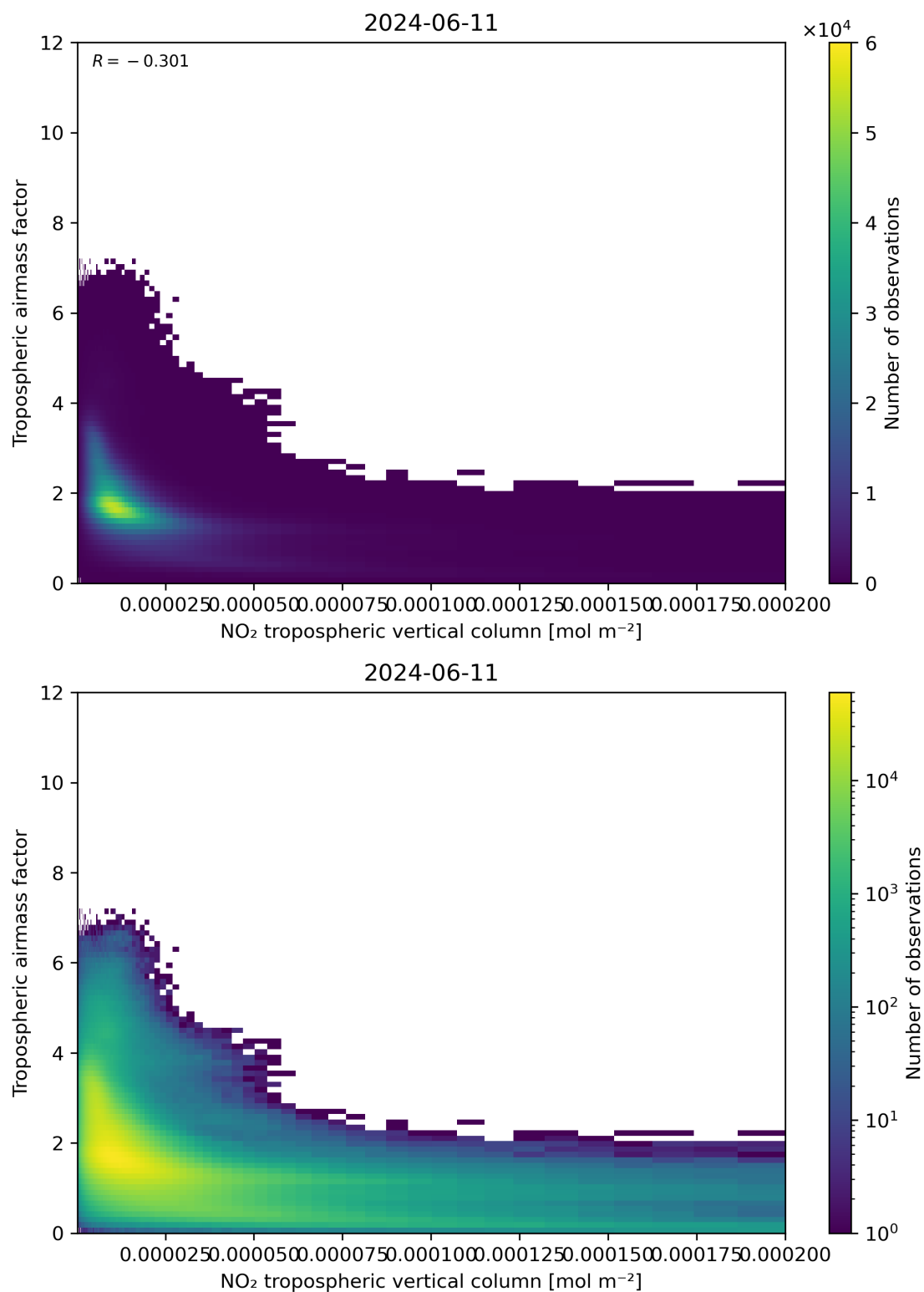
Figure 123: Scatter density plot of “NO 2 tropospheric vertical column” against “Tropospheric air mass factor” for 2024-06-10 to 2024-06-12.
