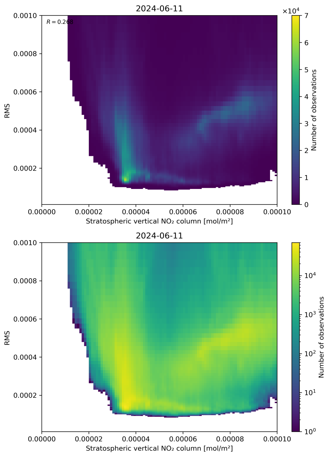
Figure 102: Scatter density plot of “Stratospheric vertical NO 2 column” against “RMS” for 2024-06-10 to 2024-06-12.
