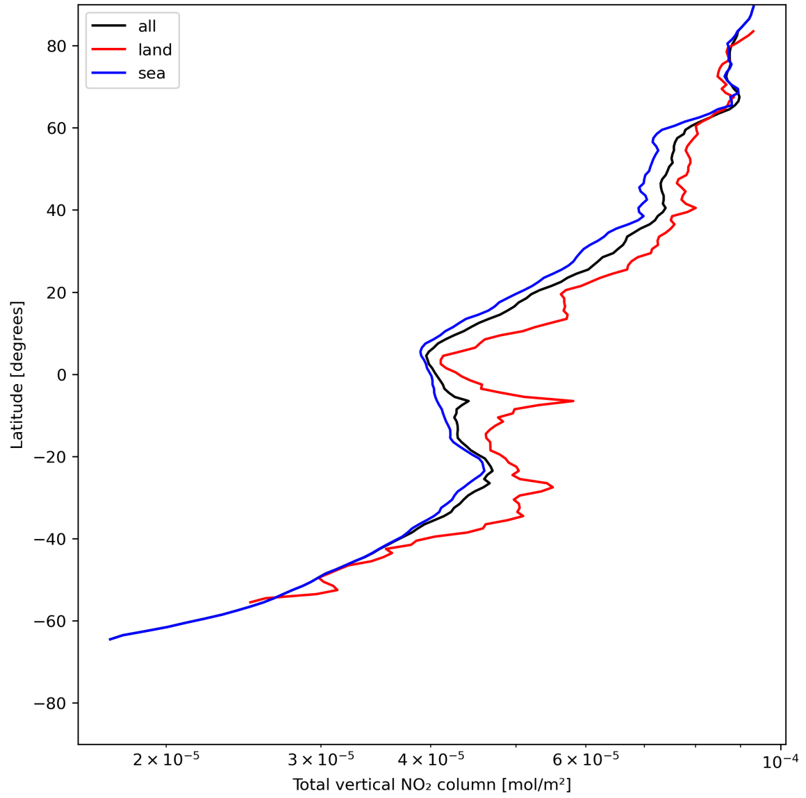
Figure 21: Zonal average of “Total vertical NO 2 column” for 2024-06-10 to 2024-06-12.
