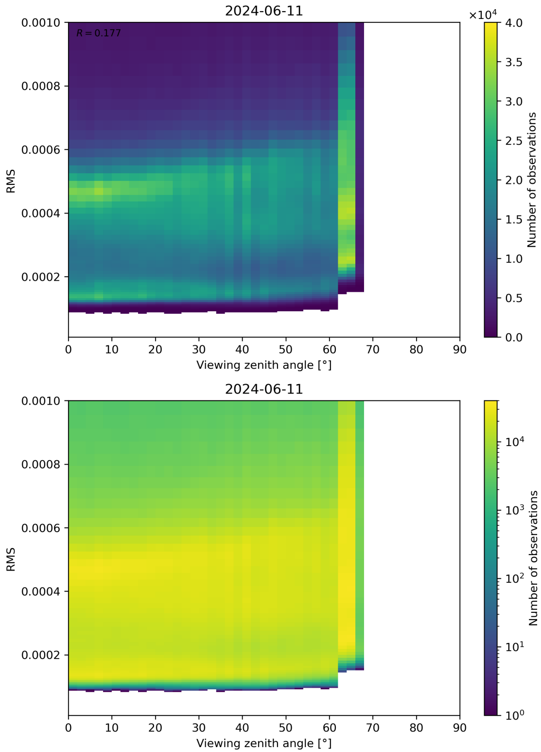
Figure 171: Scatter density plot of “Viewing zenith angle” against “RMS” for 2024-06-10 to 2024-06-12.
