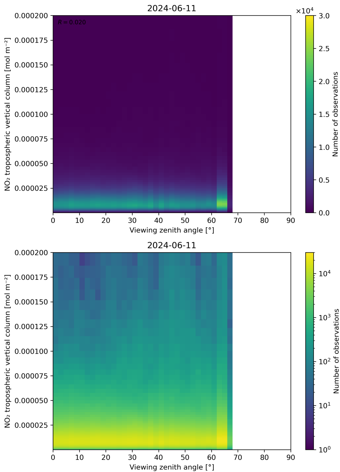
Figure 169: Scatter density plot of “Viewing zenith angle” against “NO 2 tropospheric vertical column” for 2024-06-10 to 2024-06-12.
