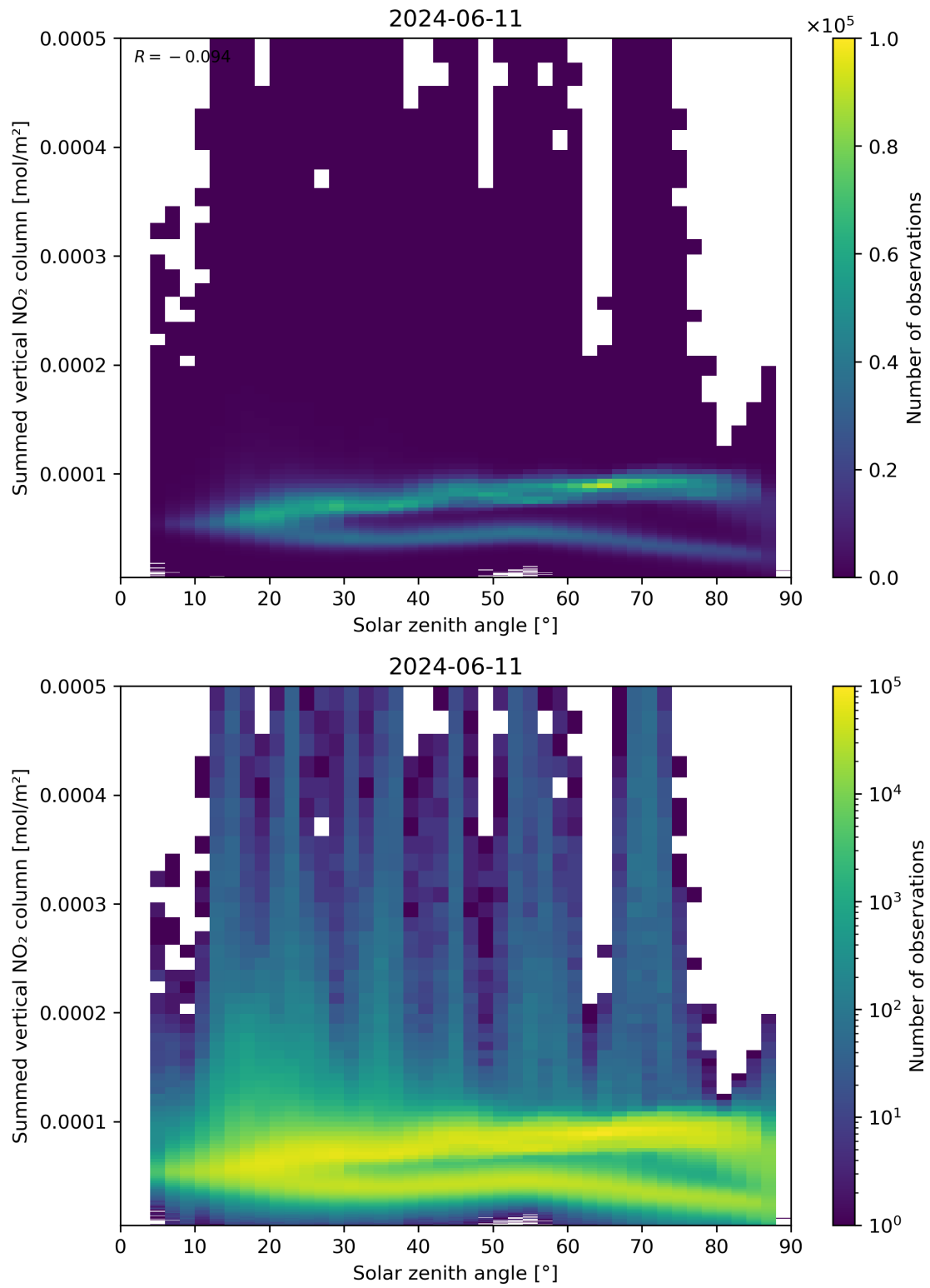
Figure 151: Scatter density plot of “Solar zenith angle” against “Summed vertical NO 2 column” for 2024-06-10 to 2024-06-12.
