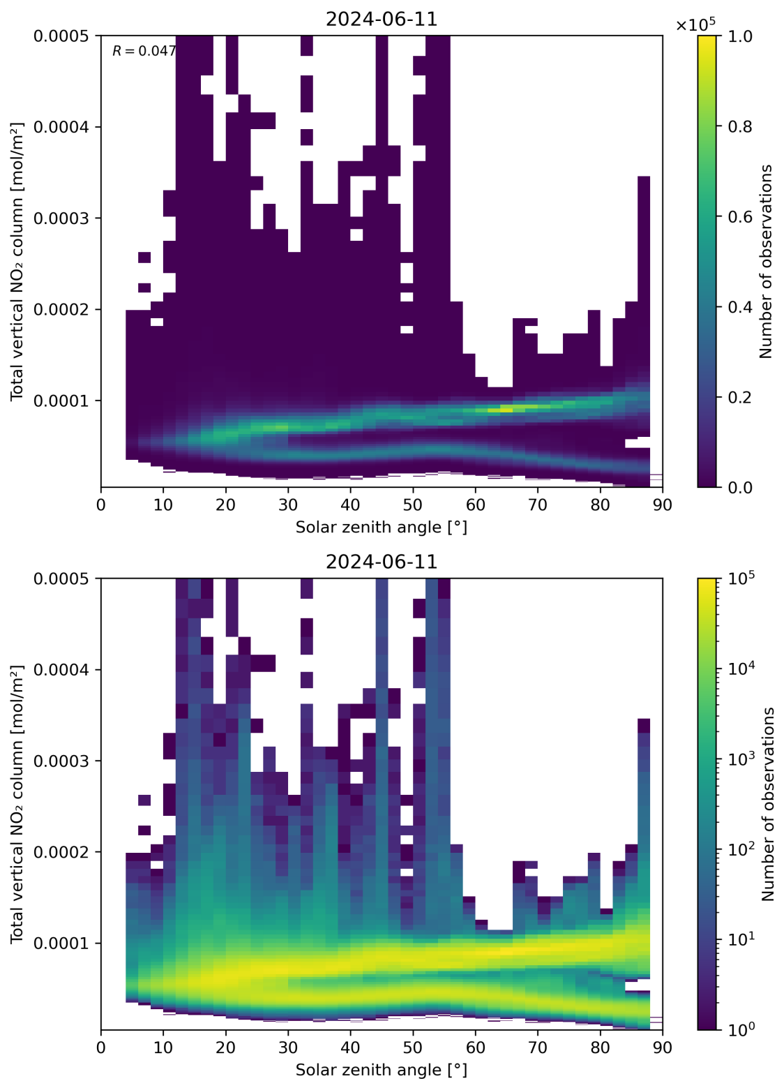
Figure 153: Scatter density plot of “Solar zenith angle” against “Total vertical NO 2 column” for 2024-06-10 to 2024-06-12.
