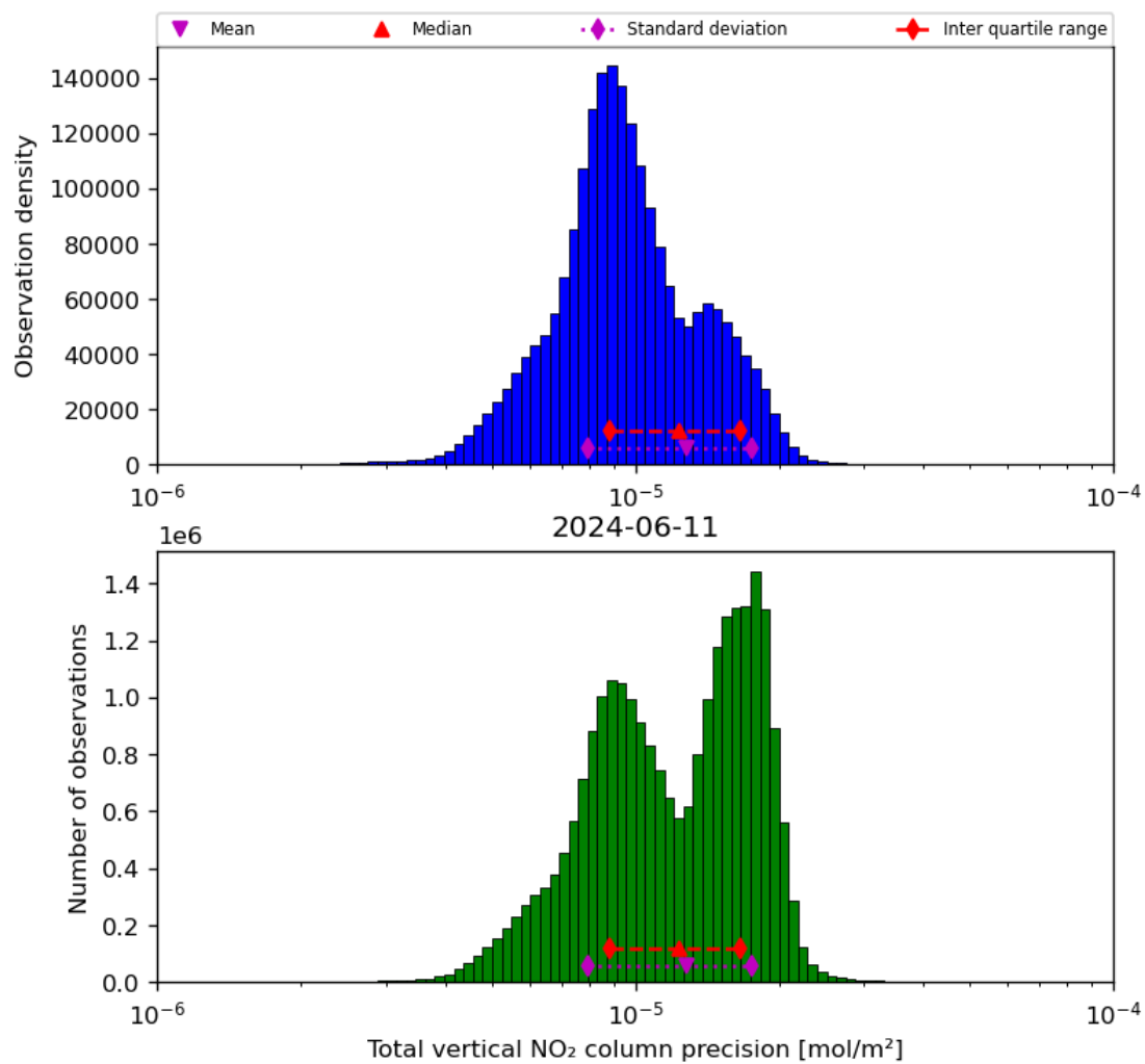
Figure 39: Histogram of “Total vertical NO 2 column precision” for 2024-06-10 to 2024-06-12
