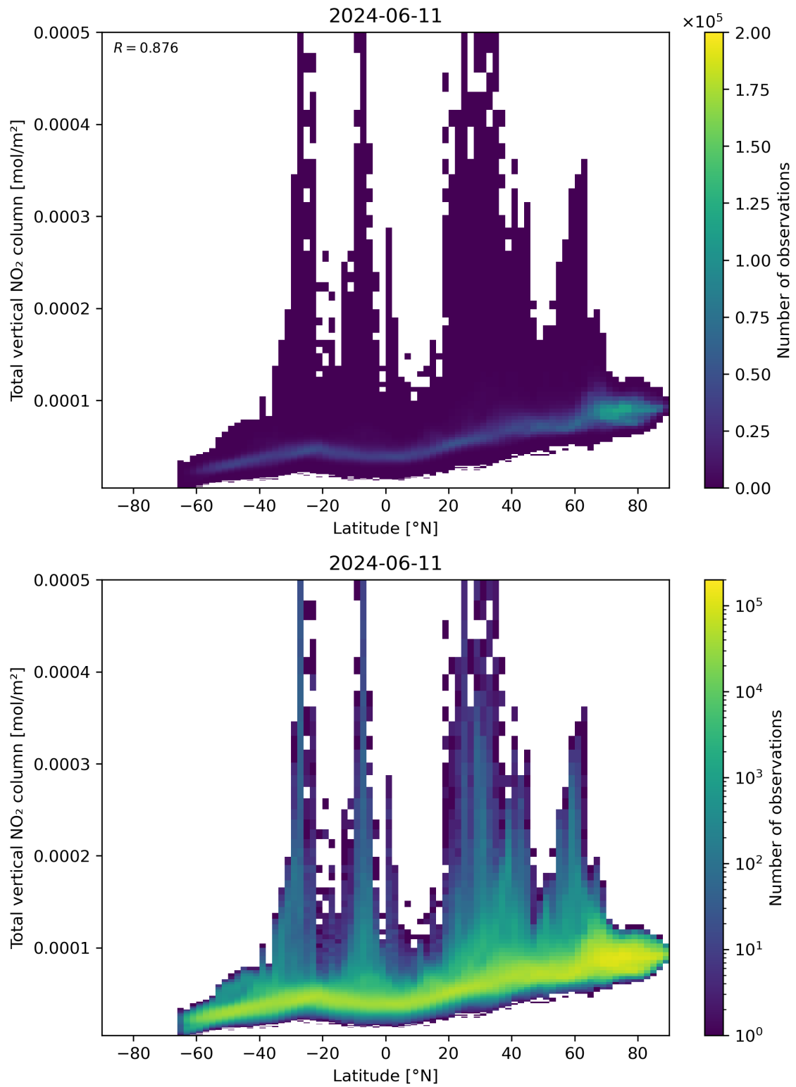
Figure 90: Scatter density plot of “Latitude” against “Total vertical NO 2 column” for 2024-06-10 to 2024-06-12.
