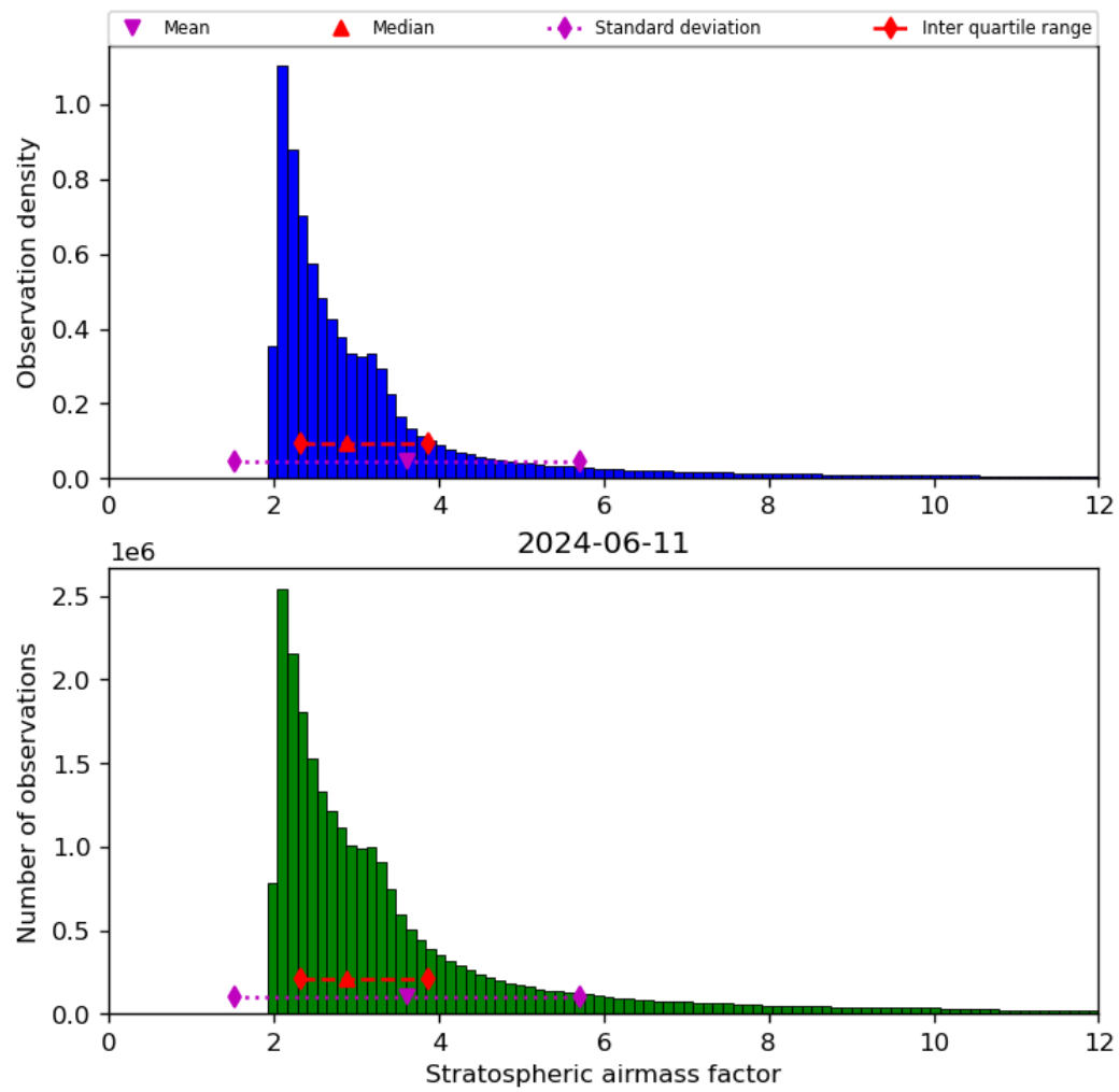
Figure 44: Histogram of “Stratospheric airmass factor” for 2024-06-10 to 2024-06-12
