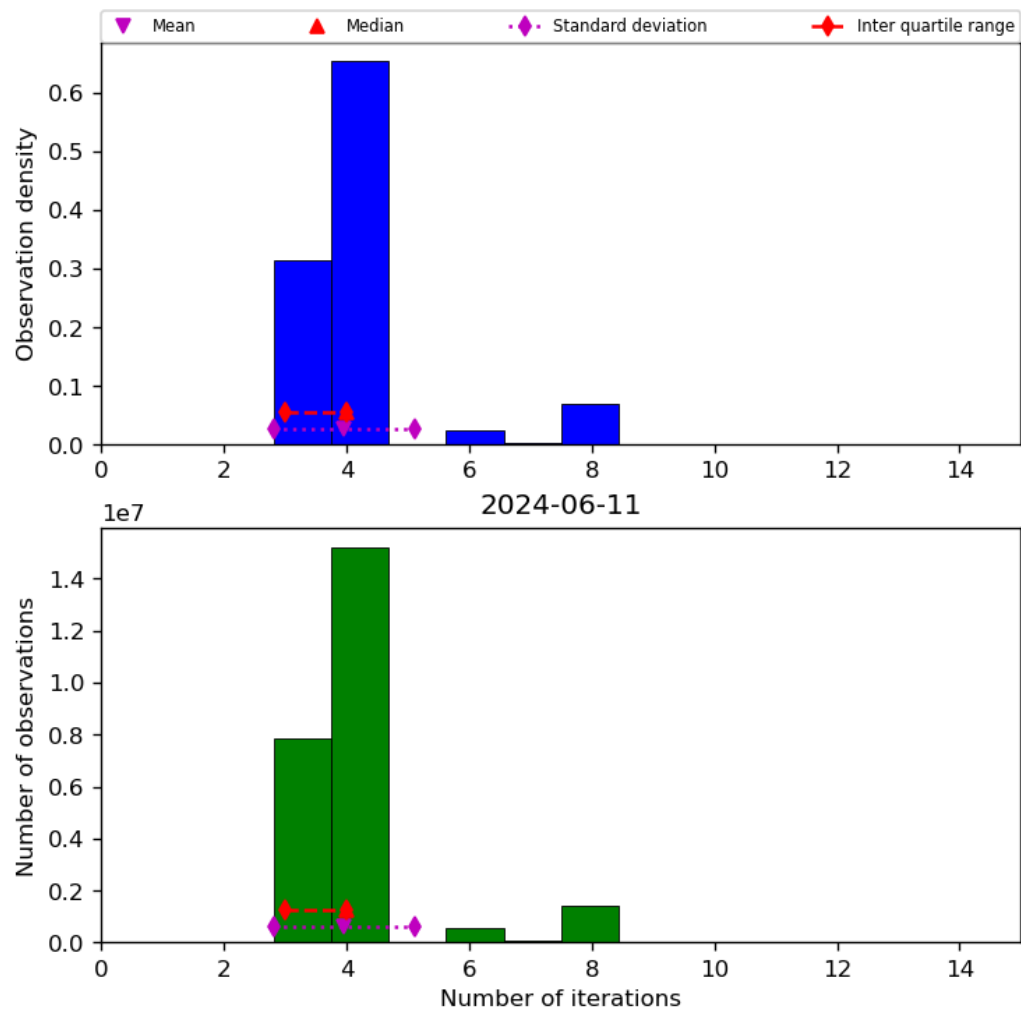
Figure 34: Histogram of “Number of iterations” for 2024-06-10 to 2024-06-12
