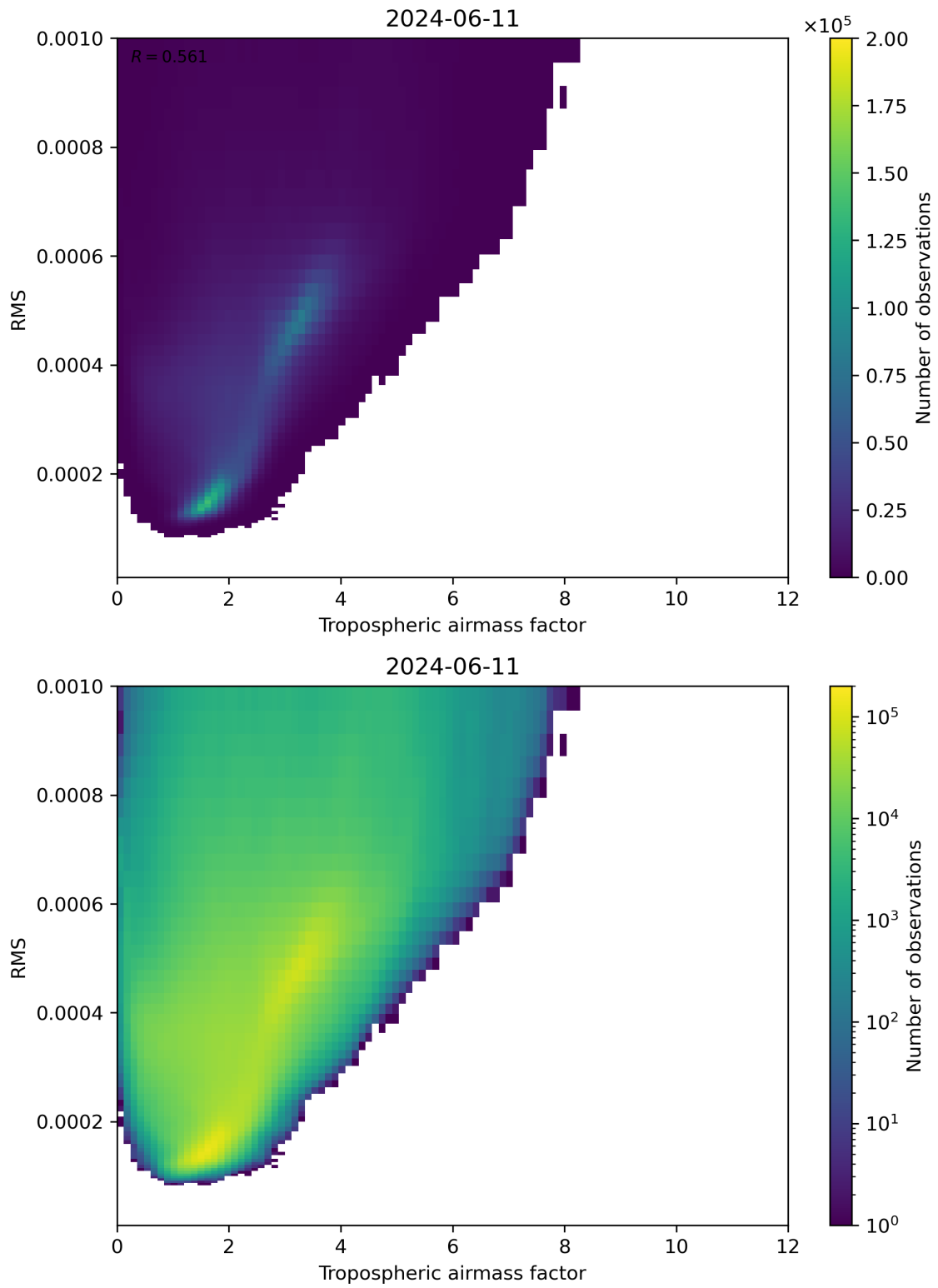
Figure 79: Scatter density plot of “Tropospheric airmass factor” against “RMS” for 2024-06-10 to 2024-06-12.
