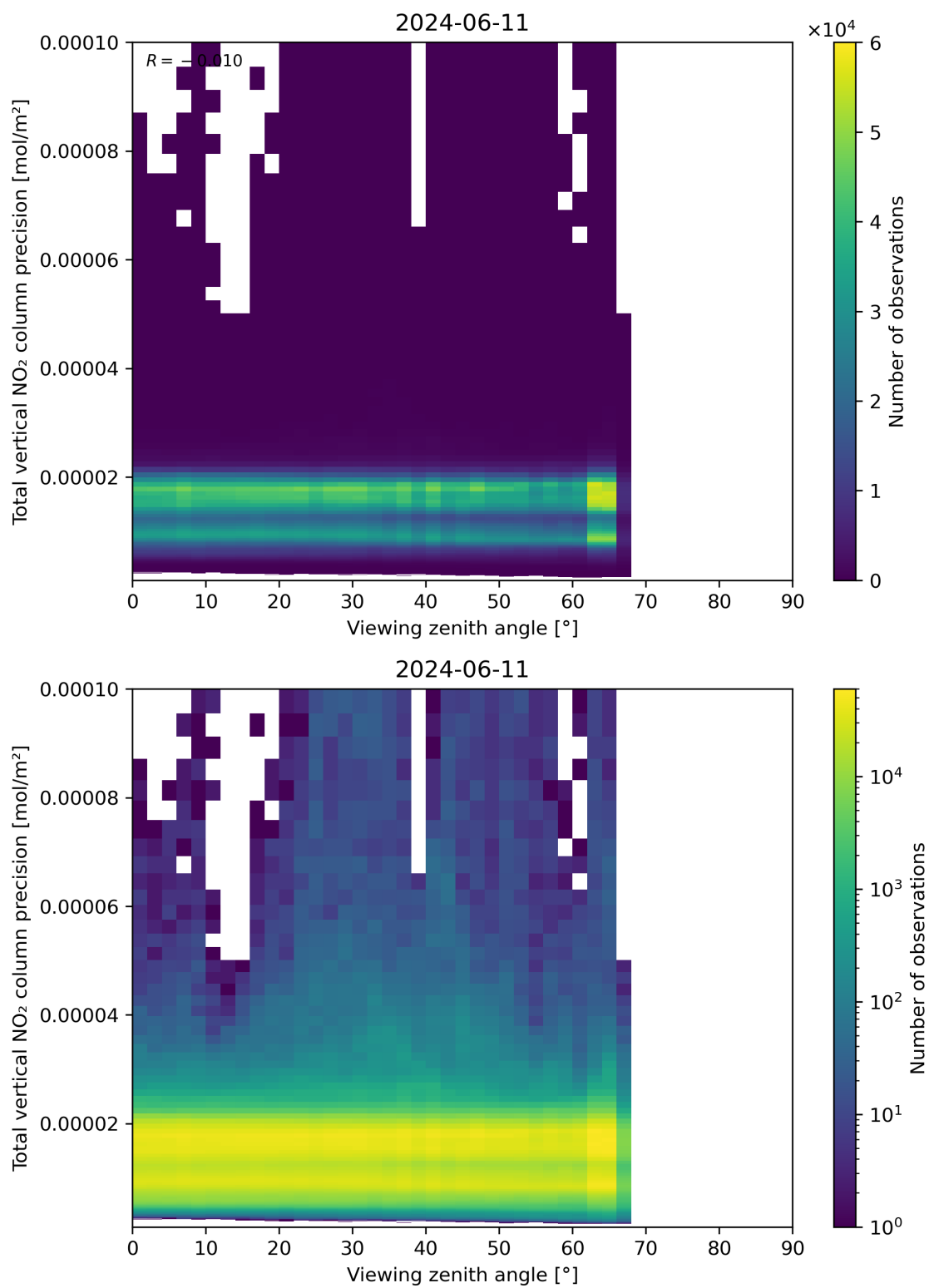
Figure 168: Scatter density plot of “Viewing zenith angle” against “Total vertical NO 2 column precision” for 2024-06-10 to 2024-06-12.
