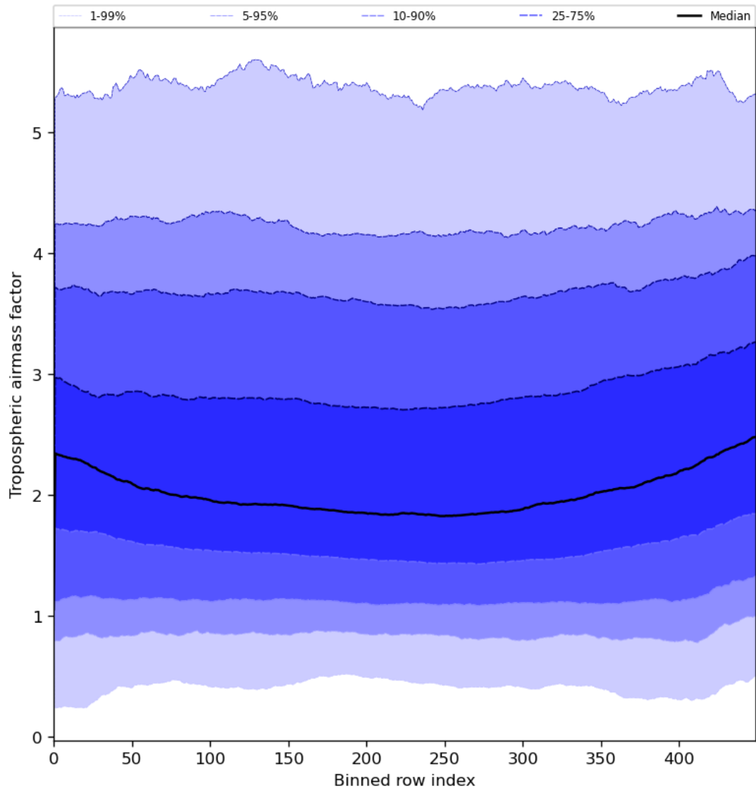
Figure 48: Along track statistics of “Tropospheric airmass factor” for 2024-06-10 to 2024-06-12
