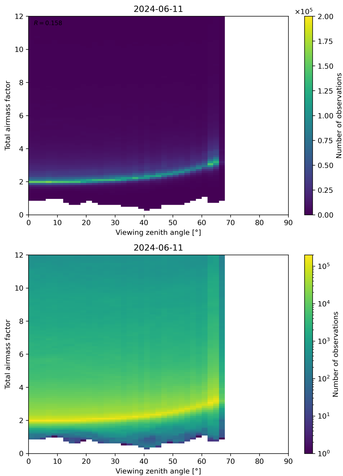
Figure 160: Scatter density plot of “Viewing zenith angle” against “Total airmass factor” for 2024-06-10 to 2024-06-12.
