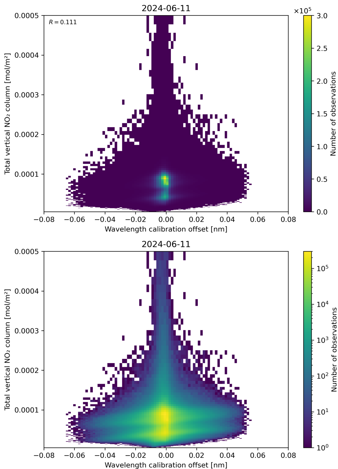
Figure 179: Scatter density plot of “Wavelength calibration offset” against “Total vertical NO 2 column” for 2024-06-10 to 2024-06-12.
