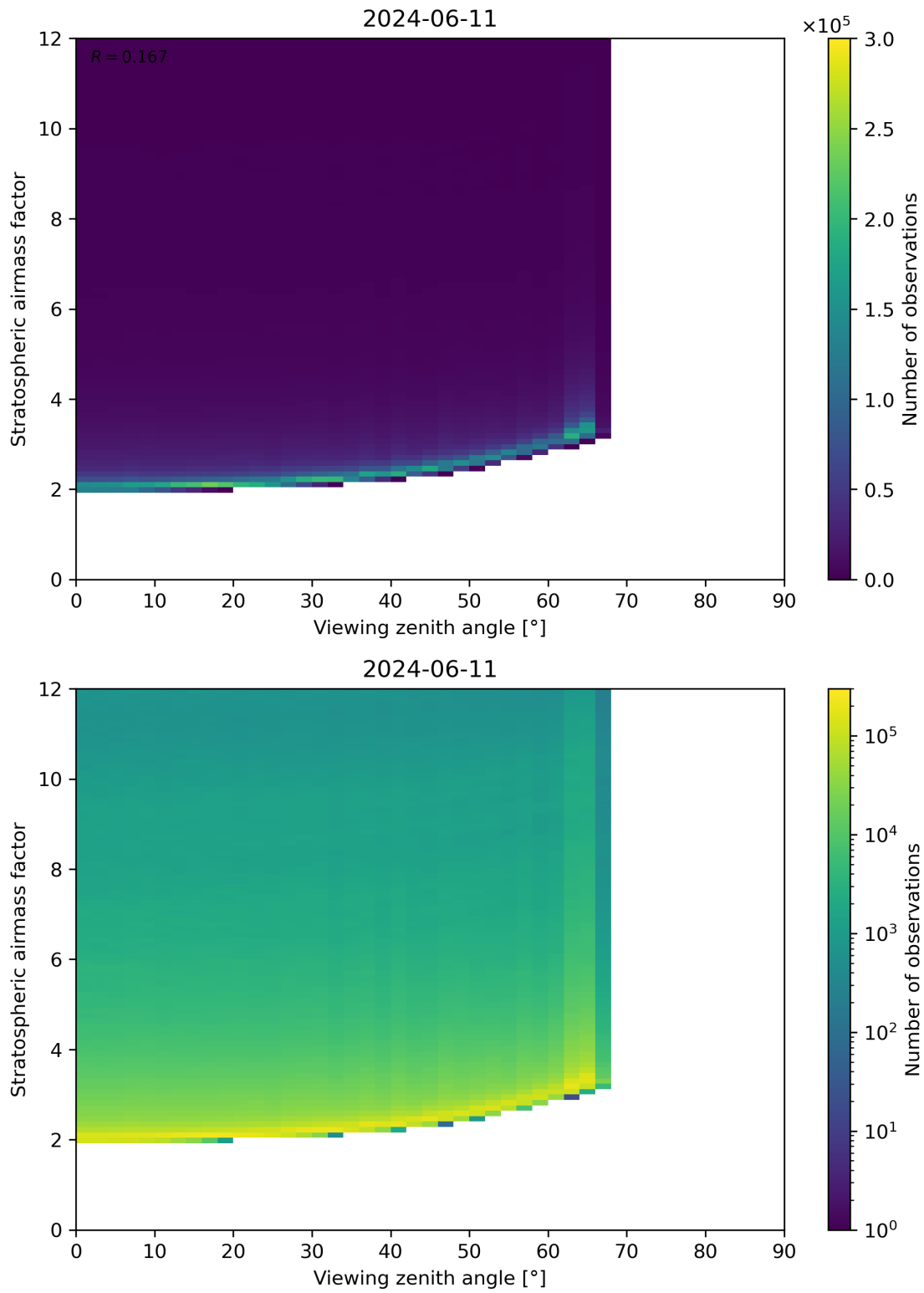
Figure 159: Scatter density plot of “Viewing zenith angle” against “Stratospheric airmass factor” for 2024-06-10 to 2024-06-12.
