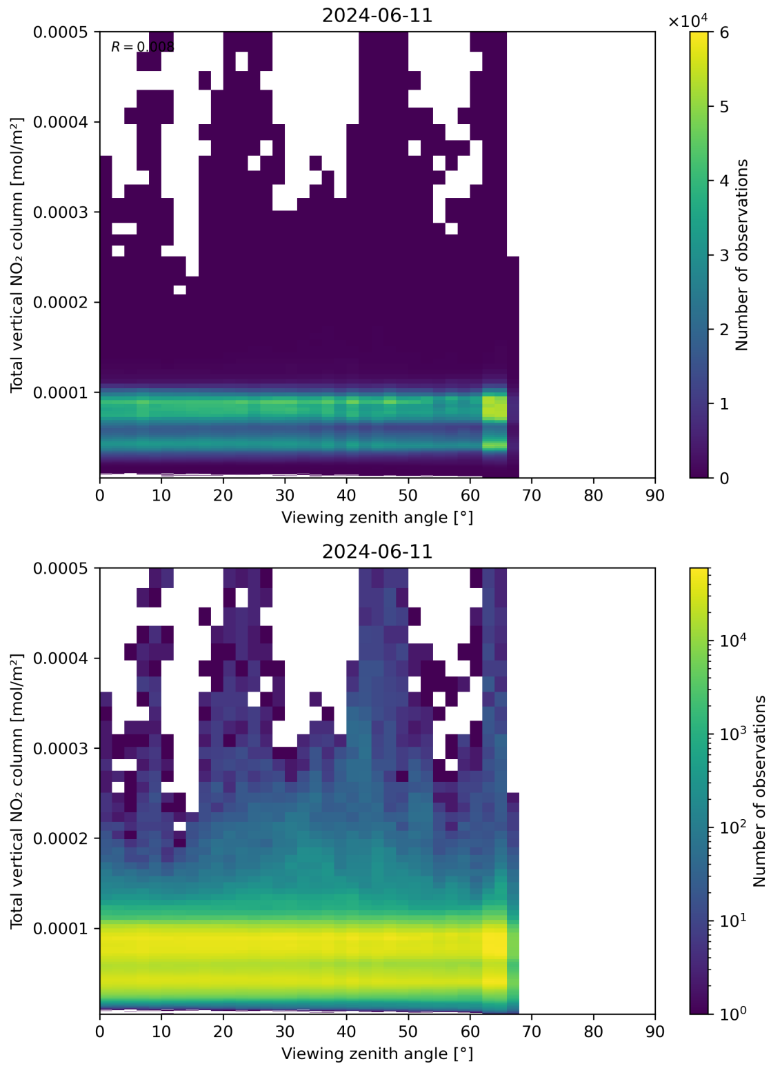
Figure 167: Scatter density plot of “Viewing zenith angle” against “Total vertical NO 2 column” for 2024-06-10 to 2024-06-12.
