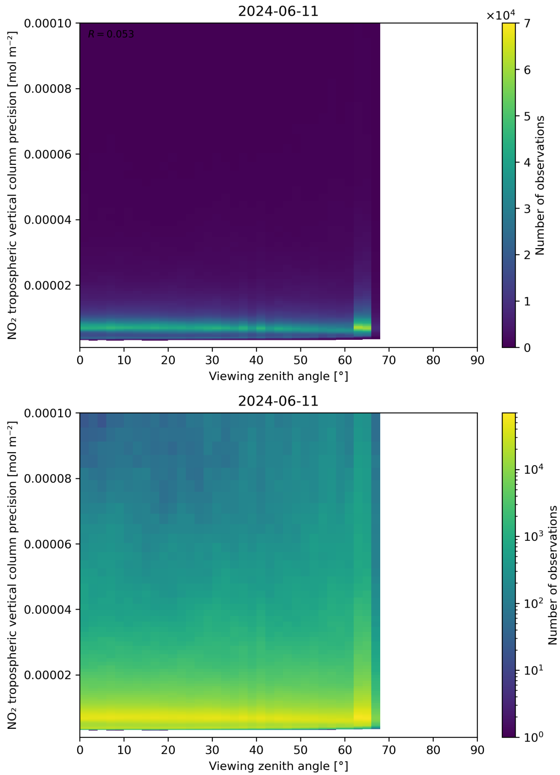
Figure 170: Scatter density plot of “Viewing zenith angle” against “NO 2 tropospheric vertical column precision” for 2024-06-10 to 2024-06-12.
