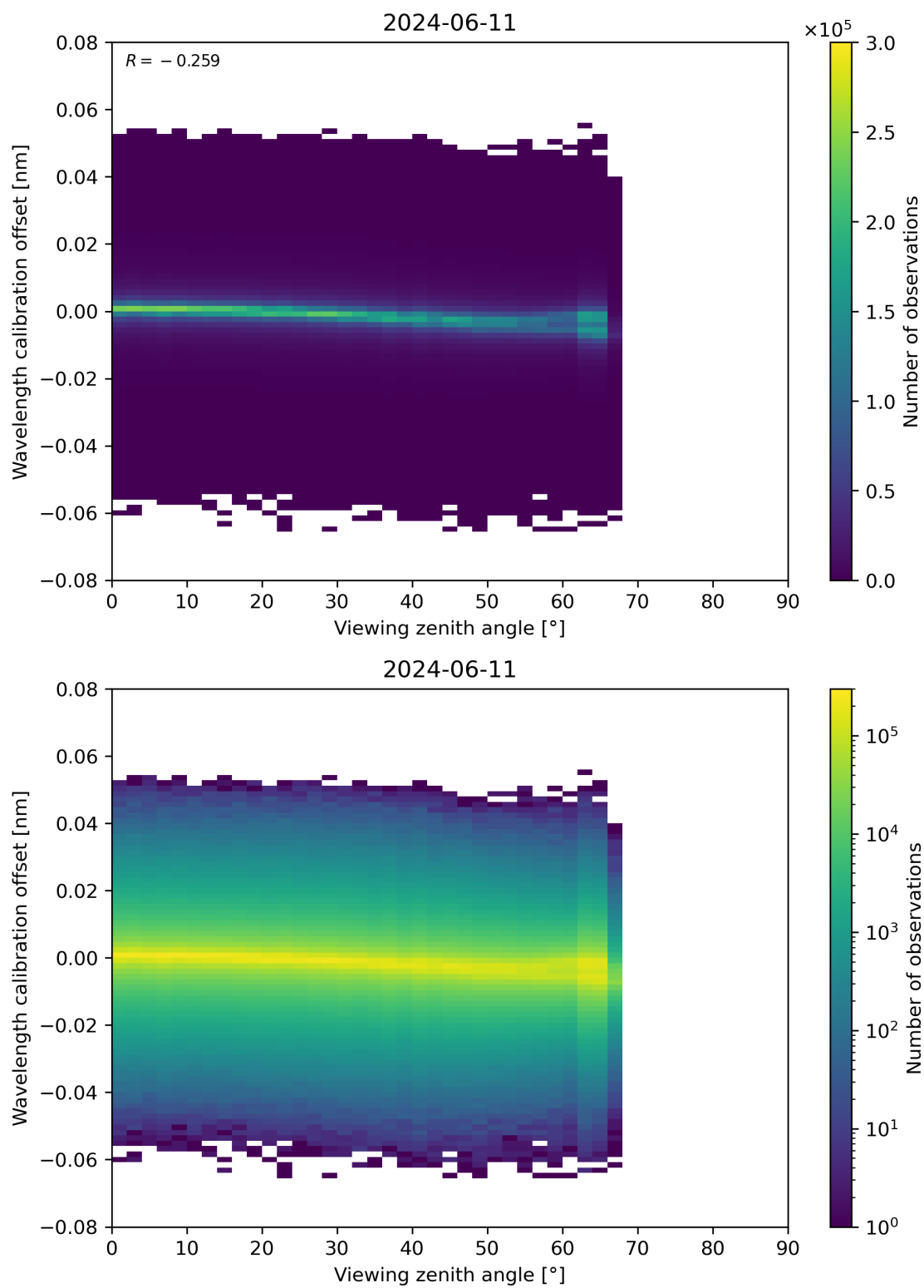
Figure 173: Scatter density plot of “Viewing zenith angle” against “Wavelength calibration offset” for 2024-06-10 to 2024-06-12.
