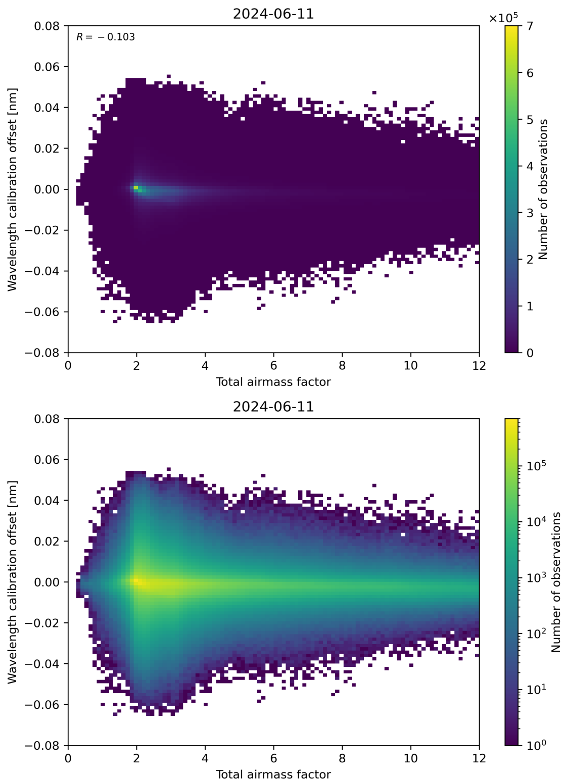
Figure 70: Scatter density plot of “Total airmass factor” against “Wavelength calibration offset” for 2024-06-10 to 2024-06-12.
