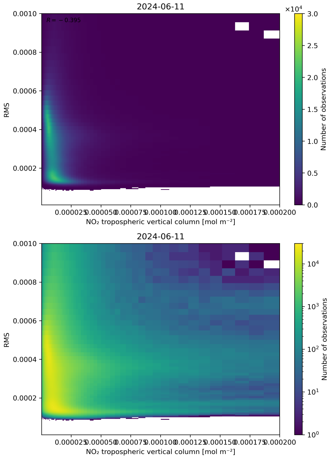
Figure 142: Scatter density plot of “NO 2 tropospheric vertical column” against “RMS” for 2024-06-10 to 2024-06-12.
