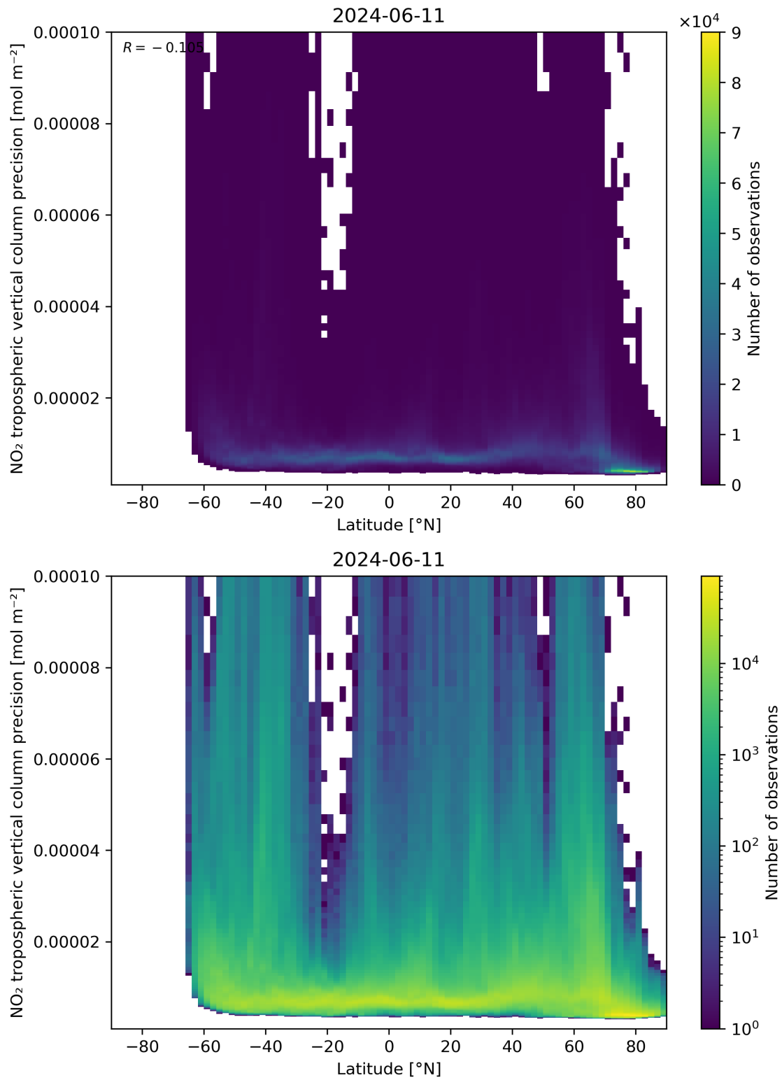
Figure 93: Scatter density plot of “Latitude” against “NO 2 tropospheric vertical column precision” for 2024-06-10 to 2024-06-12.
