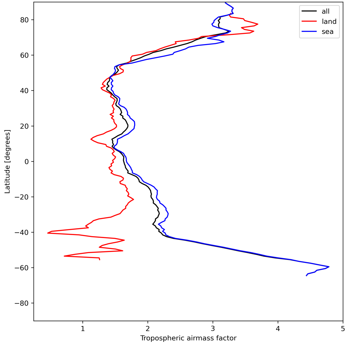
Figure 14: Zonal average of “Tropospheric airmass factor” for 2024-06-10 to 2024-06-12.
