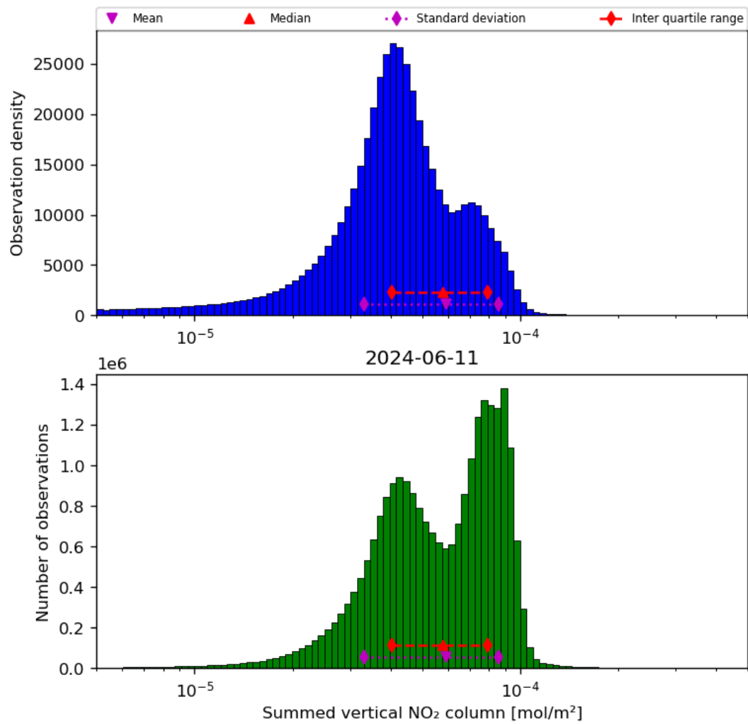
Figure 40: Histogram of “Summed vertical NO 2 column” for 2024-06-10 to 2024-06-12
