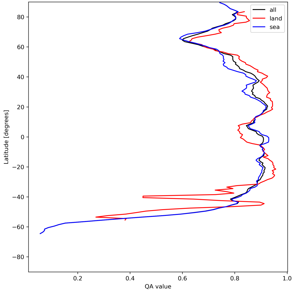
Figure 11: Zonal average of “QA value” for 2024-06-10 to 2024-06-12.
