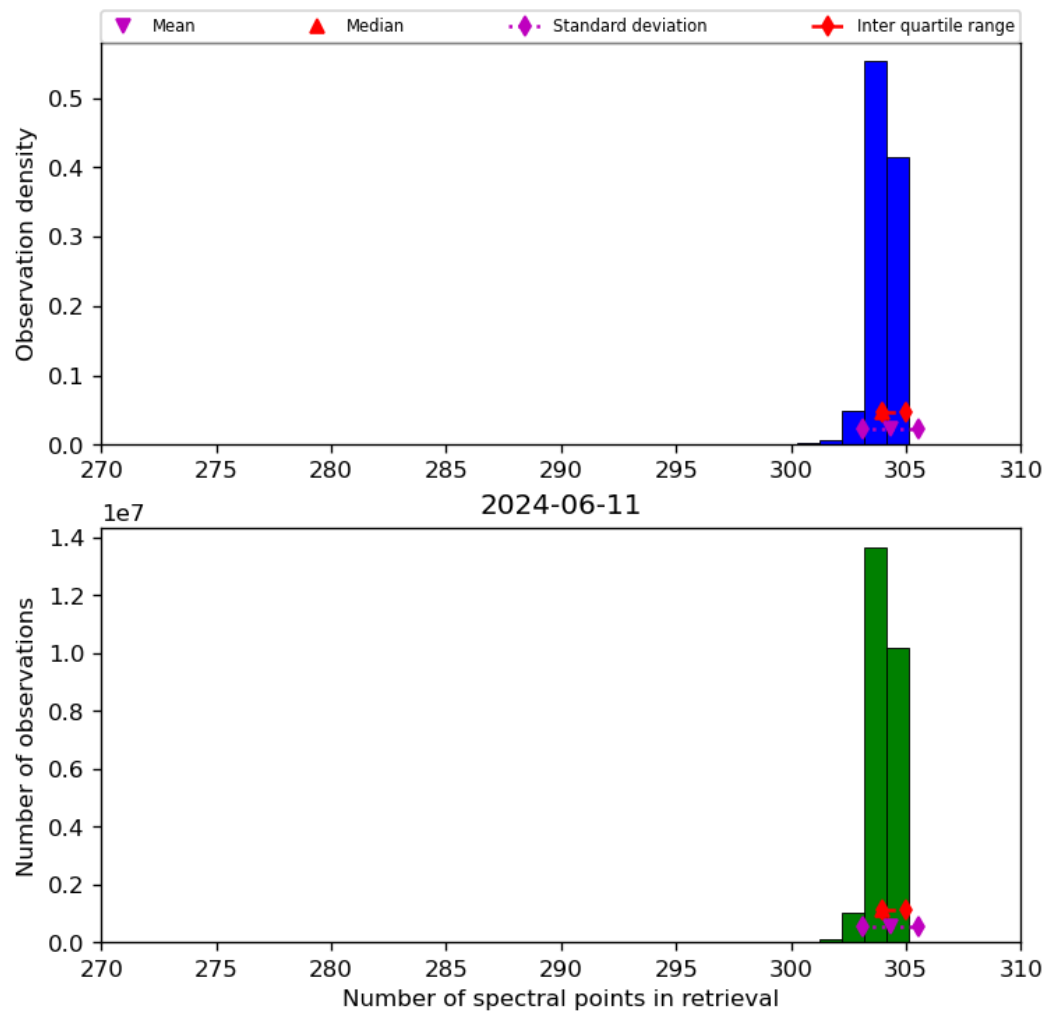
Figure 33: Histogram of “Number of spectral points in retrieval” for 2024-06-10 to 2024-06-12
