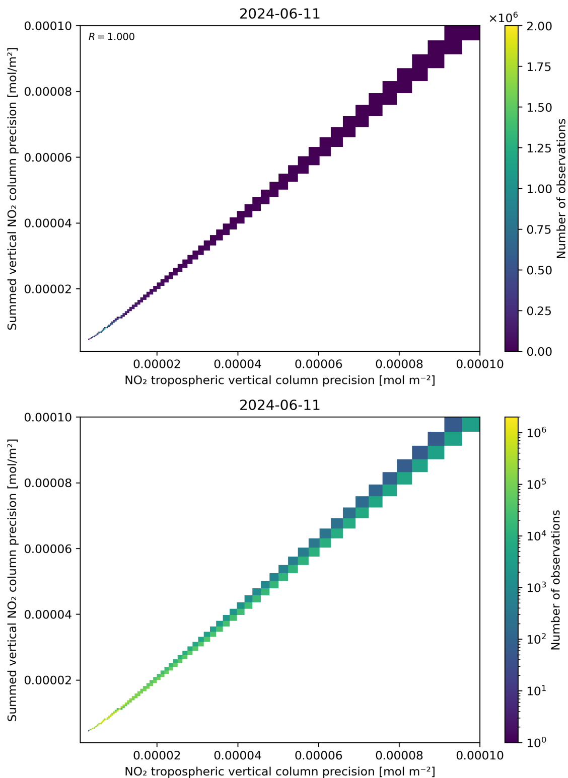
Figure 137: Scatter density plot of “NO 2 tropospheric vertical column precision” against “Summed vertical NO 2 column precision” for 2024-06-10 to 2024-06-12.
