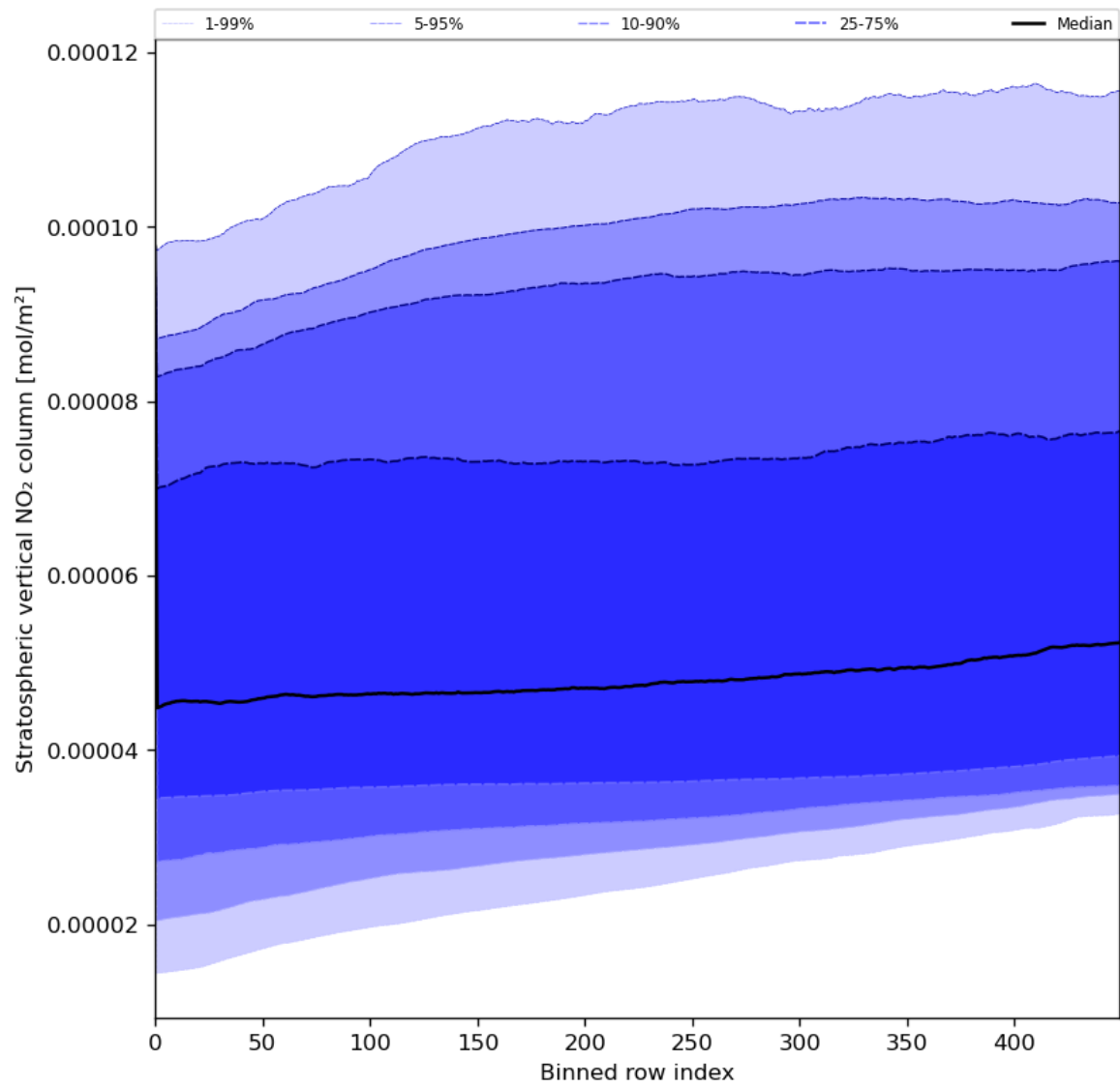
Figure 53: Along track statistics of “Stratospheric vertical NO 2 column” for 2024-06-11 to 2024-06-13
