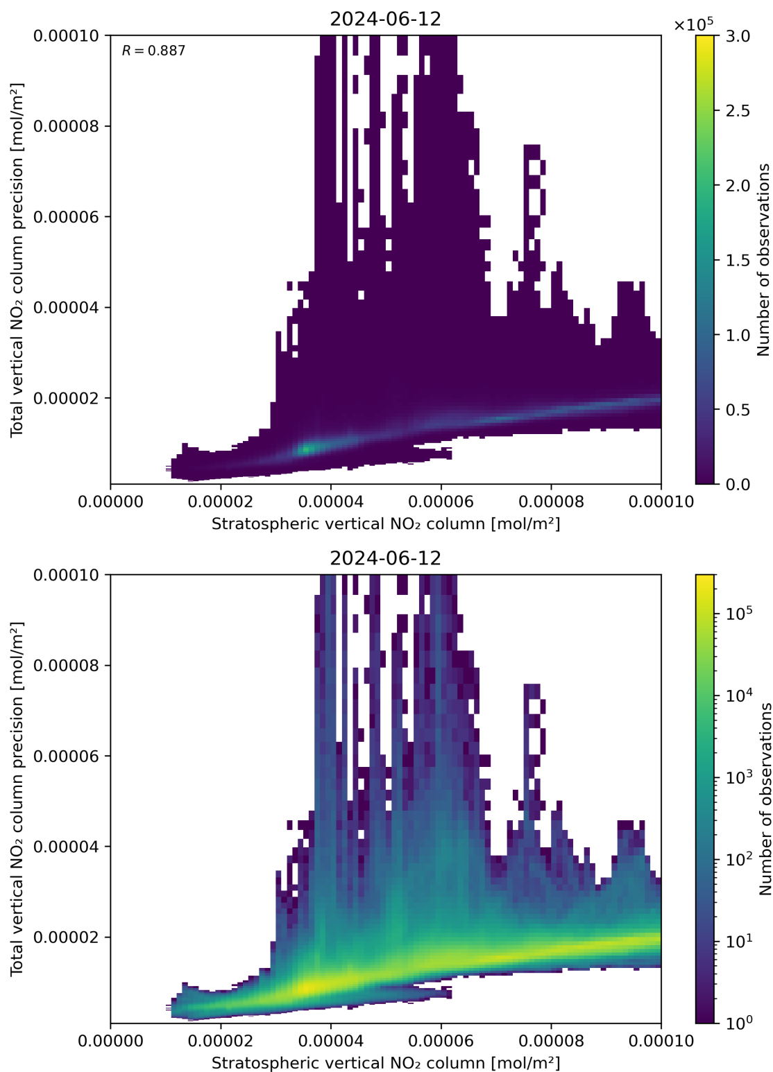
Figure 101: Scatter density plot of “Stratospheric vertical NO 2 column” against “Total vertical NO 2 column precision” for 2024-06-11 to 2024-06-13.
