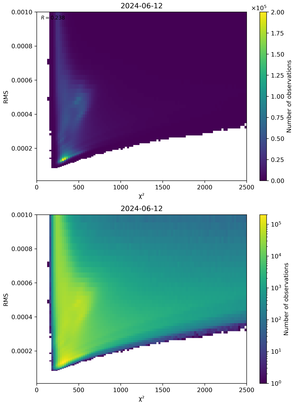
Figure 82: Scatter density plot of “ \chi^2 ” against “RMS” for 2024-06-11 to 2024-06-13.
