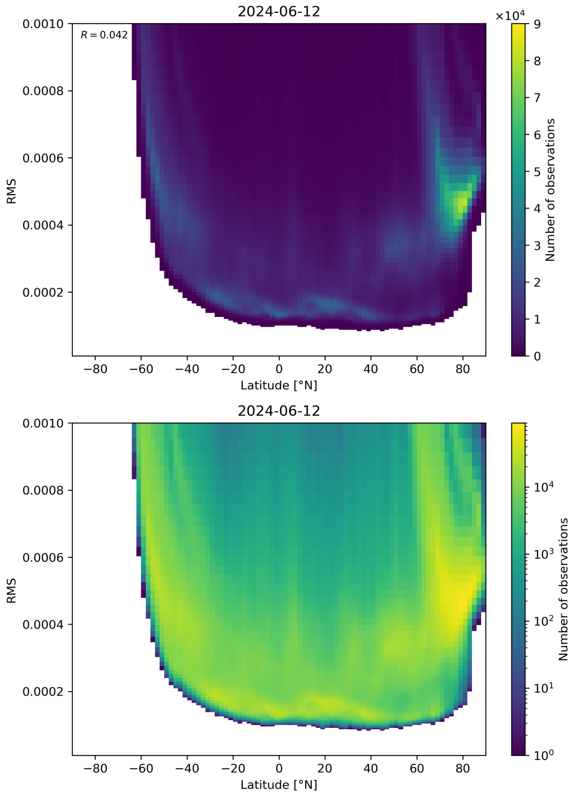
Figure 94: Scatter density plot of “Latitude” against “RMS” for 2024-06-11 to 2024-06-13.
