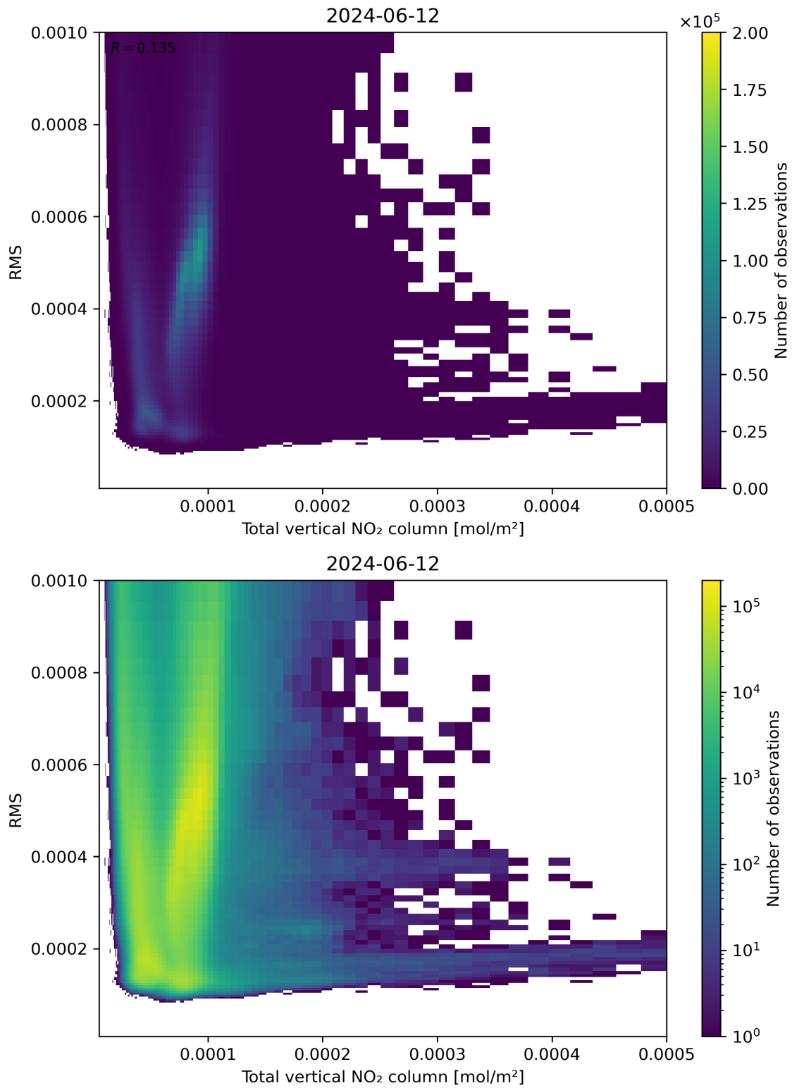
Figure 120: Scatter density plot of “Total vertical NO 2 column” against “RMS” for 2024-06-11 to 2024-06-13.
