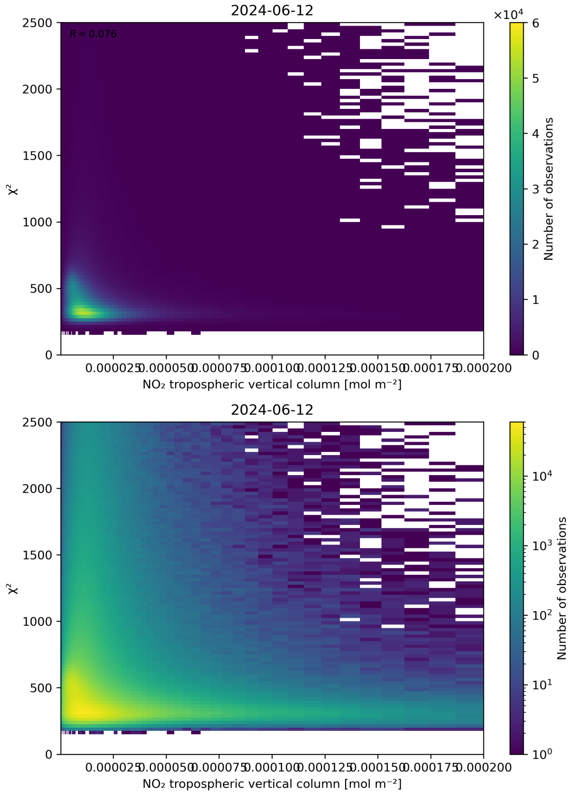
Figure 124: Scatter density plot of “NO 2 tropospheric vertical column” against “ \chi^2 ” for 2024-06-11 to 2024-06-13.
