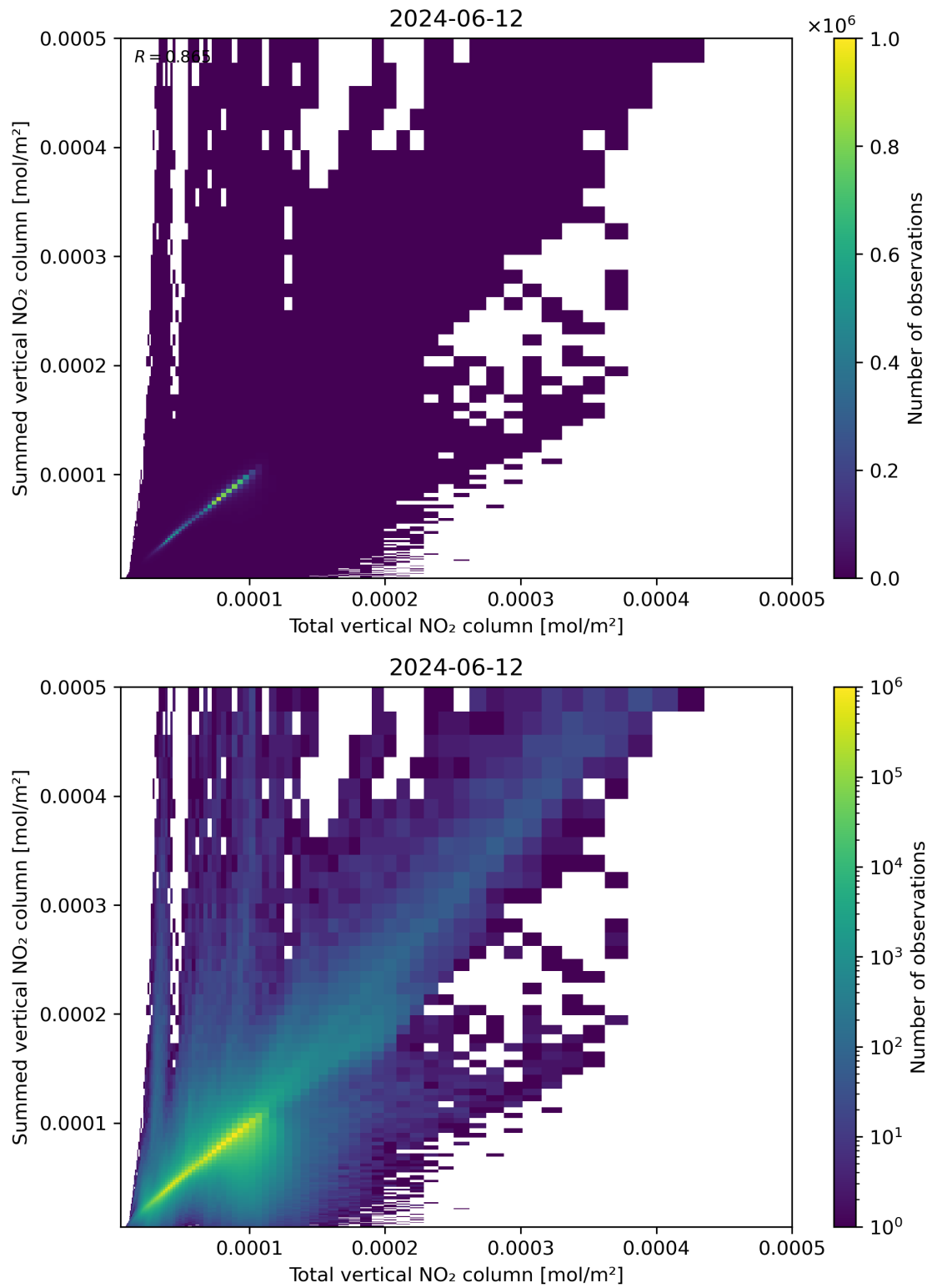
Figure 112: Scatter density plot of “Total vertical NO 2 column” against “Summed vertical NO 2 column” for 2024-06-11 to 2024-06-13.
