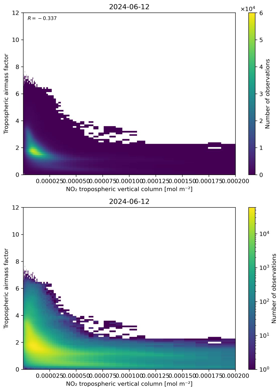
Figure 123: Scatter density plot of “NO 2 tropospheric vertical column” against “Tropospheric airmass factor” for 2024-06-11 to 2024-06-13.
