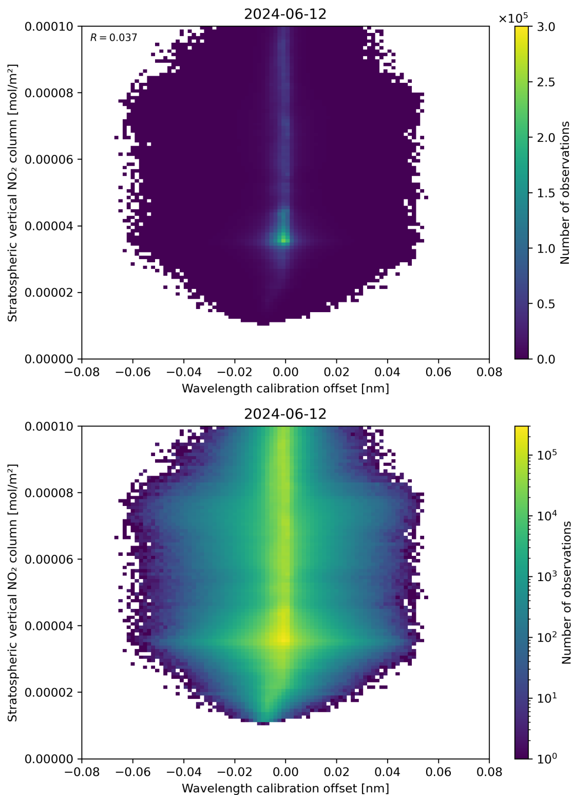
Figure 176: Scatter density plot of “Wavelength calibration offset” against “Stratospheric vertical NO 2 column” for 2024-06-11 to 2024-06-13.
