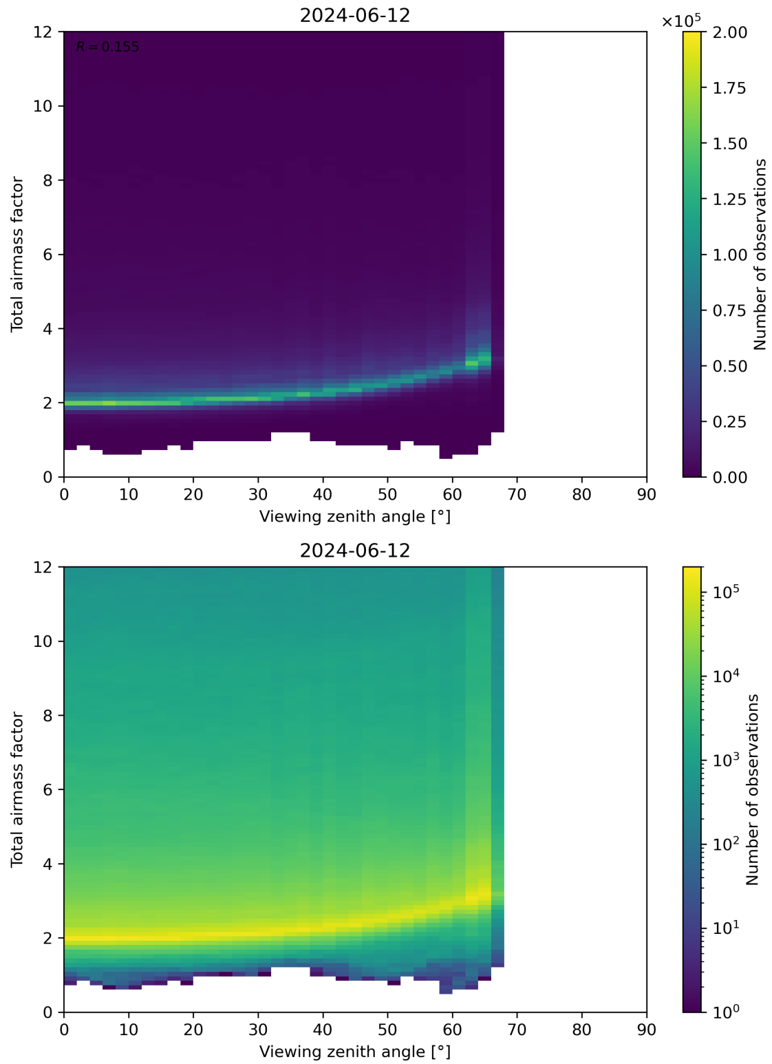
Figure 160: Scatter density plot of “Viewing zenith angle” against “Total airmass factor” for 2024-06-11 to 2024-06-13.
