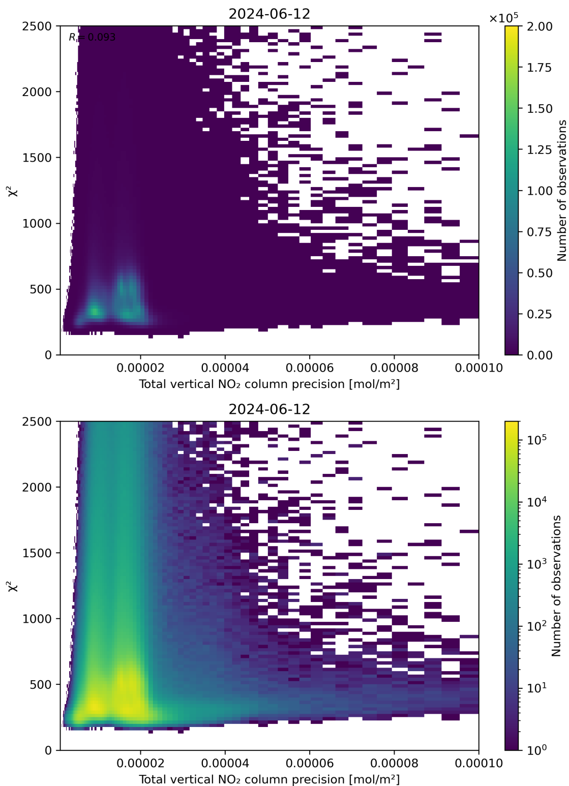
Figure 116: Scatter density plot of “Total vertical NO 2 column precision” against “ \chi^2 ” for 2024-06-11 to 2024-06-13.
