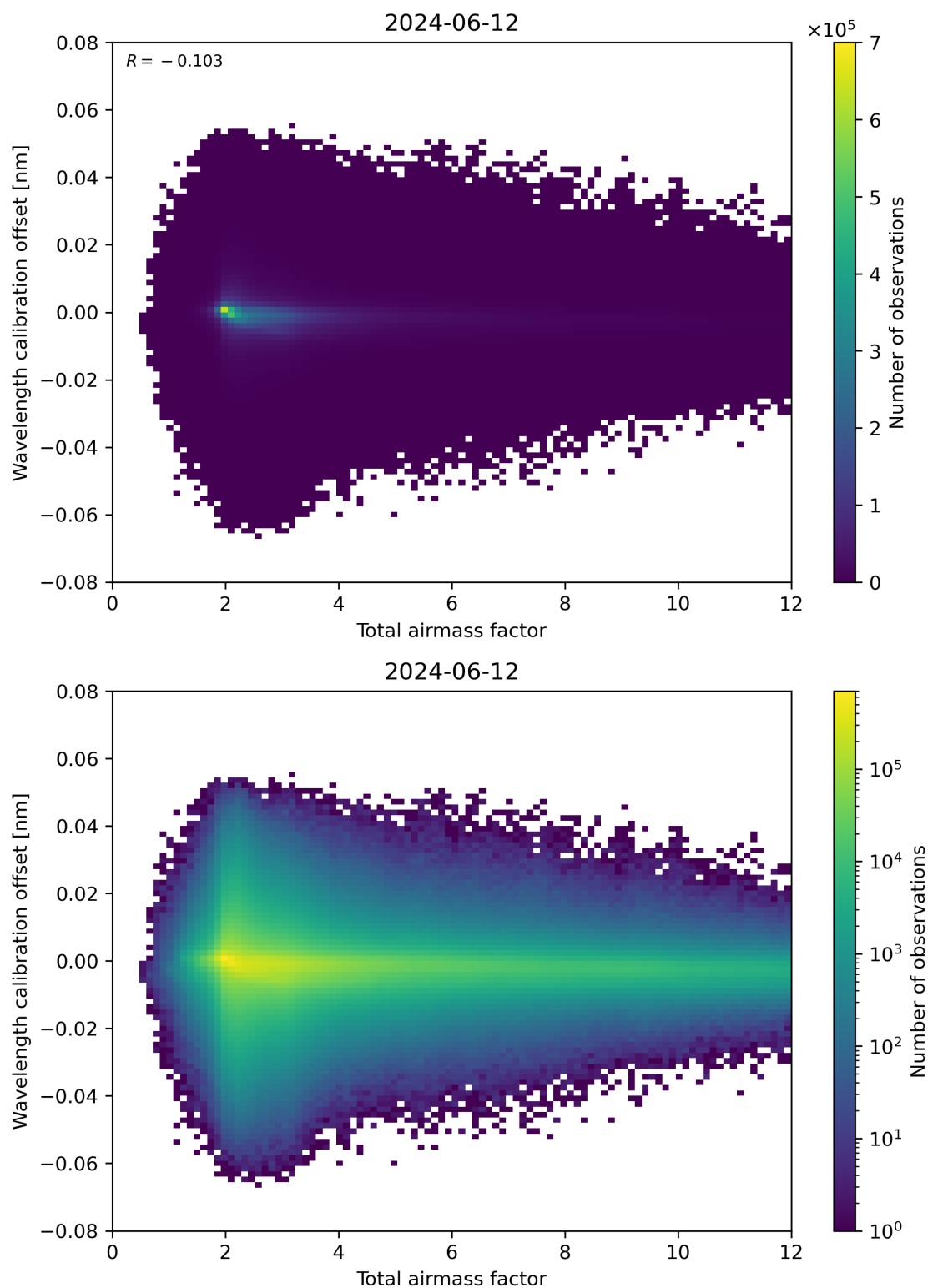
Figure 70: Scatter density plot of “Total airmass factor” against “Wavelength calibration offset” for 2024-06-11 to 2024-06-13.
