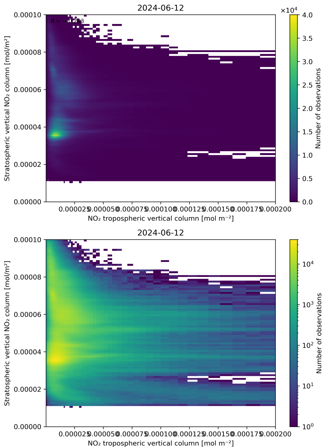
Figure 125: Scatter density plot of “NO 2 tropospheric vertical column” against “Stratospheric vertical NO 2 column” for 2024-06-11 to 2024-06-13.
