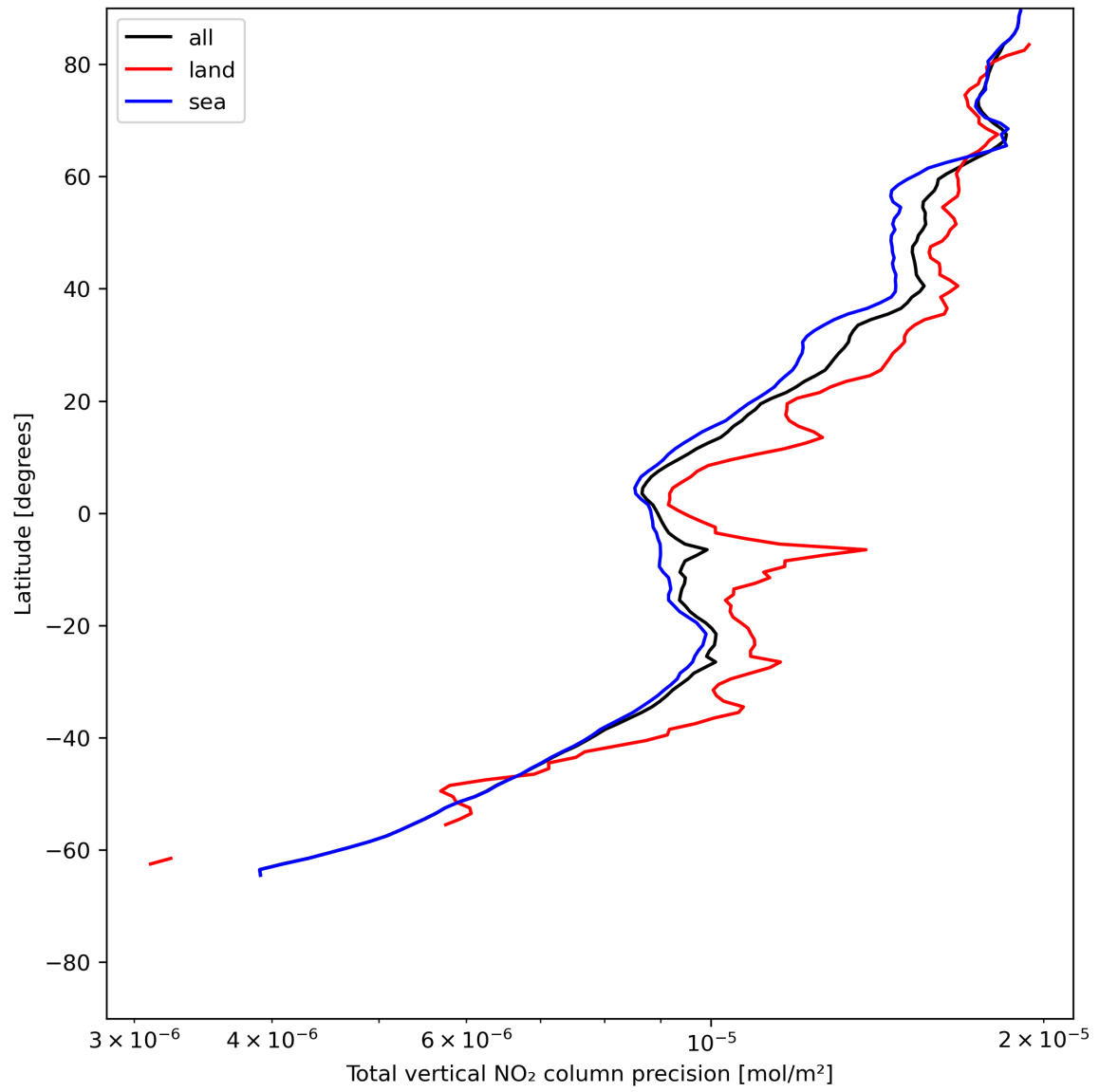
Figure 22: Zonal average of “Total vertical NO 2 column precision” for 2024-06-11 to 2024-06-13.
