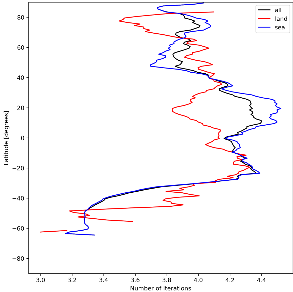
Figure 17: Zonal average of “Number of iterations” for 2024-06-11 to 2024-06-13.
