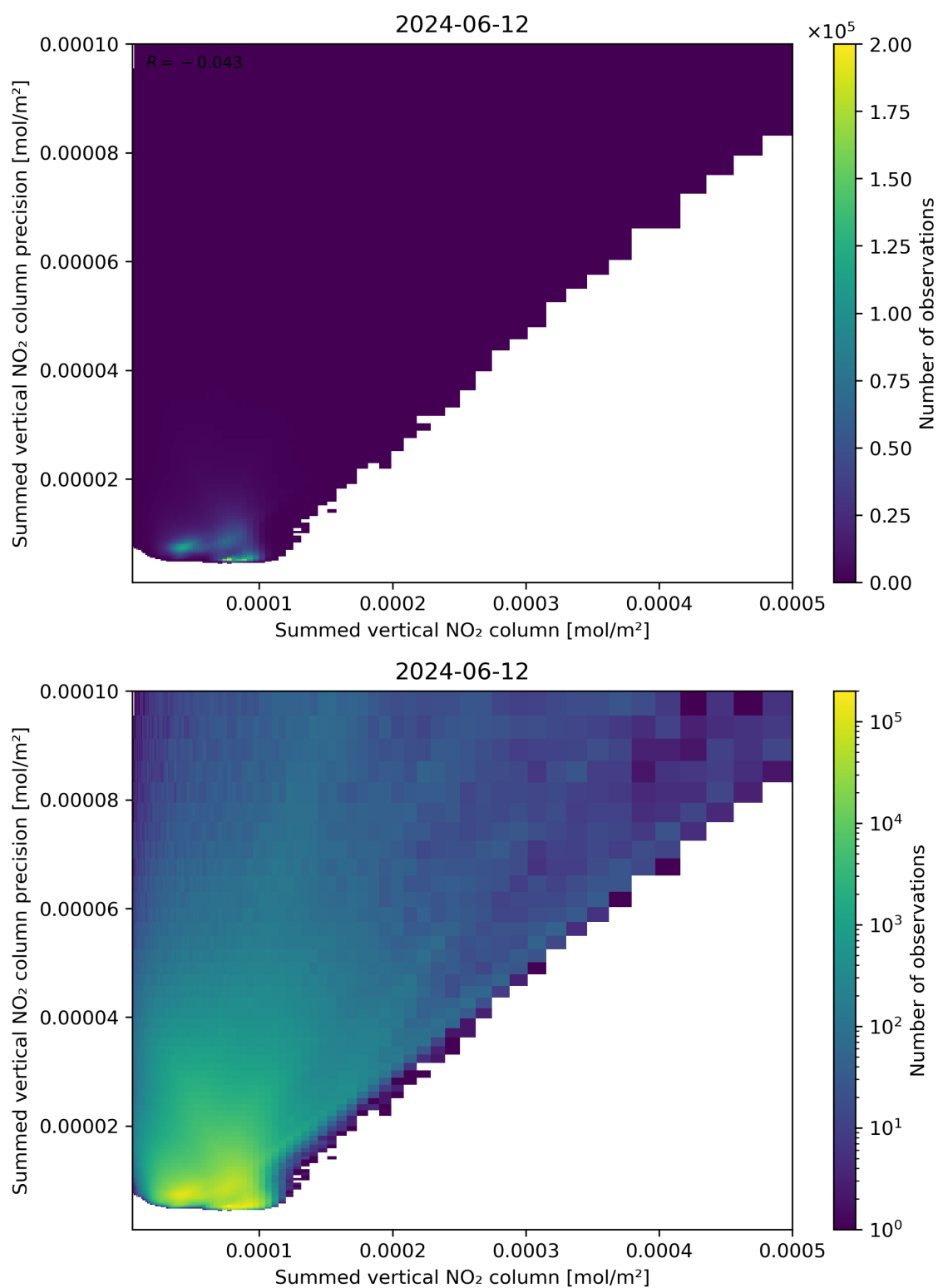
Figure 105: Scatter density plot of “Summed vertical NO 2 column” against “Summed vertical NO 2 column precision” for 2024-06-11 to 2024-06-13.
