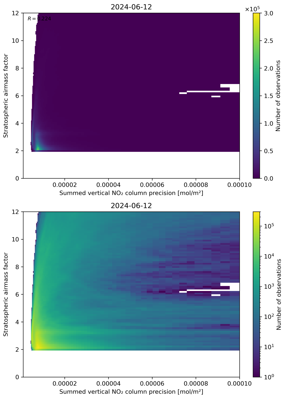
Figure 106: Scatter density plot of “Summed vertical NO 2 column precision” against “Stratospheric airmass factor” for 2024-06-11 to 2024-06-13.
