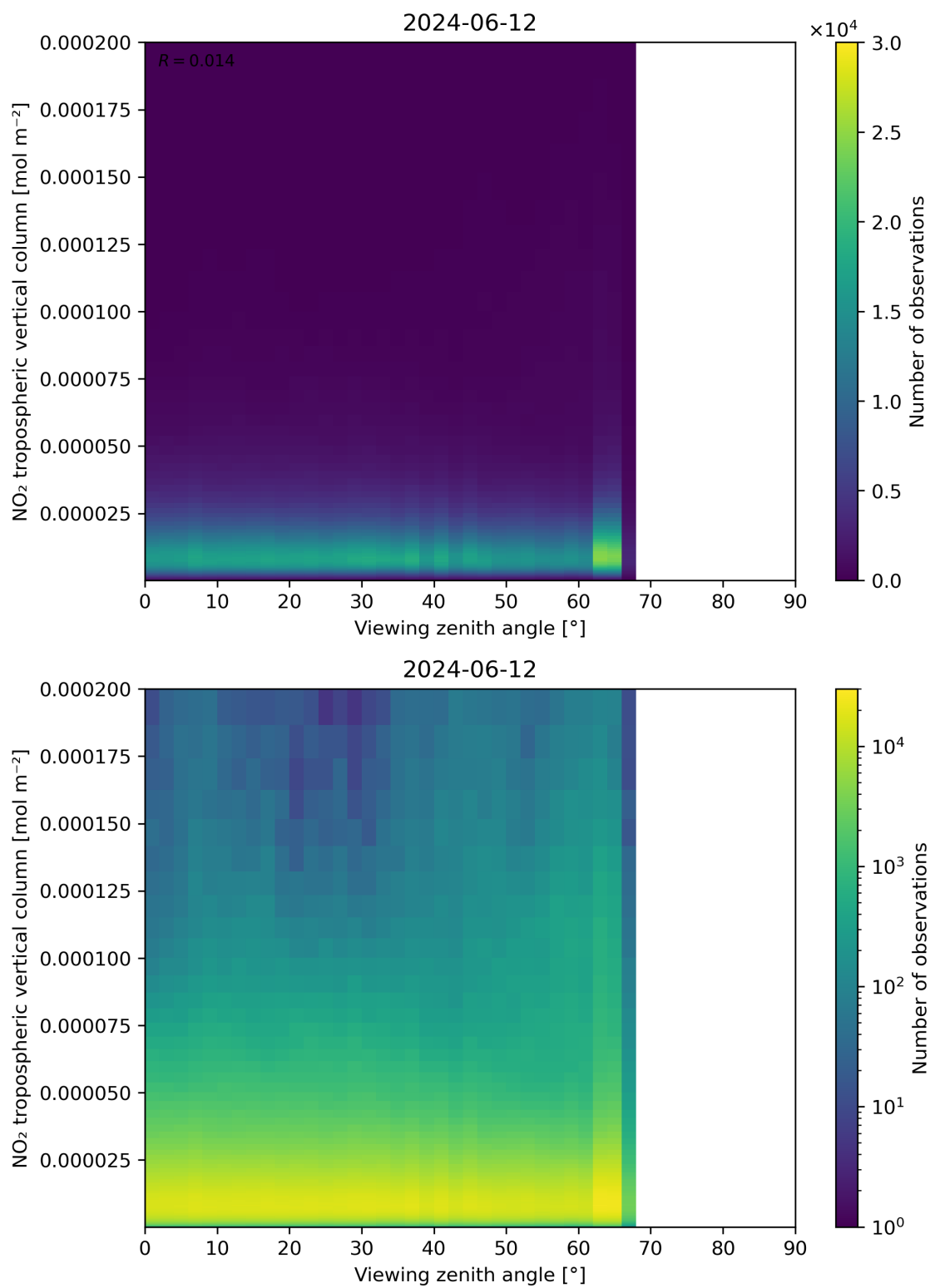
Figure 169: Scatter density plot of “Viewing zenith angle” against “NO 2 tropospheric vertical column” for 2024-06-11 to 2024-06-13.
