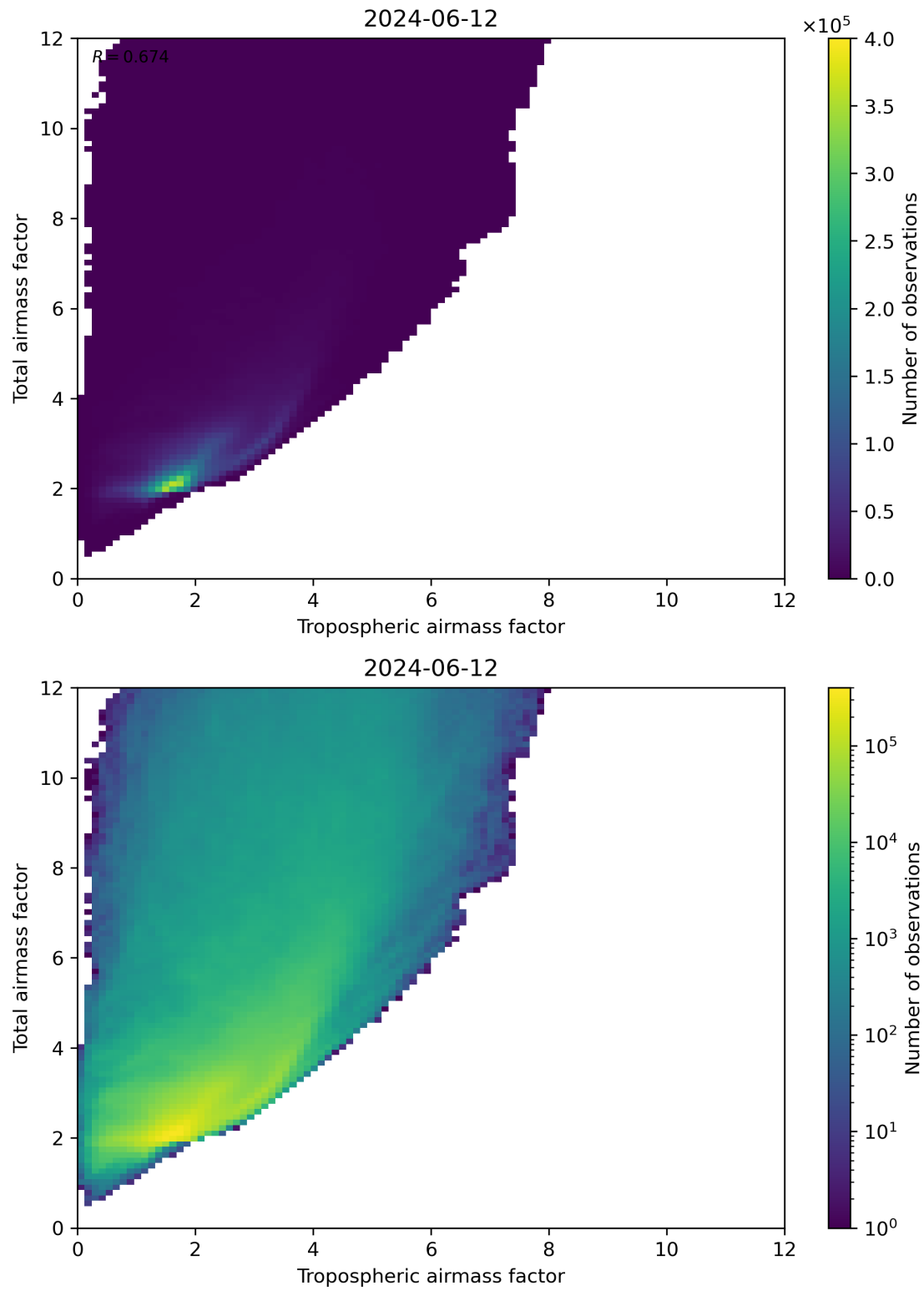
Figure 72: Scatter density plot of “Tropospheric airmass factor” against “Total airmass factor” for 2024-06-11 to 2024-06-13.
