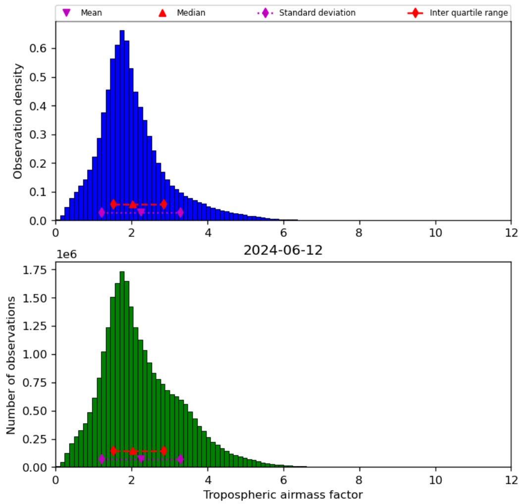
Figure 31: Histogram of “Tropospheric airmass factor” for 2024-06-11 to 2024-06-13
