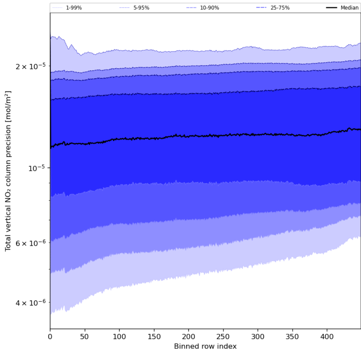
Figure 56: Along track statistics of “Total vertical NO 2 column precision” for 2024-06-11 to 2024-06-13
