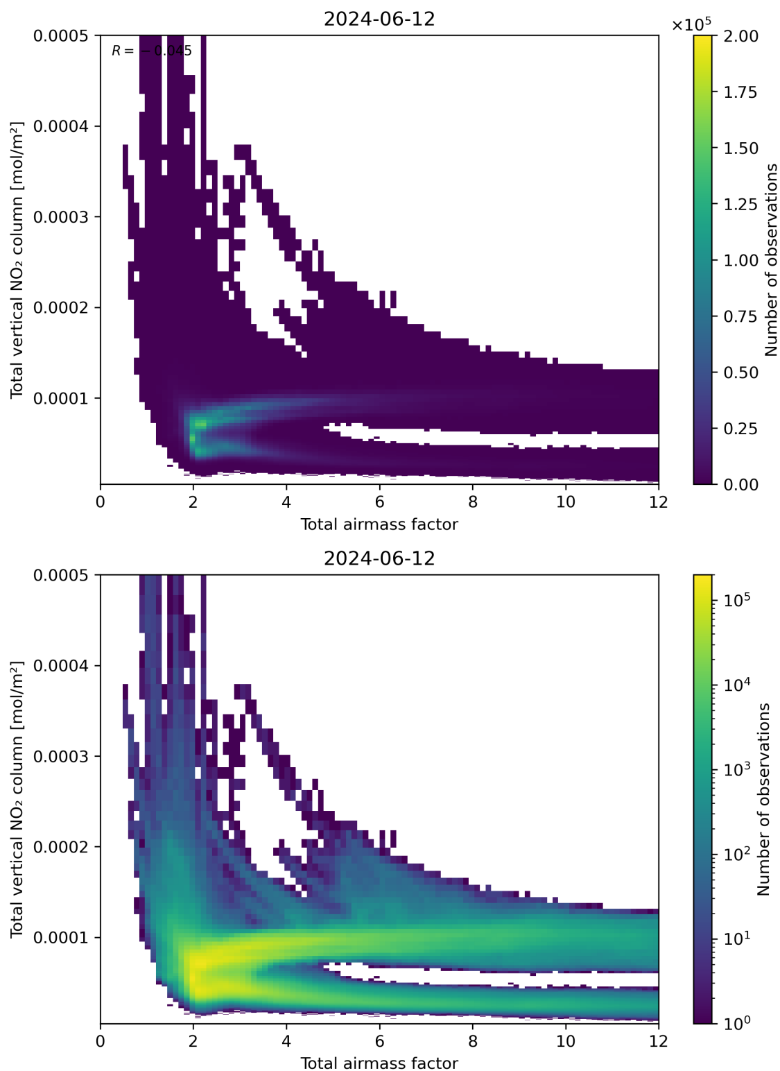
Figure 67: Scatter density plot of “Total airmass factor” against “Total vertical NO 2 column” for 2024-06-11 to 2024-06-13.
