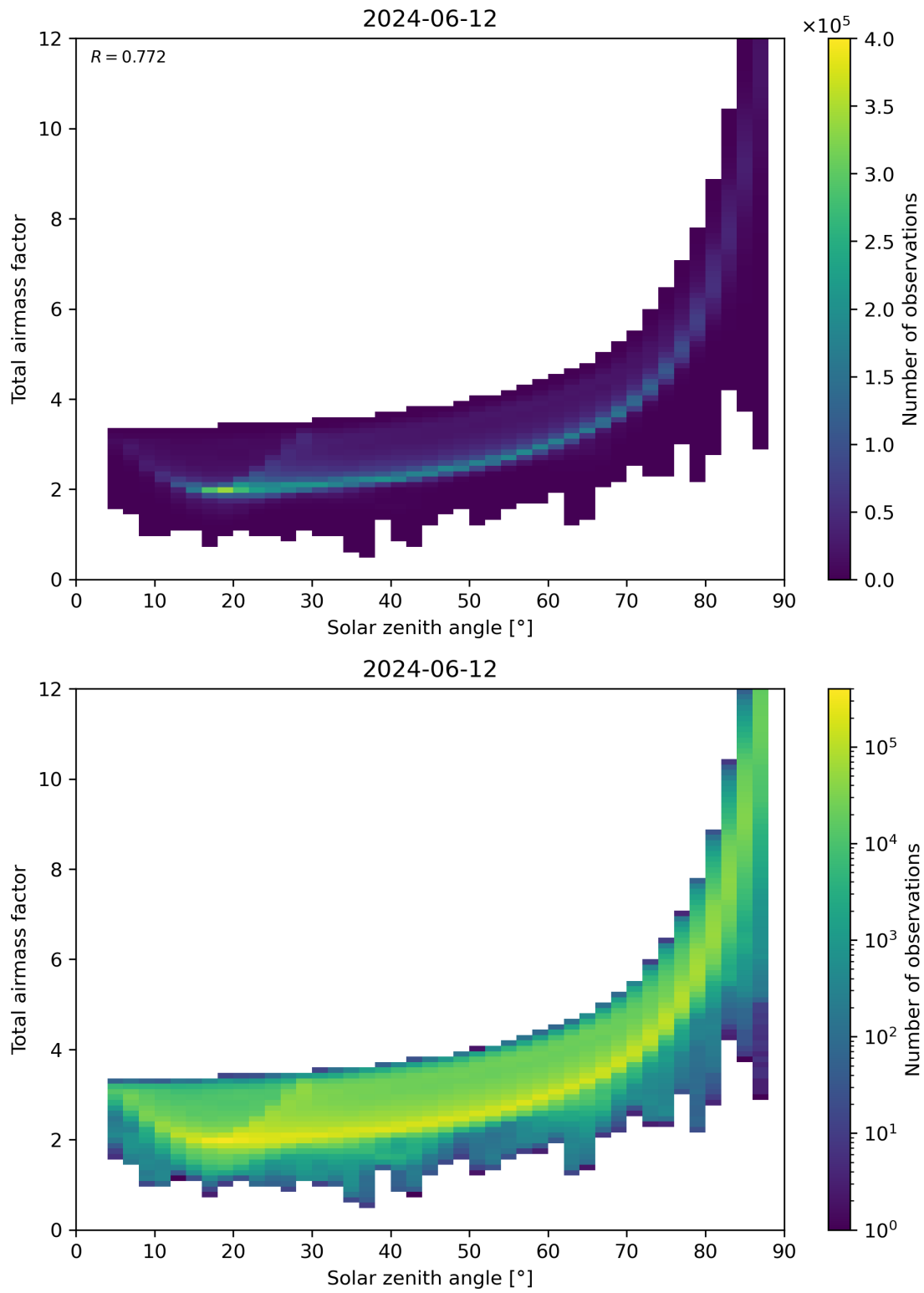
Figure 146: Scatter density plot of “Solar zenith angle” against “Total air mass factor” for 2024-06-11 to 2024-06-13.
