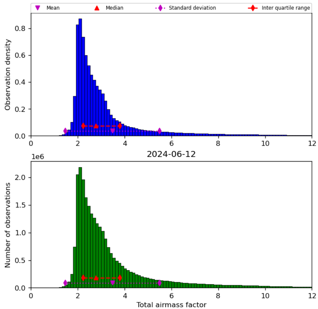
Figure 32: Histogram of “Total airmass factor” for 2024-06-11 to 2024-06-13
