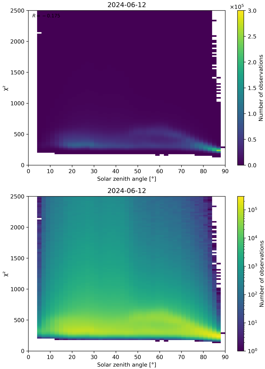
Figure 148: Scatter density plot of “Solar zenith angle” against “ \chi^2 ” for 2024-06-11 to 2024-06-13.
