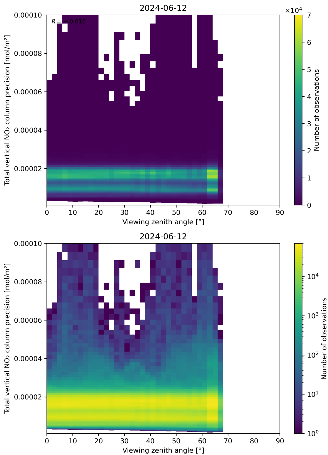
Figure 168: Scatter density plot of “Viewing zenith angle” against “Total vertical NO 2 column precision” for 2024-06-11 to 2024-06-13.
