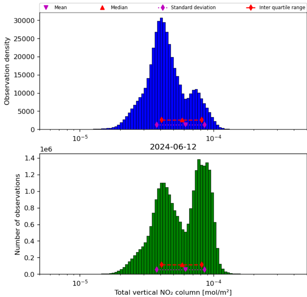
Figure 38: Histogram of “Total vertical NO 2 column” for 2024-06-11 to 2024-06-13
