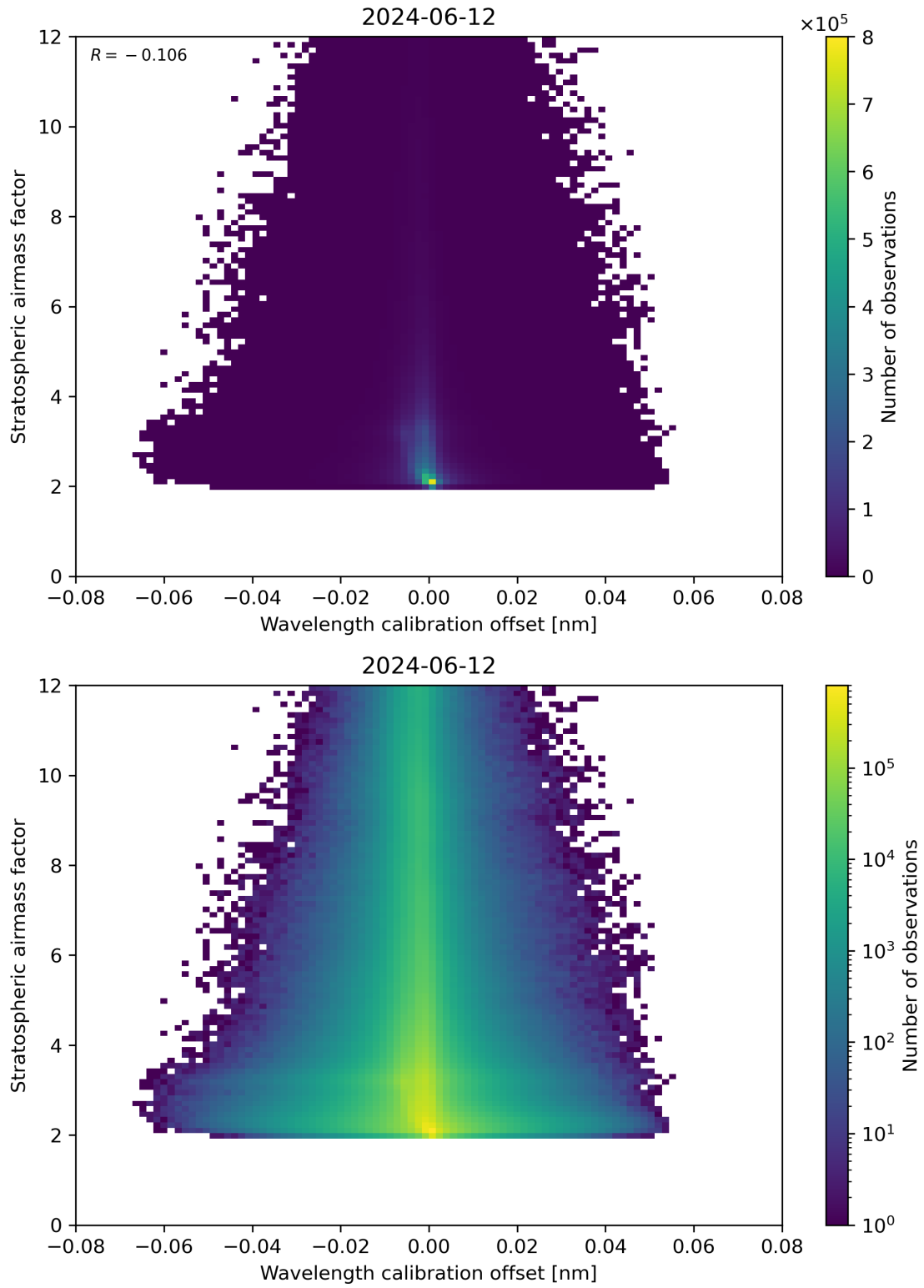
Figure 174: Scatter density plot of “Wavelength calibration offset” against “Stratospheric airmass factor” for 2024-06-11 to 2024-06-13.
