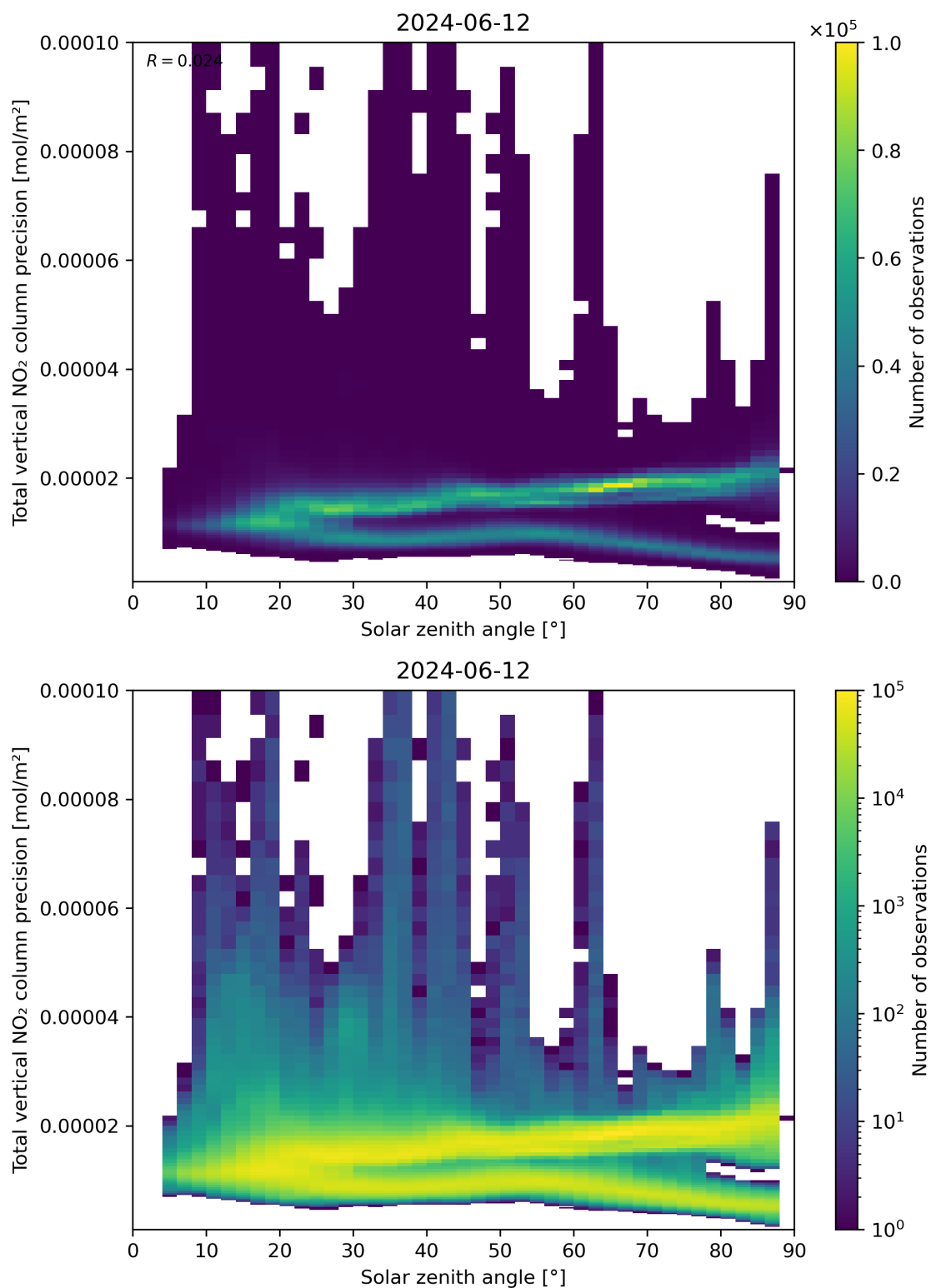
Figure 154: Scatter density plot of “Solar zenith angle” against “Total vertical NO 2 column precision” for 2024-06-11 to 2024-06-13.
