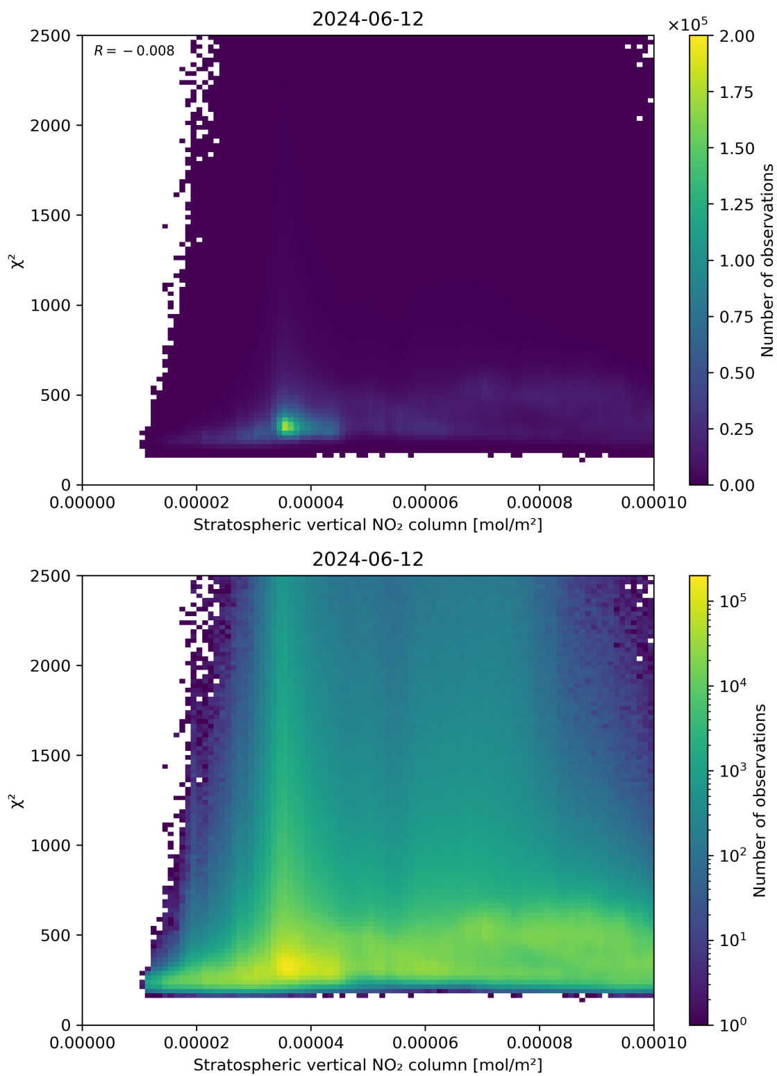
Figure 97: Scatter density plot of “Stratospheric vertical NO 2 column” against “ \chi^2 ” for 2024-06-11 to 2024-06-13.
