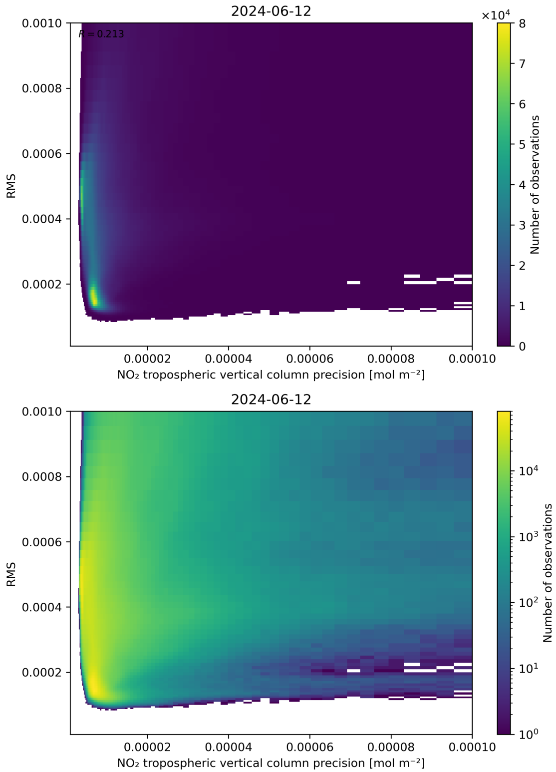
Figure 140: Scatter density plot of “NO 2 tropospheric vertical column precision” against “RMS” for 2024-06-11 to 2024-06-13.
