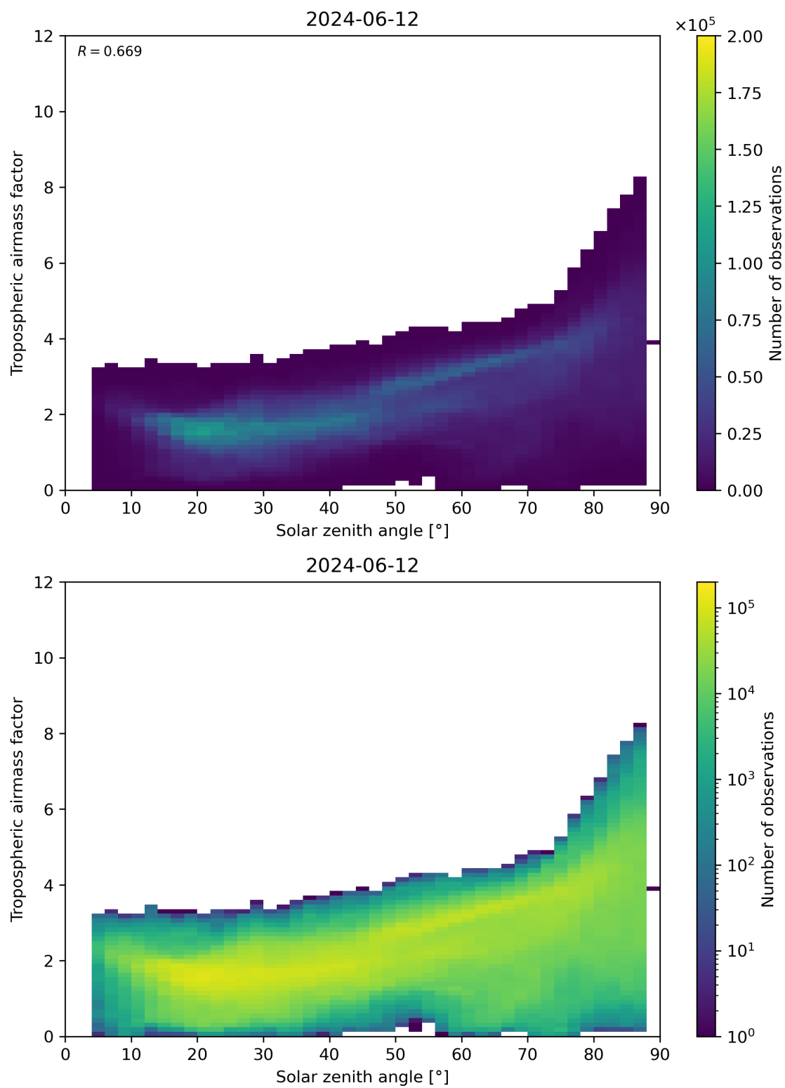
Figure 147: Scatter density plot of “Solar zenith angle” against “Tropospheric airmass factor” for 2024-06-11 to 2024-06-13.
