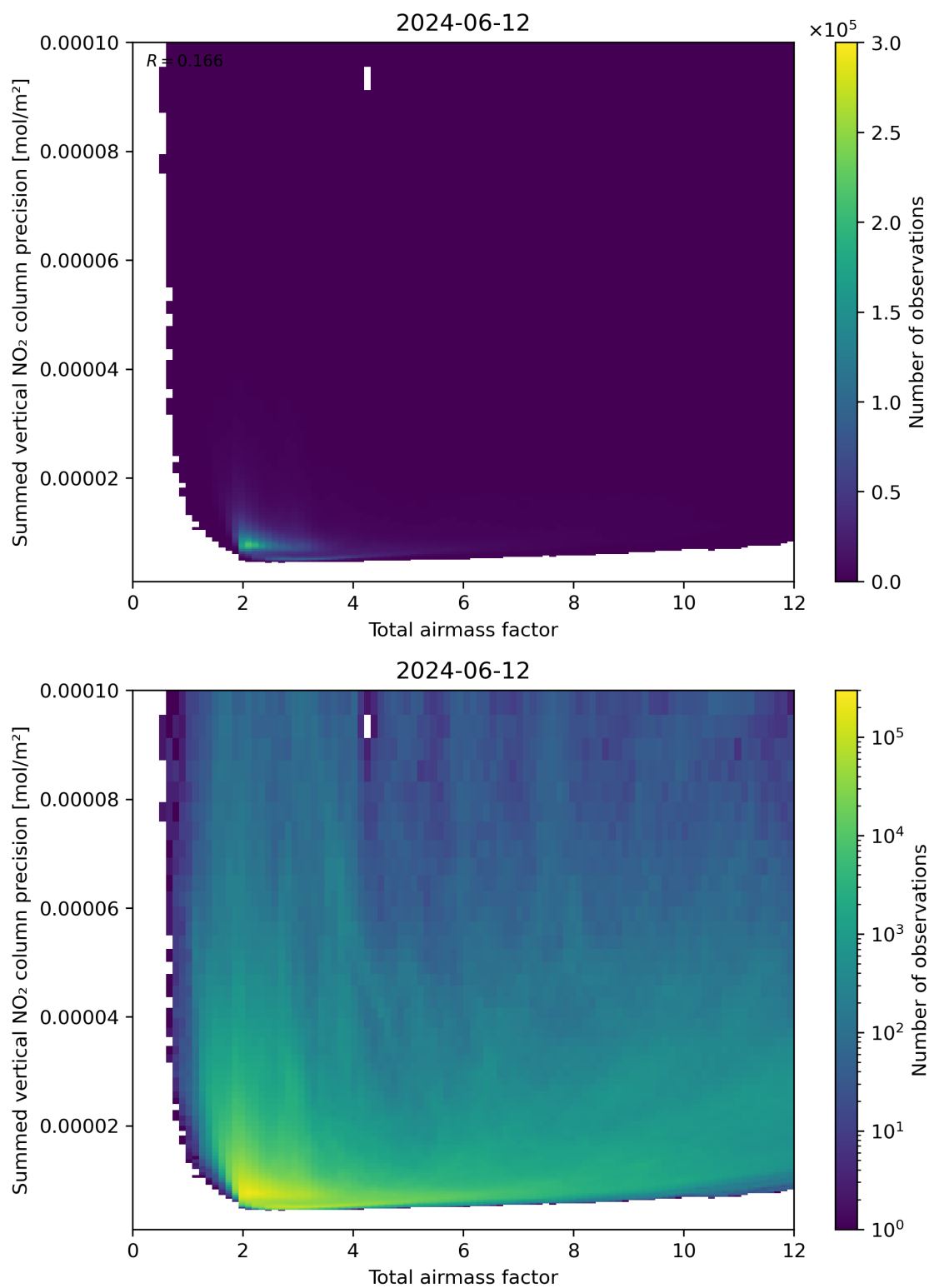
Figure 66: Scatter density plot of “Total airmass factor” against “Summed vertical NO 2 column precision” for 2024-06-11 to 2024-06-13.
