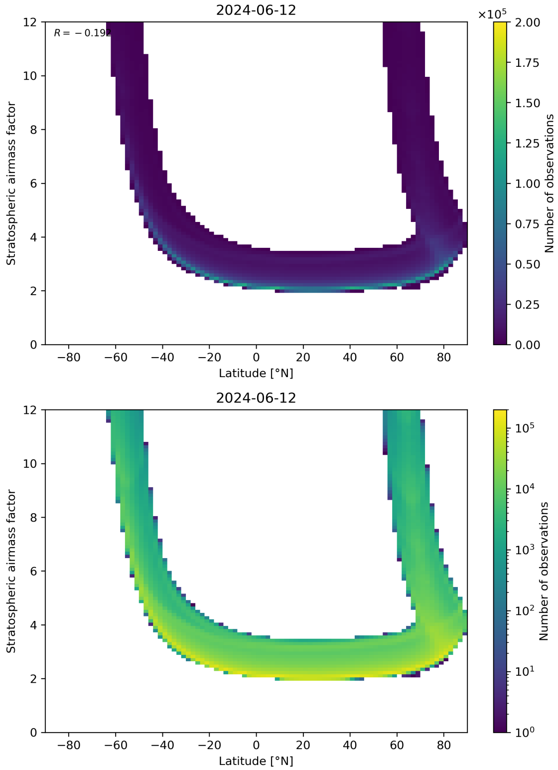
Figure 83: Scatter density plot of “Latitude” against “Stratospheric air mass factor” for 2024-06-11 to 2024-06-13.
