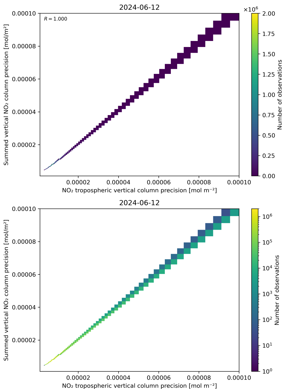
Figure 137: Scatter density plot of “NO 2 tropospheric vertical column precision” against “Summed vertical NO 2 column precision” for 2024-06-11 to 2024-06-13.
