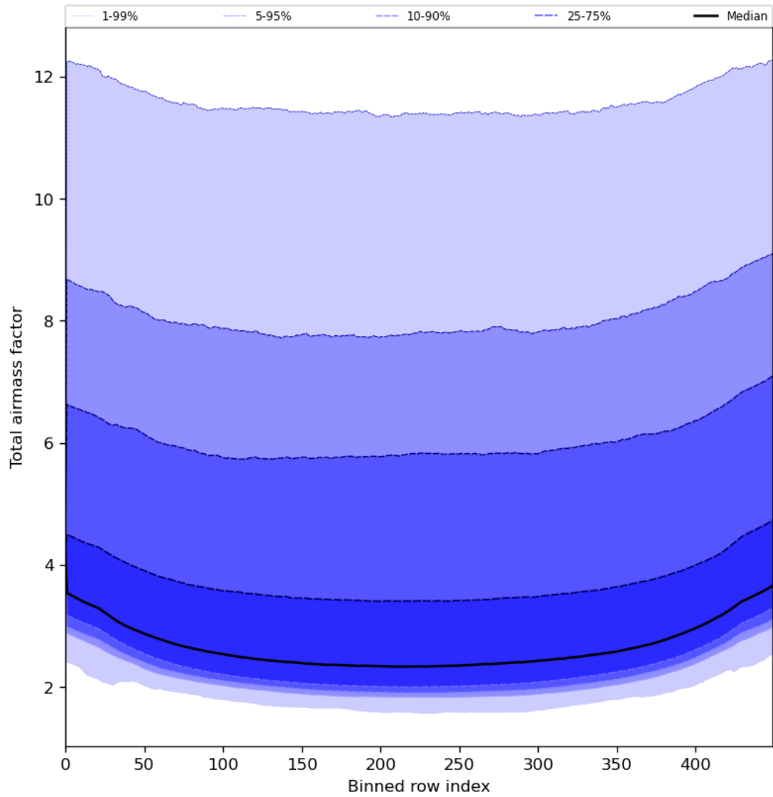
Figure 49: Along track statistics of “Total airmass factor” for 2024-06-11 to 2024-06-13
