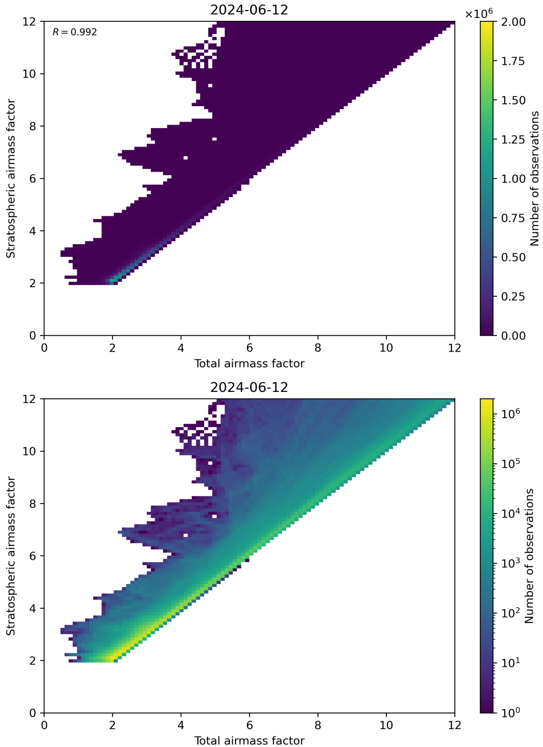
Figure 62: Scatter density plot of “Total airmass factor” against “Stratospheric airmass factor” for 2024-06-11 to 2024-06-13.
