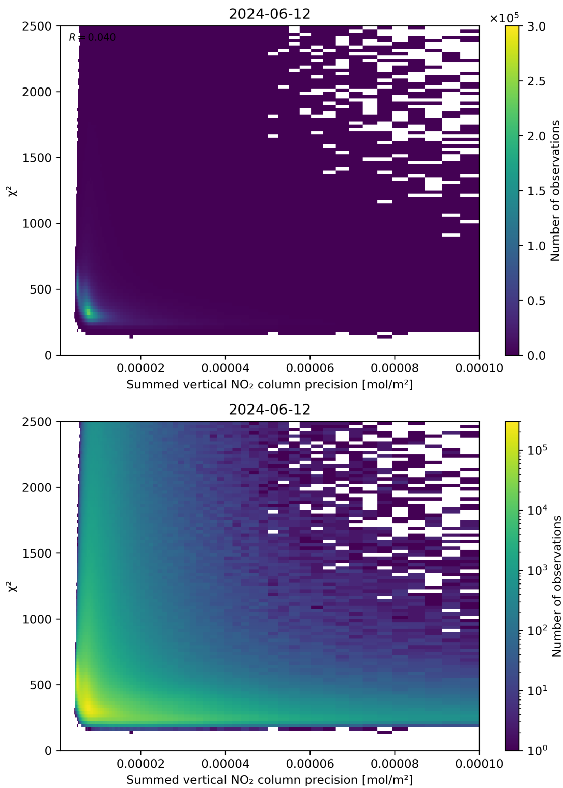
Figure 107: Scatter density plot of “Summed vertical NO 2 column precision” against “ \chi^2 ” for 2024-06-11 to 2024-06-13.
