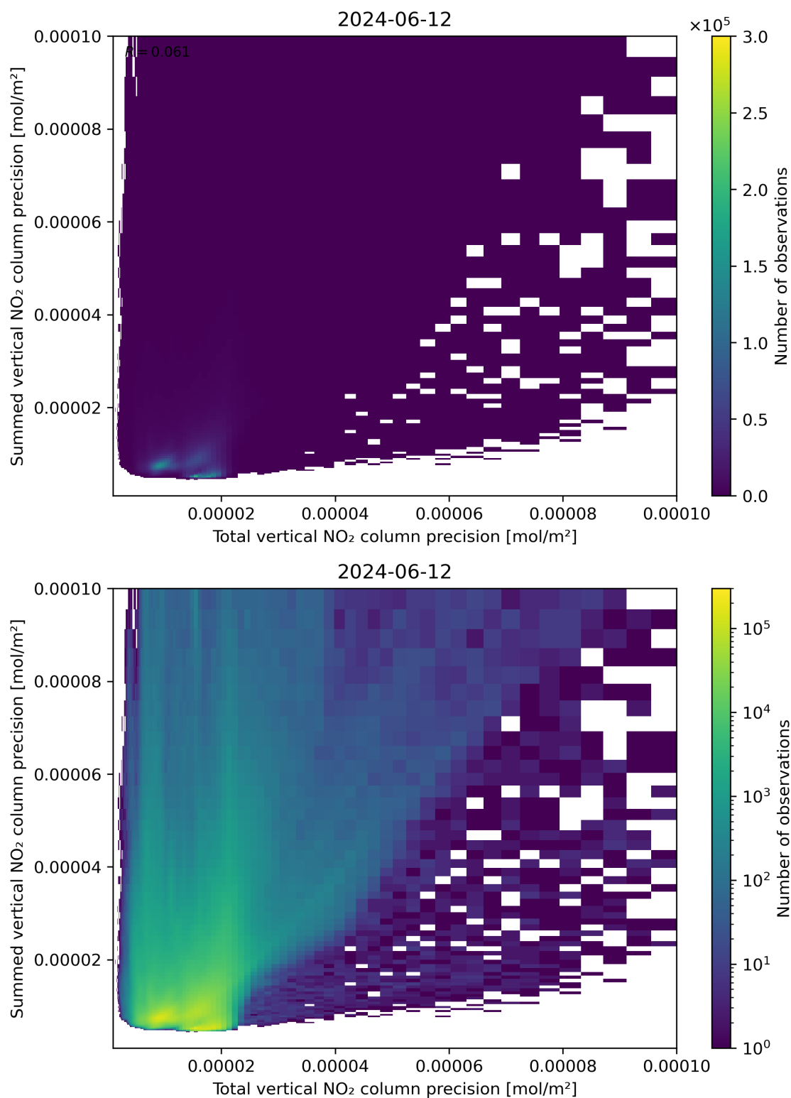
Figure 118: Scatter density plot of “Total vertical NO 2 column precision” against “Summed vertical NO 2 column precision” for 2024-06-11 to 2024-06-13.
