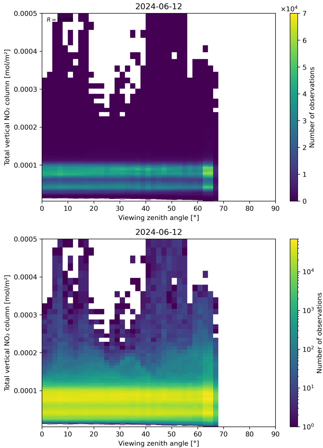
Figure 167: Scatter density plot of “Viewing zenith angle” against “Total vertical NO 2 column” for 2024-06-11 to 2024-06-13.
