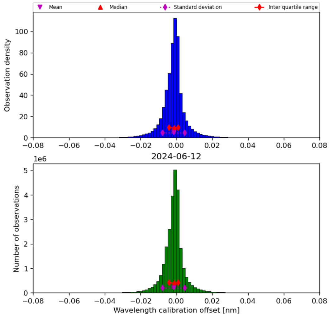
Figure 35: Histogram of “Wavelength calibration offset” for 2024-06-11 to 2024-06-13
