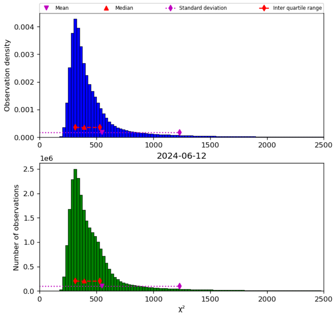
Figure 42: Histogram of “ \chi^2 ” for 2024-06-11 to 2024-06-13
