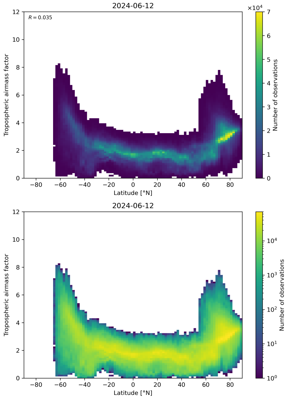
Figure 85: Scatter density plot of “Latitude” against “Tropospheric airmass factor” for 2024-06-11 to 2024-06-13.
