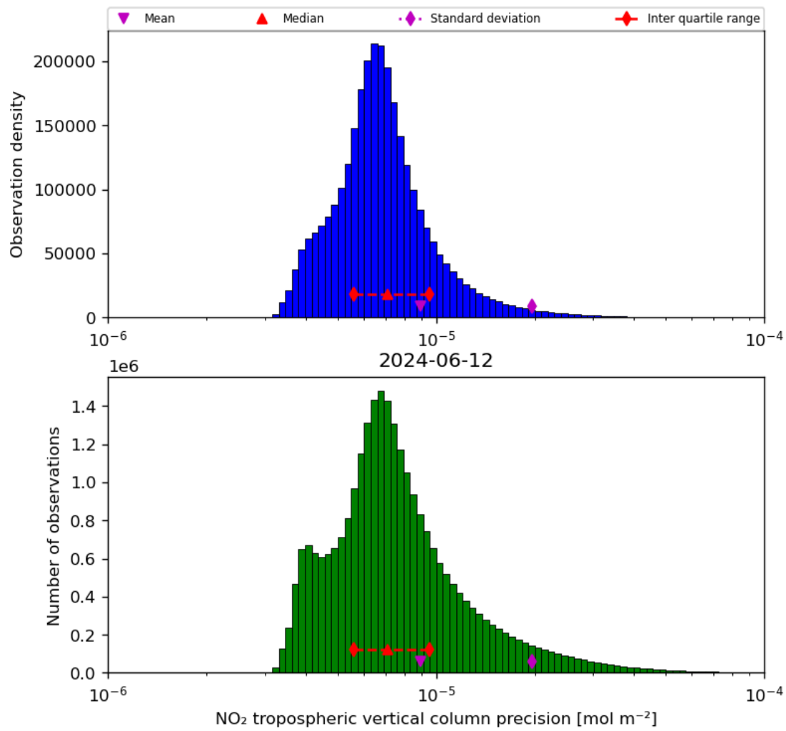
Figure 30: Histogram of “NO 2 tropospheric vertical column precision” for 2024-06-11 to 2024-06-13
