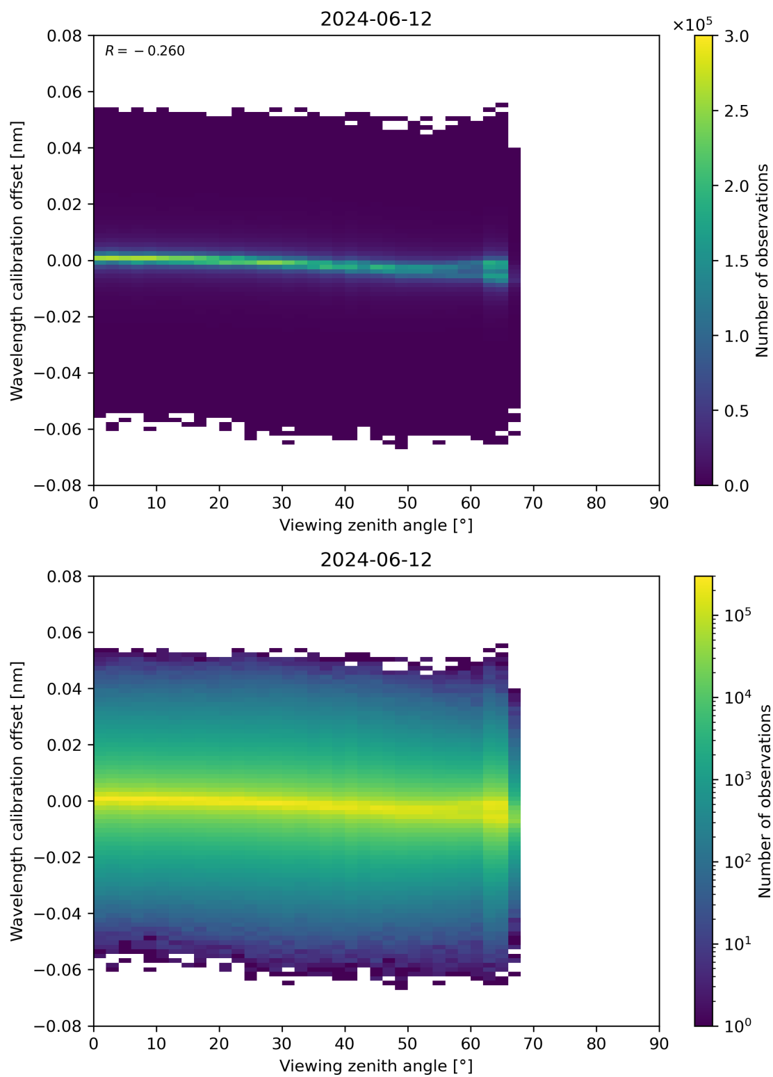
Figure 173: Scatter density plot of “Viewing zenith angle” against “Wavelength calibration offset” for 2024-06-11 to 2024-06-13.
