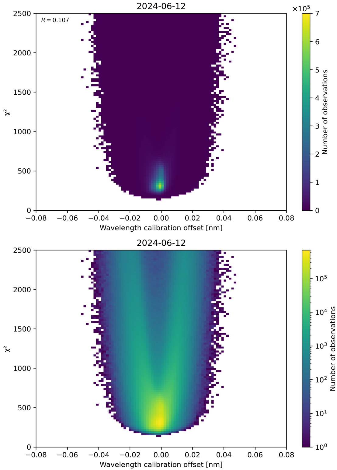
Figure 175: Scatter density plot of “Wavelength calibration offset” against “ \chi^2 ” for 2024-06-11 to 2024-06-13.
