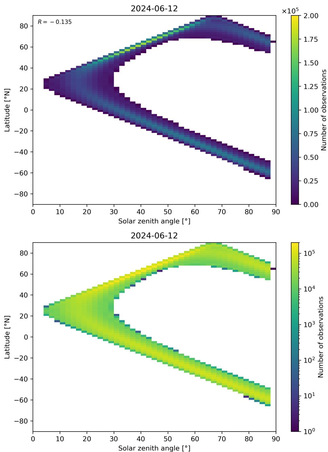
Figure 149: Scatter density plot of “Solar zenith angle” against “Latitude” for 2024-06-11 to 2024-06-13.
