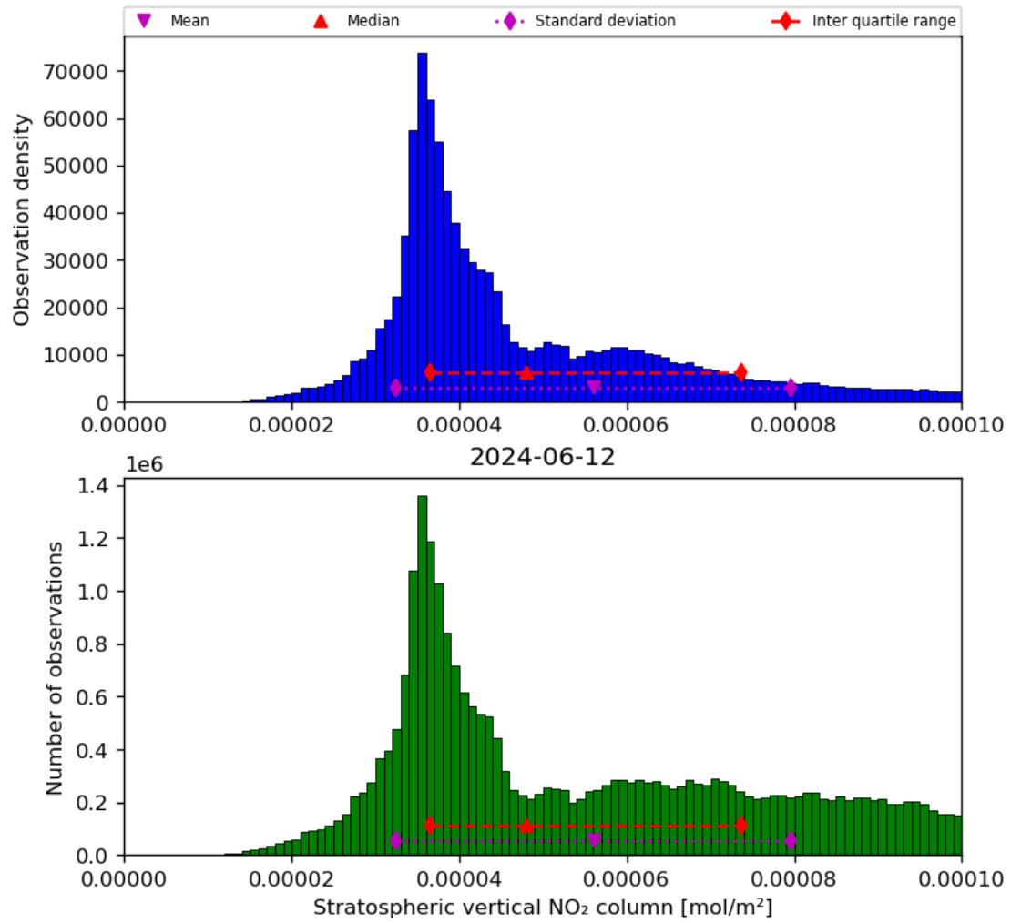
Figure 36: Histogram of “Stratospheric vertical NO 2 column” for 2024-06-11 to 2024-06-13
