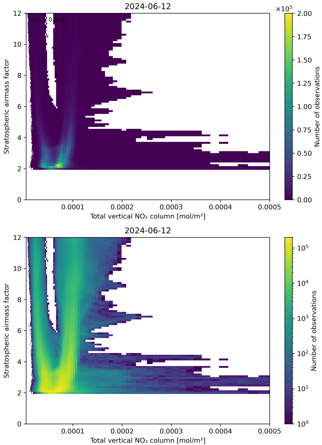
Figure 110: Scatter density plot of “Total vertical NO 2 column” against “Stratospheric airmass factor” for 2024-06-11 to 2024-06-13.
