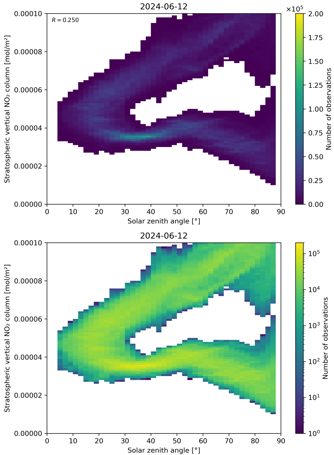
Figure 150: Scatter density plot of “Solar zenith angle” against “Stratospheric vertical NO 2 column” for 2024-06-11 to 2024-06-13.
