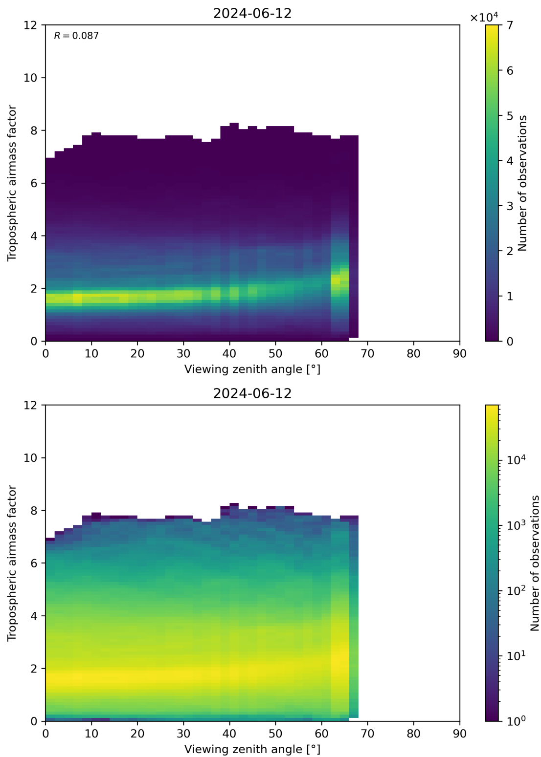
Figure 161: Scatter density plot of “Viewing zenith angle” against “Tropospheric airmass factor” for 2024-06-11 to 2024-06-13.
