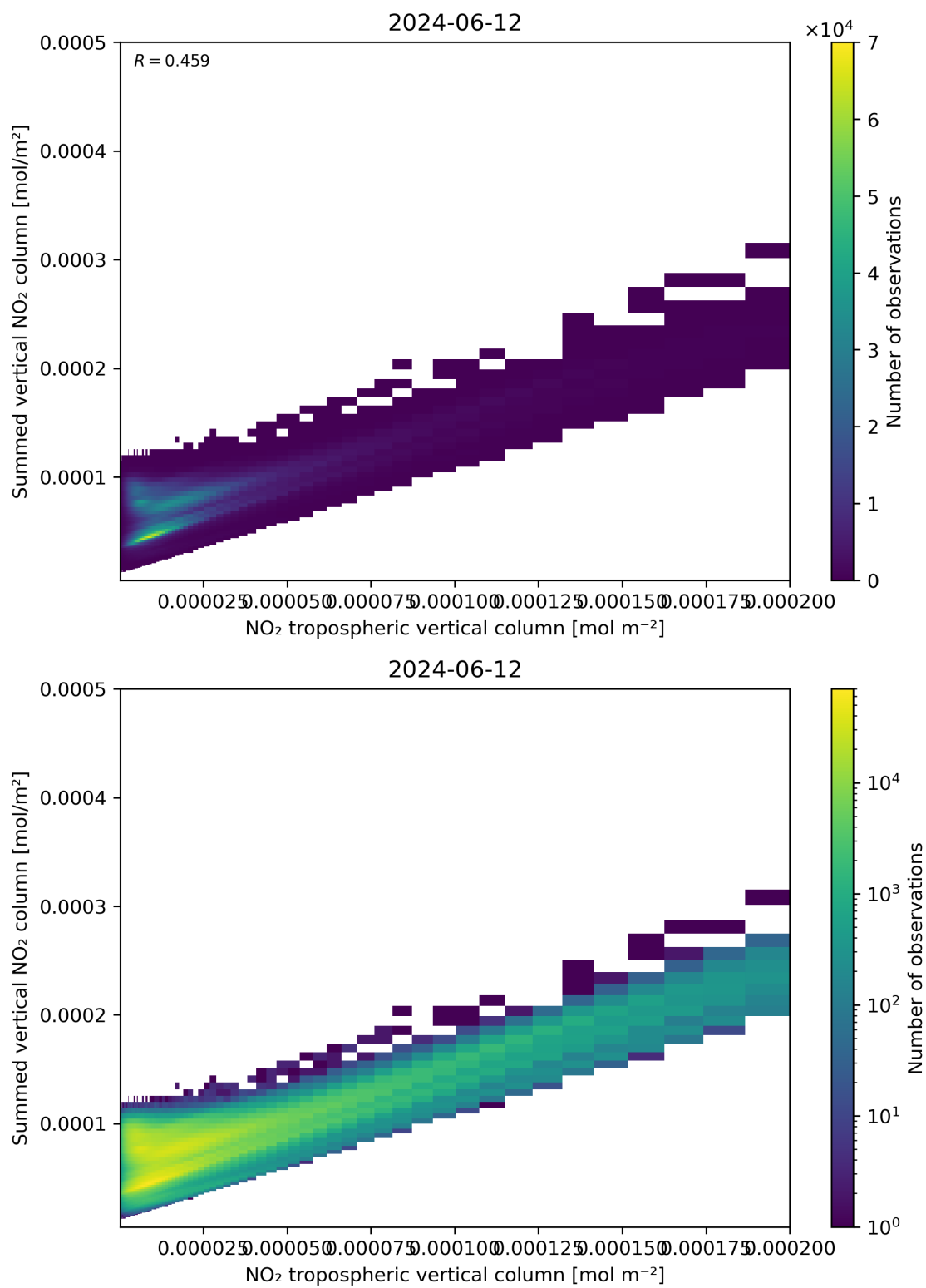
Figure 126: Scatter density plot of “NO 2 tropospheric vertical column” against “Summed vertical NO 2 column” for 2024-06-11 to 2024-06-13.
