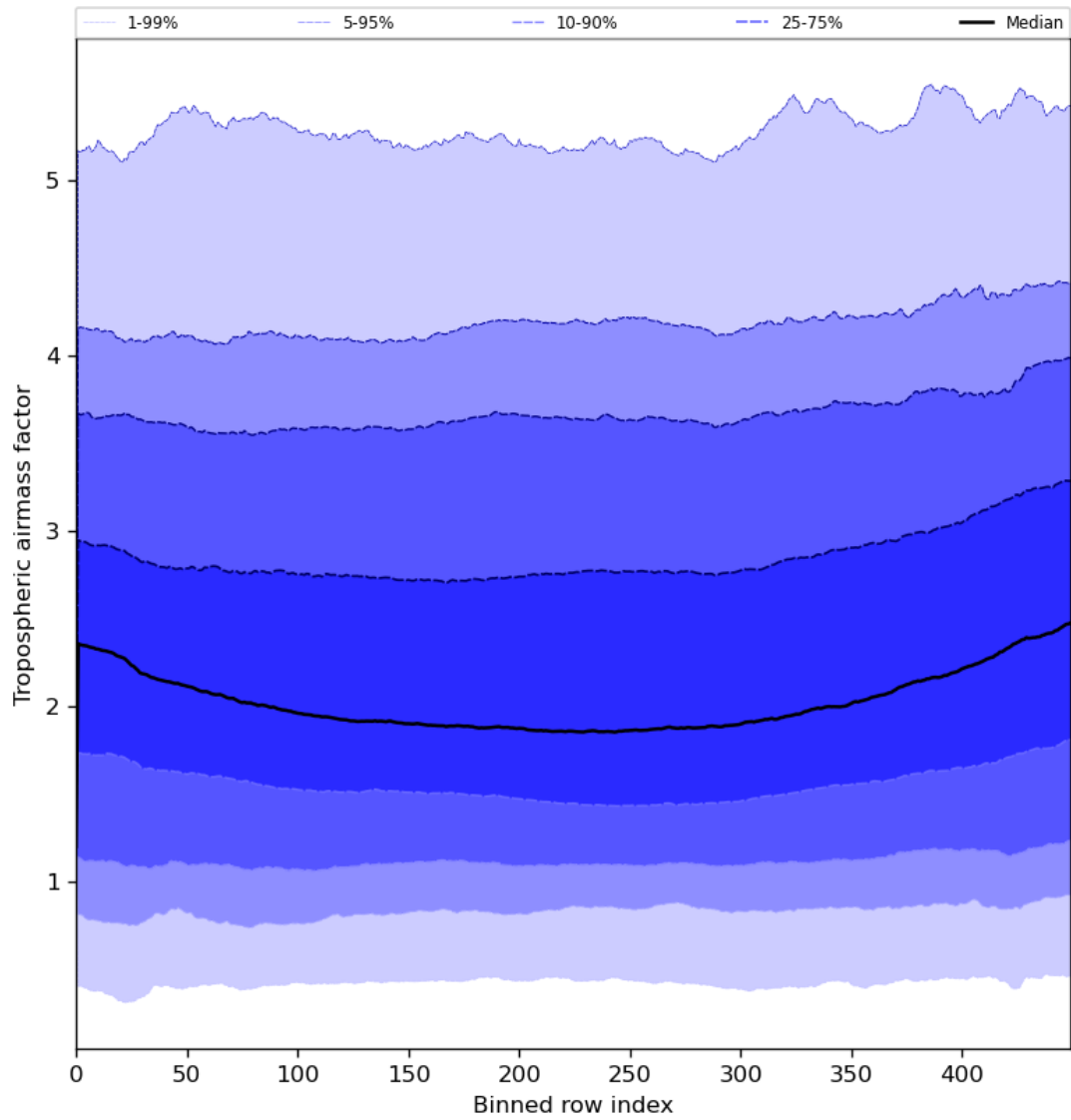
Figure 48: Along track statistics of “Tropospheric airmass factor” for 2024-06-11 to 2024-06-13
