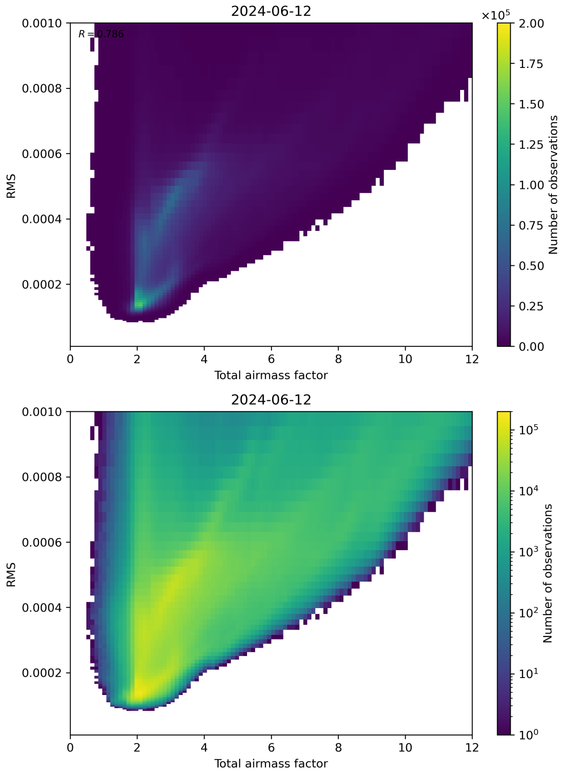
Figure 69: Scatter density plot of “Total airmass factor” against “RMS” for 2024-06-11 to 2024-06-13.
