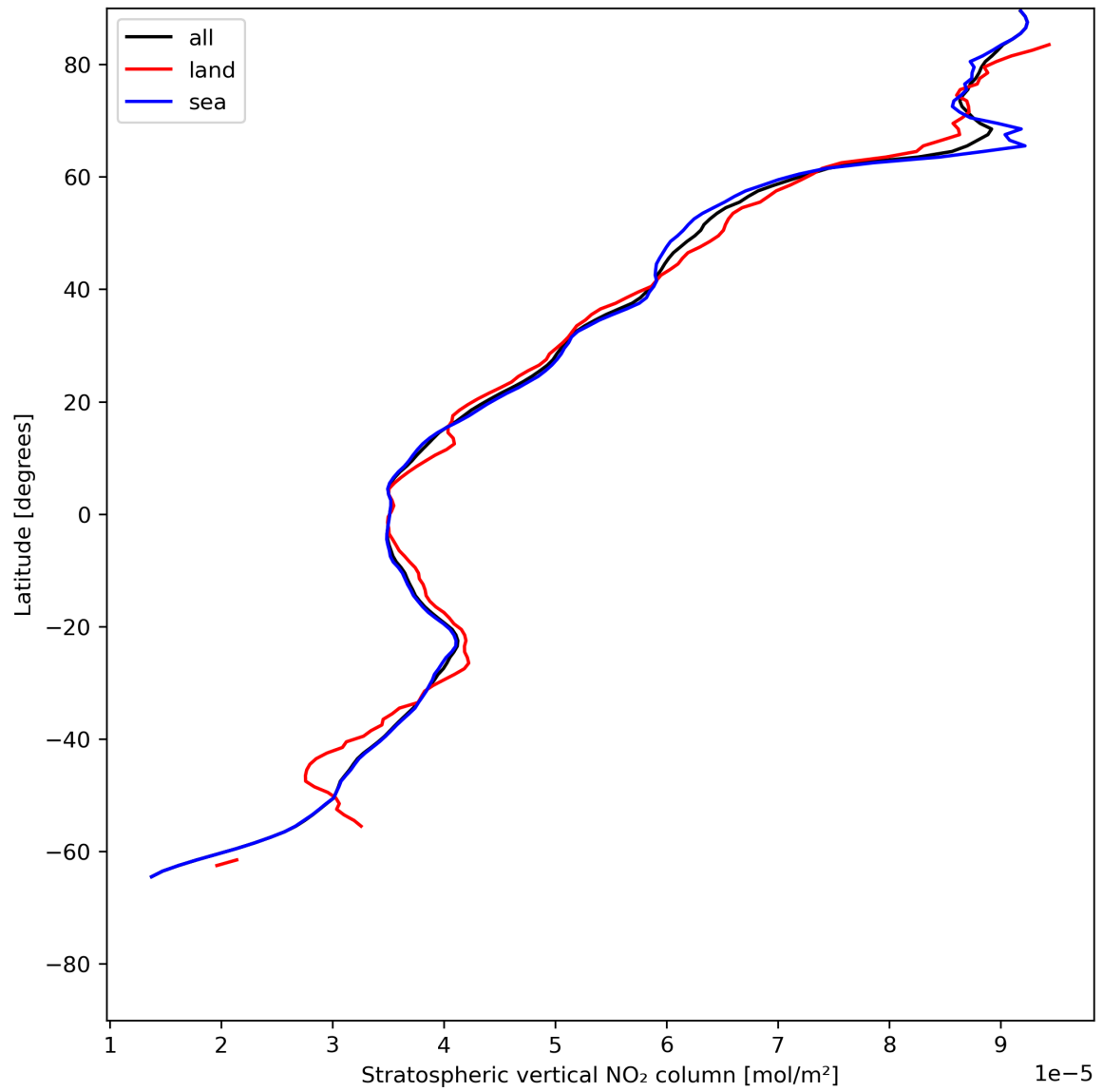
Figure 19: Zonal average of “Stratospheric vertical NO 2 column” for 2024-06-11 to 2024-06-13.
