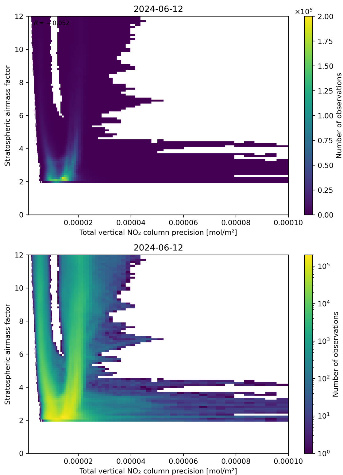
Figure 115: Scatter density plot of “Total vertical NO 2 column precision” against “Stratospheric air mass factor” for 2024-06-11 to 2024-06-13.
