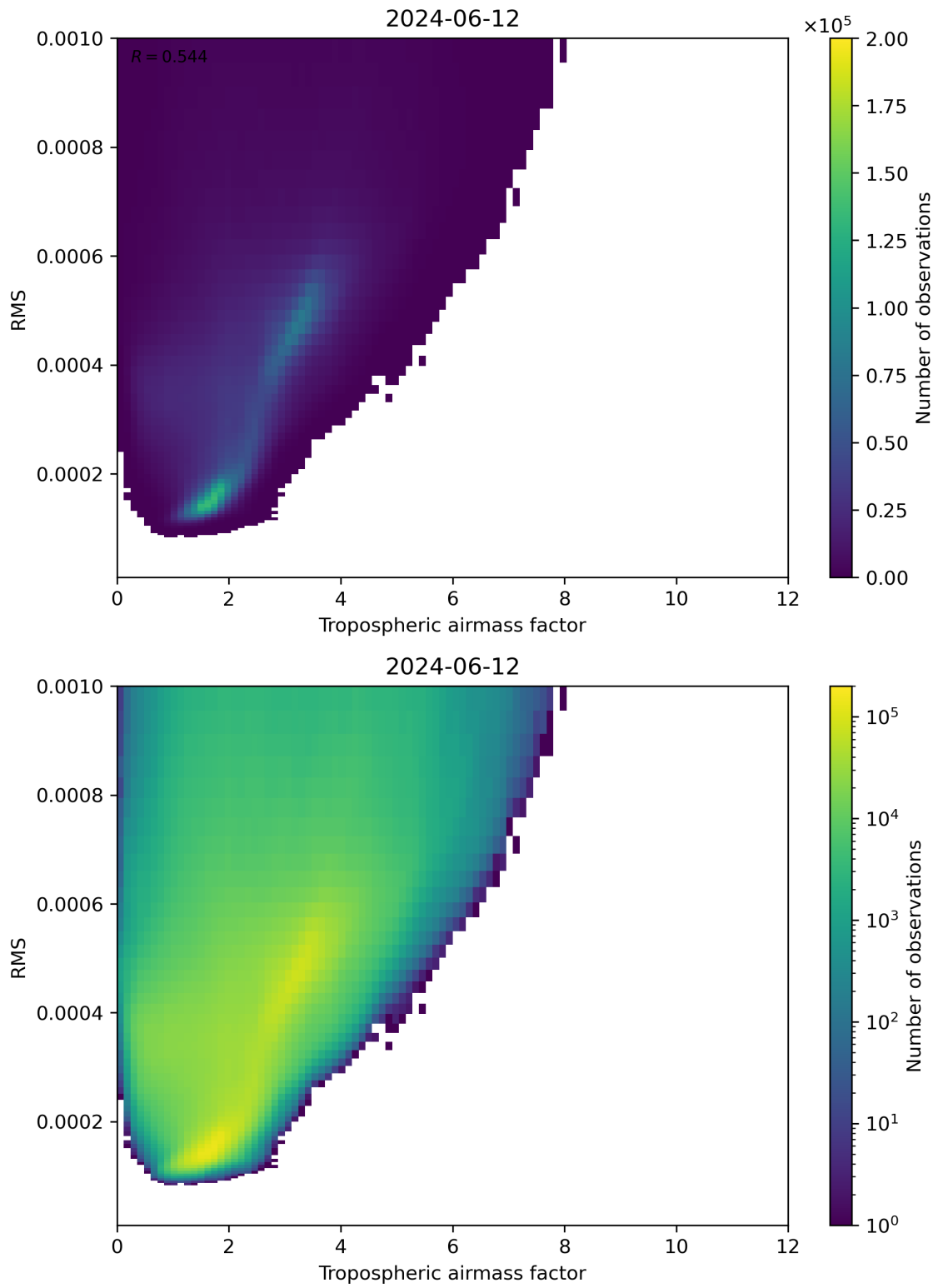
Figure 79: Scatter density plot of “Tropospheric airmass factor” against “RMS” for 2024-06-11 to 2024-06-13.
