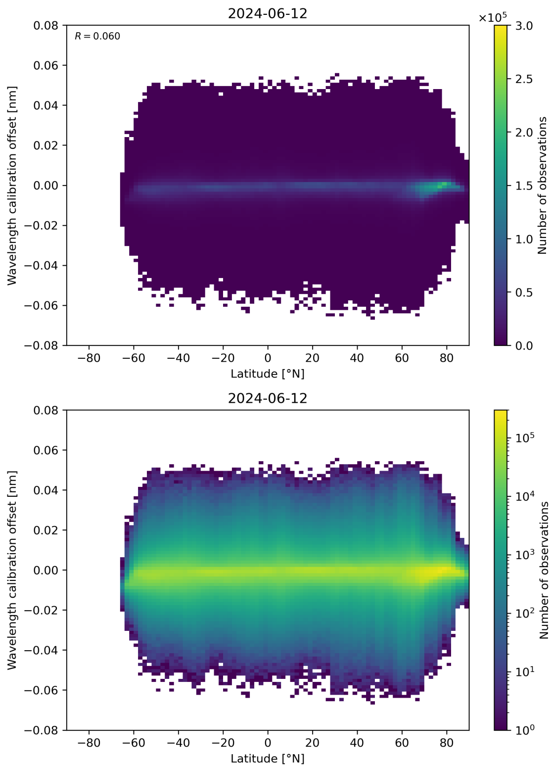
Figure 95: Scatter density plot of “Latitude” against “Wavelength calibration offset” for 2024-06-11 to 2024-06-13.
