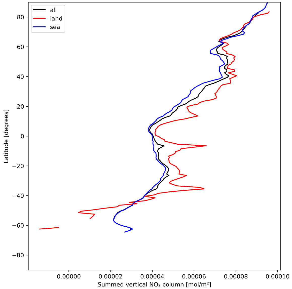
Figure 23: Zonal average of “Summed vertical NO 2 column” for 2024-06-11 to 2024-06-13.
