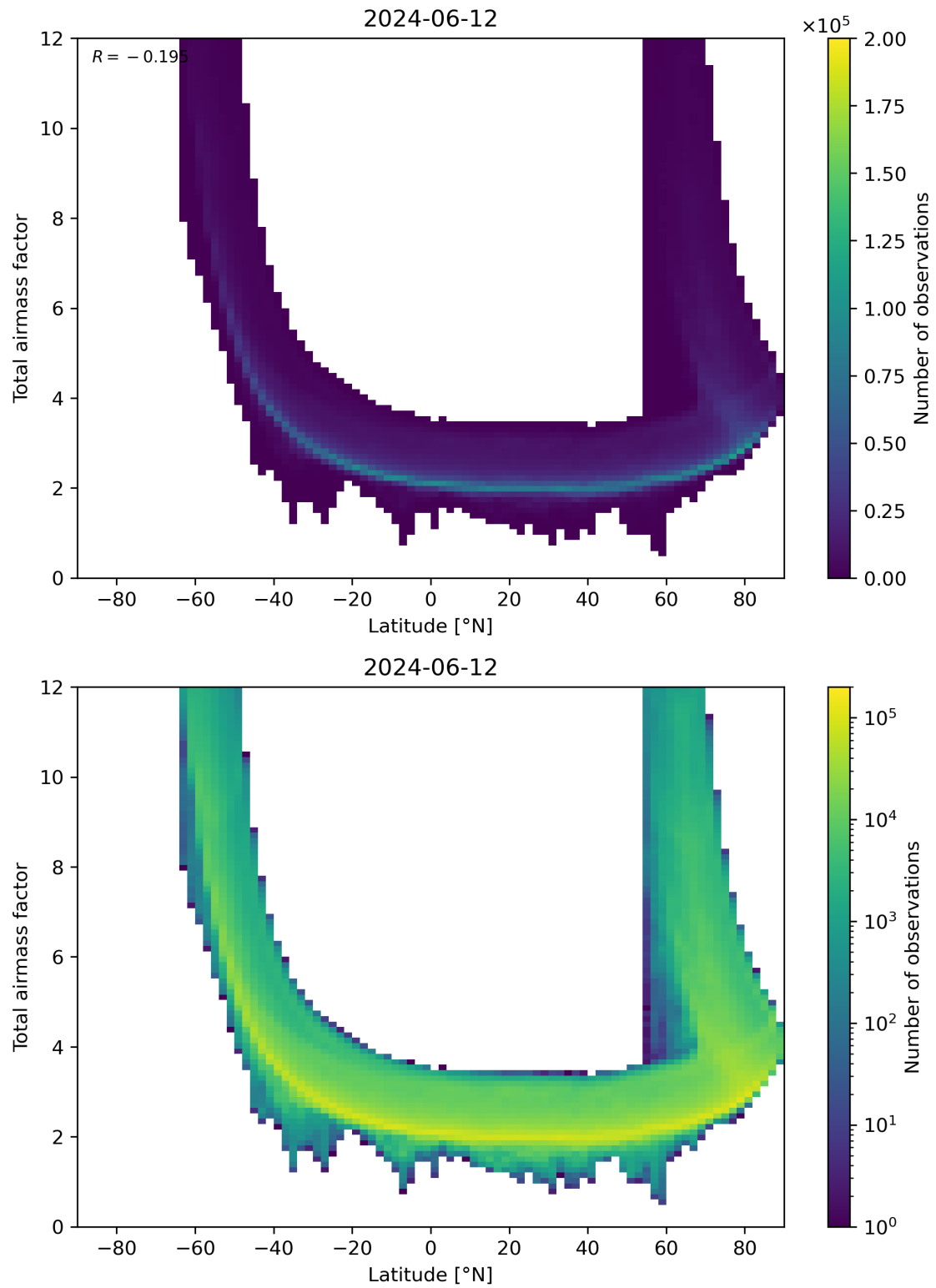
Figure 84: Scatter density plot of “Latitude” against “Total airmass factor” for 2024-06-11 to 2024-06-13.
