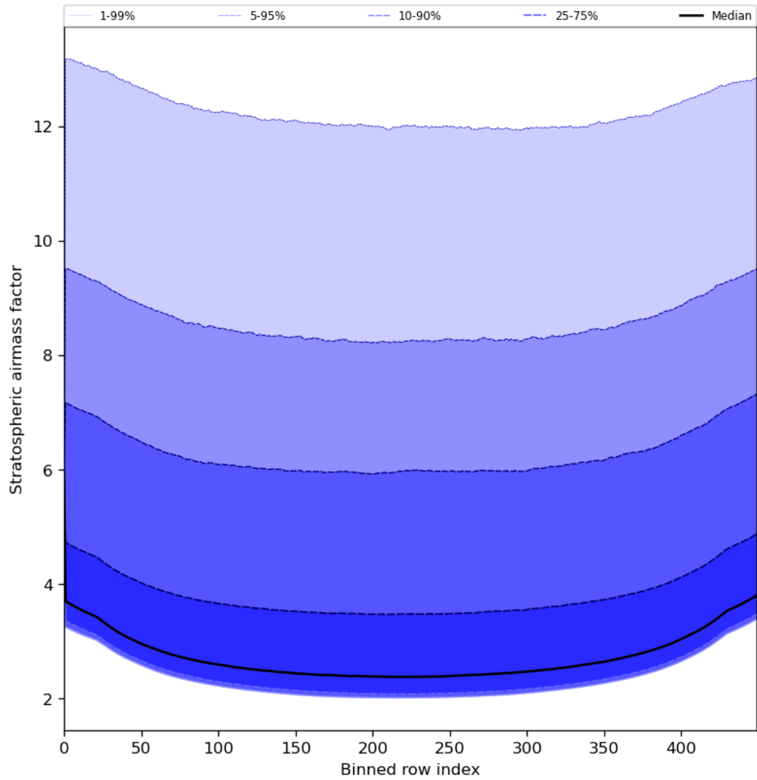
Figure 61: Along track statistics of “Stratospheric airmass factor” for 2024-06-11 to 2024-06-13
