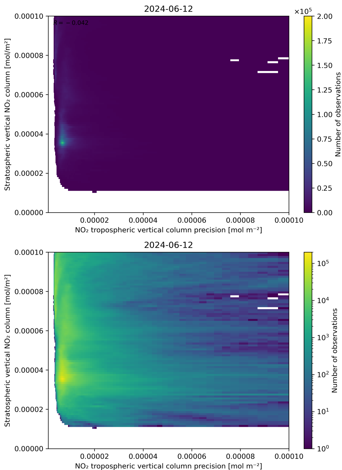
Figure 135: Scatter density plot of “NO 2 tropospheric vertical column precision” against “Stratospheric vertical NO 2 column” for 2024-06-11 to 2024-06-13.
