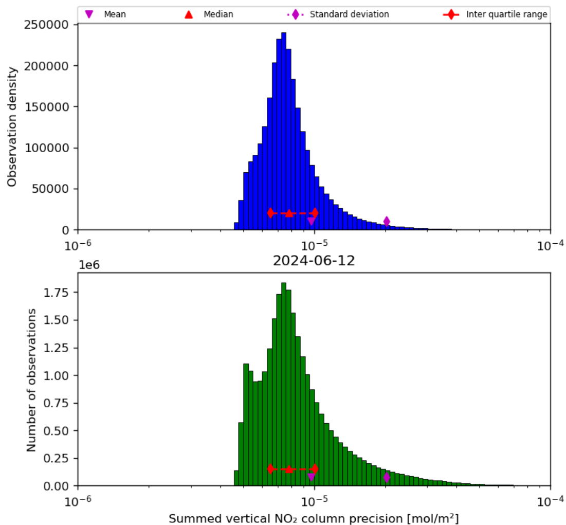
Figure 41: Histogram of "Summed vertical NO 2 column precision" for 2024-06-11 to 2024-06-13
