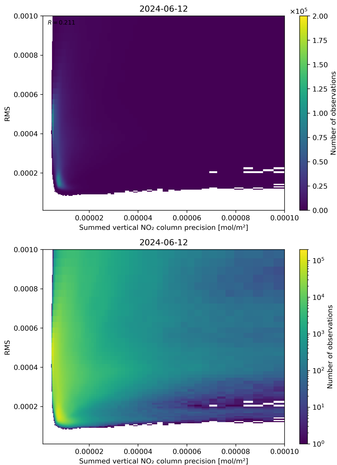
Figure 108: Scatter density plot of “Summed vertical NO 2 column precision” against “RMS” for 2024-06-11 to 2024-06-13.
