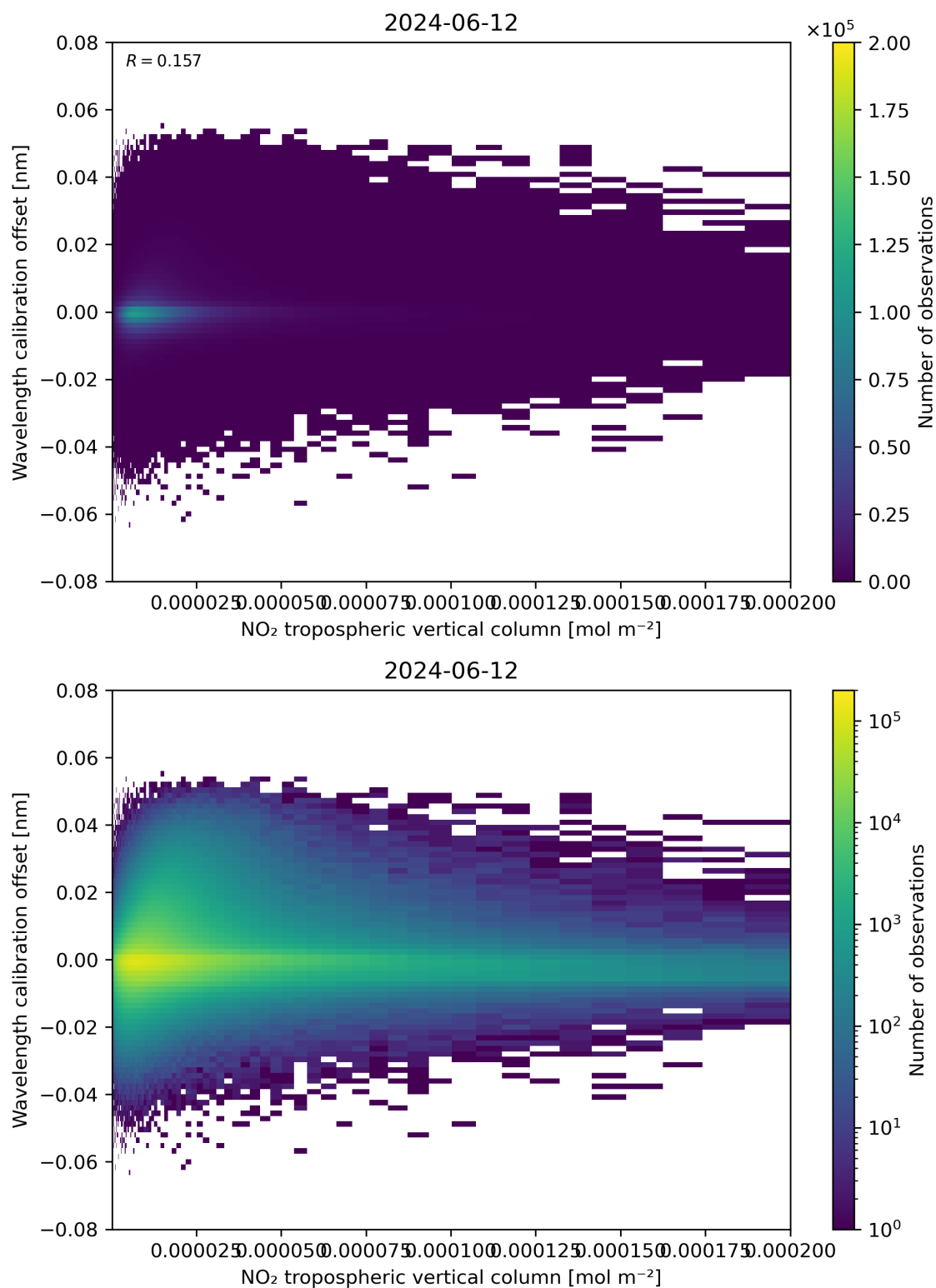
Figure 143: Scatter density plot of “NO 2 tropospheric vertical column” against “Wavelength calibration offset” for 2024-06-11 to 2024-06-13.
