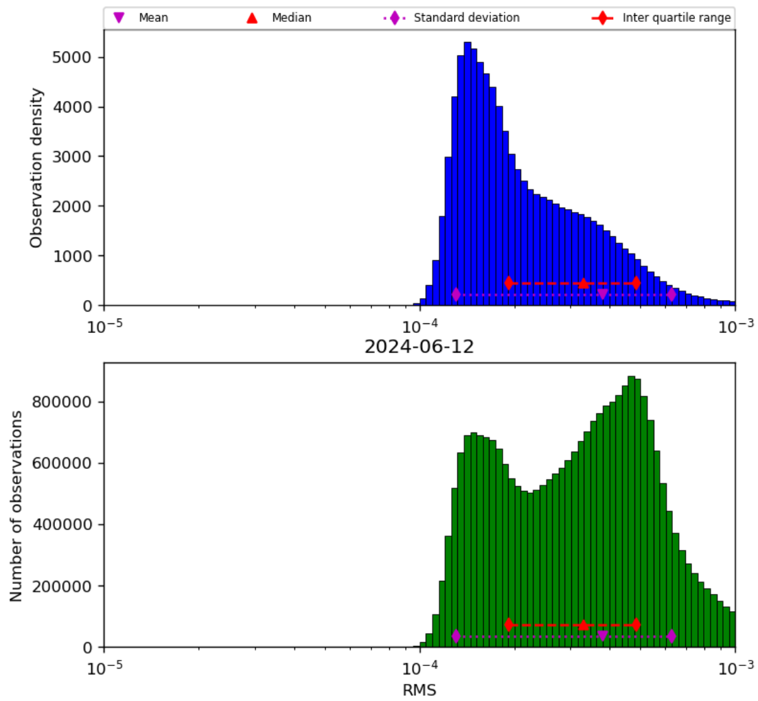
Figure 43: Histogram of “RMS” for 2024-06-11 to 2024-06-13
