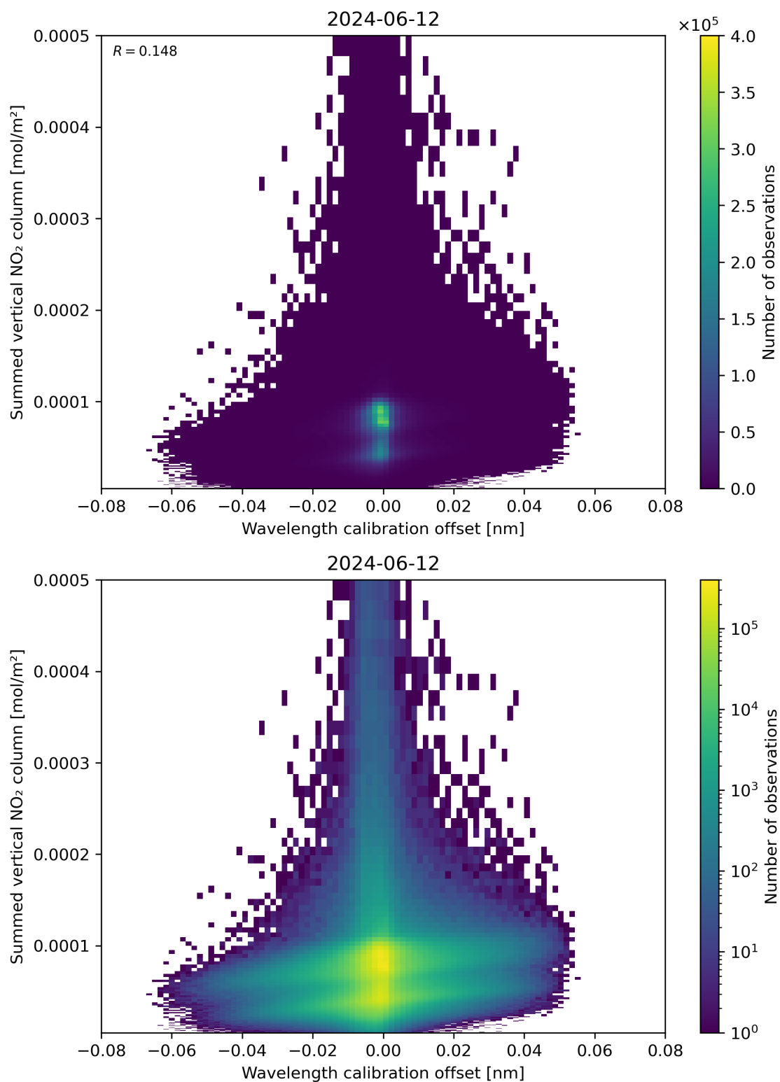
Figure 177: Scatter density plot of “Wavelength calibration offset” against “Summed vertical NO 2 column” for 2024-06-11 to 2024-06-13.
