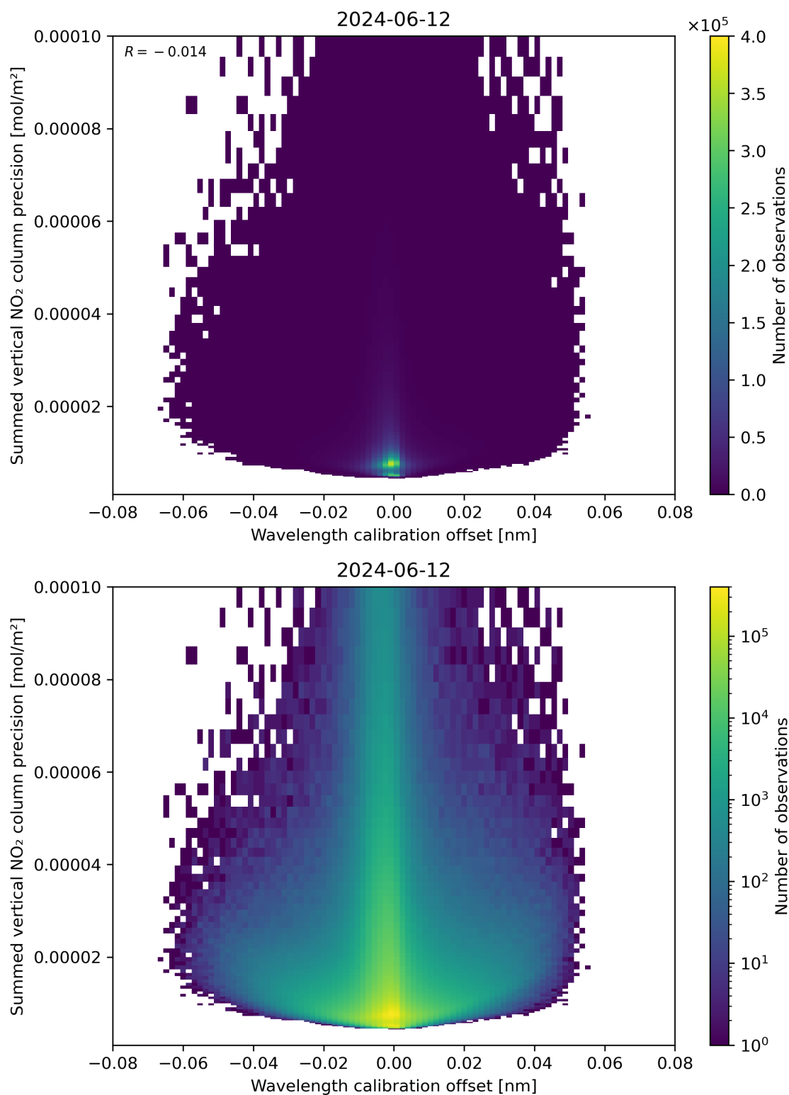
Figure 178: Scatter density plot of “Wavelength calibration offset” against “Summed vertical NO 2 column precision” for 2024-06-11 to 2024-06-13.
