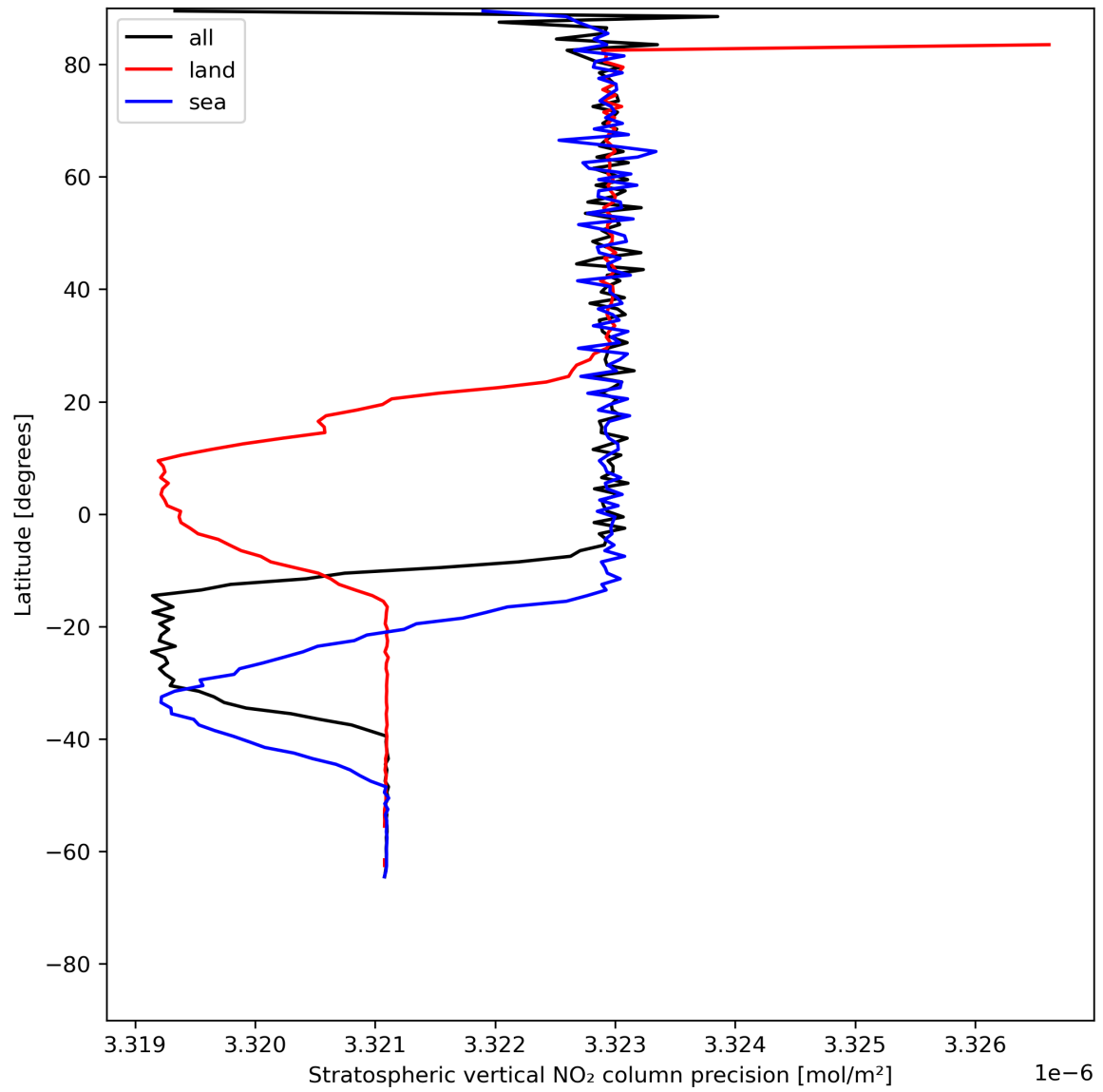
Figure 20: Zonal average of “Stratospheric vertical NO 2 column precision” for 2024-06-11 to 2024-06-13.
