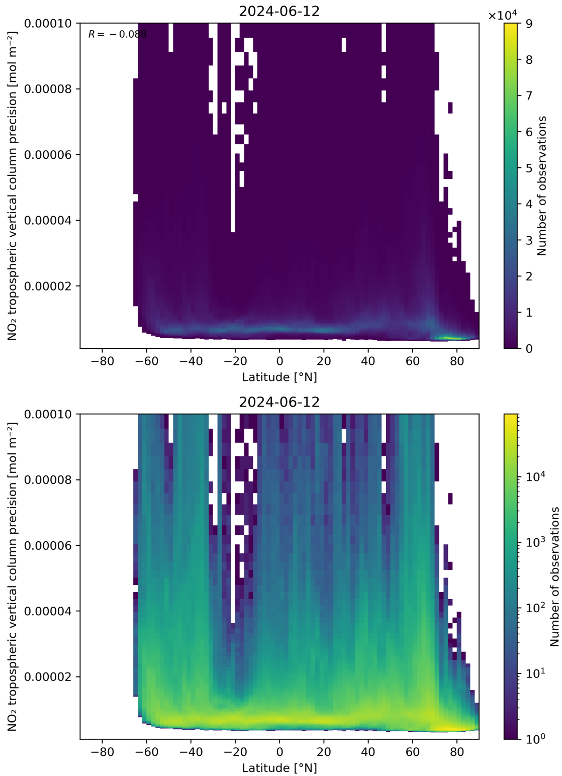
Figure 93: Scatter density plot of “Latitude” against “NO 2 tropospheric vertical column precision” for 2024-06-11 to 2024-06-13.
