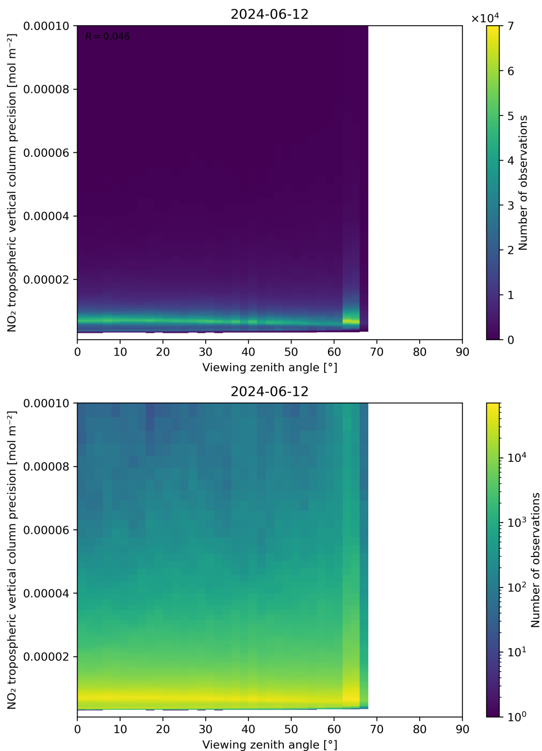
Figure 170: Scatter density plot of “Viewing zenith angle” against “NO 2 tropospheric vertical column precision” for 2024-06-11 to 2024-06-13.
