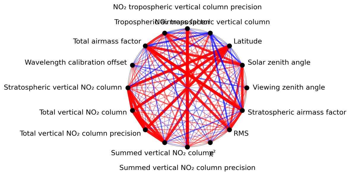
Figure 1: Map of correlation graph for 2024-06-11 to 2024-06-13.
