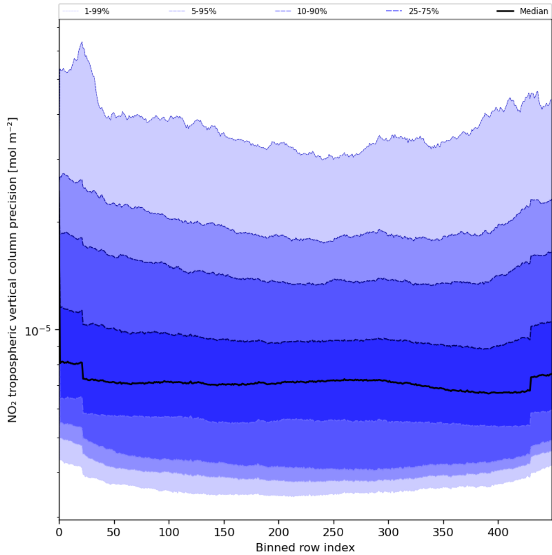
Figure 47: Along track statistics of “NO 2 tropospheric vertical column precision” for 2024-06-11 to 2024-06-13
