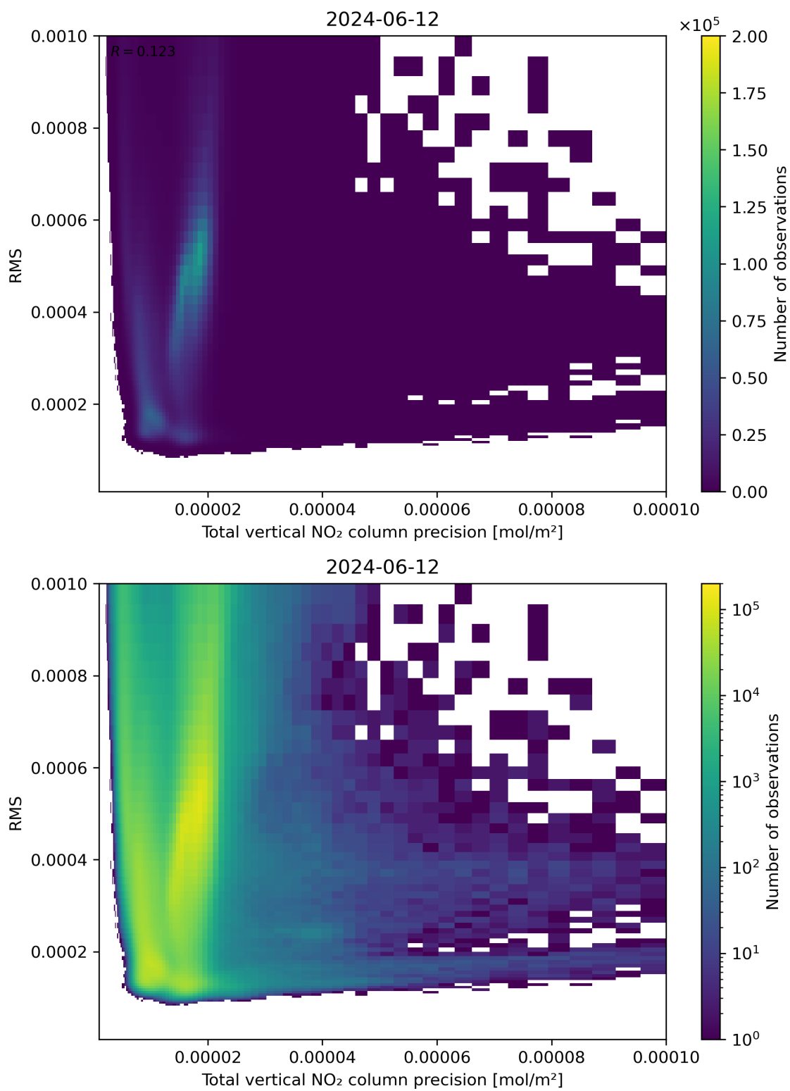
Figure 119: Scatter density plot of “Total vertical NO 2 column precision” against “RMS” for 2024-06-11 to 2024-06-13.
