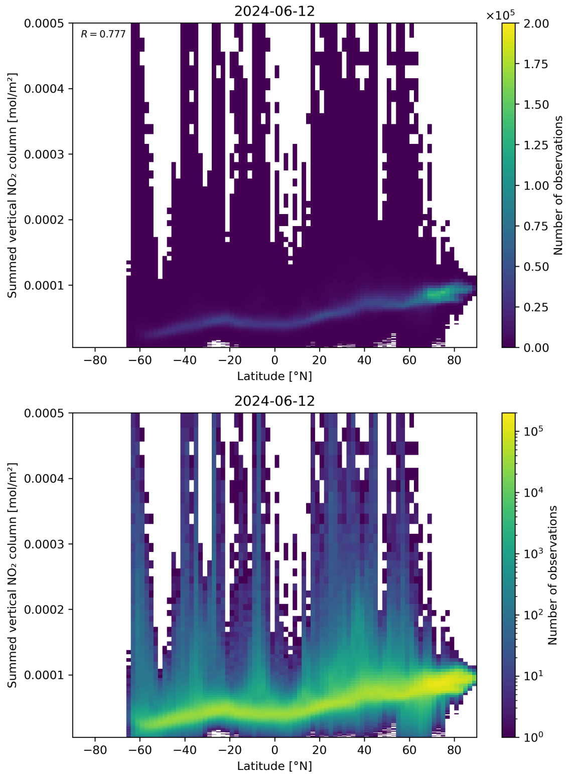
Figure 88: Scatter density plot of “Latitude” against “Summed vertical NO 2 column” for 2024-06-11 to 2024-06-13.
