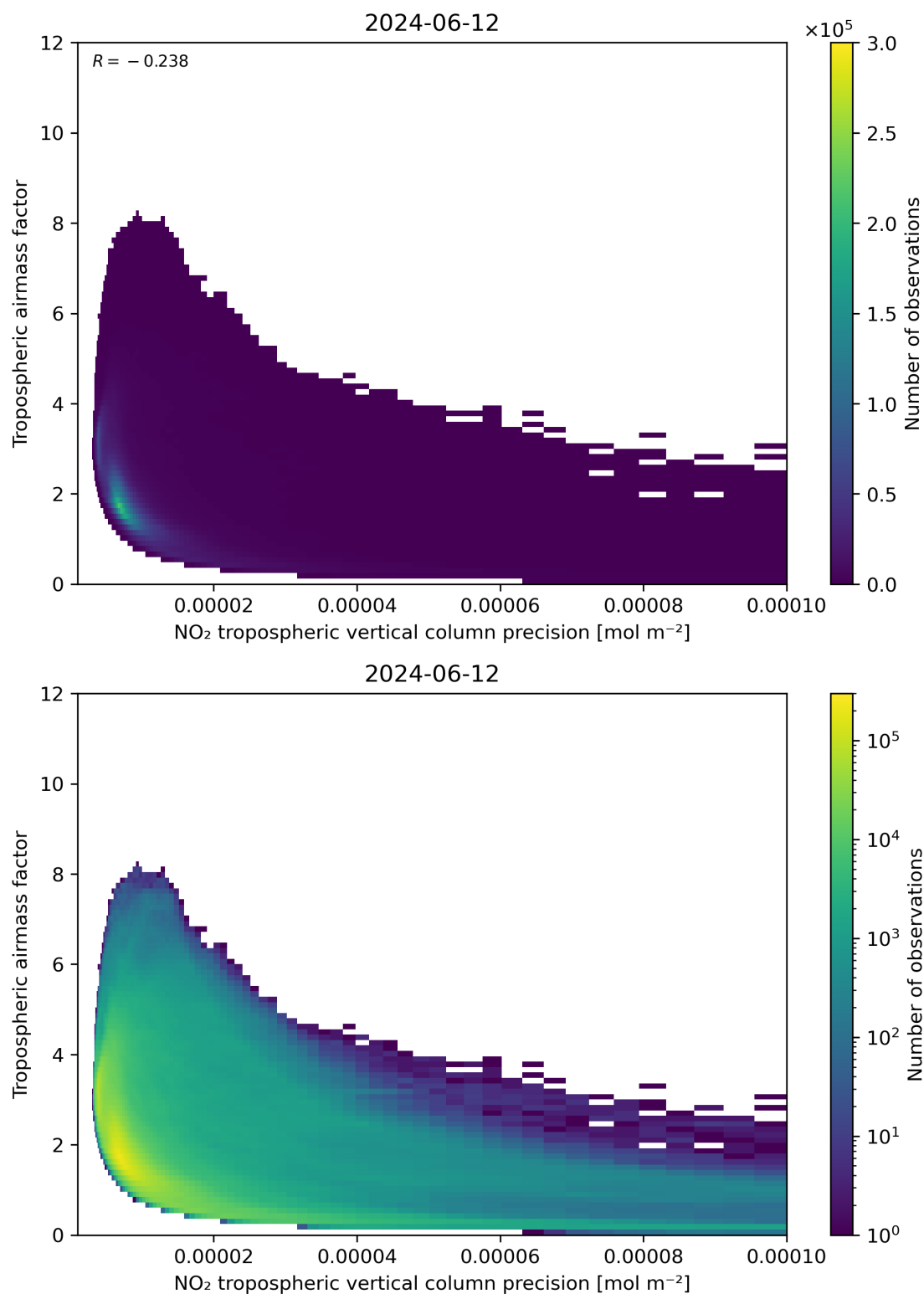
Figure 133: Scatter density plot of “NO 2 tropospheric vertical column precision” against “Tropospheric airmass factor” for 2024-06-11 to 2024-06-13.
