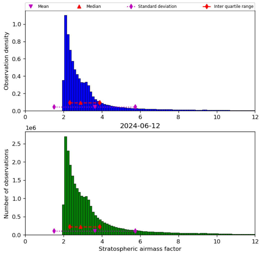
Figure 44: Histogram of “Stratospheric airmass factor” for 2024-06-11 to 2024-06-13
