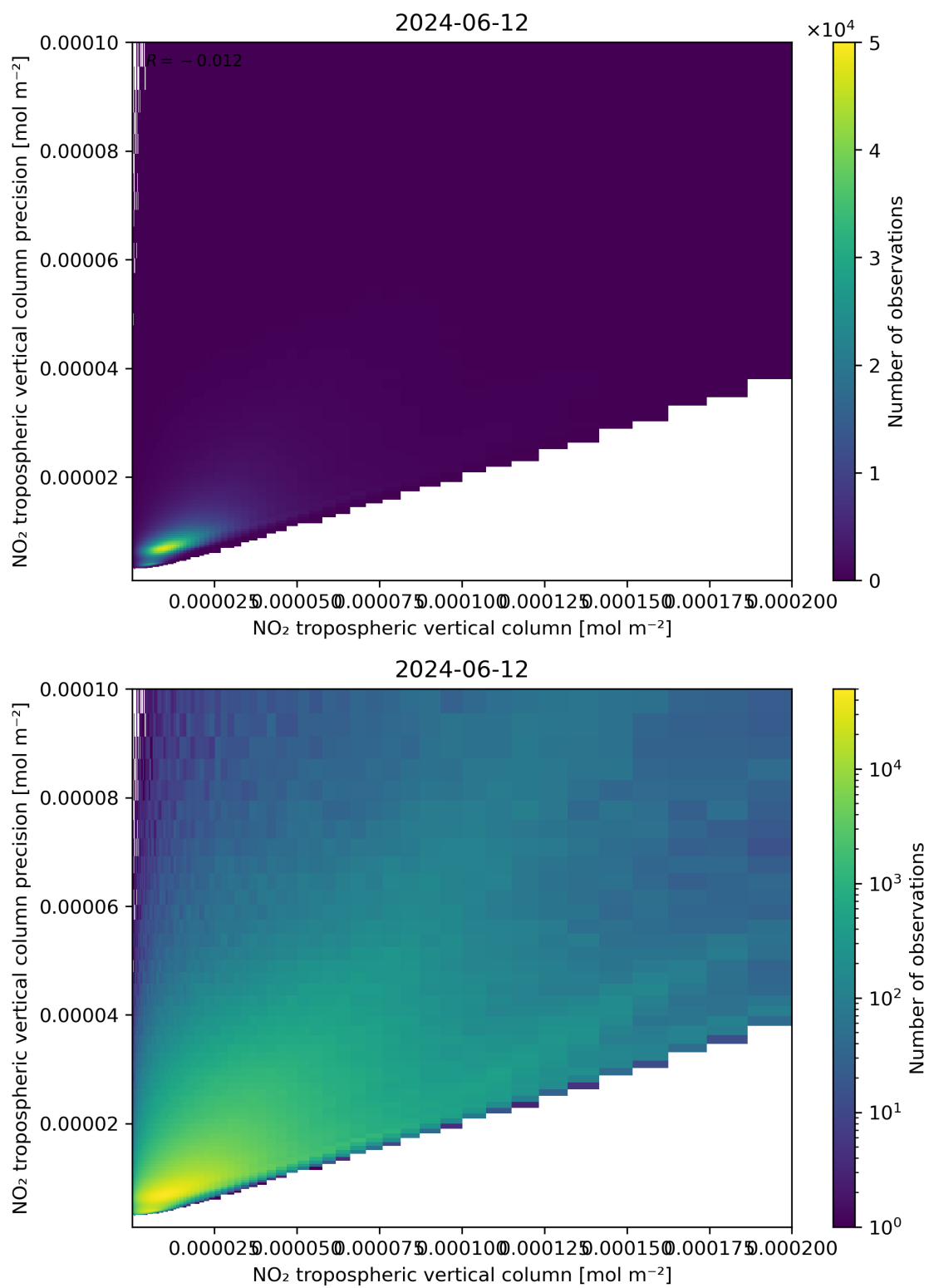
Figure 130: Scatter density plot of “NO 2 tropospheric vertical column” against “NO 2 tropospheric vertical column precision” for 2024-06-11 to 2024-06-13.
