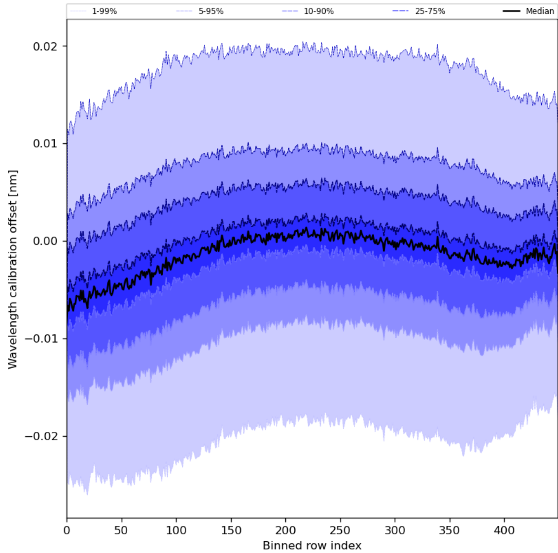
Figure 52: Along track statistics of “Wavelength calibration offset” for 2024-06-11 to 2024-06-13
