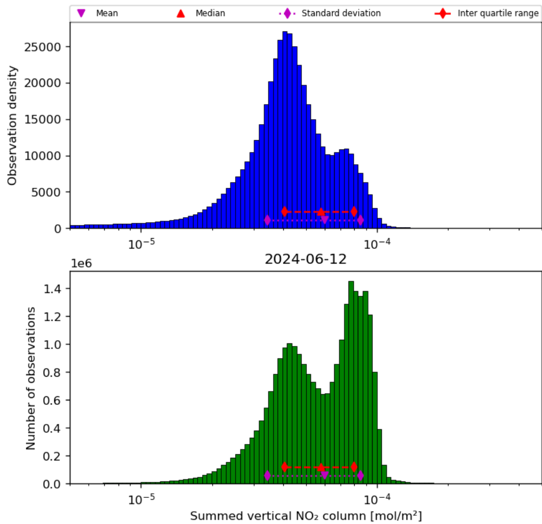
Figure 40: Histogram of “Summed vertical NO 2 column” for 2024-06-11 to 2024-06-13
