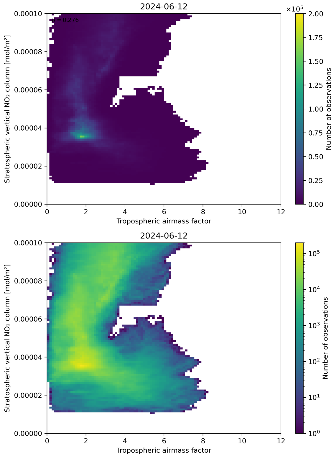
Figure 74: Scatter density plot of “Tropospheric air mass factor” against “Stratospheric vertical NO 2 column” for 2024-06-11 to 2024-06-13.
