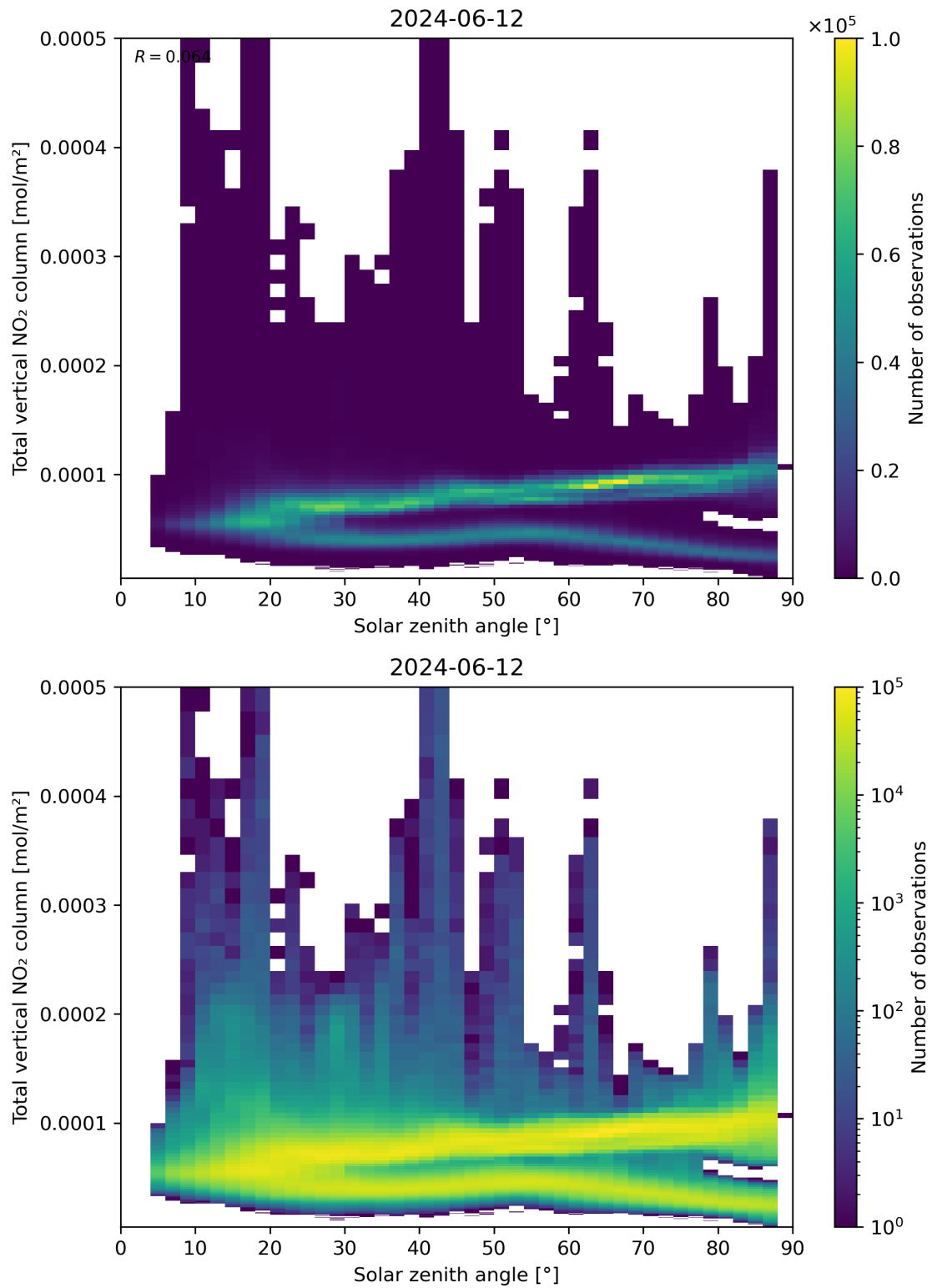
Figure 153: Scatter density plot of “Solar zenith angle” against “Total vertical NO 2 column” for 2024-06-11 to 2024-06-13.
