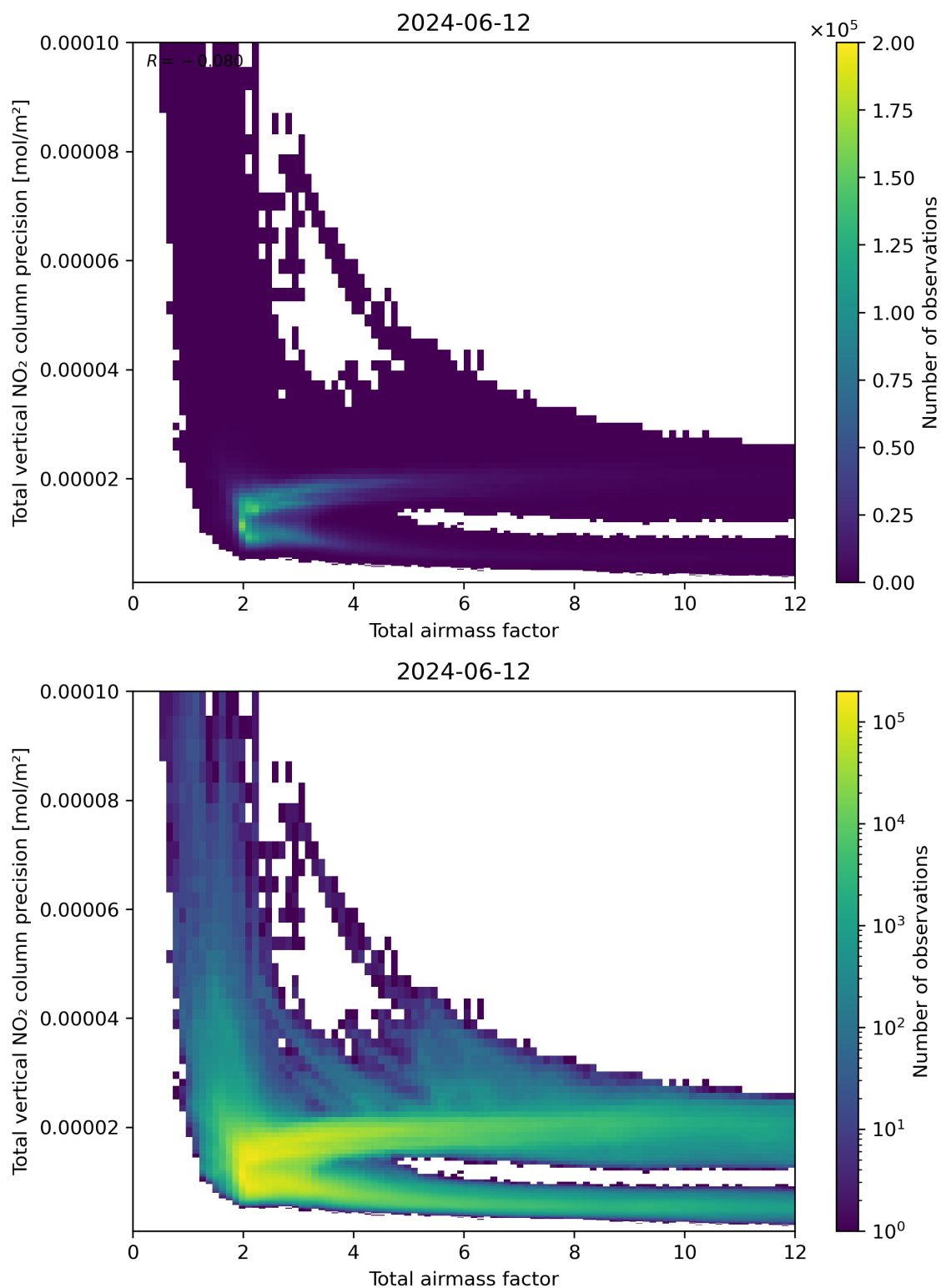
Figure 68: Scatter density plot of “Total airmass factor” against “Total vertical NO 2 column precision” for 2024-06-11 to 2024-06-13.
