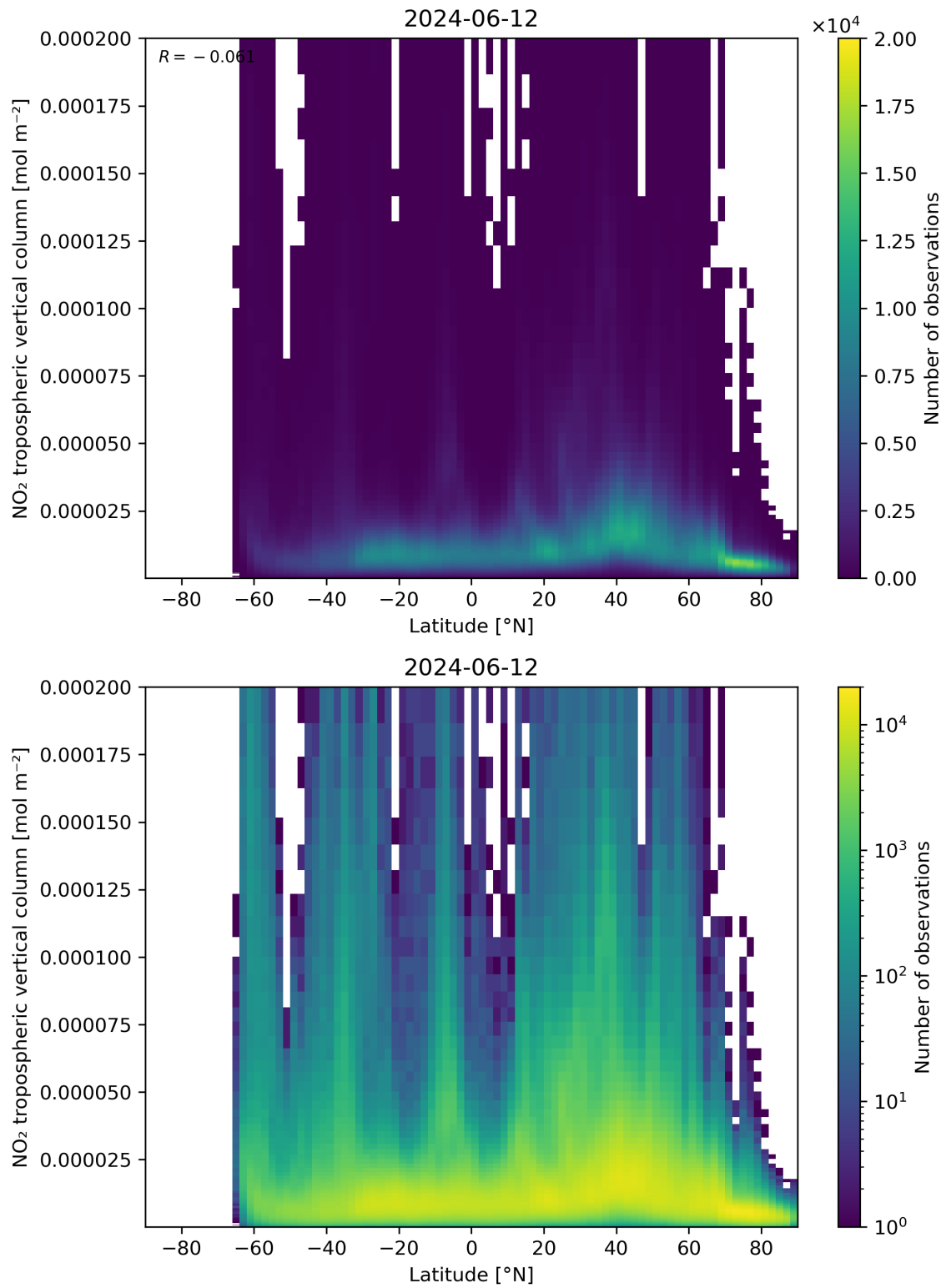
Figure 92: Scatter density plot of “Latitude” against “NO 2 tropospheric vertical column” for 2024-06-11 to 2024-06-13.
