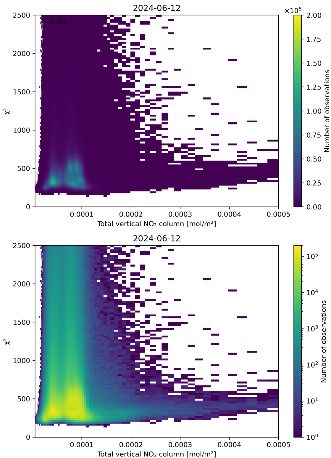
Figure 111: Scatter density plot of “Total vertical NO 2 column” against “ \chi^2 ” for 2024-06-11 to 2024-06-13.
