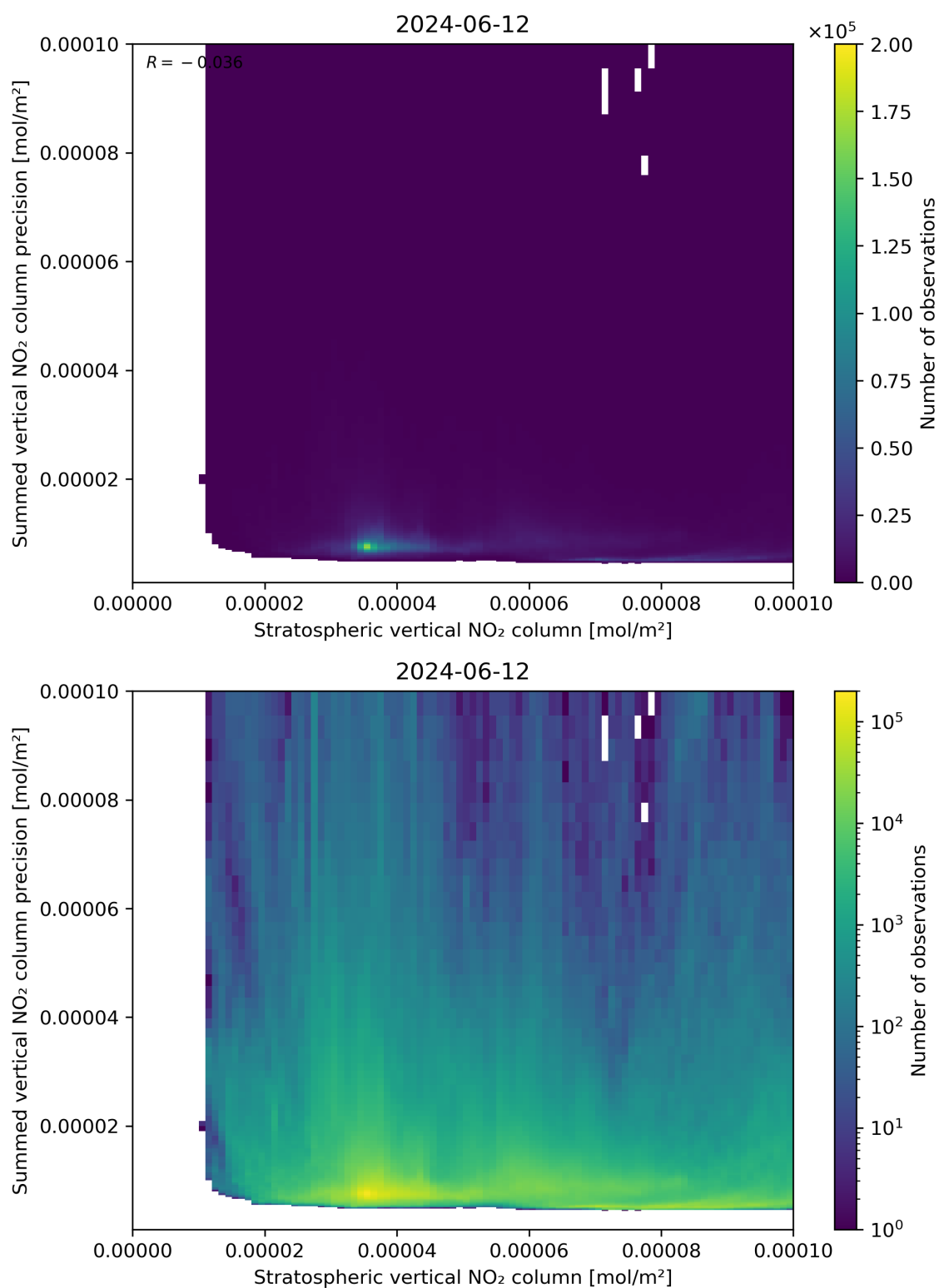
Figure 99: Scatter density plot of “Stratospheric vertical NO 2 column” against “Summed vertical NO 2 column precision” for 2024-06-11 to 2024-06-13.
