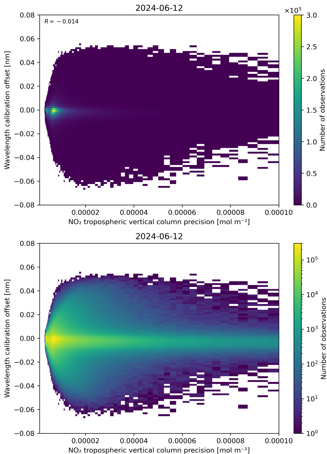
Figure 141: Scatter density plot of “NO 2 tropospheric vertical column precision” against “Wavelength calibration offset” for 2024-06-11 to 2024-06-13.
