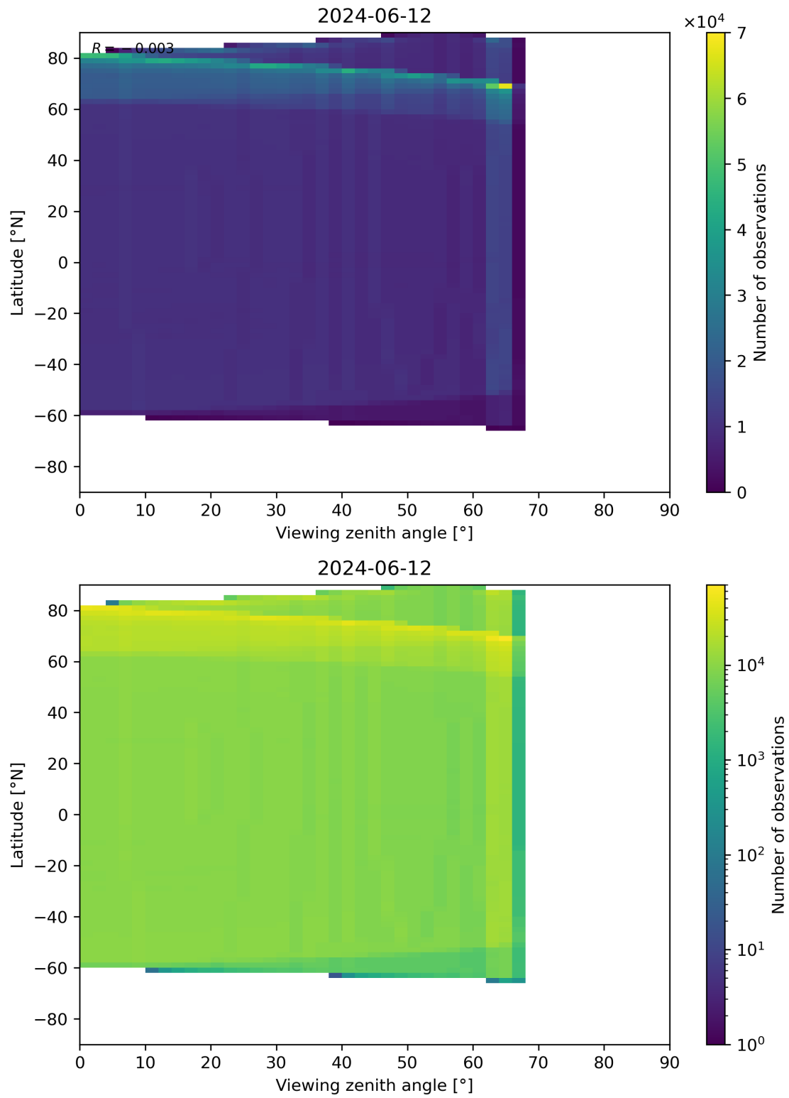
Figure 163: Scatter density plot of “Viewing zenith angle” against “Latitude” for 2024-06-11 to 2024-06-13.
