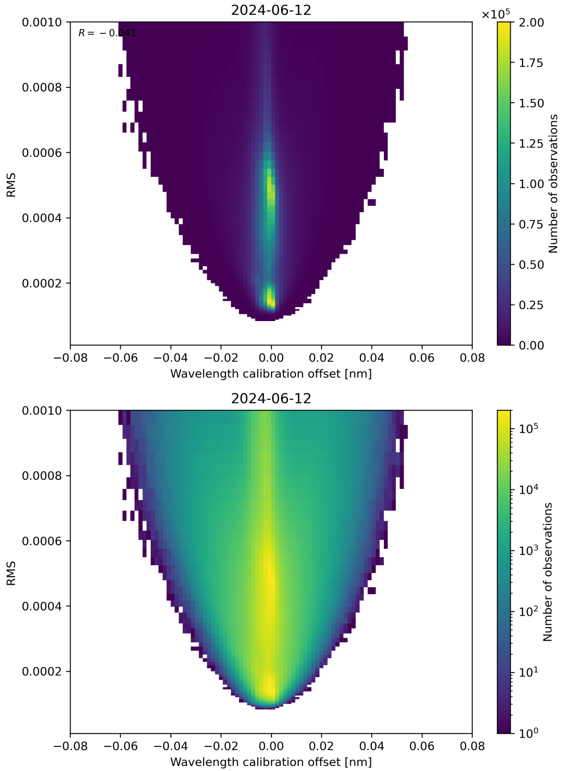
Figure 181: Scatter density plot of “Wavelength calibration offset” against “RMS” for 2024-06-11 to 2024-06-13.
