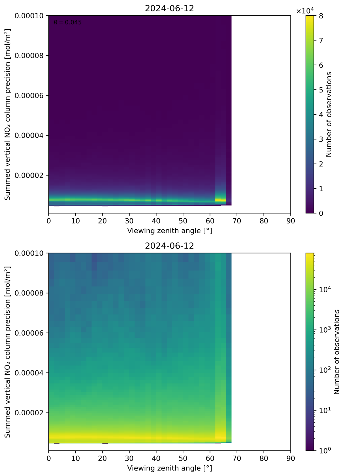
Figure 166: Scatter density plot of “Viewing zenith angle” against “Summed vertical NO 2 column precision” for 2024-06-11 to 2024-06-13.
