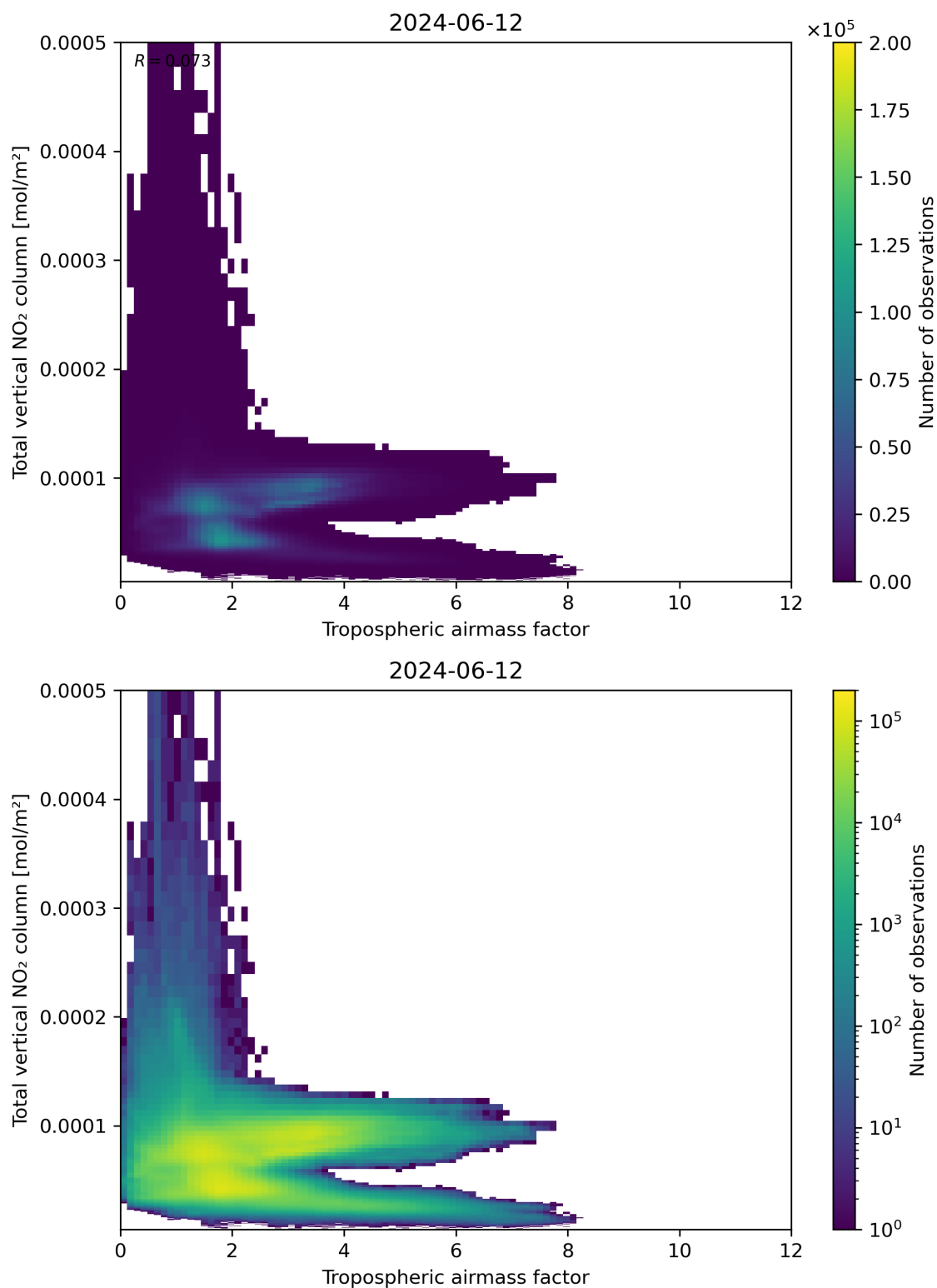
Figure 77: Scatter density plot of “Tropospheric airmass factor” against “Total vertical NO 2 column” for 2024-06-11 to 2024-06-13.
