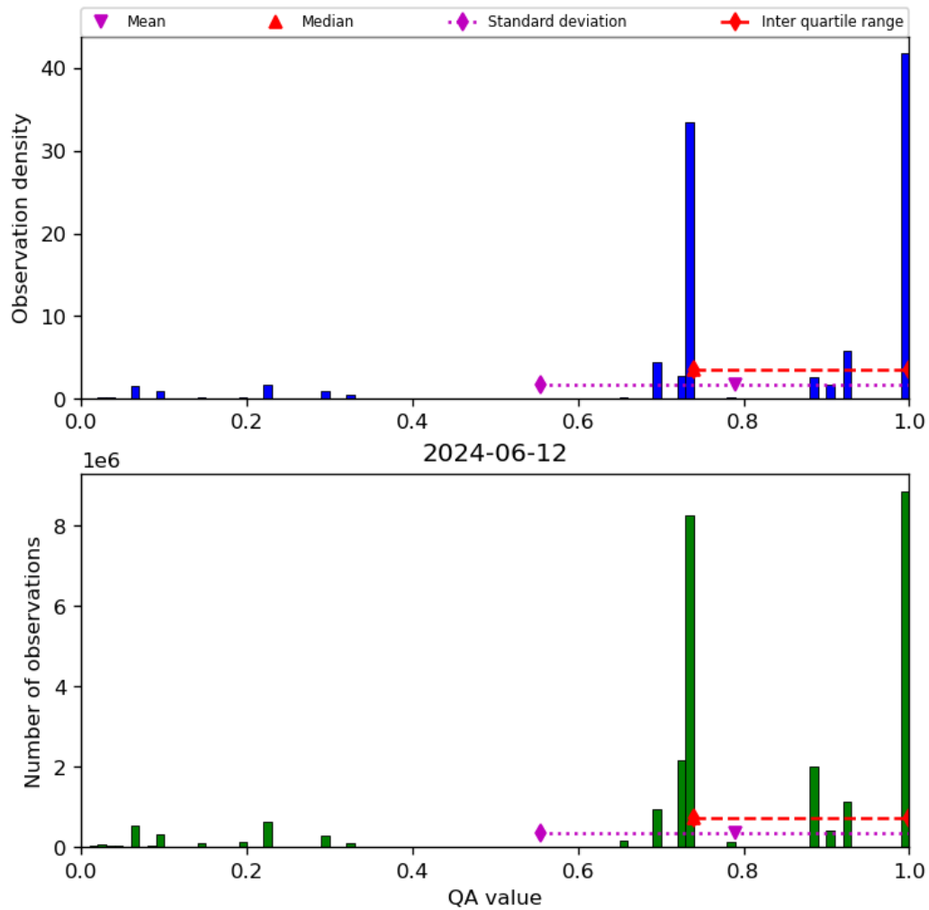
Figure 28: Histogram of “QA value” for 2024-06-11 to 2024-06-13
