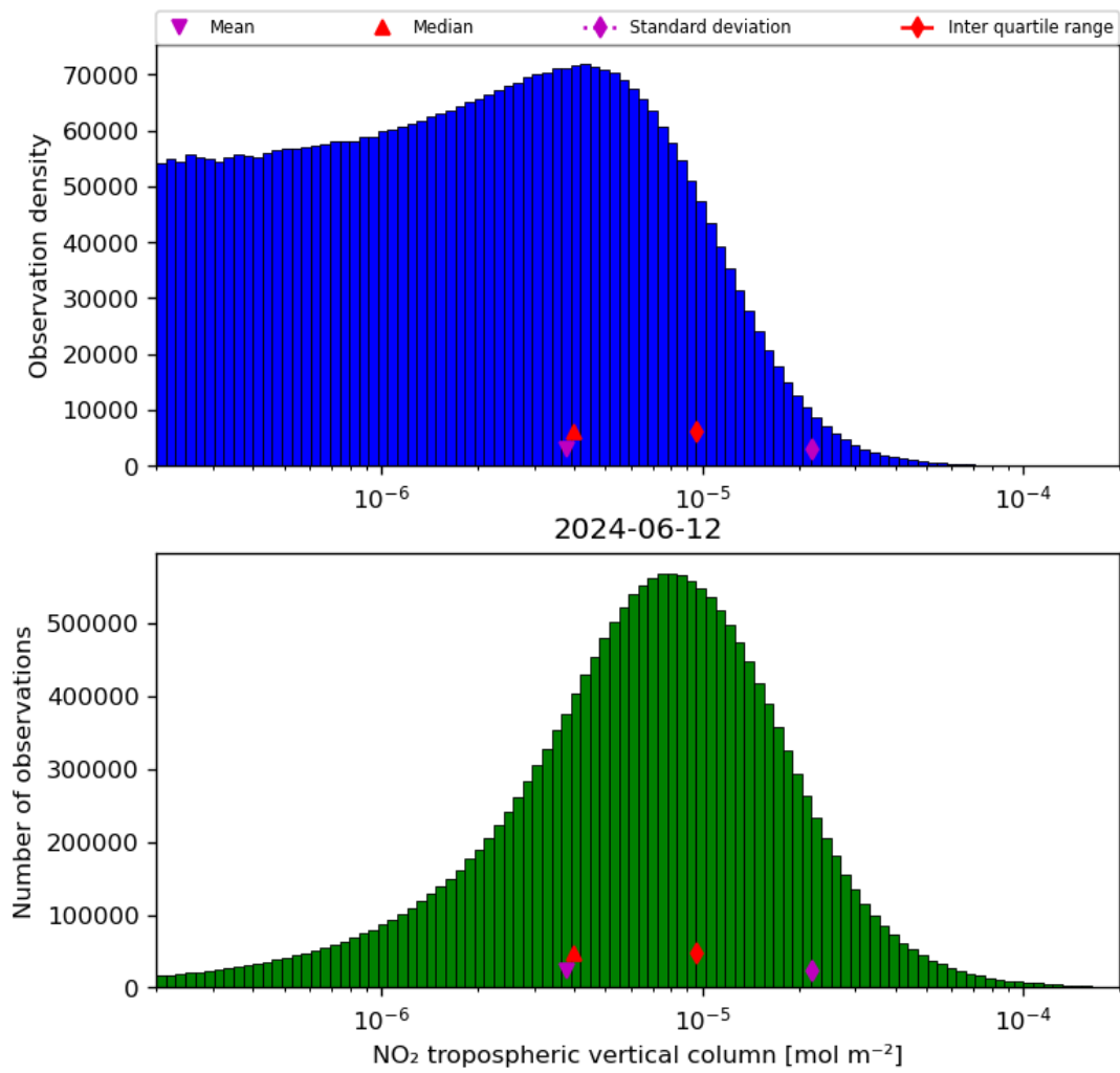
Figure 29: Histogram of “NO 2 tropospheric vertical column” for 2024-06-11 to 2024-06-13
