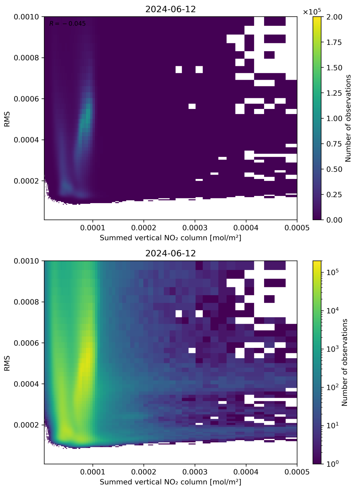
Figure 109: Scatter density plot of “Summed vertical NO 2 column” against “RMS” for 2024-06-11 to 2024-06-13.
