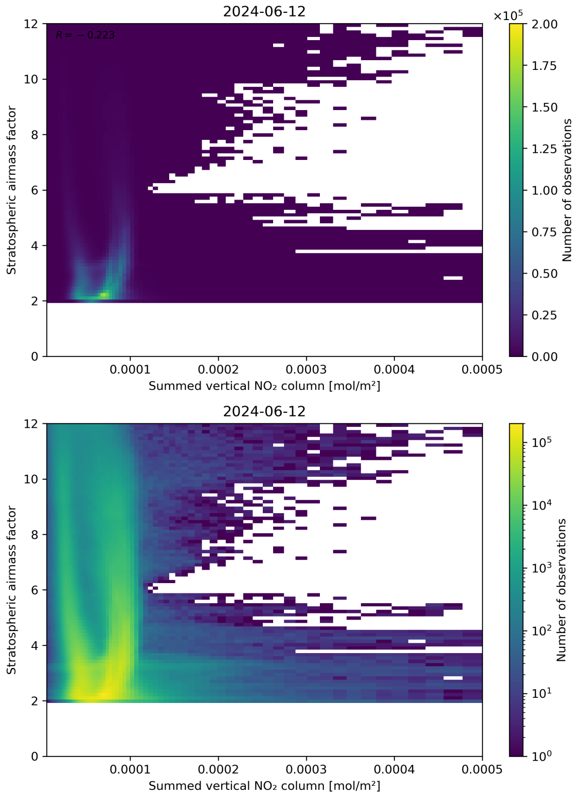
Figure 103: Scatter density plot of “Summed vertical NO 2 column” against “Stratospheric air mass factor” for 2024-06-11 to 2024-06-13.
