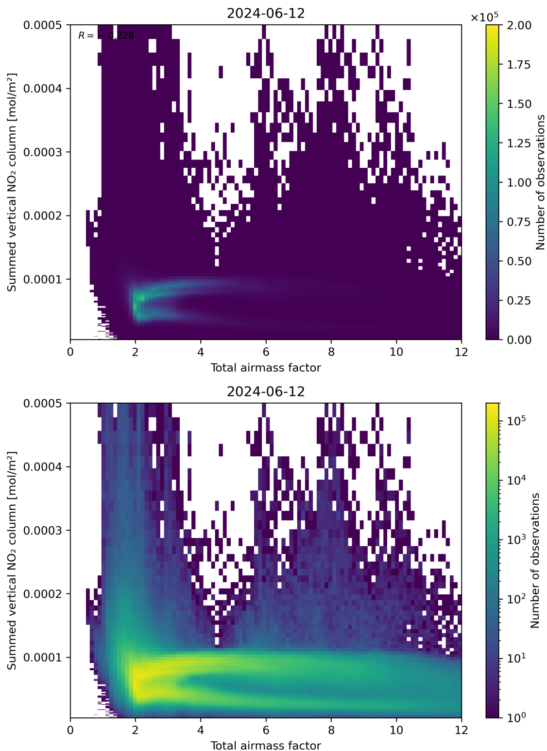
Figure 65: Scatter density plot of “Total airmass factor” against “Summed vertical NO 2 column” for 2024-06-11 to 2024-06-13.
