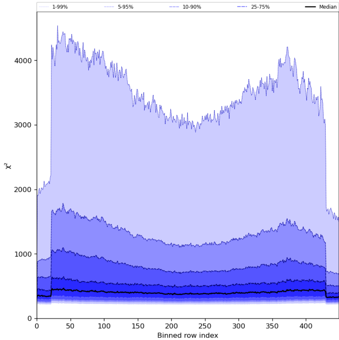
Figure 59: Along track statistics of “ \chi^2 ” for 2024-06-11 to 2024-06-13
