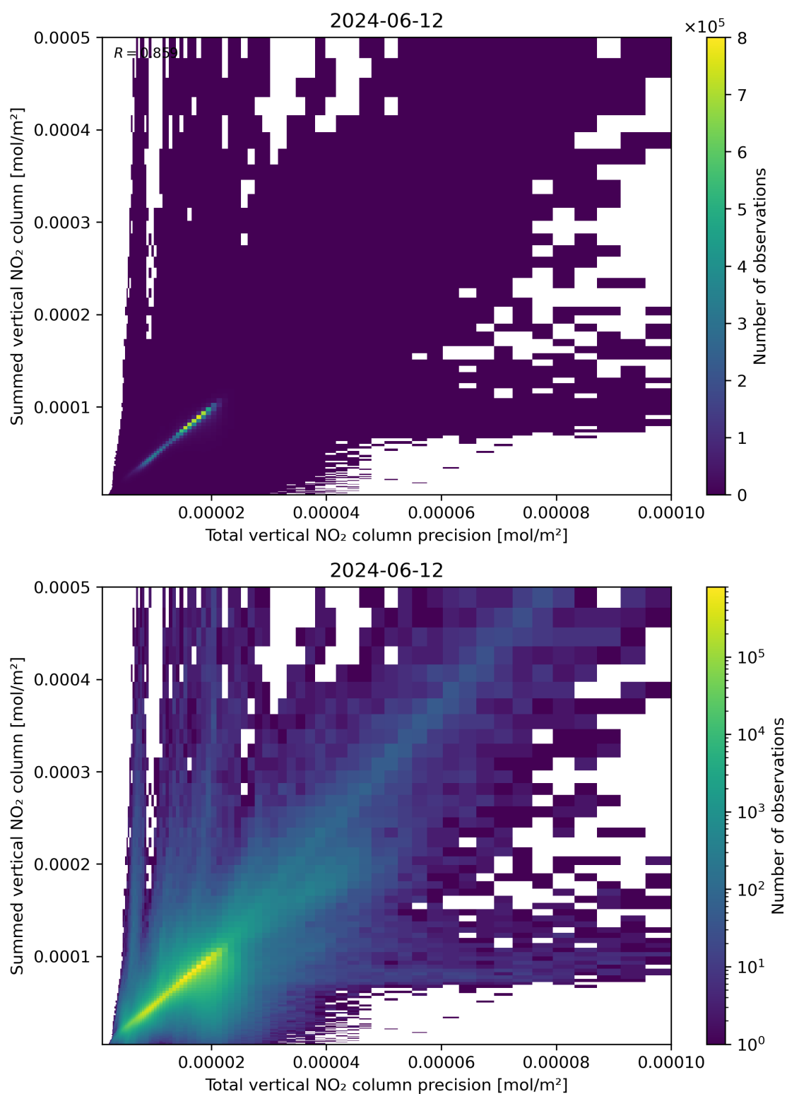
Figure 117: Scatter density plot of “Total vertical NO 2 column precision” against “Summed vertical NO 2 column” for 2024-06-11 to 2024-06-13.
