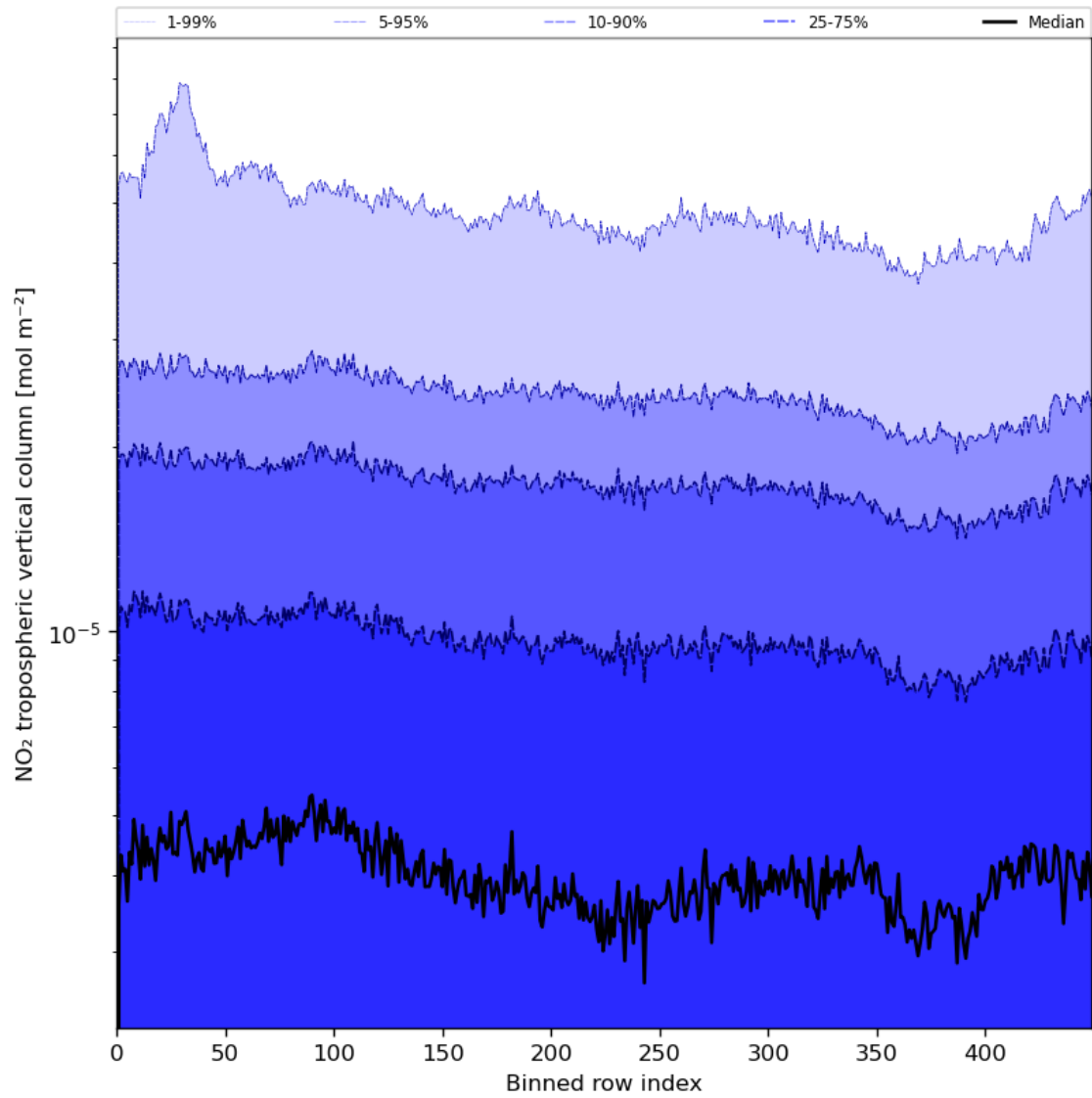
Figure 46: Along track statistics of “NO 2 tropospheric vertical column” for 2024-06-11 to 2024-06-13
