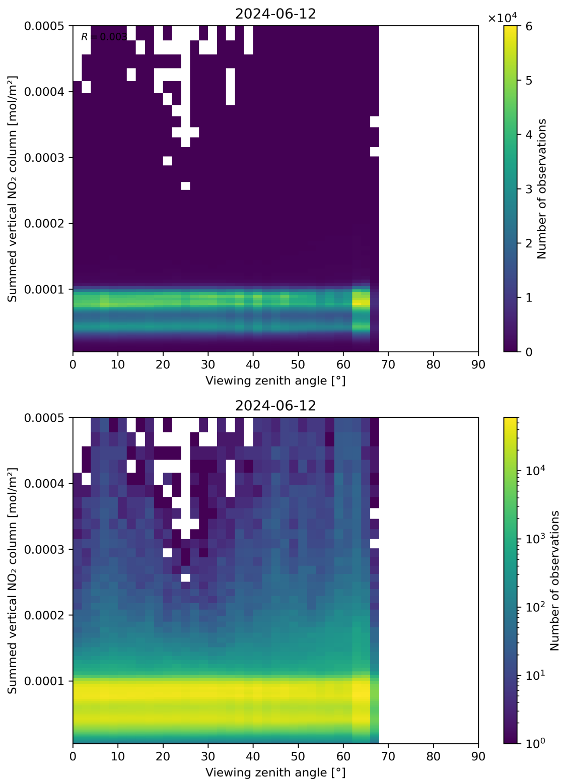
Figure 165: Scatter density plot of “Viewing zenith angle” against “Summed vertical NO 2 column” for 2024-06-11 to 2024-06-13.
