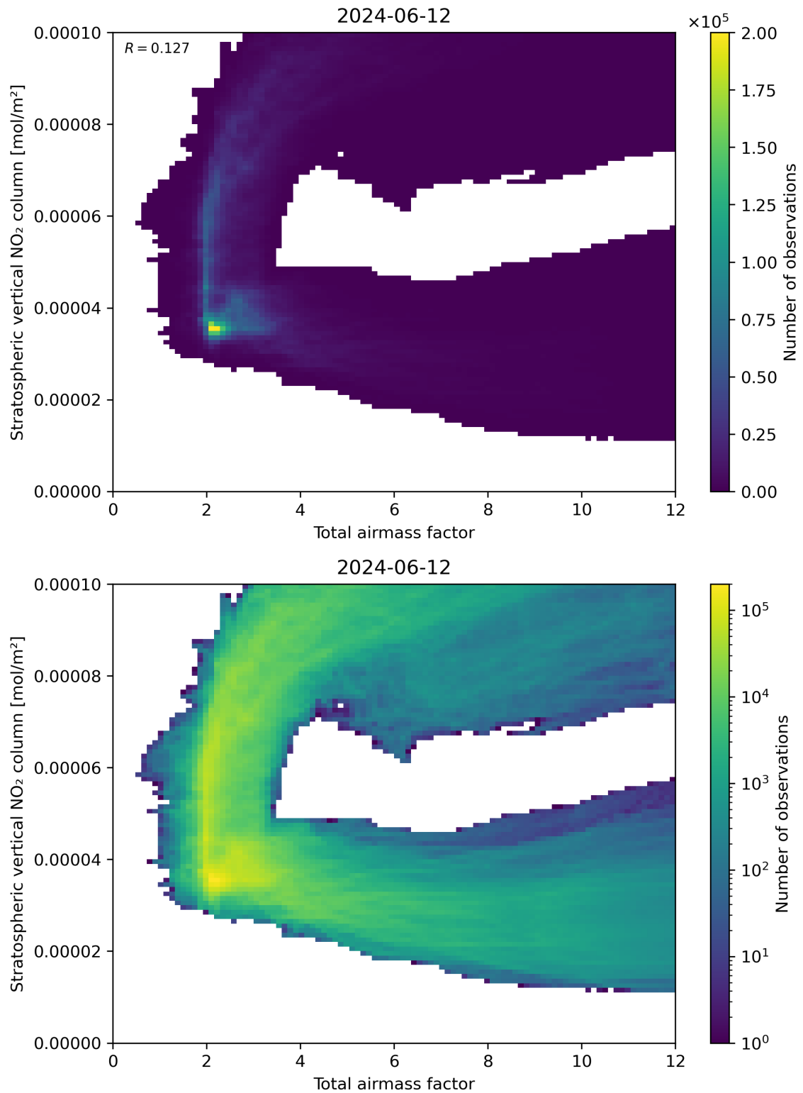
Figure 64: Scatter density plot of “Total airmass factor” against “Stratospheric vertical NO 2 column” for 2024-06-11 to 2024-06-13.
