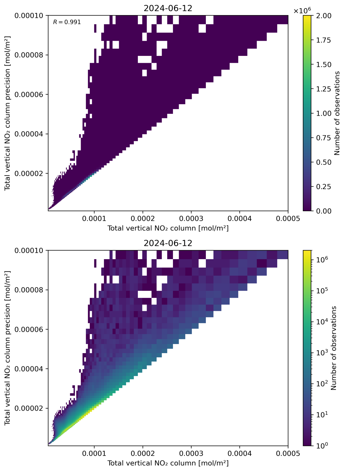
Figure 114: Scatter density plot of “Total vertical NO 2 column” against “Total vertical NO 2 column precision” for 2024-06-11 to 2024-06-13.
