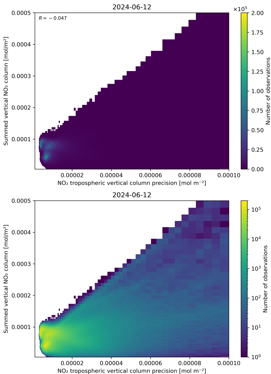
Figure 136: Scatter density plot of “NO 2 tropospheric vertical column precision” against “Summed vertical NO 2 column” for 2024-06-11 to 2024-06-13.
