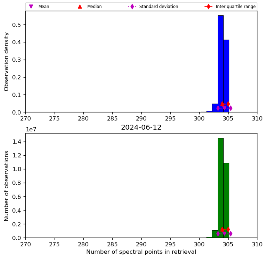
Figure 33: Histogram of “Number of spectral points in retrieval” for 2024-06-11 to 2024-06-13
