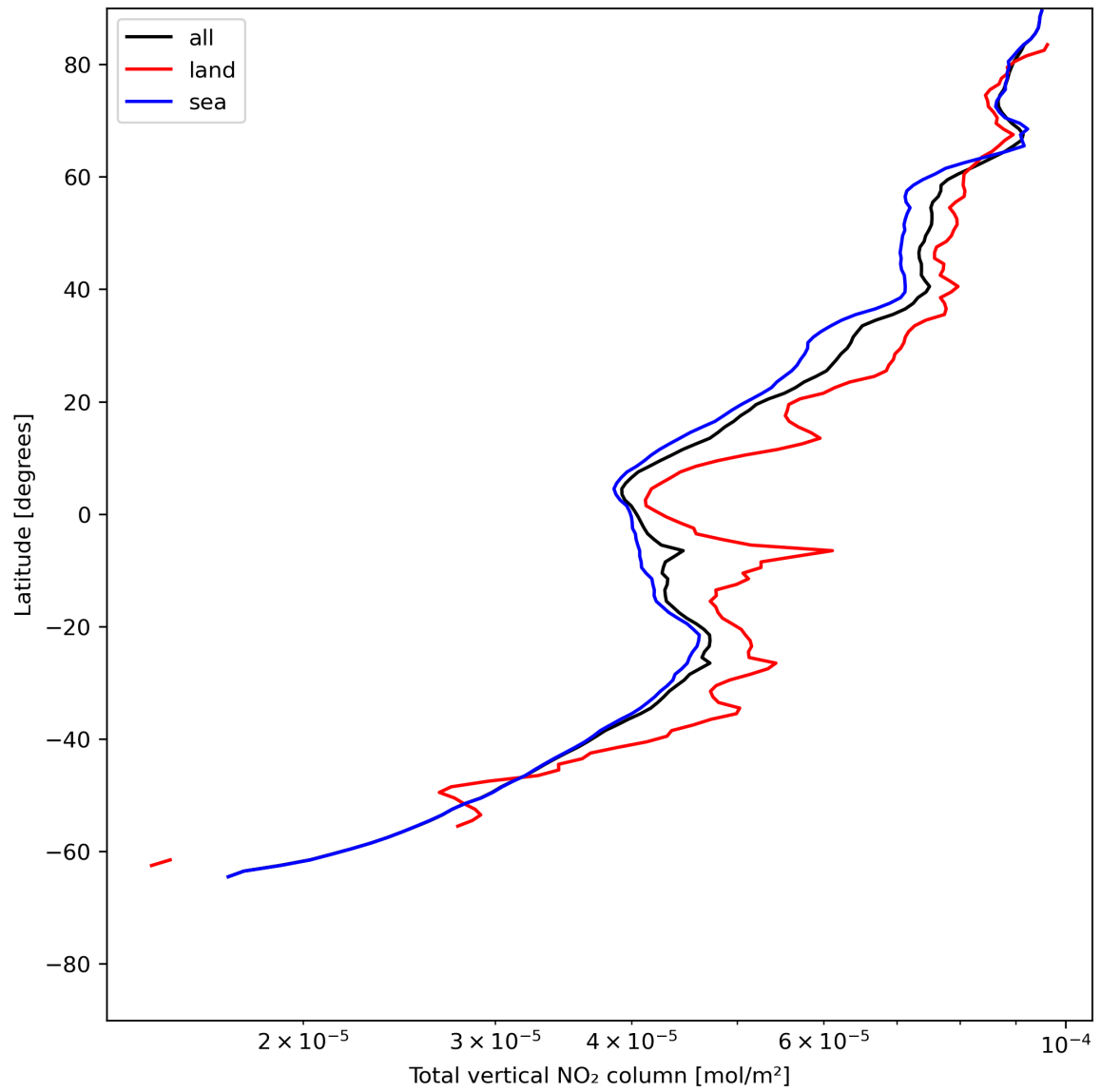
Figure 21: Zonal average of “Total vertical NO 2 column” for 2024-06-11 to 2024-06-13.
