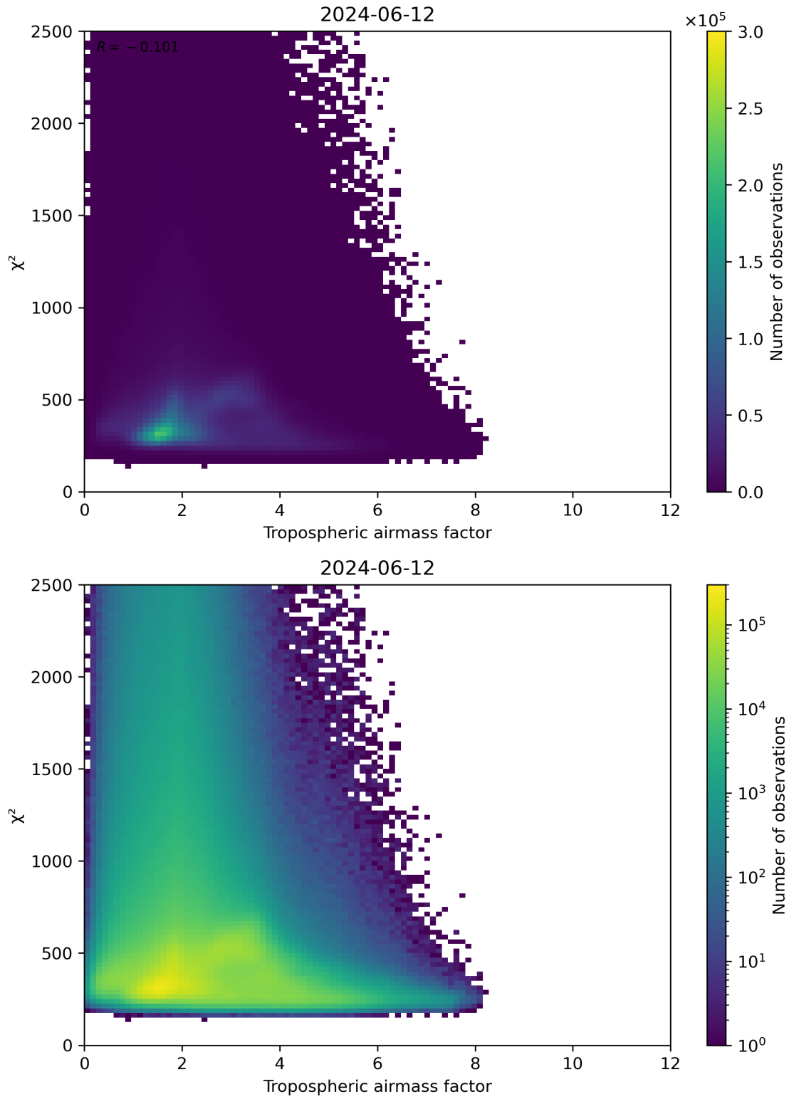
Figure 73: Scatter density plot of “Tropospheric airmass factor” against “ \chi^2 ” for 2024-06-11 to 2024-06-13.
