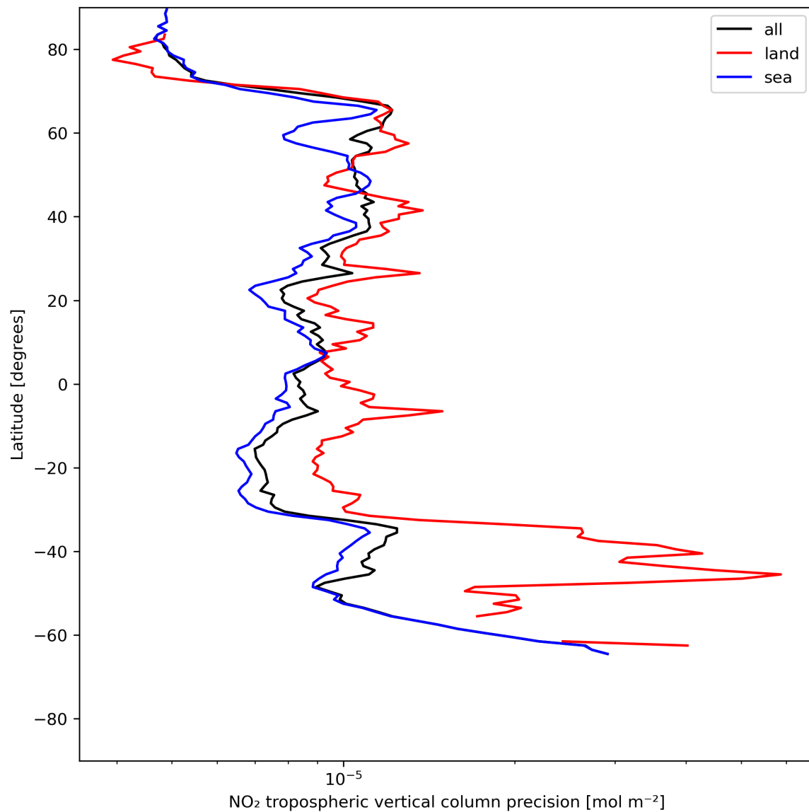
Figure 13: Zonal average of “NO 2 tropospheric vertical column precision” for 2024-06-11 to 2024-06-13.
