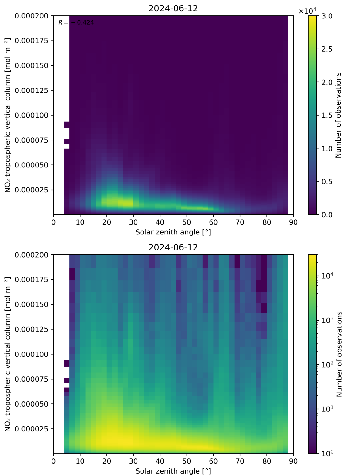
Figure 155: Scatter density plot of “Solar zenith angle” against “NO 2 tropospheric vertical column” for 2024-06-11 to 2024-06-13.
