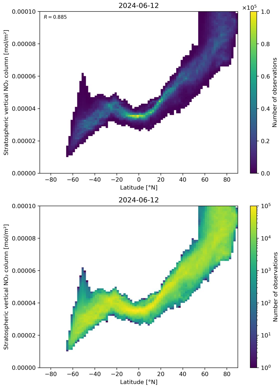
Figure 87: Scatter density plot of “Latitude” against “Stratospheric vertical NO 2 column” for 2024-06-11 to 2024-06-13.
