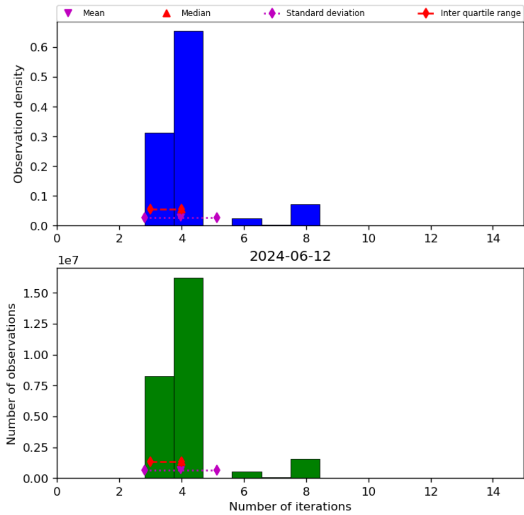
Figure 34: Histogram of “Number of iterations” for 2024-06-11 to 2024-06-13
