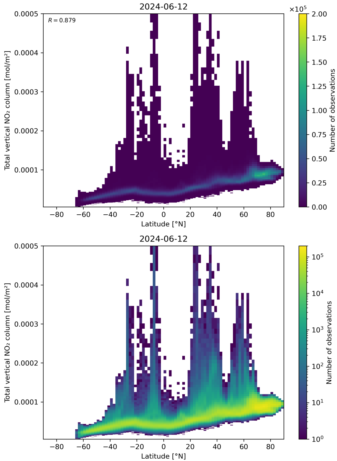
Figure 90: Scatter density plot of “Latitude” against “Total vertical NO 2 column” for 2024-06-11 to 2024-06-13.
