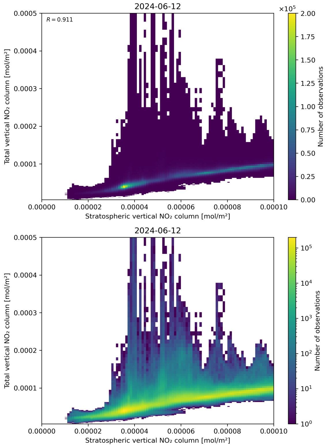
Figure 100: Scatter density plot of “Stratospheric vertical NO 2 column” against “Total vertical NO 2 column” for 2024-06-11 to 2024-06-13.
