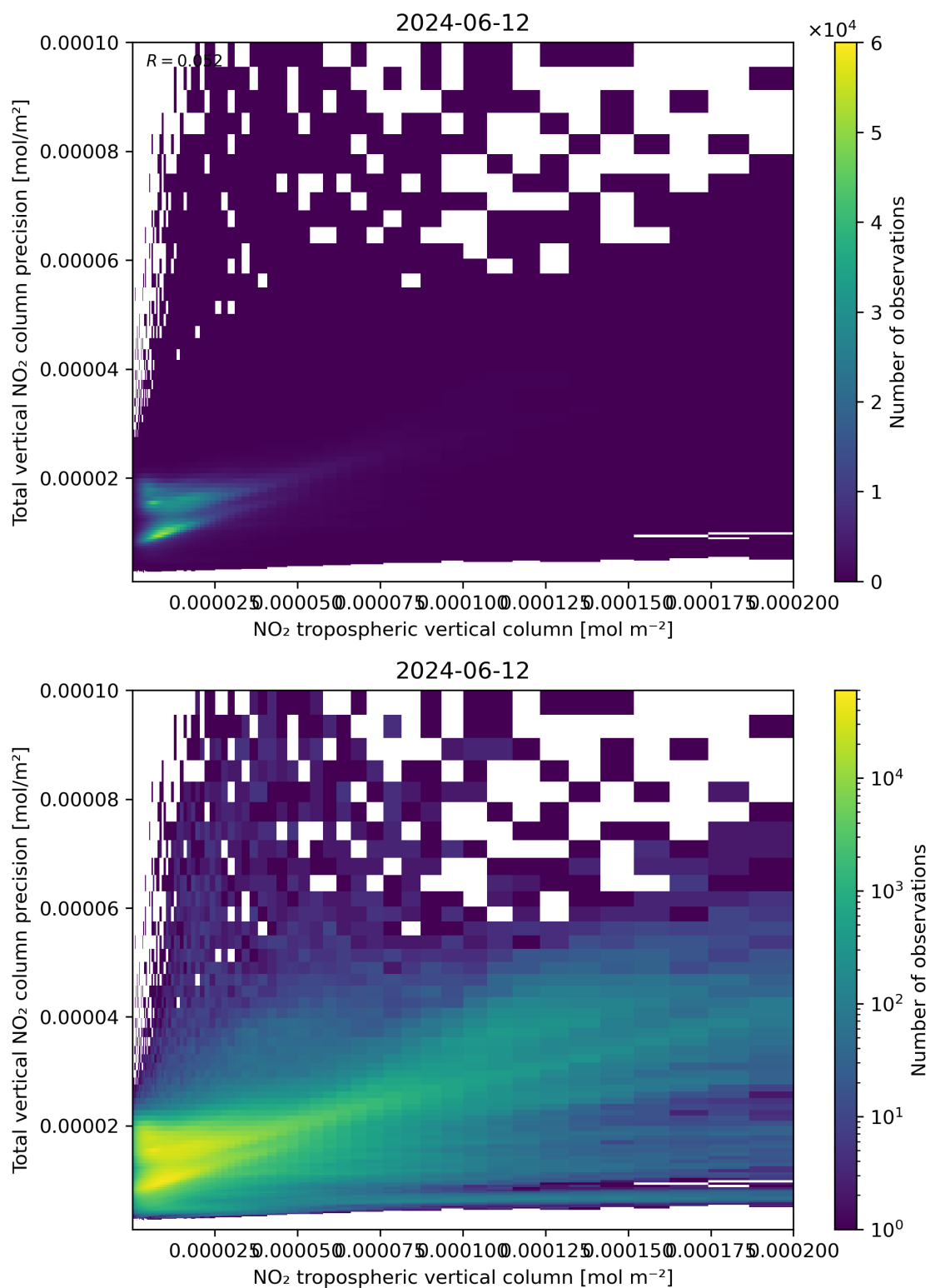
Figure 129: Scatter density plot of “NO 2 tropospheric vertical column” against “Total vertical NO 2 column precision” for 2024-06-11 to 2024-06-13.
