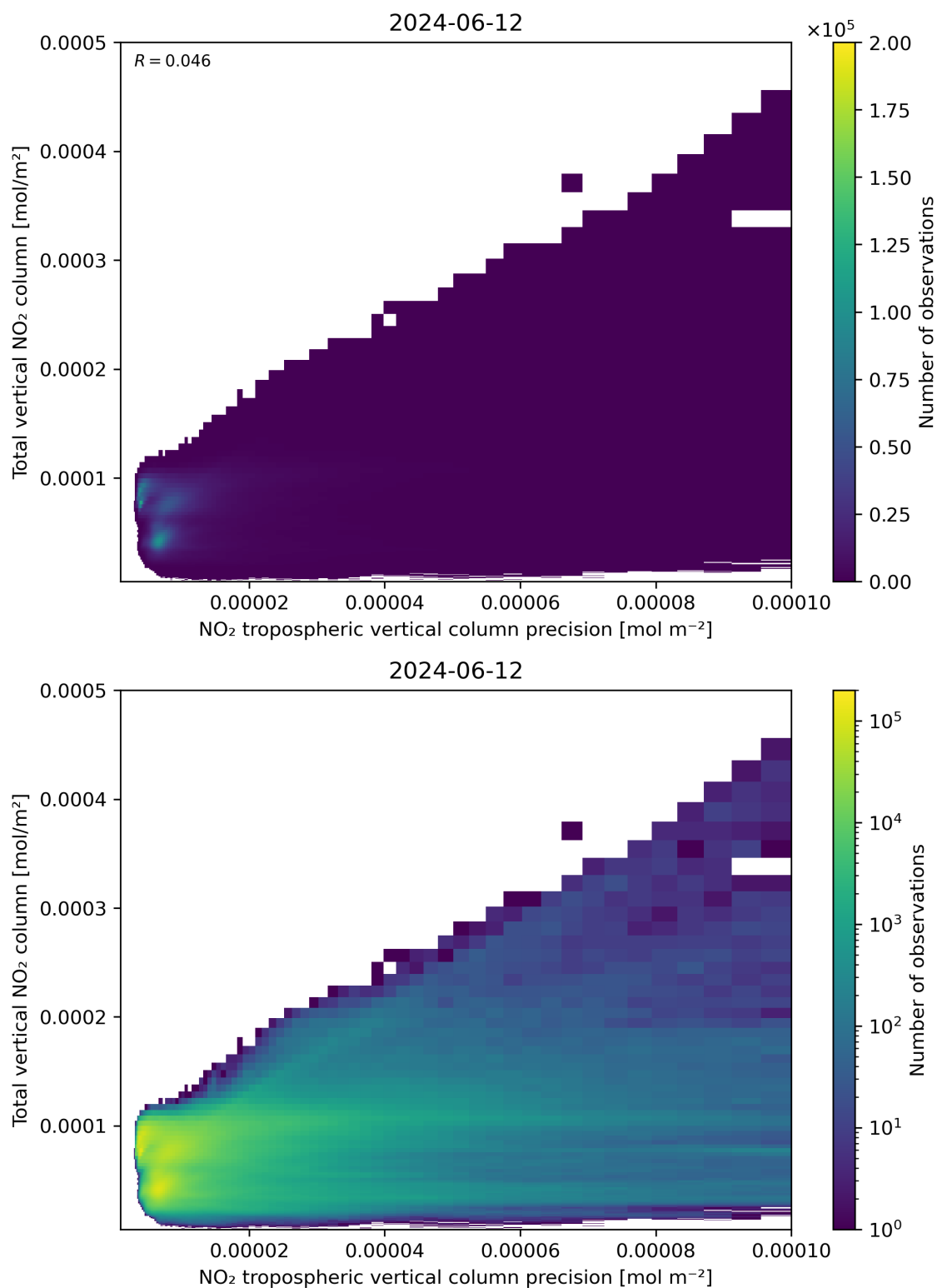
Figure 138: Scatter density plot of “NO 2 tropospheric vertical column precision” against “Total vertical NO 2 column” for 2024-06-11 to 2024-06-13.
