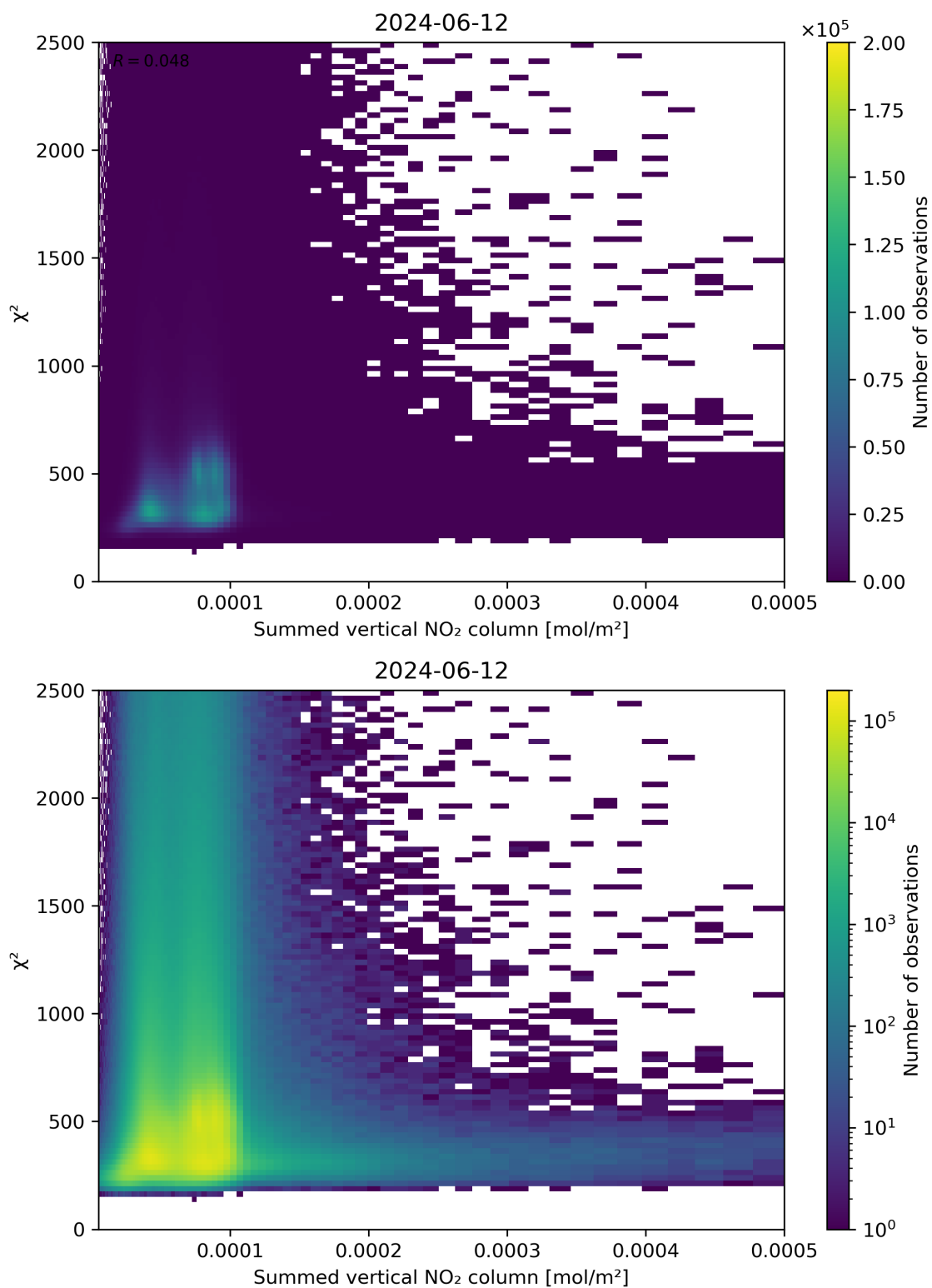
Figure 104: Scatter density plot of “Summed vertical NO 2 column” against “ \chi^2 ” for 2024-06-11 to 2024-06-13.
