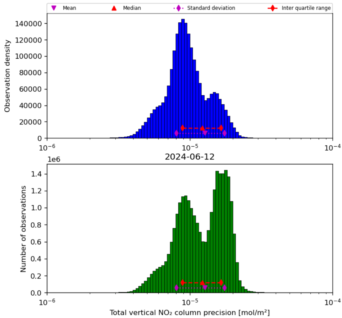
Figure 39: Histogram of “Total vertical NO 2 column precision” for 2024-06-11 to 2024-06-13
