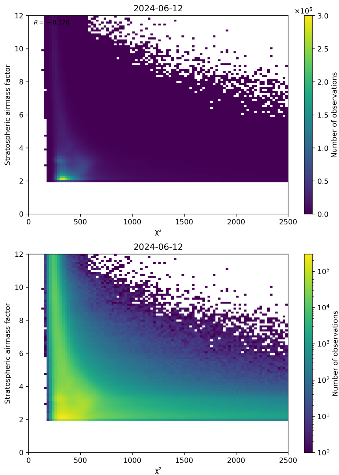
Figure 81: Scatter density plot of “ \chi^2 ” against “Stratospheric airmass factor” for 2024-06-11 to 2024-06-13.
