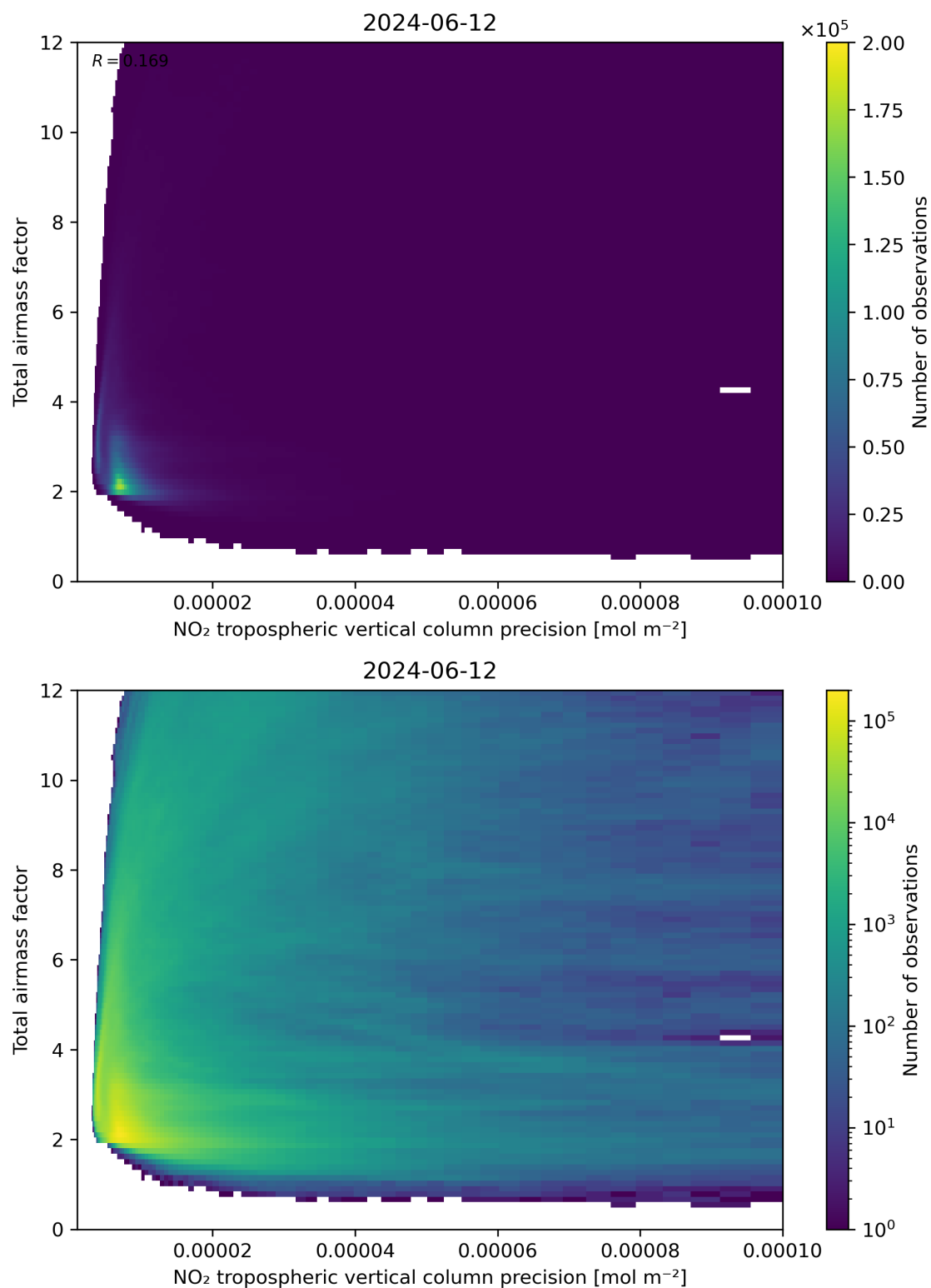
Figure 132: Scatter density plot of “NO 2 tropospheric vertical column precision” against “Total air mass factor” for 2024-06-11 to 2024-06-13.
