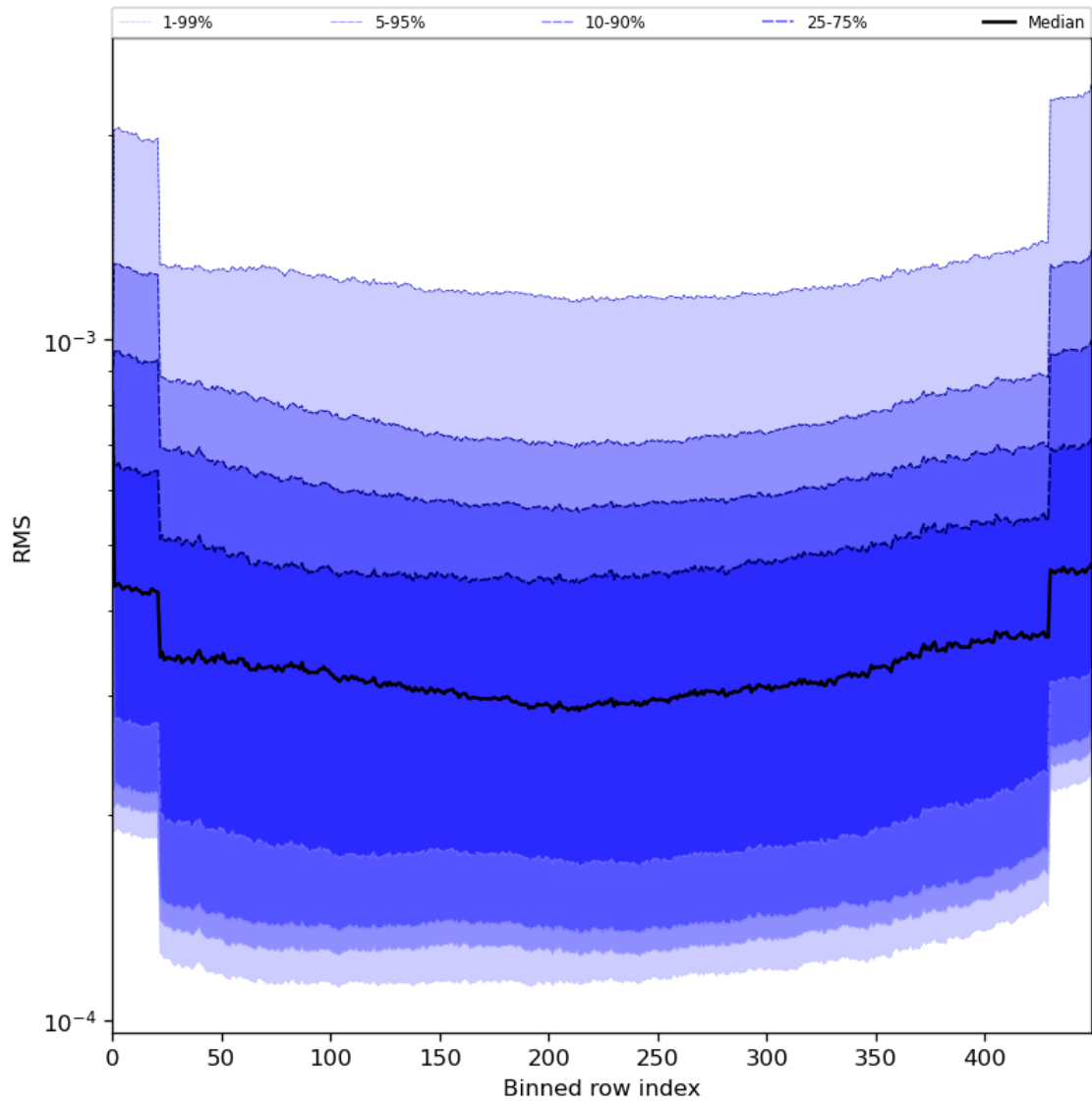
Figure 60: Along track statistics of “RMS” for 2024-06-11 to 2024-06-13
