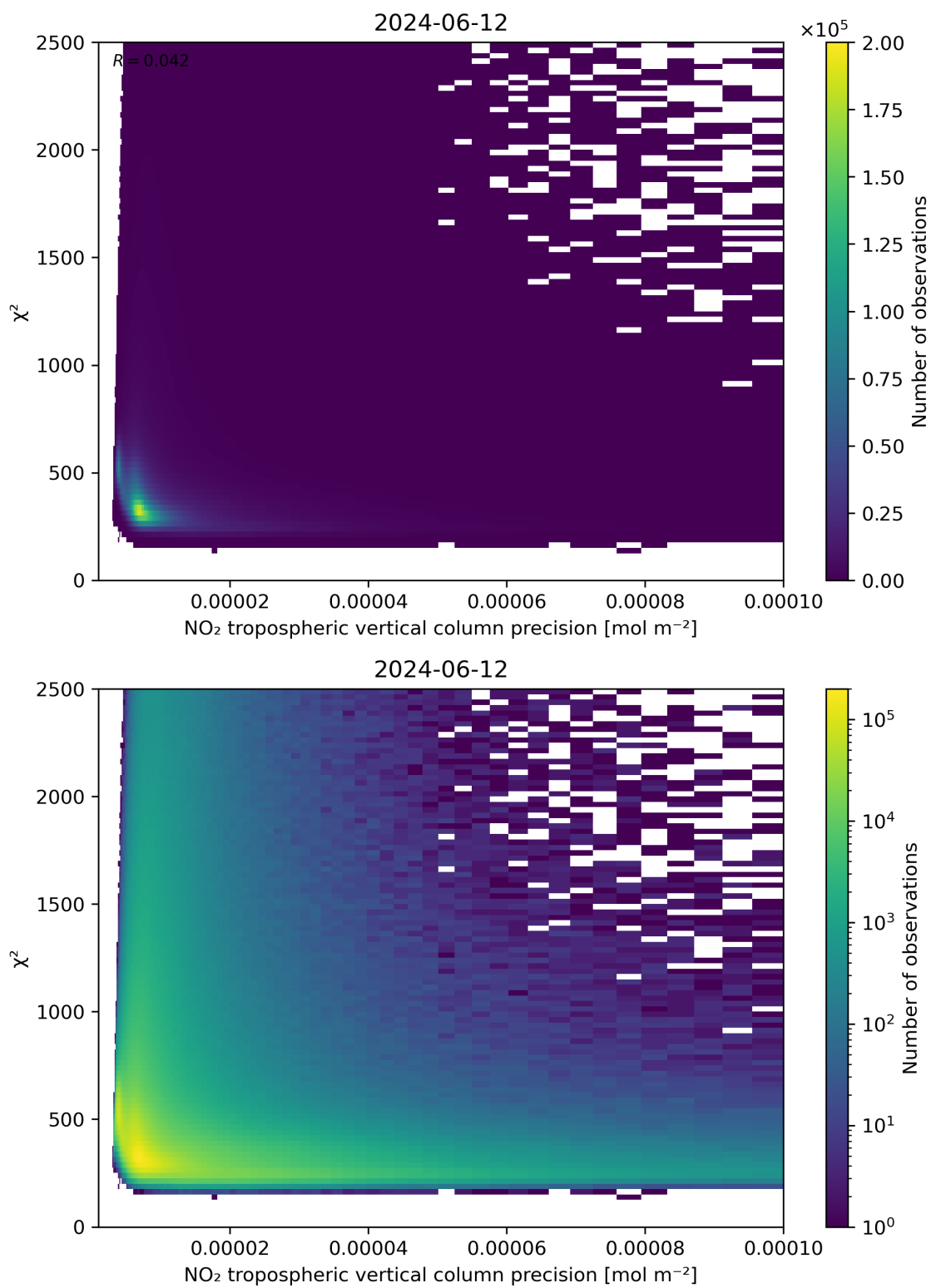
Figure 134: Scatter density plot of “NO 2 tropospheric vertical column precision” against “ \chi^2 ” for 2024-06-11 to 2024-06-13.
