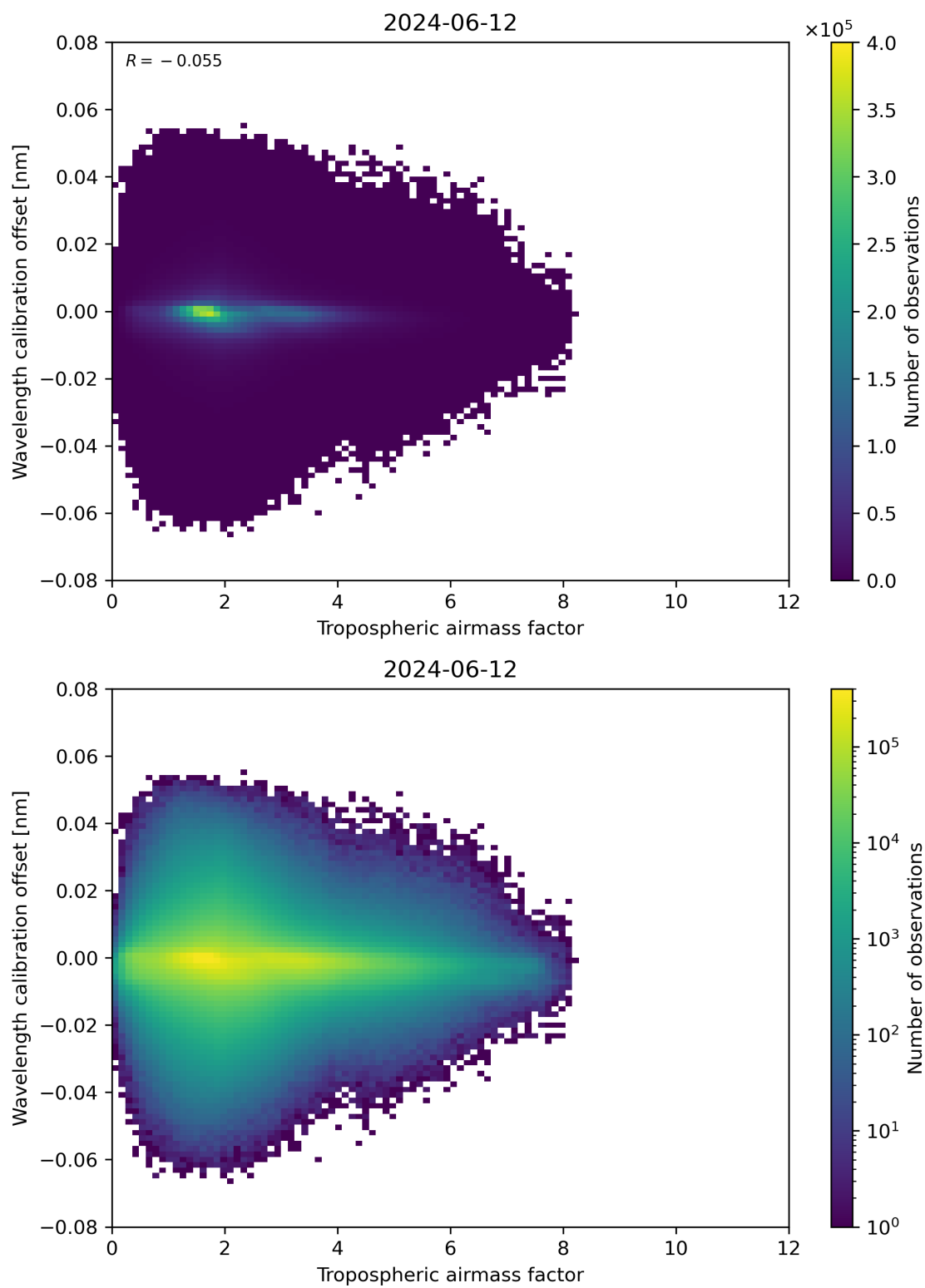
Figure 80: Scatter density plot of “Tropospheric airmass factor” against “Wavelength calibration offset” for 2024-06-11 to 2024-06-13.
