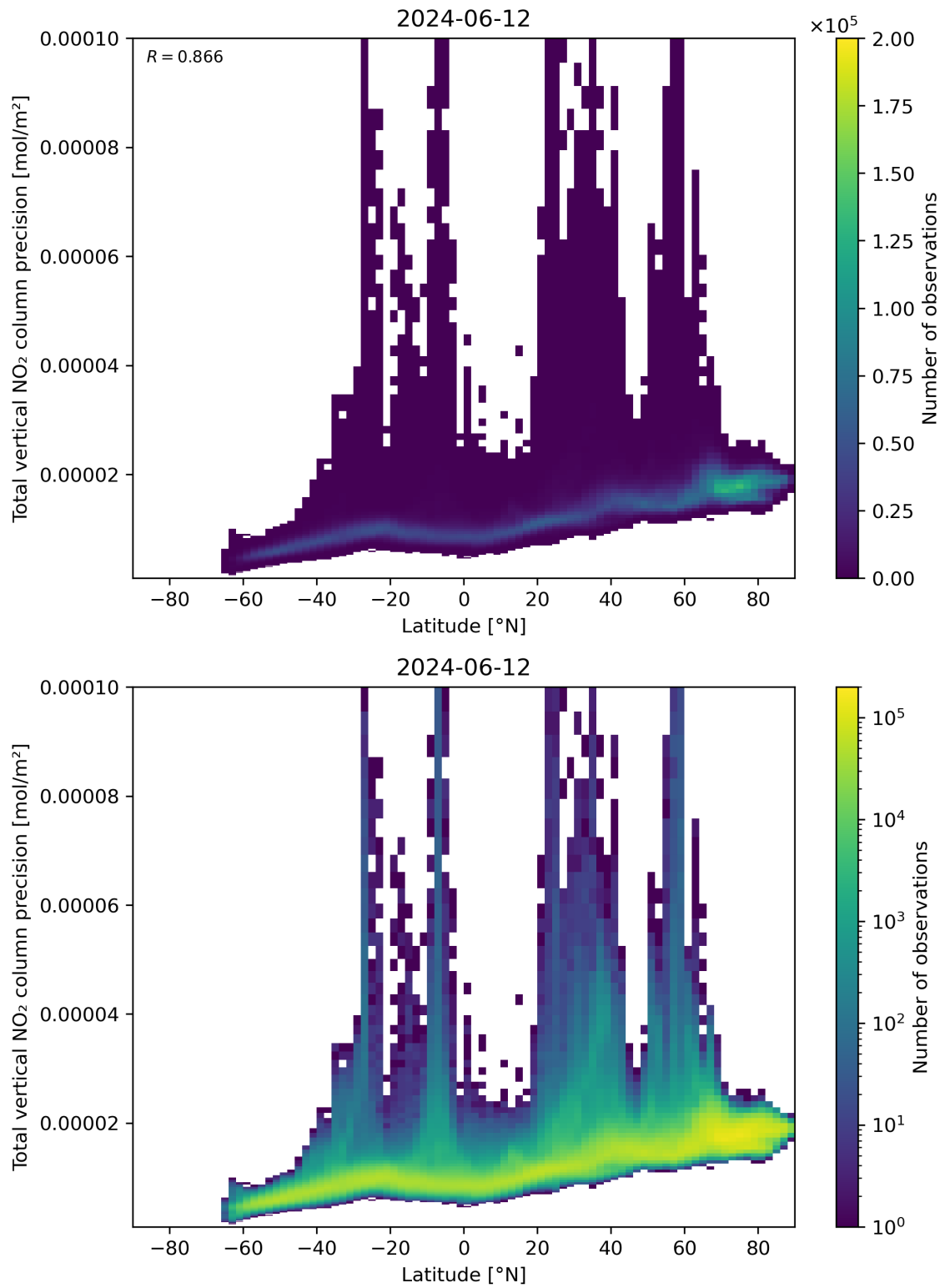
Figure 91: Scatter density plot of “Latitude” against “Total vertical NO 2 column precision” for 2024-06-11 to 2024-06-13.
