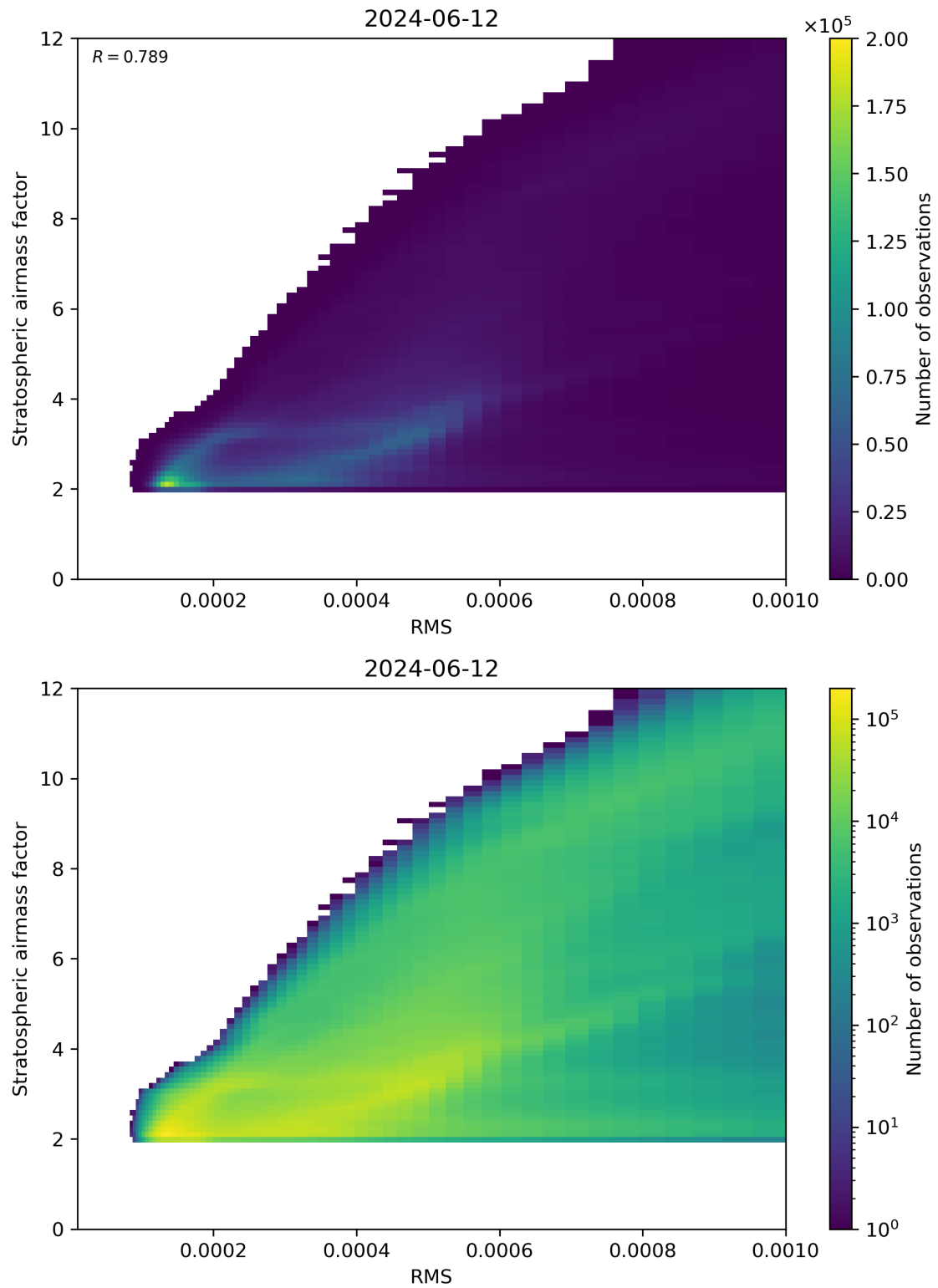
Figure 144: Scatter density plot of “RMS” against “Stratospheric airmass factor” for 2024-06-11 to 2024-06-13.
