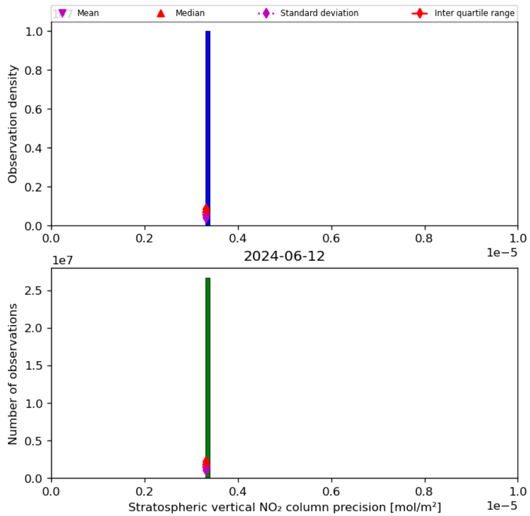
Figure 37: Histogram of “Stratospheric vertical NO 2 column precision” for 2024-06-11 to 2024-06-13
