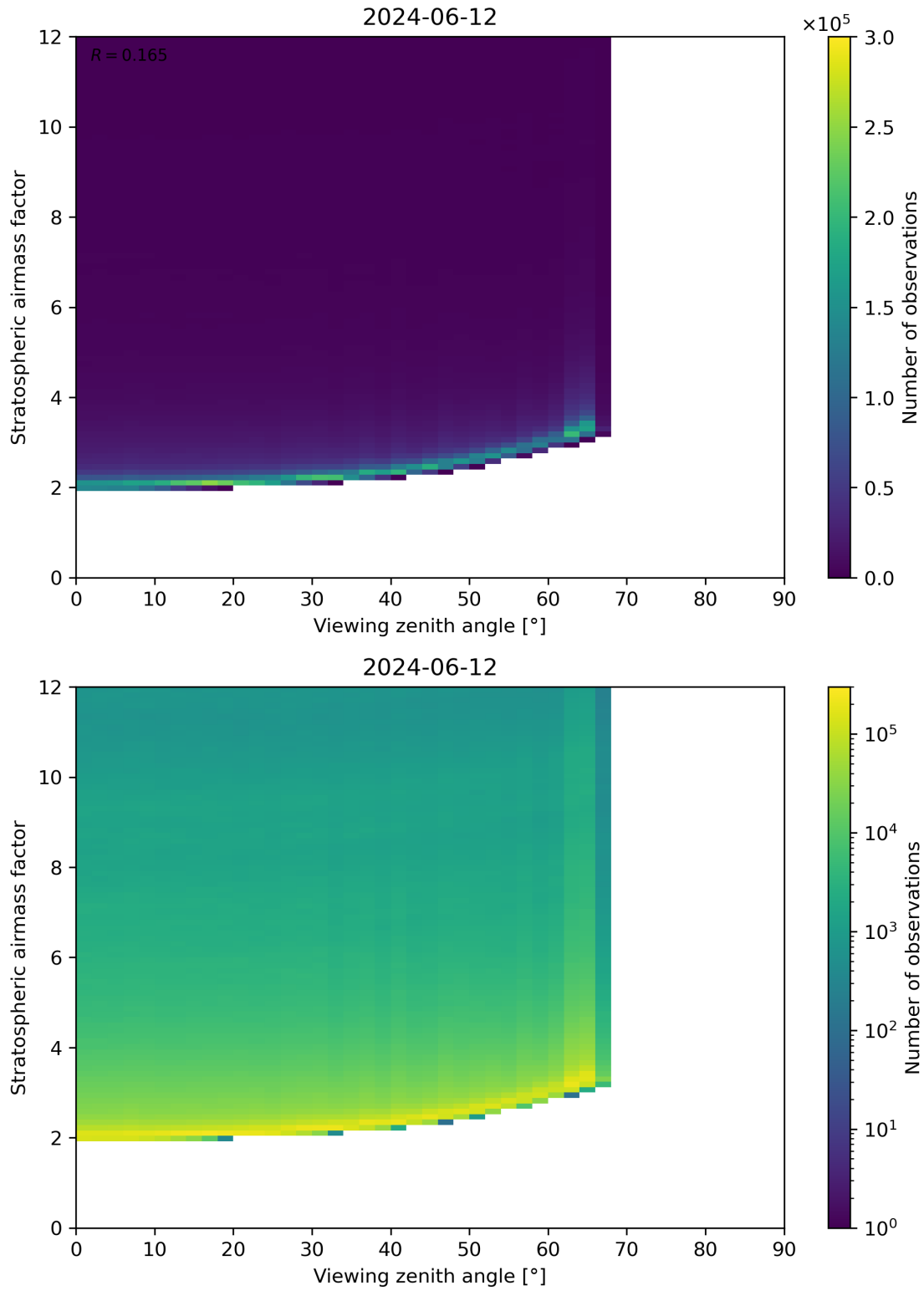
Figure 159: Scatter density plot of “Viewing zenith angle” against “Stratospheric airmass factor” for 2024-06-11 to 2024-06-13.
