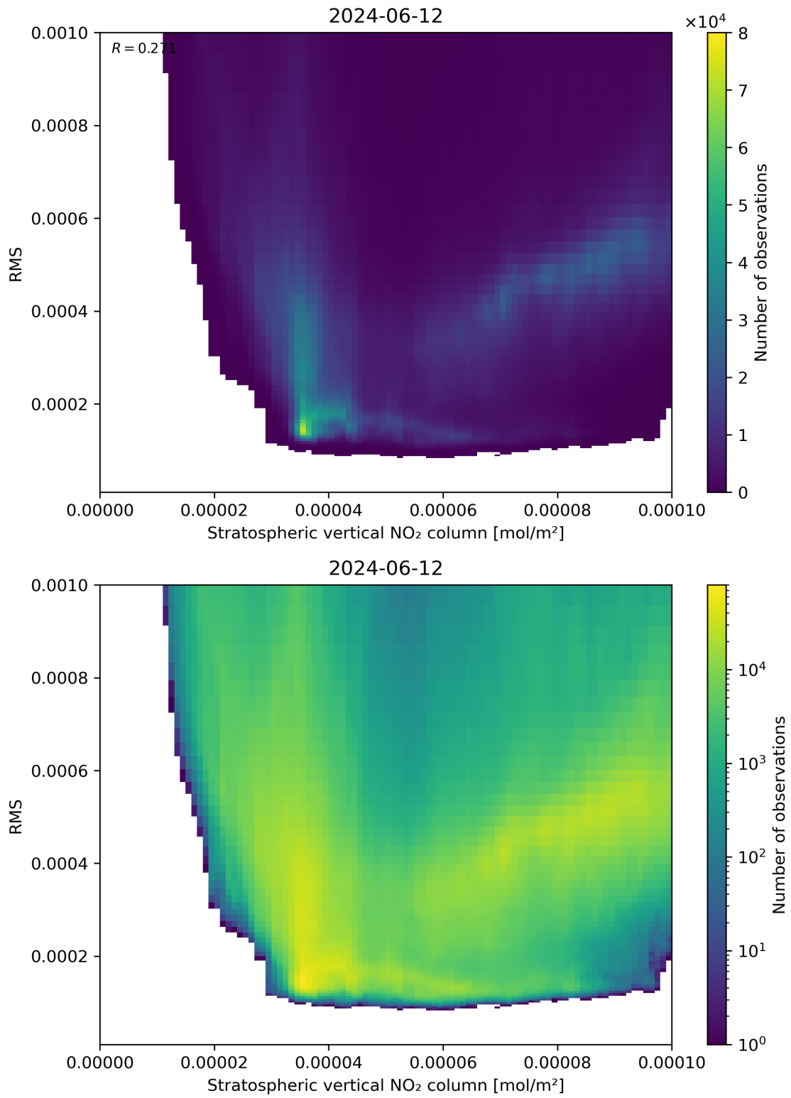
Figure 102: Scatter density plot of “Stratospheric vertical NO 2 column” against “RMS” for 2024-06-11 to 2024-06-13.
