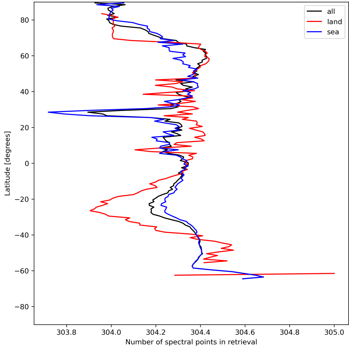
Figure 16: Zonal average of “Number of spectral points in retrieval” for 2024-06-11 to 2024-06-13.
