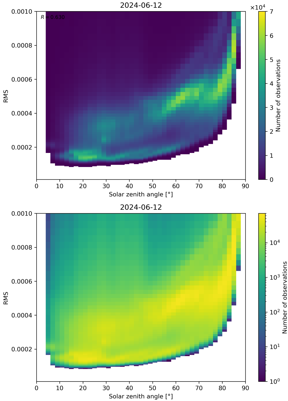
Figure 157: Scatter density plot of “Solar zenith angle” against “RMS” for 2024-06-11 to 2024-06-13.
