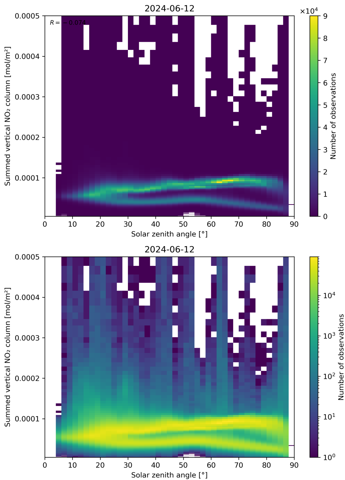
Figure 151: Scatter density plot of “Solar zenith angle” against “Summed vertical NO 2 column” for 2024-06-11 to 2024-06-13.
