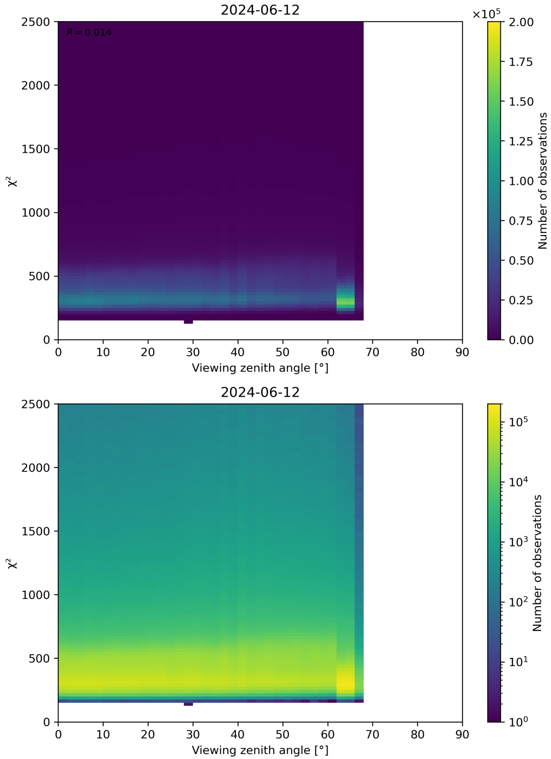
Figure 162: Scatter density plot of “Viewing zenith angle” against “ \chi^2 ” for 2024-06-11 to 2024-06-13.
