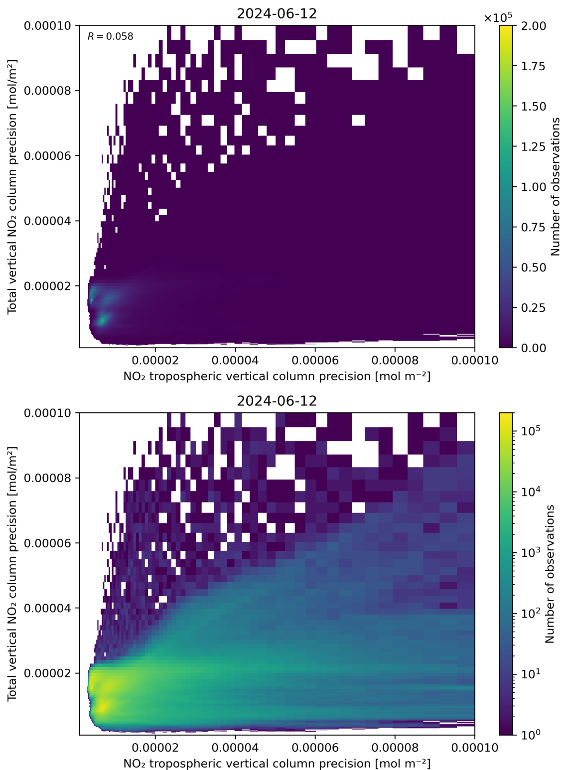
Figure 139: Scatter density plot of “NO 2 tropospheric vertical column precision” against “Total vertical NO 2 column precision” for 2024-06-11 to 2024-06-13.
