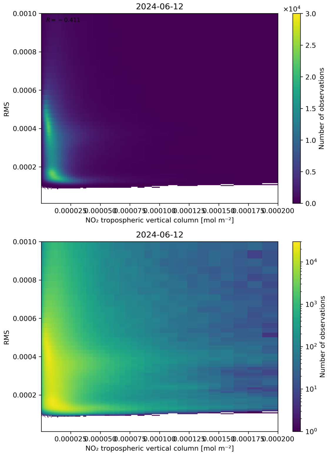
Figure 142: Scatter density plot of “NO 2 tropospheric vertical column” against “RMS” for 2024-06-11 to 2024-06-13.
