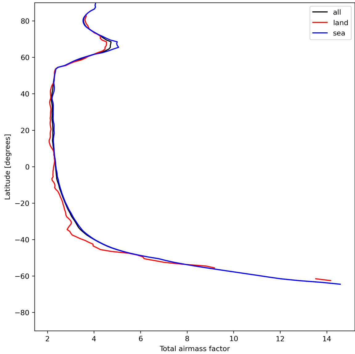
Figure 15: Zonal average of “Total airmass factor” for 2024-06-11 to 2024-06-13.
