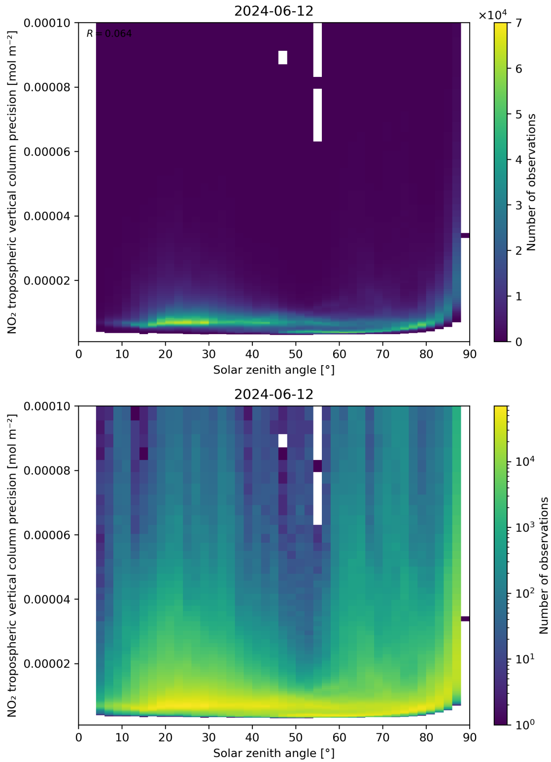
Figure 156: Scatter density plot of “Solar zenith angle” against “NO 2 tropospheric vertical column precision” for 2024-06-11 to 2024-06-13.
