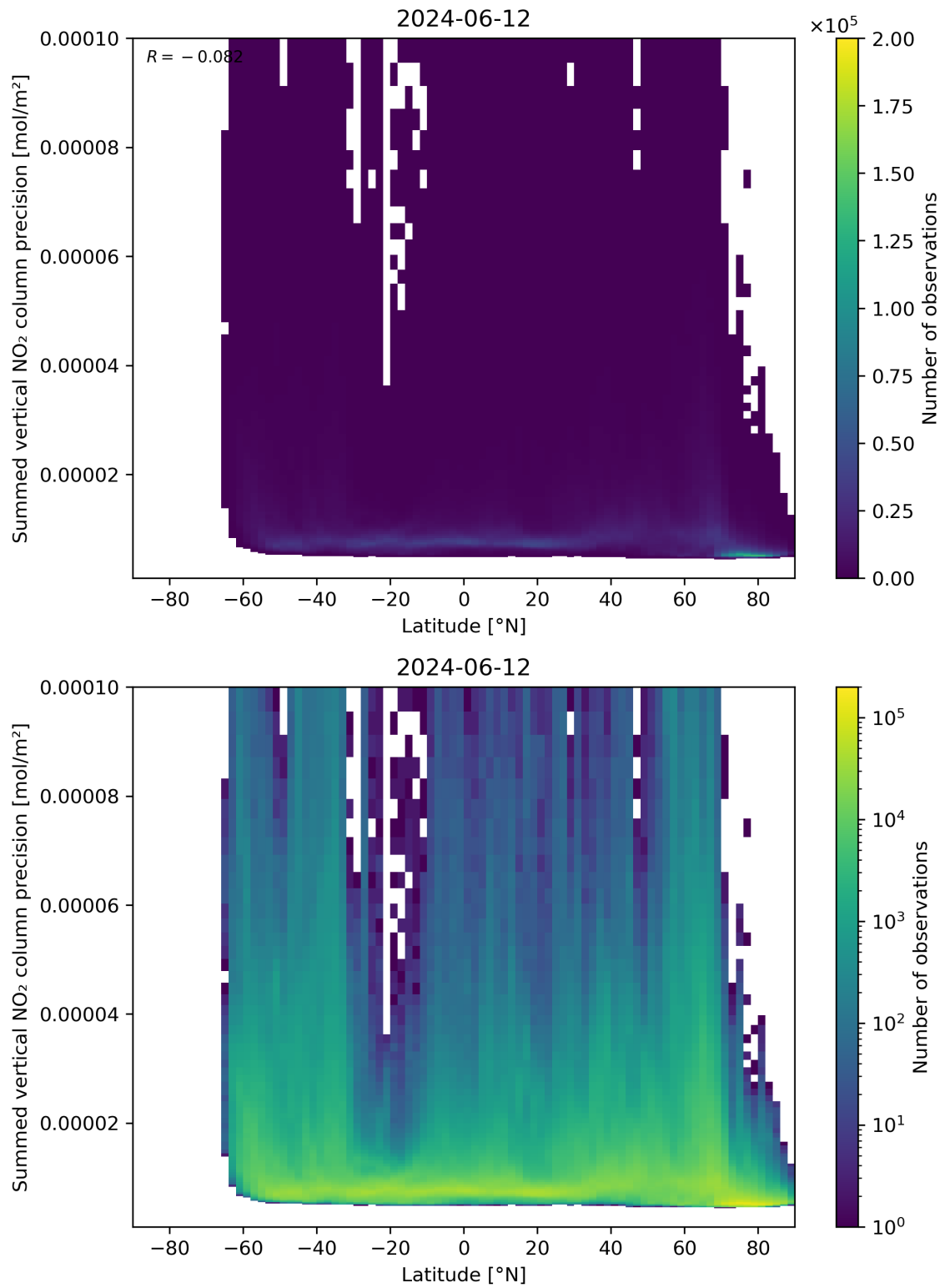
Figure 89: Scatter density plot of “Latitude” against “Summed vertical NO 2 column precision” for 2024-06-11 to 2024-06-13.
