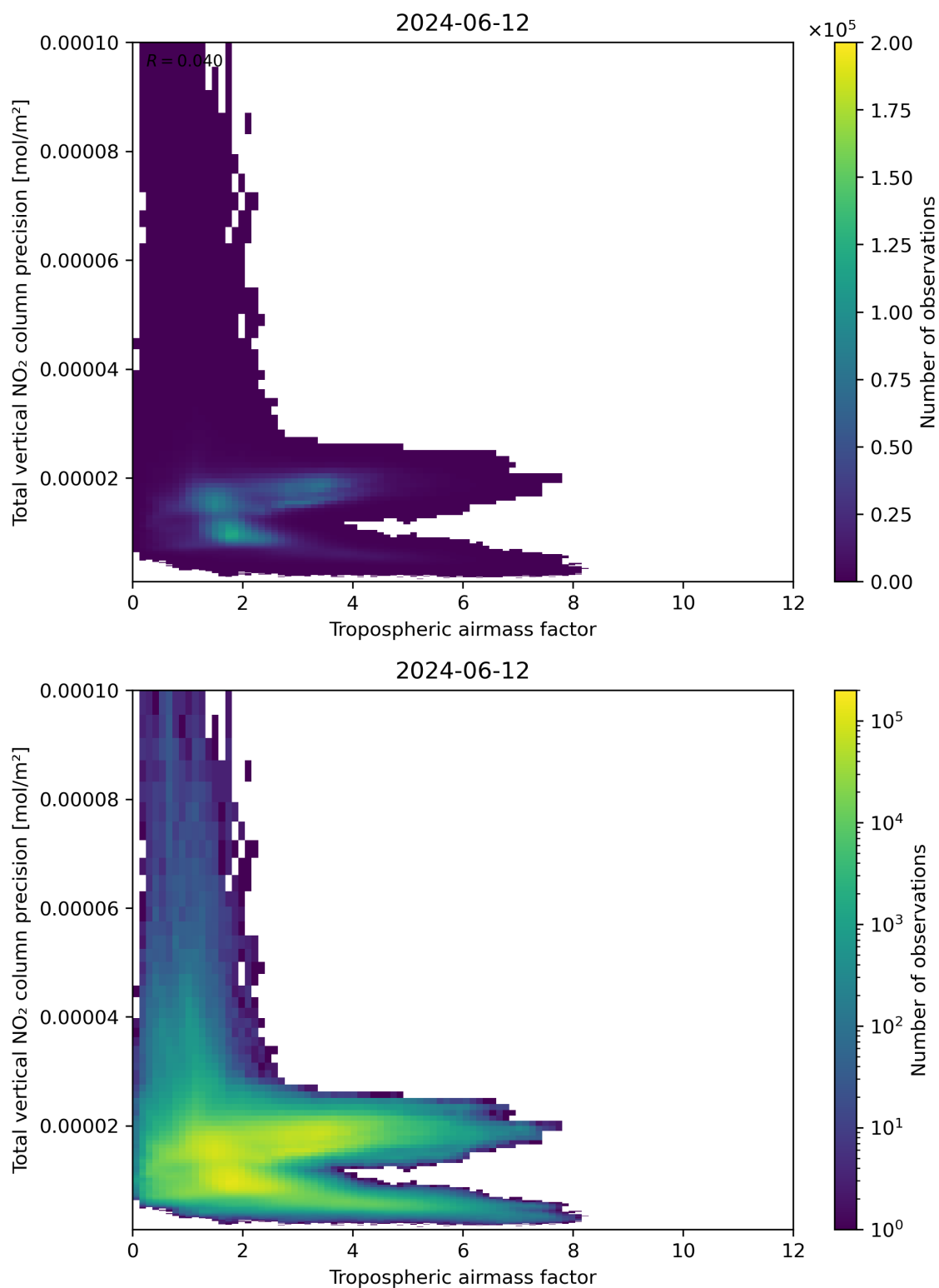
Figure 78: Scatter density plot of “Tropospheric air mass factor” against “Total vertical NO 2 column precision” for 2024-06-11 to 2024-06-13.
