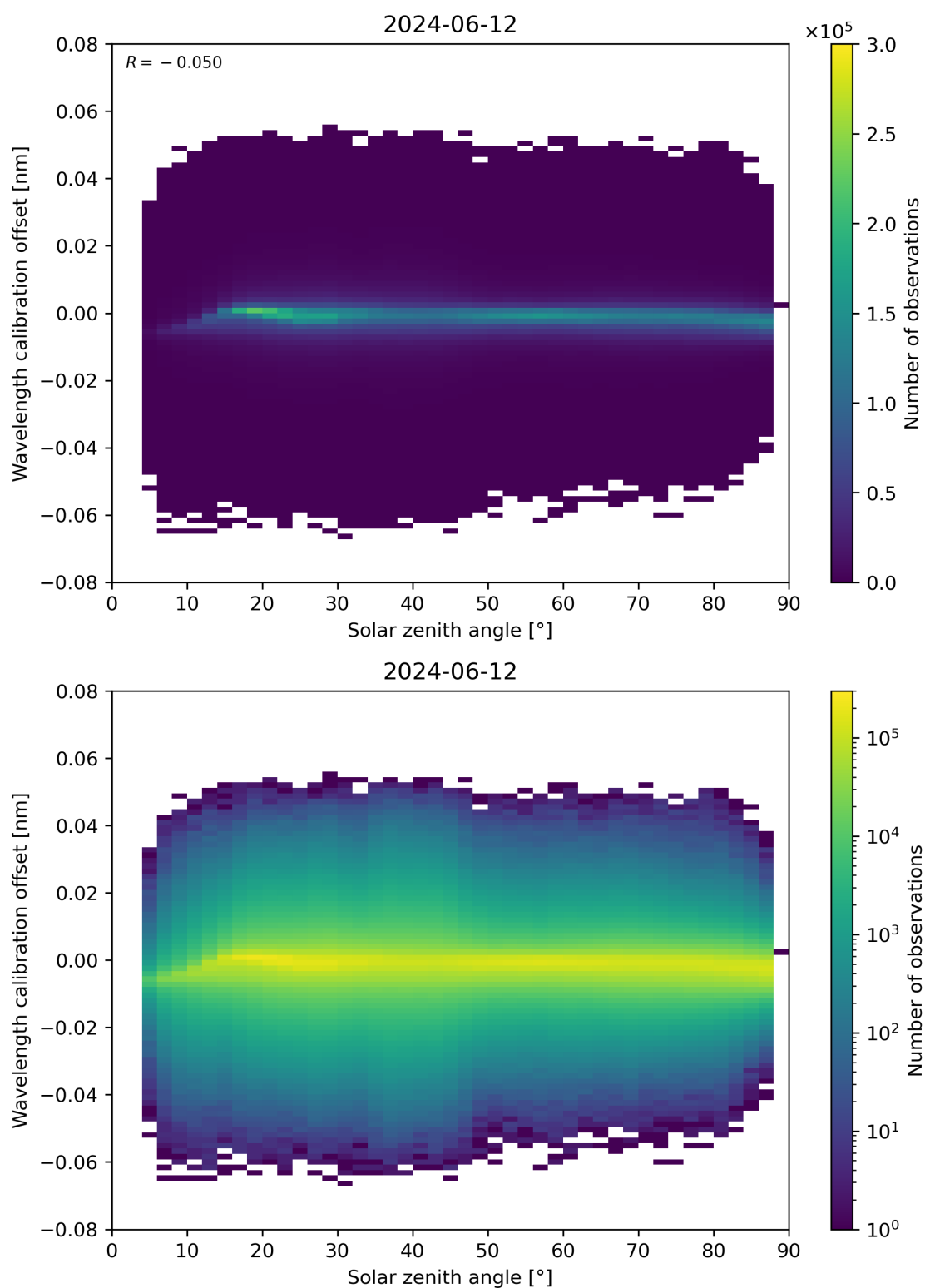
Figure 158: Scatter density plot of “Solar zenith angle” against “Wavelength calibration offset” for 2024-06-11 to 2024-06-13.
