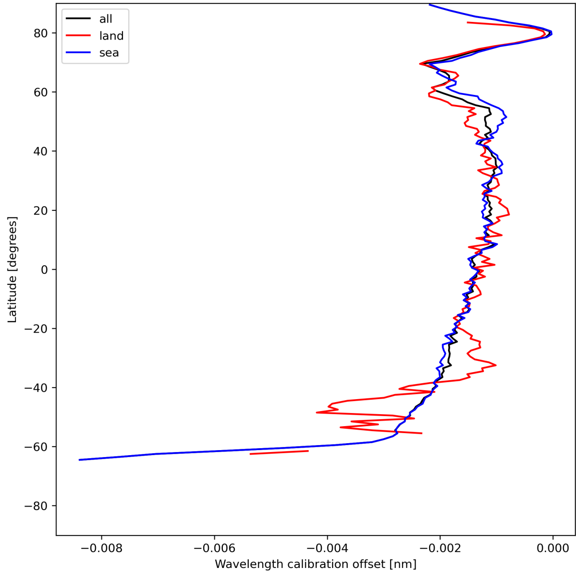
Figure 18: Zonal average of “Wavelength calibration offset” for 2024-06-11 to 2024-06-13.
