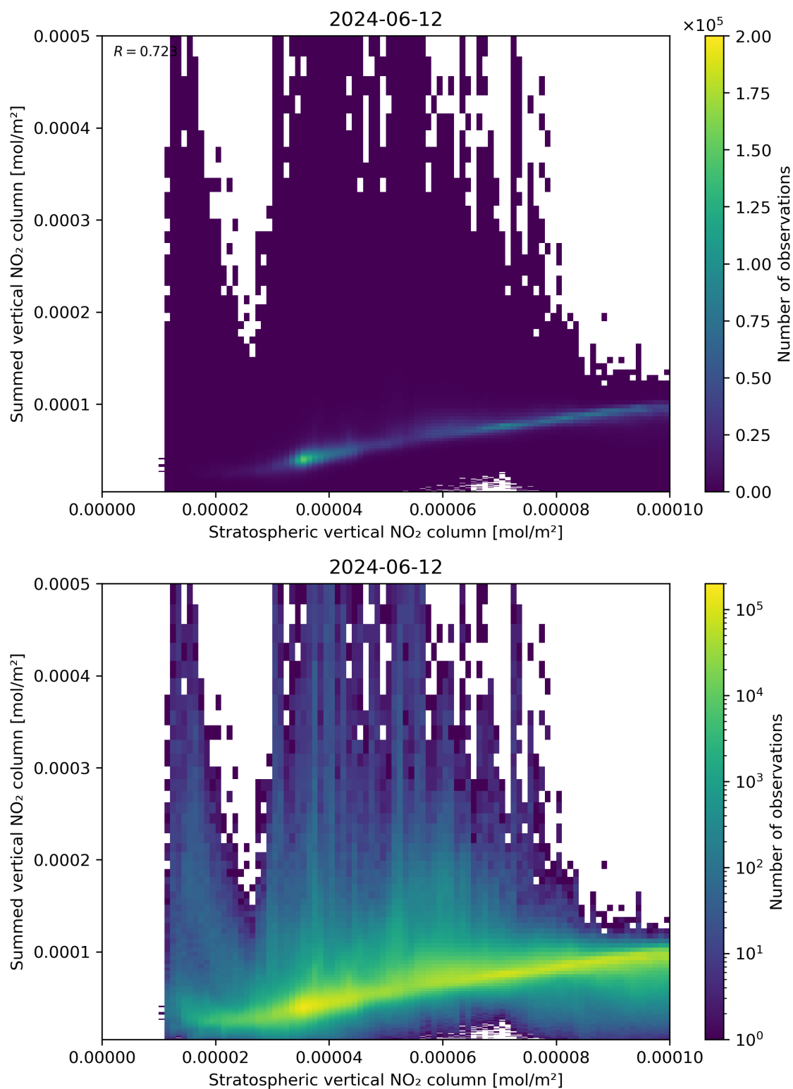
Figure 98: Scatter density plot of “Stratospheric vertical NO 2 column” against “Summed vertical NO 2 column” for 2024-06-11 to 2024-06-13.
