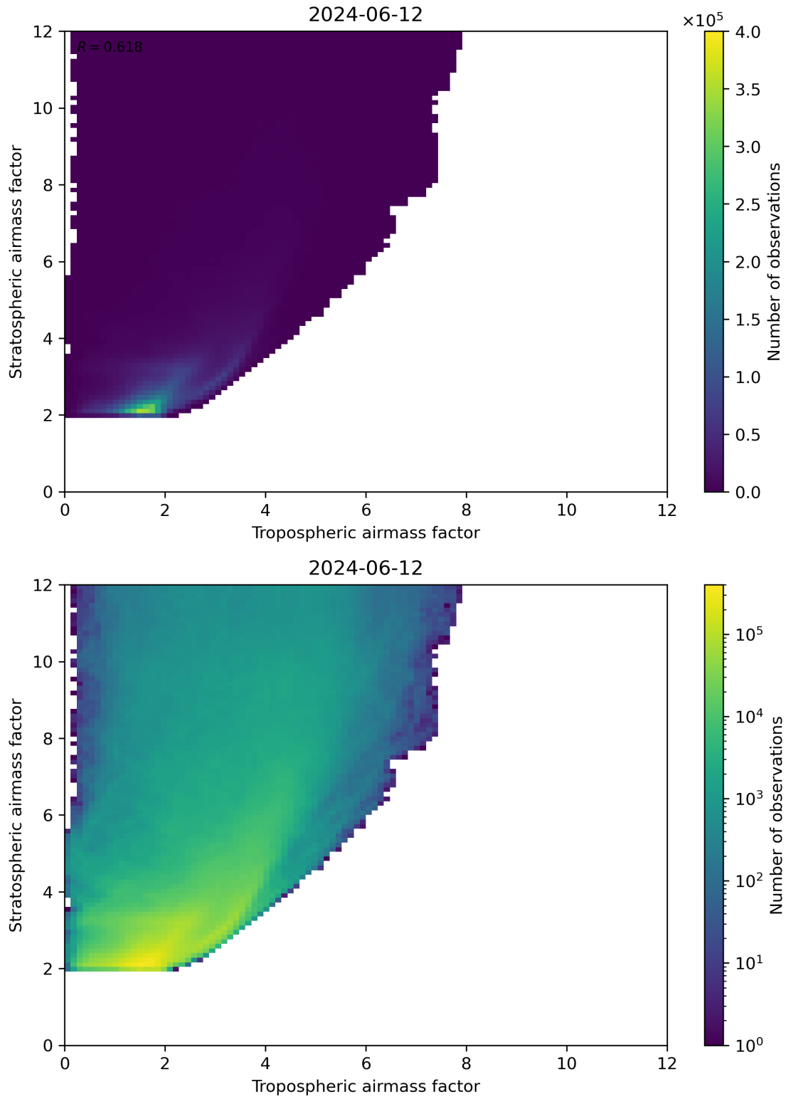
Figure 71: Scatter density plot of “Tropospheric airmass factor” against “Stratospheric airmass factor” for 2024-06-11 to 2024-06-13.
