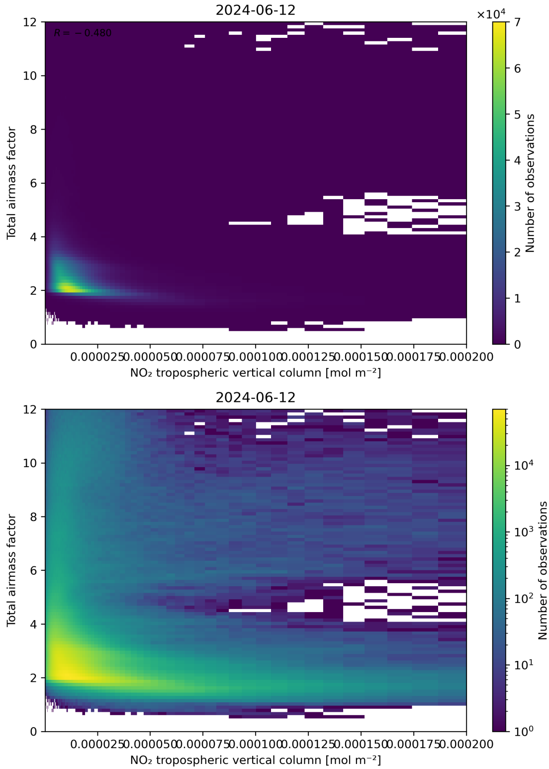
Figure 122: Scatter density plot of “NO 2 tropospheric vertical column” against “Total air mass factor” for 2024-06-11 to 2024-06-13.
