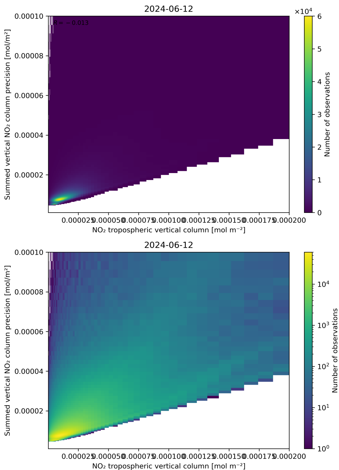
Figure 127: Scatter density plot of “NO 2 tropospheric vertical column” against “Summed vertical NO 2 column precision” for 2024-06-11 to 2024-06-13.
