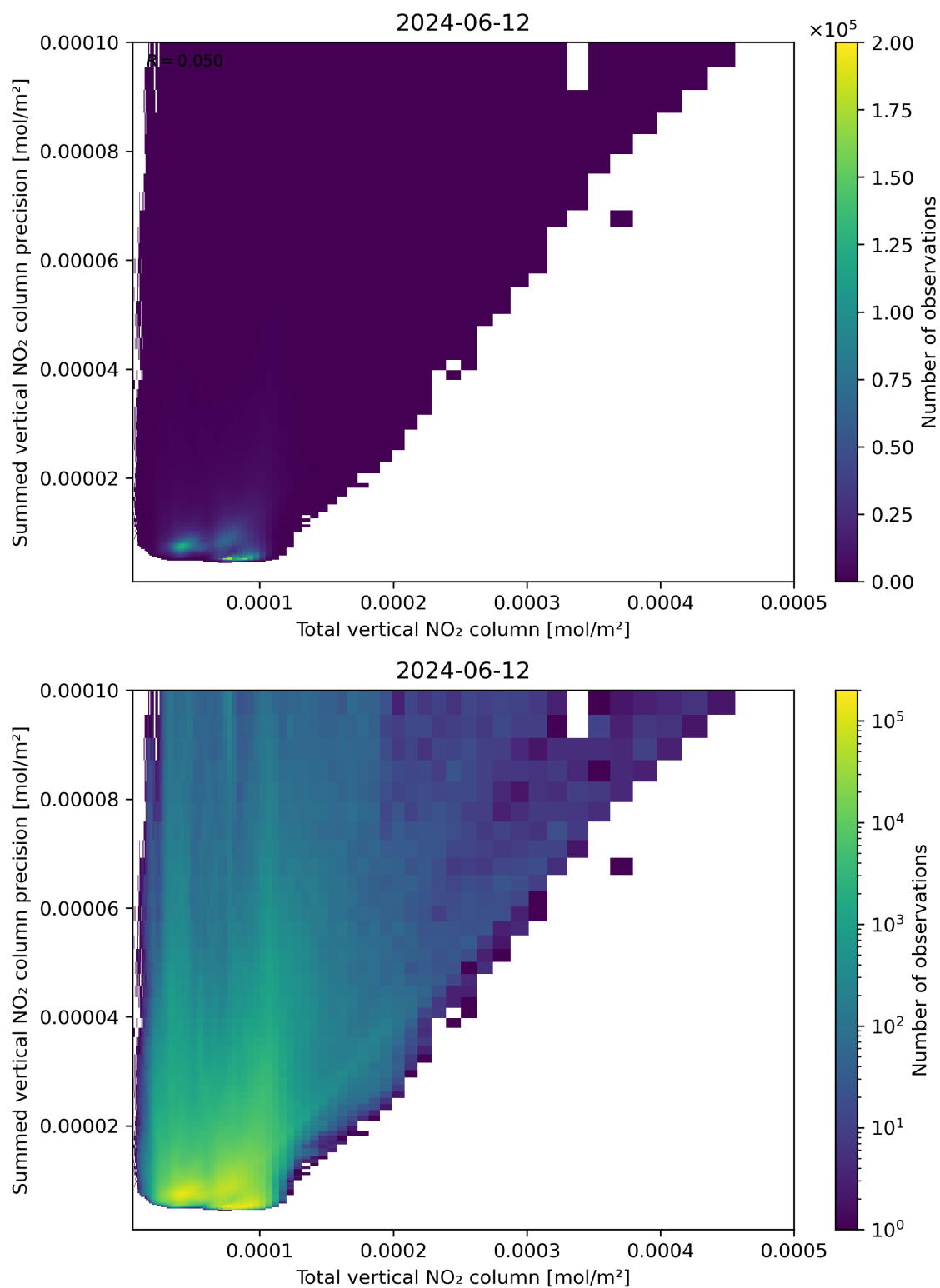
Figure 113: Scatter density plot of “Total vertical NO 2 column” against “Summed vertical NO 2 column precision” for 2024-06-11 to 2024-06-13.
