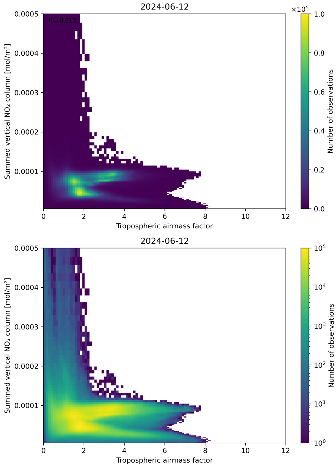
Figure 75: Scatter density plot of “Tropospheric airmass factor” against “Summed vertical NO 2 column” for 2024-06-11 to 2024-06-13.
