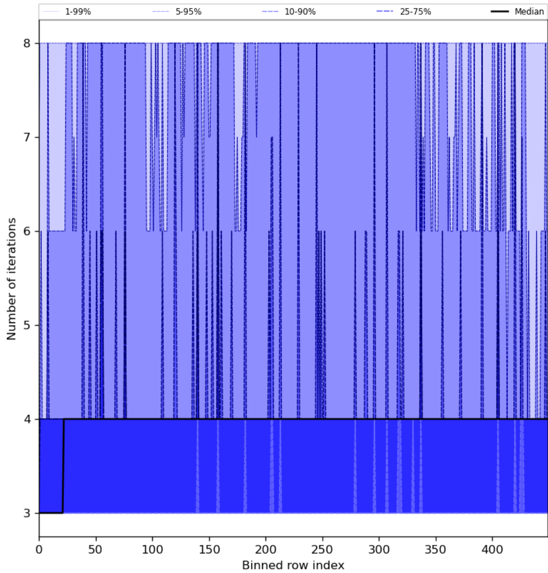
Figure 51: Along track statistics of “Number of iterations” for 2024-06-11 to 2024-06-13
