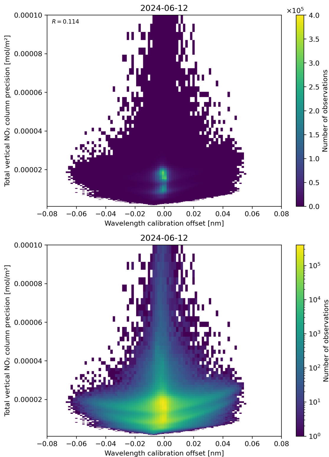
Figure 180: Scatter density plot of “Wavelength calibration offset” against “Total vertical NO 2 column precision” for 2024-06-11 to 2024-06-13.
