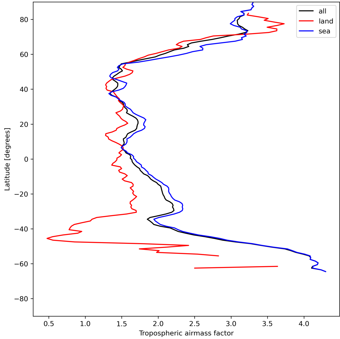
Figure 14: Zonal average of “Tropospheric airmass factor” for 2024-06-11 to 2024-06-13.
