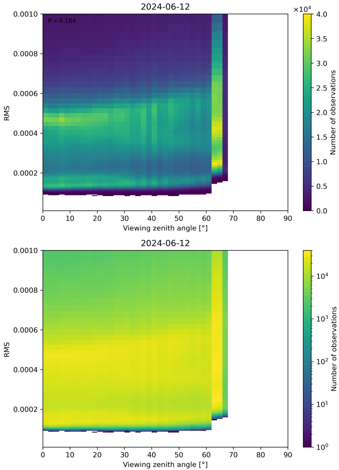
Figure 171: Scatter density plot of “Viewing zenith angle” against “RMS” for 2024-06-11 to 2024-06-13.
