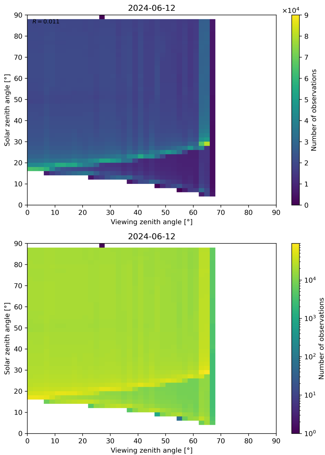
Figure 172: Scatter density plot of “Viewing zenith angle” against “Solar zenith angle” for 2024-06-11 to 2024-06-13.
