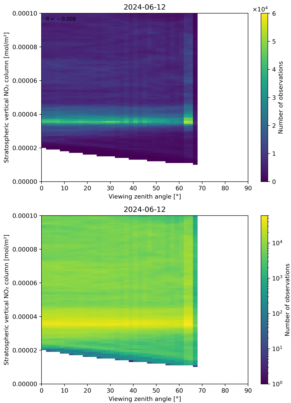
Figure 164: Scatter density plot of “Viewing zenith angle” against “Stratospheric vertical NO 2 column” for 2024-06-11 to 2024-06-13.
