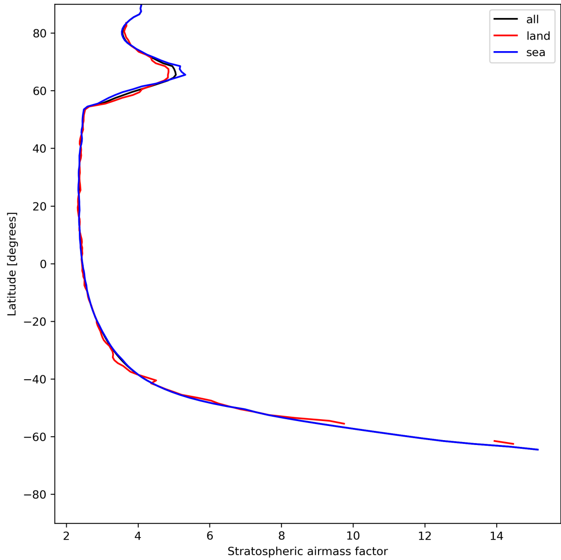
Figure 27: Zonal average of “Stratospheric air mass factor” for 2024-06-11 to 2024-06-13.
