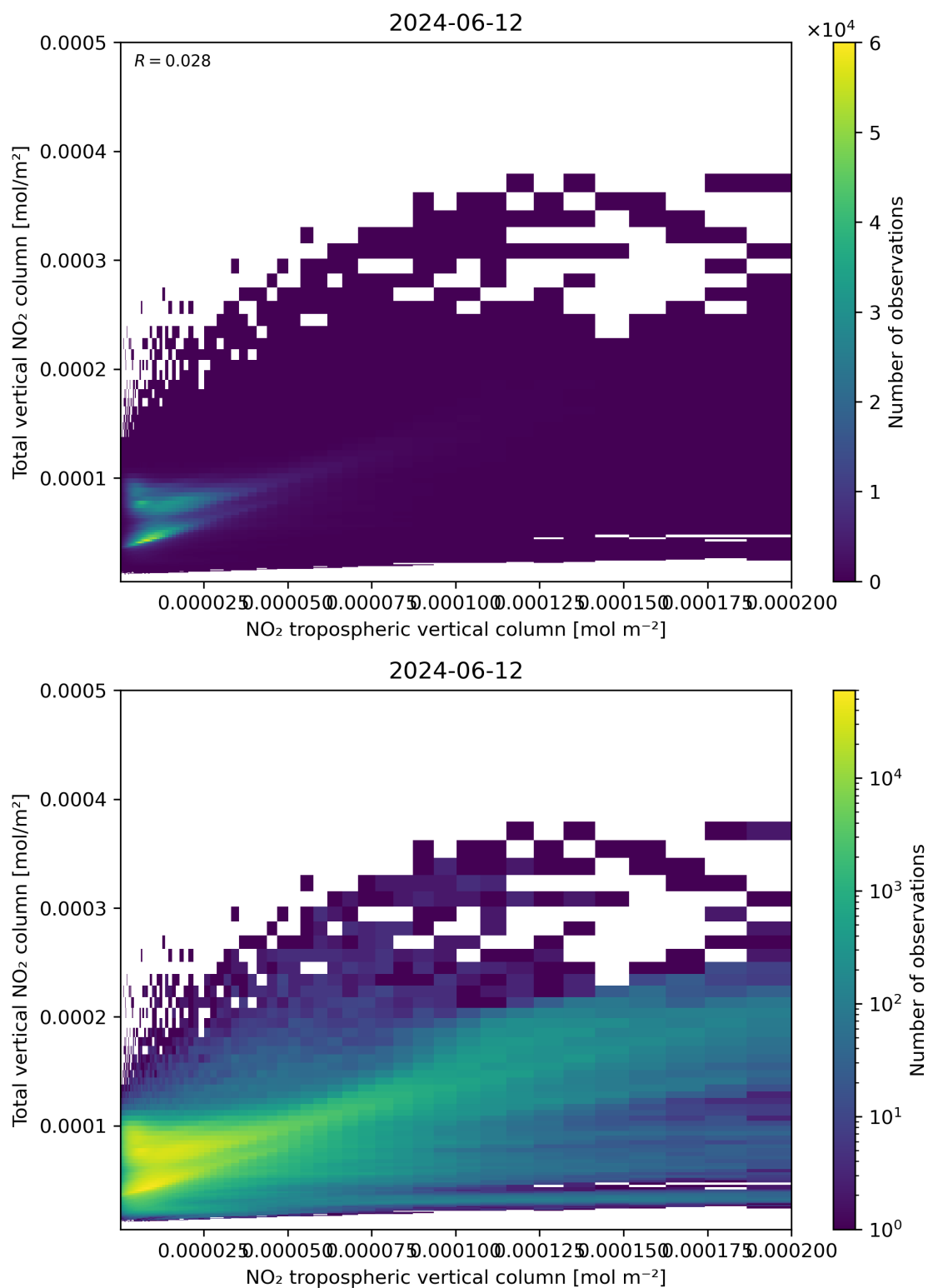
Figure 128: Scatter density plot of “NO 2 tropospheric vertical column” against “Total vertical NO 2 column” for 2024-06-11 to 2024-06-13.
