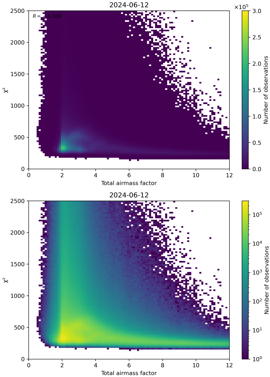
Figure 63: Scatter density plot of “Total airmass factor” against “ \chi^2 ” for 2024-06-11 to 2024-06-13.
