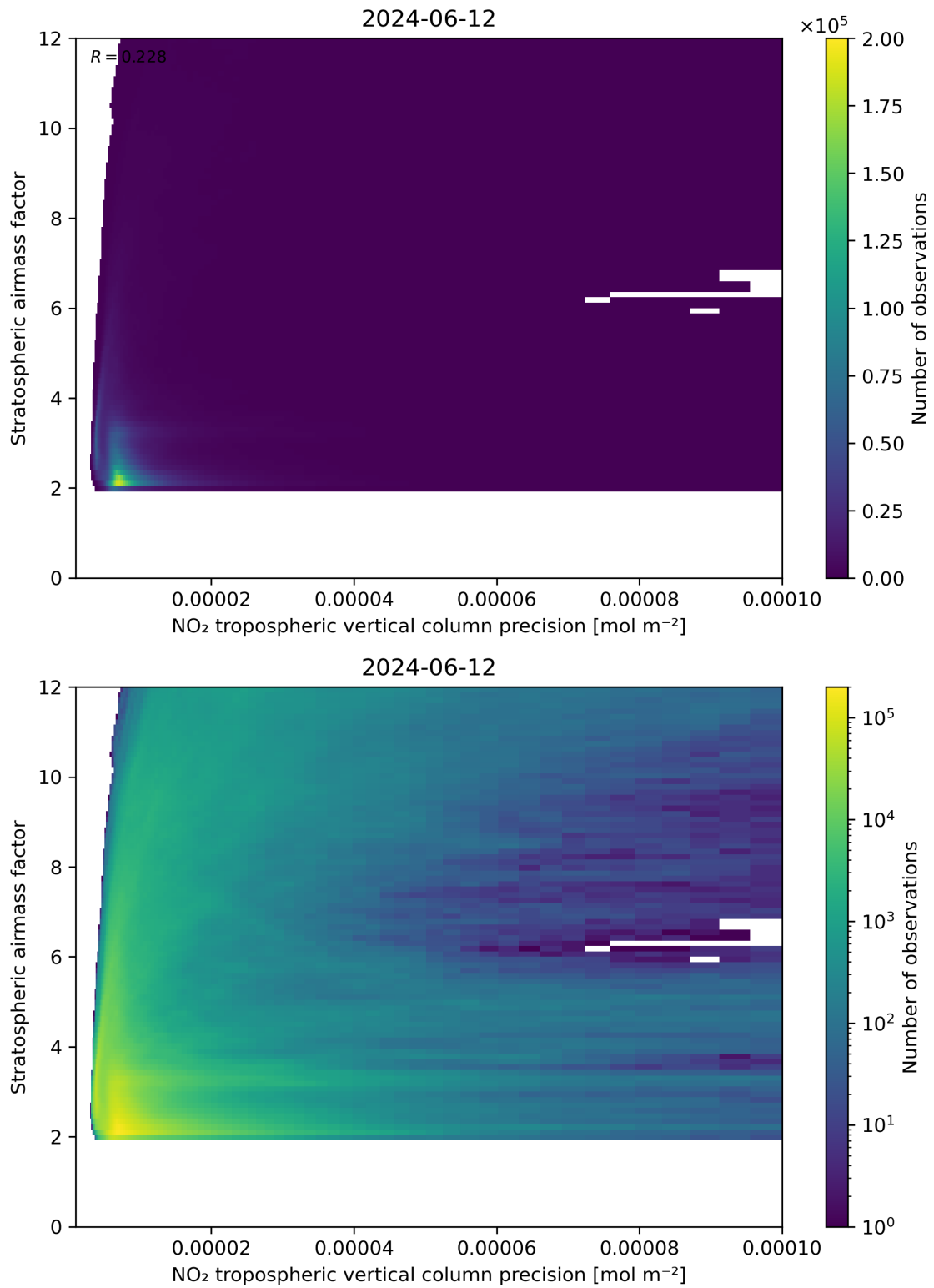
Figure 131: Scatter density plot of “NO 2 tropospheric vertical column precision” against “Stratospheric airmass factor” for 2024-06-11 to 2024-06-13.
