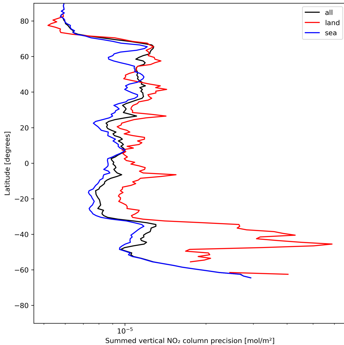
Figure 24: Zonal average of “Summed vertical NO 2 column precision” for 2024-06-11 to 2024-06-13.
