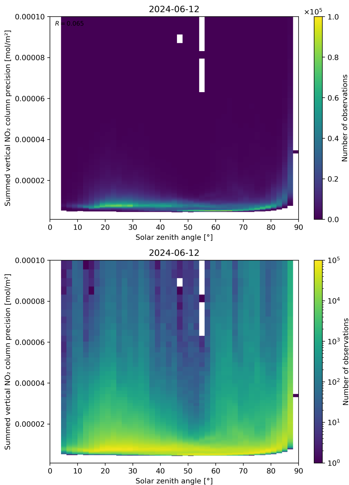
Figure 152: Scatter density plot of “Solar zenith angle” against “Summed vertical NO 2 column precision” for 2024-06-11 to 2024-06-13.
