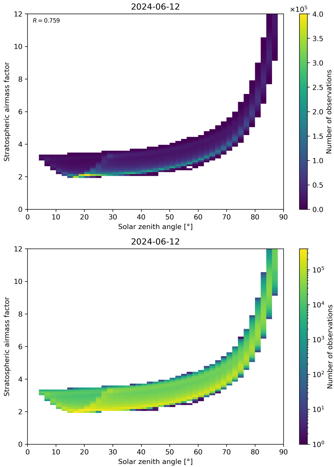
Figure 145: Scatter density plot of “Solar zenith angle” against “Stratospheric airmass factor” for 2024-06-11 to 2024-06-13.
