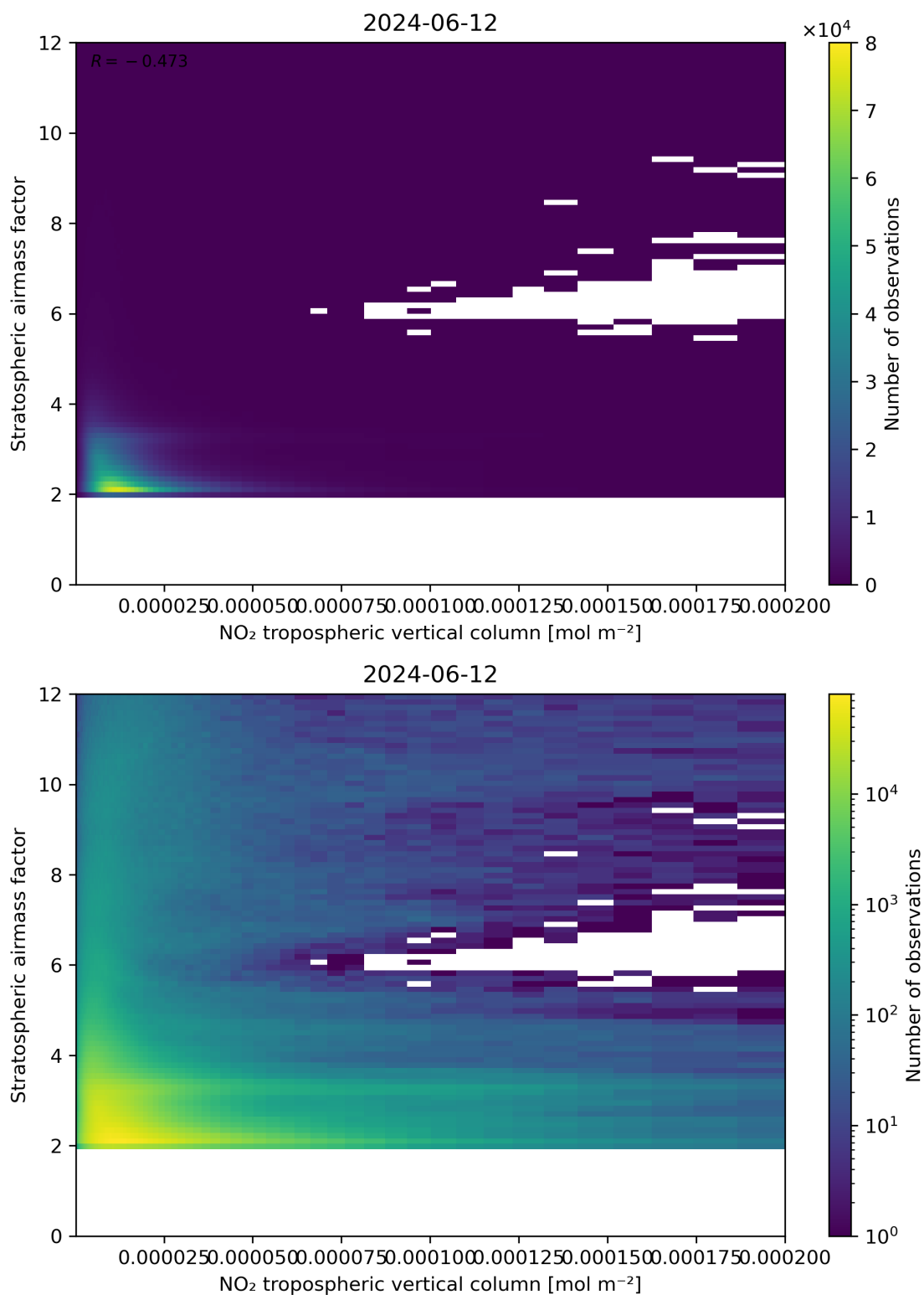
Figure 121: Scatter density plot of “NO 2 tropospheric vertical column” against “Stratospheric air mass factor” for 2024-06-11 to 2024-06-13.
