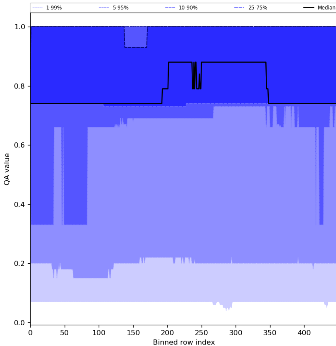
Figure 45: Along track statistics of “QA value” for 2024-06-11 to 2024-06-13
