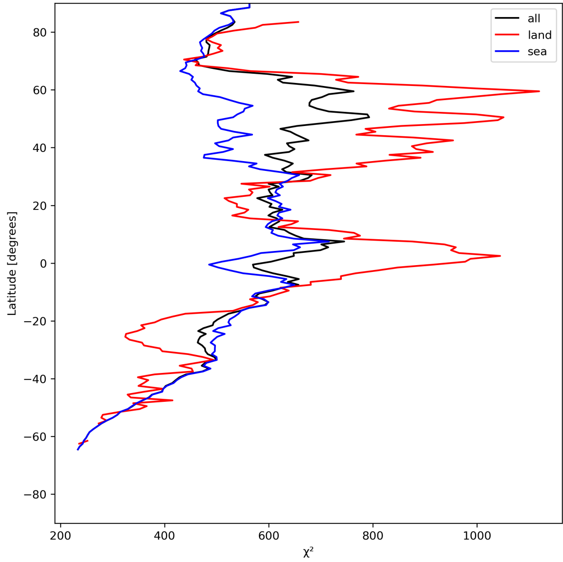
Figure 25: Zonal average of “ \chi^2 ” for 2024-06-11 to 2024-06-13.
