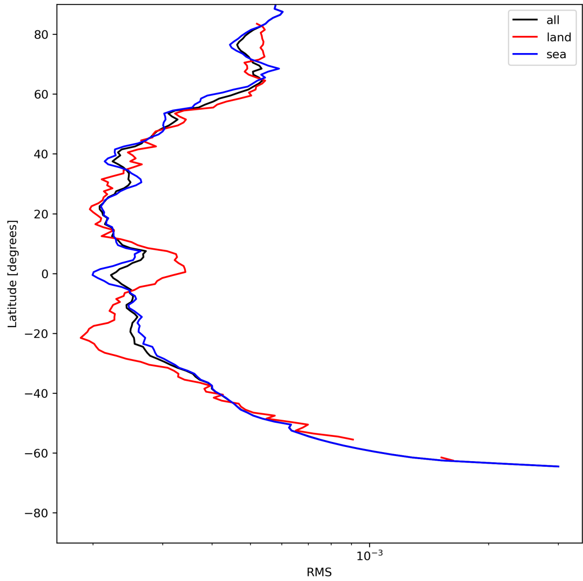
Figure 26: Zonal average of “RMS” for 2024-06-11 to 2024-06-13.
