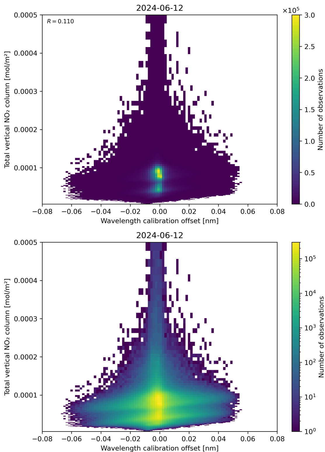
Figure 179: Scatter density plot of “Wavelength calibration offset” against “Total vertical NO 2 column” for 2024-06-11 to 2024-06-13.
