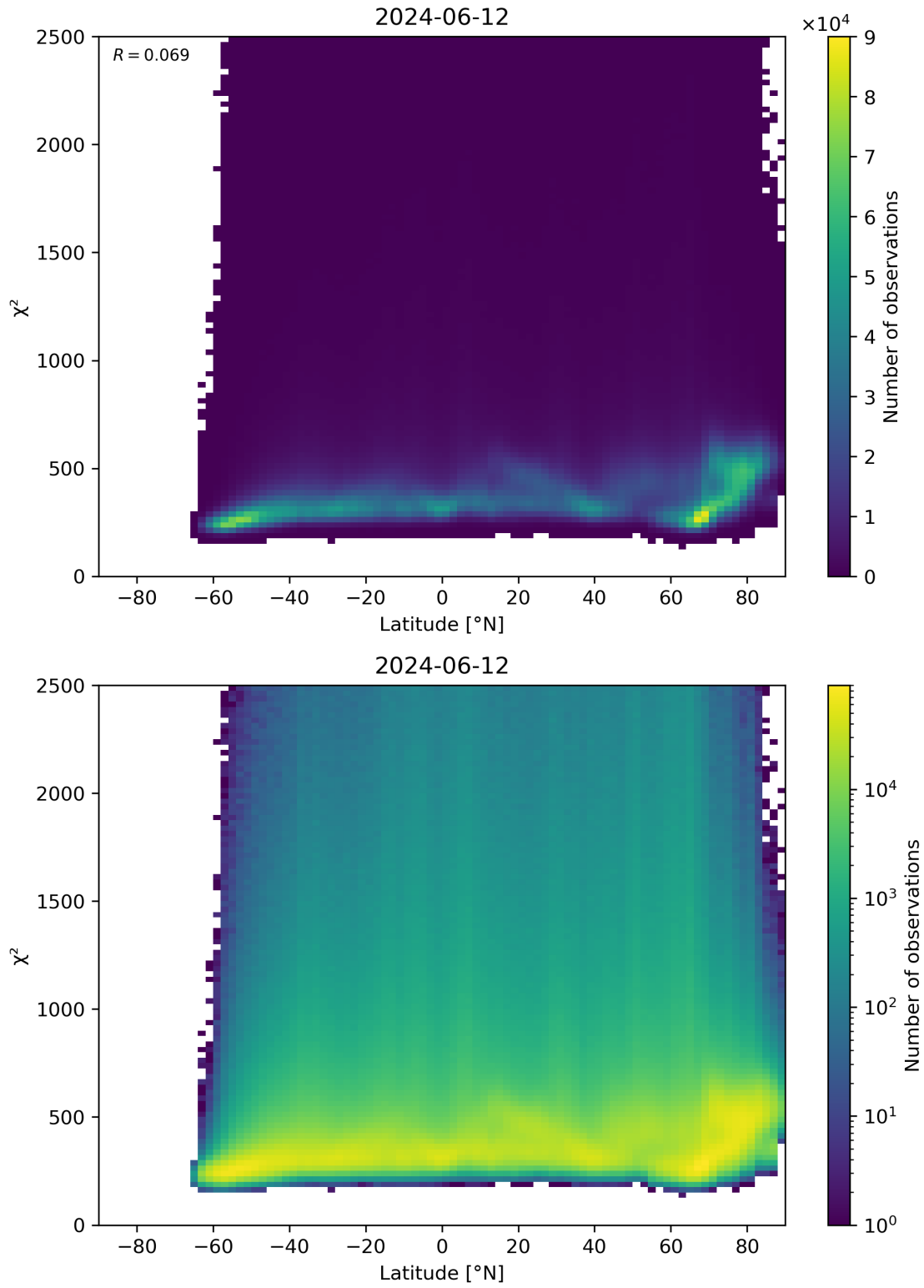
Figure 86: Scatter density plot of “Latitude” against “ \chi^2 ” for 2024-06-11 to 2024-06-13.
