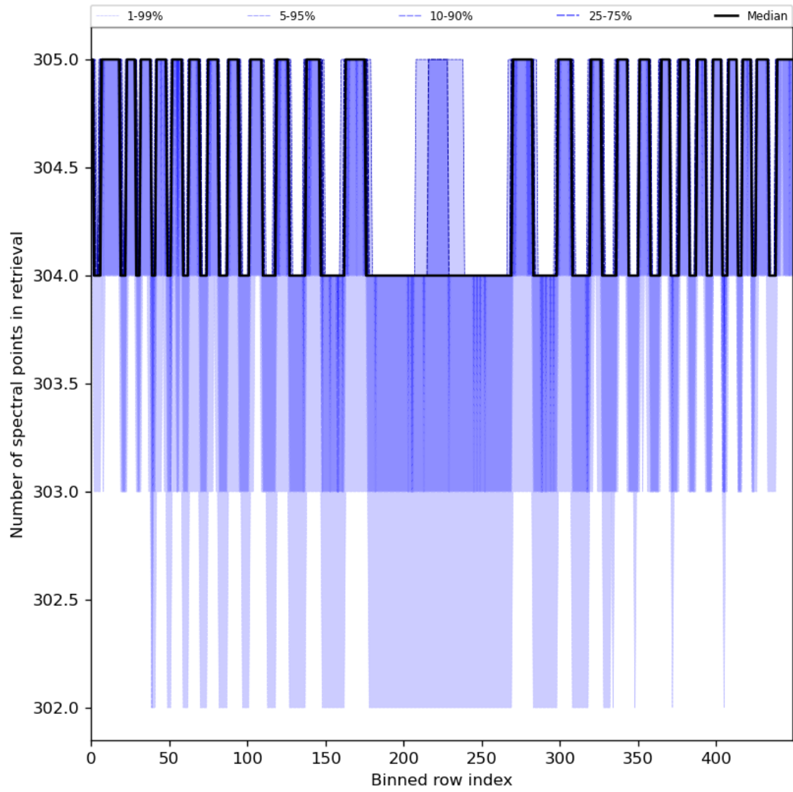
Figure 50: Along track statistics of “Number of spectral points in retrieval” for 2024-06-11 to 2024-06-13
