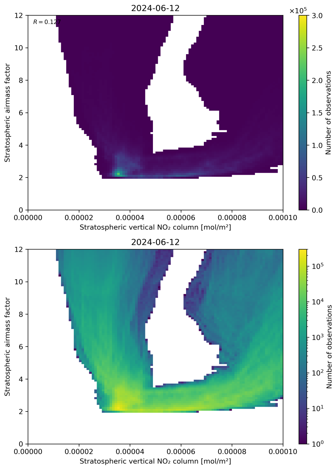
Figure 96: Scatter density plot of “Stratospheric vertical NO 2 column” against “Stratospheric airmass factor” for 2024-06-11 to 2024-06-13.
