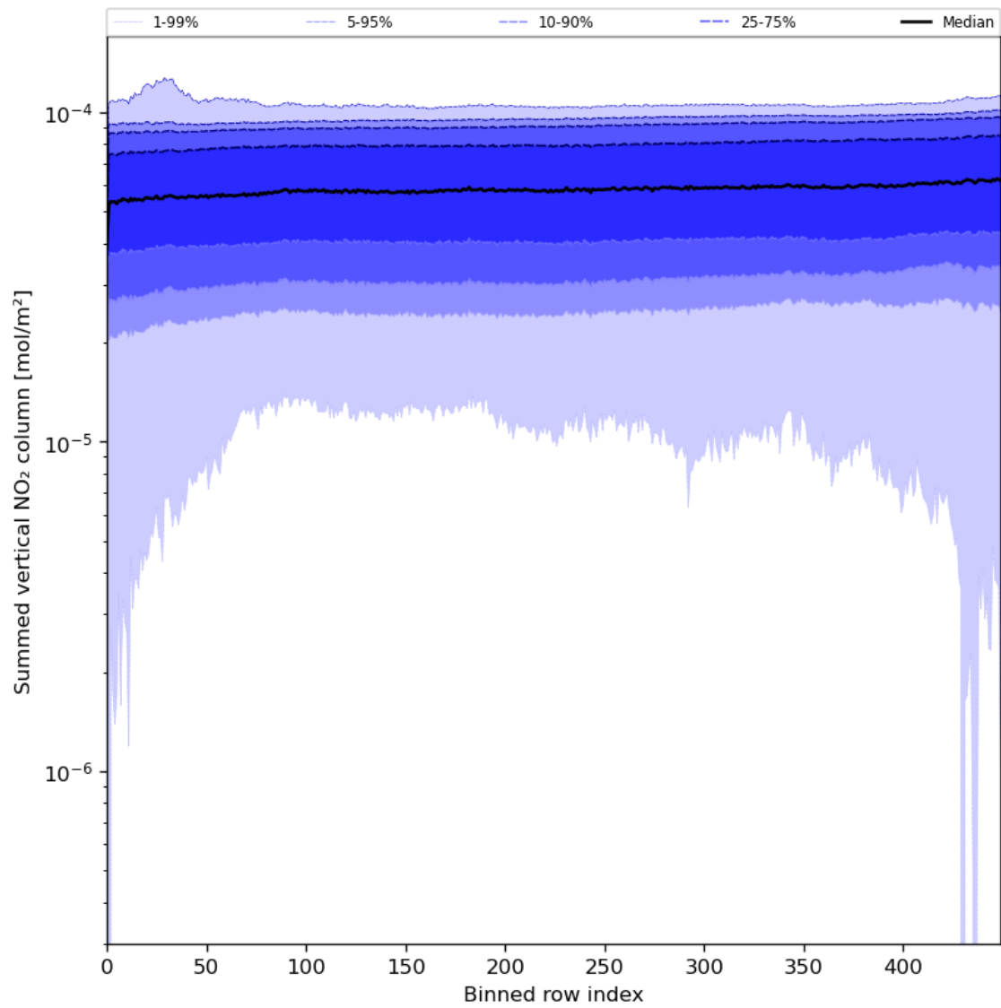
Figure 57: Along track statistics of “Summed vertical NO 2 column” for 2024-06-11 to 2024-06-13
