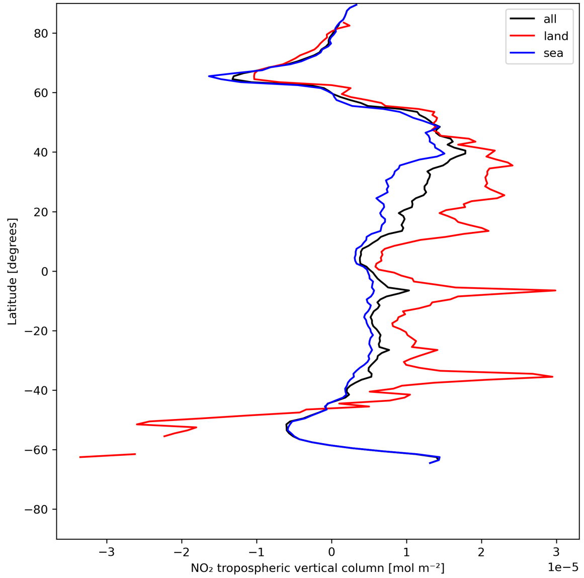
Figure 12: Zonal average of “NO 2 tropospheric vertical column” for 2024-06-11 to 2024-06-13.
