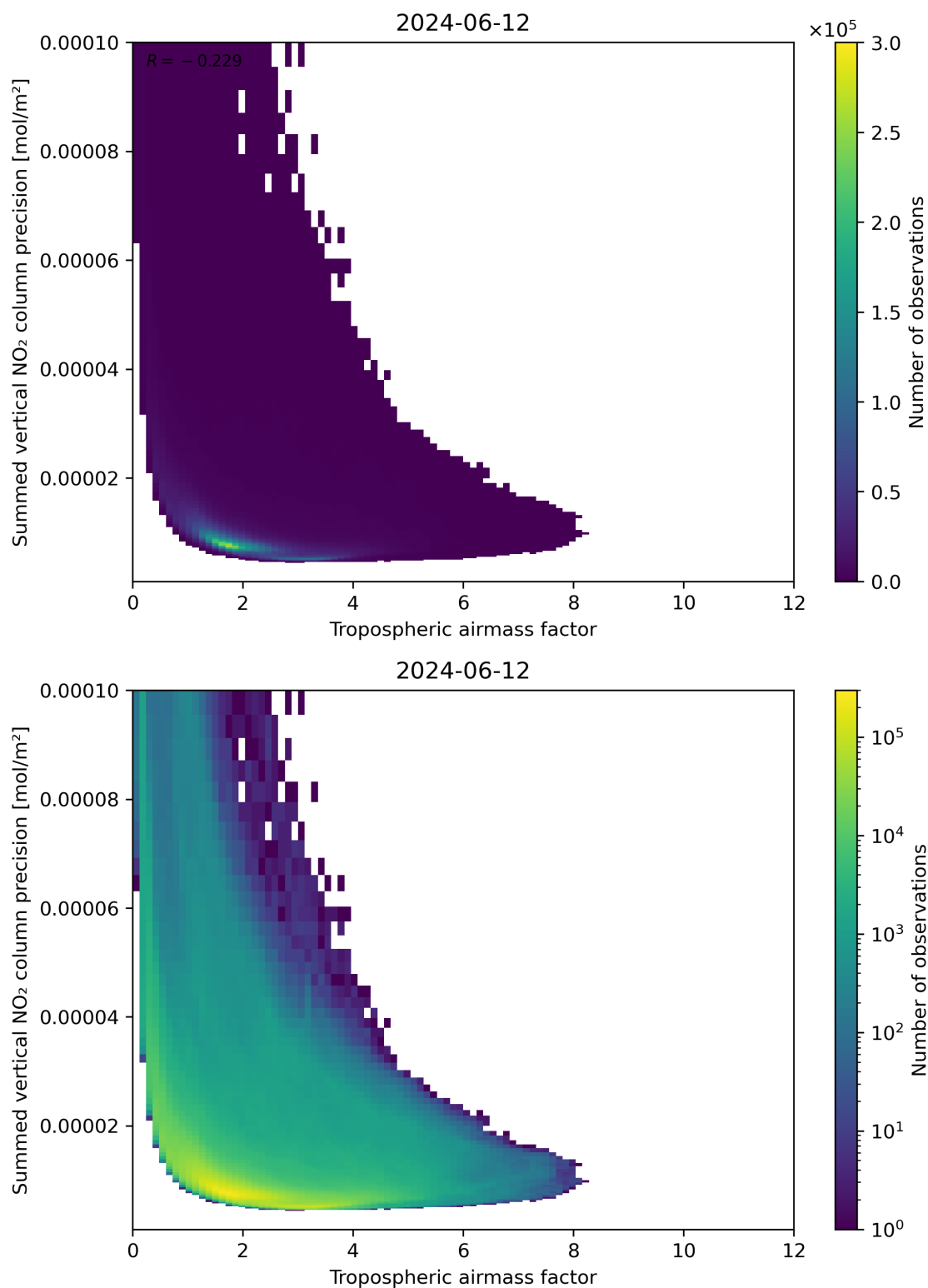
Figure 76: Scatter density plot of “Tropospheric air mass factor” against “Summed vertical NO 2 column precision” for 2024-06-11 to 2024-06-13.
