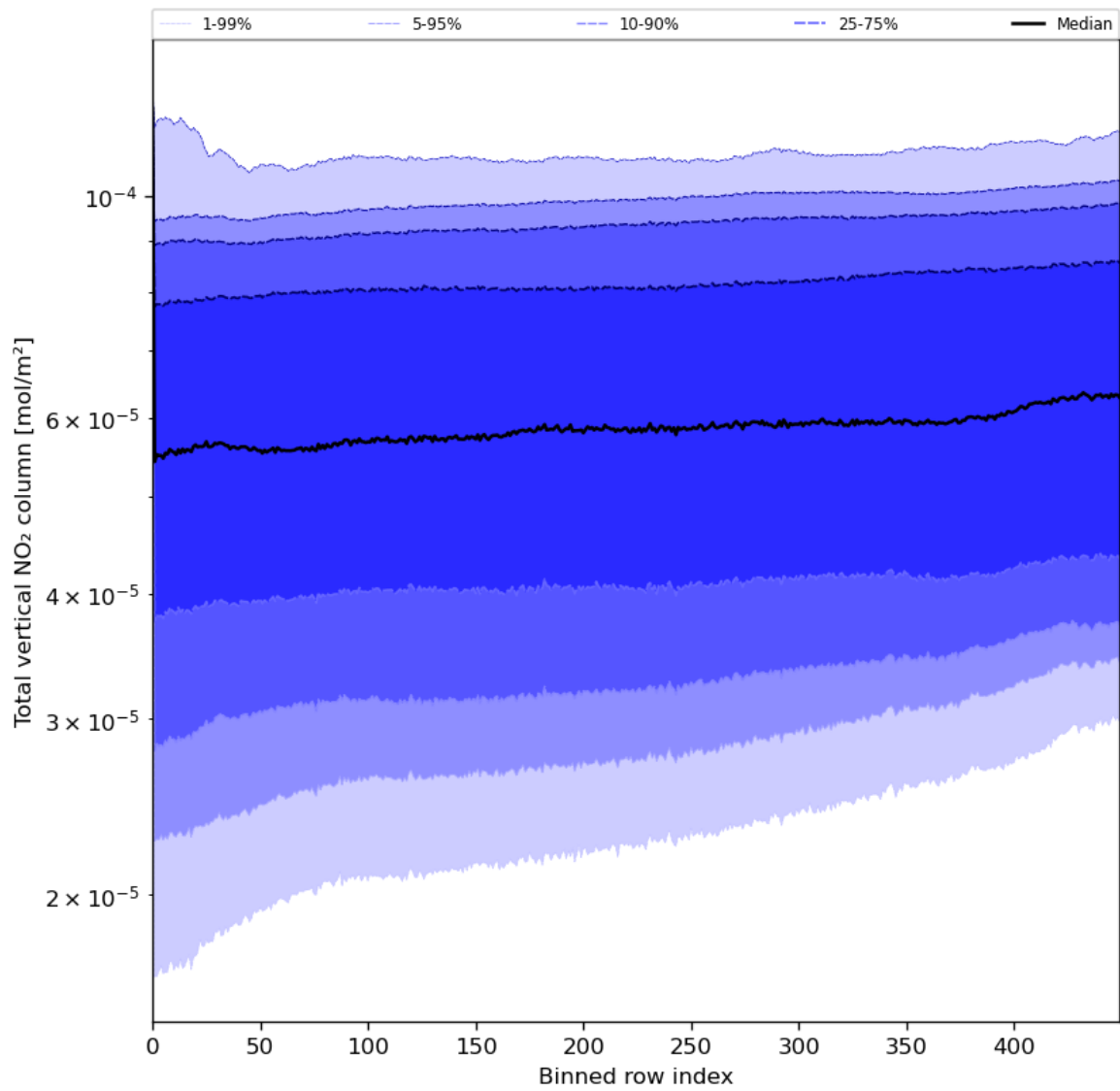
Figure 55: Along track statistics of “Total vertical NO 2 column” for 2024-06-11 to 2024-06-13
