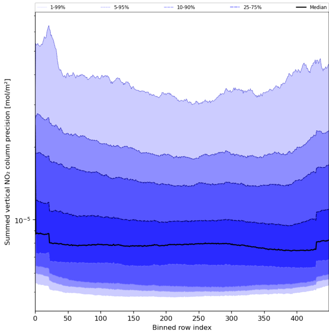
Figure 58: Along track statistics of “Summed vertical NO 2 column precision” for 2024-06-11 to 2024-06-13
