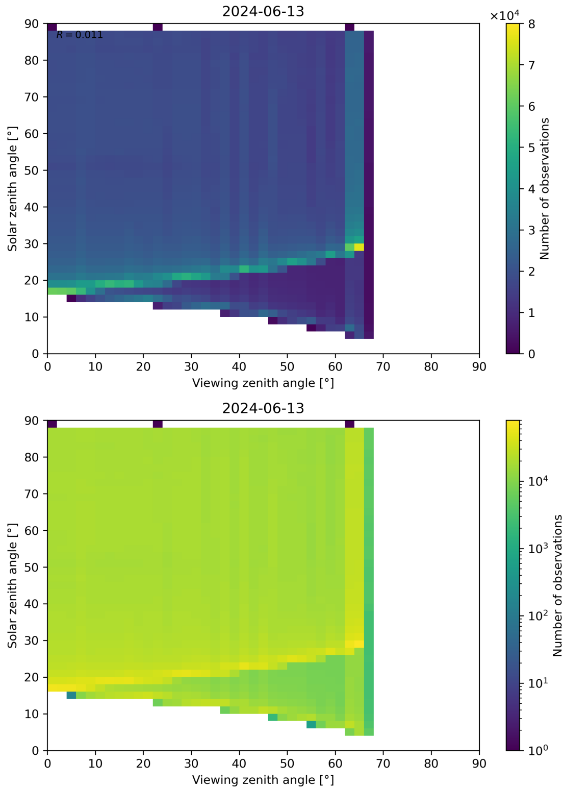
Figure 172: Scatter density plot of “Viewing zenith angle” against “Solar zenith angle” for 2024-06-13 to 2024-06-14.
