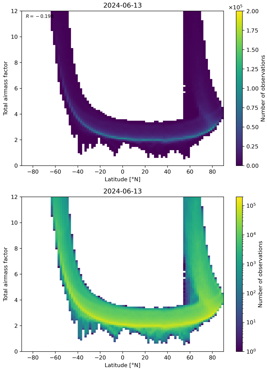
Figure 84: Scatter density plot of “Latitude” against “Total airmass factor” for 2024-06-13 to 2024-06-14.
