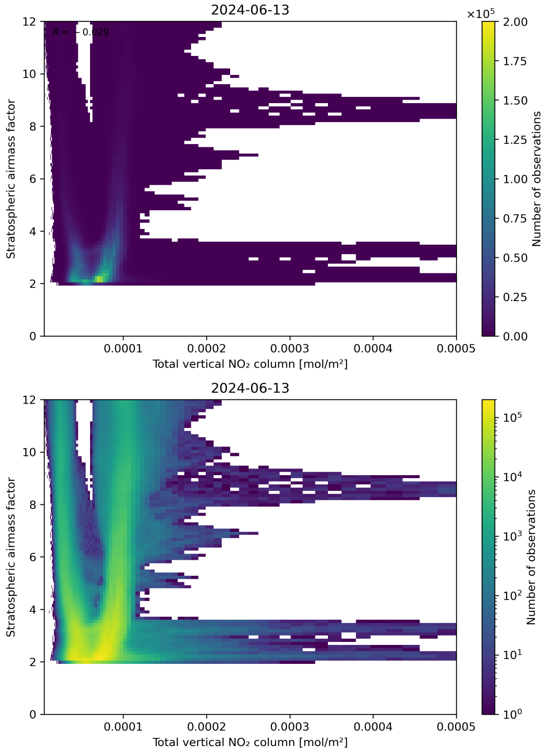
Figure 110: Scatter density plot of “Total vertical NO 2 column” against “Stratospheric airmass factor” for 2024-06-13 to 2024-06-14.
