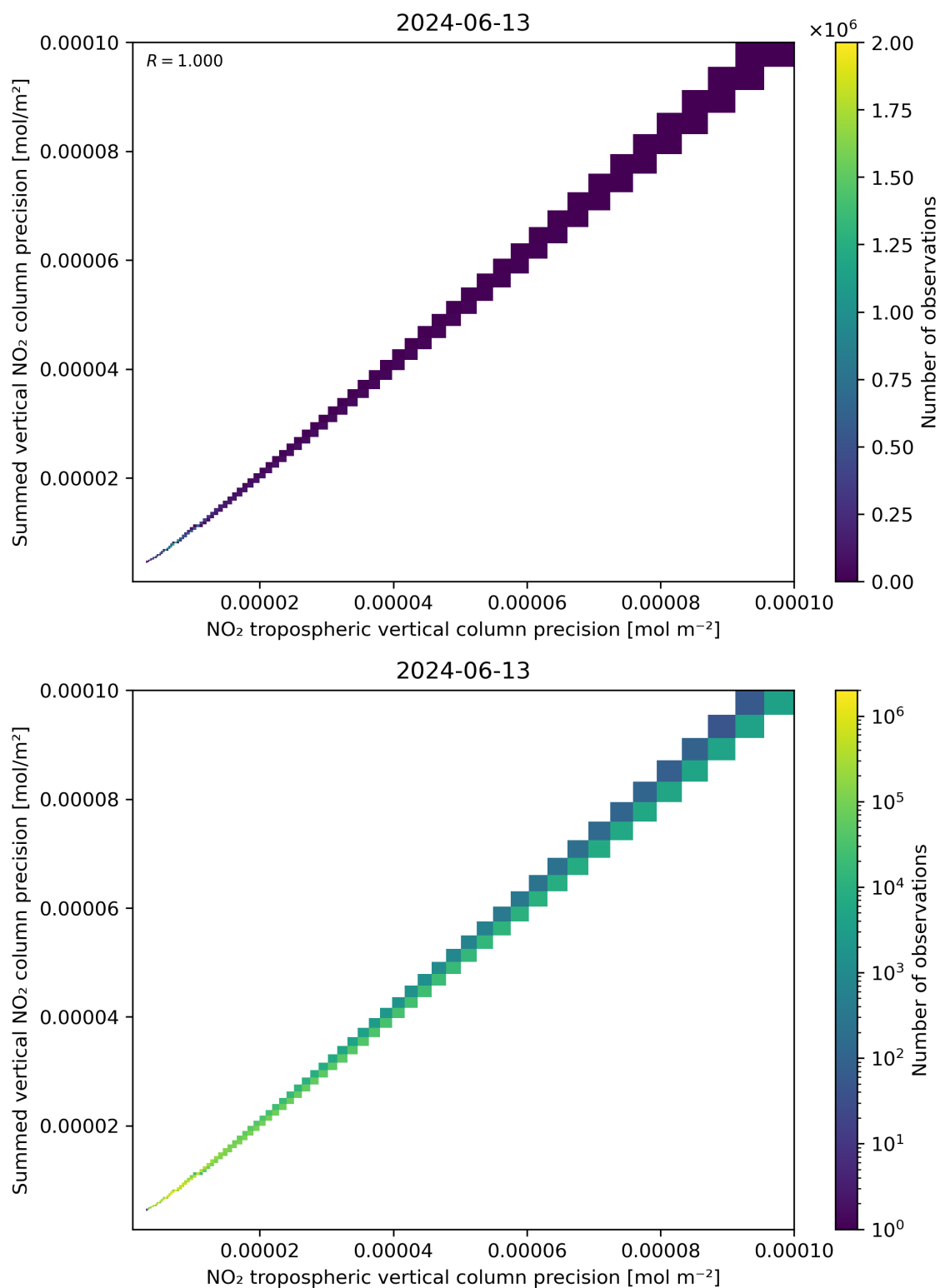
Figure 137: Scatter density plot of “NO 2 tropospheric vertical column precision” against “Summed vertical NO 2 column precision” for 2024-06-13 to 2024-06-14.
