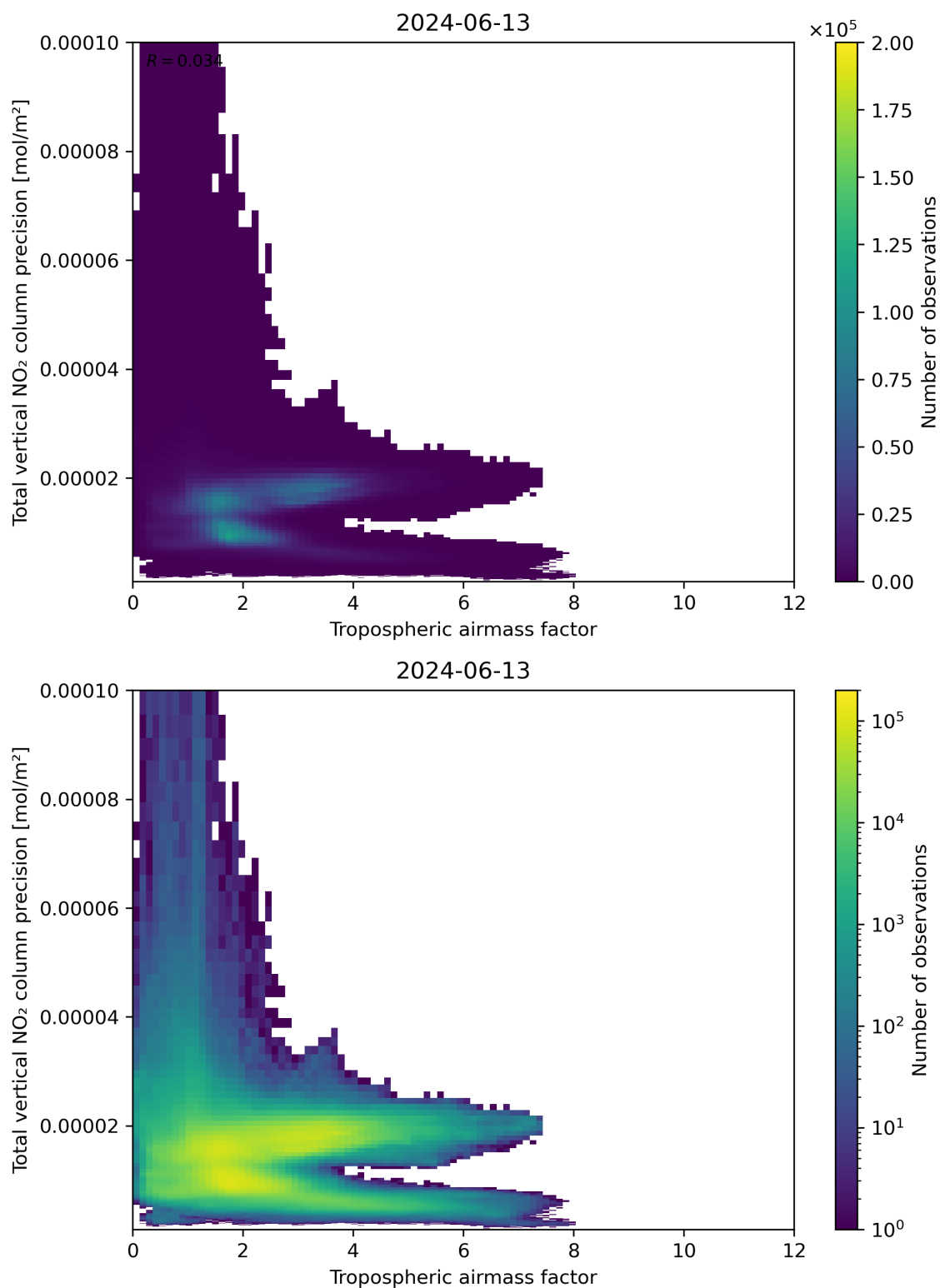
Figure 78: Scatter density plot of “Tropospheric air mass factor” against “Total vertical NO 2 column precision” for 2024-06-13 to 2024-06-14.
