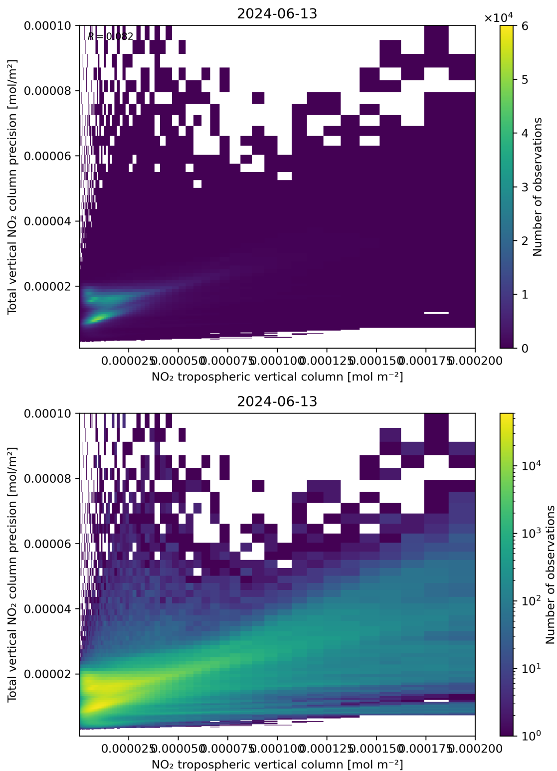
Figure 129: Scatter density plot of “NO 2 tropospheric vertical column” against “Total vertical NO 2 column precision” for 2024-06-13 to 2024-06-14.
