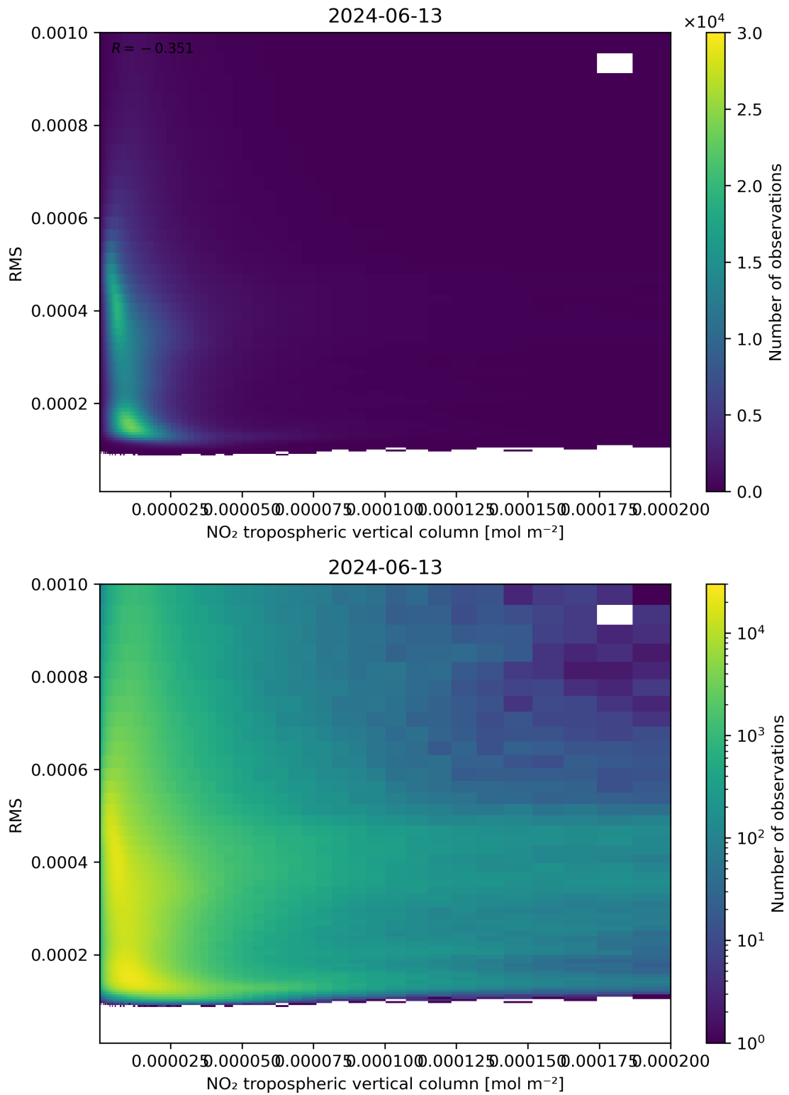
Figure 142: Scatter density plot of “NO 2 tropospheric vertical column” against “RMS” for 2024-06-13 to 2024-06-14.
