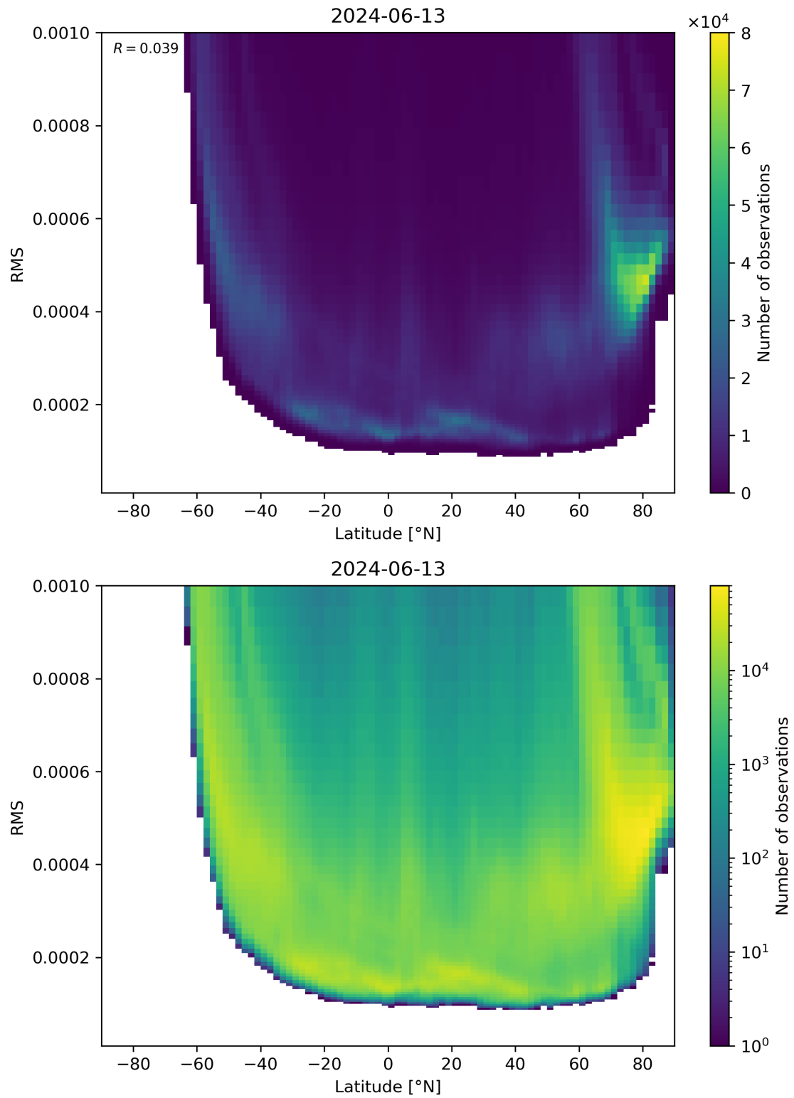
Figure 94: Scatter density plot of “Latitude” against “RMS” for 2024-06-13 to 2024-06-14.
