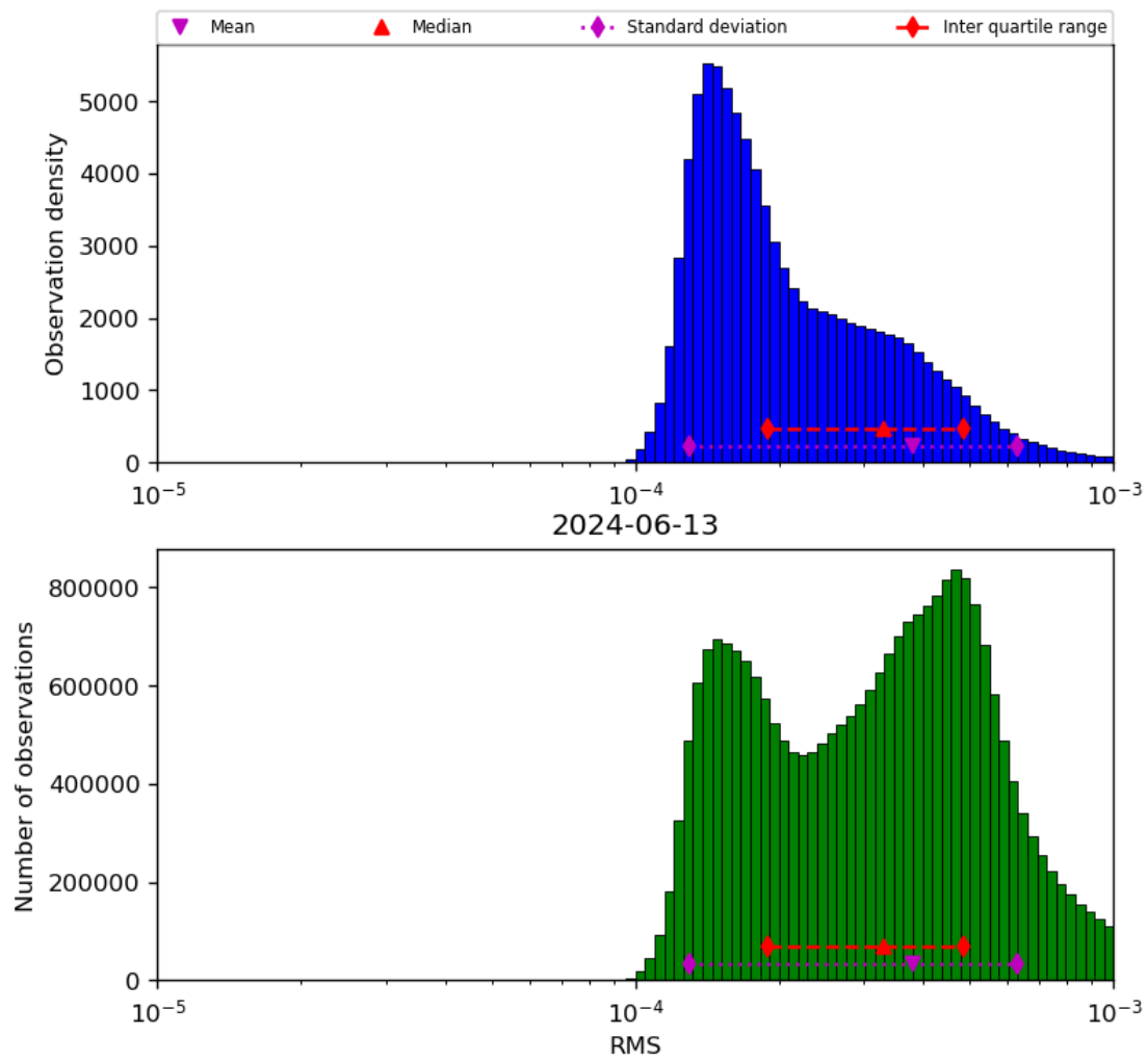
Figure 43: Histogram of “RMS” for 2024-06-13 to 2024-06-14
