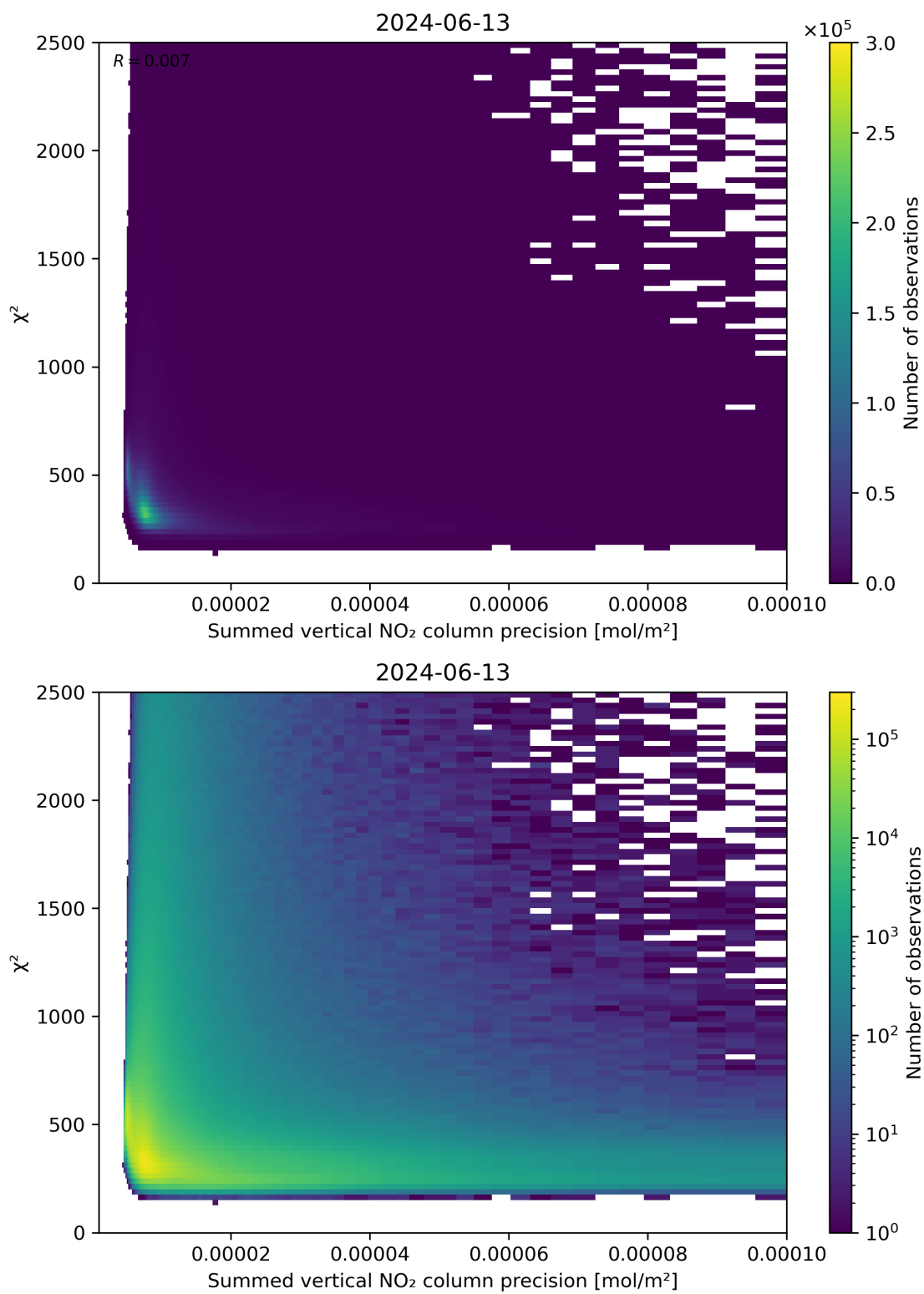
Figure 107: Scatter density plot of “Summed vertical NO 2 column precision” against “ \chi^2 ” for 2024-06-13 to 2024-06-14.
