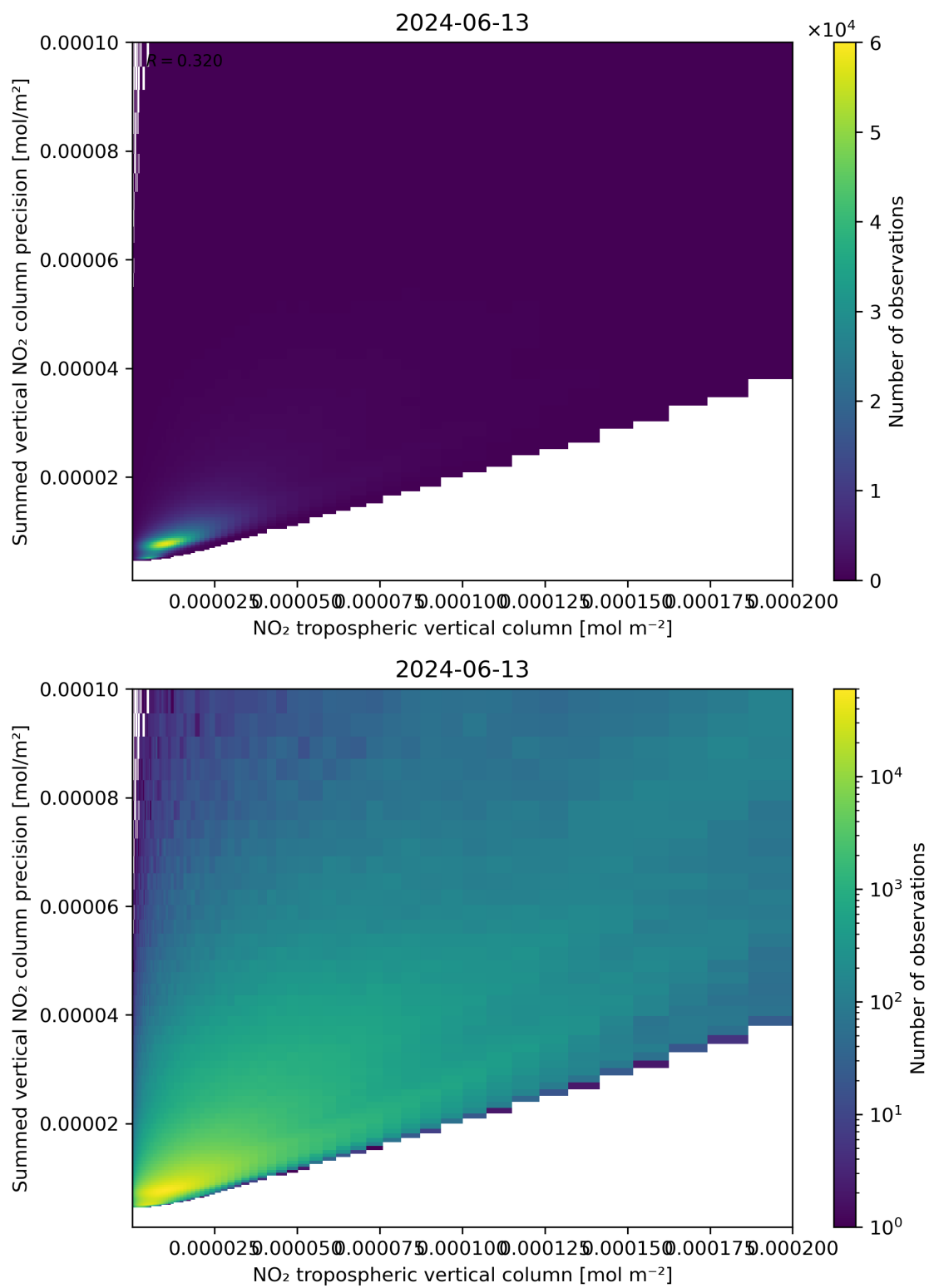
Figure 127: Scatter density plot of “NO 2 tropospheric vertical column” against “Summed vertical NO 2 column precision” for 2024-06-13 to 2024-06-14.
