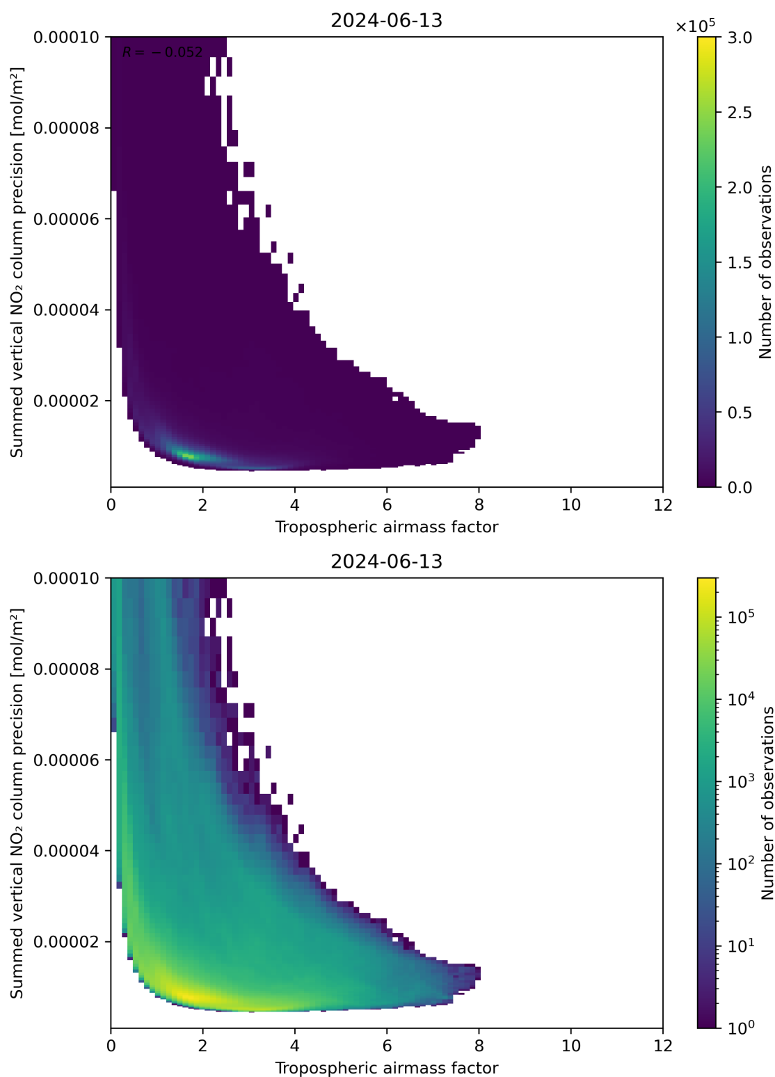
Figure 76: Scatter density plot of “Tropospheric air mass factor” against “Summed vertical NO 2 column precision” for 2024-06-13 to 2024-06-14.
