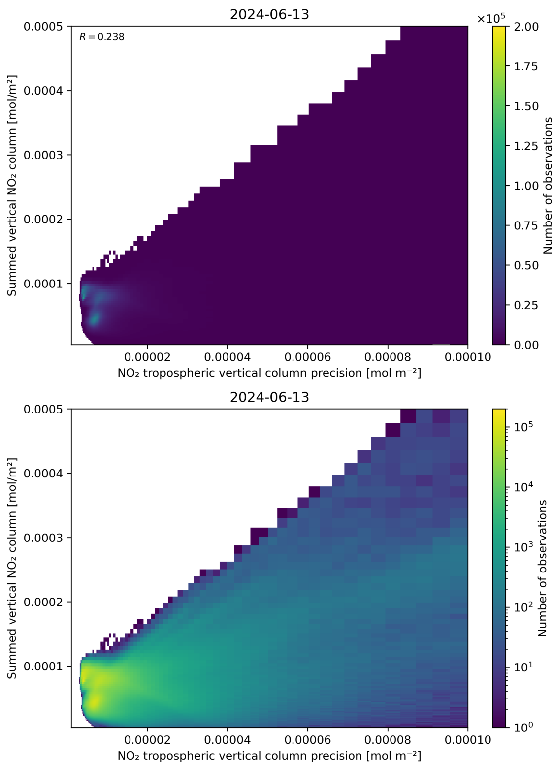
Figure 136: Scatter density plot of “NO 2 tropospheric vertical column precision” against “Summed vertical NO 2 column” for 2024-06-13 to 2024-06-14.
