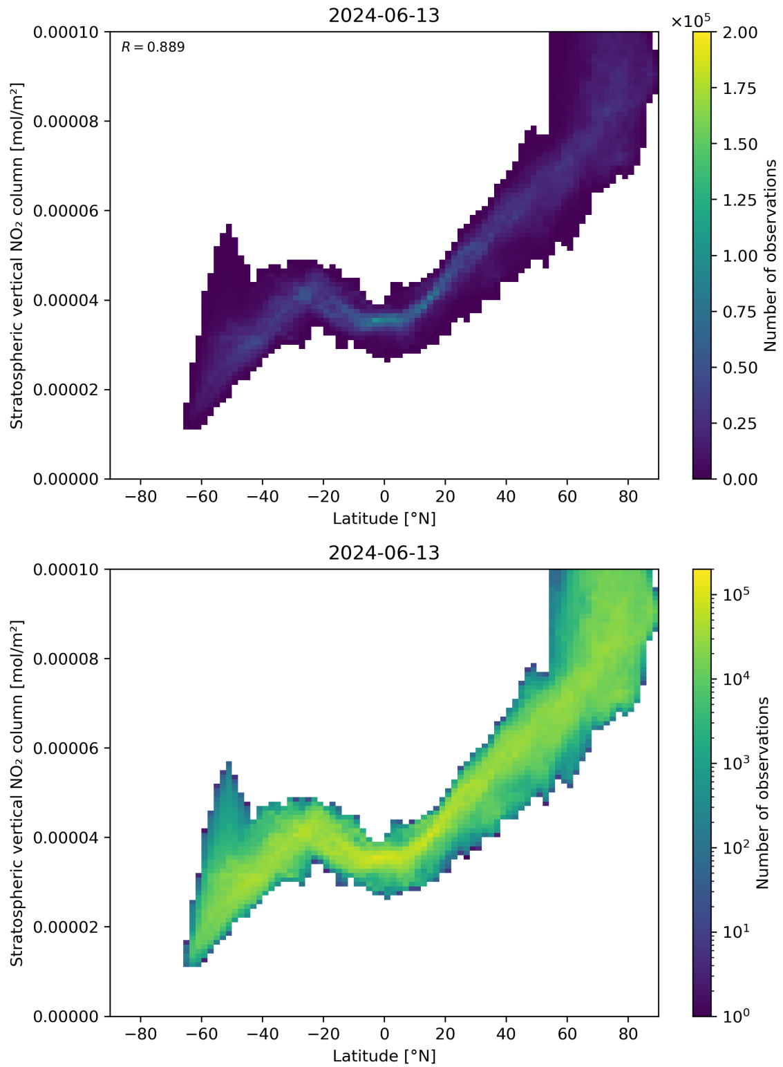
Figure 87: Scatter density plot of “Latitude” against “Stratospheric vertical NO 2 column” for 2024-06-13 to 2024-06-14.
