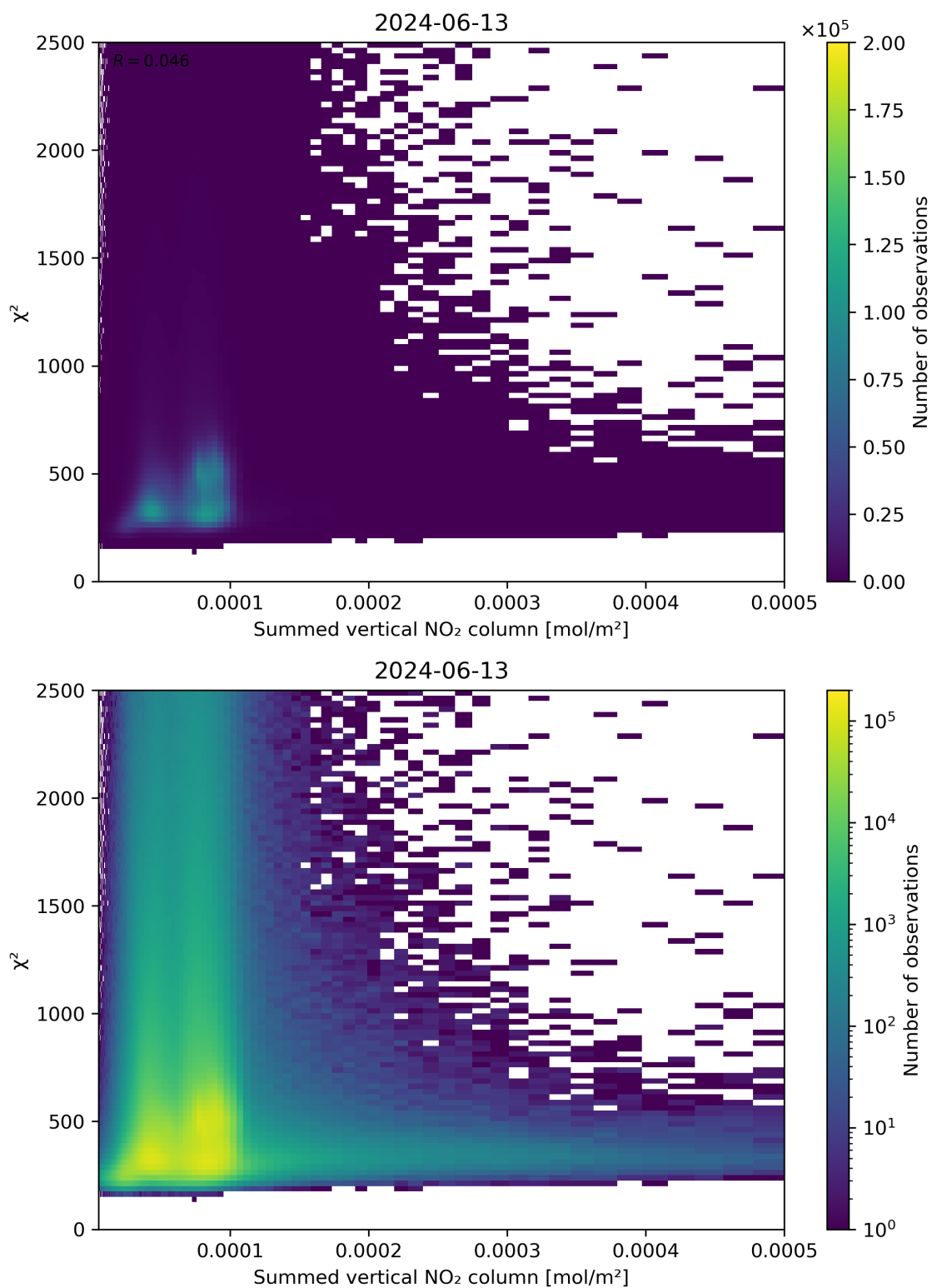
Figure 104: Scatter density plot of “Summed vertical NO 2 column” against “ \chi^2 ” for 2024-06-13 to 2024-06-14.
