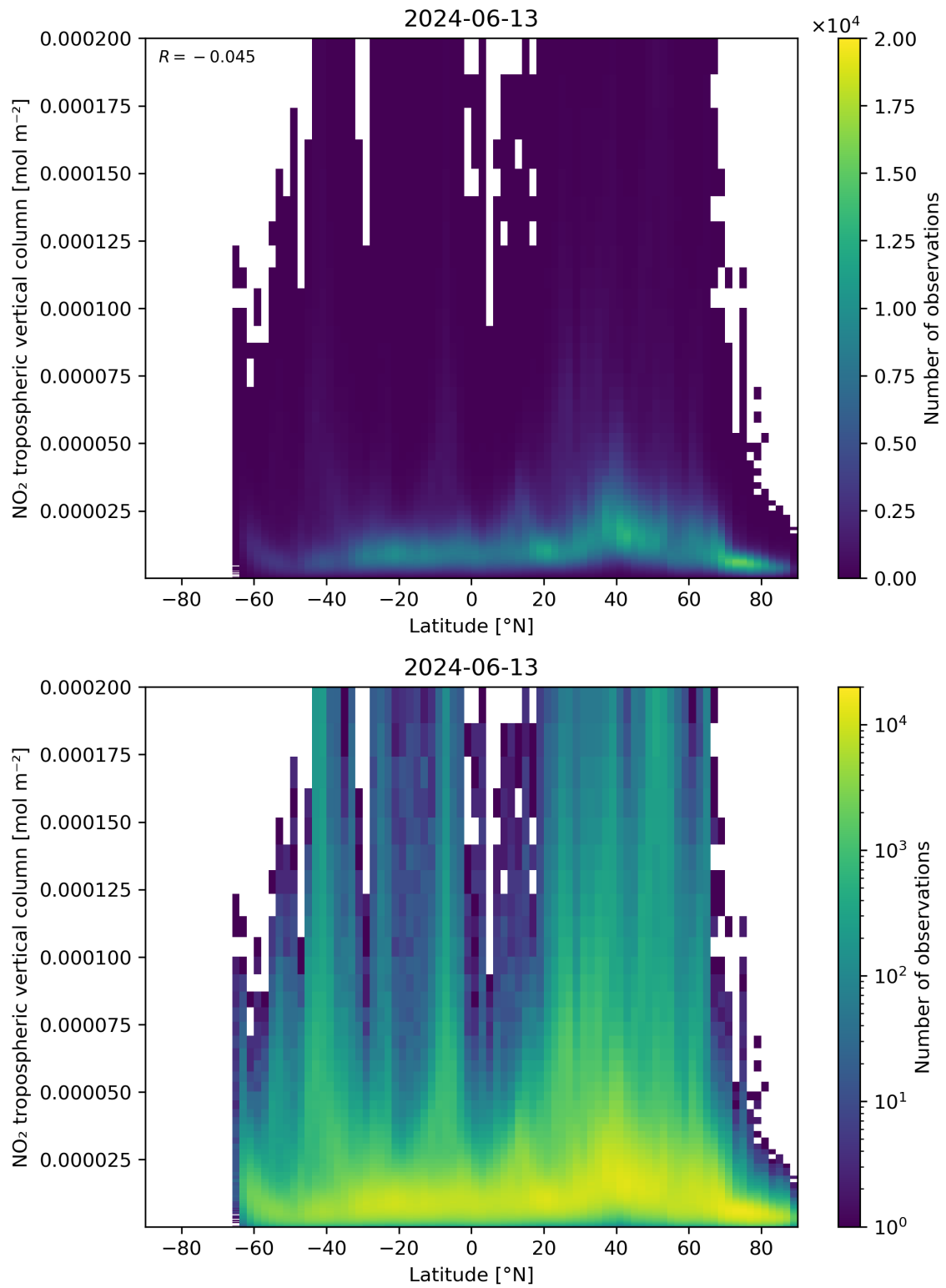
Figure 92: Scatter density plot of “Latitude” against “NO 2 tropospheric vertical column” for 2024-06-13 to 2024-06-14.
