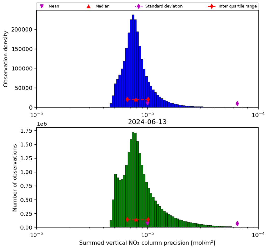
Figure 41: Histogram of “Summed vertical NO 2 column precision” for 2024-06-13 to 2024-06-14
