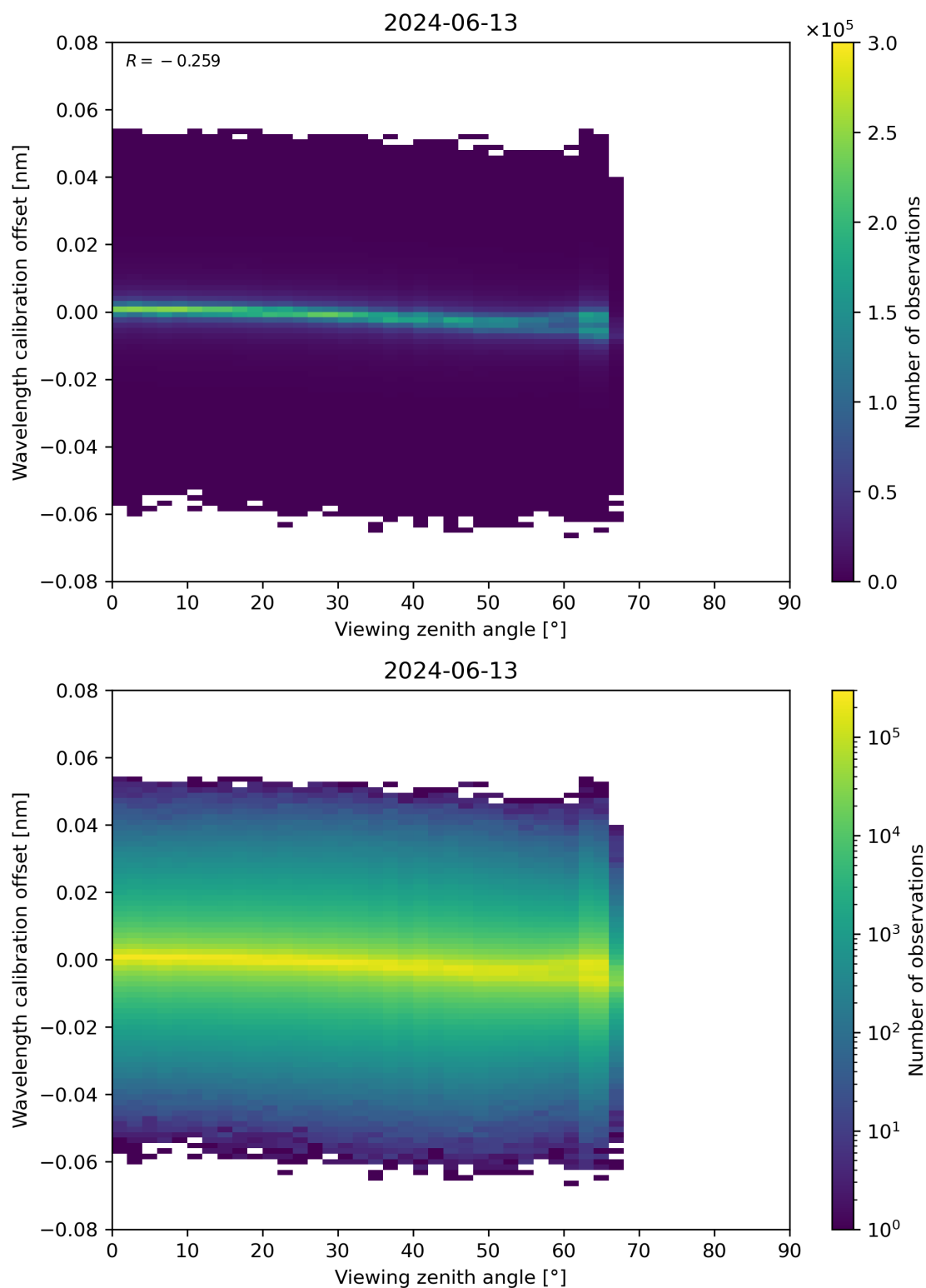
Figure 173: Scatter density plot of “Viewing zenith angle” against “Wavelength calibration offset” for 2024-06-13 to 2024-06-14.
