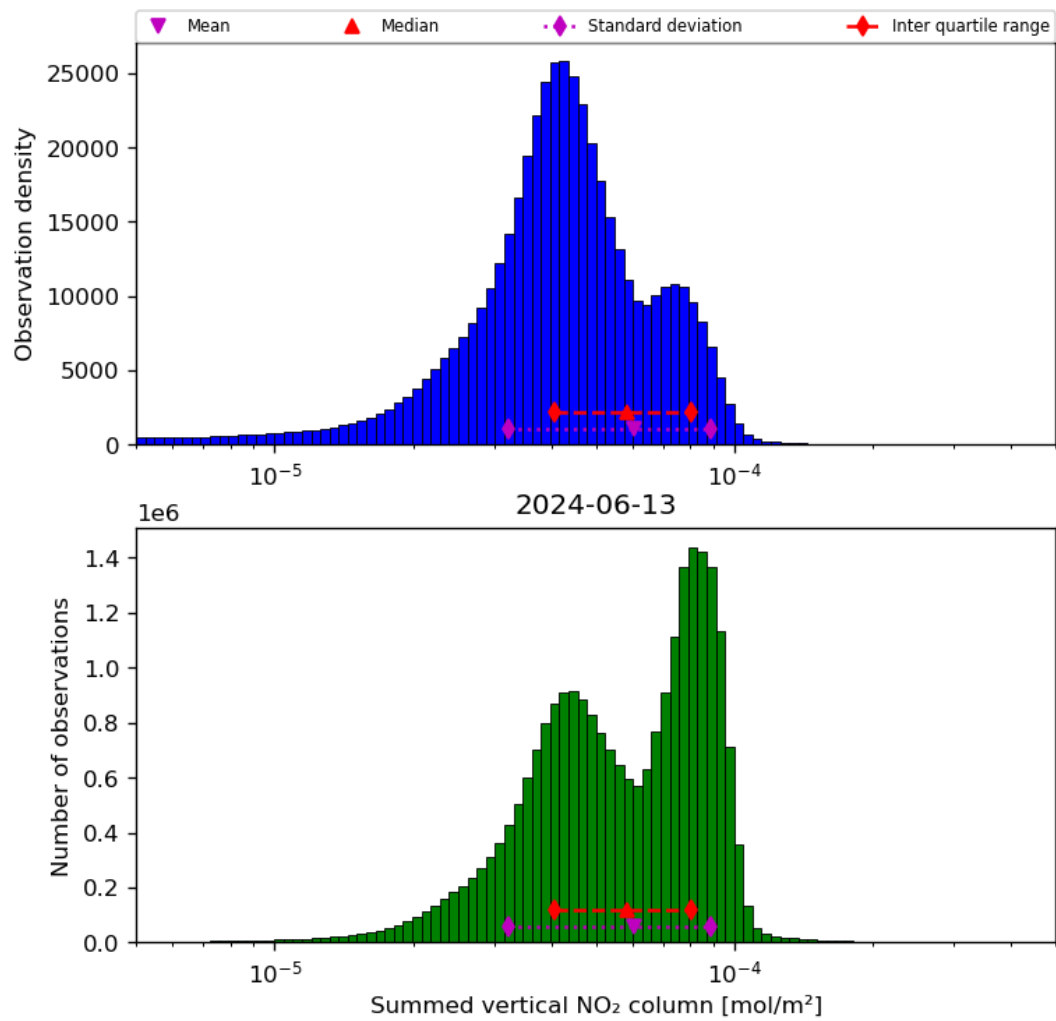
Figure 40: Histogram of “Summed vertical NO 2 column” for 2024-06-13 to 2024-06-14
