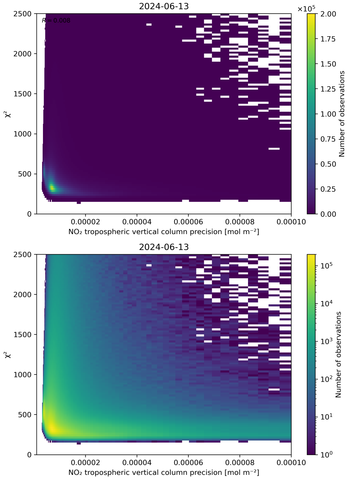
Figure 134: Scatter density plot of “NO 2 tropospheric vertical column precision” against “ \chi^2 ” for 2024-06-13 to 2024-06-14.
