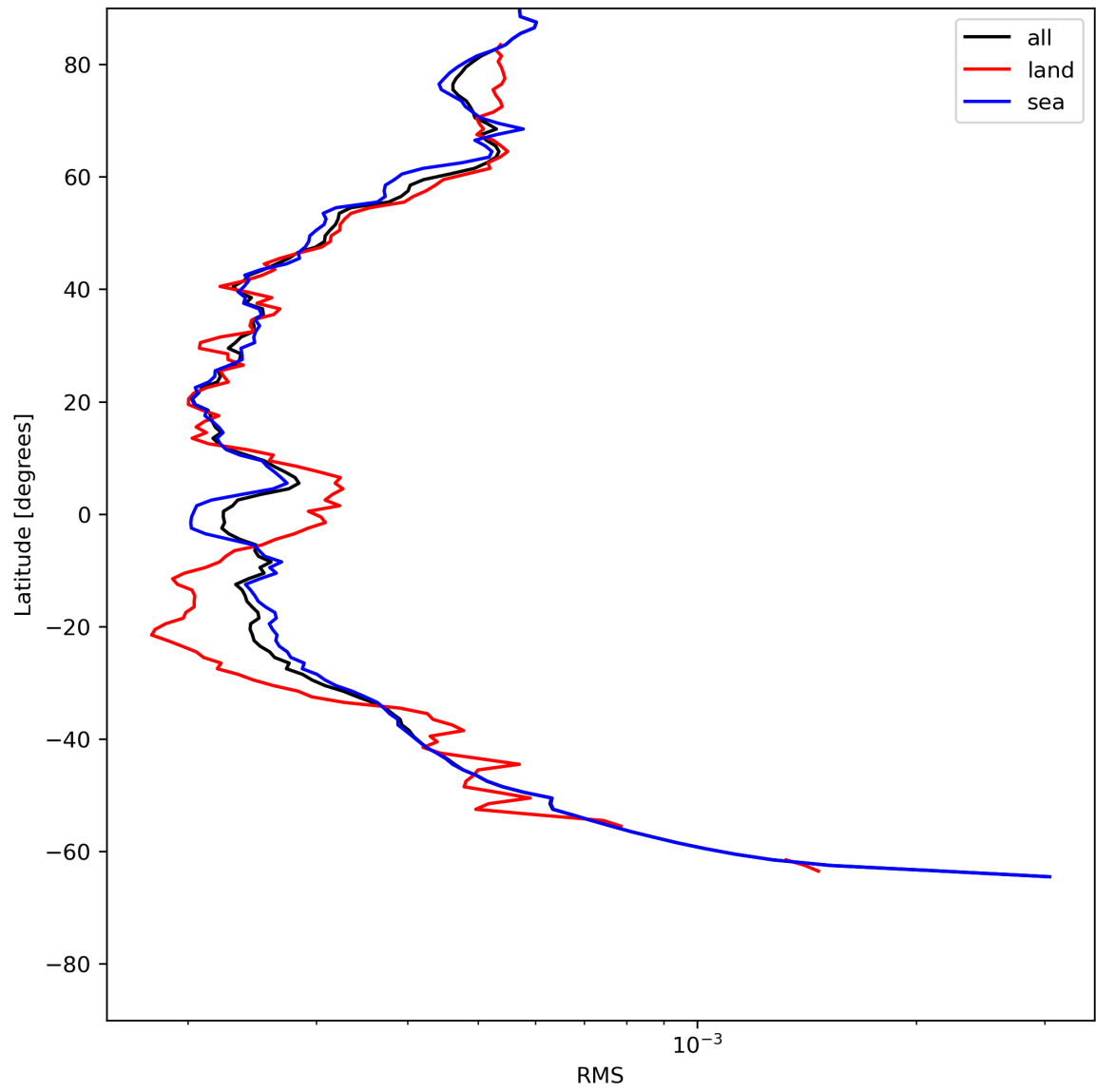
Figure 26: Zonal average of “RMS” for 2024-06-13 to 2024-06-14.
