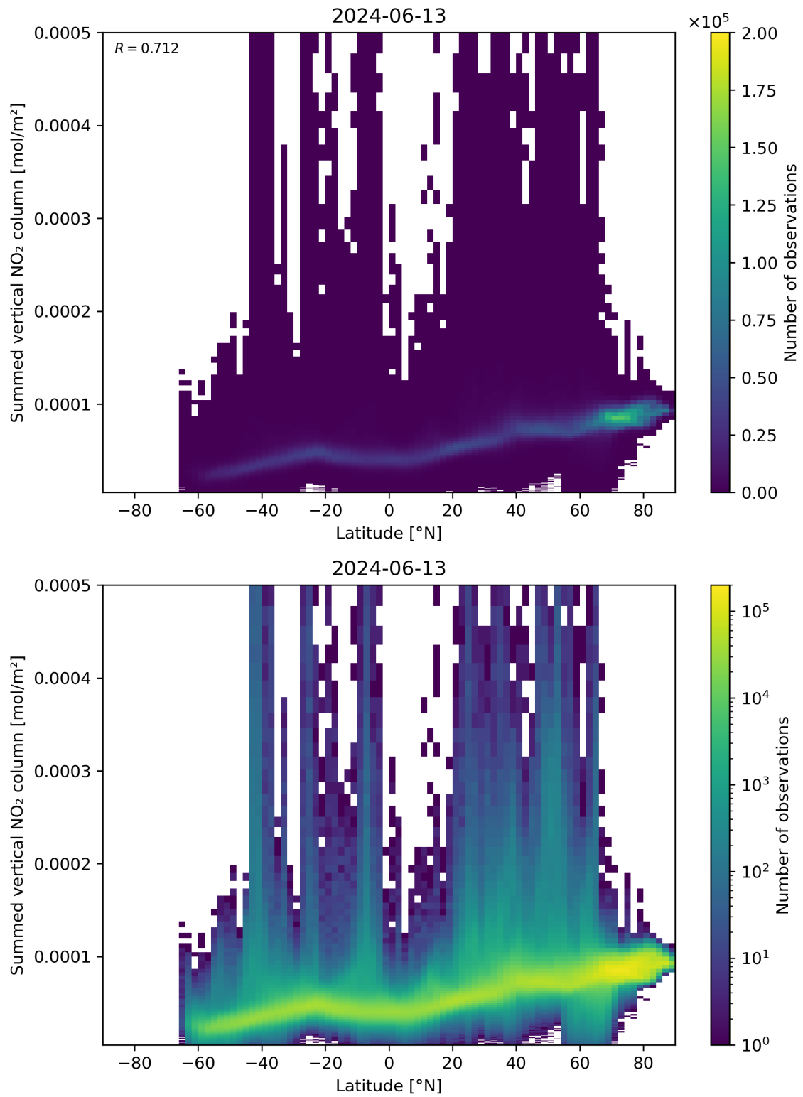
Figure 88: Scatter density plot of “Latitude” against “Summed vertical NO 2 column” for 2024-06-13 to 2024-06-14.
