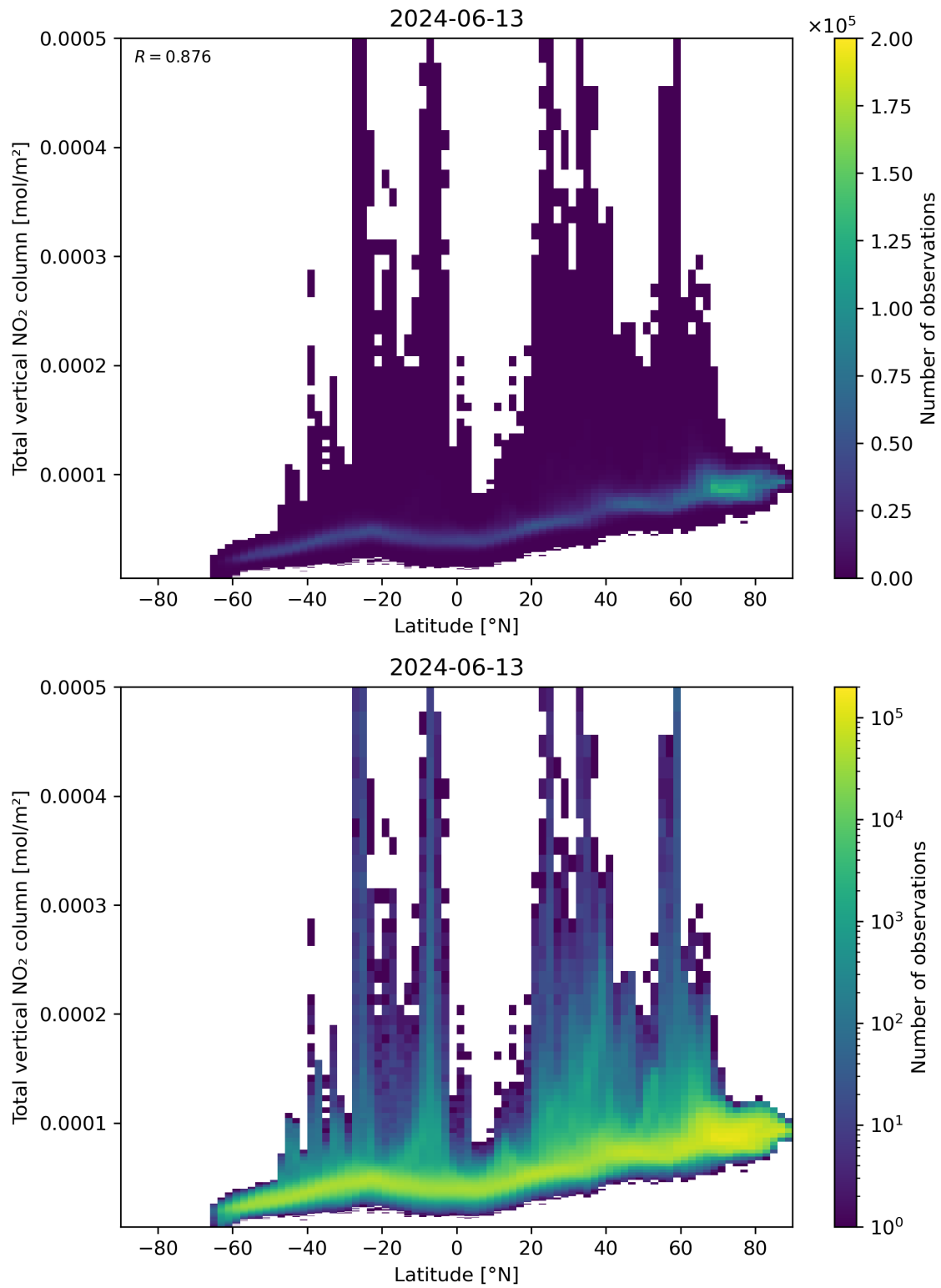
Figure 90: Scatter density plot of “Latitude” against “Total vertical NO 2 column” for 2024-06-13 to 2024-06-14.
