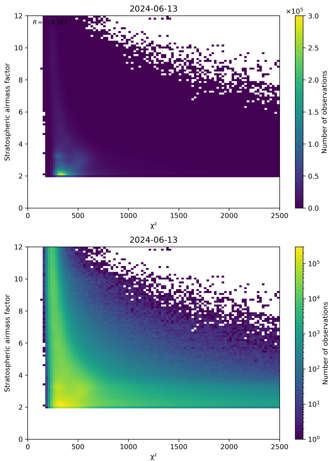
Figure 81: Scatter density plot of “ \chi^2 ” against “Stratospheric airmass factor” for 2024-06-13 to 2024-06-14.
