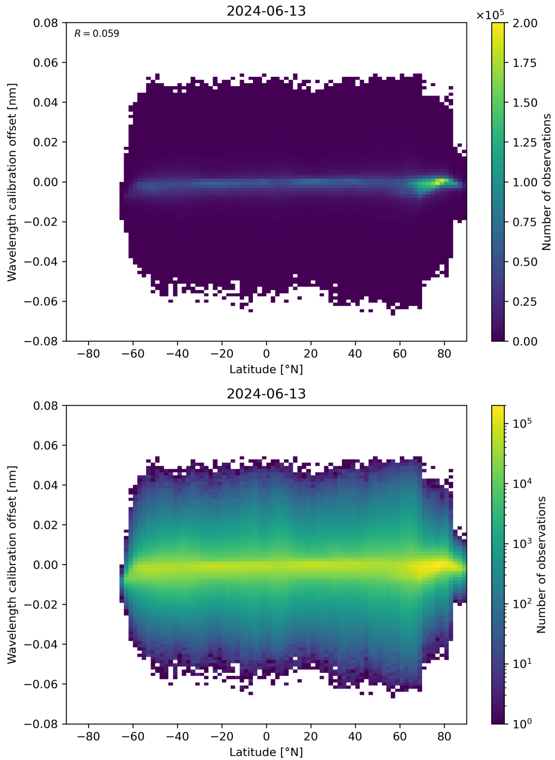
Figure 95: Scatter density plot of “Latitude” against “Wavelength calibration offset” for 2024-06-13 to 2024-06-14.
