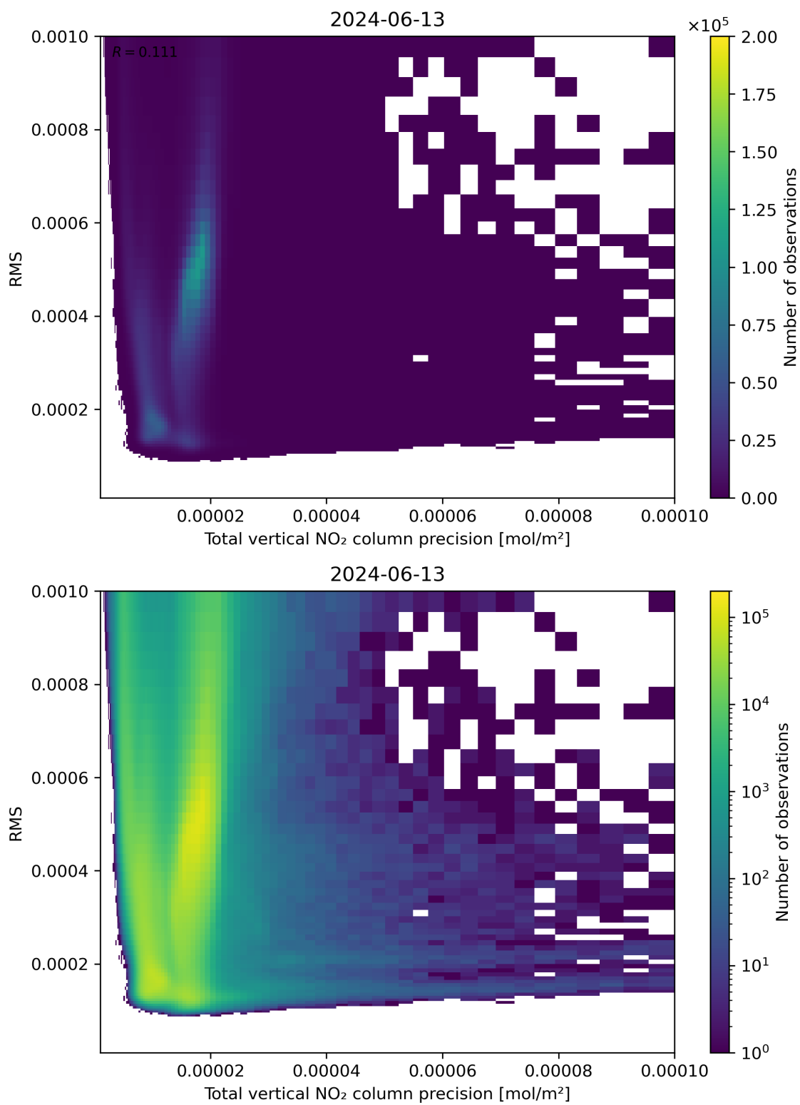
Figure 119: Scatter density plot of “Total vertical NO 2 column precision” against “RMS” for 2024-06-13 to 2024-06-14.
