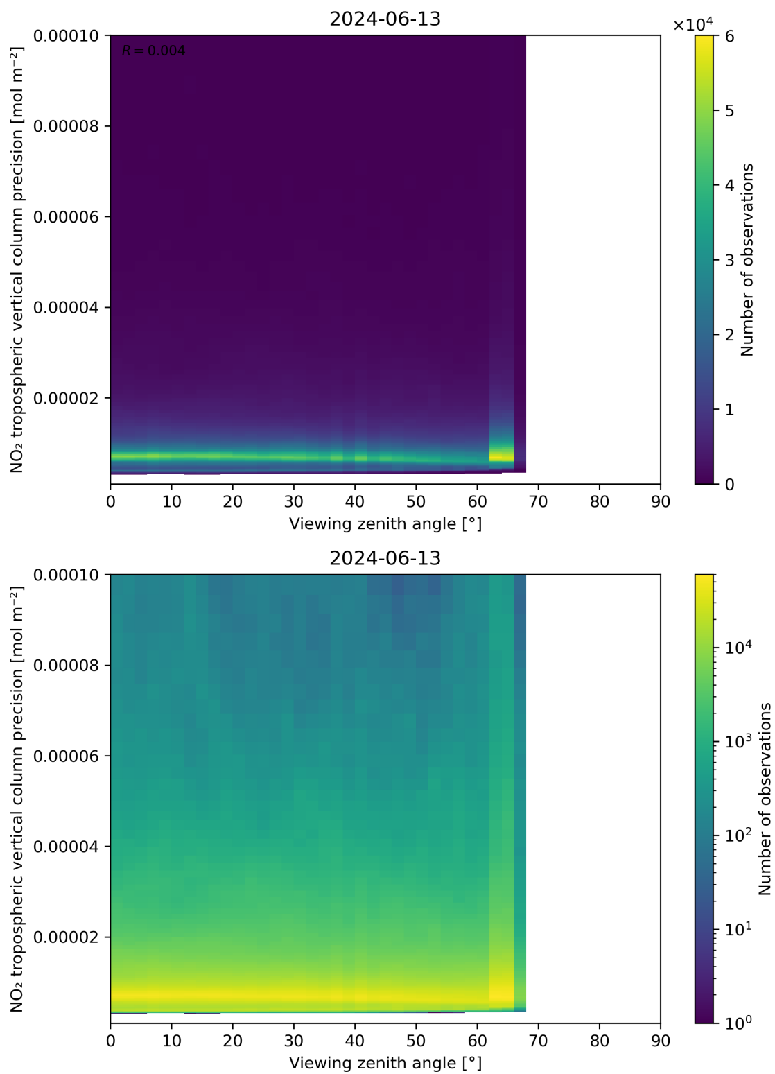
Figure 170: Scatter density plot of “Viewing zenith angle” against “NO 2 tropospheric vertical column precision” for 2024-06-13 to 2024-06-14.
