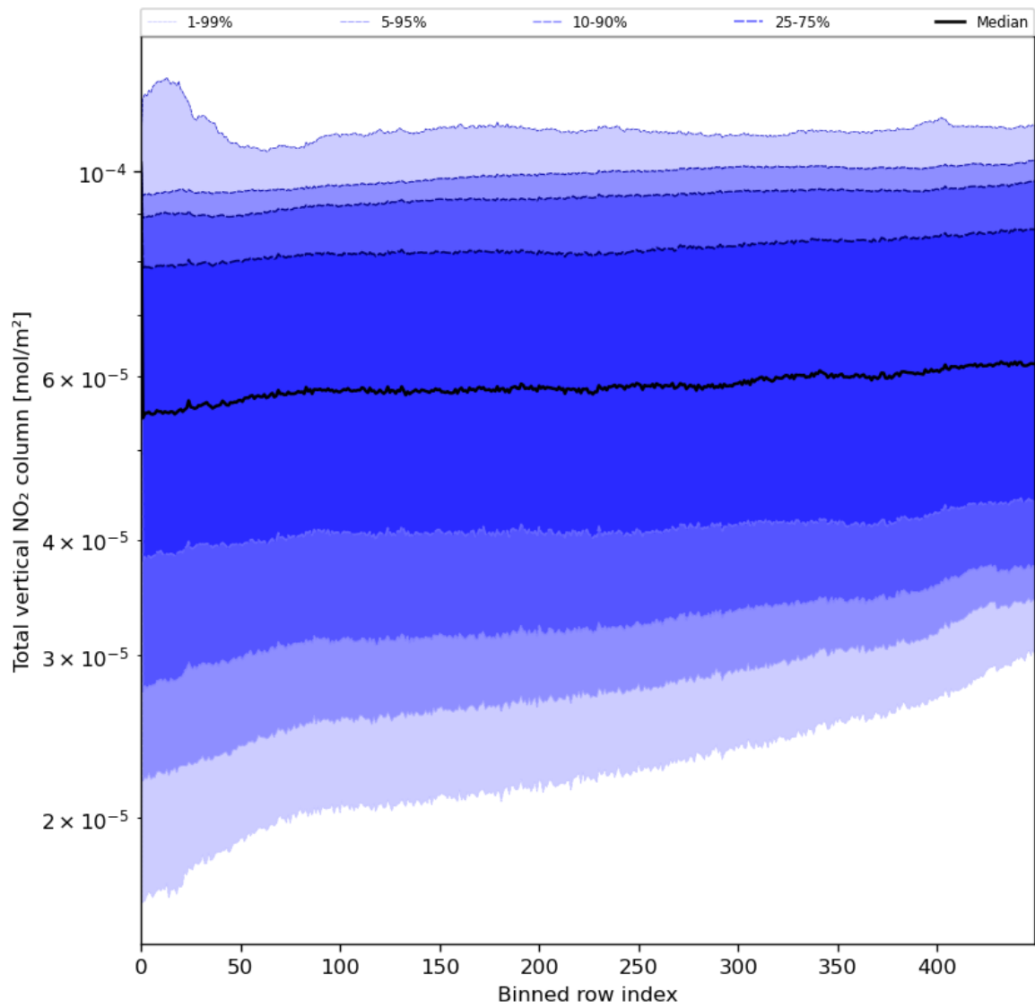
Figure 55: Along track statistics of “Total vertical NO 2 column” for 2024-06-13 to 2024-06-14
