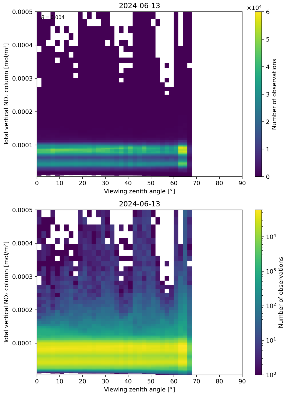
Figure 167: Scatter density plot of “Viewing zenith angle” against “Total vertical NO 2 column” for 2024-06-13 to 2024-06-14.
