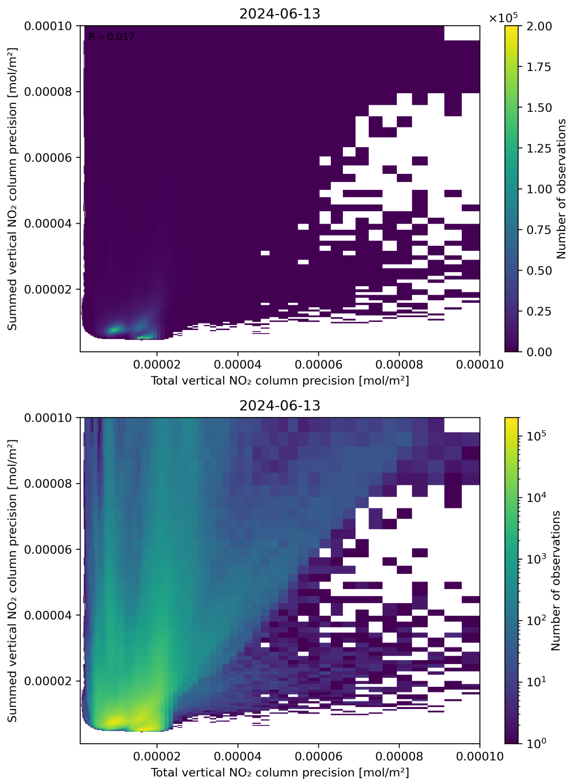
Figure 118: Scatter density plot of “Total vertical NO 2 column precision” against “Summed vertical NO 2 column precision” for 2024-06-13 to 2024-06-14.
