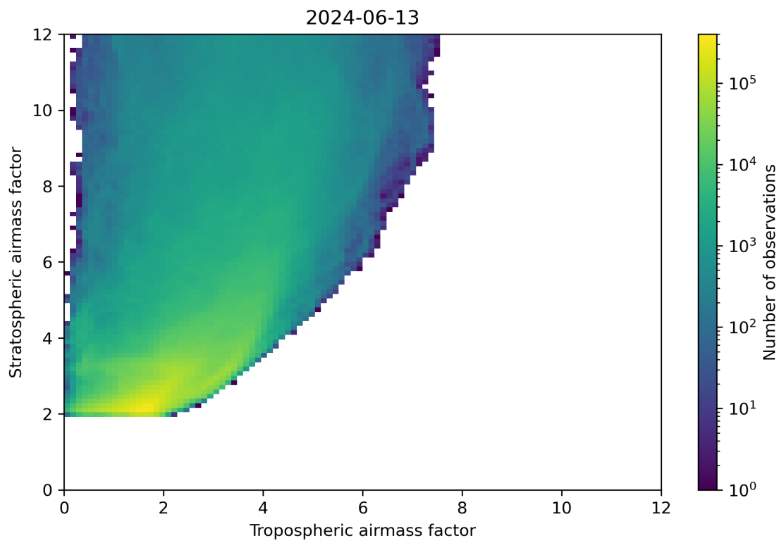
Figure 71: Scatter density plot of “Tropospheric airmass factor” against “Stratospheric airmass factor” for 2024-06-13 to 2024-06-14.
