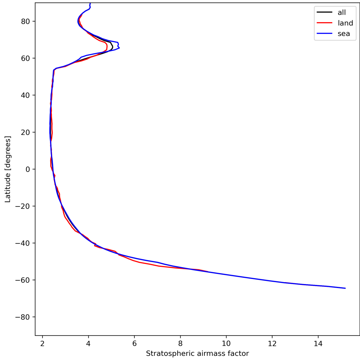
Figure 27: Zonal average of “Stratospheric airmass factor” for 2024-06-13 to 2024-06-14.
