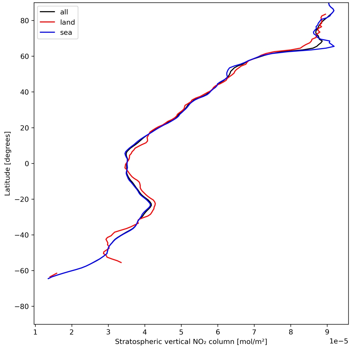
Figure 19: Zonal average of “Stratospheric vertical NO 2 column” for 2024-06-13 to 2024-06-14.
