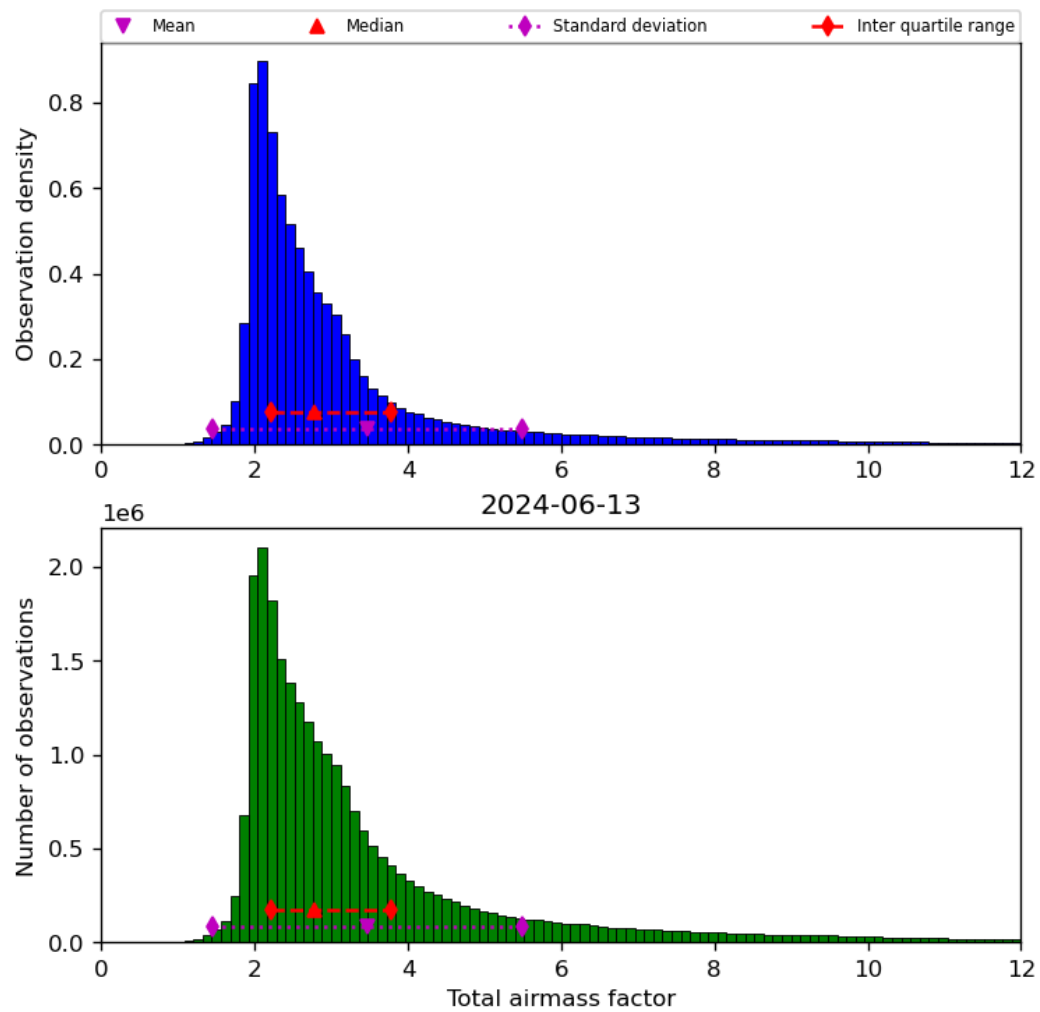
Figure 32: Histogram of “Total airmass factor” for 2024-06-13 to 2024-06-14
