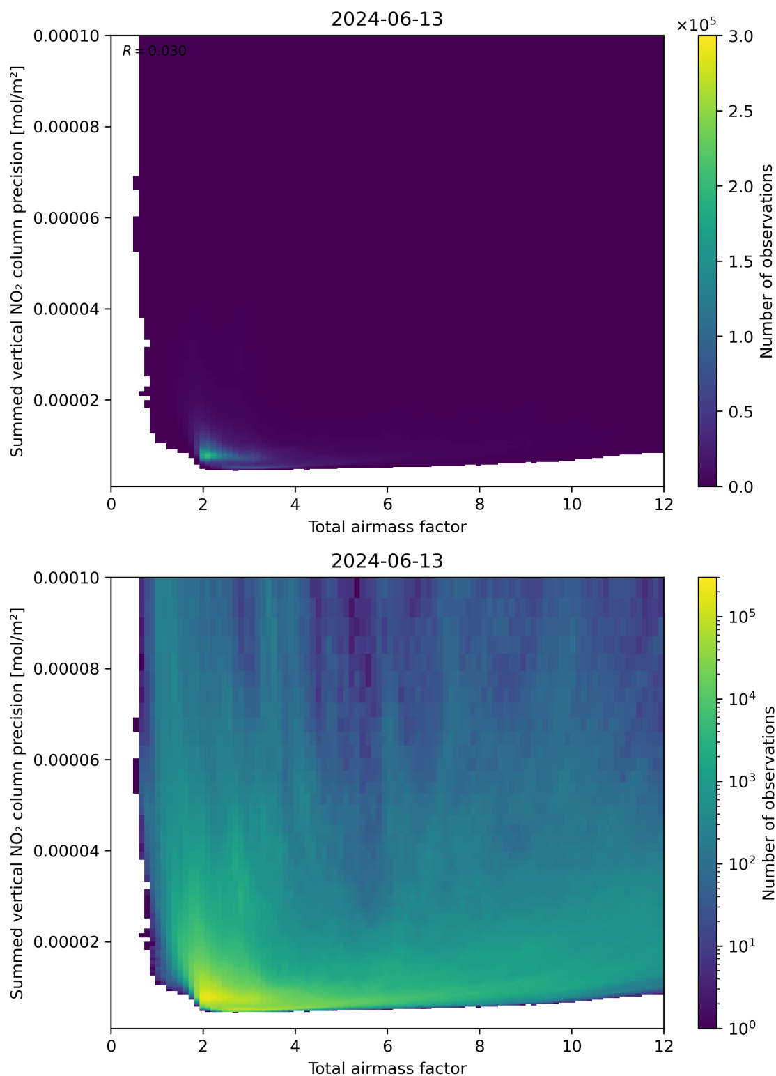
Figure 66: Scatter density plot of “Total airmass factor” against “Summed vertical NO 2 column precision” for 2024-06-13 to 2024-06-14.
