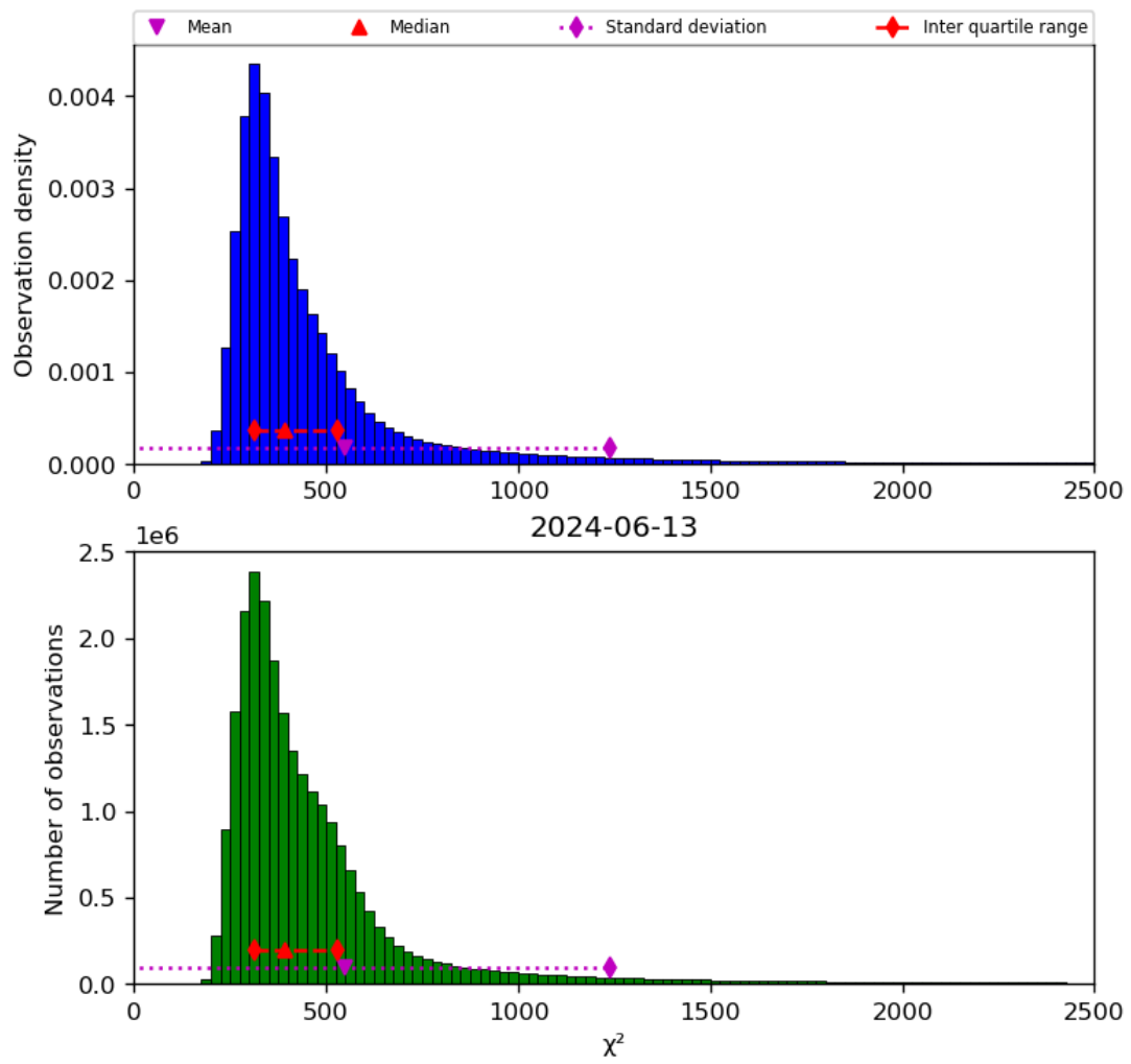
Figure 42: Histogram of " \chi^2 " for 2024-06-13 to 2024-06-14
