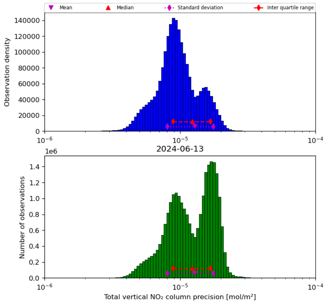
Figure 39: Histogram of “Total vertical NO 2 column precision” for 2024-06-13 to 2024-06-14
