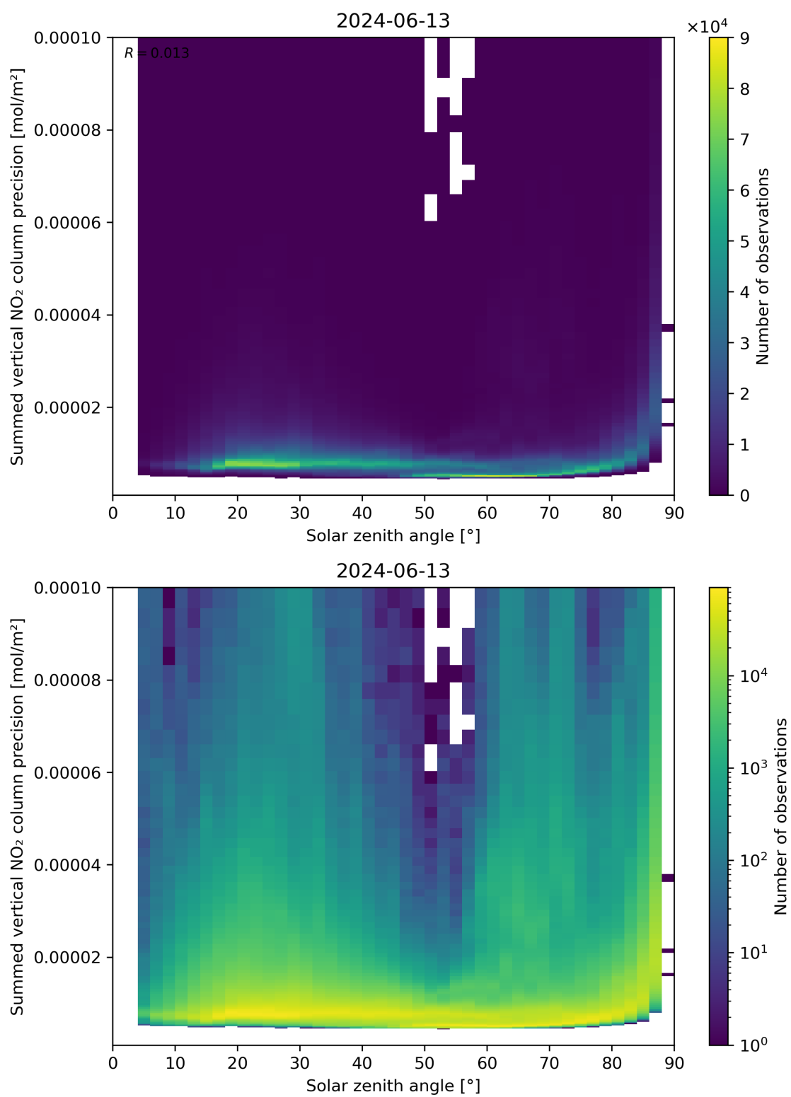
Figure 152: Scatter density plot of “Solar zenith angle” against “Summed vertical NO 2 column precision” for 2024-06-13 to 2024-06-14.
