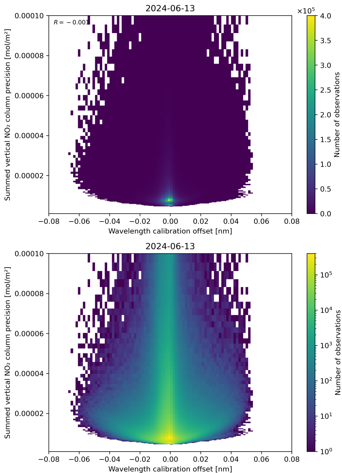
Figure 178: Scatter density plot of “Wavelength calibration offset” against “Summed vertical NO 2 column precision” for 2024-06-13 to 2024-06-14.
