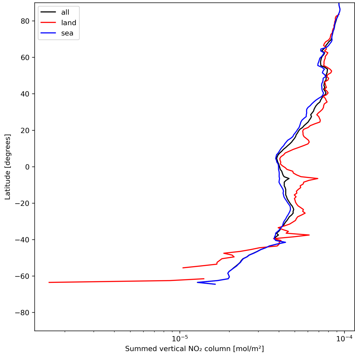
Figure 23: Zonal average of “Summed vertical NO 2 column” for 2024-06-13 to 2024-06-14.
