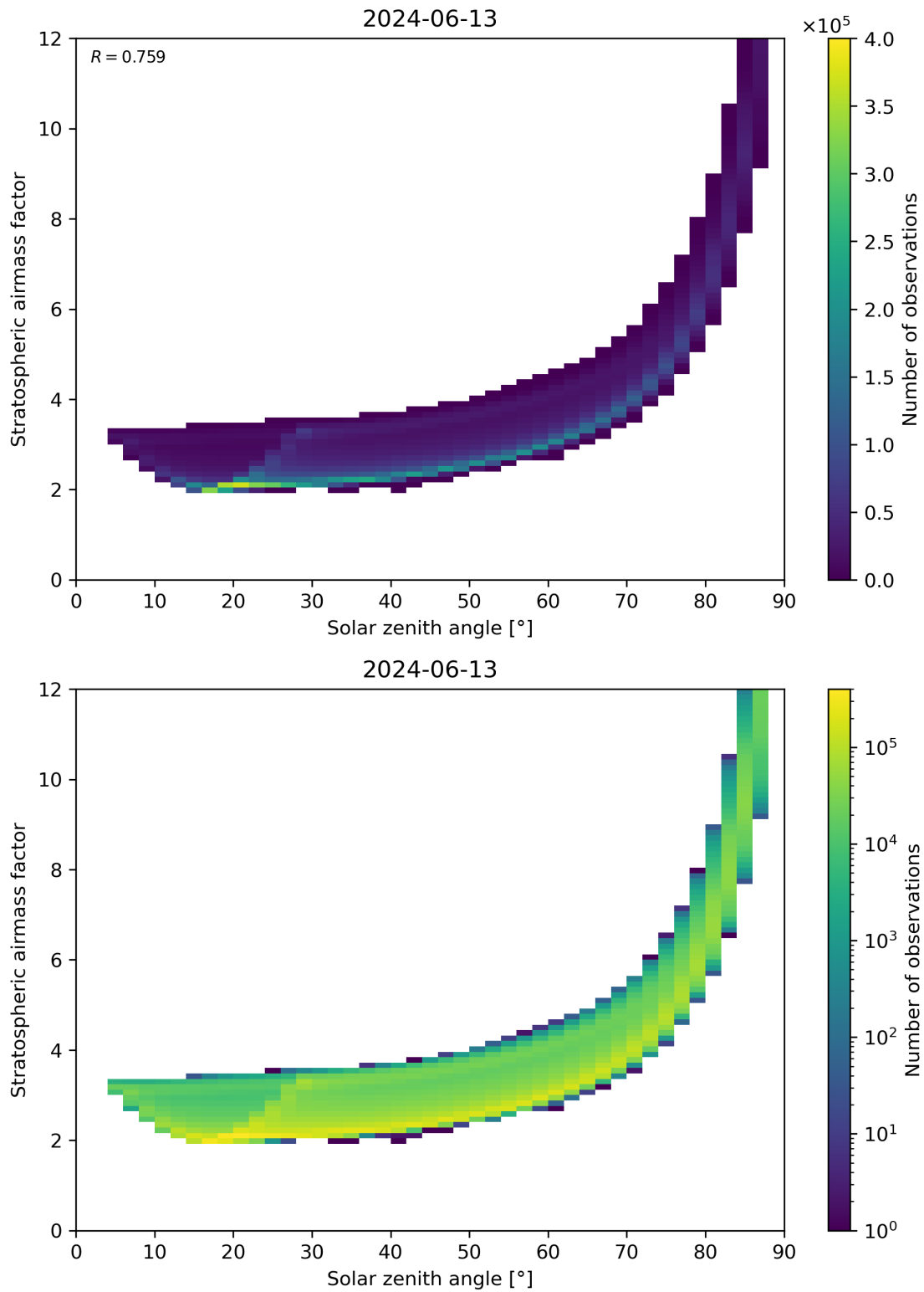
Figure 145: Scatter density plot of “Solar zenith angle” against “Stratospheric airmass factor” for 2024-06-13 to 2024-06-14.
