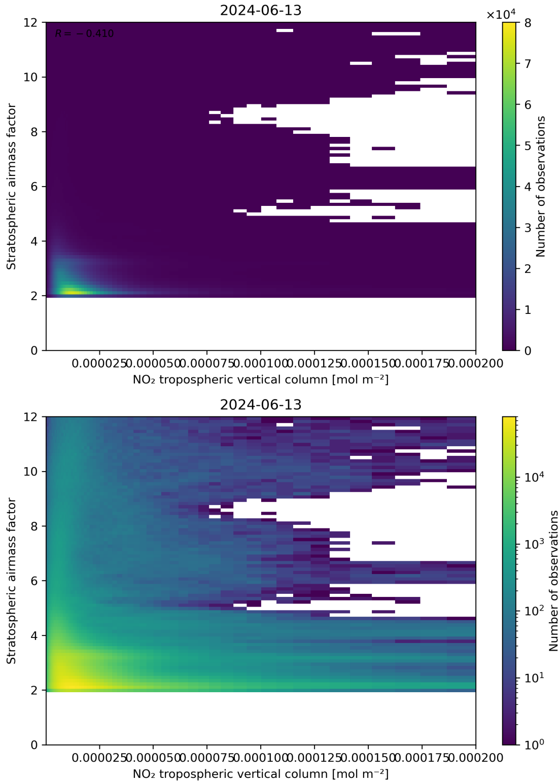
Figure 121: Scatter density plot of “NO 2 tropospheric vertical column” against “Stratospheric air mass factor” for 2024-06-13 to 2024-06-14.
