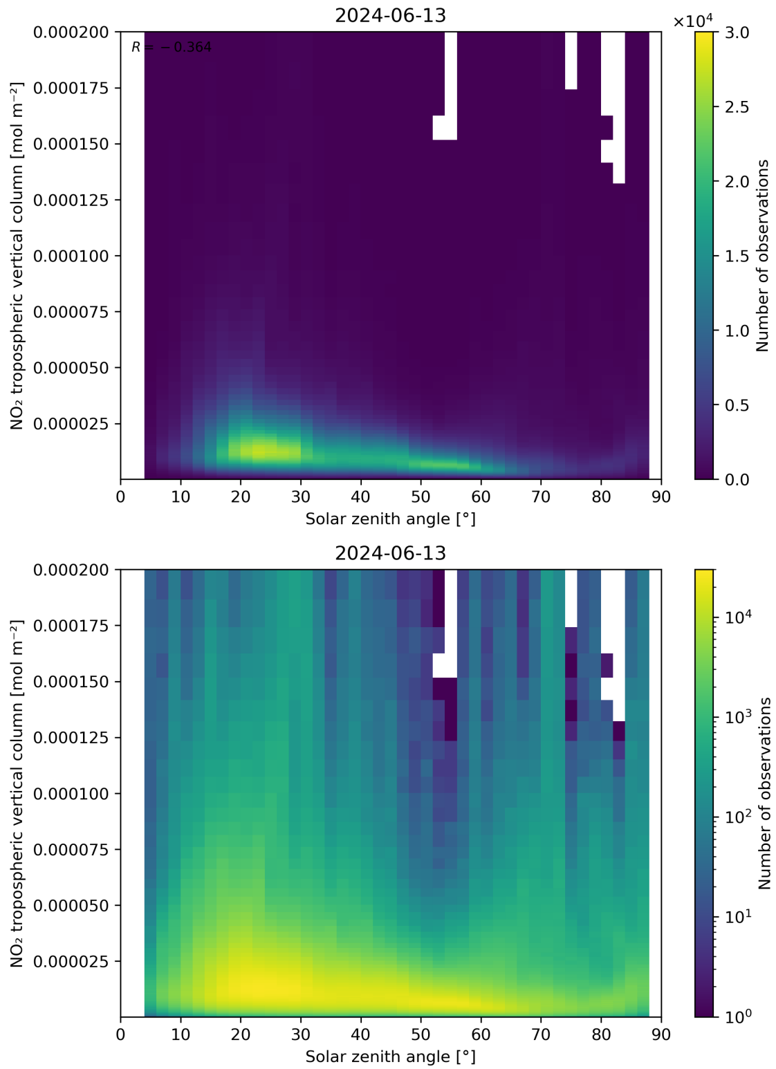
Figure 155: Scatter density plot of “Solar zenith angle” against “NO 2 tropospheric vertical column” for 2024-06-13 to 2024-06-14.
