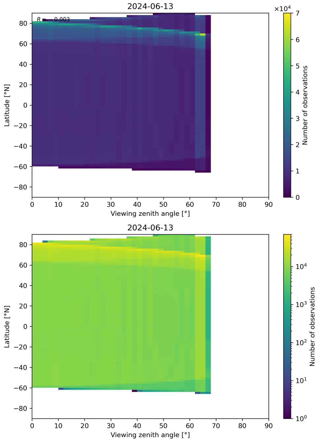
Figure 163: Scatter density plot of “Viewing zenith angle” against “Latitude” for 2024-06-13 to 2024-06-14.
