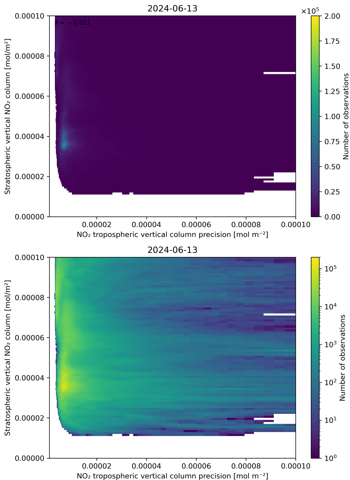
Figure 135: Scatter density plot of “NO 2 tropospheric vertical column precision” against “Stratospheric vertical NO 2 column” for 2024-06-13 to 2024-06-14.
