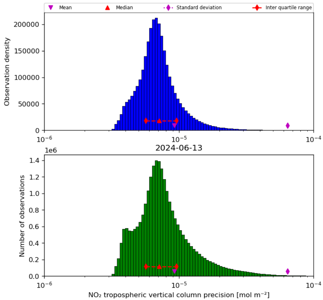
Figure 30: Histogram of “NO 2 tropospheric vertical column precision” for 2024-06-13 to 2024-06-14
