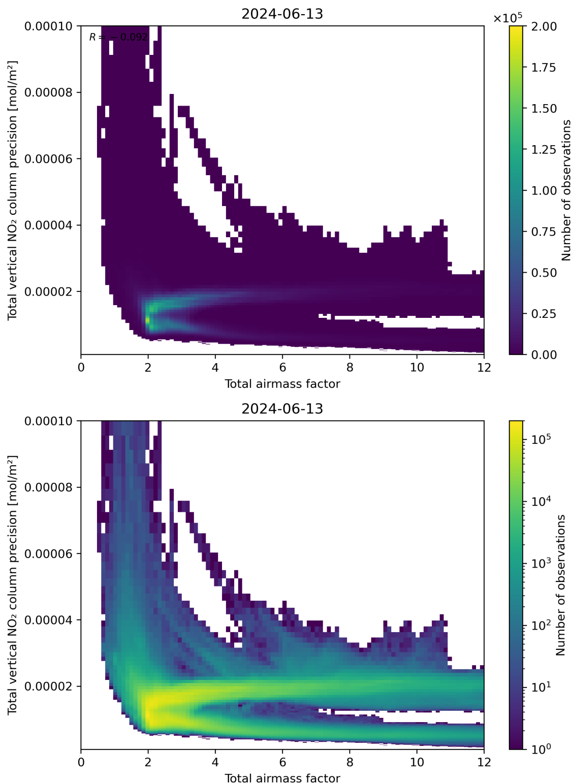
Figure 68: Scatter density plot of “Total airmass factor” against “Total vertical NO 2 column precision” for 2024-06-13 to 2024-06-14.
