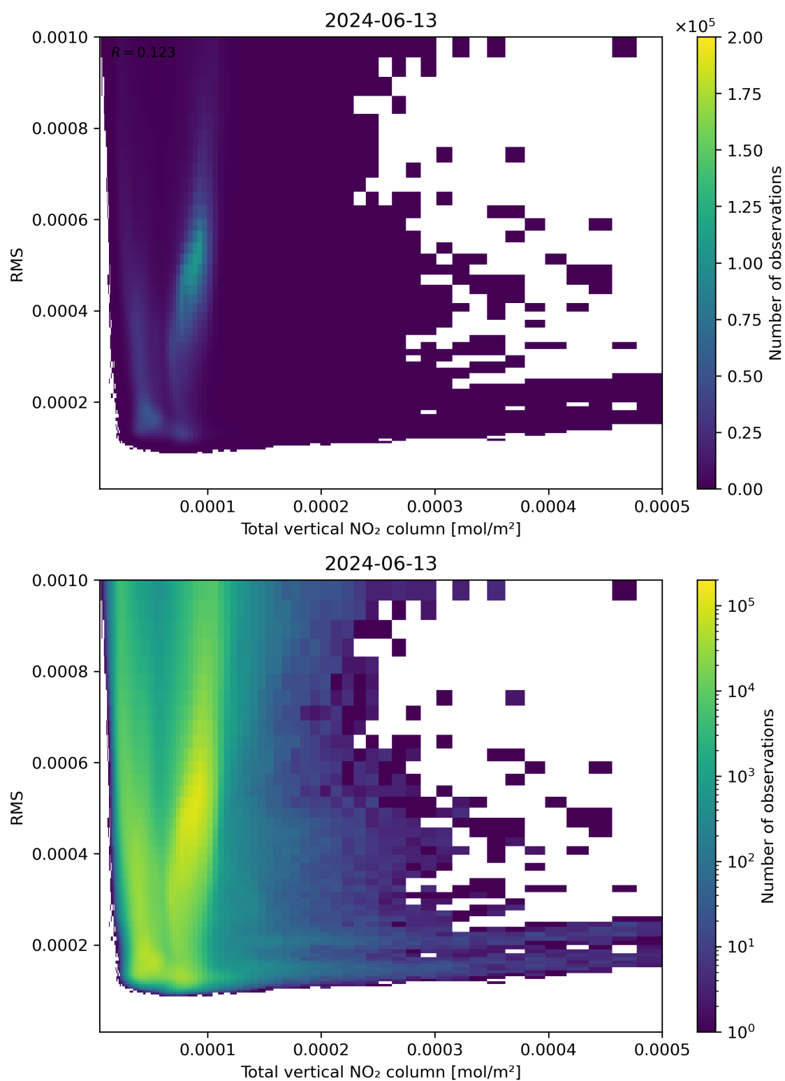
Figure 120: Scatter density plot of “Total vertical NO 2 column” against “RMS” for 2024-06-13 to 2024-06-14.
