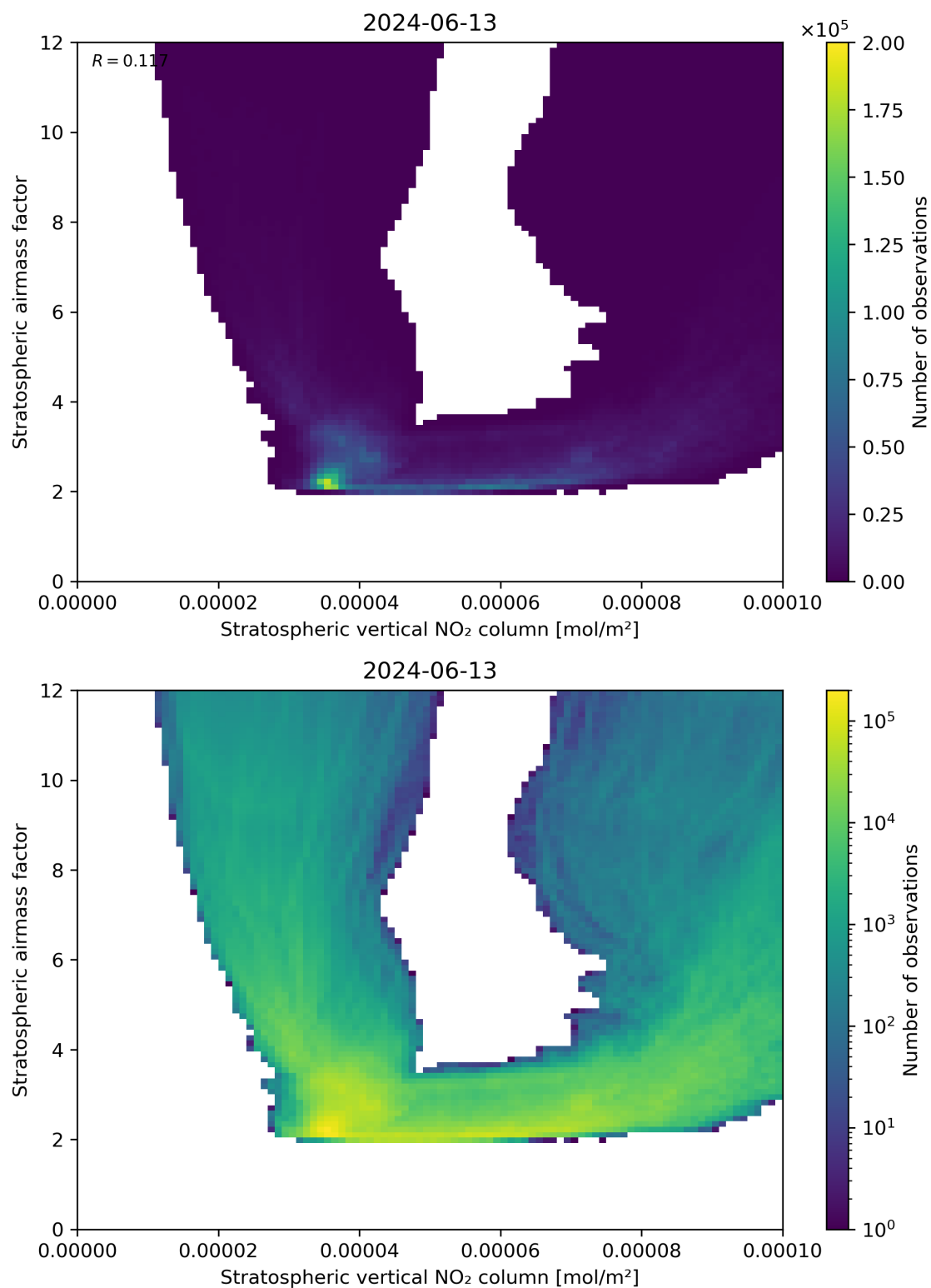
Figure 96: Scatter density plot of “Stratospheric vertical NO 2 column” against “Stratospheric airmass factor” for 2024-06-13 to 2024-06-14.
