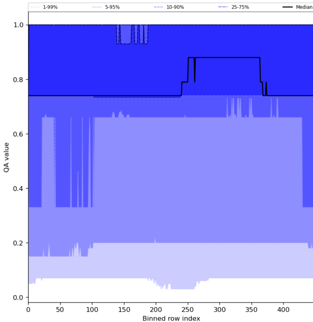
Figure 45: Along track statistics of “QA value” for 2024-06-13 to 2024-06-14
