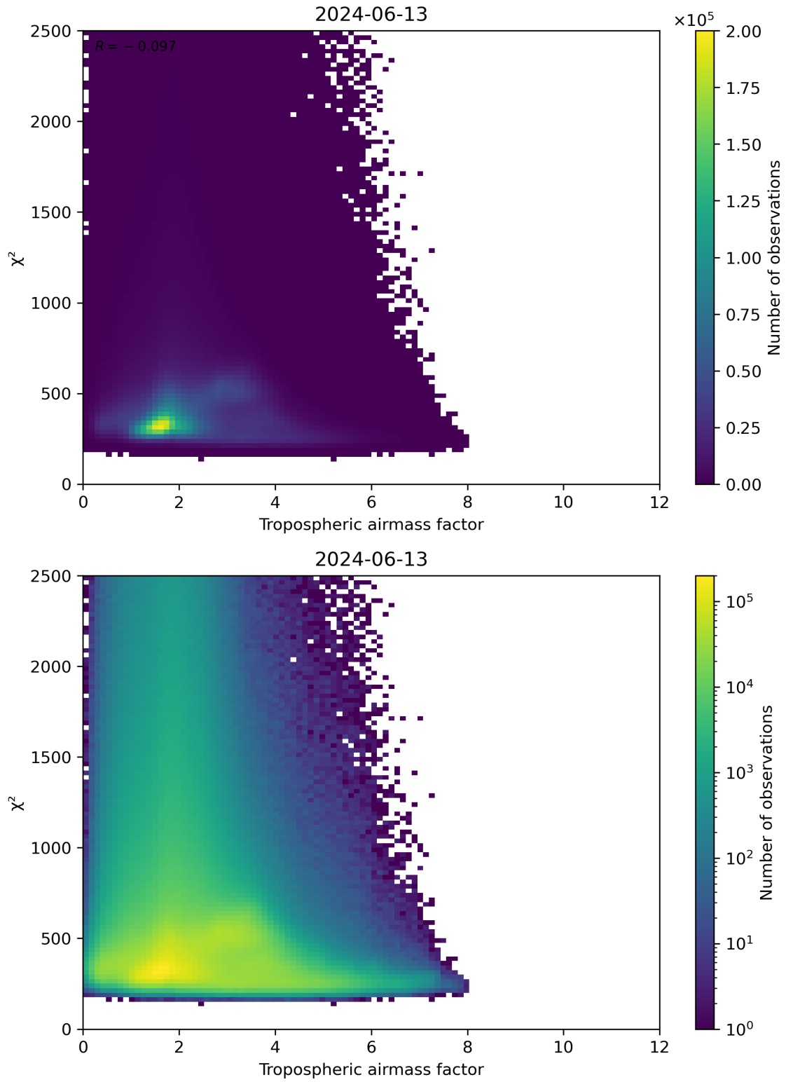
Figure 73: Scatter density plot of “Tropospheric airmass factor” against “ \chi^2 ” for 2024-06-13 to 2024-06-14.
