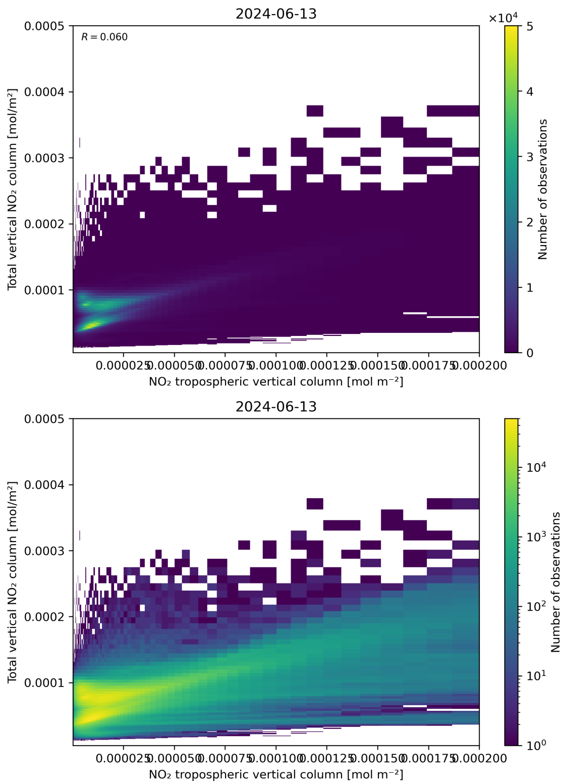
Figure 128: Scatter density plot of “NO 2 tropospheric vertical column” against “Total vertical NO 2 column” for 2024-06-13 to 2024-06-14.
