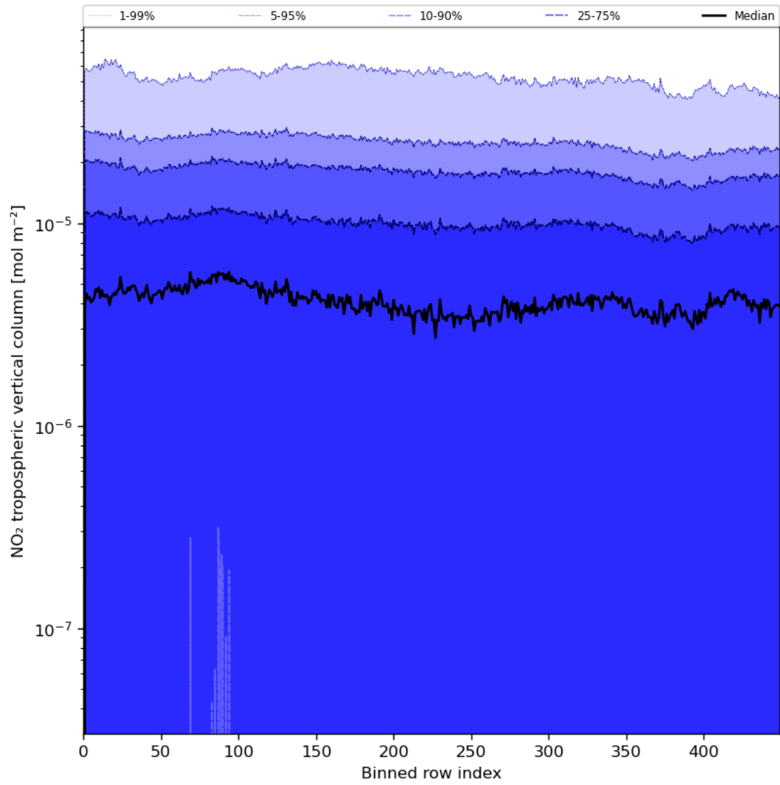
Figure 46: Along track statistics of “NO 2 tropospheric vertical column” for 2024-06-13 to 2024-06-14
