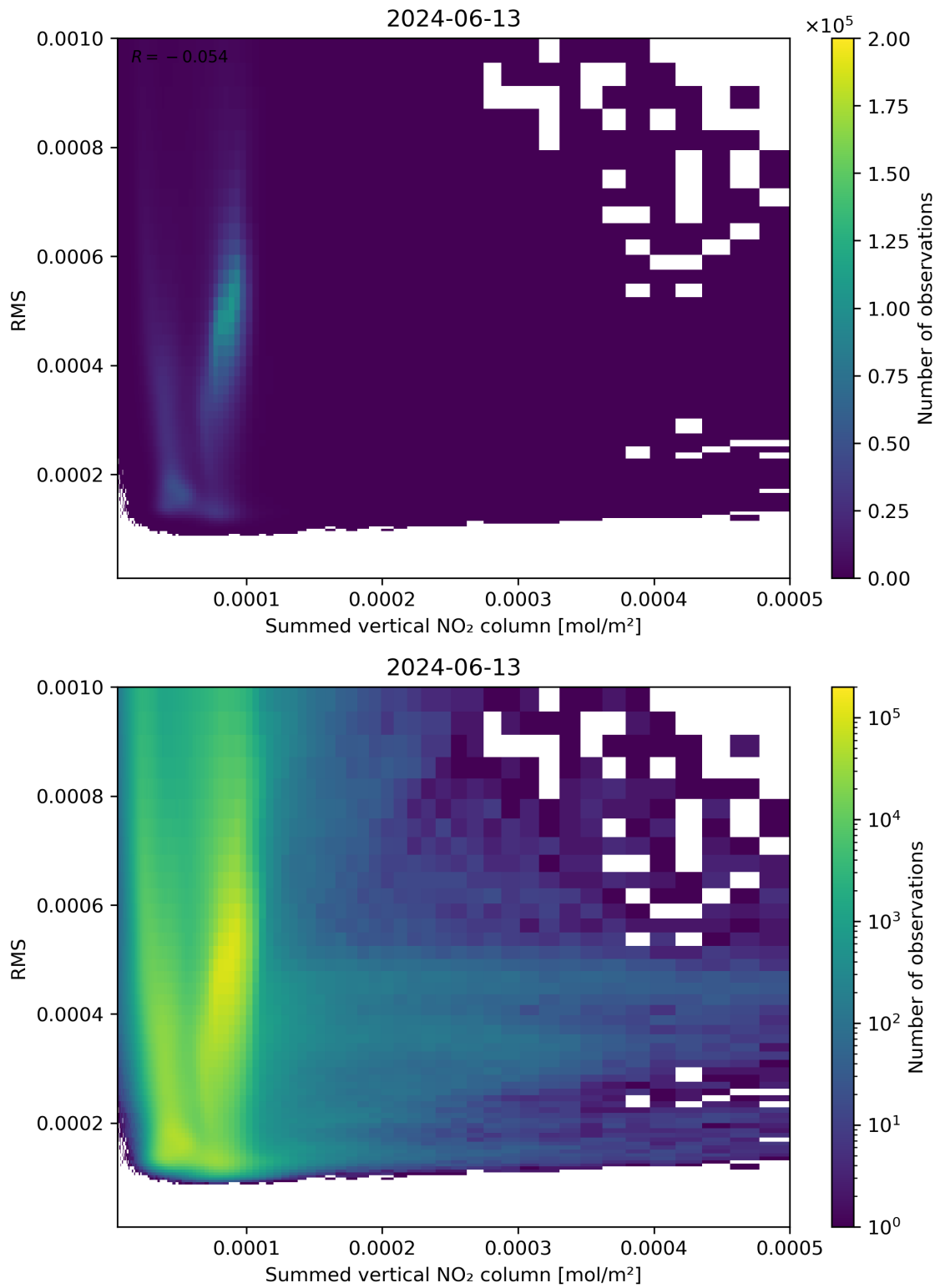
Figure 109: Scatter density plot of “Summed vertical NO 2 column” against “RMS” for 2024-06-13 to 2024-06-14.
