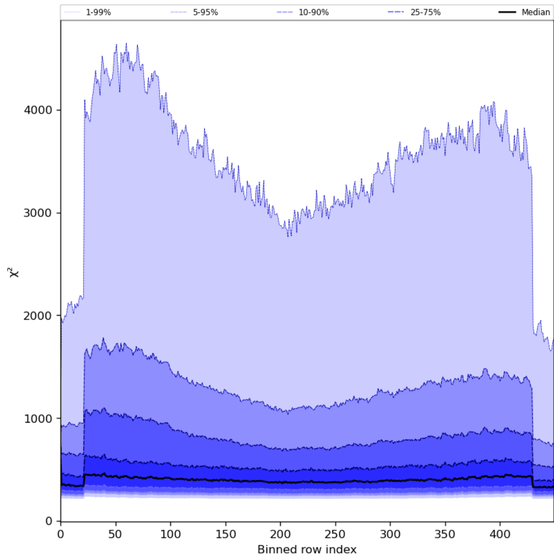
Figure 59: Along track statistics of “ \chi^2 ” for 2024-06-13 to 2024-06-14
