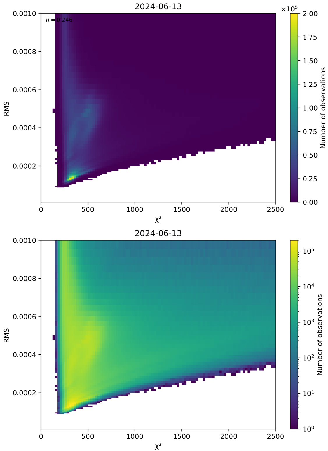
Figure 82: Scatter density plot of “ \chi^2 ” against “RMS” for 2024-06-13 to 2024-06-14.
