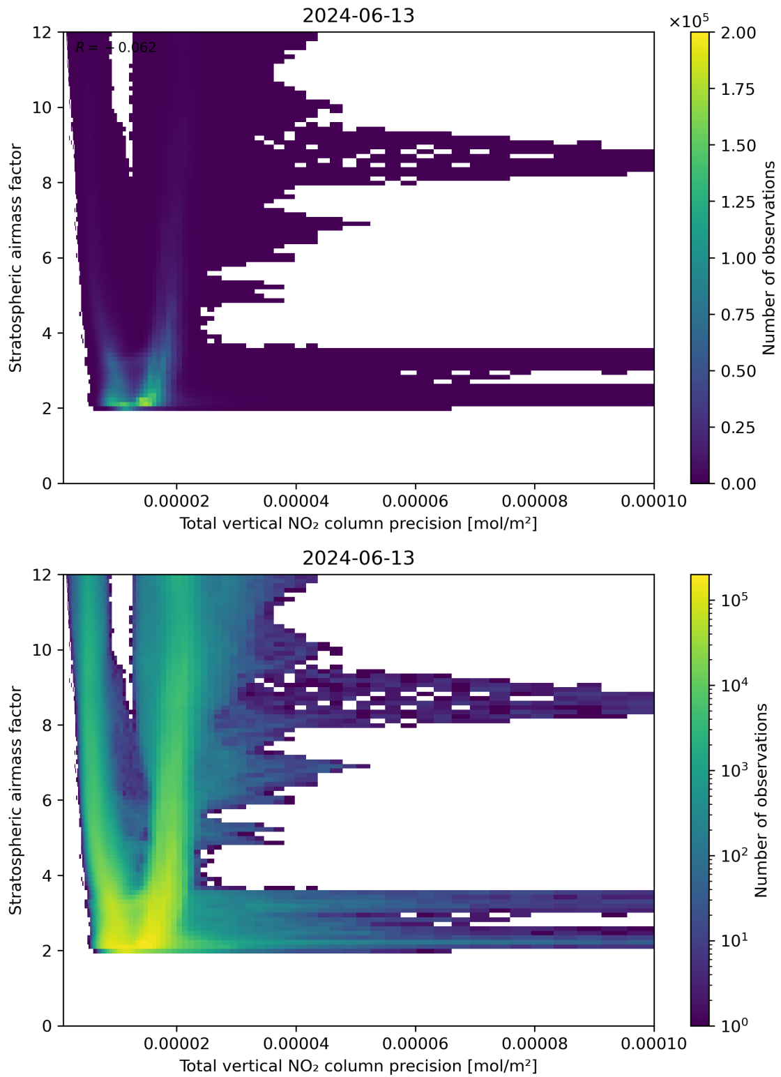
Figure 115: Scatter density plot of “Total vertical NO 2 column precision” against “Stratospheric air mass factor” for 2024-06-13 to 2024-06-14.
