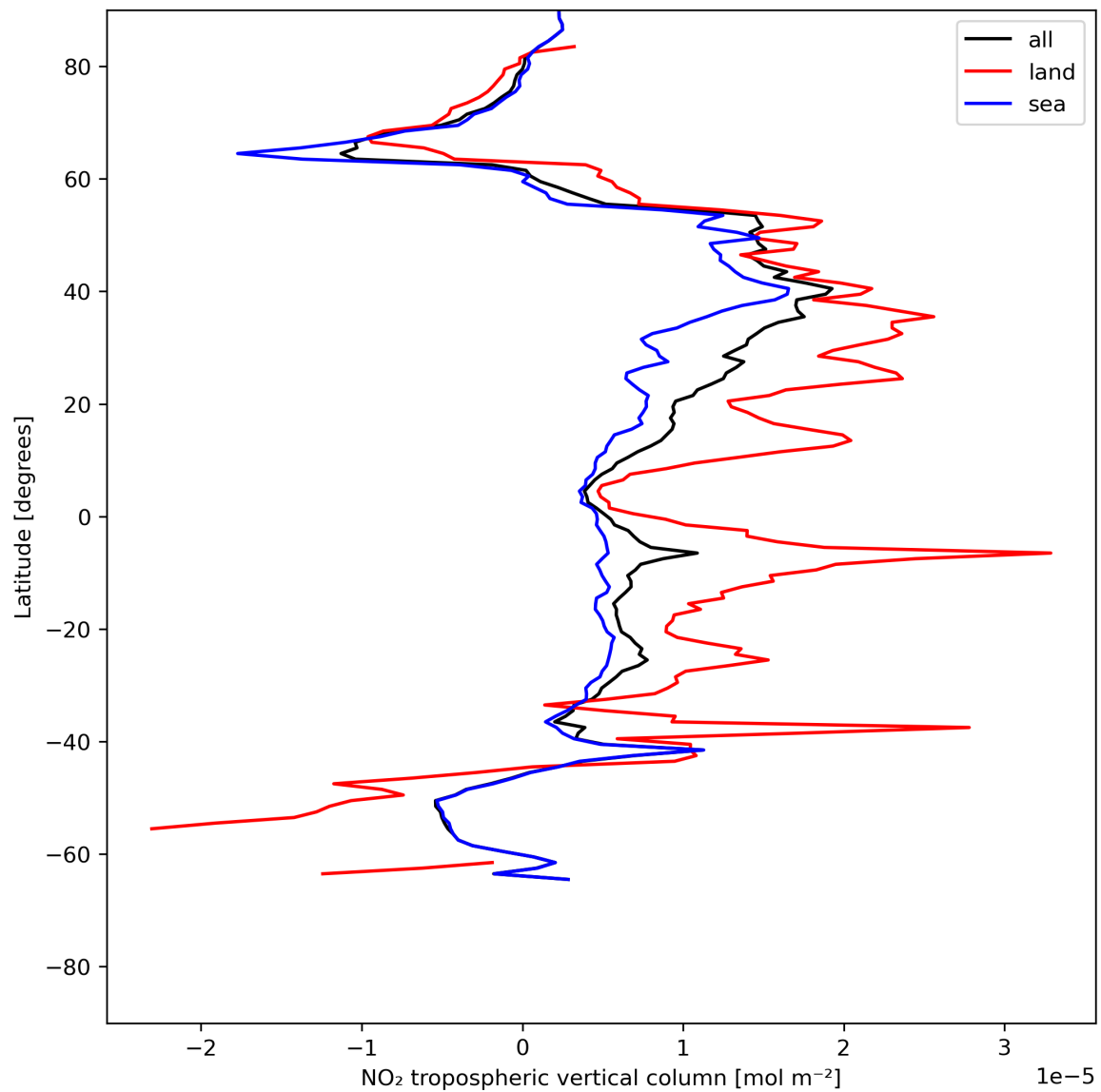
Figure 12: Zonal average of “NO 2 tropospheric vertical column” for 2024-06-13 to 2024-06-14.
