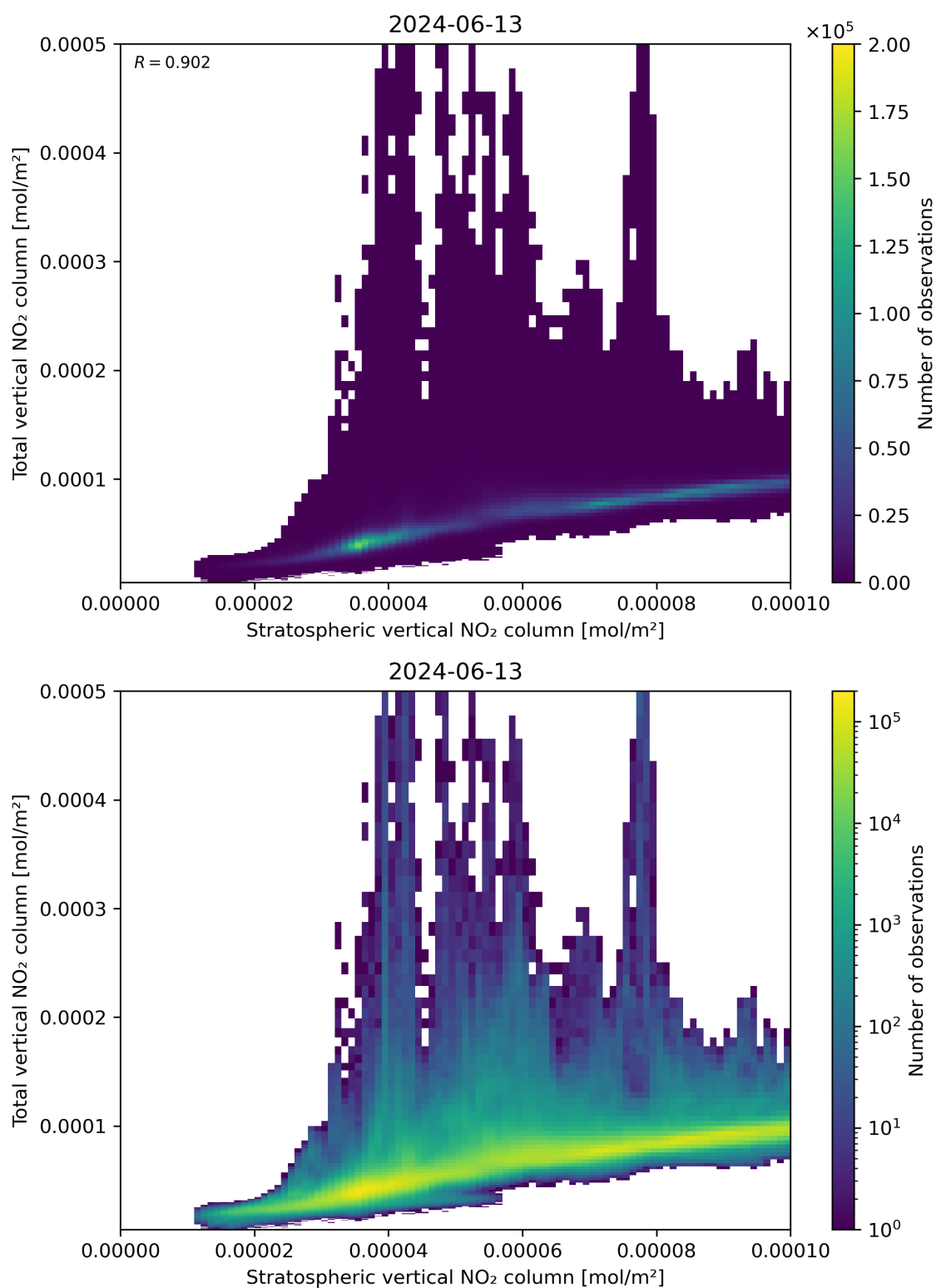
Figure 100: Scatter density plot of “Stratospheric vertical NO 2 column” against “Total vertical NO 2 column” for 2024-06-13 to 2024-06-14.
