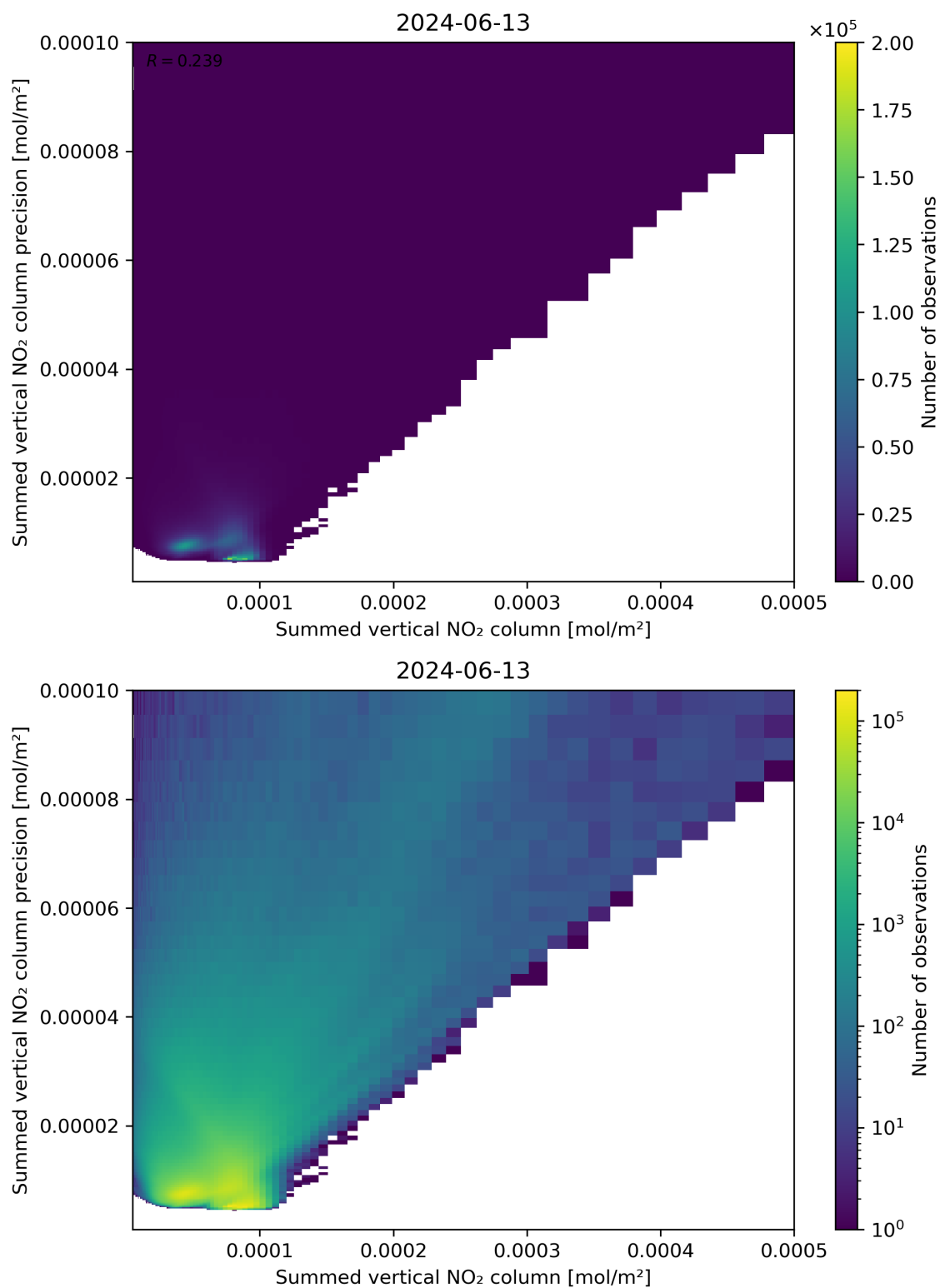
Figure 105: Scatter density plot of “Summed vertical NO 2 column” against “Summed vertical NO 2 column precision” for 2024-06-13 to 2024-06-14.
