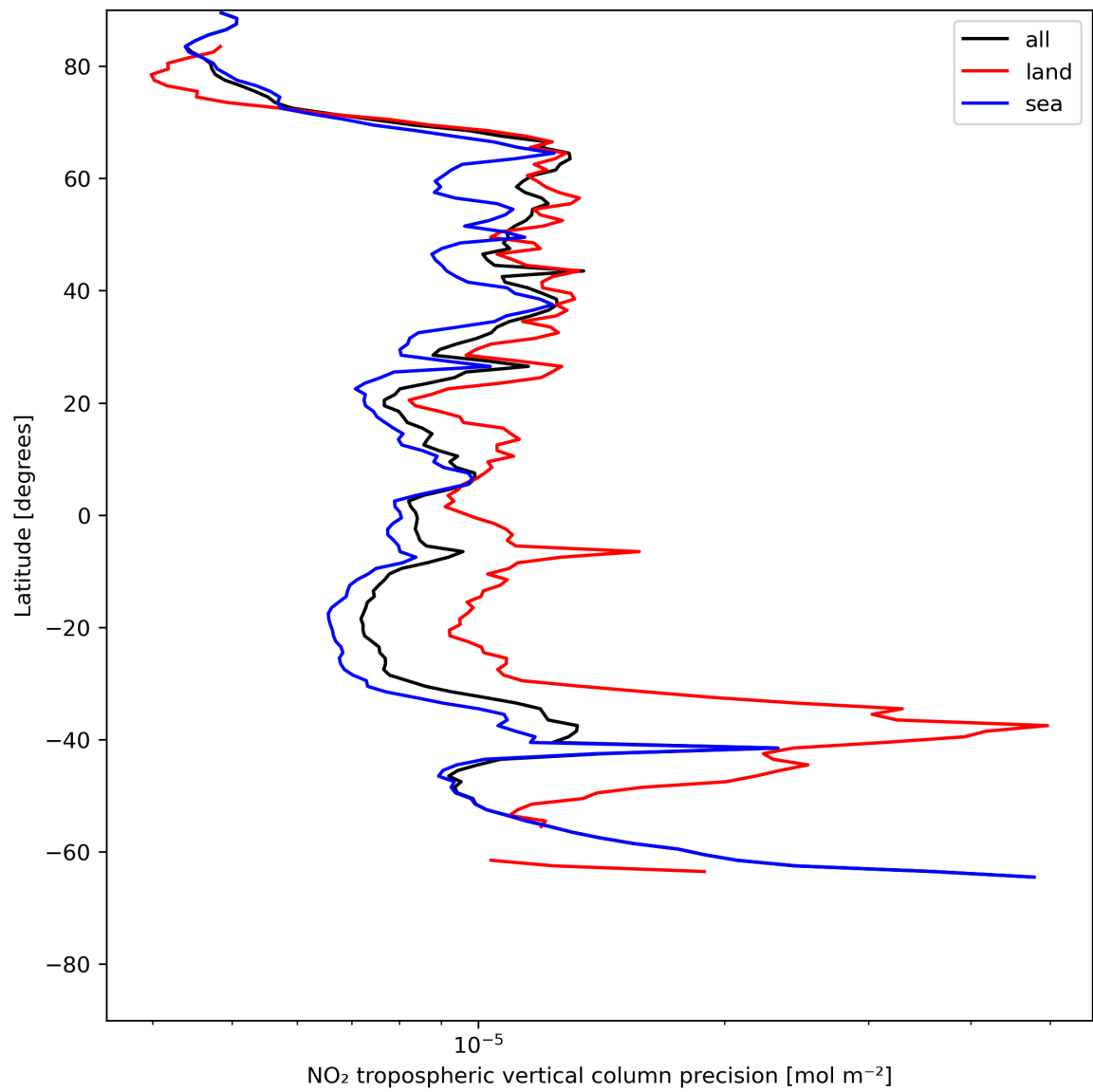
Figure 13: Zonal average of “NO 2 tropospheric vertical column precision” for 2024-06-13 to 2024-06-14.
