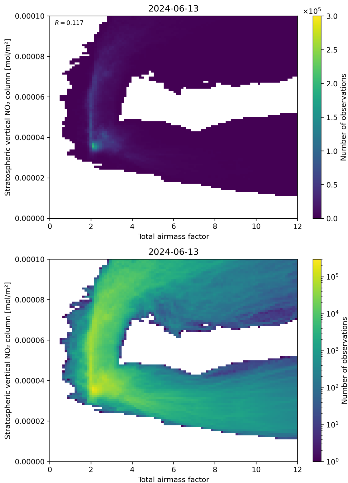
Figure 64: Scatter density plot of “Total airmass factor” against “Stratospheric vertical \text{NO}_2 column” for 2024-06-13 to 2024-06-14.
