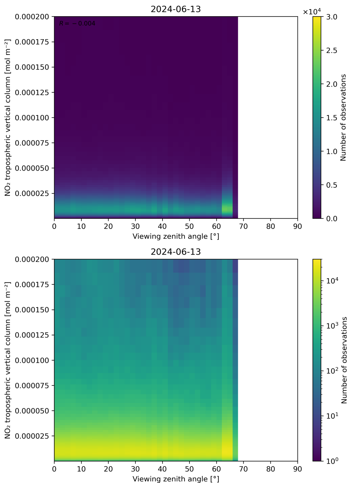
Figure 169: Scatter density plot of “Viewing zenith angle” against “NO 2 tropospheric vertical column” for 2024-06-13 to 2024-06-14.
