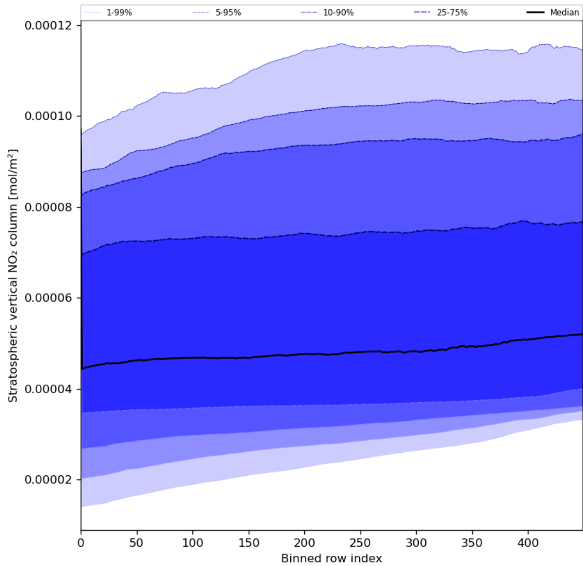
Figure 53: Along track statistics of “Stratospheric vertical NO 2 column” for 2024-06-13 to 2024-06-14
