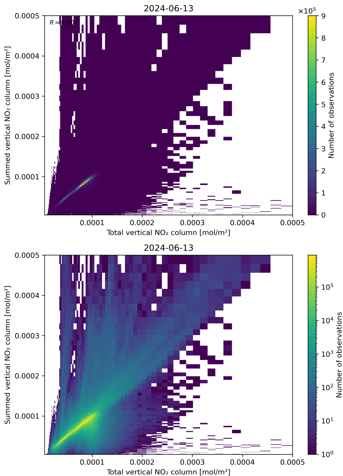
Figure 112: Scatter density plot of “Total vertical NO 2 column” against “Summed vertical NO 2 column” for 2024-06-13 to 2024-06-14.
