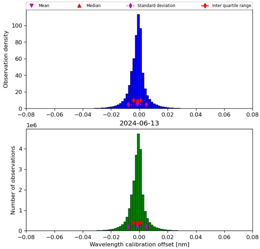
Figure 35: Histogram of “Wavelength calibration offset” for 2024-06-13 to 2024-06-14
