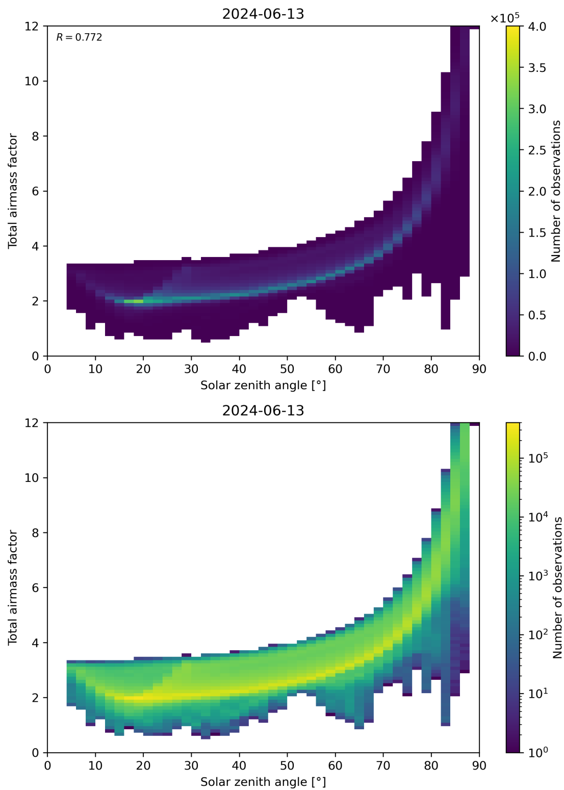
Figure 146: Scatter density plot of “Solar zenith angle” against “Total air mass factor” for 2024-06-13 to 2024-06-14.
