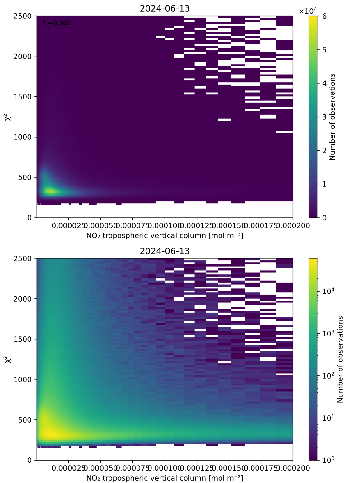
Figure 124: Scatter density plot of “NO 2 tropospheric vertical column” against “ \chi^2 ” for 2024-06-13 to 2024-06-14.
