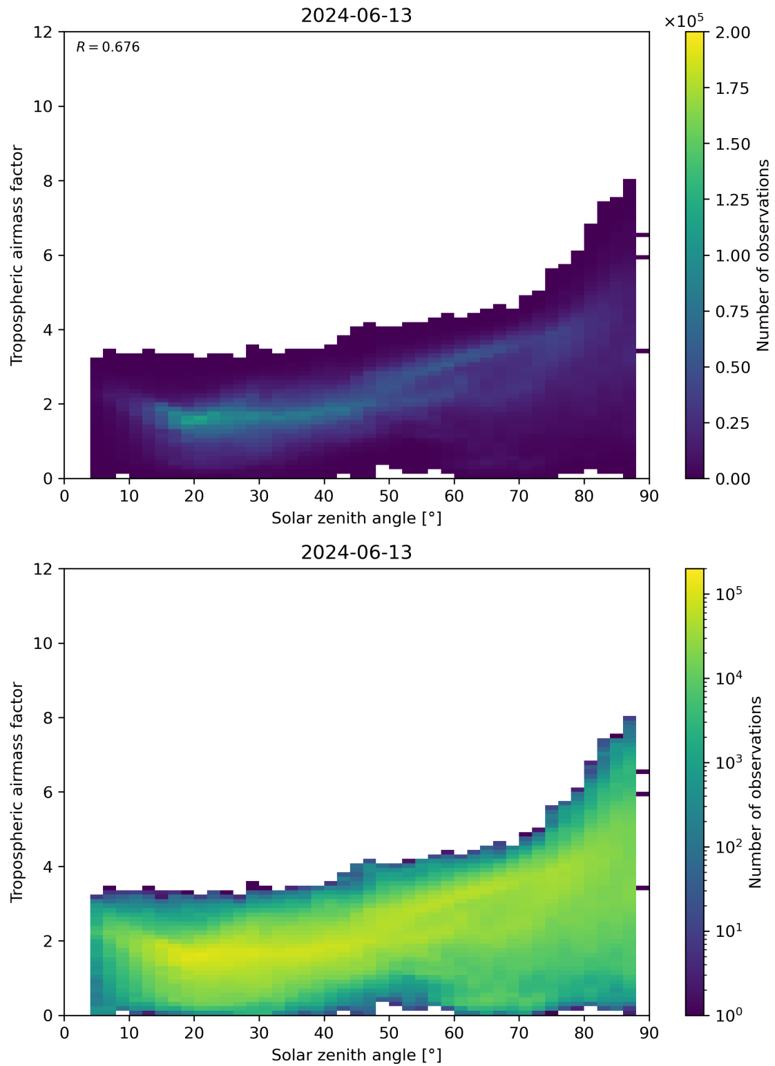
Figure 147: Scatter density plot of “Solar zenith angle” against “Tropospheric airmass factor” for 2024-06-13 to 2024-06-14.
