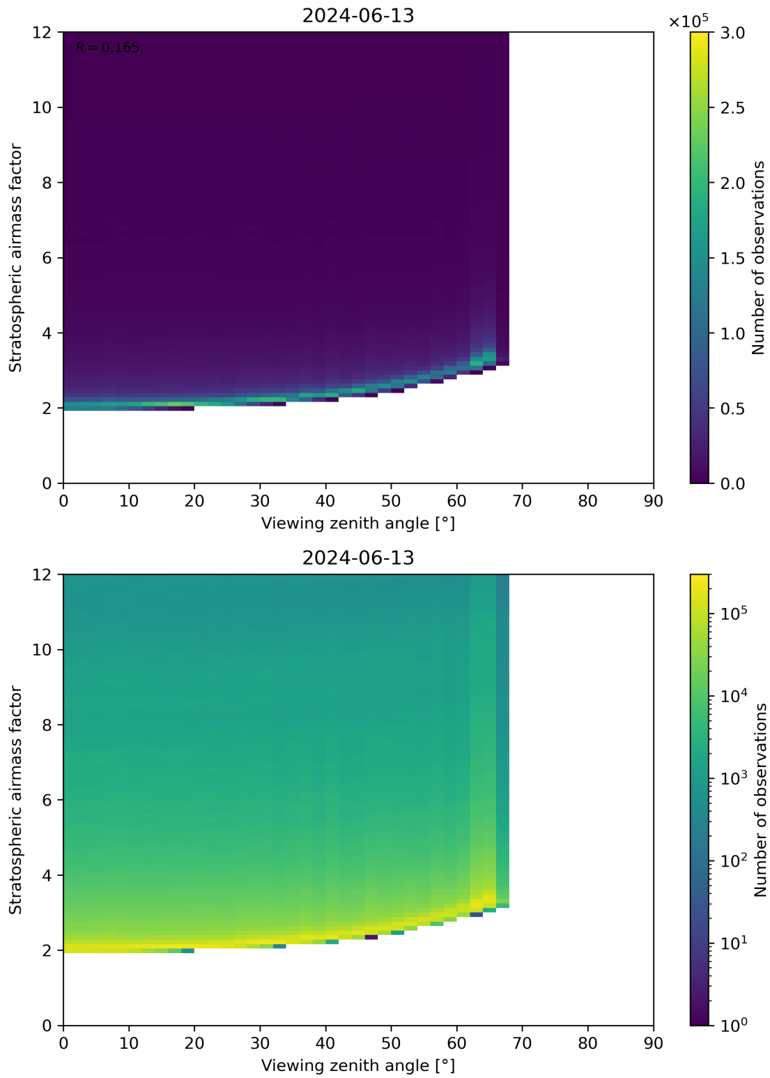
Figure 159: Scatter density plot of “Viewing zenith angle” against “Stratospheric airmass factor” for 2024-06-13 to 2024-06-14.
