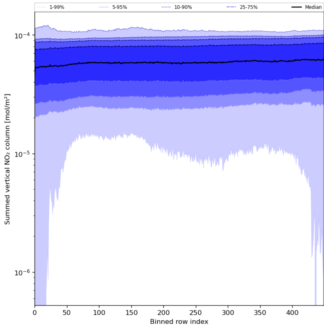
Figure 57: Along track statistics of “Summed vertical NO 2 column” for 2024-06-13 to 2024-06-14
