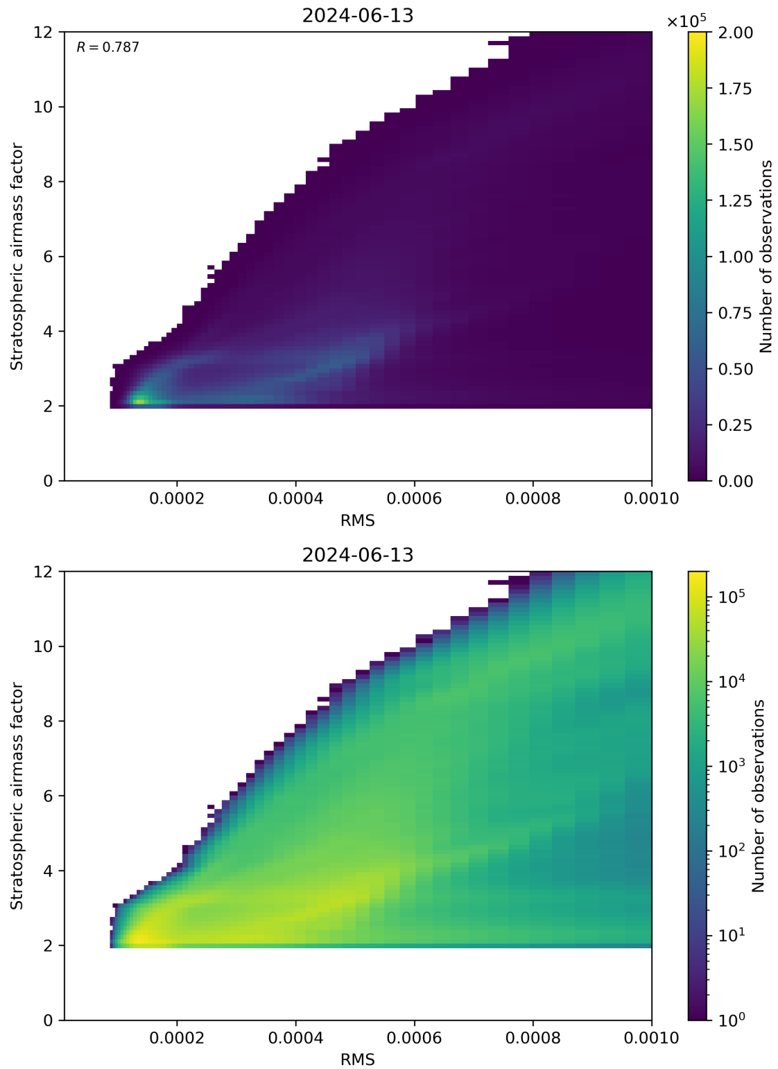
Figure 144: Scatter density plot of “RMS” against “Stratospheric airmass factor” for 2024-06-13 to 2024-06-14.
