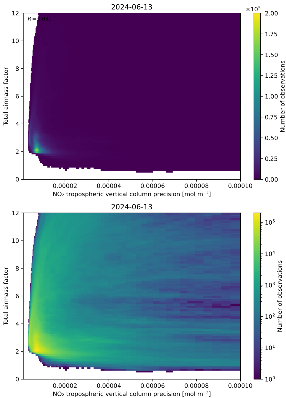
Figure 132: Scatter density plot of “NO 2 tropospheric vertical column precision” against “Total air mass factor” for 2024-06-13 to 2024-06-14.
