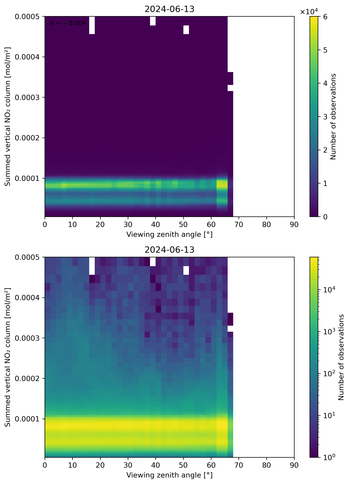
Figure 165: Scatter density plot of “Viewing zenith angle” against “Summed vertical NO 2 column” for 2024-06-13 to 2024-06-14.
