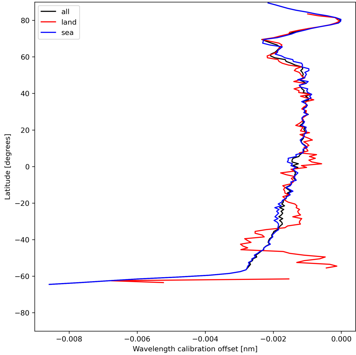
Figure 18: Zonal average of “Wavelength calibration offset” for 2024-06-13 to 2024-06-14.
