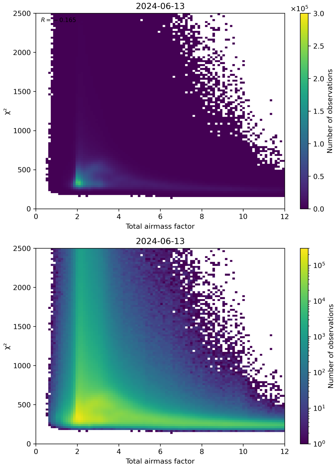
Figure 63: Scatter density plot of “Total airmass factor” against “ \chi^2 ” for 2024-06-13 to 2024-06-14.
