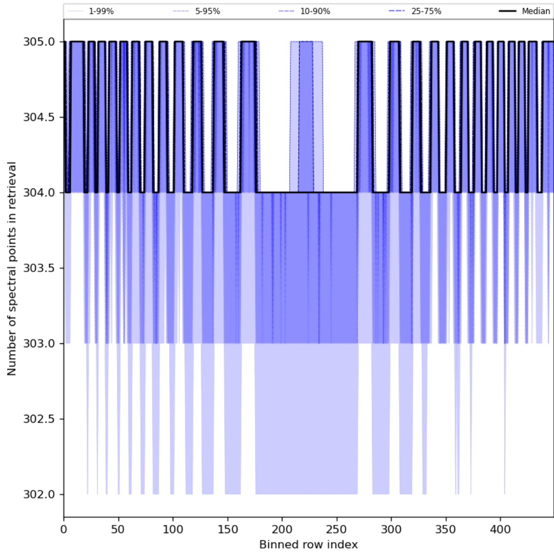
Figure 50: Along track statistics of “Number of spectral points in retrieval” for 2024-06-13 to 2024-06-14
