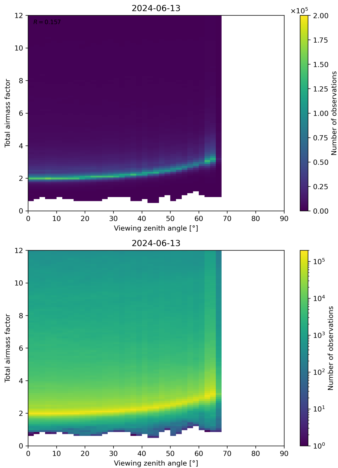
Figure 160: Scatter density plot of “Viewing zenith angle” against “Total airmass factor” for 2024-06-13 to 2024-06-14.
