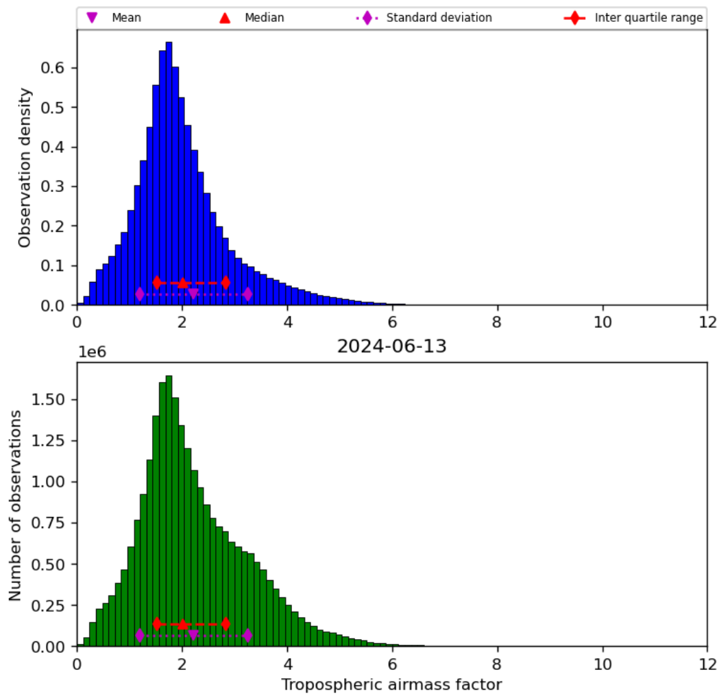
Figure 31: Histogram of “Tropospheric airmass factor” for 2024-06-13 to 2024-06-14
