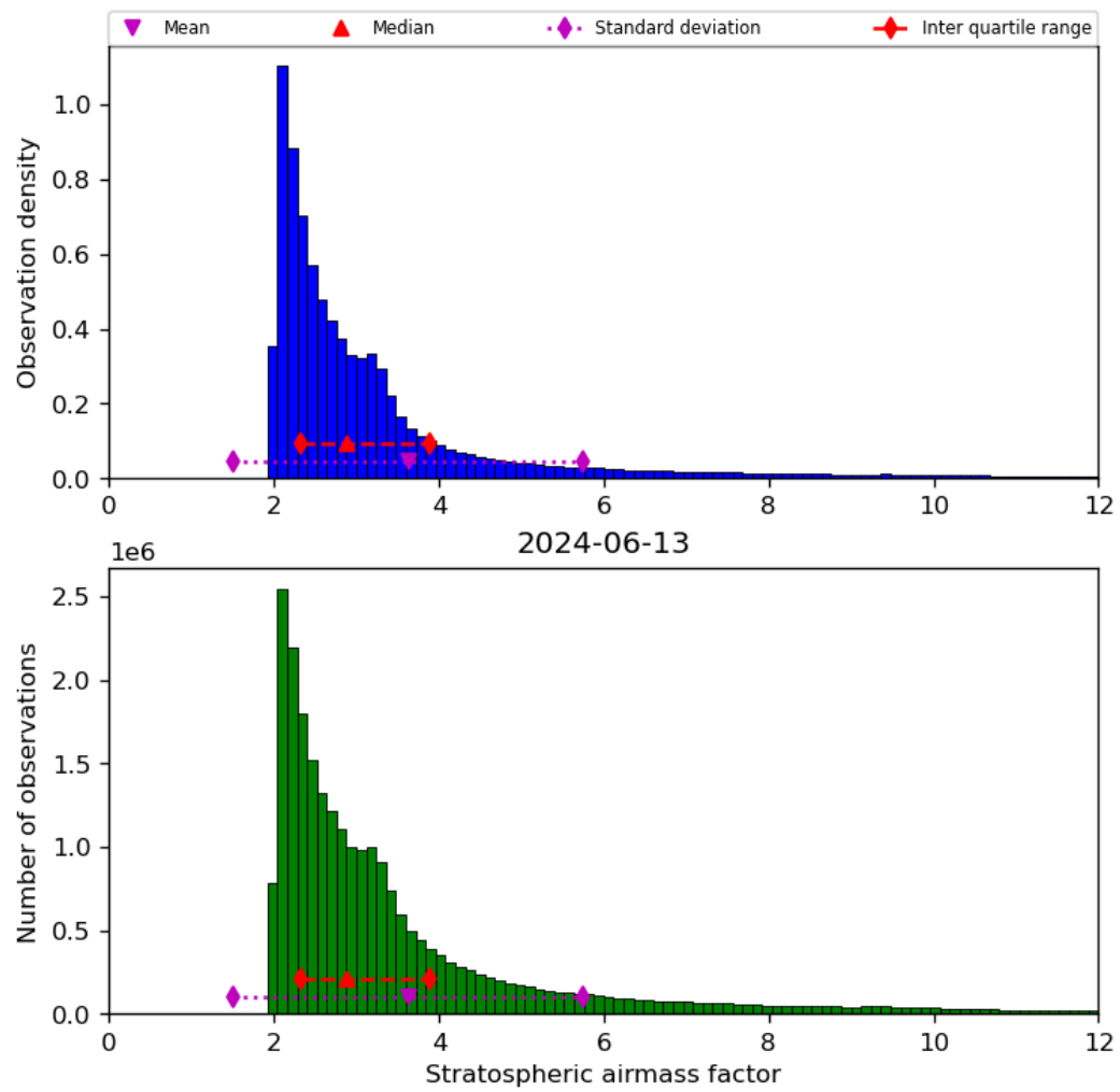
Figure 44: Histogram of “Stratospheric airmass factor” for 2024-06-13 to 2024-06-14
