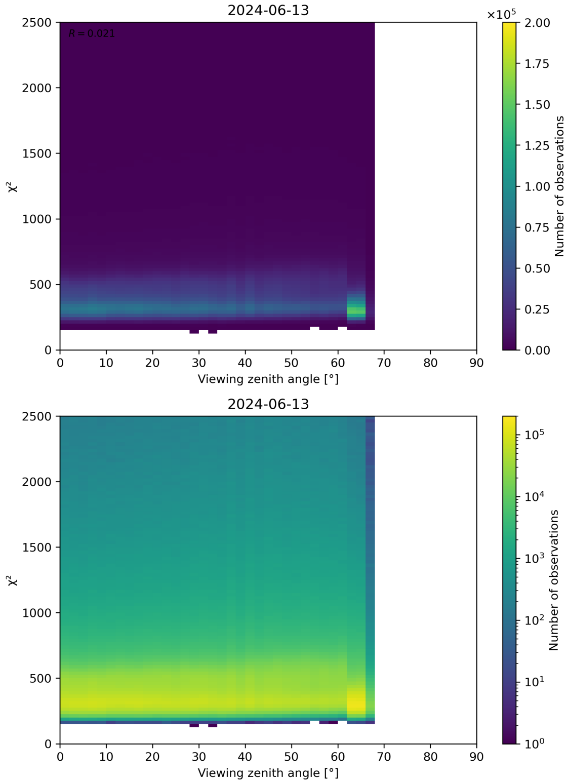
Figure 162: Scatter density plot of “Viewing zenith angle” against “ \chi^2 ” for 2024-06-13 to 2024-06-14.
