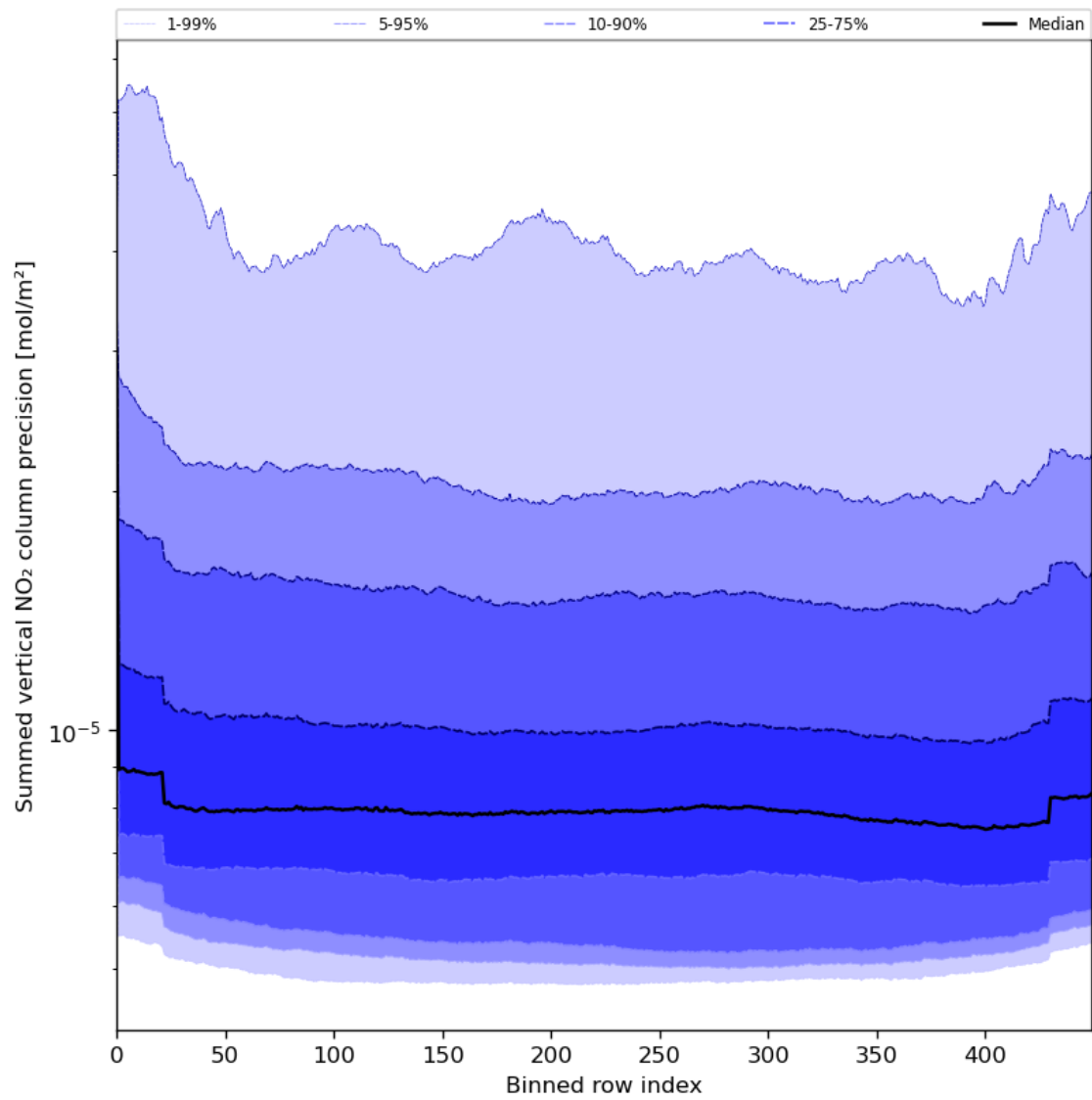
Figure 58: Along track statistics of “Summed vertical NO 2 column precision” for 2024-06-13 to 2024-06-14
