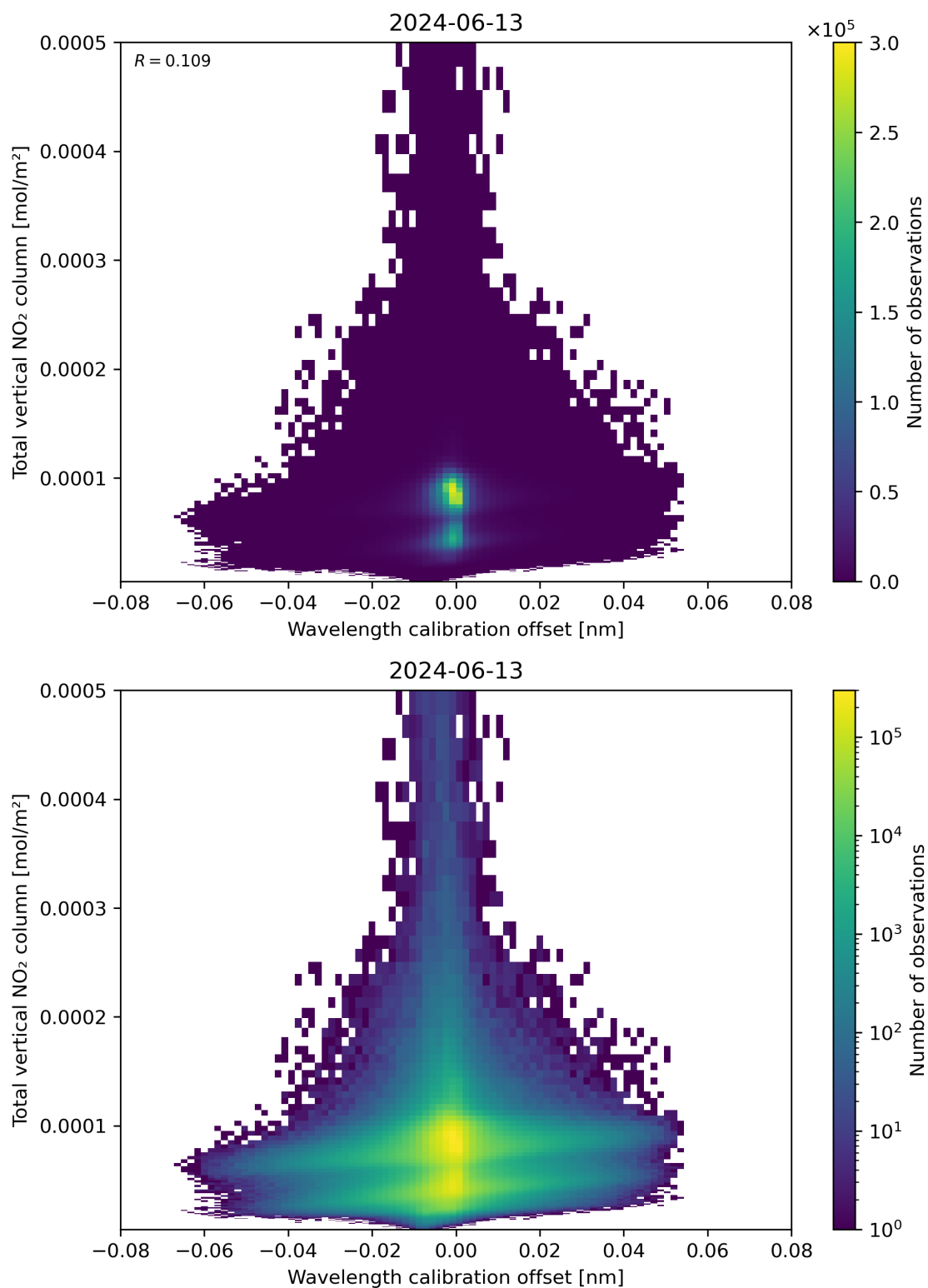
Figure 179: Scatter density plot of “Wavelength calibration offset” against “Total vertical NO 2 column” for 2024-06-13 to 2024-06-14.
