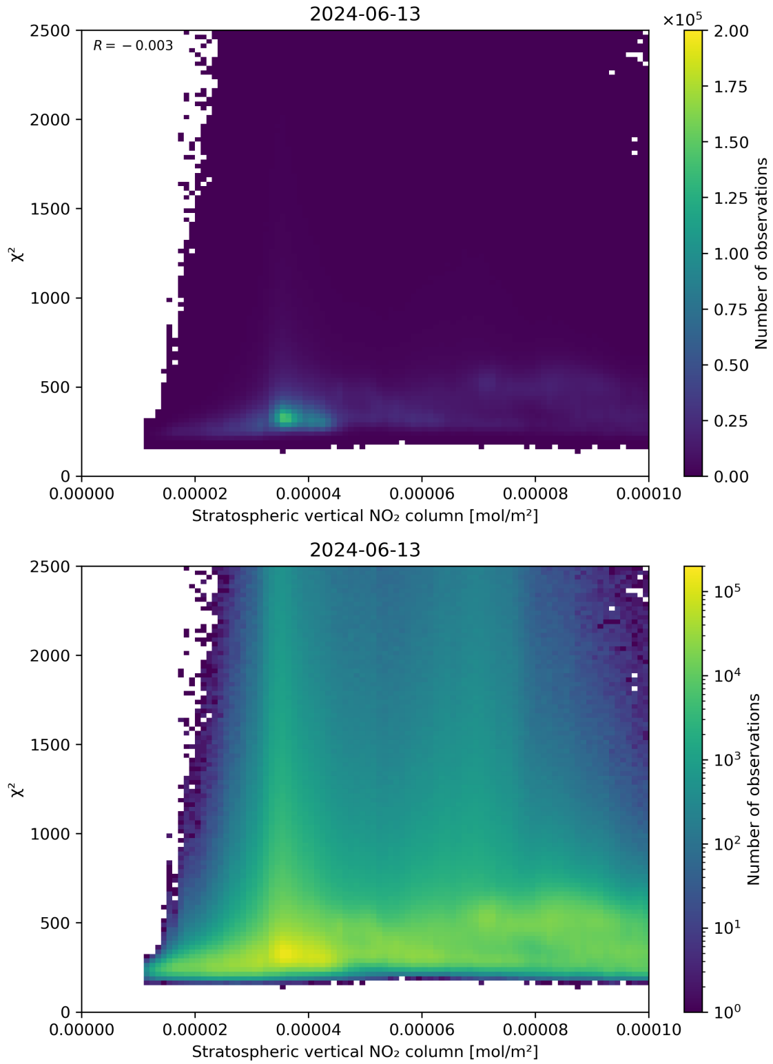
Figure 97: Scatter density plot of “Stratospheric vertical NO 2 column” against “ \chi^2 ” for 2024-06-13 to 2024-06-14.
