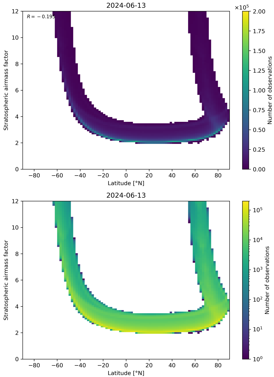
Figure 83: Scatter density plot of “Latitude” against “Stratospheric air mass factor” for 2024-06-13 to 2024-06-14.
