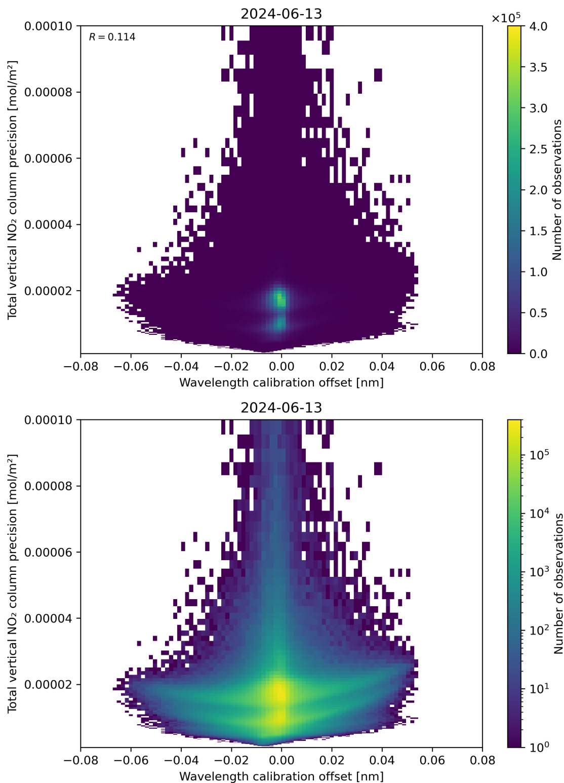
Figure 180: Scatter density plot of “Wavelength calibration offset” against “Total vertical NO 2 column precision” for 2024-06-13 to 2024-06-14.
