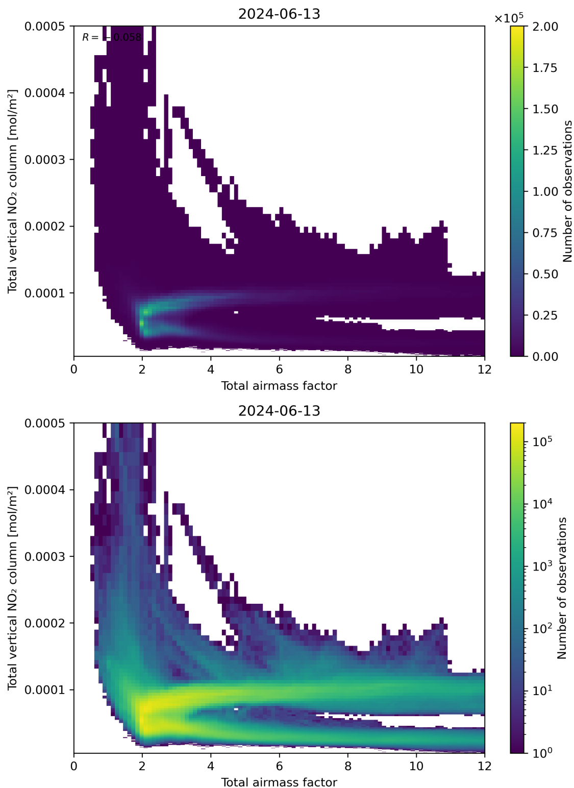
Figure 67: Scatter density plot of “Total airmass factor” against “Total vertical NO 2 column” for 2024-06-13 to 2024-06-14.
