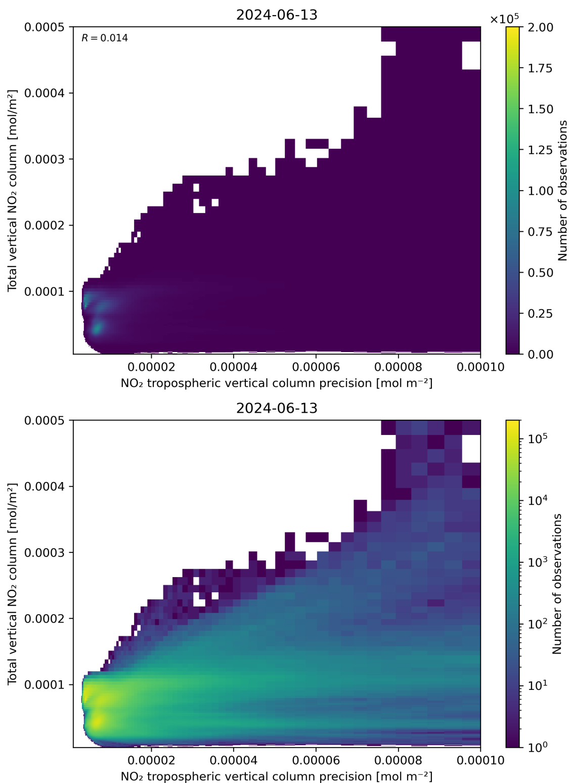
Figure 138: Scatter density plot of “NO 2 tropospheric vertical column precision” against “Total vertical NO 2 column” for 2024-06-13 to 2024-06-14.
