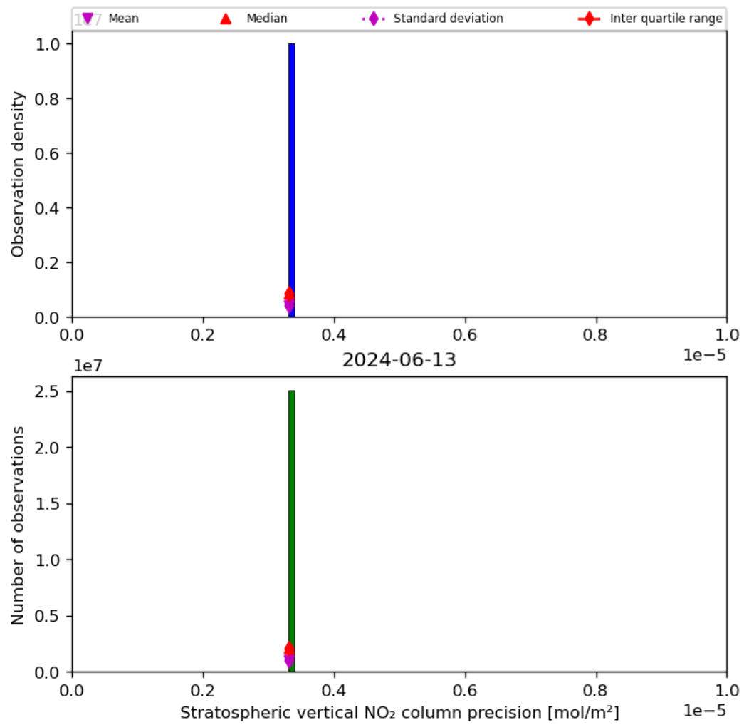
Figure 37: Histogram of “Stratospheric vertical NO 2 column precision” for 2024-06-13 to 2024-06-14
