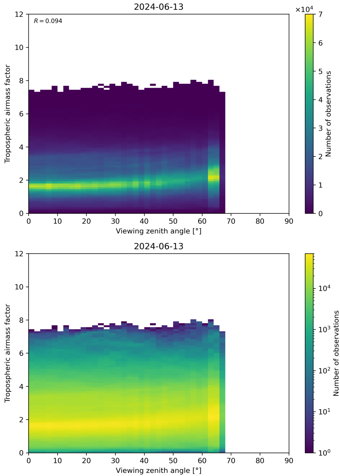
Figure 161: Scatter density plot of “Viewing zenith angle” against “Tropospheric airmass factor” for 2024-06-13 to 2024-06-14.
