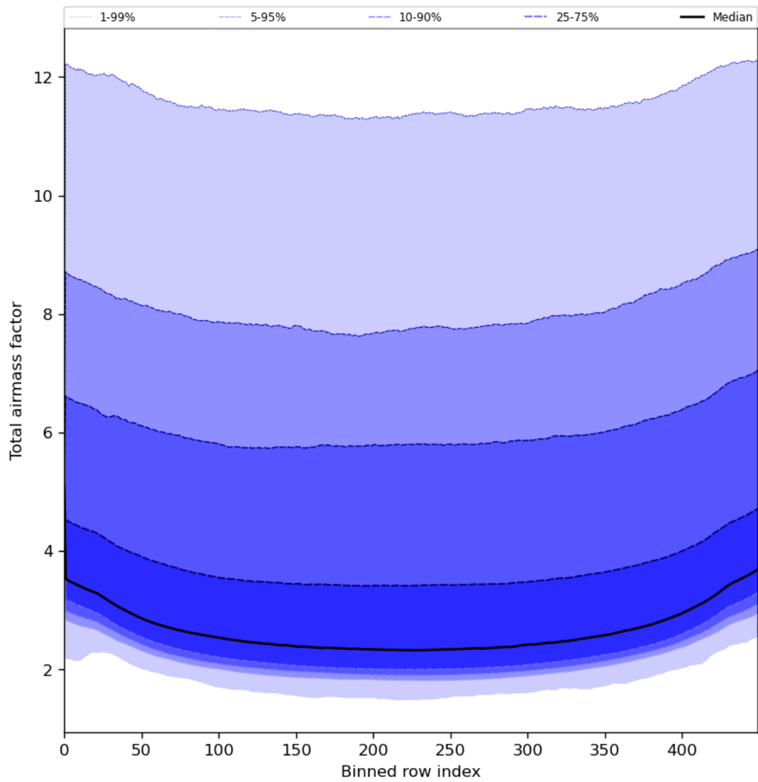
Figure 49: Along track statistics of “Total airmass factor” for 2024-06-13 to 2024-06-14
