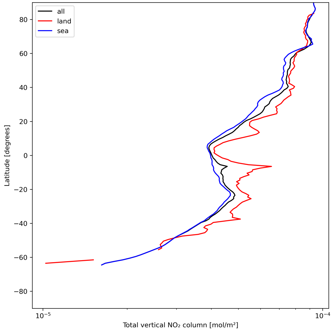
Figure 21: Zonal average of “Total vertical NO 2 column” for 2024-06-13 to 2024-06-14.
