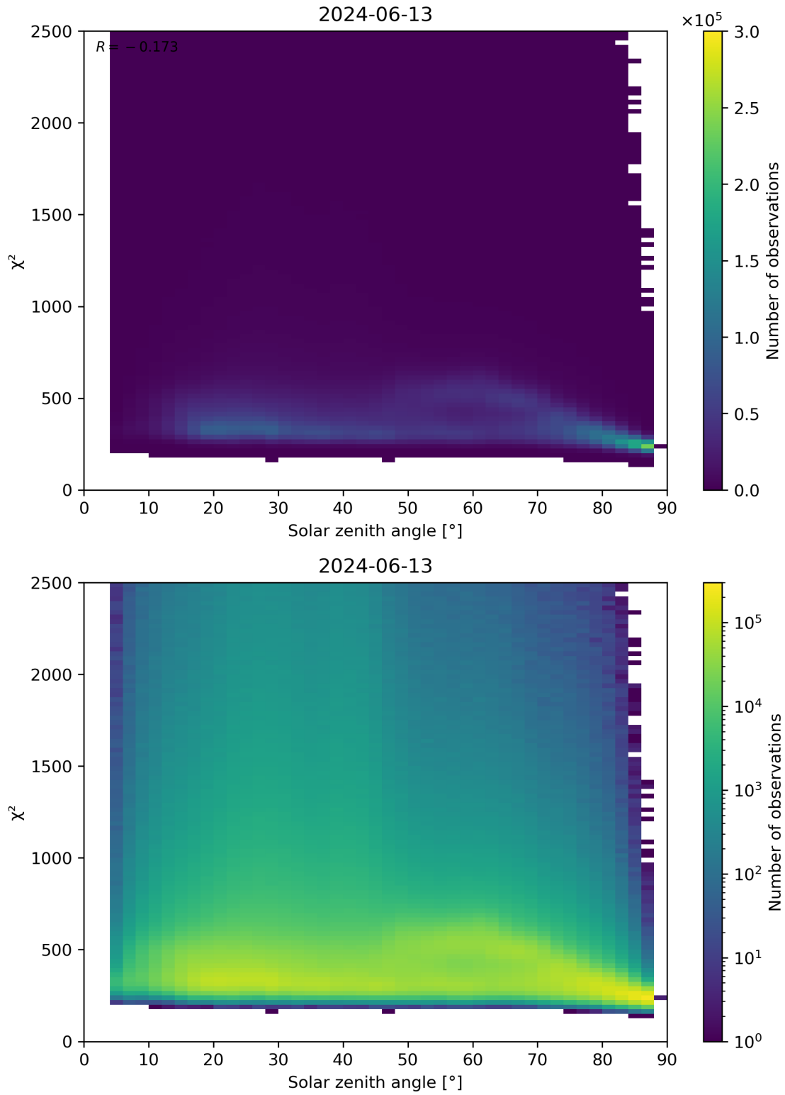
Figure 148: Scatter density plot of “Solar zenith angle” against “ \chi^2 ” for 2024-06-13 to 2024-06-14.
