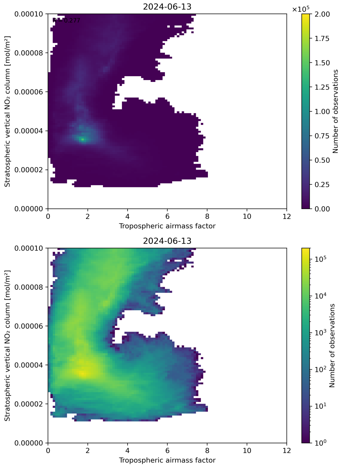
Figure 74: Scatter density plot of “Tropospheric air mass factor” against “Stratospheric vertical NO 2 column” for 2024-06-13 to 2024-06-14.
