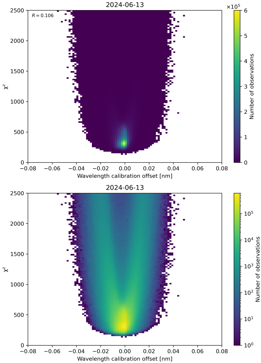
Figure 175: Scatter density plot of “Wavelength calibration offset” against “ \chi^2 ” for 2024-06-13 to 2024-06-14.
