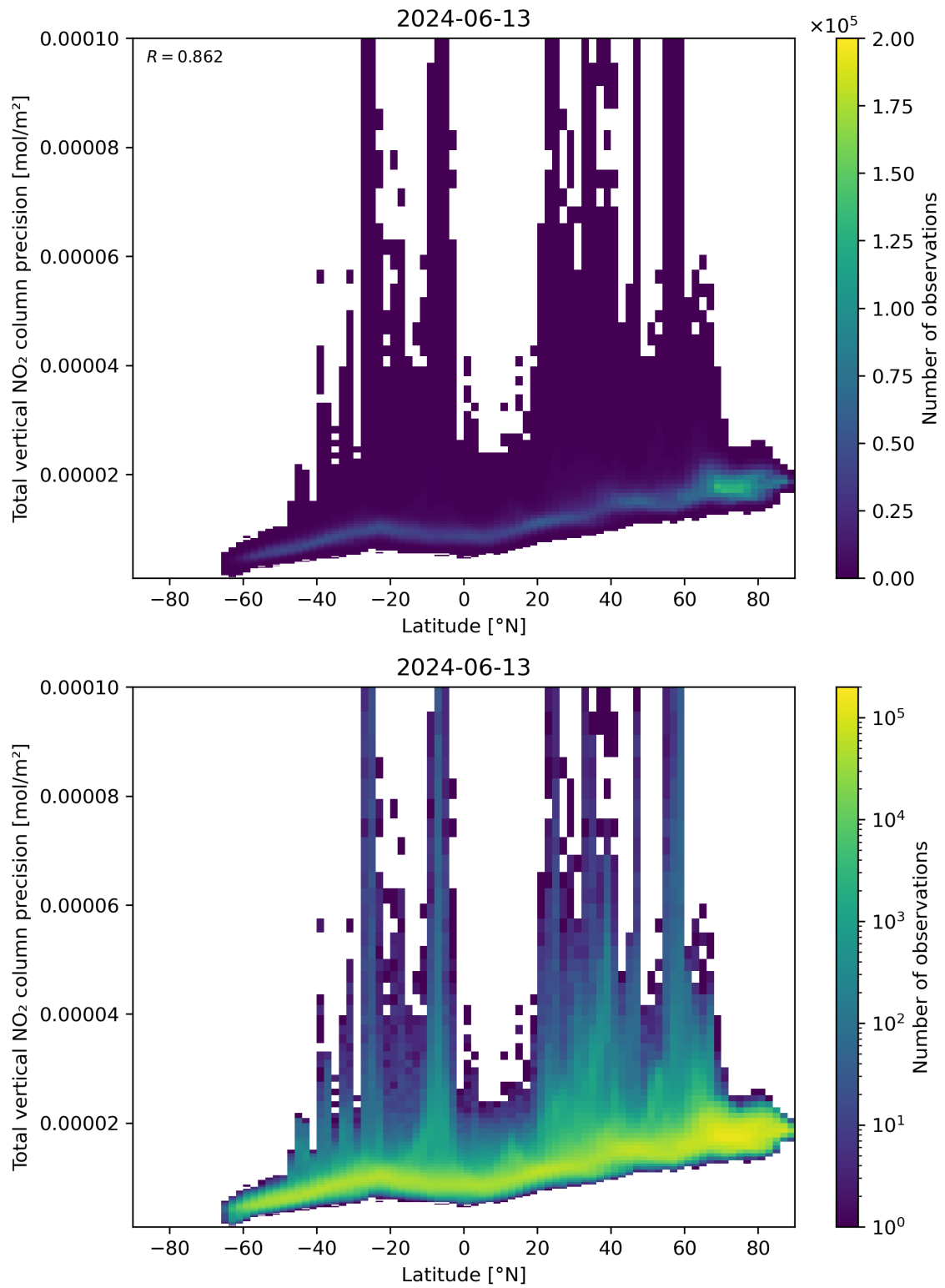
Figure 91: Scatter density plot of “Latitude” against “Total vertical NO 2 column precision” for 2024-06-13 to 2024-06-14.
