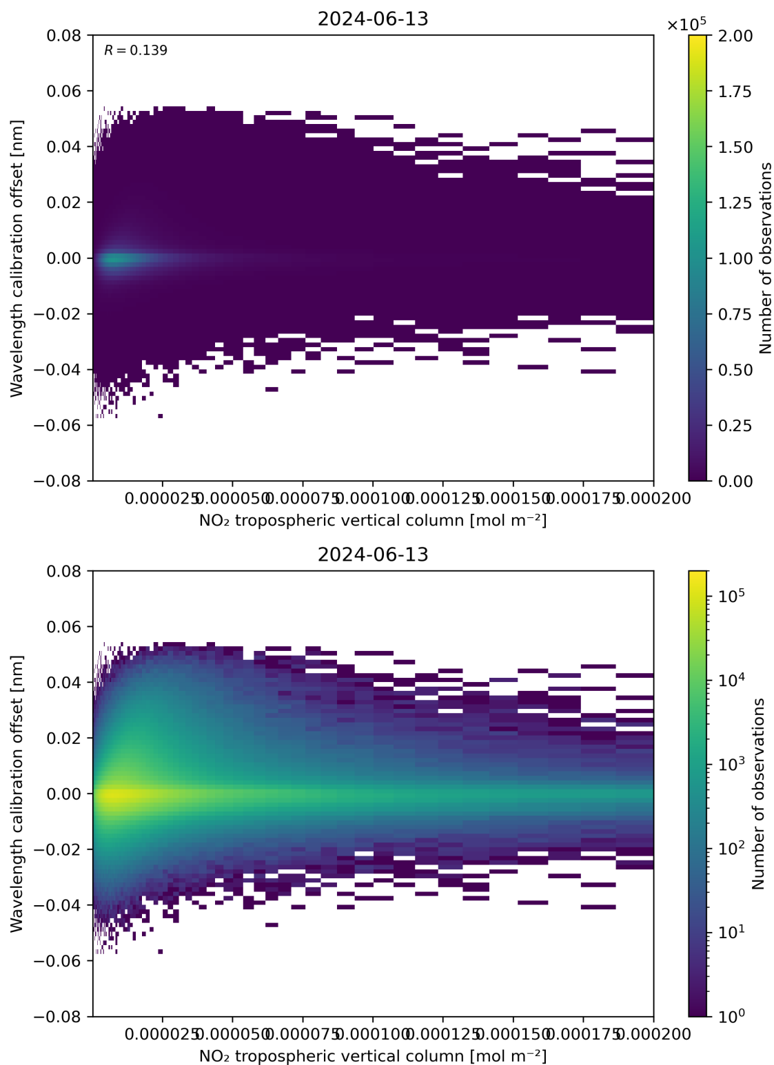
Figure 143: Scatter density plot of “NO 2 tropospheric vertical column” against “Wavelength calibration offset” for 2024-06-13 to 2024-06-14.
