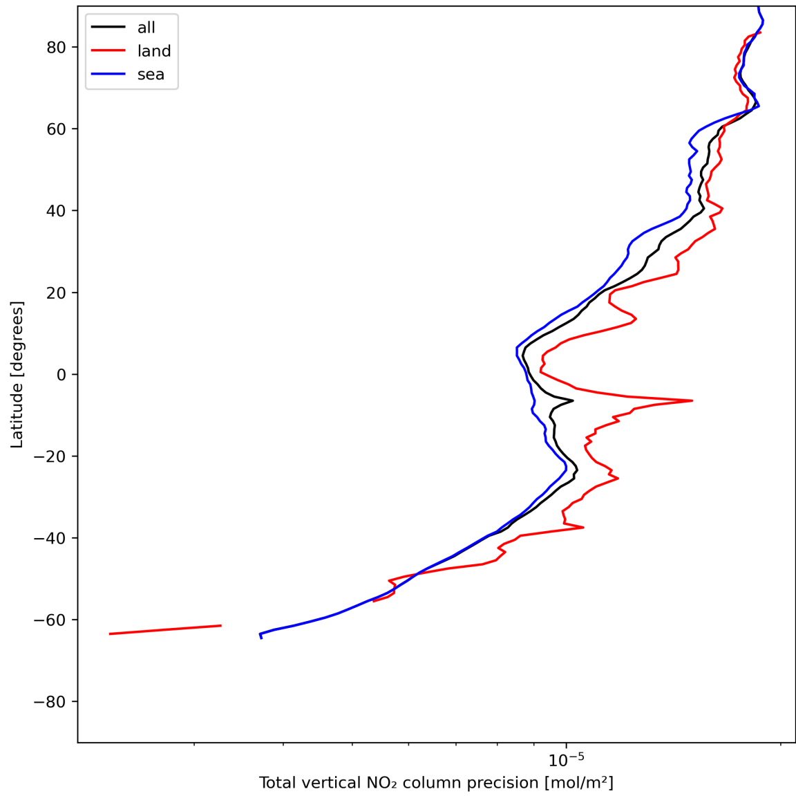
Figure 22: Zonal average of “Total vertical NO 2 column precision” for 2024-06-13 to 2024-06-14.
