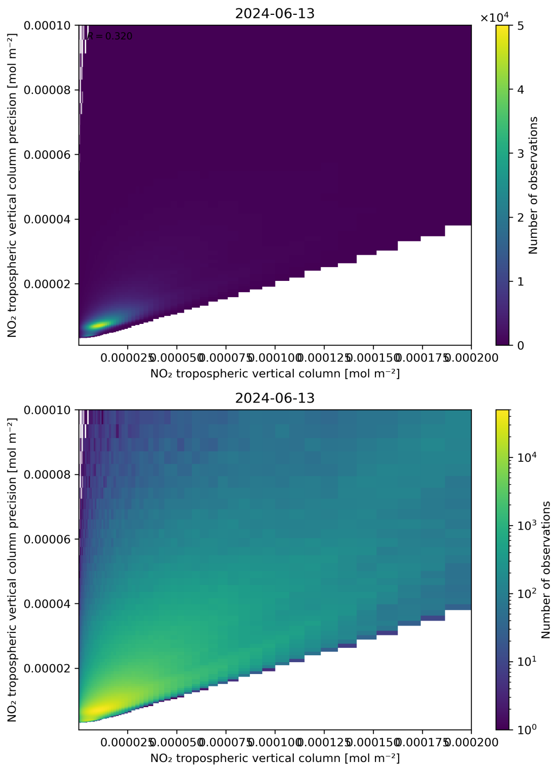
Figure 130: Scatter density plot of “NO 2 tropospheric vertical column” against “NO 2 tropospheric vertical column precision” for 2024-06-13 to 2024-06-14.
