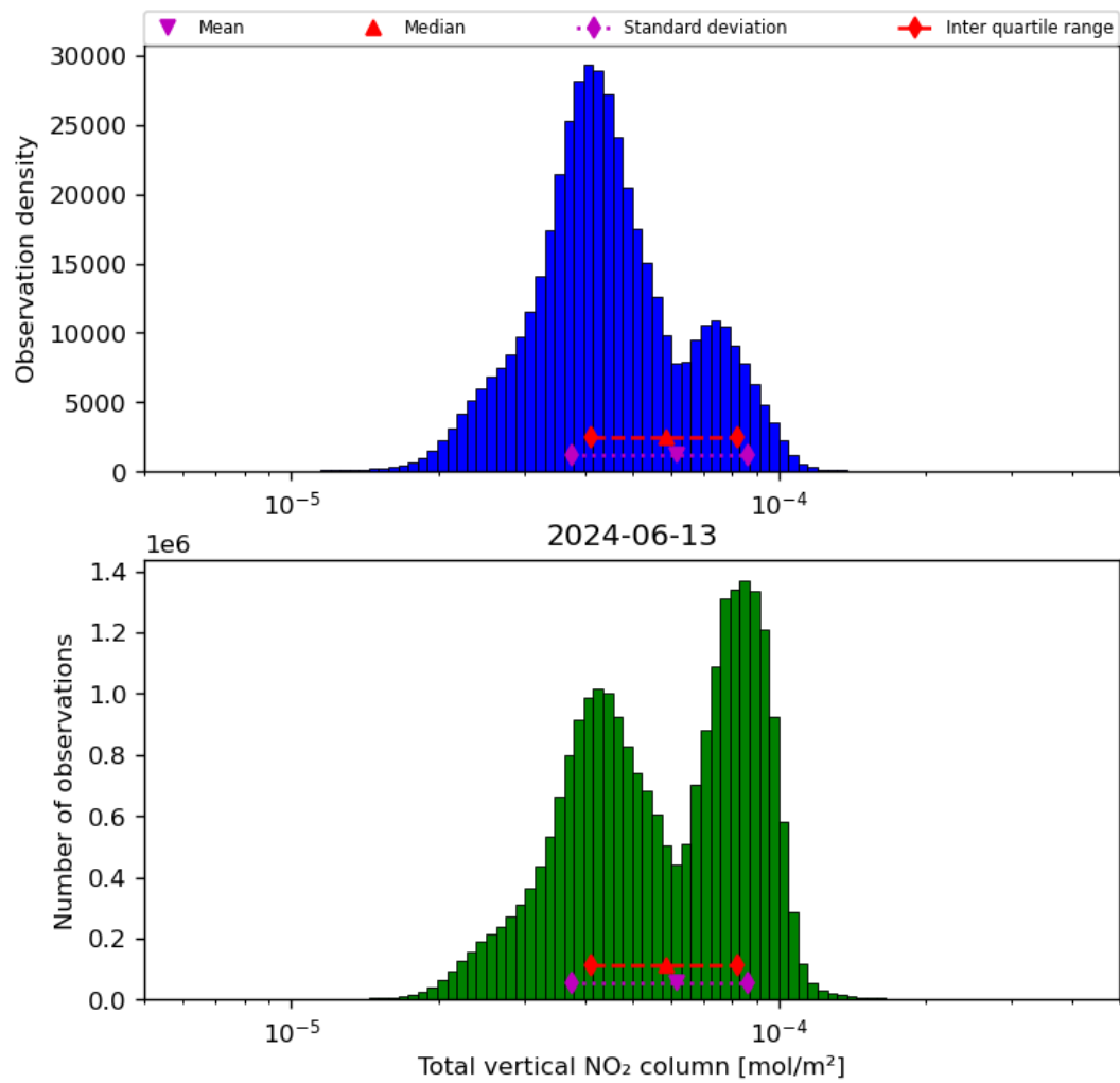
Figure 38: Histogram of “Total vertical NO 2 column” for 2024-06-13 to 2024-06-14
