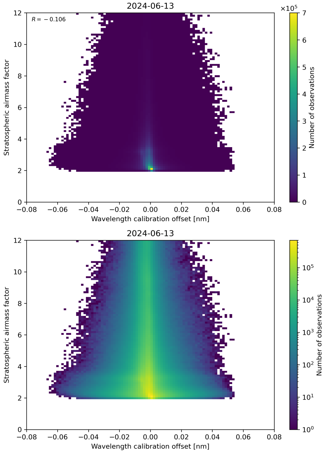
Figure 174: Scatter density plot of “Wavelength calibration offset” against “Stratospheric air mass factor” for 2024-06-13 to 2024-06-14.
