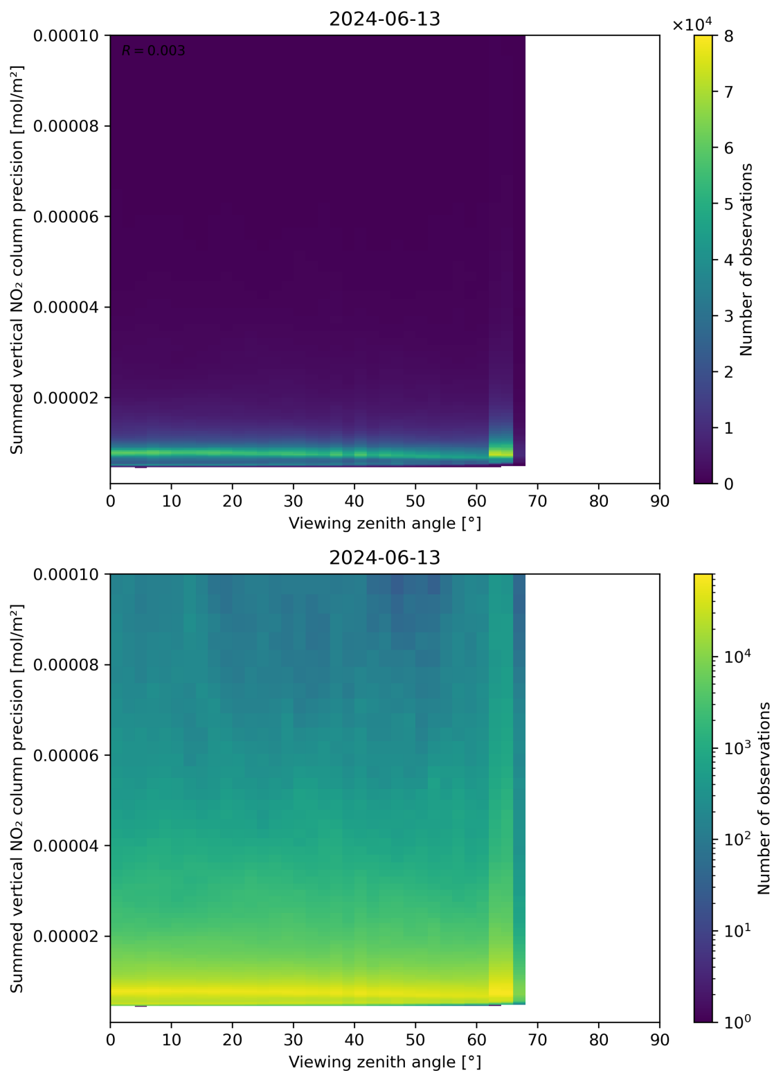
Figure 166: Scatter density plot of “Viewing zenith angle” against “Summed vertical NO 2 column precision” for 2024-06-13 to 2024-06-14.
