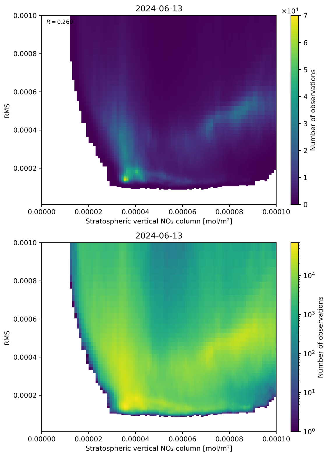
Figure 102: Scatter density plot of “Stratospheric vertical NO 2 column” against “RMS” for 2024-06-13 to 2024-06-14.
