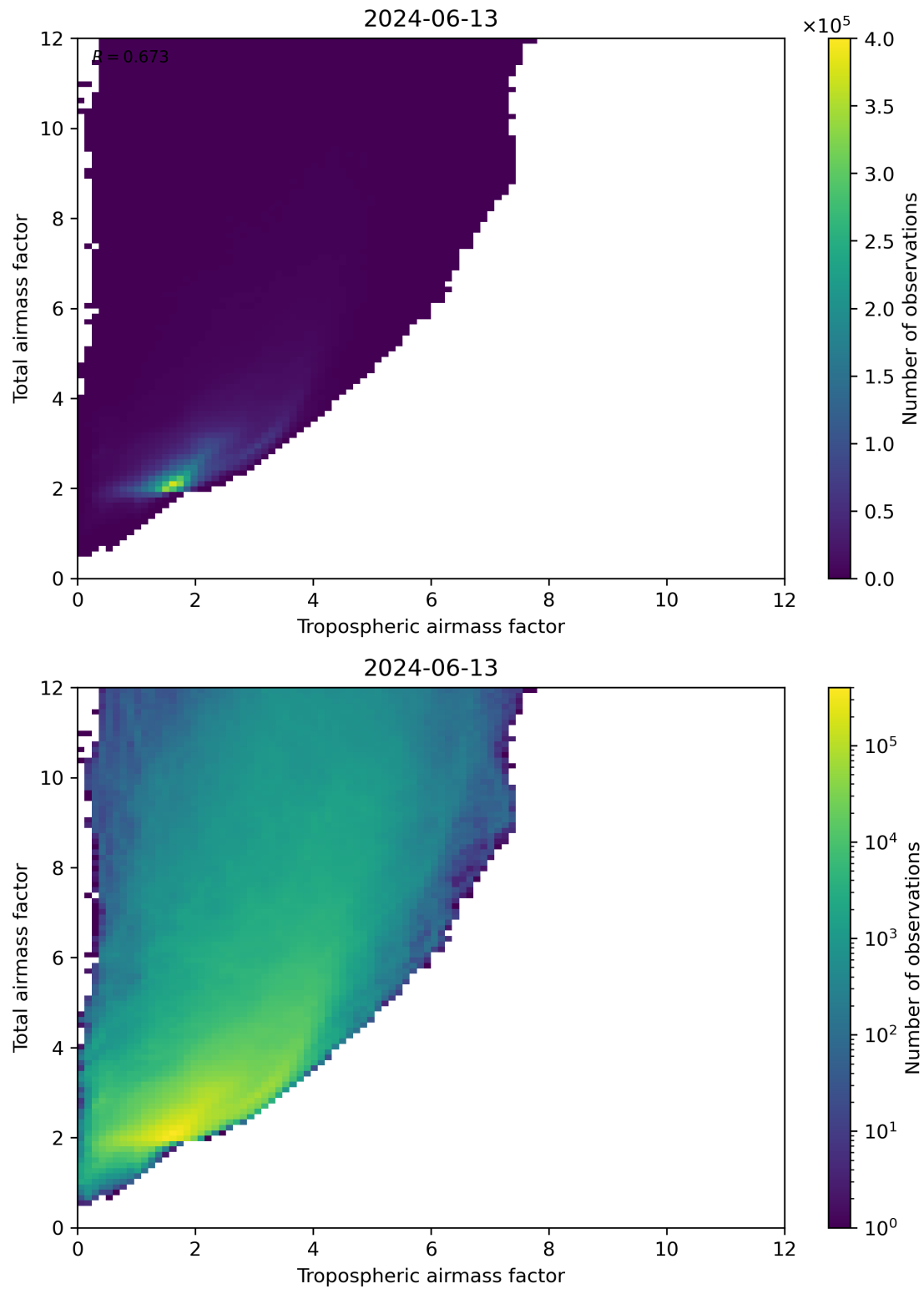
Figure 72: Scatter density plot of “Tropospheric airmass factor” against “Total airmass factor” for 2024-06-13 to 2024-06-14.
