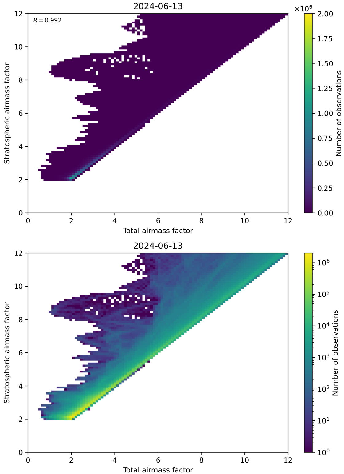
Figure 62: Scatter density plot of “Total airmass factor” against “Stratospheric airmass factor” for 2024-06-13 to 2024-06-14.
