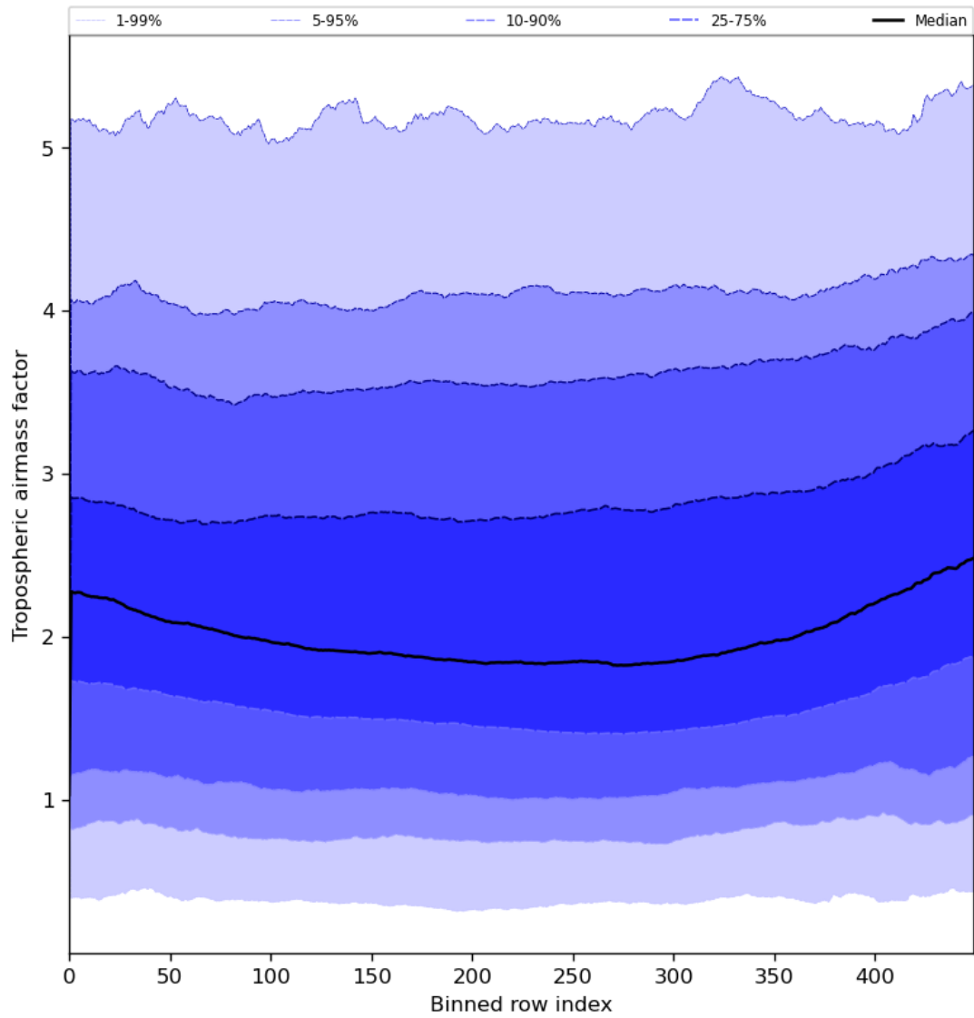
Figure 48: Along track statistics of “Tropospheric airmass factor” for 2024-06-13 to 2024-06-14
