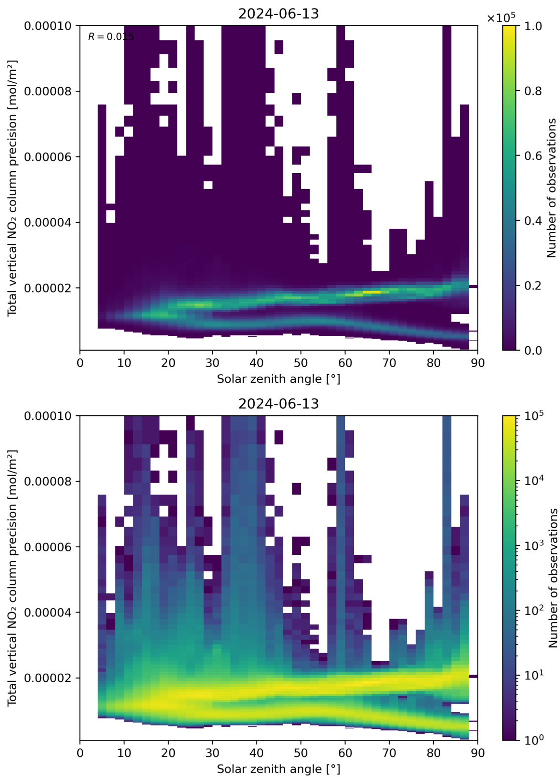
Figure 154: Scatter density plot of “Solar zenith angle” against “Total vertical NO 2 column precision” for 2024-06-13 to 2024-06-14.
