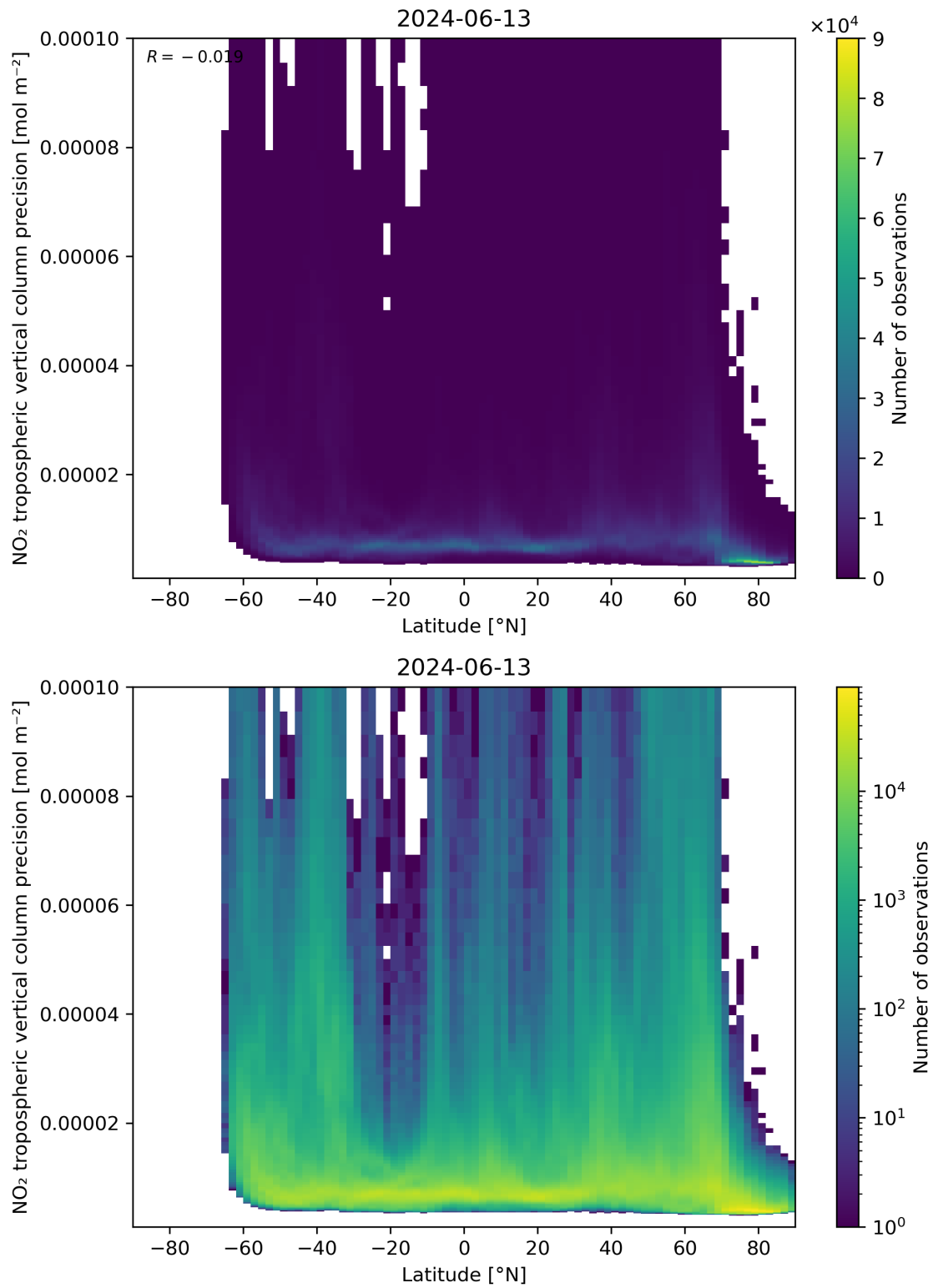
Figure 93: Scatter density plot of “Latitude” against “NO 2 tropospheric vertical column precision” for 2024-06-13 to 2024-06-14.
