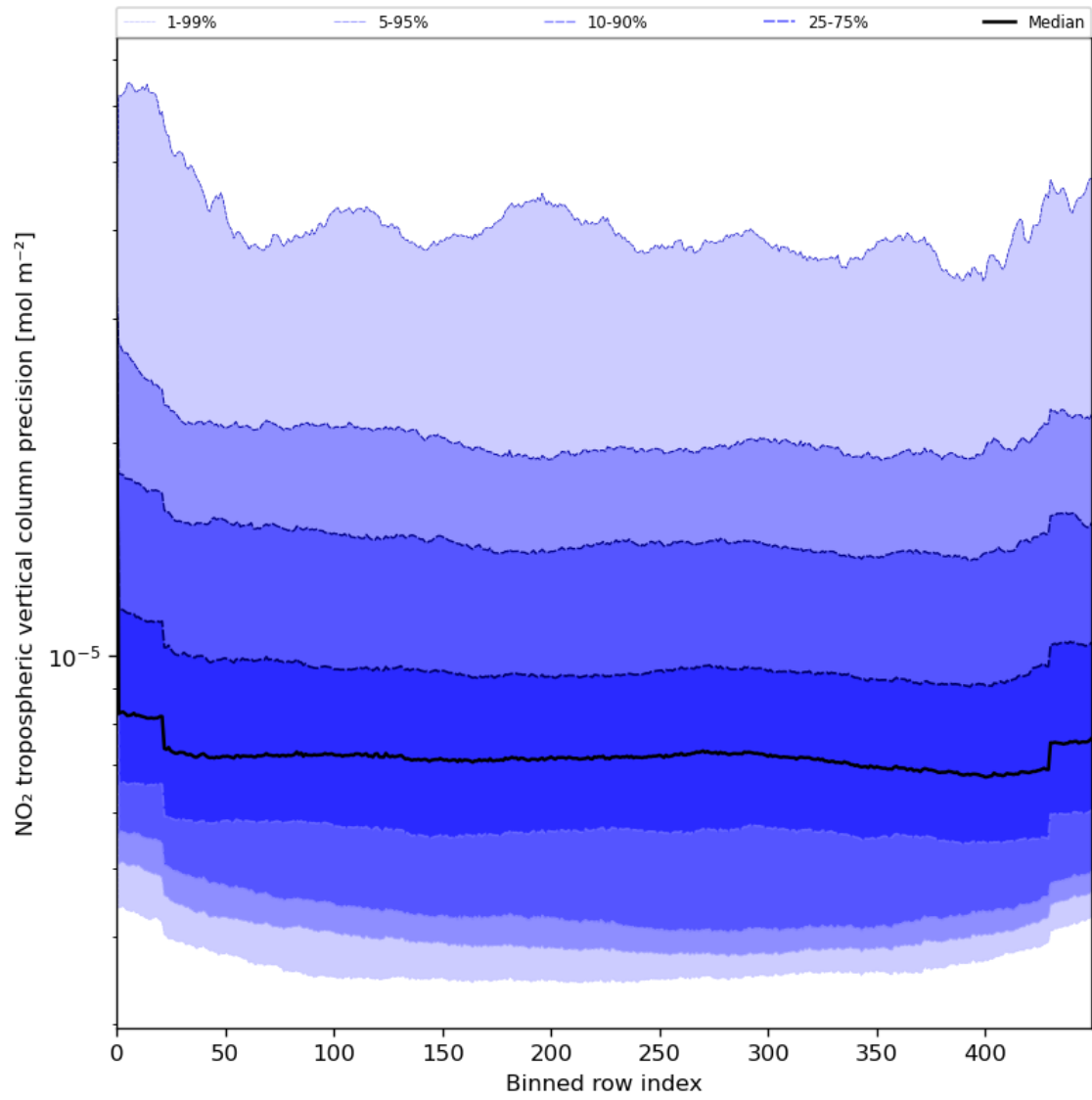
Figure 47: Along track statistics of “NO 2 tropospheric vertical column precision” for 2024-06-13 to 2024-06-14
