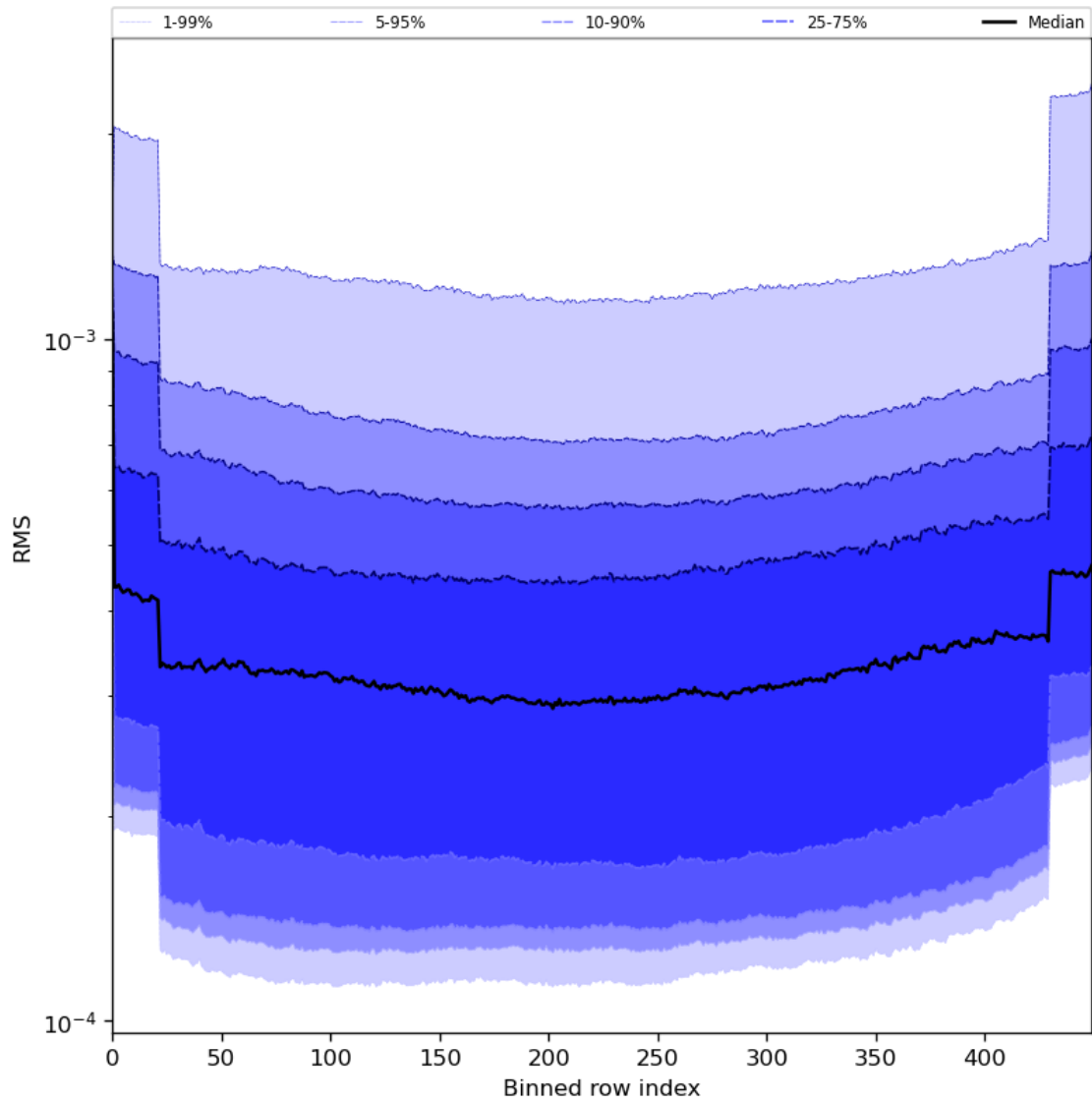
Figure 60: Along track statistics of “RMS” for 2024-06-13 to 2024-06-14
