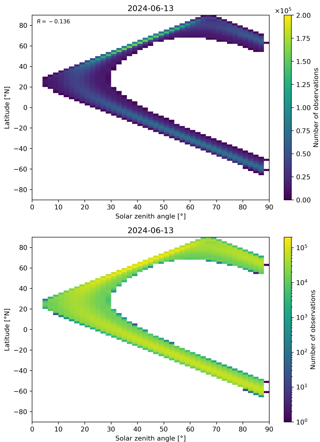
Figure 149: Scatter density plot of “Solar zenith angle” against “Latitude” for 2024-06-13 to 2024-06-14.
