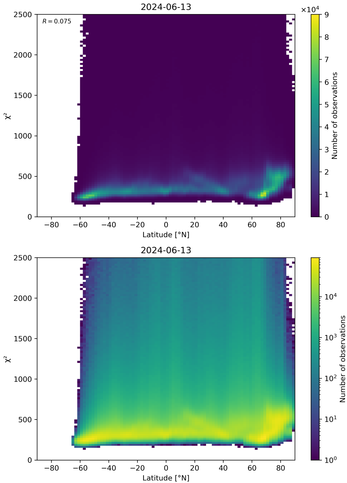
Figure 86: Scatter density plot of “Latitude” against “ \chi^2 ” for 2024-06-13 to 2024-06-14.
