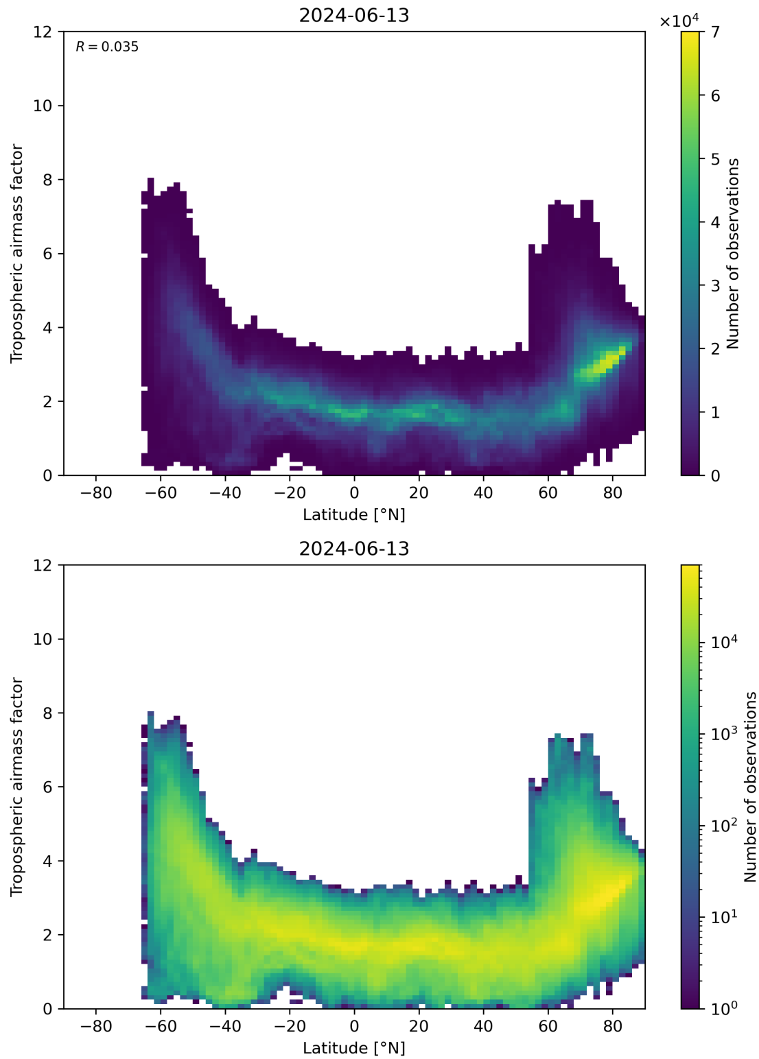
Figure 85: Scatter density plot of “Latitude” against “Tropospheric airmass factor” for 2024-06-13 to 2024-06-14.
