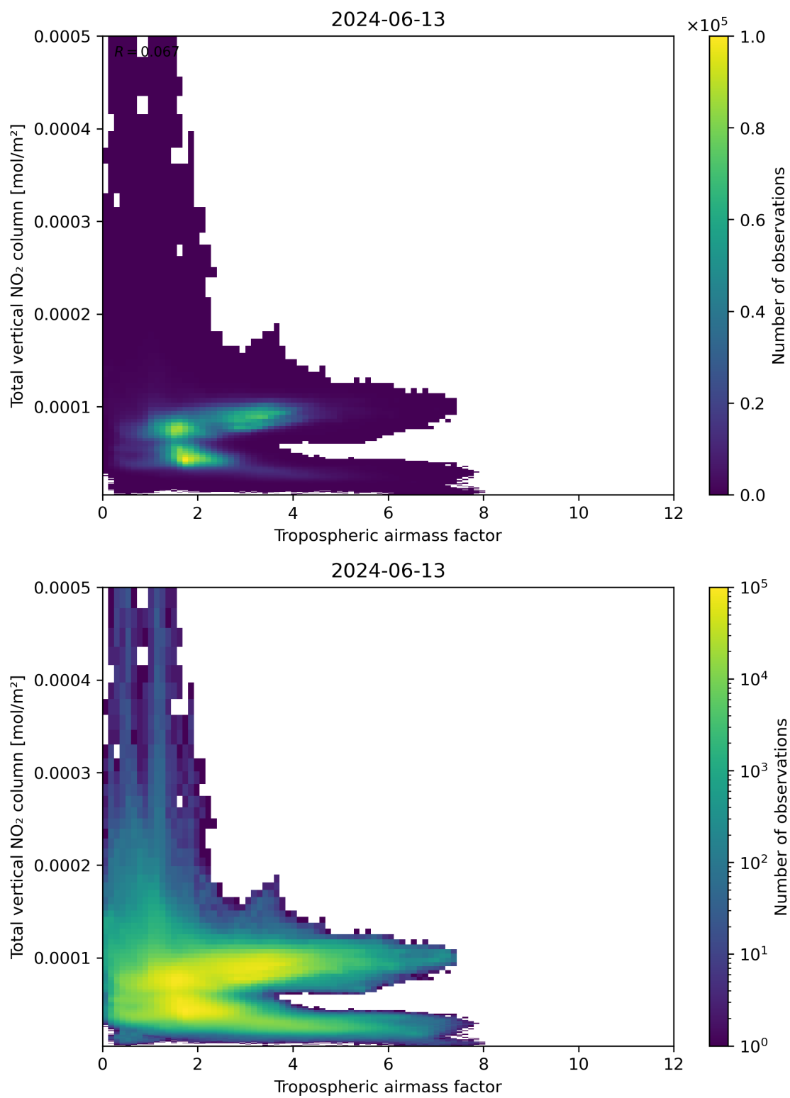
Figure 77: Scatter density plot of “Tropospheric airmass factor” against “Total vertical NO 2 column” for 2024-06-13 to 2024-06-14.
