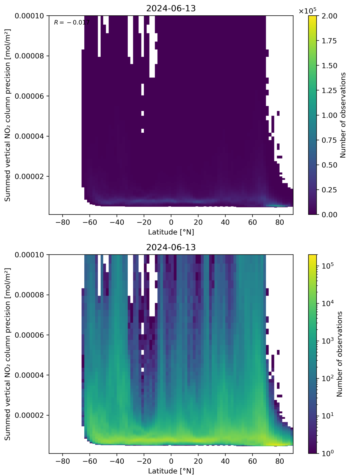
Figure 89: Scatter density plot of “Latitude” against “Summed vertical NO 2 column precision” for 2024-06-13 to 2024-06-14.
