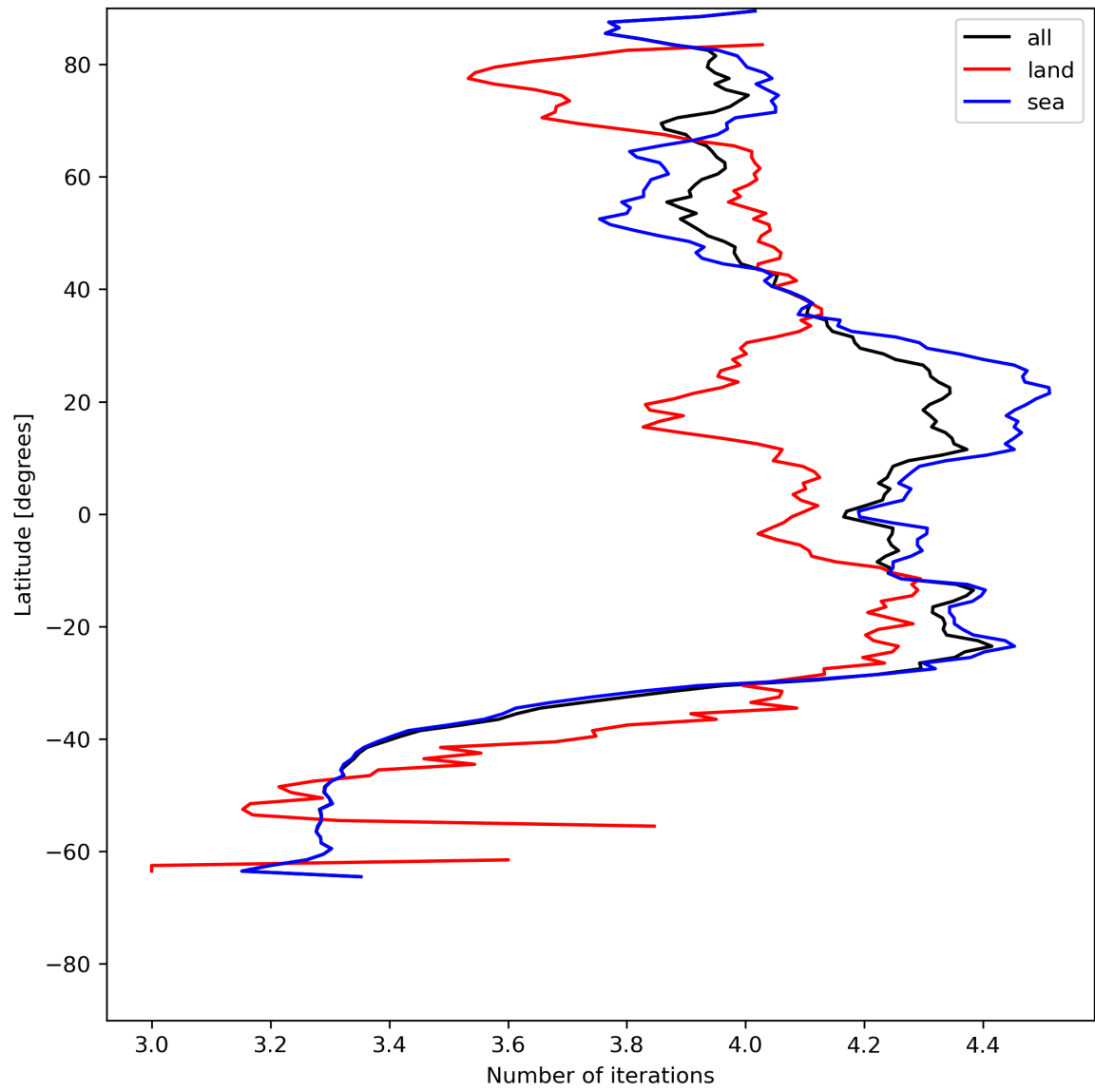
Figure 17: Zonal average of “Number of iterations” for 2024-06-13 to 2024-06-14.
