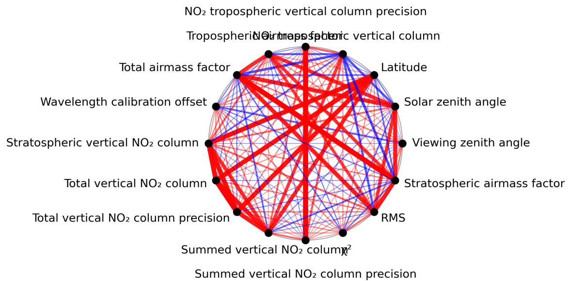
Figure 1: Map of correlation graph for 2024-06-13 to 2024-06-14.
