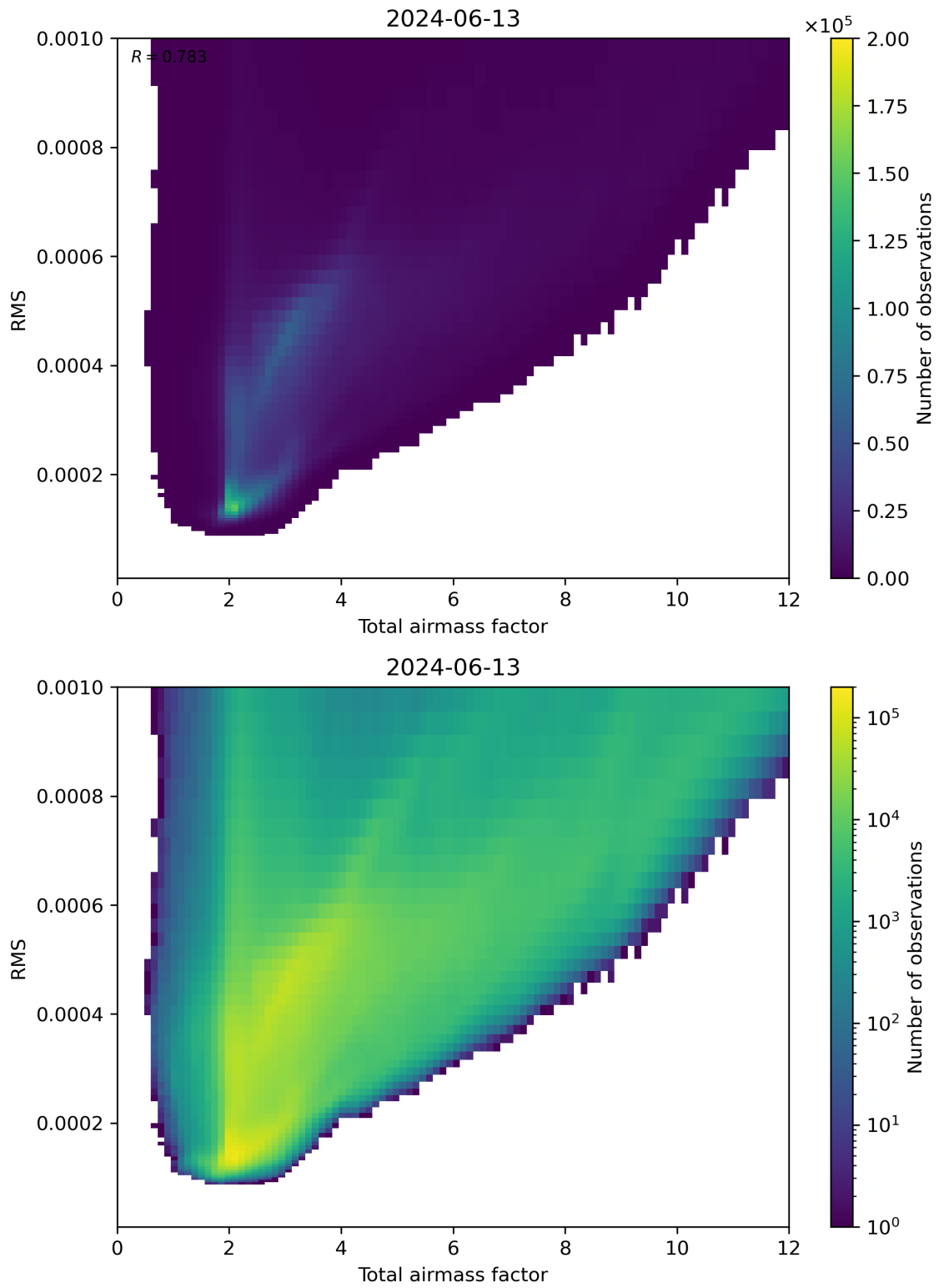
Figure 69: Scatter density plot of “Total airmass factor” against “RMS” for 2024-06-13 to 2024-06-14.
