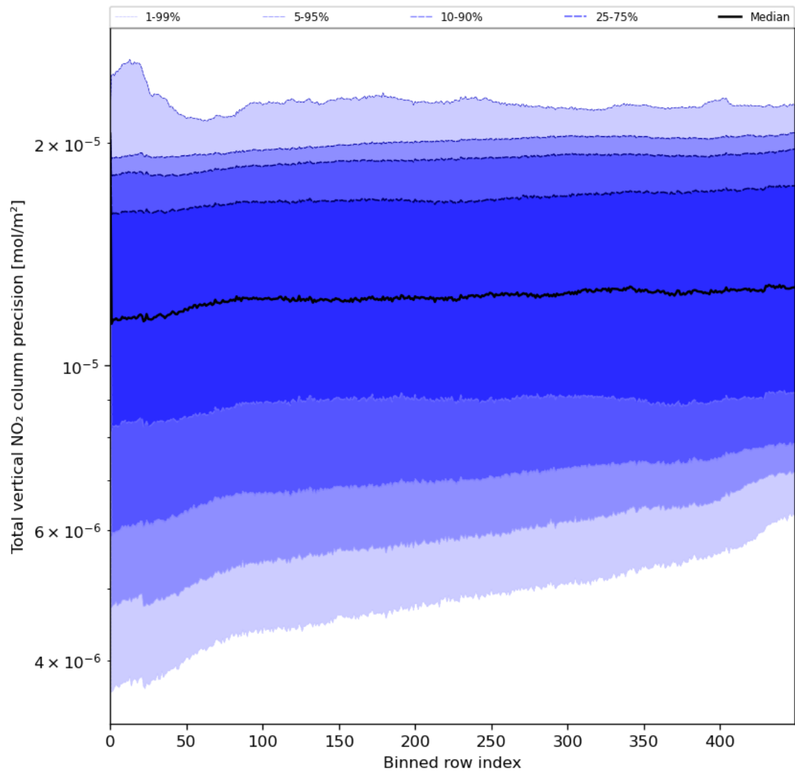
Figure 56: Along track statistics of “Total vertical NO 2 column precision” for 2024-06-13 to 2024-06-14
