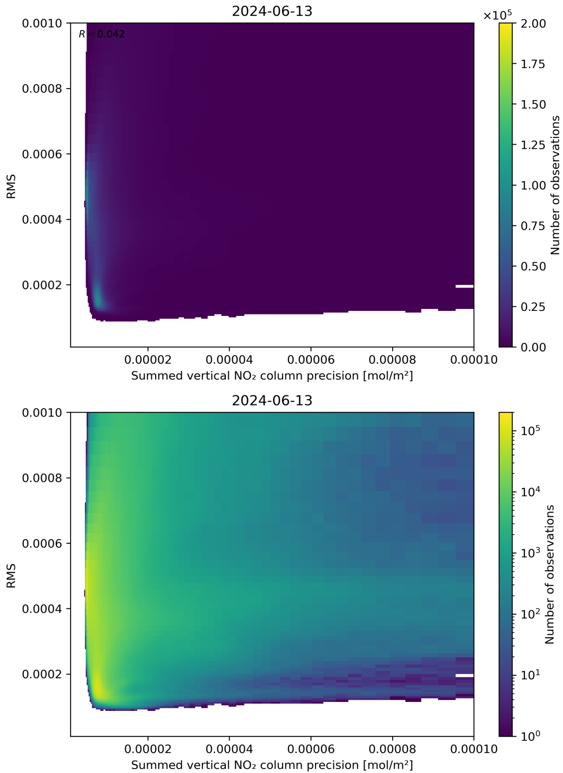
Figure 108: Scatter density plot of “Summed vertical NO 2 column precision” against “RMS” for 2024-06-13 to 2024-06-14.
