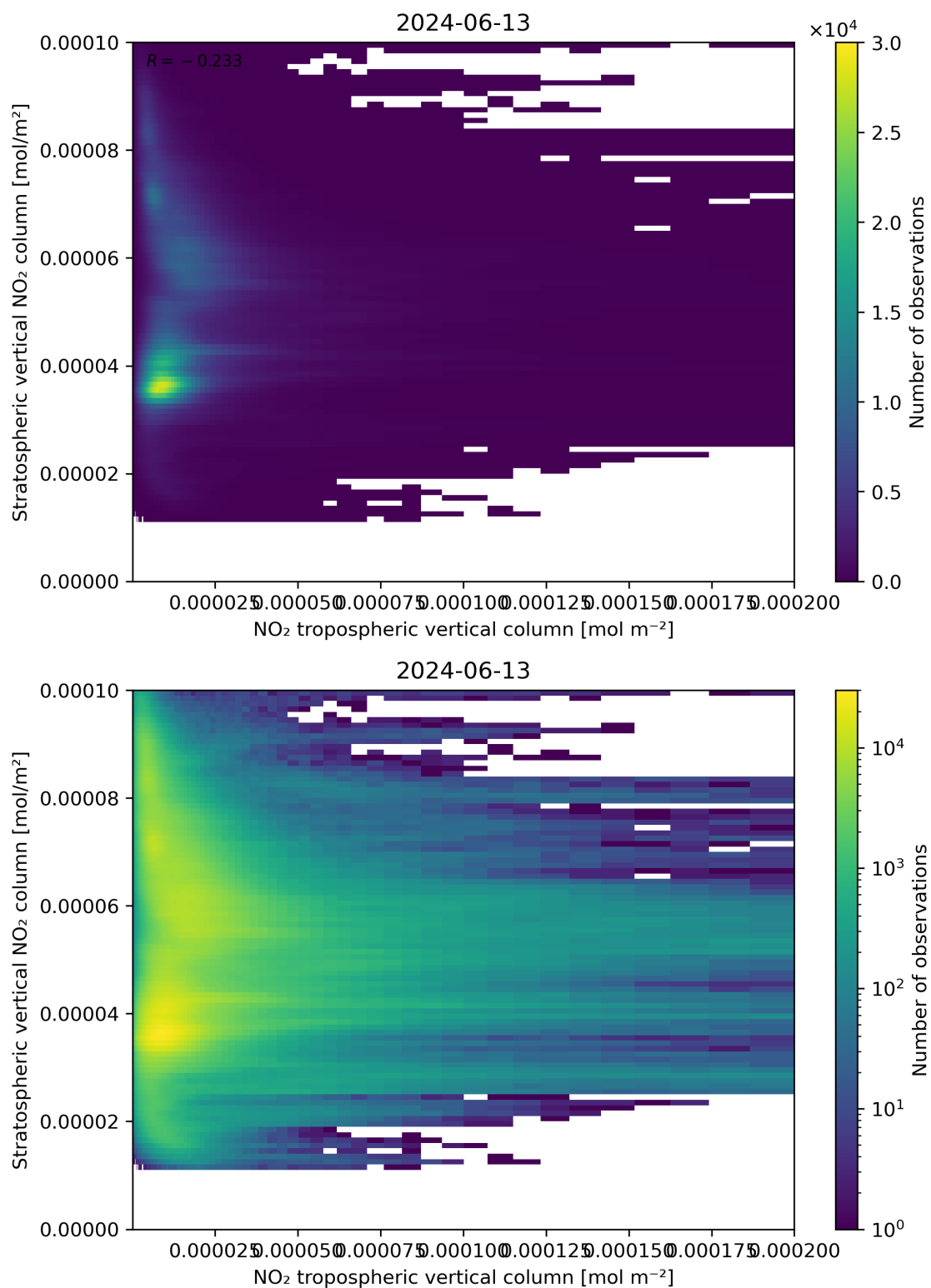
Figure 125: Scatter density plot of “NO 2 tropospheric vertical column” against “Stratospheric vertical NO 2 column” for 2024-06-13 to 2024-06-14.
