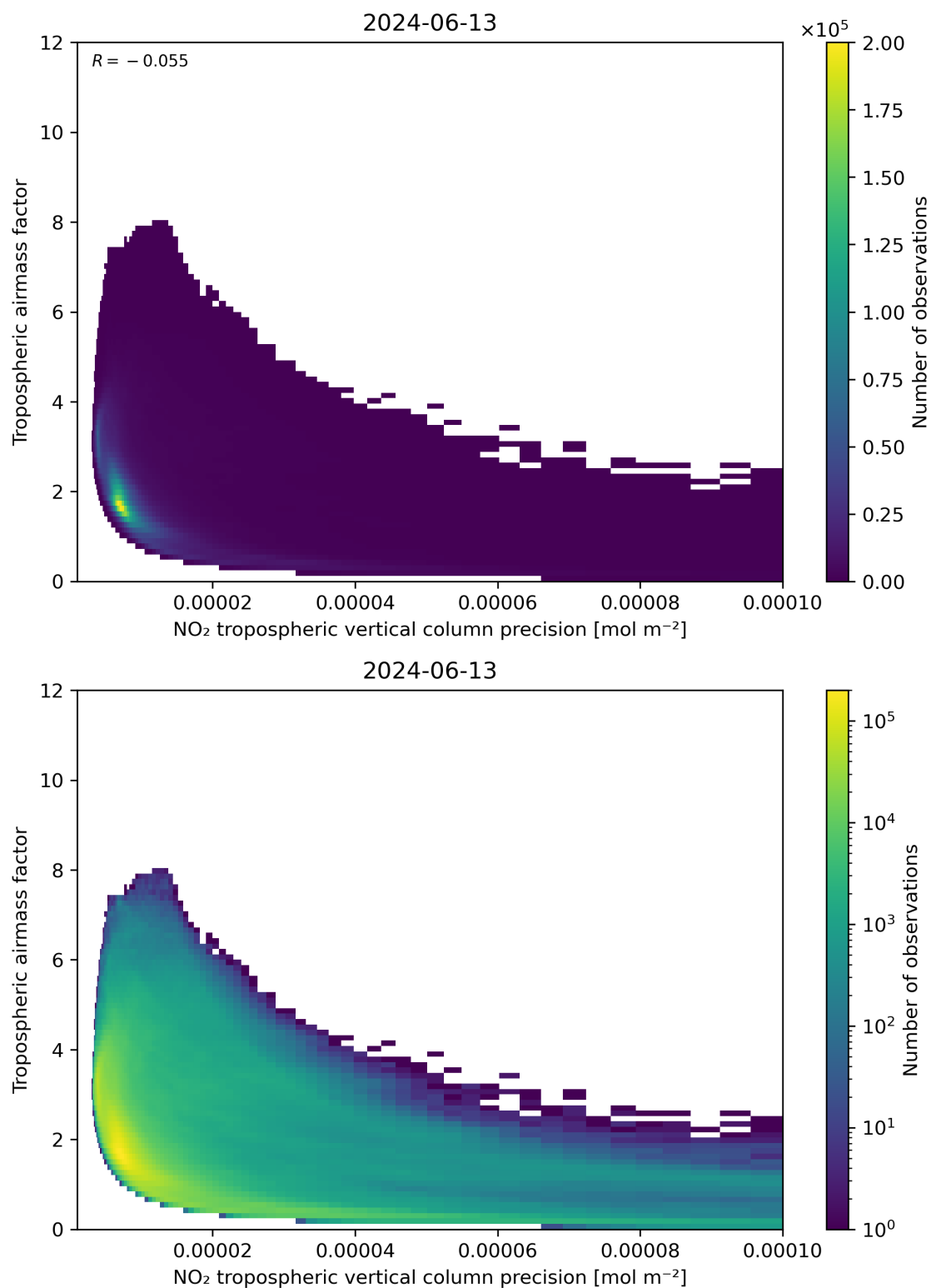
Figure 133: Scatter density plot of “NO 2 tropospheric vertical column precision” against “Tropospheric airmass factor” for 2024-06-13 to 2024-06-14.
