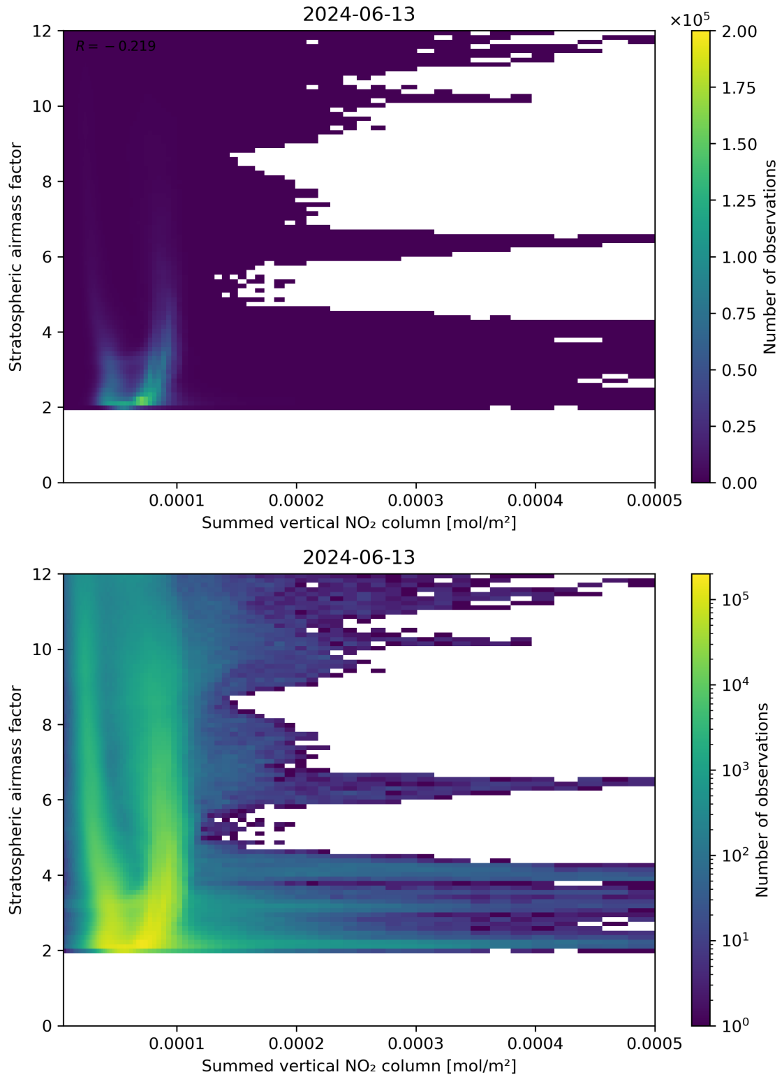
Figure 103: Scatter density plot of “Summed vertical NO 2 column” against “Stratospheric air mass factor” for 2024-06-13 to 2024-06-14.
