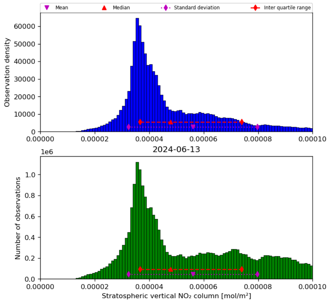
Figure 36: Histogram of “Stratospheric vertical NO 2 column” for 2024-06-13 to 2024-06-14
