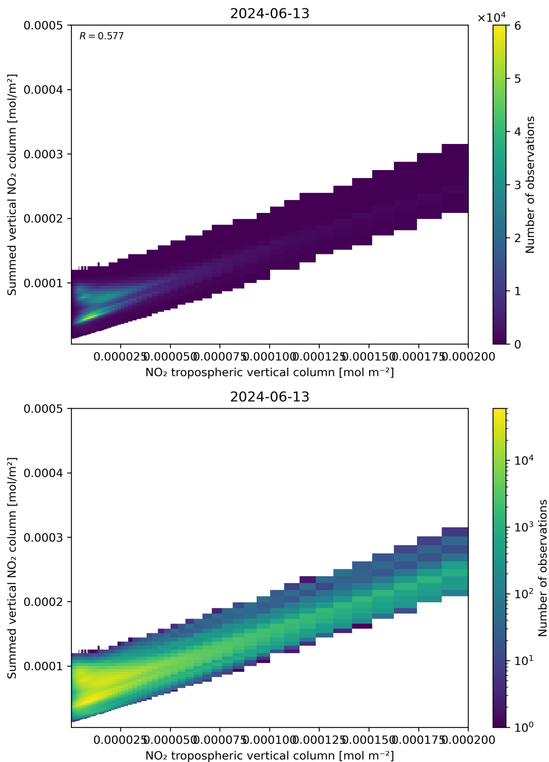
Figure 126: Scatter density plot of “NO 2 tropospheric vertical column” against “Summed vertical NO 2 column” for 2024-06-13 to 2024-06-14.
