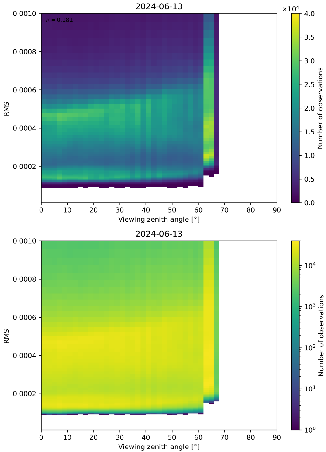
Figure 171: Scatter density plot of “Viewing zenith angle” against “RMS” for 2024-06-13 to 2024-06-14.
