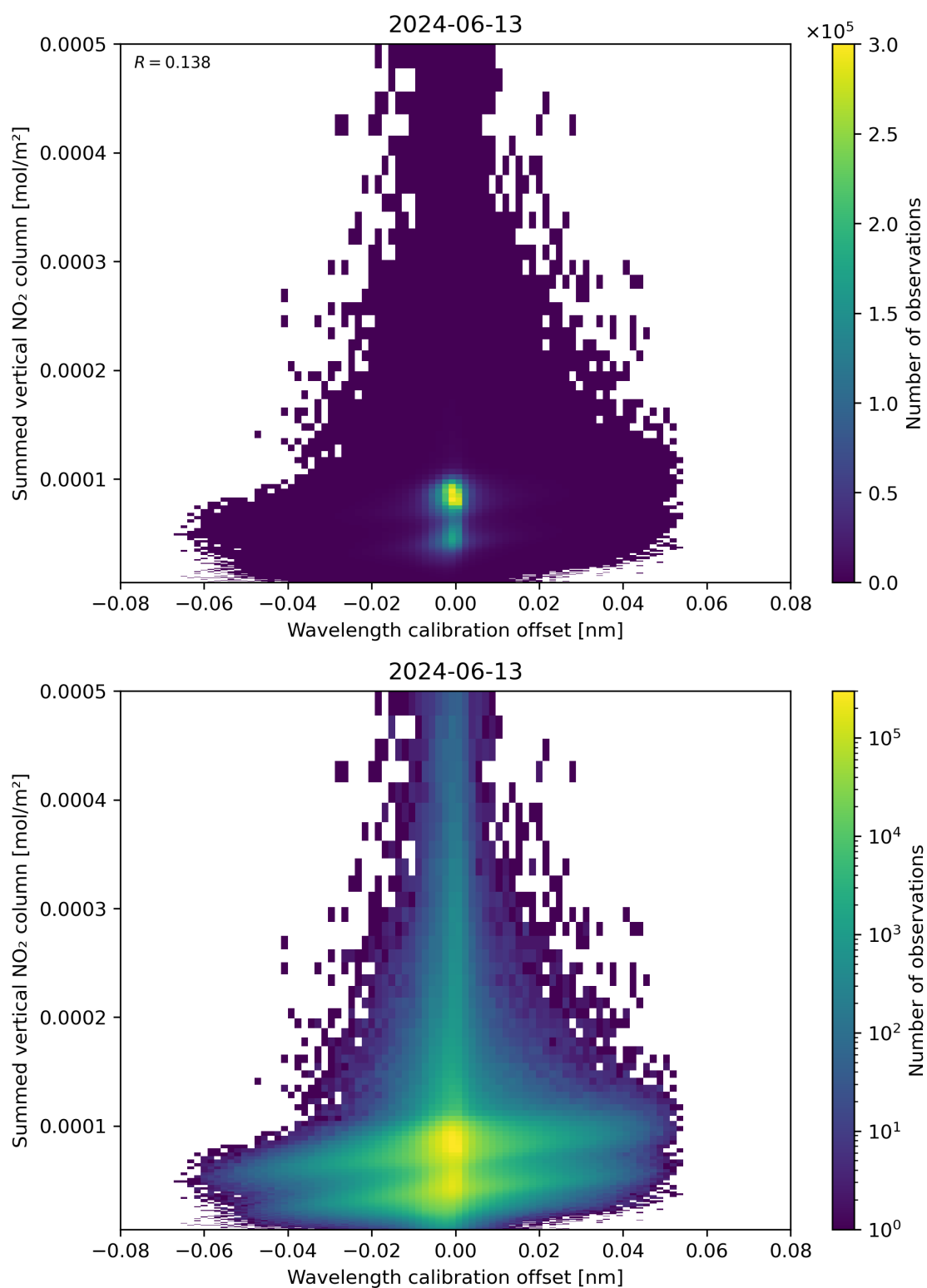
Figure 177: Scatter density plot of “Wavelength calibration offset” against “Summed vertical NO 2 column” for 2024-06-13 to 2024-06-14.
