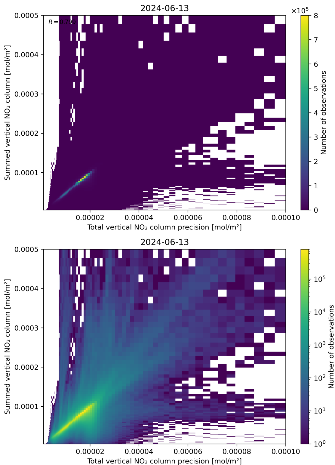
Figure 117: Scatter density plot of “Total vertical NO 2 column precision” against “Summed vertical NO 2 column” for 2024-06-13 to 2024-06-14.
