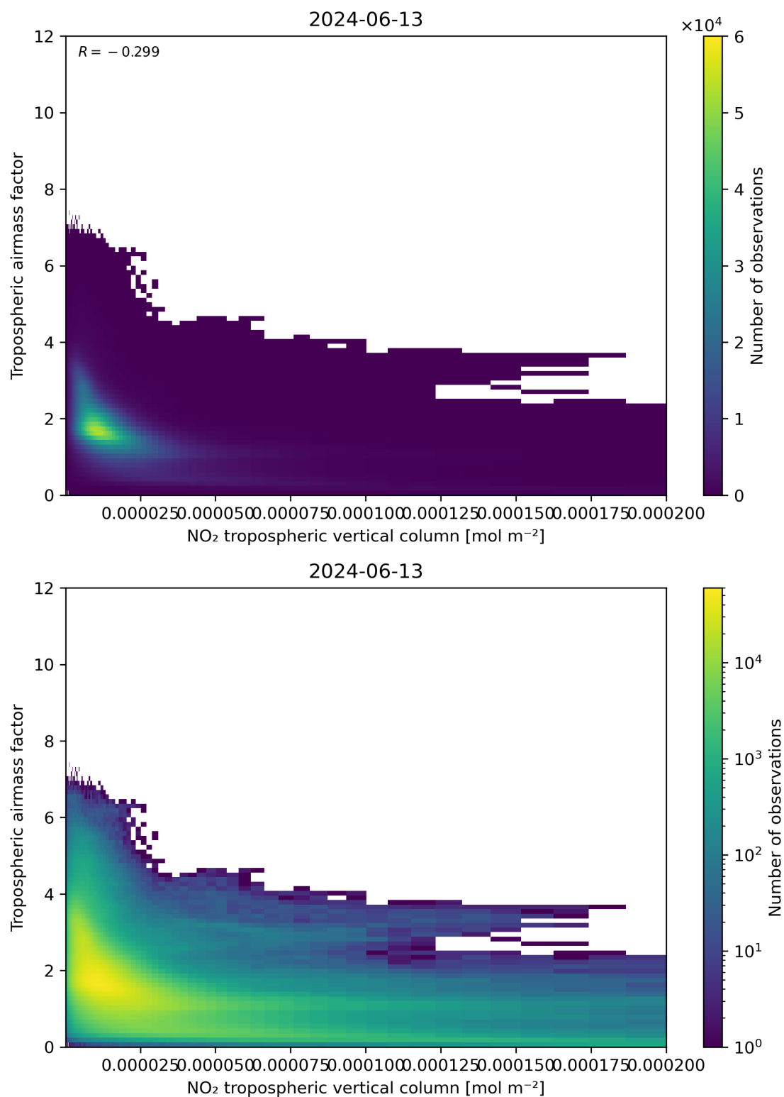
Figure 123: Scatter density plot of “NO 2 tropospheric vertical column” against “Tropospheric air mass factor” for 2024-06-13 to 2024-06-14.
