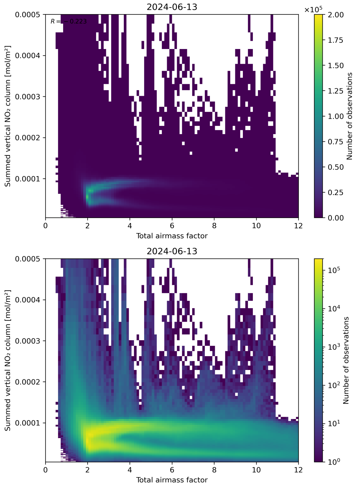
Figure 65: Scatter density plot of “Total airmass factor” against “Summed vertical NO 2 column” for 2024-06-13 to 2024-06-14.
