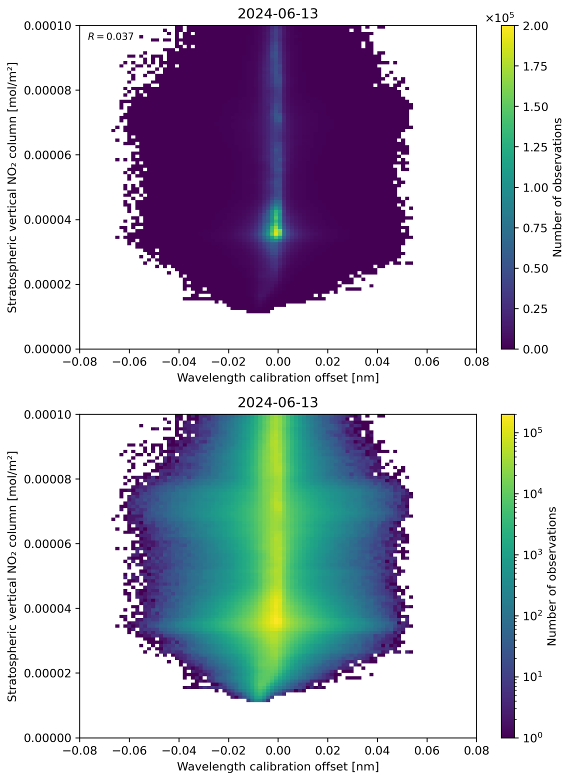
Figure 176: Scatter density plot of “Wavelength calibration offset” against “Stratospheric vertical NO 2 column” for 2024-06-13 to 2024-06-14.
