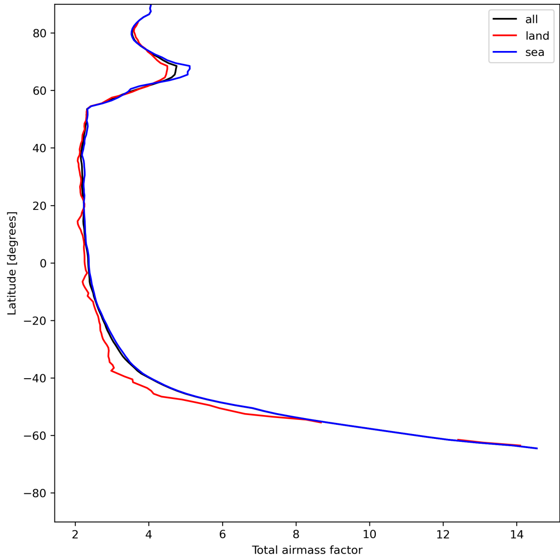
Figure 15: Zonal average of “Total airmass factor” for 2024-06-13 to 2024-06-14.
