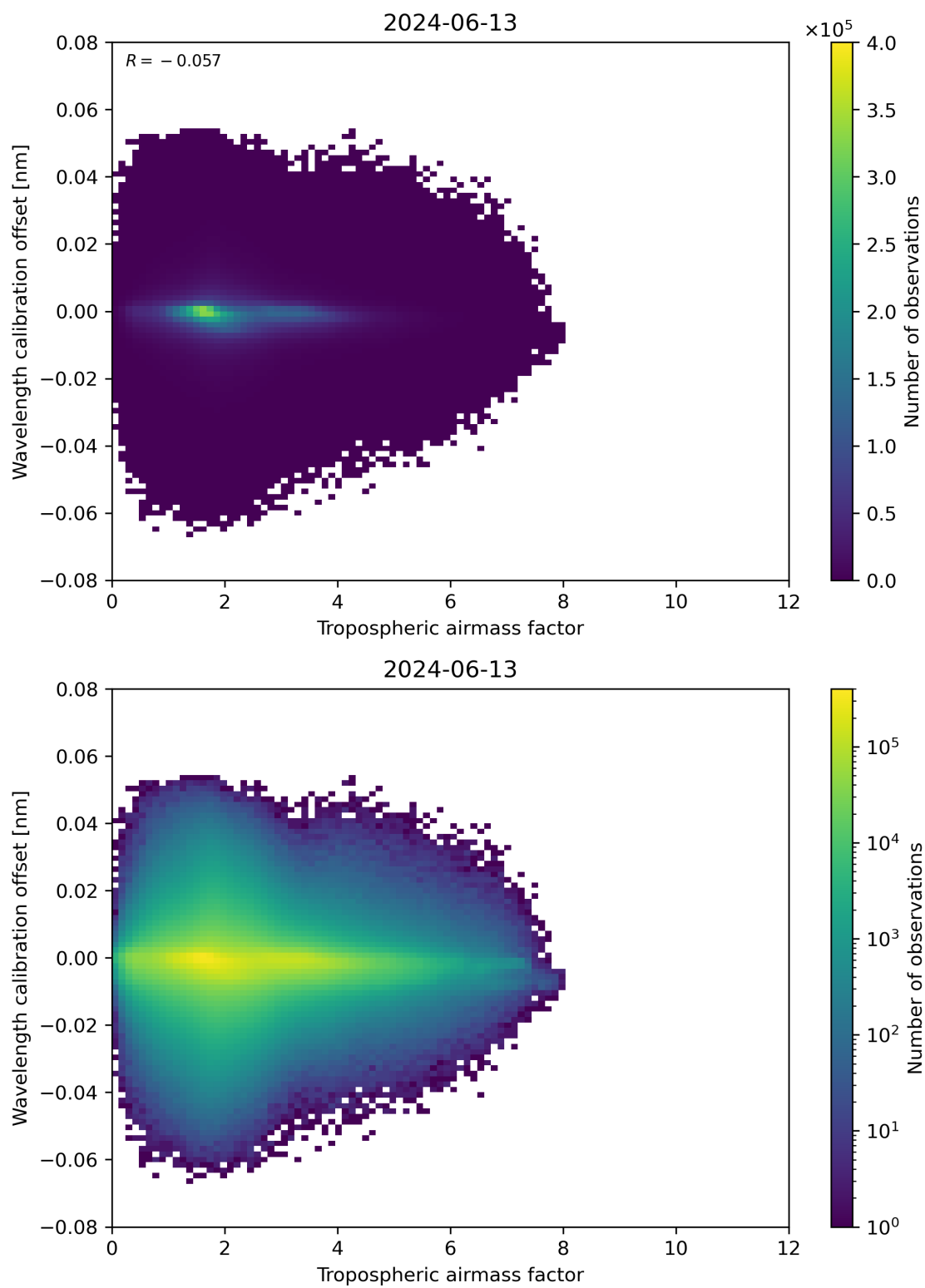
Figure 80: Scatter density plot of “Tropospheric air mass factor” against “Wavelength calibration offset” for 2024-06-13 to 2024-06-14.
