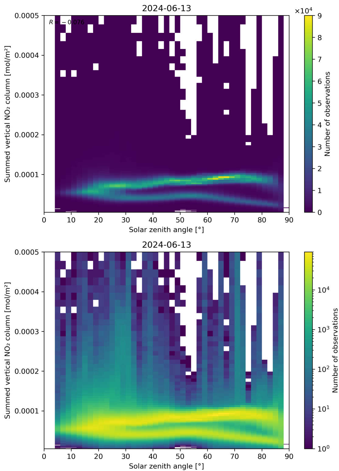
Figure 151: Scatter density plot of “Solar zenith angle” against “Summed vertical NO 2 column” for 2024-06-13 to 2024-06-14.
