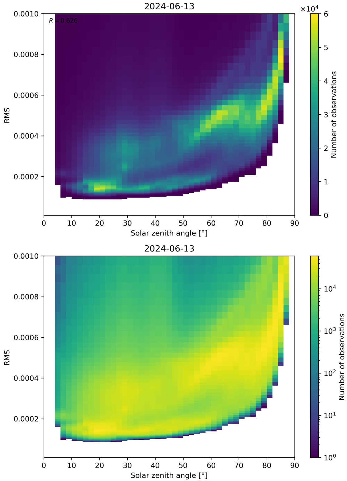
Figure 157: Scatter density plot of “Solar zenith angle” against “RMS” for 2024-06-13 to 2024-06-14.
