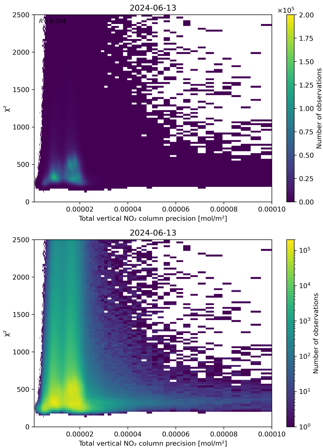
Figure 116: Scatter density plot of “Total vertical NO 2 column precision” against “ \chi^2 ” for 2024-06-13 to 2024-06-14.
