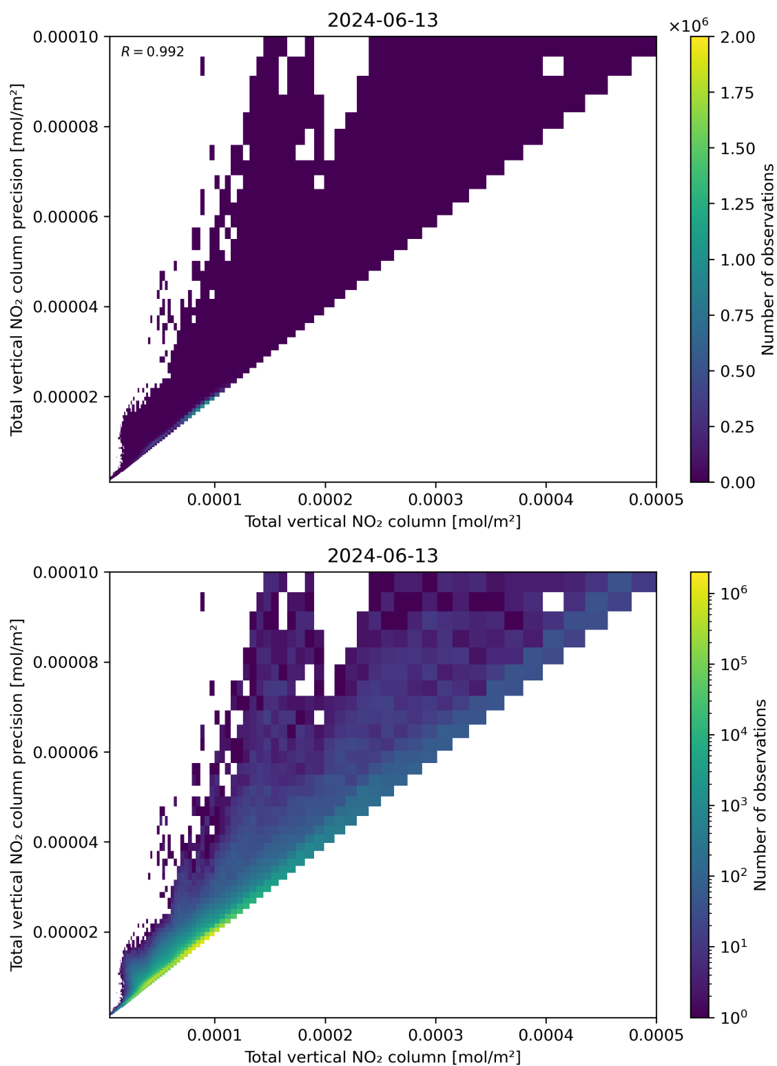
Figure 114: Scatter density plot of “Total vertical NO 2 column” against “Total vertical NO 2 column precision” for 2024-06-13 to 2024-06-14.
