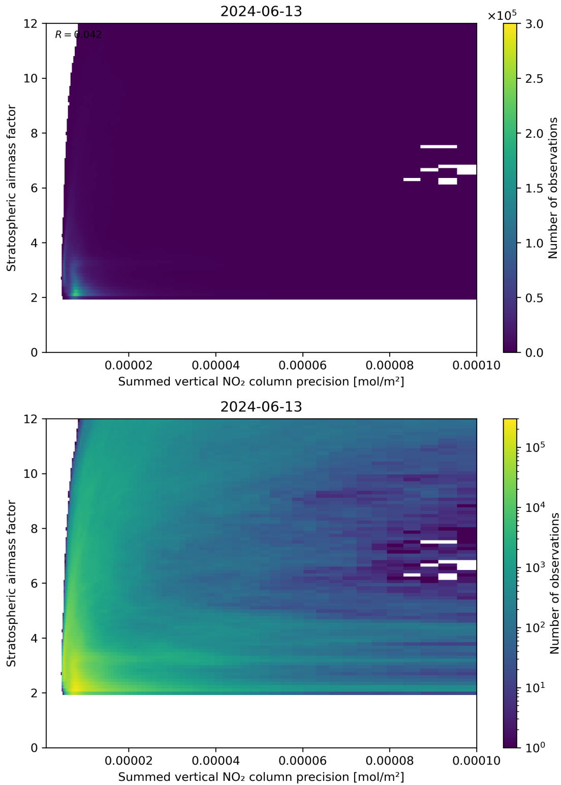
Figure 106: Scatter density plot of “Summed vertical NO 2 column precision” against “Stratospheric airmass factor” for 2024-06-13 to 2024-06-14.
