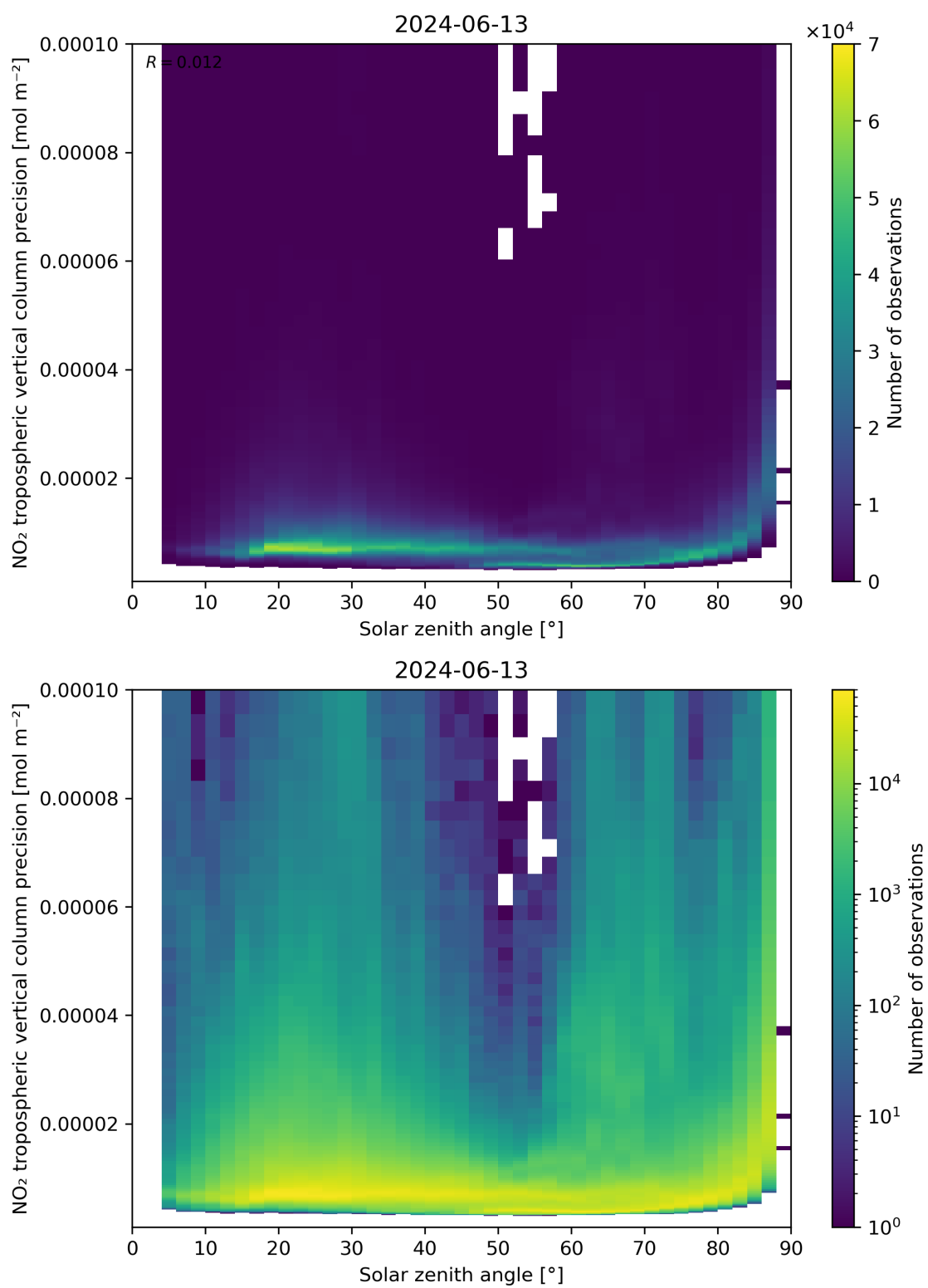
Figure 156: Scatter density plot of “Solar zenith angle” against “NO 2 tropospheric vertical column precision” for 2024-06-13 to 2024-06-14.
