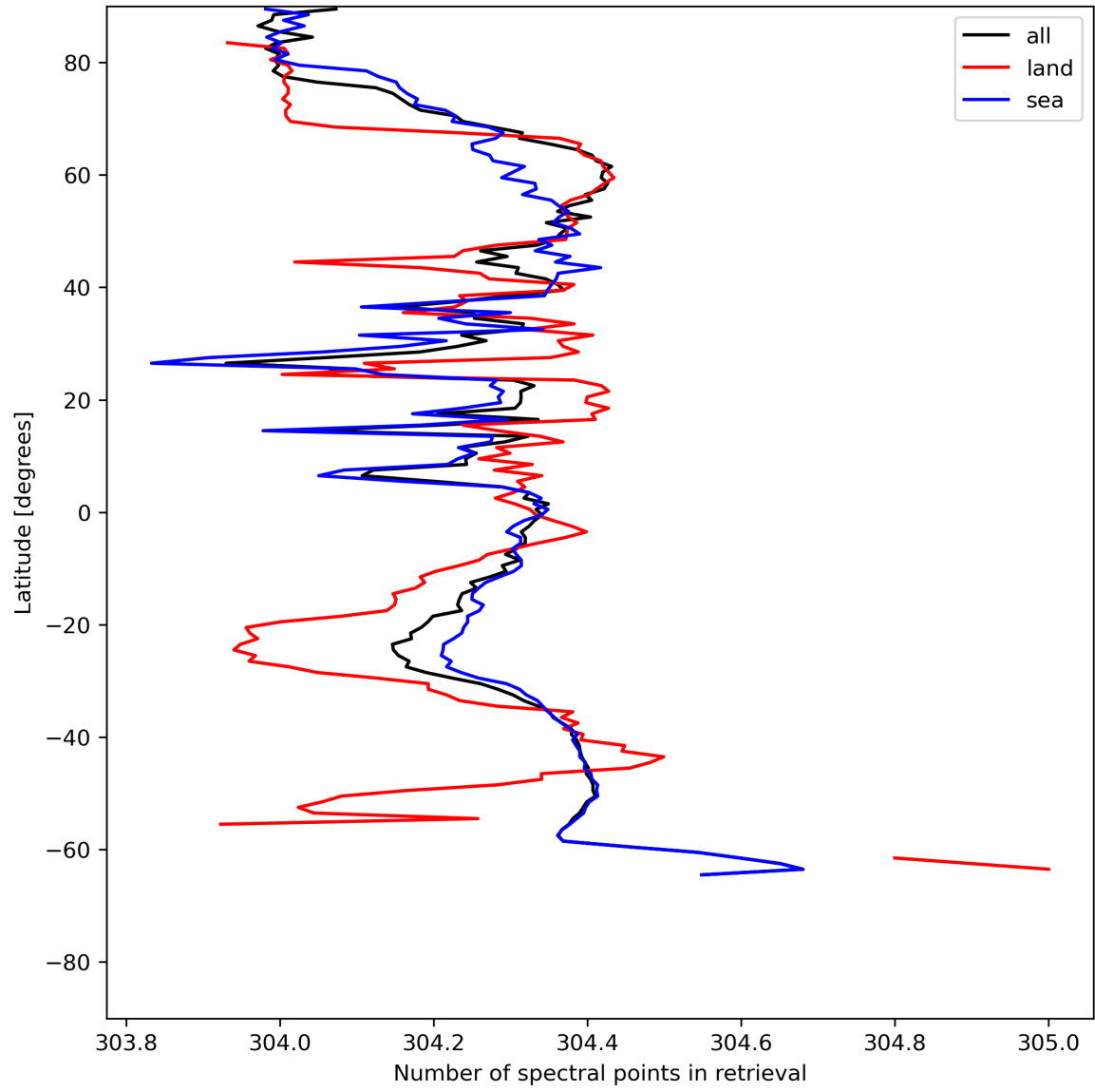
Figure 16: Zonal average of “Number of spectral points in retrieval” for 2024-06-13 to 2024-06-14.
