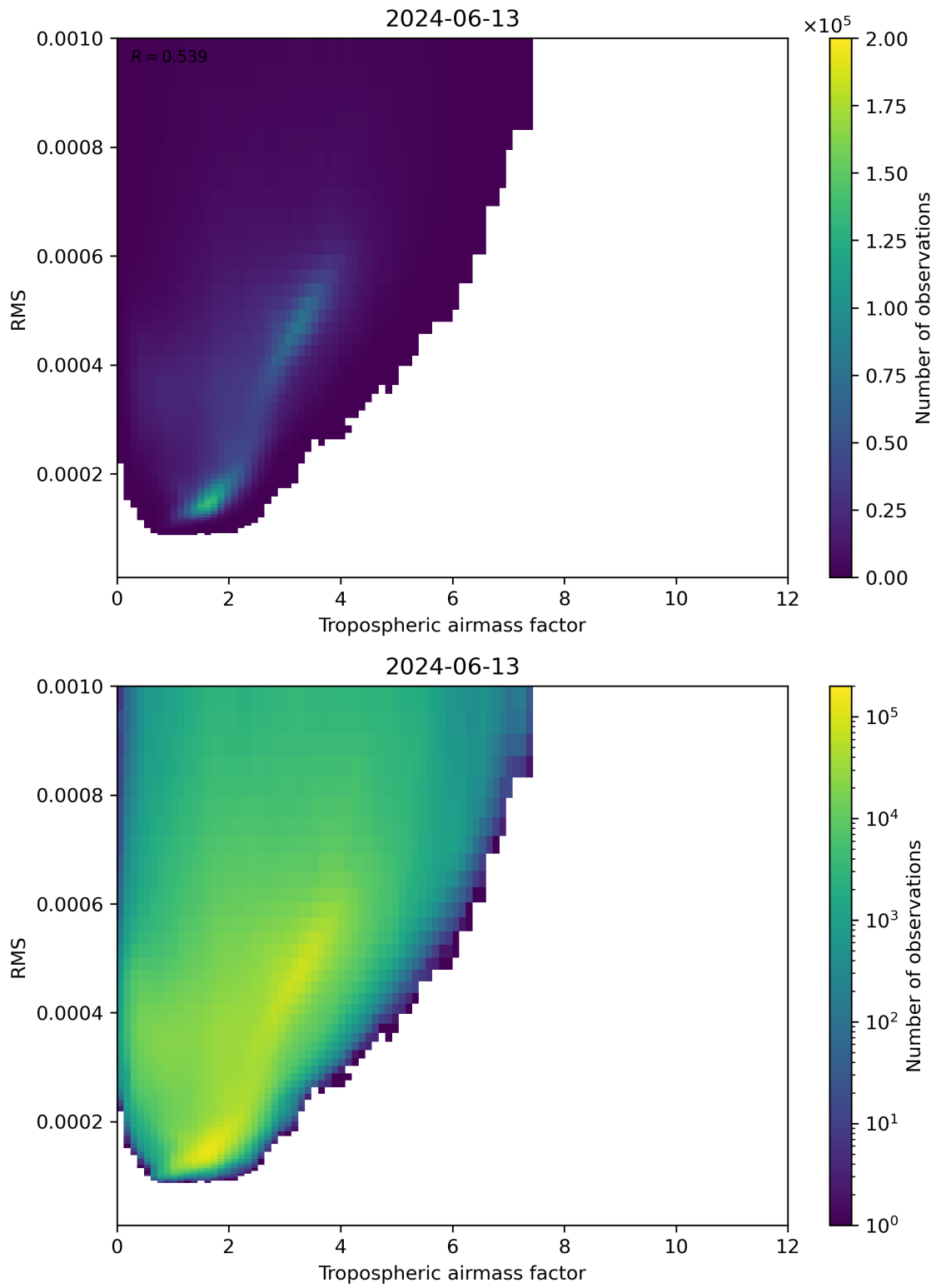
Figure 79: Scatter density plot of “Tropospheric airmass factor” against “RMS” for 2024-06-13 to 2024-06-14.
