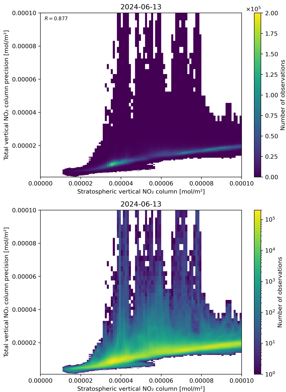
Figure 101: Scatter density plot of “Stratospheric vertical NO 2 column” against “Total vertical NO 2 column precision” for 2024-06-13 to 2024-06-14.
