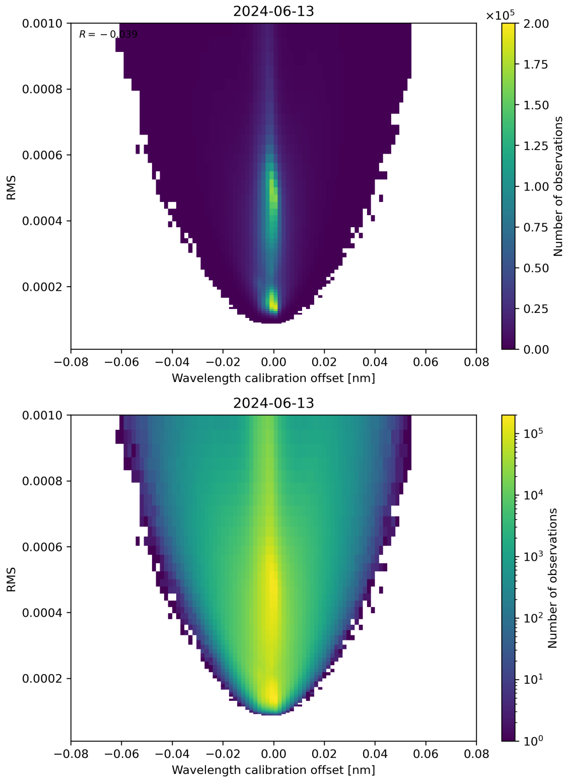
Figure 181: Scatter density plot of “Wavelength calibration offset” against “RMS” for 2024-06-13 to 2024-06-14.
