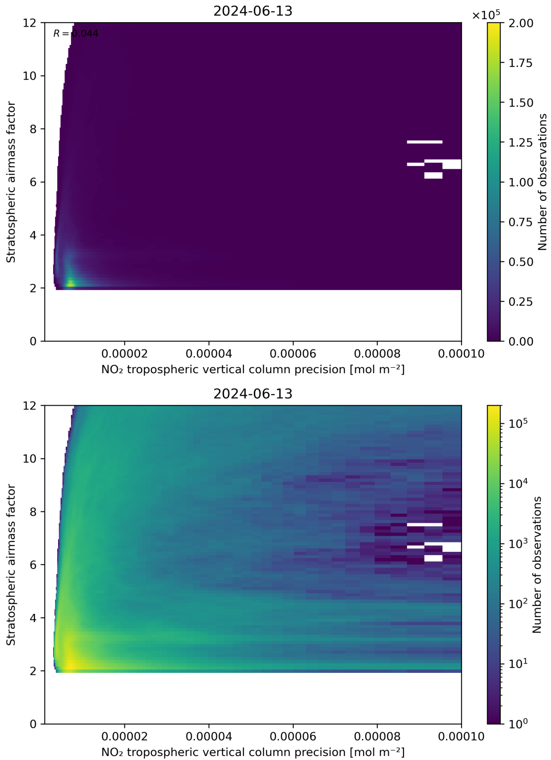
Figure 131: Scatter density plot of “NO 2 tropospheric vertical column precision” against “Stratospheric airmass factor” for 2024-06-13 to 2024-06-14.
