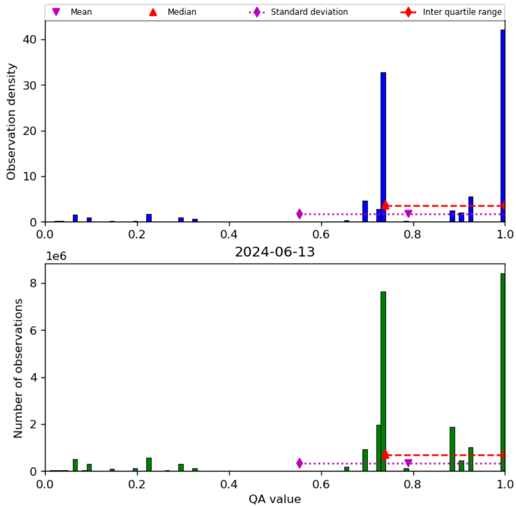
Figure 28: Histogram of “QA value” for 2024-06-13 to 2024-06-14
