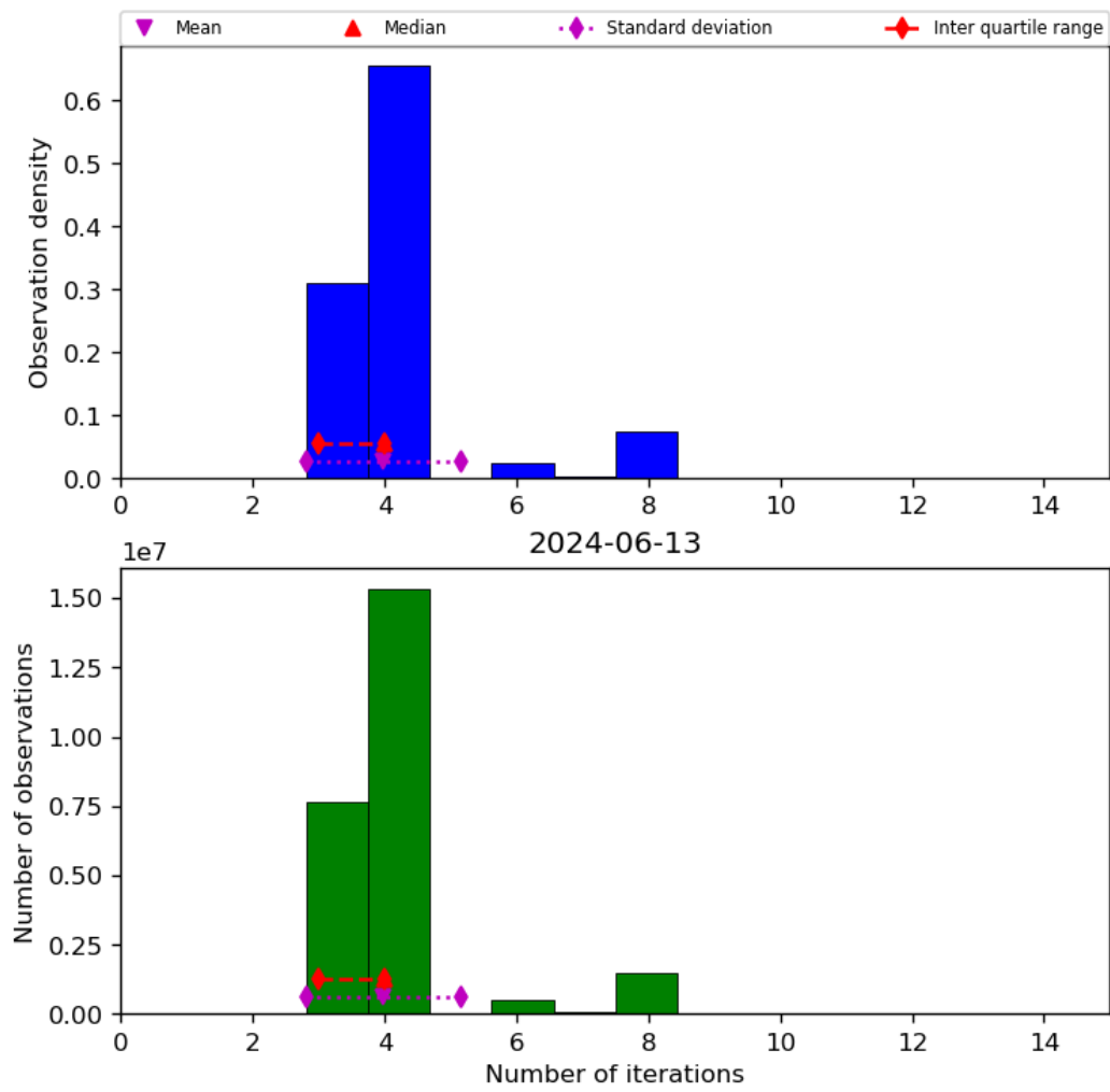
Figure 34: Histogram of “Number of iterations” for 2024-06-13 to 2024-06-14
