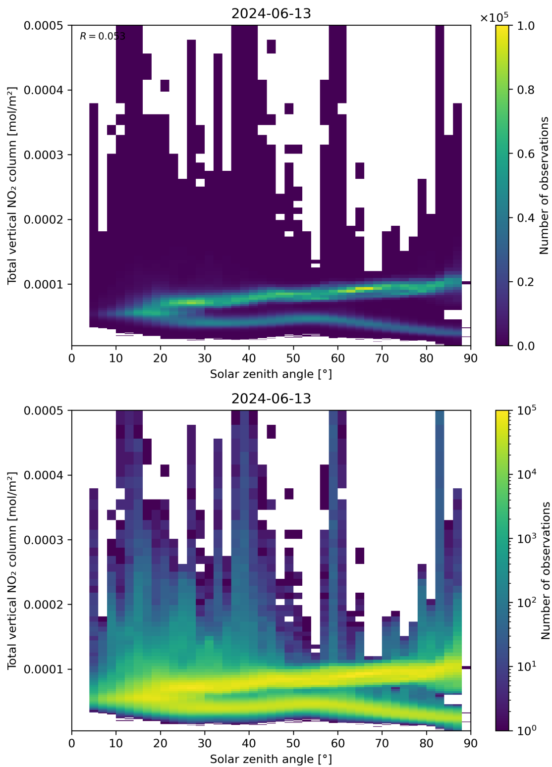
Figure 153: Scatter density plot of “Solar zenith angle” against “Total vertical NO 2 column” for 2024-06-13 to 2024-06-14.
