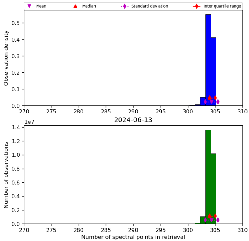
Figure 33: Histogram of “Number of spectral points in retrieval” for 2024-06-13 to 2024-06-14
