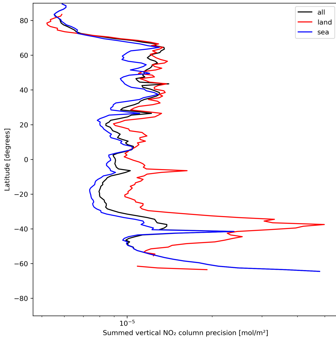
Figure 24: Zonal average of “Summed vertical NO 2 column precision” for 2024-06-13 to 2024-06-14.
