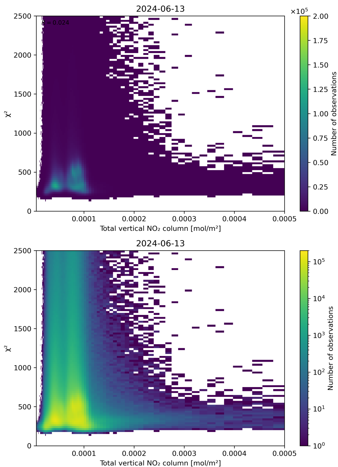
Figure 111: Scatter density plot of “Total vertical NO 2 column” against “ \chi^2 ” for 2024-06-13 to 2024-06-14.
