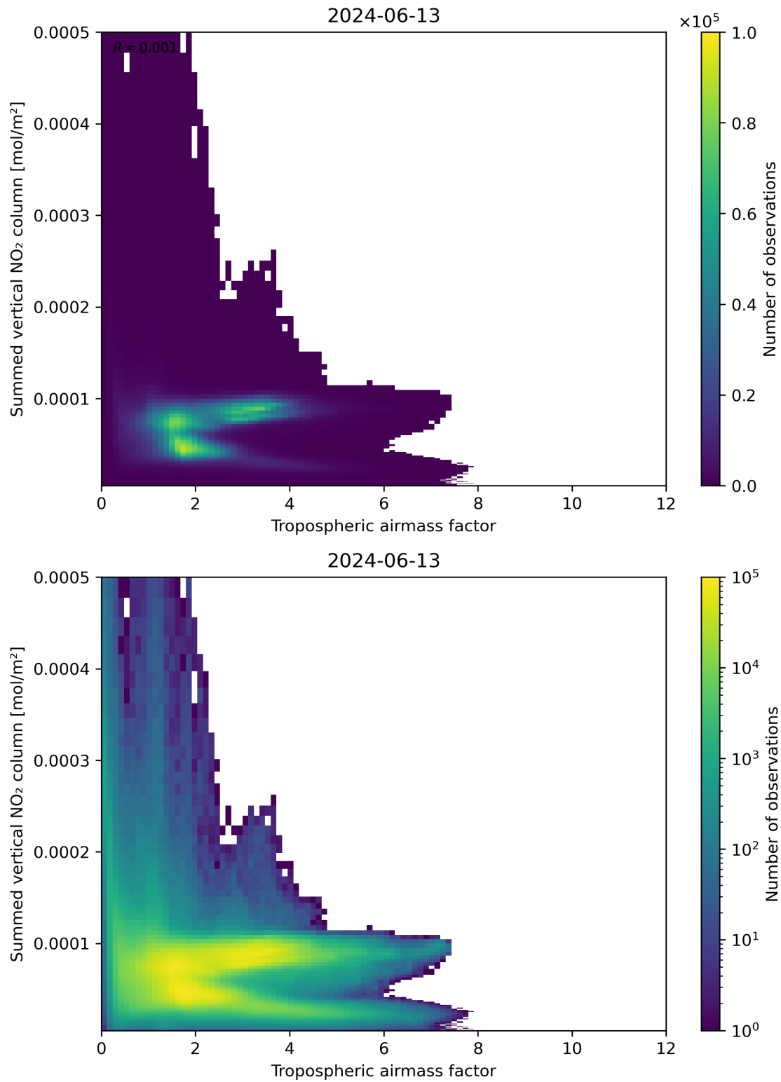
Figure 75: Scatter density plot of “Tropospheric airmass factor” against “Summed vertical NO 2 column” for 2024-06-13 to 2024-06-14.
