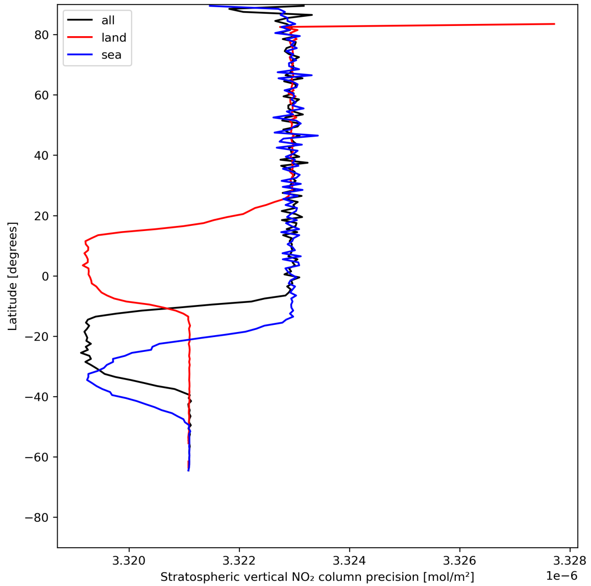
Figure 20: Zonal average of “Stratospheric vertical NO 2 column precision” for 2024-06-13 to 2024-06-14.
