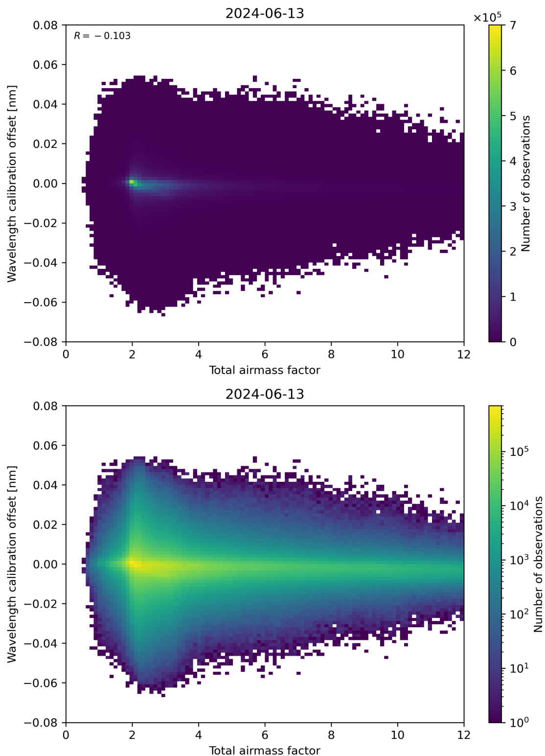
Figure 70: Scatter density plot of “Total airmass factor” against “Wavelength calibration offset” for 2024-06-13 to 2024-06-14.
