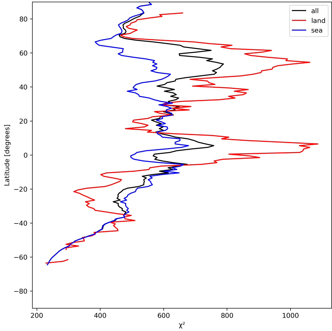
Figure 25: Zonal average of “ \chi^2 ” for 2024-06-13 to 2024-06-14.
