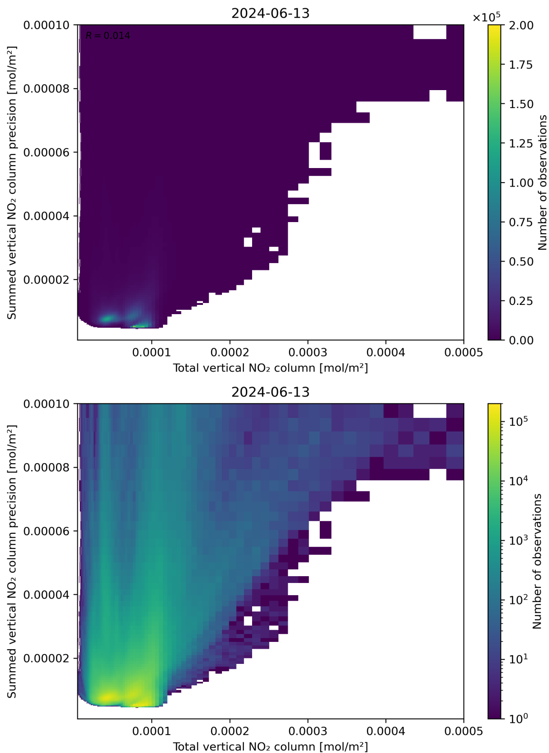
Figure 113: Scatter density plot of “Total vertical NO 2 column” against “Summed vertical NO 2 column precision” for 2024-06-13 to 2024-06-14.
