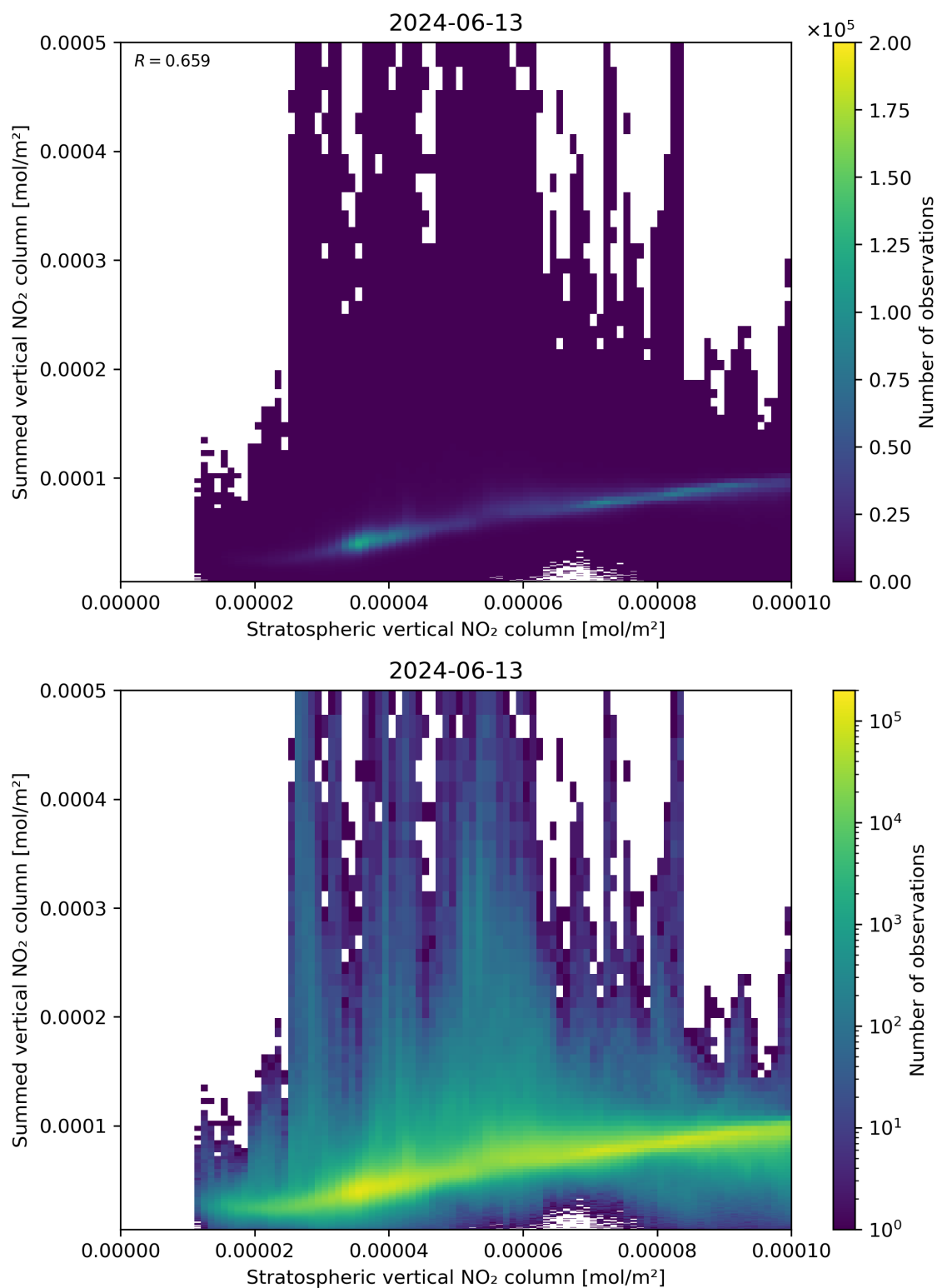
Figure 98: Scatter density plot of “Stratospheric vertical NO 2 column” against “Summed vertical NO 2 column” for 2024-06-13 to 2024-06-14.
