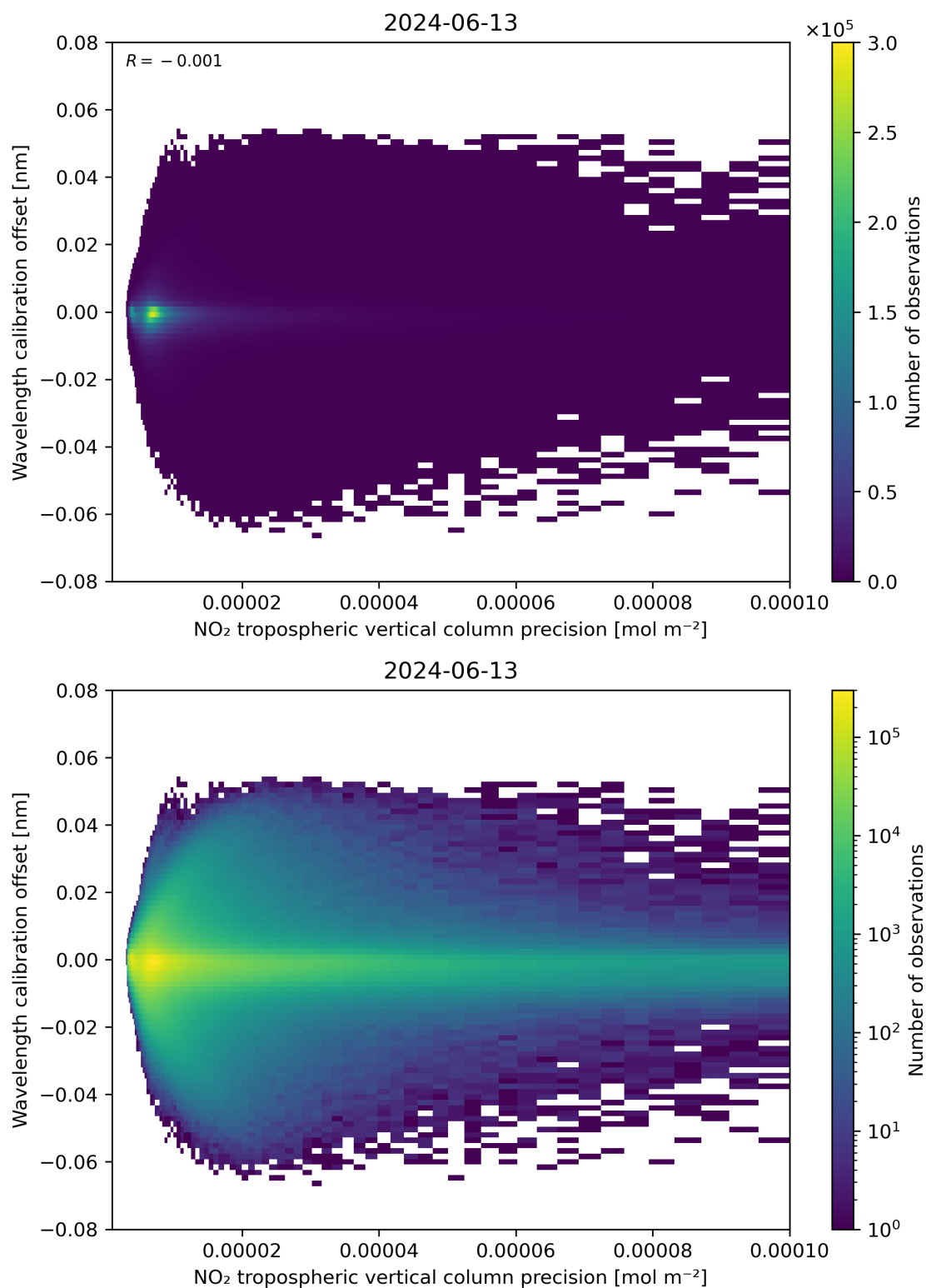
Figure 141: Scatter density plot of “NO 2 tropospheric vertical column precision” against “Wavelength calibration offset” for 2024-06-13 to 2024-06-14.
