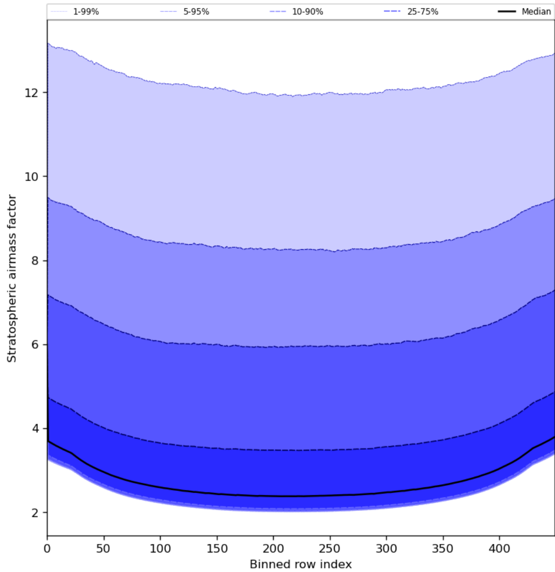
Figure 61: Along track statistics of “Stratospheric airmass factor” for 2024-06-13 to 2024-06-14
