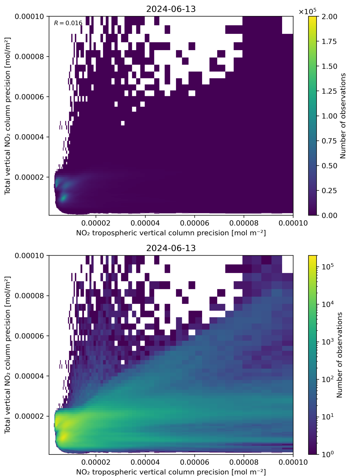
Figure 139: Scatter density plot of “NO 2 tropospheric vertical column precision” against “Total vertical NO 2 column precision” for 2024-06-13 to 2024-06-14.
