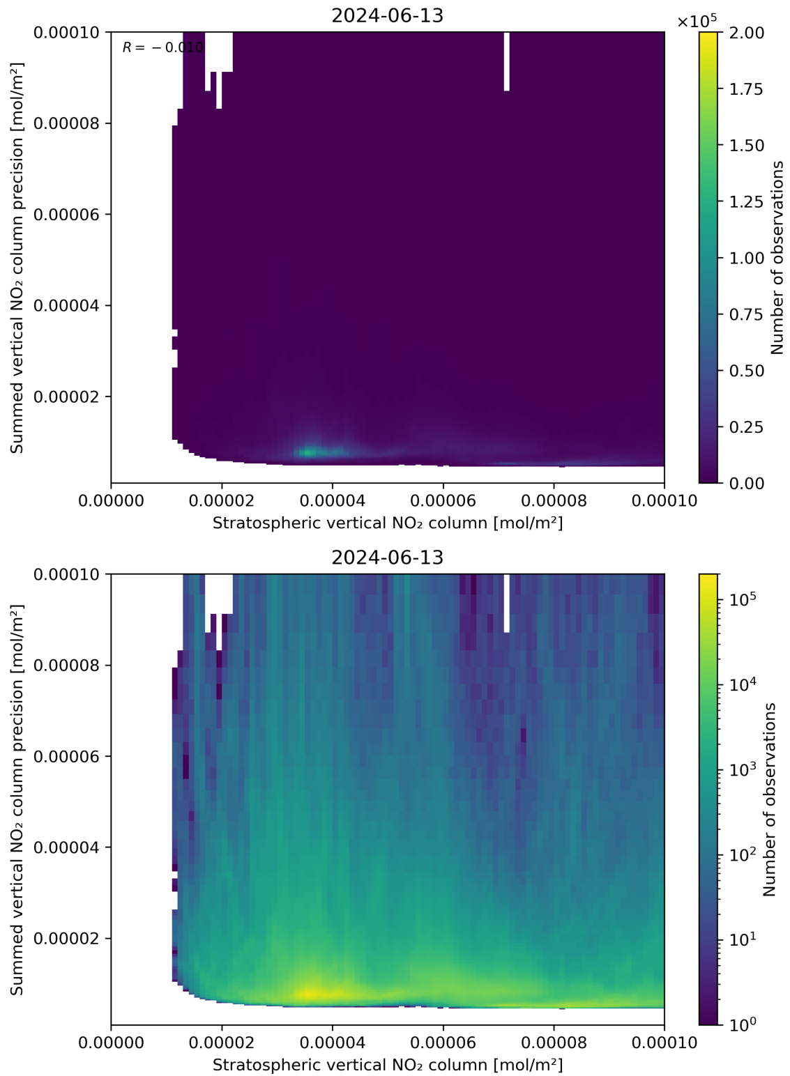
Figure 99: Scatter density plot of “Stratospheric vertical NO 2 column” against “Summed vertical NO 2 column precision” for 2024-06-13 to 2024-06-14.
