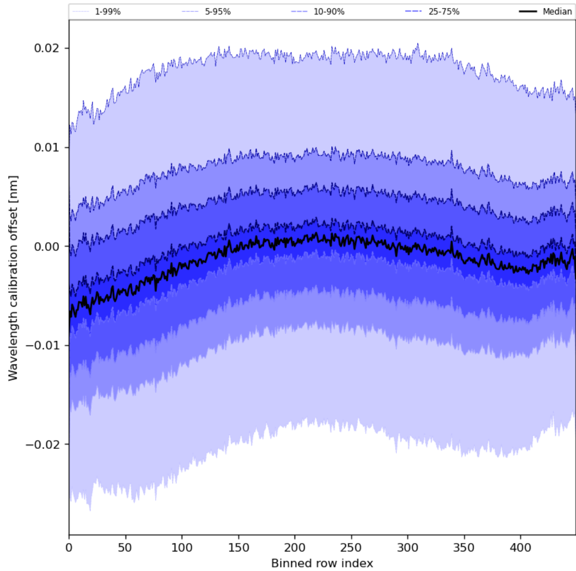
Figure 52: Along track statistics of “Wavelength calibration offset” for 2024-06-13 to 2024-06-14
