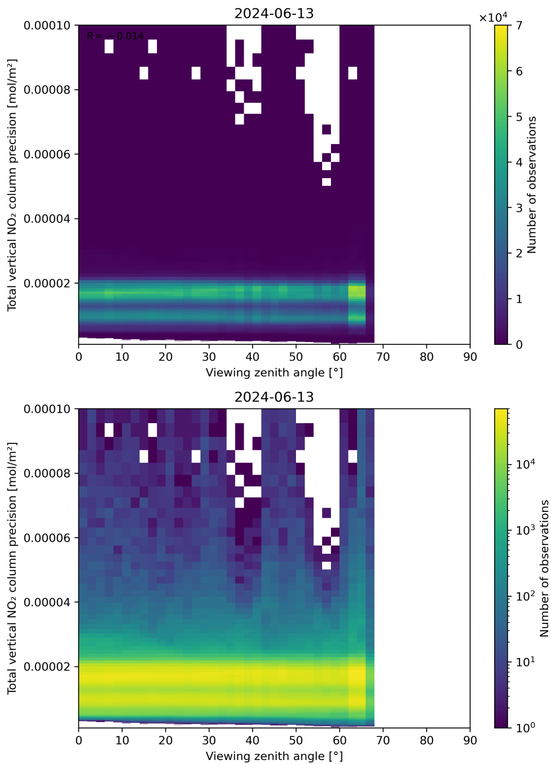
Figure 168: Scatter density plot of “Viewing zenith angle” against “Total vertical NO 2 column precision” for 2024-06-13 to 2024-06-14.
