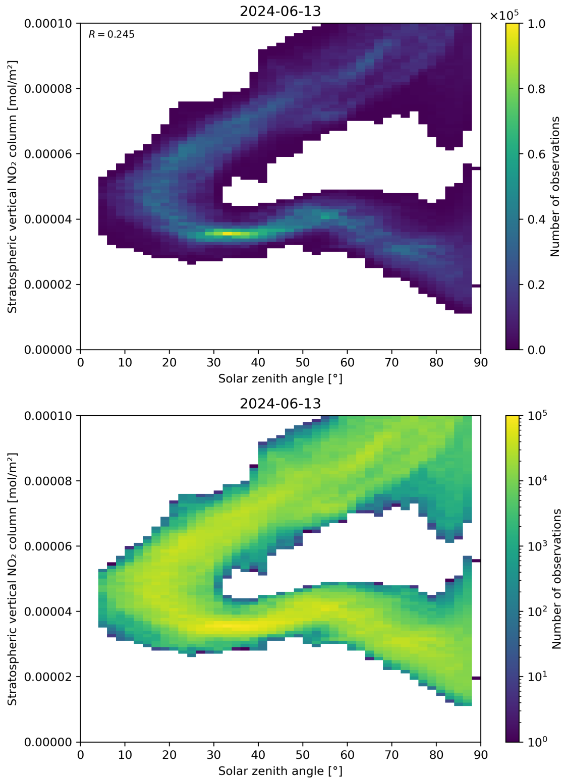
Figure 150: Scatter density plot of “Solar zenith angle” against “Stratospheric vertical NO 2 column” for 2024-06-13 to 2024-06-14.
