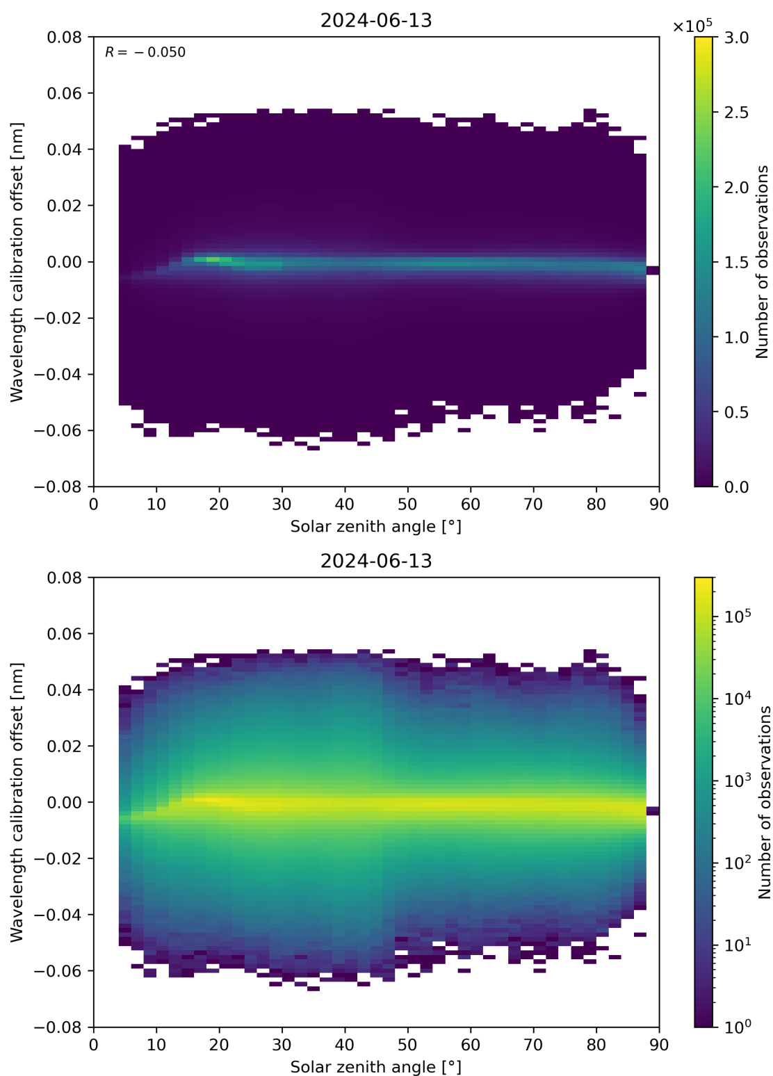
Figure 158: Scatter density plot of “Solar zenith angle” against “Wavelength calibration offset” for 2024-06-13 to 2024-06-14.
