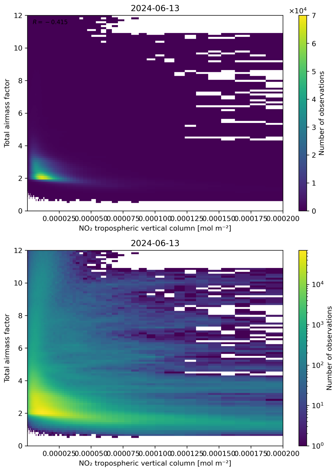
Figure 122: Scatter density plot of “NO 2 tropospheric vertical column” against “Total air mass factor” for 2024-06-13 to 2024-06-14.
