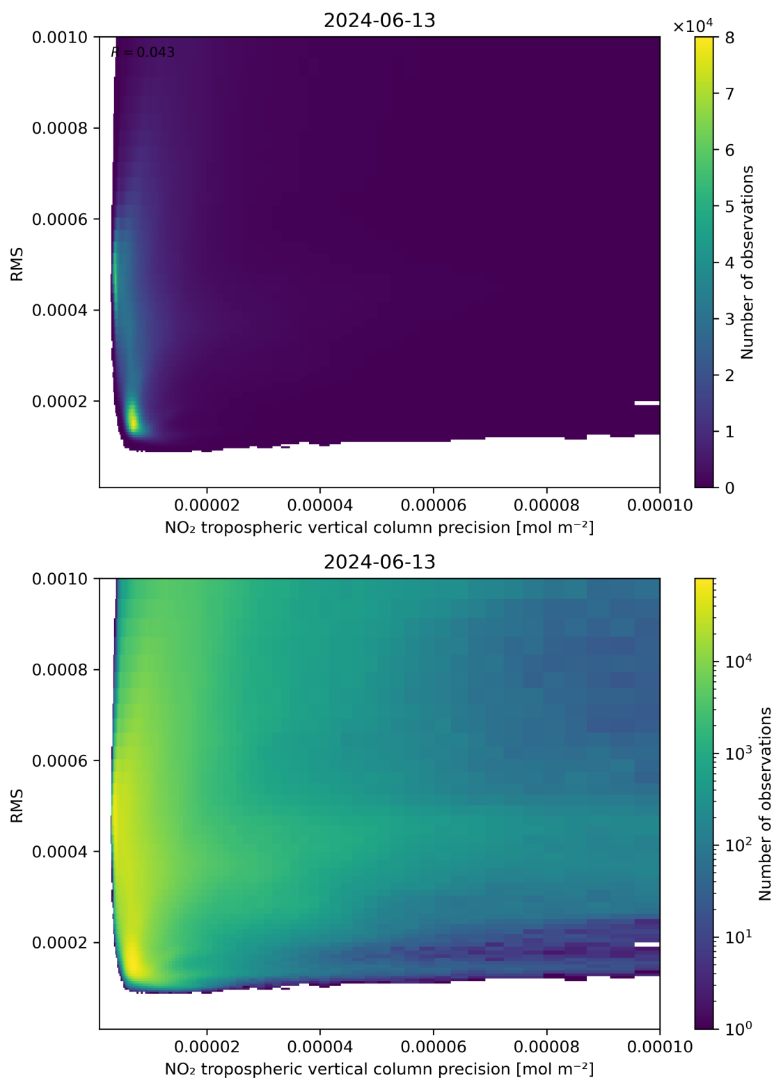
Figure 140: Scatter density plot of “NO 2 tropospheric vertical column precision” against “RMS” for 2024-06-13 to 2024-06-14.
