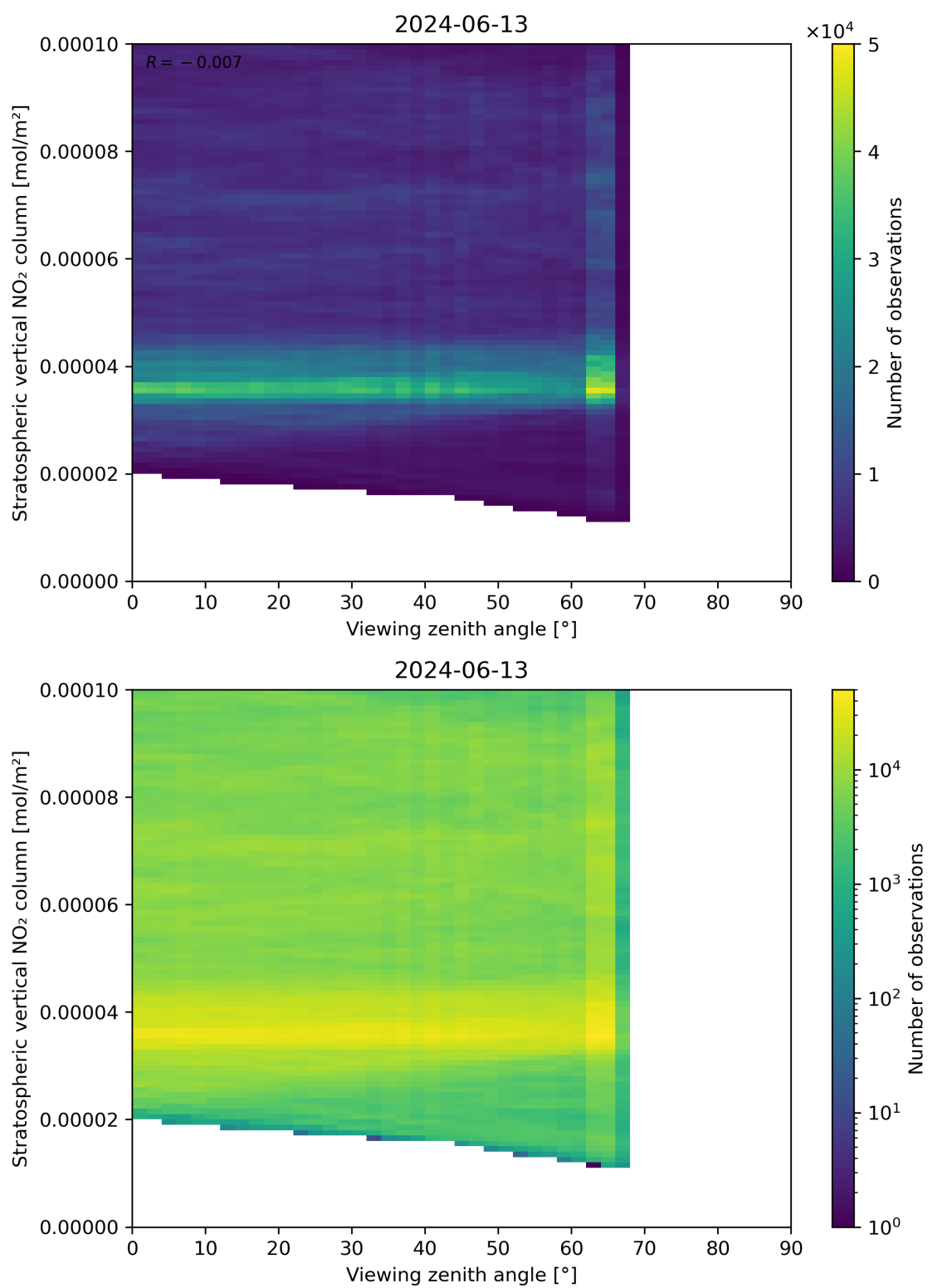
Figure 164: Scatter density plot of “Viewing zenith angle” against “Stratospheric vertical NO 2 column” for 2024-06-13 to 2024-06-14.
