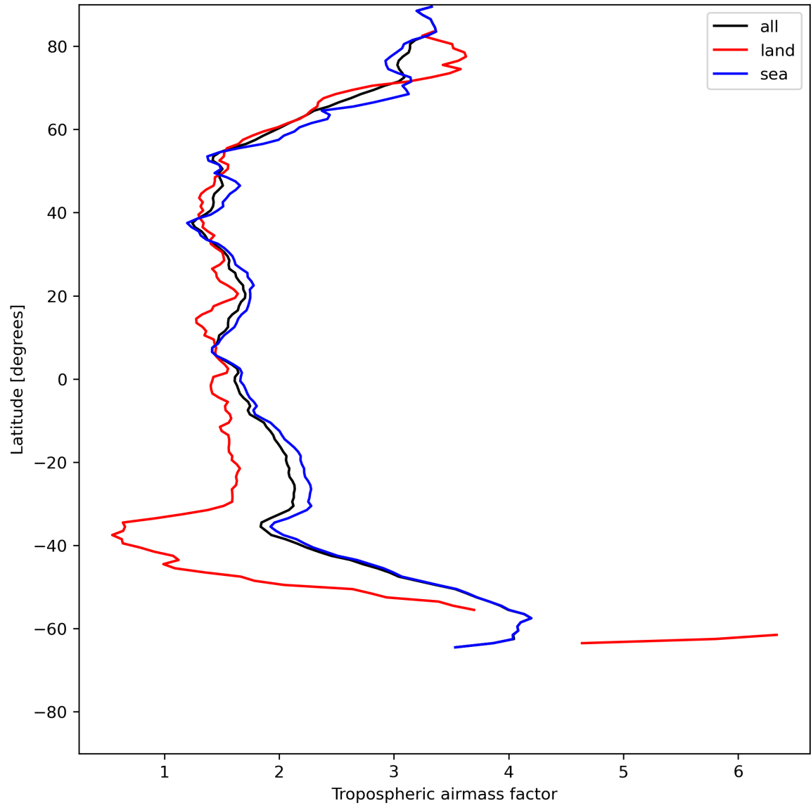
Figure 14: Zonal average of “Tropospheric airmass factor” for 2024-06-13 to 2024-06-14.
