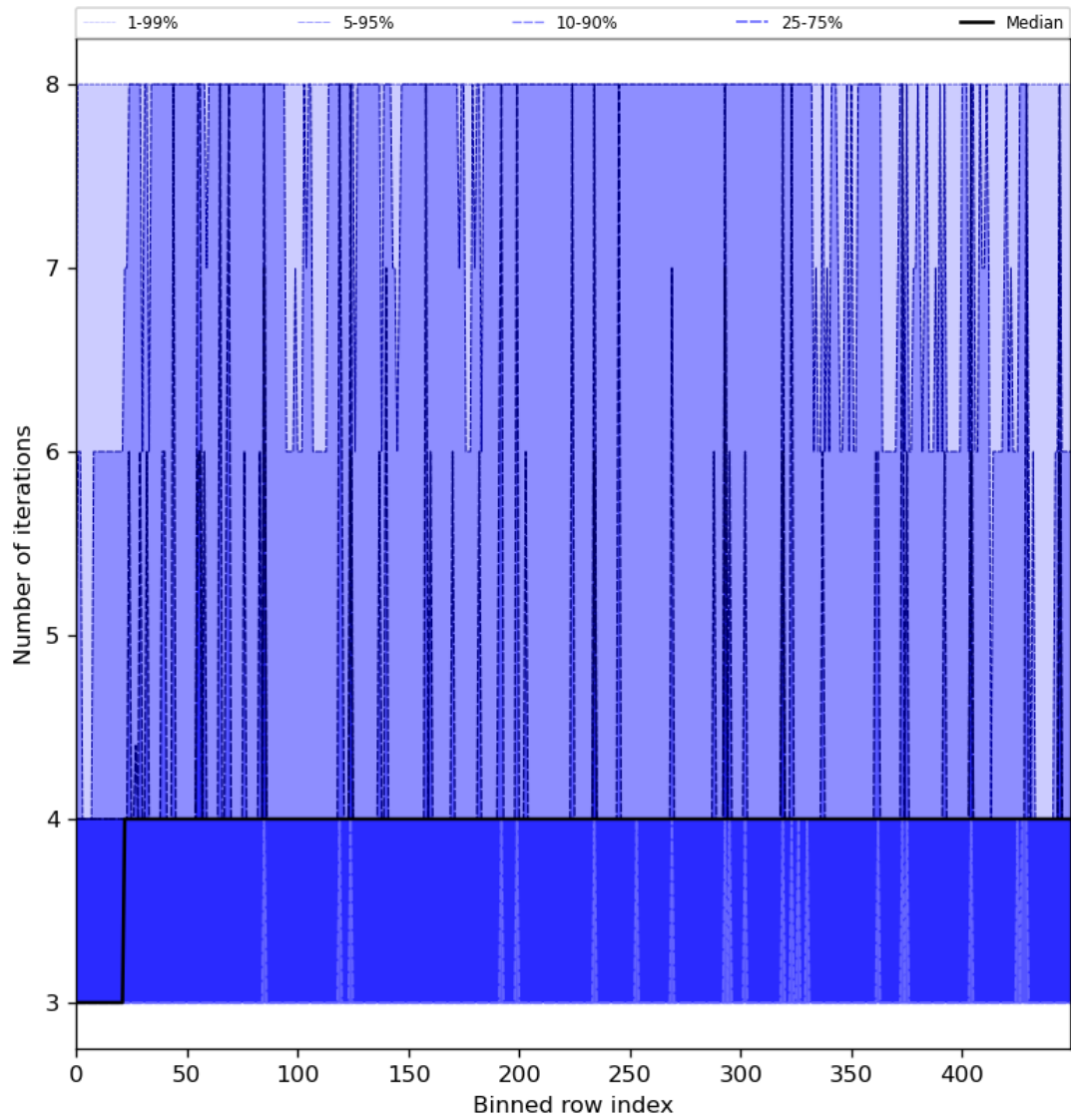
Figure 51: Along track statistics of “Number of iterations” for 2024-06-13 to 2024-06-14
