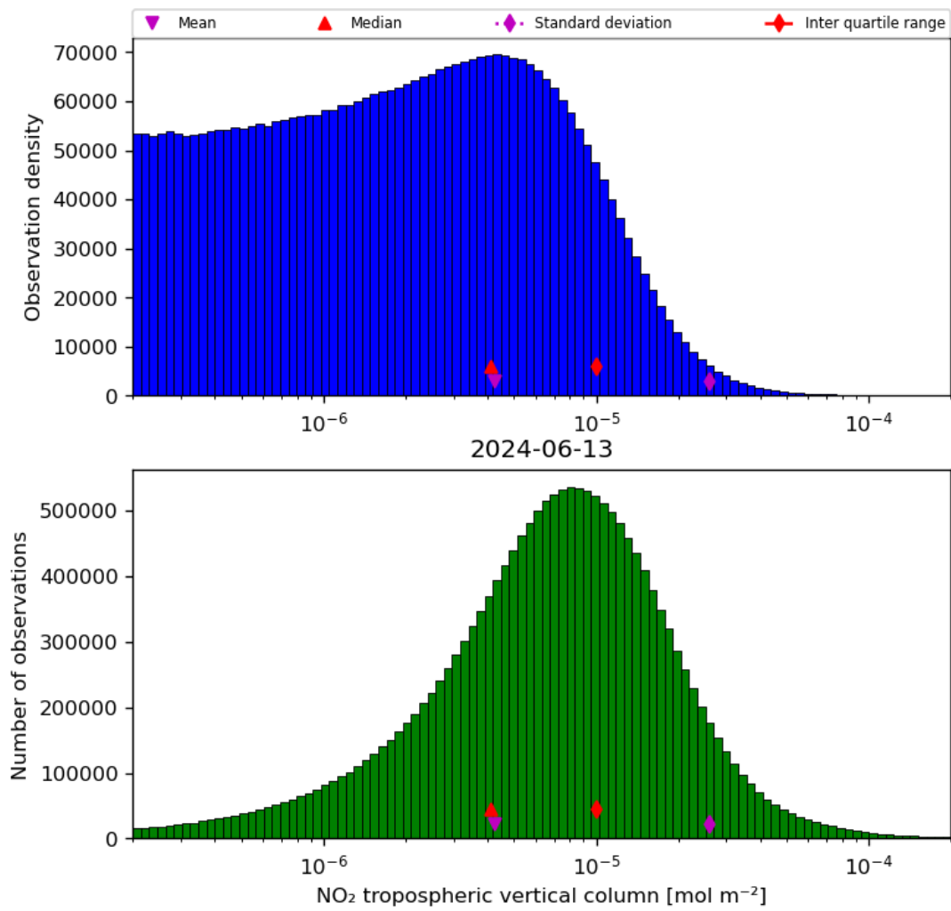
Figure 29: Histogram of “NO 2 tropospheric vertical column” for 2024-06-13 to 2024-06-14
