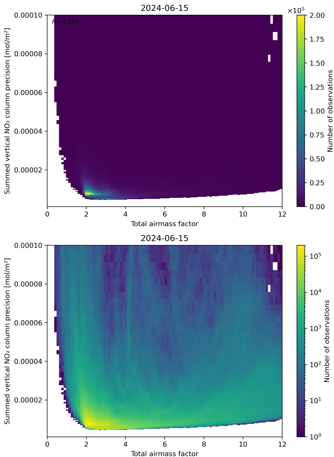
Figure 66: Scatter density plot of “Total airmass factor” against “Summed vertical NO 2 column precision” for 2024-06-14 to 2024-06-16.
