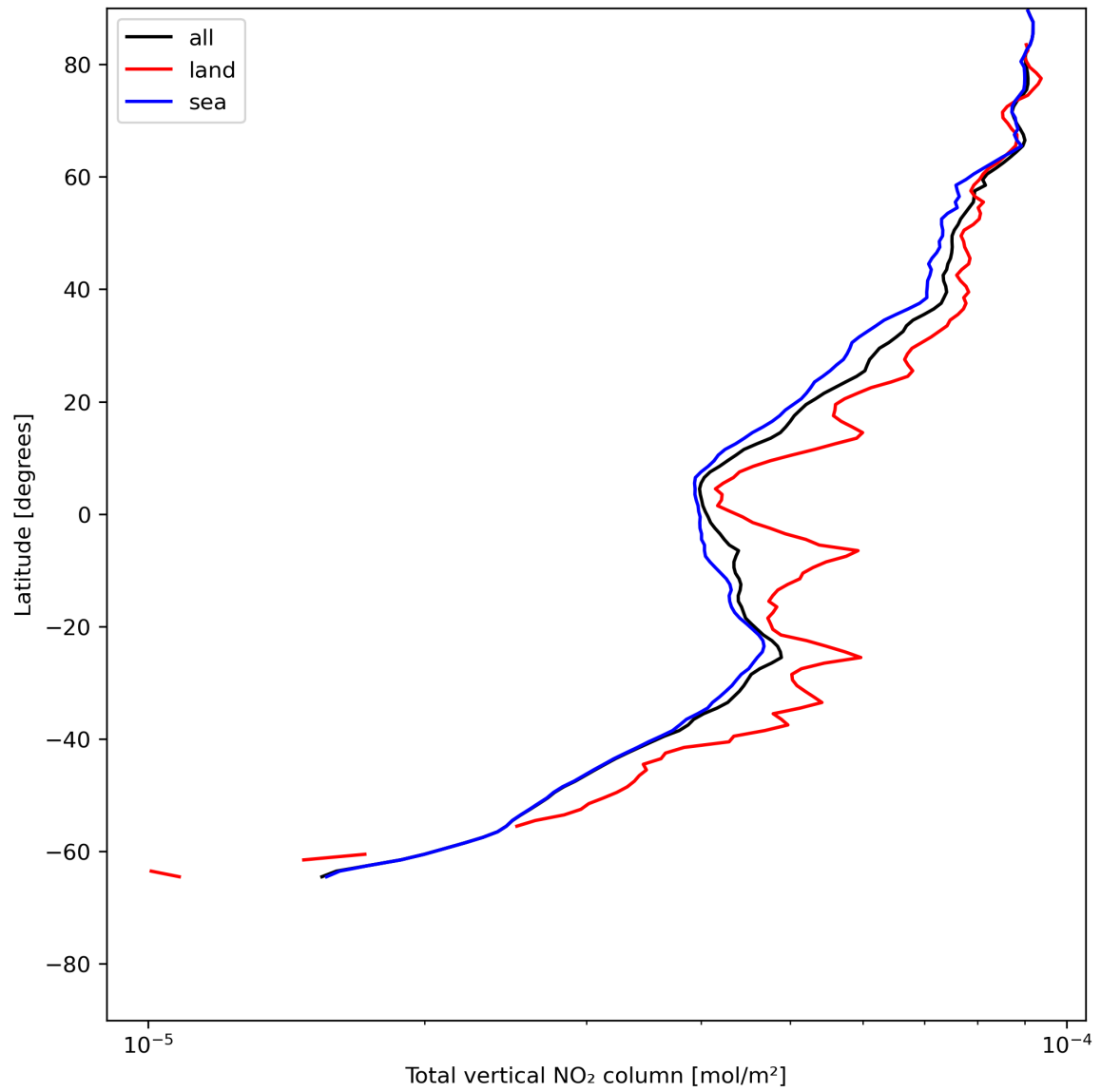
Figure 21: Zonal average of “Total vertical NO 2 column” for 2024-06-14 to 2024-06-16.
