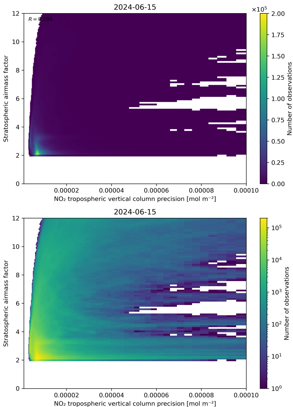
Figure 131: Scatter density plot of “NO 2 tropospheric vertical column precision” against “Stratospheric airmass factor” for 2024-06-14 to 2024-06-16.
