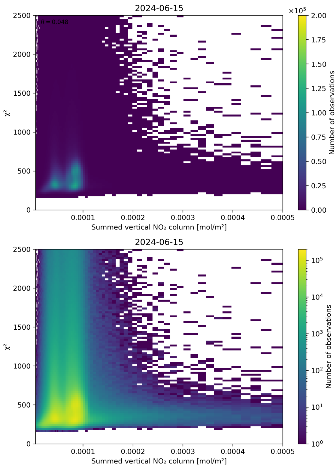
Figure 104: Scatter density plot of “Summed vertical NO 2 column” against “ \chi^2 ” for 2024-06-14 to 2024-06-16.
