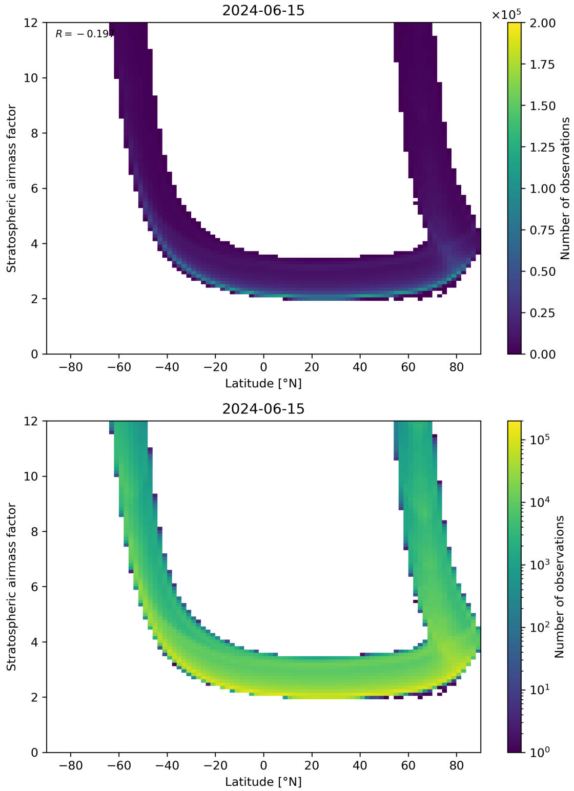
Figure 83: Scatter density plot of “Latitude” against “Stratospheric air mass factor” for 2024-06-14 to 2024-06-16.
