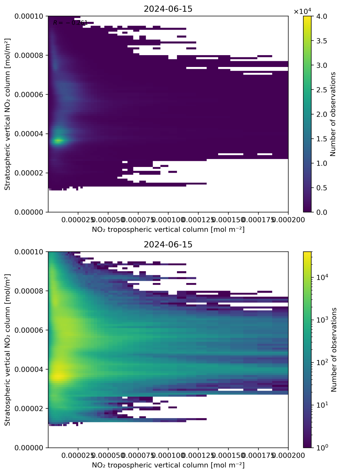
Figure 125: Scatter density plot of “NO 2 tropospheric vertical column” against “Stratospheric vertical NO 2 column” for 2024-06-14 to 2024-06-16.
