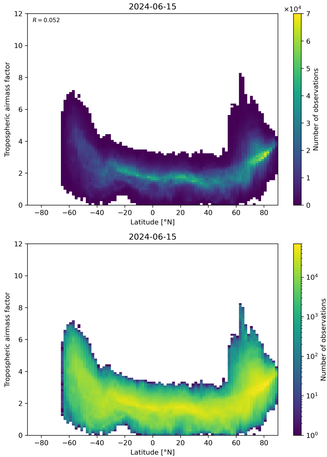
Figure 85: Scatter density plot of “Latitude” against “Tropospheric airmass factor” for 2024-06-14 to 2024-06-16.
