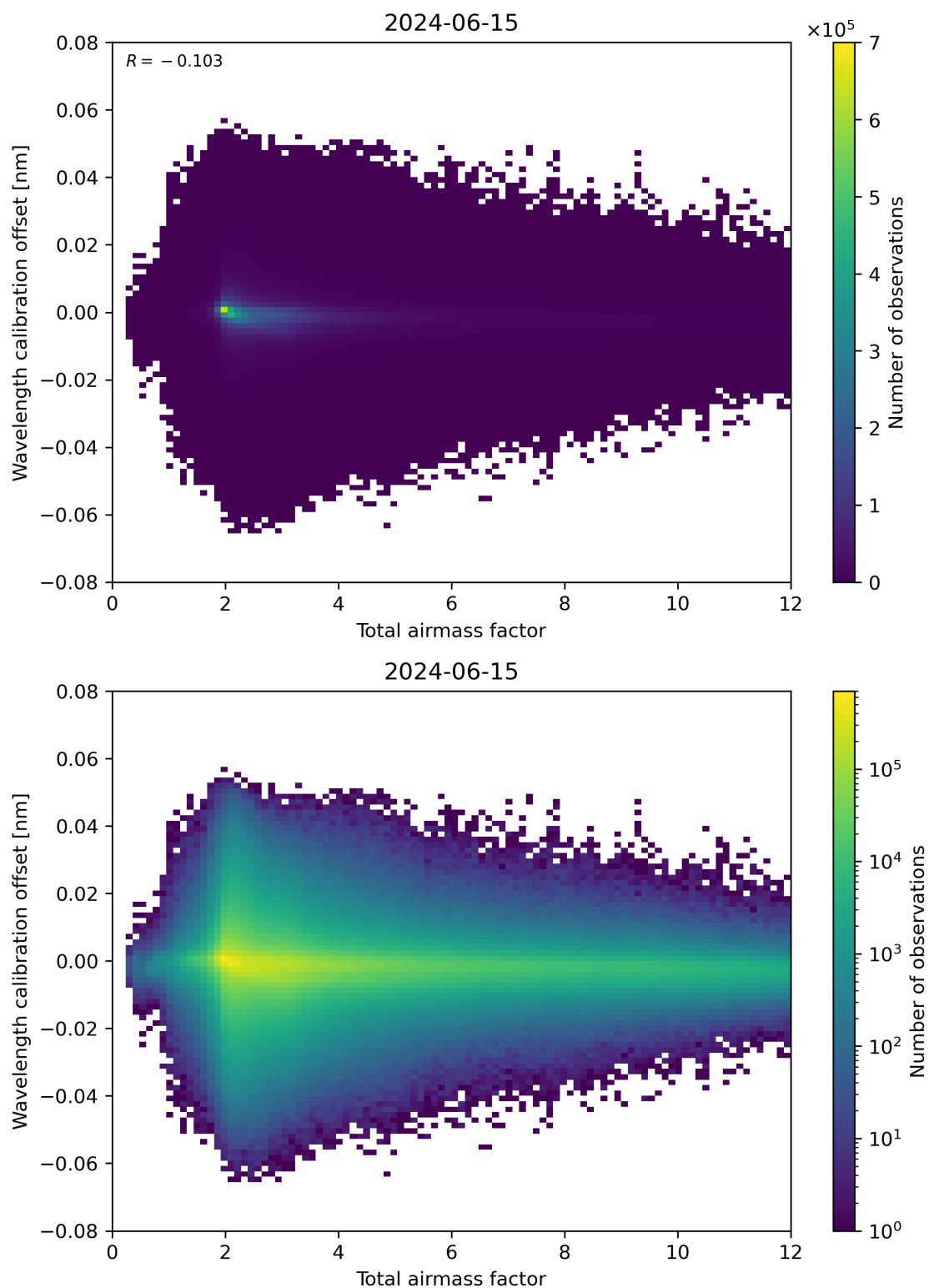
Figure 70: Scatter density plot of “Total airmass factor” against “Wavelength calibration offset” for 2024-06-14 to 2024-06-16.
