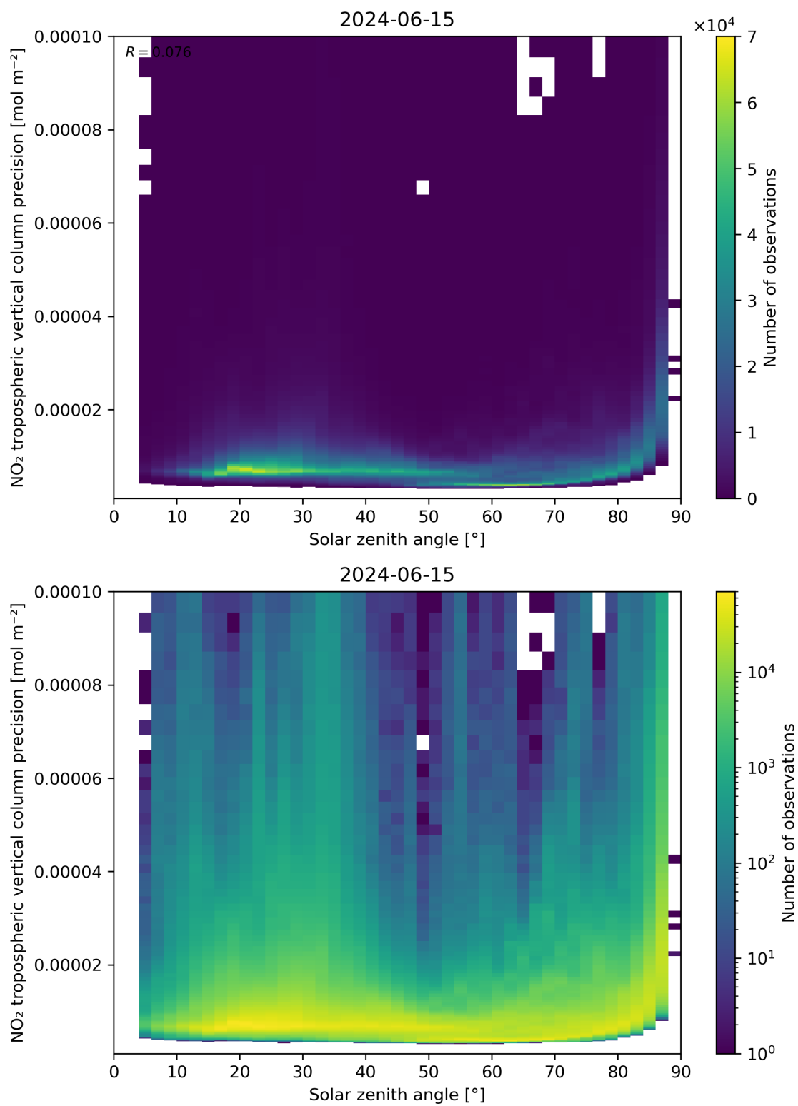
Figure 156: Scatter density plot of “Solar zenith angle” against “NO 2 tropospheric vertical column precision” for 2024-06-14 to 2024-06-16.
