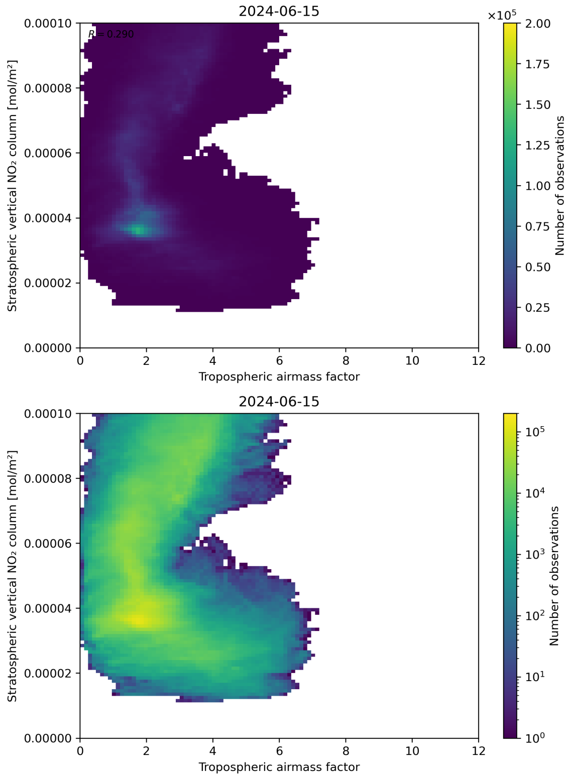
Figure 74: Scatter density plot of “Tropospheric air mass factor” against “Stratospheric vertical NO 2 column” for 2024-06-14 to 2024-06-16.
