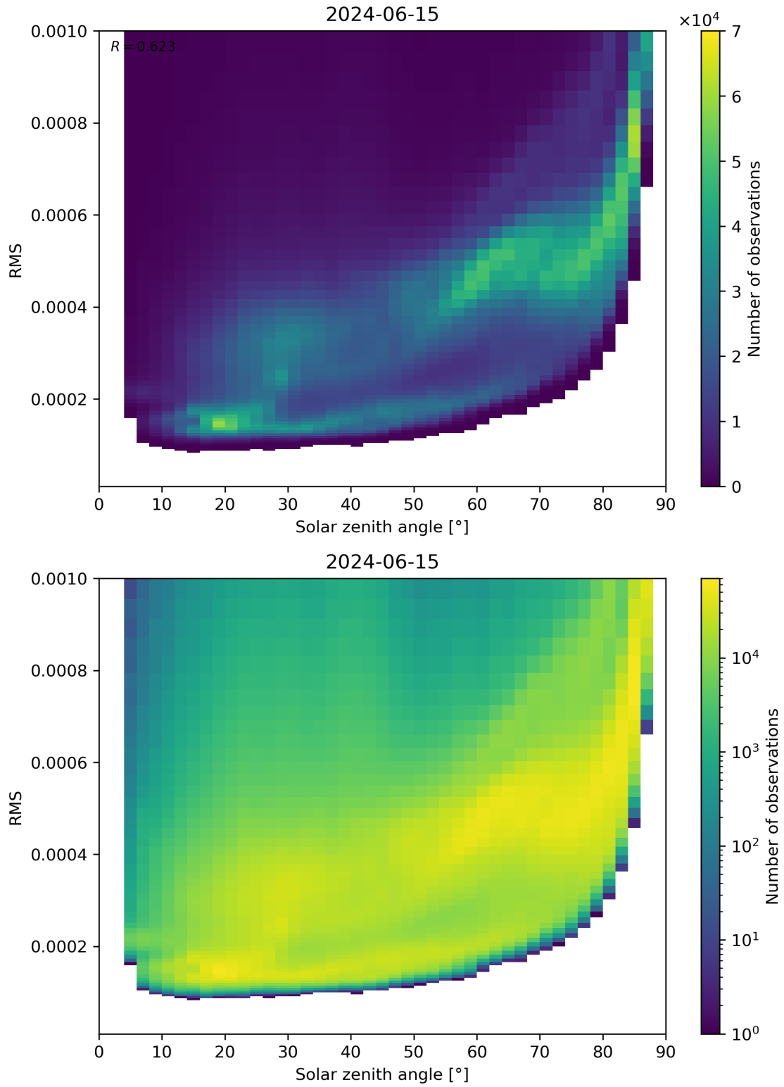
Figure 157: Scatter density plot of “Solar zenith angle” against “RMS” for 2024-06-14 to 2024-06-16.
