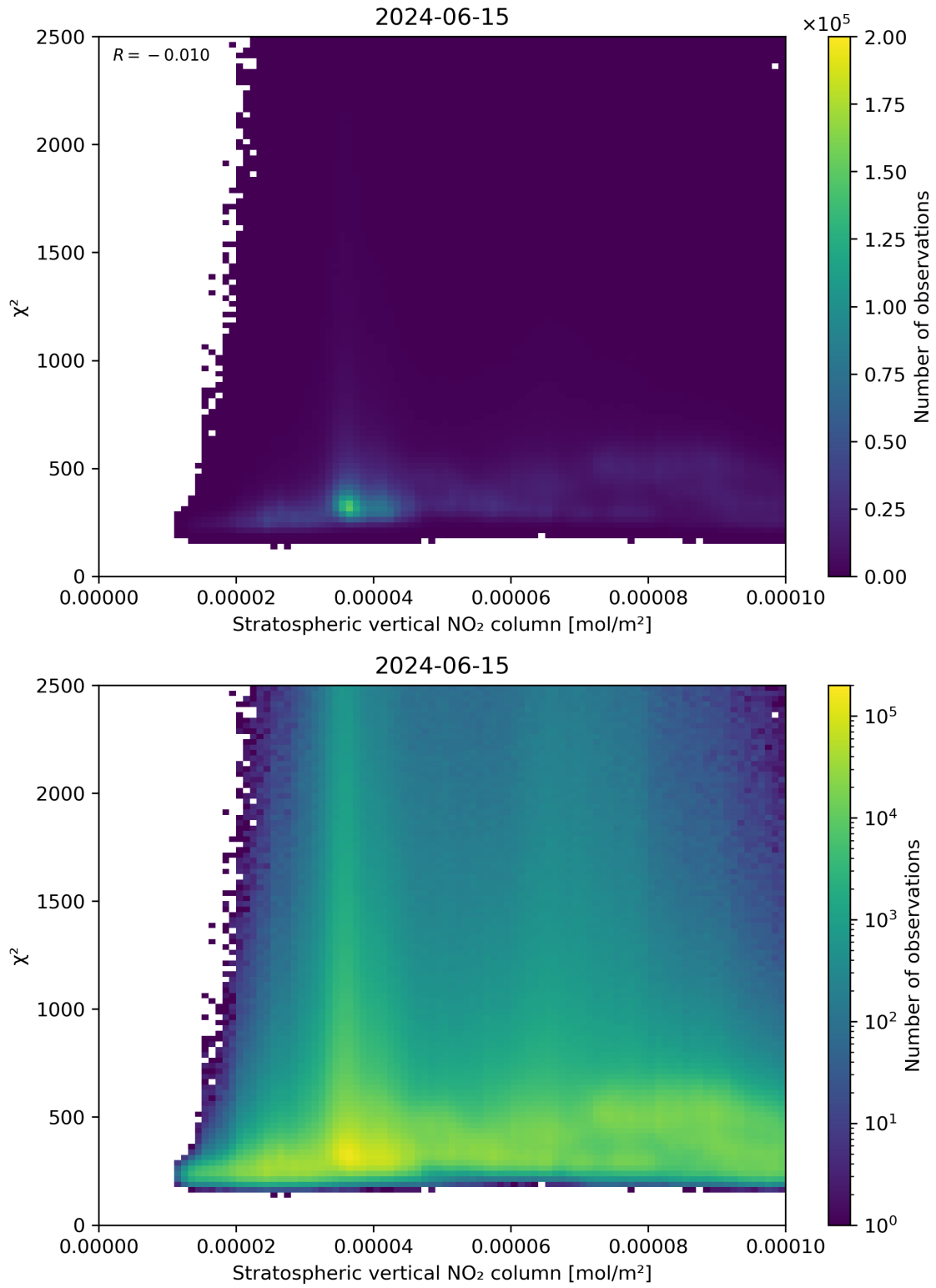
Figure 97: Scatter density plot of “Stratospheric vertical NO 2 column” against “ \chi^2 ” for 2024-06-14 to 2024-06-16.
