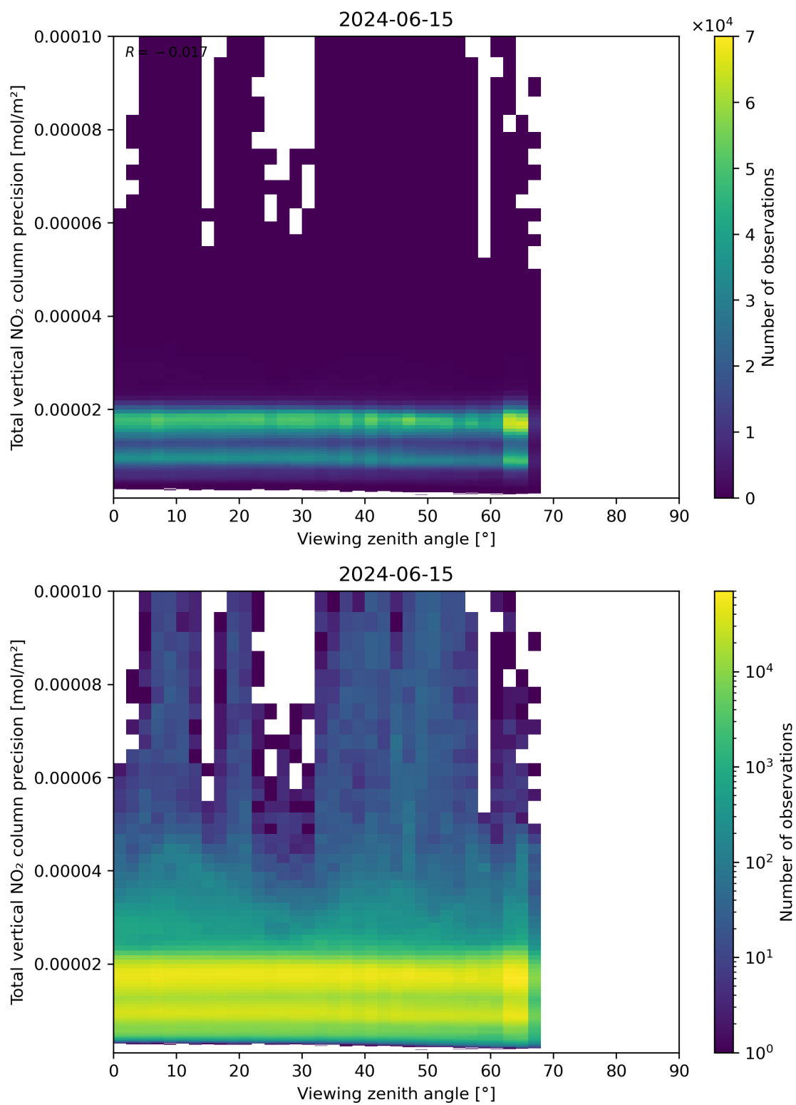
Figure 168: Scatter density plot of “Viewing zenith angle” against “Total vertical NO 2 column precision” for 2024-06-14 to 2024-06-16.
