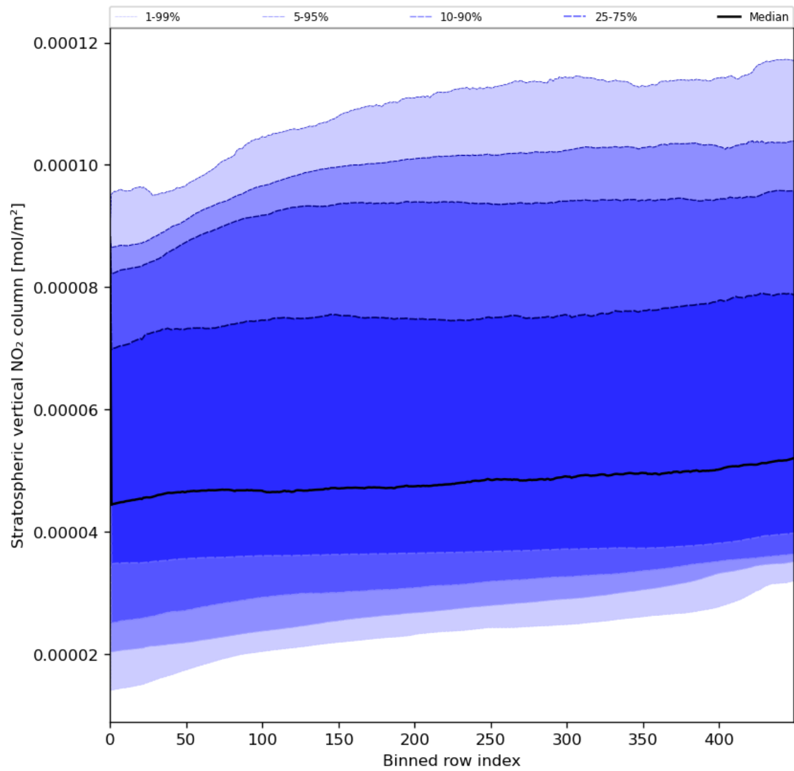
Figure 53: Along track statistics of “Stratospheric vertical NO 2 column” for 2024-06-14 to 2024-06-16
