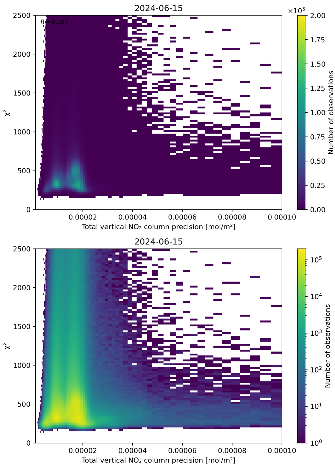
Figure 116: Scatter density plot of “Total vertical NO 2 column precision” against “ \chi^2 ” for 2024-06-14 to 2024-06-16.
