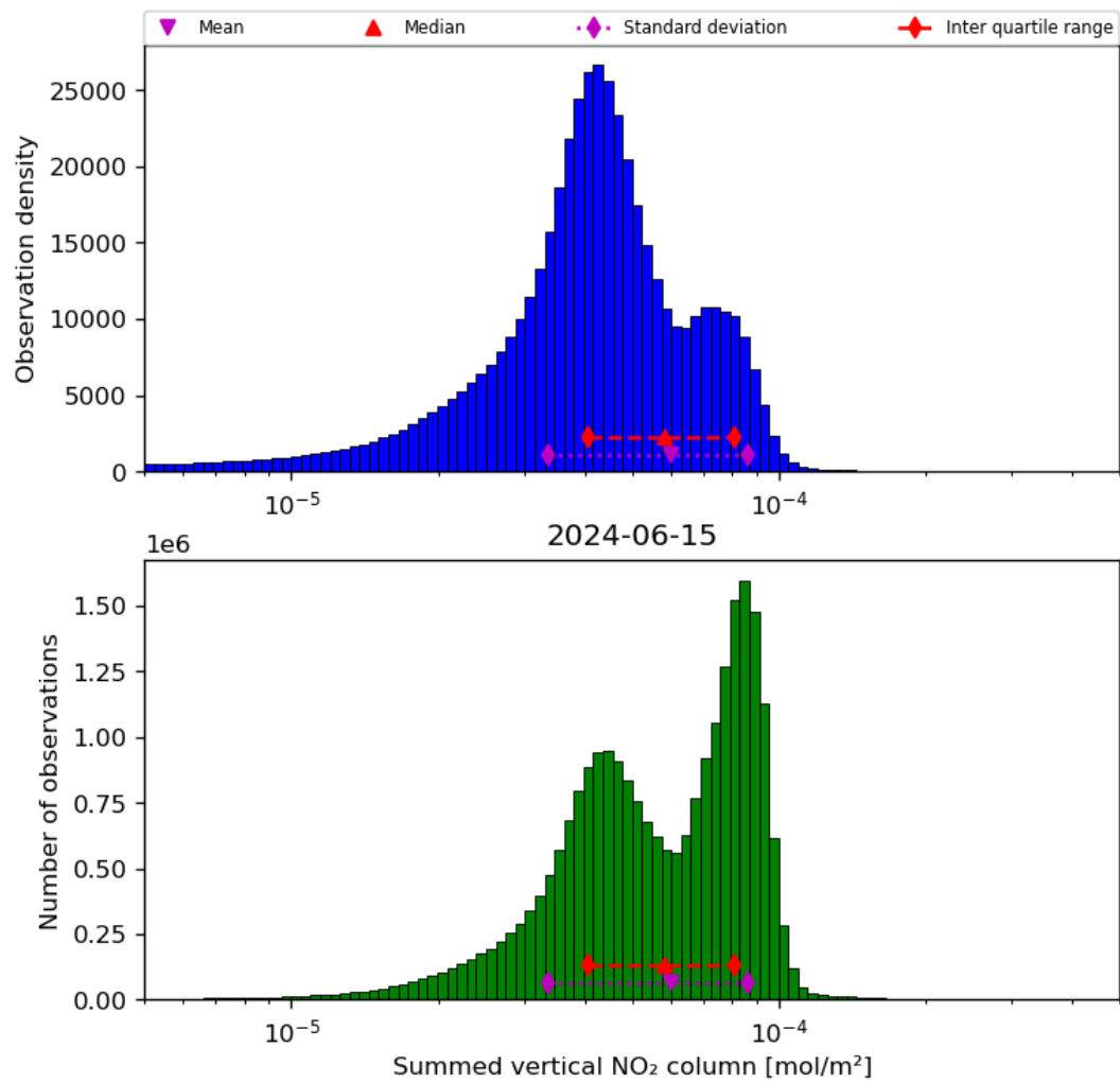
Figure 40: Histogram of “Summed vertical NO 2 column” for 2024-06-14 to 2024-06-16
