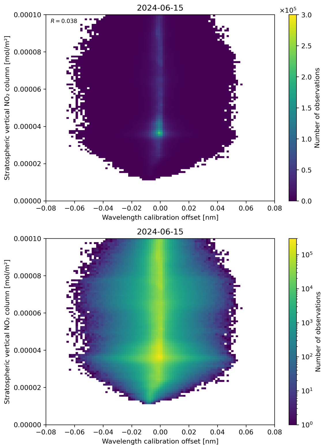
Figure 176: Scatter density plot of “Wavelength calibration offset” against “Stratospheric vertical NO 2 column” for 2024-06-14 to 2024-06-16.
