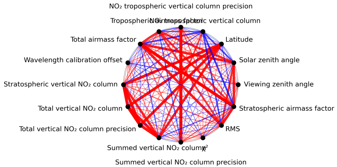
Figure 1: Map of correlation graph for 2024-06-14 to 2024-06-16.
