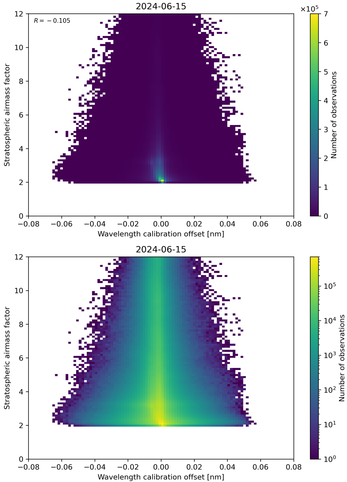
Figure 174: Scatter density plot of “Wavelength calibration offset” against “Stratospheric airmass factor” for 2024-06-14 to 2024-06-16.
