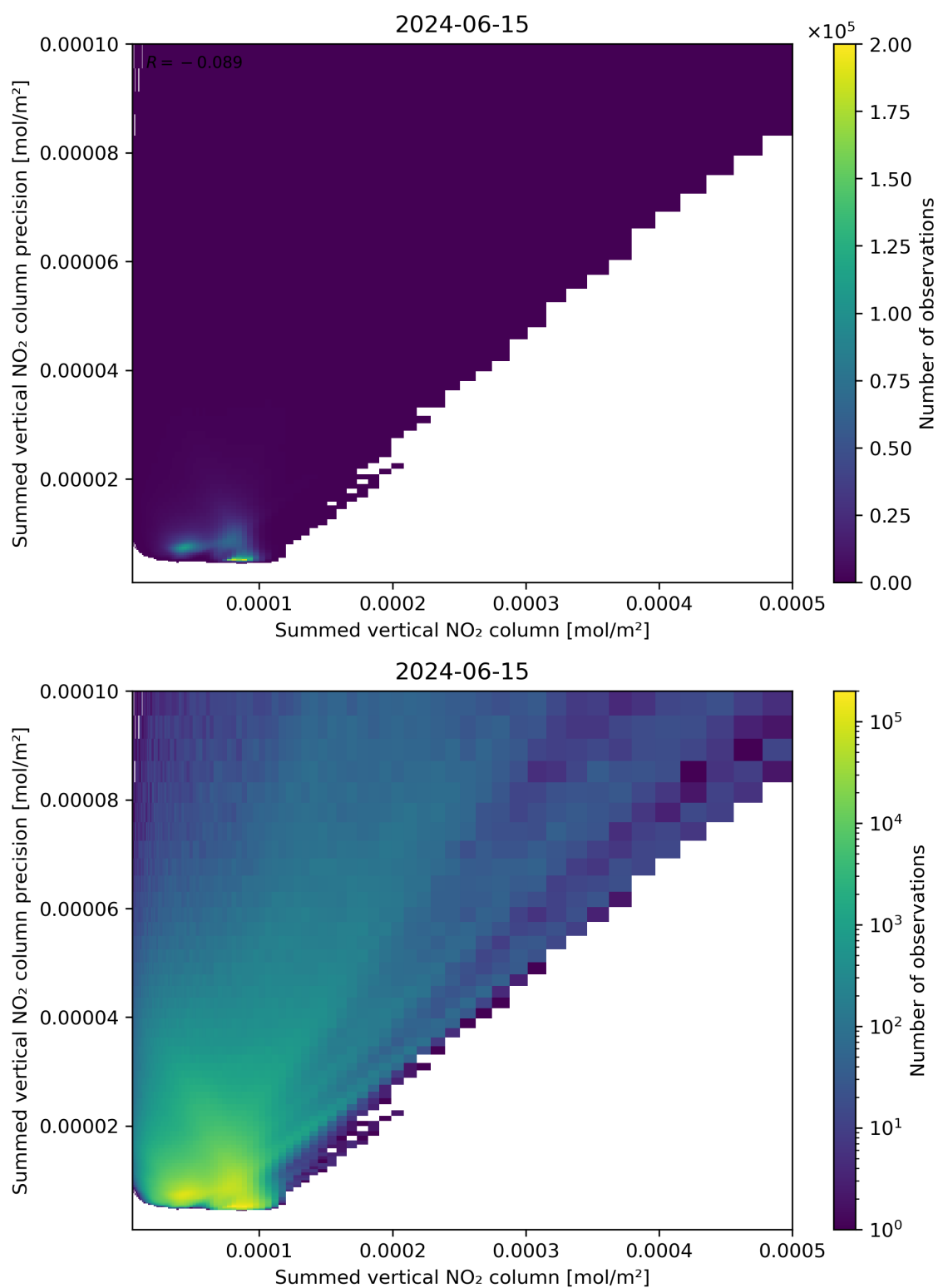
Figure 105: Scatter density plot of “Summed vertical NO 2 column” against “Summed vertical NO 2 column precision” for 2024-06-14 to 2024-06-16.
