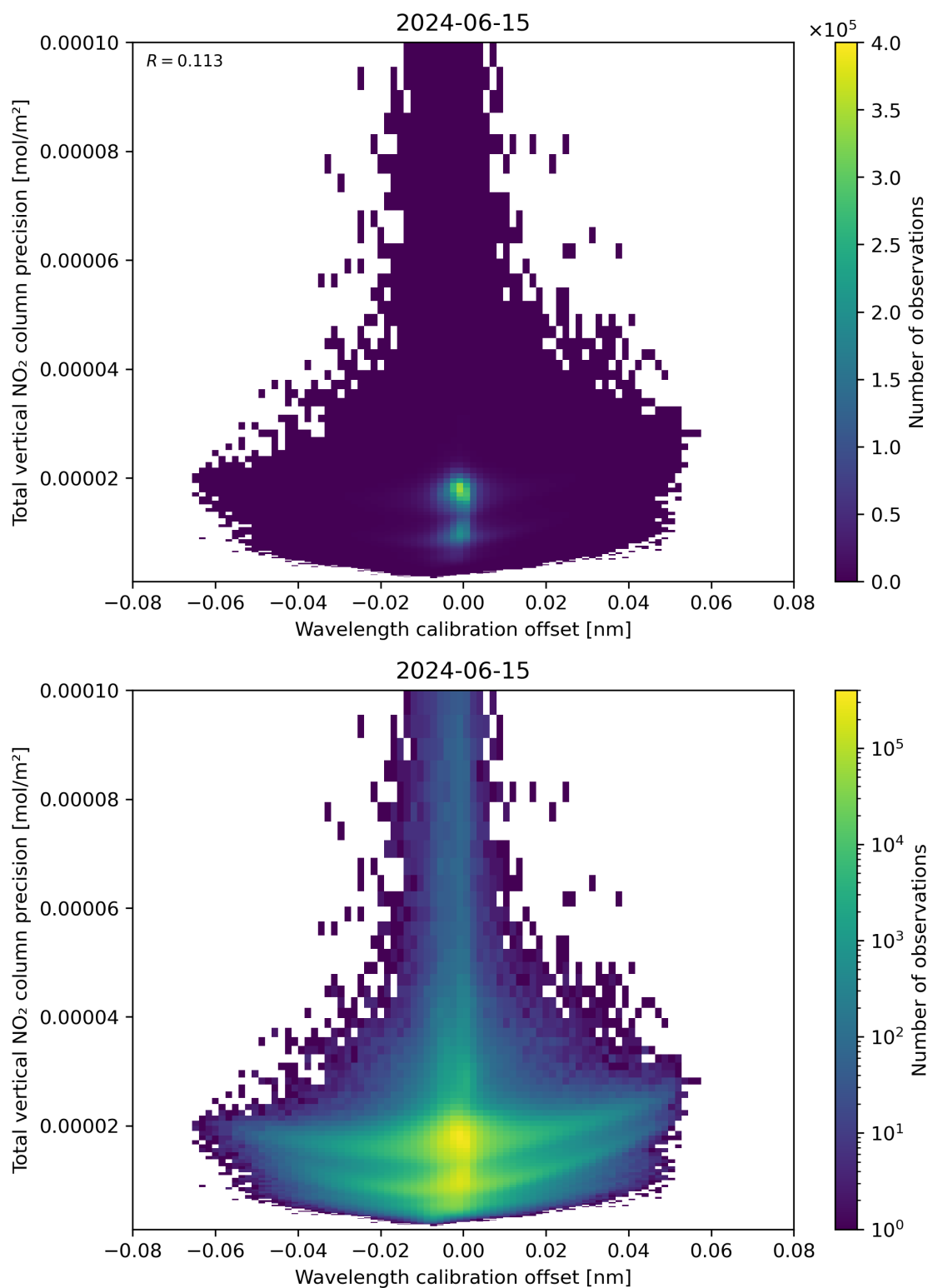
Figure 180: Scatter density plot of “Wavelength calibration offset” against “Total vertical NO 2 column precision” for 2024-06-14 to 2024-06-16.
