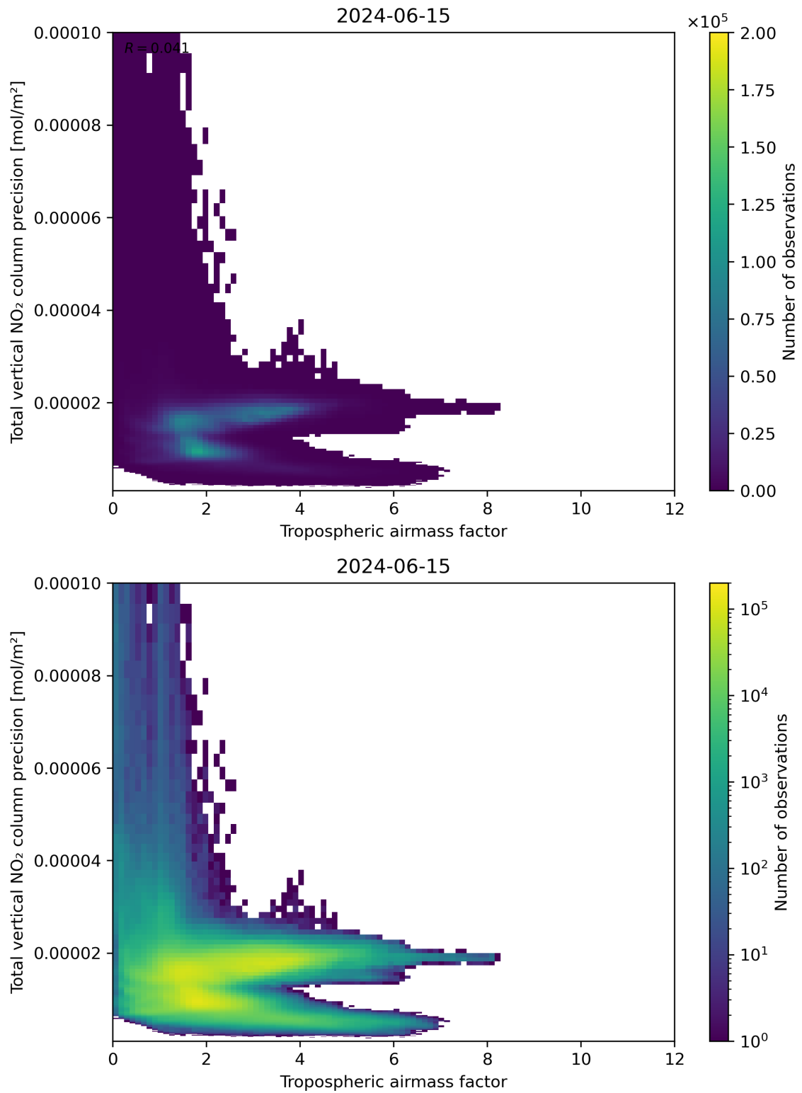
Figure 78: Scatter density plot of “Tropospheric air mass factor” against “Total vertical NO 2 column precision” for 2024-06-14 to 2024-06-16.
