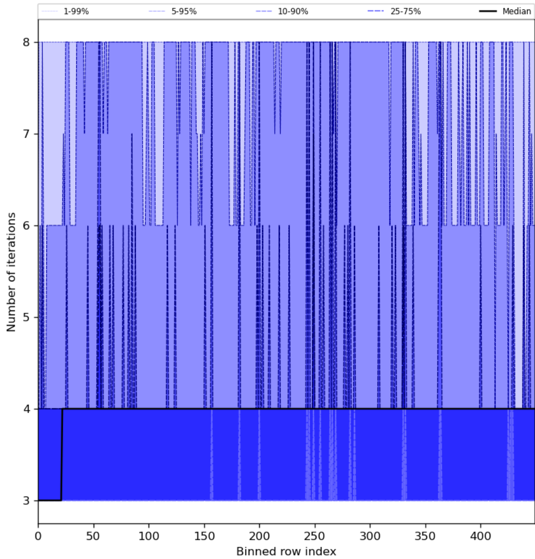
Figure 51: Along track statistics of “Number of iterations” for 2024-06-14 to 2024-06-16
