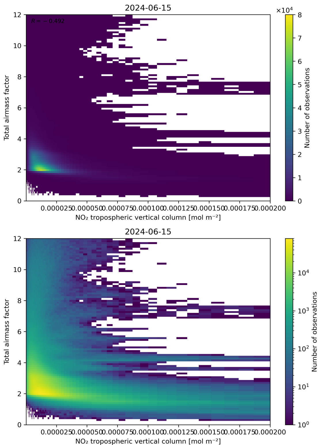
Figure 122: Scatter density plot of “NO 2 tropospheric vertical column” against “Total air mass factor” for 2024-06-14 to 2024-06-16.
