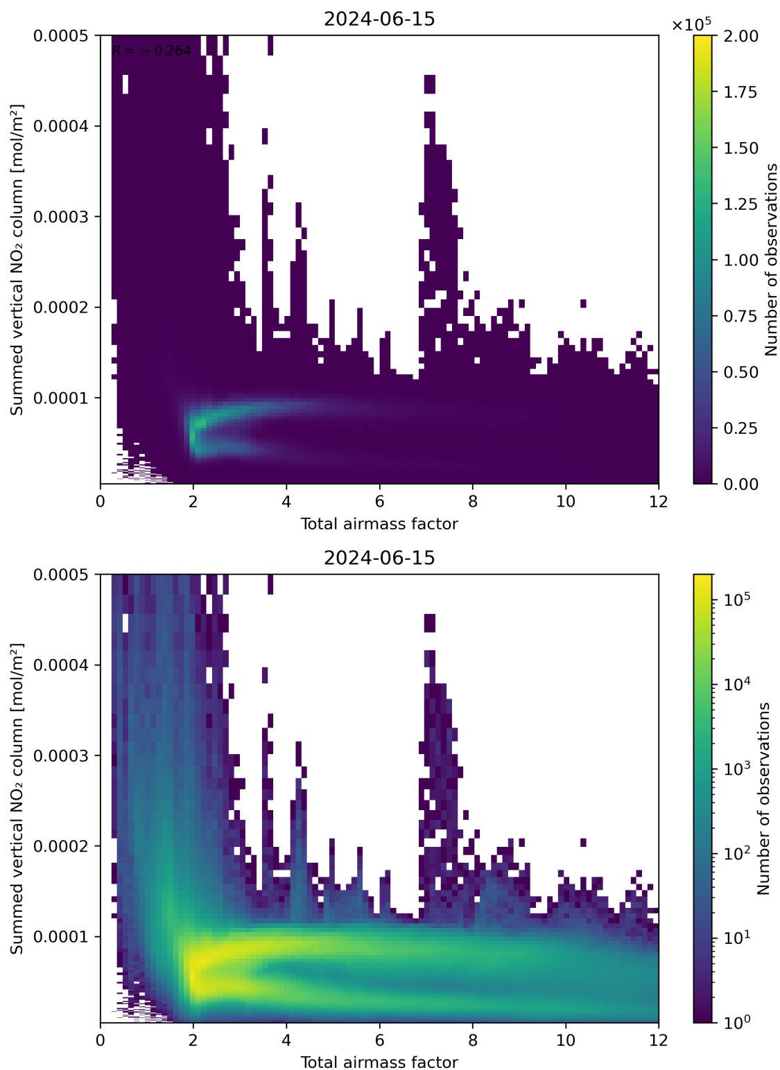
Figure 65: Scatter density plot of “Total airmass factor” against “Summed vertical NO 2 column” for 2024-06-14 to 2024-06-16.
