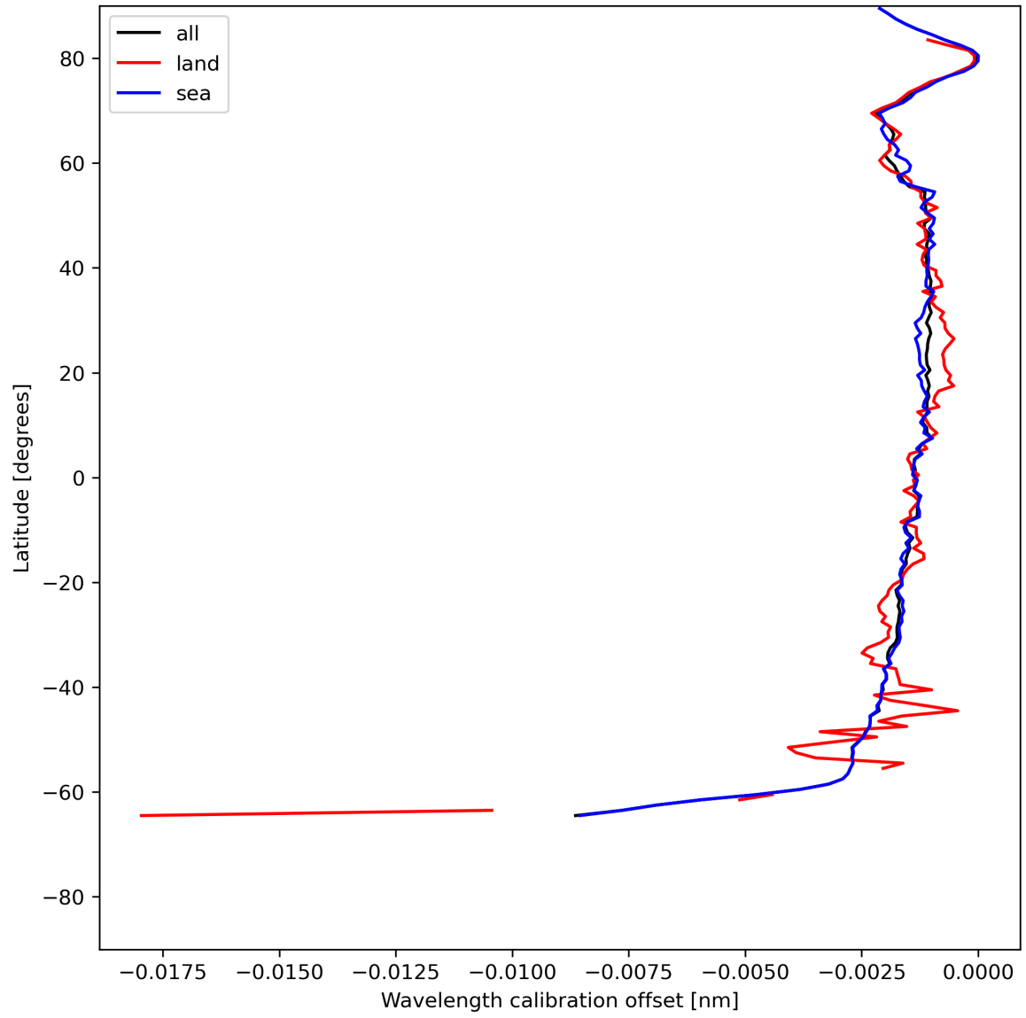
Figure 18: Zonal average of “Wavelength calibration offset” for 2024-06-14 to 2024-06-16.
