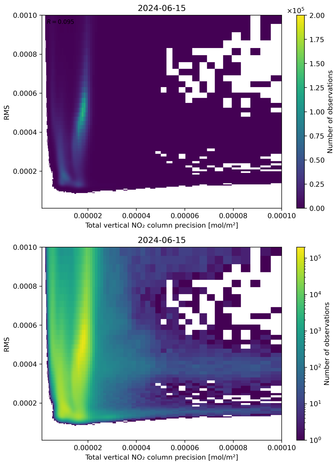
Figure 119: Scatter density plot of “Total vertical NO 2 column precision” against “RMS” for 2024-06-14 to 2024-06-16.
