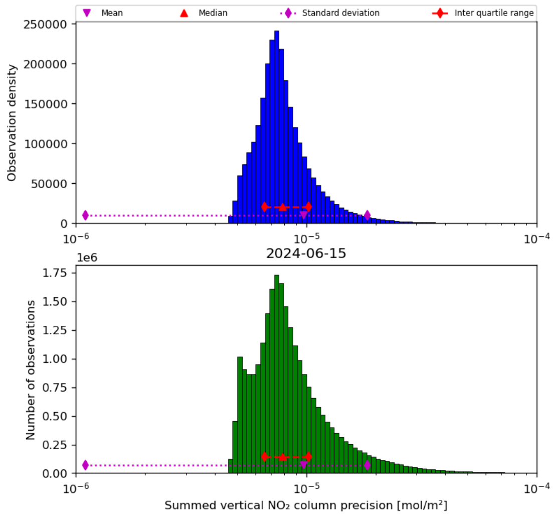
Figure 41: Histogram of "Summed vertical NO 2 column precision" for 2024-06-14 to 2024-06-16
