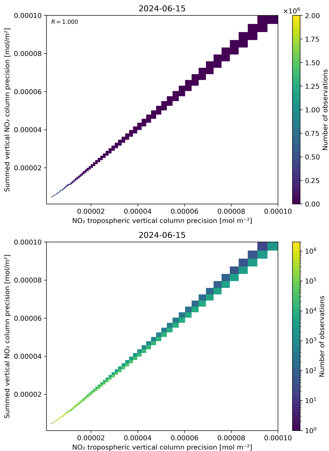
Figure 137: Scatter density plot of “NO 2 tropospheric vertical column precision” against “Summed vertical NO 2 column precision” for 2024-06-14 to 2024-06-16.
