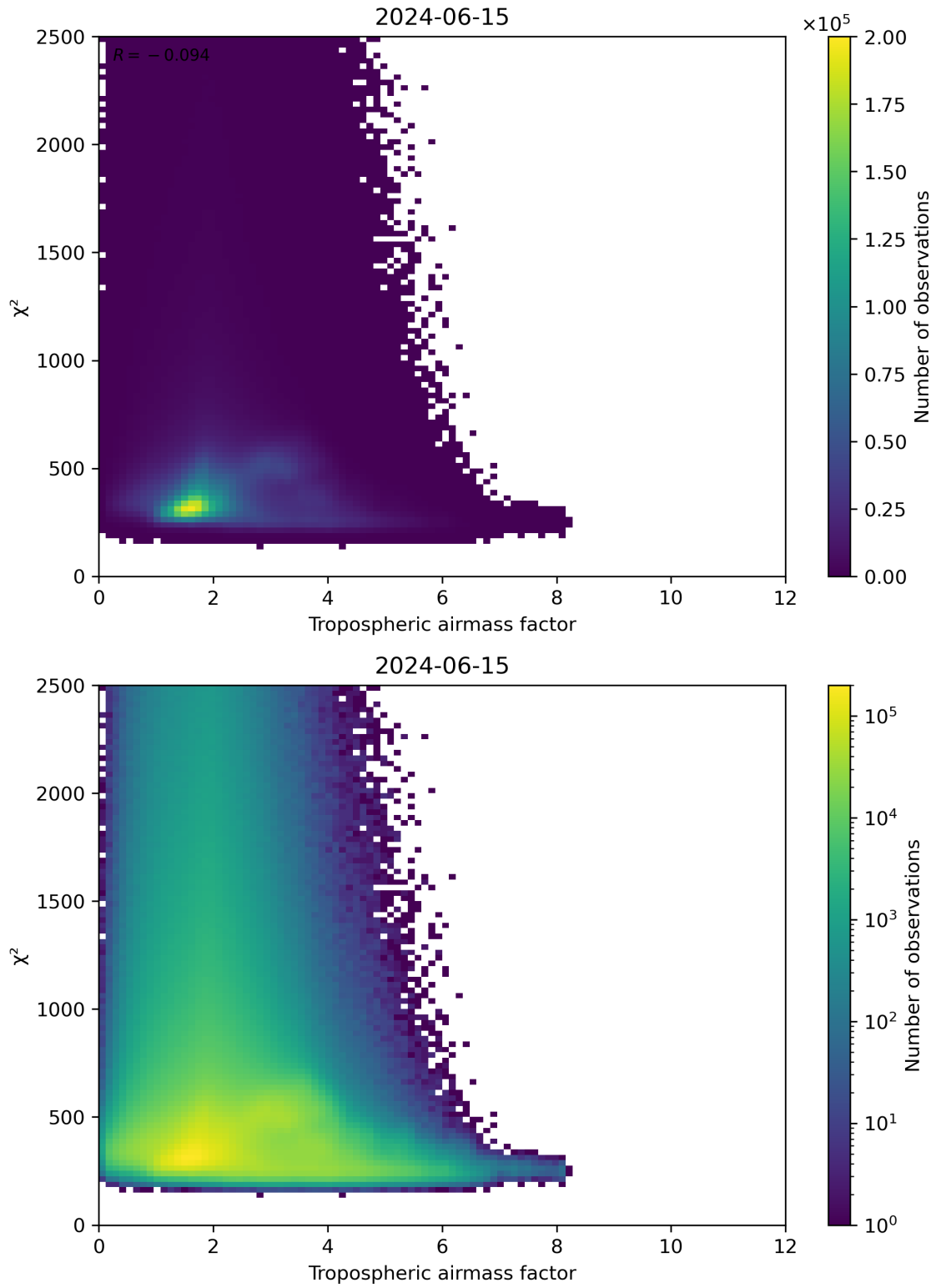
Figure 73: Scatter density plot of “Tropospheric airmass factor” against “ \chi^2 ” for 2024-06-14 to 2024-06-16.
