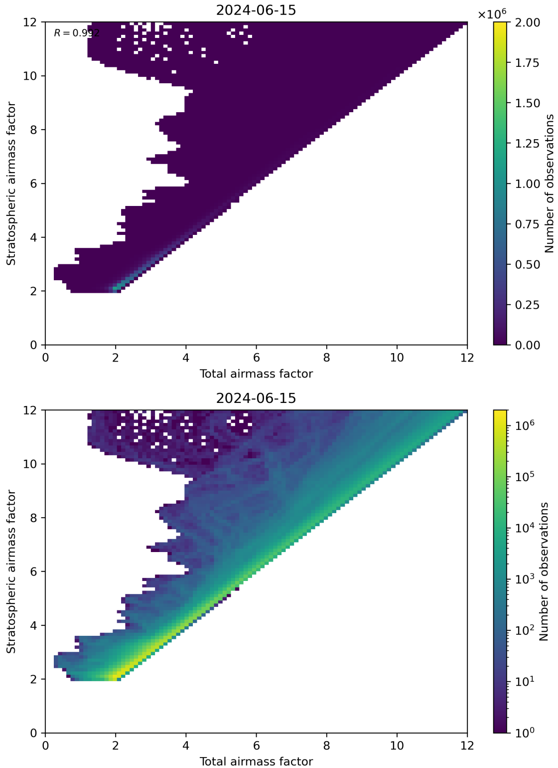
Figure 62: Scatter density plot of “Total airmass factor” against “Stratospheric airmass factor” for 2024-06-14 to 2024-06-16.
