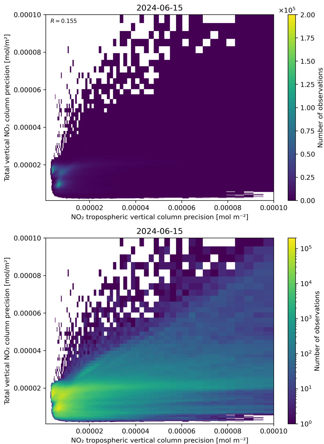
Figure 139: Scatter density plot of “NO 2 tropospheric vertical column precision” against “Total vertical NO 2 column precision” for 2024-06-14 to 2024-06-16.
