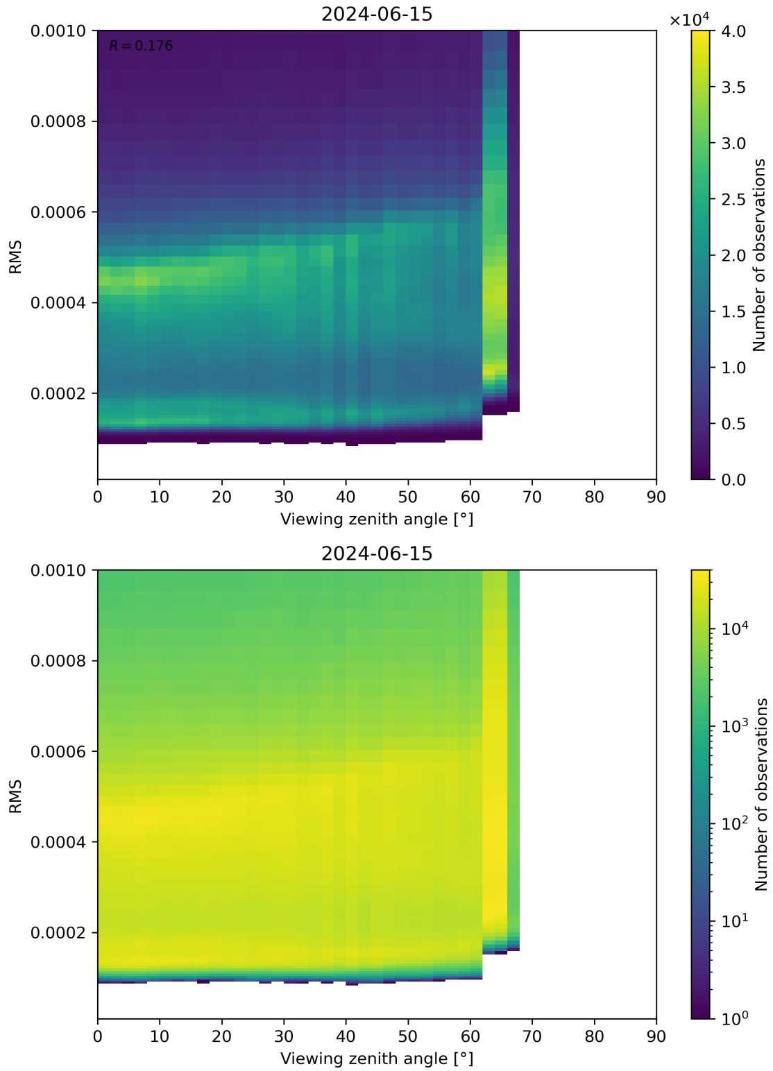
Figure 171: Scatter density plot of “Viewing zenith angle” against “RMS” for 2024-06-14 to 2024-06-16.
