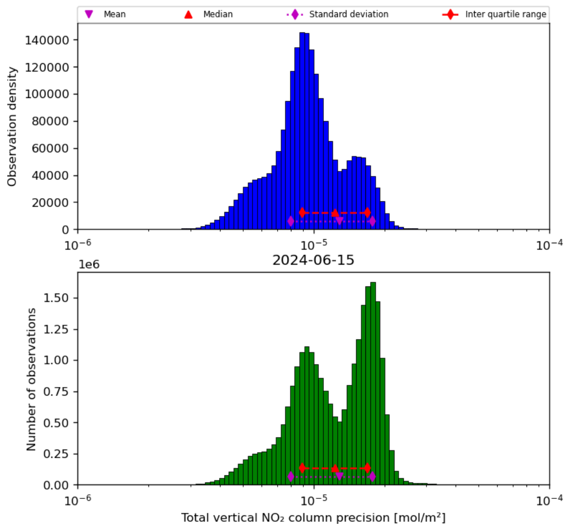
Figure 39: Histogram of “Total vertical NO 2 column precision” for 2024-06-14 to 2024-06-16
