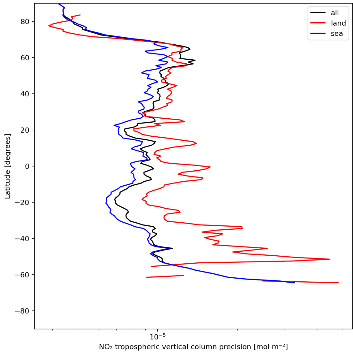
Figure 13: Zonal average of “NO 2 tropospheric vertical column precision” for 2024-06-14 to 2024-06-16.
