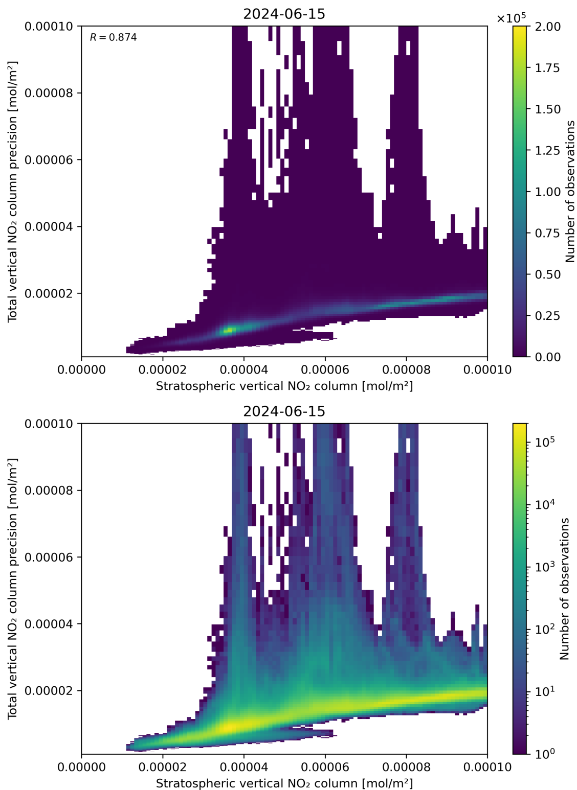
Figure 101: Scatter density plot of “Stratospheric vertical NO 2 column” against “Total vertical NO 2 column precision” for 2024-06-14 to 2024-06-16.
