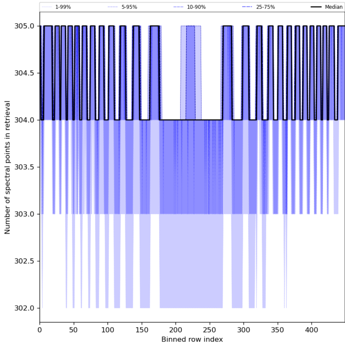
Figure 50: Along track statistics of “Number of spectral points in retrieval” for 2024-06-14 to 2024-06-16
