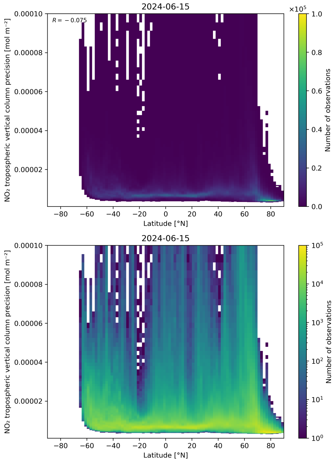
Figure 93: Scatter density plot of “Latitude” against “NO 2 tropospheric vertical column precision” for 2024-06-14 to 2024-06-16.
