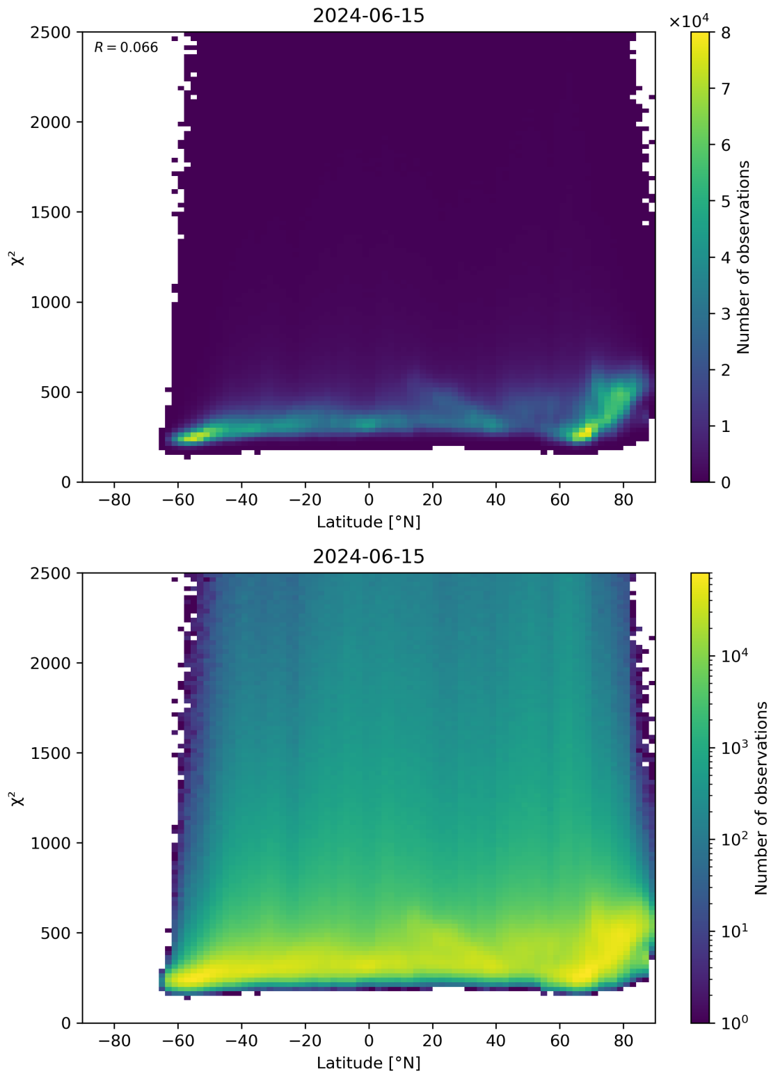
Figure 86: Scatter density plot of “Latitude” against “ \chi^2 ” for 2024-06-14 to 2024-06-16.
