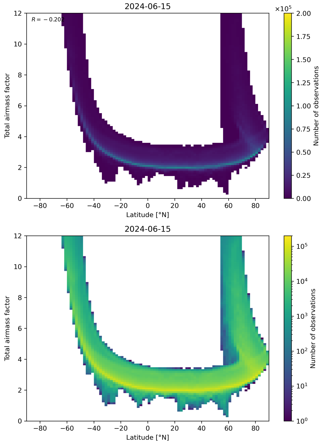
Figure 84: Scatter density plot of “Latitude” against “Total airmass factor” for 2024-06-14 to 2024-06-16.
