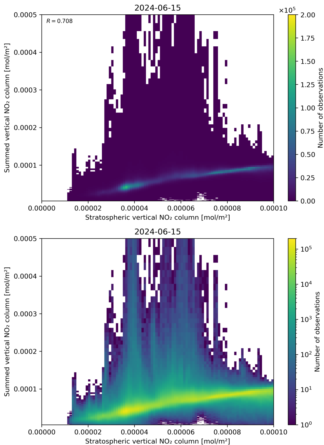
Figure 98: Scatter density plot of “Stratospheric vertical NO 2 column” against “Summed vertical NO 2 column” for 2024-06-14 to 2024-06-16.
