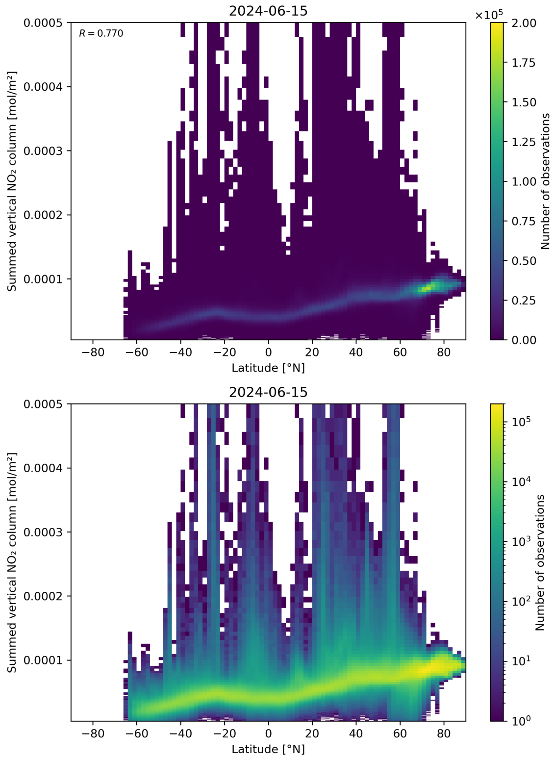
Figure 88: Scatter density plot of “Latitude” against “Summed vertical NO 2 column” for 2024-06-14 to 2024-06-16.
