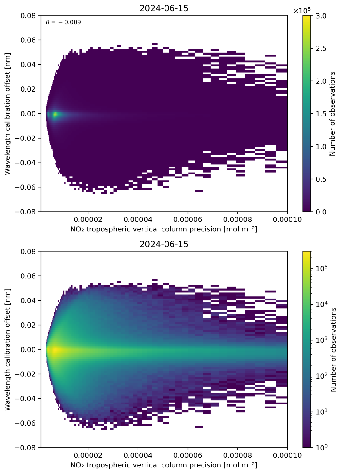
Figure 141: Scatter density plot of “NO 2 tropospheric vertical column precision” against “Wavelength calibration offset” for 2024-06-14 to 2024-06-16.
