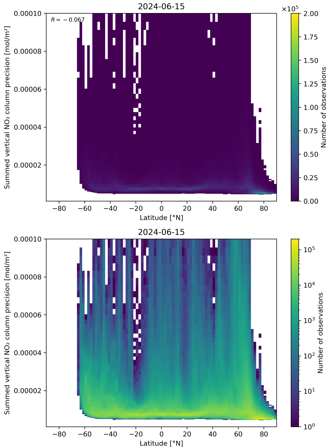
Figure 89: Scatter density plot of “Latitude” against “Summed vertical NO 2 column precision” for 2024-06-14 to 2024-06-16.
