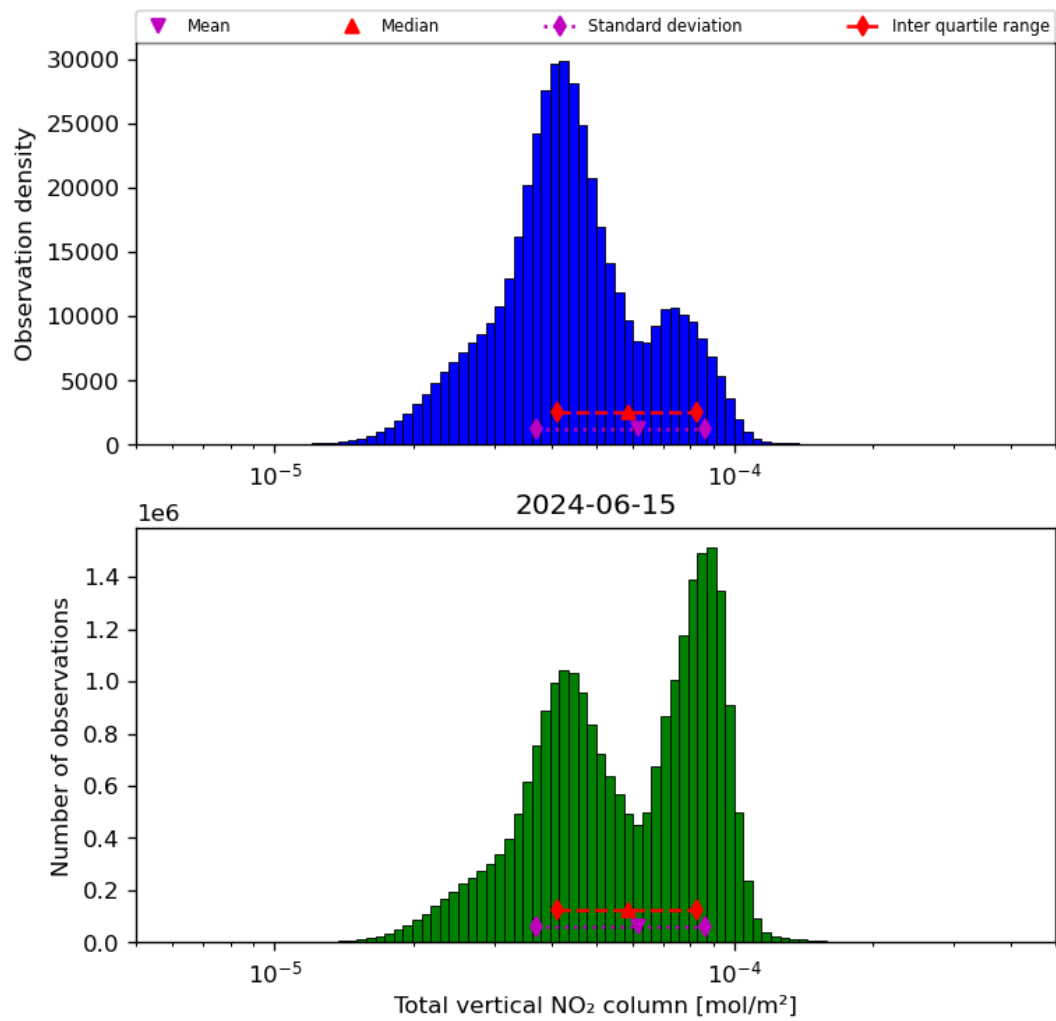
Figure 38: Histogram of “Total vertical NO 2 column” for 2024-06-14 to 2024-06-16
