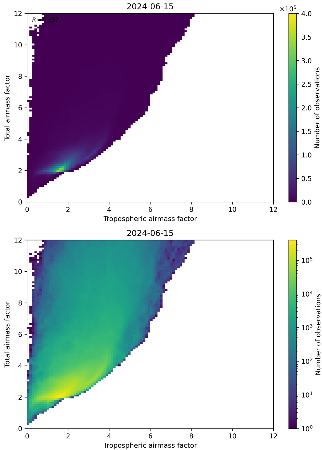
Figure 72: Scatter density plot of “Tropospheric airmass factor” against “Total airmass factor” for 2024-06-14 to 2024-06-16.
