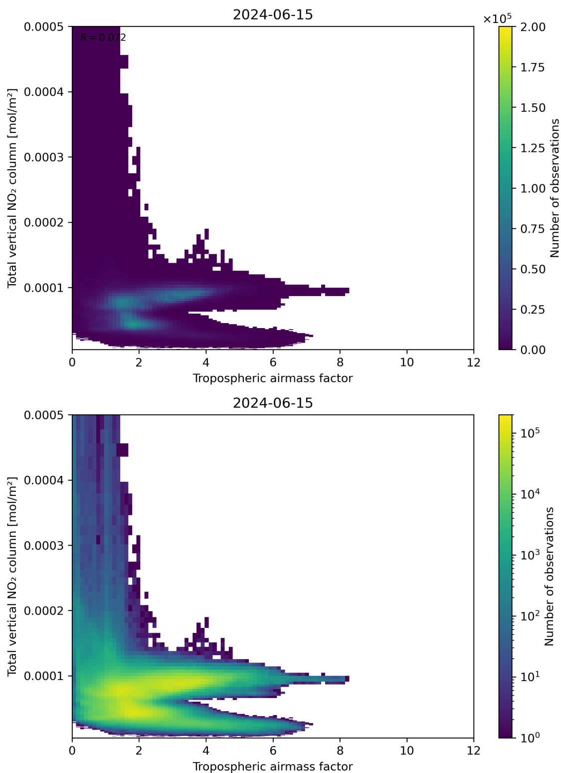
Figure 77: Scatter density plot of “Tropospheric airmass factor” against “Total vertical NO 2 column” for 2024-06-14 to 2024-06-16.
