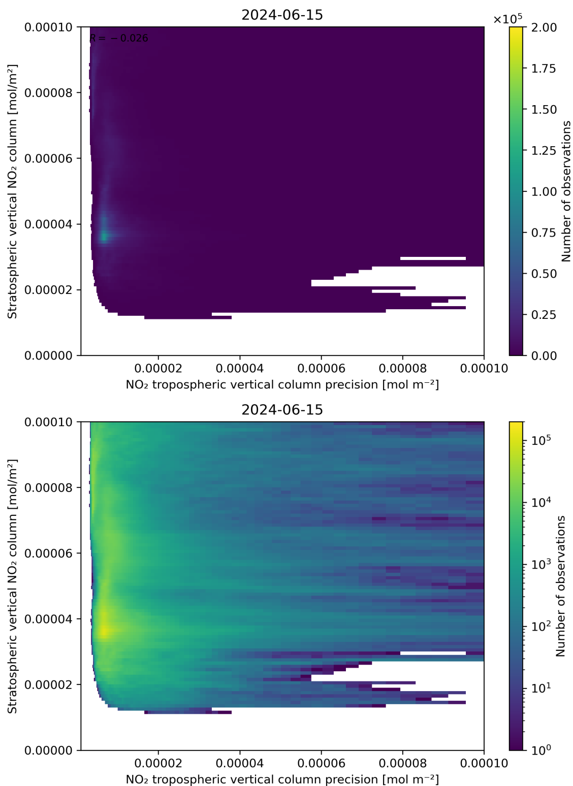
Figure 135: Scatter density plot of “NO 2 tropospheric vertical column precision” against “Stratospheric vertical NO 2 column” for 2024-06-14 to 2024-06-16.
