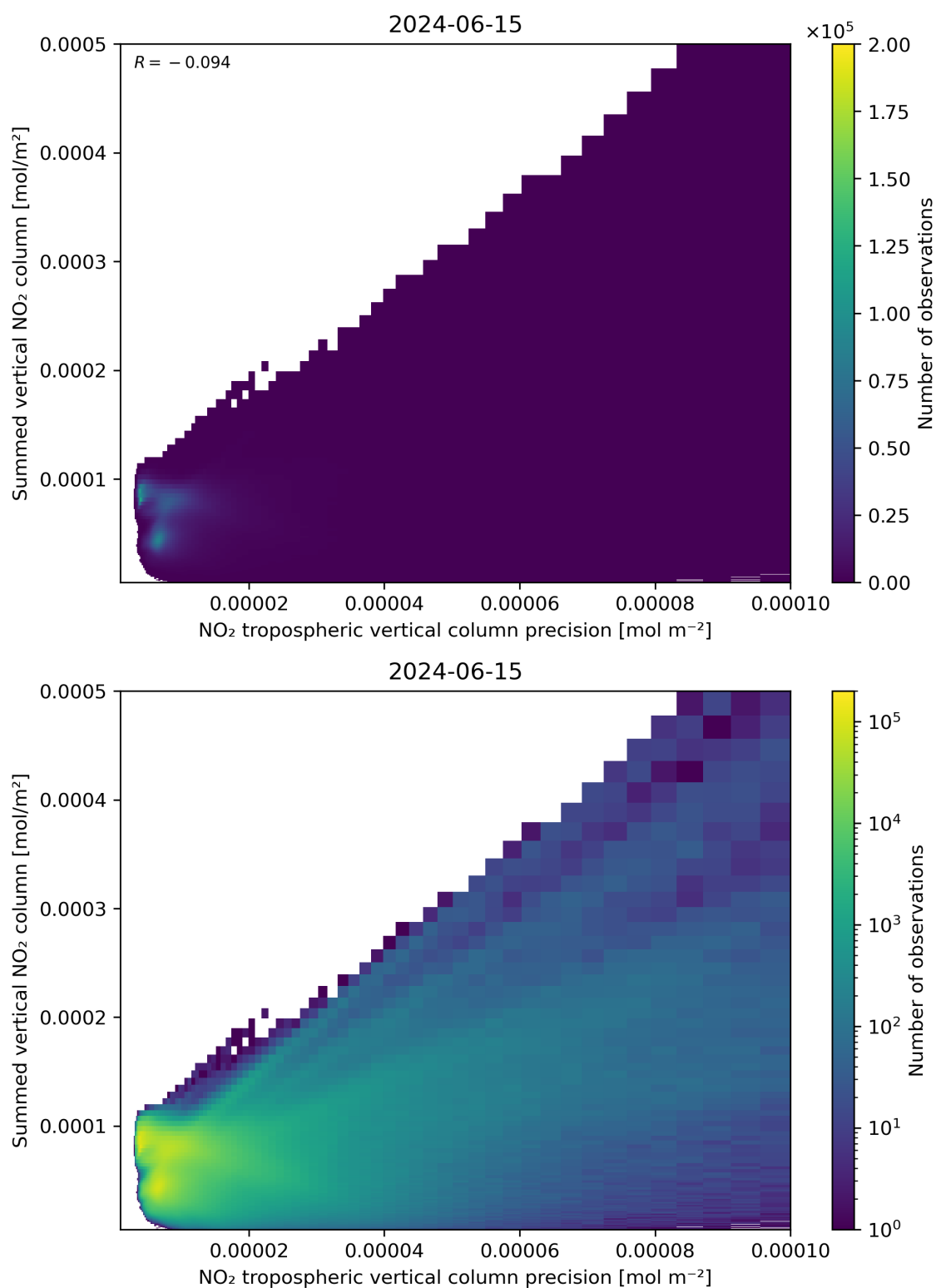
Figure 136: Scatter density plot of “NO 2 tropospheric vertical column precision” against “Summed vertical NO 2 column” for 2024-06-14 to 2024-06-16.
