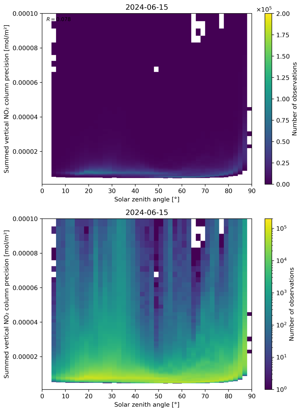
Figure 152: Scatter density plot of “Solar zenith angle” against “Summed vertical NO 2 column precision” for 2024-06-14 to 2024-06-16.
