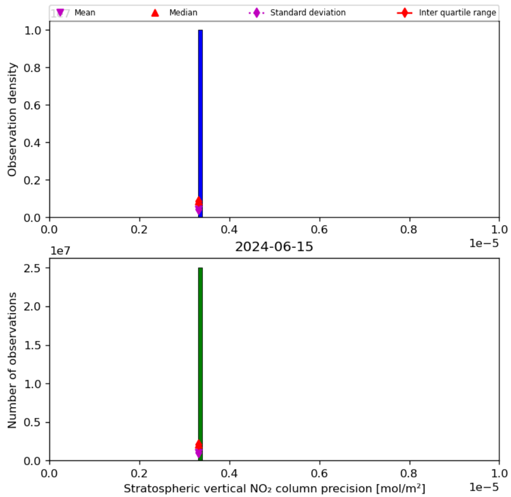
Figure 37: Histogram of “Stratospheric vertical NO 2 column precision” for 2024-06-14 to 2024-06-16
