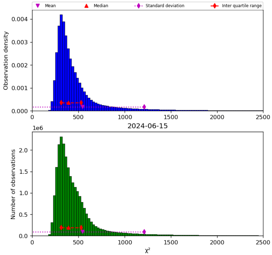
Figure 42: Histogram of “ \chi^2 ” for 2024-06-14 to 2024-06-16
