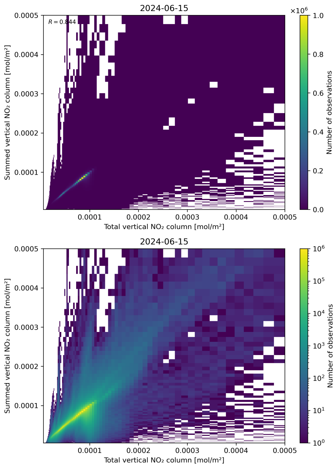
Figure 112: Scatter density plot of “Total vertical NO 2 column” against “Summed vertical NO 2 column” for 2024-06-14 to 2024-06-16.
