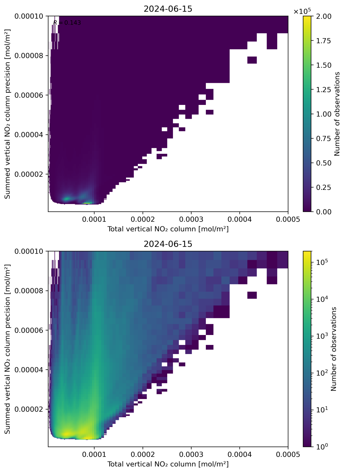
Figure 113: Scatter density plot of “Total vertical NO 2 column” against “Summed vertical NO 2 column precision” for 2024-06-14 to 2024-06-16.
