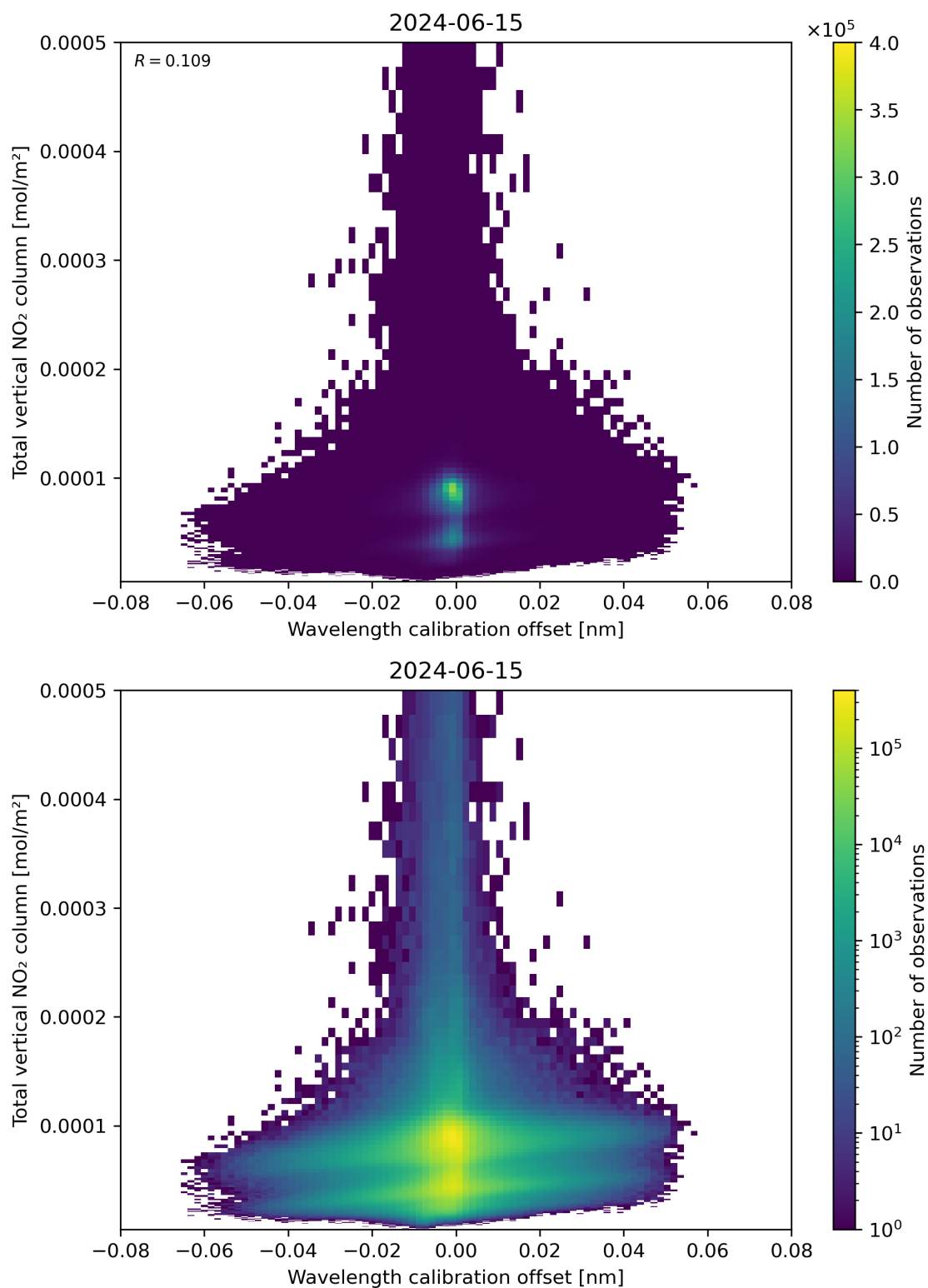
Figure 179: Scatter density plot of “Wavelength calibration offset” against “Total vertical NO 2 column” for 2024-06-14 to 2024-06-16.
