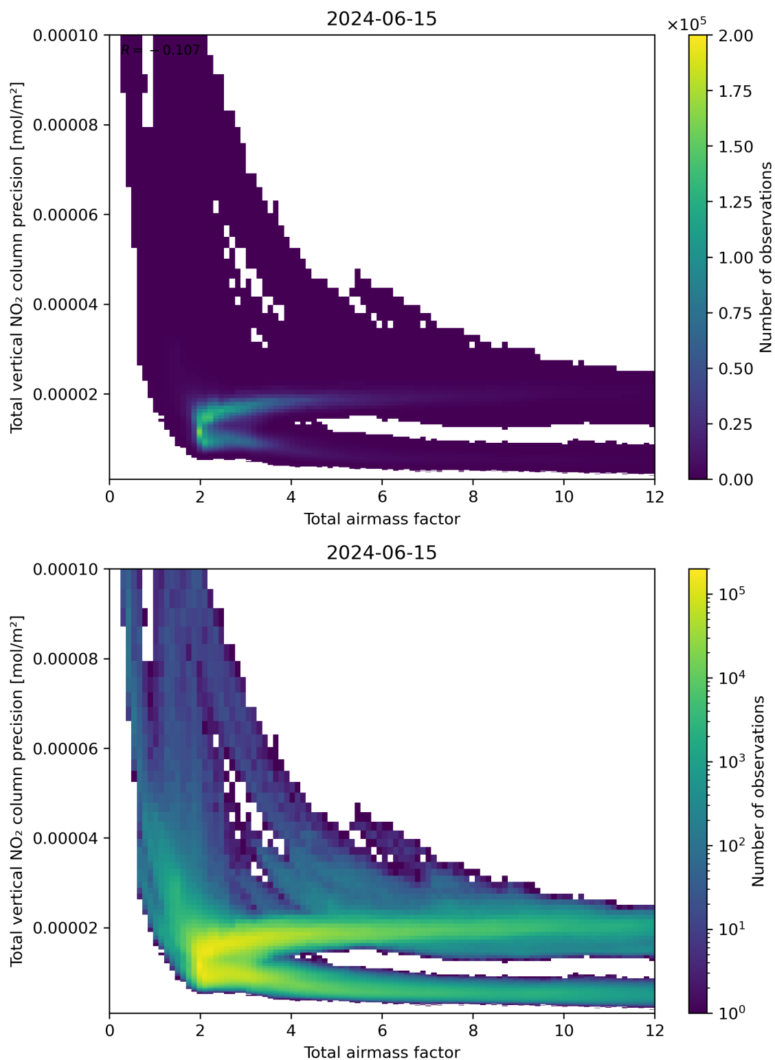
Figure 68: Scatter density plot of “Total airmass factor” against “Total vertical NO 2 column precision” for 2024-06-14 to 2024-06-16.
