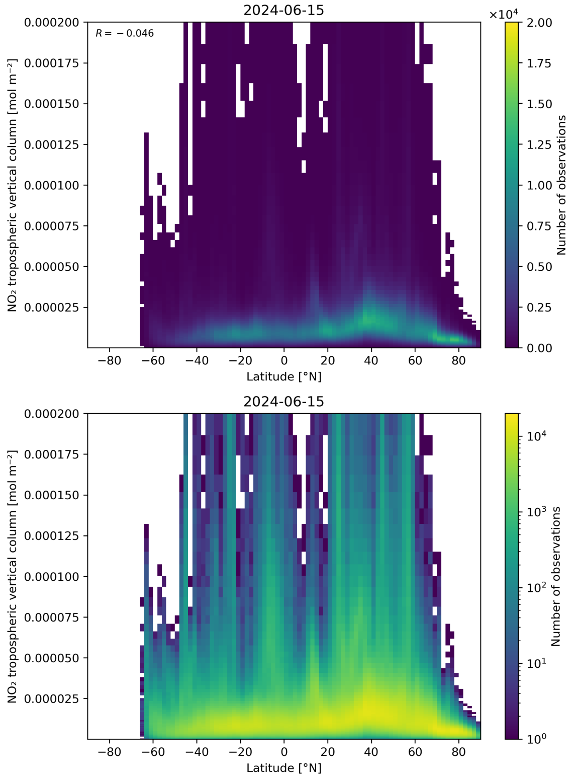
Figure 92: Scatter density plot of “Latitude” against “NO 2 tropospheric vertical column” for 2024-06-14 to 2024-06-16.
