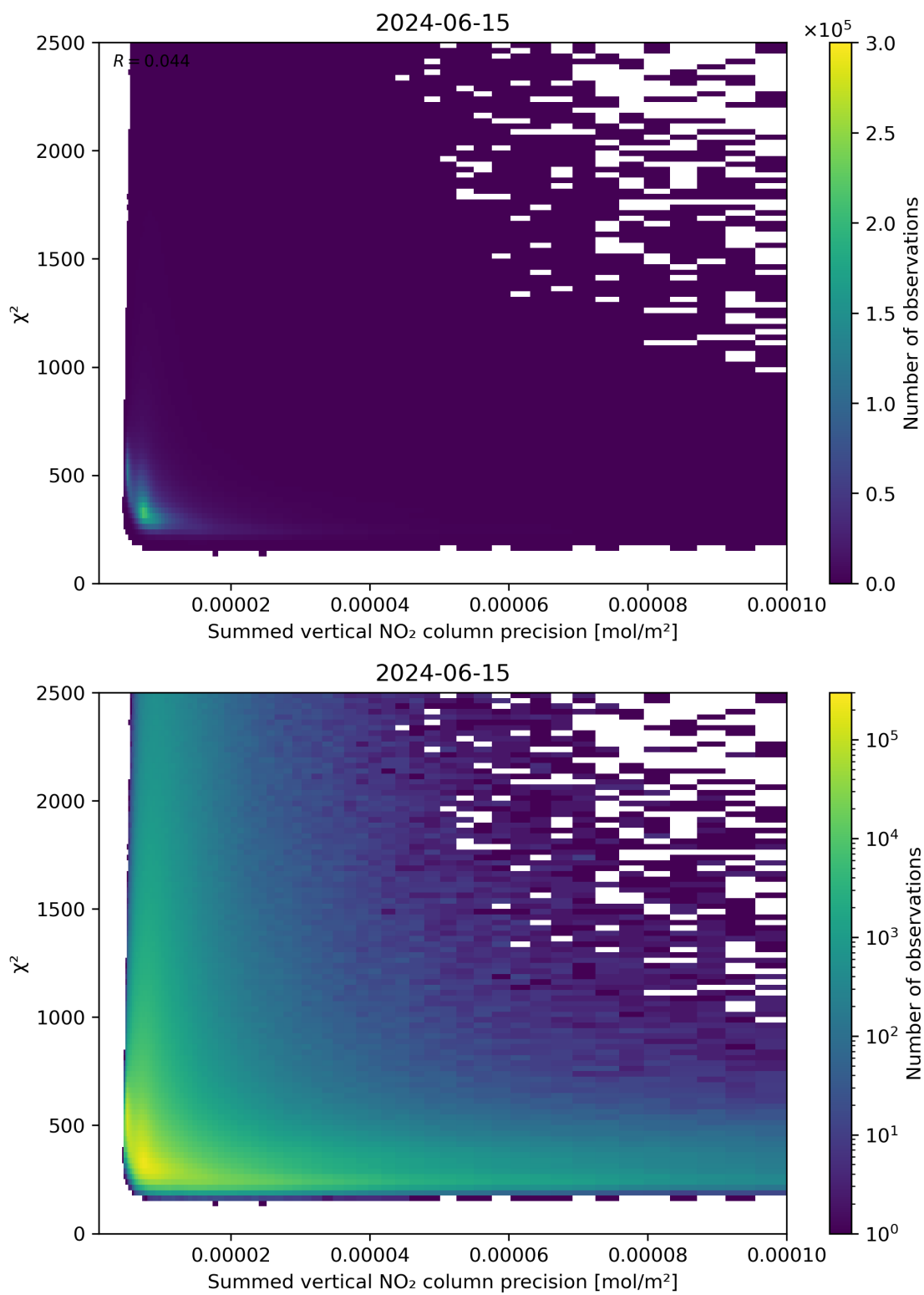
Figure 107: Scatter density plot of “Summed vertical NO 2 column precision” against “ \chi^2 ” for 2024-06-14 to 2024-06-16.
