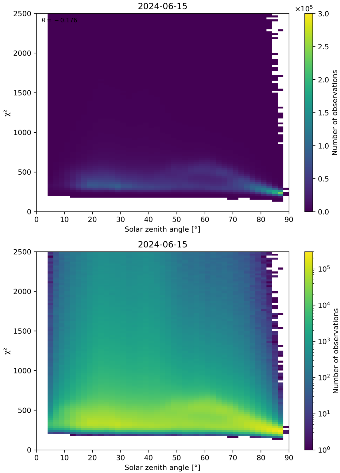
Figure 148: Scatter density plot of “Solar zenith angle” against “ \chi^2 ” for 2024-06-14 to 2024-06-16.
