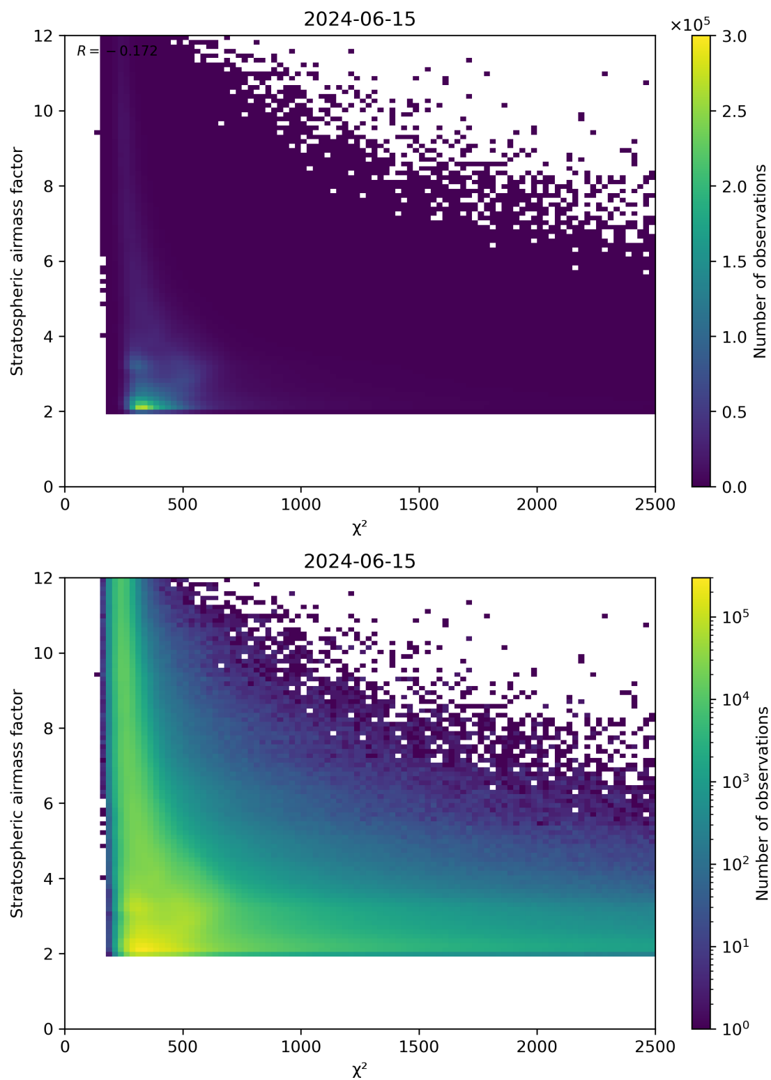
Figure 81: Scatter density plot of “ \chi^2 ” against “Stratospheric airmass factor” for 2024-06-14 to 2024-06-16.
