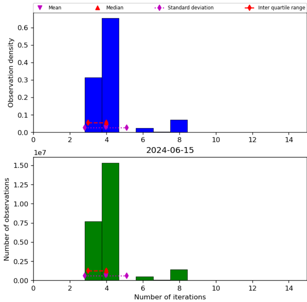
Figure 34: Histogram of “Number of iterations” for 2024-06-14 to 2024-06-16
