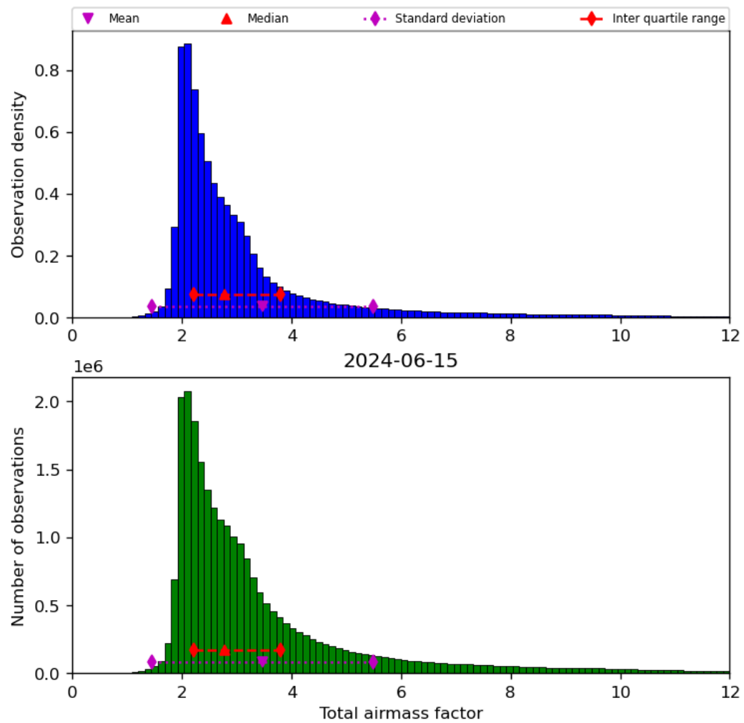
Figure 32: Histogram of “Total airmass factor” for 2024-06-14 to 2024-06-16
