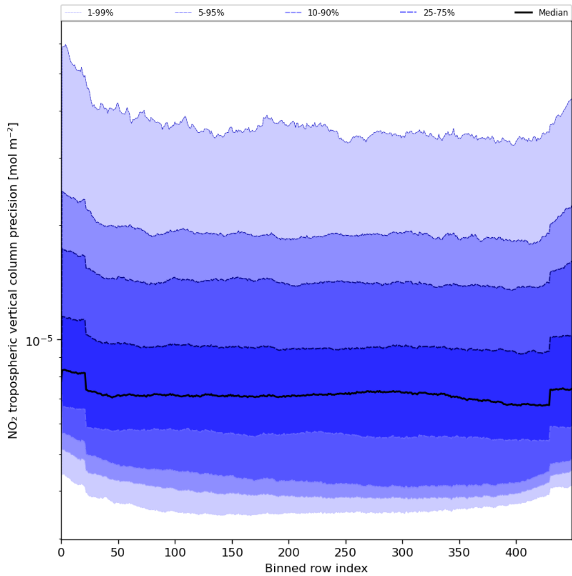
Figure 47: Along track statistics of “NO 2 tropospheric vertical column precision” for 2024-06-14 to 2024-06-16
