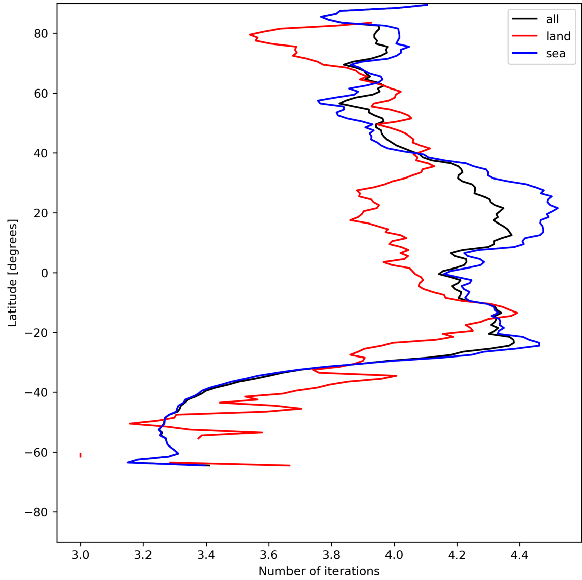
Figure 17: Zonal average of “Number of iterations” for 2024-06-14 to 2024-06-16.
