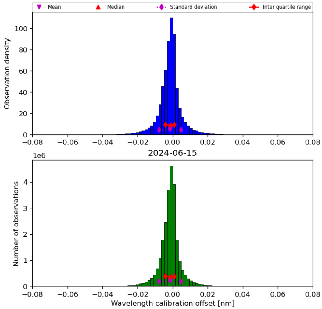
Figure 35: Histogram of “Wavelength calibration offset” for 2024-06-14 to 2024-06-16
