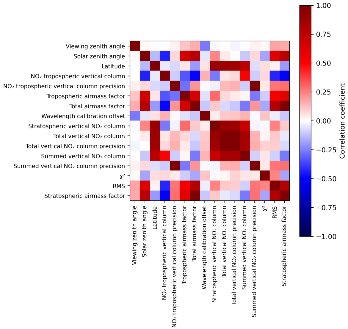
Figure 2: Map of correlation matrix for 2024-06-14 to 2024-06-16.
