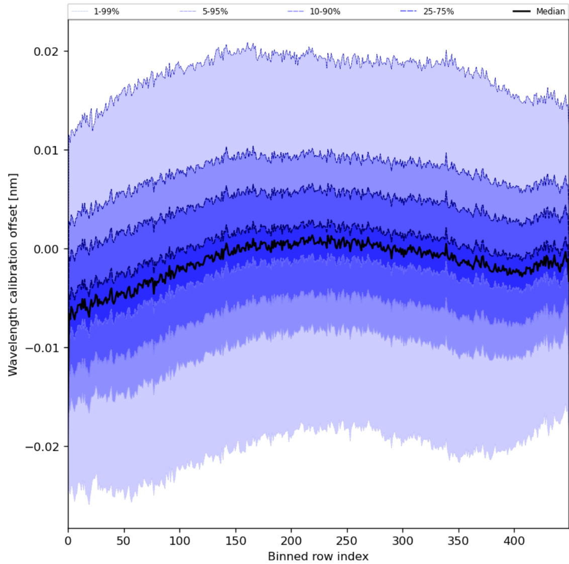
Figure 52: Along track statistics of “Wavelength calibration offset” for 2024-06-14 to 2024-06-16
