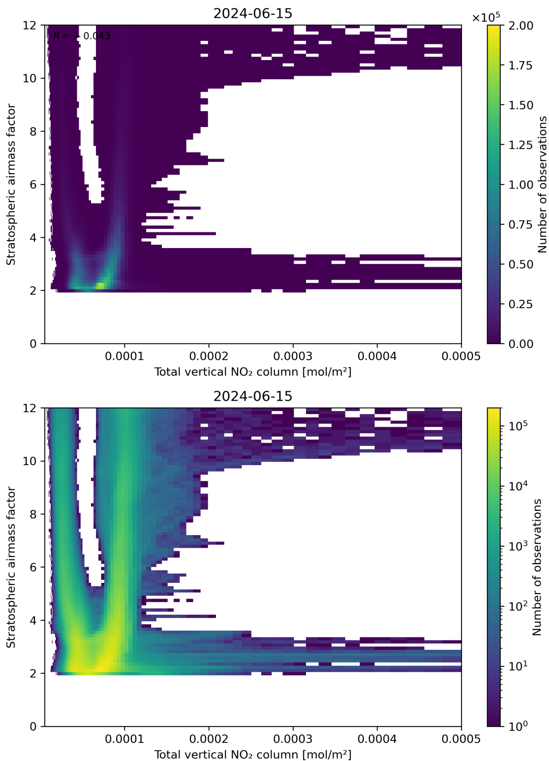
Figure 110: Scatter density plot of “Total vertical NO 2 column” against “Stratospheric airmass factor” for 2024-06-14 to 2024-06-16.
