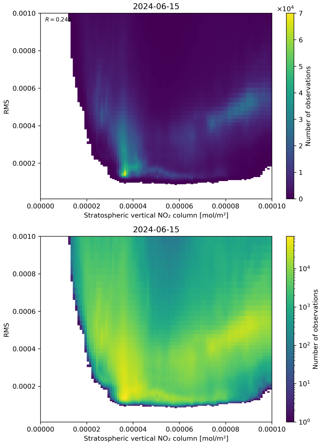
Figure 102: Scatter density plot of “Stratospheric vertical NO 2 column” against “RMS” for 2024-06-14 to 2024-06-16.
