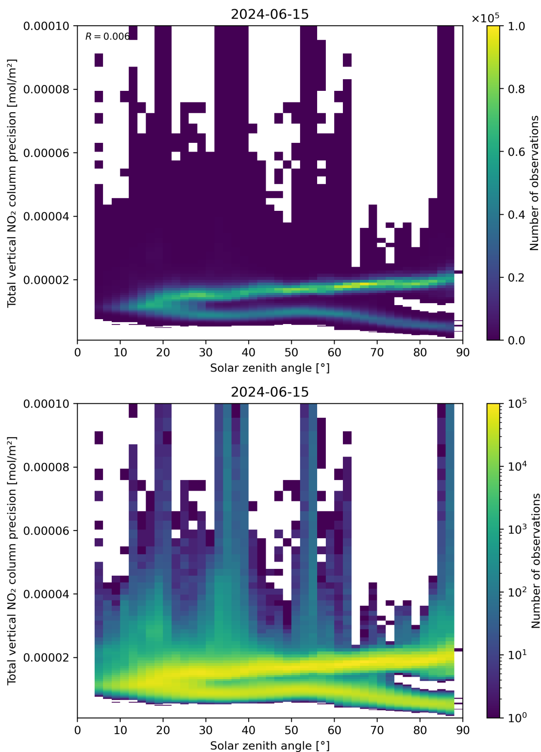
Figure 154: Scatter density plot of “Solar zenith angle” against “Total vertical NO 2 column precision” for 2024-06-14 to 2024-06-16.
