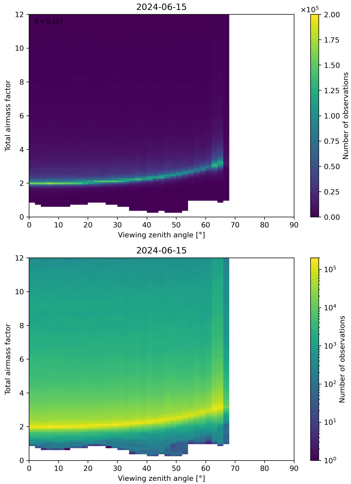
Figure 160: Scatter density plot of “Viewing zenith angle” against “Total airmass factor” for 2024-06-14 to 2024-06-16.
