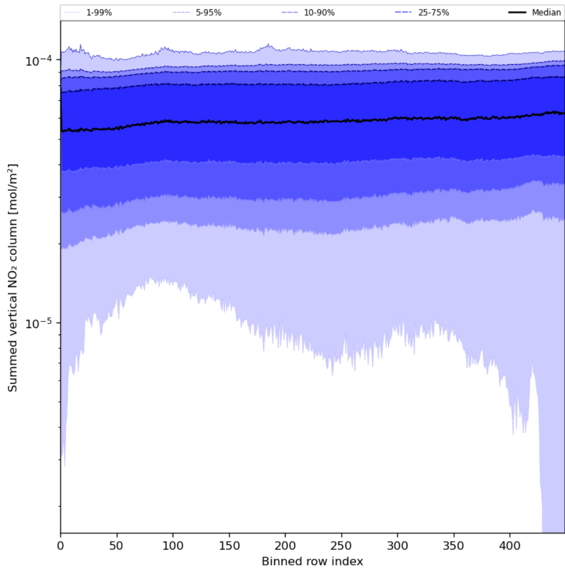
Figure 57: Along track statistics of “Summed vertical NO 2 column” for 2024-06-14 to 2024-06-16
