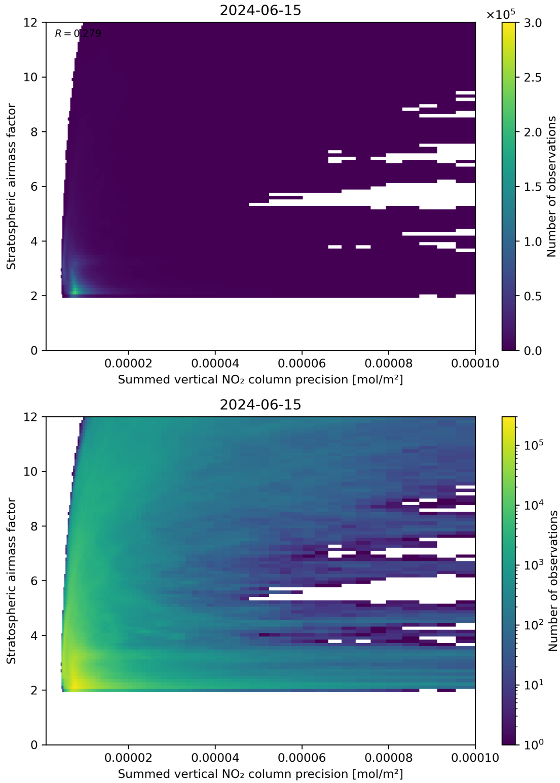
Figure 106: Scatter density plot of “Summed vertical NO 2 column precision” against “Stratospheric airmass factor” for 2024-06-14 to 2024-06-16.
