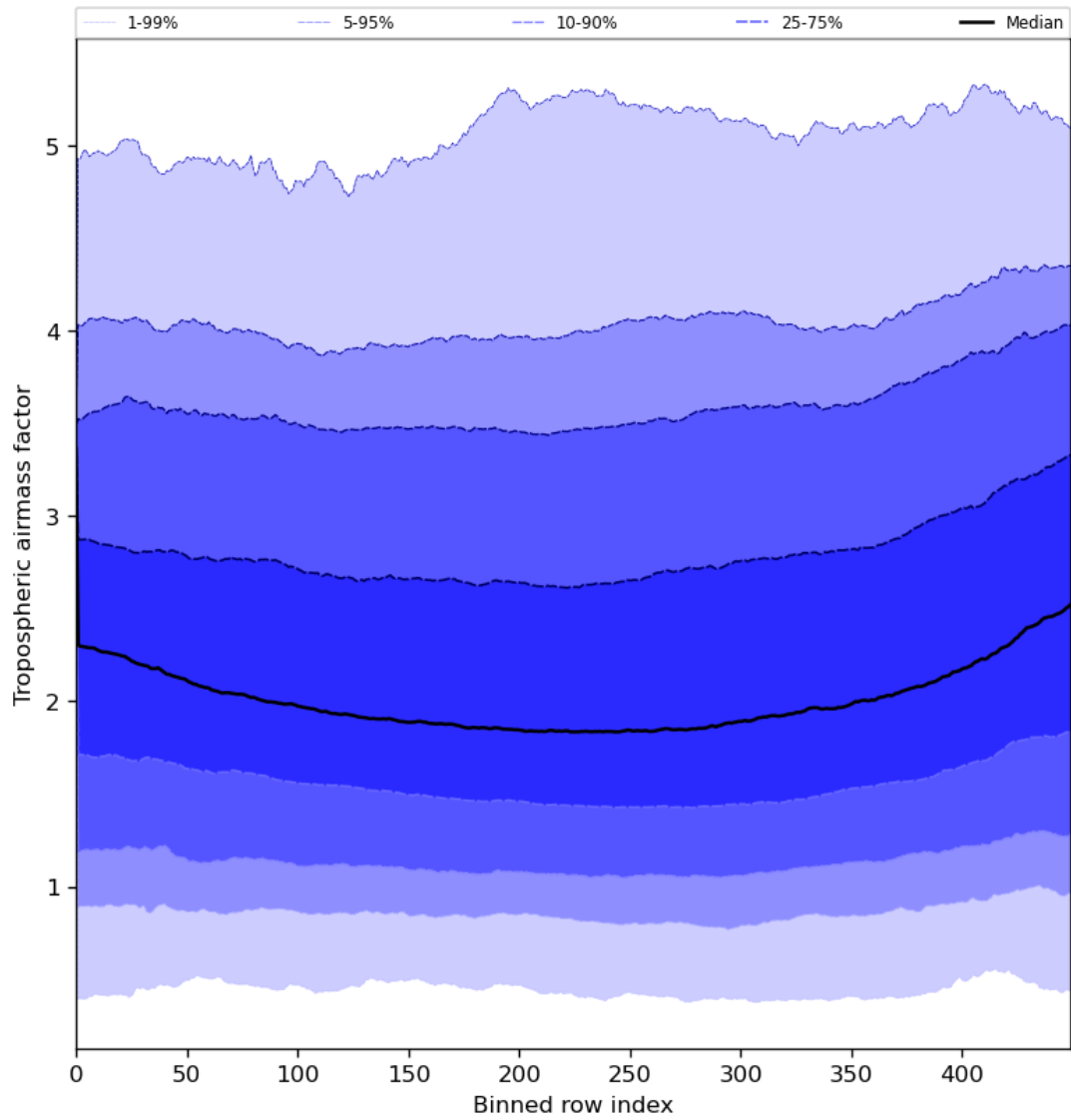
Figure 48: Along track statistics of “Tropospheric airmass factor” for 2024-06-14 to 2024-06-16
