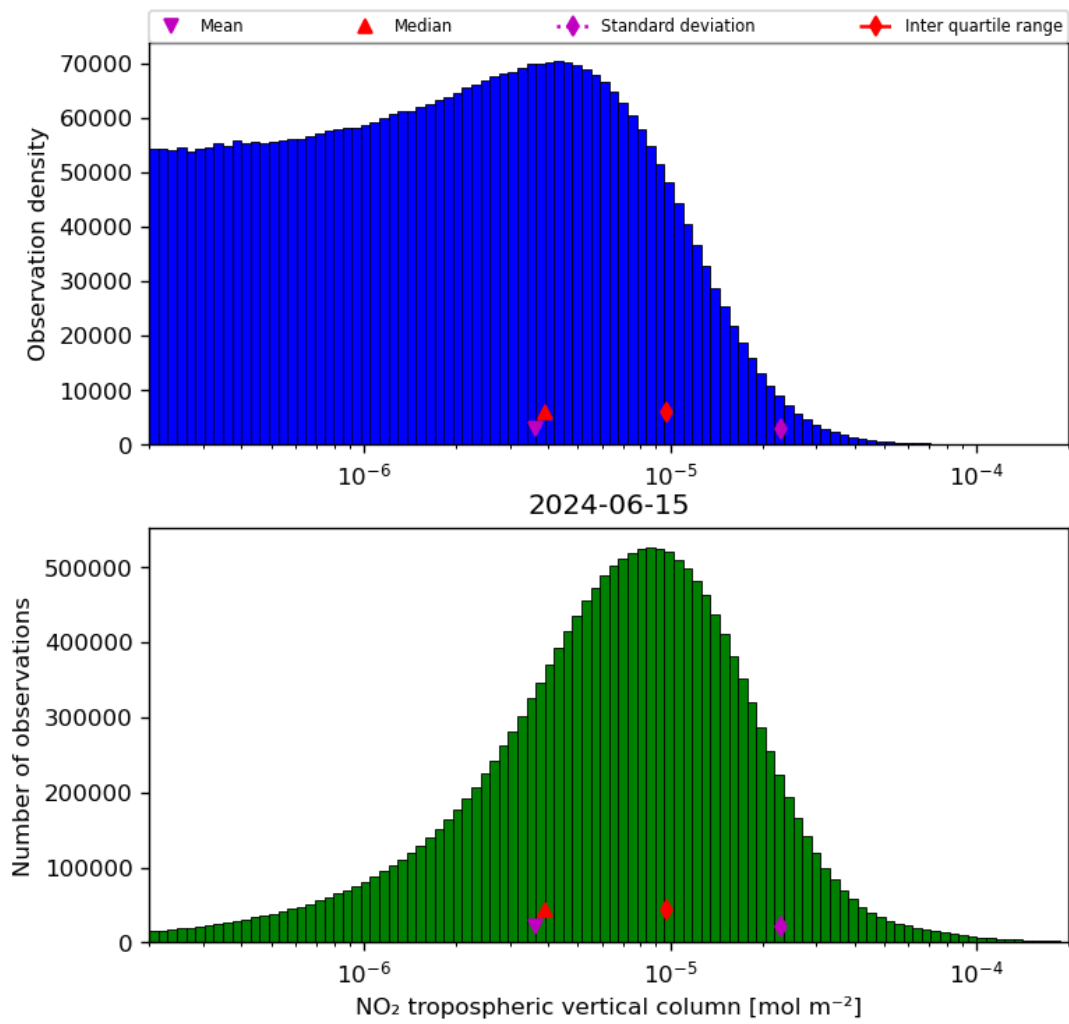
Figure 29: Histogram of “NO 2 tropospheric vertical column” for 2024-06-14 to 2024-06-16
