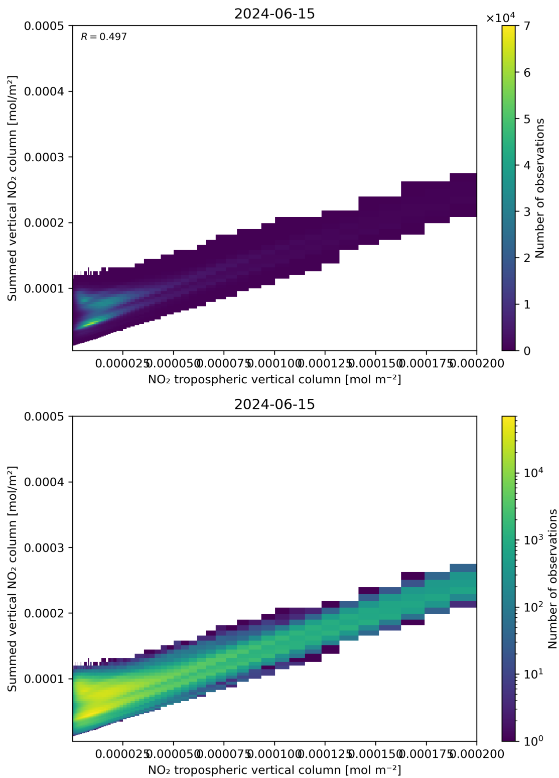
Figure 126: Scatter density plot of “NO 2 tropospheric vertical column” against “Summed vertical NO 2 column” for 2024-06-14 to 2024-06-16.
