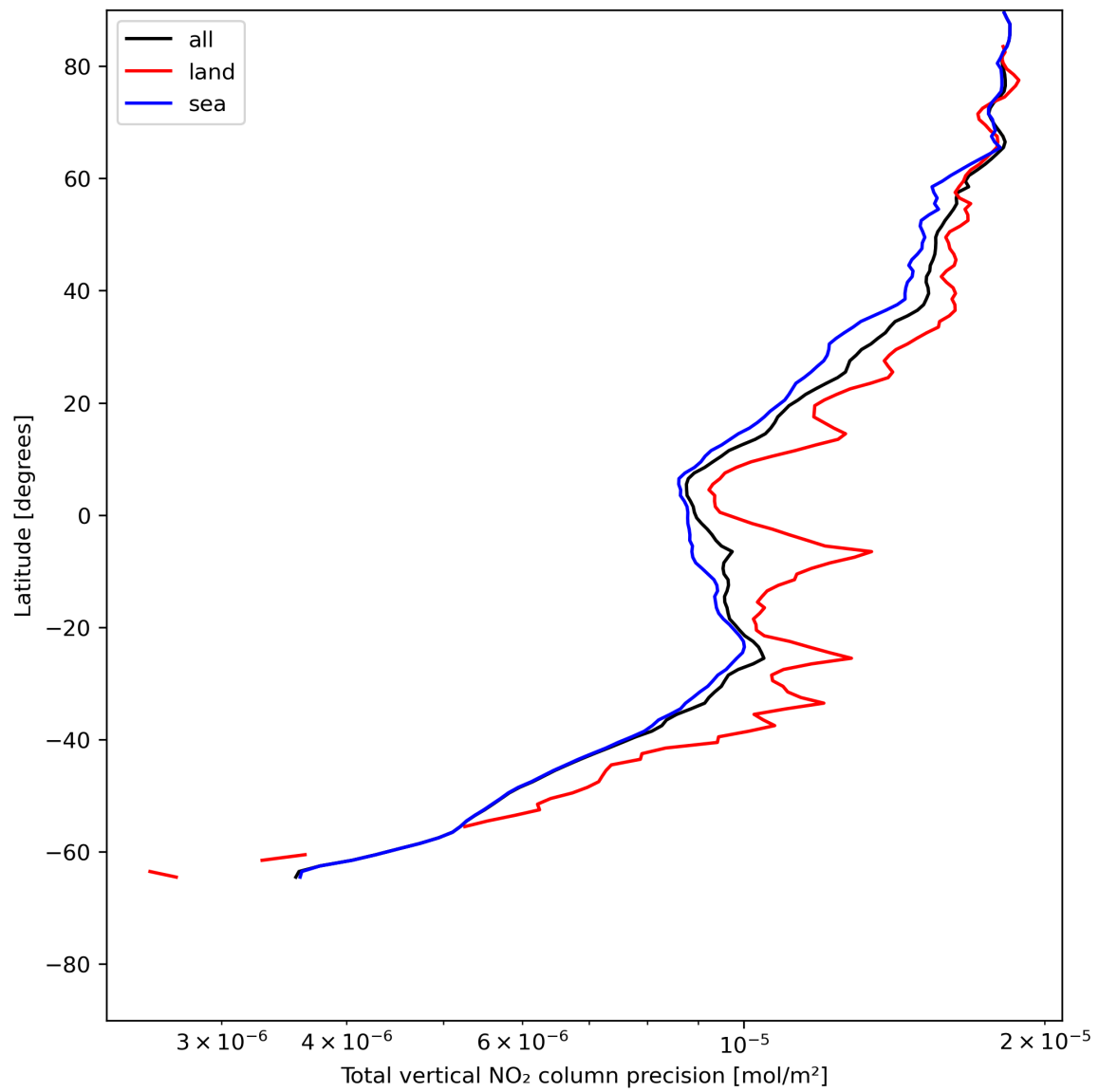
Figure 22: Zonal average of “Total vertical NO 2 column precision” for 2024-06-14 to 2024-06-16.
