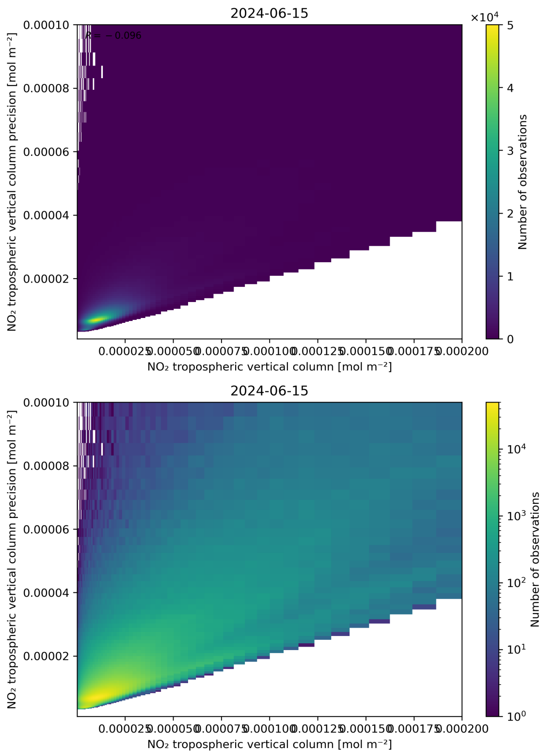
Figure 130: Scatter density plot of “NO 2 tropospheric vertical column” against “NO 2 tropospheric vertical column precision” for 2024-06-14 to 2024-06-16.
