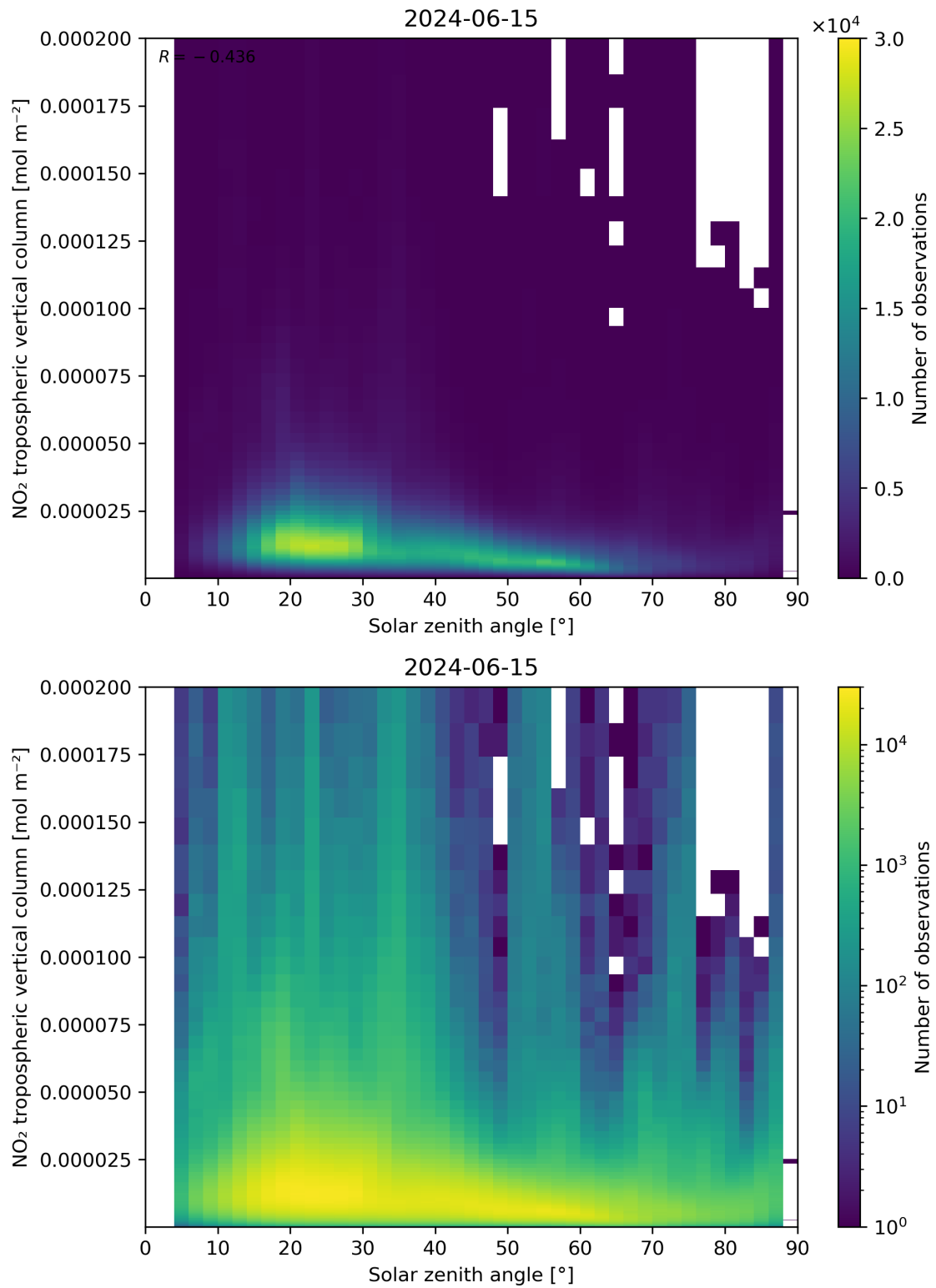
Figure 155: Scatter density plot of “Solar zenith angle” against “NO 2 tropospheric vertical column” for 2024-06-14 to 2024-06-16.
