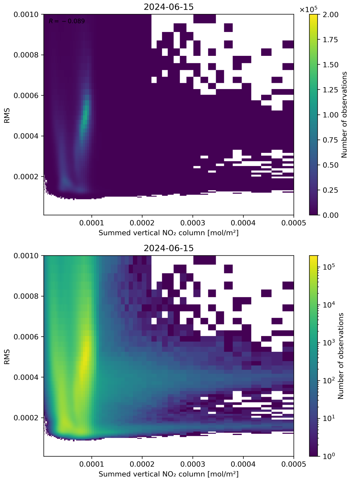
Figure 109: Scatter density plot of “Summed vertical NO 2 column” against “RMS” for 2024-06-14 to 2024-06-16.
