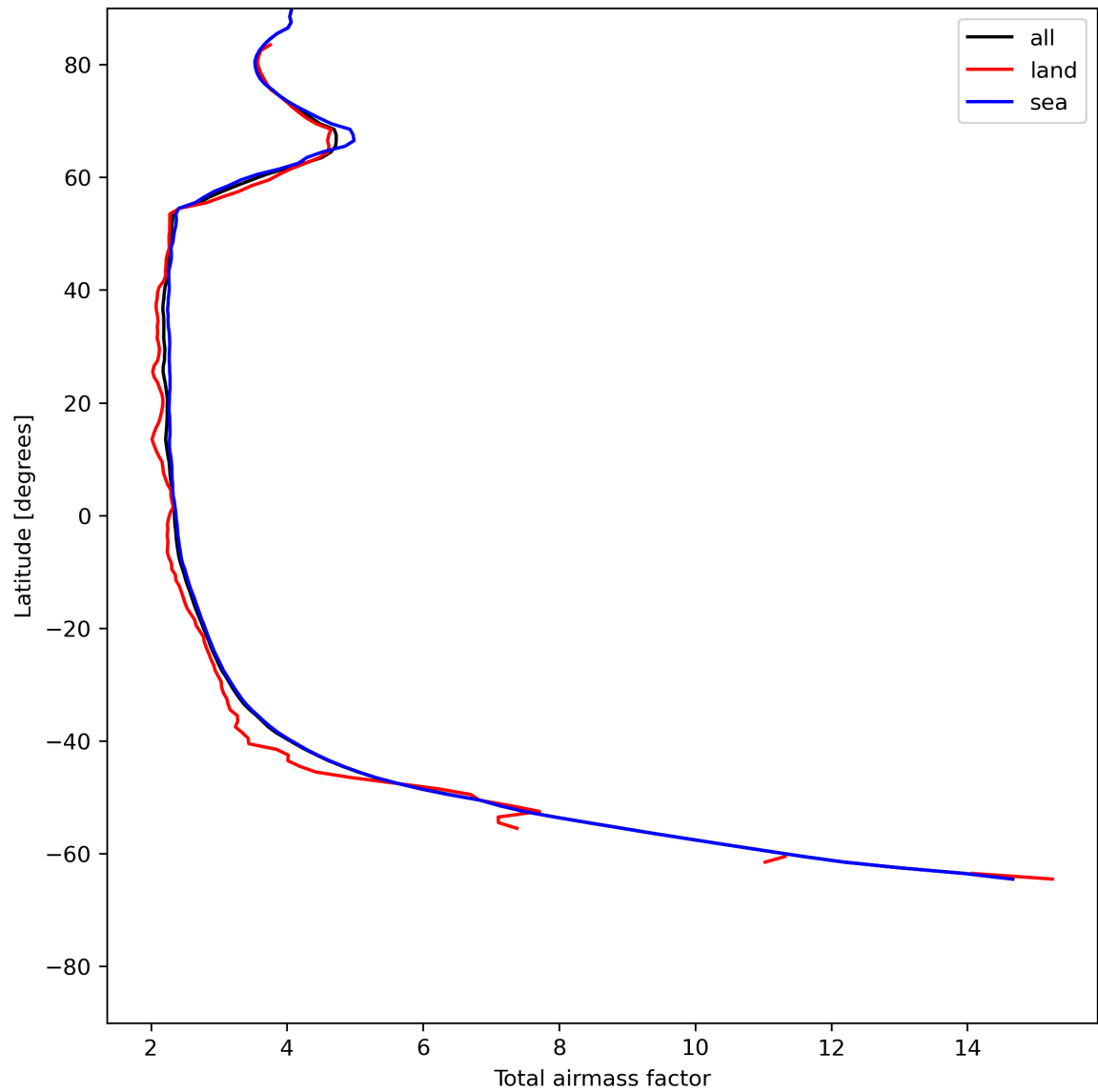
Figure 15: Zonal average of “Total airmass factor” for 2024-06-14 to 2024-06-16.
