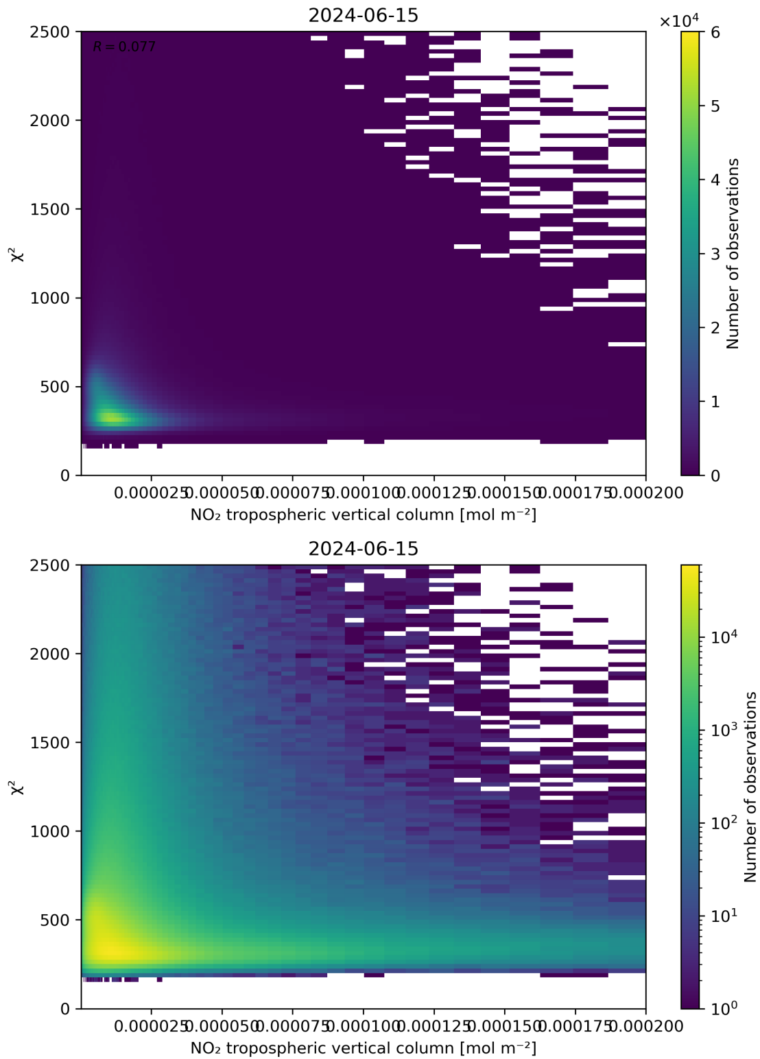
Figure 124: Scatter density plot of “NO 2 tropospheric vertical column” against “ \chi^2 ” for 2024-06-14 to 2024-06-16.
