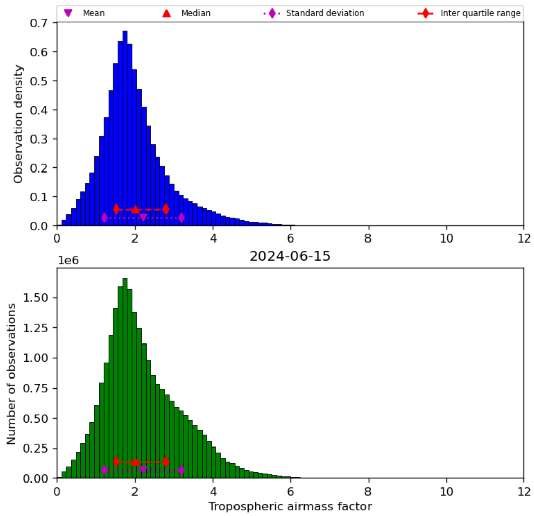
Figure 31: Histogram of “Tropospheric airmass factor” for 2024-06-14 to 2024-06-16
