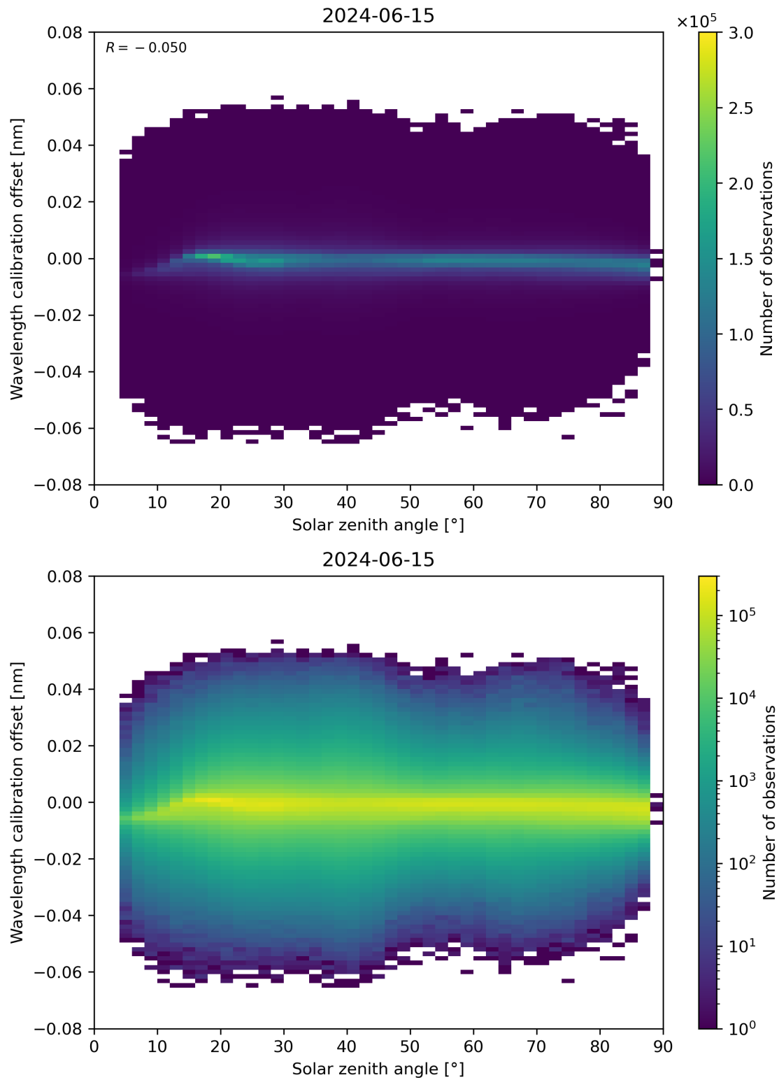
Figure 158: Scatter density plot of “Solar zenith angle” against “Wavelength calibration offset” for 2024-06-14 to 2024-06-16.
