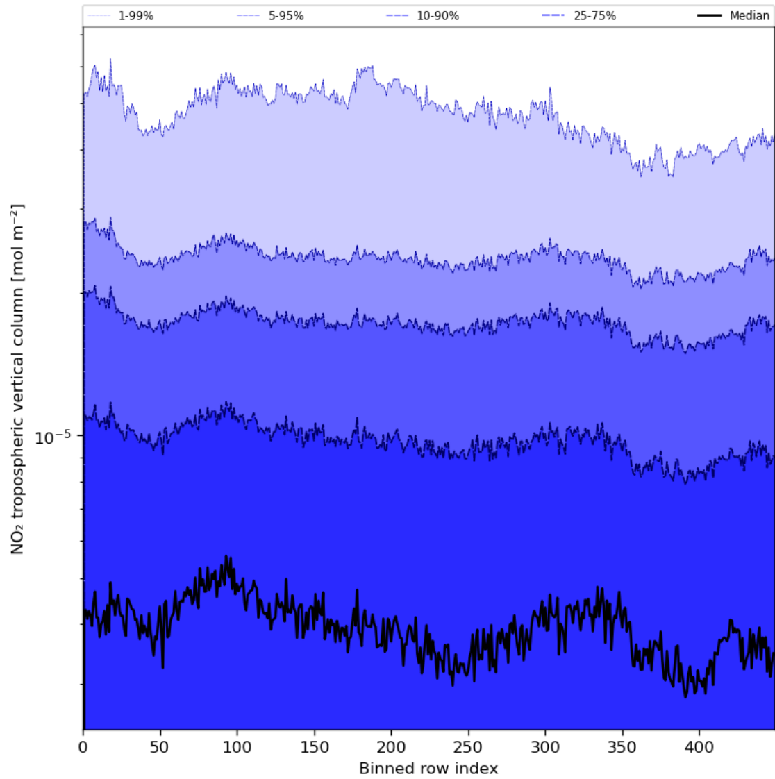
Figure 46: Along track statistics of “NO 2 tropospheric vertical column” for 2024-06-14 to 2024-06-16
