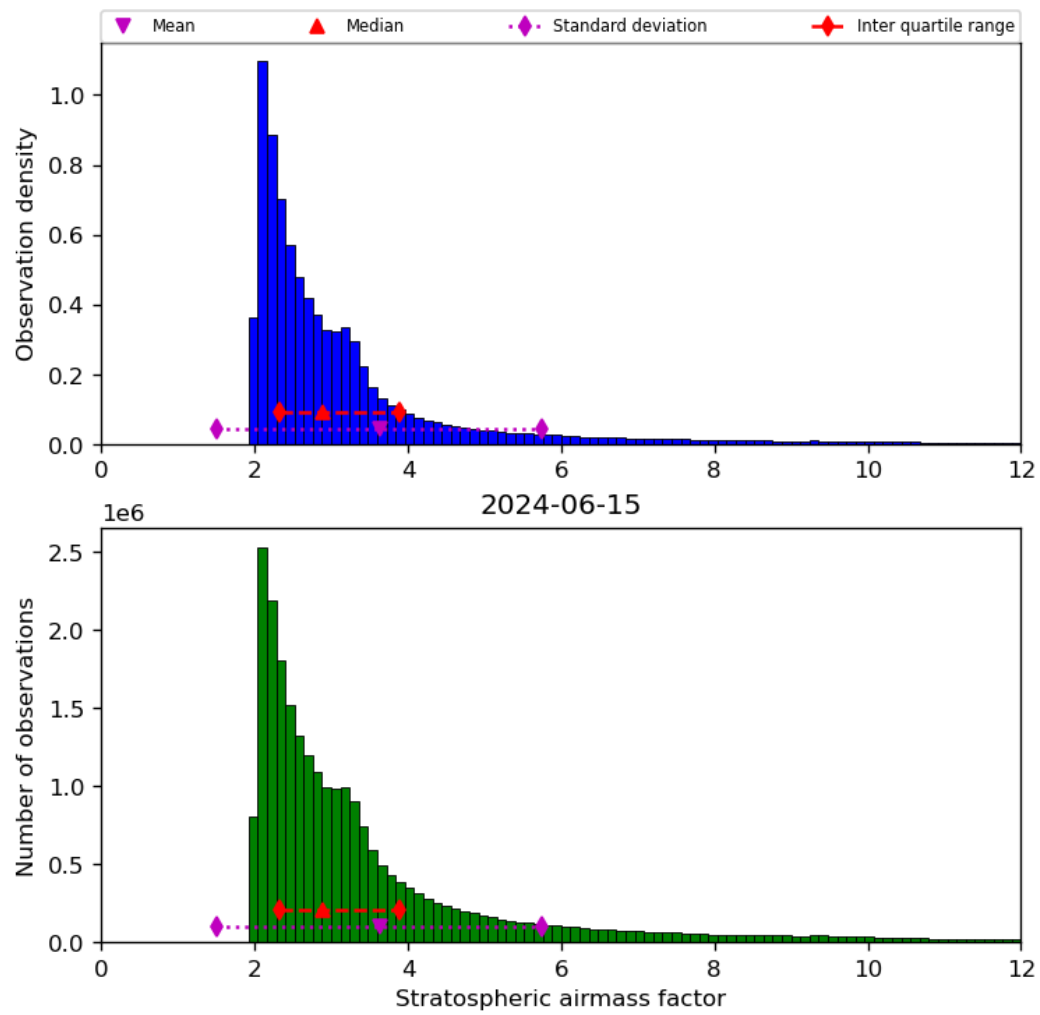
Figure 44: Histogram of “Stratospheric airmass factor” for 2024-06-14 to 2024-06-16
