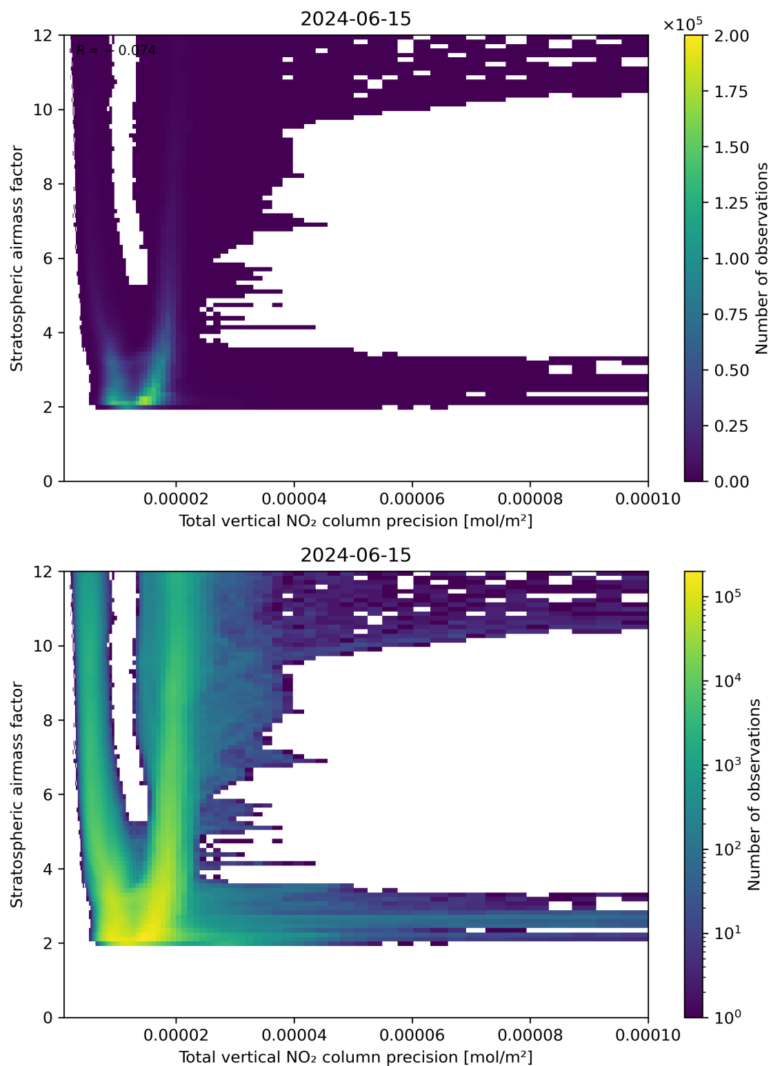
Figure 115: Scatter density plot of “Total vertical NO 2 column precision” against “Stratospheric airmass factor” for 2024-06-14 to 2024-06-16.
