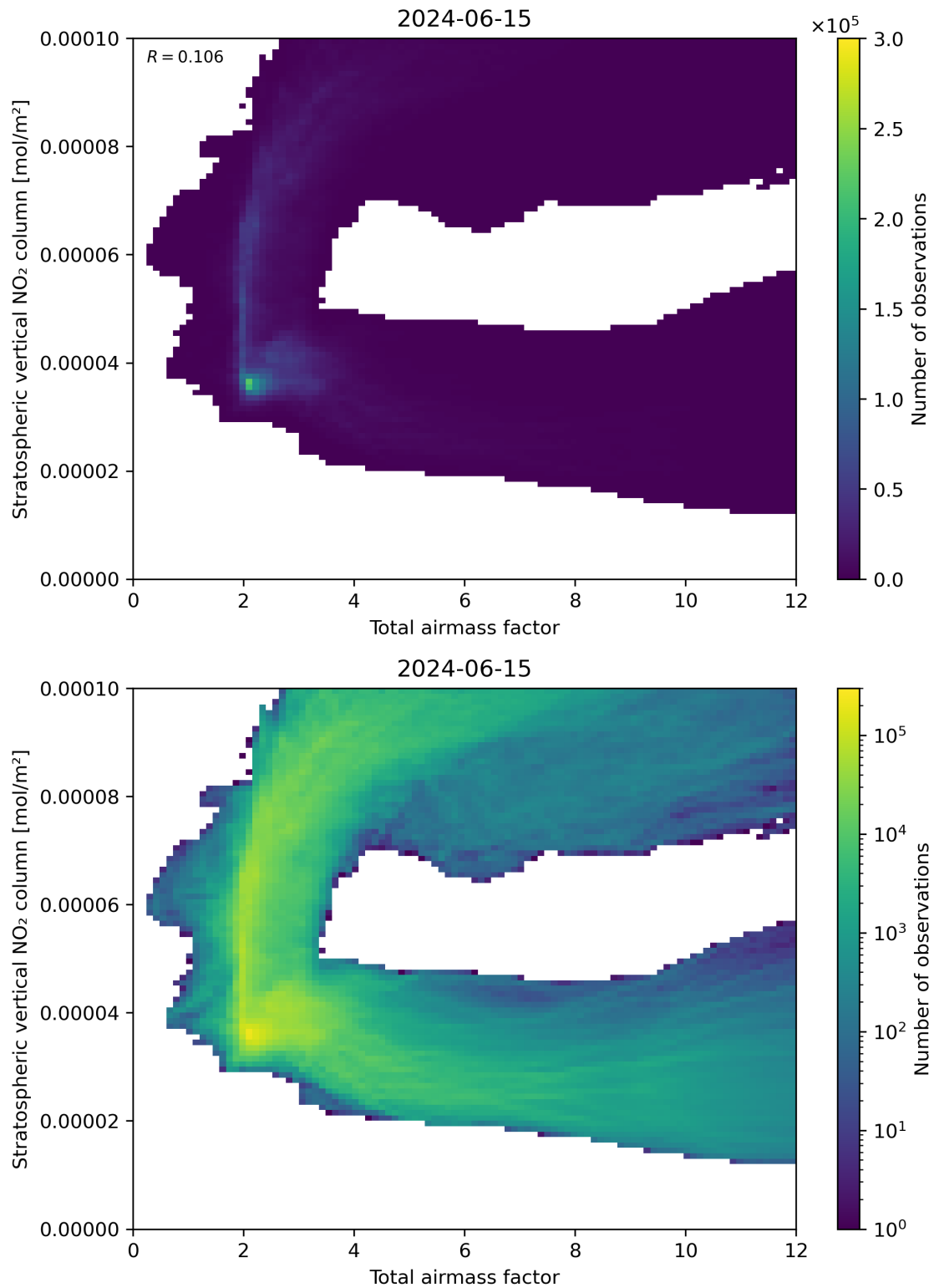
Figure 64: Scatter density plot of “Total airmass factor” against “Stratospheric vertical NO 2 column” for 2024-06-14 to 2024-06-16.
