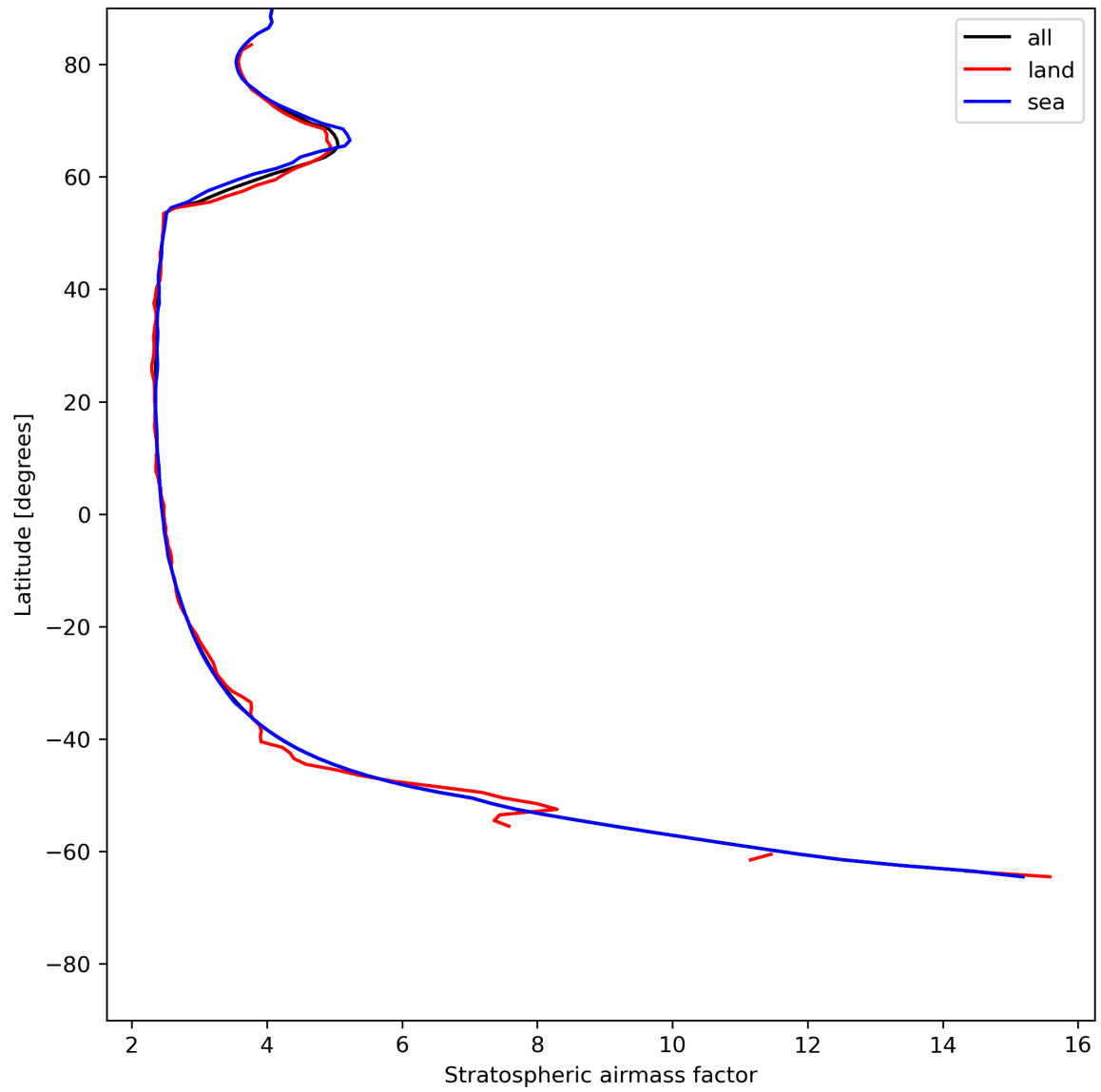
Figure 27: Zonal average of “Stratospheric air mass factor” for 2024-06-14 to 2024-06-16.
