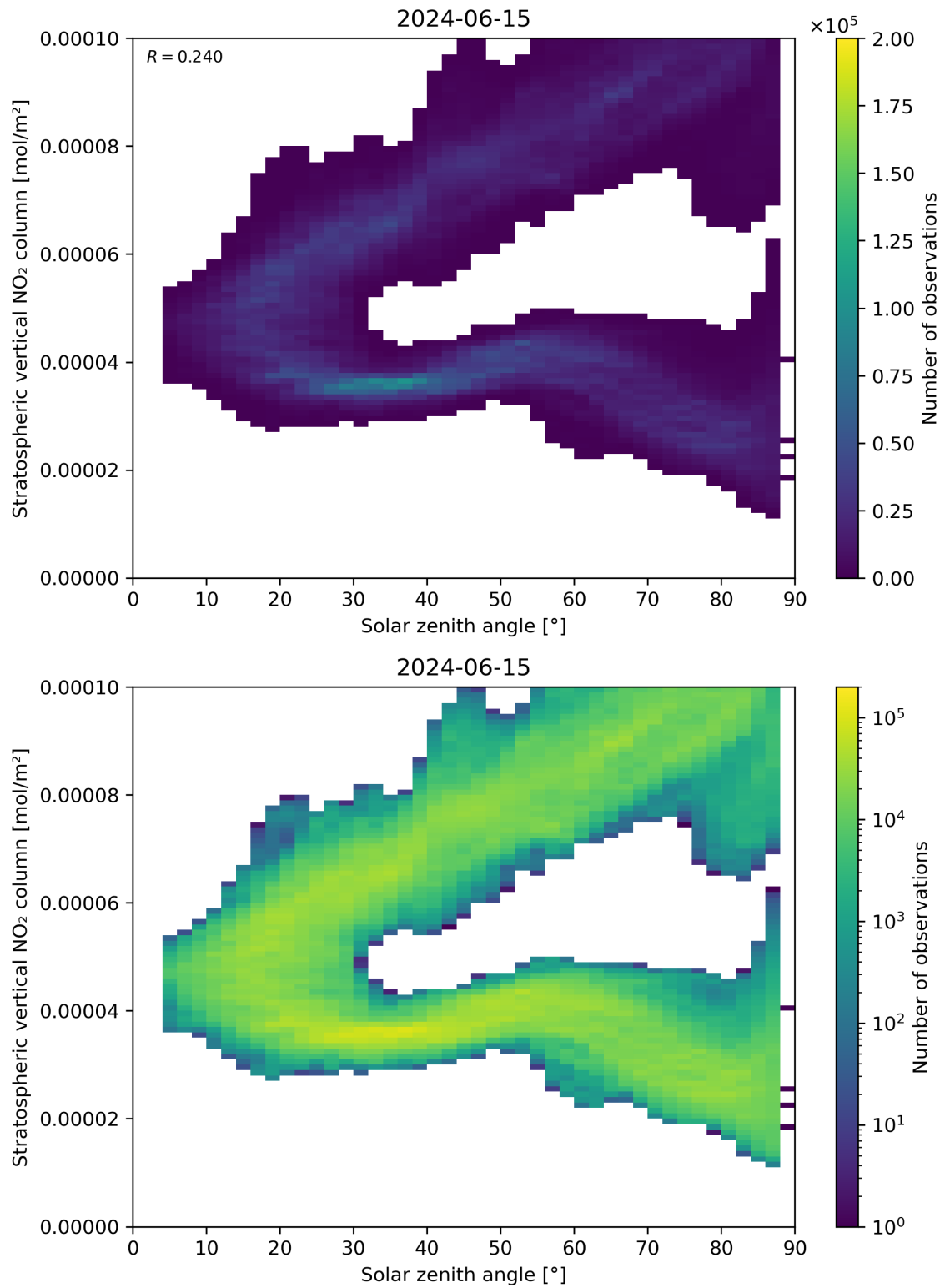
Figure 150: Scatter density plot of “Solar zenith angle” against “Stratospheric vertical NO 2 column” for 2024-06-14 to 2024-06-16.
