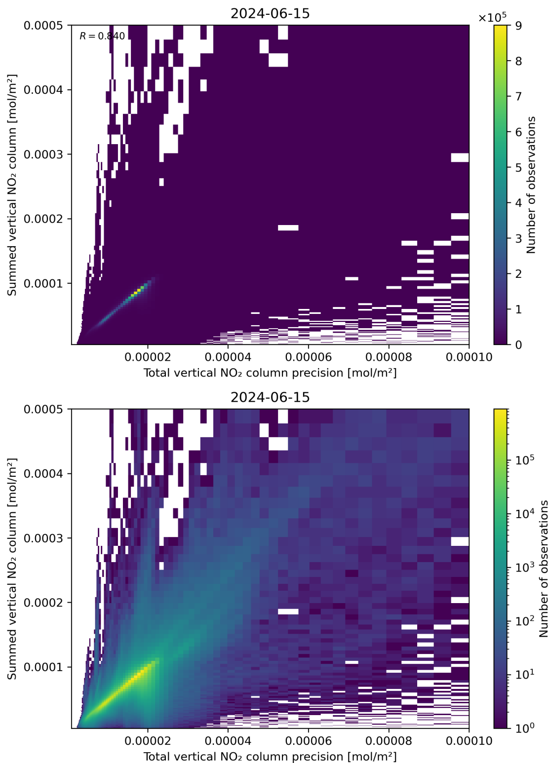
Figure 117: Scatter density plot of “Total vertical NO 2 column precision” against “Summed vertical NO 2 column” for 2024-06-14 to 2024-06-16.
