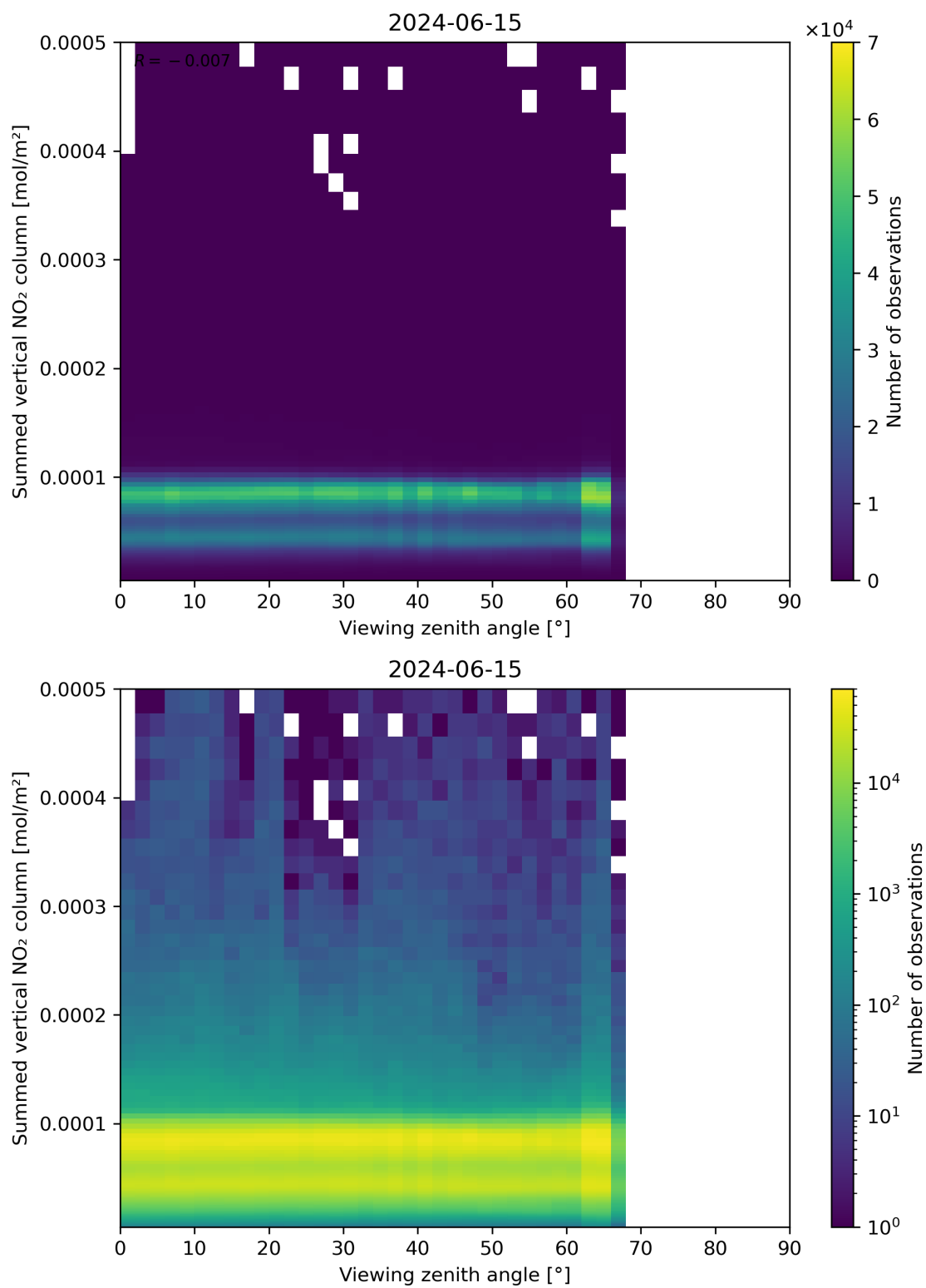
Figure 165: Scatter density plot of “Viewing zenith angle” against “Summed vertical NO 2 column” for 2024-06-14 to 2024-06-16.
