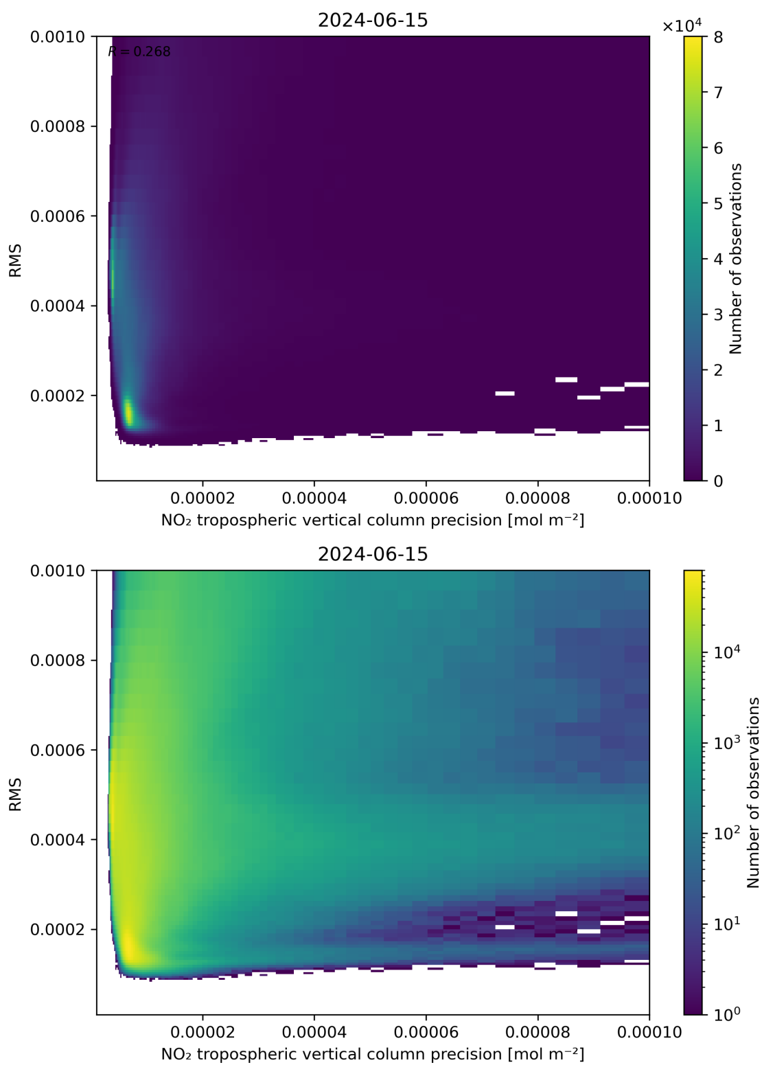
Figure 140: Scatter density plot of “NO 2 tropospheric vertical column precision” against “RMS” for 2024-06-14 to 2024-06-16.
