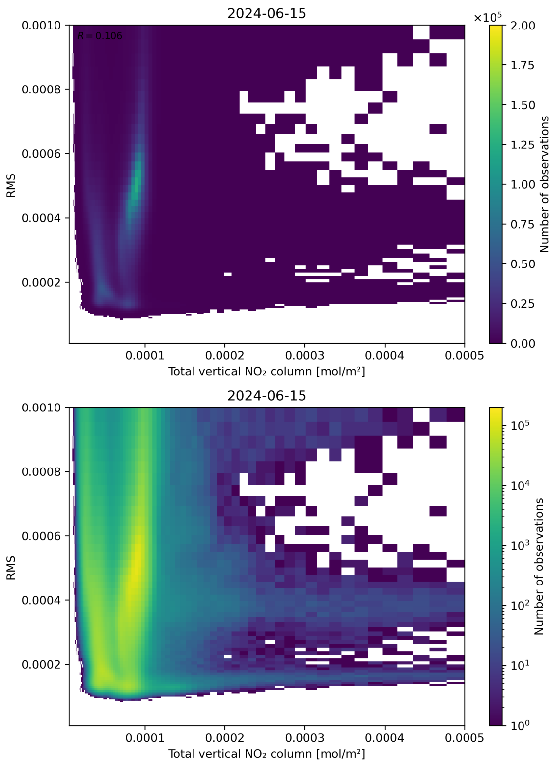
Figure 120: Scatter density plot of “Total vertical NO 2 column” against “RMS” for 2024-06-14 to 2024-06-16.
