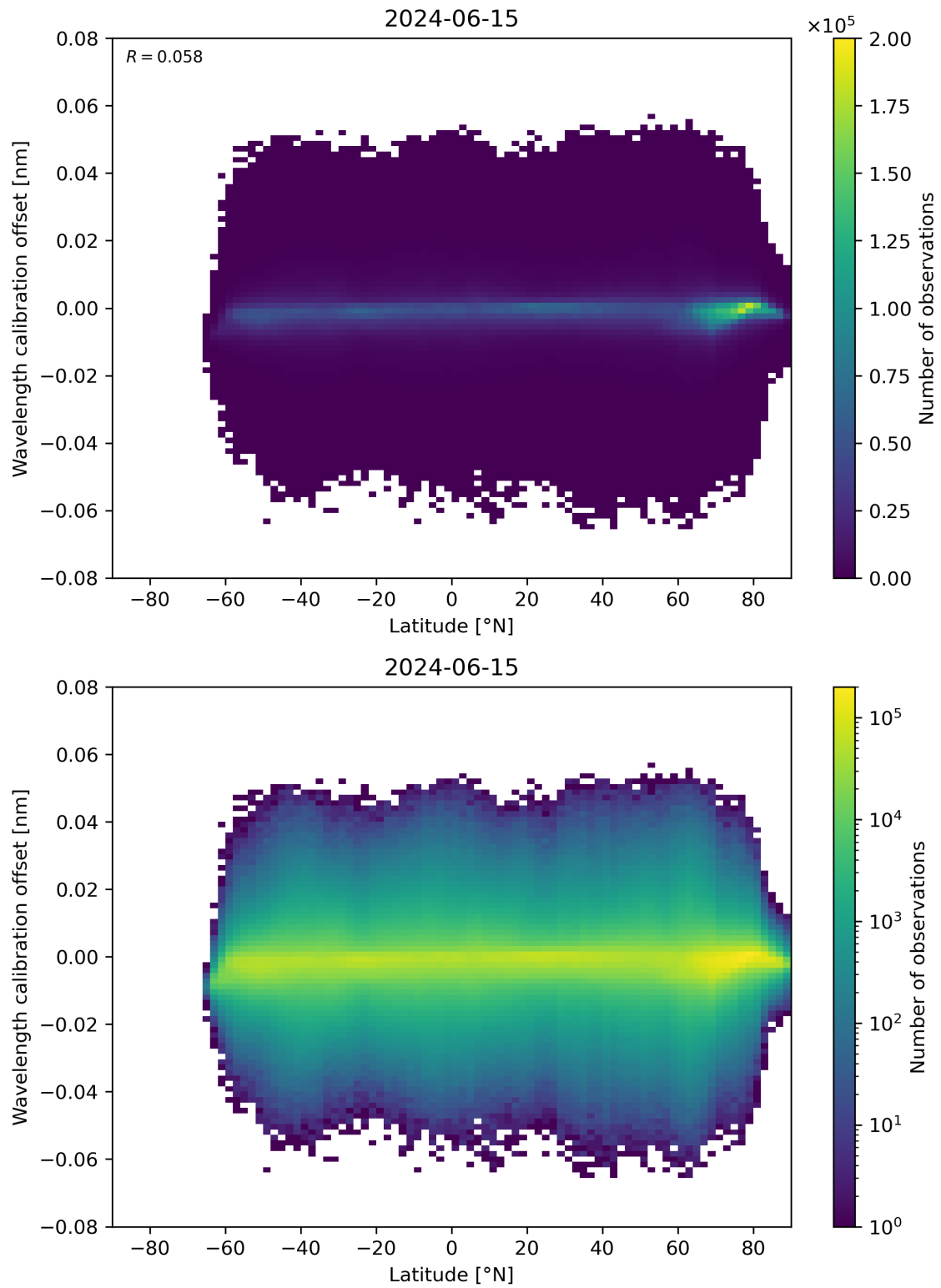
Figure 95: Scatter density plot of “Latitude” against “Wavelength calibration offset” for 2024-06-14 to 2024-06-16.
