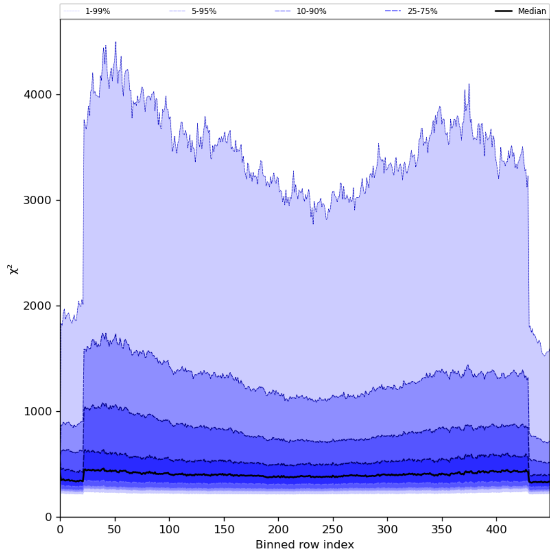
Figure 59: Along track statistics of “ \chi^2 ” for 2024-06-14 to 2024-06-16
