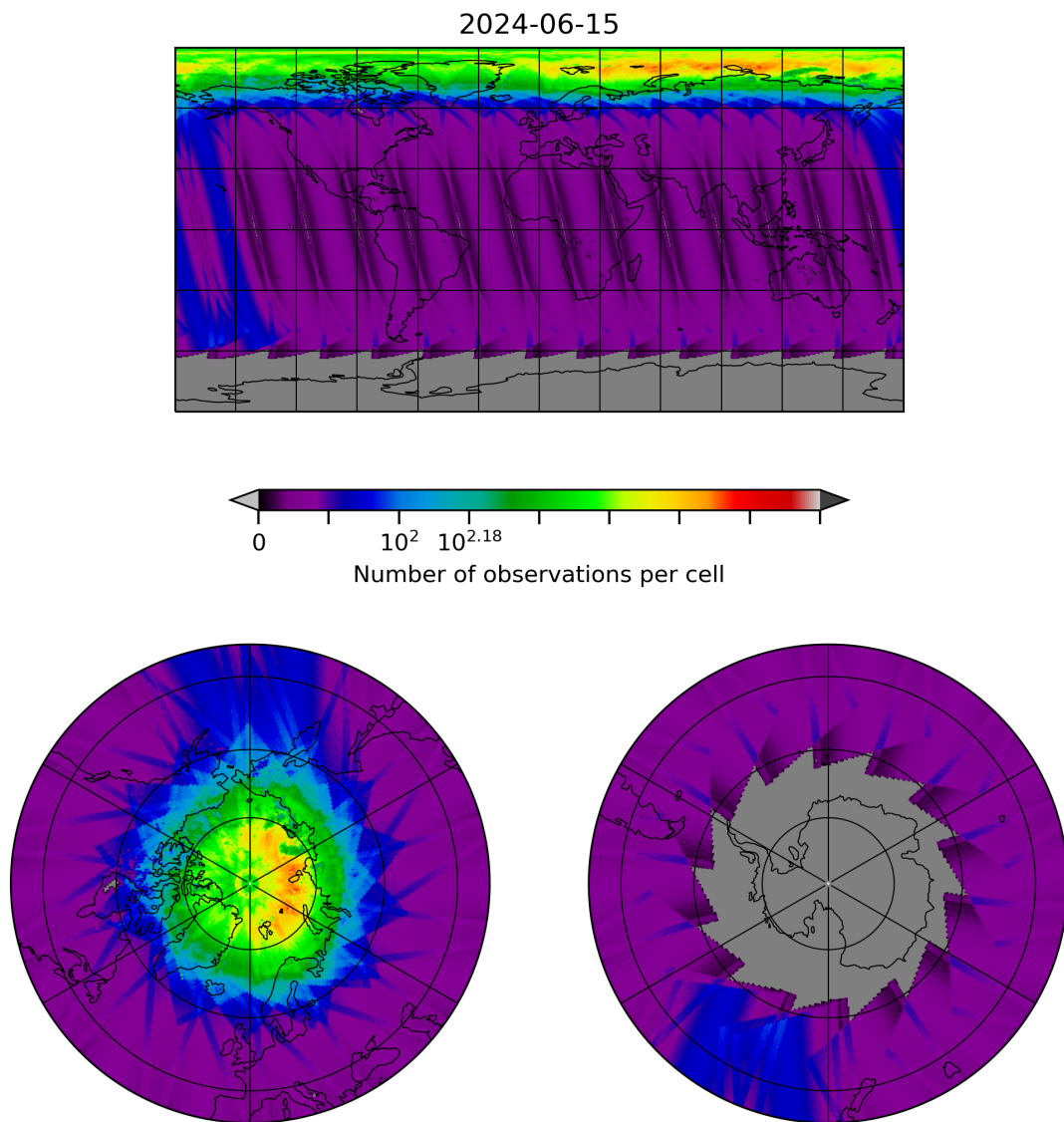
Figure 10: Map of the number of observations for 2024-06-14 to 2024-06-16
