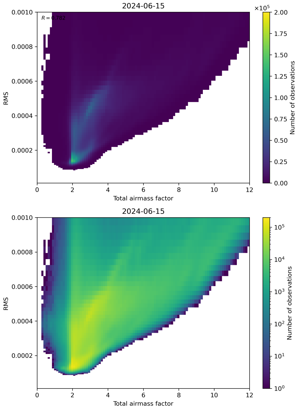
Figure 69: Scatter density plot of “Total airmass factor” against “RMS” for 2024-06-14 to 2024-06-16.
