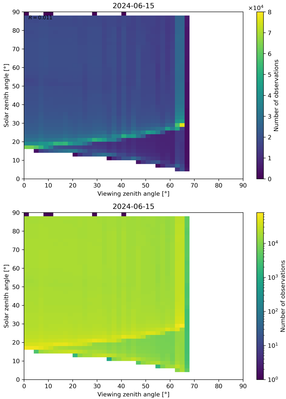
Figure 172: Scatter density plot of “Viewing zenith angle” against “Solar zenith angle” for 2024-06-14 to 2024-06-16.
