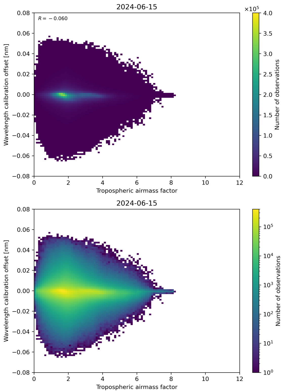
Figure 80: Scatter density plot of “Tropospheric airmass factor” against “Wavelength calibration offset” for 2024-06-14 to 2024-06-16.
