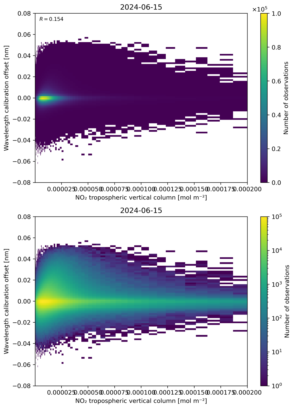
Figure 143: Scatter density plot of “NO 2 tropospheric vertical column” against “Wavelength calibration offset” for 2024-06-14 to 2024-06-16.
