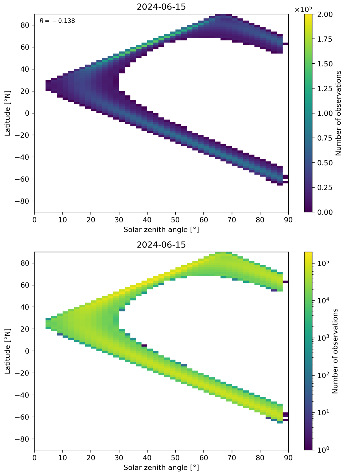
Figure 149: Scatter density plot of “Solar zenith angle” against “Latitude” for 2024-06-14 to 2024-06-16.
