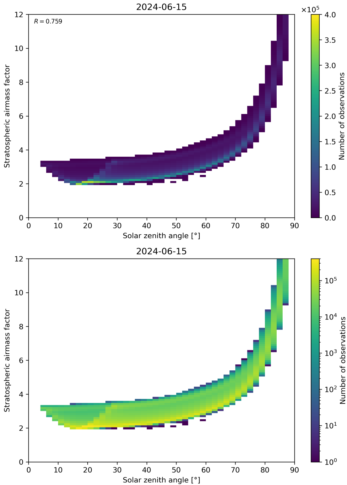
Figure 145: Scatter density plot of “Solar zenith angle” against “Stratospheric airmass factor” for 2024-06-14 to 2024-06-16.
