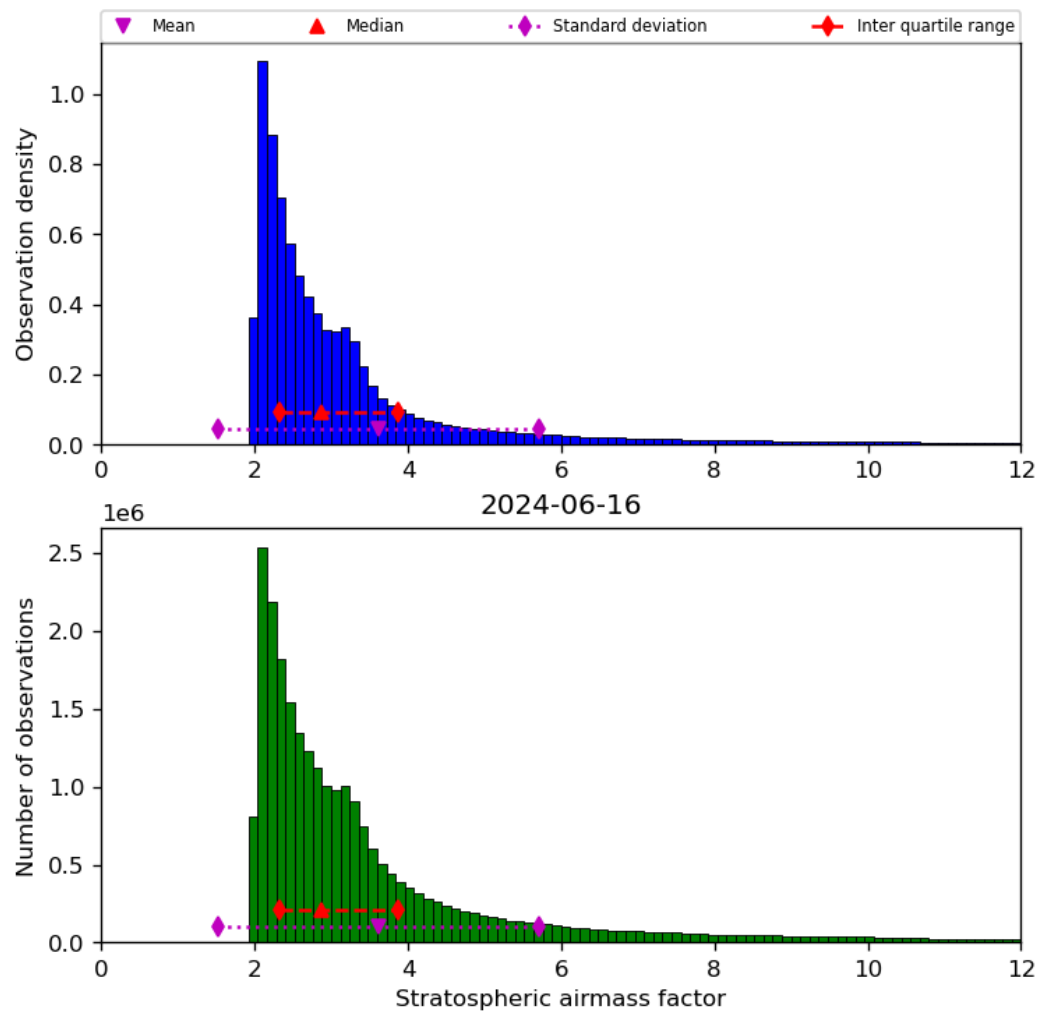
Figure 44: Histogram of “Stratospheric airmass factor” for 2024-06-15 to 2024-06-17
