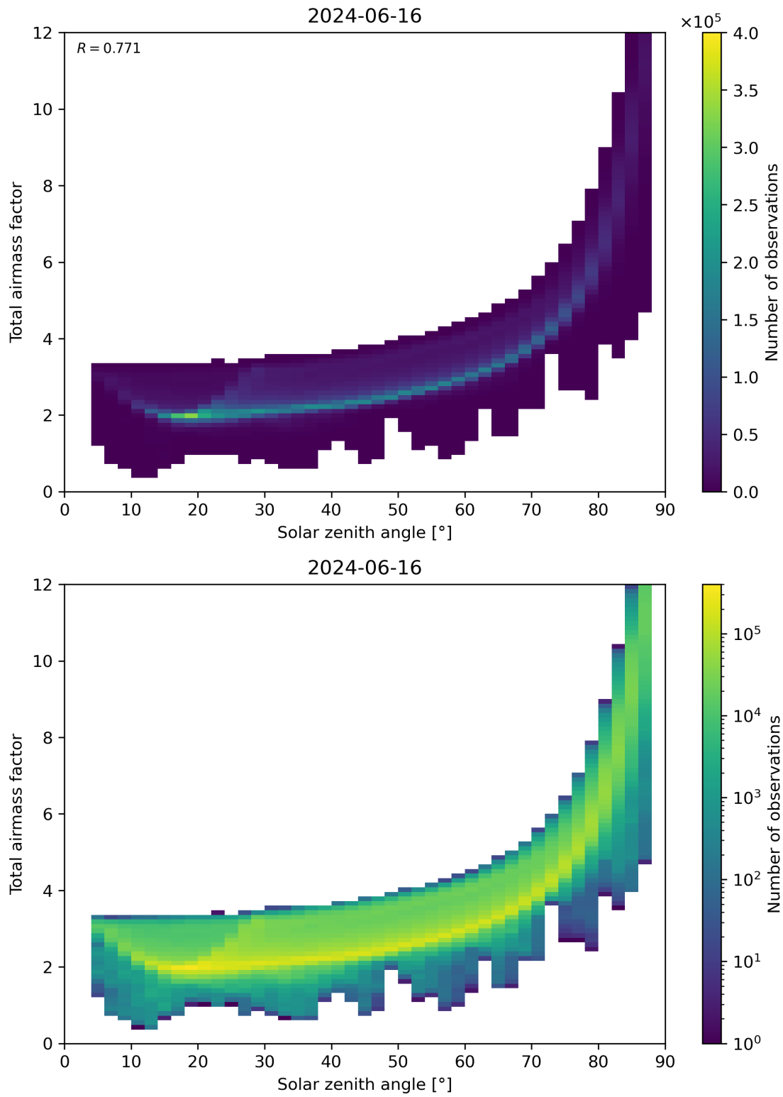
Figure 146: Scatter density plot of “Solar zenith angle” against “Total air mass factor” for 2024-06-15 to 2024-06-17.
