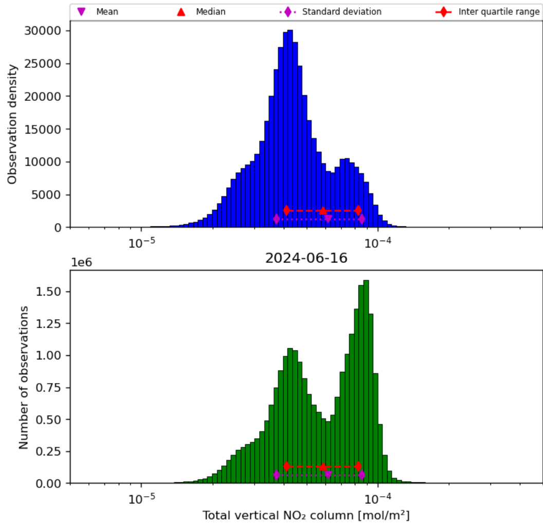
Figure 38: Histogram of “Total vertical NO 2 column” for 2024-06-15 to 2024-06-17
