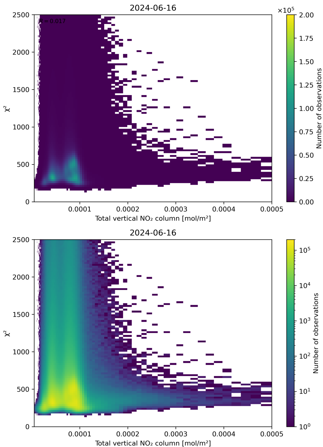
Figure 111: Scatter density plot of “Total vertical NO 2 column” against “ \chi^2 ” for 2024-06-15 to 2024-06-17.
