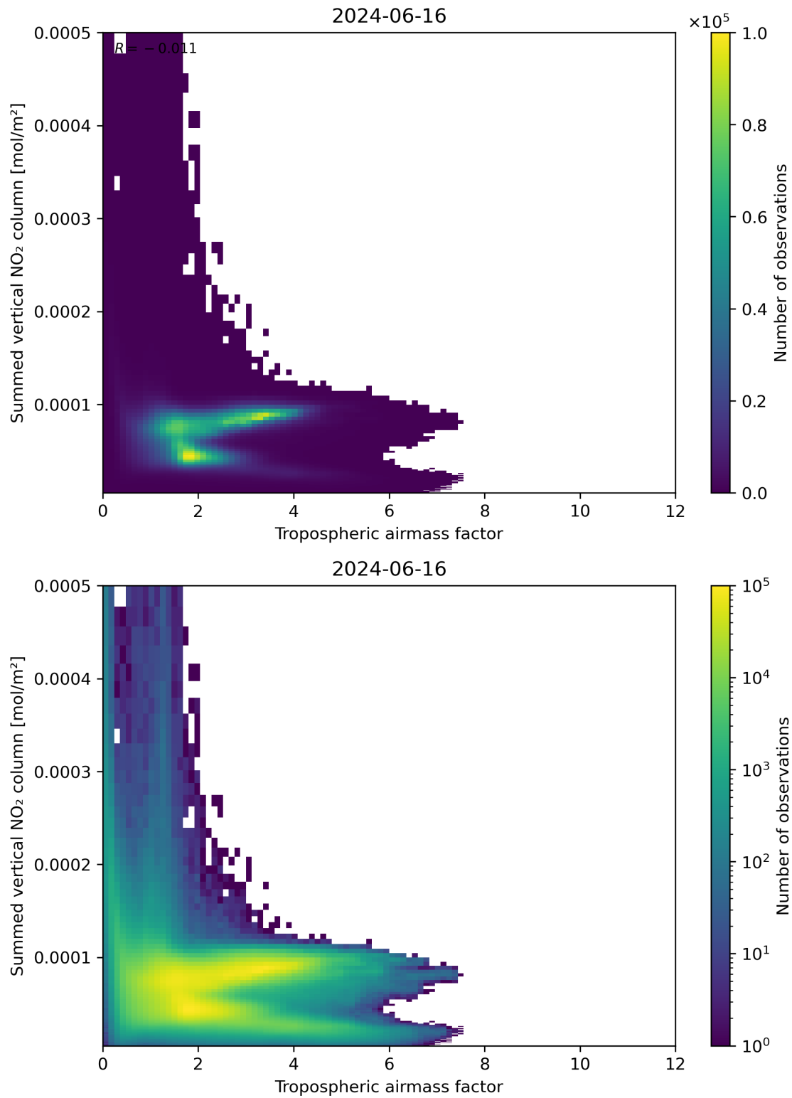
Figure 75: Scatter density plot of “Tropospheric airmass factor” against “Summed vertical NO 2 column” for 2024-06-15 to 2024-06-17.
