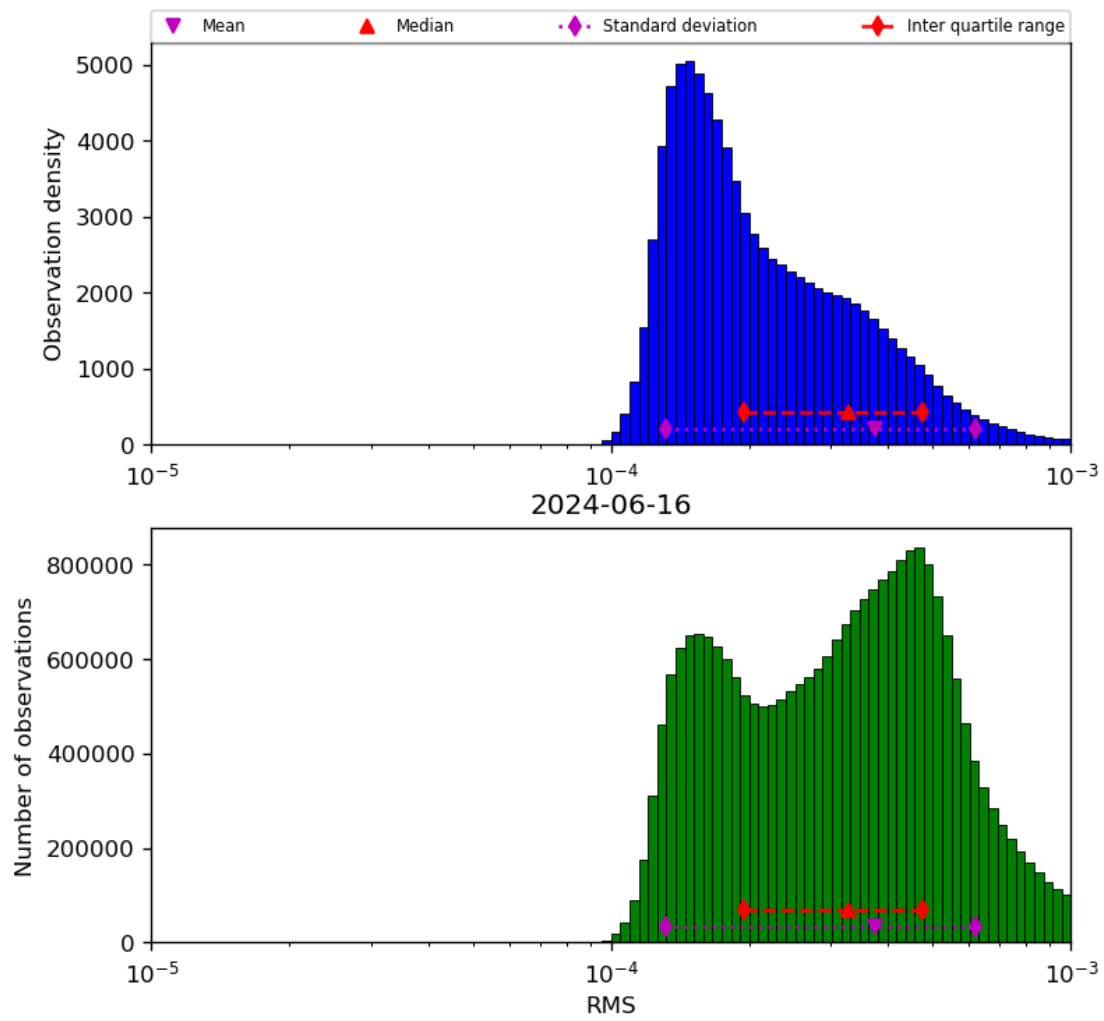
Figure 43: Histogram of “RMS” for 2024-06-15 to 2024-06-17
