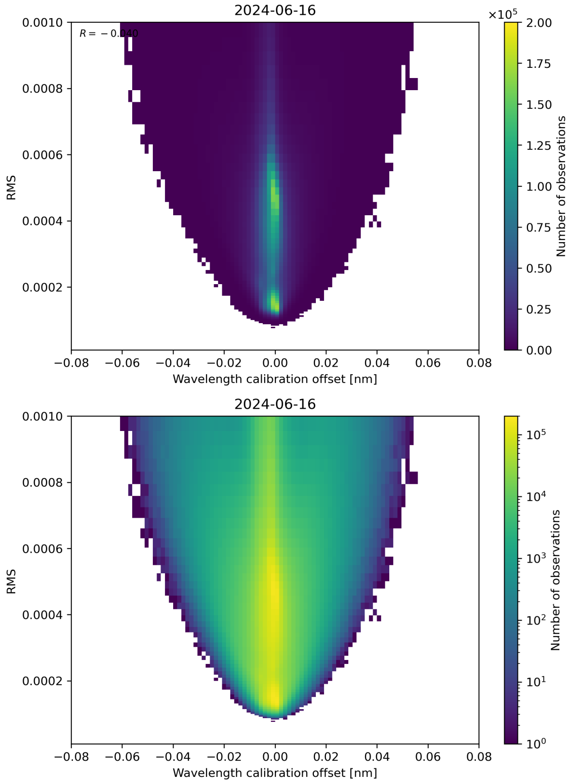
Figure 181: Scatter density plot of “Wavelength calibration offset” against “RMS” for 2024-06-15 to 2024-06-17.
