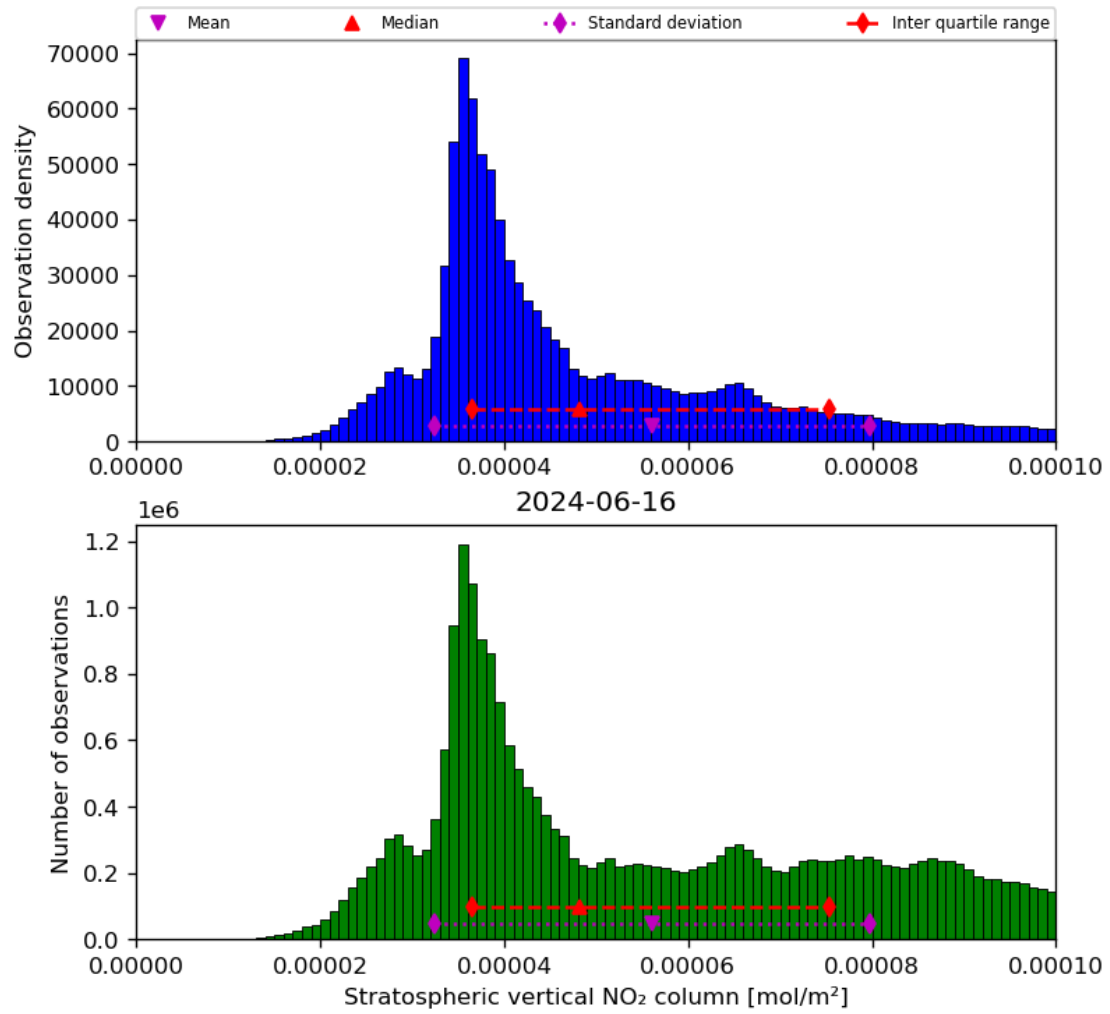
Figure 36: Histogram of “Stratospheric vertical NO 2 column” for 2024-06-15 to 2024-06-17
