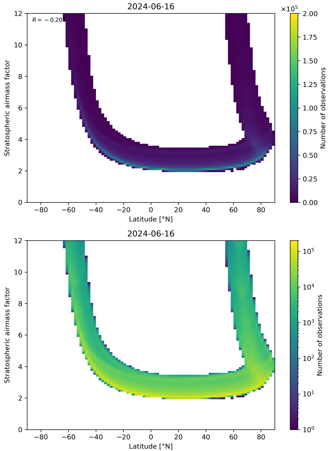
Figure 83: Scatter density plot of “Latitude” against “Stratospheric air mass factor” for 2024-06-15 to 2024-06-17.
