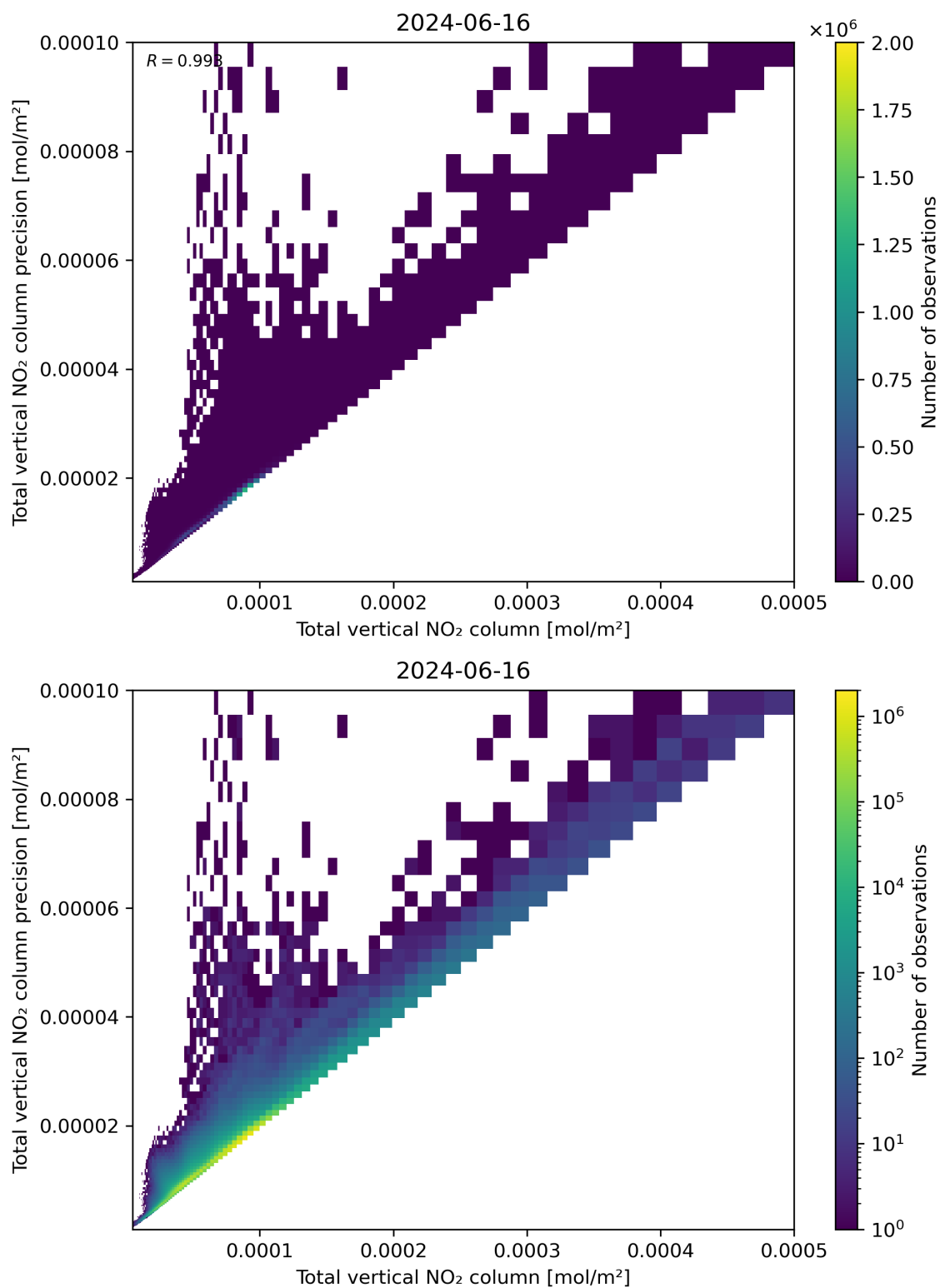
Figure 114: Scatter density plot of “Total vertical NO 2 column” against “Total vertical NO 2 column precision” for 2024-06-15 to 2024-06-17.
