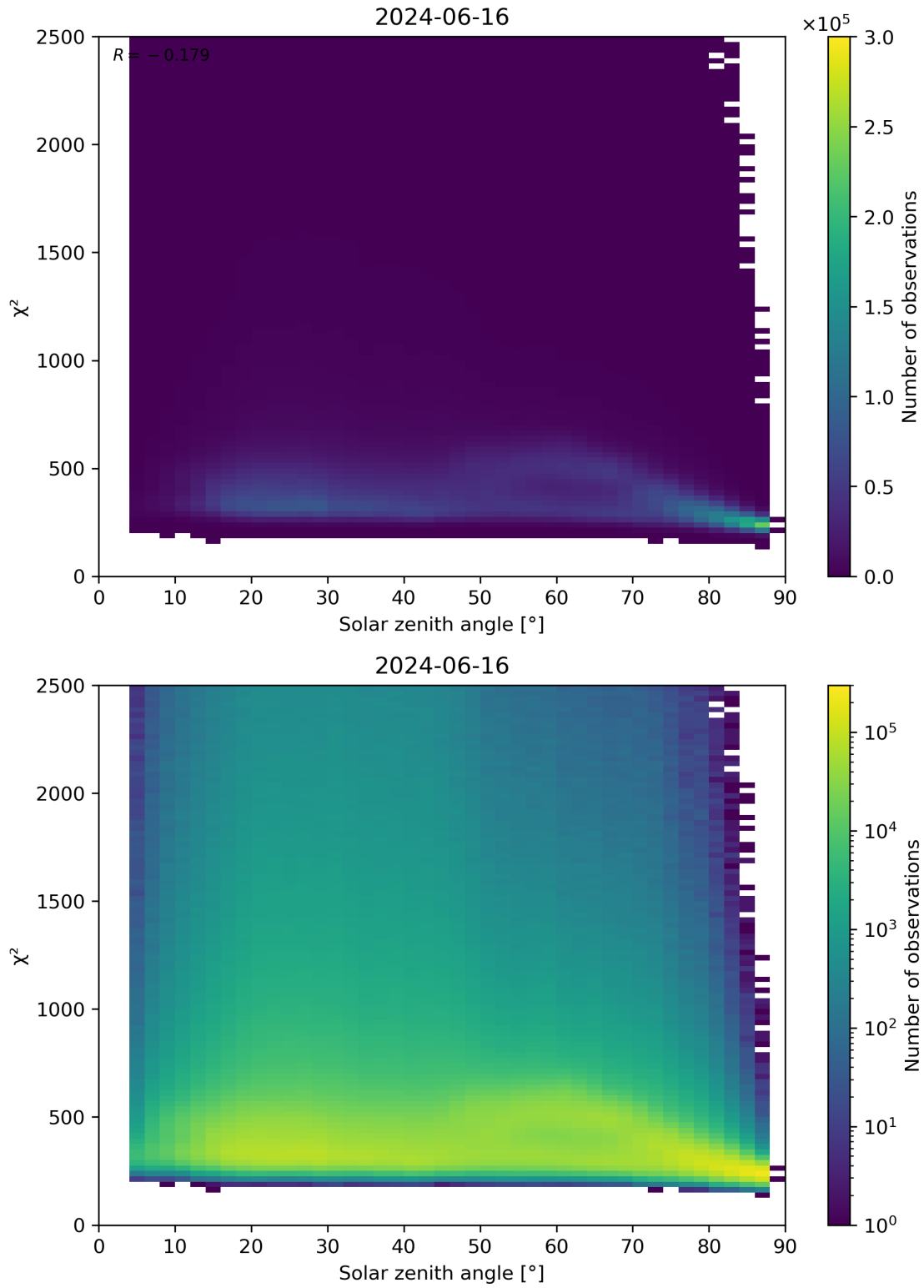
Figure 148: Scatter density plot of “Solar zenith angle” against “ \chi^2 ” for 2024-06-15 to 2024-06-17.
