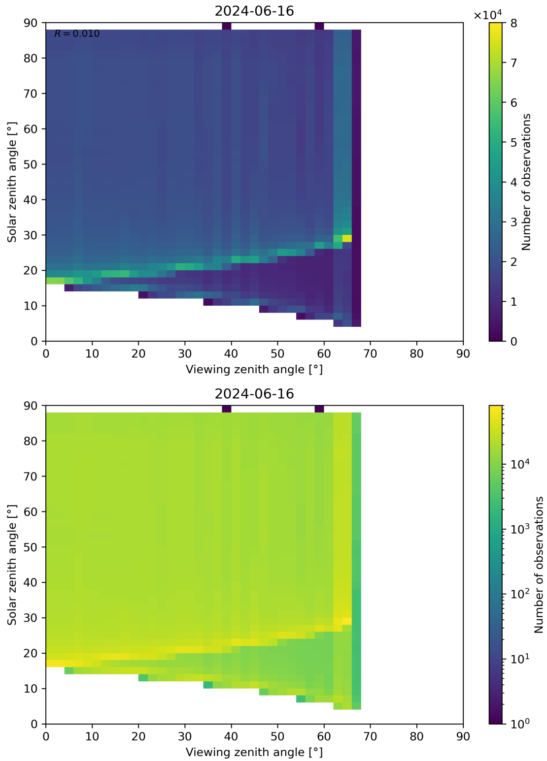
Figure 172: Scatter density plot of “Viewing zenith angle” against “Solar zenith angle” for 2024-06-15 to 2024-06-17.
