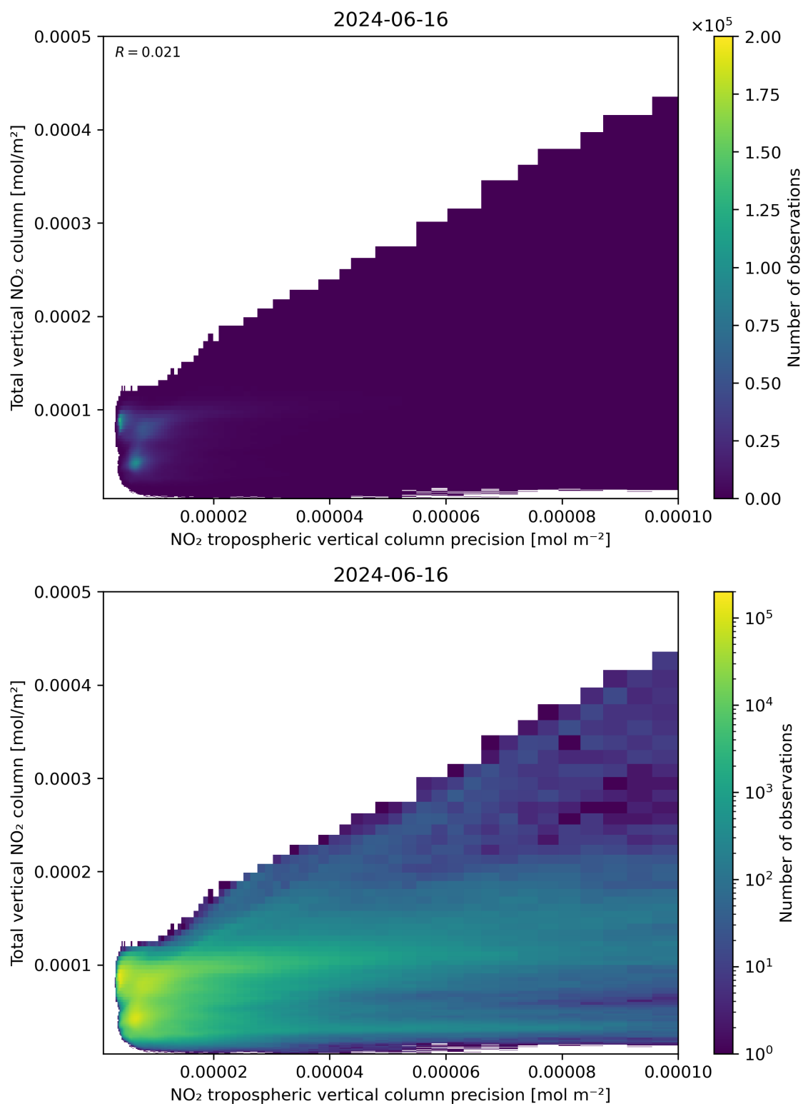
Figure 138: Scatter density plot of “NO 2 tropospheric vertical column precision” against “Total vertical NO 2 column” for 2024-06-15 to 2024-06-17.
