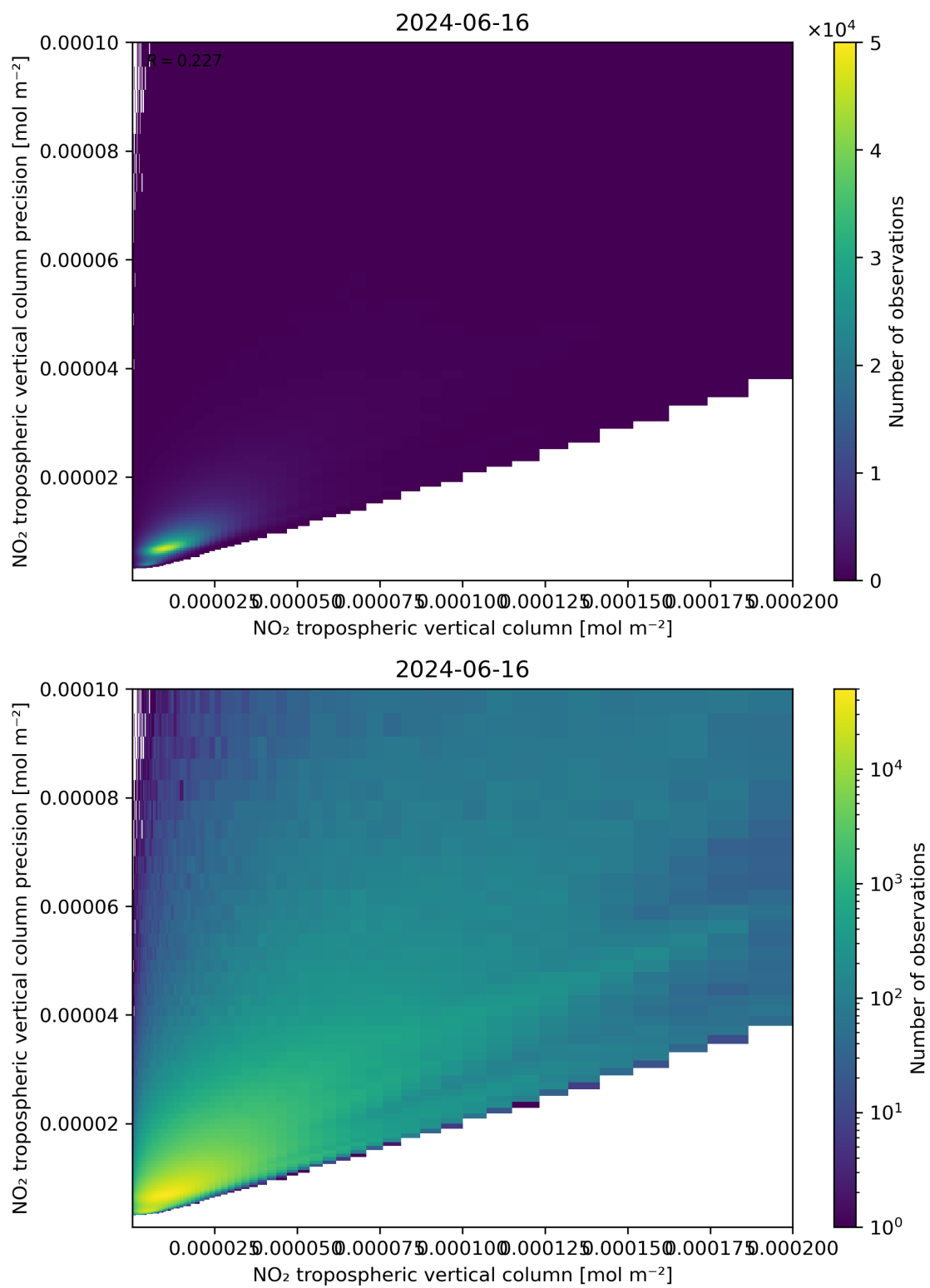
Figure 130: Scatter density plot of “NO 2 tropospheric vertical column” against “NO 2 tropospheric vertical column precision” for 2024-06-15 to 2024-06-17.
