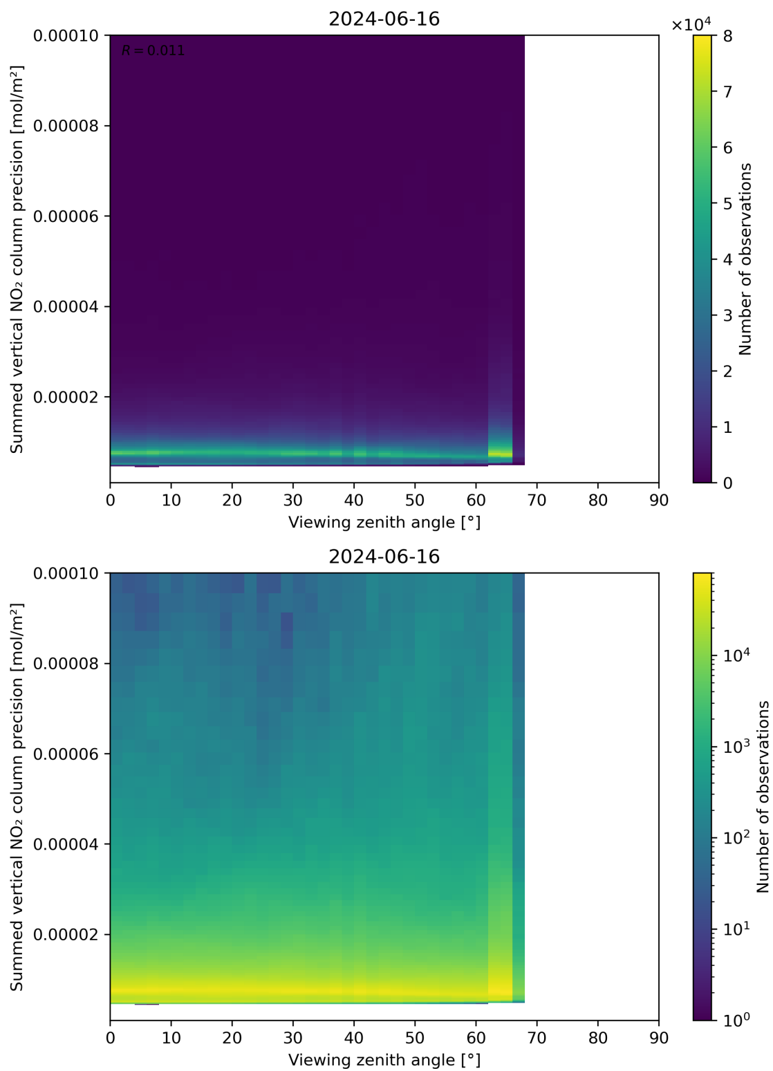
Figure 166: Scatter density plot of “Viewing zenith angle” against “Summed vertical NO 2 column precision” for 2024-06-15 to 2024-06-17.
