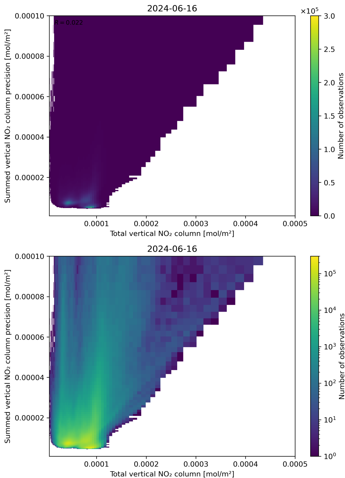
Figure 113: Scatter density plot of “Total vertical NO 2 column” against “Summed vertical NO 2 column precision” for 2024-06-15 to 2024-06-17.
