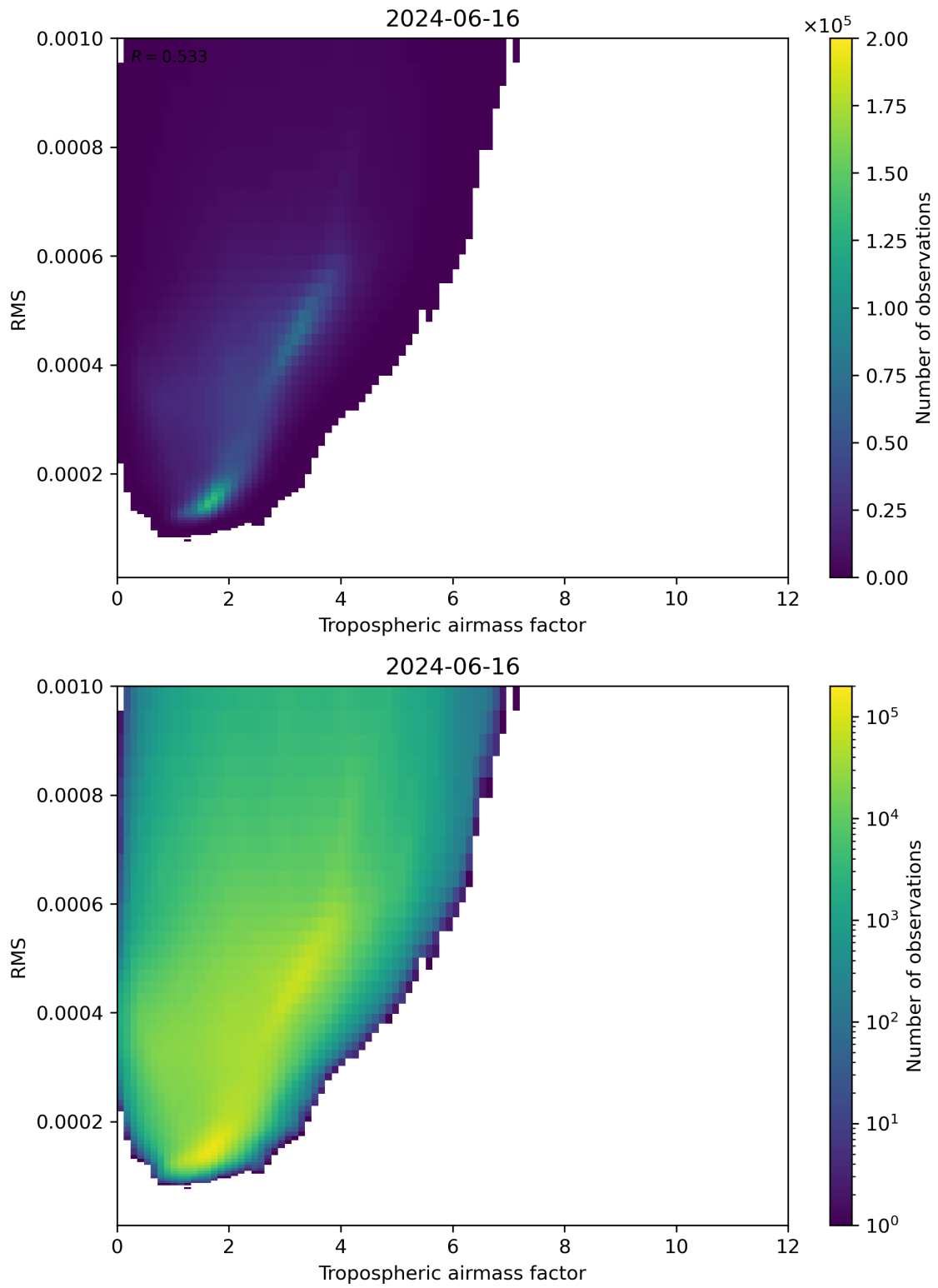
Figure 79: Scatter density plot of “Tropospheric airmass factor” against “RMS” for 2024-06-15 to 2024-06-17.
