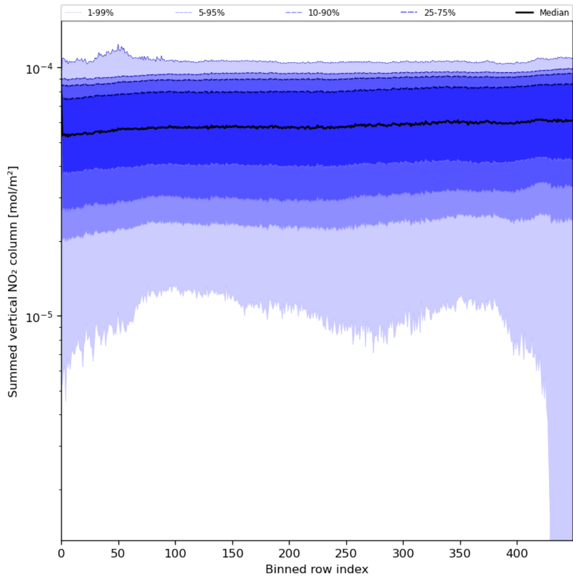
Figure 57: Along track statistics of “Summed vertical NO 2 column” for 2024-06-15 to 2024-06-17
