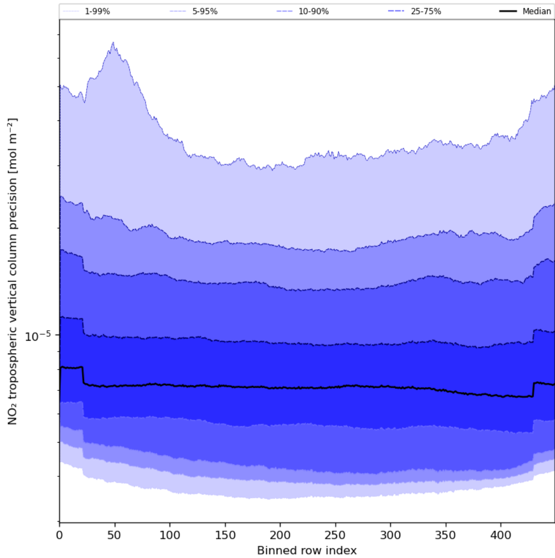
Figure 47: Along track statistics of “NO 2 tropospheric vertical column precision” for 2024-06-15 to 2024-06-17
