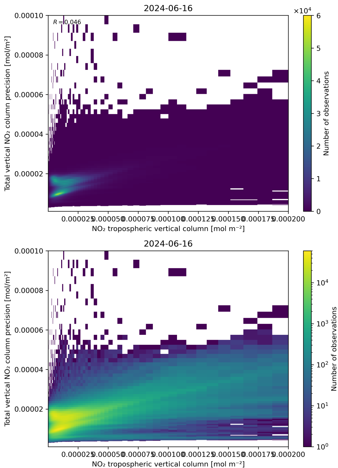
Figure 129: Scatter density plot of “NO 2 tropospheric vertical column” against “Total vertical NO 2 column precision” for 2024-06-15 to 2024-06-17.
