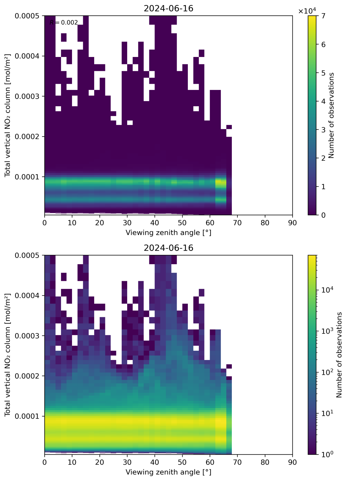
Figure 167: Scatter density plot of “Viewing zenith angle” against “Total vertical NO 2 column” for 2024-06-15 to 2024-06-17.
