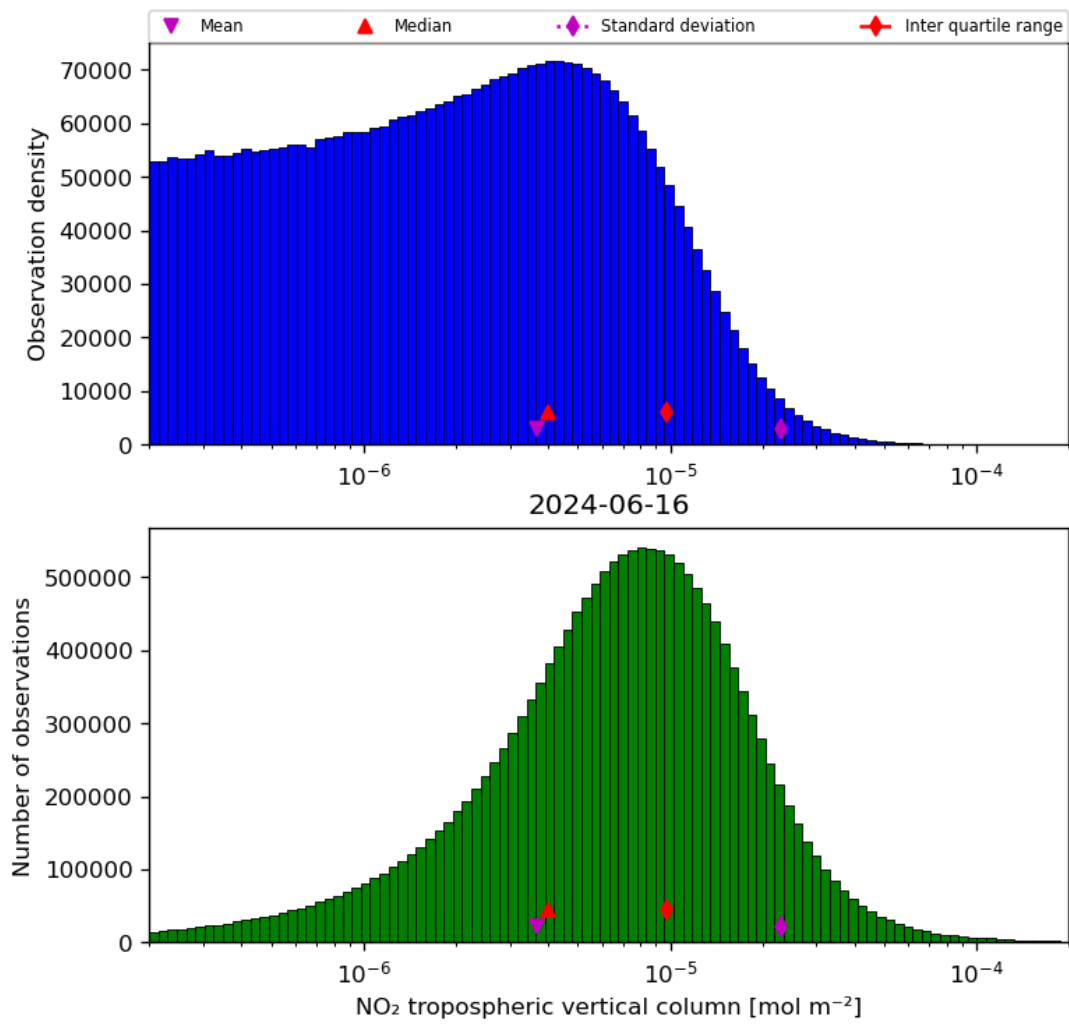
Figure 29: Histogram of “NO 2 tropospheric vertical column” for 2024-06-15 to 2024-06-17
