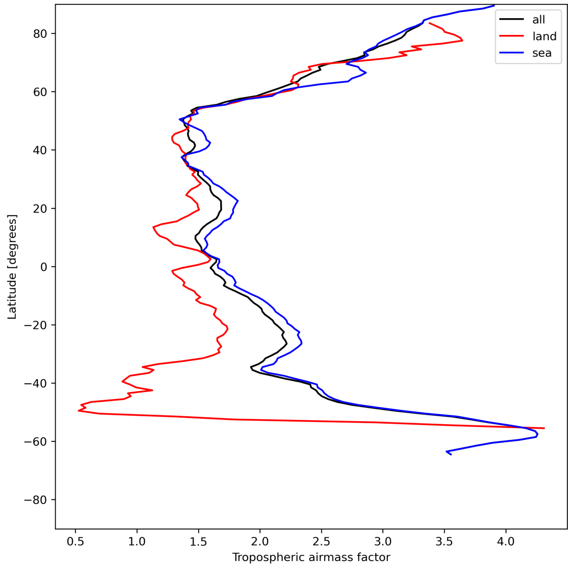
Figure 14: Zonal average of “Tropospheric airmass factor” for 2024-06-15 to 2024-06-17.
