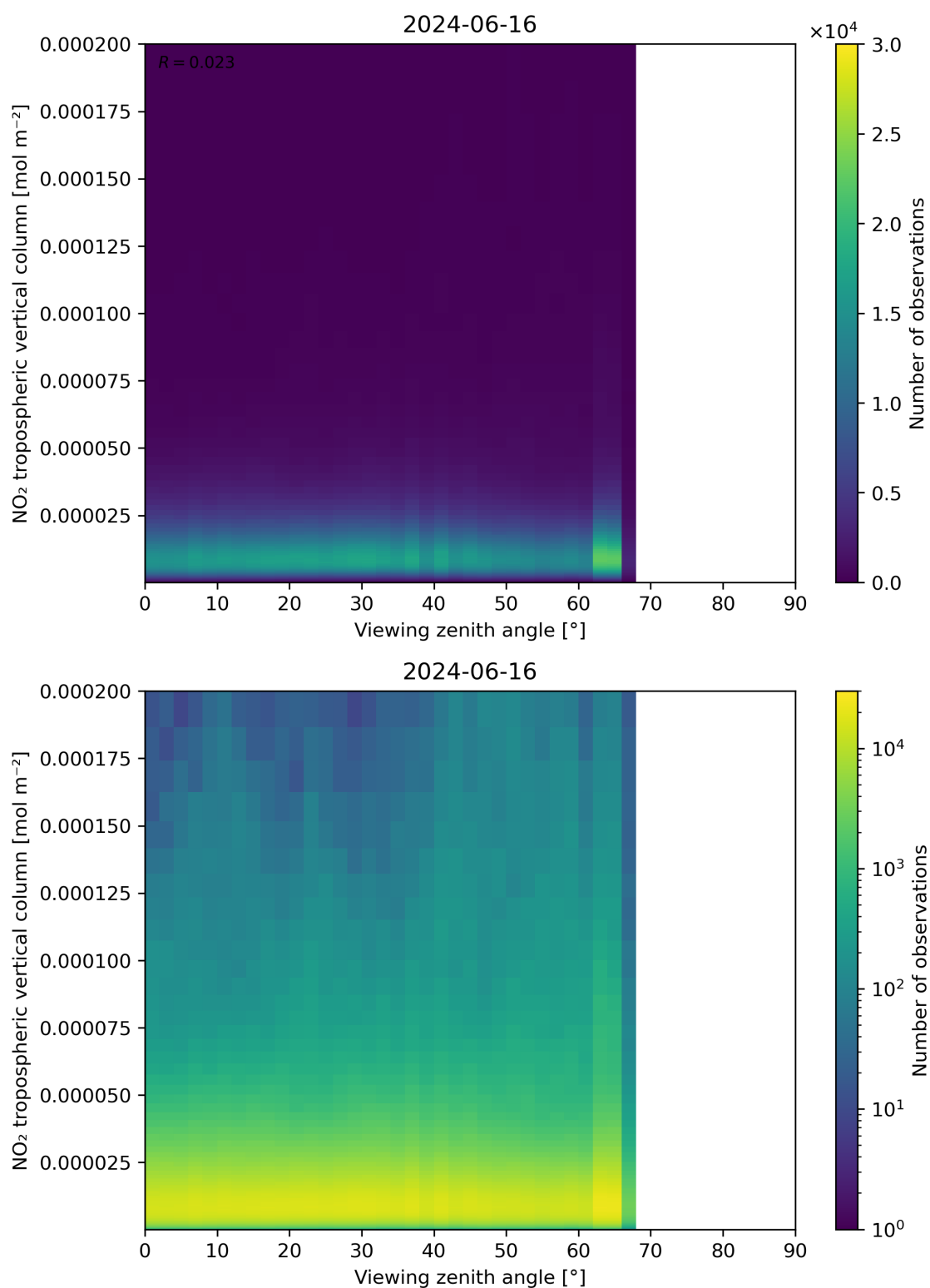
Figure 169: Scatter density plot of “Viewing zenith angle” against “NO 2 tropospheric vertical column” for 2024-06-15 to 2024-06-17.
