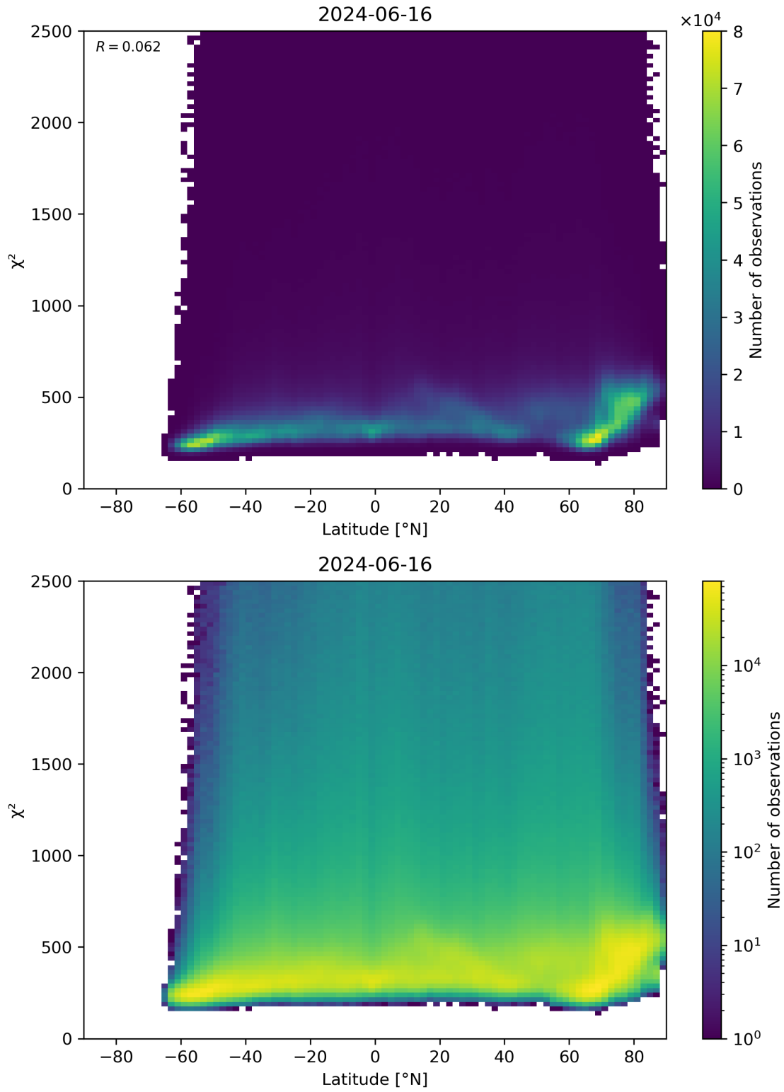
Figure 86: Scatter density plot of “Latitude” against “ \chi^2 ” for 2024-06-15 to 2024-06-17.
