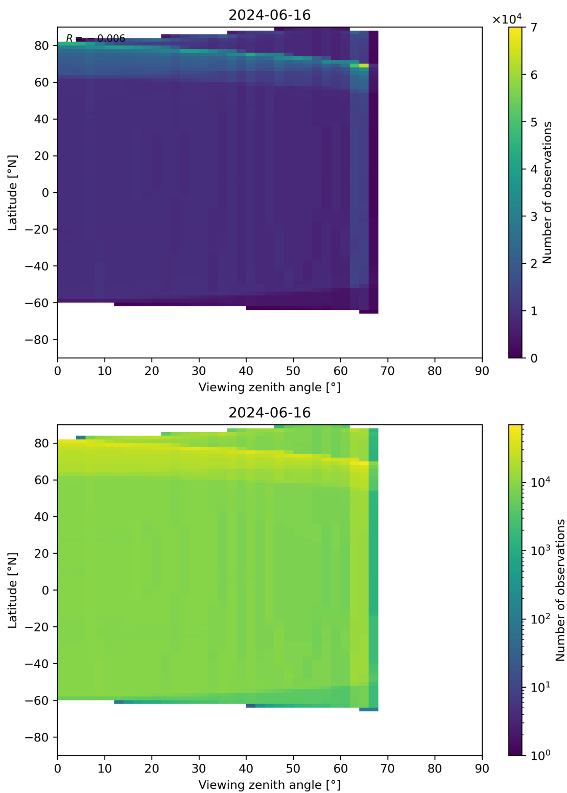
Figure 163: Scatter density plot of “Viewing zenith angle” against “Latitude” for 2024-06-15 to 2024-06-17.
