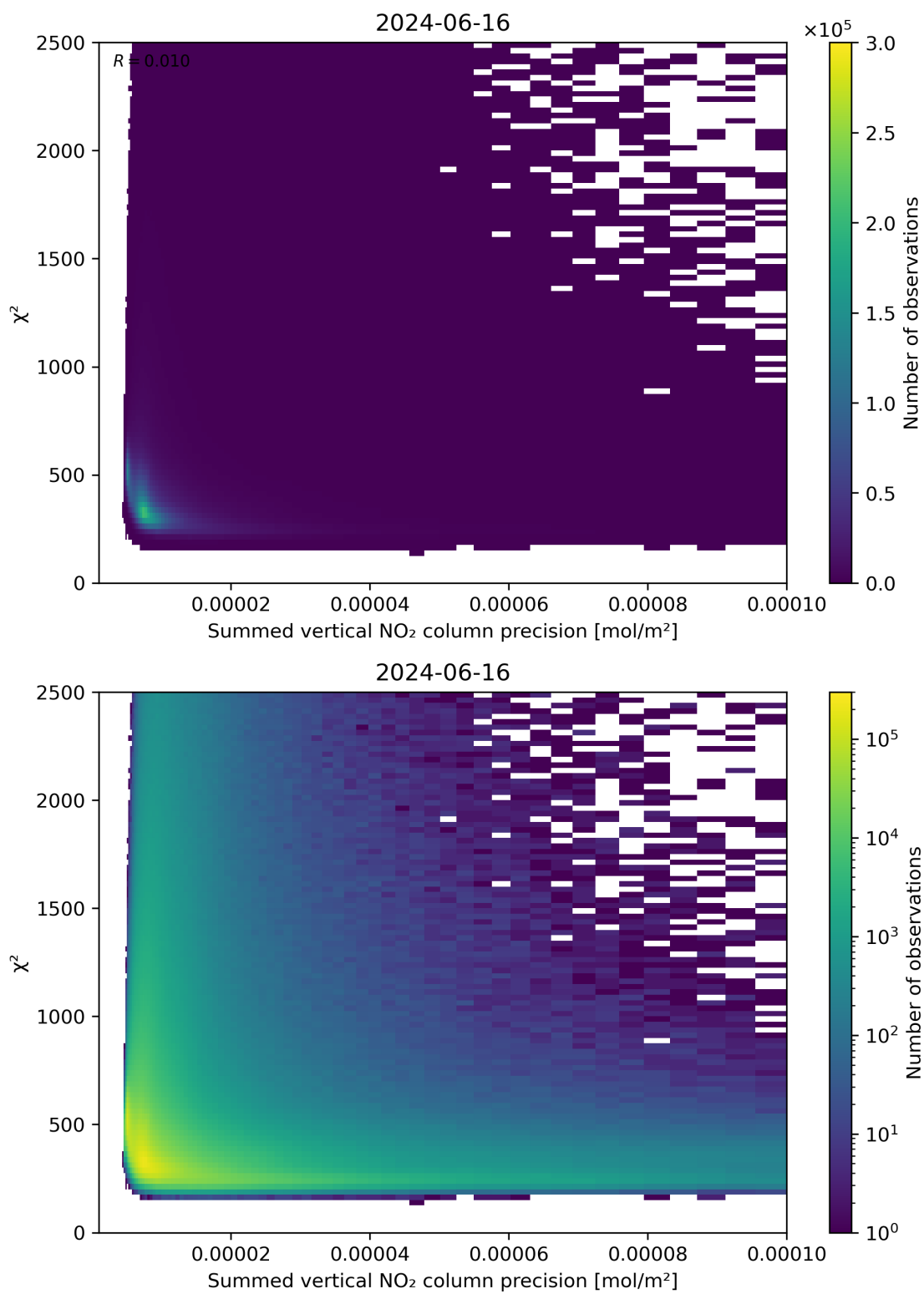
Figure 107: Scatter density plot of “Summed vertical NO 2 column precision” against “ \chi^2 ” for 2024-06-15 to 2024-06-17.
