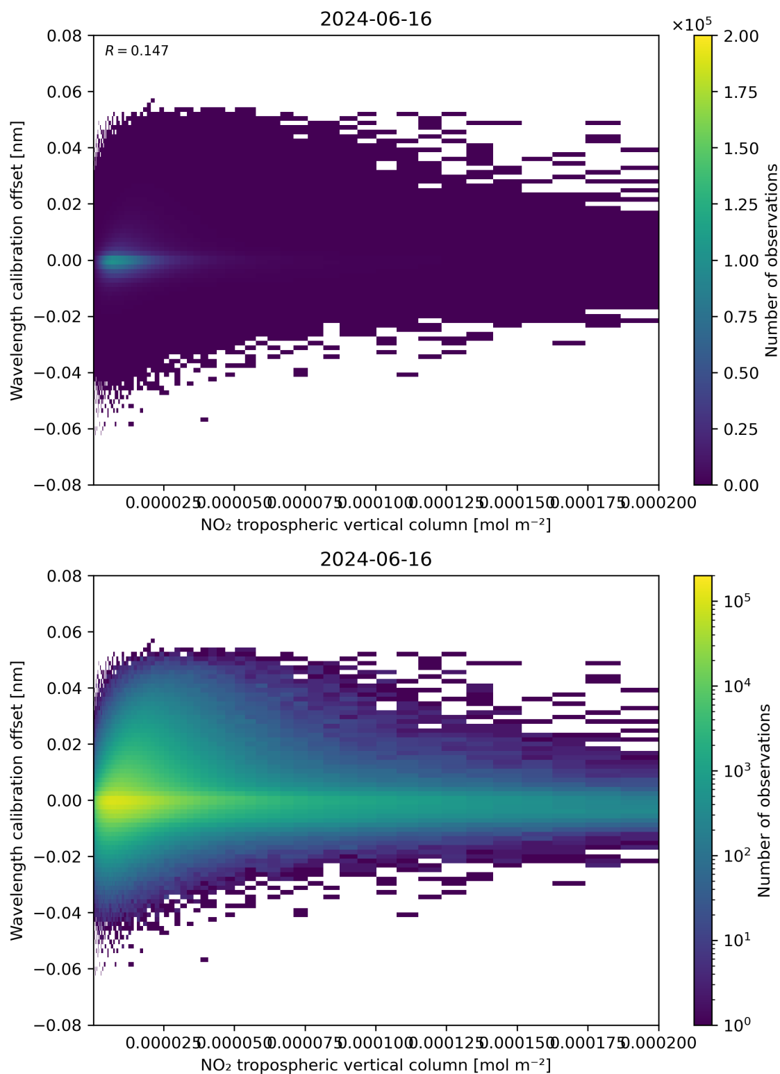
Figure 143: Scatter density plot of “NO 2 tropospheric vertical column” against “Wavelength calibration offset” for 2024-06-15 to 2024-06-17.
