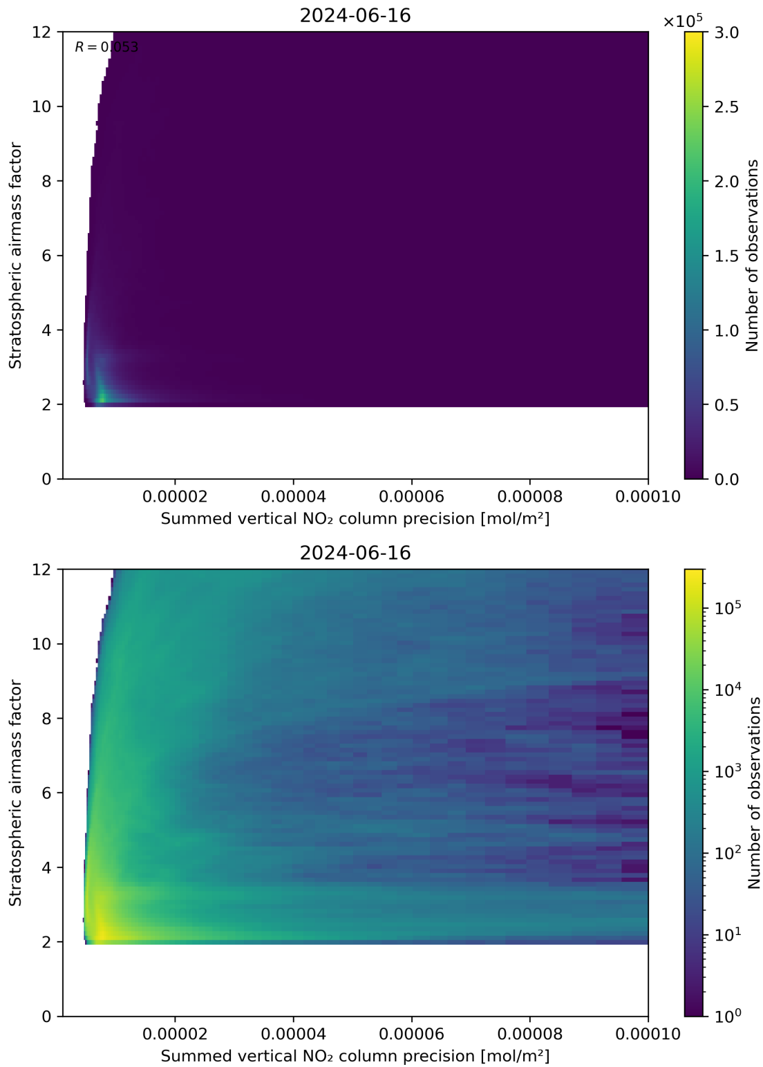
Figure 106: Scatter density plot of “Summed vertical NO 2 column precision” against “Stratospheric airmass factor” for 2024-06-15 to 2024-06-17.
