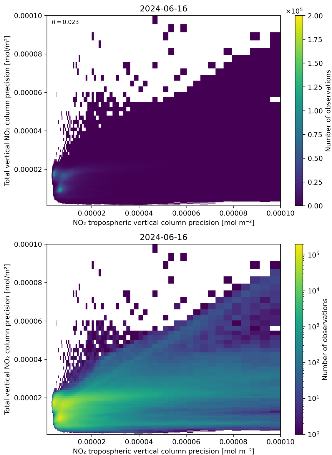
Figure 139: Scatter density plot of “NO 2 tropospheric vertical column precision” against “Total vertical NO 2 column precision” for 2024-06-15 to 2024-06-17.
