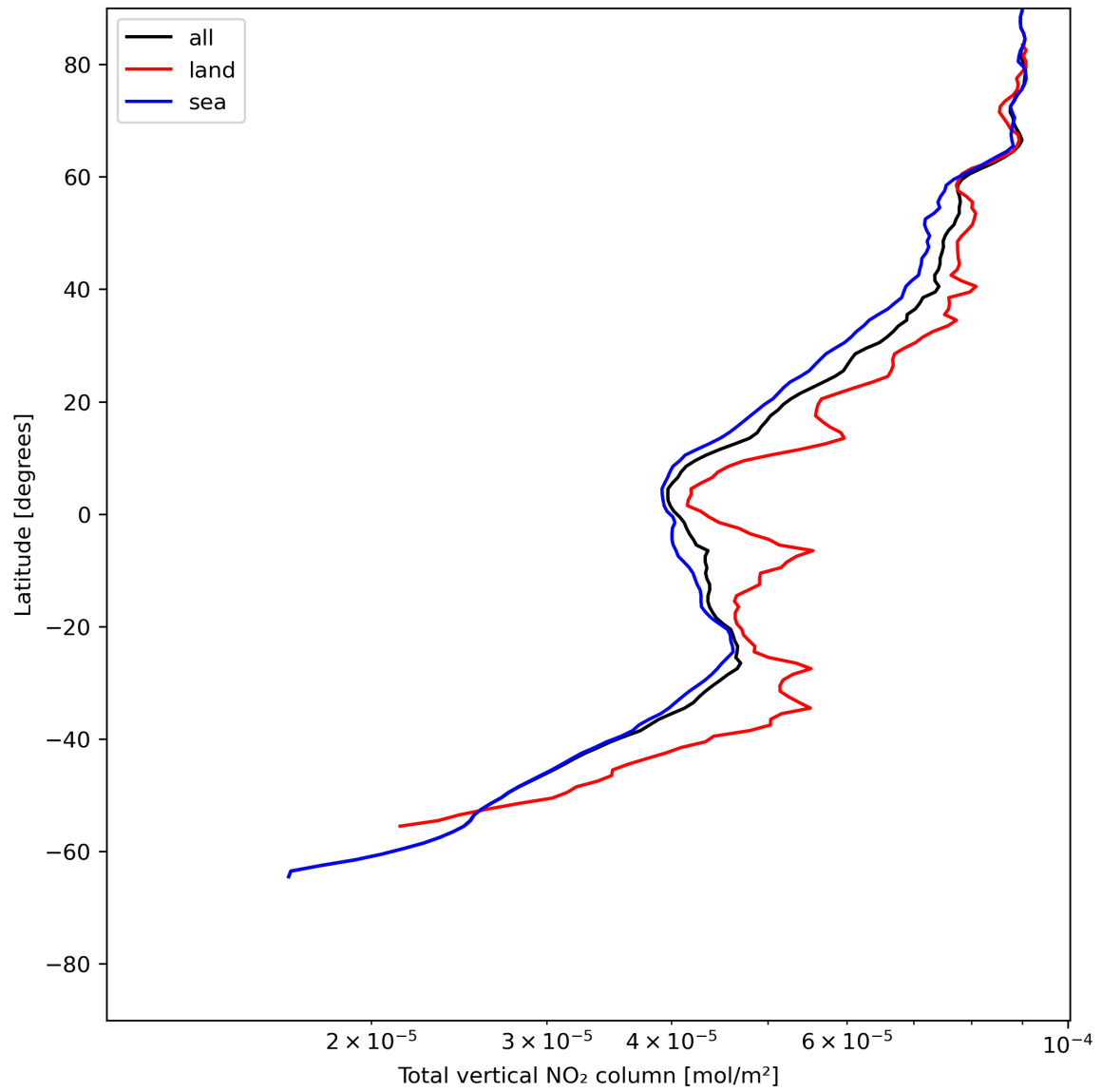
Figure 21: Zonal average of “Total vertical NO 2 column” for 2024-06-15 to 2024-06-17.
