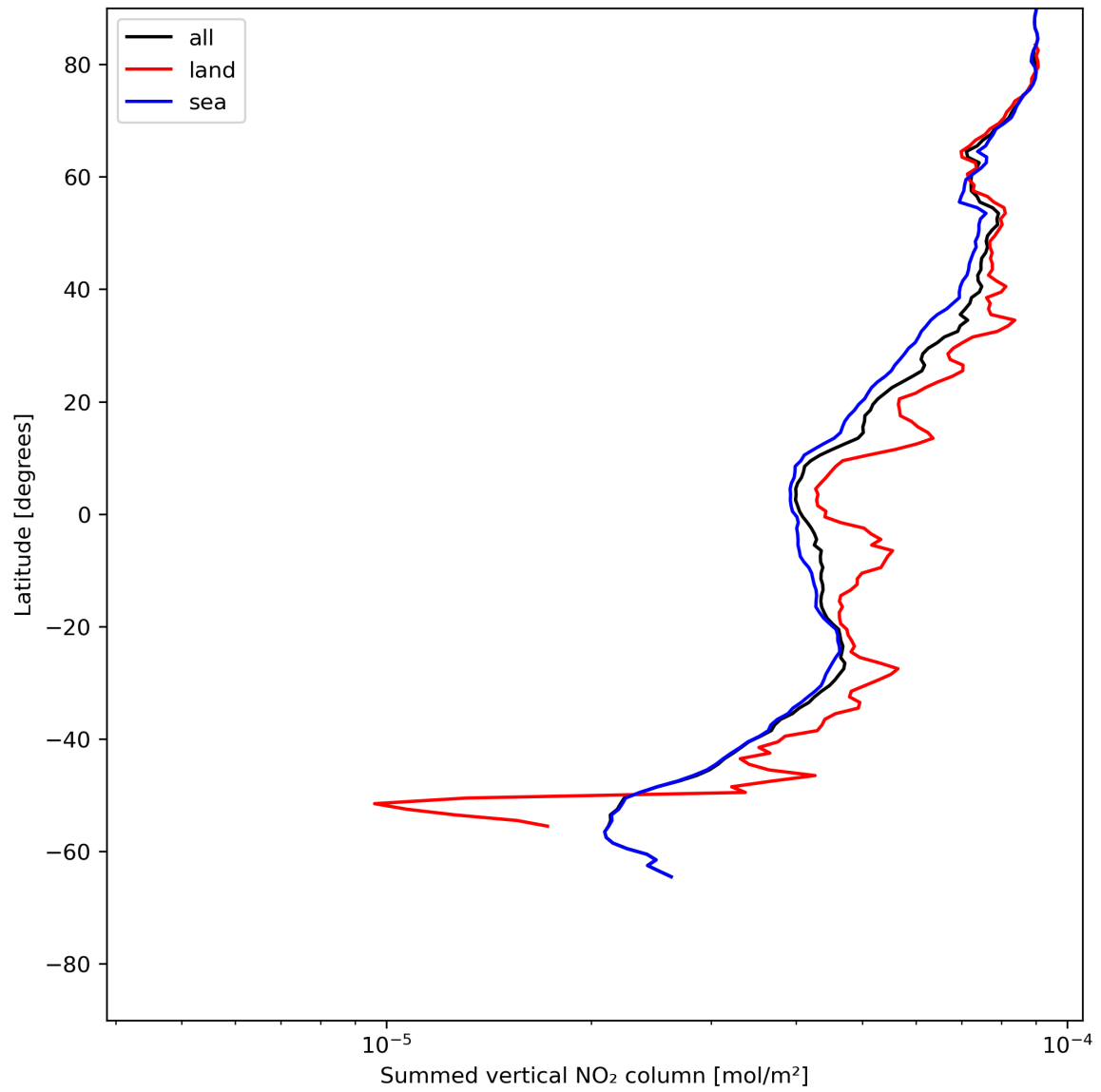
Figure 23: Zonal average of “Summed vertical NO 2 column” for 2024-06-15 to 2024-06-17.
