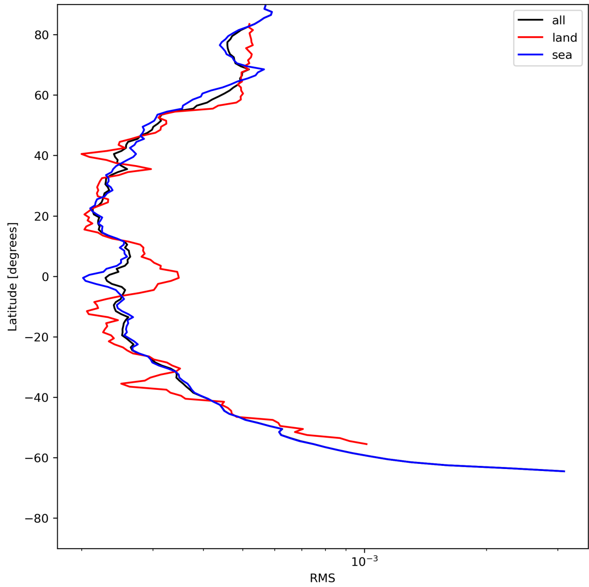
Figure 26: Zonal average of “RMS” for 2024-06-15 to 2024-06-17.
