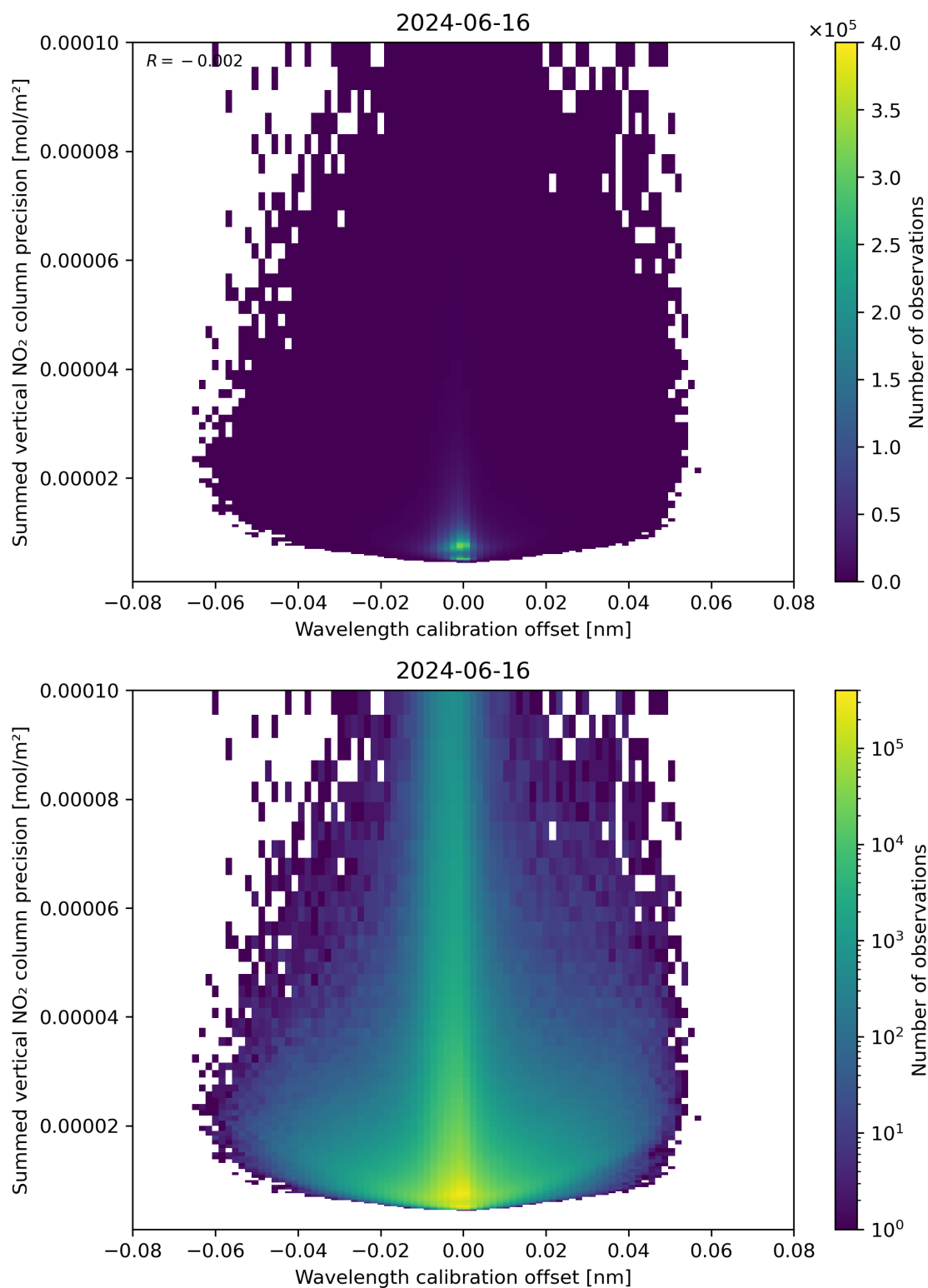
Figure 178: Scatter density plot of “Wavelength calibration offset” against “Summed vertical NO 2 column precision” for 2024-06-15 to 2024-06-17.
