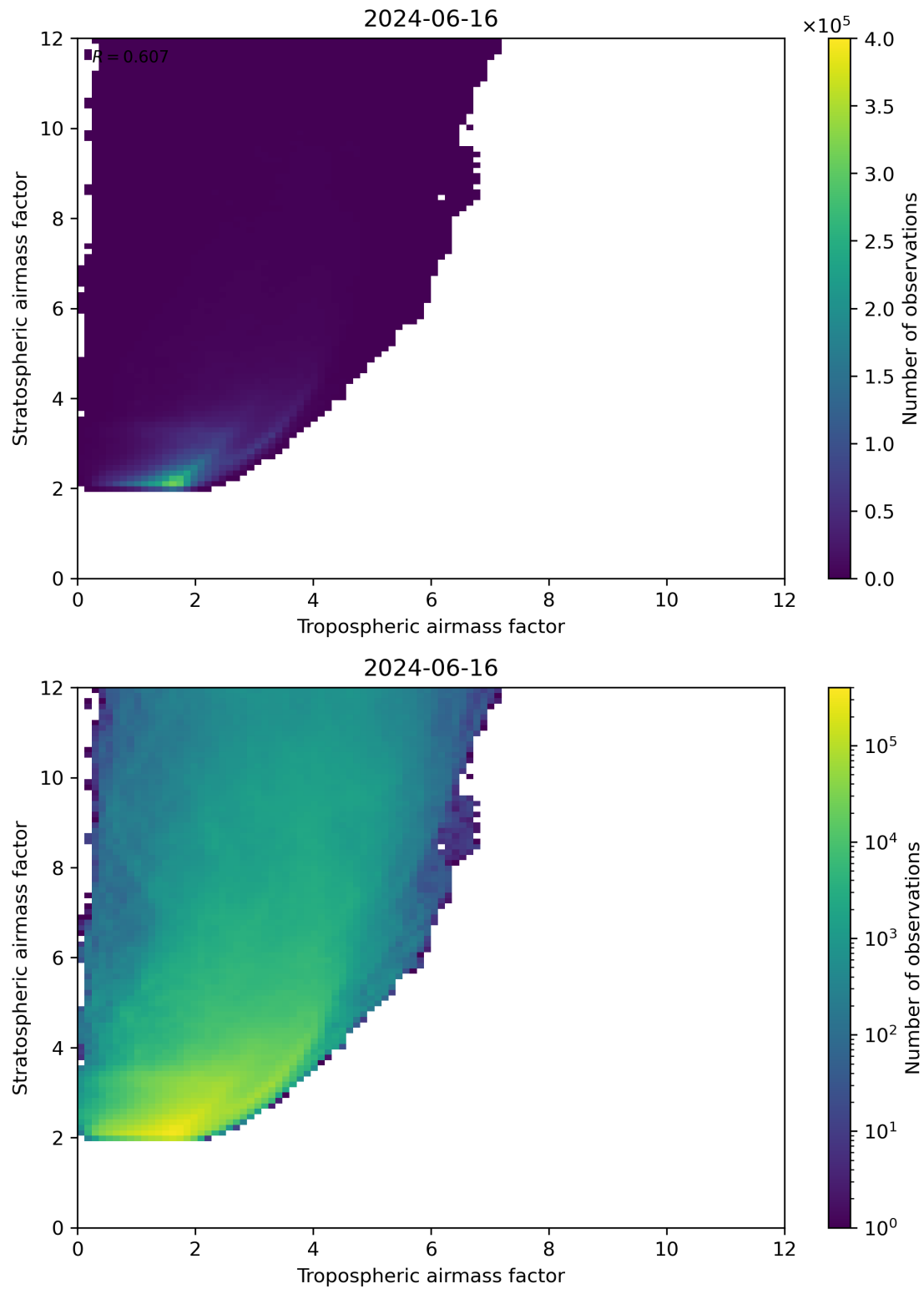
Figure 71: Scatter density plot of “Tropospheric airmass factor” against “Stratospheric airmass factor” for 2024-06-15 to 2024-06-17.
