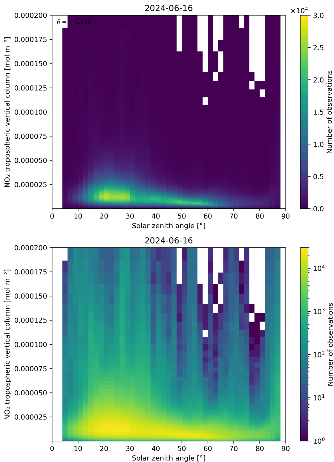
Figure 155: Scatter density plot of “Solar zenith angle” against “NO 2 tropospheric vertical column” for 2024-06-15 to 2024-06-17.
