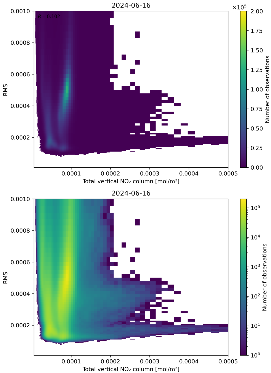
Figure 120: Scatter density plot of “Total vertical NO 2 column” against “RMS” for 2024-06-15 to 2024-06-17.
