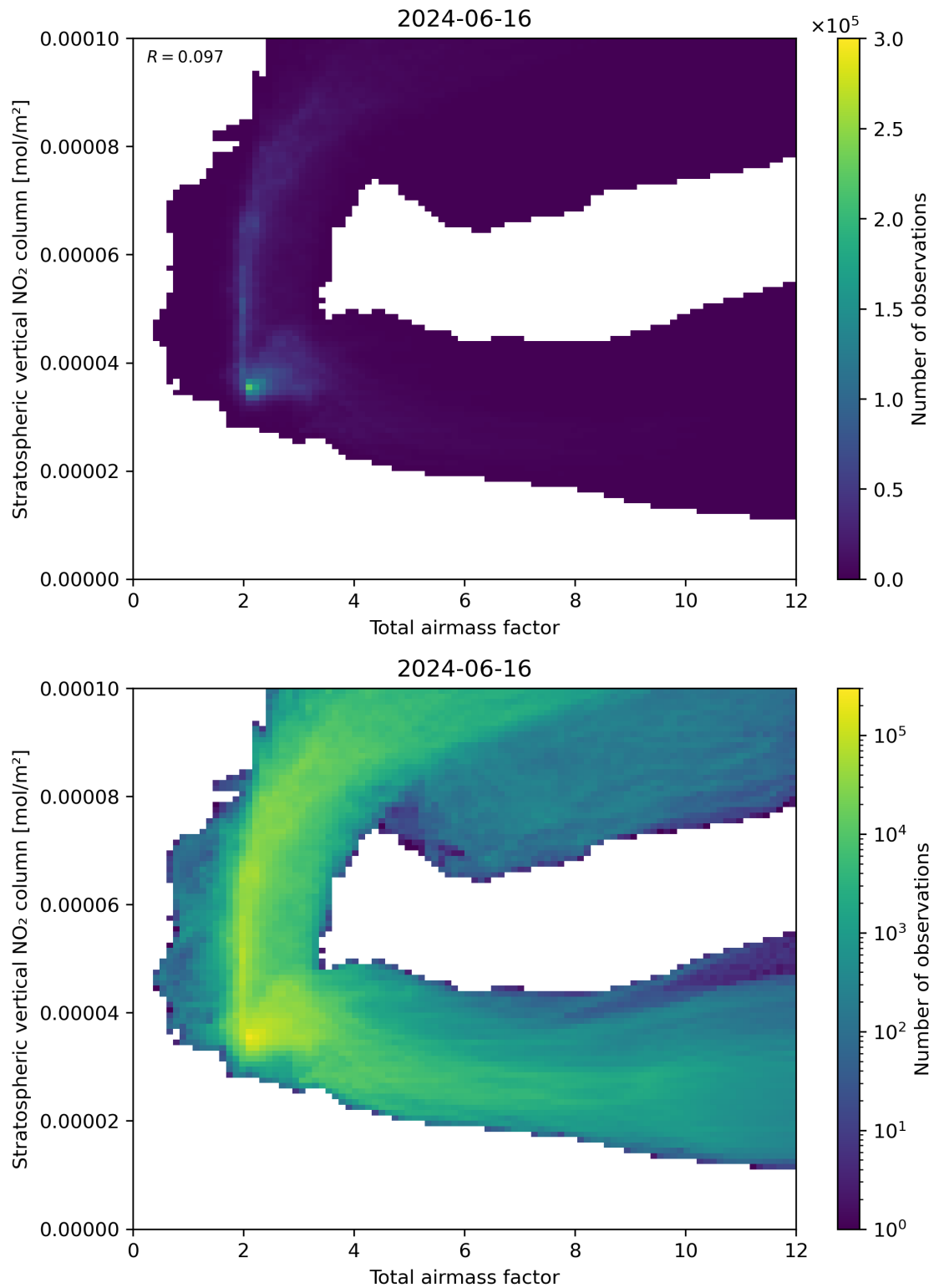
Figure 64: Scatter density plot of “Total airmass factor” against “Stratospheric vertical NO 2 column” for 2024-06-15 to 2024-06-17.
