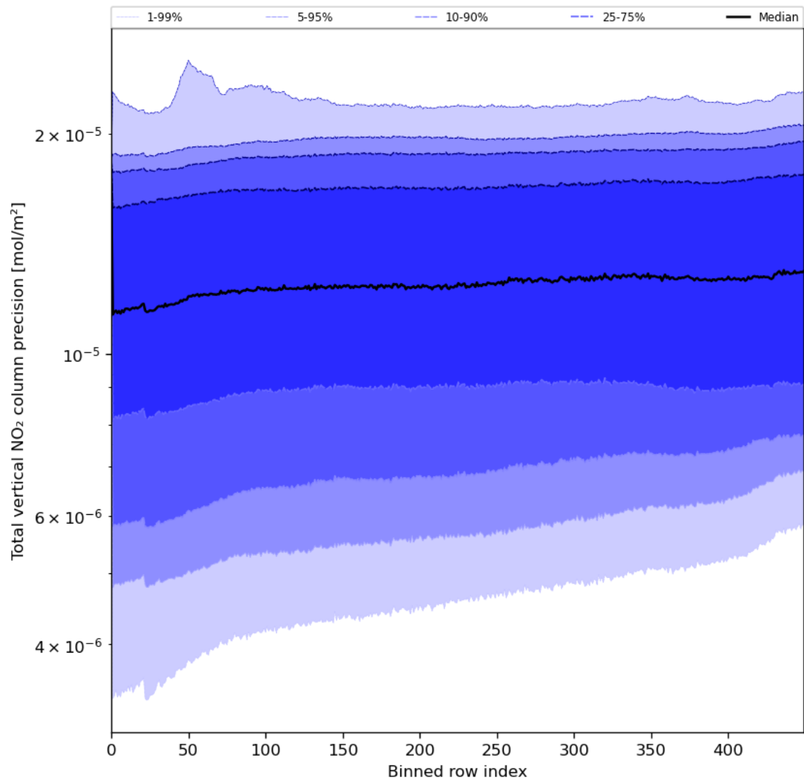
Figure 56: Along track statistics of “Total vertical NO 2 column precision” for 2024-06-15 to 2024-06-17
