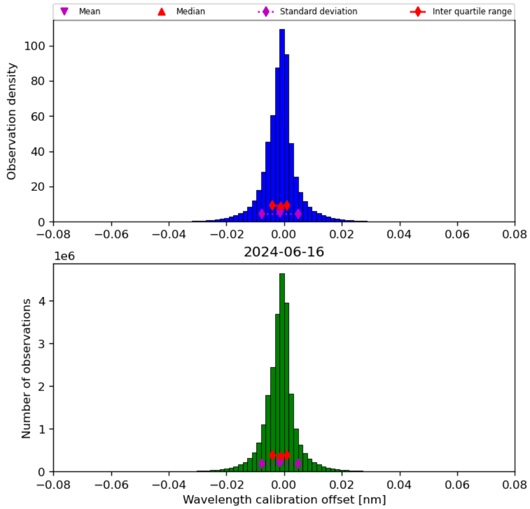
Figure 35: Histogram of “Wavelength calibration offset” for 2024-06-15 to 2024-06-17
