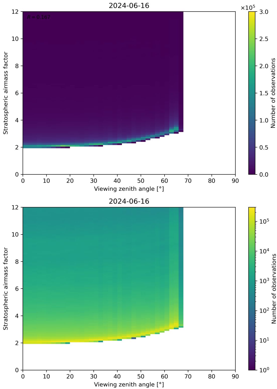
Figure 159: Scatter density plot of “Viewing zenith angle” against “Stratospheric airmass factor” for 2024-06-15 to 2024-06-17.
