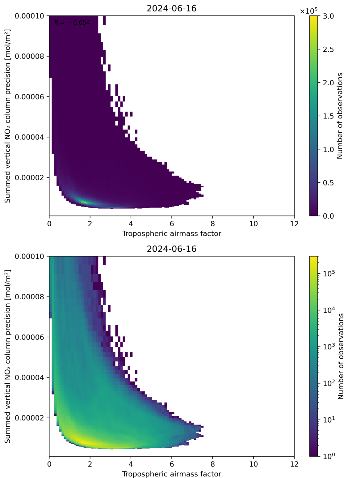
Figure 76: Scatter density plot of “Tropospheric air mass factor” against “Summed vertical NO 2 column precision” for 2024-06-15 to 2024-06-17.
