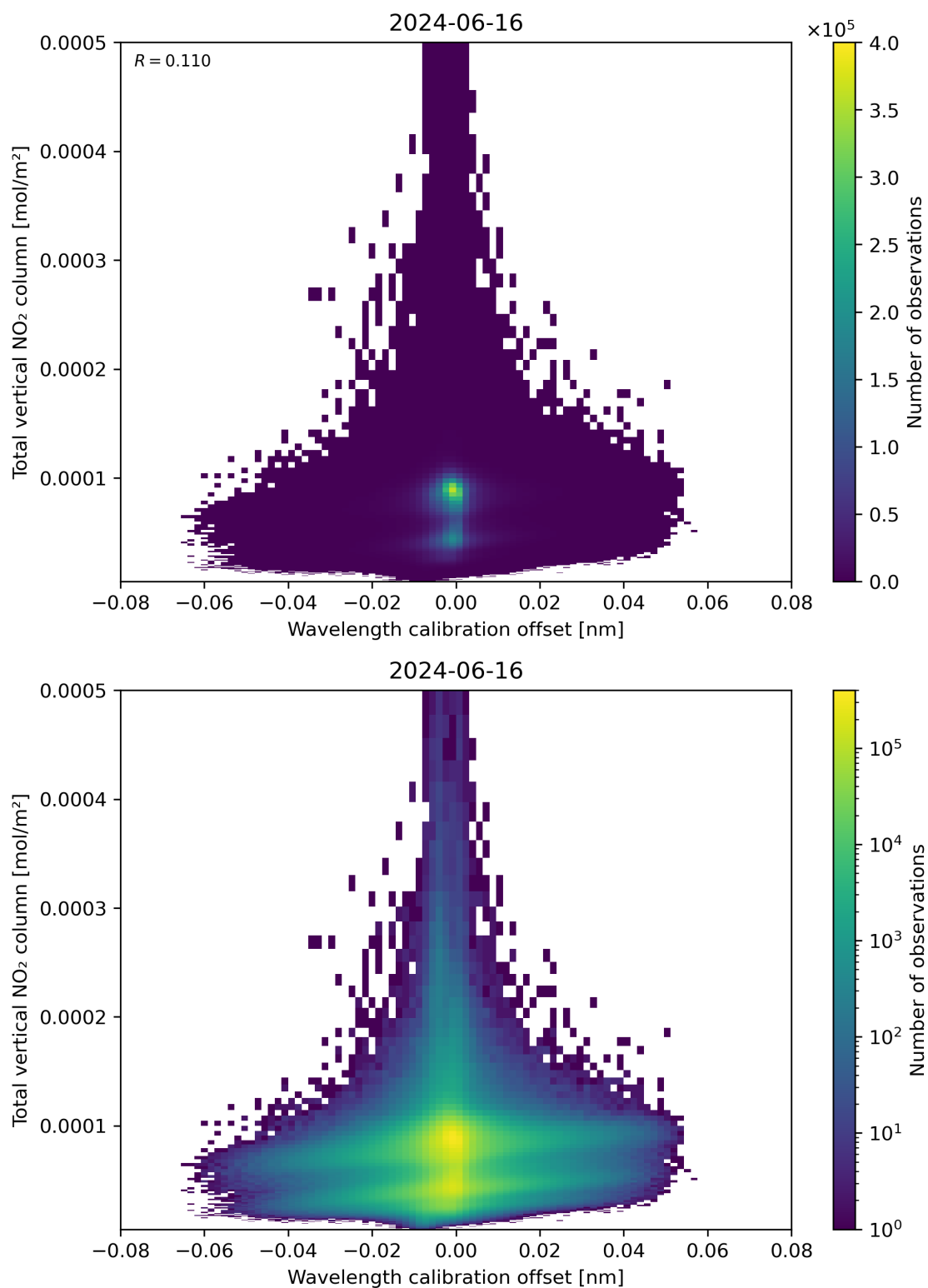
Figure 179: Scatter density plot of “Wavelength calibration offset” against “Total vertical NO 2 column” for 2024-06-15 to 2024-06-17.
