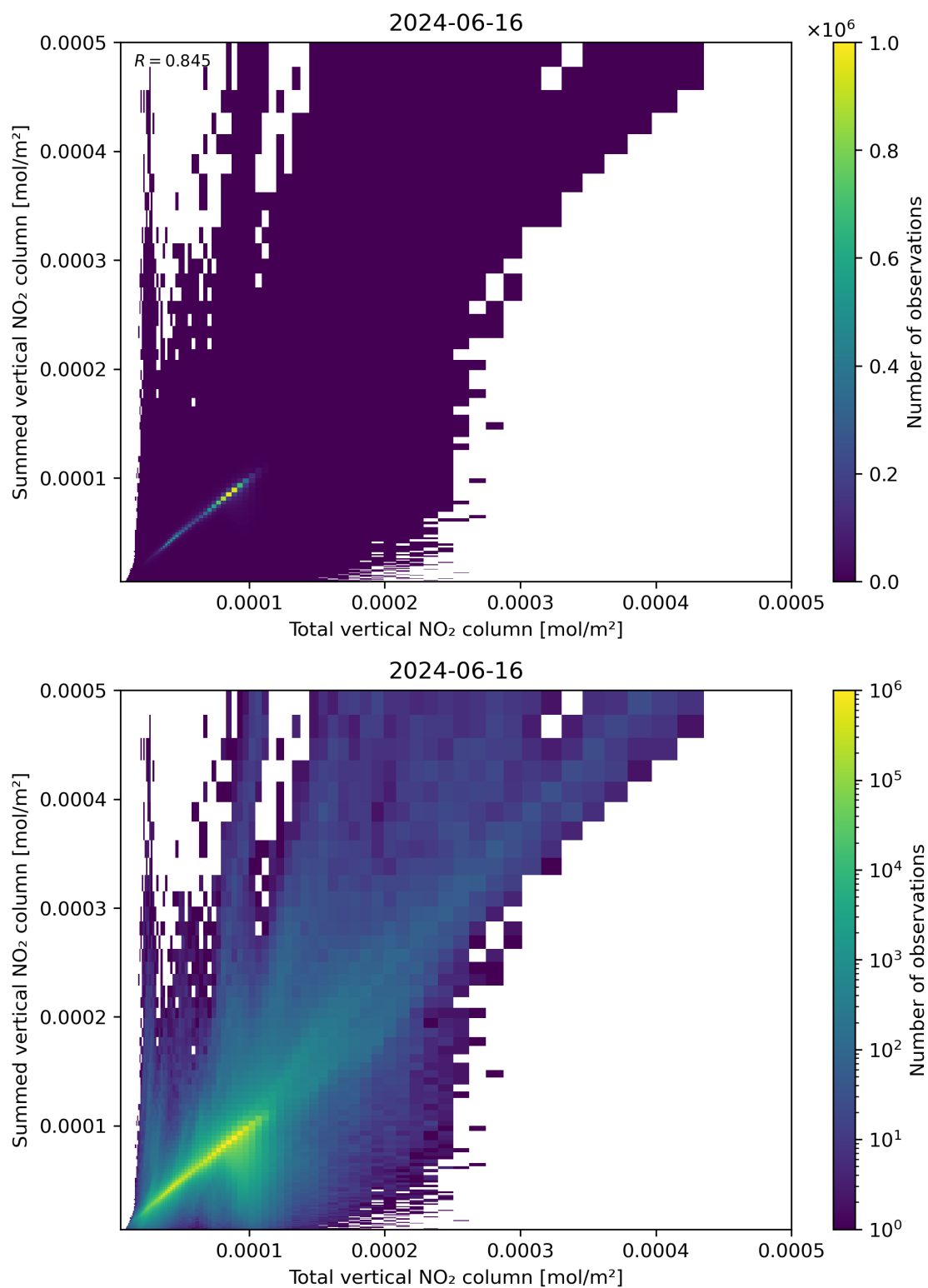
Figure 112: Scatter density plot of “Total vertical NO 2 column” against “Summed vertical NO 2 column” for 2024-06-15 to 2024-06-17.
