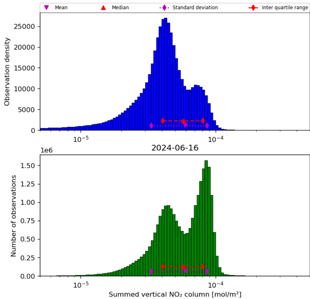
Figure 40: Histogram of “Summed vertical NO 2 column” for 2024-06-15 to 2024-06-17
