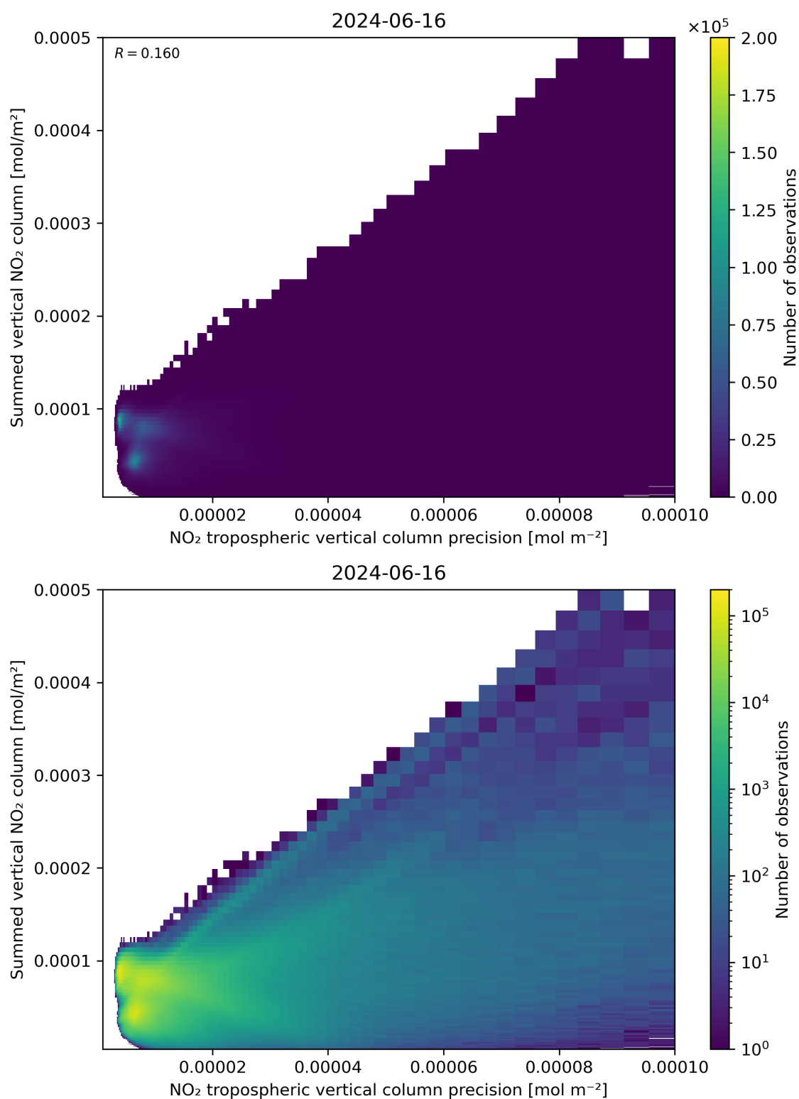
Figure 136: Scatter density plot of “NO 2 tropospheric vertical column precision” against “Summed vertical NO 2 column” for 2024-06-15 to 2024-06-17.
