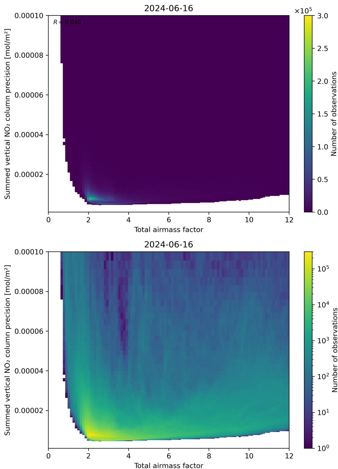
Figure 66: Scatter density plot of “Total airmass factor” against “Summed vertical NO 2 column precision” for 2024-06-15 to 2024-06-17.
