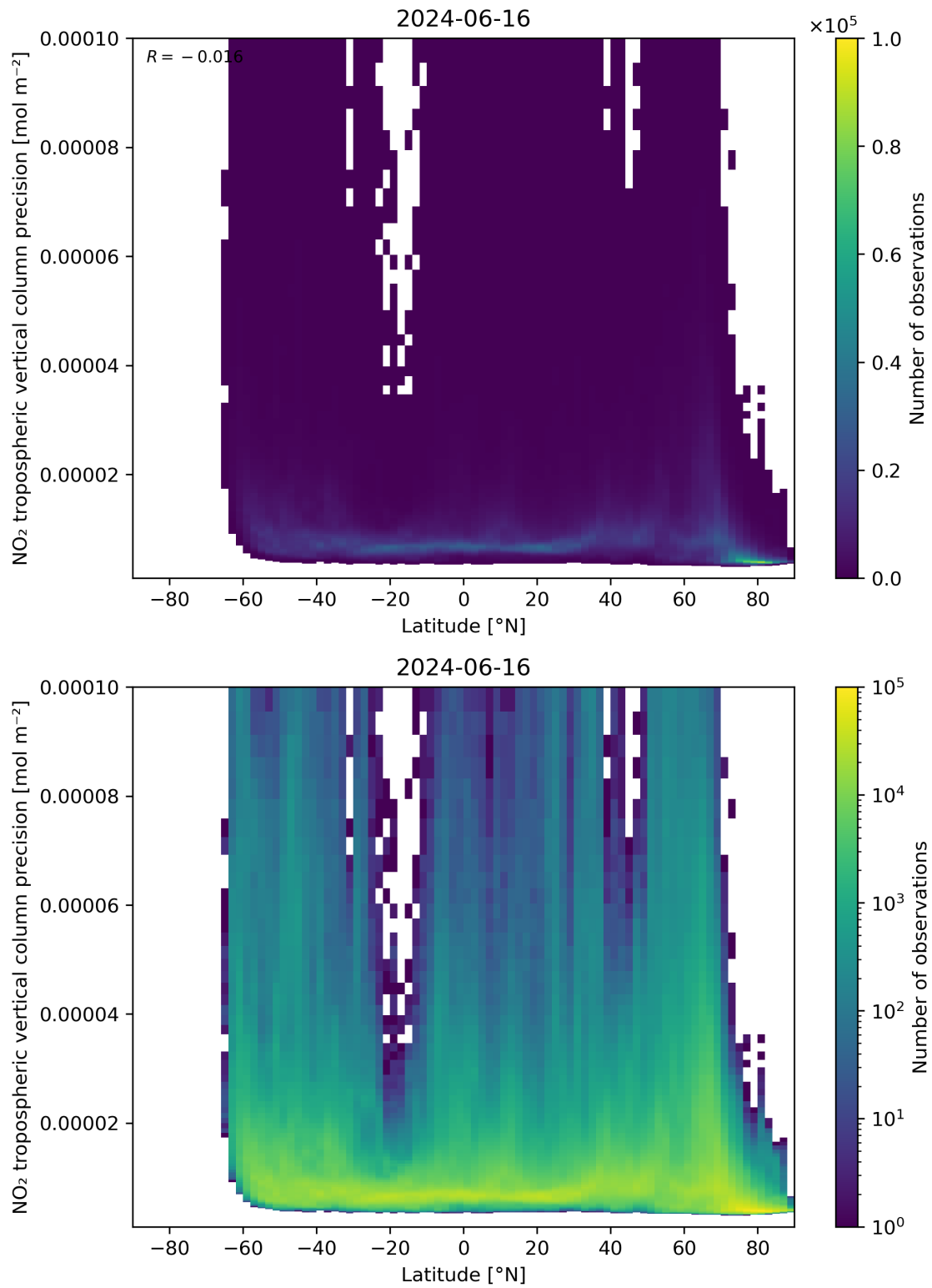
Figure 93: Scatter density plot of “Latitude” against “NO 2 tropospheric vertical column precision” for 2024-06-15 to 2024-06-17.
