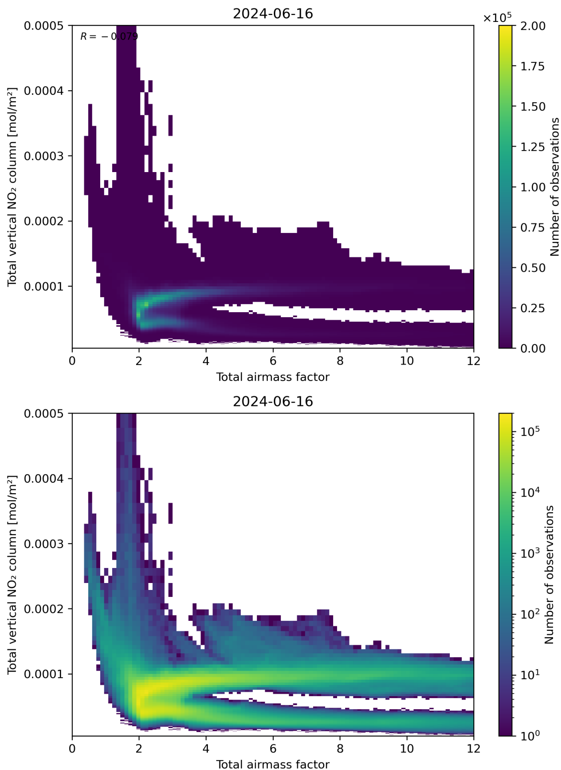
Figure 67: Scatter density plot of “Total airmass factor” against “Total vertical NO 2 column” for 2024-06-15 to 2024-06-17.
