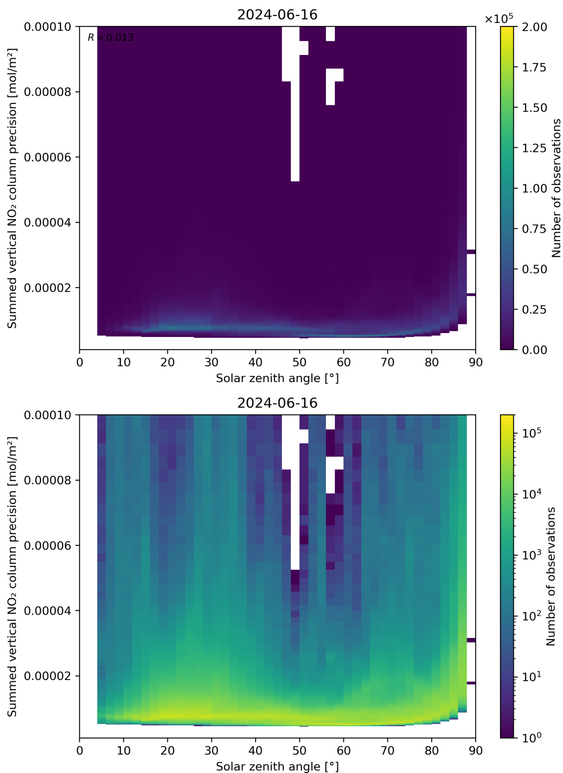
Figure 152: Scatter density plot of “Solar zenith angle” against “Summed vertical NO 2 column precision” for 2024-06-15 to 2024-06-17.
