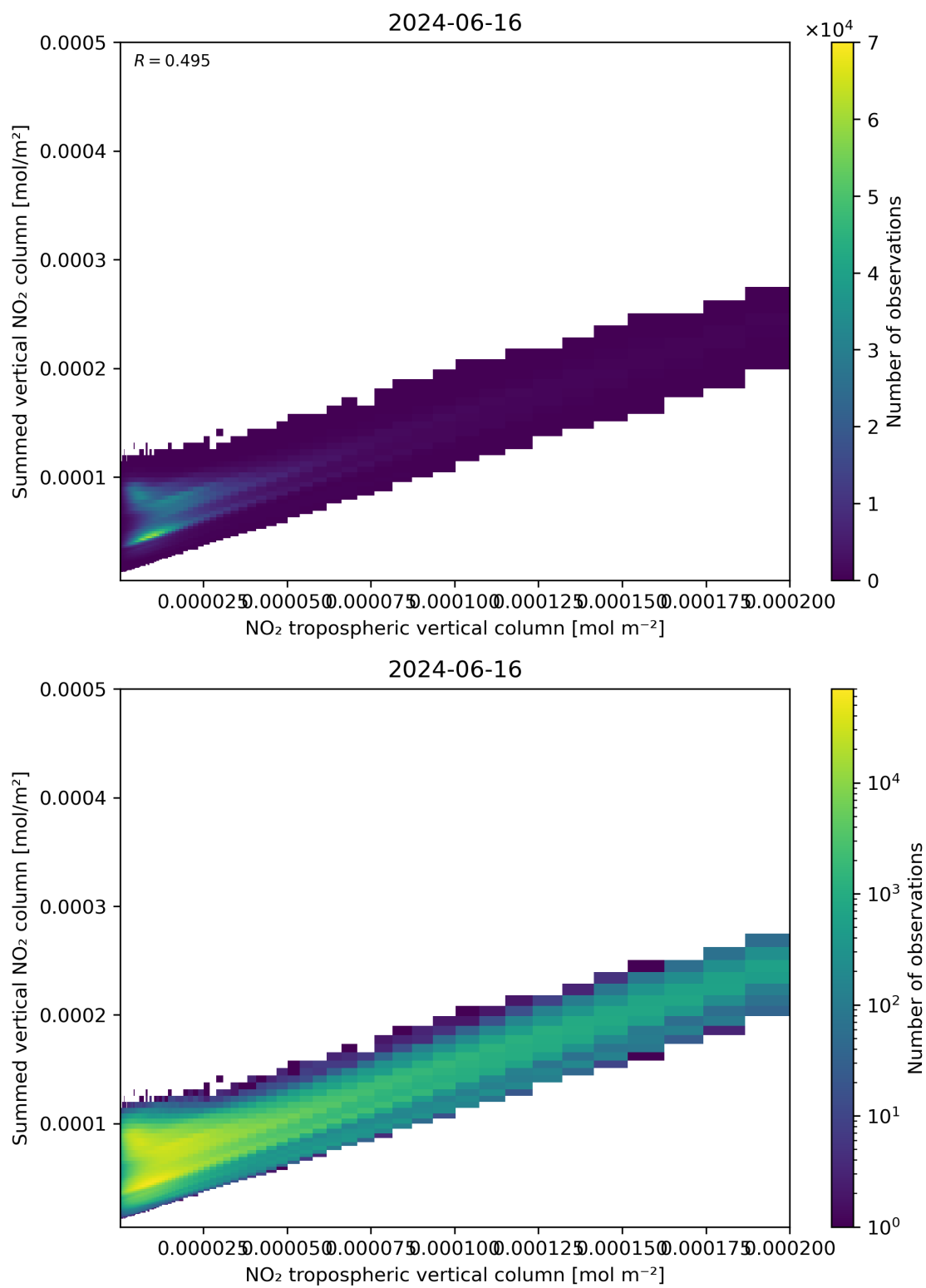
Figure 126: Scatter density plot of “NO 2 tropospheric vertical column” against “Summed vertical NO 2 column” for 2024-06-15 to 2024-06-17.
