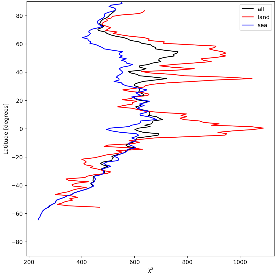
Figure 25: Zonal average of “ \chi^2 ” for 2024-06-15 to 2024-06-17.
