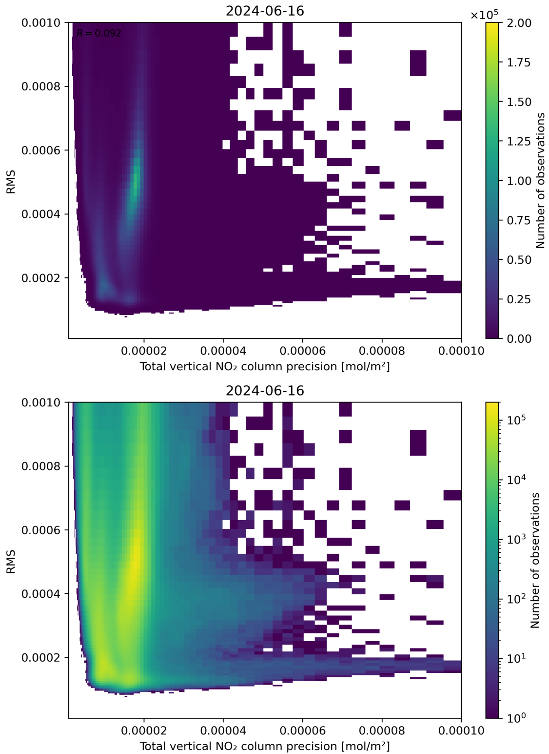
Figure 119: Scatter density plot of “Total vertical NO 2 column precision” against “RMS” for 2024-06-15 to 2024-06-17.
