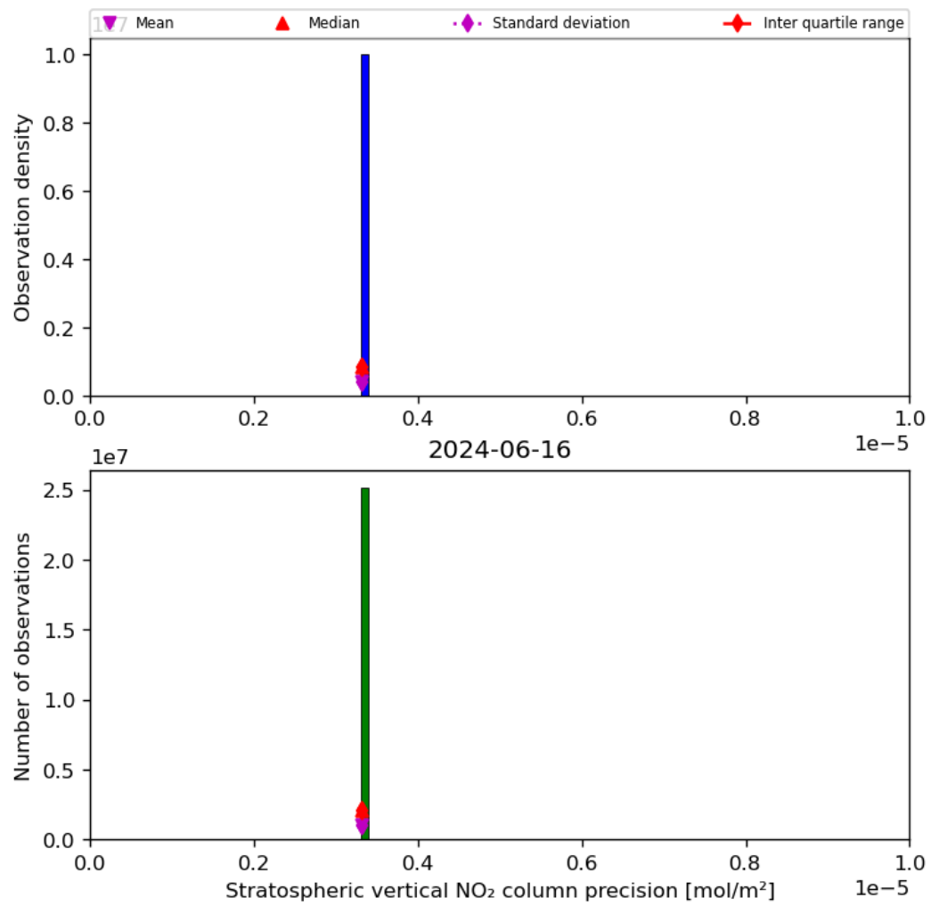
Figure 37: Histogram of “Stratospheric vertical NO 2 column precision” for 2024-06-15 to 2024-06-17
