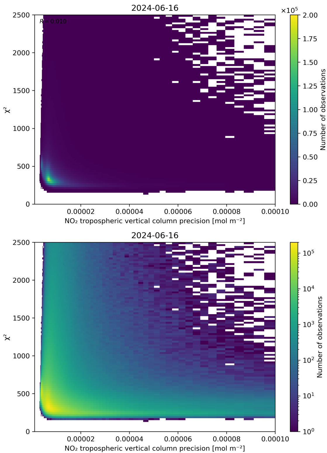
Figure 134: Scatter density plot of “NO 2 tropospheric vertical column precision” against “ \chi^2 ” for 2024-06-15 to 2024-06-17.
