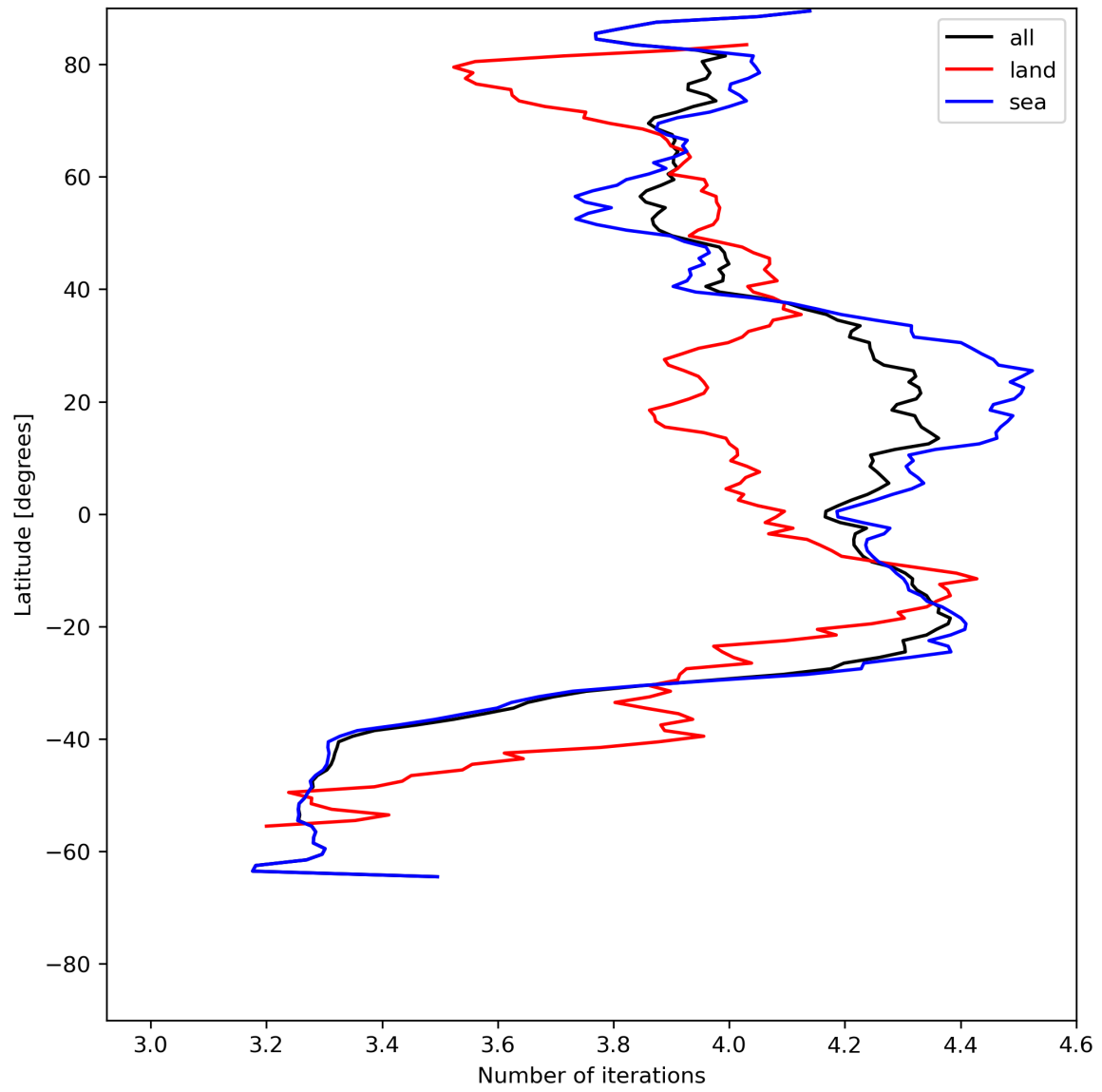
Figure 17: Zonal average of “Number of iterations” for 2024-06-15 to 2024-06-17.
