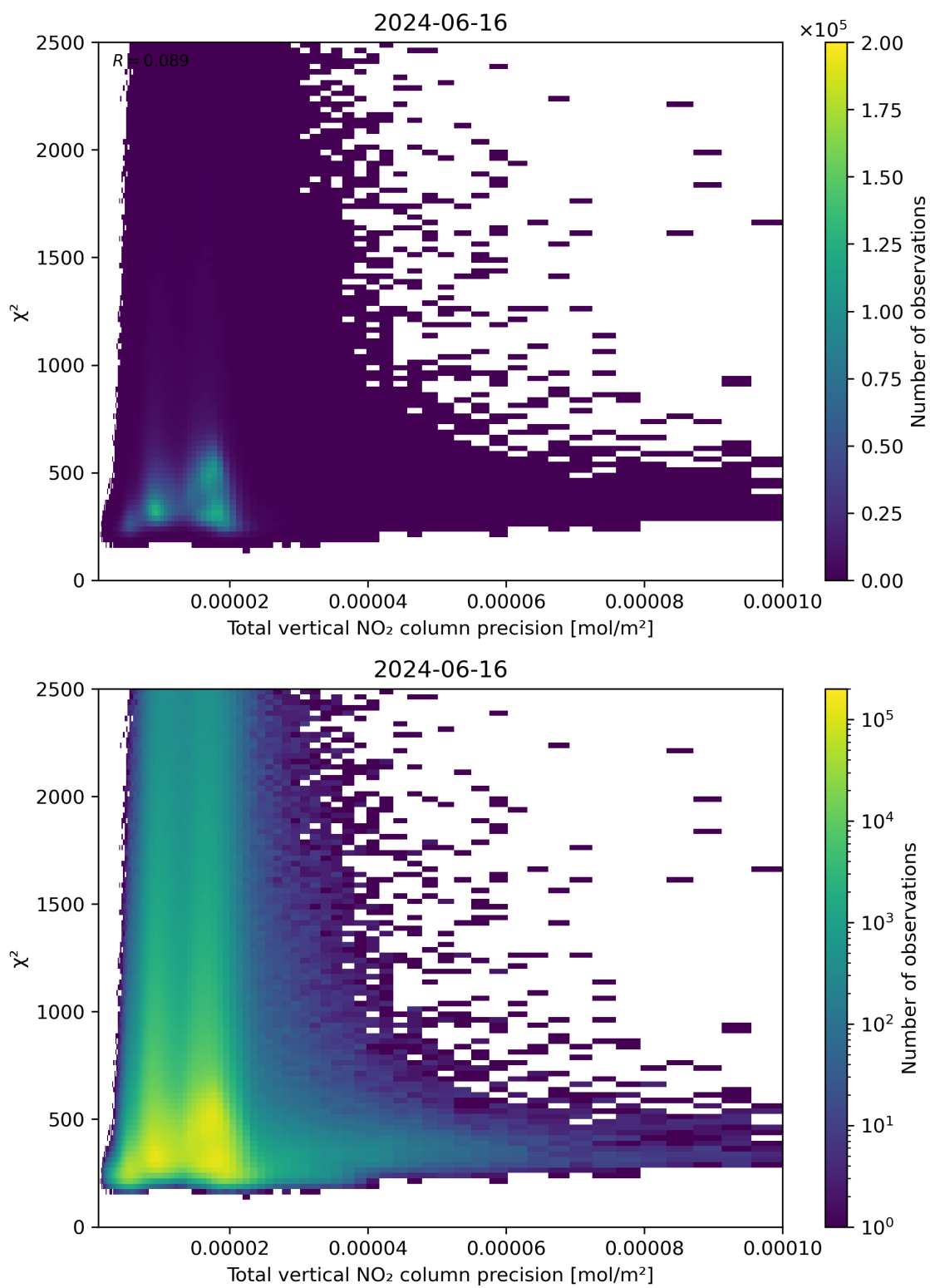
Figure 116: Scatter density plot of “Total vertical NO 2 column precision” against “ \chi^2 ” for 2024-06-15 to 2024-06-17.
