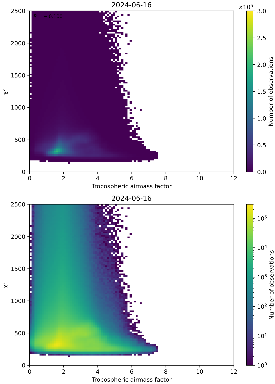
Figure 73: Scatter density plot of “Tropospheric airmass factor” against “ \chi^2 ” for 2024-06-15 to 2024-06-17.
