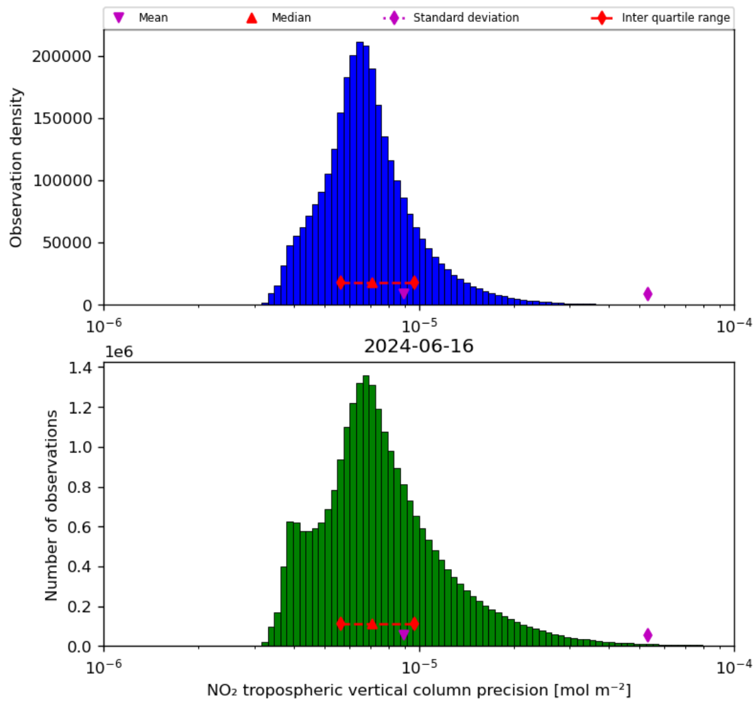
Figure 30: Histogram of “NO 2 tropospheric vertical column precision” for 2024-06-15 to 2024-06-17
