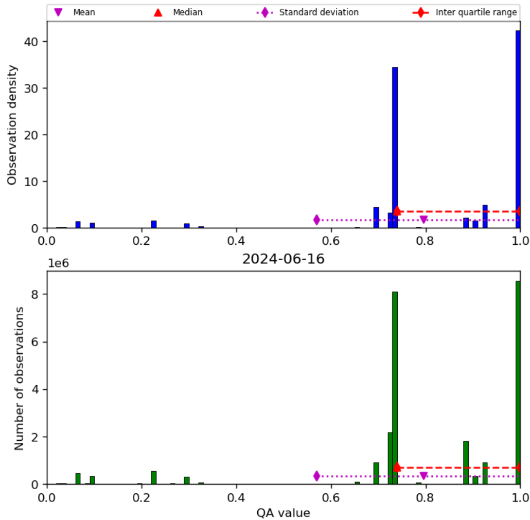
Figure 28: Histogram of “QA value” for 2024-06-15 to 2024-06-17
