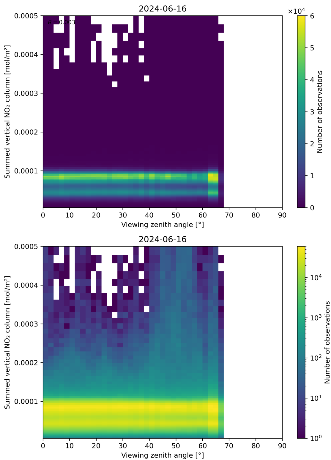
Figure 165: Scatter density plot of “Viewing zenith angle” against “Summed vertical NO 2 column” for 2024-06-15 to 2024-06-17.
