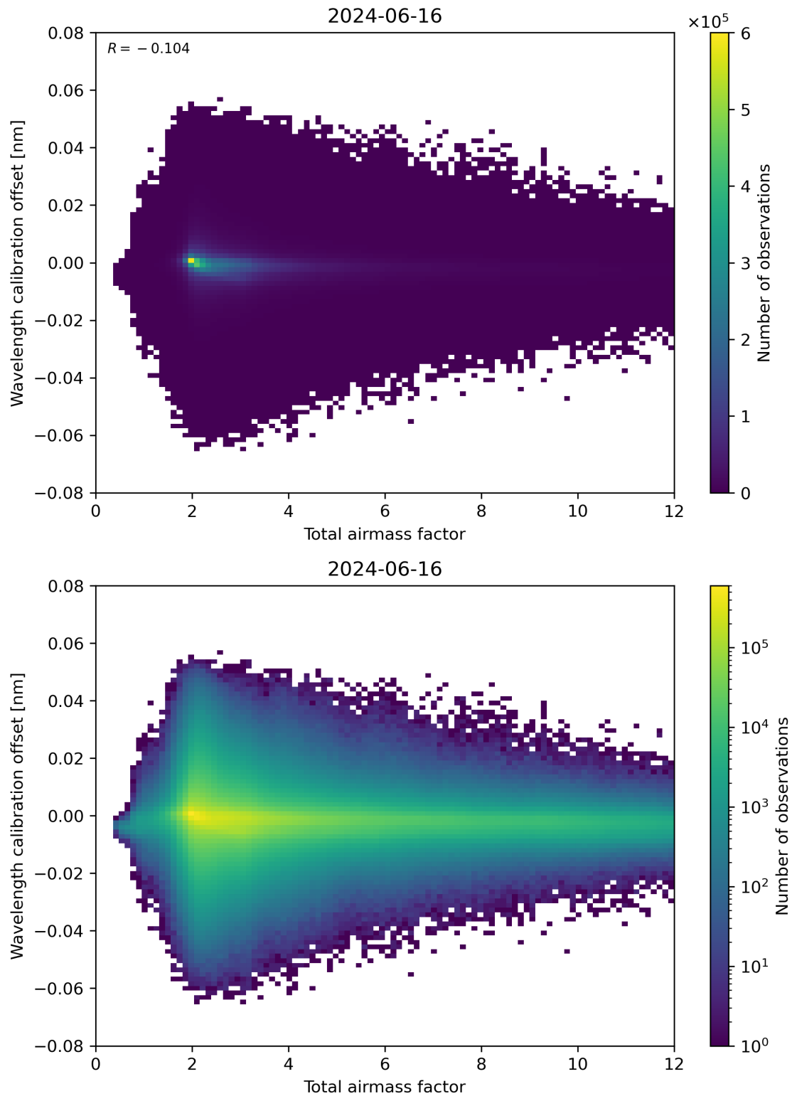
Figure 70: Scatter density plot of “Total airmass factor” against “Wavelength calibration offset” for 2024-06-15 to 2024-06-17.
