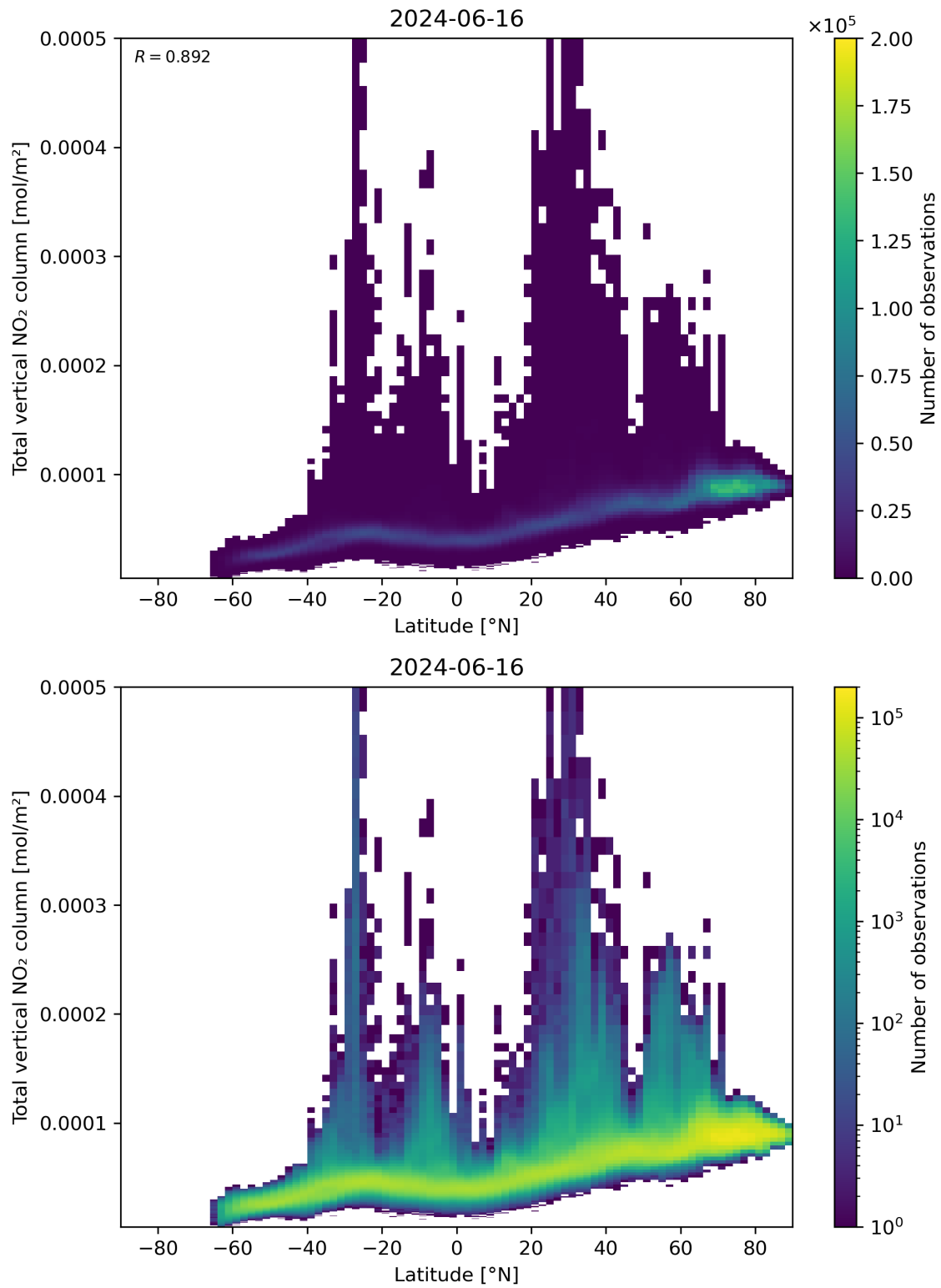
Figure 90: Scatter density plot of “Latitude” against “Total vertical NO 2 column” for 2024-06-15 to 2024-06-17.
