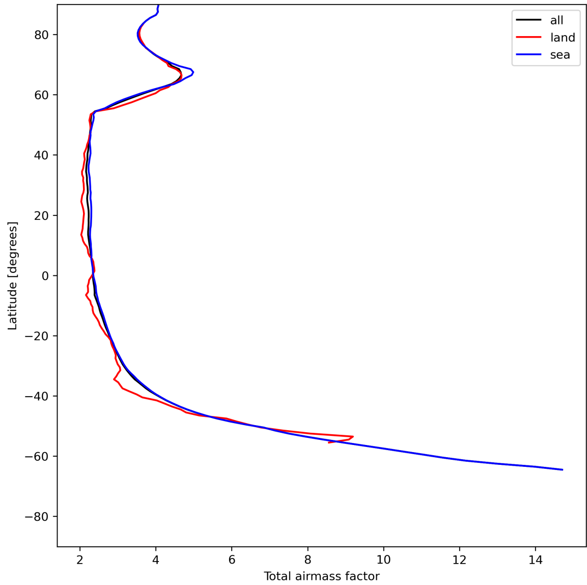
Figure 15: Zonal average of “Total airmass factor” for 2024-06-15 to 2024-06-17.
