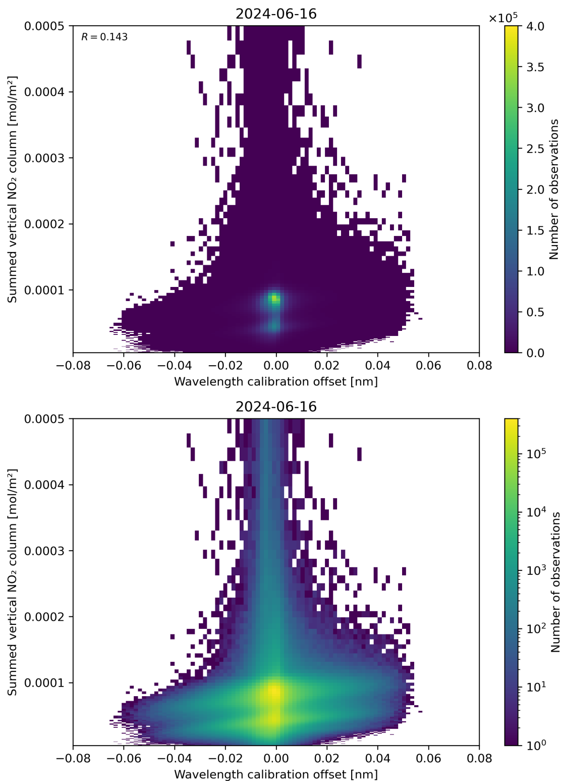
Figure 177: Scatter density plot of “Wavelength calibration offset” against “Summed vertical NO 2 column” for 2024-06-15 to 2024-06-17.
