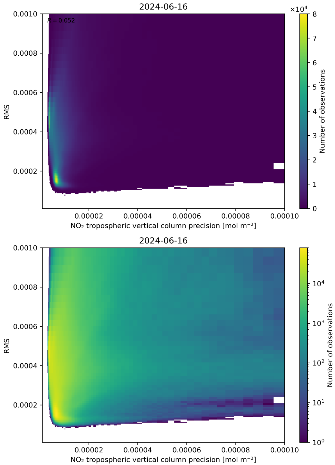
Figure 140: Scatter density plot of “NO 2 tropospheric vertical column precision” against “RMS” for 2024-06-15 to 2024-06-17.
