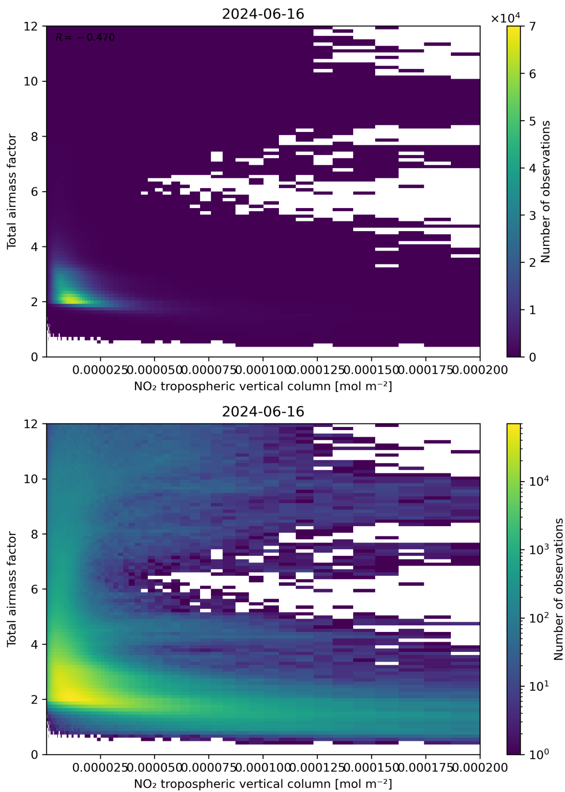
Figure 122: Scatter density plot of “NO 2 tropospheric vertical column” against “Total air mass factor” for 2024-06-15 to 2024-06-17.
