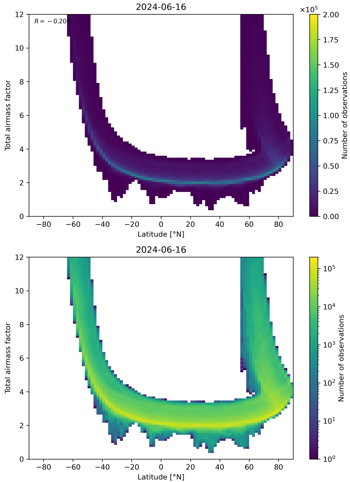
Figure 84: Scatter density plot of “Latitude” against “Total airmass factor” for 2024-06-15 to 2024-06-17.
