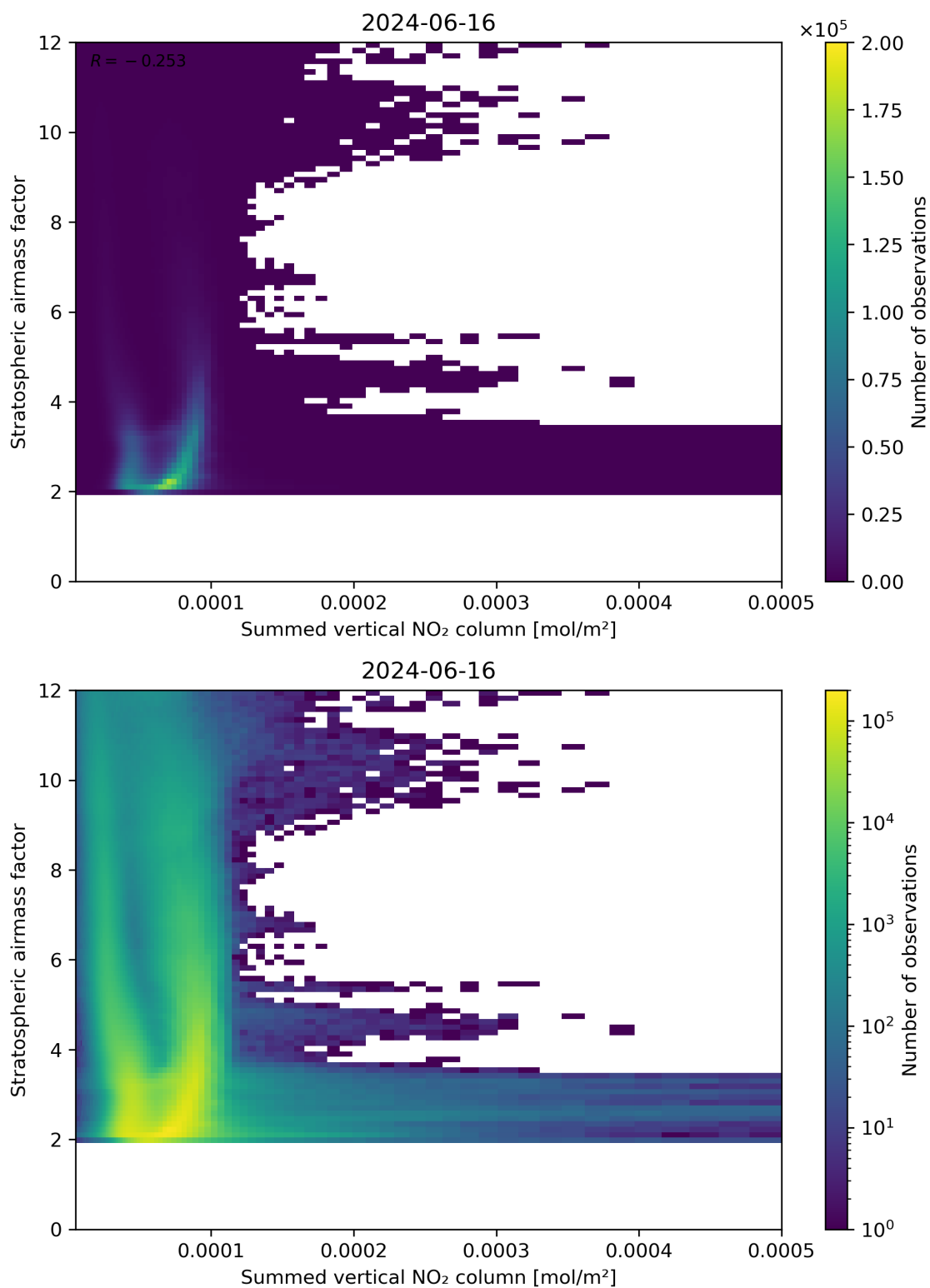
Figure 103: Scatter density plot of “Summed vertical NO 2 column” against “Stratospheric air mass factor” for 2024-06-15 to 2024-06-17.
