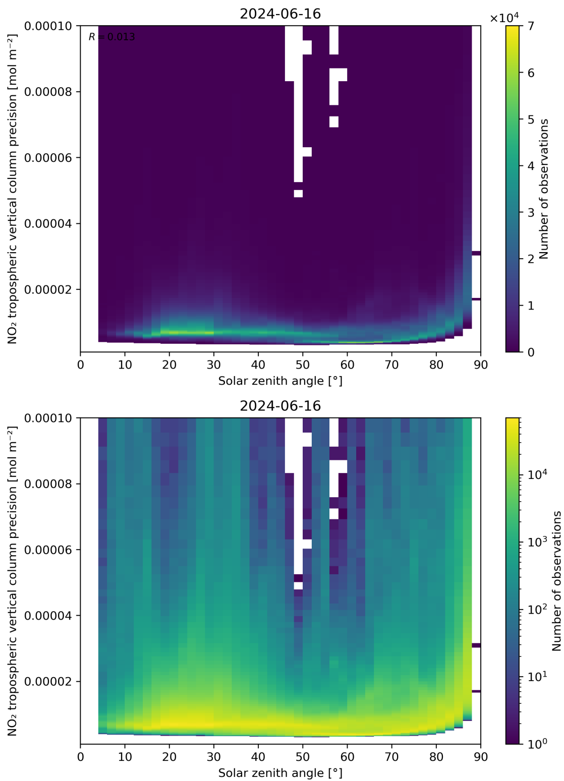
Figure 156: Scatter density plot of “Solar zenith angle” against “NO 2 tropospheric vertical column precision” for 2024-06-15 to 2024-06-17.
