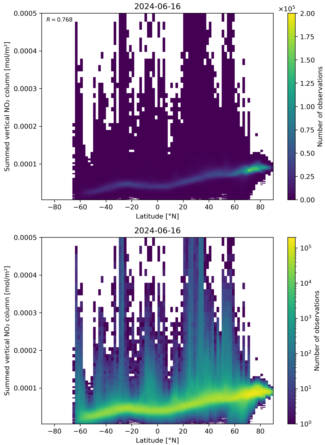
Figure 88: Scatter density plot of “Latitude” against “Summed vertical NO 2 column” for 2024-06-15 to 2024-06-17.
