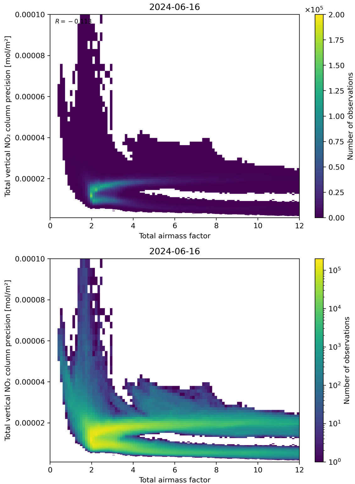
Figure 68: Scatter density plot of “Total airmass factor” against “Total vertical NO 2 column precision” for 2024-06-15 to 2024-06-17.
