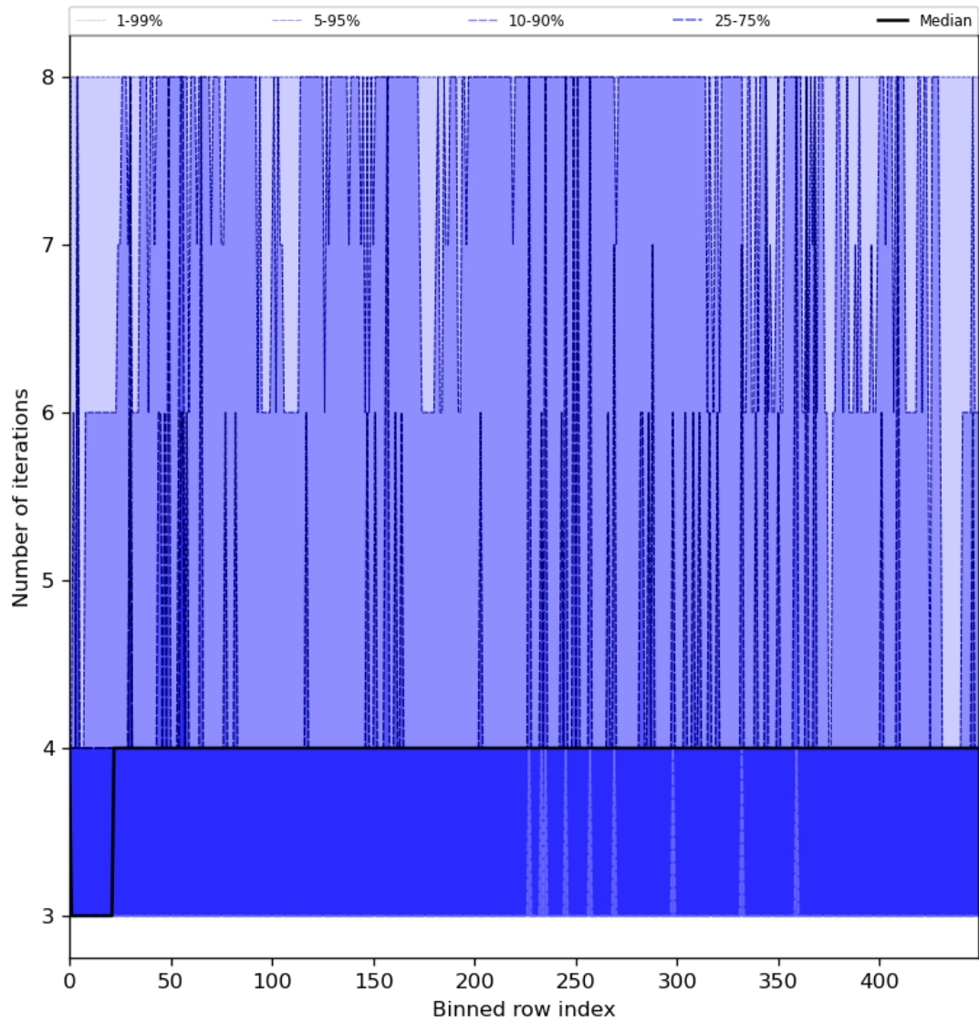
Figure 51: Along track statistics of “Number of iterations” for 2024-06-15 to 2024-06-17
