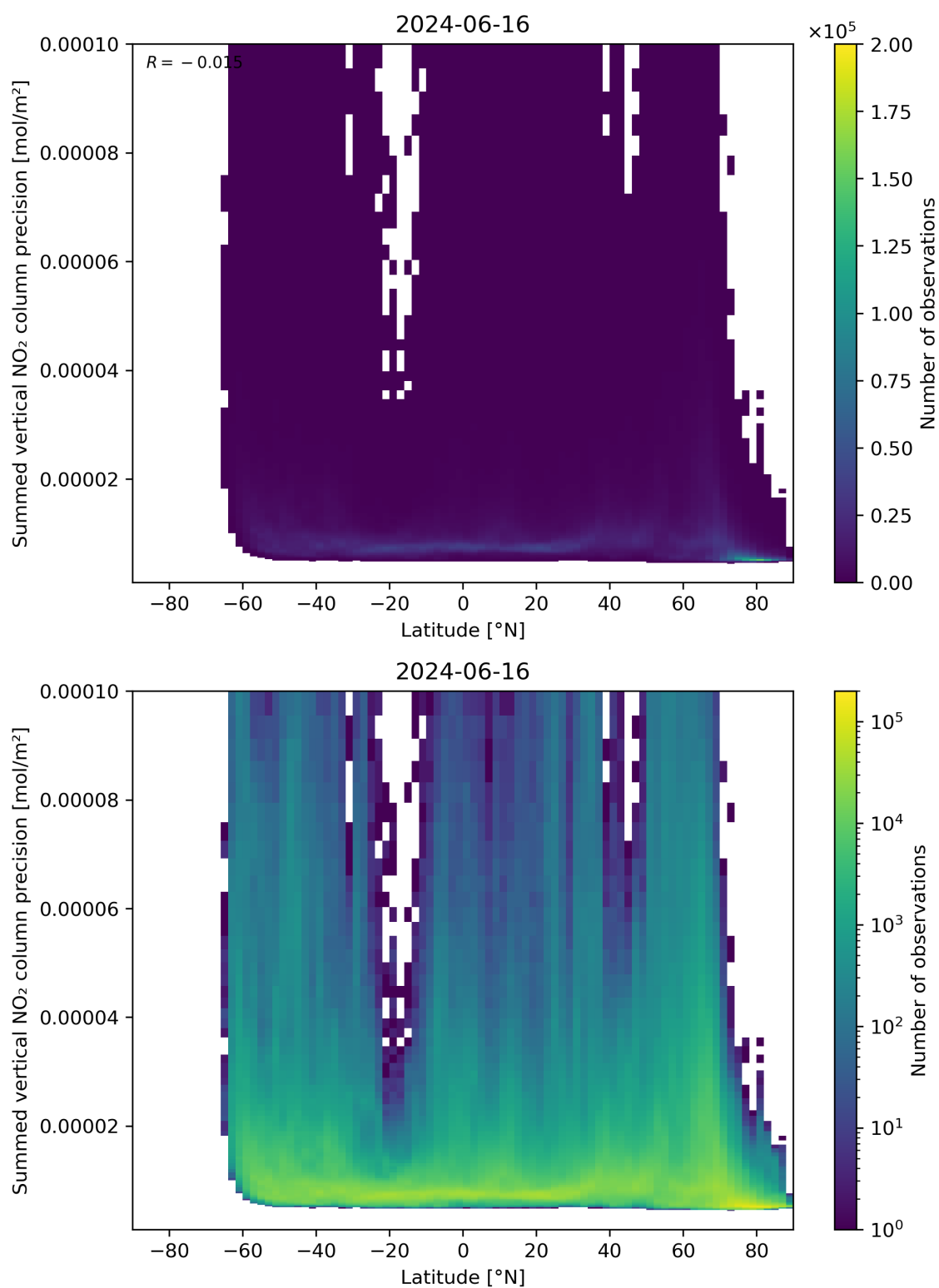
Figure 89: Scatter density plot of “Latitude” against “Summed vertical NO 2 column precision” for 2024-06-15 to 2024-06-17.
