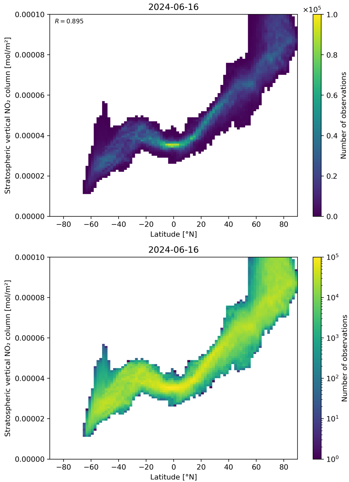
Figure 87: Scatter density plot of “Latitude” against “Stratospheric vertical NO 2 column” for 2024-06-15 to 2024-06-17.
