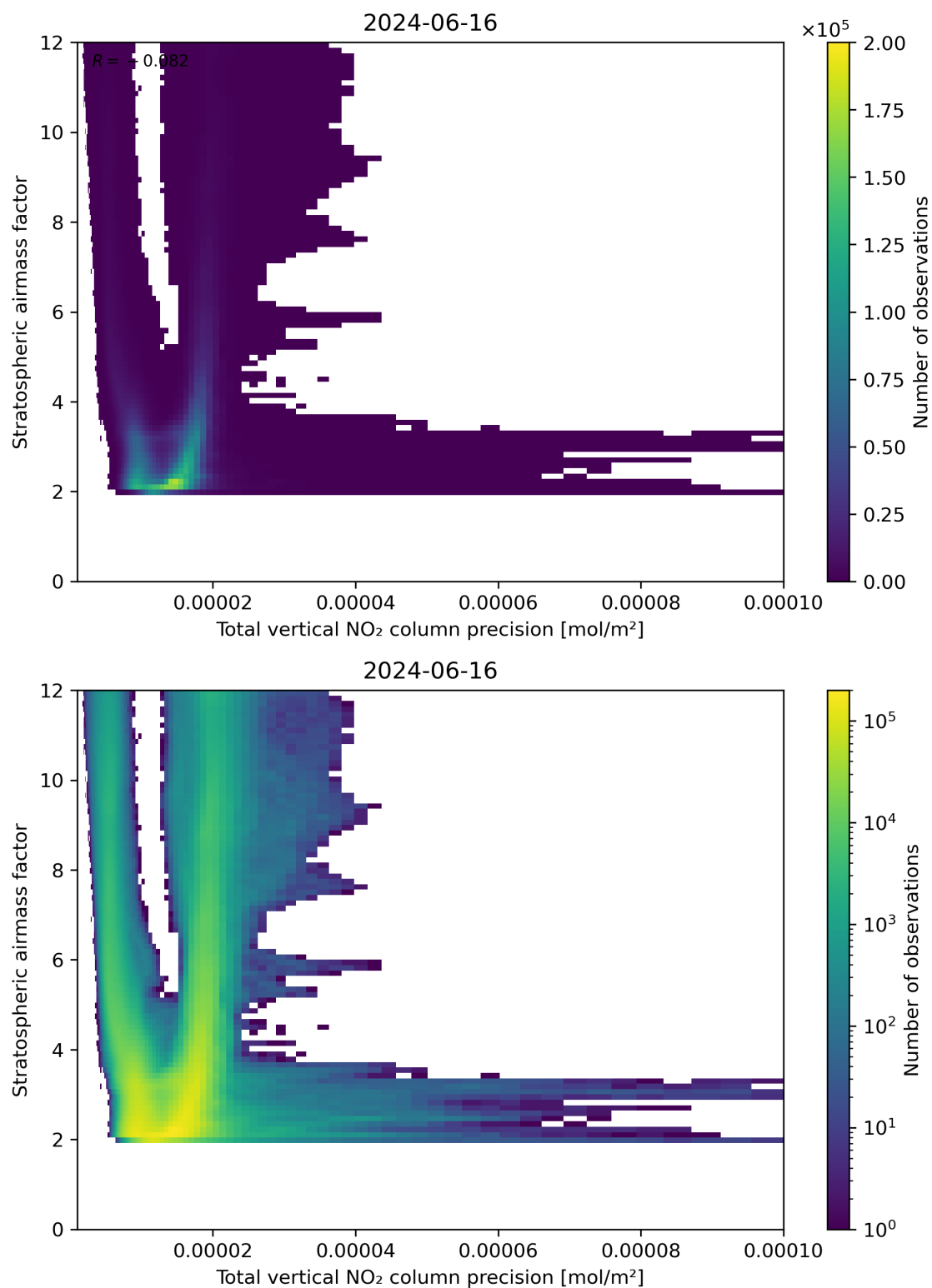
Figure 115: Scatter density plot of “Total vertical NO 2 column precision” against “Stratospheric air mass factor” for 2024-06-15 to 2024-06-17.
