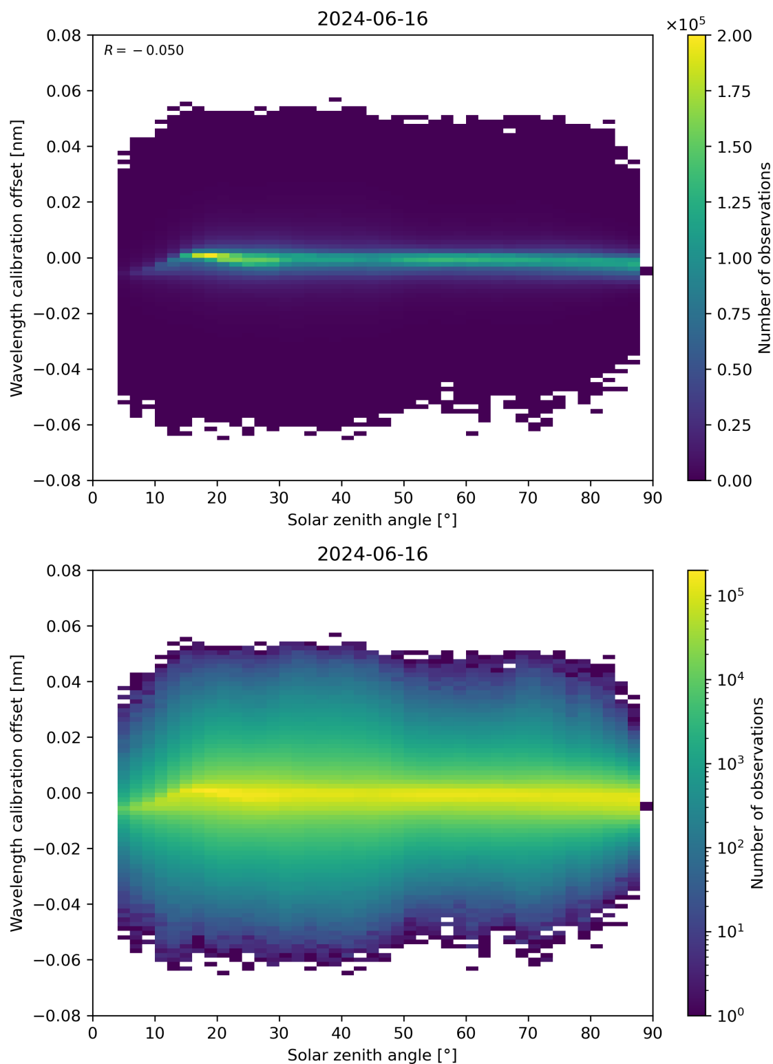
Figure 158: Scatter density plot of “Solar zenith angle” against “Wavelength calibration offset” for 2024-06-15 to 2024-06-17.
