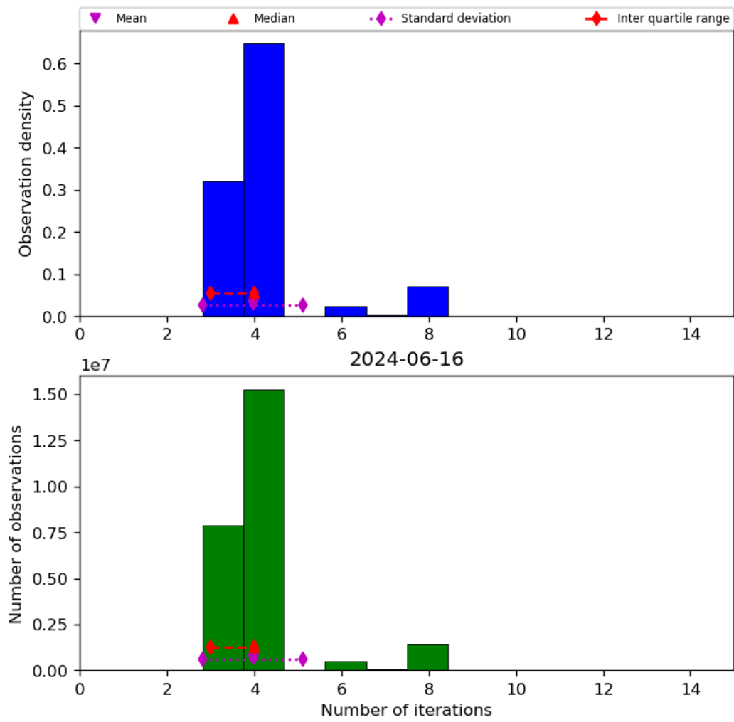
Figure 34: Histogram of “Number of iterations” for 2024-06-15 to 2024-06-17
