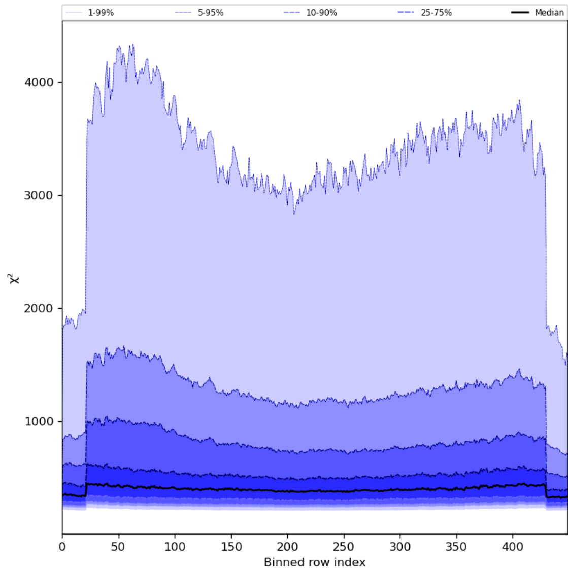
Figure 59: Along track statistics of “ \chi^2 ” for 2024-06-15 to 2024-06-17
