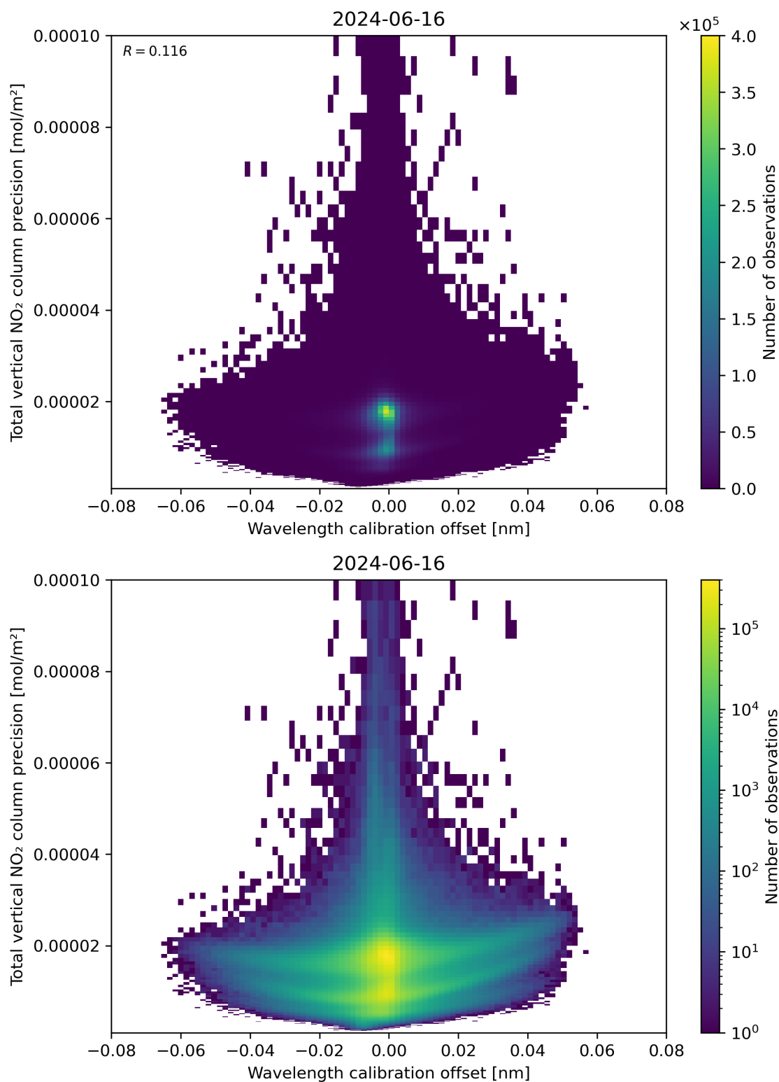
Figure 180: Scatter density plot of “Wavelength calibration offset” against “Total vertical NO 2 column precision” for 2024-06-15 to 2024-06-17.
