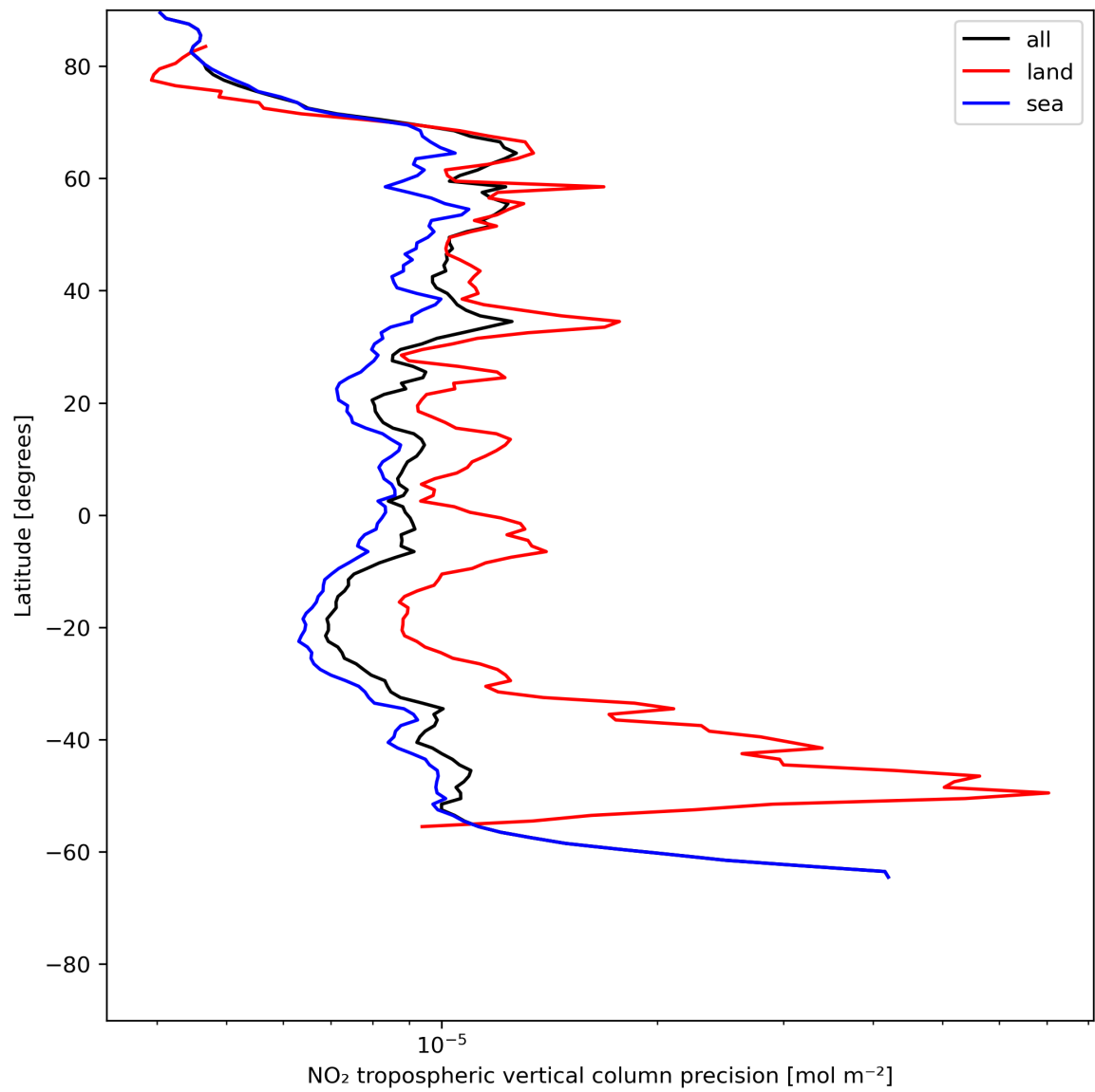
Figure 13: Zonal average of “NO 2 tropospheric vertical column precision” for 2024-06-15 to 2024-06-17.
