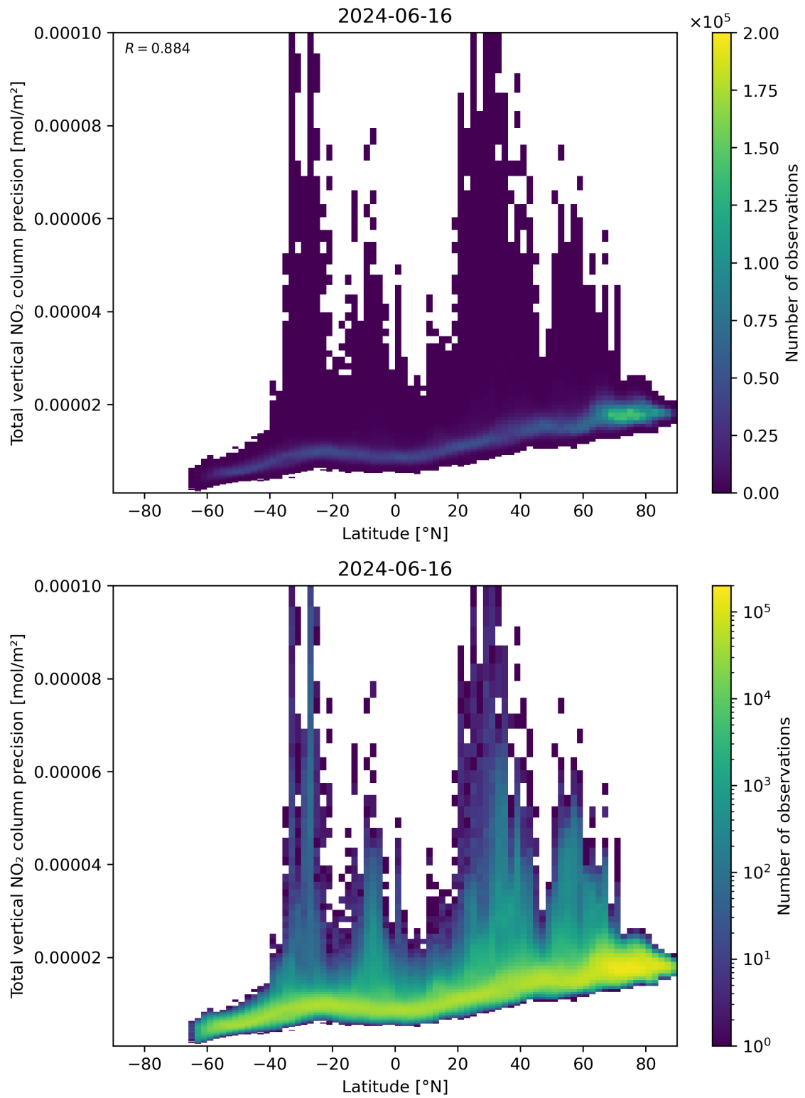
Figure 91: Scatter density plot of “Latitude” against “Total vertical NO 2 column precision” for 2024-06-15 to 2024-06-17.
