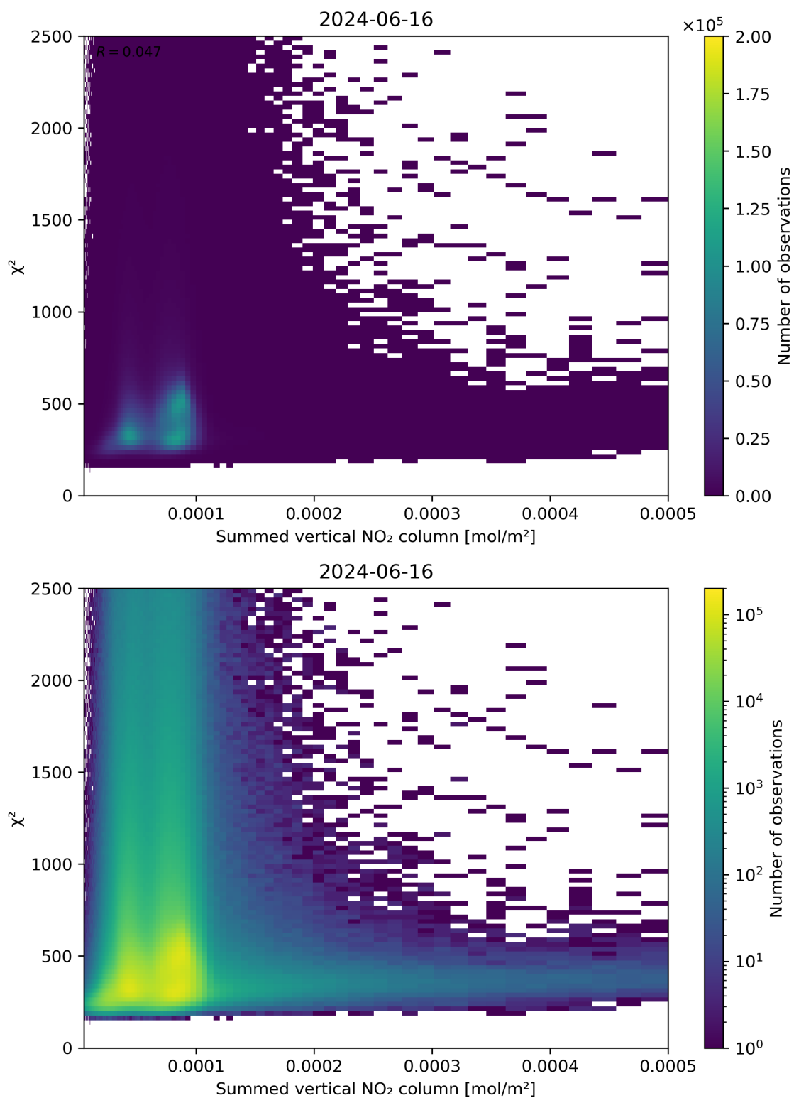
Figure 104: Scatter density plot of “Summed vertical NO 2 column” against “ \chi^2 ” for 2024-06-15 to 2024-06-17.
