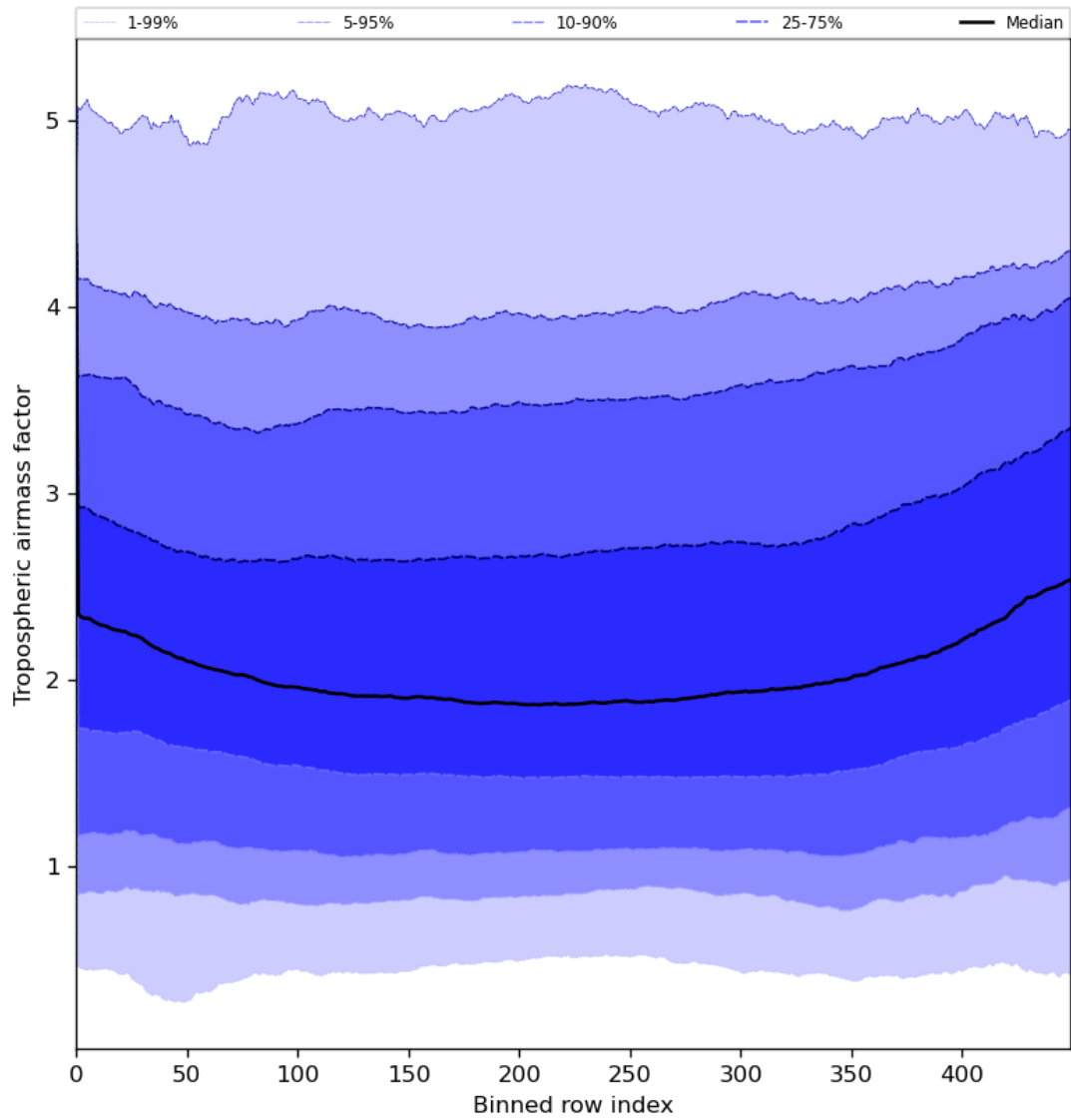
Figure 48: Along track statistics of “Tropospheric air mass factor” for 2024-06-15 to 2024-06-17
