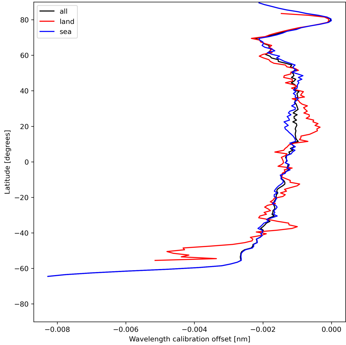
Figure 18: Zonal average of “Wavelength calibration offset” for 2024-06-15 to 2024-06-17.
