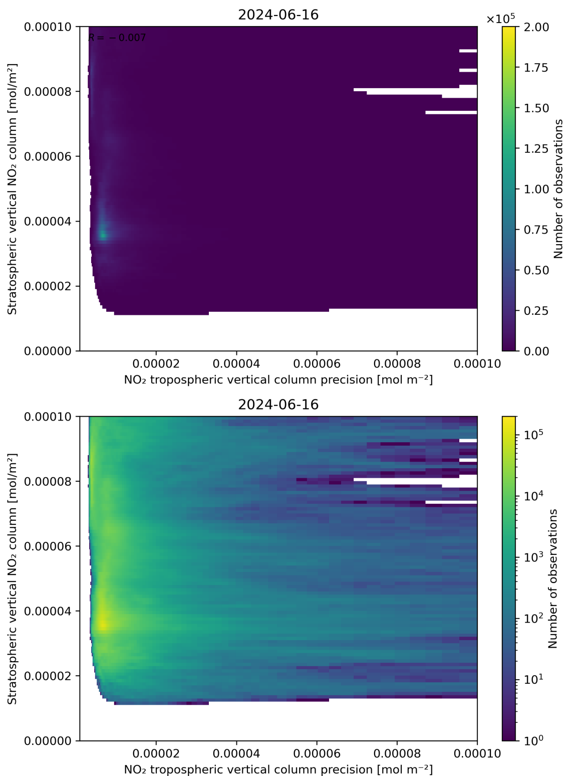
Figure 135: Scatter density plot of “NO 2 tropospheric vertical column precision” against “Stratospheric vertical NO 2 column” for 2024-06-15 to 2024-06-17.
