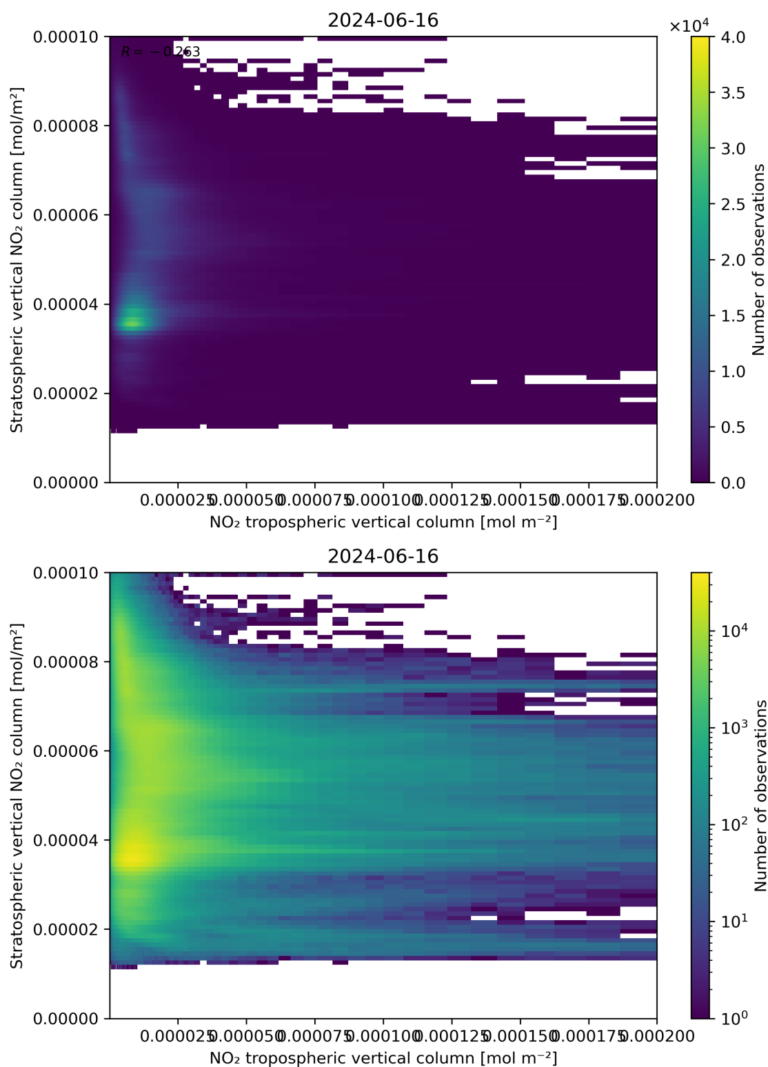
Figure 125: Scatter density plot of “NO 2 tropospheric vertical column” against “Stratospheric vertical NO 2 column” for 2024-06-15 to 2024-06-17.
