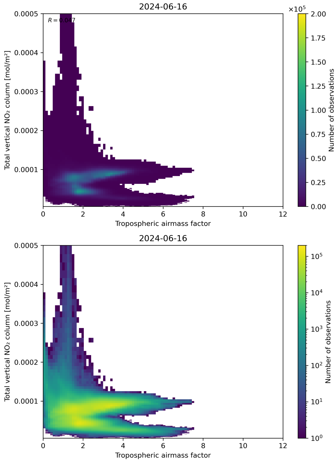
Figure 77: Scatter density plot of “Tropospheric airmass factor” against “Total vertical NO 2 column” for 2024-06-15 to 2024-06-17.
