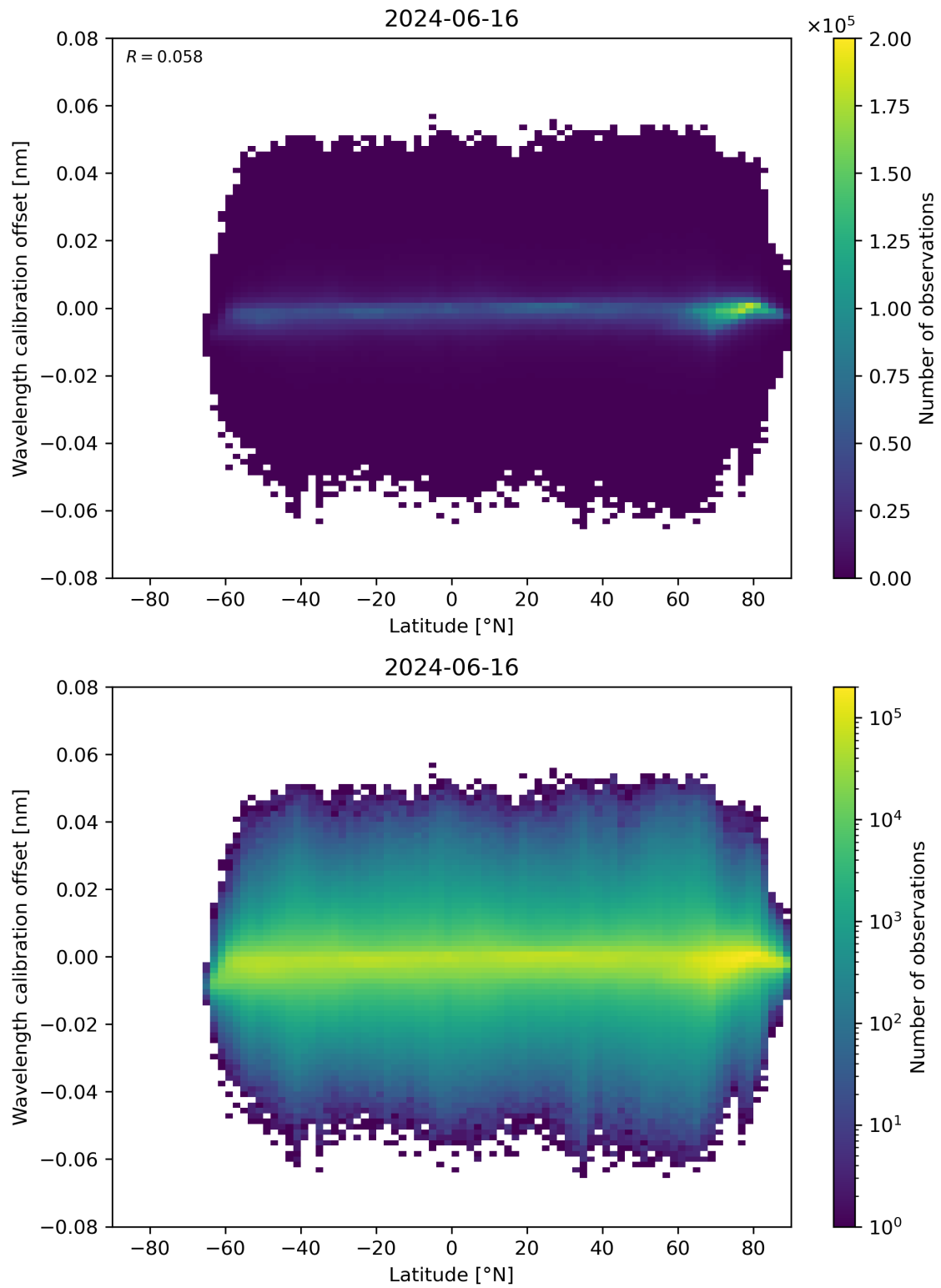
Figure 95: Scatter density plot of “Latitude” against “Wavelength calibration offset” for 2024-06-15 to 2024-06-17.
