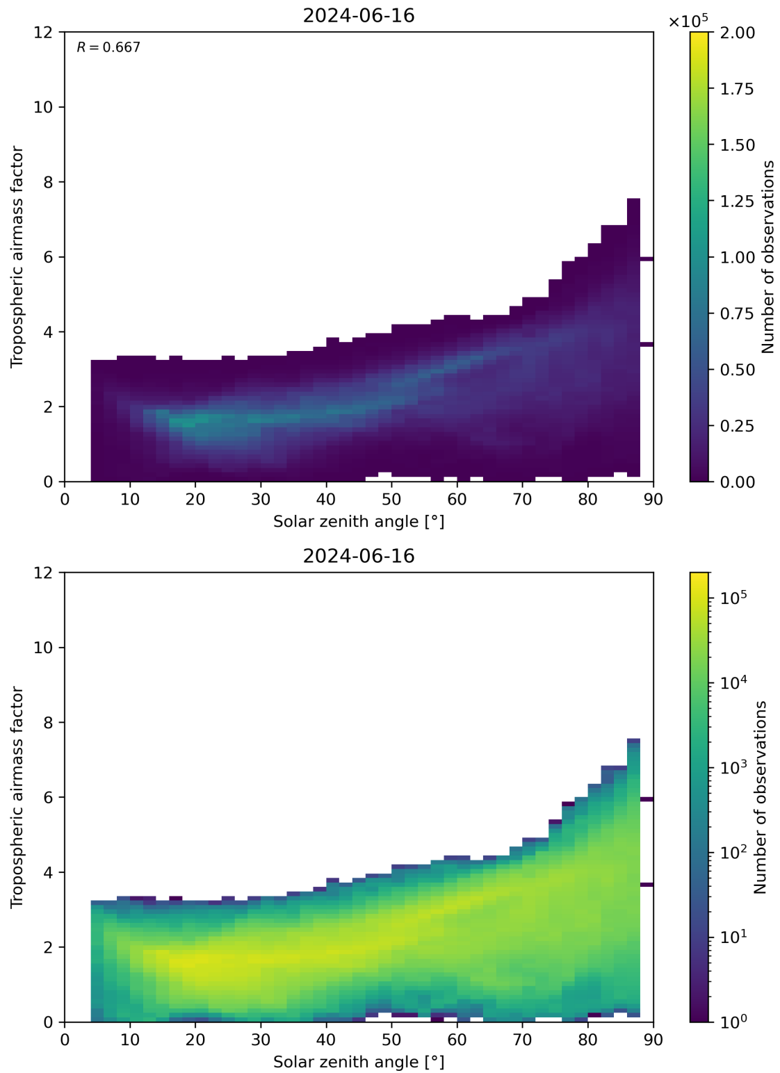
Figure 147: Scatter density plot of “Solar zenith angle” against “Tropospheric airmass factor” for 2024-06-15 to 2024-06-17.
