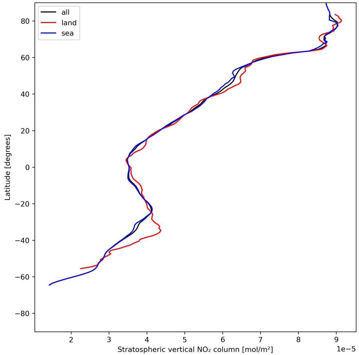
Figure 19: Zonal average of “Stratospheric vertical NO 2 column” for 2024-06-15 to 2024-06-17.
