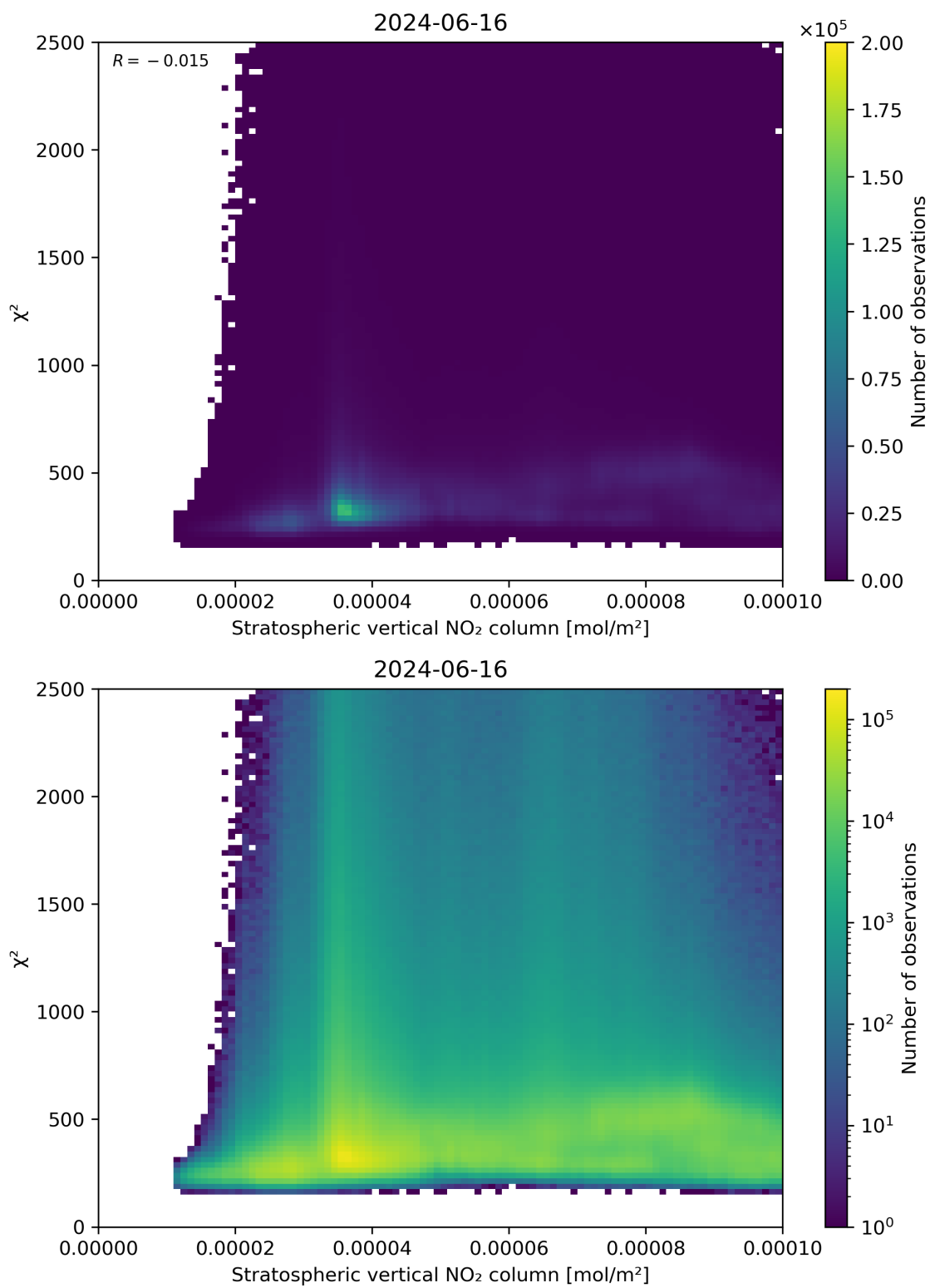
Figure 97: Scatter density plot of “Stratospheric vertical NO 2 column” against “ \chi^2 ” for 2024-06-15 to 2024-06-17.
