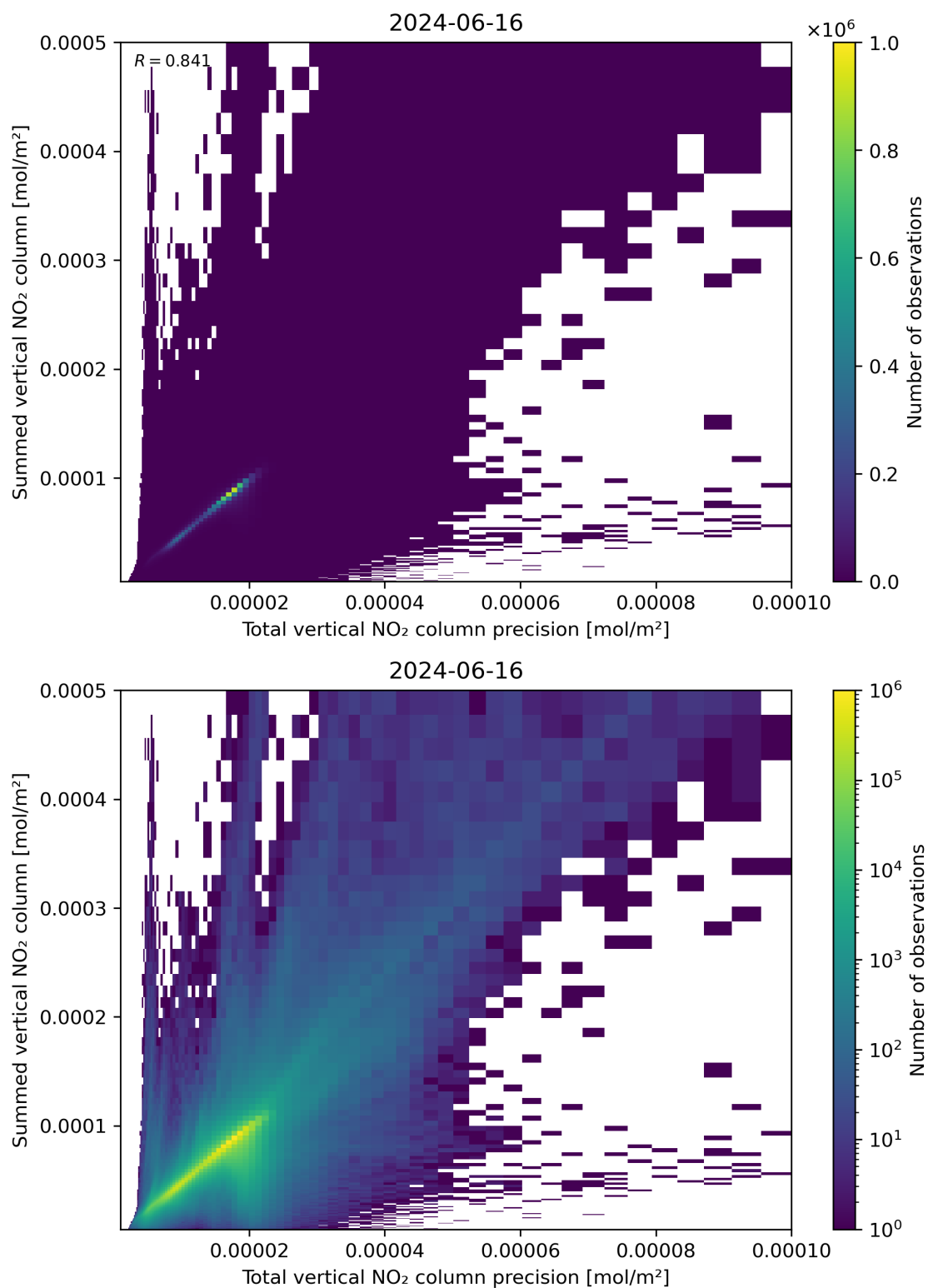
Figure 117: Scatter density plot of “Total vertical NO 2 column precision” against “Summed vertical NO 2 column” for 2024-06-15 to 2024-06-17.
