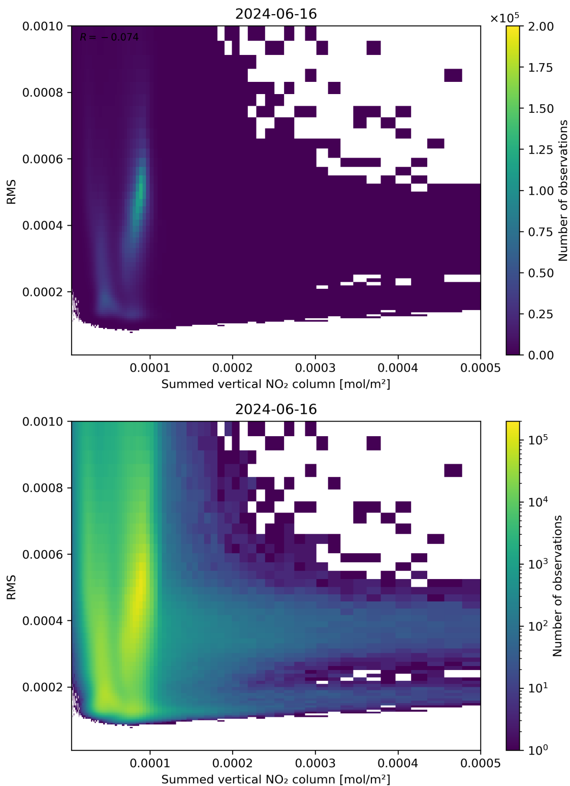
Figure 109: Scatter density plot of “Summed vertical NO 2 column” against “RMS” for 2024-06-15 to 2024-06-17.
