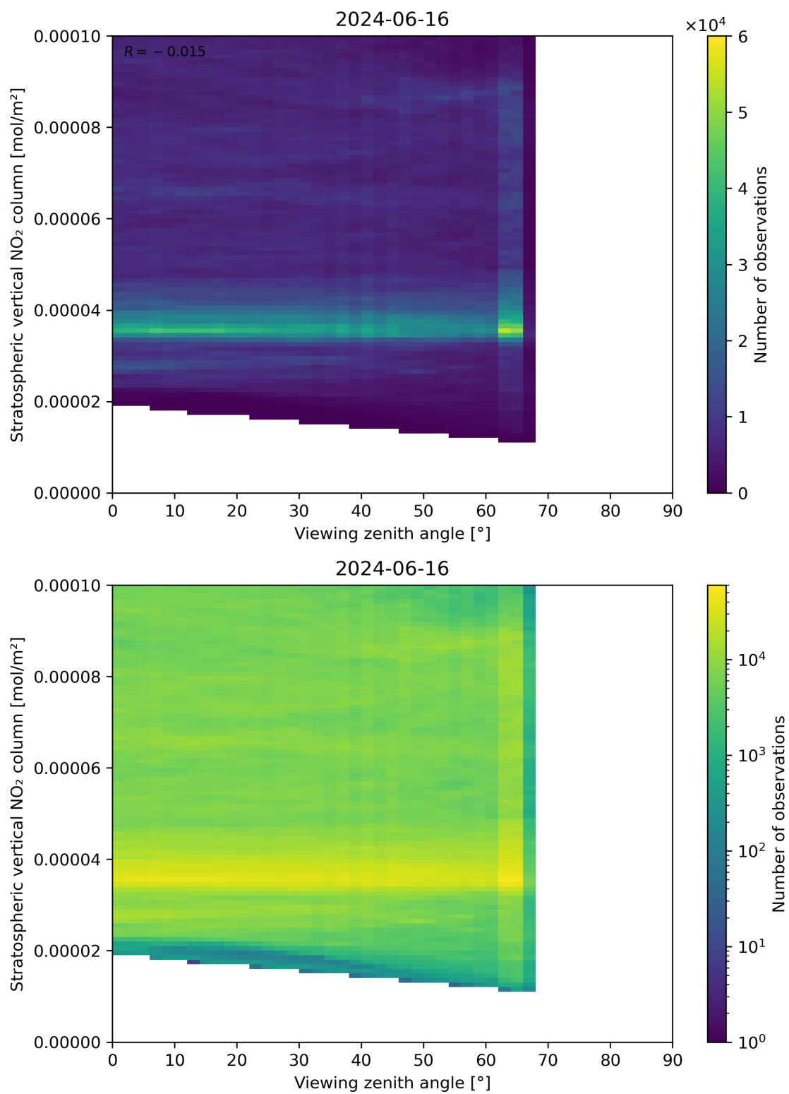
Figure 164: Scatter density plot of “Viewing zenith angle” against “Stratospheric vertical NO 2 column” for 2024-06-15 to 2024-06-17.
