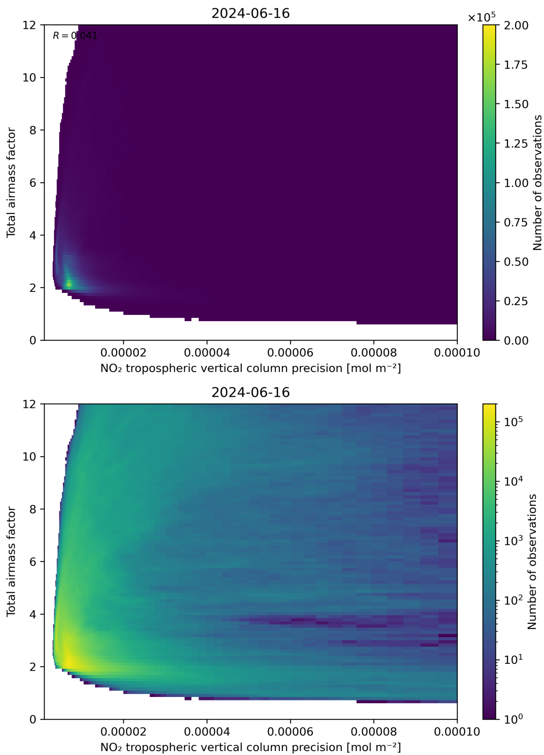
Figure 132: Scatter density plot of “NO 2 tropospheric vertical column precision” against “Total air mass factor” for 2024-06-15 to 2024-06-17.
