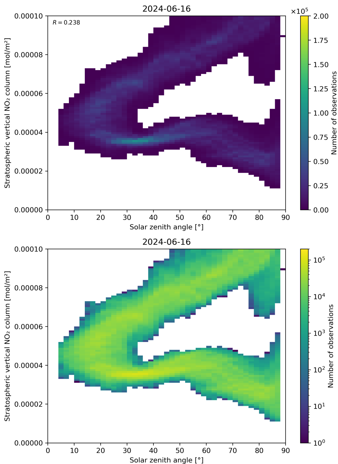
Figure 150: Scatter density plot of “Solar zenith angle” against “Stratospheric vertical NO 2 column” for 2024-06-15 to 2024-06-17.
