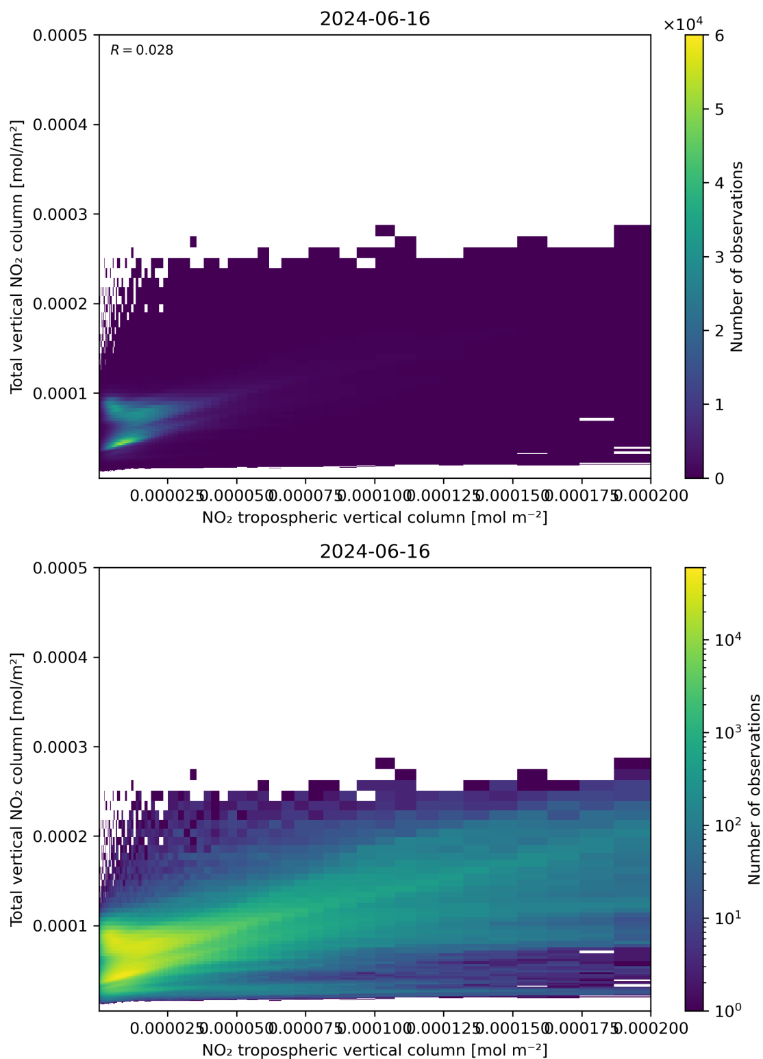
Figure 128: Scatter density plot of “NO 2 tropospheric vertical column” against “Total vertical NO 2 column” for 2024-06-15 to 2024-06-17.
