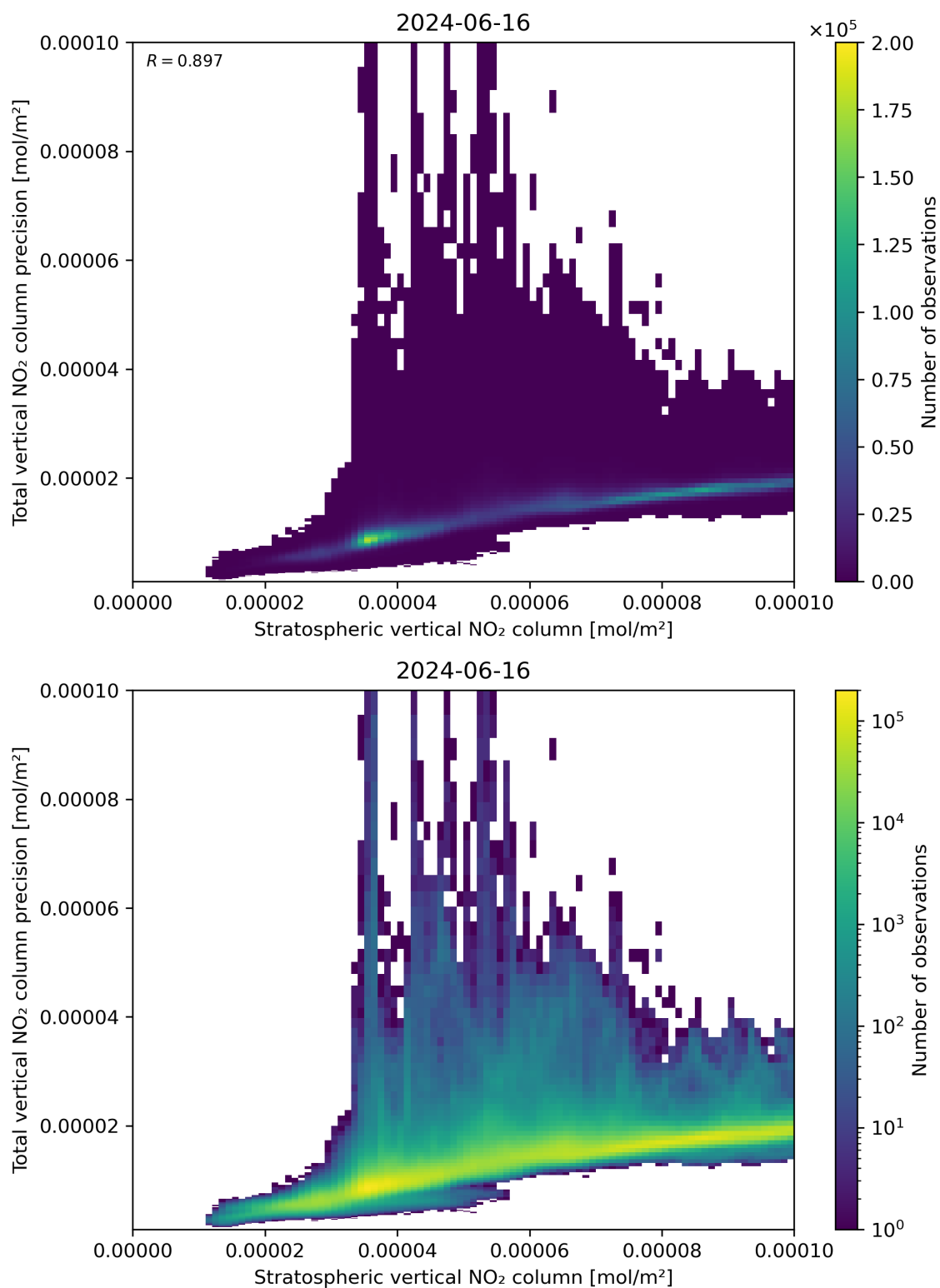
Figure 101: Scatter density plot of “Stratospheric vertical NO 2 column” against “Total vertical NO 2 column precision” for 2024-06-15 to 2024-06-17.
