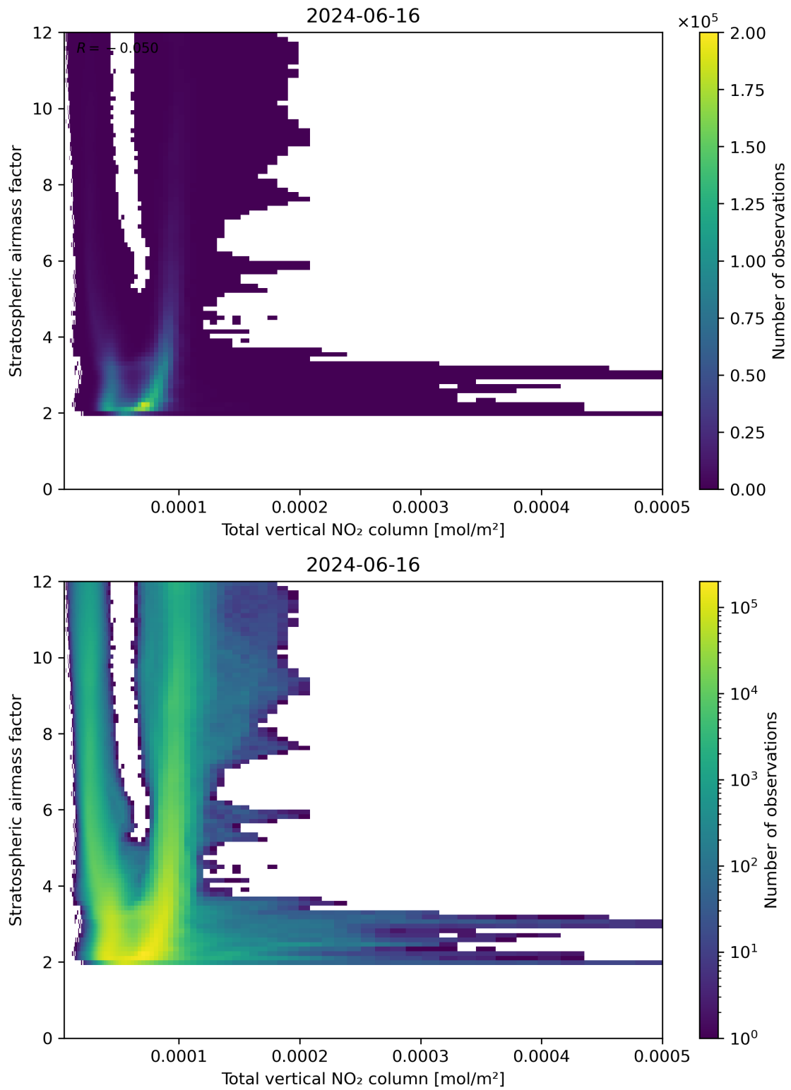
Figure 110: Scatter density plot of “Total vertical NO 2 column” against “Stratospheric air mass factor” for 2024-06-15 to 2024-06-17.
