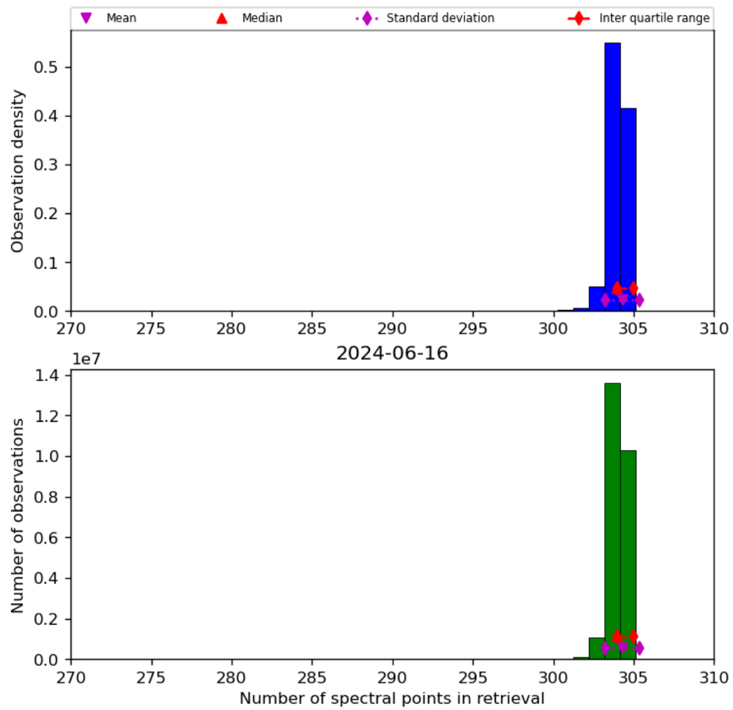
Figure 33: Histogram of “Number of spectral points in retrieval” for 2024-06-15 to 2024-06-17
