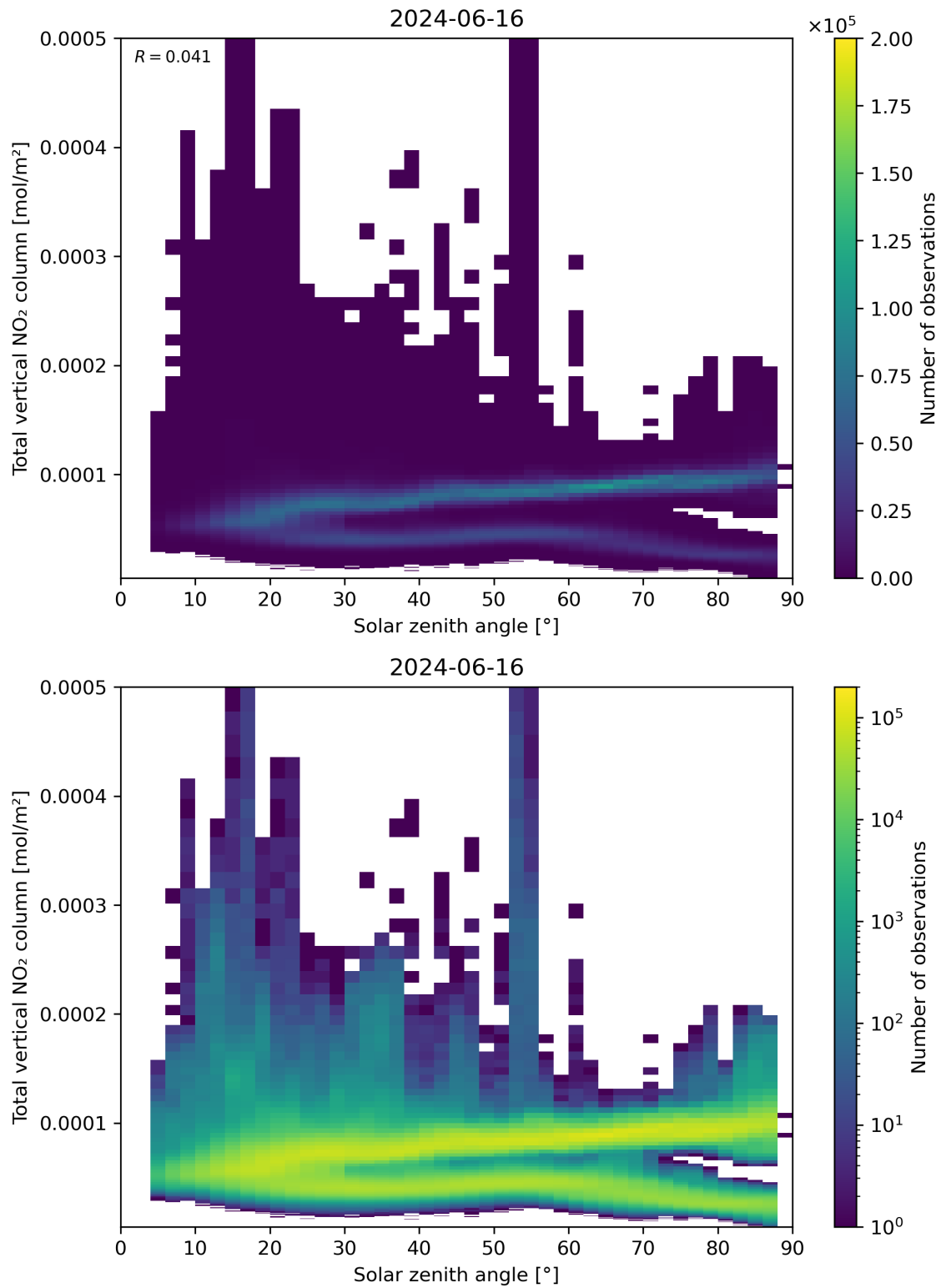
Figure 153: Scatter density plot of “Solar zenith angle” against “Total vertical NO 2 column” for 2024-06-15 to 2024-06-17.
