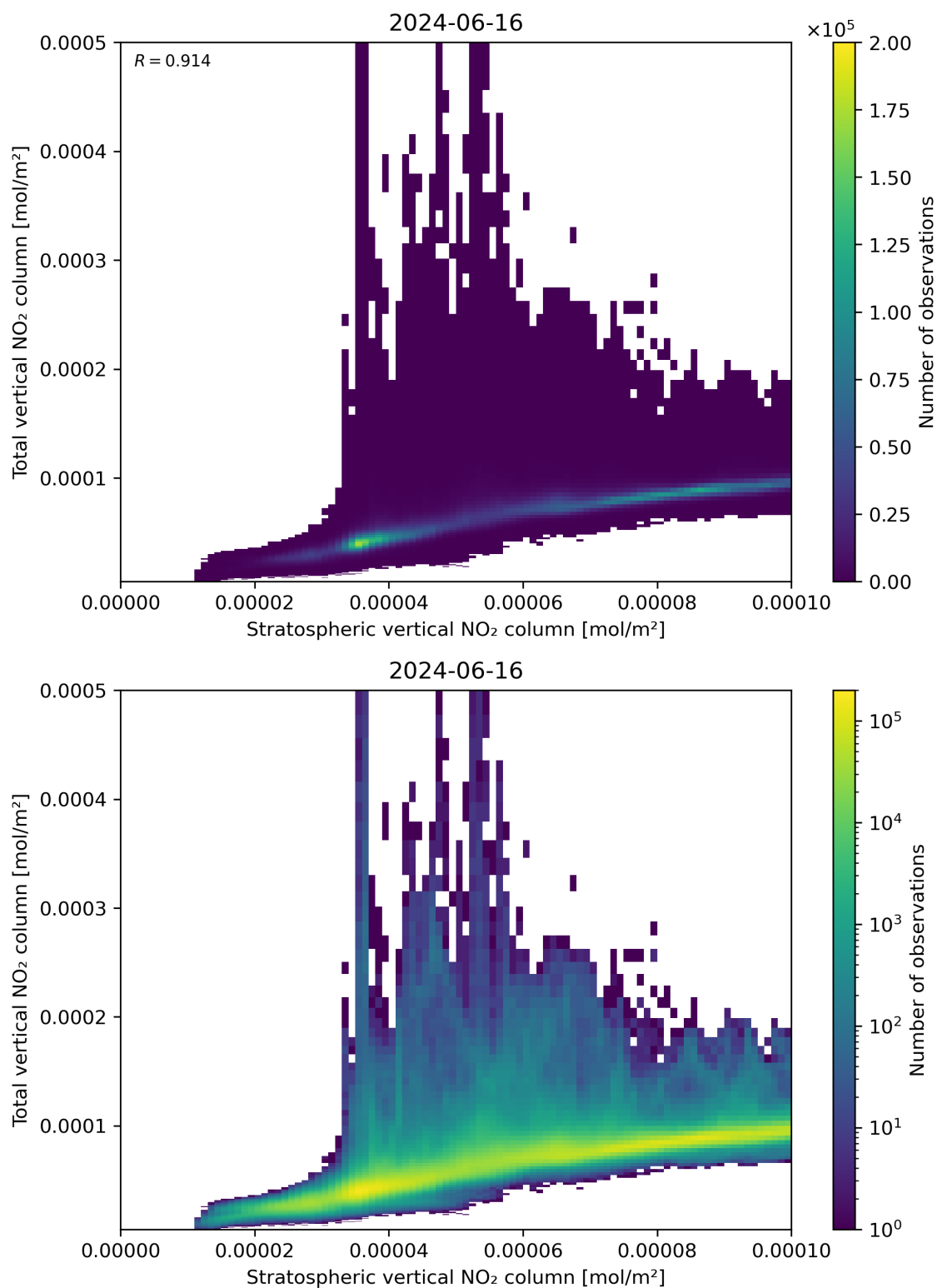
Figure 100: Scatter density plot of “Stratospheric vertical NO 2 column” against “Total vertical NO 2 column” for 2024-06-15 to 2024-06-17.
