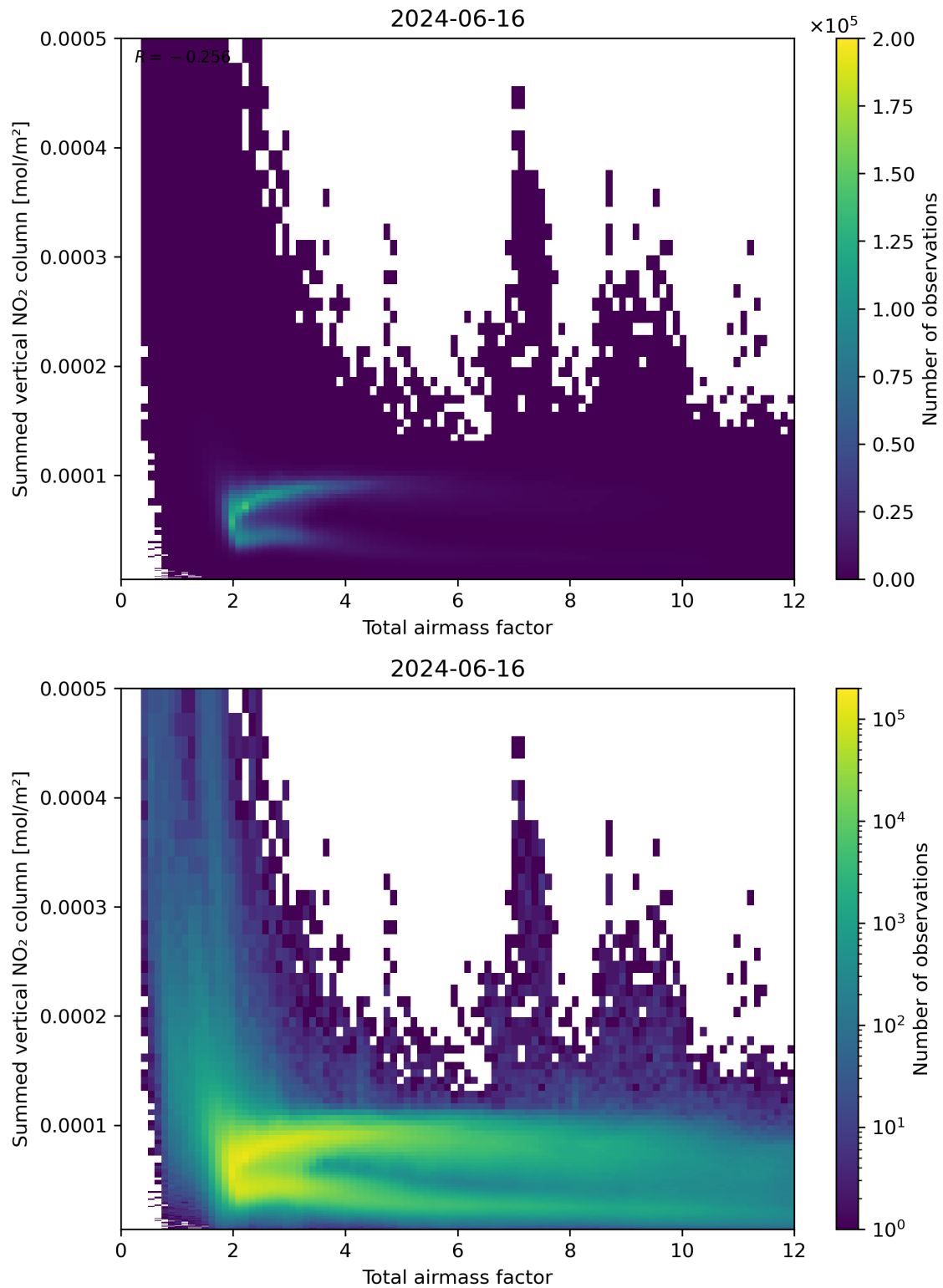
Figure 65: Scatter density plot of “Total airmass factor” against “Summed vertical NO 2 column” for 2024-06-15 to 2024-06-17.
