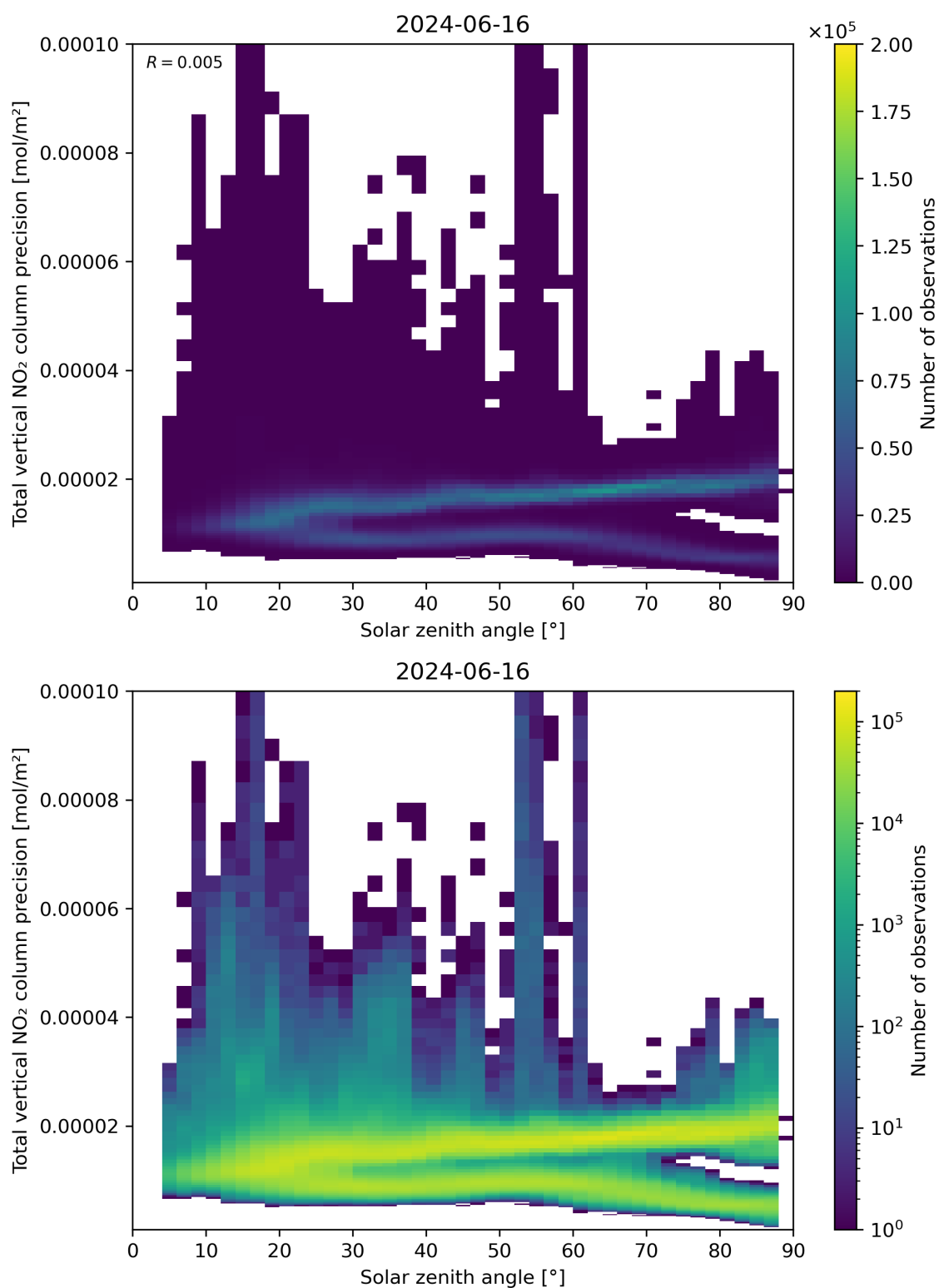
Figure 154: Scatter density plot of “Solar zenith angle” against “Total vertical NO 2 column precision” for 2024-06-15 to 2024-06-17.
