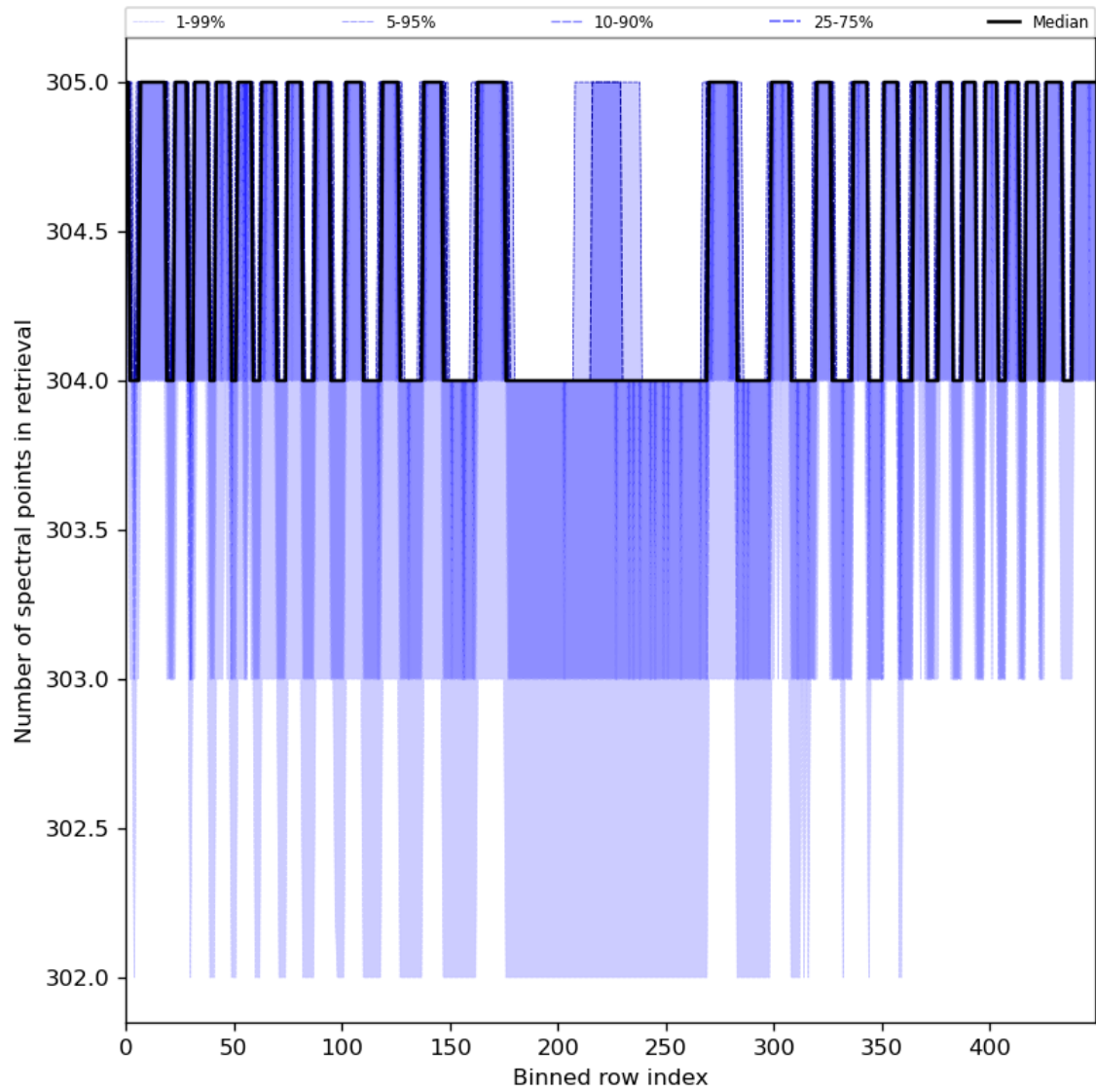
Figure 50: Along track statistics of “Number of spectral points in retrieval” for 2024-06-15 to 2024-06-17
