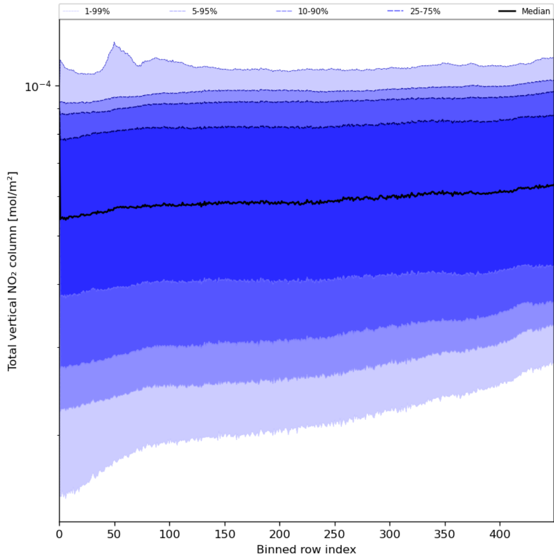
Figure 55: Along track statistics of “Total vertical NO 2 column” for 2024-06-15 to 2024-06-17
