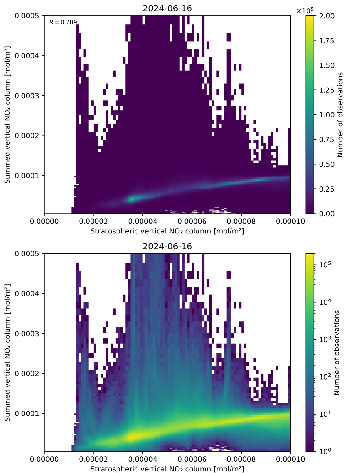
Figure 98: Scatter density plot of “Stratospheric vertical NO 2 column” against “Summed vertical NO 2 column” for 2024-06-15 to 2024-06-17.
