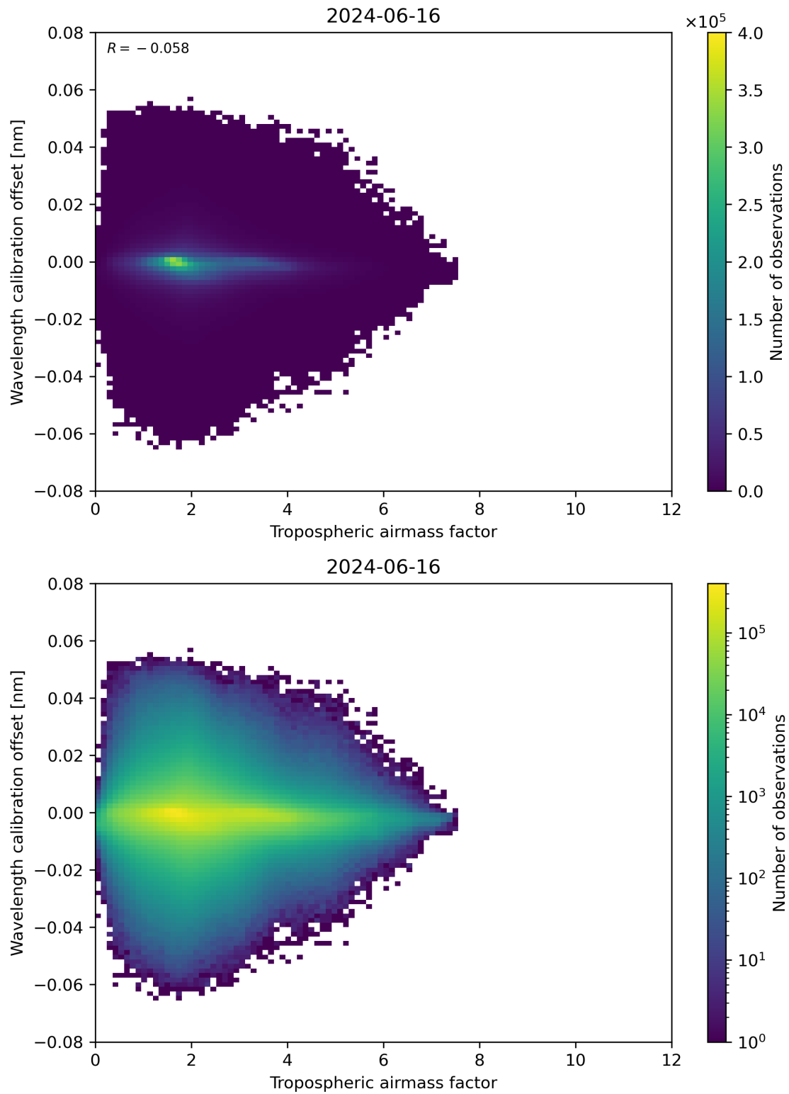
Figure 80: Scatter density plot of “Tropospheric airmass factor” against “Wavelength calibration offset” for 2024-06-15 to 2024-06-17.
