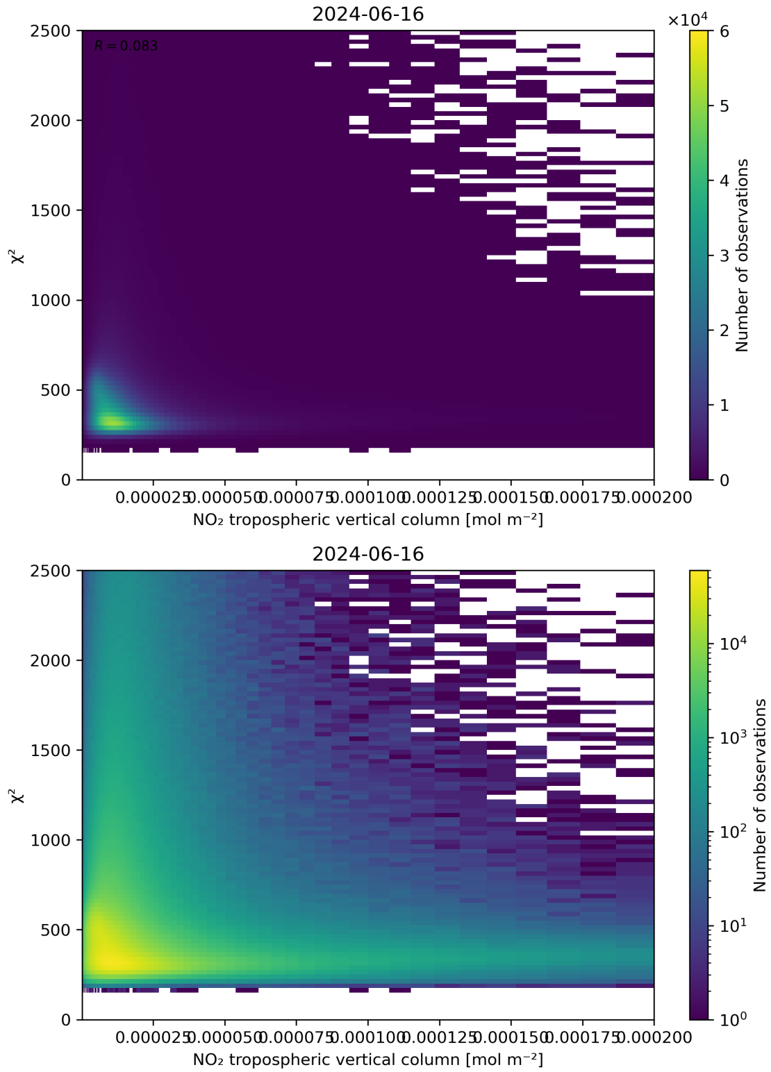
Figure 124: Scatter density plot of “NO 2 tropospheric vertical column” against “ \chi^2 ” for 2024-06-15 to 2024-06-17.
