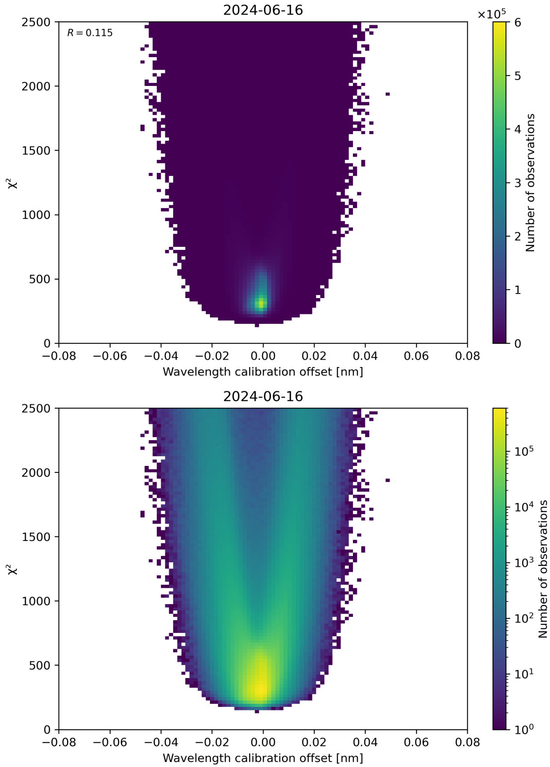
Figure 175: Scatter density plot of “Wavelength calibration offset” against “ \chi^2 ” for 2024-06-15 to 2024-06-17.
