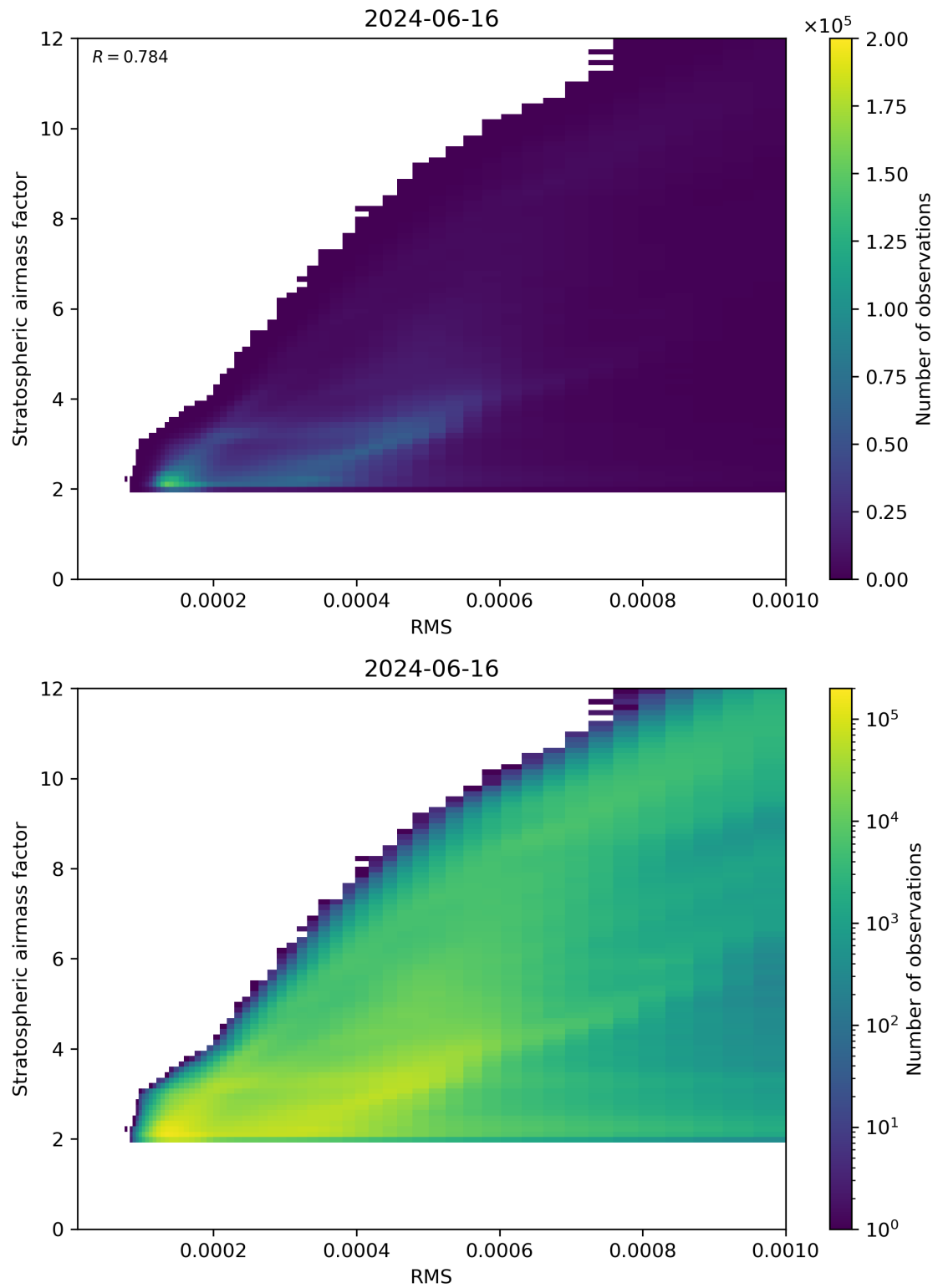
Figure 144: Scatter density plot of “RMS” against “Stratospheric airmass factor” for 2024-06-15 to 2024-06-17.
