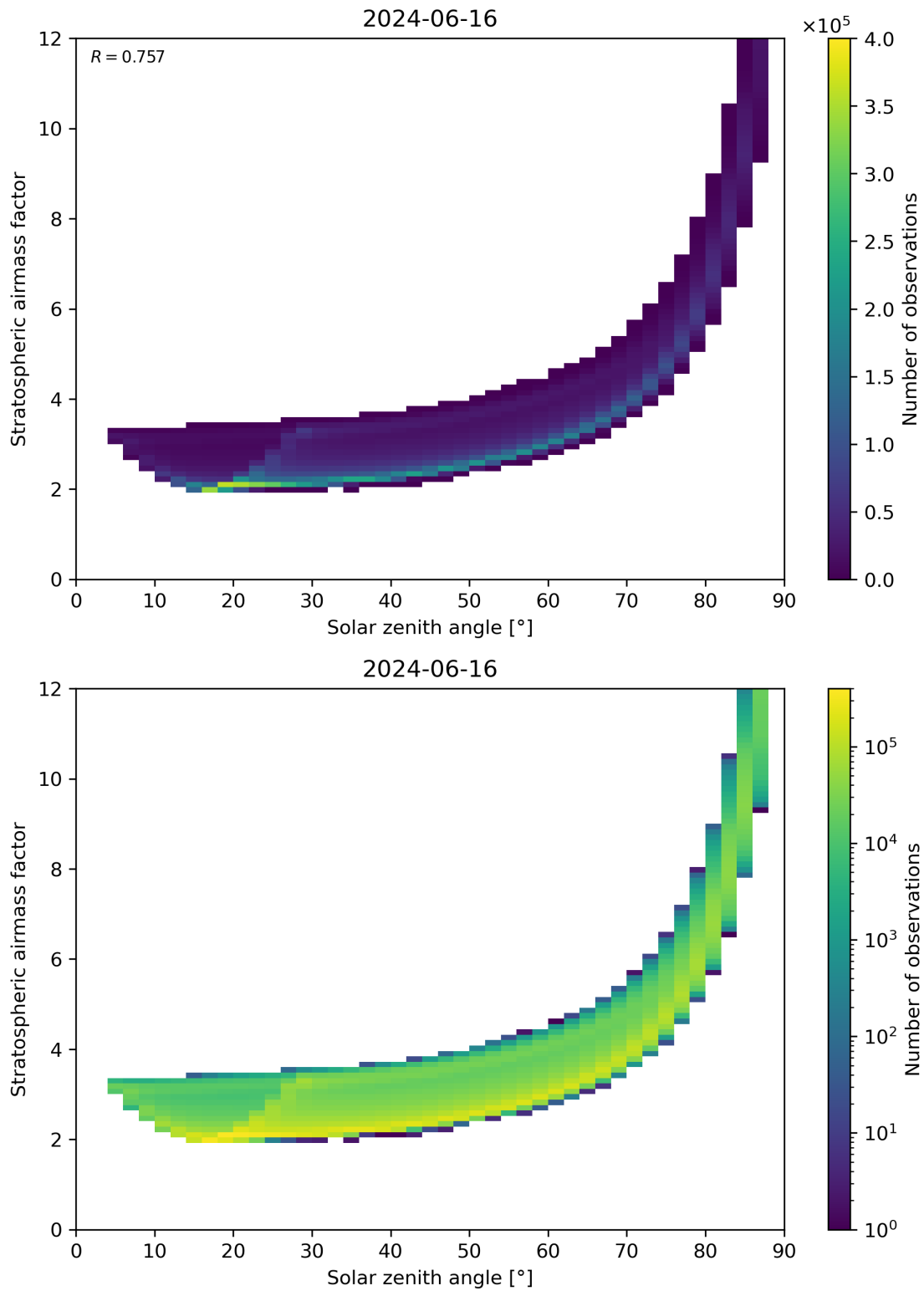
Figure 145: Scatter density plot of “Solar zenith angle” against “Stratospheric airmass factor” for 2024-06-15 to 2024-06-17.
