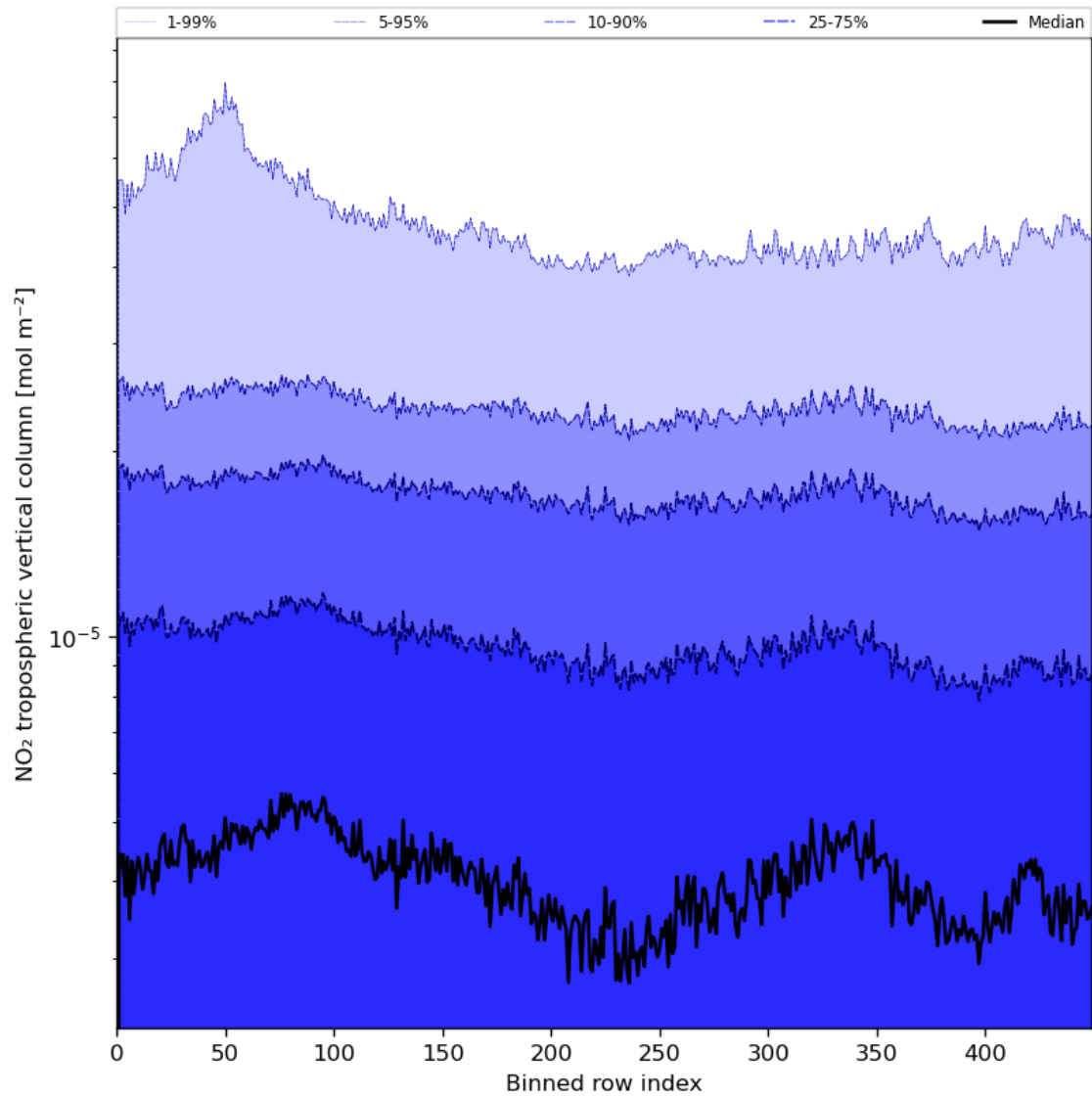
Figure 46: Along track statistics of “NO 2 tropospheric vertical column” for 2024-06-15 to 2024-06-17
