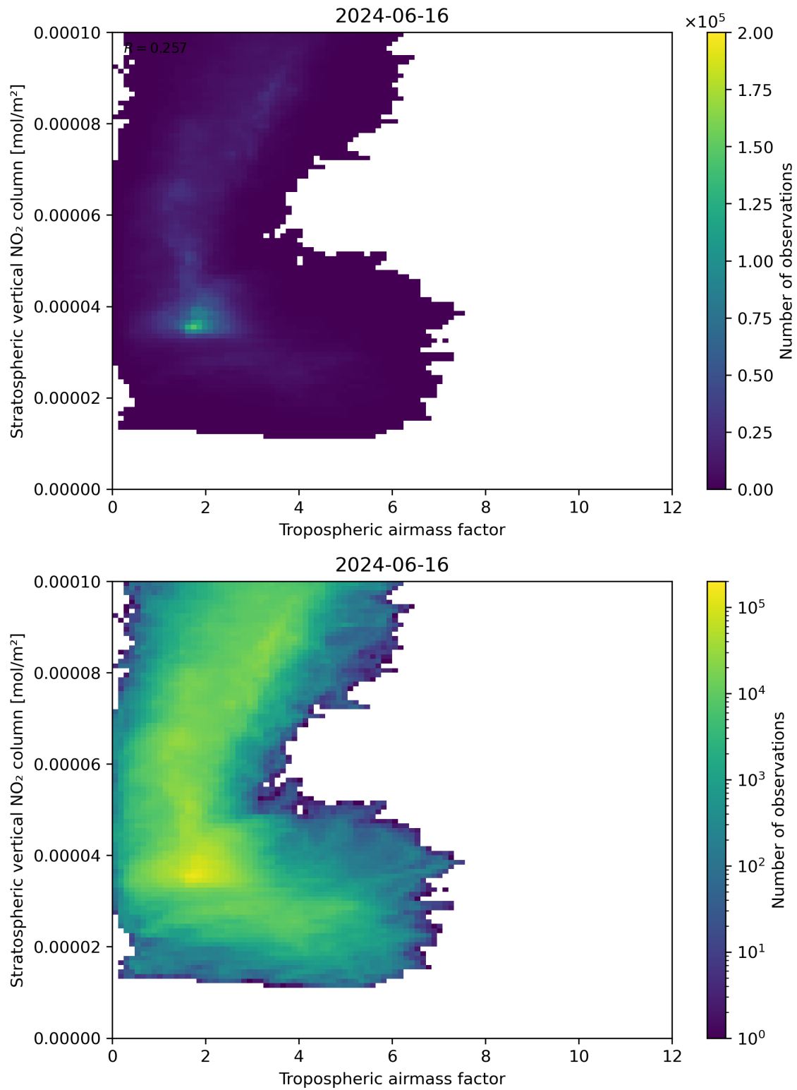
Figure 74: Scatter density plot of “Tropospheric air mass factor” against “Stratospheric vertical NO 2 column” for 2024-06-15 to 2024-06-17.
