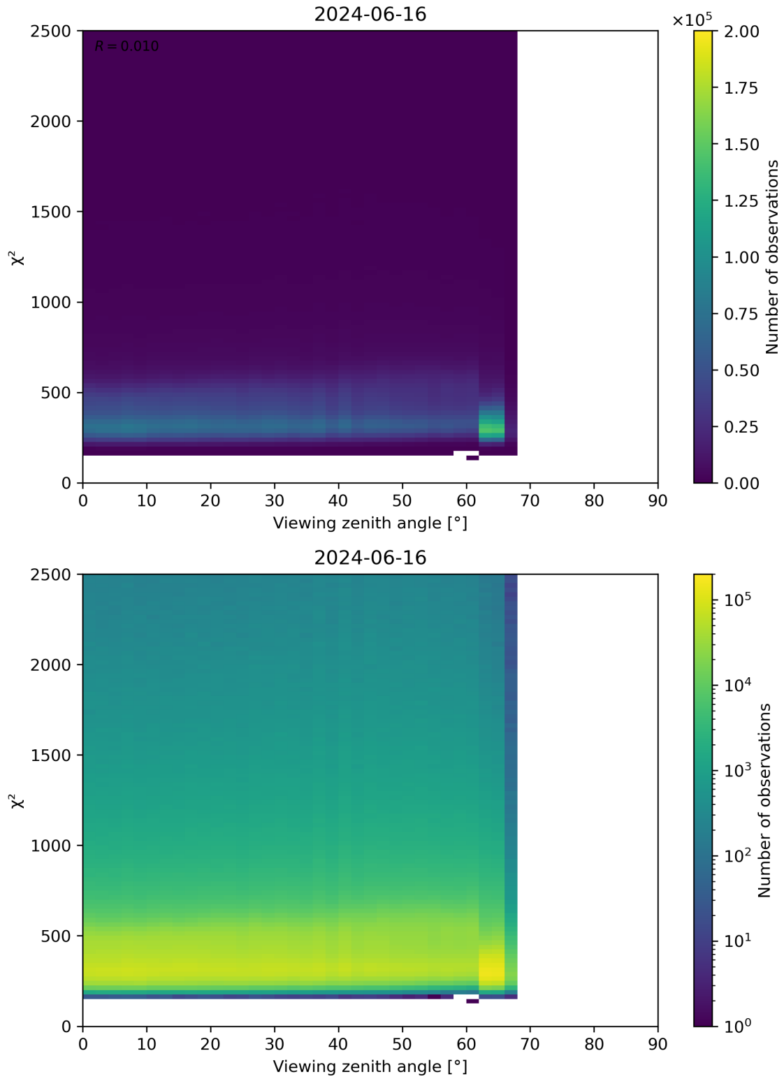
Figure 162: Scatter density plot of “Viewing zenith angle” against “ \chi^2 ” for 2024-06-15 to 2024-06-17.
