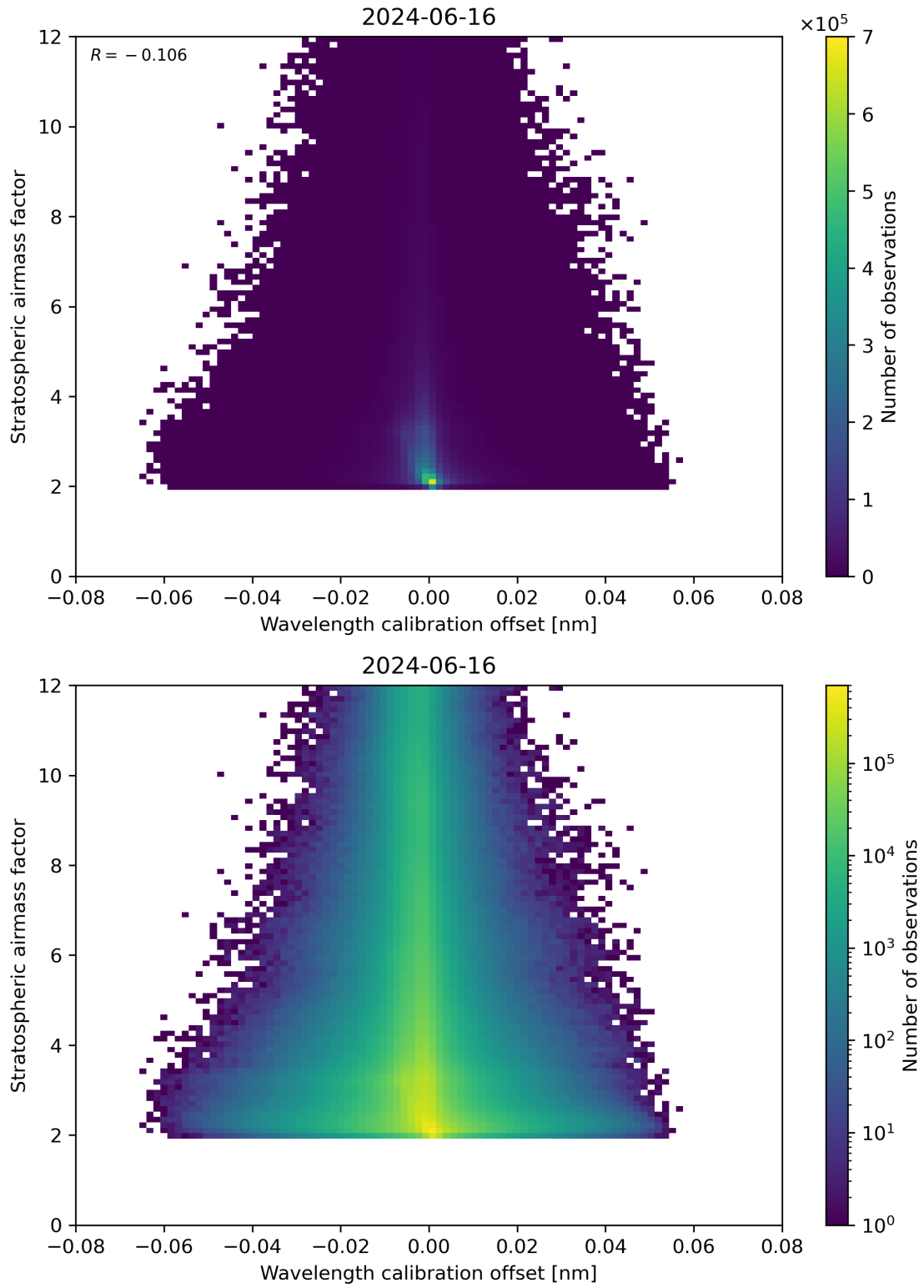
Figure 174: Scatter density plot of “Wavelength calibration offset” against “Stratospheric air mass factor” for 2024-06-15 to 2024-06-17.
