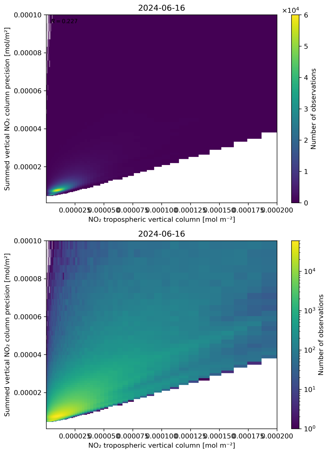
Figure 127: Scatter density plot of “NO 2 tropospheric vertical column” against “Summed vertical NO 2 column precision” for 2024-06-15 to 2024-06-17.
