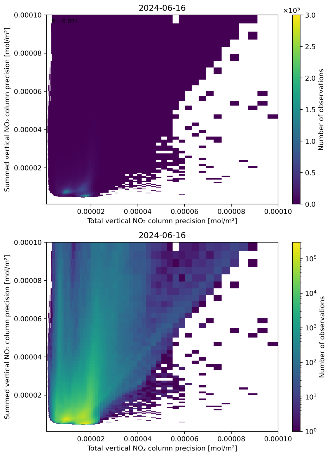
Figure 118: Scatter density plot of “Total vertical NO 2 column precision” against “Summed vertical NO 2 column precision” for 2024-06-15 to 2024-06-17.
