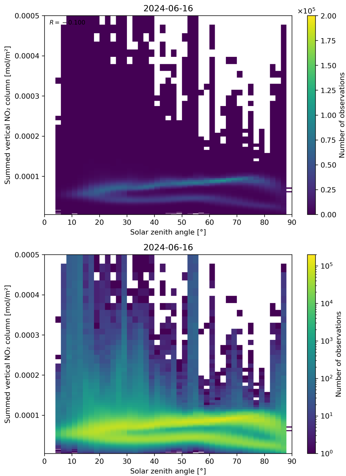
Figure 151: Scatter density plot of “Solar zenith angle” against “Summed vertical NO 2 column” for 2024-06-15 to 2024-06-17.
