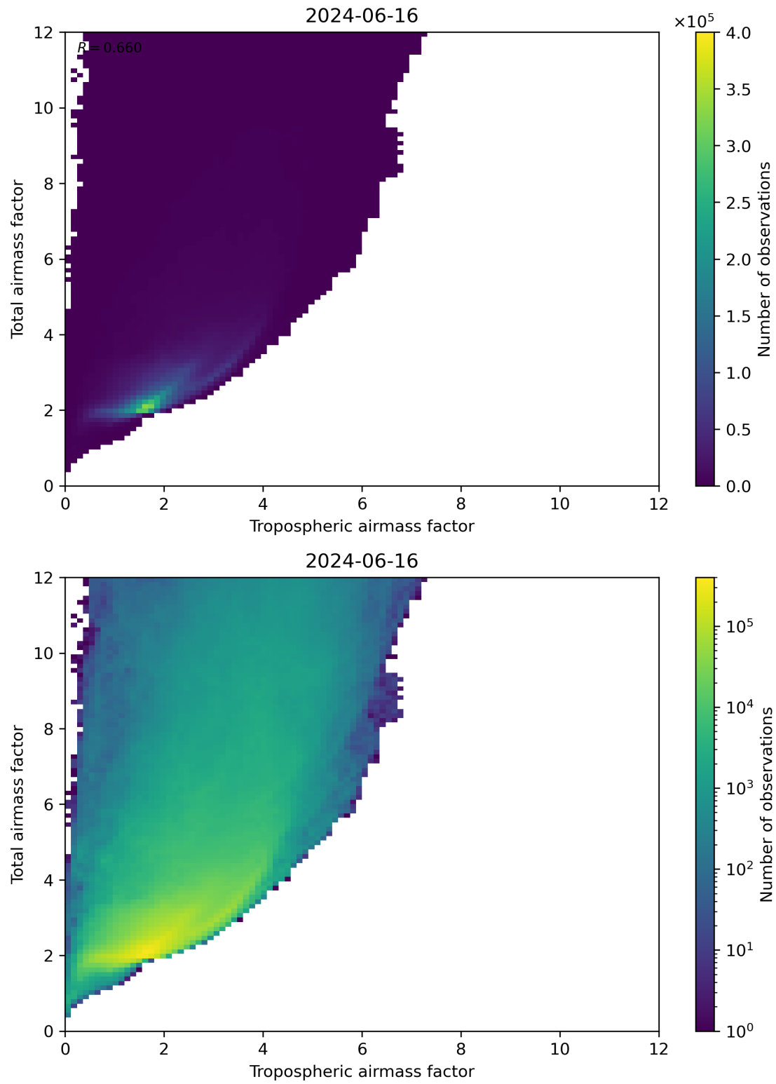
Figure 72: Scatter density plot of “Tropospheric airmass factor” against “Total airmass factor” for 2024-06-15 to 2024-06-17.
