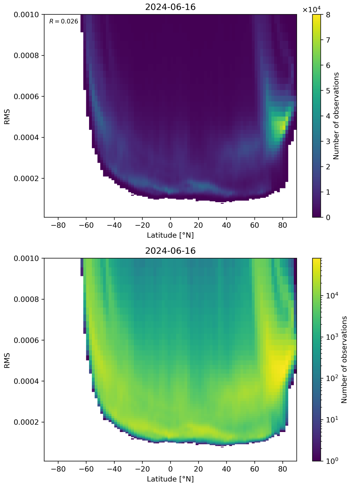
Figure 94: Scatter density plot of “Latitude” against “RMS” for 2024-06-15 to 2024-06-17.
