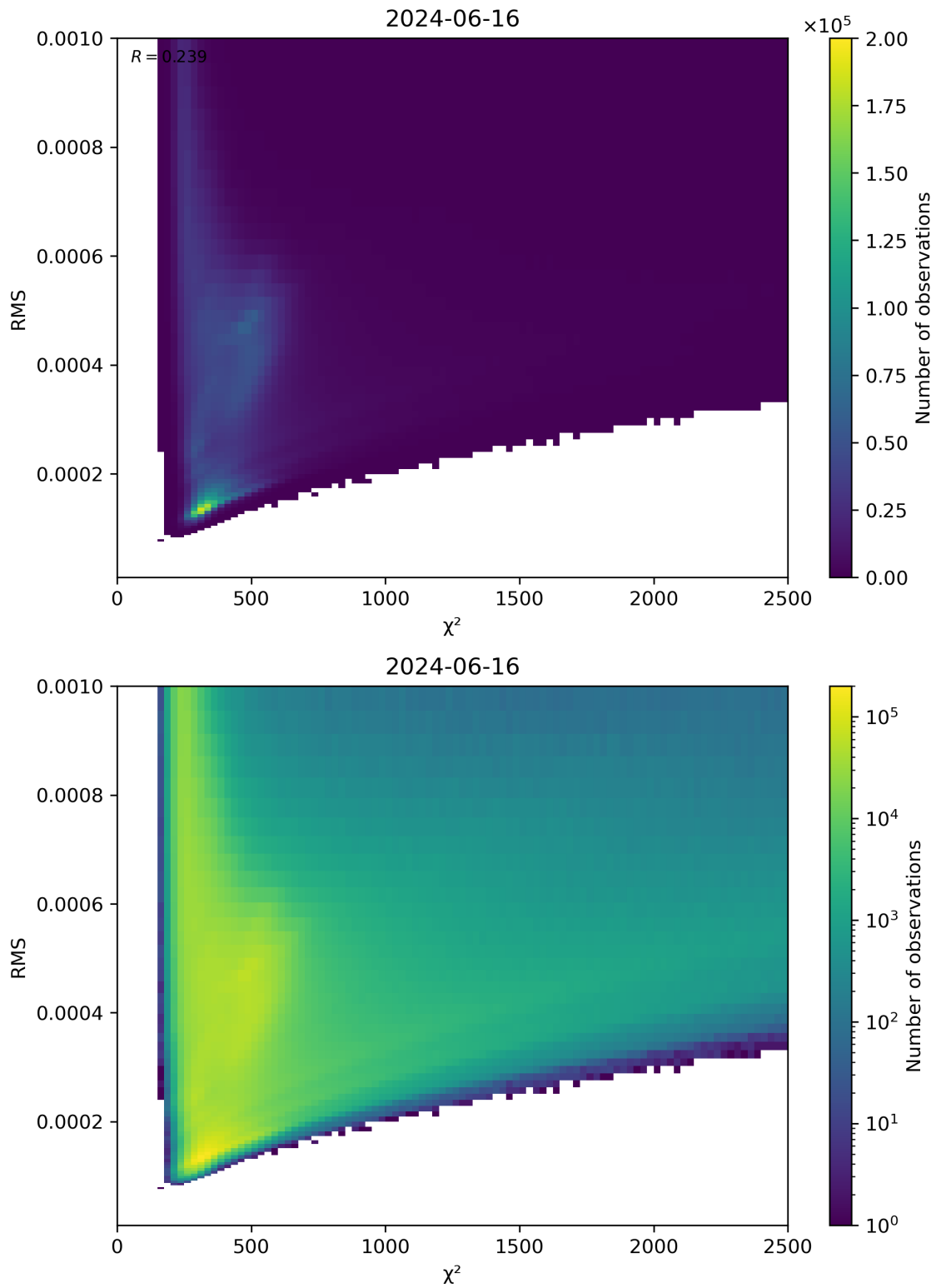
Figure 82: Scatter density plot of “ \chi^2 ” against “RMS” for 2024-06-15 to 2024-06-17.
