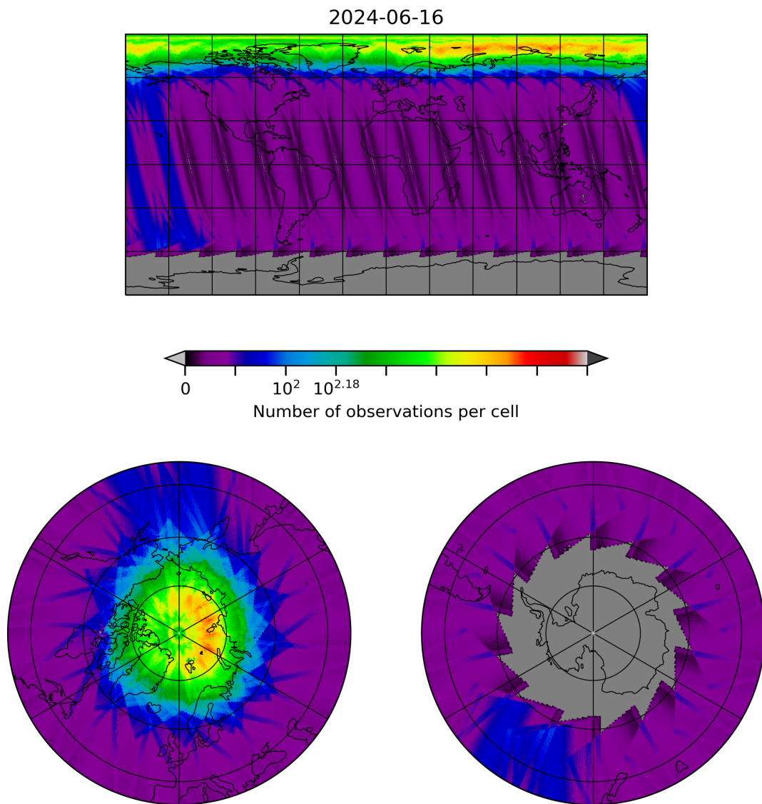
Figure 10: Map of the number of observations for 2024-06-15 to 2024-06-17
