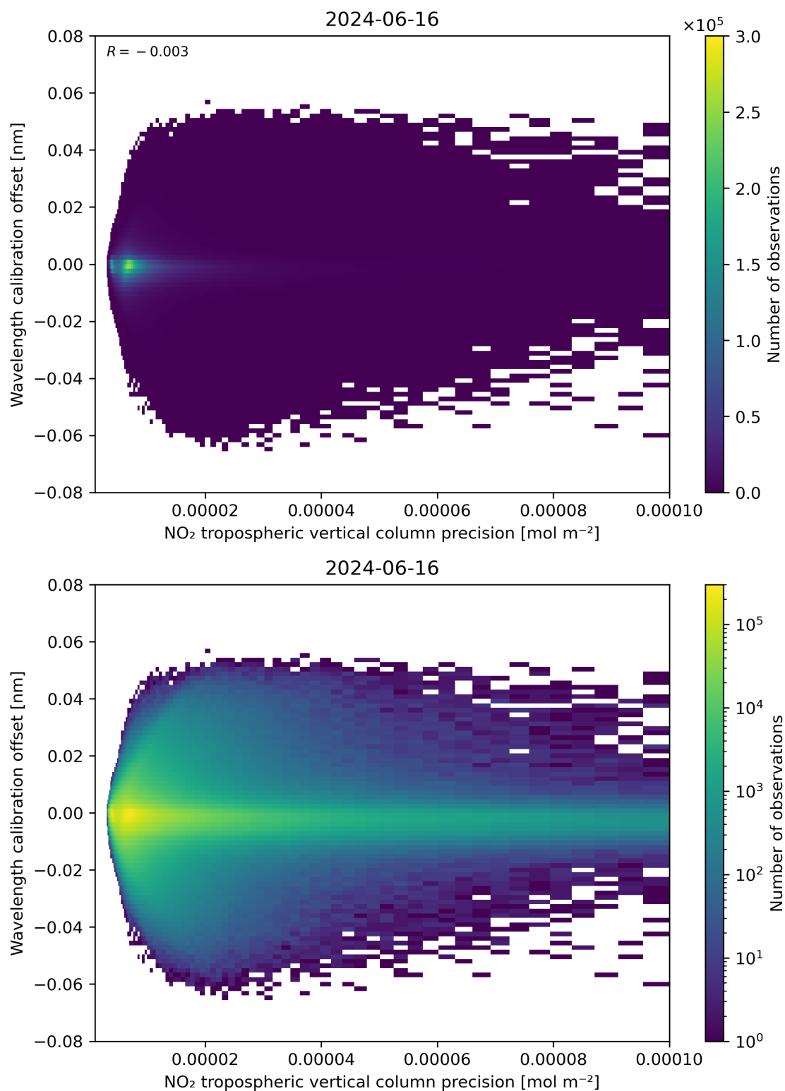
Figure 141: Scatter density plot of “NO 2 tropospheric vertical column precision” against “Wavelength calibration offset” for 2024-06-15 to 2024-06-17.
