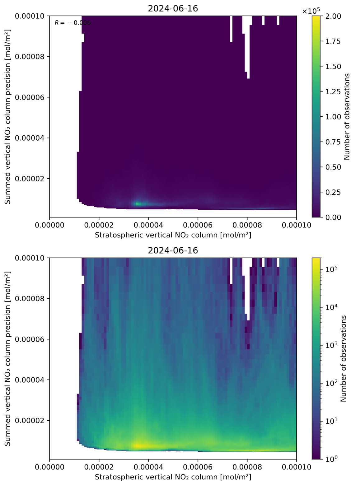
Figure 99: Scatter density plot of “Stratospheric vertical NO 2 column” against “Summed vertical NO 2 column precision” for 2024-06-15 to 2024-06-17.
