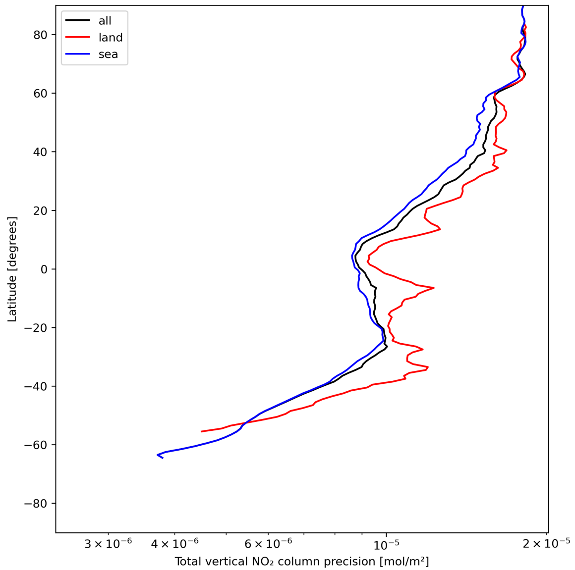
Figure 22: Zonal average of “Total vertical NO 2 column precision” for 2024-06-15 to 2024-06-17.
