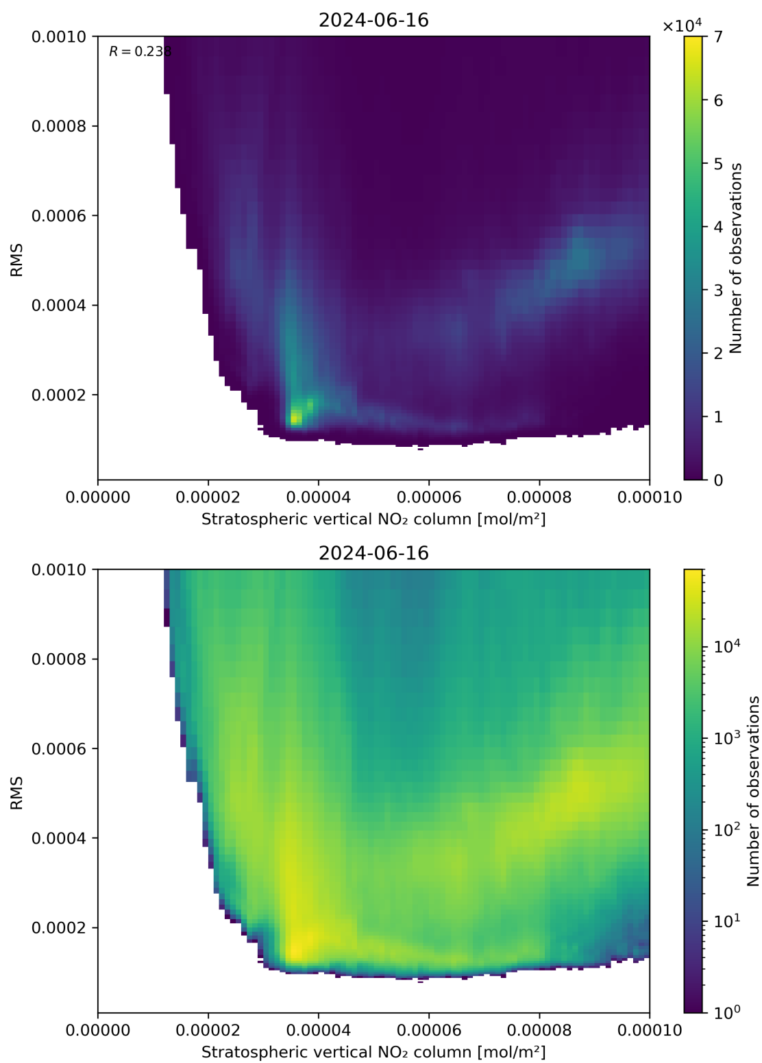
Figure 102: Scatter density plot of “Stratospheric vertical NO 2 column” against “RMS” for 2024-06-15 to 2024-06-17.
