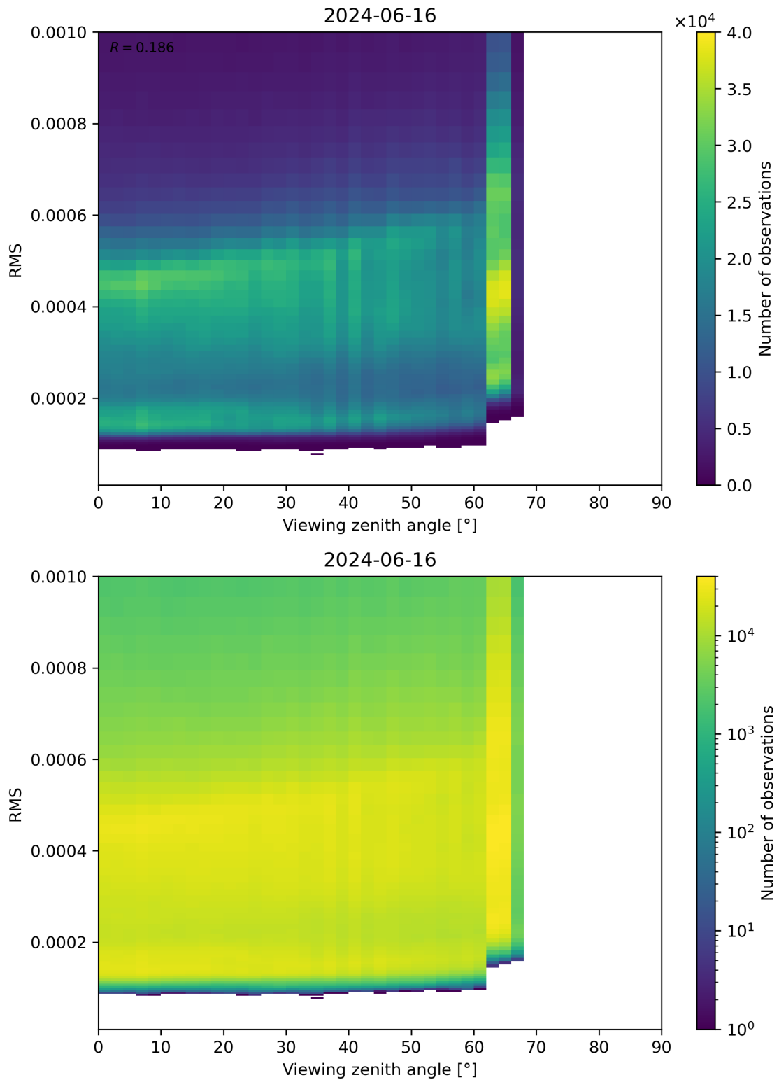
Figure 171: Scatter density plot of “Viewing zenith angle” against “RMS” for 2024-06-15 to 2024-06-17.
