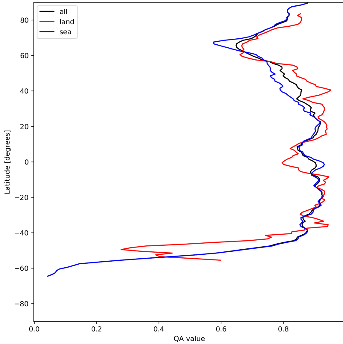
Figure 11: Zonal average of “QA value” for 2024-06-15 to 2024-06-17.
