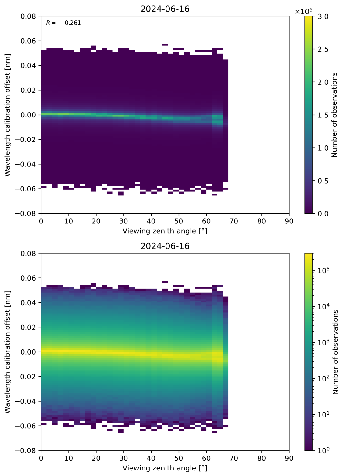
Figure 173: Scatter density plot of “Viewing zenith angle” against “Wavelength calibration offset” for 2024-06-15 to 2024-06-17.
