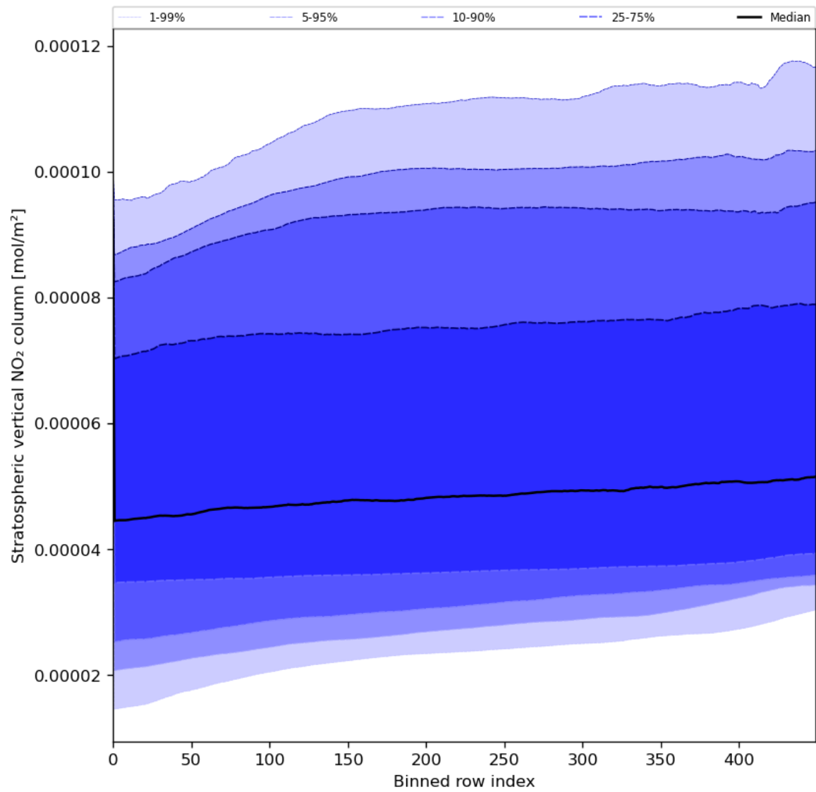
Figure 53: Along track statistics of “Stratospheric vertical NO 2 column” for 2024-06-15 to 2024-06-17
