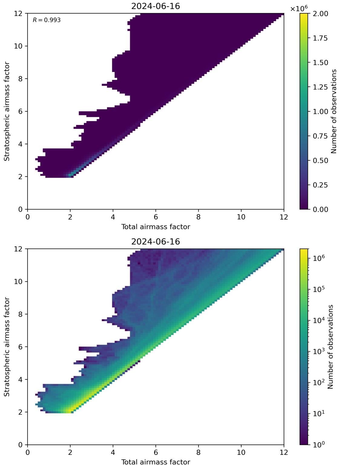
Figure 62: Scatter density plot of “Total airmass factor” against “Stratospheric airmass factor” for 2024-06-15 to 2024-06-17.
