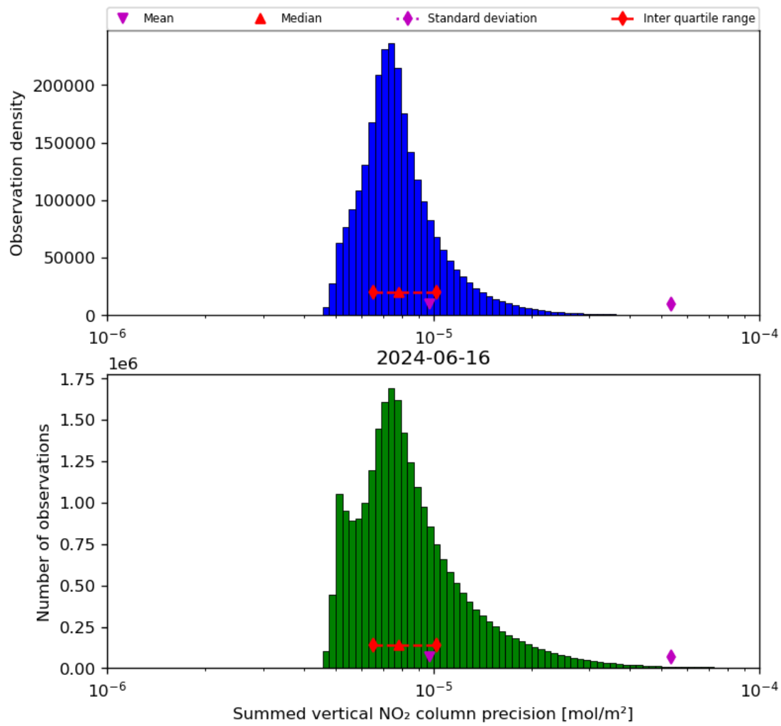
Figure 41: Histogram of "Summed vertical NO 2 column precision" for 2024-06-15 to 2024-06-17
