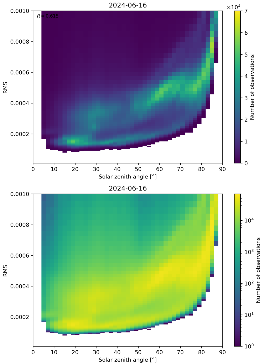
Figure 157: Scatter density plot of “Solar zenith angle” against “RMS” for 2024-06-15 to 2024-06-17.
