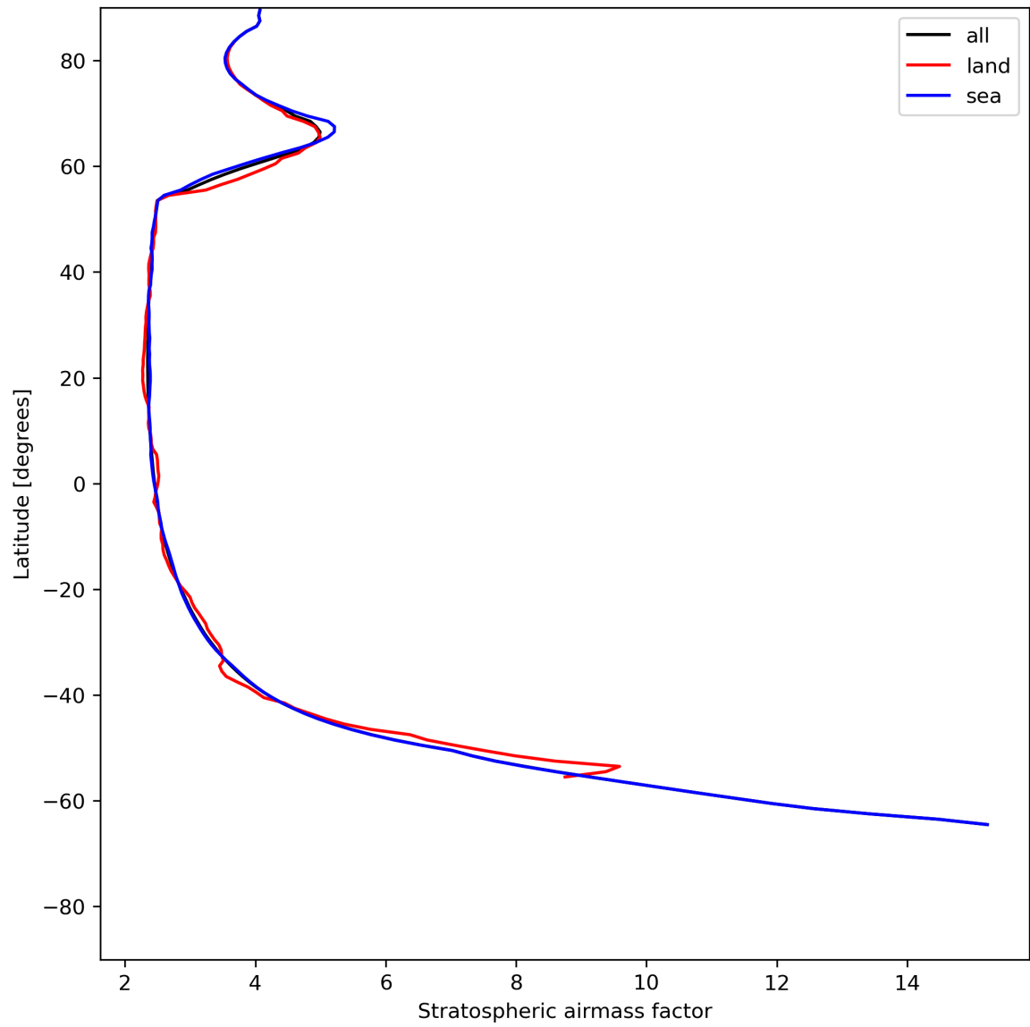
Figure 27: Zonal average of “Stratospheric airmass factor” for 2024-06-15 to 2024-06-17.
