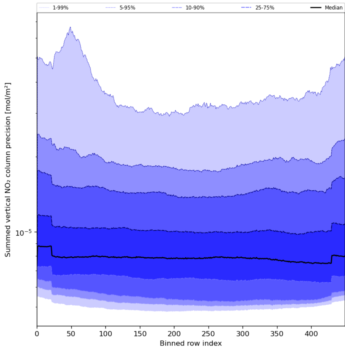
Figure 58: Along track statistics of “Summed vertical NO 2 column precision” for 2024-06-15 to 2024-06-17
