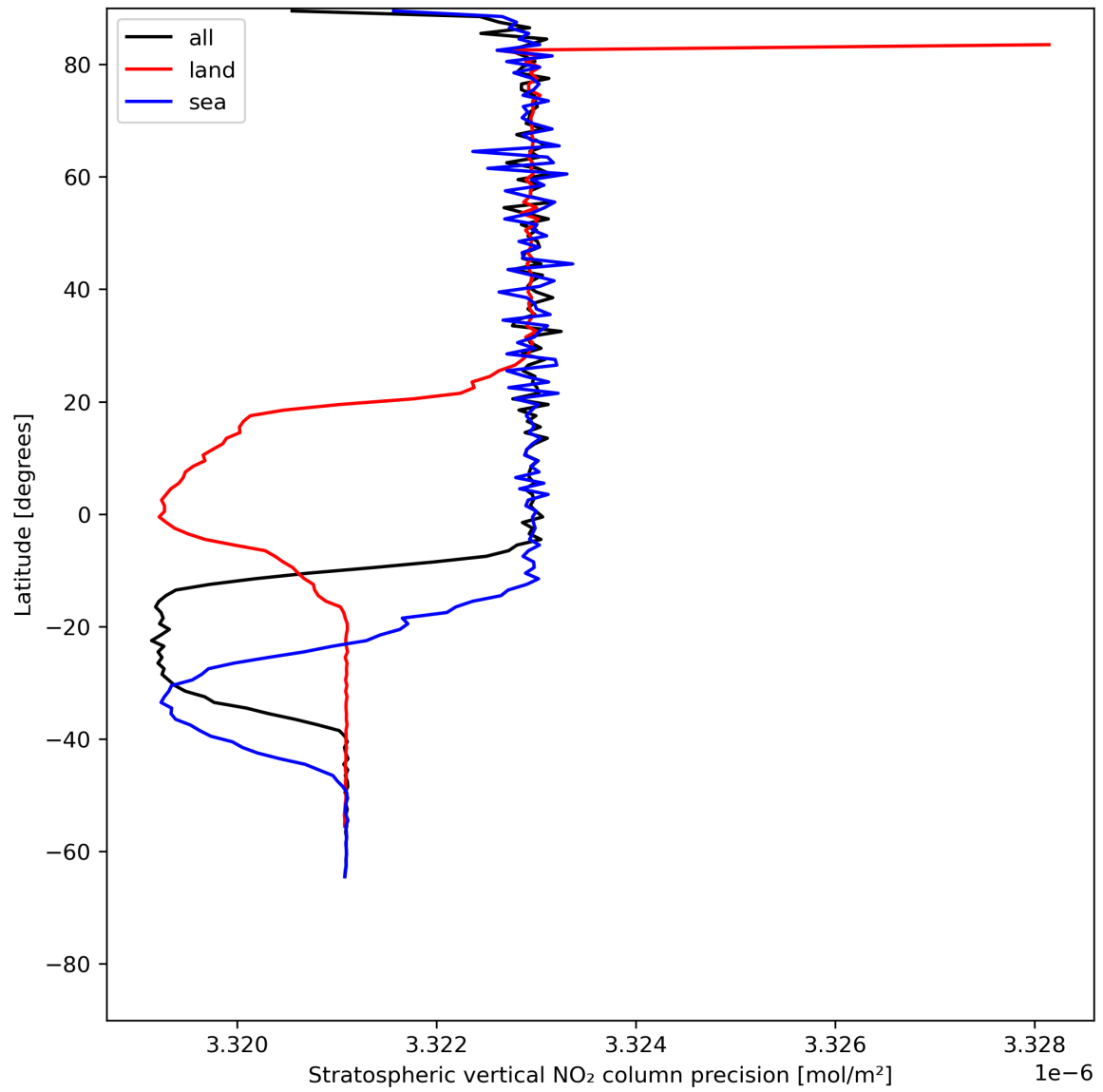
Figure 20: Zonal average of “Stratospheric vertical NO 2 column precision” for 2024-06-15 to 2024-06-17.
