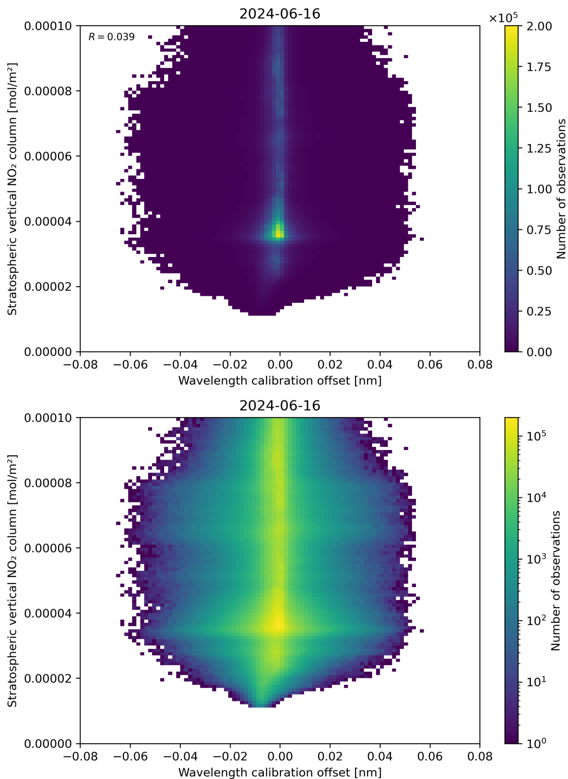
Figure 176: Scatter density plot of “Wavelength calibration offset” against “Stratospheric vertical NO 2 column” for 2024-06-15 to 2024-06-17.
