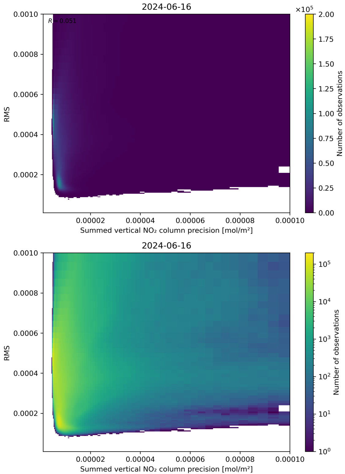
Figure 108: Scatter density plot of “Summed vertical NO 2 column precision” against “RMS” for 2024-06-15 to 2024-06-17.
