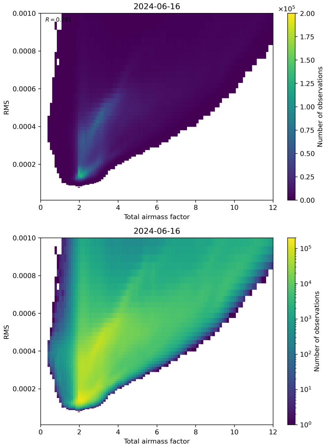
Figure 69: Scatter density plot of “Total airmass factor” against “RMS” for 2024-06-15 to 2024-06-17.
