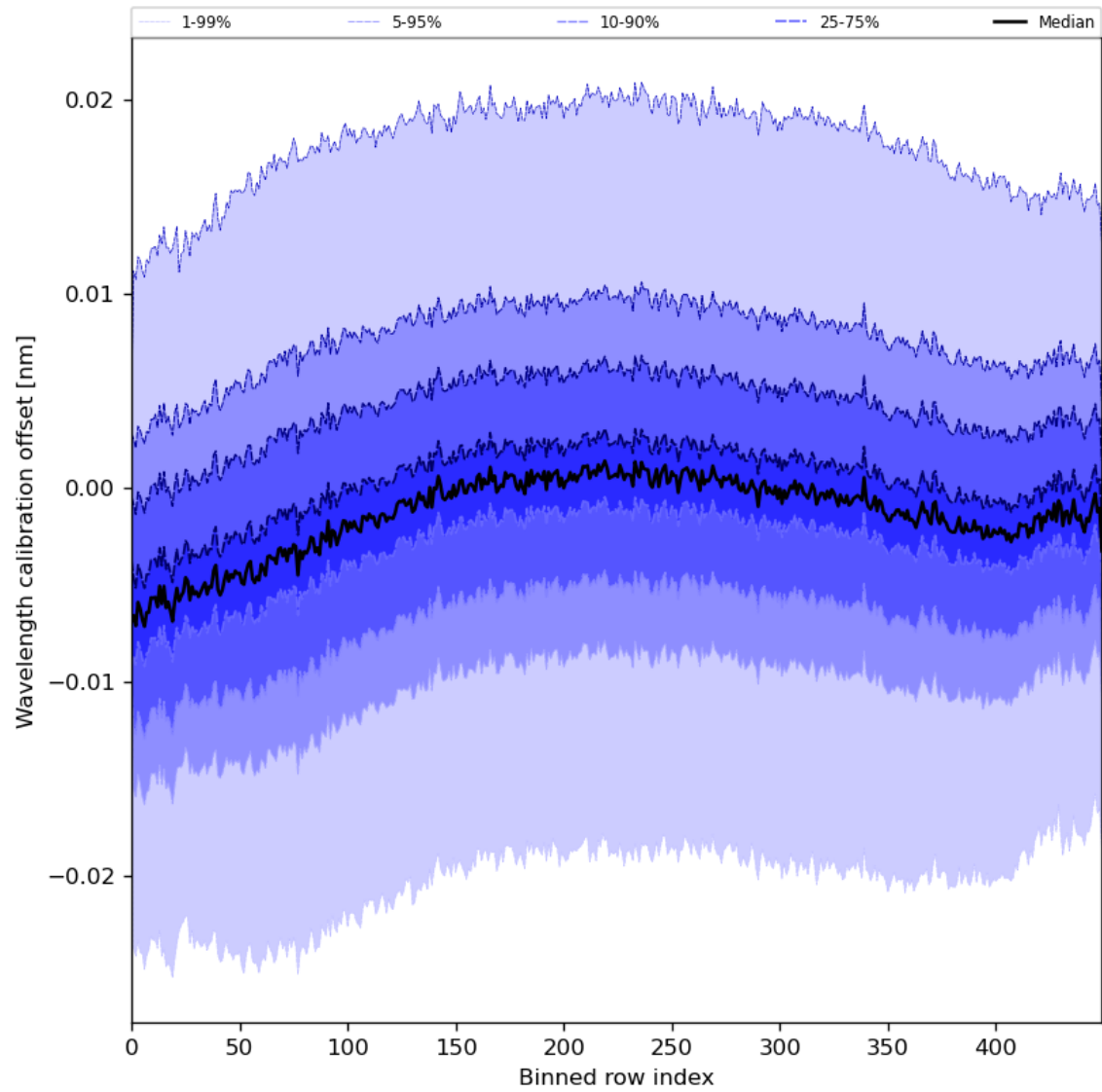
Figure 52: Along track statistics of “Wavelength calibration offset” for 2024-06-15 to 2024-06-17
