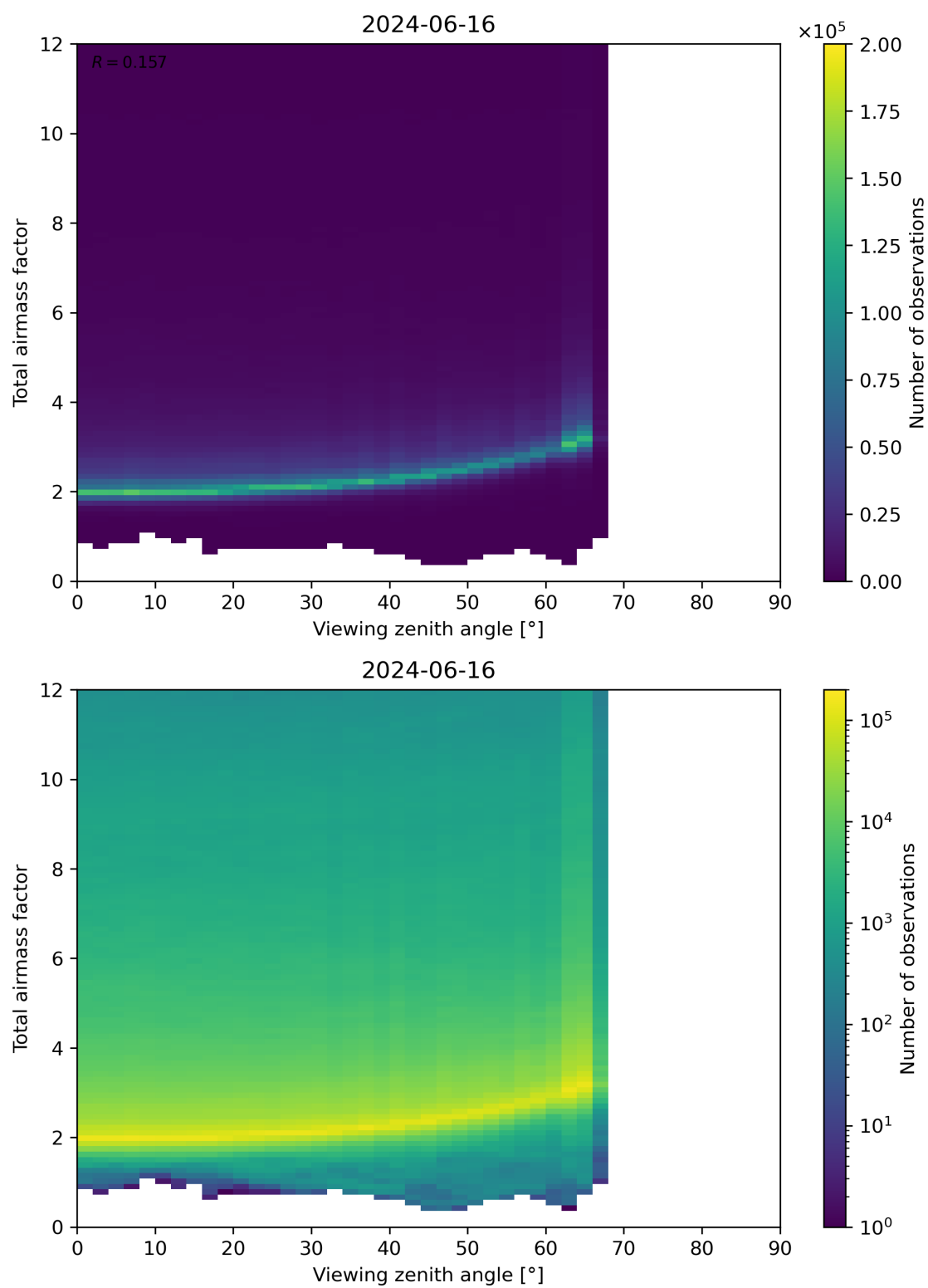
Figure 160: Scatter density plot of “Viewing zenith angle” against “Total airmass factor” for 2024-06-15 to 2024-06-17.
