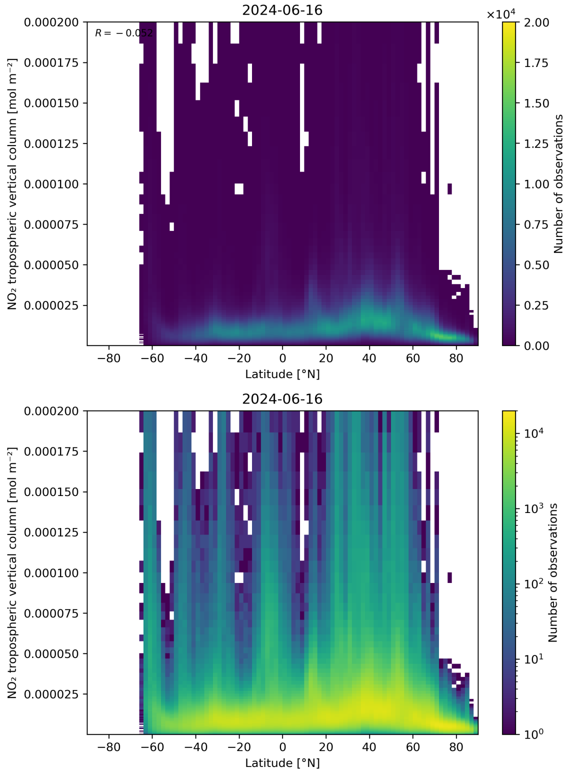
Figure 92: Scatter density plot of “Latitude” against “NO 2 tropospheric vertical column” for 2024-06-15 to 2024-06-17.
