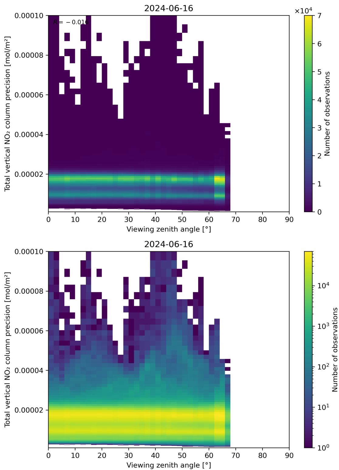
Figure 168: Scatter density plot of “Viewing zenith angle” against “Total vertical NO 2 column precision” for 2024-06-15 to 2024-06-17.
