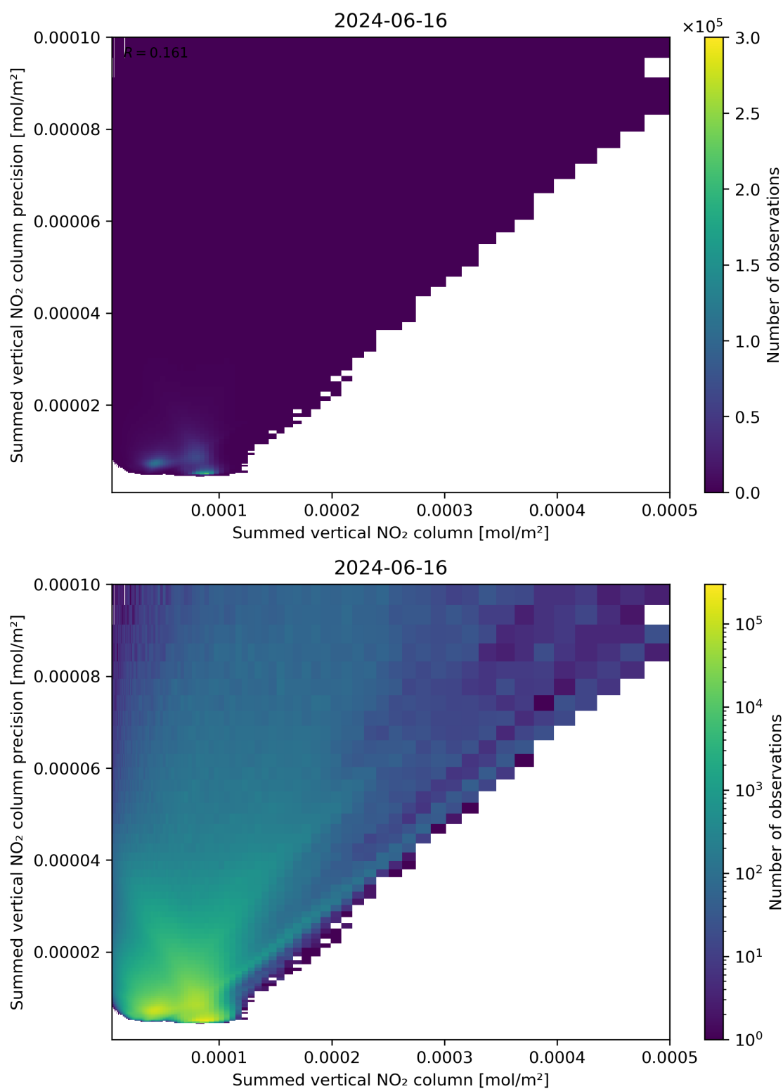
Figure 105: Scatter density plot of “Summed vertical NO 2 column” against “Summed vertical NO 2 column precision” for 2024-06-15 to 2024-06-17.
