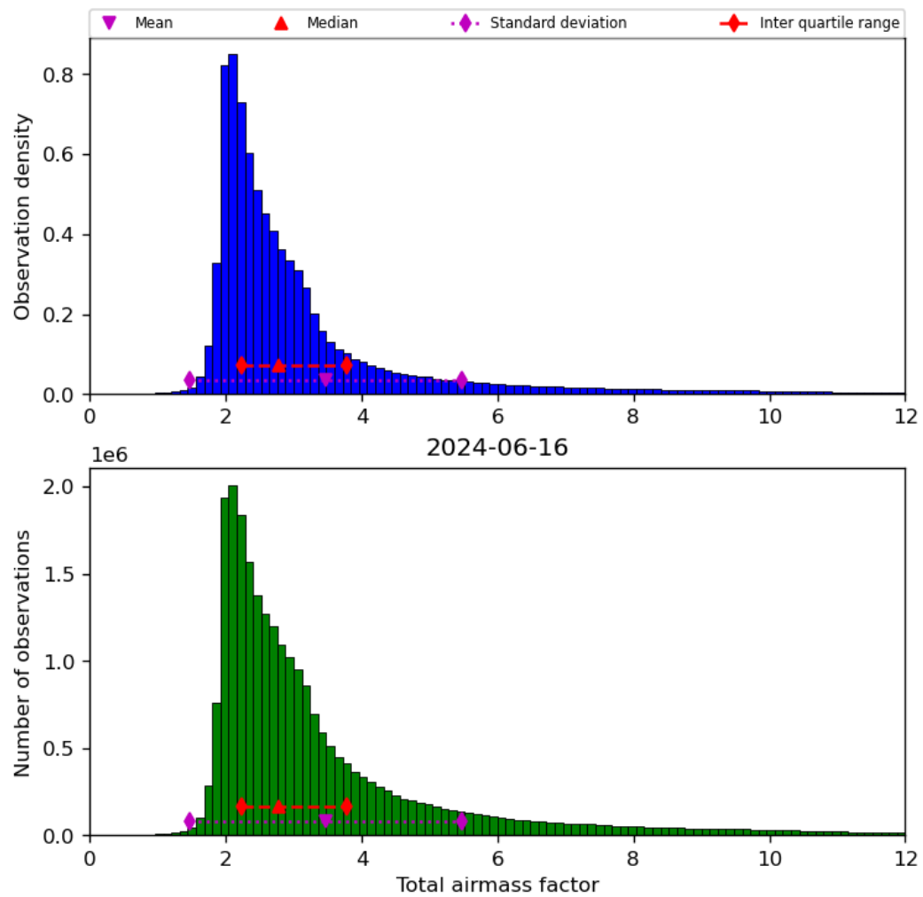
Figure 32: Histogram of “Total airmass factor” for 2024-06-15 to 2024-06-17
