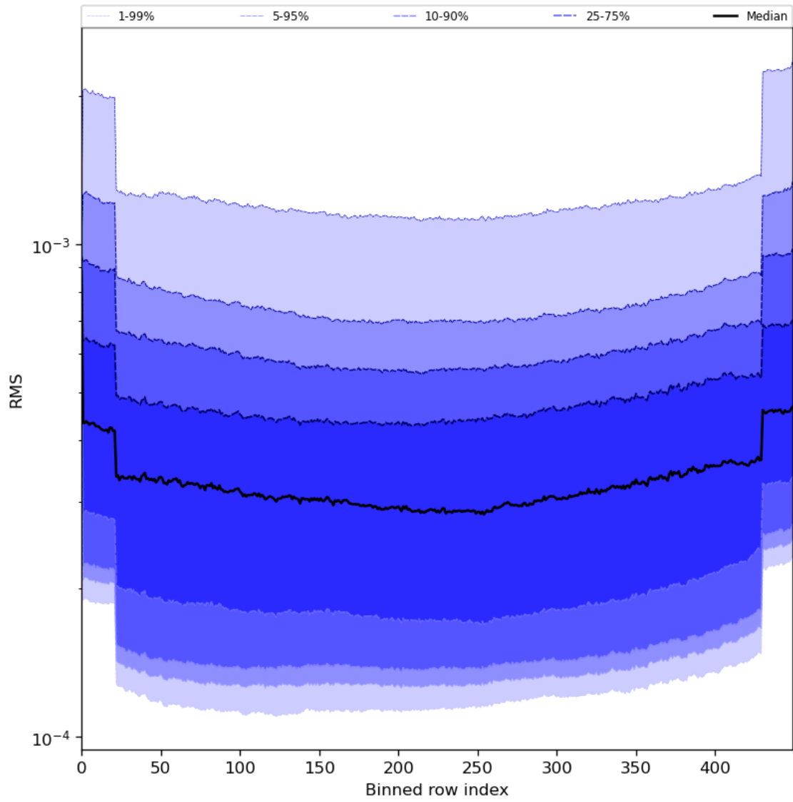
Figure 60: Along track statistics of “RMS” for 2024-06-15 to 2024-06-17
