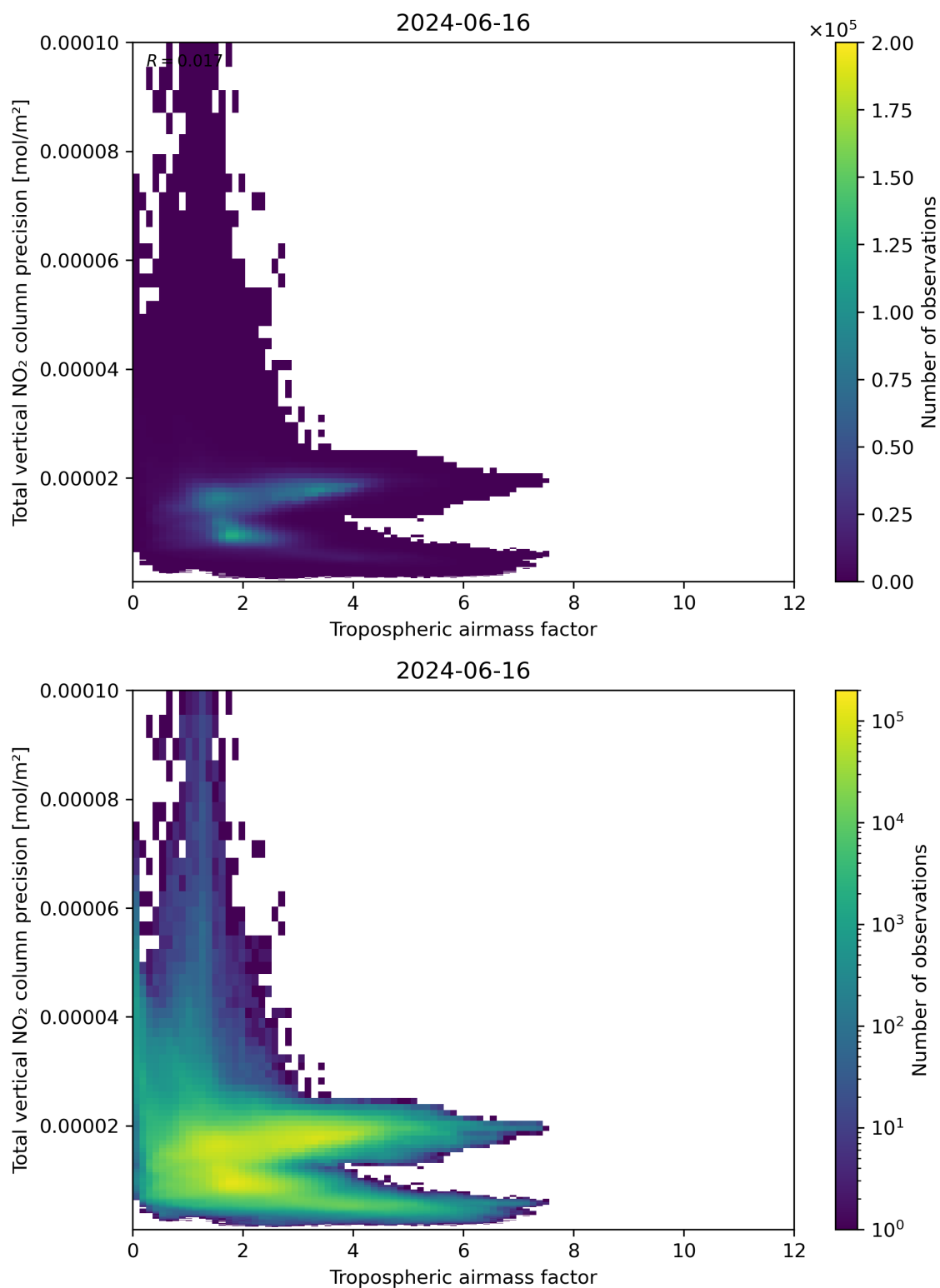
Figure 78: Scatter density plot of “Tropospheric air mass factor” against “Total vertical NO 2 column precision” for 2024-06-15 to 2024-06-17.
