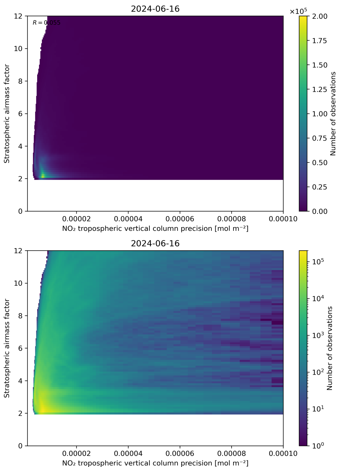
Figure 131: Scatter density plot of “NO 2 tropospheric vertical column precision” against “Stratospheric airmass factor” for 2024-06-15 to 2024-06-17.
