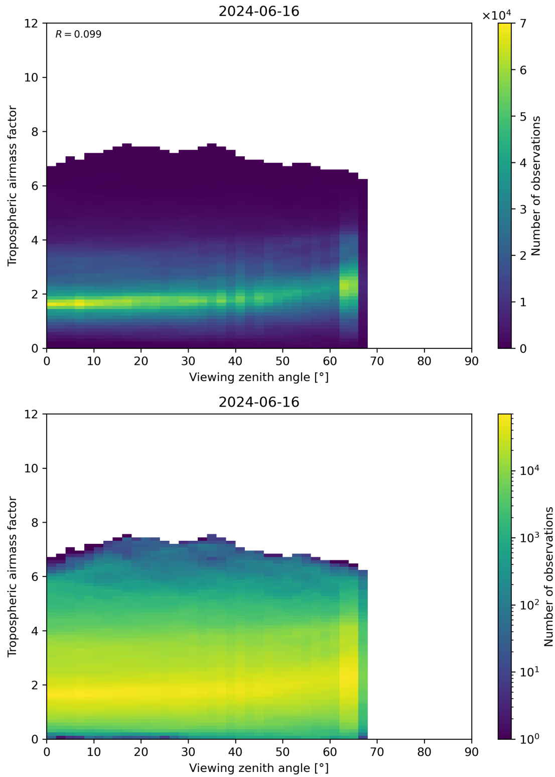
Figure 161: Scatter density plot of “Viewing zenith angle” against “Tropospheric airmass factor” for 2024-06-15 to 2024-06-17.
