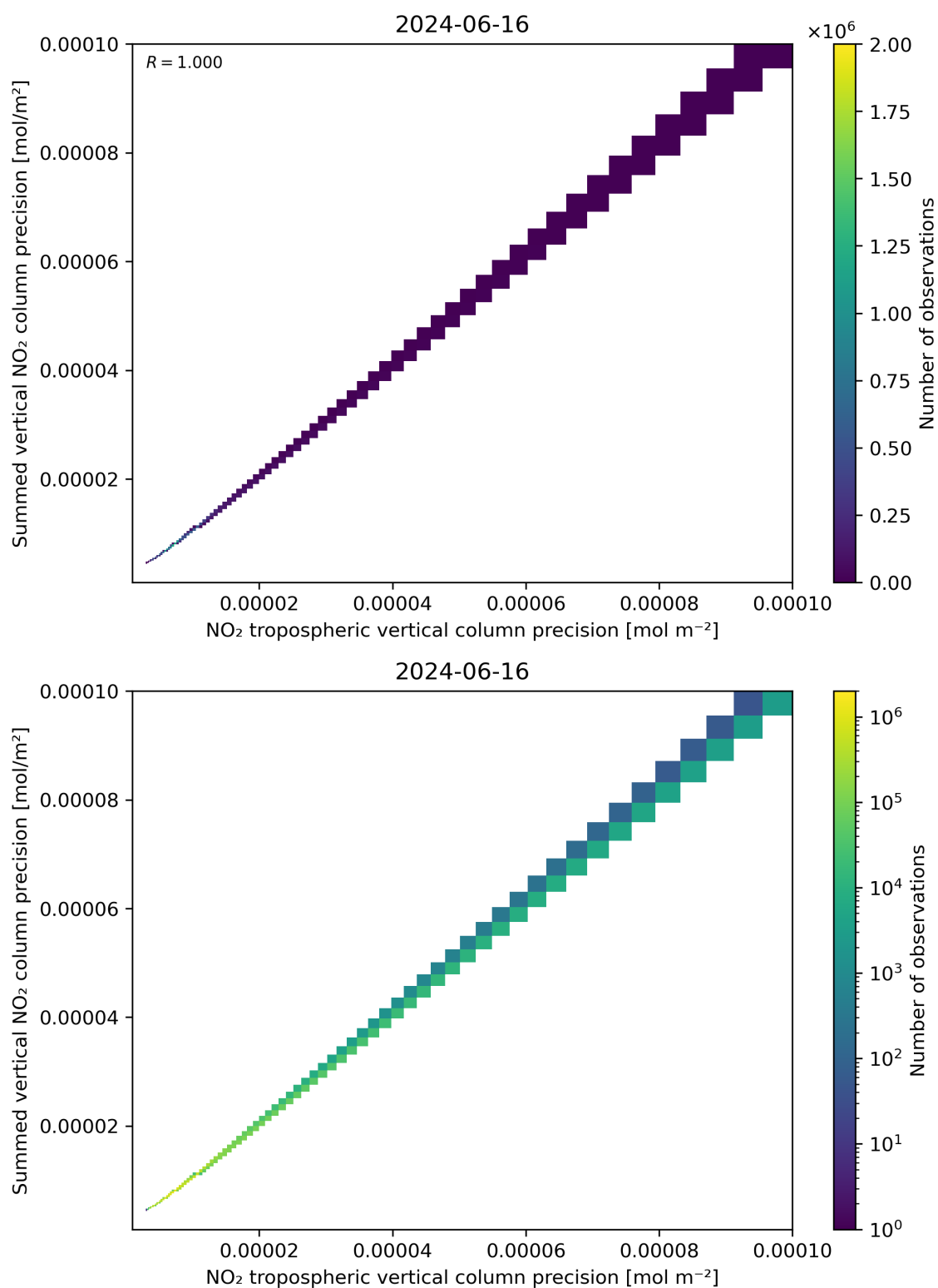
Figure 137: Scatter density plot of “NO 2 tropospheric vertical column precision” against “Summed vertical NO 2 column precision” for 2024-06-15 to 2024-06-17.
