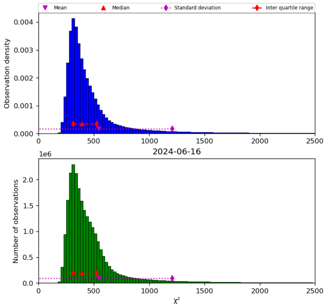
Figure 42: Histogram of “ \chi^2 ” for 2024-06-15 to 2024-06-17
