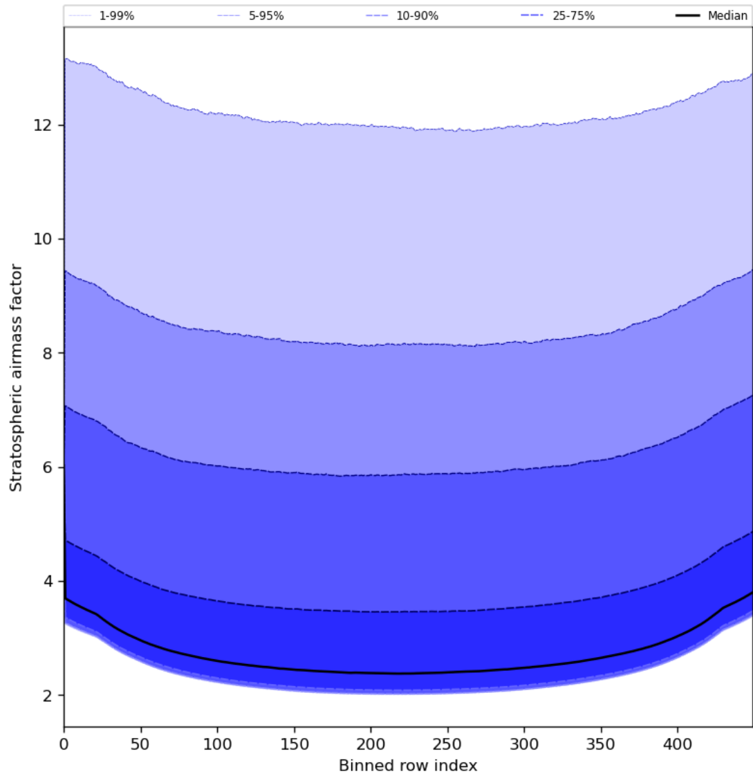
Figure 61: Along track statistics of “Stratospheric airmass factor” for 2024-06-15 to 2024-06-17
