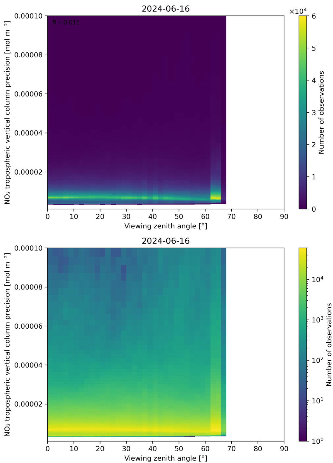
Figure 170: Scatter density plot of “Viewing zenith angle” against “NO 2 tropospheric vertical column precision” for 2024-06-15 to 2024-06-17.
