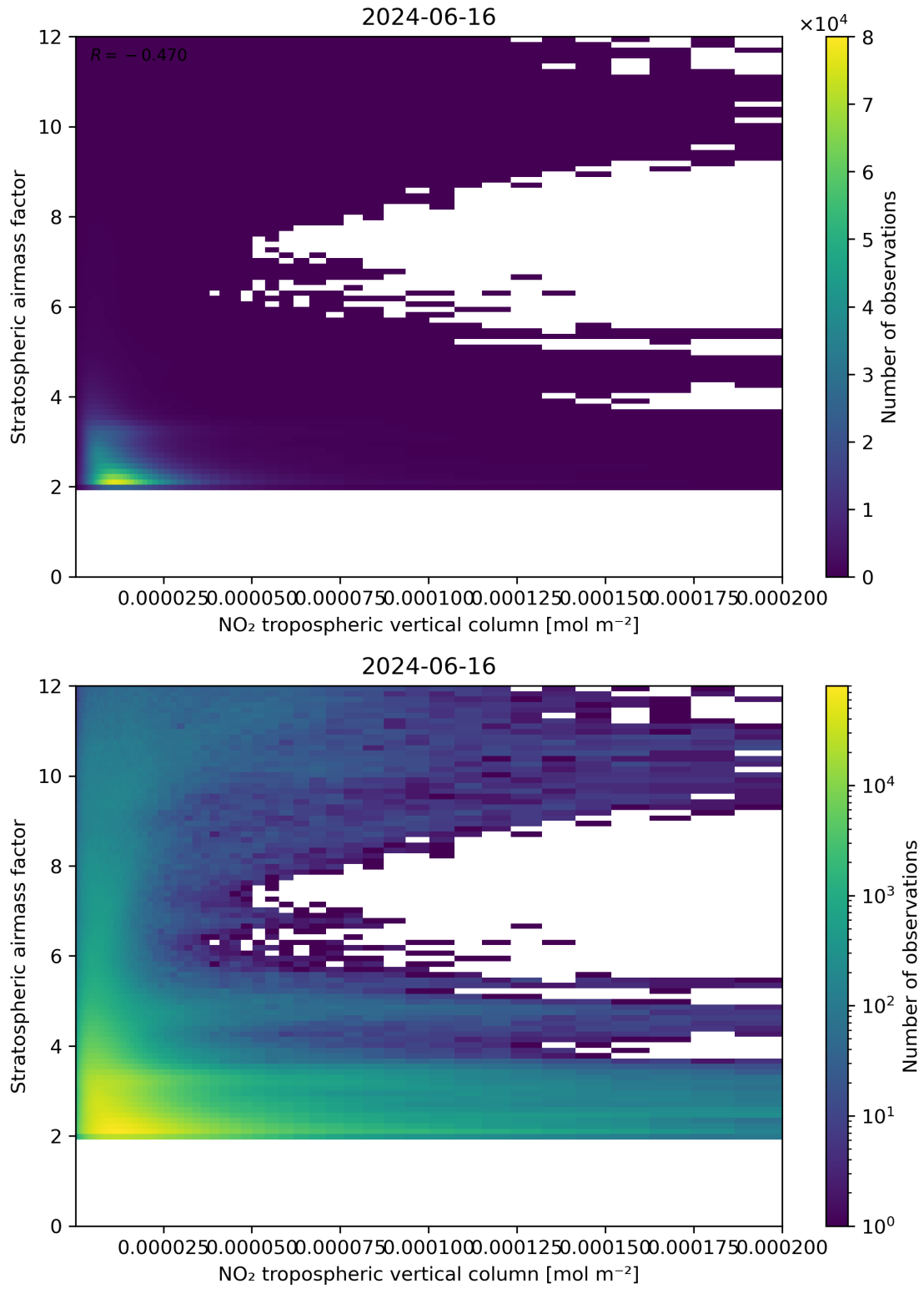
Figure 121: Scatter density plot of “NO 2 tropospheric vertical column” against “Stratospheric air mass factor” for 2024-06-15 to 2024-06-17.
