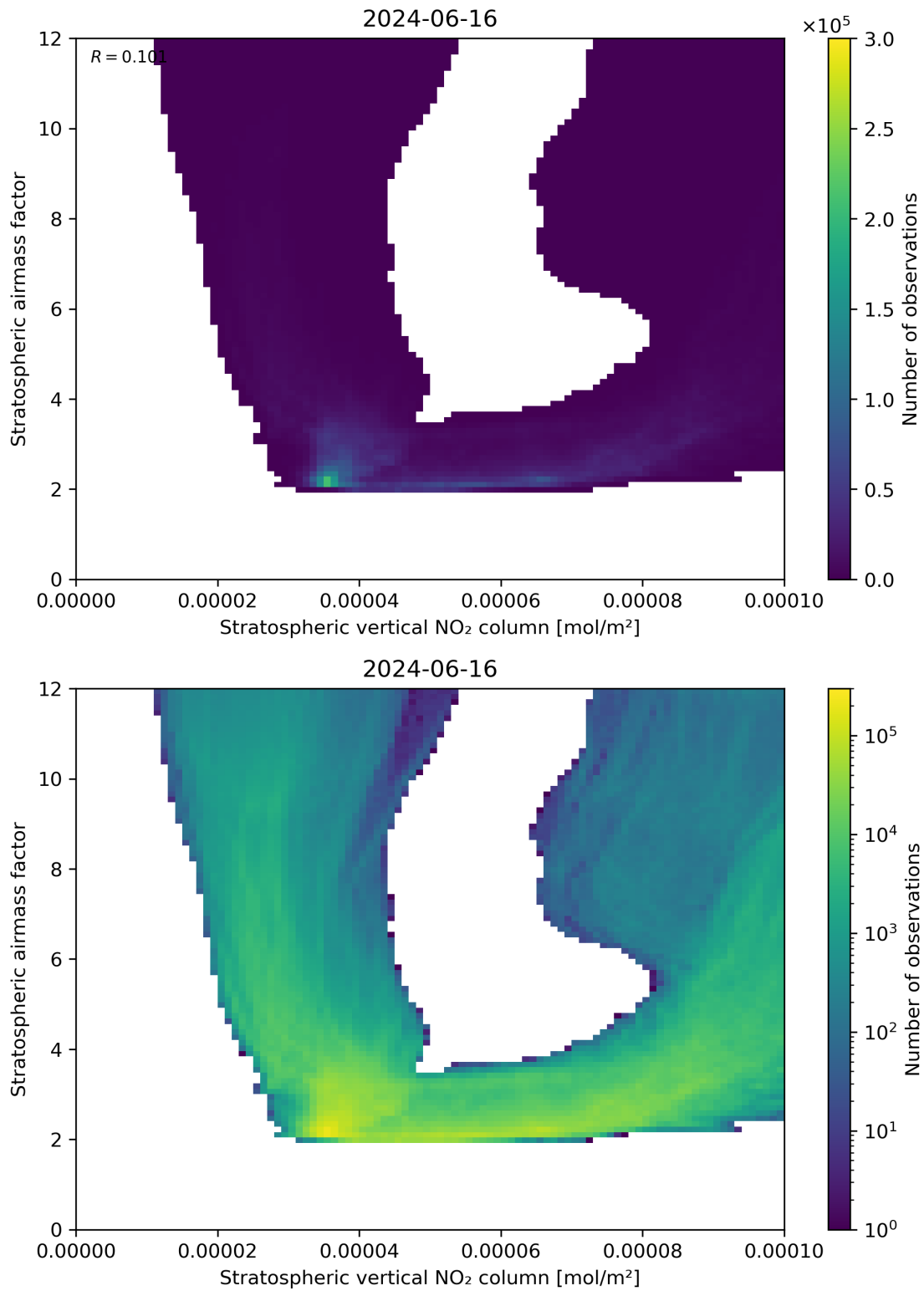
Figure 96: Scatter density plot of “Stratospheric vertical NO 2 column” against “Stratospheric airmass factor” for 2024-06-15 to 2024-06-17.
