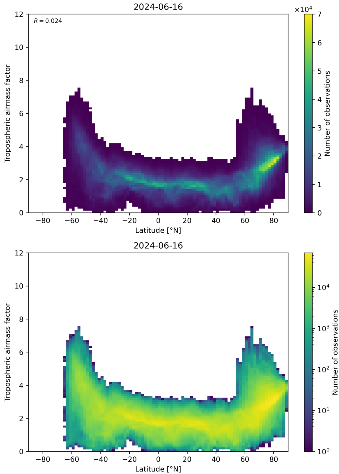
Figure 85: Scatter density plot of “Latitude” against “Tropospheric airmass factor” for 2024-06-15 to 2024-06-17.
