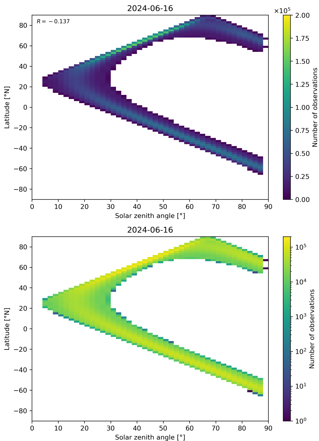
Figure 149: Scatter density plot of “Solar zenith angle” against “Latitude” for 2024-06-15 to 2024-06-17.
