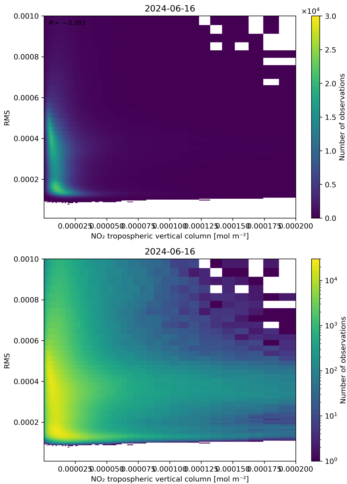
Figure 142: Scatter density plot of “NO 2 tropospheric vertical column” against “RMS” for 2024-06-15 to 2024-06-17.
