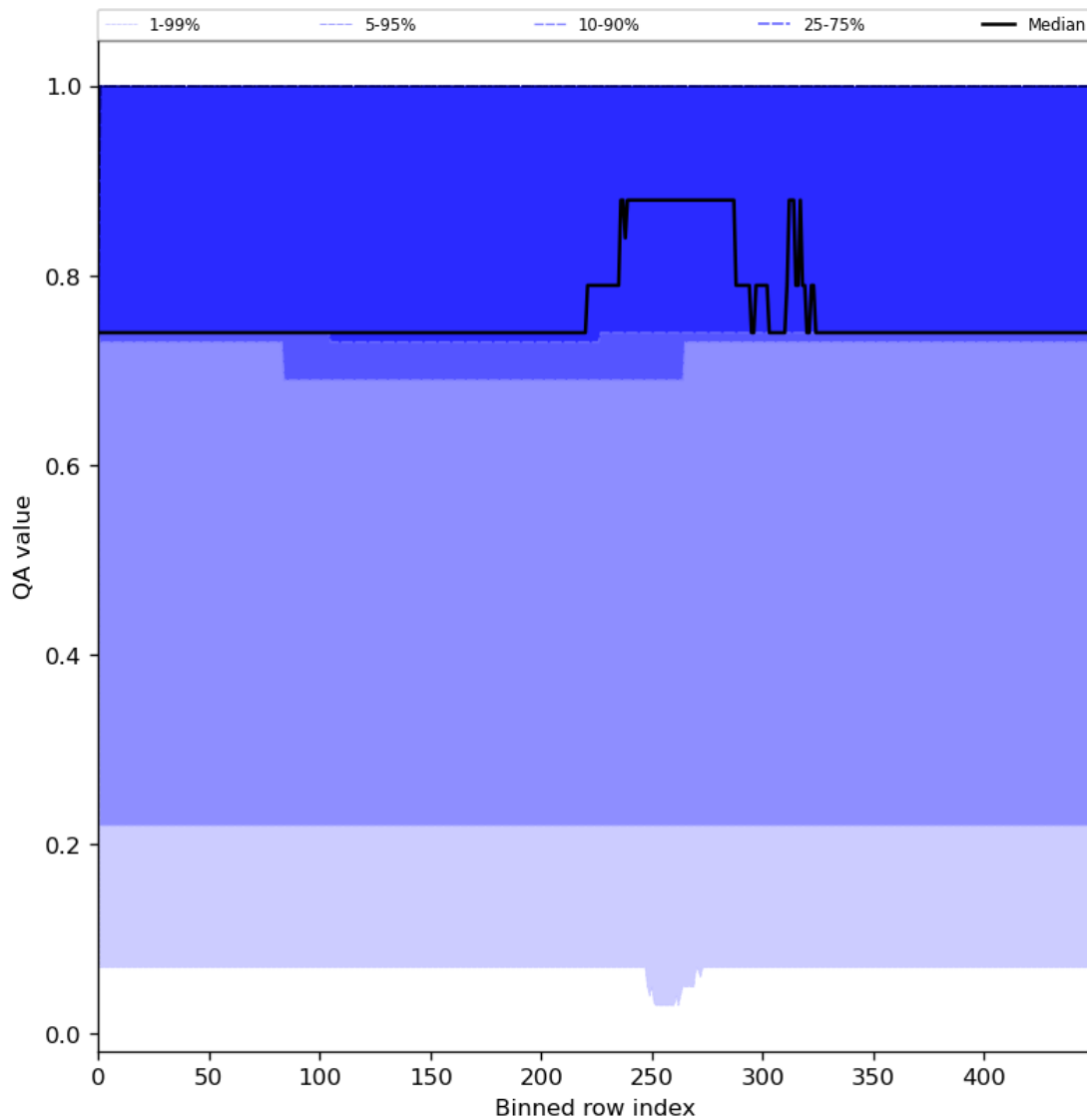
Figure 45: Along track statistics of “QA value” for 2024-06-15 to 2024-06-17
