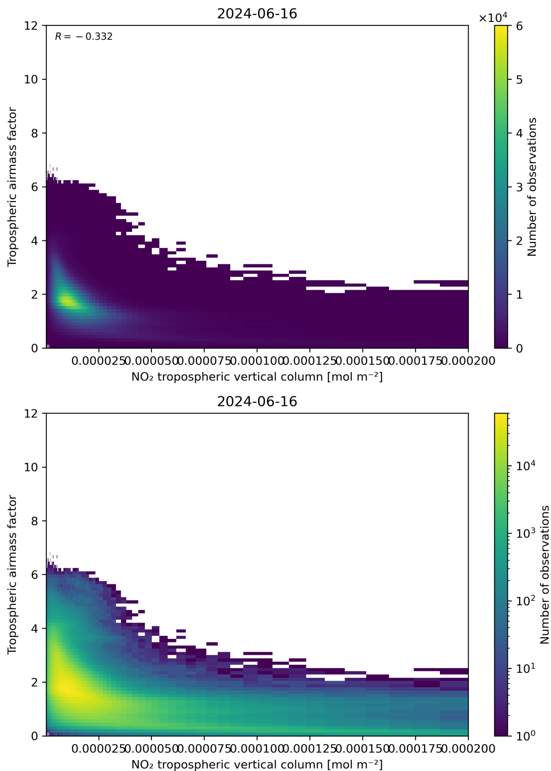
Figure 123: Scatter density plot of “NO 2 tropospheric vertical column” against “Tropospheric air mass factor” for 2024-06-15 to 2024-06-17.
