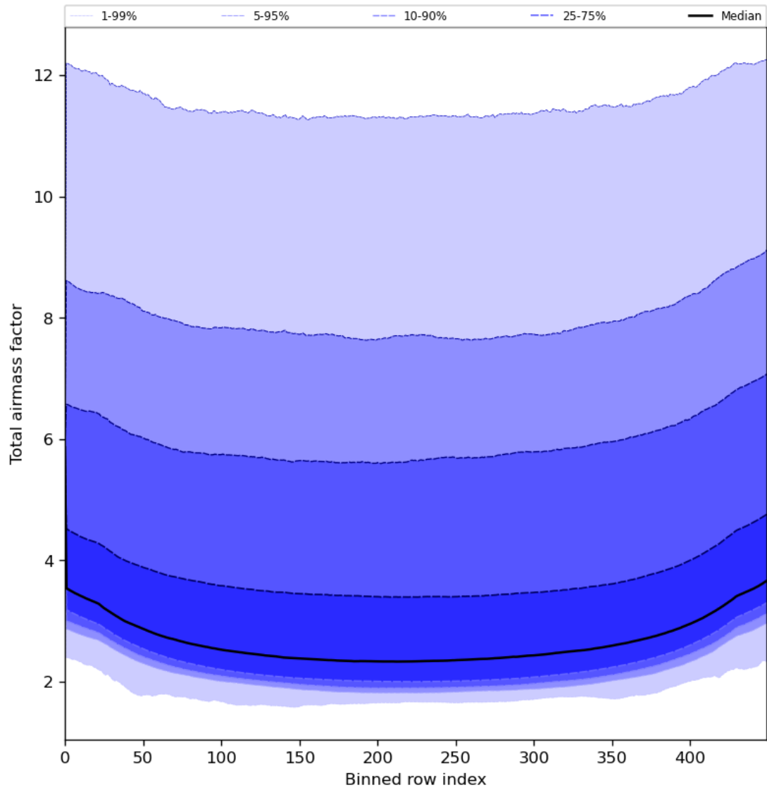
Figure 49: Along track statistics of “Total airmass factor” for 2024-06-15 to 2024-06-17
