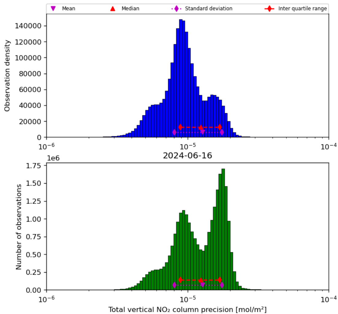
Figure 39: Histogram of “Total vertical NO 2 column precision” for 2024-06-15 to 2024-06-17
