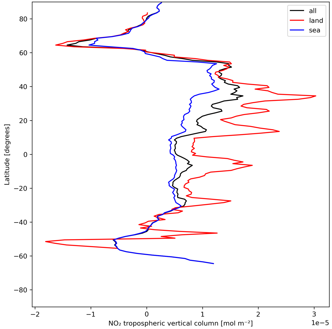
Figure 12: Zonal average of “NO 2 tropospheric vertical column” for 2024-06-15 to 2024-06-17.
