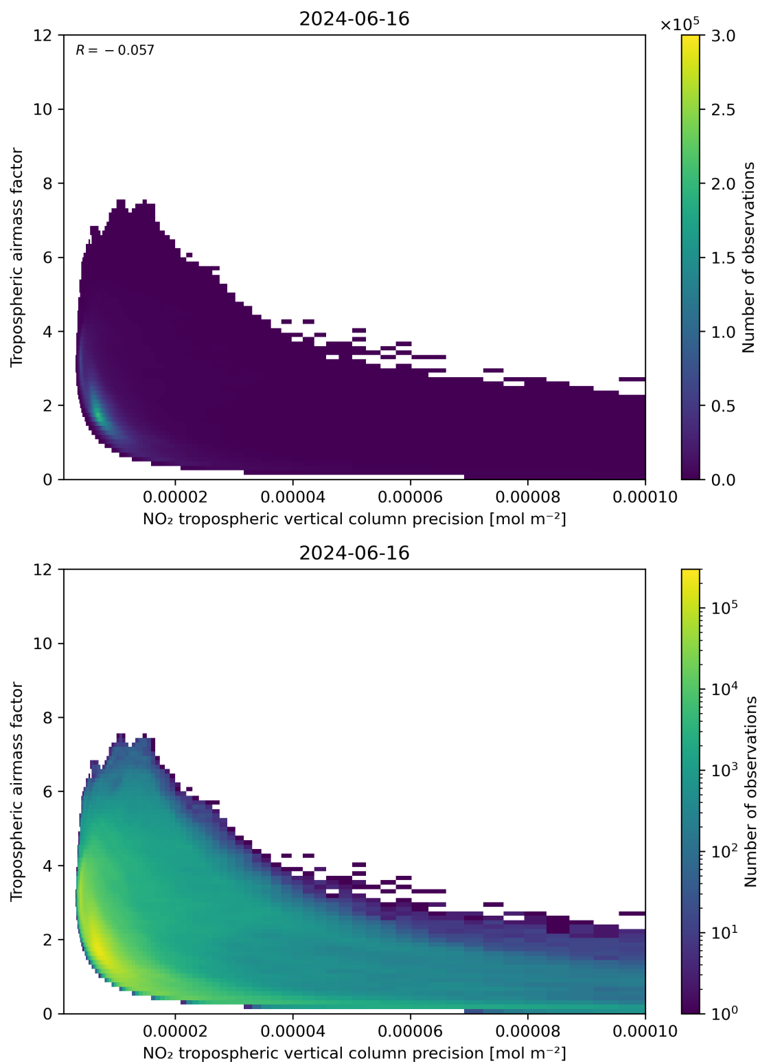
Figure 133: Scatter density plot of “NO 2 tropospheric vertical column precision” against “Tropospheric airmass factor” for 2024-06-15 to 2024-06-17.
