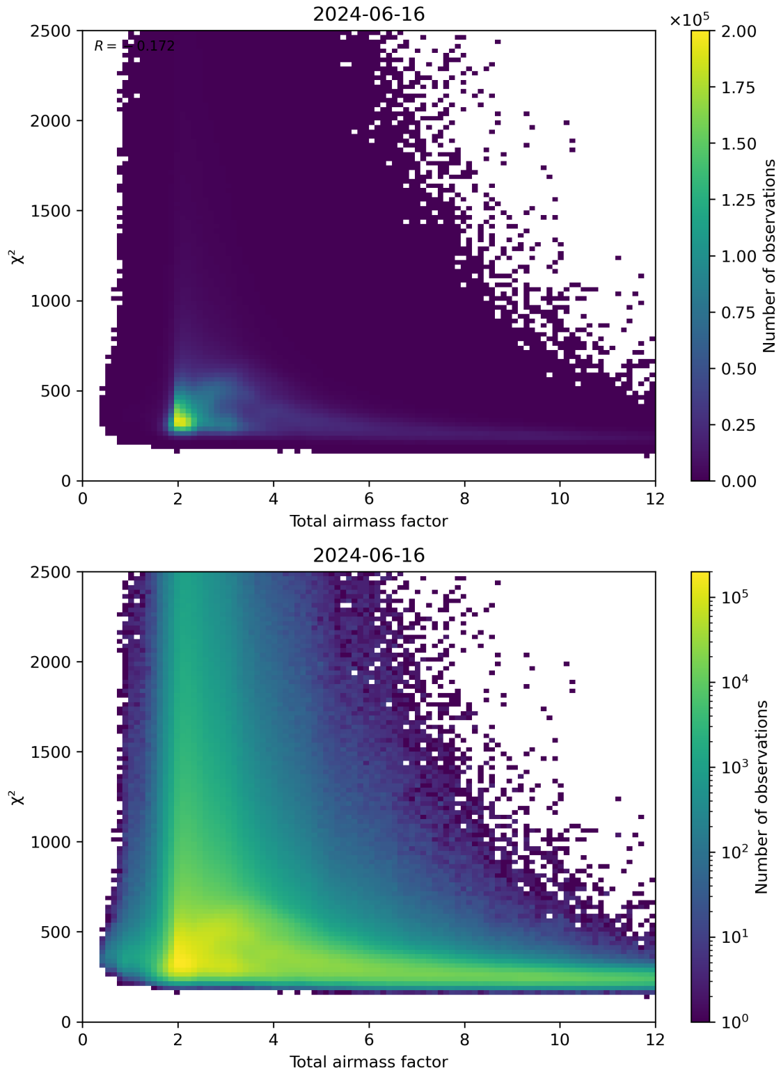
Figure 63: Scatter density plot of “Total airmass factor” against “ \chi^2 ” for 2024-06-15 to 2024-06-17.
