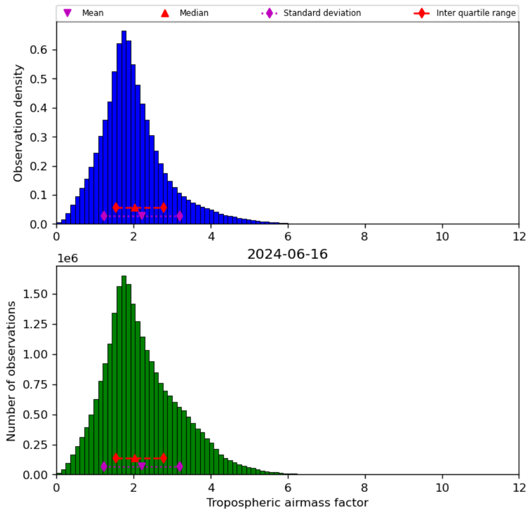
Figure 31: Histogram of “Tropospheric airmass factor” for 2024-06-15 to 2024-06-17
