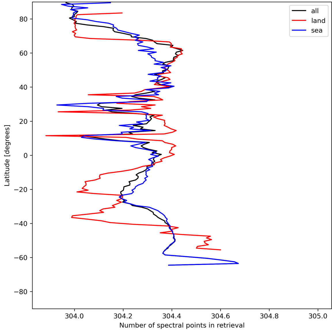
Figure 16: Zonal average of “Number of spectral points in retrieval” for 2024-06-15 to 2024-06-17.
