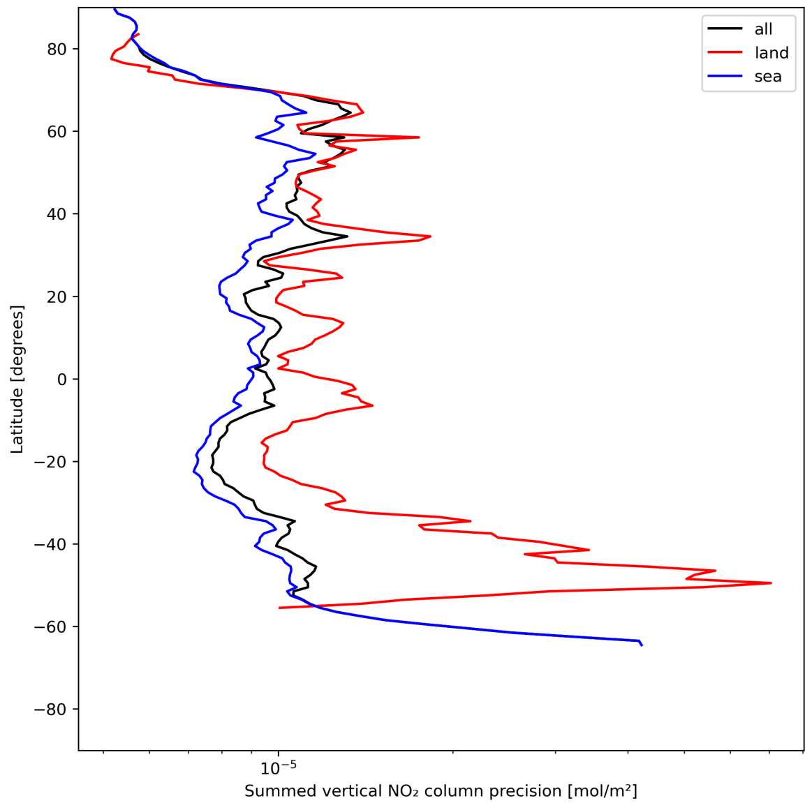
Figure 24: Zonal average of “Summed vertical NO 2 column precision” for 2024-06-15 to 2024-06-17.
