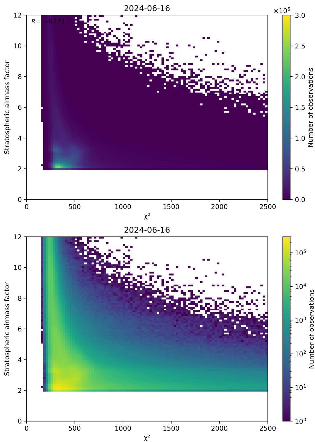
Figure 81: Scatter density plot of “ \chi^2 ” against “Stratospheric airmass factor” for 2024-06-15 to 2024-06-17.
