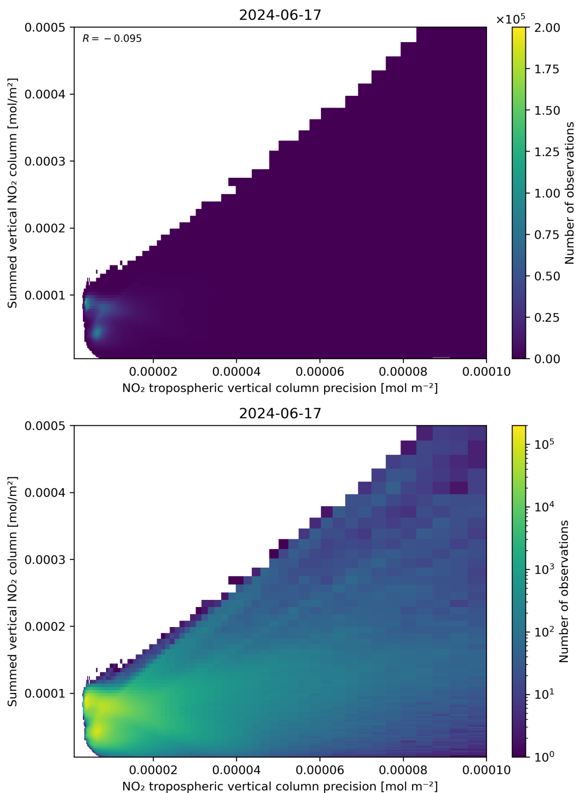
Figure 136: Scatter density plot of “NO 2 tropospheric vertical column precision” against “Summed vertical NO 2 column” for 2024-06-16 to 2024-06-18.
