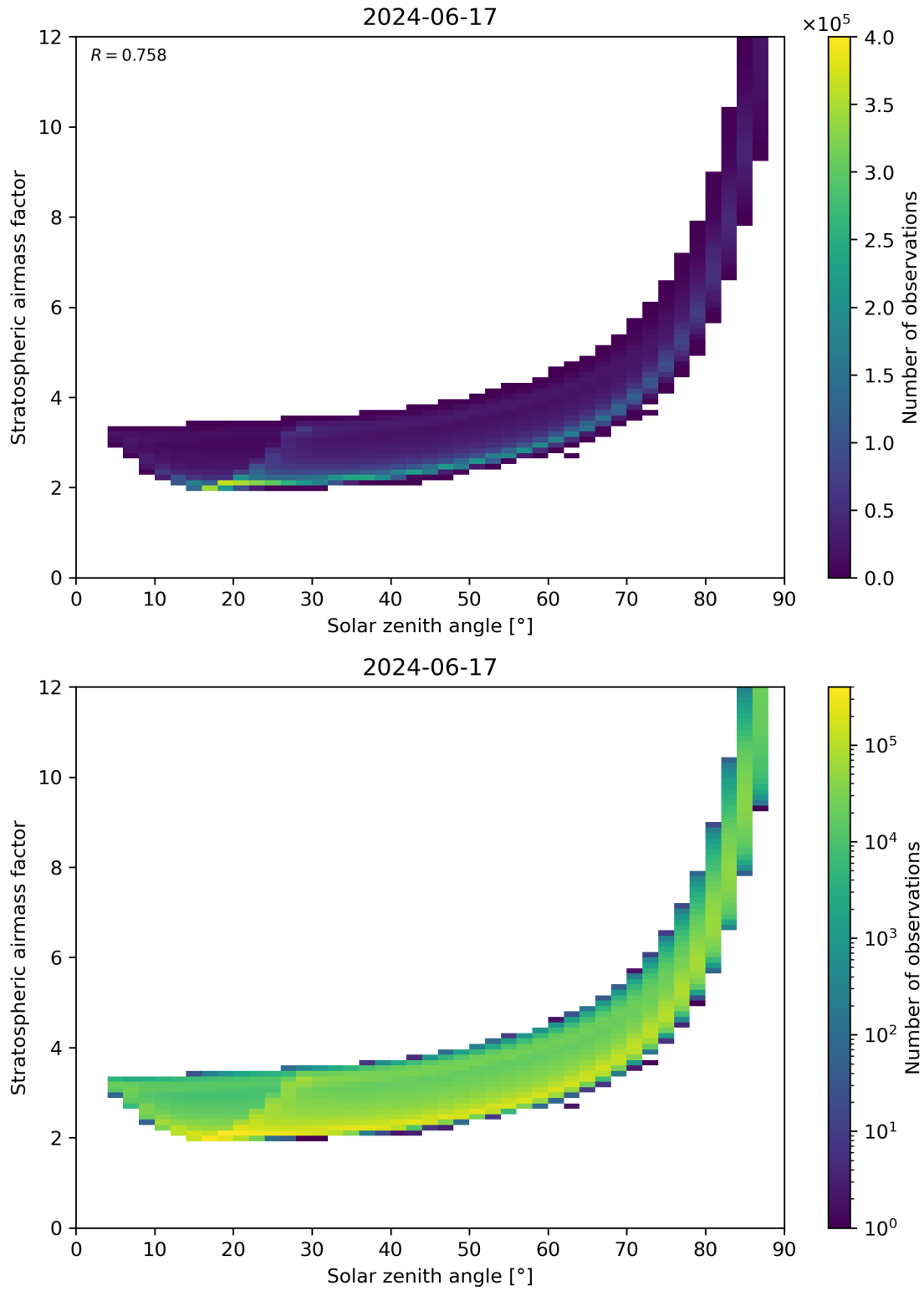
Figure 145: Scatter density plot of “Solar zenith angle” against “Stratospheric airmass factor” for 2024-06-16 to 2024-06-18.
