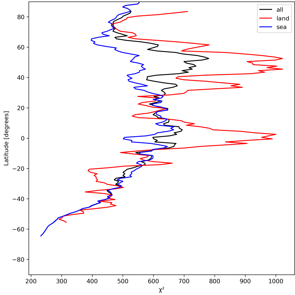
Figure 25: Zonal average of “ \chi^2 ” for 2024-06-16 to 2024-06-18.
