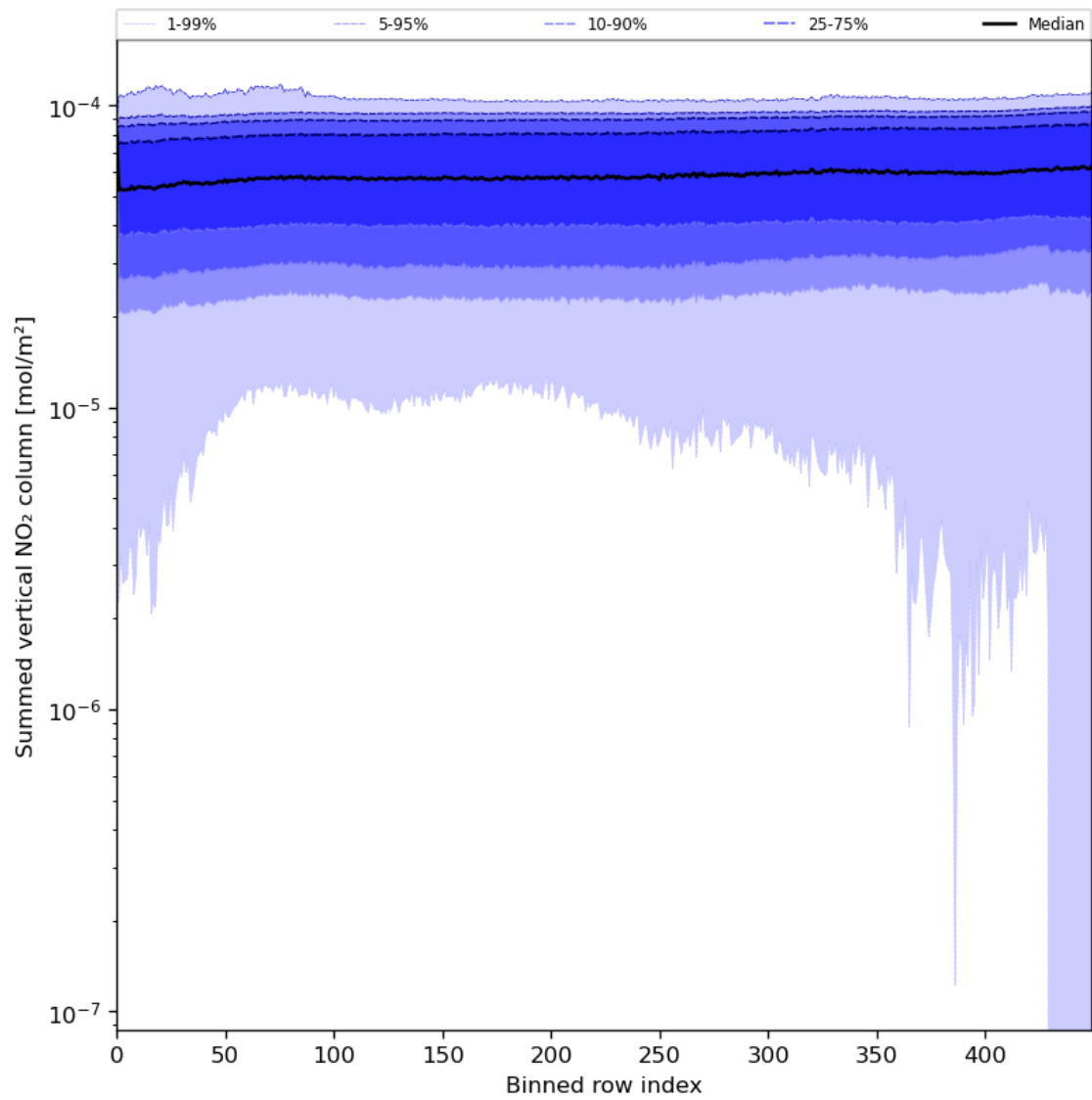
Figure 57: Along track statistics of “Summed vertical NO 2 column” for 2024-06-16 to 2024-06-18
