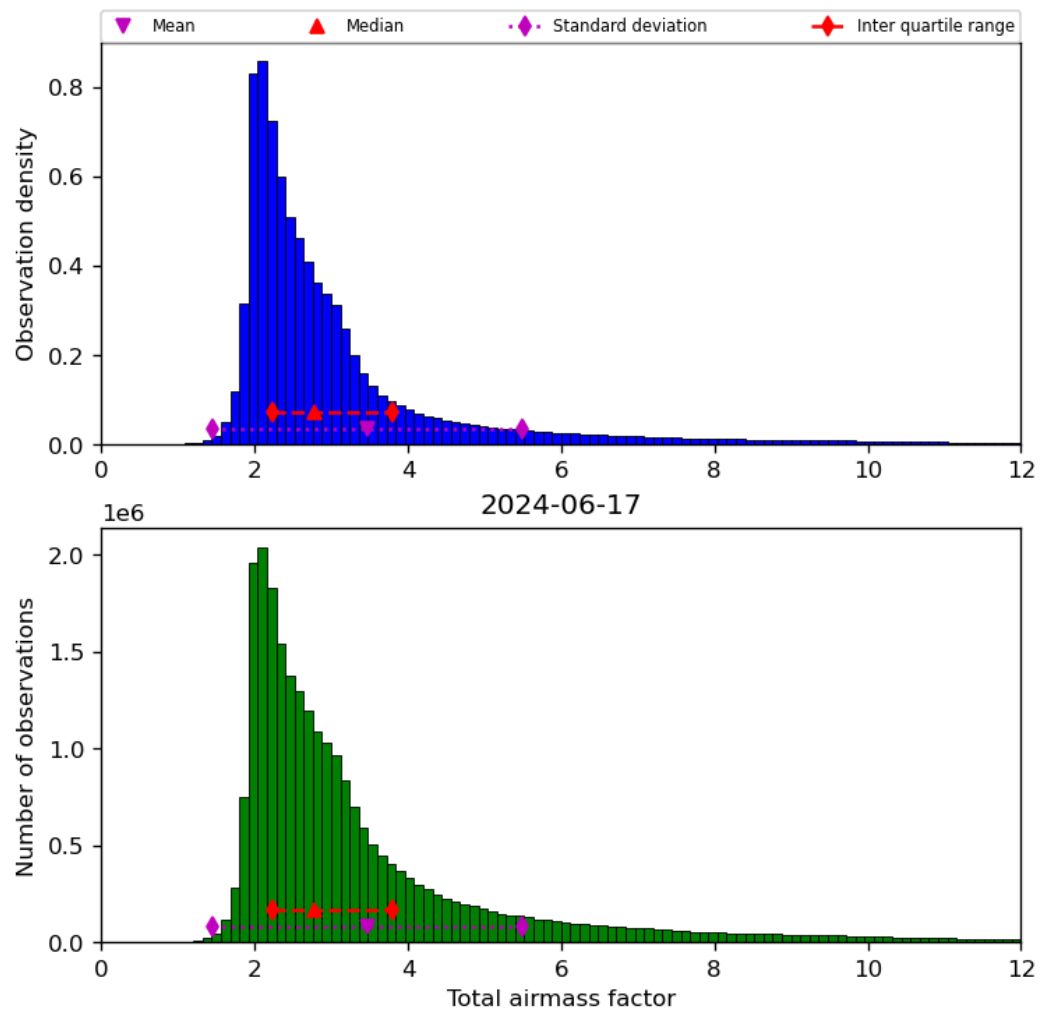
Figure 32: Histogram of “Total airmass factor” for 2024-06-16 to 2024-06-18
