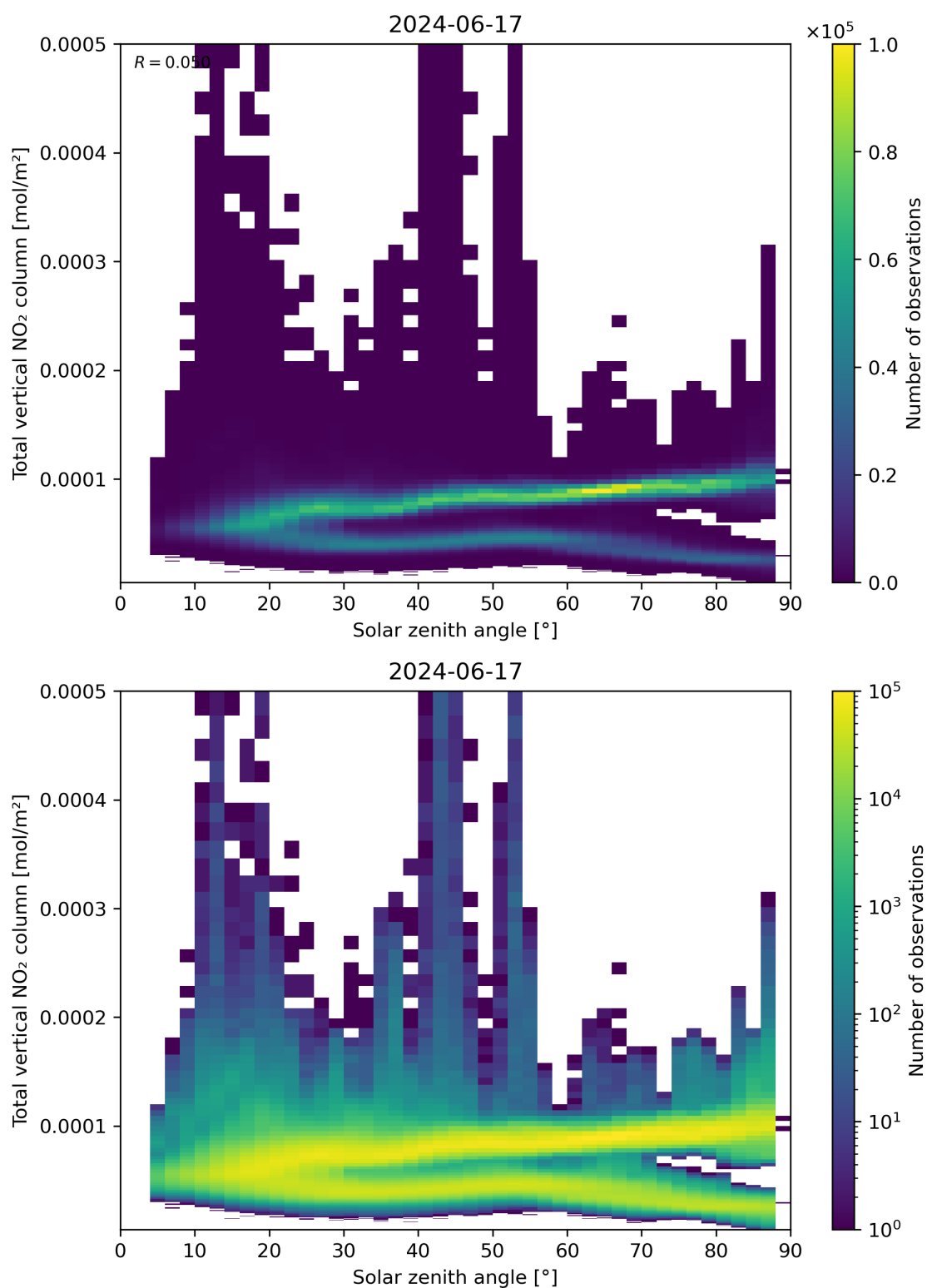
Figure 153: Scatter density plot of “Solar zenith angle” against “Total vertical NO 2 column” for 2024-06-16 to 2024-06-18.
