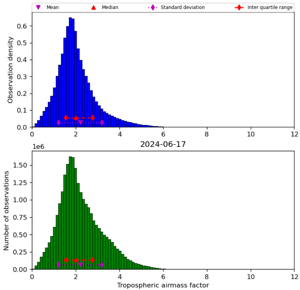
Figure 31: Histogram of “Tropospheric airmass factor” for 2024-06-16 to 2024-06-18
