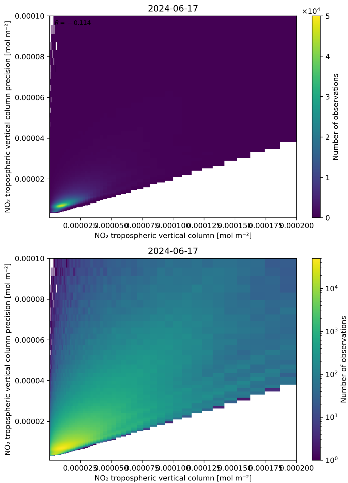
Figure 130: Scatter density plot of “NO 2 tropospheric vertical column” against “NO 2 tropospheric vertical column precision” for 2024-06-16 to 2024-06-18.
