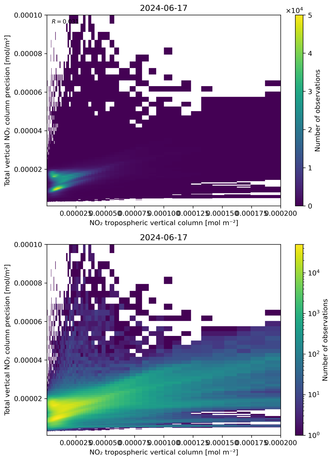
Figure 129: Scatter density plot of “NO 2 tropospheric vertical column” against “Total vertical NO 2 column precision” for 2024-06-16 to 2024-06-18.
