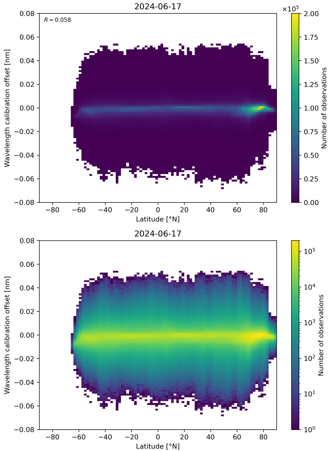
Figure 95: Scatter density plot of “Latitude” against “Wavelength calibration offset” for 2024-06-16 to 2024-06-18.
