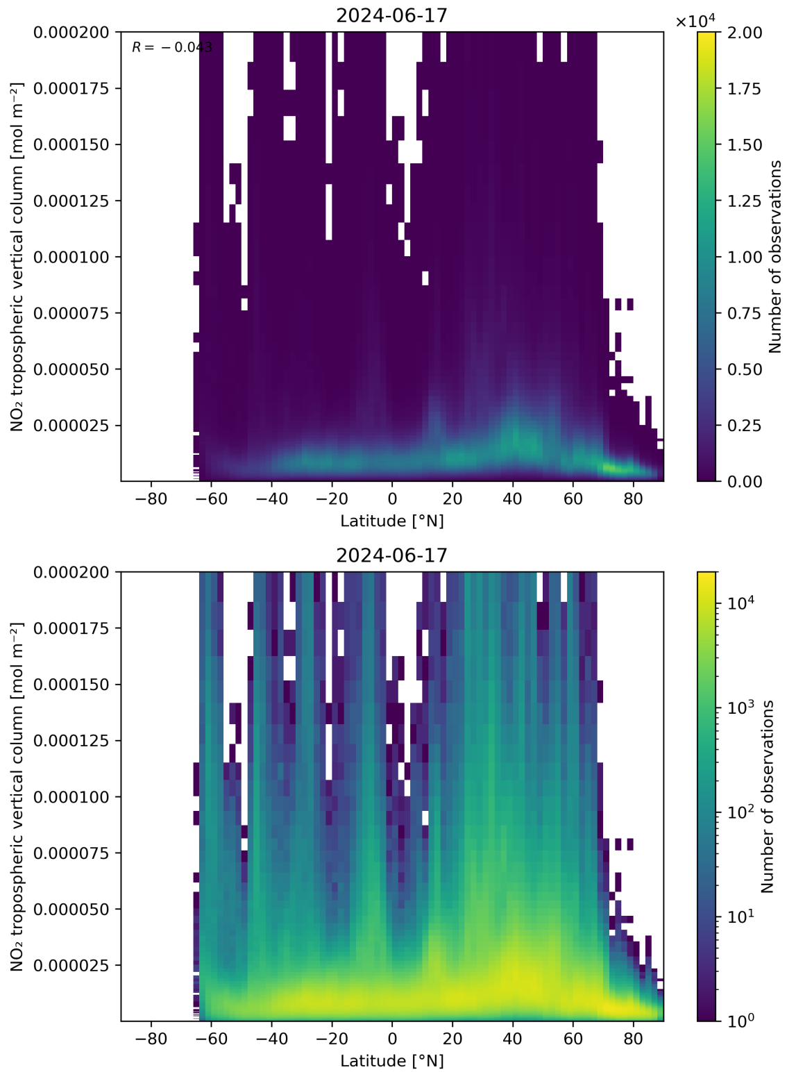
Figure 92: Scatter density plot of “Latitude” against “NO 2 tropospheric vertical column” for 2024-06-16 to 2024-06-18.
