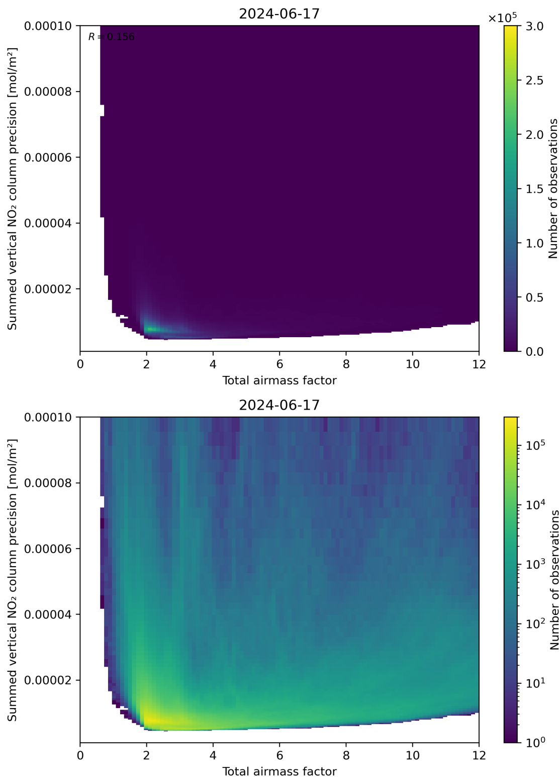
Figure 66: Scatter density plot of “Total airmass factor” against “Summed vertical NO 2 column precision” for 2024-06-16 to 2024-06-18.
