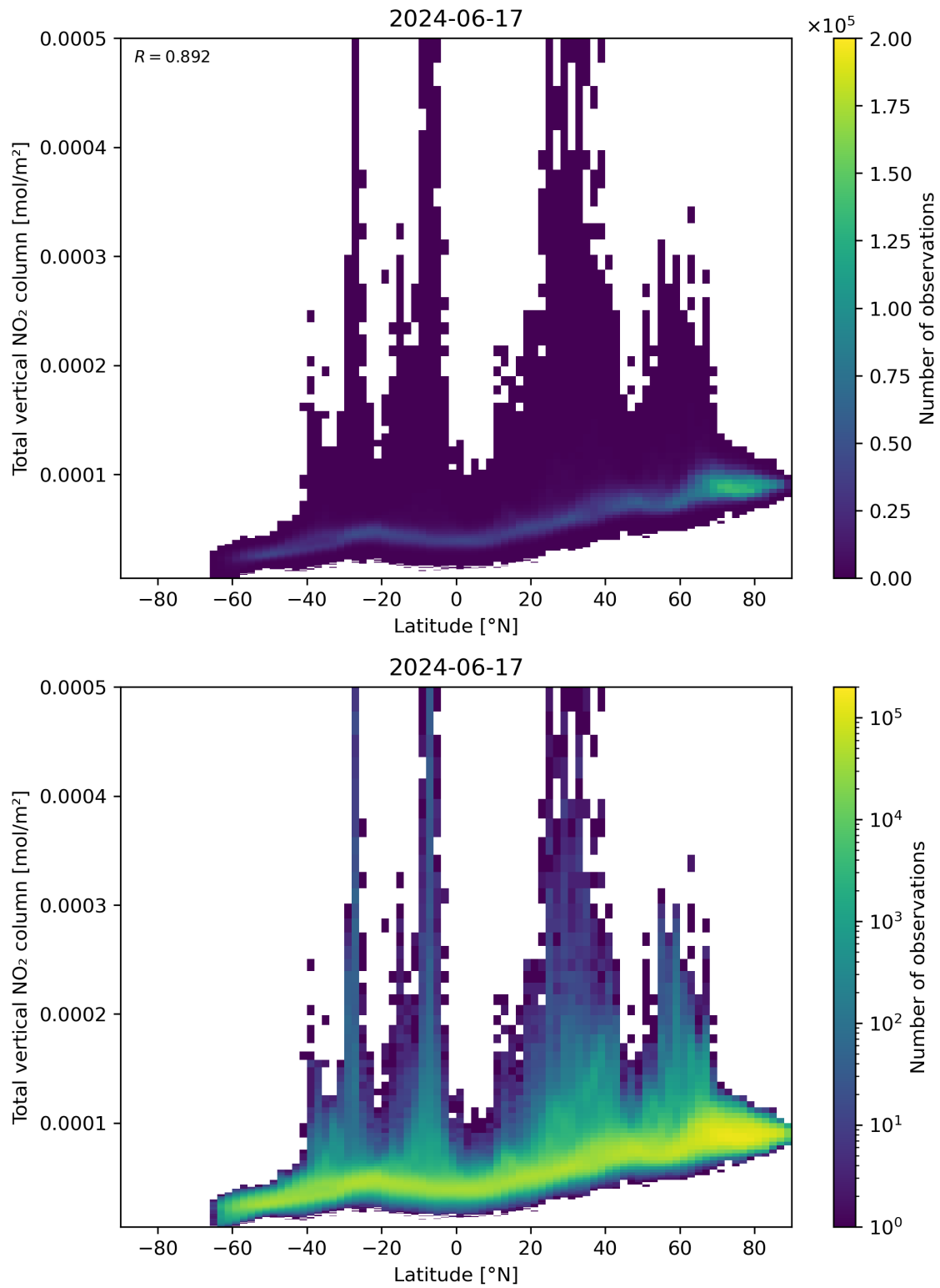
Figure 90: Scatter density plot of “Latitude” against “Total vertical NO 2 column” for 2024-06-16 to 2024-06-18.
