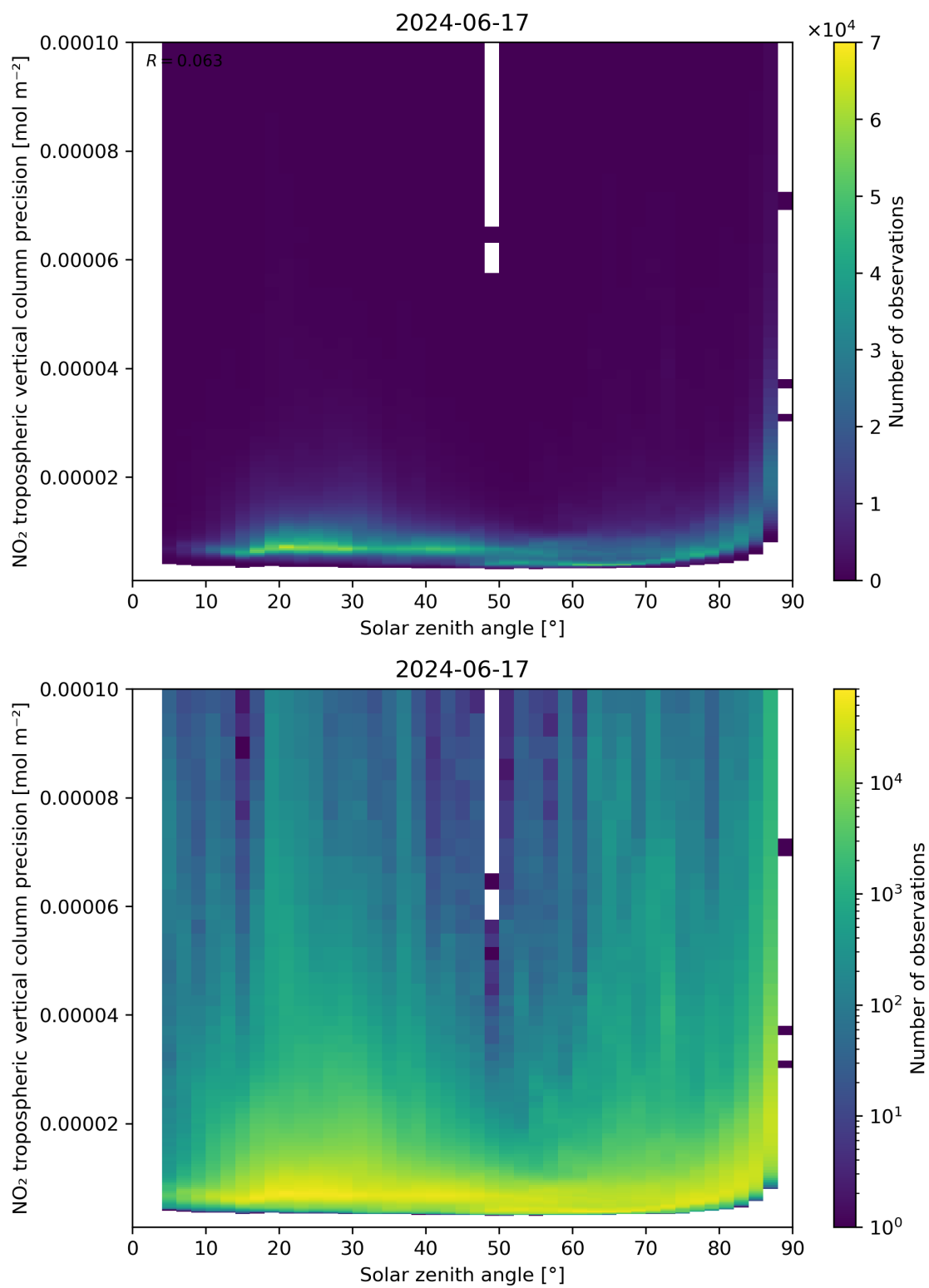
Figure 156: Scatter density plot of “Solar zenith angle” against “NO 2 tropospheric vertical column precision” for 2024-06-16 to 2024-06-18.
