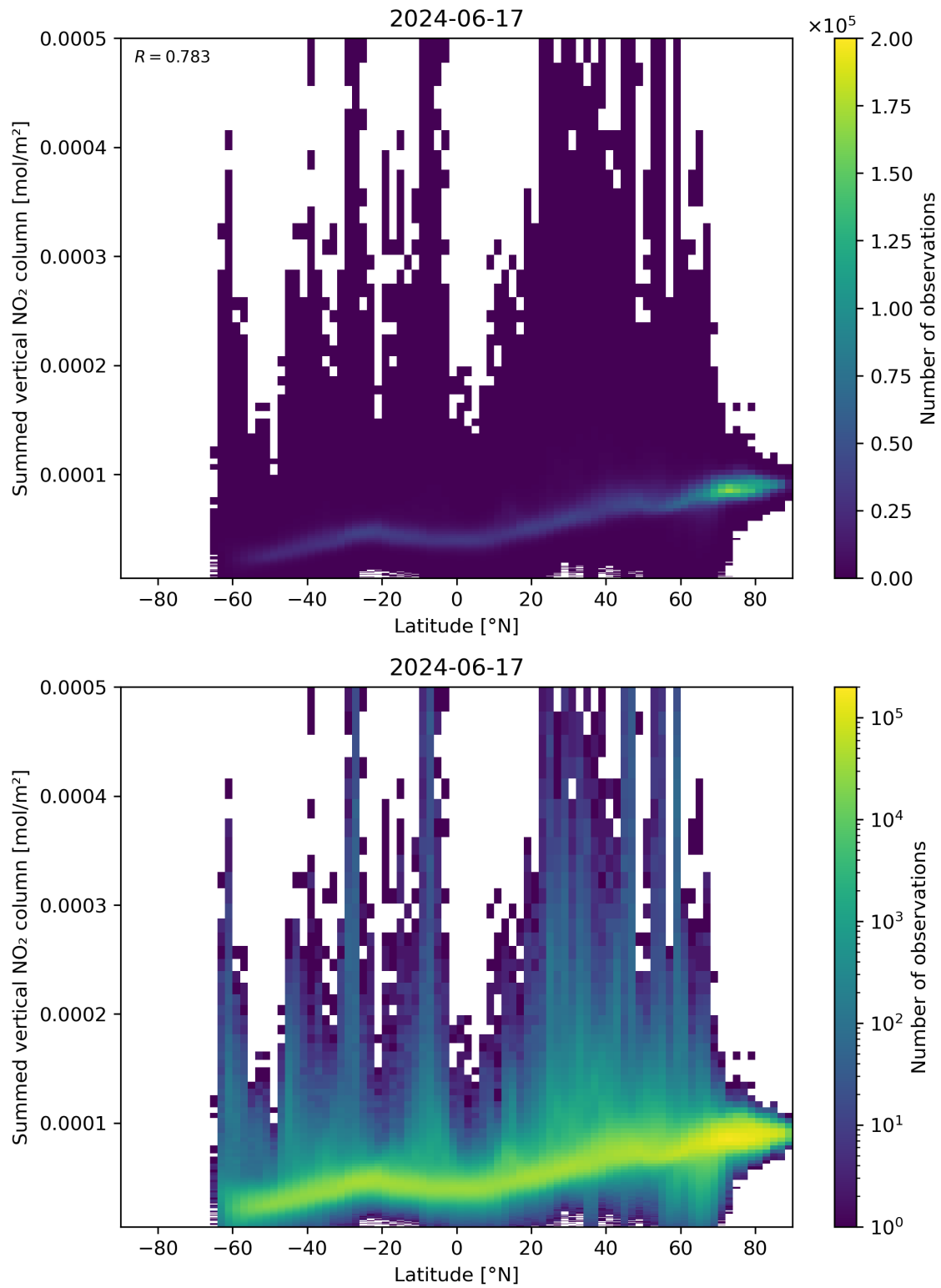
Figure 88: Scatter density plot of “Latitude” against “Summed vertical NO 2 column” for 2024-06-16 to 2024-06-18.
