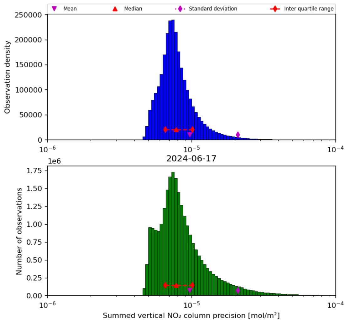
Figure 41: Histogram of "Summed vertical NO 2 column precision" for 2024-06-16 to 2024-06-18
