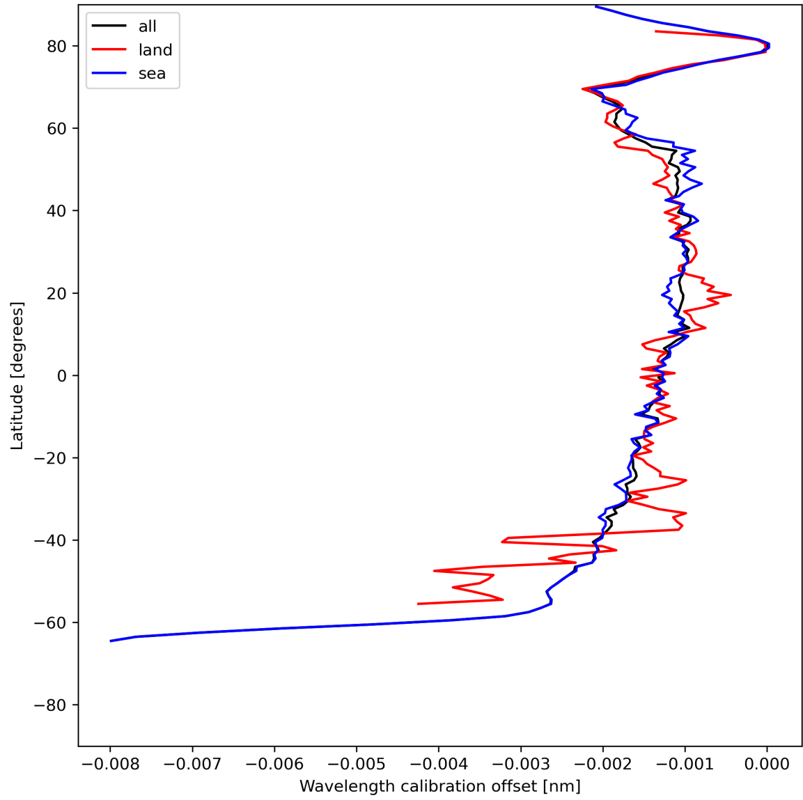
Figure 18: Zonal average of “Wavelength calibration offset” for 2024-06-16 to 2024-06-18.
