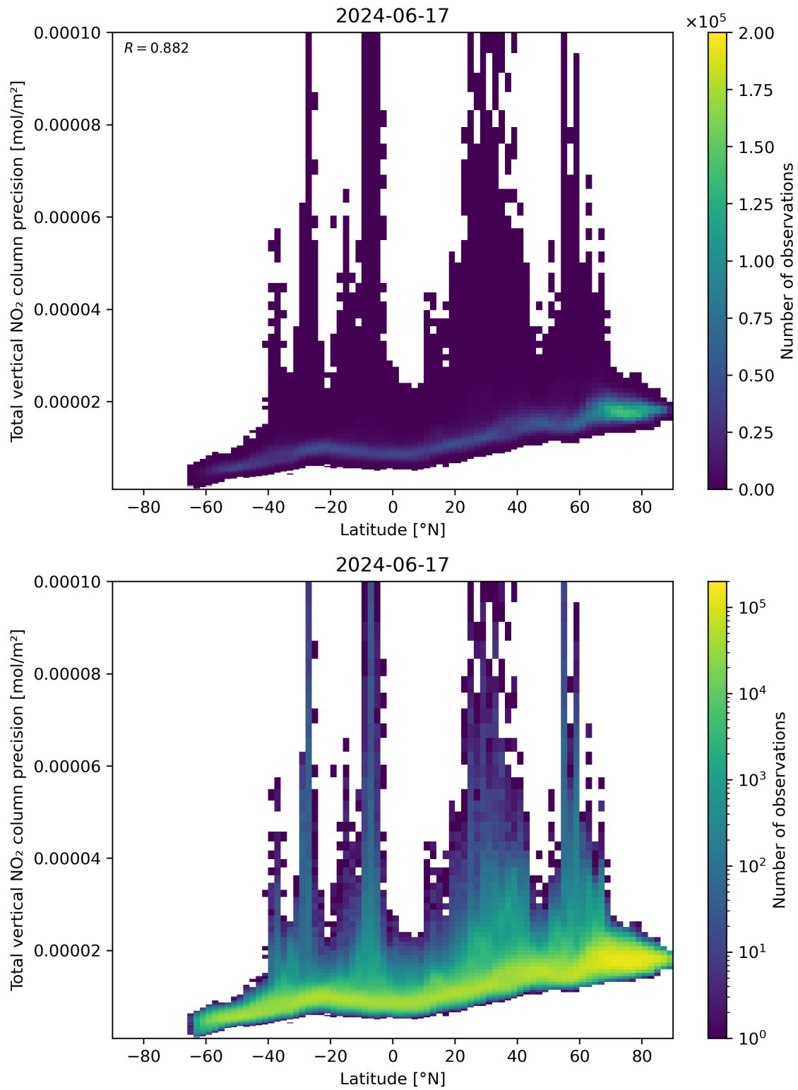
Figure 91: Scatter density plot of “Latitude” against “Total vertical NO 2 column precision” for 2024-06-16 to 2024-06-18.
