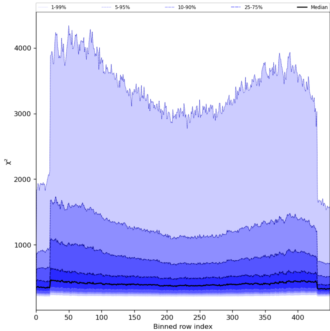
Figure 59: Along track statistics of “ \chi^2 ” for 2024-06-16 to 2024-06-18
