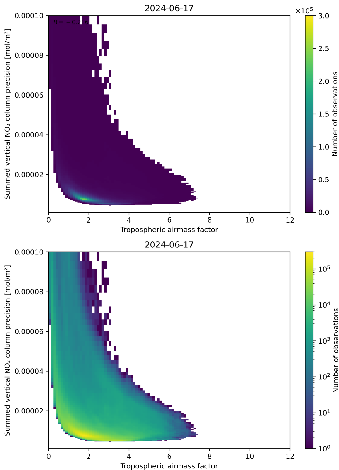
Figure 76: Scatter density plot of “Tropospheric air mass factor” against “Summed vertical NO 2 column precision” for 2024-06-16 to 2024-06-18.
