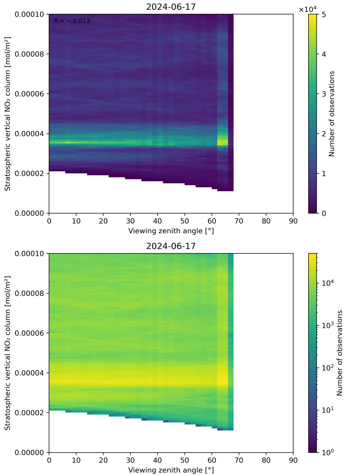
Figure 164: Scatter density plot of “Viewing zenith angle” against “Stratospheric vertical NO 2 column” for 2024-06-16 to 2024-06-18.
