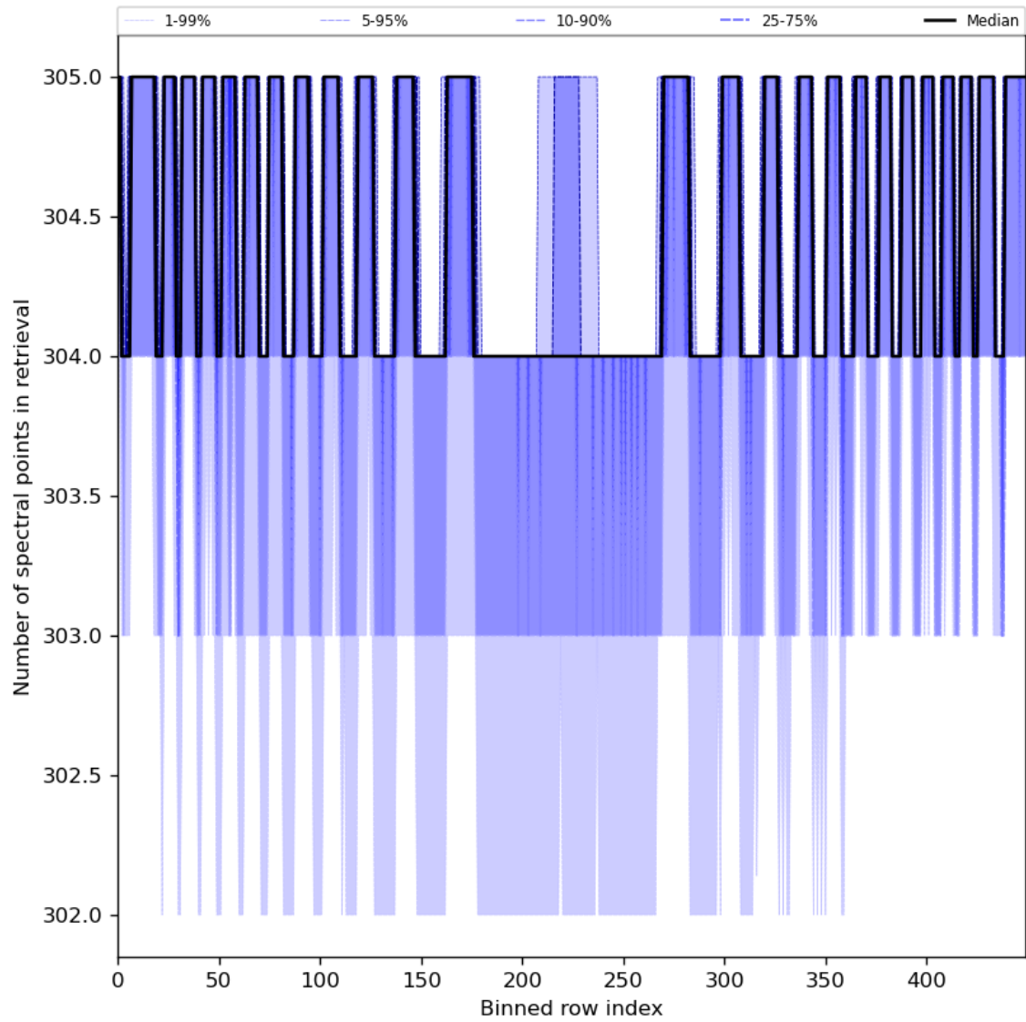
Figure 50: Along track statistics of “Number of spectral points in retrieval” for 2024-06-16 to 2024-06-18
