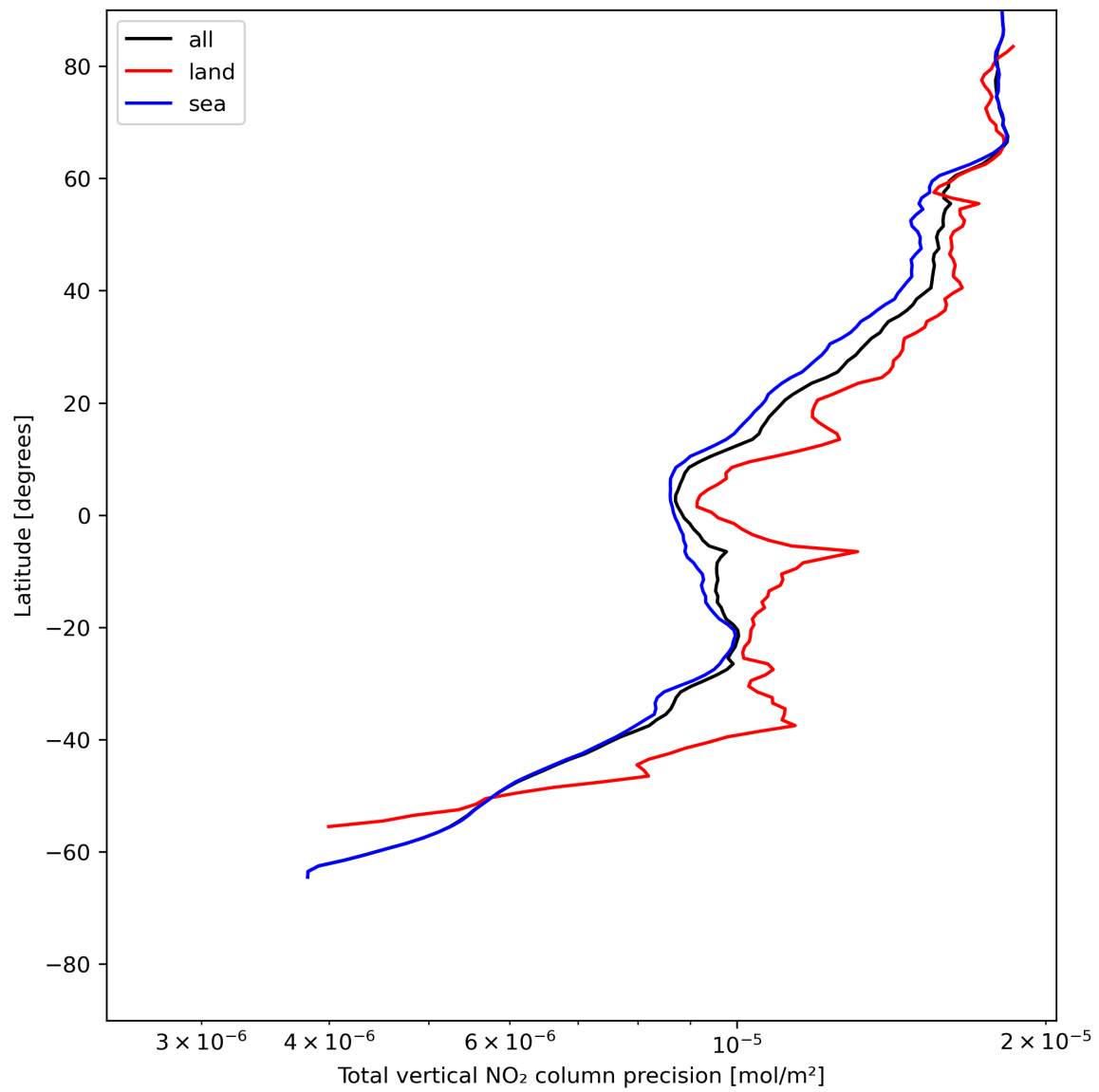
Figure 22: Zonal average of “Total vertical NO 2 column precision” for 2024-06-16 to 2024-06-18.
