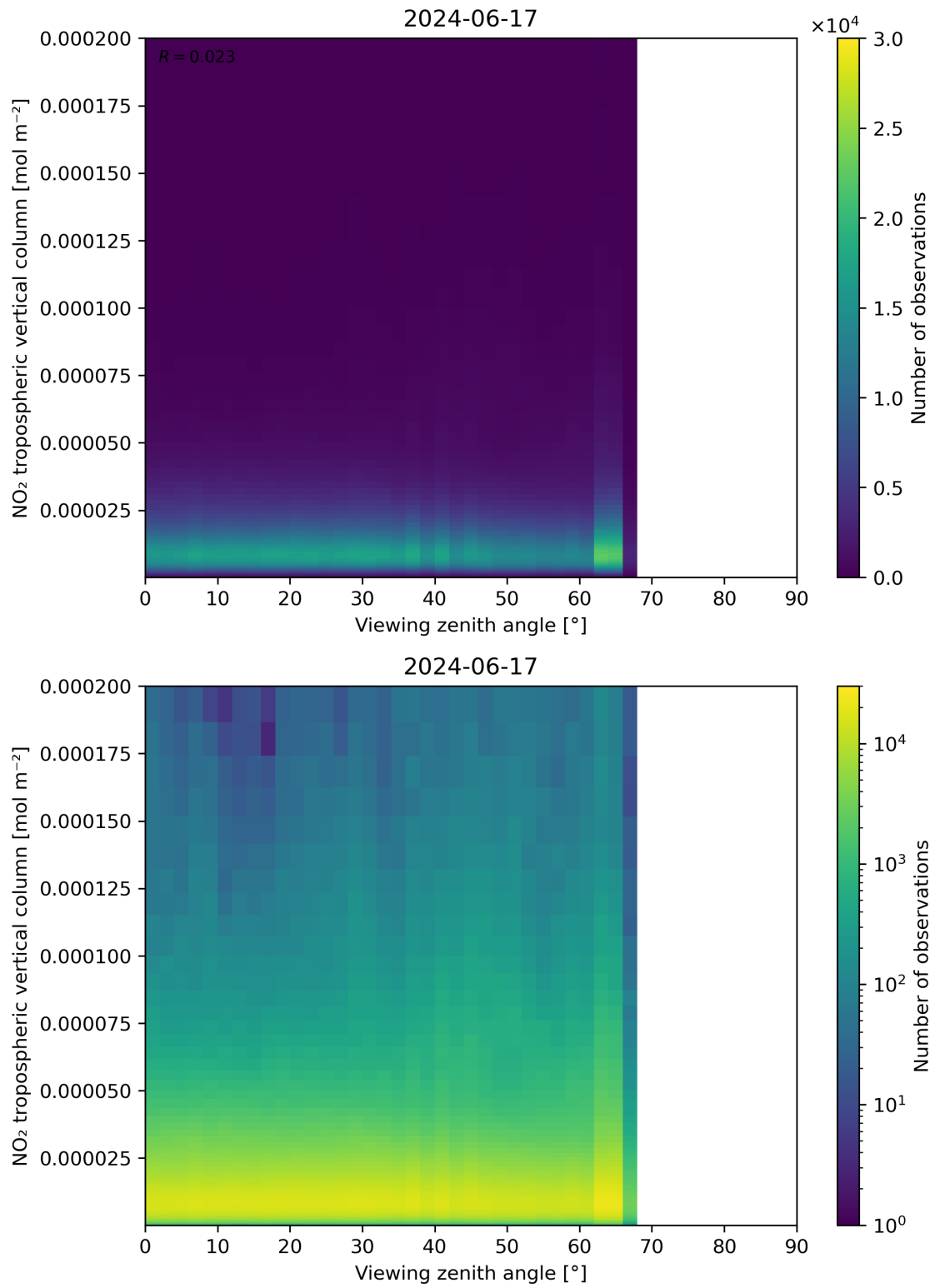
Figure 169: Scatter density plot of “Viewing zenith angle” against “NO 2 tropospheric vertical column” for 2024-06-16 to 2024-06-18.
