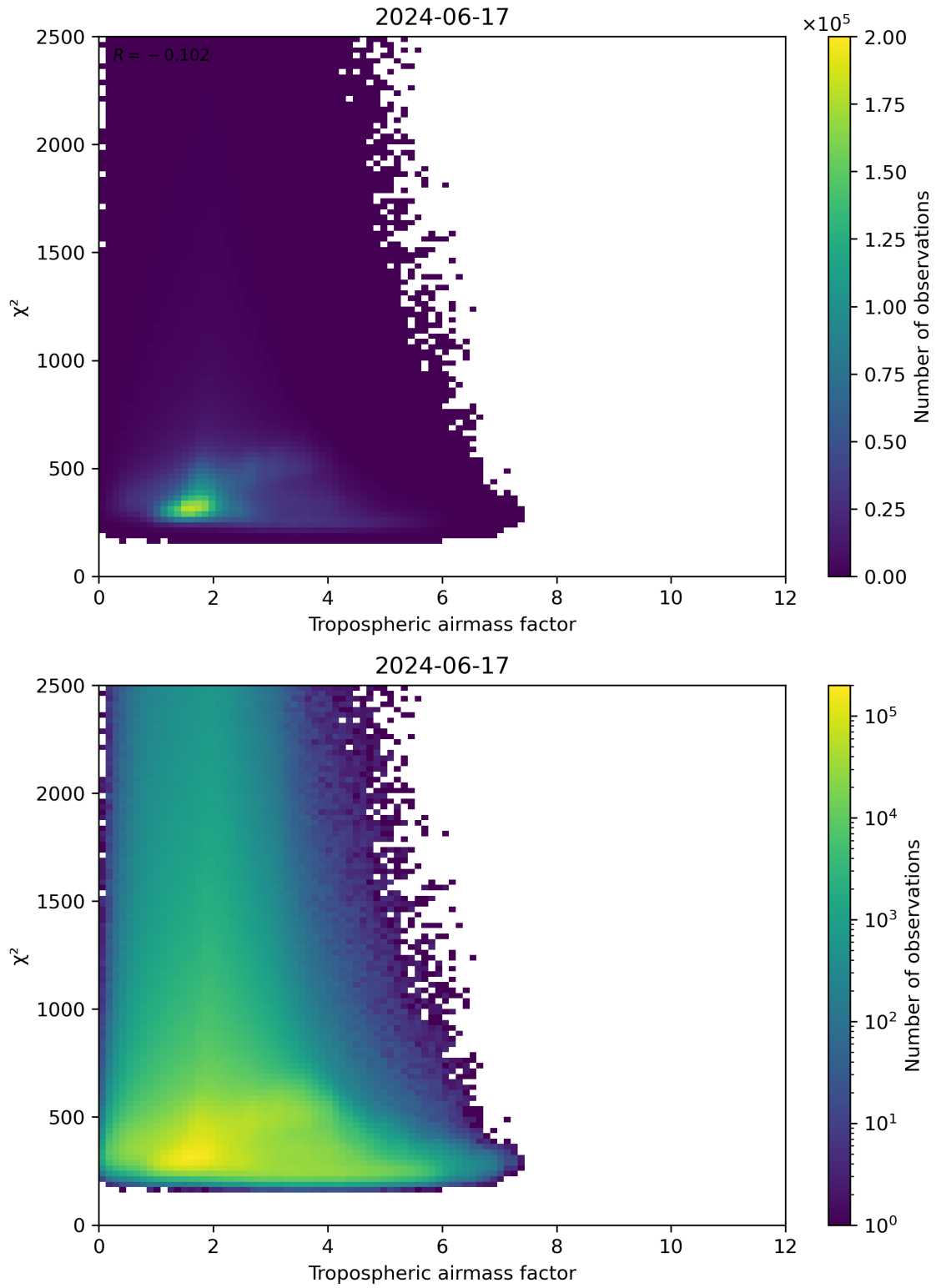
Figure 73: Scatter density plot of “Tropospheric airmass factor” against “ \chi^2 ” for 2024-06-16 to 2024-06-18.
