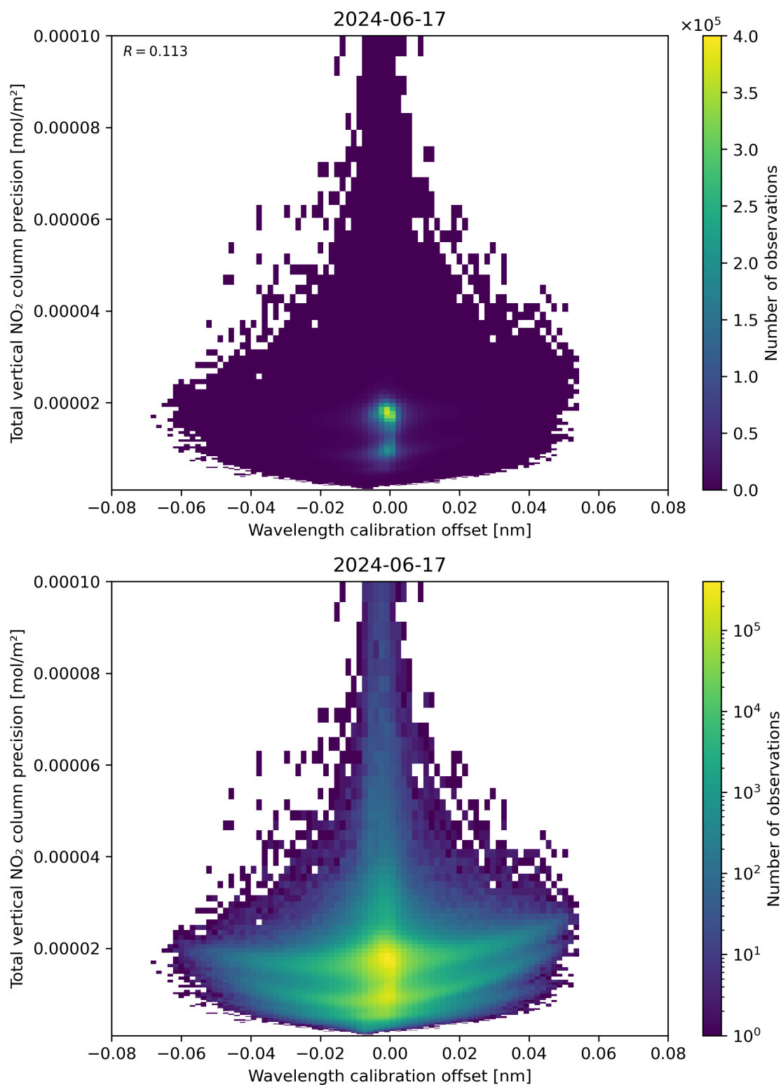
Figure 180: Scatter density plot of “Wavelength calibration offset” against “Total vertical NO 2 column precision” for 2024-06-16 to 2024-06-18.
