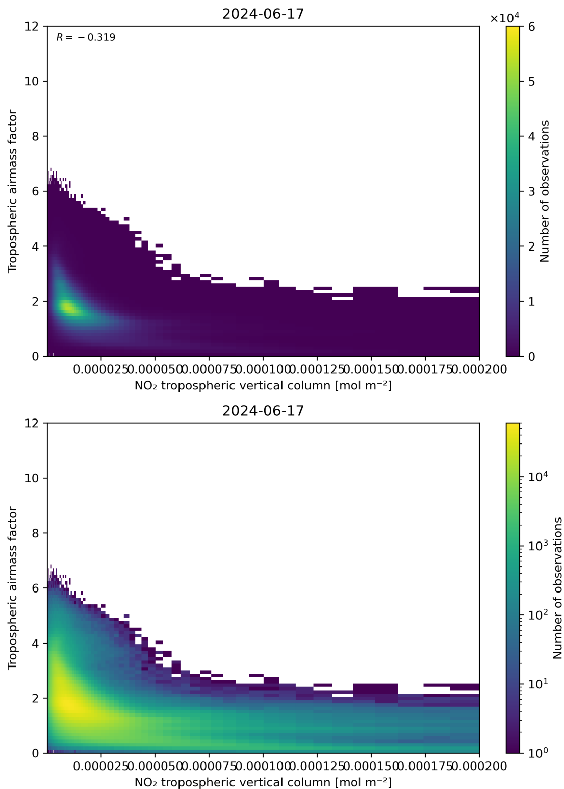
Figure 123: Scatter density plot of “NO 2 tropospheric vertical column” against “Tropospheric air mass factor” for 2024-06-16 to 2024-06-18.
