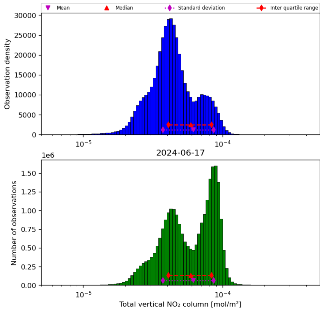
Figure 38: Histogram of “Total vertical NO 2 column” for 2024-06-16 to 2024-06-18
