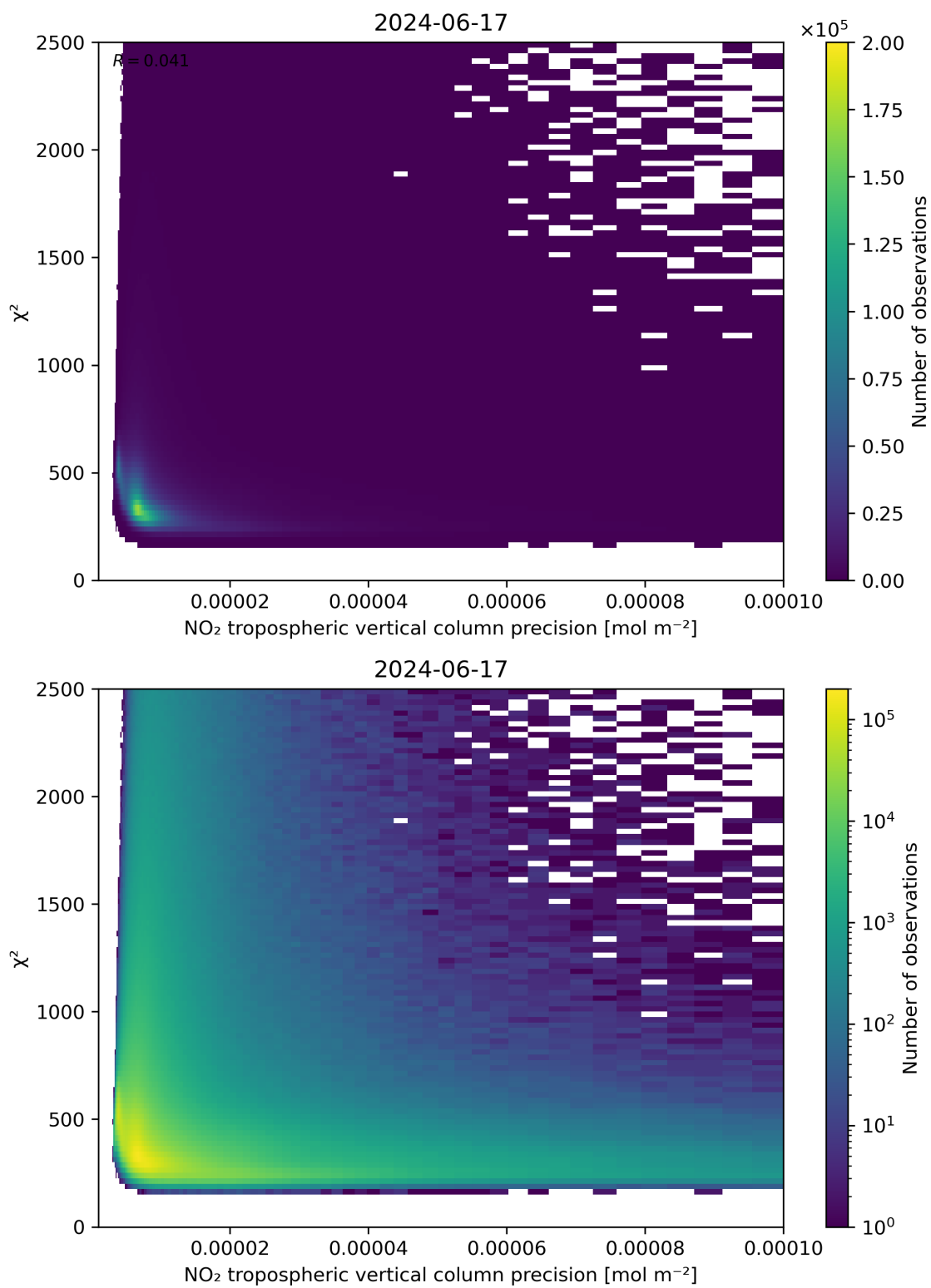
Figure 134: Scatter density plot of “NO 2 tropospheric vertical column precision” against “ \chi^2 ” for 2024-06-16 to 2024-06-18.
