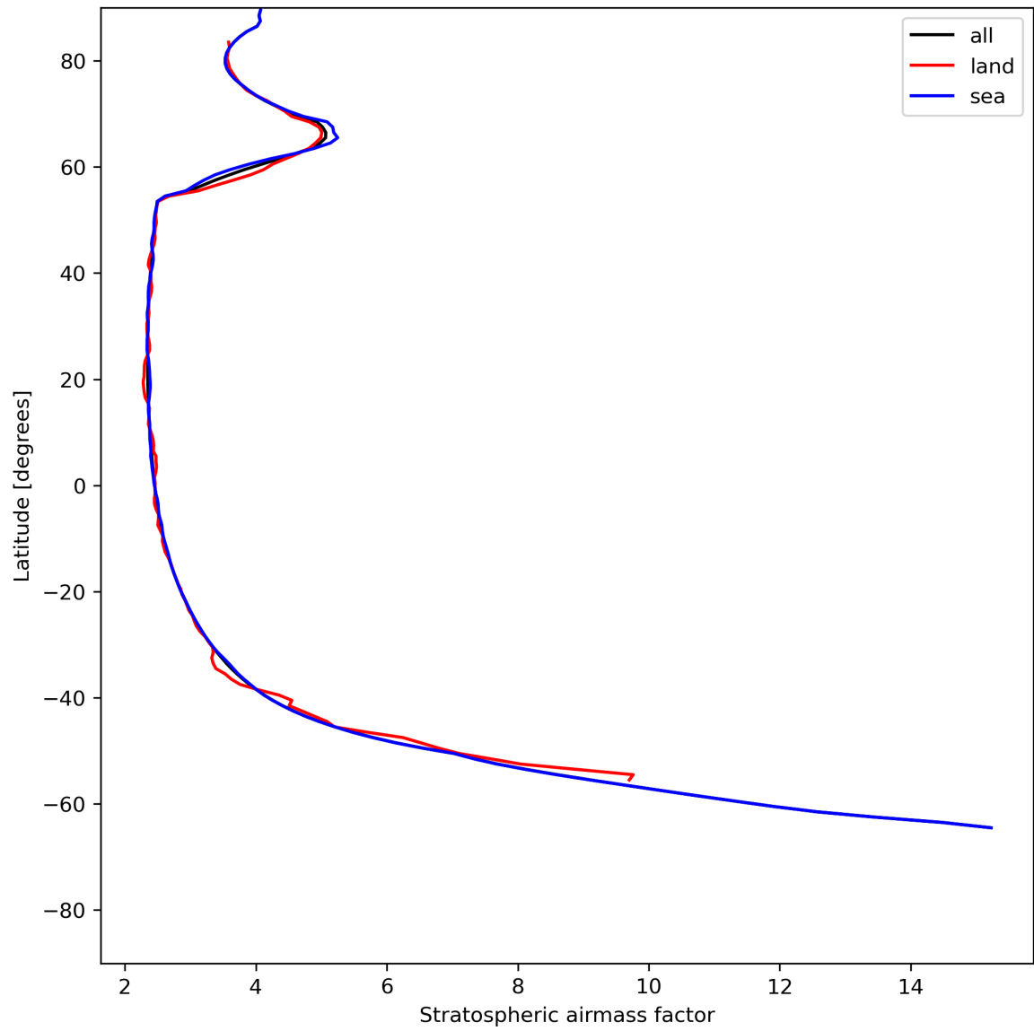
Figure 27: Zonal average of “Stratospheric air mass factor” for 2024-06-16 to 2024-06-18.
