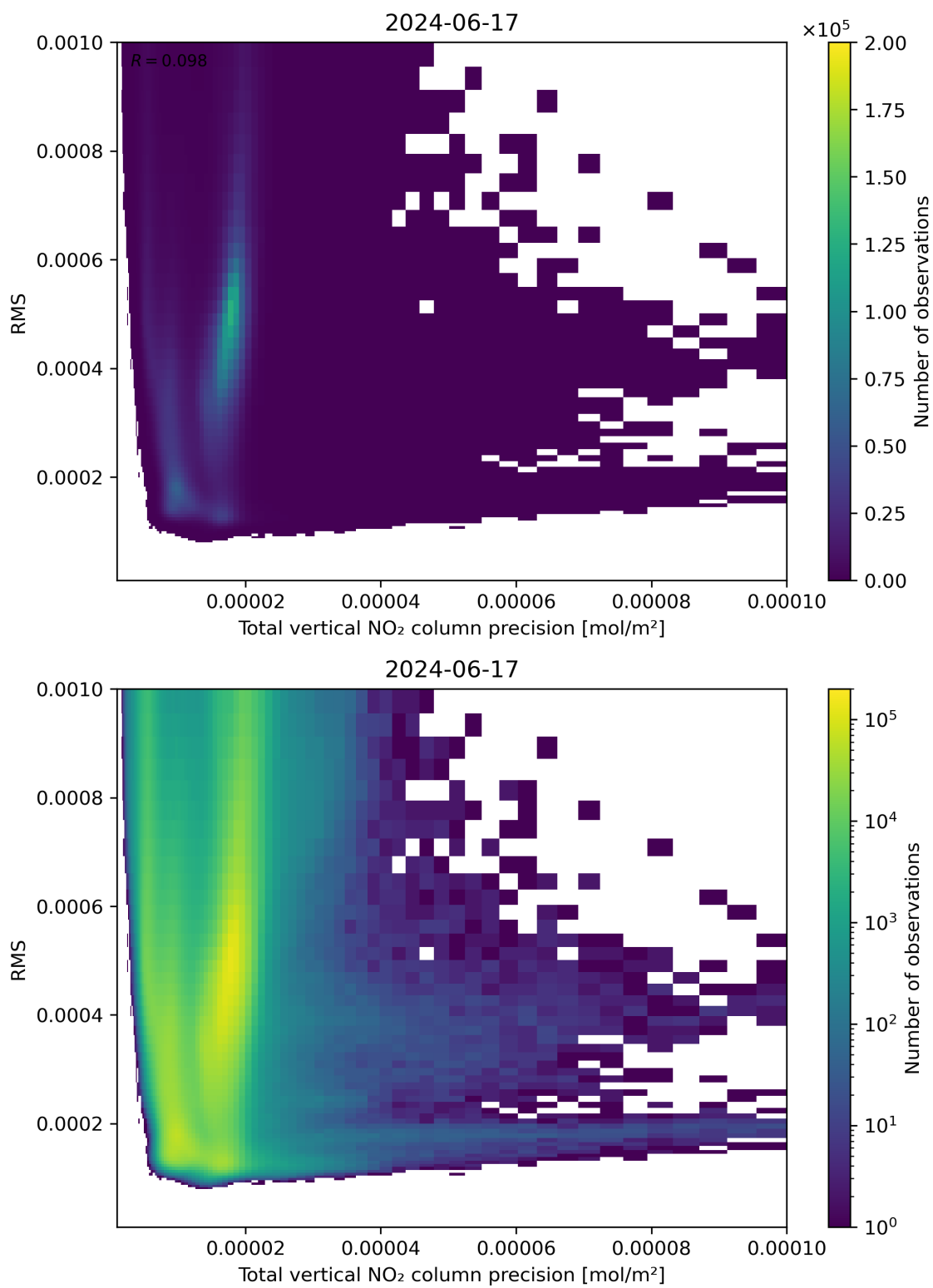
Figure 119: Scatter density plot of “Total vertical NO 2 column precision” against “RMS” for 2024-06-16 to 2024-06-18.
