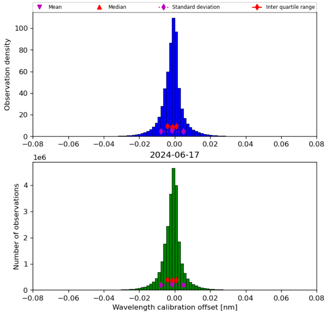
Figure 35: Histogram of “Wavelength calibration offset” for 2024-06-16 to 2024-06-18
