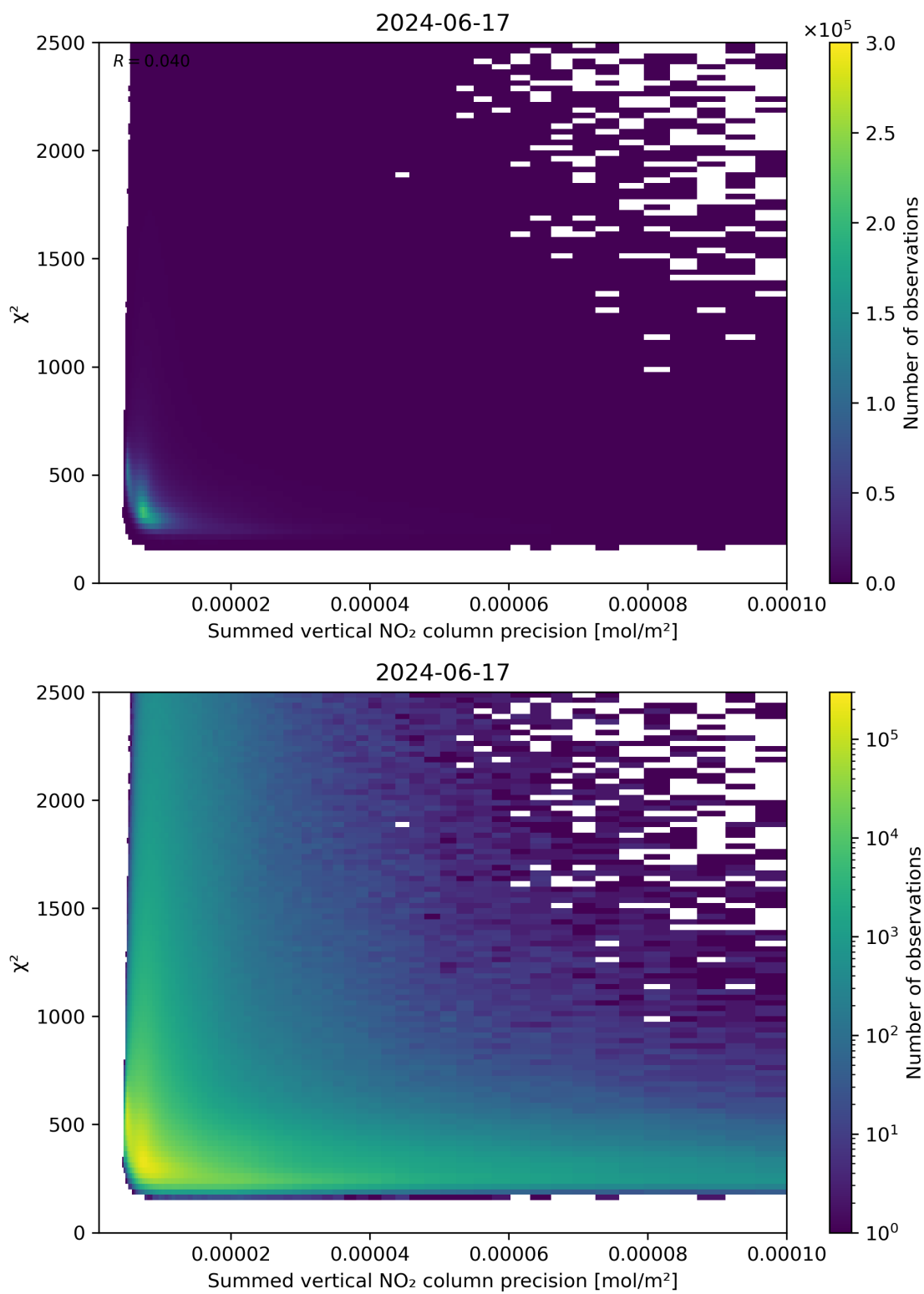
Figure 107: Scatter density plot of “Summed vertical NO 2 column precision” against “ \chi^2 ” for 2024-06-16 to 2024-06-18.
