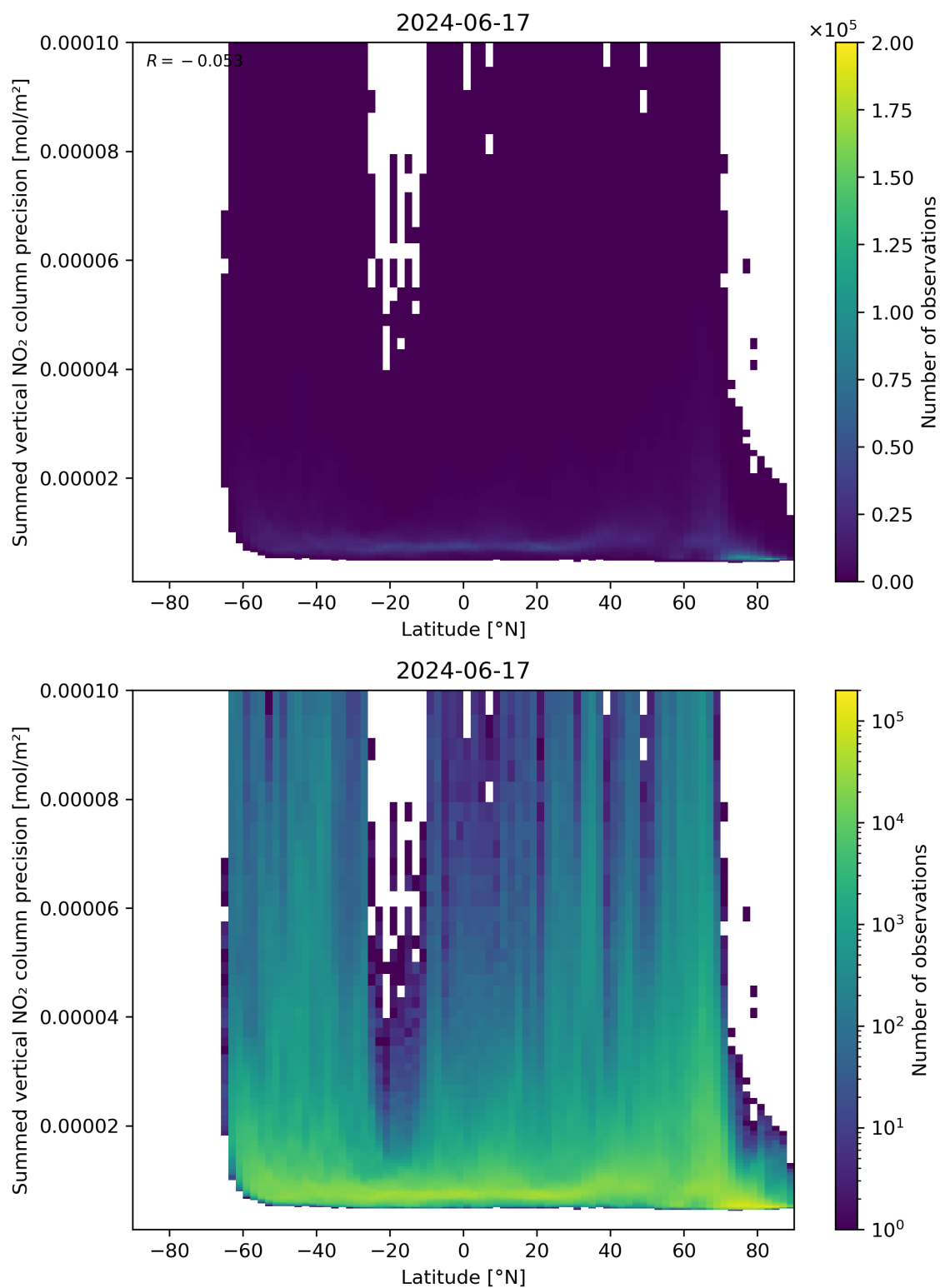
Figure 89: Scatter density plot of “Latitude” against “Summed vertical NO 2 column precision” for 2024-06-16 to 2024-06-18.
