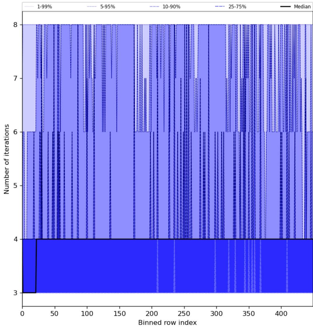
Figure 51: Along track statistics of “Number of iterations” for 2024-06-16 to 2024-06-18
