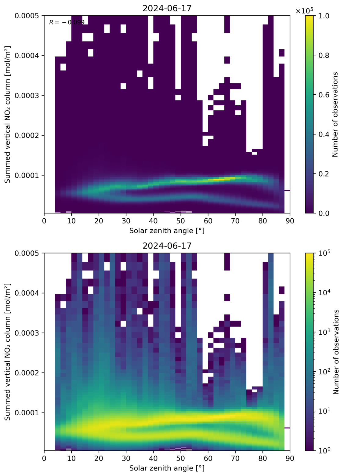
Figure 151: Scatter density plot of “Solar zenith angle” against “Summed vertical NO 2 column” for 2024-06-16 to 2024-06-18.
