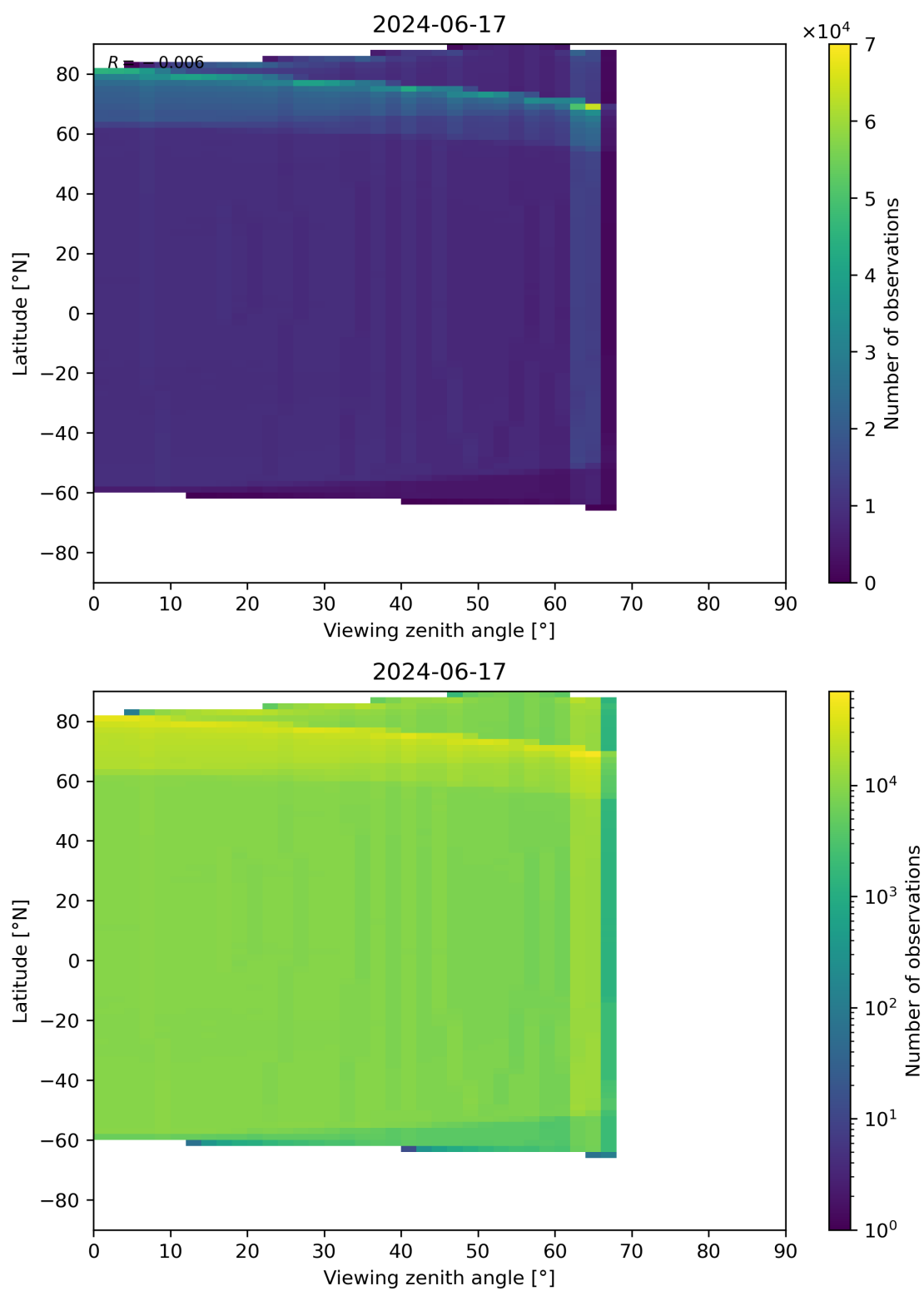
Figure 163: Scatter density plot of “Viewing zenith angle” against “Latitude” for 2024-06-16 to 2024-06-18.
