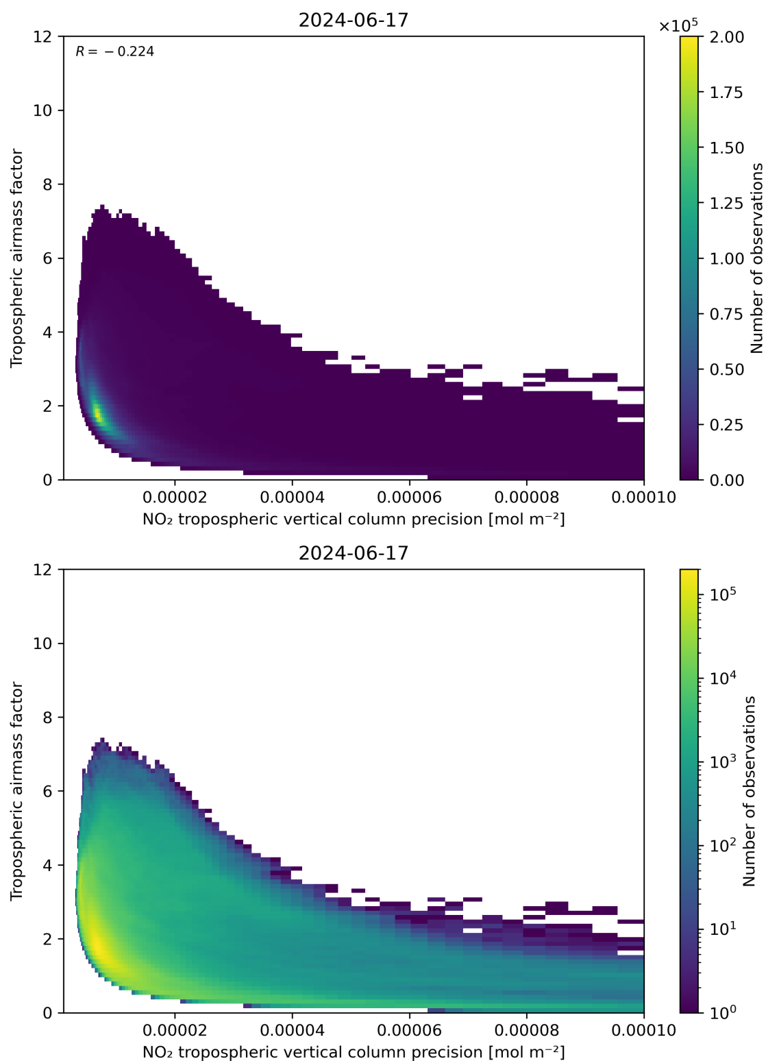
Figure 133: Scatter density plot of “NO 2 tropospheric vertical column precision” against “Tropospheric airmass factor” for 2024-06-16 to 2024-06-18.
