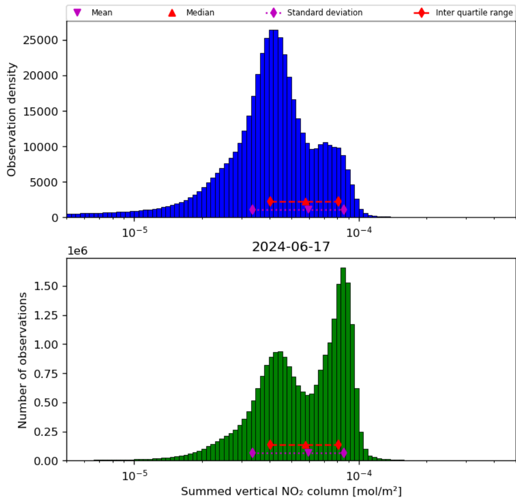
Figure 40: Histogram of “Summed vertical NO 2 column” for 2024-06-16 to 2024-06-18
