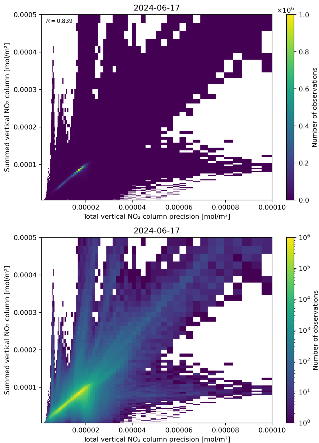
Figure 117: Scatter density plot of “Total vertical NO 2 column precision” against “Summed vertical NO 2 column” for 2024-06-16 to 2024-06-18.
