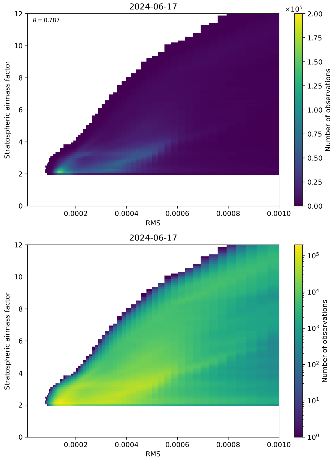
Figure 144: Scatter density plot of “RMS” against “Stratospheric airmass factor” for 2024-06-16 to 2024-06-18.
