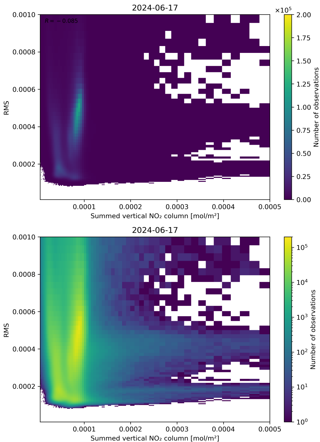
Figure 109: Scatter density plot of “Summed vertical NO 2 column” against “RMS” for 2024-06-16 to 2024-06-18.
