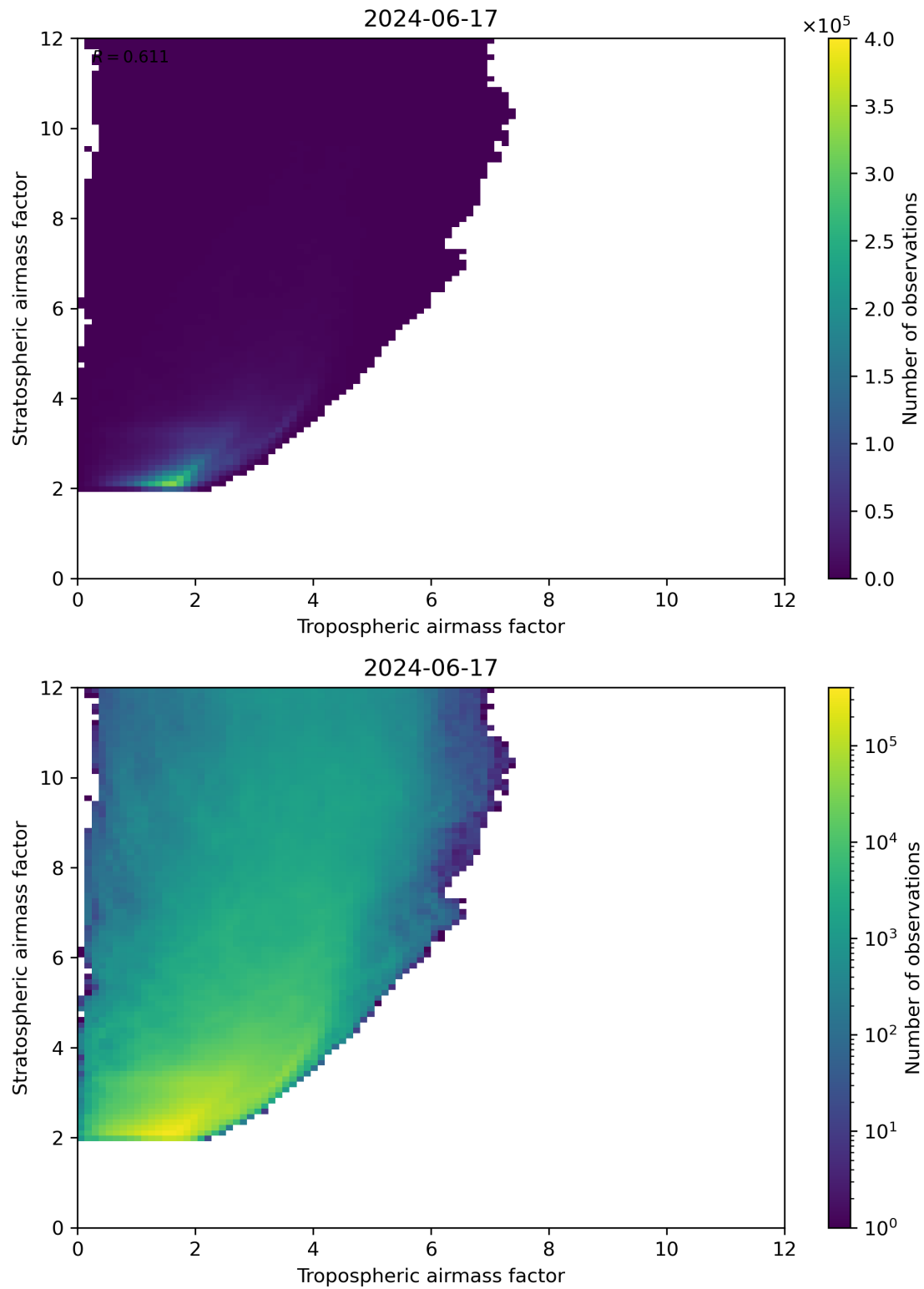
Figure 71: Scatter density plot of “Tropospheric airmass factor” against “Stratospheric airmass factor” for 2024-06-16 to 2024-06-18.
