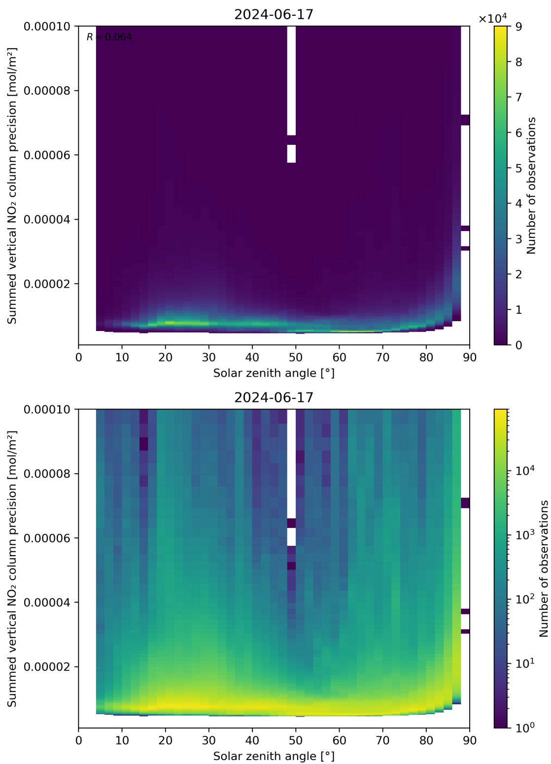
Figure 152: Scatter density plot of “Solar zenith angle” against “Summed vertical NO 2 column precision” for 2024-06-16 to 2024-06-18.
