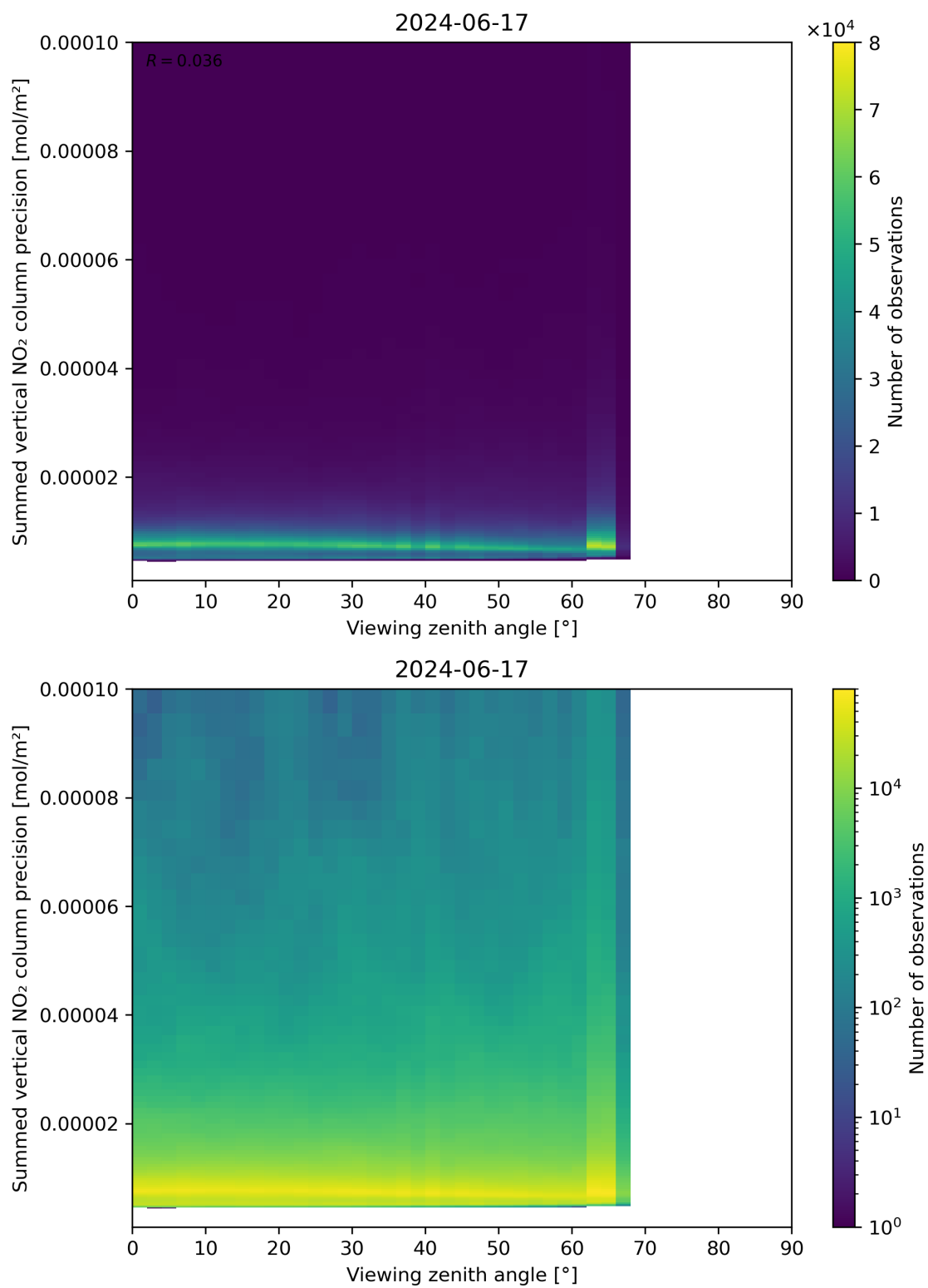
Figure 166: Scatter density plot of “Viewing zenith angle” against “Summed vertical NO 2 column precision” for 2024-06-16 to 2024-06-18.
