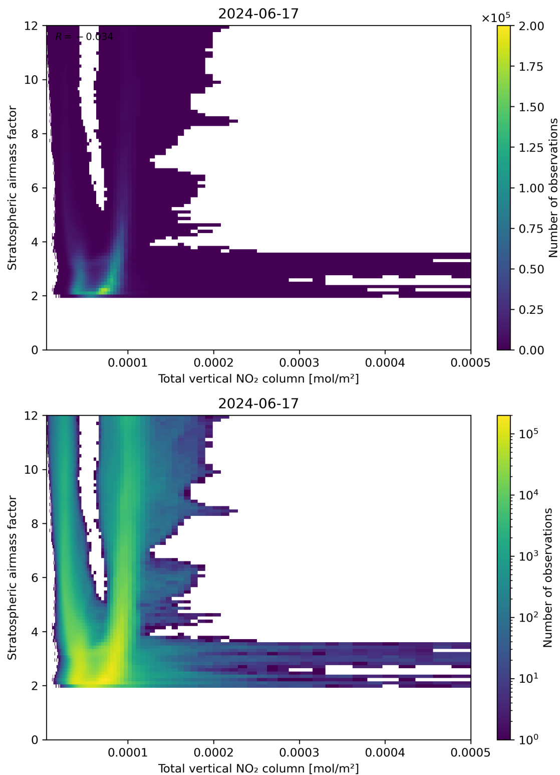
Figure 110: Scatter density plot of “Total vertical NO 2 column” against “Stratospheric airmass factor” for 2024-06-16 to 2024-06-18.
