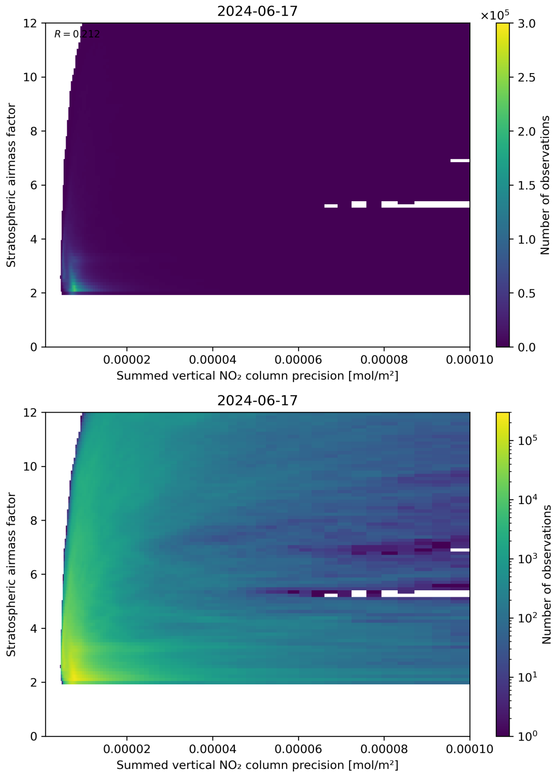
Figure 106: Scatter density plot of “Summed vertical NO 2 column precision” against “Stratospheric airmass factor” for 2024-06-16 to 2024-06-18.
