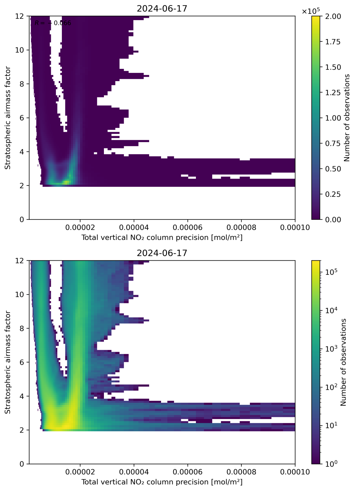
Figure 115: Scatter density plot of “Total vertical NO 2 column precision” against “Stratospheric air mass factor” for 2024-06-16 to 2024-06-18.
