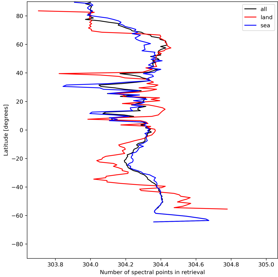
Figure 16: Zonal average of “Number of spectral points in retrieval” for 2024-06-16 to 2024-06-18.
