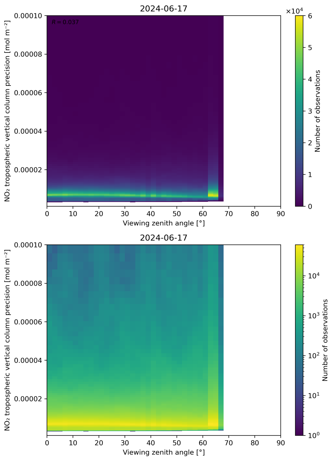
Figure 170: Scatter density plot of “Viewing zenith angle” against “NO 2 tropospheric vertical column precision” for 2024-06-16 to 2024-06-18.
