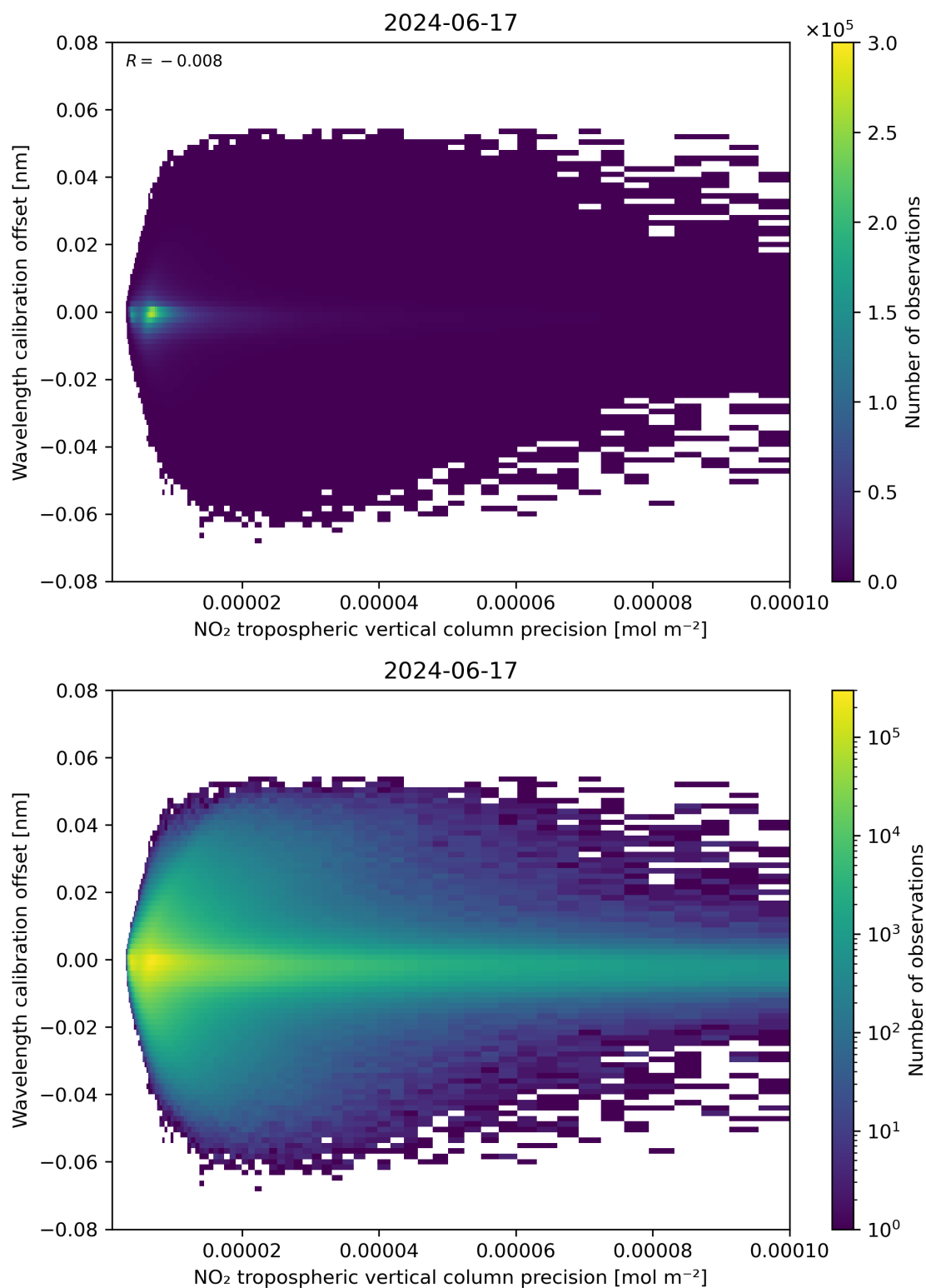
Figure 141: Scatter density plot of “NO 2 tropospheric vertical column precision” against “Wavelength calibration offset” for 2024-06-16 to 2024-06-18.
