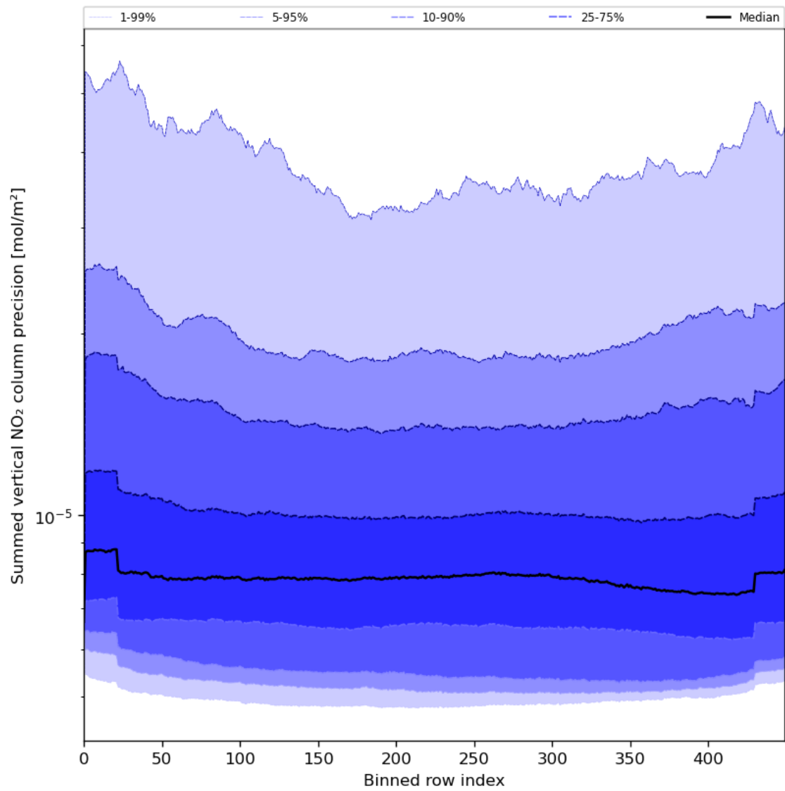
Figure 58: Along track statistics of “Summed vertical NO 2 column precision” for 2024-06-16 to 2024-06-18
