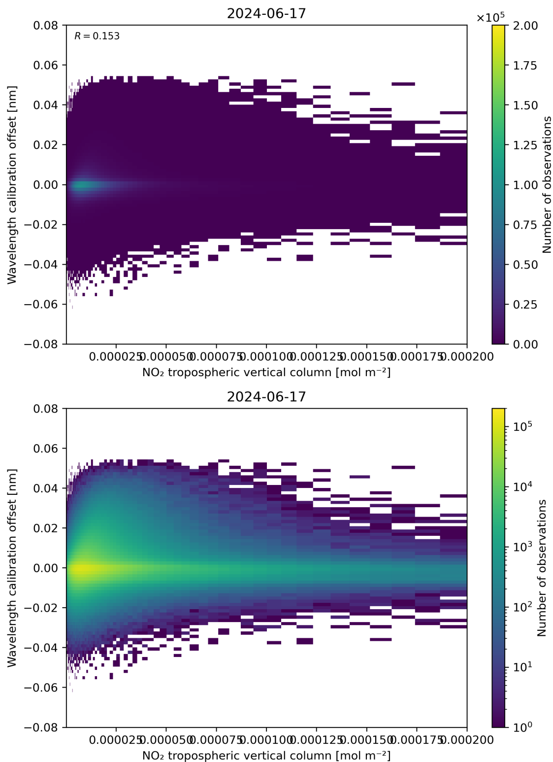
Figure 143: Scatter density plot of “NO 2 tropospheric vertical column” against “Wavelength calibration offset” for 2024-06-16 to 2024-06-18.
