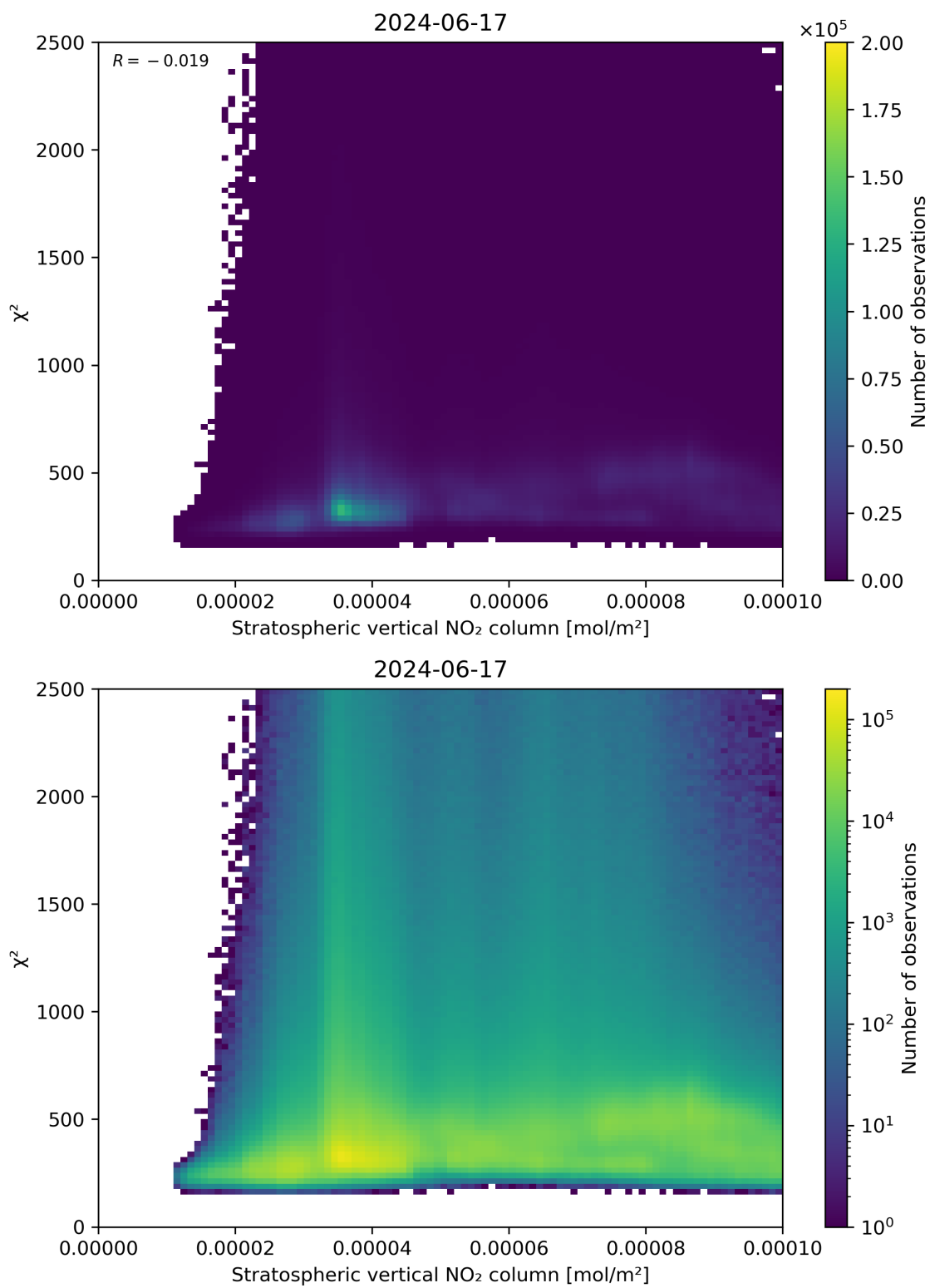
Figure 97: Scatter density plot of “Stratospheric vertical NO 2 column” against “ \chi^2 ” for 2024-06-16 to 2024-06-18.
