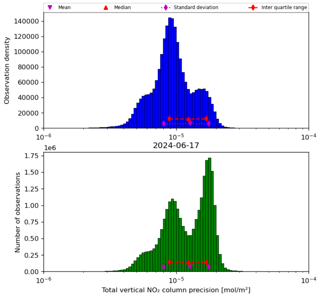
Figure 39: Histogram of “Total vertical NO 2 column precision” for 2024-06-16 to 2024-06-18
