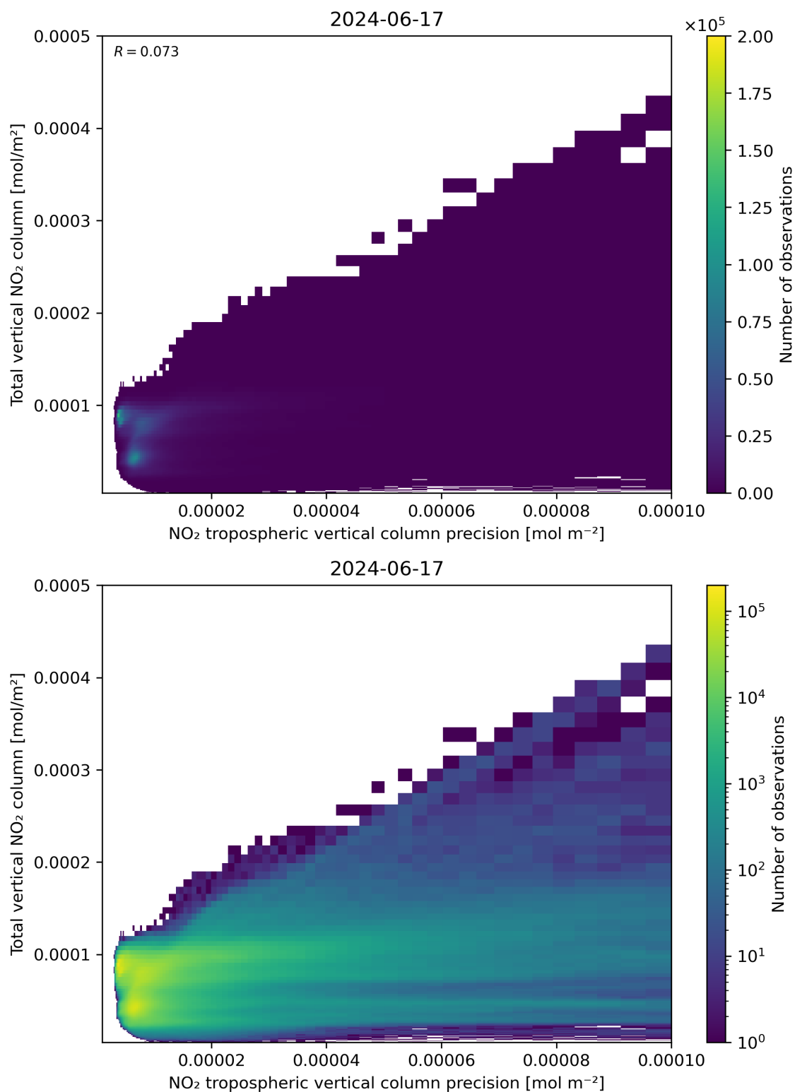
Figure 138: Scatter density plot of “NO 2 tropospheric vertical column precision” against “Total vertical NO 2 column” for 2024-06-16 to 2024-06-18.
