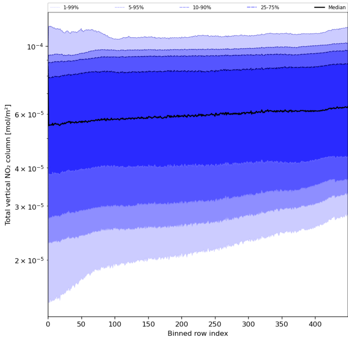
Figure 55: Along track statistics of “Total vertical NO 2 column” for 2024-06-16 to 2024-06-18
