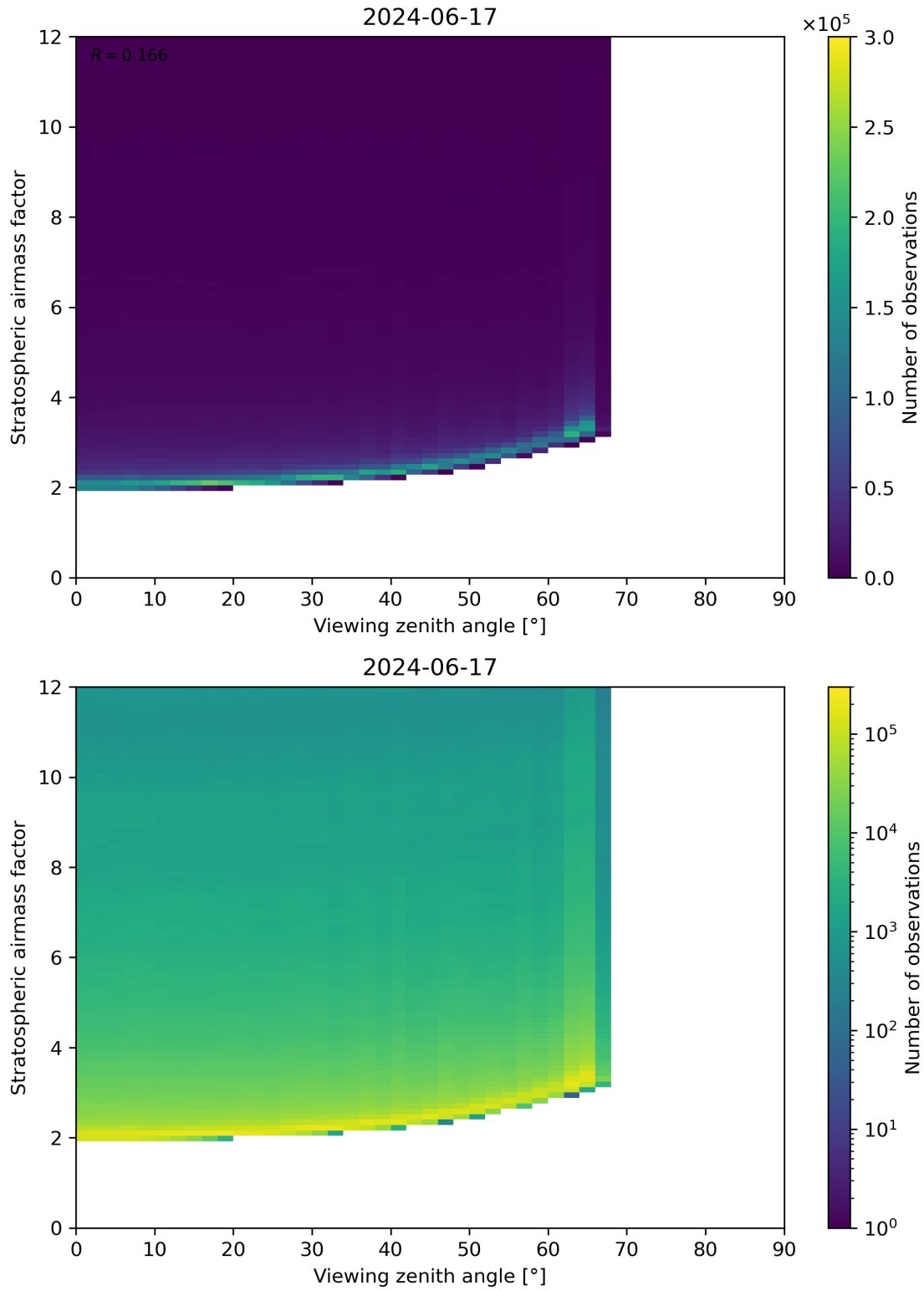
Figure 159: Scatter density plot of “Viewing zenith angle” against “Stratospheric airmass factor” for 2024-06-16 to 2024-06-18.
