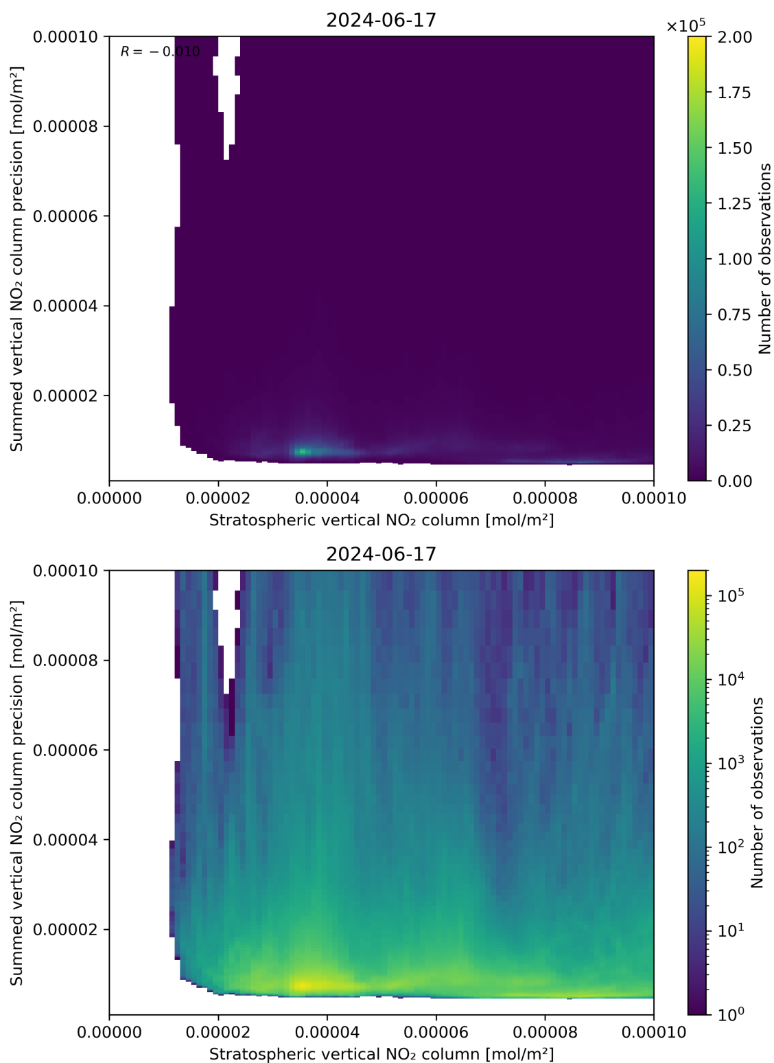
Figure 99: Scatter density plot of “Stratospheric vertical NO 2 column” against “Summed vertical NO 2 column precision” for 2024-06-16 to 2024-06-18.
