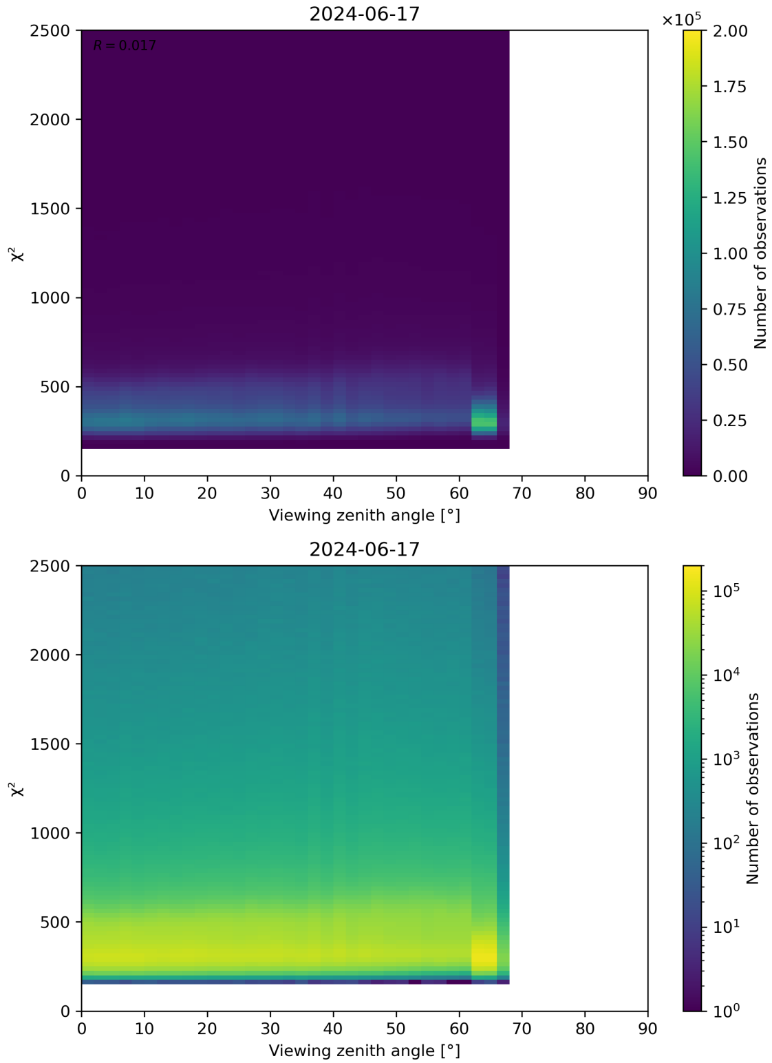
Figure 162: Scatter density plot of “Viewing zenith angle” against “ \chi^2 ” for 2024-06-16 to 2024-06-18.
