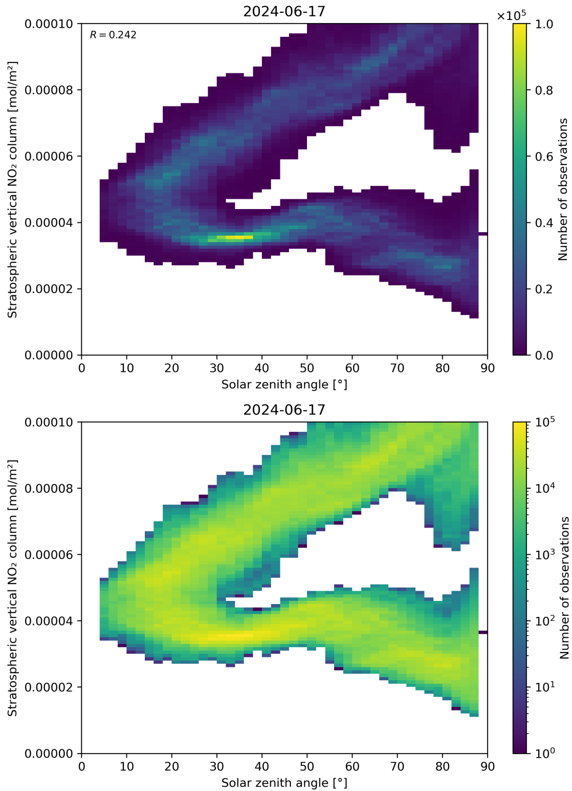
Figure 150: Scatter density plot of “Solar zenith angle” against “Stratospheric vertical NO 2 column” for 2024-06-16 to 2024-06-18.
