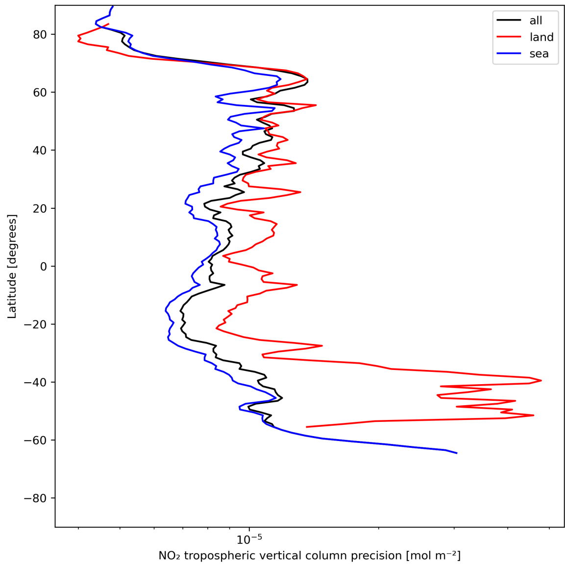
Figure 13: Zonal average of “NO 2 tropospheric vertical column precision” for 2024-06-16 to 2024-06-18.
