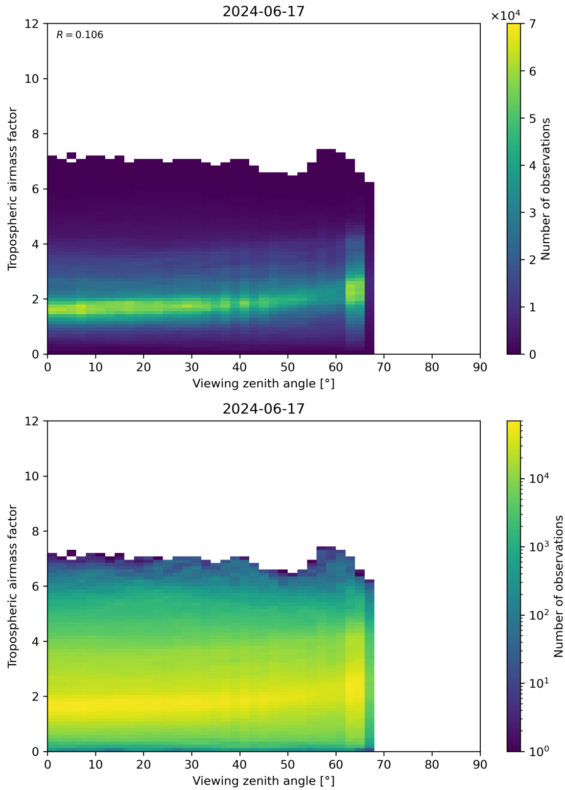
Figure 161: Scatter density plot of “Viewing zenith angle” against “Tropospheric airmass factor” for 2024-06-16 to 2024-06-18.
