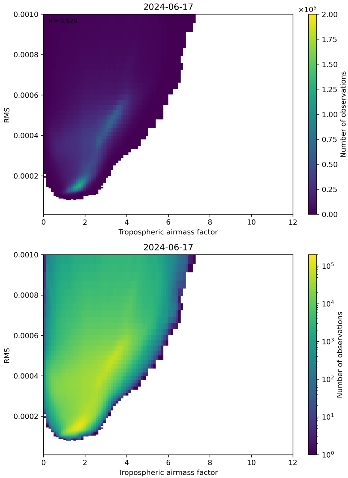
Figure 79: Scatter density plot of “Tropospheric airmass factor” against “RMS” for 2024-06-16 to 2024-06-18.
