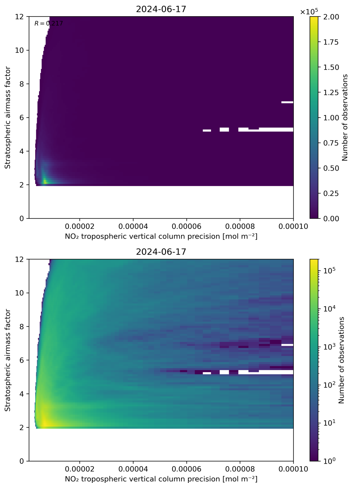
Figure 131: Scatter density plot of “NO 2 tropospheric vertical column precision” against “Stratospheric airmass factor” for 2024-06-16 to 2024-06-18.
