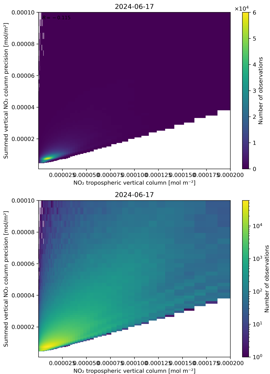
Figure 127: Scatter density plot of “NO 2 tropospheric vertical column” against “Summed vertical NO 2 column precision” for 2024-06-16 to 2024-06-18.
