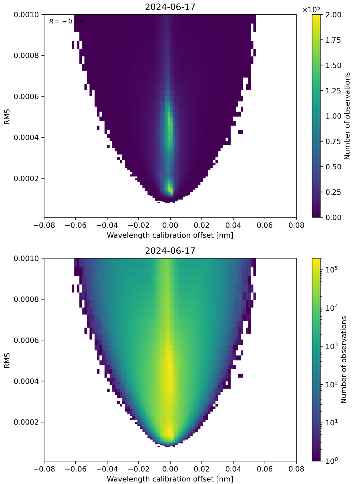
Figure 181: Scatter density plot of “Wavelength calibration offset” against “RMS” for 2024-06-16 to 2024-06-18.
