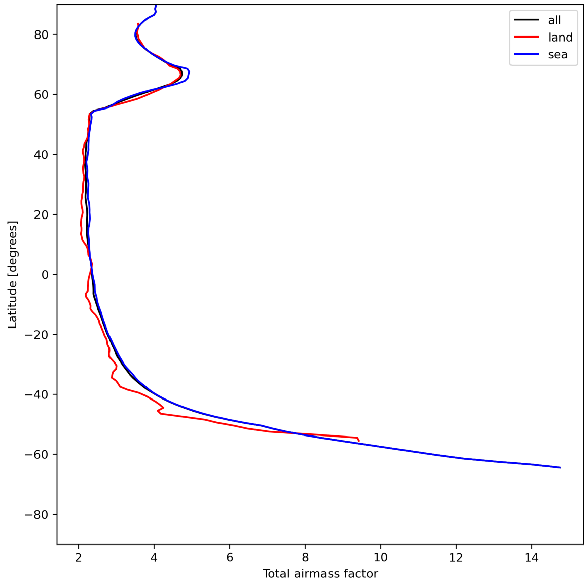
Figure 15: Zonal average of “Total airmass factor” for 2024-06-16 to 2024-06-18.
