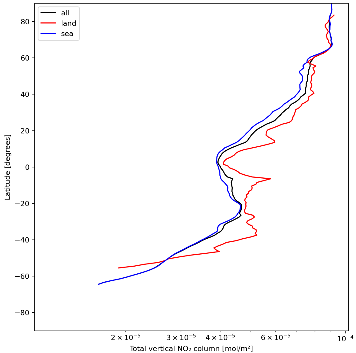
Figure 21: Zonal average of “Total vertical NO 2 column” for 2024-06-16 to 2024-06-18.
