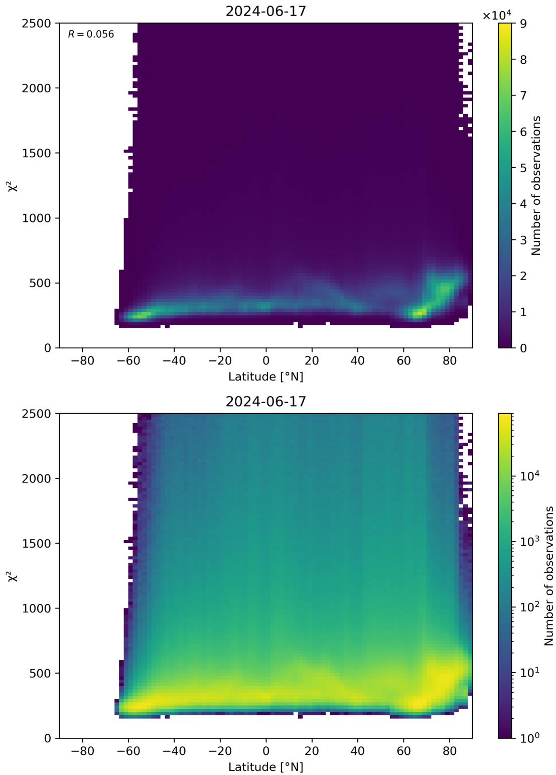
Figure 86: Scatter density plot of “Latitude” against “ \chi^2 ” for 2024-06-16 to 2024-06-18.
