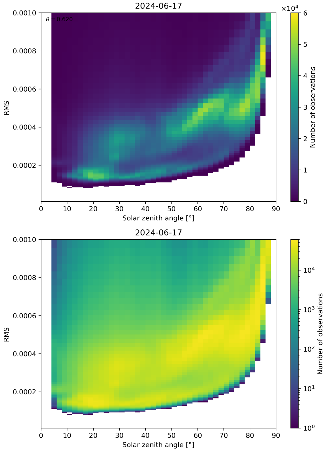
Figure 157: Scatter density plot of “Solar zenith angle” against “RMS” for 2024-06-16 to 2024-06-18.
