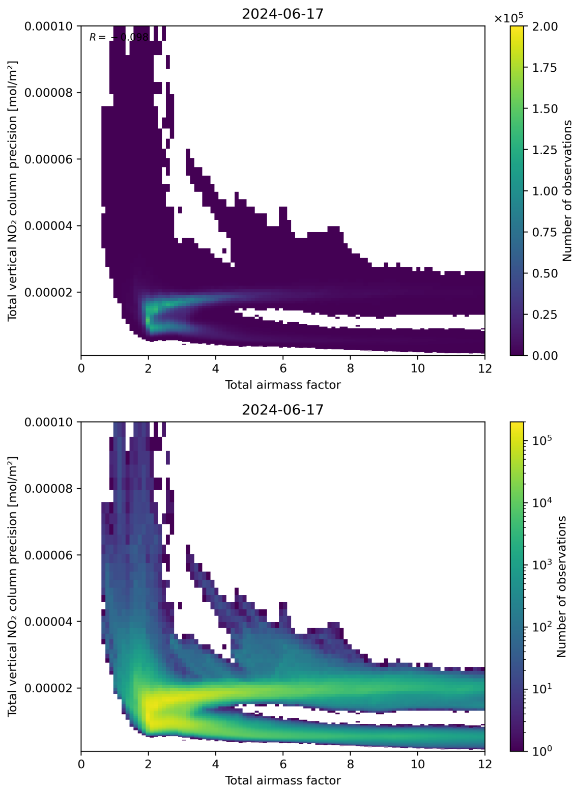
Figure 68: Scatter density plot of “Total airmass factor” against “Total vertical NO 2 column precision” for 2024-06-16 to 2024-06-18.
