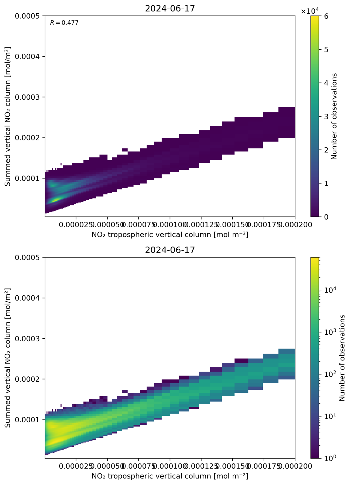
Figure 126: Scatter density plot of “NO 2 tropospheric vertical column” against “Summed vertical NO 2 column” for 2024-06-16 to 2024-06-18.
