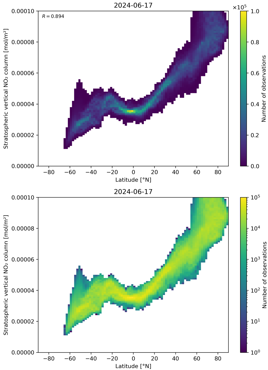
Figure 87: Scatter density plot of “Latitude” against “Stratospheric vertical NO 2 column” for 2024-06-16 to 2024-06-18.
