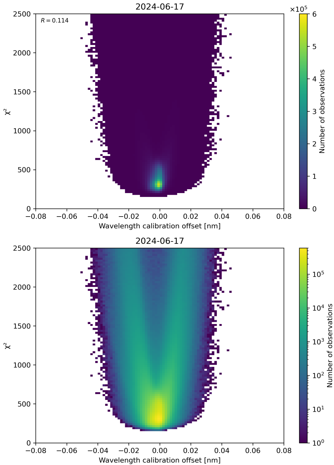
Figure 175: Scatter density plot of “Wavelength calibration offset” against “ \chi^2 ” for 2024-06-16 to 2024-06-18.
