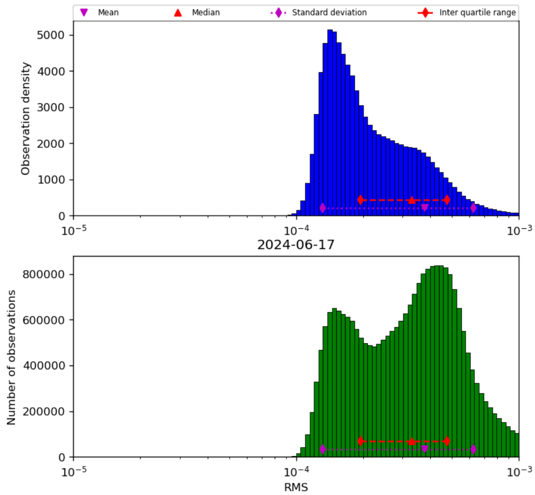
Figure 43: Histogram of “RMS” for 2024-06-16 to 2024-06-18
