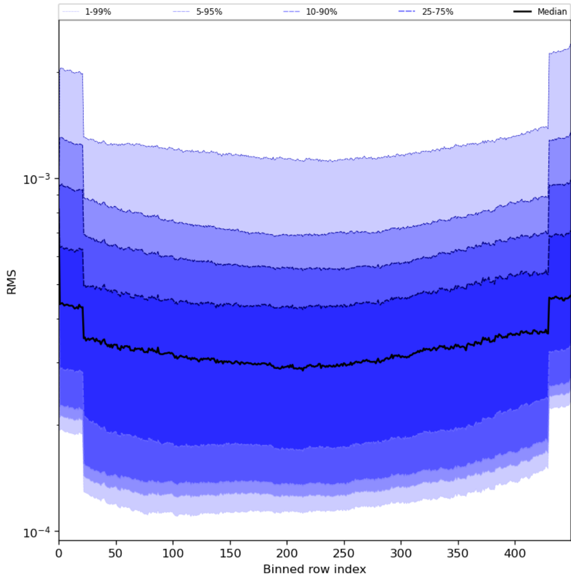
Figure 60: Along track statistics of “RMS” for 2024-06-16 to 2024-06-18
