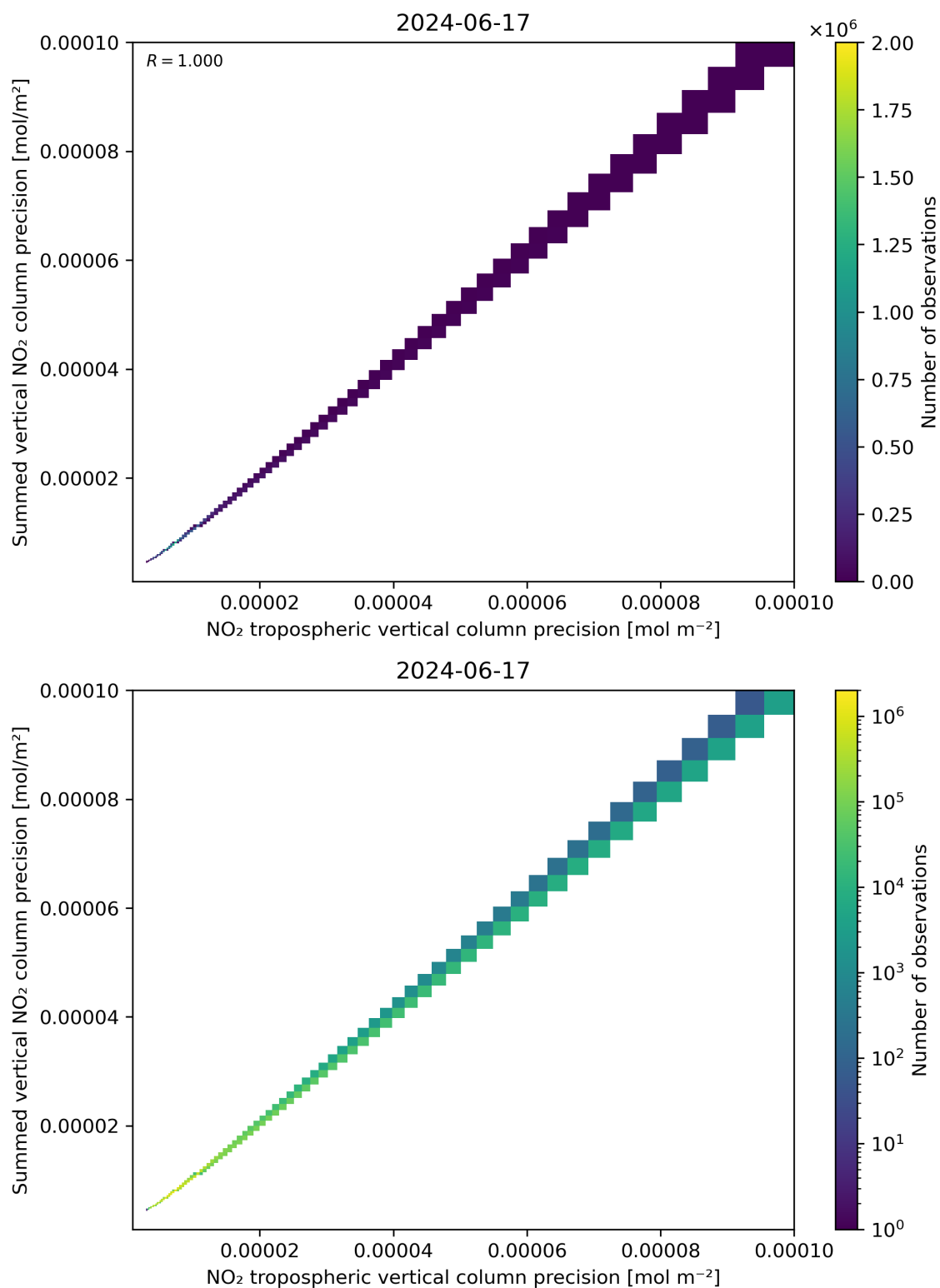
Figure 137: Scatter density plot of “NO 2 tropospheric vertical column precision” against “Summed vertical NO 2 column precision” for 2024-06-16 to 2024-06-18.
