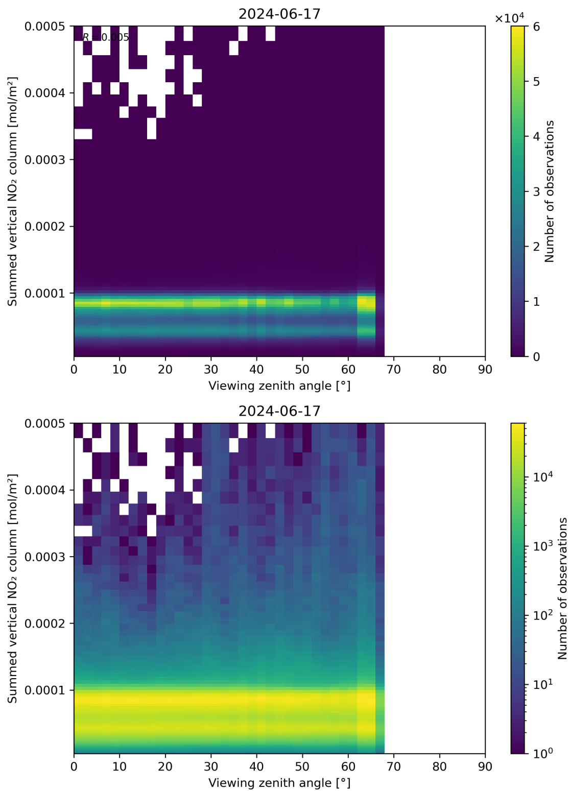
Figure 165: Scatter density plot of “Viewing zenith angle” against “Summed vertical NO 2 column” for 2024-06-16 to 2024-06-18.
