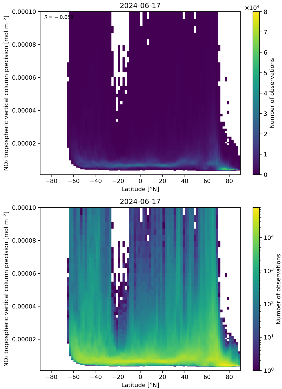
Figure 93: Scatter density plot of “Latitude” against “NO 2 tropospheric vertical column precision” for 2024-06-16 to 2024-06-18.
