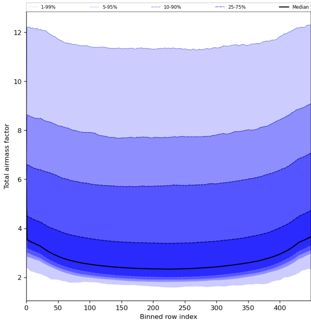
Figure 49: Along track statistics of “Total airmass factor” for 2024-06-16 to 2024-06-18
