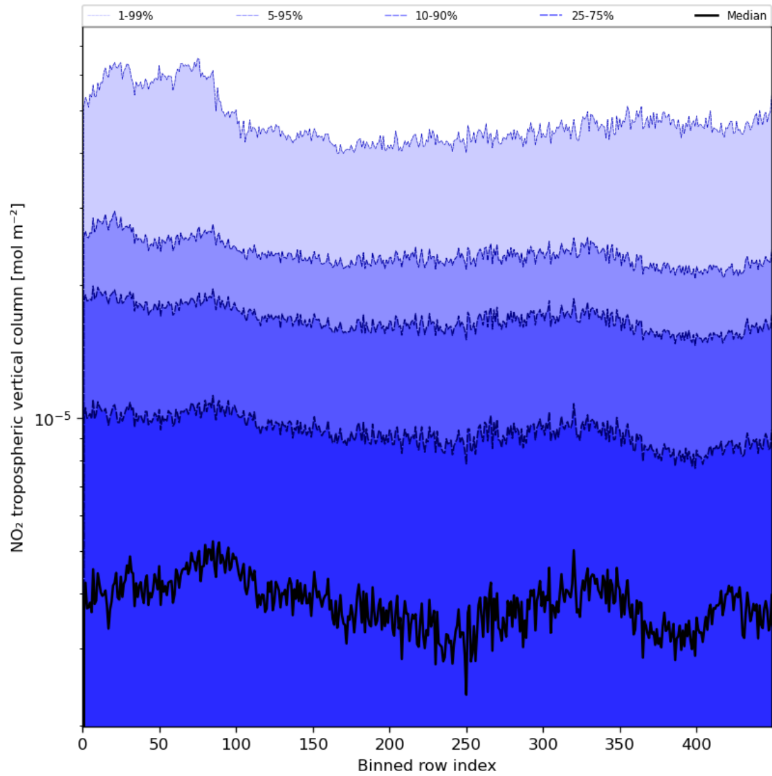
Figure 46: Along track statistics of “NO 2 tropospheric vertical column” for 2024-06-16 to 2024-06-18
