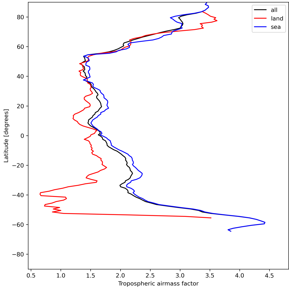
Figure 14: Zonal average of “Tropospheric airmass factor” for 2024-06-16 to 2024-06-18.
