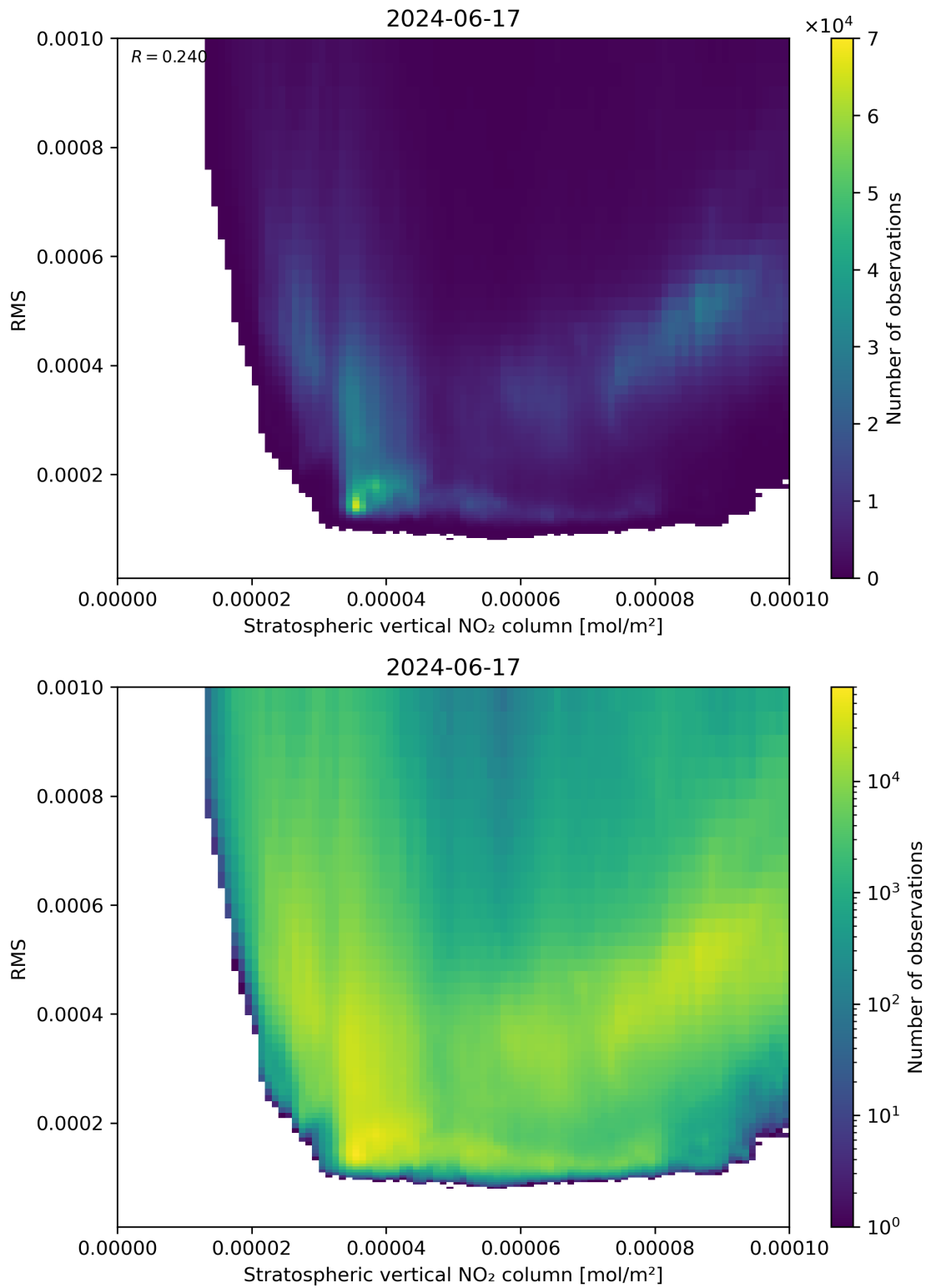
Figure 102: Scatter density plot of “Stratospheric vertical NO 2 column” against “RMS” for 2024-06-16 to 2024-06-18.
