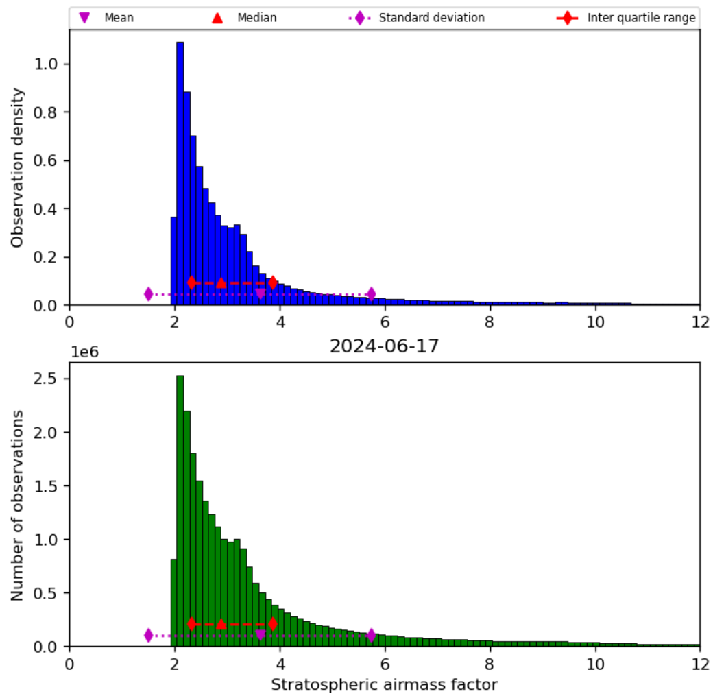
Figure 44: Histogram of “Stratospheric airmass factor” for 2024-06-16 to 2024-06-18
