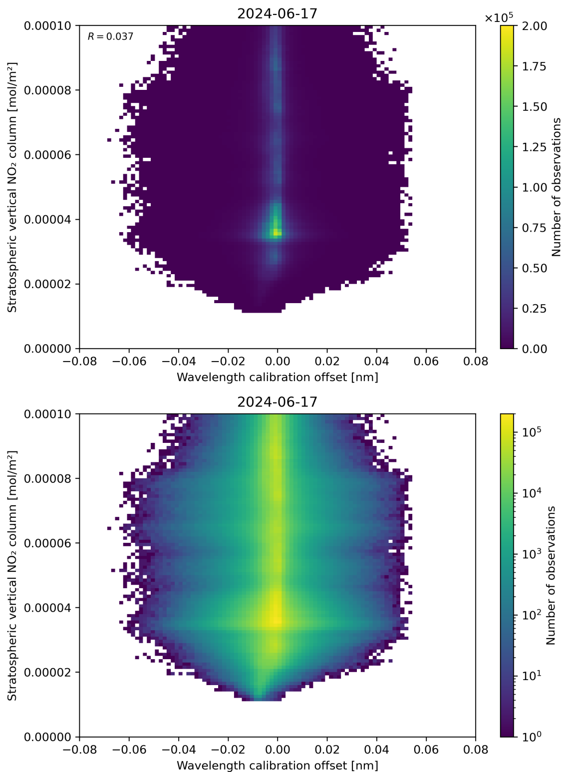
Figure 176: Scatter density plot of “Wavelength calibration offset” against “Stratospheric vertical NO 2 column” for 2024-06-16 to 2024-06-18.
