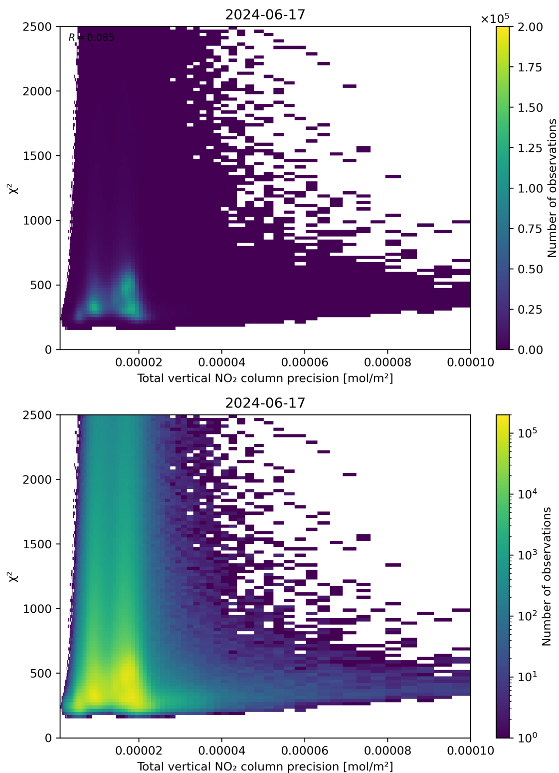
Figure 116: Scatter density plot of “Total vertical NO 2 column precision” against “ \chi^2 ” for 2024-06-16 to 2024-06-18.
