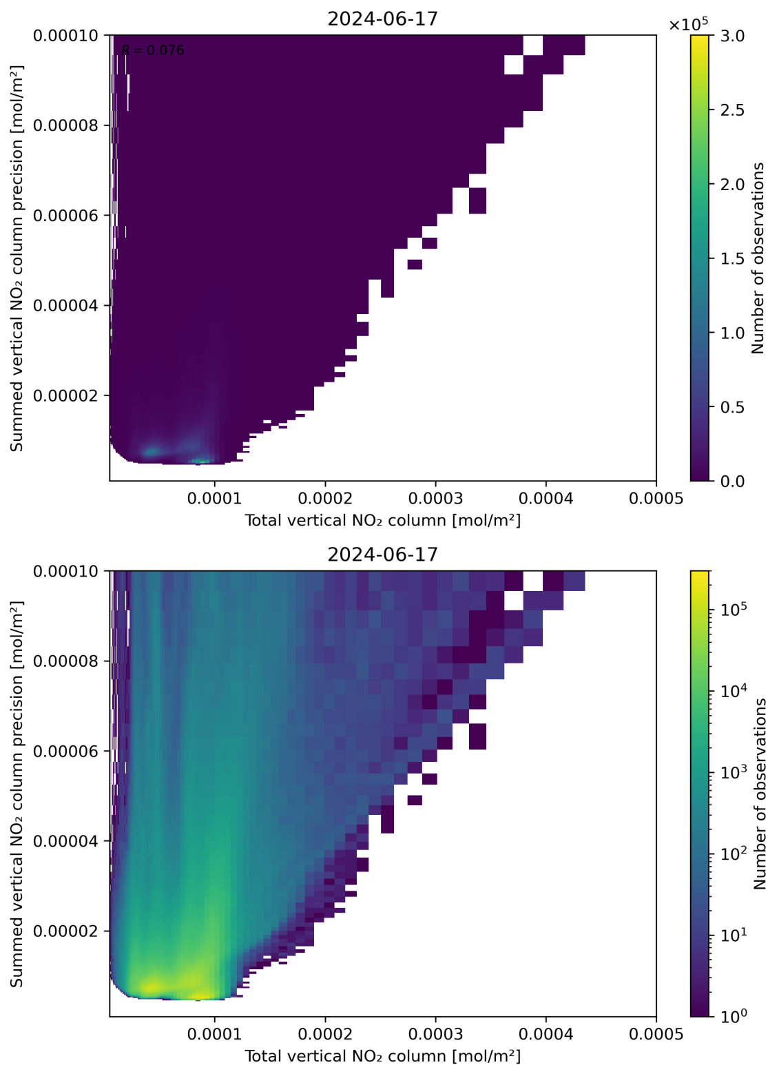
Figure 113: Scatter density plot of “Total vertical NO 2 column” against “Summed vertical NO 2 column precision” for 2024-06-16 to 2024-06-18.
