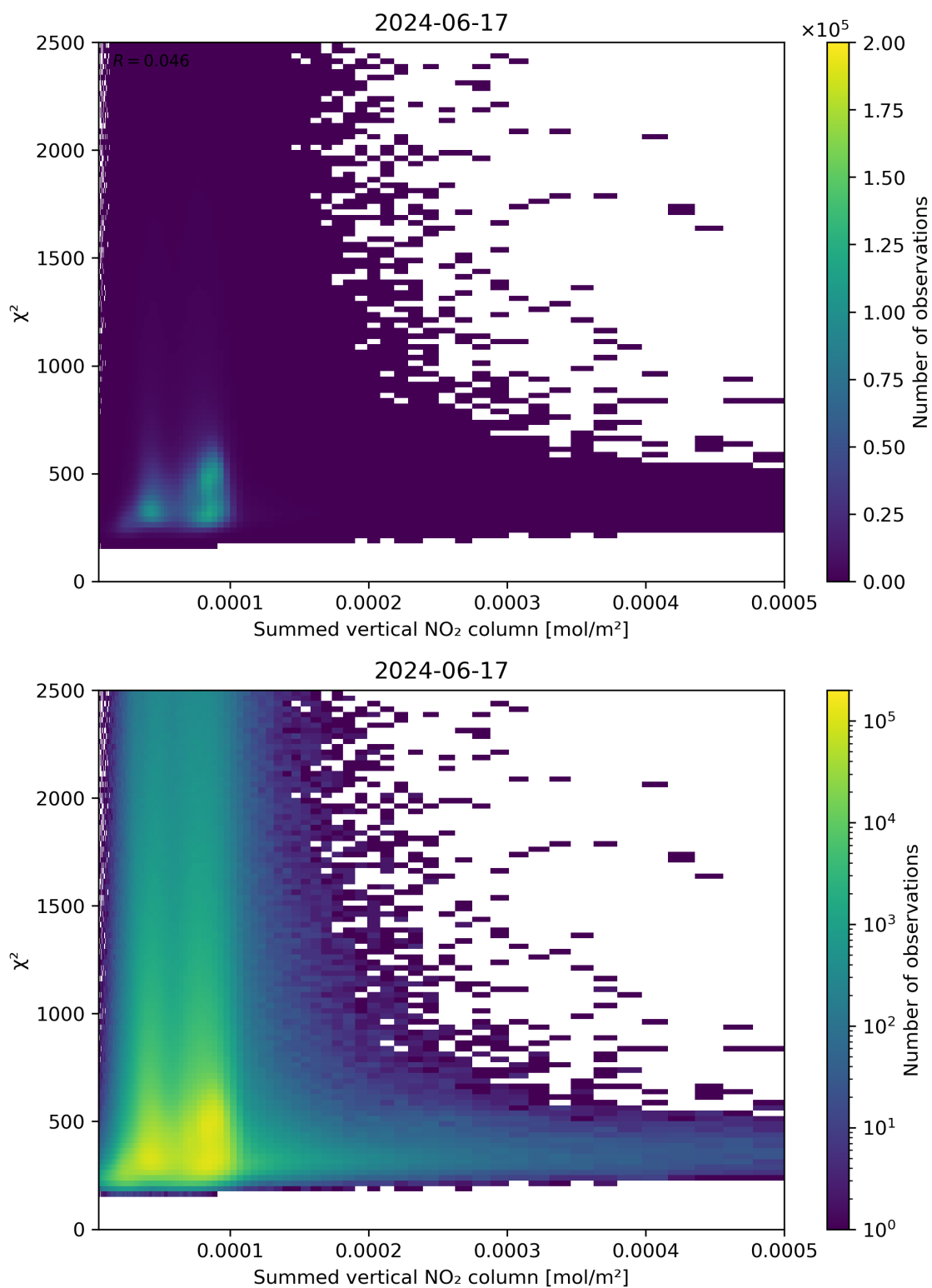
Figure 104: Scatter density plot of “Summed vertical NO 2 column” against “ \chi^2 ” for 2024-06-16 to 2024-06-18.
