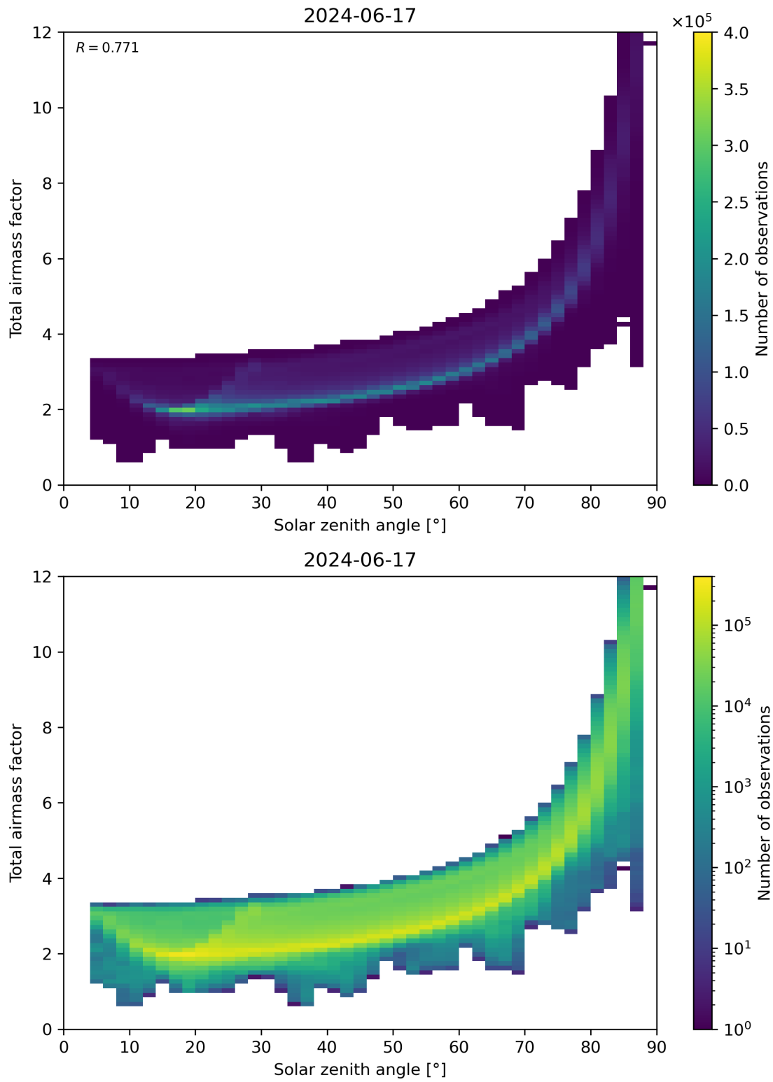
Figure 146: Scatter density plot of “Solar zenith angle” against “Total air mass factor” for 2024-06-16 to 2024-06-18.
