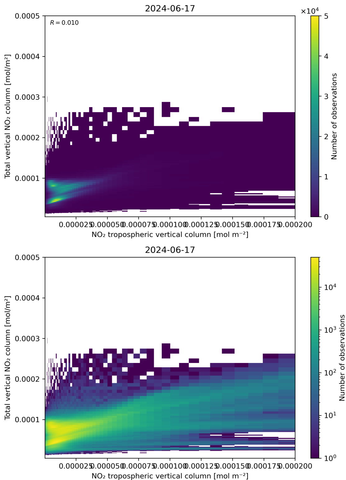
Figure 128: Scatter density plot of “NO 2 tropospheric vertical column” against “Total vertical NO 2 column” for 2024-06-16 to 2024-06-18.
