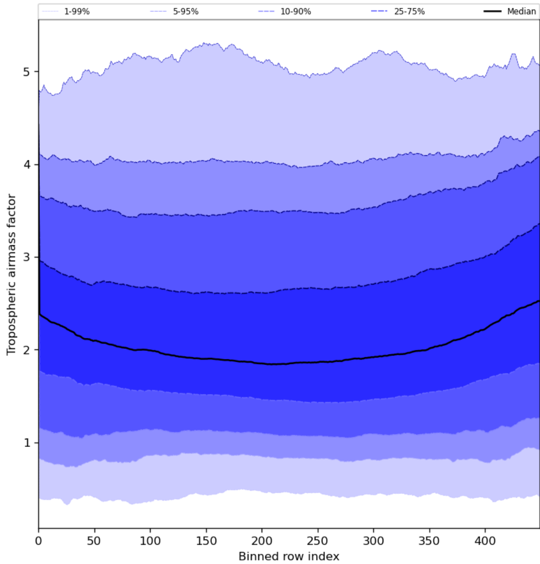
Figure 48: Along track statistics of “Tropospheric air mass factor” for 2024-06-16 to 2024-06-18
