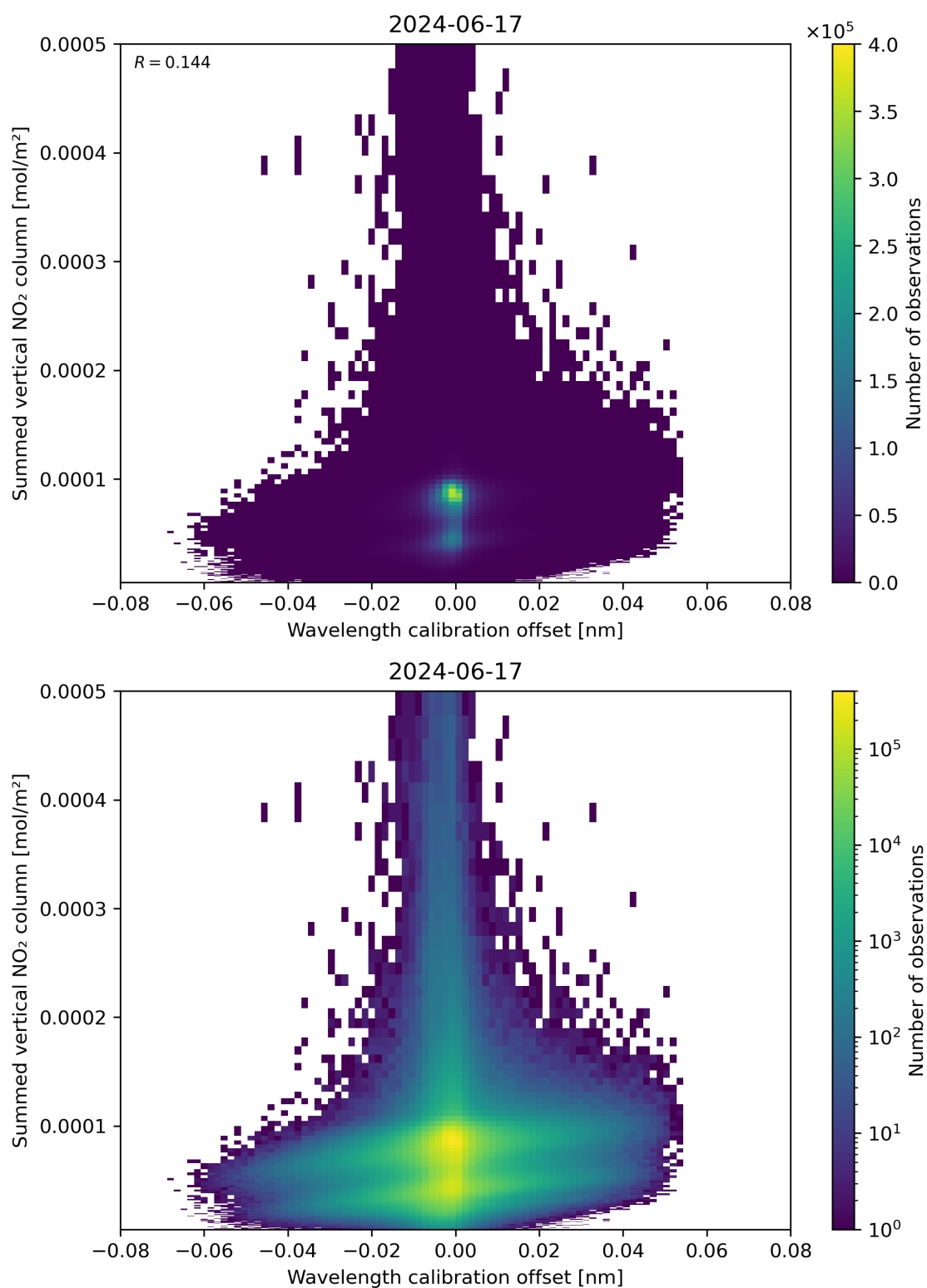
Figure 177: Scatter density plot of “Wavelength calibration offset” against “Summed vertical NO 2 column” for 2024-06-16 to 2024-06-18.
