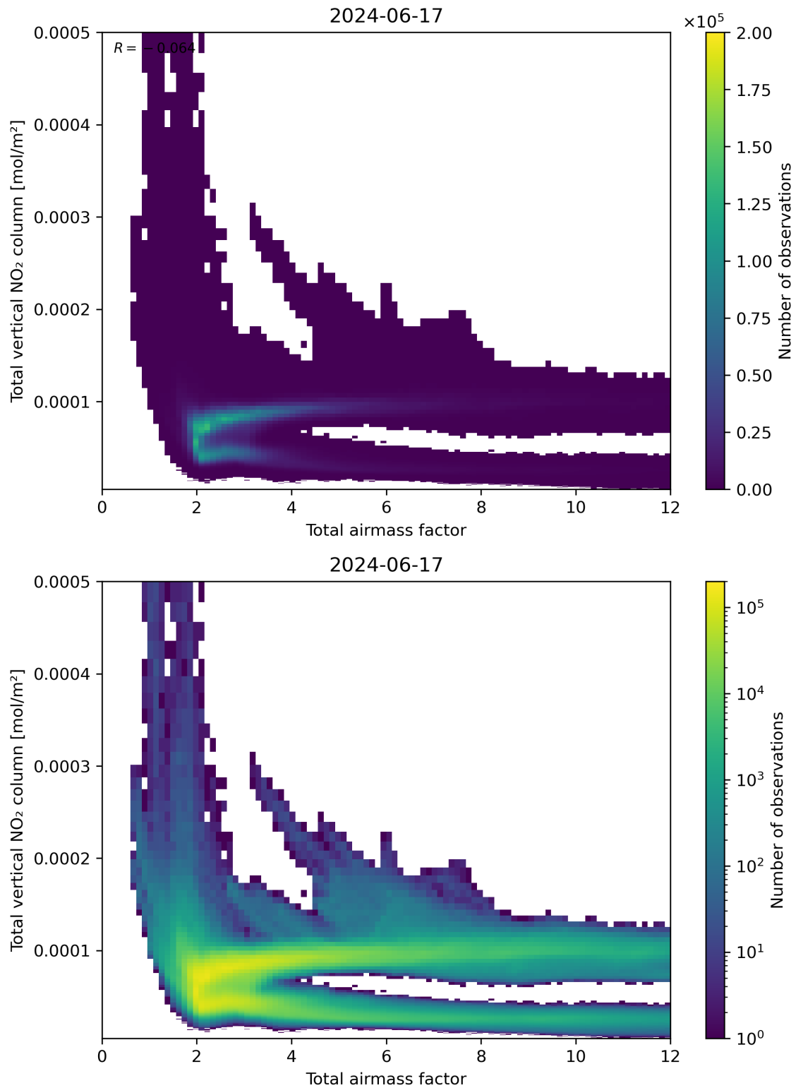
Figure 67: Scatter density plot of “Total airmass factor” against “Total vertical NO 2 column” for 2024-06-16 to 2024-06-18.
