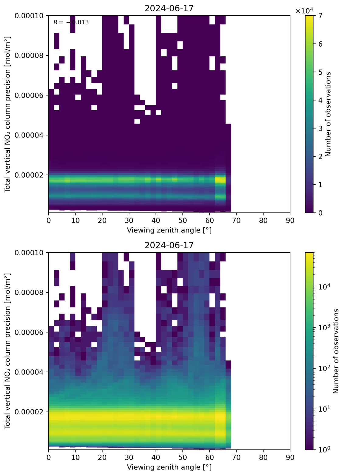
Figure 168: Scatter density plot of “Viewing zenith angle” against “Total vertical NO 2 column precision” for 2024-06-16 to 2024-06-18.
