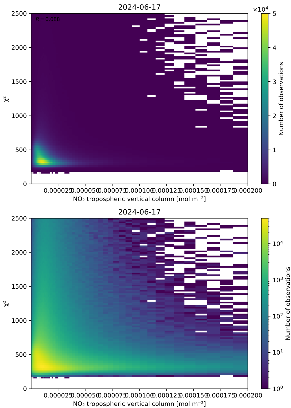
Figure 124: Scatter density plot of “NO 2 tropospheric vertical column” against “ \chi^2 ” for 2024-06-16 to 2024-06-18.
