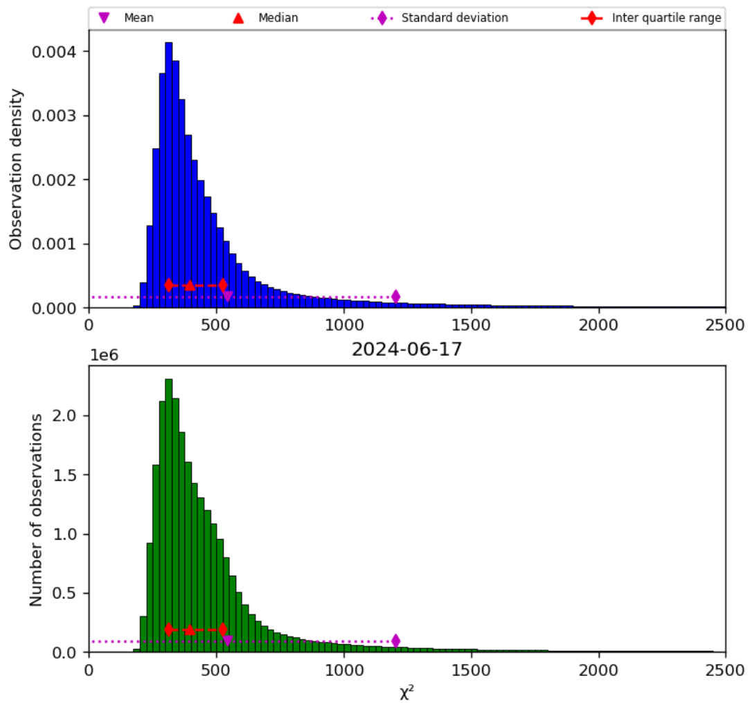
Figure 42: Histogram of “ \chi^2 ” for 2024-06-16 to 2024-06-18
