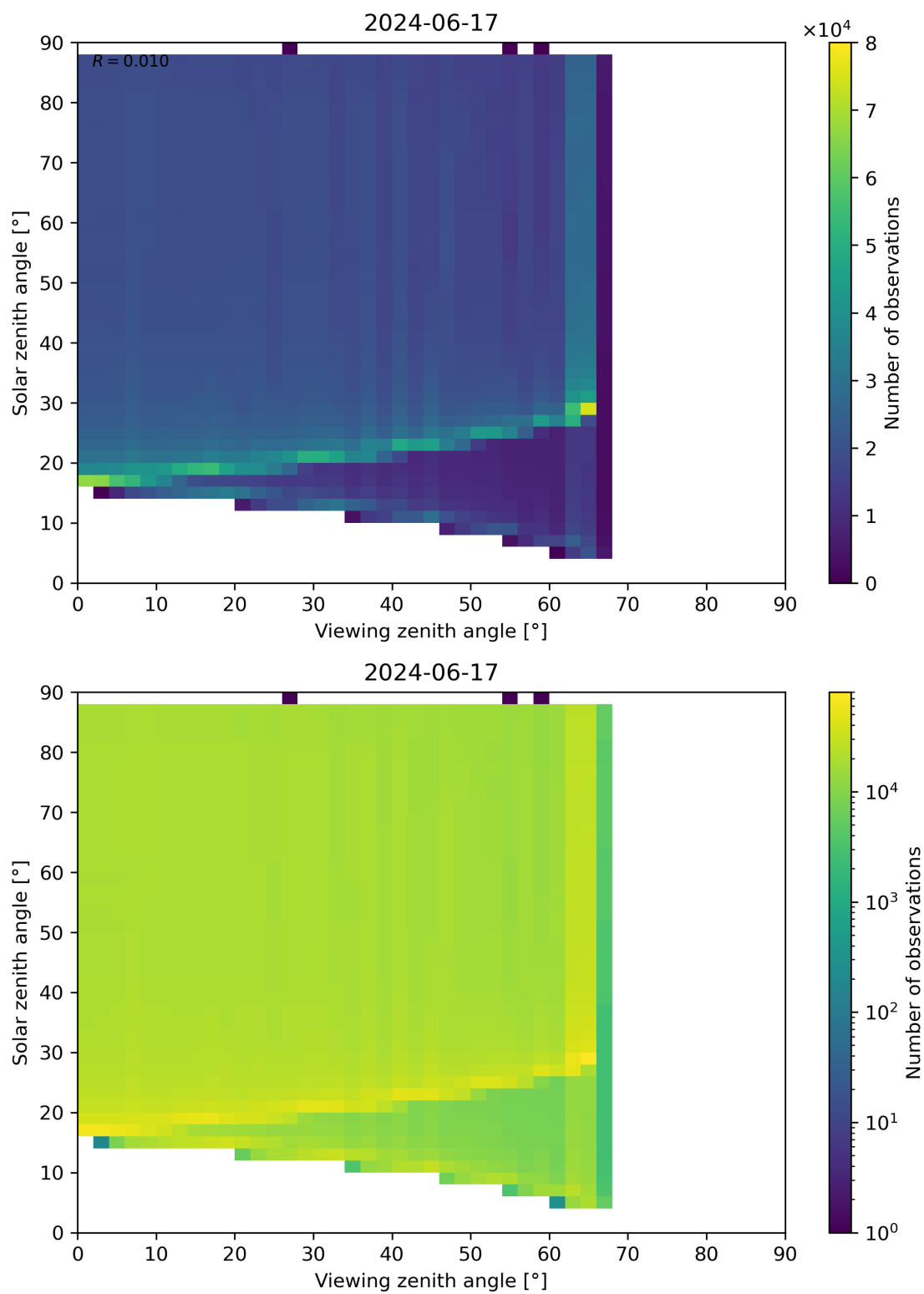
Figure 172: Scatter density plot of “Viewing zenith angle” against “Solar zenith angle” for 2024-06-16 to 2024-06-18.
