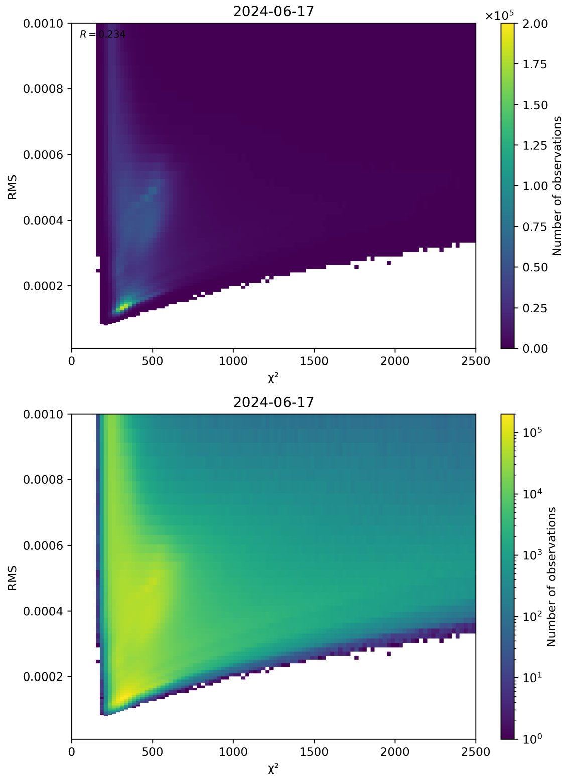
Figure 82: Scatter density plot of “ \chi^2 ” against “RMS” for 2024-06-16 to 2024-06-18.
