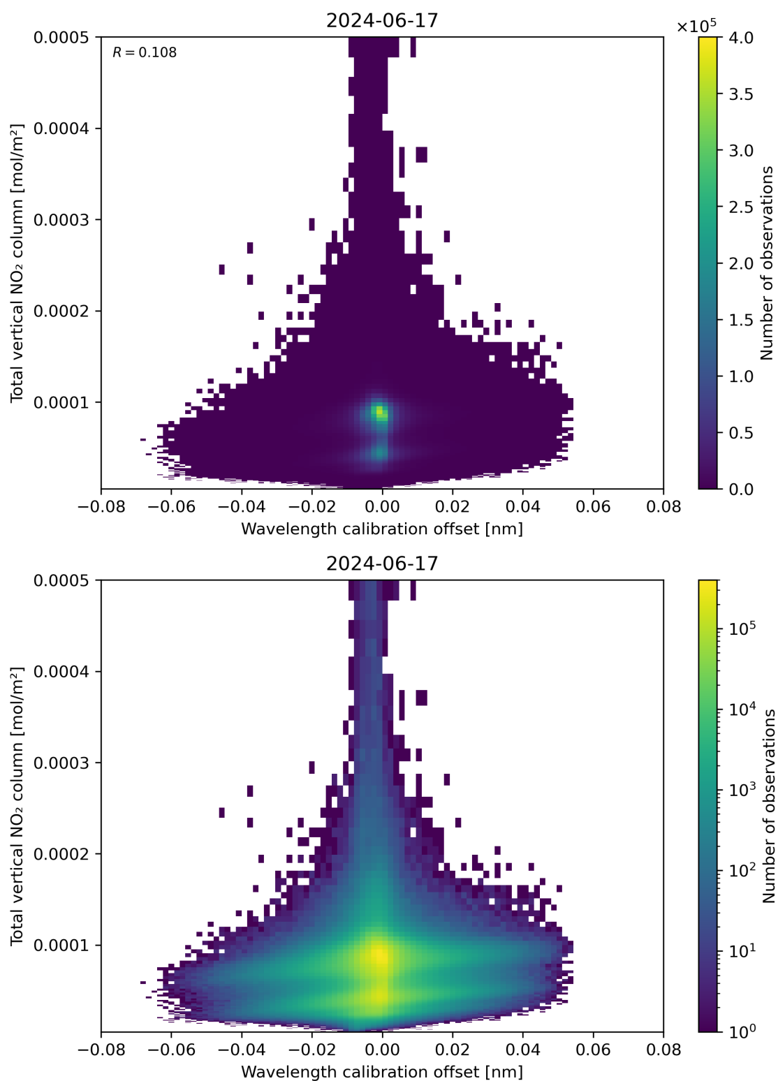
Figure 179: Scatter density plot of “Wavelength calibration offset” against “Total vertical NO 2 column” for 2024-06-16 to 2024-06-18.
