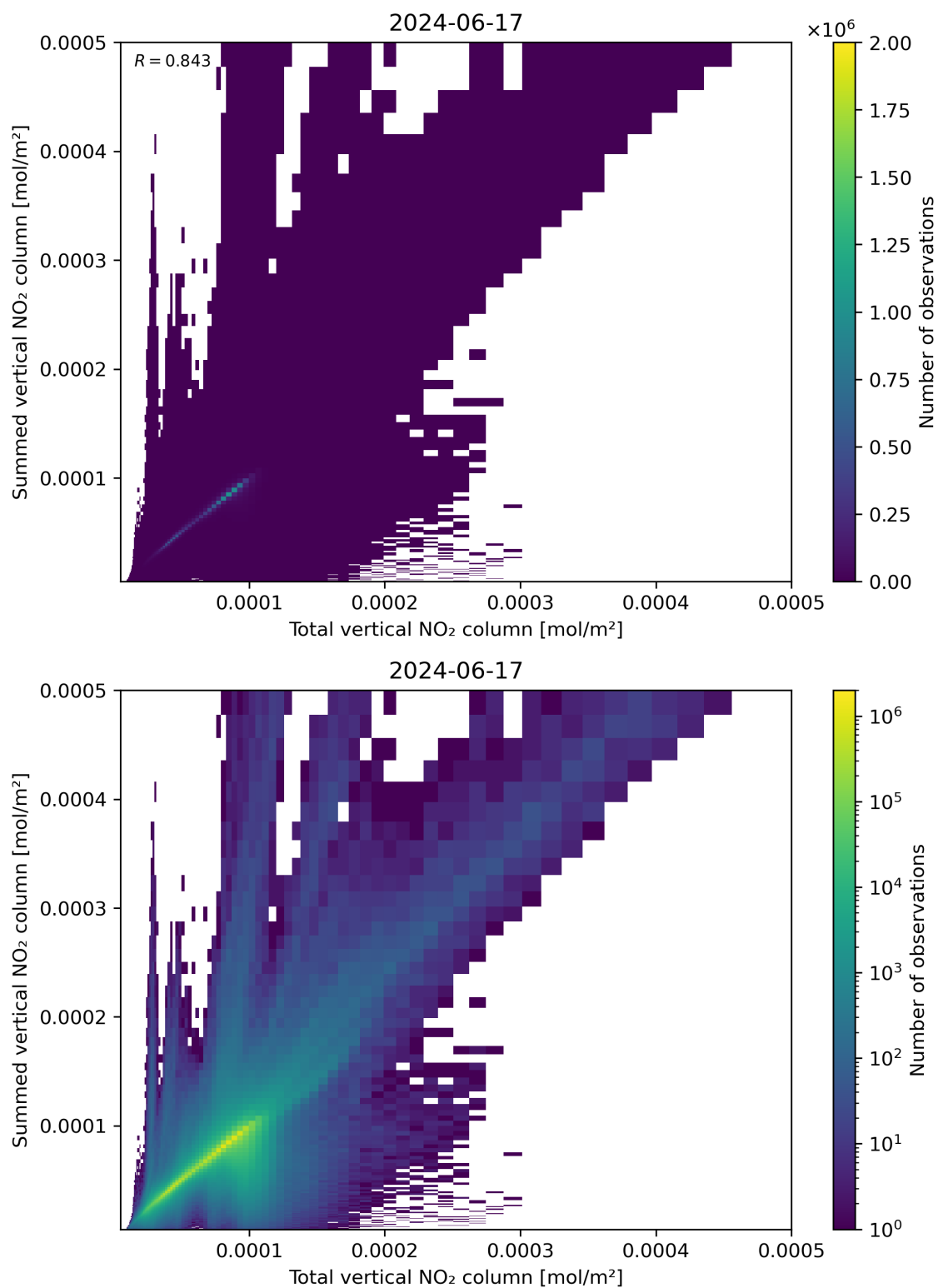
Figure 112: Scatter density plot of “Total vertical NO 2 column” against “Summed vertical NO 2 column” for 2024-06-16 to 2024-06-18.
