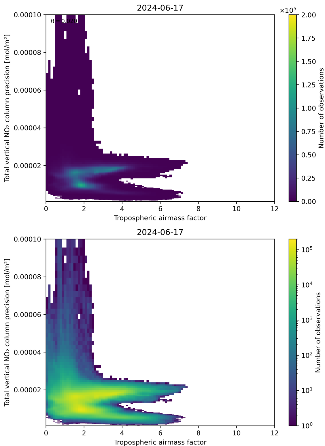
Figure 78: Scatter density plot of “Tropospheric air mass factor” against “Total vertical NO 2 column precision” for 2024-06-16 to 2024-06-18.
