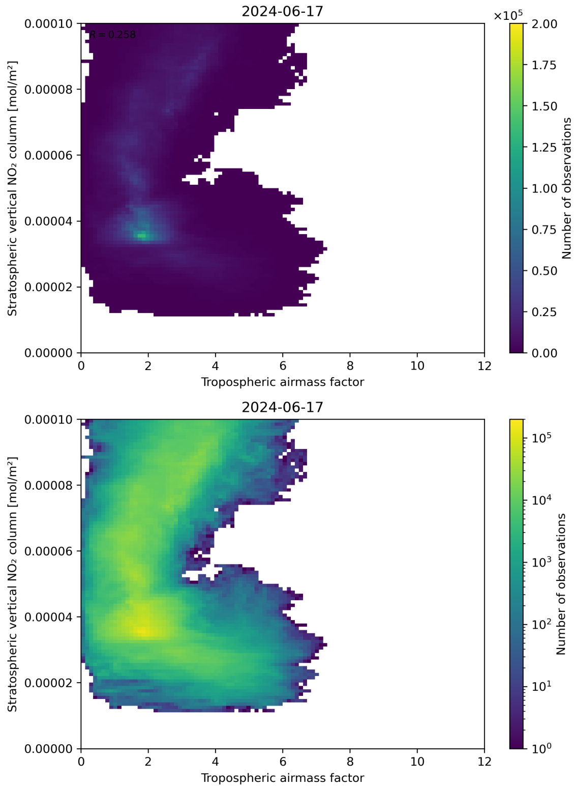
Figure 74: Scatter density plot of “Tropospheric air mass factor” against “Stratospheric vertical NO 2 column” for 2024-06-16 to 2024-06-18.
