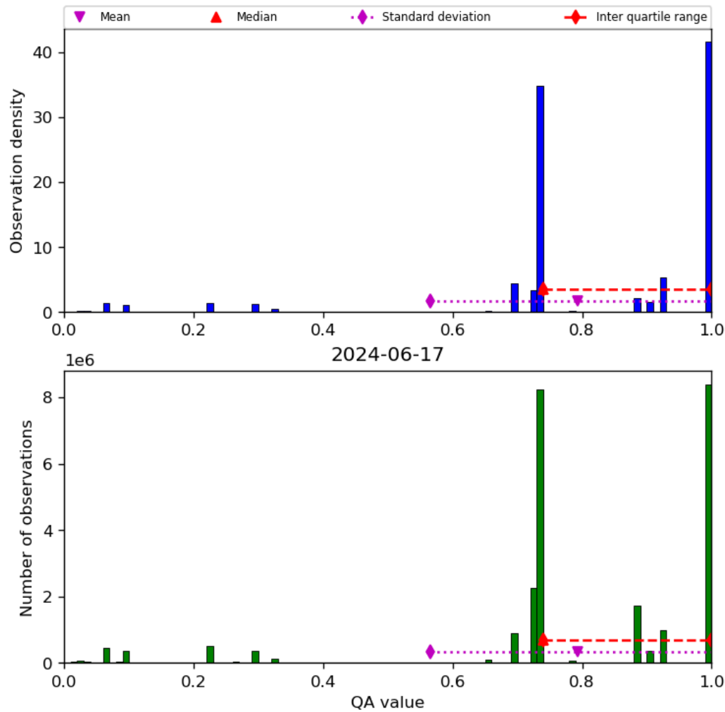
Figure 28: Histogram of “QA value” for 2024-06-16 to 2024-06-18
