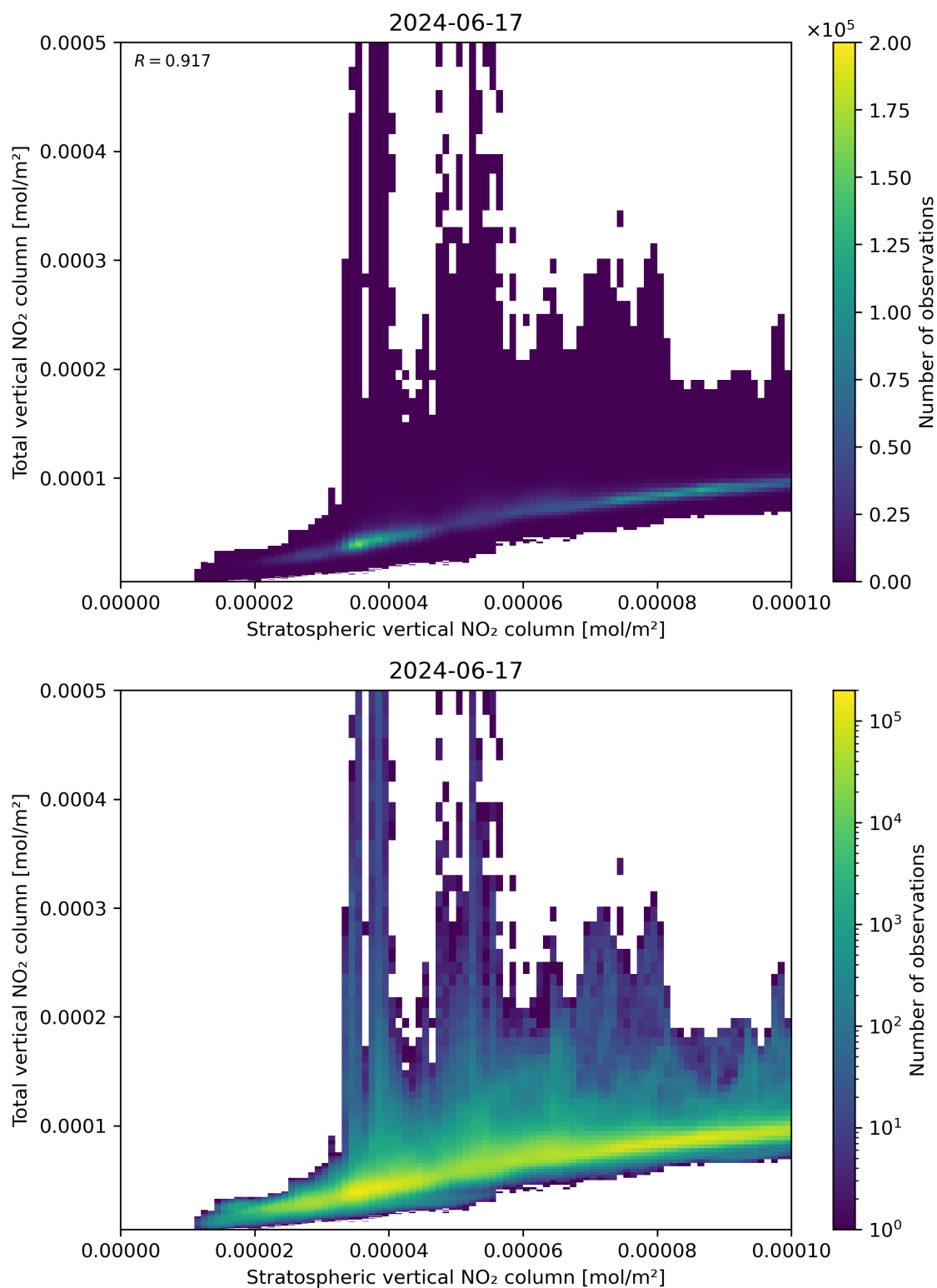
Figure 100: Scatter density plot of “Stratospheric vertical NO 2 column” against “Total vertical NO 2 column” for 2024-06-16 to 2024-06-18.
