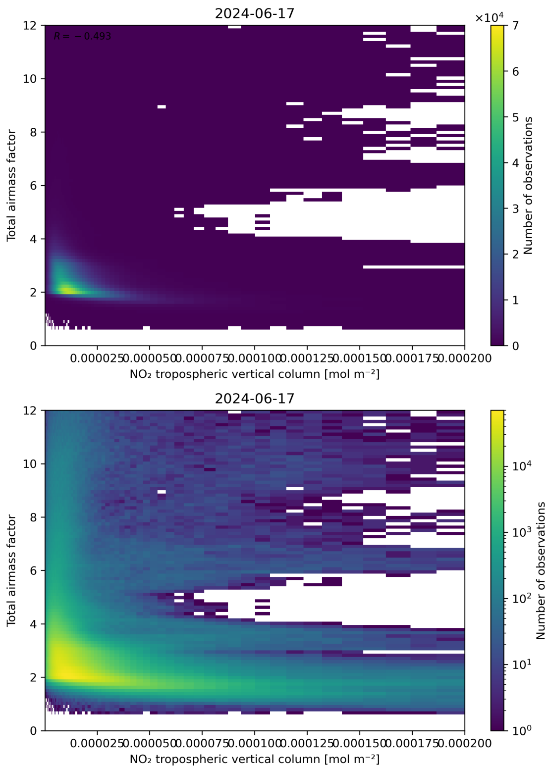
Figure 122: Scatter density plot of “NO 2 tropospheric vertical column” against “Total air mass factor” for 2024-06-16 to 2024-06-18.
