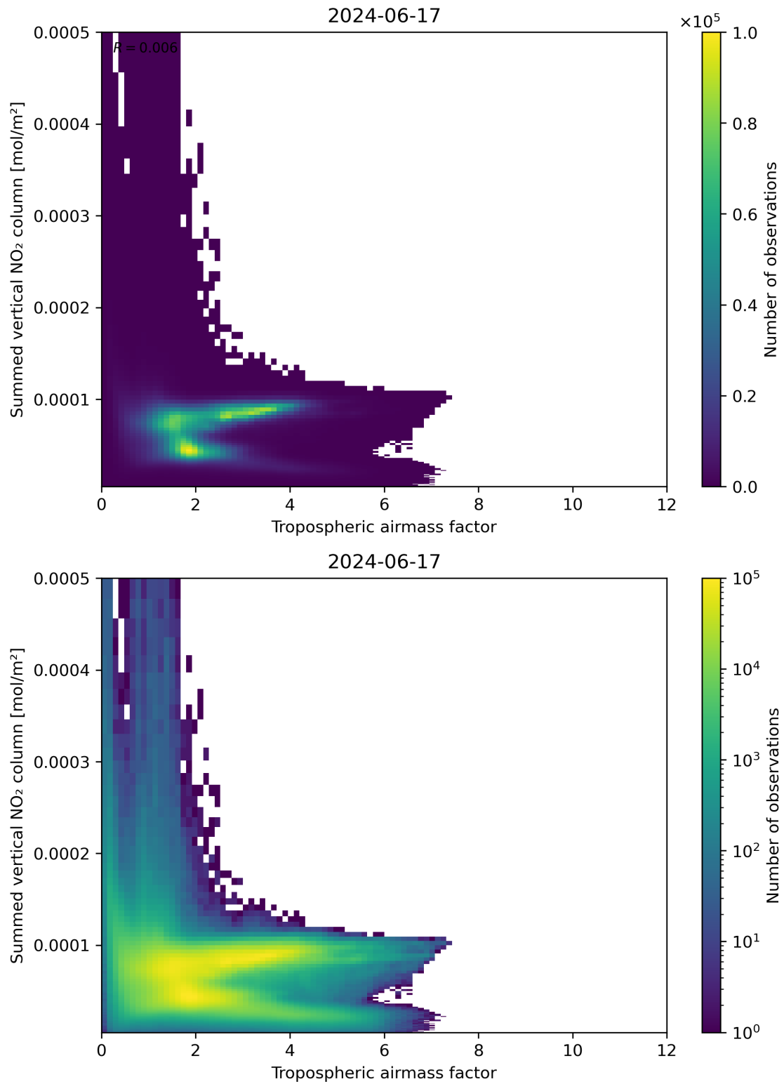
Figure 75: Scatter density plot of “Tropospheric airmass factor” against “Summed vertical NO 2 column” for 2024-06-16 to 2024-06-18.
