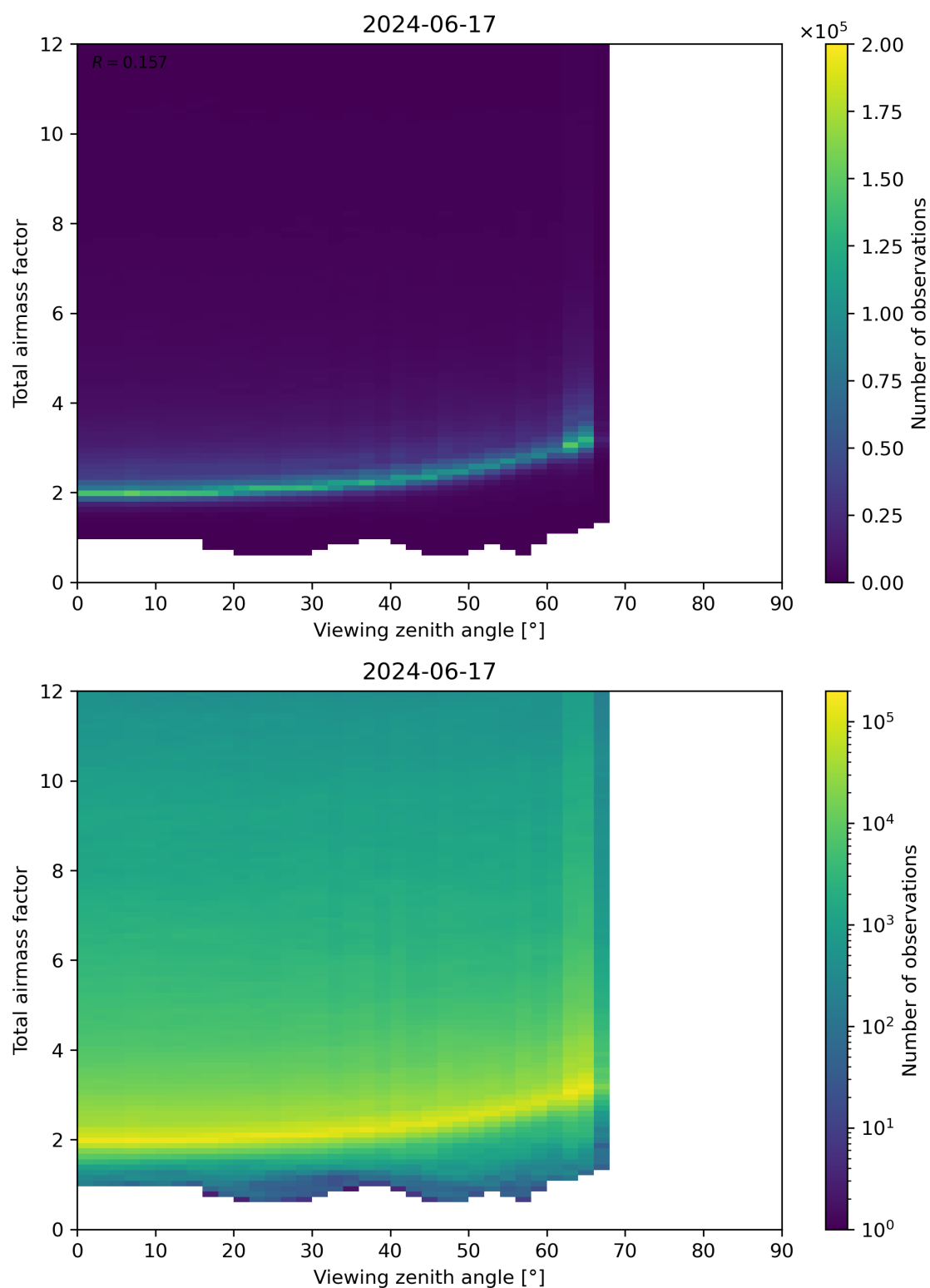
Figure 160: Scatter density plot of “Viewing zenith angle” against “Total airmass factor” for 2024-06-16 to 2024-06-18.
