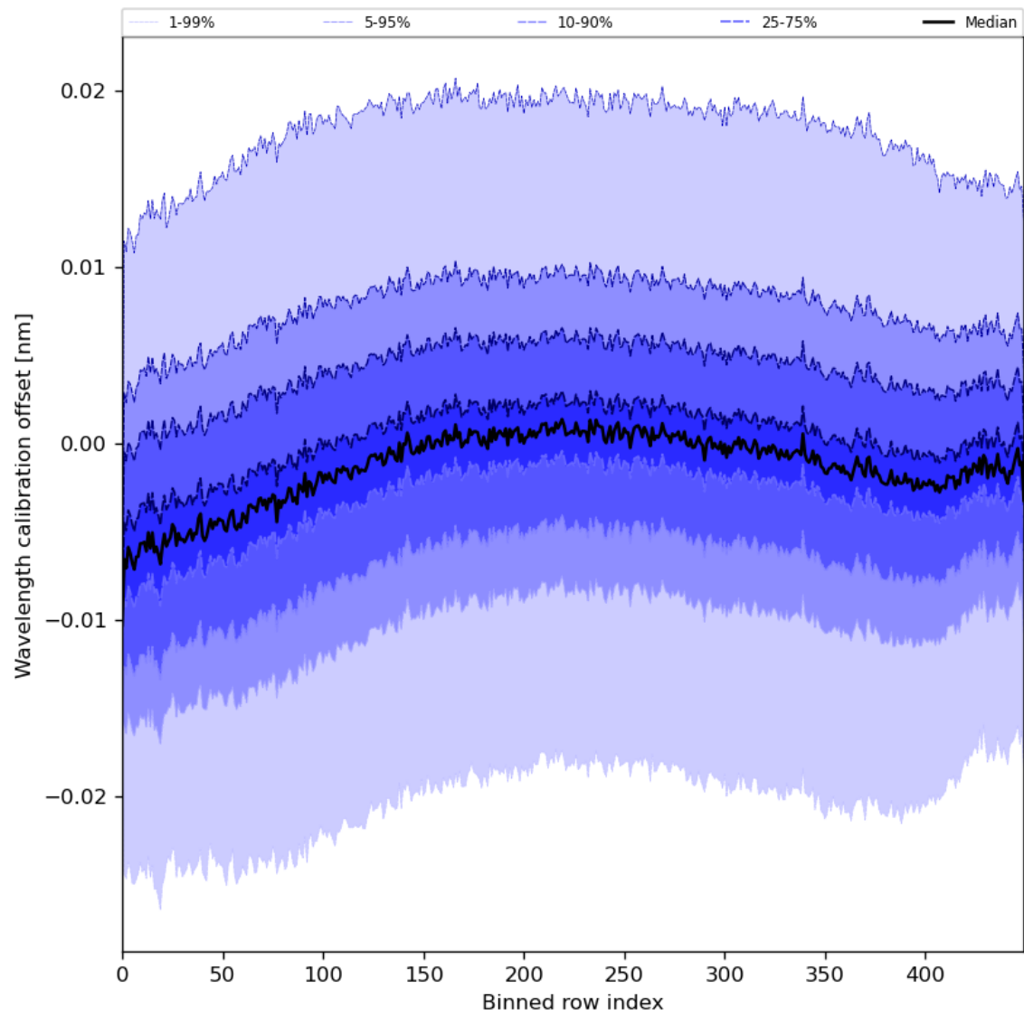
Figure 52: Along track statistics of “Wavelength calibration offset” for 2024-06-16 to 2024-06-18
