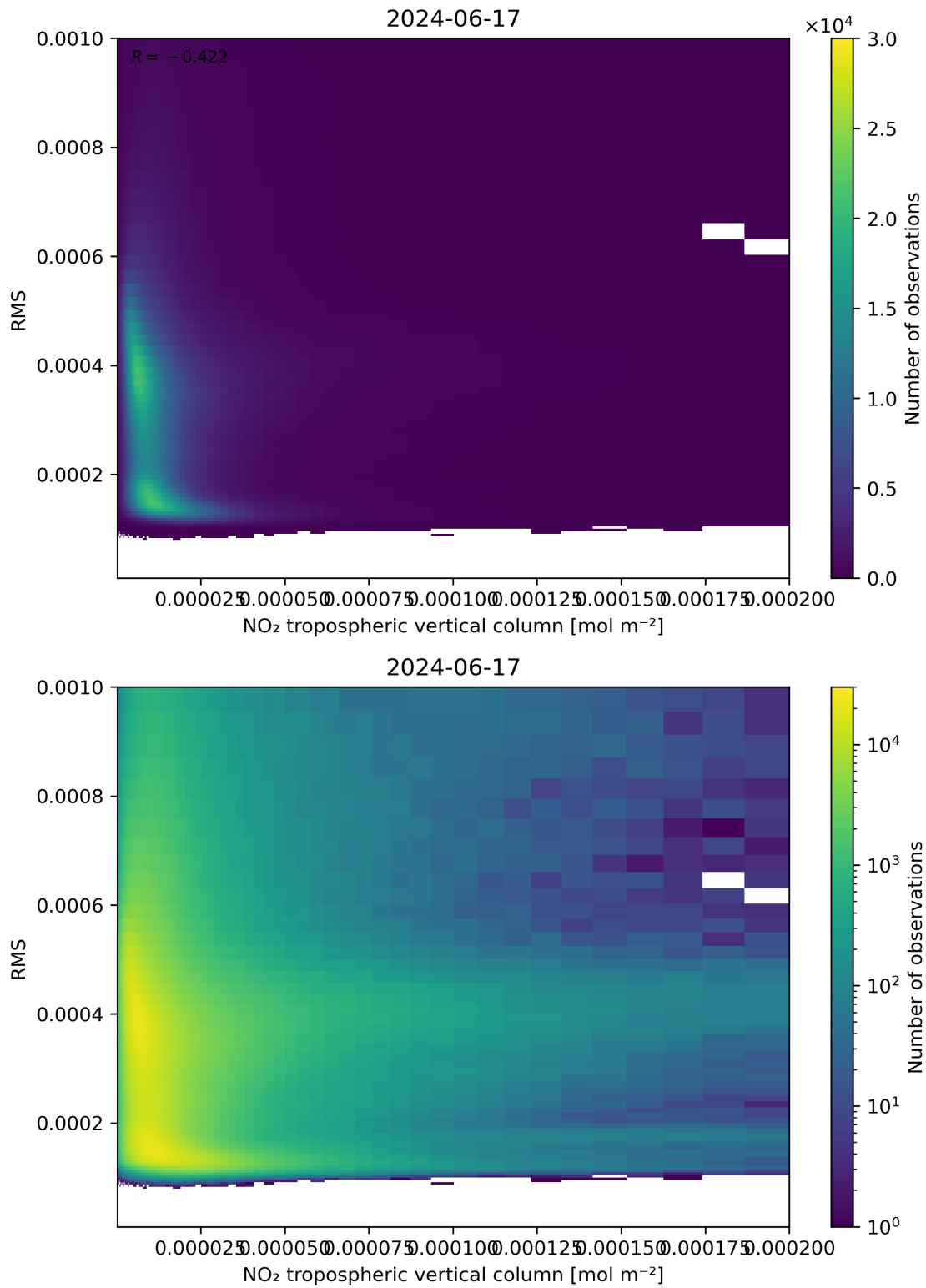
Figure 142: Scatter density plot of “NO 2 tropospheric vertical column” against “RMS” for 2024-06-16 to 2024-06-18.
