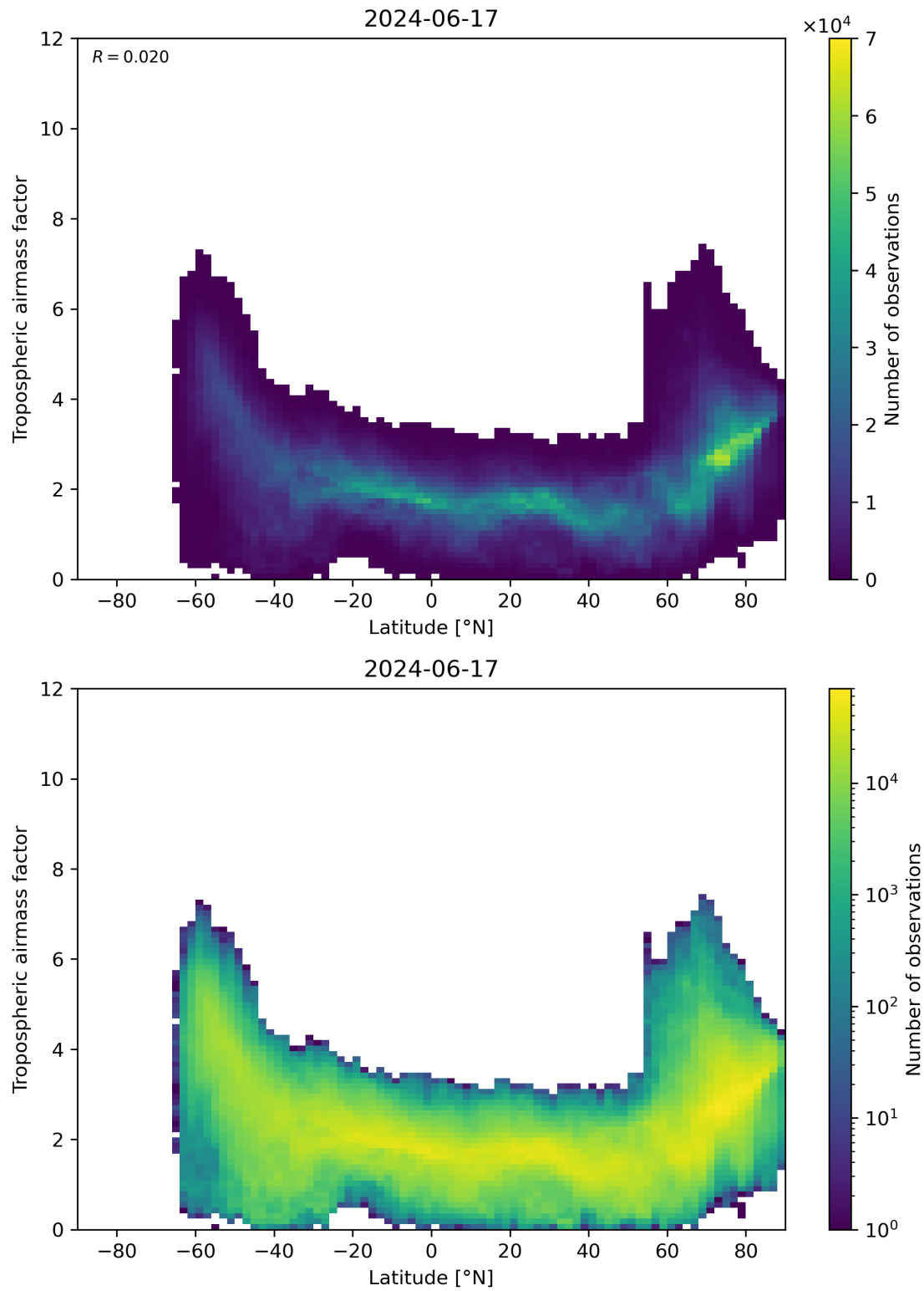
Figure 85: Scatter density plot of “Latitude” against “Tropospheric airmass factor” for 2024-06-16 to 2024-06-18.
