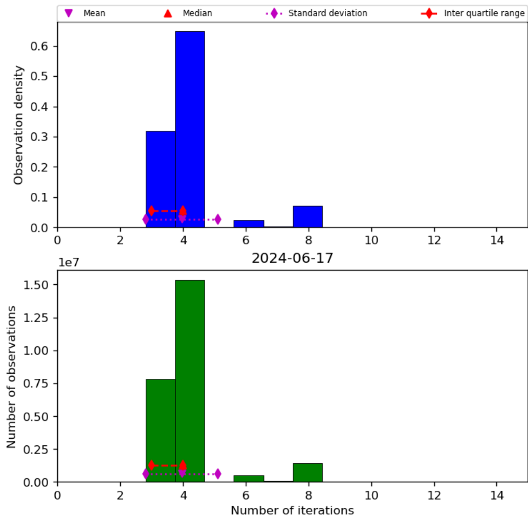
Figure 34: Histogram of “Number of iterations” for 2024-06-16 to 2024-06-18
