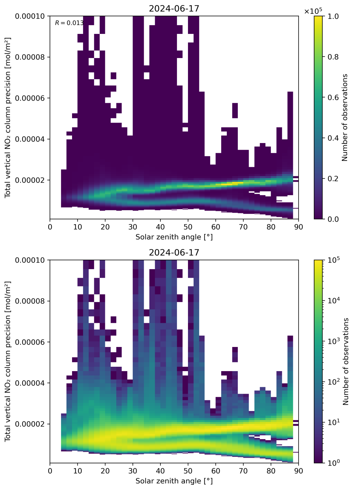
Figure 154: Scatter density plot of “Solar zenith angle” against “Total vertical NO 2 column precision” for 2024-06-16 to 2024-06-18.
