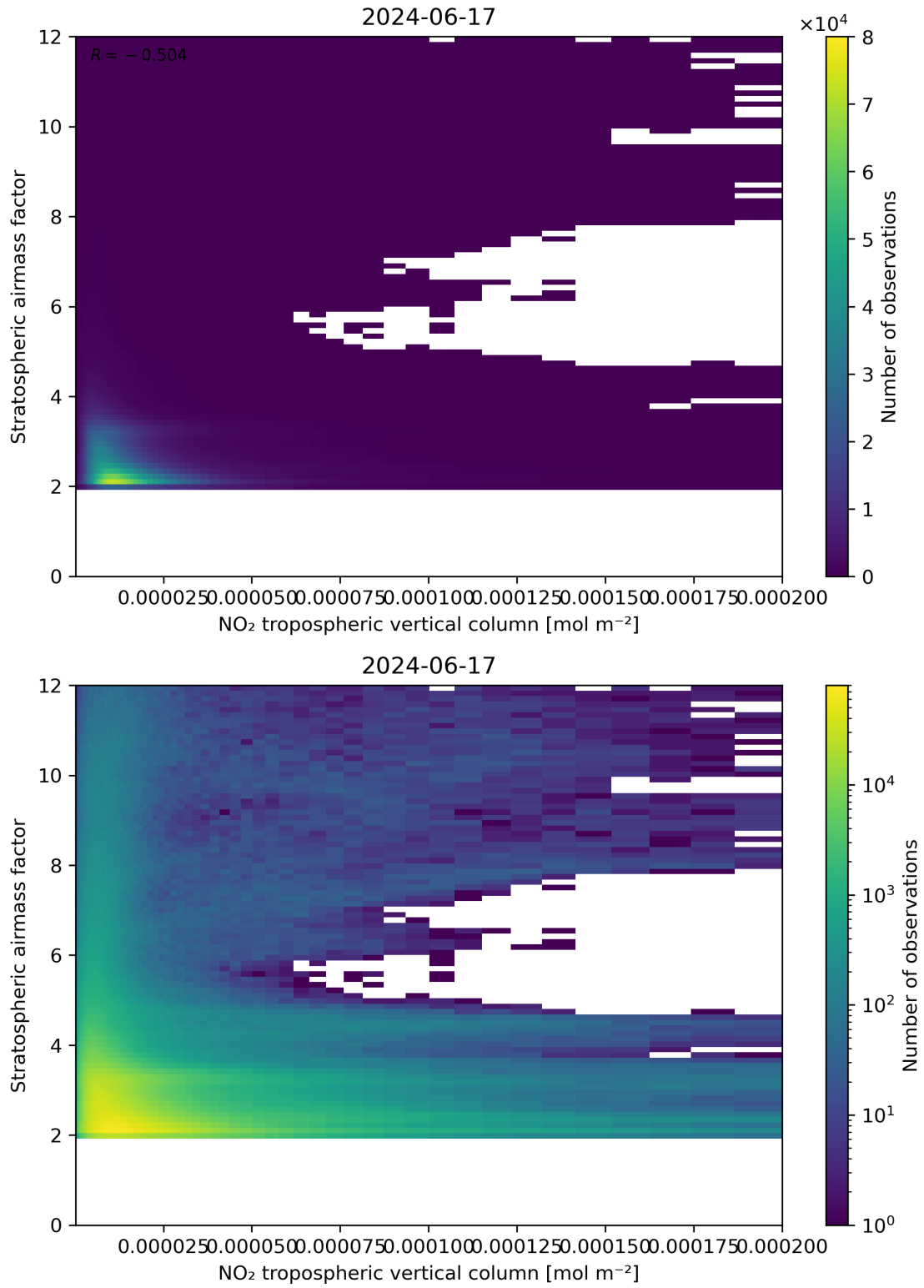
Figure 121: Scatter density plot of “NO 2 tropospheric vertical column” against “Stratospheric air mass factor” for 2024-06-16 to 2024-06-18.
