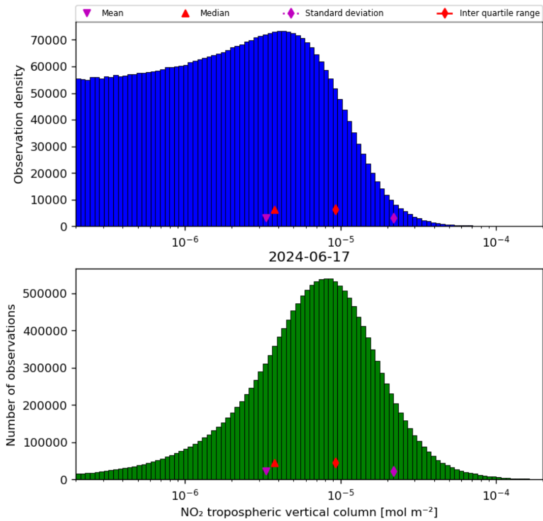
Figure 29: Histogram of “NO 2 tropospheric vertical column” for 2024-06-16 to 2024-06-18
