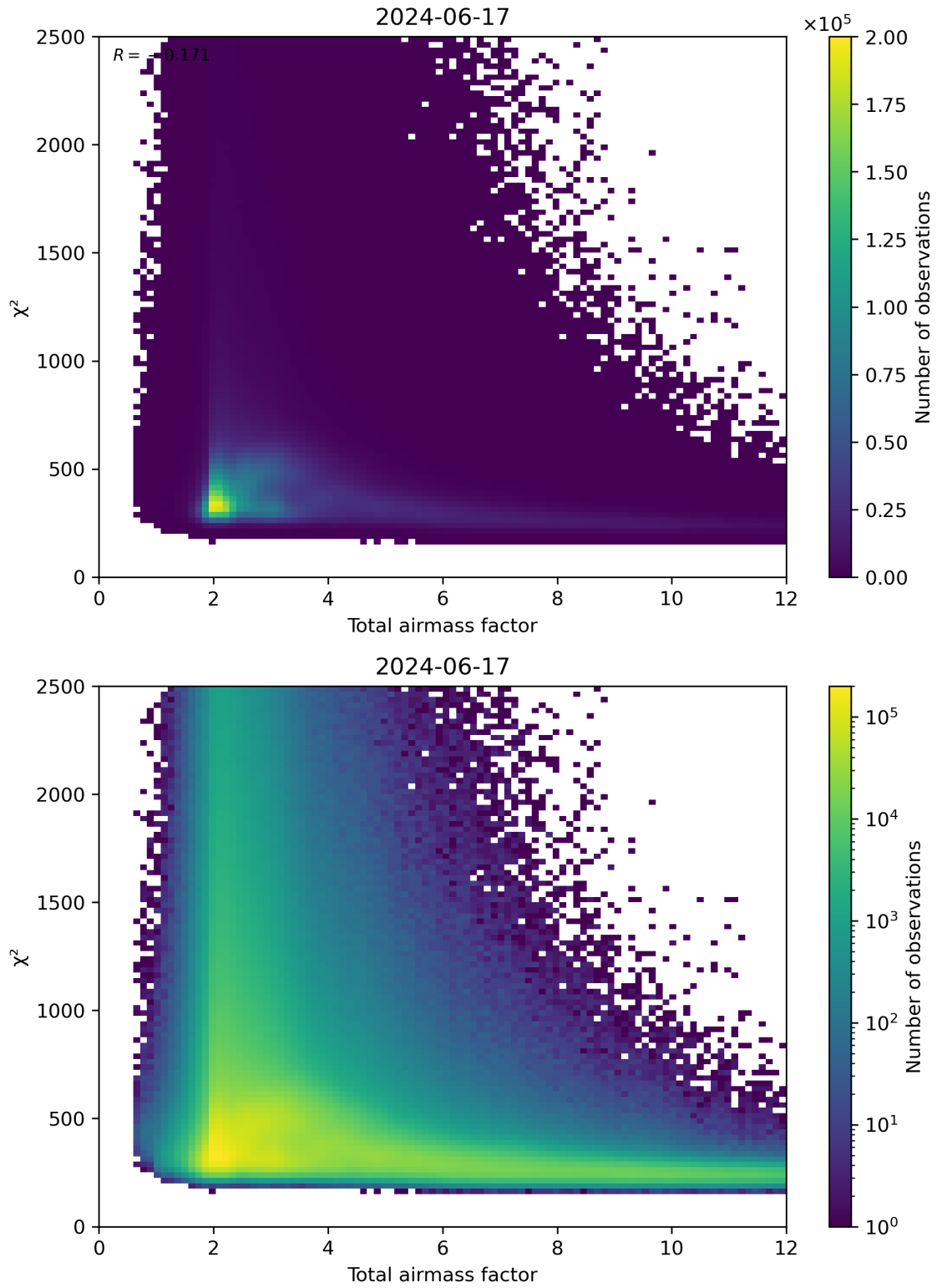
Figure 63: Scatter density plot of “Total airmass factor” against “ \chi^2 ” for 2024-06-16 to 2024-06-18.
