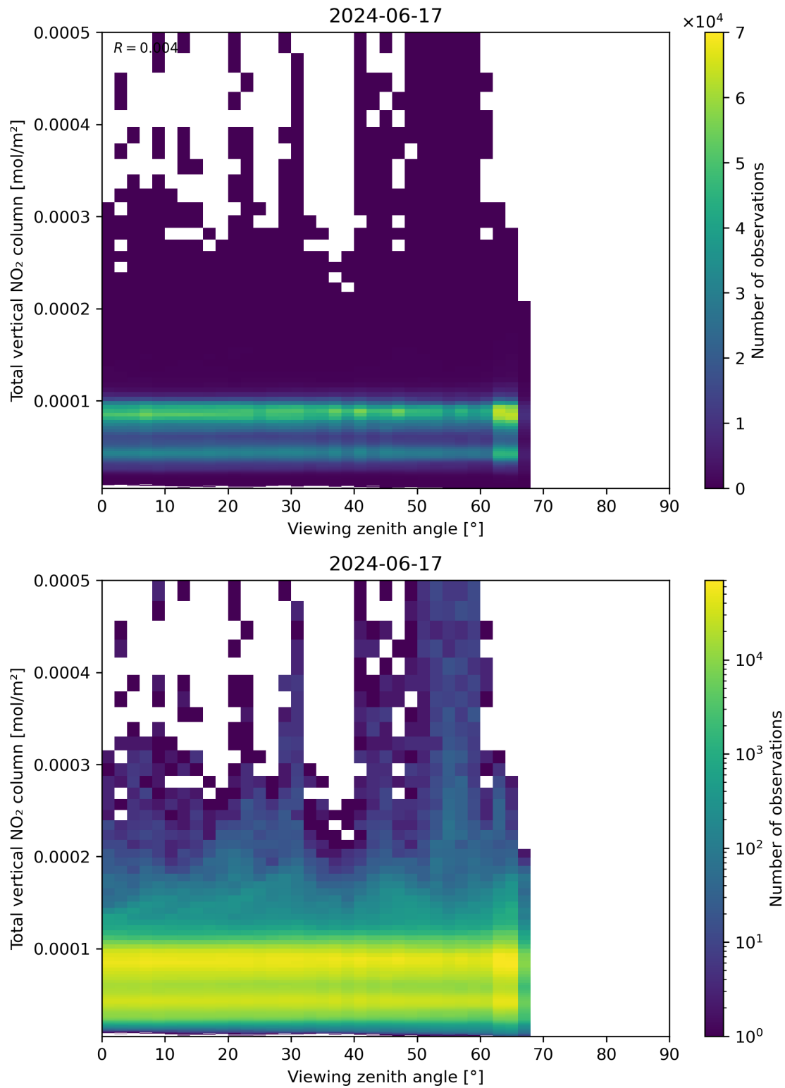
Figure 167: Scatter density plot of “Viewing zenith angle” against “Total vertical NO 2 column” for 2024-06-16 to 2024-06-18.
