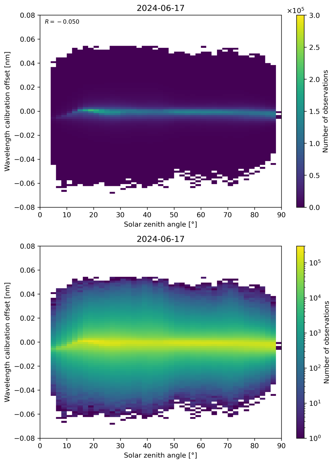
Figure 158: Scatter density plot of “Solar zenith angle” against “Wavelength calibration offset” for 2024-06-16 to 2024-06-18.
