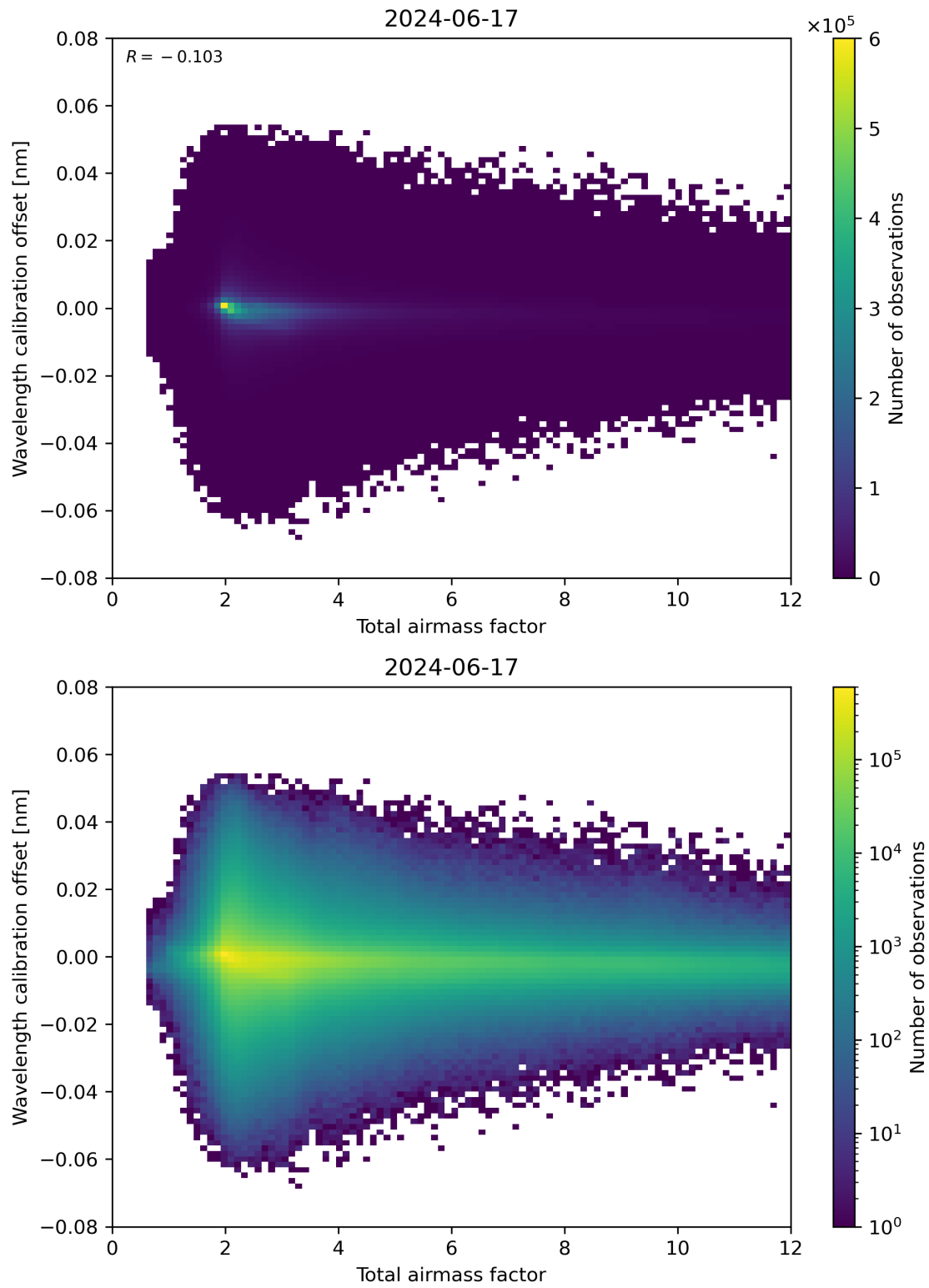
Figure 70: Scatter density plot of “Total airmass factor” against “Wavelength calibration offset” for 2024-06-16 to 2024-06-18.
