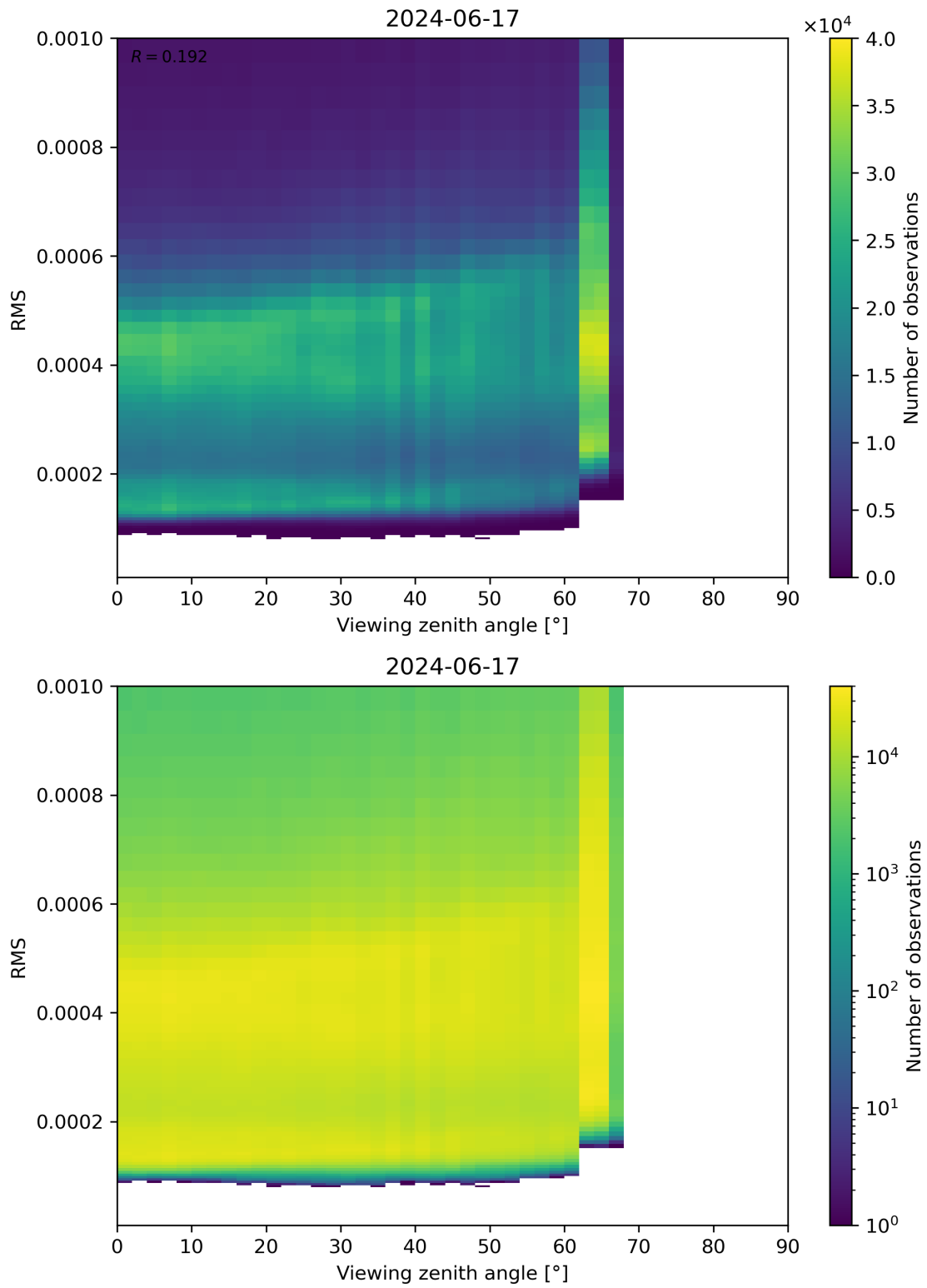
Figure 171: Scatter density plot of “Viewing zenith angle” against “RMS” for 2024-06-16 to 2024-06-18.
