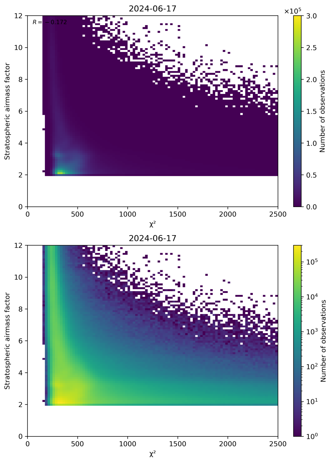
Figure 81: Scatter density plot of “ \chi^2 ” against “Stratospheric airmass factor” for 2024-06-16 to 2024-06-18.
