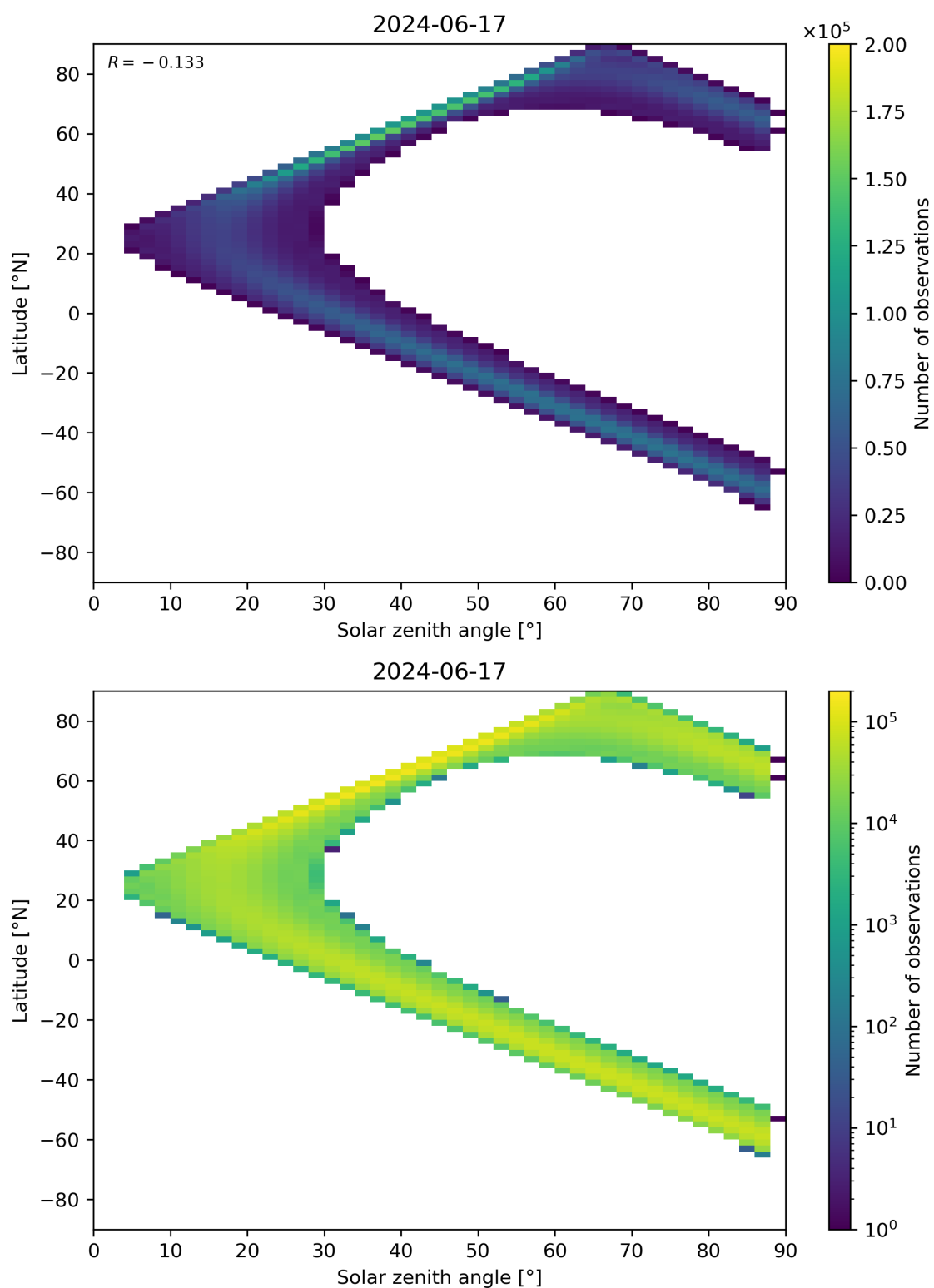
Figure 149: Scatter density plot of “Solar zenith angle” against “Latitude” for 2024-06-16 to 2024-06-18.
