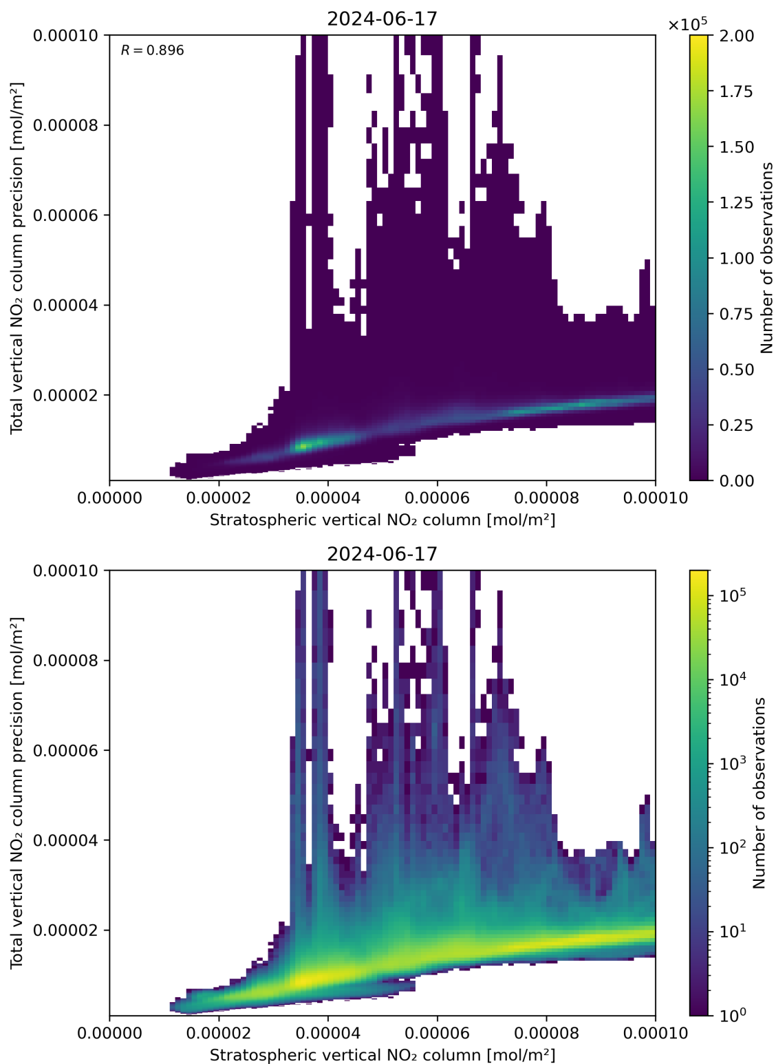
Figure 101: Scatter density plot of “Stratospheric vertical NO 2 column” against “Total vertical NO 2 column precision” for 2024-06-16 to 2024-06-18.
