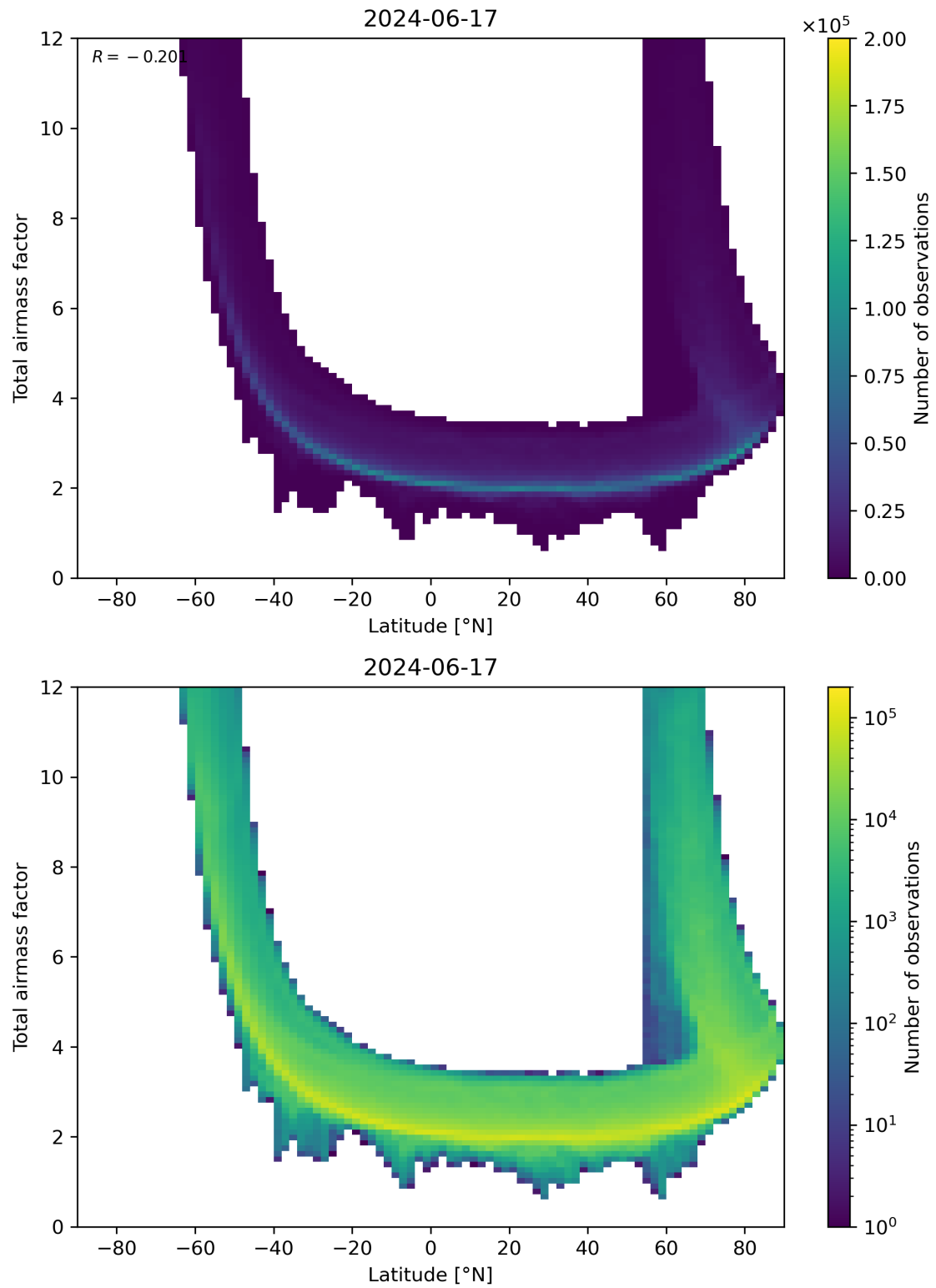
Figure 84: Scatter density plot of “Latitude” against “Total airmass factor” for 2024-06-16 to 2024-06-18.
