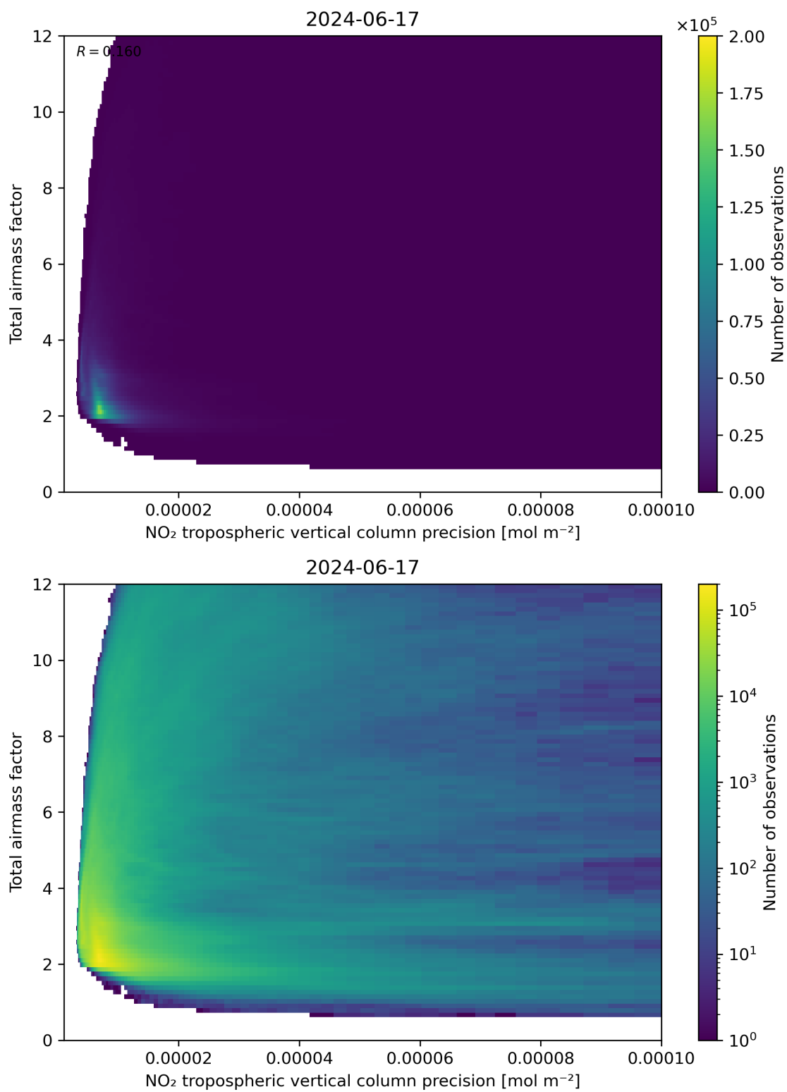
Figure 132: Scatter density plot of “NO 2 tropospheric vertical column precision” against “Total air mass factor” for 2024-06-16 to 2024-06-18.
