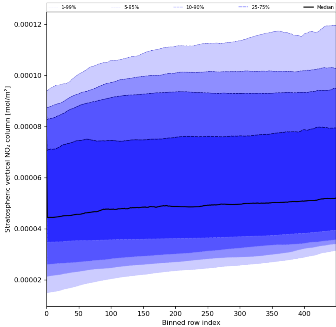
Figure 53: Along track statistics of “Stratospheric vertical NO 2 column” for 2024-06-16 to 2024-06-18
