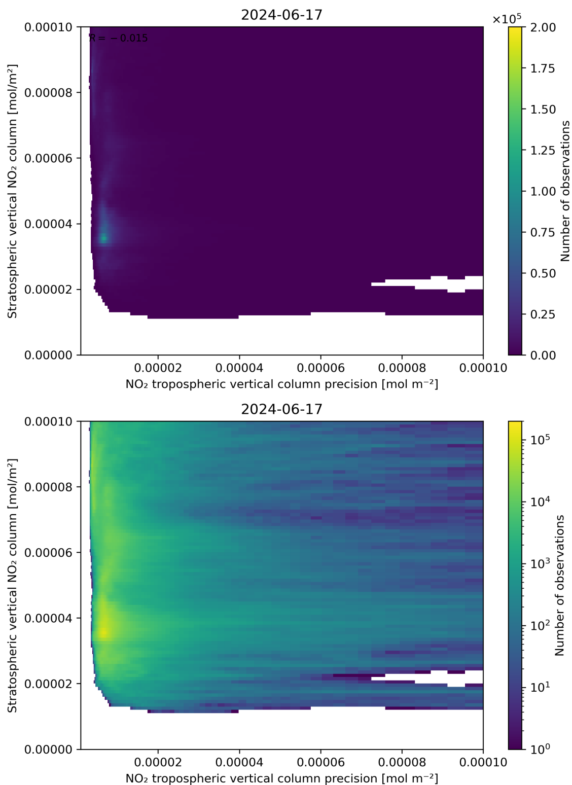
Figure 135: Scatter density plot of “NO 2 tropospheric vertical column precision” against “Stratospheric vertical NO 2 column” for 2024-06-16 to 2024-06-18.
