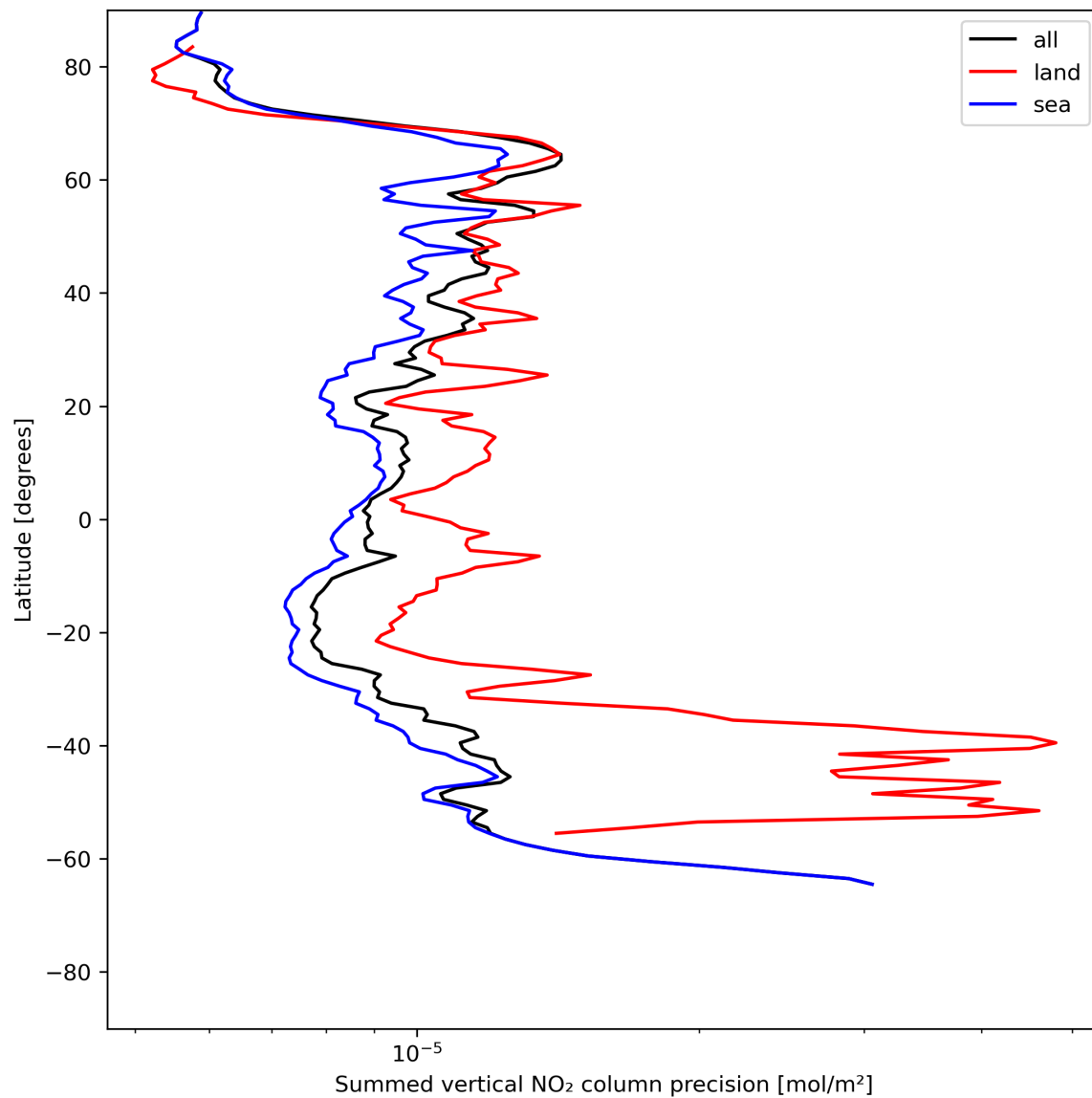
Figure 24: Zonal average of “Summed vertical NO 2 column precision” for 2024-06-16 to 2024-06-18.
