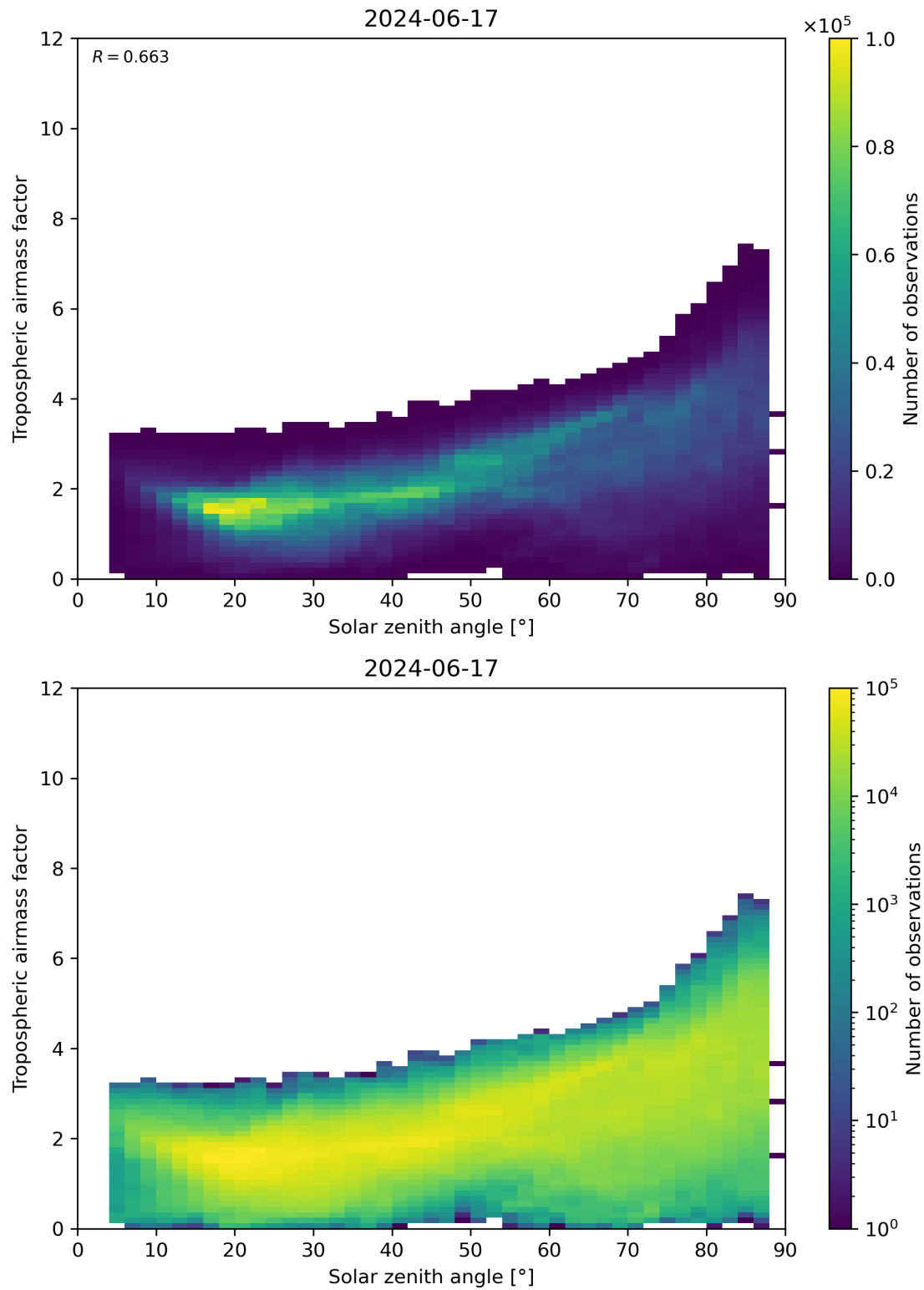
Figure 147: Scatter density plot of “Solar zenith angle” against “Tropospheric airmass factor” for 2024-06-16 to 2024-06-18.
