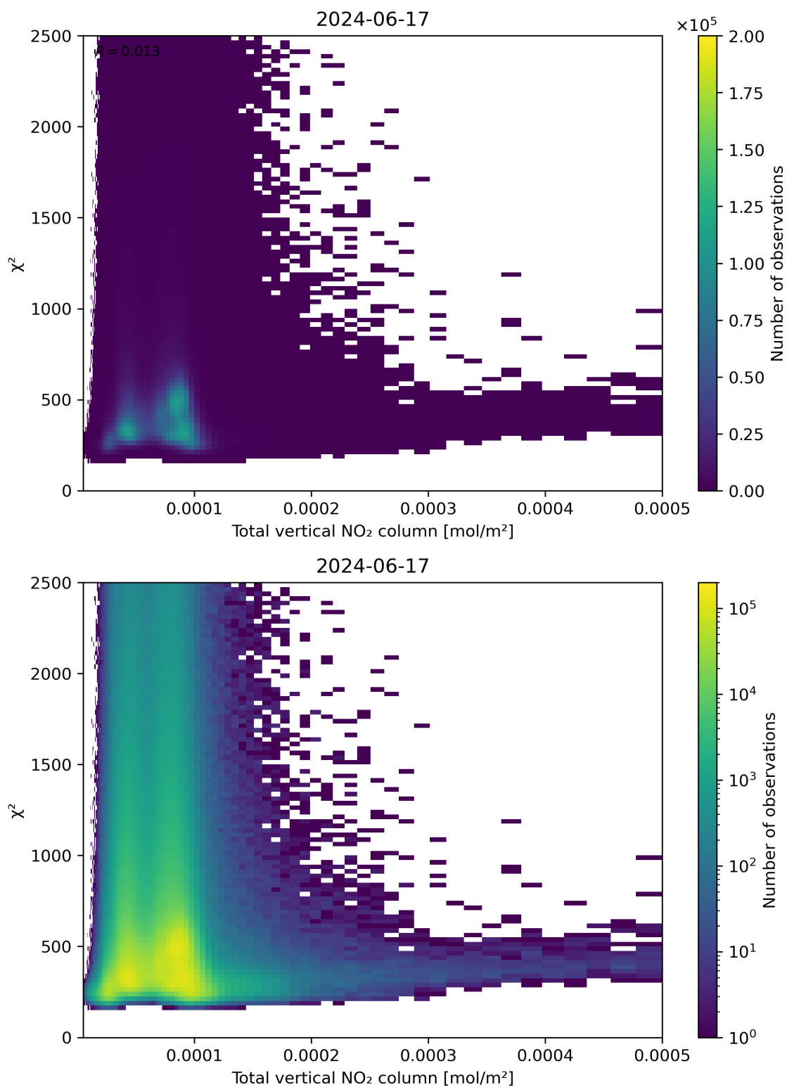
Figure 111: Scatter density plot of “Total vertical NO 2 column” against “ \chi^2 ” for 2024-06-16 to 2024-06-18.
