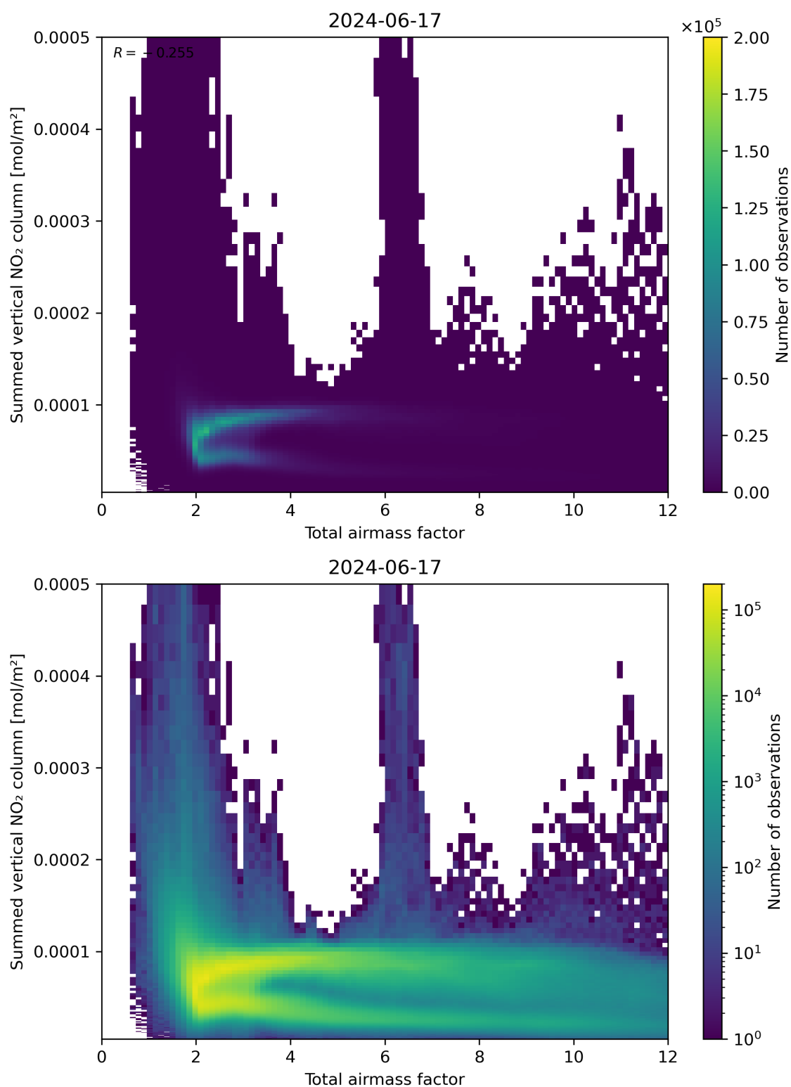
Figure 65: Scatter density plot of “Total airmass factor” against “Summed vertical NO 2 column” for 2024-06-16 to 2024-06-18.
