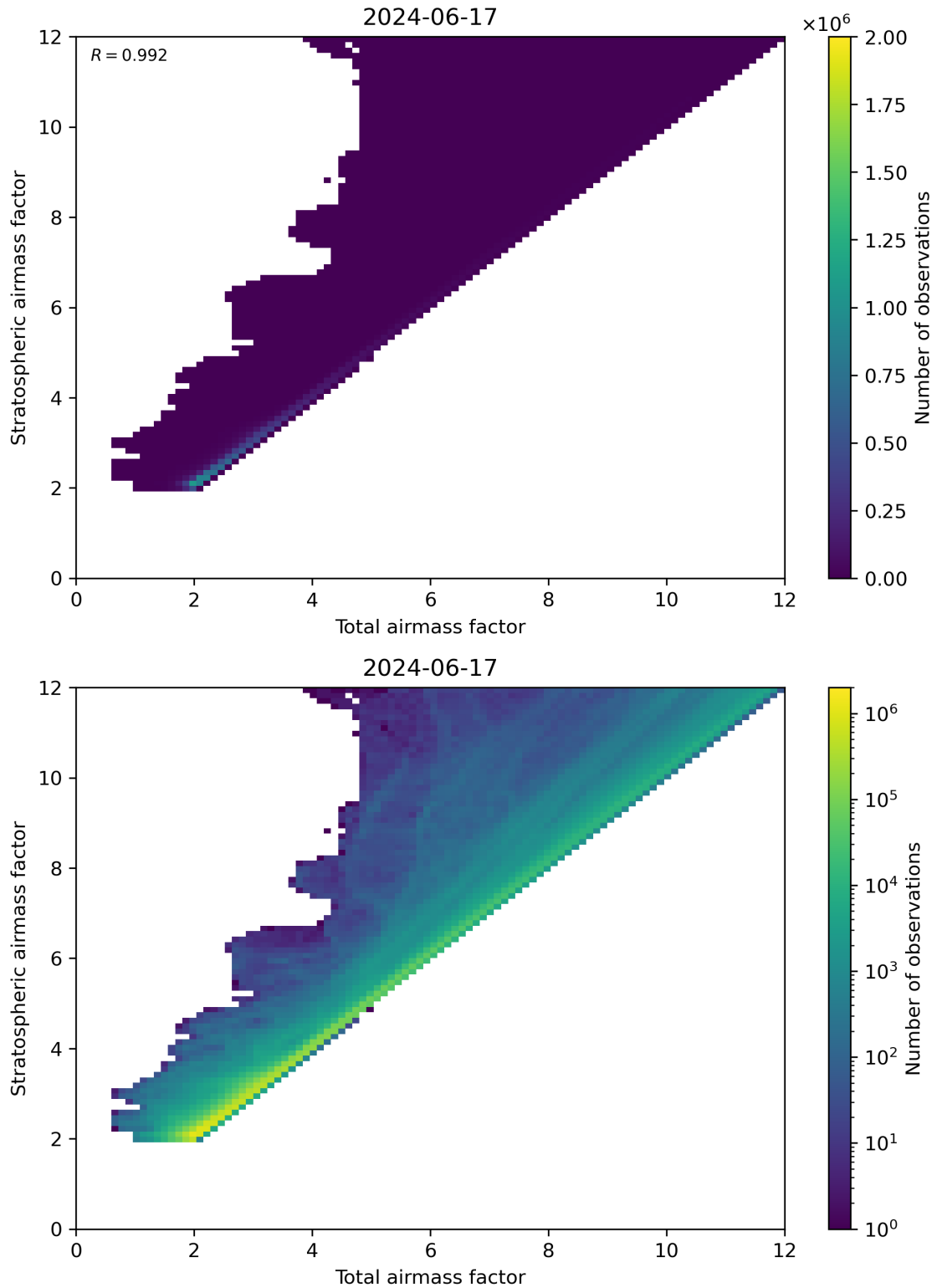
Figure 62: Scatter density plot of “Total airmass factor” against “Stratospheric airmass factor” for 2024-06-16 to 2024-06-18.
