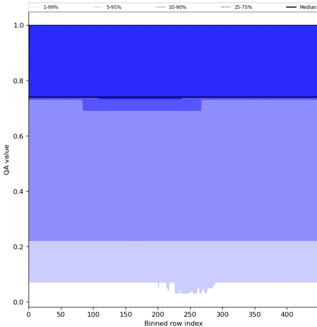
Figure 45: Along track statistics of “QA value” for 2024-06-16 to 2024-06-18
