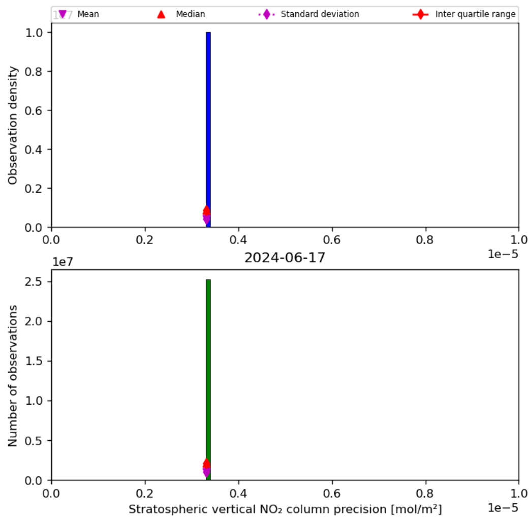
Figure 37: Histogram of “Stratospheric vertical NO 2 column precision” for 2024-06-16 to 2024-06-18
