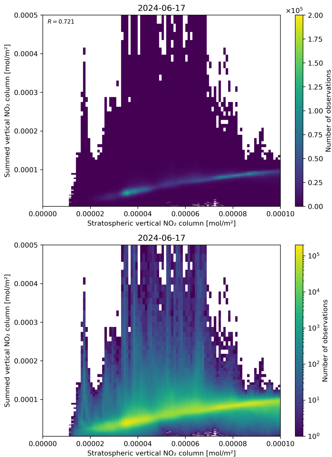
Figure 98: Scatter density plot of “Stratospheric vertical NO 2 column” against “Summed vertical NO 2 column” for 2024-06-16 to 2024-06-18.
