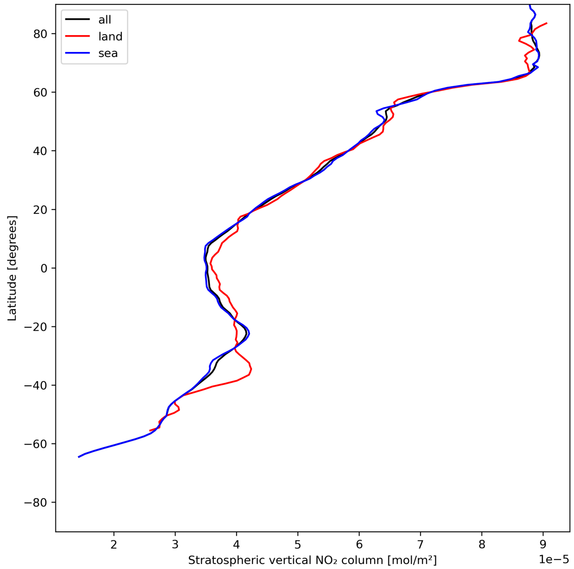
Figure 19: Zonal average of “Stratospheric vertical NO 2 column” for 2024-06-16 to 2024-06-18.
