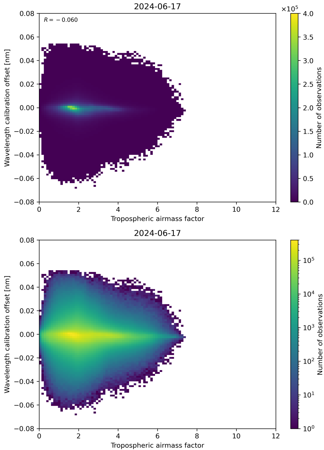
Figure 80: Scatter density plot of “Tropospheric airmass factor” against “Wavelength calibration offset” for 2024-06-16 to 2024-06-18.
