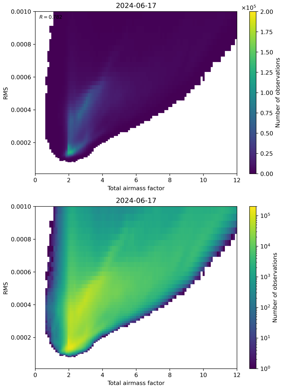
Figure 69: Scatter density plot of “Total airmass factor” against “RMS” for 2024-06-16 to 2024-06-18.
