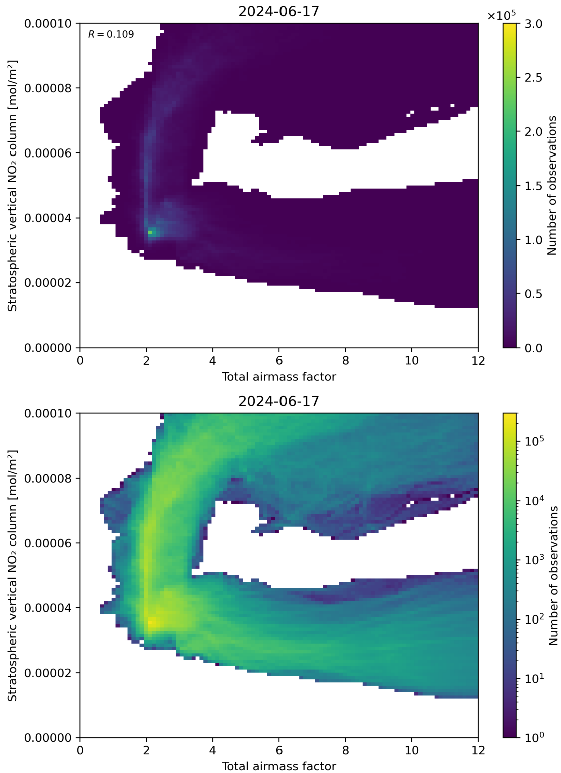
Figure 64: Scatter density plot of “Total airmass factor” against “Stratospheric vertical NO 2 column” for 2024-06-16 to 2024-06-18.
