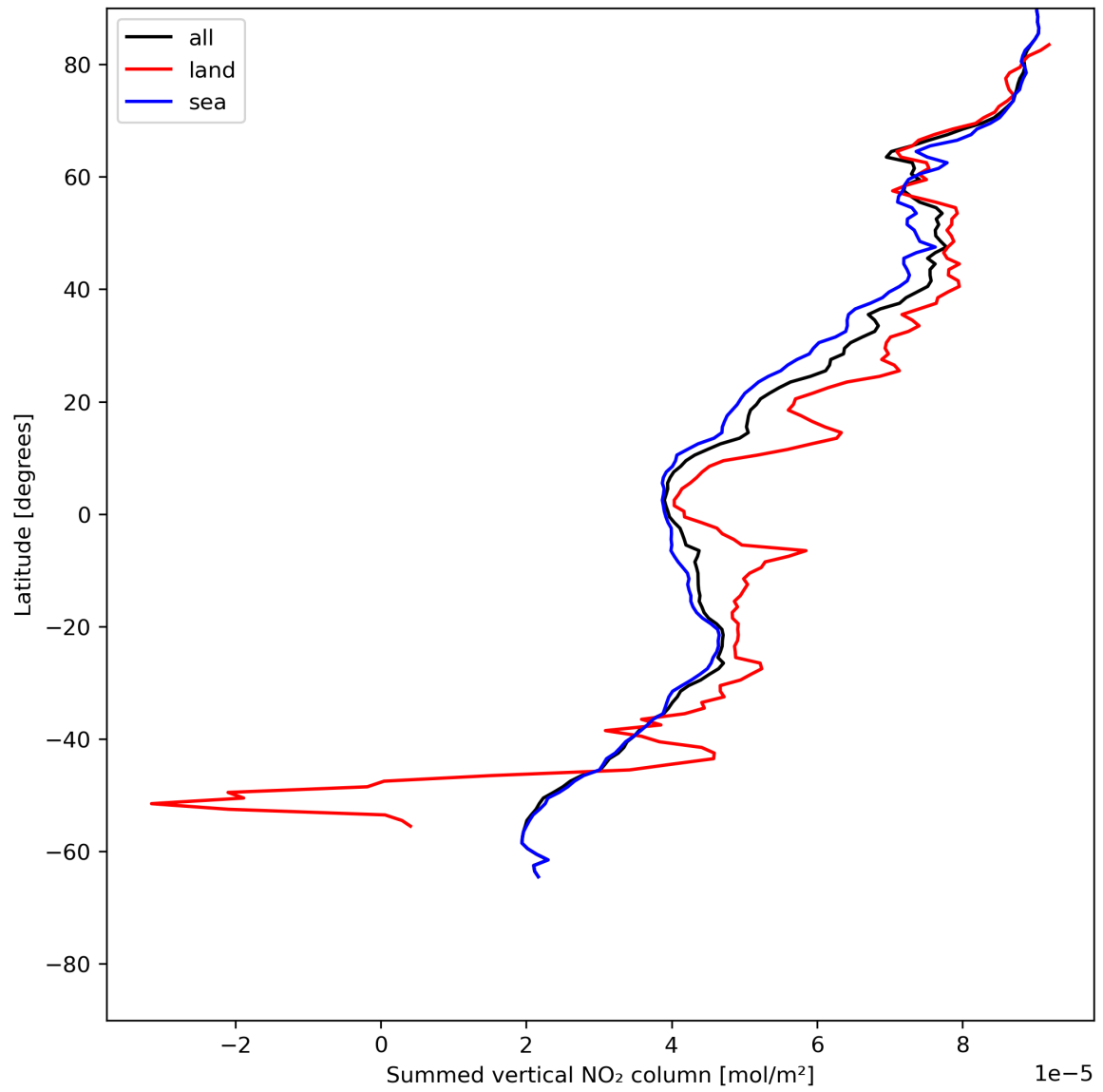
Figure 23: Zonal average of “Summed vertical NO 2 column” for 2024-06-16 to 2024-06-18.
