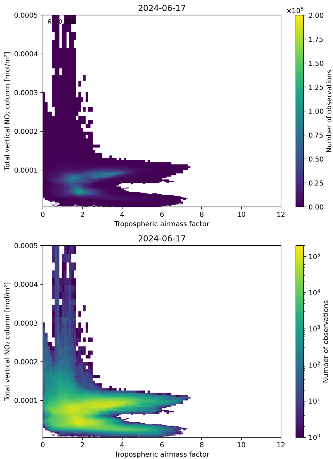
Figure 77: Scatter density plot of “Tropospheric airmass factor” against “Total vertical NO 2 column” for 2024-06-16 to 2024-06-18.
