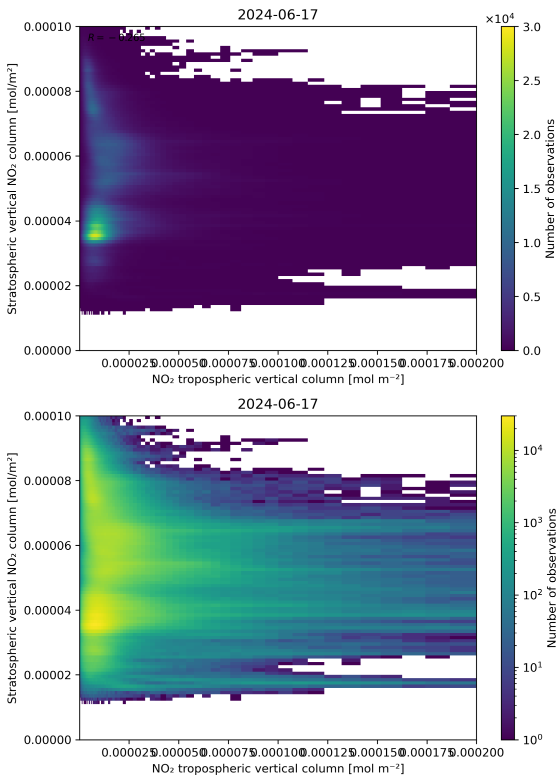
Figure 125: Scatter density plot of “NO 2 tropospheric vertical column” against “Stratospheric vertical NO 2 column” for 2024-06-16 to 2024-06-18.
