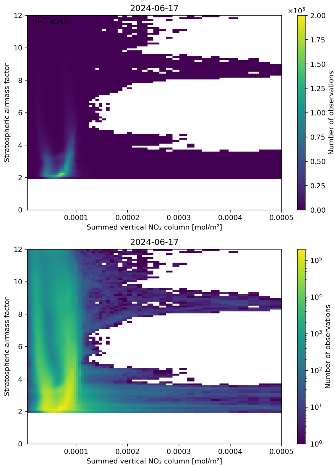
Figure 103: Scatter density plot of “Summed vertical NO 2 column” against “Stratospheric air mass factor” for 2024-06-16 to 2024-06-18.
