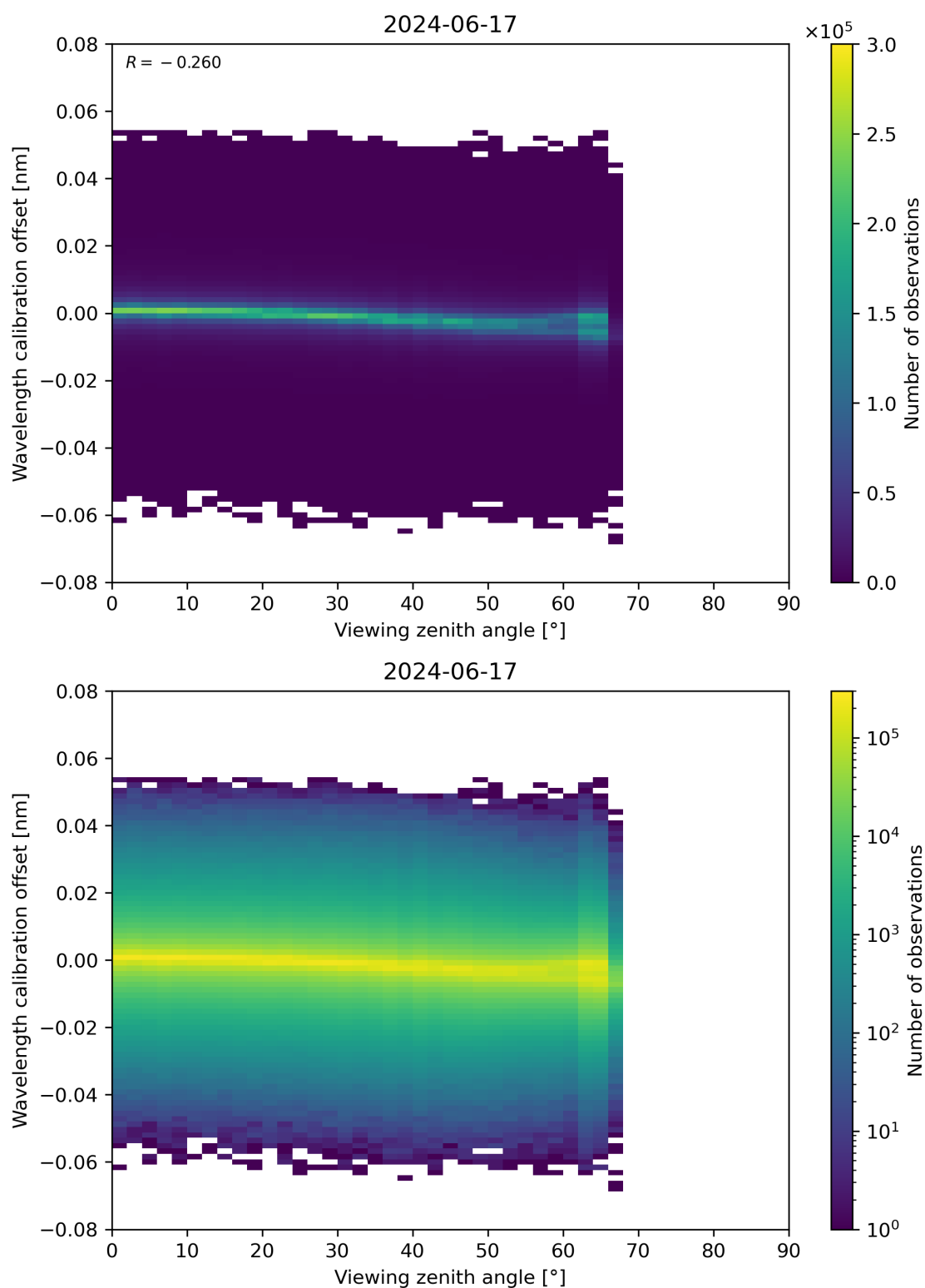
Figure 173: Scatter density plot of “Viewing zenith angle” against “Wavelength calibration offset” for 2024-06-16 to 2024-06-18.
