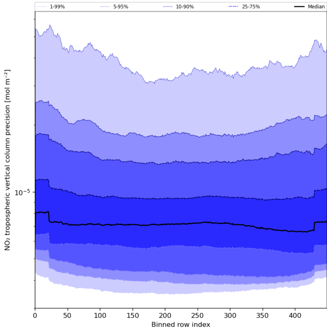
Figure 47: Along track statistics of “NO 2 tropospheric vertical column precision” for 2024-06-16 to 2024-06-18
