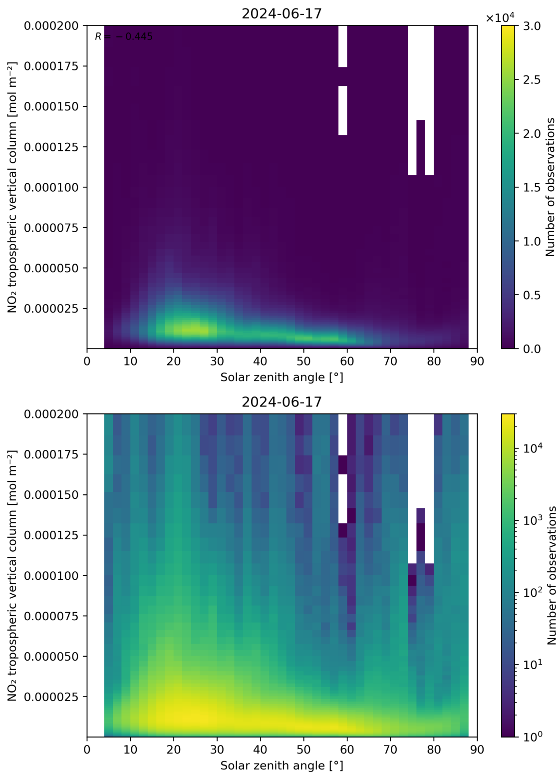
Figure 155: Scatter density plot of “Solar zenith angle” against “NO 2 tropospheric vertical column” for 2024-06-16 to 2024-06-18.
