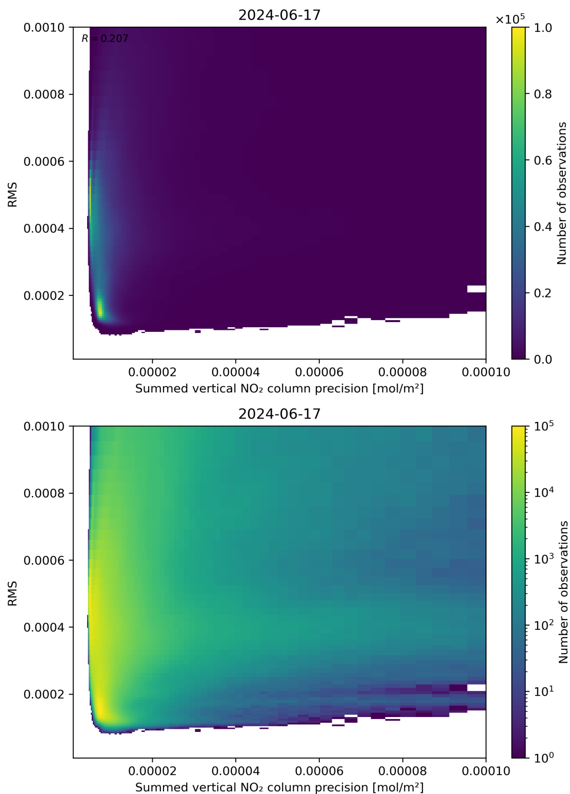
Figure 108: Scatter density plot of “Summed vertical NO 2 column precision” against “RMS” for 2024-06-16 to 2024-06-18.
