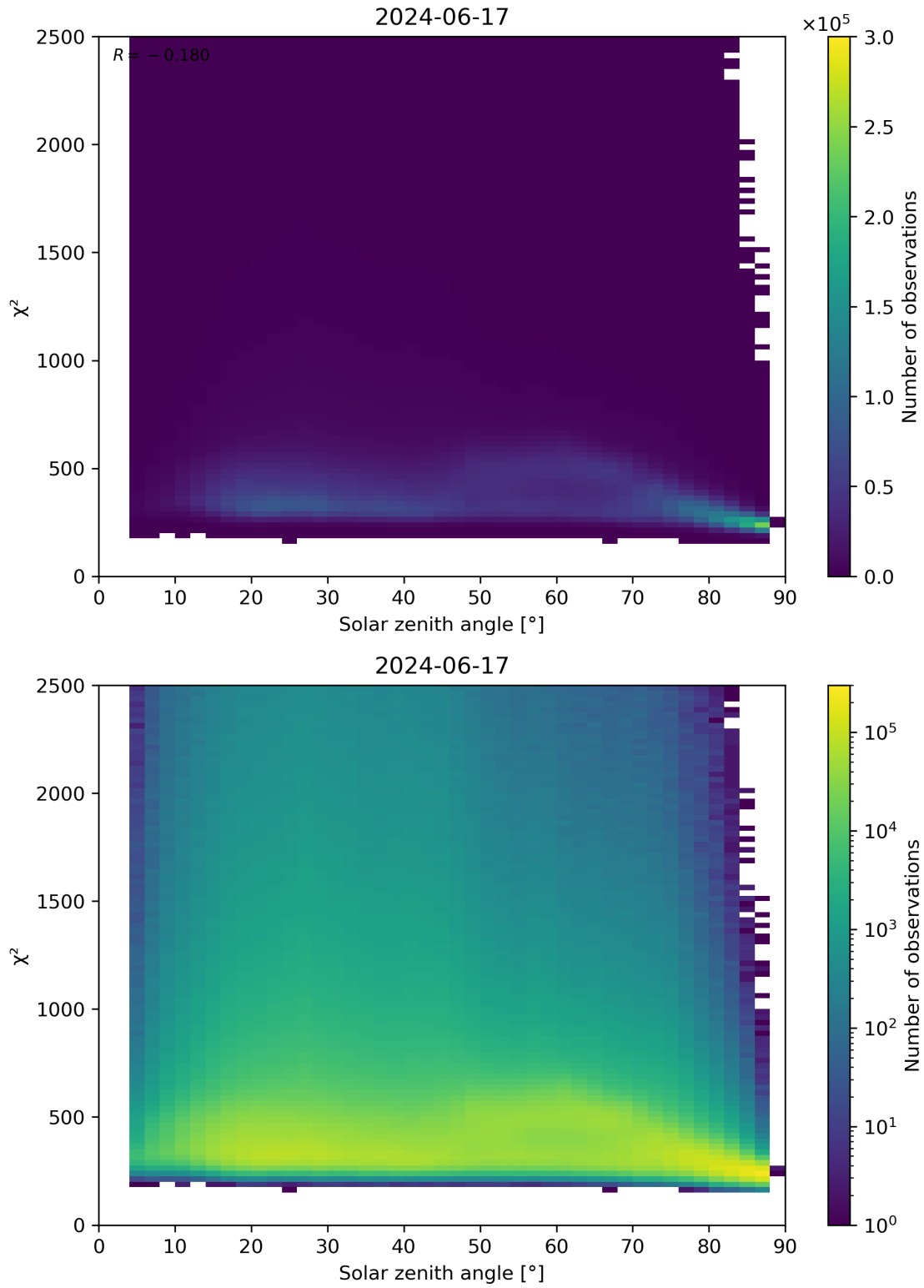
Figure 148: Scatter density plot of “Solar zenith angle” against “ \chi^2 ” for 2024-06-16 to 2024-06-18.
