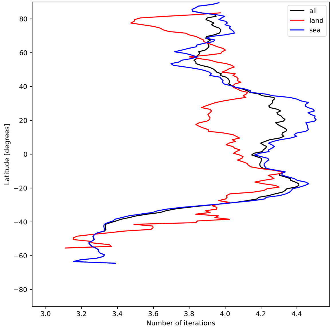
Figure 17: Zonal average of “Number of iterations” for 2024-06-16 to 2024-06-18.
