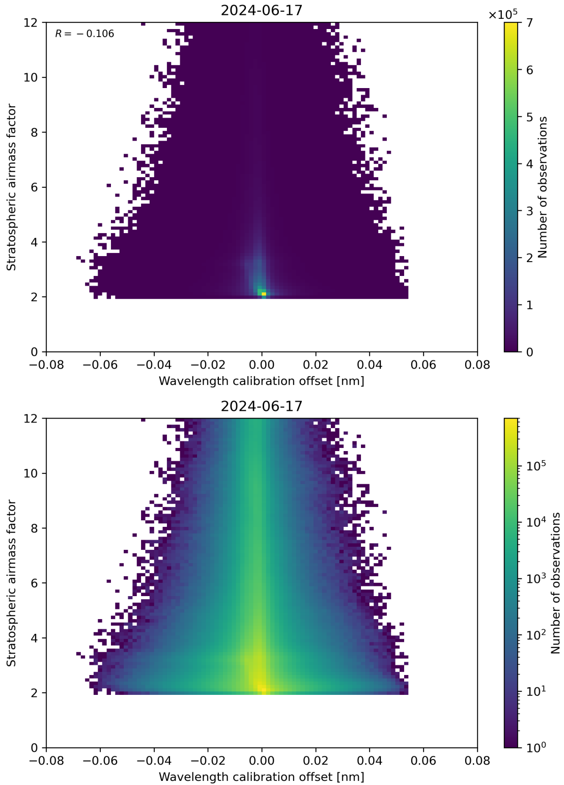
Figure 174: Scatter density plot of “Wavelength calibration offset” against “Stratospheric air mass factor” for 2024-06-16 to 2024-06-18.
