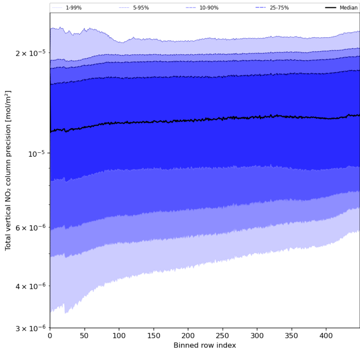
Figure 56: Along track statistics of “Total vertical NO 2 column precision” for 2024-06-16 to 2024-06-18
