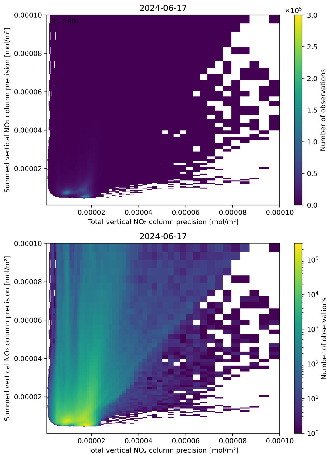
Figure 118: Scatter density plot of “Total vertical NO 2 column precision” against “Summed vertical NO 2 column precision” for 2024-06-16 to 2024-06-18.
