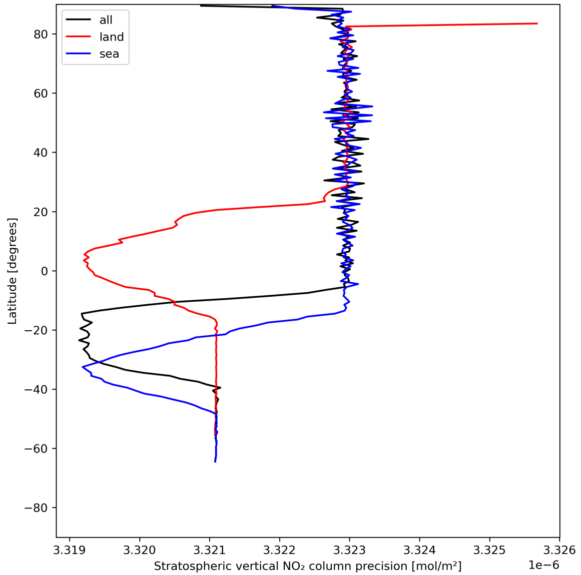
Figure 20: Zonal average of “Stratospheric vertical NO 2 column precision” for 2024-06-16 to 2024-06-18.
