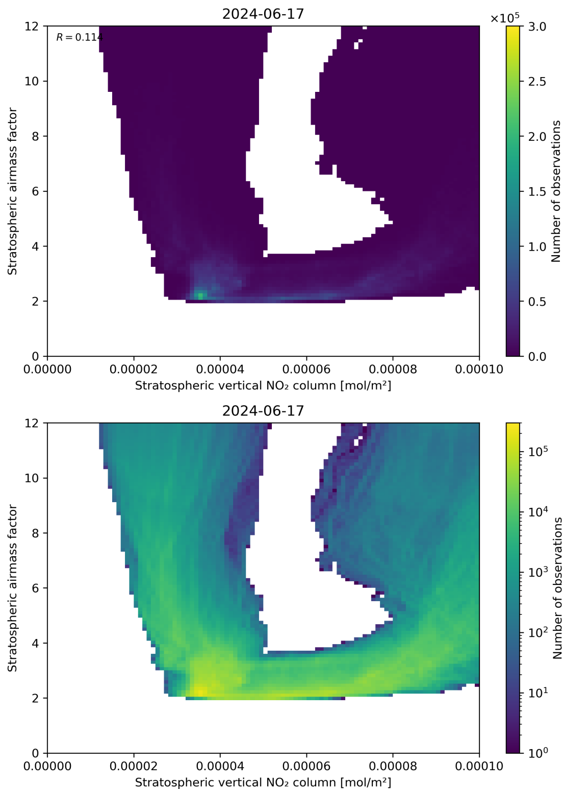
Figure 96: Scatter density plot of “Stratospheric vertical NO 2 column” against “Stratospheric airmass factor” for 2024-06-16 to 2024-06-18.
