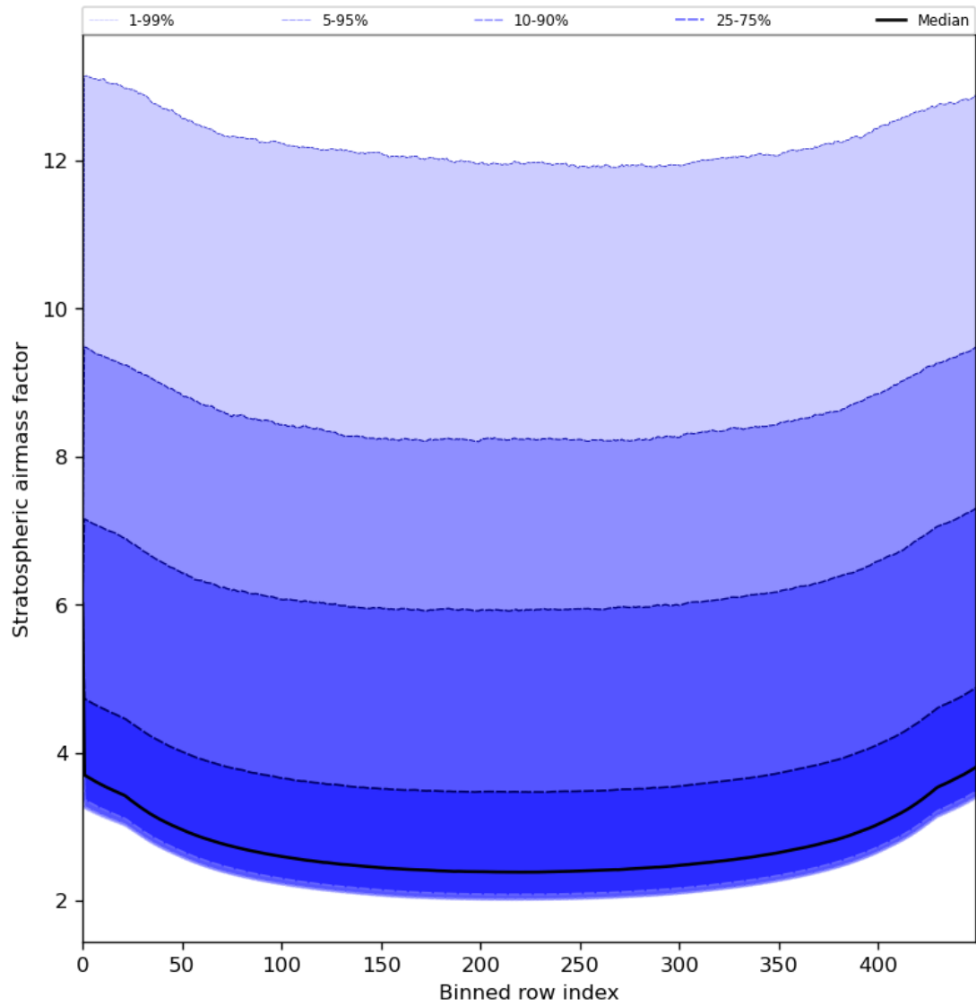
Figure 61: Along track statistics of “Stratospheric airmass factor” for 2024-06-16 to 2024-06-18
