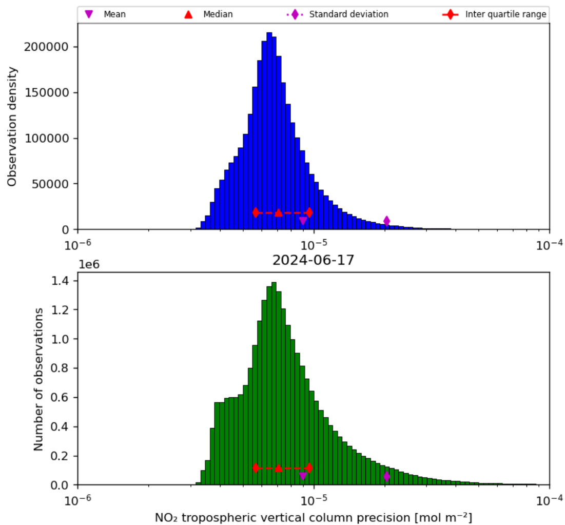
Figure 30: Histogram of “NO 2 tropospheric vertical column precision” for 2024-06-16 to 2024-06-18
