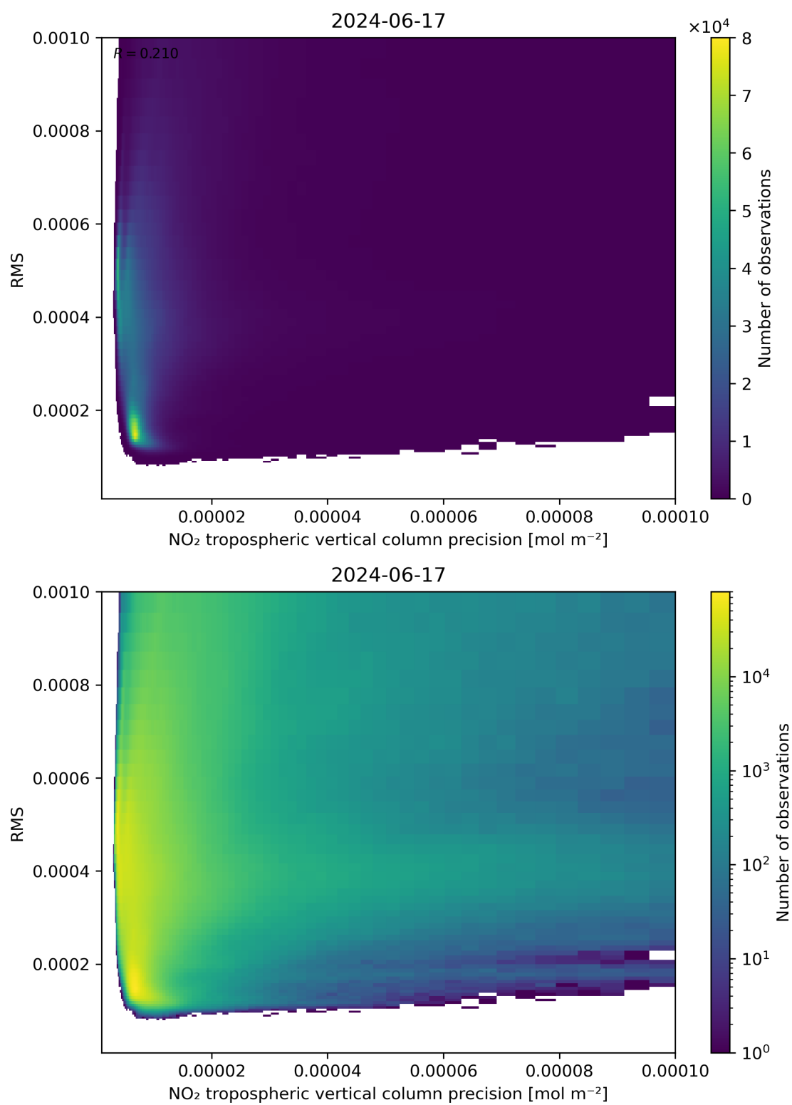
Figure 140: Scatter density plot of “NO 2 tropospheric vertical column precision” against “RMS” for 2024-06-16 to 2024-06-18.
