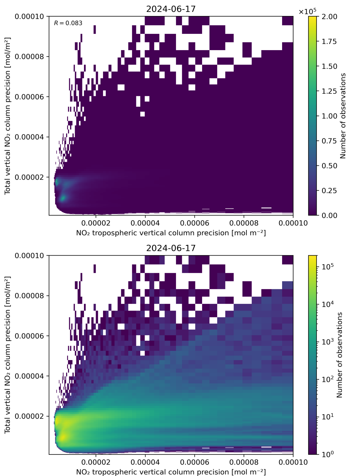
Figure 139: Scatter density plot of “NO 2 tropospheric vertical column precision” against “Total vertical NO 2 column precision” for 2024-06-16 to 2024-06-18.
