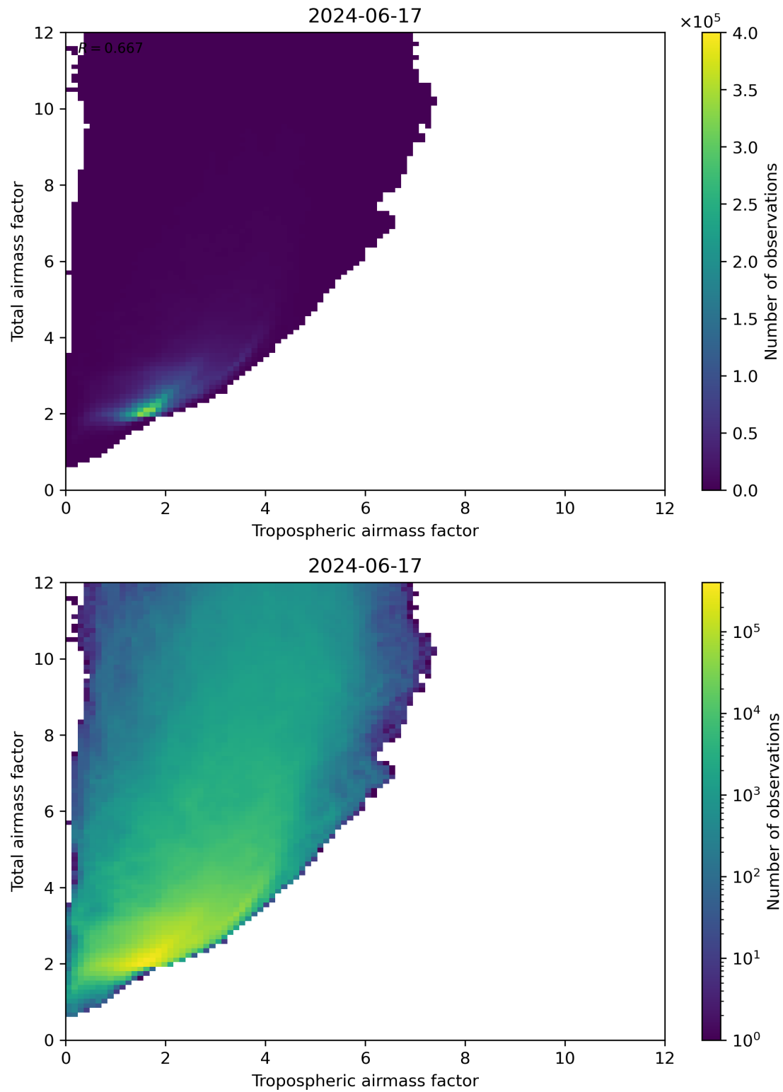
Figure 72: Scatter density plot of “Tropospheric airmass factor” against “Total airmass factor” for 2024-06-16 to 2024-06-18.
