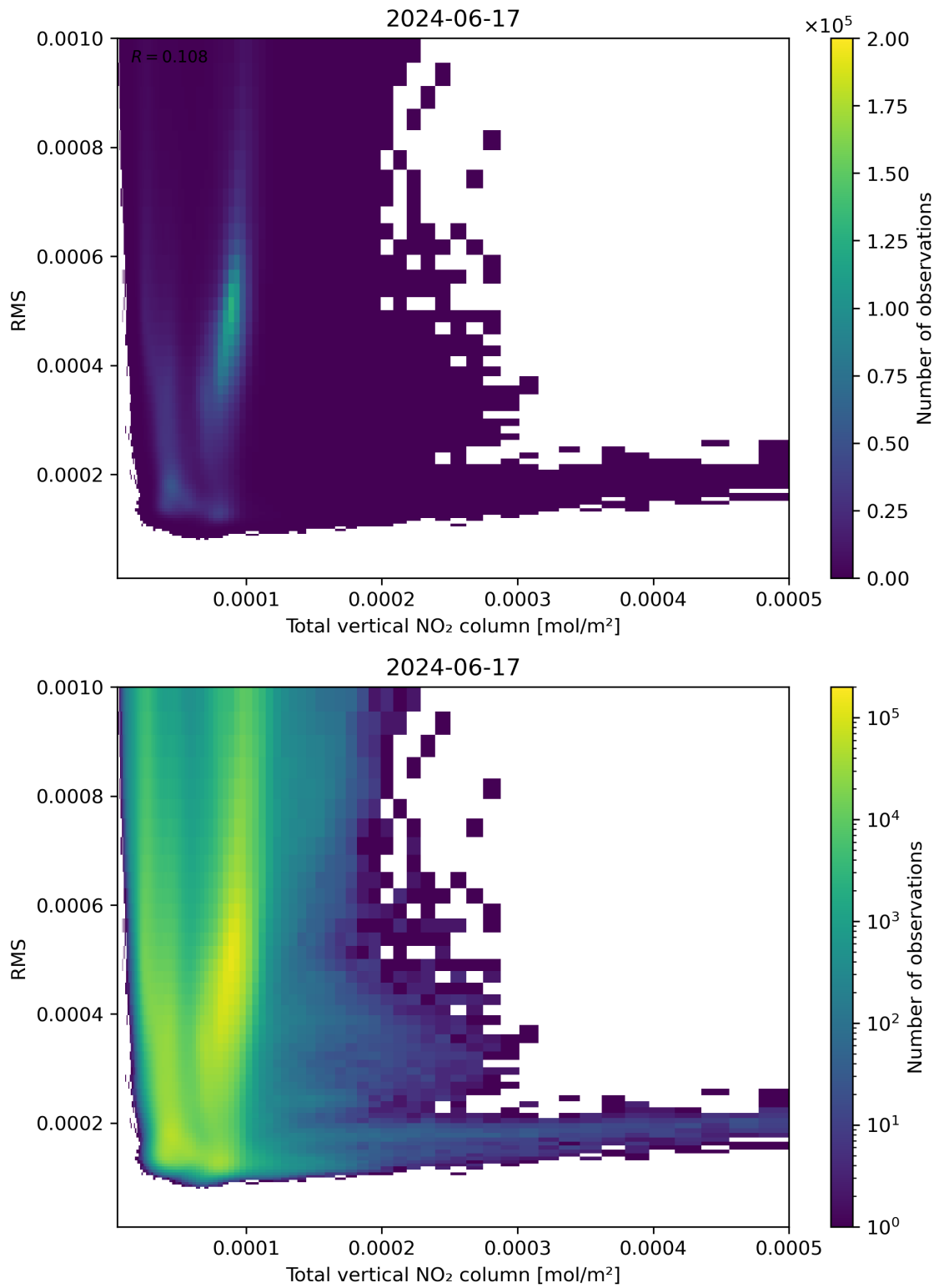
Figure 120: Scatter density plot of “Total vertical NO 2 column” against “RMS” for 2024-06-16 to 2024-06-18.
