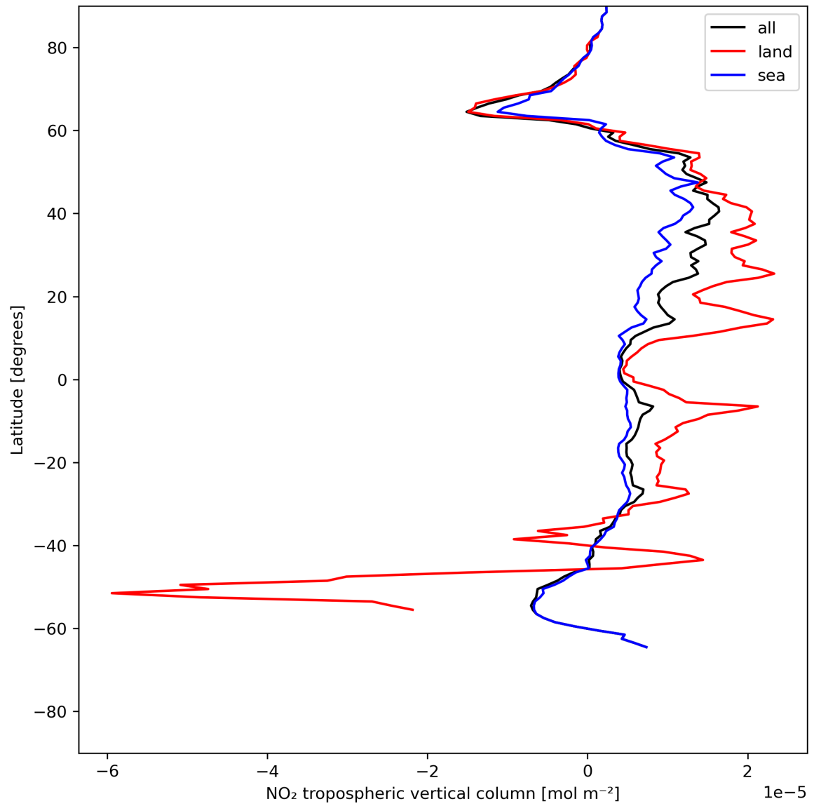
Figure 12: Zonal average of “NO 2 tropospheric vertical column” for 2024-06-16 to 2024-06-18.
