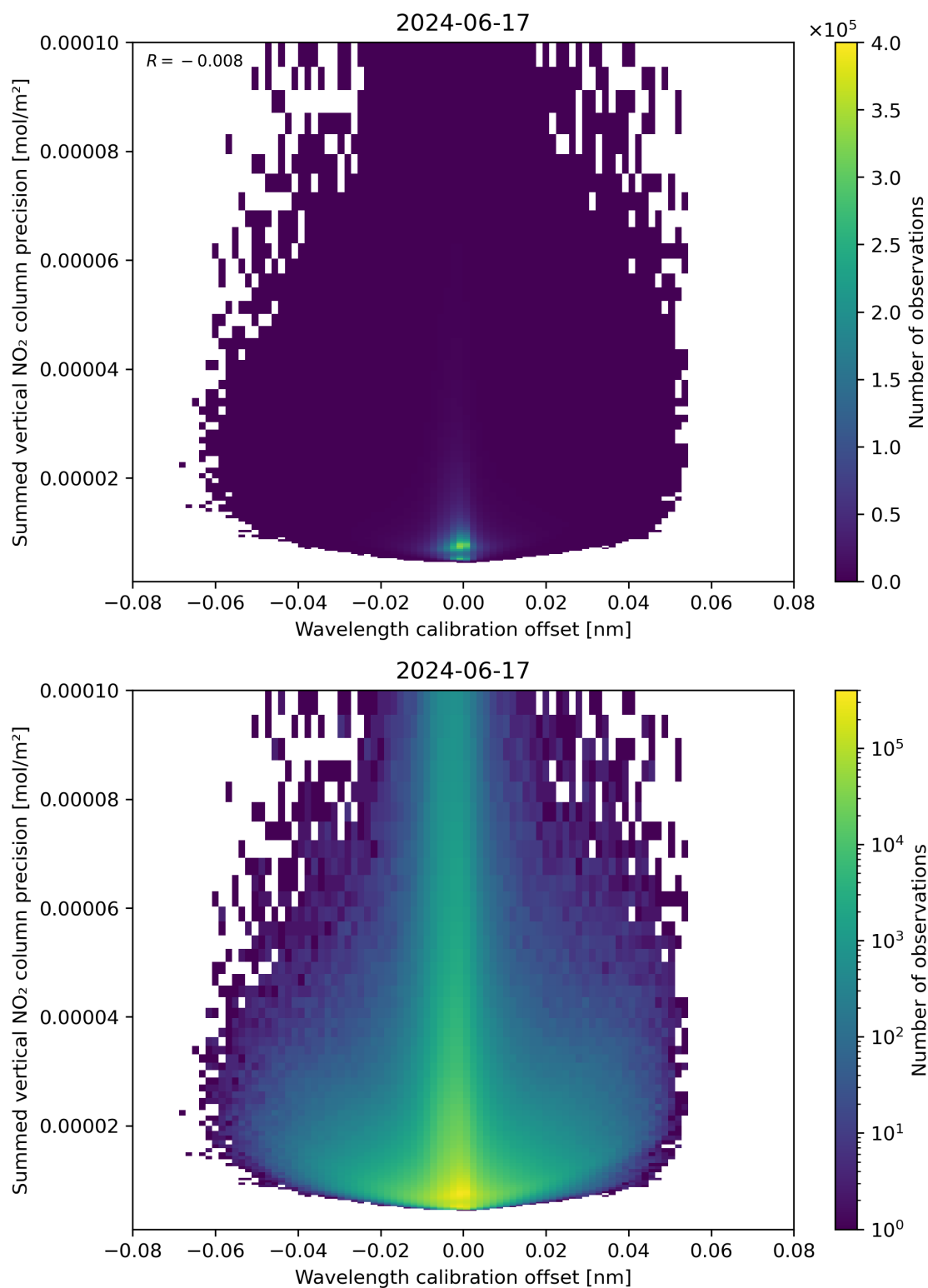
Figure 178: Scatter density plot of “Wavelength calibration offset” against “Summed vertical NO 2 column precision” for 2024-06-16 to 2024-06-18.
