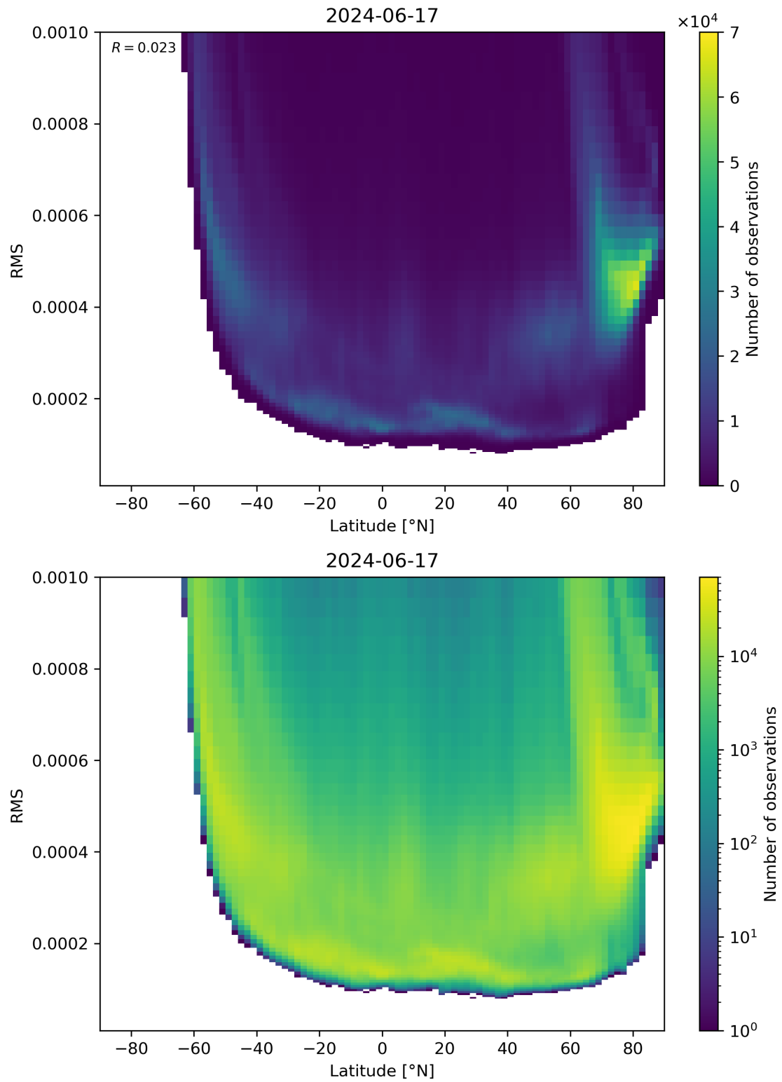
Figure 94: Scatter density plot of “Latitude” against “RMS” for 2024-06-16 to 2024-06-18.
