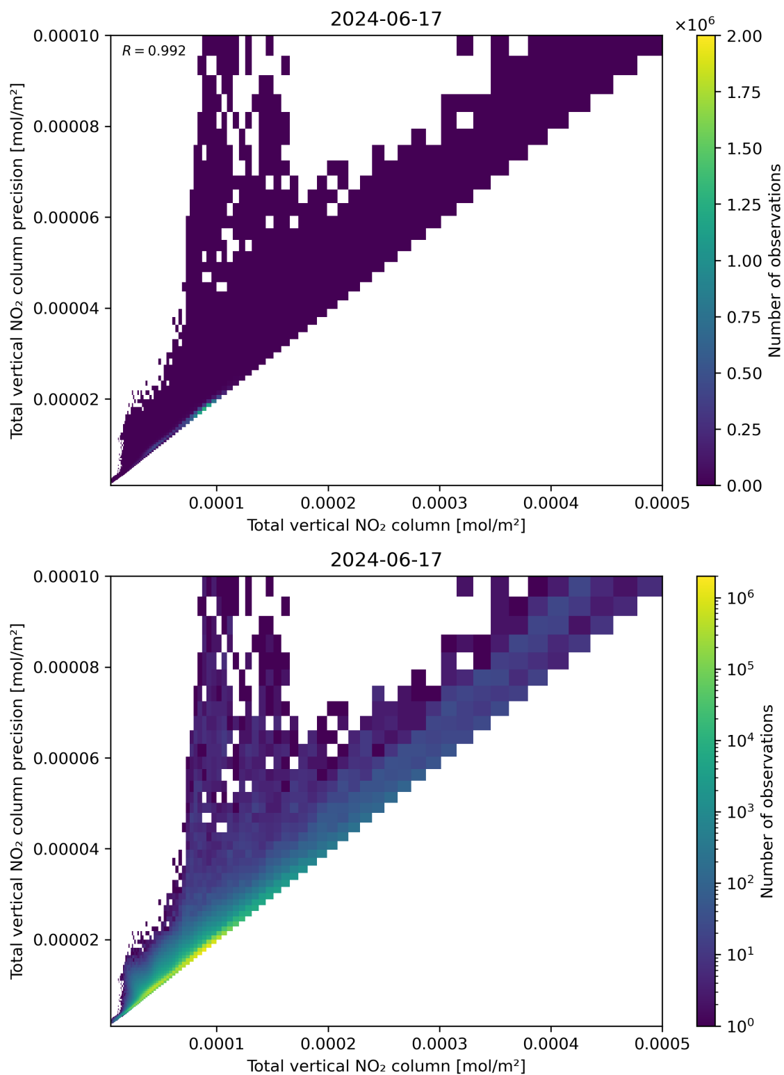
Figure 114: Scatter density plot of “Total vertical NO 2 column” against “Total vertical NO 2 column precision” for 2024-06-16 to 2024-06-18.
