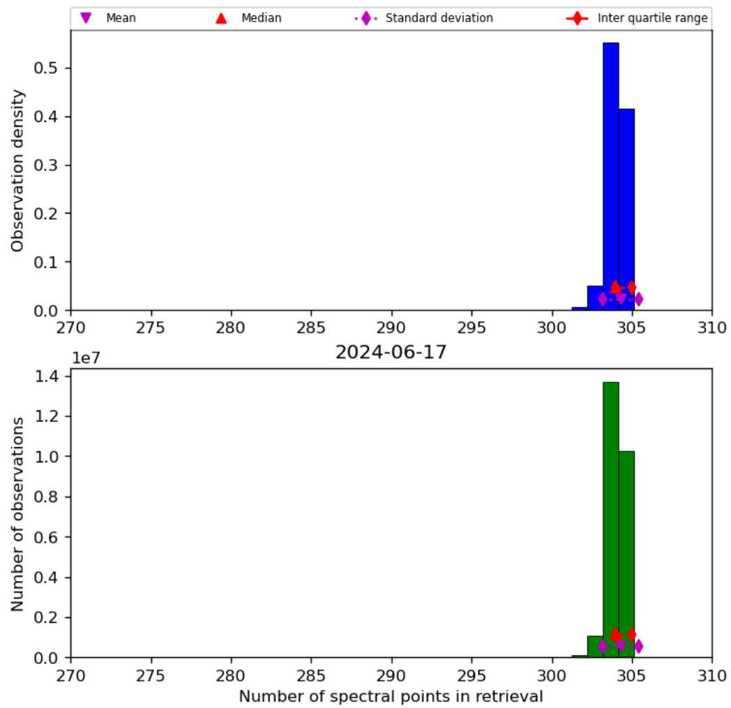
Figure 33: Histogram of “Number of spectral points in retrieval” for 2024-06-16 to 2024-06-18
