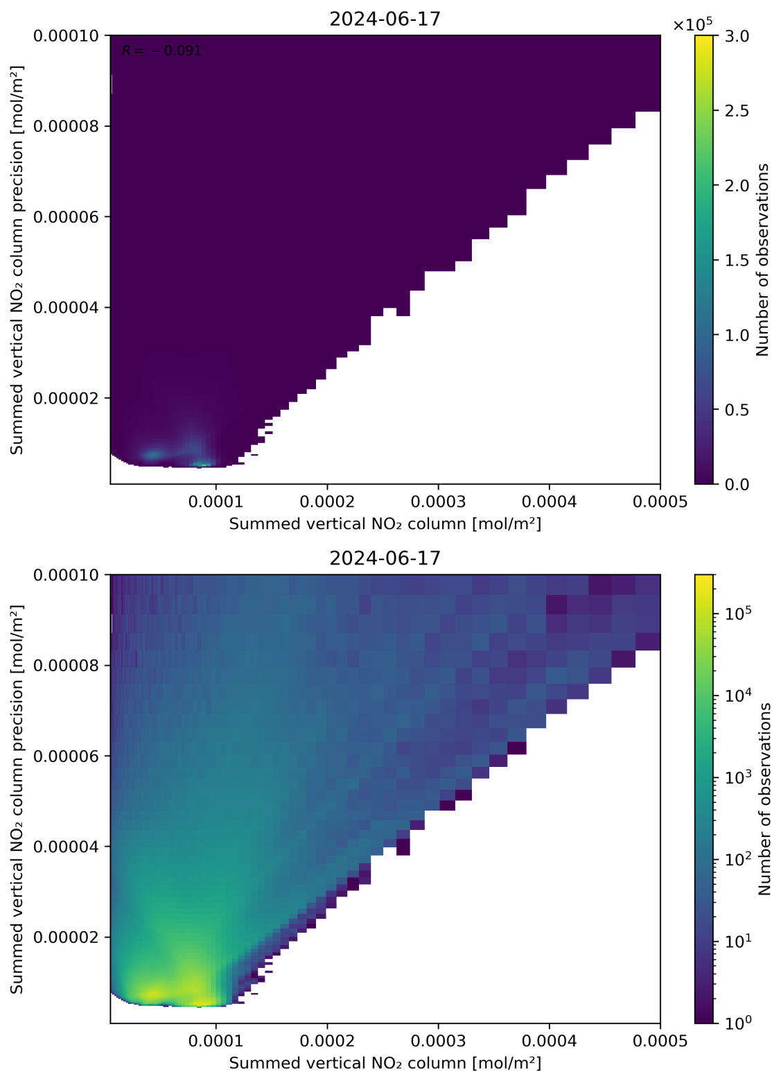
Figure 105: Scatter density plot of “Summed vertical NO 2 column” against “Summed vertical NO 2 column precision” for 2024-06-16 to 2024-06-18.
