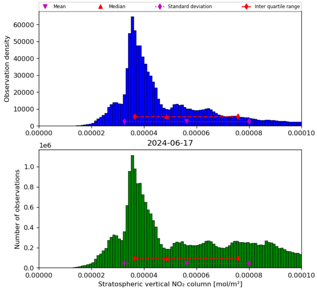
Figure 36: Histogram of “Stratospheric vertical NO 2 column” for 2024-06-16 to 2024-06-18
