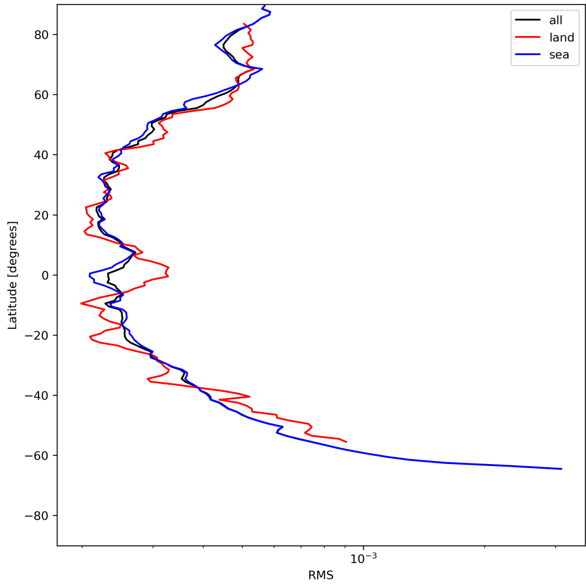
Figure 26: Zonal average of “RMS” for 2024-06-16 to 2024-06-18.
