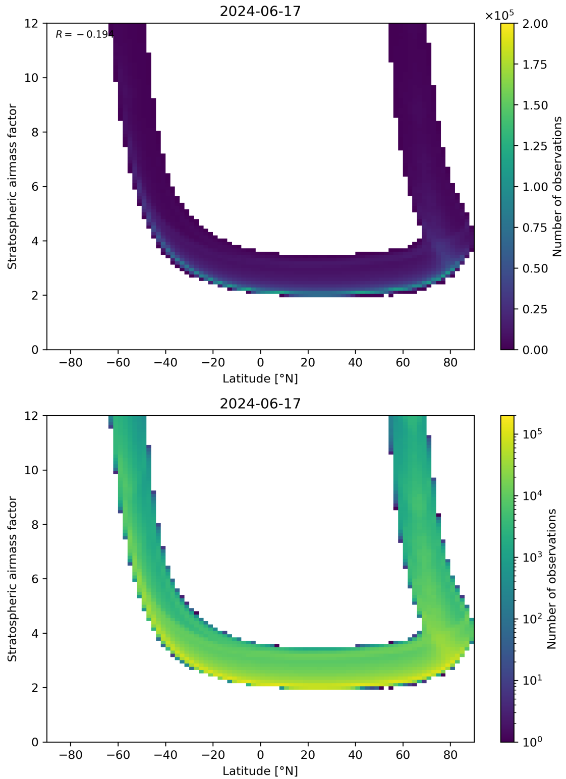
Figure 83: Scatter density plot of “Latitude” against “Stratospheric air mass factor” for 2024-06-16 to 2024-06-18.
