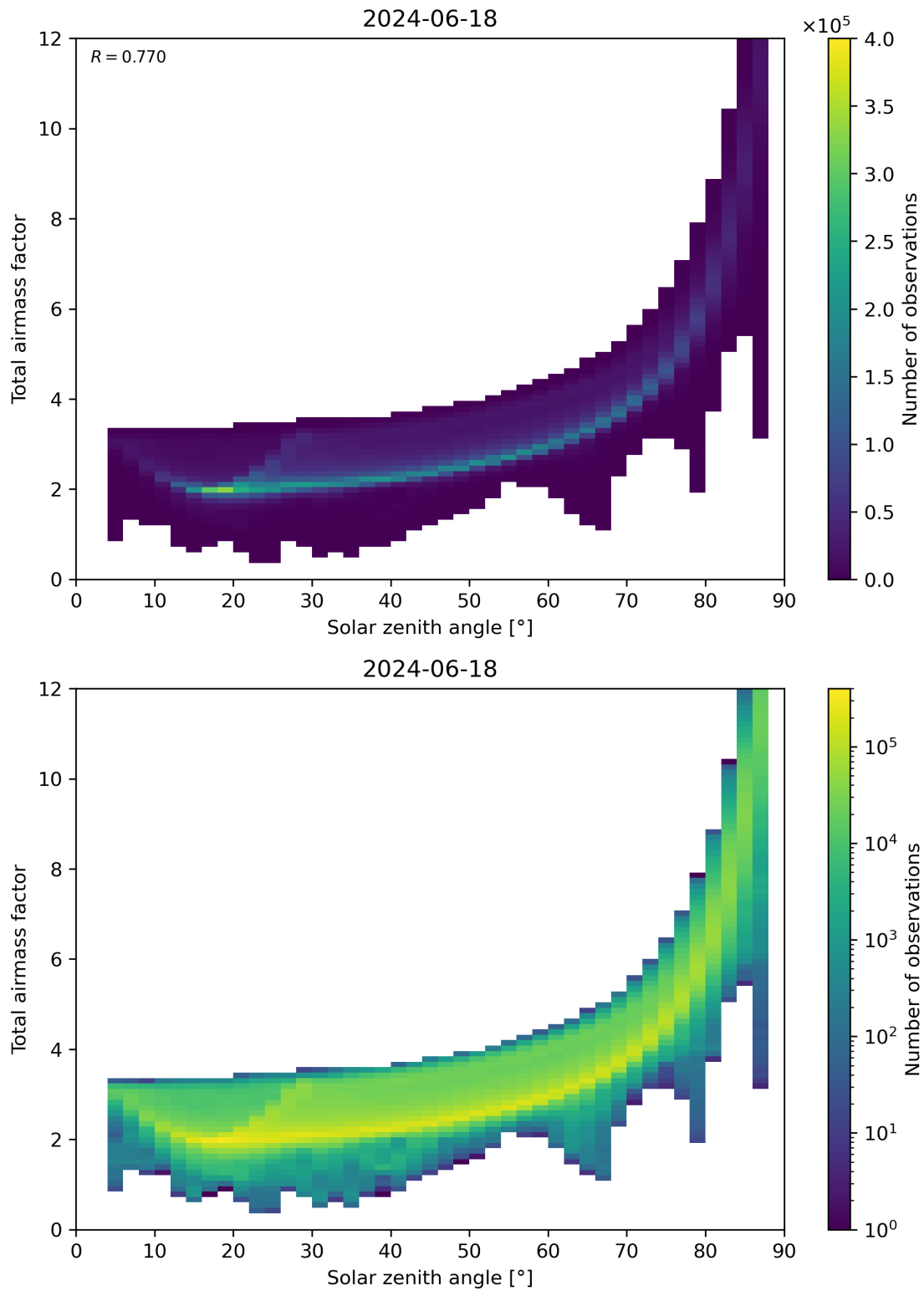
Figure 146: Scatter density plot of “Solar zenith angle” against “Total air mass factor” for 2024-06-17 to 2024-06-19.
