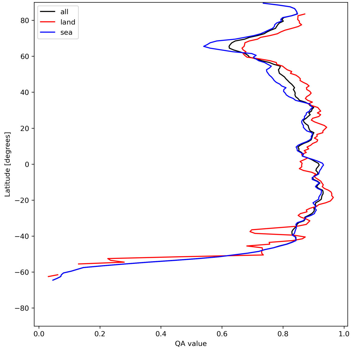
Figure 11: Zonal average of “QA value” for 2024-06-17 to 2024-06-19.
