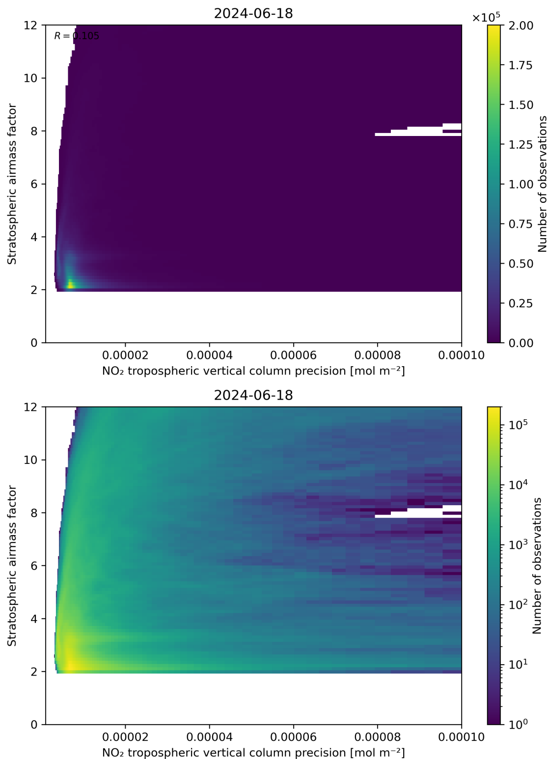
Figure 131: Scatter density plot of “NO 2 tropospheric vertical column precision” against “Stratospheric airmass factor” for 2024-06-17 to 2024-06-19.
