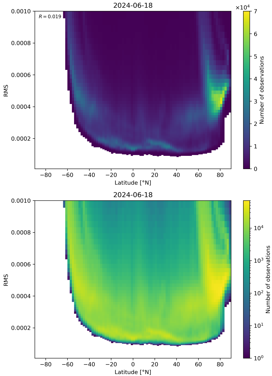
Figure 94: Scatter density plot of “Latitude” against “RMS” for 2024-06-17 to 2024-06-19.
