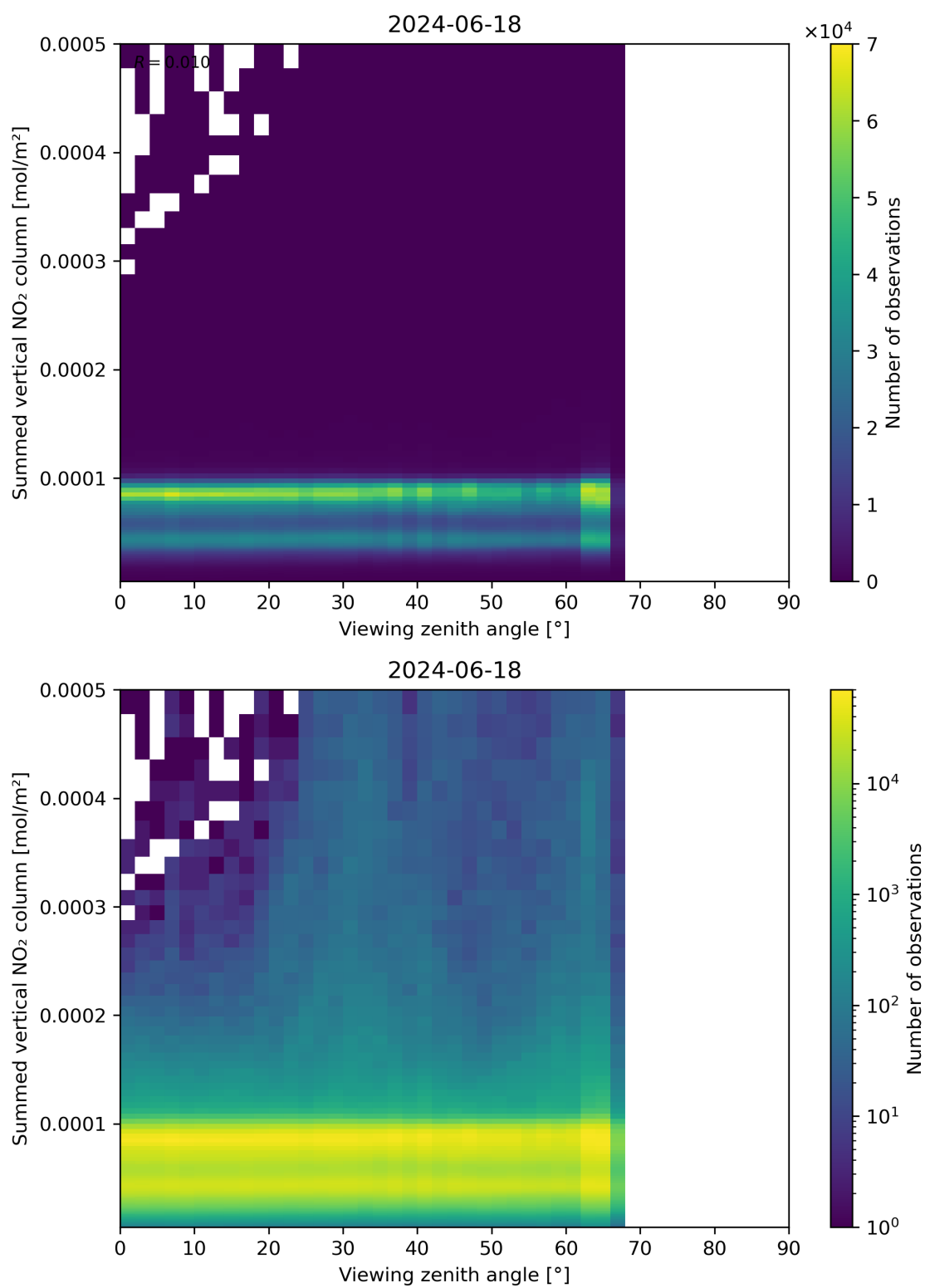
Figure 165: Scatter density plot of “Viewing zenith angle” against “Summed vertical NO 2 column” for 2024-06-17 to 2024-06-19.
