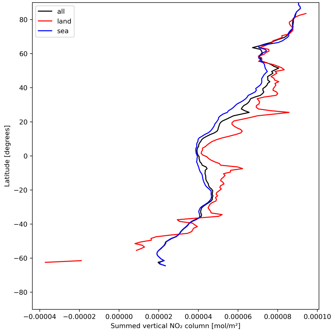
Figure 23: Zonal average of “Summed vertical NO 2 column” for 2024-06-17 to 2024-06-19.
