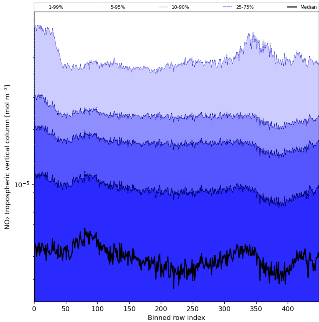
Figure 46: Along track statistics of “NO 2 tropospheric vertical column” for 2024-06-17 to 2024-06-19
