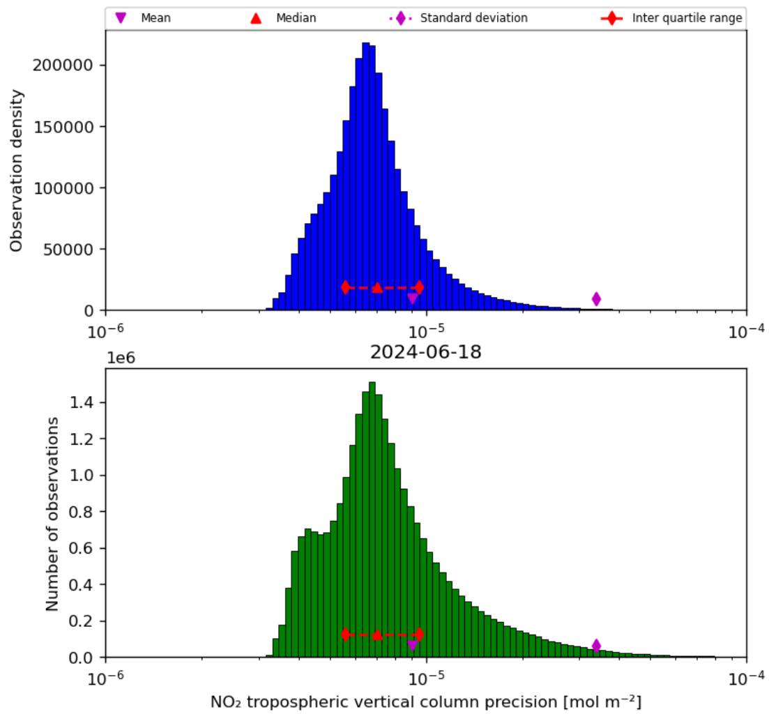
Figure 30: Histogram of “NO 2 tropospheric vertical column precision” for 2024-06-17 to 2024-06-19
