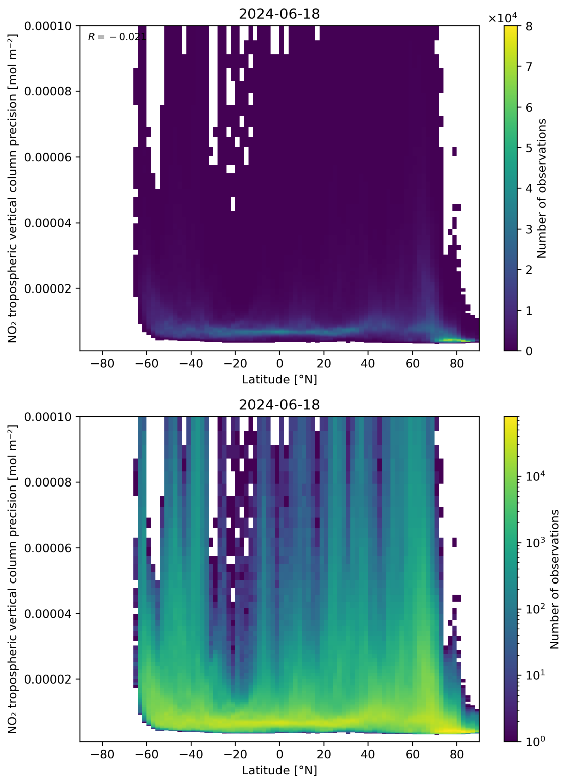
Figure 93: Scatter density plot of “Latitude” against “NO 2 tropospheric vertical column precision” for 2024-06-17 to 2024-06-19.
