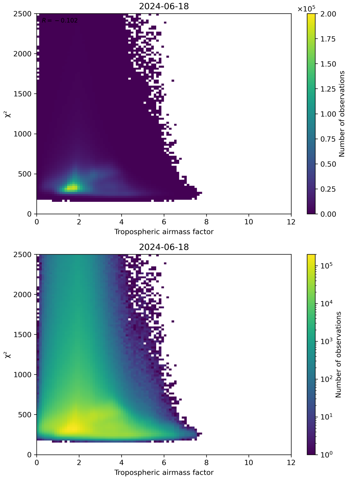
Figure 73: Scatter density plot of “Tropospheric airmass factor” against “ \chi^2 ” for 2024-06-17 to 2024-06-19.
