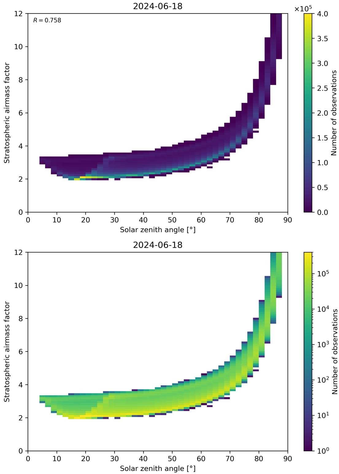
Figure 145: Scatter density plot of “Solar zenith angle” against “Stratospheric airmass factor” for 2024-06-17 to 2024-06-19.
