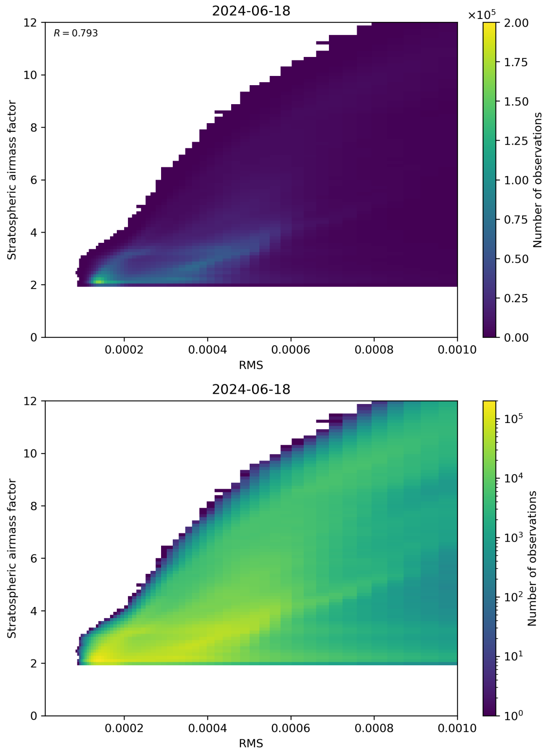
Figure 144: Scatter density plot of “RMS” against “Stratospheric airmass factor” for 2024-06-17 to 2024-06-19.
