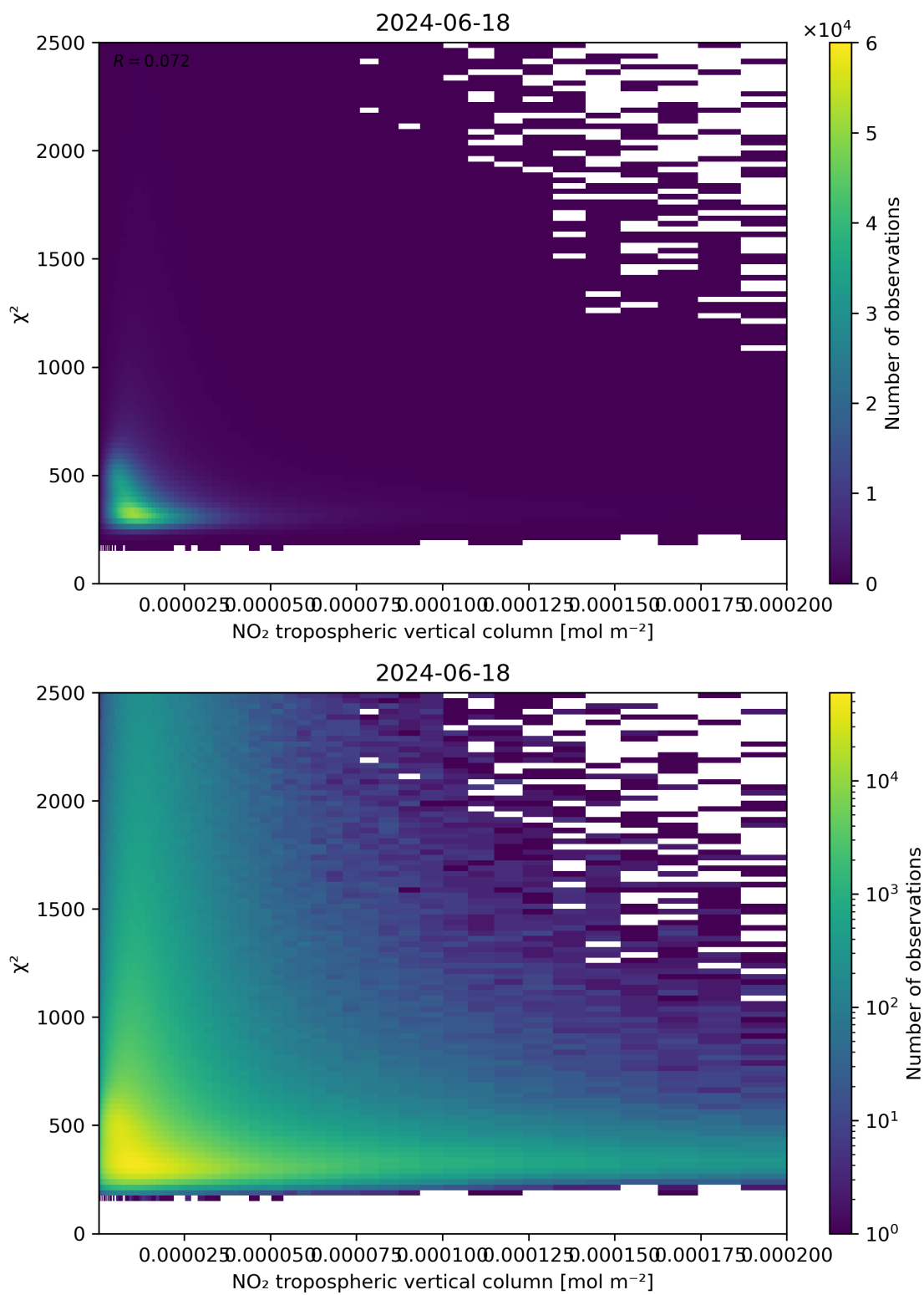
Figure 124: Scatter density plot of “NO 2 tropospheric vertical column” against “ \chi^2 ” for 2024-06-17 to 2024-06-19.
