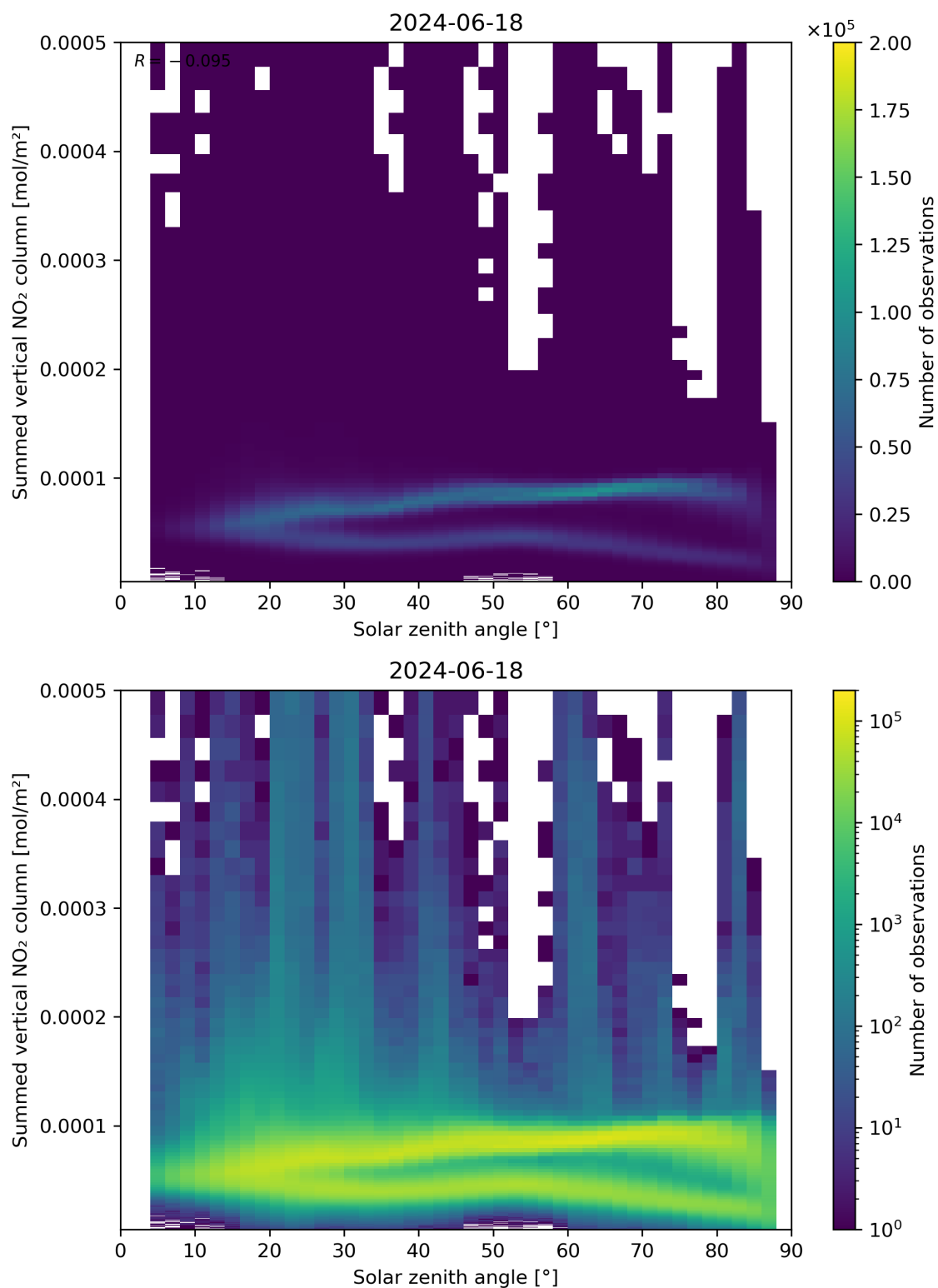
Figure 151: Scatter density plot of “Solar zenith angle” against “Summed vertical NO 2 column” for 2024-06-17 to 2024-06-19.
