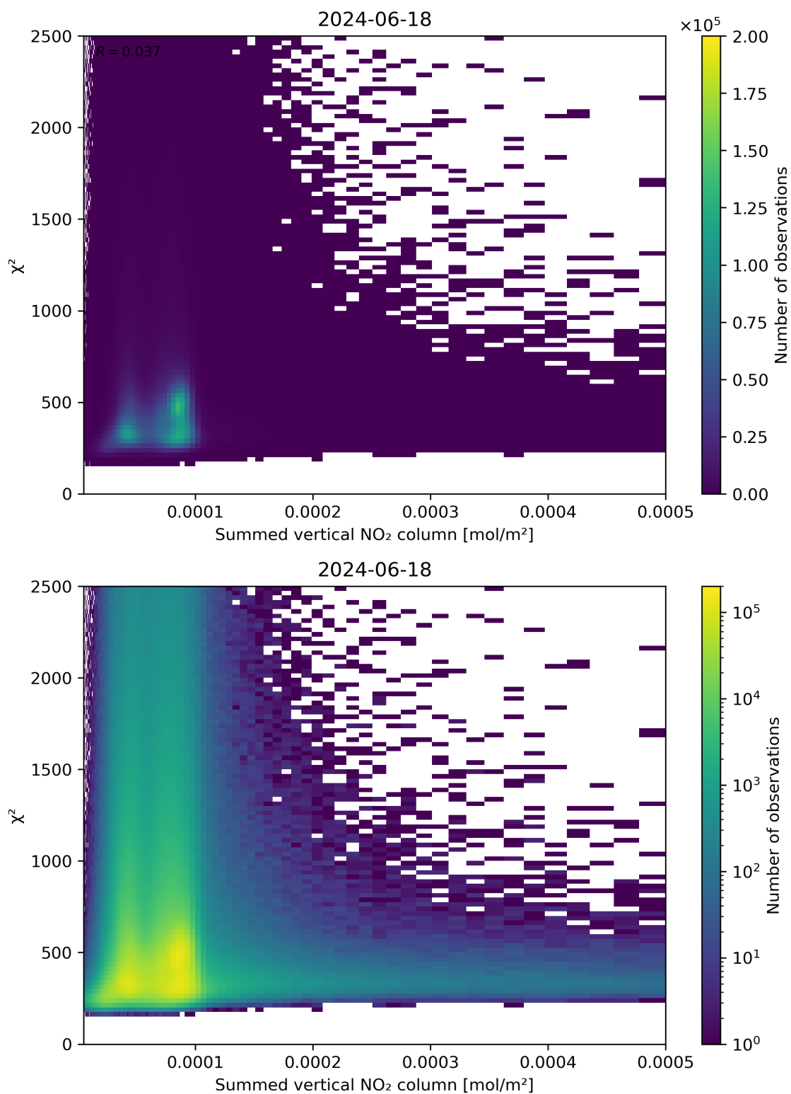
Figure 104: Scatter density plot of “Summed vertical NO 2 column” against “ \chi^2 ” for 2024-06-17 to 2024-06-19.
