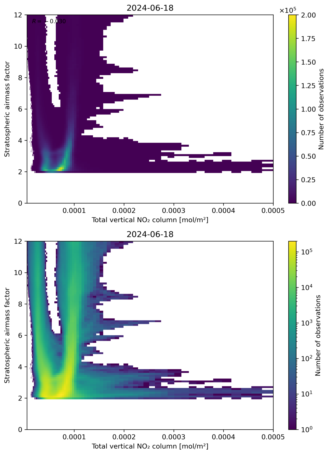
Figure 110: Scatter density plot of “Total vertical NO 2 column” against “Stratospheric airmass factor” for 2024-06-17 to 2024-06-19.
