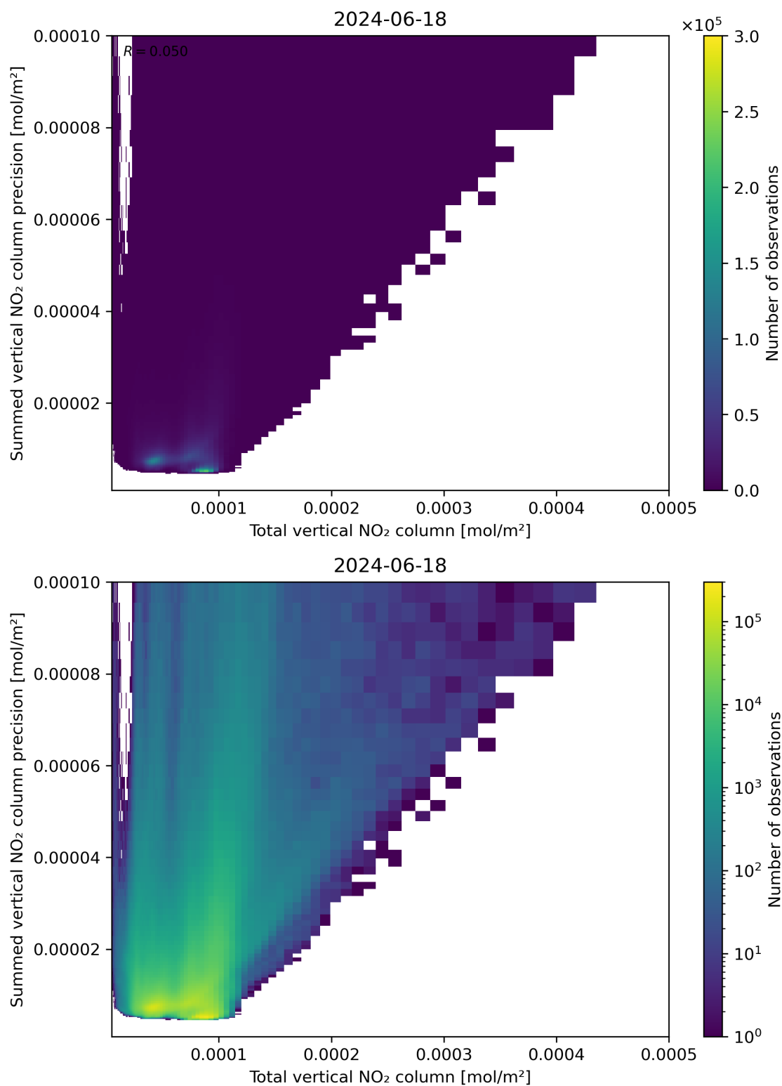
Figure 113: Scatter density plot of “Total vertical NO 2 column” against “Summed vertical NO 2 column precision” for 2024-06-17 to 2024-06-19.
