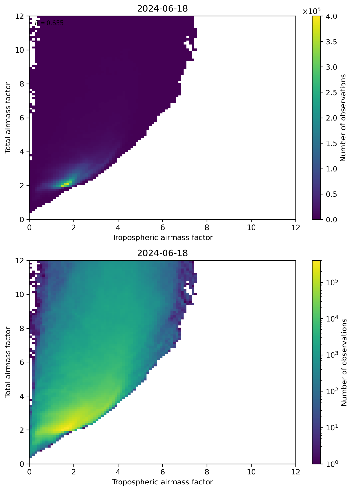
Figure 72: Scatter density plot of “Tropospheric airmass factor” against “Total airmass factor” for 2024-06-17 to 2024-06-19.
