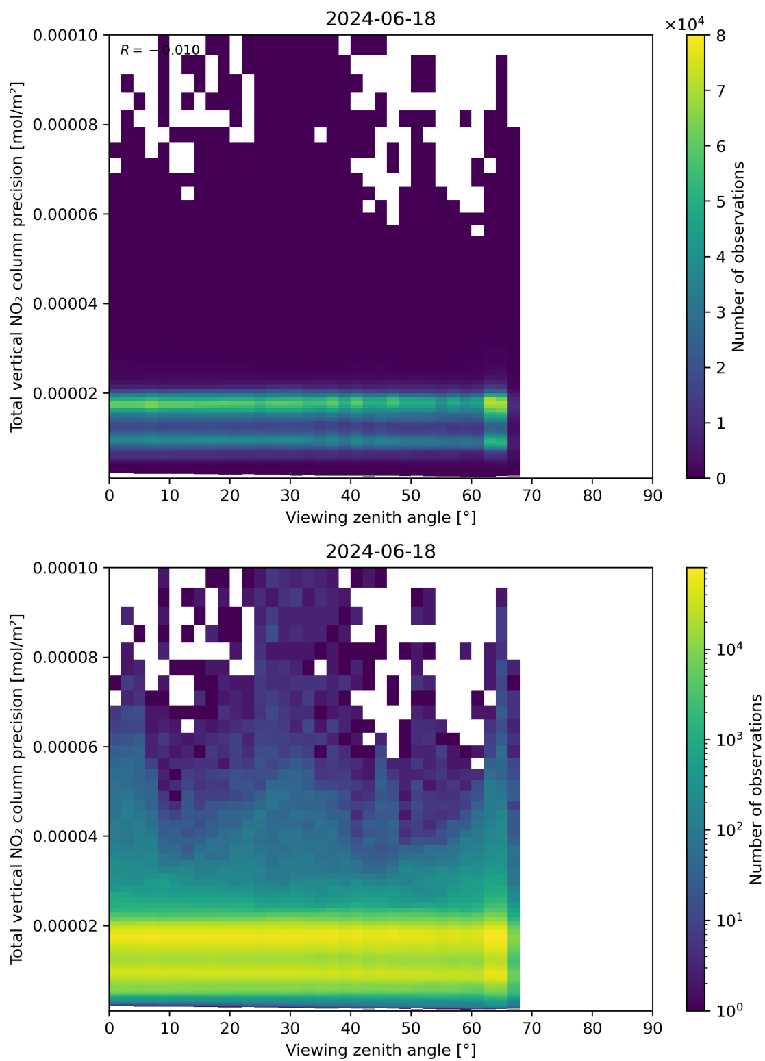
Figure 168: Scatter density plot of “Viewing zenith angle” against “Total vertical NO 2 column precision” for 2024-06-17 to 2024-06-19.
