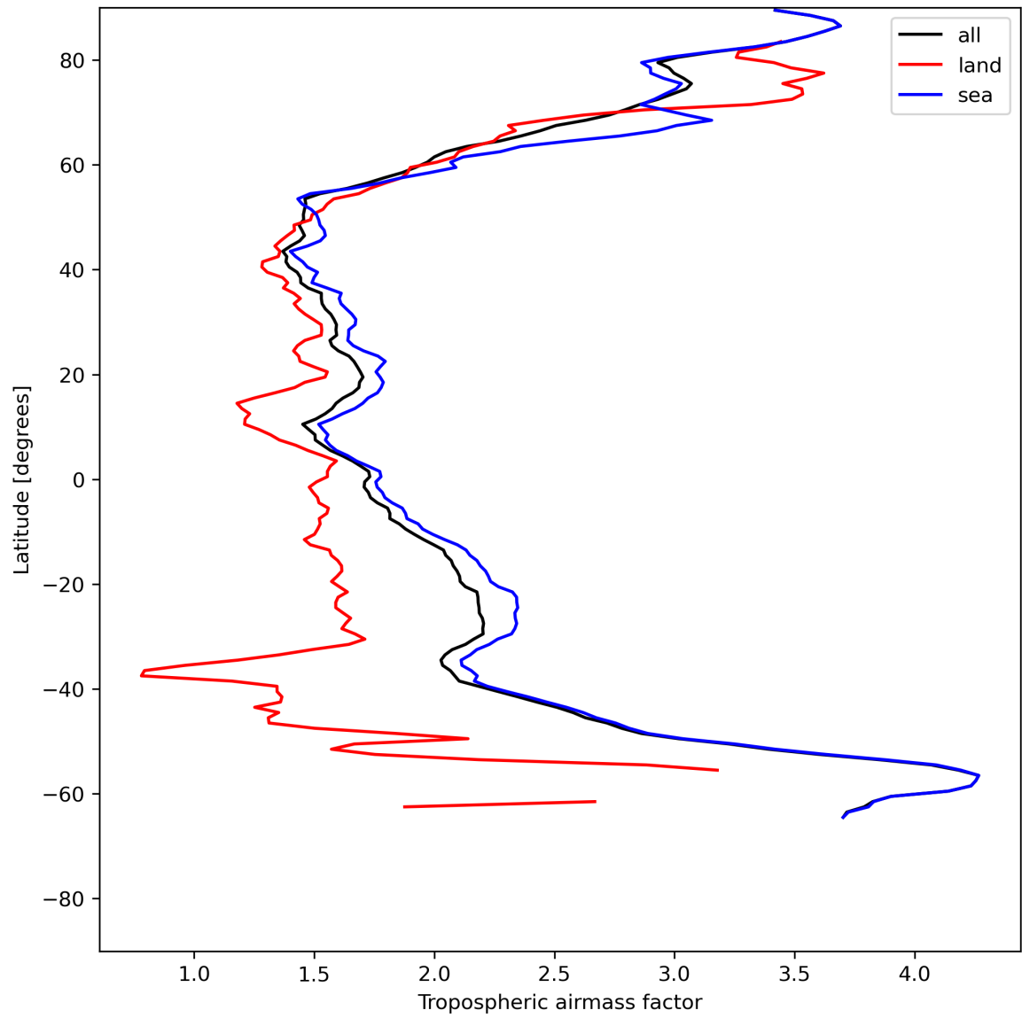
Figure 14: Zonal average of “Tropospheric airmass factor” for 2024-06-17 to 2024-06-19.
