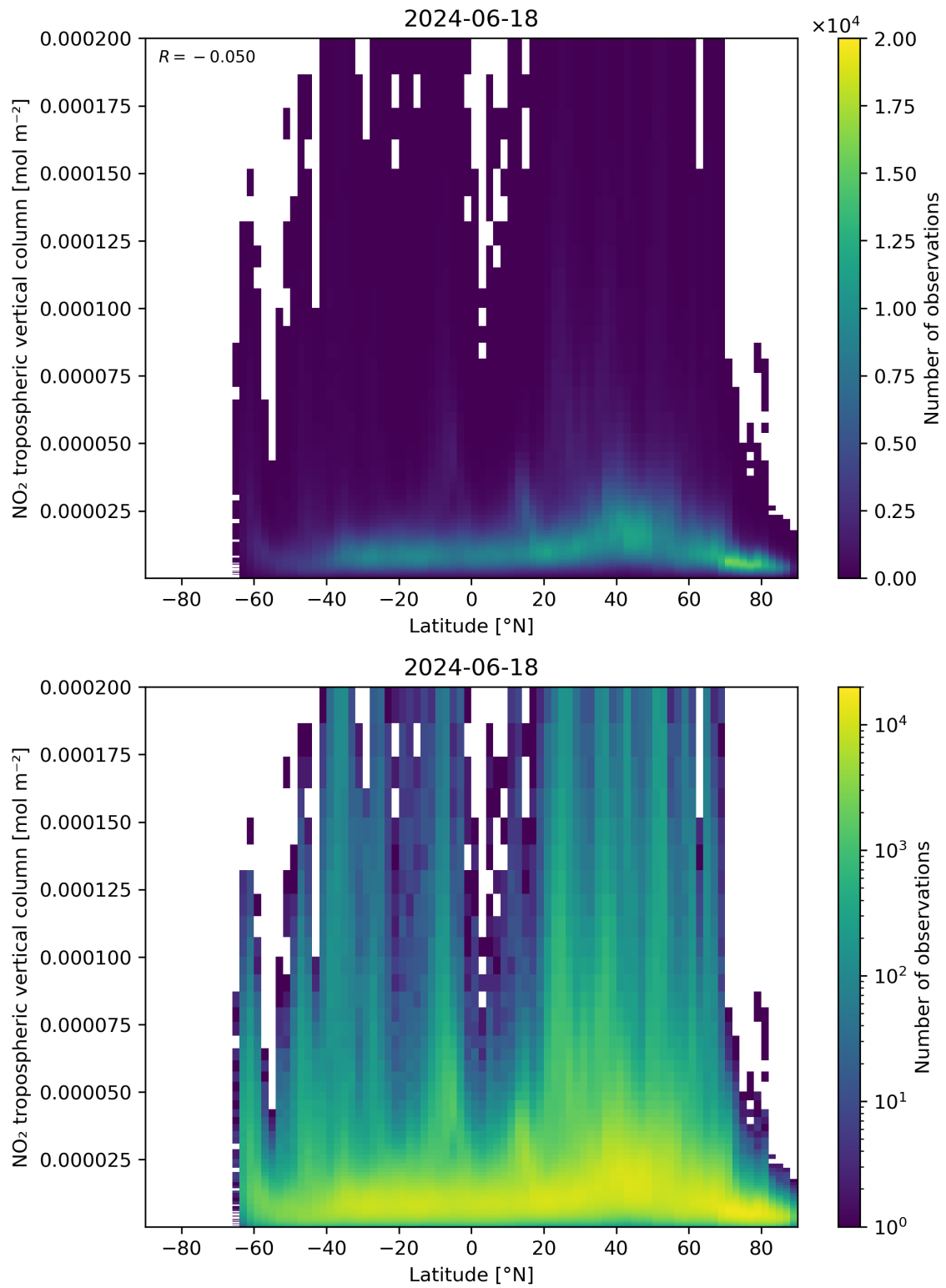
Figure 92: Scatter density plot of “Latitude” against “NO 2 tropospheric vertical column” for 2024-06-17 to 2024-06-19.
