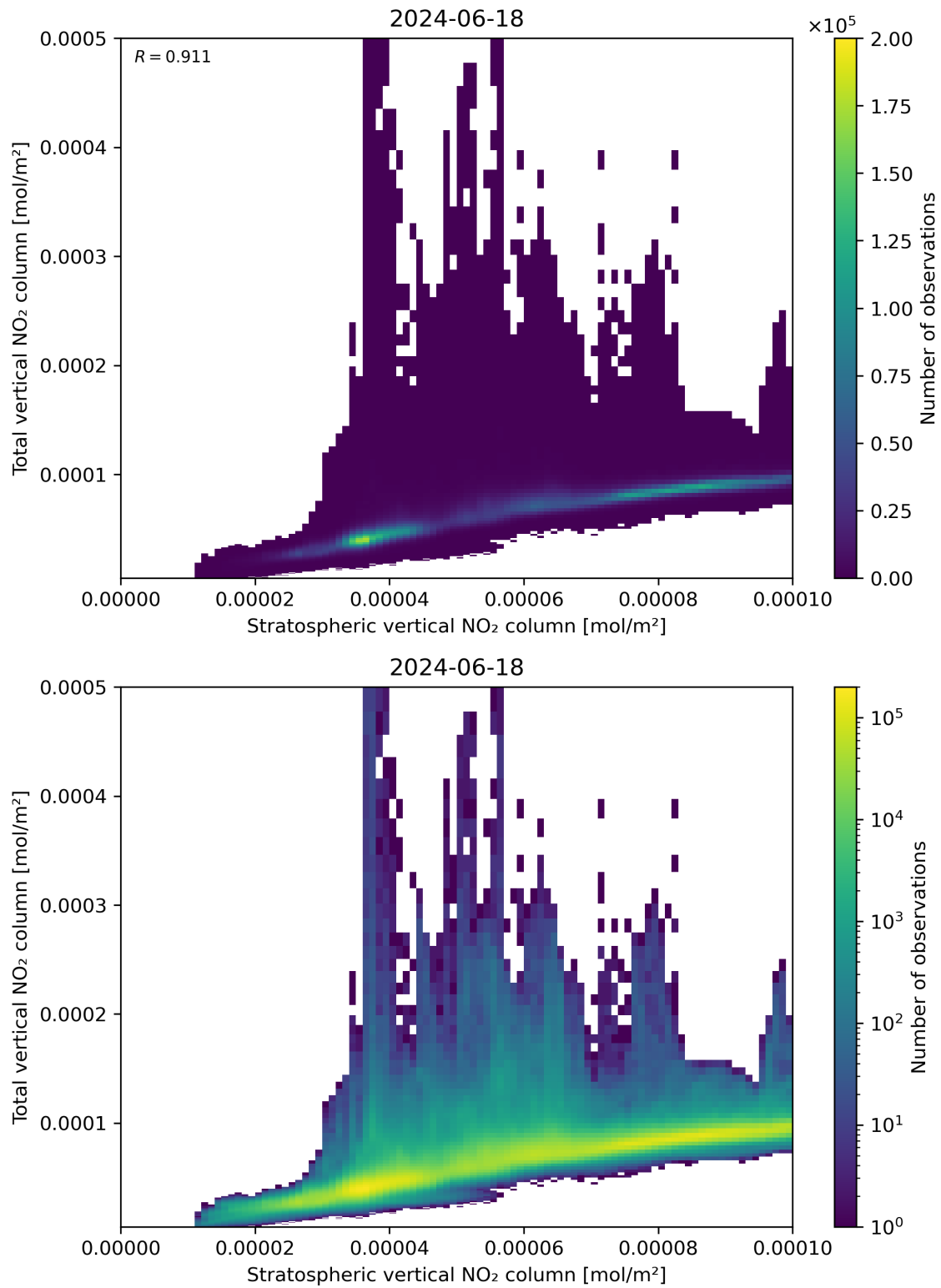
Figure 100: Scatter density plot of “Stratospheric vertical NO 2 column” against “Total vertical NO 2 column” for 2024-06-17 to 2024-06-19.
