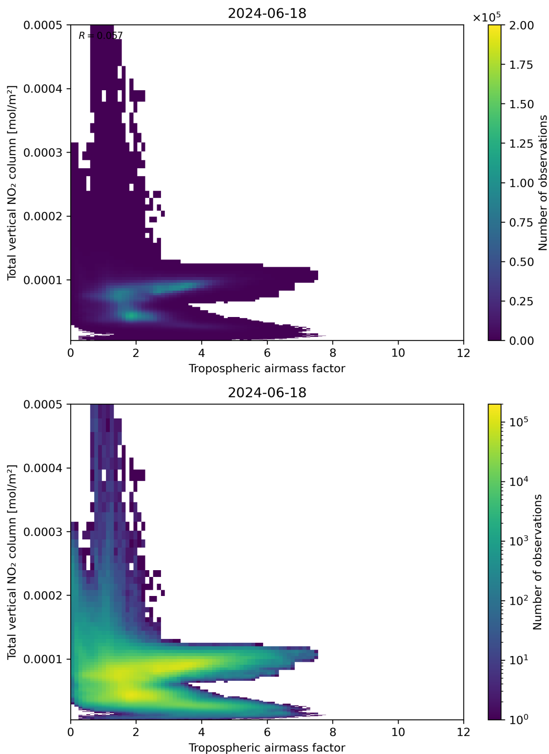
Figure 77: Scatter density plot of “Tropospheric airmass factor” against “Total vertical \text{NO}_2 column” for 2024-06-17 to 2024-06-19.
