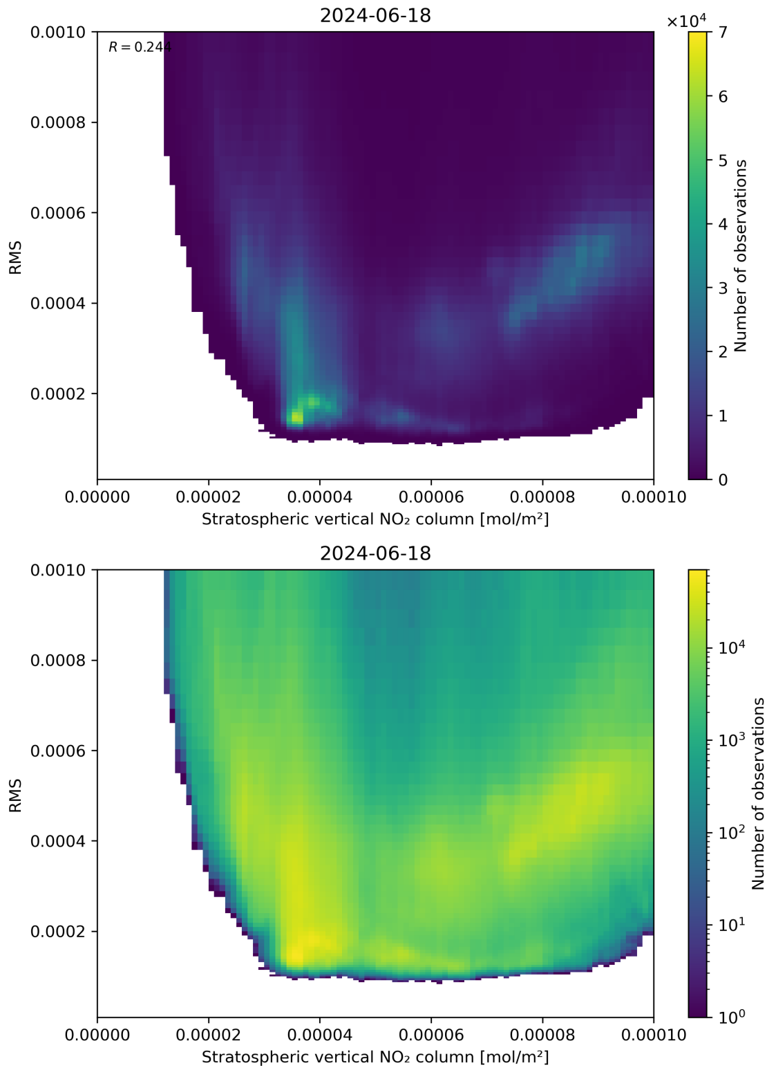
Figure 102: Scatter density plot of “Stratospheric vertical NO 2 column” against “RMS” for 2024-06-17 to 2024-06-19.
