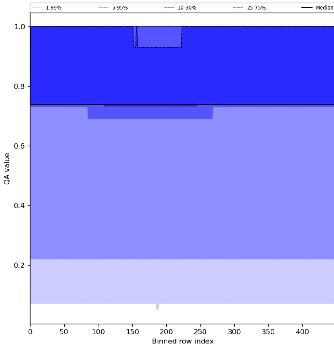
Figure 45: Along track statistics of “QA value” for 2024-06-17 to 2024-06-19
