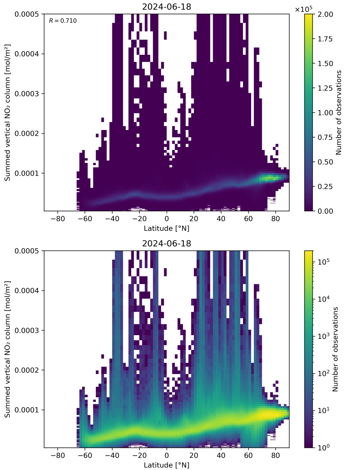
Figure 88: Scatter density plot of “Latitude” against “Summed vertical NO 2 column” for 2024-06-17 to 2024-06-19.
