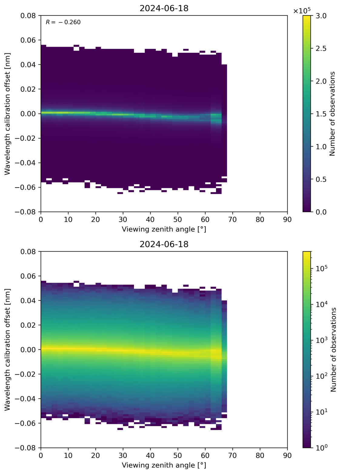
Figure 173: Scatter density plot of “Viewing zenith angle” against “Wavelength calibration offset” for 2024-06-17 to 2024-06-19.
