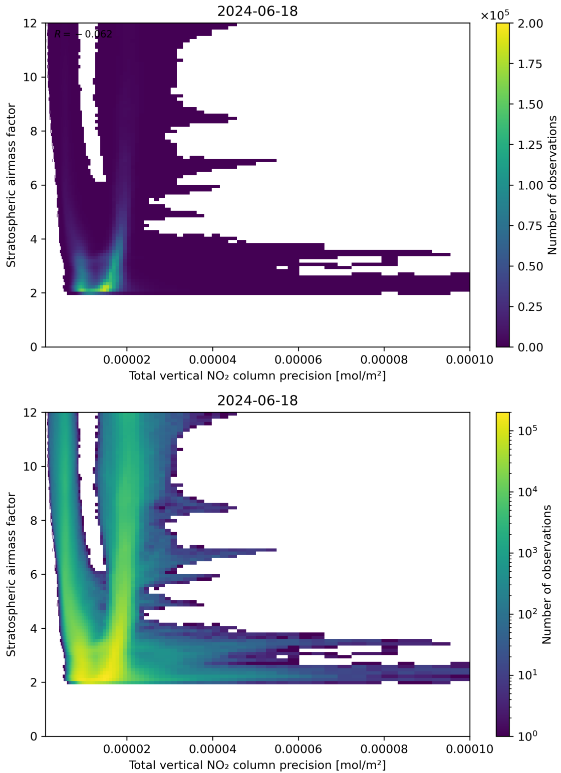
Figure 115: Scatter density plot of “Total vertical NO 2 column precision” against “Stratospheric air mass factor” for 2024-06-17 to 2024-06-19.
