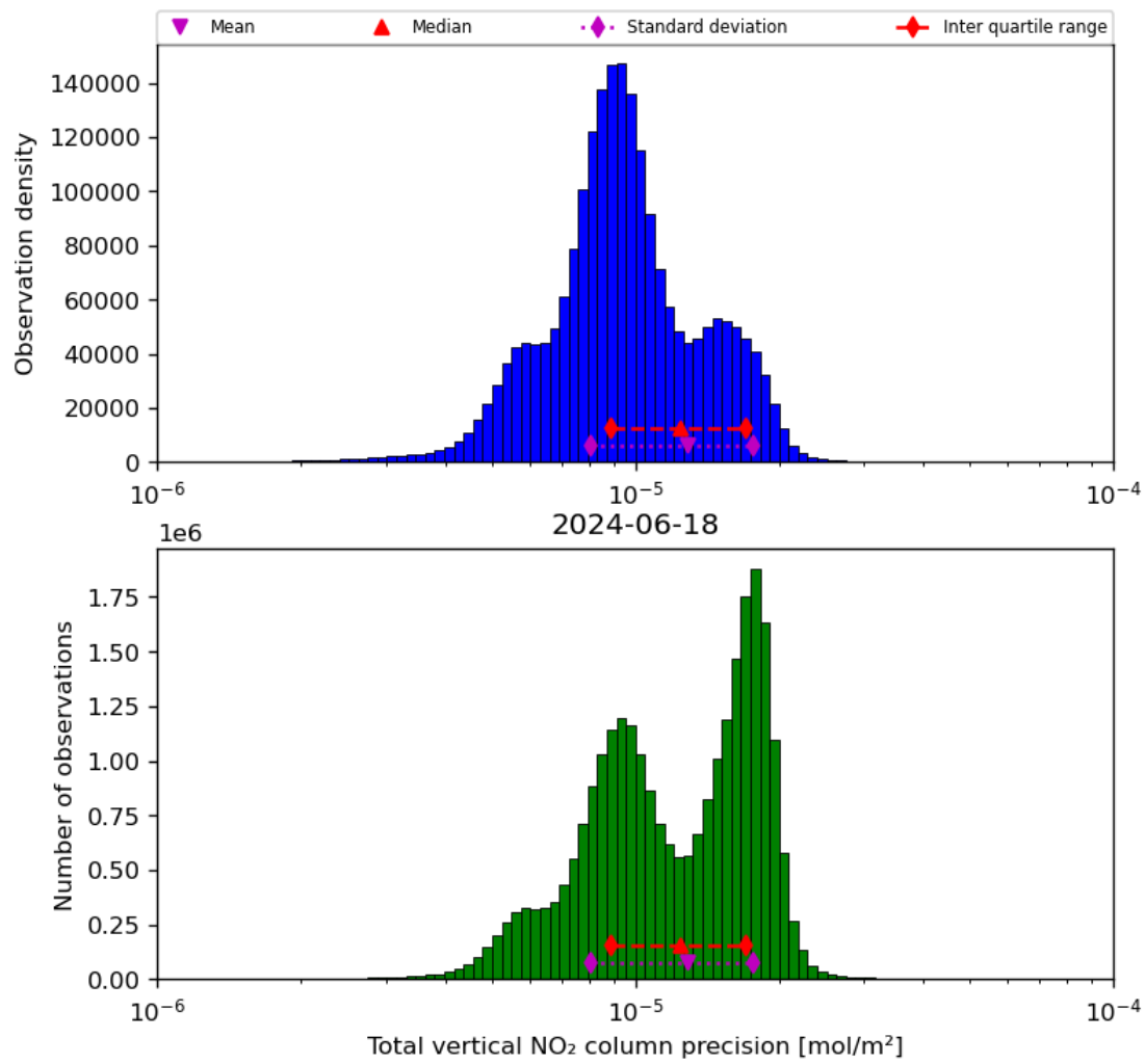
Figure 39: Histogram of “Total vertical NO 2 column precision” for 2024-06-17 to 2024-06-19
