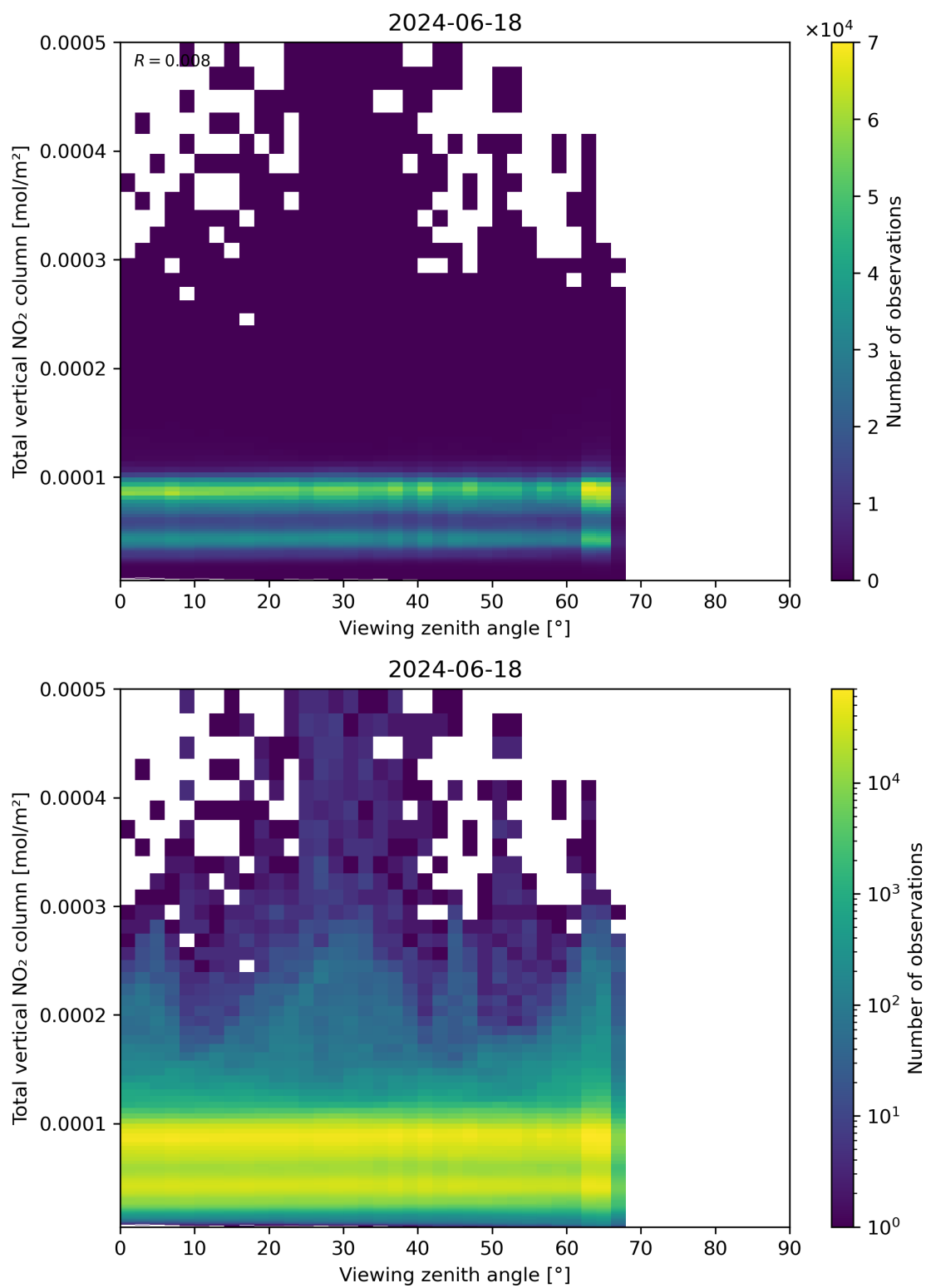
Figure 167: Scatter density plot of “Viewing zenith angle” against “Total vertical NO 2 column” for 2024-06-17 to 2024-06-19.
