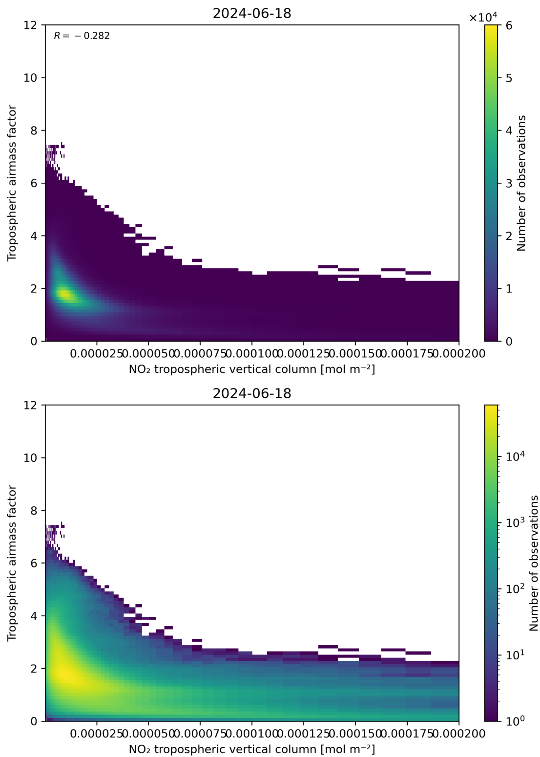
Figure 123: Scatter density plot of “NO 2 tropospheric vertical column” against “Tropospheric airmass factor” for 2024-06-17 to 2024-06-19.
