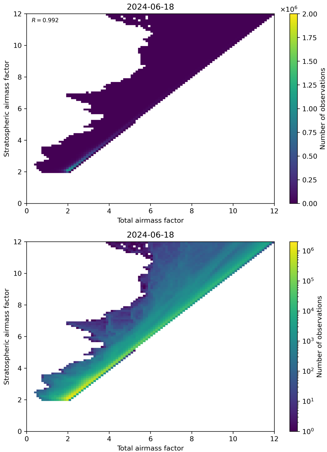
Figure 62: Scatter density plot of “Total airmass factor” against “Stratospheric airmass factor” for 2024-06-17 to 2024-06-19.
