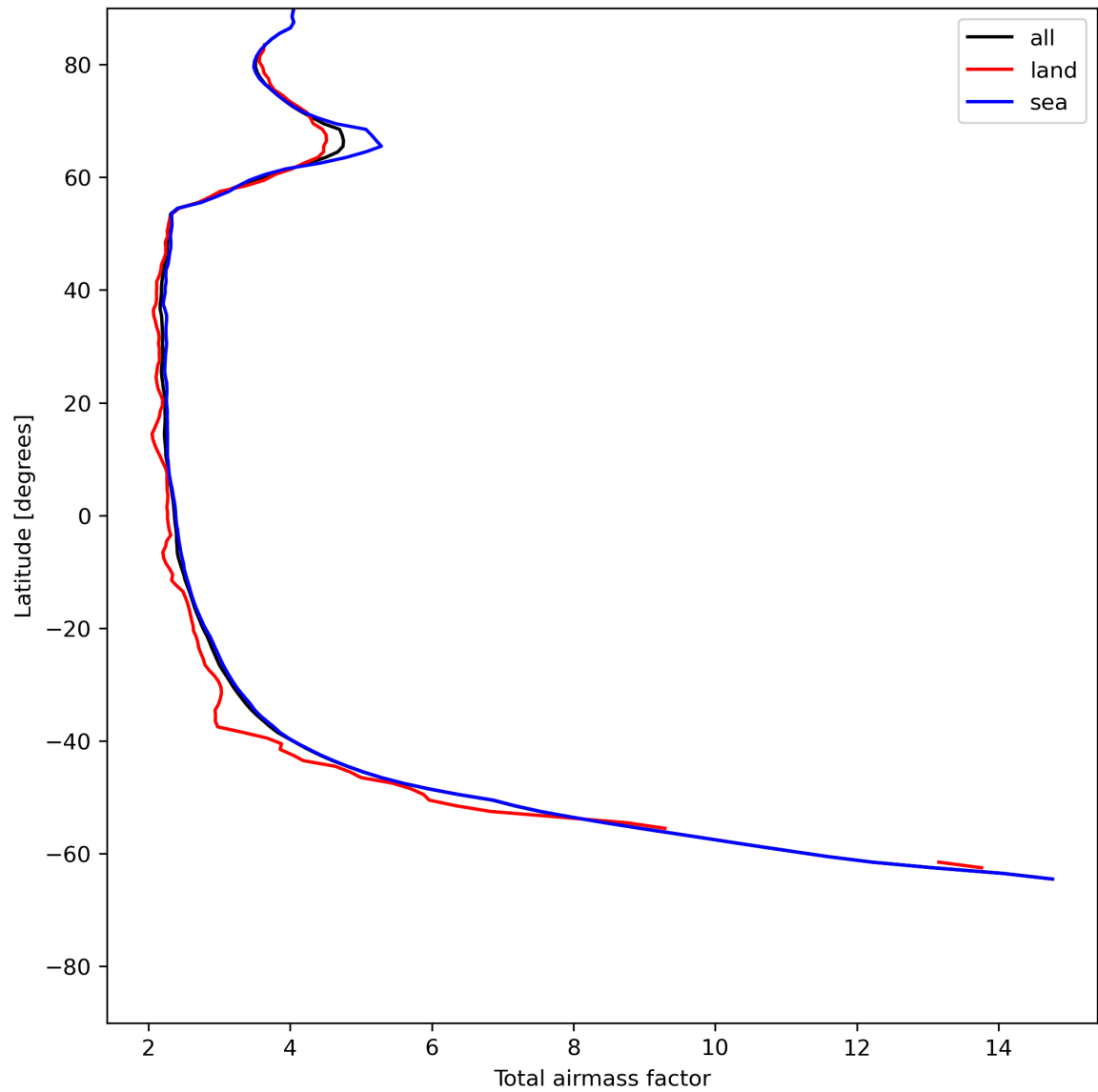
Figure 15: Zonal average of “Total airmass factor” for 2024-06-17 to 2024-06-19.
