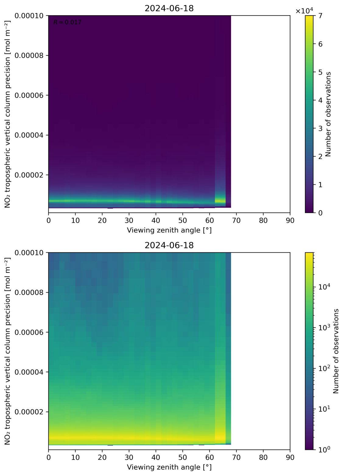
Figure 170: Scatter density plot of “Viewing zenith angle” against “NO 2 tropospheric vertical column precision” for 2024-06-17 to 2024-06-19.
