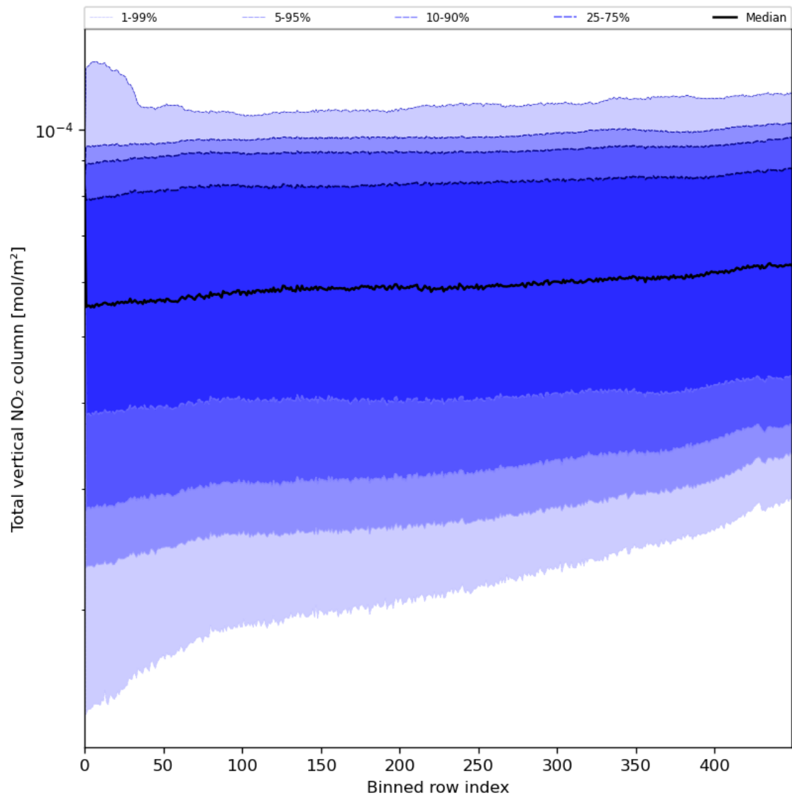
Figure 55: Along track statistics of “Total vertical NO 2 column” for 2024-06-17 to 2024-06-19
