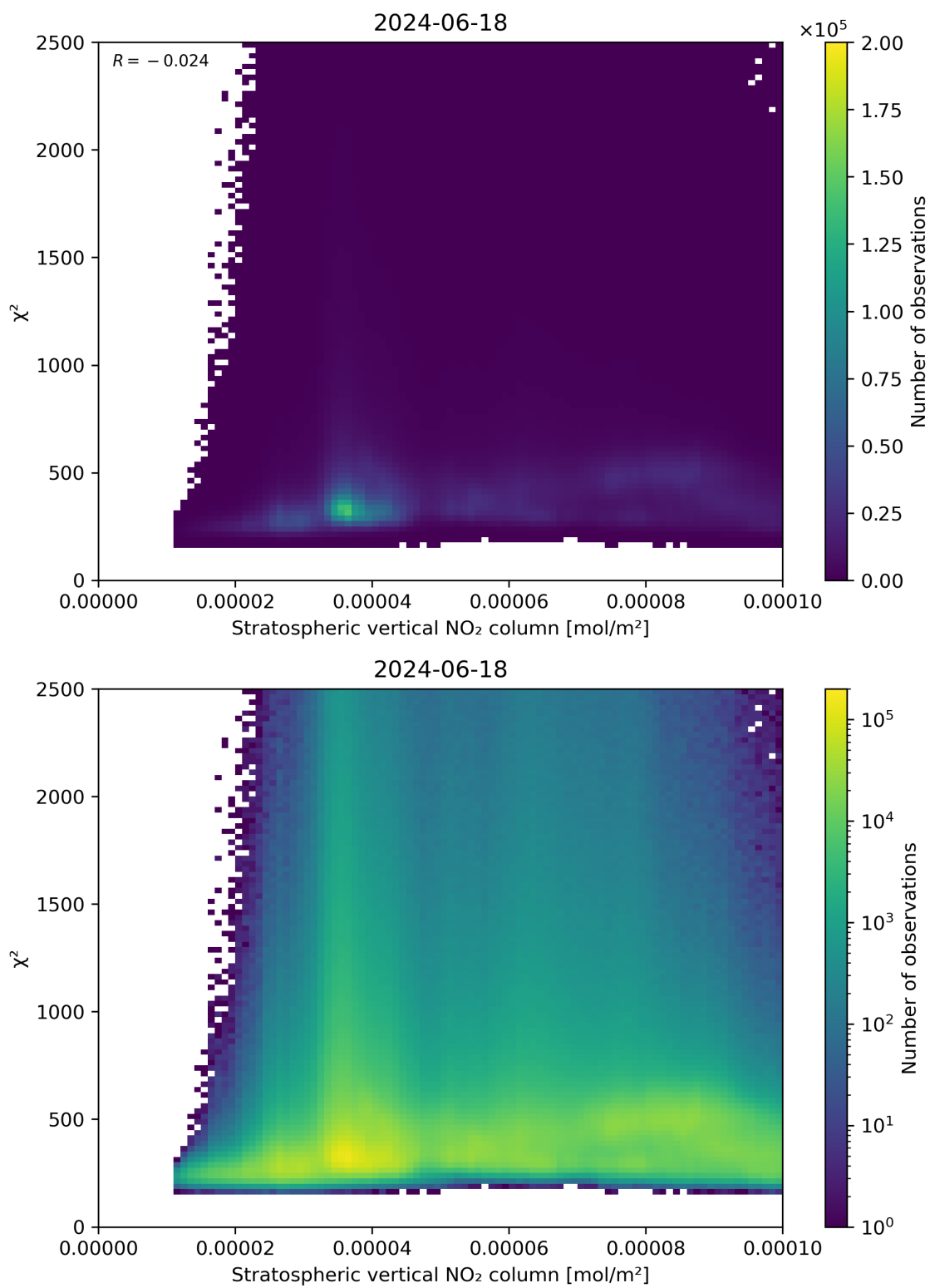
Figure 97: Scatter density plot of “Stratospheric vertical NO 2 column” against “ \chi^2 ” for 2024-06-17 to 2024-06-19.
