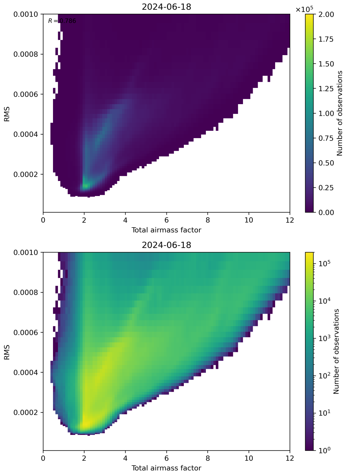
Figure 69: Scatter density plot of “Total airmass factor” against “RMS” for 2024-06-17 to 2024-06-19.
