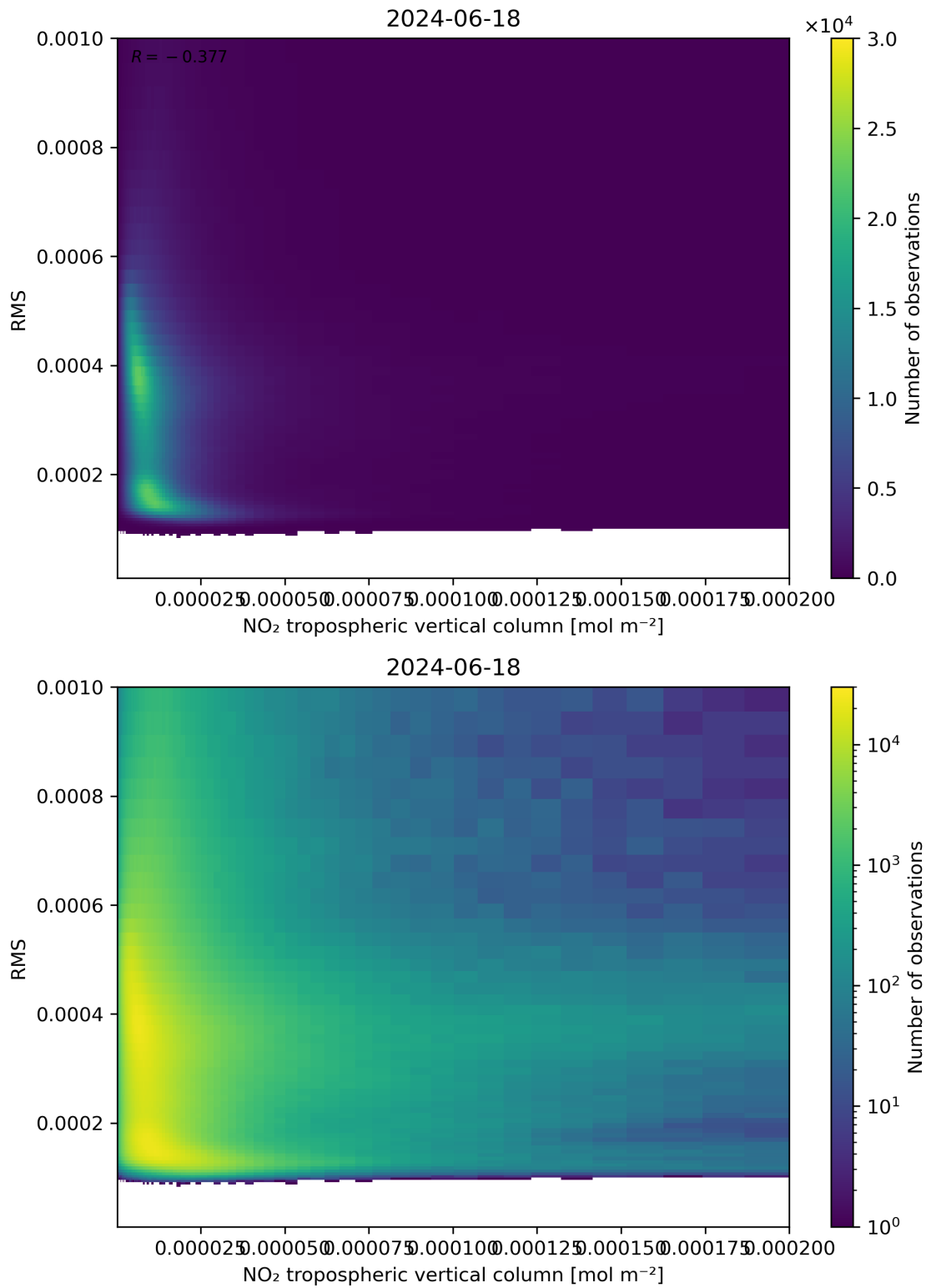
Figure 142: Scatter density plot of “NO 2 tropospheric vertical column” against “RMS” for 2024-06-17 to 2024-06-19.
