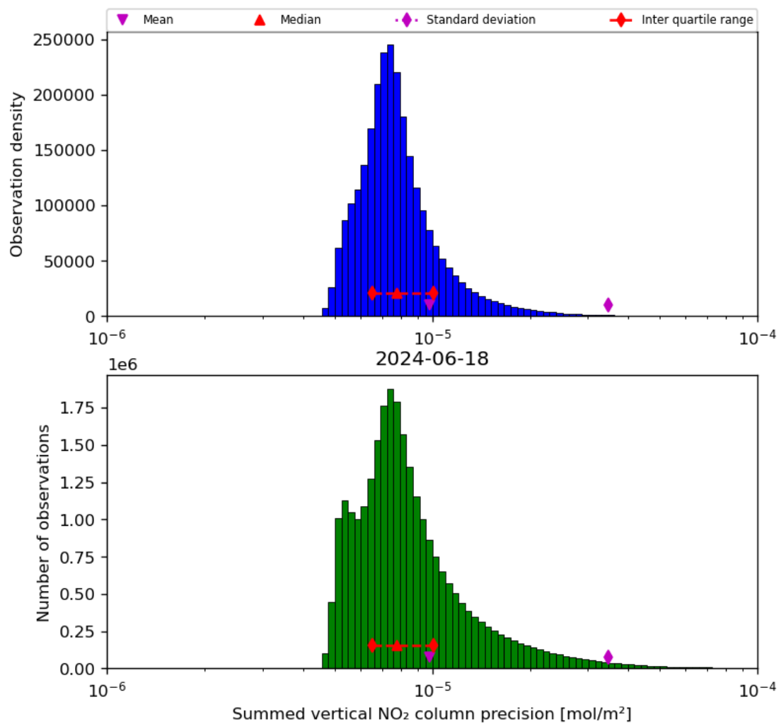
Figure 41: Histogram of "Summed vertical NO 2 column precision" for 2024-06-17 to 2024-06-19
