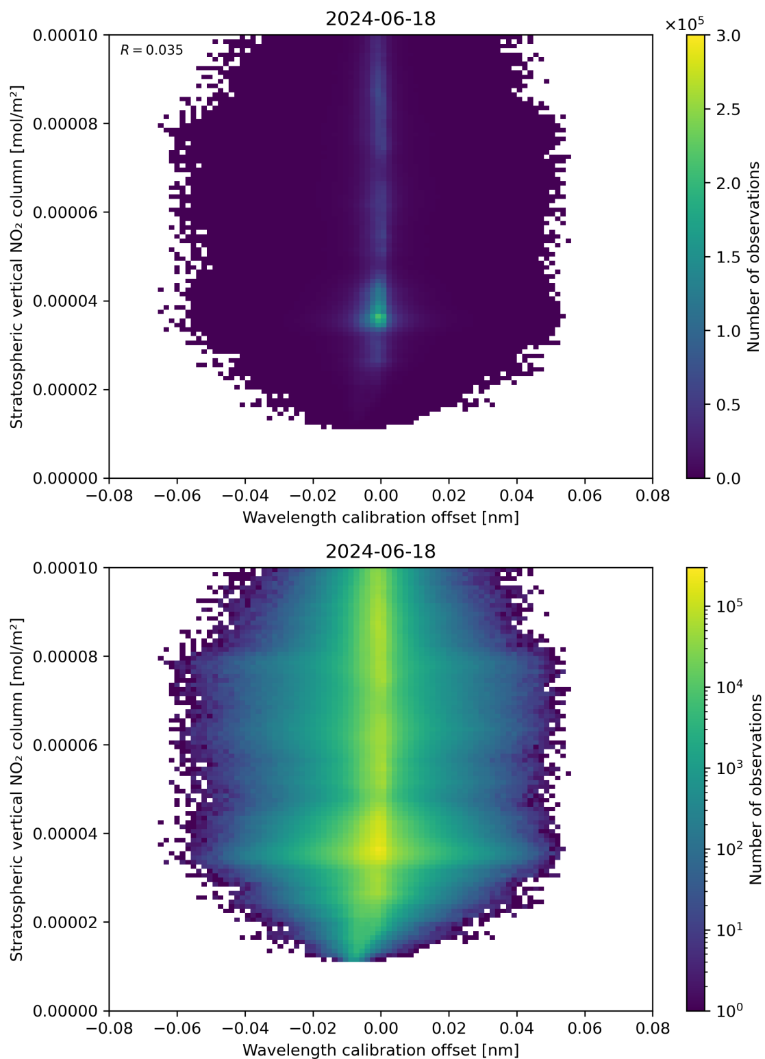
Figure 176: Scatter density plot of “Wavelength calibration offset” against “Stratospheric vertical NO 2 column” for 2024-06-17 to 2024-06-19.
