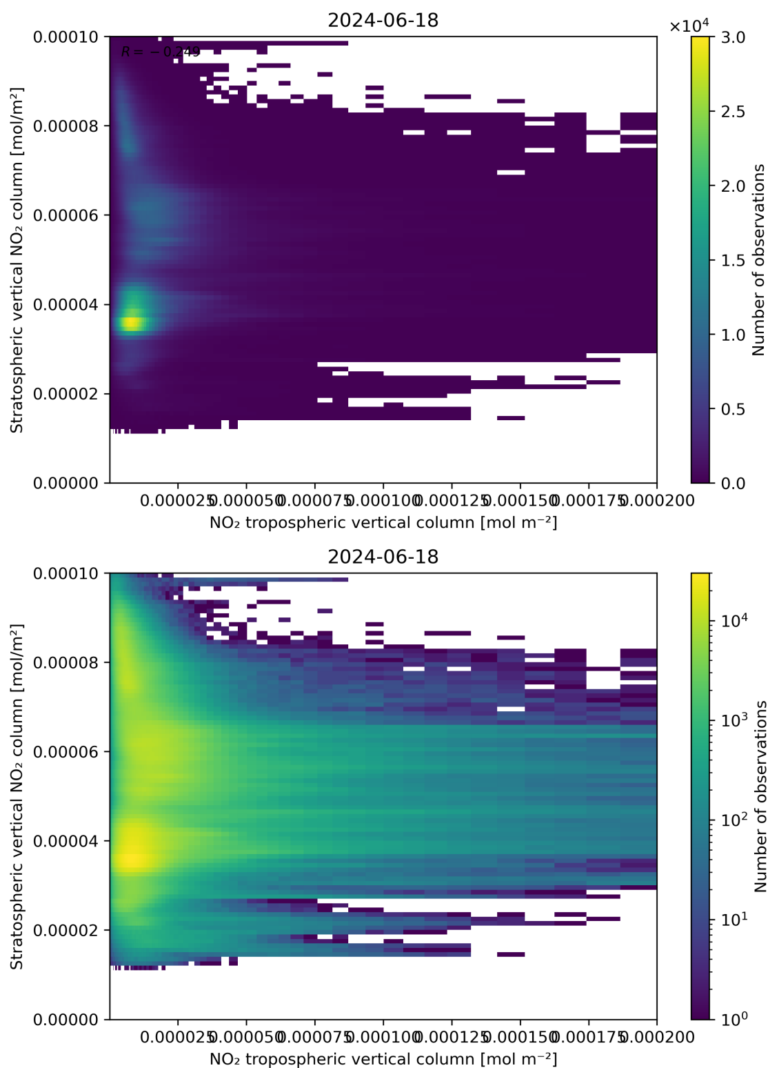
Figure 125: Scatter density plot of “NO 2 tropospheric vertical column” against “Stratospheric vertical NO 2 column” for 2024-06-17 to 2024-06-19.
