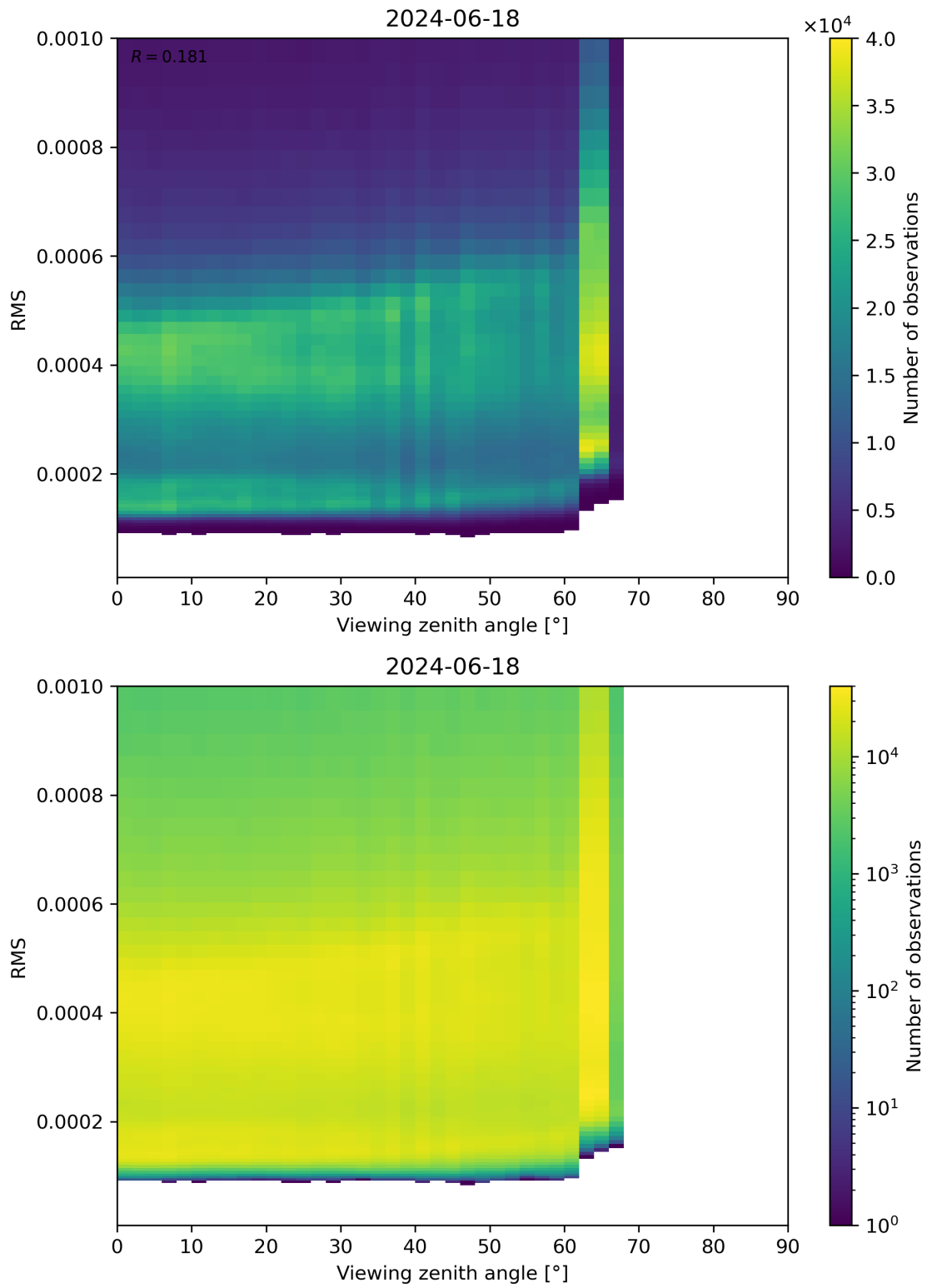
Figure 171: Scatter density plot of “Viewing zenith angle” against “RMS” for 2024-06-17 to 2024-06-19.
