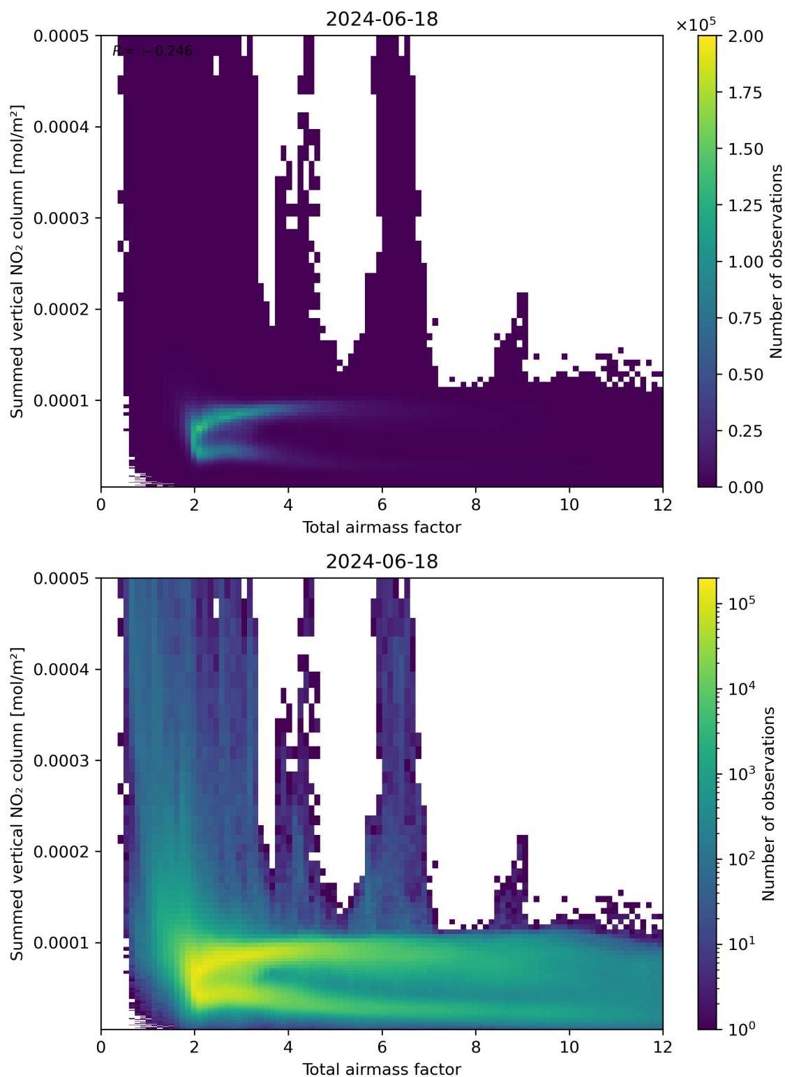
Figure 65: Scatter density plot of “Total airmass factor” against “Summed vertical NO 2 column” for 2024-06-17 to 2024-06-19.
