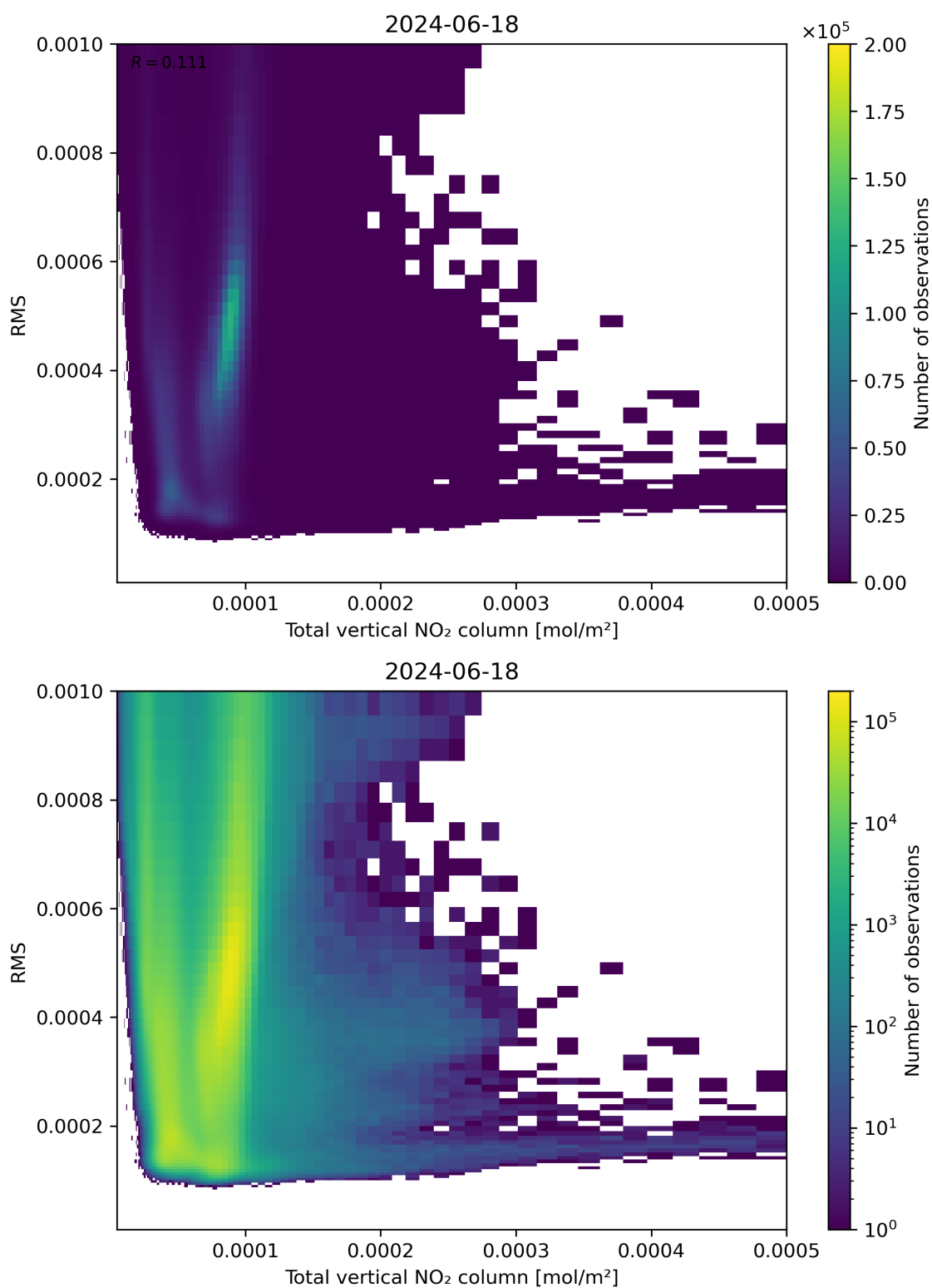
Figure 120: Scatter density plot of “Total vertical NO 2 column” against “RMS” for 2024-06-17 to 2024-06-19.
