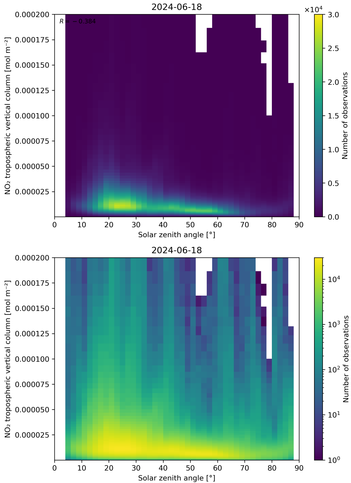
Figure 155: Scatter density plot of “Solar zenith angle” against “NO 2 tropospheric vertical column” for 2024-06-17 to 2024-06-19.
