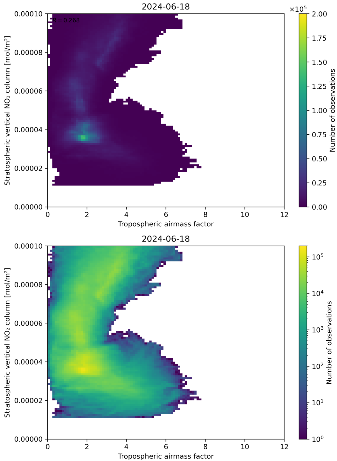
Figure 74: Scatter density plot of “Tropospheric air mass factor” against “Stratospheric vertical NO 2 column” for 2024-06-17 to 2024-06-19.
