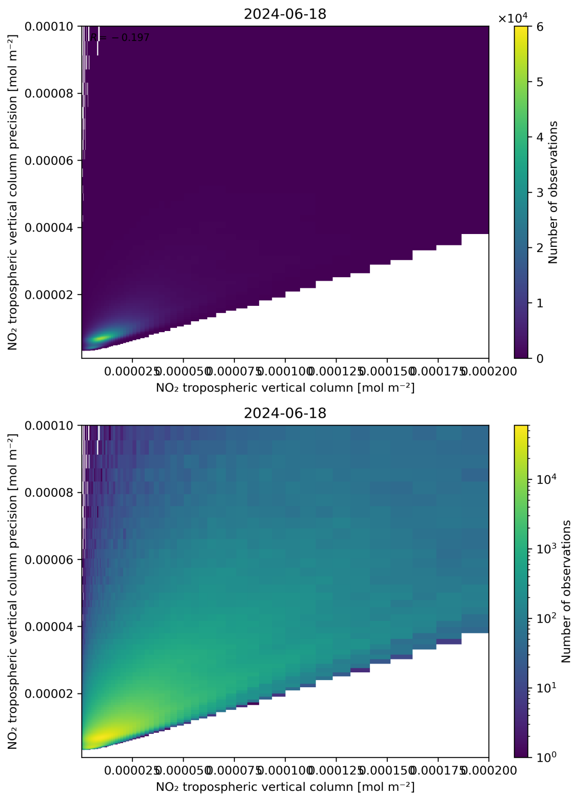
Figure 130: Scatter density plot of “NO 2 tropospheric vertical column” against “NO 2 tropospheric vertical column precision” for 2024-06-17 to 2024-06-19.
