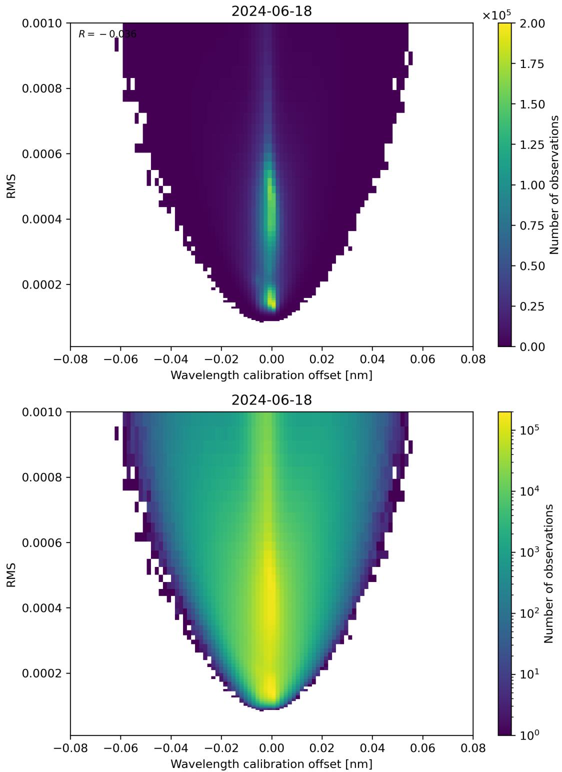
Figure 181: Scatter density plot of “Wavelength calibration offset” against “RMS” for 2024-06-17 to 2024-06-19.
