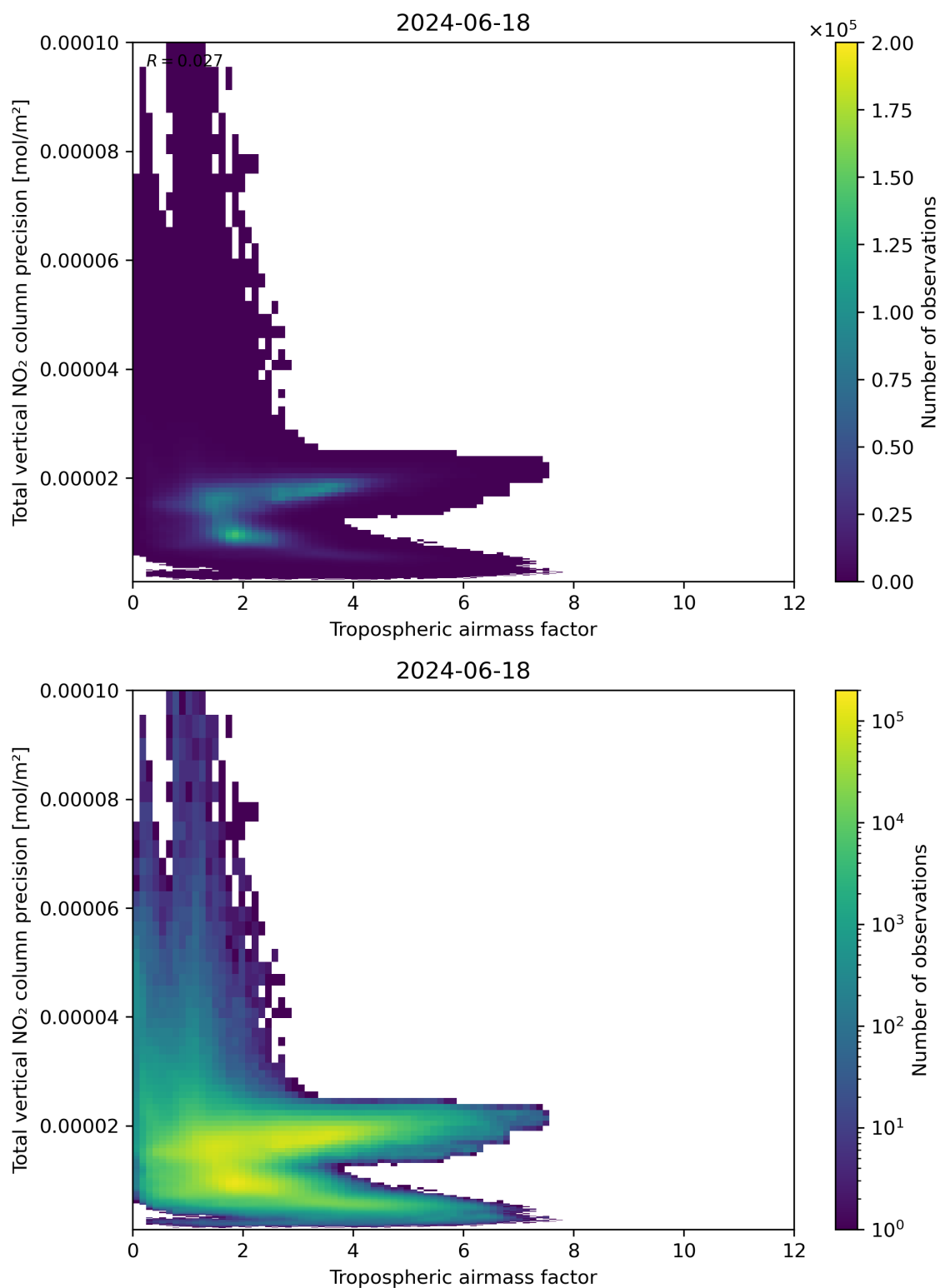
Figure 78: Scatter density plot of “Tropospheric air mass factor” against “Total vertical NO 2 column precision” for 2024-06-17 to 2024-06-19.
