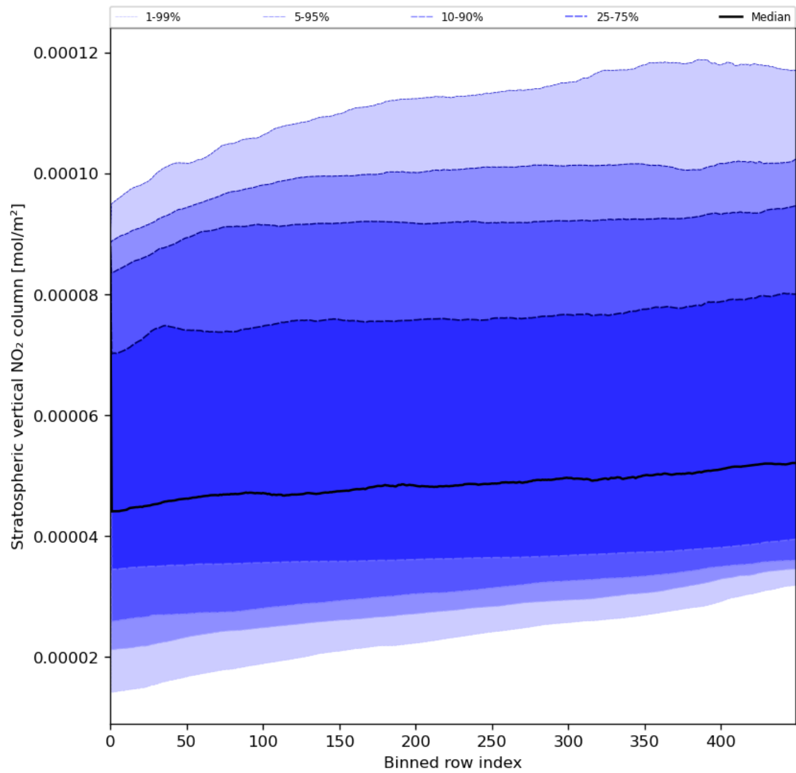
Figure 53: Along track statistics of “Stratospheric vertical NO 2 column” for 2024-06-17 to 2024-06-19
