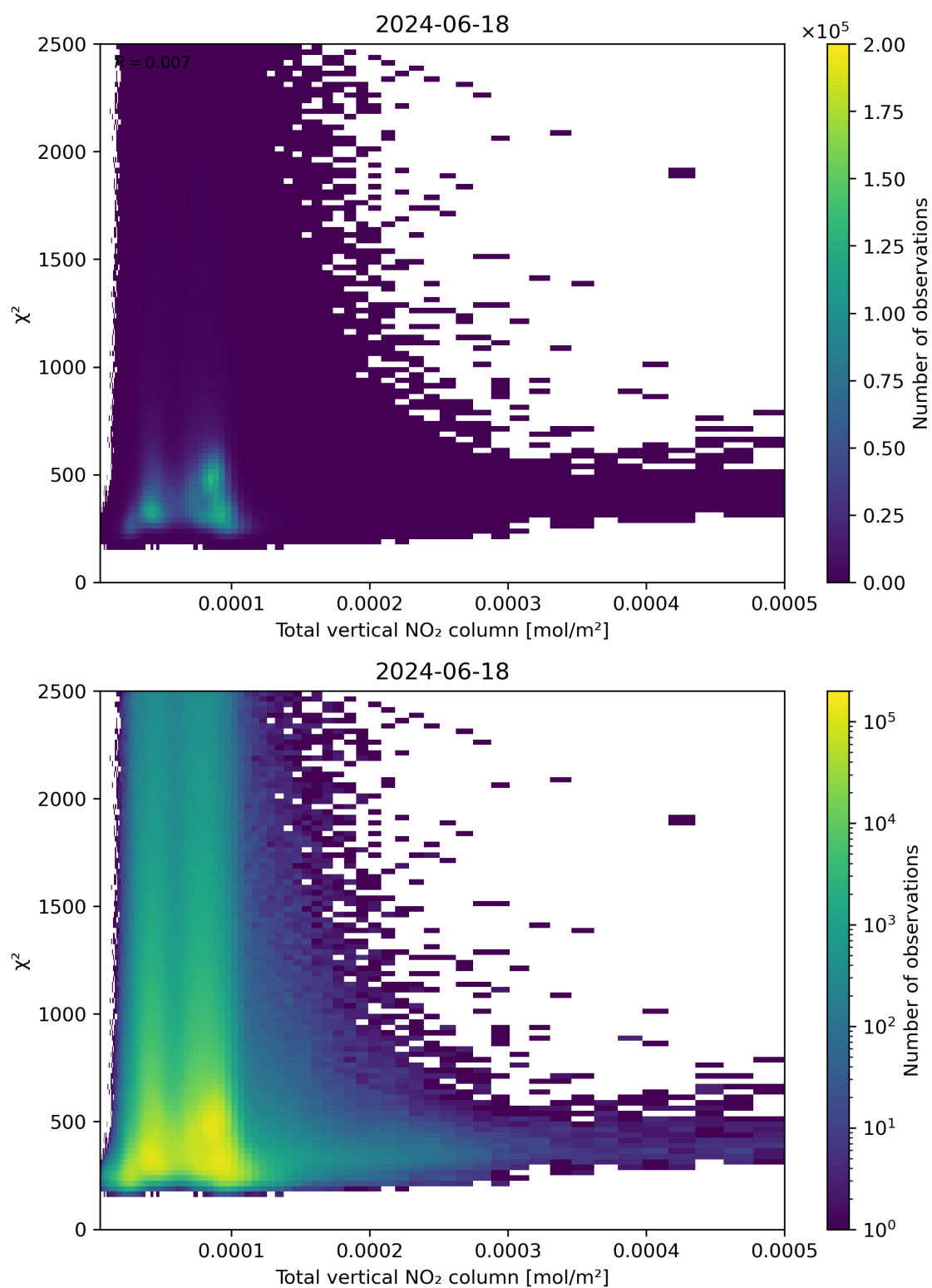
Figure 111: Scatter density plot of “Total vertical NO 2 column” against “ \chi^2 ” for 2024-06-17 to 2024-06-19.
