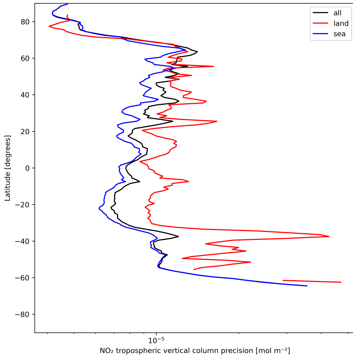
Figure 13: Zonal average of “NO 2 tropospheric vertical column precision” for 2024-06-17 to 2024-06-19.
