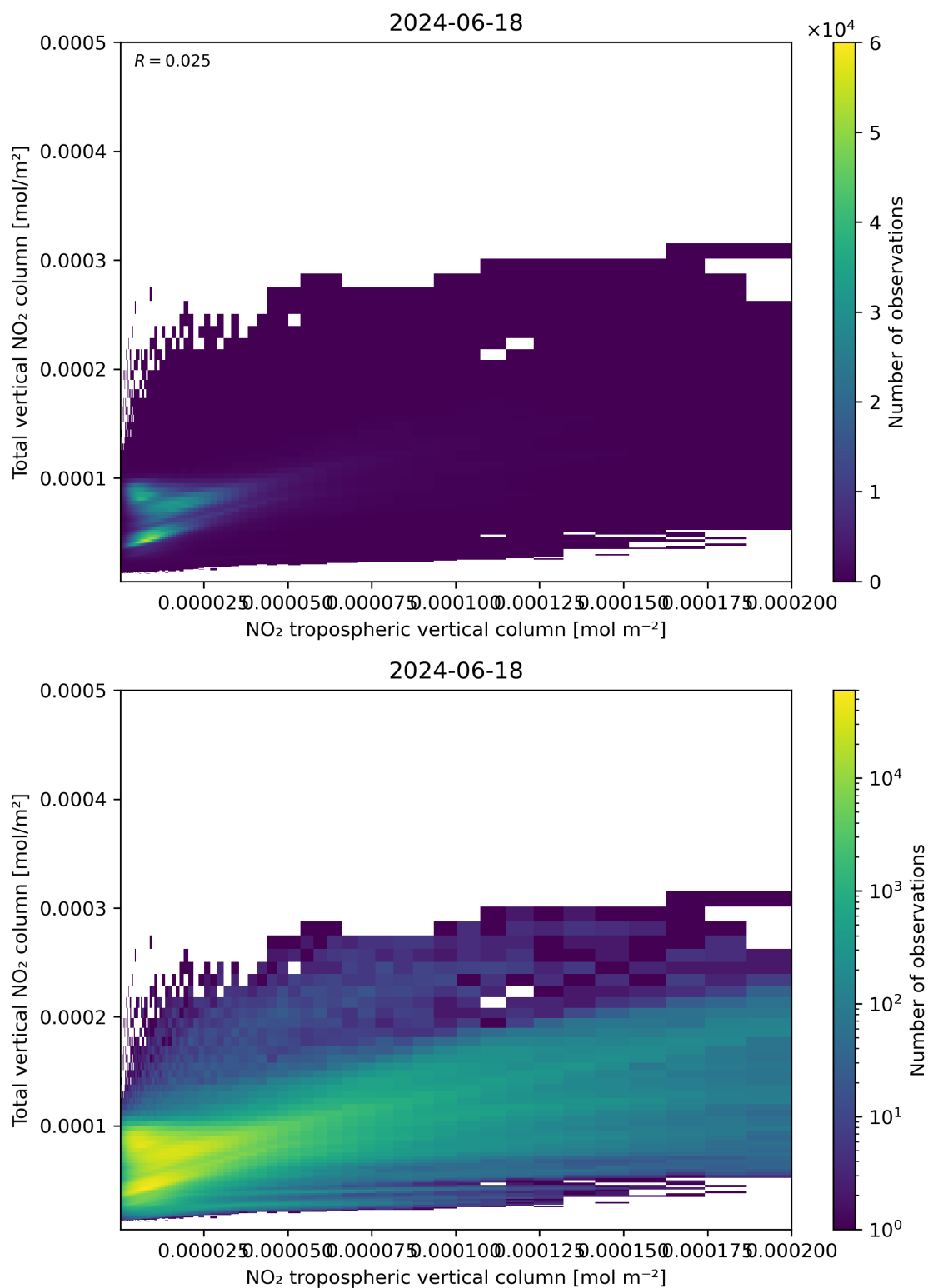
Figure 128: Scatter density plot of “NO 2 tropospheric vertical column” against “Total vertical NO 2 column” for 2024-06-17 to 2024-06-19.
