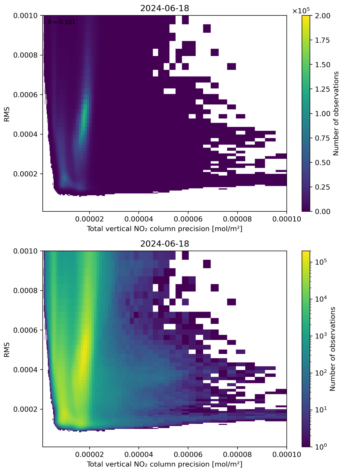
Figure 119: Scatter density plot of “Total vertical NO 2 column precision” against “RMS” for 2024-06-17 to 2024-06-19.
