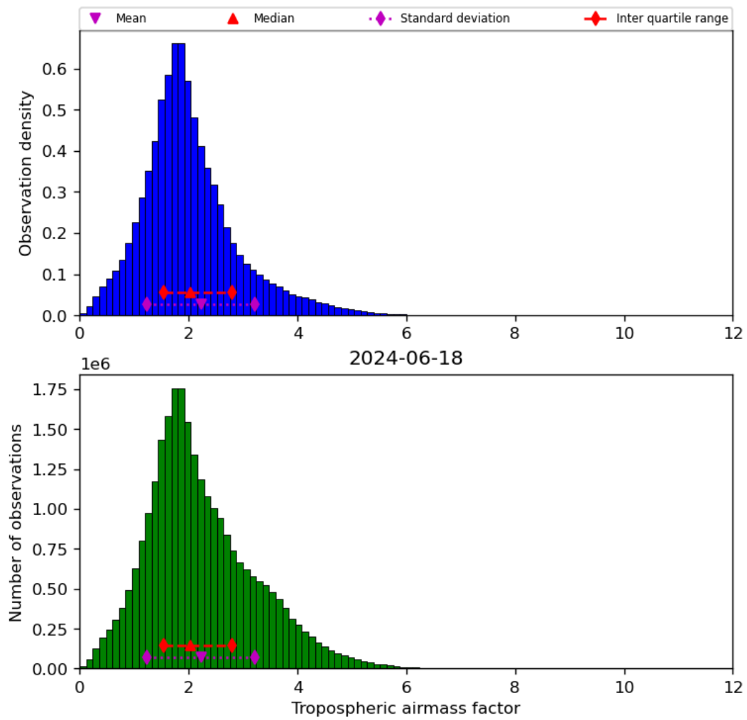
Figure 31: Histogram of “Tropospheric airmass factor” for 2024-06-17 to 2024-06-19
