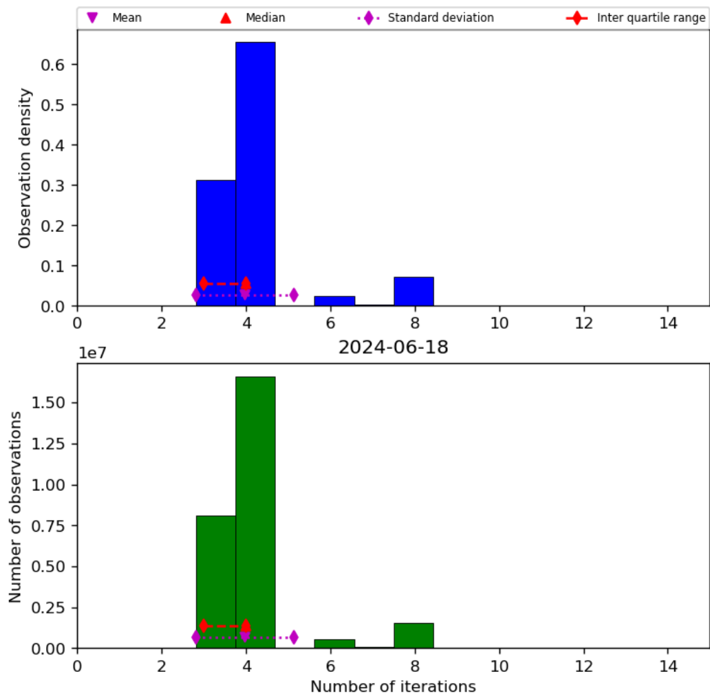
Figure 34: Histogram of “Number of iterations” for 2024-06-17 to 2024-06-19
