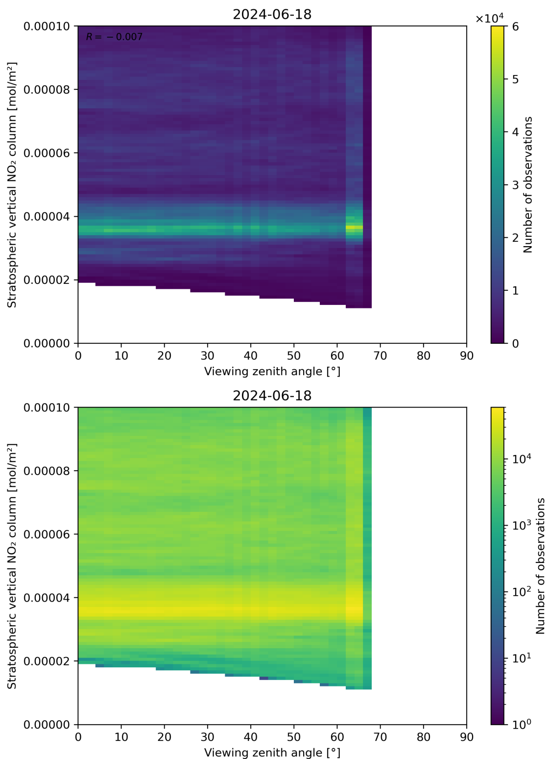
Figure 164: Scatter density plot of “Viewing zenith angle” against “Stratospheric vertical NO 2 column” for 2024-06-17 to 2024-06-19.
