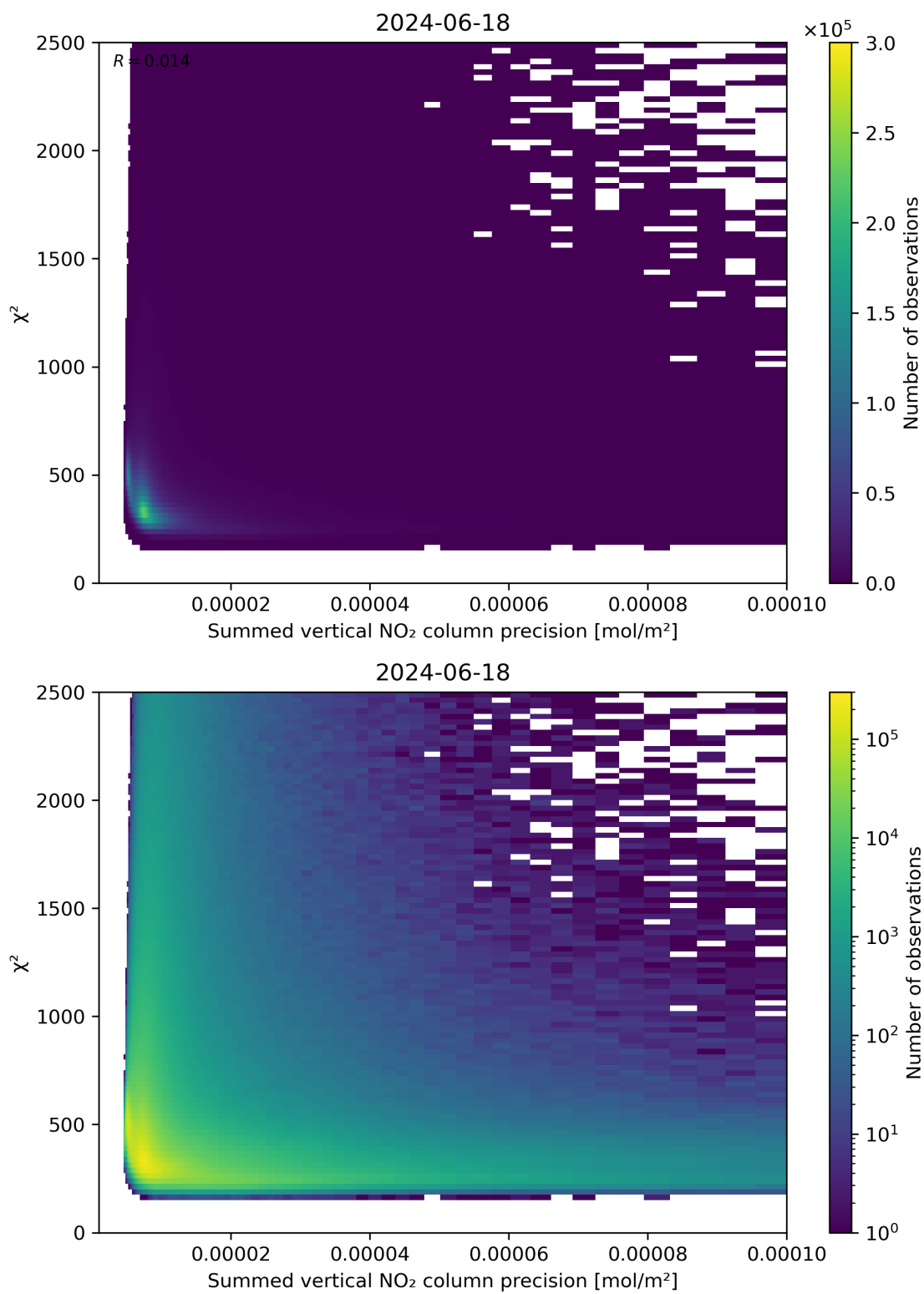
Figure 107: Scatter density plot of “Summed vertical NO 2 column precision” against “ \chi^2 ” for 2024-06-17 to 2024-06-19.
