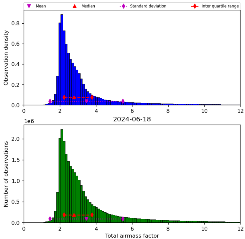
Figure 32: Histogram of “Total airmass factor” for 2024-06-17 to 2024-06-19
