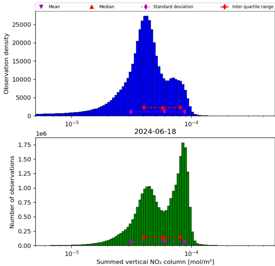
Figure 40: Histogram of “Summed vertical NO 2 column” for 2024-06-17 to 2024-06-19
