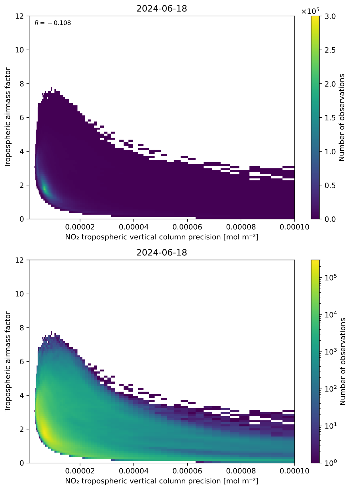
Figure 133: Scatter density plot of “NO 2 tropospheric vertical column precision” against “Tropospheric air mass factor” for 2024-06-17 to 2024-06-19.
