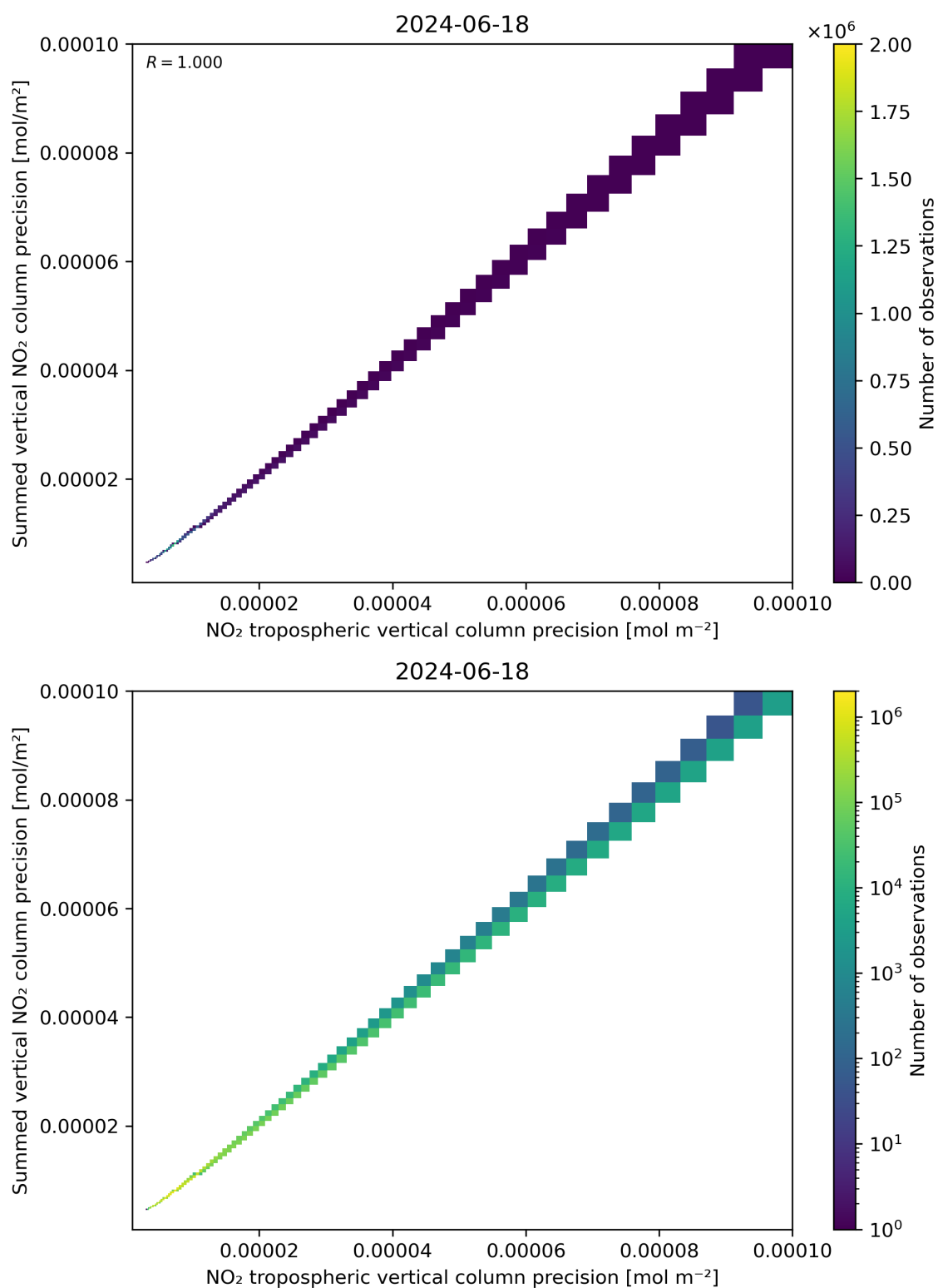
Figure 137: Scatter density plot of “NO 2 tropospheric vertical column precision” against “Summed vertical NO 2 column precision” for 2024-06-17 to 2024-06-19.
