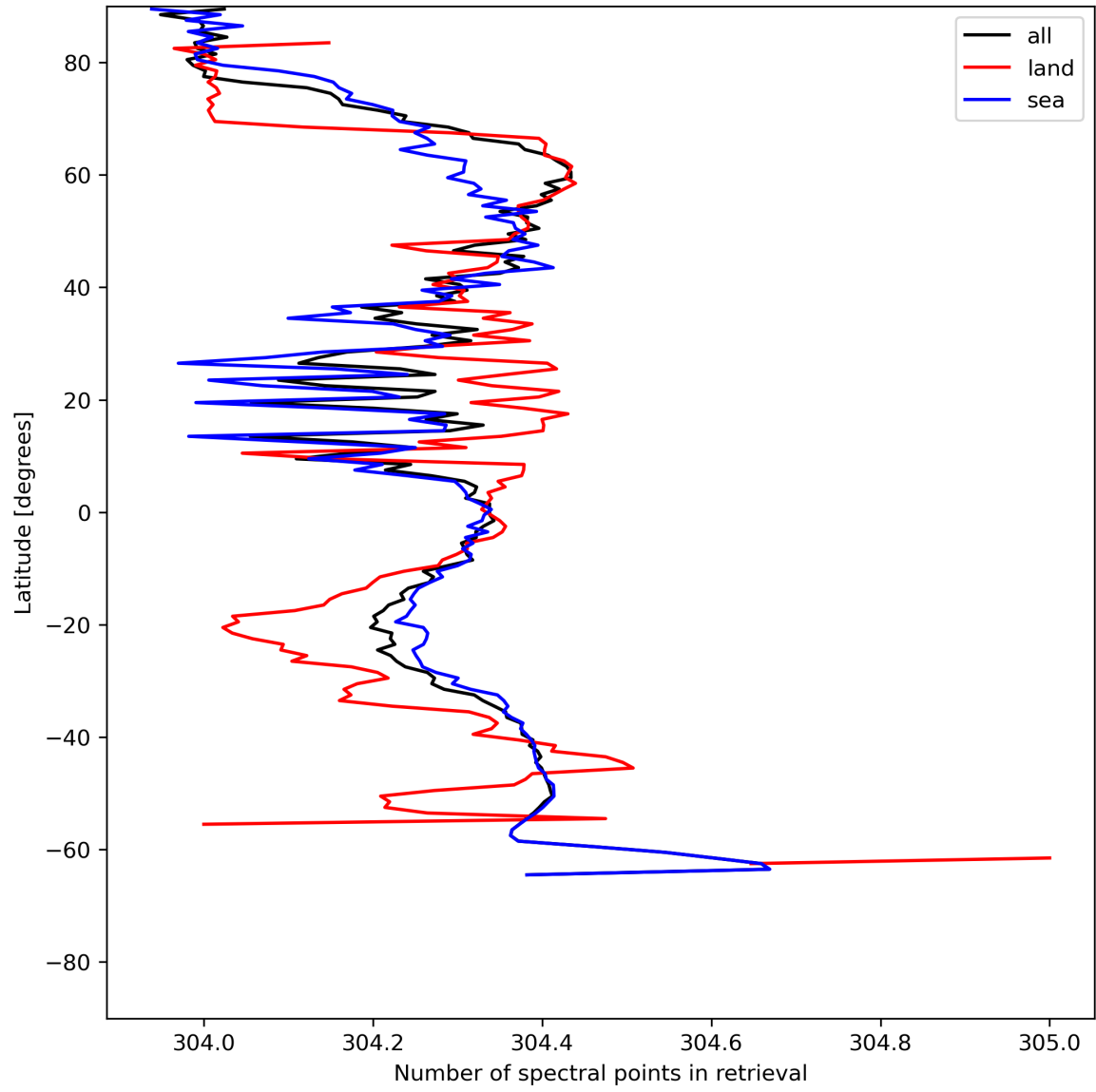
Figure 16: Zonal average of “Number of spectral points in retrieval” for 2024-06-17 to 2024-06-19.
