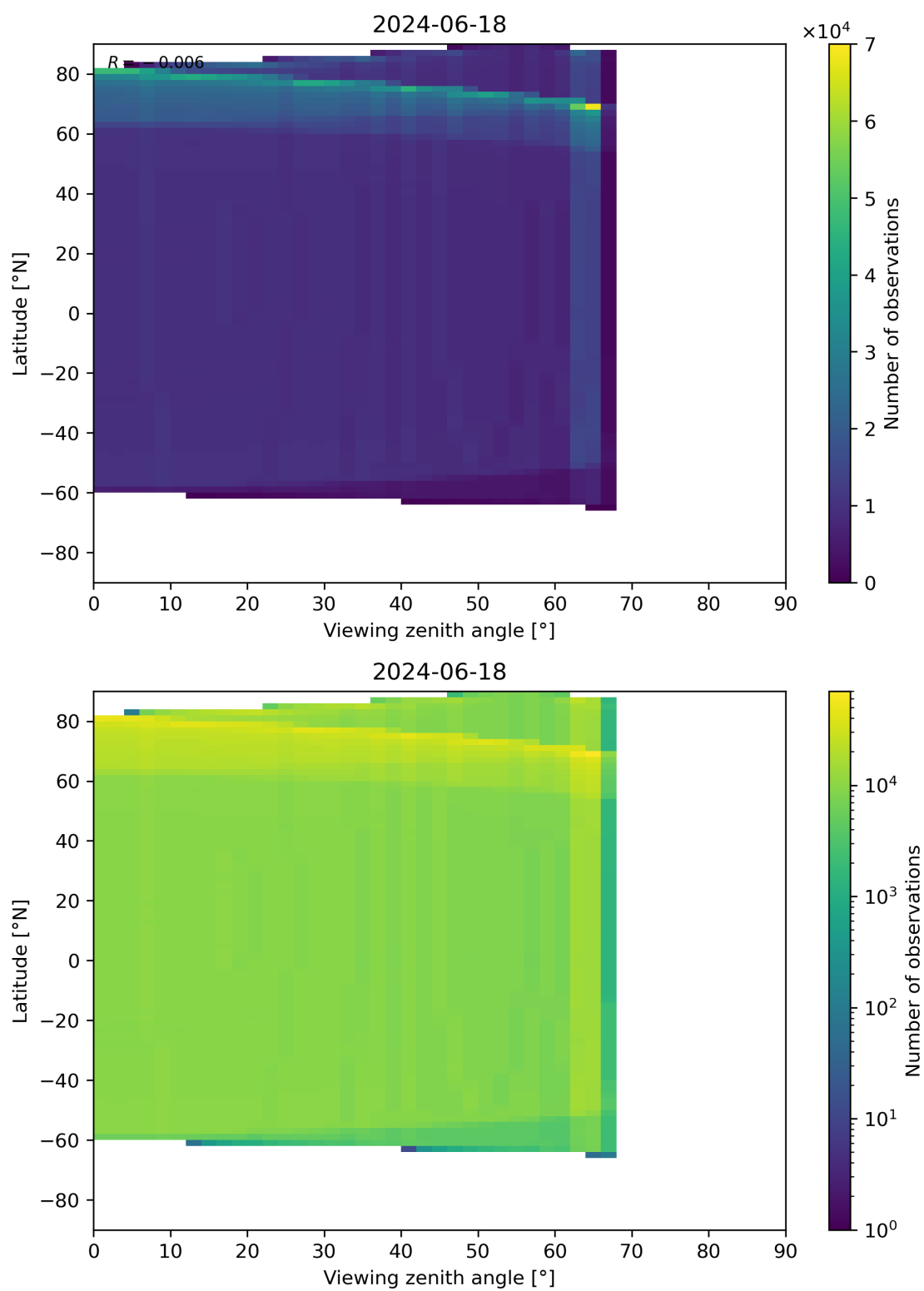
Figure 163: Scatter density plot of “Viewing zenith angle” against “Latitude” for 2024-06-17 to 2024-06-19.
