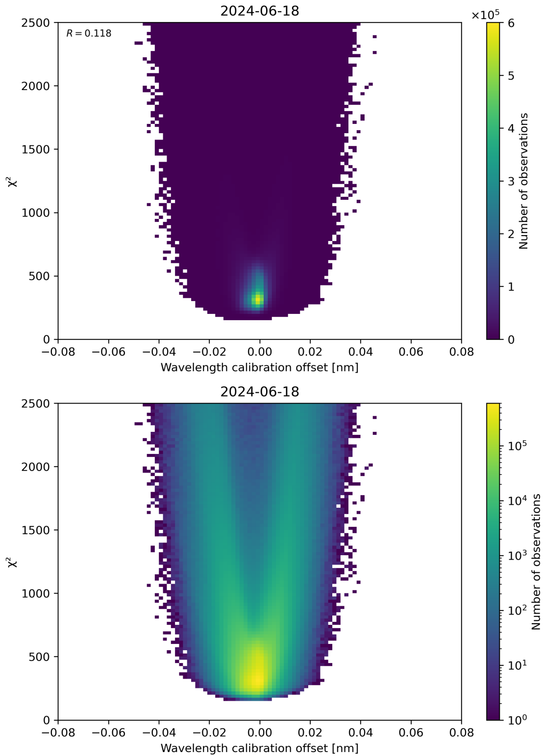
Figure 175: Scatter density plot of “Wavelength calibration offset” against “ \chi^2 ” for 2024-06-17 to 2024-06-19.
