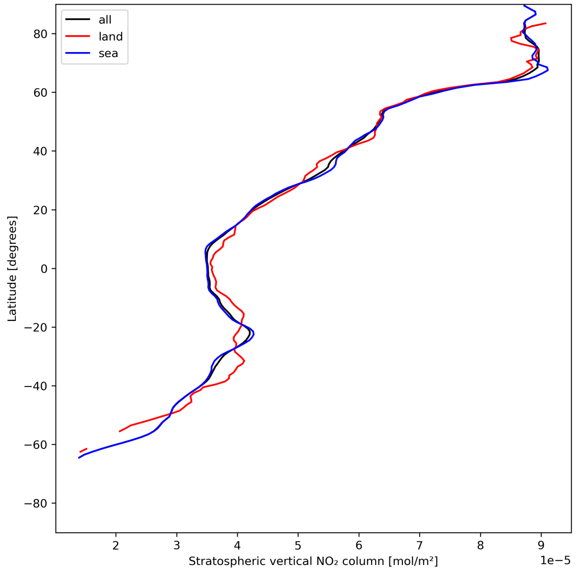
Figure 19: Zonal average of “Stratospheric vertical NO 2 column” for 2024-06-17 to 2024-06-19.
