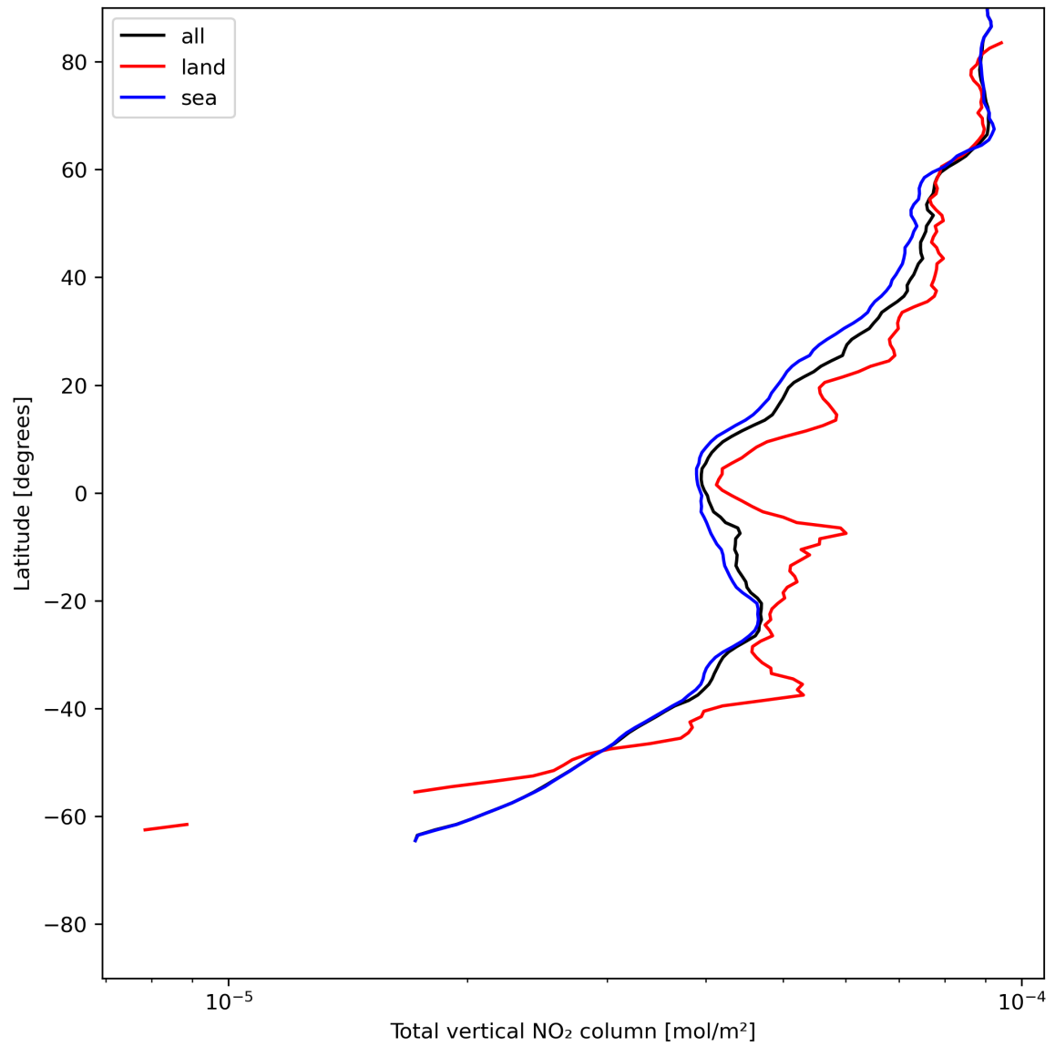
Figure 21: Zonal average of “Total vertical NO 2 column” for 2024-06-17 to 2024-06-19.
