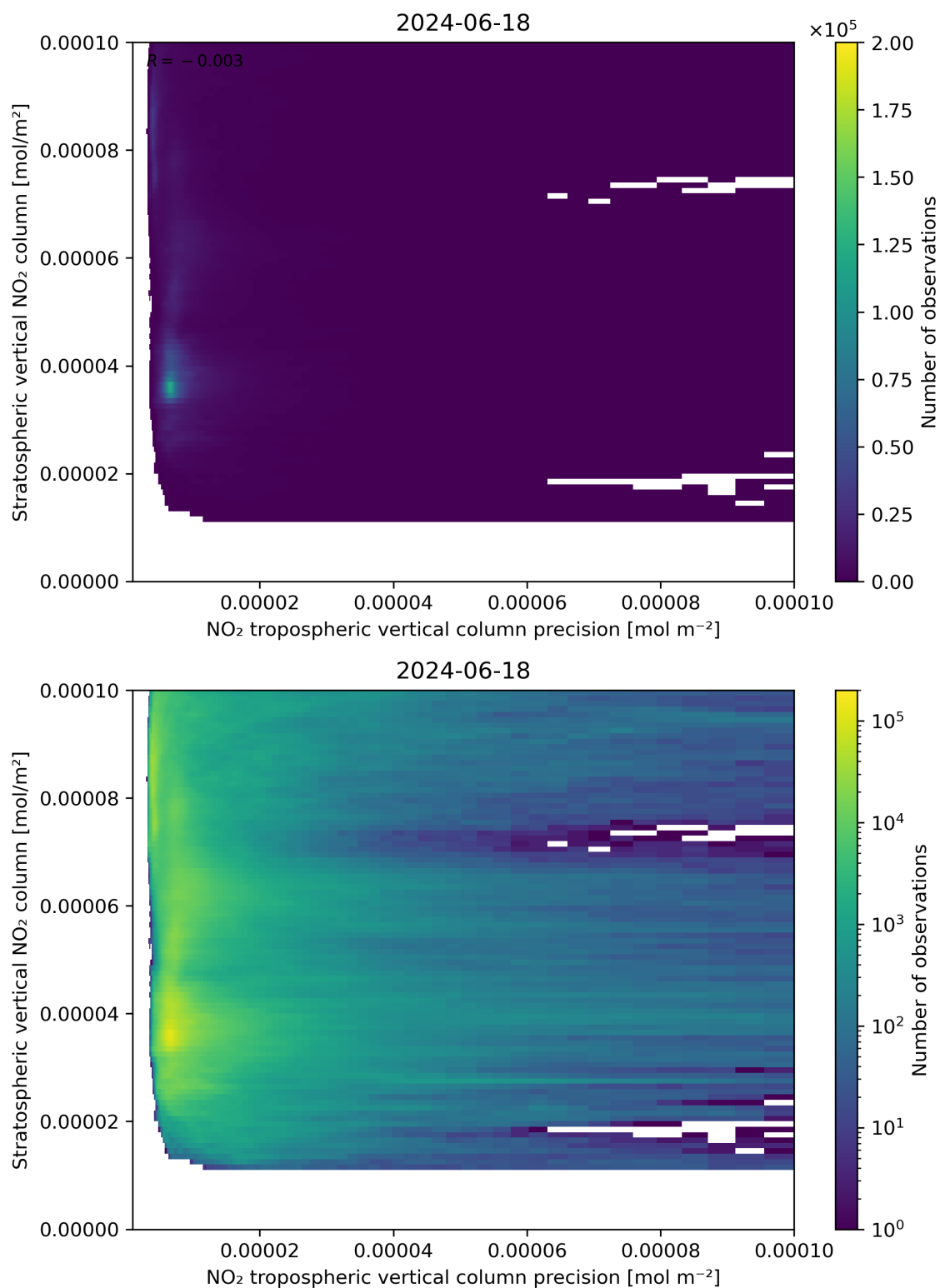
Figure 135: Scatter density plot of “NO 2 tropospheric vertical column precision” against “Stratospheric vertical NO 2 column” for 2024-06-17 to 2024-06-19.
