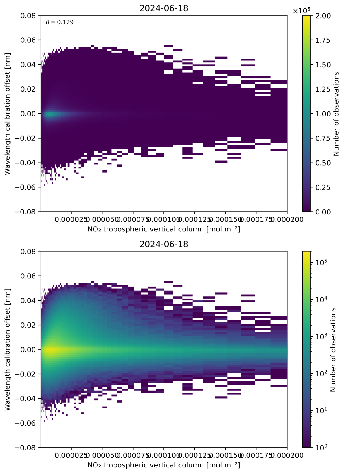
Figure 143: Scatter density plot of “NO 2 tropospheric vertical column” against “Wavelength calibration offset” for 2024-06-17 to 2024-06-19.
