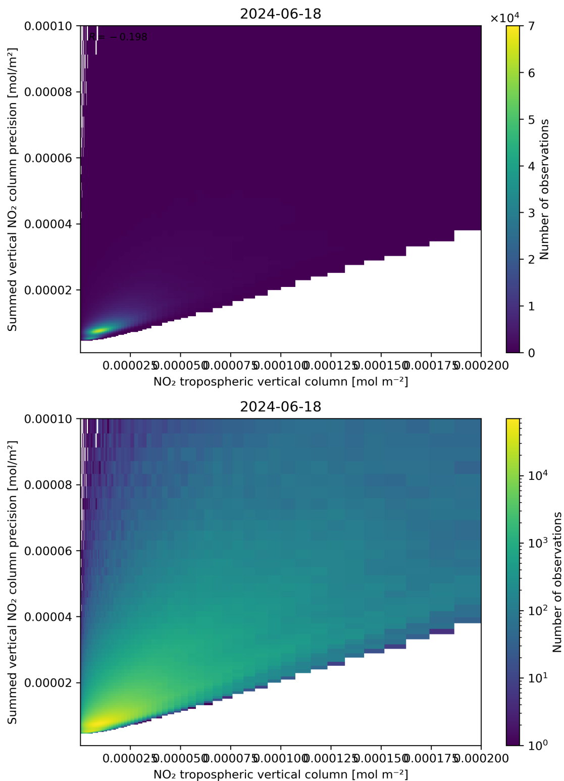
Figure 127: Scatter density plot of “NO 2 tropospheric vertical column” against “Summed vertical NO 2 column precision” for 2024-06-17 to 2024-06-19.
