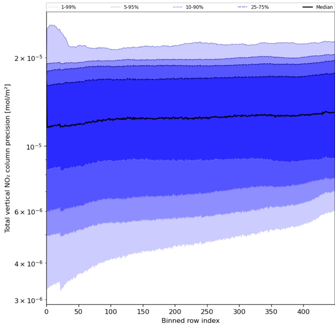
Figure 56: Along track statistics of “Total vertical NO 2 column precision” for 2024-06-17 to 2024-06-19
