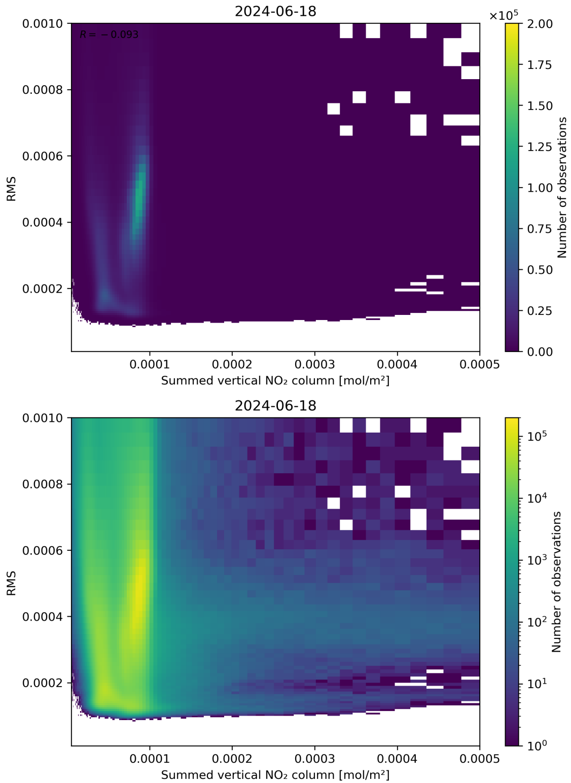
Figure 109: Scatter density plot of “Summed vertical NO 2 column” against “RMS” for 2024-06-17 to 2024-06-19.
