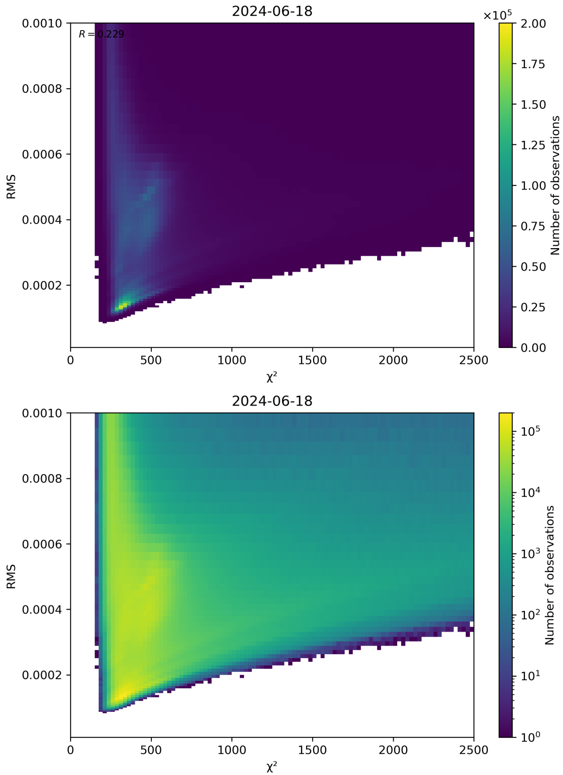
Figure 82: Scatter density plot of “ \chi^2 ” against “RMS” for 2024-06-17 to 2024-06-19.
