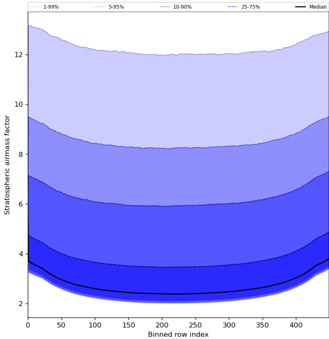
Figure 61: Along track statistics of “Stratospheric airmass factor” for 2024-06-17 to 2024-06-19
