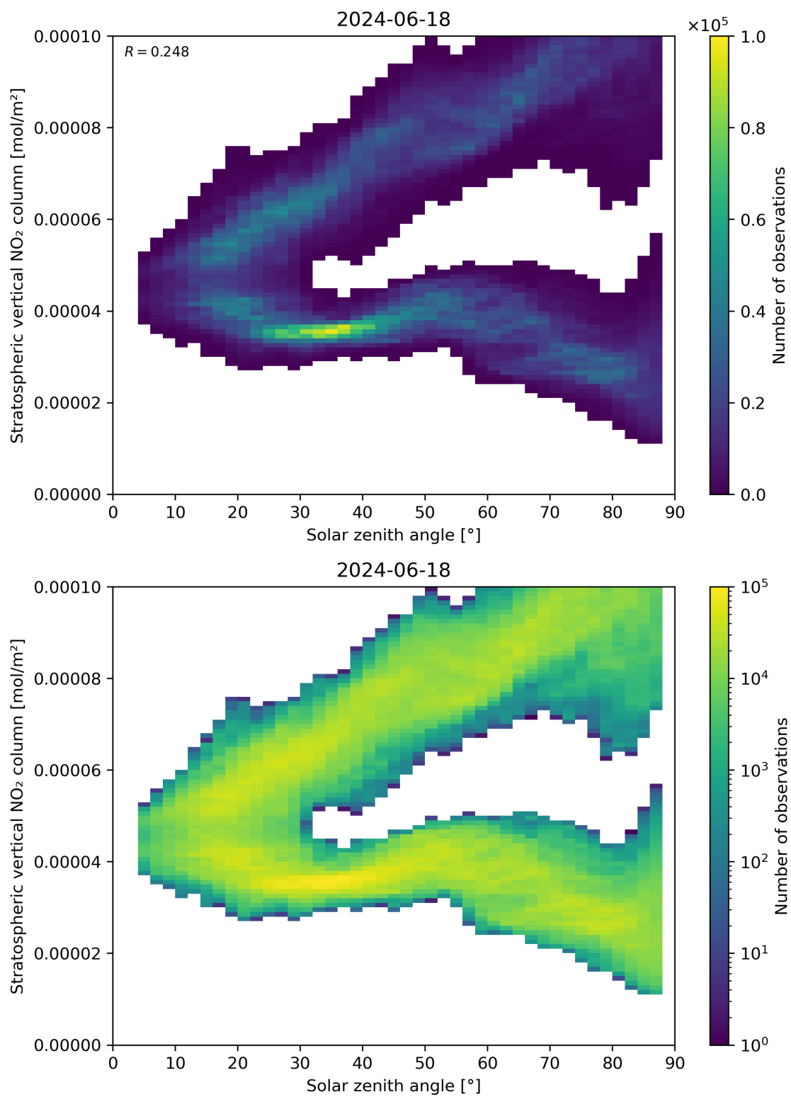
Figure 150: Scatter density plot of “Solar zenith angle” against “Stratospheric vertical NO 2 column” for 2024-06-17 to 2024-06-19.
