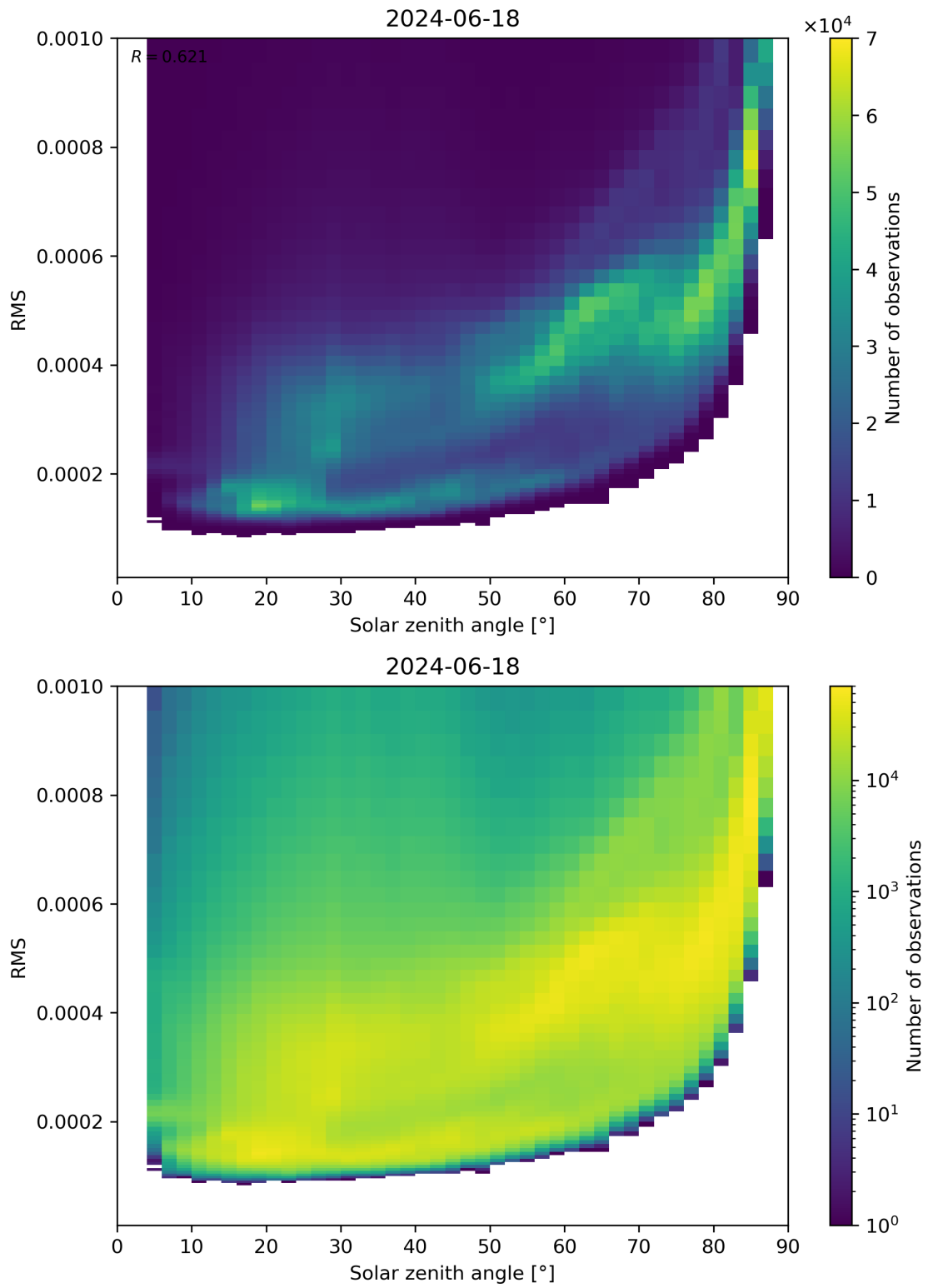
Figure 157: Scatter density plot of “Solar zenith angle” against “RMS” for 2024-06-17 to 2024-06-19.
