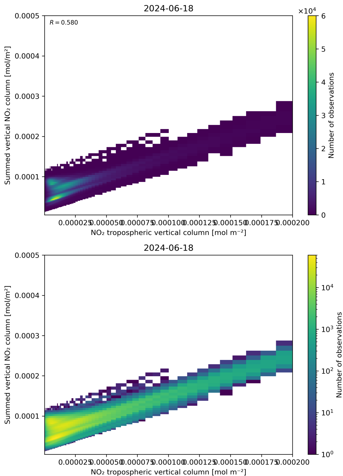
Figure 126: Scatter density plot of “NO 2 tropospheric vertical column” against “Summed vertical NO 2 column” for 2024-06-17 to 2024-06-19.
