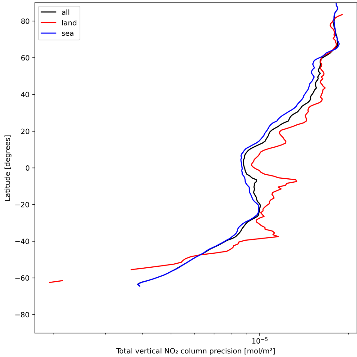
Figure 22: Zonal average of “Total vertical NO 2 column precision” for 2024-06-17 to 2024-06-19.
