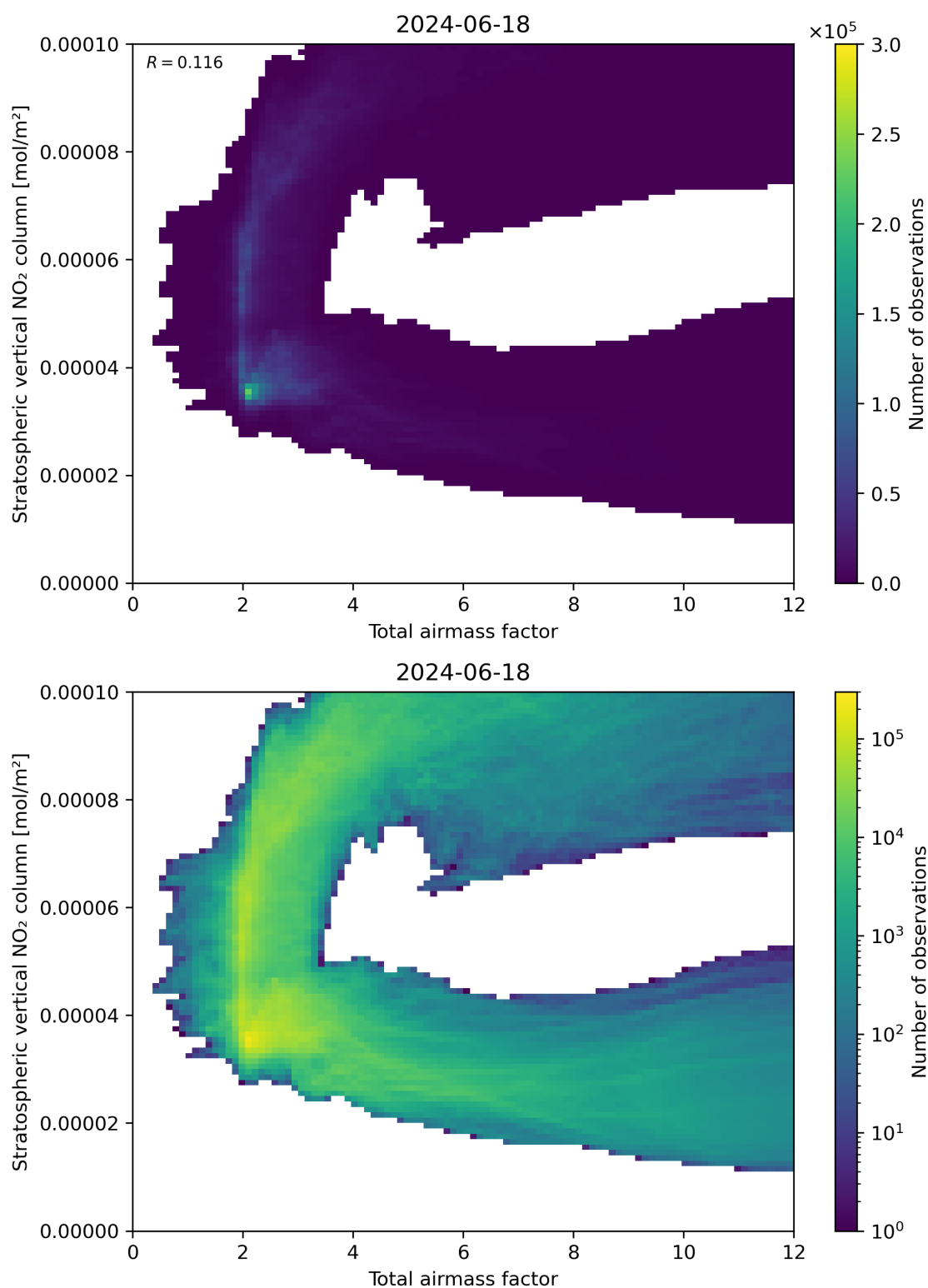
Figure 64: Scatter density plot of “Total airmass factor” against “Stratospheric vertical NO 2 column” for 2024-06-17 to 2024-06-19.
