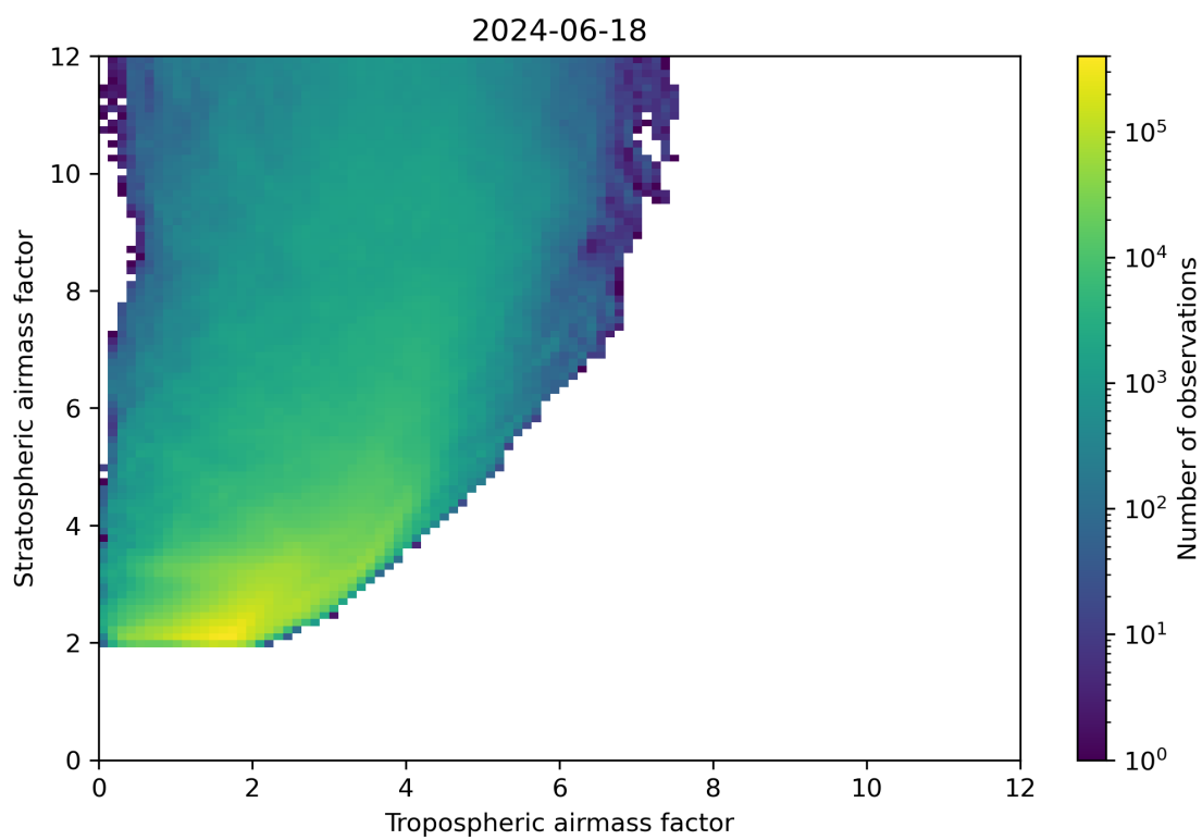
Figure 71: Scatter density plot of “Tropospheric airmass factor” against “Stratospheric airmass factor” for 2024-06-17 to 2024-06-19.
