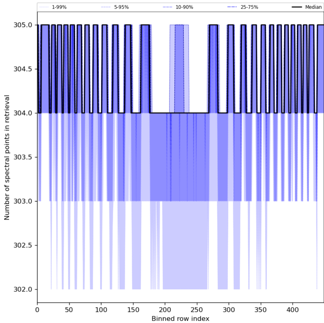
Figure 50: Along track statistics of “Number of spectral points in retrieval” for 2024-06-17 to 2024-06-19
