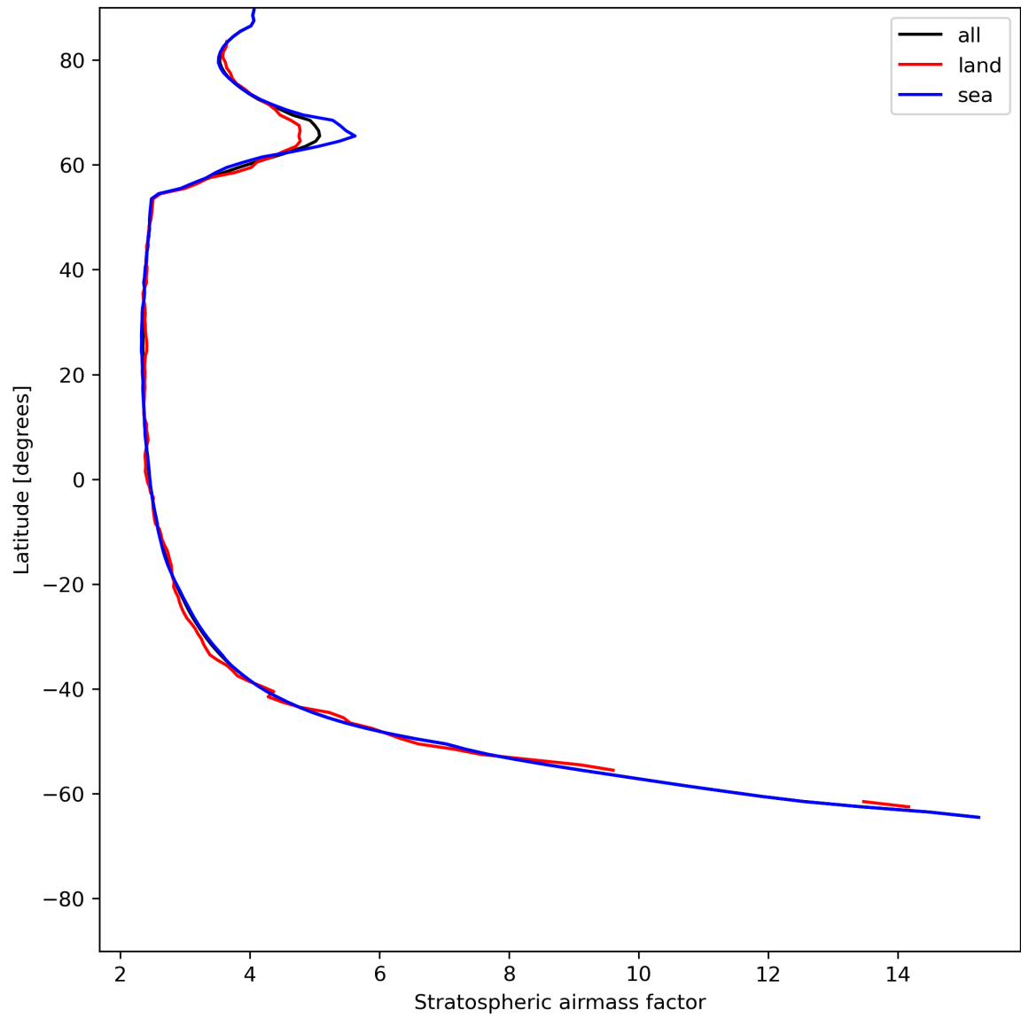
Figure 27: Zonal average of “Stratospheric airmass factor” for 2024-06-17 to 2024-06-19.
