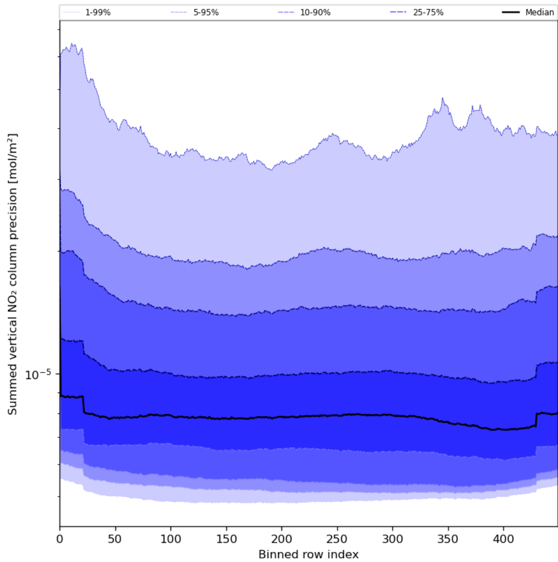
Figure 58: Along track statistics of “Summed vertical NO 2 column precision” for 2024-06-17 to 2024-06-19
