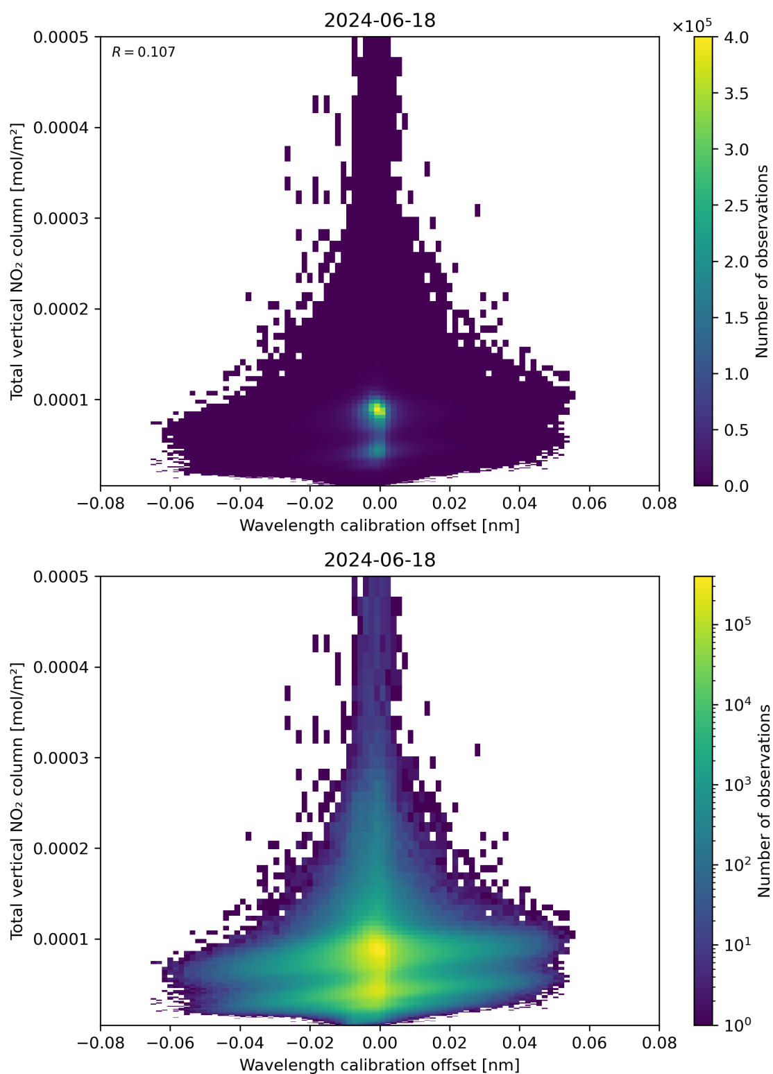
Figure 179: Scatter density plot of “Wavelength calibration offset” against “Total vertical NO 2 column” for 2024-06-17 to 2024-06-19.
