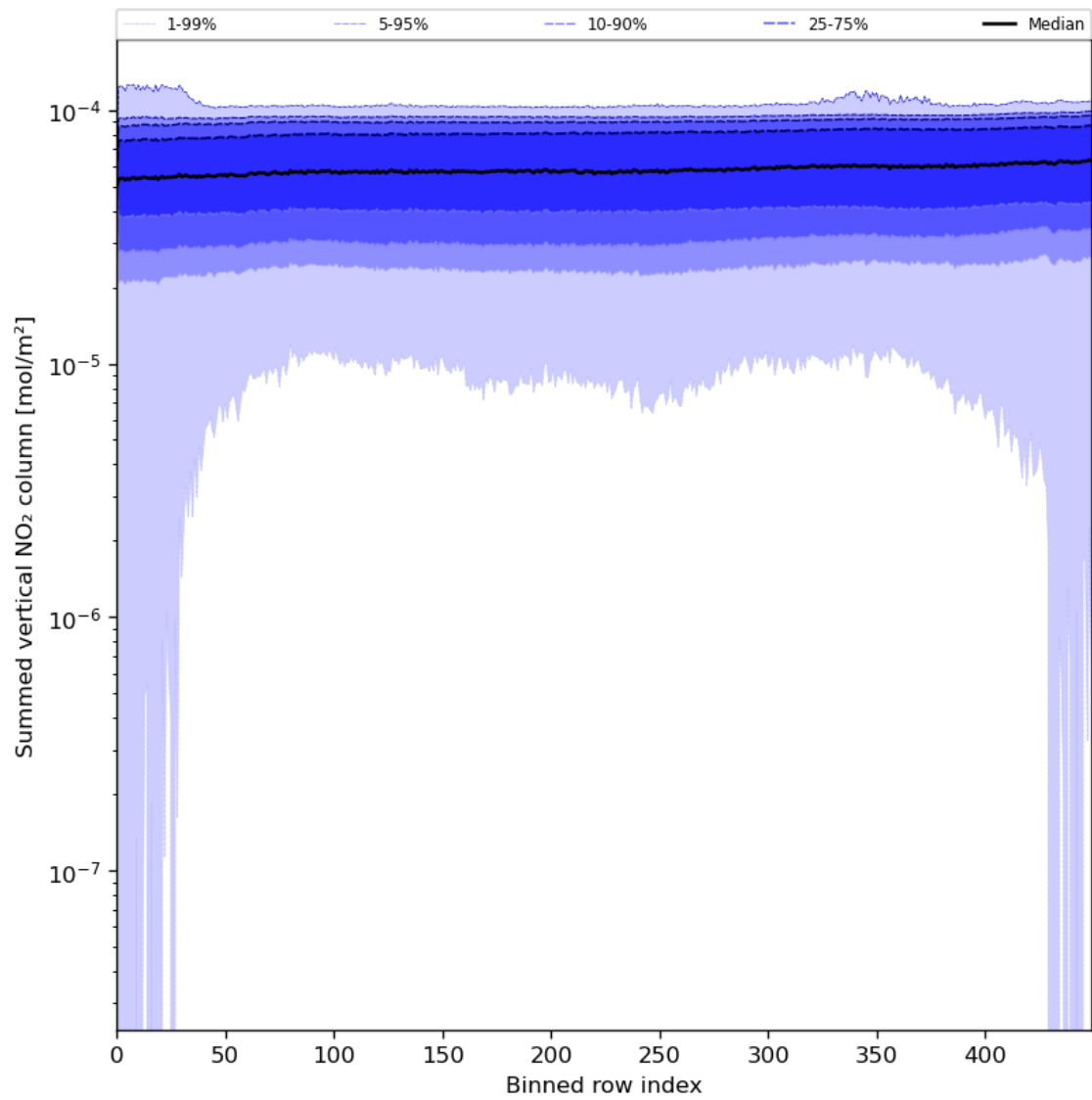
Figure 57: Along track statistics of “Summed vertical NO 2 column” for 2024-06-17 to 2024-06-19
