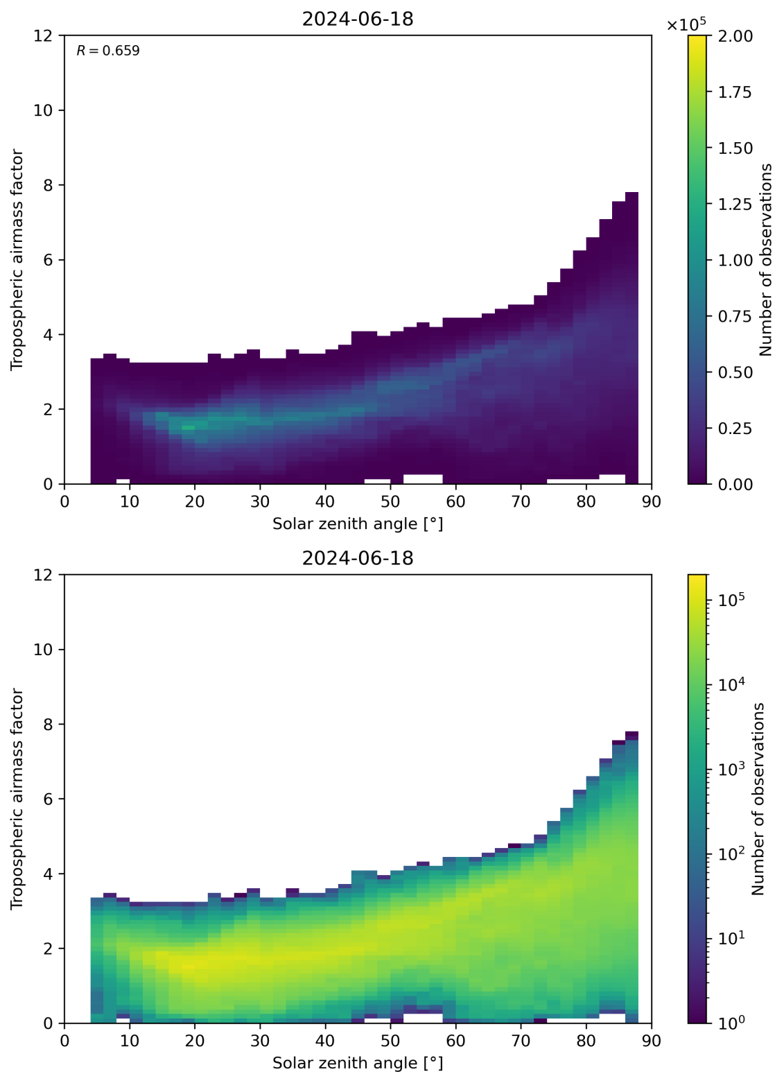
Figure 147: Scatter density plot of “Solar zenith angle” against “Tropospheric airmass factor” for 2024-06-17 to 2024-06-19.
