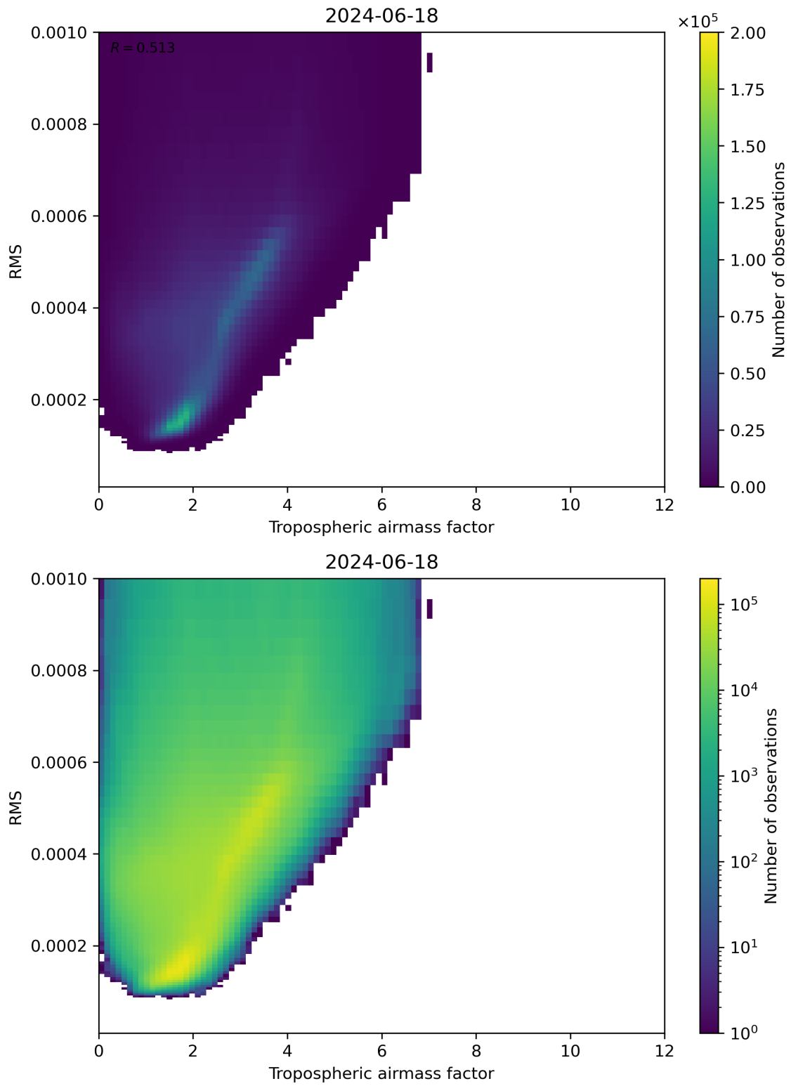
Figure 79: Scatter density plot of “Tropospheric airmass factor” against “RMS” for 2024-06-17 to 2024-06-19.
