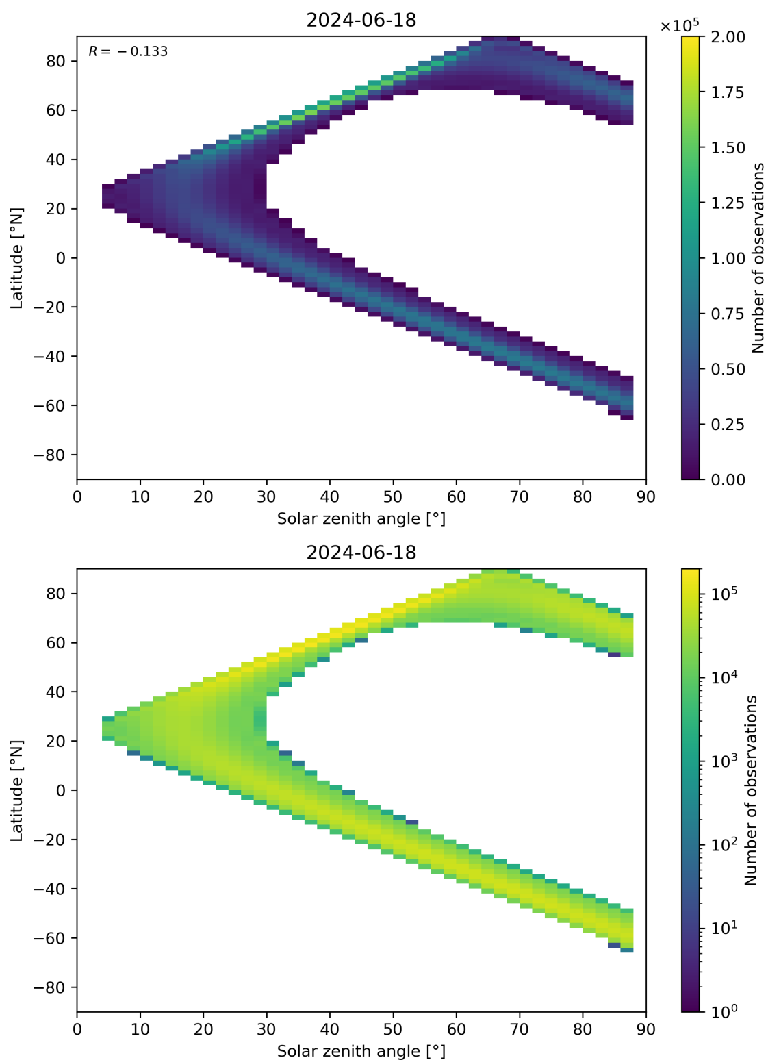
Figure 149: Scatter density plot of “Solar zenith angle” against “Latitude” for 2024-06-17 to 2024-06-19.
