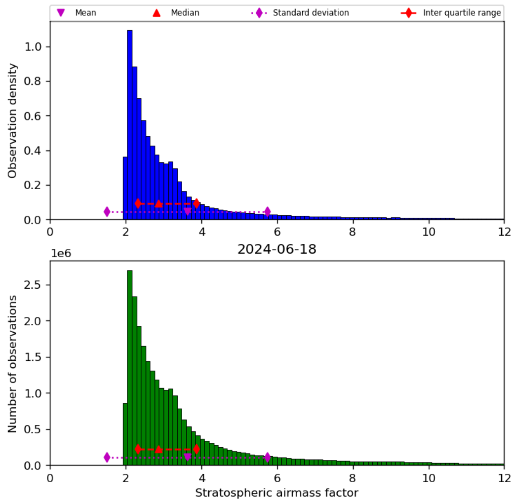
Figure 44: Histogram of “Stratospheric airmass factor” for 2024-06-17 to 2024-06-19
