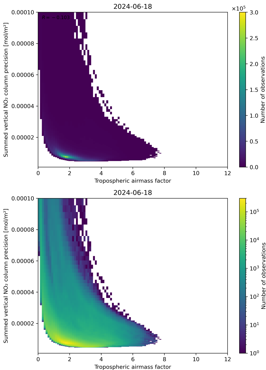
Figure 76: Scatter density plot of “Tropospheric air mass factor” against “Summed vertical NO 2 column precision” for 2024-06-17 to 2024-06-19.
