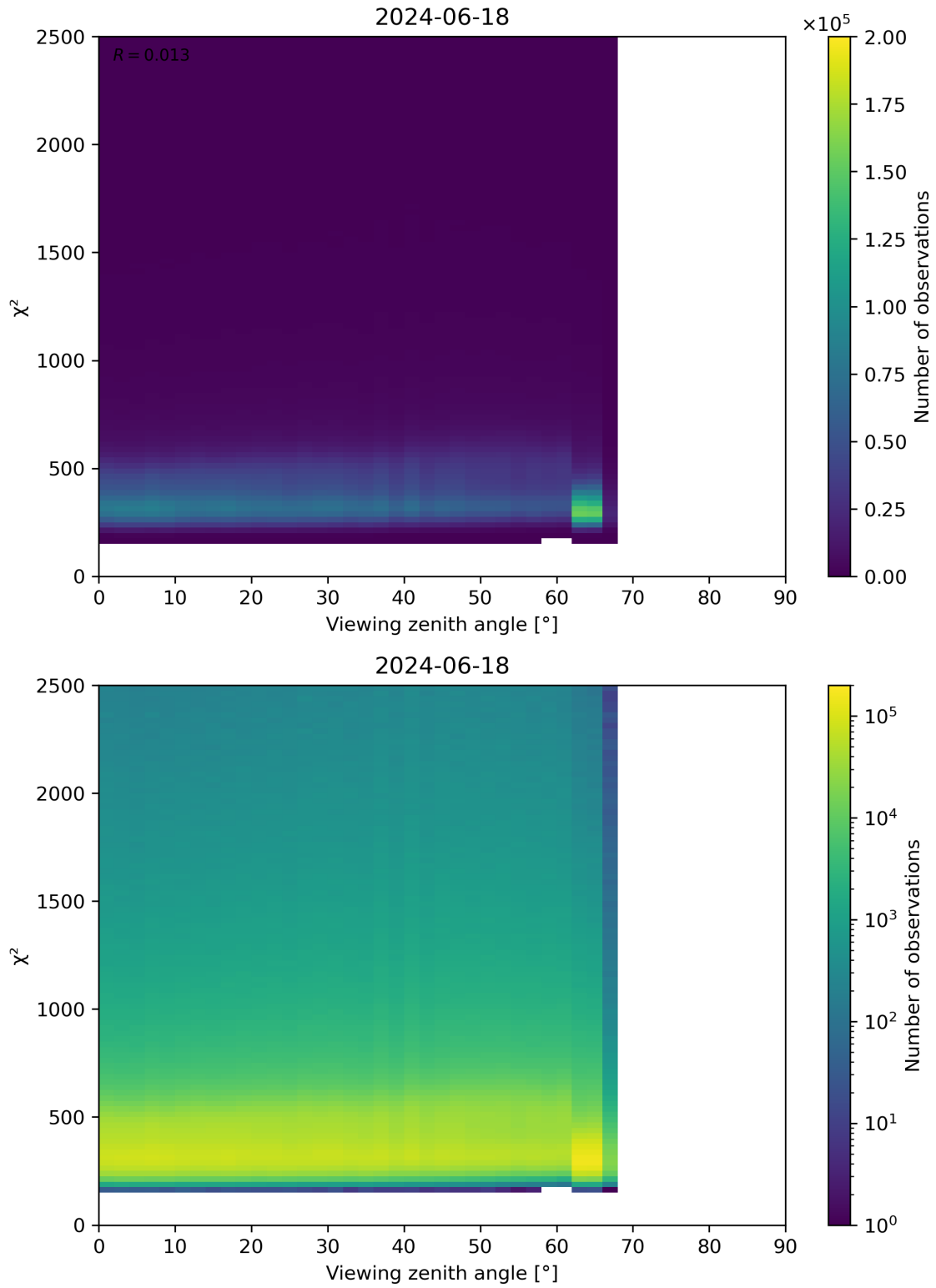
Figure 162: Scatter density plot of “Viewing zenith angle” against “ \chi^2 ” for 2024-06-17 to 2024-06-19.
