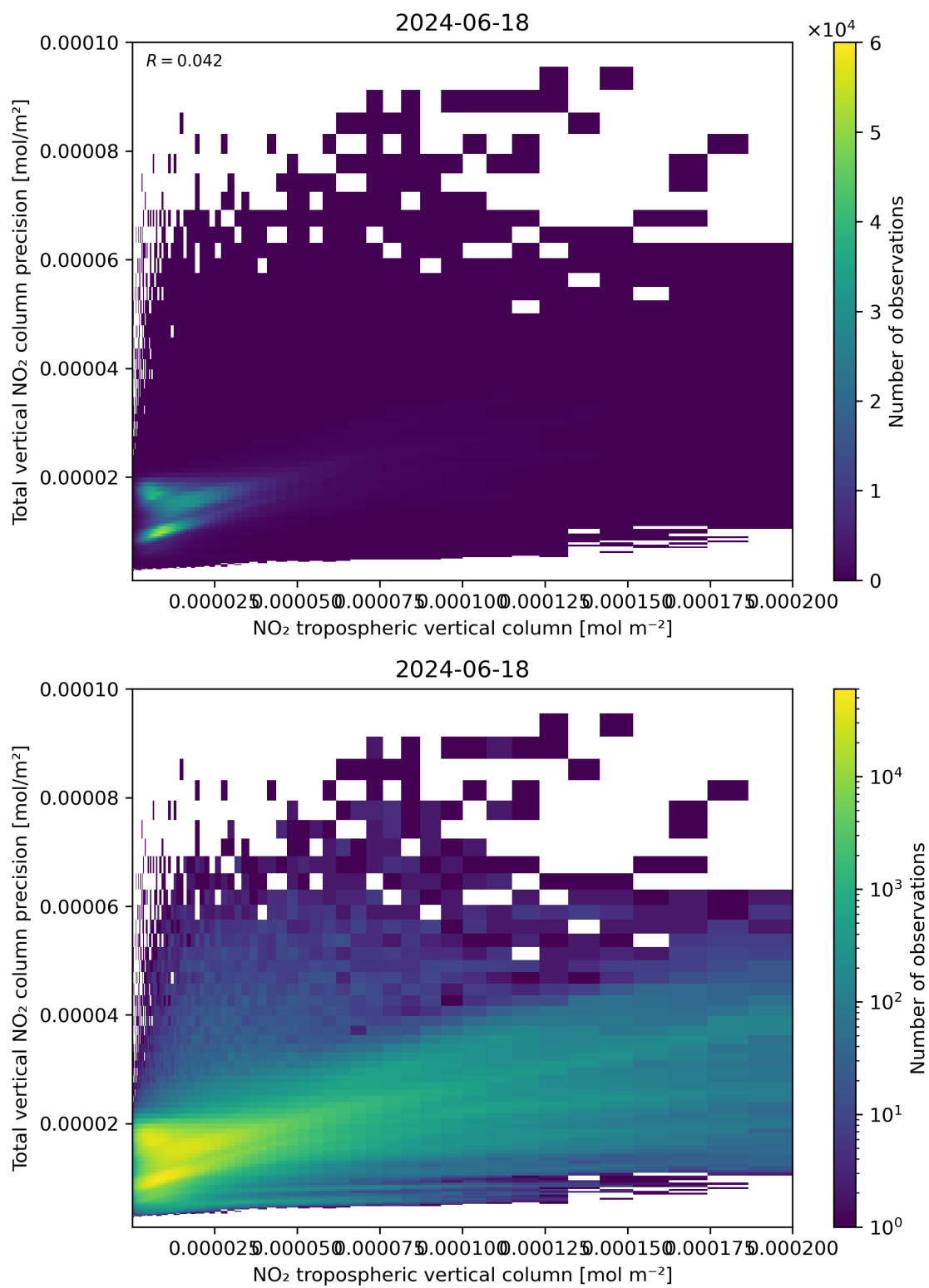
Figure 129: Scatter density plot of “NO 2 tropospheric vertical column” against “Total vertical NO 2 column precision” for 2024-06-17 to 2024-06-19.
