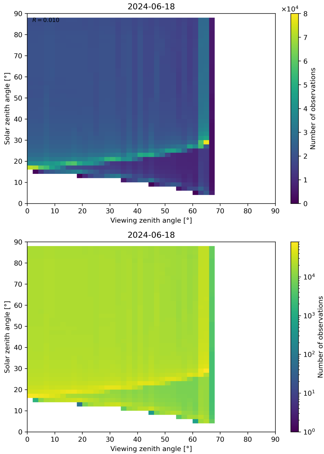
Figure 172: Scatter density plot of “Viewing zenith angle” against “Solar zenith angle” for 2024-06-17 to 2024-06-19.
