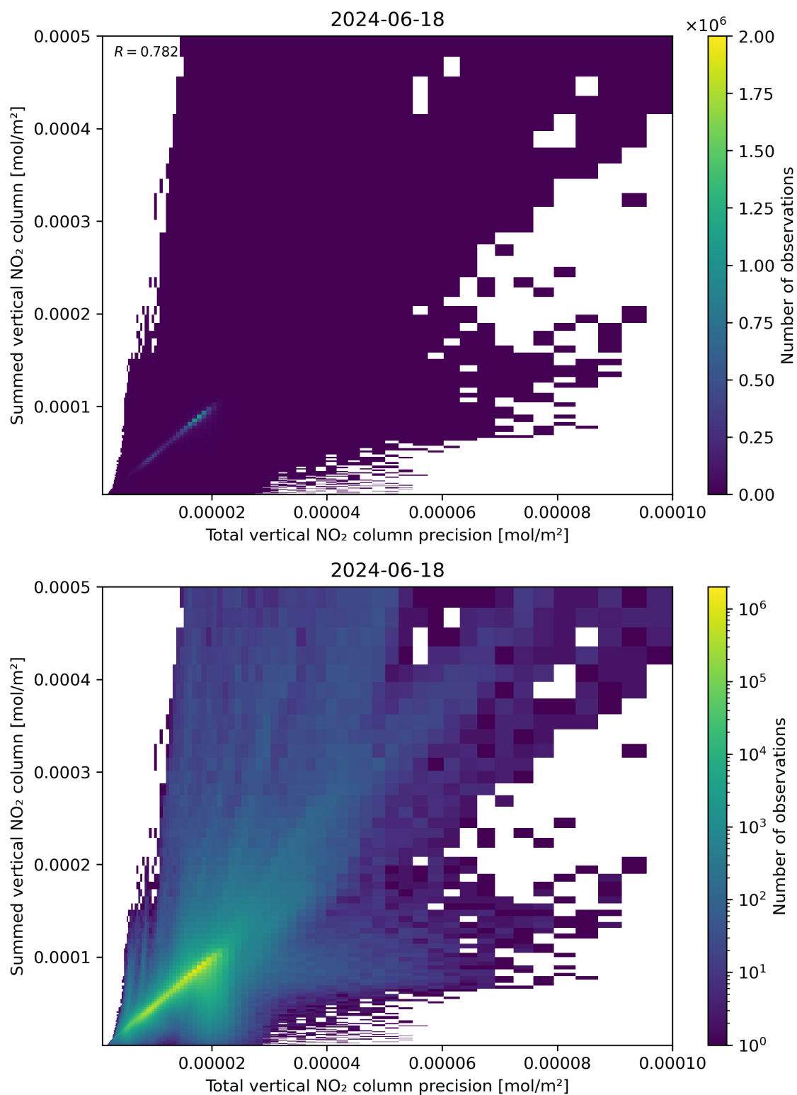
Figure 117: Scatter density plot of “Total vertical NO 2 column precision” against “Summed vertical NO 2 column” for 2024-06-17 to 2024-06-19.
