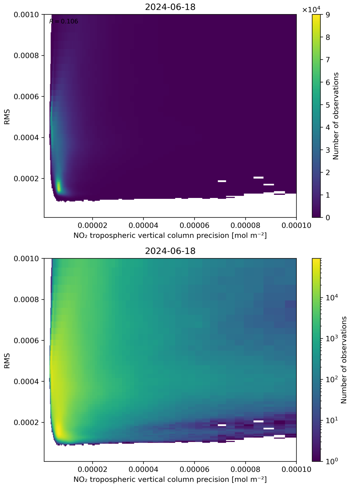
Figure 140: Scatter density plot of “NO 2 tropospheric vertical column precision” against “RMS” for 2024-06-17 to 2024-06-19.
