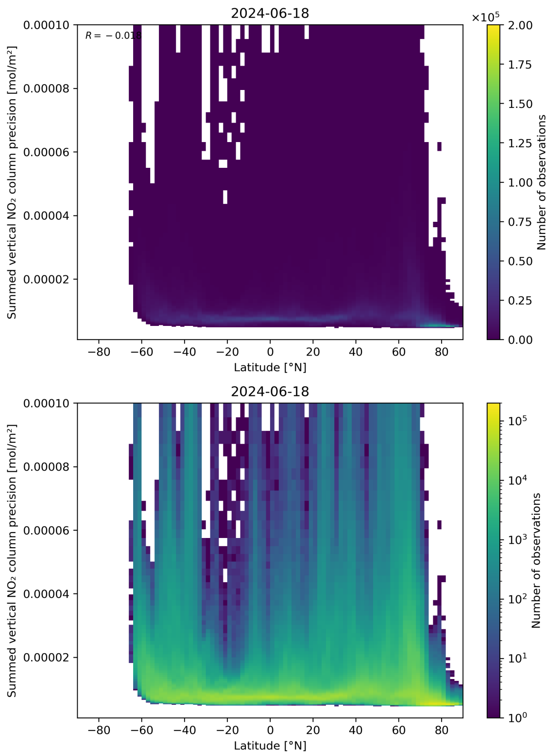
Figure 89: Scatter density plot of “Latitude” against “Summed vertical NO 2 column precision” for 2024-06-17 to 2024-06-19.
