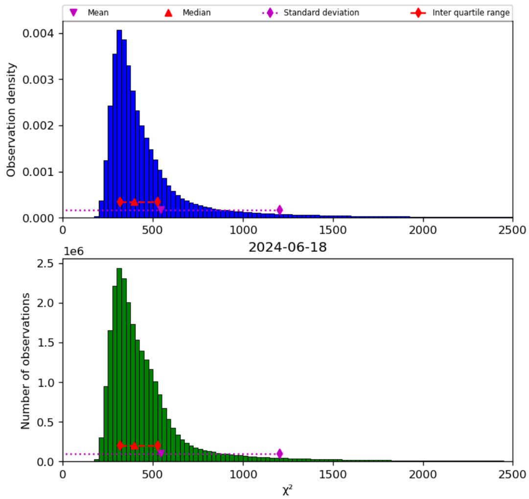
Figure 42: Histogram of “ \chi^2 ” for 2024-06-17 to 2024-06-19
