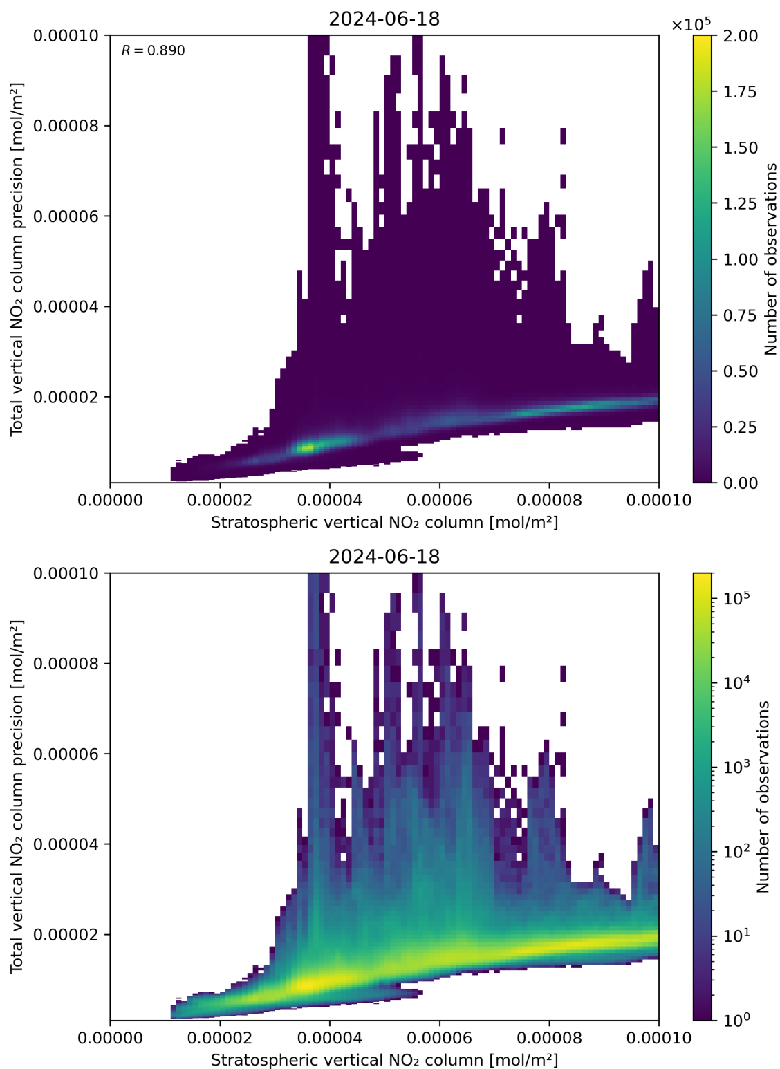
Figure 101: Scatter density plot of “Stratospheric vertical NO 2 column” against “Total vertical NO 2 column precision” for 2024-06-17 to 2024-06-19.
