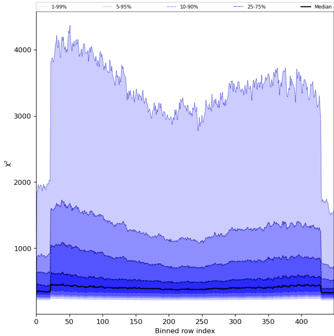
Figure 59: Along track statistics of “ \chi^2 ” for 2024-06-17 to 2024-06-19
