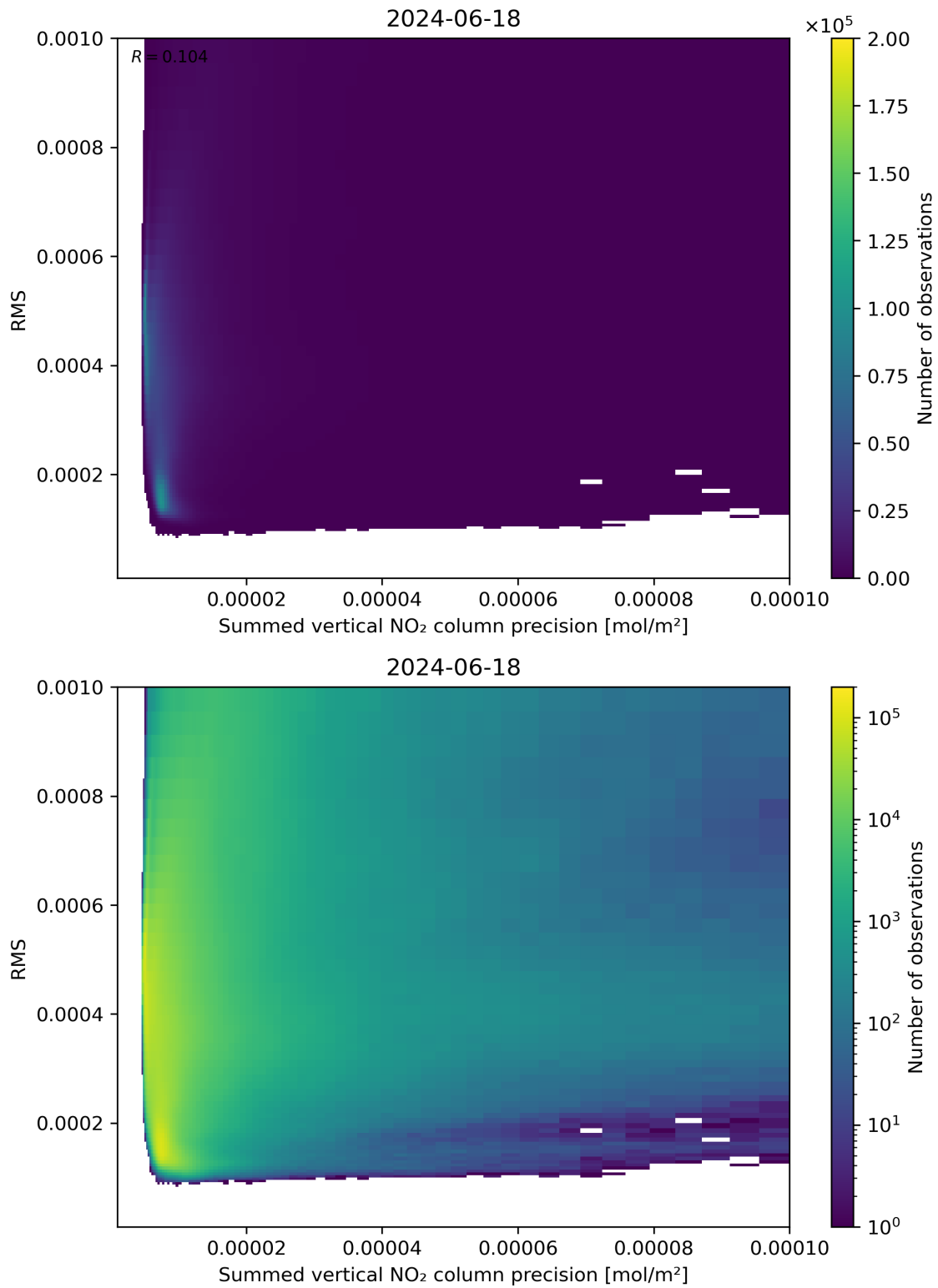
Figure 108: Scatter density plot of “Summed vertical NO 2 column precision” against “RMS” for 2024-06-17 to 2024-06-19.
