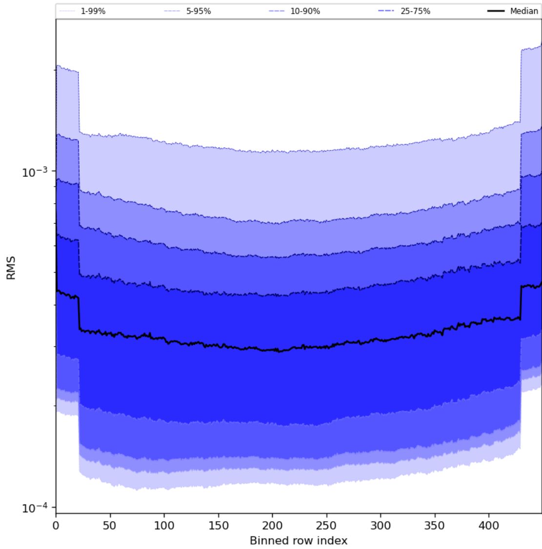
Figure 60: Along track statistics of “RMS” for 2024-06-17 to 2024-06-19
