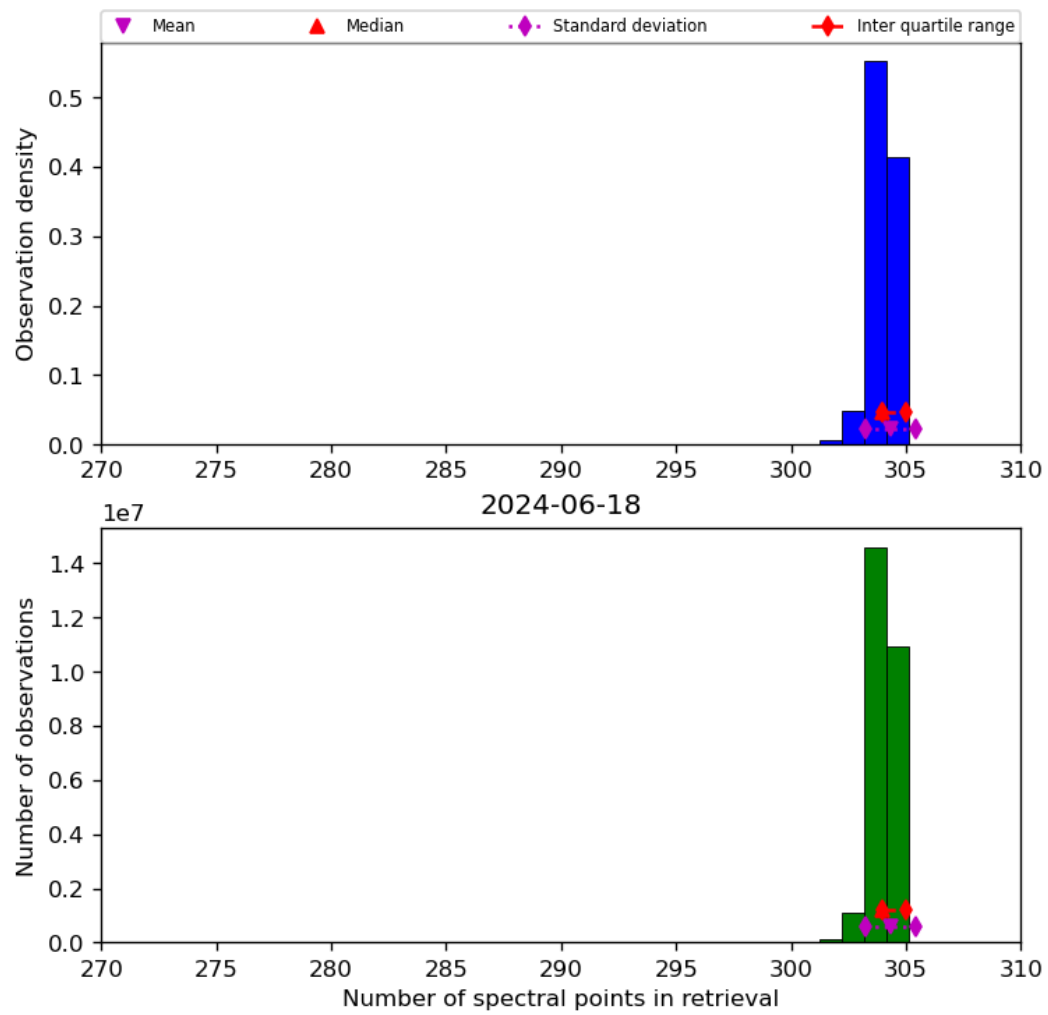
Figure 33: Histogram of “Number of spectral points in retrieval” for 2024-06-17 to 2024-06-19
