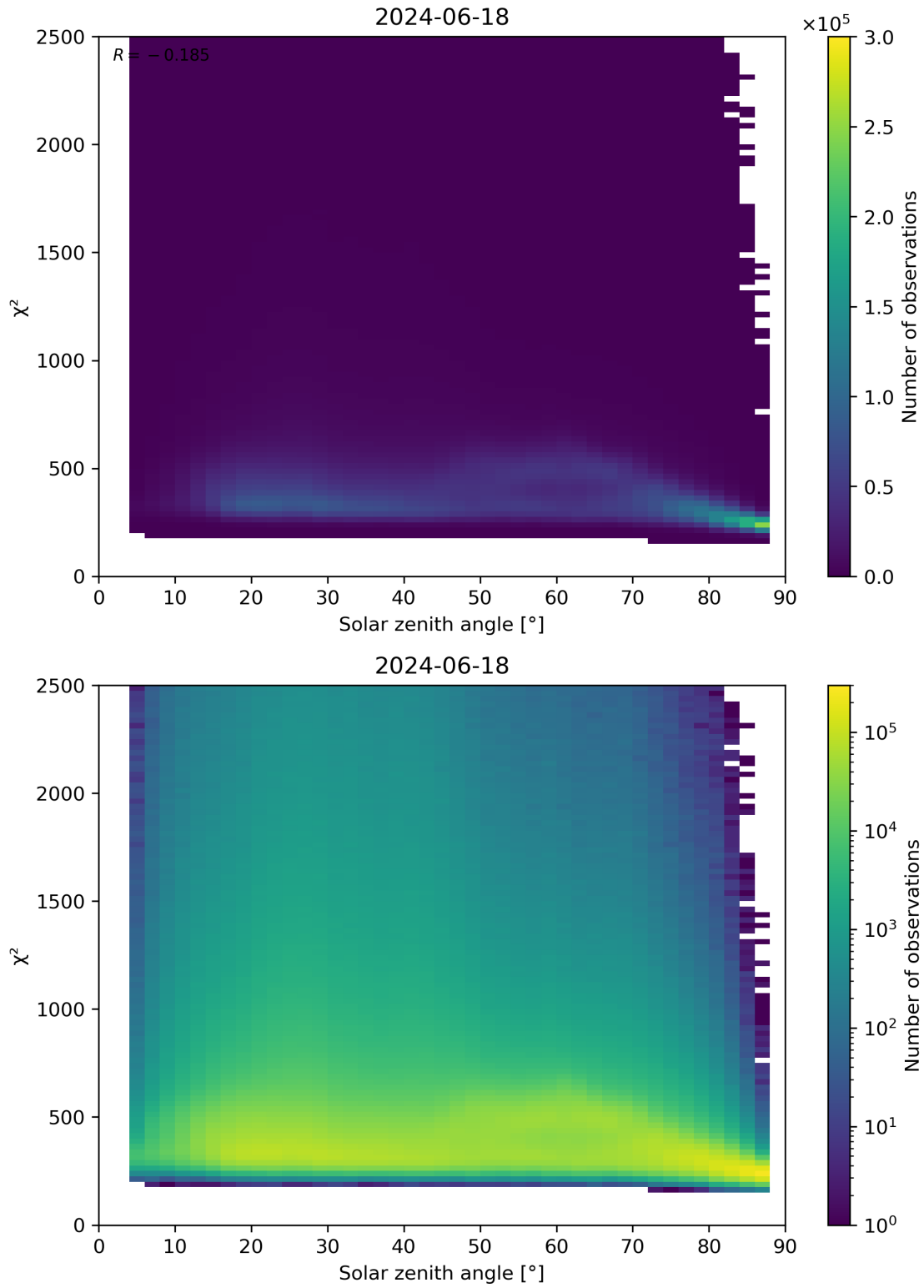
Figure 148: Scatter density plot of “Solar zenith angle” against “ \chi^2 ” for 2024-06-17 to 2024-06-19.
