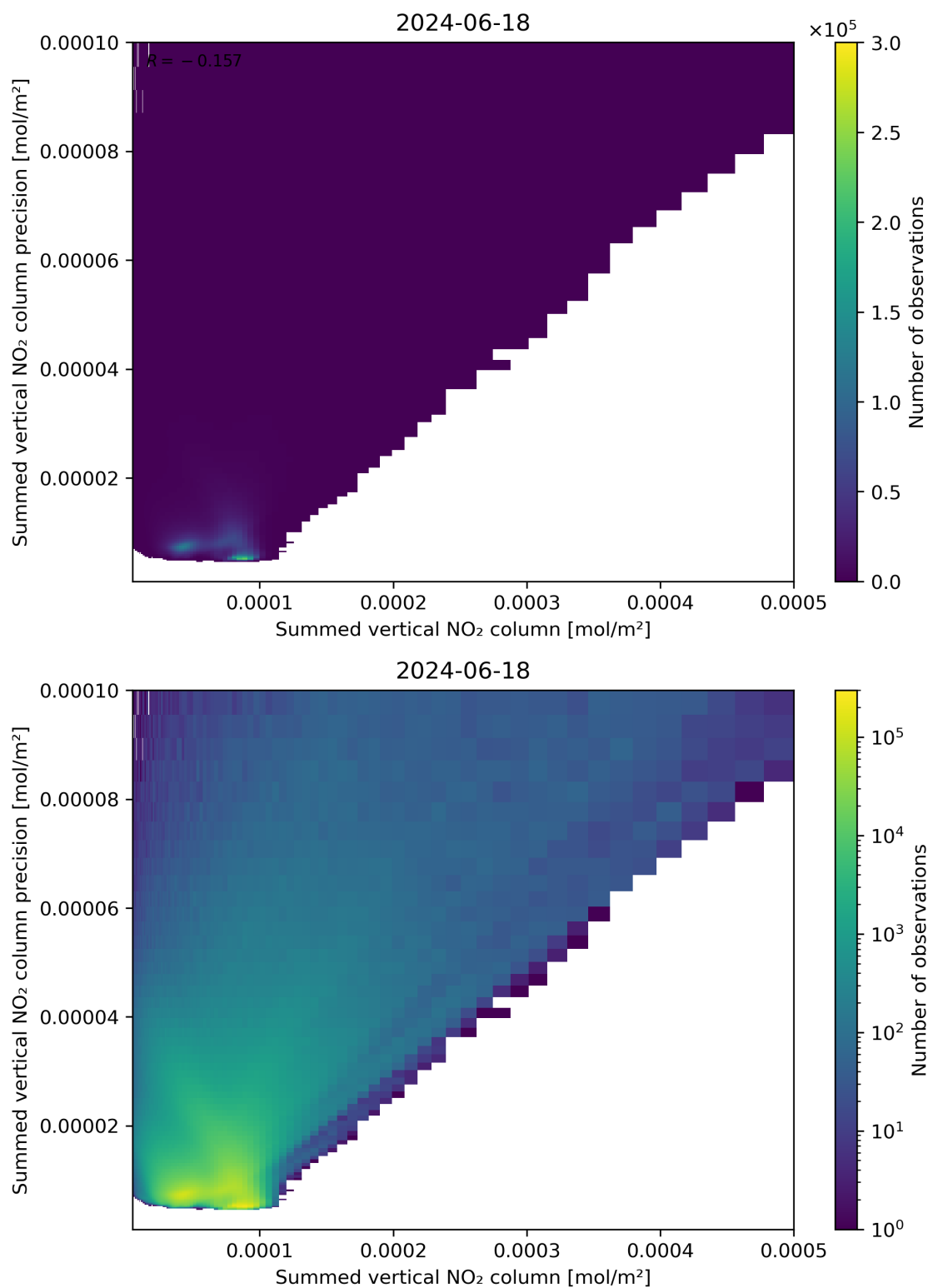
Figure 105: Scatter density plot of “Summed vertical NO 2 column” against “Summed vertical NO 2 column precision” for 2024-06-17 to 2024-06-19.
