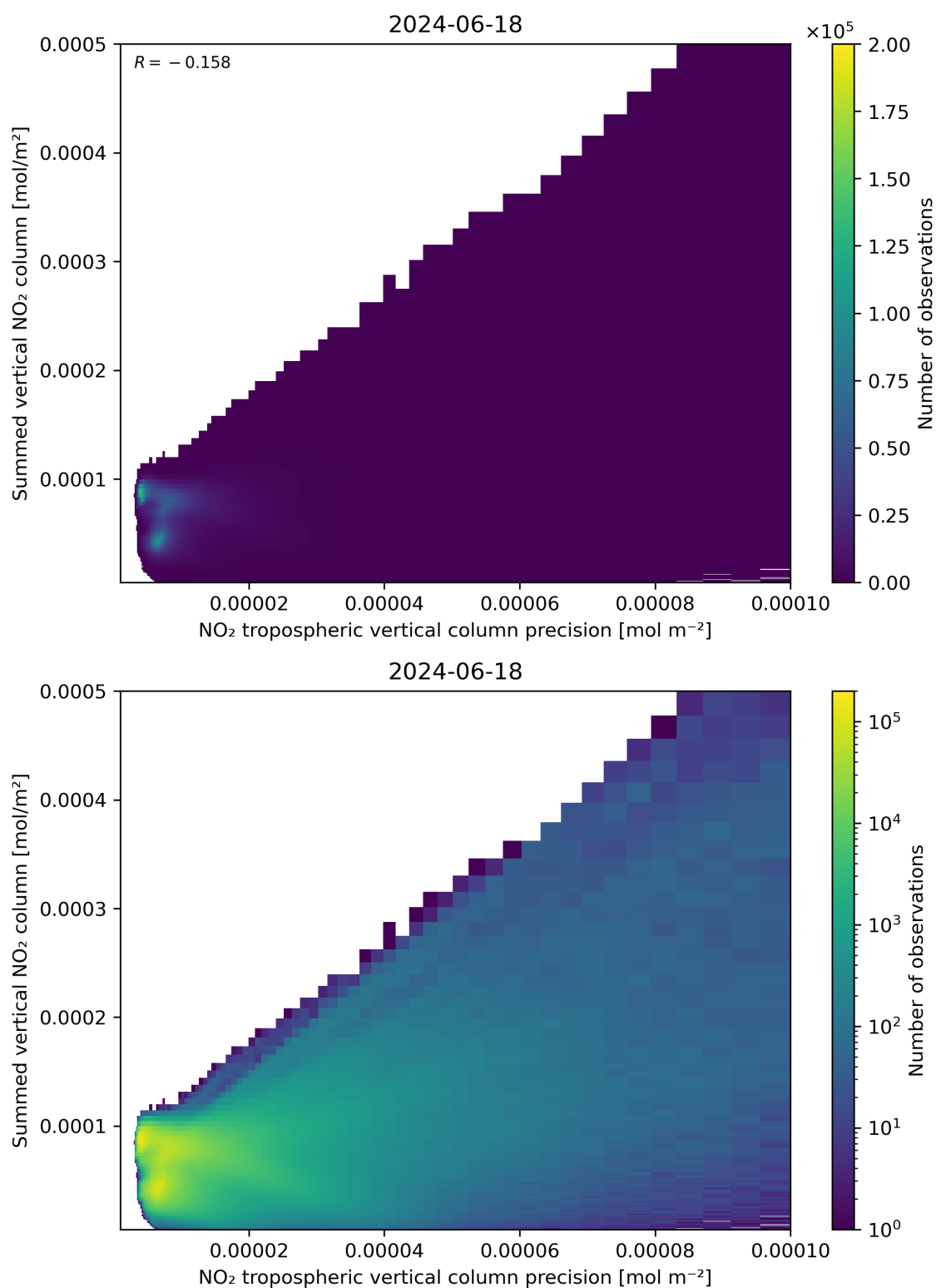
Figure 136: Scatter density plot of “NO 2 tropospheric vertical column precision” against “Summed vertical NO 2 column” for 2024-06-17 to 2024-06-19.
