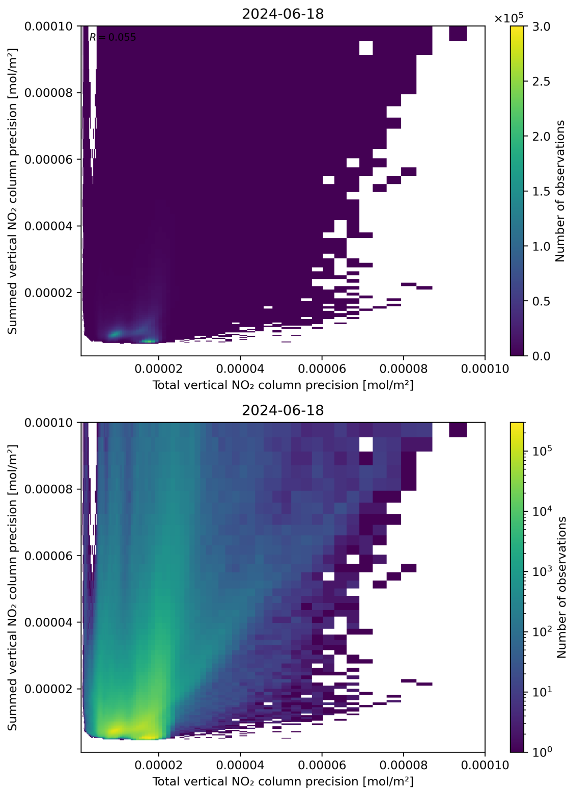
Figure 118: Scatter density plot of “Total vertical NO 2 column precision” against “Summed vertical NO 2 column precision” for 2024-06-17 to 2024-06-19.
