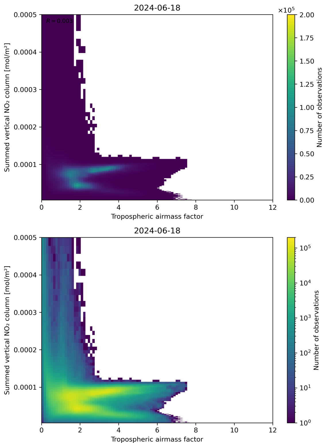
Figure 75: Scatter density plot of “Tropospheric air mass factor” against “Summed vertical NO 2 column” for 2024-06-17 to 2024-06-19.
