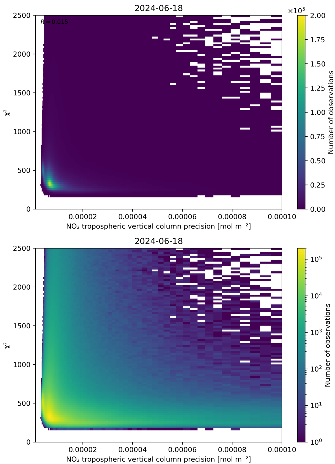
Figure 134: Scatter density plot of “NO 2 tropospheric vertical column precision” against “ \chi^2 ” for 2024-06-17 to 2024-06-19.
