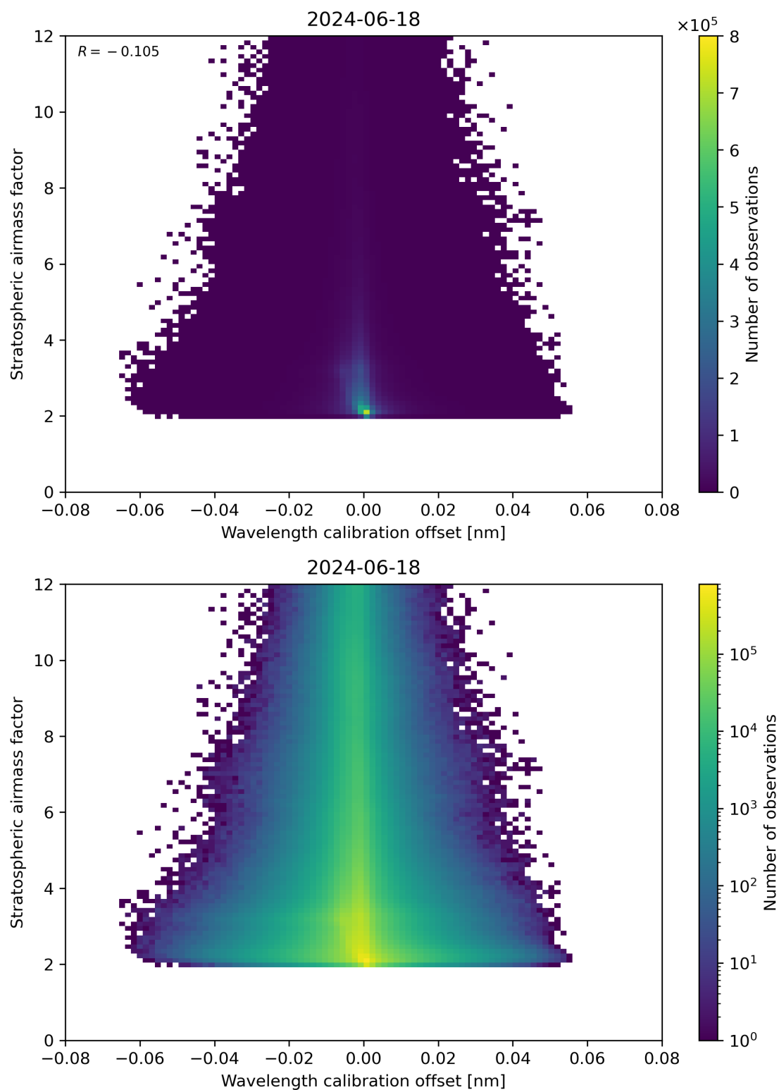
Figure 174: Scatter density plot of “Wavelength calibration offset” against “Stratospheric air mass factor” for 2024-06-17 to 2024-06-19.
