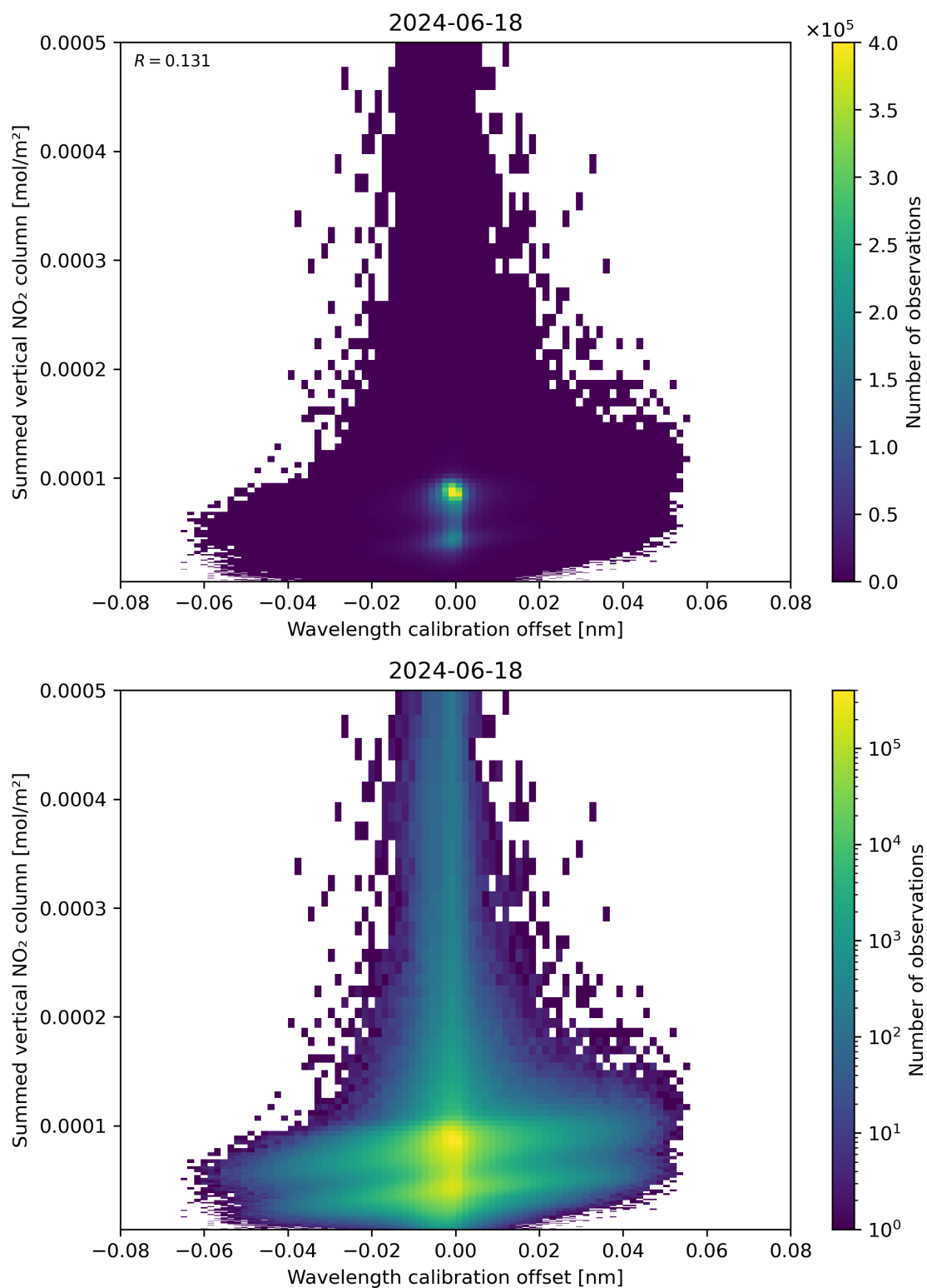
Figure 177: Scatter density plot of “Wavelength calibration offset” against “Summed vertical NO 2 column” for 2024-06-17 to 2024-06-19.
