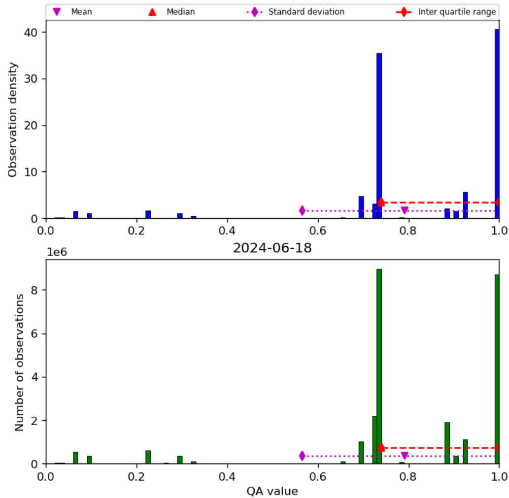
Figure 28: Histogram of “QA value” for 2024-06-17 to 2024-06-19
