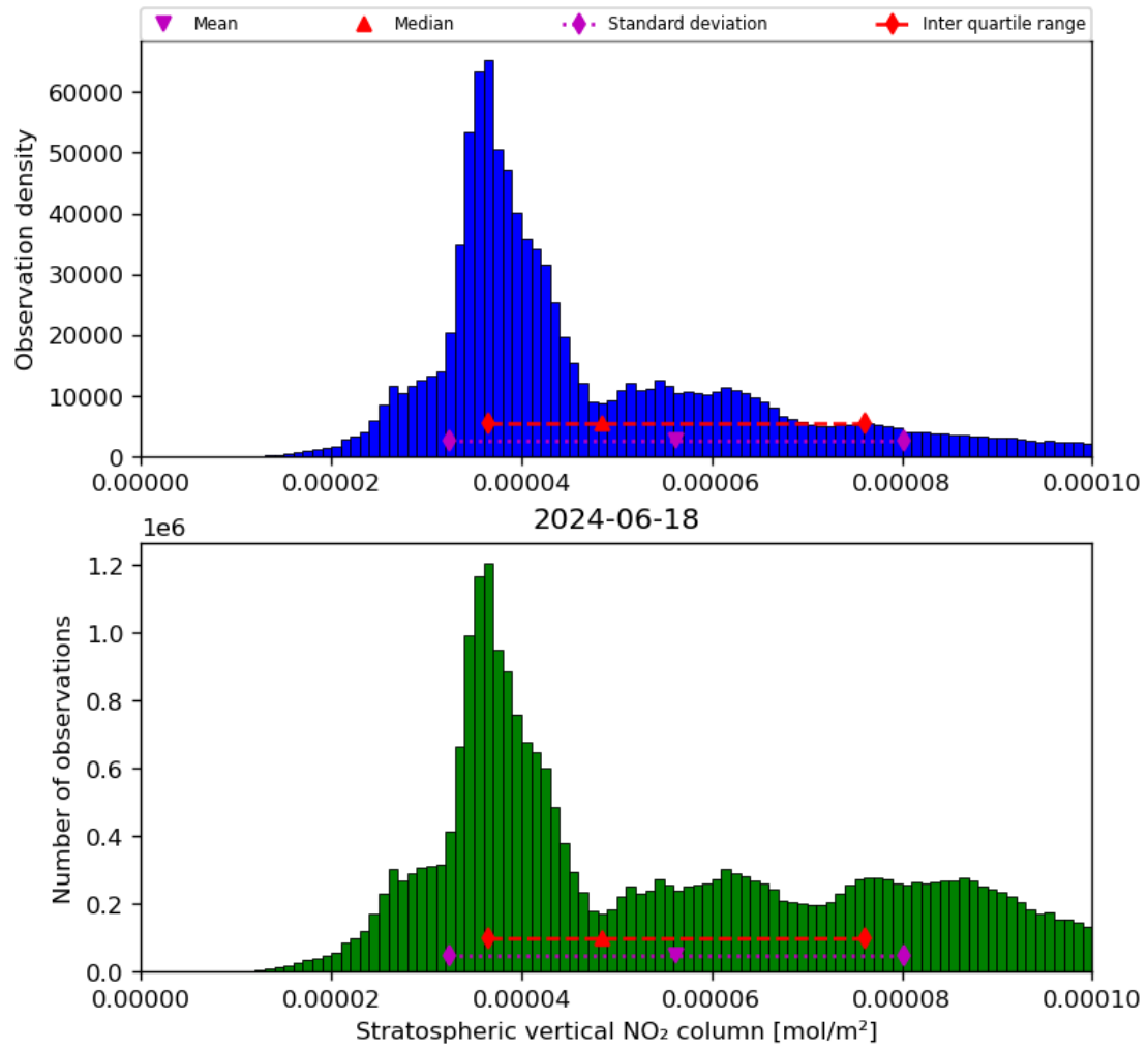
Figure 36: Histogram of “Stratospheric vertical NO 2 column” for 2024-06-17 to 2024-06-19
