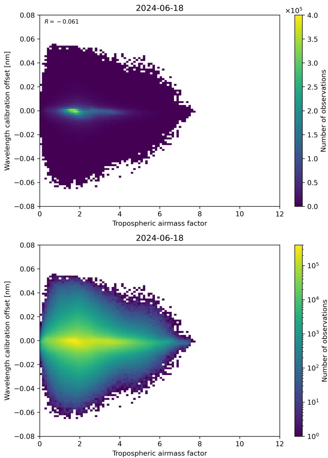
Figure 80: Scatter density plot of “Tropospheric airmass factor” against “Wavelength calibration offset” for 2024-06-17 to 2024-06-19.
