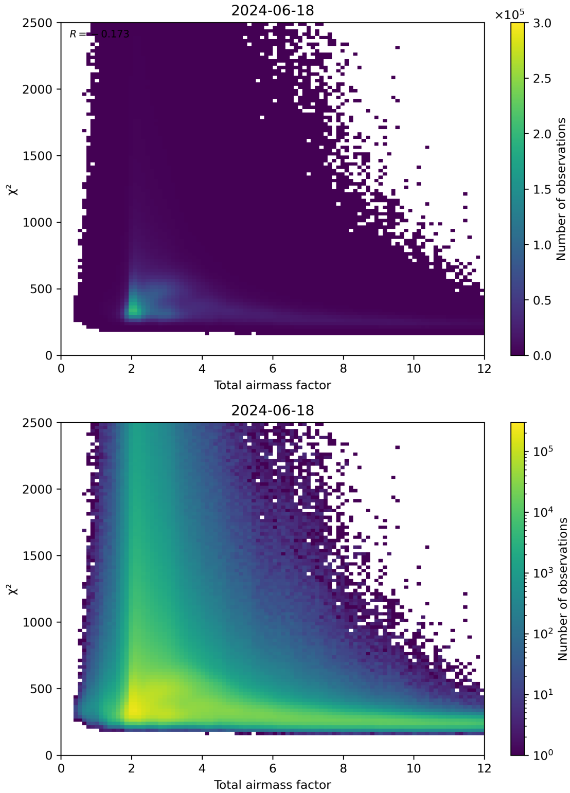
Figure 63: Scatter density plot of “Total airmass factor” against “ \chi^2 ” for 2024-06-17 to 2024-06-19.
