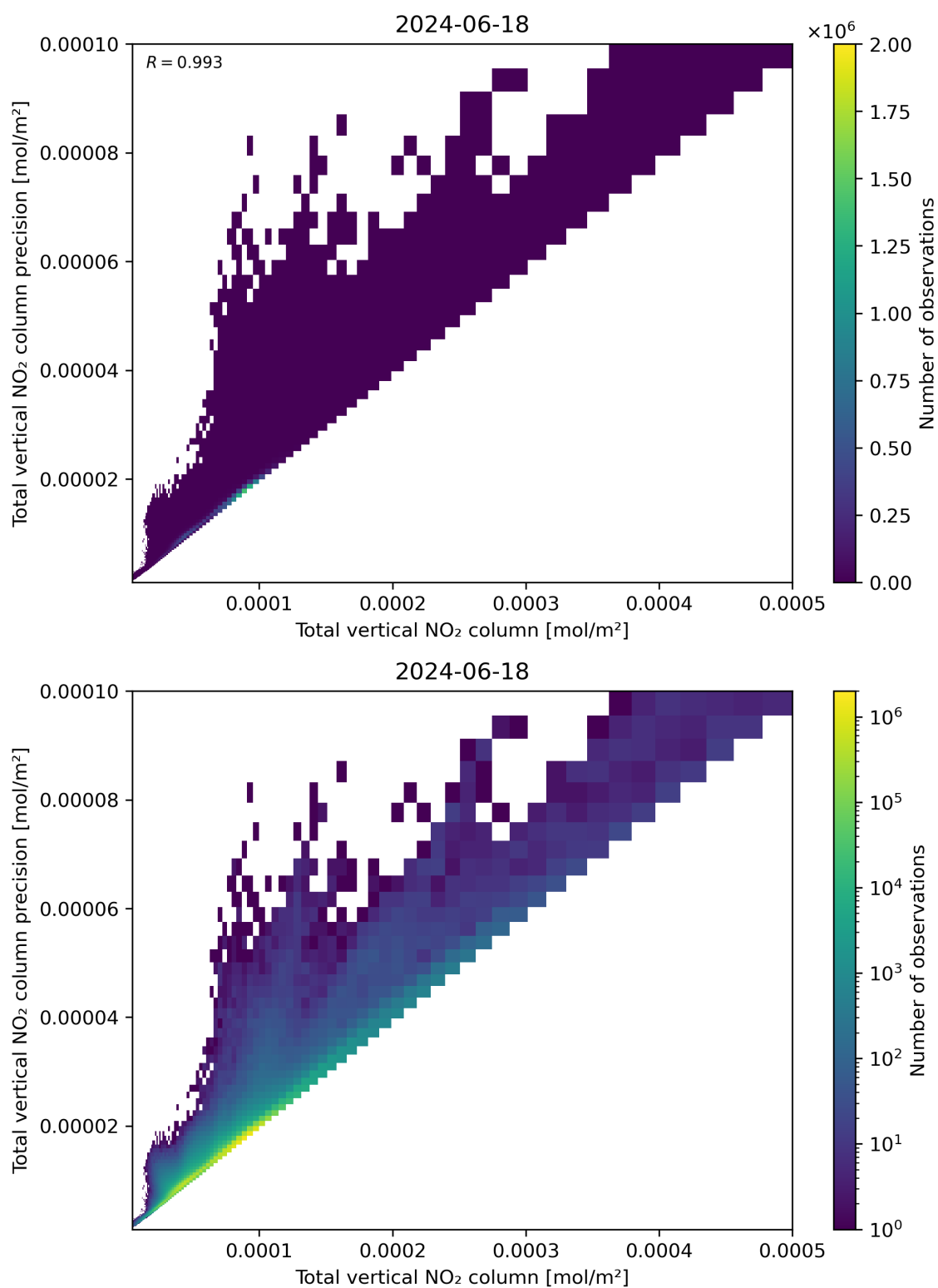
Figure 114: Scatter density plot of “Total vertical NO 2 column” against “Total vertical NO 2 column precision” for 2024-06-17 to 2024-06-19.
