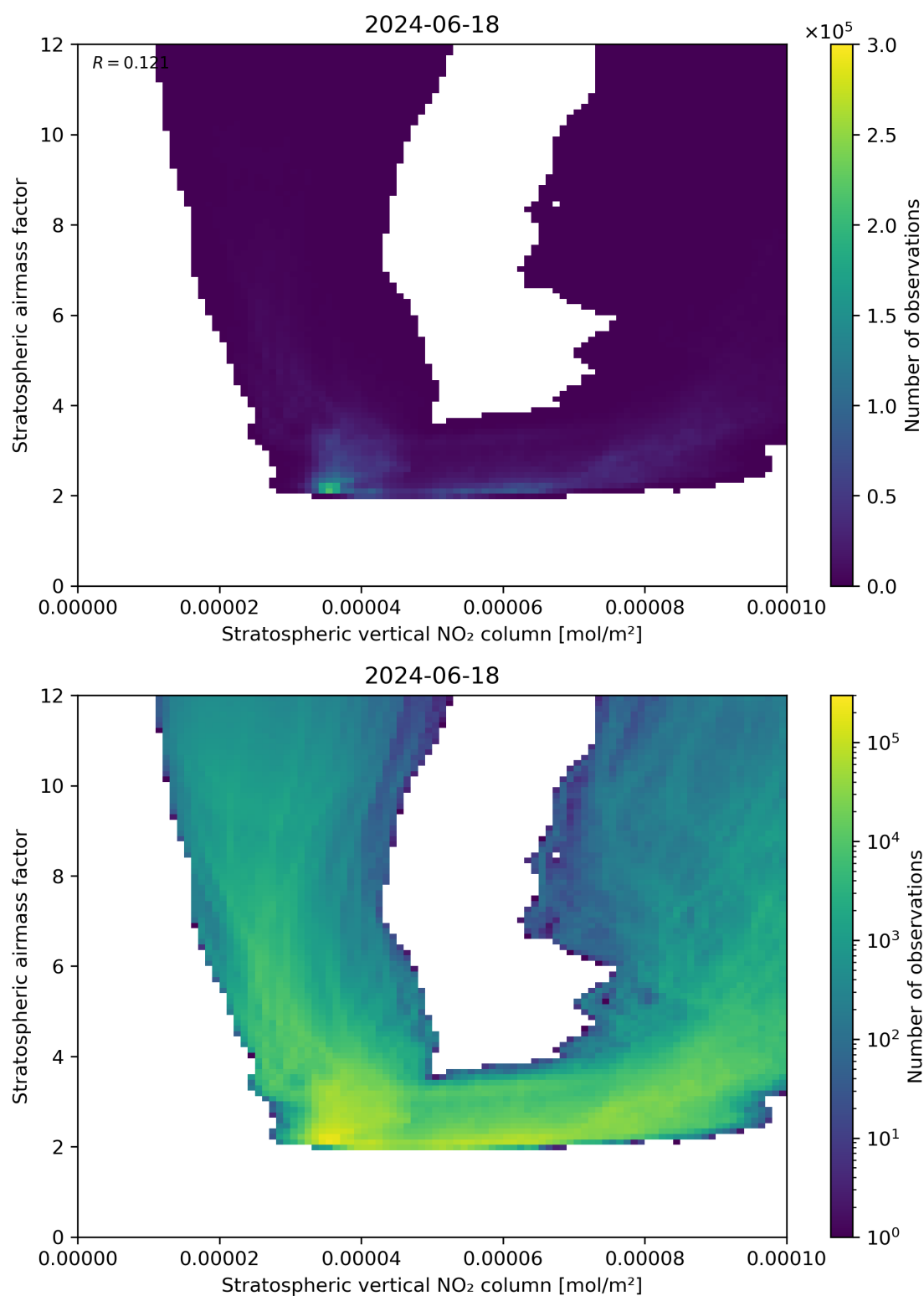
Figure 96: Scatter density plot of “Stratospheric vertical NO 2 column” against “Stratospheric airmass factor” for 2024-06-17 to 2024-06-19.
