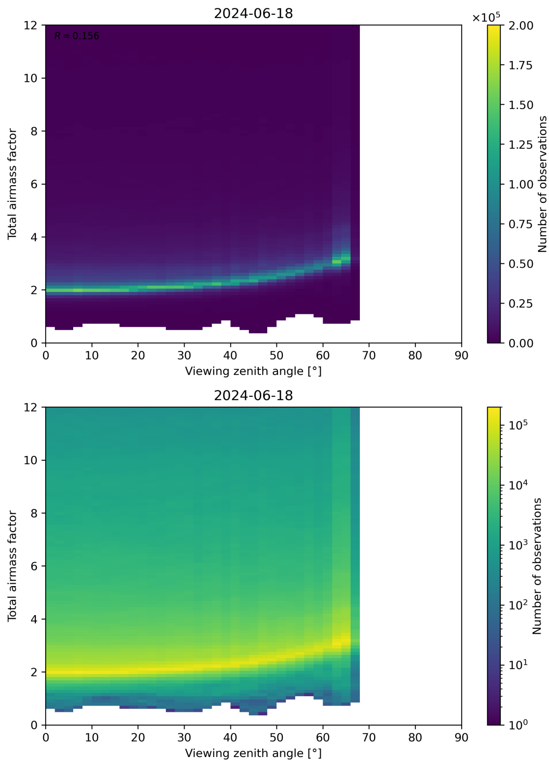
Figure 160: Scatter density plot of “Viewing zenith angle” against “Total airmass factor” for 2024-06-17 to 2024-06-19.
