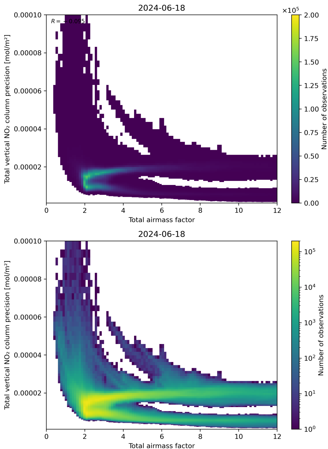
Figure 68: Scatter density plot of “Total airmass factor” against “Total vertical NO 2 column precision” for 2024-06-17 to 2024-06-19.
