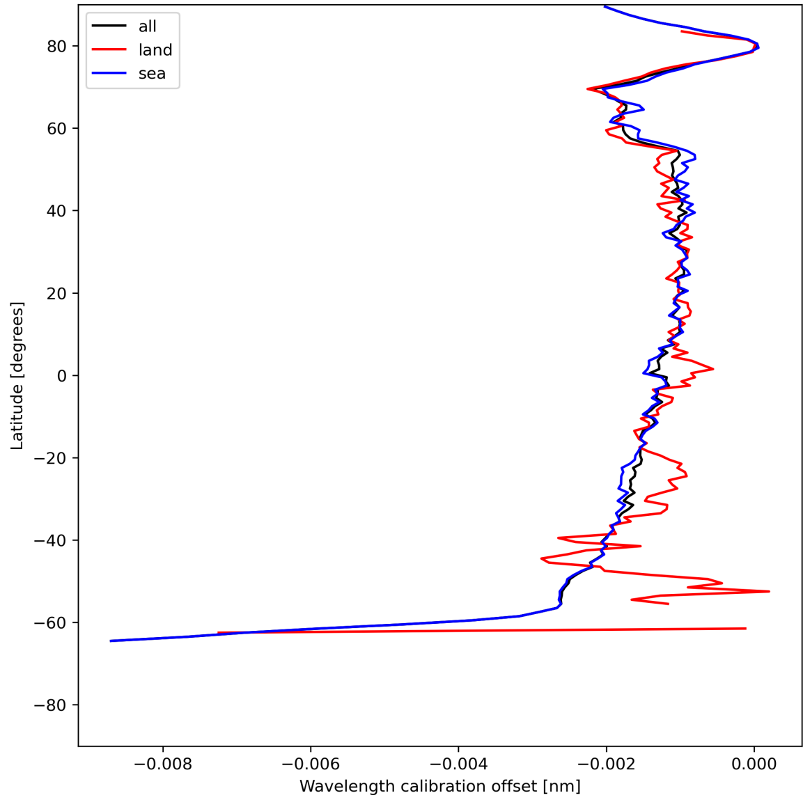
Figure 18: Zonal average of “Wavelength calibration offset” for 2024-06-17 to 2024-06-19.
