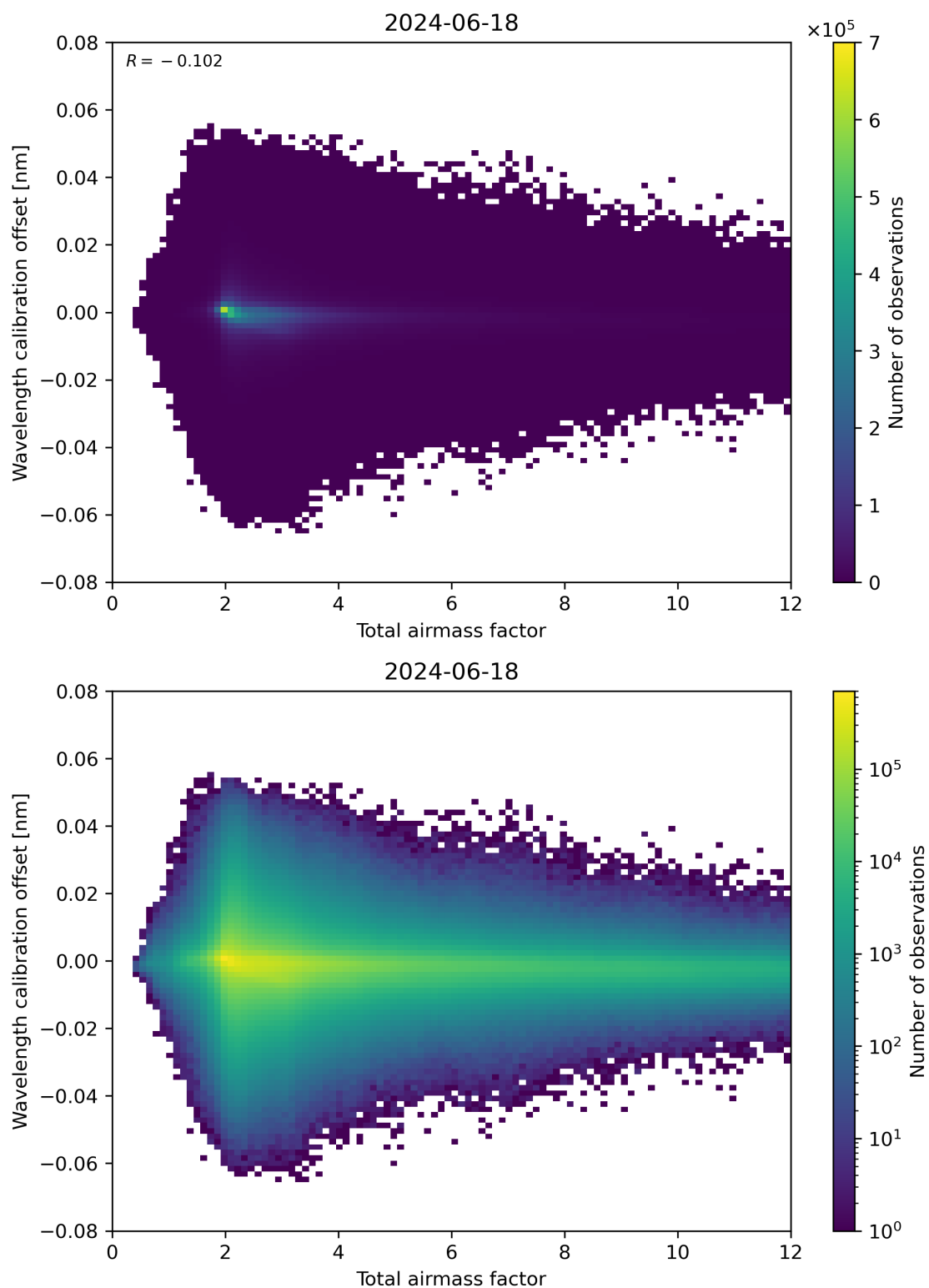
Figure 70: Scatter density plot of “Total airmass factor” against “Wavelength calibration offset” for 2024-06-17 to 2024-06-19.
