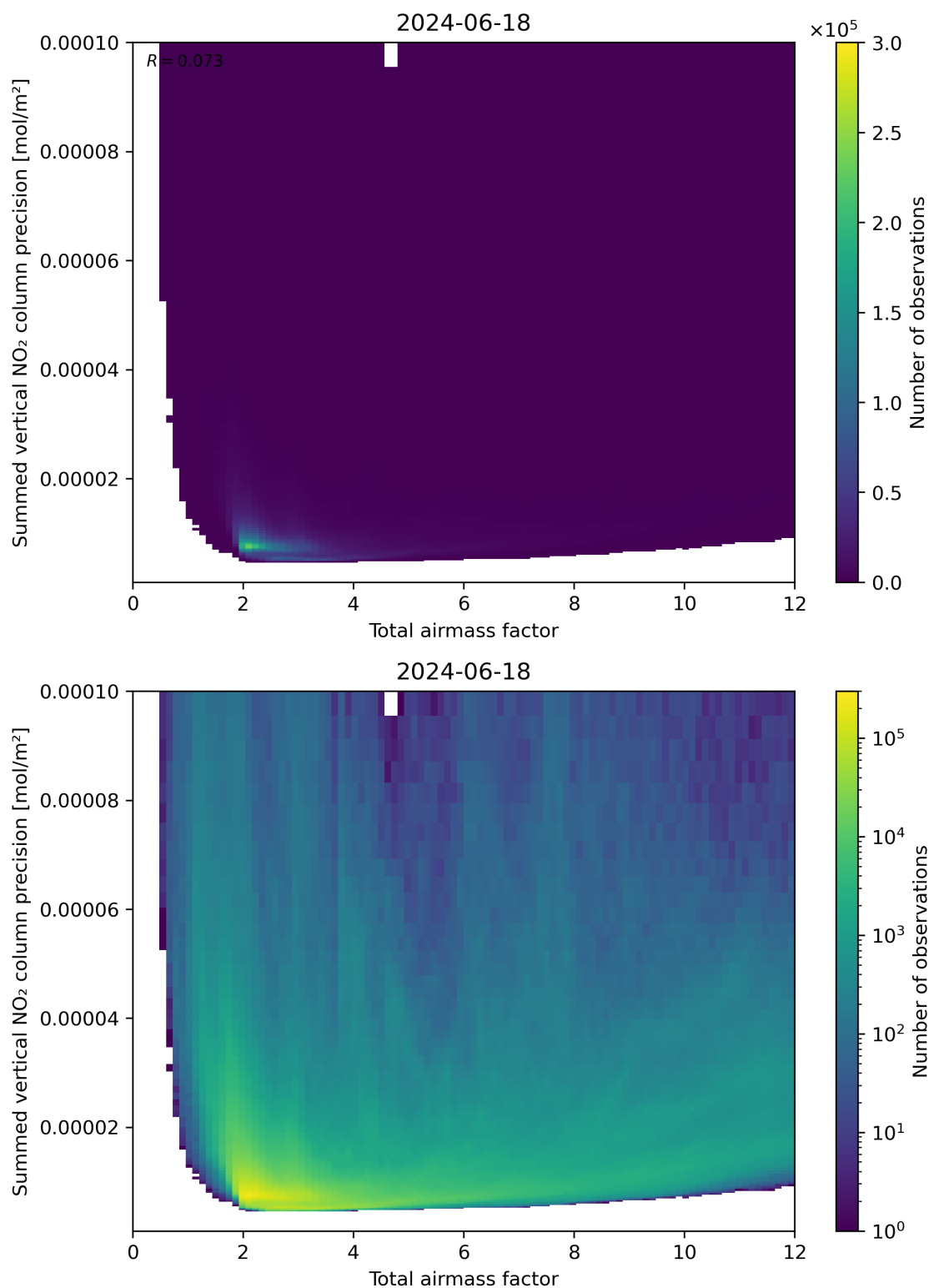
Figure 66: Scatter density plot of “Total airmass factor” against “Summed vertical NO 2 column precision” for 2024-06-17 to 2024-06-19.
