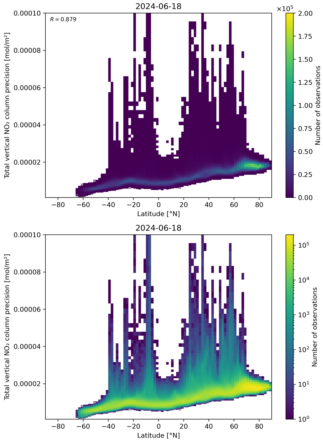
Figure 91: Scatter density plot of “Latitude” against “Total vertical NO 2 column precision” for 2024-06-17 to 2024-06-19.
