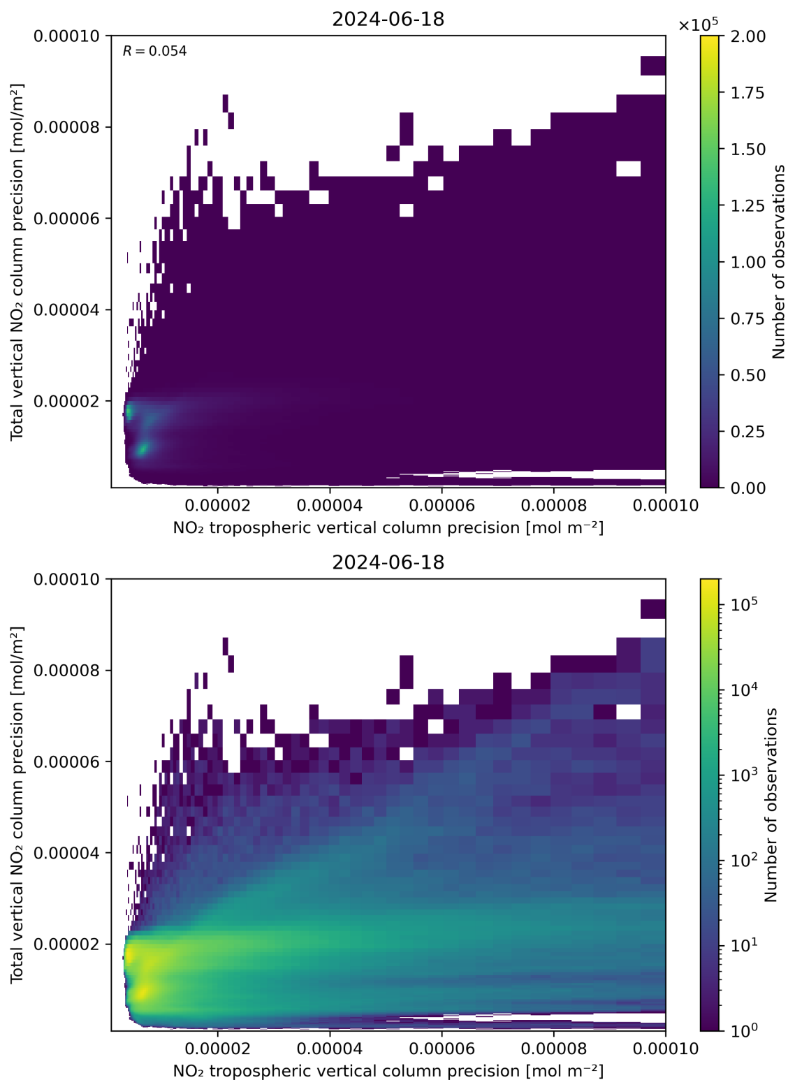
Figure 139: Scatter density plot of “NO 2 tropospheric vertical column precision” against “Total vertical NO 2 column precision” for 2024-06-17 to 2024-06-19.
