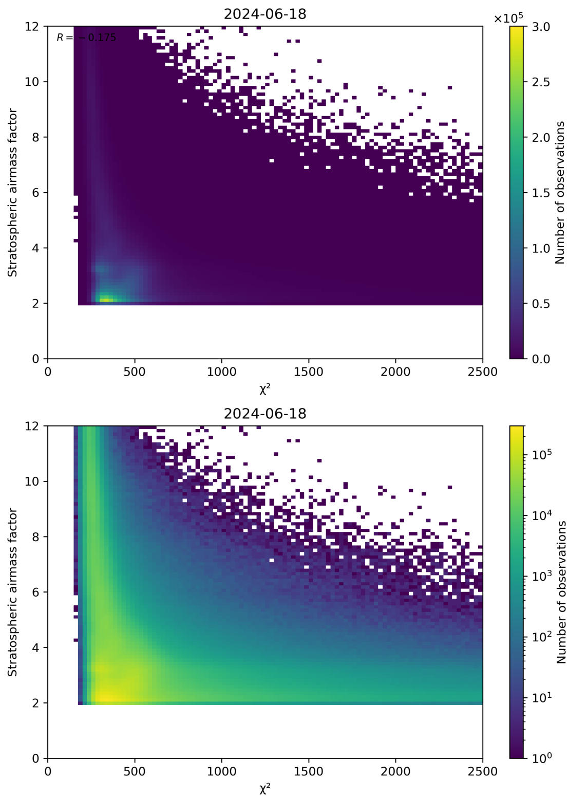
Figure 81: Scatter density plot of “ \chi^2 ” against “Stratospheric air mass factor” for 2024-06-17 to 2024-06-19.
