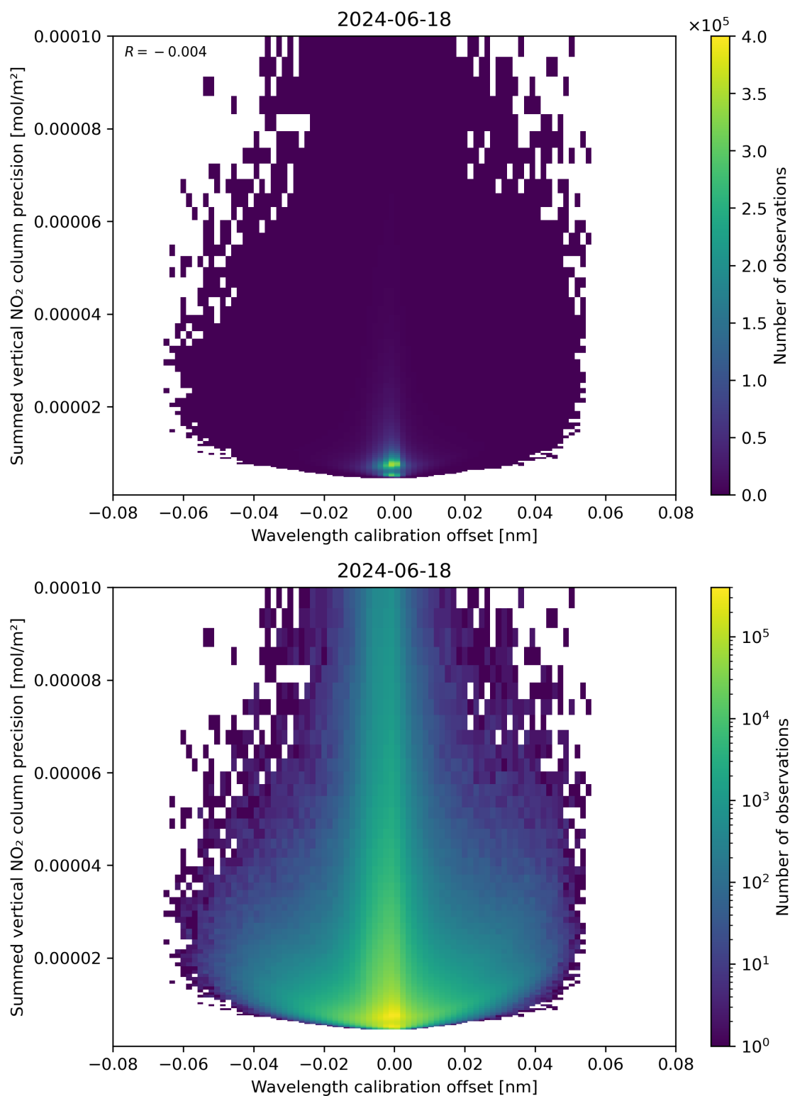
Figure 178: Scatter density plot of “Wavelength calibration offset” against “Summed vertical NO 2 column precision” for 2024-06-17 to 2024-06-19.
