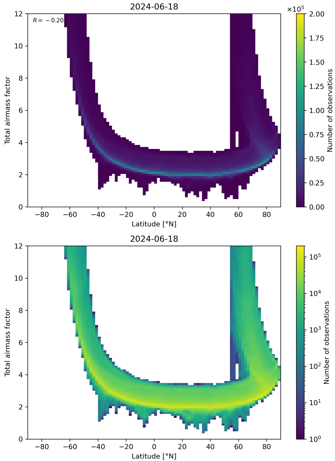
Figure 84: Scatter density plot of “Latitude” against “Total airmass factor” for 2024-06-17 to 2024-06-19.
