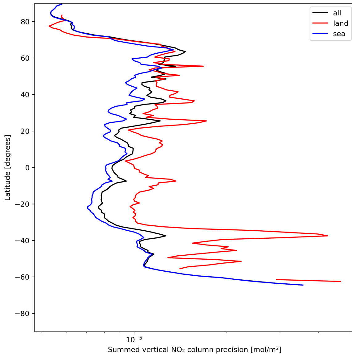
Figure 24: Zonal average of “Summed vertical NO 2 column precision” for 2024-06-17 to 2024-06-19.
