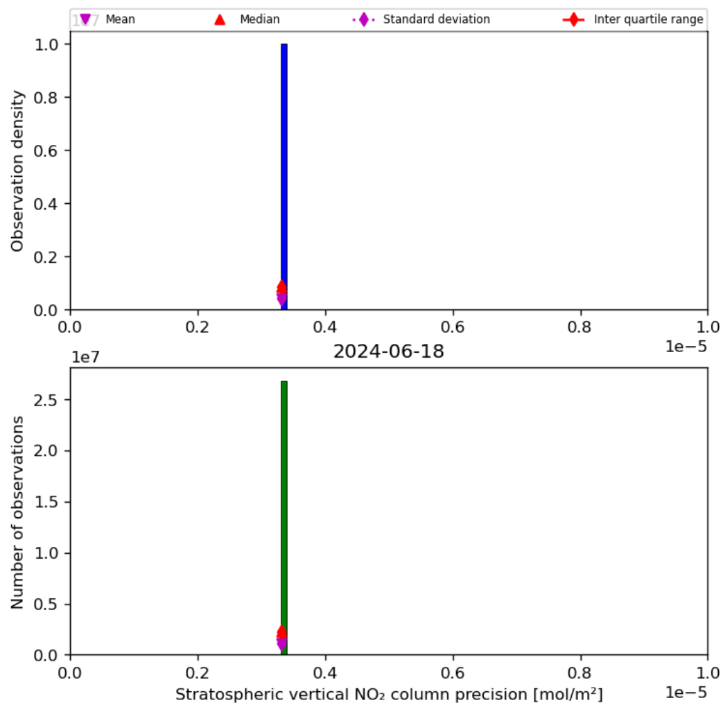
Figure 37: Histogram of “Stratospheric vertical NO 2 column precision” for 2024-06-17 to 2024-06-19
