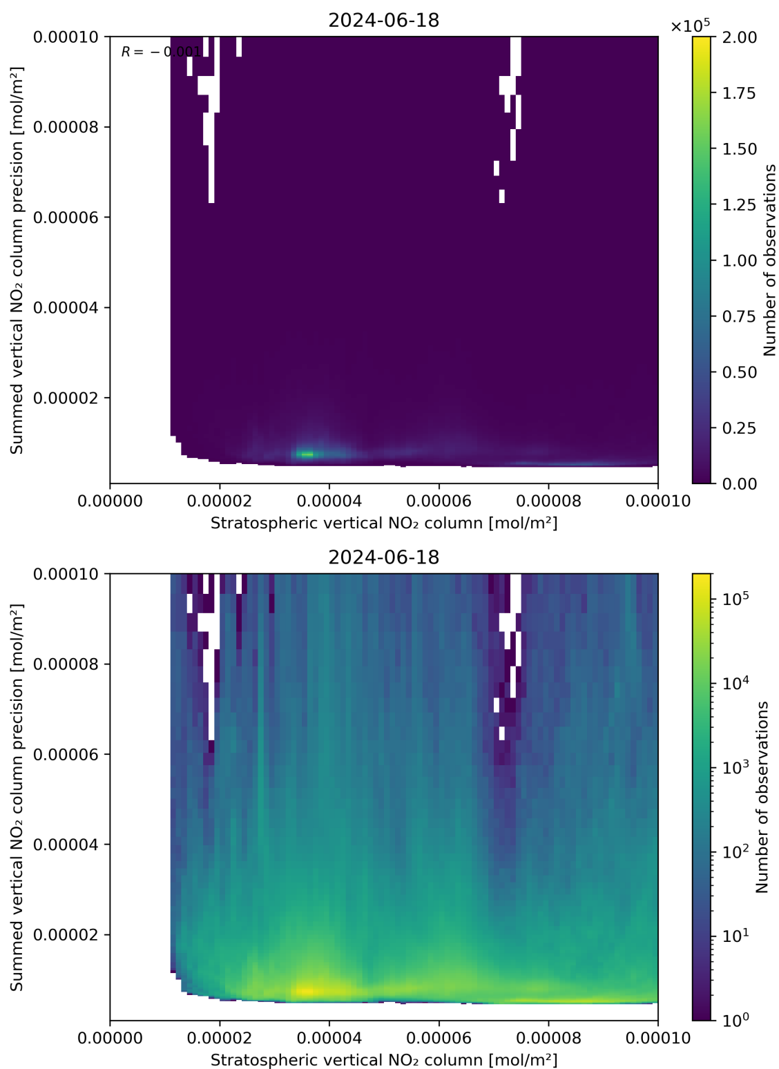
Figure 99: Scatter density plot of “Stratospheric vertical NO 2 column” against “Summed vertical NO 2 column precision” for 2024-06-17 to 2024-06-19.
