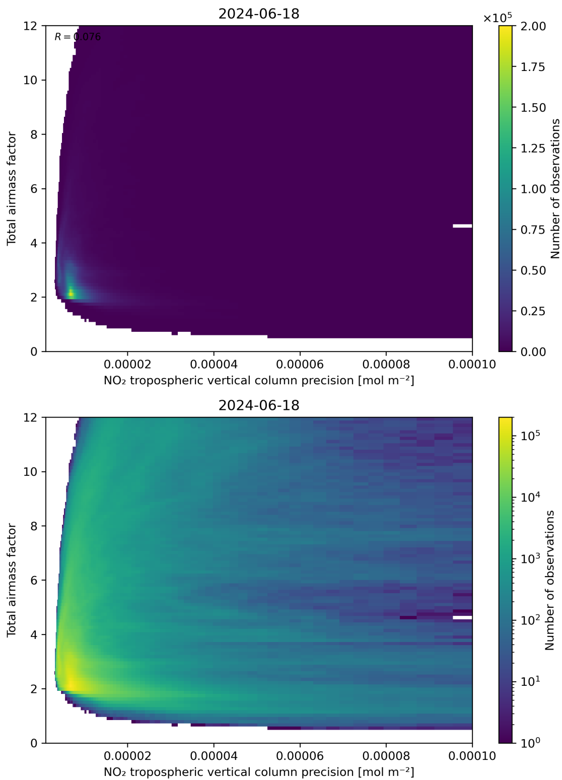
Figure 132: Scatter density plot of “NO 2 tropospheric vertical column precision” against “Total air mass factor” for 2024-06-17 to 2024-06-19.
