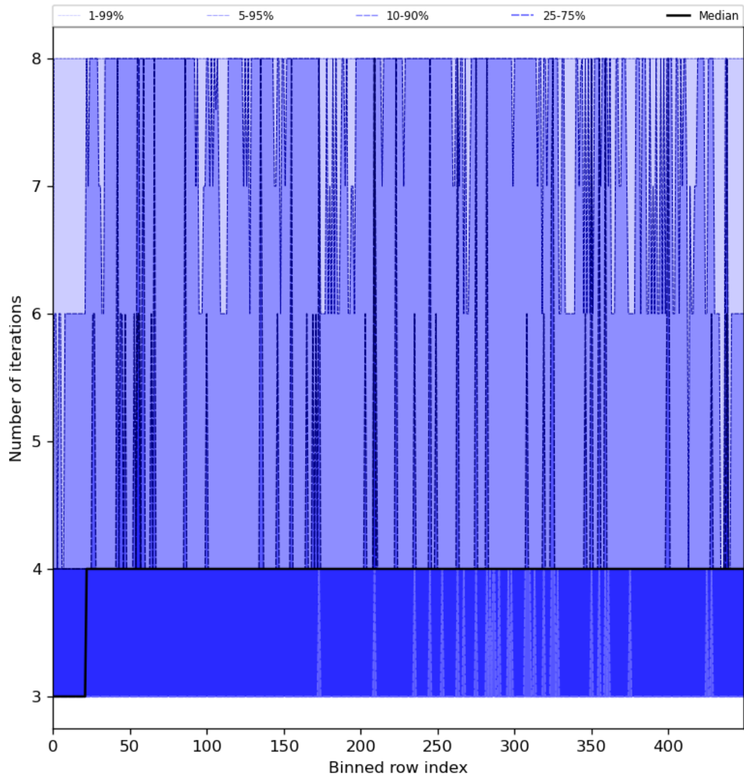
Figure 51: Along track statistics of “Number of iterations” for 2024-06-17 to 2024-06-19
