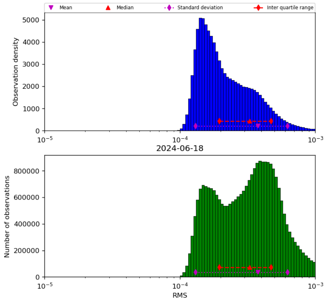
Figure 43: Histogram of “RMS” for 2024-06-17 to 2024-06-19
