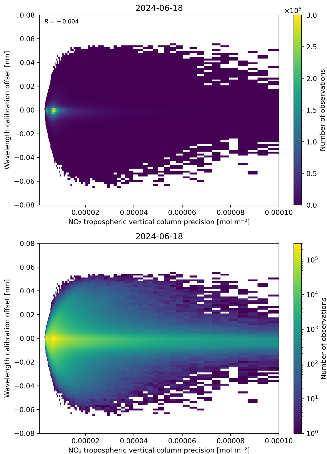
Figure 141: Scatter density plot of “NO 2 tropospheric vertical column precision” against “Wavelength calibration offset” for 2024-06-17 to 2024-06-19.
