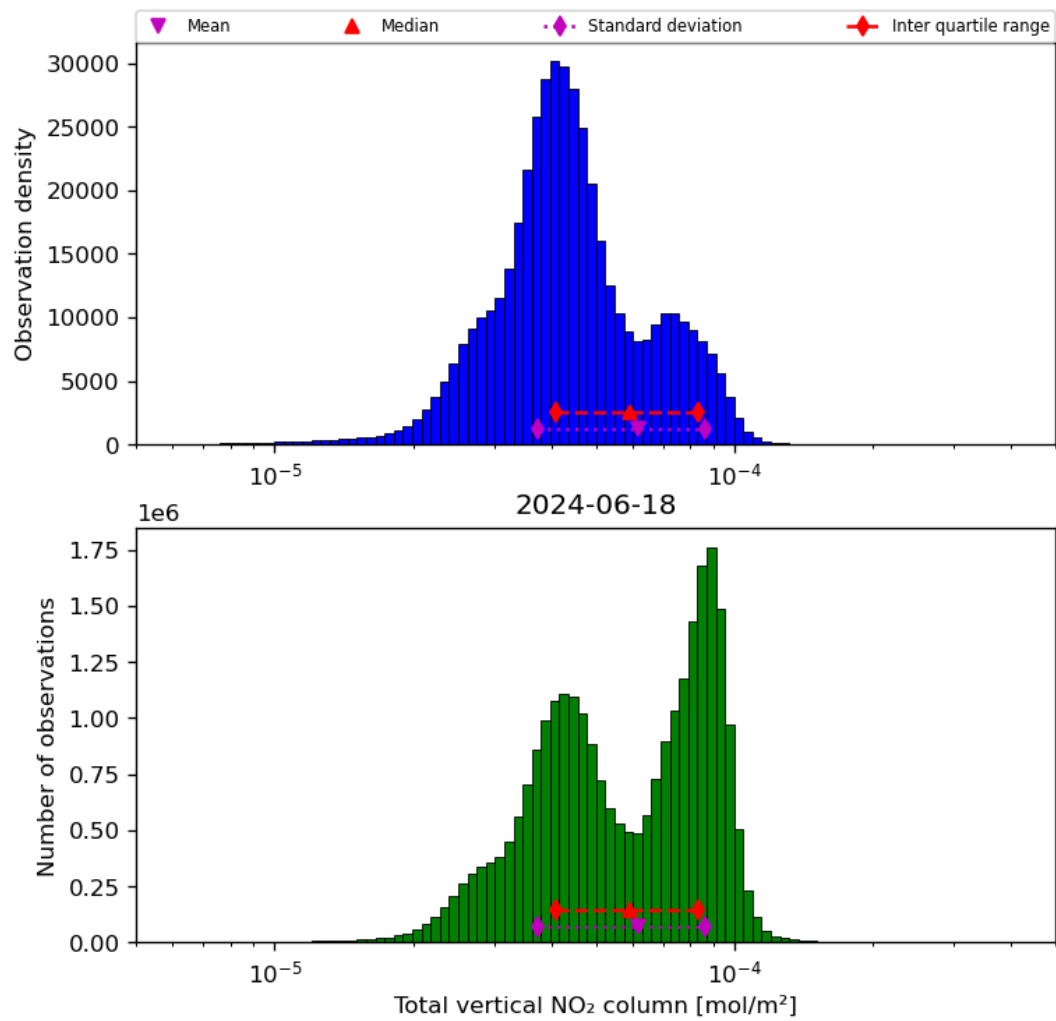
Figure 38: Histogram of “Total vertical NO 2 column” for 2024-06-17 to 2024-06-19
