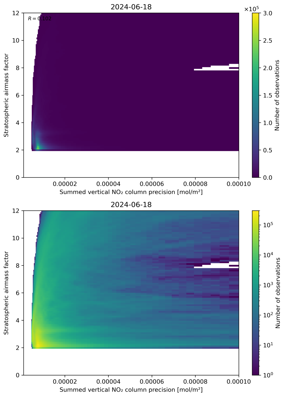
Figure 106: Scatter density plot of “Summed vertical NO 2 column precision” against “Stratospheric airmass factor” for 2024-06-17 to 2024-06-19.
