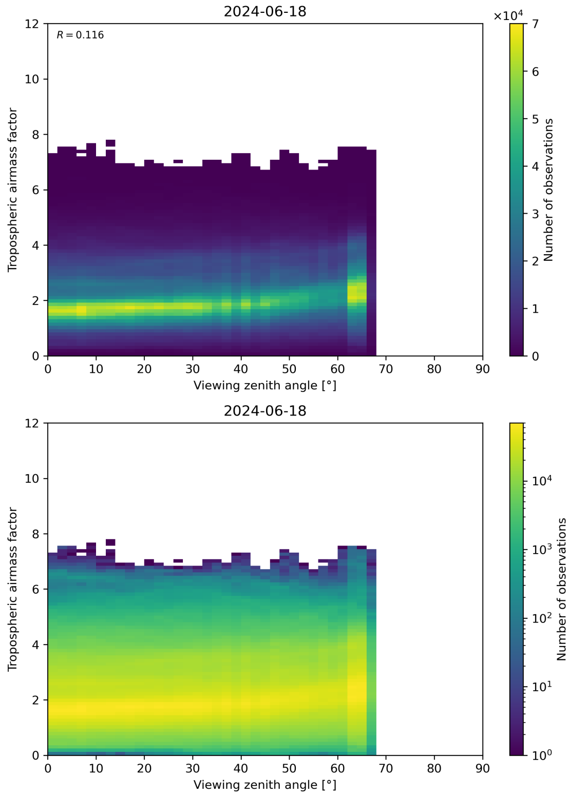
Figure 161: Scatter density plot of “Viewing zenith angle” against “Tropospheric airmass factor” for 2024-06-17 to 2024-06-19.
