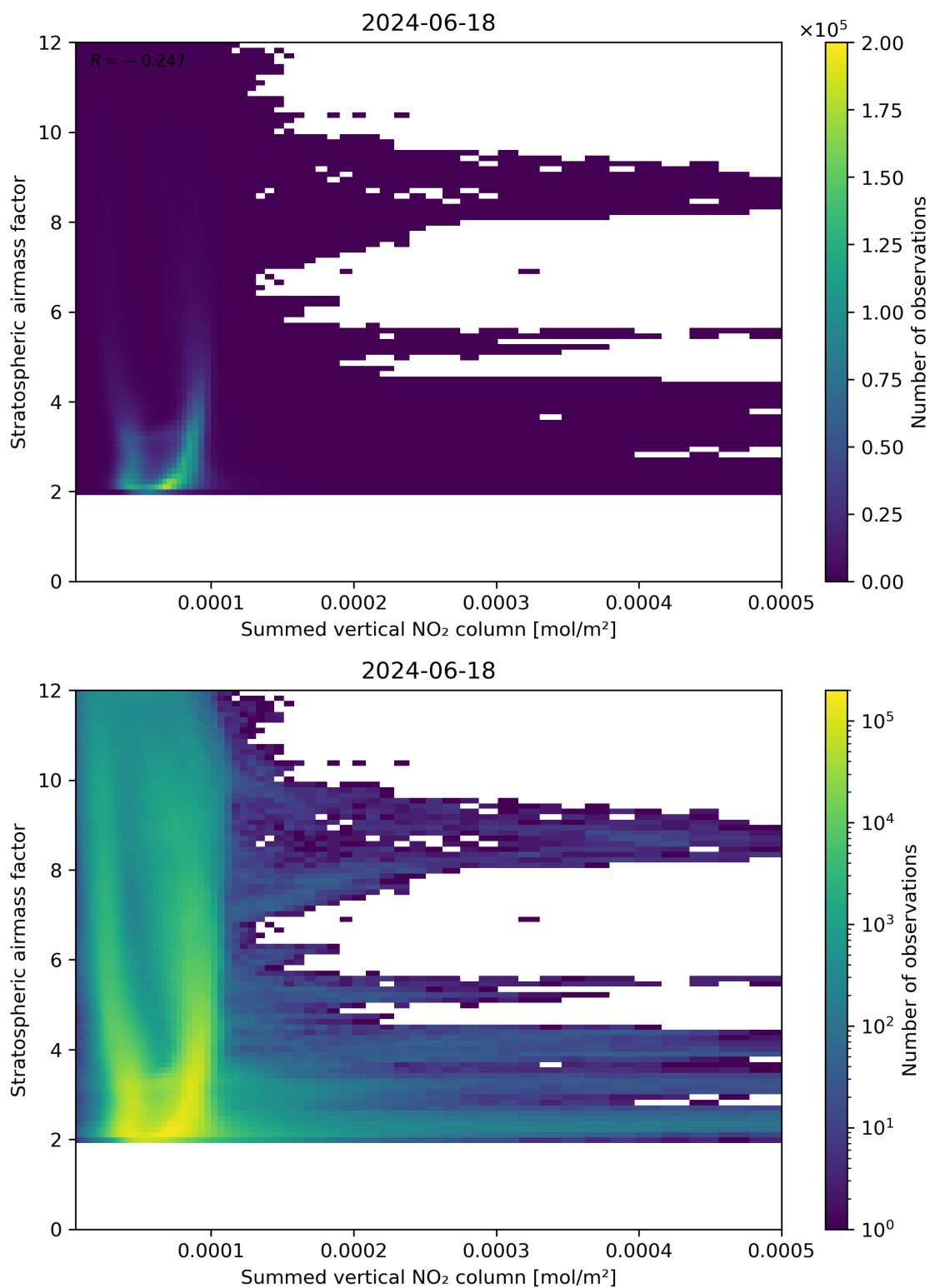
Figure 103: Scatter density plot of “Summed vertical NO 2 column” against “Stratospheric air mass factor” for 2024-06-17 to 2024-06-19.
