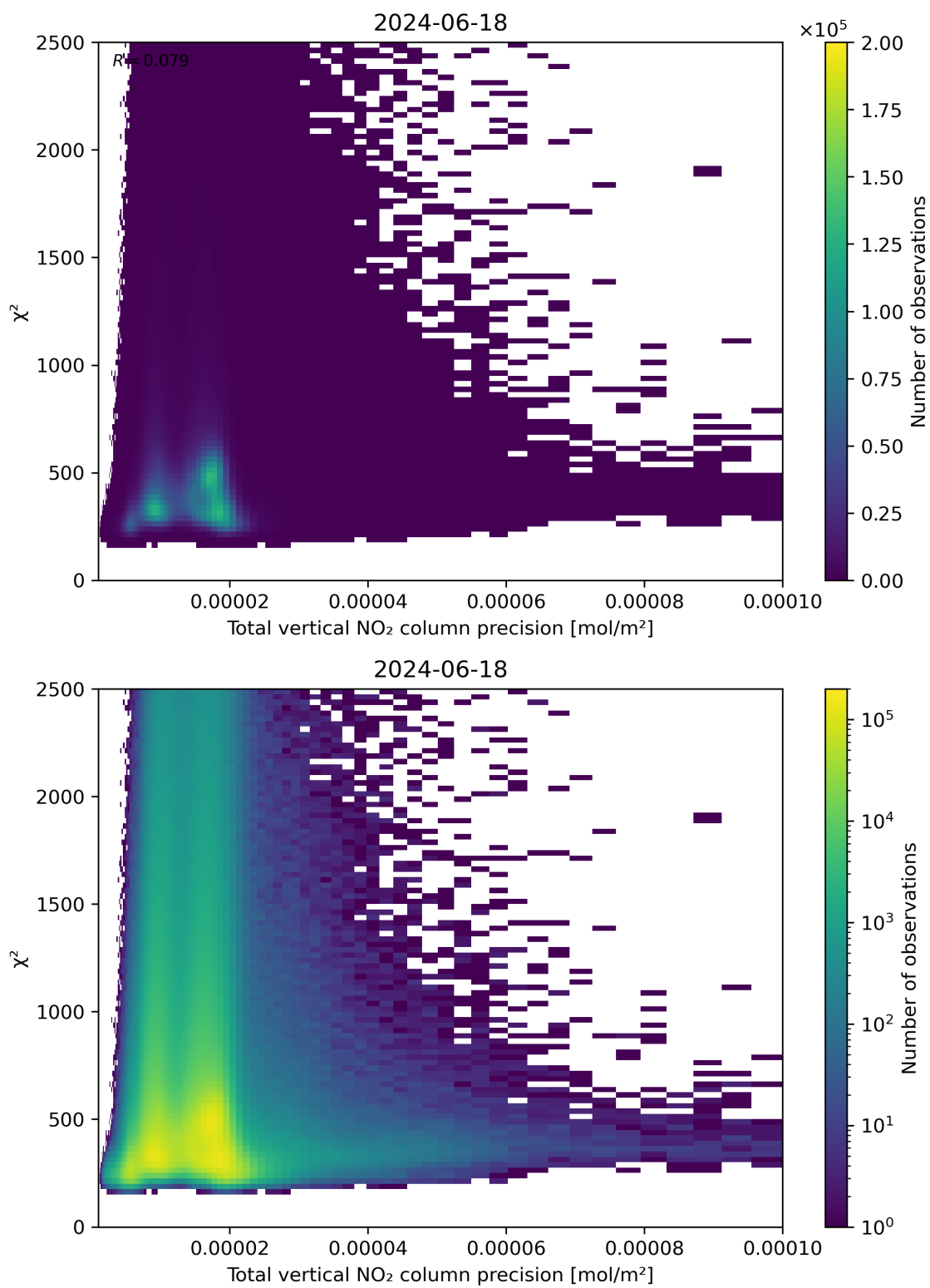
Figure 116: Scatter density plot of “Total vertical NO 2 column precision” against “ \chi^2 ” for 2024-06-17 to 2024-06-19.
