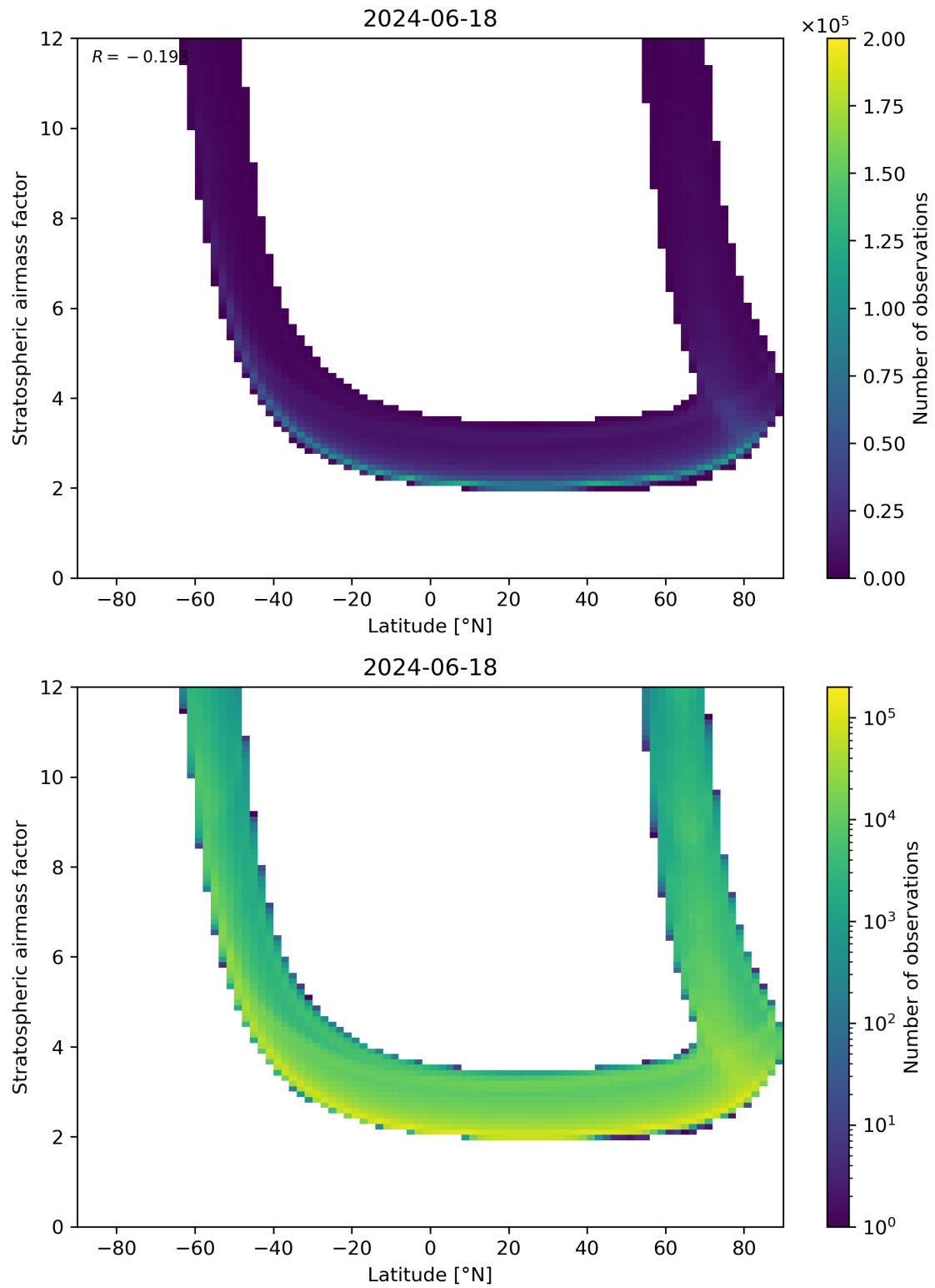
Figure 83: Scatter density plot of “Latitude” against “Stratospheric airmass factor” for 2024-06-17 to 2024-06-19.
