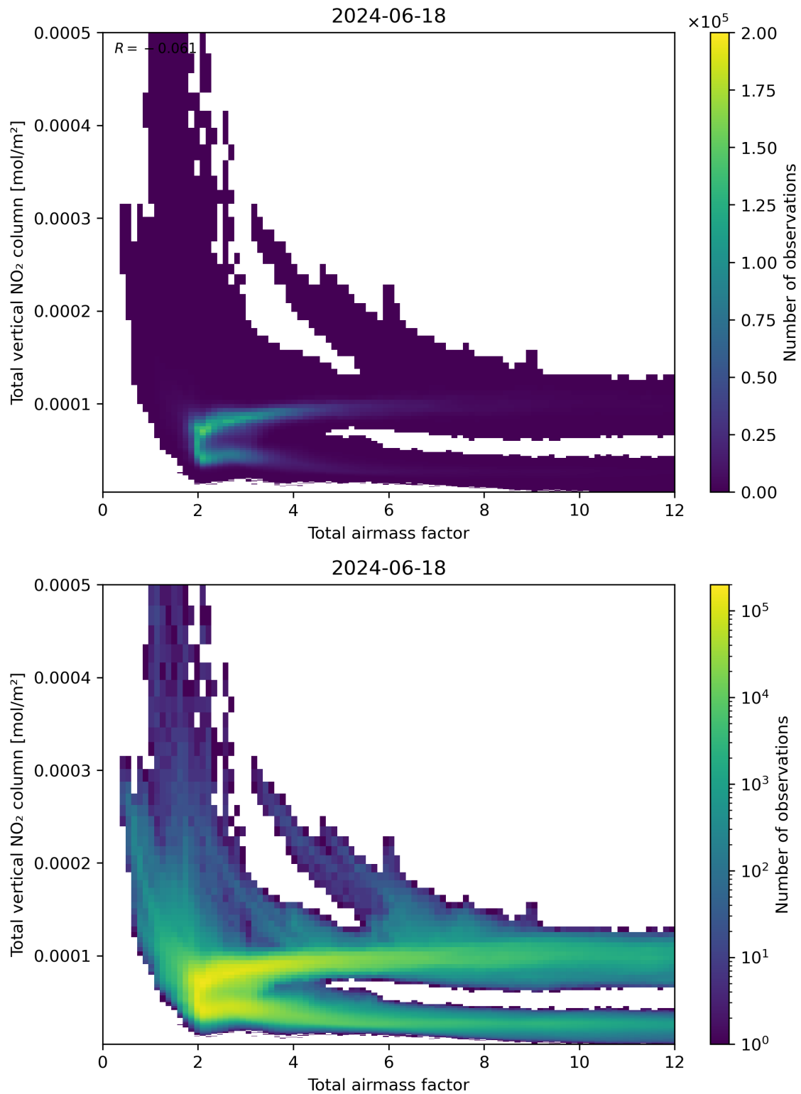
Figure 67: Scatter density plot of “Total airmass factor” against “Total vertical NO 2 column” for 2024-06-17 to 2024-06-19.
