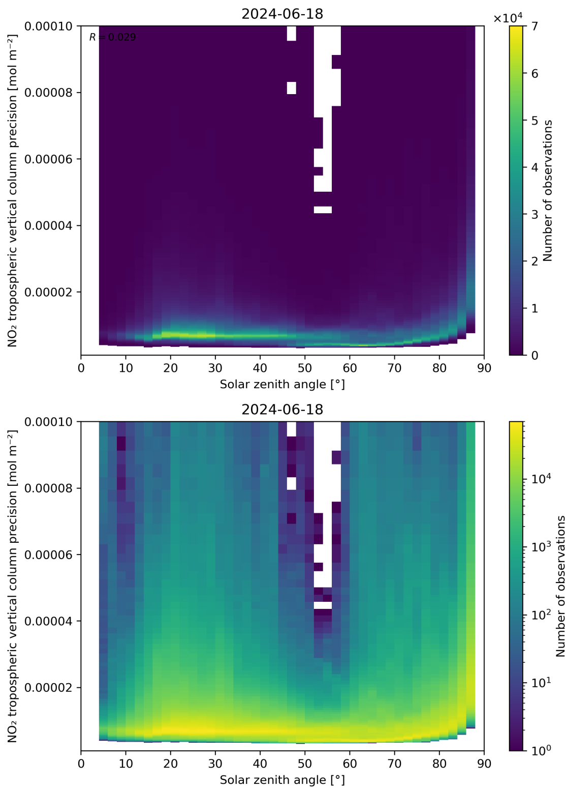
Figure 156: Scatter density plot of “Solar zenith angle” against “NO 2 tropospheric vertical column precision” for 2024-06-17 to 2024-06-19.
