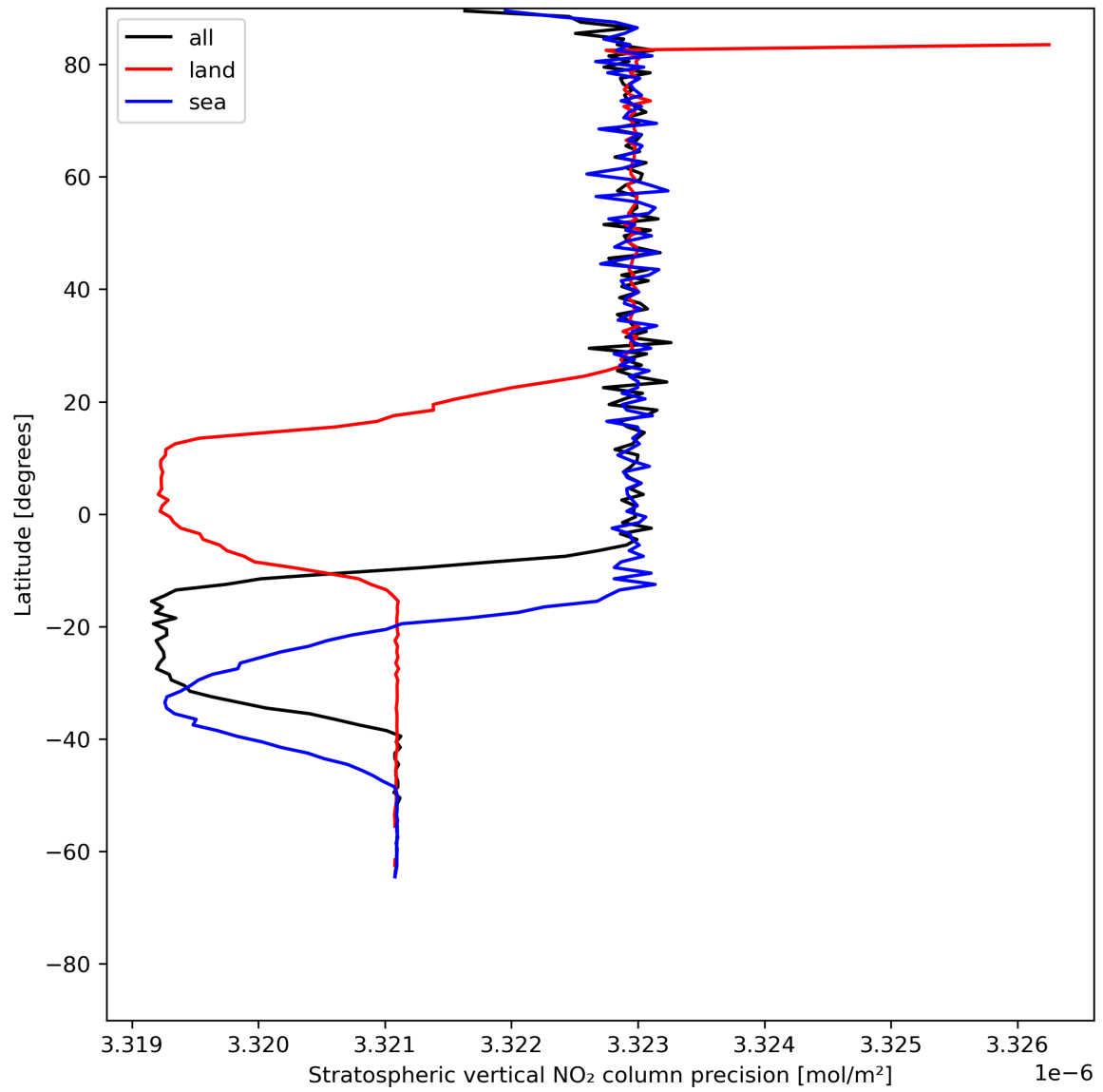
Figure 20: Zonal average of “Stratospheric vertical NO 2 column precision” for 2024-06-17 to 2024-06-19.
