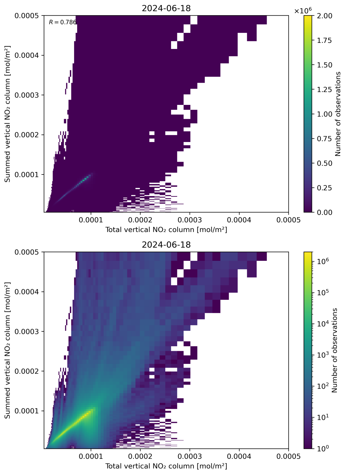
Figure 112: Scatter density plot of “Total vertical NO 2 column” against “Summed vertical NO 2 column” for 2024-06-17 to 2024-06-19.
