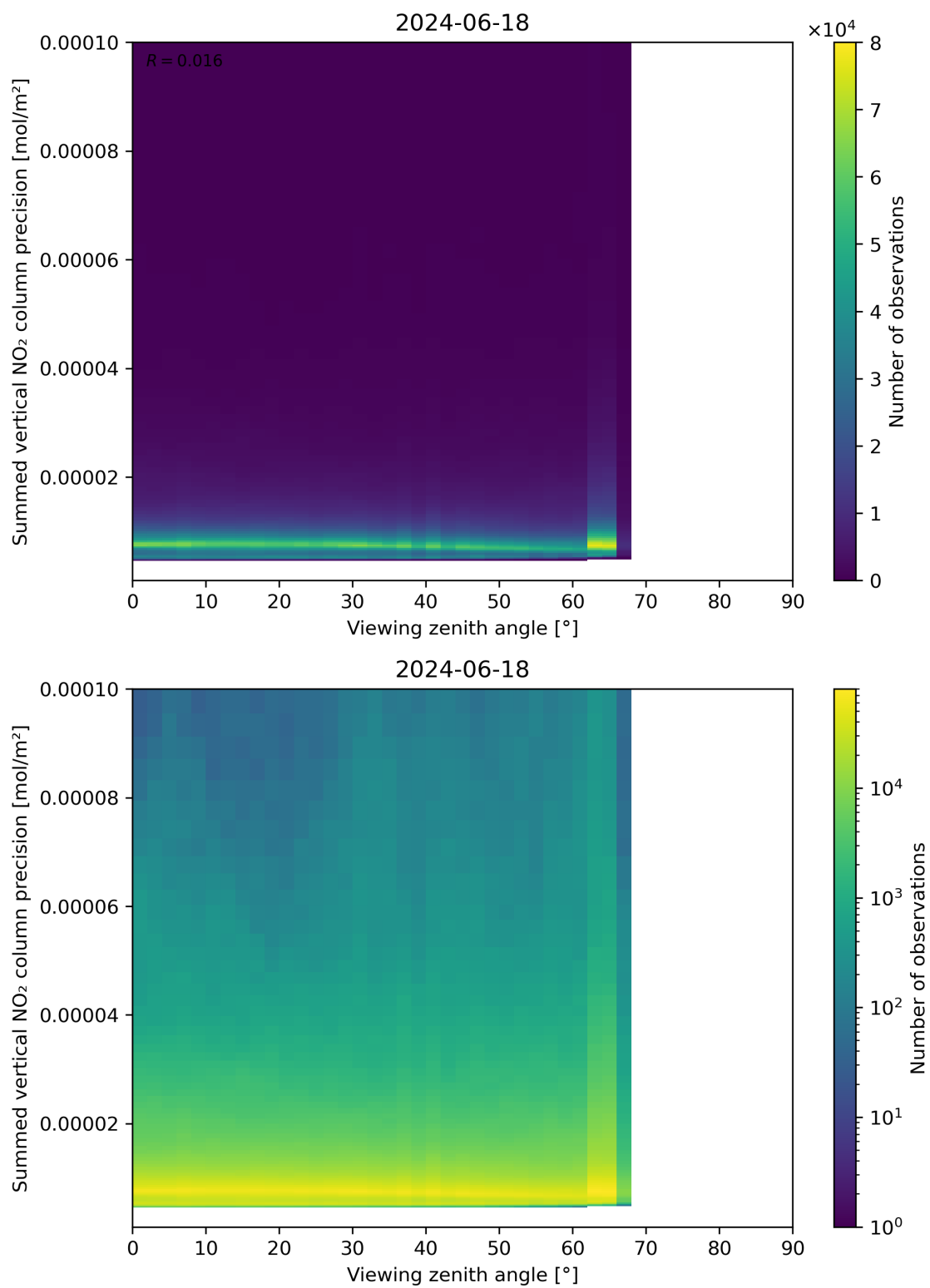
Figure 166: Scatter density plot of “Viewing zenith angle” against “Summed vertical NO 2 column precision” for 2024-06-17 to 2024-06-19.
