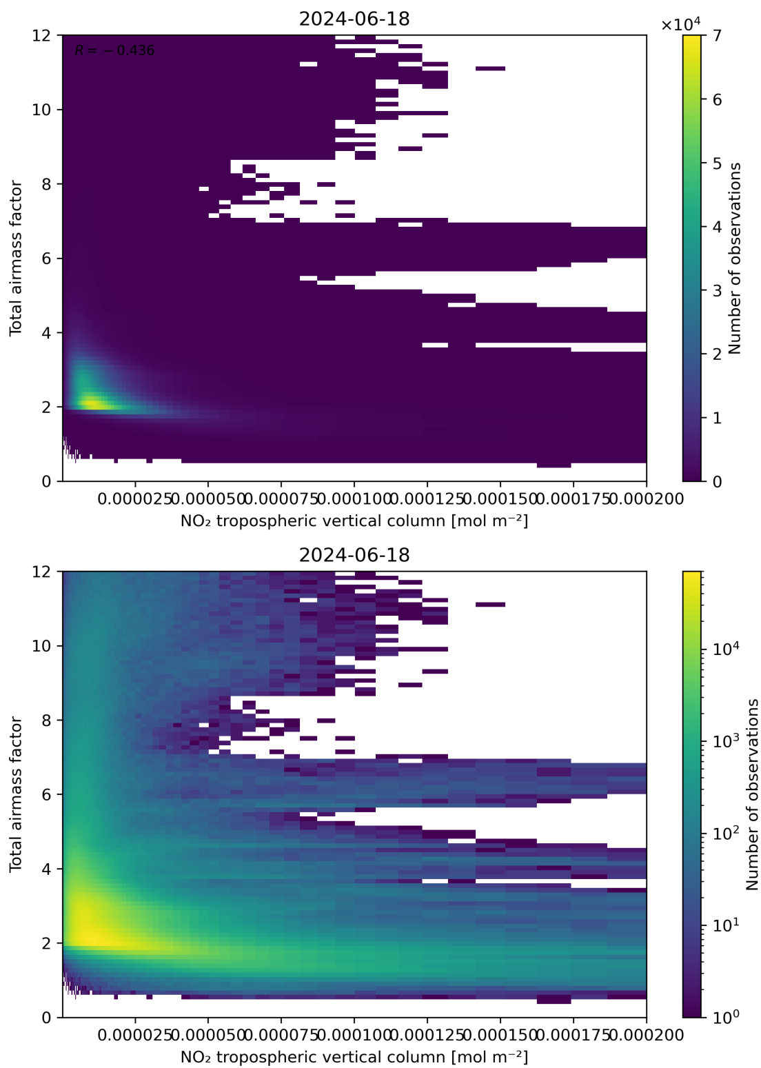
Figure 122: Scatter density plot of “NO 2 tropospheric vertical column” against “Total air mass factor” for 2024-06-17 to 2024-06-19.
