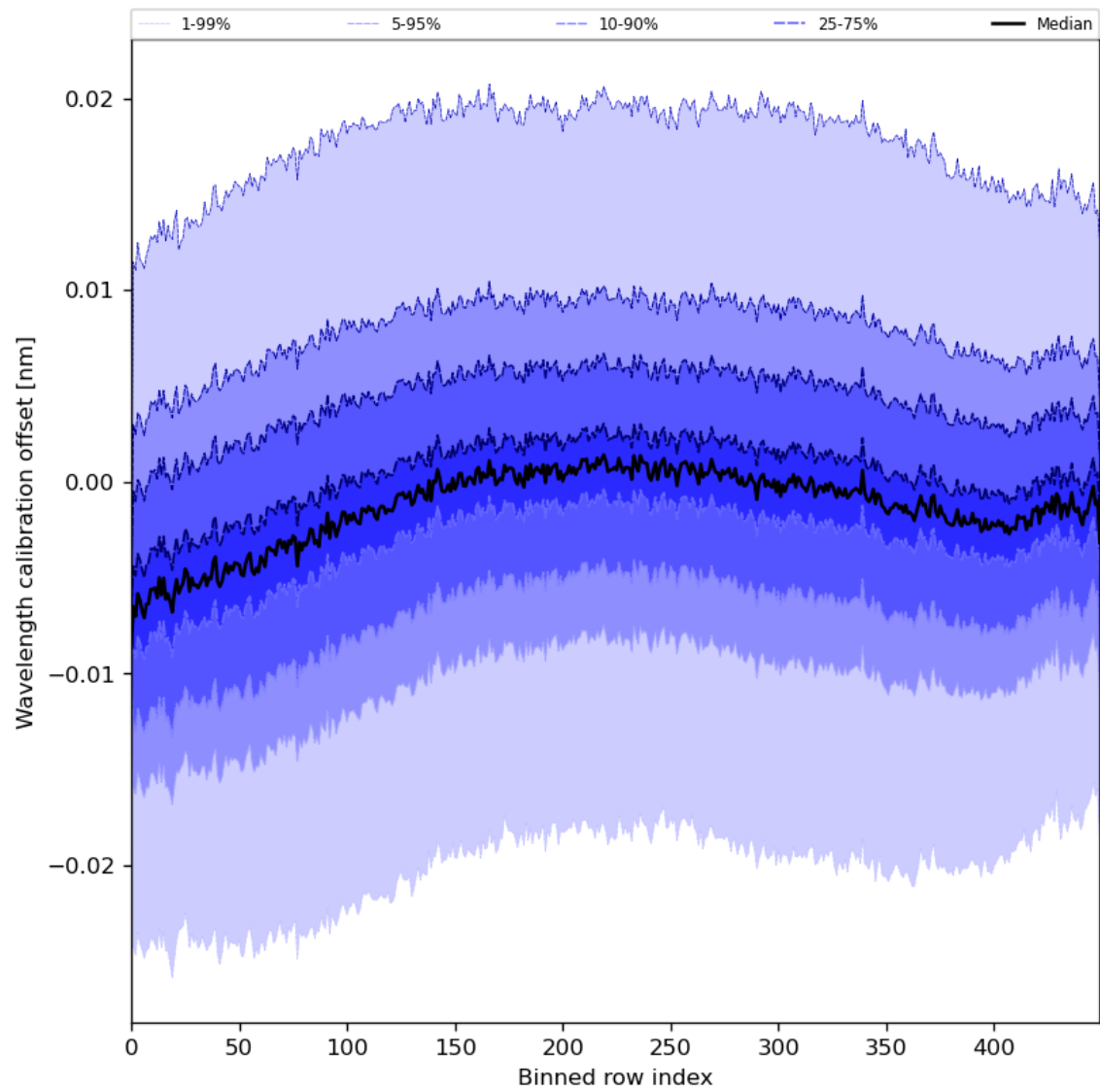
Figure 52: Along track statistics of “Wavelength calibration offset” for 2024-06-17 to 2024-06-19
