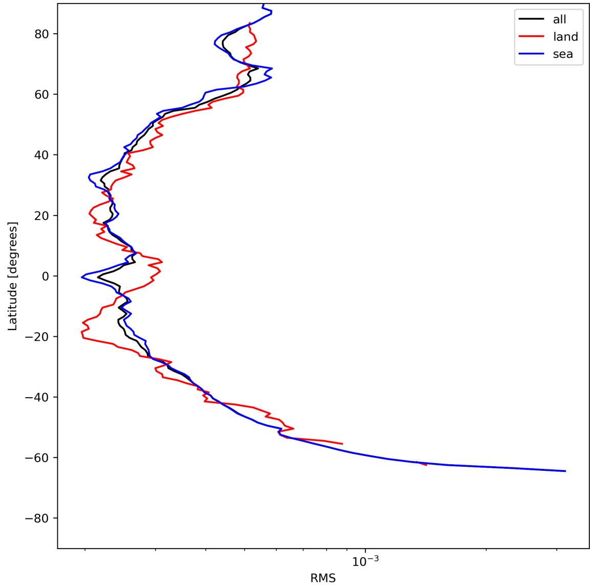
Figure 26: Zonal average of “RMS” for 2024-06-17 to 2024-06-19.
