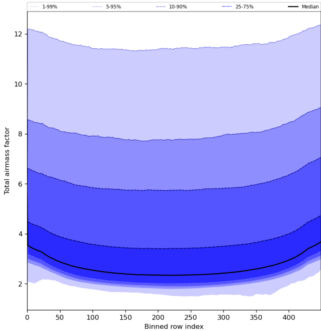
Figure 49: Along track statistics of “Total airmass factor” for 2024-06-17 to 2024-06-19
