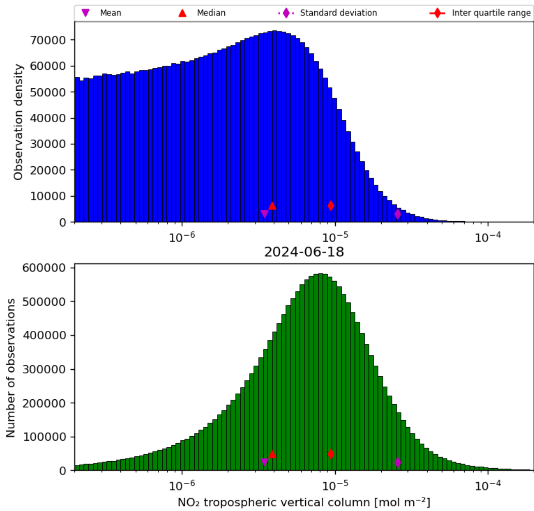
Figure 29: Histogram of “NO 2 tropospheric vertical column” for 2024-06-17 to 2024-06-19
