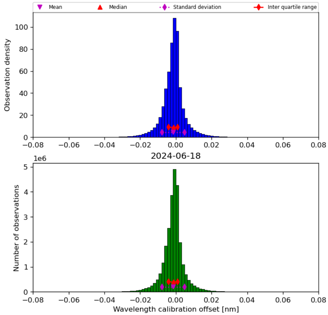
Figure 35: Histogram of “Wavelength calibration offset” for 2024-06-17 to 2024-06-19
