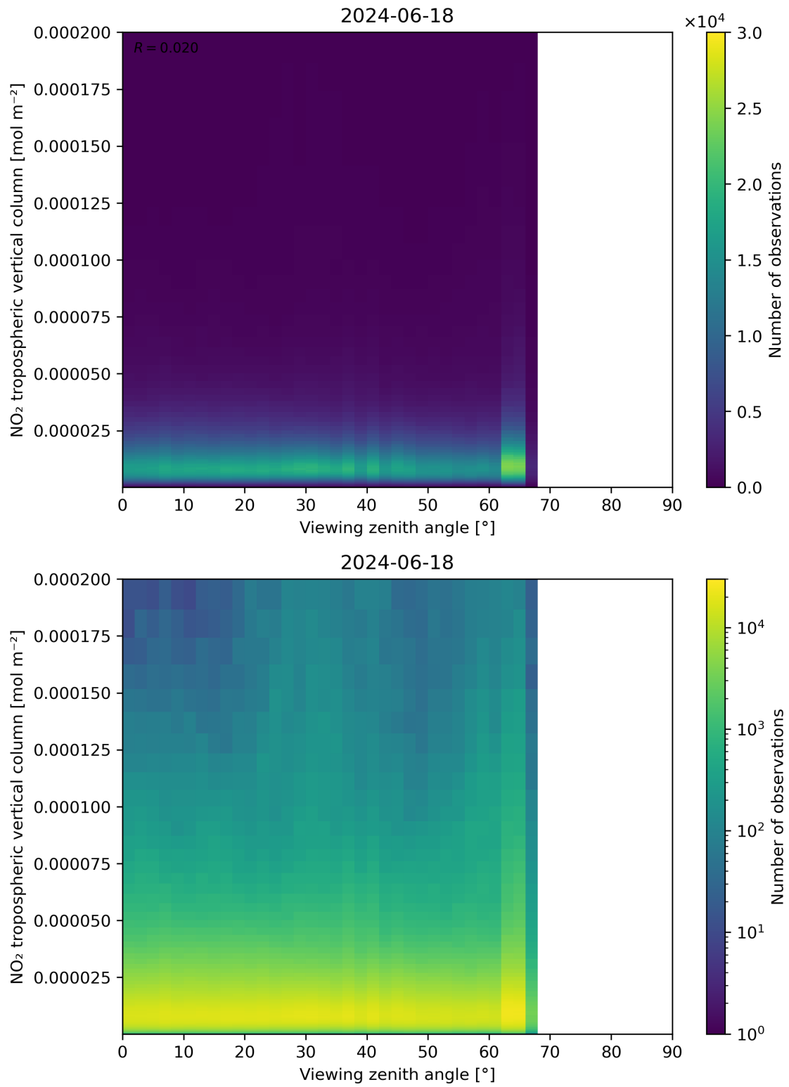
Figure 169: Scatter density plot of “Viewing zenith angle” against “NO 2 tropospheric vertical column” for 2024-06-17 to 2024-06-19.
