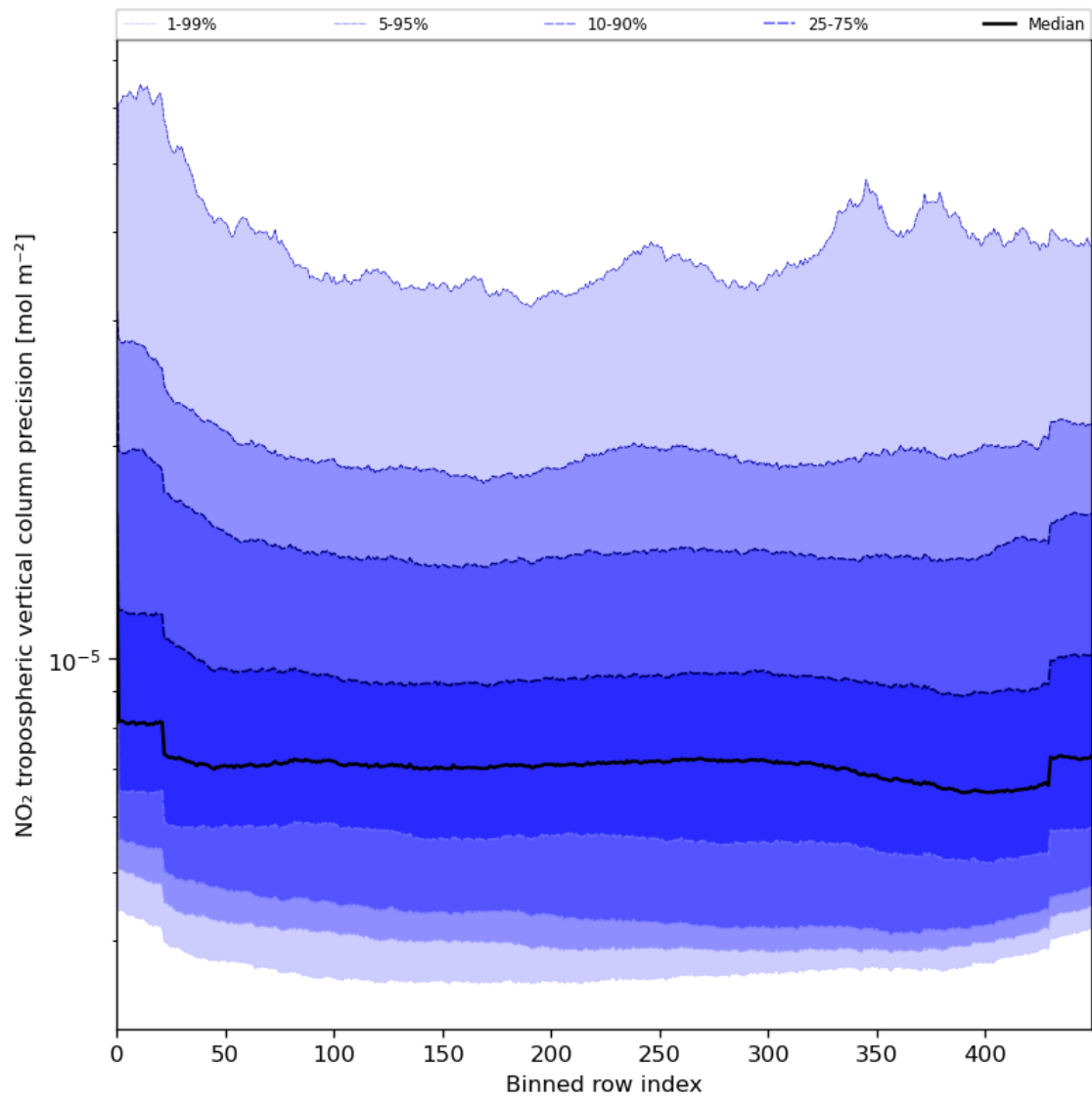
Figure 47: Along track statistics of “NO 2 tropospheric vertical column precision” for 2024-06-17 to 2024-06-19
