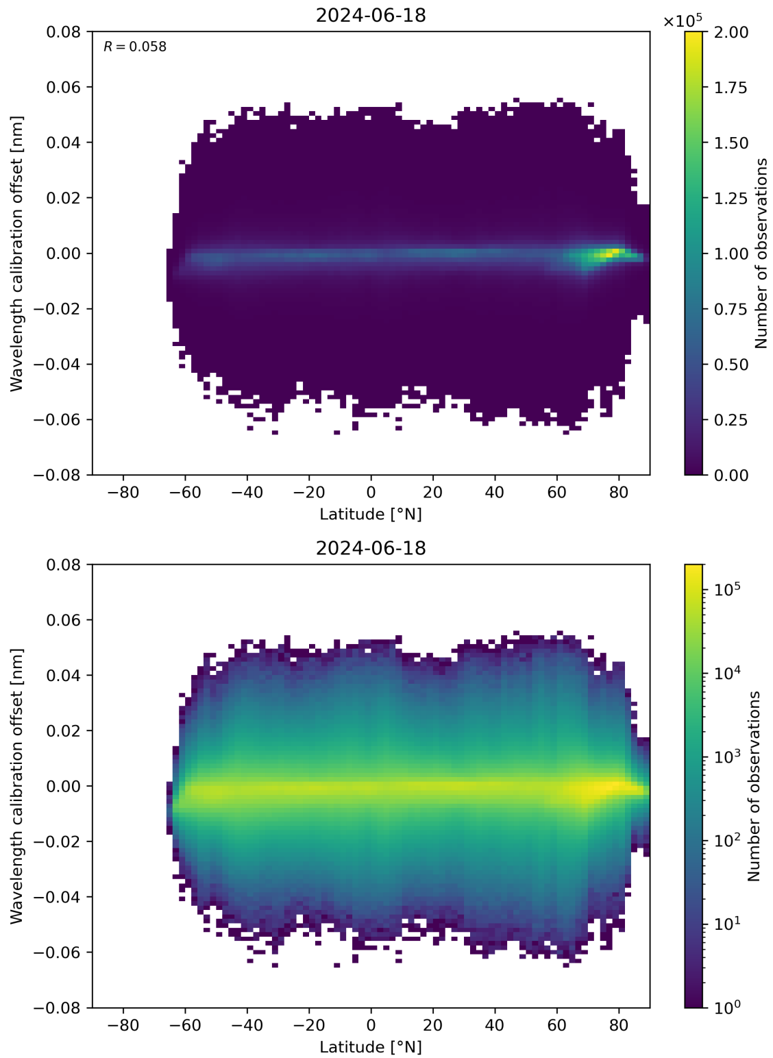
Figure 95: Scatter density plot of “Latitude” against “Wavelength calibration offset” for 2024-06-17 to 2024-06-19.
