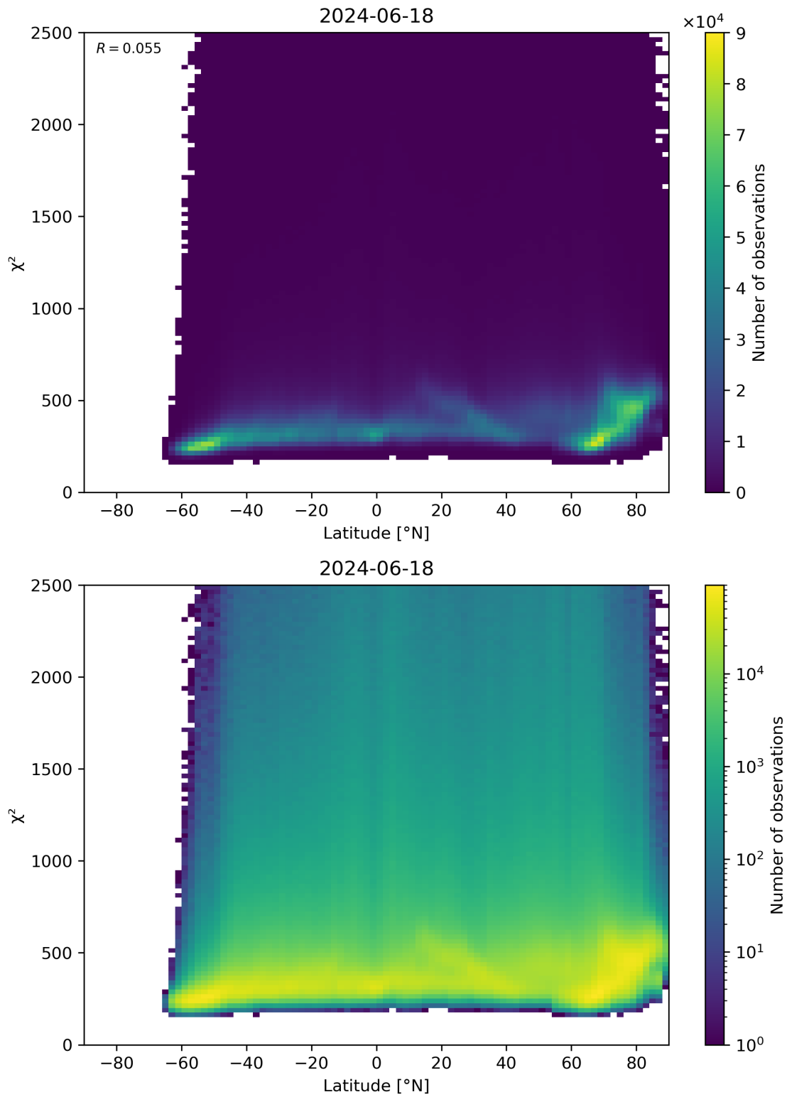
Figure 86: Scatter density plot of “Latitude” against “ \chi^2 ” for 2024-06-17 to 2024-06-19.
