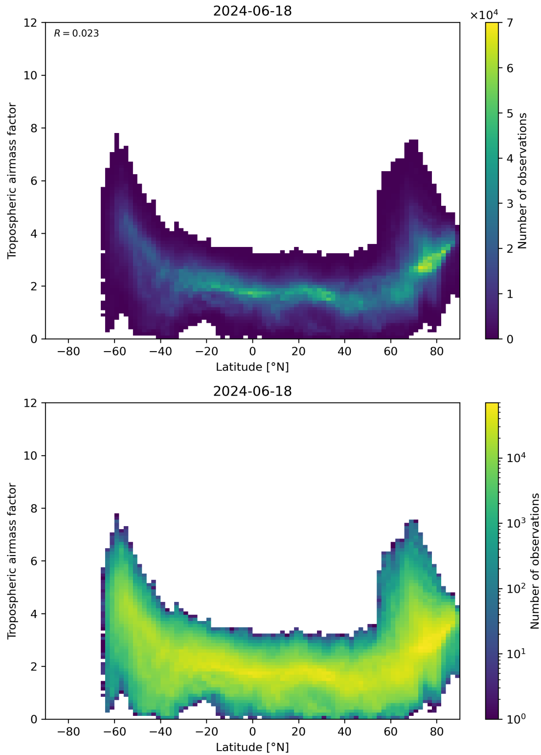
Figure 85: Scatter density plot of “Latitude” against “Tropospheric airmass factor” for 2024-06-17 to 2024-06-19.
