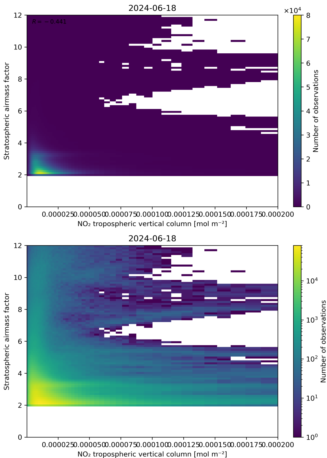
Figure 121: Scatter density plot of “NO 2 tropospheric vertical column” against “Stratospheric air mass factor” for 2024-06-17 to 2024-06-19.
