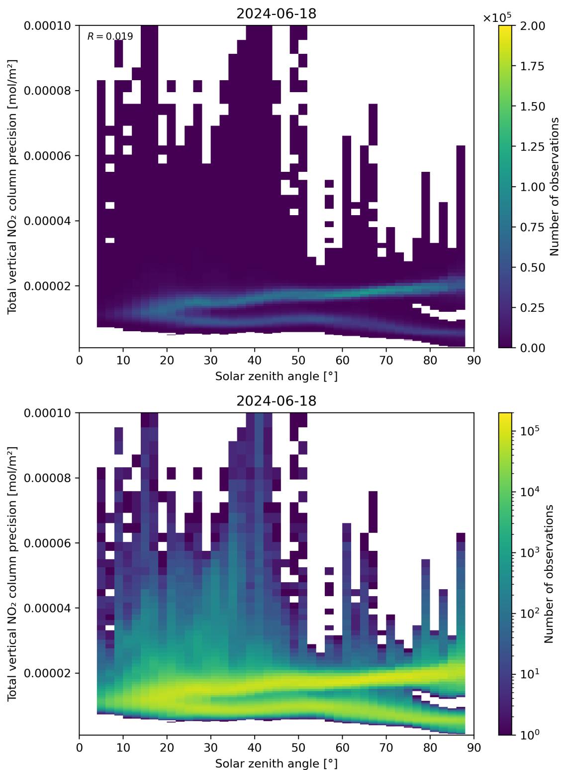
Figure 154: Scatter density plot of “Solar zenith angle” against “Total vertical NO 2 column precision” for 2024-06-17 to 2024-06-19.
