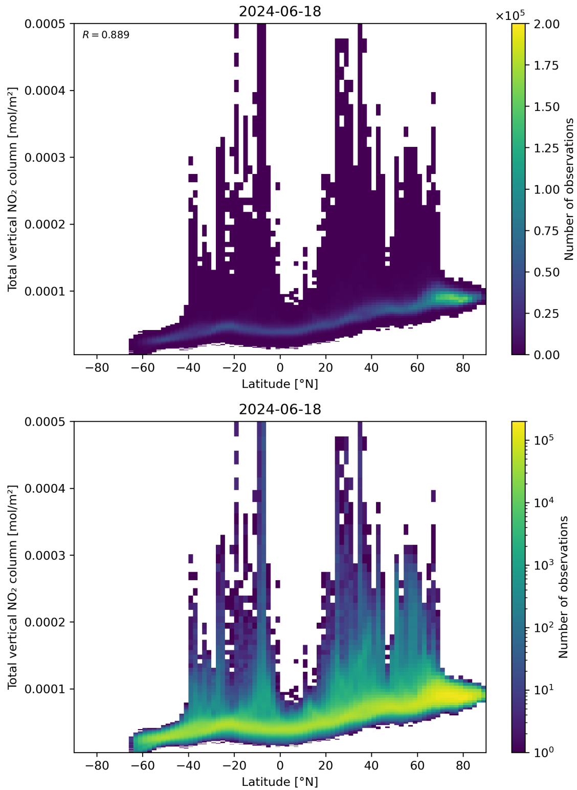
Figure 90: Scatter density plot of “Latitude” against “Total vertical NO 2 column” for 2024-06-17 to 2024-06-19.
