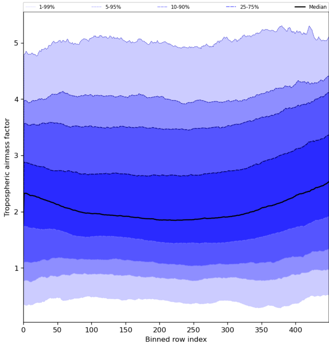
Figure 48: Along track statistics of “Tropospheric airmass factor” for 2024-06-17 to 2024-06-19
