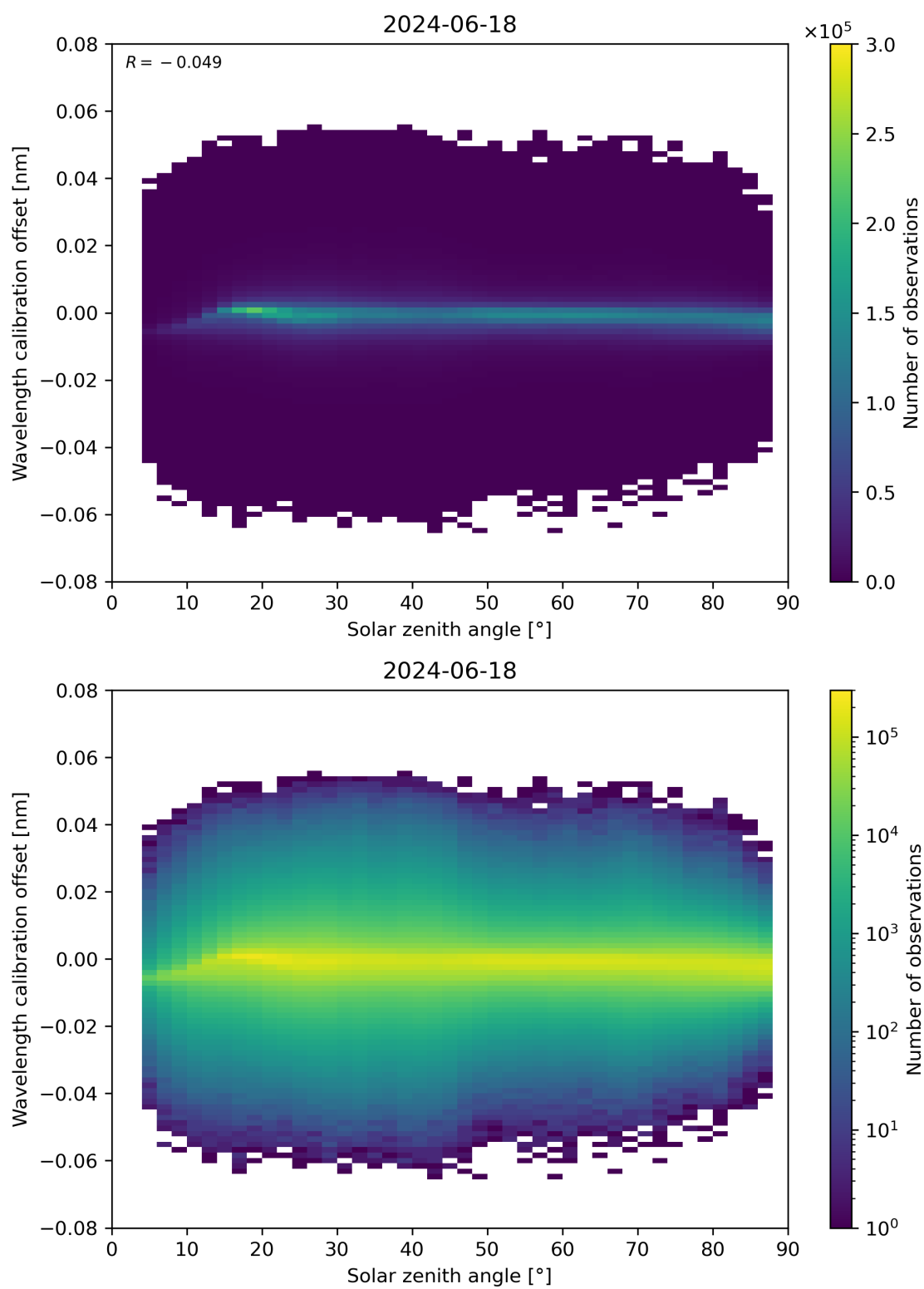
Figure 158: Scatter density plot of “Solar zenith angle” against “Wavelength calibration offset” for 2024-06-17 to 2024-06-19.
