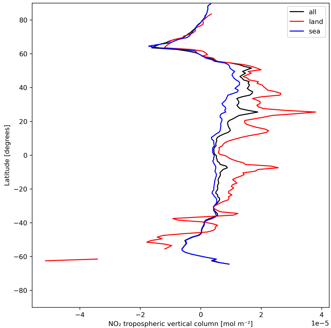
Figure 12: Zonal average of “NO 2 tropospheric vertical column” for 2024-06-17 to 2024-06-19.
