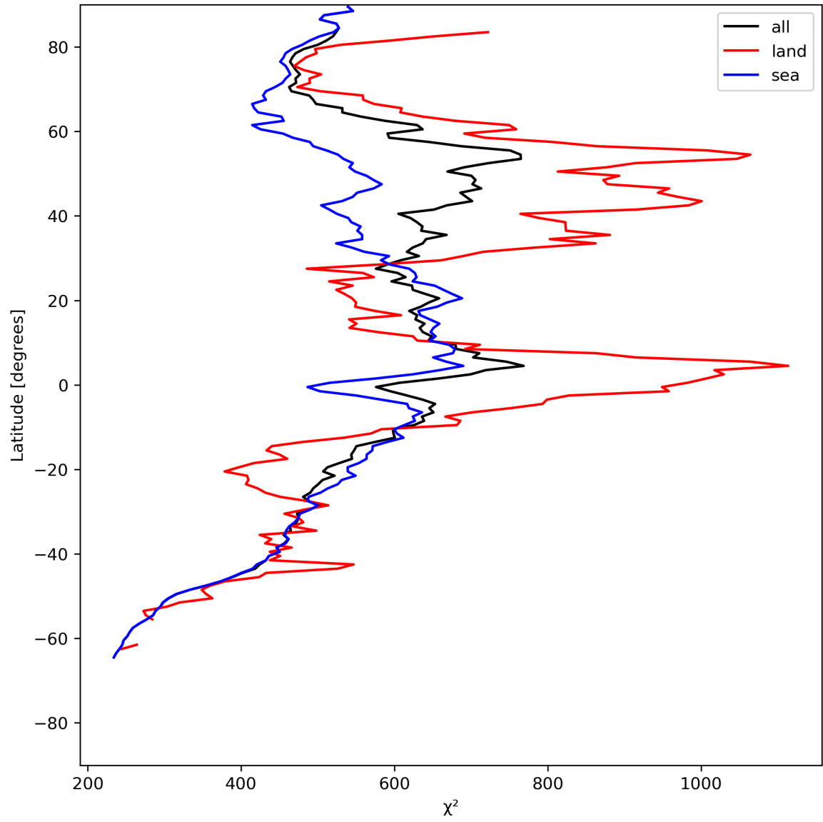
Figure 25: Zonal average of “ \chi^2 ” for 2024-06-17 to 2024-06-19.
