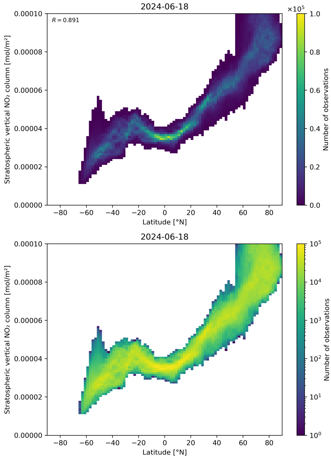
Figure 87: Scatter density plot of “Latitude” against “Stratospheric vertical NO 2 column” for 2024-06-17 to 2024-06-19.
