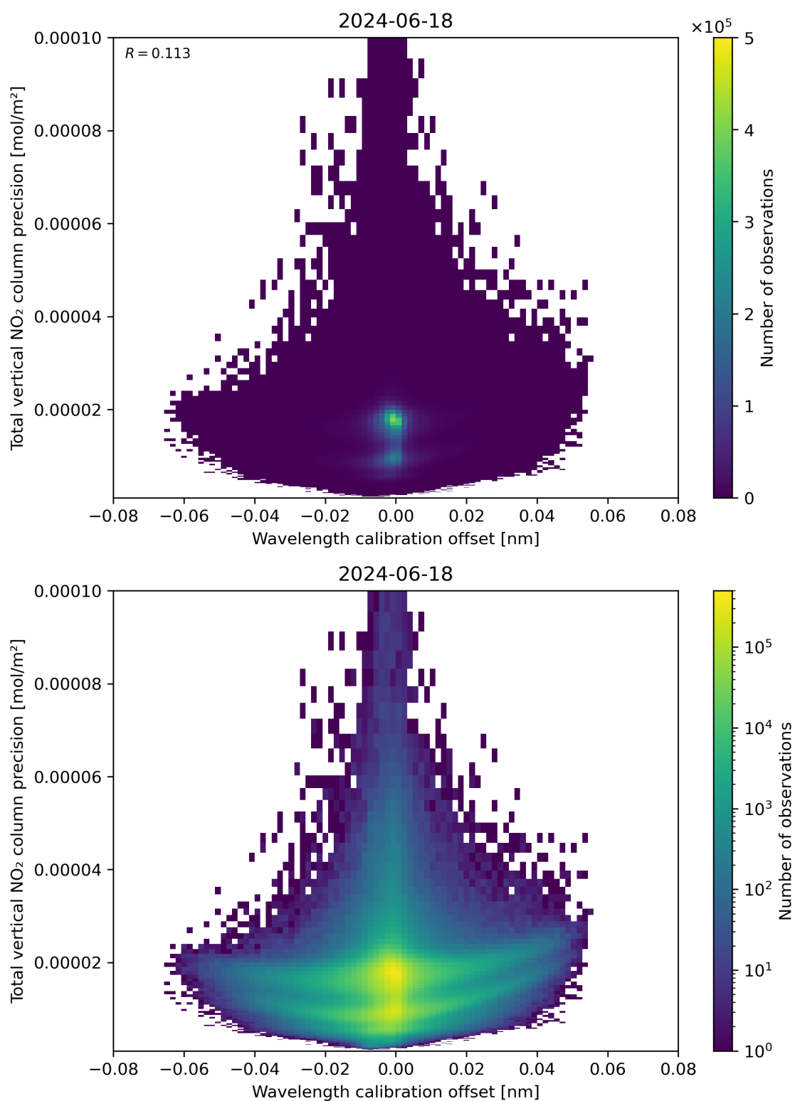
Figure 180: Scatter density plot of “Wavelength calibration offset” against “Total vertical NO 2 column precision” for 2024-06-17 to 2024-06-19.
