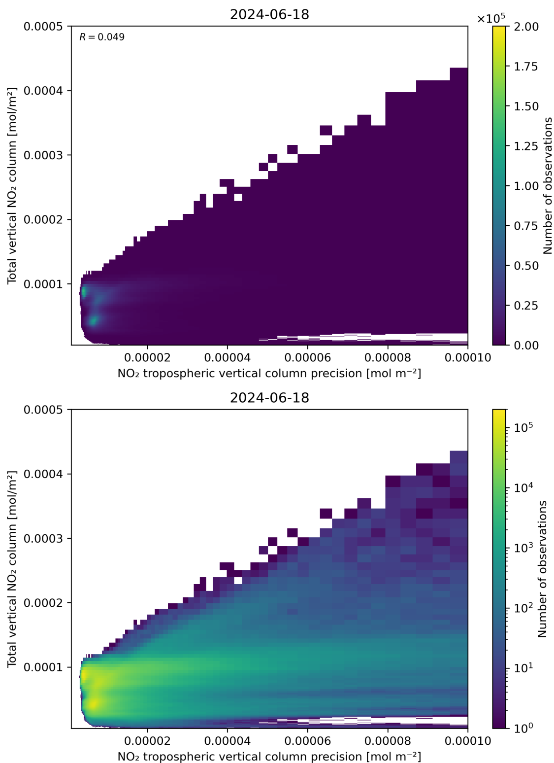
Figure 138: Scatter density plot of “NO 2 tropospheric vertical column precision” against “Total vertical NO 2 column” for 2024-06-17 to 2024-06-19.
