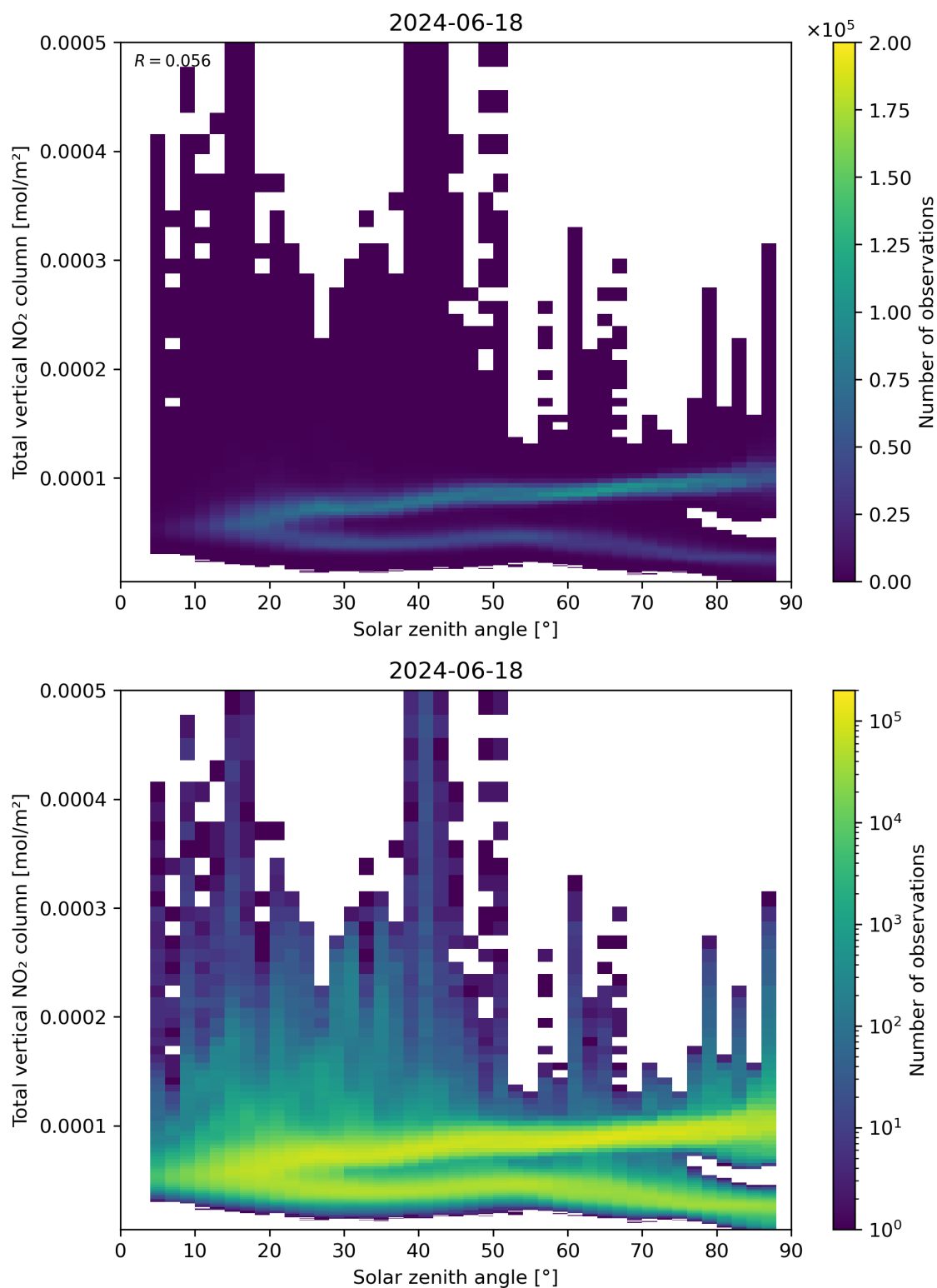
Figure 153: Scatter density plot of “Solar zenith angle” against “Total vertical NO 2 column” for 2024-06-17 to 2024-06-19.
