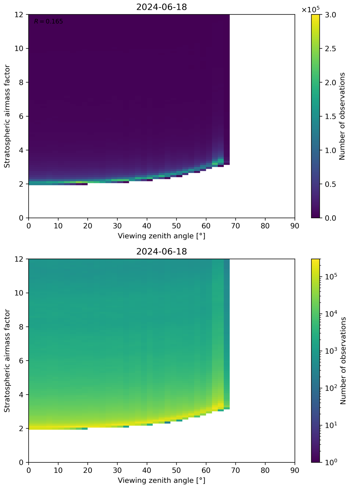
Figure 159: Scatter density plot of “Viewing zenith angle” against “Stratospheric airmass factor” for 2024-06-17 to 2024-06-19.
