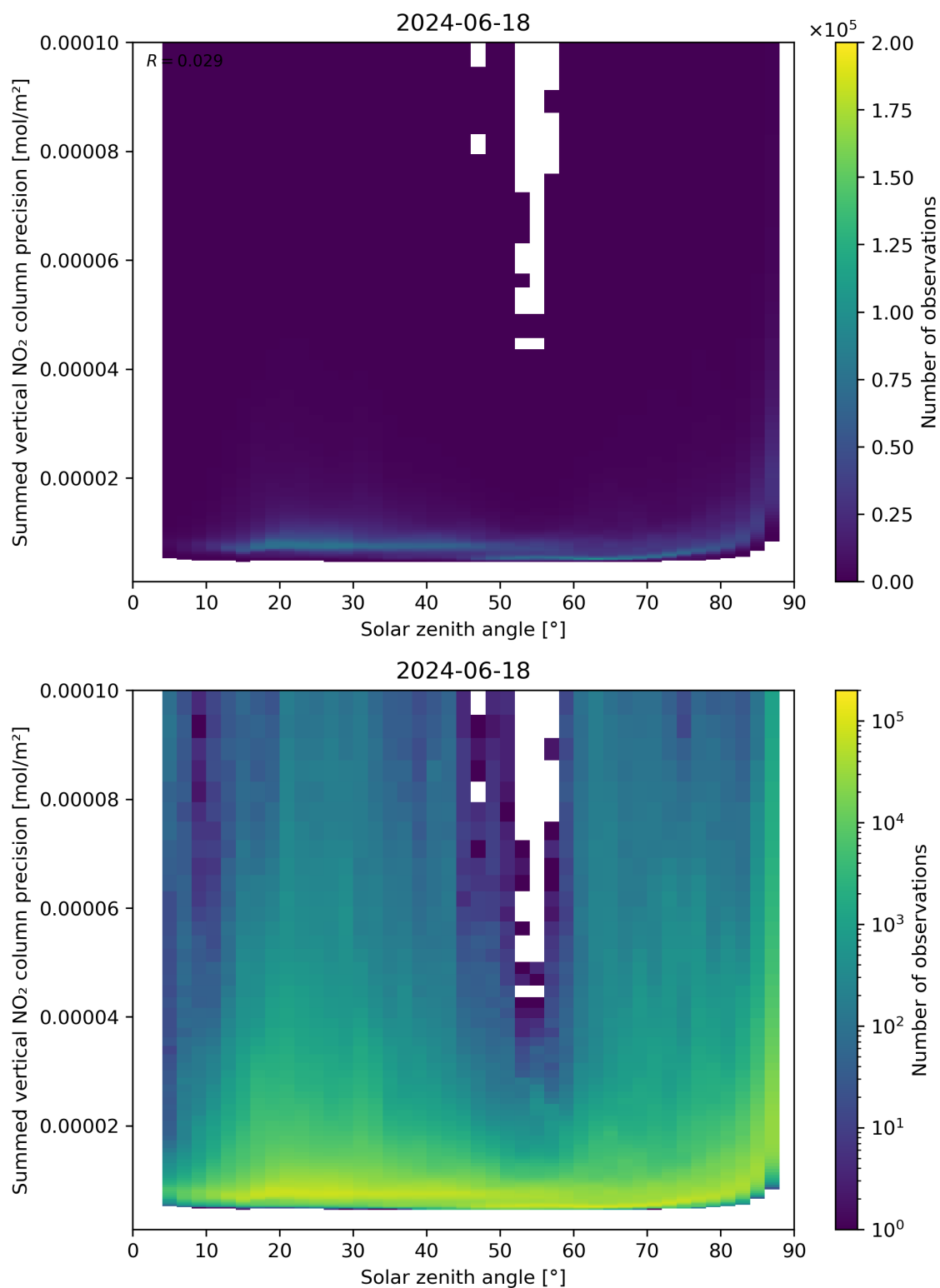
Figure 152: Scatter density plot of “Solar zenith angle” against “Summed vertical NO 2 column precision” for 2024-06-17 to 2024-06-19.
