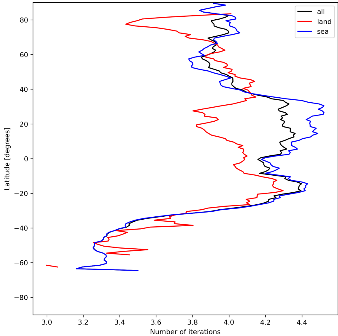
Figure 17: Zonal average of “Number of iterations” for 2024-06-17 to 2024-06-19.
