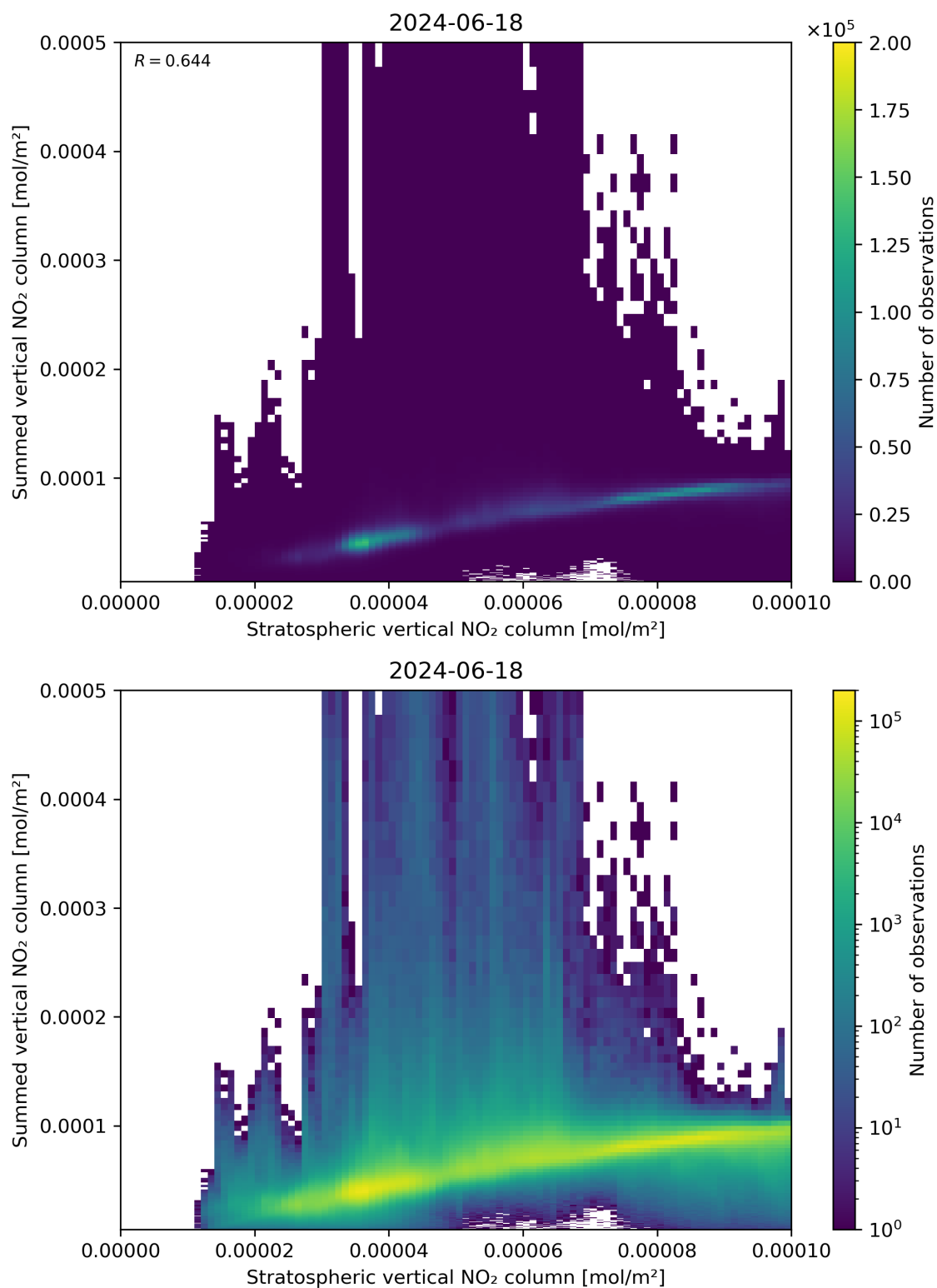
Figure 98: Scatter density plot of “Stratospheric vertical NO 2 column” against “Summed vertical NO 2 column” for 2024-06-17 to 2024-06-19.
