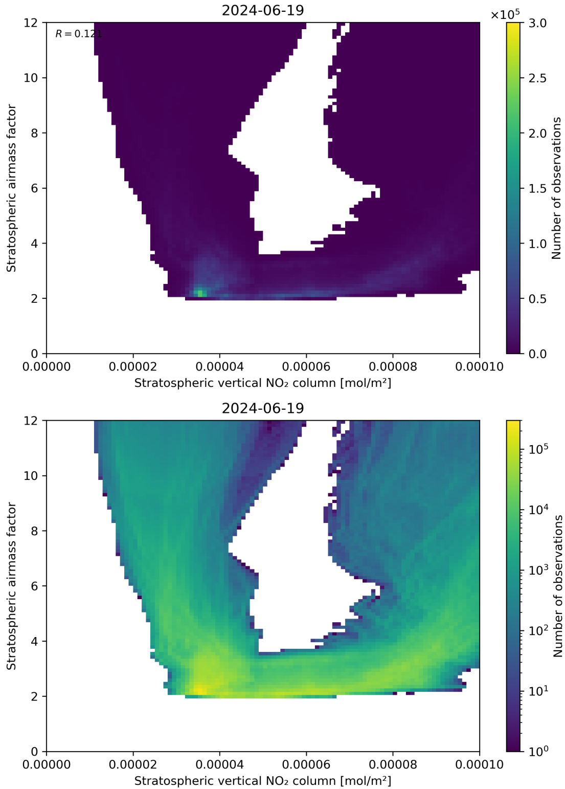
Figure 96: Scatter density plot of “Stratospheric vertical NO 2 column” against “Stratospheric airmass factor” for 2024-06-19 to 2024-06-20.
