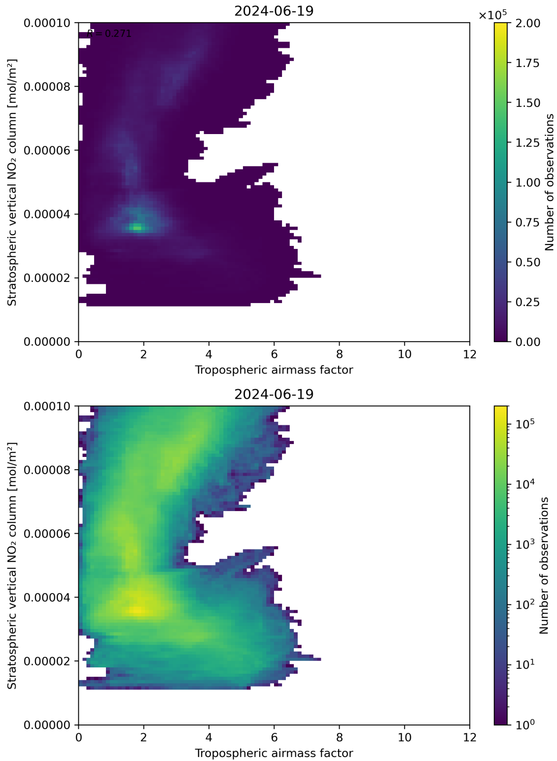
Figure 74: Scatter density plot of “Tropospheric airmass factor” against “Stratospheric vertical \text{NO}_2 column” for 2024-06-19 to 2024-06-20.
