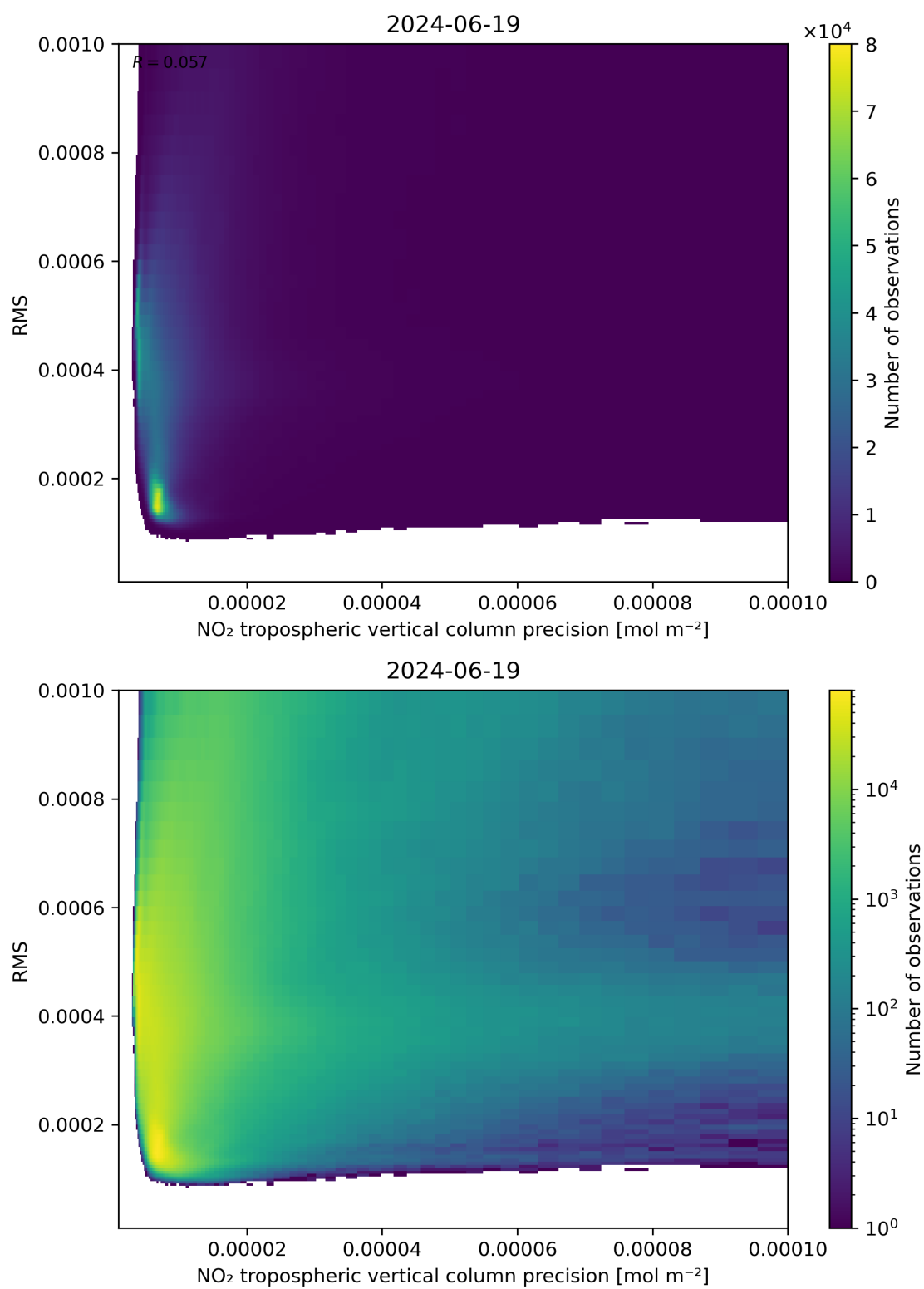
Figure 140: Scatter density plot of “NO 2 tropospheric vertical column precision” against “RMS” for 2024-06-19 to 2024-06-20.
