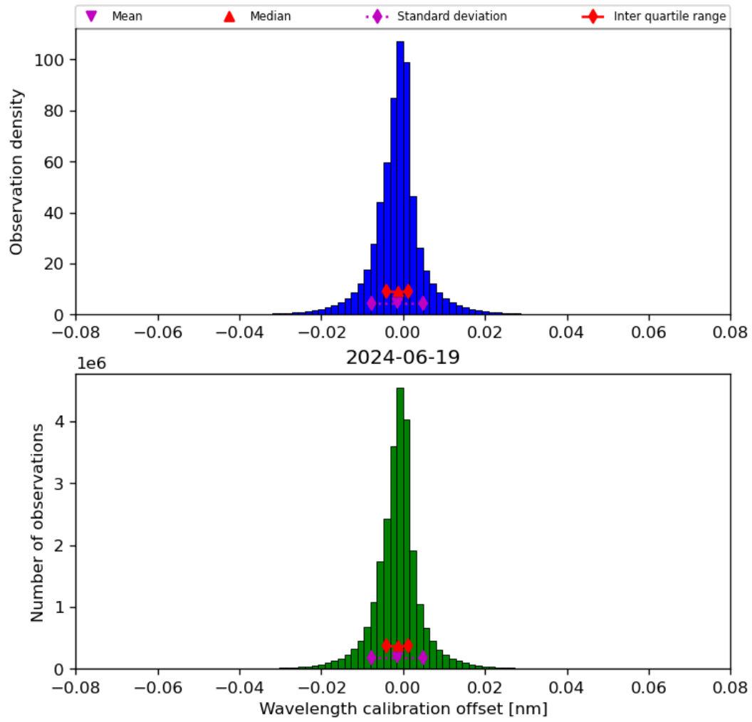
Figure 35: Histogram of “Wavelength calibration offset” for 2024-06-19 to 2024-06-20
