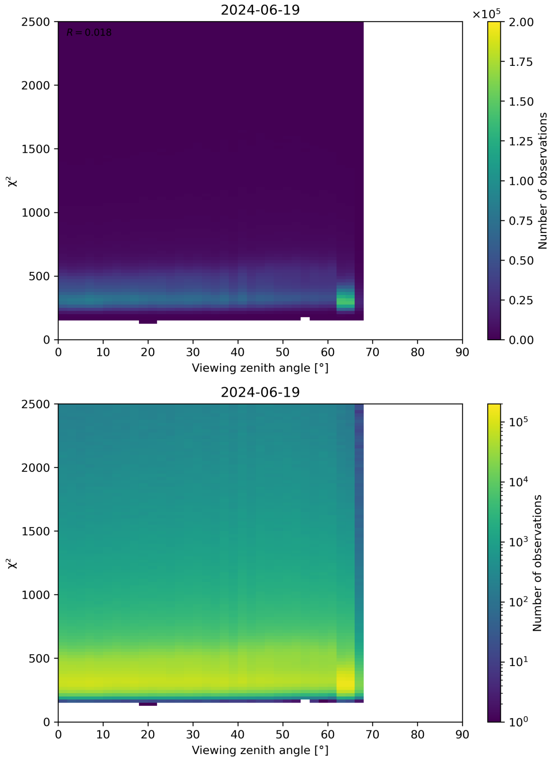
Figure 162: Scatter density plot of “Viewing zenith angle” against “ \chi^2 ” for 2024-06-19 to 2024-06-20.
