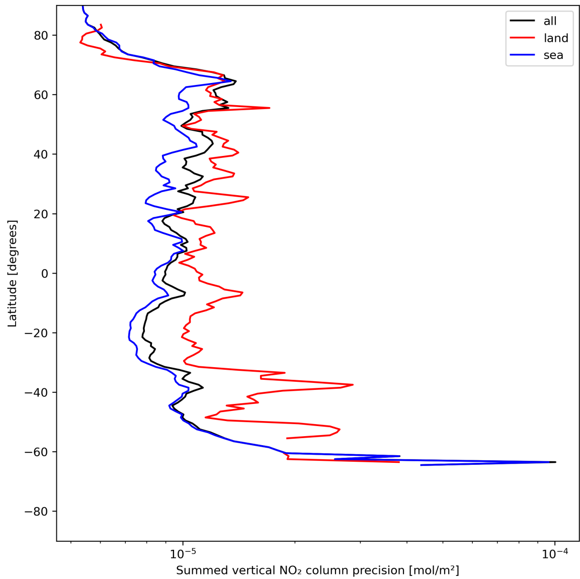
Figure 24: Zonal average of “Summed vertical NO 2 column precision” for 2024-06-19 to 2024-06-20.
