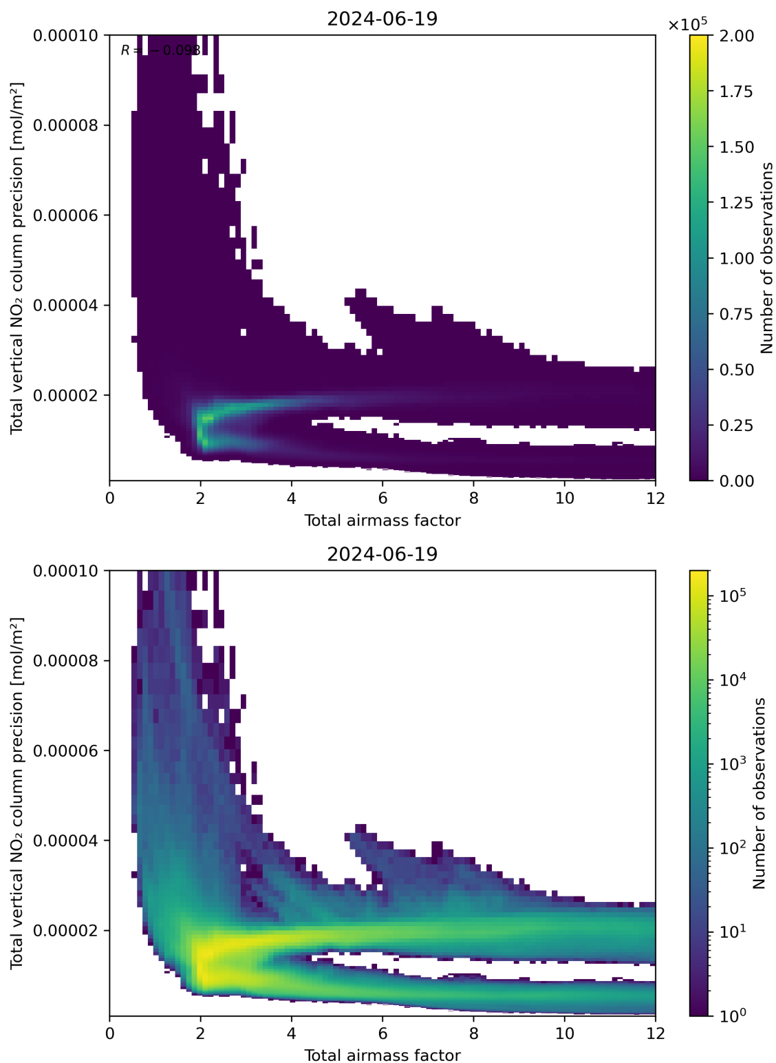
Figure 68: Scatter density plot of “Total airmass factor” against “Total vertical NO 2 column precision” for 2024-06-19 to 2024-06-20.
