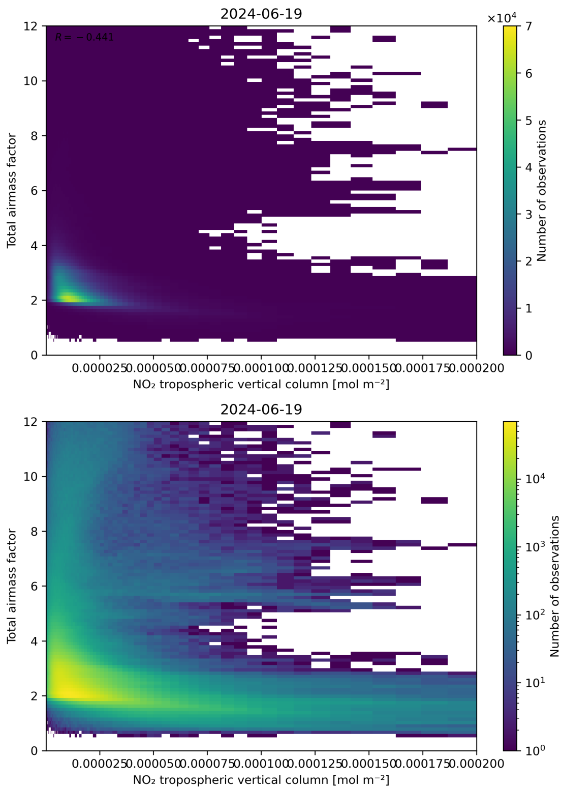
Figure 122: Scatter density plot of “NO 2 tropospheric vertical column” against “Total air mass factor” for 2024-06-19 to 2024-06-20.
