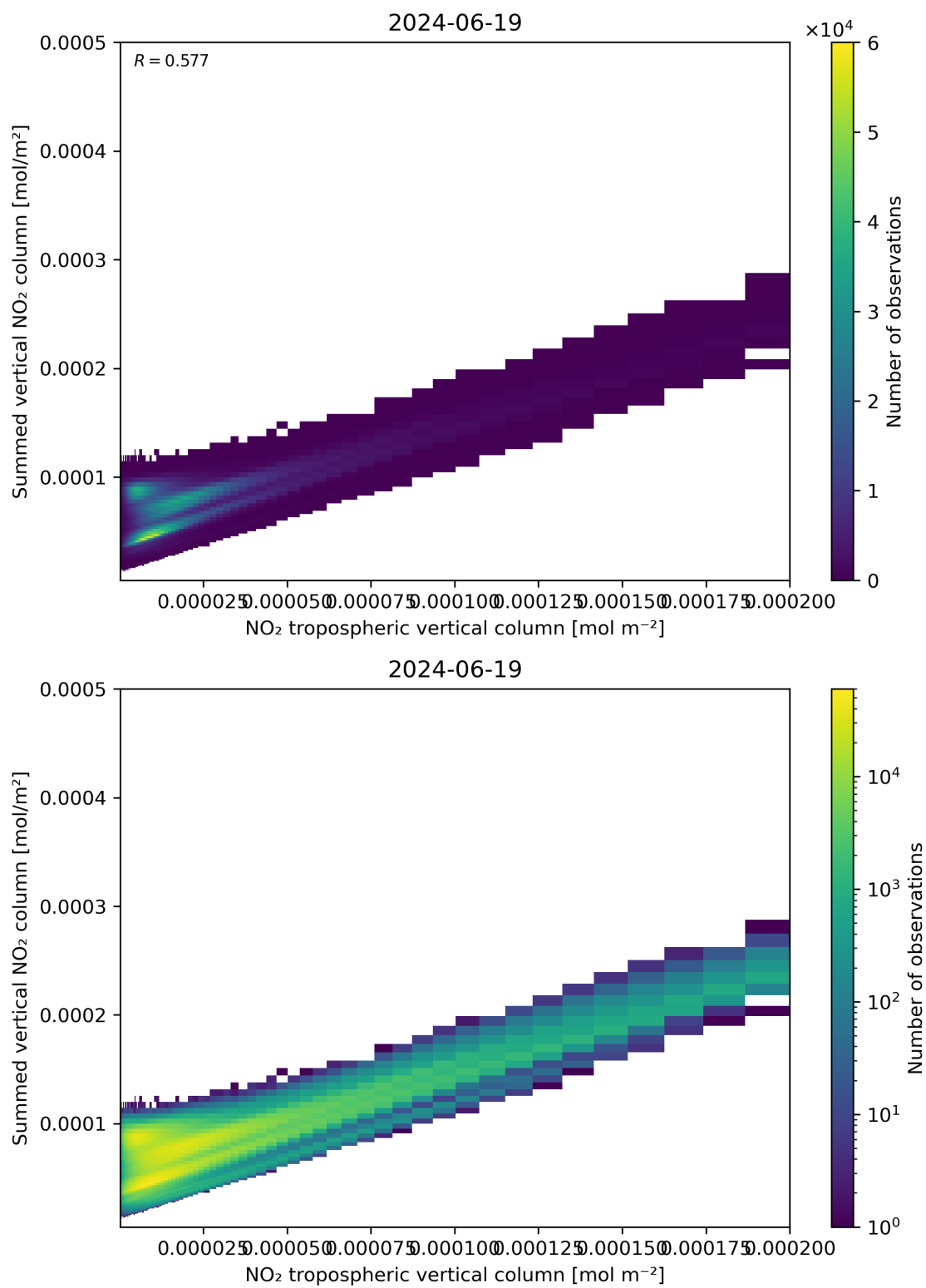
Figure 126: Scatter density plot of “NO 2 tropospheric vertical column” against “Summed vertical NO 2 column” for 2024-06-19 to 2024-06-20.
