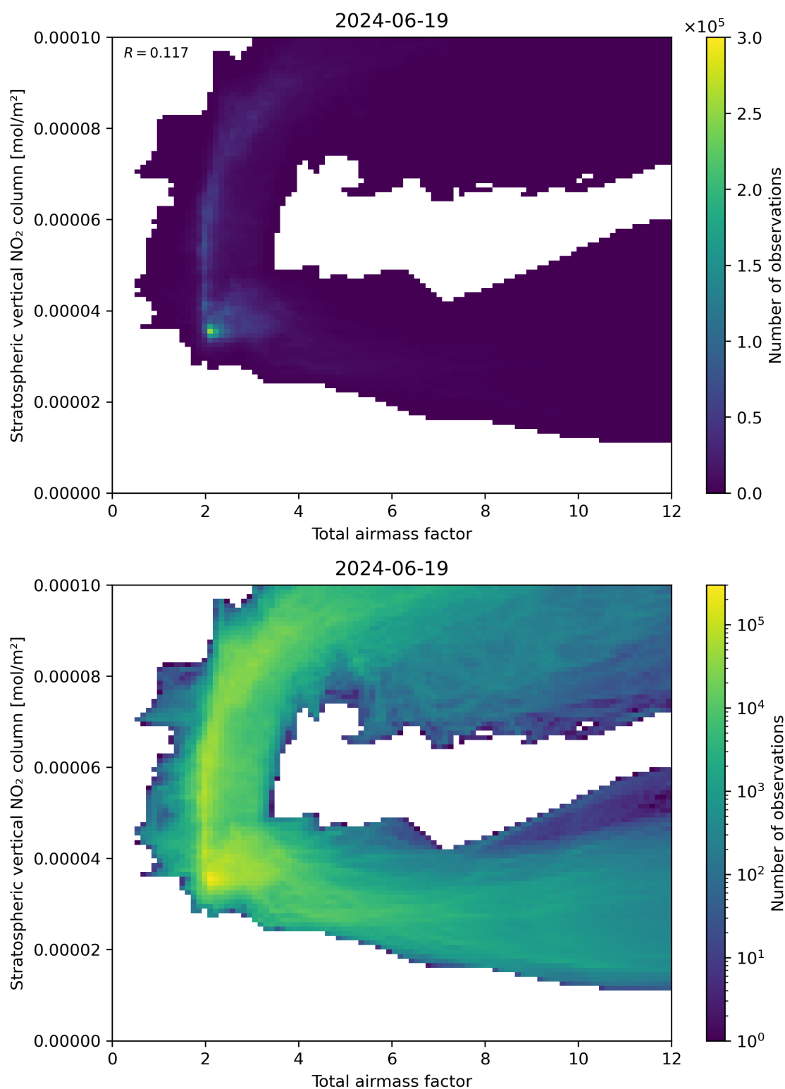
Figure 64: Scatter density plot of “Total airmass factor” against “Stratospheric vertical NO 2 column” for 2024-06-19 to 2024-06-20.
