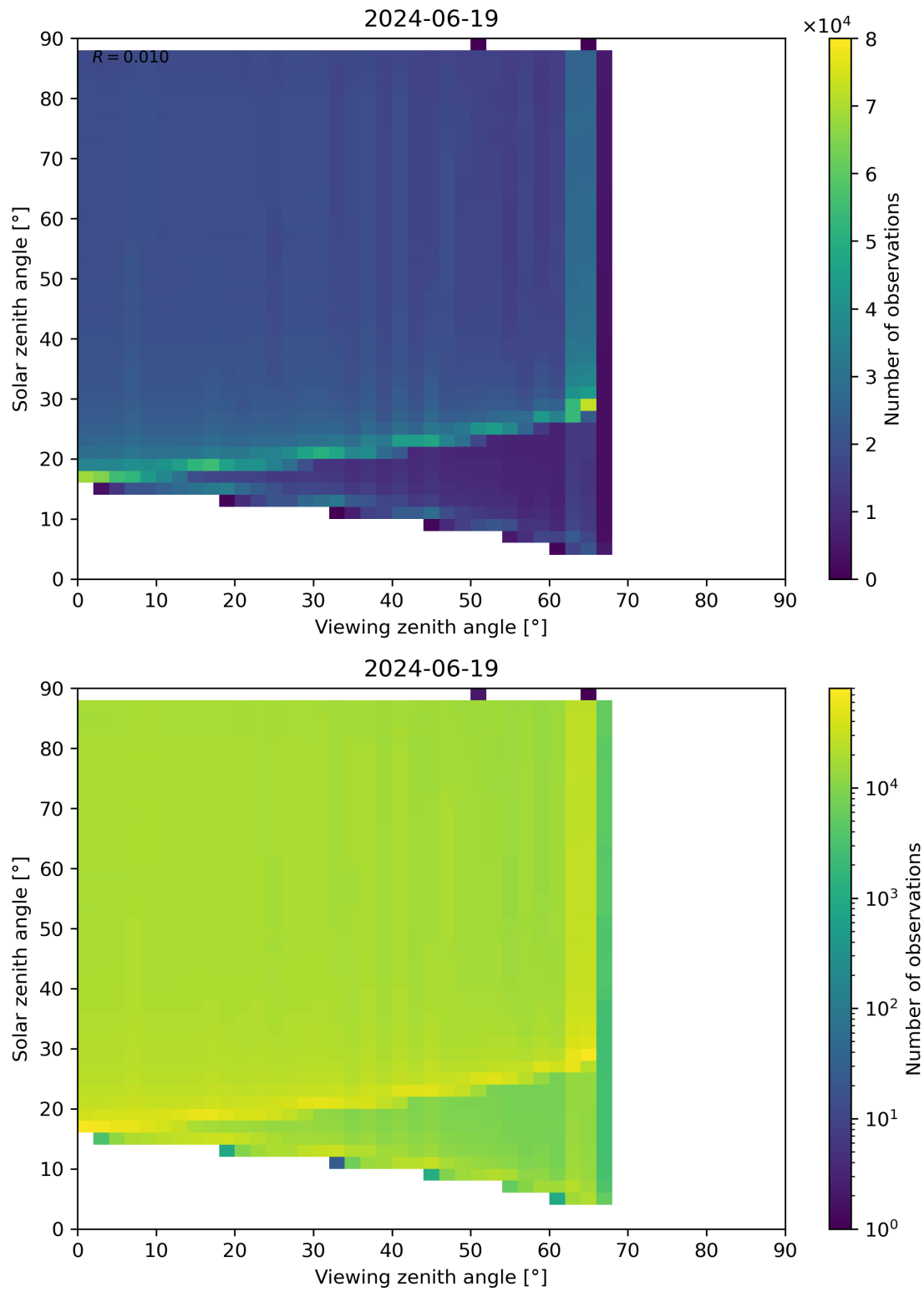
Figure 172: Scatter density plot of “Viewing zenith angle” against “Solar zenith angle” for 2024-06-19 to 2024-06-20.
