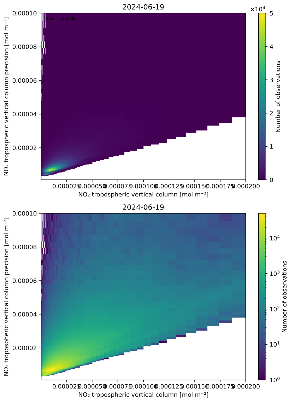
Figure 130: Scatter density plot of “NO 2 tropospheric vertical column” against “NO 2 tropospheric vertical column precision” for 2024-06-19 to 2024-06-20.
