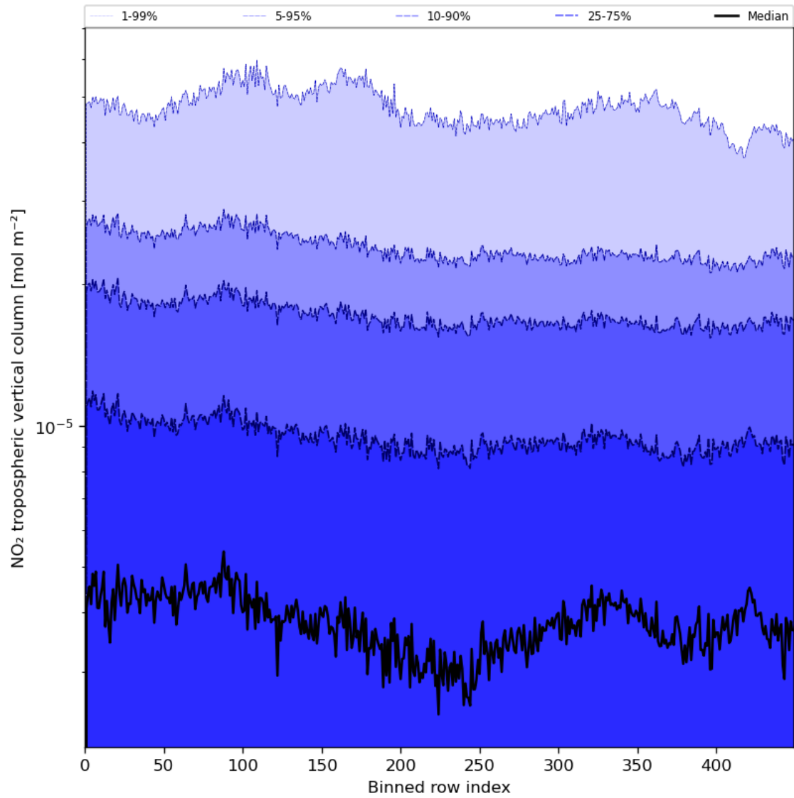
Figure 46: Along track statistics of “NO 2 tropospheric vertical column” for 2024-06-19 to 2024-06-20
