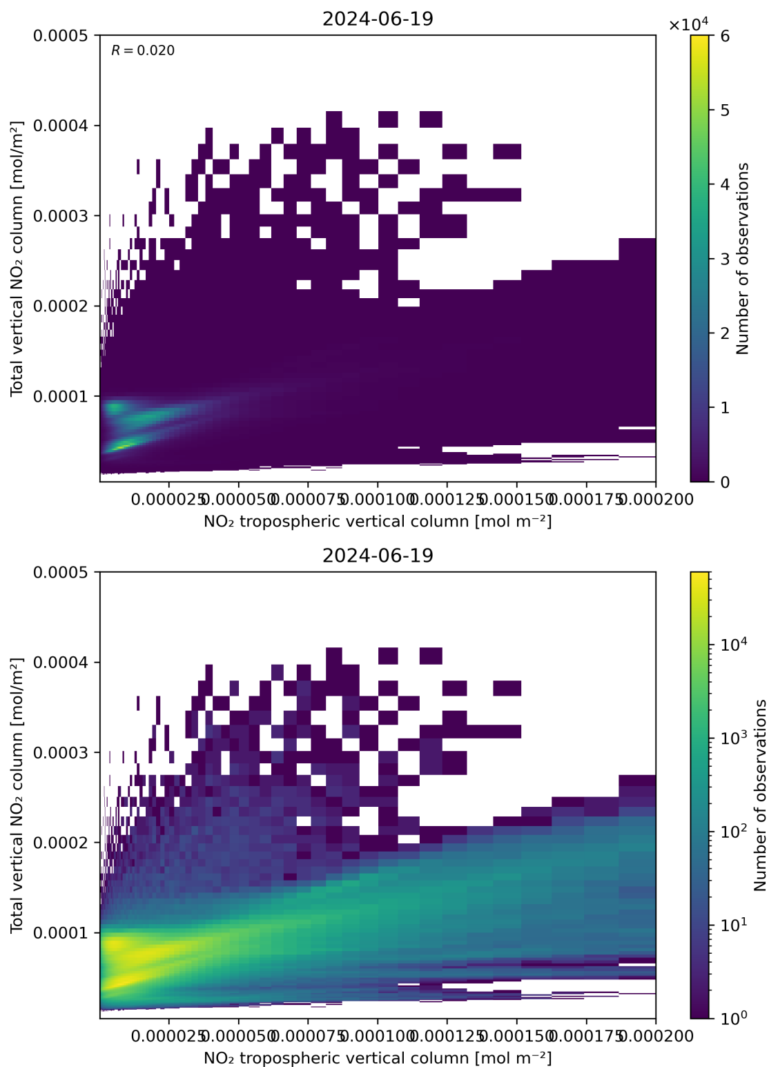
Figure 128: Scatter density plot of “NO 2 tropospheric vertical column” against “Total vertical NO 2 column” for 2024-06-19 to 2024-06-20.
