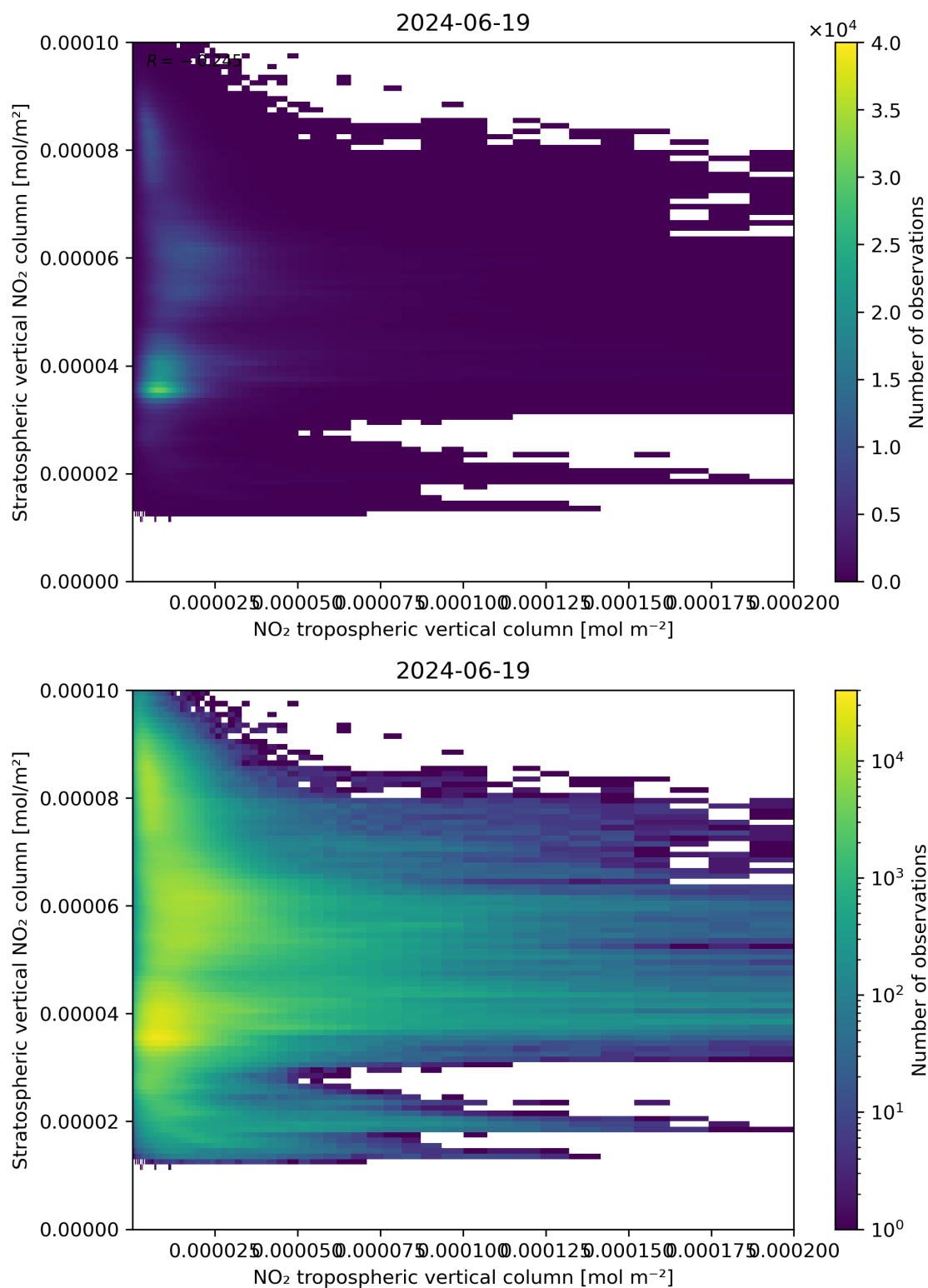
Figure 125: Scatter density plot of “NO 2 tropospheric vertical column” against “Stratospheric vertical NO 2 column” for 2024-06-19 to 2024-06-20.
