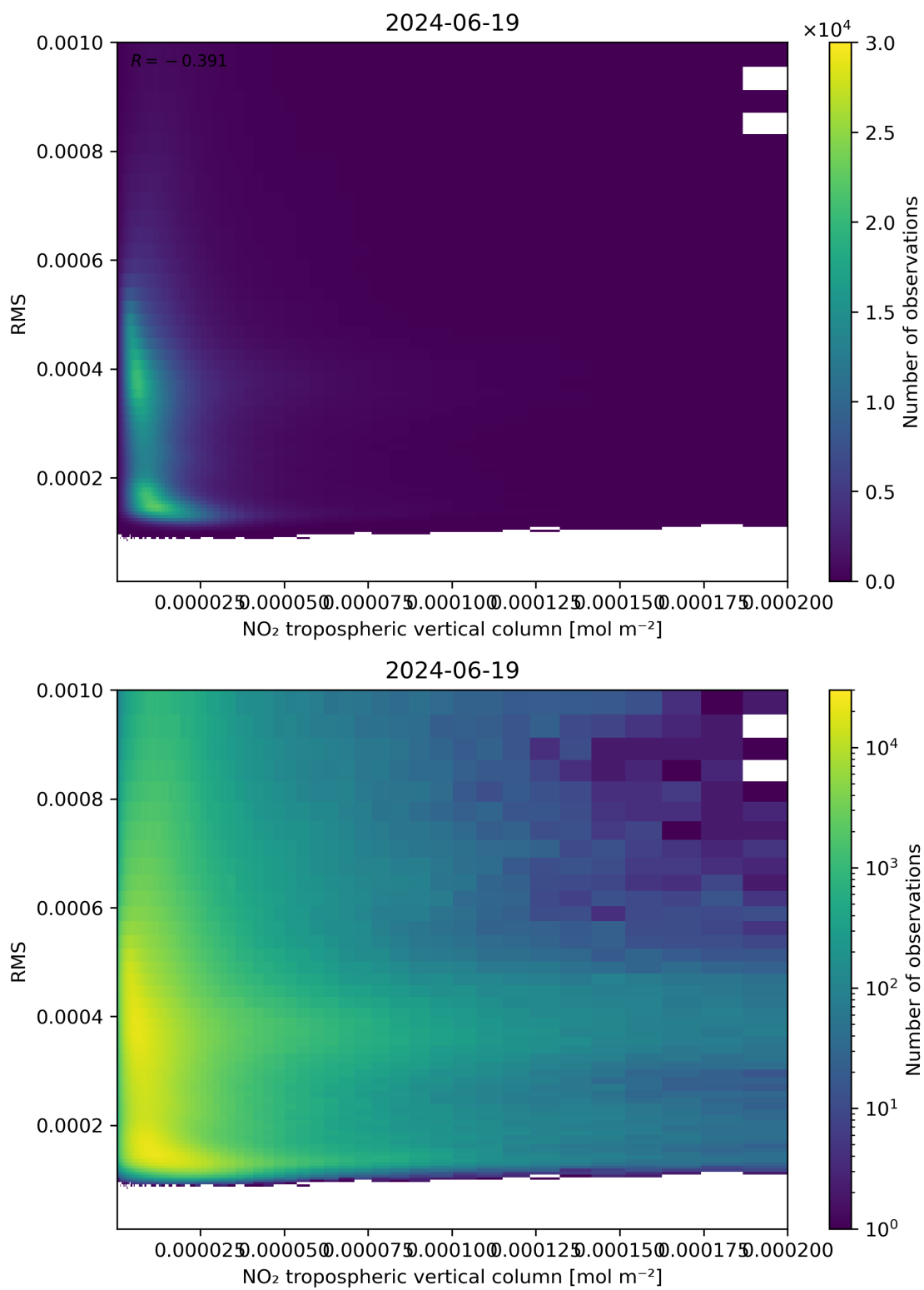
Figure 142: Scatter density plot of “NO 2 tropospheric vertical column” against “RMS” for 2024-06-19 to 2024-06-20.
