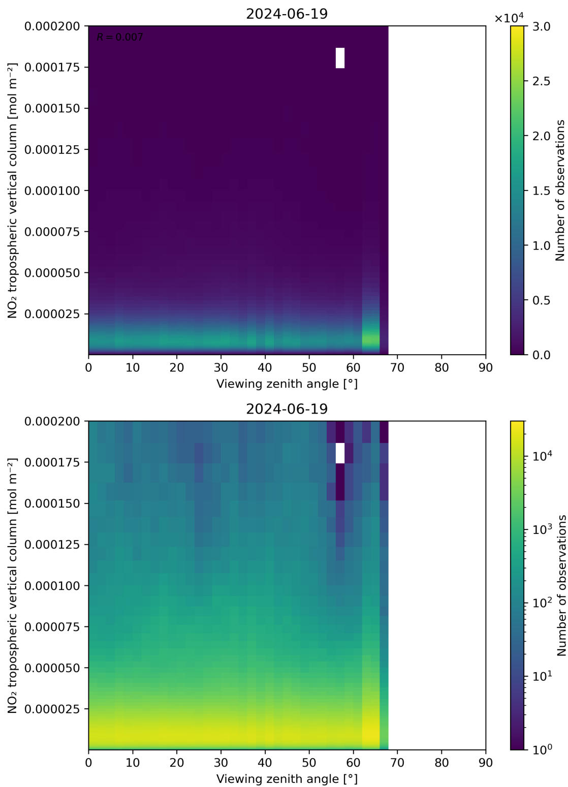
Figure 169: Scatter density plot of “Viewing zenith angle” against “NO 2 tropospheric vertical column” for 2024-06-19 to 2024-06-20.
