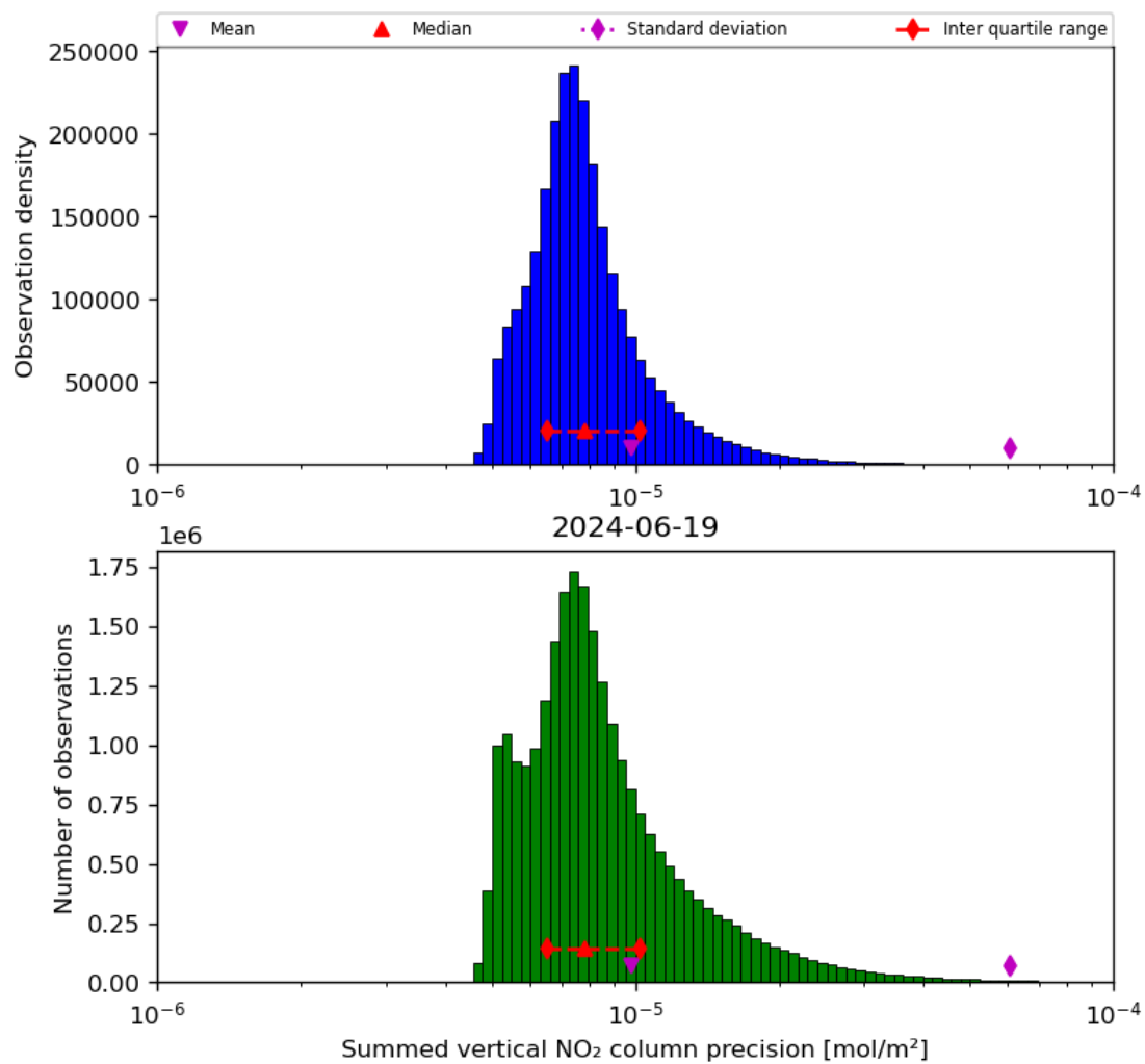
Figure 41: Histogram of “Summed vertical NO 2 column precision” for 2024-06-19 to 2024-06-20
