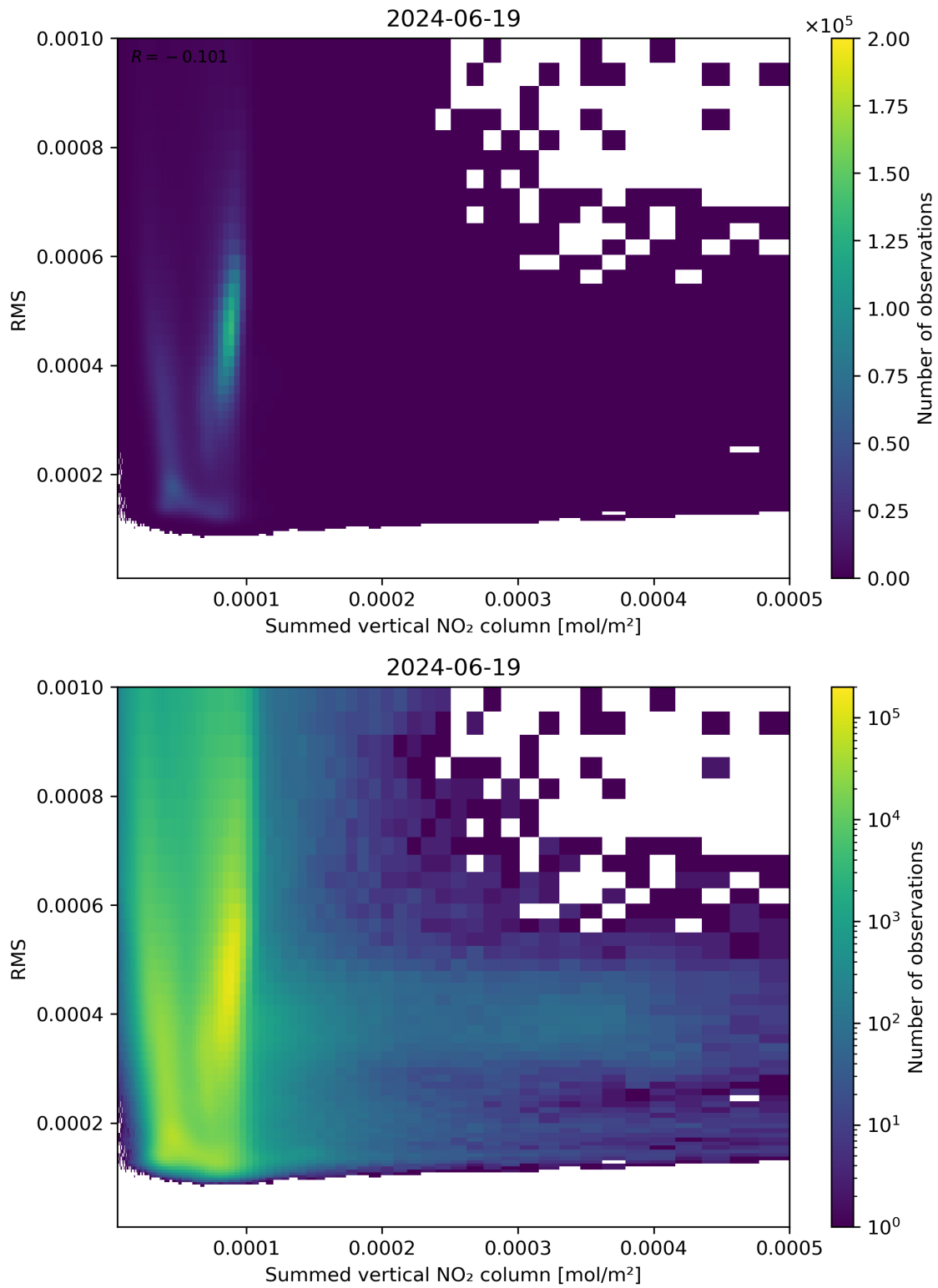
Figure 109: Scatter density plot of “Summed vertical NO 2 column” against “RMS” for 2024-06-19 to 2024-06-20.
