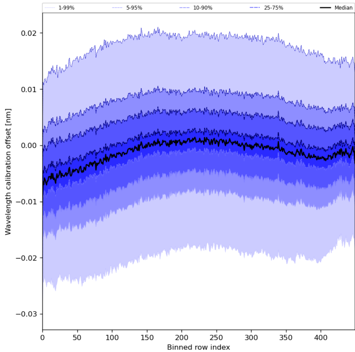
Figure 52: Along track statistics of “Wavelength calibration offset” for 2024-06-19 to 2024-06-20
