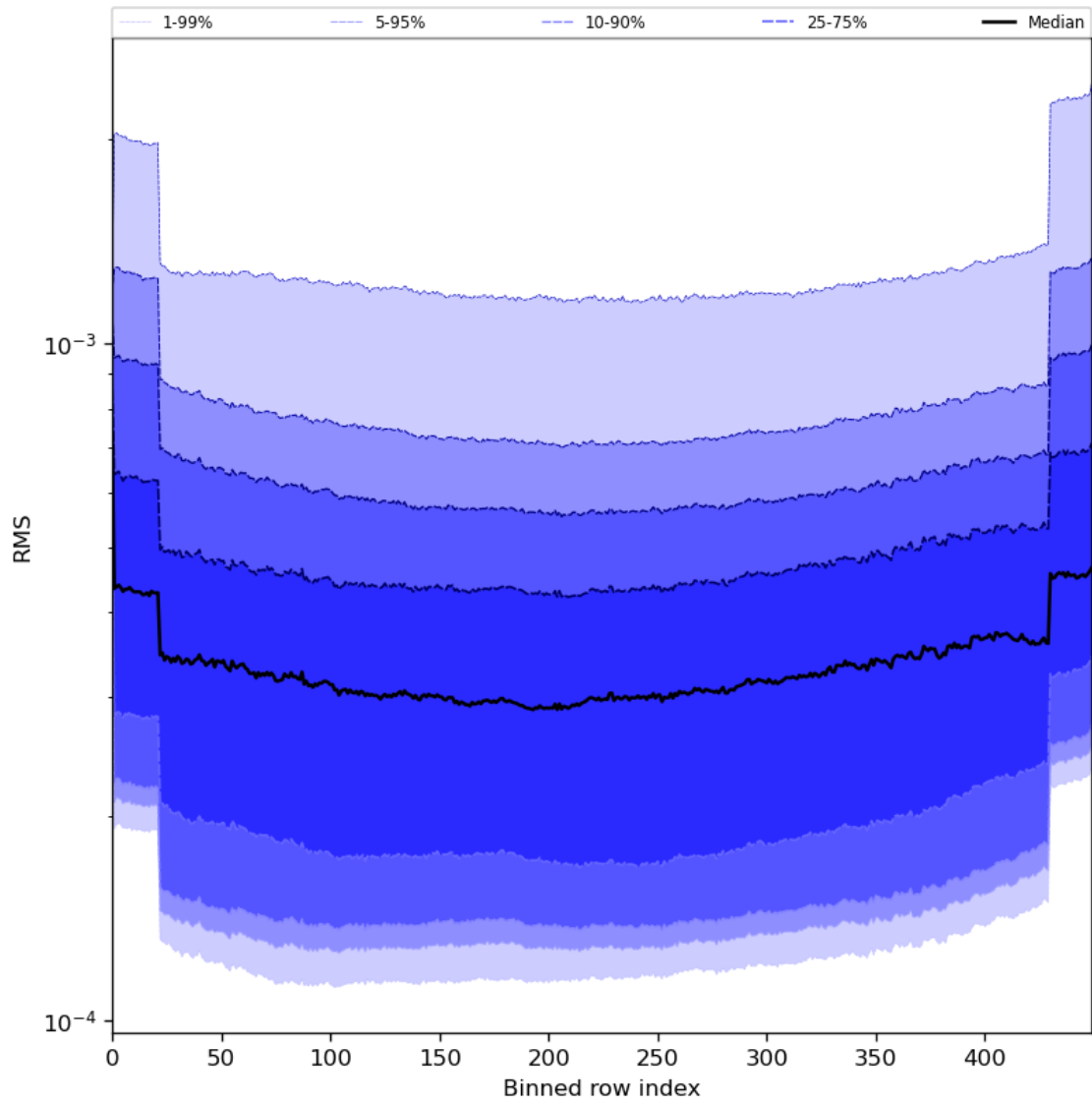
Figure 60: Along track statistics of “RMS” for 2024-06-19 to 2024-06-20
