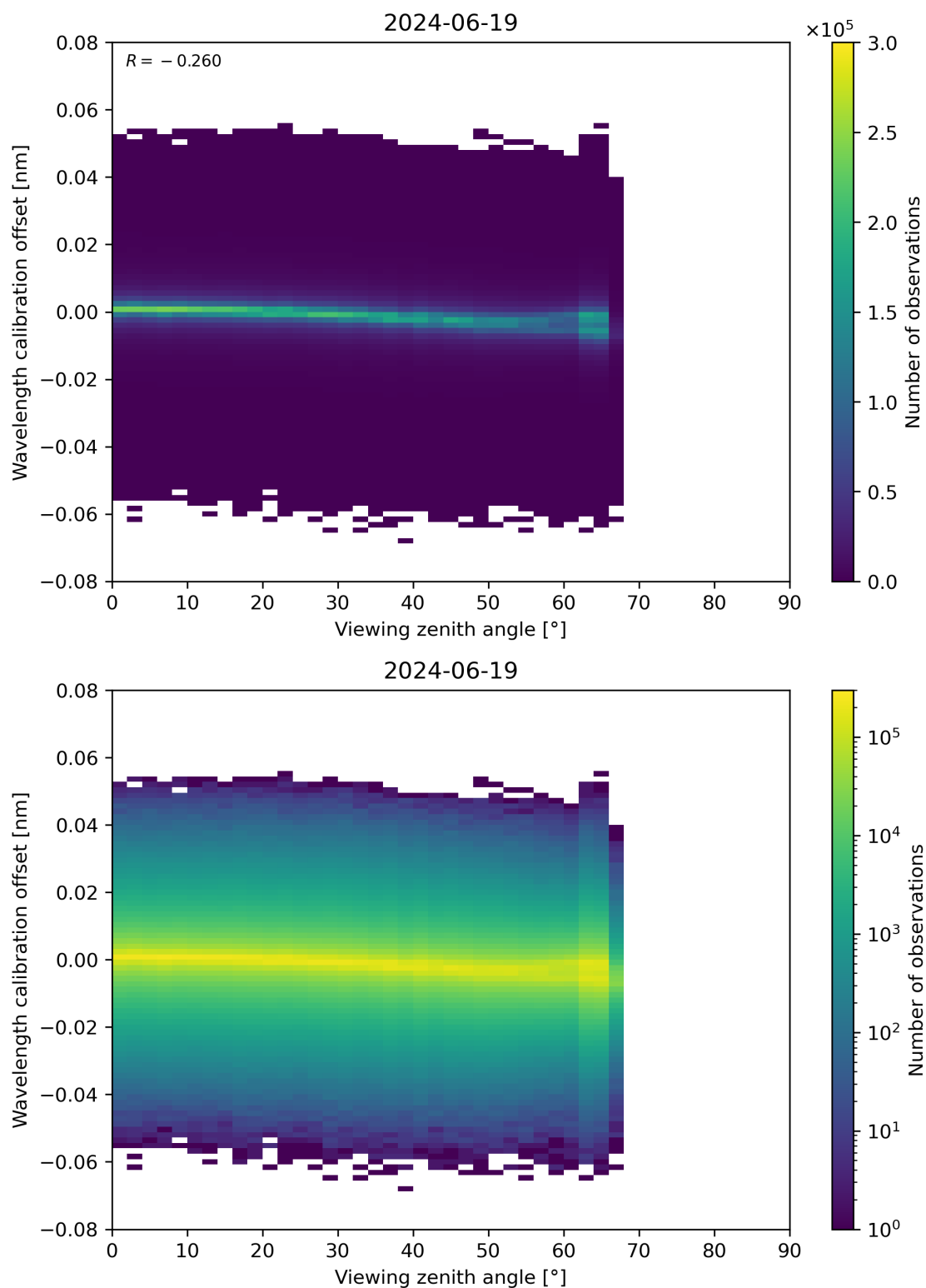
Figure 173: Scatter density plot of “Viewing zenith angle” against “Wavelength calibration offset” for 2024-06-19 to 2024-06-20.
