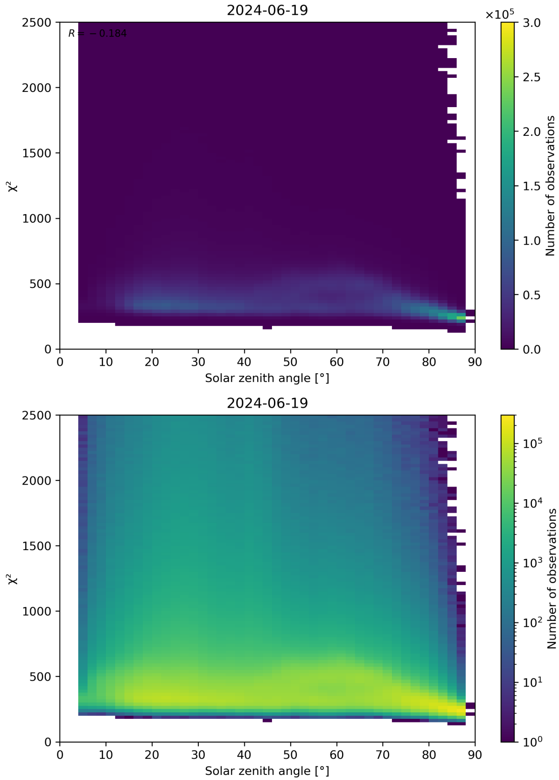
Figure 148: Scatter density plot of “Solar zenith angle” against “ \chi^2 ” for 2024-06-19 to 2024-06-20.
