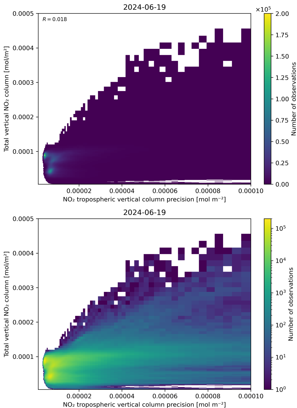
Figure 138: Scatter density plot of “NO 2 tropospheric vertical column precision” against “Total vertical NO 2 column” for 2024-06-19 to 2024-06-20.
