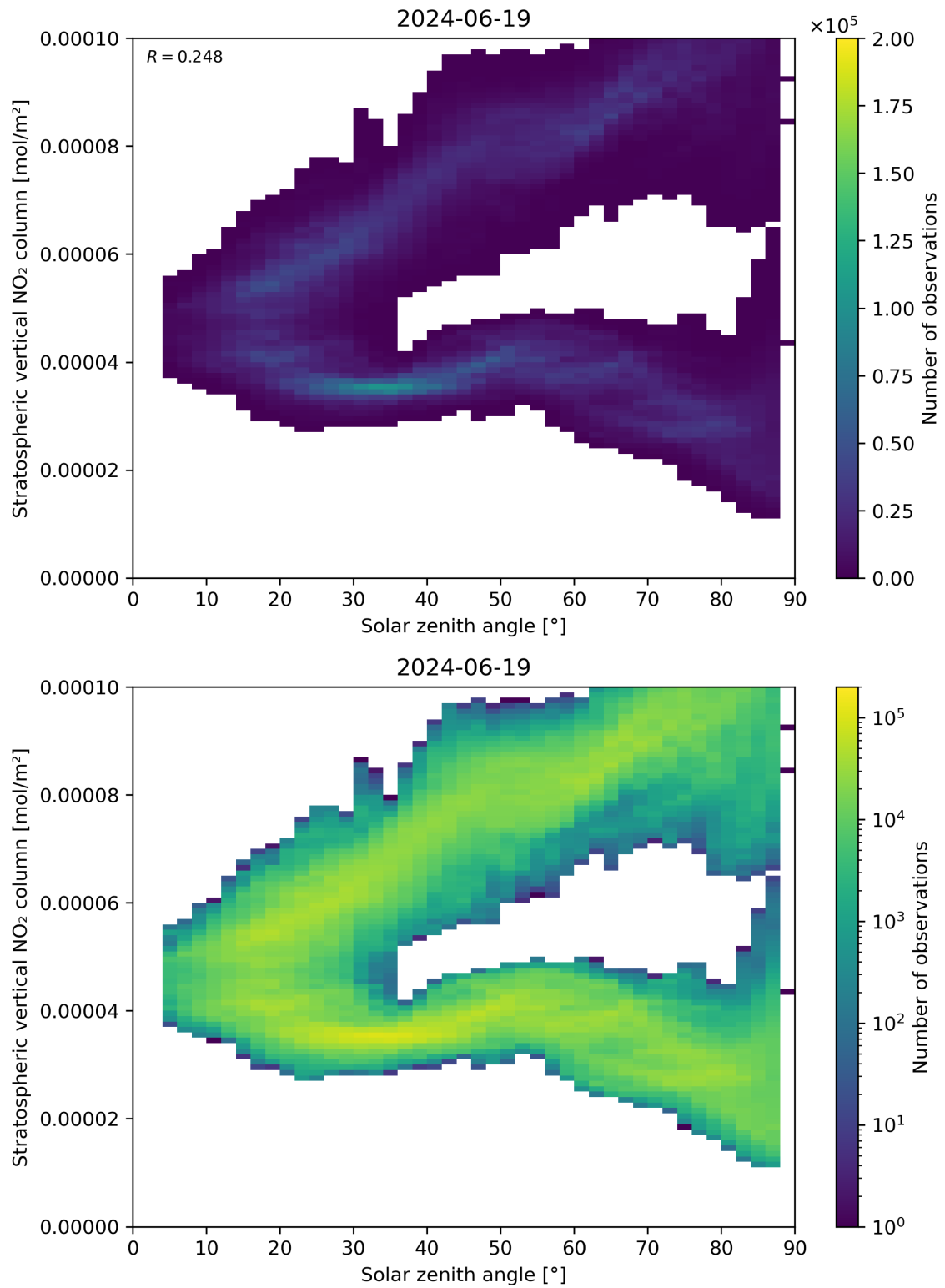
Figure 150: Scatter density plot of “Solar zenith angle” against “Stratospheric vertical NO 2 column” for 2024-06-19 to 2024-06-20.
