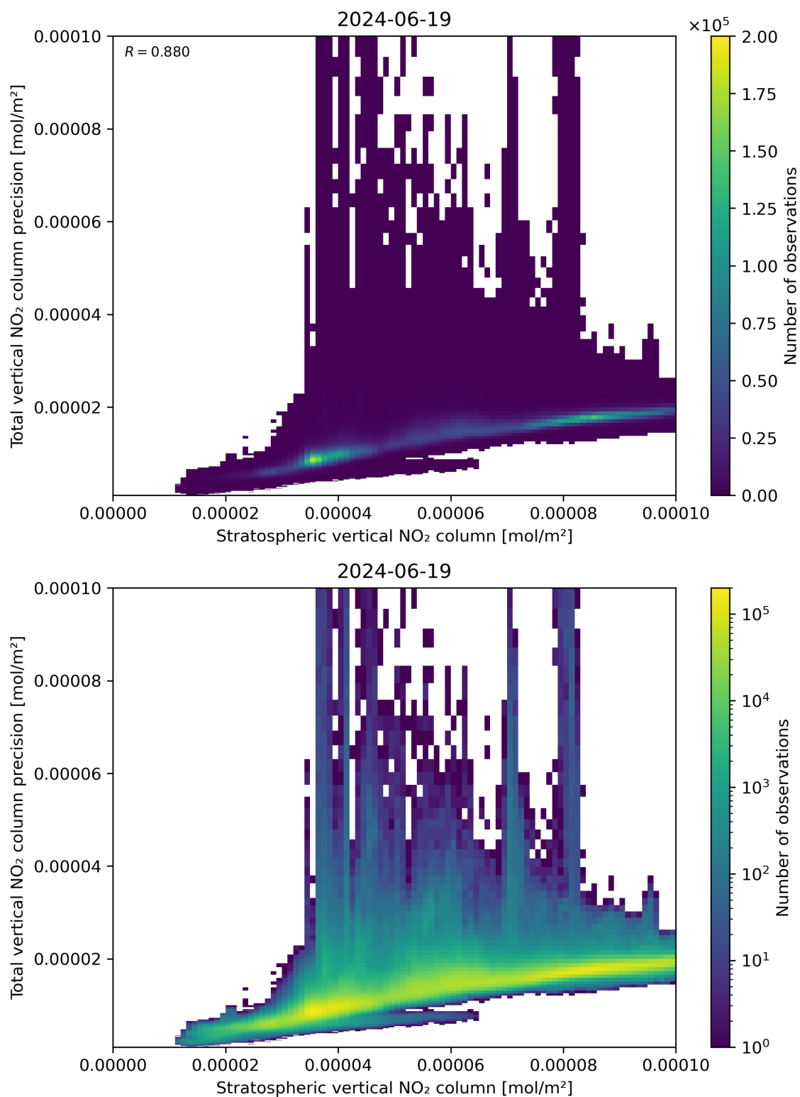
Figure 101: Scatter density plot of “Stratospheric vertical NO 2 column” against “Total vertical NO 2 column precision” for 2024-06-19 to 2024-06-20.
