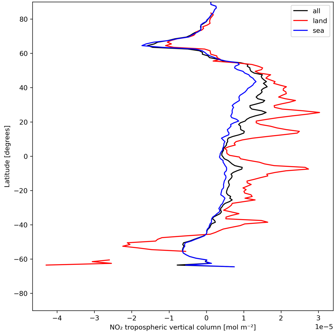
Figure 12: Zonal average of “NO 2 tropospheric vertical column” for 2024-06-19 to 2024-06-20.
