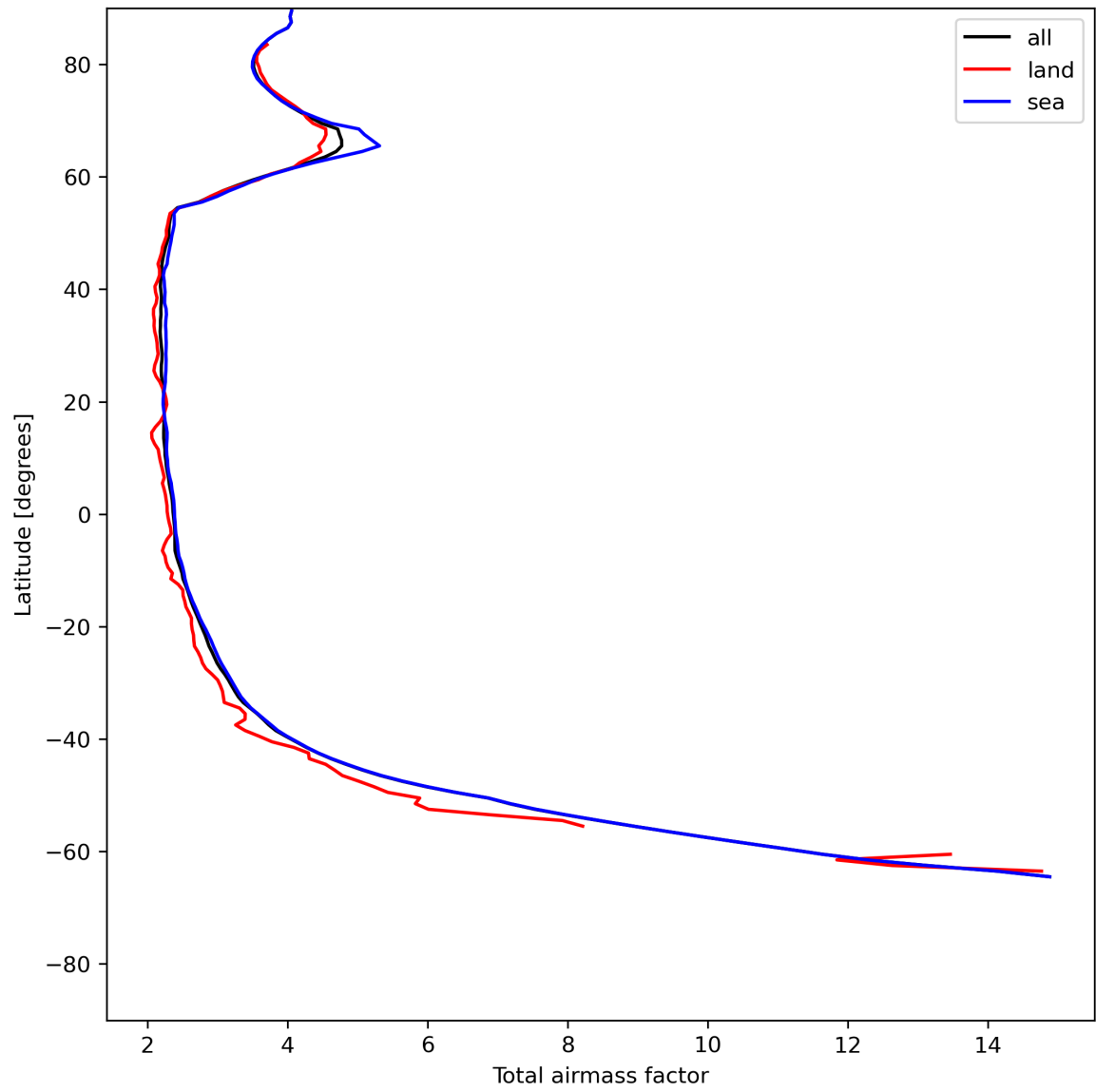
Figure 15: Zonal average of “Total airmass factor” for 2024-06-19 to 2024-06-20.
