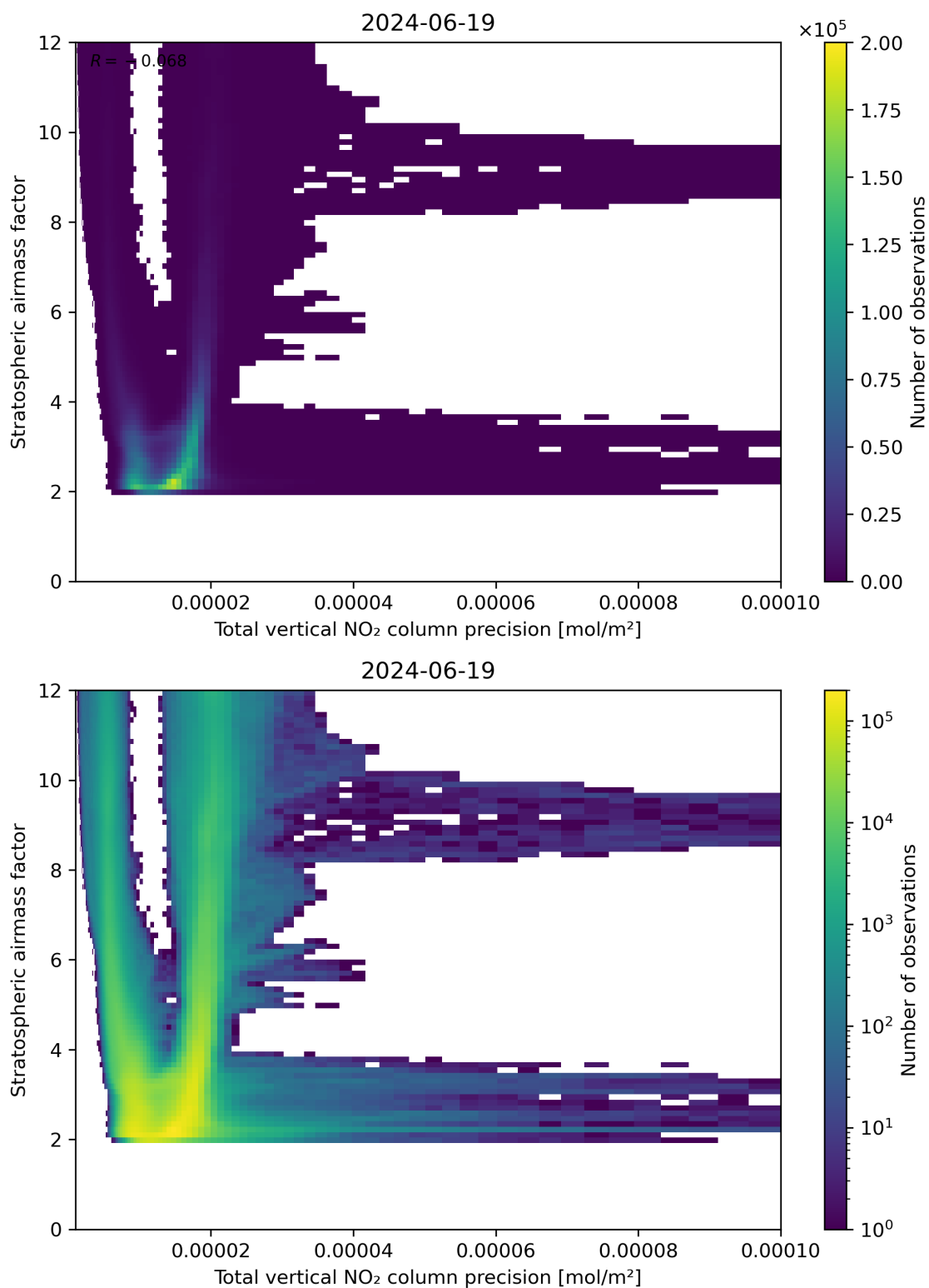
Figure 115: Scatter density plot of “Total vertical NO 2 column precision” against “Stratospheric air mass factor” for 2024-06-19 to 2024-06-20.
