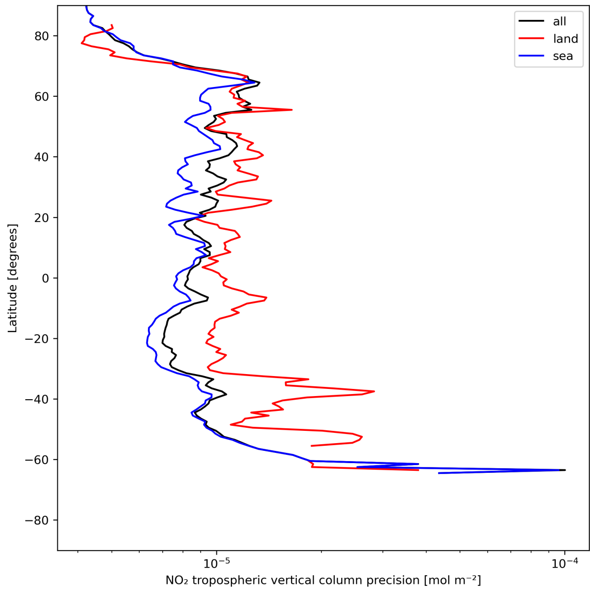
Figure 13: Zonal average of “NO 2 tropospheric vertical column precision” for 2024-06-19 to 2024-06-20.
