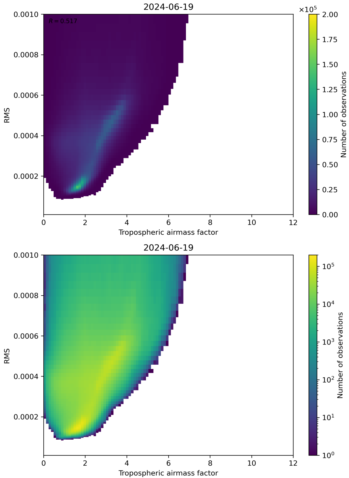
Figure 79: Scatter density plot of “Tropospheric airmass factor” against “RMS” for 2024-06-19 to 2024-06-20.
