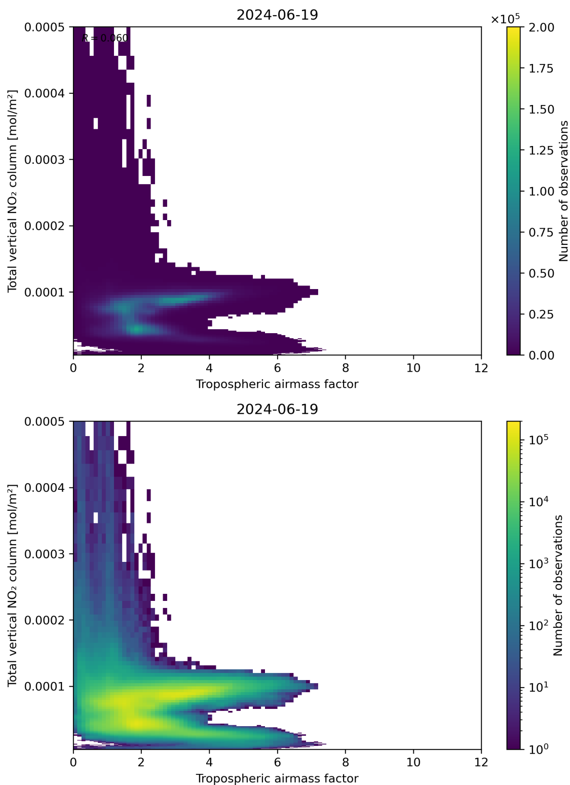
Figure 77: Scatter density plot of “Tropospheric airmass factor” against “Total vertical \text{NO}_2 column” for 2024-06-19 to 2024-06-20.
