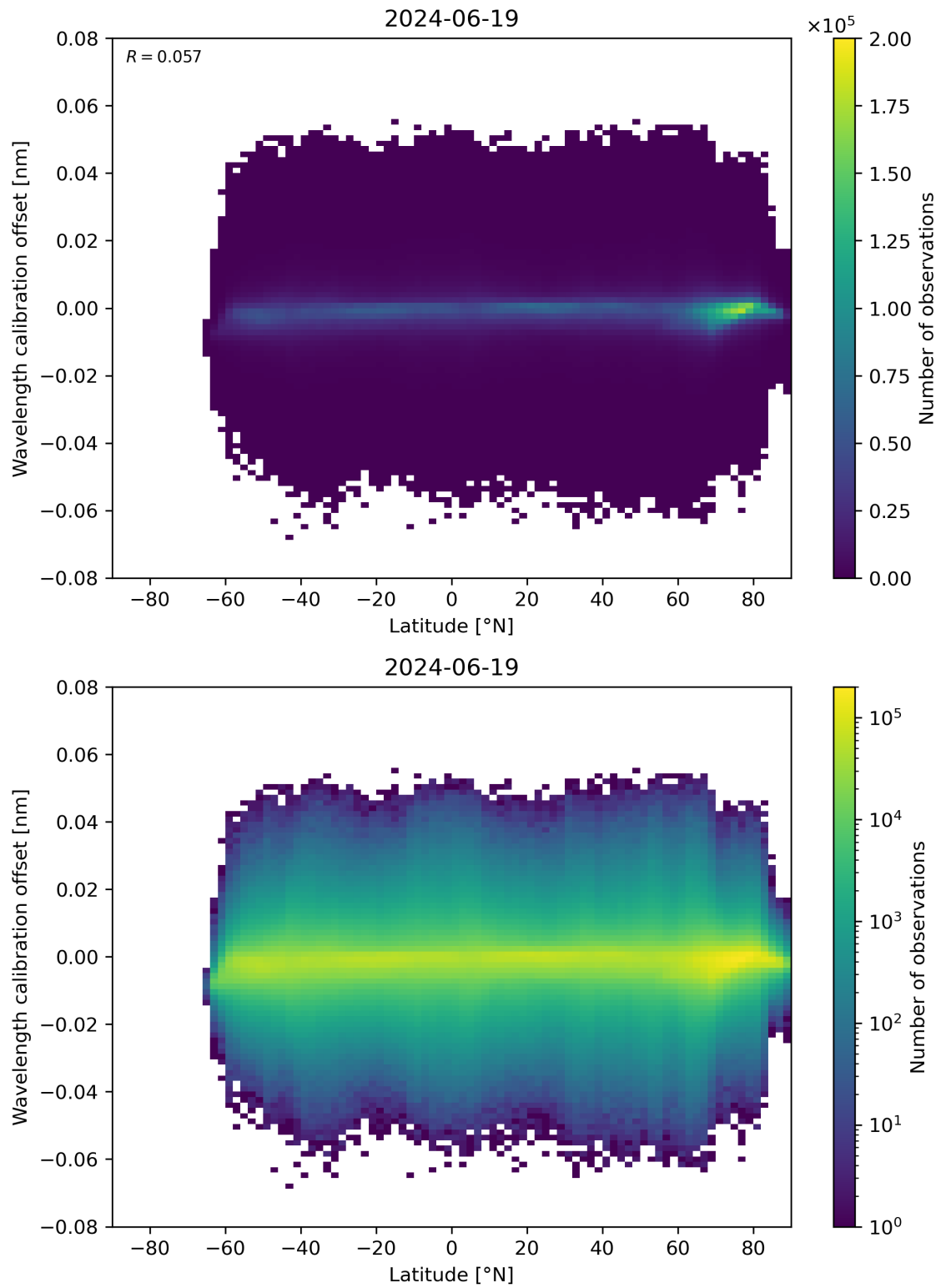
Figure 95: Scatter density plot of “Latitude” against “Wavelength calibration offset” for 2024-06-19 to 2024-06-20.
