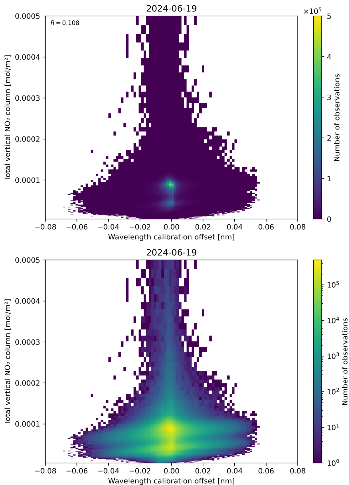
Figure 179: Scatter density plot of “Wavelength calibration offset” against “Total vertical NO 2 column” for 2024-06-19 to 2024-06-20.
