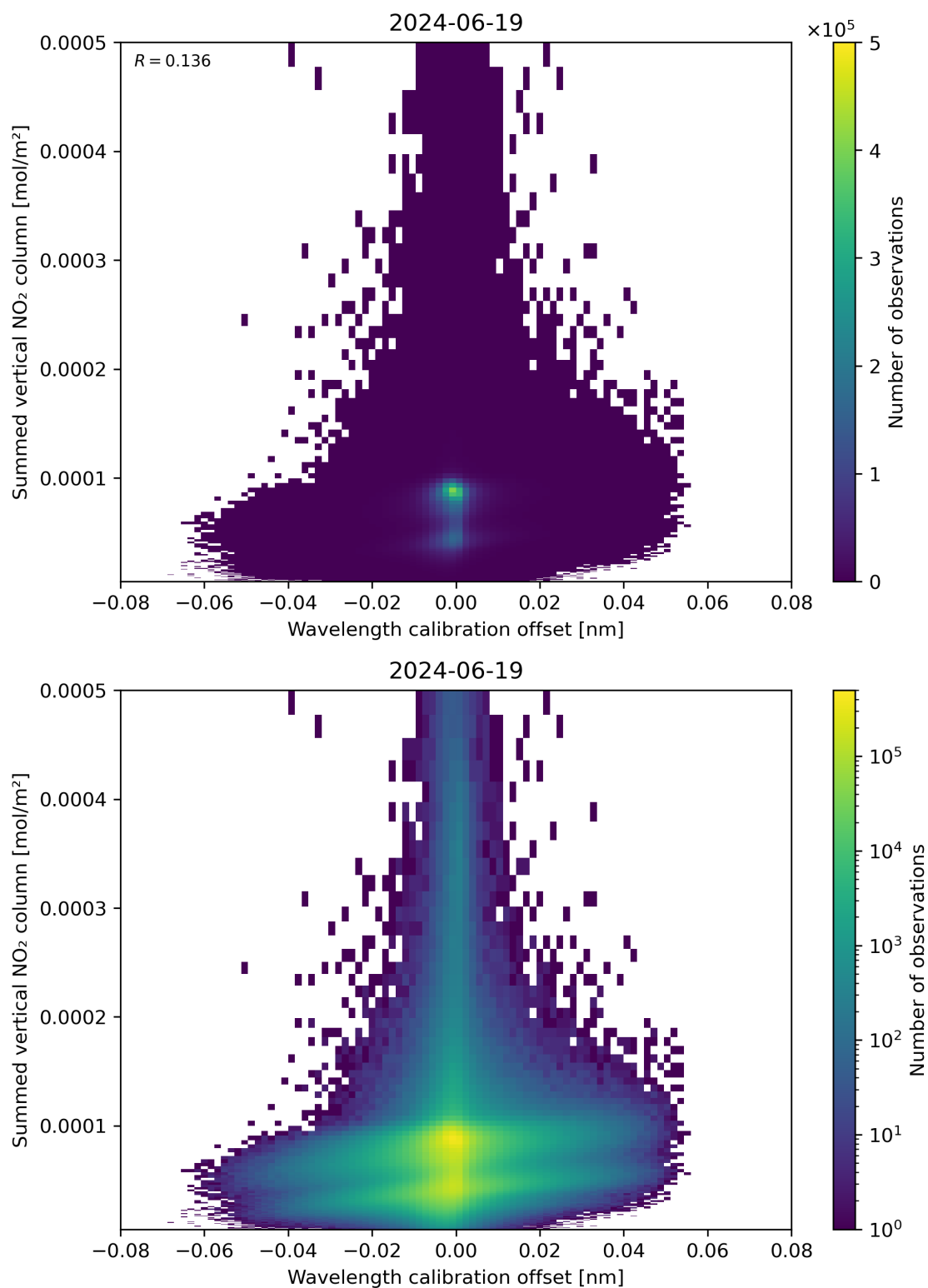
Figure 177: Scatter density plot of “Wavelength calibration offset” against “Summed vertical NO 2 column” for 2024-06-19 to 2024-06-20.
