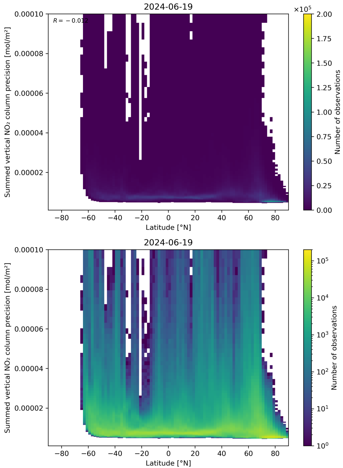
Figure 89: Scatter density plot of “Latitude” against “Summed vertical NO 2 column precision” for 2024-06-19 to 2024-06-20.
