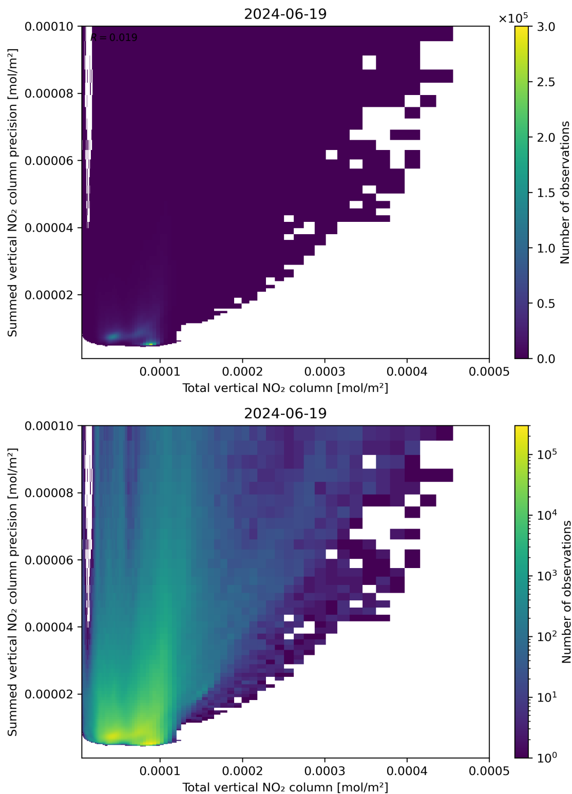
Figure 113: Scatter density plot of “Total vertical NO 2 column” against “Summed vertical NO 2 column precision” for 2024-06-19 to 2024-06-20.
