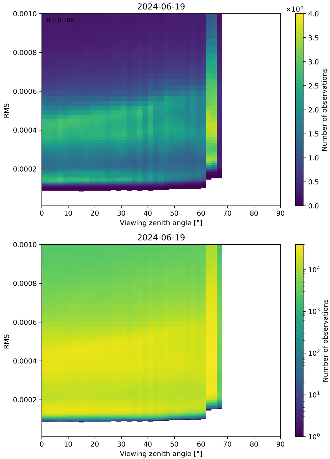
Figure 171: Scatter density plot of “Viewing zenith angle” against “RMS” for 2024-06-19 to 2024-06-20.
