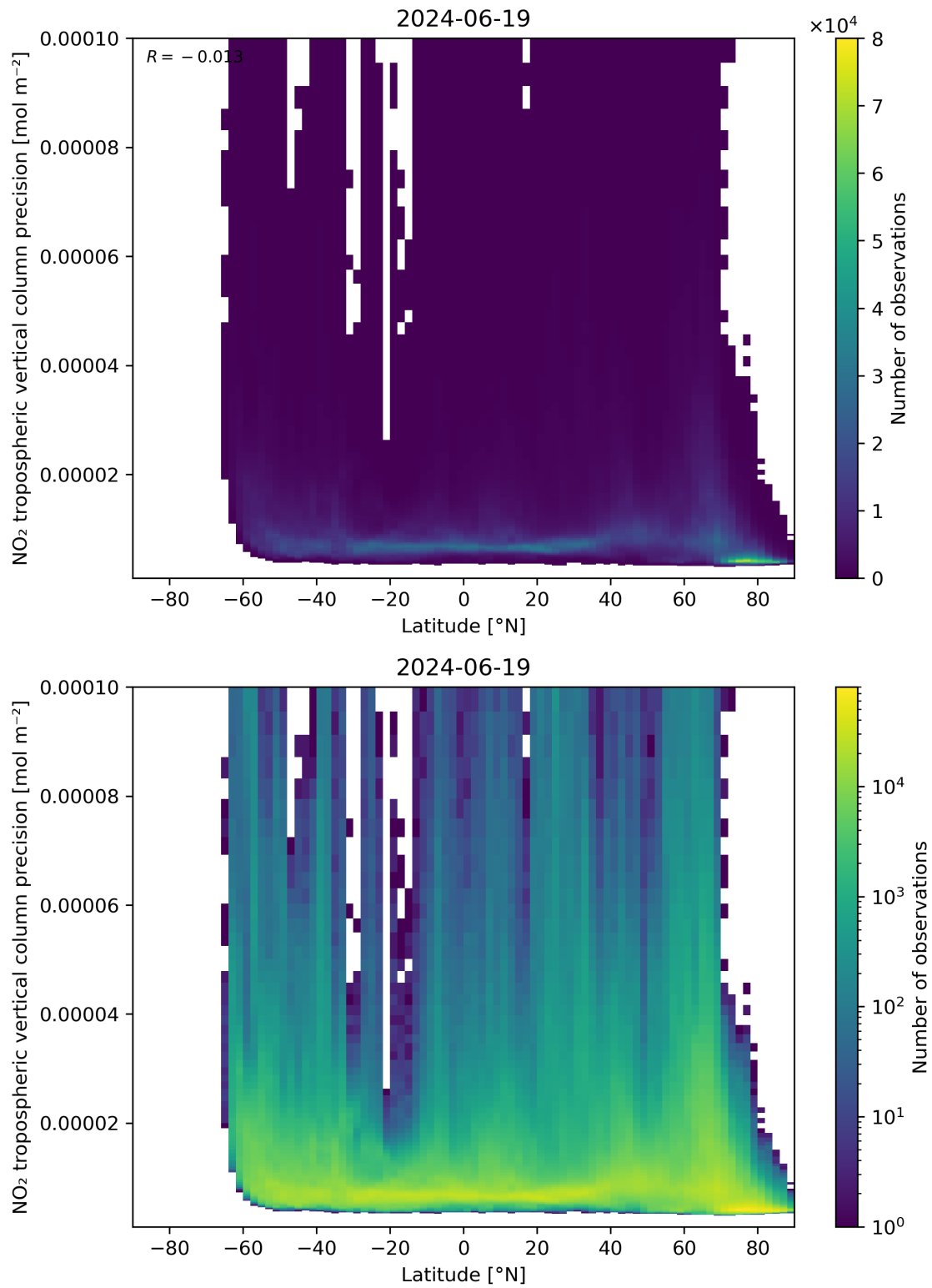
Figure 93: Scatter density plot of “Latitude” against “NO 2 tropospheric vertical column precision” for 2024-06-19 to 2024-06-20.
