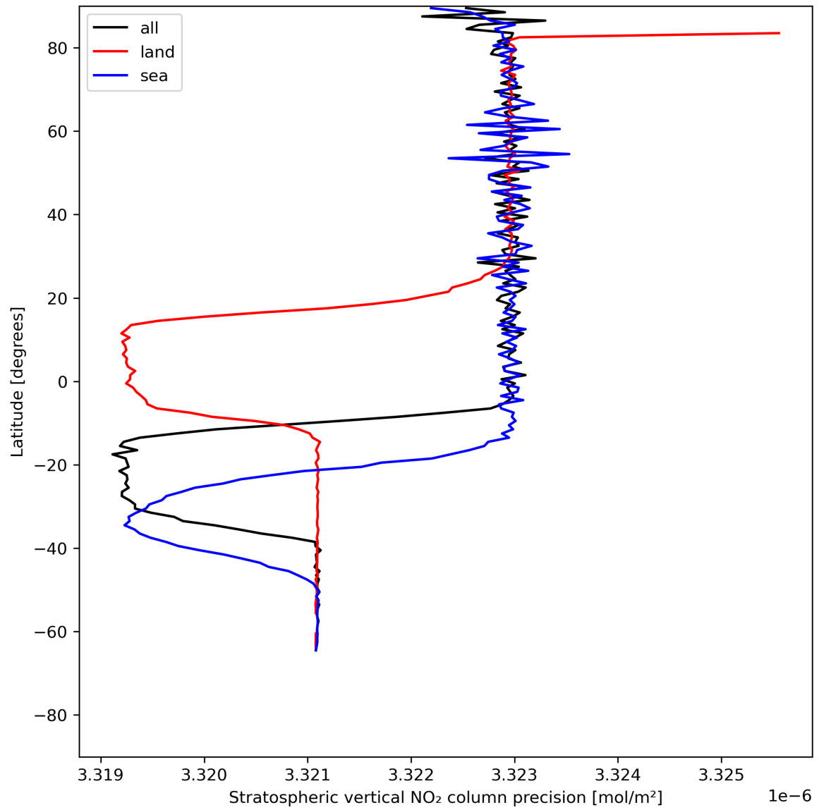
Figure 20: Zonal average of “Stratospheric vertical NO 2 column precision” for 2024-06-19 to 2024-06-20.
