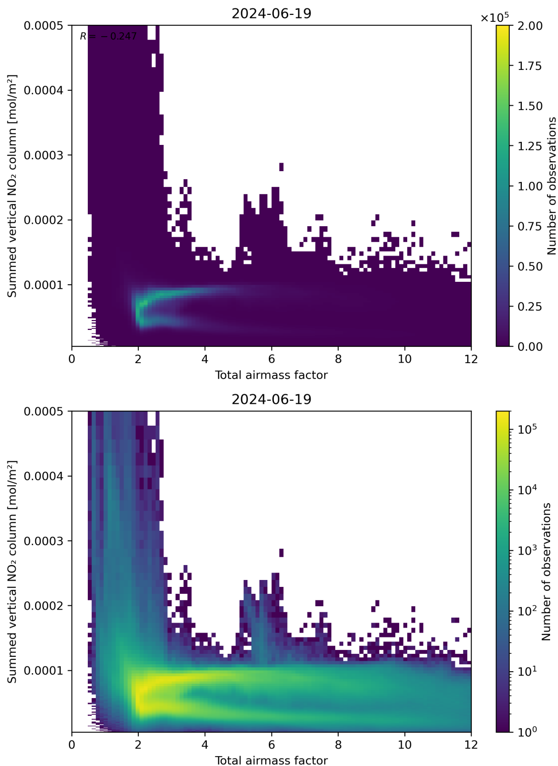
Figure 65: Scatter density plot of “Total airmass factor” against “Summed vertical NO 2 column” for 2024-06-19 to 2024-06-20.
