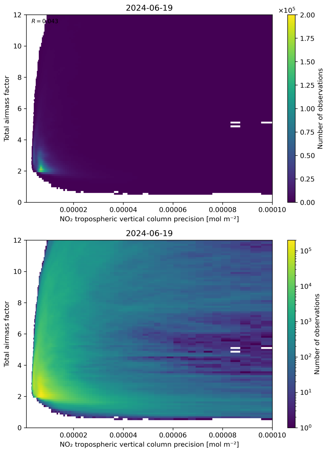
Figure 132: Scatter density plot of “NO 2 tropospheric vertical column precision” against “Total air mass factor” for 2024-06-19 to 2024-06-20.
