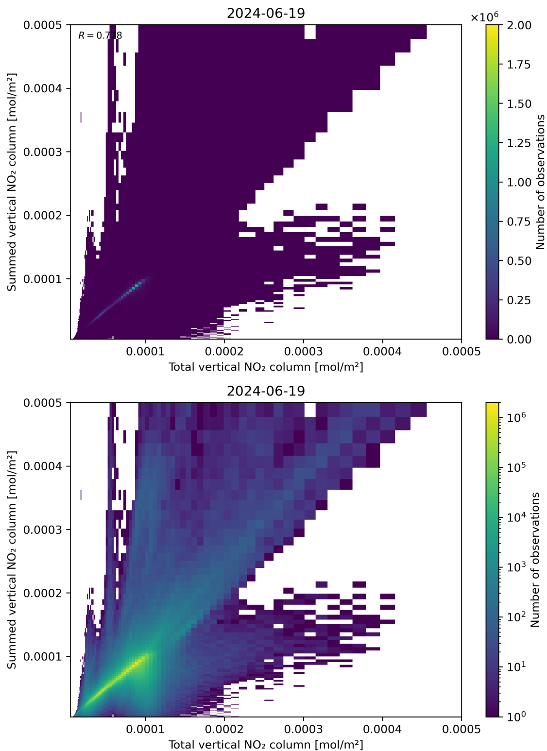
Figure 112: Scatter density plot of “Total vertical NO 2 column” against “Summed vertical NO 2 column” for 2024-06-19 to 2024-06-20.
