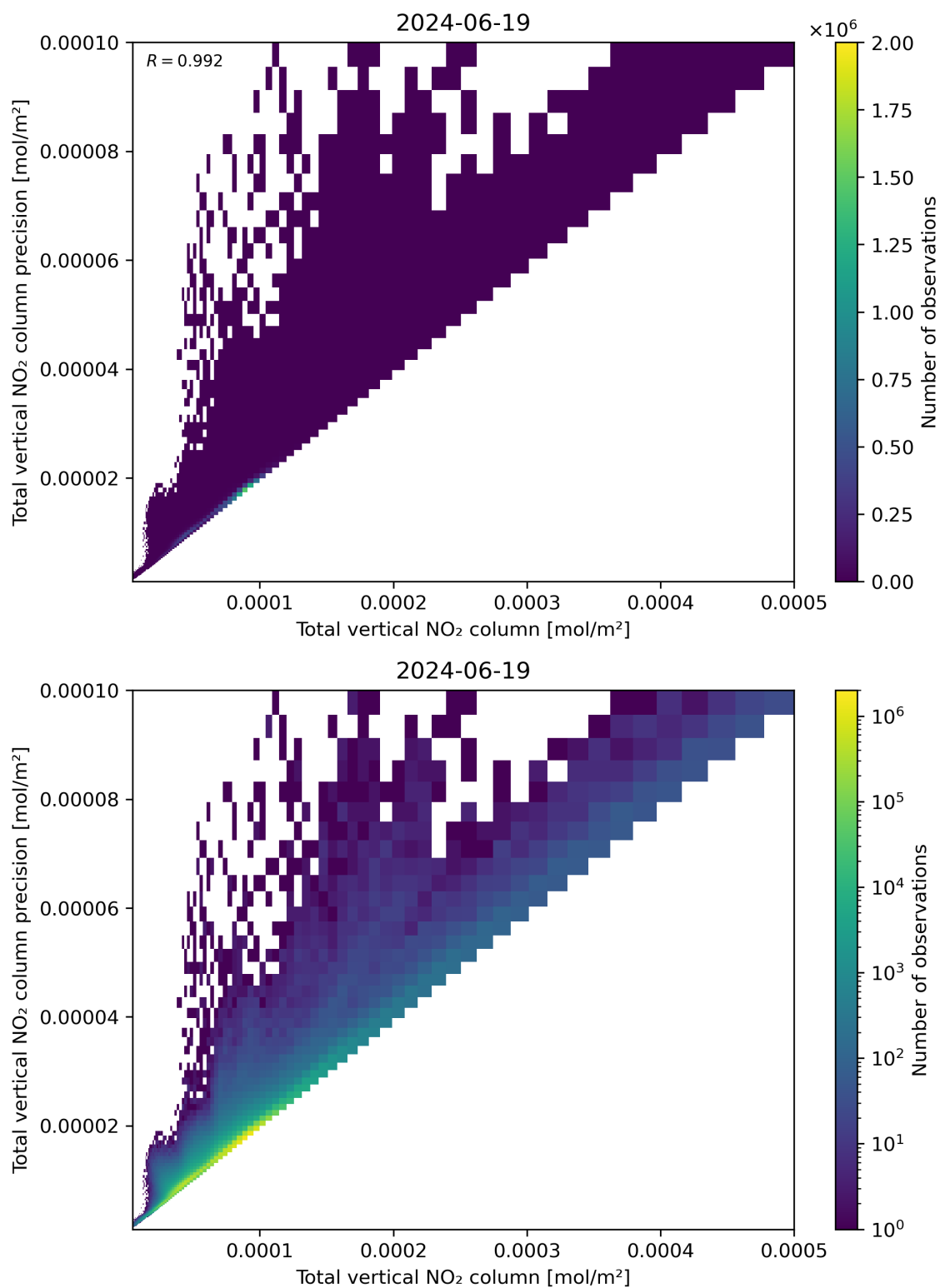
Figure 114: Scatter density plot of “Total vertical NO 2 column” against “Total vertical NO 2 column precision” for 2024-06-19 to 2024-06-20.
