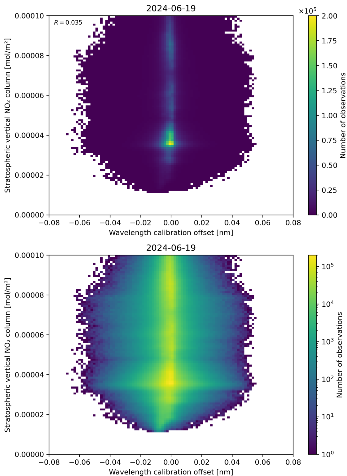
Figure 176: Scatter density plot of “Wavelength calibration offset” against “Stratospheric vertical NO 2 column” for 2024-06-19 to 2024-06-20.
