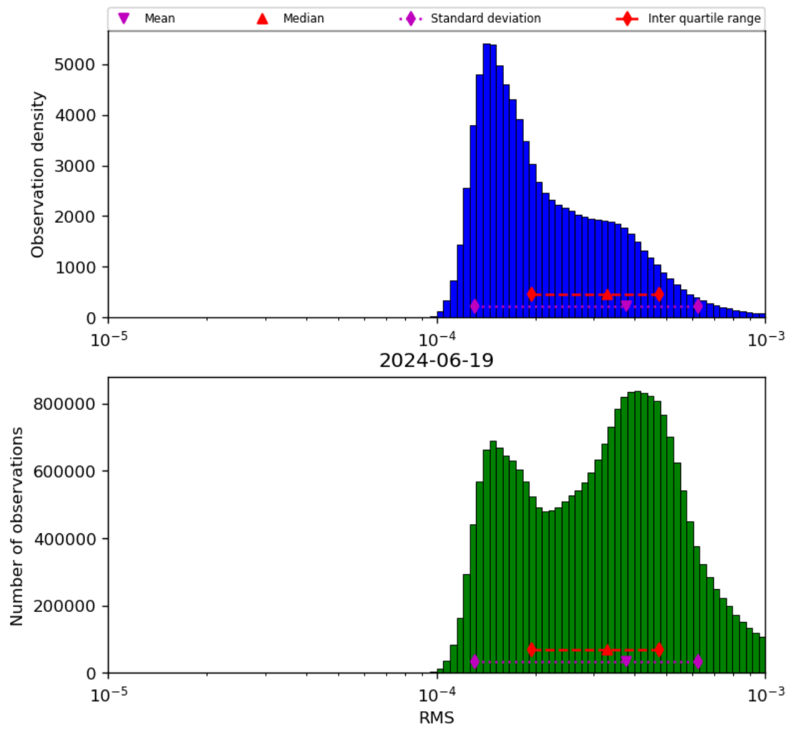
Figure 43: Histogram of “RMS” for 2024-06-19 to 2024-06-20
