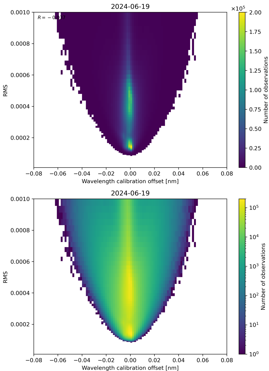
Figure 181: Scatter density plot of “Wavelength calibration offset” against “RMS” for 2024-06-19 to 2024-06-20.
