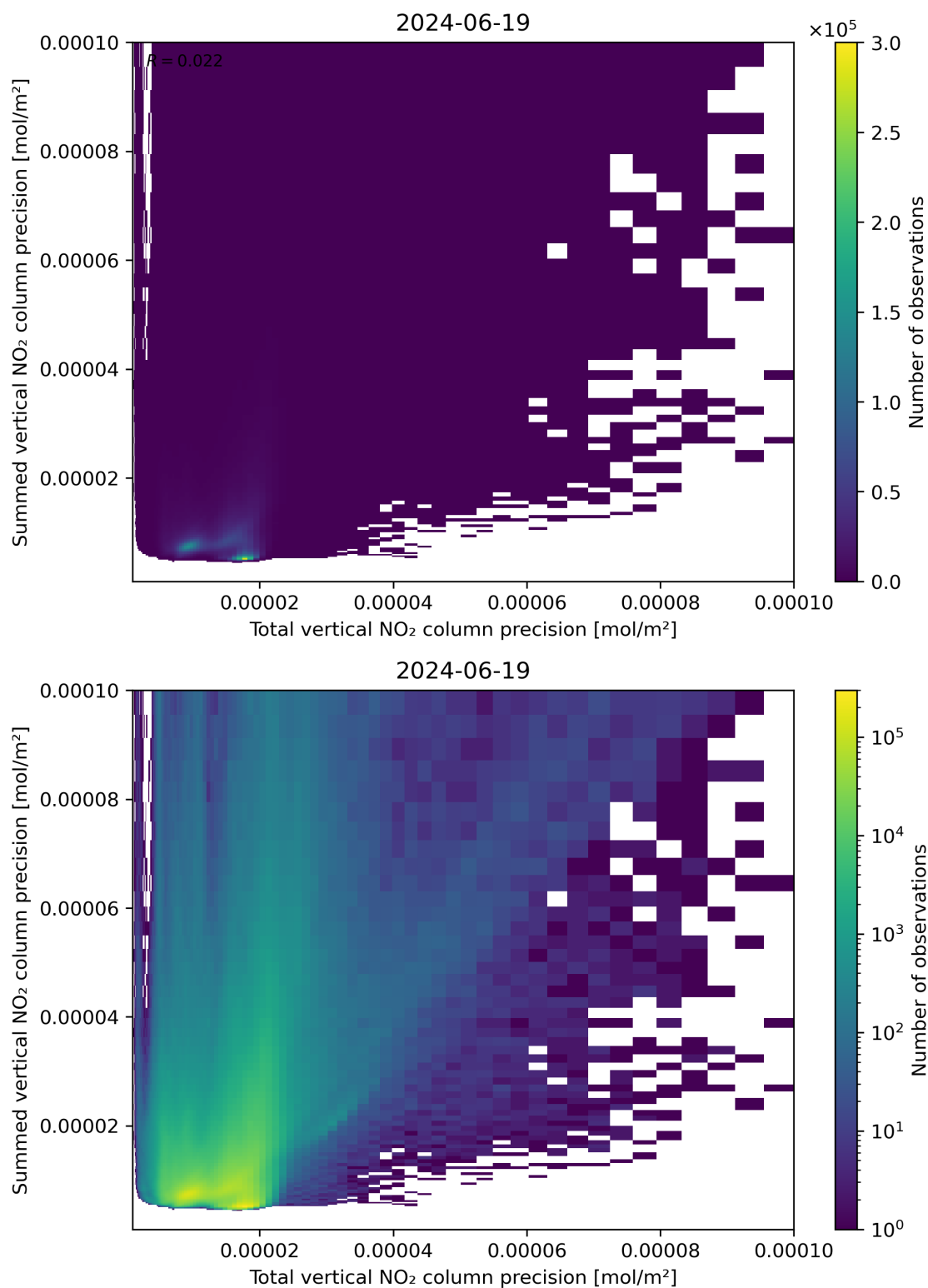
Figure 118: Scatter density plot of “Total vertical NO 2 column precision” against “Summed vertical NO 2 column precision” for 2024-06-19 to 2024-06-20.
