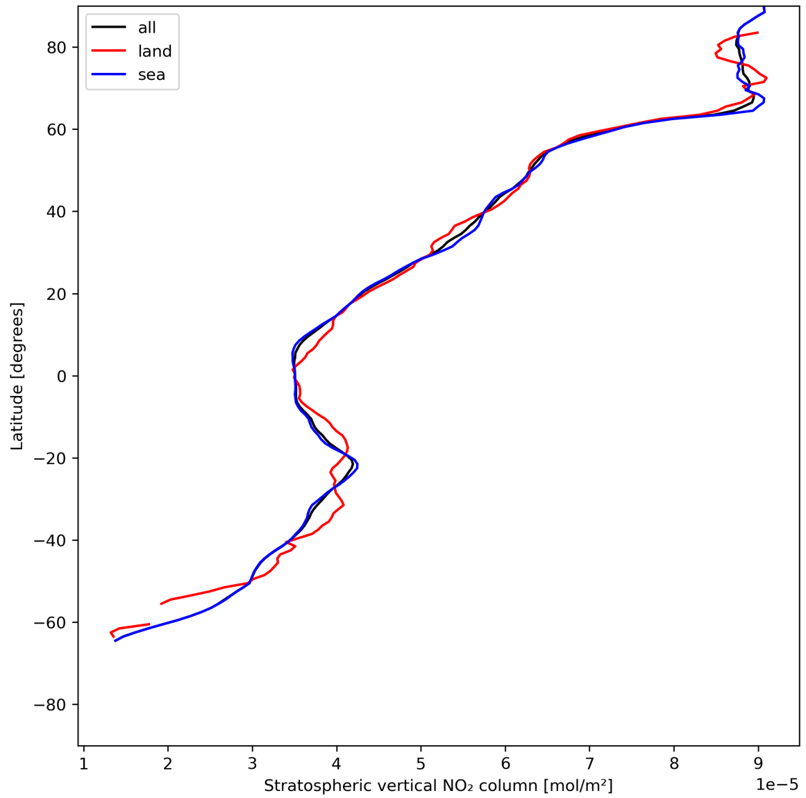
Figure 19: Zonal average of “Stratospheric vertical NO 2 column” for 2024-06-19 to 2024-06-20.
