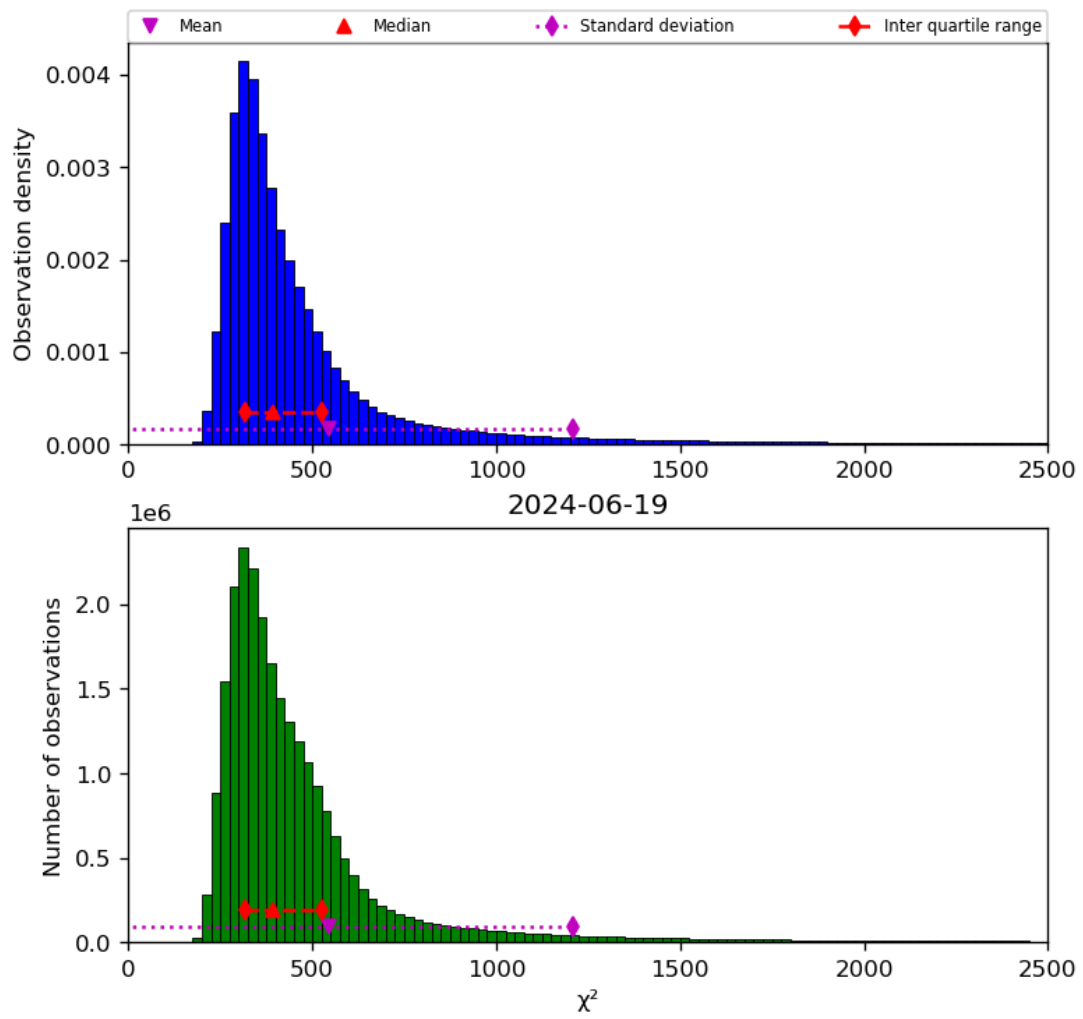
Figure 42: Histogram of “ \chi^2 ” for 2024-06-19 to 2024-06-20
