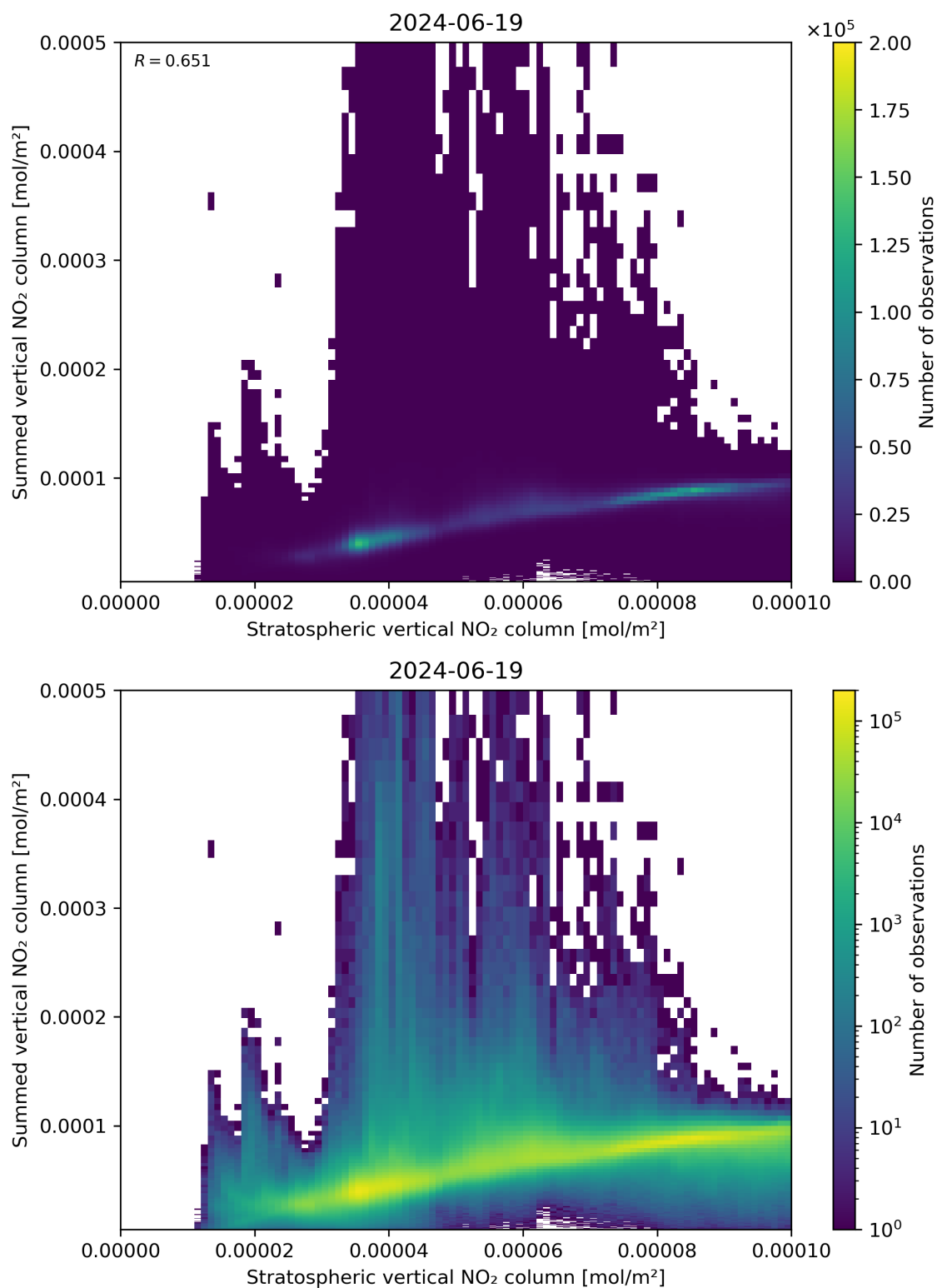
Figure 98: Scatter density plot of “Stratospheric vertical NO 2 column” against “Summed vertical NO 2 column” for 2024-06-19 to 2024-06-20.
