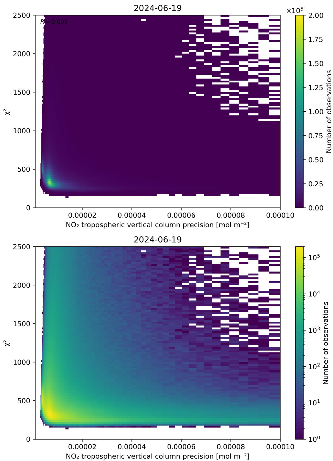
Figure 134: Scatter density plot of “NO 2 tropospheric vertical column precision” against “ \chi^2 ” for 2024-06-19 to 2024-06-20.
