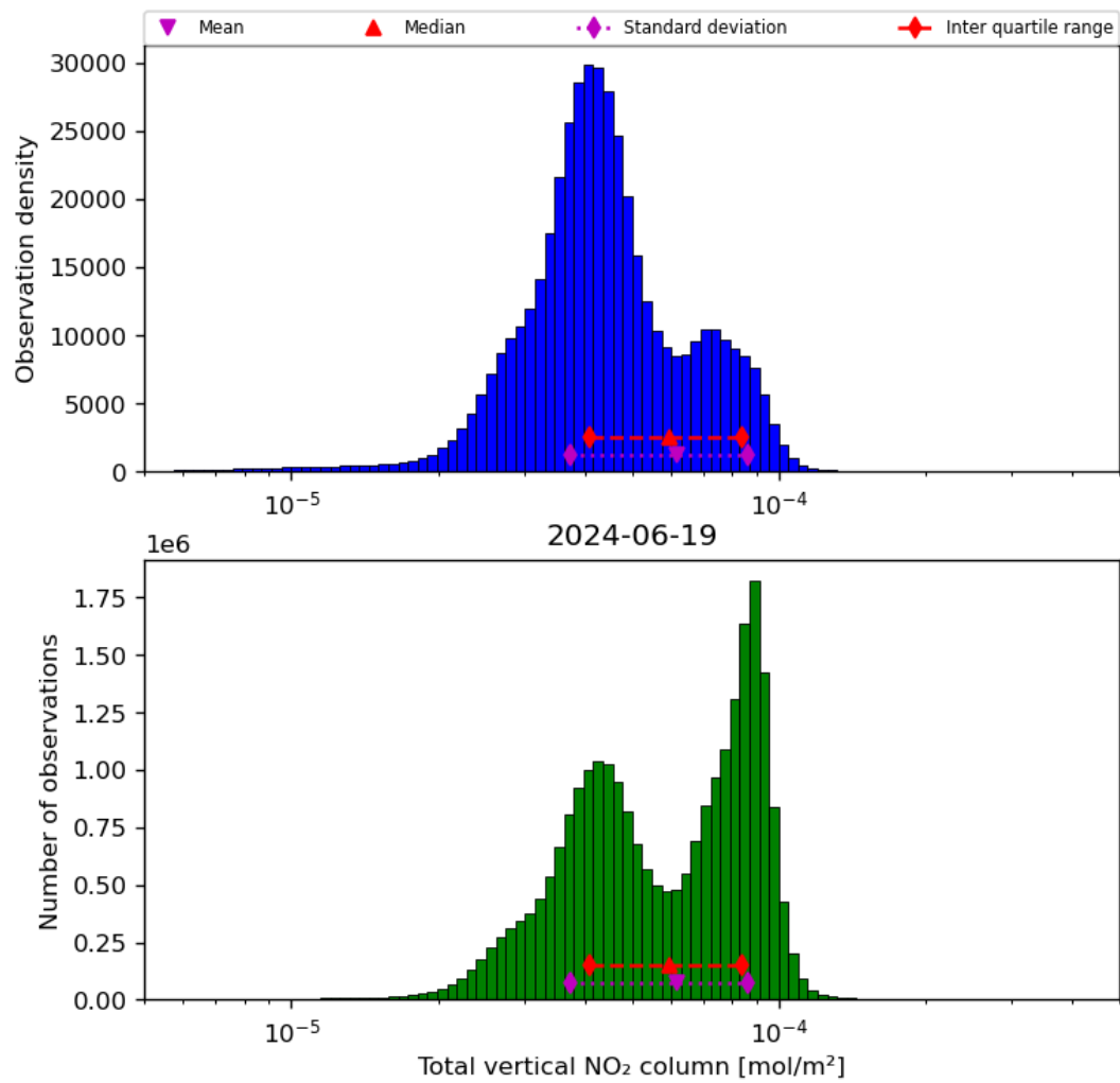
Figure 38: Histogram of “Total vertical NO 2 column” for 2024-06-19 to 2024-06-20
