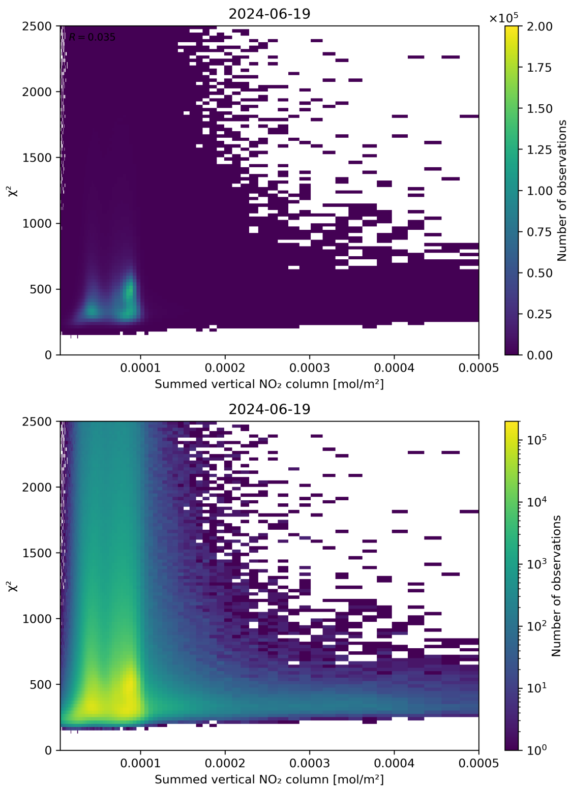
Figure 104: Scatter density plot of “Summed vertical NO 2 column” against “ \chi^2 ” for 2024-06-19 to 2024-06-20.
