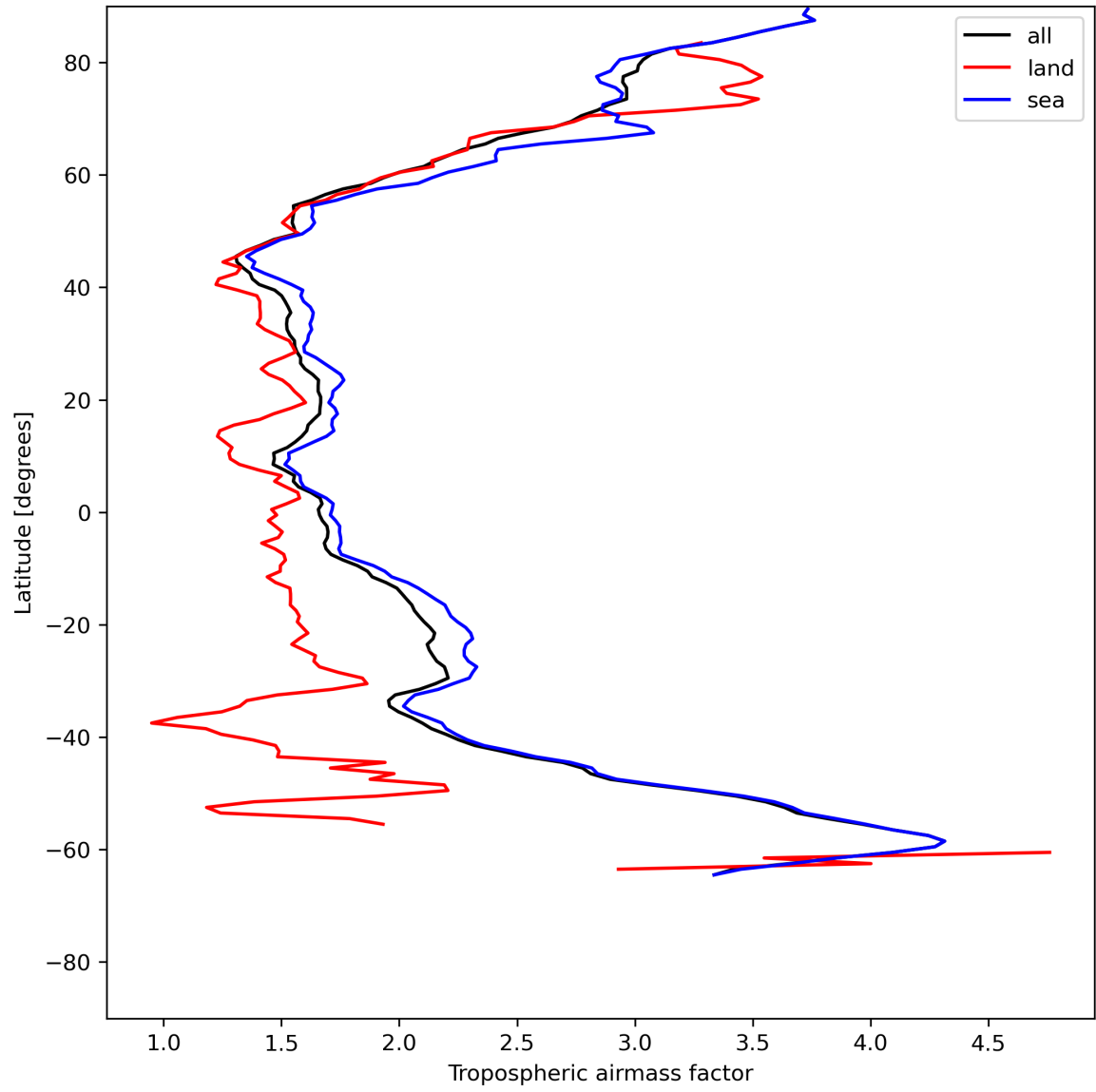
Figure 14: Zonal average of “Tropospheric airmass factor” for 2024-06-19 to 2024-06-20.
