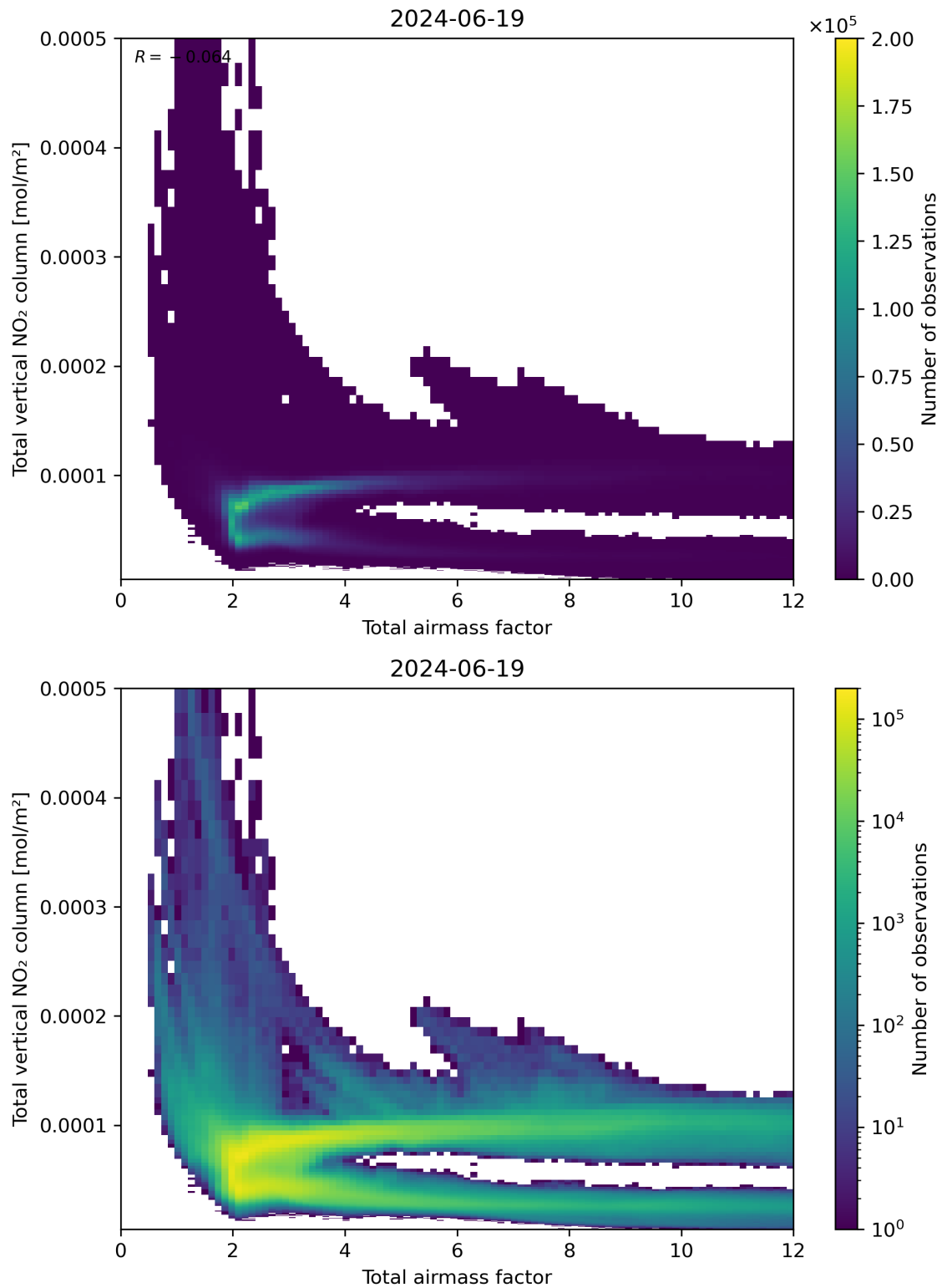
Figure 67: Scatter density plot of “Total airmass factor” against “Total vertical NO 2 column” for 2024-06-19 to 2024-06-20.
