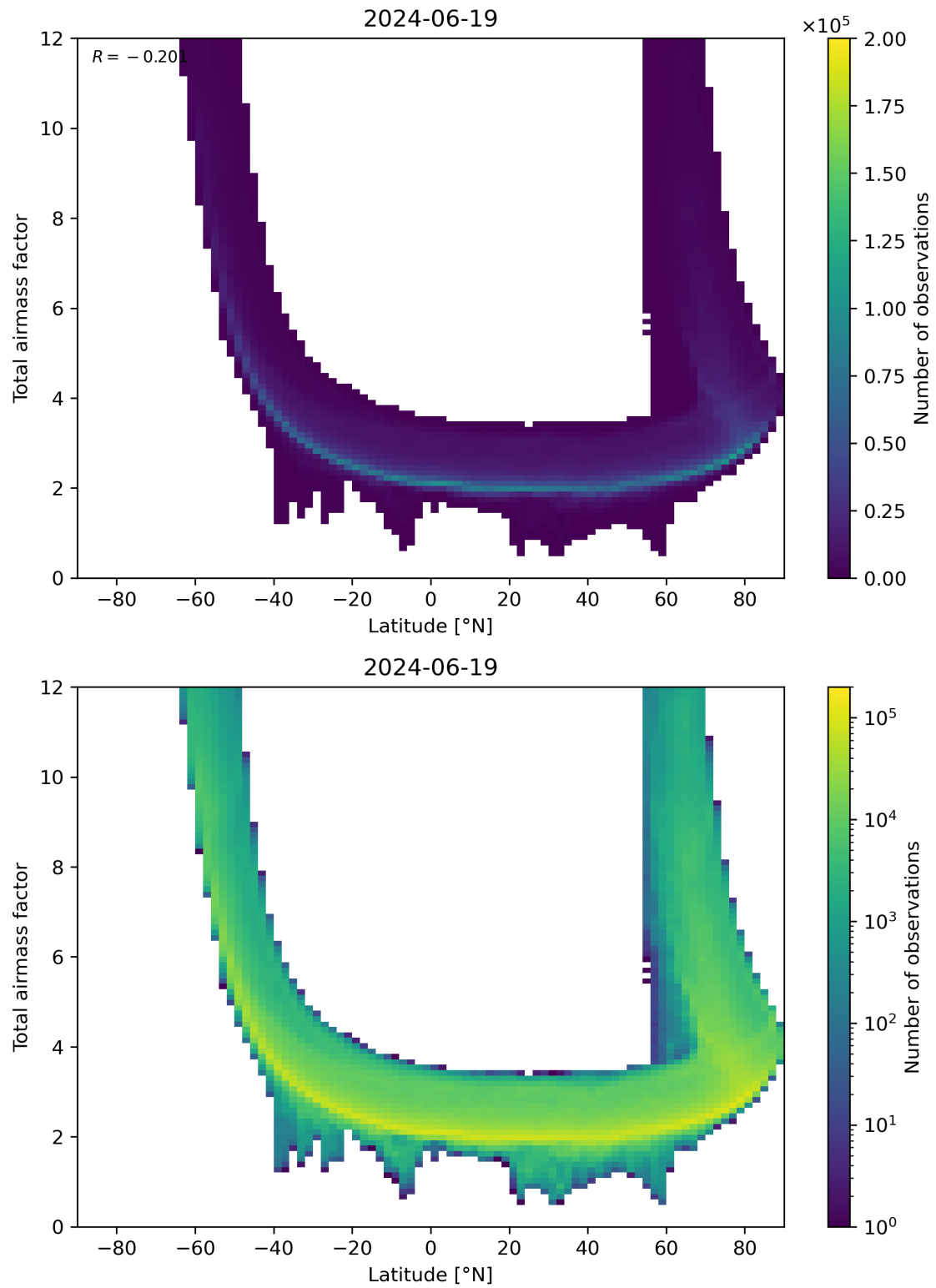
Figure 84: Scatter density plot of “Latitude” against “Total airmass factor” for 2024-06-19 to 2024-06-20.
