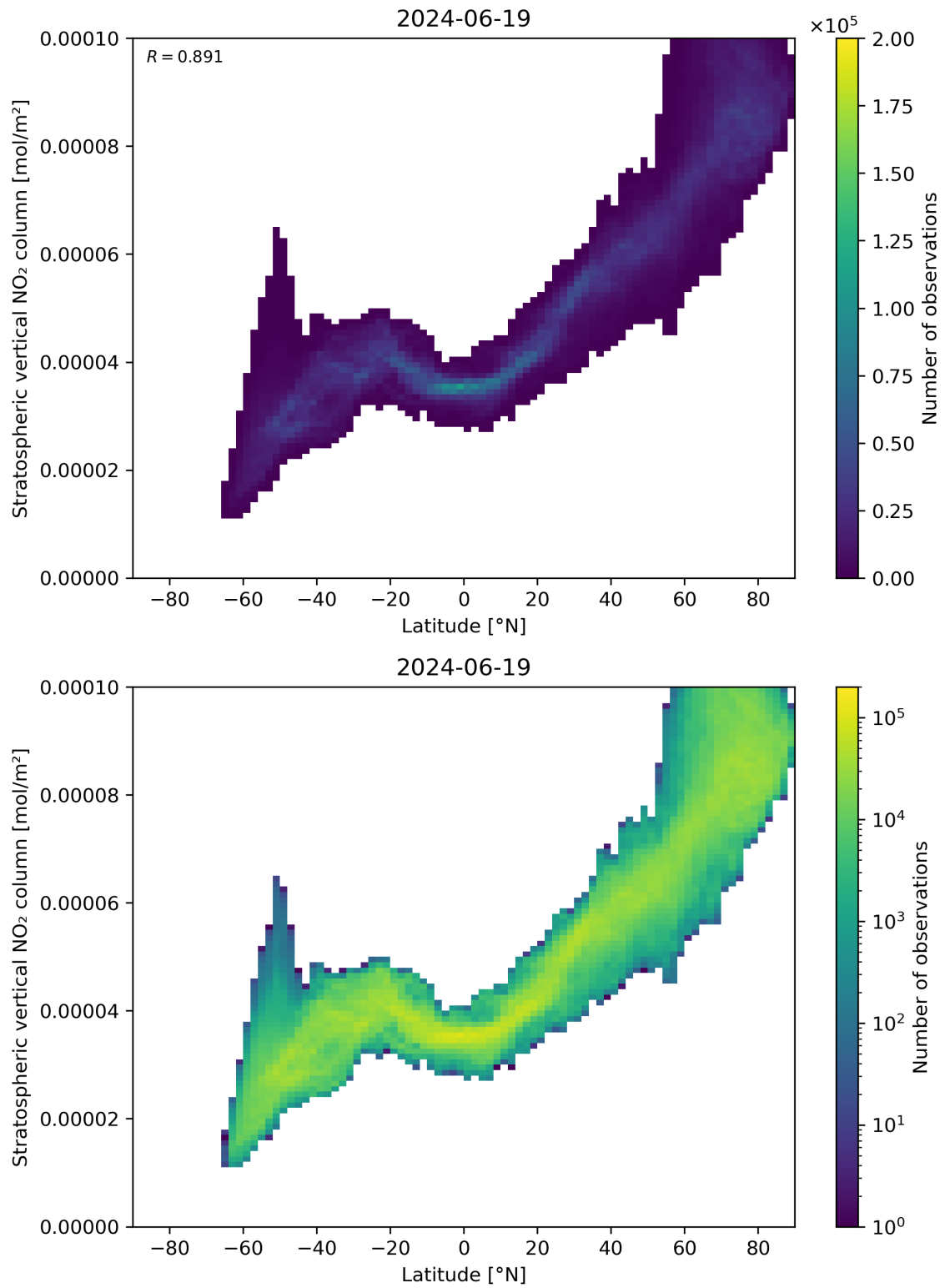
Figure 87: Scatter density plot of “Latitude” against “Stratospheric vertical NO 2 column” for 2024-06-19 to 2024-06-20.
