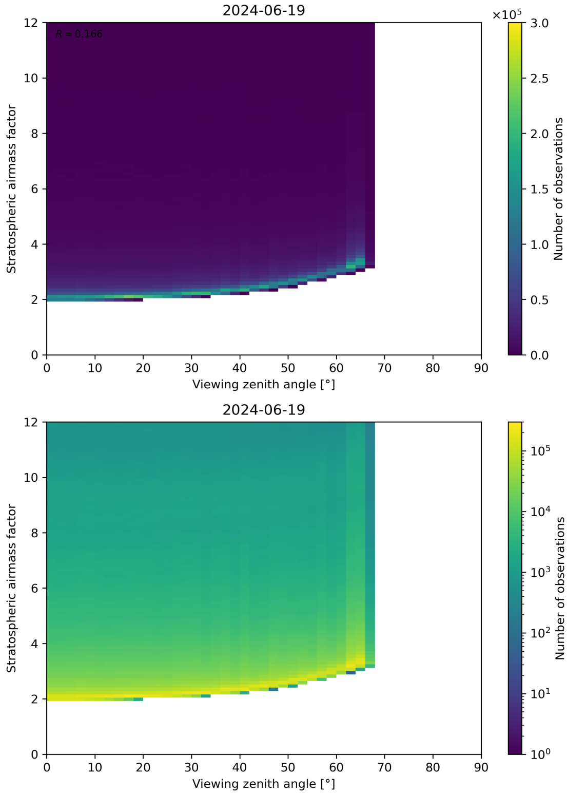
Figure 159: Scatter density plot of “Viewing zenith angle” against “Stratospheric airmass factor” for 2024-06-19 to 2024-06-20.
