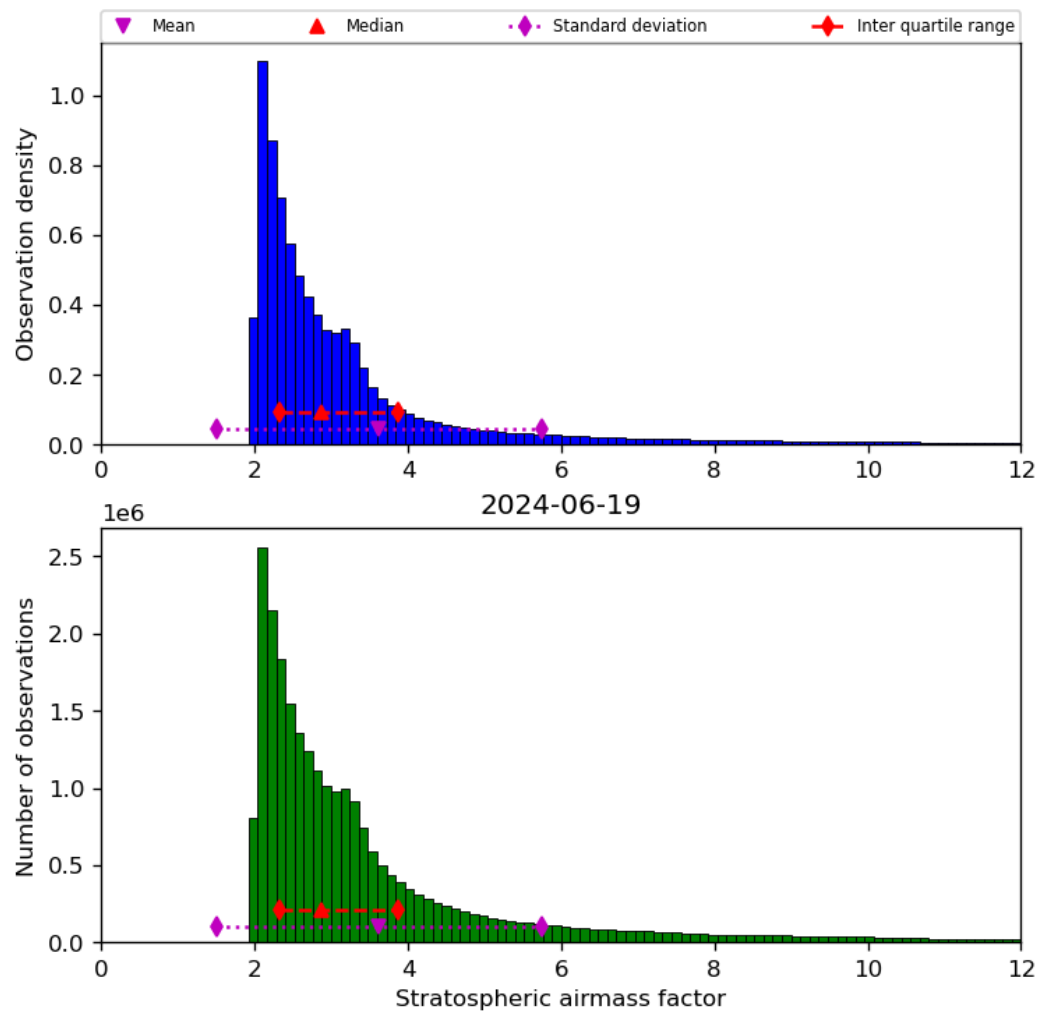
Figure 44: Histogram of “Stratospheric airmass factor” for 2024-06-19 to 2024-06-20
