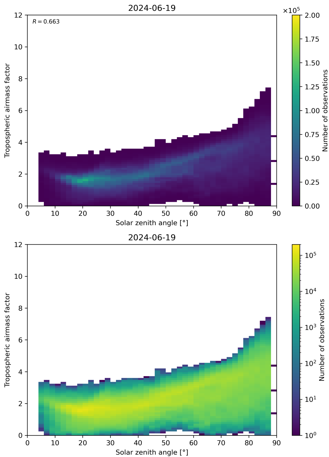
Figure 147: Scatter density plot of “Solar zenith angle” against “Tropospheric airmass factor” for 2024-06-19 to 2024-06-20.
