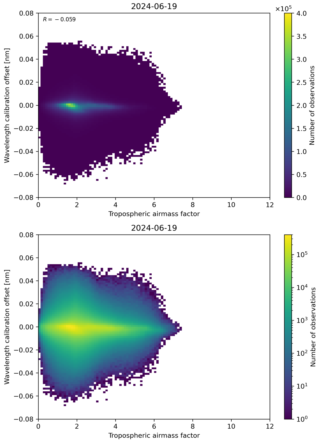
Figure 80: Scatter density plot of “Tropospheric airmass factor” against “Wavelength calibration offset” for 2024-06-19 to 2024-06-20.
