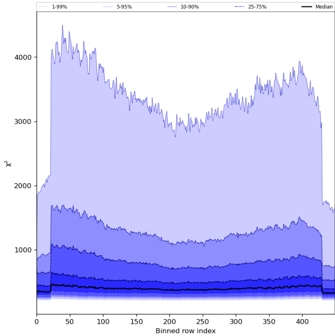
Figure 59: Along track statistics of “ \chi^2 ” for 2024-06-19 to 2024-06-20
