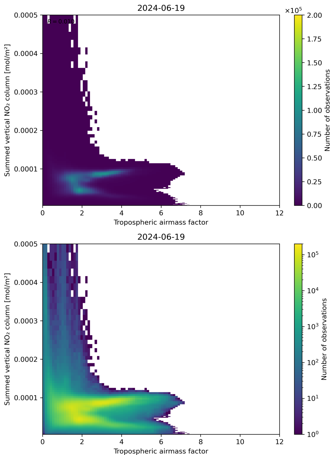
Figure 75: Scatter density plot of “Tropospheric airmass factor” against “Summed vertical NO 2 column” for 2024-06-19 to 2024-06-20.
