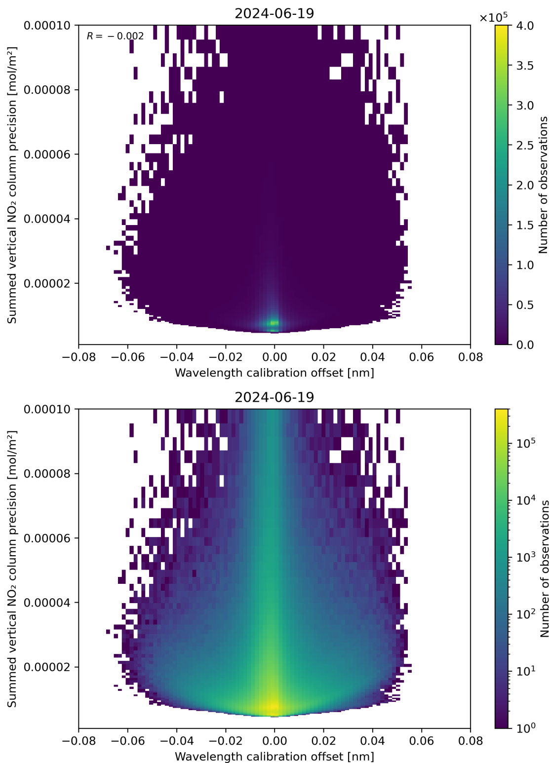
Figure 178: Scatter density plot of “Wavelength calibration offset” against “Summed vertical NO 2 column precision” for 2024-06-19 to 2024-06-20.
