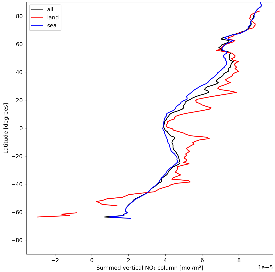
Figure 23: Zonal average of “Summed vertical NO 2 column” for 2024-06-19 to 2024-06-20.
