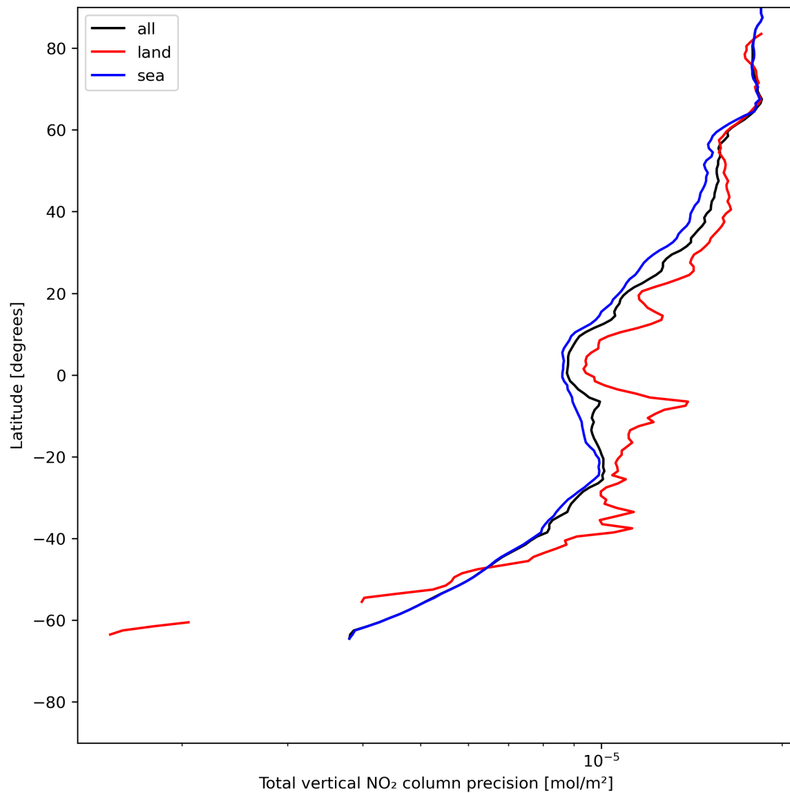
Figure 22: Zonal average of “Total vertical NO 2 column precision” for 2024-06-19 to 2024-06-20.
