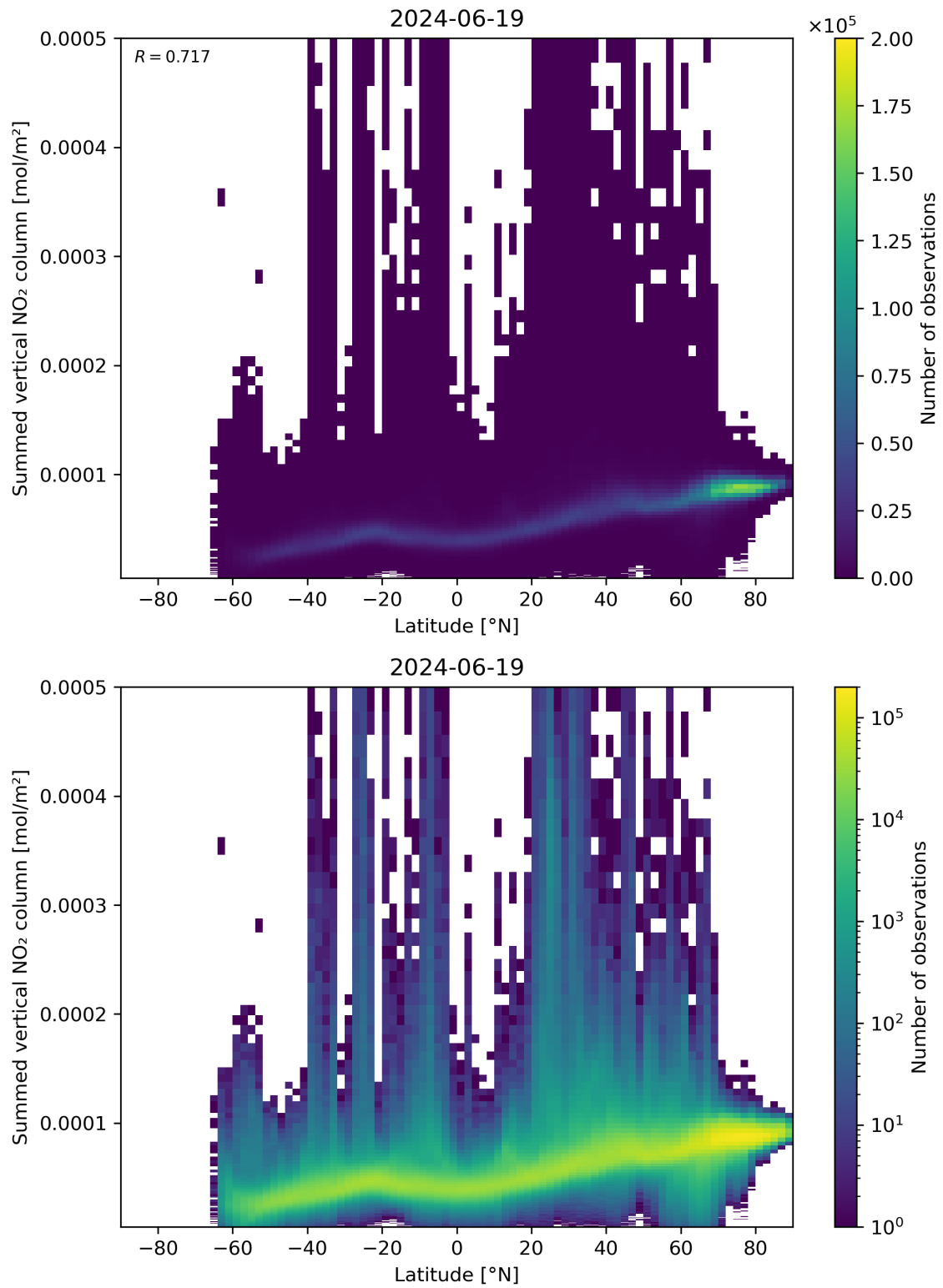
Figure 88: Scatter density plot of “Latitude” against “Summed vertical NO 2 column” for 2024-06-19 to 2024-06-20.
