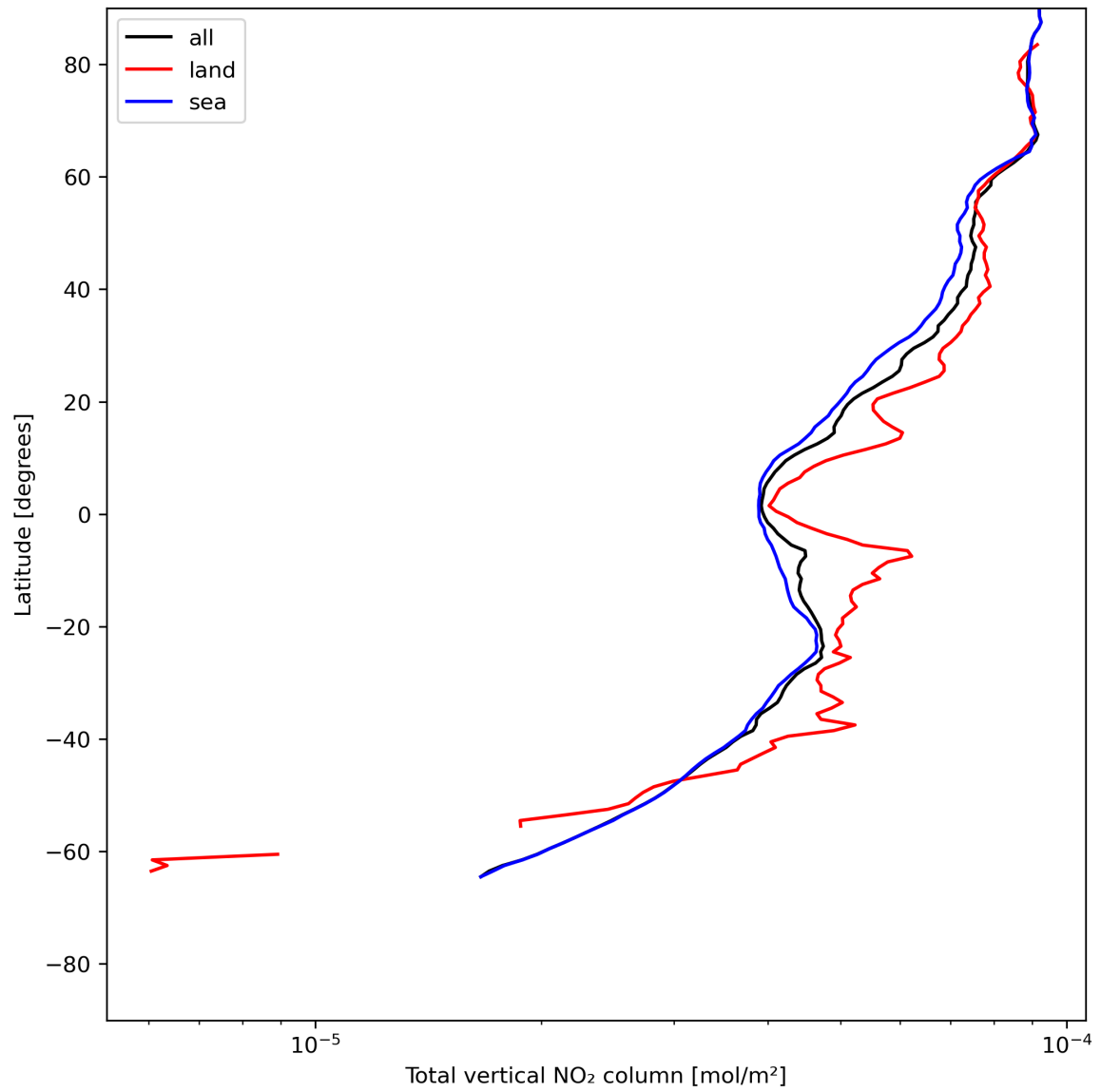
Figure 21: Zonal average of “Total vertical NO 2 column” for 2024-06-19 to 2024-06-20.
