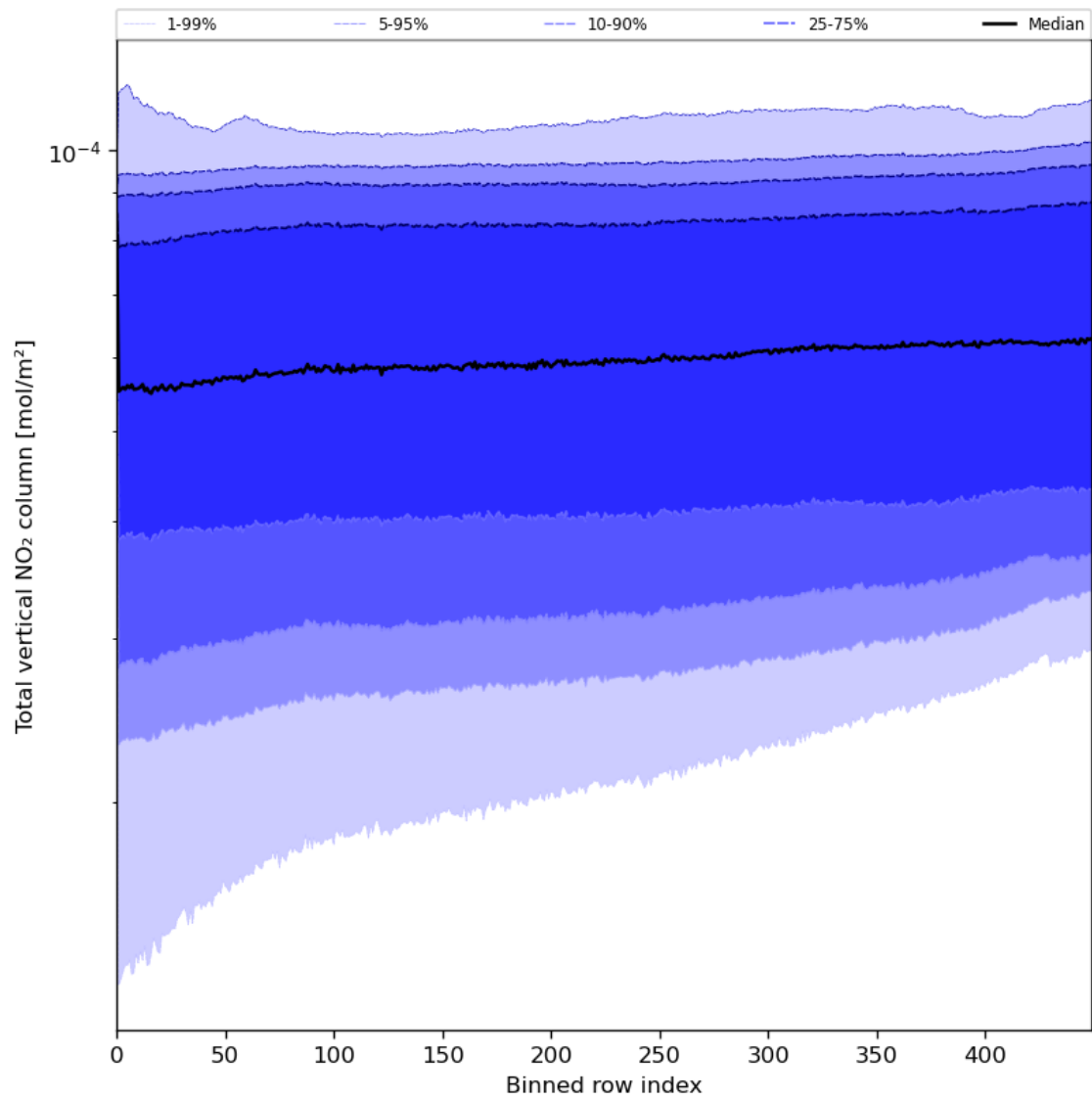
Figure 55: Along track statistics of “Total vertical NO 2 column” for 2024-06-19 to 2024-06-20
