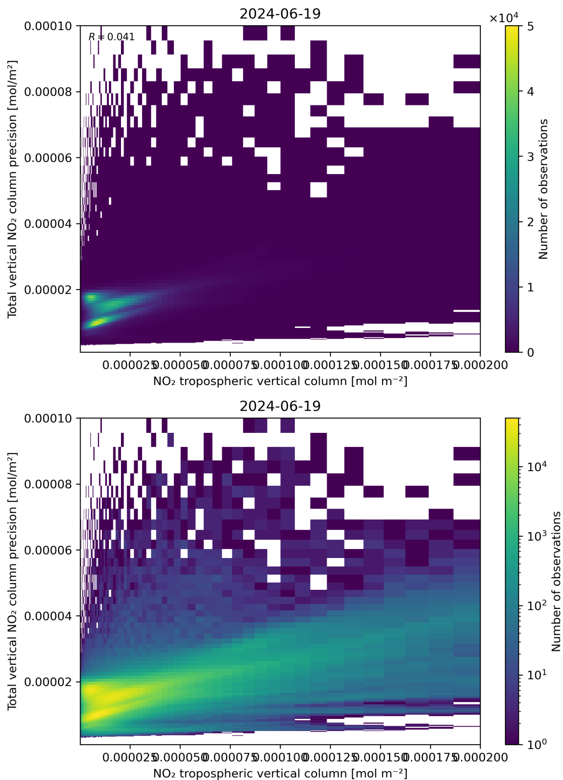
Figure 129: Scatter density plot of “NO 2 tropospheric vertical column” against “Total vertical NO 2 column precision” for 2024-06-19 to 2024-06-20.
