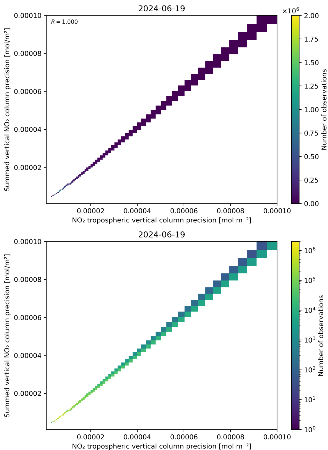
Figure 137: Scatter density plot of “NO 2 tropospheric vertical column precision” against “Summed vertical NO 2 column precision” for 2024-06-19 to 2024-06-20.
