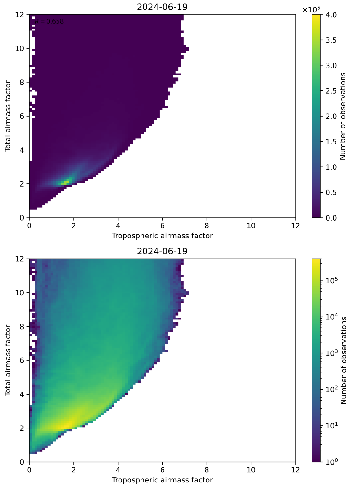
Figure 72: Scatter density plot of “Tropospheric airmass factor” against “Total airmass factor” for 2024-06-19 to 2024-06-20.
