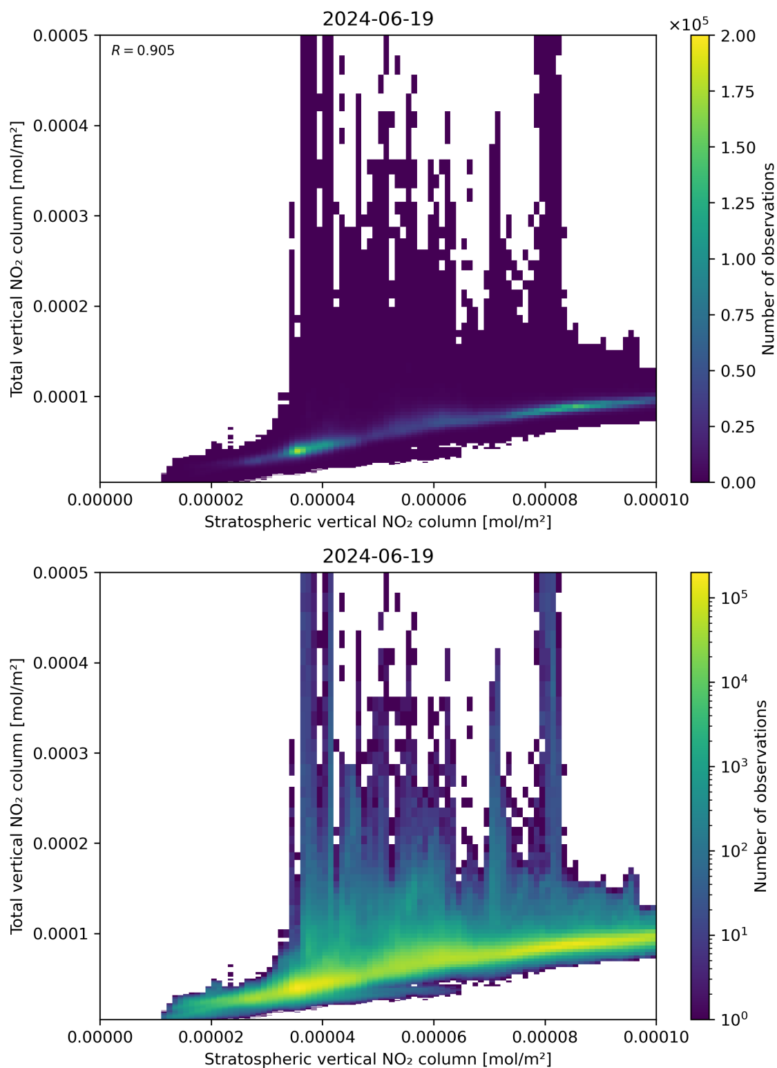
Figure 100: Scatter density plot of “Stratospheric vertical NO 2 column” against “Total vertical NO 2 column” for 2024-06-19 to 2024-06-20.
