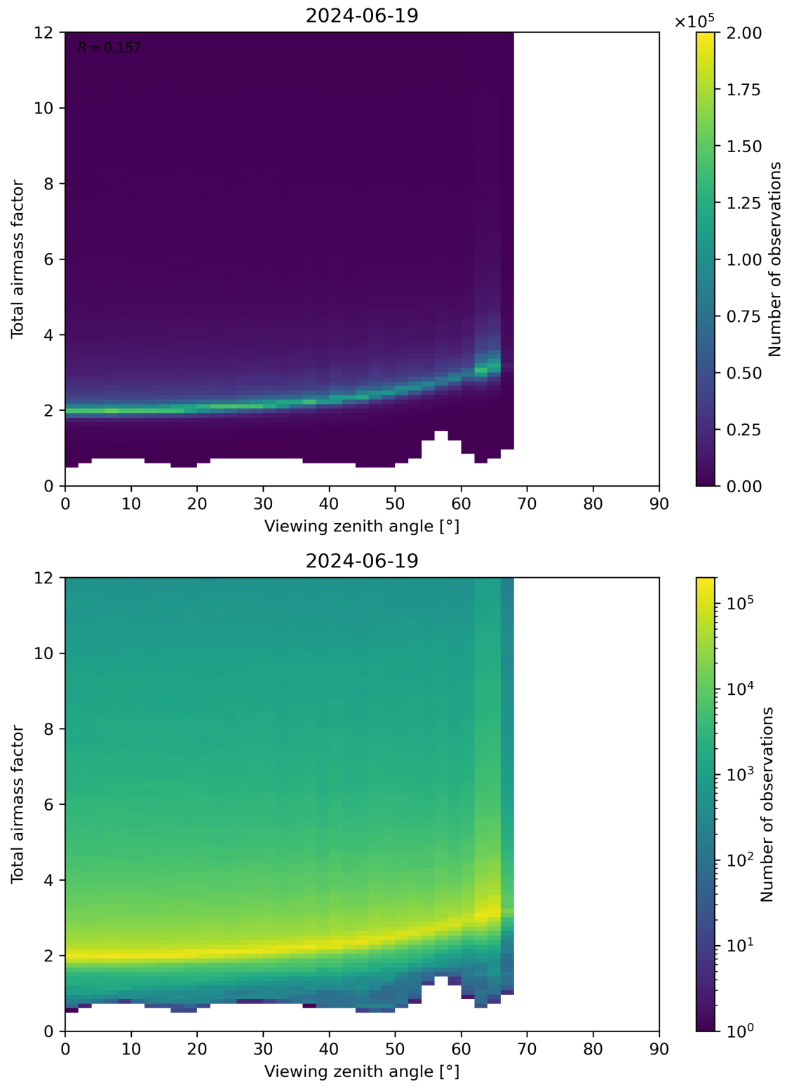
Figure 160: Scatter density plot of “Viewing zenith angle” against “Total airmass factor” for 2024-06-19 to 2024-06-20.
