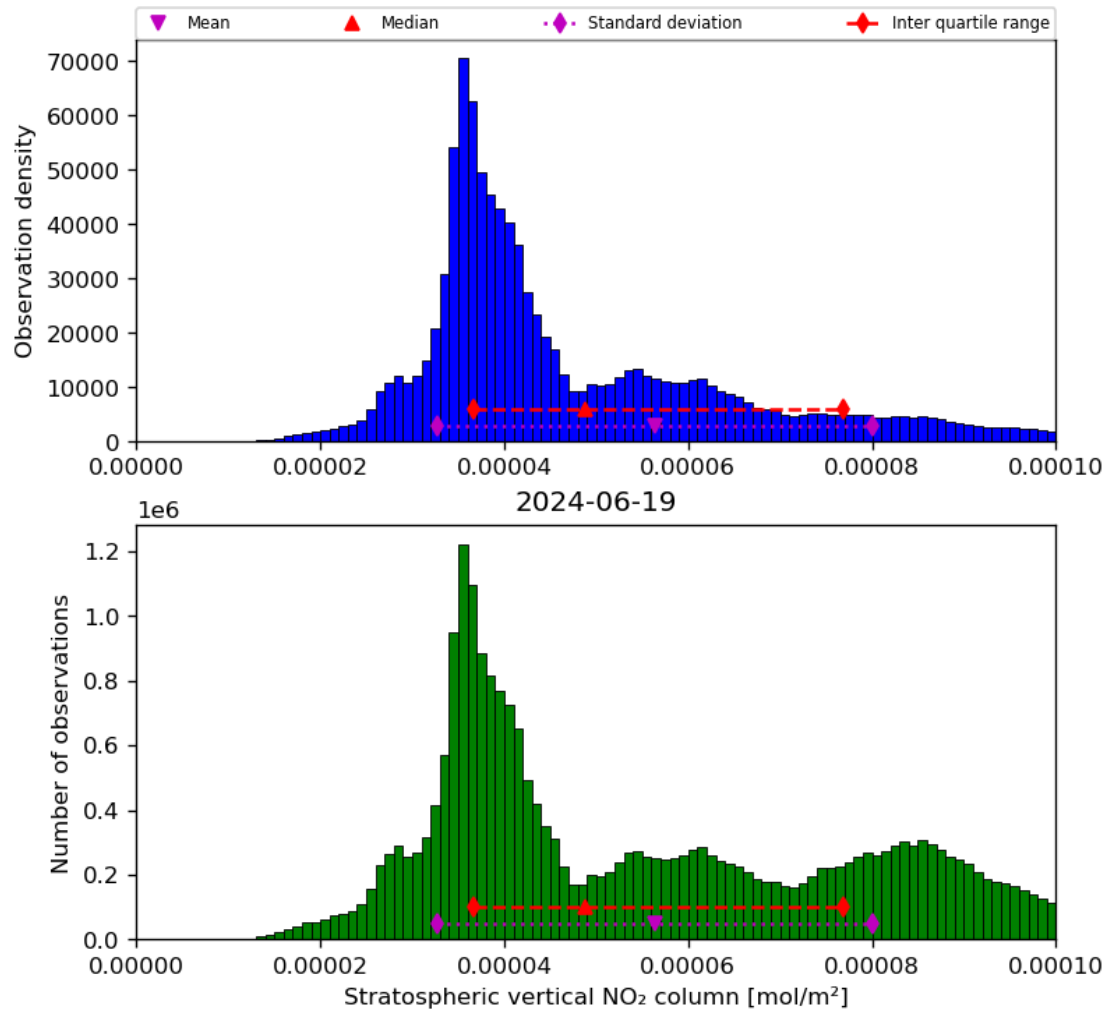
Figure 36: Histogram of “Stratospheric vertical NO 2 column” for 2024-06-19 to 2024-06-20
