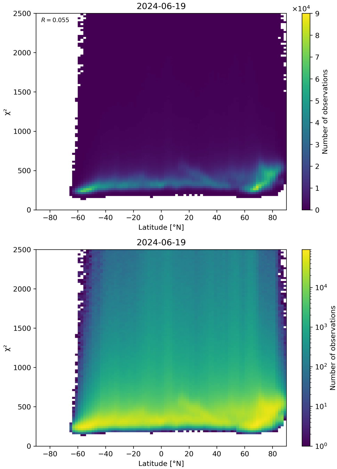
Figure 86: Scatter density plot of “Latitude” against “ \chi^2 ” for 2024-06-19 to 2024-06-20.
