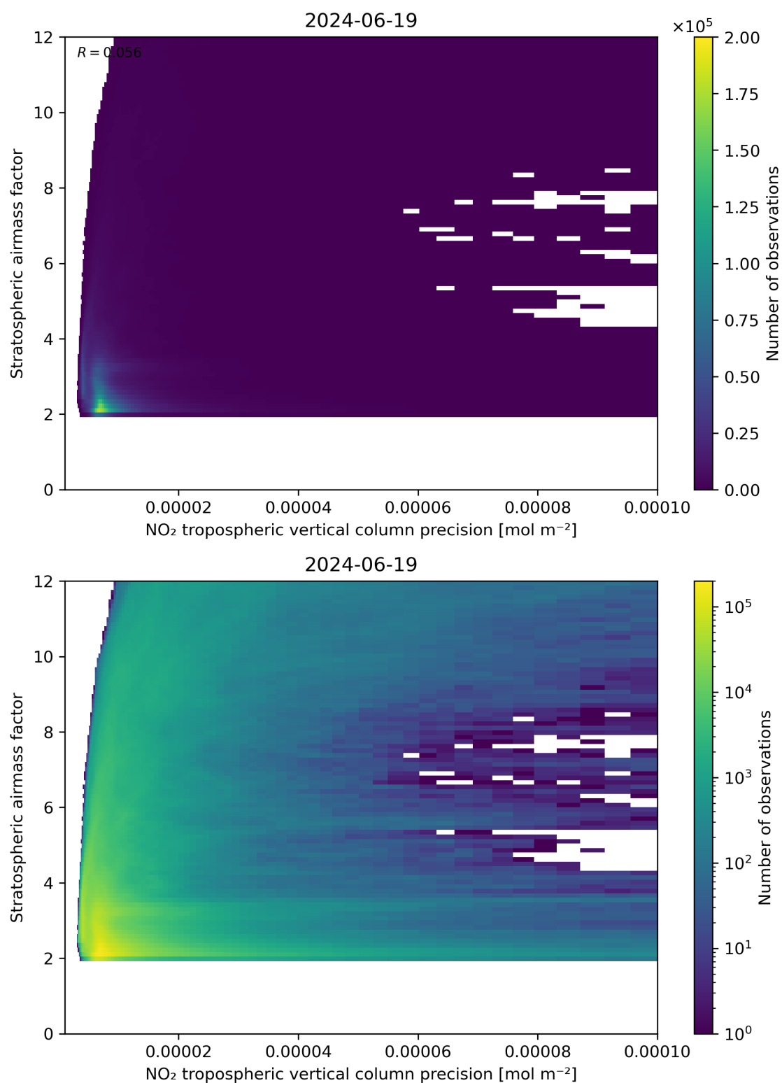
Figure 131: Scatter density plot of “NO 2 tropospheric vertical column precision” against “Stratospheric airmass factor” for 2024-06-19 to 2024-06-20.
