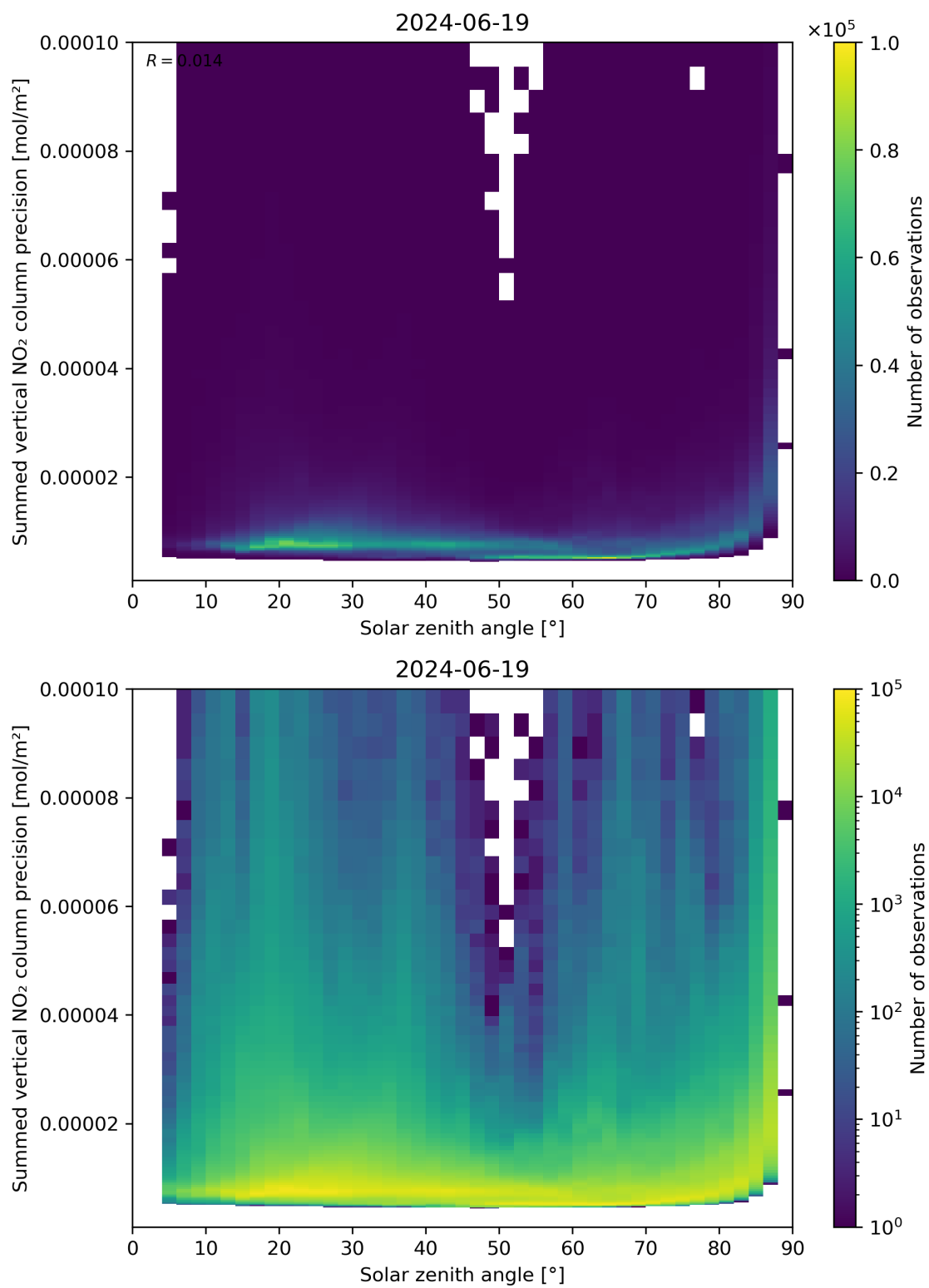
Figure 152: Scatter density plot of “Solar zenith angle” against “Summed vertical NO 2 column precision” for 2024-06-19 to 2024-06-20.
