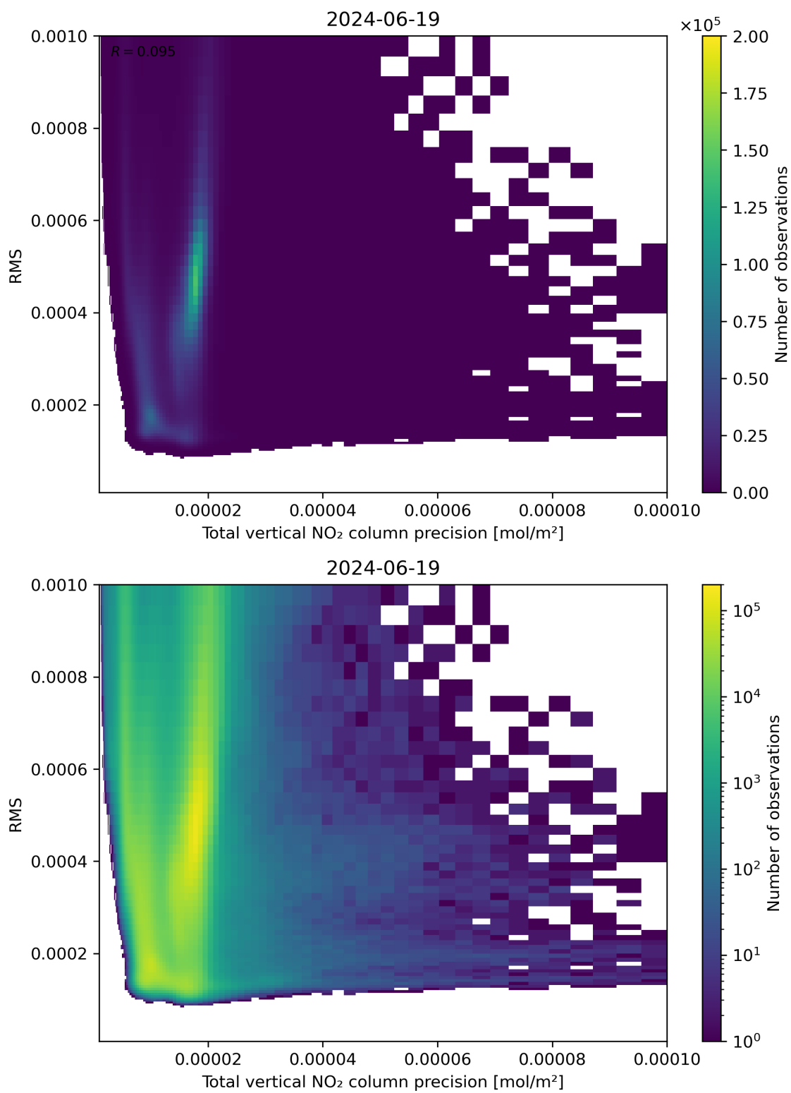
Figure 119: Scatter density plot of “Total vertical NO 2 column precision” against “RMS” for 2024-06-19 to 2024-06-20.
