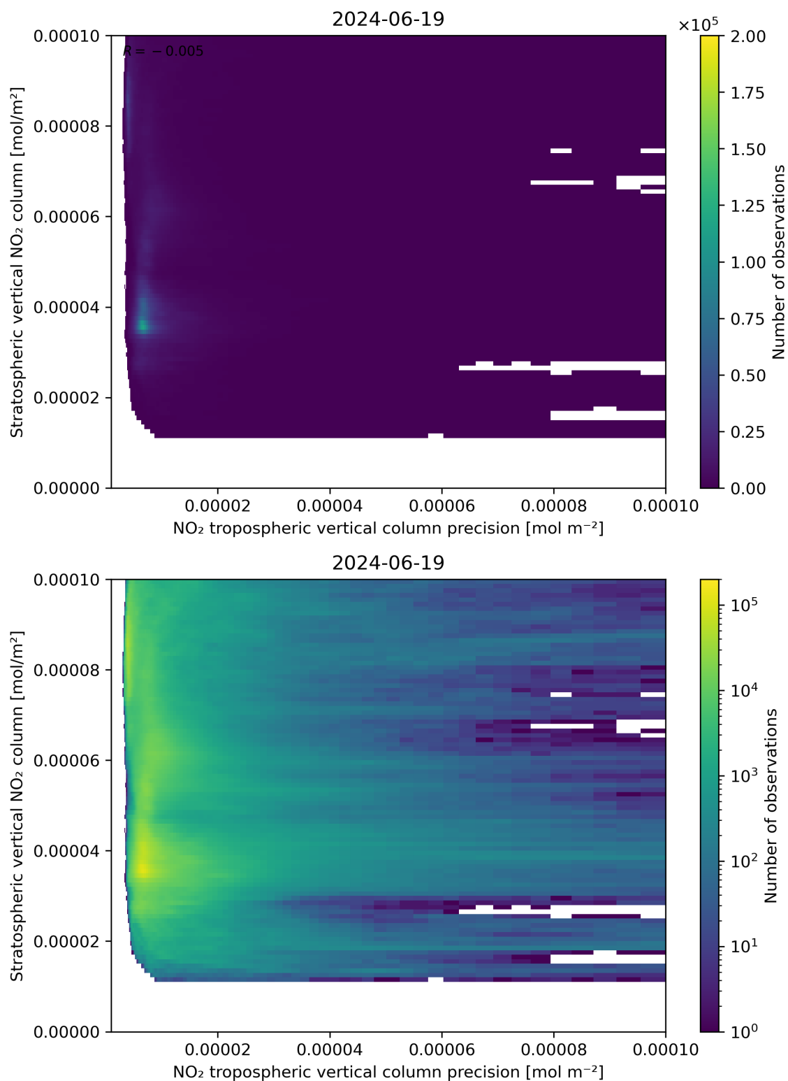
Figure 135: Scatter density plot of “NO 2 tropospheric vertical column precision” against “Stratospheric vertical NO 2 column” for 2024-06-19 to 2024-06-20.
