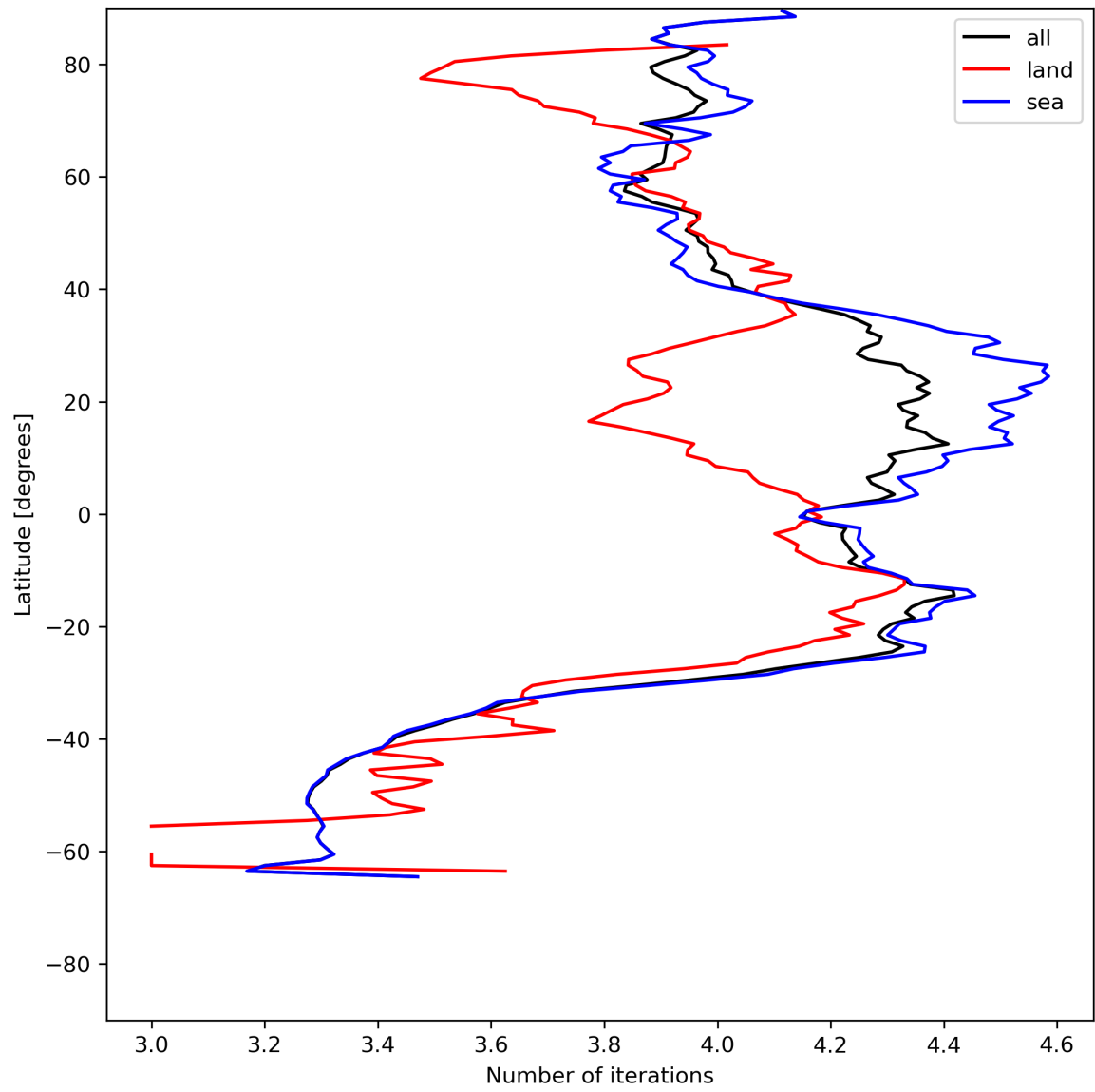
Figure 17: Zonal average of “Number of iterations” for 2024-06-19 to 2024-06-20.
