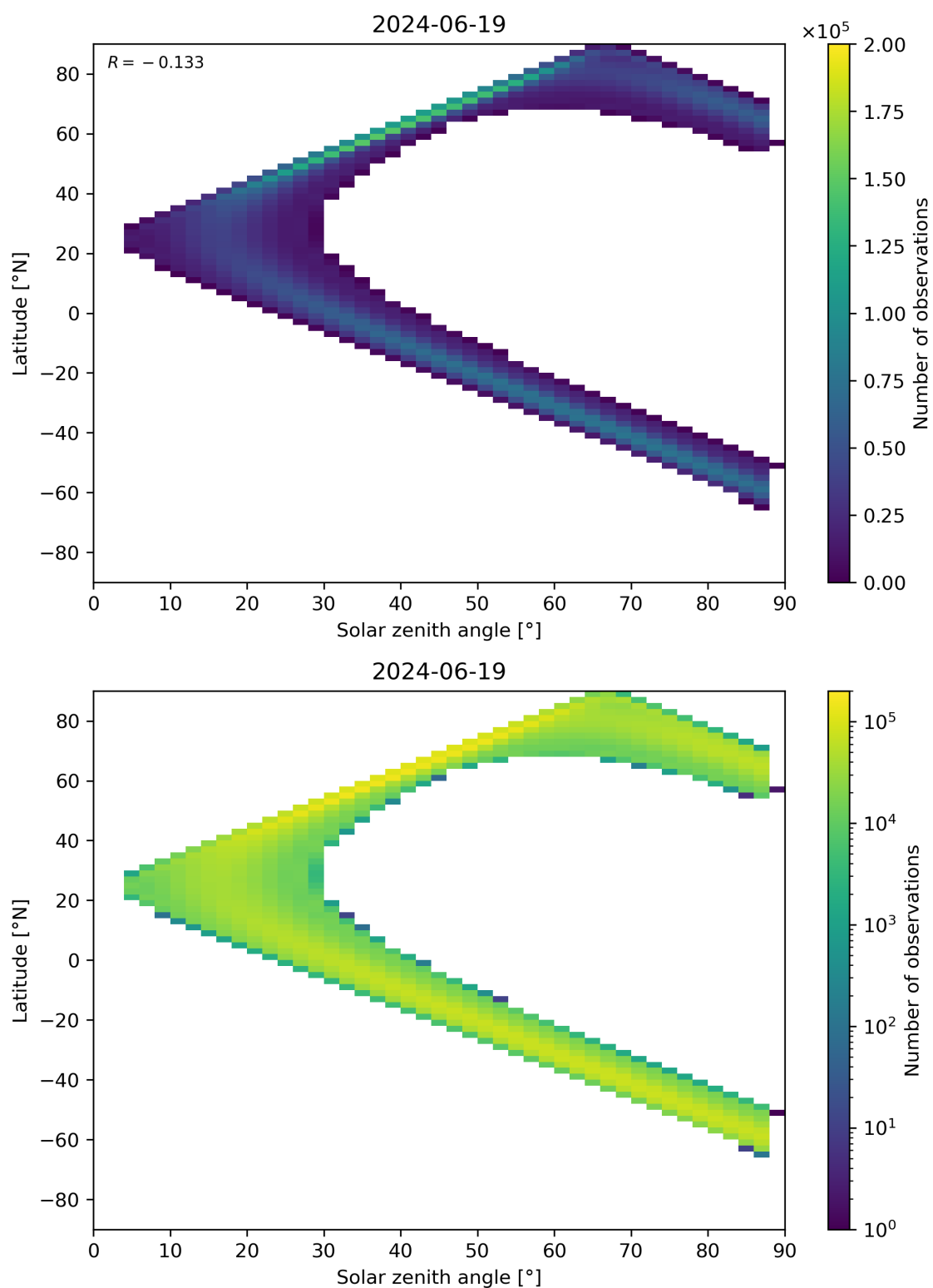
Figure 149: Scatter density plot of “Solar zenith angle” against “Latitude” for 2024-06-19 to 2024-06-20.
