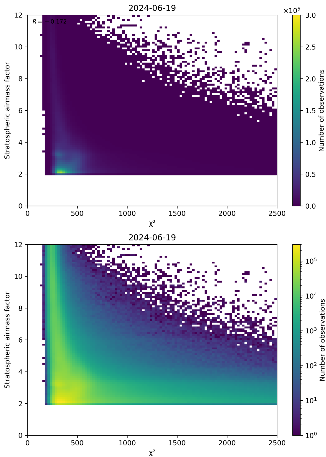
Figure 81: Scatter density plot of “ \chi^2 ” against “Stratospheric airmass factor” for 2024-06-19 to 2024-06-20.
