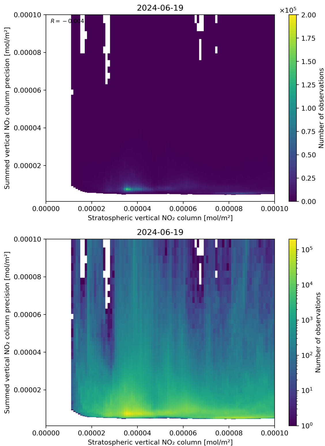
Figure 99: Scatter density plot of “Stratospheric vertical NO 2 column” against “Summed vertical NO 2 column precision” for 2024-06-19 to 2024-06-20.
