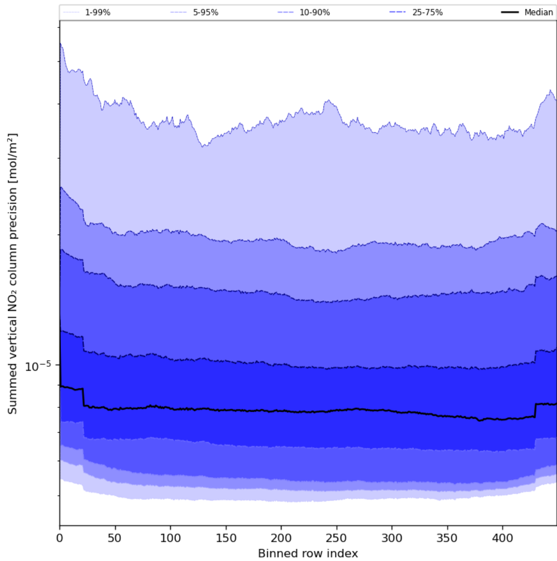
Figure 58: Along track statistics of “Summed vertical NO 2 column precision” for 2024-06-19 to 2024-06-20
