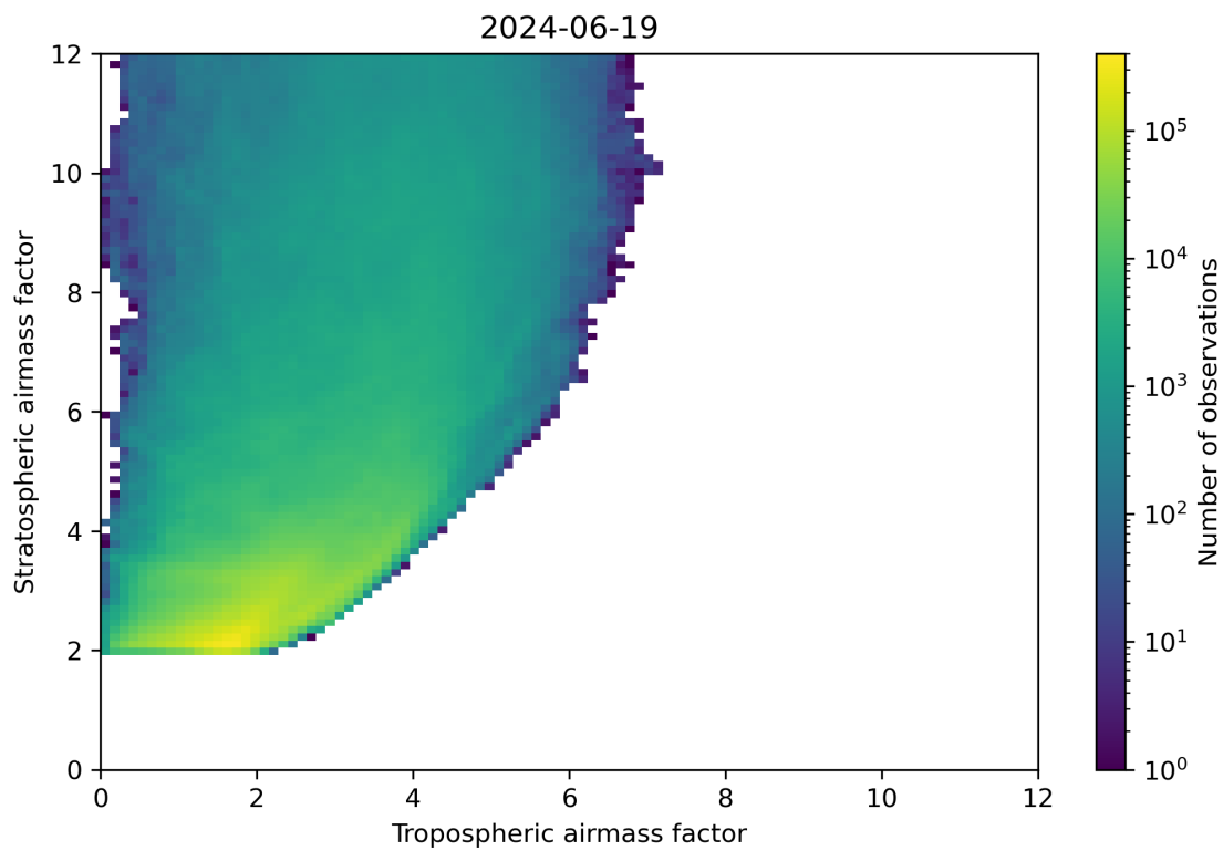
Figure 71: Scatter density plot of “Tropospheric airmass factor” against “Stratospheric airmass factor” for 2024-06-19 to 2024-06-20.
