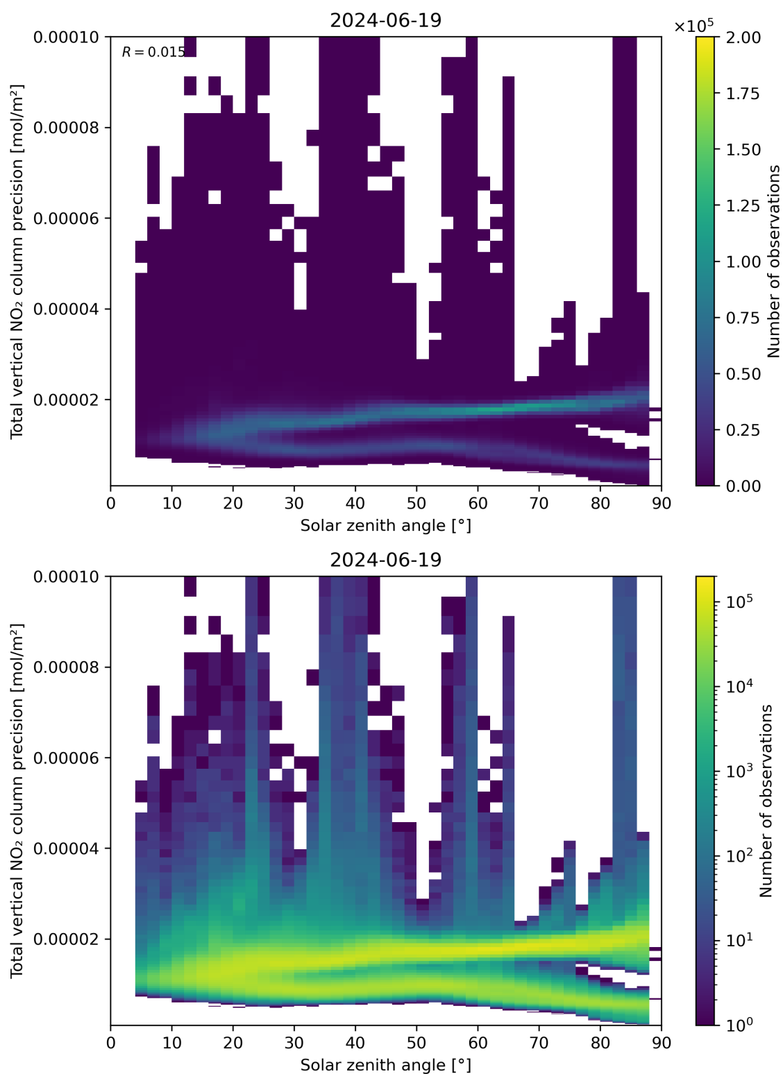
Figure 154: Scatter density plot of “Solar zenith angle” against “Total vertical NO 2 column precision” for 2024-06-19 to 2024-06-20.
