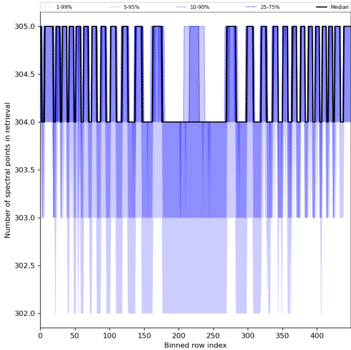
Figure 50: Along track statistics of “Number of spectral points in retrieval” for 2024-06-19 to 2024-06-20
