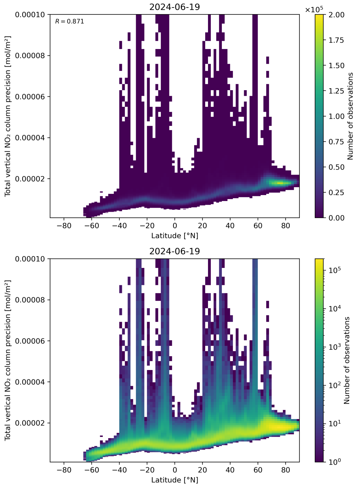
Figure 91: Scatter density plot of “Latitude” against “Total vertical NO 2 column precision” for 2024-06-19 to 2024-06-20.
