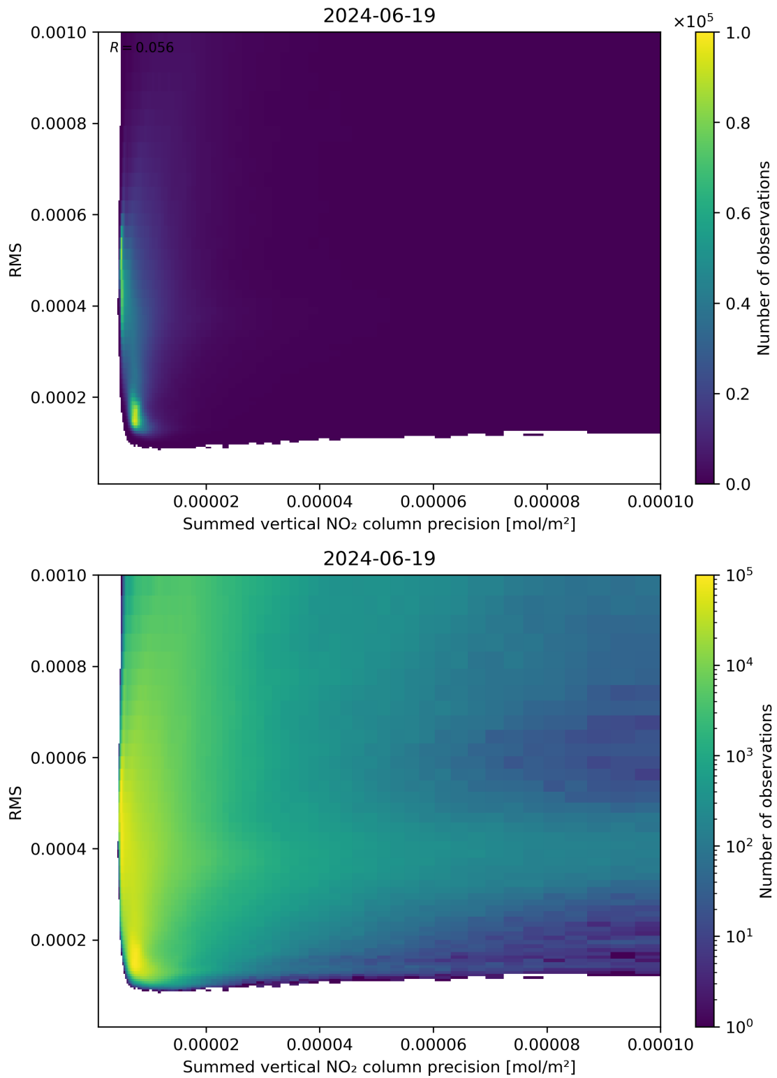
Figure 108: Scatter density plot of “Summed vertical NO 2 column precision” against “RMS” for 2024-06-19 to 2024-06-20.
