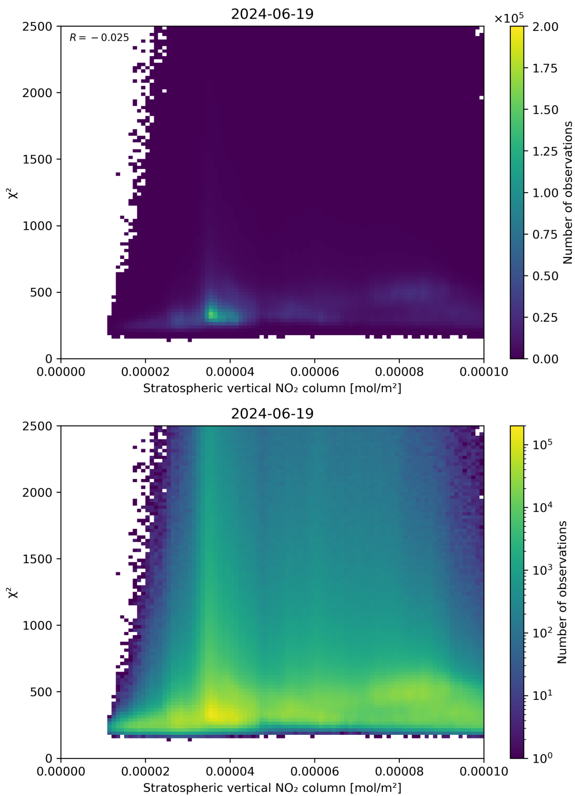
Figure 97: Scatter density plot of “Stratospheric vertical NO 2 column” against “ \chi^2 ” for 2024-06-19 to 2024-06-20.
