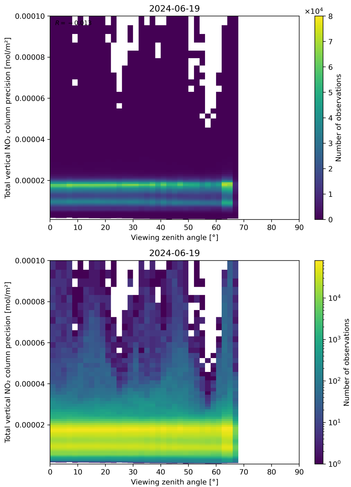
Figure 168: Scatter density plot of “Viewing zenith angle” against “Total vertical NO 2 column precision” for 2024-06-19 to 2024-06-20.
