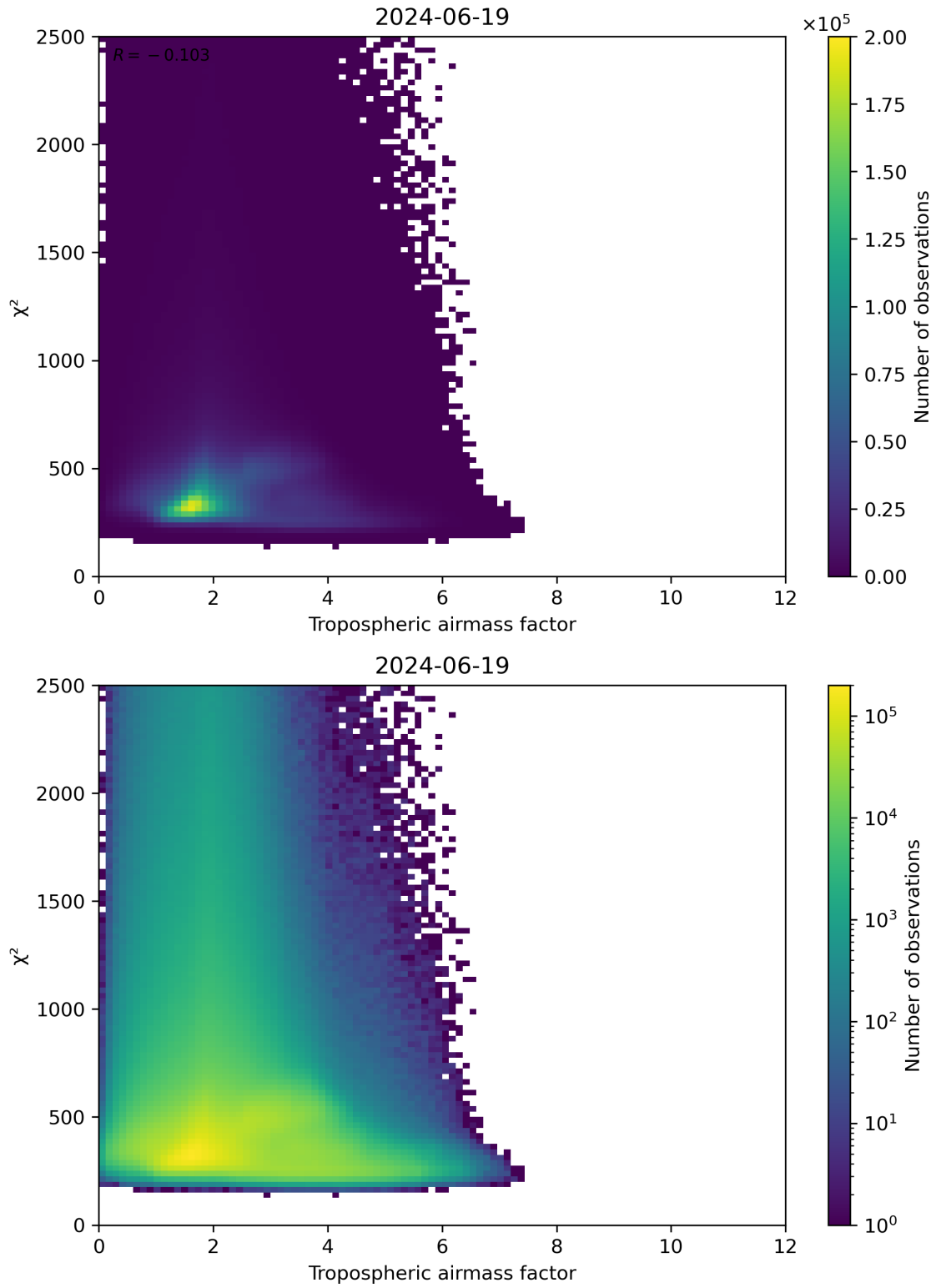
Figure 73: Scatter density plot of “Tropospheric airmass factor” against “ \chi^2 ” for 2024-06-19 to 2024-06-20.
