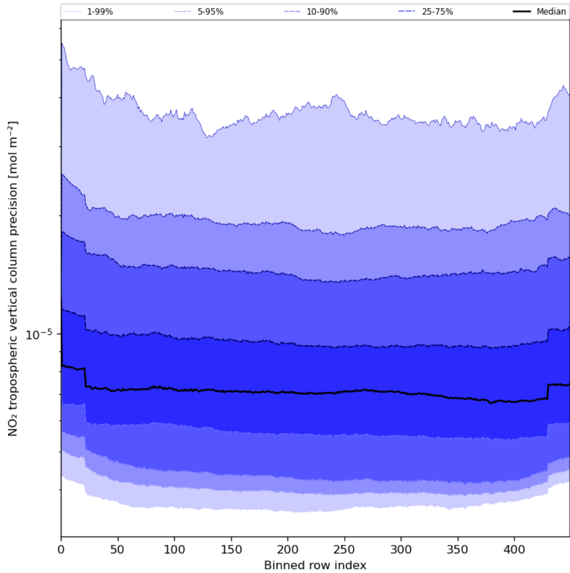
Figure 47: Along track statistics of “NO 2 tropospheric vertical column precision” for 2024-06-19 to 2024-06-20
