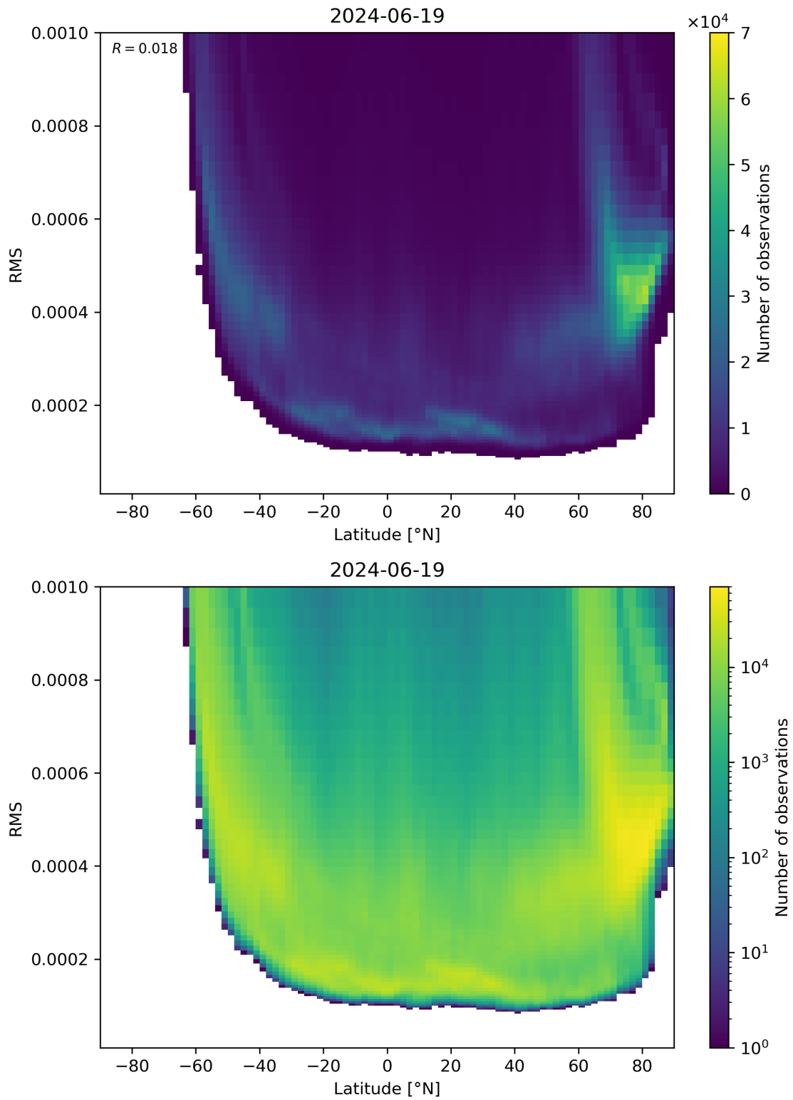
Figure 94: Scatter density plot of “Latitude” against “RMS” for 2024-06-19 to 2024-06-20.
