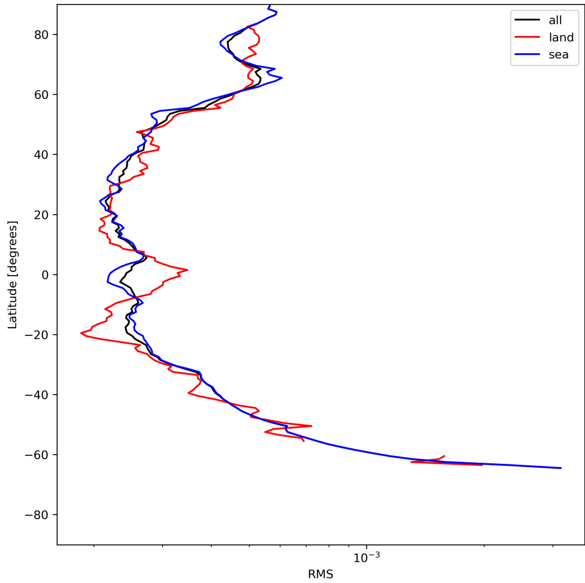
Figure 26: Zonal average of “RMS” for 2024-06-19 to 2024-06-20.
