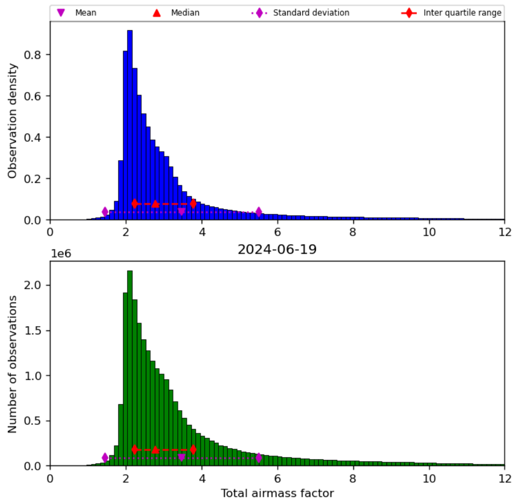
Figure 32: Histogram of “Total airmass factor” for 2024-06-19 to 2024-06-20
