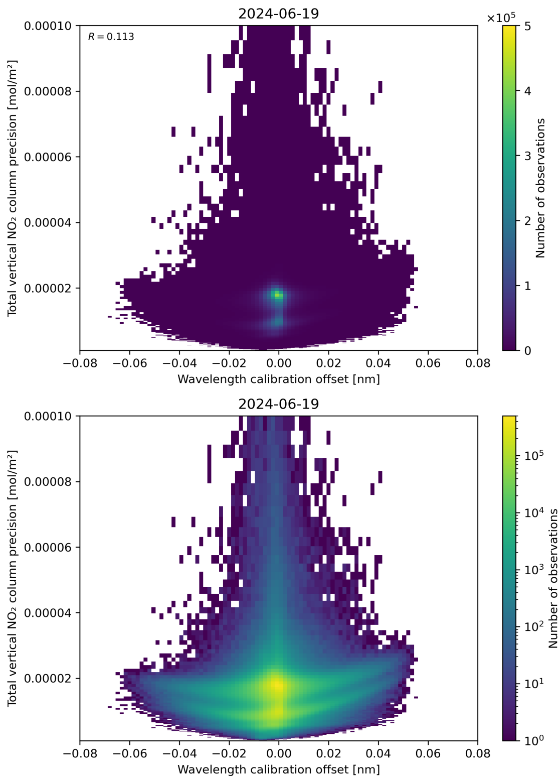
Figure 180: Scatter density plot of “Wavelength calibration offset” against “Total vertical NO 2 column precision” for 2024-06-19 to 2024-06-20.
