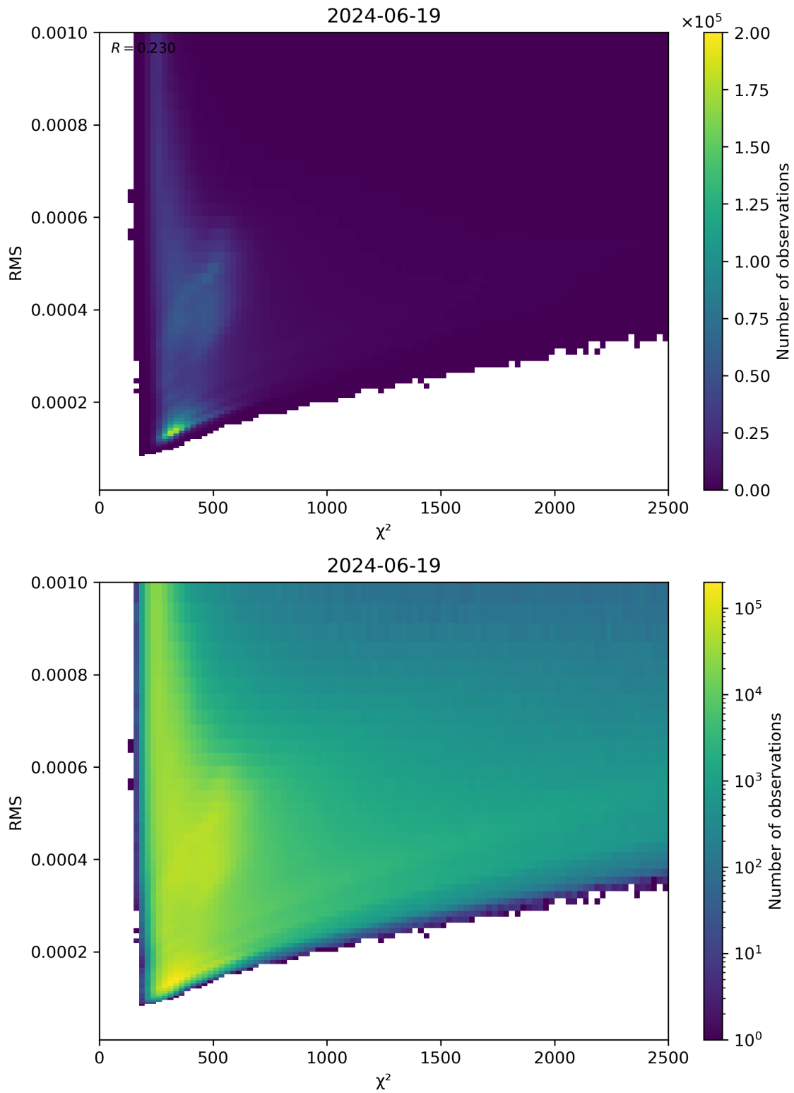
Figure 82: Scatter density plot of “ \chi^2 ” against “RMS” for 2024-06-19 to 2024-06-20.
