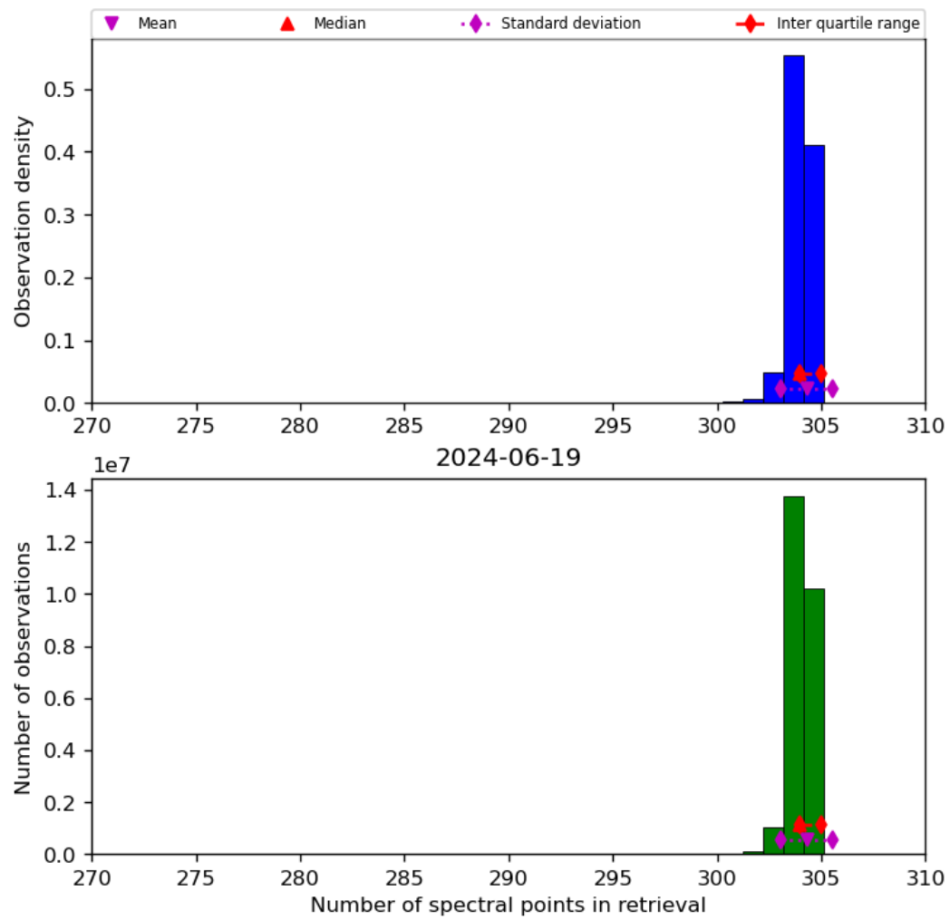
Figure 33: Histogram of “Number of spectral points in retrieval” for 2024-06-19 to 2024-06-20
