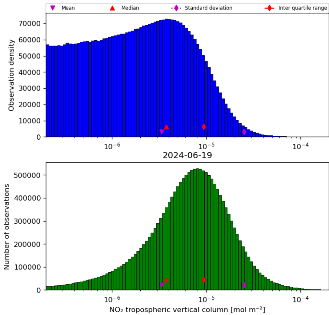
Figure 29: Histogram of “NO 2 tropospheric vertical column” for 2024-06-19 to 2024-06-20
