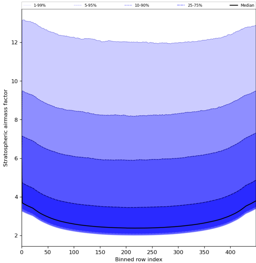
Figure 61: Along track statistics of “Stratospheric airmass factor” for 2024-06-19 to 2024-06-20
