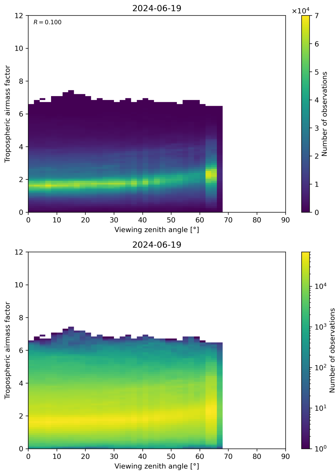
Figure 161: Scatter density plot of “Viewing zenith angle” against “Tropospheric airmass factor” for 2024-06-19 to 2024-06-20.
