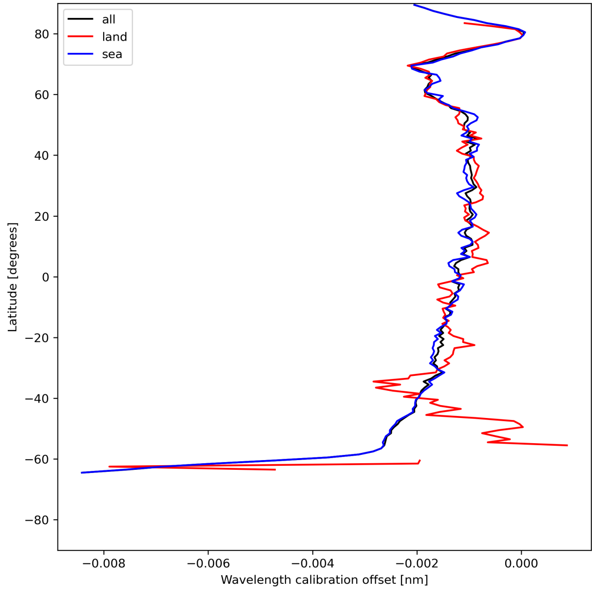
Figure 18: Zonal average of “Wavelength calibration offset” for 2024-06-19 to 2024-06-20.
