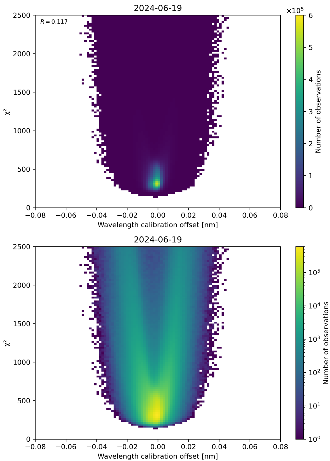
Figure 175: Scatter density plot of “Wavelength calibration offset” against “ \chi^2 ” for 2024-06-19 to 2024-06-20.
