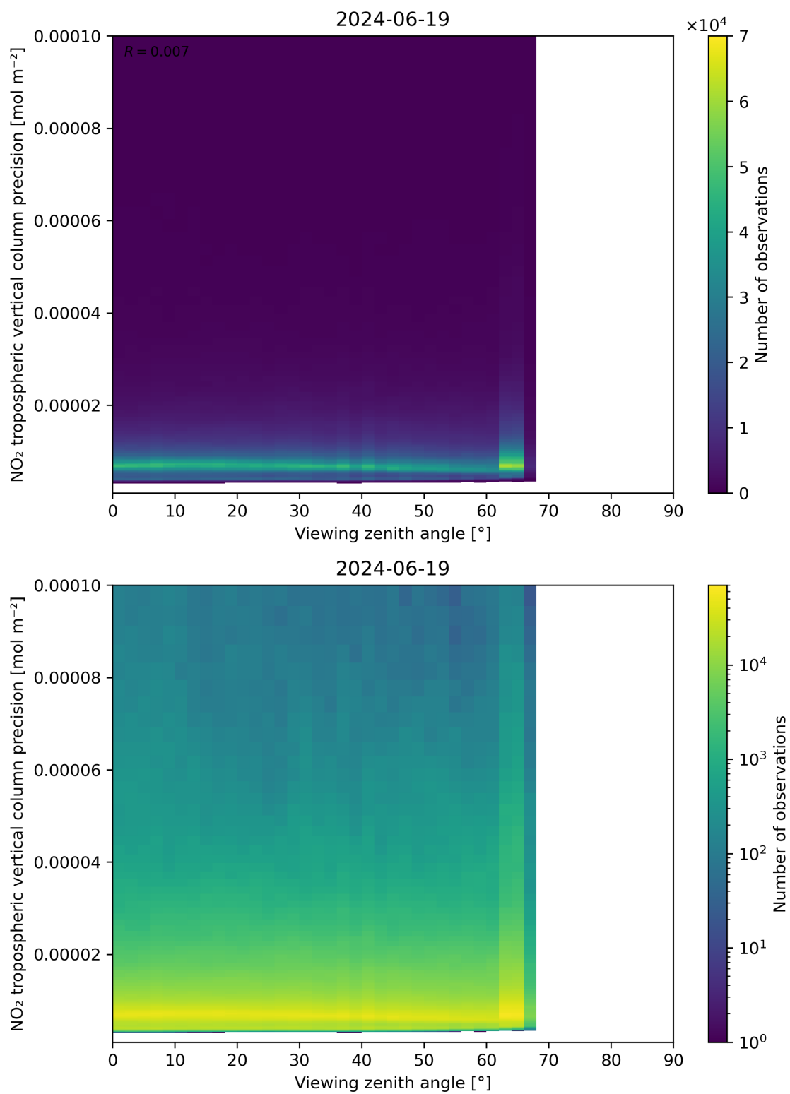
Figure 170: Scatter density plot of “Viewing zenith angle” against “NO 2 tropospheric vertical column precision” for 2024-06-19 to 2024-06-20.
