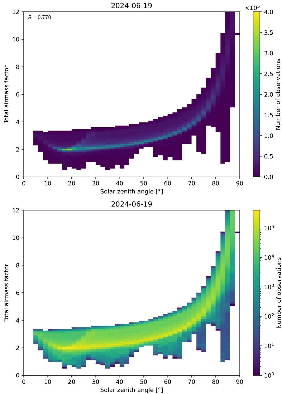
Figure 146: Scatter density plot of “Solar zenith angle” against “Total air mass factor” for 2024-06-19 to 2024-06-20.
