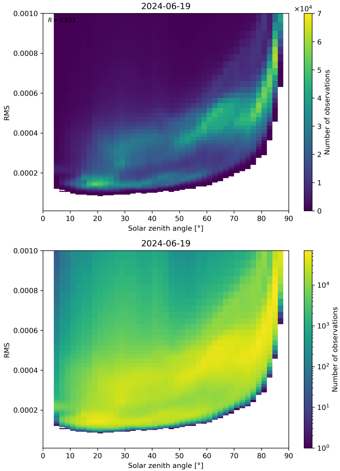
Figure 157: Scatter density plot of “Solar zenith angle” against “RMS” for 2024-06-19 to 2024-06-20.
