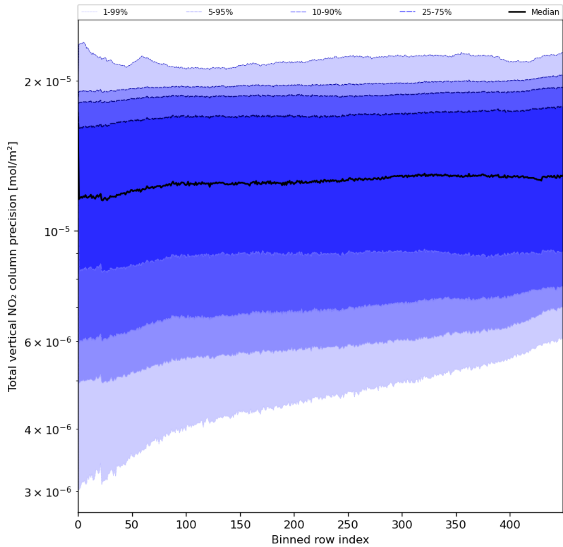
Figure 56: Along track statistics of “Total vertical NO 2 column precision” for 2024-06-19 to 2024-06-20
