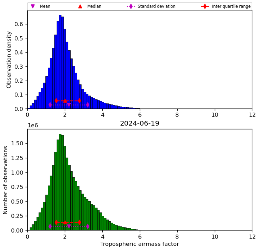
Figure 31: Histogram of “Tropospheric airmass factor” for 2024-06-19 to 2024-06-20
