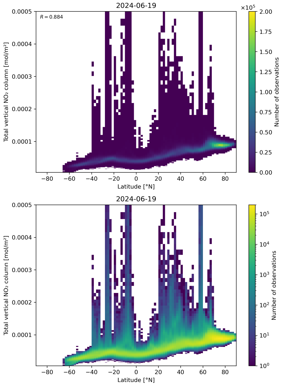
Figure 90: Scatter density plot of “Latitude” against “Total vertical NO 2 column” for 2024-06-19 to 2024-06-20.
