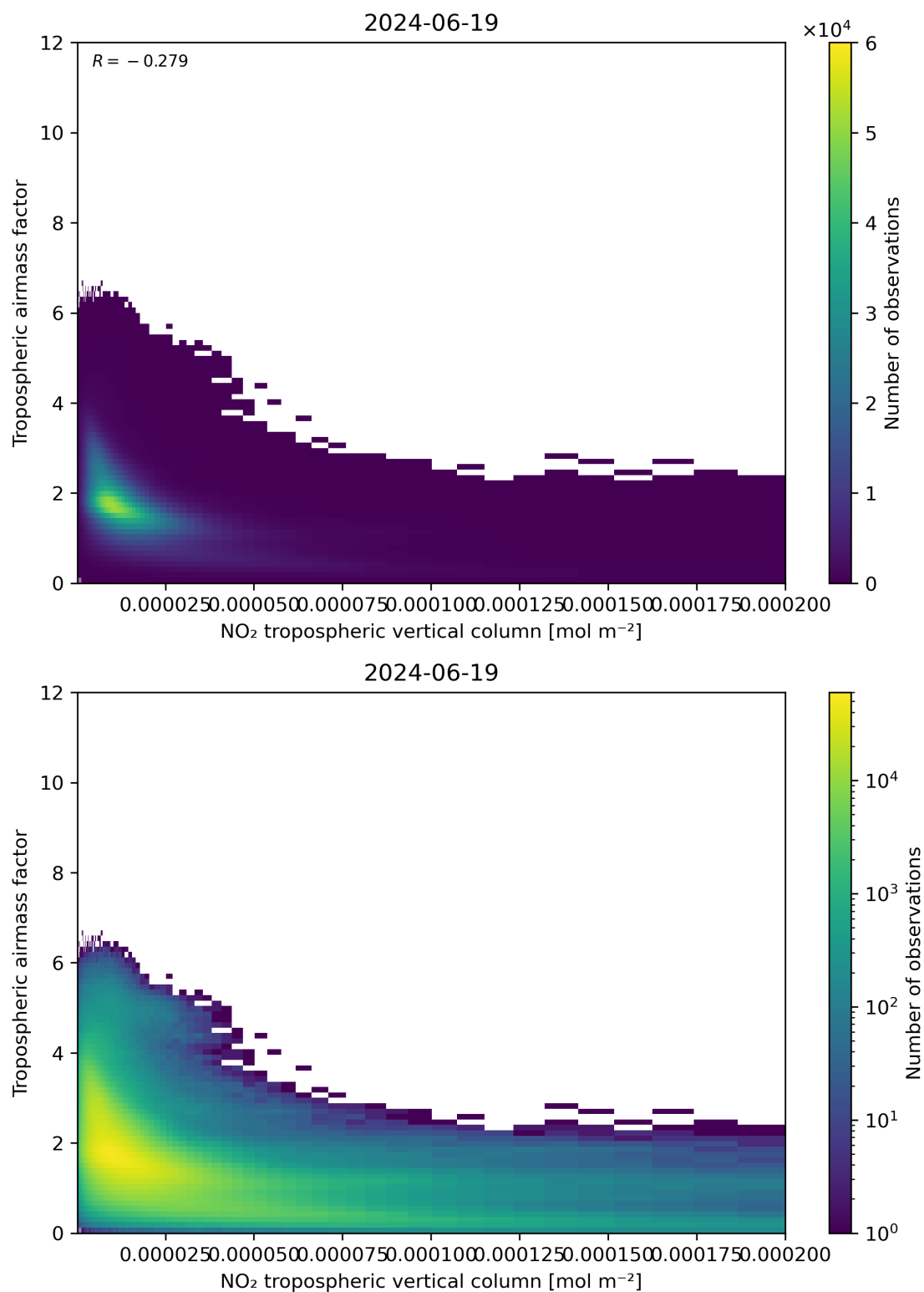
Figure 123: Scatter density plot of “NO 2 tropospheric vertical column” against “Tropospheric airmass factor” for 2024-06-19 to 2024-06-20.
