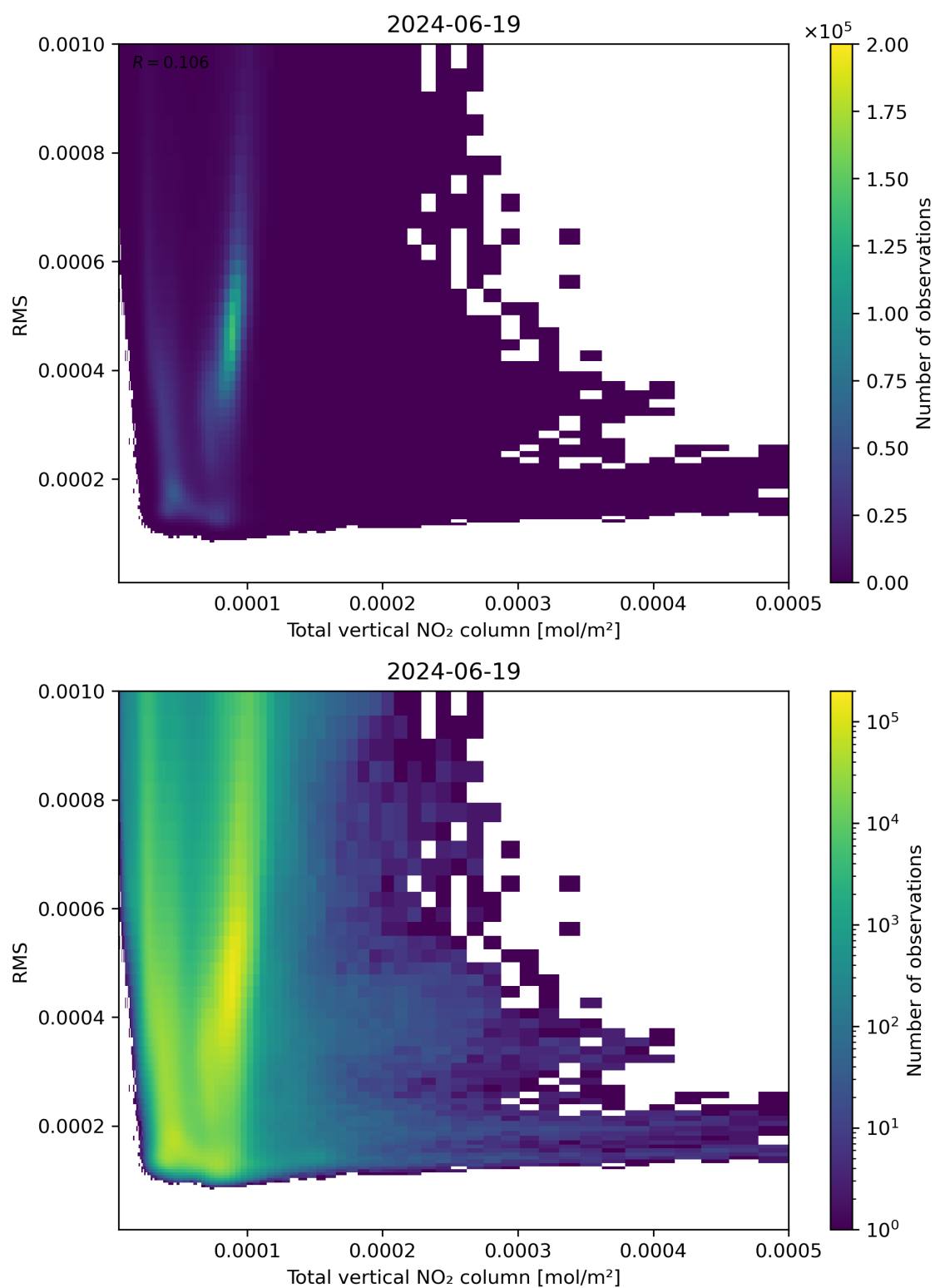
Figure 120: Scatter density plot of “Total vertical NO 2 column” against “RMS” for 2024-06-19 to 2024-06-20.
