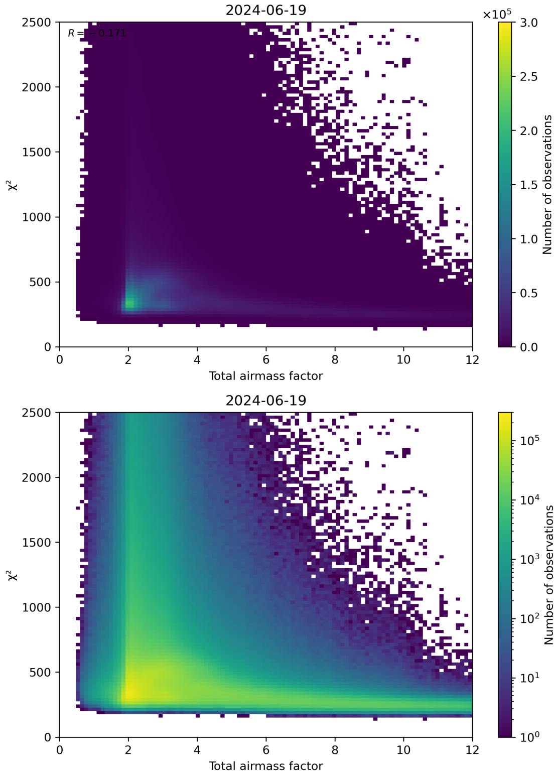
Figure 63: Scatter density plot of “Total airmass factor” against “ \chi^2 ” for 2024-06-19 to 2024-06-20.
