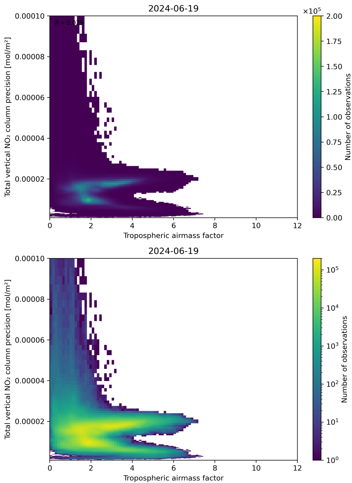
Figure 78: Scatter density plot of “Tropospheric air mass factor” against “Total vertical NO 2 column precision” for 2024-06-19 to 2024-06-20.
