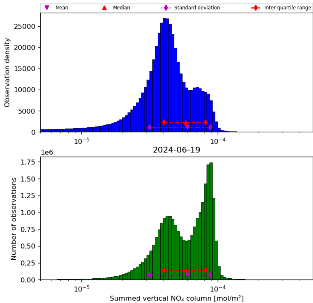
Figure 40: Histogram of “Summed vertical NO 2 column” for 2024-06-19 to 2024-06-20
