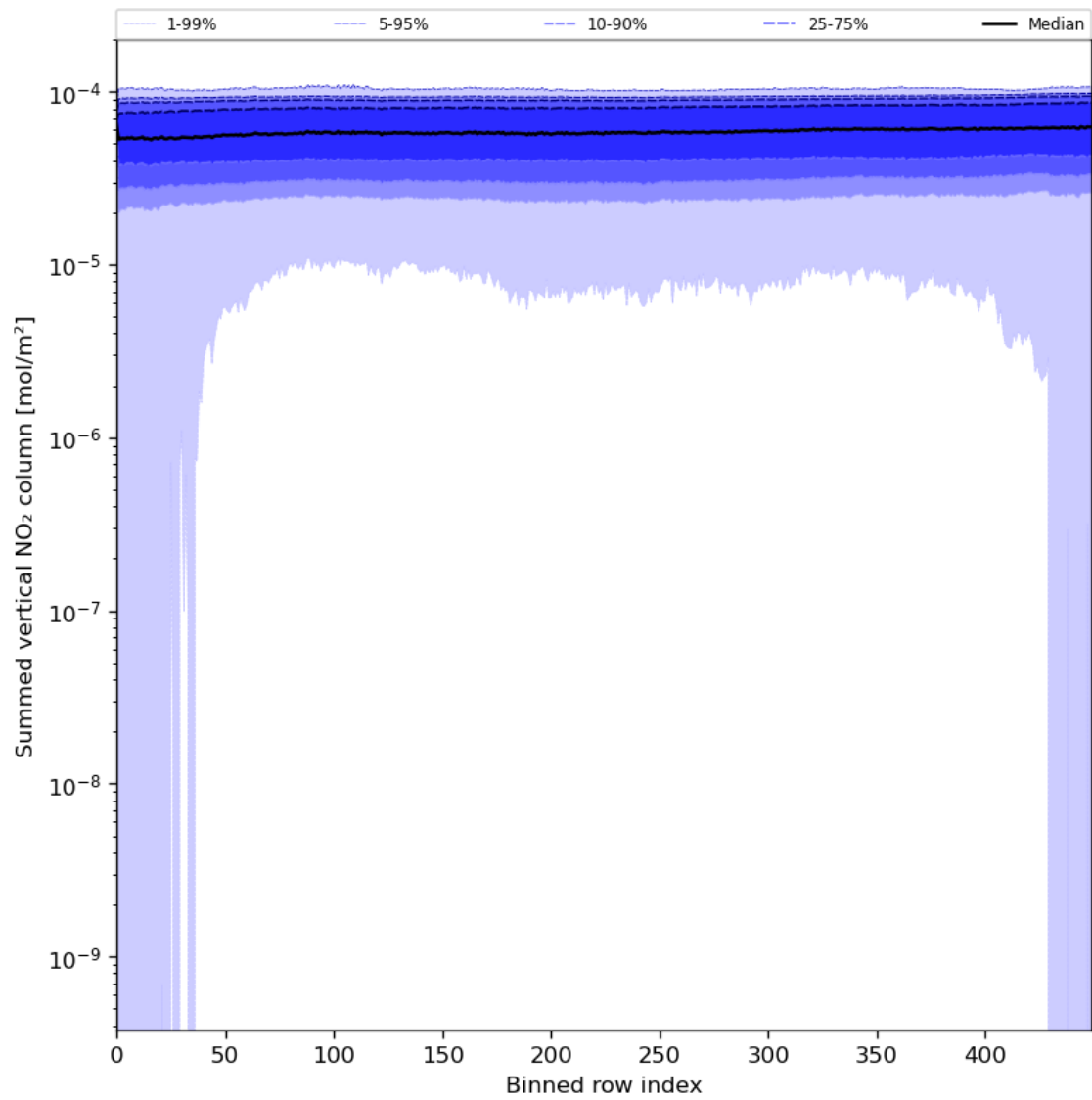
Figure 57: Along track statistics of “Summed vertical NO 2 column” for 2024-06-19 to 2024-06-20
