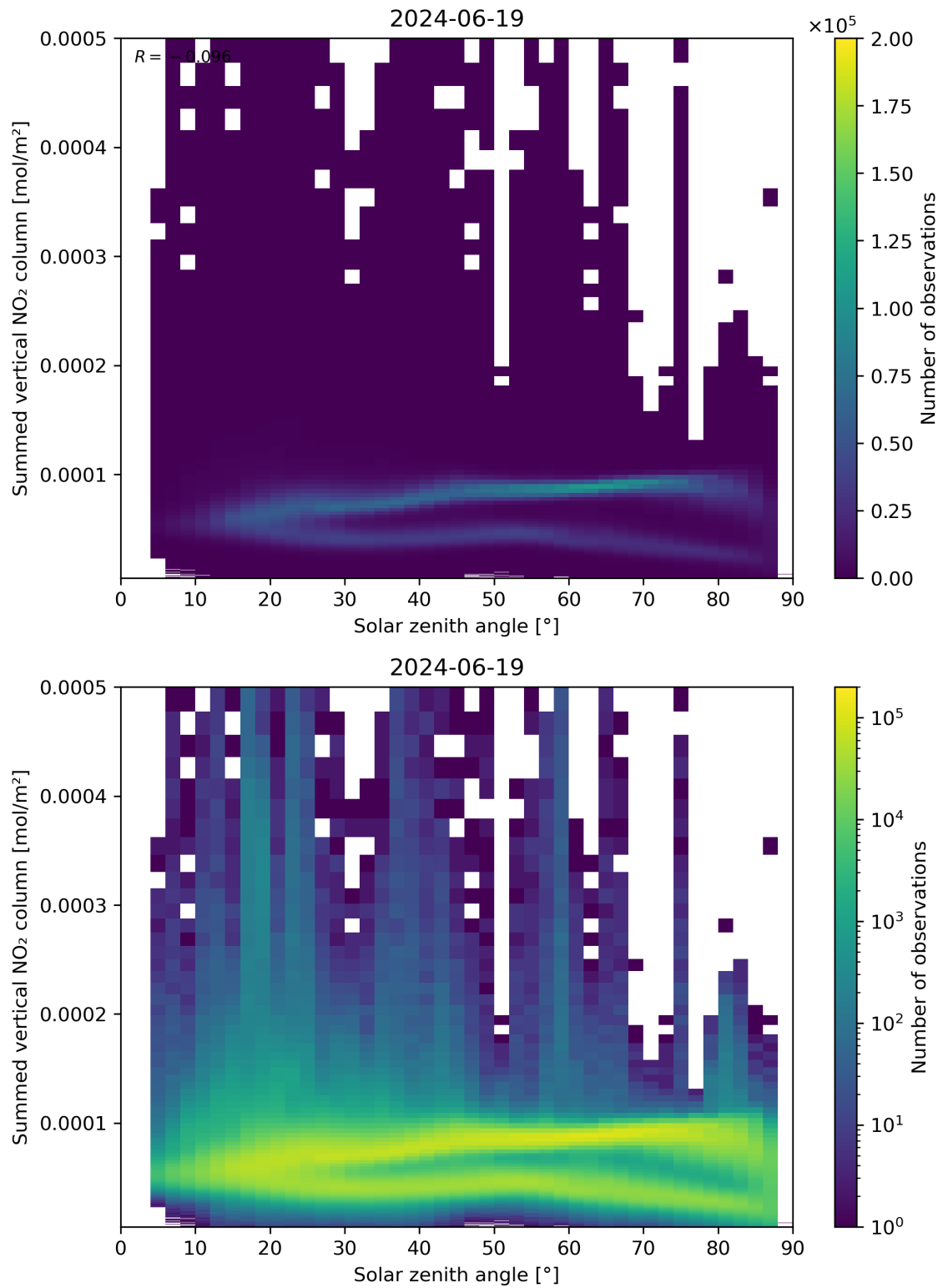
Figure 151: Scatter density plot of “Solar zenith angle” against “Summed vertical NO 2 column” for 2024-06-19 to 2024-06-20.
