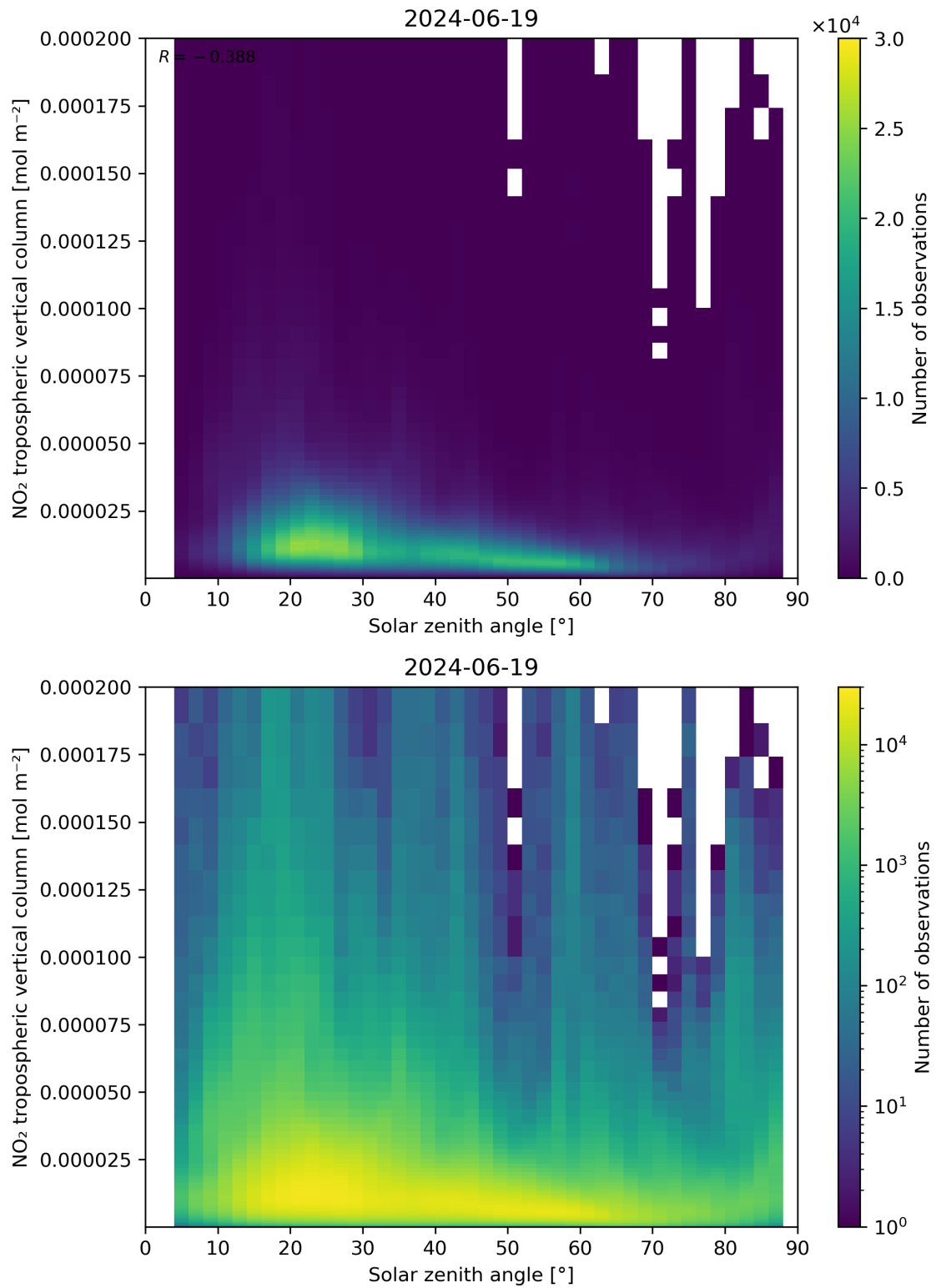
Figure 155: Scatter density plot of “Solar zenith angle” against “NO 2 tropospheric vertical column” for 2024-06-19 to 2024-06-20.
