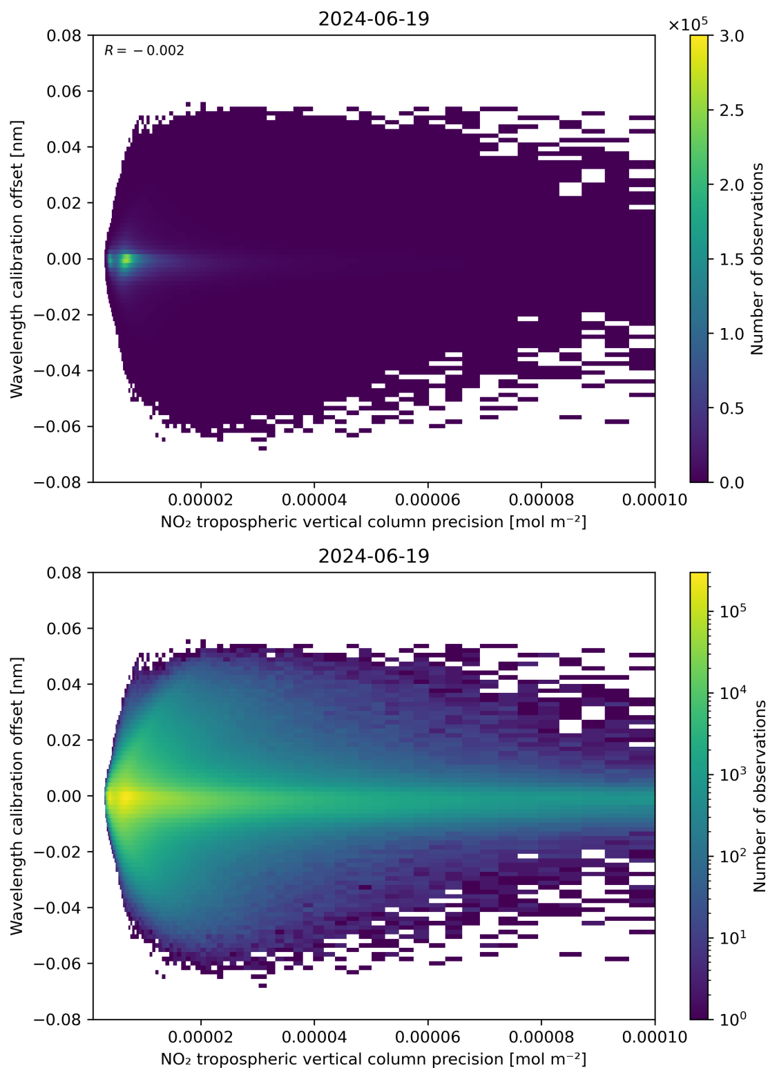
Figure 141: Scatter density plot of “NO 2 tropospheric vertical column precision” against “Wavelength calibration offset” for 2024-06-19 to 2024-06-20.
