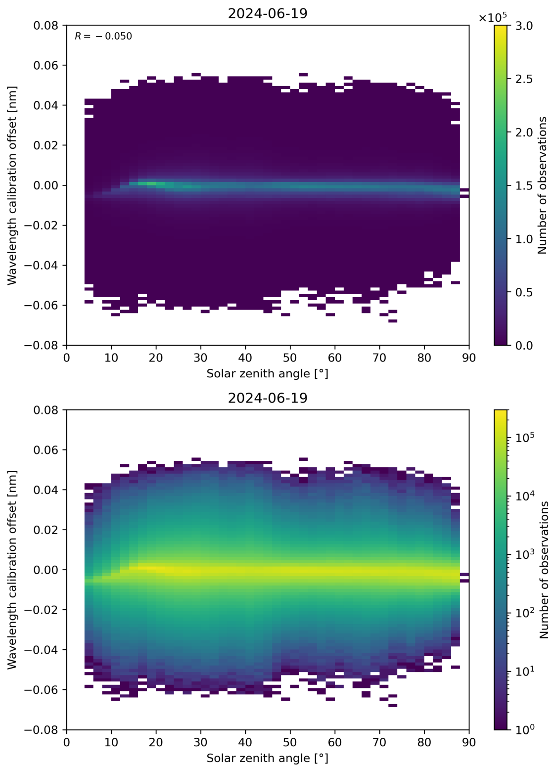
Figure 158: Scatter density plot of “Solar zenith angle” against “Wavelength calibration offset” for 2024-06-19 to 2024-06-20.
