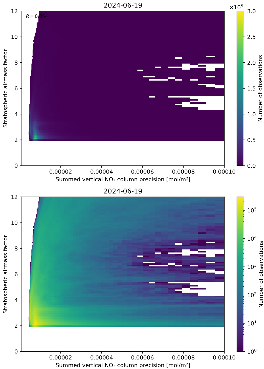
Figure 106: Scatter density plot of “Summed vertical NO 2 column precision” against “Stratospheric airmass factor” for 2024-06-19 to 2024-06-20.
