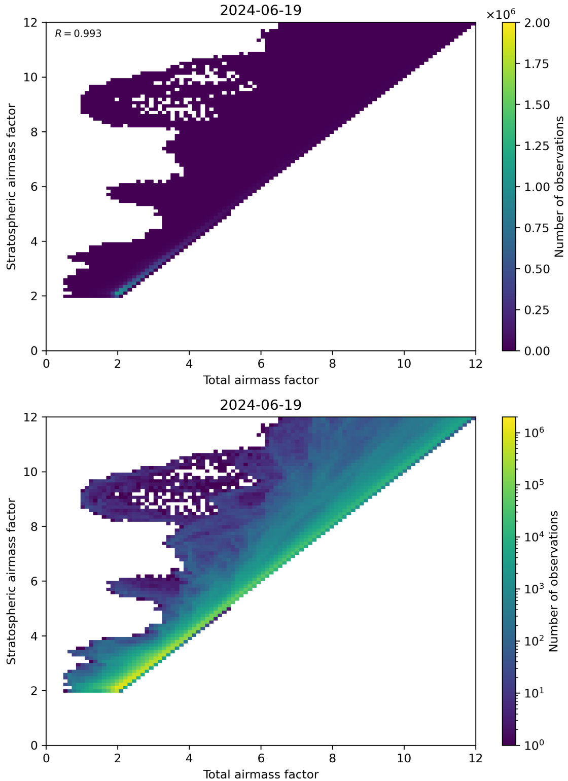
Figure 62: Scatter density plot of “Total airmass factor” against “Stratospheric airmass factor” for 2024-06-19 to 2024-06-20.
