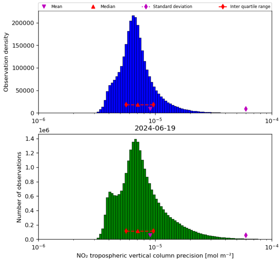
Figure 30: Histogram of “NO 2 tropospheric vertical column precision” for 2024-06-19 to 2024-06-20
