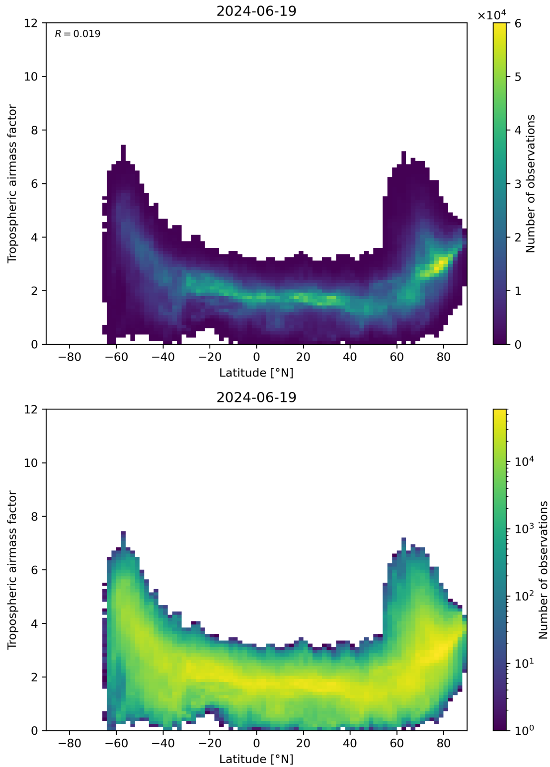
Figure 85: Scatter density plot of “Latitude” against “Tropospheric airmass factor” for 2024-06-19 to 2024-06-20.
