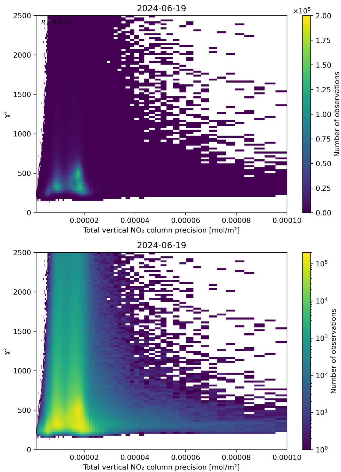
Figure 116: Scatter density plot of “Total vertical NO 2 column precision” against “ \chi^2 ” for 2024-06-19 to 2024-06-20.
