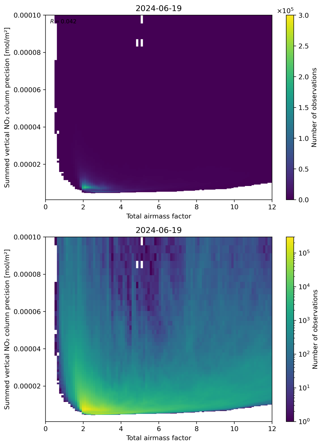
Figure 66: Scatter density plot of “Total airmass factor” against “Summed vertical NO 2 column precision” for 2024-06-19 to 2024-06-20.
