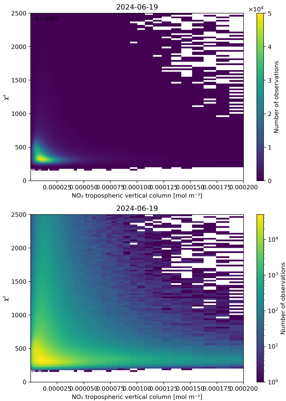
Figure 124: Scatter density plot of “NO 2 tropospheric vertical column” against “ \chi^2 ” for 2024-06-19 to 2024-06-20.
