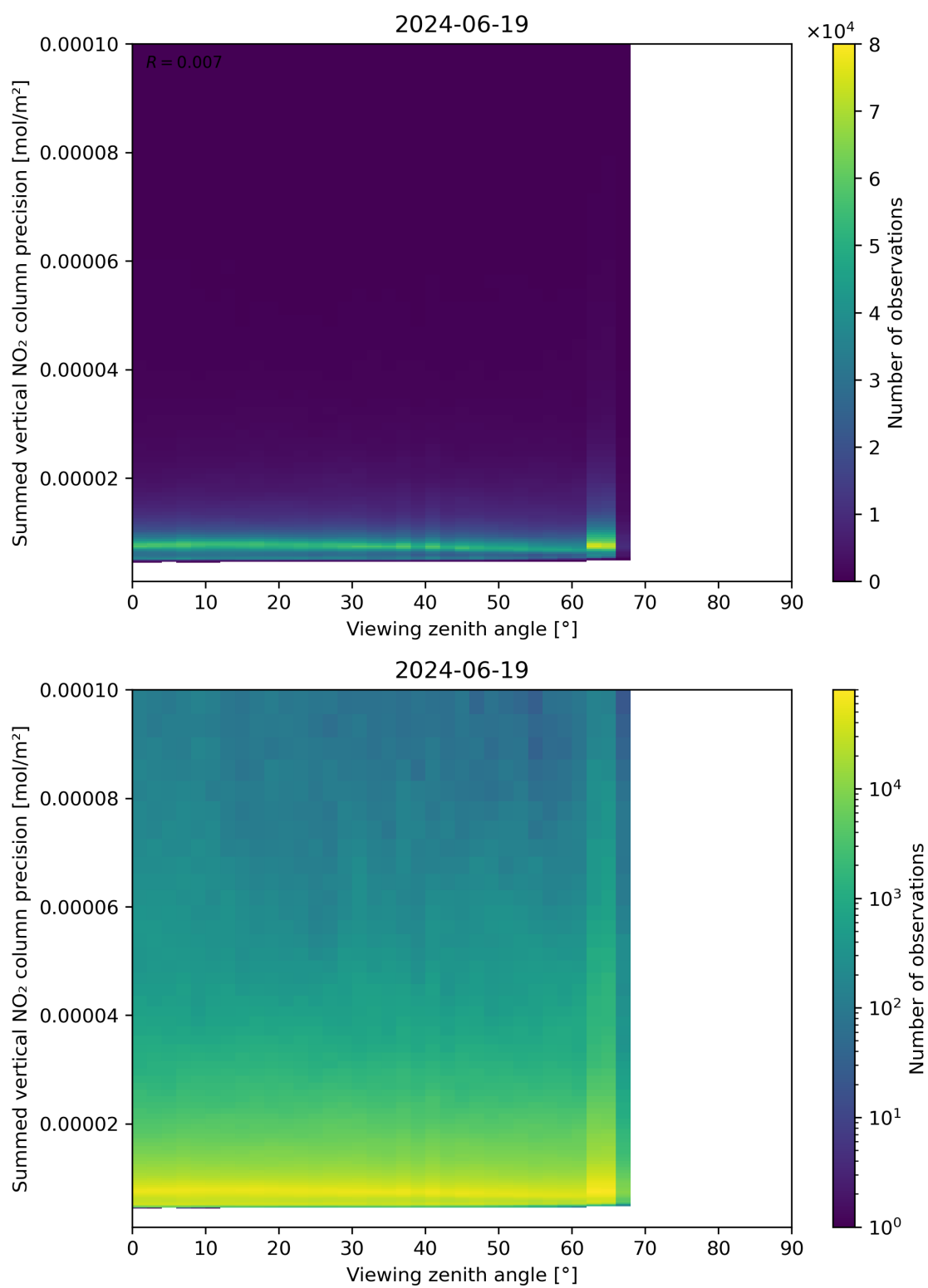
Figure 166: Scatter density plot of “Viewing zenith angle” against “Summed vertical NO 2 column precision” for 2024-06-19 to 2024-06-20.
