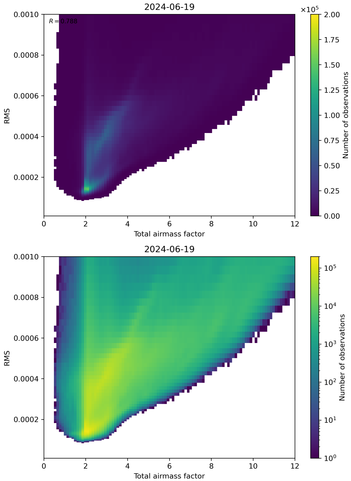
Figure 69: Scatter density plot of “Total airmass factor” against “RMS” for 2024-06-19 to 2024-06-20.
