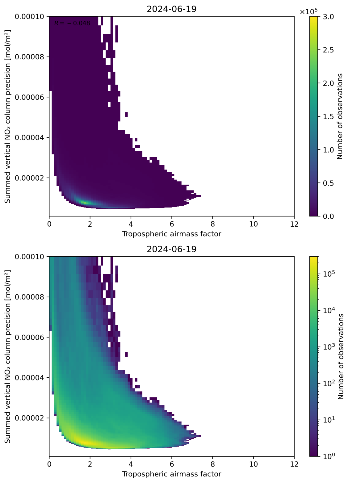
Figure 76: Scatter density plot of “Tropospheric air mass factor” against “Summed vertical NO 2 column precision” for 2024-06-19 to 2024-06-20.
