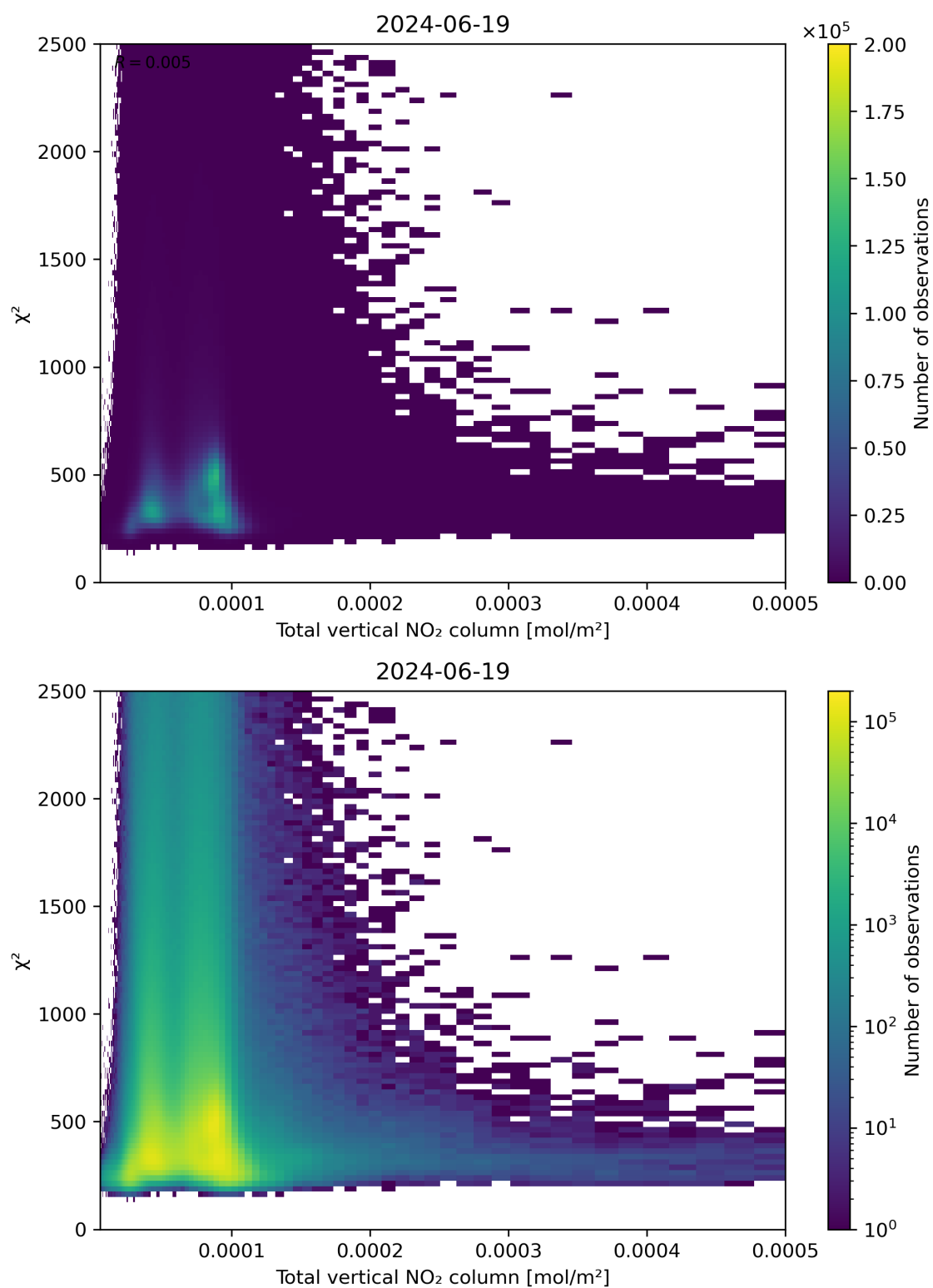
Figure 111: Scatter density plot of “Total vertical NO 2 column” against “ \chi^2 ” for 2024-06-19 to 2024-06-20.
