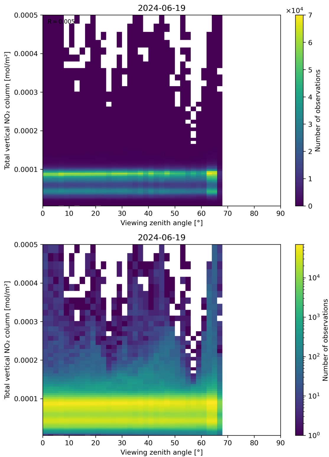
Figure 167: Scatter density plot of “Viewing zenith angle” against “Total vertical NO 2 column” for 2024-06-19 to 2024-06-20.
