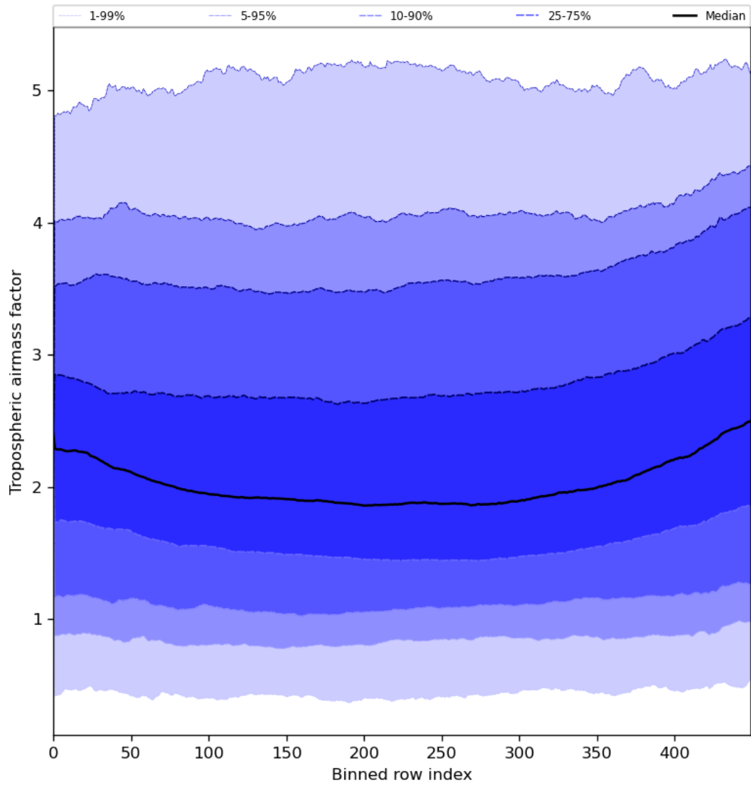
Figure 48: Along track statistics of “Tropospheric airmass factor” for 2024-06-19 to 2024-06-20
