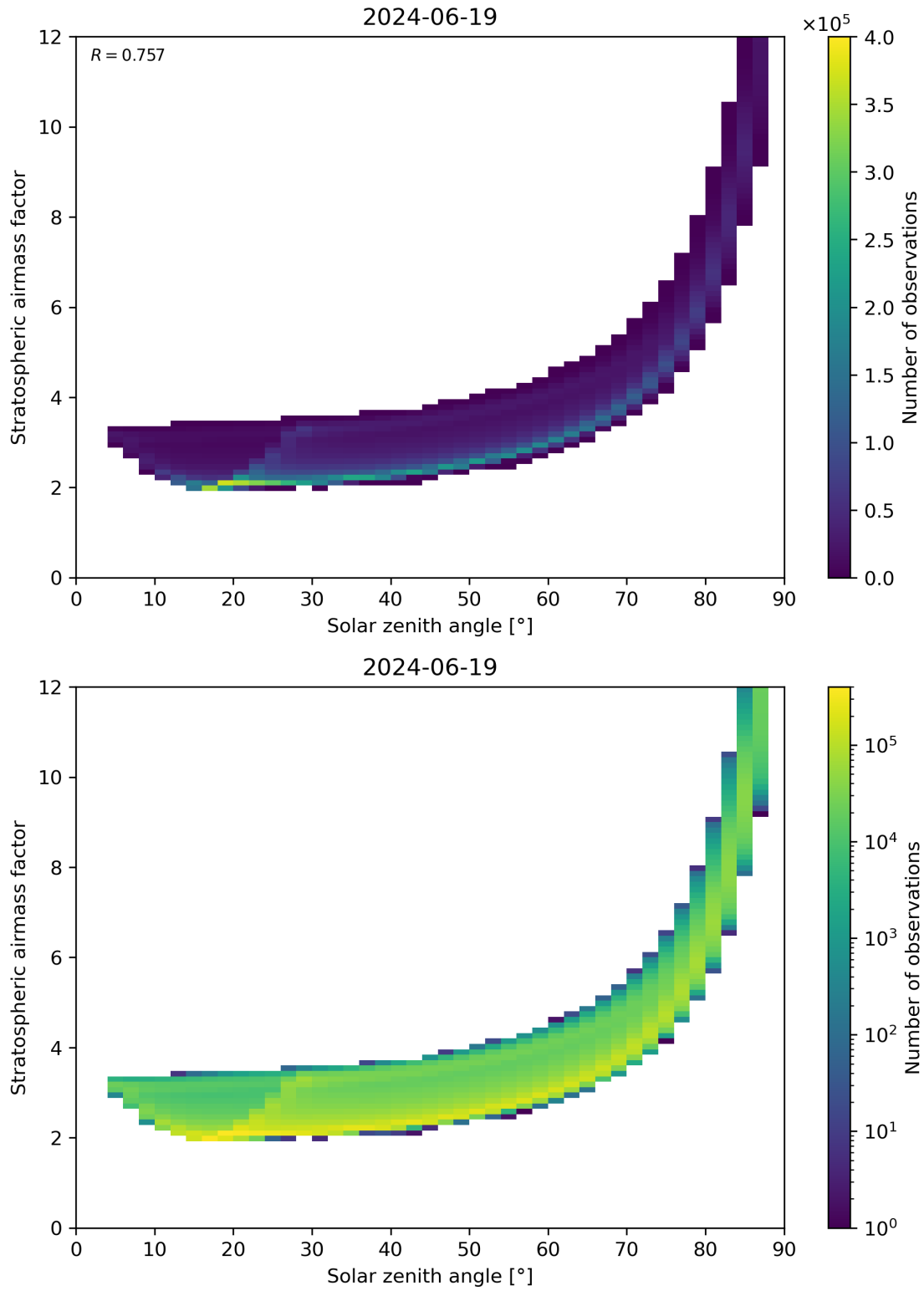
Figure 145: Scatter density plot of “Solar zenith angle” against “Stratospheric airmass factor” for 2024-06-19 to 2024-06-20.
