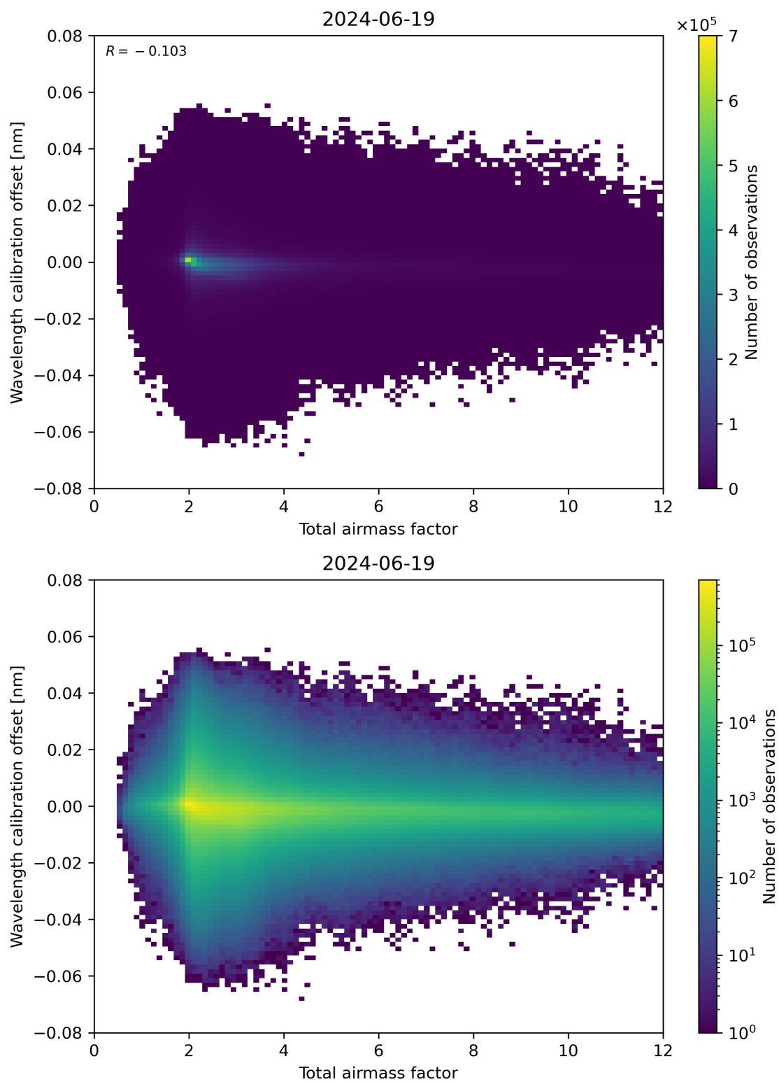
Figure 70: Scatter density plot of “Total airmass factor” against “Wavelength calibration offset” for 2024-06-19 to 2024-06-20.
