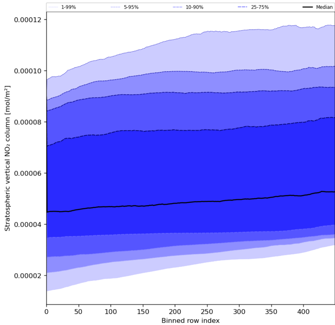
Figure 53: Along track statistics of “Stratospheric vertical NO 2 column” for 2024-06-19 to 2024-06-20
