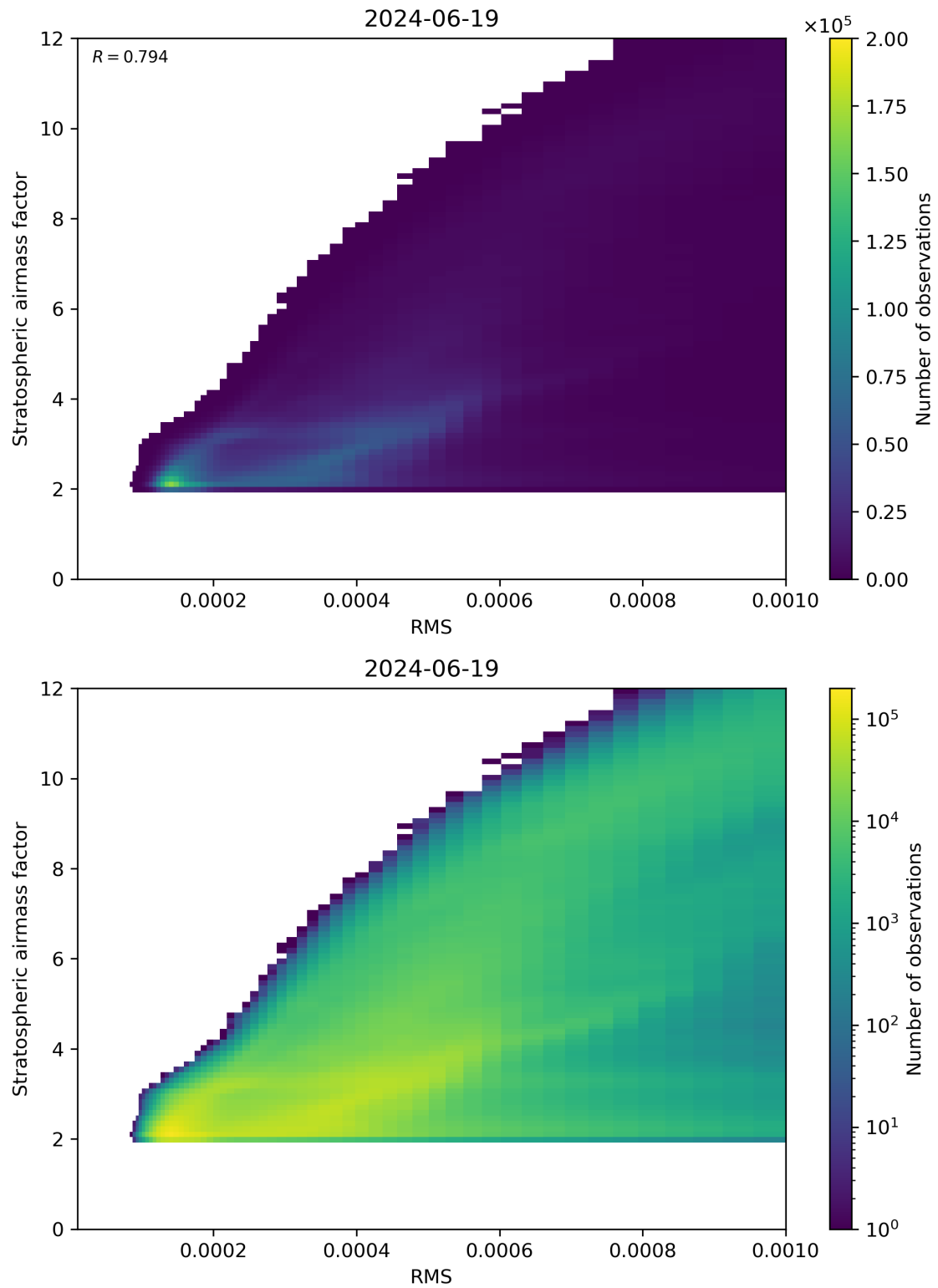
Figure 144: Scatter density plot of “RMS” against “Stratospheric airmass factor” for 2024-06-19 to 2024-06-20.
