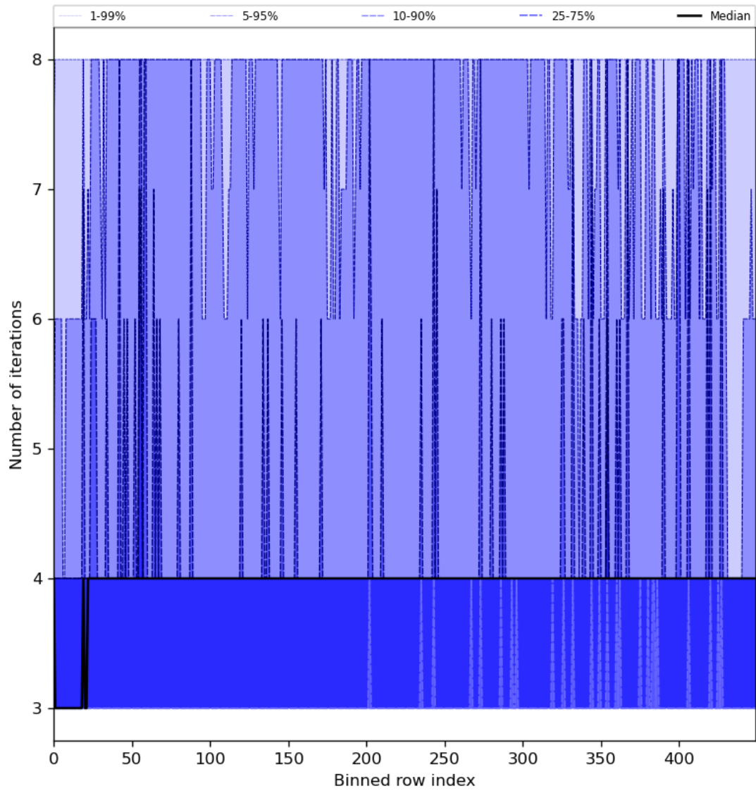
Figure 51: Along track statistics of “Number of iterations” for 2024-06-19 to 2024-06-20
