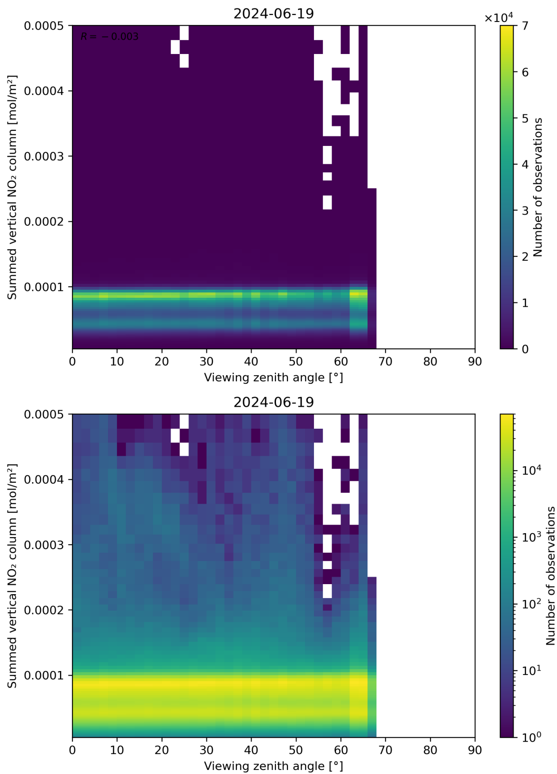
Figure 165: Scatter density plot of “Viewing zenith angle” against “Summed vertical NO 2 column” for 2024-06-19 to 2024-06-20.
