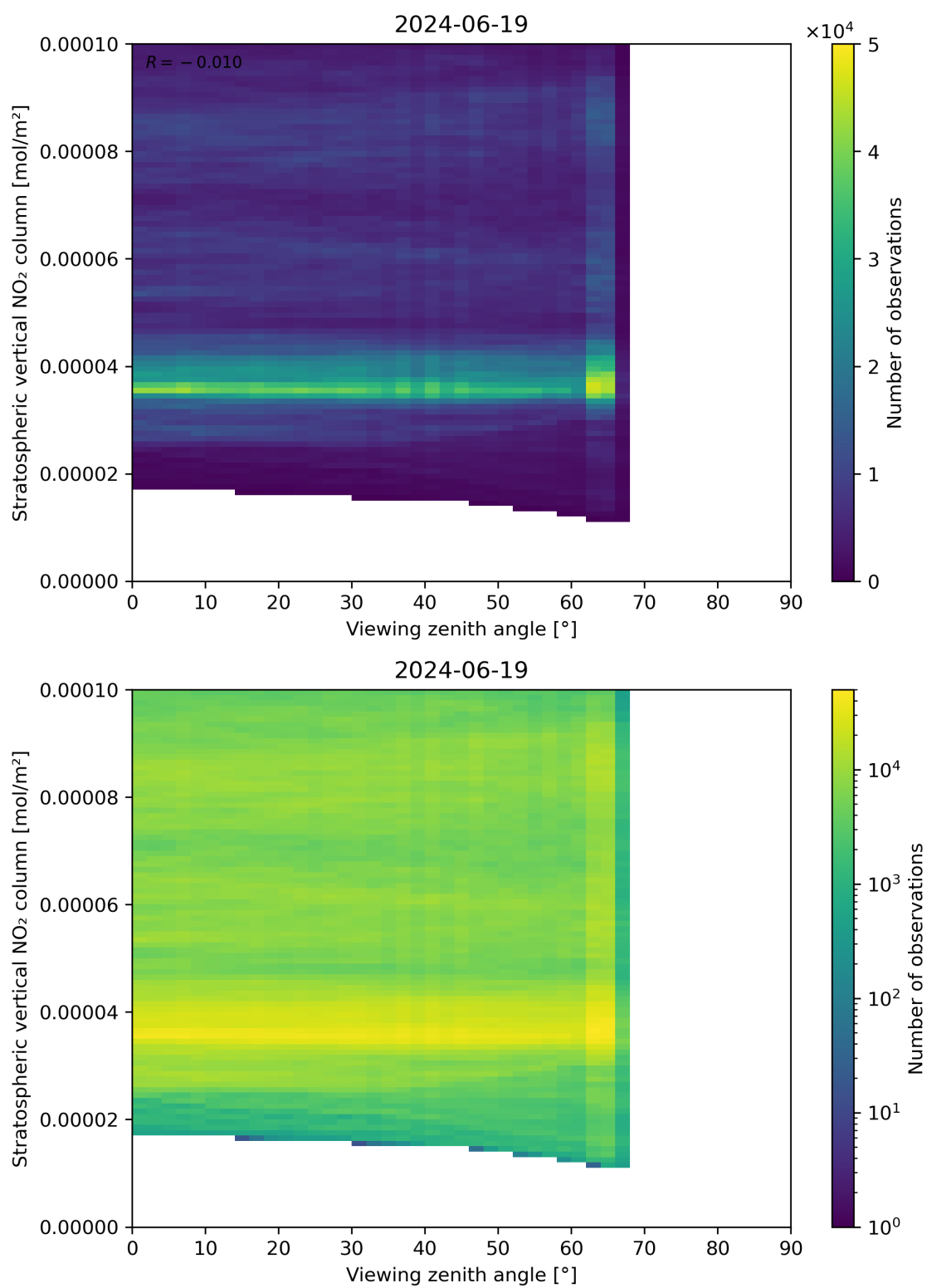
Figure 164: Scatter density plot of “Viewing zenith angle” against “Stratospheric vertical NO 2 column” for 2024-06-19 to 2024-06-20.
