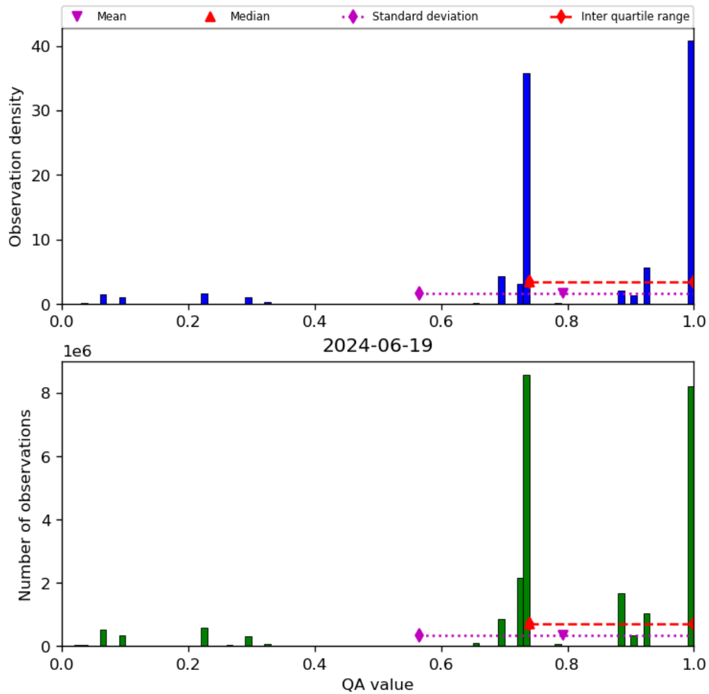
Figure 28: Histogram of “QA value” for 2024-06-19 to 2024-06-20
