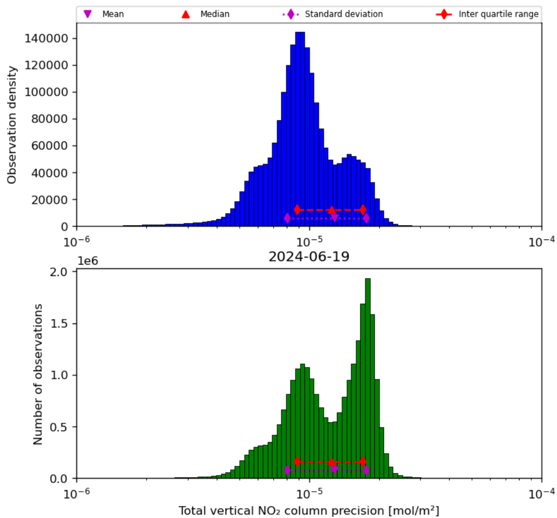
Figure 39: Histogram of “Total vertical NO 2 column precision” for 2024-06-19 to 2024-06-20
