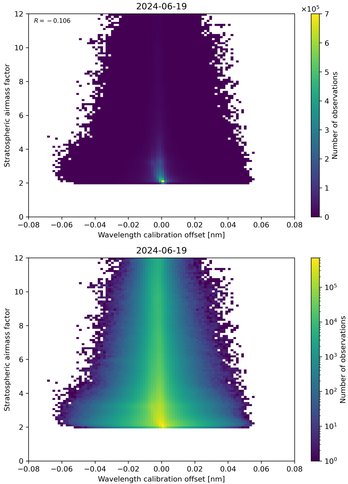
Figure 174: Scatter density plot of “Wavelength calibration offset” against “Stratospheric airmass factor” for 2024-06-19 to 2024-06-20.
