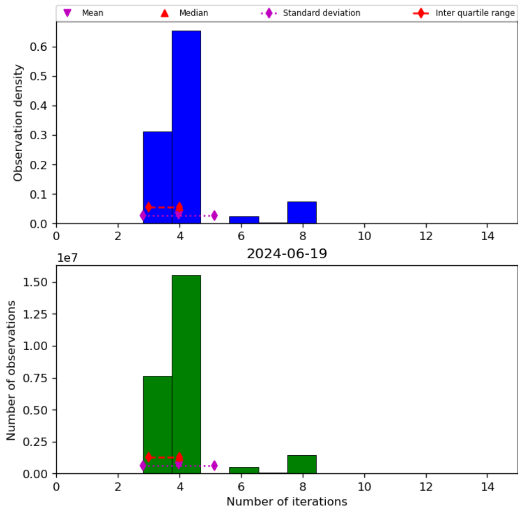
Figure 34: Histogram of “Number of iterations” for 2024-06-19 to 2024-06-20
