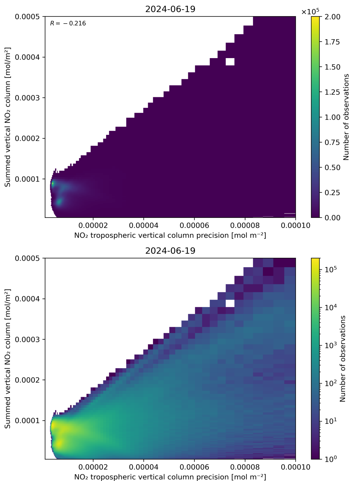
Figure 136: Scatter density plot of “NO 2 tropospheric vertical column precision” against “Summed vertical NO 2 column” for 2024-06-19 to 2024-06-20.
