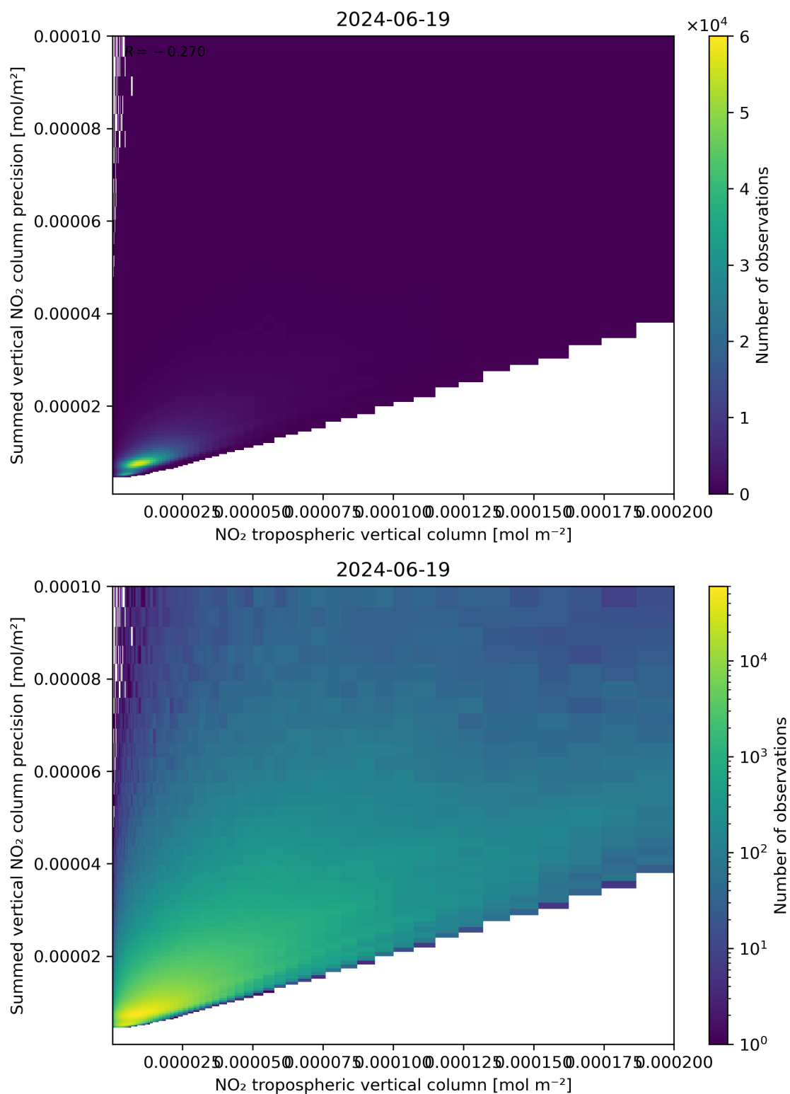
Figure 127: Scatter density plot of “NO 2 tropospheric vertical column” against “Summed vertical NO 2 column precision” for 2024-06-19 to 2024-06-20.
