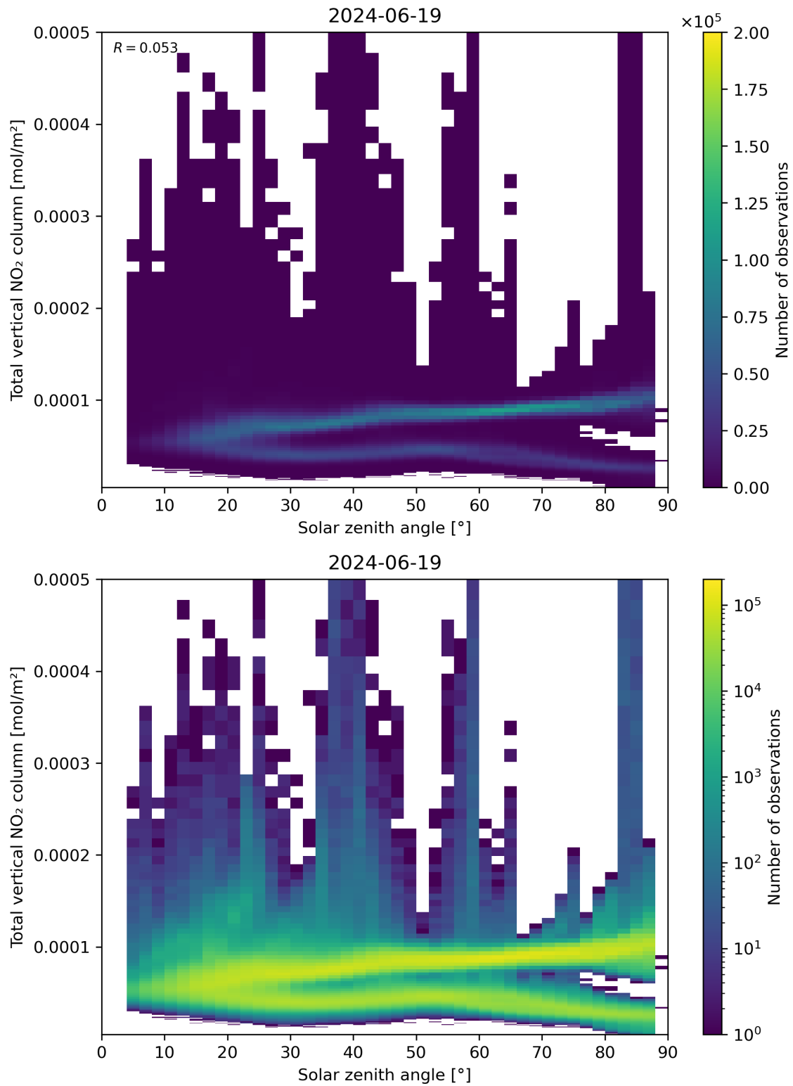
Figure 153: Scatter density plot of “Solar zenith angle” against “Total vertical NO 2 column” for 2024-06-19 to 2024-06-20.
