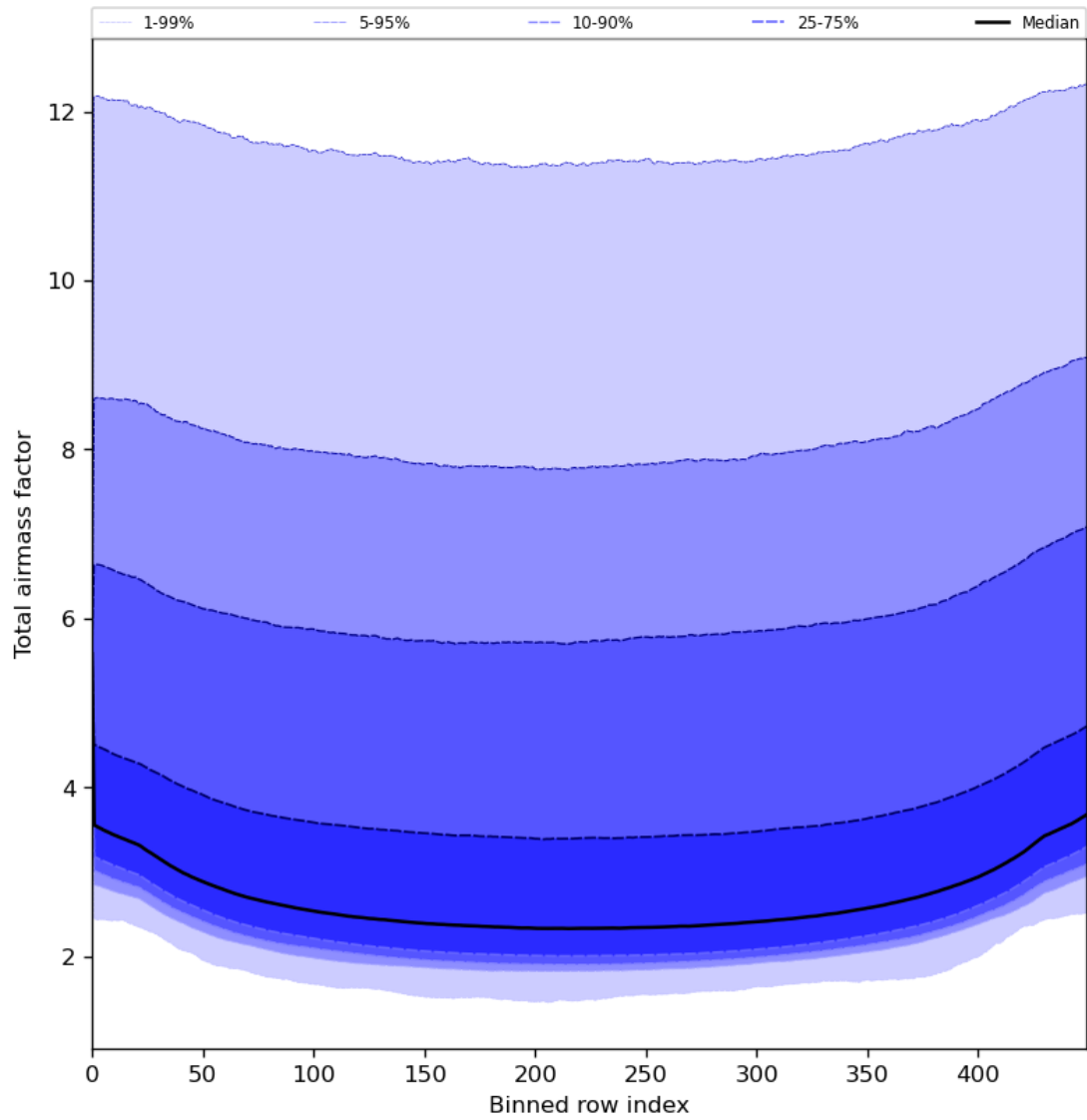
Figure 49: Along track statistics of “Total airmass factor” for 2024-06-19 to 2024-06-20
