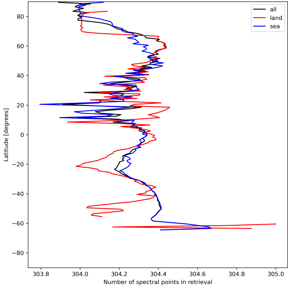
Figure 16: Zonal average of “Number of spectral points in retrieval” for 2024-06-19 to 2024-06-20.
