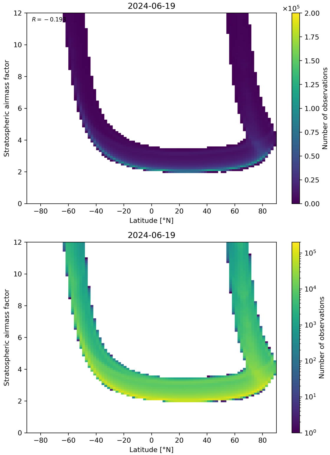
Figure 83: Scatter density plot of “Latitude” against “Stratospheric air mass factor” for 2024-06-19 to 2024-06-20.
