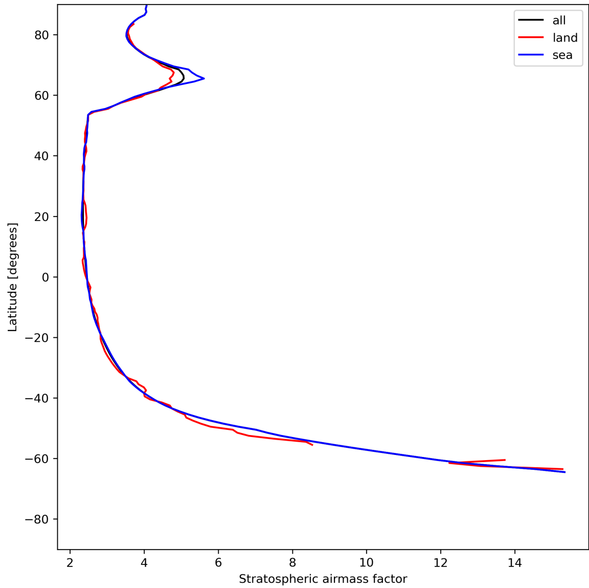
Figure 27: Zonal average of “Stratospheric airmass factor” for 2024-06-19 to 2024-06-20.
