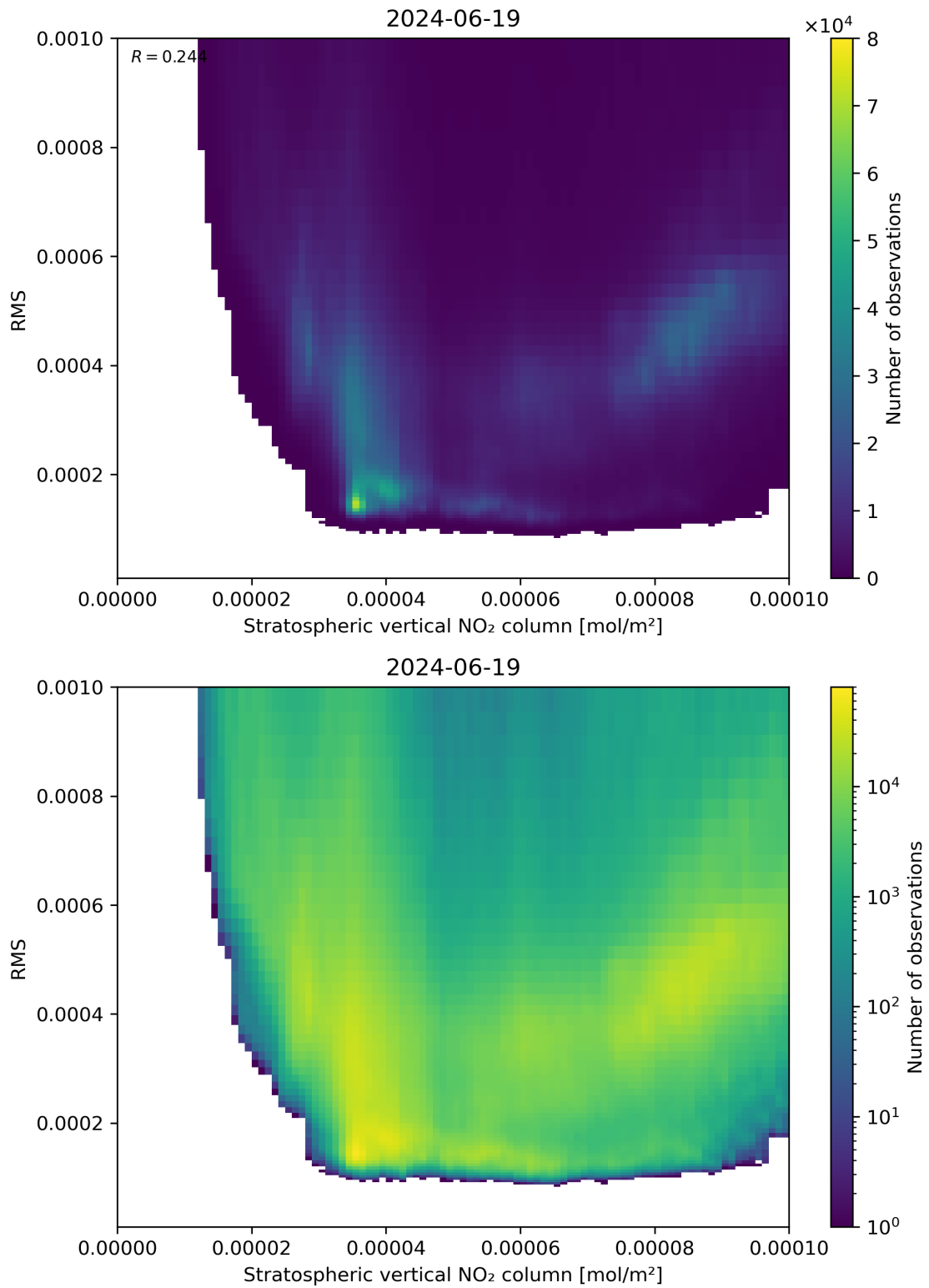
Figure 102: Scatter density plot of “Stratospheric vertical NO 2 column” against “RMS” for 2024-06-19 to 2024-06-20.
