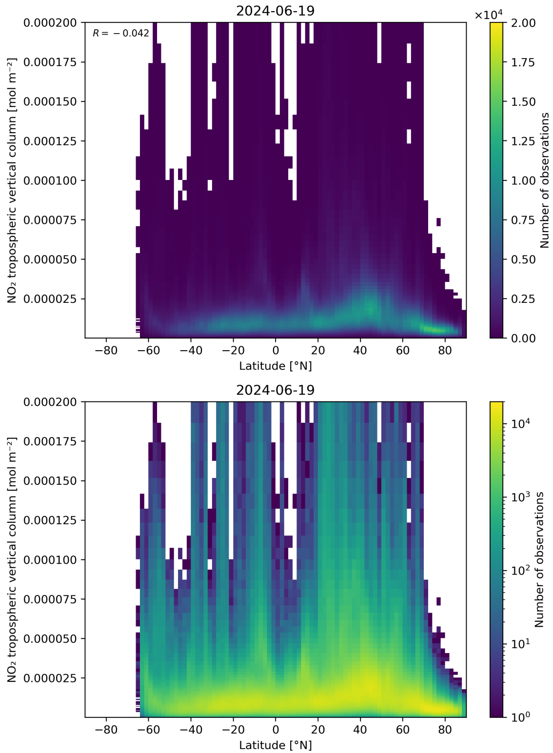
Figure 92: Scatter density plot of “Latitude” against “NO 2 tropospheric vertical column” for 2024-06-19 to 2024-06-20.
