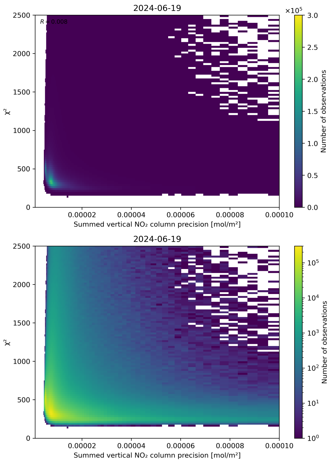
Figure 107: Scatter density plot of “Summed vertical NO 2 column precision” against “ \chi^2 ” for 2024-06-19 to 2024-06-20.
