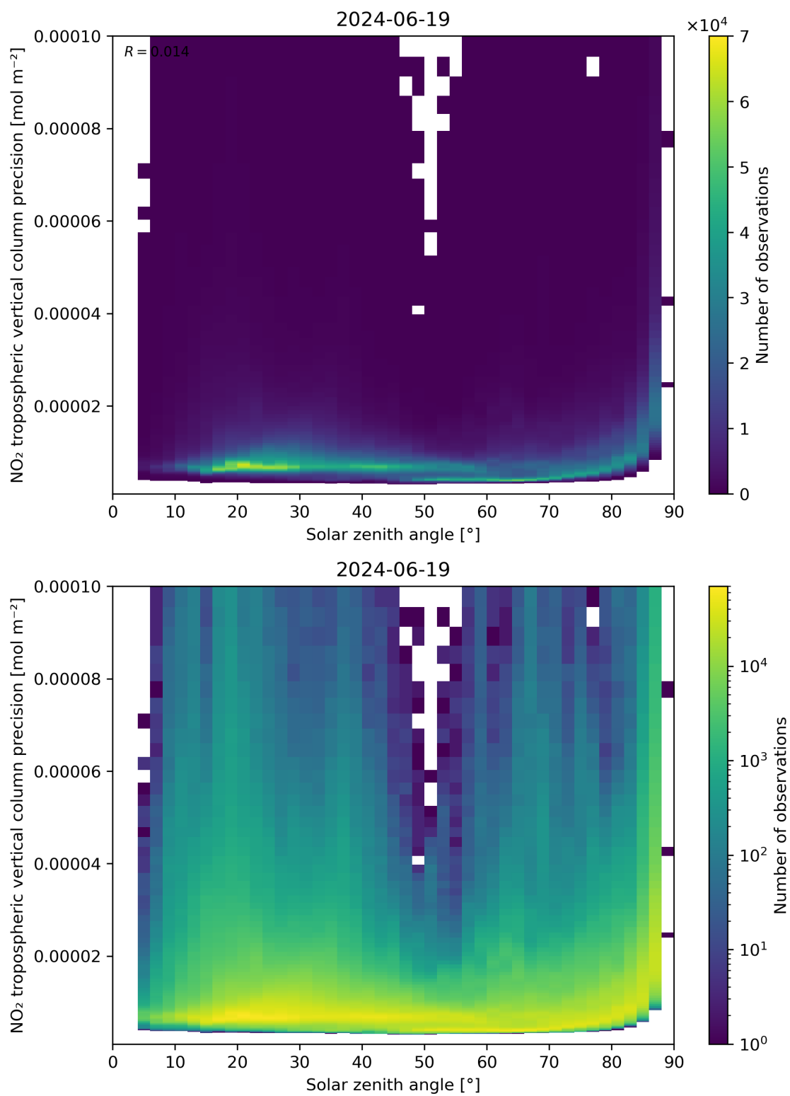
Figure 156: Scatter density plot of “Solar zenith angle” against “NO 2 tropospheric vertical column precision” for 2024-06-19 to 2024-06-20.
