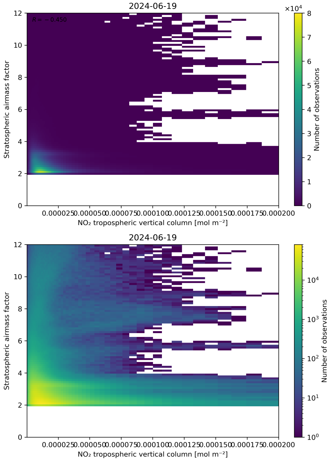
Figure 121: Scatter density plot of “NO 2 tropospheric vertical column” against “Stratospheric air mass factor” for 2024-06-19 to 2024-06-20.
