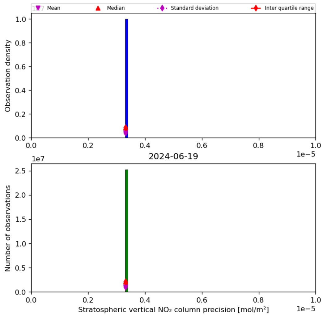
Figure 37: Histogram of “Stratospheric vertical NO 2 column precision” for 2024-06-19 to 2024-06-20
