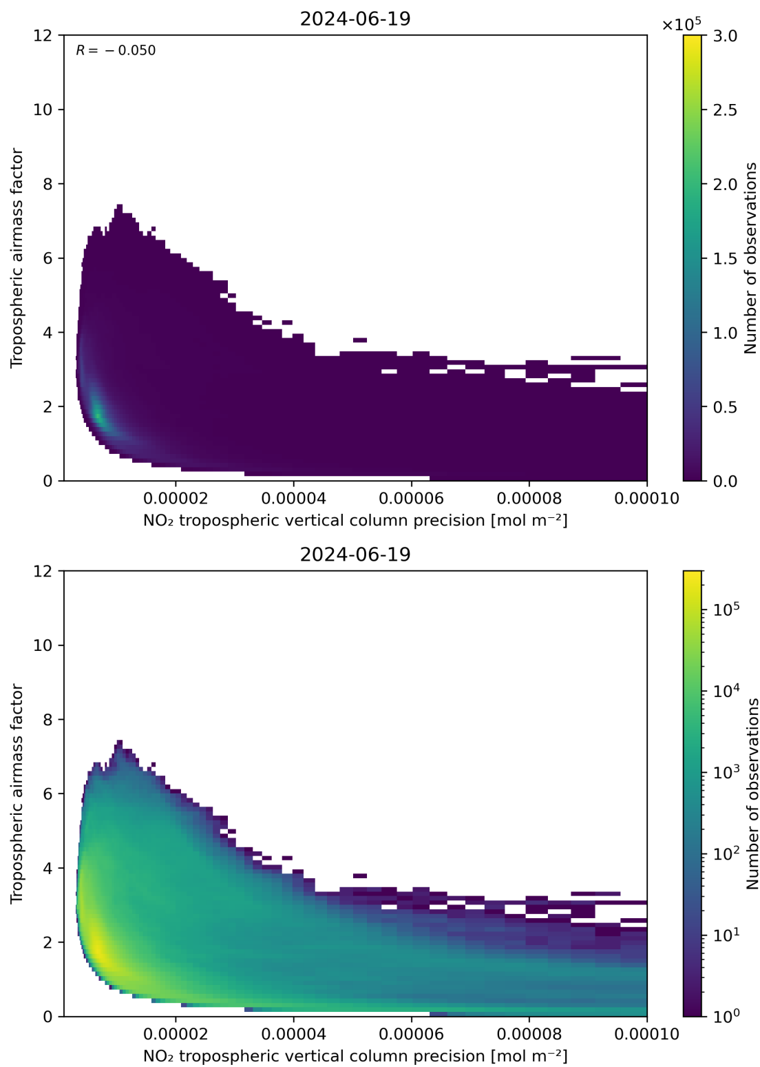
Figure 133: Scatter density plot of “NO 2 tropospheric vertical column precision” against “Tropospheric airmass factor” for 2024-06-19 to 2024-06-20.
