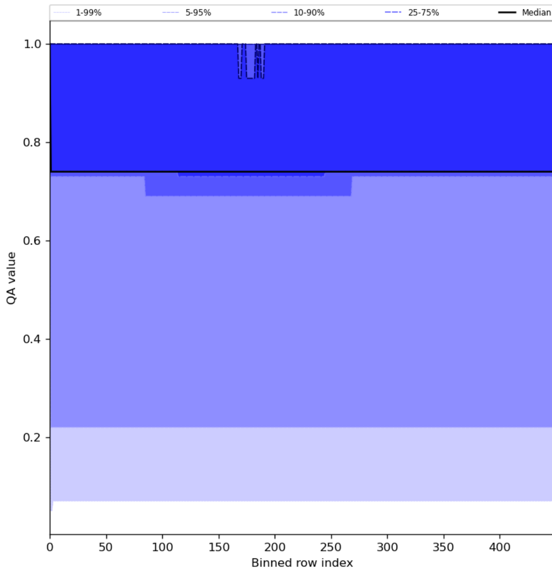
Figure 45: Along track statistics of “QA value” for 2024-06-19 to 2024-06-20
