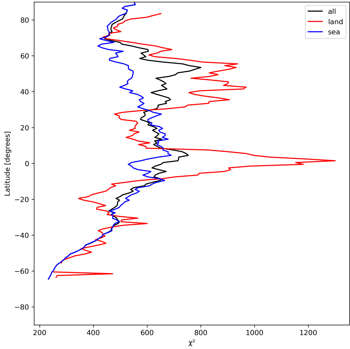
Figure 25: Zonal average of “ \chi^2 ” for 2024-06-19 to 2024-06-20.
