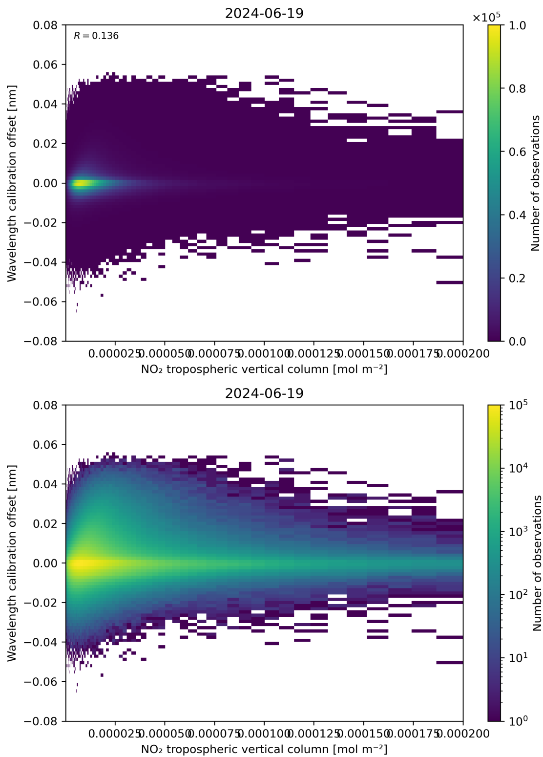
Figure 143: Scatter density plot of “NO 2 tropospheric vertical column” against “Wavelength calibration offset” for 2024-06-19 to 2024-06-20.
