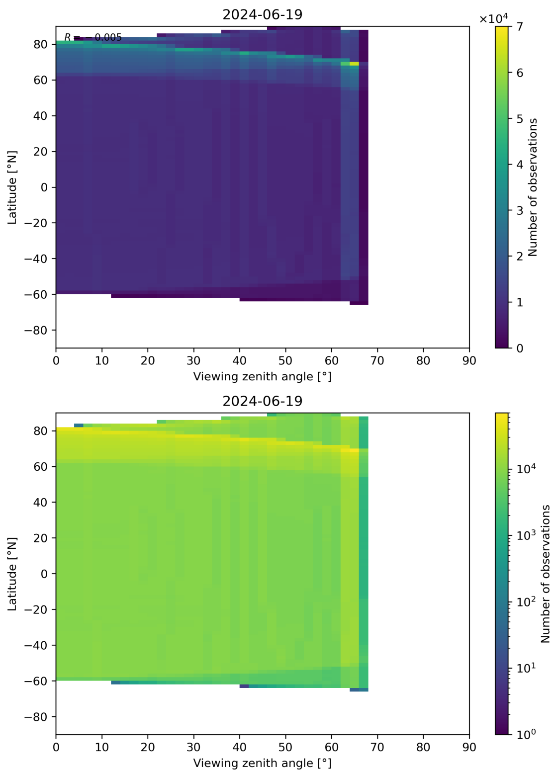
Figure 163: Scatter density plot of “Viewing zenith angle” against “Latitude” for 2024-06-19 to 2024-06-20.
