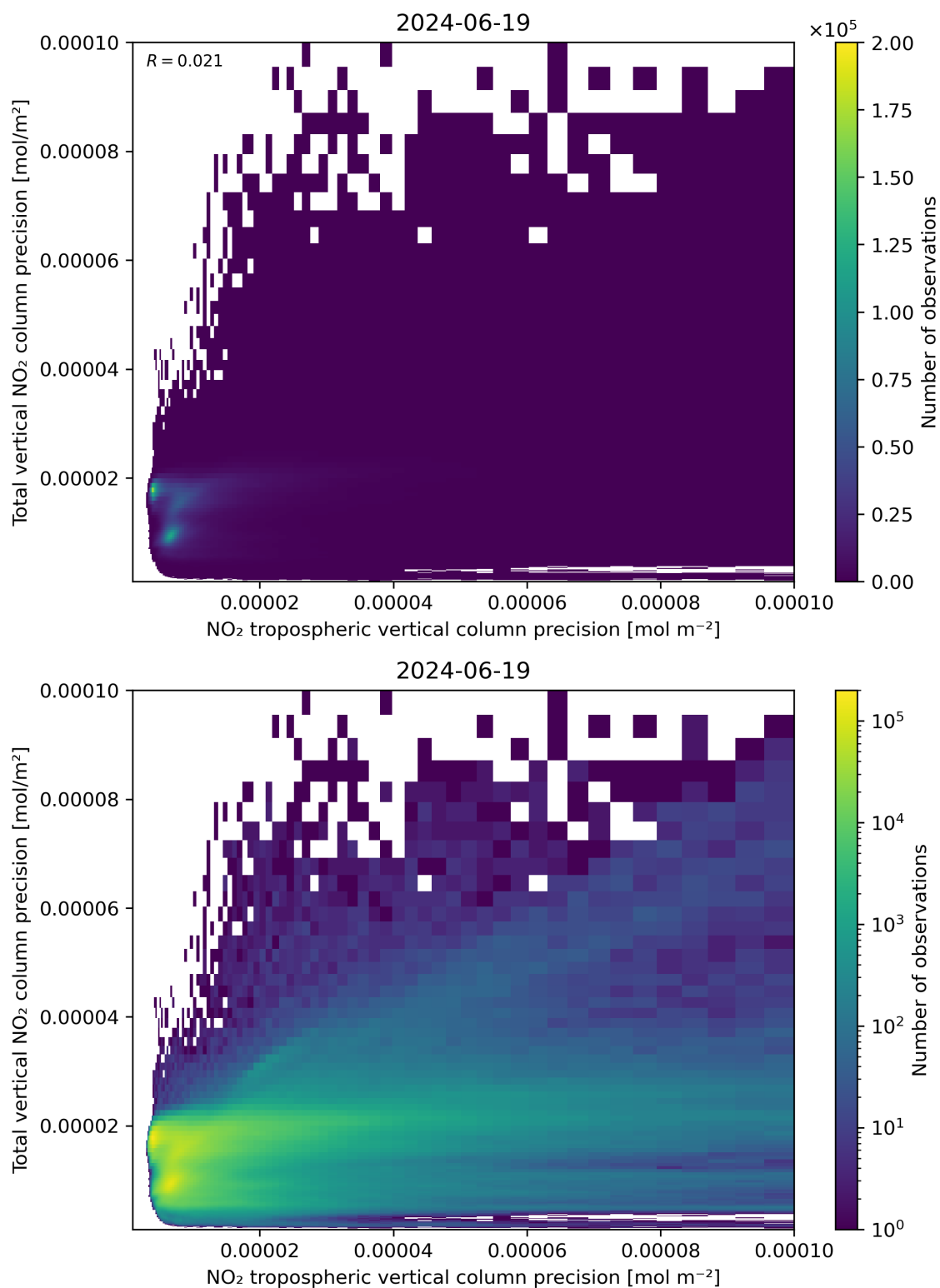
Figure 139: Scatter density plot of “NO 2 tropospheric vertical column precision” against “Total vertical NO 2 column precision” for 2024-06-19 to 2024-06-20.
