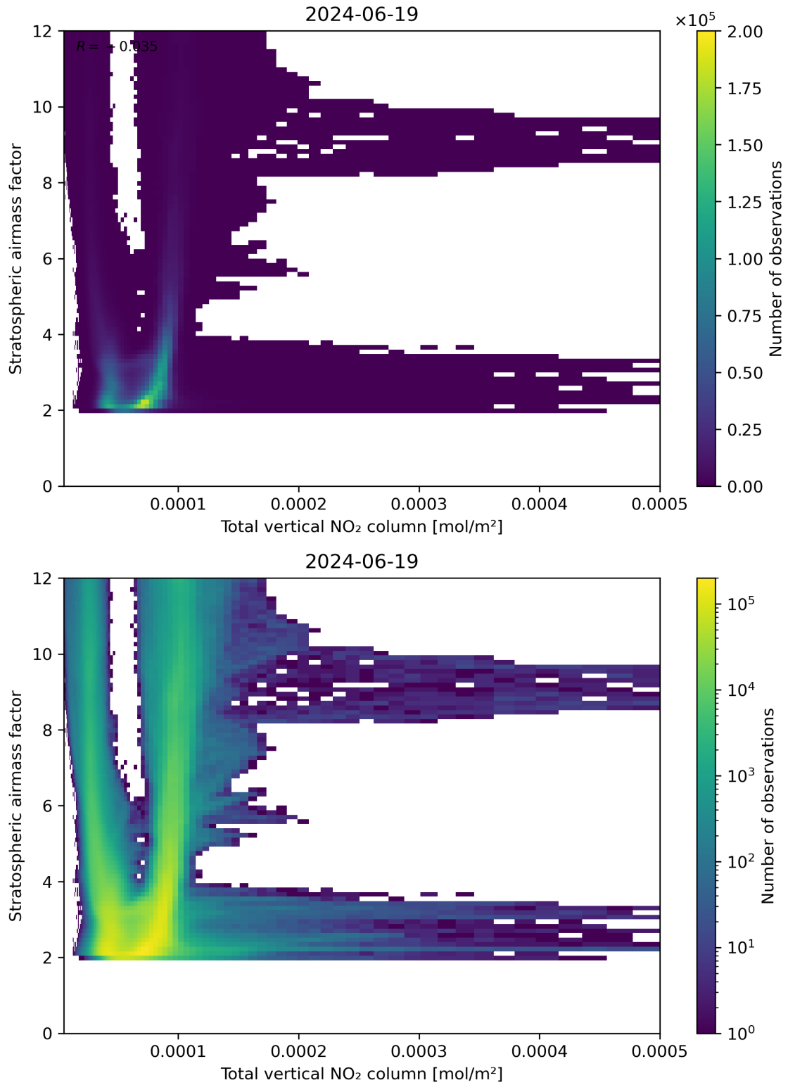
Figure 110: Scatter density plot of “Total vertical NO 2 column” against “Stratospheric airmass factor” for 2024-06-19 to 2024-06-20.
