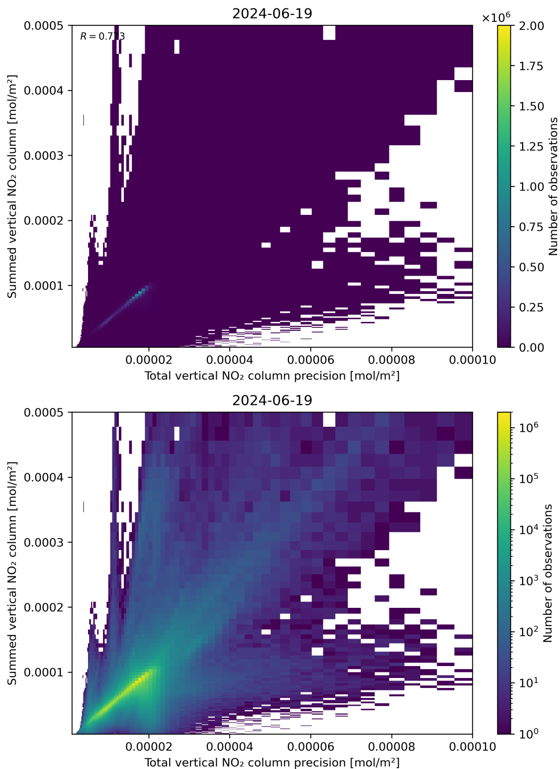
Figure 117: Scatter density plot of “Total vertical NO 2 column precision” against “Summed vertical NO 2 column” for 2024-06-19 to 2024-06-20.
