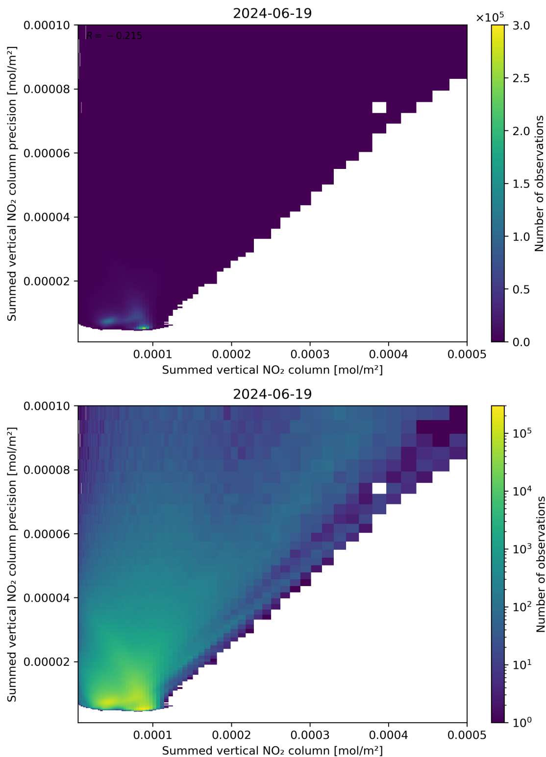
Figure 105: Scatter density plot of “Summed vertical NO 2 column” against “Summed vertical NO 2 column precision” for 2024-06-19 to 2024-06-20.
