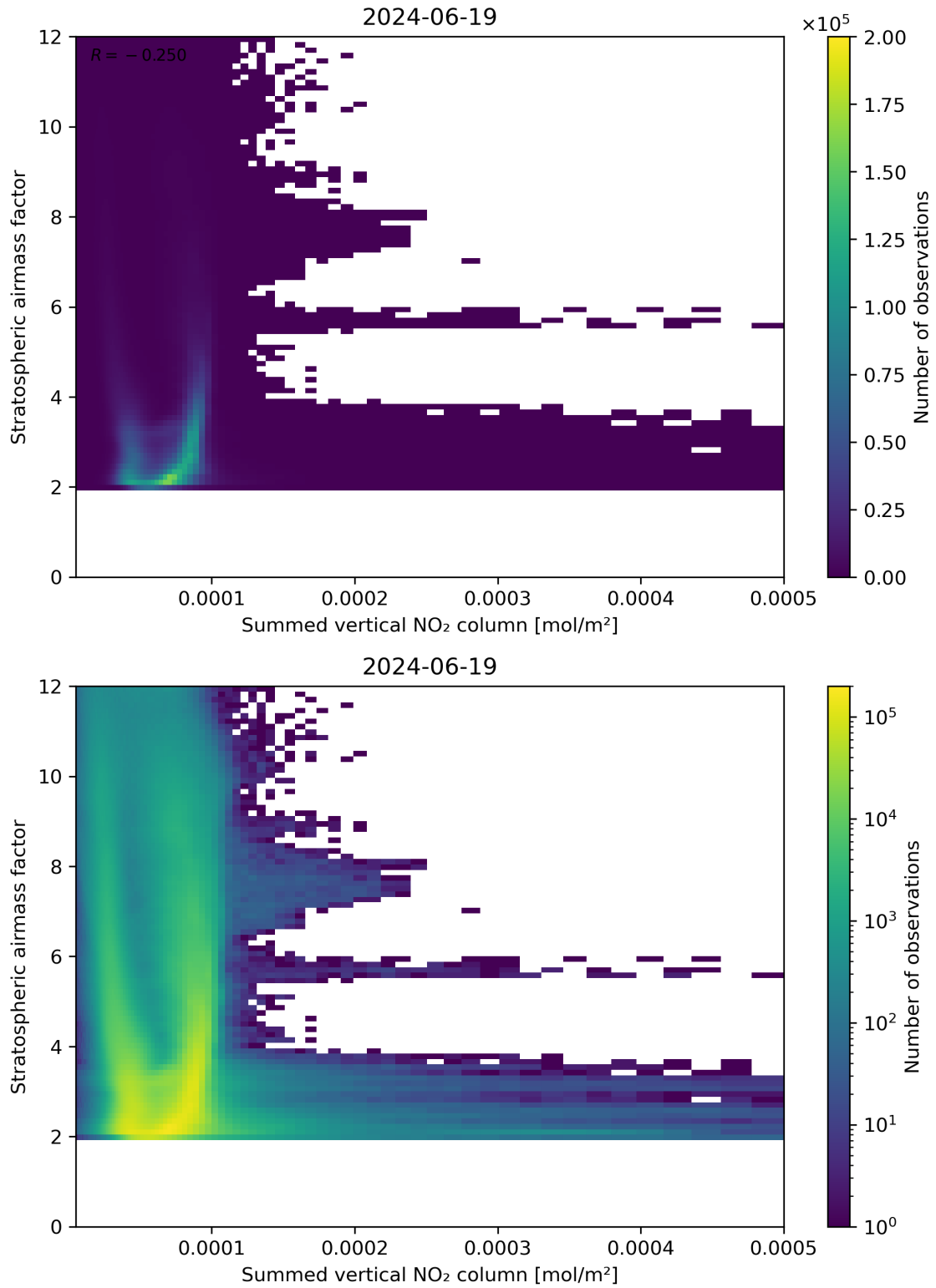
Figure 103: Scatter density plot of “Summed vertical NO 2 column” against “Stratospheric air mass factor” for 2024-06-19 to 2024-06-20.
