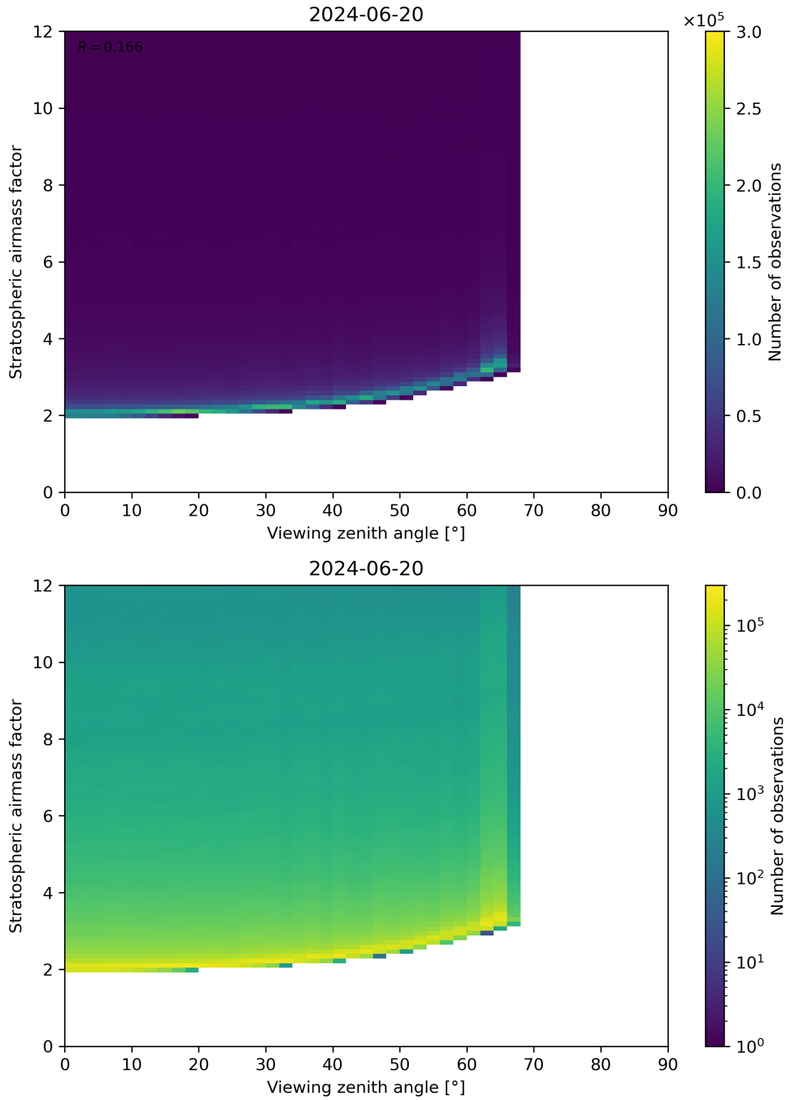
Figure 159: Scatter density plot of “Viewing zenith angle” against “Stratospheric airmass factor” for 2024-06-19 to 2024-06-21.
