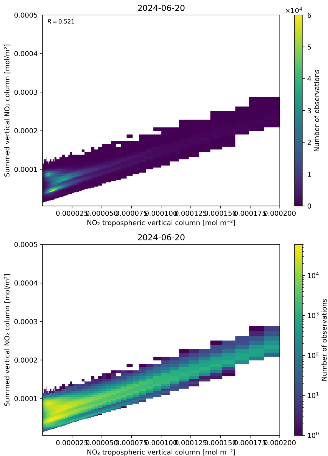
Figure 126: Scatter density plot of “NO 2 tropospheric vertical column” against “Summed vertical NO 2 column” for 2024-06-19 to 2024-06-21.
