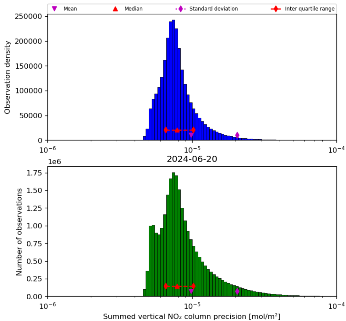
Figure 41: Histogram of “Summed vertical NO 2 column precision” for 2024-06-19 to 2024-06-21
