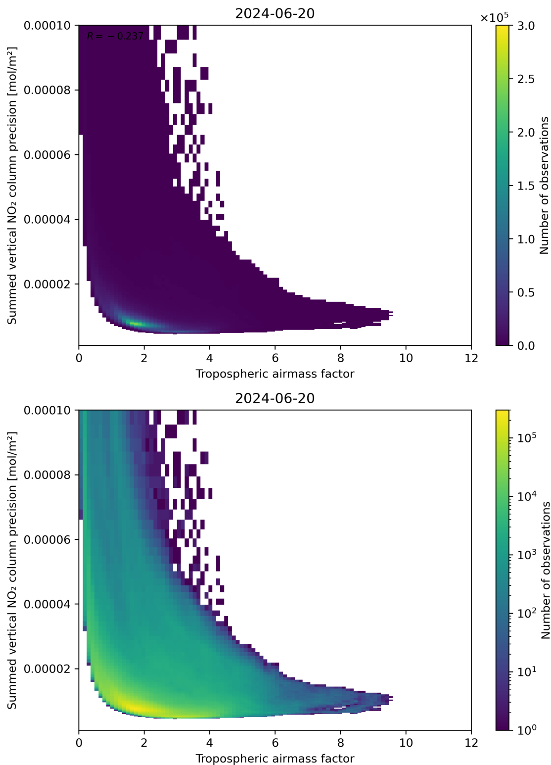
Figure 76: Scatter density plot of “Tropospheric air mass factor” against “Summed vertical NO 2 column precision” for 2024-06-19 to 2024-06-21.
