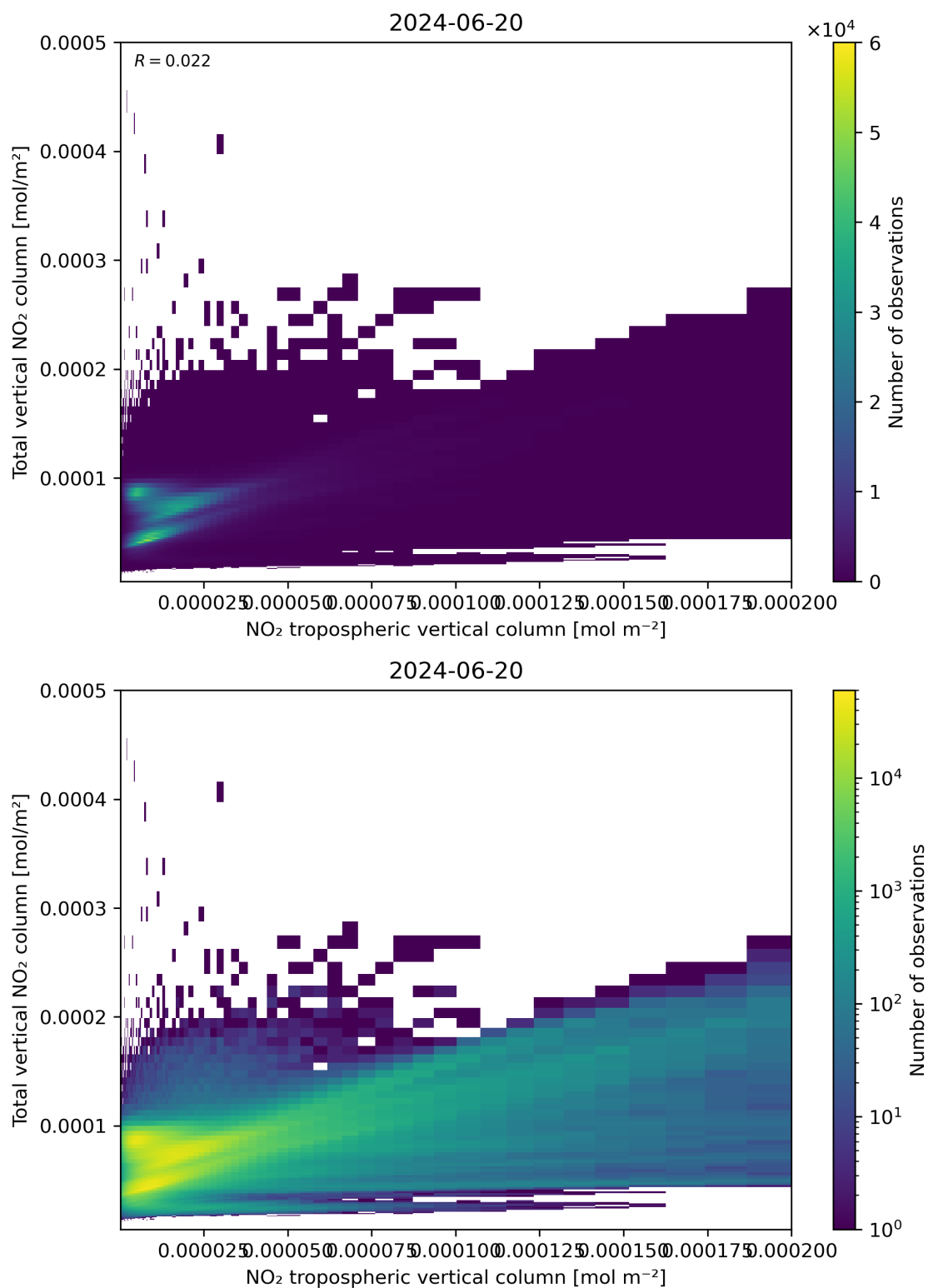
Figure 128: Scatter density plot of “NO 2 tropospheric vertical column” against “Total vertical NO 2 column” for 2024-06-19 to 2024-06-21.
