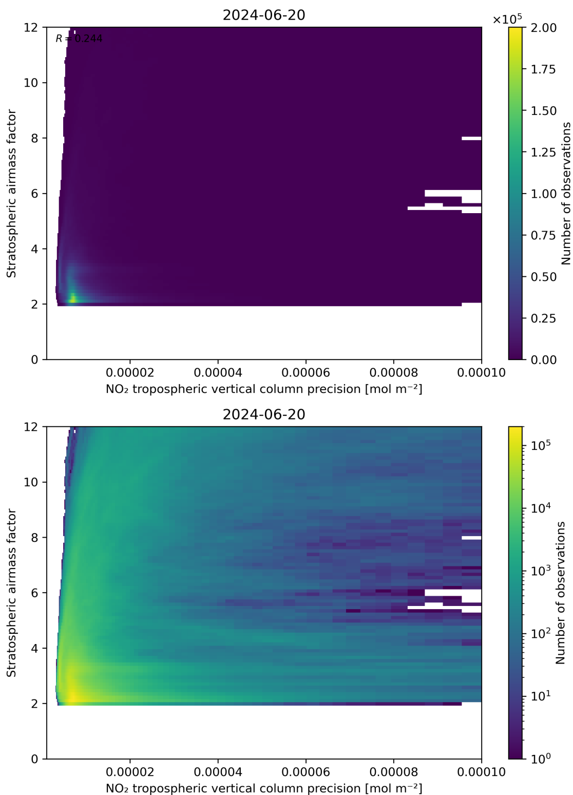
Figure 131: Scatter density plot of “NO 2 tropospheric vertical column precision” against “Stratospheric airmass factor” for 2024-06-19 to 2024-06-21.
