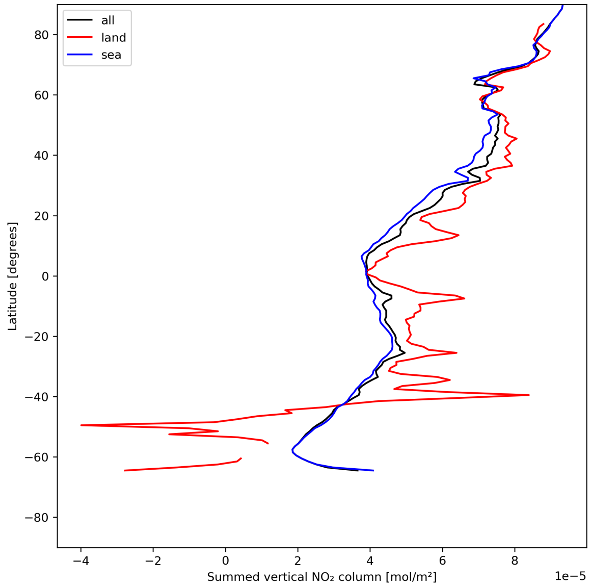
Figure 23: Zonal average of “Summed vertical NO 2 column” for 2024-06-19 to 2024-06-21.
