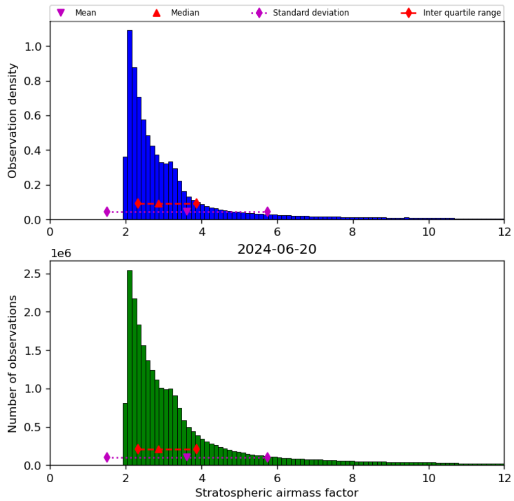
Figure 44: Histogram of “Stratospheric airmass factor” for 2024-06-19 to 2024-06-21
