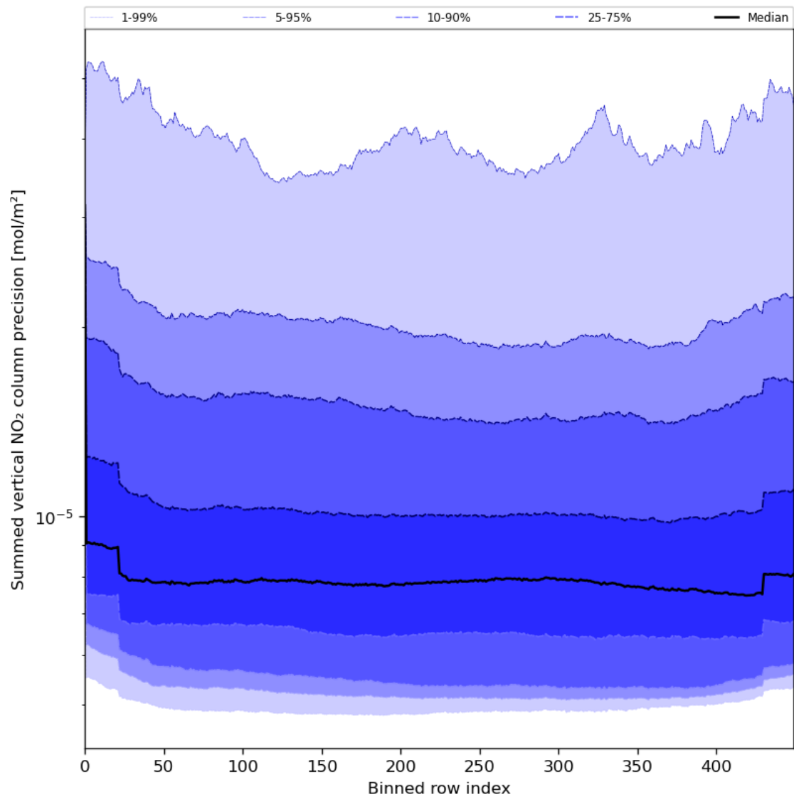
Figure 58: Along track statistics of “Summed vertical NO 2 column precision” for 2024-06-19 to 2024-06-21
