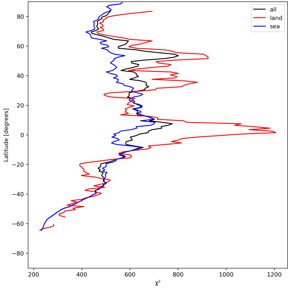
Figure 25: Zonal average of “ \chi^2 ” for 2024-06-19 to 2024-06-21.
