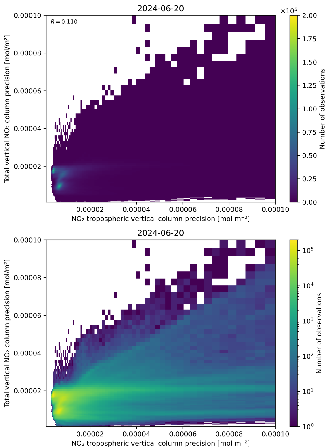
Figure 139: Scatter density plot of “NO 2 tropospheric vertical column precision” against “Total vertical NO 2 column precision” for 2024-06-19 to 2024-06-21.
