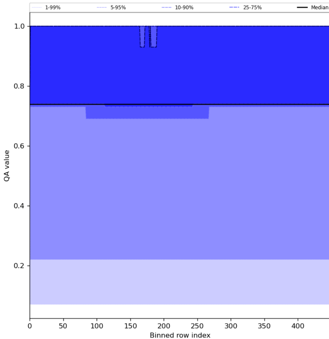
Figure 45: Along track statistics of “QA value” for 2024-06-19 to 2024-06-21
