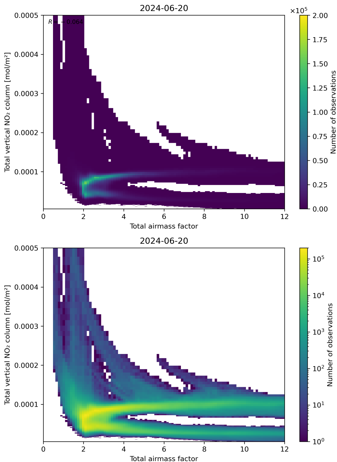
Figure 67: Scatter density plot of “Total airmass factor” against “Total vertical NO 2 column” for 2024-06-19 to 2024-06-21.
