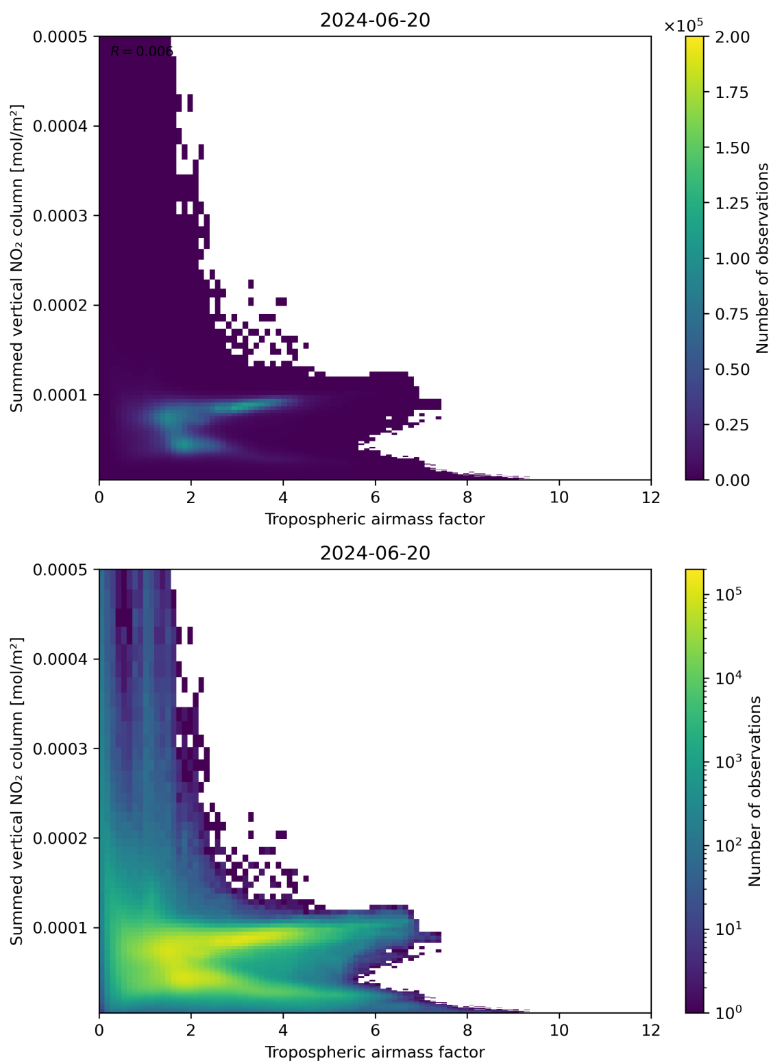
Figure 75: Scatter density plot of “Tropospheric airmass factor” against “Summed vertical NO 2 column” for 2024-06-19 to 2024-06-21.
