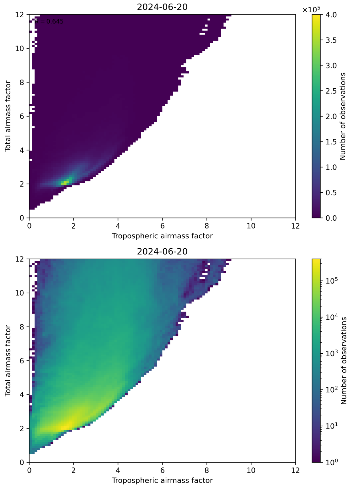
Figure 72: Scatter density plot of “Tropospheric airmass factor” against “Total airmass factor” for 2024-06-19 to 2024-06-21.
