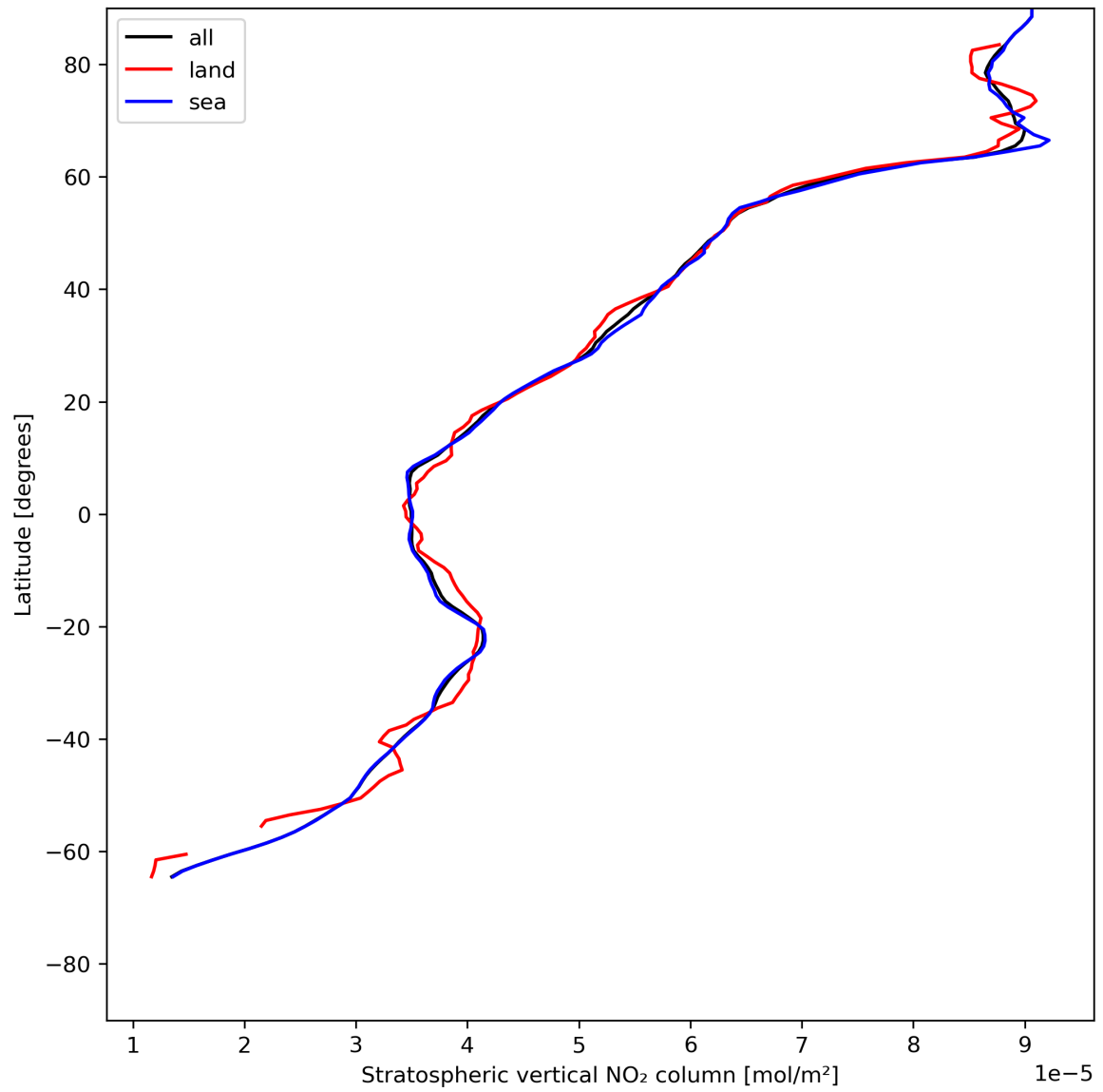
Figure 19: Zonal average of “Stratospheric vertical NO 2 column” for 2024-06-19 to 2024-06-21.
