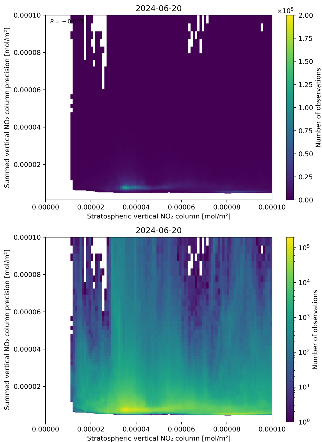
Figure 99: Scatter density plot of “Stratospheric vertical NO 2 column” against “Summed vertical NO 2 column precision” for 2024-06-19 to 2024-06-21.
