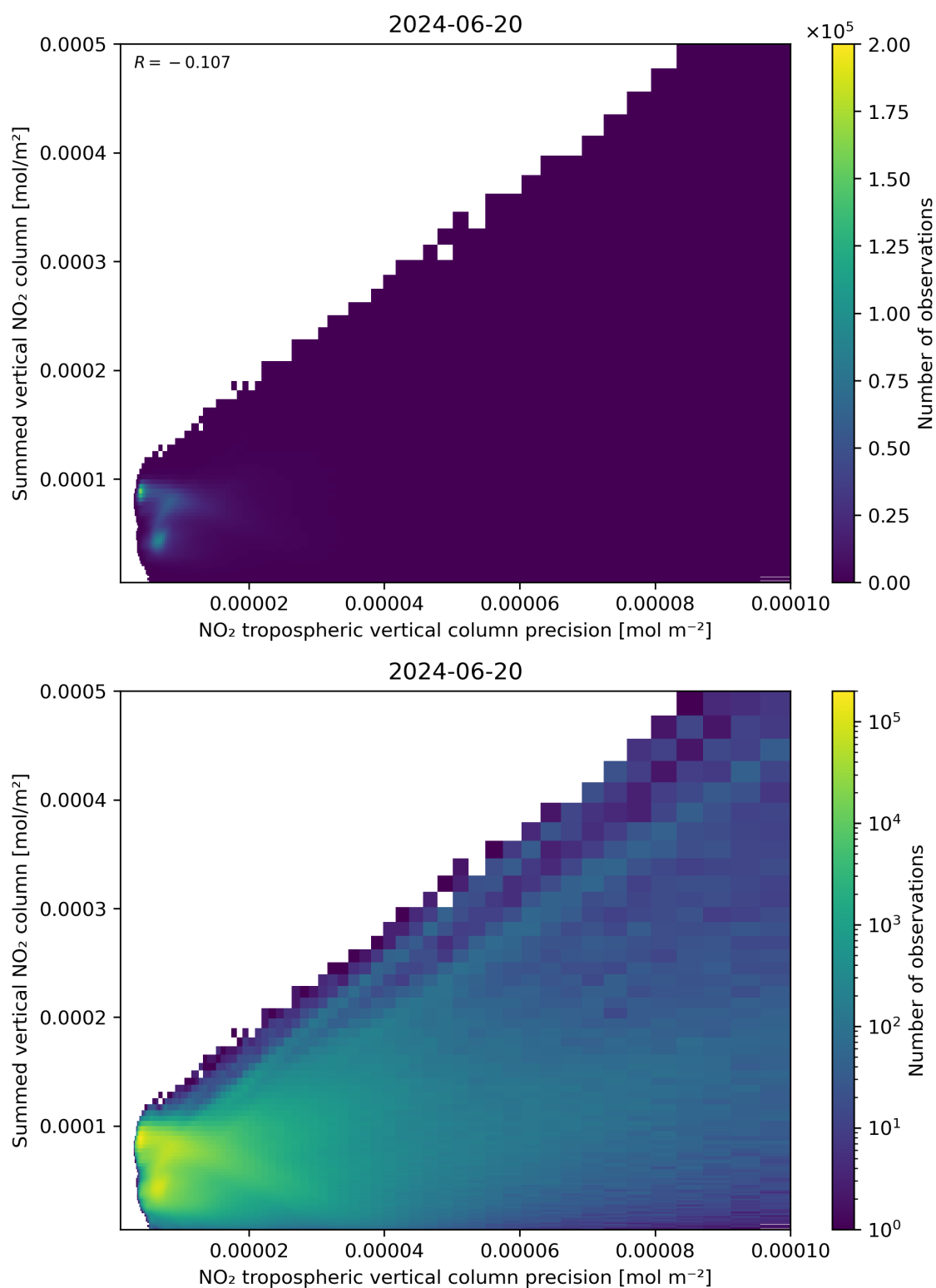
Figure 136: Scatter density plot of “NO 2 tropospheric vertical column precision” against “Summed vertical NO 2 column” for 2024-06-19 to 2024-06-21.
