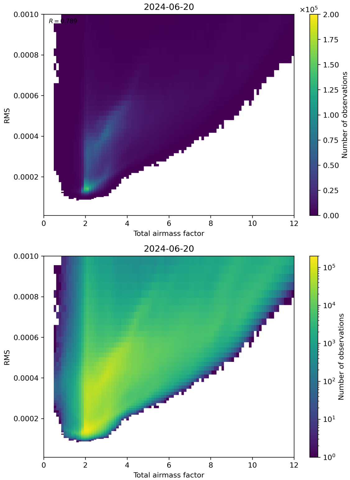
Figure 69: Scatter density plot of “Total airmass factor” against “RMS” for 2024-06-19 to 2024-06-21.
