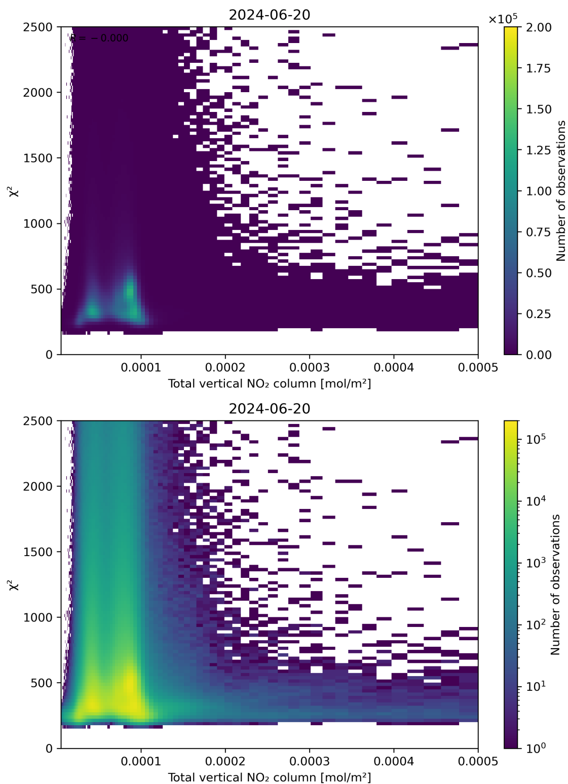
Figure 111: Scatter density plot of “Total vertical NO 2 column” against “ \chi^2 ” for 2024-06-19 to 2024-06-21.
