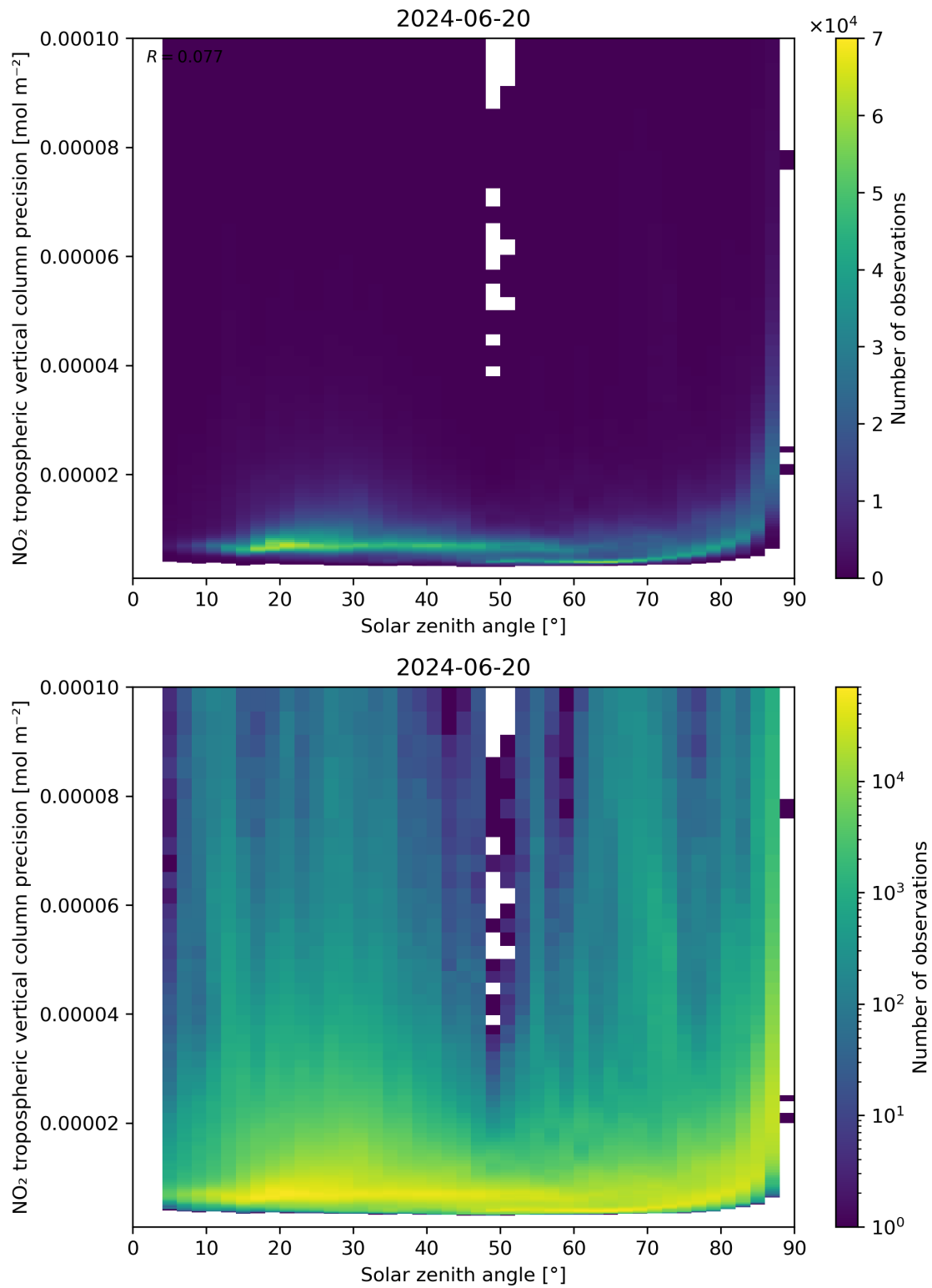
Figure 156: Scatter density plot of “Solar zenith angle” against “NO 2 tropospheric vertical column precision” for 2024-06-19 to 2024-06-21.
