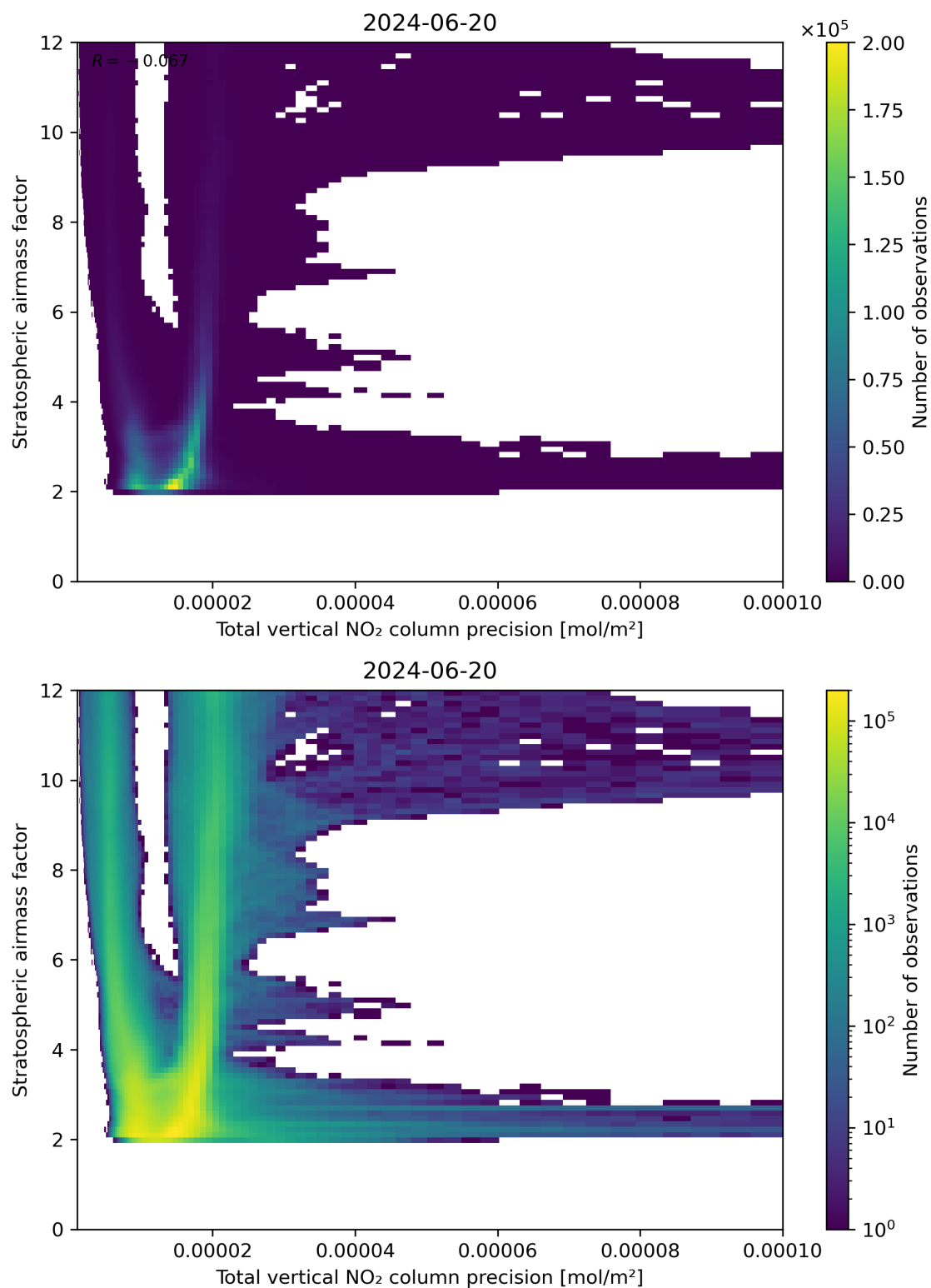
Figure 115: Scatter density plot of “Total vertical NO 2 column precision” against “Stratospheric airmass factor” for 2024-06-19 to 2024-06-21.
