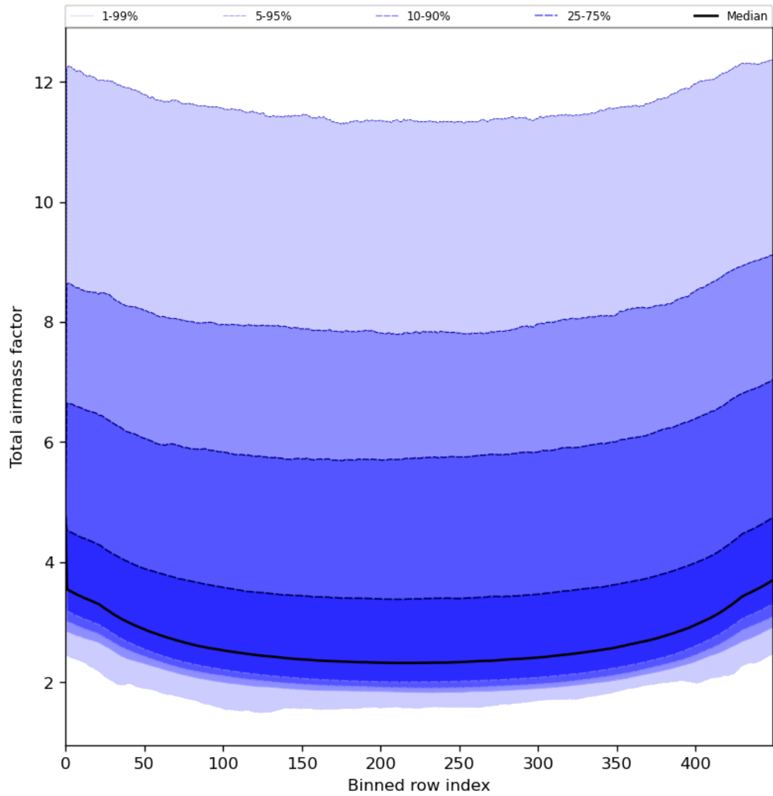
Figure 49: Along track statistics of “Total airmass factor” for 2024-06-19 to 2024-06-21
