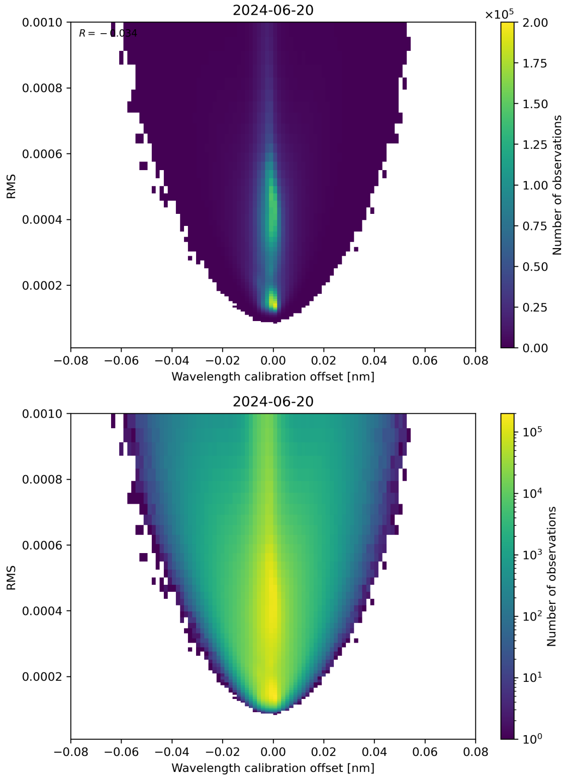
Figure 181: Scatter density plot of “Wavelength calibration offset” against “RMS” for 2024-06-19 to 2024-06-21.
