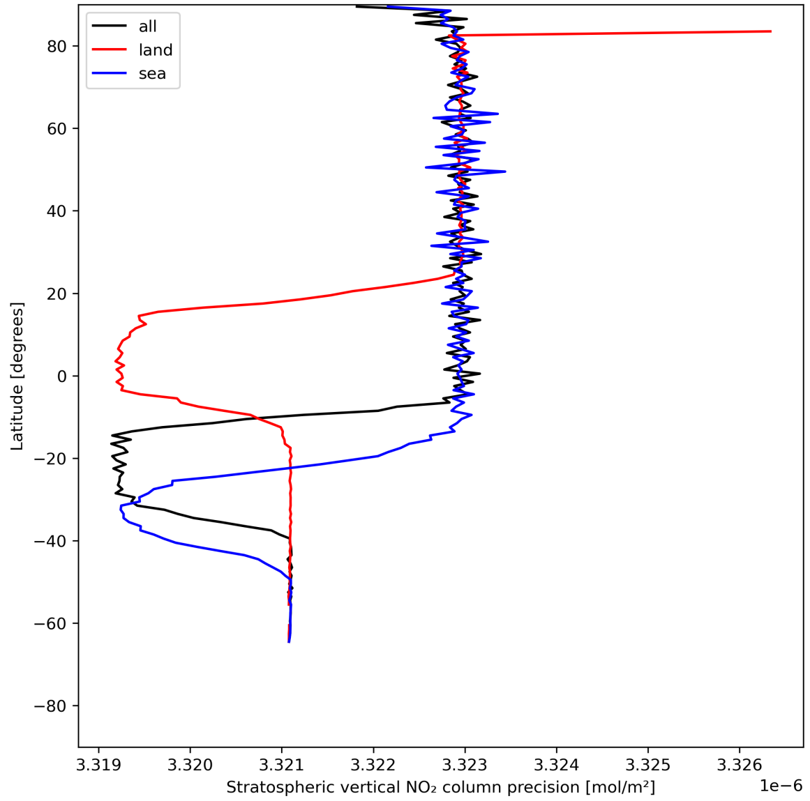
Figure 20: Zonal average of “Stratospheric vertical NO 2 column precision” for 2024-06-19 to 2024-06-21.
