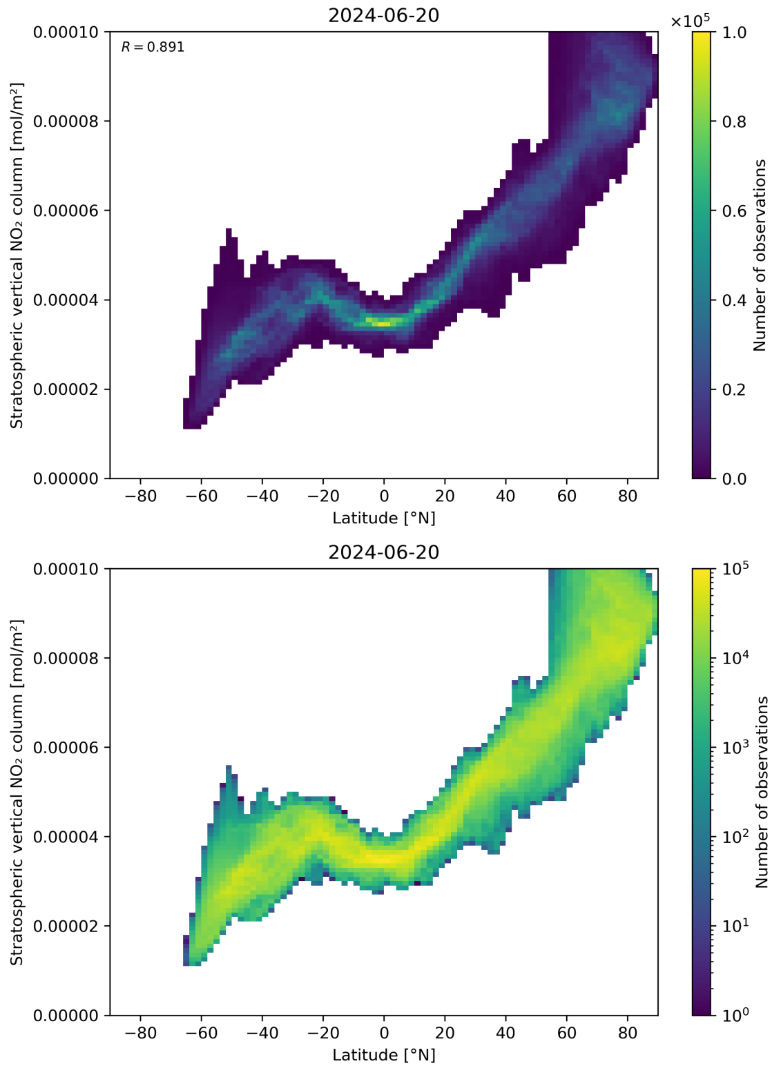
Figure 87: Scatter density plot of “Latitude” against “Stratospheric vertical NO 2 column” for 2024-06-19 to 2024-06-21.
