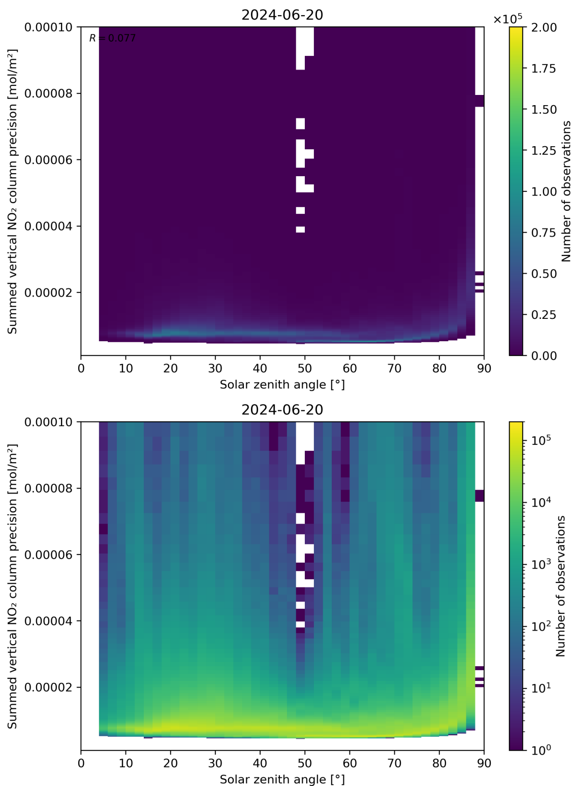
Figure 152: Scatter density plot of “Solar zenith angle” against “Summed vertical NO 2 column precision” for 2024-06-19 to 2024-06-21.
