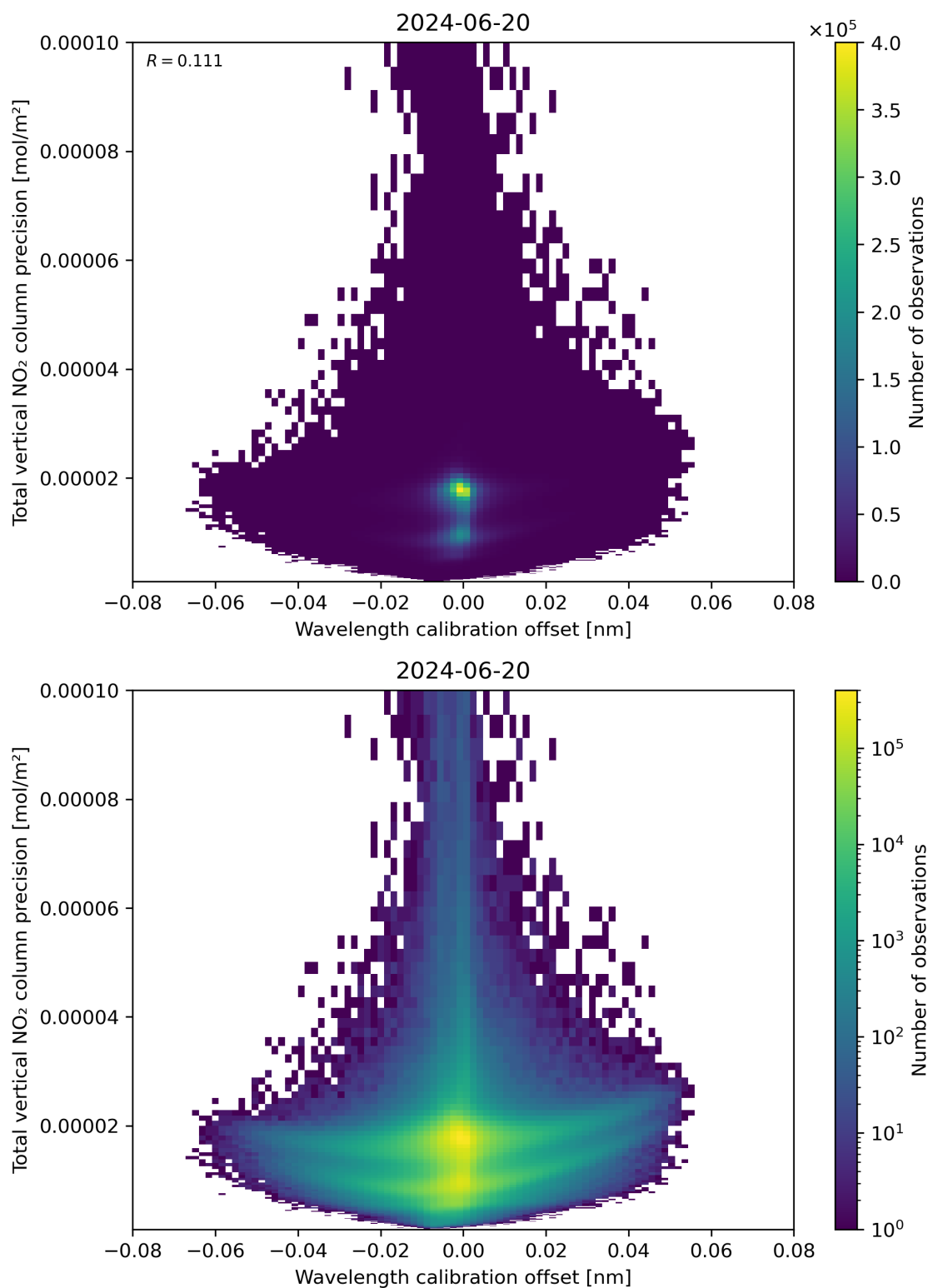
Figure 180: Scatter density plot of “Wavelength calibration offset” against “Total vertical NO 2 column precision” for 2024-06-19 to 2024-06-21.
