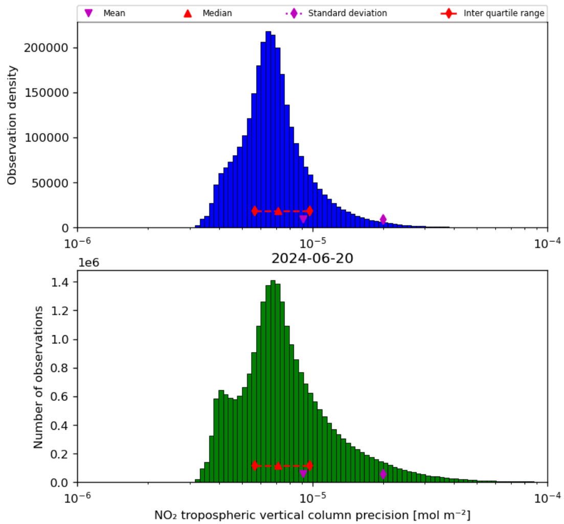
Figure 30: Histogram of “NO 2 tropospheric vertical column precision” for 2024-06-19 to 2024-06-21
