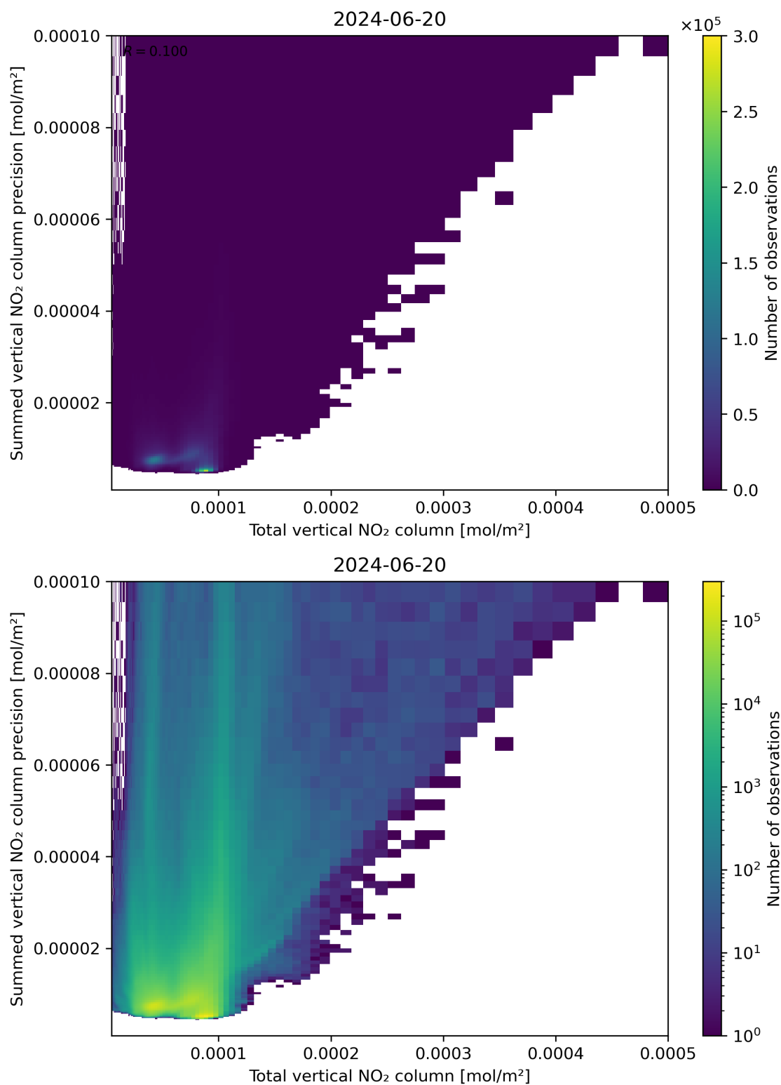
Figure 113: Scatter density plot of “Total vertical NO 2 column” against “Summed vertical NO 2 column precision” for 2024-06-19 to 2024-06-21.
