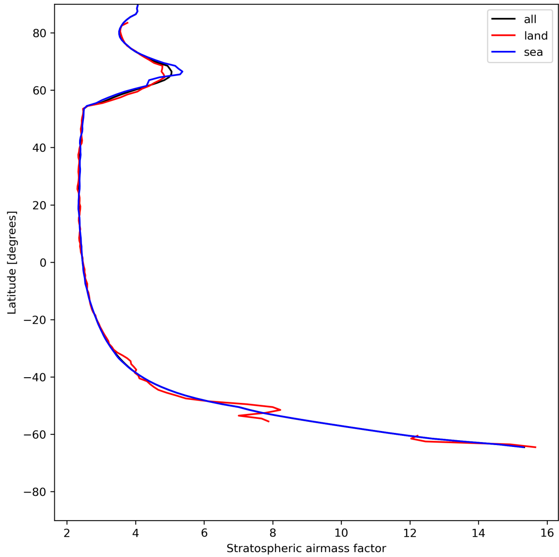
Figure 27: Zonal average of “Stratospheric air mass factor” for 2024-06-19 to 2024-06-21.
