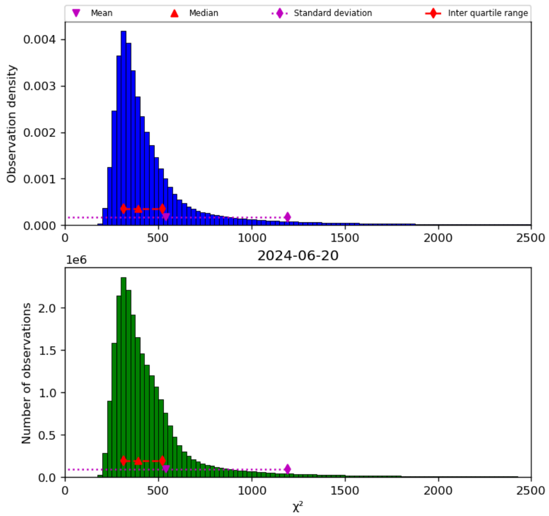
Figure 42: Histogram of “ \chi^2 ” for 2024-06-19 to 2024-06-21
