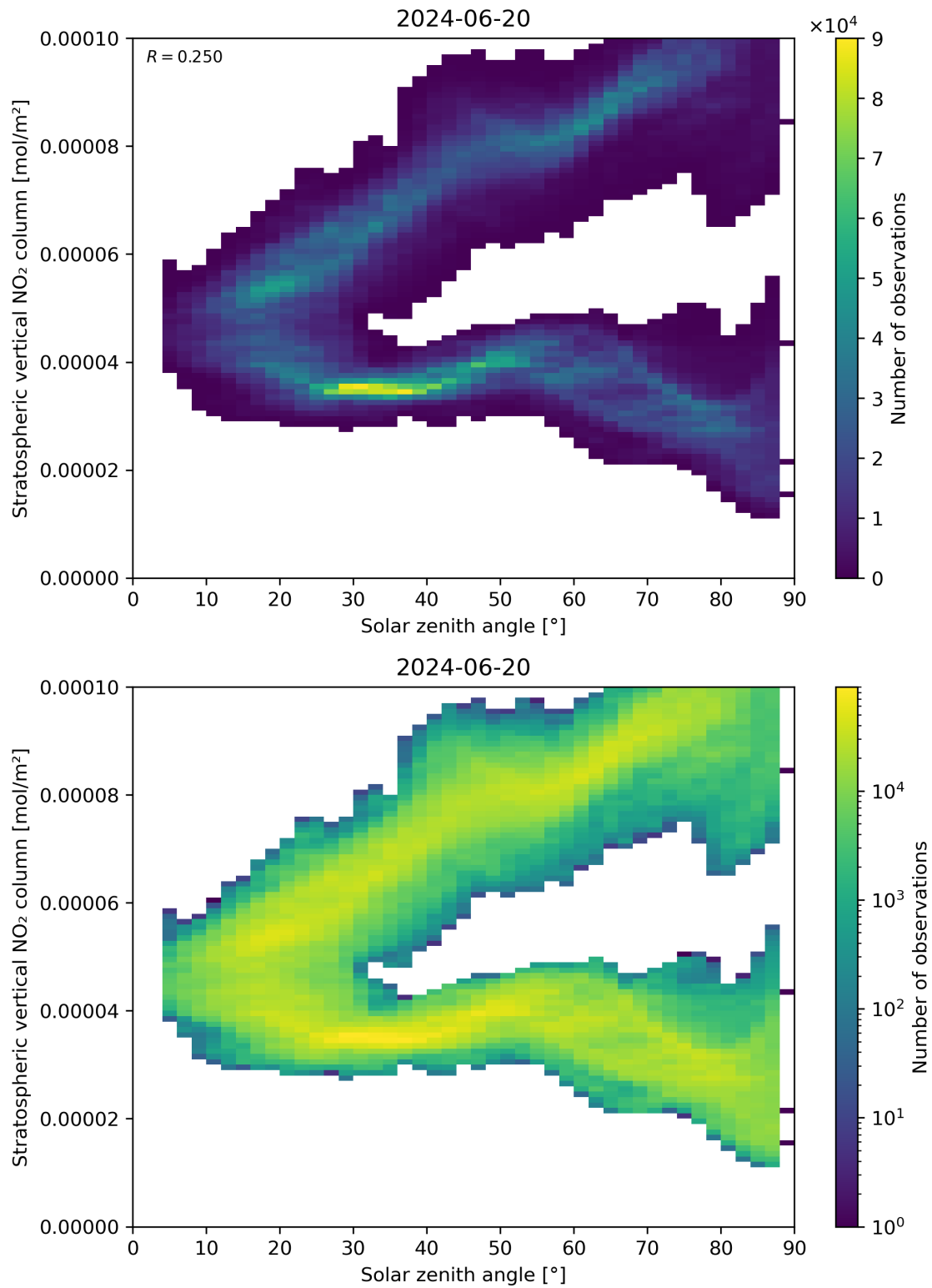
Figure 150: Scatter density plot of “Solar zenith angle” against “Stratospheric vertical NO 2 column” for 2024-06-19 to 2024-06-21.
