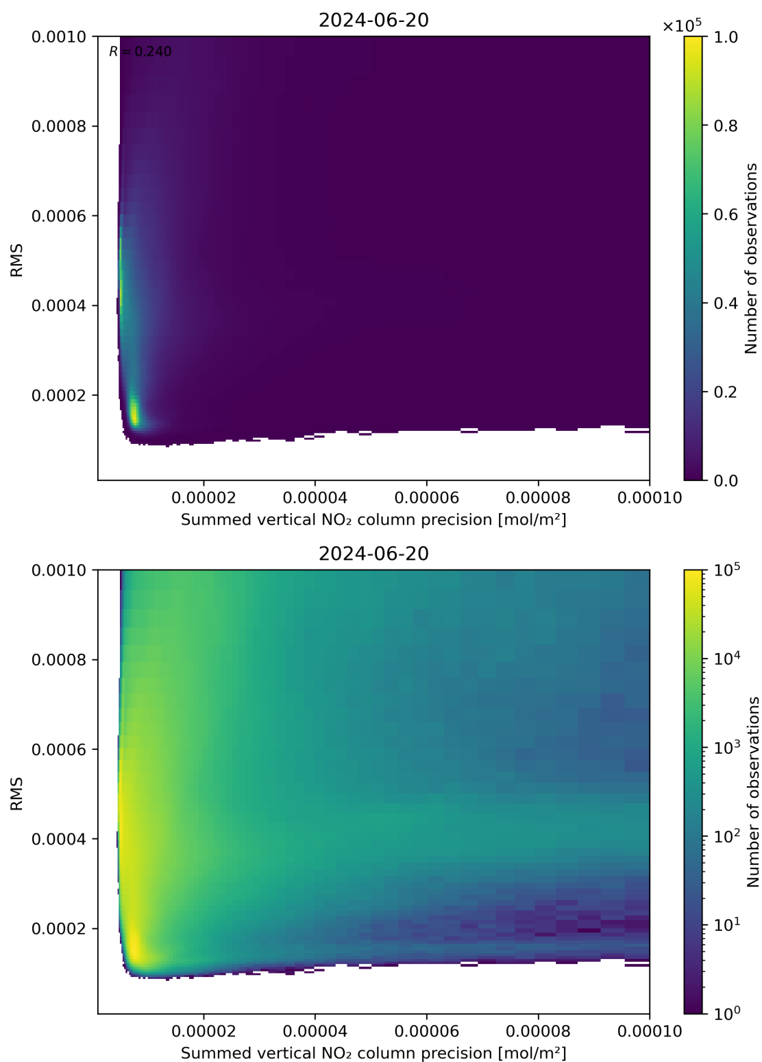
Figure 108: Scatter density plot of “Summed vertical NO 2 column precision” against “RMS” for 2024-06-19 to 2024-06-21.
