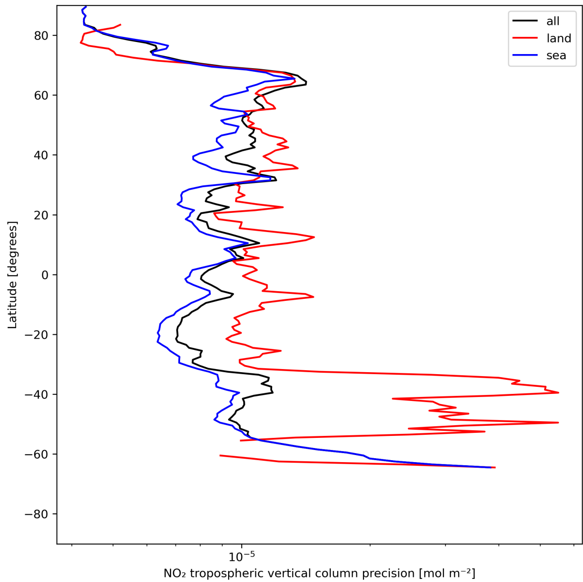
Figure 13: Zonal average of “NO 2 tropospheric vertical column precision” for 2024-06-19 to 2024-06-21.
