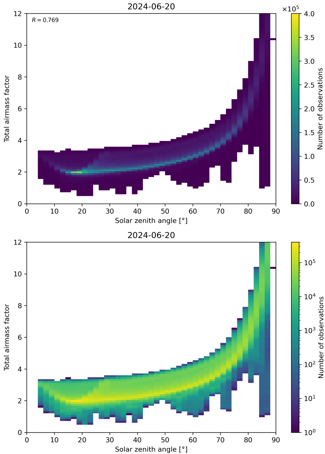
Figure 146: Scatter density plot of “Solar zenith angle” against “Total air mass factor” for 2024-06-19 to 2024-06-21.
