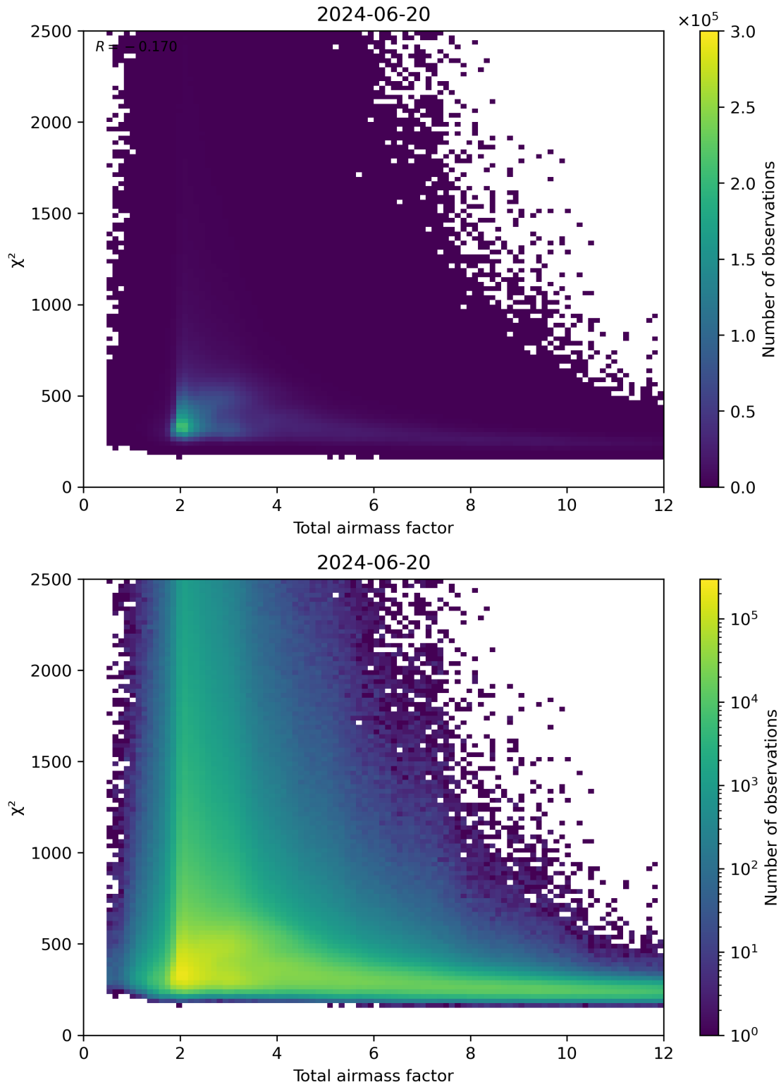
Figure 63: Scatter density plot of “Total airmass factor” against “ \chi^2 ” for 2024-06-19 to 2024-06-21.
