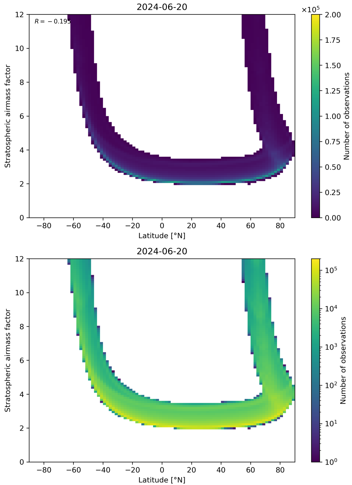
Figure 83: Scatter density plot of “Latitude” against “Stratospheric air mass factor” for 2024-06-19 to 2024-06-21.
