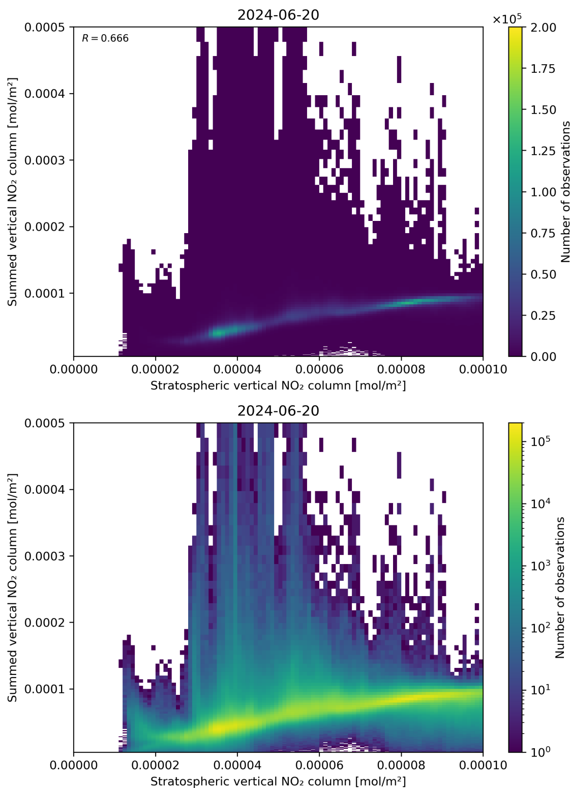
Figure 98: Scatter density plot of “Stratospheric vertical NO 2 column” against “Summed vertical NO 2 column” for 2024-06-19 to 2024-06-21.
