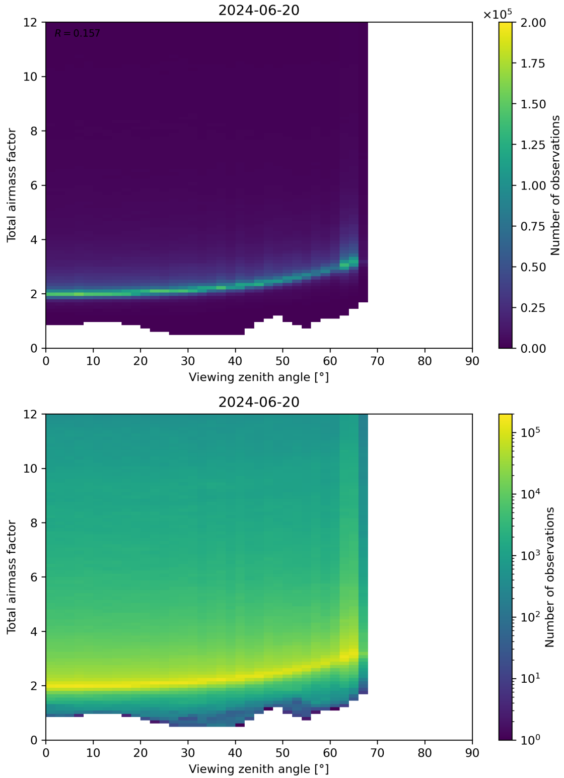
Figure 160: Scatter density plot of “Viewing zenith angle” against “Total airmass factor” for 2024-06-19 to 2024-06-21.
