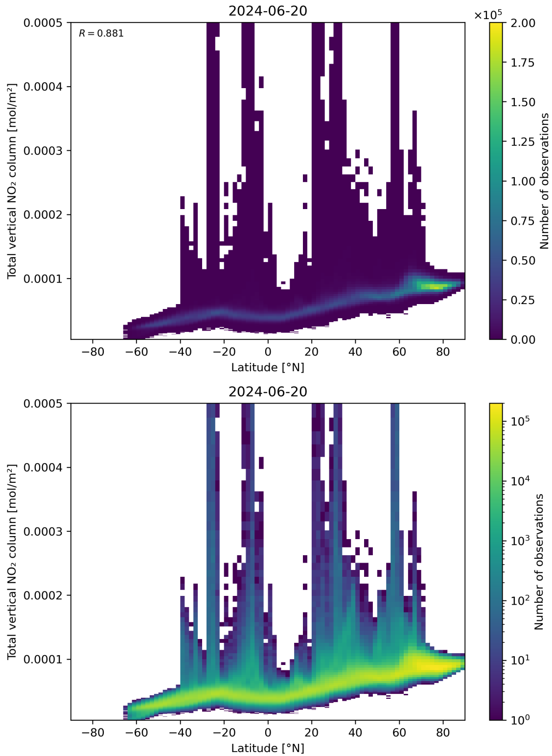
Figure 90: Scatter density plot of “Latitude” against “Total vertical NO 2 column” for 2024-06-19 to 2024-06-21.
