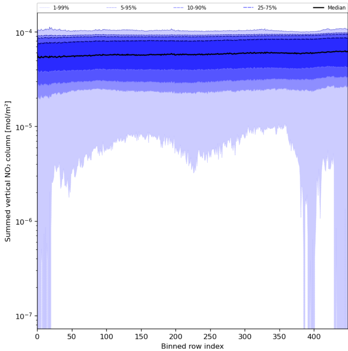
Figure 57: Along track statistics of “Summed vertical NO 2 column” for 2024-06-19 to 2024-06-21
