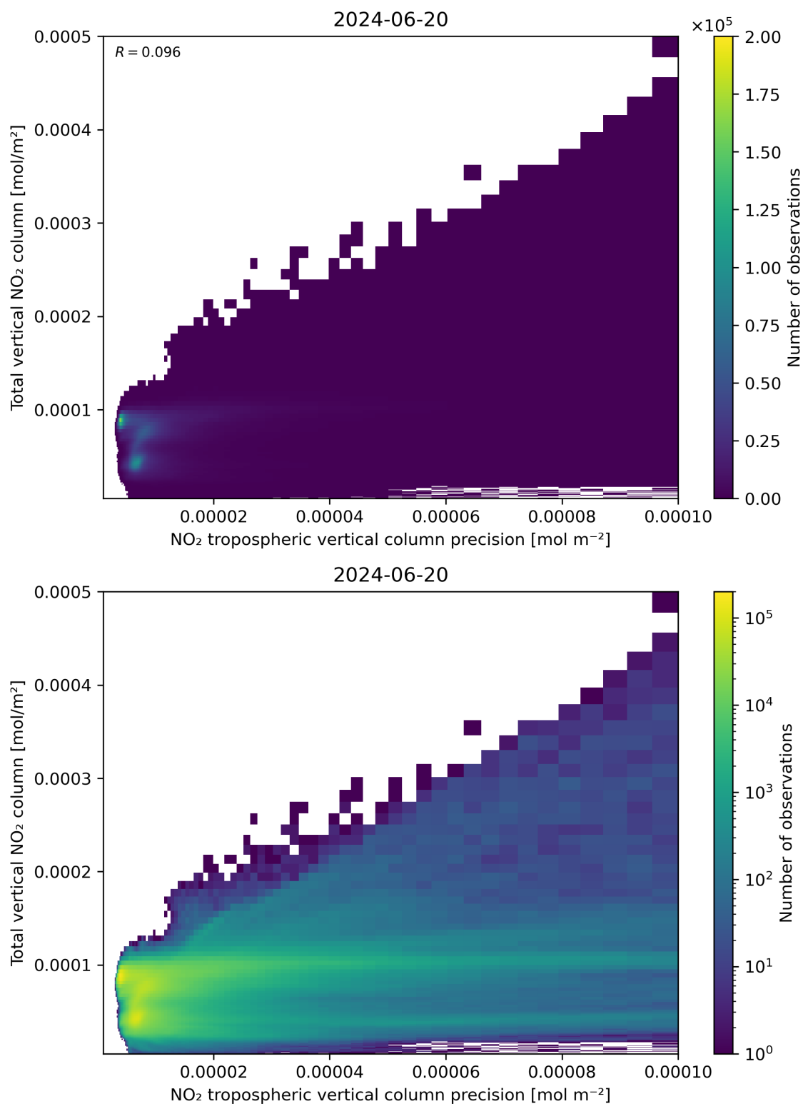
Figure 138: Scatter density plot of “NO 2 tropospheric vertical column precision” against “Total vertical NO 2 column” for 2024-06-19 to 2024-06-21.
