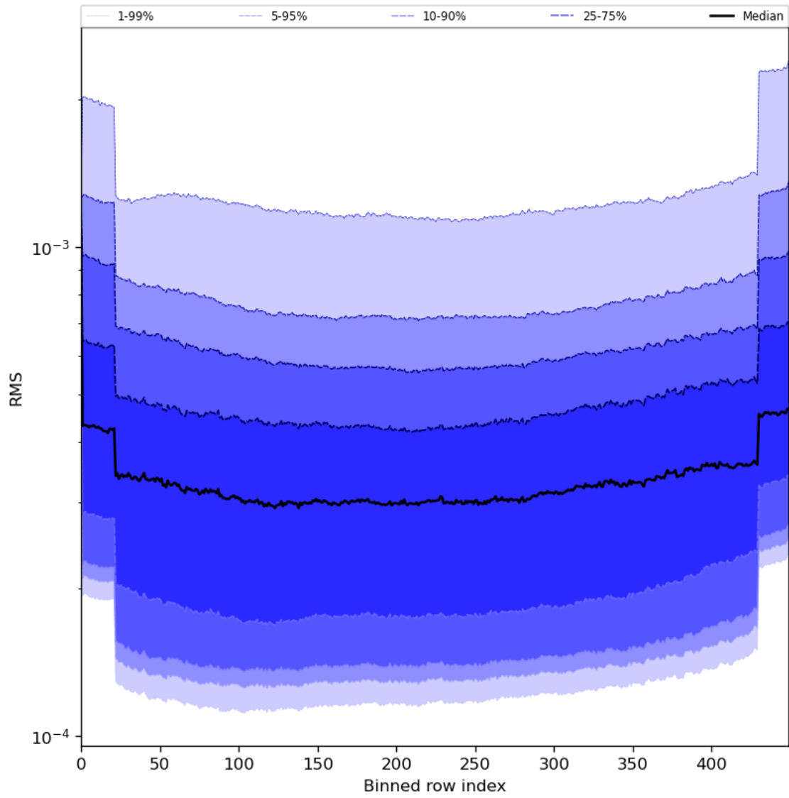
Figure 60: Along track statistics of “RMS” for 2024-06-19 to 2024-06-21
