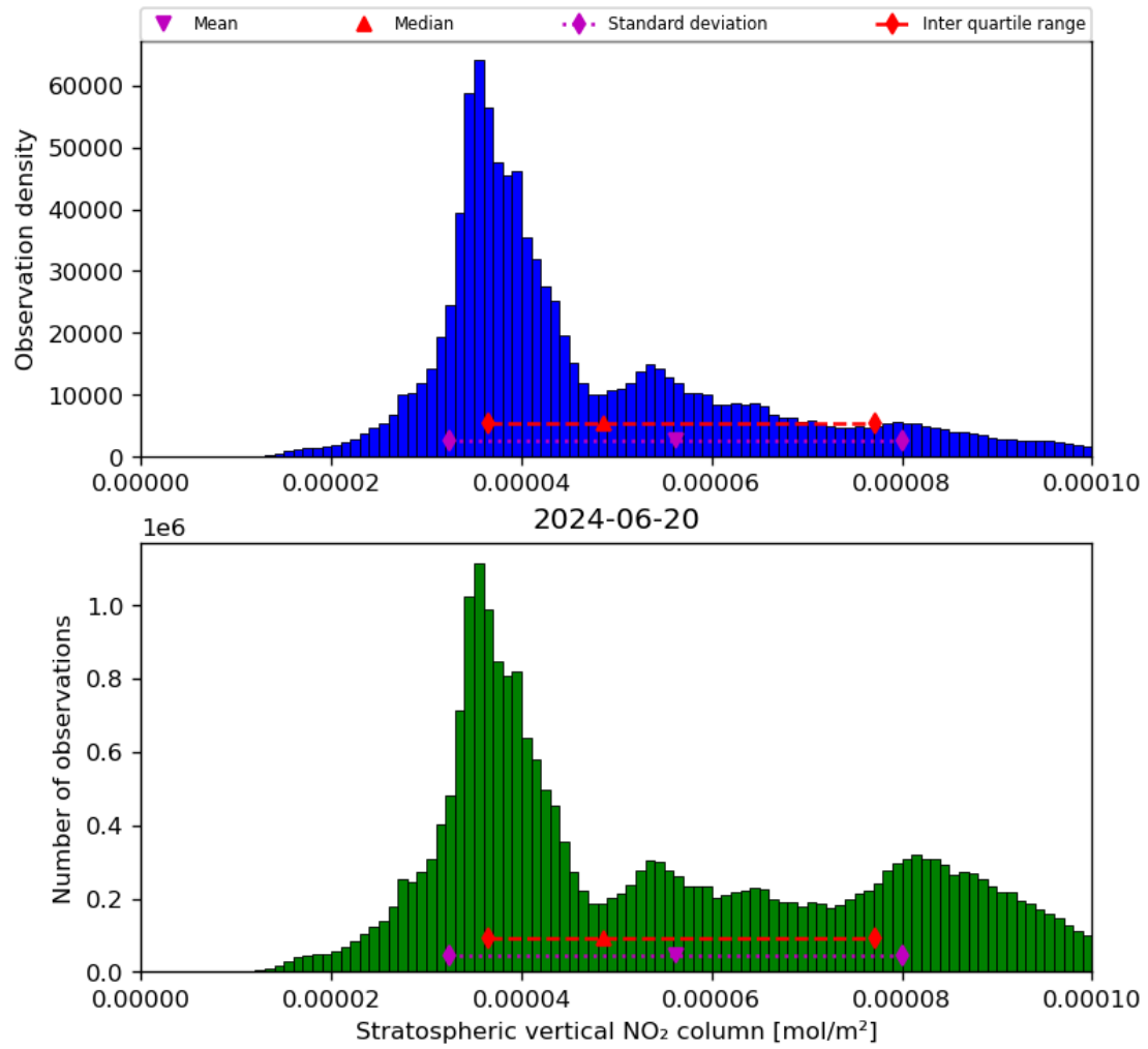
Figure 36: Histogram of “Stratospheric vertical NO 2 column” for 2024-06-19 to 2024-06-21
