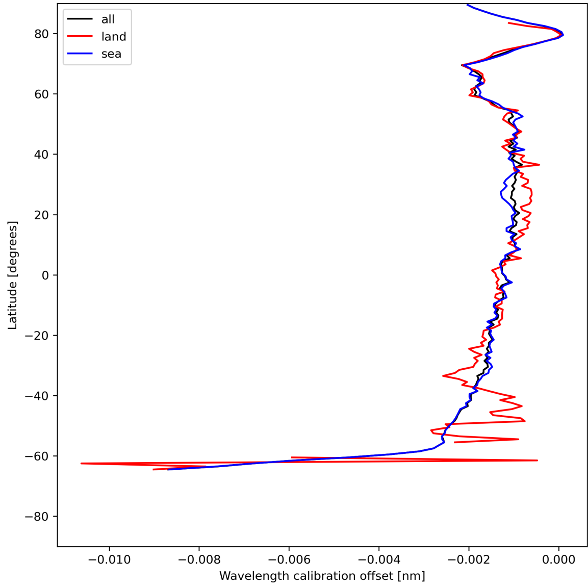
Figure 18: Zonal average of “Wavelength calibration offset” for 2024-06-19 to 2024-06-21.
