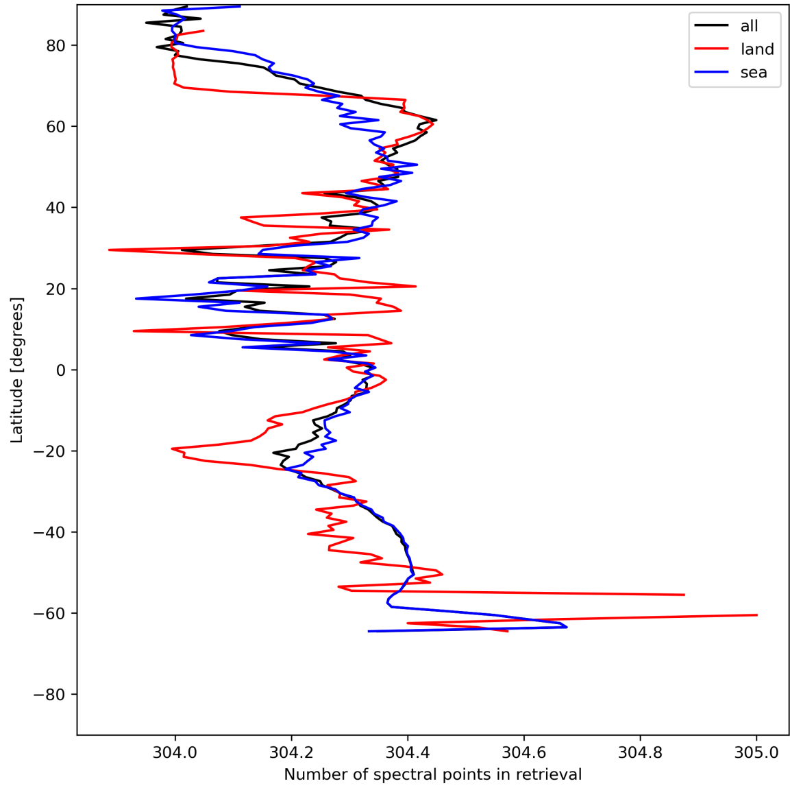
Figure 16: Zonal average of “Number of spectral points in retrieval” for 2024-06-19 to 2024-06-21.
