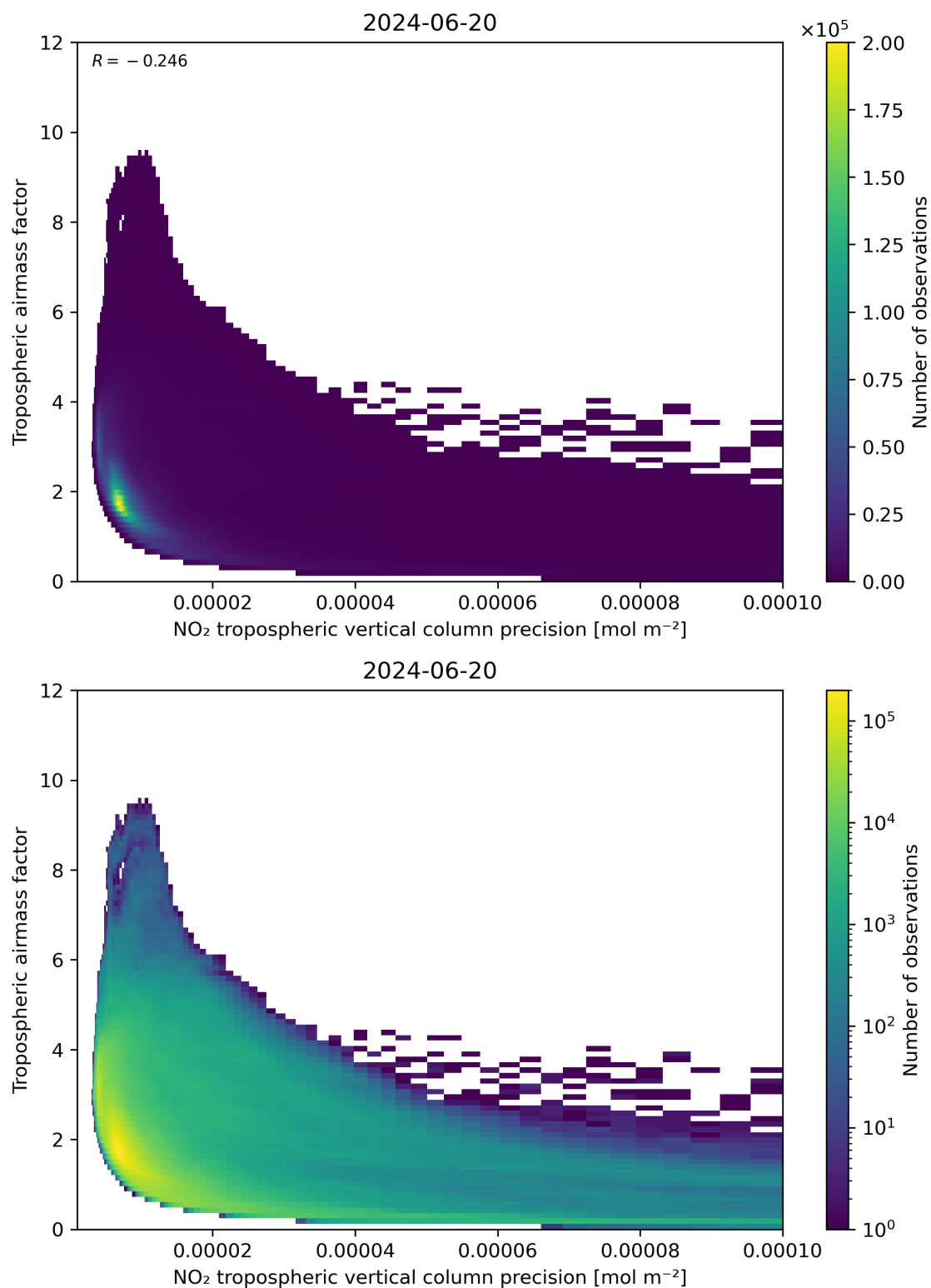
Figure 133: Scatter density plot of “NO 2 tropospheric vertical column precision” against “Tropospheric airmass factor” for 2024-06-19 to 2024-06-21.
