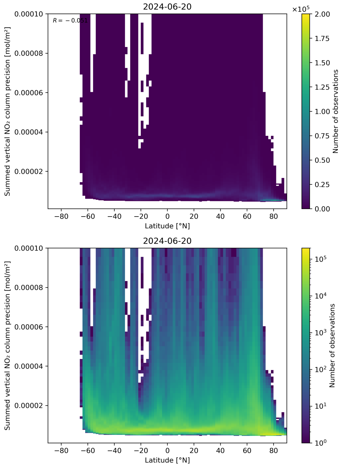
Figure 89: Scatter density plot of “Latitude” against “Summed vertical NO 2 column precision” for 2024-06-19 to 2024-06-21.
