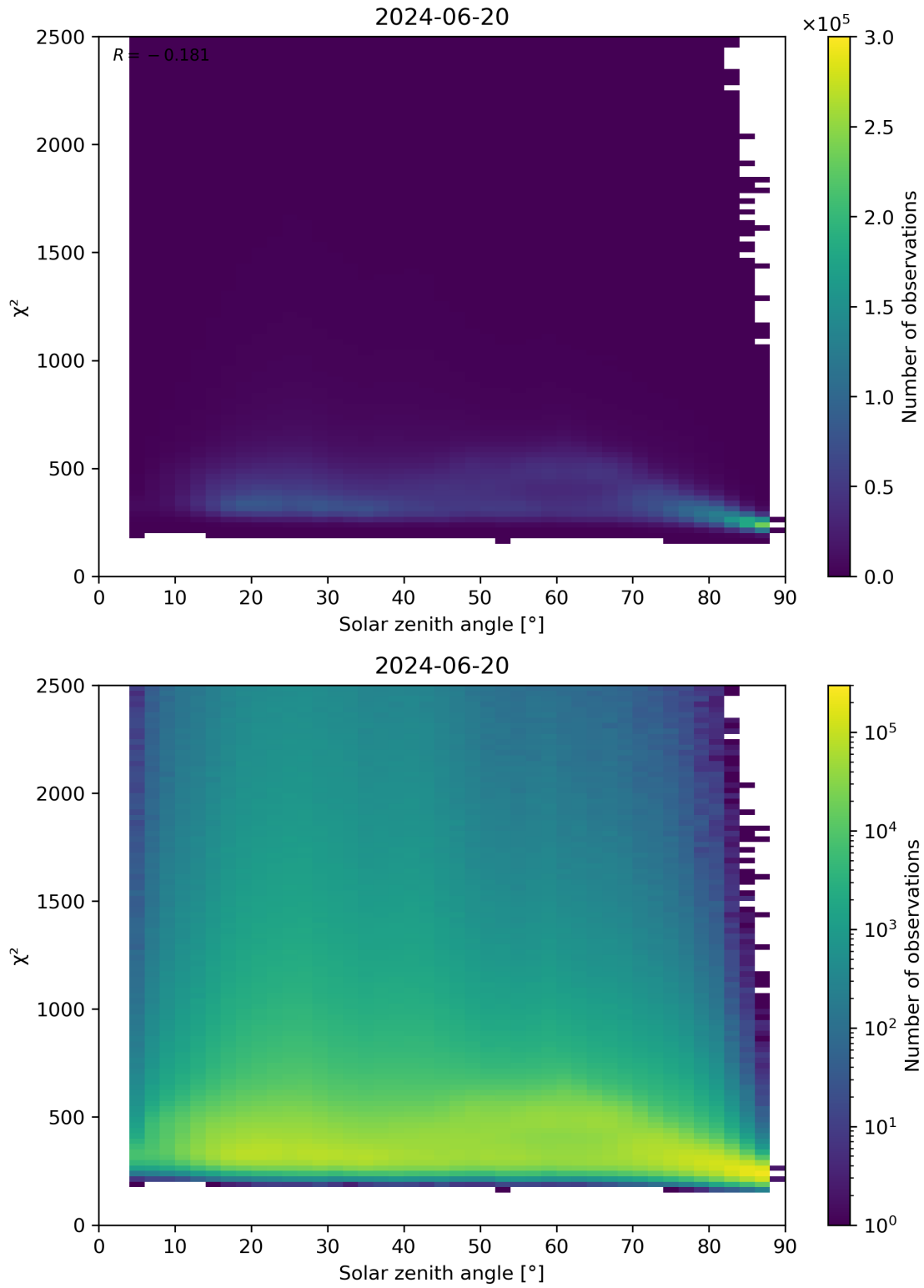
Figure 148: Scatter density plot of “Solar zenith angle” against “ \chi^2 ” for 2024-06-19 to 2024-06-21.
