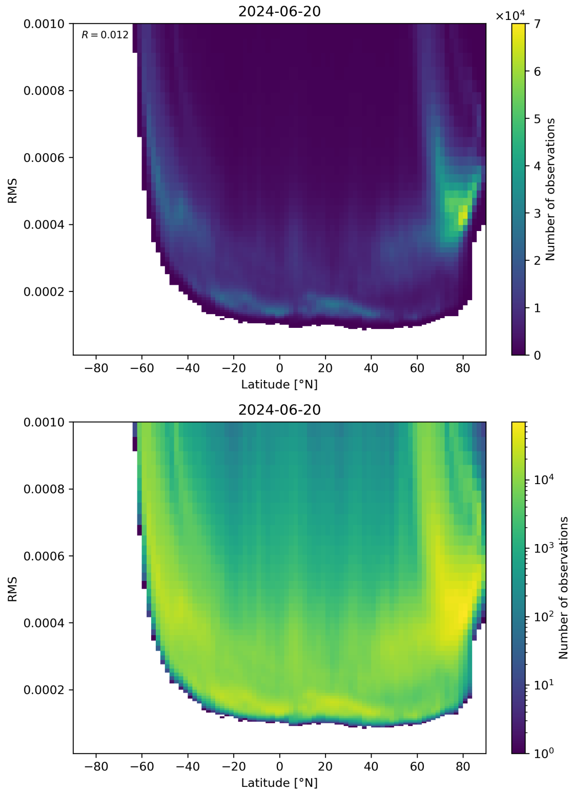
Figure 94: Scatter density plot of “Latitude” against “RMS” for 2024-06-19 to 2024-06-21.
