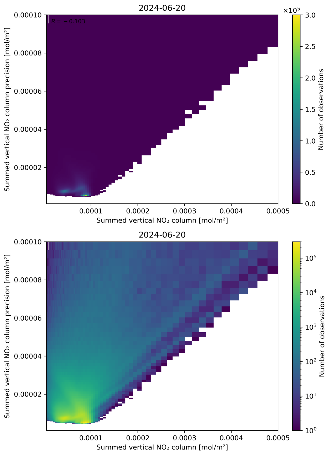
Figure 105: Scatter density plot of “Summed vertical NO 2 column” against “Summed vertical NO 2 column precision” for 2024-06-19 to 2024-06-21.
