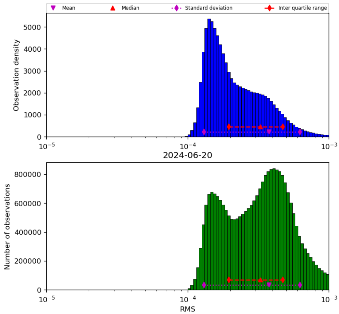
Figure 43: Histogram of “RMS” for 2024-06-19 to 2024-06-21
