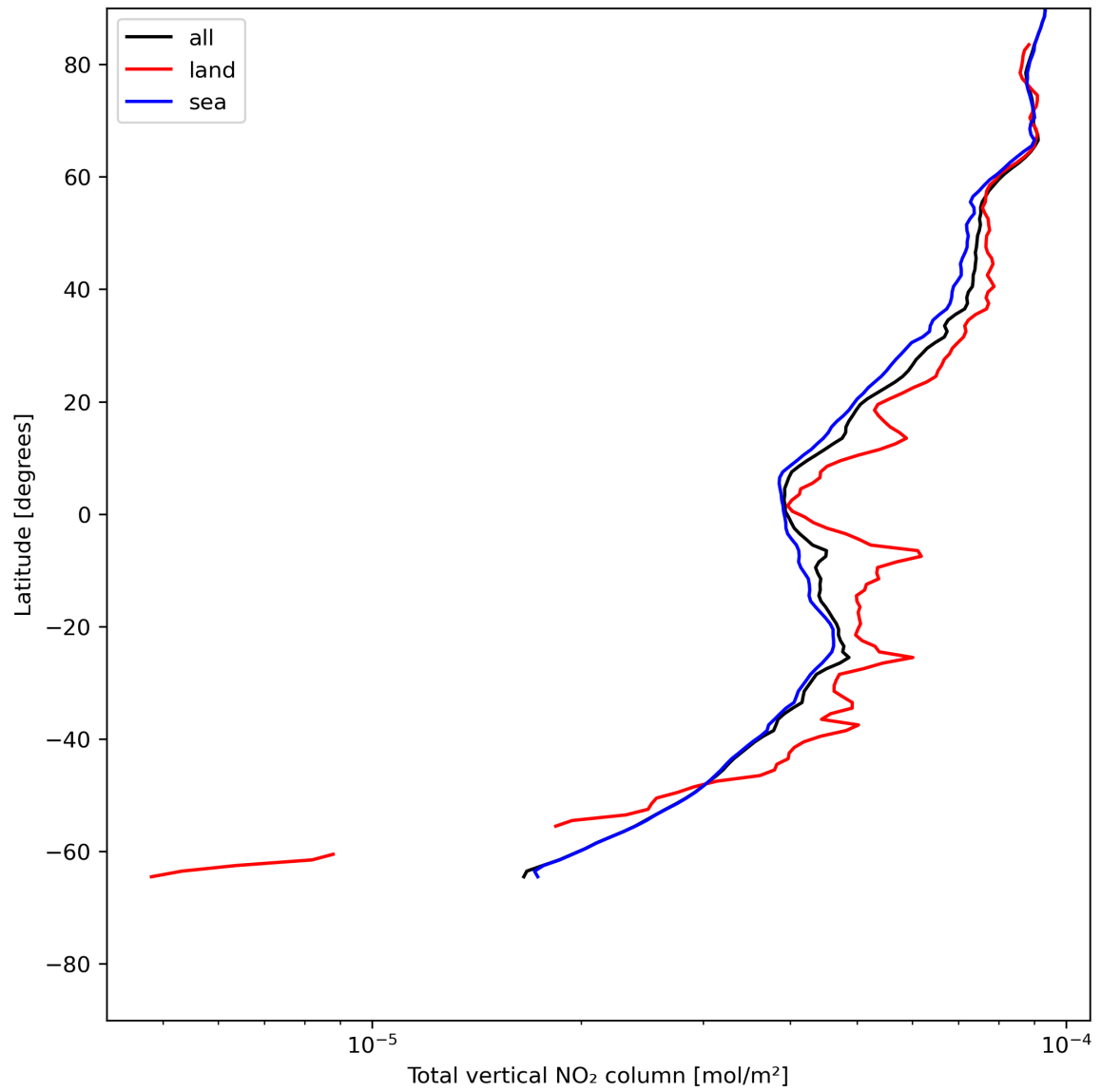
Figure 21: Zonal average of “Total vertical NO 2 column” for 2024-06-19 to 2024-06-21.
