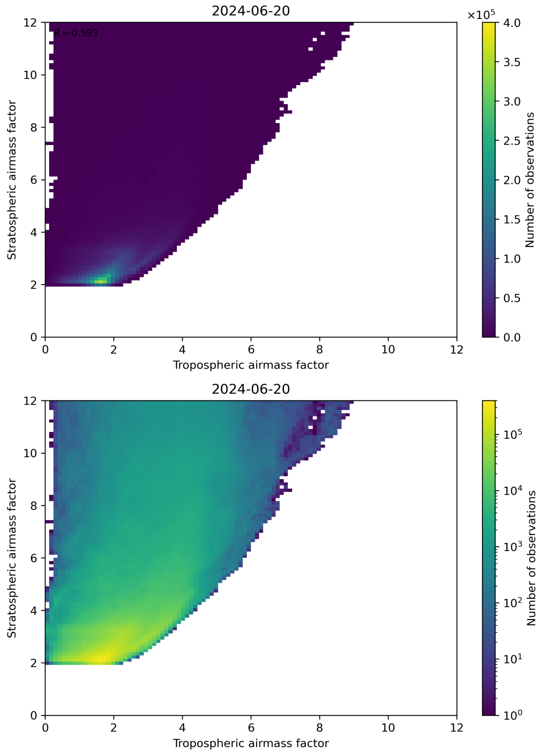
Figure 71: Scatter density plot of “Tropospheric airmass factor” against “Stratospheric airmass factor” for 2024-06-19 to 2024-06-21.
