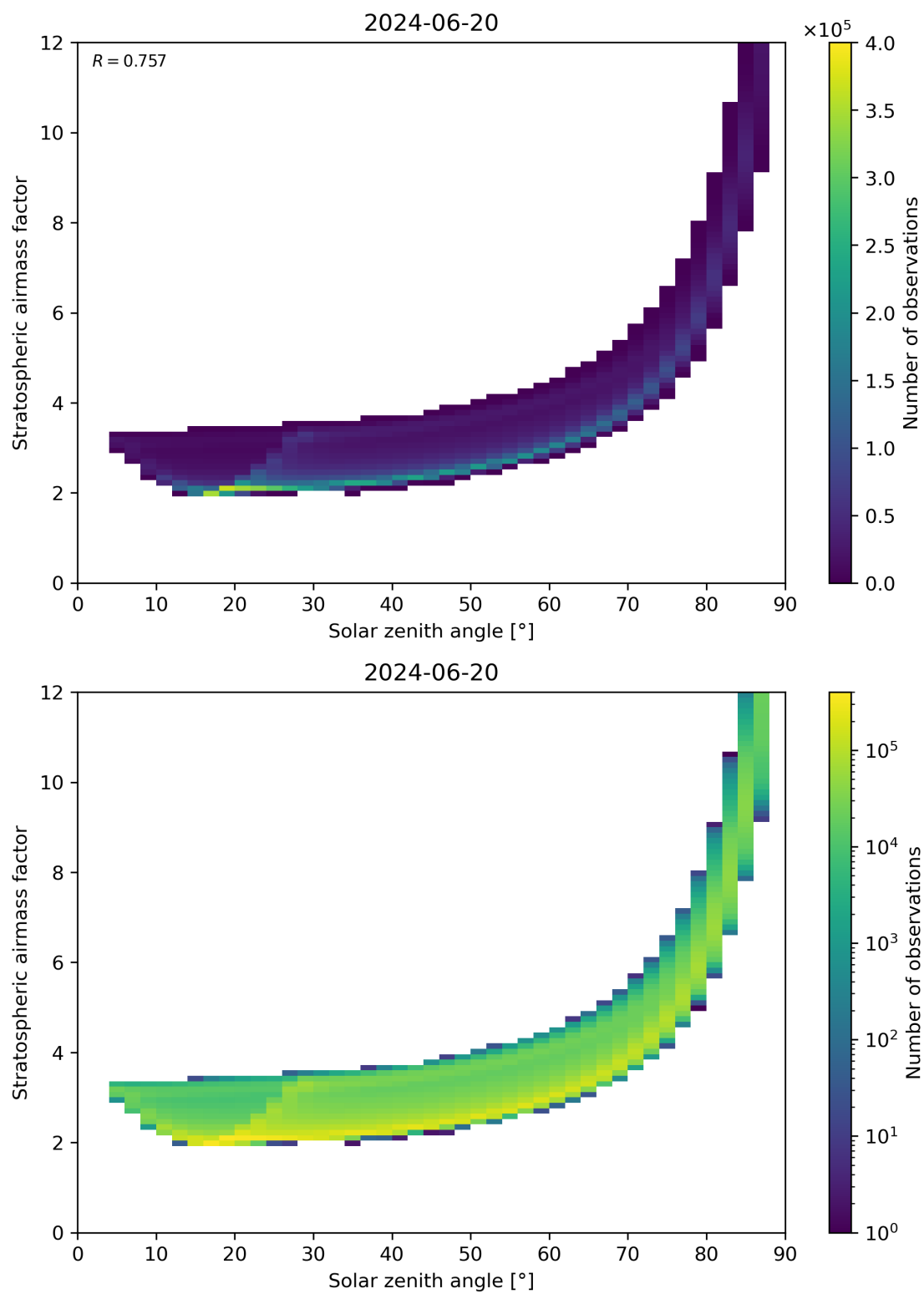
Figure 145: Scatter density plot of “Solar zenith angle” against “Stratospheric airmass factor” for 2024-06-19 to 2024-06-21.
