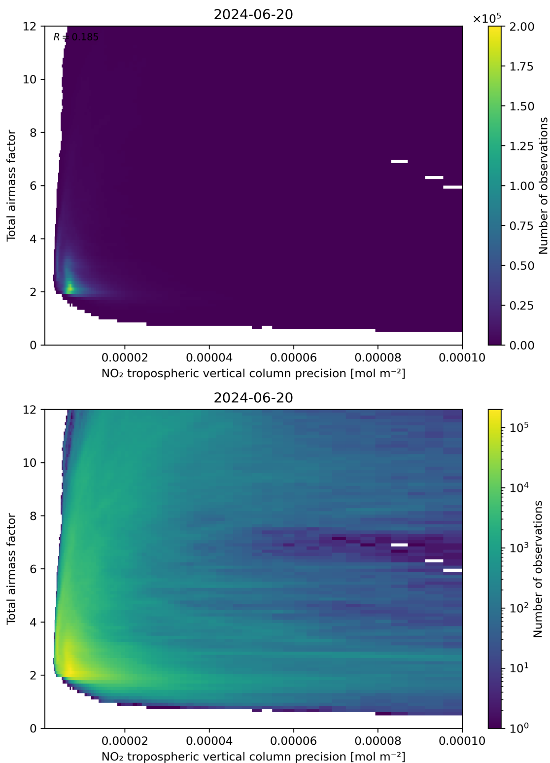
Figure 132: Scatter density plot of “NO 2 tropospheric vertical column precision” against “Total air mass factor” for 2024-06-19 to 2024-06-21.
