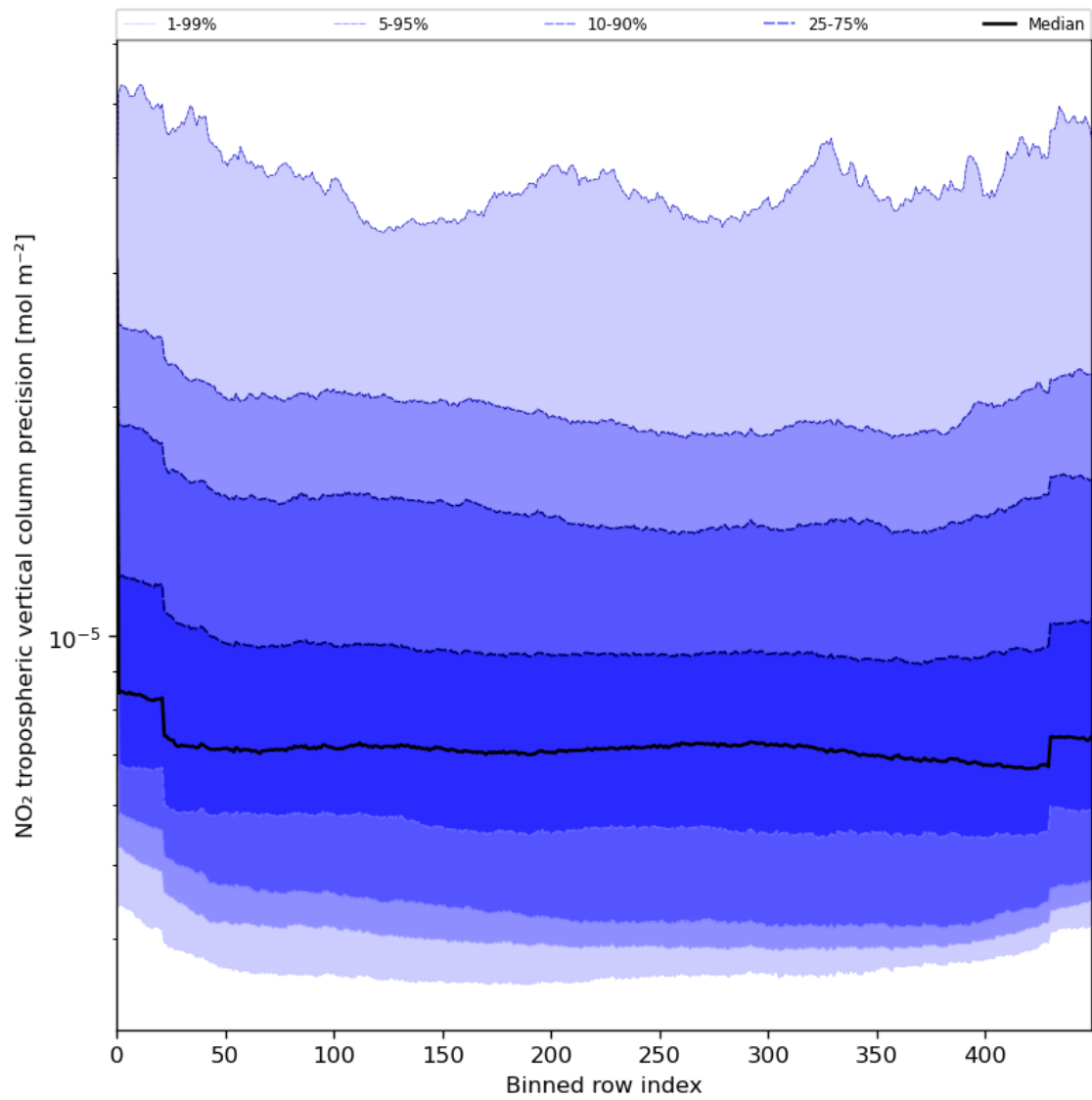
Figure 47: Along track statistics of “NO 2 tropospheric vertical column precision” for 2024-06-19 to 2024-06-21
