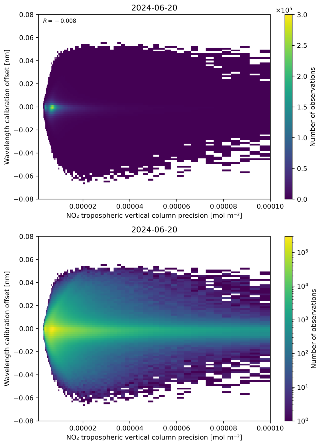
Figure 141: Scatter density plot of “NO 2 tropospheric vertical column precision” against “Wavelength calibration offset” for 2024-06-19 to 2024-06-21.
