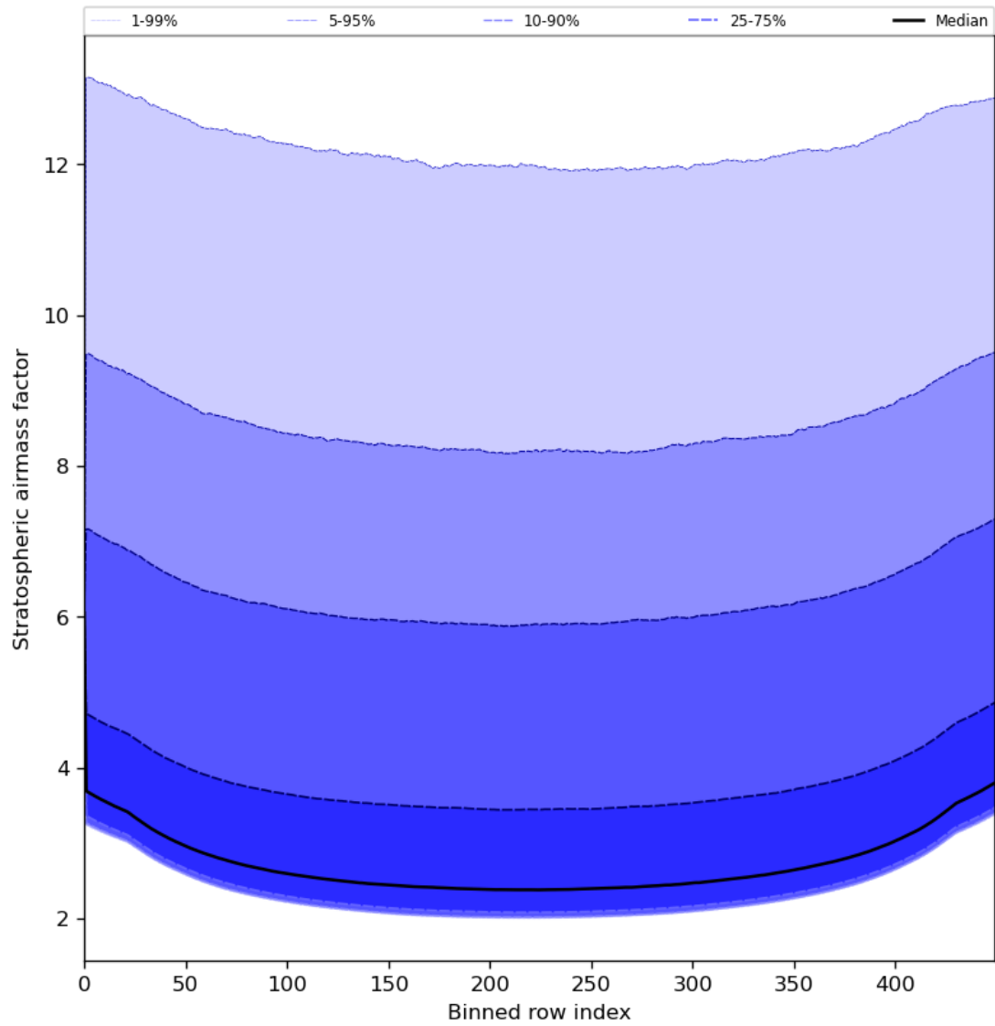
Figure 61: Along track statistics of “Stratospheric airmass factor” for 2024-06-19 to 2024-06-21
