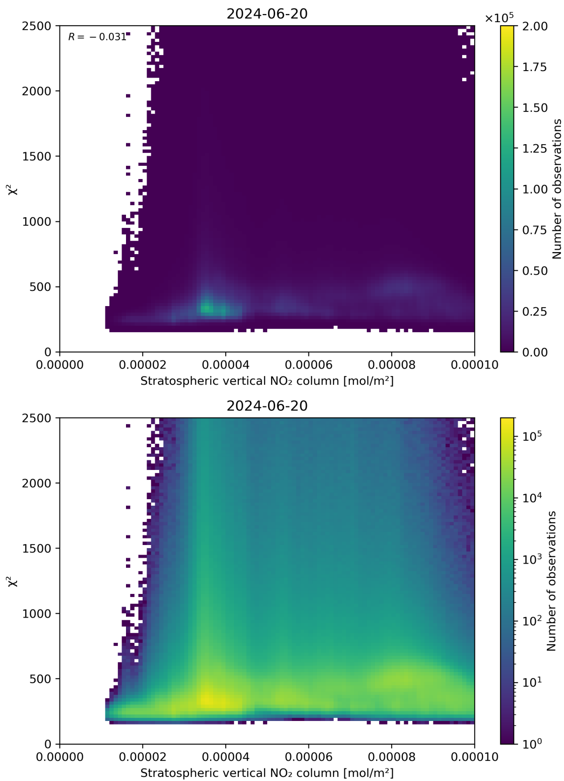
Figure 97: Scatter density plot of “Stratospheric vertical NO 2 column” against “ \chi^2 ” for 2024-06-19 to 2024-06-21.
