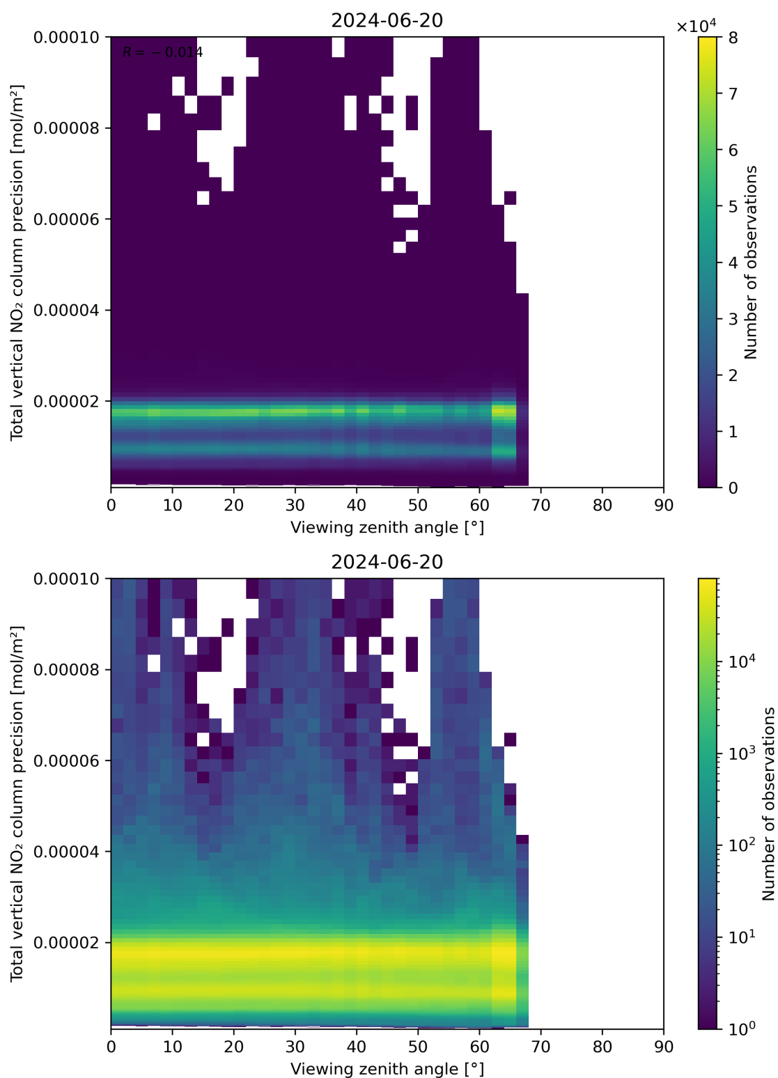
Figure 168: Scatter density plot of “Viewing zenith angle” against “Total vertical NO 2 column precision” for 2024-06-19 to 2024-06-21.
