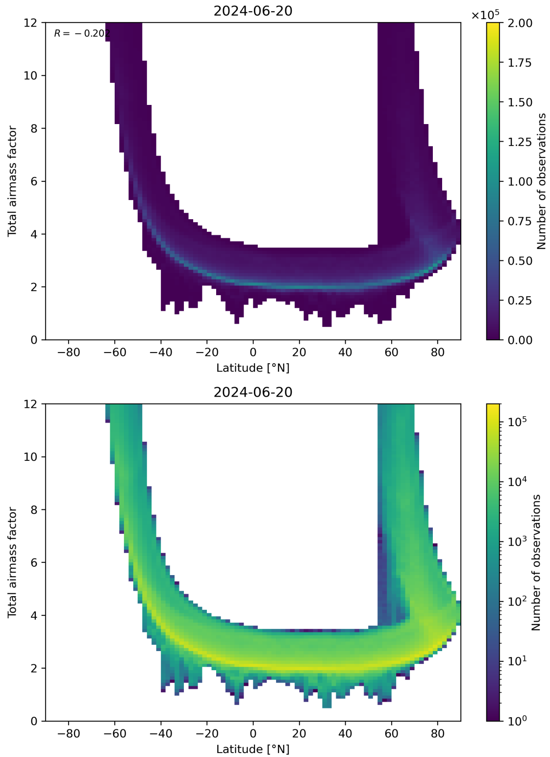
Figure 84: Scatter density plot of “Latitude” against “Total airmass factor” for 2024-06-19 to 2024-06-21.
