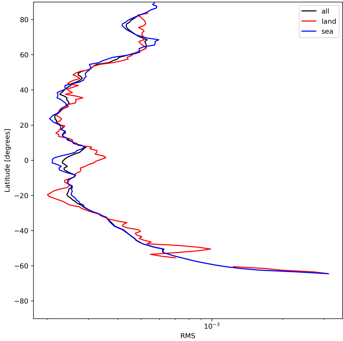
Figure 26: Zonal average of “RMS” for 2024-06-19 to 2024-06-21.
