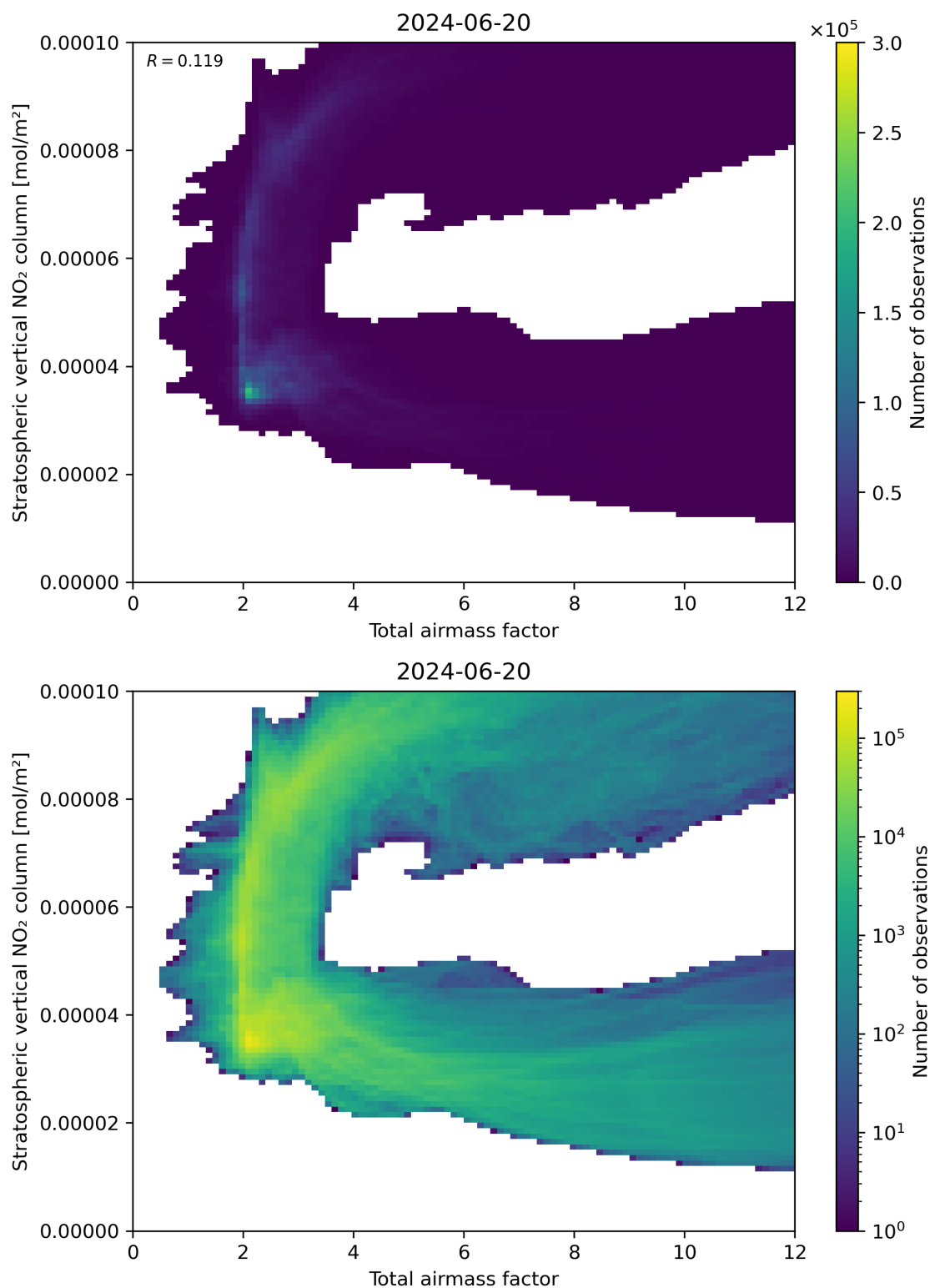
Figure 64: Scatter density plot of “Total airmass factor” against “Stratospheric vertical NO 2 column” for 2024-06-19 to 2024-06-21.
