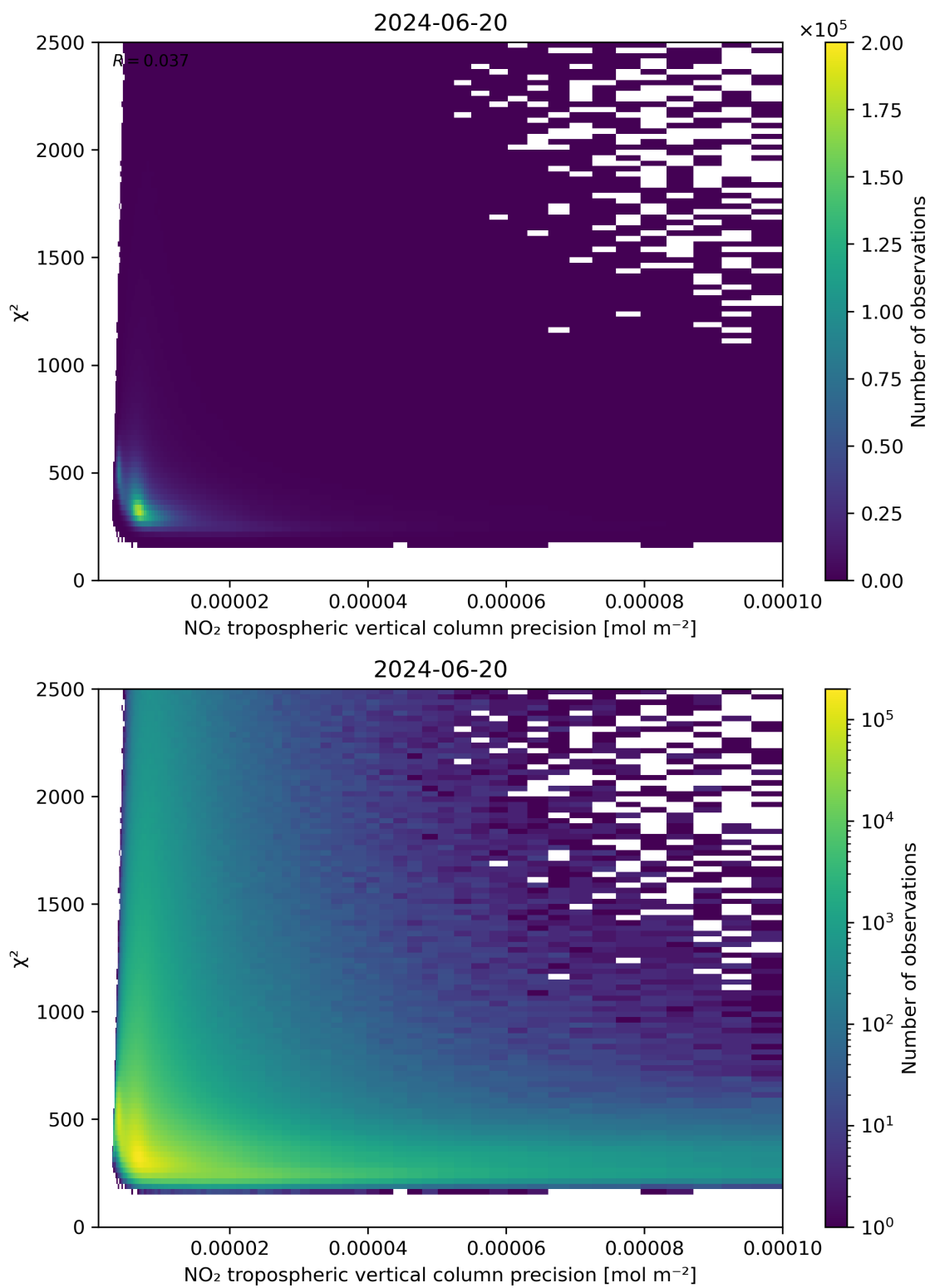
Figure 134: Scatter density plot of “NO 2 tropospheric vertical column precision” against “ \chi^2 ” for 2024-06-19 to 2024-06-21.
