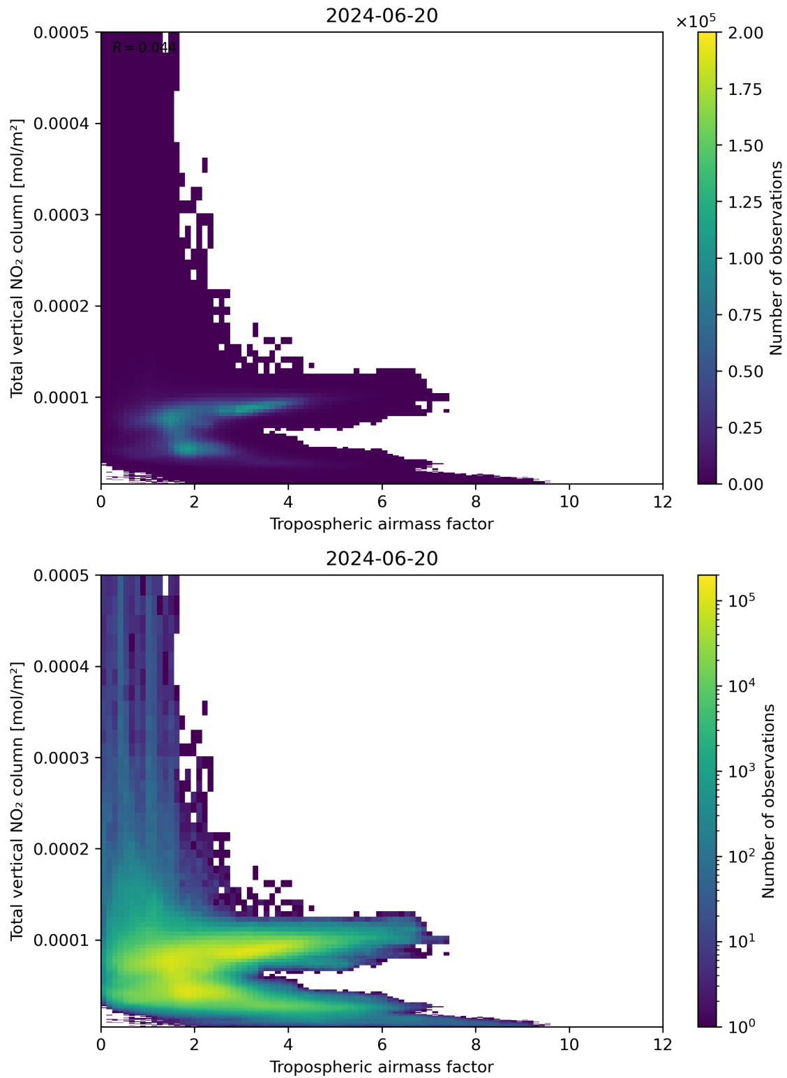
Figure 77: Scatter density plot of “Tropospheric airmass factor” against “Total vertical NO 2 column” for 2024-06-19 to 2024-06-21.
