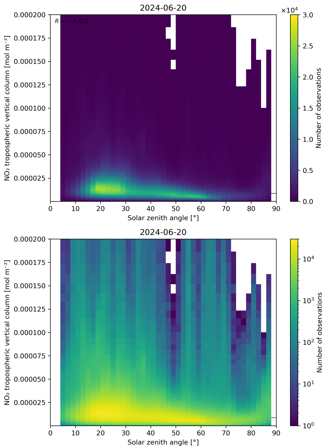
Figure 155: Scatter density plot of “Solar zenith angle” against “NO 2 tropospheric vertical column” for 2024-06-19 to 2024-06-21.
