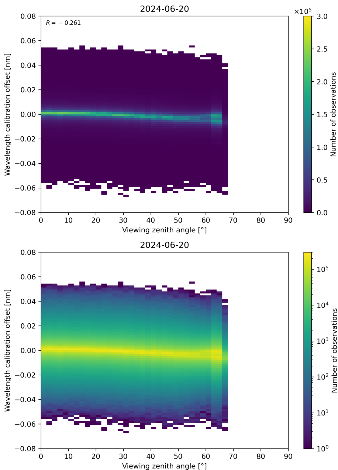
Figure 173: Scatter density plot of “Viewing zenith angle” against “Wavelength calibration offset” for 2024-06-19 to 2024-06-21.
