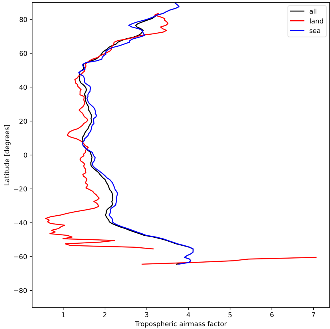
Figure 14: Zonal average of “Tropospheric airmass factor” for 2024-06-19 to 2024-06-21.
