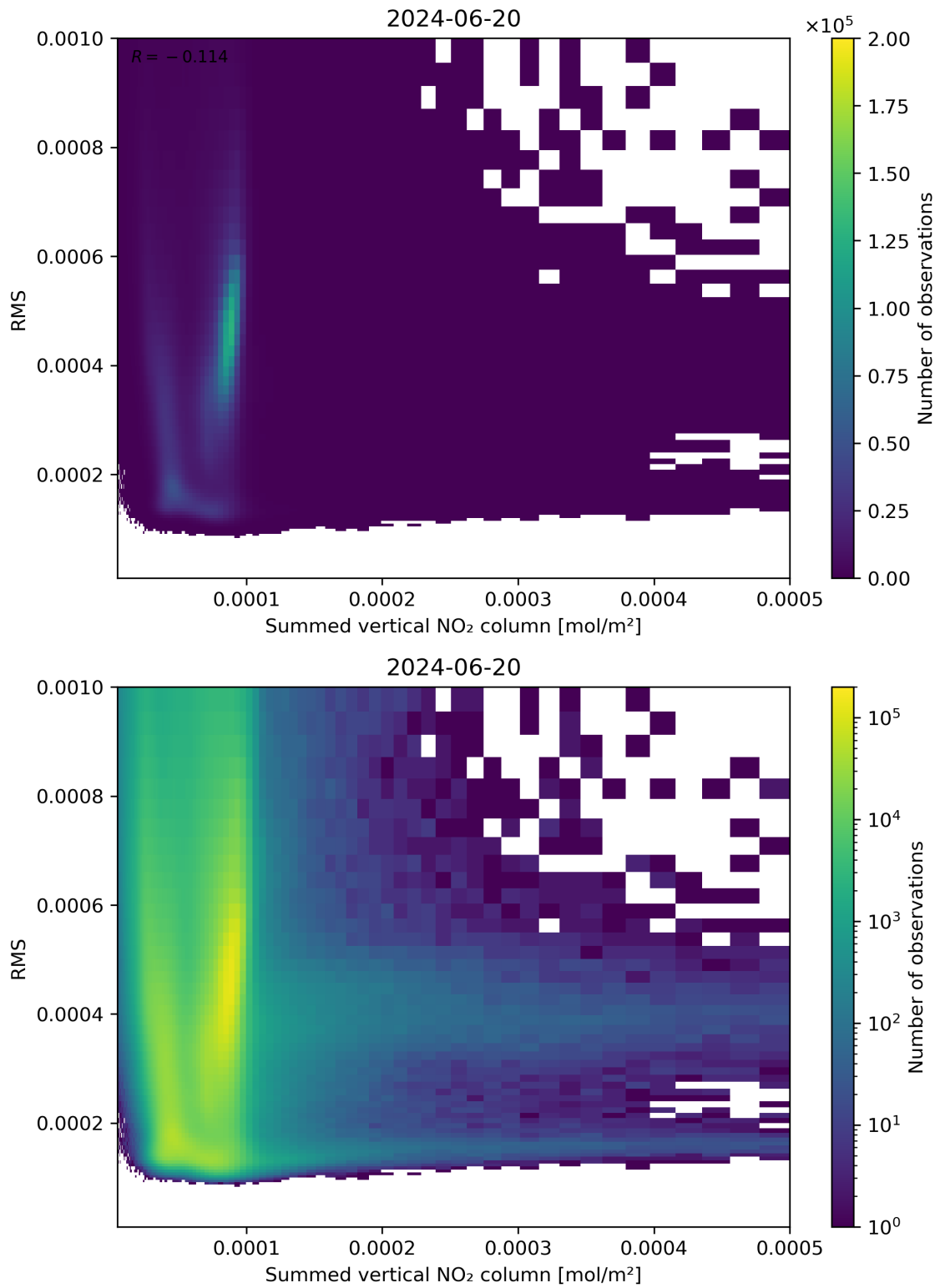
Figure 109: Scatter density plot of “Summed vertical NO 2 column” against “RMS” for 2024-06-19 to 2024-06-21.
