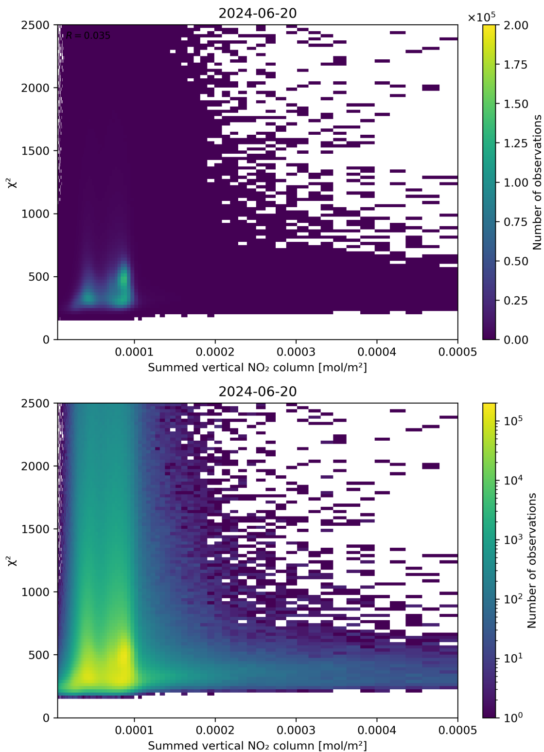
Figure 104: Scatter density plot of “Summed vertical NO 2 column” against “ \chi^2 ” for 2024-06-19 to 2024-06-21.
