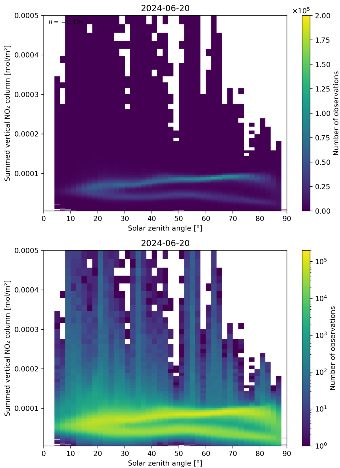
Figure 151: Scatter density plot of “Solar zenith angle” against “Summed vertical NO 2 column” for 2024-06-19 to 2024-06-21.
