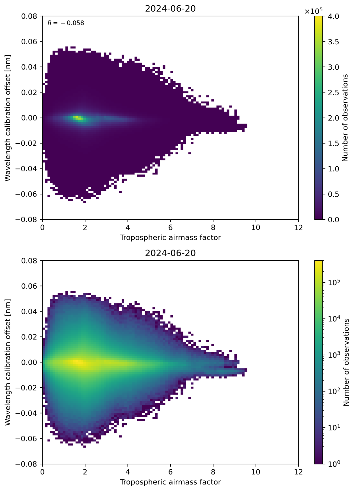
Figure 80: Scatter density plot of “Tropospheric airmass factor” against “Wavelength calibration offset” for 2024-06-19 to 2024-06-21.
