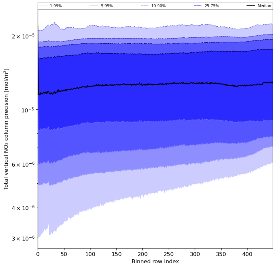
Figure 56: Along track statistics of “Total vertical NO 2 column precision” for 2024-06-19 to 2024-06-21
