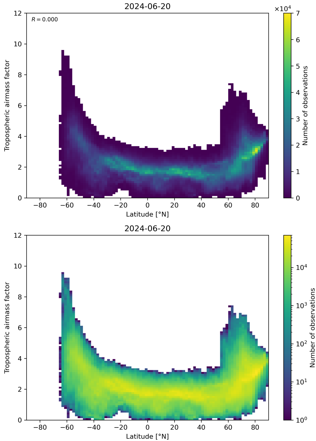
Figure 85: Scatter density plot of “Latitude” against “Tropospheric air mass factor” for 2024-06-19 to 2024-06-21.
