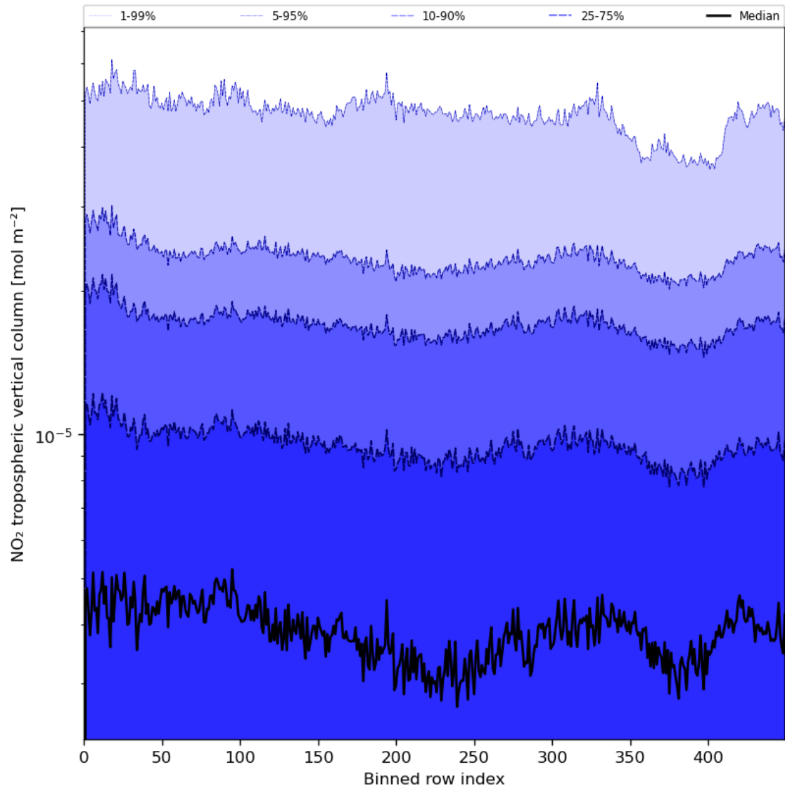
Figure 46: Along track statistics of “NO 2 tropospheric vertical column” for 2024-06-19 to 2024-06-21
