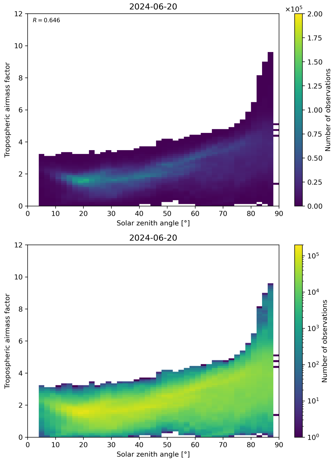
Figure 147: Scatter density plot of “Solar zenith angle” against “Tropospheric airmass factor” for 2024-06-19 to 2024-06-21.
