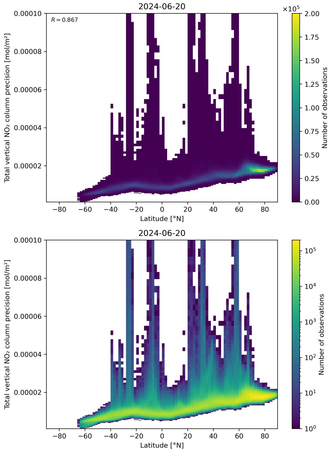
Figure 91: Scatter density plot of “Latitude” against “Total vertical NO 2 column precision” for 2024-06-19 to 2024-06-21.
