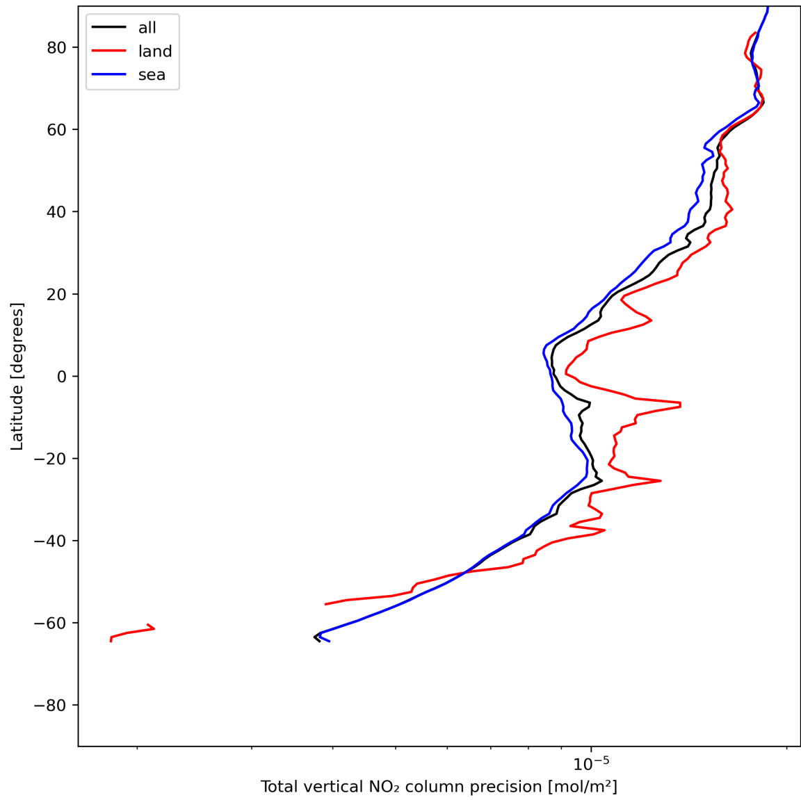
Figure 22: Zonal average of “Total vertical NO 2 column precision” for 2024-06-19 to 2024-06-21.
