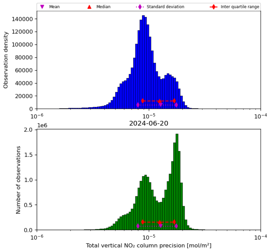
Figure 39: Histogram of “Total vertical NO 2 column precision” for 2024-06-19 to 2024-06-21
