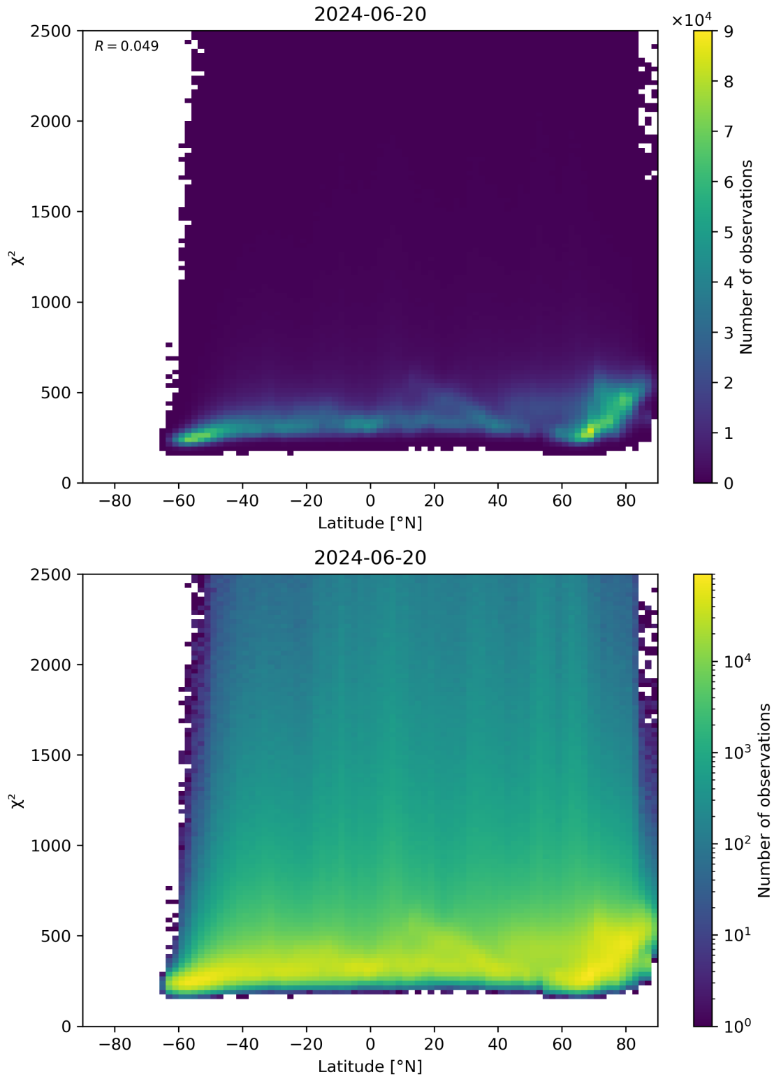
Figure 86: Scatter density plot of “Latitude” against “ \chi^2 ” for 2024-06-19 to 2024-06-21.
