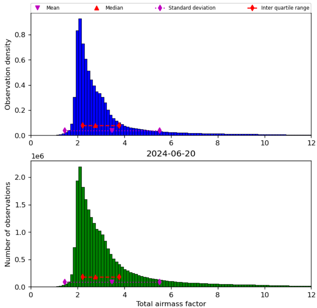
Figure 32: Histogram of “Total airmass factor” for 2024-06-19 to 2024-06-21
