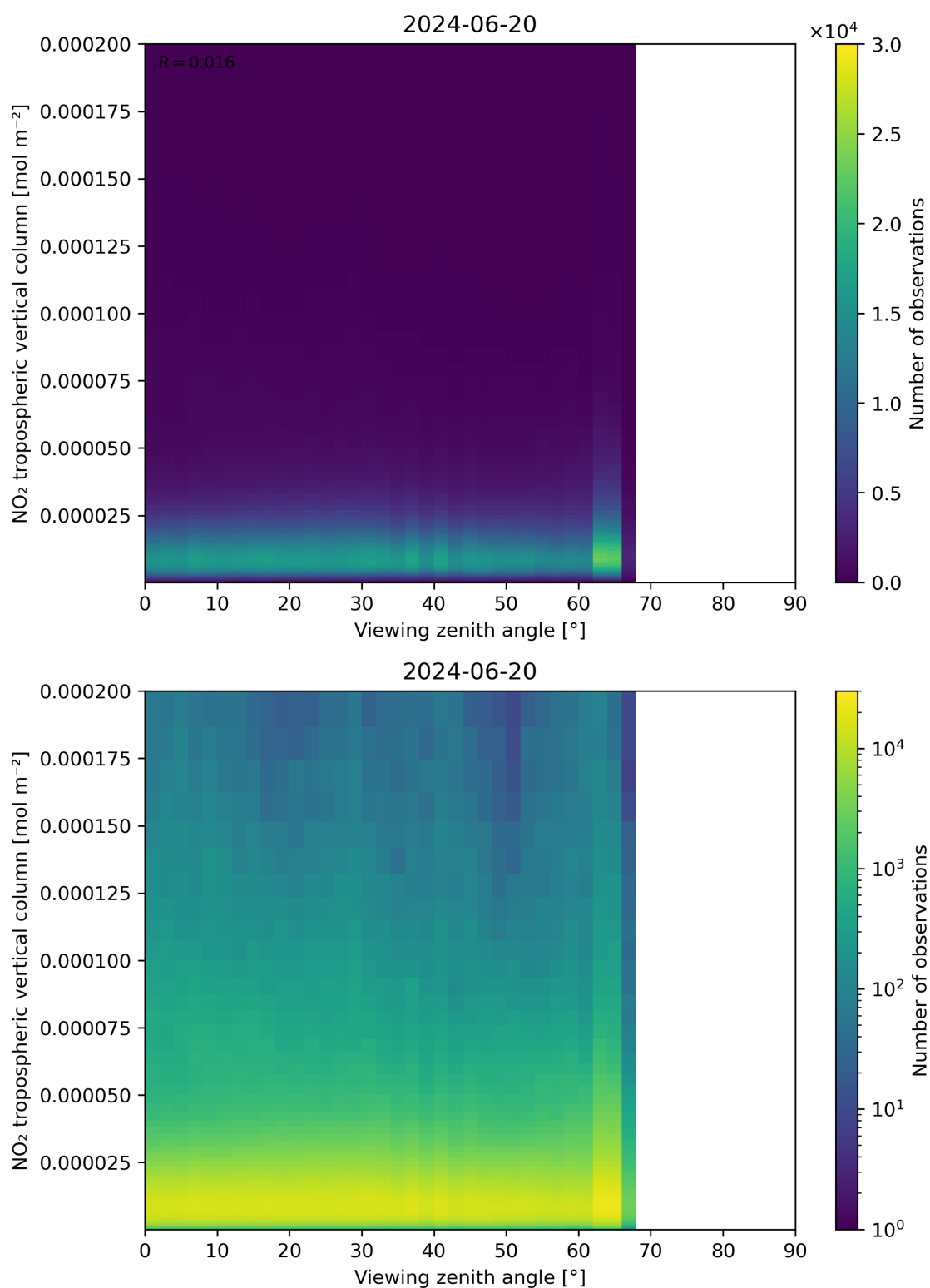
Figure 169: Scatter density plot of “Viewing zenith angle” against “NO 2 tropospheric vertical column” for 2024-06-19 to 2024-06-21.
