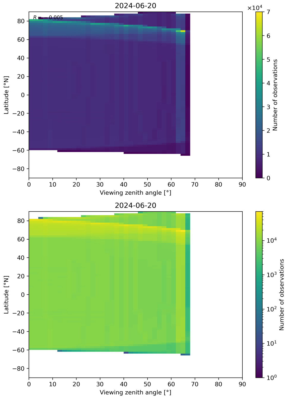
Figure 163: Scatter density plot of “Viewing zenith angle” against “Latitude” for 2024-06-19 to 2024-06-21.
