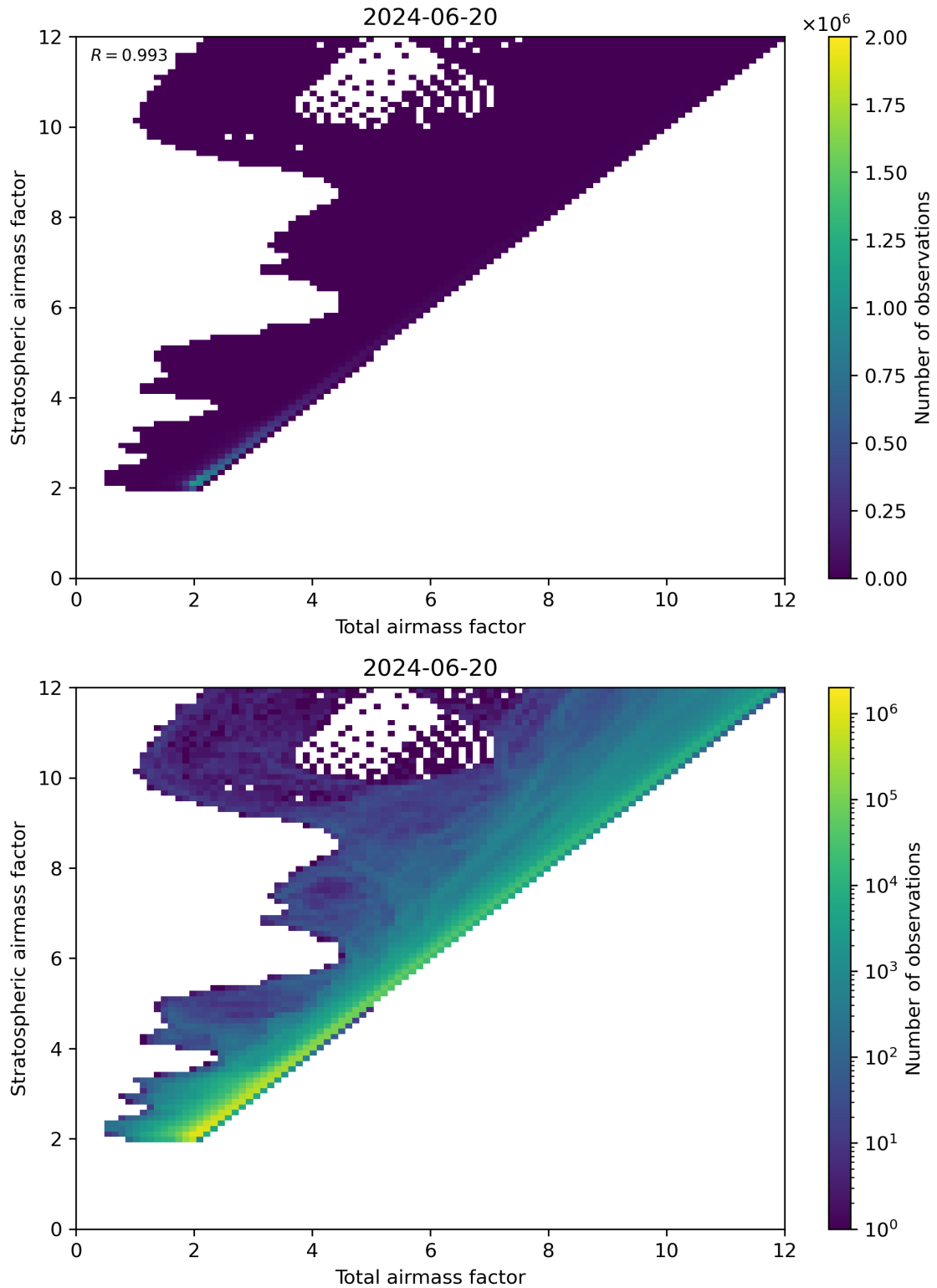
Figure 62: Scatter density plot of “Total airmass factor” against “Stratospheric airmass factor” for 2024-06-19 to 2024-06-21.
