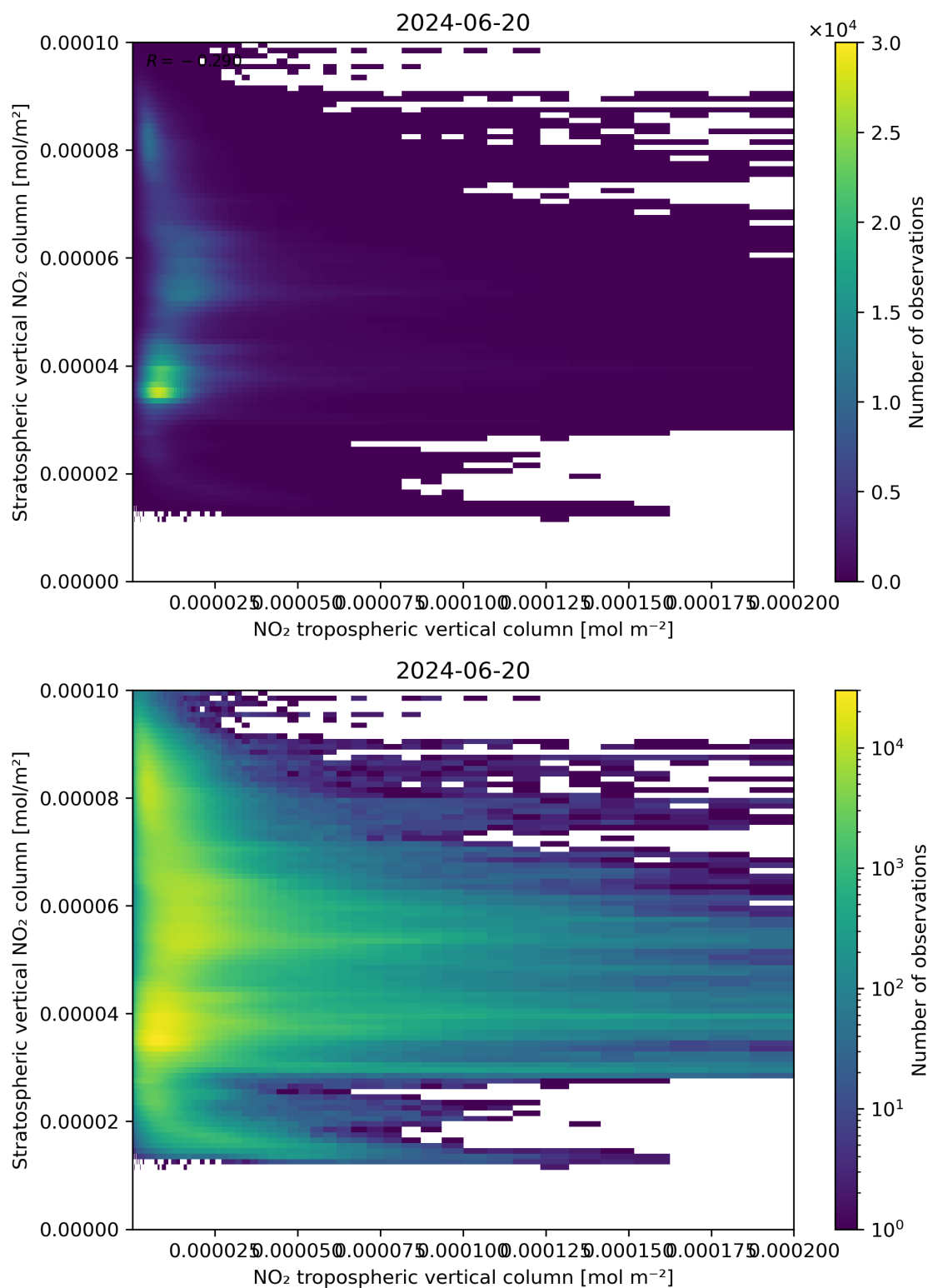
Figure 125: Scatter density plot of “NO 2 tropospheric vertical column” against “Stratospheric vertical NO 2 column” for 2024-06-19 to 2024-06-21.
