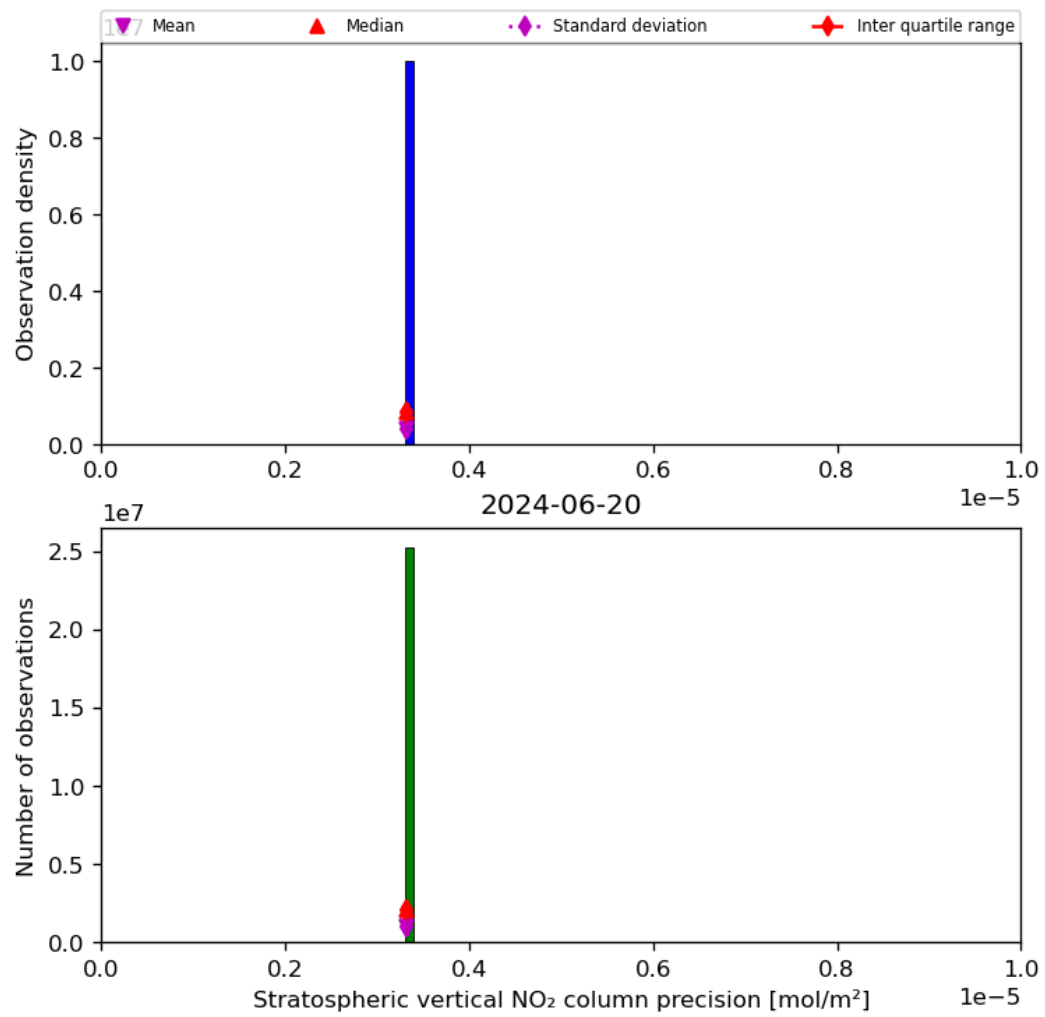
Figure 37: Histogram of “Stratospheric vertical NO 2 column precision” for 2024-06-19 to 2024-06-21
