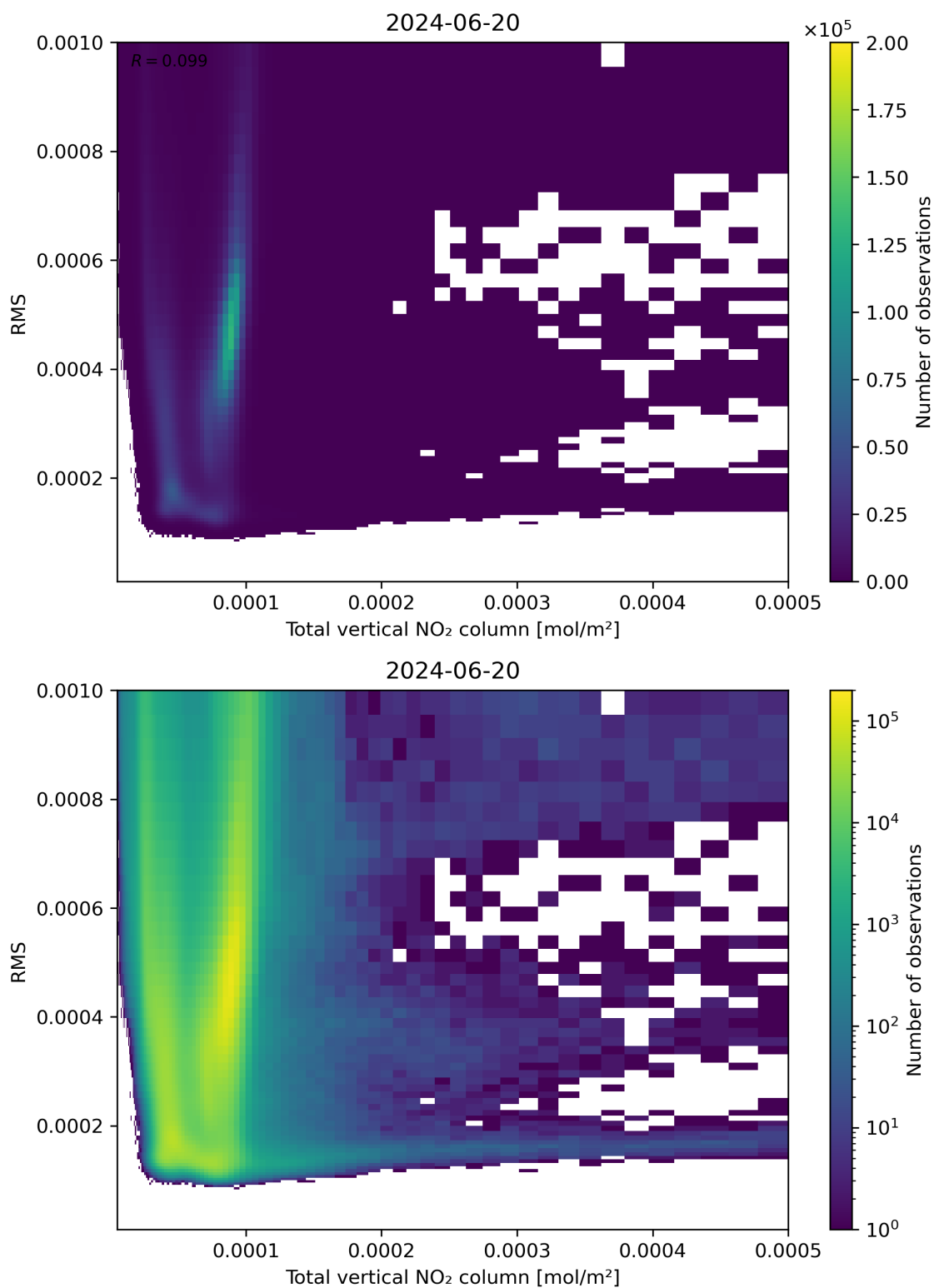
Figure 120: Scatter density plot of “Total vertical NO 2 column” against “RMS” for 2024-06-19 to 2024-06-21.
