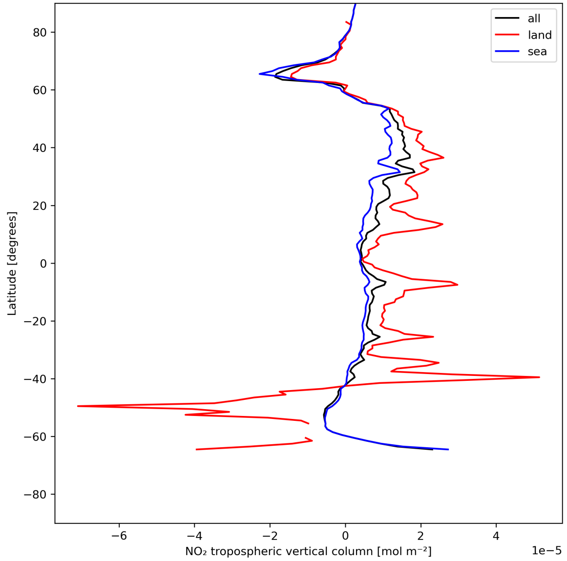
Figure 12: Zonal average of “NO 2 tropospheric vertical column” for 2024-06-19 to 2024-06-21.
