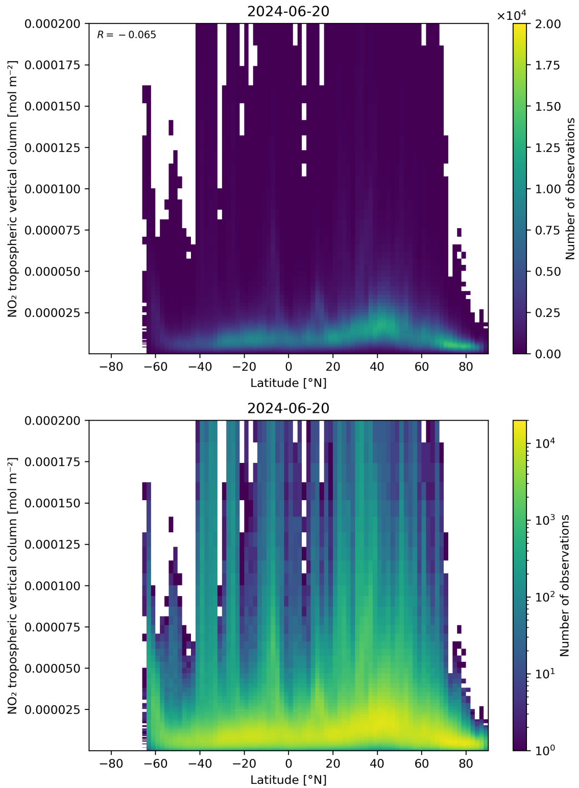
Figure 92: Scatter density plot of “Latitude” against “NO 2 tropospheric vertical column” for 2024-06-19 to 2024-06-21.
