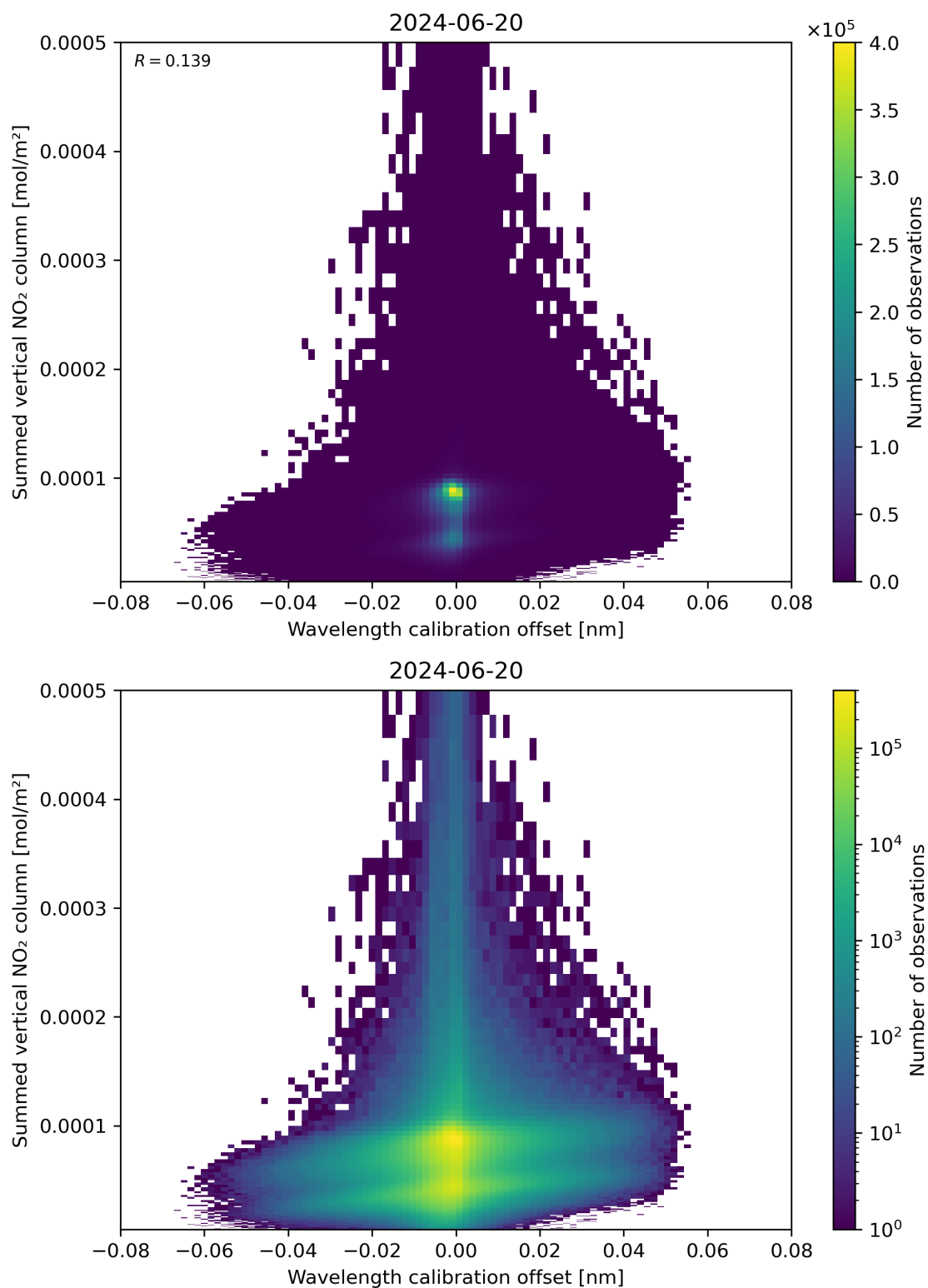
Figure 177: Scatter density plot of “Wavelength calibration offset” against “Summed vertical NO 2 column” for 2024-06-19 to 2024-06-21.
