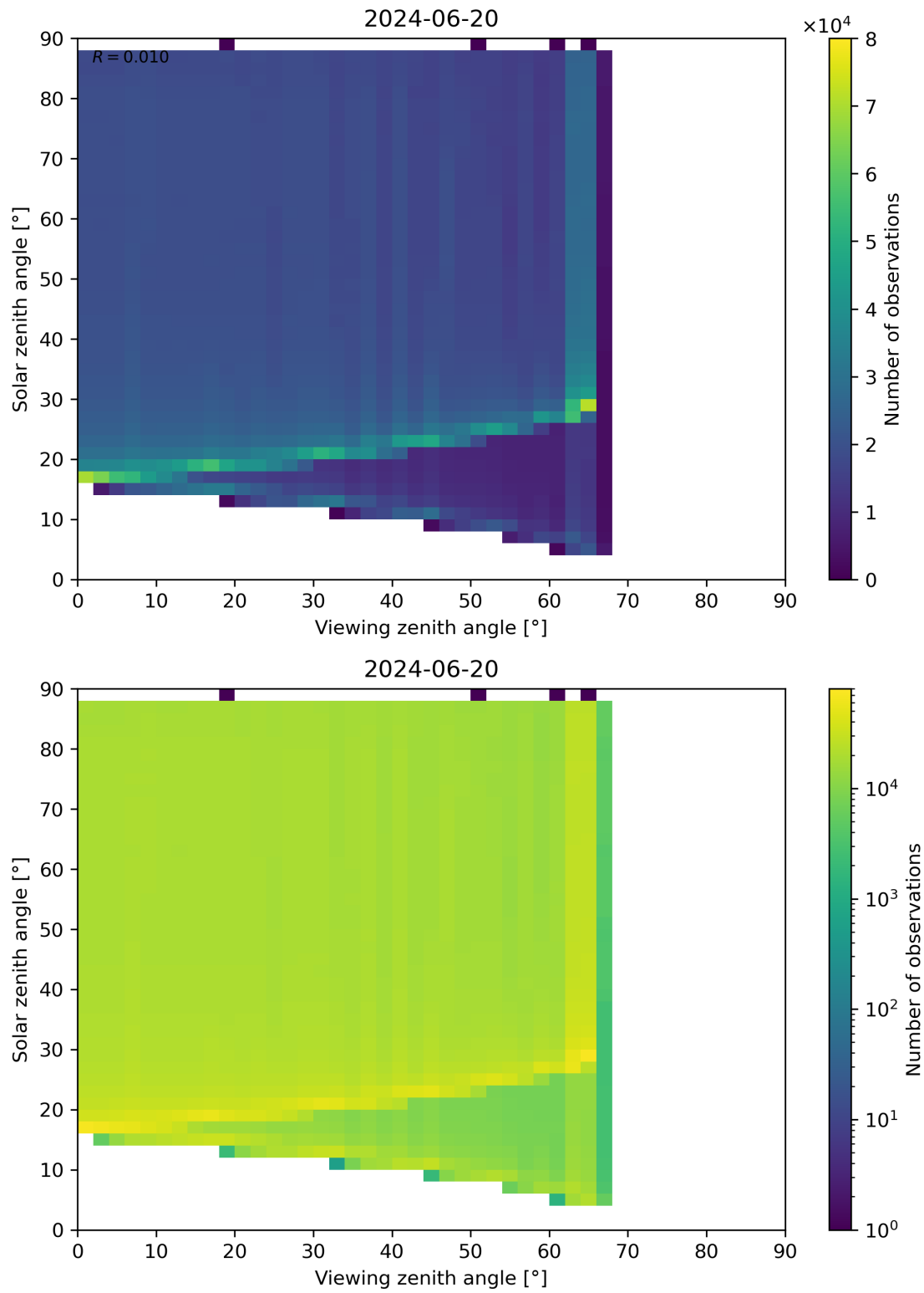
Figure 172: Scatter density plot of “Viewing zenith angle” against “Solar zenith angle” for 2024-06-19 to 2024-06-21.
