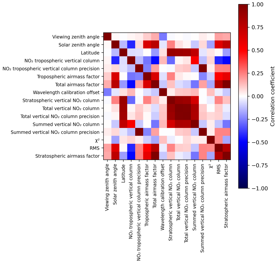
Figure 2: Map of correlation matrix for 2024-06-19 to 2024-06-21.
