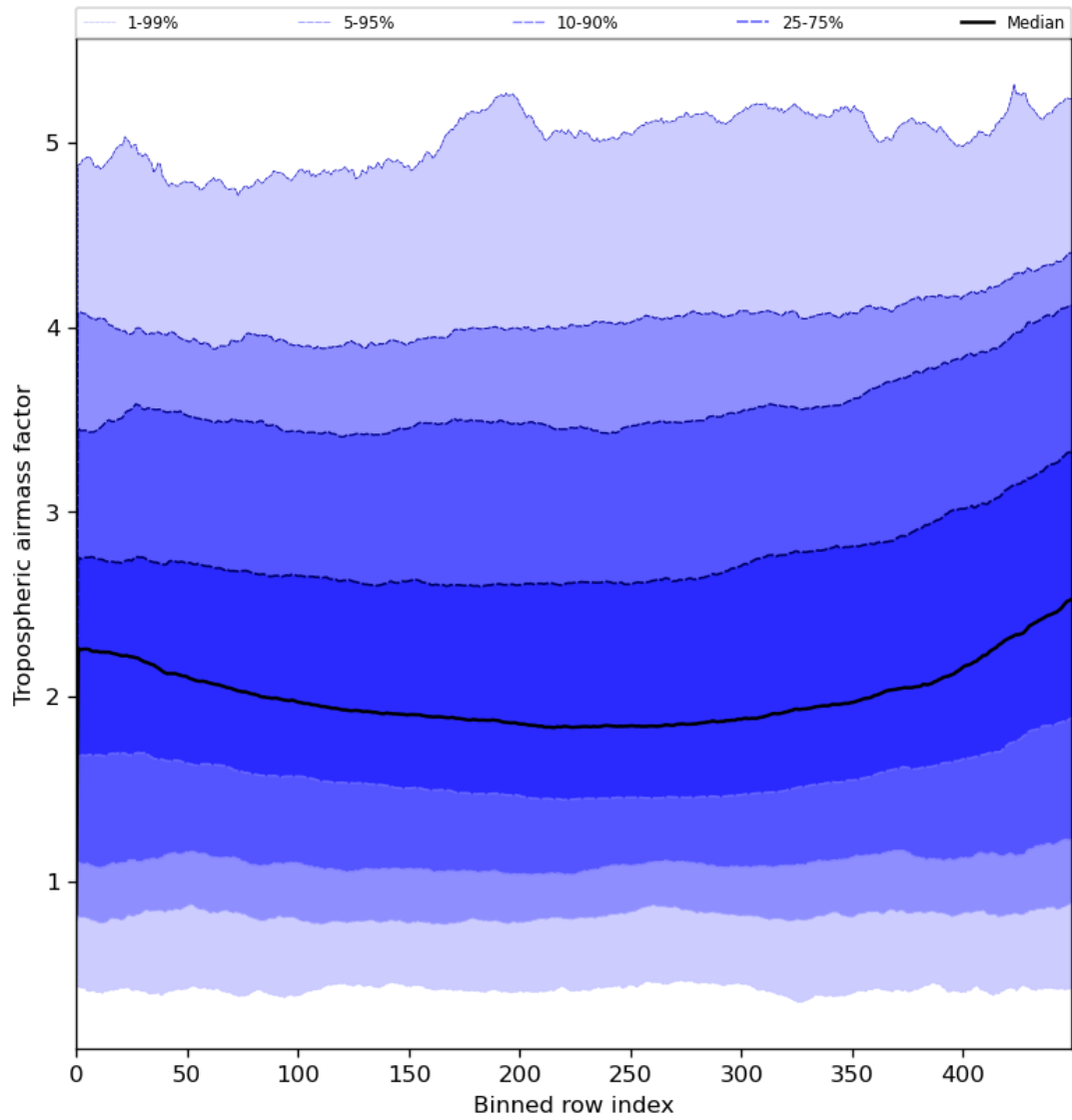
Figure 48: Along track statistics of “Tropospheric airmass factor” for 2024-06-19 to 2024-06-21
