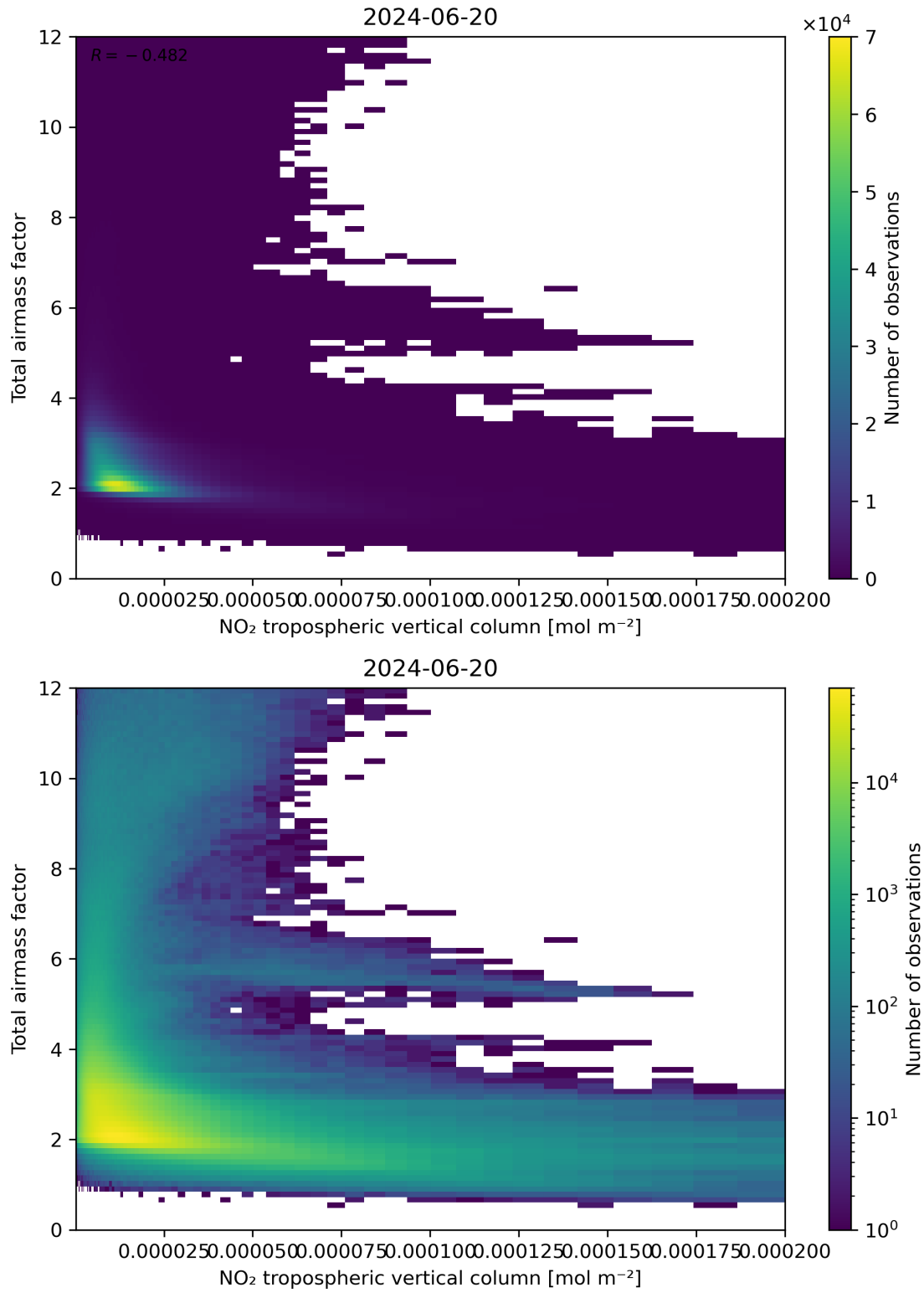
Figure 122: Scatter density plot of “NO 2 tropospheric vertical column” against “Total airmass factor” for 2024-06-19 to 2024-06-21.
