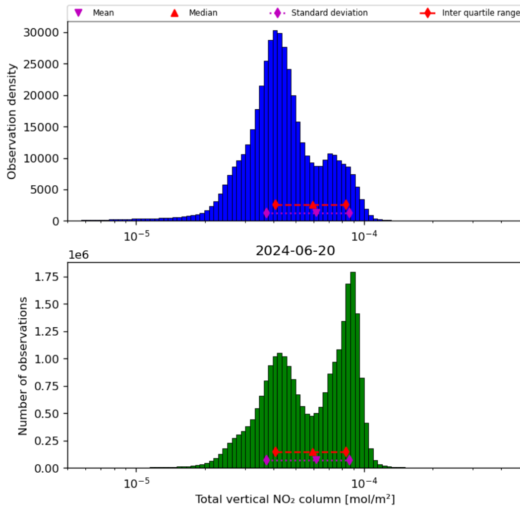
Figure 38: Histogram of “Total vertical NO 2 column” for 2024-06-19 to 2024-06-21
