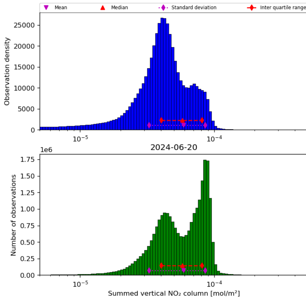
Figure 40: Histogram of “Summed vertical NO 2 column” for 2024-06-19 to 2024-06-21
