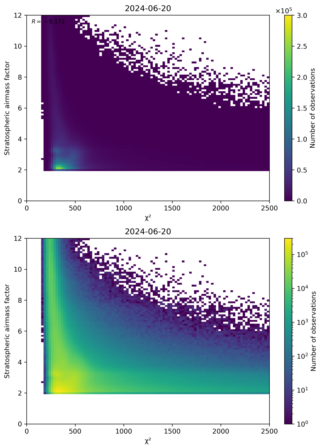
Figure 81: Scatter density plot of “ \chi^2 ” against “Stratospheric air mass factor” for 2024-06-19 to 2024-06-21.
