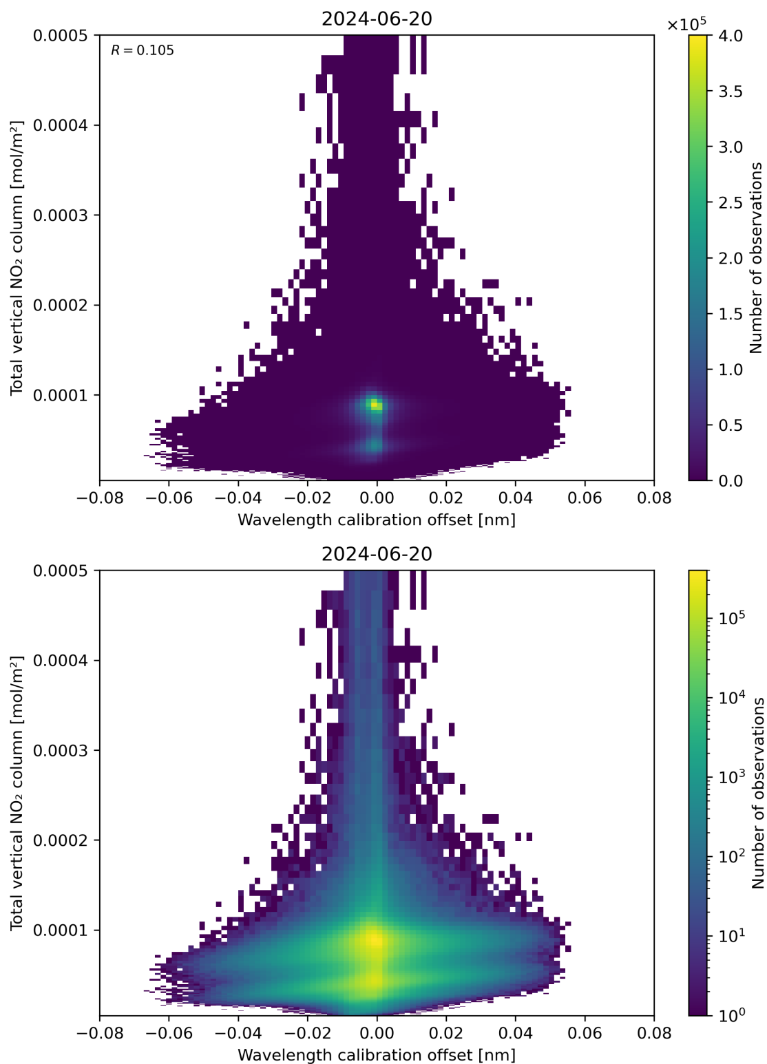
Figure 179: Scatter density plot of “Wavelength calibration offset” against “Total vertical NO 2 column” for 2024-06-19 to 2024-06-21.
