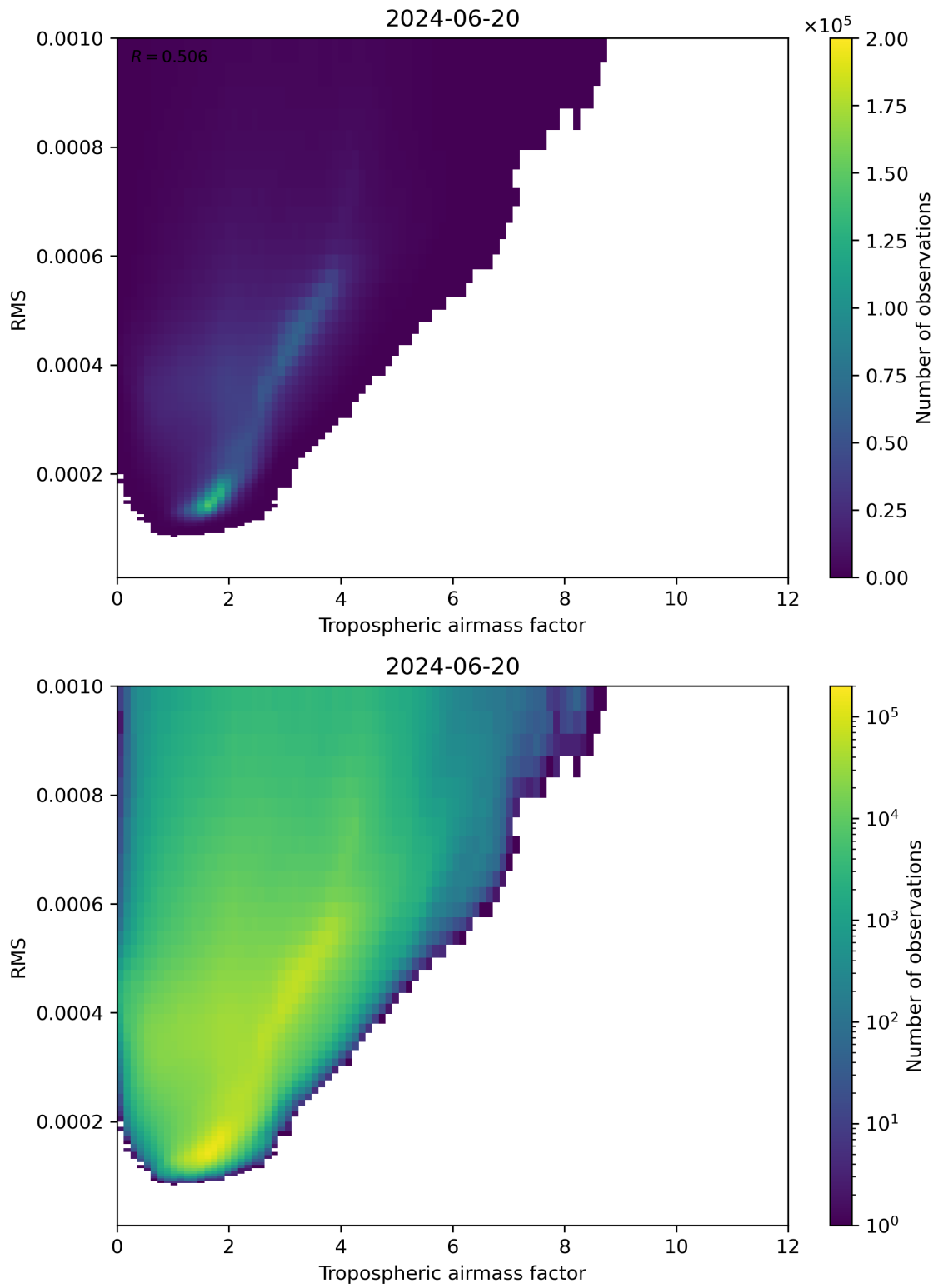
Figure 79: Scatter density plot of “Tropospheric airmass factor” against “RMS” for 2024-06-19 to 2024-06-21.
