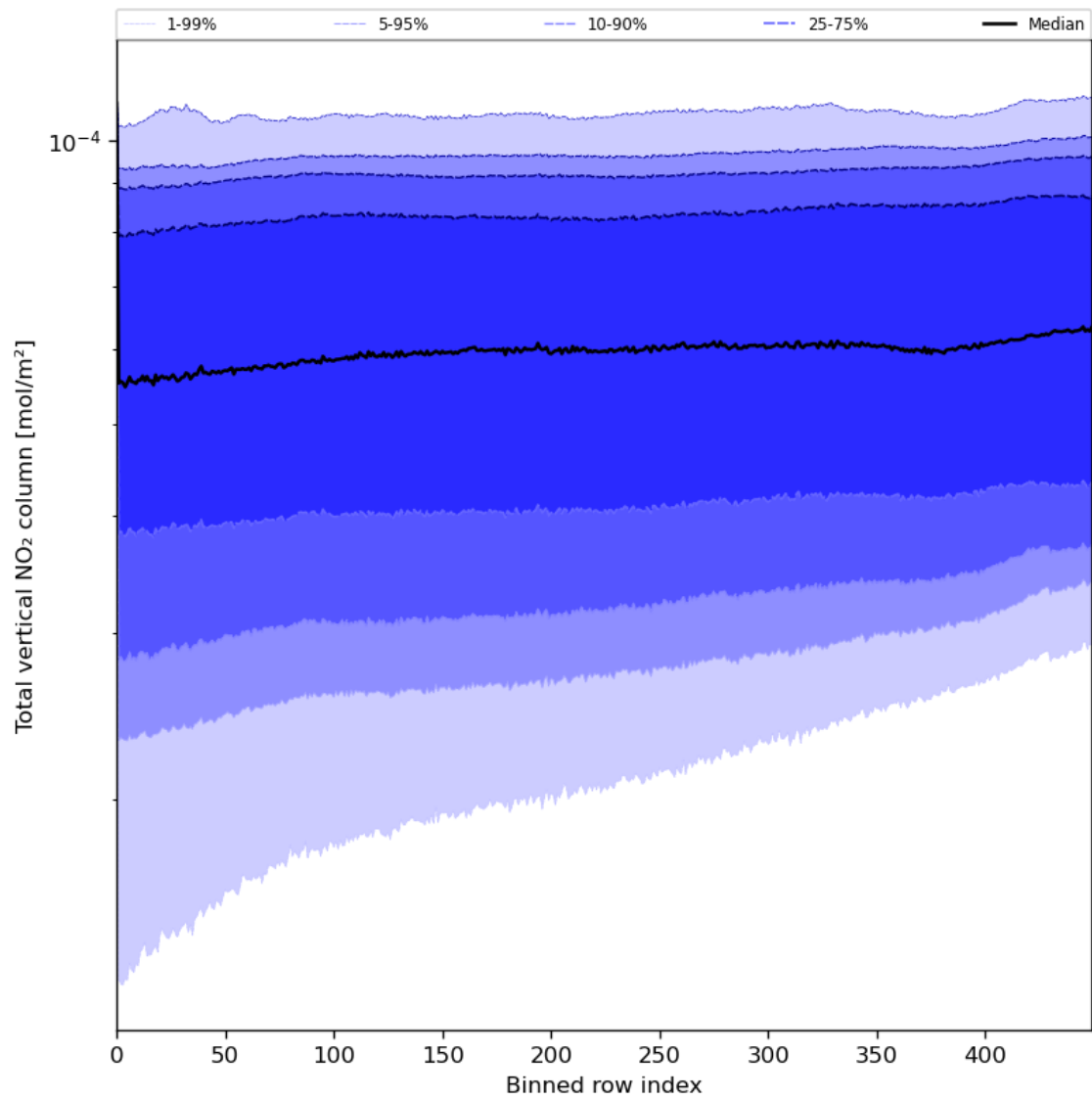
Figure 55: Along track statistics of “Total vertical NO 2 column” for 2024-06-19 to 2024-06-21
