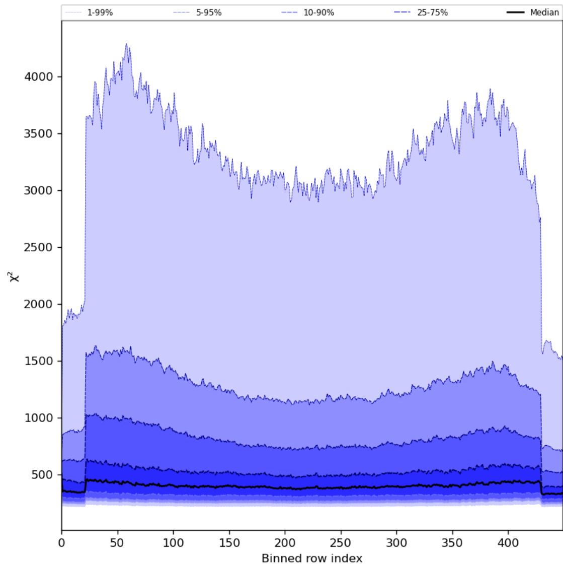
Figure 59: Along track statistics of “ \chi^2 ” for 2024-06-19 to 2024-06-21
