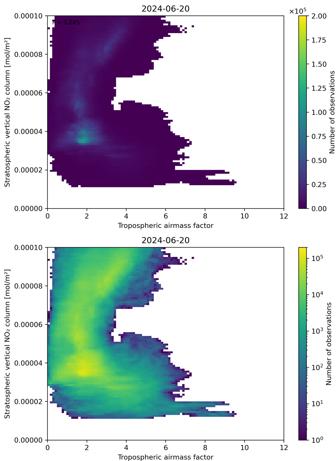
Figure 74: Scatter density plot of “Tropospheric air mass factor” against “Stratospheric vertical NO 2 column” for 2024-06-19 to 2024-06-21.
