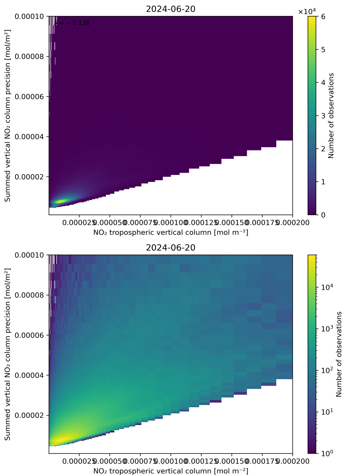
Figure 127: Scatter density plot of “NO 2 tropospheric vertical column” against “Summed vertical NO 2 column precision” for 2024-06-19 to 2024-06-21.
