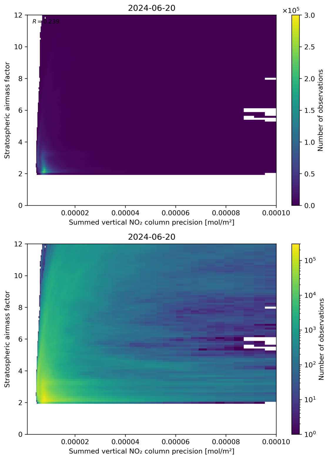
Figure 106: Scatter density plot of “Summed vertical NO 2 column precision” against “Stratospheric airmass factor” for 2024-06-19 to 2024-06-21.
