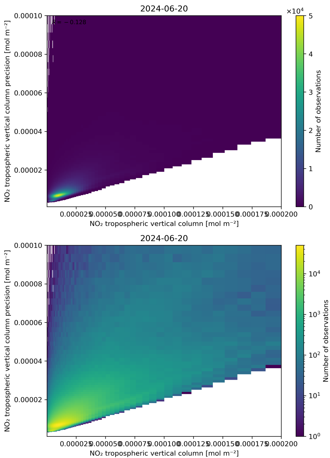
Figure 130: Scatter density plot of “NO 2 tropospheric vertical column” against “NO 2 tropospheric vertical column precision” for 2024-06-19 to 2024-06-21.
