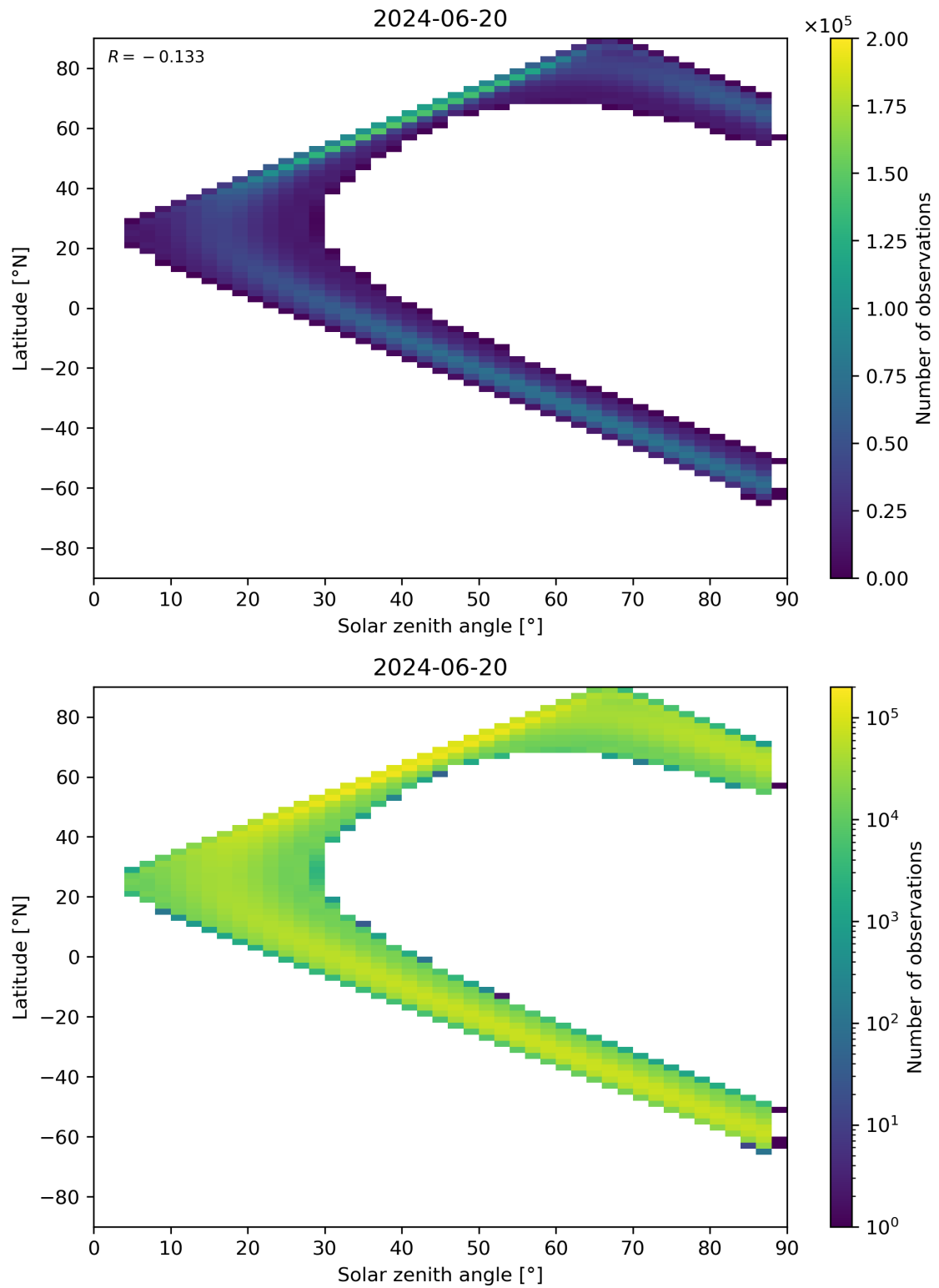
Figure 149: Scatter density plot of “Solar zenith angle” against “Latitude” for 2024-06-19 to 2024-06-21.
