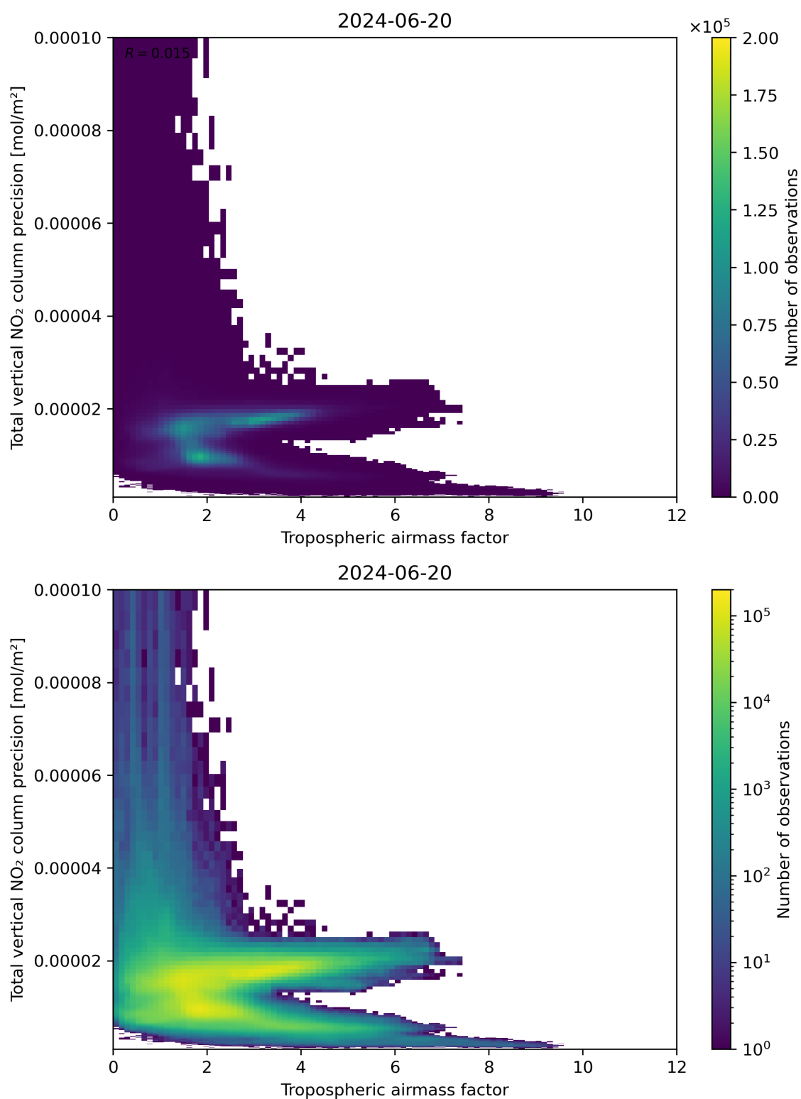
Figure 78: Scatter density plot of “Tropospheric air mass factor” against “Total vertical NO 2 column precision” for 2024-06-19 to 2024-06-21.
