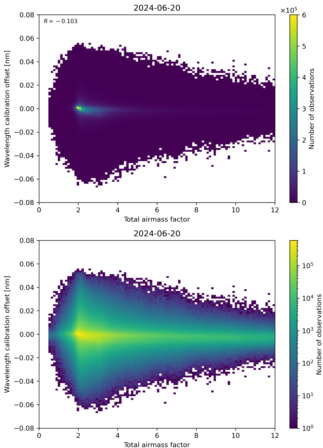
Figure 70: Scatter density plot of “Total airmass factor” against “Wavelength calibration offset” for 2024-06-19 to 2024-06-21.
