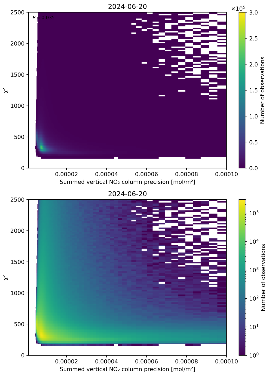
Figure 107: Scatter density plot of “Summed vertical NO 2 column precision” against “ \chi^2 ” for 2024-06-19 to 2024-06-21.
