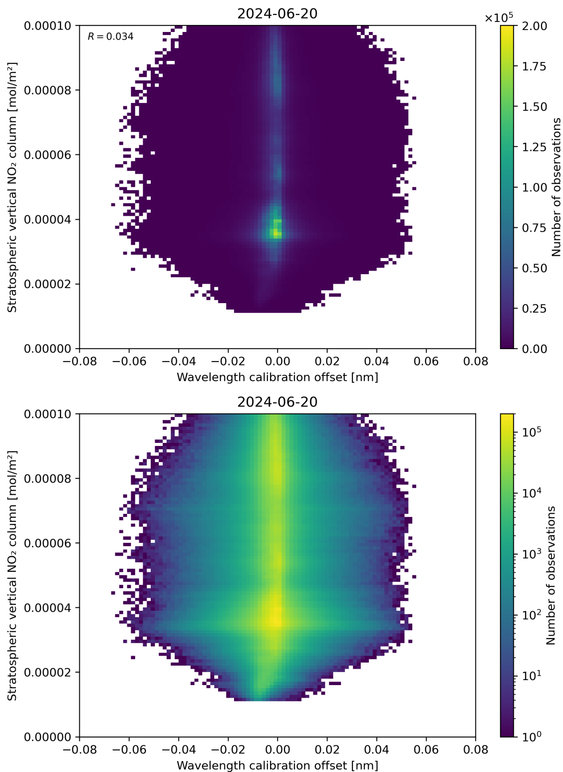
Figure 176: Scatter density plot of “Wavelength calibration offset” against “Stratospheric vertical NO 2 column” for 2024-06-19 to 2024-06-21.
