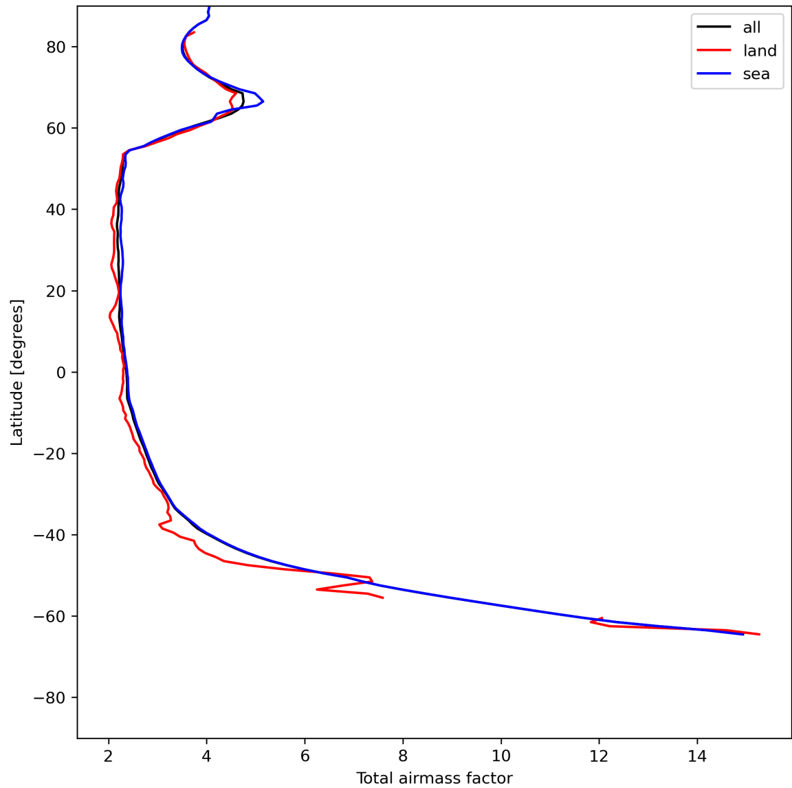
Figure 15: Zonal average of “Total airmass factor” for 2024-06-19 to 2024-06-21.
