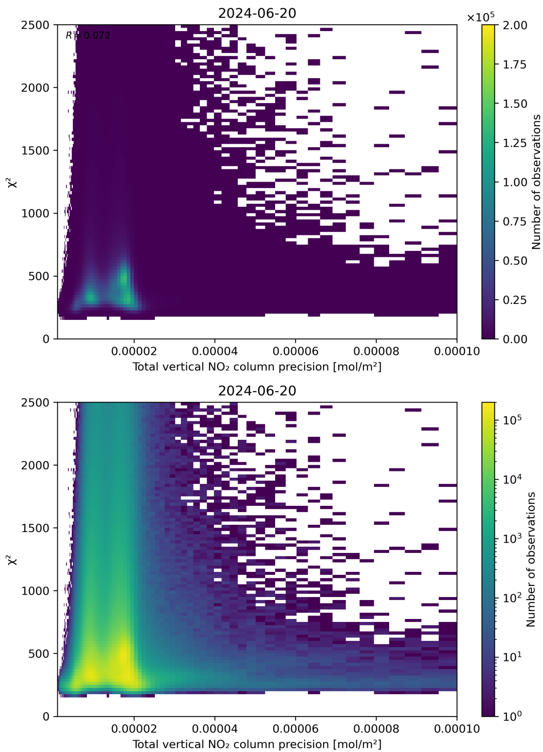
Figure 116: Scatter density plot of “Total vertical NO 2 column precision” against “ \chi^2 ” for 2024-06-19 to 2024-06-21.
