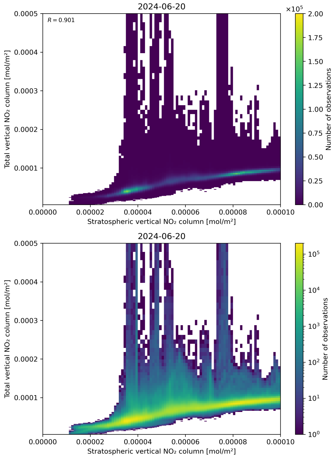
Figure 100: Scatter density plot of “Stratospheric vertical NO 2 column” against “Total vertical NO 2 column” for 2024-06-19 to 2024-06-21.
