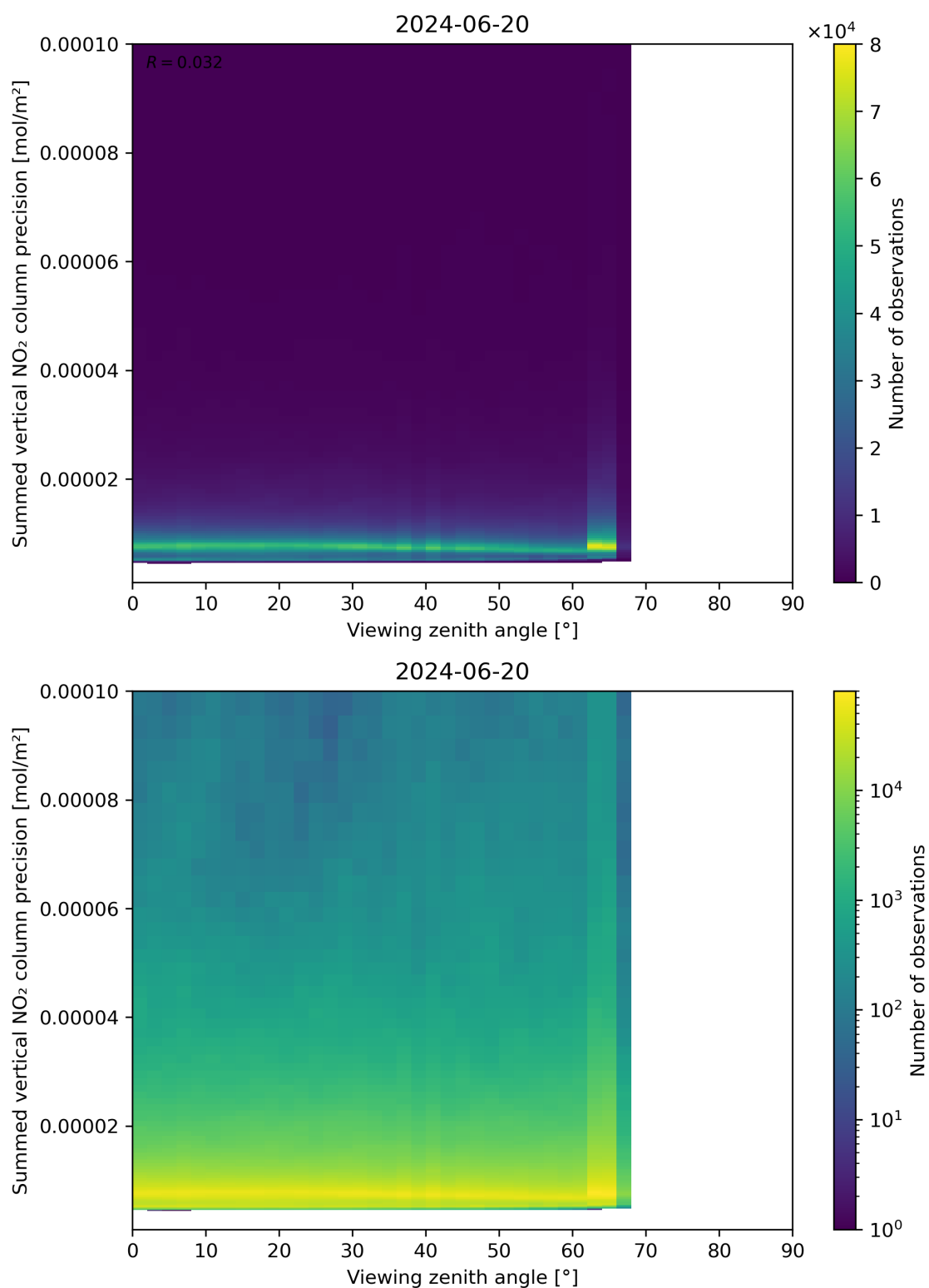
Figure 166: Scatter density plot of “Viewing zenith angle” against “Summed vertical NO 2 column precision” for 2024-06-19 to 2024-06-21.
