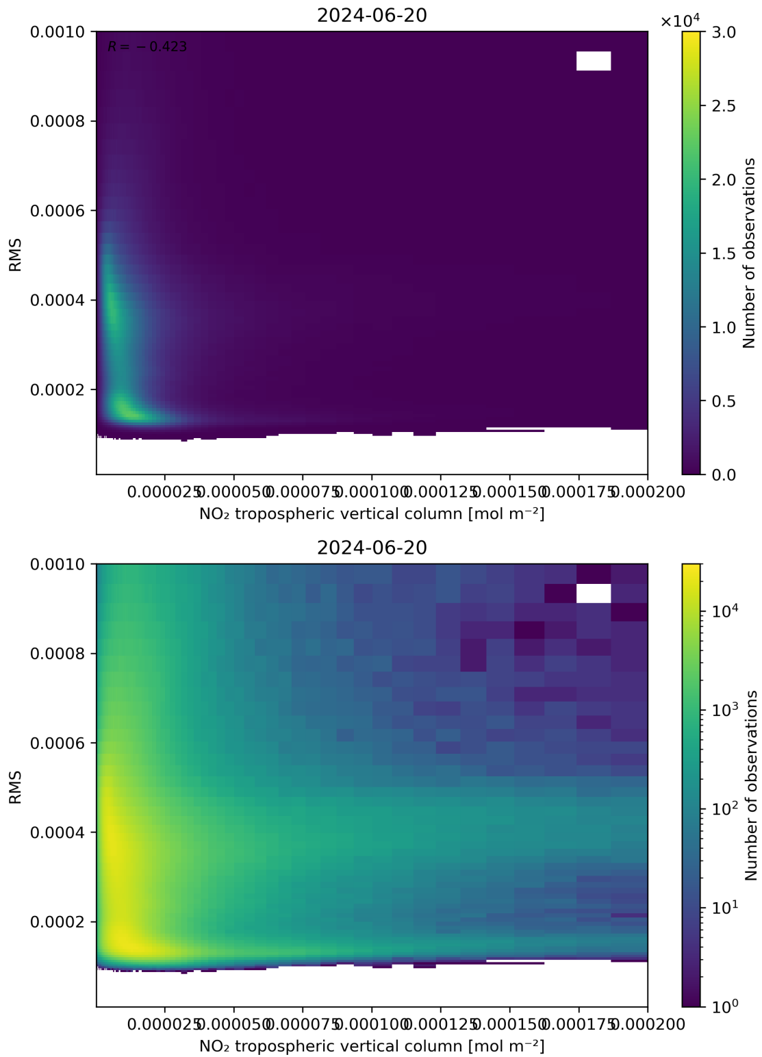
Figure 142: Scatter density plot of “NO 2 tropospheric vertical column” against “RMS” for 2024-06-19 to 2024-06-21.
