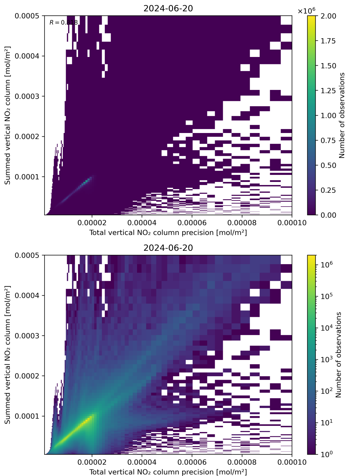
Figure 117: Scatter density plot of “Total vertical NO 2 column precision” against “Summed vertical NO 2 column” for 2024-06-19 to 2024-06-21.
