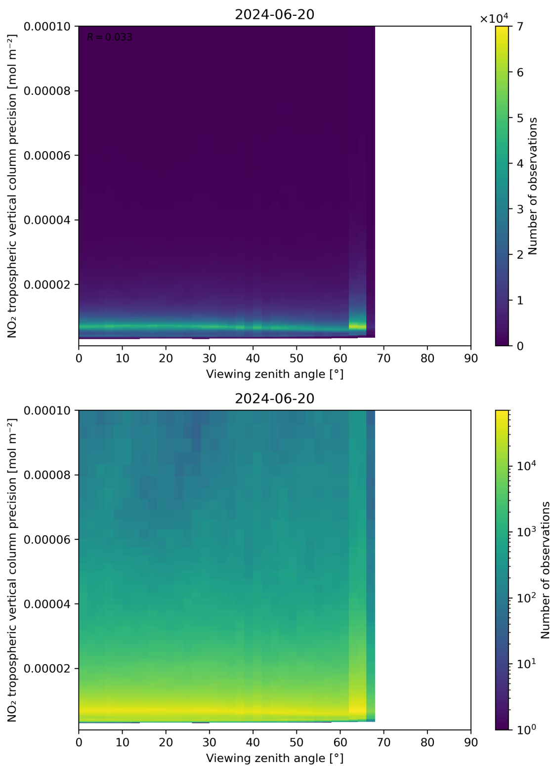
Figure 170: Scatter density plot of “Viewing zenith angle” against “NO 2 tropospheric vertical column precision” for 2024-06-19 to 2024-06-21.
