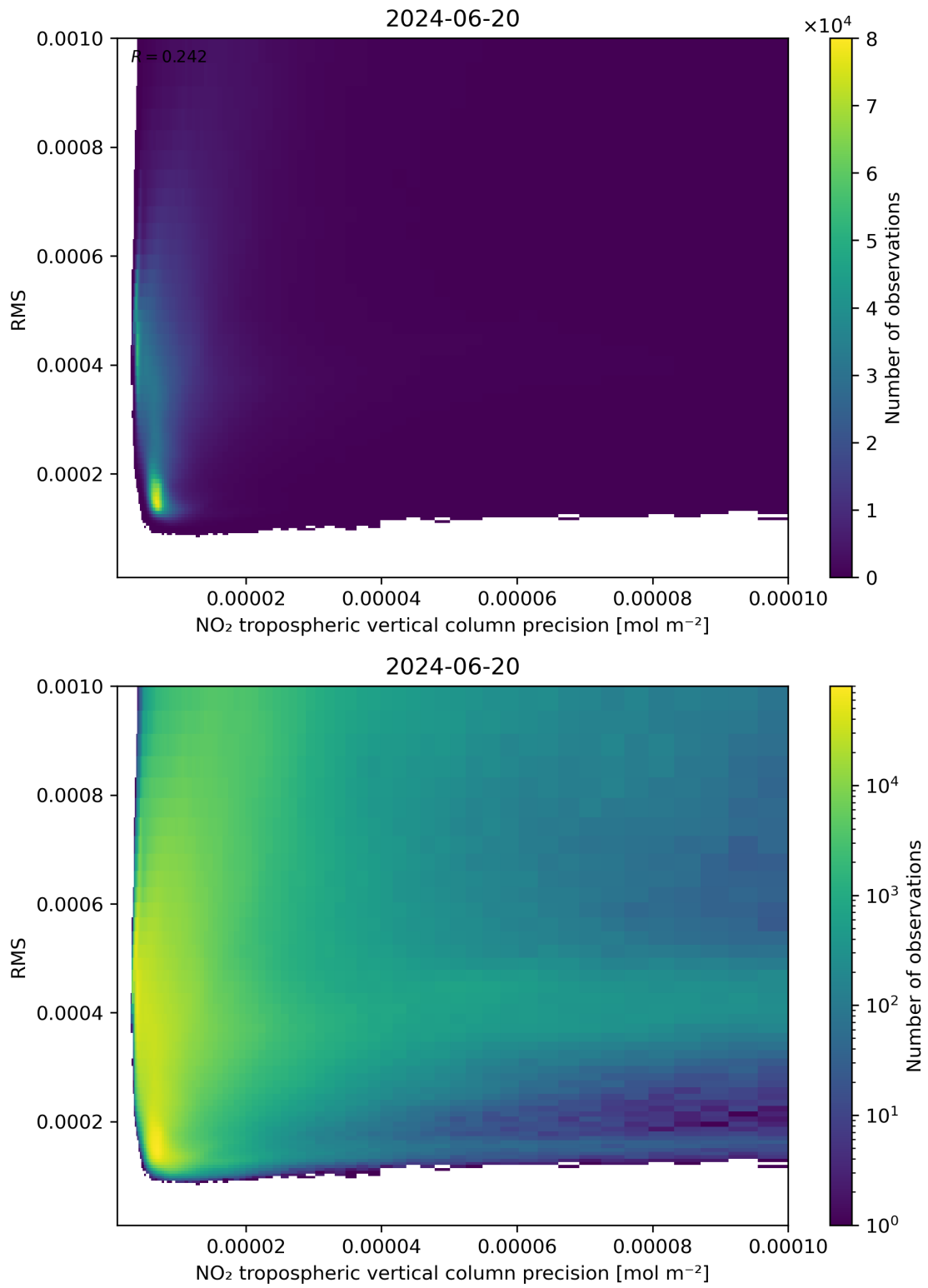
Figure 140: Scatter density plot of “NO 2 tropospheric vertical column precision” against “RMS” for 2024-06-19 to 2024-06-21.
