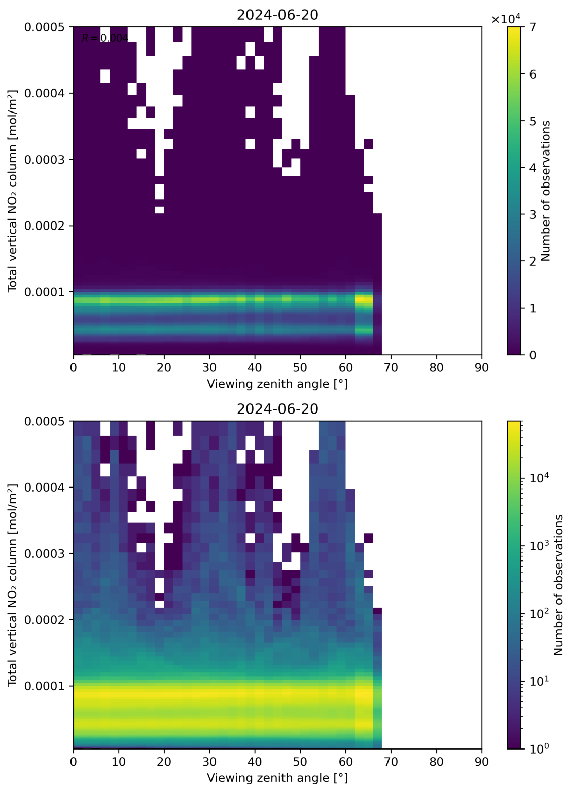
Figure 167: Scatter density plot of “Viewing zenith angle” against “Total vertical NO 2 column” for 2024-06-19 to 2024-06-21.
