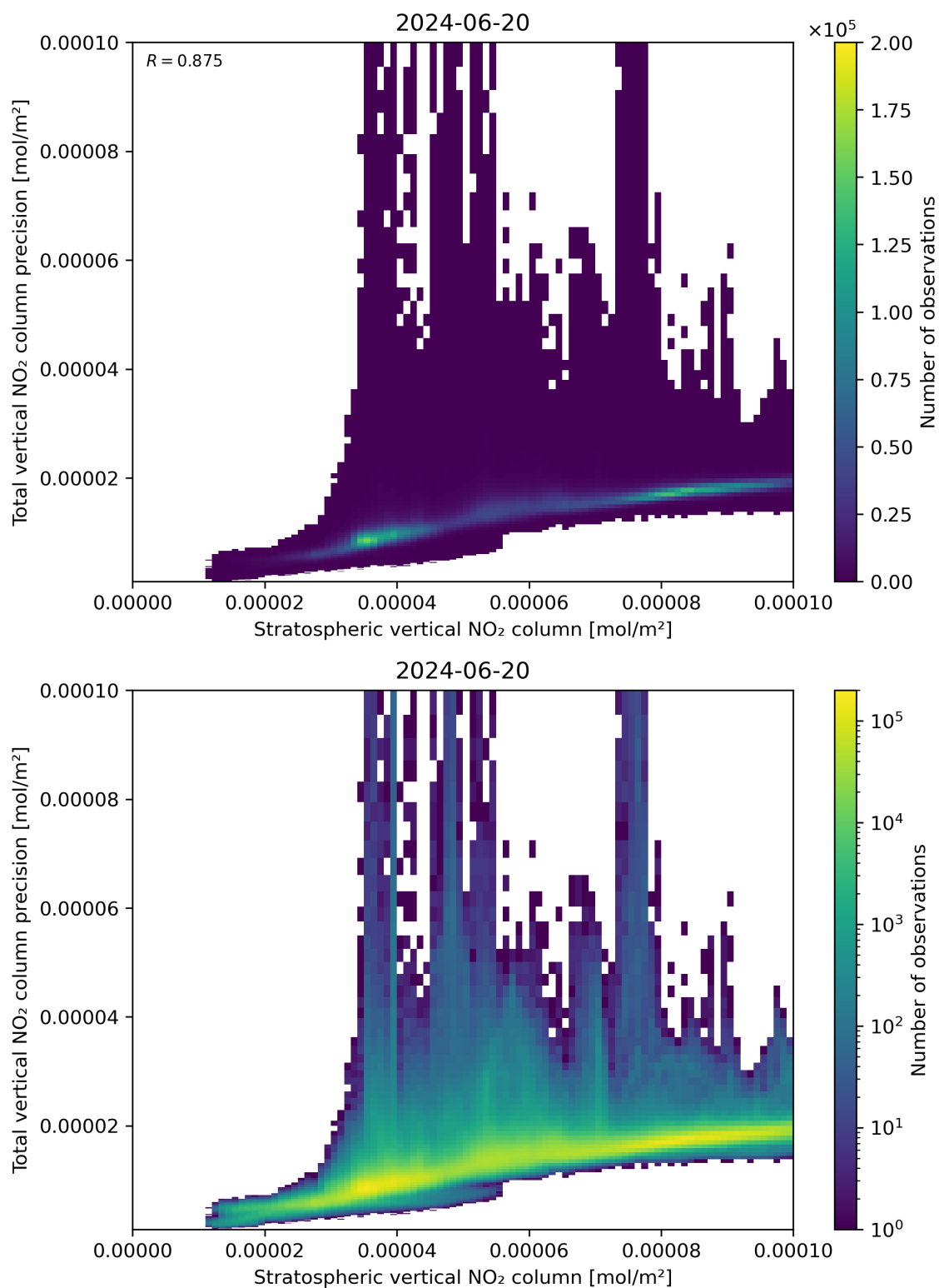
Figure 101: Scatter density plot of “Stratospheric vertical NO 2 column” against “Total vertical NO 2 column precision” for 2024-06-19 to 2024-06-21.
