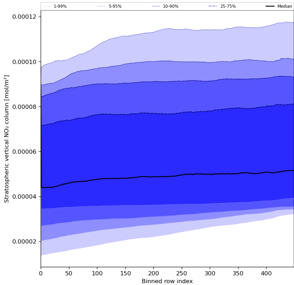
Figure 53: Along track statistics of “Stratospheric vertical NO 2 column” for 2024-06-19 to 2024-06-21
