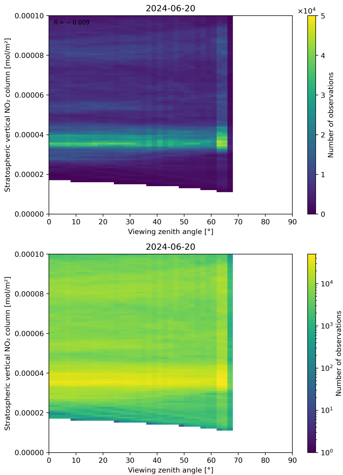
Figure 164: Scatter density plot of “Viewing zenith angle” against “Stratospheric vertical NO 2 column” for 2024-06-19 to 2024-06-21.
