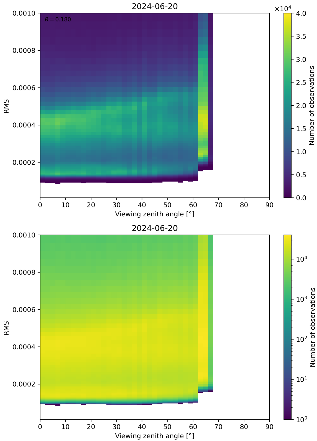
Figure 171: Scatter density plot of “Viewing zenith angle” against “RMS” for 2024-06-19 to 2024-06-21.
