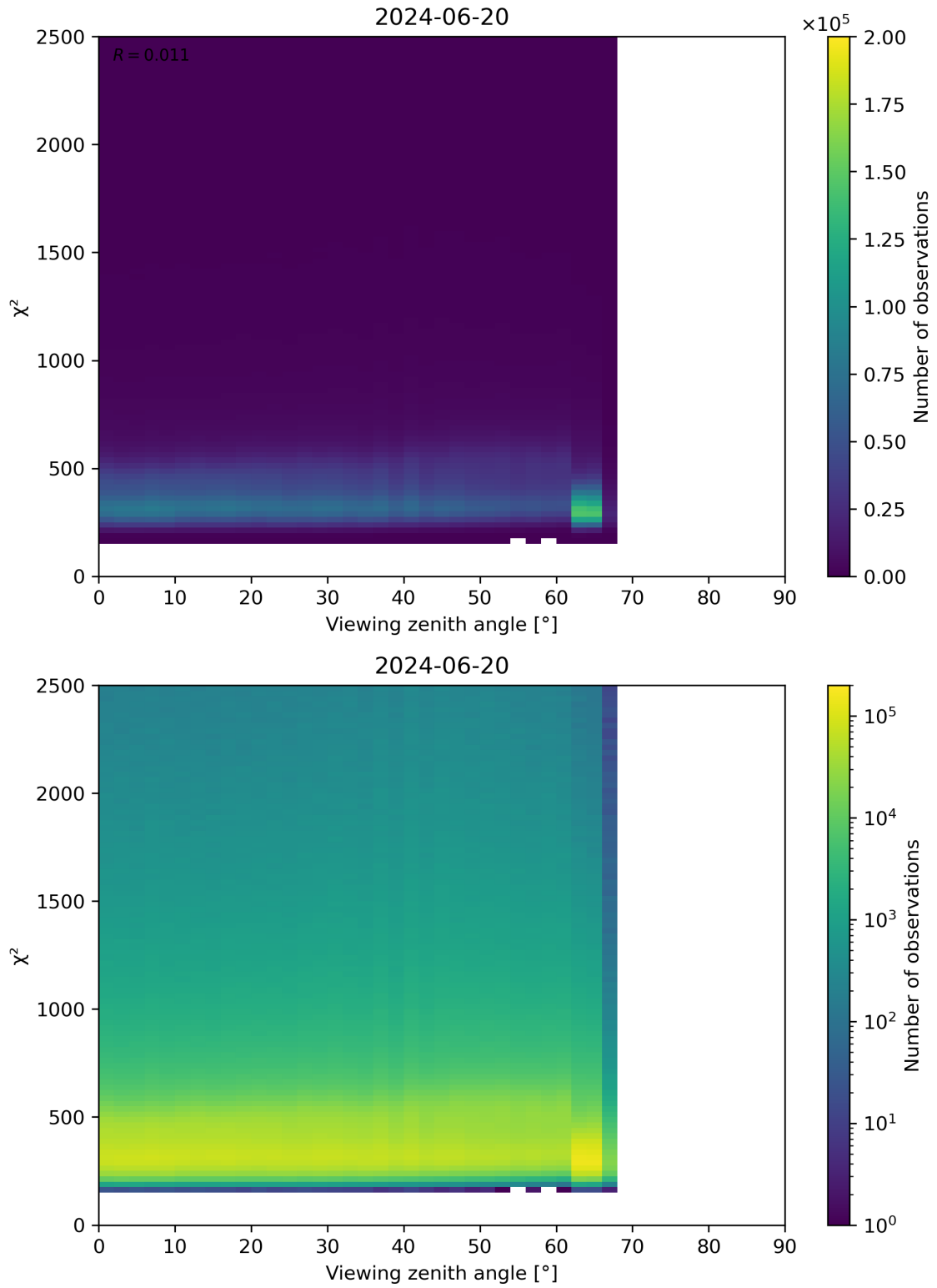
Figure 162: Scatter density plot of “Viewing zenith angle” against “ \chi^2 ” for 2024-06-19 to 2024-06-21.
