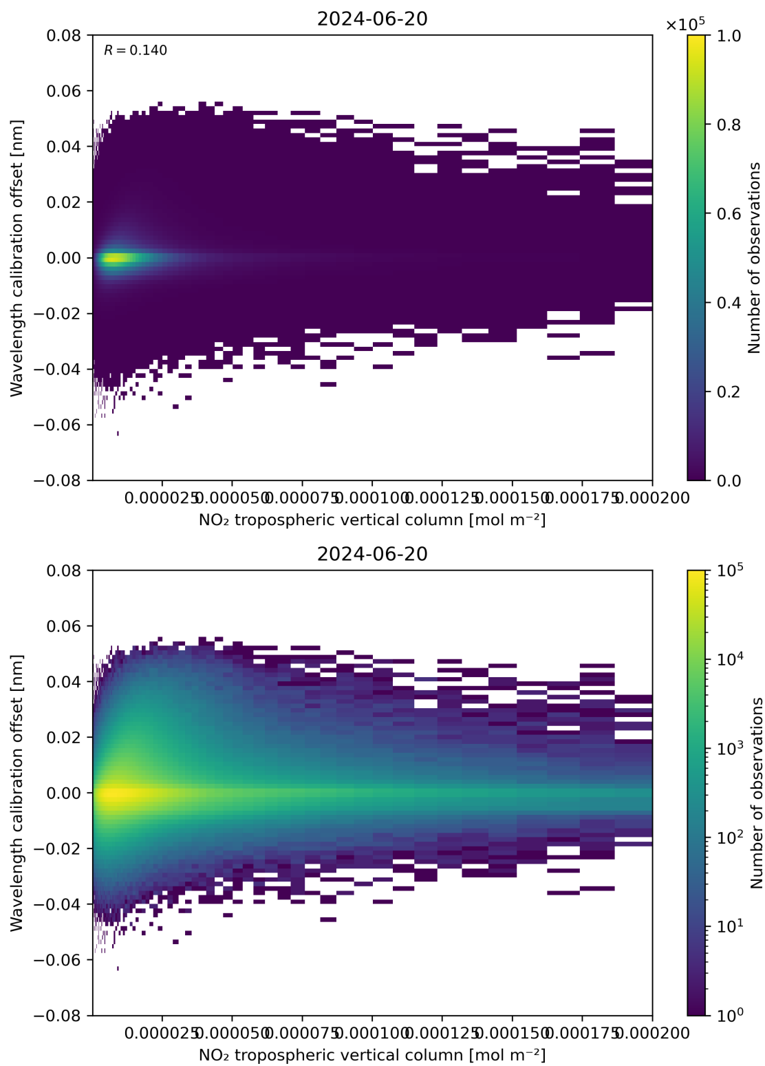
Figure 143: Scatter density plot of “NO 2 tropospheric vertical column” against “Wavelength calibration offset” for 2024-06-19 to 2024-06-21.
