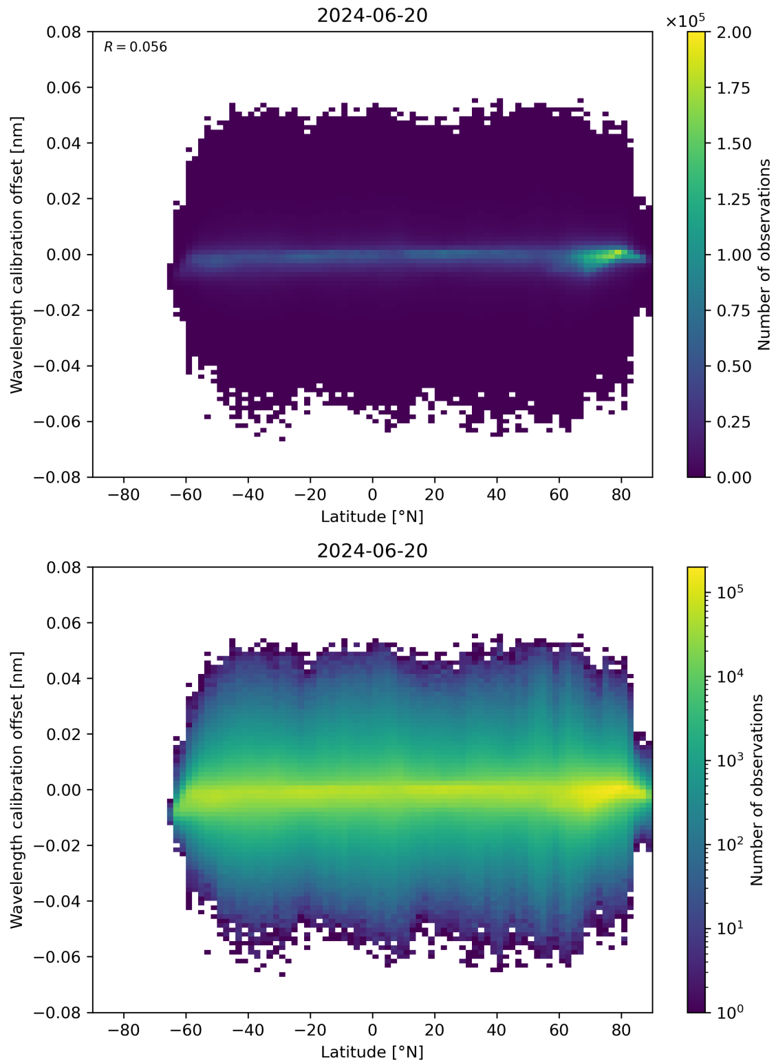
Figure 95: Scatter density plot of “Latitude” against “Wavelength calibration offset” for 2024-06-19 to 2024-06-21.
