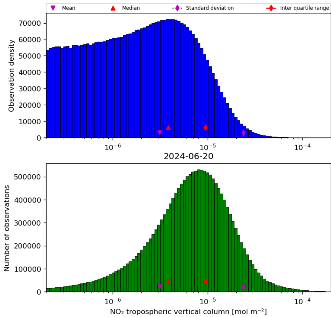
Figure 29: Histogram of “NO 2 tropospheric vertical column” for 2024-06-19 to 2024-06-21
