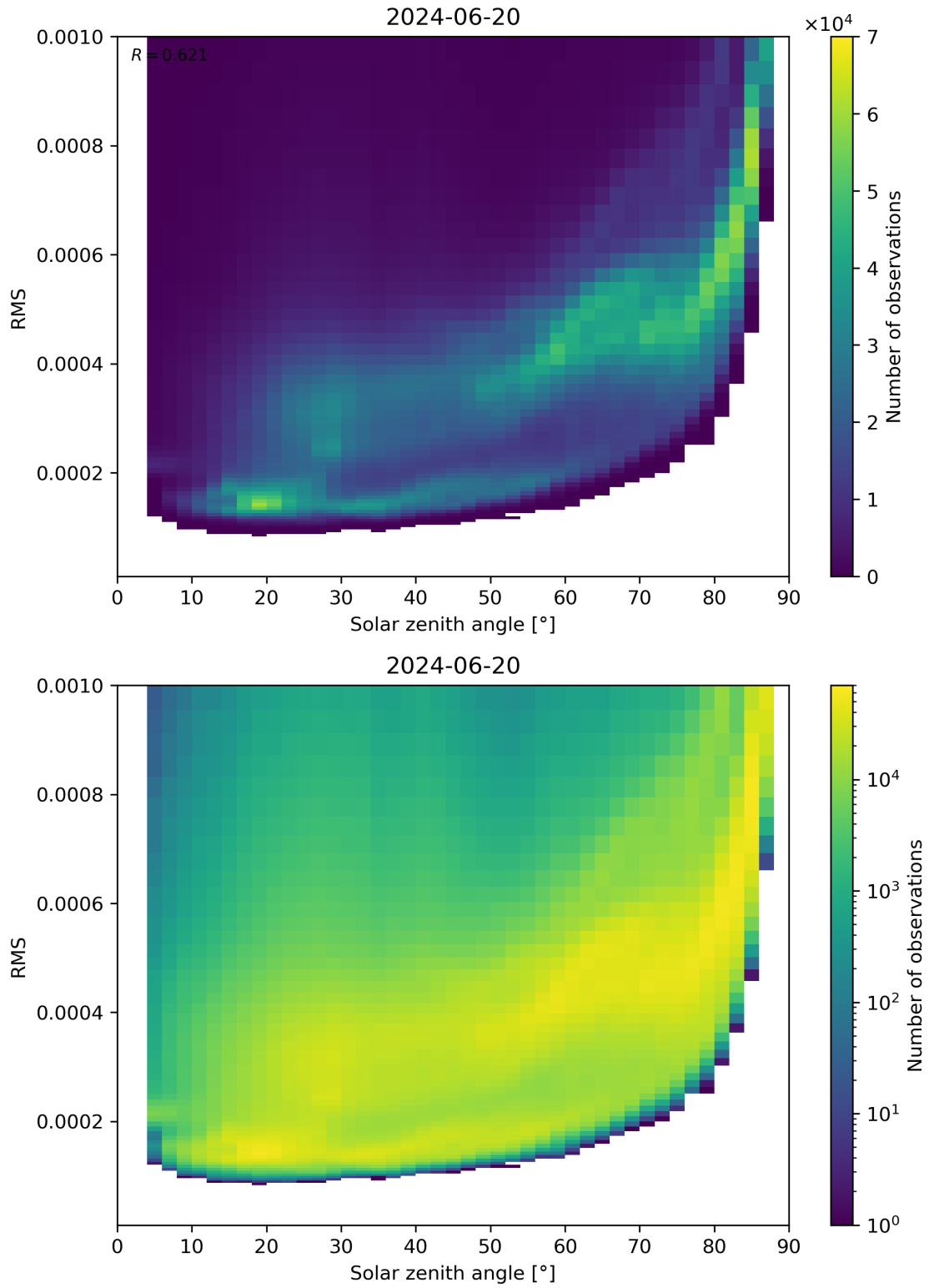
Figure 157: Scatter density plot of “Solar zenith angle” against “RMS” for 2024-06-19 to 2024-06-21.
