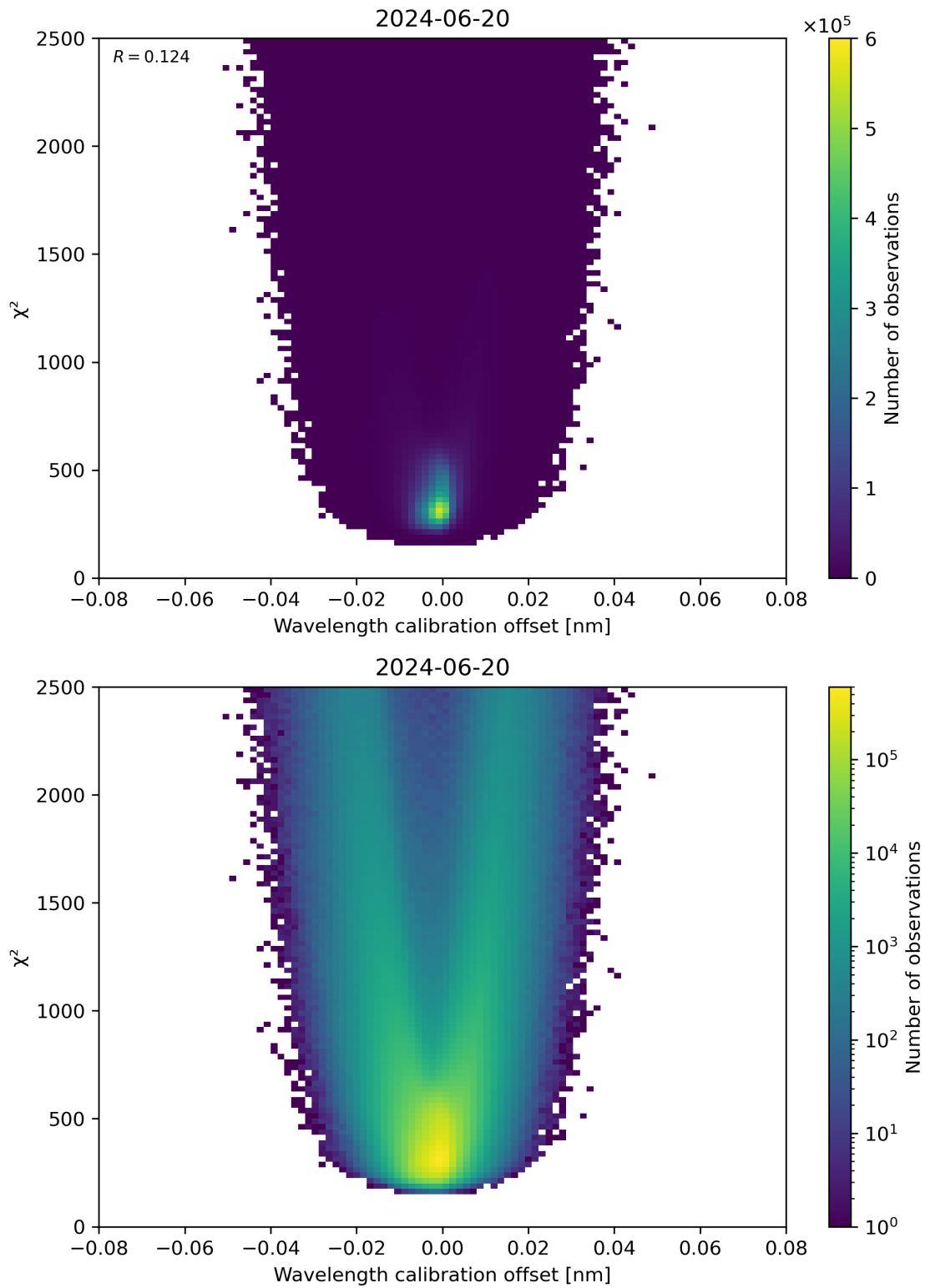
Figure 175: Scatter density plot of “Wavelength calibration offset” against “ \chi^2 ” for 2024-06-19 to 2024-06-21.
