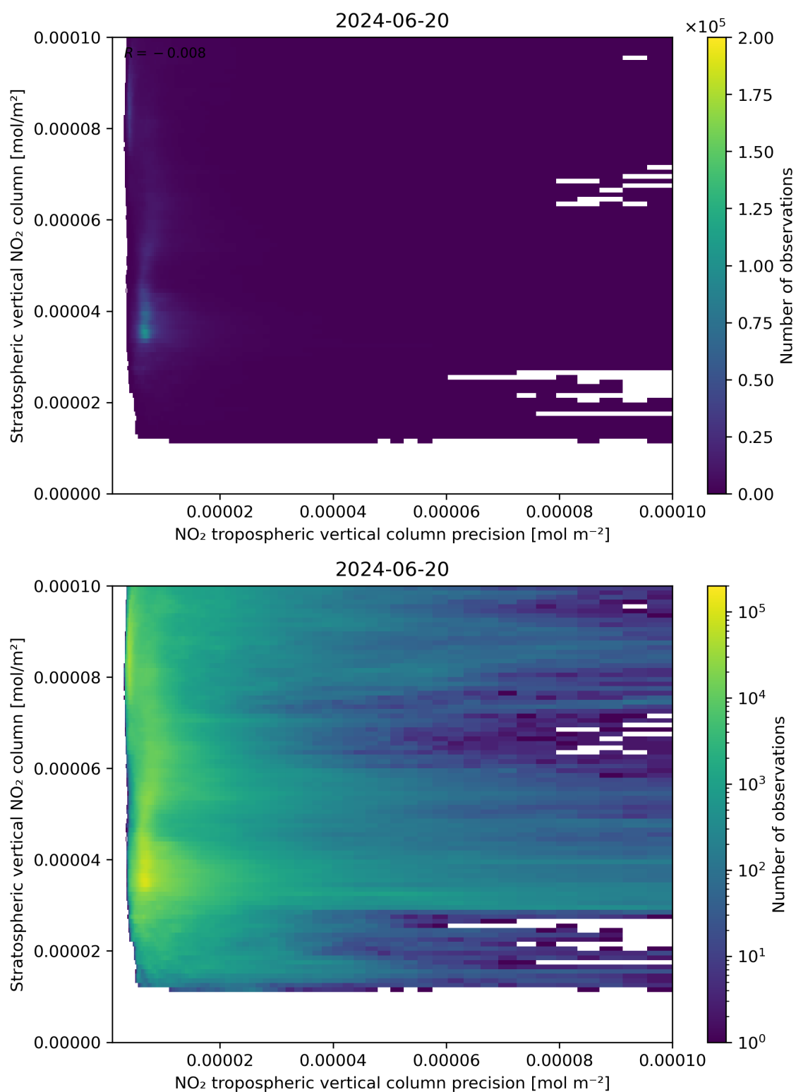
Figure 135: Scatter density plot of “NO 2 tropospheric vertical column precision” against “Stratospheric vertical NO 2 column” for 2024-06-19 to 2024-06-21.
