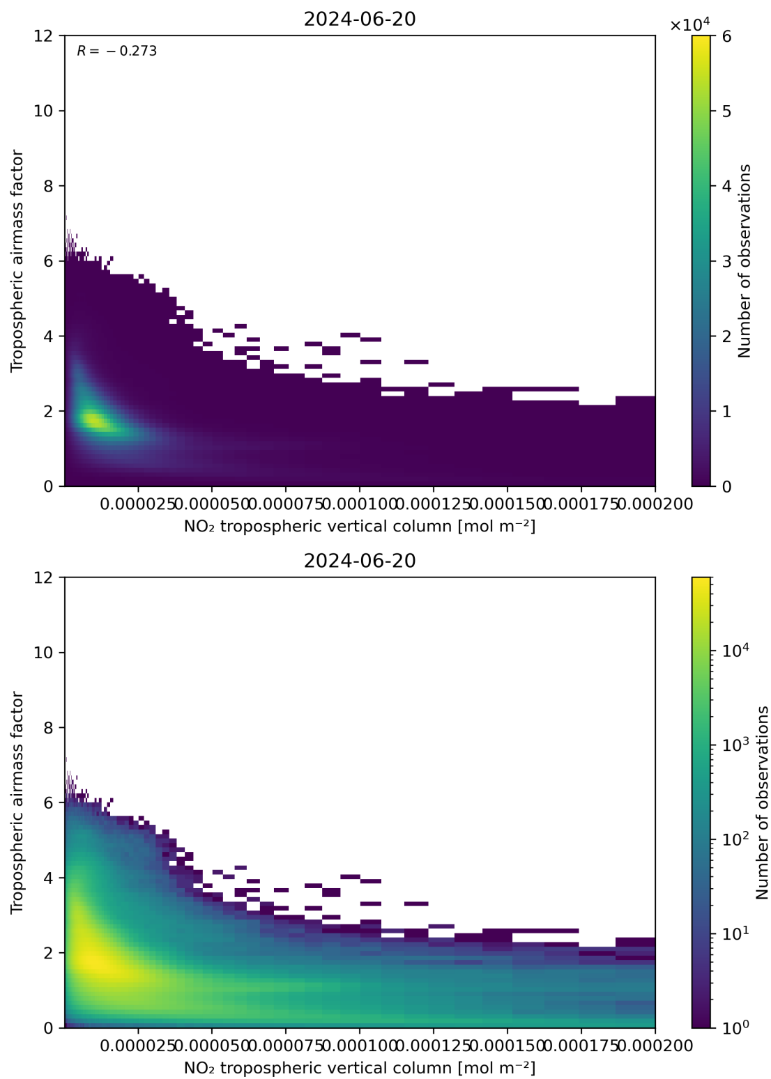
Figure 123: Scatter density plot of “NO 2 tropospheric vertical column” against “Tropospheric air mass factor” for 2024-06-19 to 2024-06-21.
