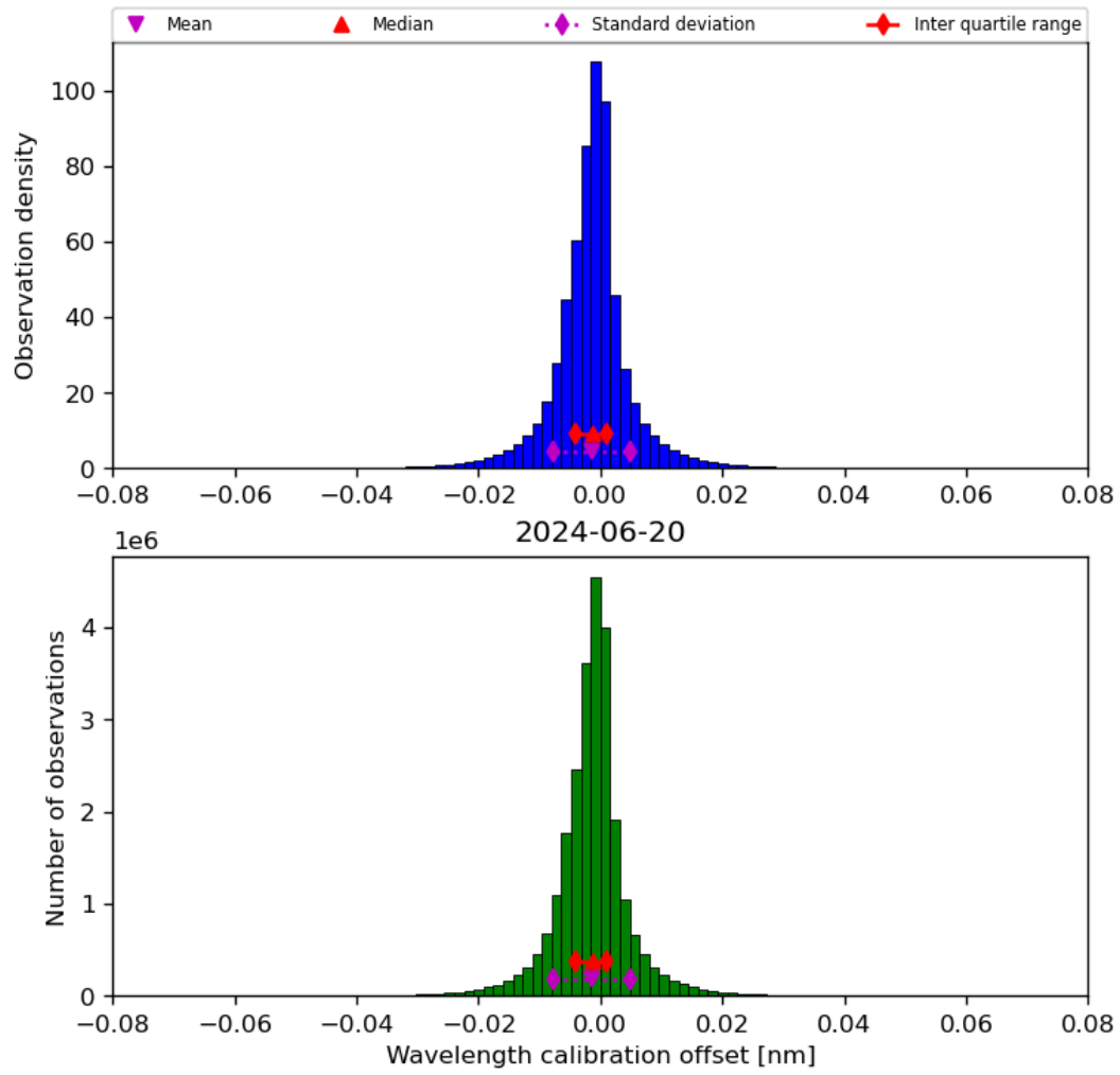
Figure 35: Histogram of “Wavelength calibration offset” for 2024-06-19 to 2024-06-21
