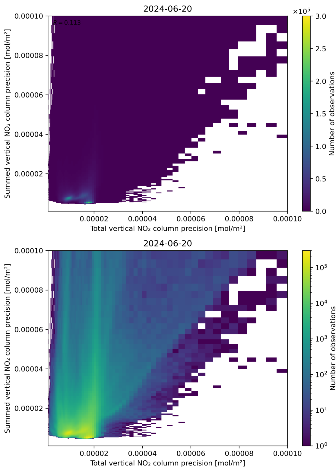
Figure 118: Scatter density plot of “Total vertical NO 2 column precision” against “Summed vertical NO 2 column precision” for 2024-06-19 to 2024-06-21.
