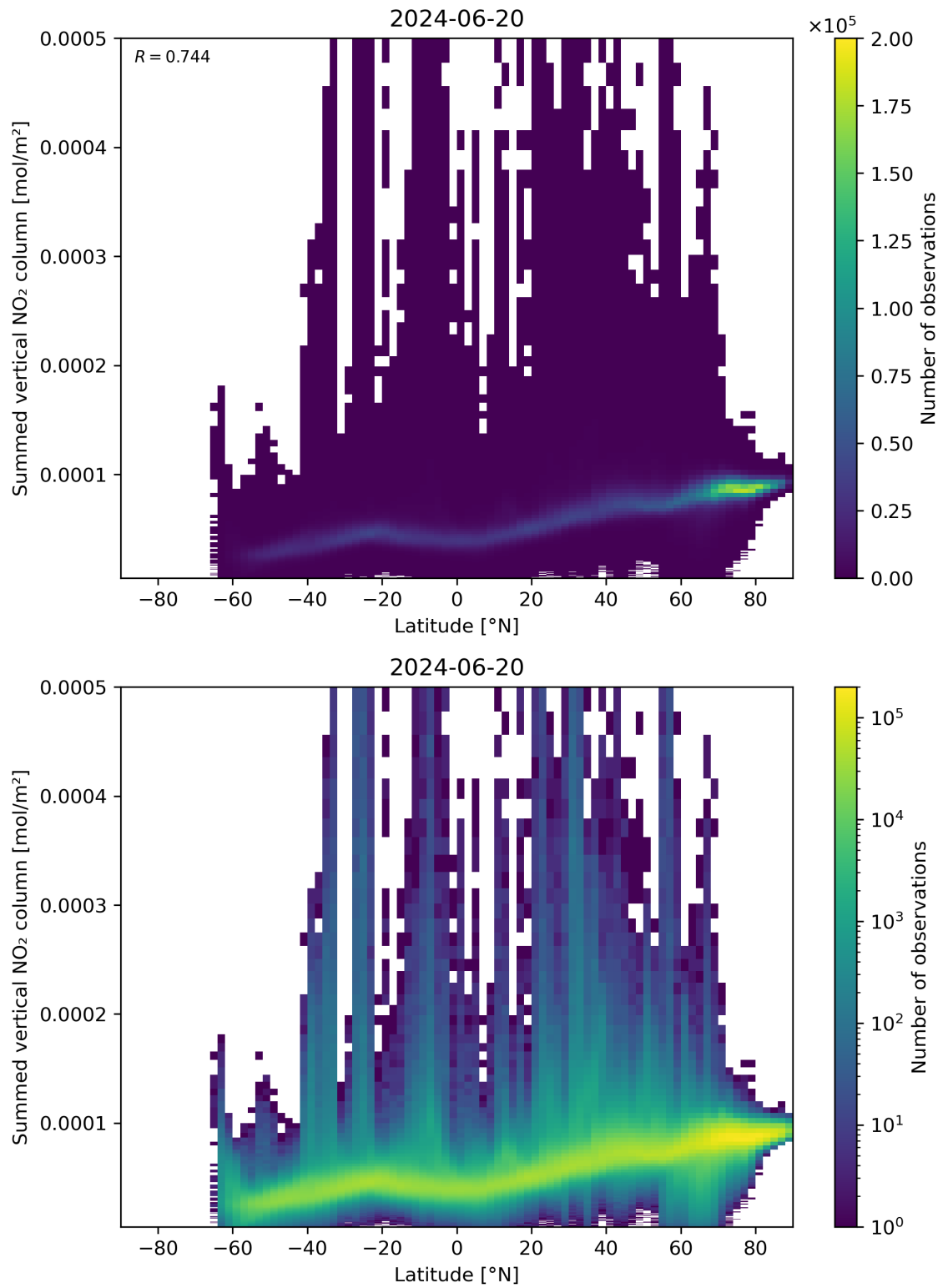
Figure 88: Scatter density plot of “Latitude” against “Summed vertical NO 2 column” for 2024-06-19 to 2024-06-21.
