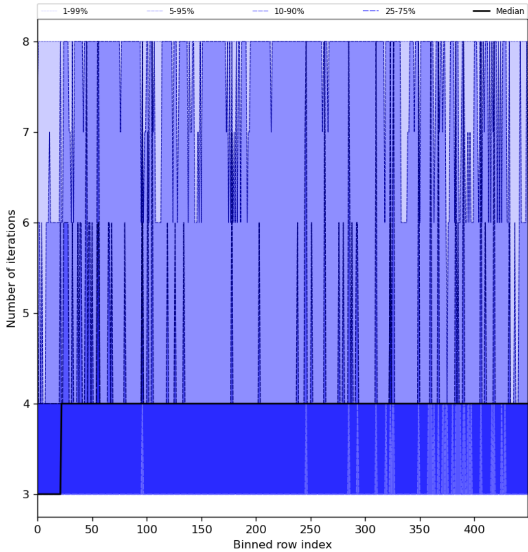
Figure 51: Along track statistics of “Number of iterations” for 2024-06-19 to 2024-06-21
