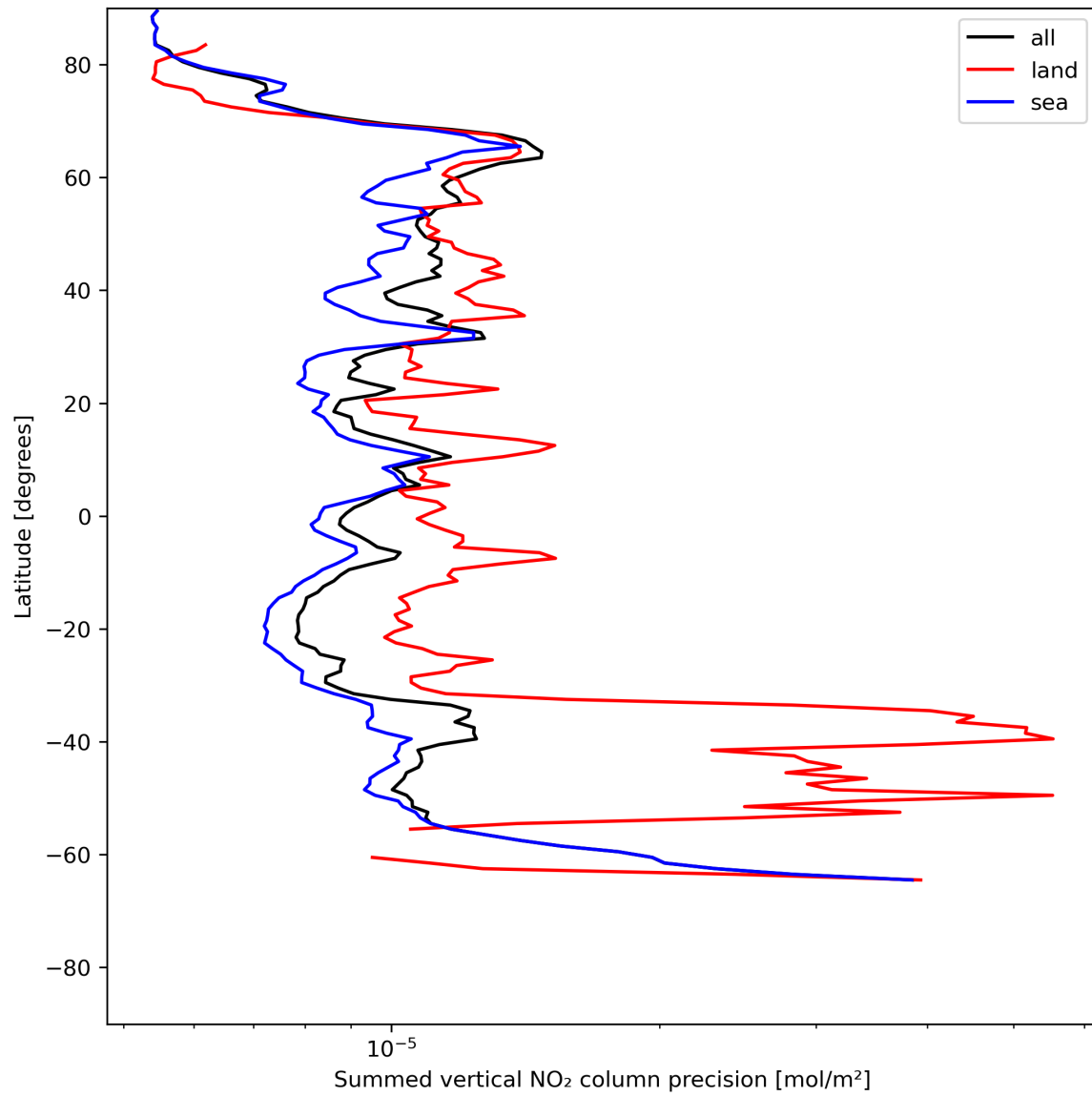
Figure 24: Zonal average of “Summed vertical NO 2 column precision” for 2024-06-19 to 2024-06-21.
