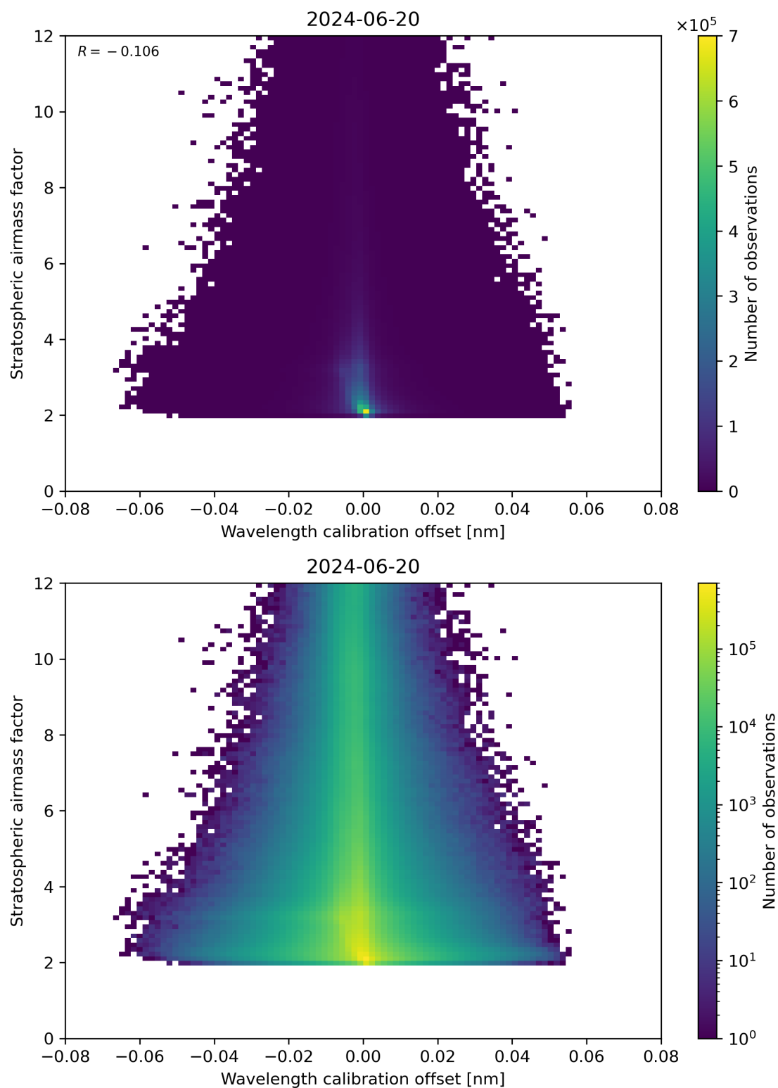
Figure 174: Scatter density plot of “Wavelength calibration offset” against “Stratospheric air mass factor” for 2024-06-19 to 2024-06-21.
