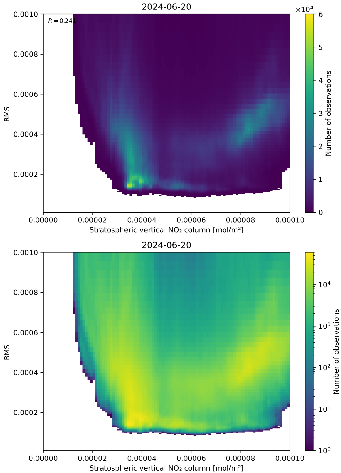
Figure 102: Scatter density plot of “Stratospheric vertical NO 2 column” against “RMS” for 2024-06-19 to 2024-06-21.
