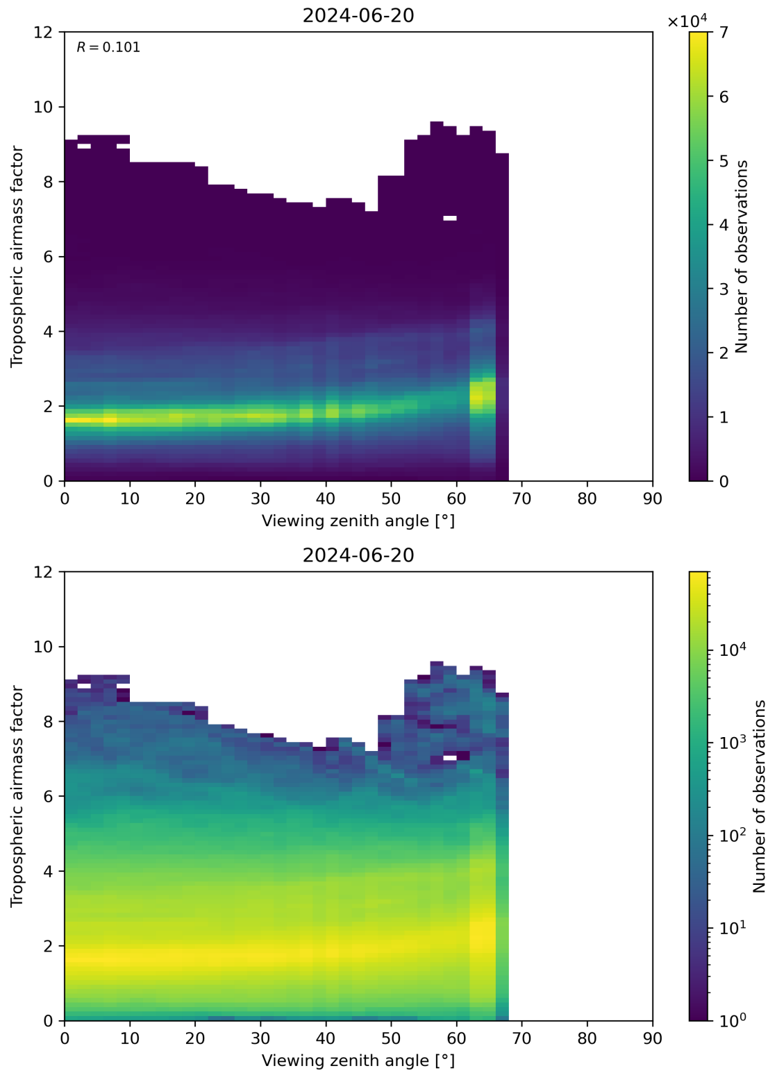
Figure 161: Scatter density plot of “Viewing zenith angle” against “Tropospheric airmass factor” for 2024-06-19 to 2024-06-21.
