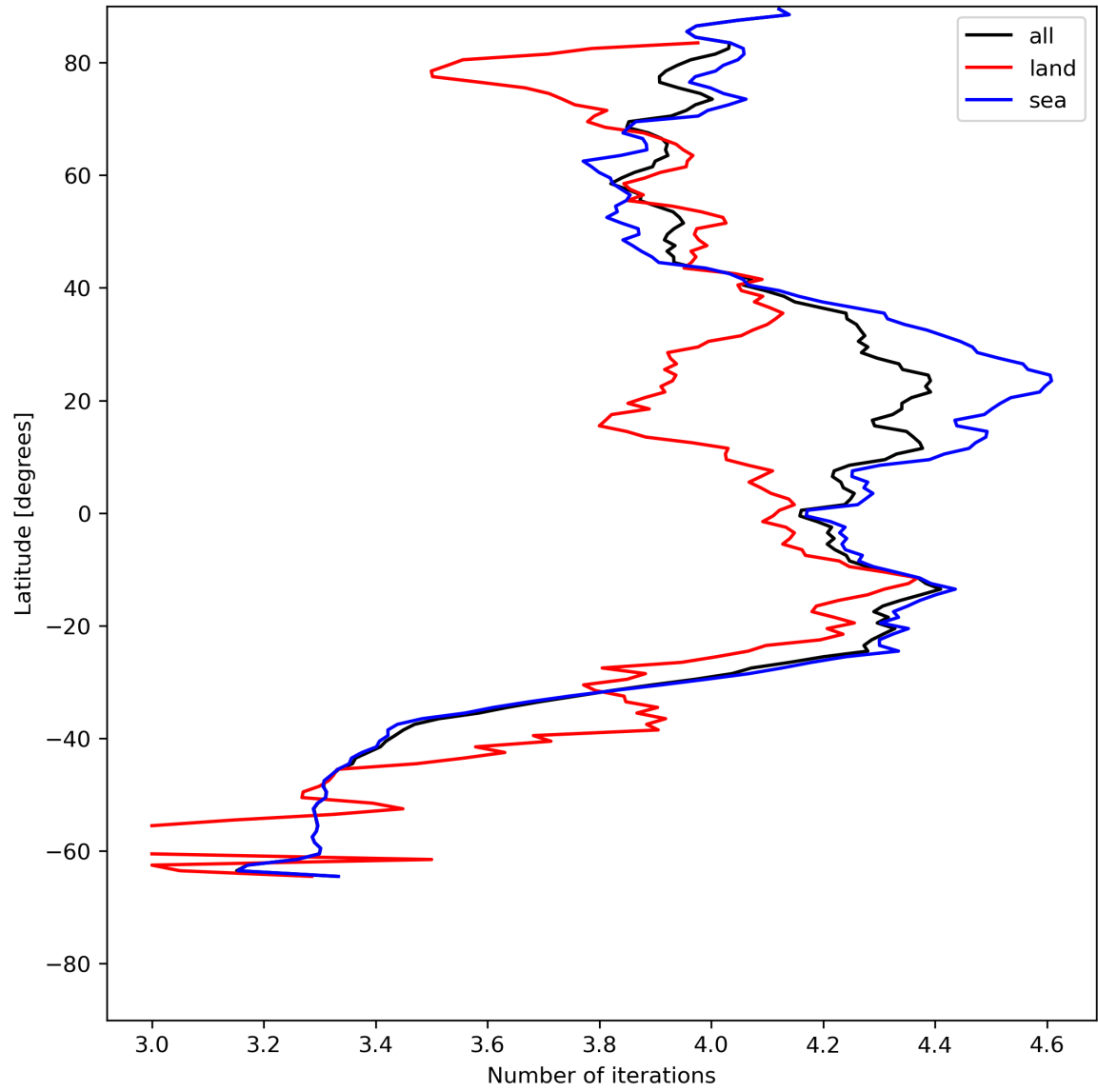
Figure 17: Zonal average of “Number of iterations” for 2024-06-19 to 2024-06-21.
