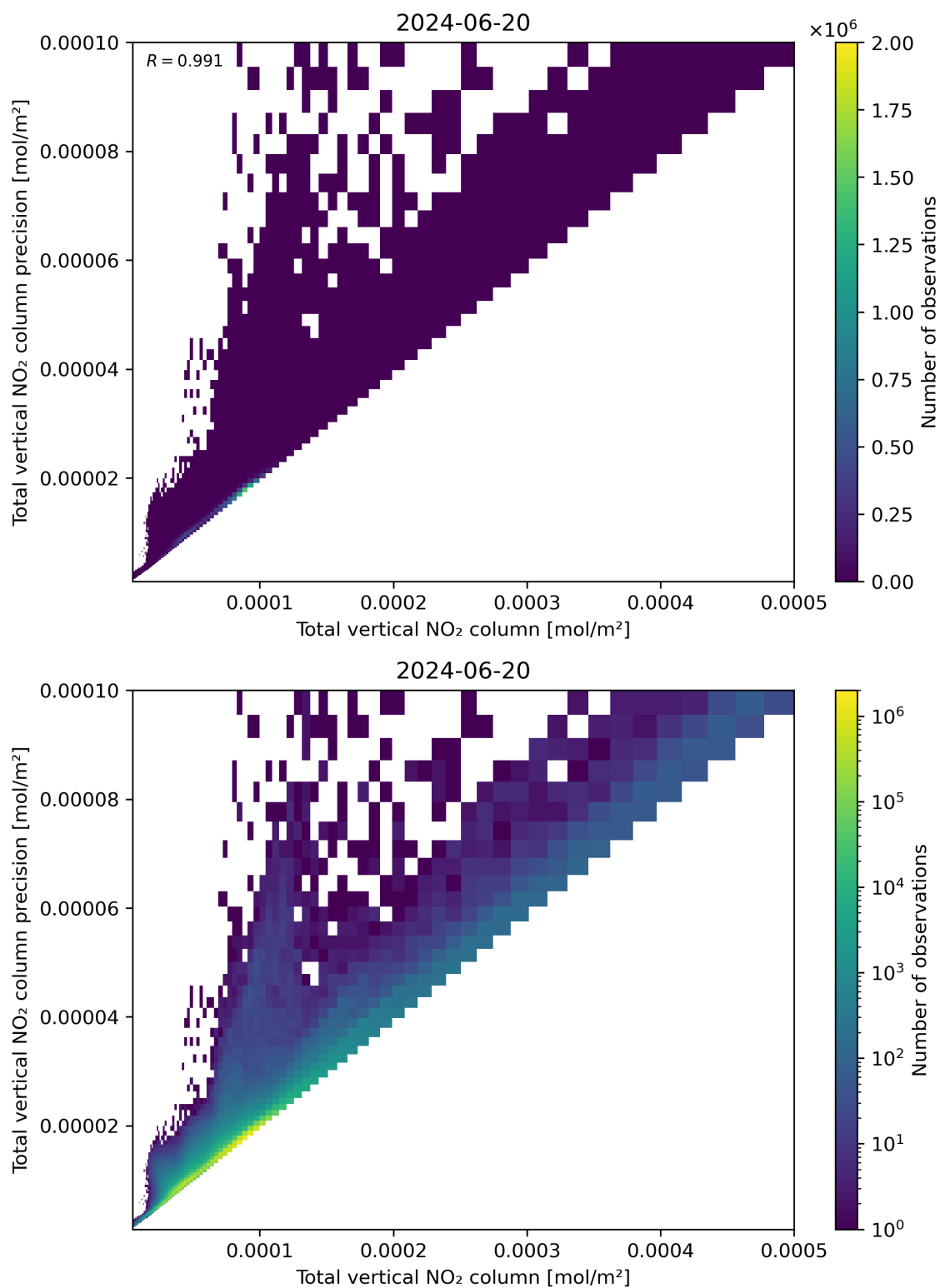
Figure 114: Scatter density plot of “Total vertical NO 2 column” against “Total vertical NO 2 column precision” for 2024-06-19 to 2024-06-21.
