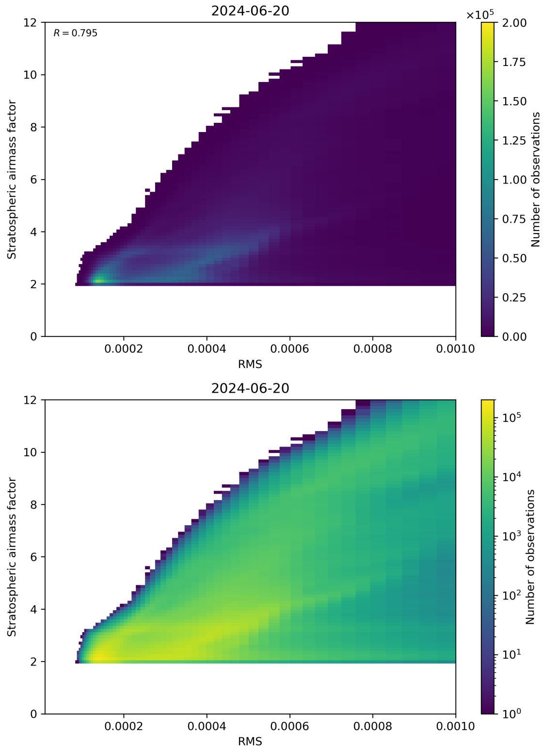
Figure 144: Scatter density plot of “RMS” against “Stratospheric airmass factor” for 2024-06-19 to 2024-06-21.
