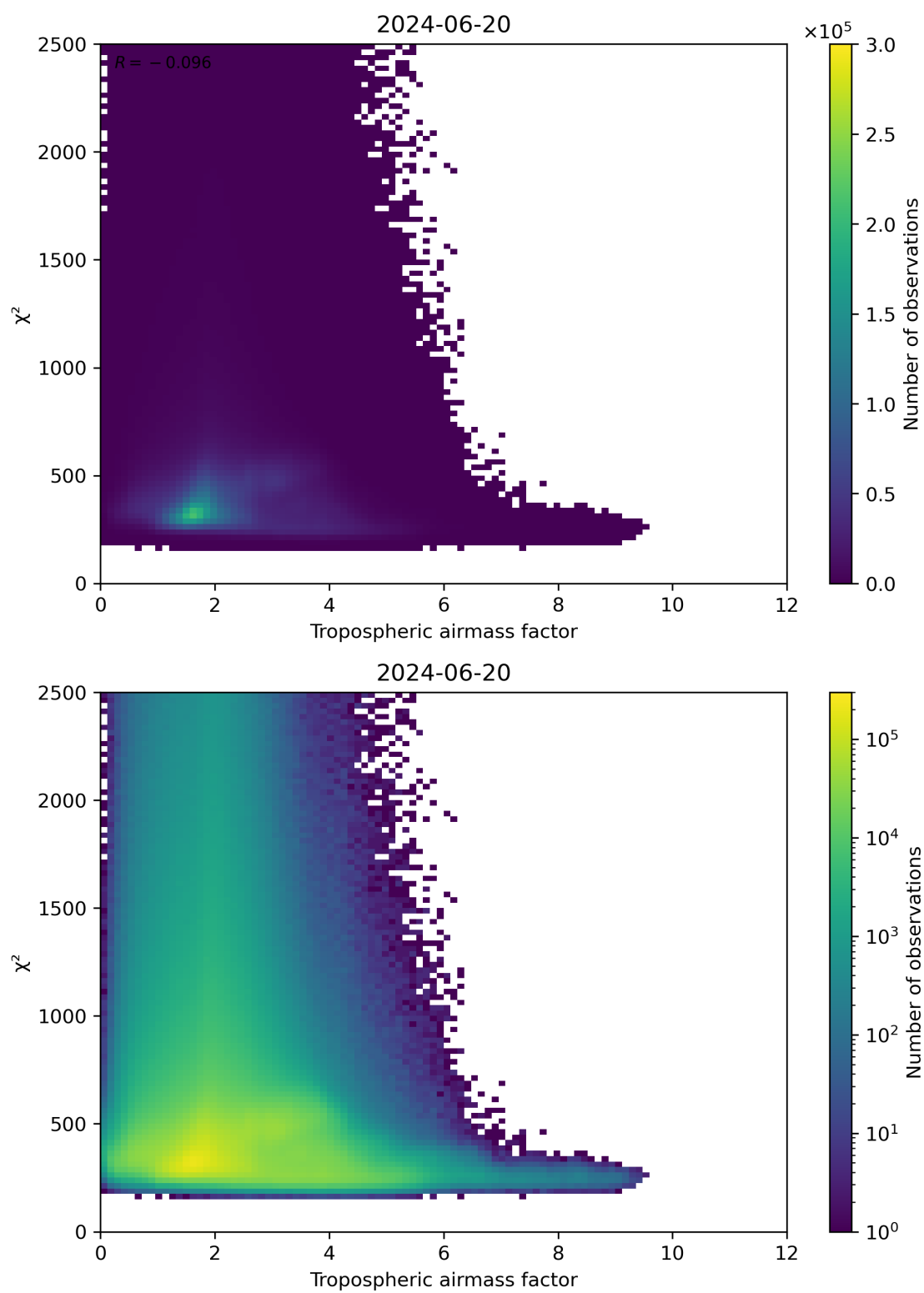
Figure 73: Scatter density plot of “Tropospheric airmass factor” against “ \chi^2 ” for 2024-06-19 to 2024-06-21.
