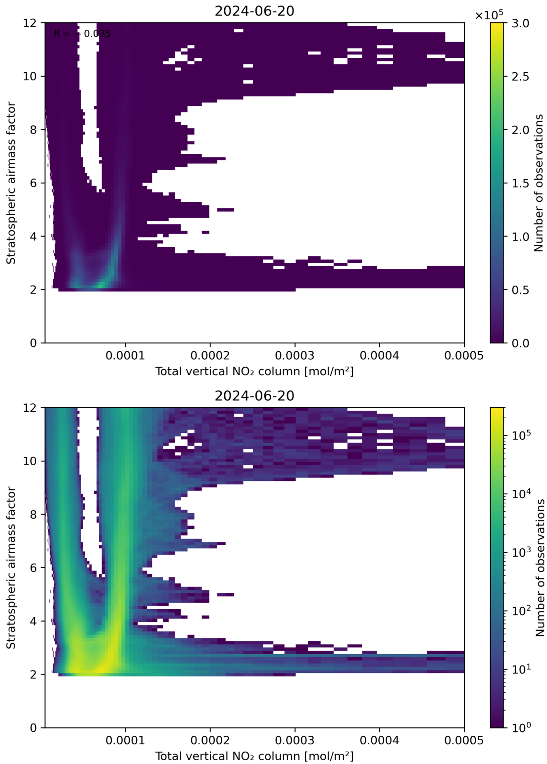
Figure 110: Scatter density plot of “Total vertical NO 2 column” against “Stratospheric airmass factor” for 2024-06-19 to 2024-06-21.
