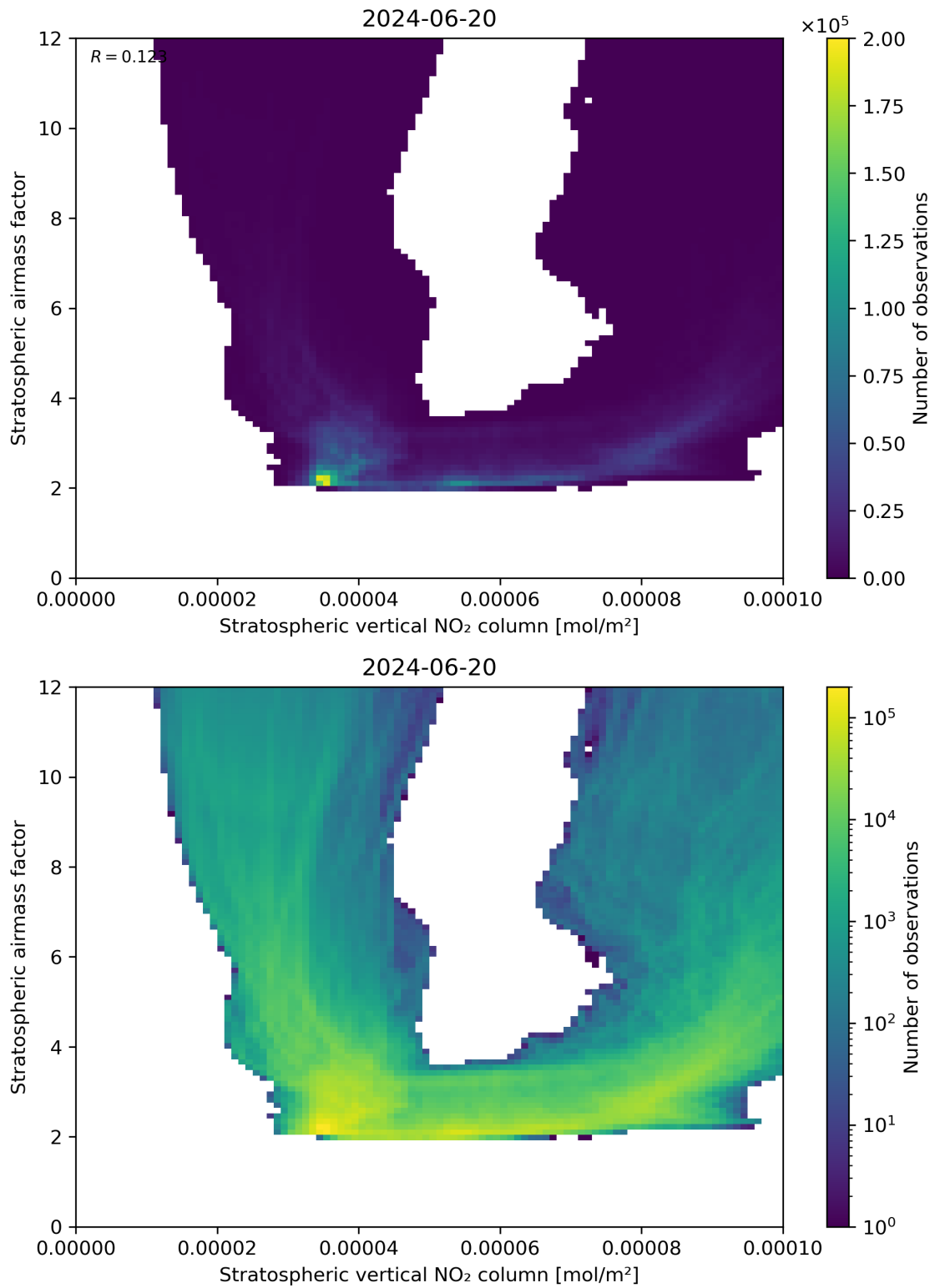
Figure 96: Scatter density plot of “Stratospheric vertical NO 2 column” against “Stratospheric airmass factor” for 2024-06-19 to 2024-06-21.
