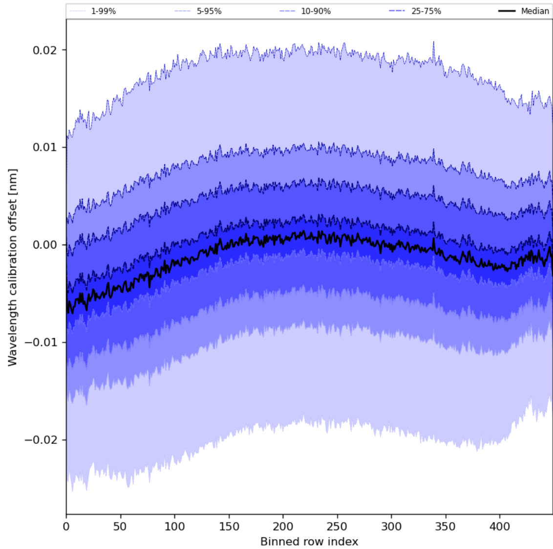
Figure 52: Along track statistics of “Wavelength calibration offset” for 2024-06-19 to 2024-06-21
