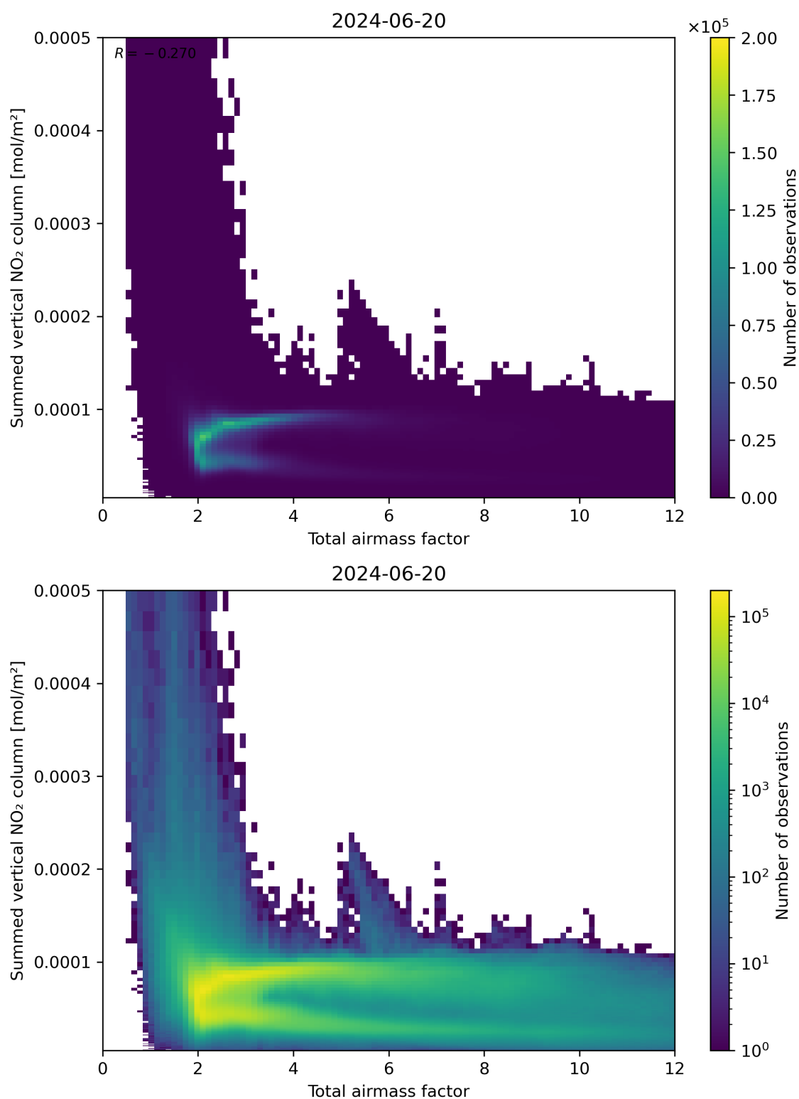
Figure 65: Scatter density plot of “Total airmass factor” against “Summed vertical NO 2 column” for 2024-06-19 to 2024-06-21.
