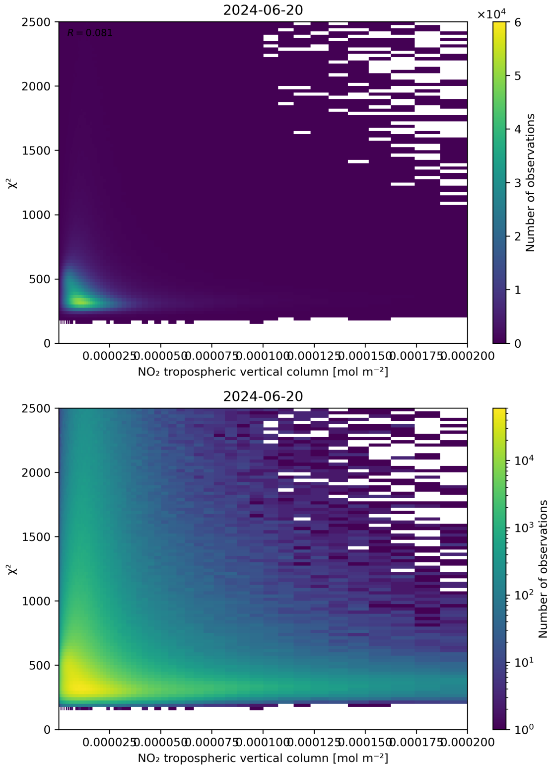
Figure 124: Scatter density plot of “NO 2 tropospheric vertical column” against “ \chi^2 ” for 2024-06-19 to 2024-06-21.
