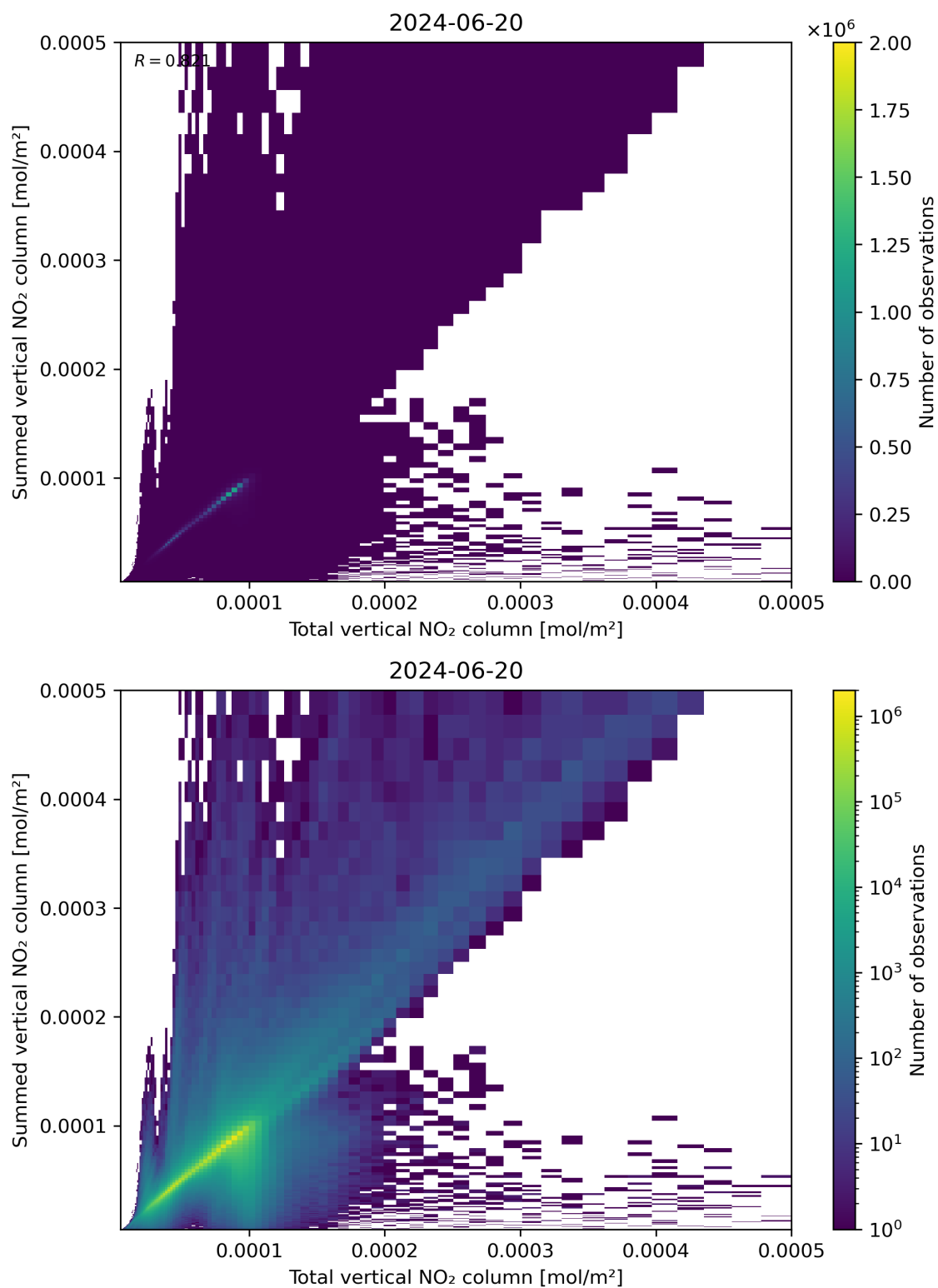
Figure 112: Scatter density plot of “Total vertical NO 2 column” against “Summed vertical NO 2 column” for 2024-06-19 to 2024-06-21.
