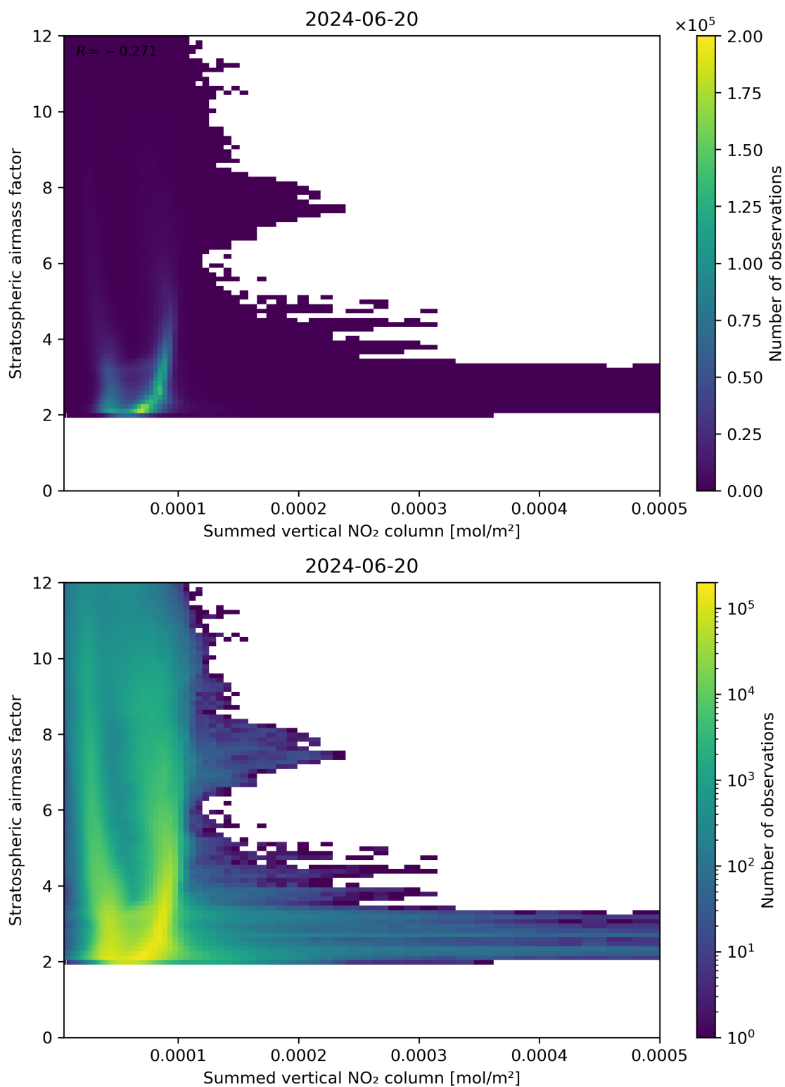
Figure 103: Scatter density plot of “Summed vertical NO 2 column” against “Stratospheric air mass factor” for 2024-06-19 to 2024-06-21.
