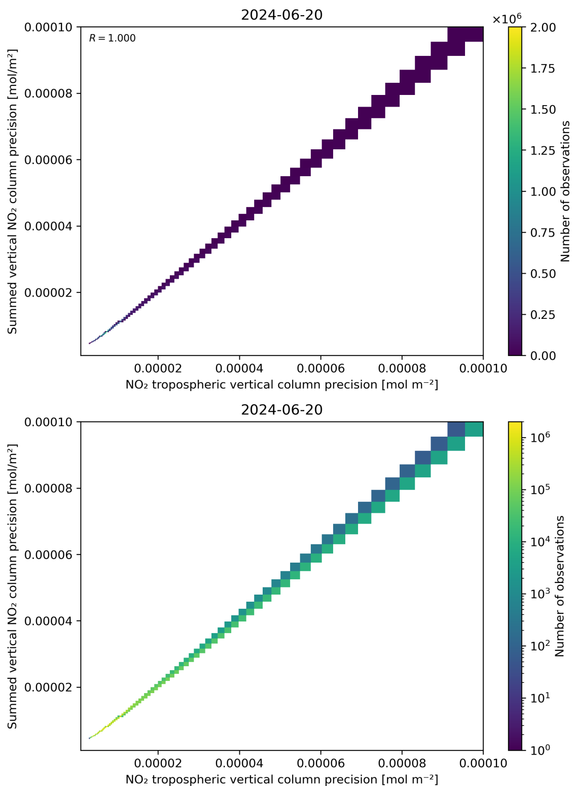
Figure 137: Scatter density plot of “NO 2 tropospheric vertical column precision” against “Summed vertical NO 2 column precision” for 2024-06-19 to 2024-06-21.
