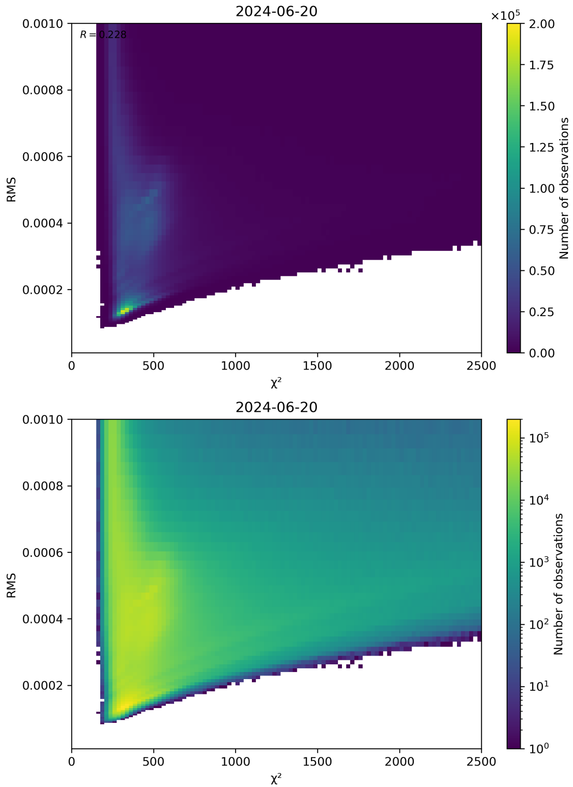
Figure 82: Scatter density plot of “ \chi^2 ” against “RMS” for 2024-06-19 to 2024-06-21.
