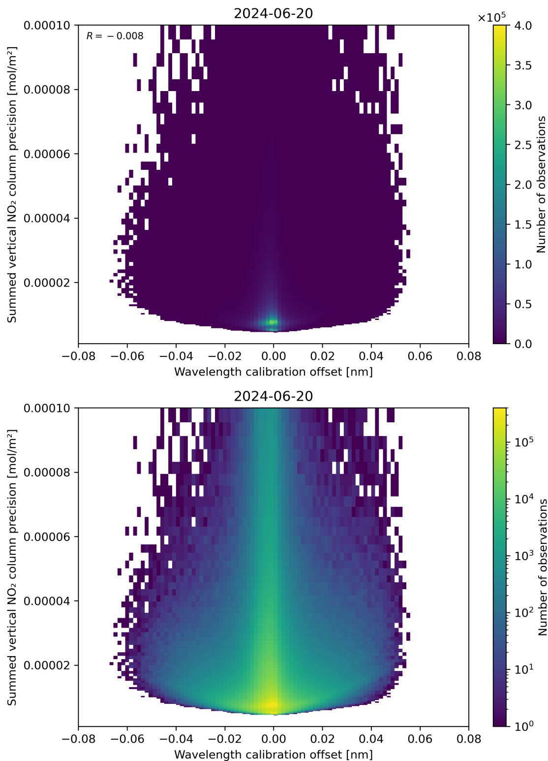
Figure 178: Scatter density plot of “Wavelength calibration offset” against “Summed vertical NO 2 column precision” for 2024-06-19 to 2024-06-21.
