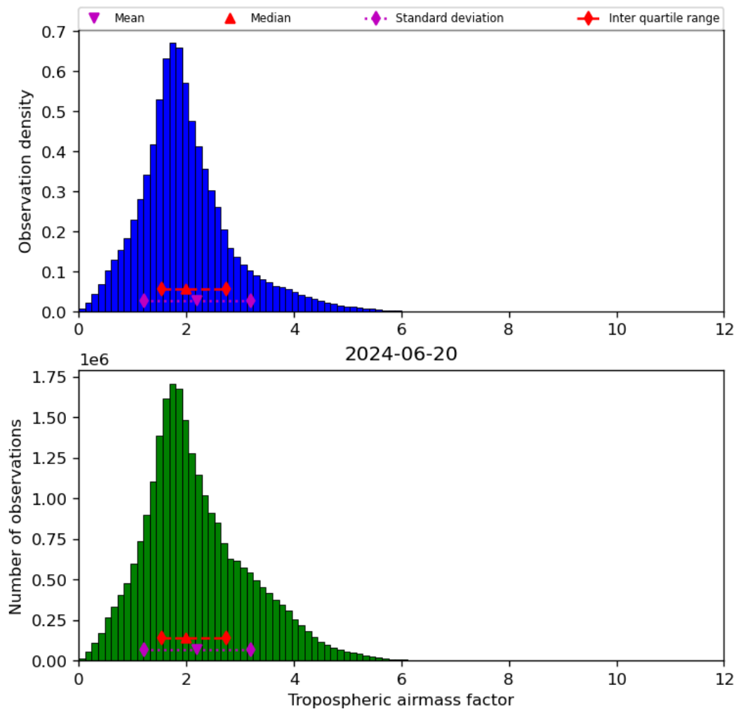
Figure 31: Histogram of “Tropospheric airmass factor” for 2024-06-19 to 2024-06-21
