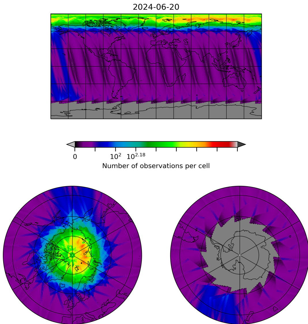
Figure 10: Map of the number of observations for 2024-06-19 to 2024-06-21
