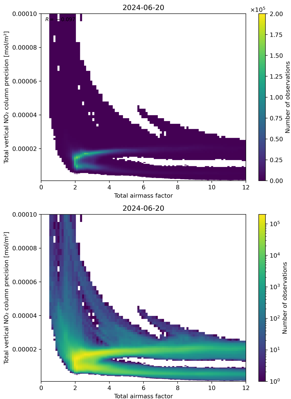
Figure 68: Scatter density plot of “Total airmass factor” against “Total vertical NO 2 column precision” for 2024-06-19 to 2024-06-21.
