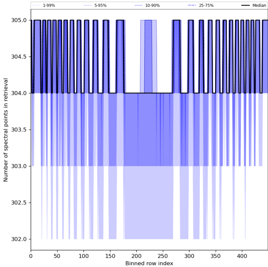
Figure 50: Along track statistics of “Number of spectral points in retrieval” for 2024-06-19 to 2024-06-21
