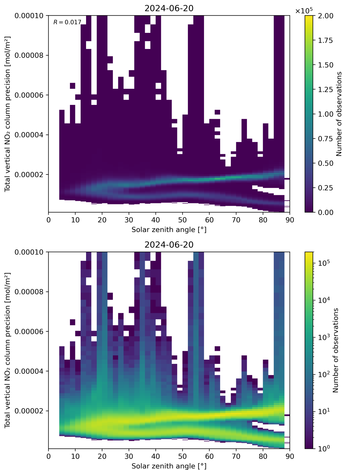
Figure 154: Scatter density plot of “Solar zenith angle” against “Total vertical NO 2 column precision” for 2024-06-19 to 2024-06-21.
