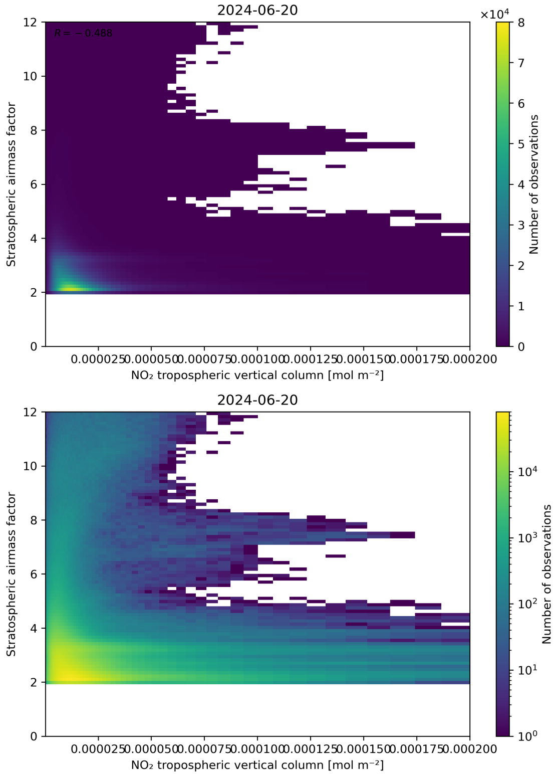
Figure 121: Scatter density plot of “NO 2 tropospheric vertical column” against “Stratospheric airmass factor” for 2024-06-19 to 2024-06-21.
