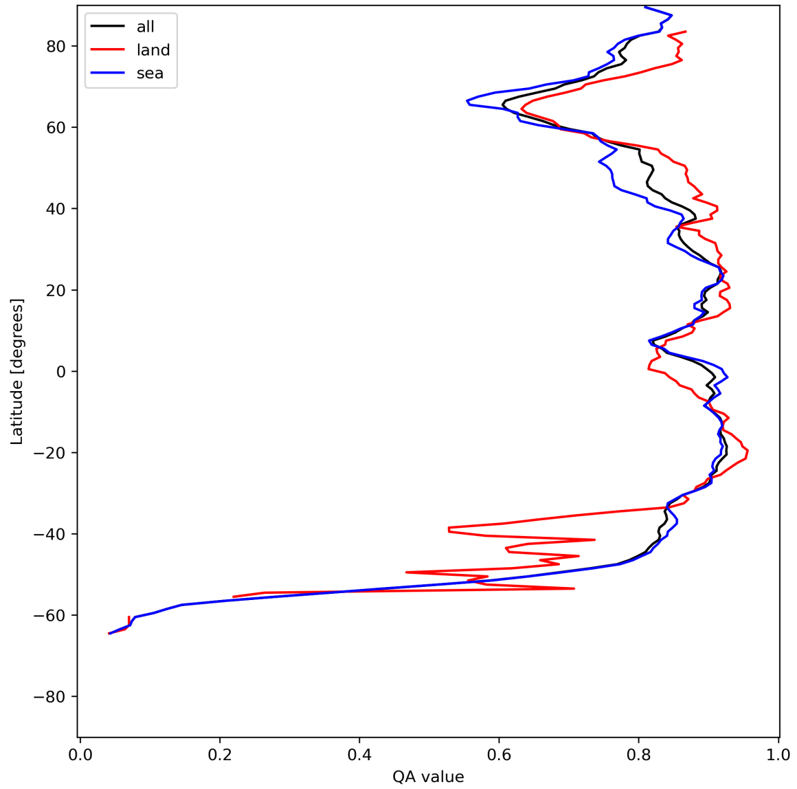
Figure 11: Zonal average of “QA value” for 2024-06-19 to 2024-06-21.
