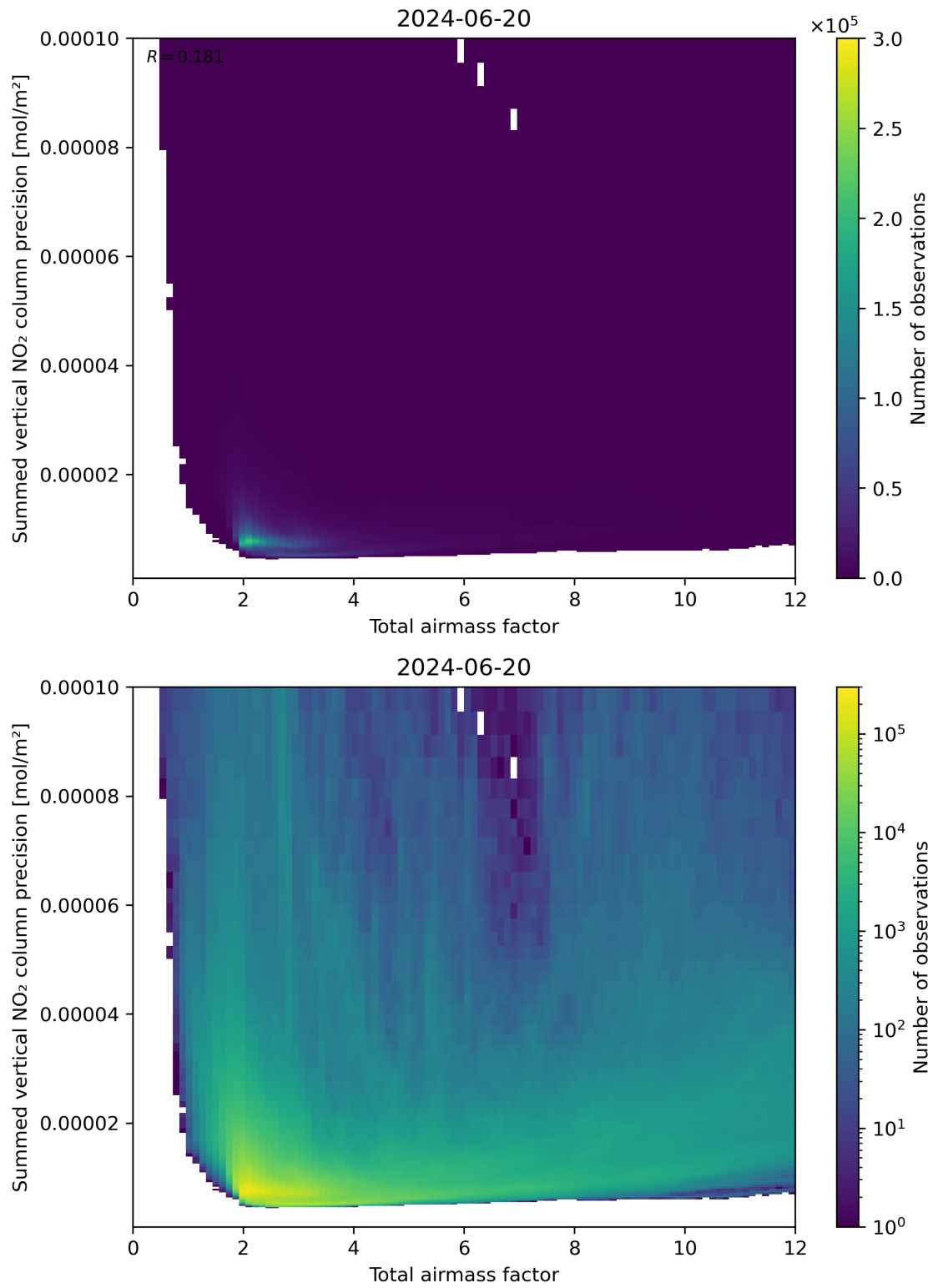
Figure 66: Scatter density plot of “Total airmass factor” against “Summed vertical NO 2 column precision” for 2024-06-19 to 2024-06-21.
