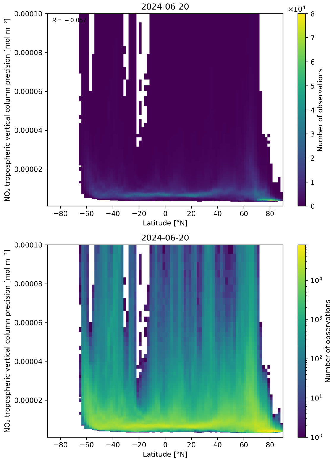
Figure 93: Scatter density plot of “Latitude” against “NO 2 tropospheric vertical column precision” for 2024-06-19 to 2024-06-21.
