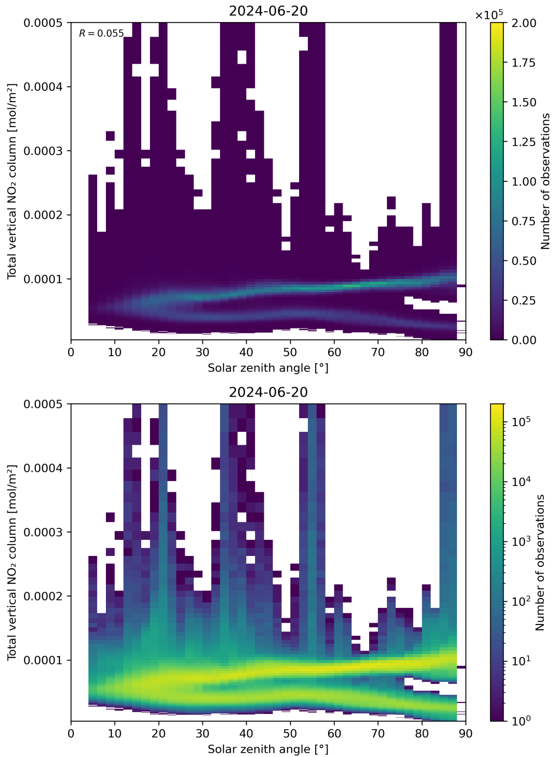
Figure 153: Scatter density plot of “Solar zenith angle” against “Total vertical NO 2 column” for 2024-06-19 to 2024-06-21.
