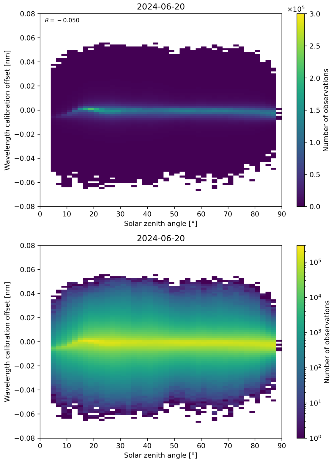
Figure 158: Scatter density plot of “Solar zenith angle” against “Wavelength calibration offset” for 2024-06-19 to 2024-06-21.
