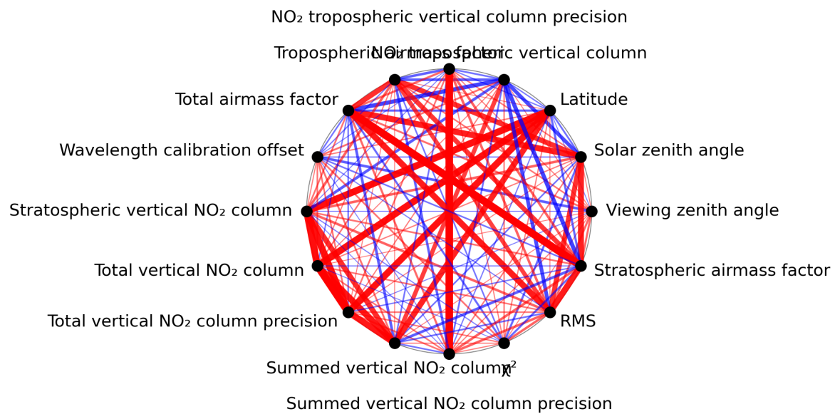
Figure 1: Map of correlation graph for 2024-06-19 to 2024-06-21.
