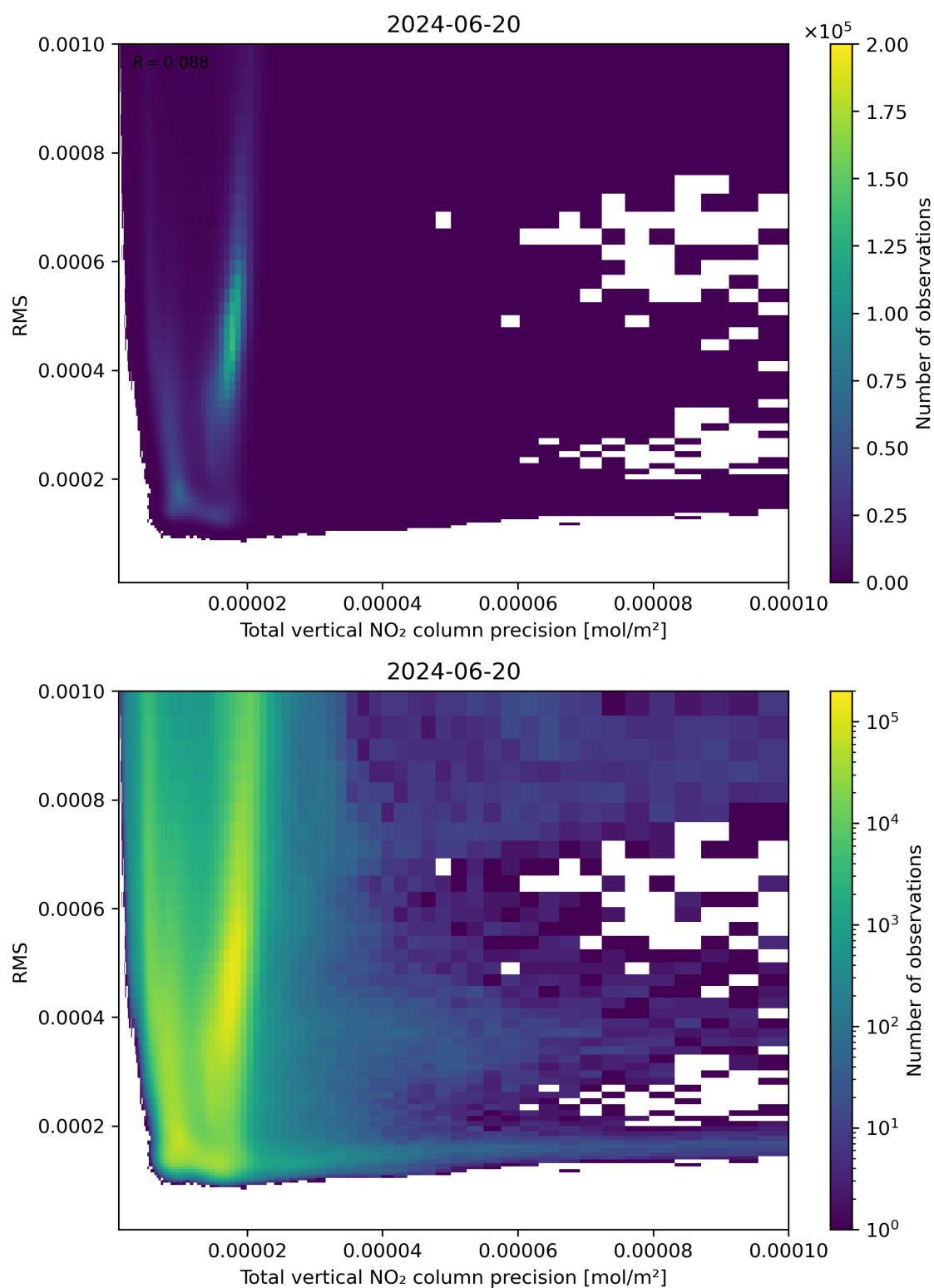
Figure 119: Scatter density plot of “Total vertical NO 2 column precision” against “RMS” for 2024-06-19 to 2024-06-21.
