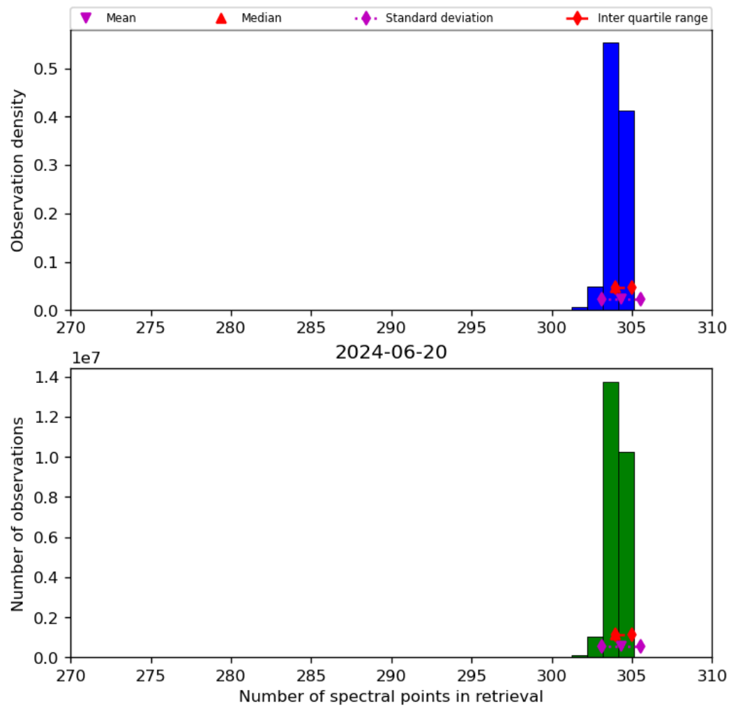
Figure 33: Histogram of “Number of spectral points in retrieval” for 2024-06-19 to 2024-06-21
