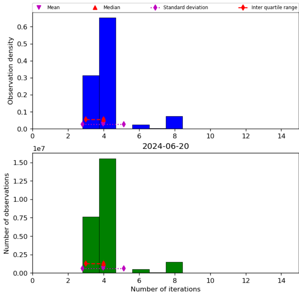
Figure 34: Histogram of “Number of iterations” for 2024-06-19 to 2024-06-21
