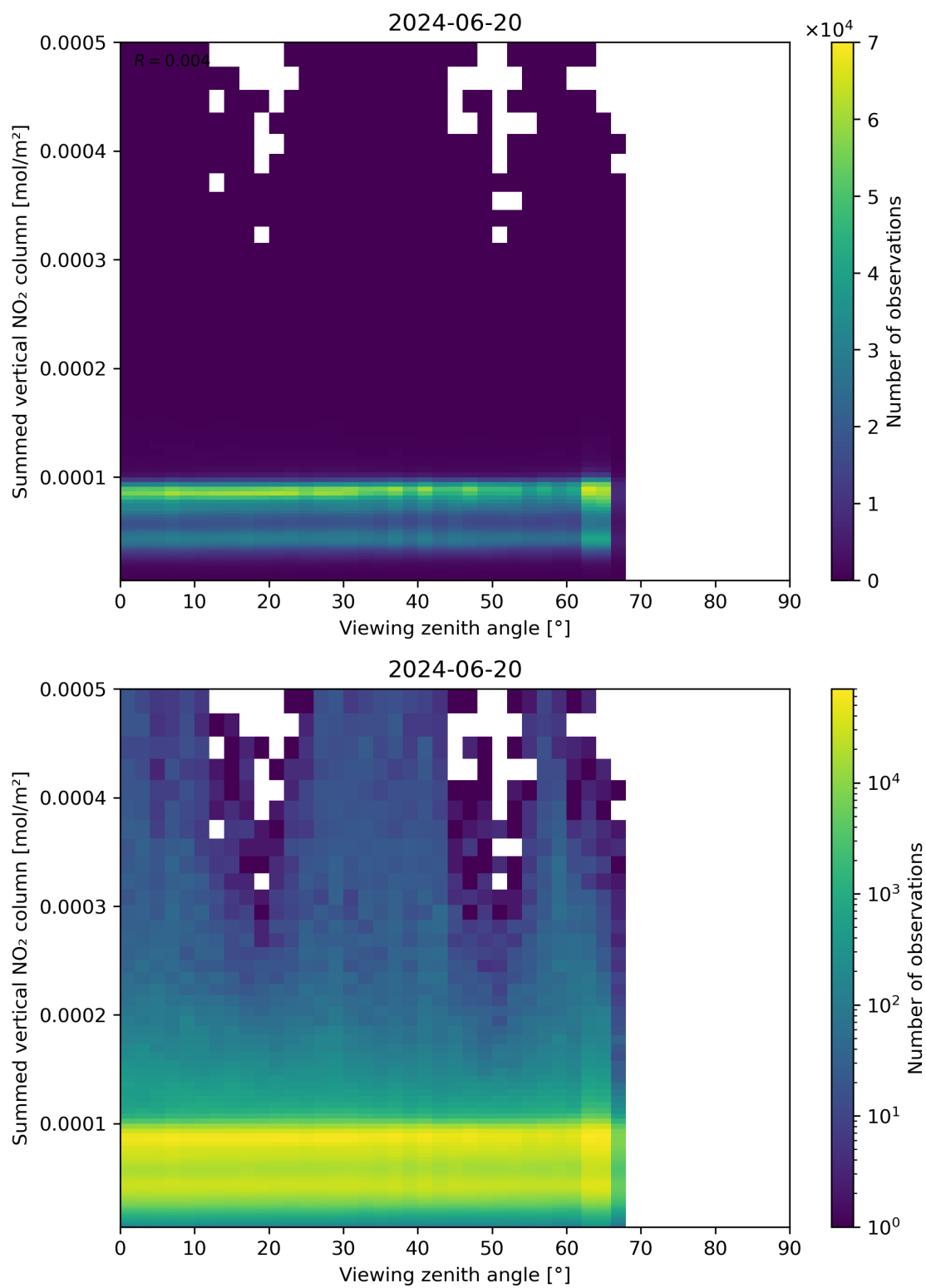
Figure 165: Scatter density plot of “Viewing zenith angle” against “Summed vertical NO 2 column” for 2024-06-19 to 2024-06-21.
