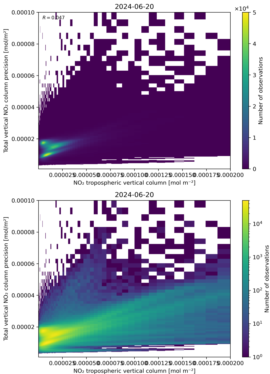
Figure 129: Scatter density plot of “NO 2 tropospheric vertical column” against “Total vertical NO 2 column precision” for 2024-06-19 to 2024-06-21.
