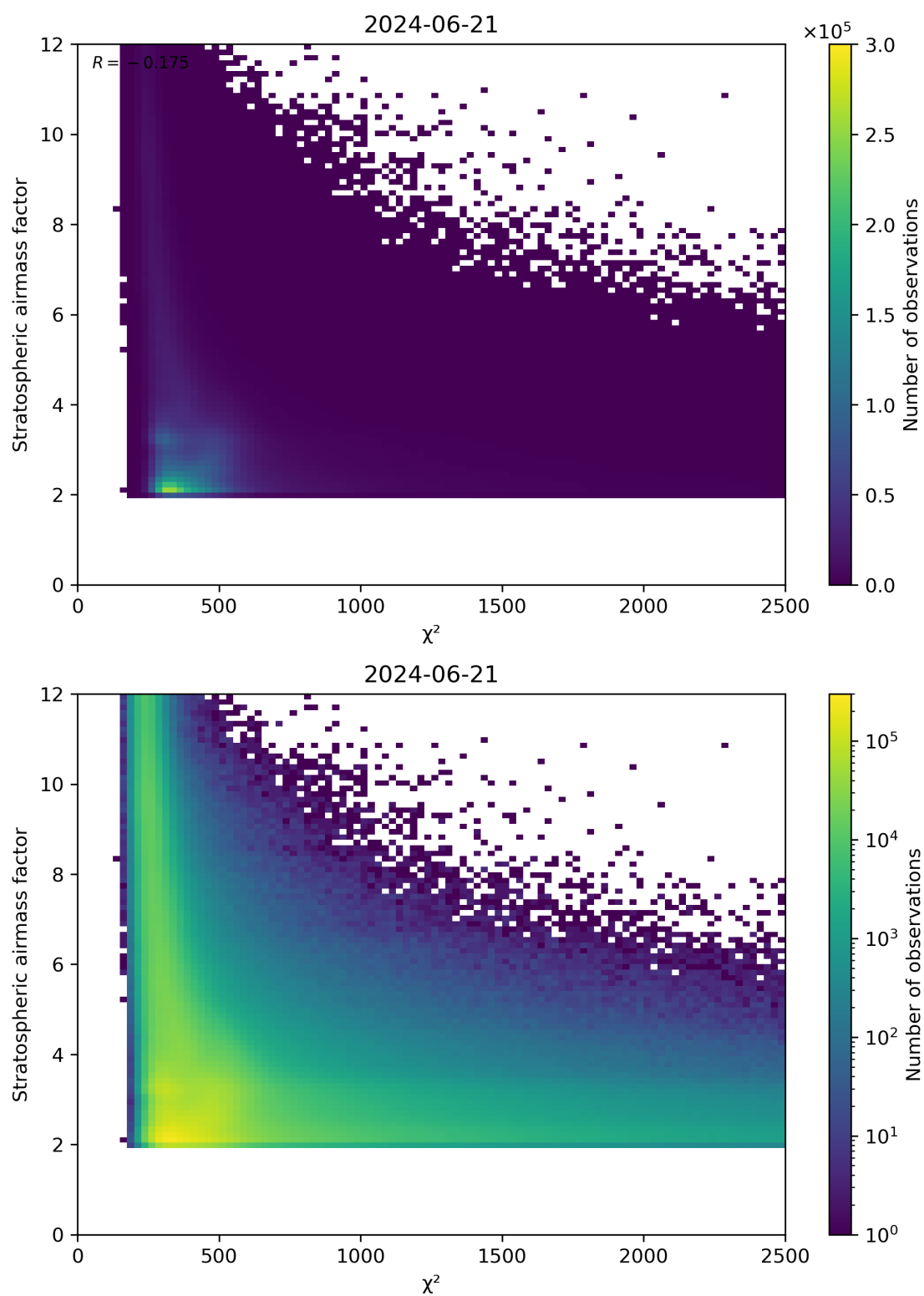
Figure 81: Scatter density plot of “ \chi^2 ” against “Stratospheric airmass factor” for 2024-06-20 to 2024-06-22.
