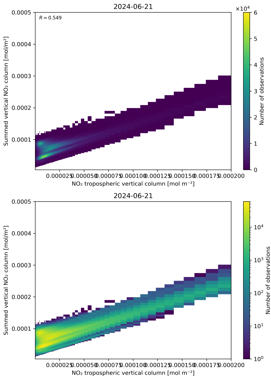
Figure 126: Scatter density plot of “NO 2 tropospheric vertical column” against “Summed vertical NO 2 column” for 2024-06-20 to 2024-06-22.
