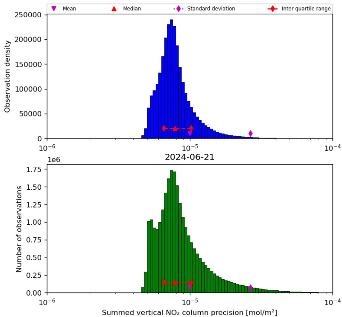
Figure 41: Histogram of "Summed vertical NO 2 column precision" for 2024-06-20 to 2024-06-22
