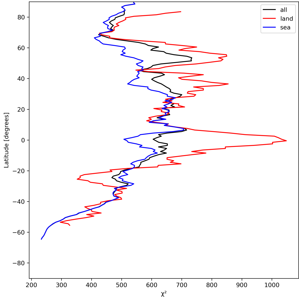
Figure 25: Zonal average of “ \chi^2 ” for 2024-06-20 to 2024-06-22.
