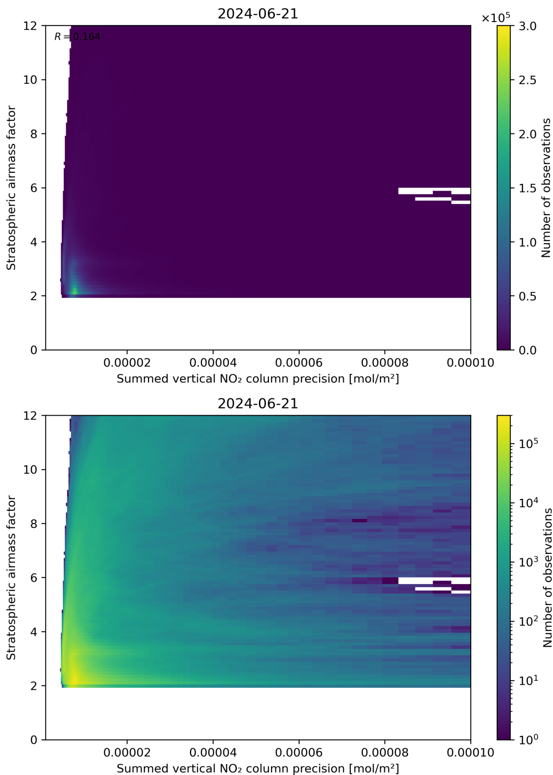
Figure 106: Scatter density plot of “Summed vertical NO 2 column precision” against “Stratospheric airmass factor” for 2024-06-20 to 2024-06-22.
