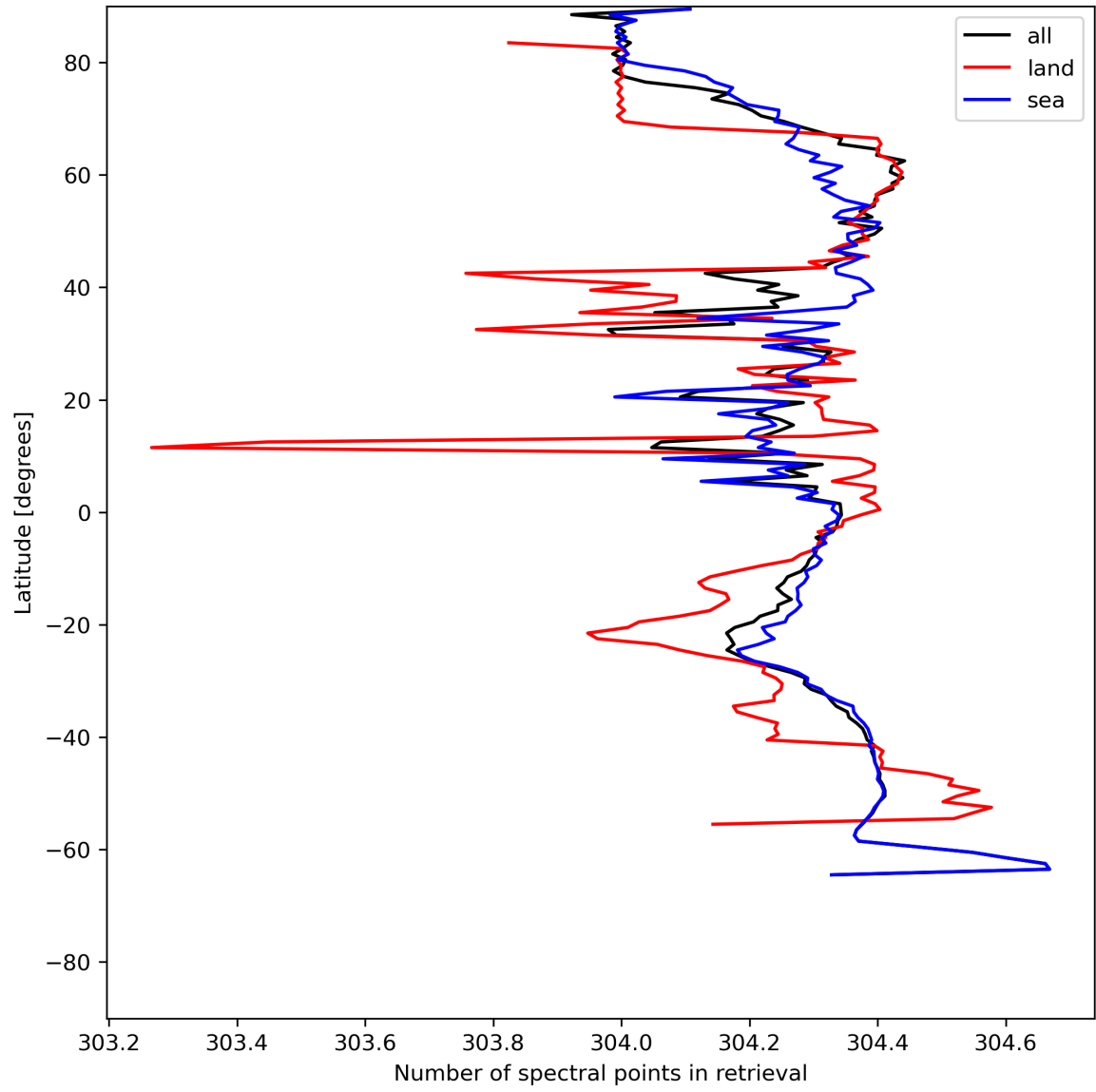
Figure 16: Zonal average of “Number of spectral points in retrieval” for 2024-06-20 to 2024-06-22.
