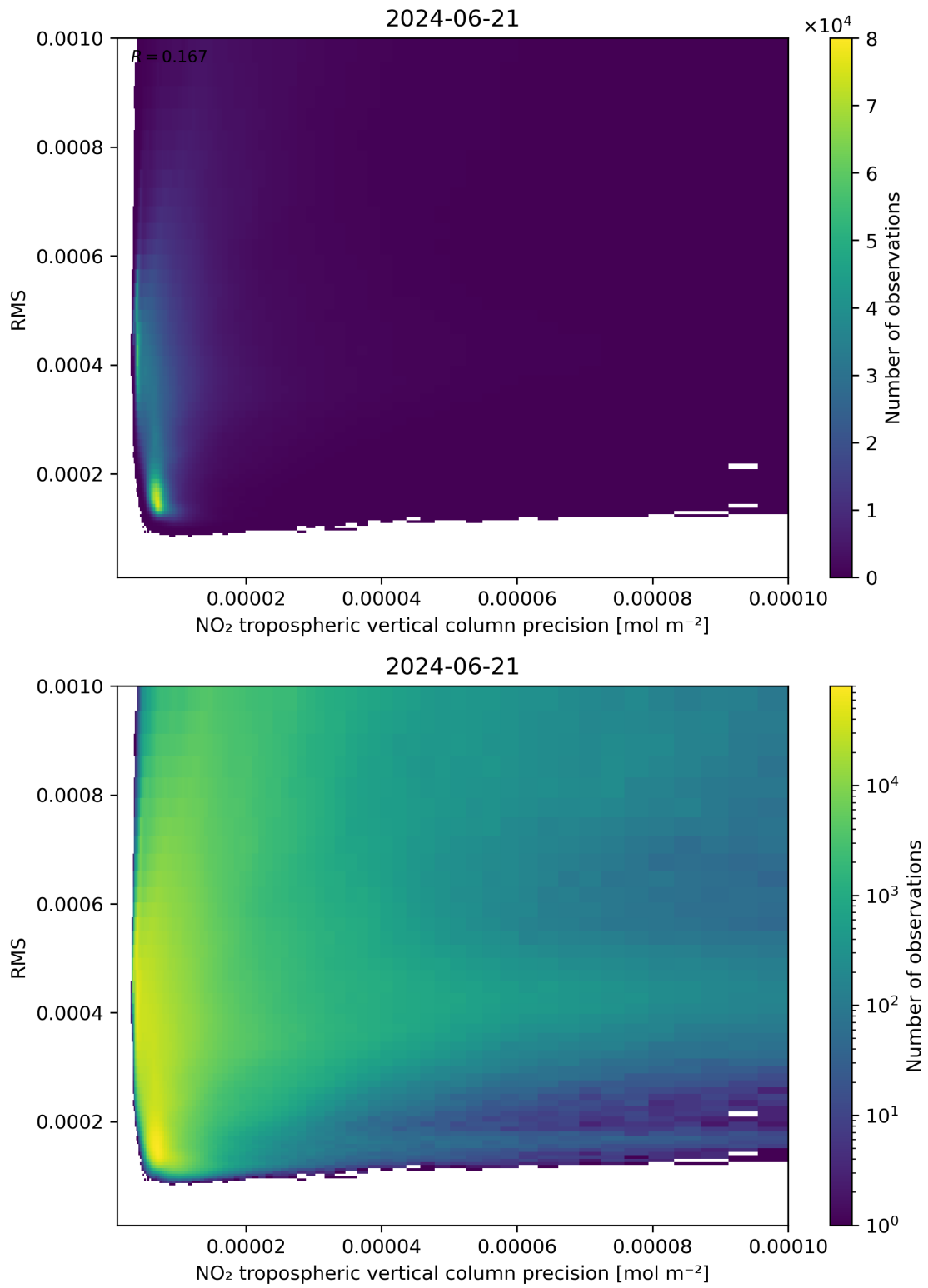
Figure 140: Scatter density plot of “NO 2 tropospheric vertical column precision” against “RMS” for 2024-06-20 to 2024-06-22.
