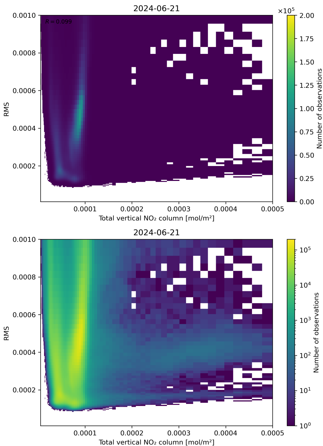
Figure 120: Scatter density plot of “Total vertical NO 2 column” against “RMS” for 2024-06-20 to 2024-06-22.
