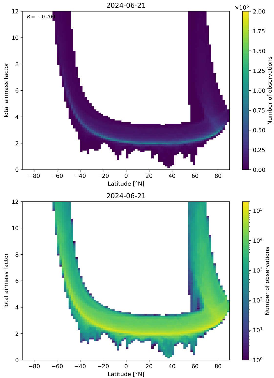
Figure 84: Scatter density plot of “Latitude” against “Total airmass factor” for 2024-06-20 to 2024-06-22.
