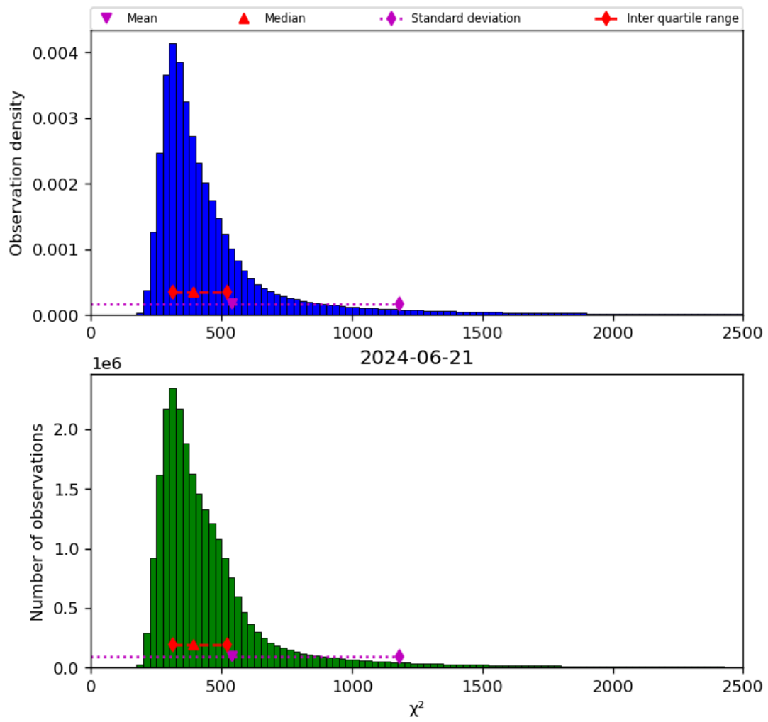
Figure 42: Histogram of “ \chi^2 ” for 2024-06-20 to 2024-06-22
