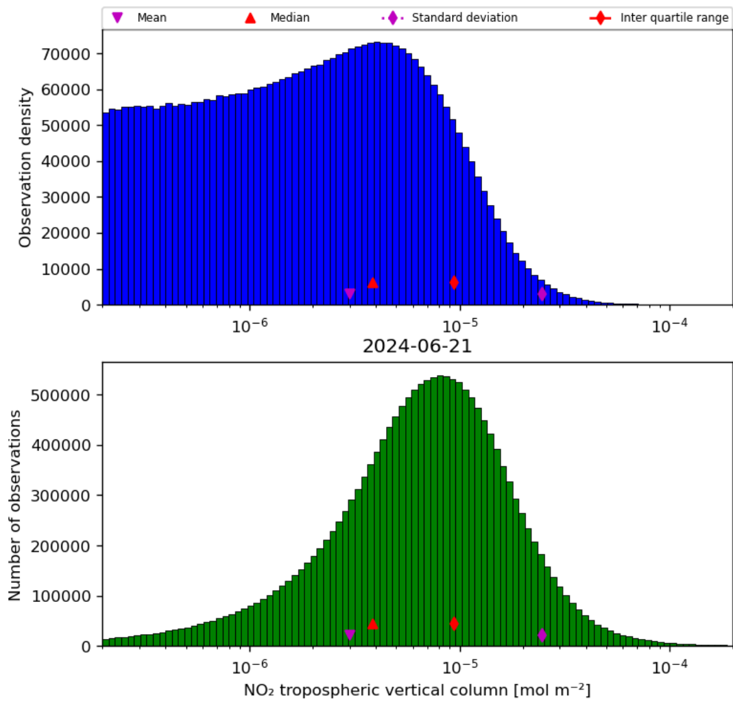
Figure 29: Histogram of “NO 2 tropospheric vertical column” for 2024-06-20 to 2024-06-22
