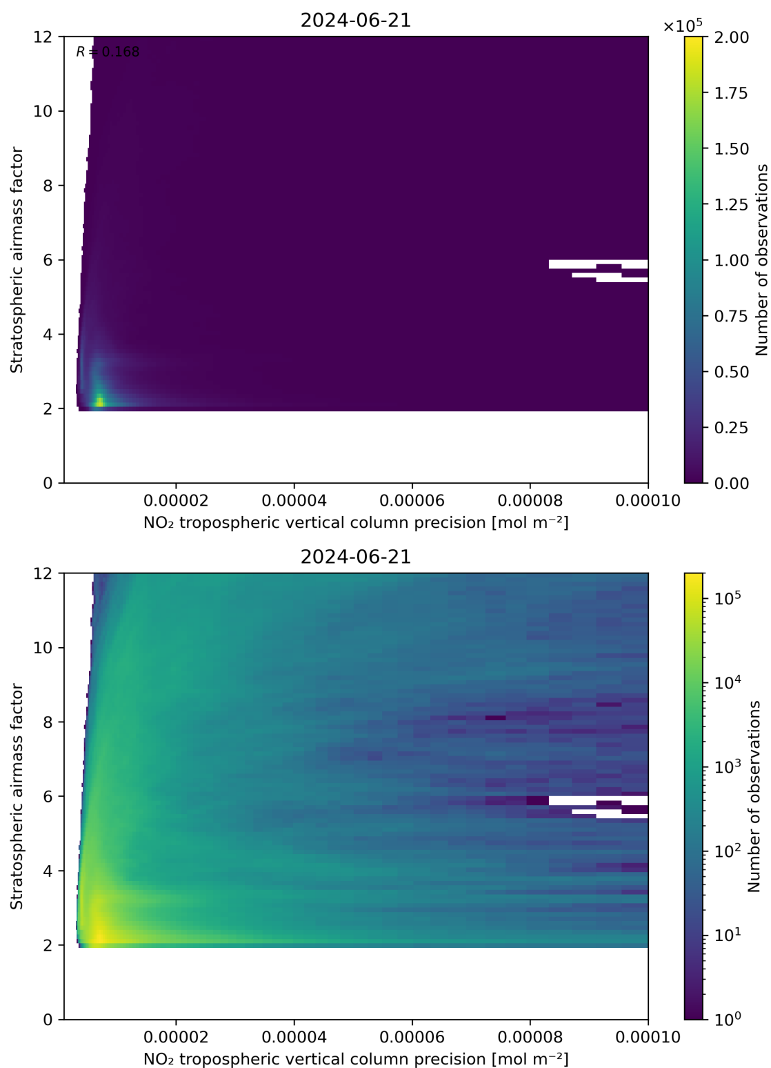
Figure 131: Scatter density plot of “NO 2 tropospheric vertical column precision” against “Stratospheric airmass factor” for 2024-06-20 to 2024-06-22.
