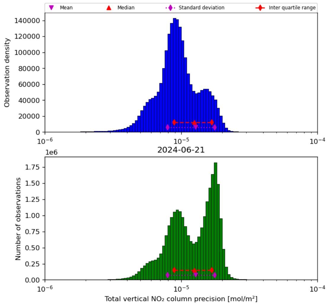
Figure 39: Histogram of “Total vertical NO 2 column precision” for 2024-06-20 to 2024-06-22
