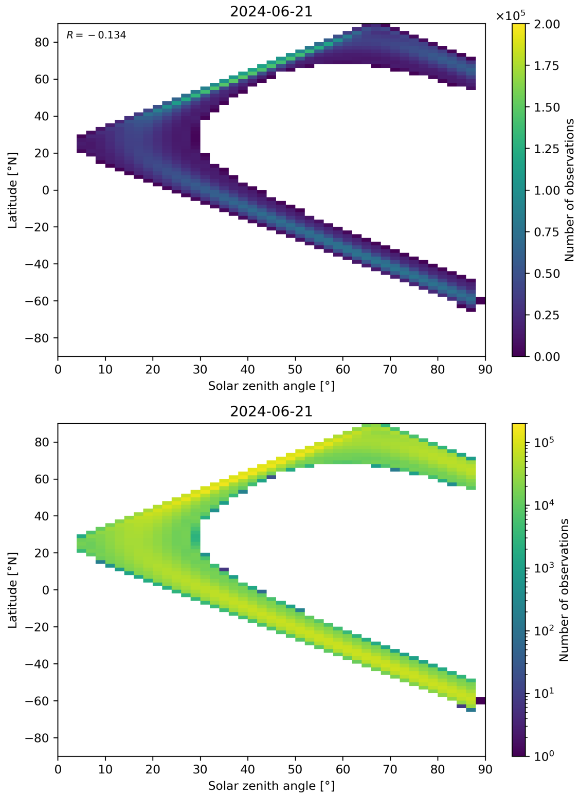
Figure 149: Scatter density plot of “Solar zenith angle” against “Latitude” for 2024-06-20 to 2024-06-22.
