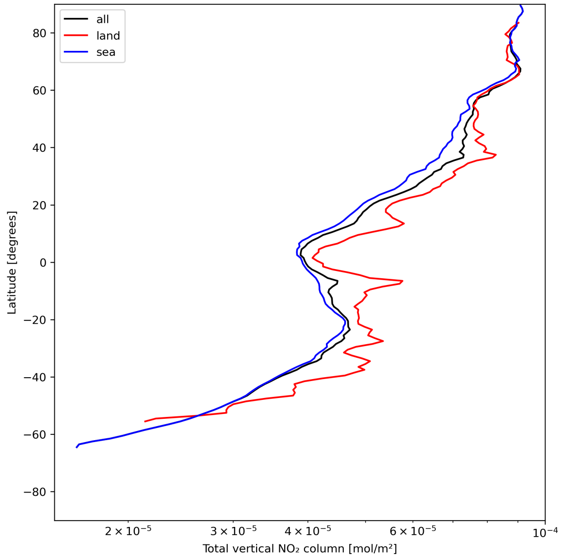
Figure 21: Zonal average of “Total vertical NO 2 column” for 2024-06-20 to 2024-06-22.
