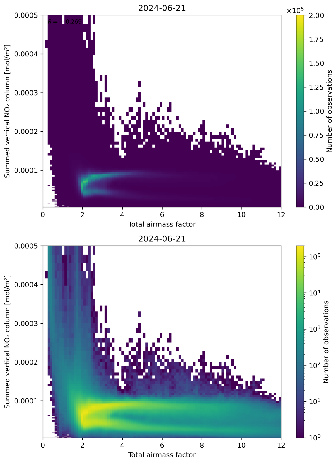
Figure 65: Scatter density plot of “Total airmass factor” against “Summed vertical NO 2 column” for 2024-06-20 to 2024-06-22.
