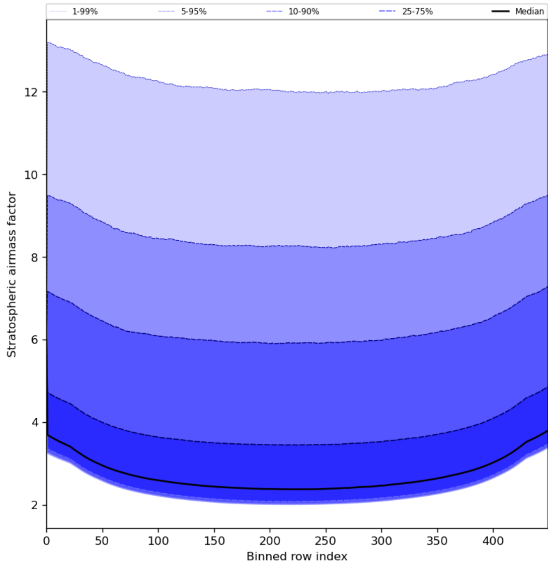
Figure 61: Along track statistics of “Stratospheric airmass factor” for 2024-06-20 to 2024-06-22
