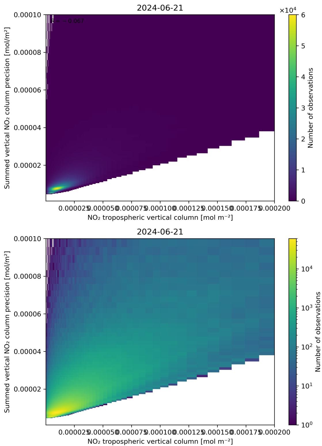
Figure 127: Scatter density plot of “NO 2 tropospheric vertical column” against “Summed vertical NO 2 column precision” for 2024-06-20 to 2024-06-22.
