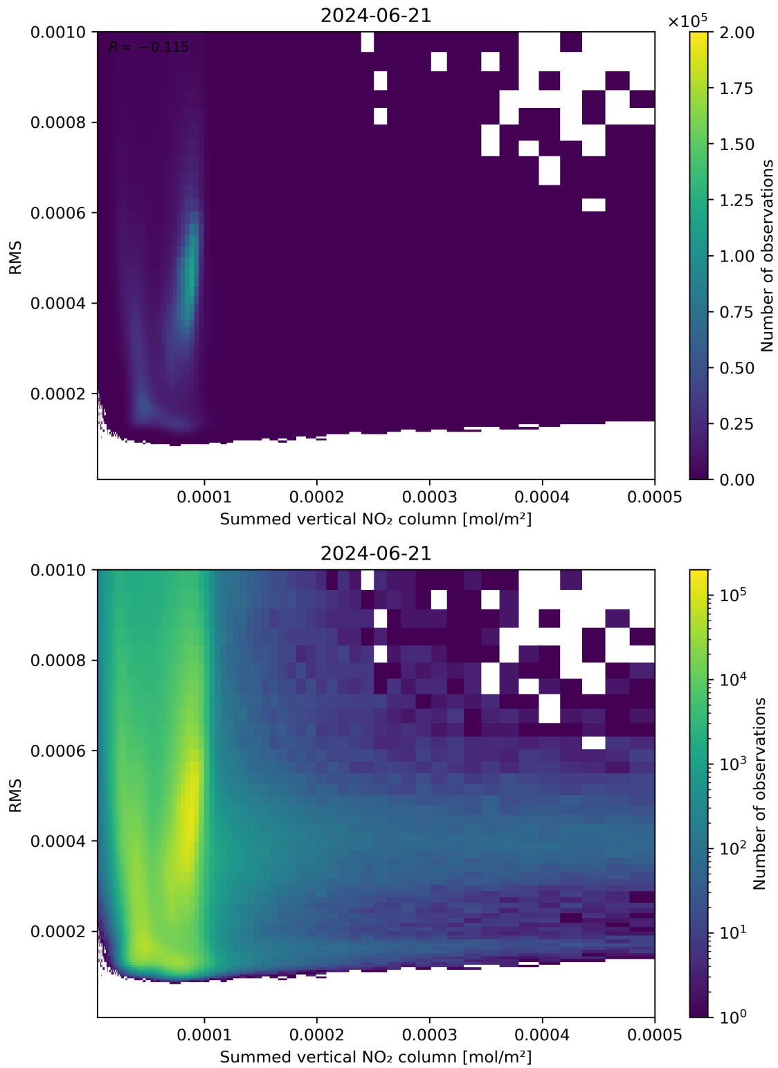
Figure 109: Scatter density plot of “Summed vertical NO 2 column” against “RMS” for 2024-06-20 to 2024-06-22.
