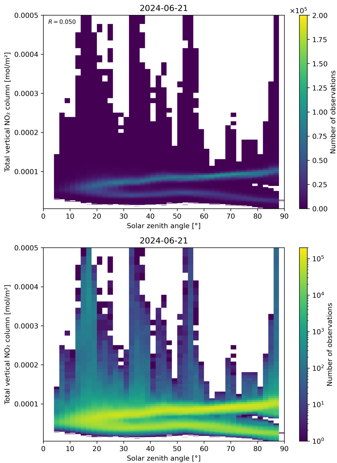
Figure 153: Scatter density plot of “Solar zenith angle” against “Total vertical NO 2 column” for 2024-06-20 to 2024-06-22.
