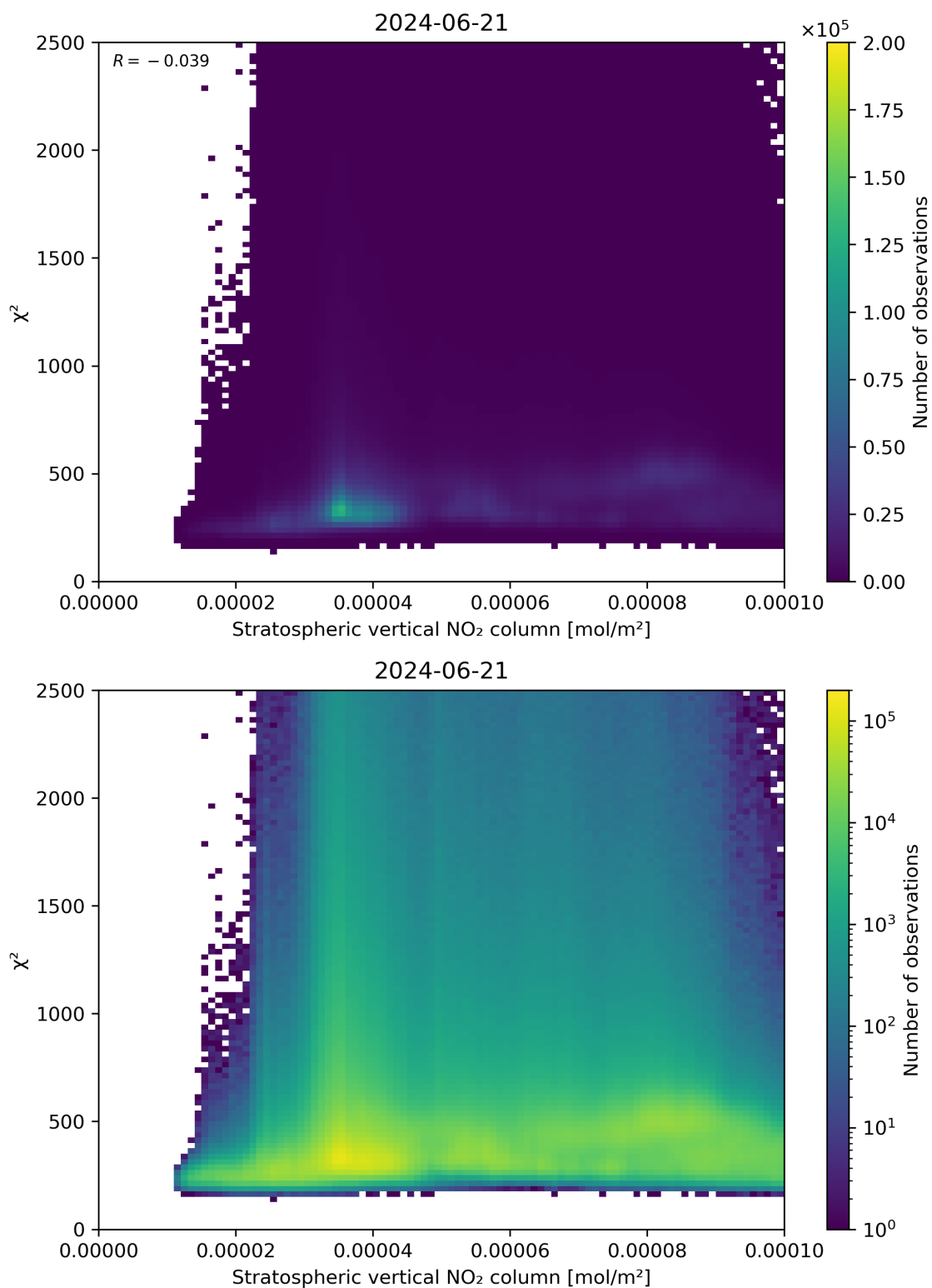
Figure 97: Scatter density plot of “Stratospheric vertical NO 2 column” against “ \chi^2 ” for 2024-06-20 to 2024-06-22.
