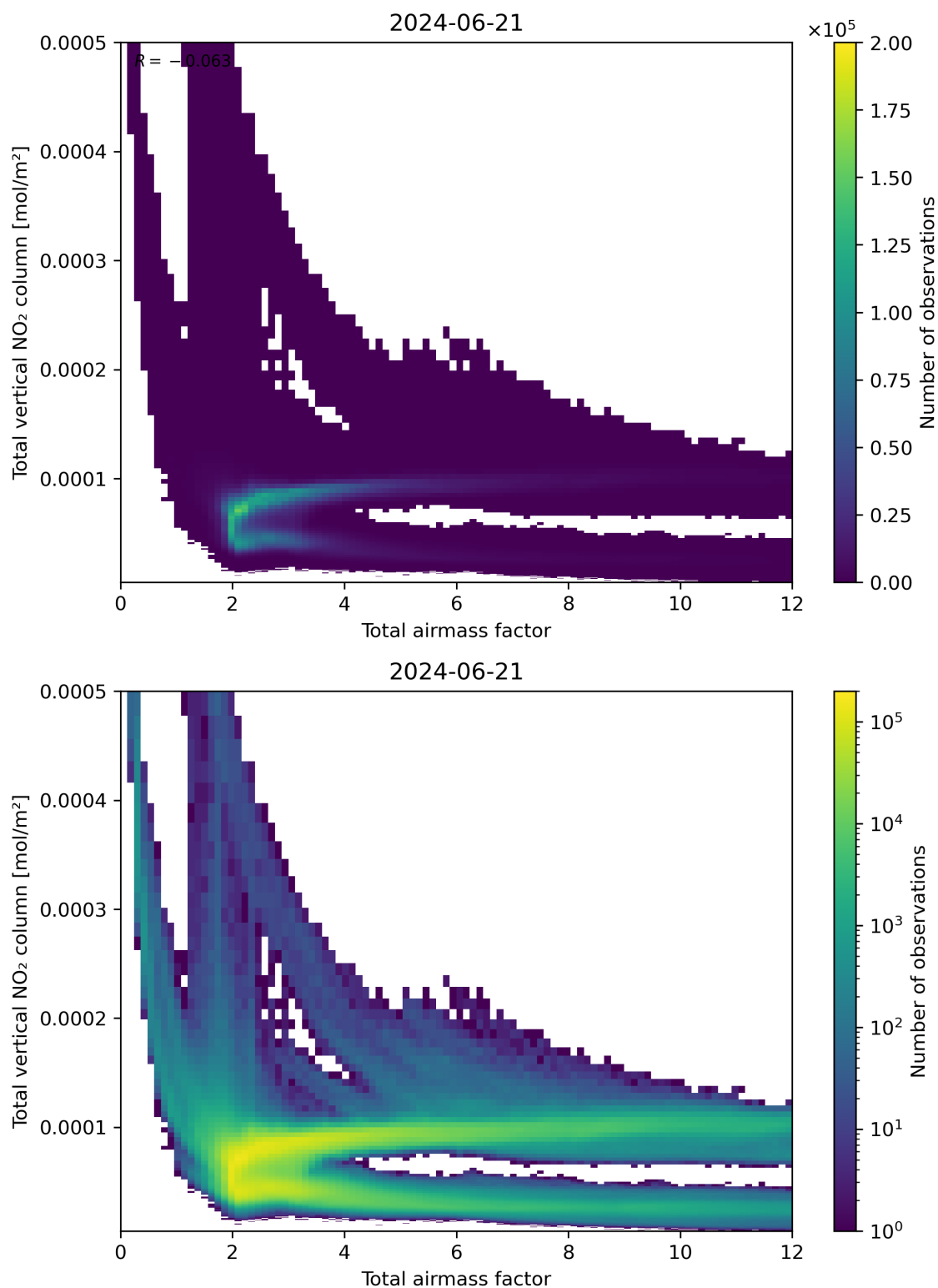
Figure 67: Scatter density plot of “Total airmass factor” against “Total vertical NO 2 column” for 2024-06-20 to 2024-06-22.
