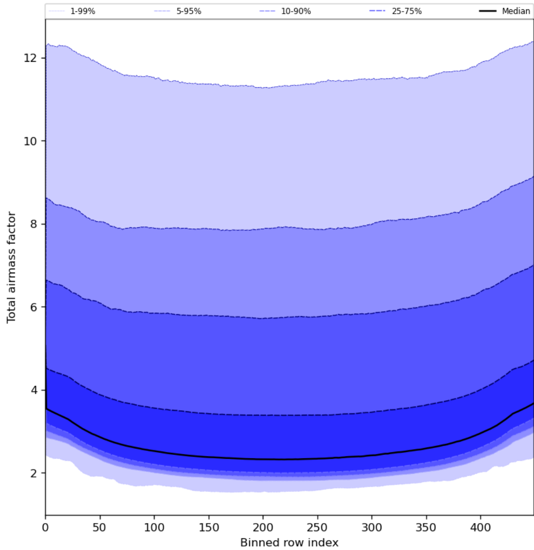
Figure 49: Along track statistics of “Total airmass factor” for 2024-06-20 to 2024-06-22
