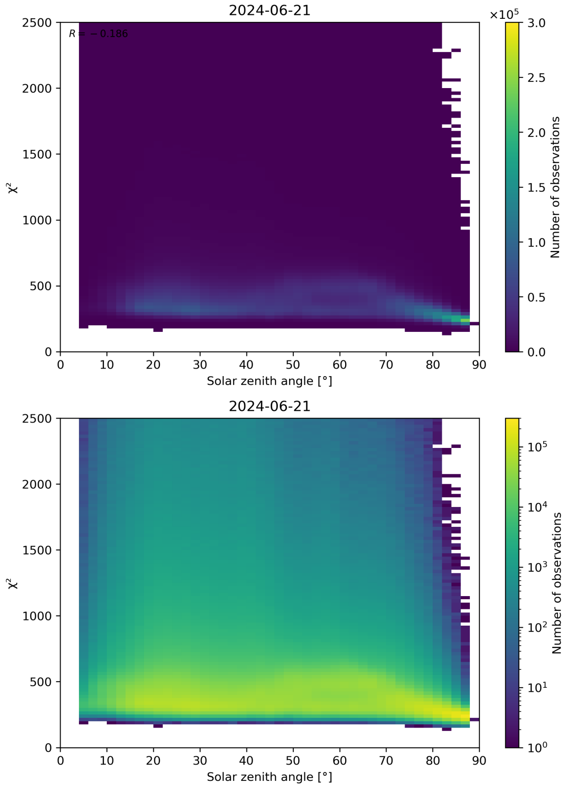
Figure 148: Scatter density plot of “Solar zenith angle” against “ \chi^2 ” for 2024-06-20 to 2024-06-22.
