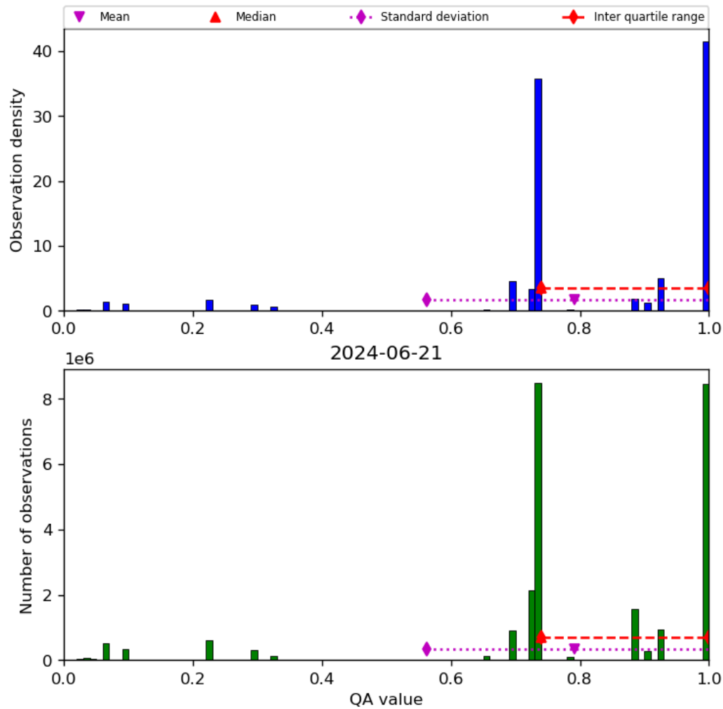
Figure 28: Histogram of “QA value” for 2024-06-20 to 2024-06-22
