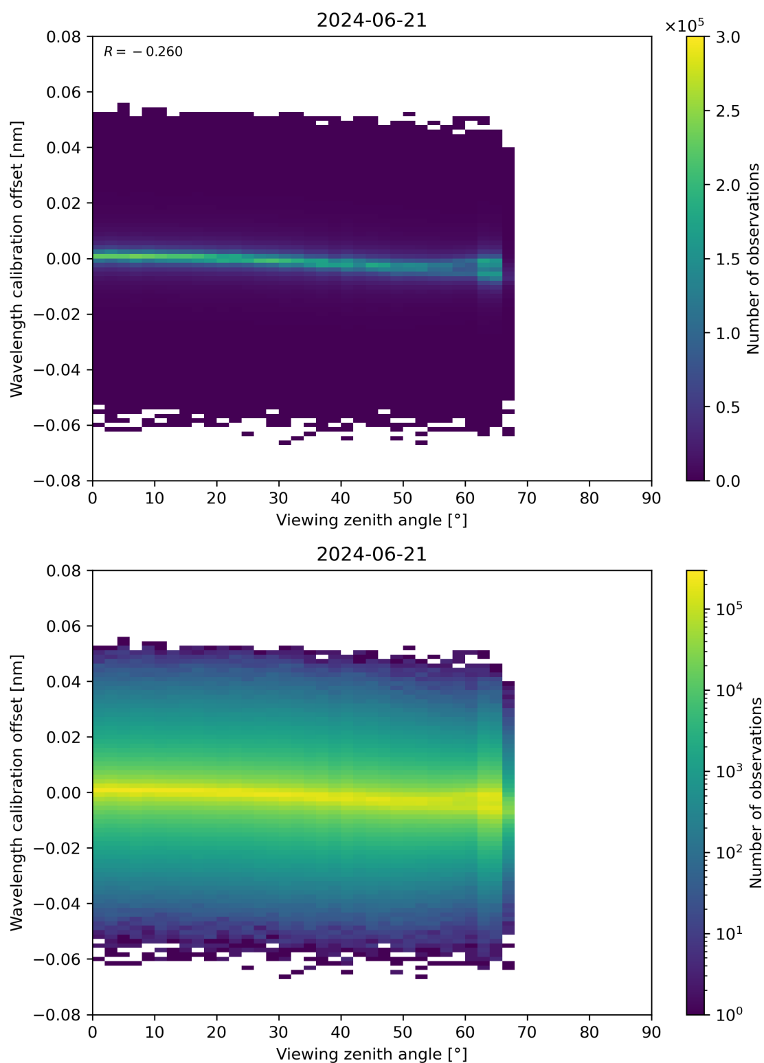
Figure 173: Scatter density plot of “Viewing zenith angle” against “Wavelength calibration offset” for 2024-06-20 to 2024-06-22.
