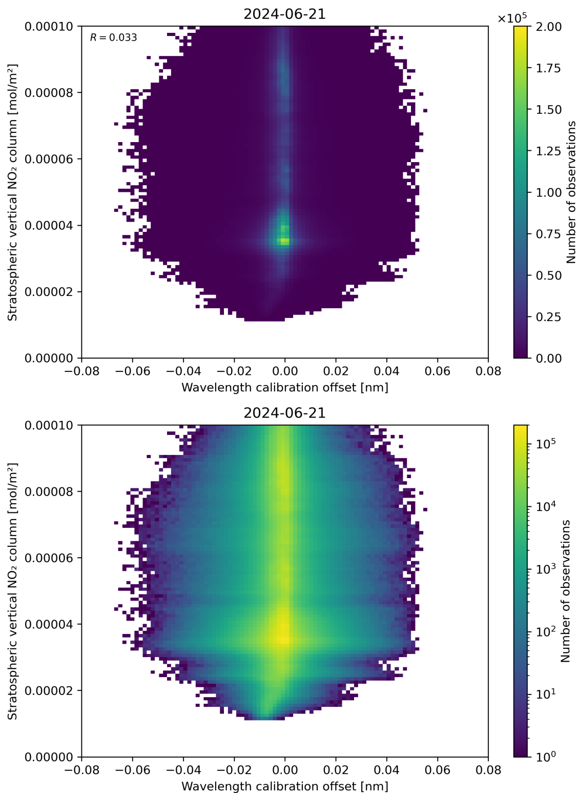
Figure 176: Scatter density plot of “Wavelength calibration offset” against “Stratospheric vertical NO 2 column” for 2024-06-20 to 2024-06-22.
