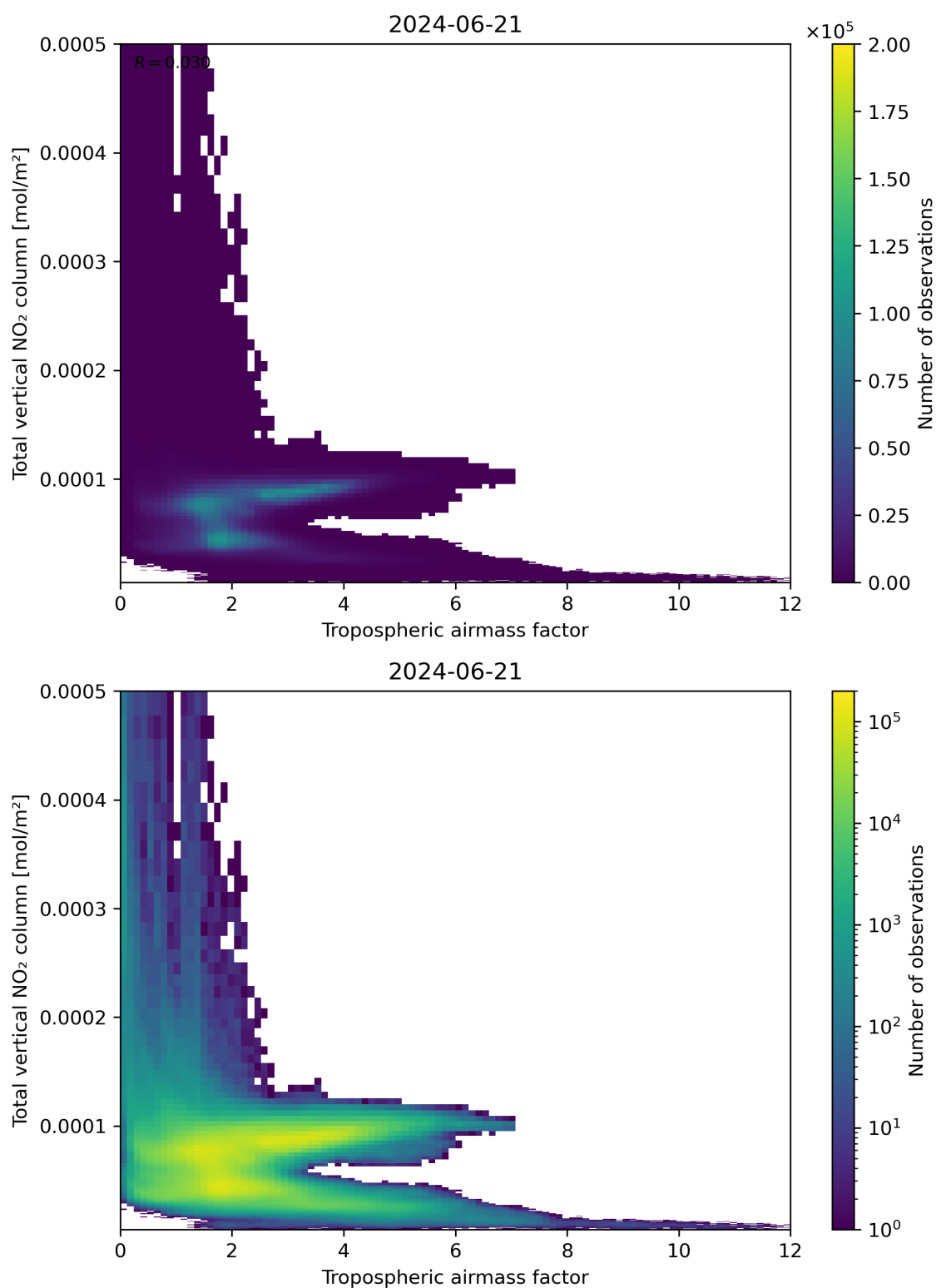
Figure 77: Scatter density plot of “Tropospheric airmass factor” against “Total vertical NO 2 column” for 2024-06-20 to 2024-06-22.
