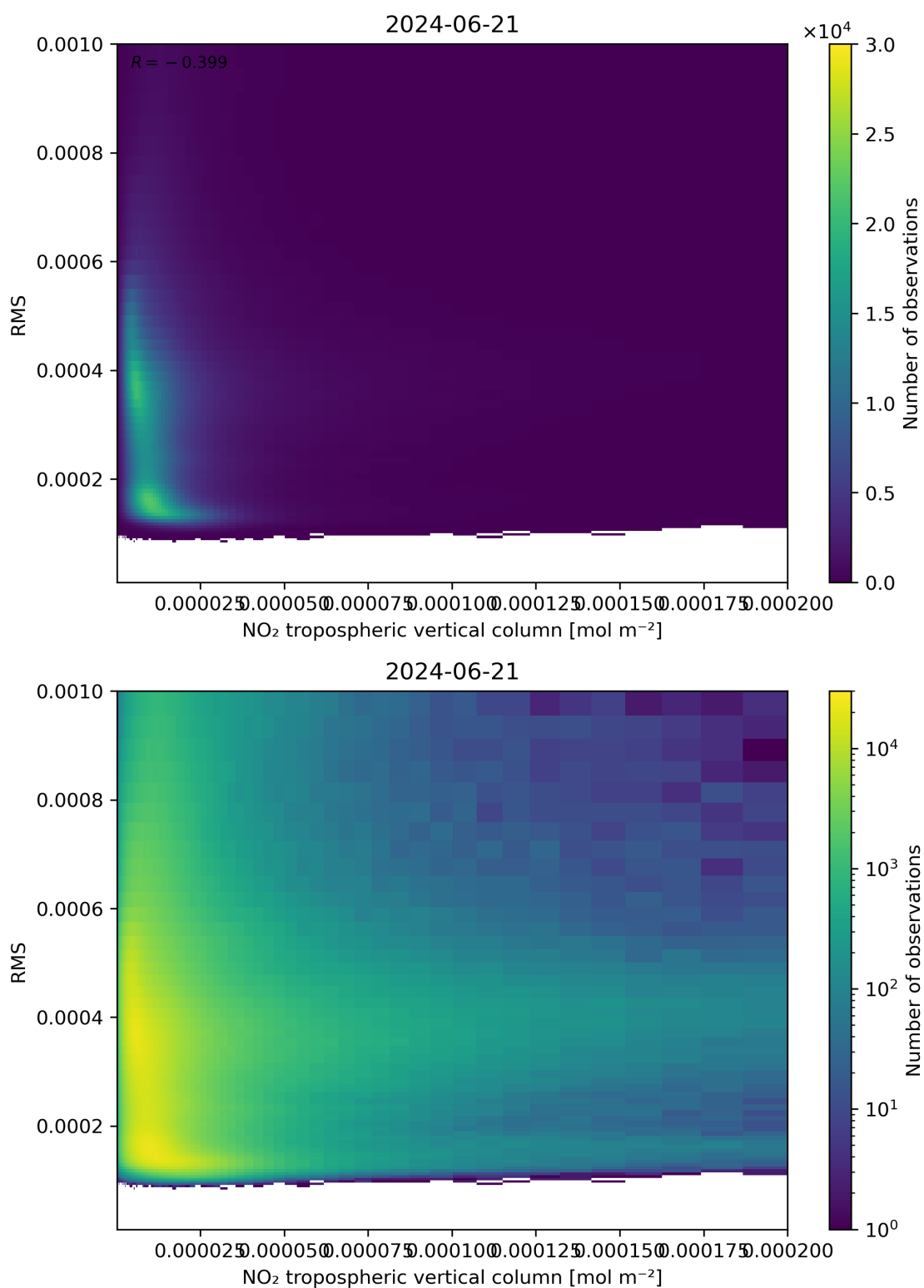
Figure 142: Scatter density plot of “NO 2 tropospheric vertical column” against “RMS” for 2024-06-20 to 2024-06-22.
