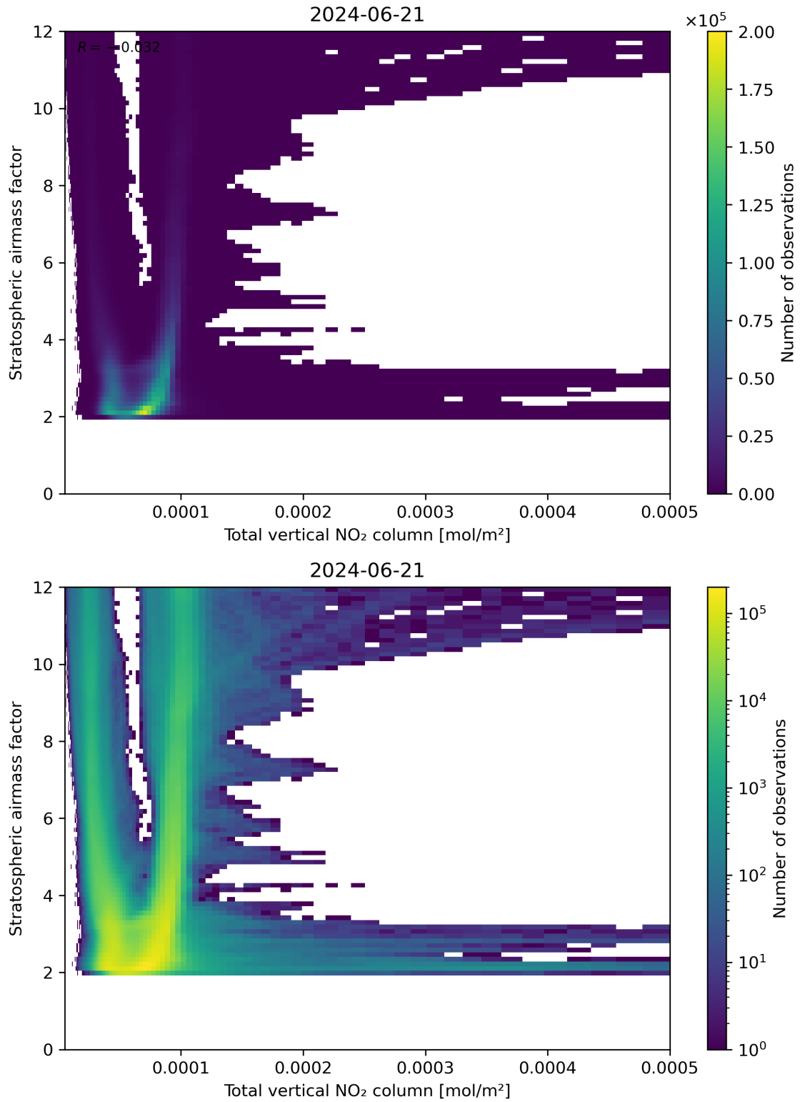
Figure 110: Scatter density plot of “Total vertical NO 2 column” against “Stratospheric airmass factor” for 2024-06-20 to 2024-06-22.
