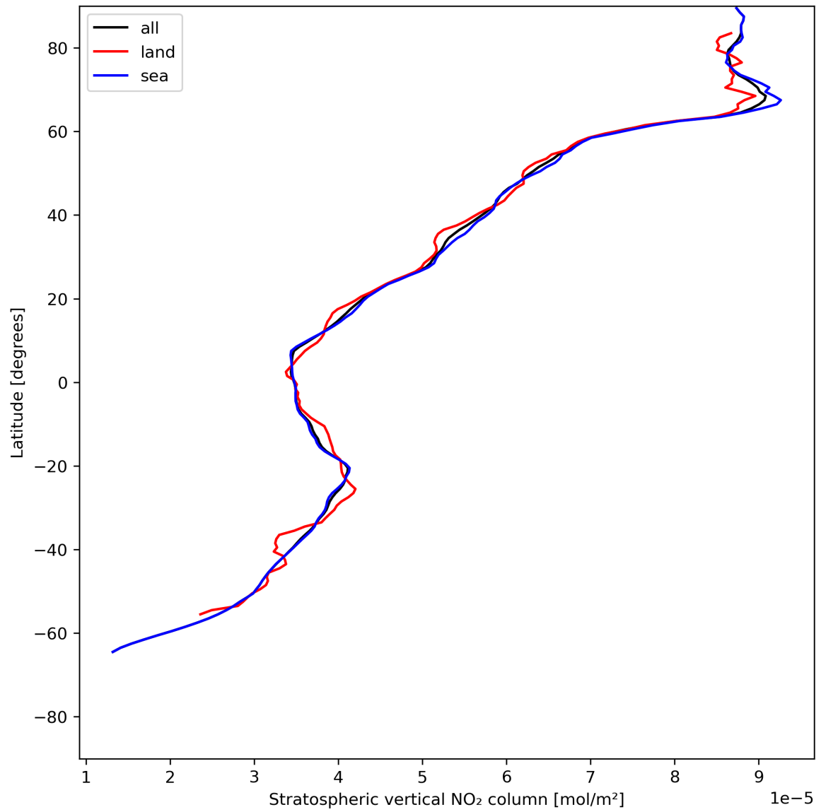
Figure 19: Zonal average of “Stratospheric vertical NO 2 column” for 2024-06-20 to 2024-06-22.
