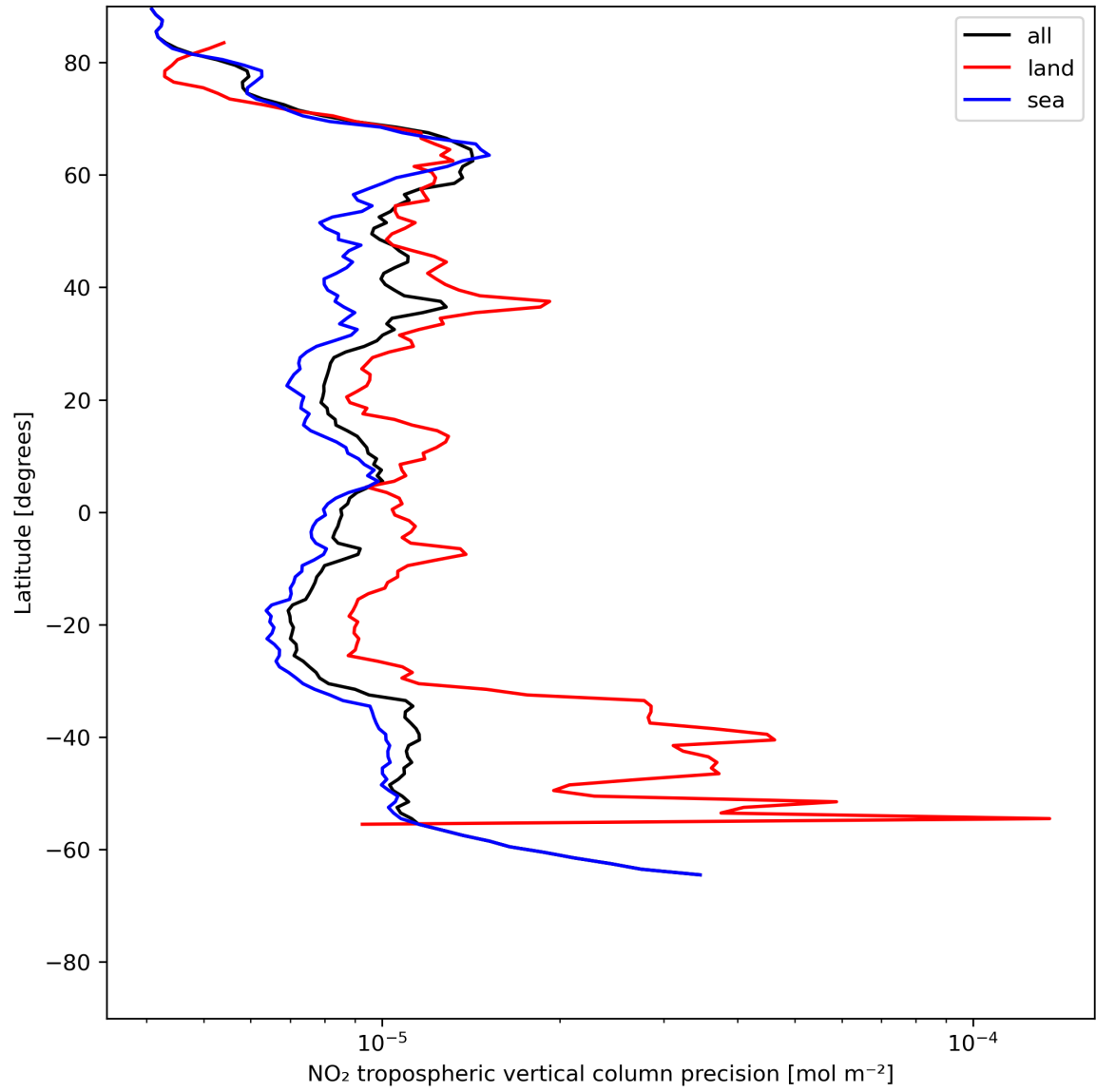
Figure 13: Zonal average of “NO 2 tropospheric vertical column precision” for 2024-06-20 to 2024-06-22.
