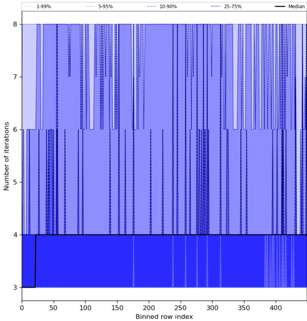
Figure 51: Along track statistics of “Number of iterations” for 2024-06-20 to 2024-06-22
