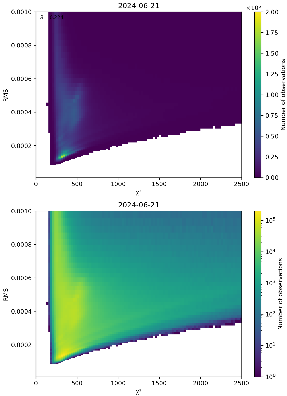
Figure 82: Scatter density plot of “ \chi^2 ” against “RMS” for 2024-06-20 to 2024-06-22.
