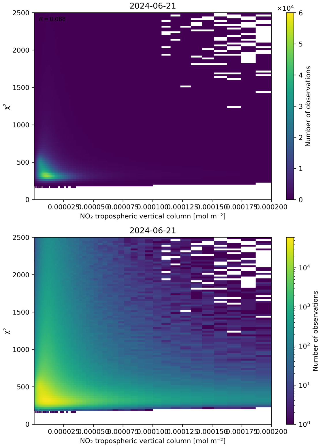
Figure 124: Scatter density plot of “NO 2 tropospheric vertical column” against “ \chi^2 ” for 2024-06-20 to 2024-06-22.
