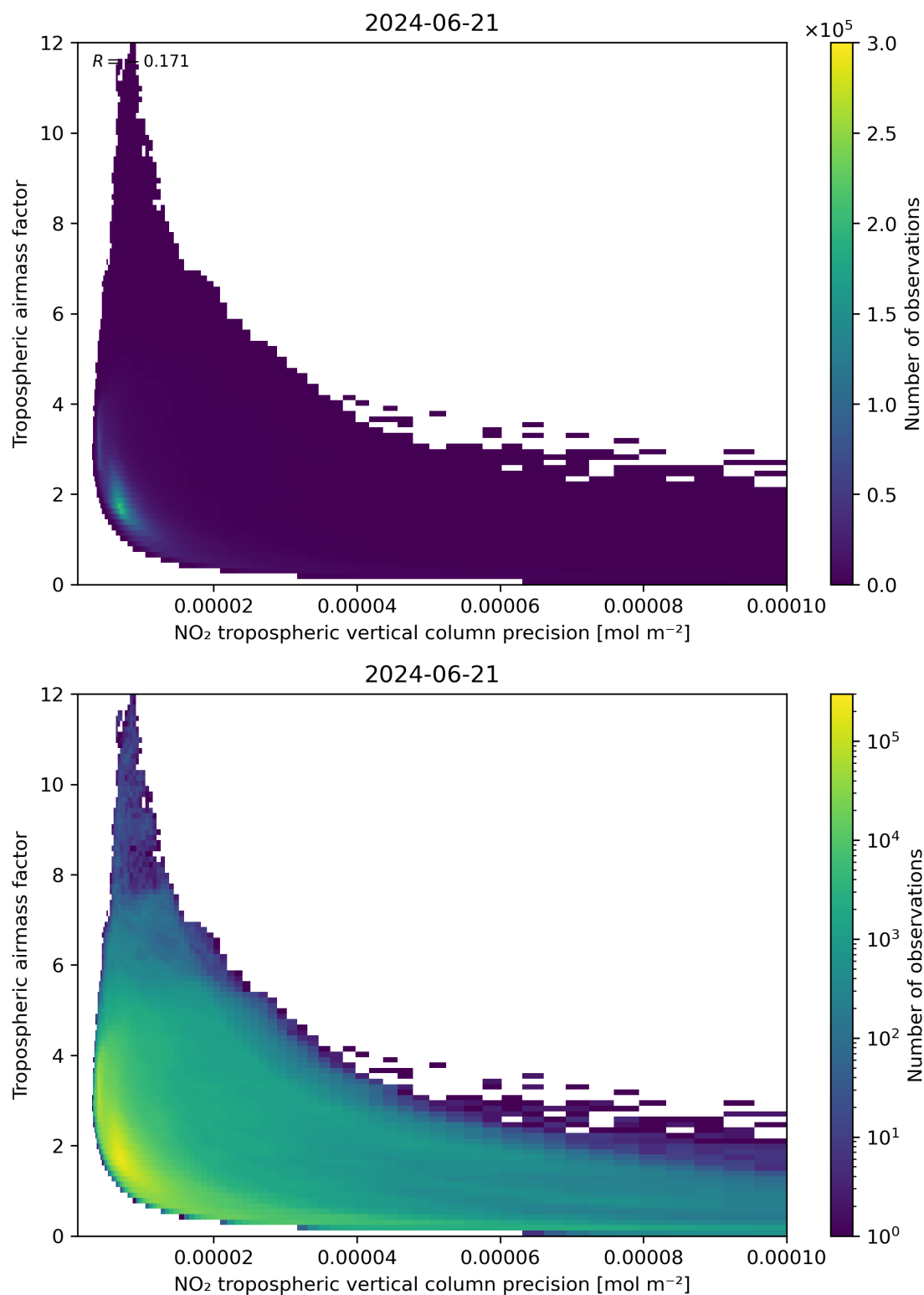
Figure 133: Scatter density plot of “NO 2 tropospheric vertical column precision” against “Tropospheric airmass factor” for 2024-06-20 to 2024-06-22.
