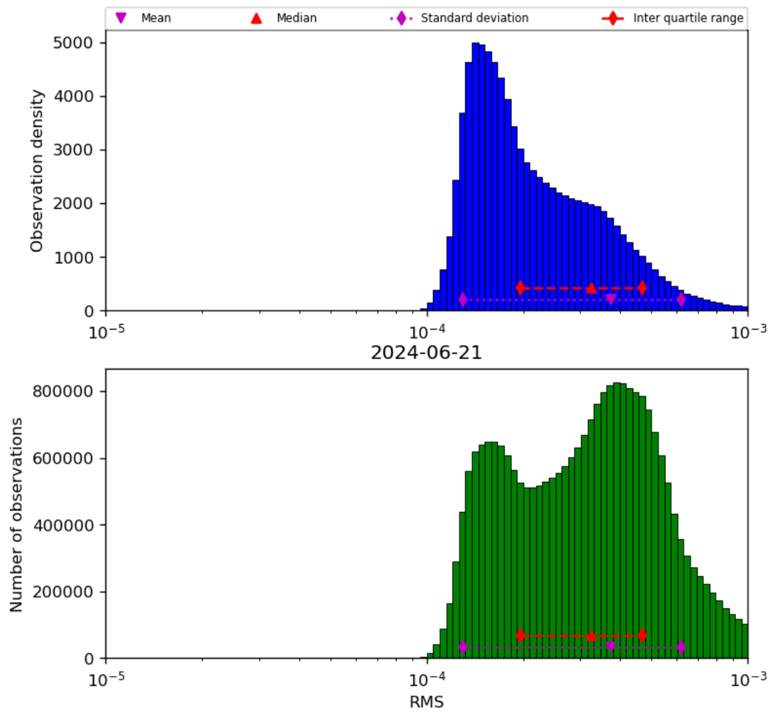
Figure 43: Histogram of “RMS” for 2024-06-20 to 2024-06-22
