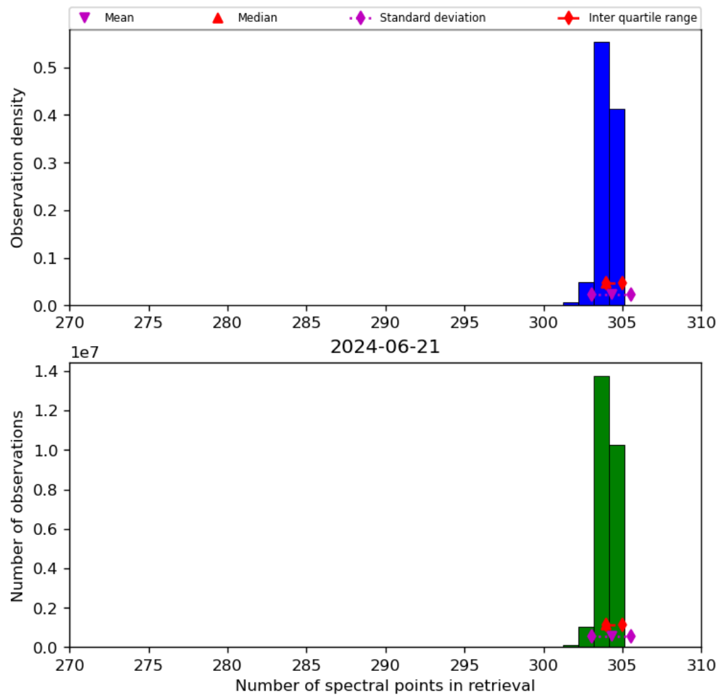
Figure 33: Histogram of “Number of spectral points in retrieval” for 2024-06-20 to 2024-06-22
