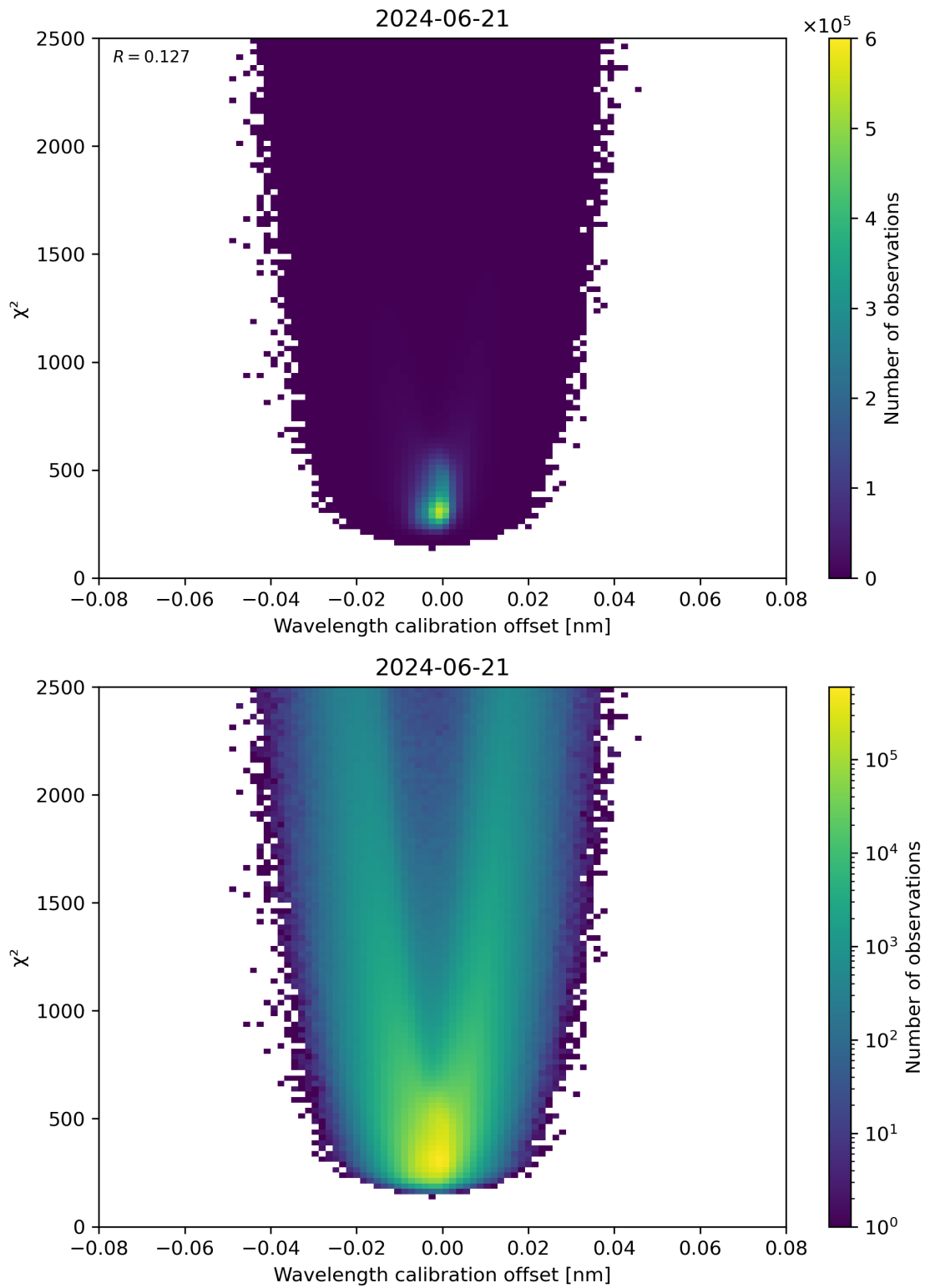
Figure 175: Scatter density plot of “Wavelength calibration offset” against “ \chi^2 ” for 2024-06-20 to 2024-06-22.
