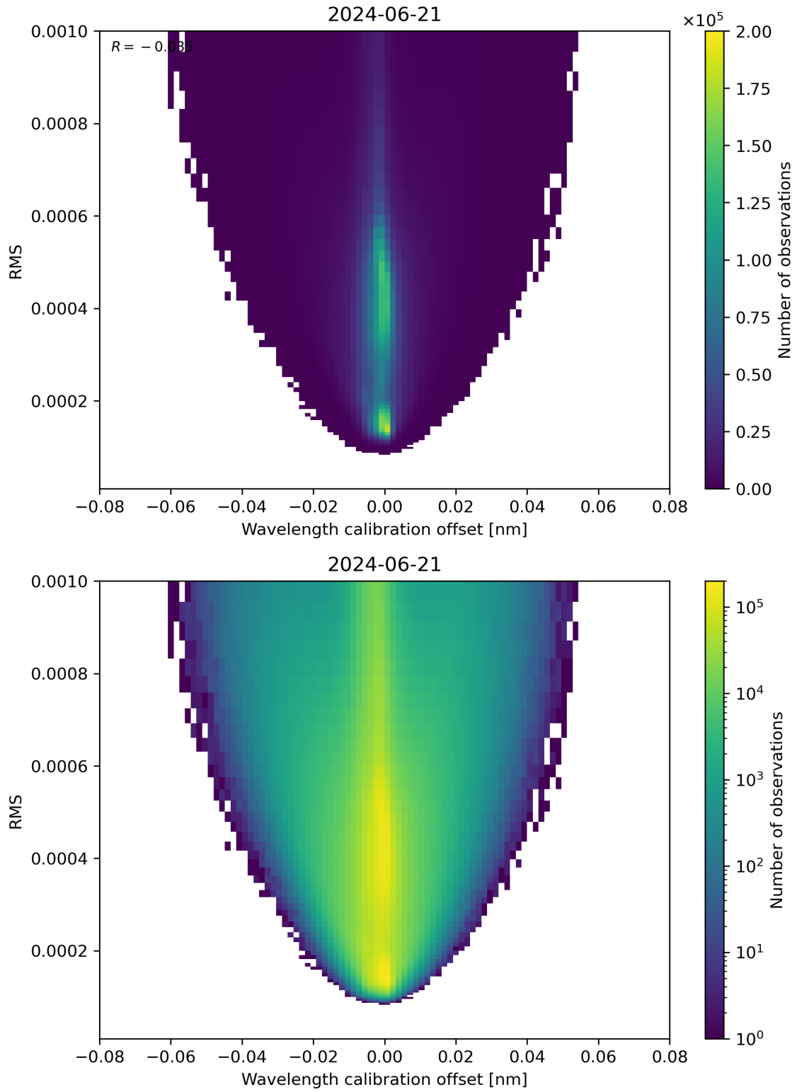
Figure 181: Scatter density plot of “Wavelength calibration offset” against “RMS” for 2024-06-20 to 2024-06-22.
