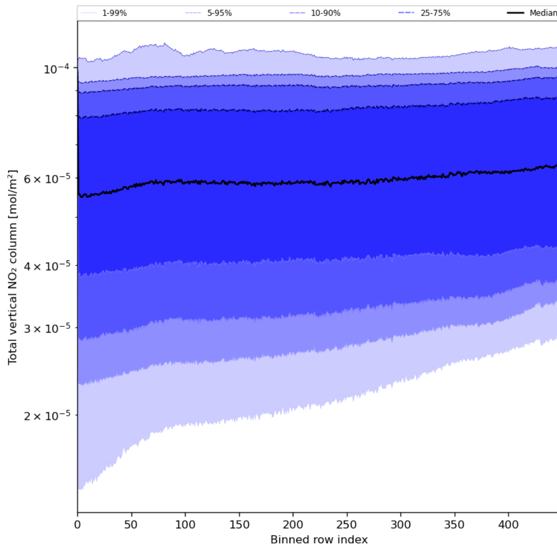
Figure 55: Along track statistics of “Total vertical NO 2 column” for 2024-06-20 to 2024-06-22
