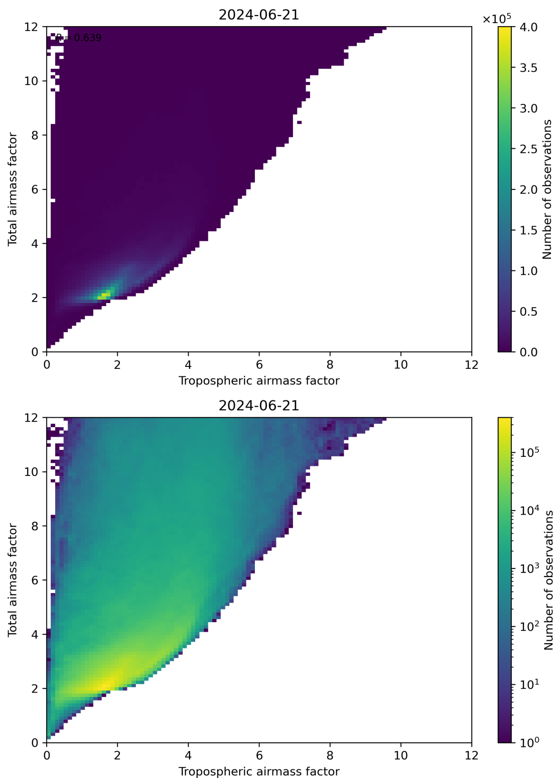
Figure 72: Scatter density plot of “Tropospheric airmass factor” against “Total airmass factor” for 2024-06-20 to 2024-06-22.
