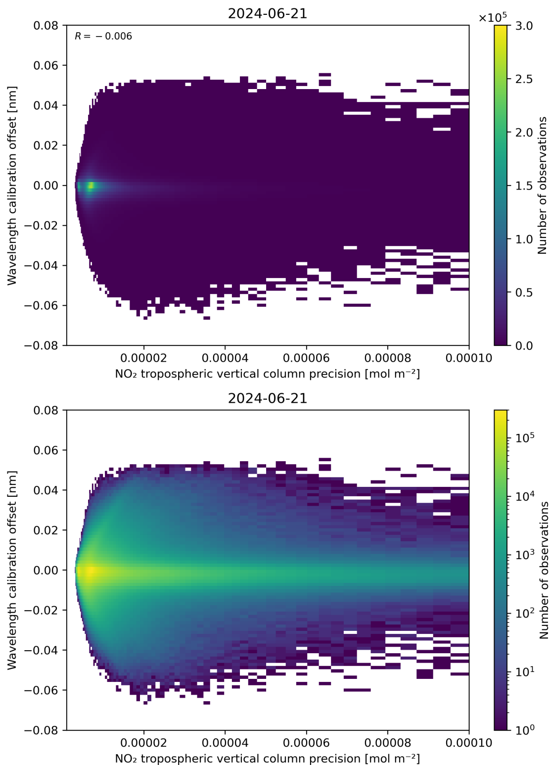
Figure 141: Scatter density plot of “NO 2 tropospheric vertical column precision” against “Wavelength calibration offset” for 2024-06-20 to 2024-06-22.
