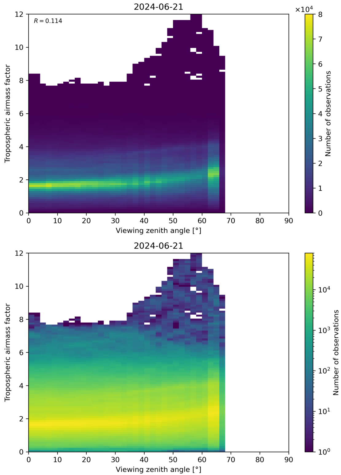
Figure 161: Scatter density plot of “Viewing zenith angle” against “Tropospheric airmass factor” for 2024-06-20 to 2024-06-22.
