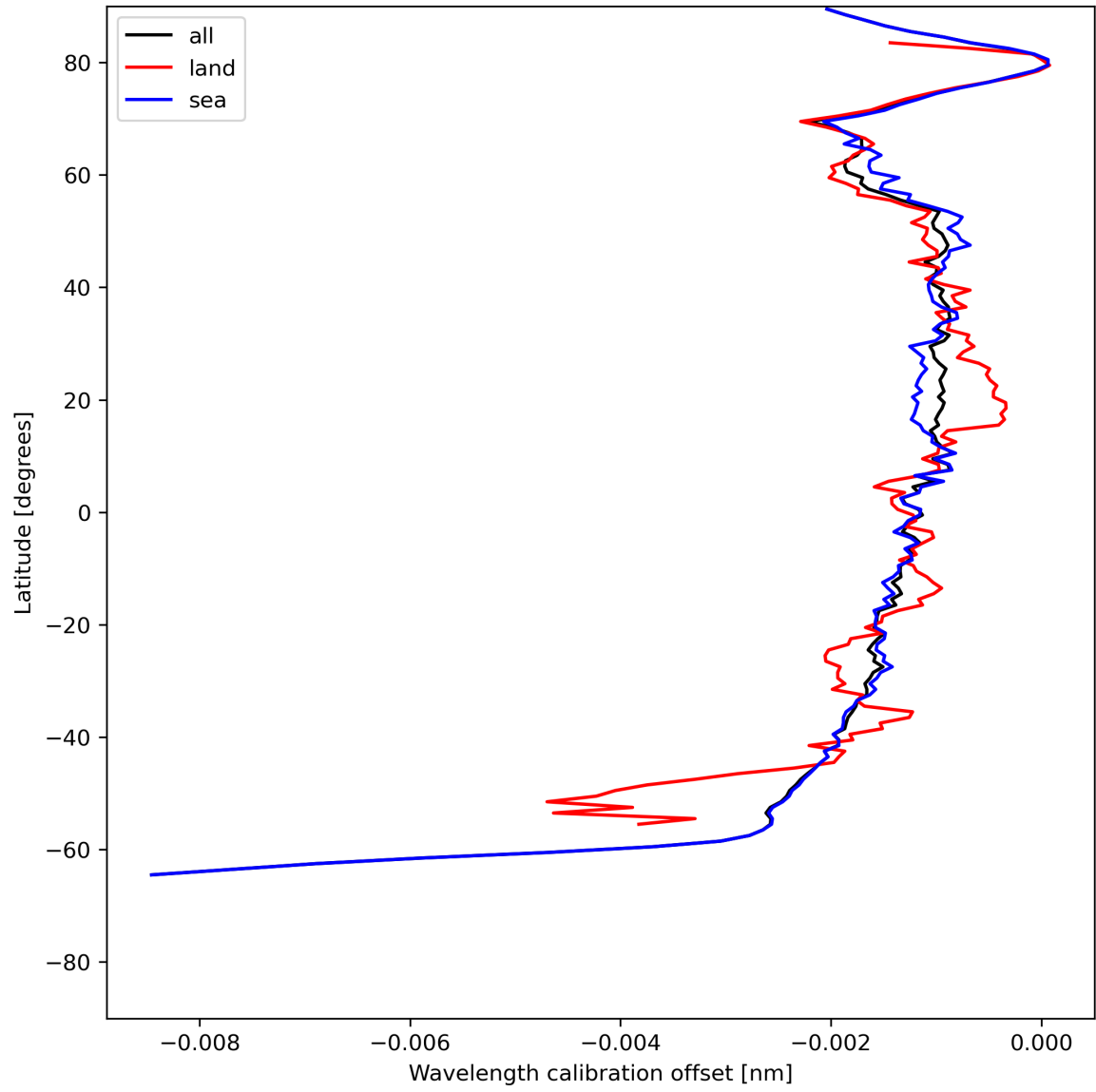
Figure 18: Zonal average of “Wavelength calibration offset” for 2024-06-20 to 2024-06-22.
