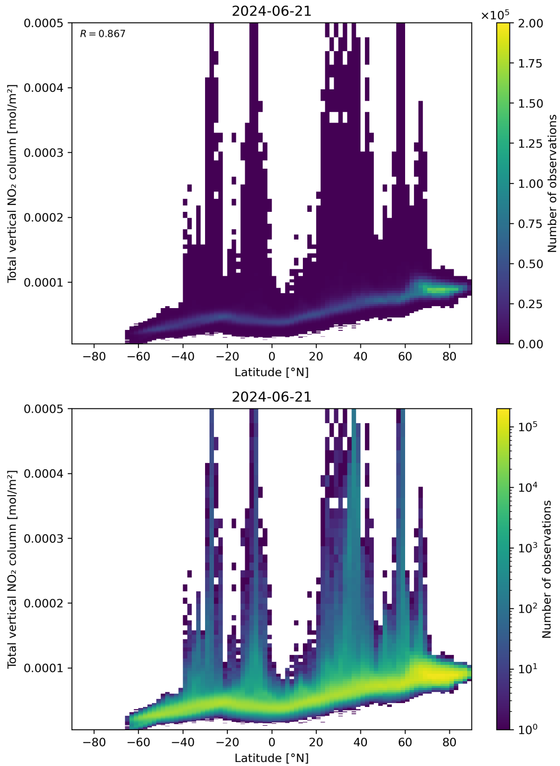
Figure 90: Scatter density plot of “Latitude” against “Total vertical NO 2 column” for 2024-06-20 to 2024-06-22.
