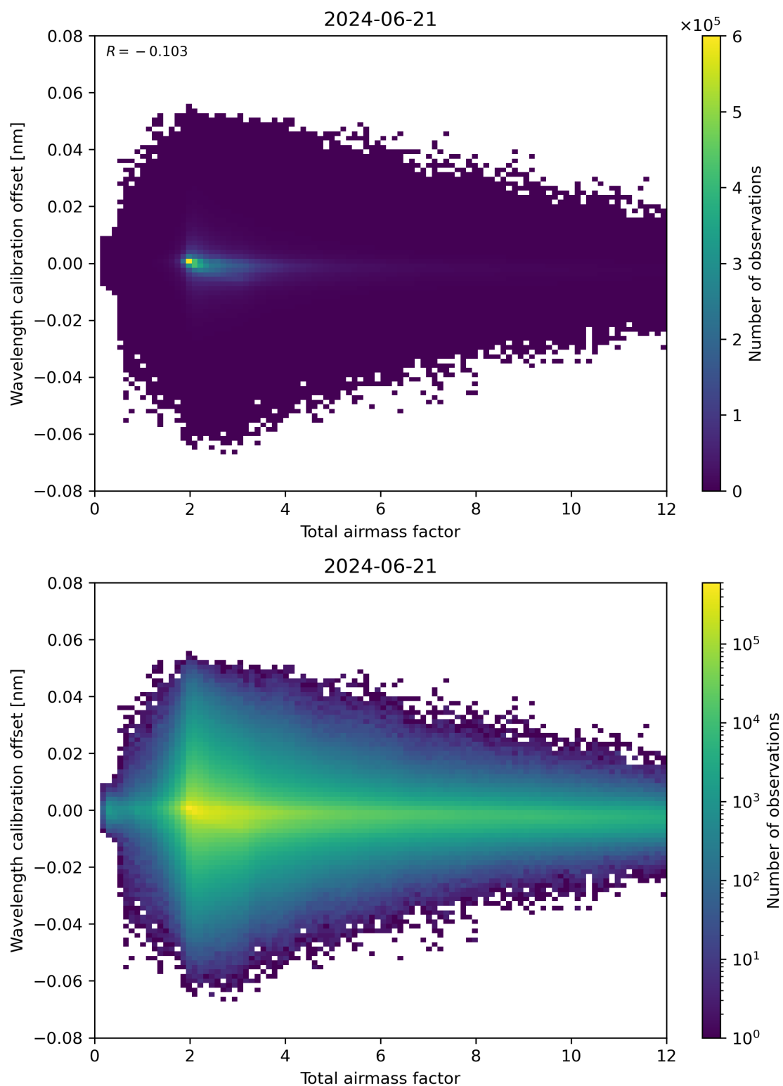
Figure 70: Scatter density plot of “Total airmass factor” against “Wavelength calibration offset” for 2024-06-20 to 2024-06-22.
