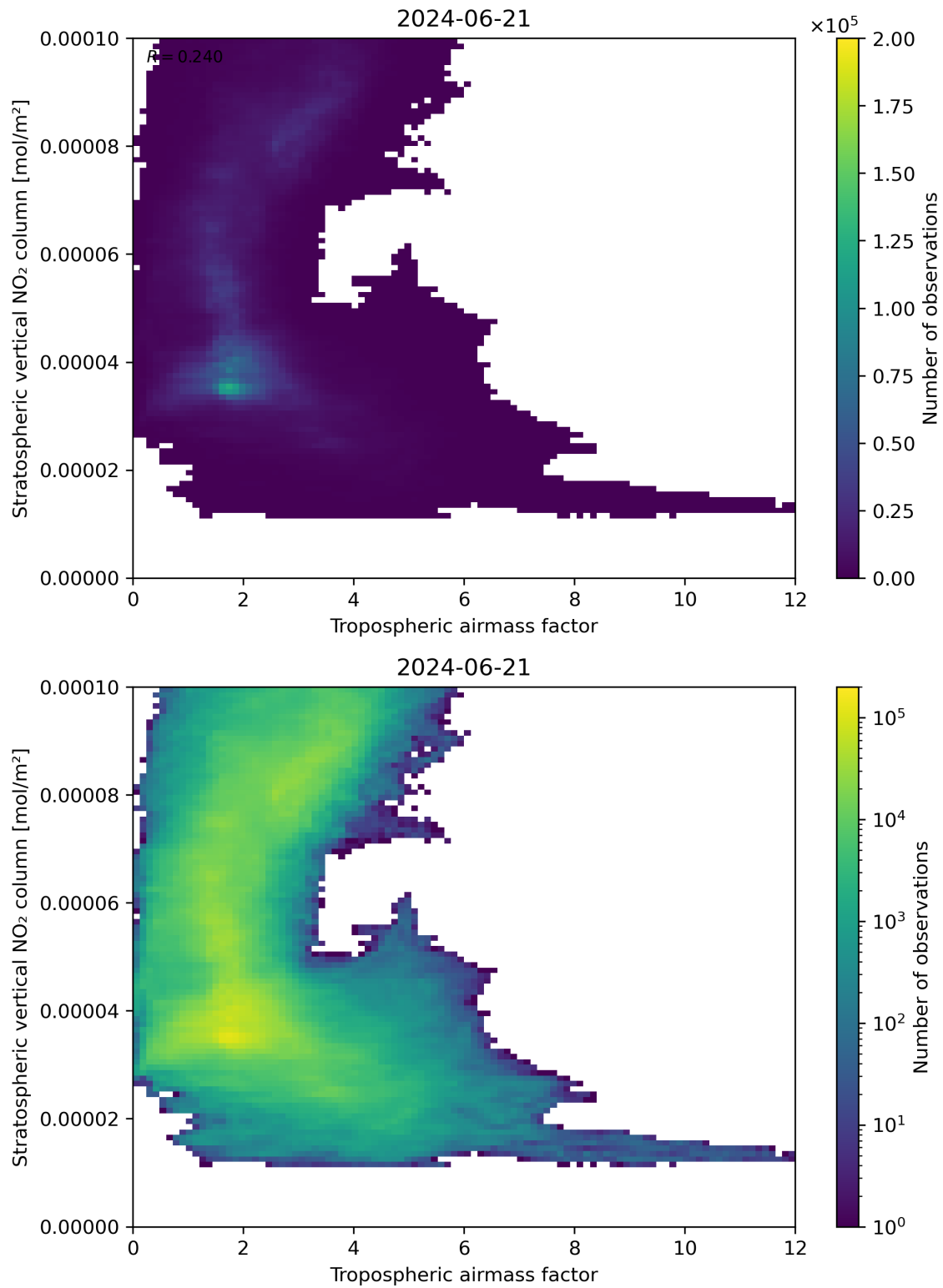
Figure 74: Scatter density plot of “Tropospheric air mass factor” against “Stratospheric vertical NO 2 column” for 2024-06-20 to 2024-06-22.
