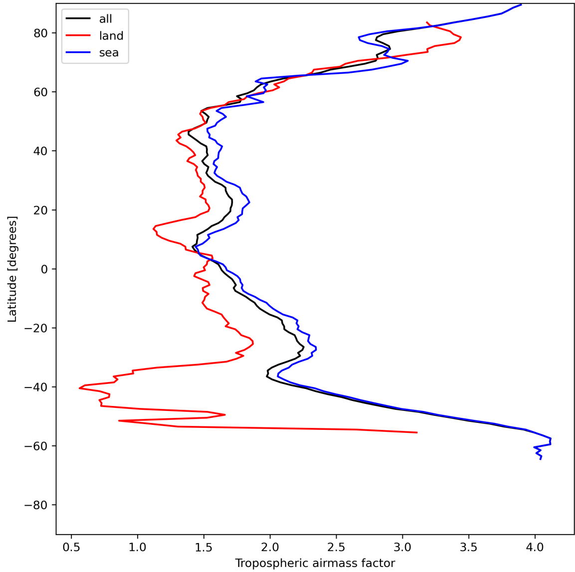
Figure 14: Zonal average of “Tropospheric airmass factor” for 2024-06-20 to 2024-06-22.
