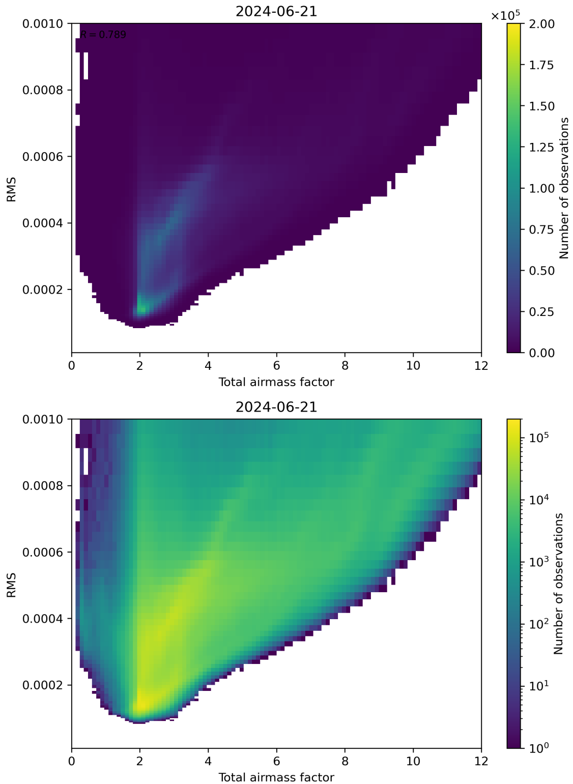
Figure 69: Scatter density plot of “Total airmass factor” against “RMS” for 2024-06-20 to 2024-06-22.
