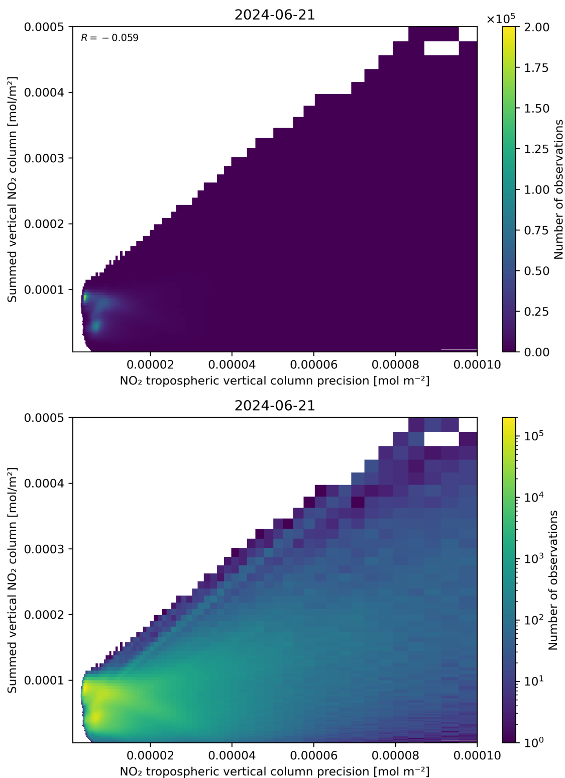
Figure 136: Scatter density plot of “NO 2 tropospheric vertical column precision” against “Summed vertical NO 2 column” for 2024-06-20 to 2024-06-22.
