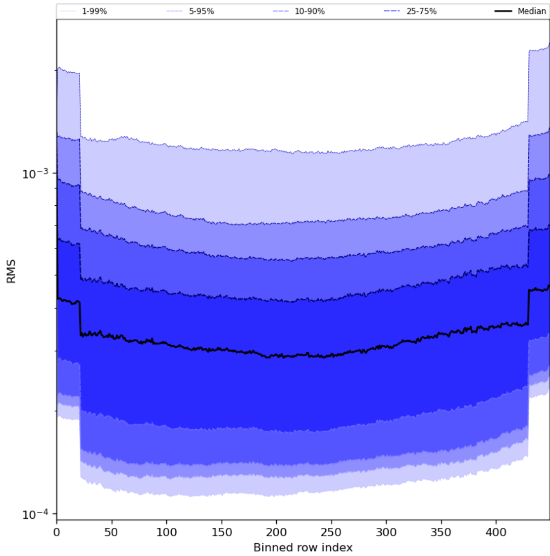
Figure 60: Along track statistics of “RMS” for 2024-06-20 to 2024-06-22
