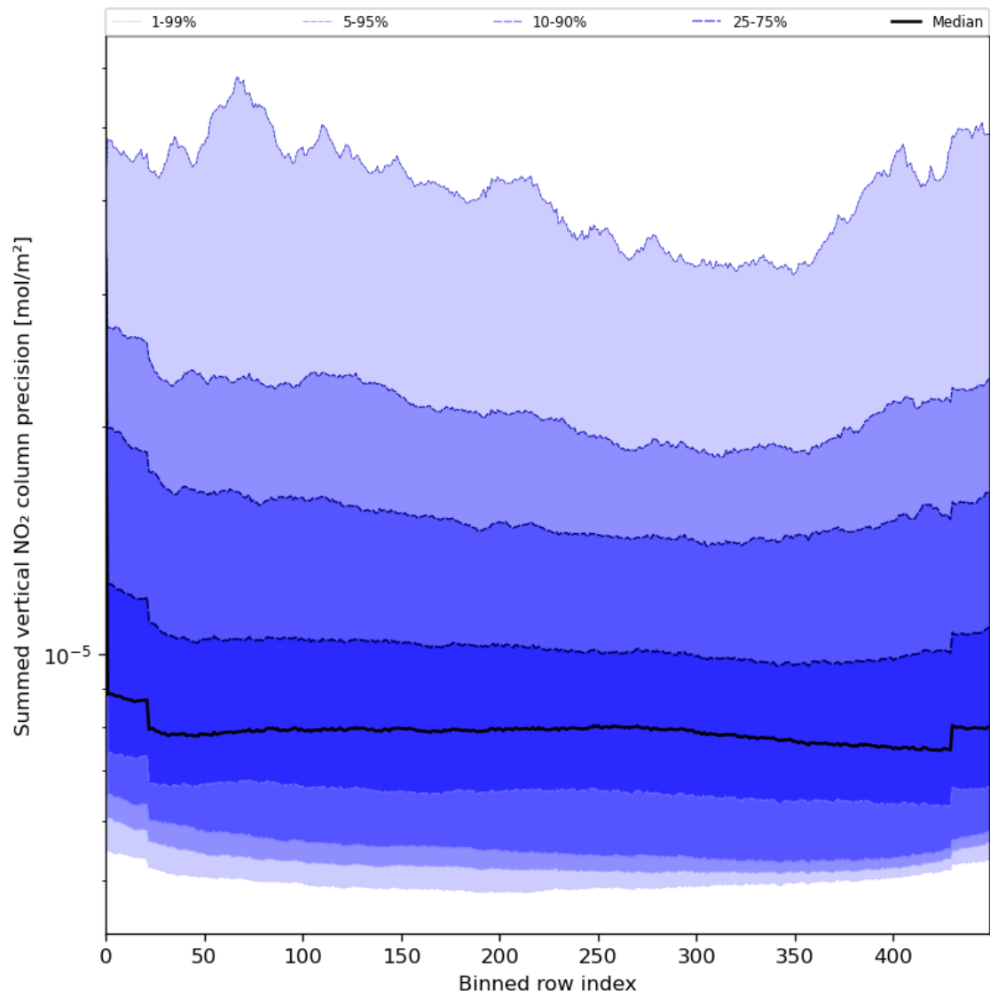
Figure 58: Along track statistics of “Summed vertical NO 2 column precision” for 2024-06-20 to 2024-06-22
