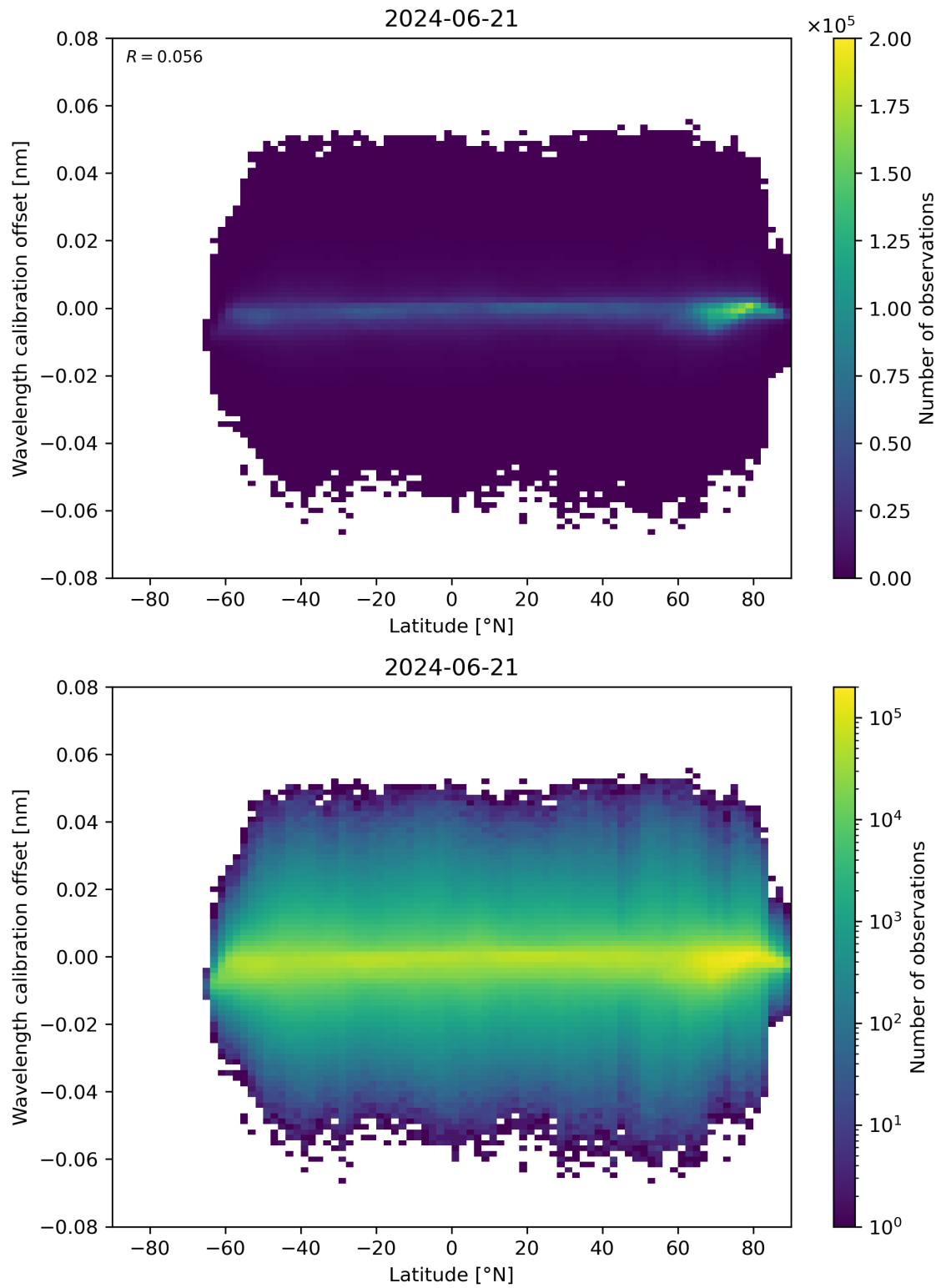
Figure 95: Scatter density plot of “Latitude” against “Wavelength calibration offset” for 2024-06-20 to 2024-06-22.
