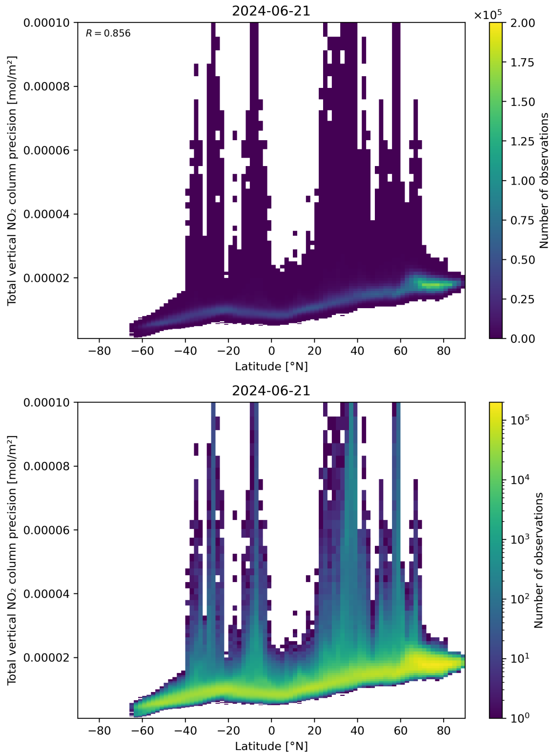
Figure 91: Scatter density plot of “Latitude” against “Total vertical NO 2 column precision” for 2024-06-20 to 2024-06-22.
