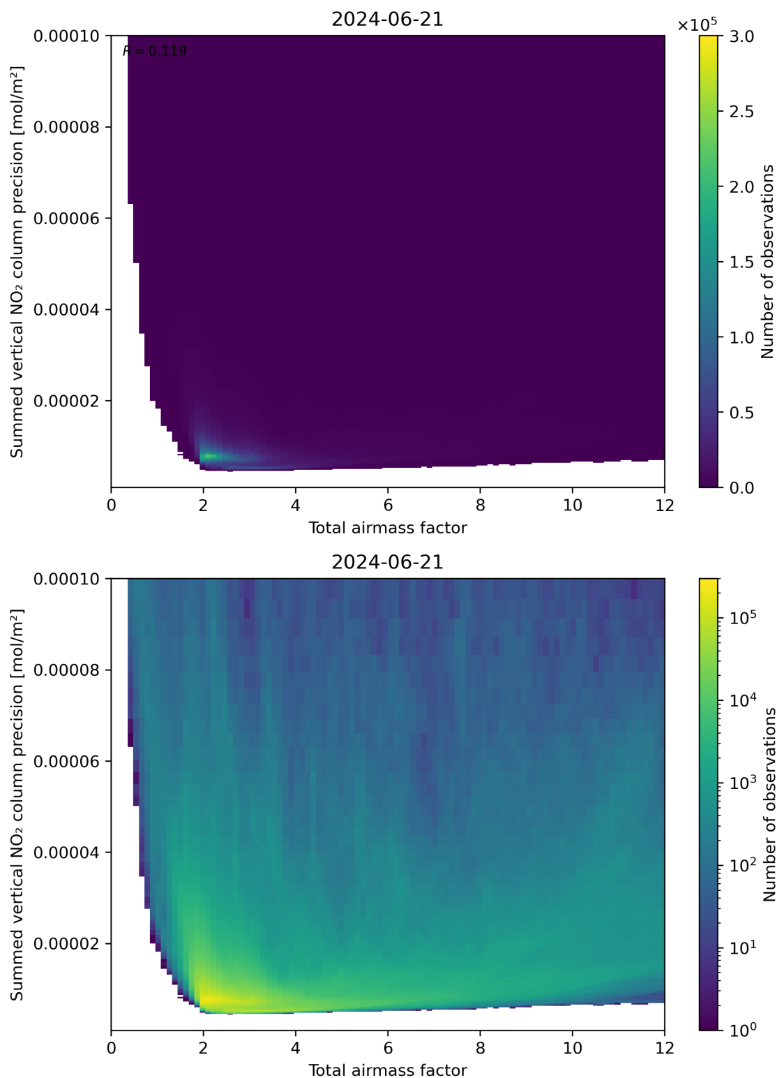
Figure 66: Scatter density plot of “Total airmass factor” against “Summed vertical NO 2 column precision” for 2024-06-20 to 2024-06-22.
