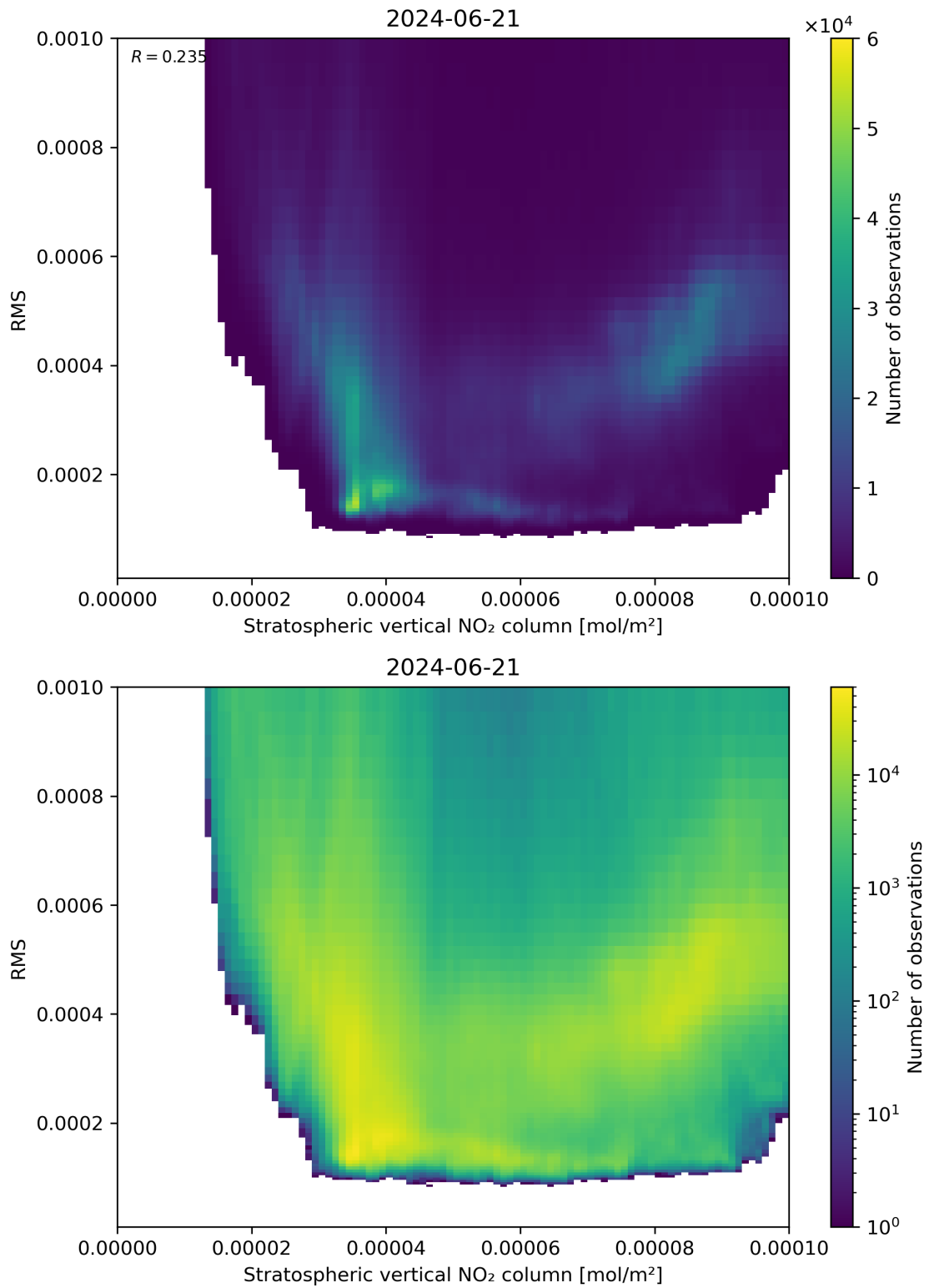
Figure 102: Scatter density plot of “Stratospheric vertical NO 2 column” against “RMS” for 2024-06-20 to 2024-06-22.
