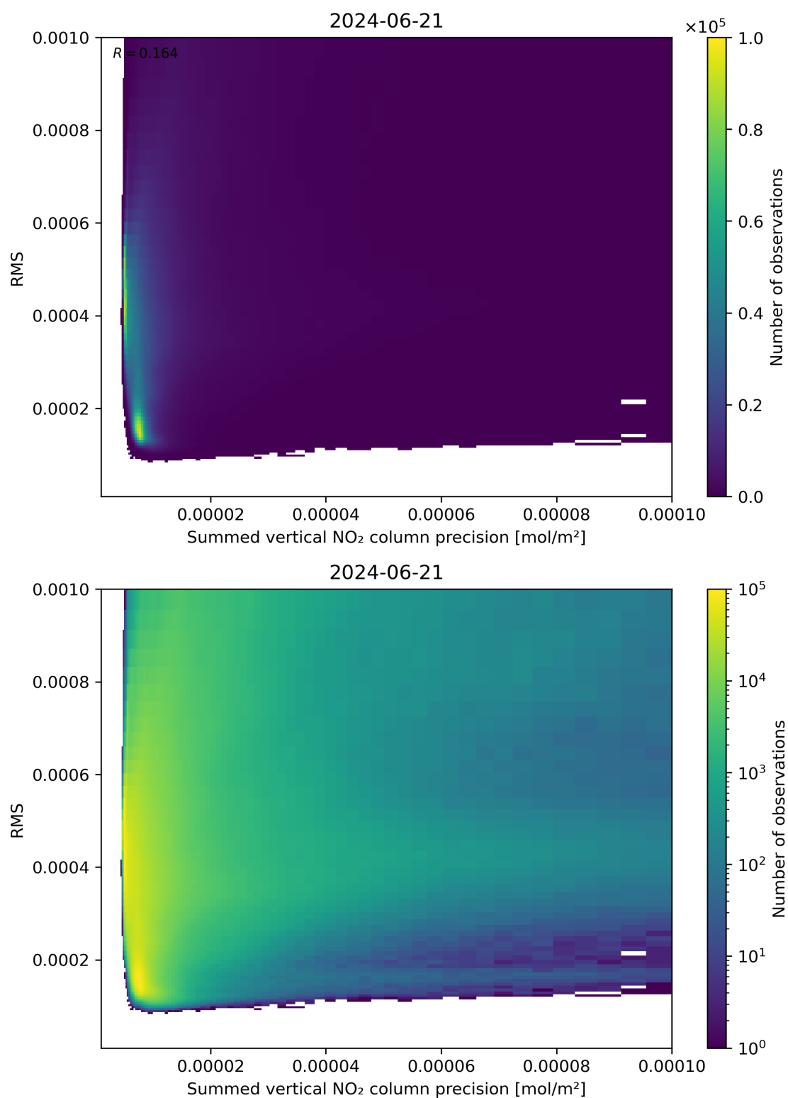
Figure 108: Scatter density plot of “Summed vertical NO 2 column precision” against “RMS” for 2024-06-20 to 2024-06-22.
