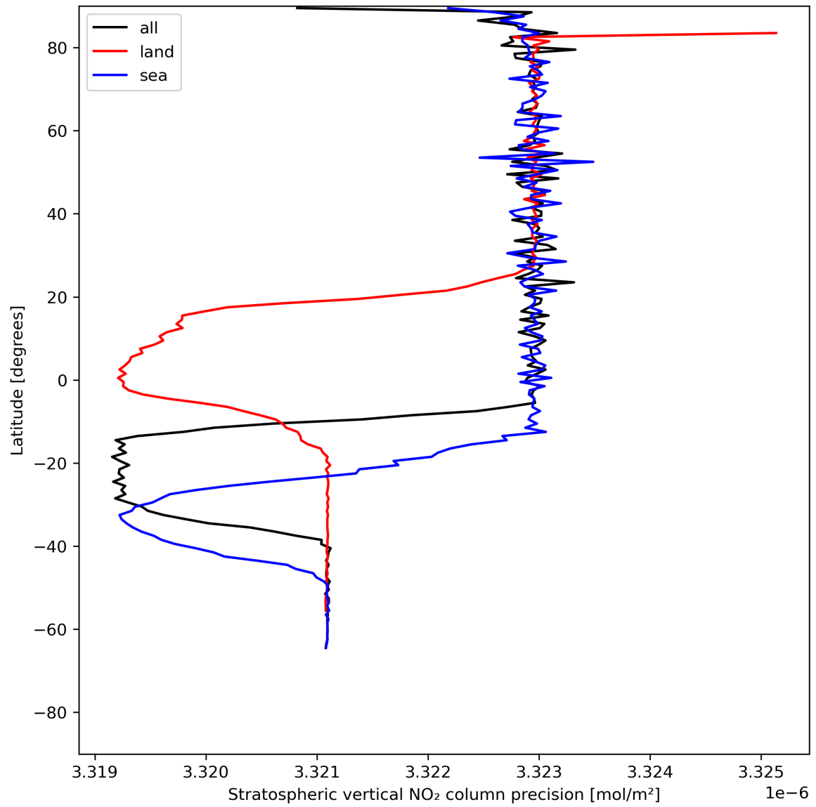
Figure 20: Zonal average of “Stratospheric vertical NO 2 column precision” for 2024-06-20 to 2024-06-22.
