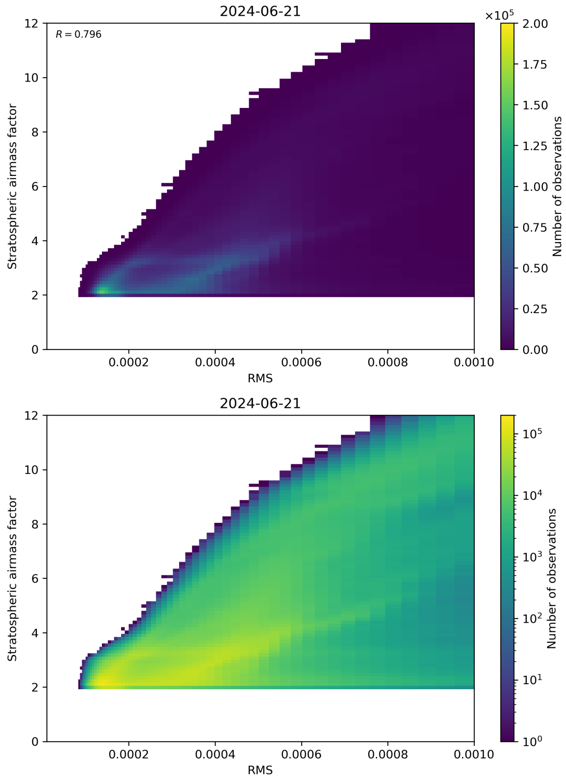
Figure 144: Scatter density plot of “RMS” against “Stratospheric airmass factor” for 2024-06-20 to 2024-06-22.
