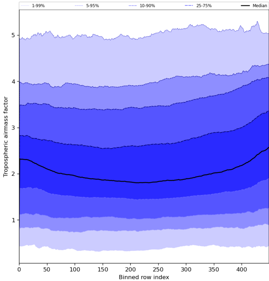
Figure 48: Along track statistics of “Tropospheric airmass factor” for 2024-06-20 to 2024-06-22
