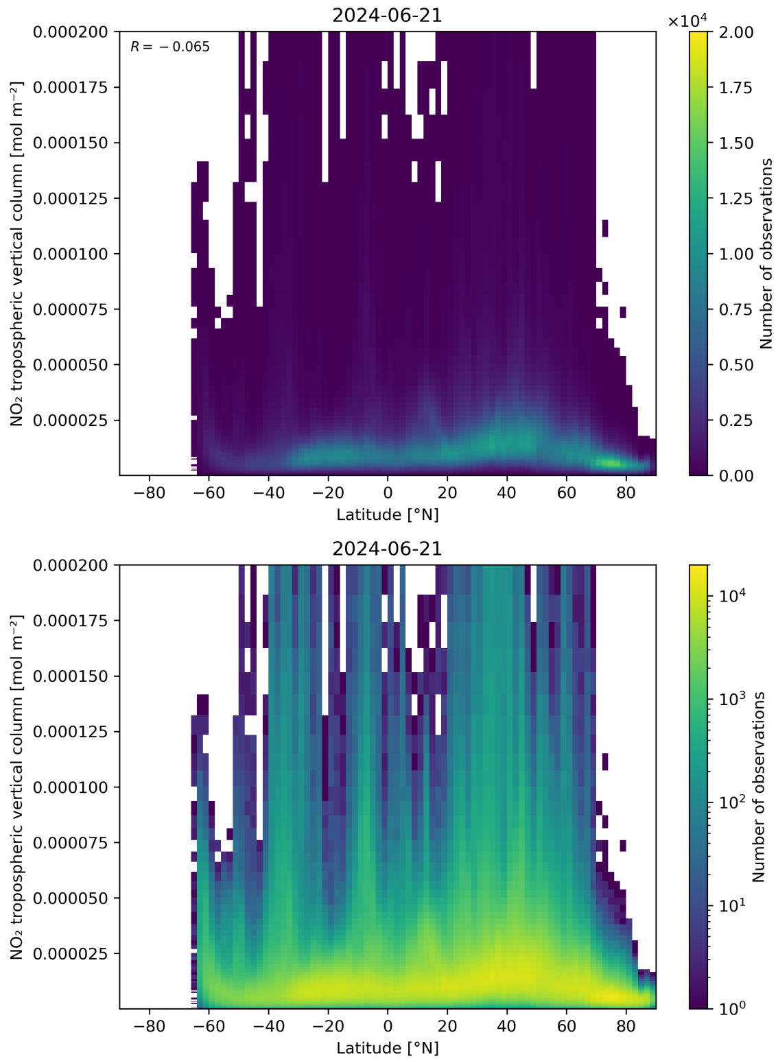
Figure 92: Scatter density plot of “Latitude” against “NO 2 tropospheric vertical column” for 2024-06-20 to 2024-06-22.
