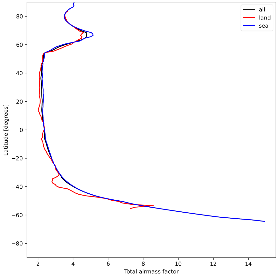
Figure 15: Zonal average of “Total airmass factor” for 2024-06-20 to 2024-06-22.
