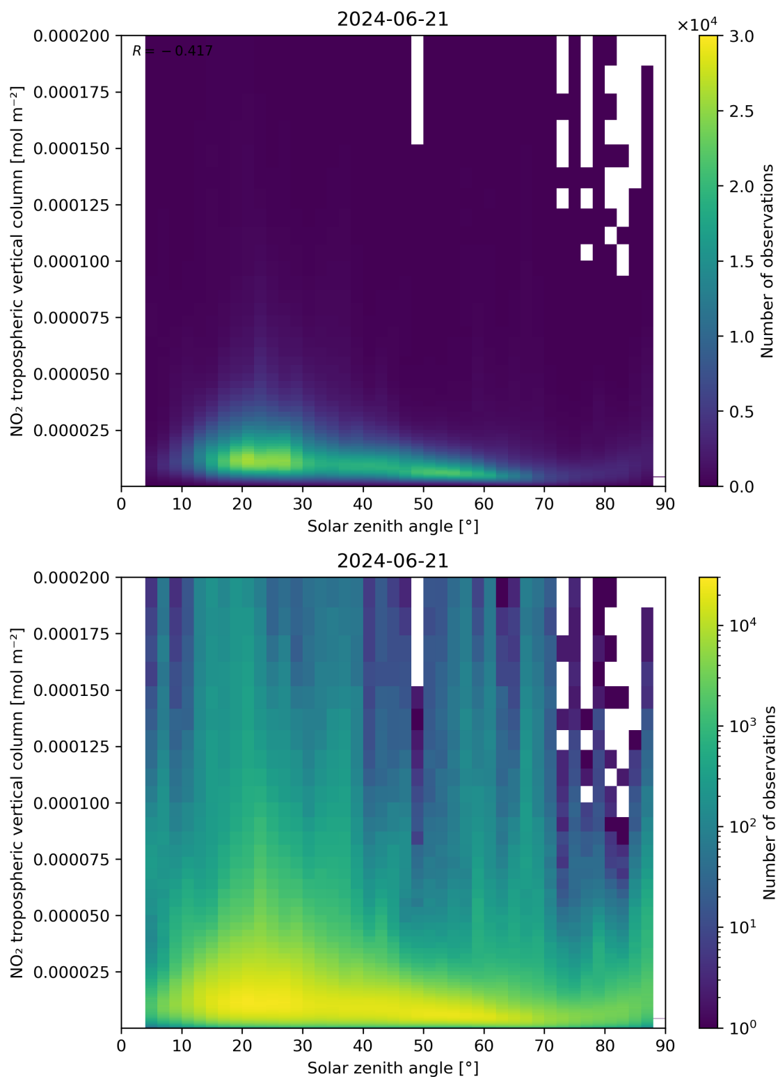
Figure 155: Scatter density plot of “Solar zenith angle” against “NO 2 tropospheric vertical column” for 2024-06-20 to 2024-06-22.
