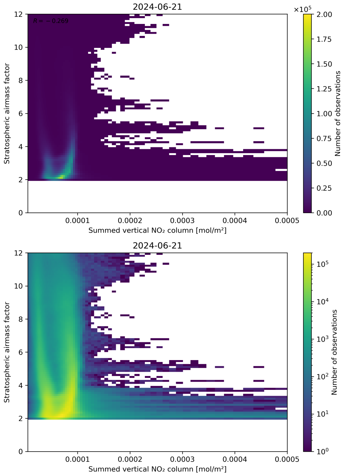
Figure 103: Scatter density plot of “Summed vertical NO 2 column” against “Stratospheric air mass factor” for 2024-06-20 to 2024-06-22.
