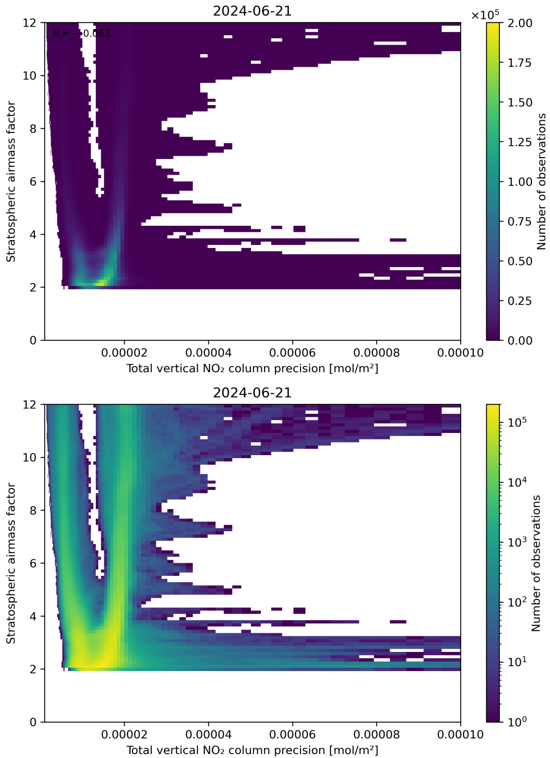
Figure 115: Scatter density plot of “Total vertical NO 2 column precision” against “Stratospheric air mass factor” for 2024-06-20 to 2024-06-22.
