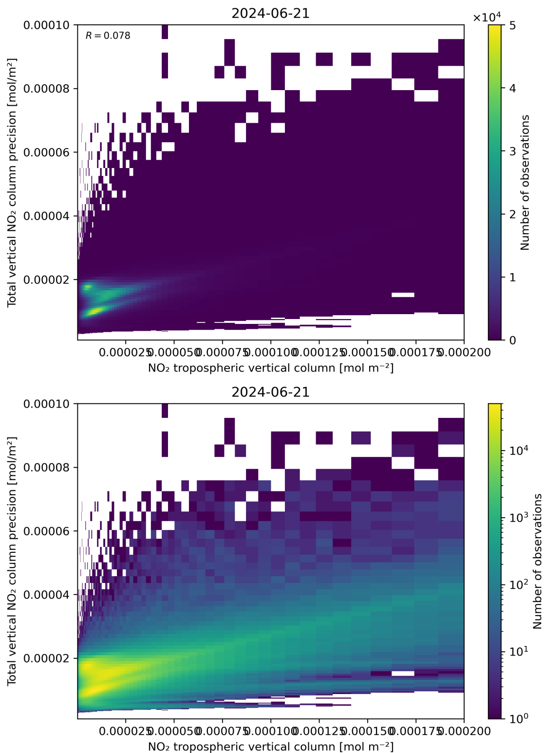
Figure 129: Scatter density plot of “NO 2 tropospheric vertical column” against “Total vertical NO 2 column precision” for 2024-06-20 to 2024-06-22.
