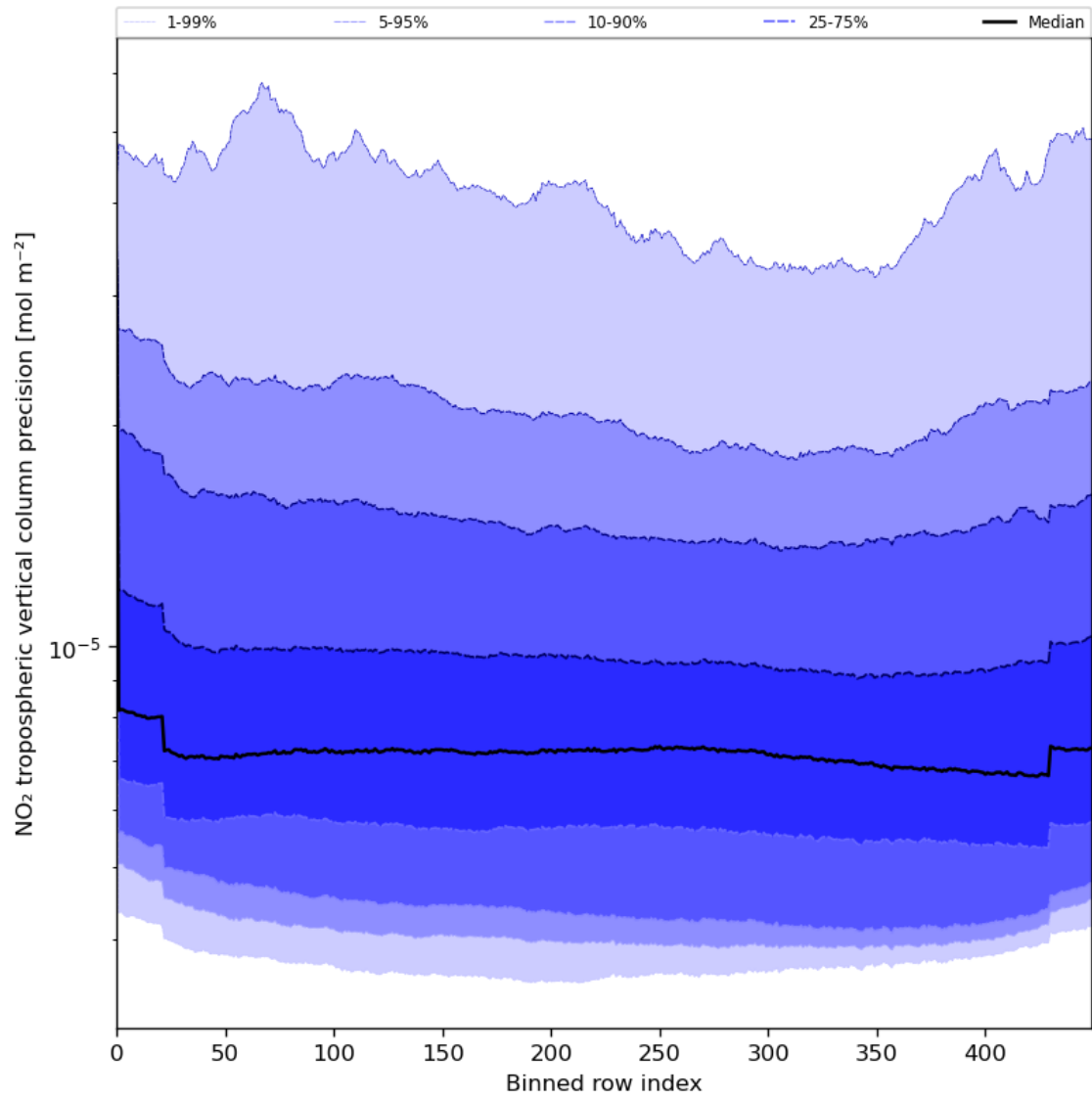
Figure 47: Along track statistics of “NO 2 tropospheric vertical column precision” for 2024-06-20 to 2024-06-22
