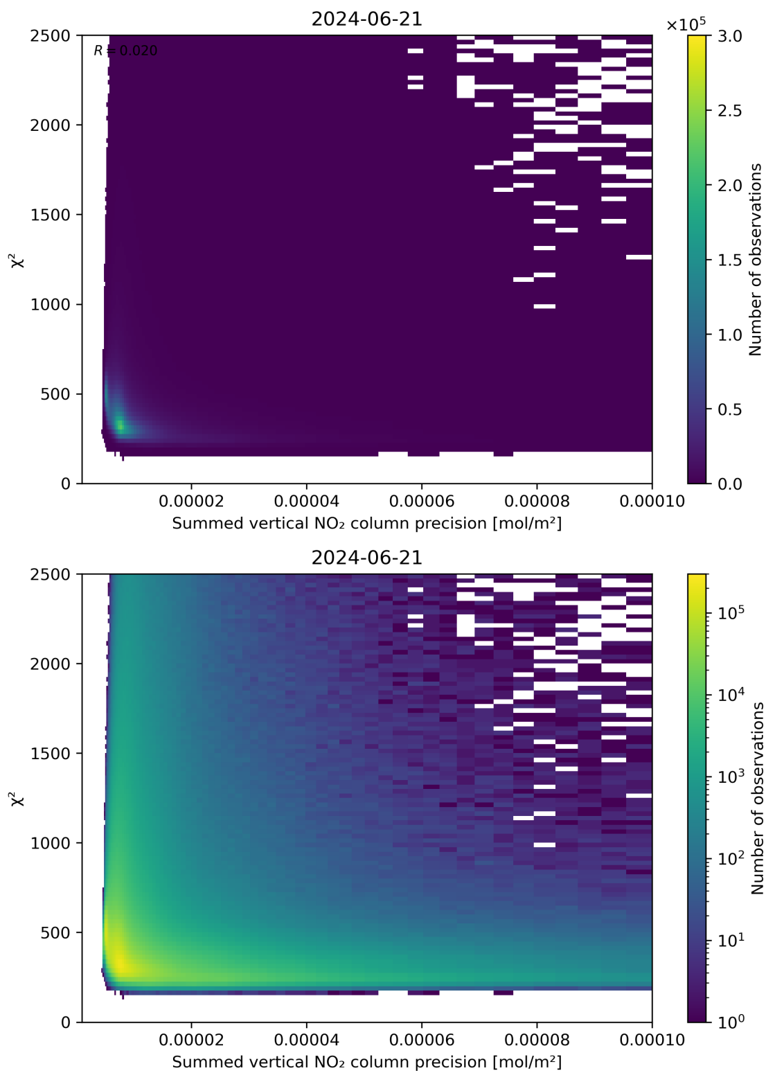
Figure 107: Scatter density plot of “Summed vertical NO 2 column precision” against “ \chi^2 ” for 2024-06-20 to 2024-06-22.
