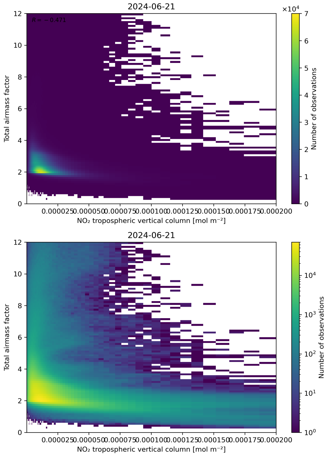
Figure 122: Scatter density plot of “NO 2 tropospheric vertical column” against “Total air mass factor” for 2024-06-20 to 2024-06-22.
