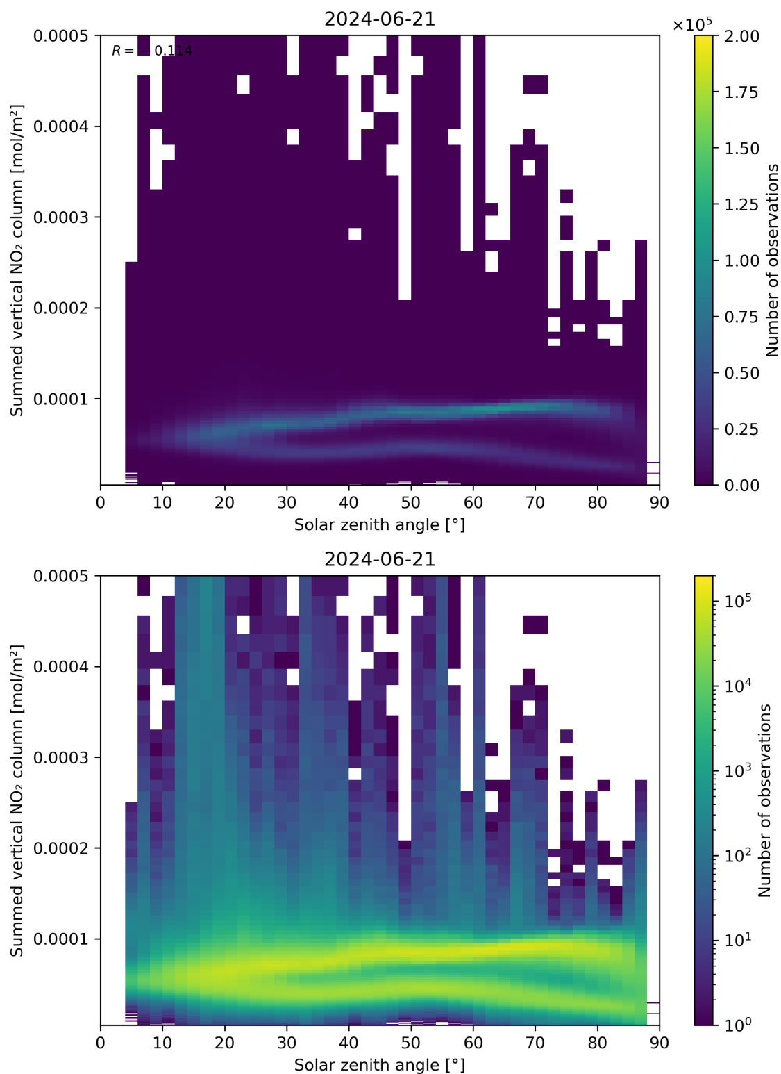
Figure 151: Scatter density plot of “Solar zenith angle” against “Summed vertical NO 2 column” for 2024-06-20 to 2024-06-22.
