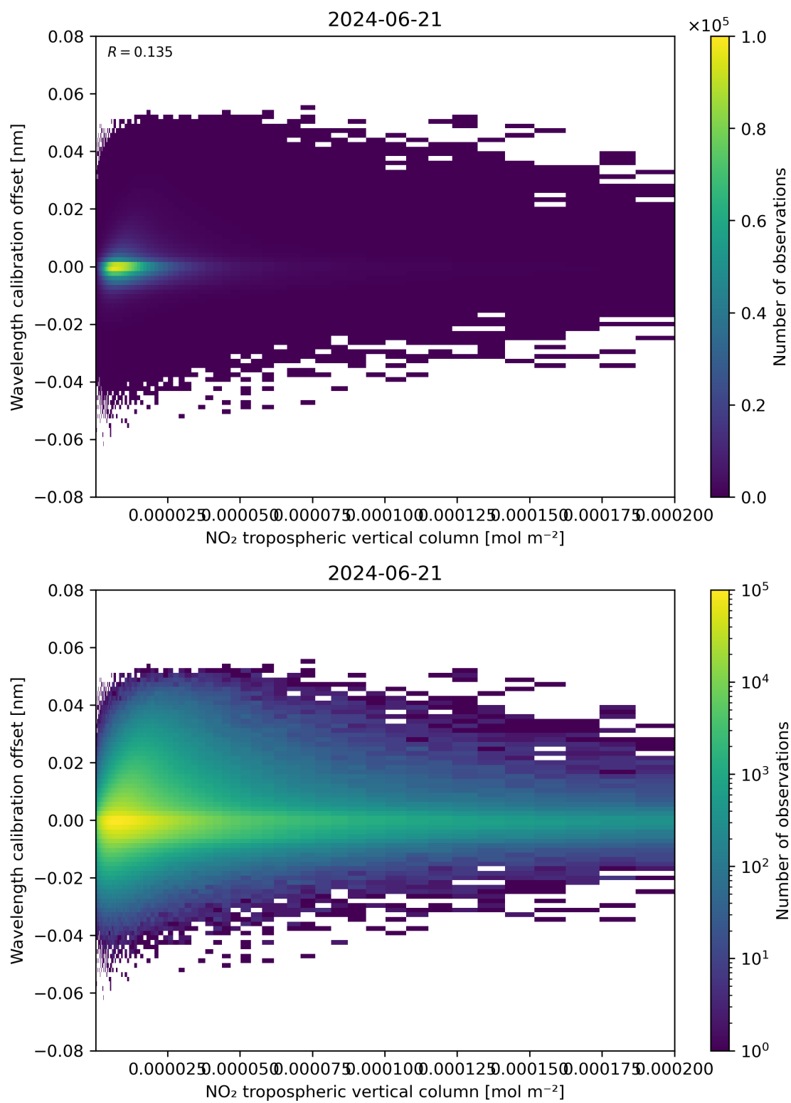
Figure 143: Scatter density plot of “NO 2 tropospheric vertical column” against “Wavelength calibration offset” for 2024-06-20 to 2024-06-22.
