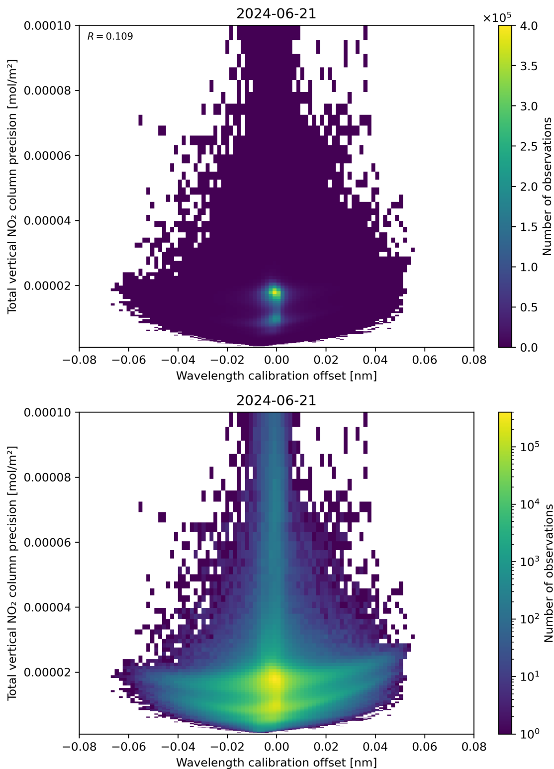
Figure 180: Scatter density plot of “Wavelength calibration offset” against “Total vertical NO 2 column precision” for 2024-06-20 to 2024-06-22.
