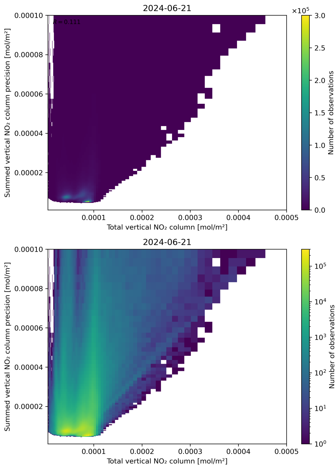
Figure 113: Scatter density plot of “Total vertical NO 2 column” against “Summed vertical NO 2 column precision” for 2024-06-20 to 2024-06-22.
