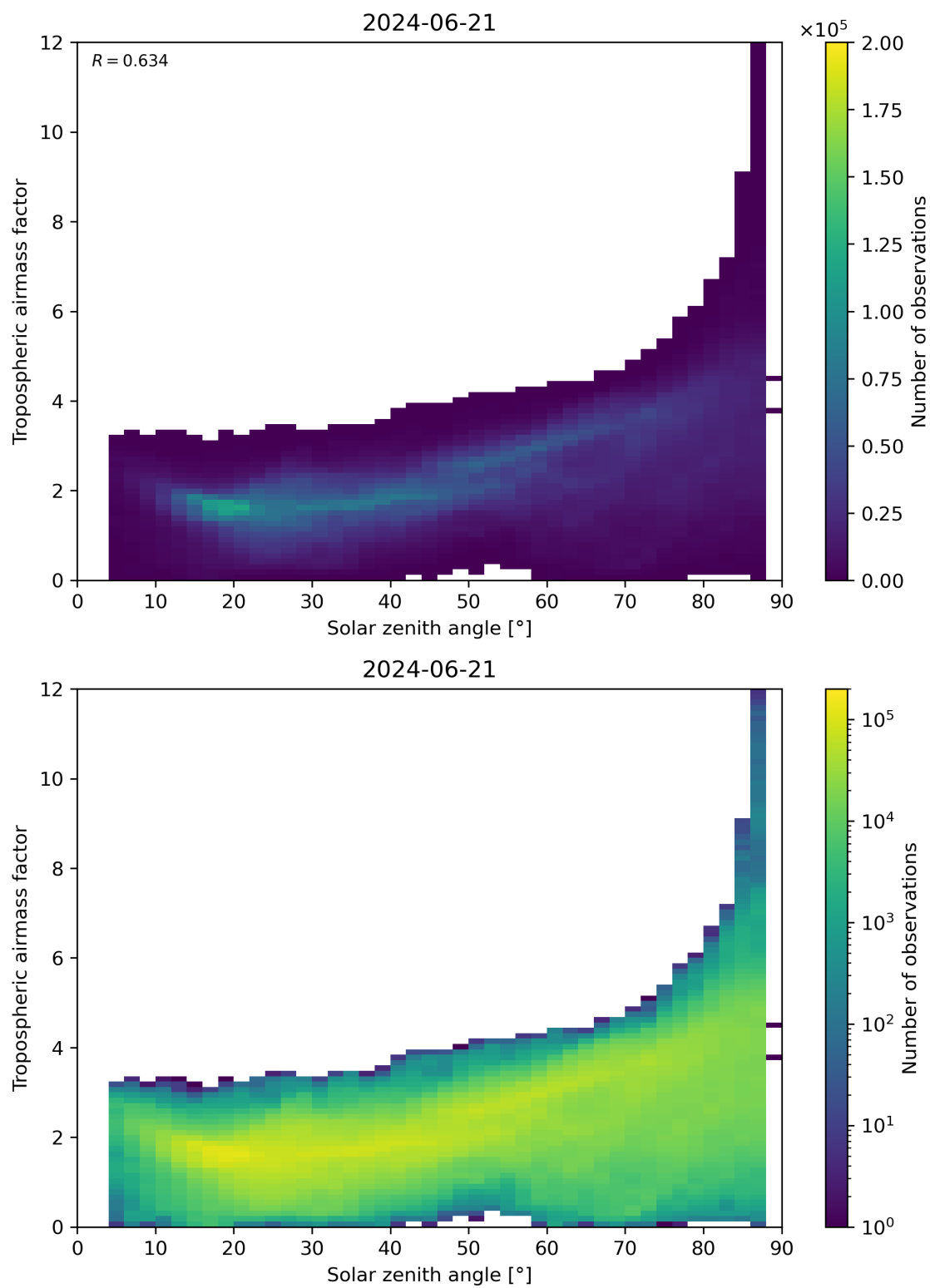
Figure 147: Scatter density plot of “Solar zenith angle” against “Tropospheric airmass factor” for 2024-06-20 to 2024-06-22.
