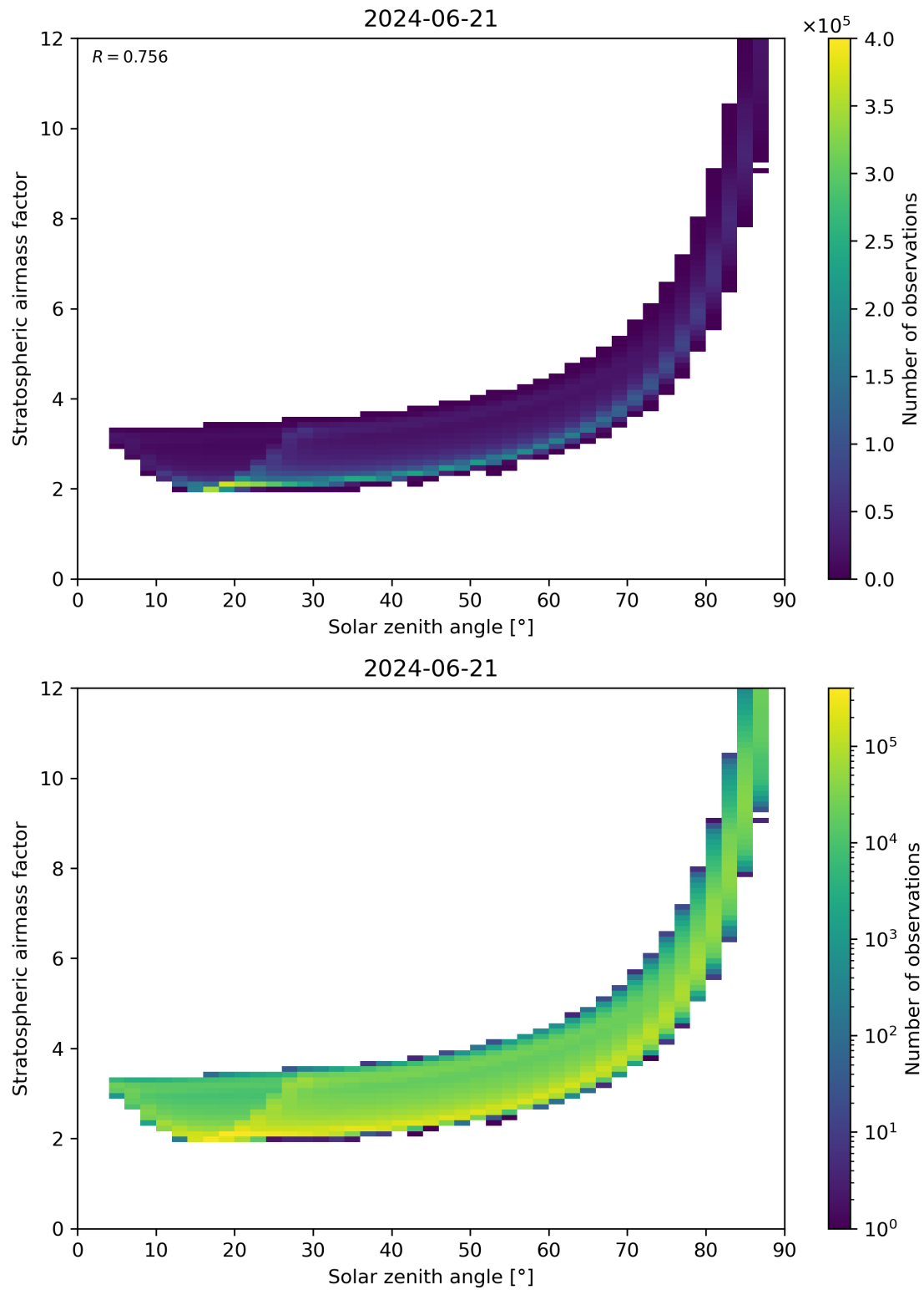
Figure 145: Scatter density plot of “Solar zenith angle” against “Stratospheric airmass factor” for 2024-06-20 to 2024-06-22.
