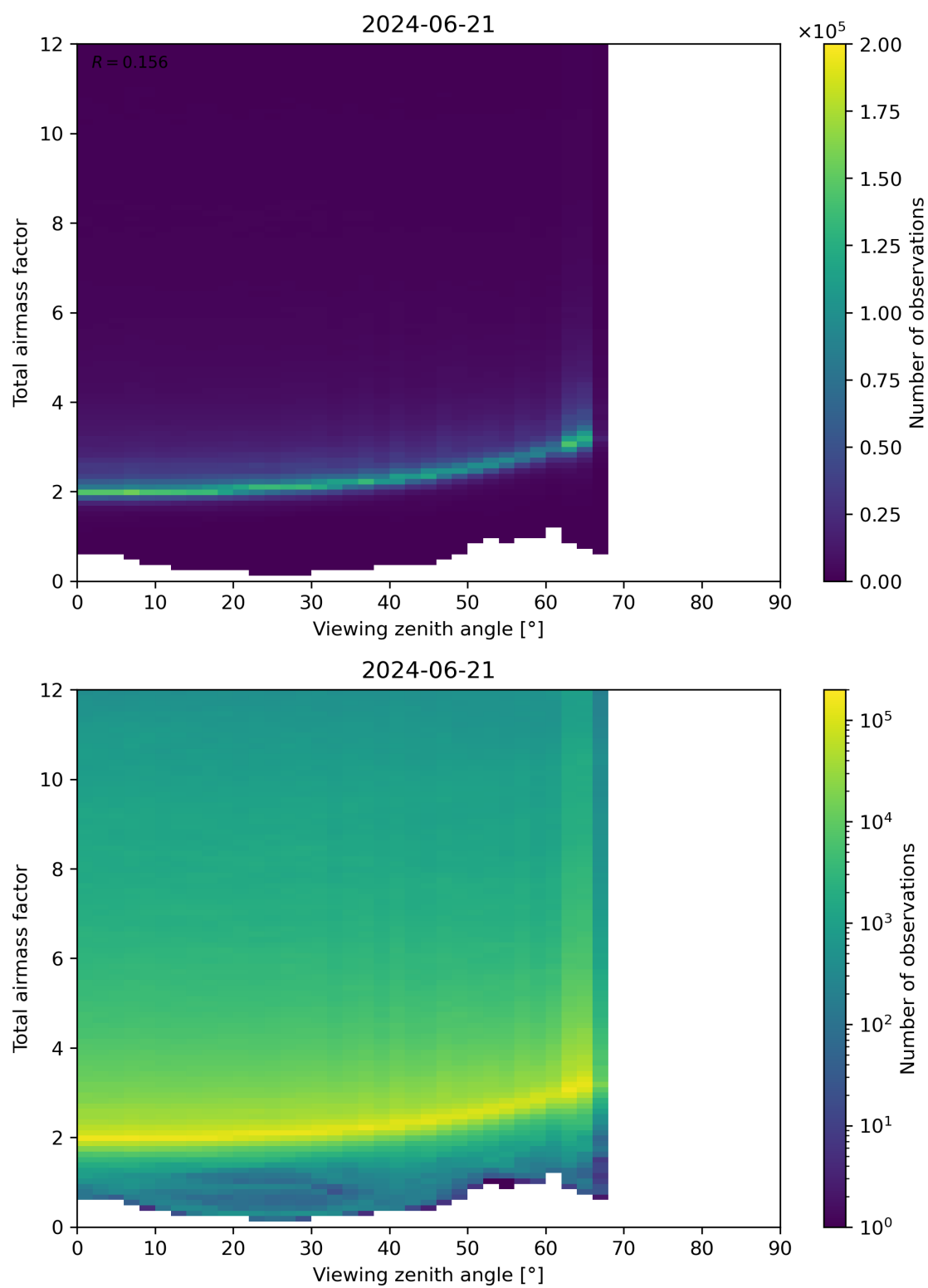
Figure 160: Scatter density plot of “Viewing zenith angle” against “Total airmass factor” for 2024-06-20 to 2024-06-22.
