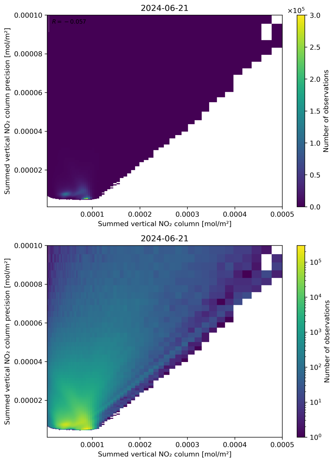
Figure 105: Scatter density plot of “Summed vertical NO 2 column” against “Summed vertical NO 2 column precision” for 2024-06-20 to 2024-06-22.
