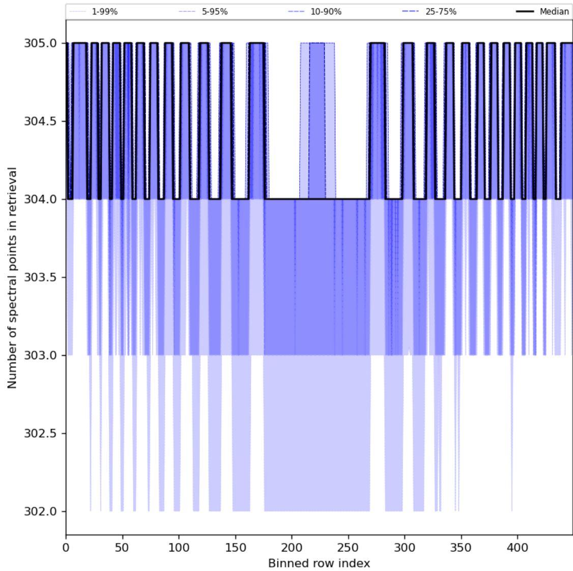
Figure 50: Along track statistics of “Number of spectral points in retrieval” for 2024-06-20 to 2024-06-22
