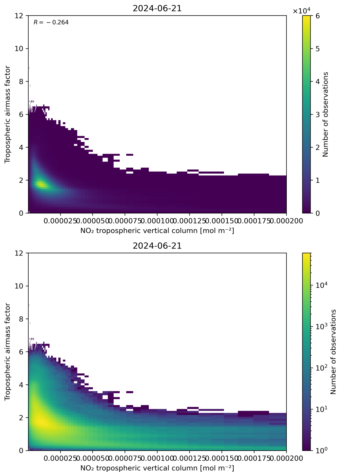
Figure 123: Scatter density plot of “NO 2 tropospheric vertical column” against “Tropospheric air mass factor” for 2024-06-20 to 2024-06-22.
