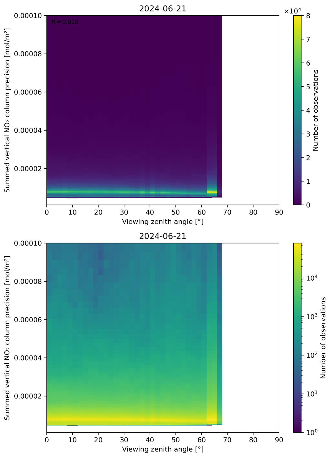
Figure 166: Scatter density plot of “Viewing zenith angle” against “Summed vertical NO 2 column precision” for 2024-06-20 to 2024-06-22.
