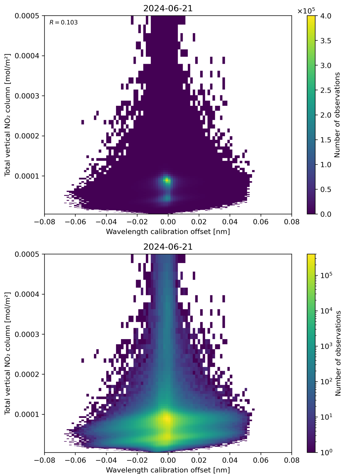
Figure 179: Scatter density plot of “Wavelength calibration offset” against “Total vertical NO 2 column” for 2024-06-20 to 2024-06-22.
