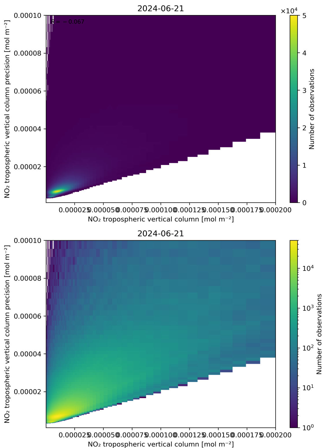
Figure 130: Scatter density plot of “NO 2 tropospheric vertical column” against “NO 2 tropospheric vertical column precision” for 2024-06-20 to 2024-06-22.
