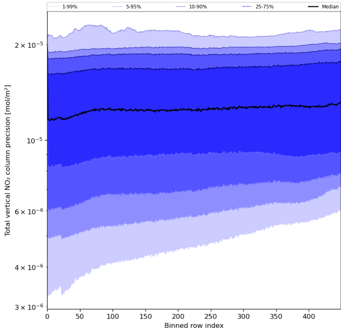
Figure 56: Along track statistics of “Total vertical NO 2 column precision” for 2024-06-20 to 2024-06-22
