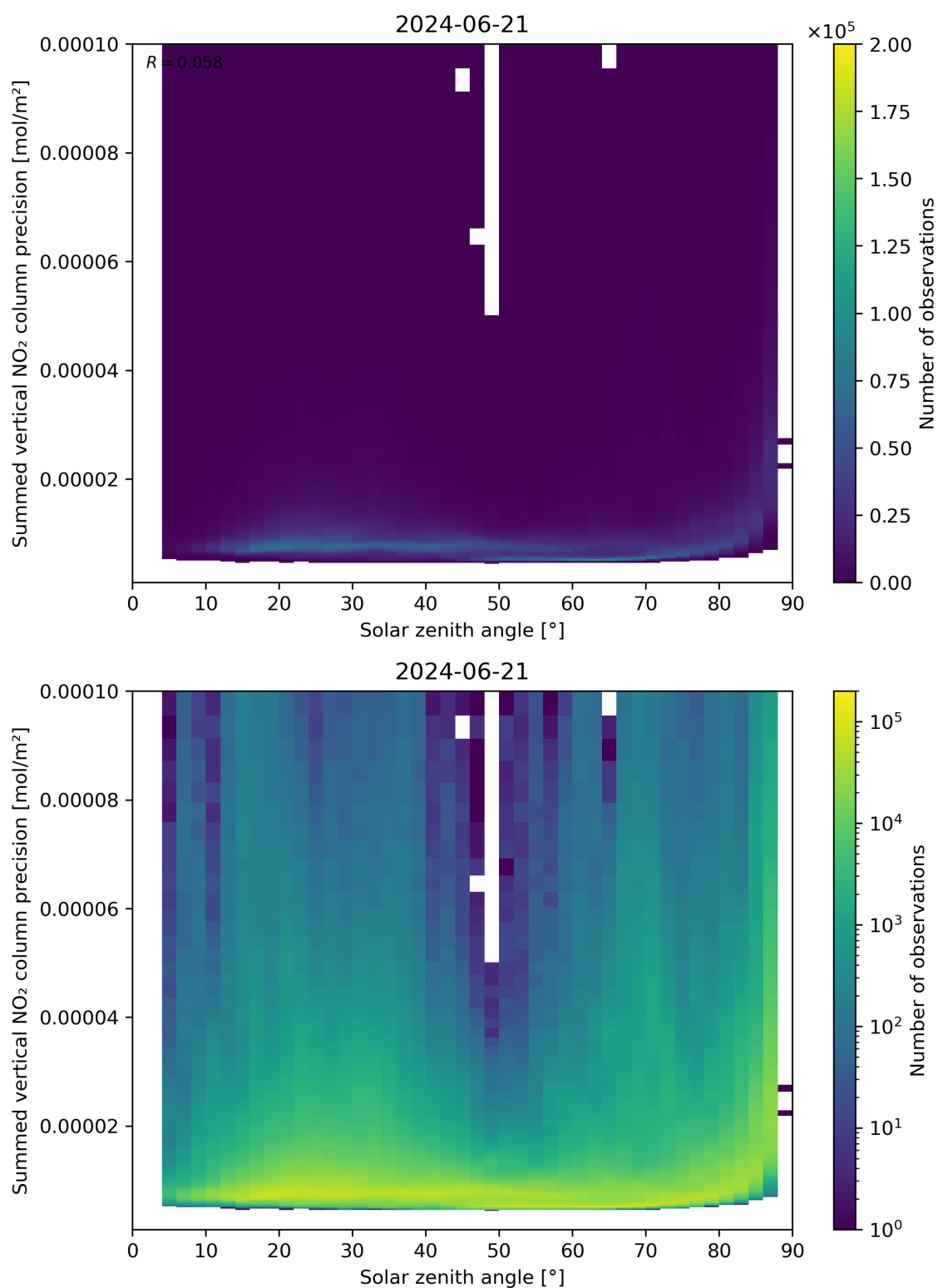
Figure 152: Scatter density plot of “Solar zenith angle” against “Summed vertical NO 2 column precision” for 2024-06-20 to 2024-06-22.
