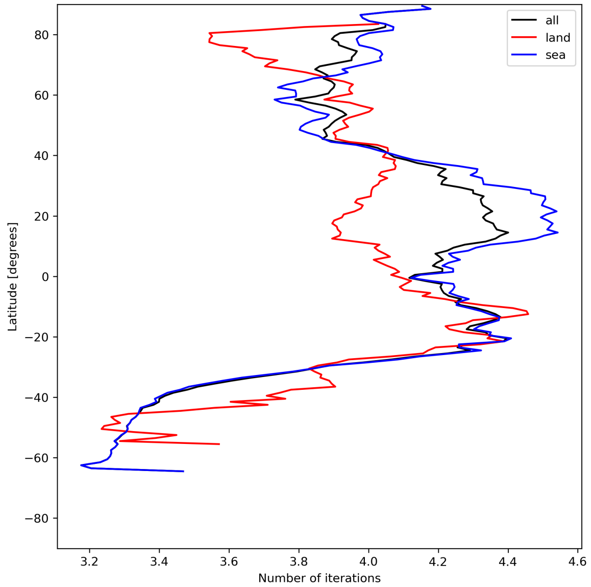
Figure 17: Zonal average of “Number of iterations” for 2024-06-20 to 2024-06-22.
