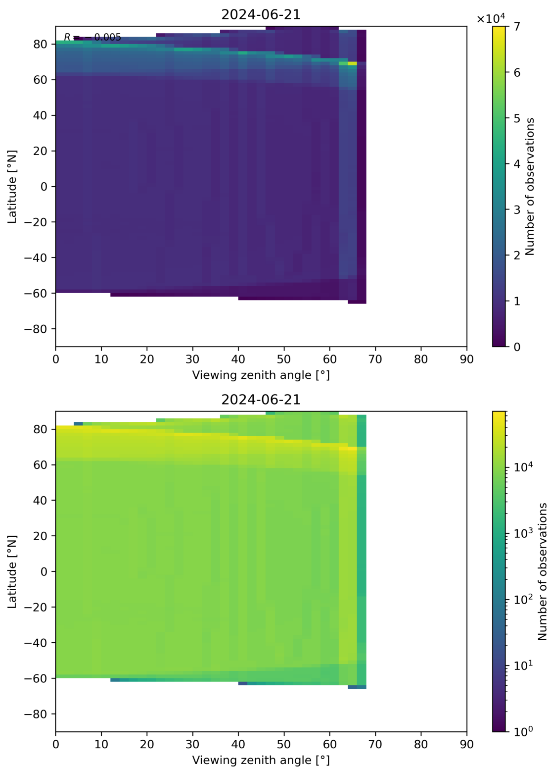
Figure 163: Scatter density plot of “Viewing zenith angle” against “Latitude” for 2024-06-20 to 2024-06-22.
