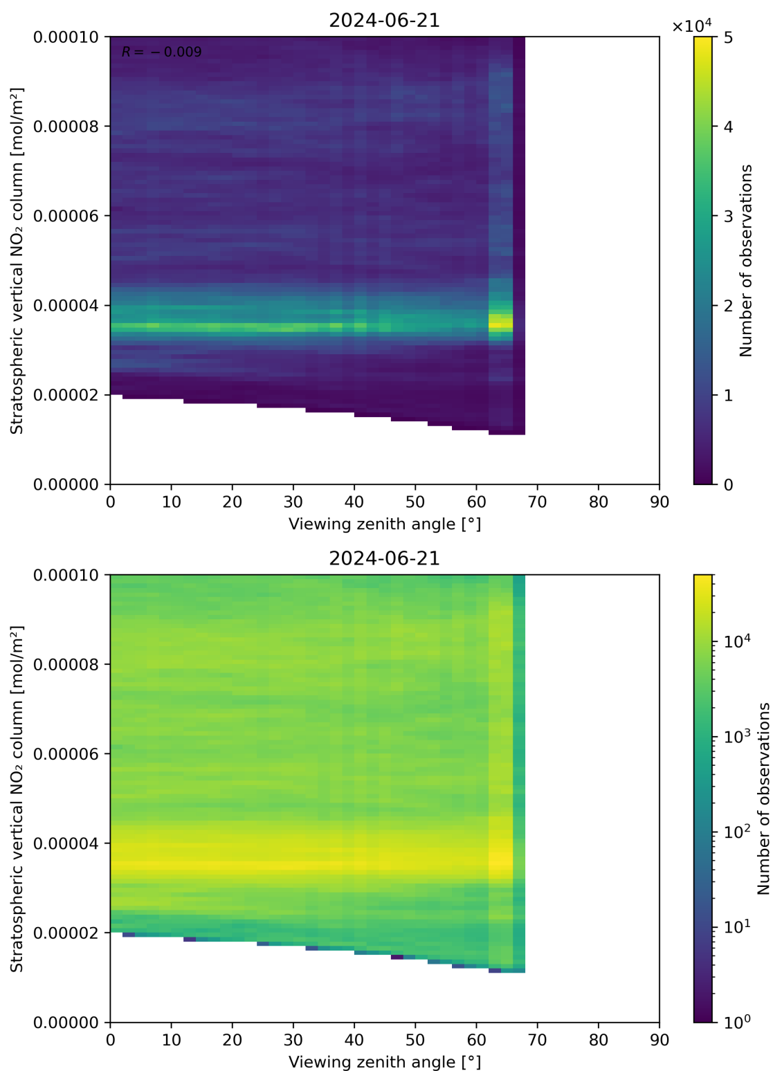
Figure 164: Scatter density plot of “Viewing zenith angle” against “Stratospheric vertical NO 2 column” for 2024-06-20 to 2024-06-22.
