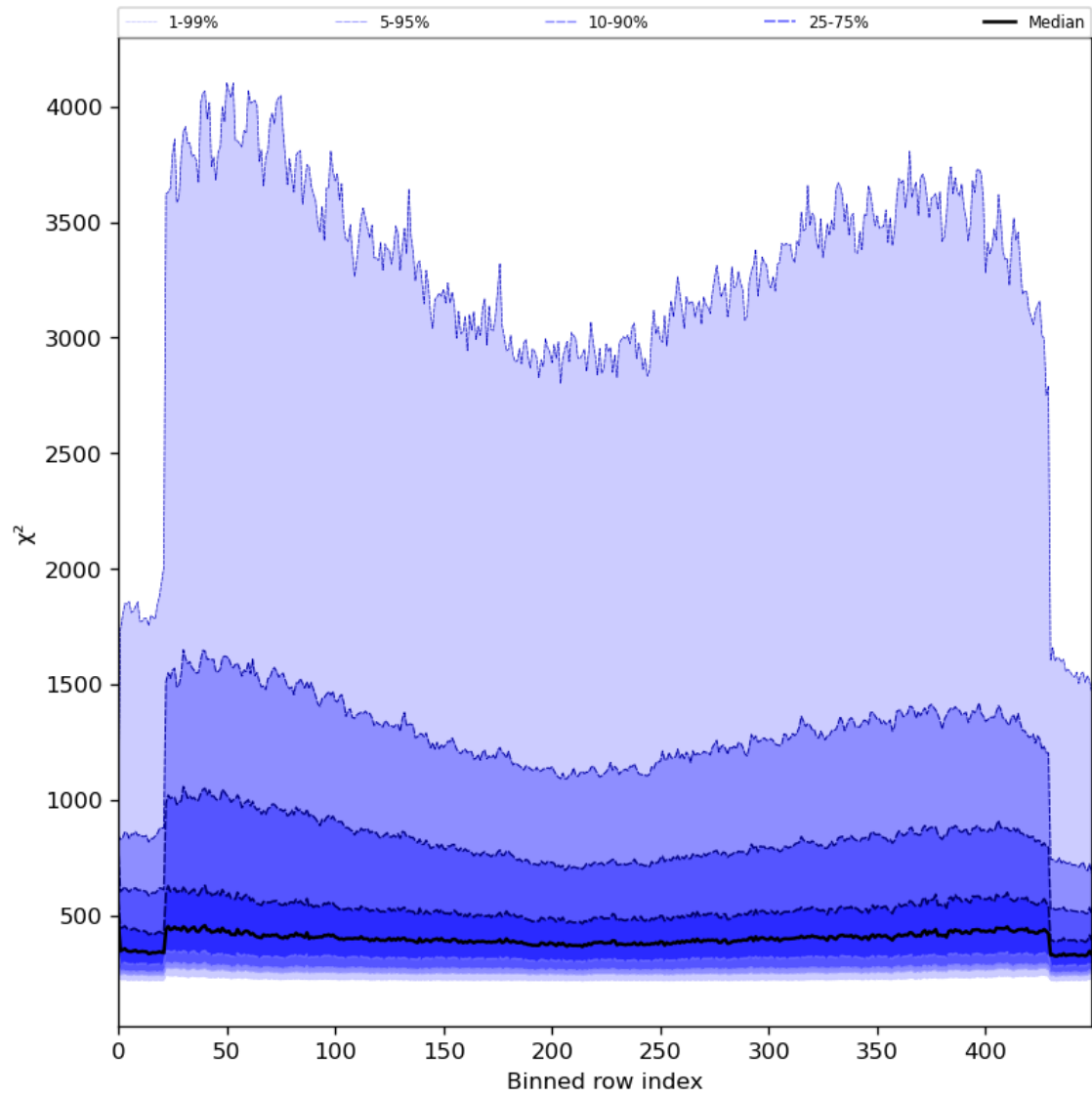
Figure 59: Along track statistics of “ \chi^2 ” for 2024-06-20 to 2024-06-22
