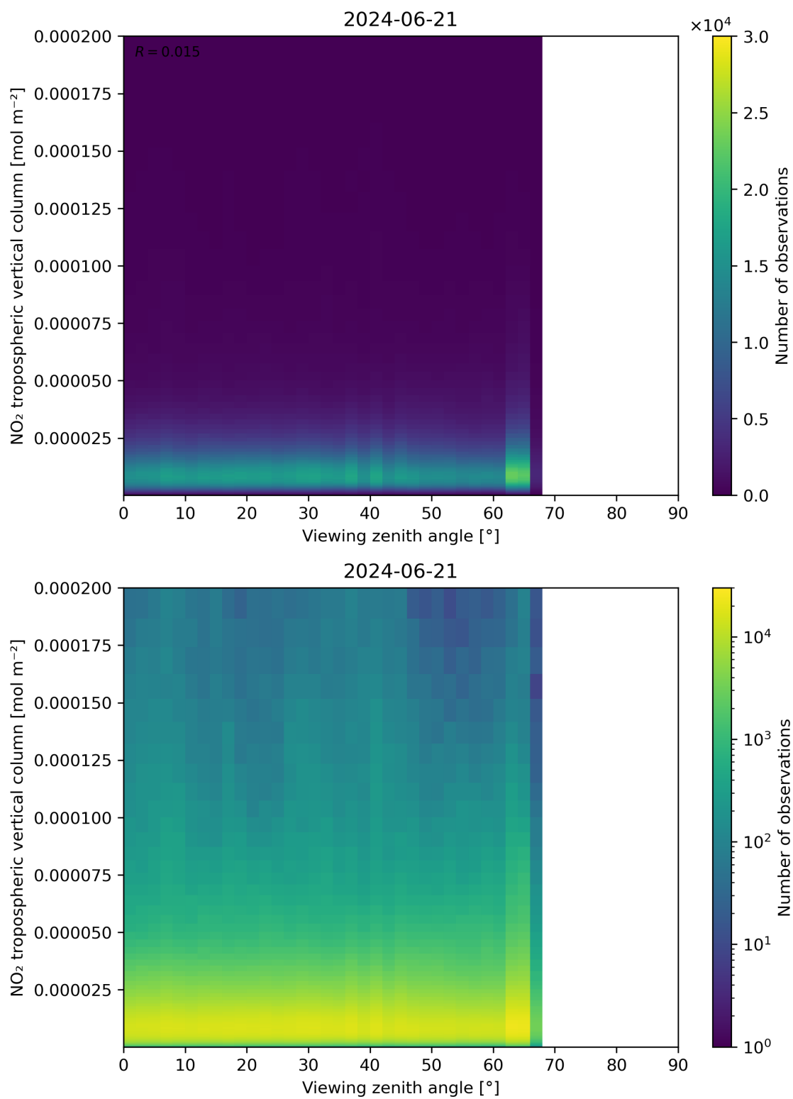
Figure 169: Scatter density plot of “Viewing zenith angle” against “NO 2 tropospheric vertical column” for 2024-06-20 to 2024-06-22.
