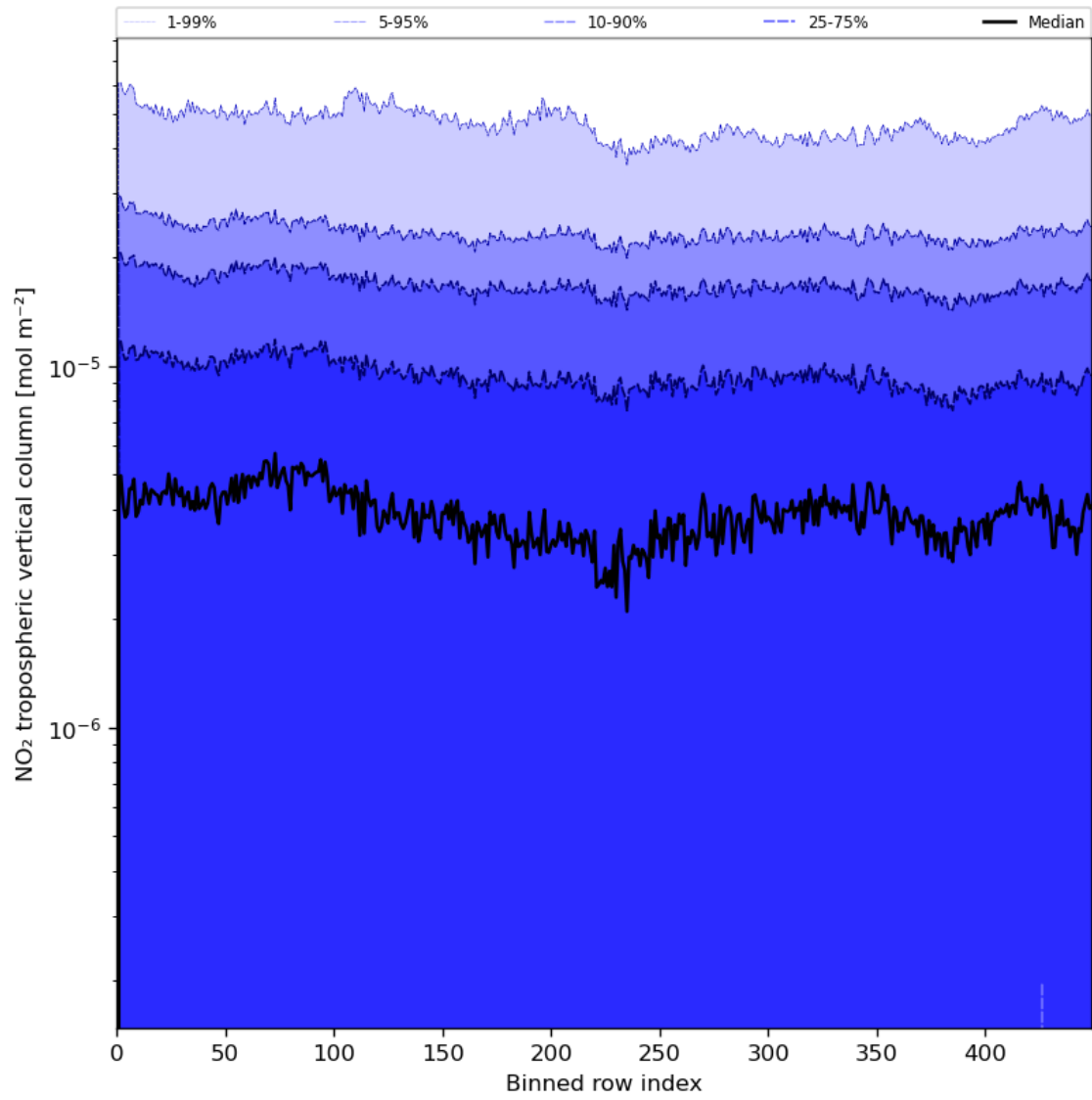
Figure 46: Along track statistics of “NO 2 tropospheric vertical column” for 2024-06-20 to 2024-06-22
