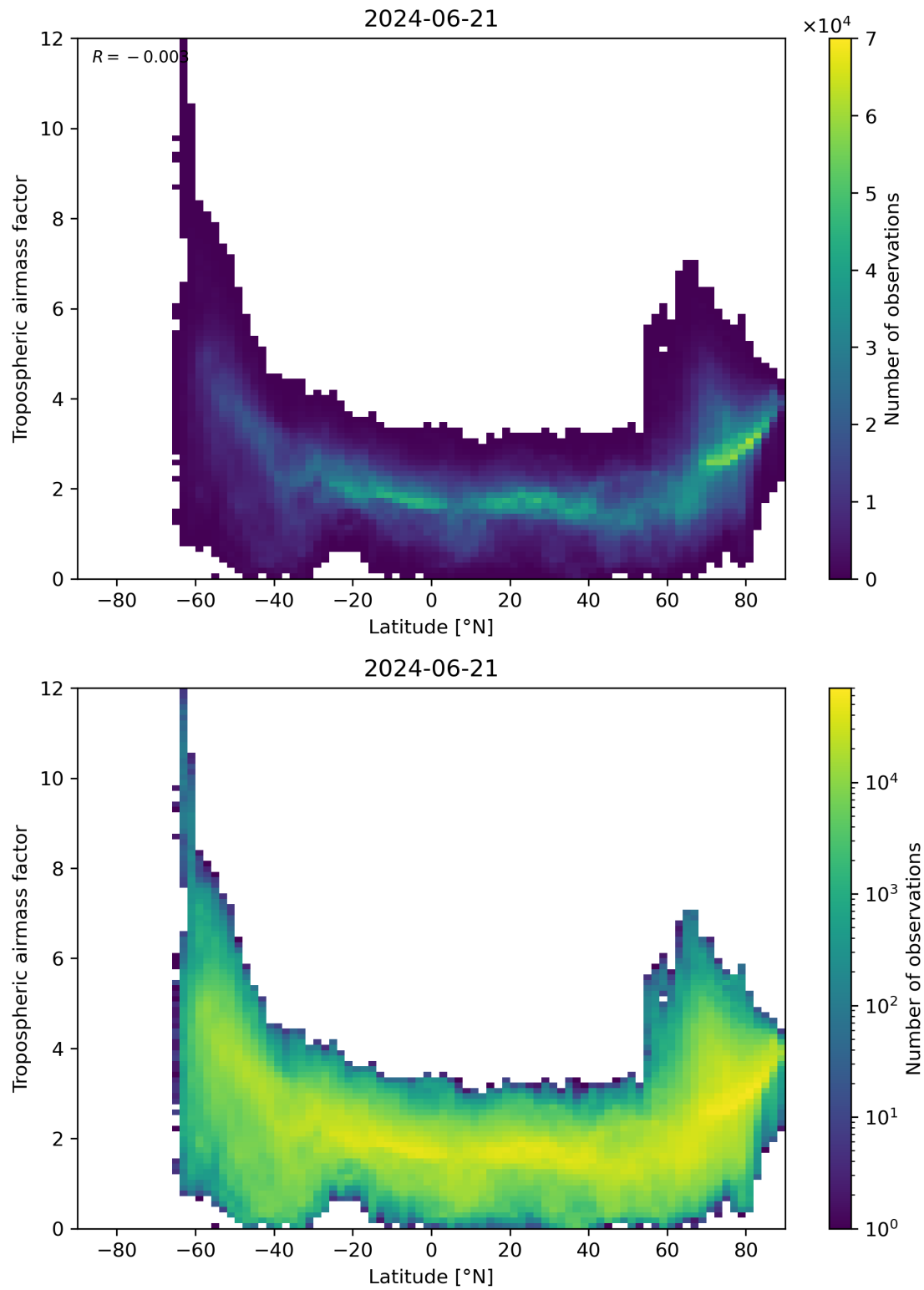
Figure 85: Scatter density plot of “Latitude” against “Tropospheric air mass factor” for 2024-06-20 to 2024-06-22.
