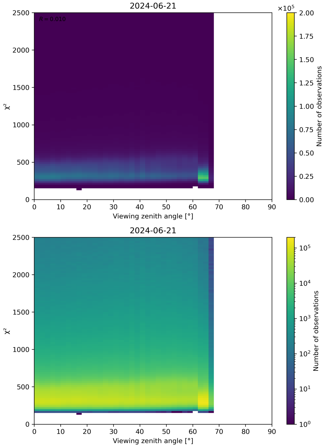
Figure 162: Scatter density plot of “Viewing zenith angle” against “ \chi^2 ” for 2024-06-20 to 2024-06-22.
