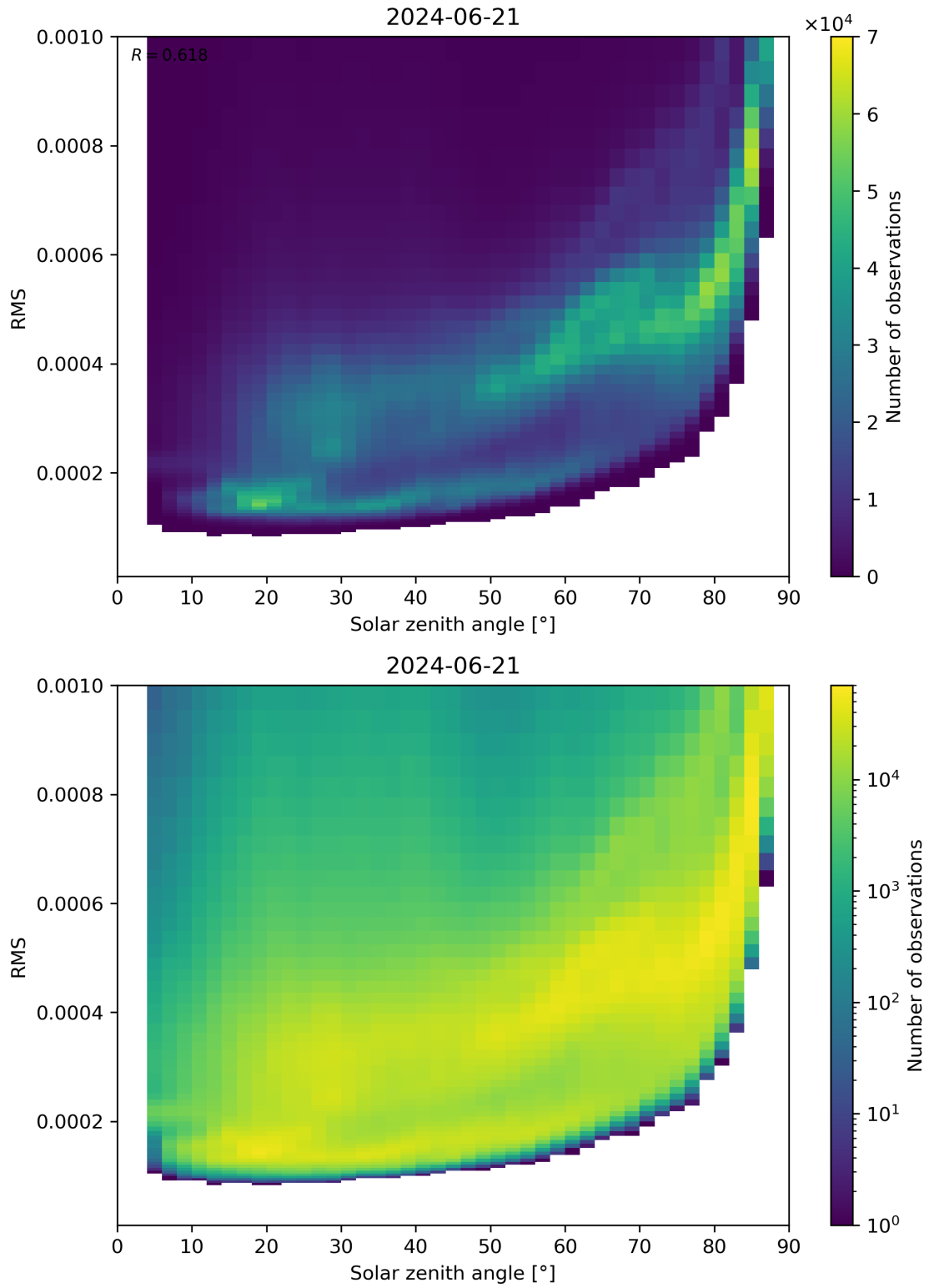
Figure 157: Scatter density plot of “Solar zenith angle” against “RMS” for 2024-06-20 to 2024-06-22.
