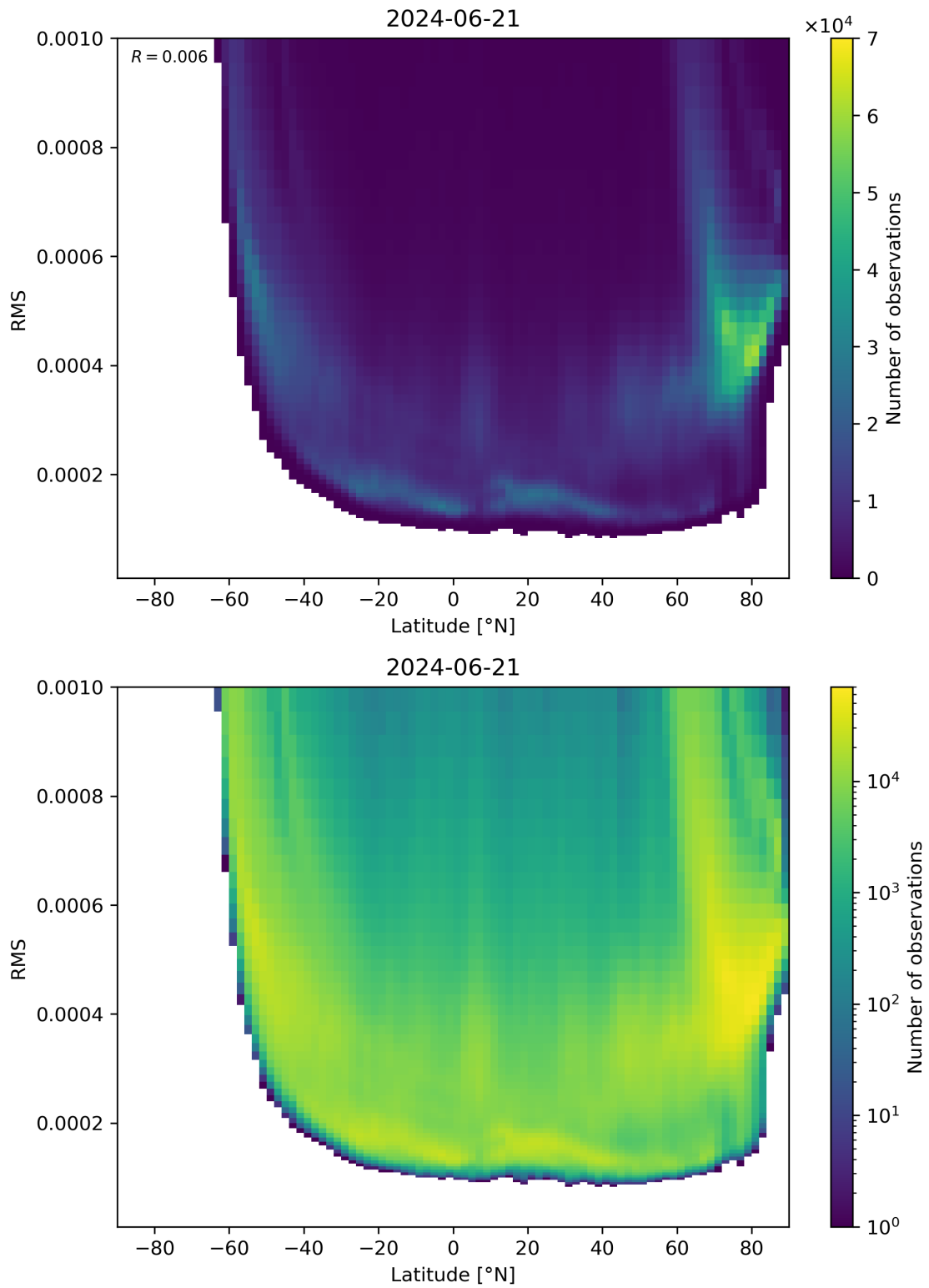
Figure 94: Scatter density plot of “Latitude” against “RMS” for 2024-06-20 to 2024-06-22.
