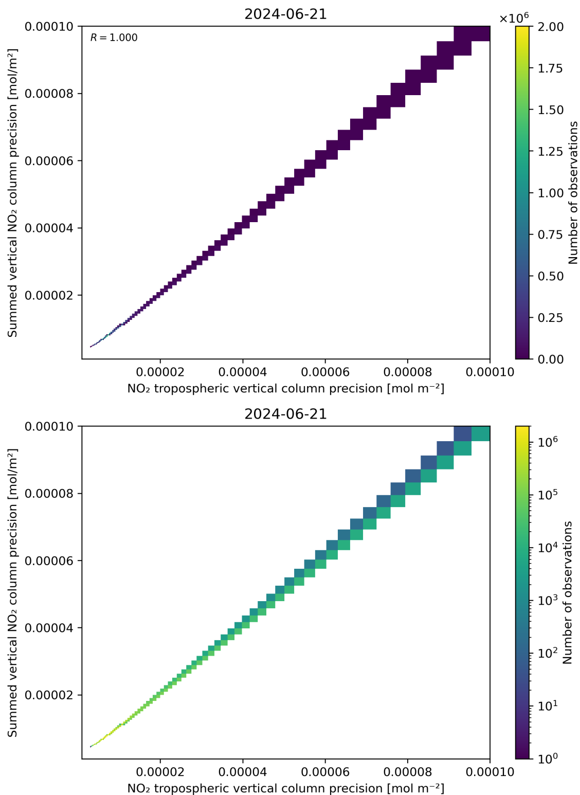
Figure 137: Scatter density plot of “NO 2 tropospheric vertical column precision” against “Summed vertical NO 2 column precision” for 2024-06-20 to 2024-06-22.
