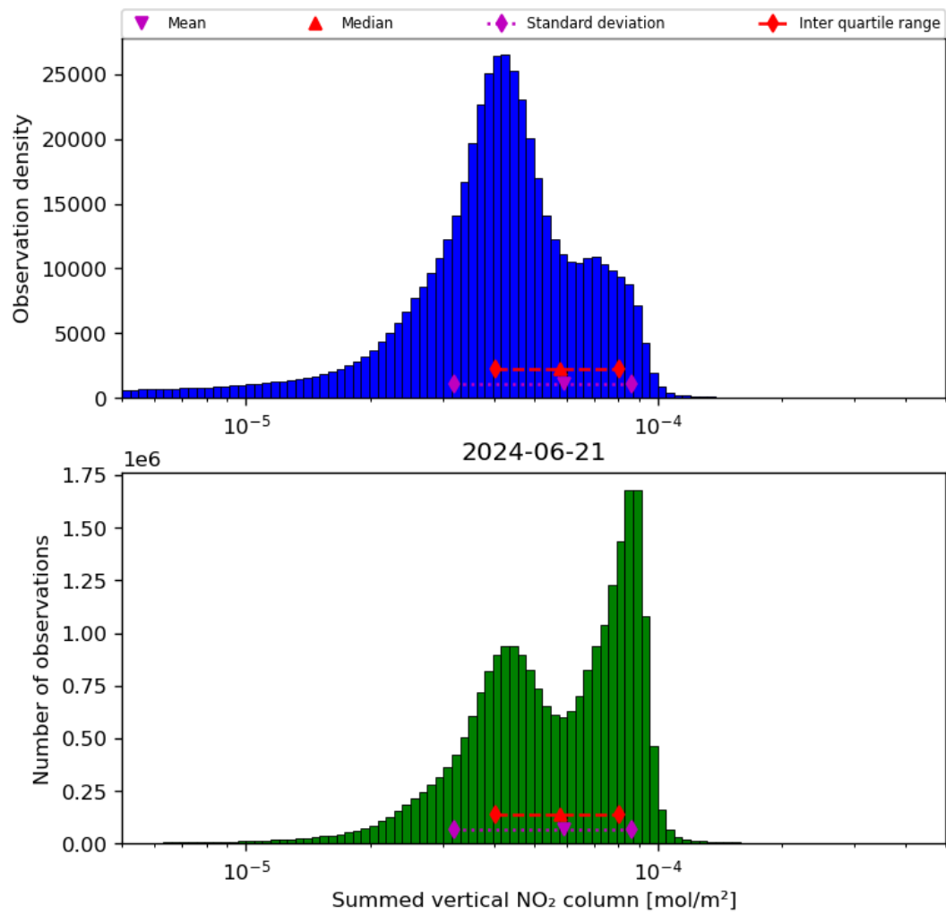
Figure 40: Histogram of “Summed vertical NO 2 column” for 2024-06-20 to 2024-06-22
