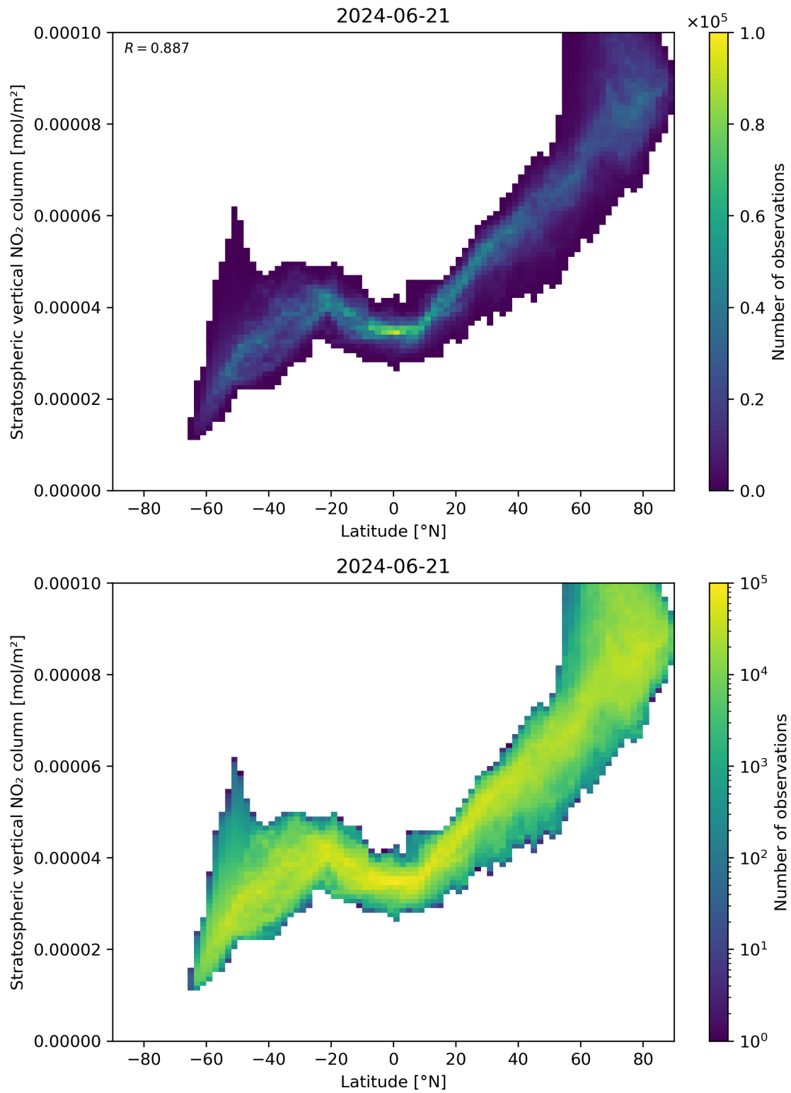
Figure 87: Scatter density plot of “Latitude” against “Stratospheric vertical \text{NO}_2 column” for 2024-06-20 to 2024-06-22.
