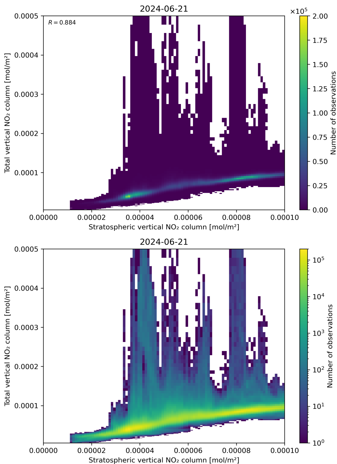
Figure 100: Scatter density plot of “Stratospheric vertical NO 2 column” against “Total vertical NO 2 column” for 2024-06-20 to 2024-06-22.
