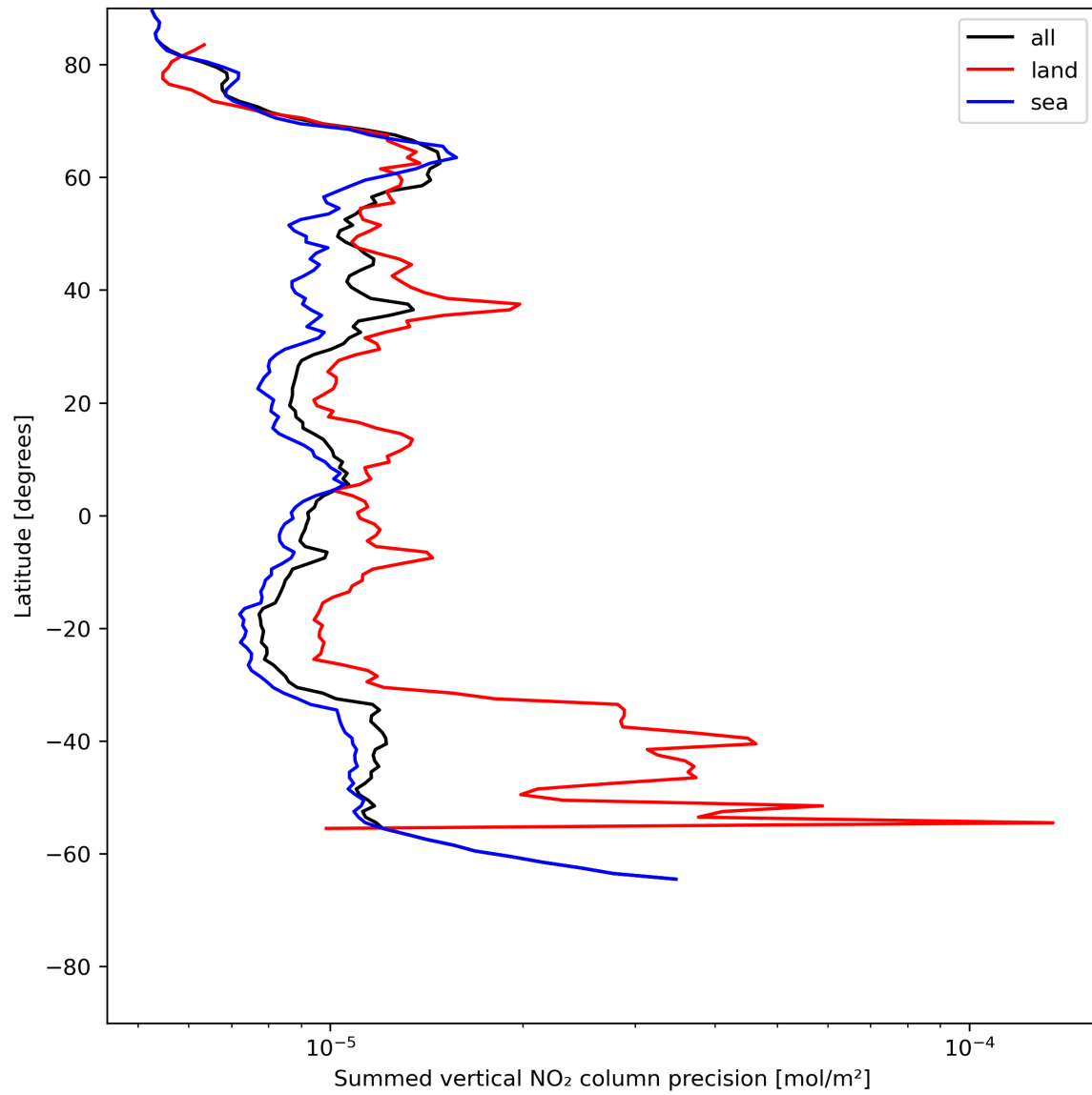
Figure 24: Zonal average of “Summed vertical NO 2 column precision” for 2024-06-20 to 2024-06-22.
