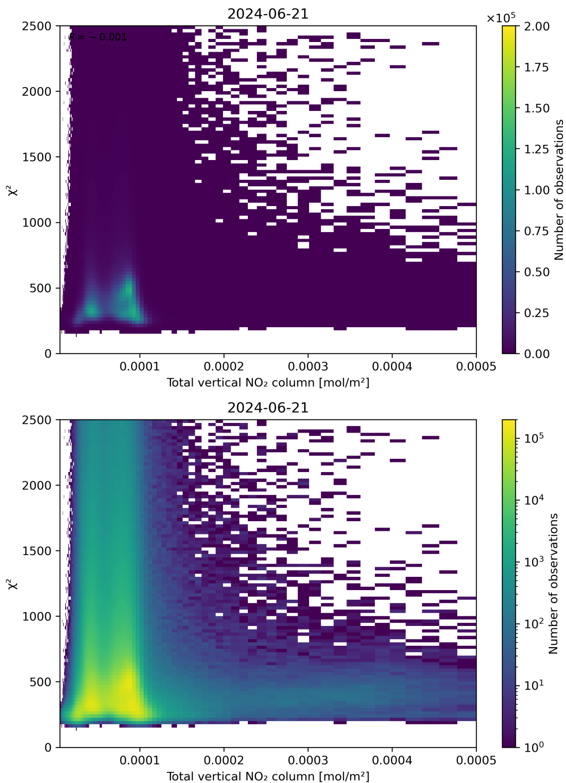
Figure 111: Scatter density plot of “Total vertical NO 2 column” against “ \chi^2 ” for 2024-06-20 to 2024-06-22.
