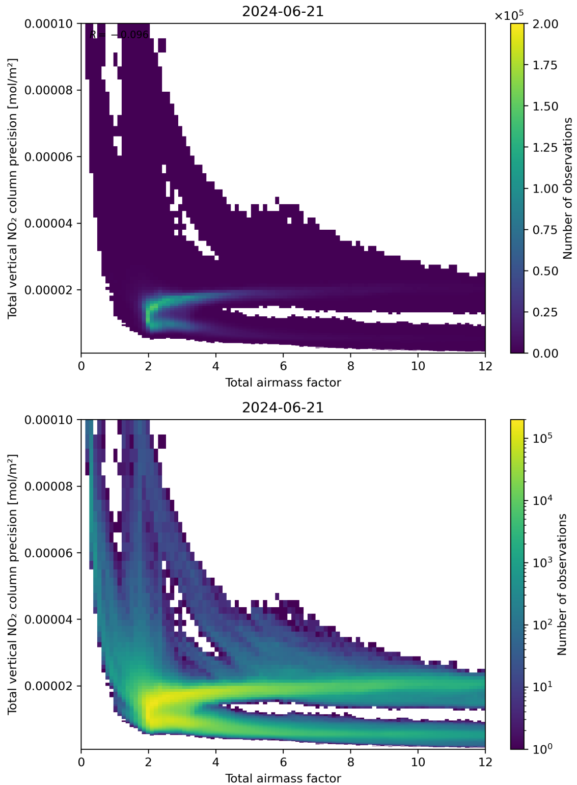
Figure 68: Scatter density plot of “Total airmass factor” against “Total vertical NO 2 column precision” for 2024-06-20 to 2024-06-22.
