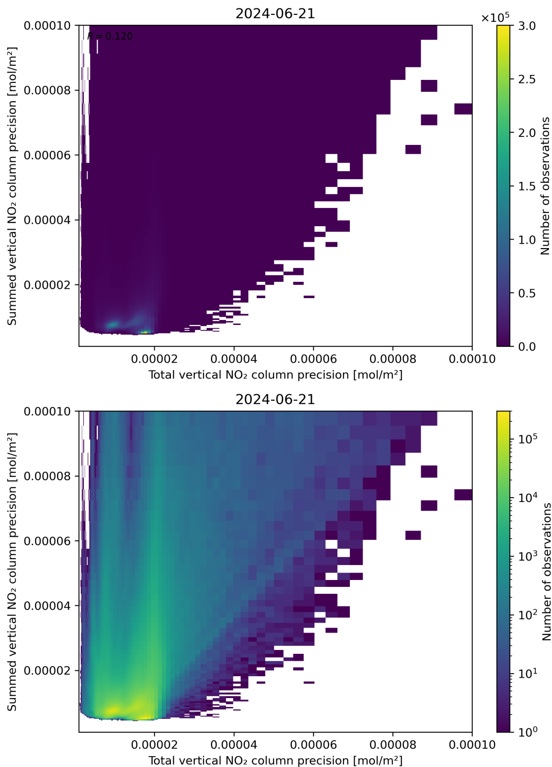
Figure 118: Scatter density plot of “Total vertical NO 2 column precision” against “Summed vertical NO 2 column precision” for 2024-06-20 to 2024-06-22.
