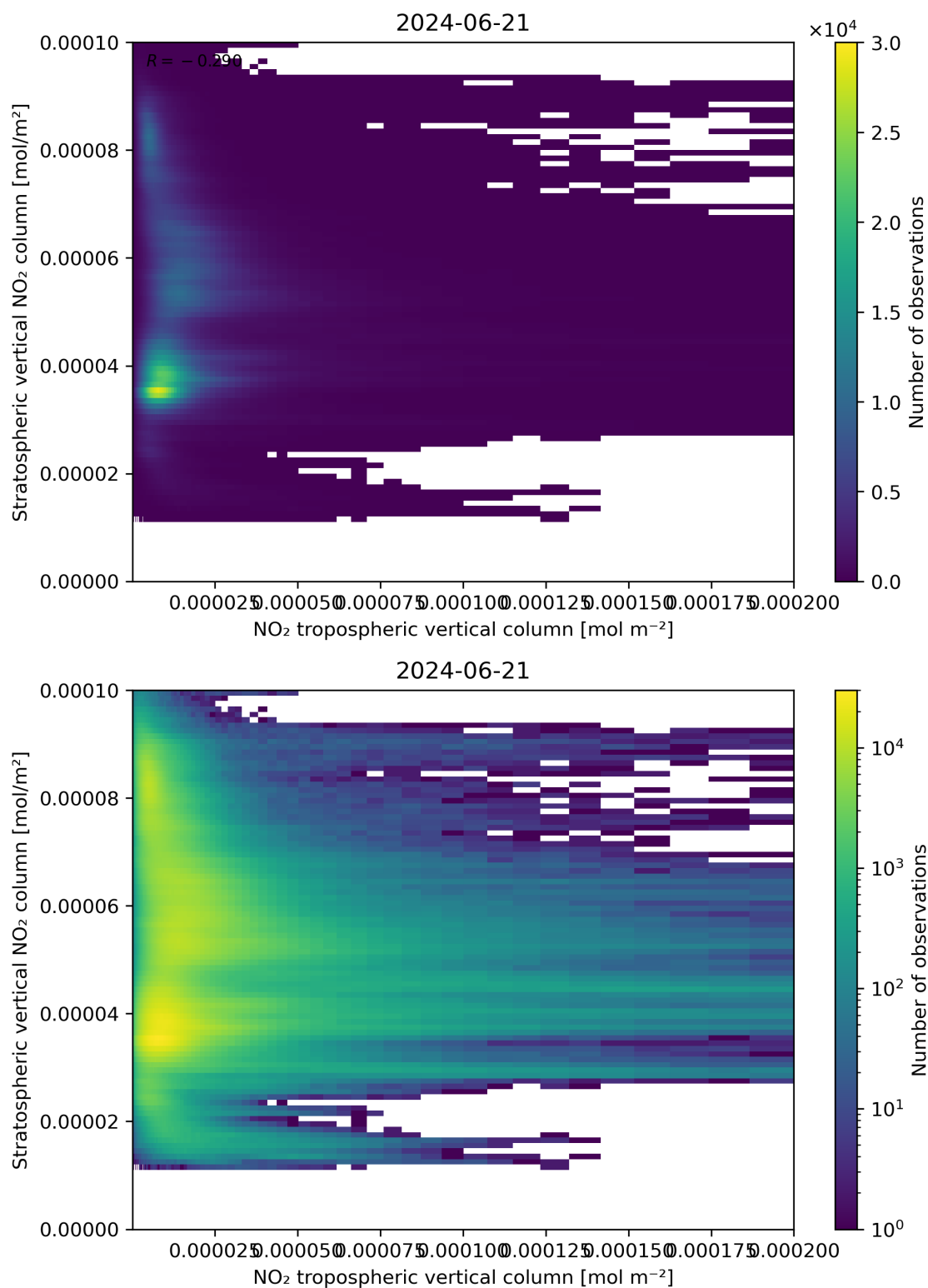
Figure 125: Scatter density plot of “NO 2 tropospheric vertical column” against “Stratospheric vertical NO 2 column” for 2024-06-20 to 2024-06-22.
