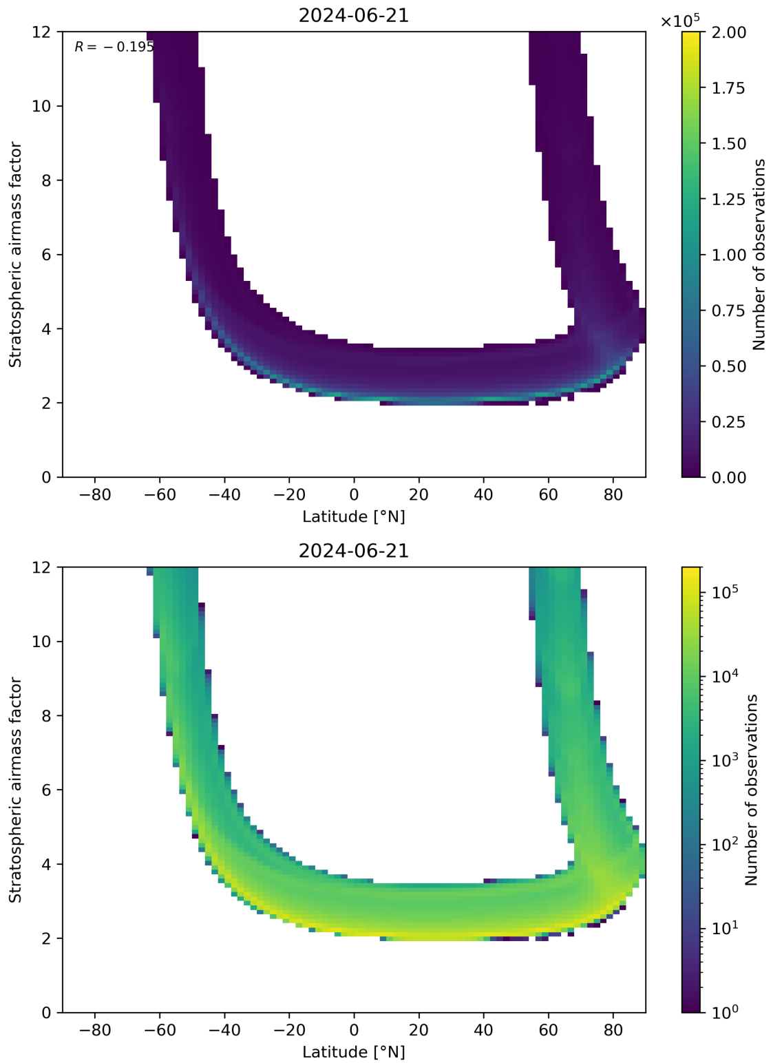
Figure 83: Scatter density plot of “Latitude” against “Stratospheric air mass factor” for 2024-06-20 to 2024-06-22.
