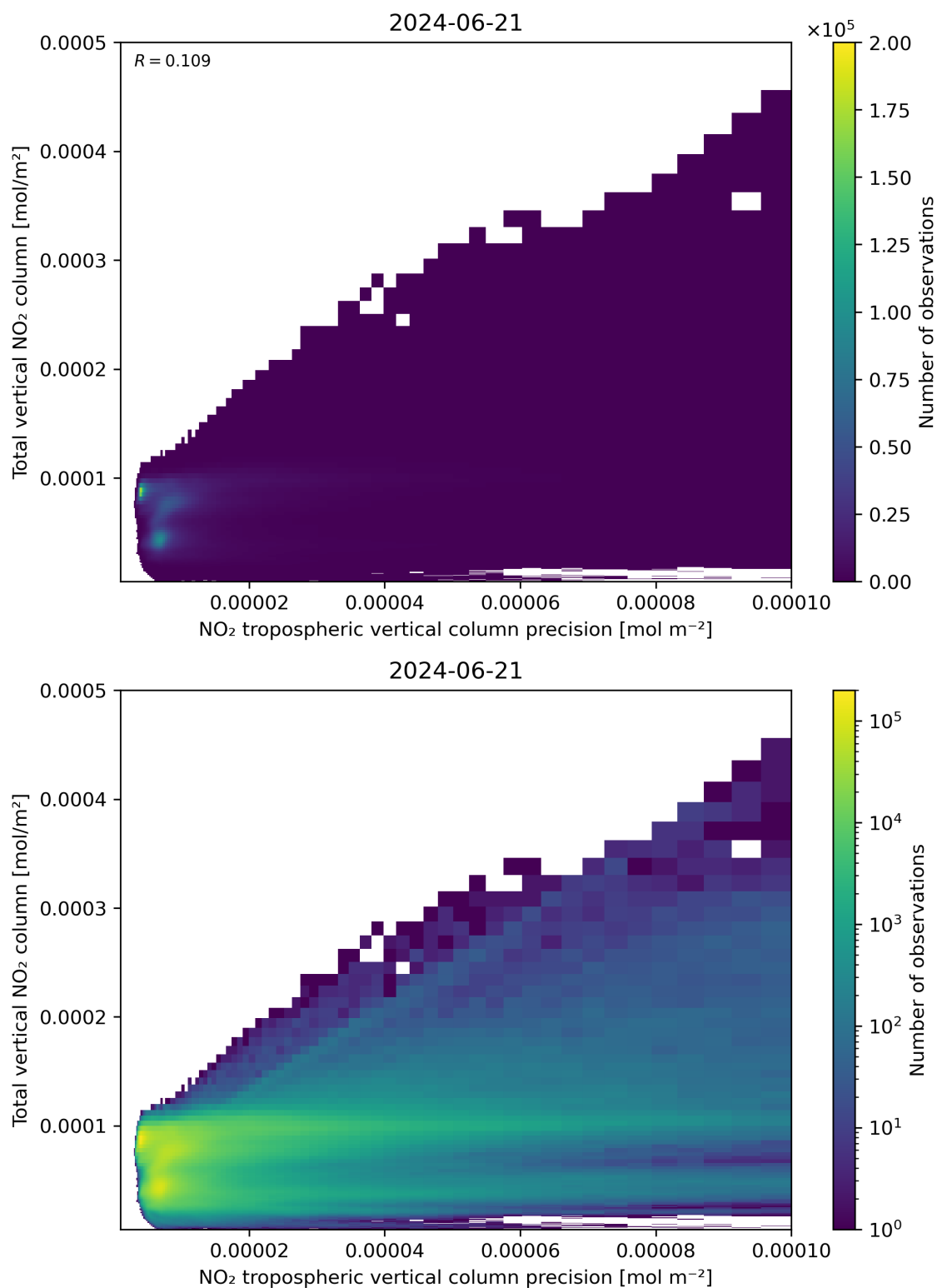
Figure 138: Scatter density plot of “NO 2 tropospheric vertical column precision” against “Total vertical NO 2 column” for 2024-06-20 to 2024-06-22.
