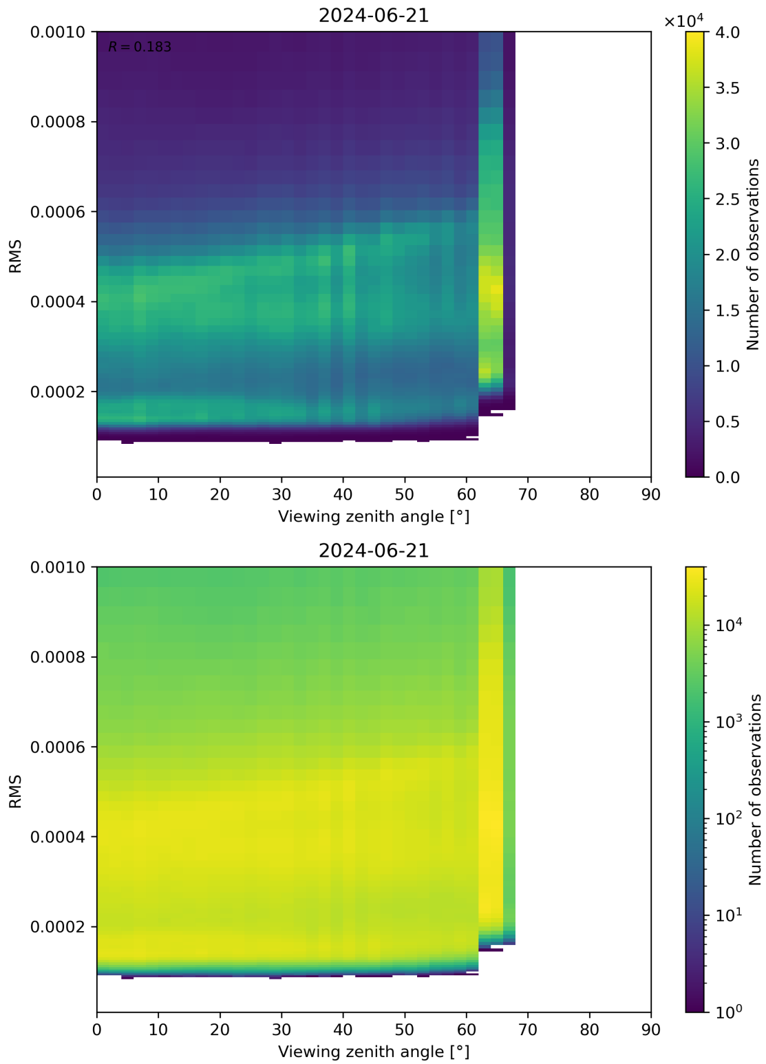
Figure 171: Scatter density plot of “Viewing zenith angle” against “RMS” for 2024-06-20 to 2024-06-22.
