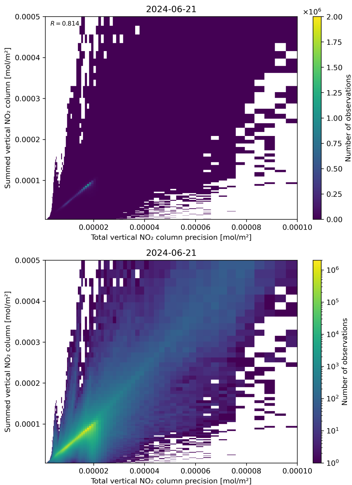
Figure 117: Scatter density plot of “Total vertical NO 2 column precision” against “Summed vertical NO 2 column” for 2024-06-20 to 2024-06-22.
