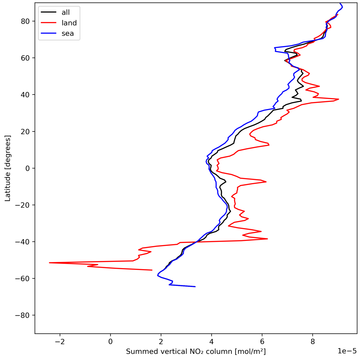
Figure 23: Zonal average of “Summed vertical NO 2 column” for 2024-06-20 to 2024-06-22.
