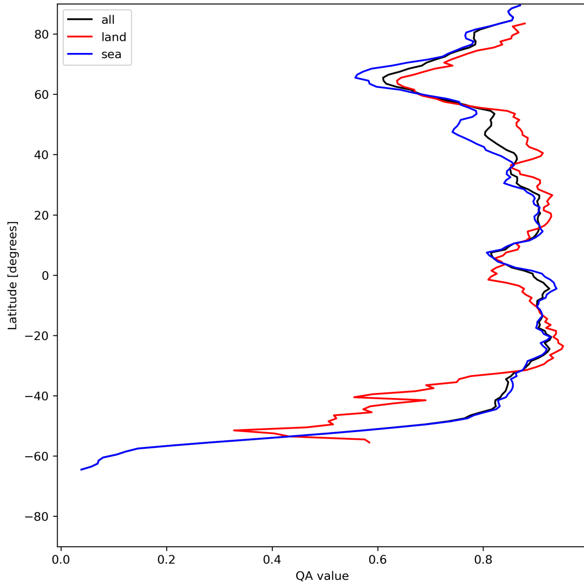
Figure 11: Zonal average of “QA value” for 2024-06-20 to 2024-06-22.
