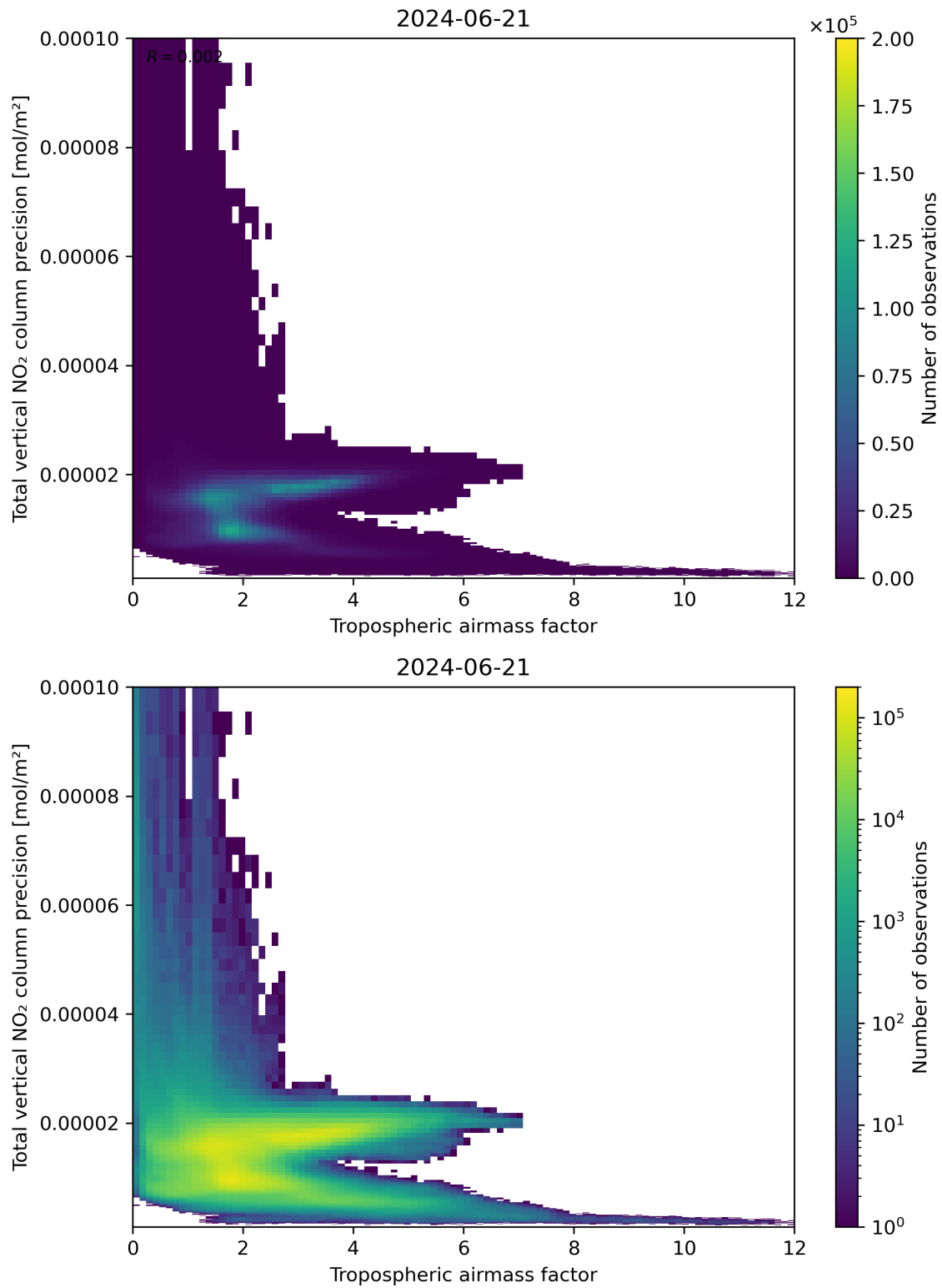
Figure 78: Scatter density plot of “Tropospheric air mass factor” against “Total vertical NO 2 column precision” for 2024-06-20 to 2024-06-22.
