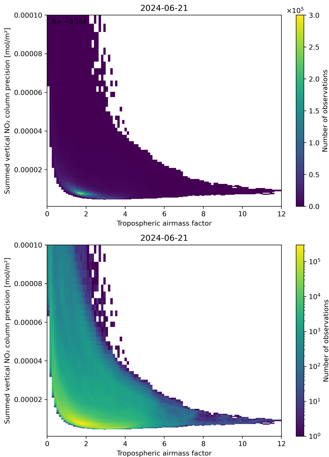
Figure 76: Scatter density plot of “Tropospheric air mass factor” against “Summed vertical NO 2 column precision” for 2024-06-20 to 2024-06-22.
