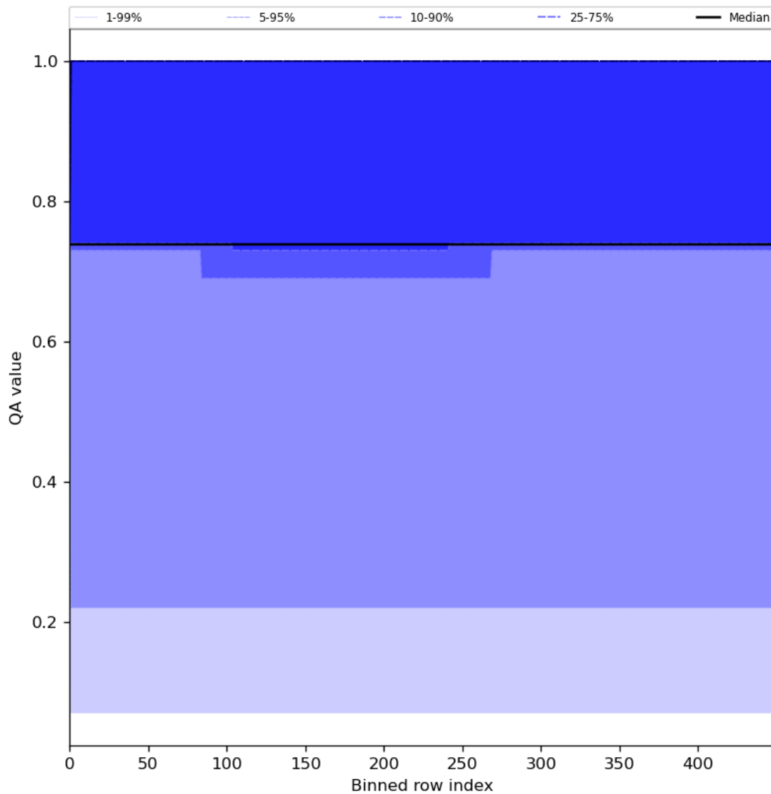
Figure 45: Along track statistics of “QA value” for 2024-06-20 to 2024-06-22
