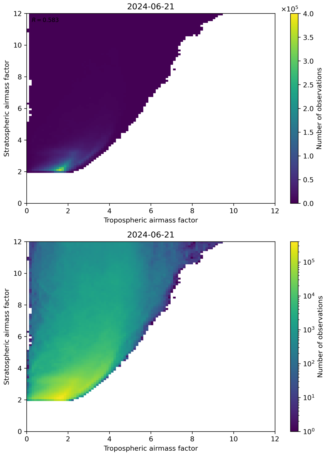
Figure 71: Scatter density plot of “Tropospheric airmass factor” against “Stratospheric airmass factor” for 2024-06-20 to 2024-06-22.
