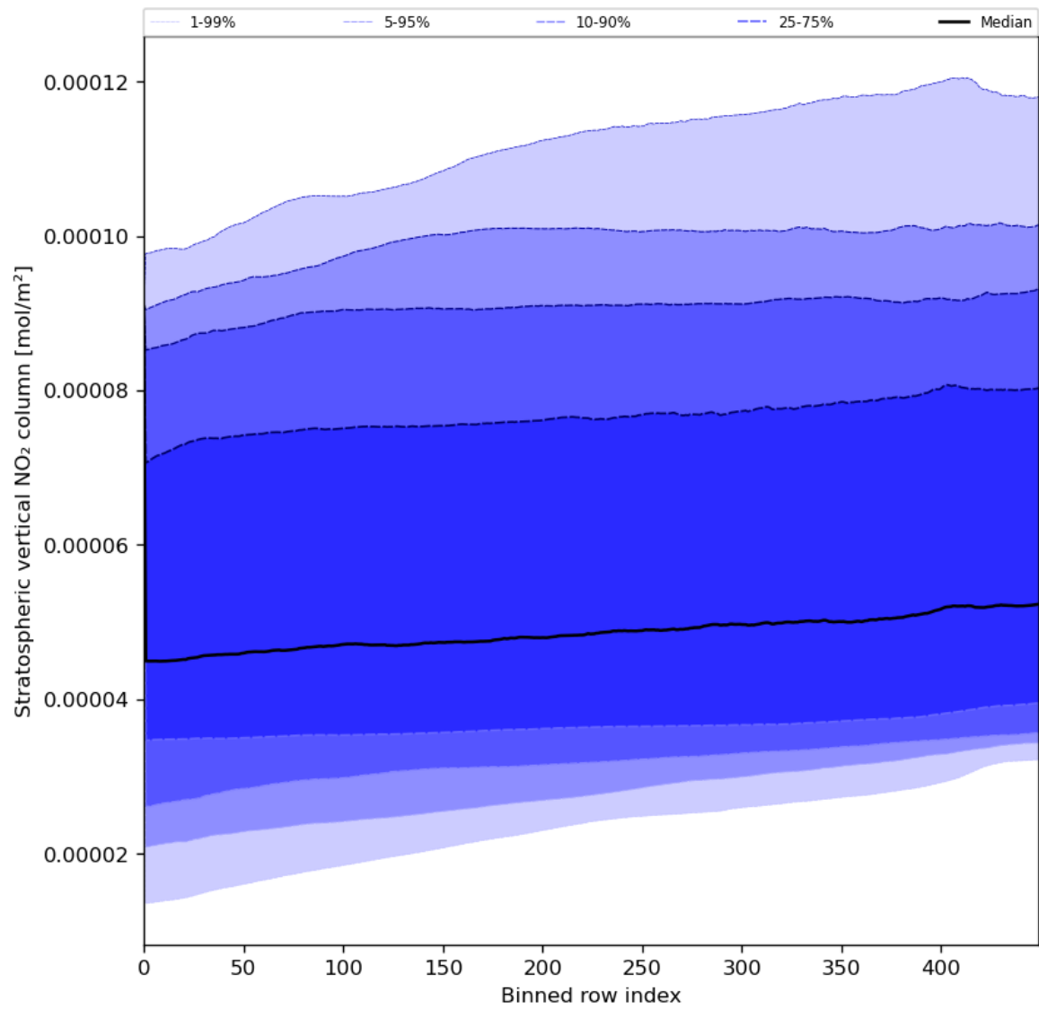
Figure 53: Along track statistics of “Stratospheric vertical NO 2 column” for 2024-06-20 to 2024-06-22
