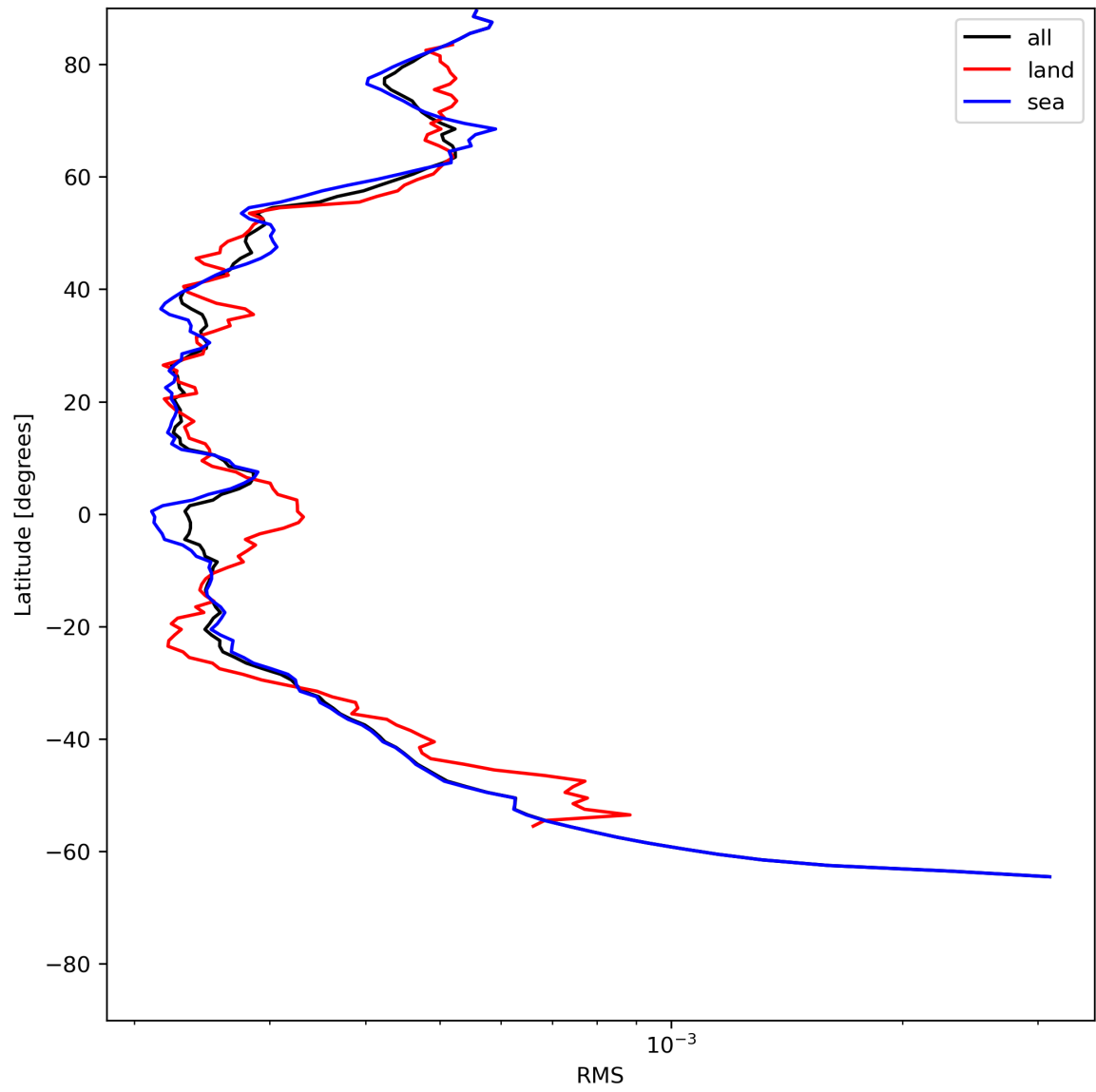
Figure 26: Zonal average of “RMS” for 2024-06-20 to 2024-06-22.
