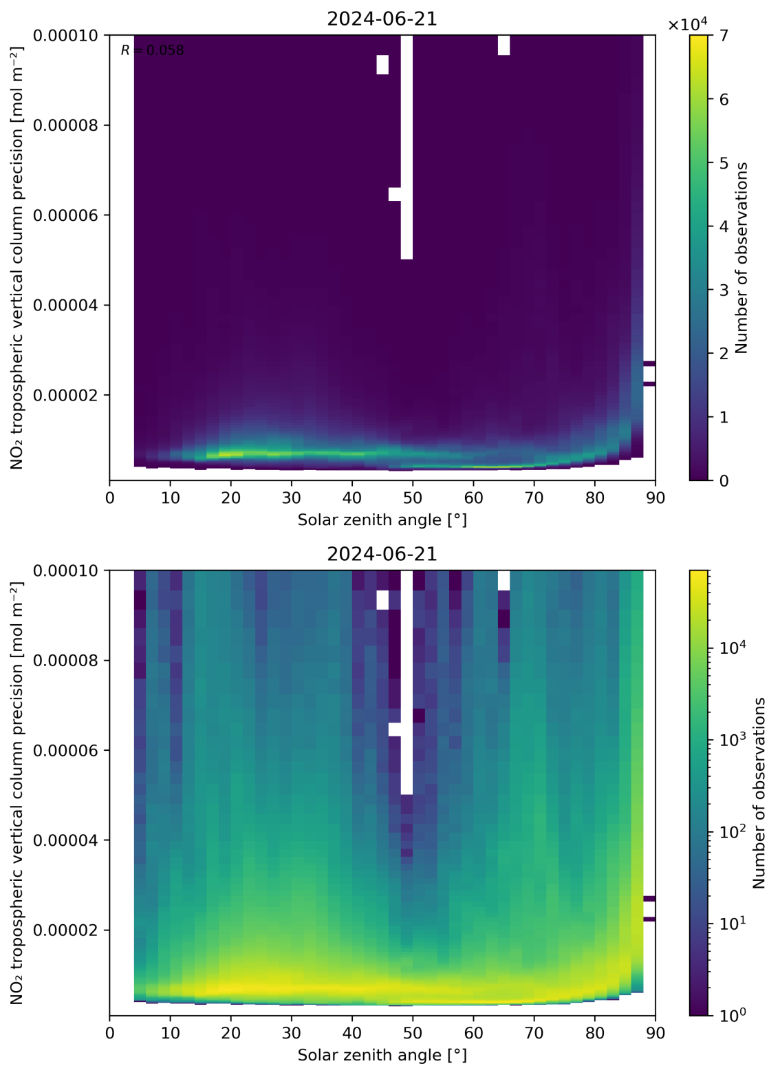
Figure 156: Scatter density plot of “Solar zenith angle” against “NO 2 tropospheric vertical column precision” for 2024-06-20 to 2024-06-22.
