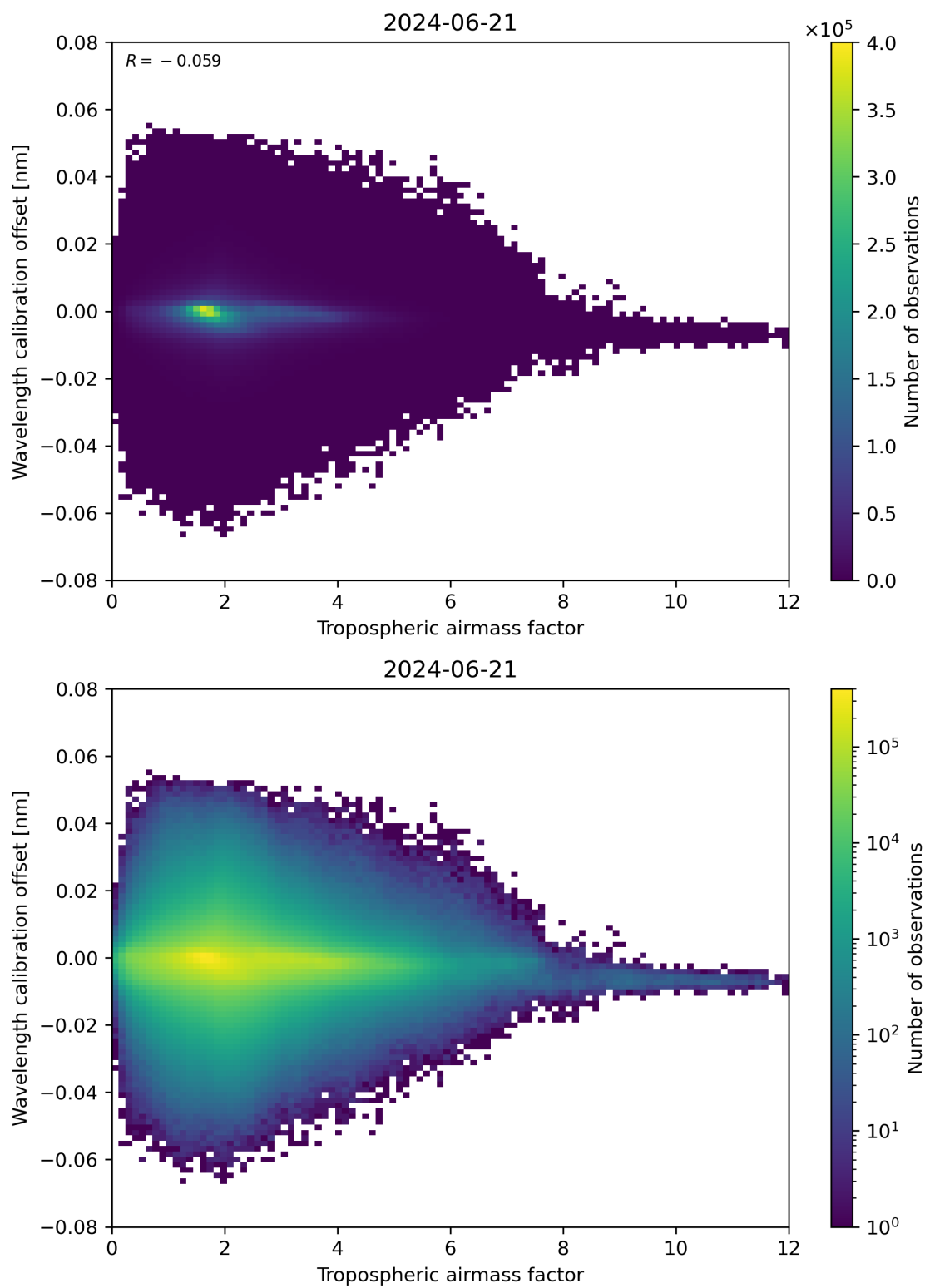
Figure 80: Scatter density plot of “Tropospheric airmass factor” against “Wavelength calibration offset” for 2024-06-20 to 2024-06-22.
