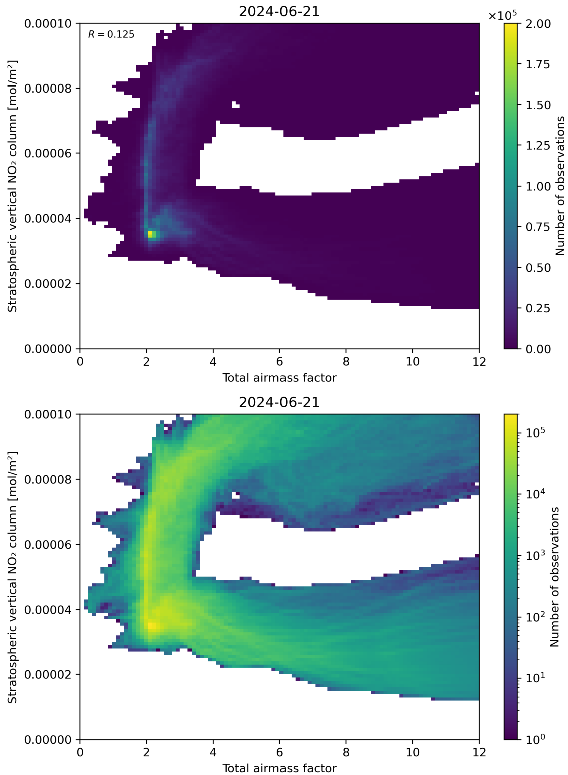
Figure 64: Scatter density plot of “Total airmass factor” against “Stratospheric vertical NO 2 column” for 2024-06-20 to 2024-06-22.
