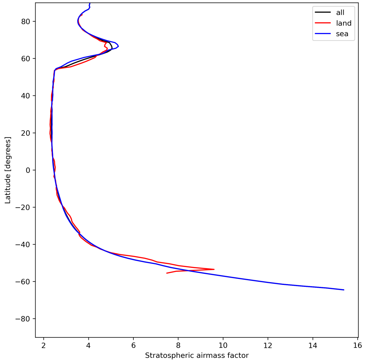
Figure 27: Zonal average of “Stratospheric airmass factor” for 2024-06-20 to 2024-06-22.
