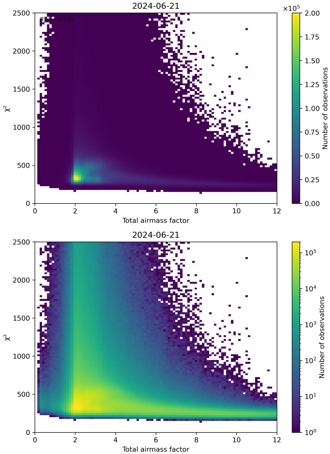
Figure 63: Scatter density plot of “Total airmass factor” against “ \chi^2 ” for 2024-06-20 to 2024-06-22.
