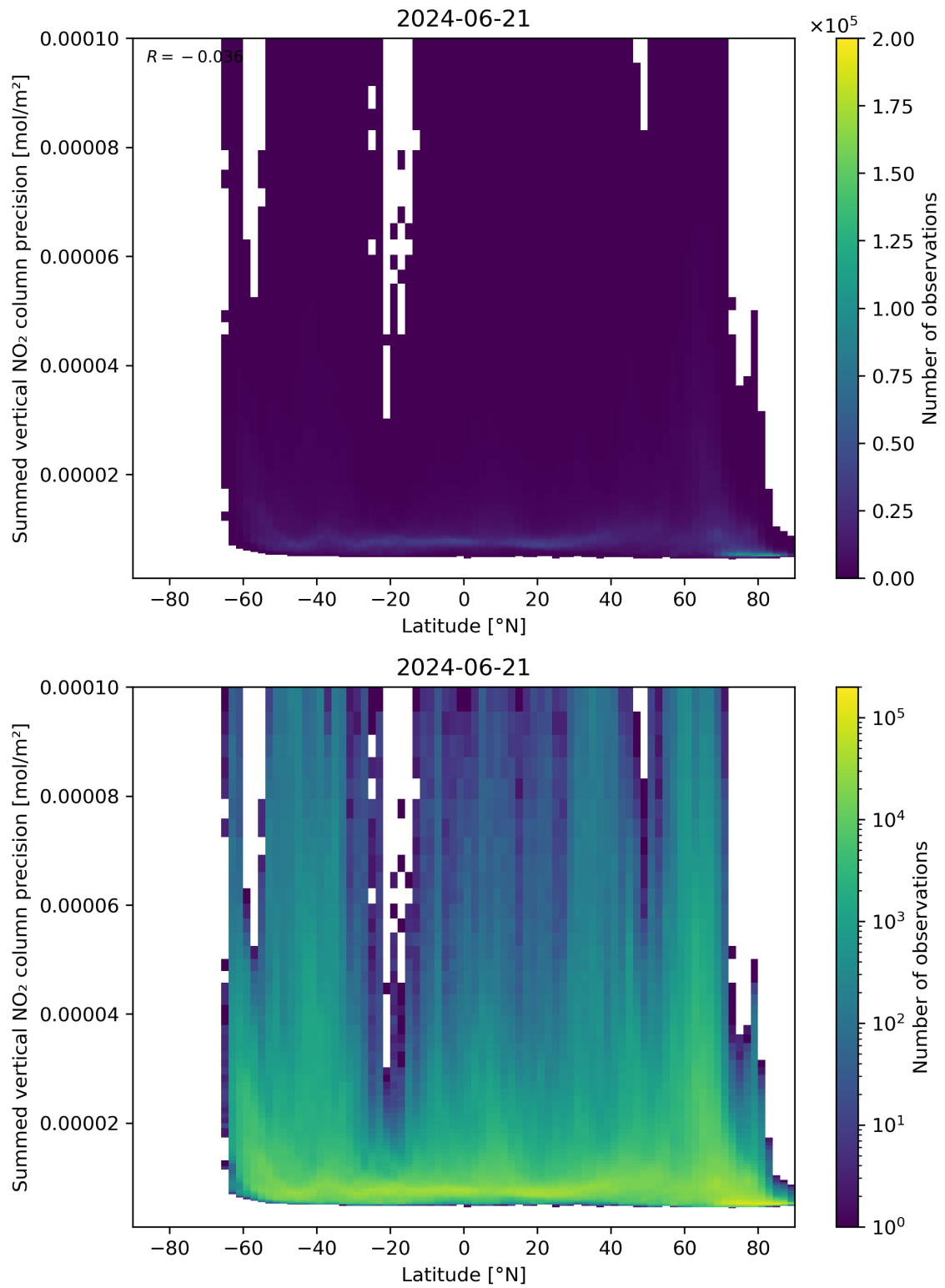
Figure 89: Scatter density plot of “Latitude” against “Summed vertical NO 2 column precision” for 2024-06-20 to 2024-06-22.
