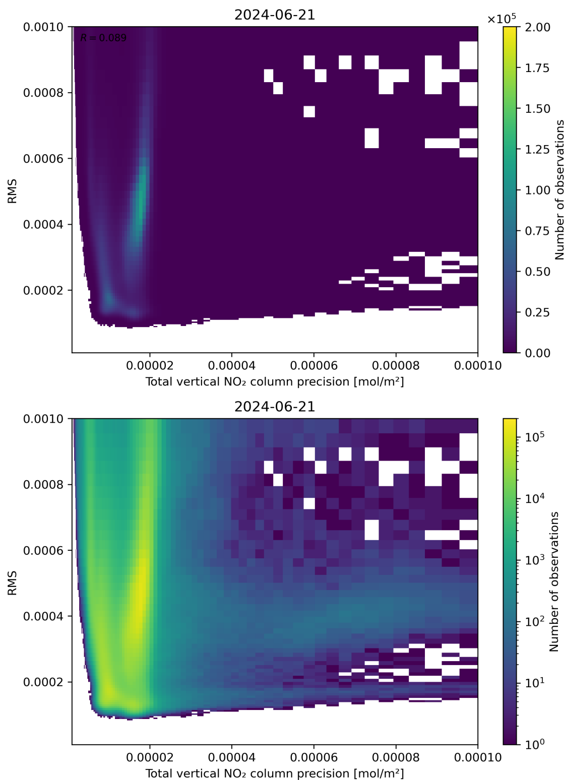
Figure 119: Scatter density plot of “Total vertical NO 2 column precision” against “RMS” for 2024-06-20 to 2024-06-22.
