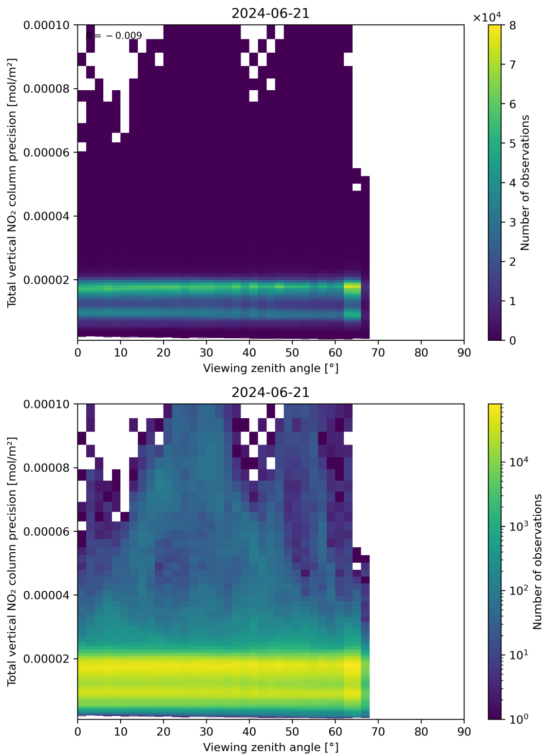
Figure 168: Scatter density plot of “Viewing zenith angle” against “Total vertical NO 2 column precision” for 2024-06-20 to 2024-06-22.
