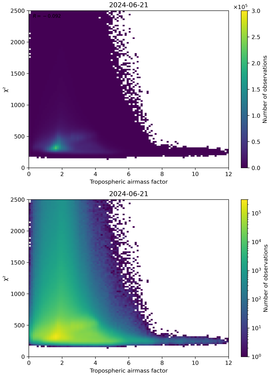
Figure 73: Scatter density plot of “Tropospheric airmass factor” against “ \chi^2 ” for 2024-06-20 to 2024-06-22.
