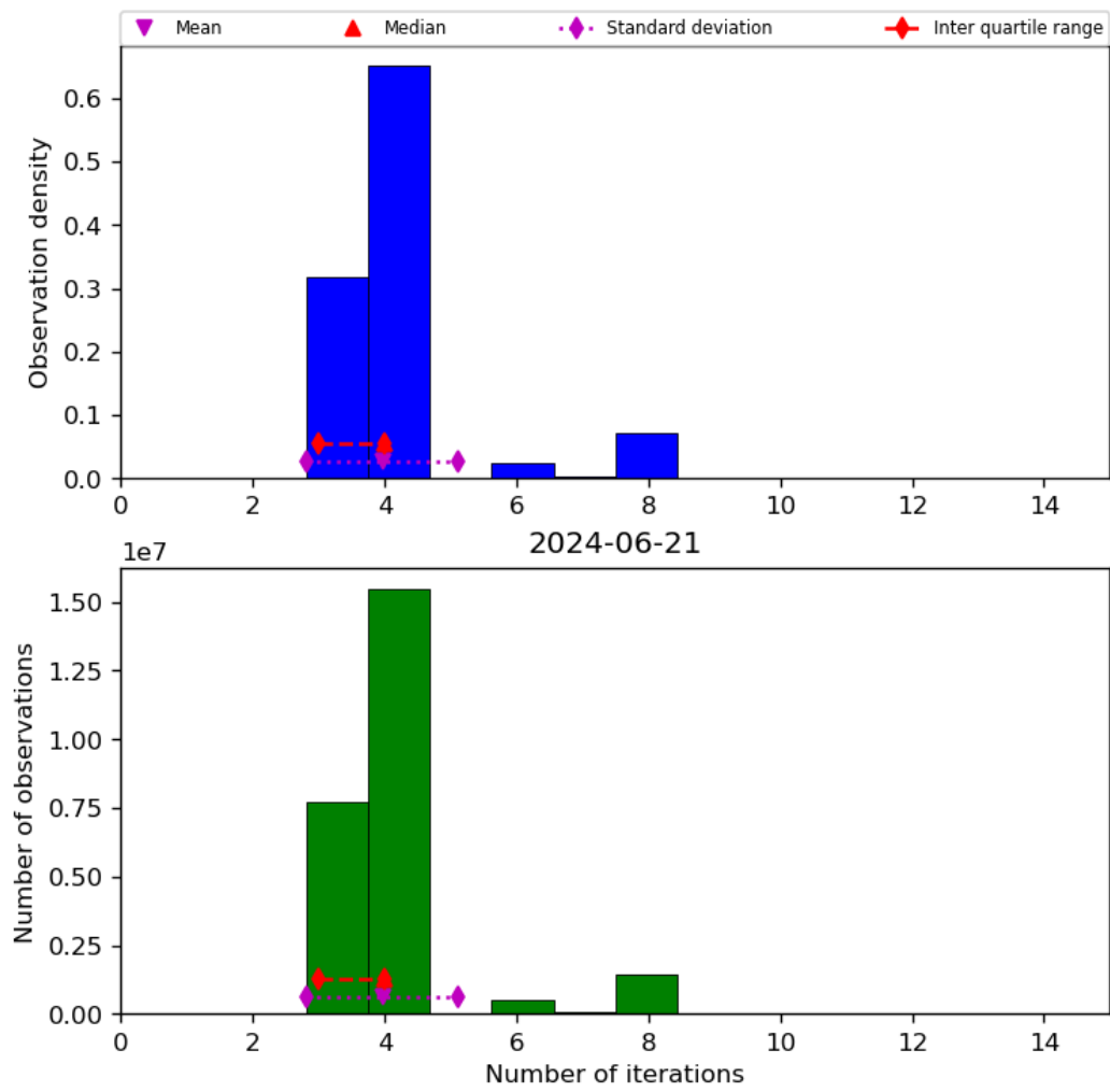
Figure 34: Histogram of “Number of iterations” for 2024-06-20 to 2024-06-22
