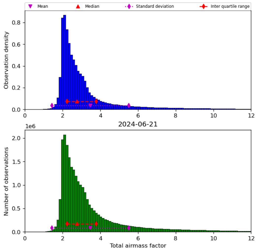
Figure 32: Histogram of “Total airmass factor” for 2024-06-20 to 2024-06-22
