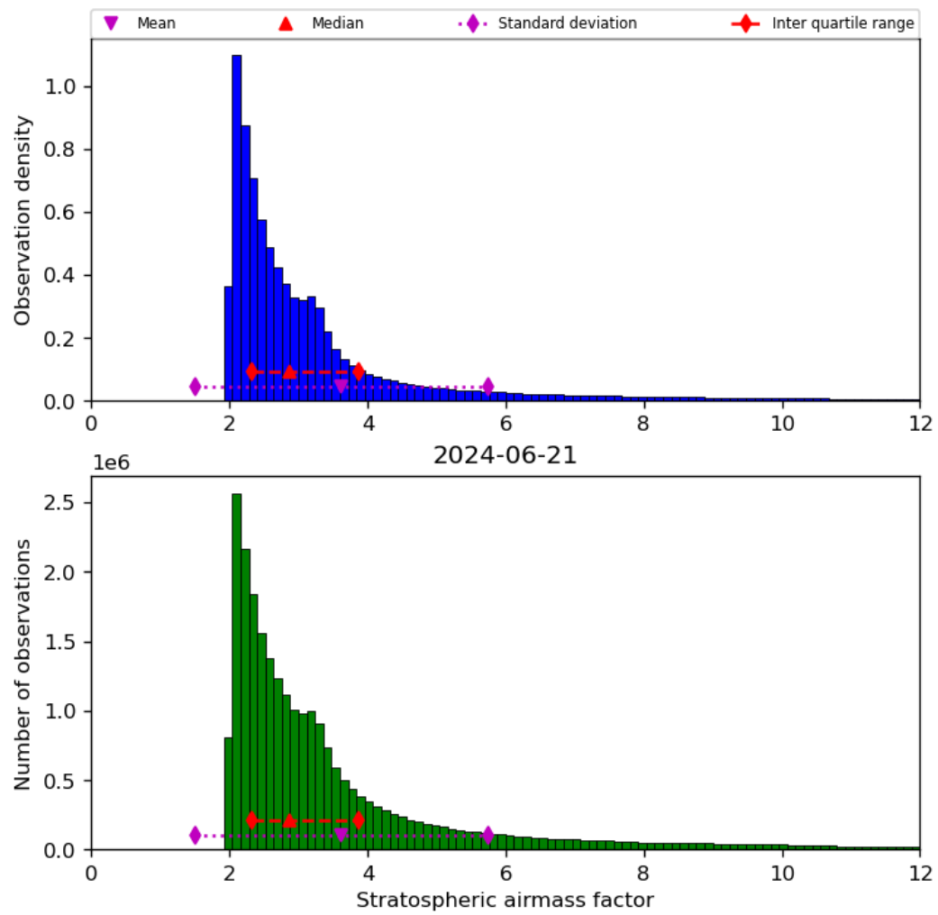
Figure 44: Histogram of “Stratospheric airmass factor” for 2024-06-20 to 2024-06-22
