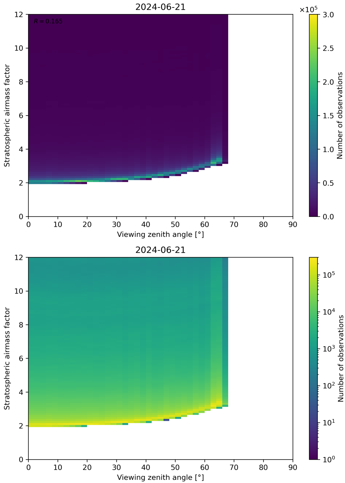
Figure 159: Scatter density plot of “Viewing zenith angle” against “Stratospheric airmass factor” for 2024-06-20 to 2024-06-22.
