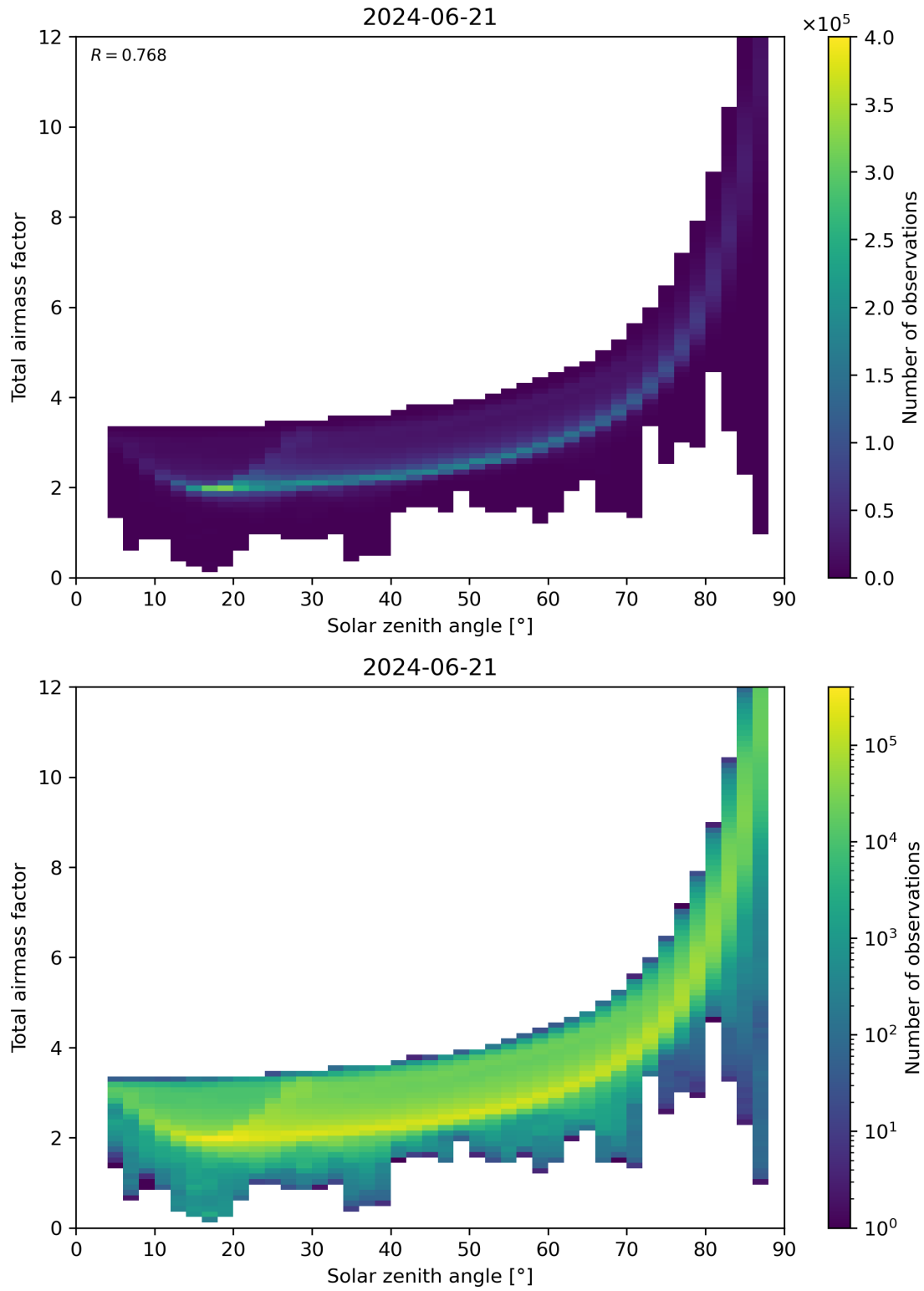
Figure 146: Scatter density plot of “Solar zenith angle” against “Total air mass factor” for 2024-06-20 to 2024-06-22.
