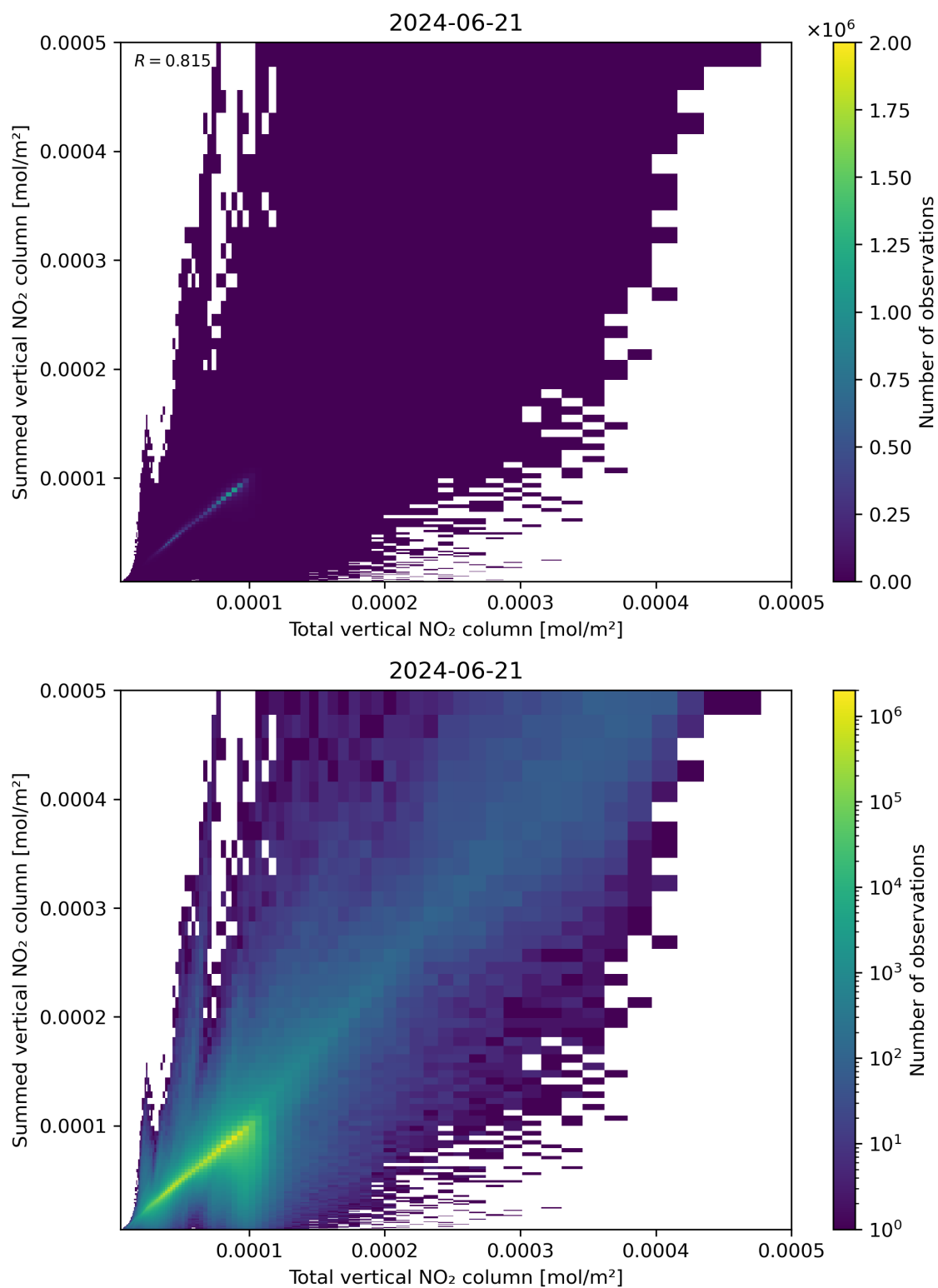
Figure 112: Scatter density plot of “Total vertical NO 2 column” against “Summed vertical NO 2 column” for 2024-06-20 to 2024-06-22.
