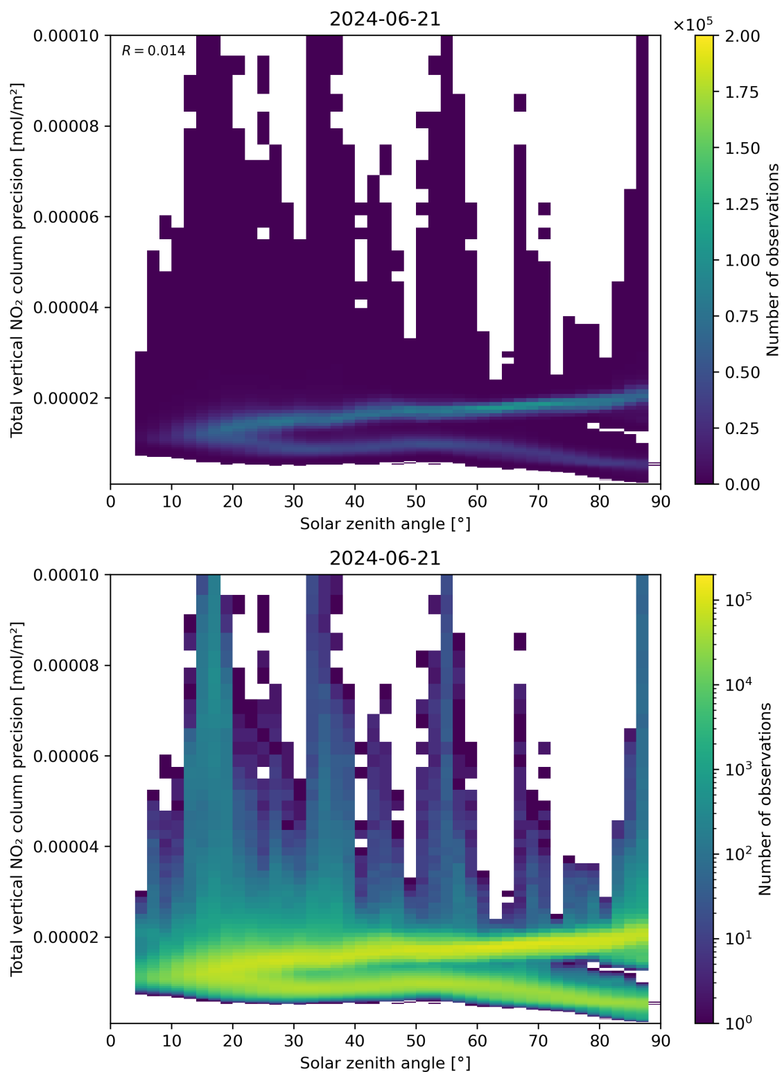
Figure 154: Scatter density plot of “Solar zenith angle” against “Total vertical NO 2 column precision” for 2024-06-20 to 2024-06-22.
