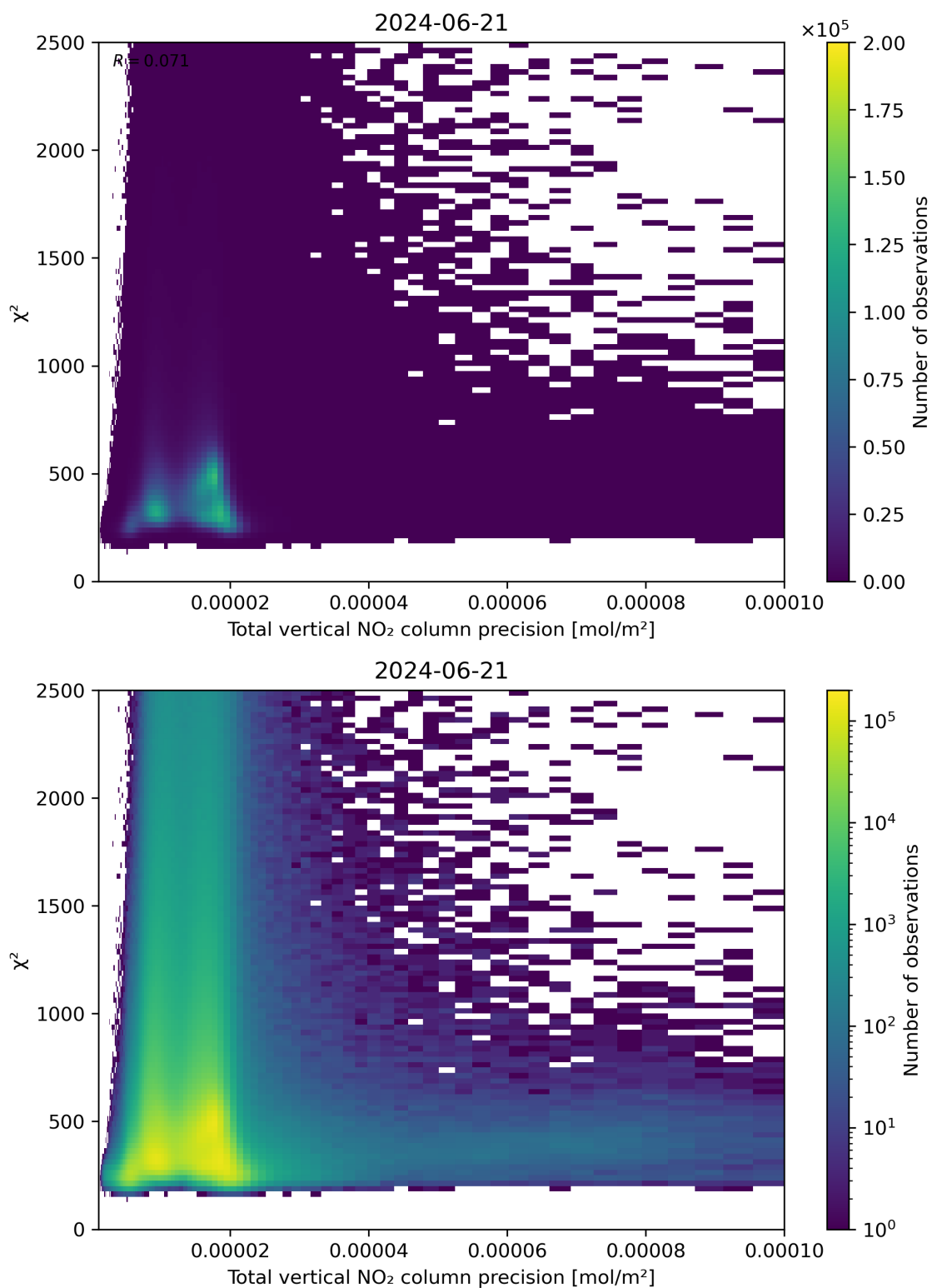
Figure 116: Scatter density plot of “Total vertical NO 2 column precision” against “ \chi^2 ” for 2024-06-20 to 2024-06-22.
