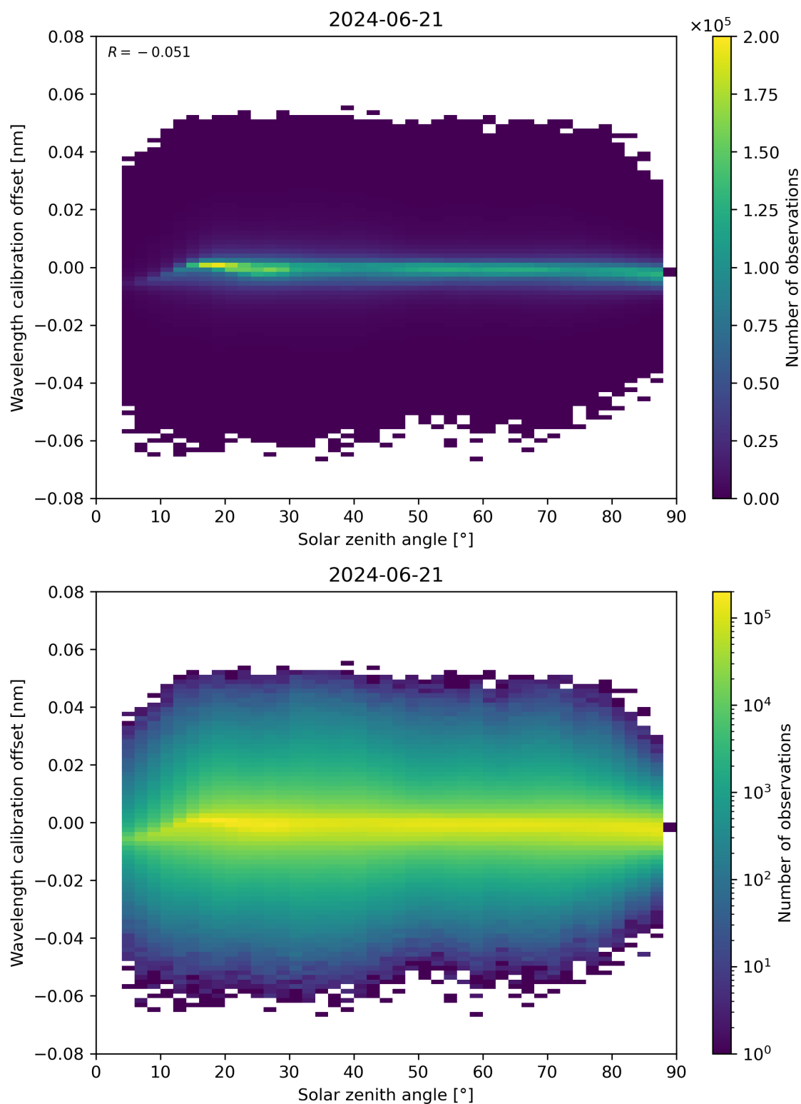
Figure 158: Scatter density plot of “Solar zenith angle” against “Wavelength calibration offset” for 2024-06-20 to 2024-06-22.
