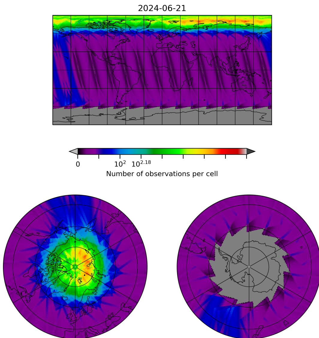
Figure 10: Map of the number of observations for 2024-06-20 to 2024-06-22
