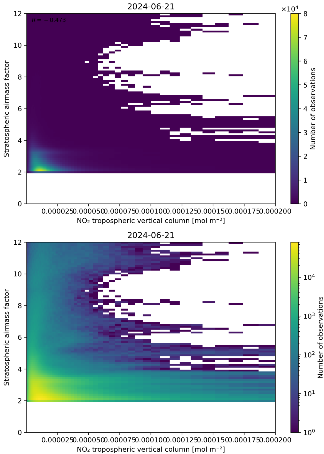
Figure 121: Scatter density plot of “NO 2 tropospheric vertical column” against “Stratospheric air mass factor” for 2024-06-20 to 2024-06-22.
