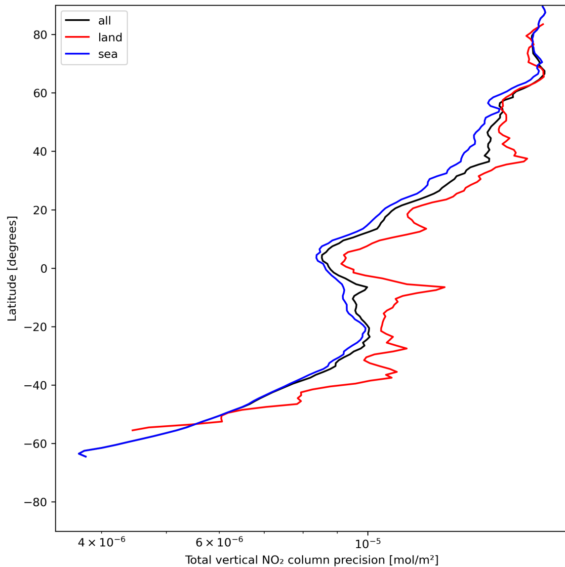
Figure 22: Zonal average of “Total vertical NO 2 column precision” for 2024-06-20 to 2024-06-22.
