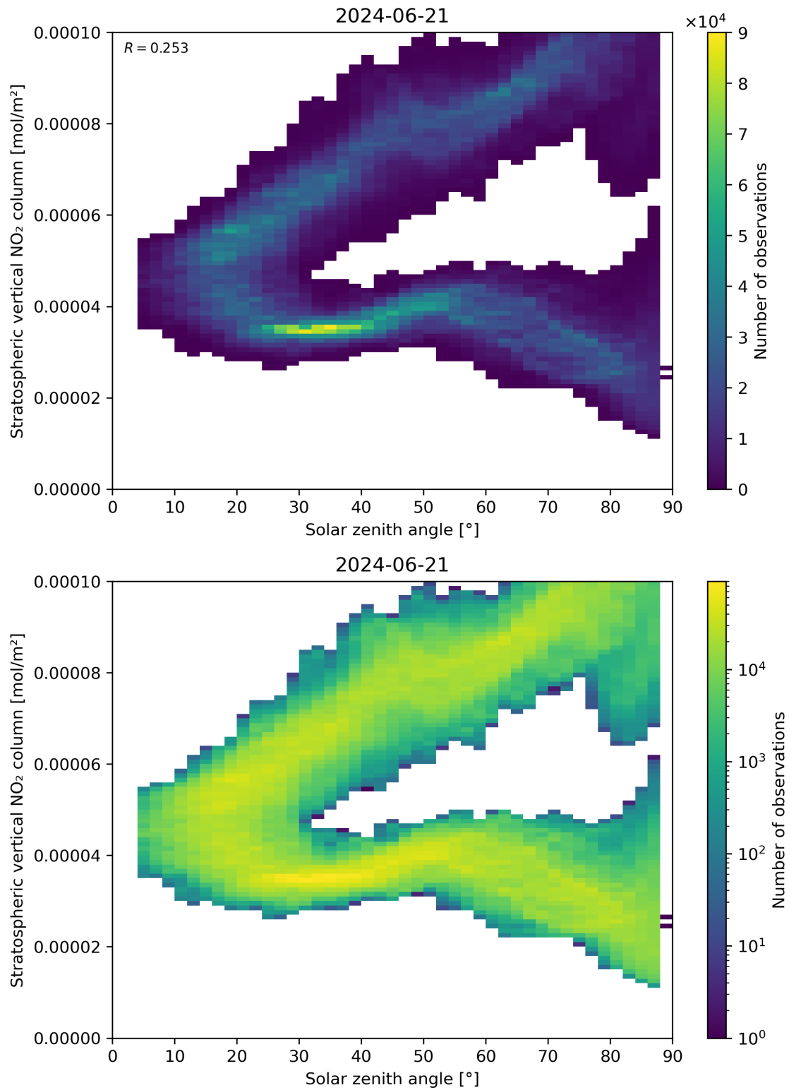
Figure 150: Scatter density plot of “Solar zenith angle” against “Stratospheric vertical NO 2 column” for 2024-06-20 to 2024-06-22.
