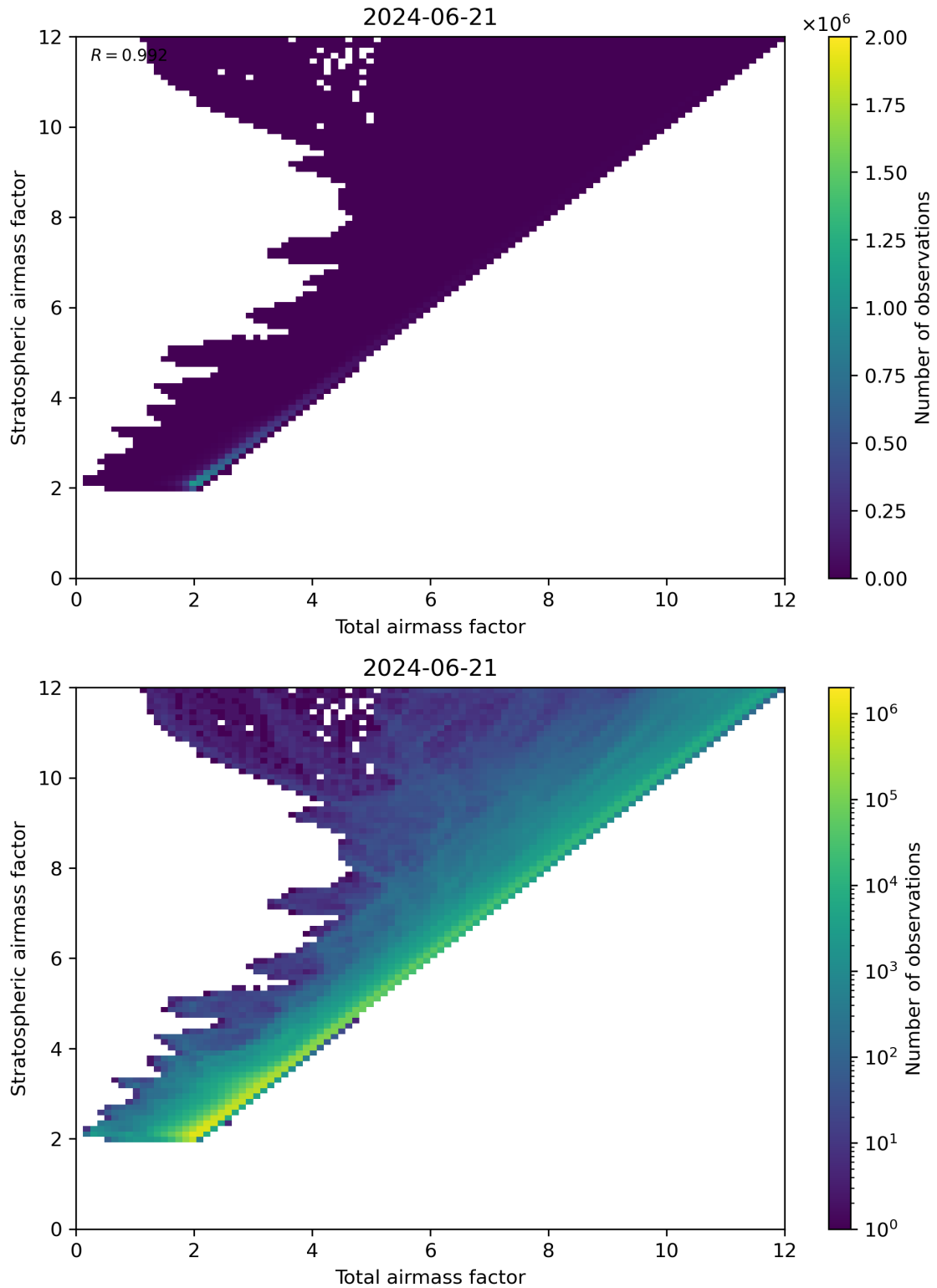
Figure 62: Scatter density plot of “Total airmass factor” against “Stratospheric airmass factor” for 2024-06-20 to 2024-06-22.
