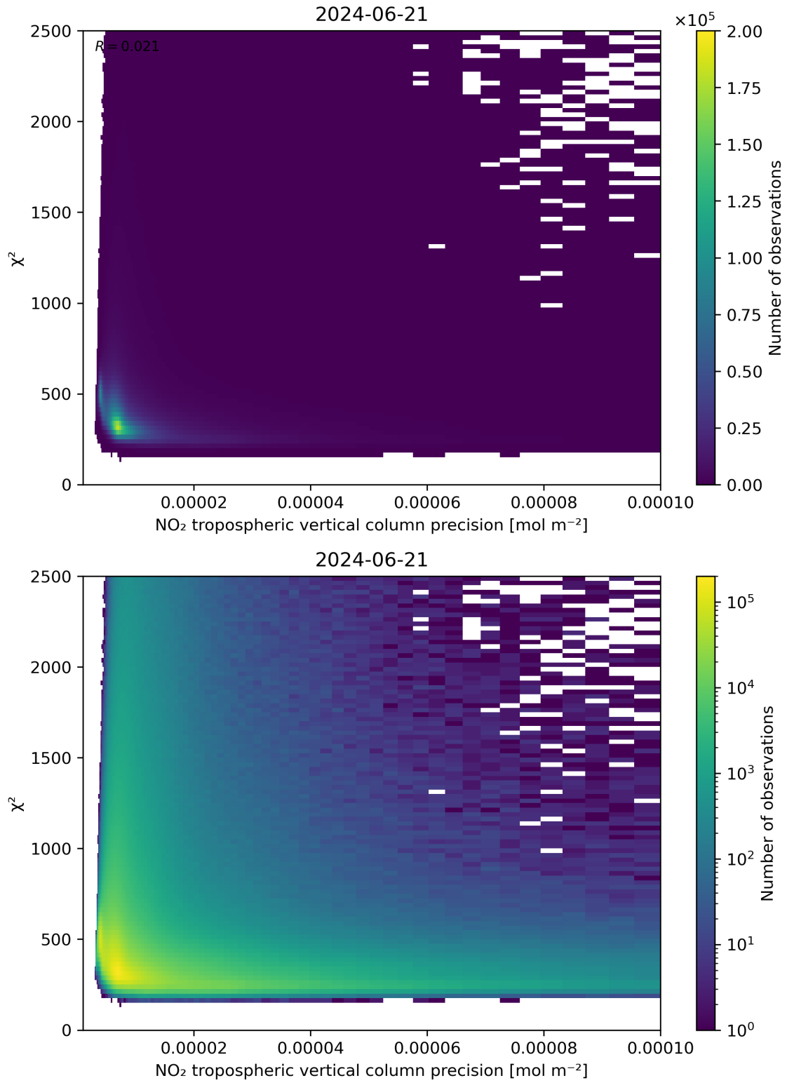
Figure 134: Scatter density plot of “NO 2 tropospheric vertical column precision” against “ \chi^2 ” for 2024-06-20 to 2024-06-22.
