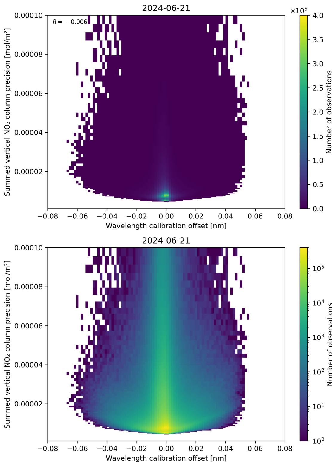
Figure 178: Scatter density plot of “Wavelength calibration offset” against “Summed vertical NO 2 column precision” for 2024-06-20 to 2024-06-22.
