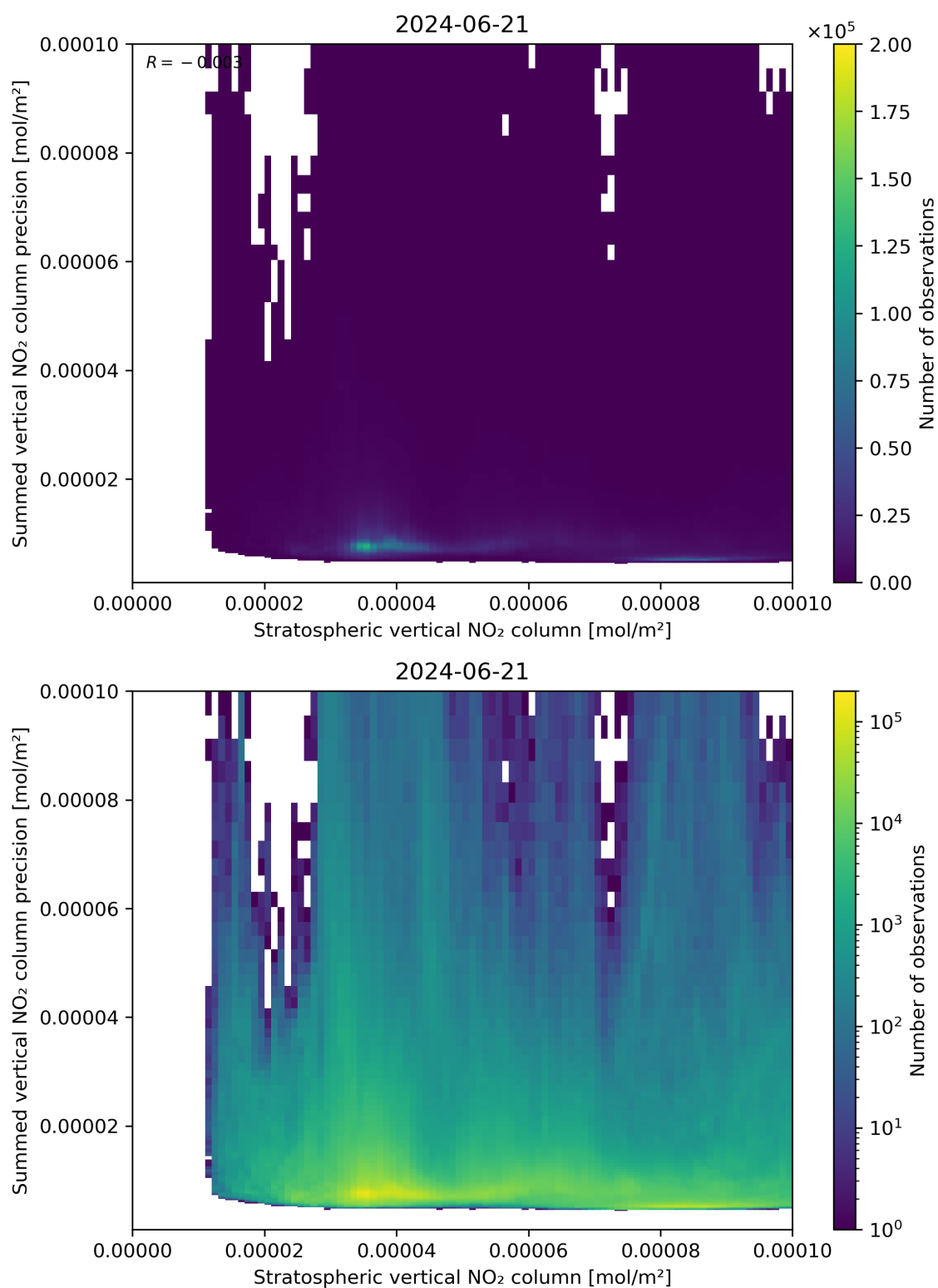
Figure 99: Scatter density plot of “Stratospheric vertical NO 2 column” against “Summed vertical NO 2 column precision” for 2024-06-20 to 2024-06-22.
