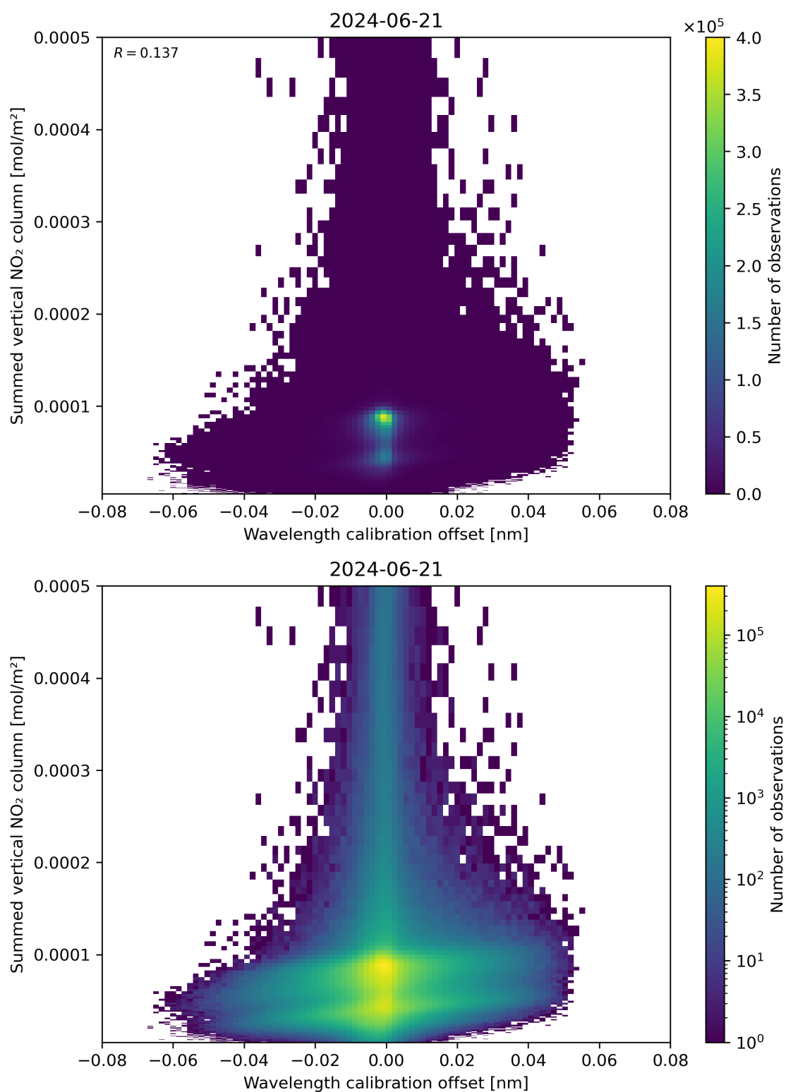
Figure 177: Scatter density plot of “Wavelength calibration offset” against “Summed vertical NO 2 column” for 2024-06-20 to 2024-06-22.
