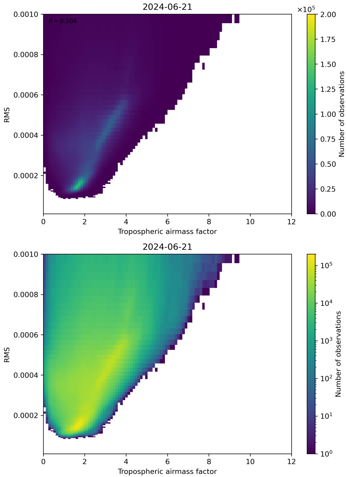
Figure 79: Scatter density plot of “Tropospheric airmass factor” against “RMS” for 2024-06-20 to 2024-06-22.
