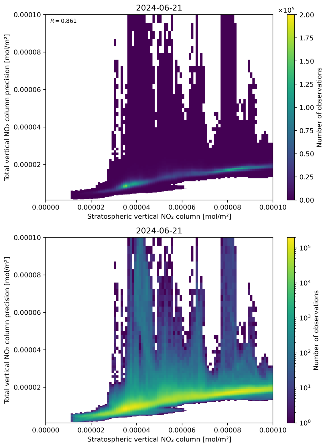
Figure 101: Scatter density plot of “Stratospheric vertical NO 2 column” against “Total vertical NO 2 column precision” for 2024-06-20 to 2024-06-22.
