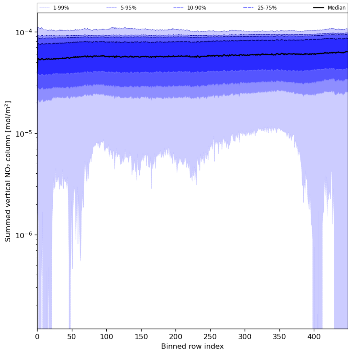
Figure 57: Along track statistics of “Summed vertical NO 2 column” for 2024-06-20 to 2024-06-22
