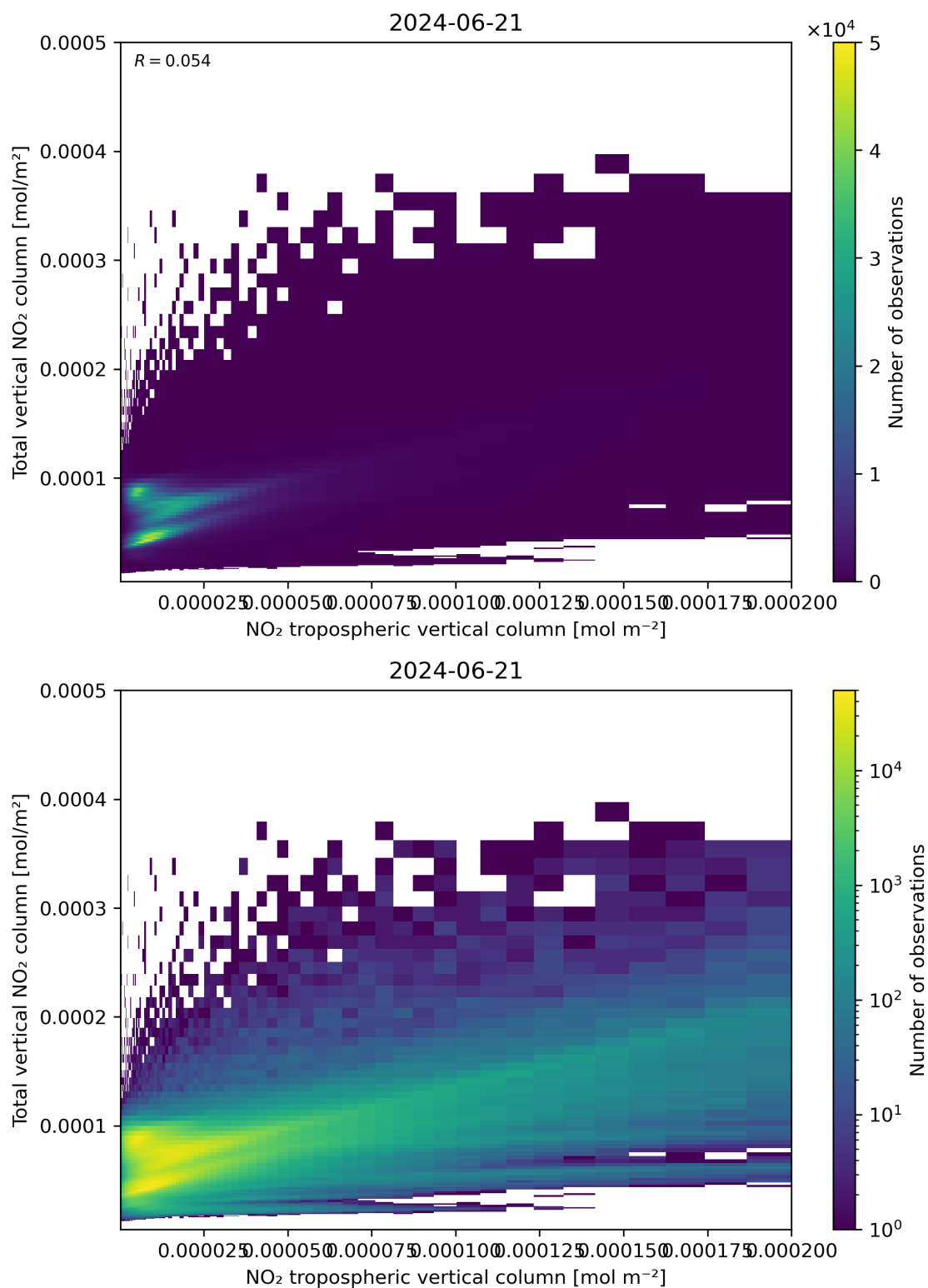
Figure 128: Scatter density plot of “NO 2 tropospheric vertical column” against “Total vertical NO 2 column” for 2024-06-20 to 2024-06-22.
