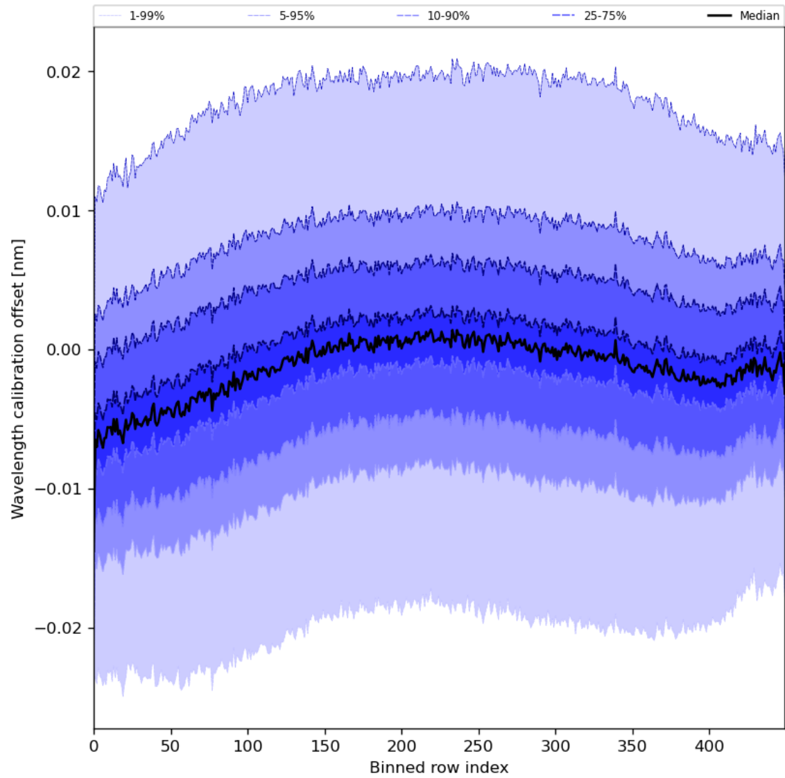
Figure 52: Along track statistics of “Wavelength calibration offset” for 2024-06-20 to 2024-06-22
