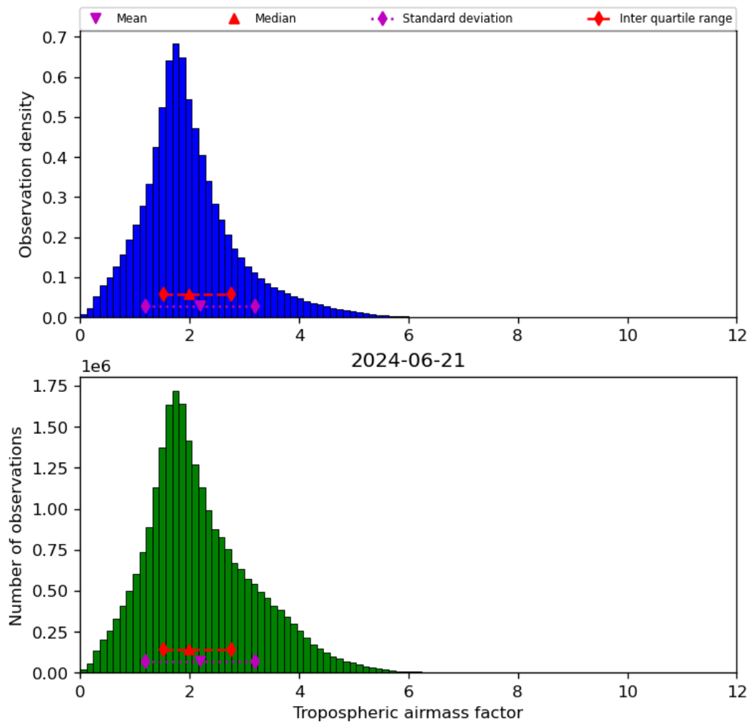
Figure 31: Histogram of “Tropospheric airmass factor” for 2024-06-20 to 2024-06-22
