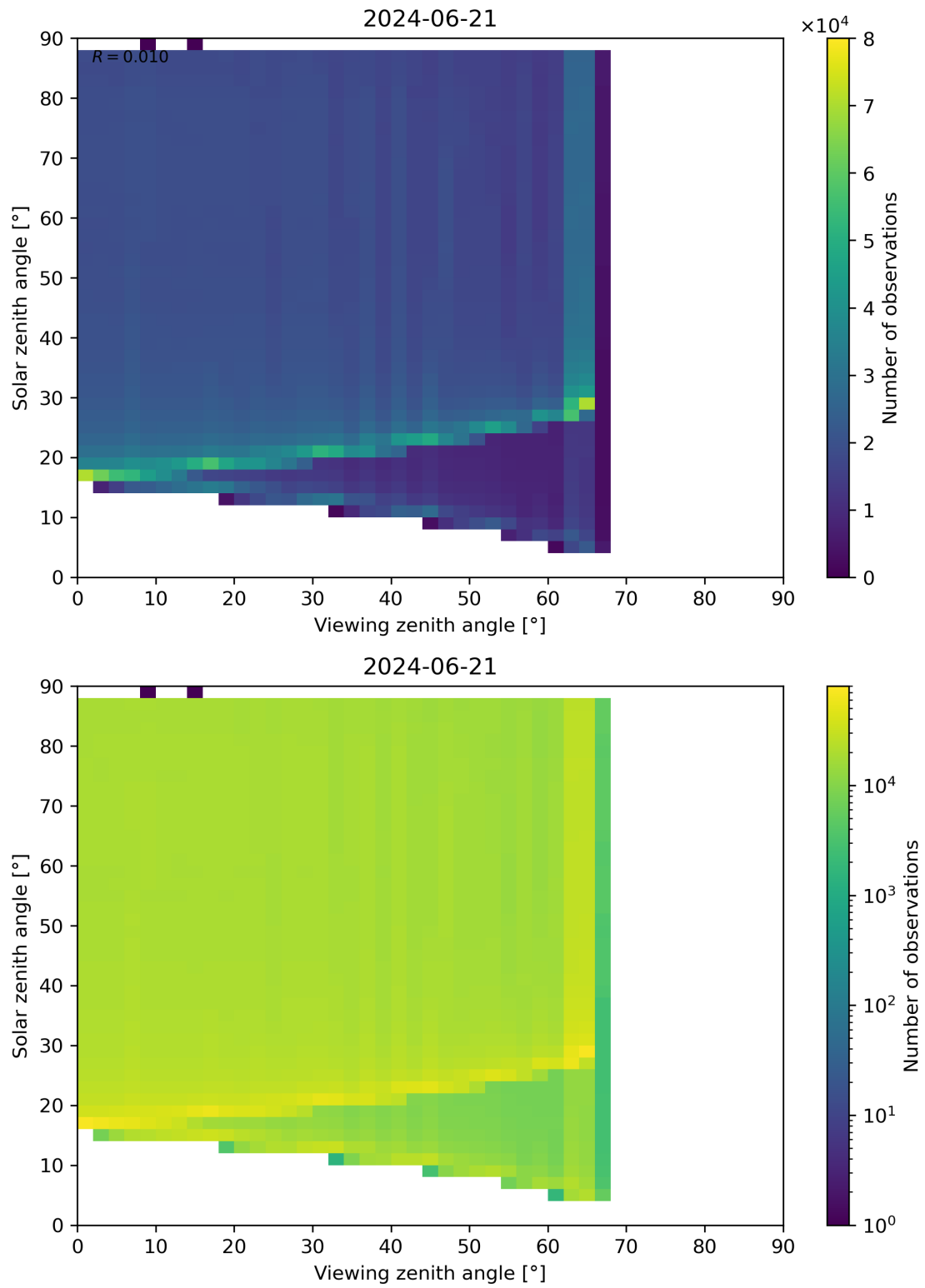
Figure 172: Scatter density plot of “Viewing zenith angle” against “Solar zenith angle” for 2024-06-20 to 2024-06-22.
