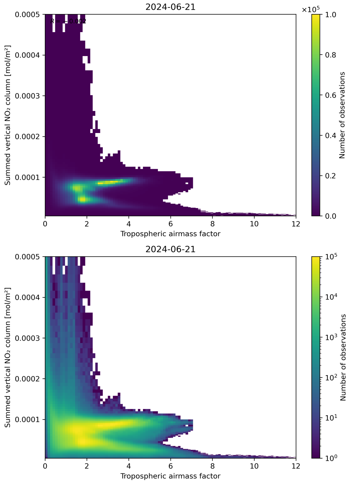
Figure 75: Scatter density plot of “Tropospheric airmass factor” against “Summed vertical NO 2 column” for 2024-06-20 to 2024-06-22.
