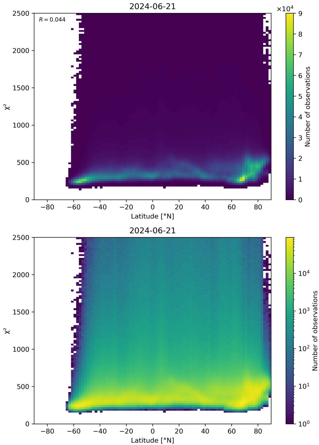
Figure 86: Scatter density plot of “Latitude” against “ \chi^2 ” for 2024-06-20 to 2024-06-22.
