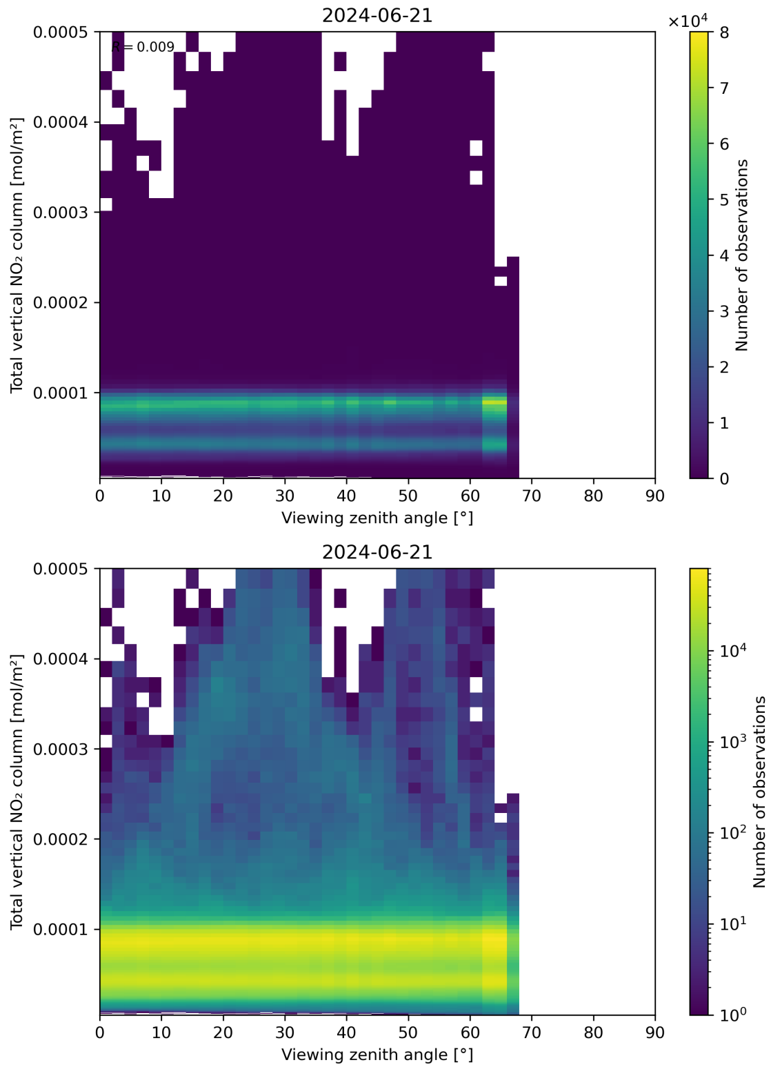
Figure 167: Scatter density plot of “Viewing zenith angle” against “Total vertical NO 2 column” for 2024-06-20 to 2024-06-22.
