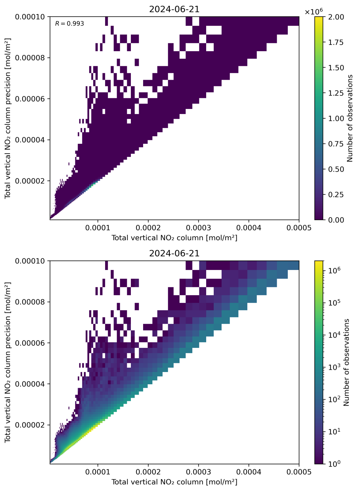
Figure 114: Scatter density plot of “Total vertical NO 2 column” against “Total vertical NO 2 column precision” for 2024-06-20 to 2024-06-22.
