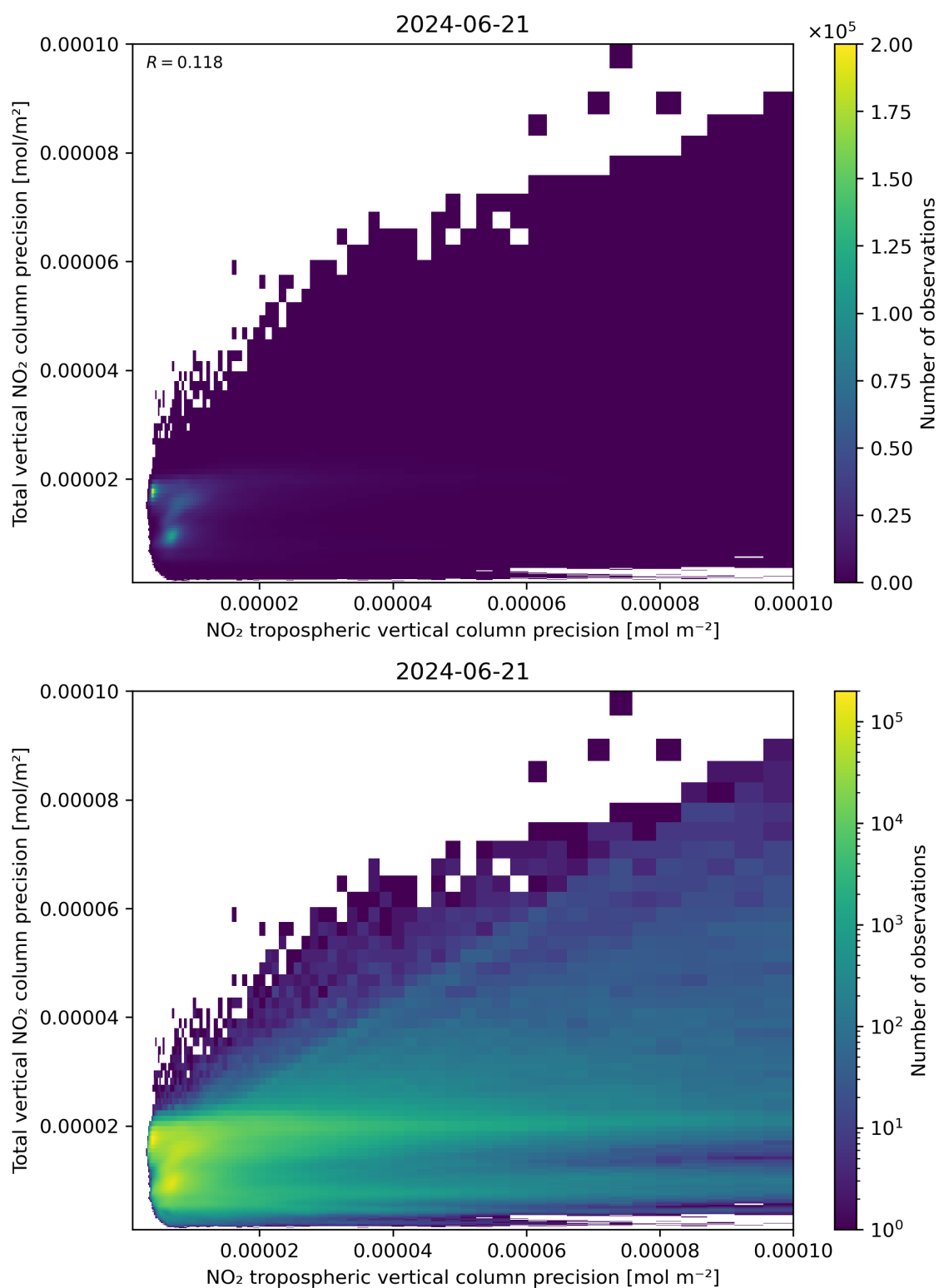
Figure 139: Scatter density plot of “NO 2 tropospheric vertical column precision” against “Total vertical NO 2 column precision” for 2024-06-20 to 2024-06-22.
