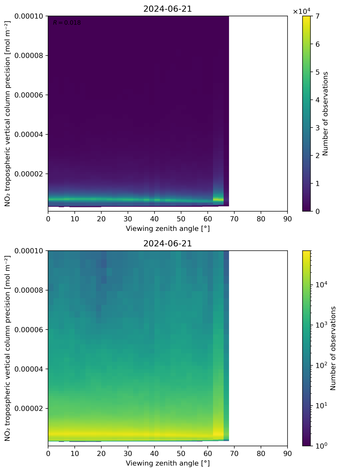
Figure 170: Scatter density plot of “Viewing zenith angle” against “NO 2 tropospheric vertical column precision” for 2024-06-20 to 2024-06-22.
