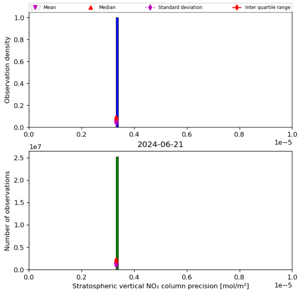
Figure 37: Histogram of “Stratospheric vertical NO 2 column precision” for 2024-06-20 to 2024-06-22
