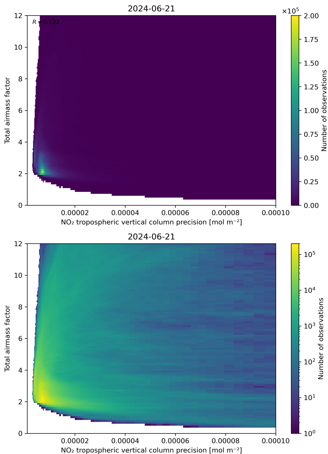
Figure 132: Scatter density plot of “NO 2 tropospheric vertical column precision” against “Total air mass factor” for 2024-06-20 to 2024-06-22.
