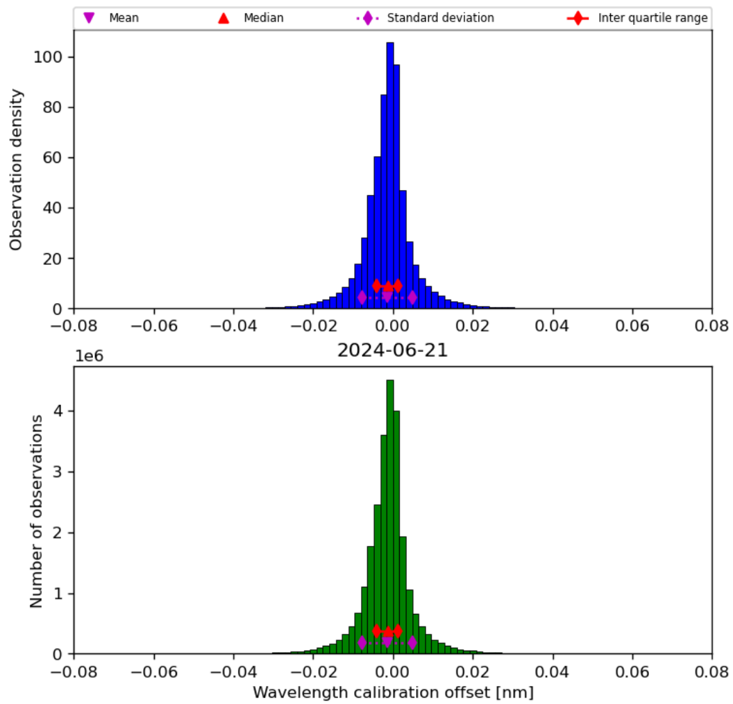
Figure 35: Histogram of “Wavelength calibration offset” for 2024-06-20 to 2024-06-22
