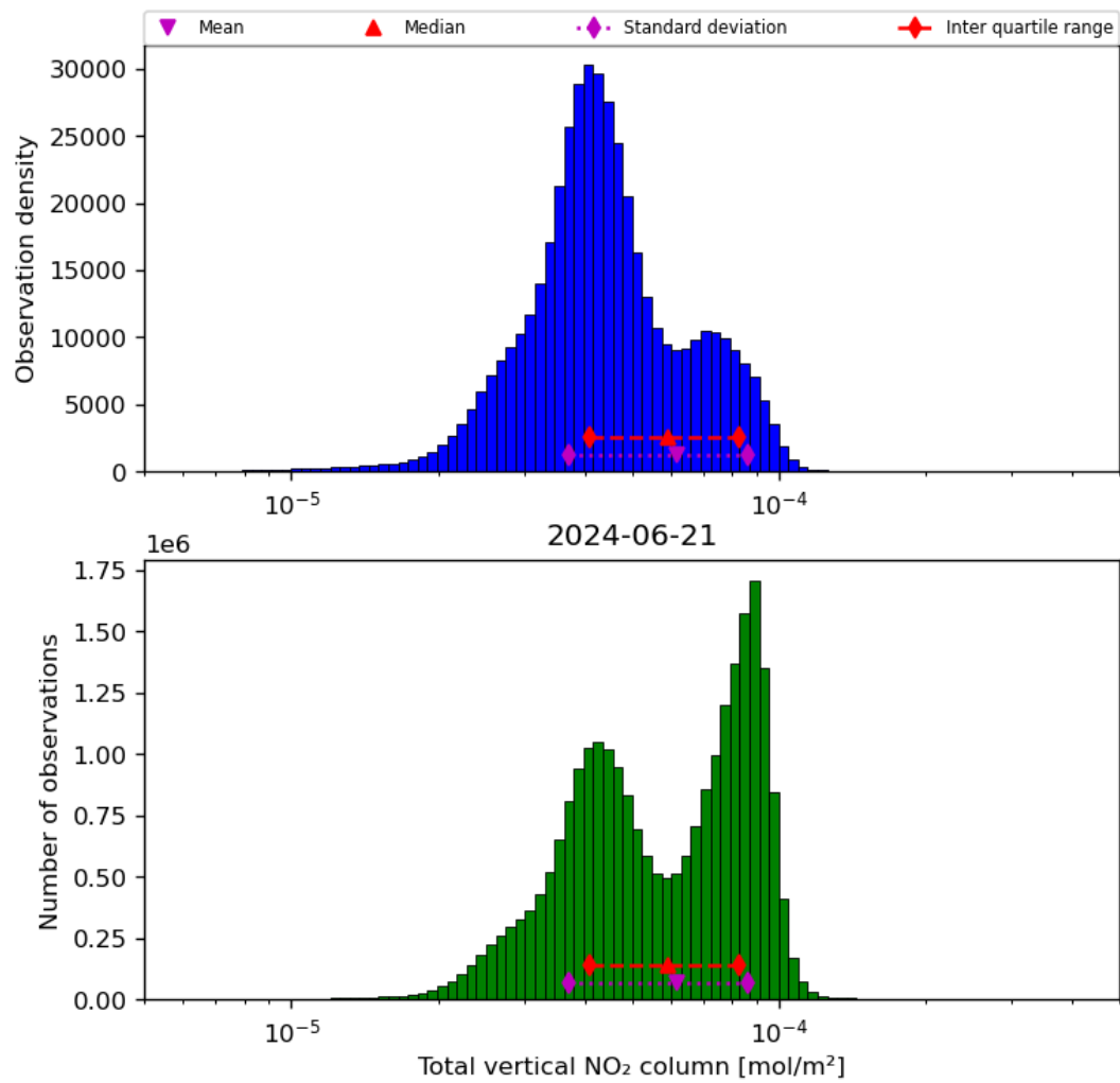
Figure 38: Histogram of “Total vertical NO 2 column” for 2024-06-20 to 2024-06-22
