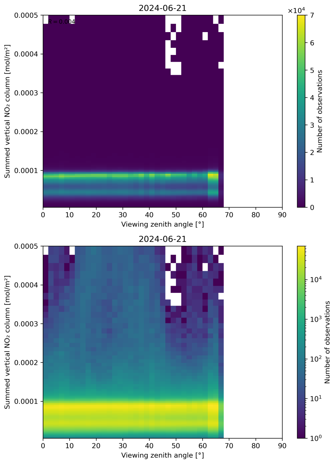
Figure 165: Scatter density plot of “Viewing zenith angle” against “Summed vertical NO 2 column” for 2024-06-20 to 2024-06-22.
