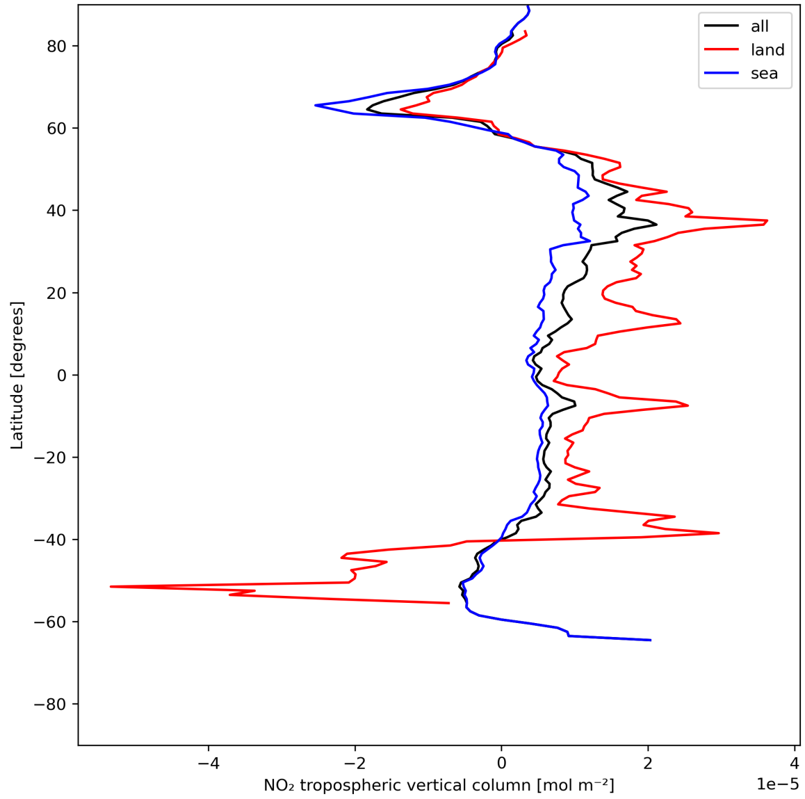
Figure 12: Zonal average of “NO 2 tropospheric vertical column” for 2024-06-20 to 2024-06-22.
