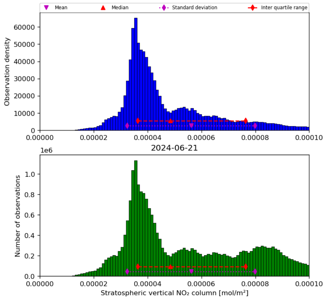
Figure 36: Histogram of “Stratospheric vertical NO 2 column” for 2024-06-20 to 2024-06-22
