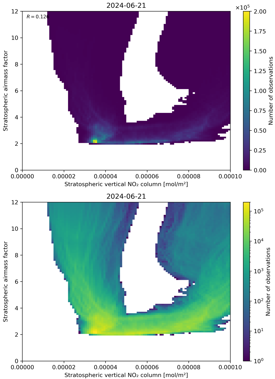
Figure 96: Scatter density plot of “Stratospheric vertical NO 2 column” against “Stratospheric airmass factor” for 2024-06-20 to 2024-06-22.
