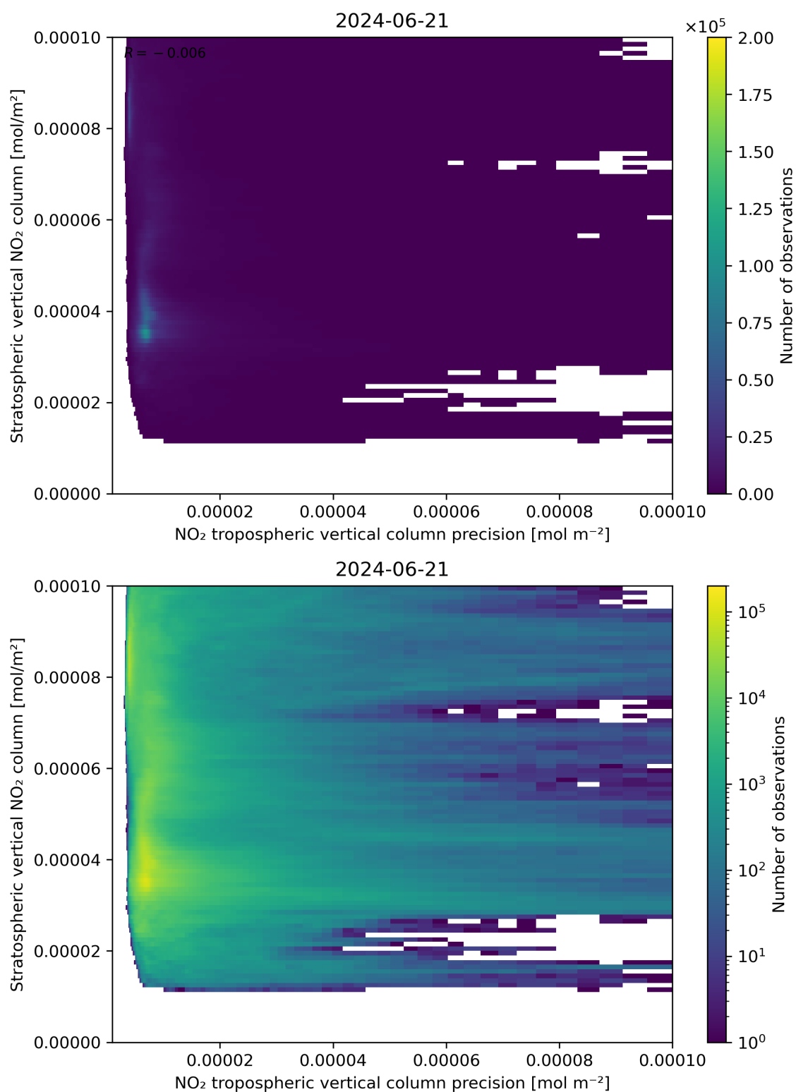
Figure 135: Scatter density plot of “NO 2 tropospheric vertical column precision” against “Stratospheric vertical NO 2 column” for 2024-06-20 to 2024-06-22.
