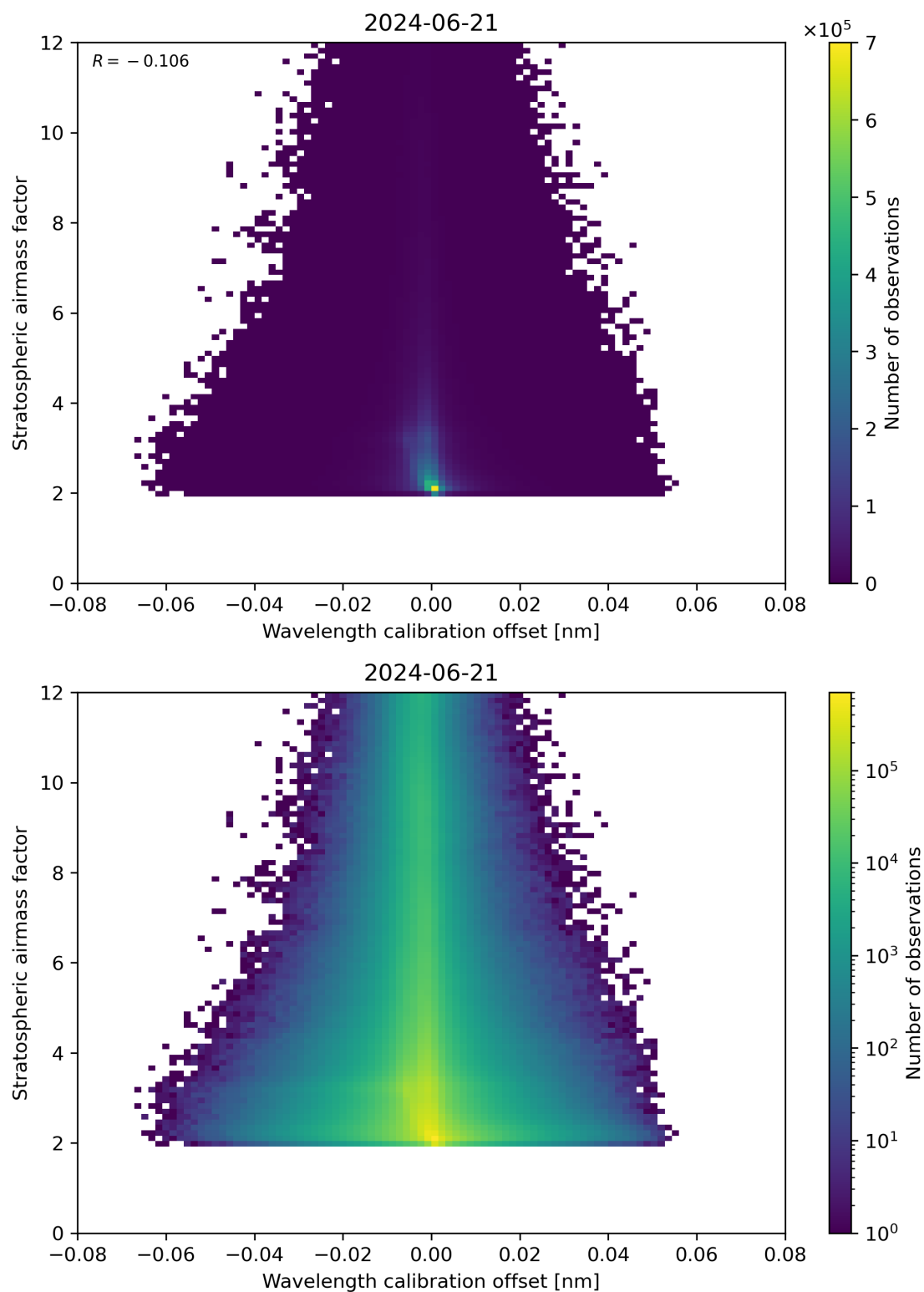
Figure 174: Scatter density plot of “Wavelength calibration offset” against “Stratospheric air mass factor” for 2024-06-20 to 2024-06-22.
