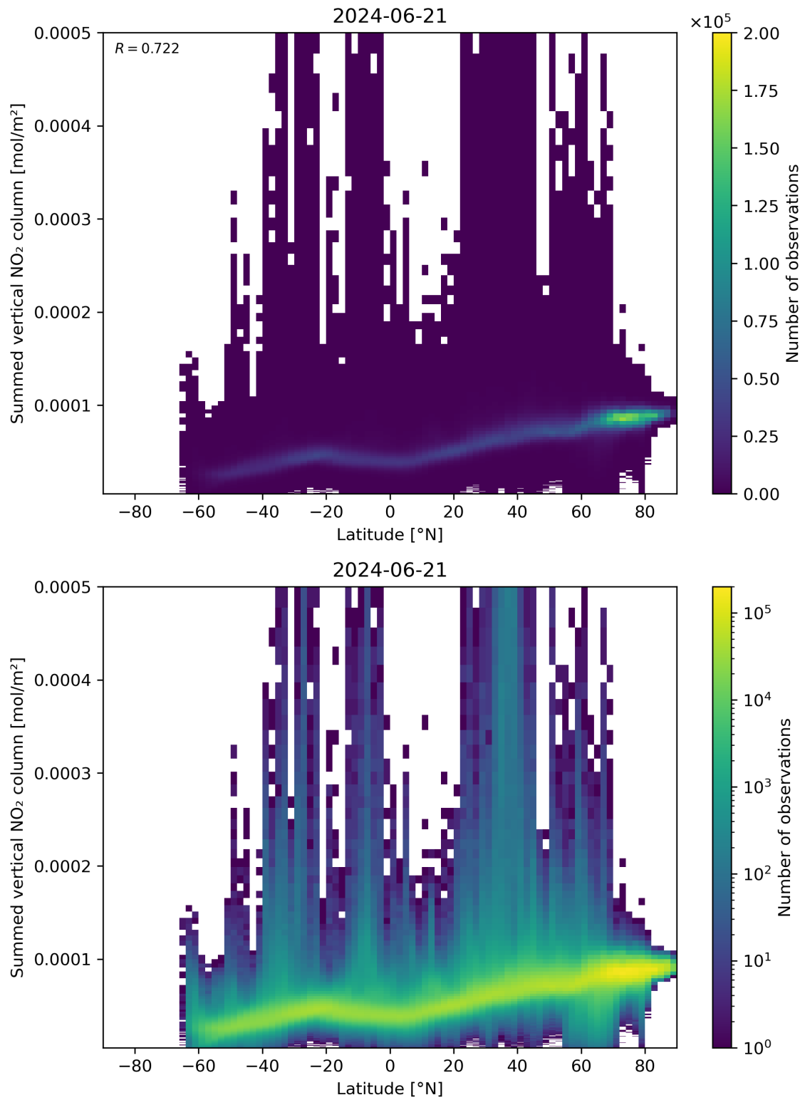
Figure 88: Scatter density plot of “Latitude” against “Summed vertical NO 2 column” for 2024-06-20 to 2024-06-22.
