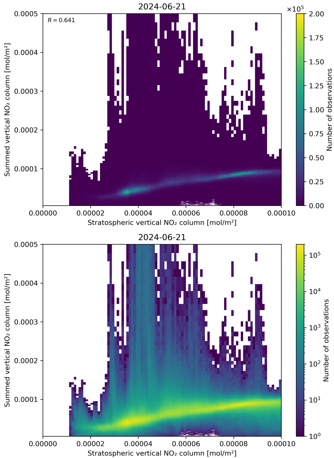
Figure 98: Scatter density plot of “Stratospheric vertical NO 2 column” against “Summed vertical NO 2 column” for 2024-06-20 to 2024-06-22.
