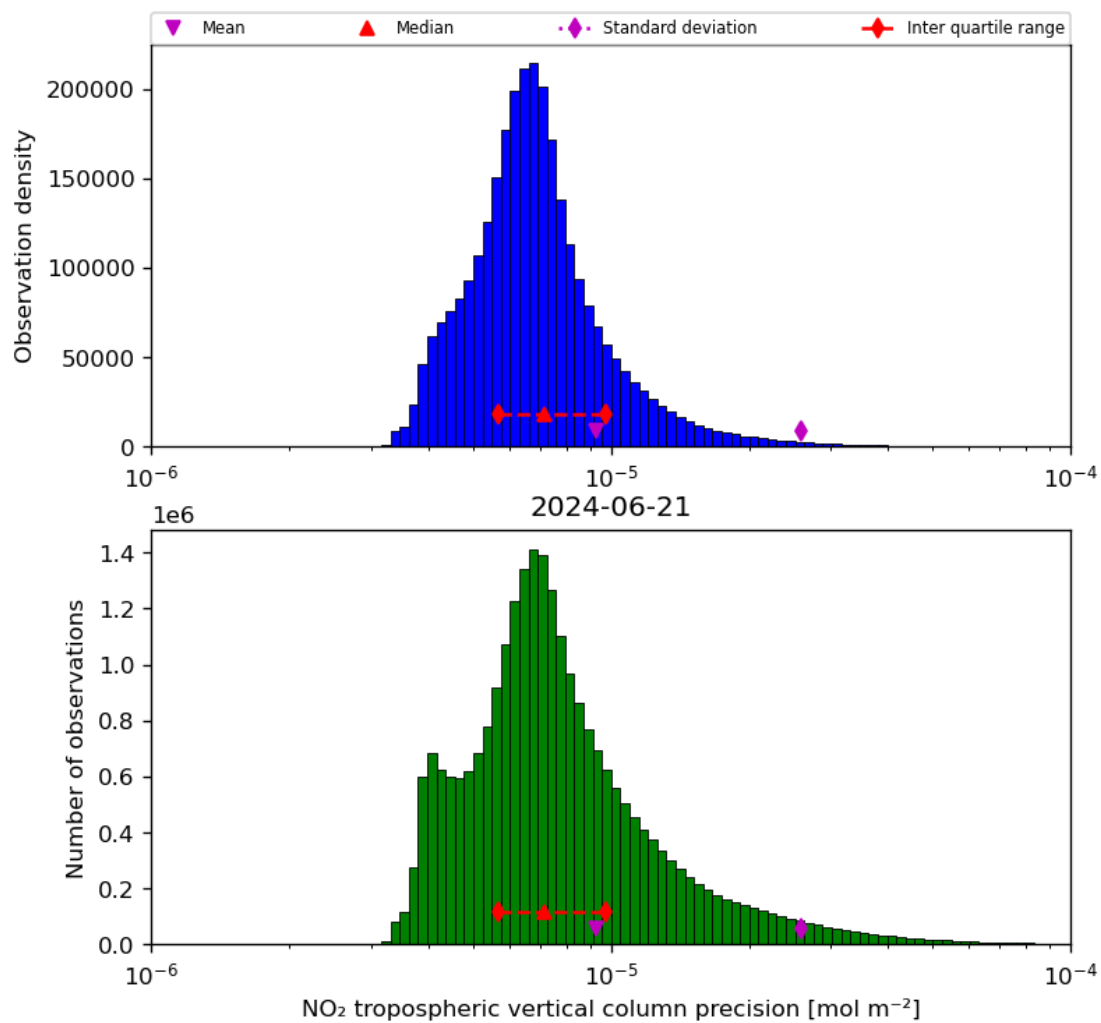
Figure 30: Histogram of “NO 2 tropospheric vertical column precision” for 2024-06-20 to 2024-06-22
