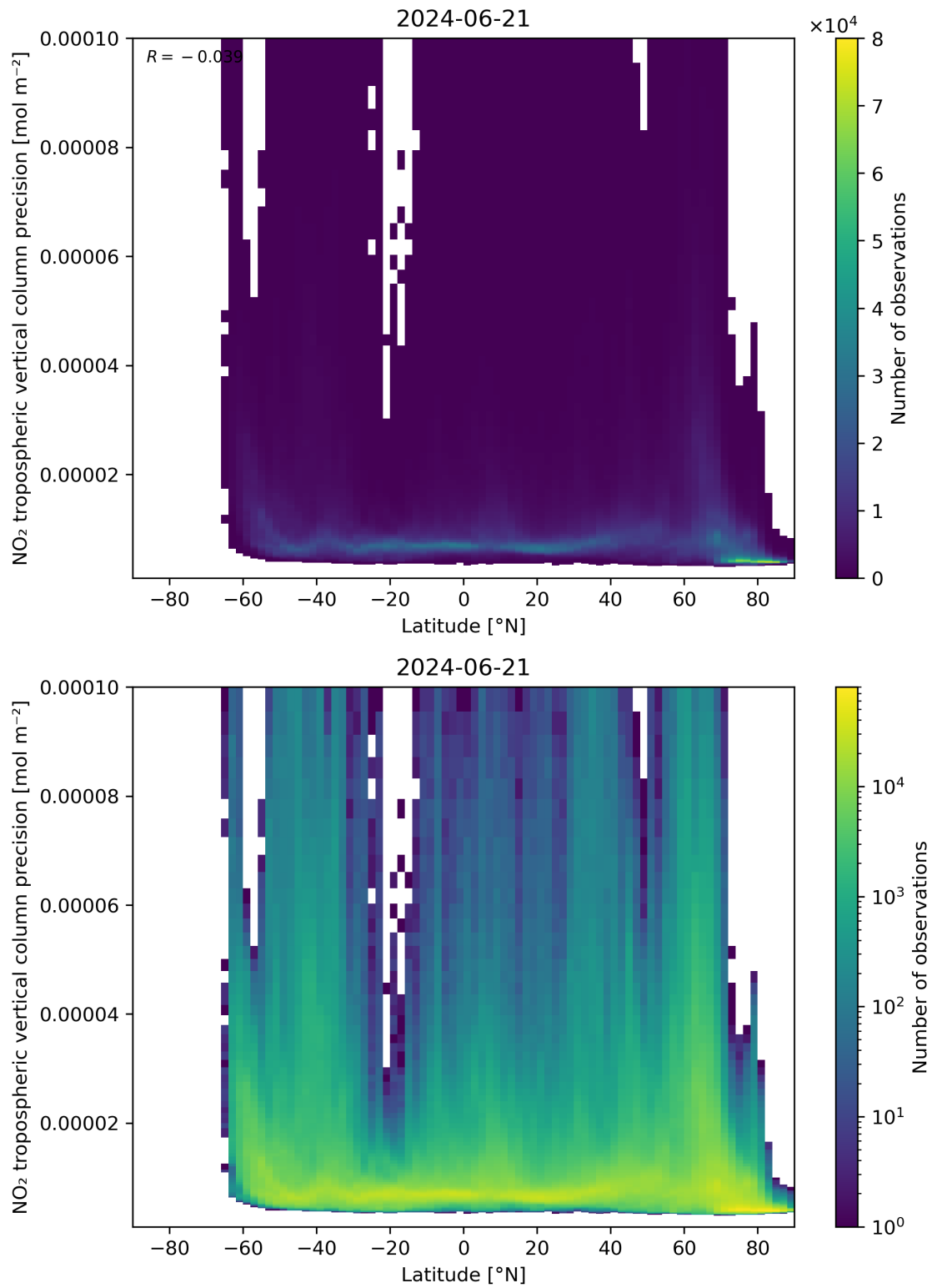
Figure 93: Scatter density plot of “Latitude” against “NO 2 tropospheric vertical column precision” for 2024-06-20 to 2024-06-22.
