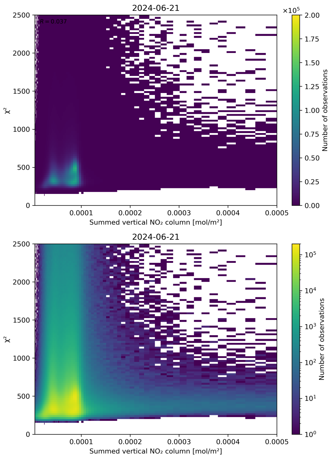
Figure 104: Scatter density plot of “Summed vertical NO 2 column” against “ \chi^2 ” for 2024-06-20 to 2024-06-22.
