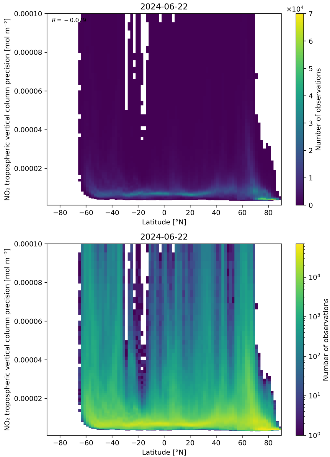
Figure 93: Scatter density plot of “Latitude” against “NO 2 tropospheric vertical column precision” for 2024-06-21 to 2024-06-23.
