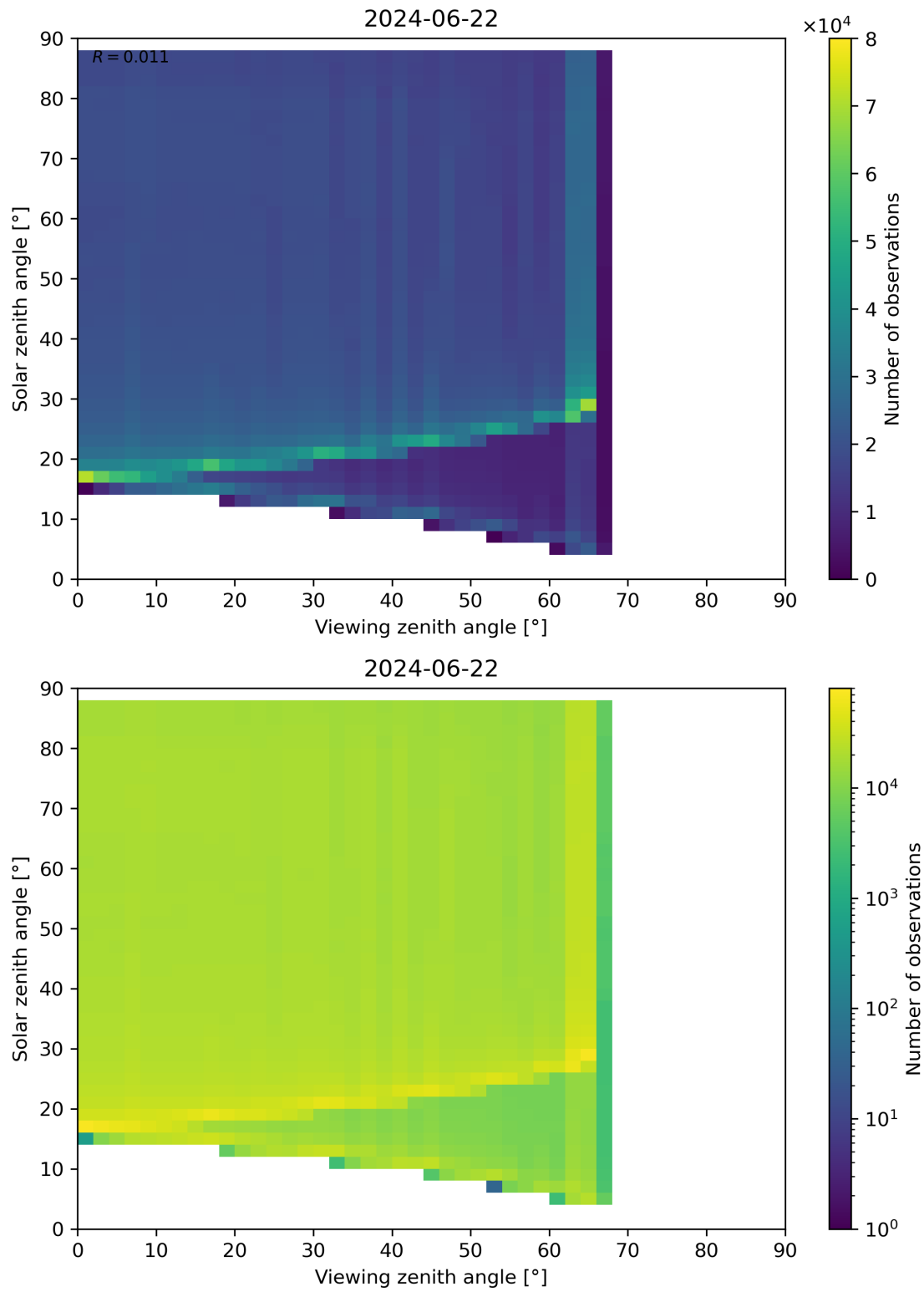
Figure 172: Scatter density plot of “Viewing zenith angle” against “Solar zenith angle” for 2024-06-21 to 2024-06-23.
