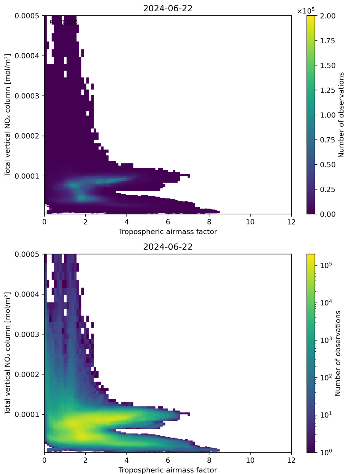
Figure 77: Scatter density plot of “Tropospheric airmass factor” against “Total vertical NO 2 column” for 2024-06-21 to 2024-06-23.
