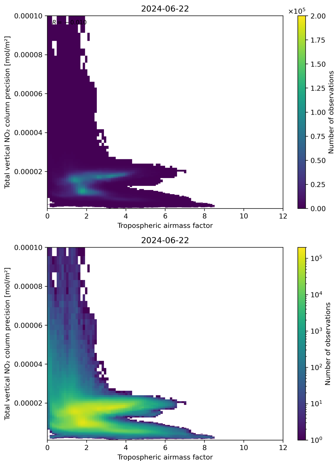
Figure 78: Scatter density plot of “Tropospheric airmass factor” against “Total vertical NO 2 column precision” for 2024-06-21 to 2024-06-23.
