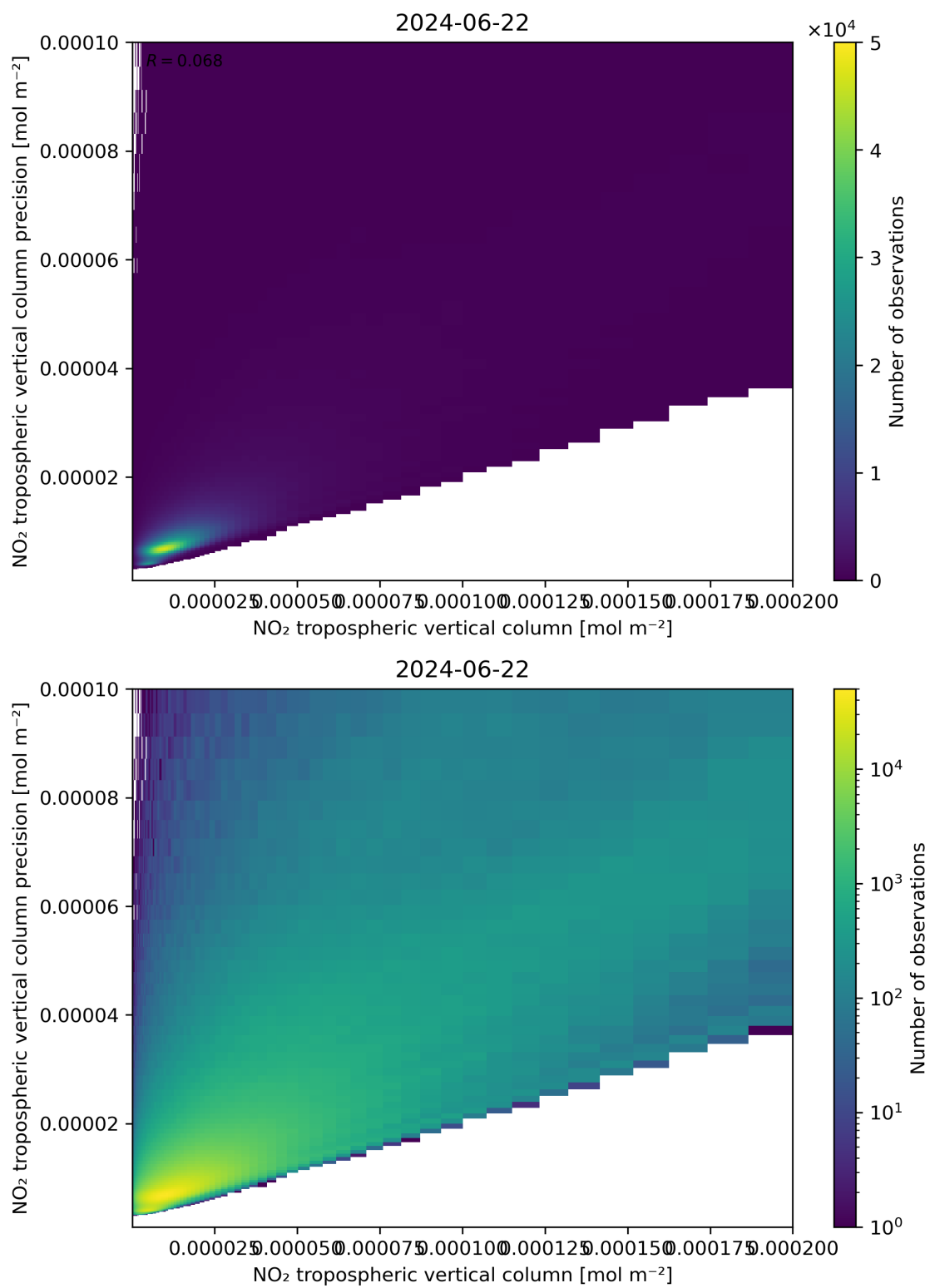
Figure 130: Scatter density plot of “NO 2 tropospheric vertical column” against “NO 2 tropospheric vertical column precision” for 2024-06-21 to 2024-06-23.
