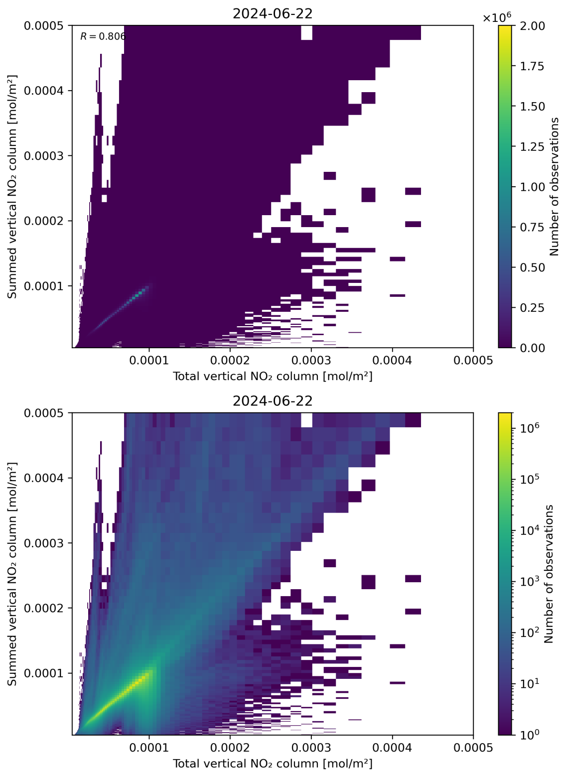
Figure 112: Scatter density plot of “Total vertical NO 2 column” against “Summed vertical NO 2 column” for 2024-06-21 to 2024-06-23.
