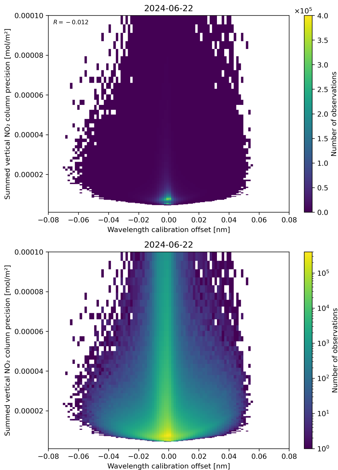
Figure 178: Scatter density plot of “Wavelength calibration offset” against “Summed vertical NO 2 column precision” for 2024-06-21 to 2024-06-23.
