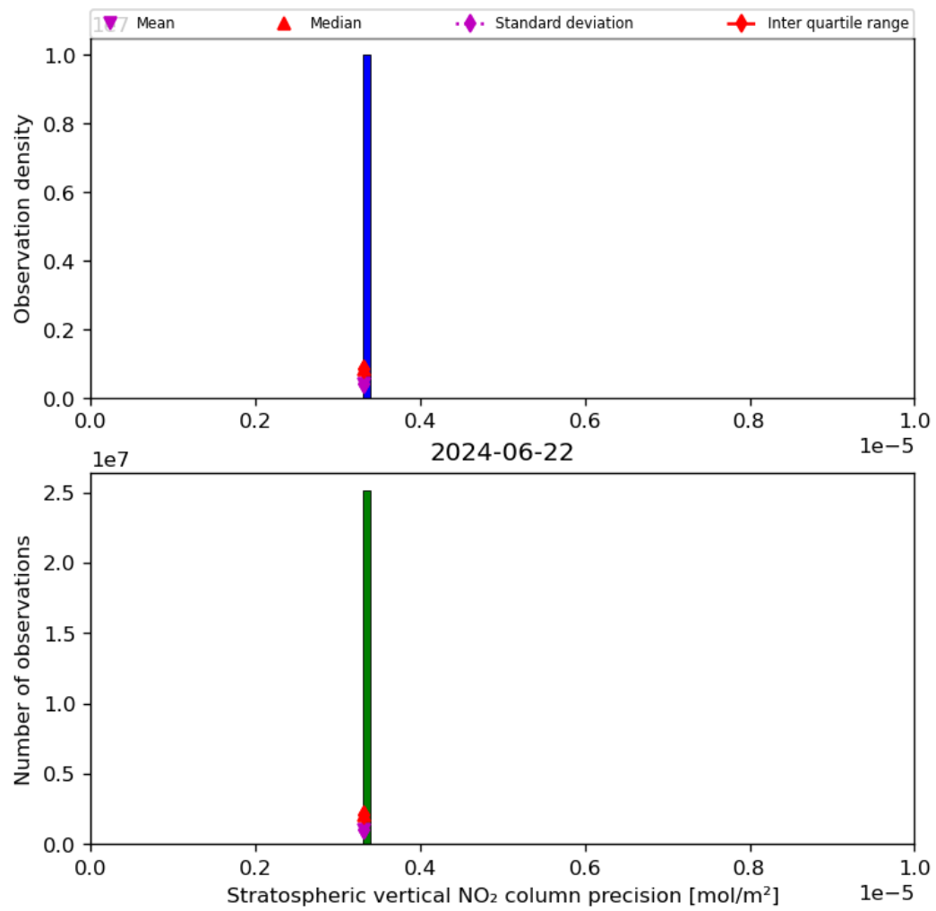
Figure 37: Histogram of “Stratospheric vertical NO 2 column precision” for 2024-06-21 to 2024-06-23
