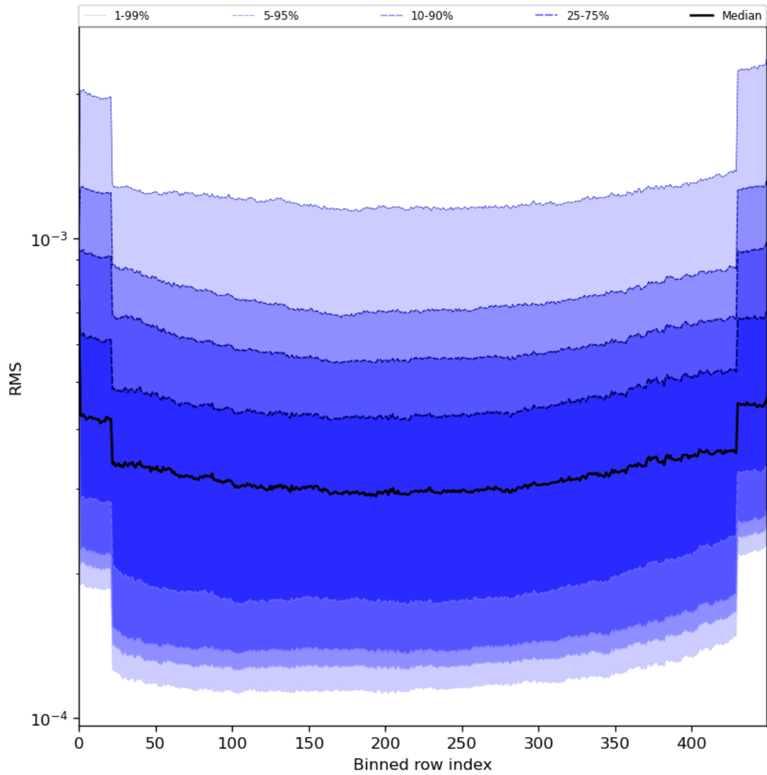
Figure 60: Along track statistics of “RMS” for 2024-06-21 to 2024-06-23
