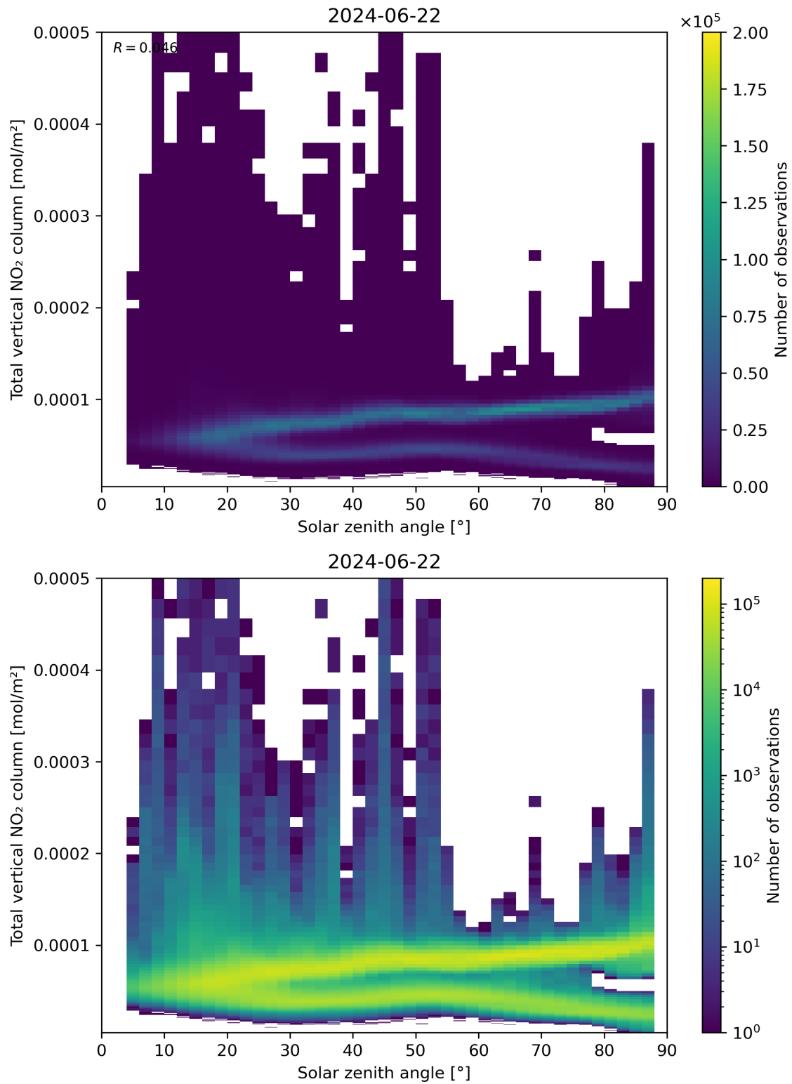
Figure 153: Scatter density plot of “Solar zenith angle” against “Total vertical NO 2 column” for 2024-06-21 to 2024-06-23.
