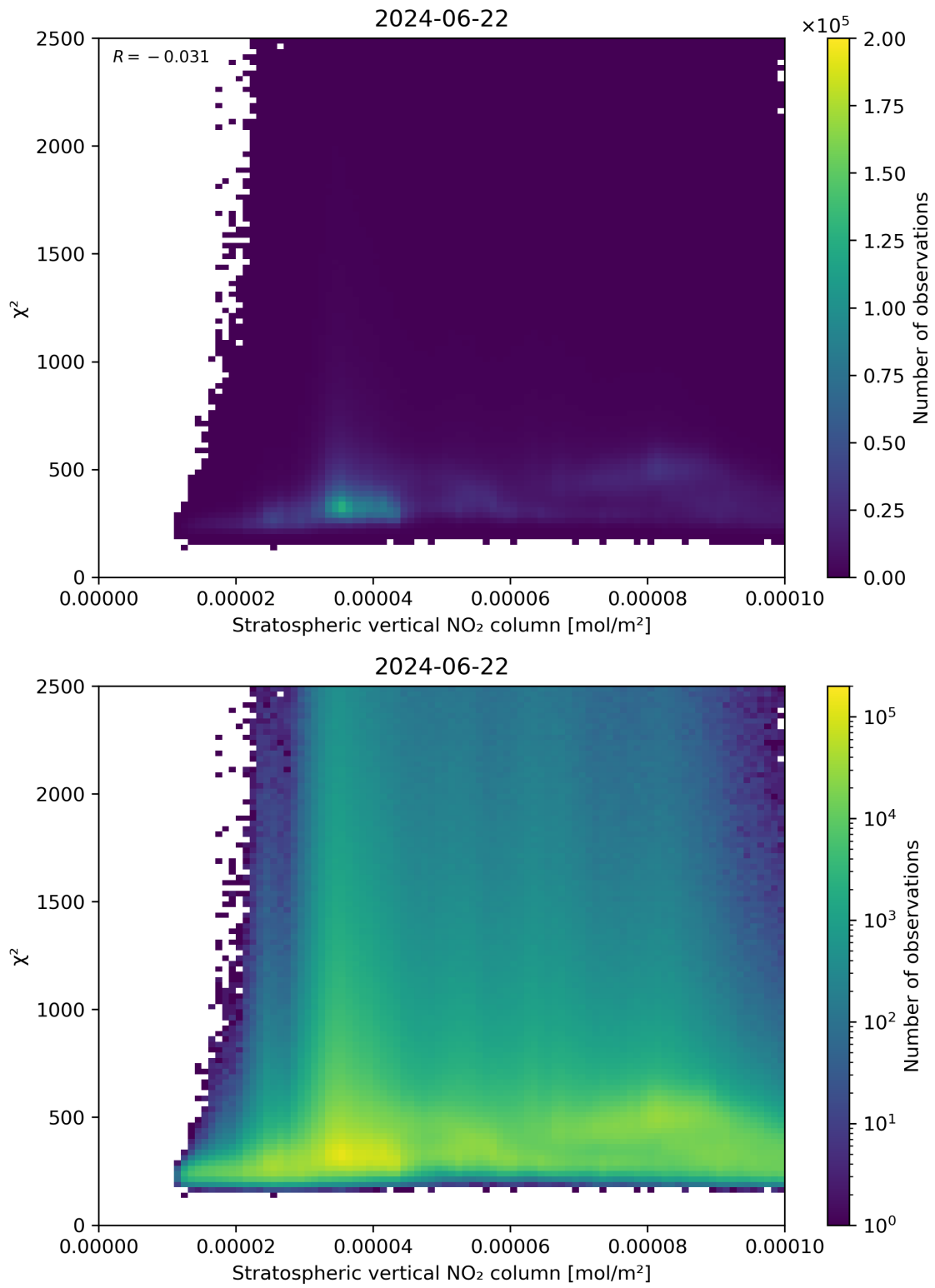
Figure 97: Scatter density plot of “Stratospheric vertical NO 2 column” against “ \chi^2 ” for 2024-06-21 to 2024-06-23.
