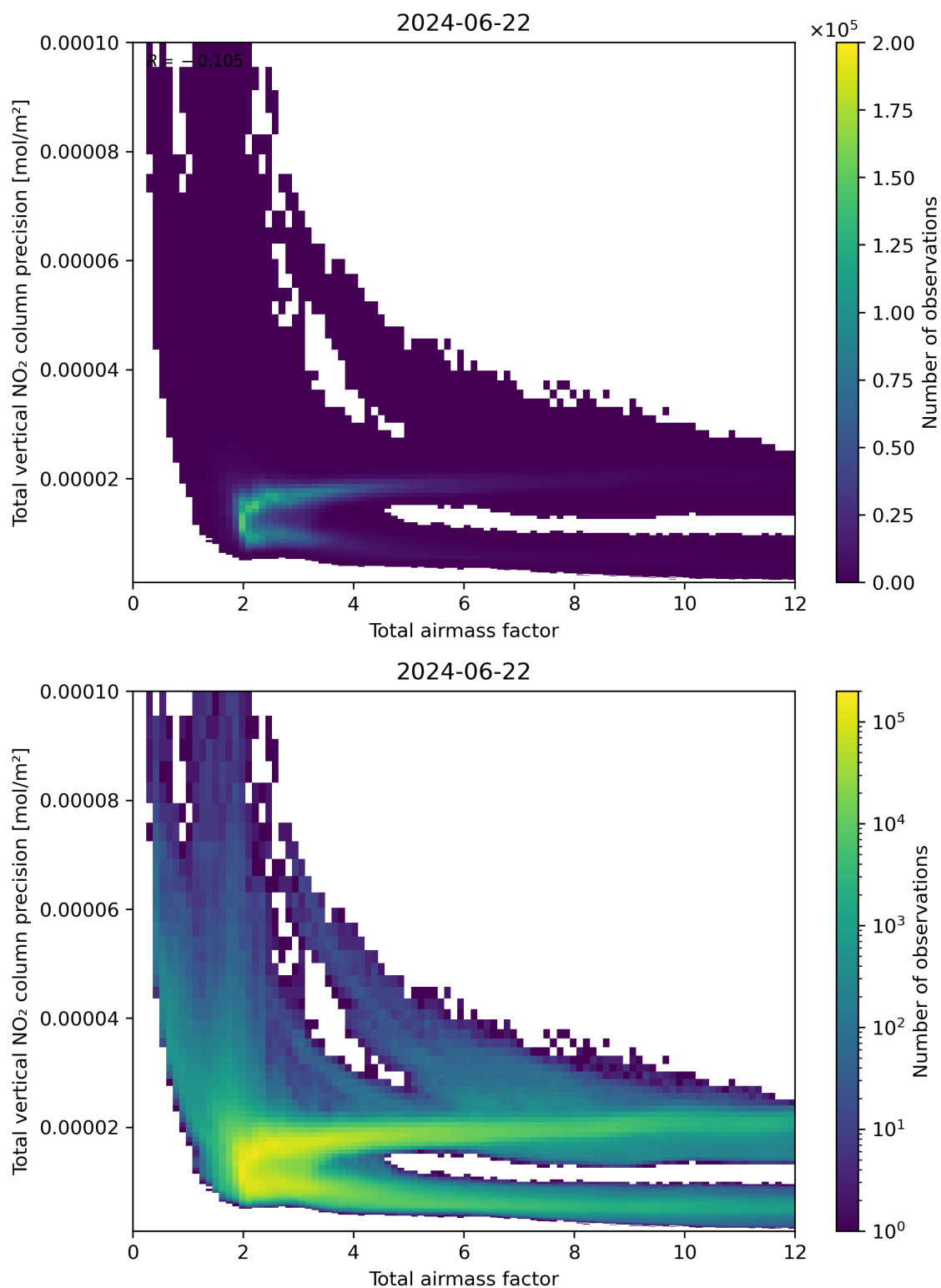
Figure 68: Scatter density plot of “Total airmass factor” against “Total vertical NO 2 column precision” for 2024-06-21 to 2024-06-23.
