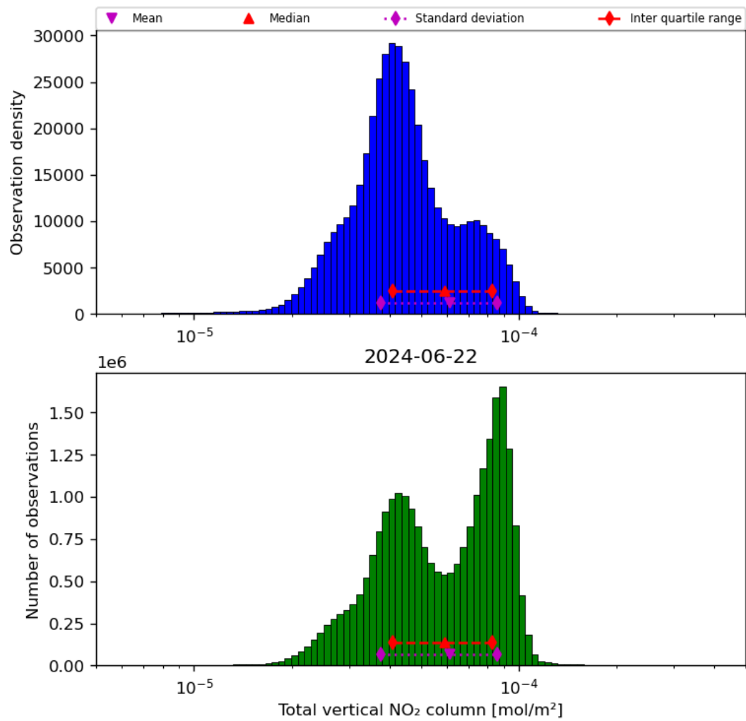
Figure 38: Histogram of “Total vertical NO 2 column” for 2024-06-21 to 2024-06-23
