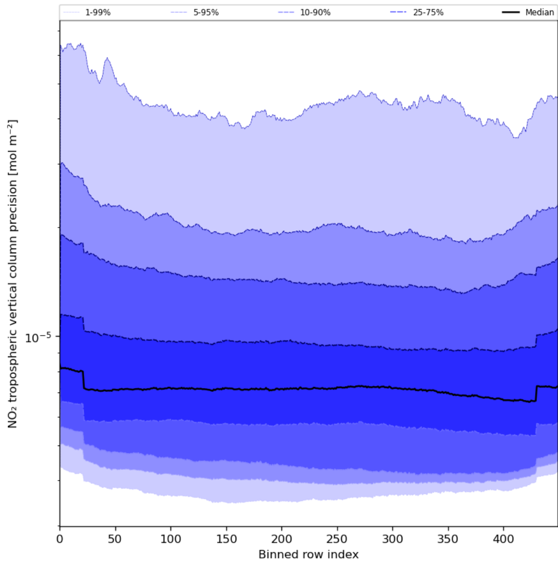
Figure 47: Along track statistics of “NO 2 tropospheric vertical column precision” for 2024-06-21 to 2024-06-23
