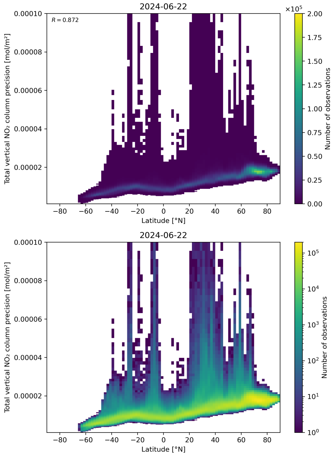
Figure 91: Scatter density plot of “Latitude” against “Total vertical NO 2 column precision” for 2024-06-21 to 2024-06-23.
