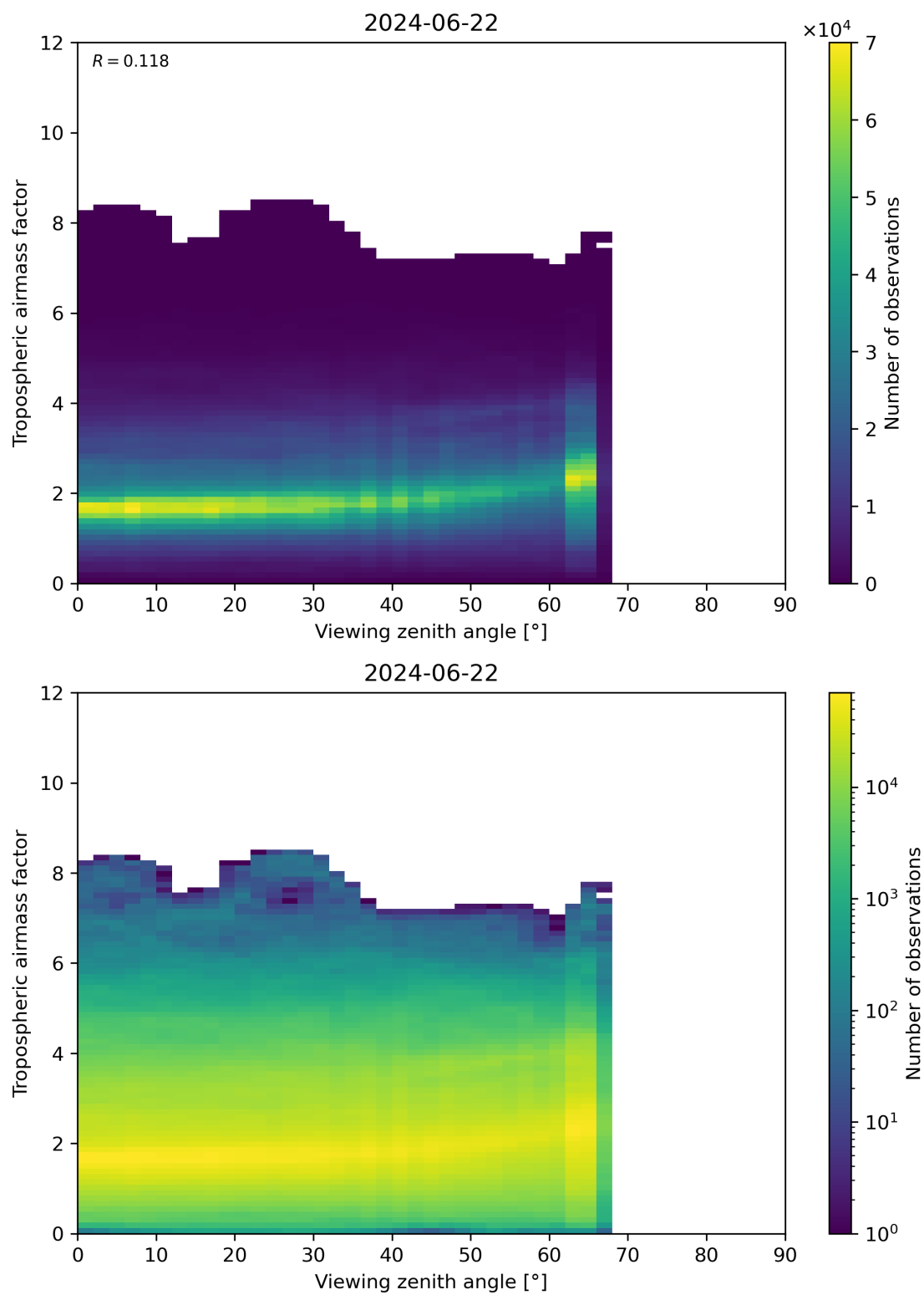
Figure 161: Scatter density plot of “Viewing zenith angle” against “Tropospheric airmass factor” for 2024-06-21 to 2024-06-23.
