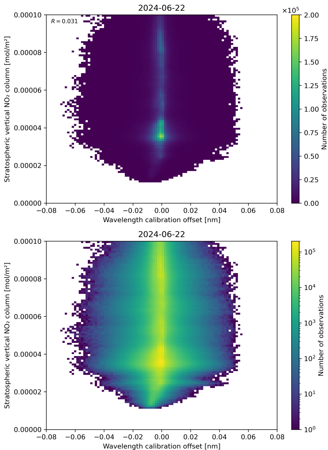
Figure 176: Scatter density plot of “Wavelength calibration offset” against “Stratospheric vertical NO 2 column” for 2024-06-21 to 2024-06-23.
