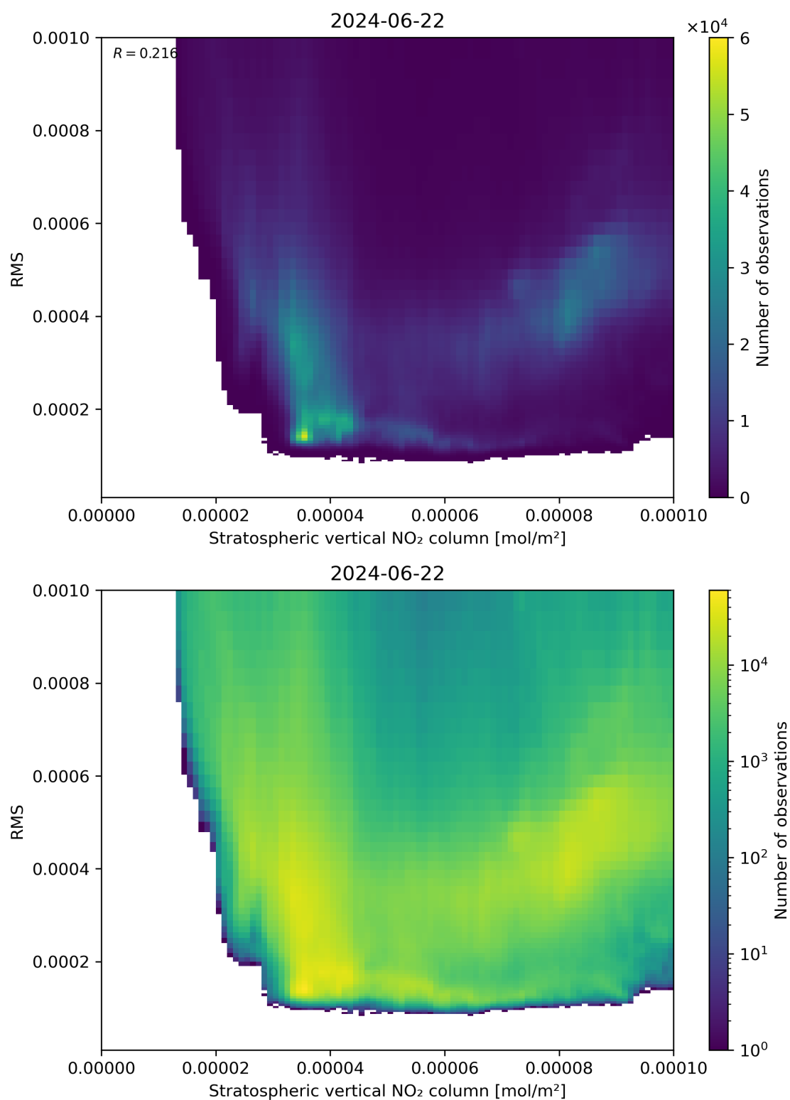
Figure 102: Scatter density plot of “Stratospheric vertical NO 2 column” against “RMS” for 2024-06-21 to 2024-06-23.
