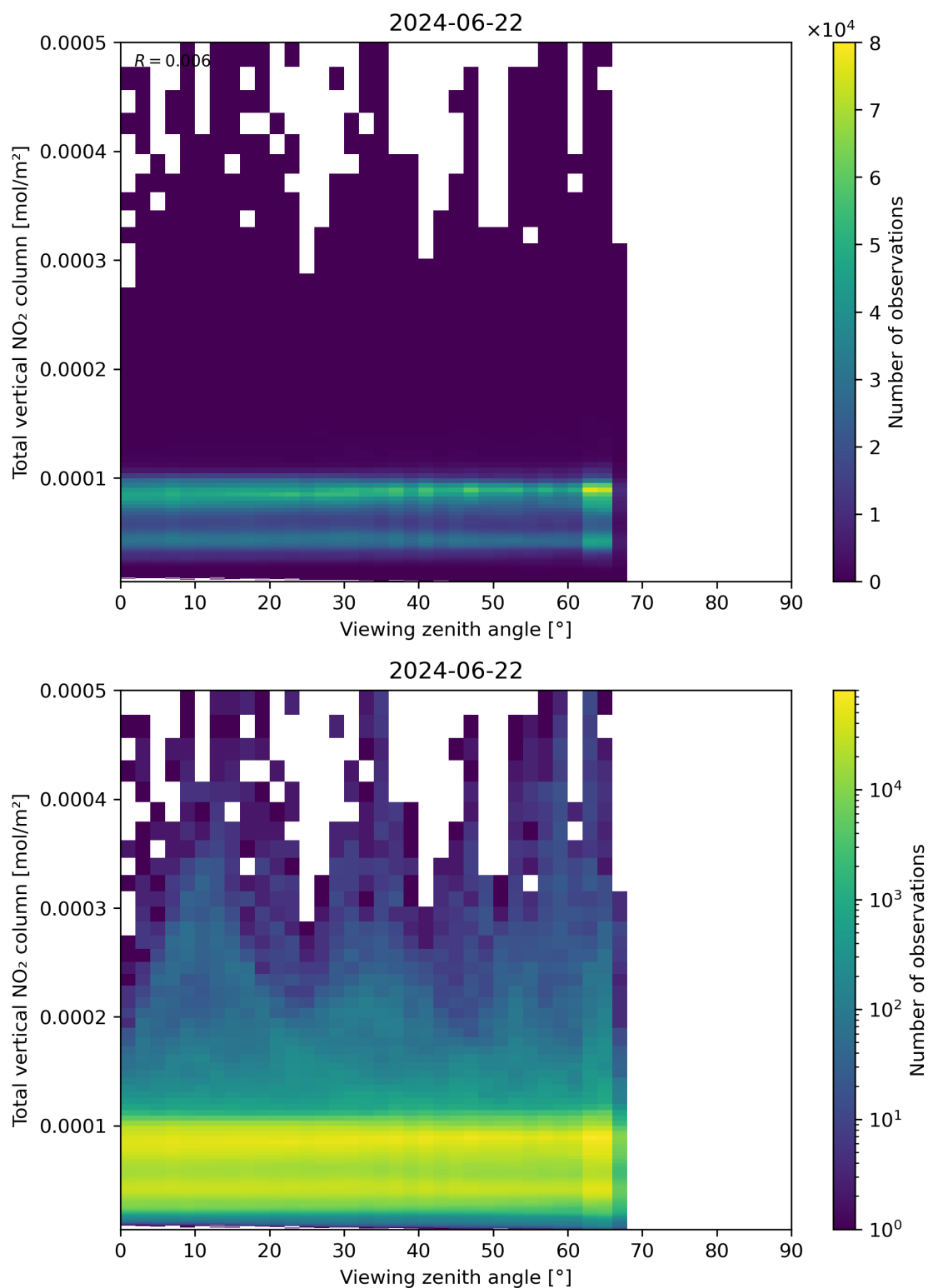
Figure 167: Scatter density plot of “Viewing zenith angle” against “Total vertical NO 2 column” for 2024-06-21 to 2024-06-23.
