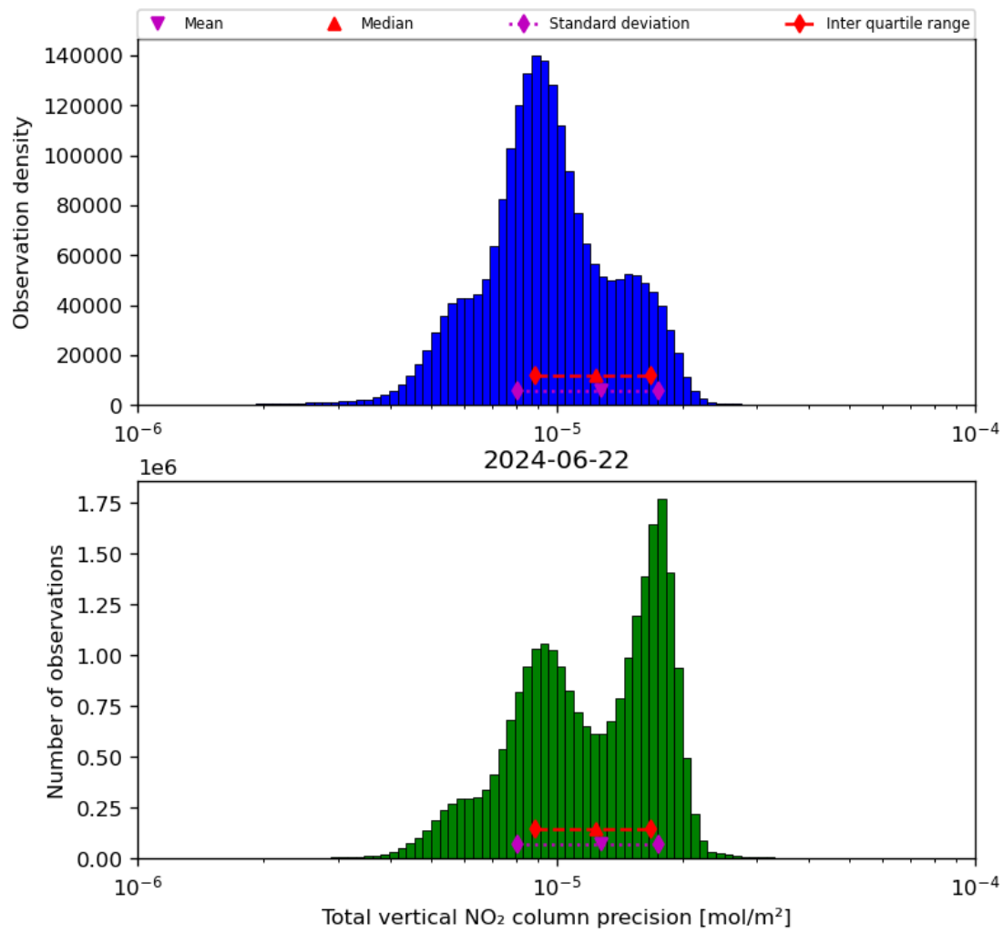
Figure 39: Histogram of “Total vertical NO 2 column precision” for 2024-06-21 to 2024-06-23
