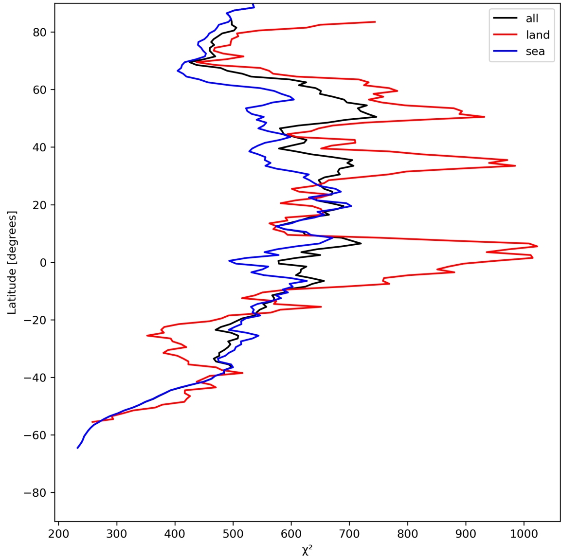
Figure 25: Zonal average of “ \chi^2 ” for 2024-06-21 to 2024-06-23.
