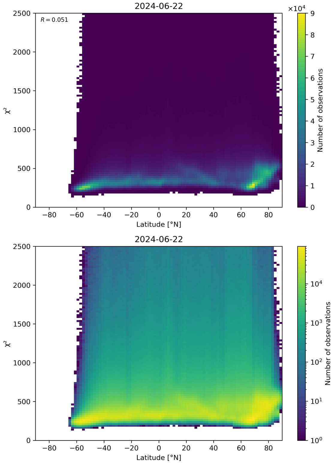
Figure 86: Scatter density plot of “Latitude” against “ \chi^2 ” for 2024-06-21 to 2024-06-23.
