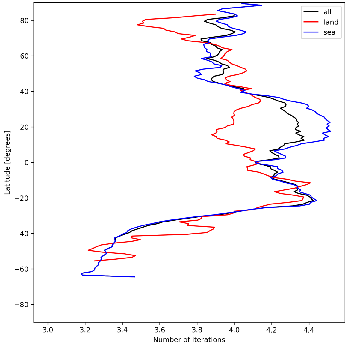
Figure 17: Zonal average of “Number of iterations” for 2024-06-21 to 2024-06-23.
