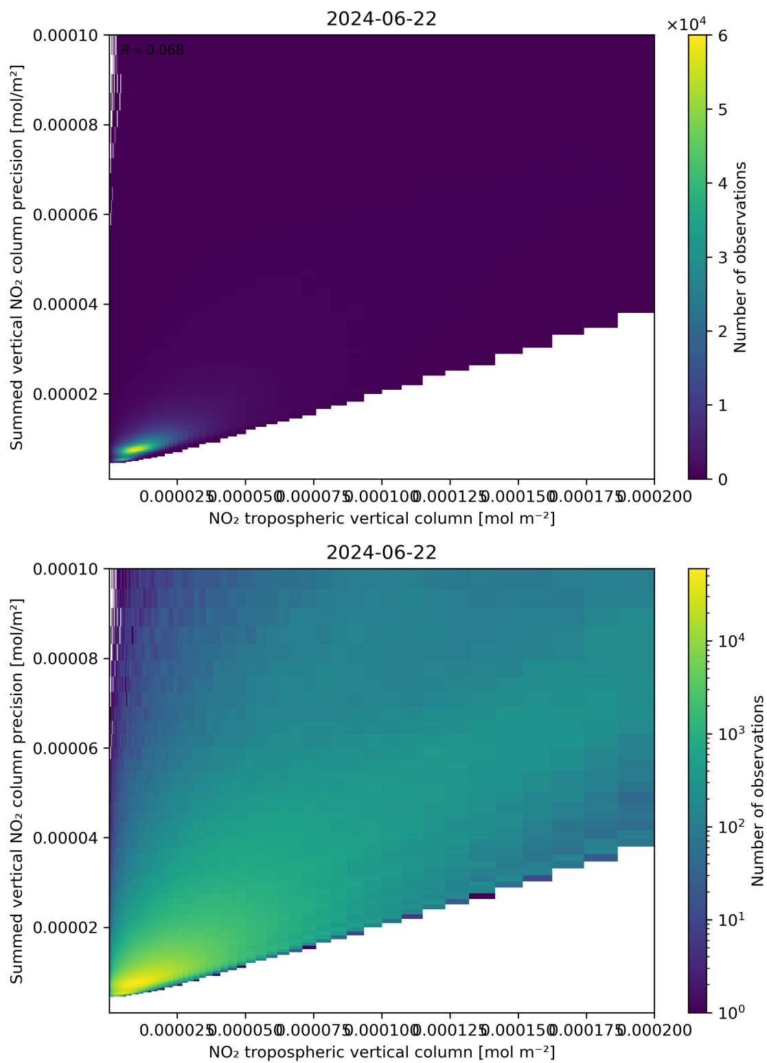
Figure 127: Scatter density plot of “NO 2 tropospheric vertical column” against “Summed vertical NO 2 column precision” for 2024-06-21 to 2024-06-23.
