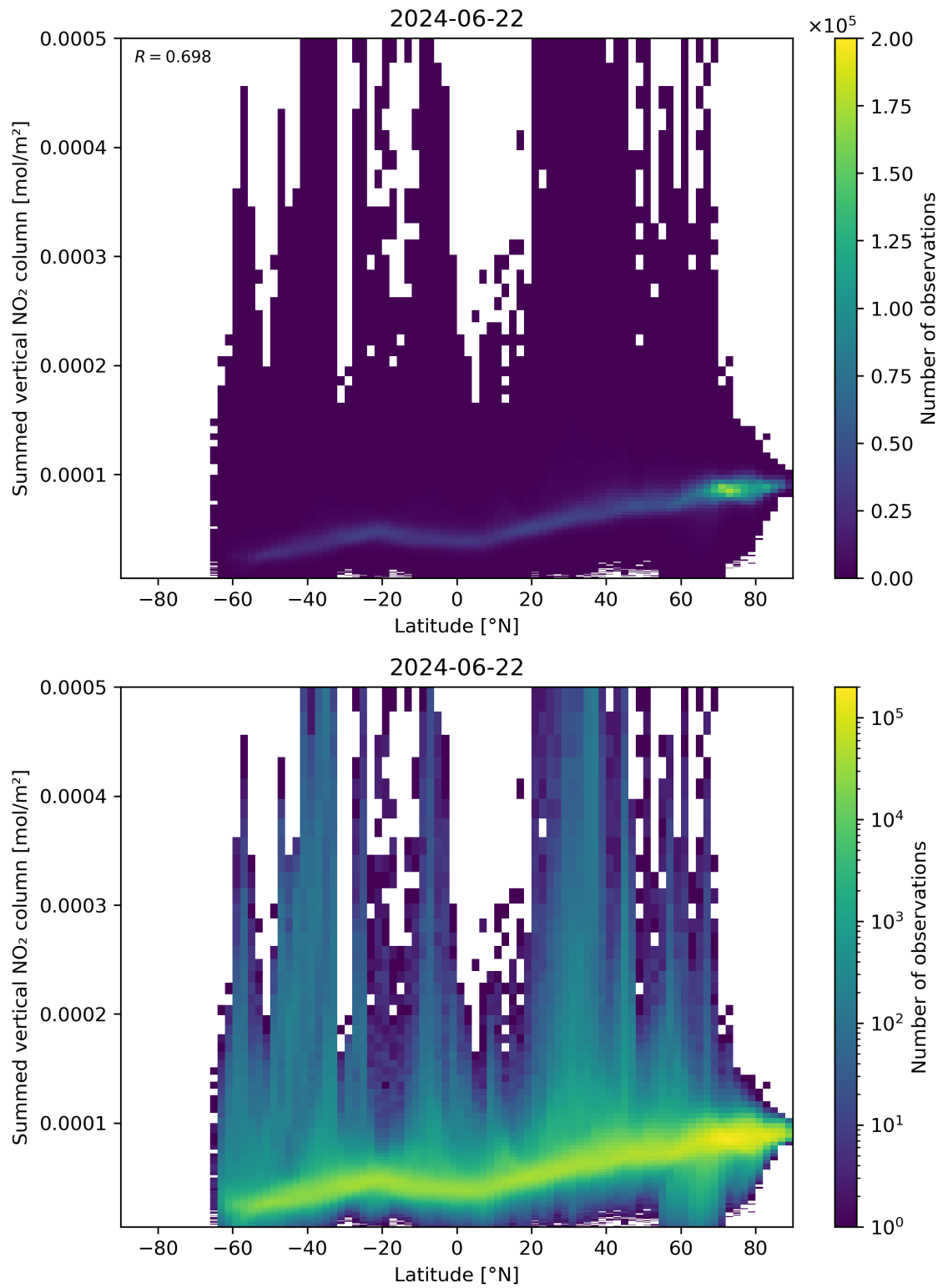
Figure 88: Scatter density plot of “Latitude” against “Summed vertical NO 2 column” for 2024-06-21 to 2024-06-23.
