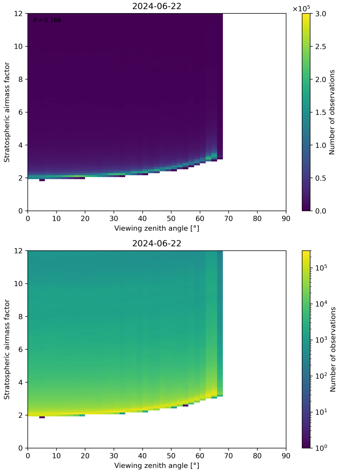
Figure 159: Scatter density plot of “Viewing zenith angle” against “Stratospheric airmass factor” for 2024-06-21 to 2024-06-23.
