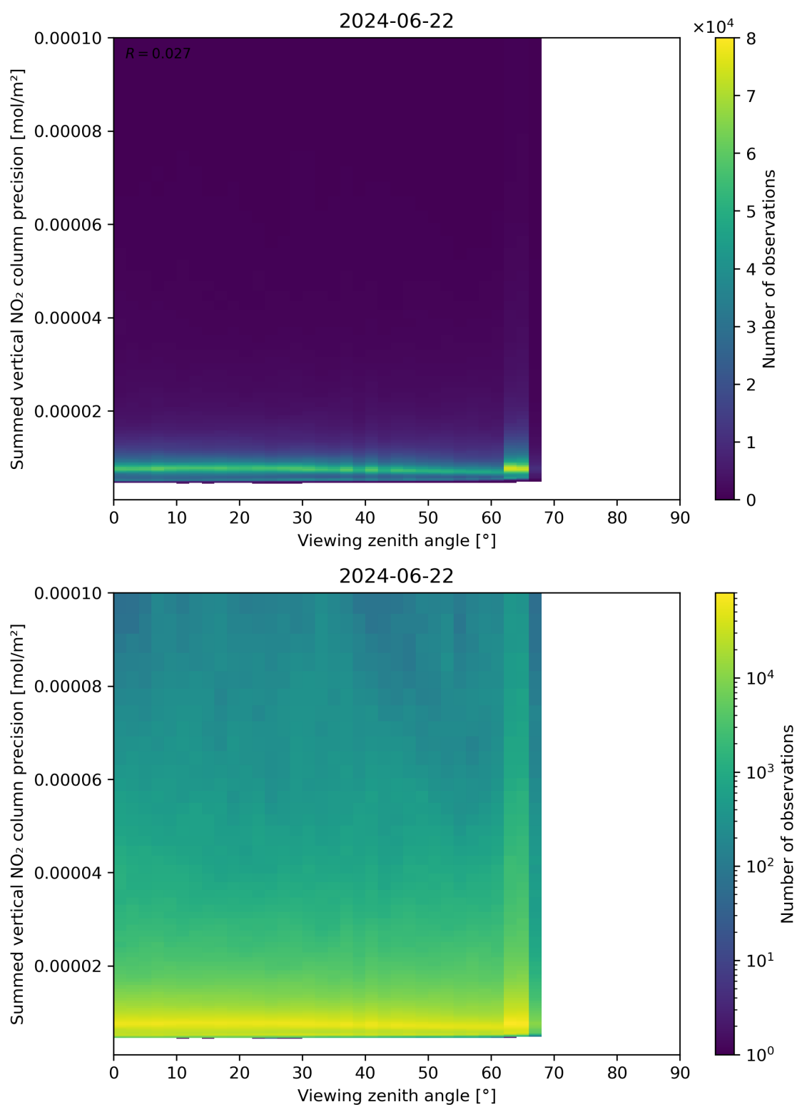
Figure 166: Scatter density plot of “Viewing zenith angle” against “Summed vertical NO 2 column precision” for 2024-06-21 to 2024-06-23.
