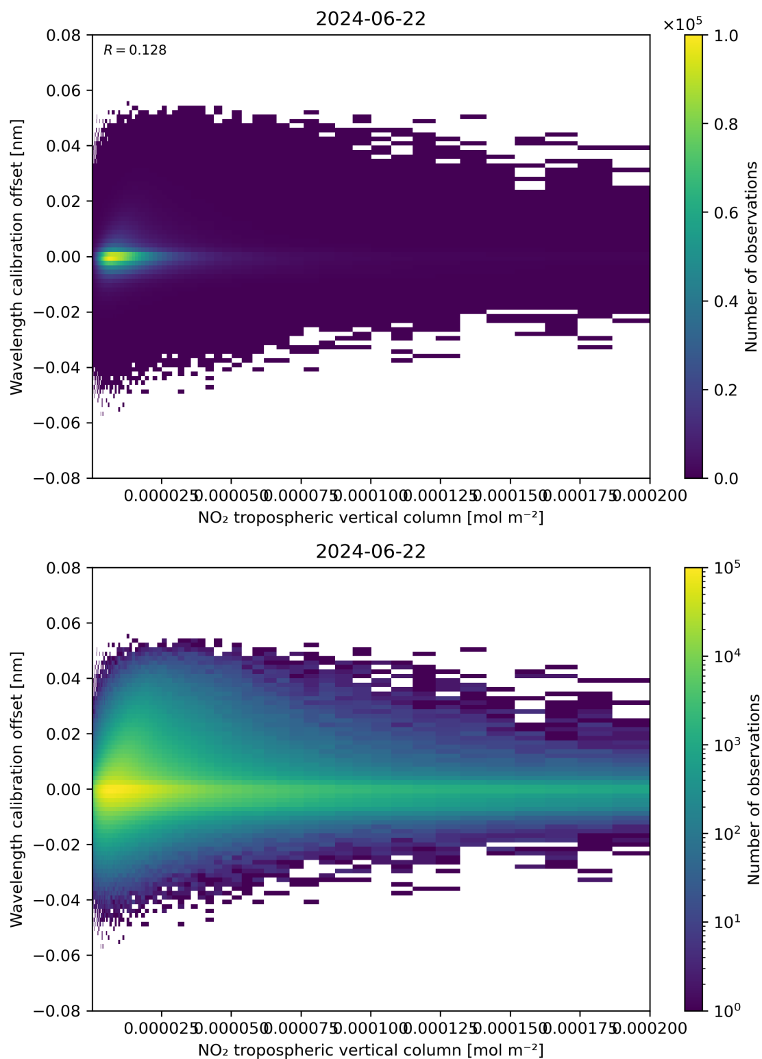
Figure 143: Scatter density plot of “NO 2 tropospheric vertical column” against “Wavelength calibration offset” for 2024-06-21 to 2024-06-23.
