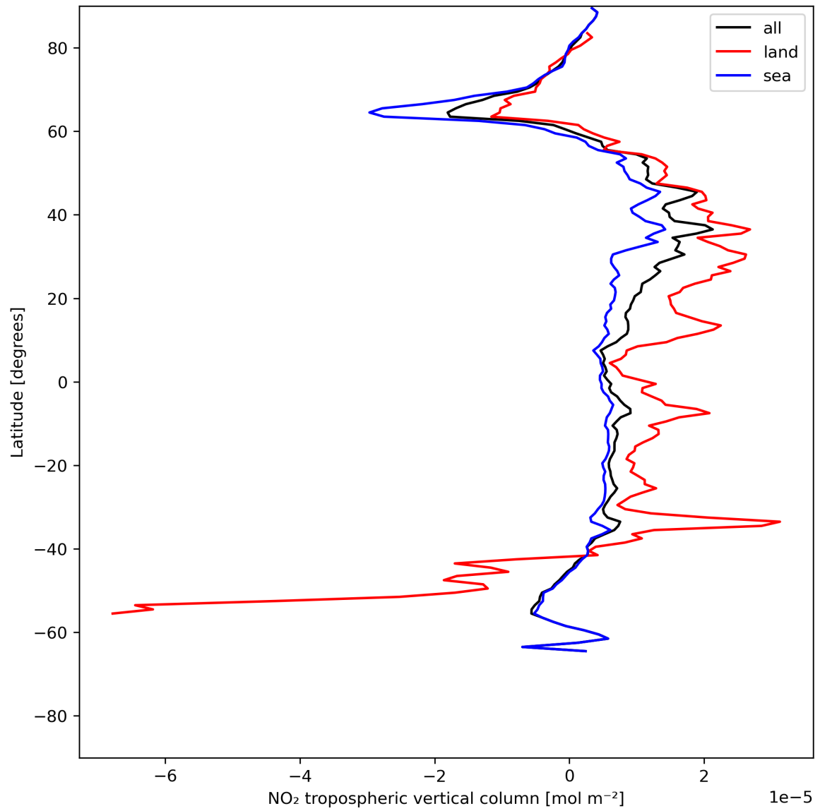
Figure 12: Zonal average of “NO 2 tropospheric vertical column” for 2024-06-21 to 2024-06-23.
