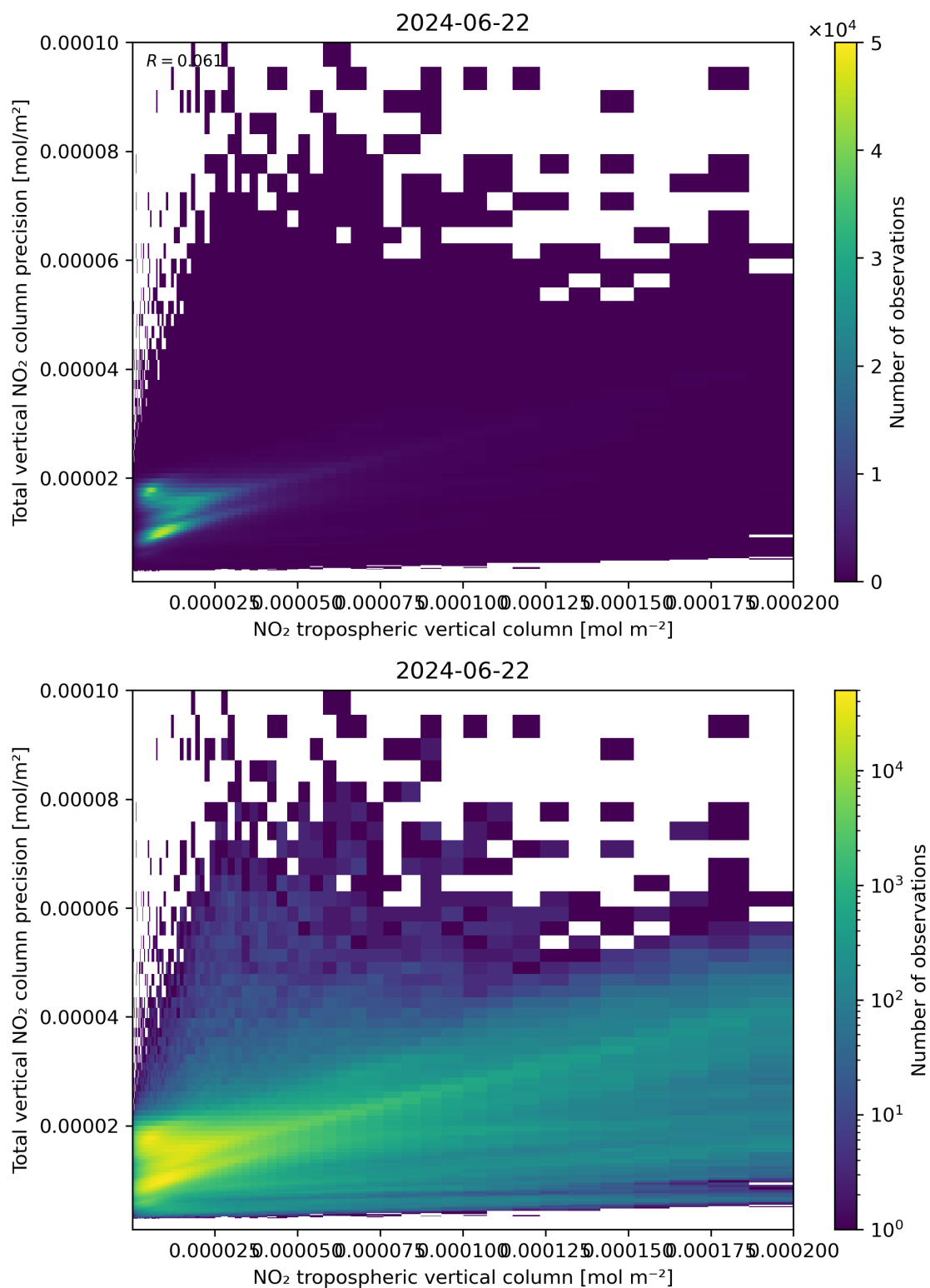
Figure 129: Scatter density plot of “NO 2 tropospheric vertical column” against “Total vertical NO 2 column precision” for 2024-06-21 to 2024-06-23.
