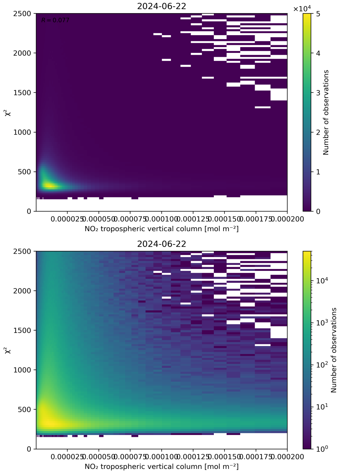
Figure 124: Scatter density plot of “NO 2 tropospheric vertical column” against “ \chi^2 ” for 2024-06-21 to 2024-06-23.
