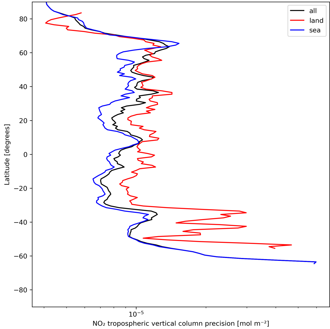
Figure 13: Zonal average of “NO 2 tropospheric vertical column precision” for 2024-06-21 to 2024-06-23.
