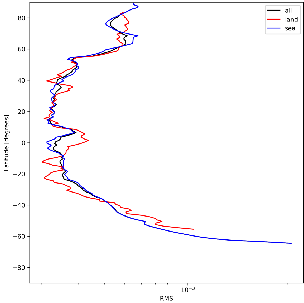
Figure 26: Zonal average of “RMS” for 2024-06-21 to 2024-06-23.
