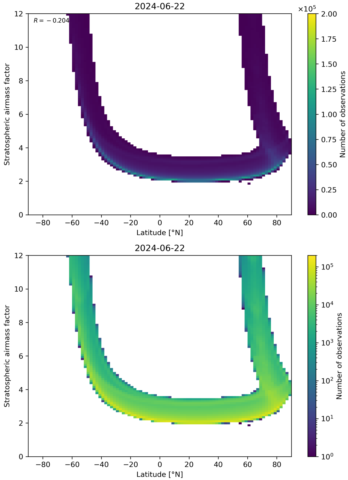
Figure 83: Scatter density plot of “Latitude” against “Stratospheric air mass factor” for 2024-06-21 to 2024-06-23.
