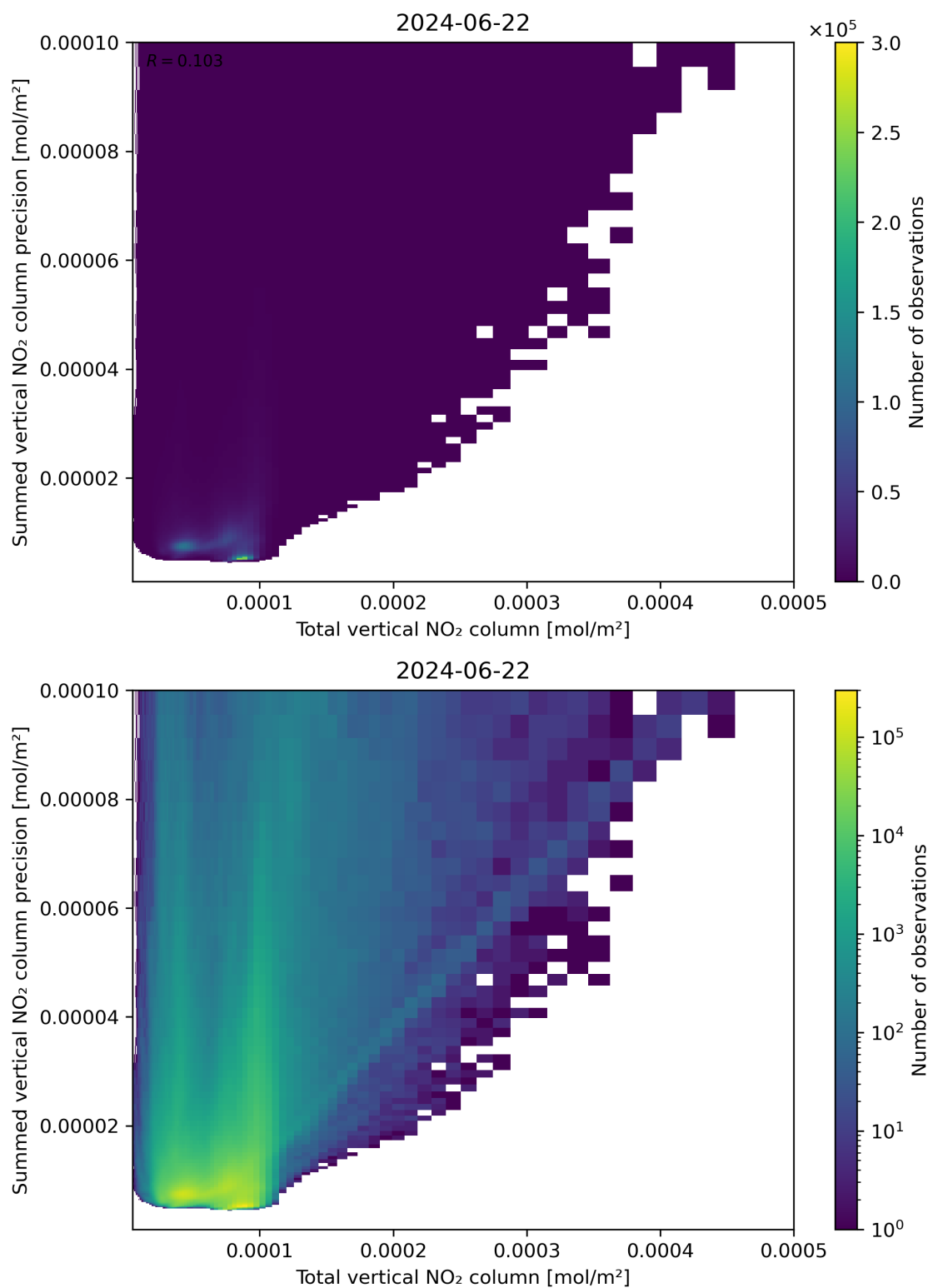
Figure 113: Scatter density plot of “Total vertical NO 2 column” against “Summed vertical NO 2 column precision” for 2024-06-21 to 2024-06-23.
