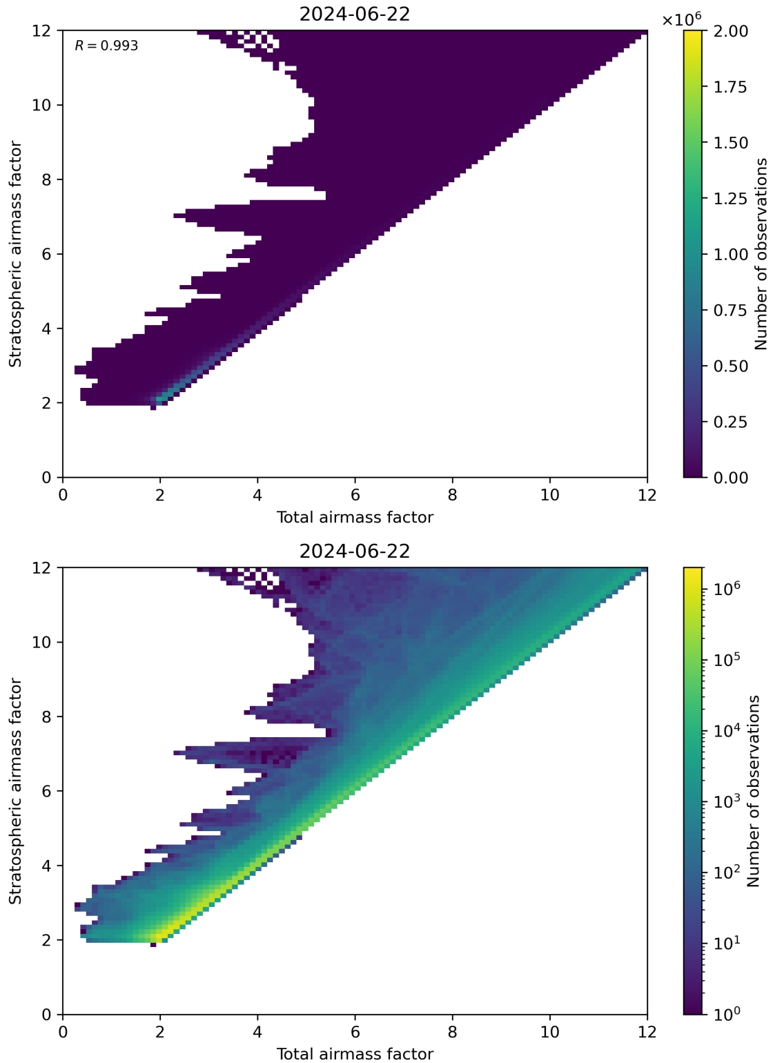
Figure 62: Scatter density plot of “Total airmass factor” against “Stratospheric airmass factor” for 2024-06-21 to 2024-06-23.
