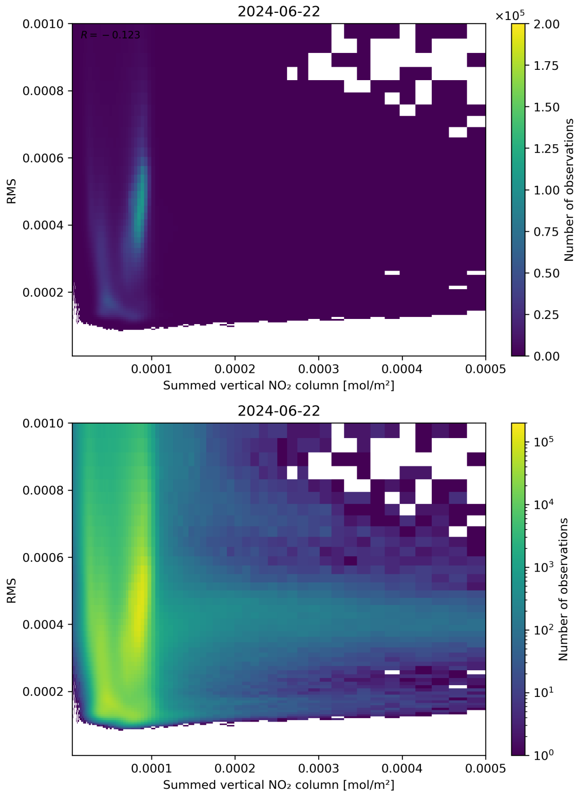
Figure 109: Scatter density plot of “Summed vertical NO 2 column” against “RMS” for 2024-06-21 to 2024-06-23.
