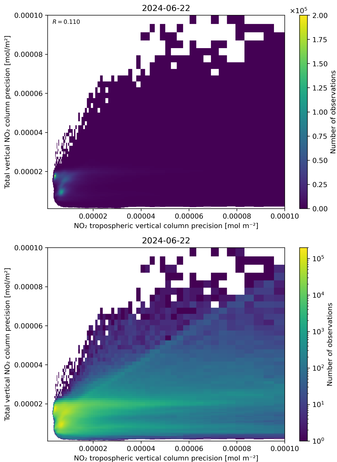
Figure 139: Scatter density plot of “NO 2 tropospheric vertical column precision” against “Total vertical NO 2 column precision” for 2024-06-21 to 2024-06-23.
