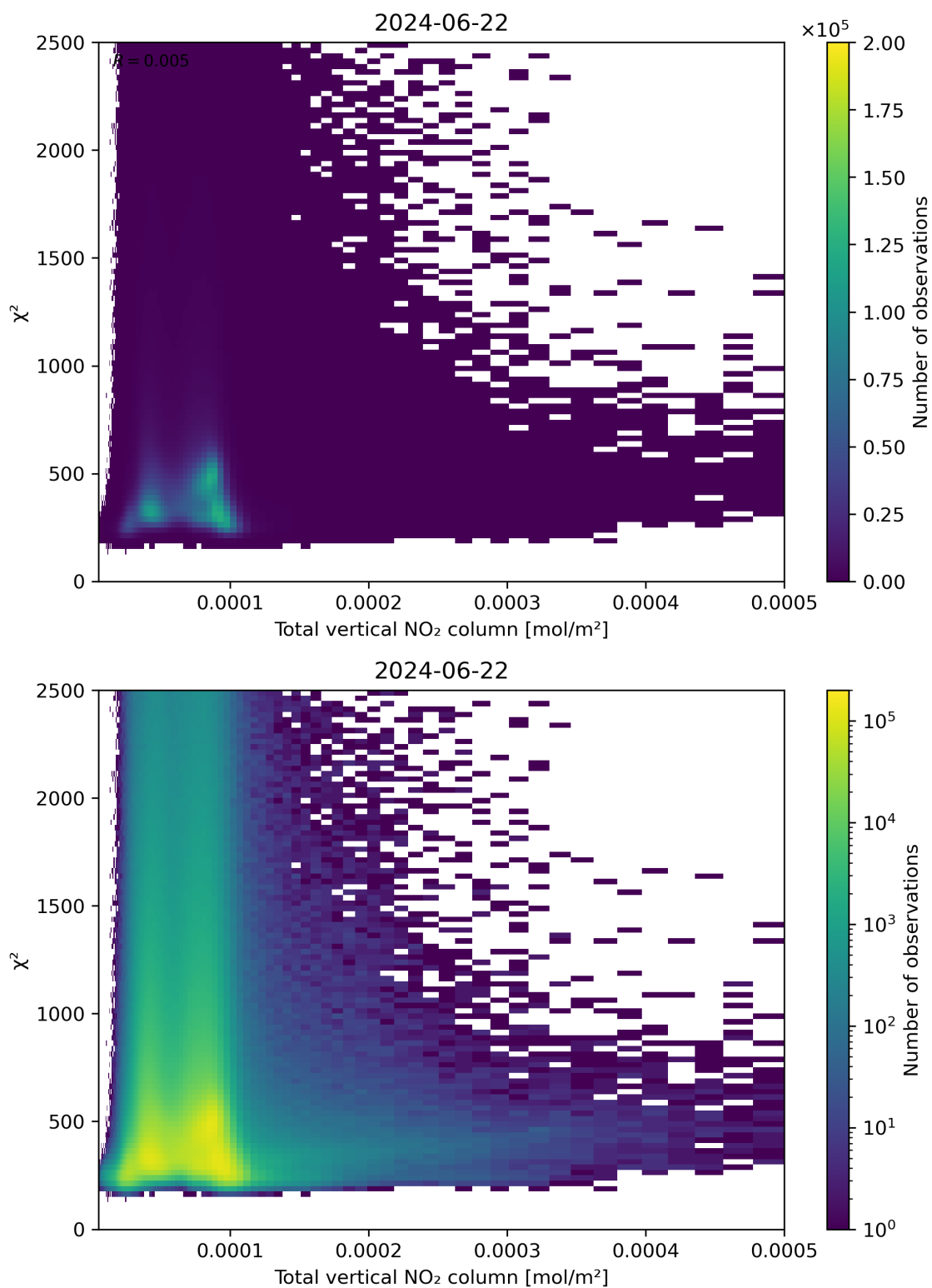
Figure 111: Scatter density plot of “Total vertical NO 2 column” against “ \chi^2 ” for 2024-06-21 to 2024-06-23.
