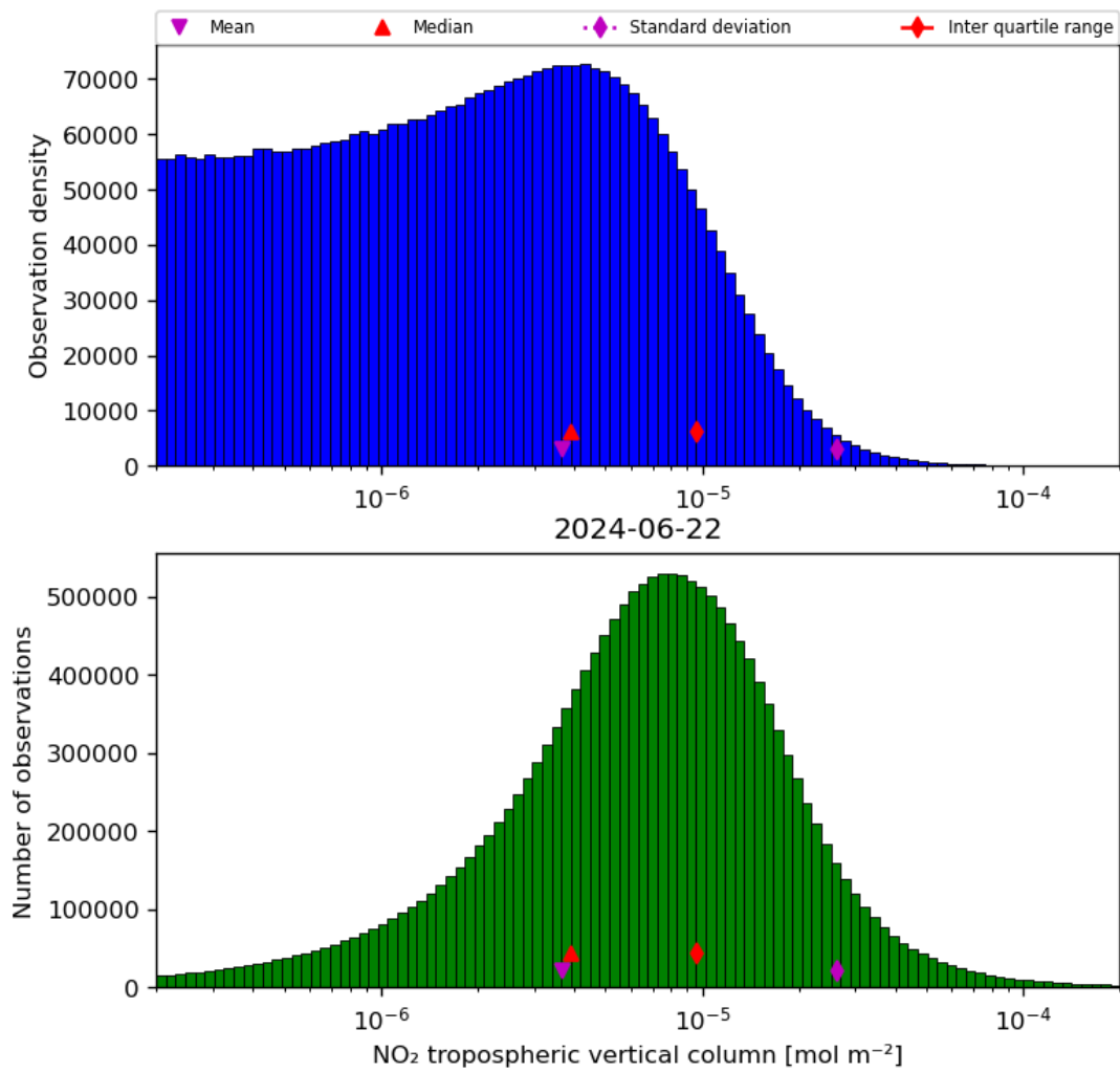
Figure 29: Histogram of “NO 2 tropospheric vertical column” for 2024-06-21 to 2024-06-23
