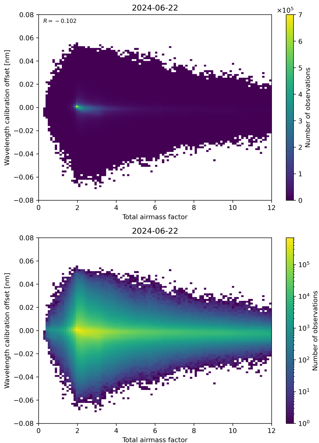
Figure 70: Scatter density plot of “Total airmass factor” against “Wavelength calibration offset” for 2024-06-21 to 2024-06-23.
