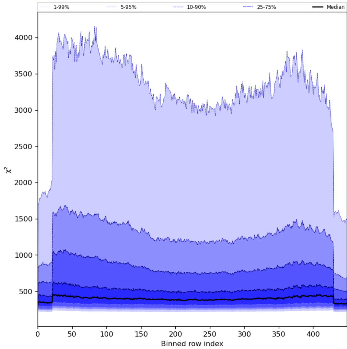
Figure 59: Along track statistics of “ \chi^2 ” for 2024-06-21 to 2024-06-23
