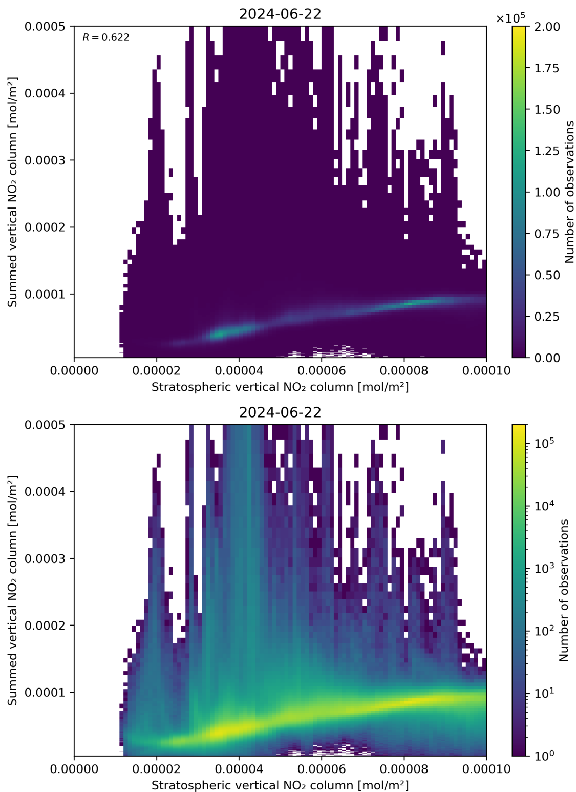
Figure 98: Scatter density plot of “Stratospheric vertical NO 2 column” against “Summed vertical NO 2 column” for 2024-06-21 to 2024-06-23.
