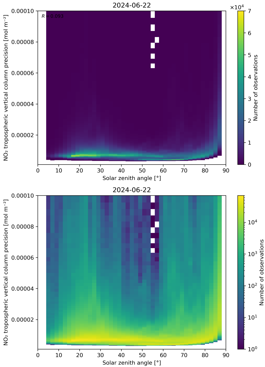
Figure 156: Scatter density plot of “Solar zenith angle” against “NO 2 tropospheric vertical column precision” for 2024-06-21 to 2024-06-23.
