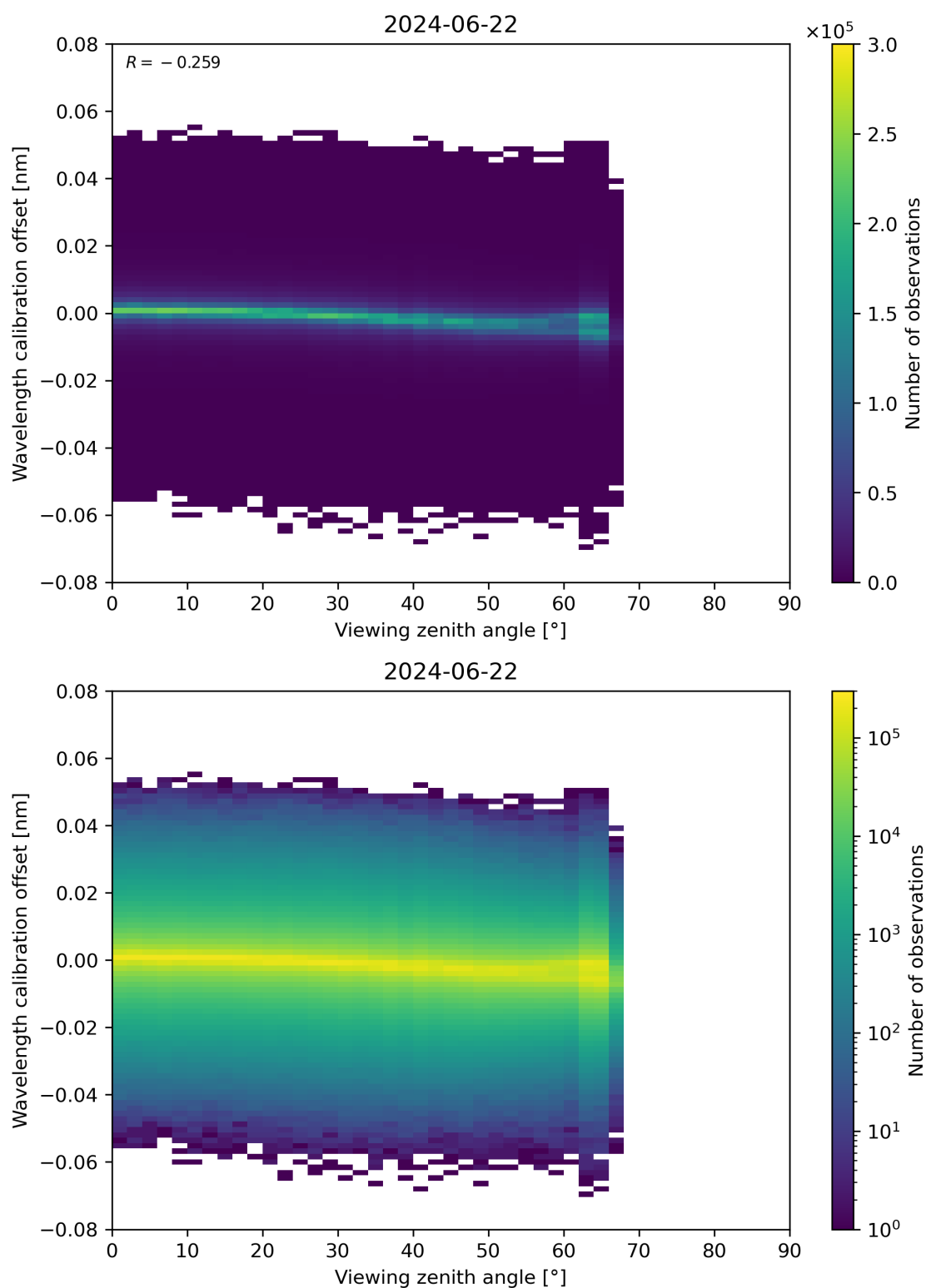
Figure 173: Scatter density plot of “Viewing zenith angle” against “Wavelength calibration offset” for 2024-06-21 to 2024-06-23.
