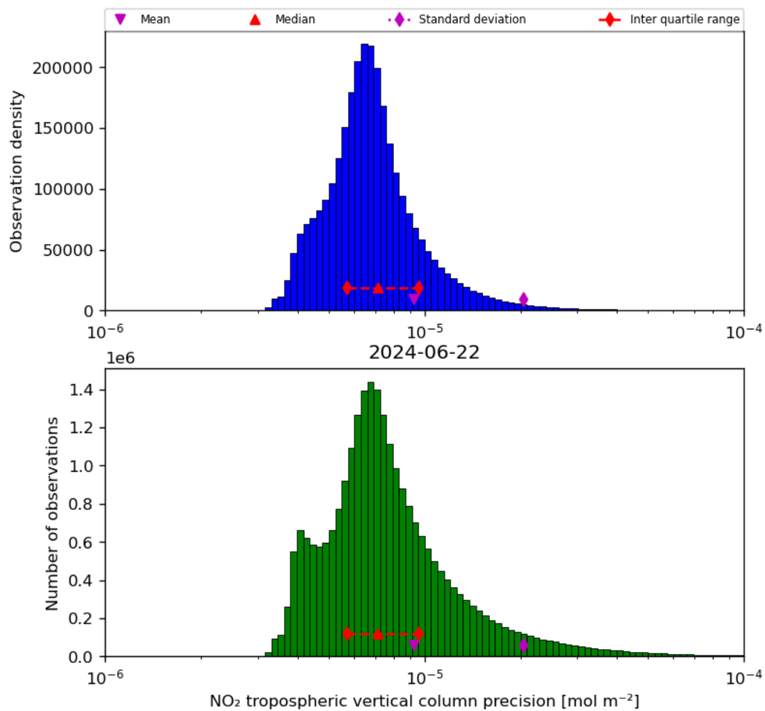
Figure 30: Histogram of “NO 2 tropospheric vertical column precision” for 2024-06-21 to 2024-06-23
