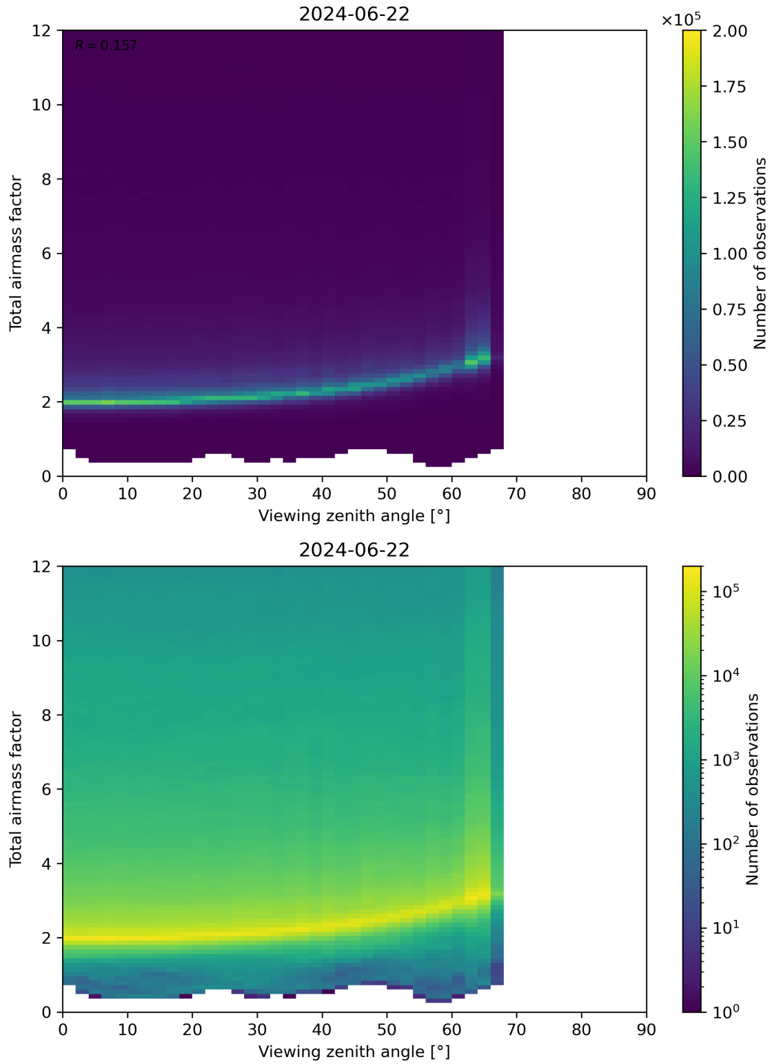
Figure 160: Scatter density plot of “Viewing zenith angle” against “Total airmass factor” for 2024-06-21 to 2024-06-23.
