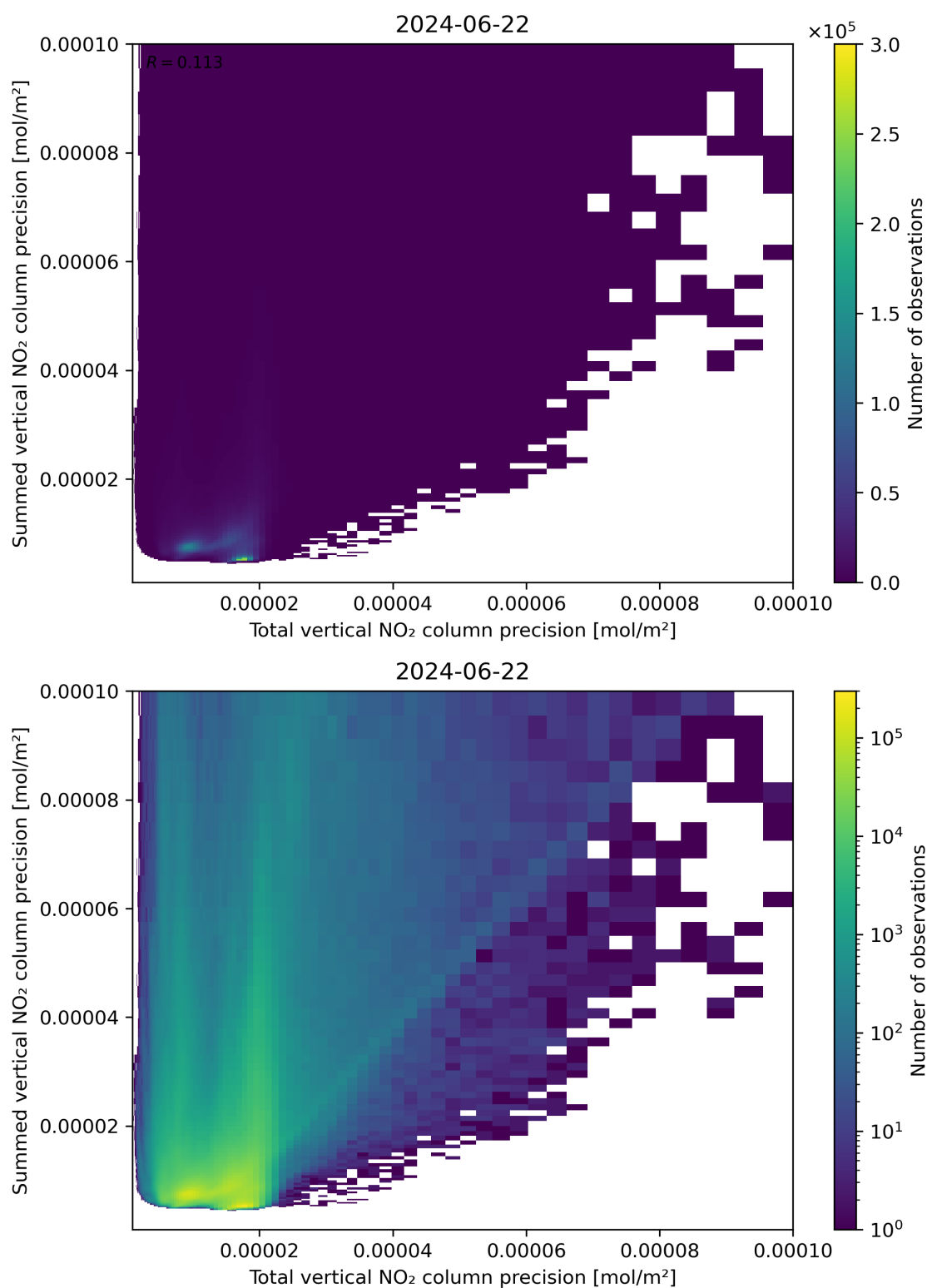
Figure 118: Scatter density plot of “Total vertical NO 2 column precision” against “Summed vertical NO 2 column precision” for 2024-06-21 to 2024-06-23.
