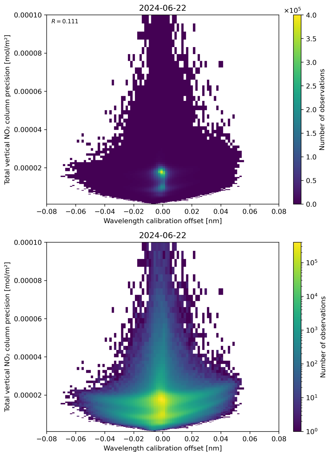
Figure 180: Scatter density plot of “Wavelength calibration offset” against “Total vertical NO 2 column precision” for 2024-06-21 to 2024-06-23.
