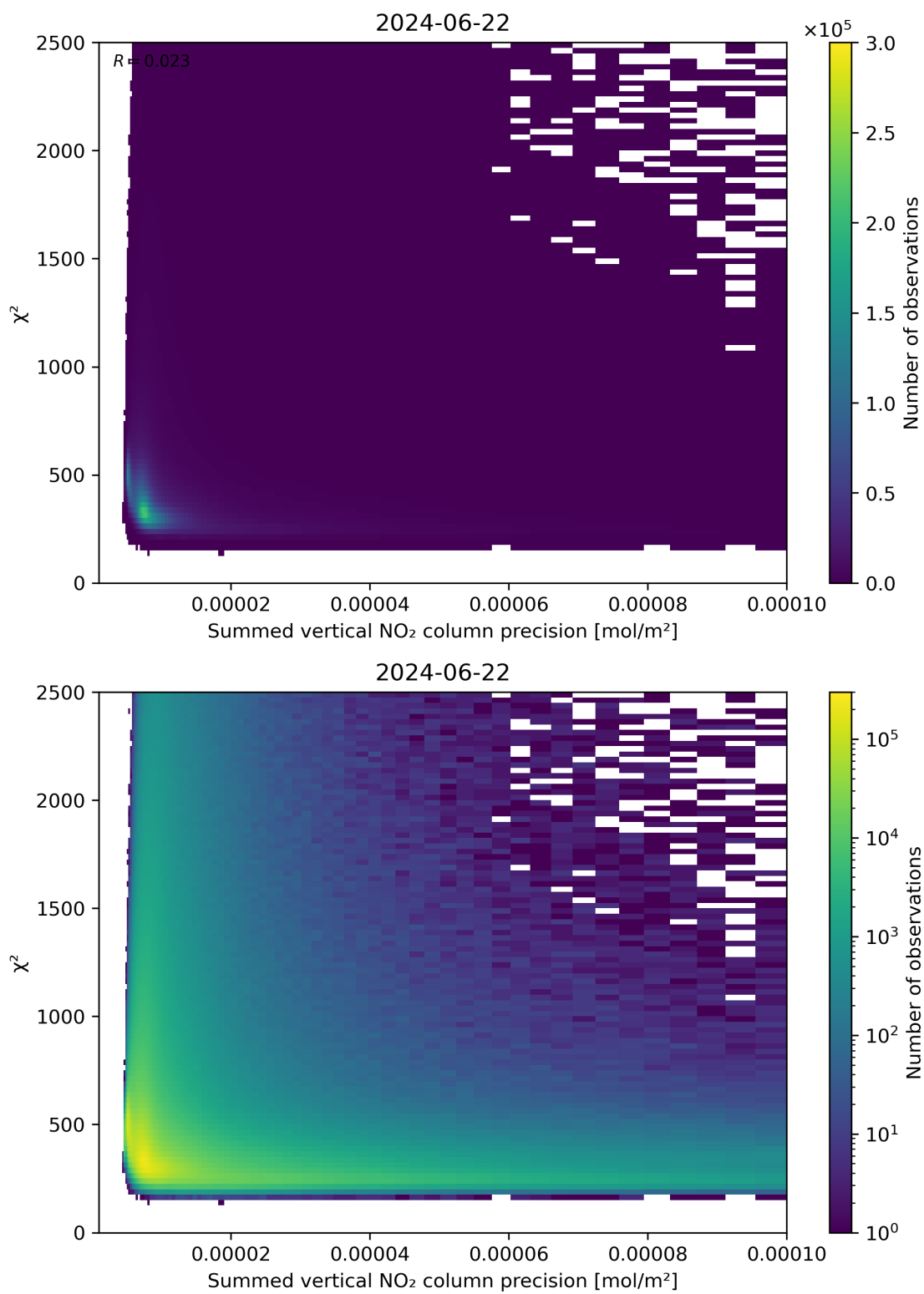
Figure 107: Scatter density plot of “Summed vertical NO 2 column precision” against “ \chi^2 ” for 2024-06-21 to 2024-06-23.
