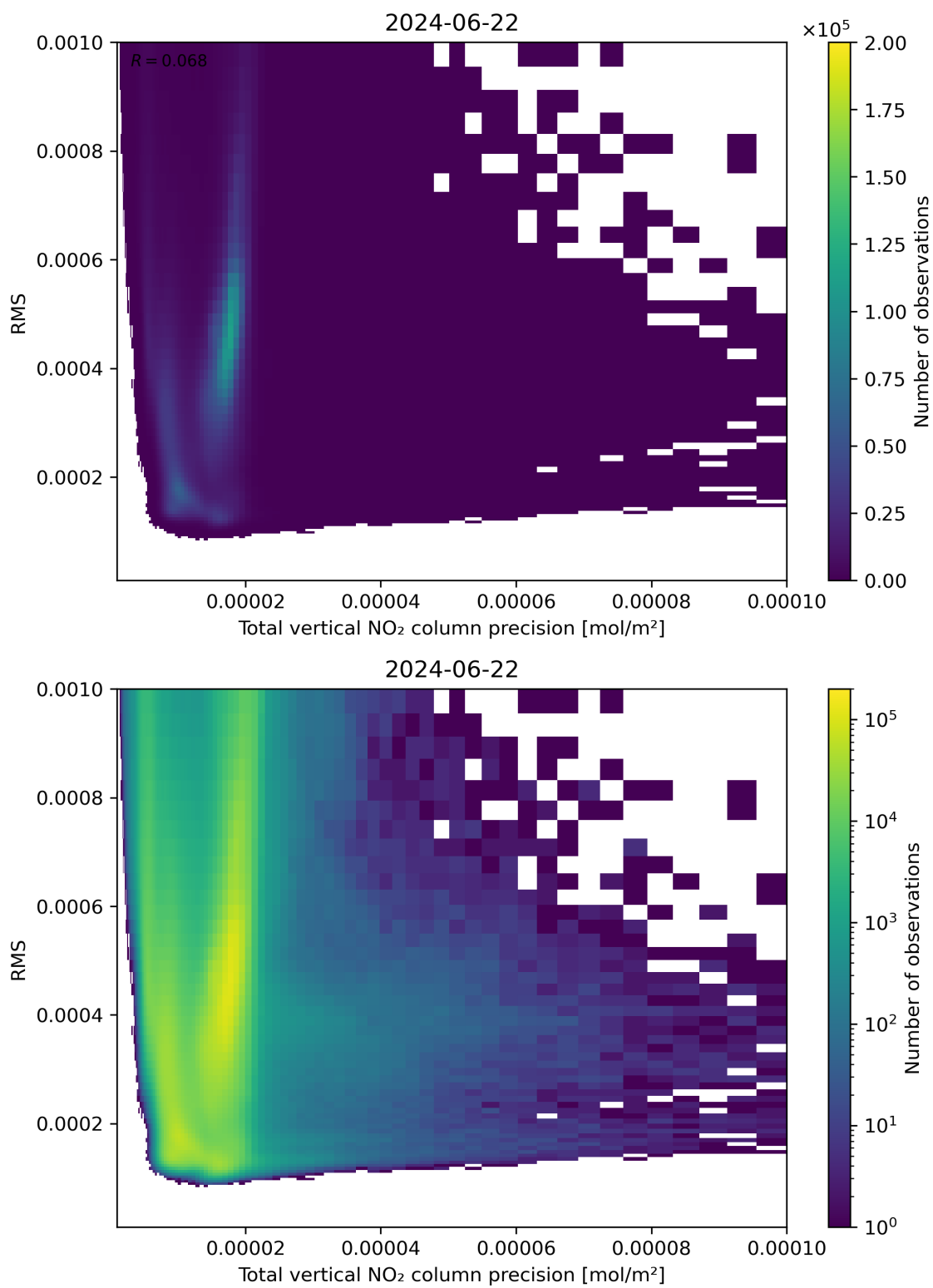
Figure 119: Scatter density plot of “Total vertical NO 2 column precision” against “RMS” for 2024-06-21 to 2024-06-23.
