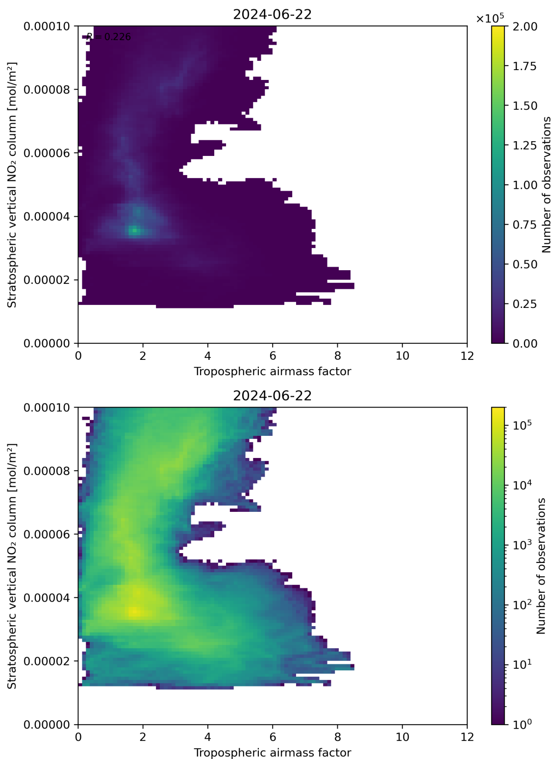
Figure 74: Scatter density plot of “Tropospheric air mass factor” against “Stratospheric vertical NO 2 column” for 2024-06-21 to 2024-06-23.
