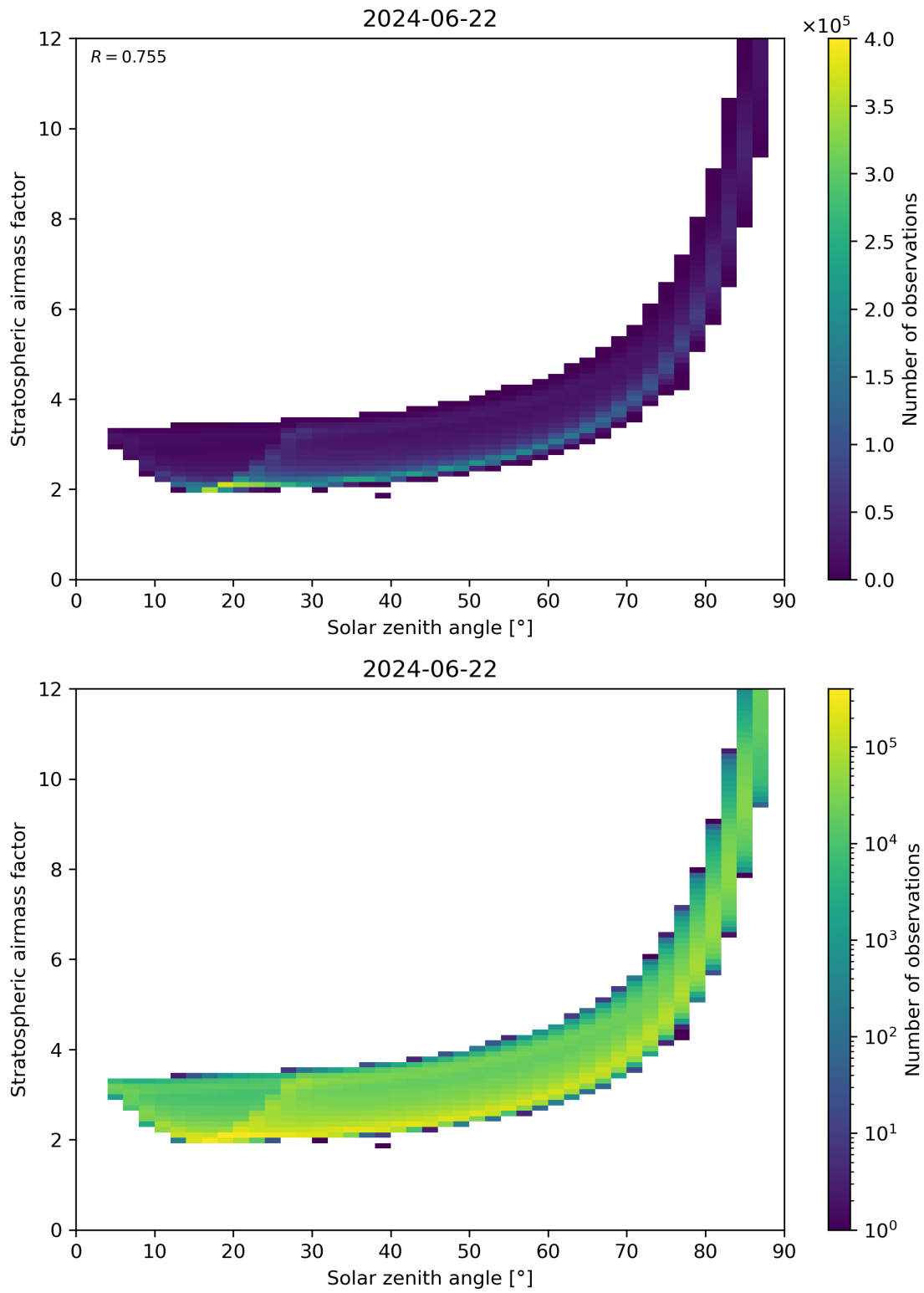
Figure 145: Scatter density plot of “Solar zenith angle” against “Stratospheric airmass factor” for 2024-06-21 to 2024-06-23.
