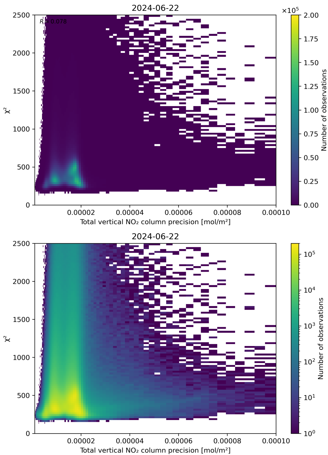
Figure 116: Scatter density plot of “Total vertical NO 2 column precision” against “ \chi^2 ” for 2024-06-21 to 2024-06-23.
