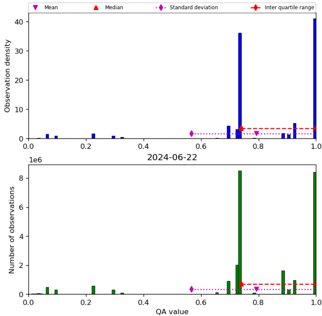
Figure 28: Histogram of “QA value” for 2024-06-21 to 2024-06-23
