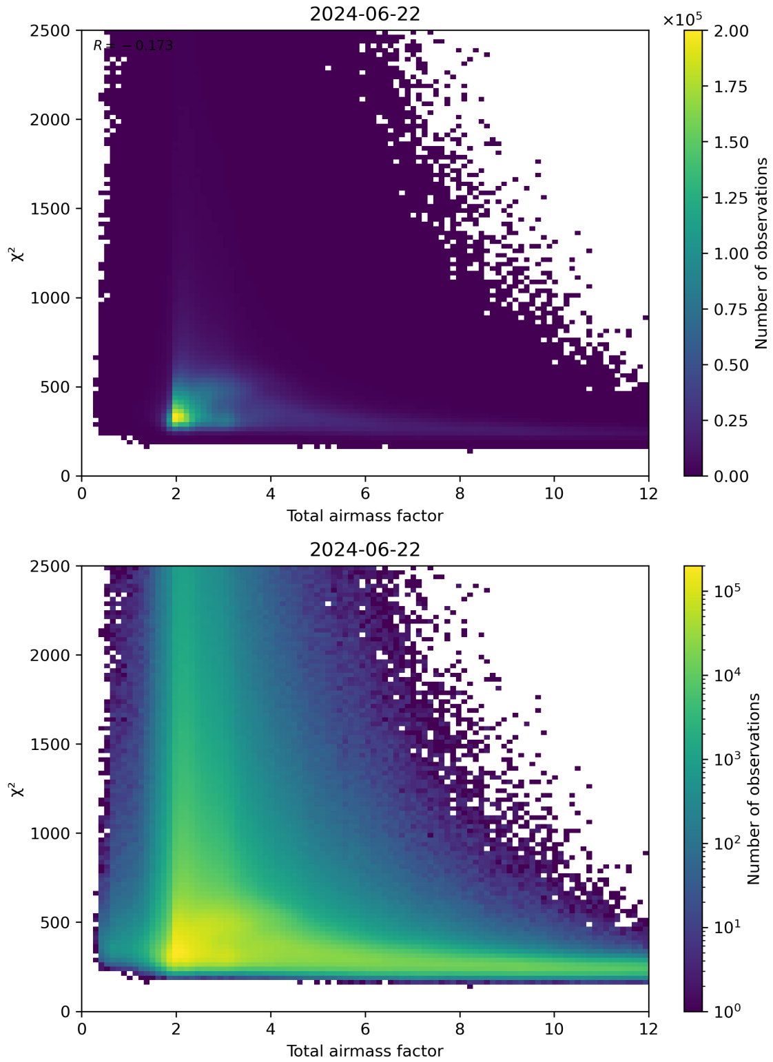
Figure 63: Scatter density plot of “Total airmass factor” against “ \chi^2 ” for 2024-06-21 to 2024-06-23.
