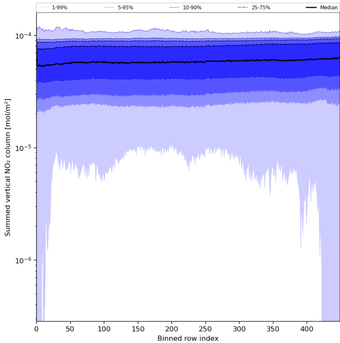
Figure 57: Along track statistics of “Summed vertical NO 2 column” for 2024-06-21 to 2024-06-23
