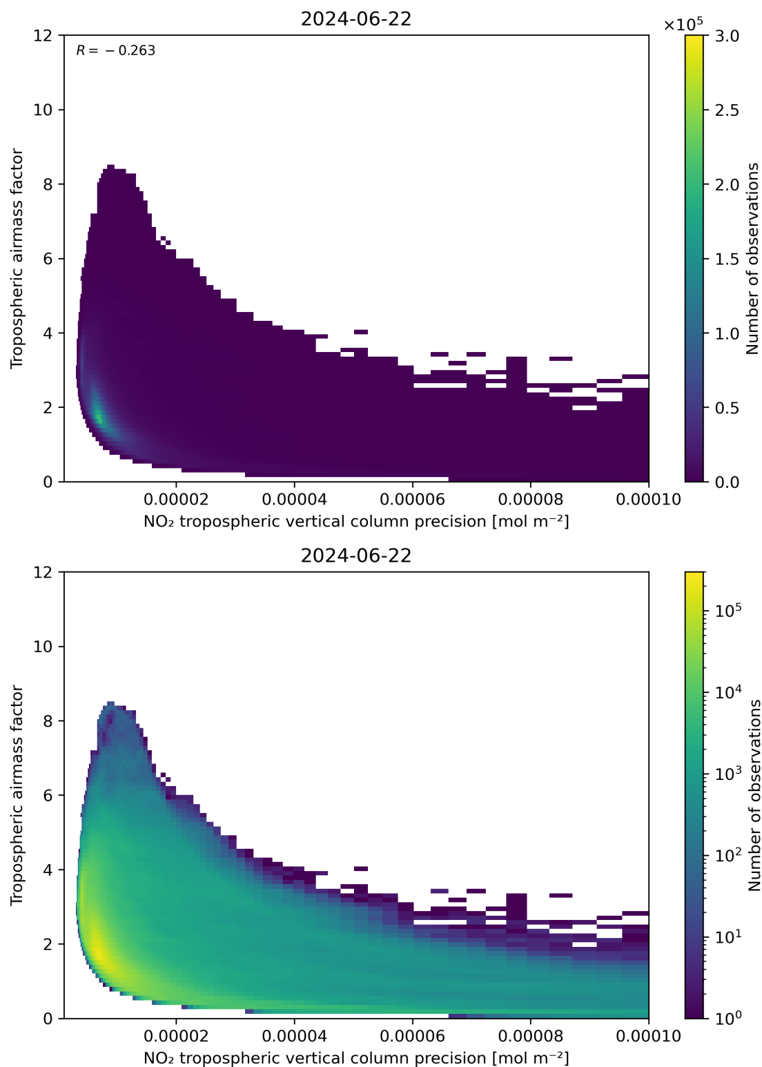
Figure 133: Scatter density plot of “NO 2 tropospheric vertical column precision” against “Tropospheric airmass factor” for 2024-06-21 to 2024-06-23.
