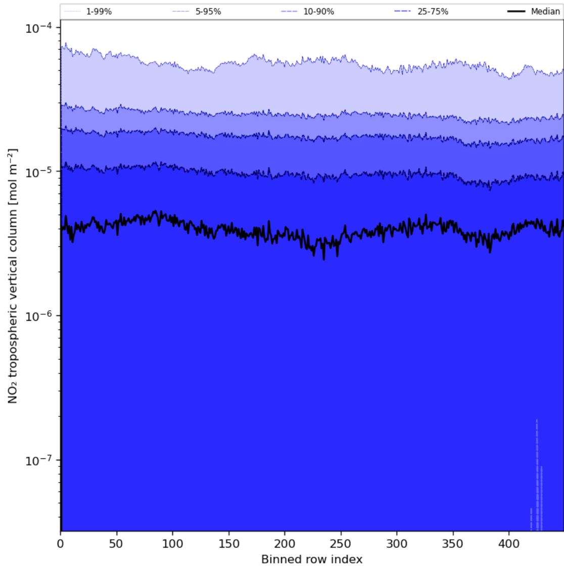
Figure 46: Along track statistics of “NO 2 tropospheric vertical column” for 2024-06-21 to 2024-06-23
