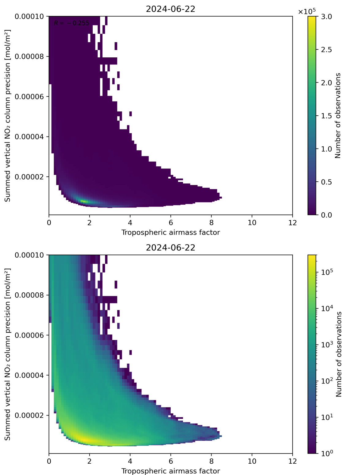
Figure 76: Scatter density plot of “Tropospheric air mass factor” against “Summed vertical NO 2 column precision” for 2024-06-21 to 2024-06-23.
