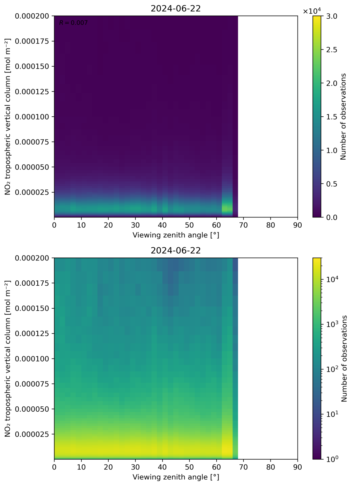
Figure 169: Scatter density plot of “Viewing zenith angle” against “NO 2 tropospheric vertical column” for 2024-06-21 to 2024-06-23.
