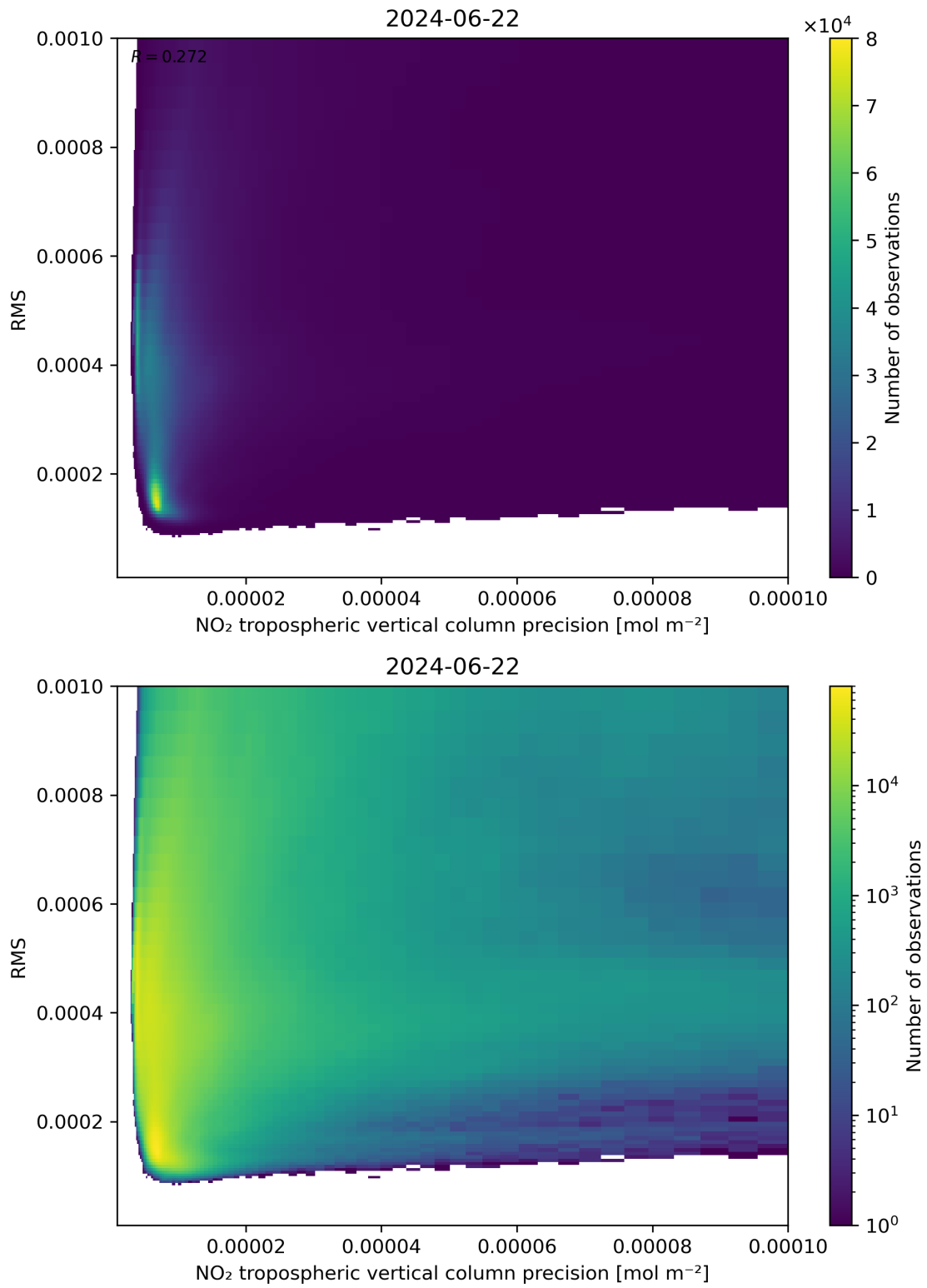
Figure 140: Scatter density plot of “NO 2 tropospheric vertical column precision” against “RMS” for 2024-06-21 to 2024-06-23.
