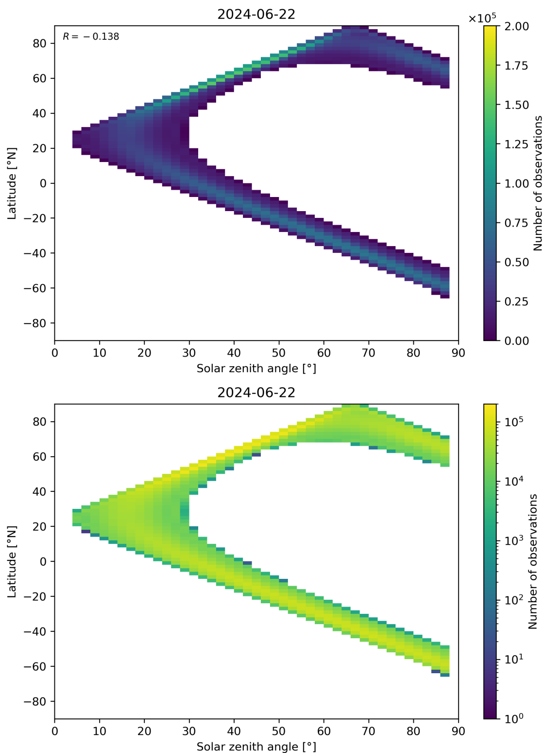
Figure 149: Scatter density plot of “Solar zenith angle” against “Latitude” for 2024-06-21 to 2024-06-23.
