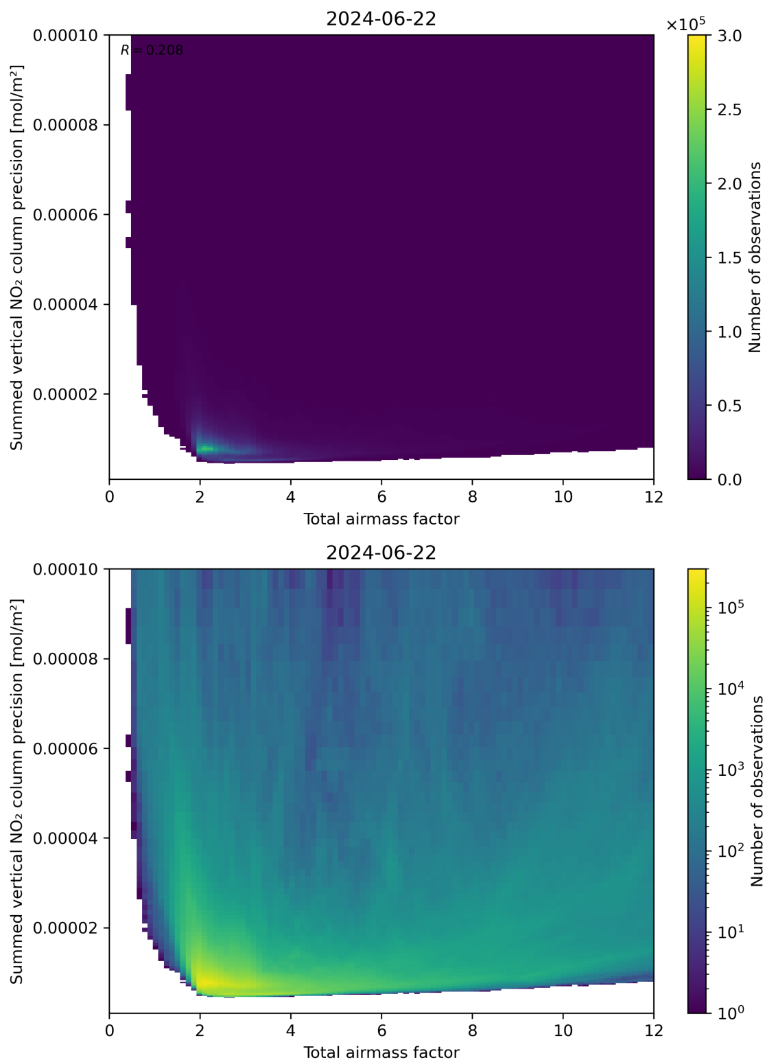
Figure 66: Scatter density plot of “Total airmass factor” against “Summed vertical NO 2 column precision” for 2024-06-21 to 2024-06-23.
