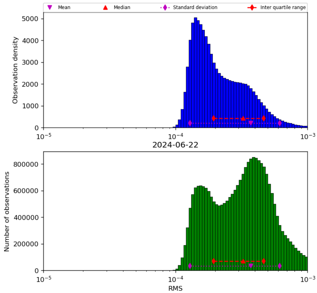
Figure 43: Histogram of “RMS” for 2024-06-21 to 2024-06-23
