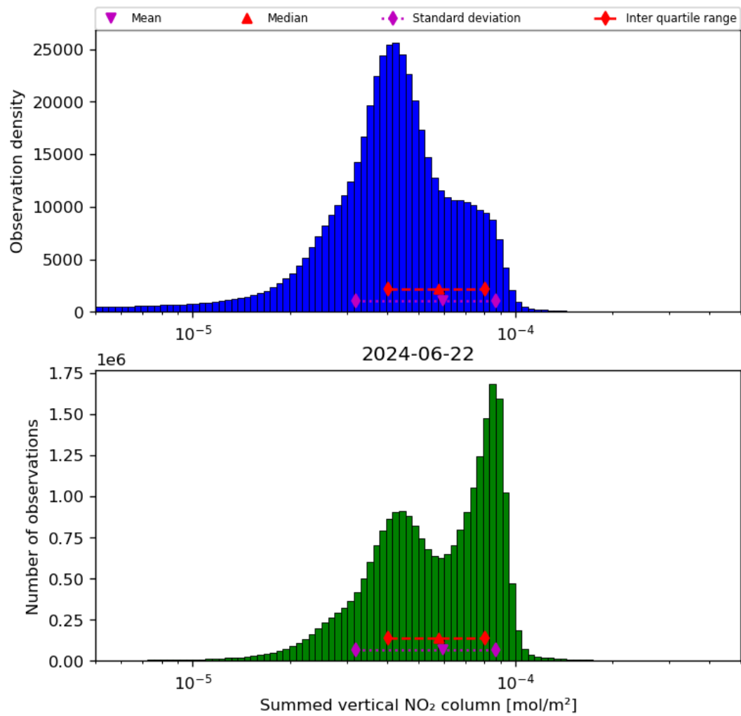
Figure 40: Histogram of “Summed vertical NO 2 column” for 2024-06-21 to 2024-06-23
