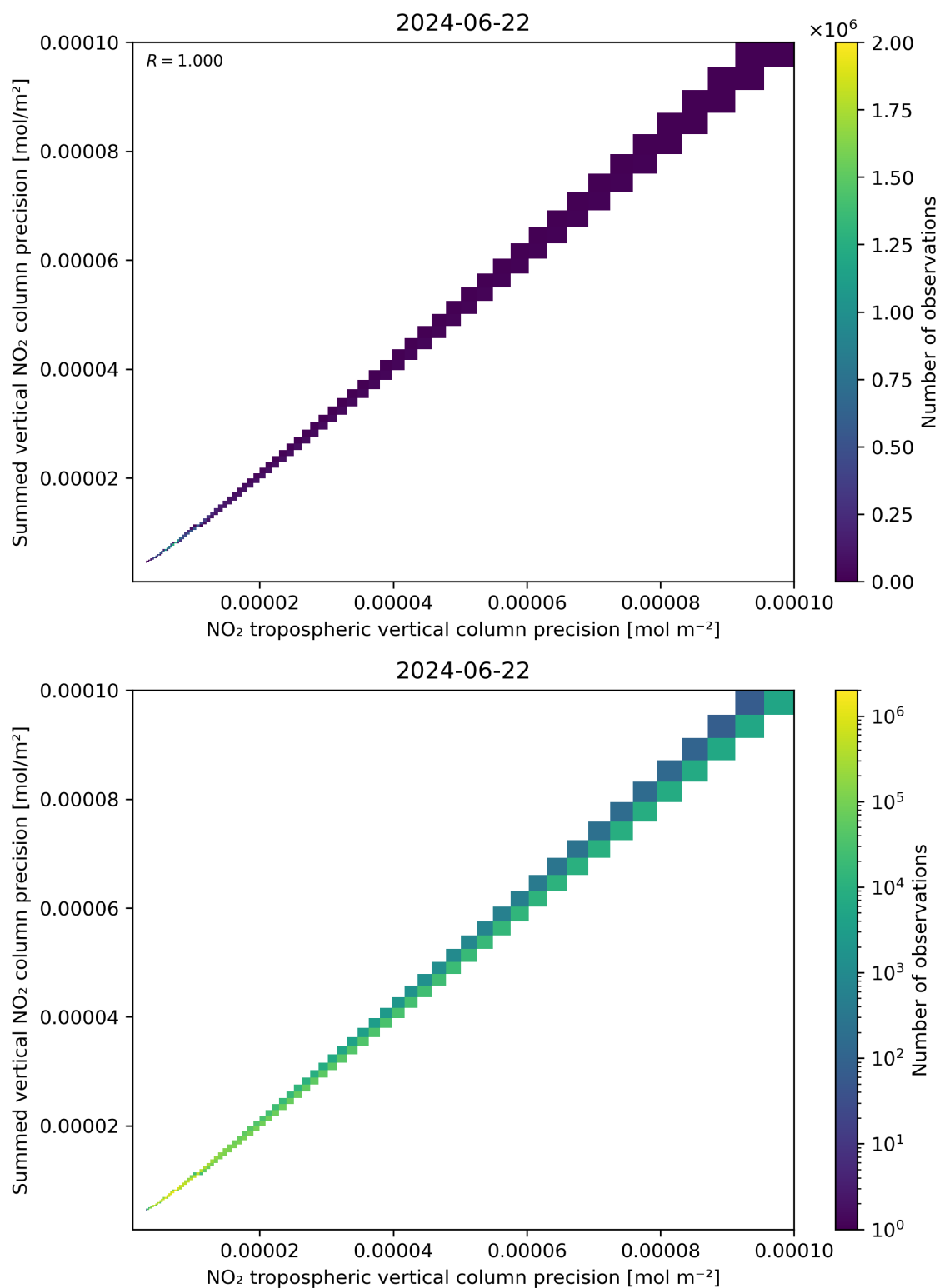
Figure 137: Scatter density plot of “NO 2 tropospheric vertical column precision” against “Summed vertical NO 2 column precision” for 2024-06-21 to 2024-06-23.
