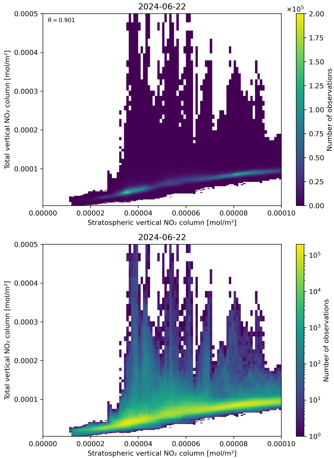
Figure 100: Scatter density plot of “Stratospheric vertical NO 2 column” against “Total vertical NO 2 column” for 2024-06-21 to 2024-06-23.
