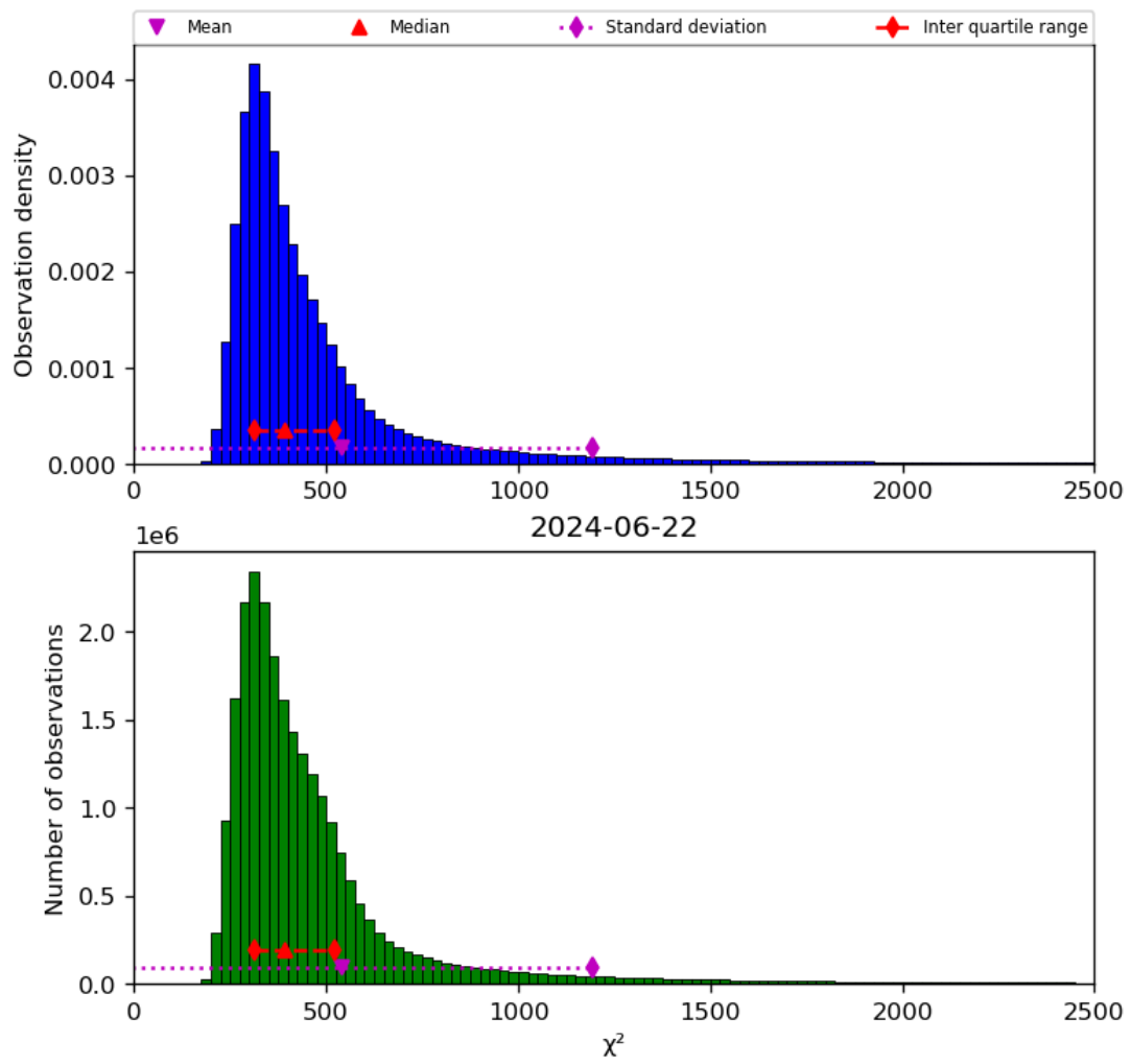
Figure 42: Histogram of “ \chi^2 ” for 2024-06-21 to 2024-06-23
