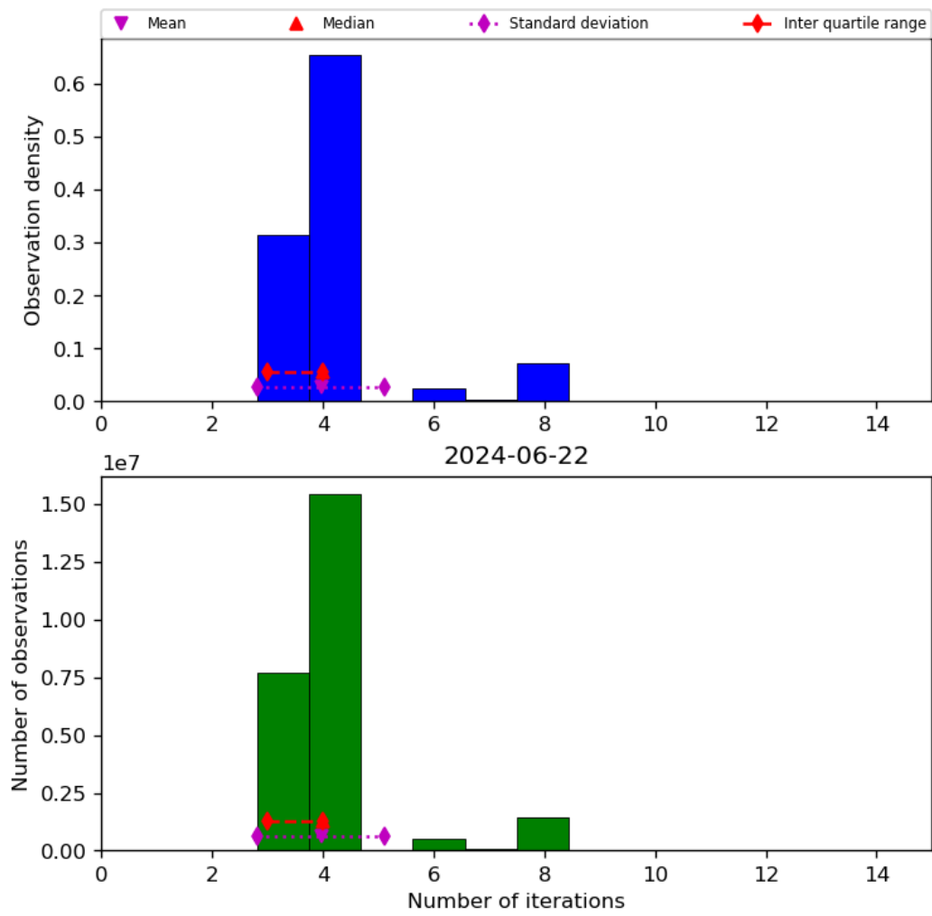
Figure 34: Histogram of “Number of iterations” for 2024-06-21 to 2024-06-23
