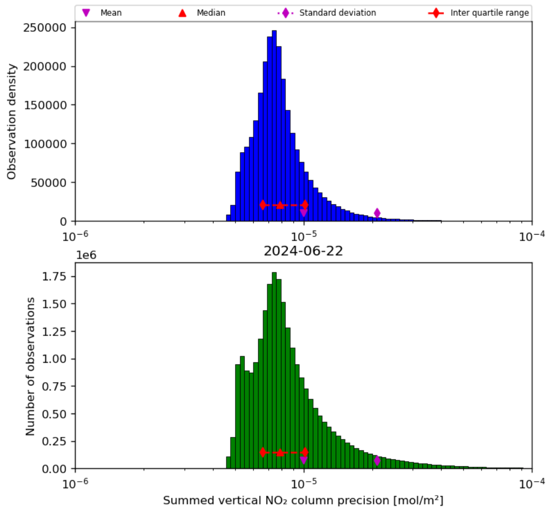
Figure 41: Histogram of "Summed vertical NO 2 column precision" for 2024-06-21 to 2024-06-23
