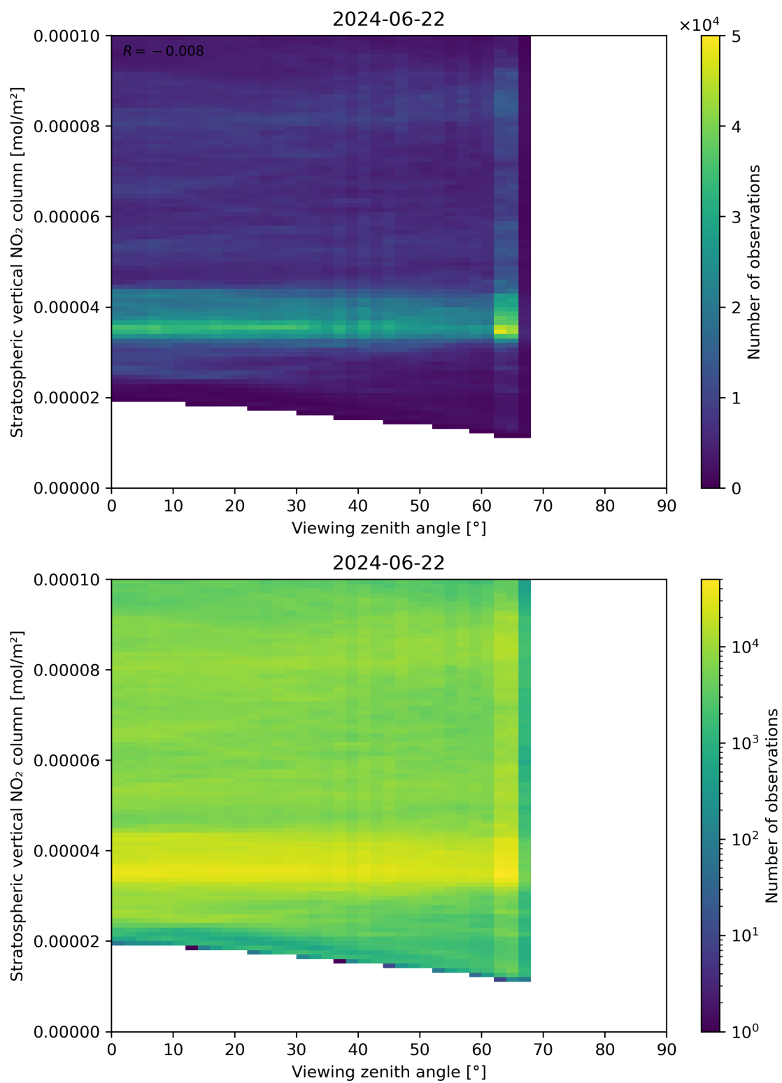
Figure 164: Scatter density plot of “Viewing zenith angle” against “Stratospheric vertical NO 2 column” for 2024-06-21 to 2024-06-23.
