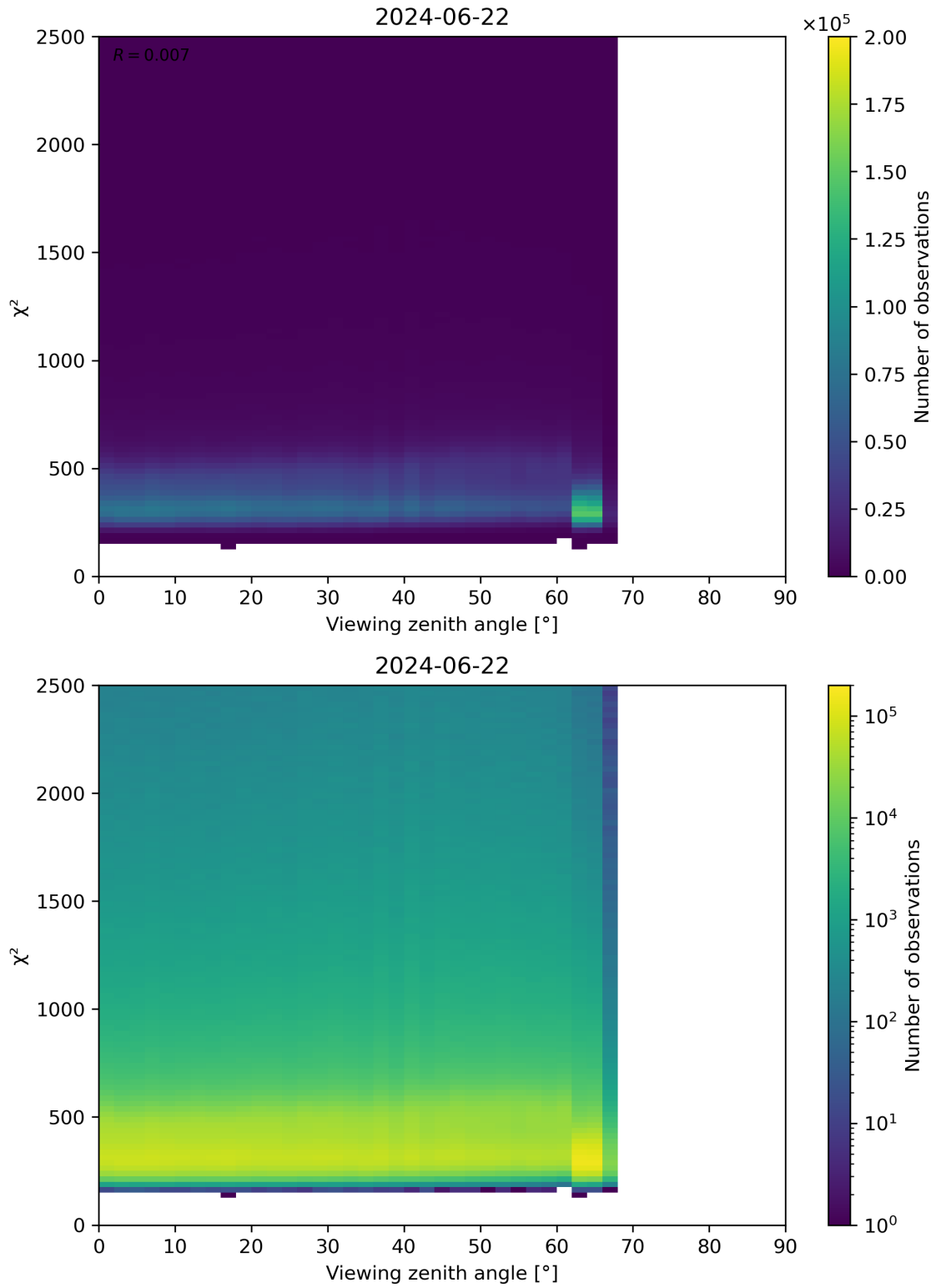
Figure 162: Scatter density plot of “Viewing zenith angle” against “ \chi^2 ” for 2024-06-21 to 2024-06-23.
