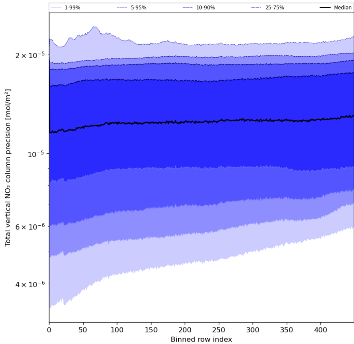
Figure 56: Along track statistics of “Total vertical NO 2 column precision” for 2024-06-21 to 2024-06-23
