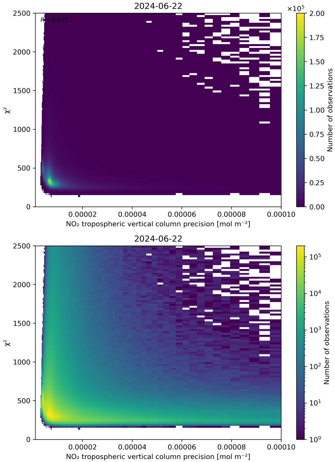
Figure 134: Scatter density plot of “NO 2 tropospheric vertical column precision” against “ \chi^2 ” for 2024-06-21 to 2024-06-23.
