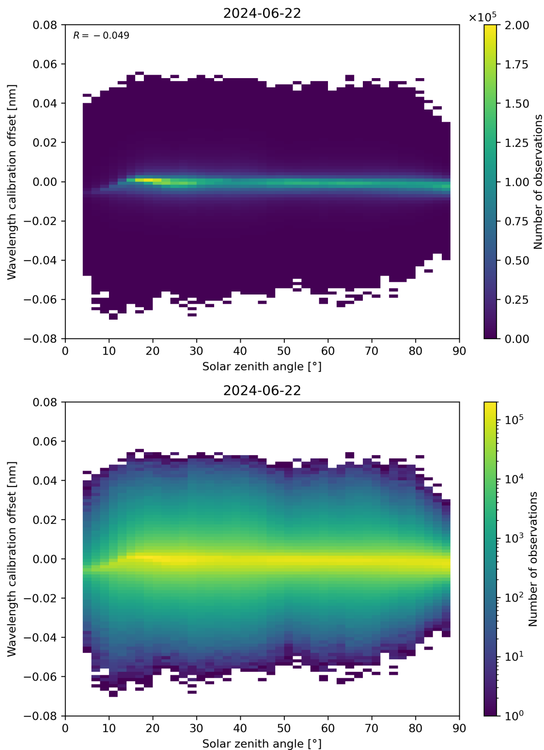
Figure 158: Scatter density plot of “Solar zenith angle” against “Wavelength calibration offset” for 2024-06-21 to 2024-06-23.
