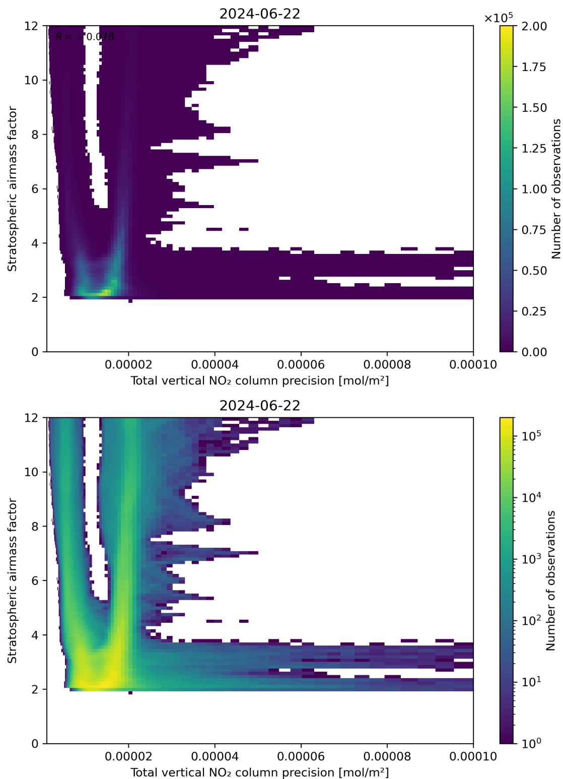
Figure 115: Scatter density plot of “Total vertical NO 2 column precision” against “Stratospheric air mass factor” for 2024-06-21 to 2024-06-23.
