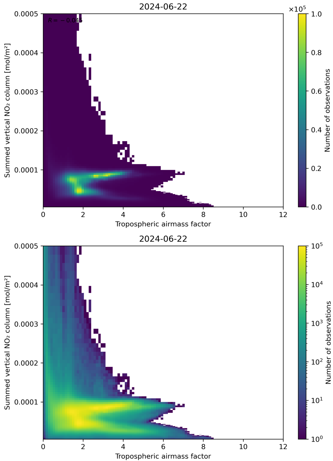
Figure 75: Scatter density plot of “Tropospheric airmass factor” against “Summed vertical NO 2 column” for 2024-06-21 to 2024-06-23.
