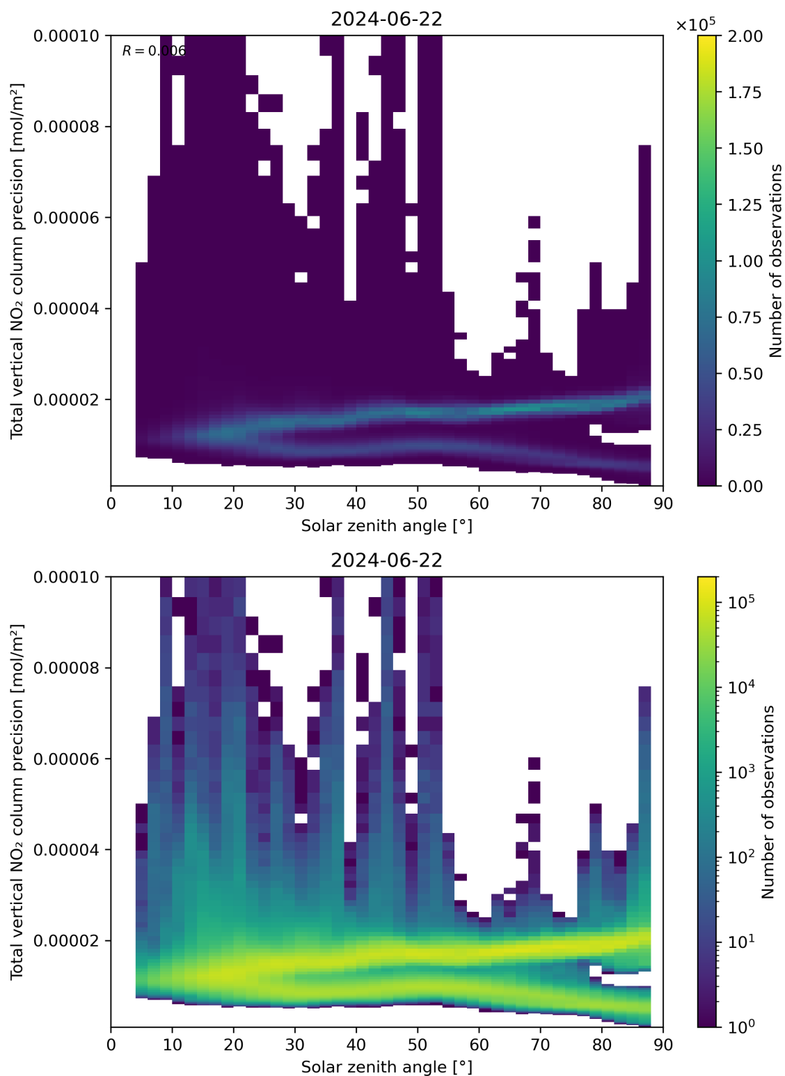
Figure 154: Scatter density plot of “Solar zenith angle” against “Total vertical NO 2 column precision” for 2024-06-21 to 2024-06-23.
