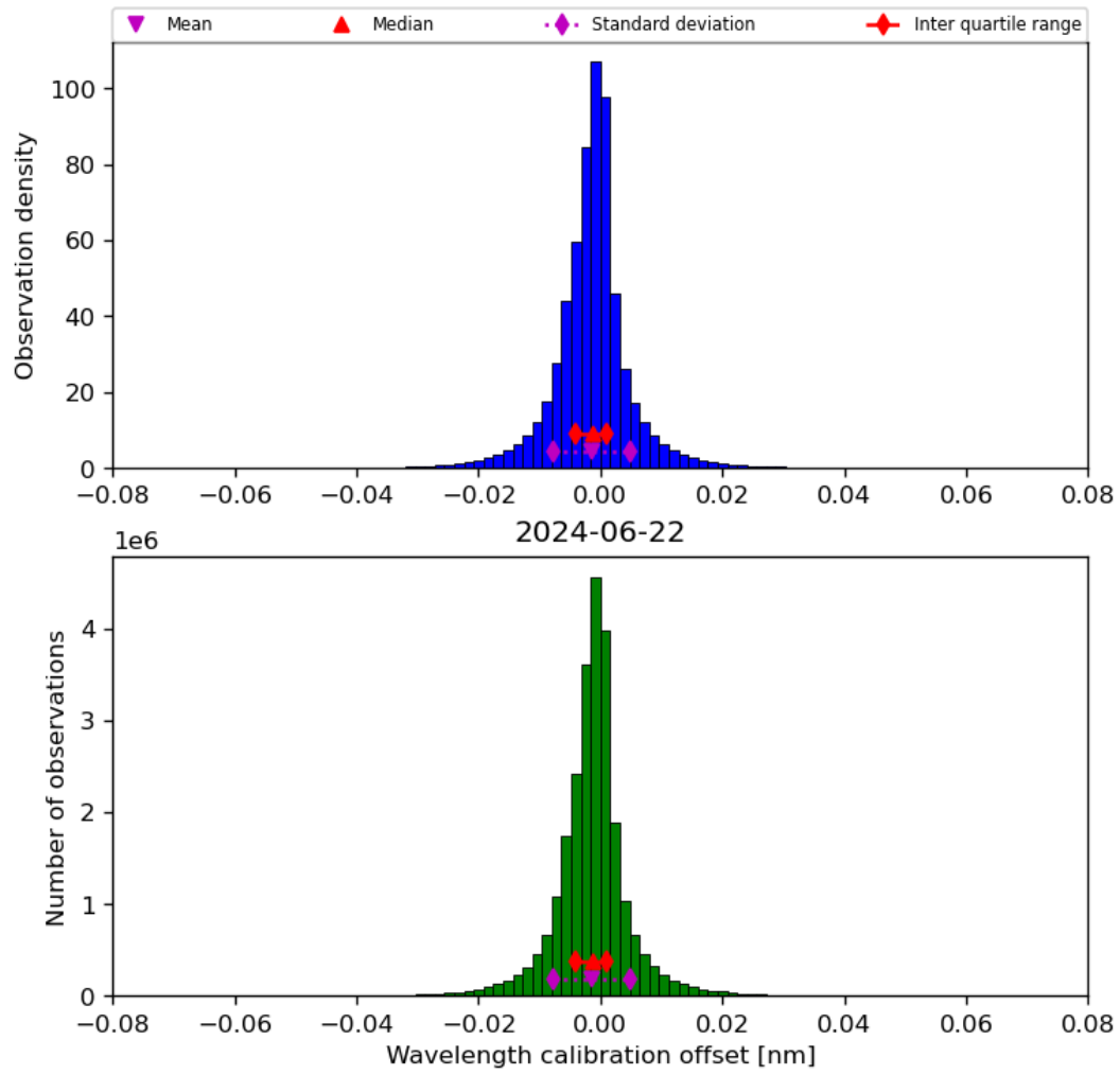
Figure 35: Histogram of “Wavelength calibration offset” for 2024-06-21 to 2024-06-23
