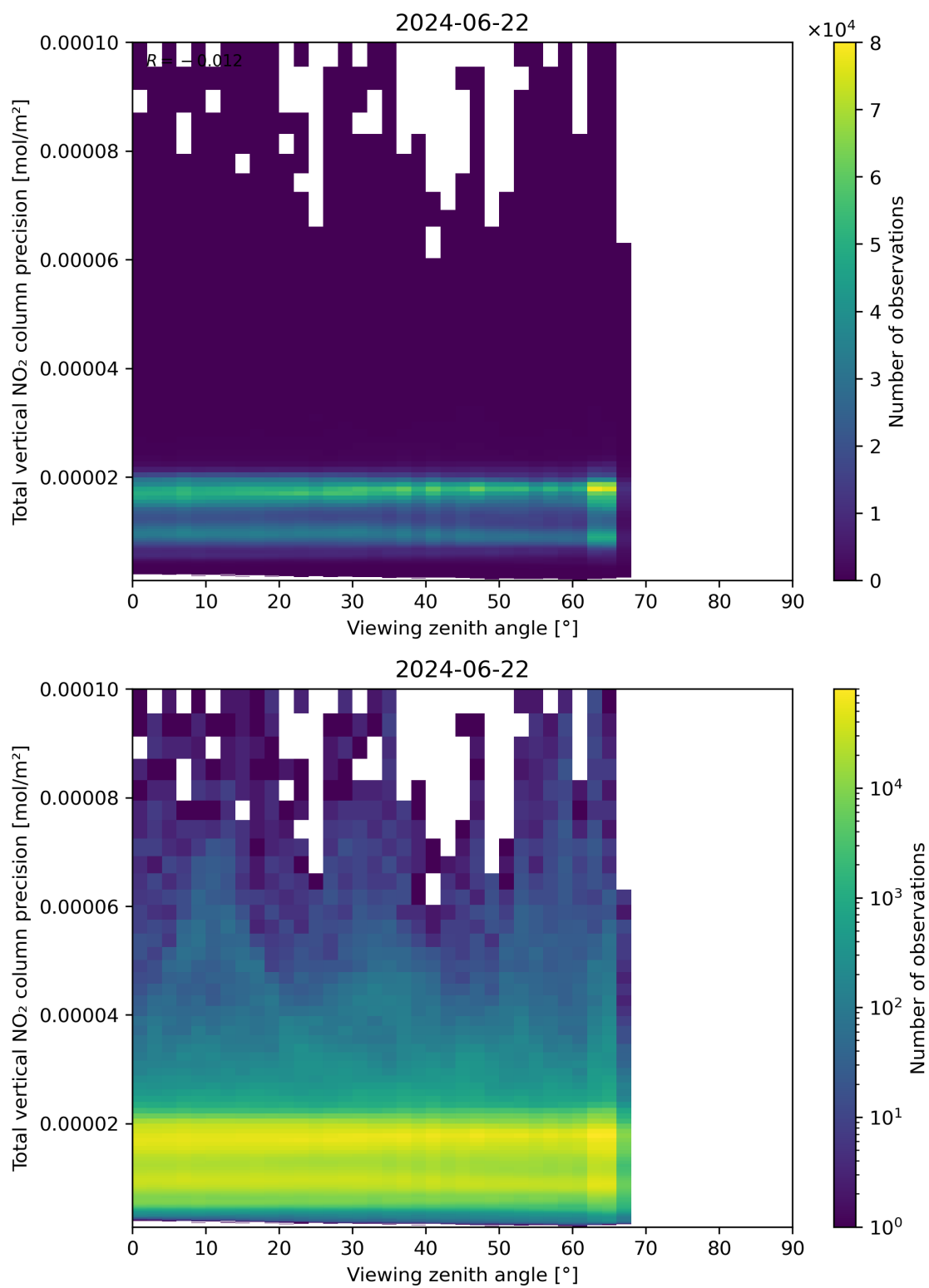
Figure 168: Scatter density plot of “Viewing zenith angle” against “Total vertical NO 2 column precision” for 2024-06-21 to 2024-06-23.
