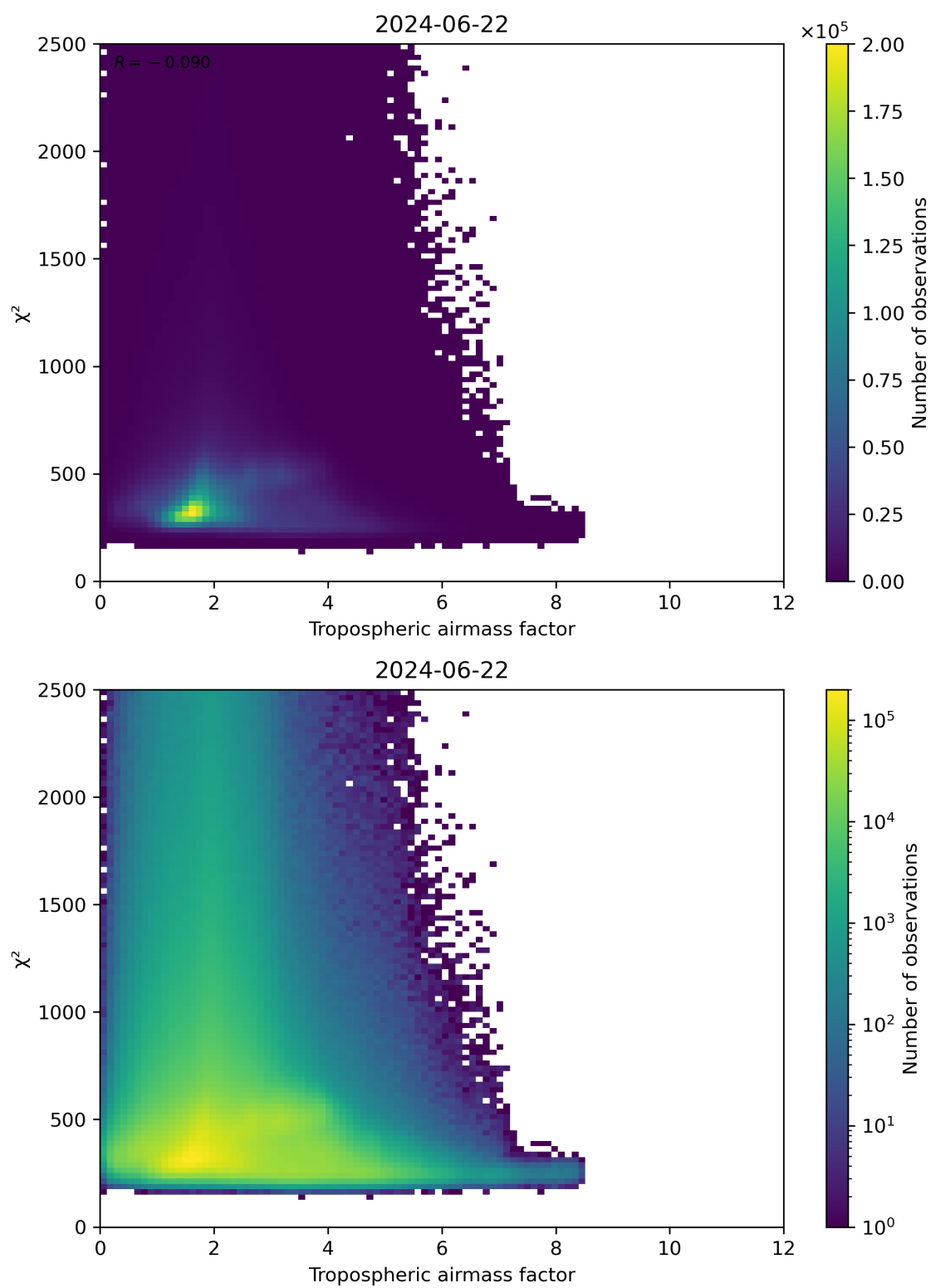
Figure 73: Scatter density plot of “Tropospheric airmass factor” against “ \chi^2 ” for 2024-06-21 to 2024-06-23.
