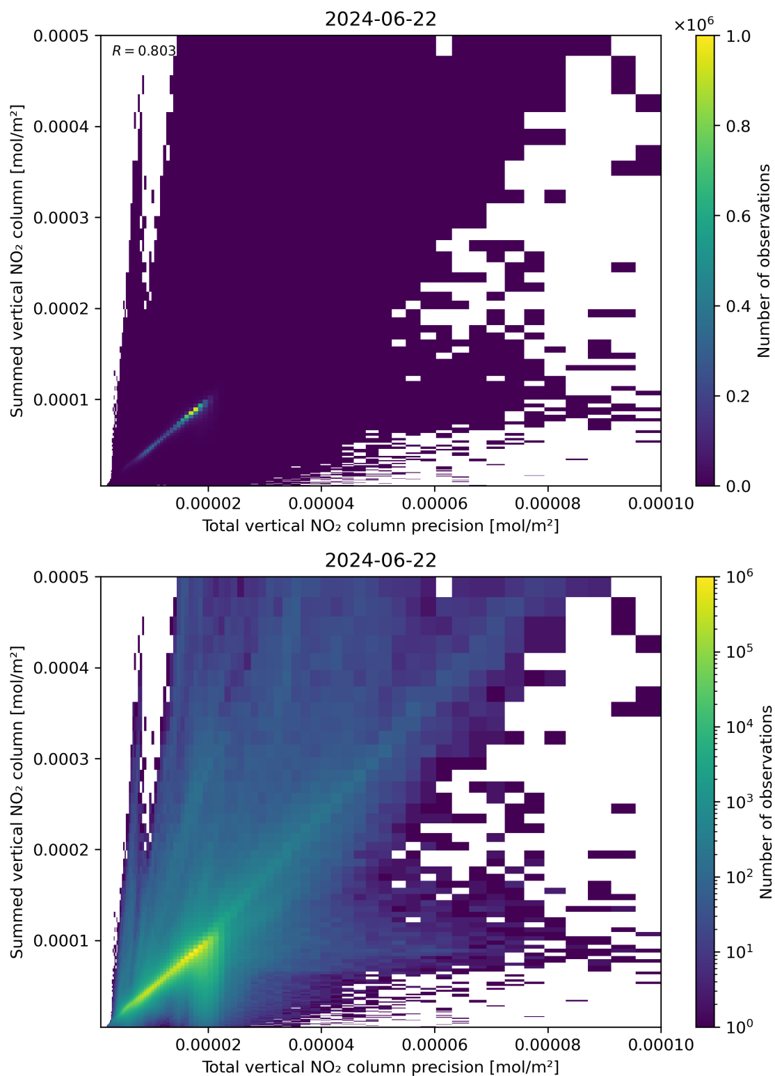
Figure 117: Scatter density plot of “Total vertical NO 2 column precision” against “Summed vertical NO 2 column” for 2024-06-21 to 2024-06-23.
