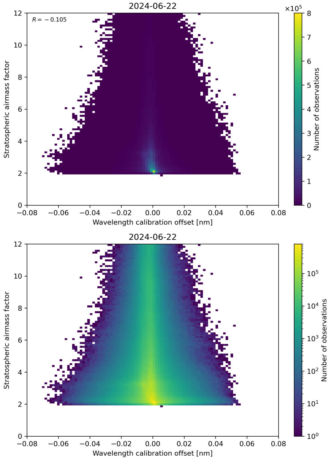
Figure 174: Scatter density plot of “Wavelength calibration offset” against “Stratospheric airmass factor” for 2024-06-21 to 2024-06-23.
