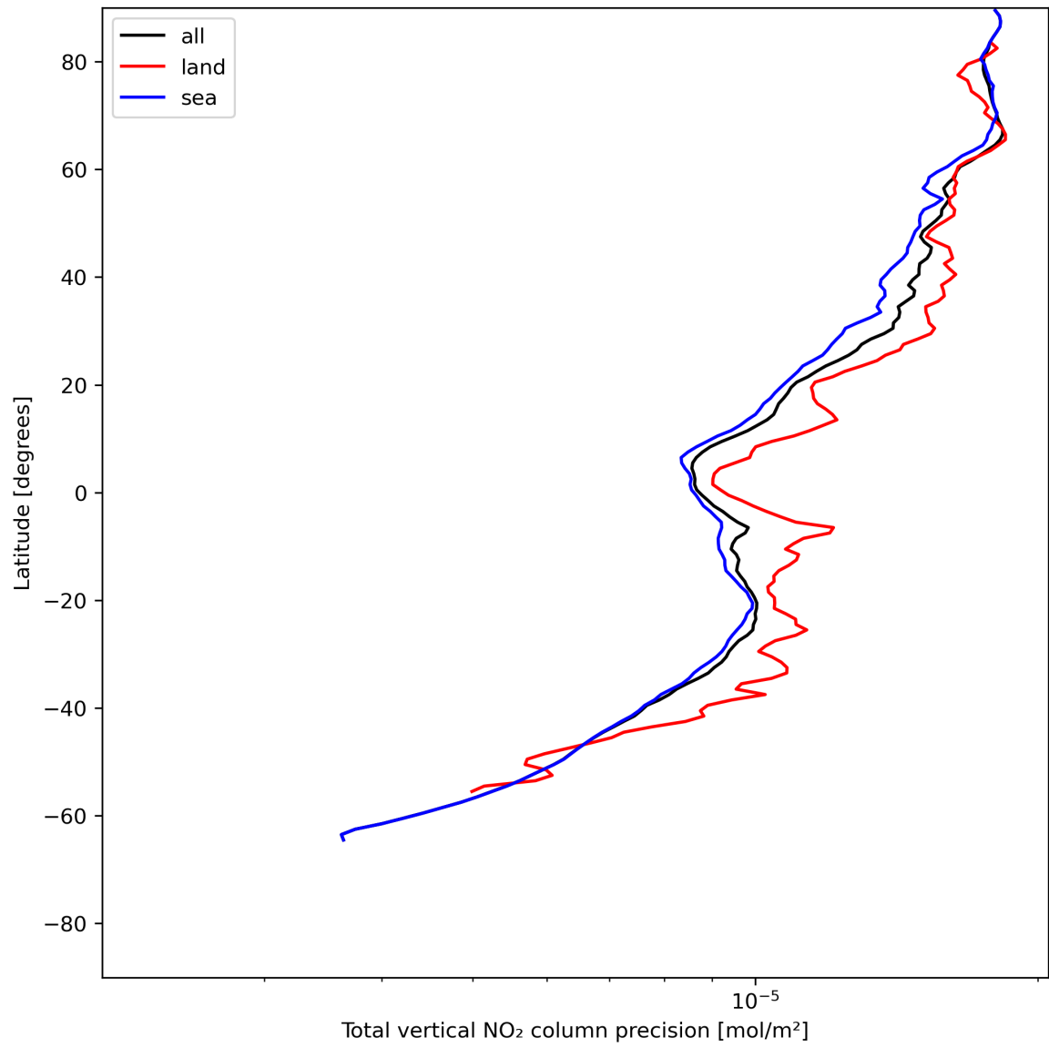
Figure 22: Zonal average of “Total vertical NO 2 column precision” for 2024-06-21 to 2024-06-23.
