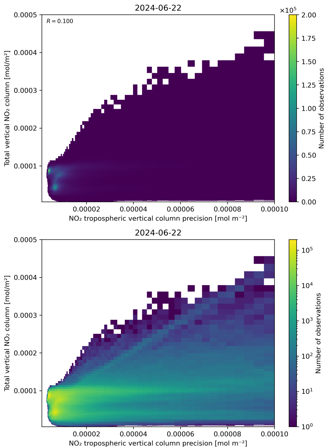
Figure 138: Scatter density plot of “NO 2 tropospheric vertical column precision” against “Total vertical NO 2 column” for 2024-06-21 to 2024-06-23.
