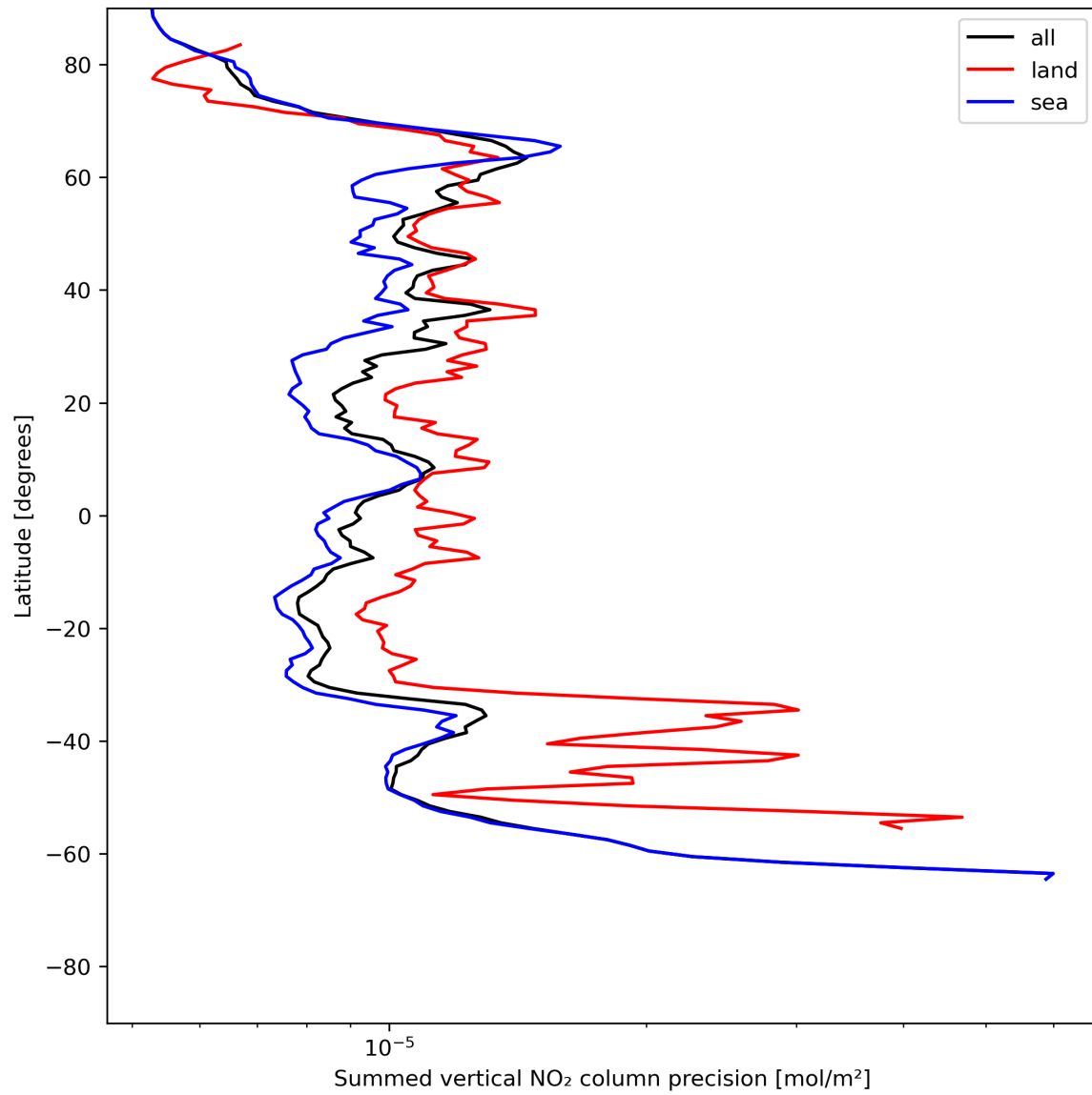
Figure 24: Zonal average of “Summed vertical NO 2 column precision” for 2024-06-21 to 2024-06-23.
