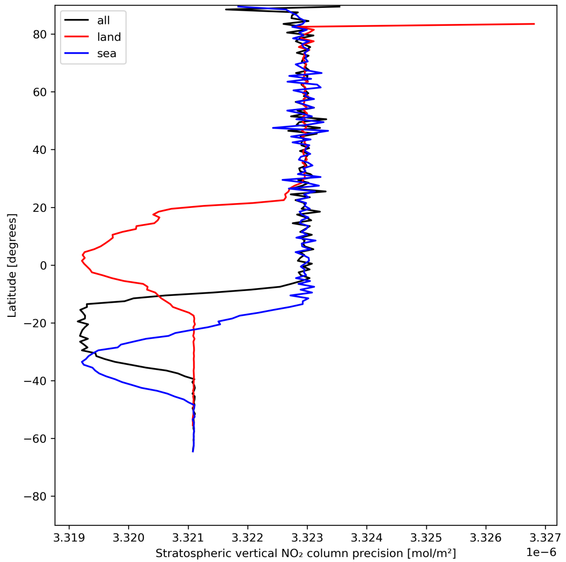
Figure 20: Zonal average of “Stratospheric vertical NO 2 column precision” for 2024-06-21 to 2024-06-23.
