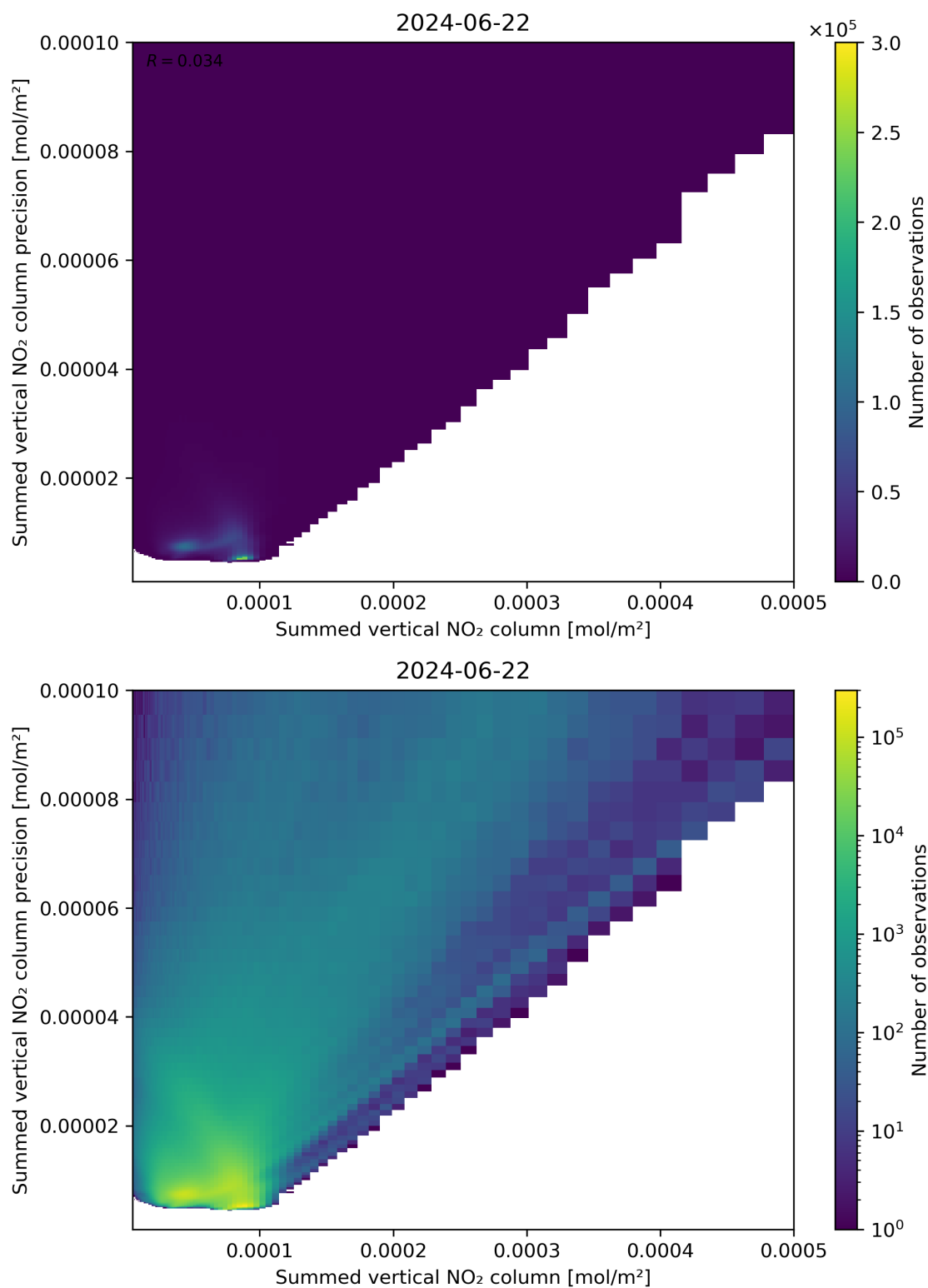
Figure 105: Scatter density plot of “Summed vertical NO 2 column” against “Summed vertical NO 2 column precision” for 2024-06-21 to 2024-06-23.
