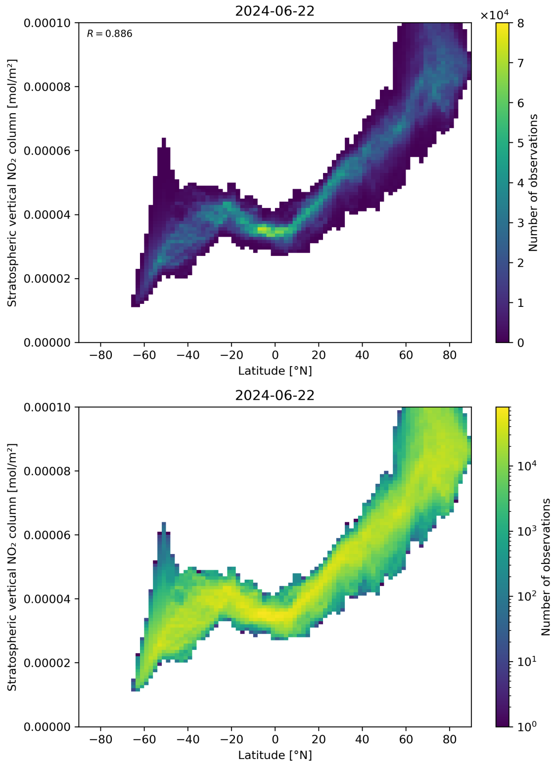
Figure 87: Scatter density plot of “Latitude” against “Stratospheric vertical NO 2 column” for 2024-06-21 to 2024-06-23.
