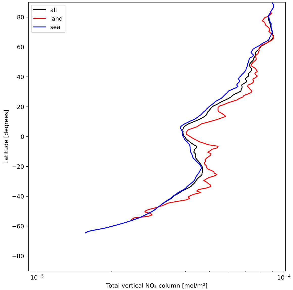
Figure 21: Zonal average of “Total vertical NO 2 column” for 2024-06-21 to 2024-06-23.
