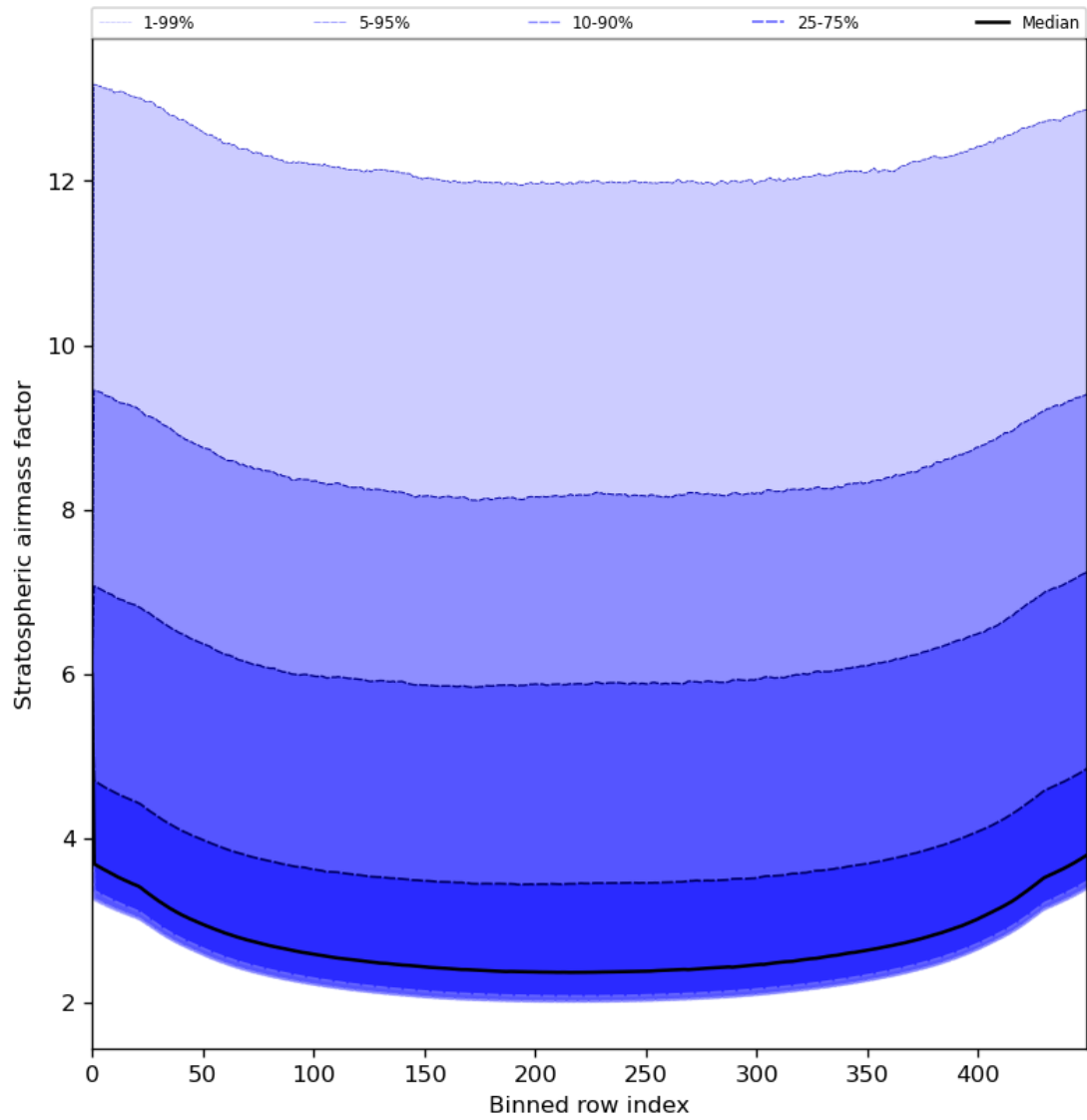
Figure 61: Along track statistics of “Stratospheric airmass factor” for 2024-06-21 to 2024-06-23
