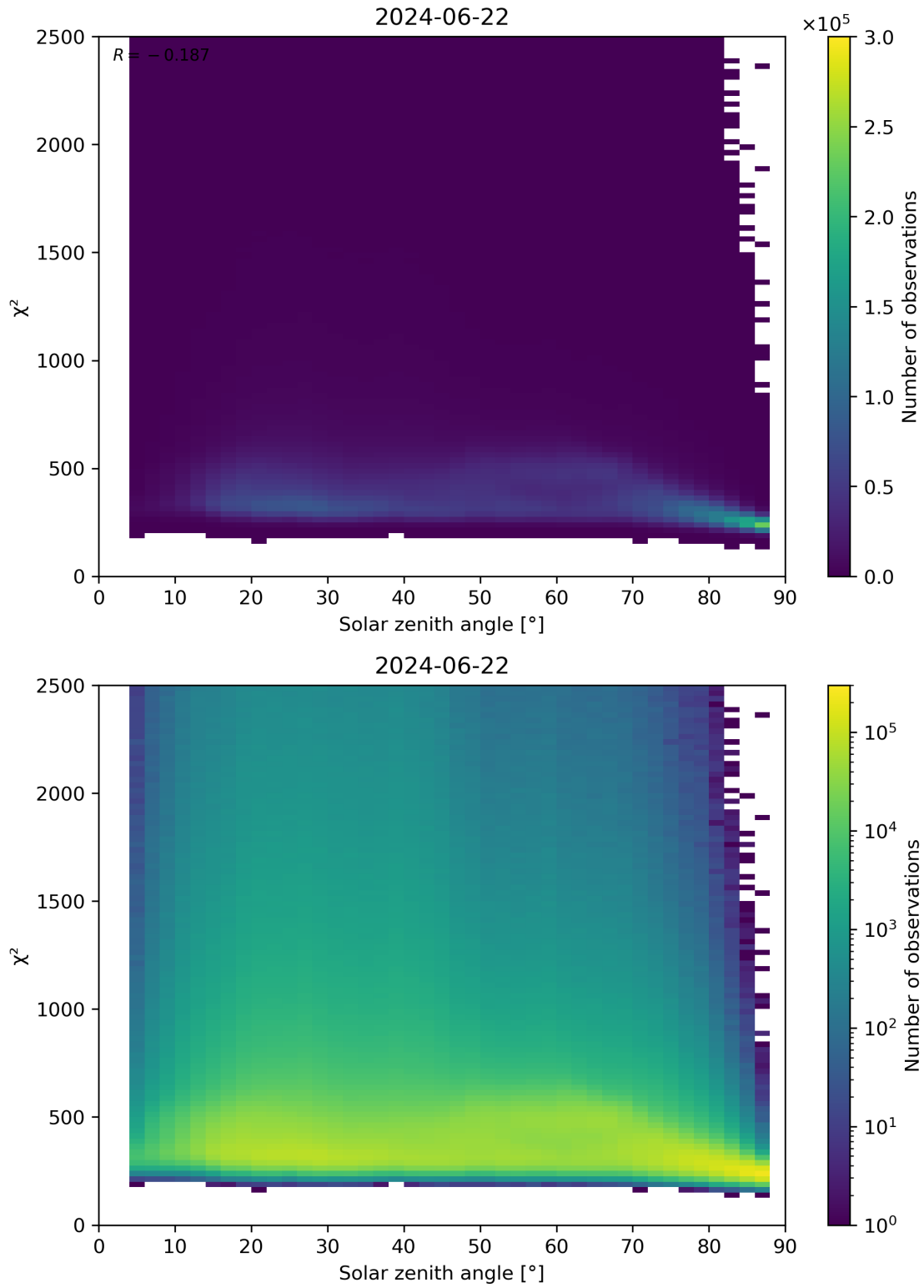
Figure 148: Scatter density plot of “Solar zenith angle” against “ \chi^2 ” for 2024-06-21 to 2024-06-23.
