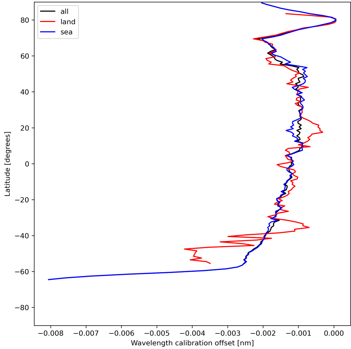
Figure 18: Zonal average of “Wavelength calibration offset” for 2024-06-21 to 2024-06-23.
