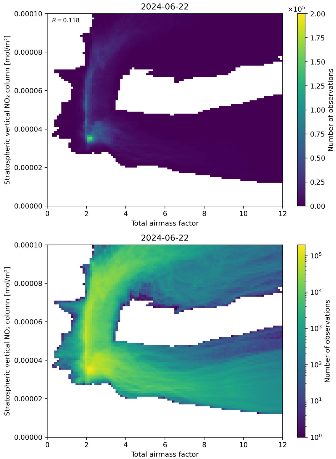
Figure 64: Scatter density plot of “Total airmass factor” against “Stratospheric vertical NO 2 column” for 2024-06-21 to 2024-06-23.
