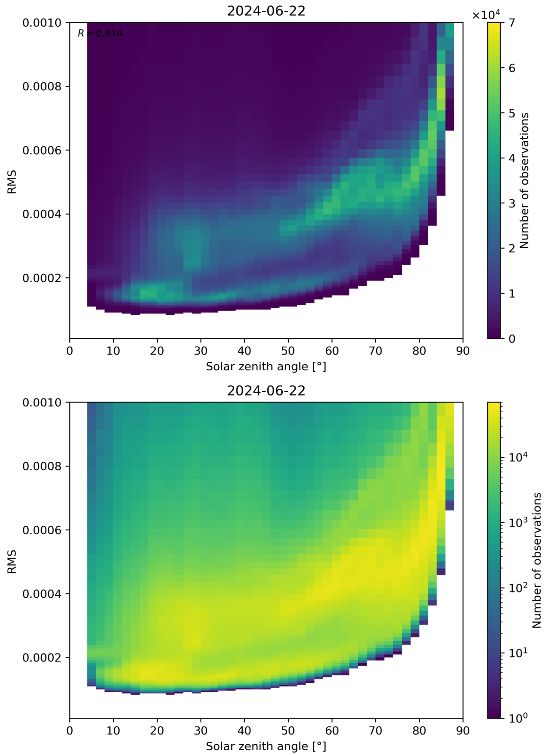
Figure 157: Scatter density plot of “Solar zenith angle” against “RMS” for 2024-06-21 to 2024-06-23.
