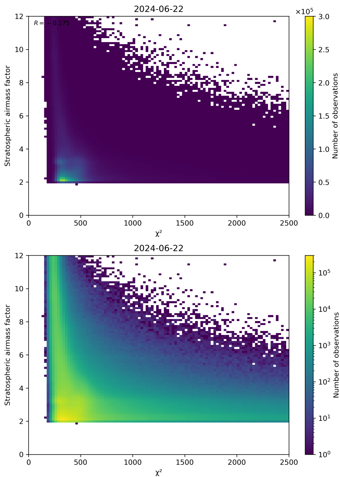
Figure 81: Scatter density plot of “ \chi^2 ” against “Stratospheric airmass factor” for 2024-06-21 to 2024-06-23.
