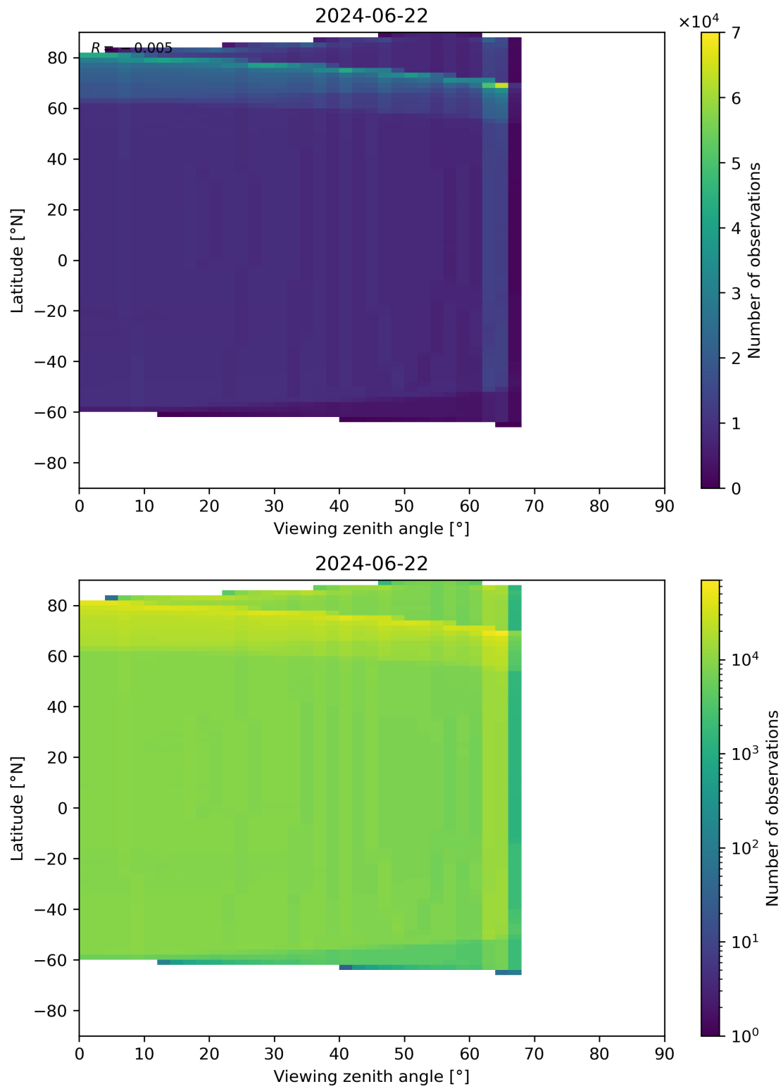
Figure 163: Scatter density plot of “Viewing zenith angle” against “Latitude” for 2024-06-21 to 2024-06-23.
