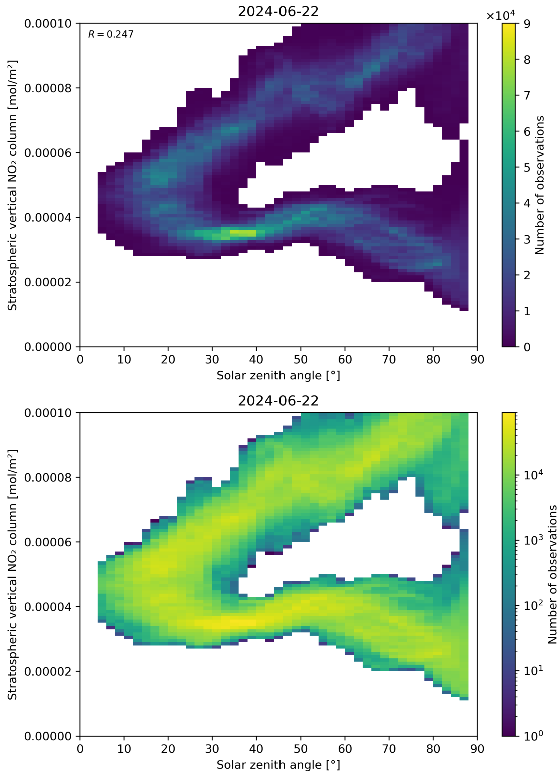
Figure 150: Scatter density plot of “Solar zenith angle” against “Stratospheric vertical NO 2 column” for 2024-06-21 to 2024-06-23.
