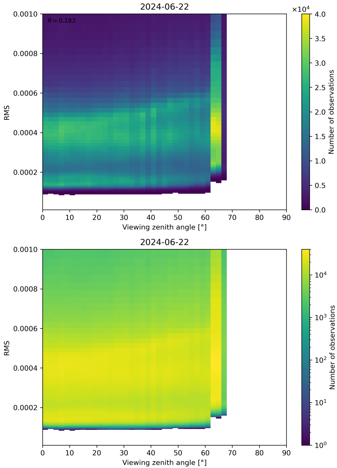
Figure 171: Scatter density plot of “Viewing zenith angle” against “RMS” for 2024-06-21 to 2024-06-23.
