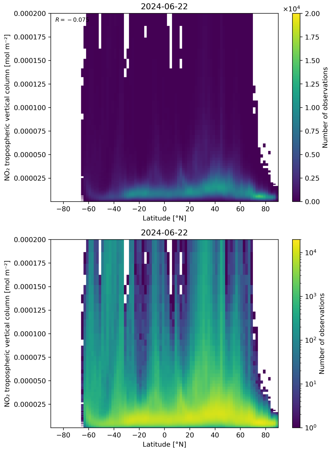
Figure 92: Scatter density plot of “Latitude” against “NO 2 tropospheric vertical column” for 2024-06-21 to 2024-06-23.
