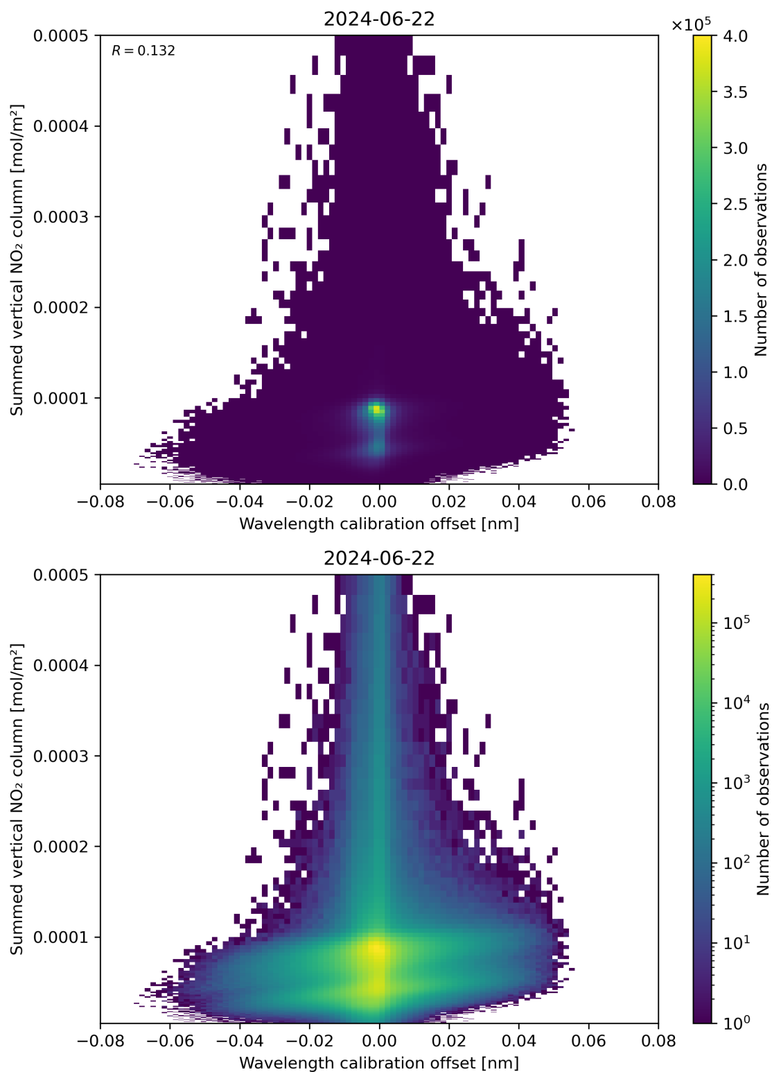
Figure 177: Scatter density plot of “Wavelength calibration offset” against “Summed vertical NO 2 column” for 2024-06-21 to 2024-06-23.
