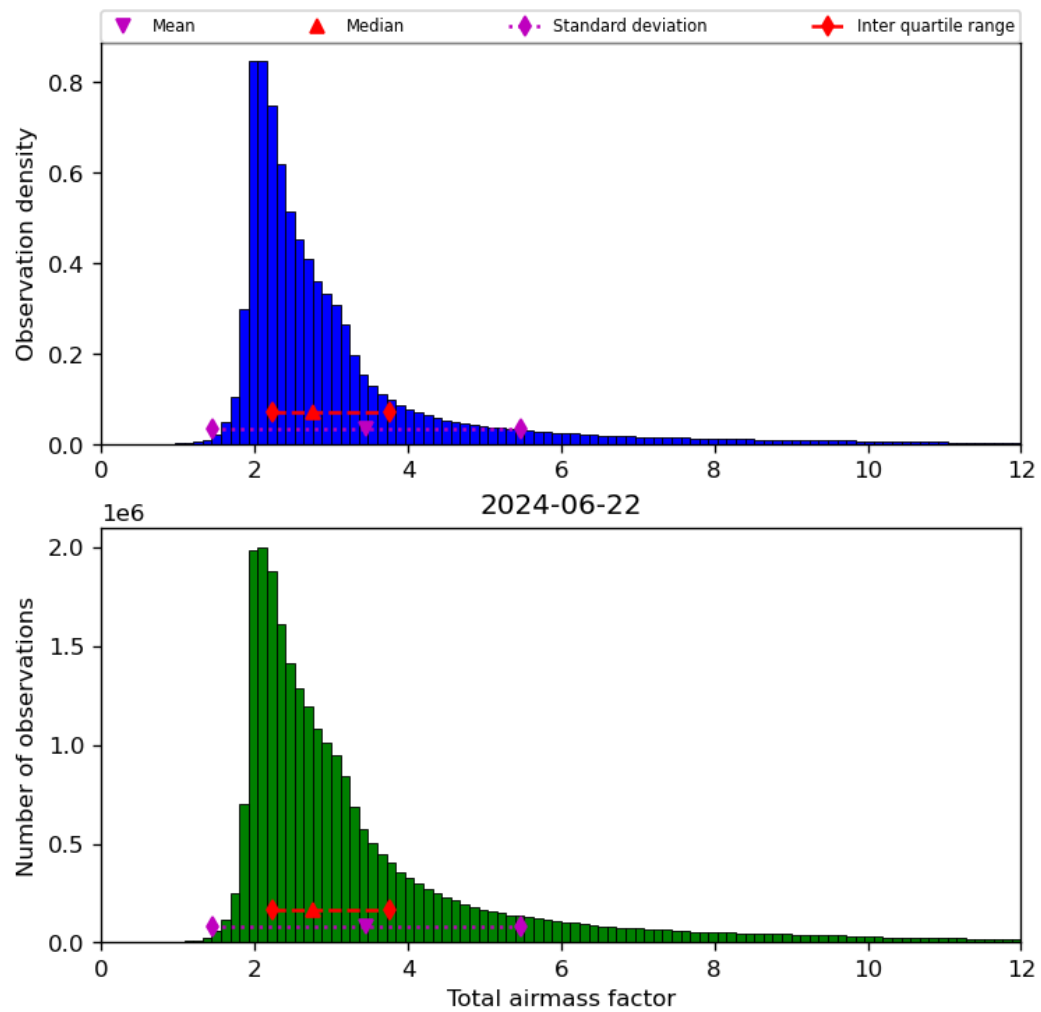
Figure 32: Histogram of “Total airmass factor” for 2024-06-21 to 2024-06-23
