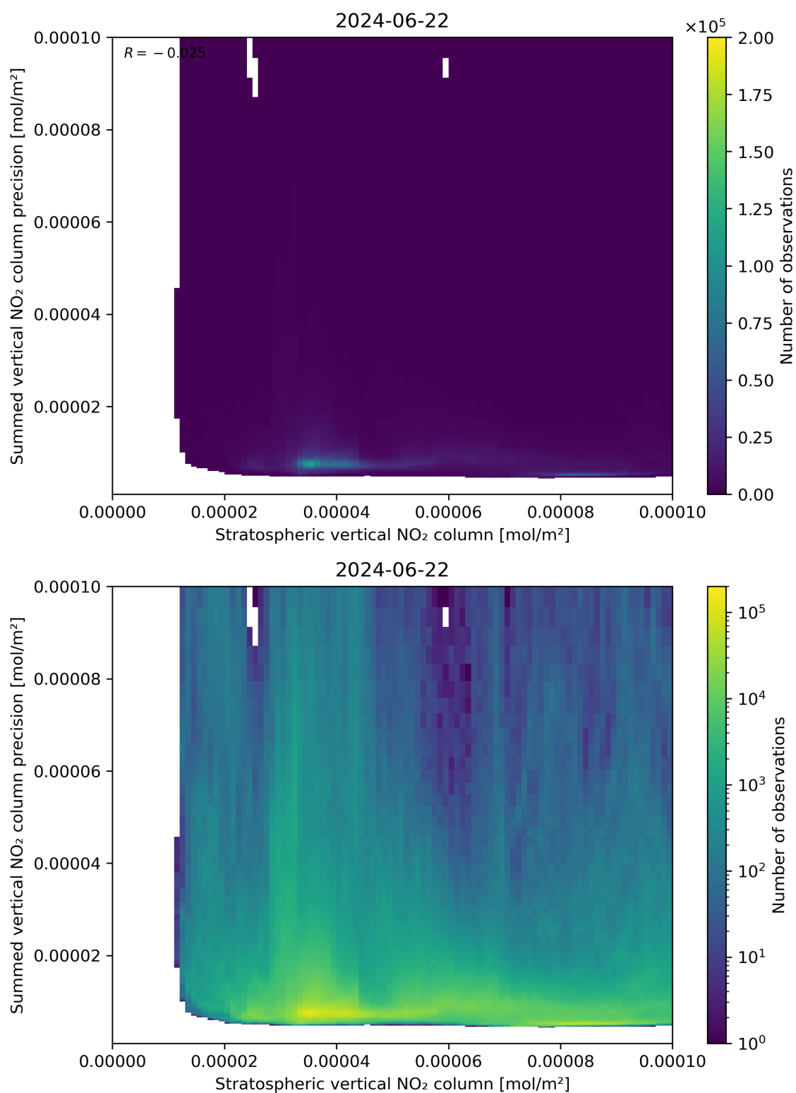
Figure 99: Scatter density plot of “Stratospheric vertical NO 2 column” against “Summed vertical NO 2 column precision” for 2024-06-21 to 2024-06-23.
