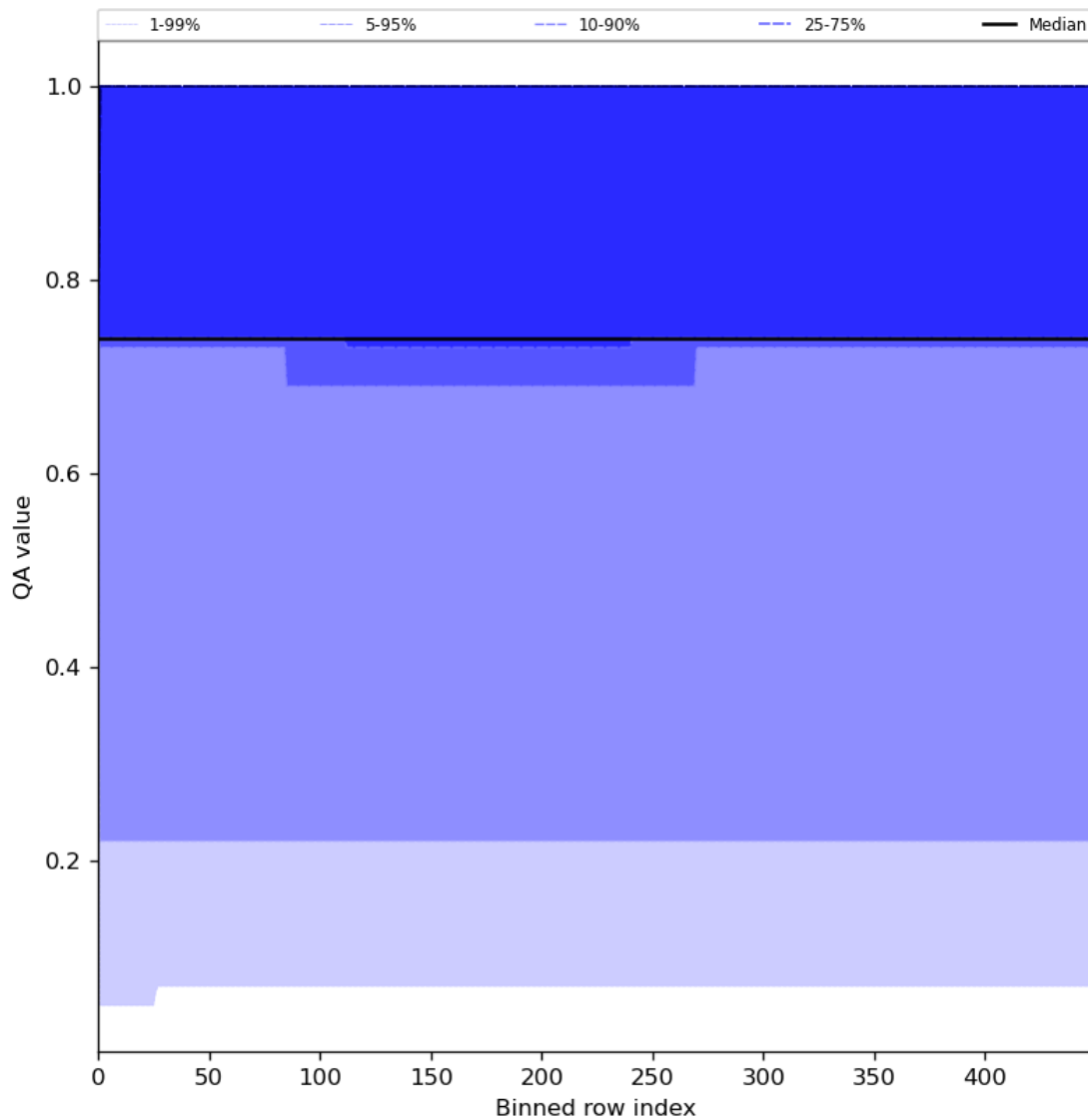
Figure 45: Along track statistics of “QA value” for 2024-06-21 to 2024-06-23
