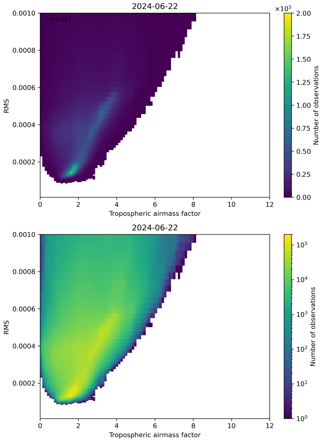
Figure 79: Scatter density plot of “Tropospheric airmass factor” against “RMS” for 2024-06-21 to 2024-06-23.
