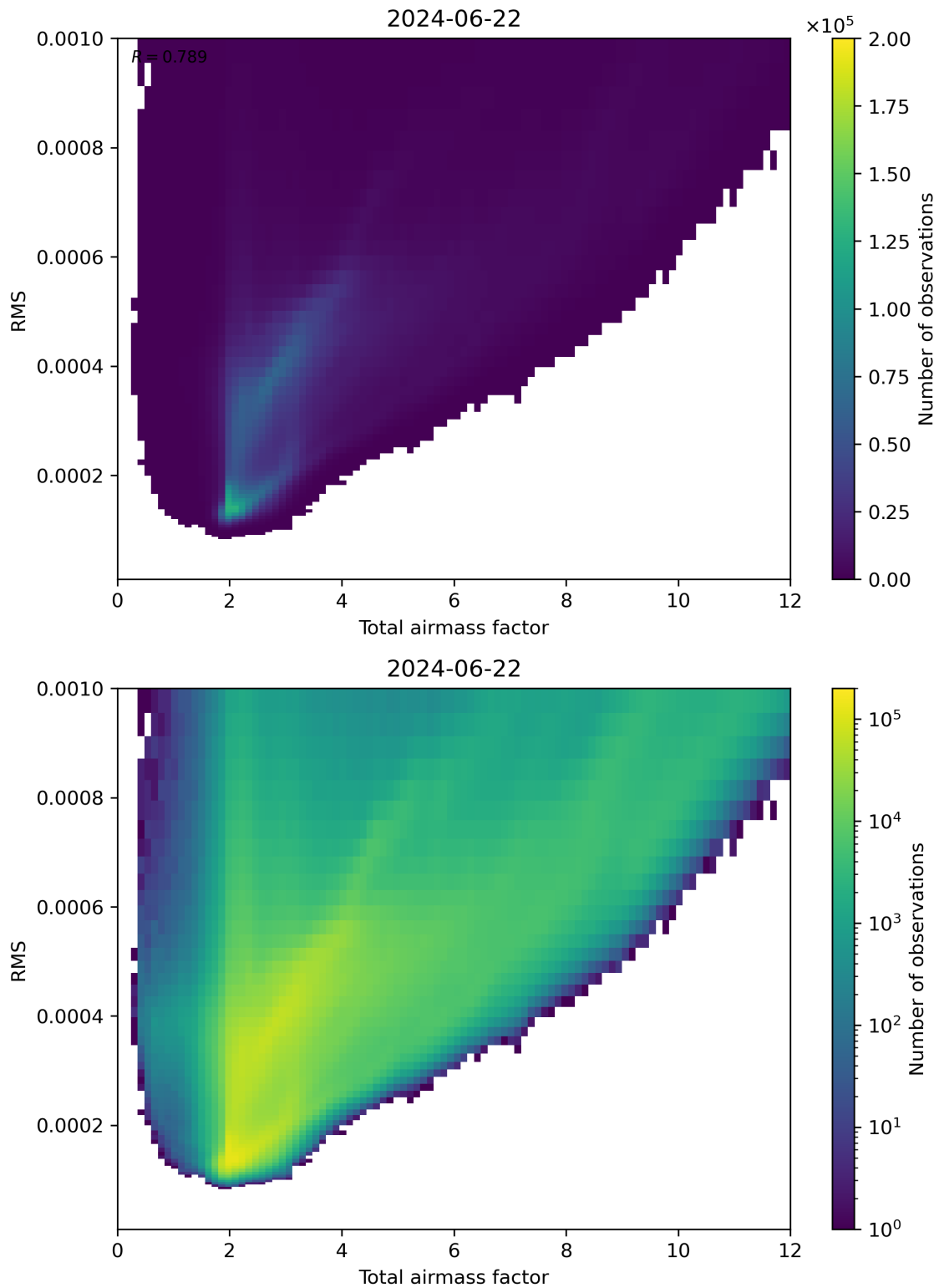
Figure 69: Scatter density plot of “Total airmass factor” against “RMS” for 2024-06-21 to 2024-06-23.
