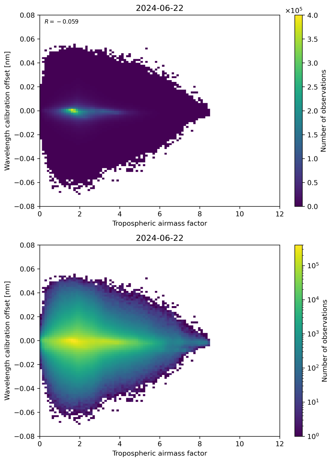
Figure 80: Scatter density plot of “Tropospheric air mass factor” against “Wavelength calibration offset” for 2024-06-21 to 2024-06-23.
