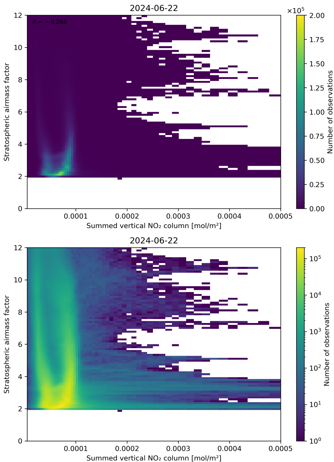
Figure 103: Scatter density plot of “Summed vertical NO 2 column” against “Stratospheric air mass factor” for 2024-06-21 to 2024-06-23.
