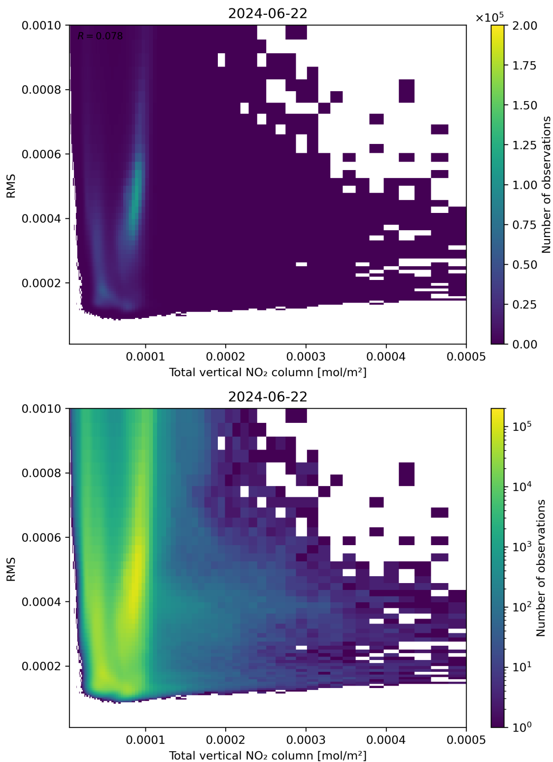
Figure 120: Scatter density plot of “Total vertical NO 2 column” against “RMS” for 2024-06-21 to 2024-06-23.
