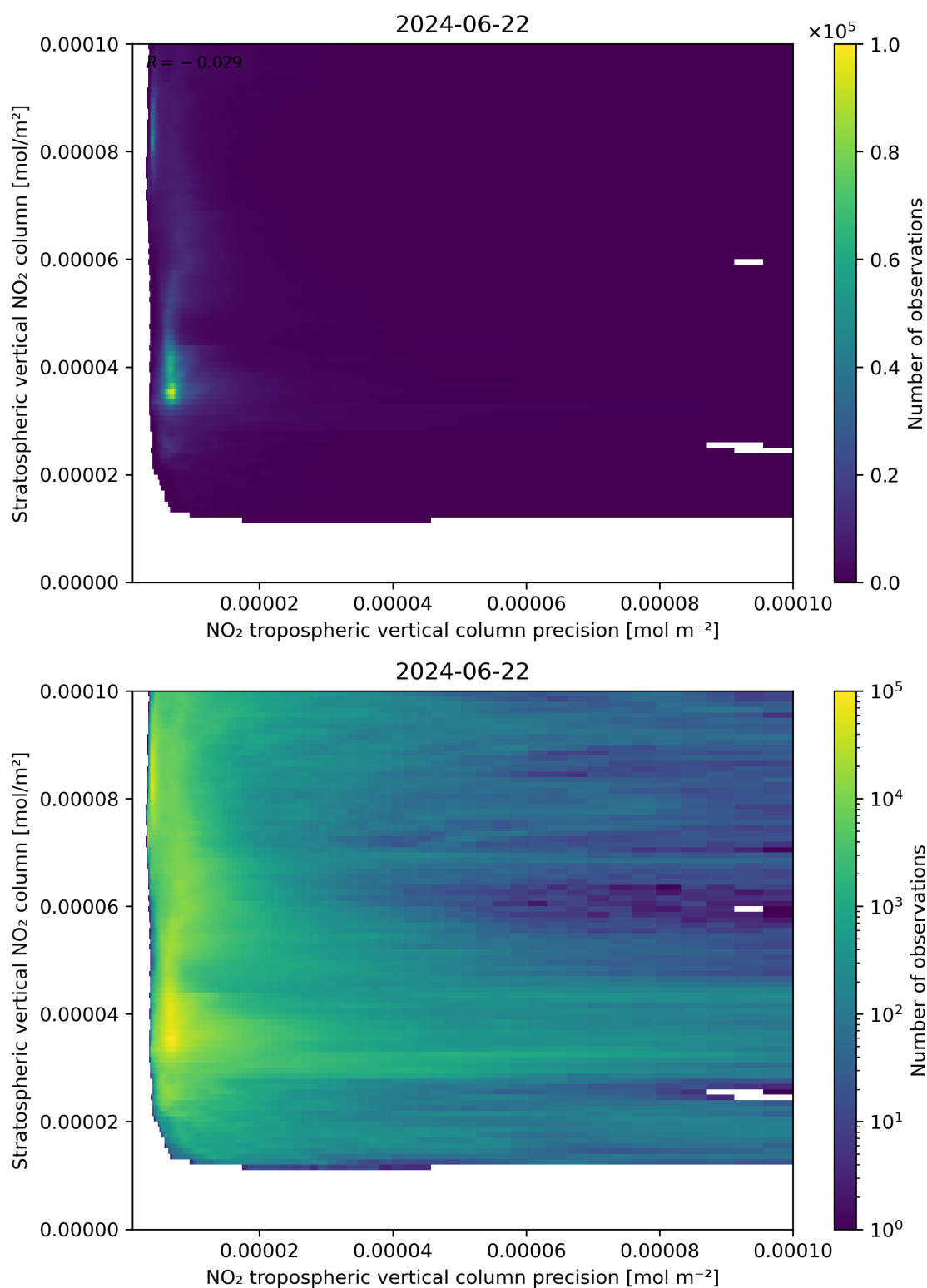
Figure 135: Scatter density plot of “NO 2 tropospheric vertical column precision” against “Stratospheric vertical NO 2 column” for 2024-06-21 to 2024-06-23.
