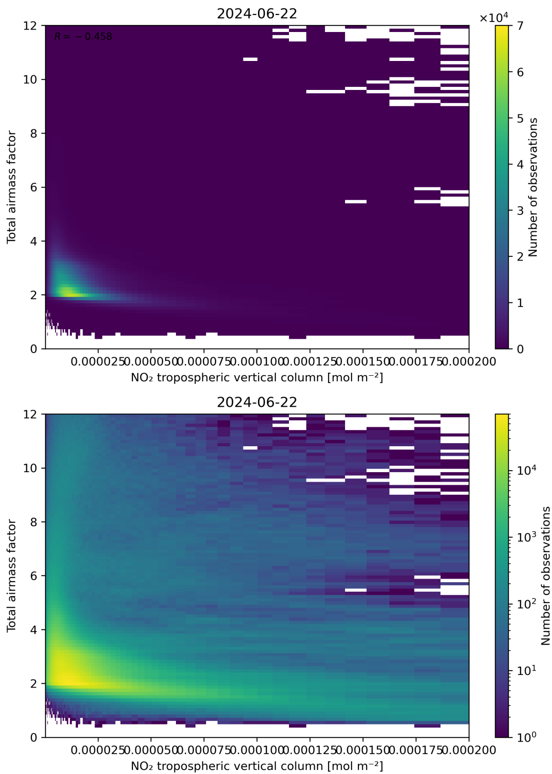
Figure 122: Scatter density plot of “NO 2 tropospheric vertical column” against “Total air mass factor” for 2024-06-21 to 2024-06-23.
