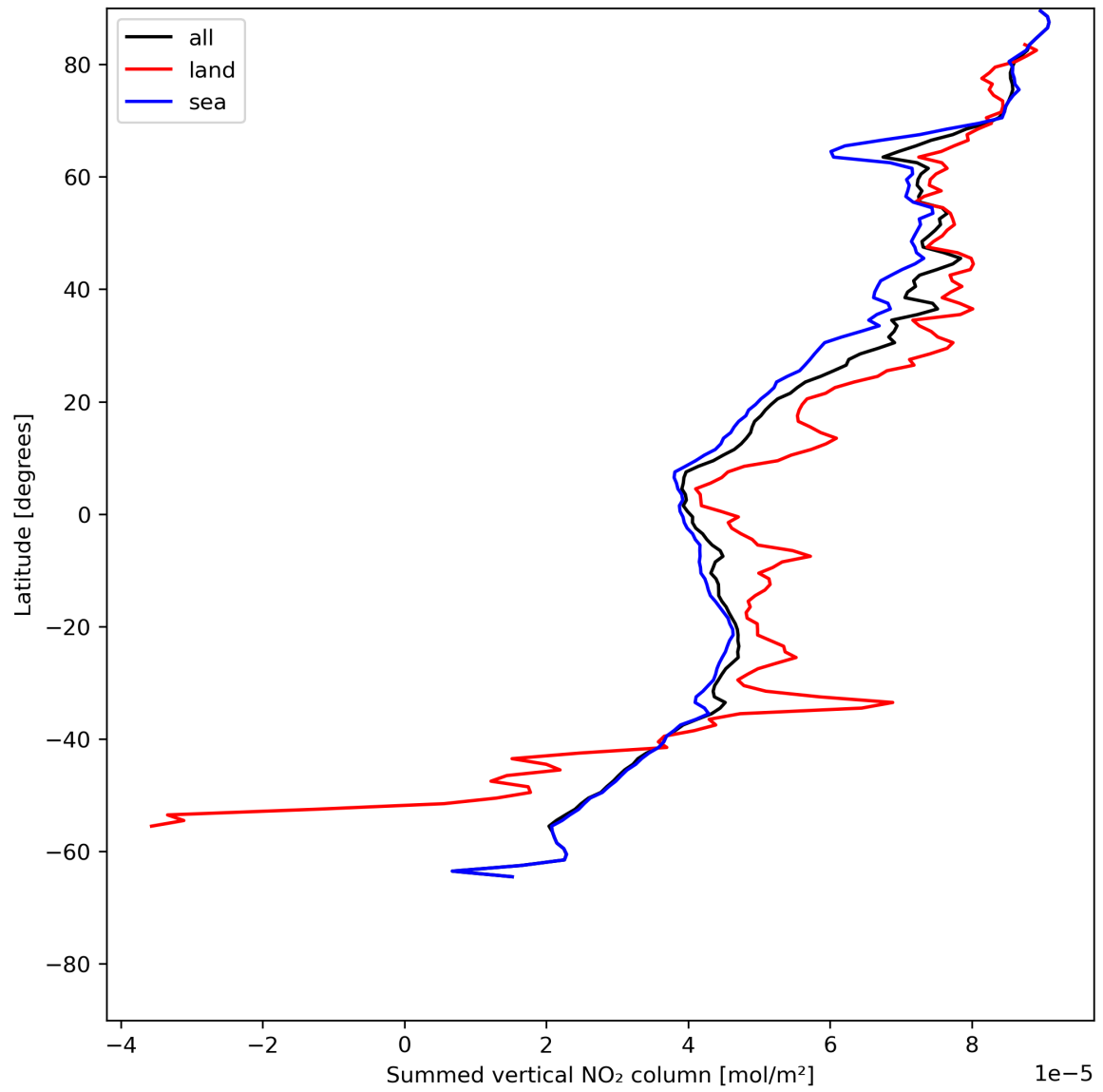
Figure 23: Zonal average of “Summed vertical NO 2 column” for 2024-06-21 to 2024-06-23.
