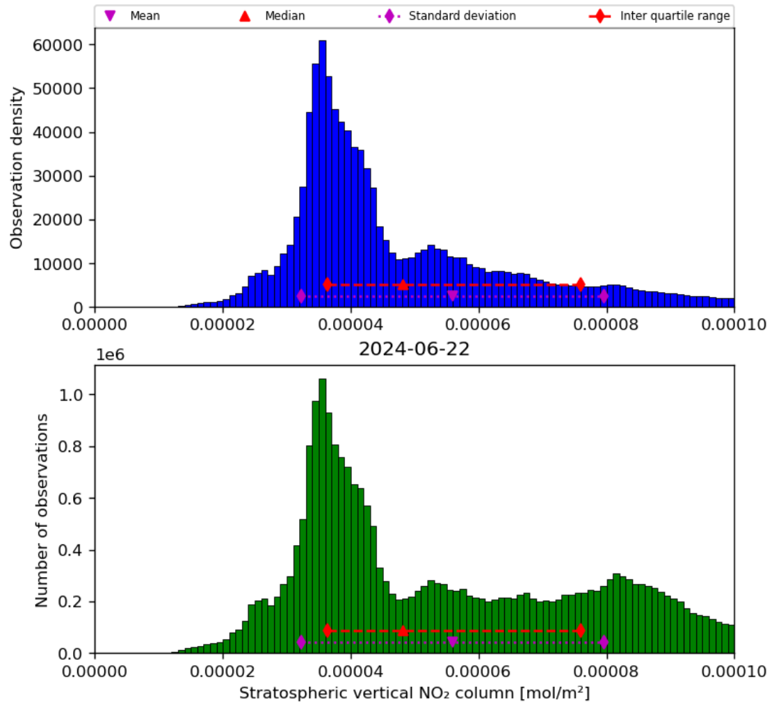
Figure 36: Histogram of “Stratospheric vertical NO 2 column” for 2024-06-21 to 2024-06-23
