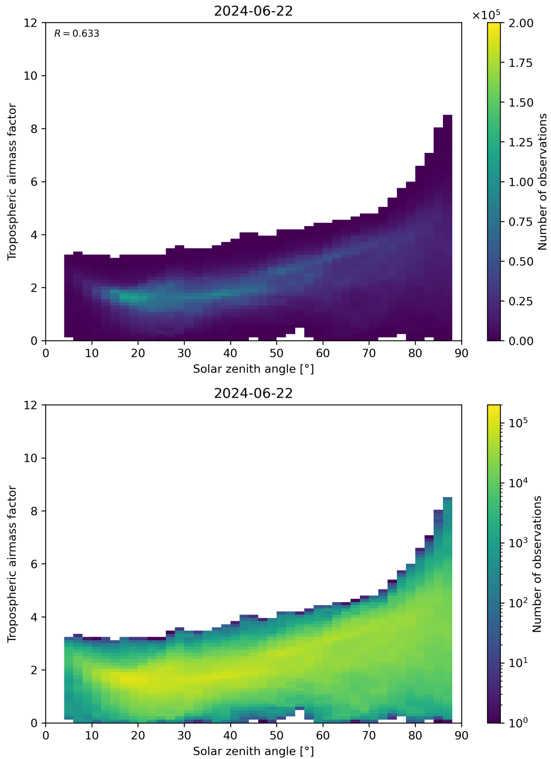
Figure 147: Scatter density plot of “Solar zenith angle” against “Tropospheric airmass factor” for 2024-06-21 to 2024-06-23.
