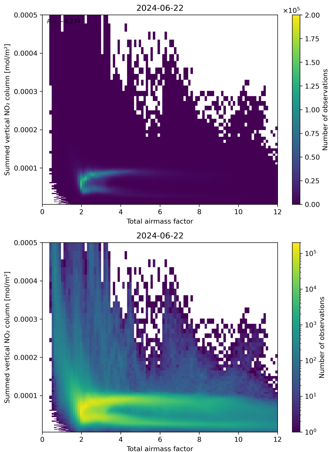
Figure 65: Scatter density plot of “Total airmass factor” against “Summed vertical NO 2 column” for 2024-06-21 to 2024-06-23.
