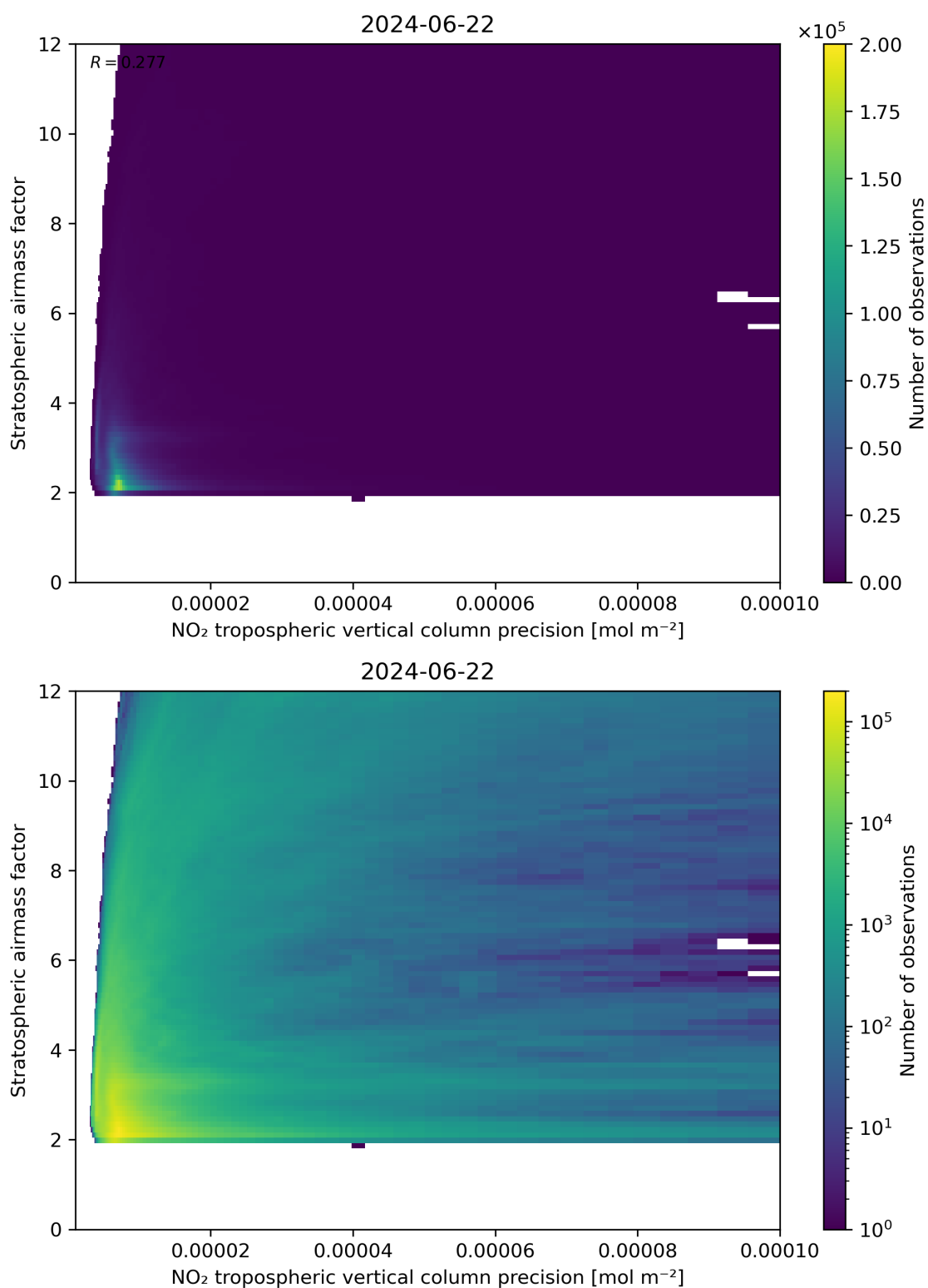
Figure 131: Scatter density plot of “NO 2 tropospheric vertical column precision” against “Stratospheric airmass factor” for 2024-06-21 to 2024-06-23.
