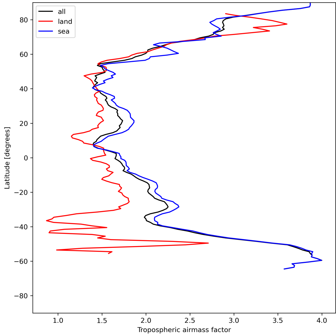
Figure 14: Zonal average of “Tropospheric airmass factor” for 2024-06-21 to 2024-06-23.
