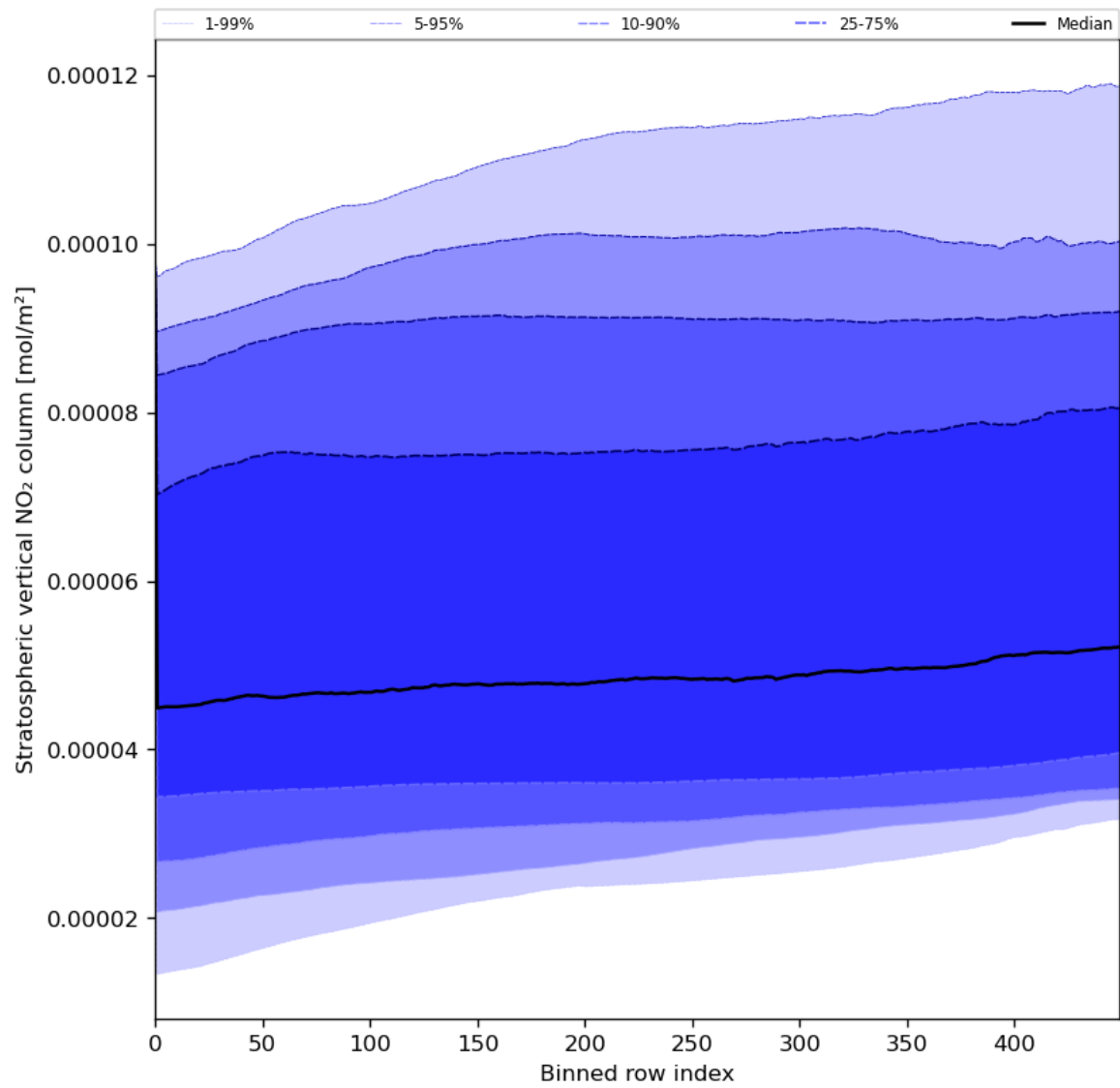
Figure 53: Along track statistics of “Stratospheric vertical NO 2 column” for 2024-06-21 to 2024-06-23
