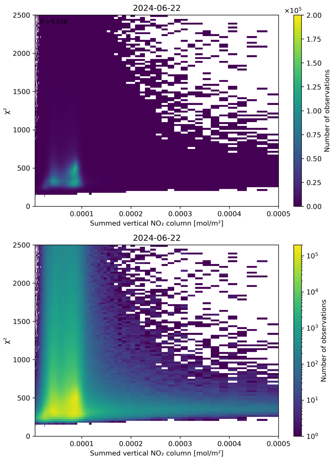
Figure 104: Scatter density plot of “Summed vertical NO 2 column” against “ \chi^2 ” for 2024-06-21 to 2024-06-23.
