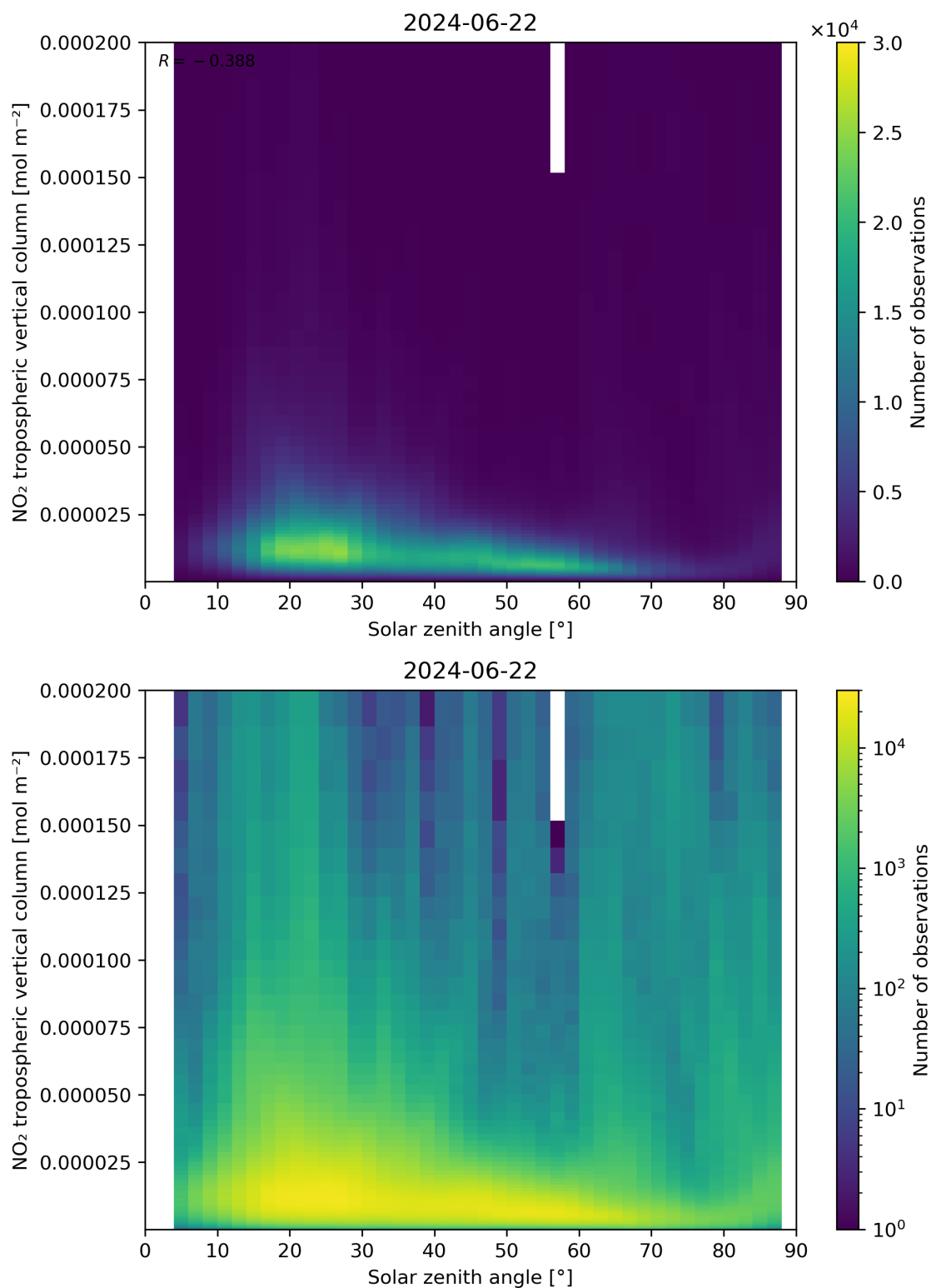
Figure 155: Scatter density plot of “Solar zenith angle” against “NO 2 tropospheric vertical column” for 2024-06-21 to 2024-06-23.
