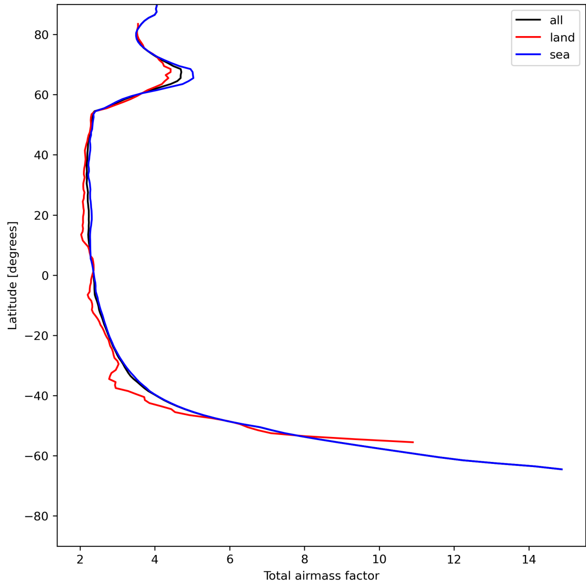
Figure 15: Zonal average of “Total airmass factor” for 2024-06-21 to 2024-06-23.
