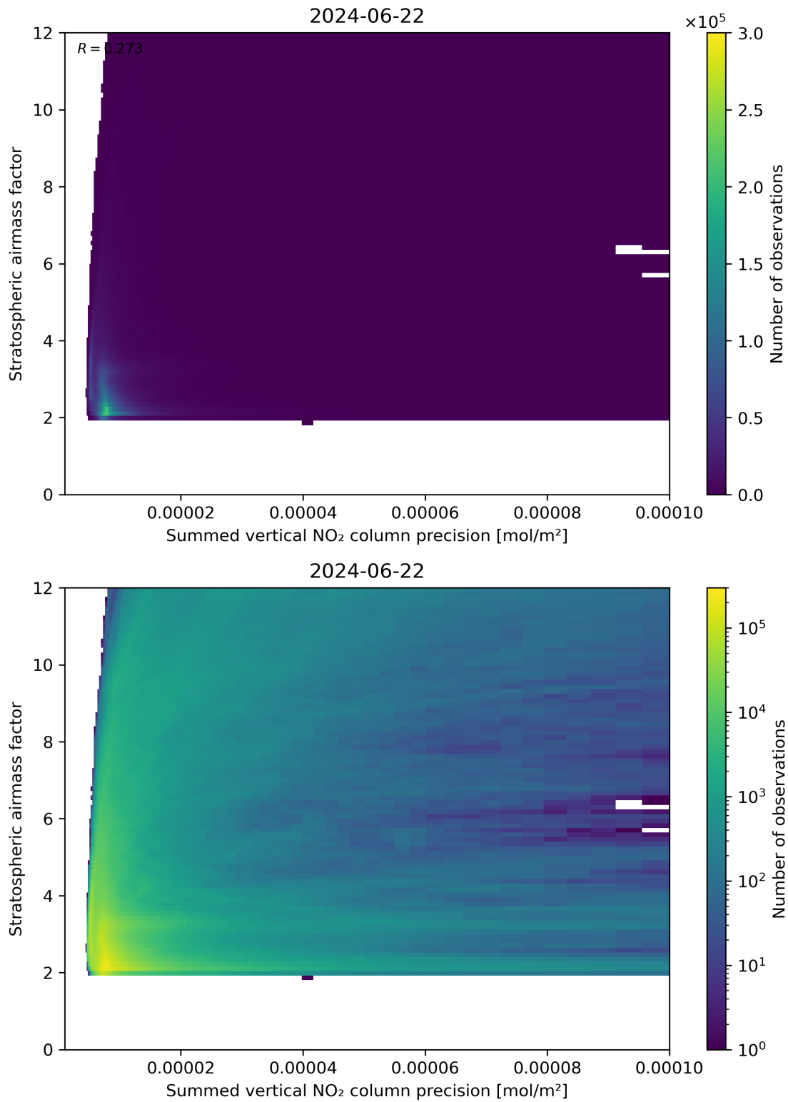
Figure 106: Scatter density plot of “Summed vertical NO 2 column precision” against “Stratospheric airmass factor” for 2024-06-21 to 2024-06-23.
