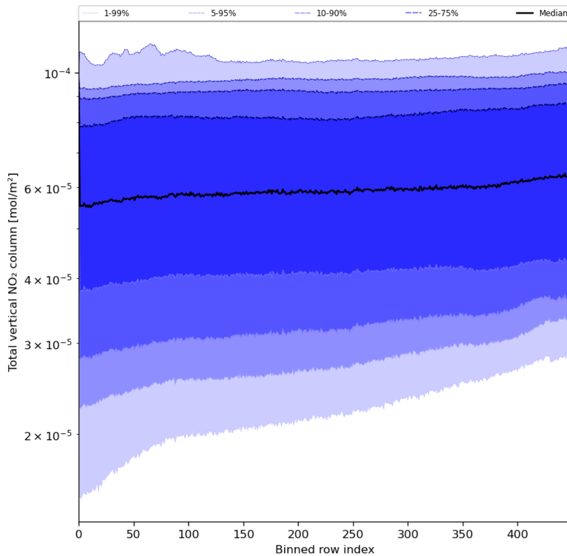
Figure 55: Along track statistics of “Total vertical NO 2 column” for 2024-06-21 to 2024-06-23
