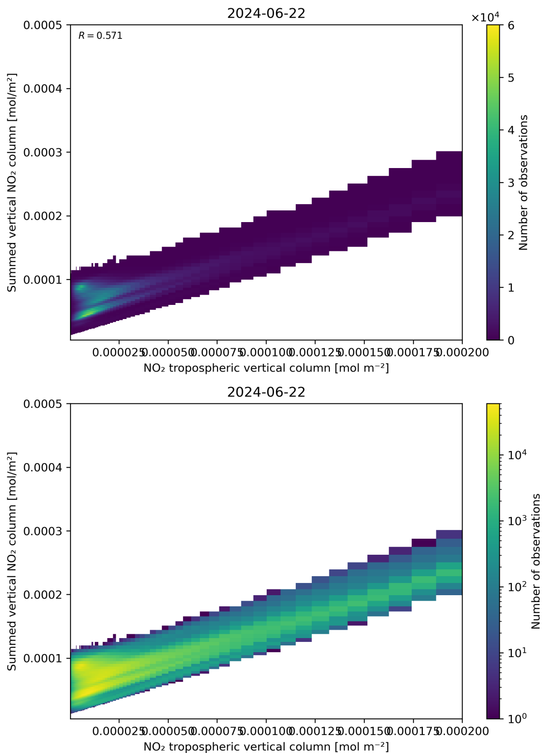
Figure 126: Scatter density plot of “NO 2 tropospheric vertical column” against “Summed vertical NO 2 column” for 2024-06-21 to 2024-06-23.
