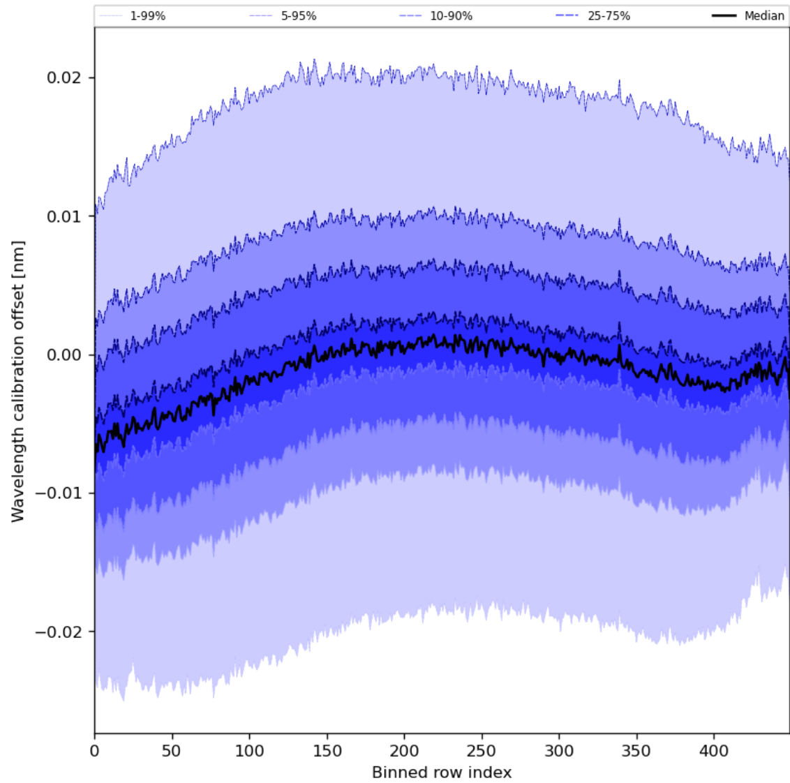
Figure 52: Along track statistics of “Wavelength calibration offset” for 2024-06-21 to 2024-06-23
