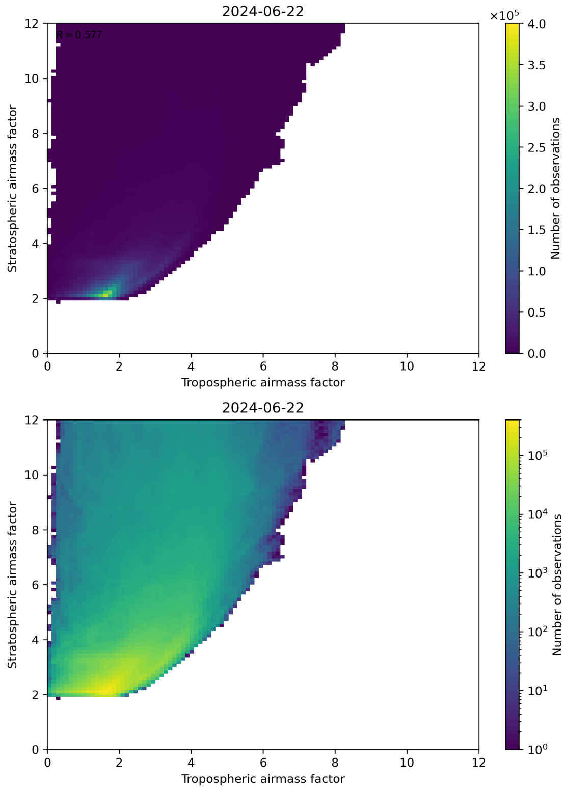
Figure 71: Scatter density plot of “Tropospheric airmass factor” against “Stratospheric airmass factor” for 2024-06-21 to 2024-06-23.
