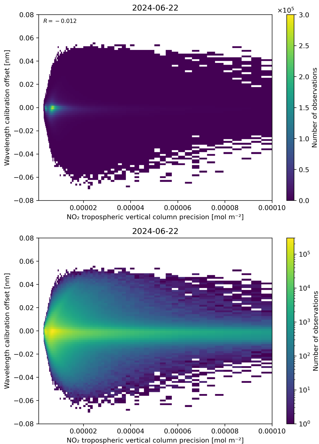
Figure 141: Scatter density plot of “NO 2 tropospheric vertical column precision” against “Wavelength calibration offset” for 2024-06-21 to 2024-06-23.
