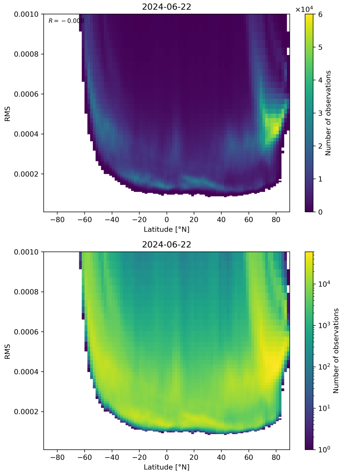
Figure 94: Scatter density plot of “Latitude” against “RMS” for 2024-06-21 to 2024-06-23.
