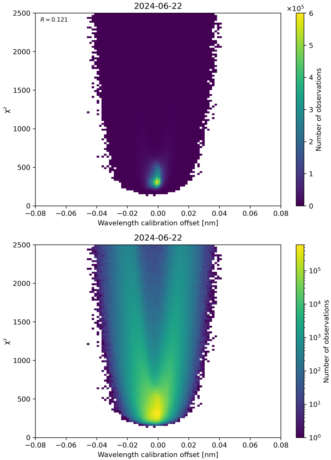
Figure 175: Scatter density plot of “Wavelength calibration offset” against “ \chi^2 ” for 2024-06-21 to 2024-06-23.
