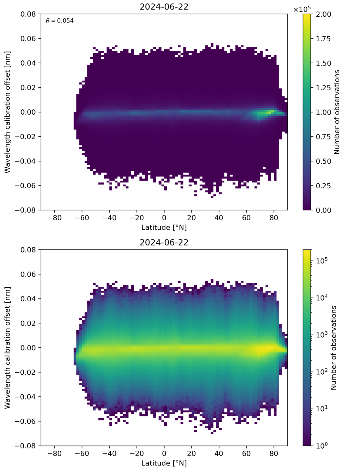
Figure 95: Scatter density plot of “Latitude” against “Wavelength calibration offset” for 2024-06-21 to 2024-06-23.
