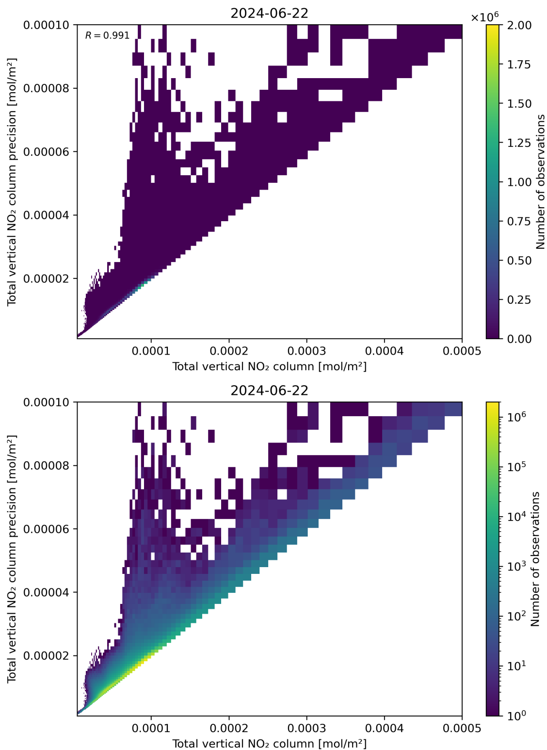
Figure 114: Scatter density plot of “Total vertical NO 2 column” against “Total vertical NO 2 column precision” for 2024-06-21 to 2024-06-23.
