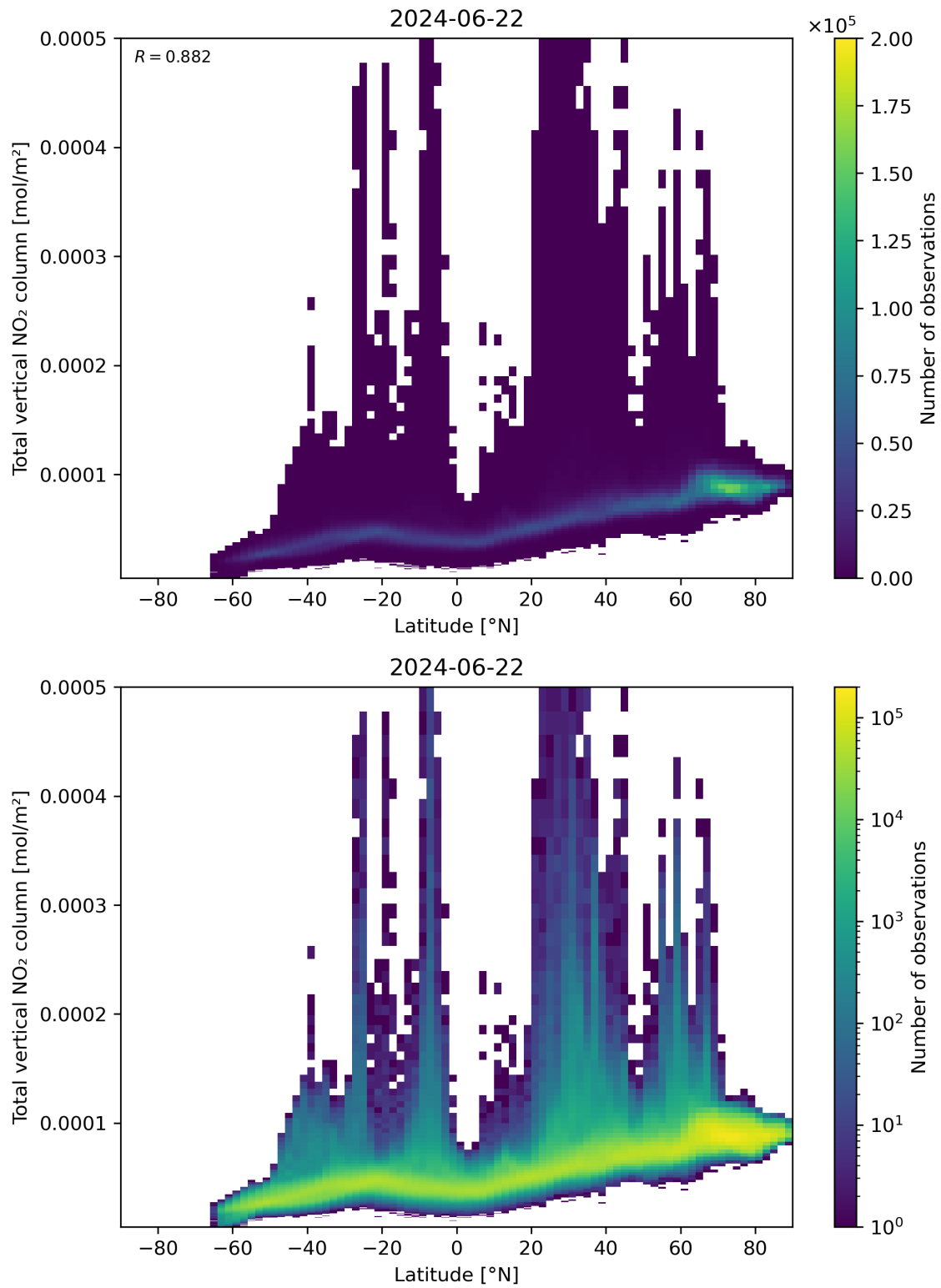
Figure 90: Scatter density plot of “Latitude” against “Total vertical NO 2 column” for 2024-06-21 to 2024-06-23.
