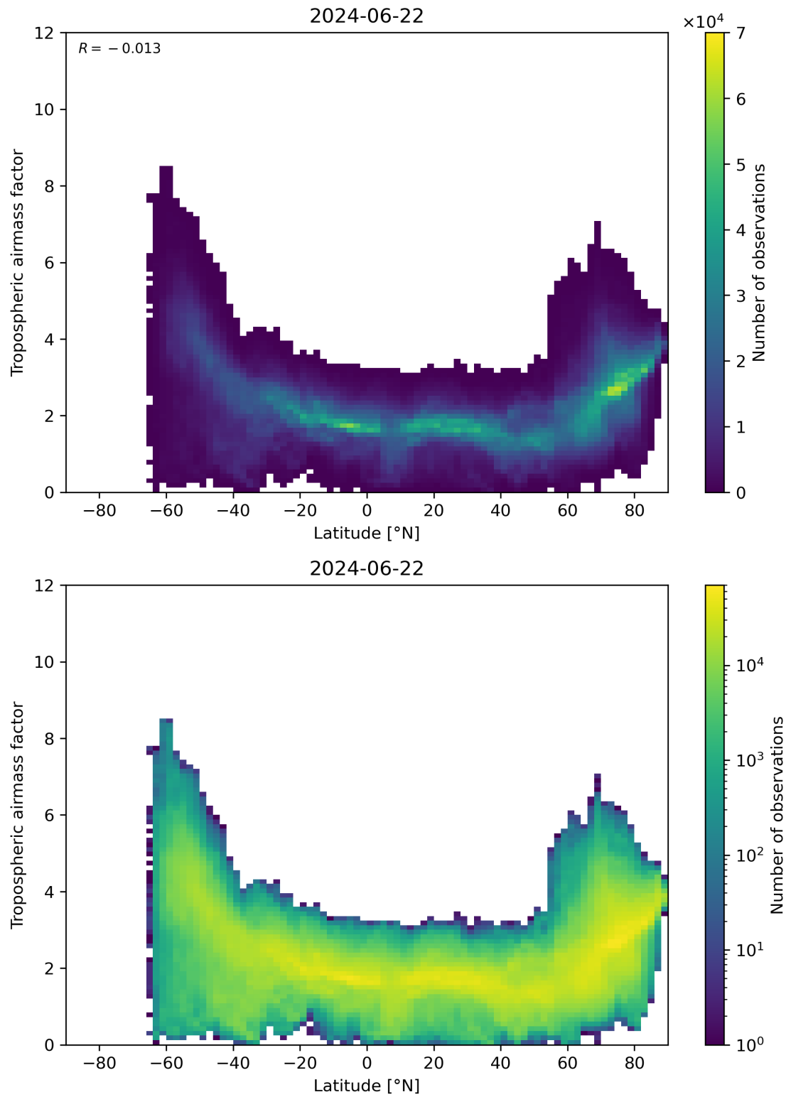
Figure 85: Scatter density plot of “Latitude” against “Tropospheric airmass factor” for 2024-06-21 to 2024-06-23.
