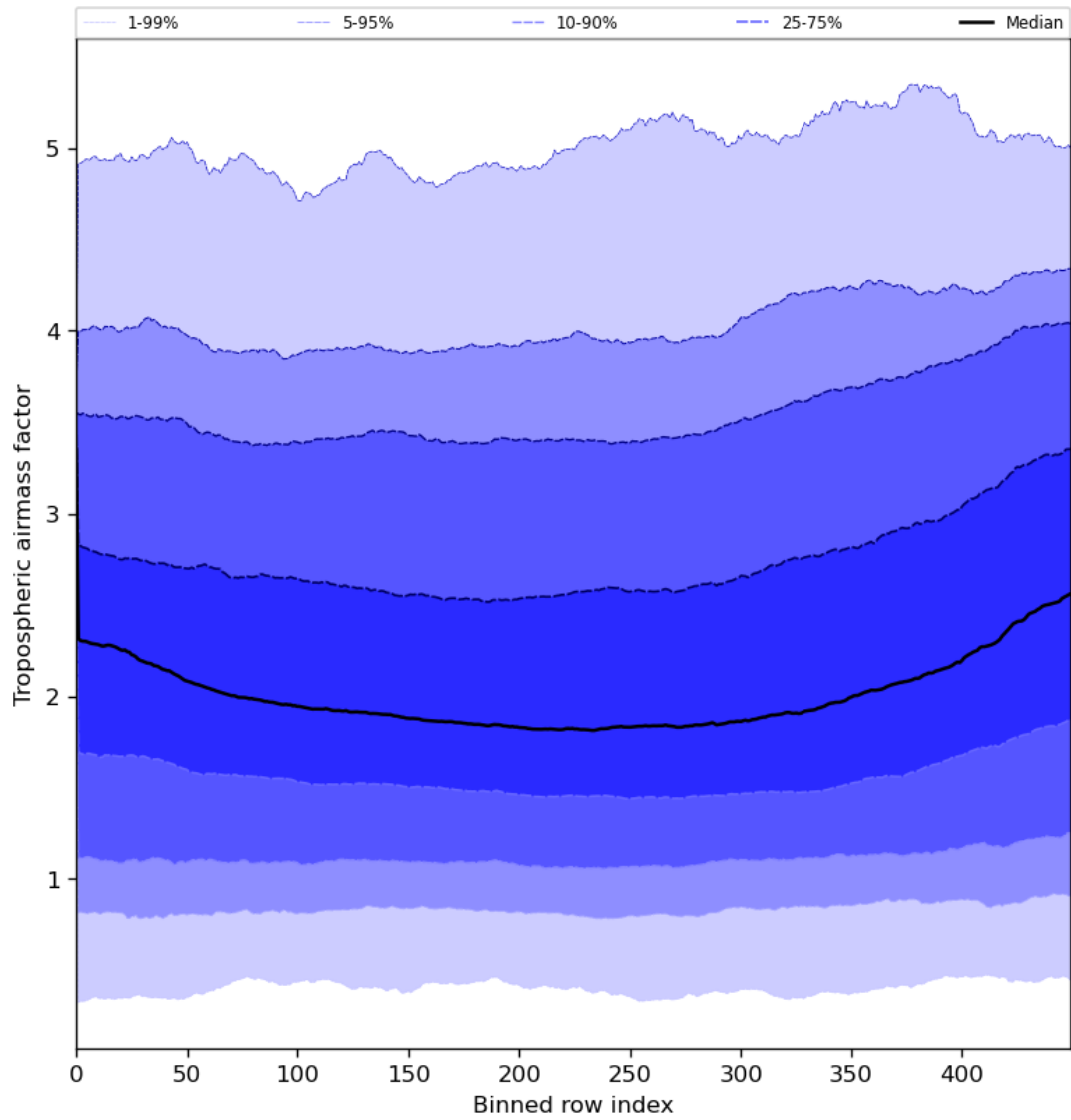
Figure 48: Along track statistics of “Tropospheric airmass factor” for 2024-06-21 to 2024-06-23
