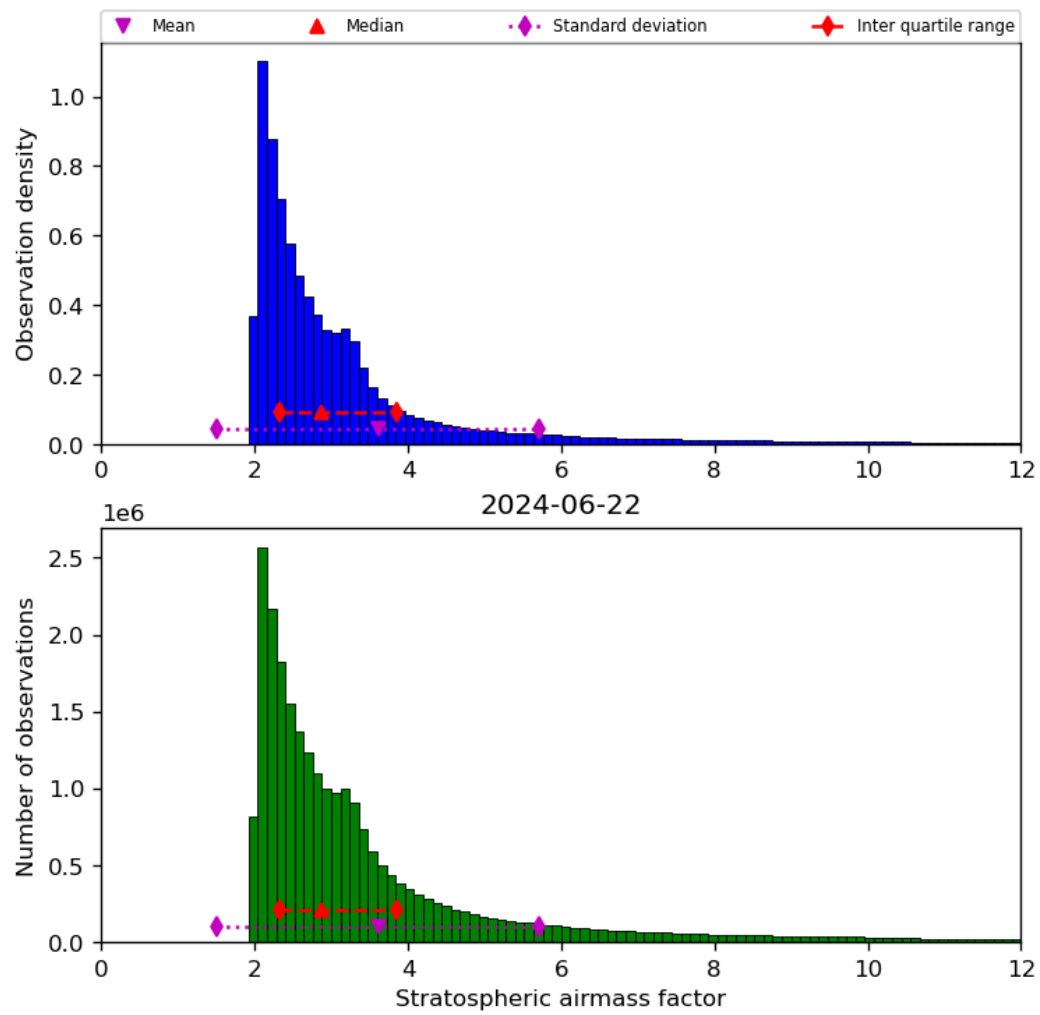
Figure 44: Histogram of “Stratospheric airmass factor” for 2024-06-21 to 2024-06-23
