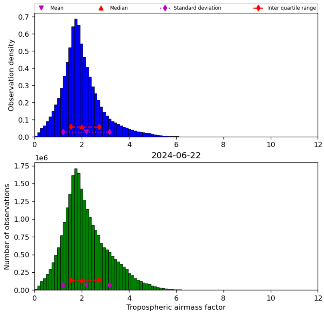
Figure 31: Histogram of “Tropospheric airmass factor” for 2024-06-21 to 2024-06-23
