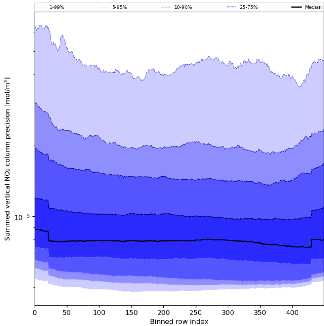
Figure 58: Along track statistics of “Summed vertical NO 2 column precision” for 2024-06-21 to 2024-06-23
