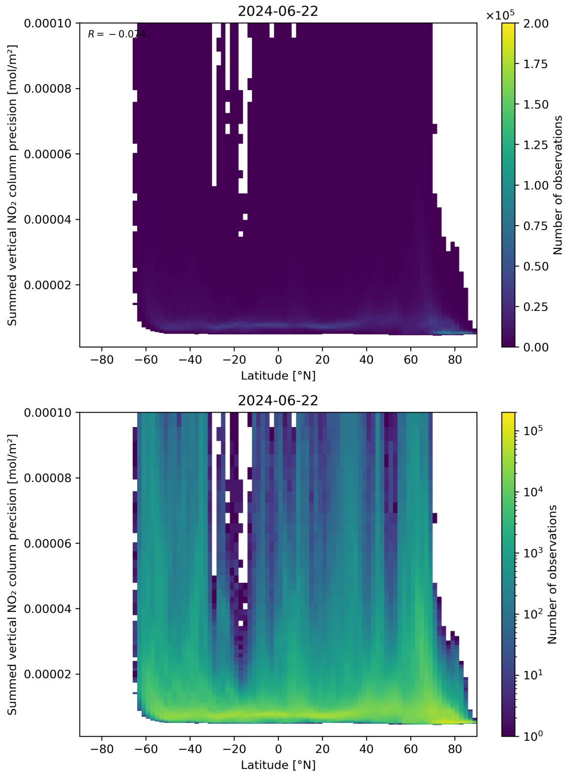
Figure 89: Scatter density plot of “Latitude” against “Summed vertical NO 2 column precision” for 2024-06-21 to 2024-06-23.
