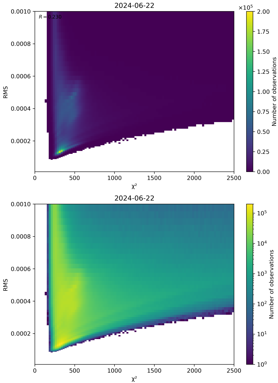
Figure 82: Scatter density plot of “ \chi^2 ” against “RMS” for 2024-06-21 to 2024-06-23.
