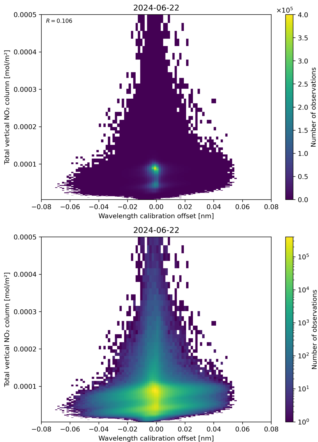
Figure 179: Scatter density plot of “Wavelength calibration offset” against “Total vertical NO 2 column” for 2024-06-21 to 2024-06-23.
