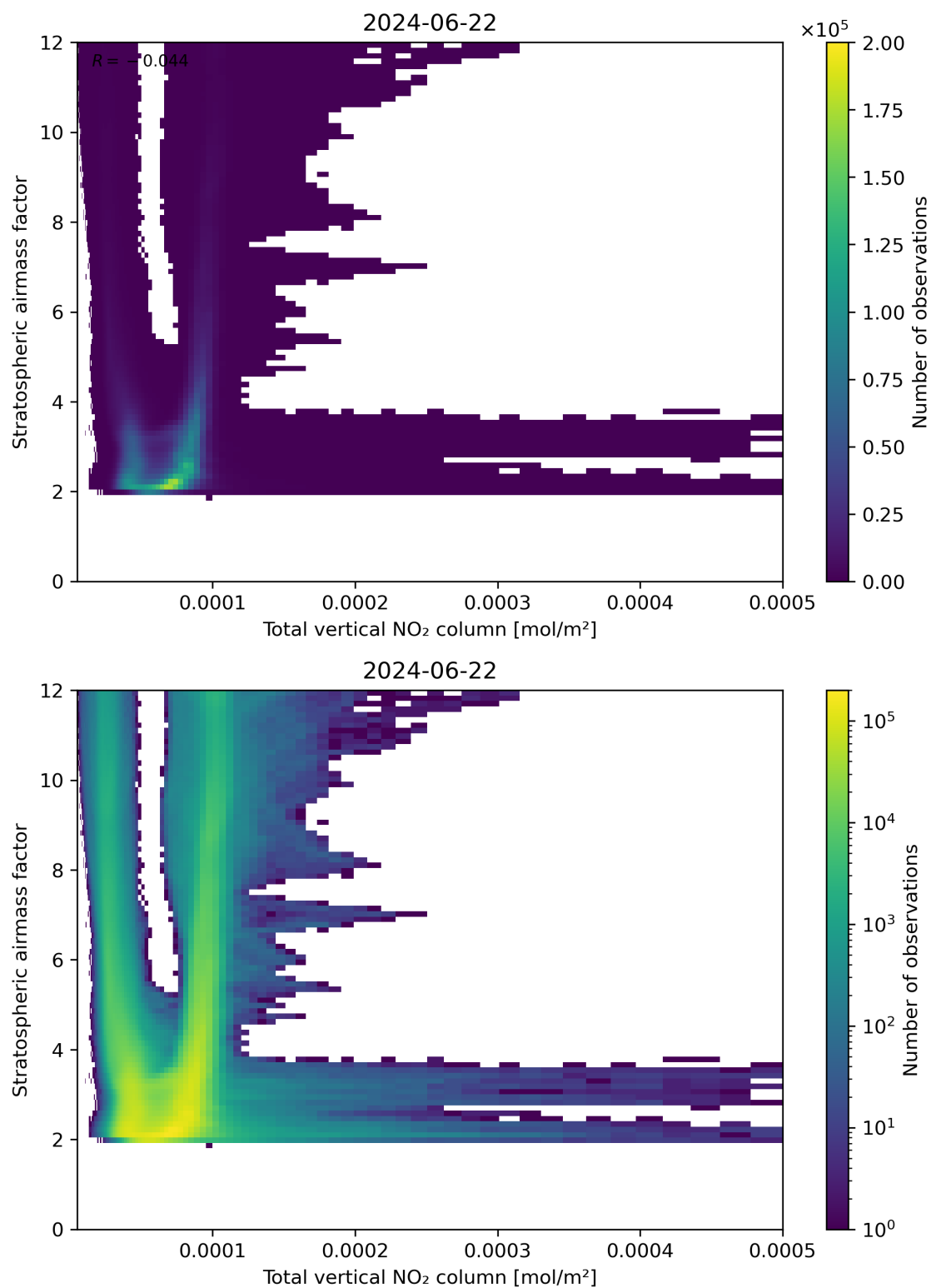
Figure 110: Scatter density plot of “Total vertical NO 2 column” against “Stratospheric airmass factor” for 2024-06-21 to 2024-06-23.
