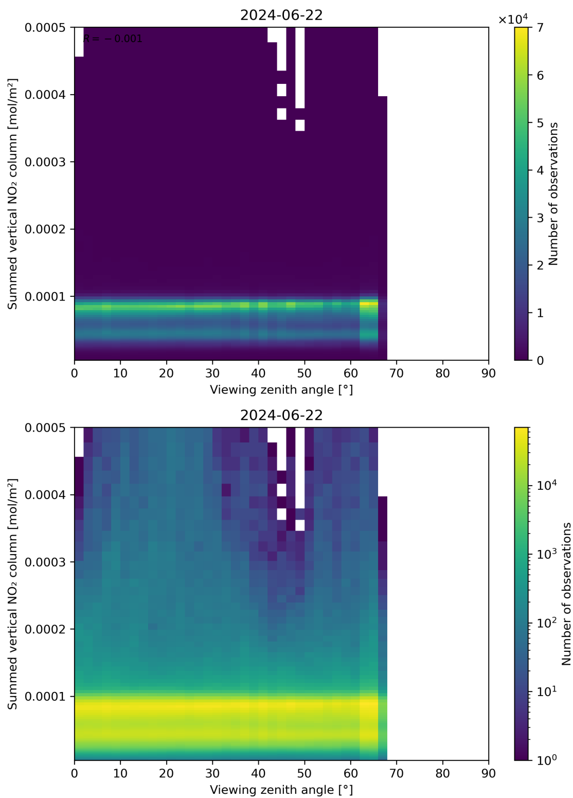
Figure 165: Scatter density plot of “Viewing zenith angle” against “Summed vertical NO 2 column” for 2024-06-21 to 2024-06-23.
