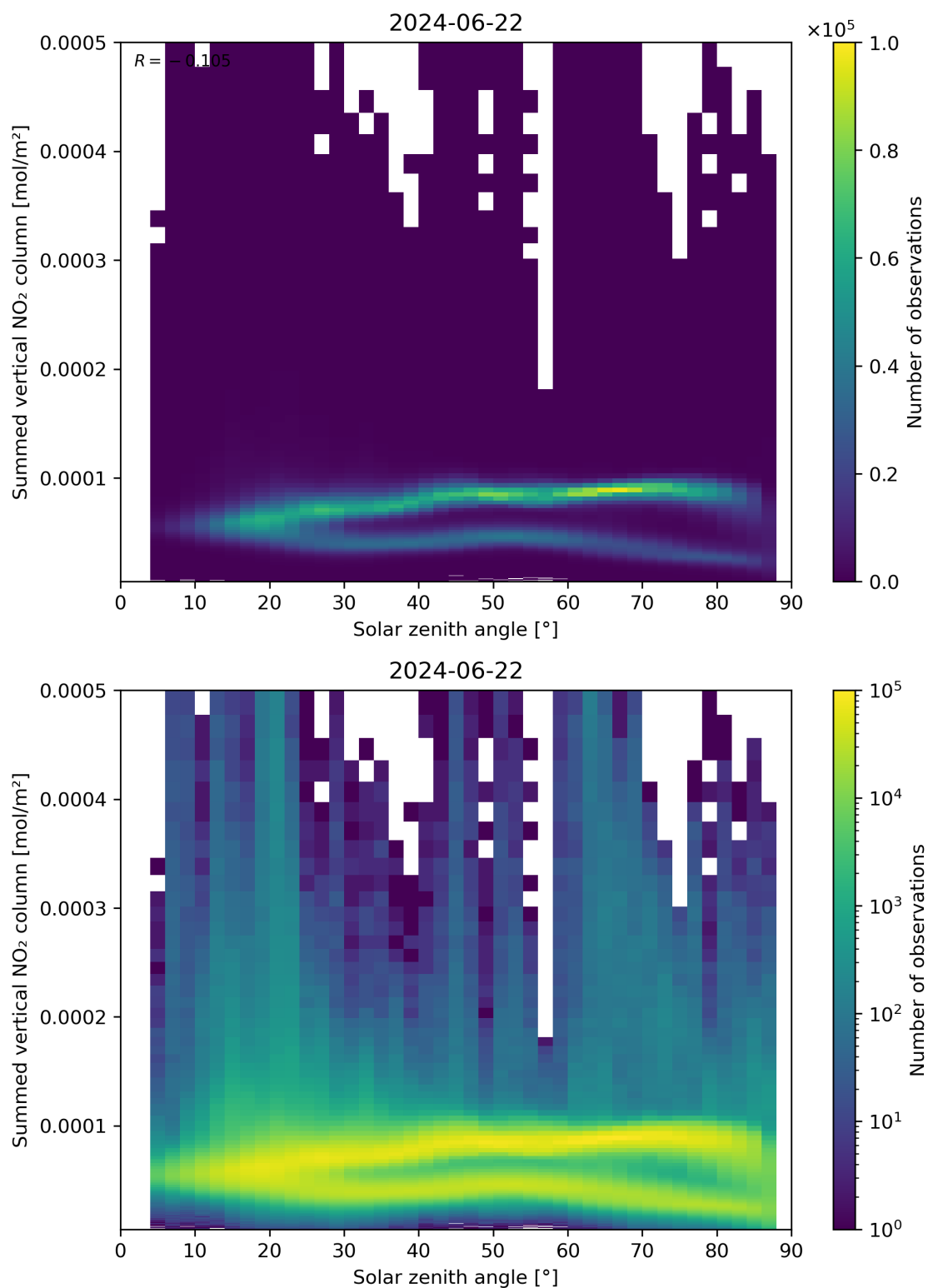
Figure 151: Scatter density plot of “Solar zenith angle” against “Summed vertical NO 2 column” for 2024-06-21 to 2024-06-23.
