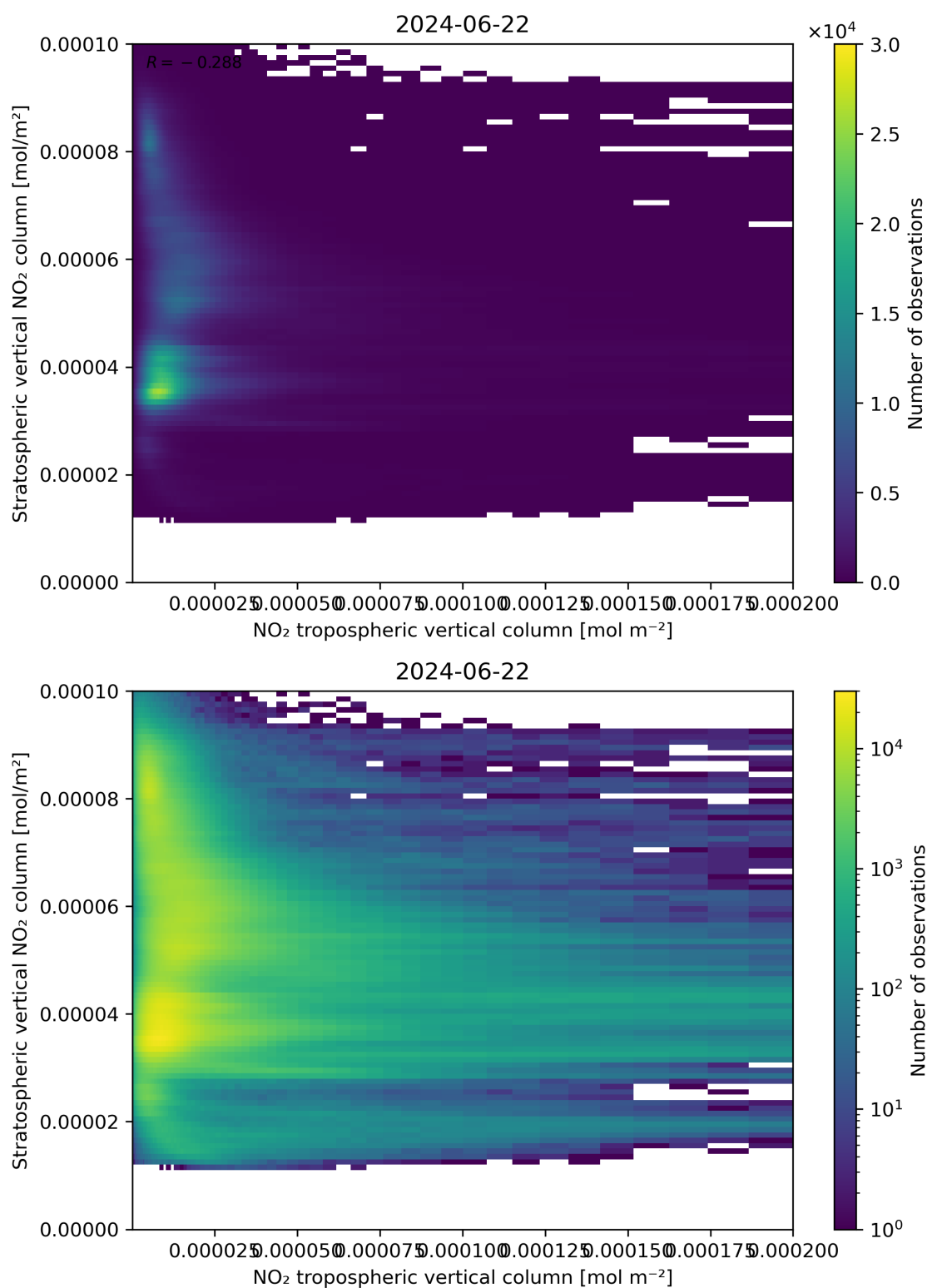
Figure 125: Scatter density plot of “NO 2 tropospheric vertical column” against “Stratospheric vertical NO 2 column” for 2024-06-21 to 2024-06-23.
