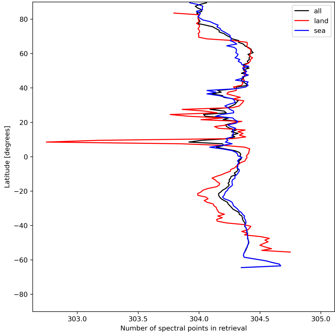
Figure 16: Zonal average of “Number of spectral points in retrieval” for 2024-06-21 to 2024-06-23.
