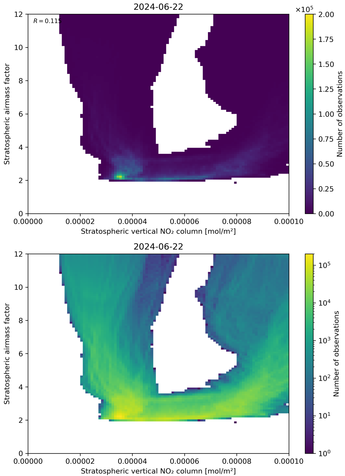
Figure 96: Scatter density plot of “Stratospheric vertical NO 2 column” against “Stratospheric airmass factor” for 2024-06-21 to 2024-06-23.
