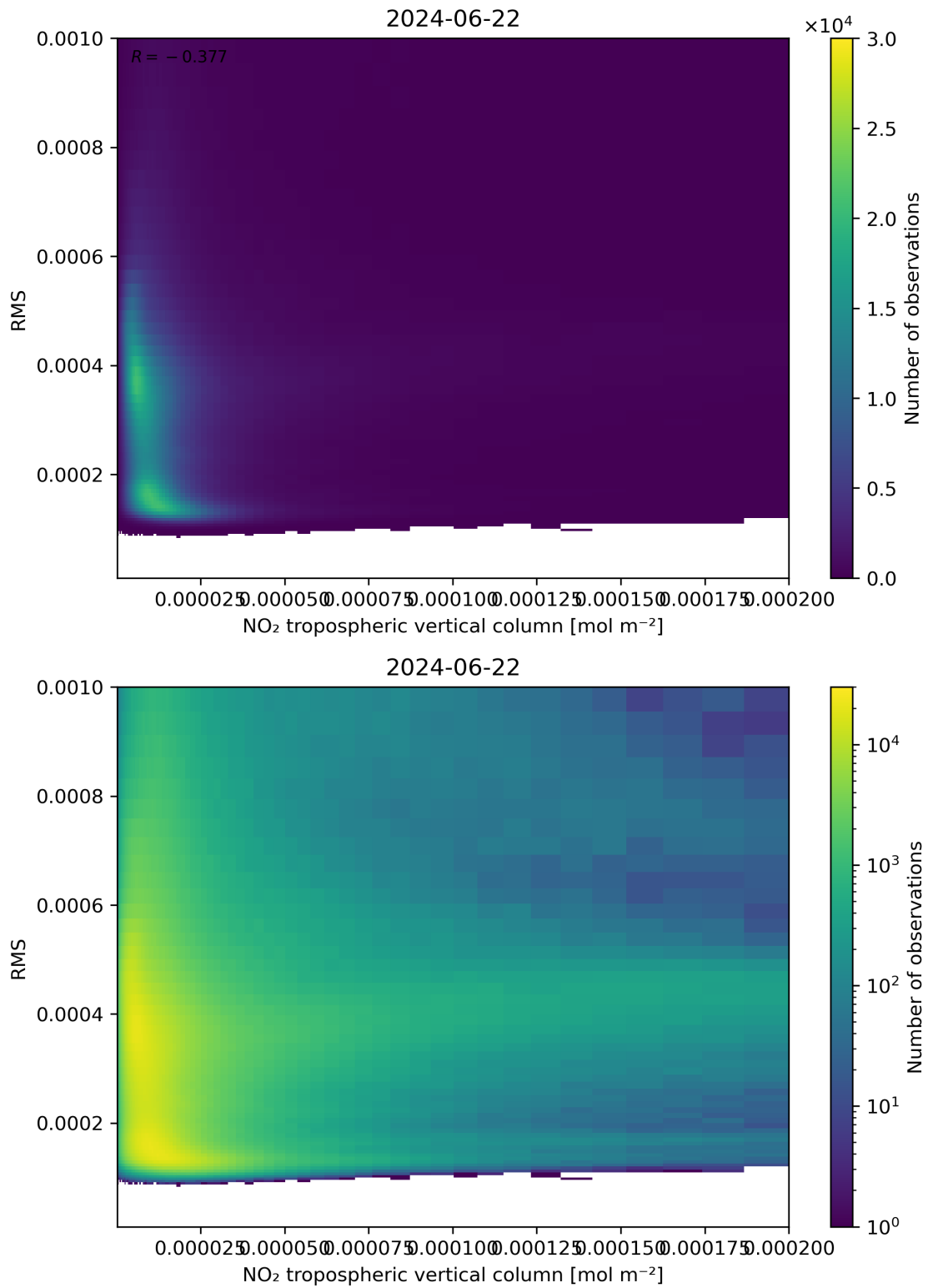
Figure 142: Scatter density plot of “NO 2 tropospheric vertical column” against “RMS” for 2024-06-21 to 2024-06-23.
