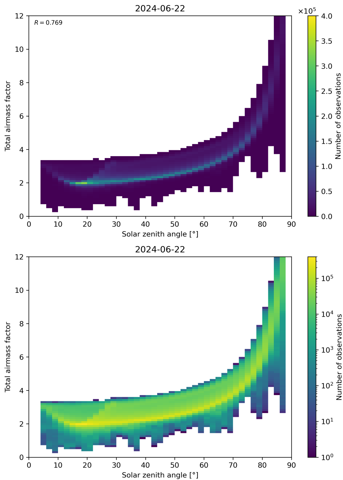
Figure 146: Scatter density plot of “Solar zenith angle” against “Total air mass factor” for 2024-06-21 to 2024-06-23.
