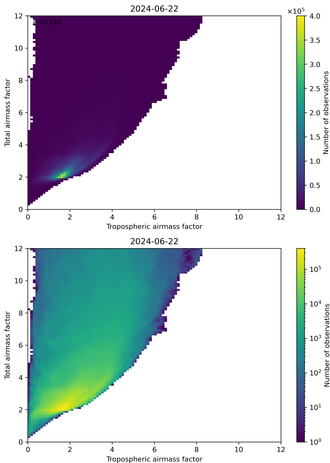
Figure 72: Scatter density plot of “Tropospheric airmass factor” against “Total airmass factor” for 2024-06-21 to 2024-06-23.
