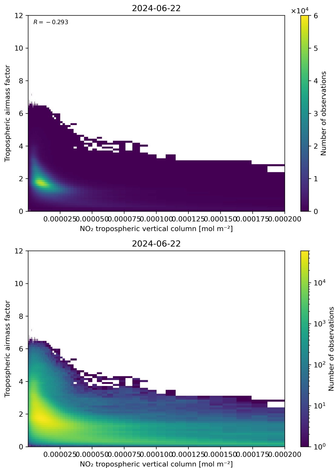
Figure 123: Scatter density plot of “NO 2 tropospheric vertical column” against “Tropospheric air mass factor” for 2024-06-21 to 2024-06-23.
