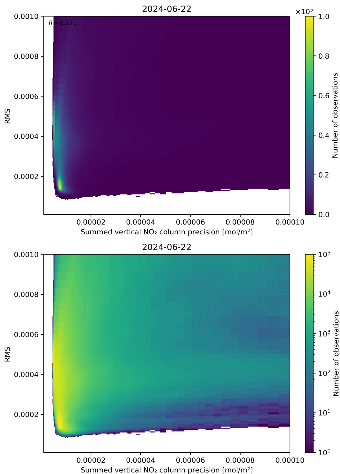
Figure 108: Scatter density plot of “Summed vertical NO 2 column precision” against “RMS” for 2024-06-21 to 2024-06-23.
