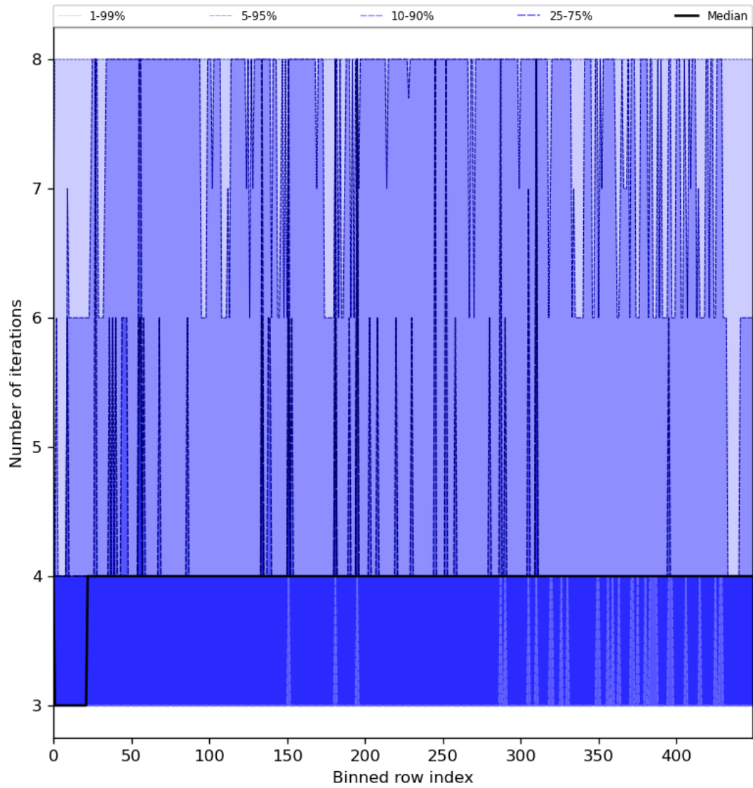
Figure 51: Along track statistics of “Number of iterations” for 2024-06-21 to 2024-06-23
