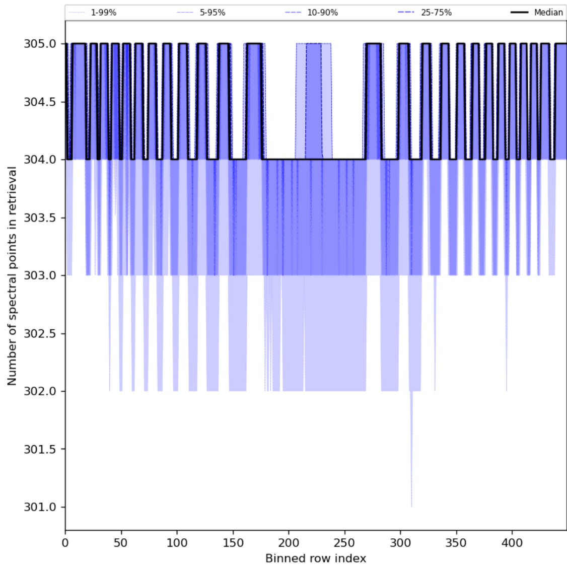
Figure 50: Along track statistics of “Number of spectral points in retrieval” for 2024-06-21 to 2024-06-23
