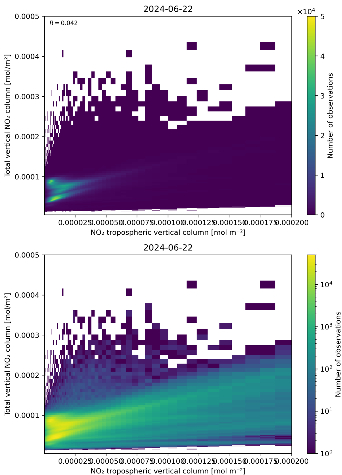
Figure 128: Scatter density plot of “NO 2 tropospheric vertical column” against “Total vertical NO 2 column” for 2024-06-21 to 2024-06-23.
