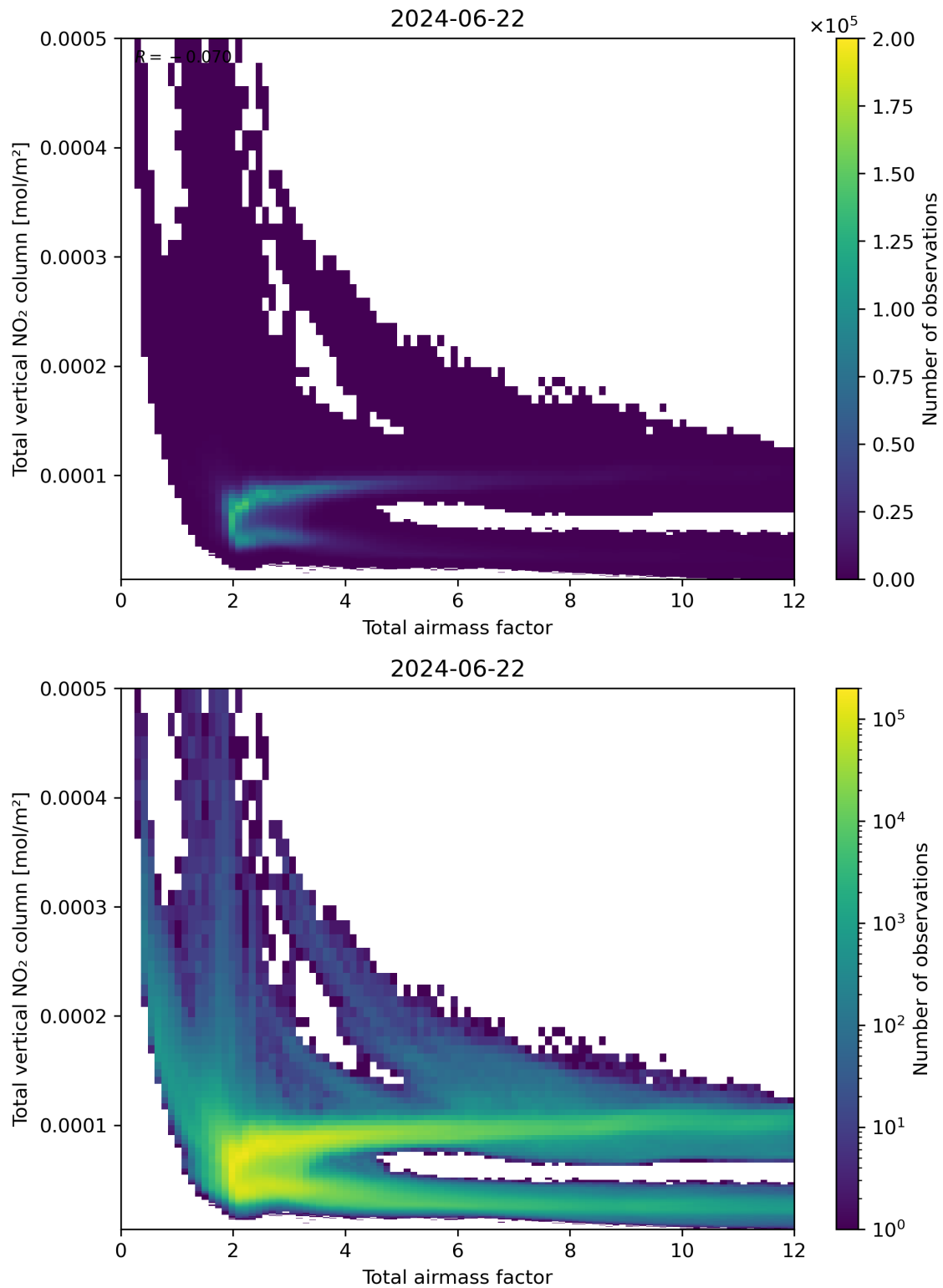
Figure 67: Scatter density plot of “Total airmass factor” against “Total vertical NO 2 column” for 2024-06-21 to 2024-06-23.
