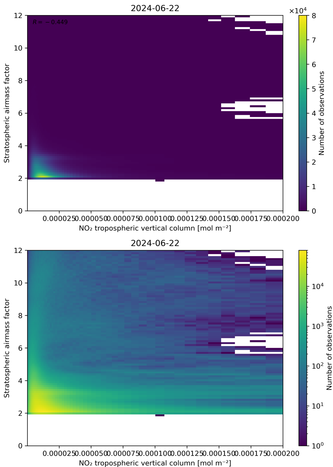
Figure 121: Scatter density plot of “NO 2 tropospheric vertical column” against “Stratospheric airmass factor” for 2024-06-21 to 2024-06-23.
