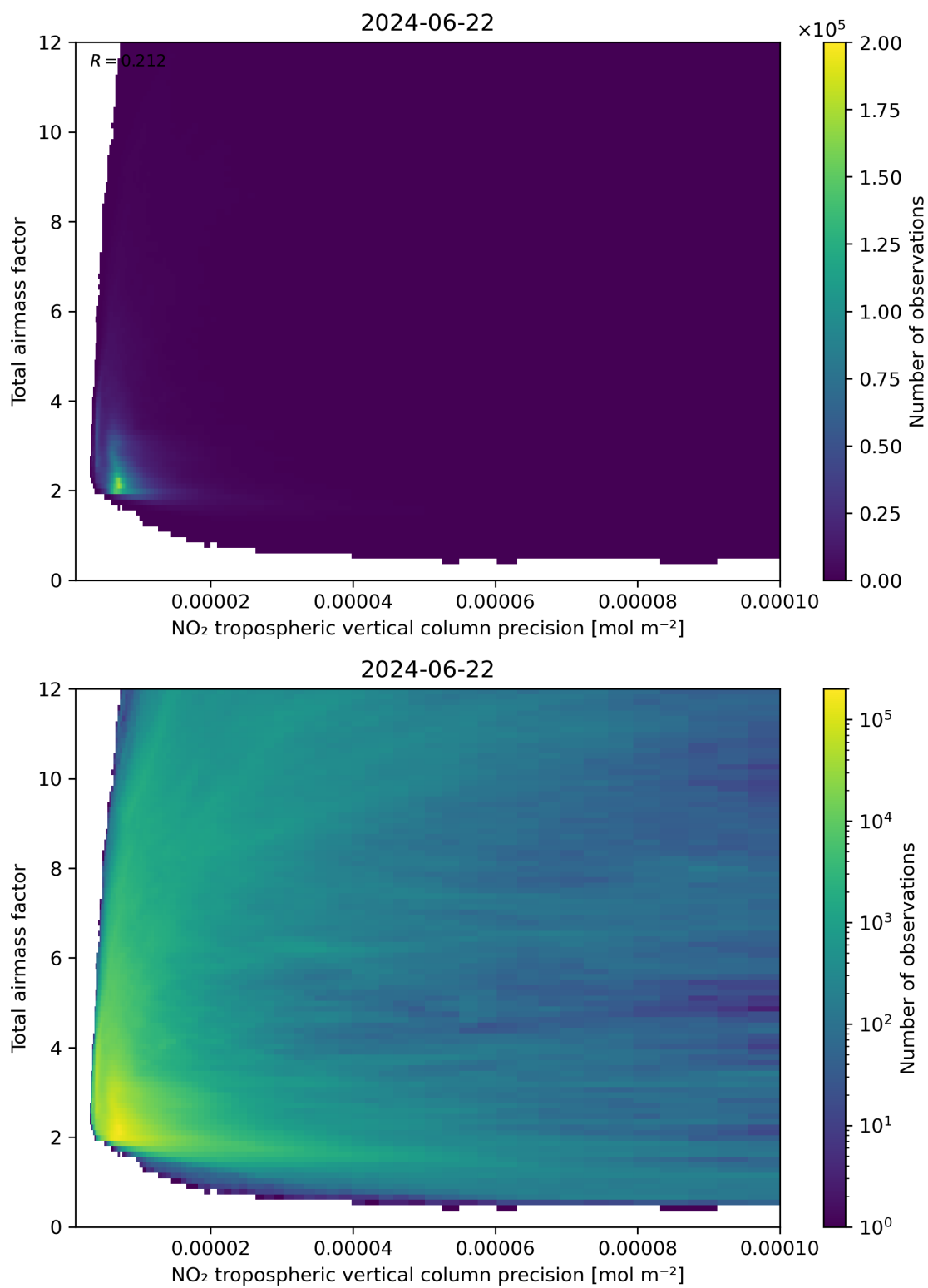
Figure 132: Scatter density plot of “NO 2 tropospheric vertical column precision” against “Total air mass factor” for 2024-06-21 to 2024-06-23.
