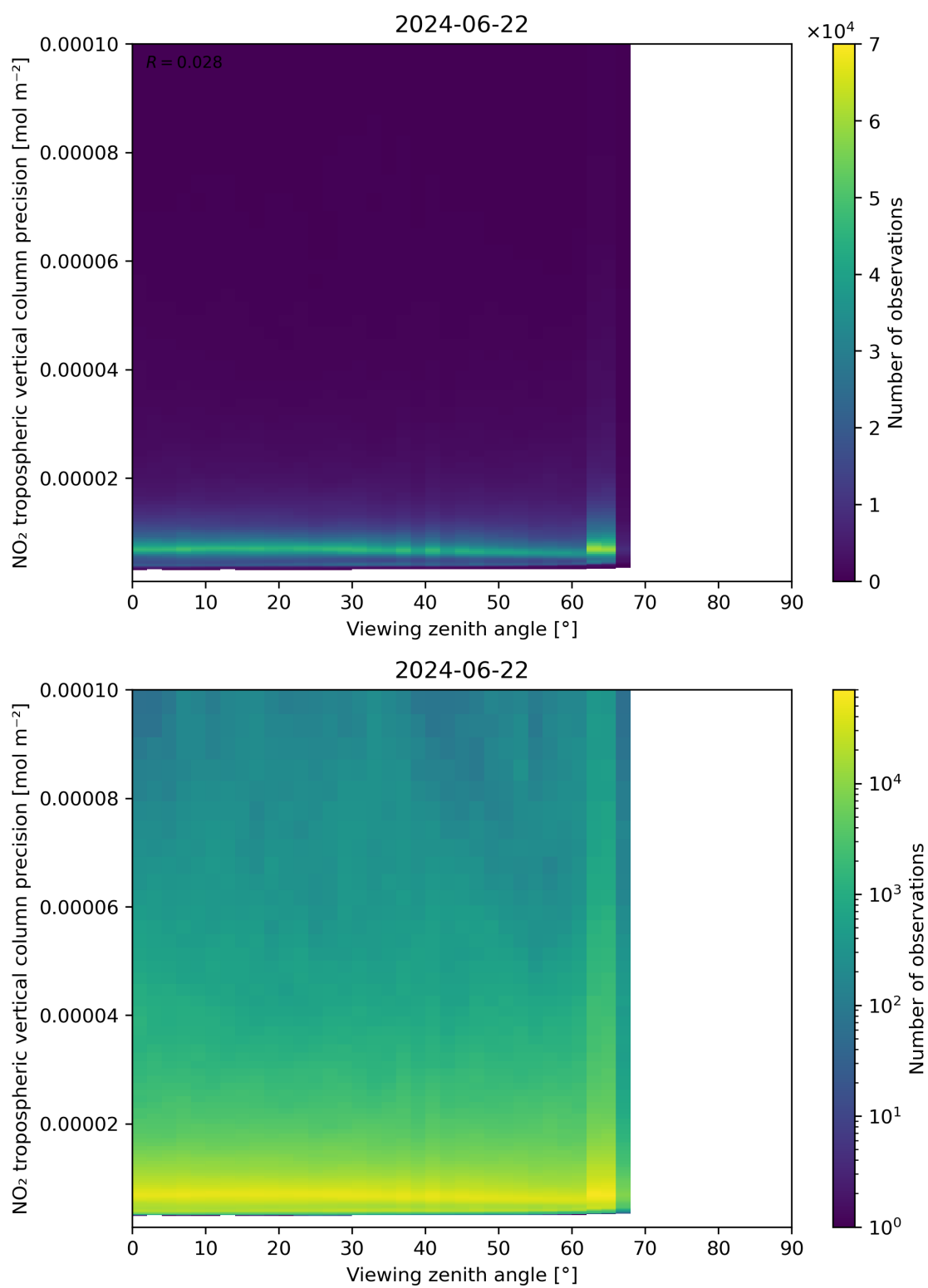
Figure 170: Scatter density plot of “Viewing zenith angle” against “NO 2 tropospheric vertical column precision” for 2024-06-21 to 2024-06-23.
