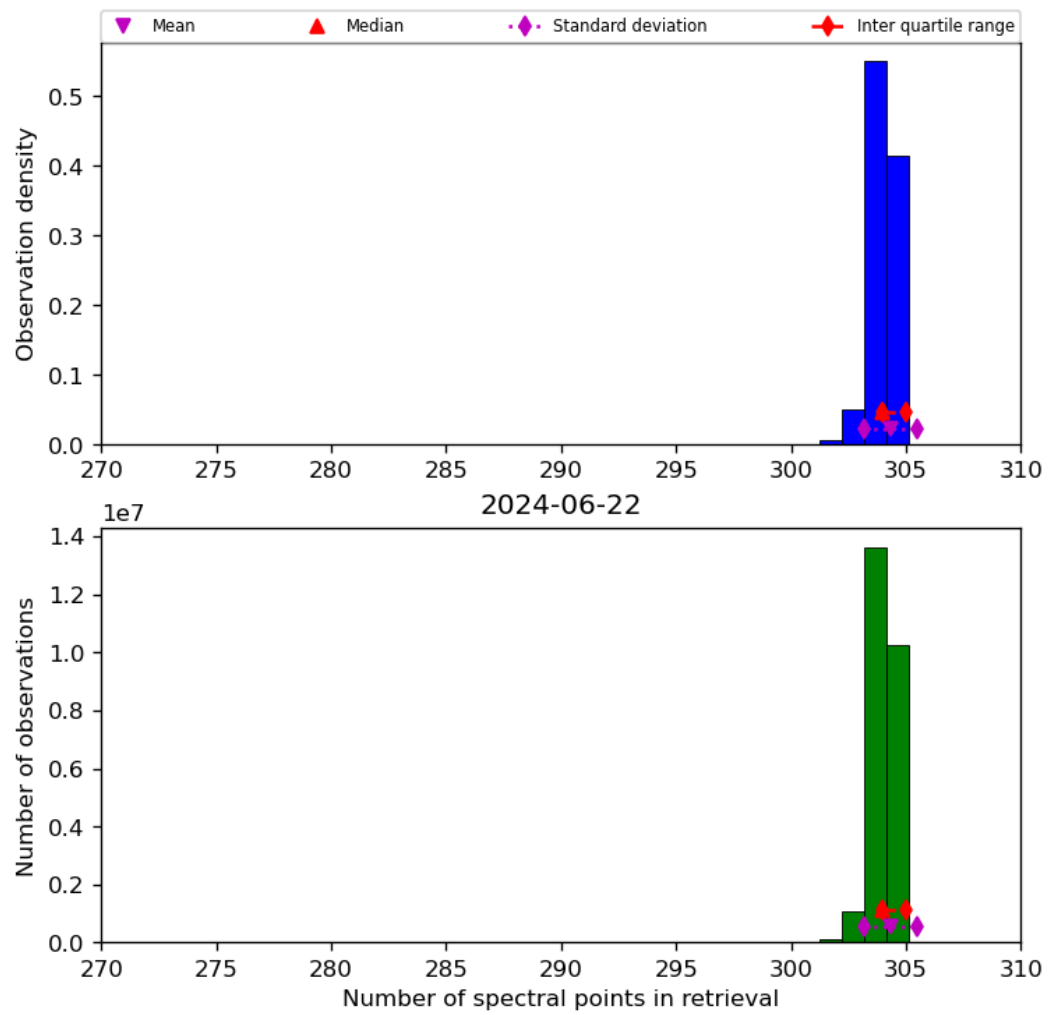
Figure 33: Histogram of “Number of spectral points in retrieval” for 2024-06-21 to 2024-06-23
