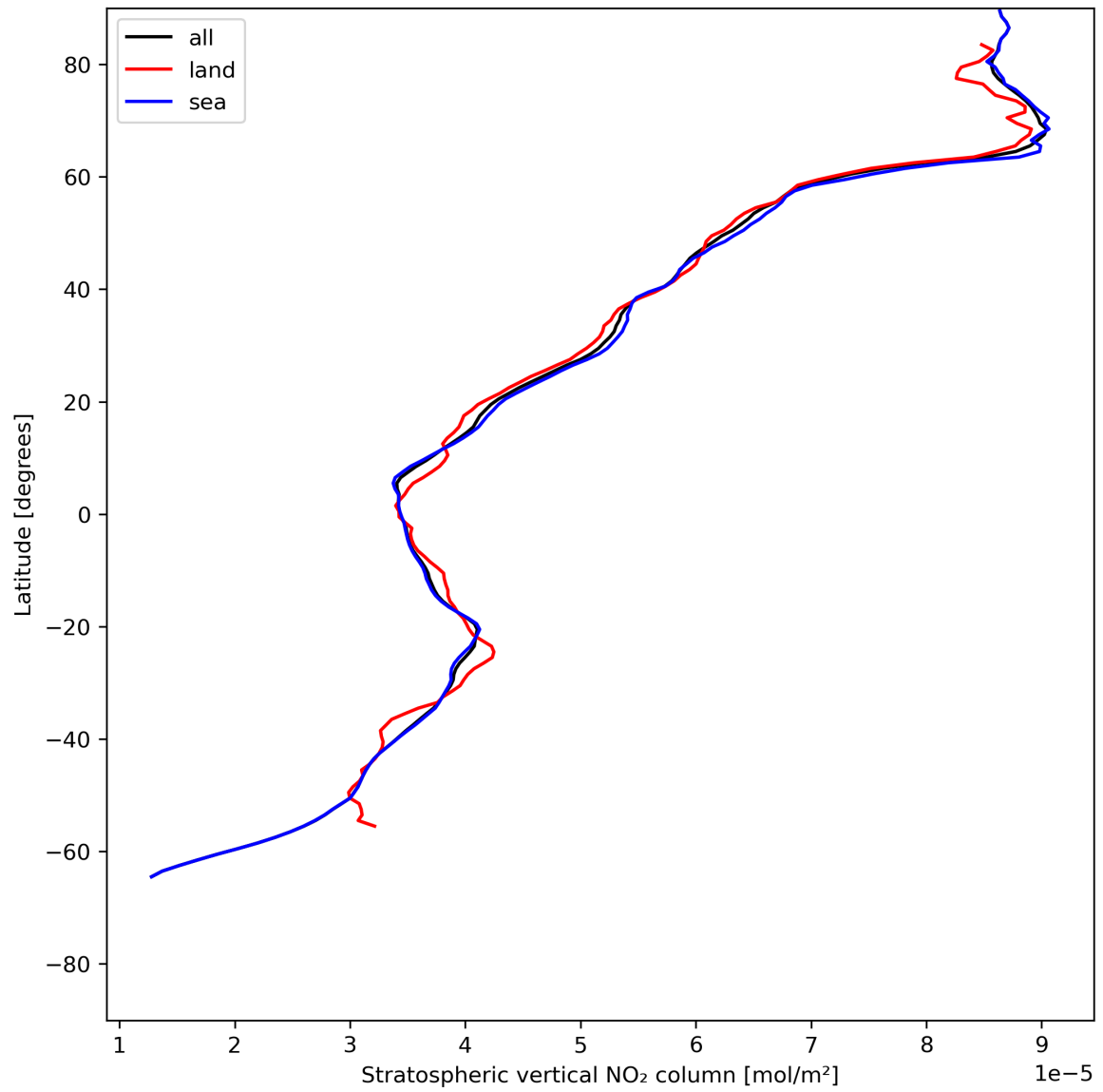
Figure 19: Zonal average of “Stratospheric vertical NO 2 column” for 2024-06-21 to 2024-06-23.
