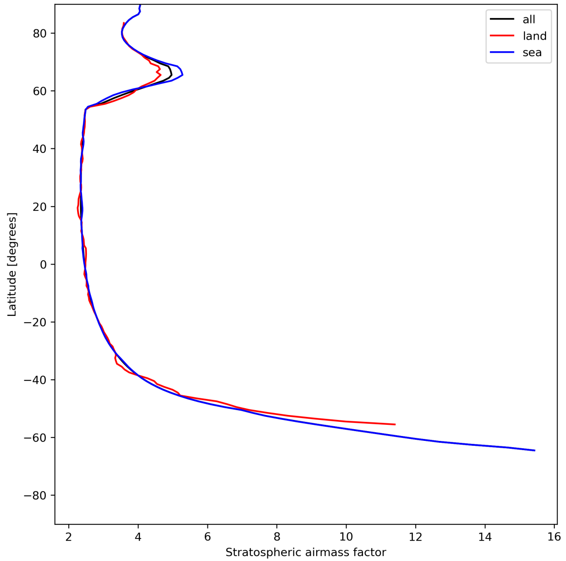
Figure 27: Zonal average of “Stratospheric airmass factor” for 2024-06-21 to 2024-06-23.
