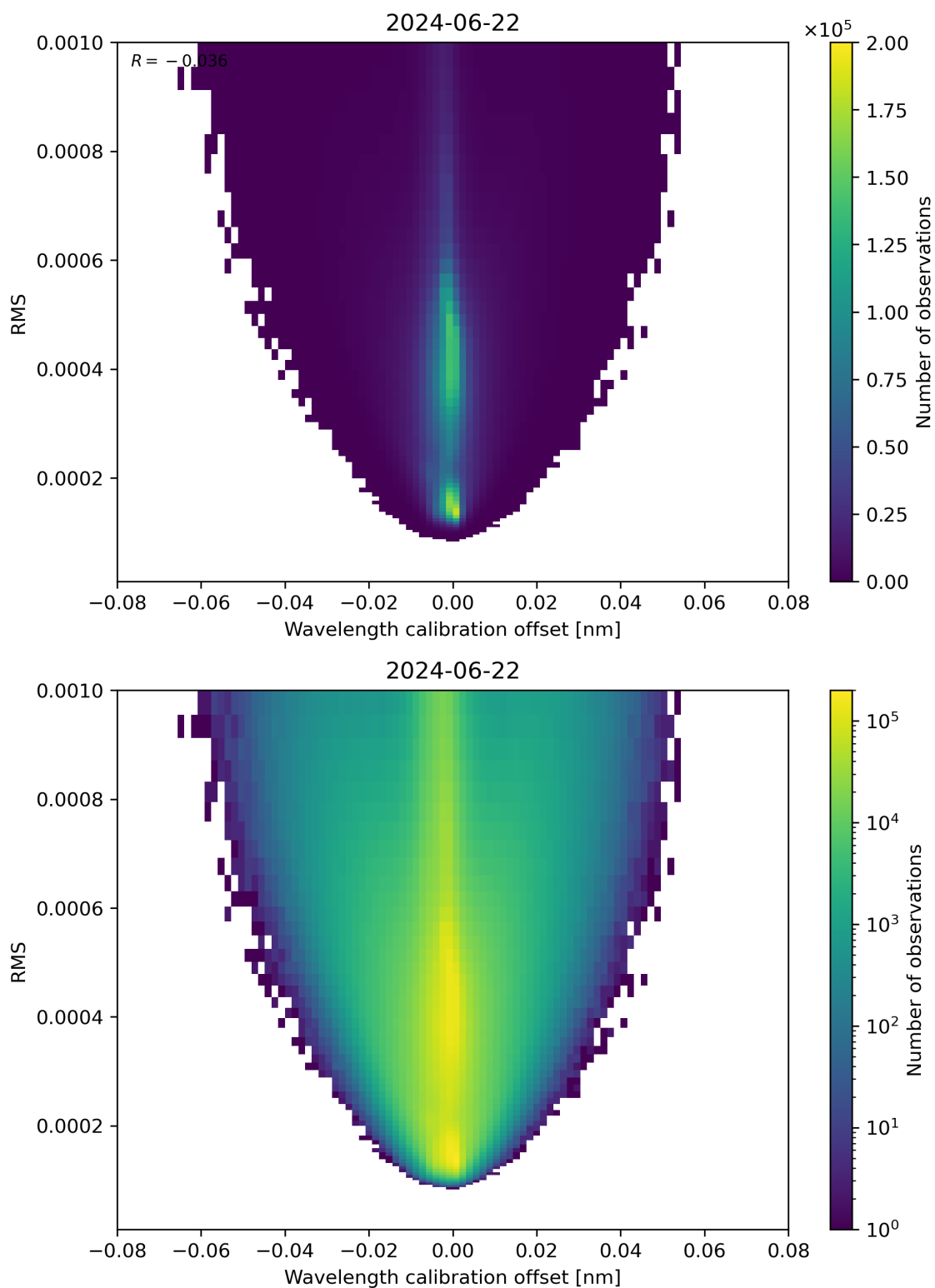
Figure 181: Scatter density plot of “Wavelength calibration offset” against “RMS” for 2024-06-21 to 2024-06-23.
