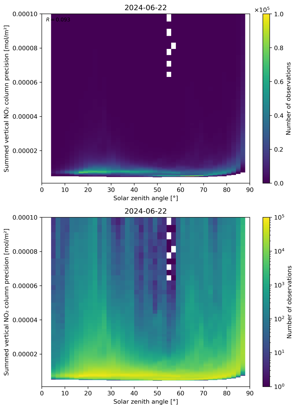
Figure 152: Scatter density plot of “Solar zenith angle” against “Summed vertical NO 2 column precision” for 2024-06-21 to 2024-06-23.
