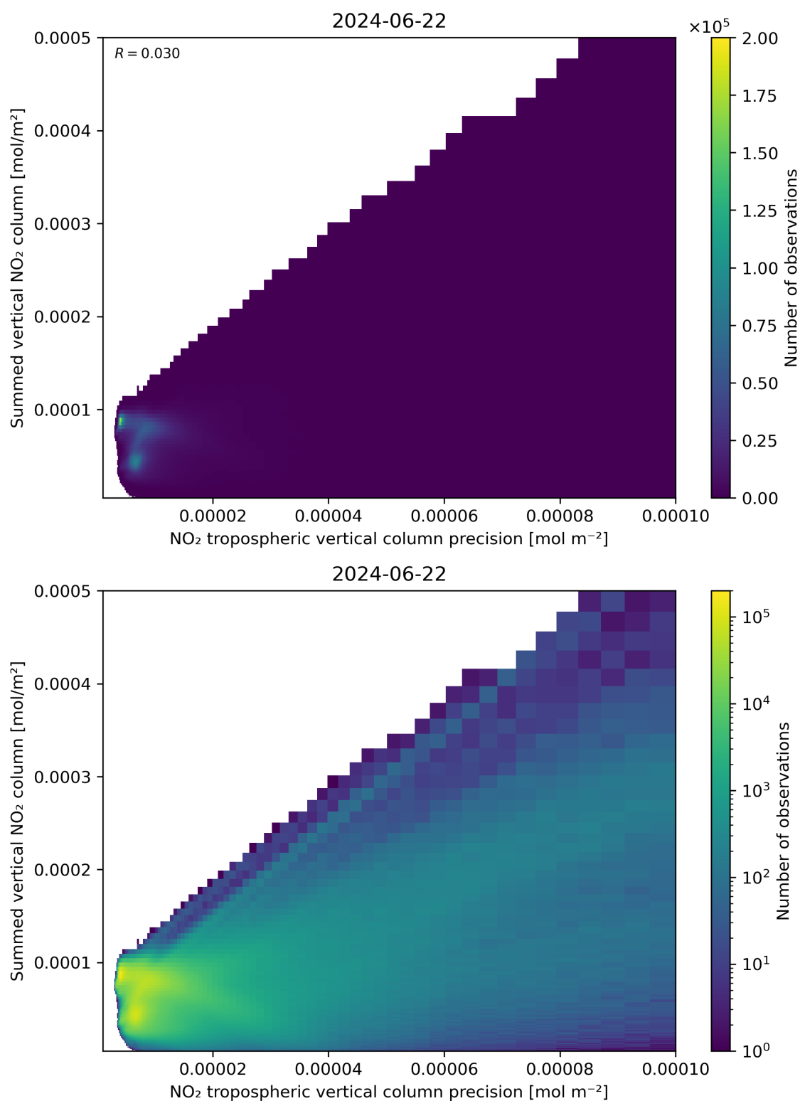
Figure 136: Scatter density plot of “NO 2 tropospheric vertical column precision” against “Summed vertical NO 2 column” for 2024-06-21 to 2024-06-23.
