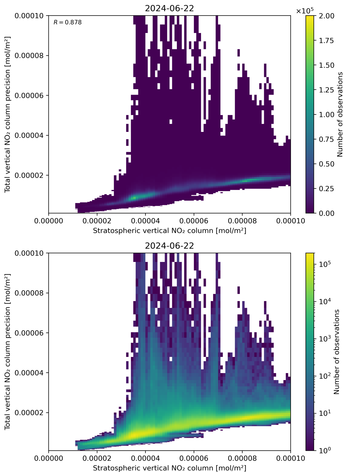
Figure 101: Scatter density plot of “Stratospheric vertical NO 2 column” against “Total vertical NO 2 column precision” for 2024-06-21 to 2024-06-23.
