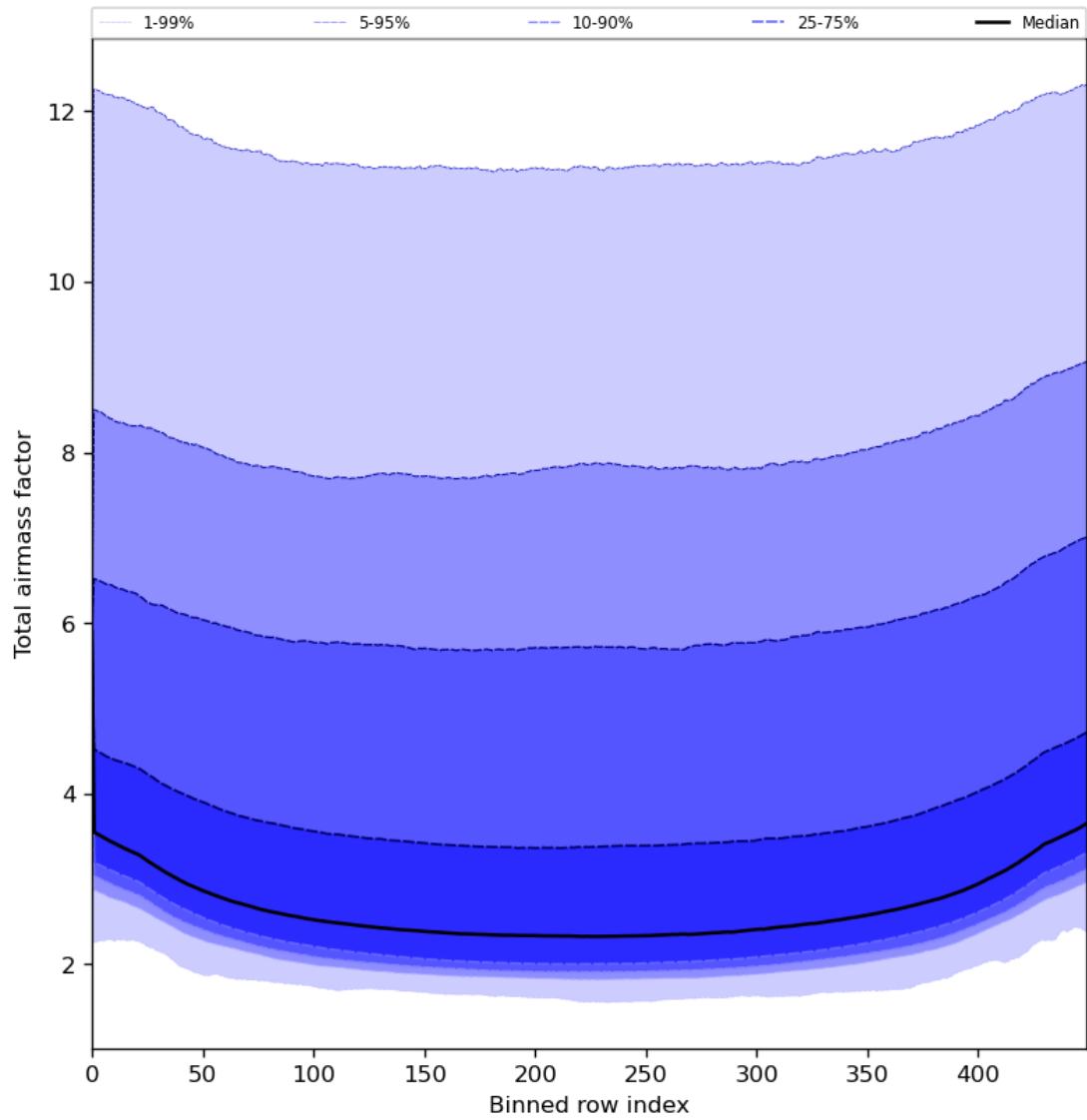
Figure 49: Along track statistics of “Total airmass factor” for 2024-06-21 to 2024-06-23
