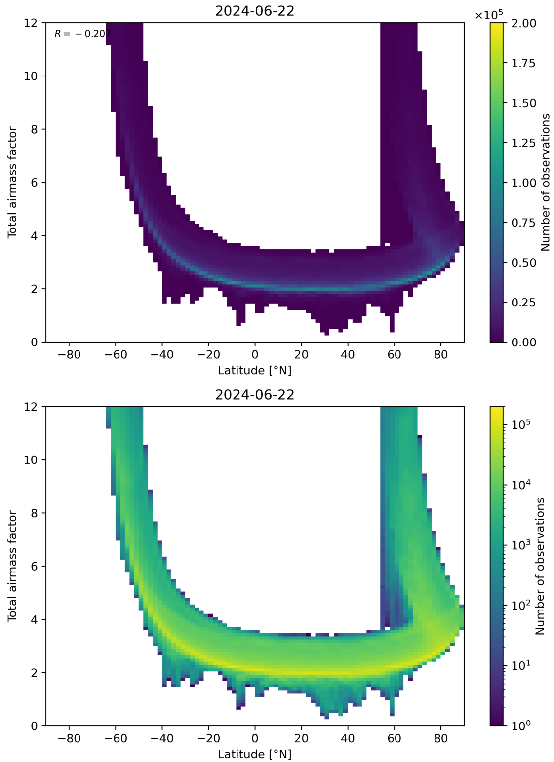
Figure 84: Scatter density plot of “Latitude” against “Total airmass factor” for 2024-06-21 to 2024-06-23.
