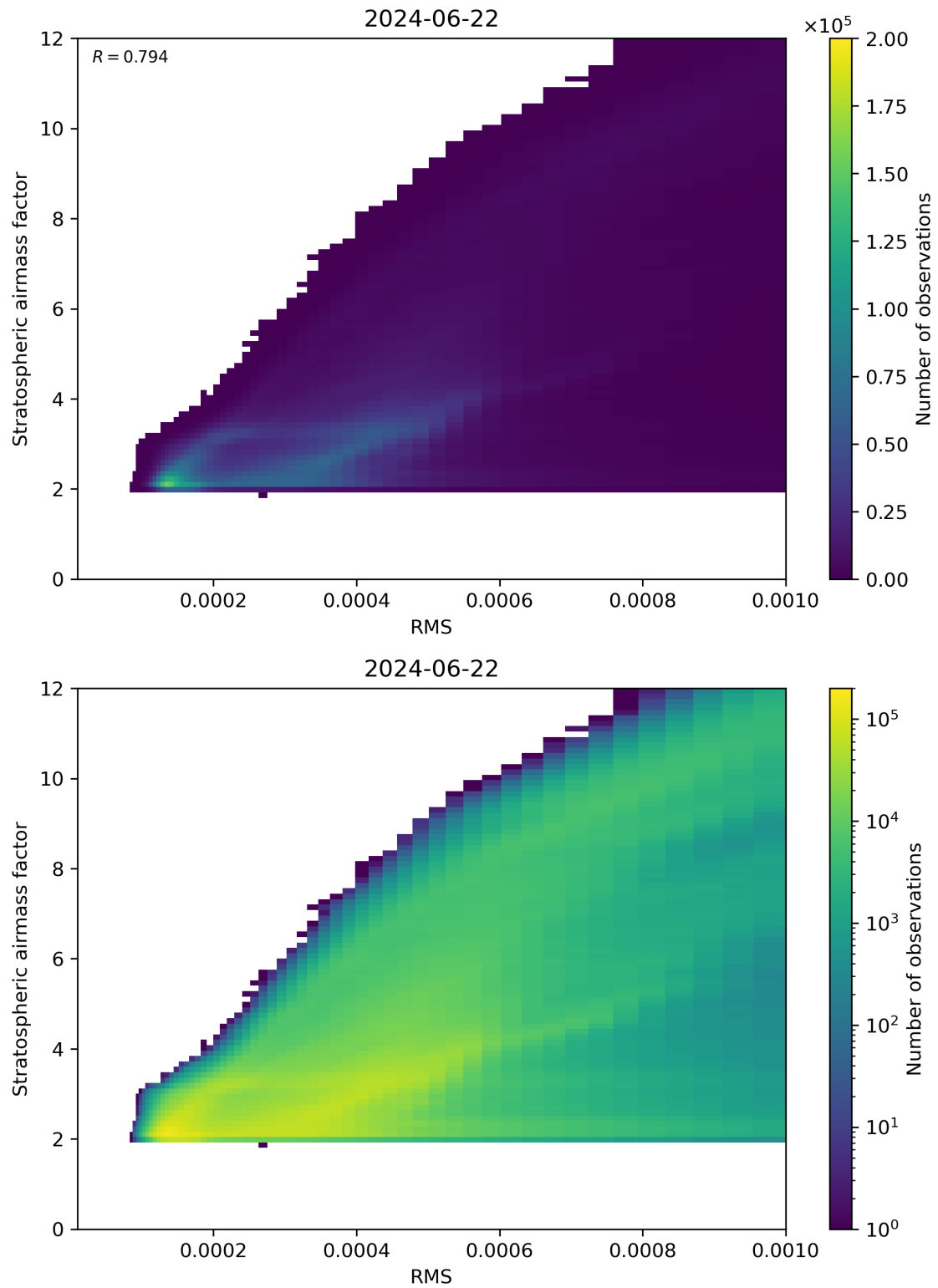
Figure 144: Scatter density plot of “RMS” against “Stratospheric airmass factor” for 2024-06-21 to 2024-06-23.
