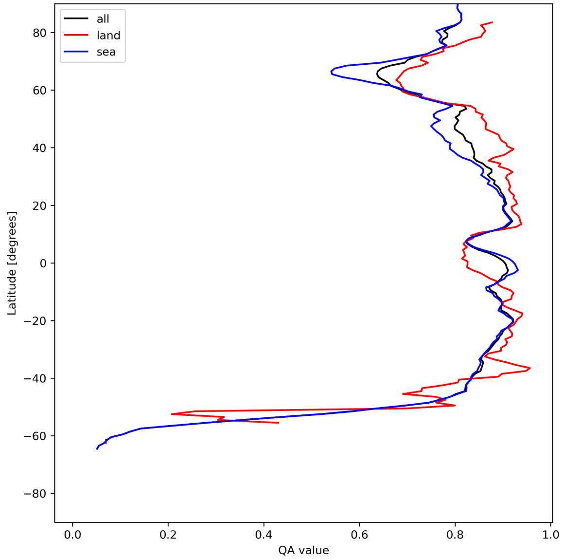
Figure 11: Zonal average of “QA value” for 2024-06-22 to 2024-06-24.
