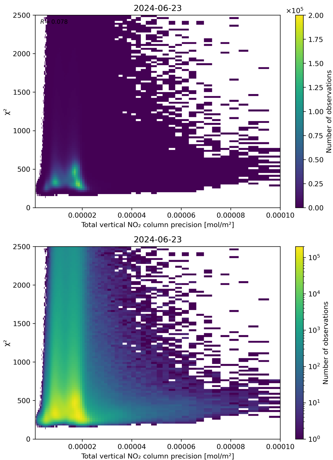
Figure 116: Scatter density plot of “Total vertical NO 2 column precision” against “ \chi^2 ” for 2024-06-22 to 2024-06-24.
