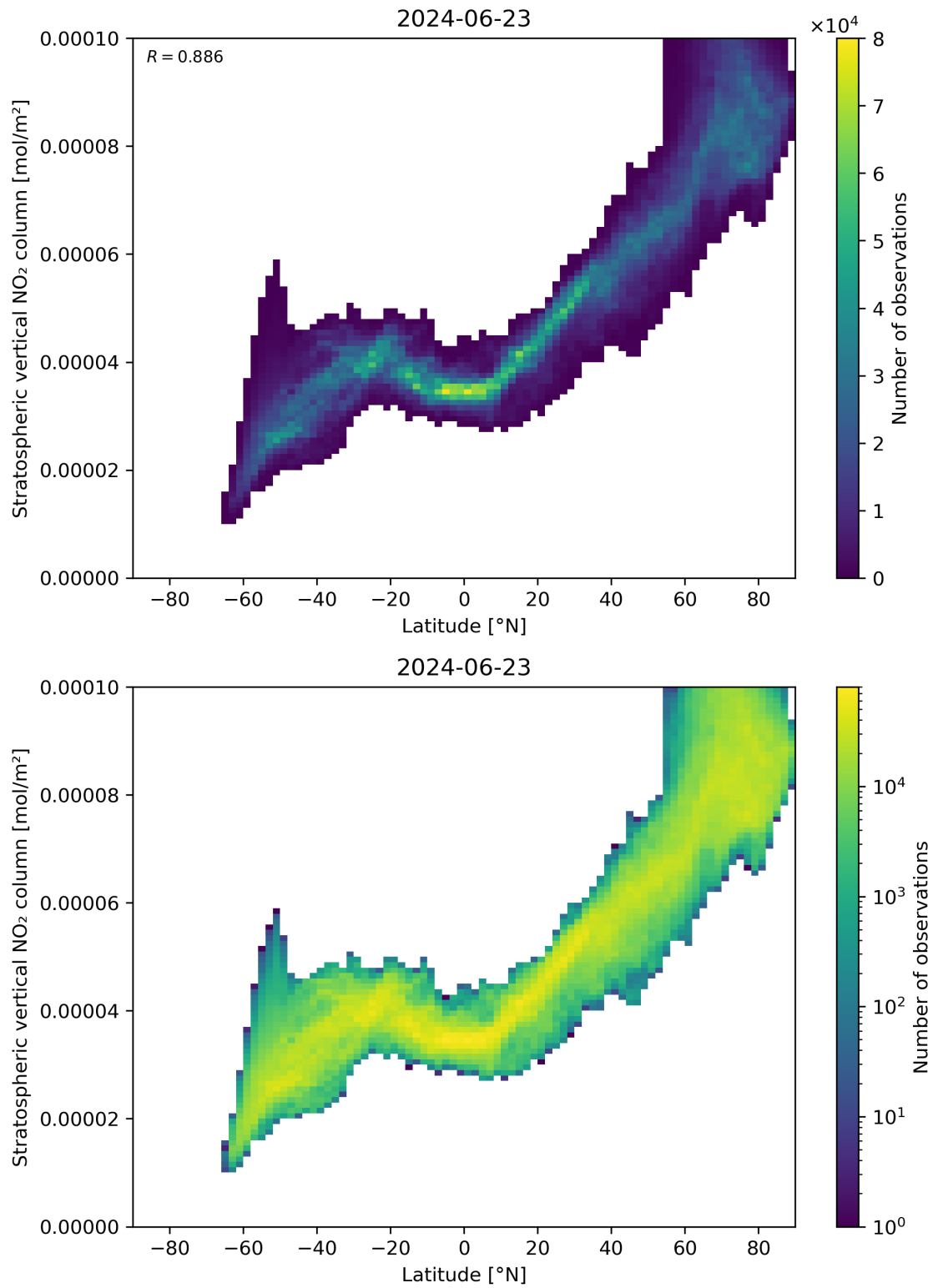
Figure 87: Scatter density plot of “Latitude” against “Stratospheric vertical NO 2 column” for 2024-06-22 to 2024-06-24.
