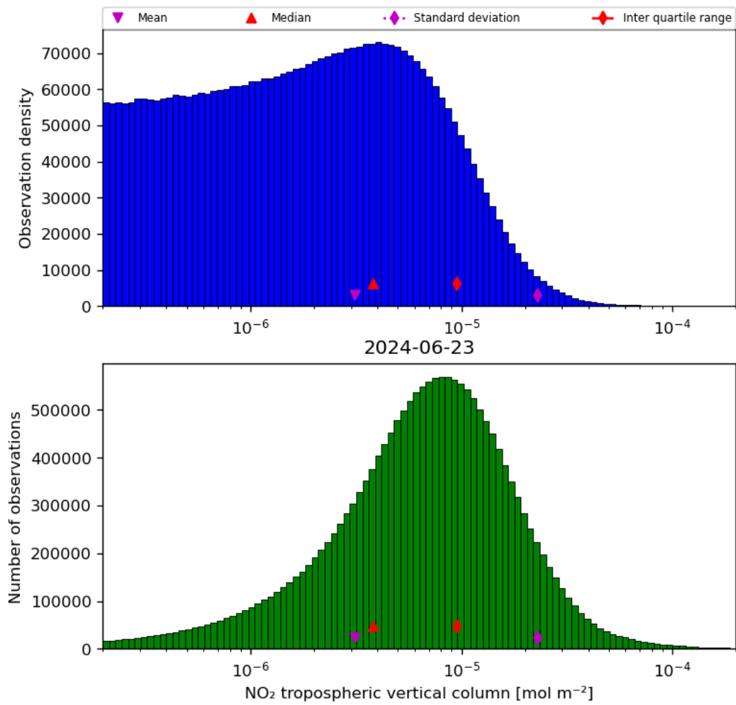
Figure 29: Histogram of “NO 2 tropospheric vertical column” for 2024-06-22 to 2024-06-24
