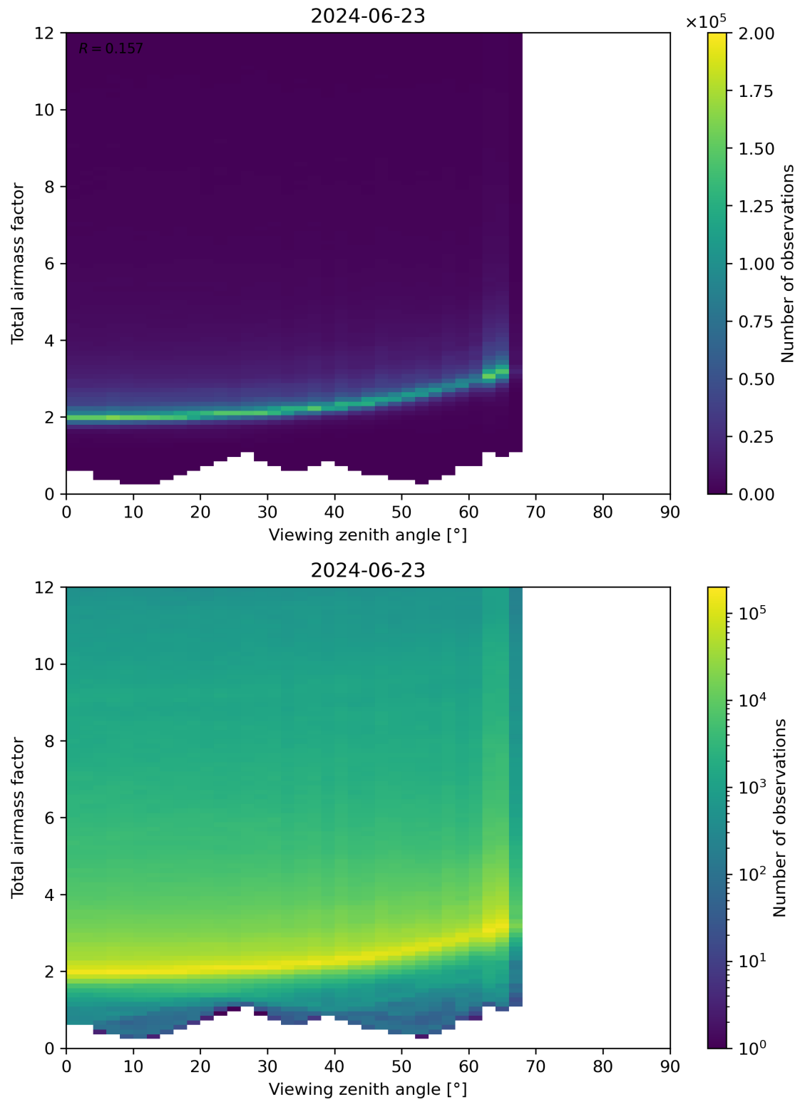
Figure 160: Scatter density plot of “Viewing zenith angle” against “Total airmass factor” for 2024-06-22 to 2024-06-24.
