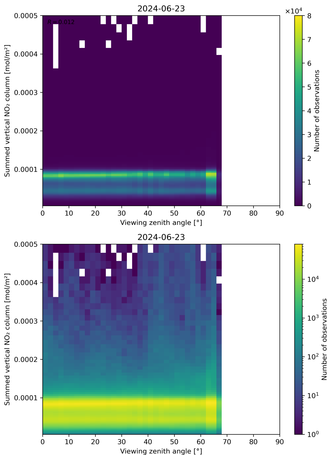
Figure 165: Scatter density plot of “Viewing zenith angle” against “Summed vertical NO 2 column” for 2024-06-22 to 2024-06-24.
