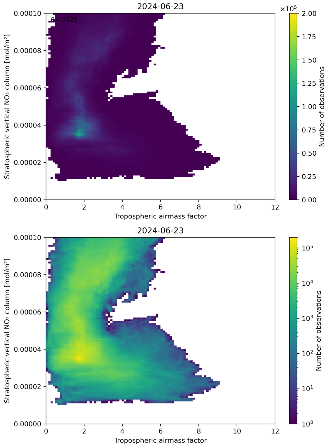
Figure 74: Scatter density plot of “Tropospheric air mass factor” against “Stratospheric vertical NO 2 column” for 2024-06-22 to 2024-06-24.
