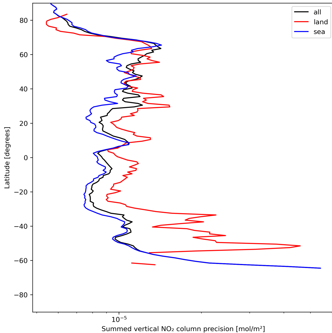
Figure 24: Zonal average of “Summed vertical NO 2 column precision” for 2024-06-22 to 2024-06-24.
