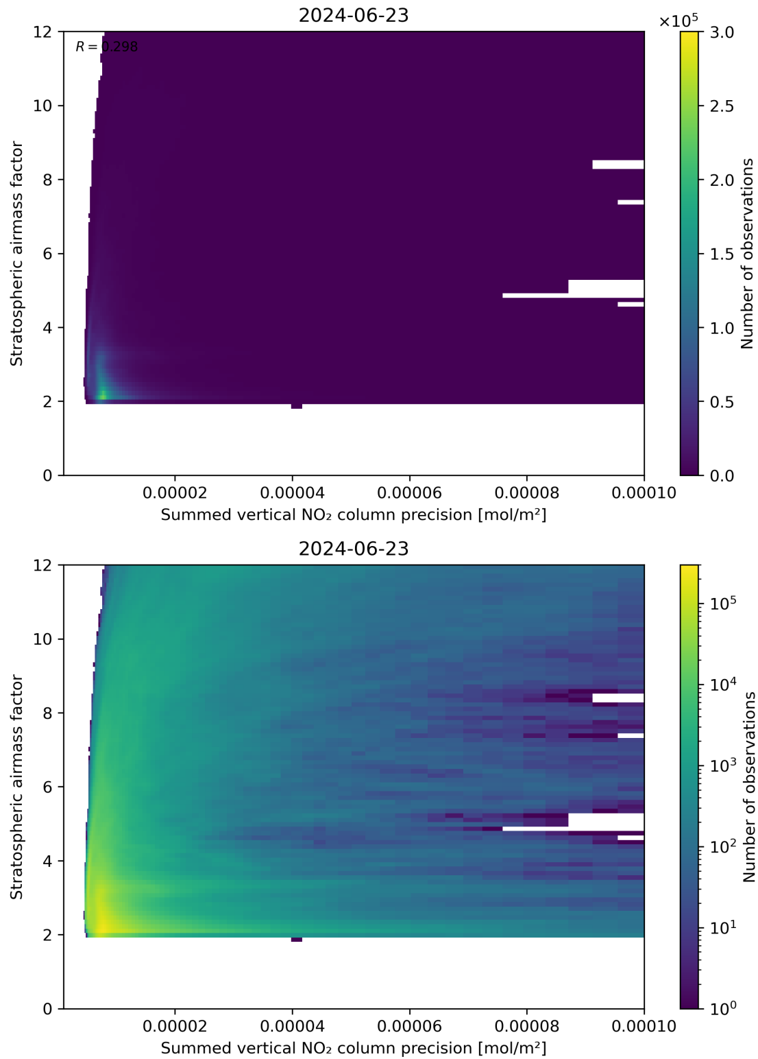
Figure 106: Scatter density plot of “Summed vertical NO 2 column precision” against “Stratospheric airmass factor” for 2024-06-22 to 2024-06-24.
