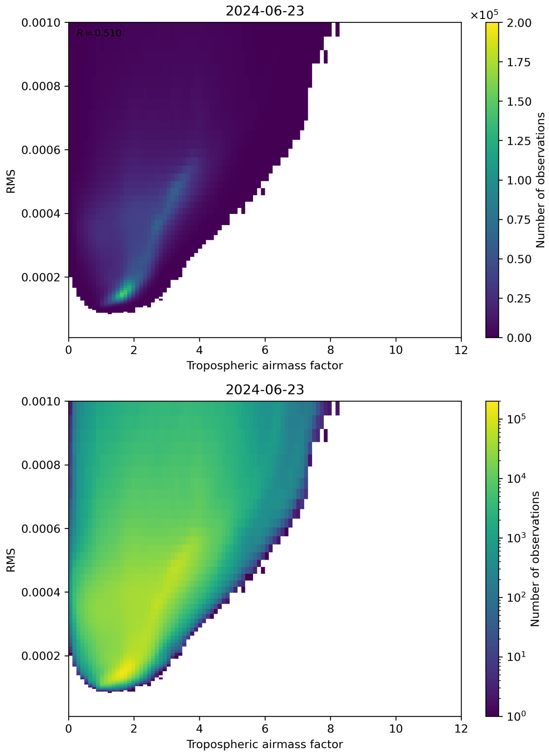
Figure 79: Scatter density plot of “Tropospheric airmass factor” against “RMS” for 2024-06-22 to 2024-06-24.
