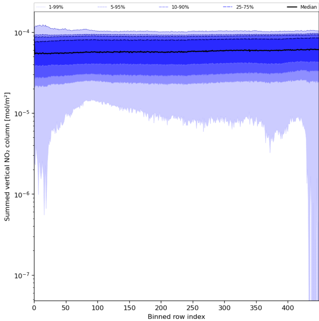
Figure 57: Along track statistics of “Summed vertical NO 2 column” for 2024-06-22 to 2024-06-24
