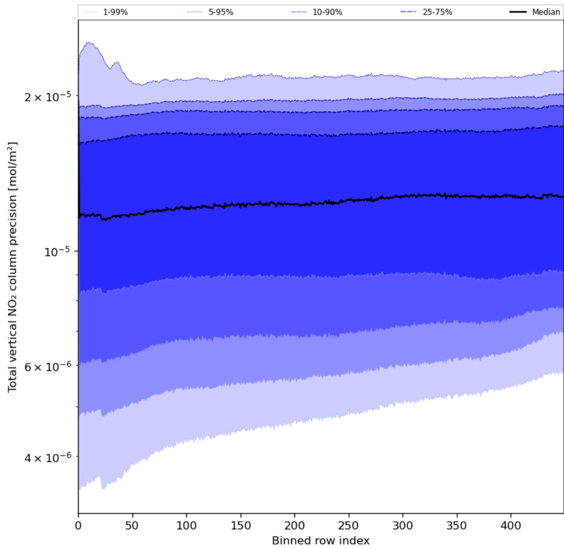
Figure 56: Along track statistics of “Total vertical NO 2 column precision” for 2024-06-22 to 2024-06-24
