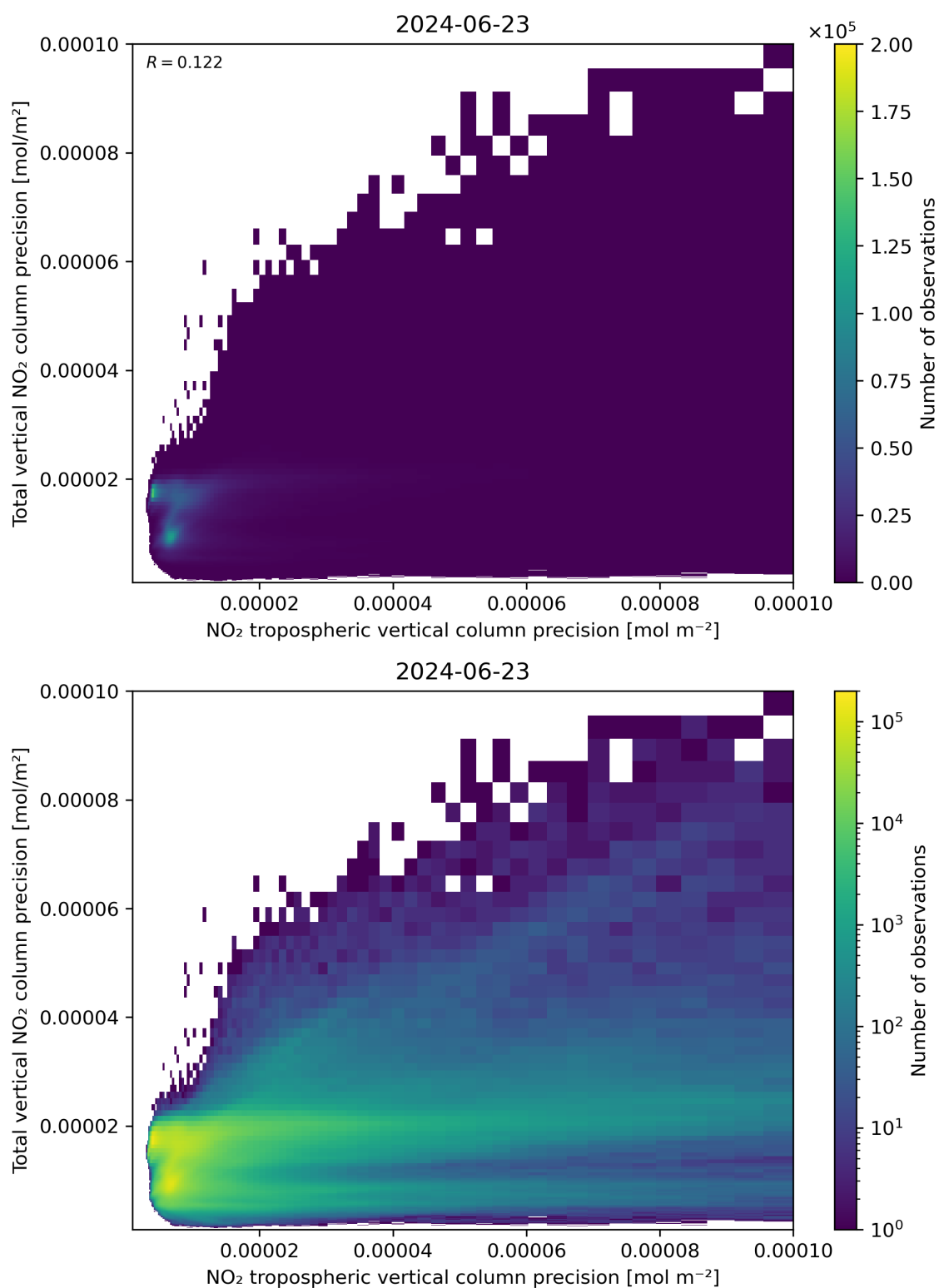
Figure 139: Scatter density plot of “NO 2 tropospheric vertical column precision” against “Total vertical NO 2 column precision” for 2024-06-22 to 2024-06-24.
