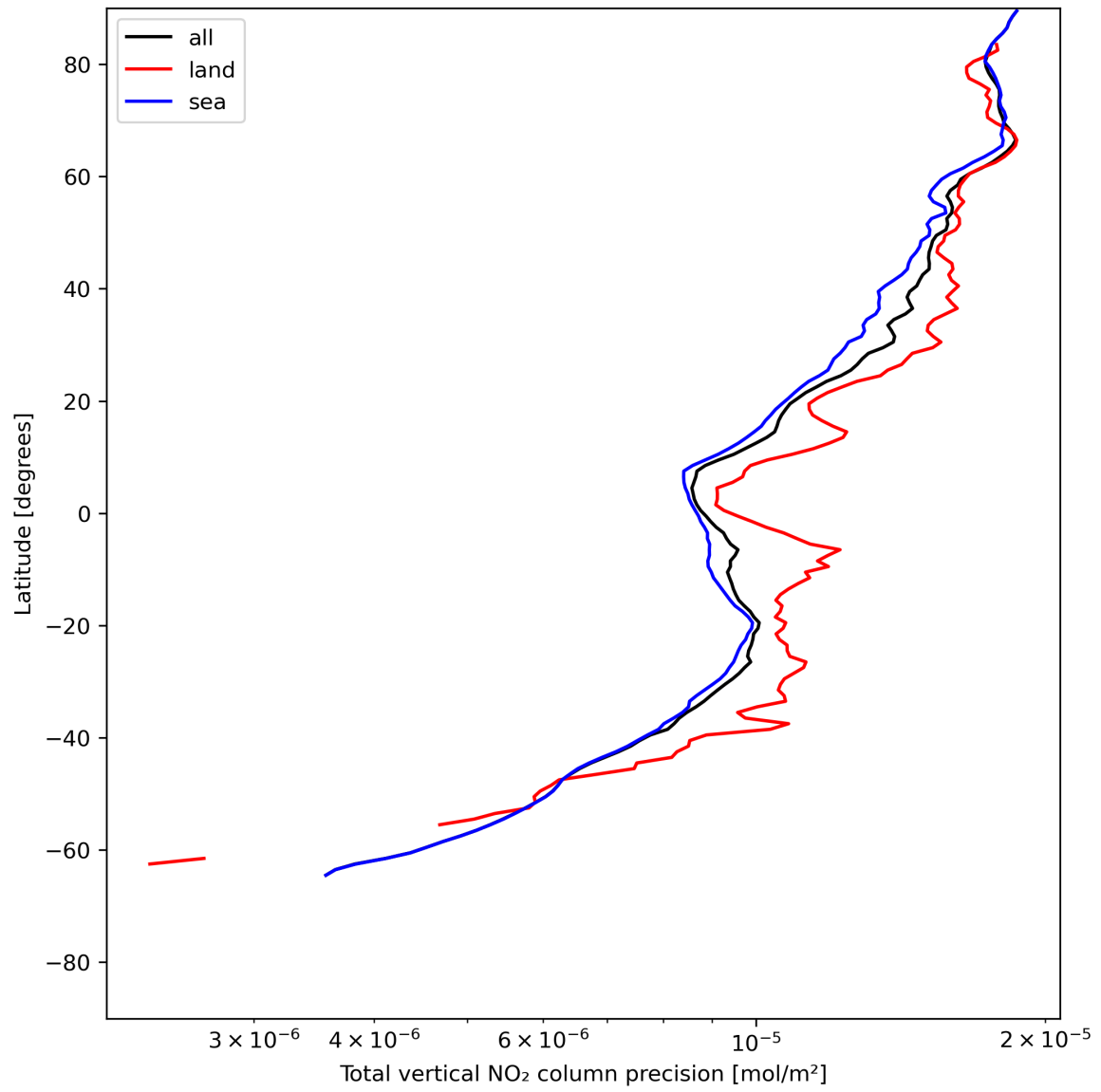
Figure 22: Zonal average of “Total vertical NO 2 column precision” for 2024-06-22 to 2024-06-24.
