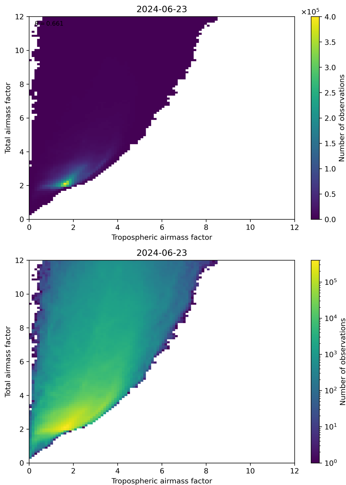
Figure 72: Scatter density plot of “Tropospheric airmass factor” against “Total airmass factor” for 2024-06-22 to 2024-06-24.
