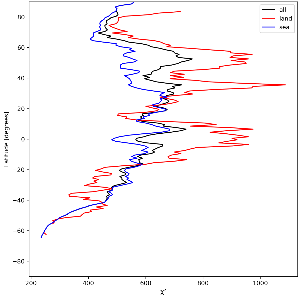
Figure 25: Zonal average of “ \chi^2 ” for 2024-06-22 to 2024-06-24.
