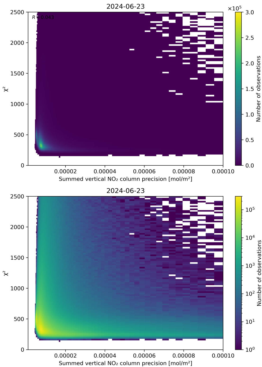
Figure 107: Scatter density plot of “Summed vertical NO 2 column precision” against “ \chi^2 ” for 2024-06-22 to 2024-06-24.
