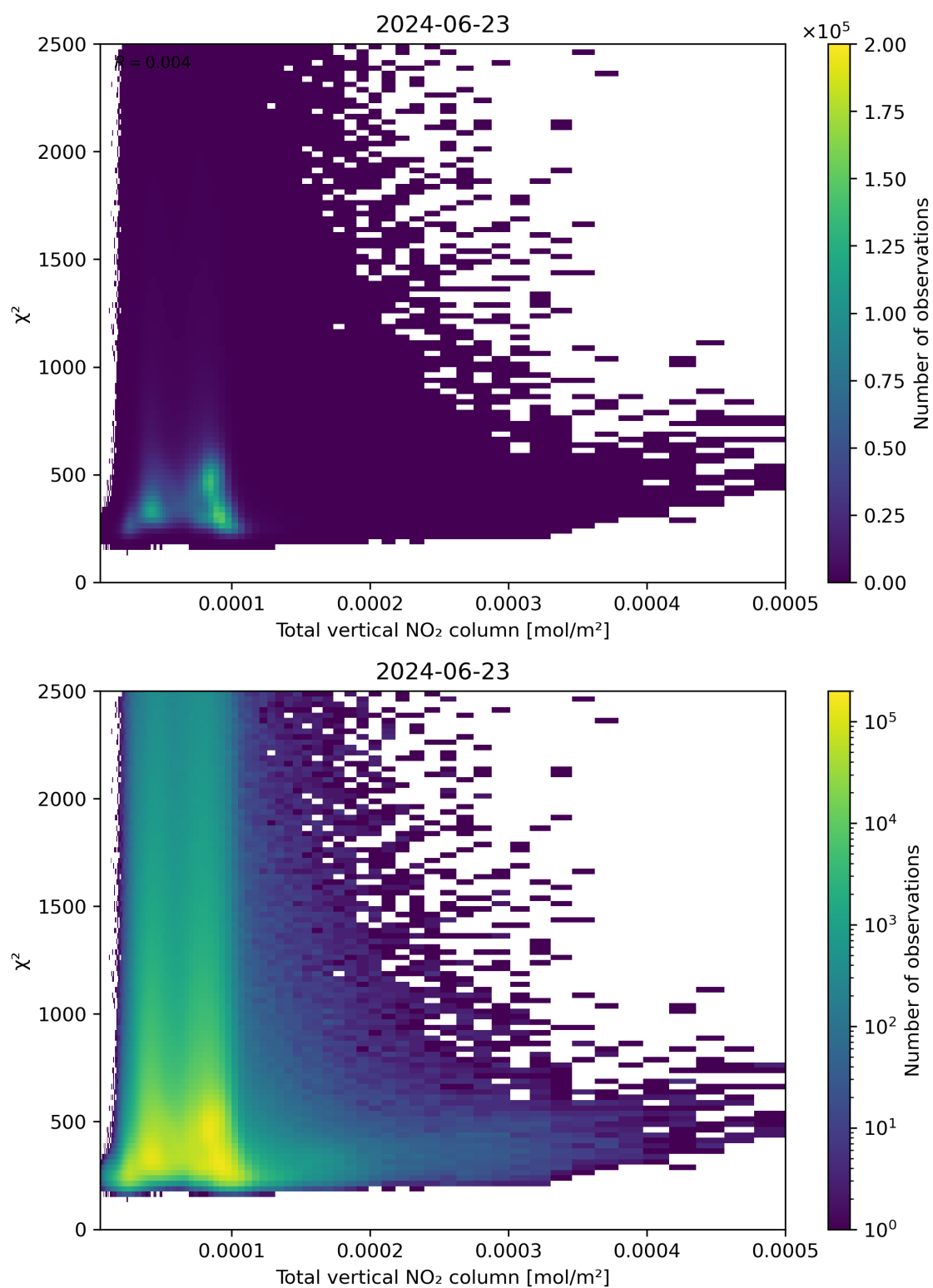
Figure 111: Scatter density plot of “Total vertical NO 2 column” against “ \chi^2 ” for 2024-06-22 to 2024-06-24.
