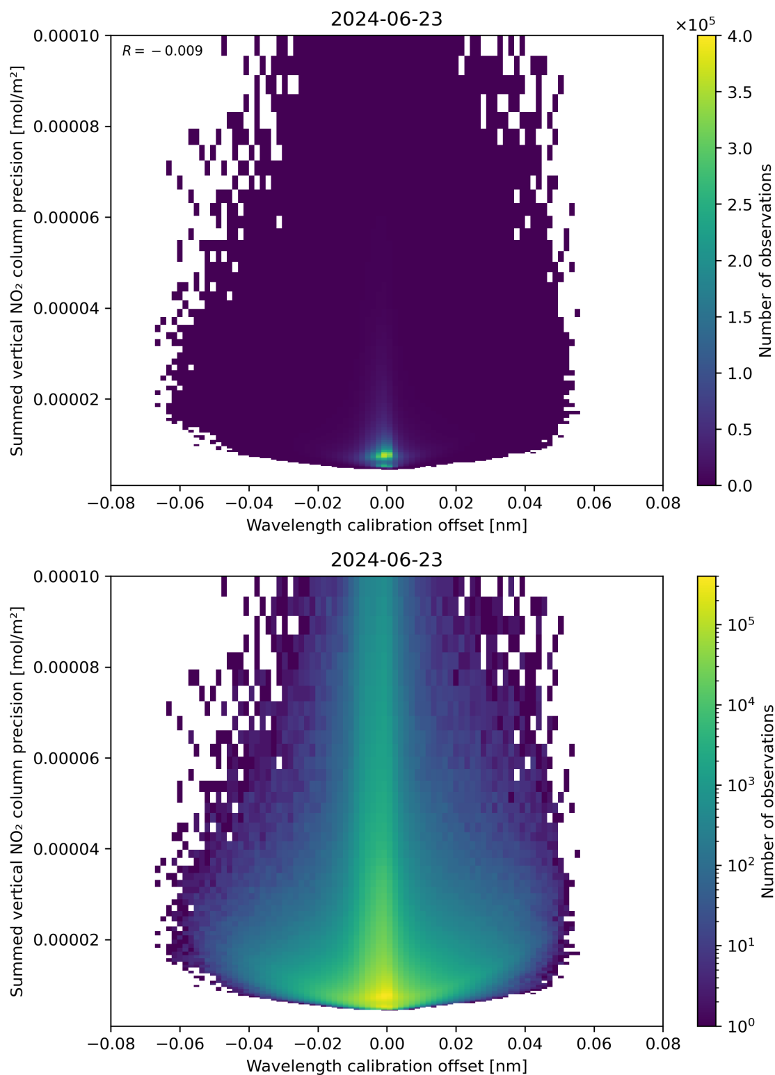
Figure 178: Scatter density plot of “Wavelength calibration offset” against “Summed vertical NO 2 column precision” for 2024-06-22 to 2024-06-24.
