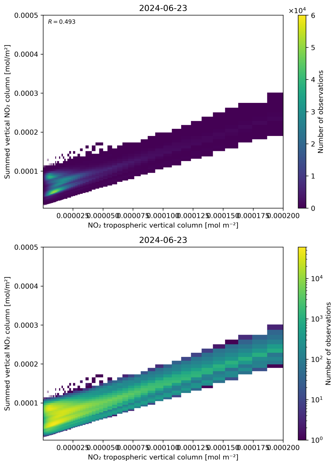
Figure 126: Scatter density plot of “NO 2 tropospheric vertical column” against “Summed vertical NO 2 column” for 2024-06-22 to 2024-06-24.
