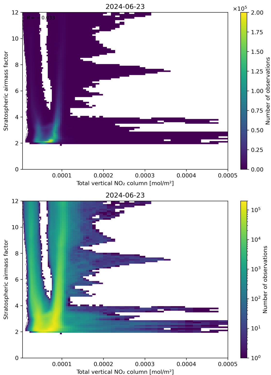
Figure 110: Scatter density plot of “Total vertical NO 2 column” against “Stratospheric airmass factor” for 2024-06-22 to 2024-06-24.
