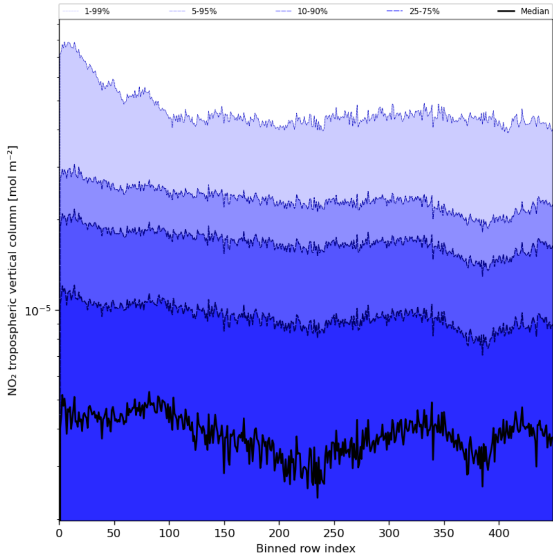
Figure 46: Along track statistics of “NO 2 tropospheric vertical column” for 2024-06-22 to 2024-06-24
