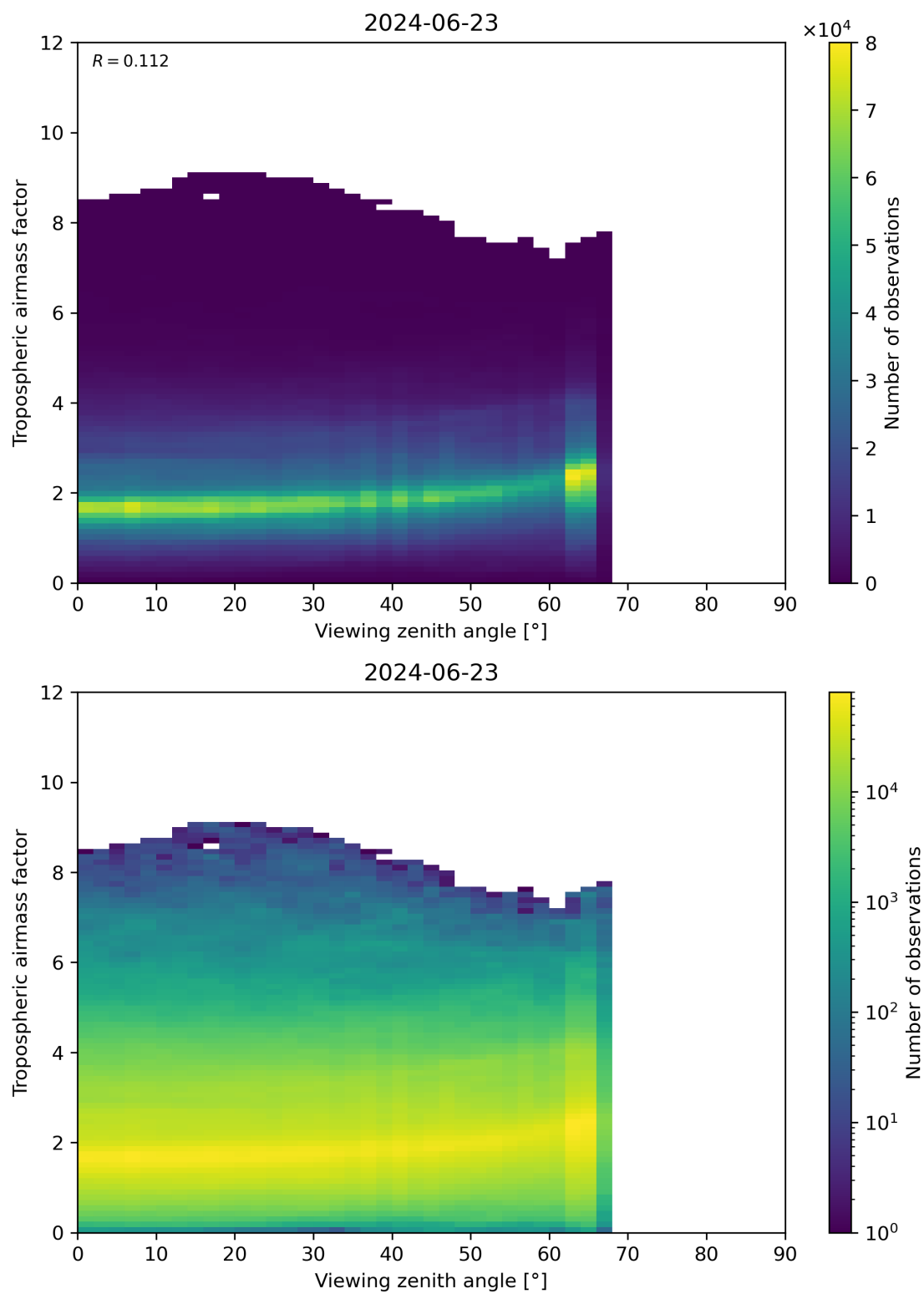
Figure 161: Scatter density plot of “Viewing zenith angle” against “Tropospheric airmass factor” for 2024-06-22 to 2024-06-24.
