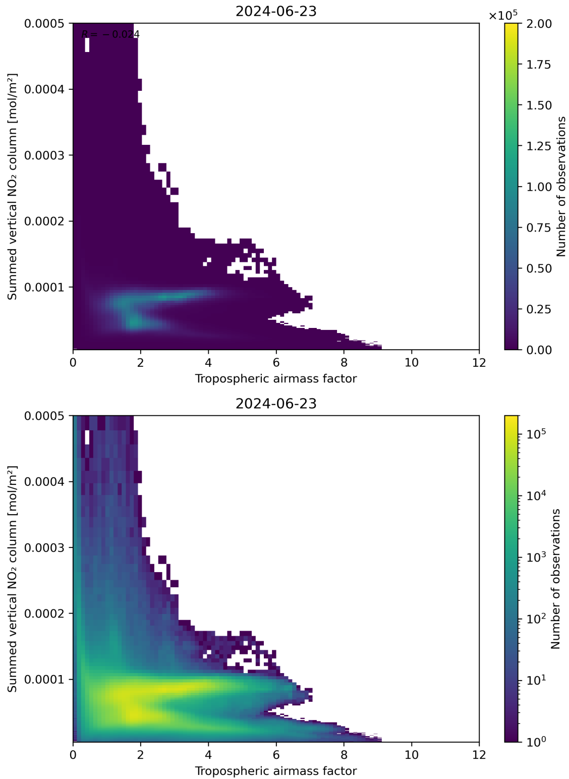
Figure 75: Scatter density plot of “Tropospheric airmass factor” against “Summed vertical NO 2 column” for 2024-06-22 to 2024-06-24.
