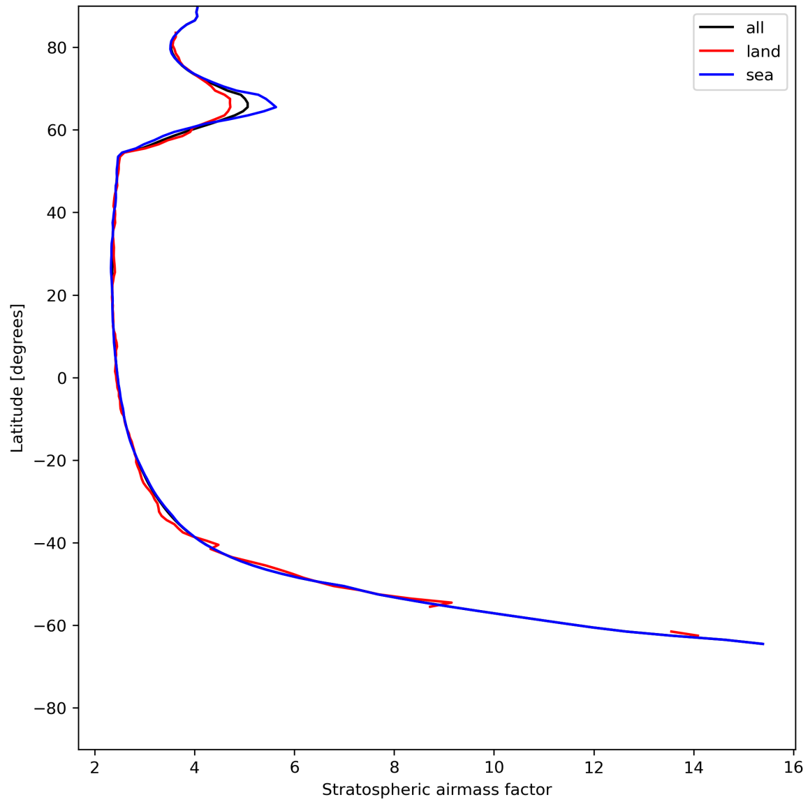
Figure 27: Zonal average of “Stratospheric airmass factor” for 2024-06-22 to 2024-06-24.
