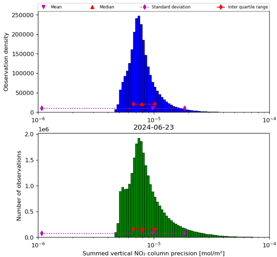
Figure 41: Histogram of “Summed vertical NO 2 column precision” for 2024-06-22 to 2024-06-24
