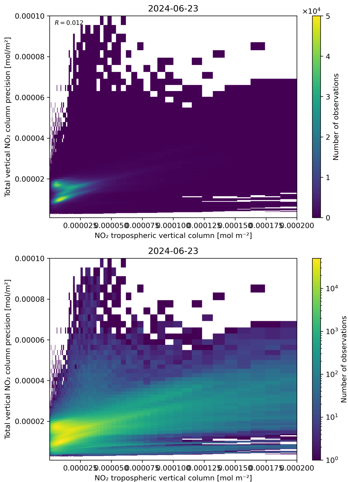
Figure 129: Scatter density plot of “NO 2 tropospheric vertical column” against “Total vertical NO 2 column precision” for 2024-06-22 to 2024-06-24.
