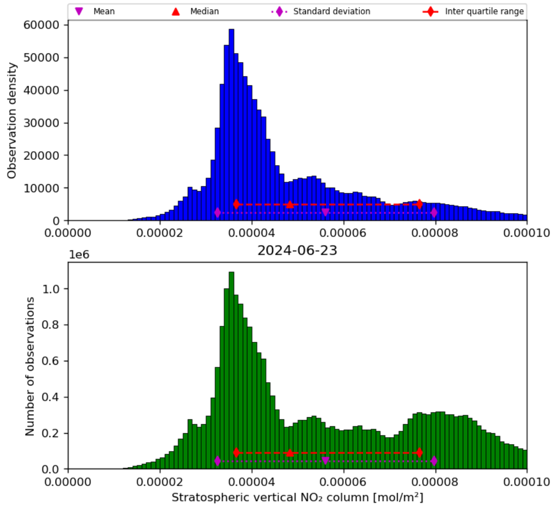
Figure 36: Histogram of “Stratospheric vertical NO 2 column” for 2024-06-22 to 2024-06-24
