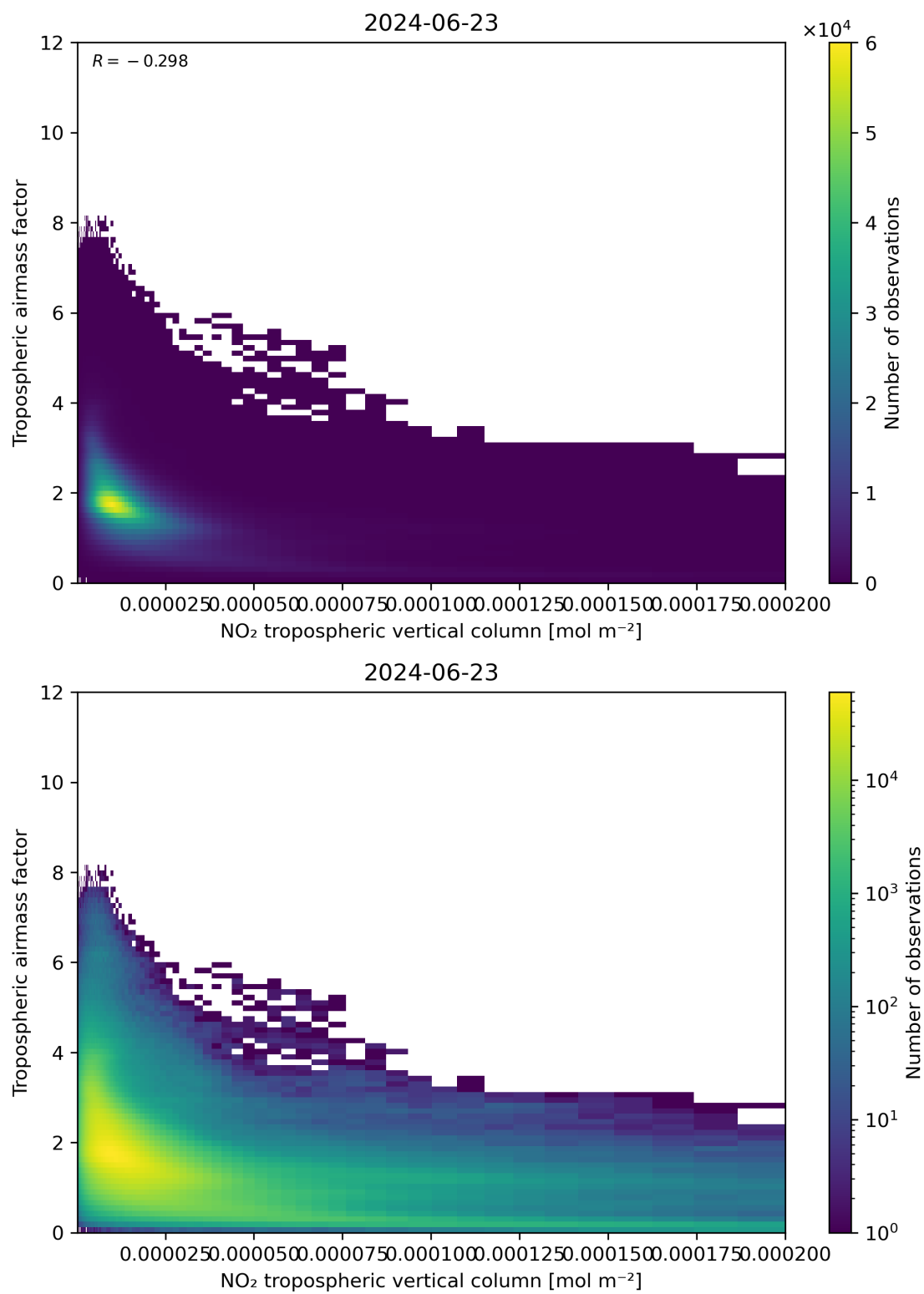
Figure 123: Scatter density plot of “NO 2 tropospheric vertical column” against “Tropospheric airmass factor” for 2024-06-22 to 2024-06-24.
