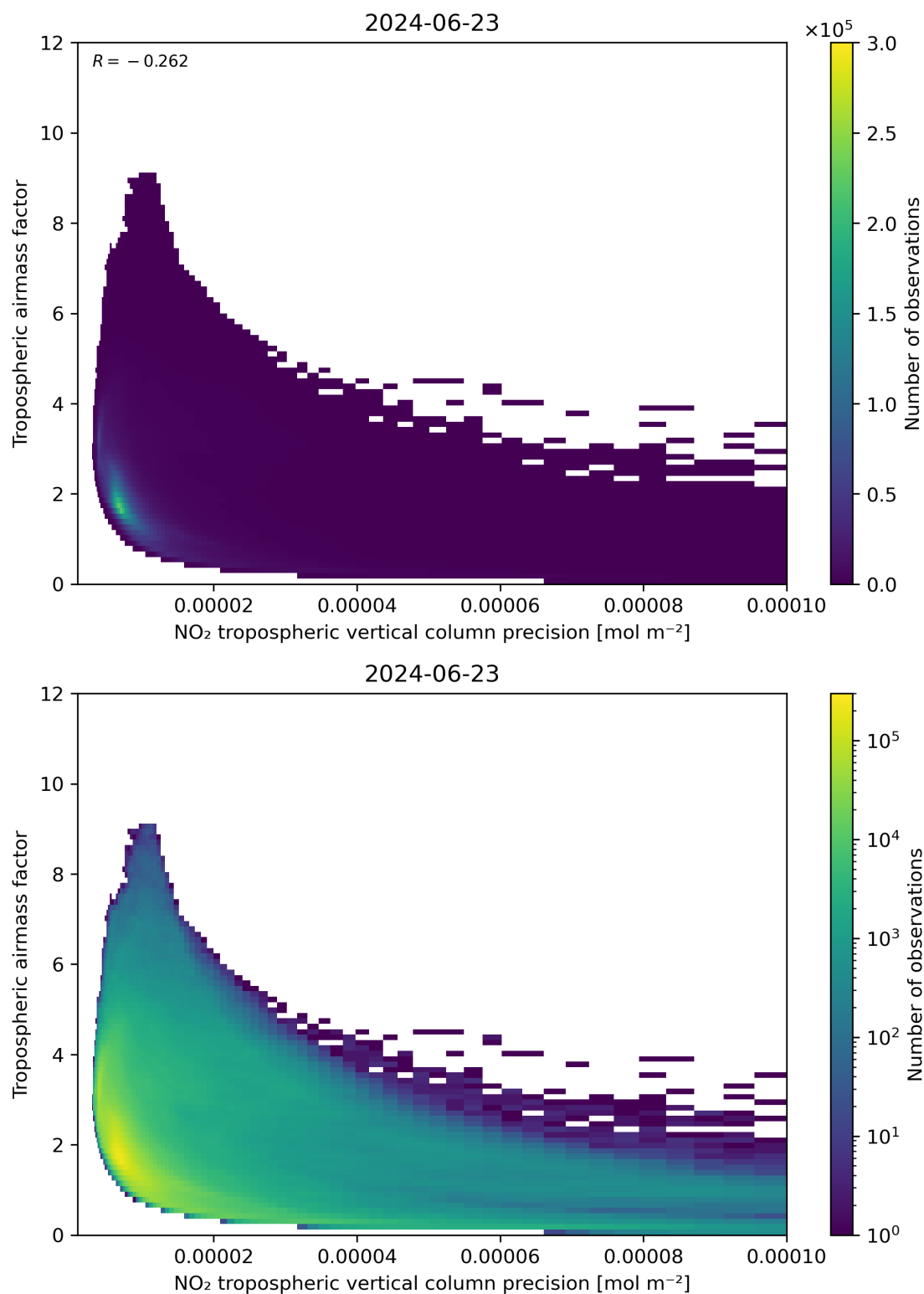
Figure 133: Scatter density plot of “NO 2 tropospheric vertical column precision” against “Tropospheric air mass factor” for 2024-06-22 to 2024-06-24.
