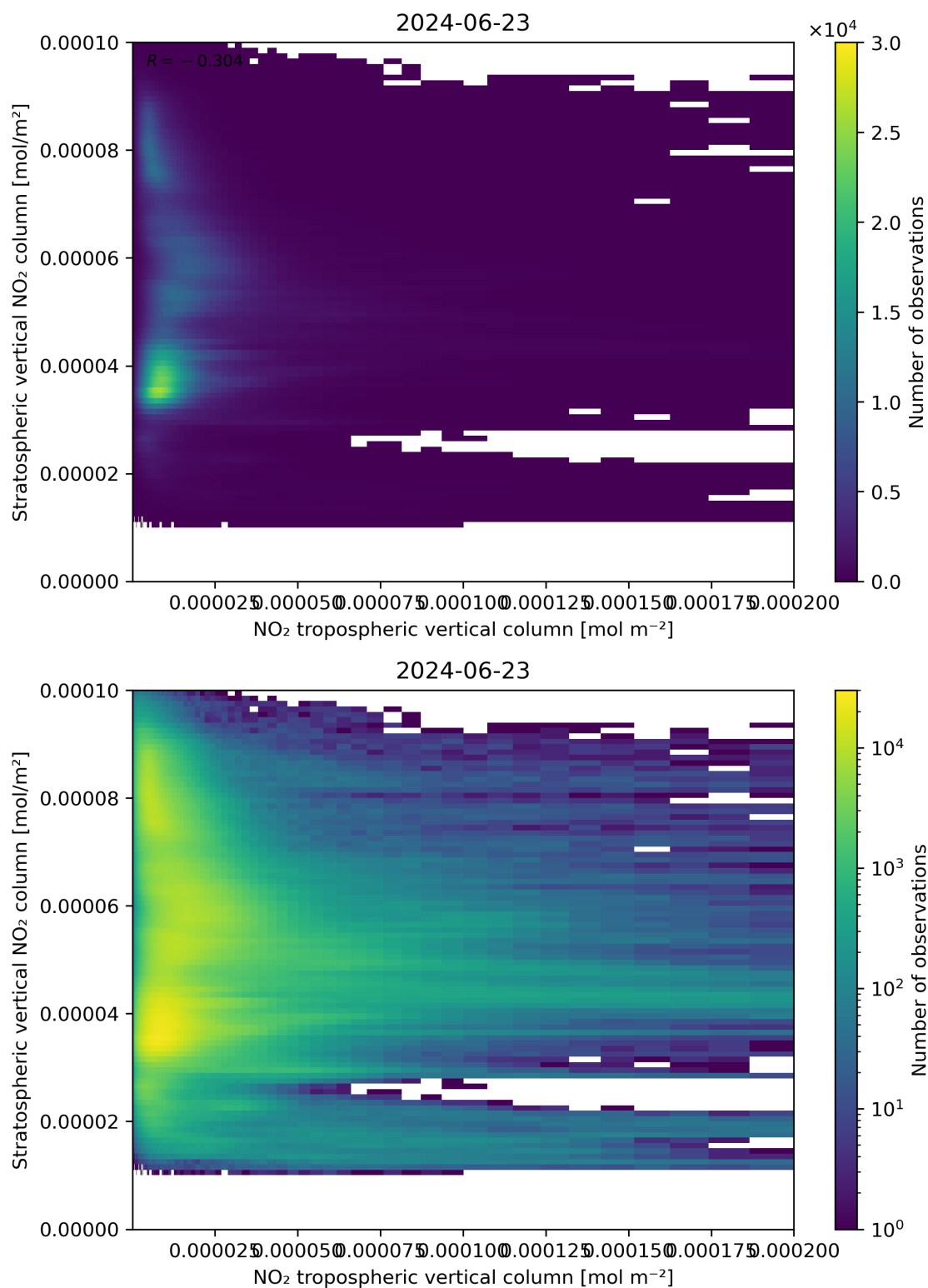
Figure 125: Scatter density plot of “NO 2 tropospheric vertical column” against “Stratospheric vertical NO 2 column” for 2024-06-22 to 2024-06-24.
