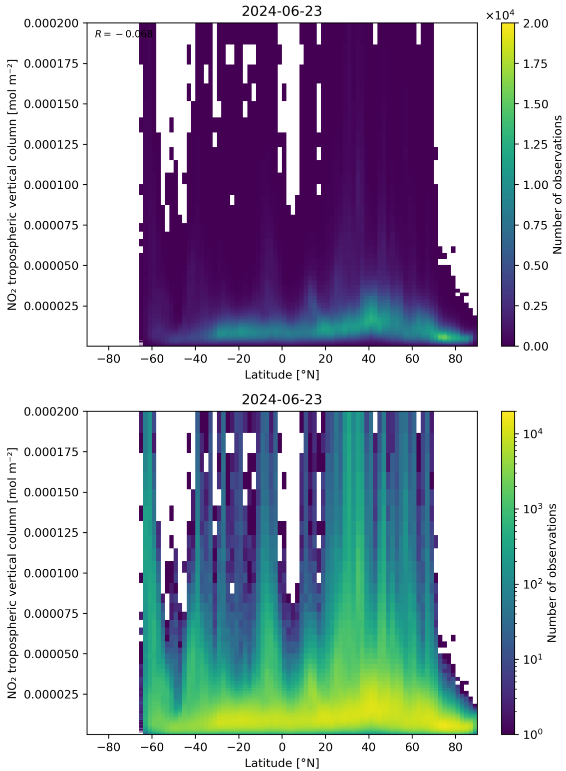
Figure 92: Scatter density plot of “Latitude” against “NO 2 tropospheric vertical column” for 2024-06-22 to 2024-06-24.
