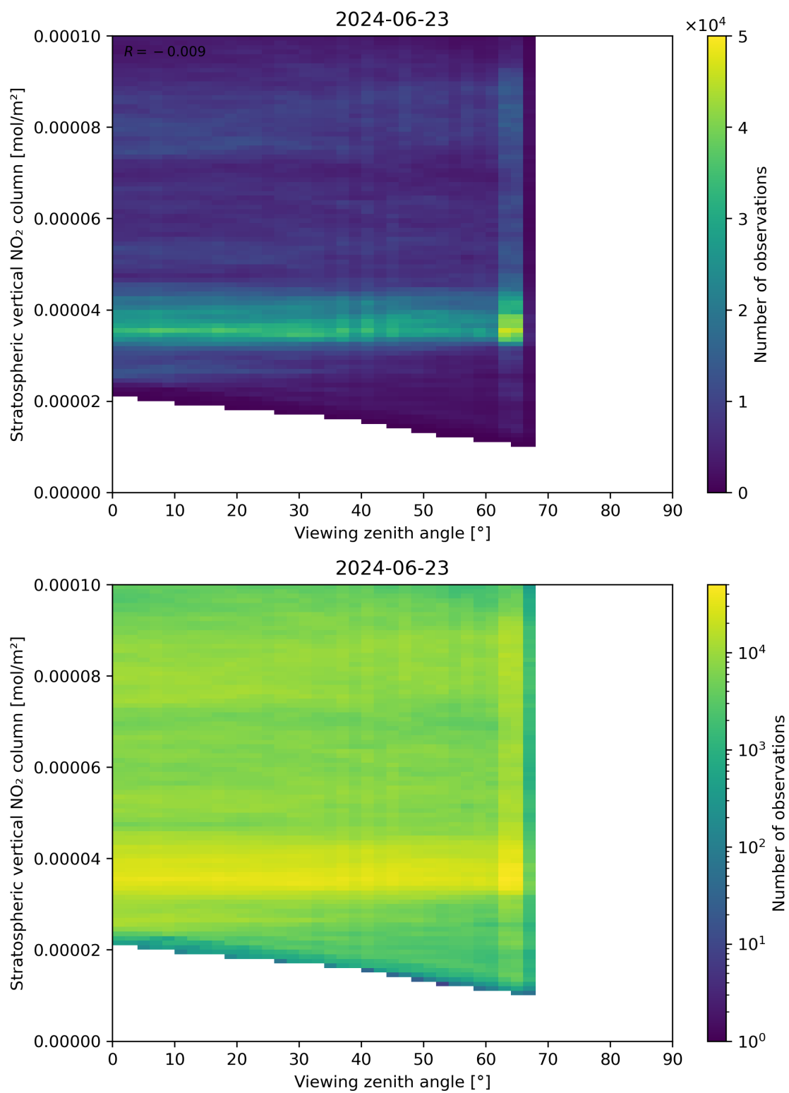
Figure 164: Scatter density plot of “Viewing zenith angle” against “Stratospheric vertical NO 2 column” for 2024-06-22 to 2024-06-24.
