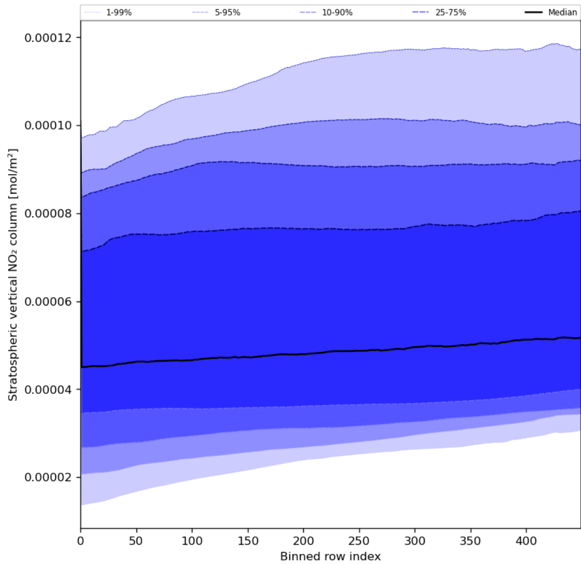
Figure 53: Along track statistics of “Stratospheric vertical NO 2 column” for 2024-06-22 to 2024-06-24
