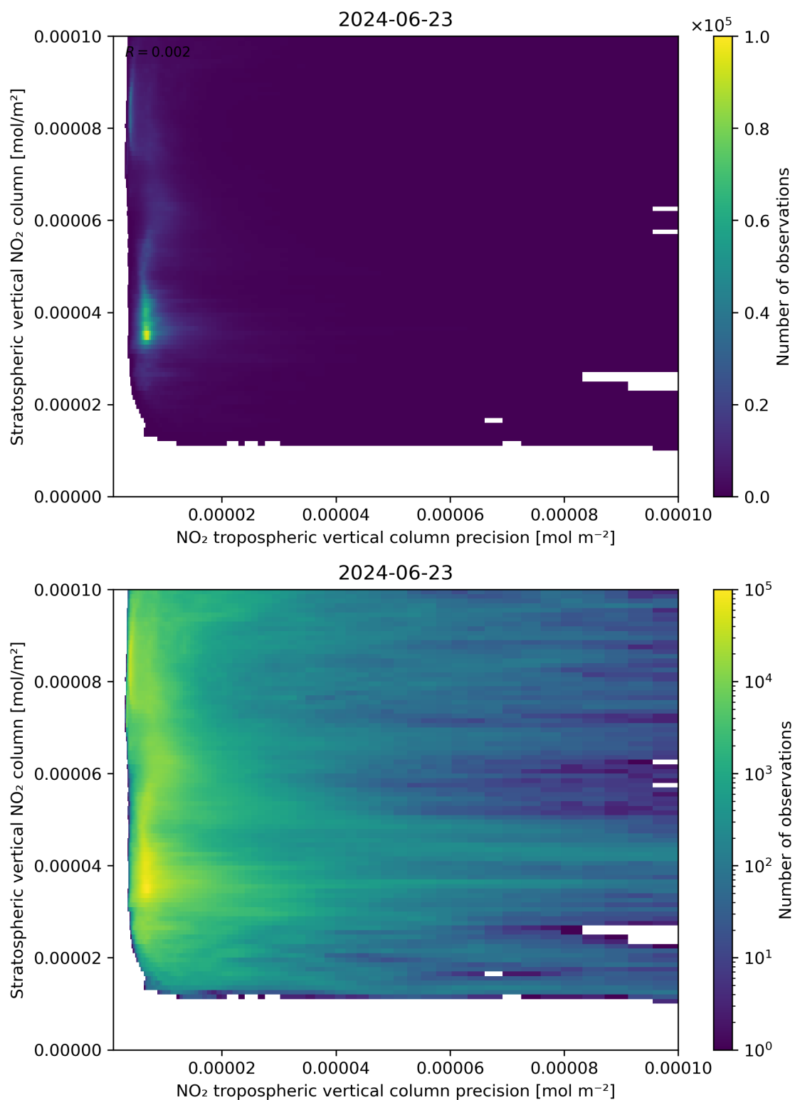
Figure 135: Scatter density plot of “NO 2 tropospheric vertical column precision” against “Stratospheric vertical NO 2 column” for 2024-06-22 to 2024-06-24.
