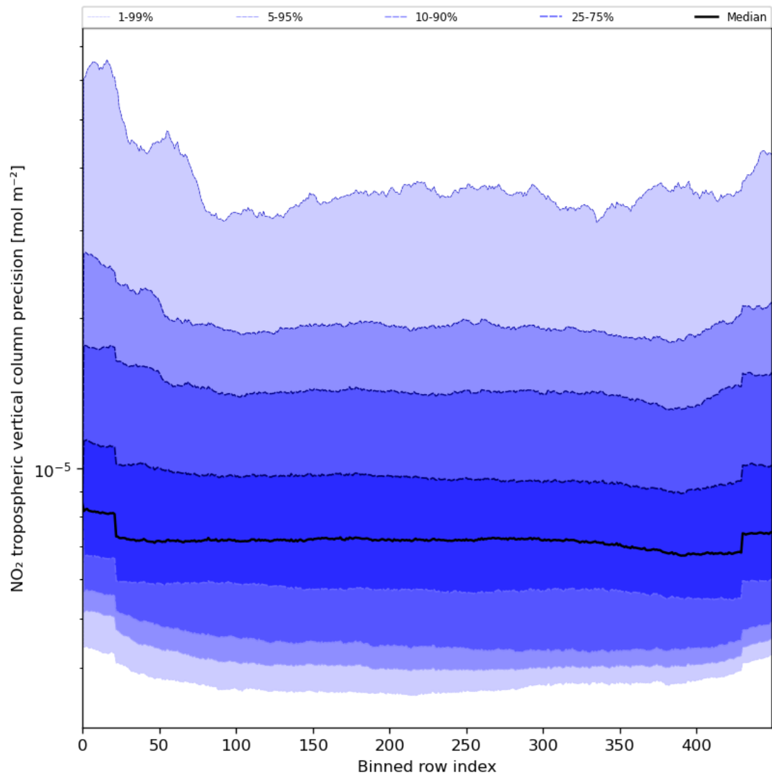
Figure 47: Along track statistics of “NO 2 tropospheric vertical column precision” for 2024-06-22 to 2024-06-24
