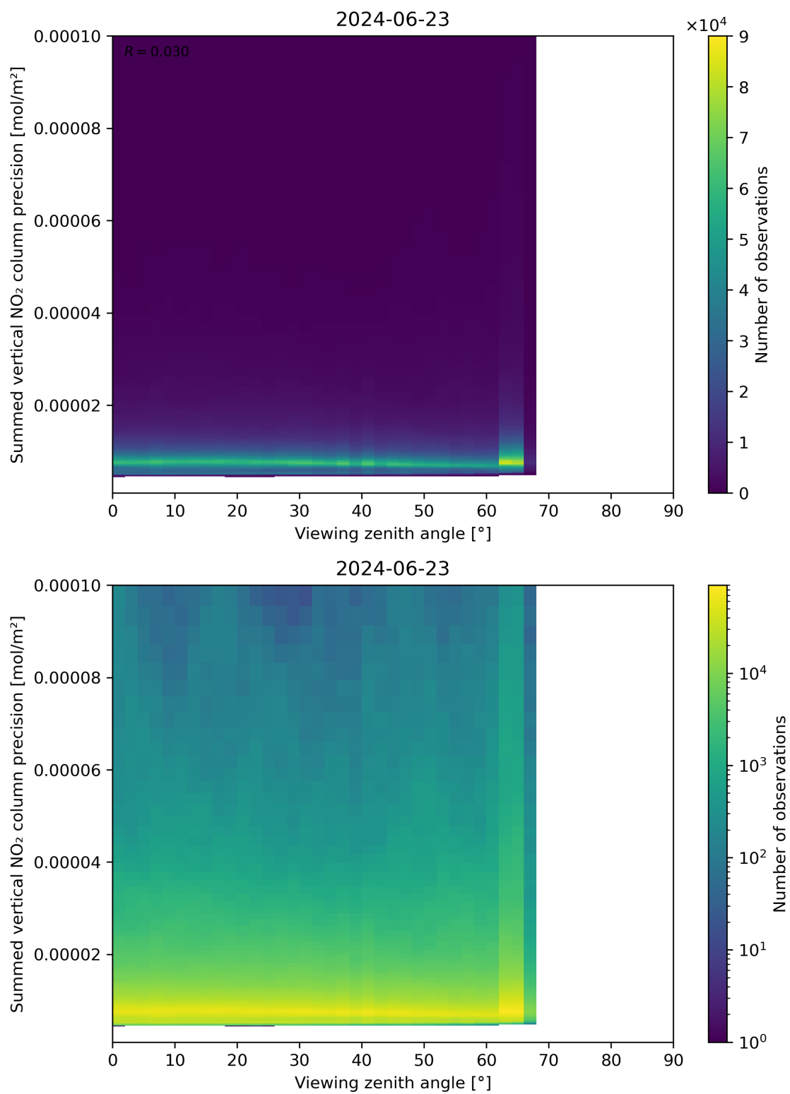
Figure 166: Scatter density plot of “Viewing zenith angle” against “Summed vertical NO 2 column precision” for 2024-06-22 to 2024-06-24.
