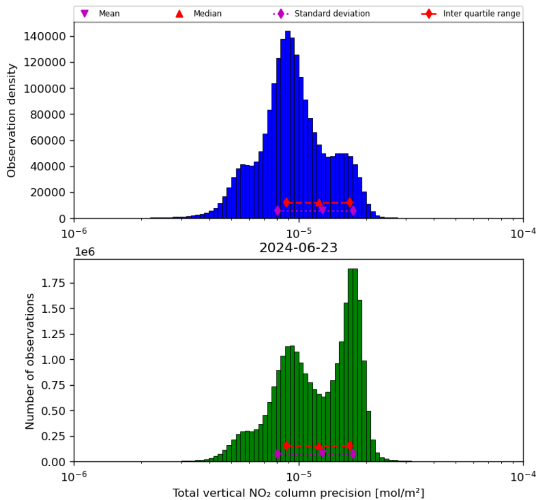
Figure 39: Histogram of "Total vertical NO 2 column precision" for 2024-06-22 to 2024-06-24
