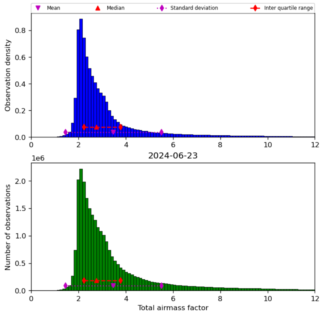
Figure 32: Histogram of “Total airmass factor” for 2024-06-22 to 2024-06-24
