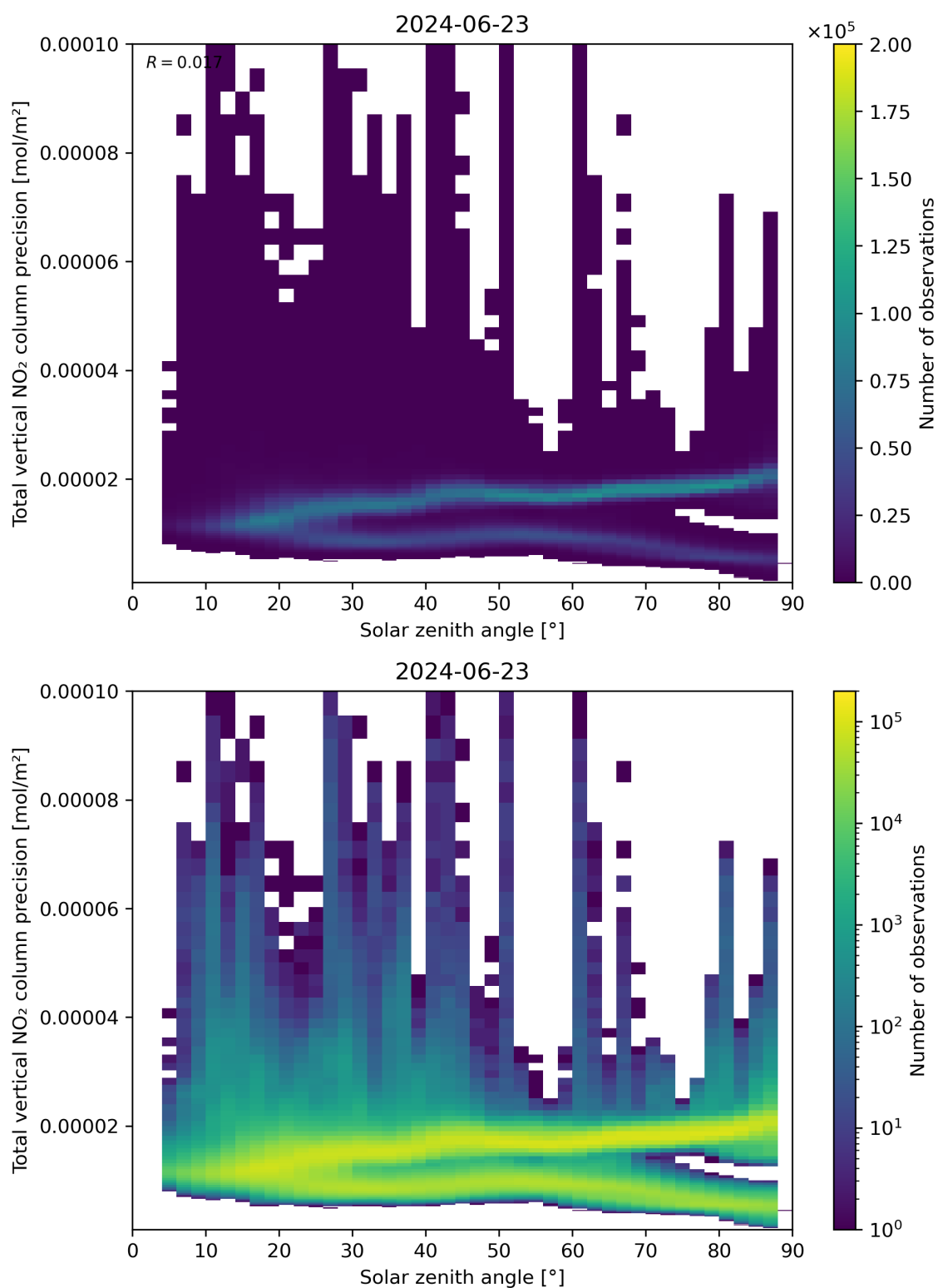
Figure 154: Scatter density plot of “Solar zenith angle” against “Total vertical NO 2 column precision” for 2024-06-22 to 2024-06-24.
