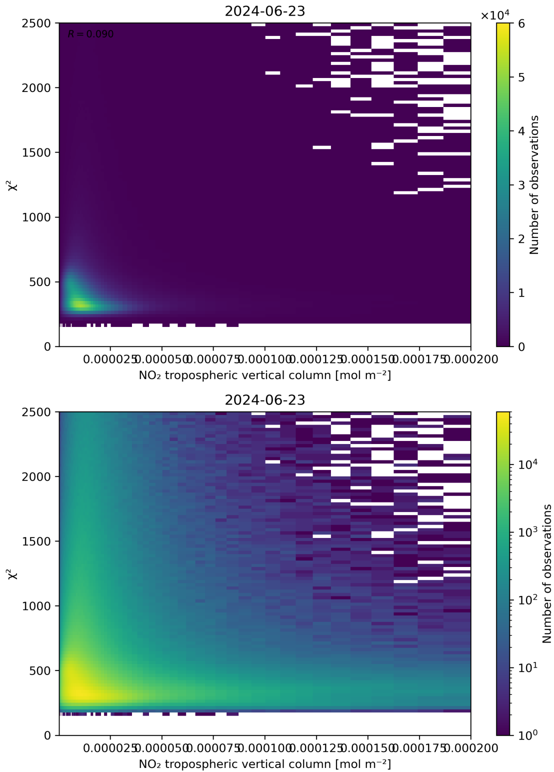
Figure 124: Scatter density plot of “NO 2 tropospheric vertical column” against “ \chi^2 ” for 2024-06-22 to 2024-06-24.
