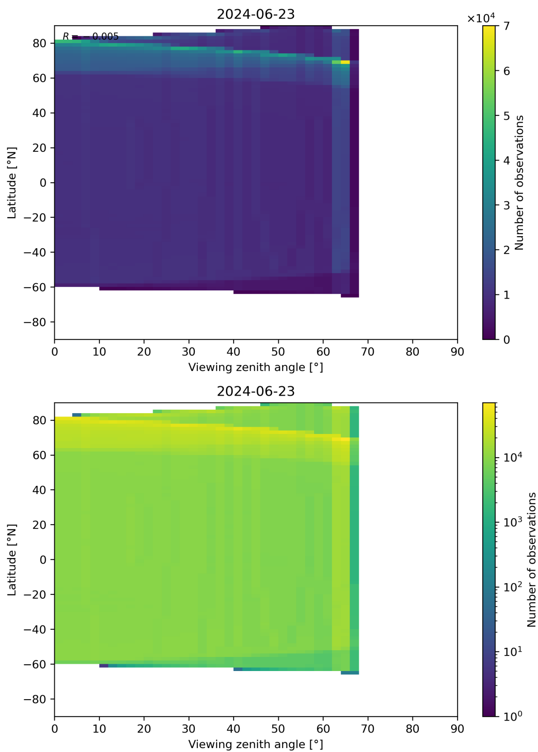
Figure 163: Scatter density plot of “Viewing zenith angle” against “Latitude” for 2024-06-22 to 2024-06-24.
