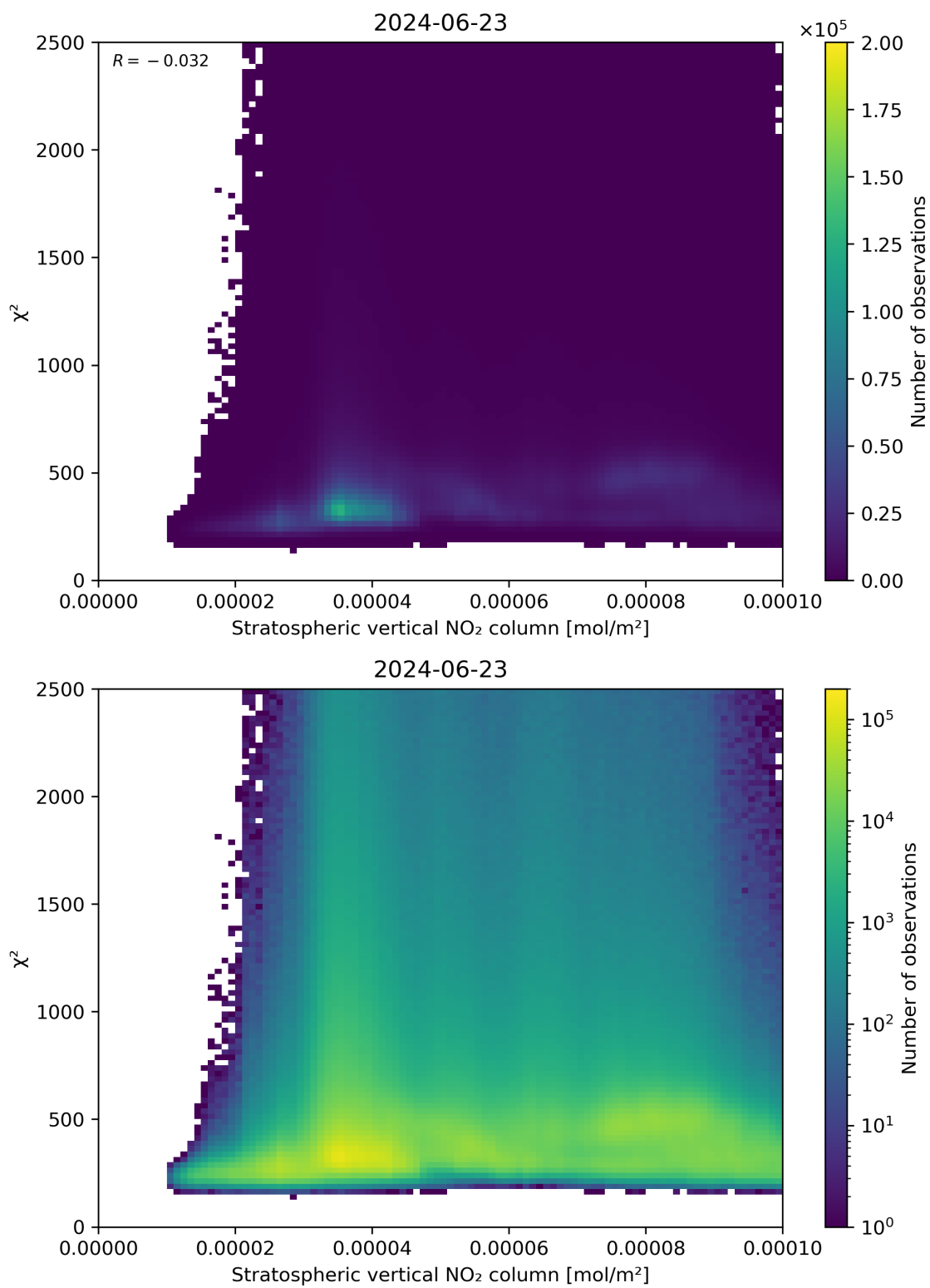
Figure 97: Scatter density plot of “Stratospheric vertical NO 2 column” against “ \chi^2 ” for 2024-06-22 to 2024-06-24.
