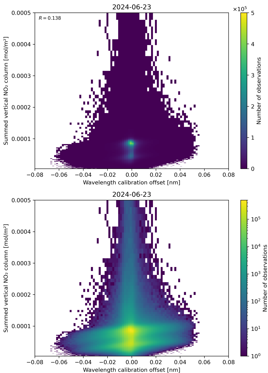
Figure 177: Scatter density plot of “Wavelength calibration offset” against “Summed vertical NO 2 column” for 2024-06-22 to 2024-06-24.
