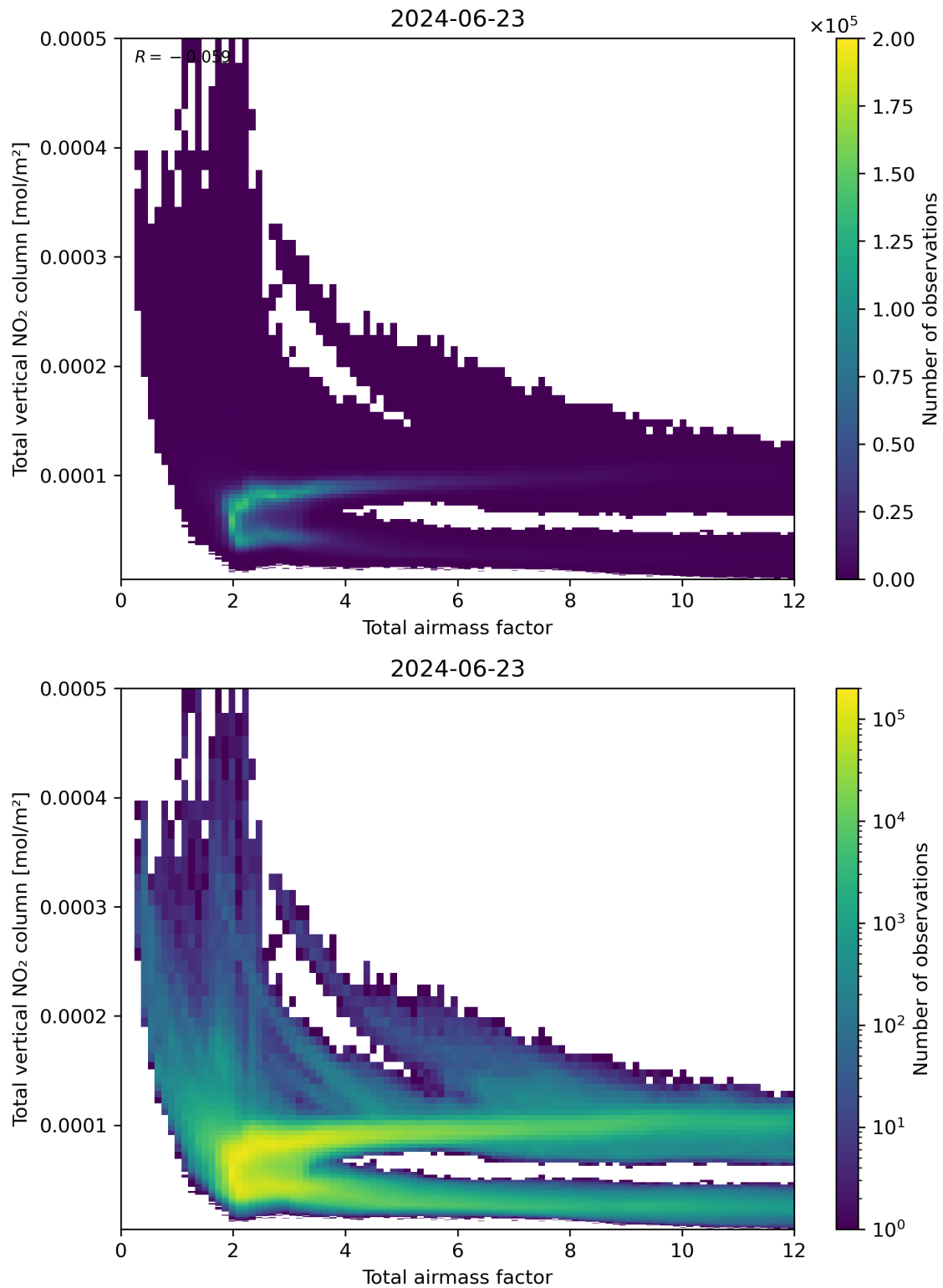
Figure 67: Scatter density plot of “Total airmass factor” against “Total vertical NO 2 column” for 2024-06-22 to 2024-06-24.
