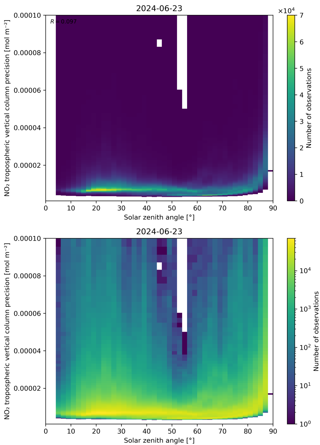
Figure 156: Scatter density plot of “Solar zenith angle” against “NO 2 tropospheric vertical column precision” for 2024-06-22 to 2024-06-24.
