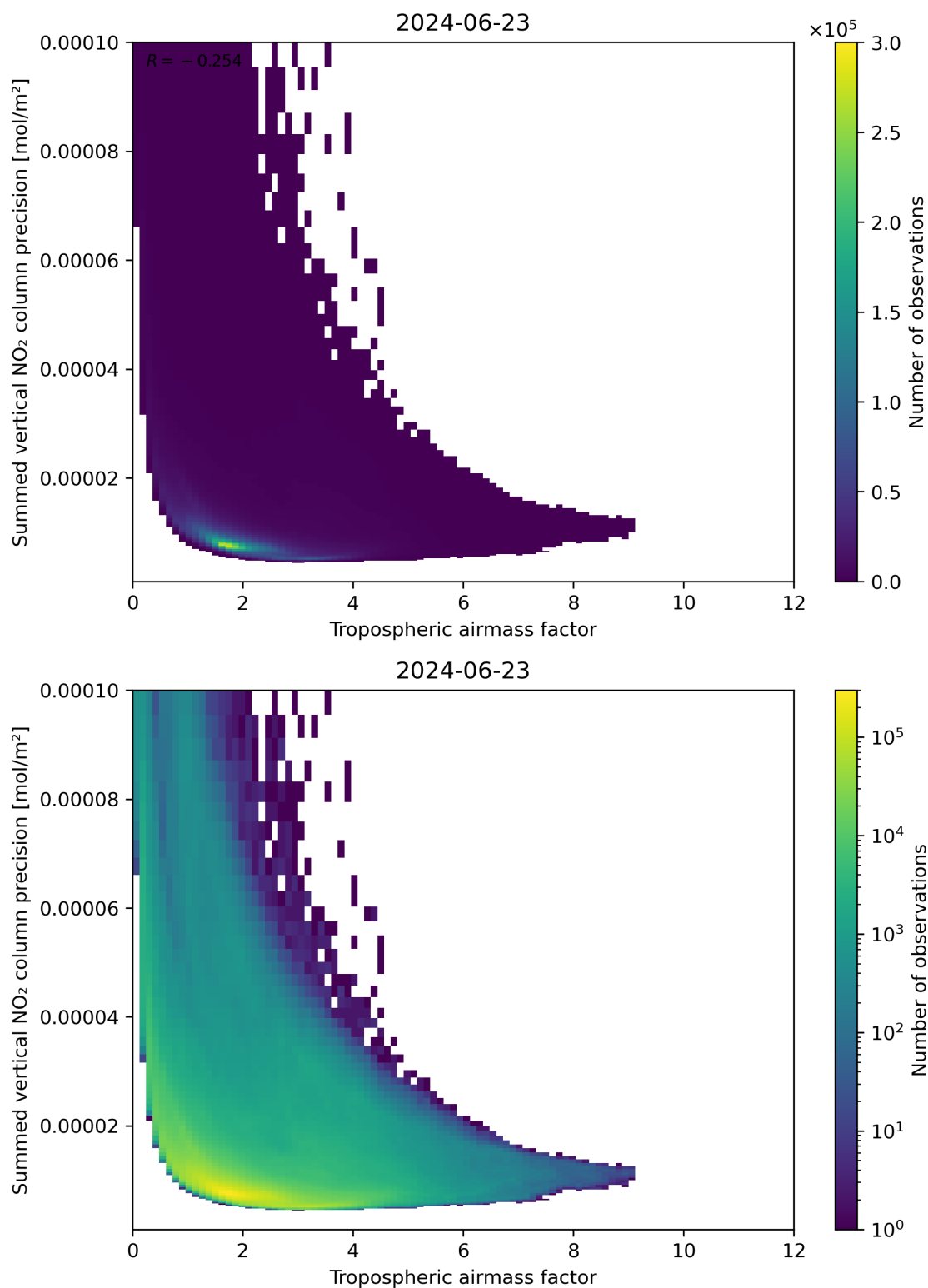
Figure 76: Scatter density plot of “Tropospheric air mass factor” against “Summed vertical NO 2 column precision” for 2024-06-22 to 2024-06-24.
