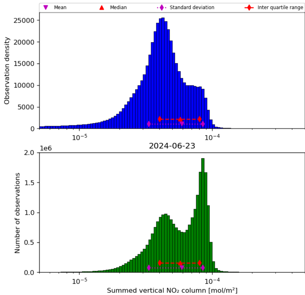
Figure 40: Histogram of “Summed vertical NO 2 column” for 2024-06-22 to 2024-06-24
