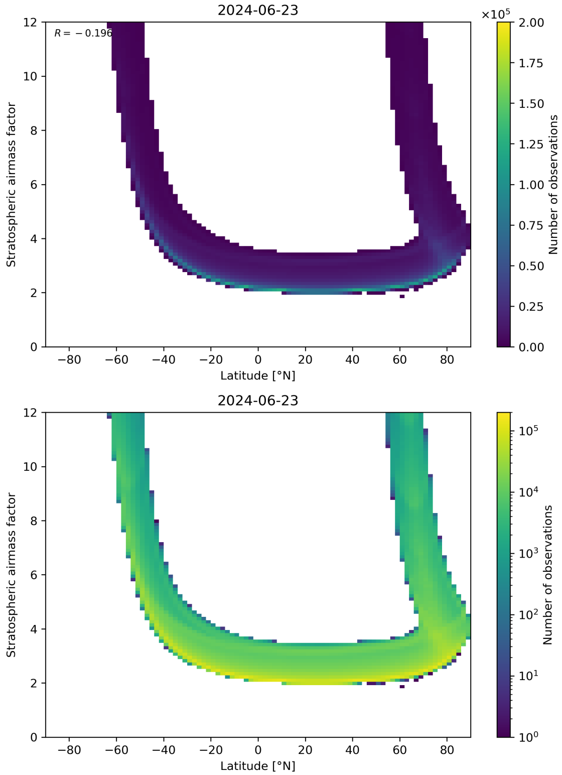
Figure 83: Scatter density plot of “Latitude” against “Stratospheric air mass factor” for 2024-06-22 to 2024-06-24.
