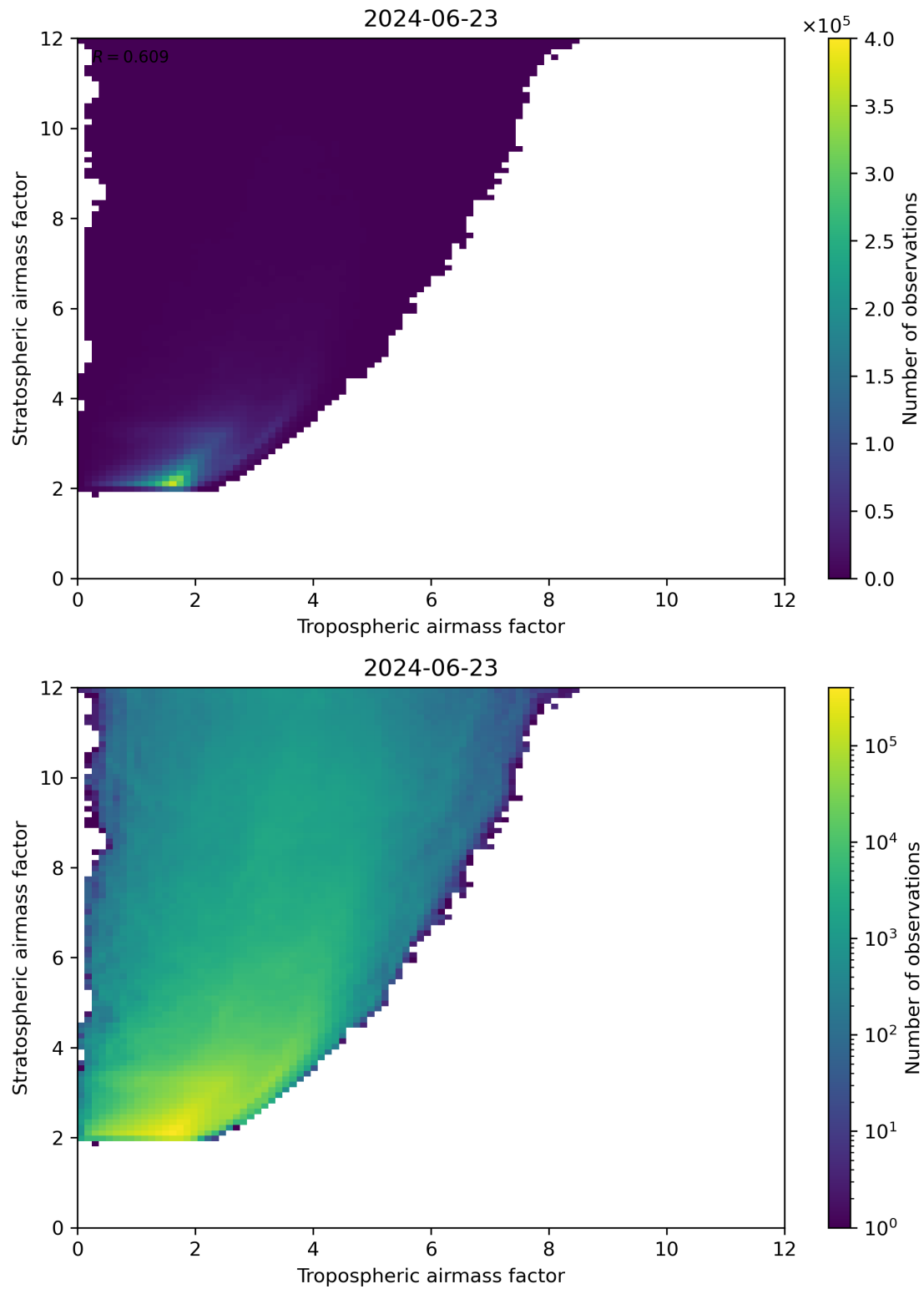
Figure 71: Scatter density plot of “Tropospheric airmass factor” against “Stratospheric airmass factor” for 2024-06-22 to 2024-06-24.
