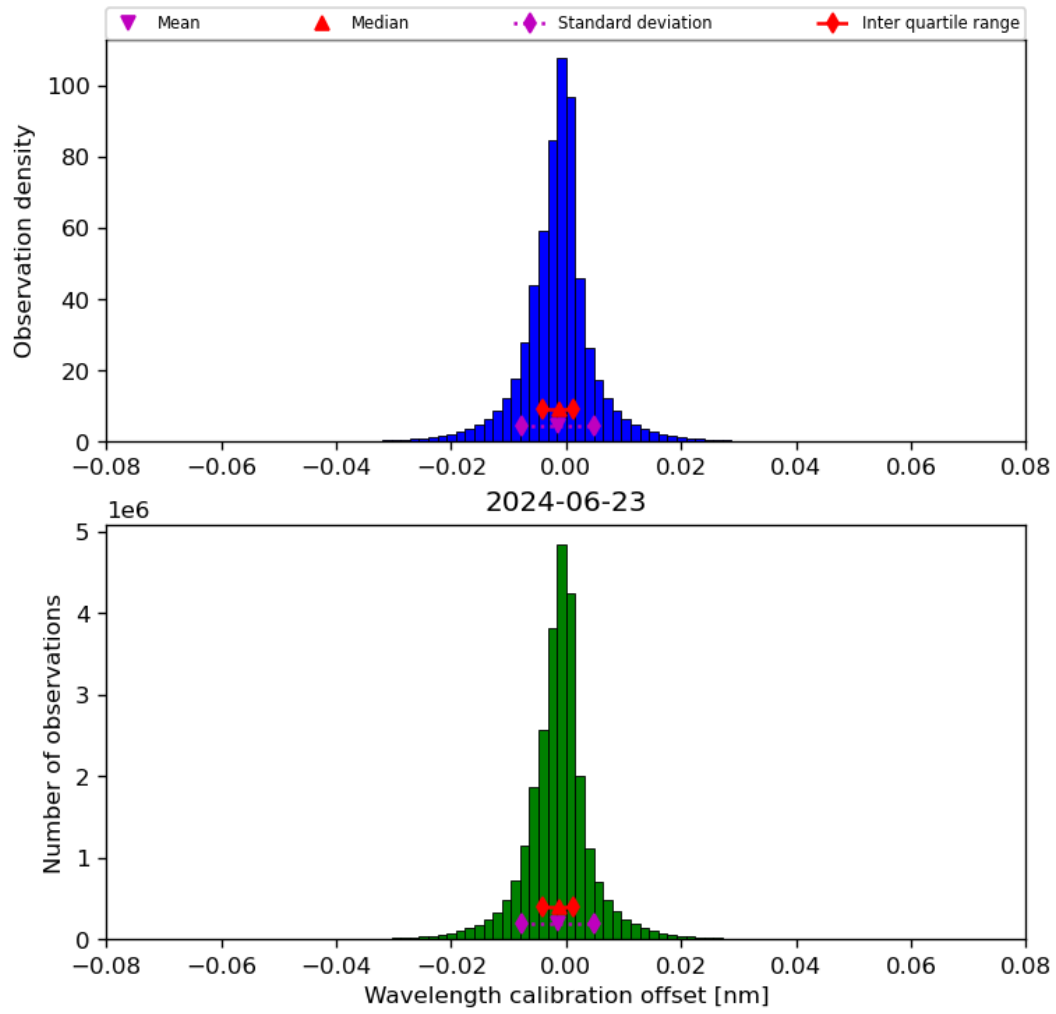
Figure 35: Histogram of “Wavelength calibration offset” for 2024-06-22 to 2024-06-24
