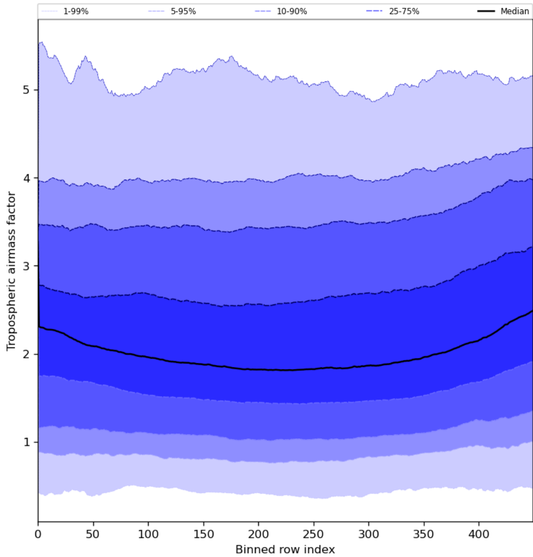
Figure 48: Along track statistics of “Tropospheric airmass factor” for 2024-06-22 to 2024-06-24
