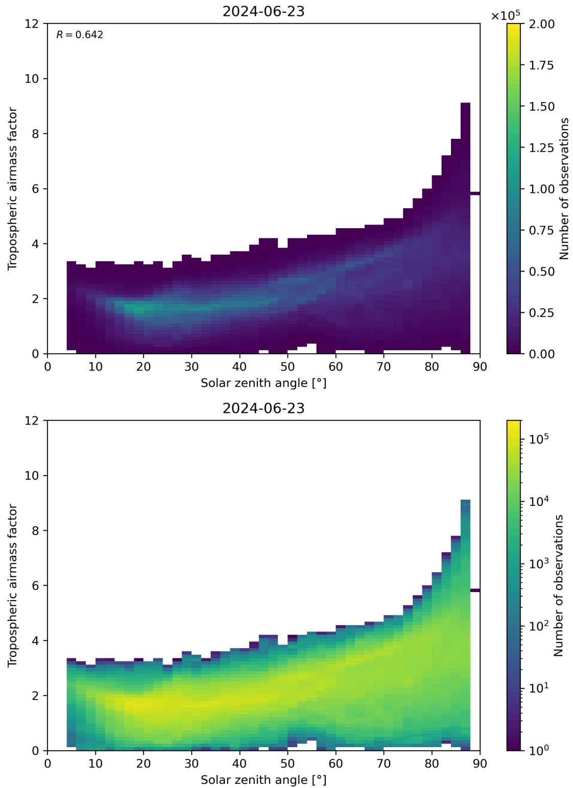
Figure 147: Scatter density plot of “Solar zenith angle” against “Tropospheric airmass factor” for 2024-06-22 to 2024-06-24.
