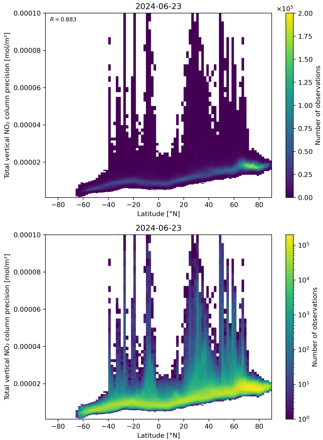
Figure 91: Scatter density plot of “Latitude” against “Total vertical NO 2 column precision” for 2024-06-22 to 2024-06-24.
