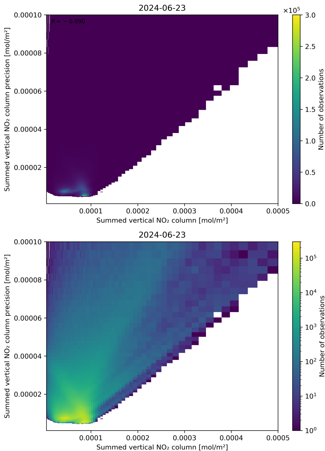
Figure 105: Scatter density plot of “Summed vertical NO 2 column” against “Summed vertical NO 2 column precision” for 2024-06-22 to 2024-06-24.
