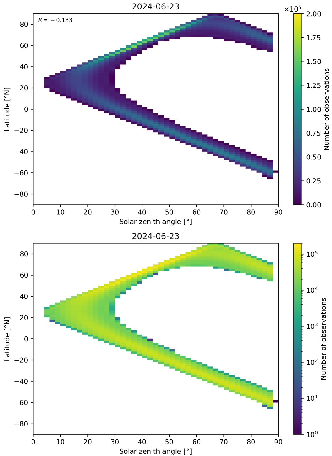
Figure 149: Scatter density plot of “Solar zenith angle” against “Latitude” for 2024-06-22 to 2024-06-24.
