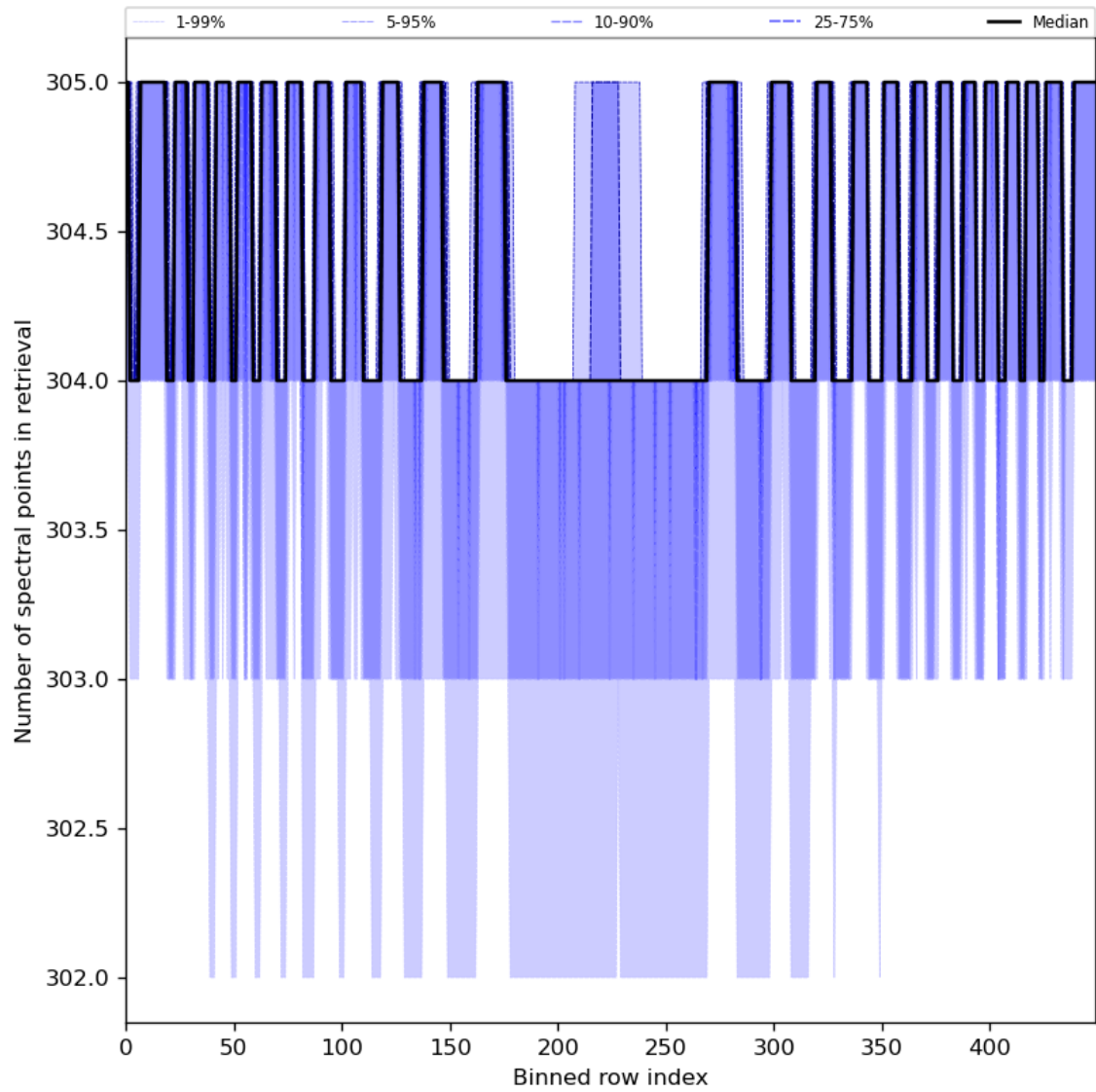
Figure 50: Along track statistics of “Number of spectral points in retrieval” for 2024-06-22 to 2024-06-24
