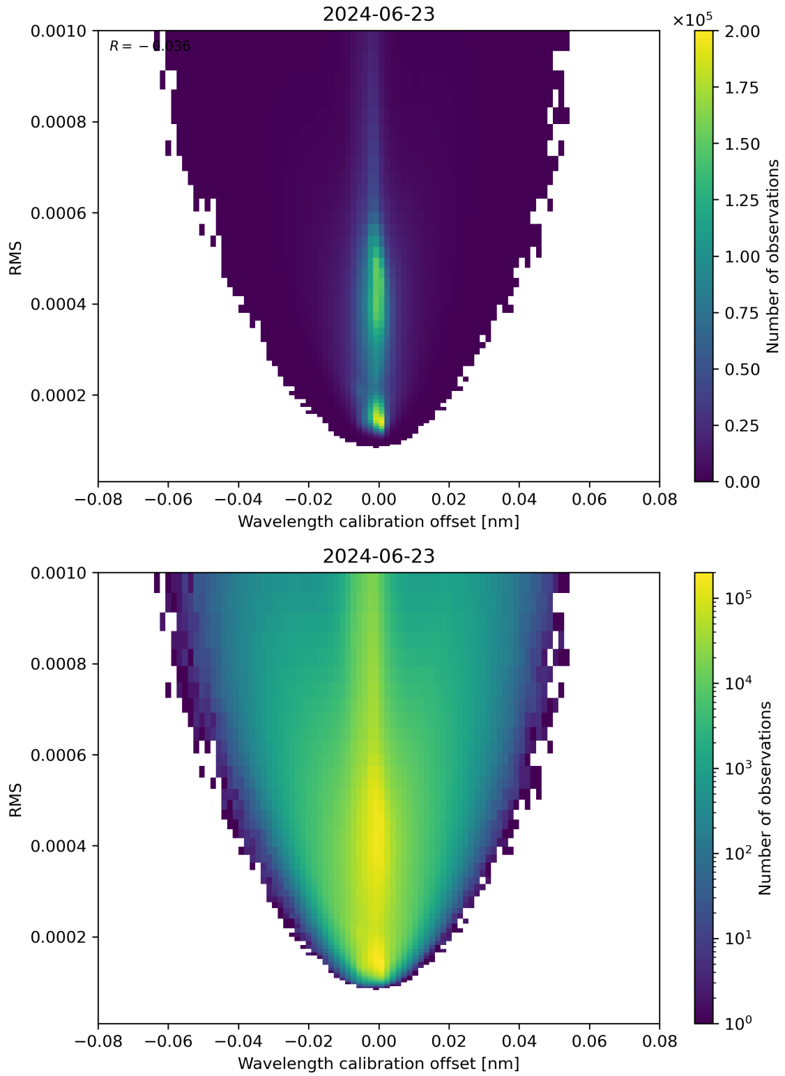
Figure 181: Scatter density plot of “Wavelength calibration offset” against “RMS” for 2024-06-22 to 2024-06-24.
