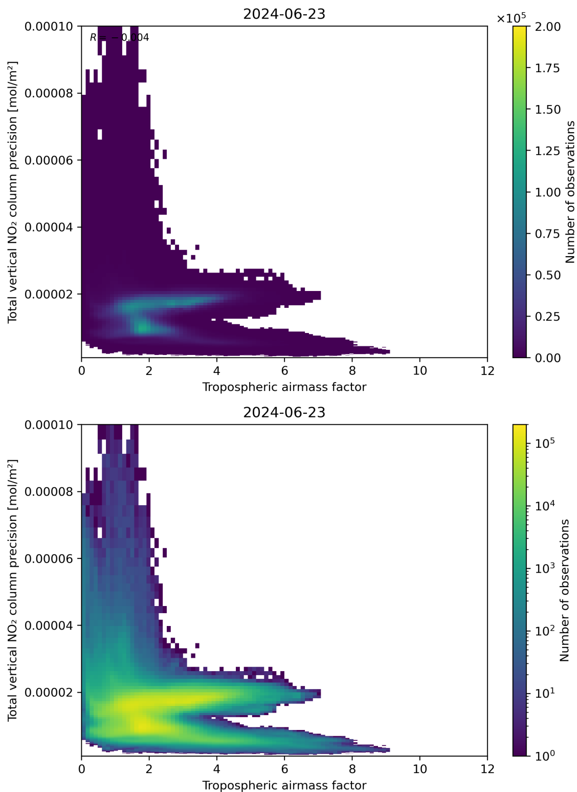
Figure 78: Scatter density plot of “Tropospheric air mass factor” against “Total vertical NO 2 column precision” for 2024-06-22 to 2024-06-24.
