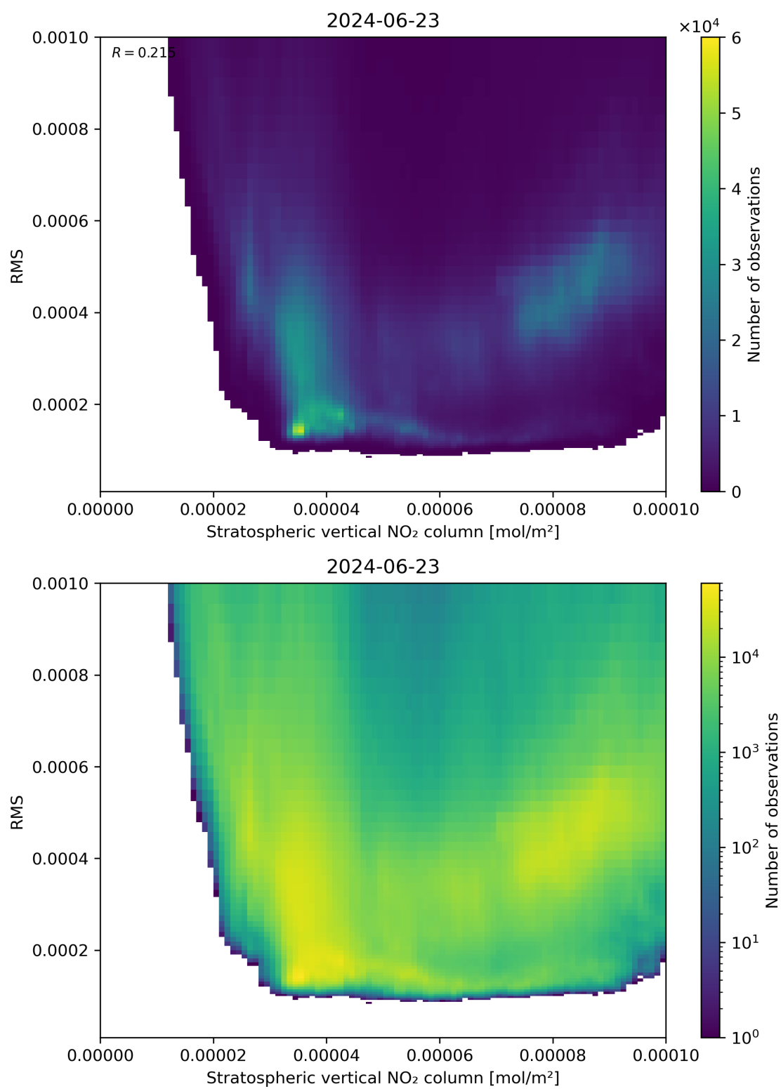
Figure 102: Scatter density plot of “Stratospheric vertical NO 2 column” against “RMS” for 2024-06-22 to 2024-06-24.
