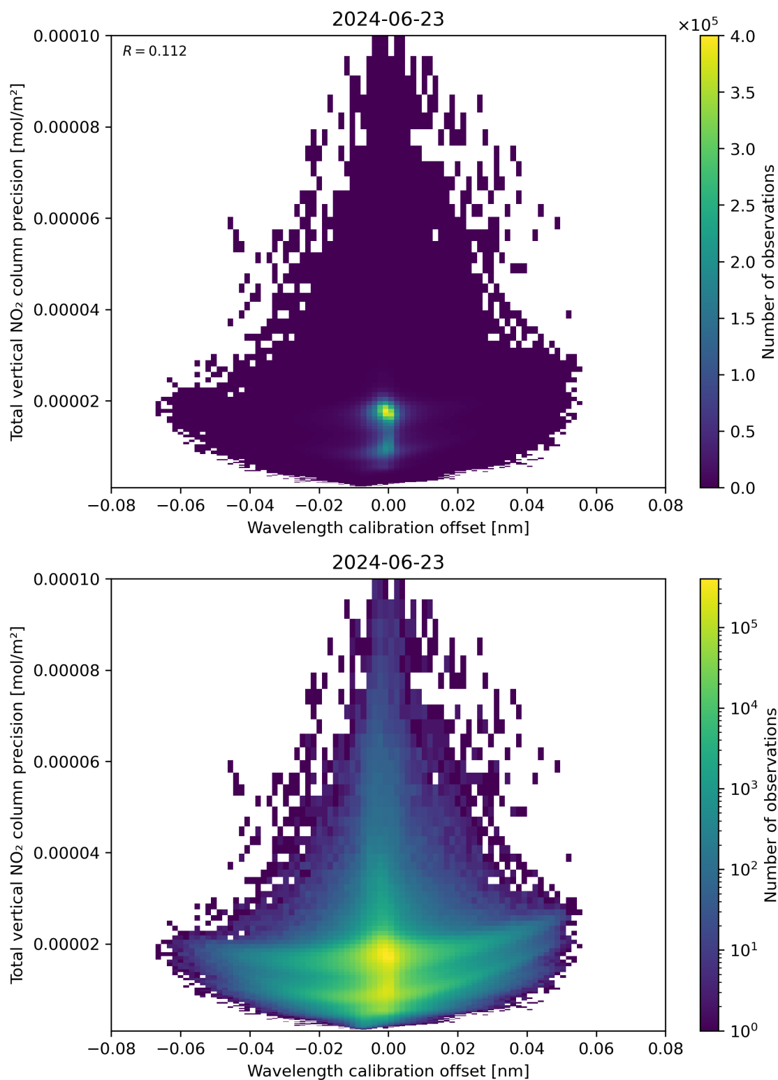
Figure 180: Scatter density plot of “Wavelength calibration offset” against “Total vertical NO 2 column precision” for 2024-06-22 to 2024-06-24.
