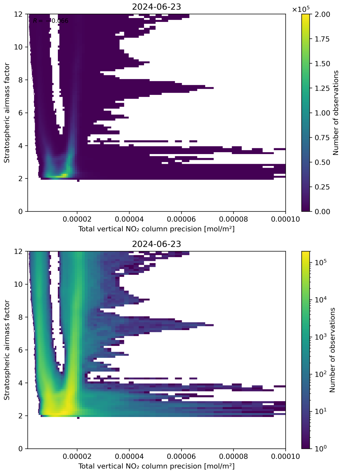
Figure 115: Scatter density plot of “Total vertical NO 2 column precision” against “Stratospheric air mass factor” for 2024-06-22 to 2024-06-24.
