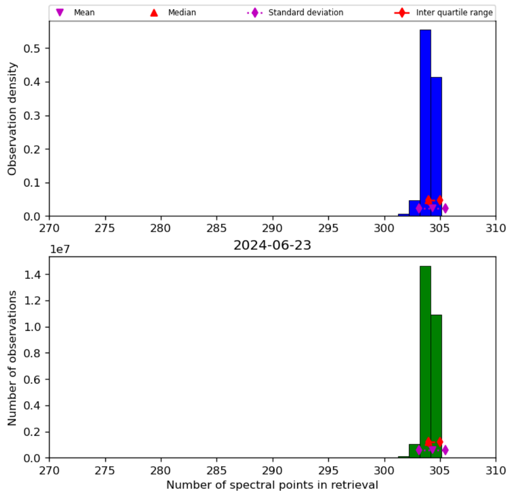
Figure 33: Histogram of “Number of spectral points in retrieval” for 2024-06-22 to 2024-06-24
