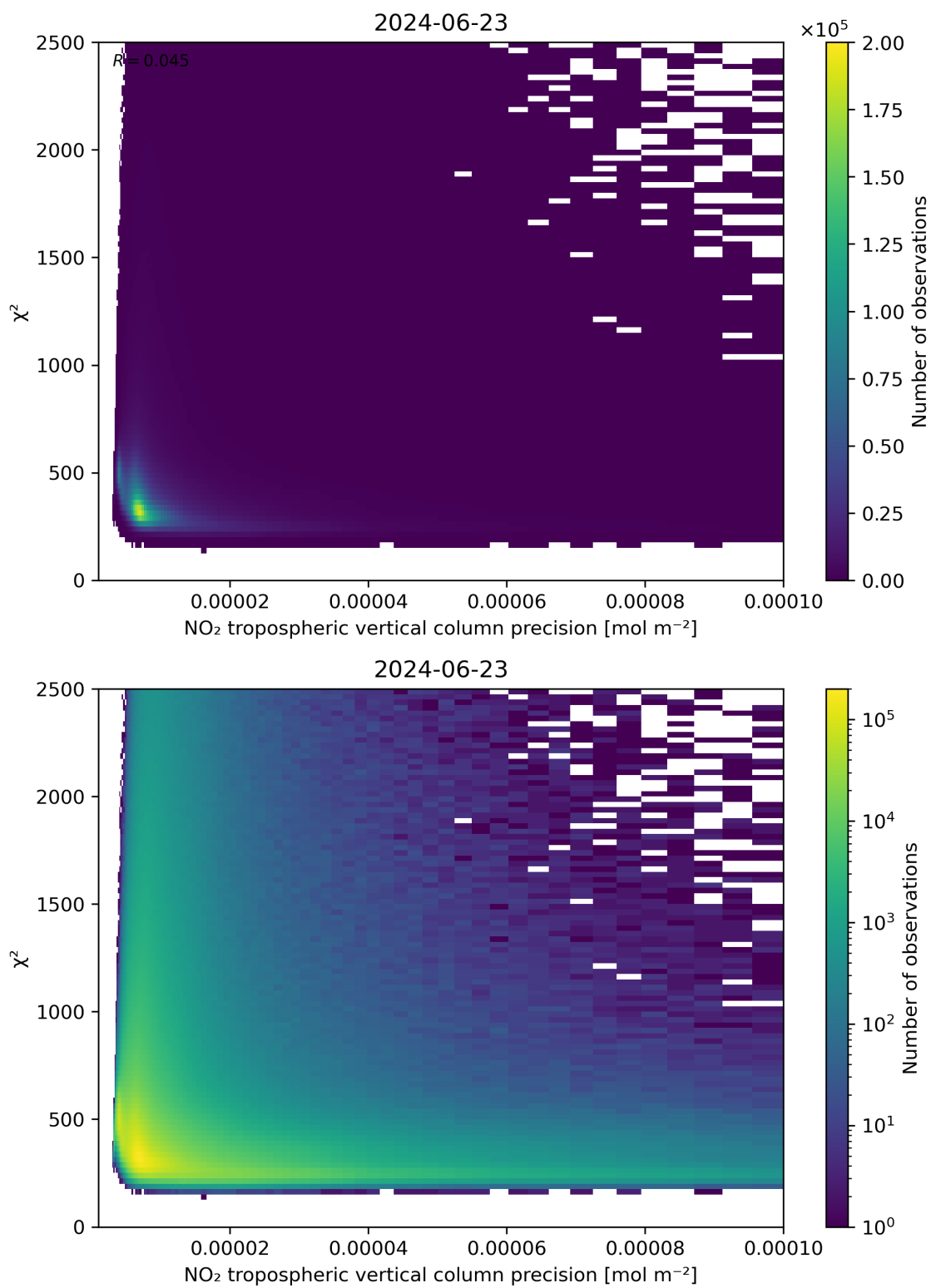
Figure 134: Scatter density plot of “NO 2 tropospheric vertical column precision” against “ \chi^2 ” for 2024-06-22 to 2024-06-24.
