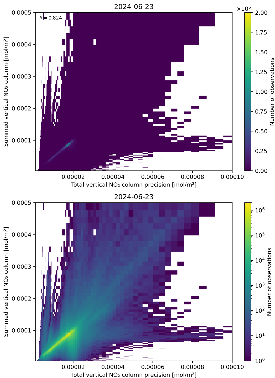
Figure 117: Scatter density plot of “Total vertical NO 2 column precision” against “Summed vertical NO 2 column” for 2024-06-22 to 2024-06-24.
