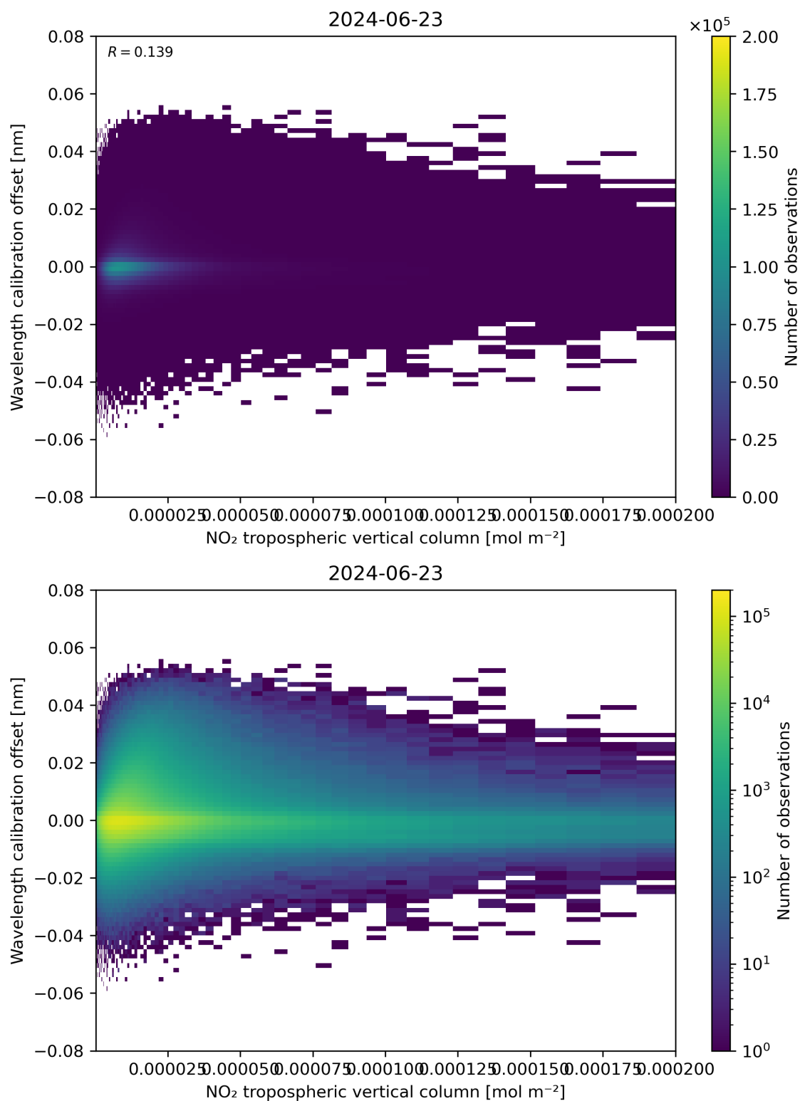
Figure 143: Scatter density plot of “NO 2 tropospheric vertical column” against “Wavelength calibration offset” for 2024-06-22 to 2024-06-24.
