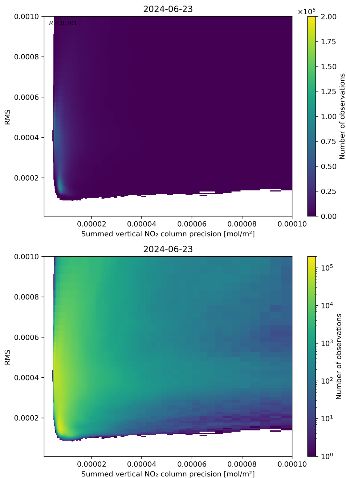
Figure 108: Scatter density plot of “Summed vertical NO 2 column precision” against “RMS” for 2024-06-22 to 2024-06-24.
