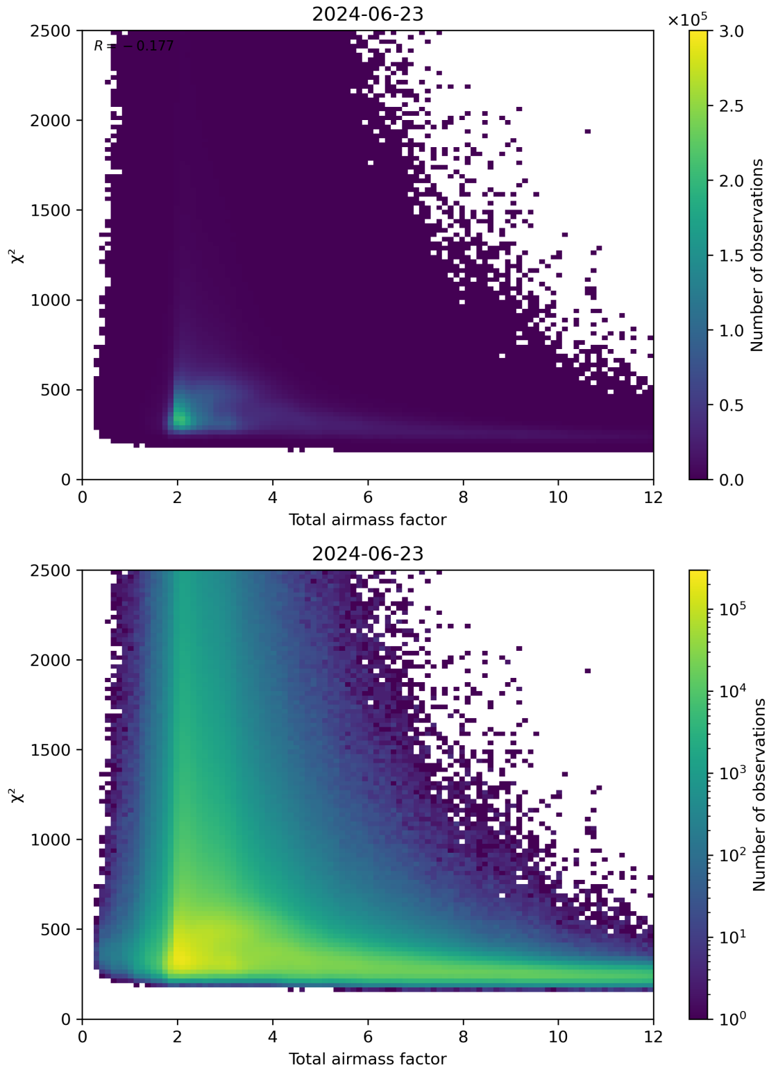
Figure 63: Scatter density plot of “Total airmass factor” against “ \chi^2 ” for 2024-06-22 to 2024-06-24.
