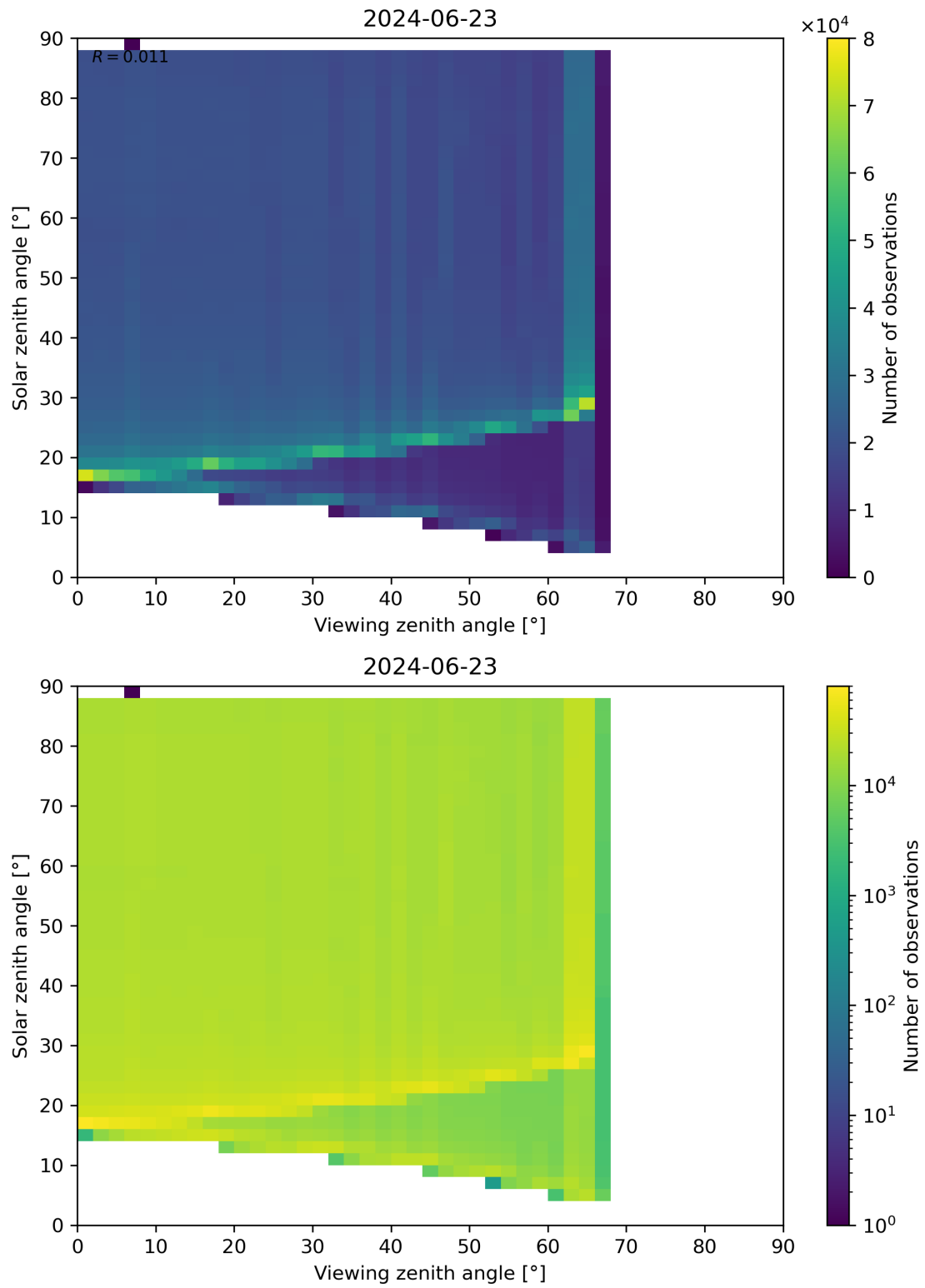
Figure 172: Scatter density plot of “Viewing zenith angle” against “Solar zenith angle” for 2024-06-22 to 2024-06-24.
