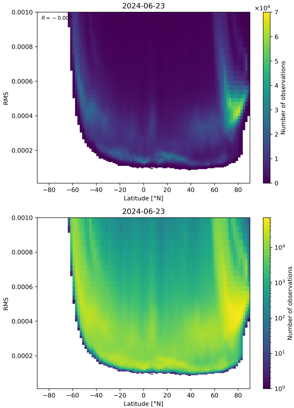
Figure 94: Scatter density plot of “Latitude” against “RMS” for 2024-06-22 to 2024-06-24.
