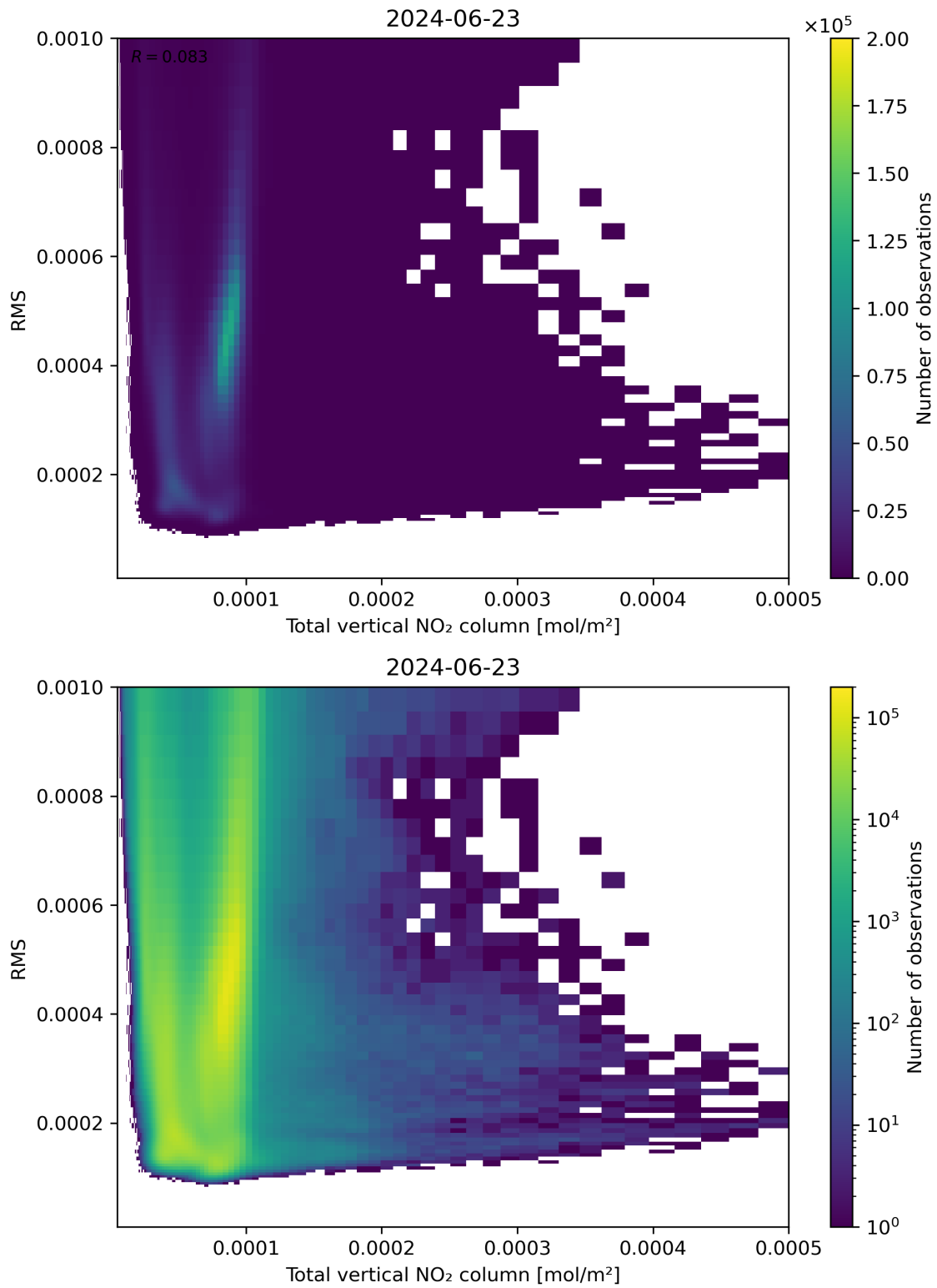
Figure 120: Scatter density plot of “Total vertical NO 2 column” against “RMS” for 2024-06-22 to 2024-06-24.
