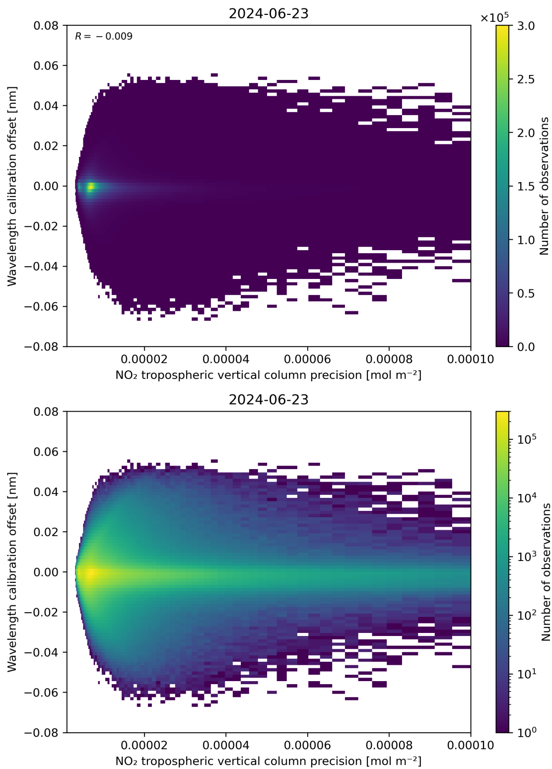
Figure 141: Scatter density plot of “NO 2 tropospheric vertical column precision” against “Wavelength calibration offset” for 2024-06-22 to 2024-06-24.
