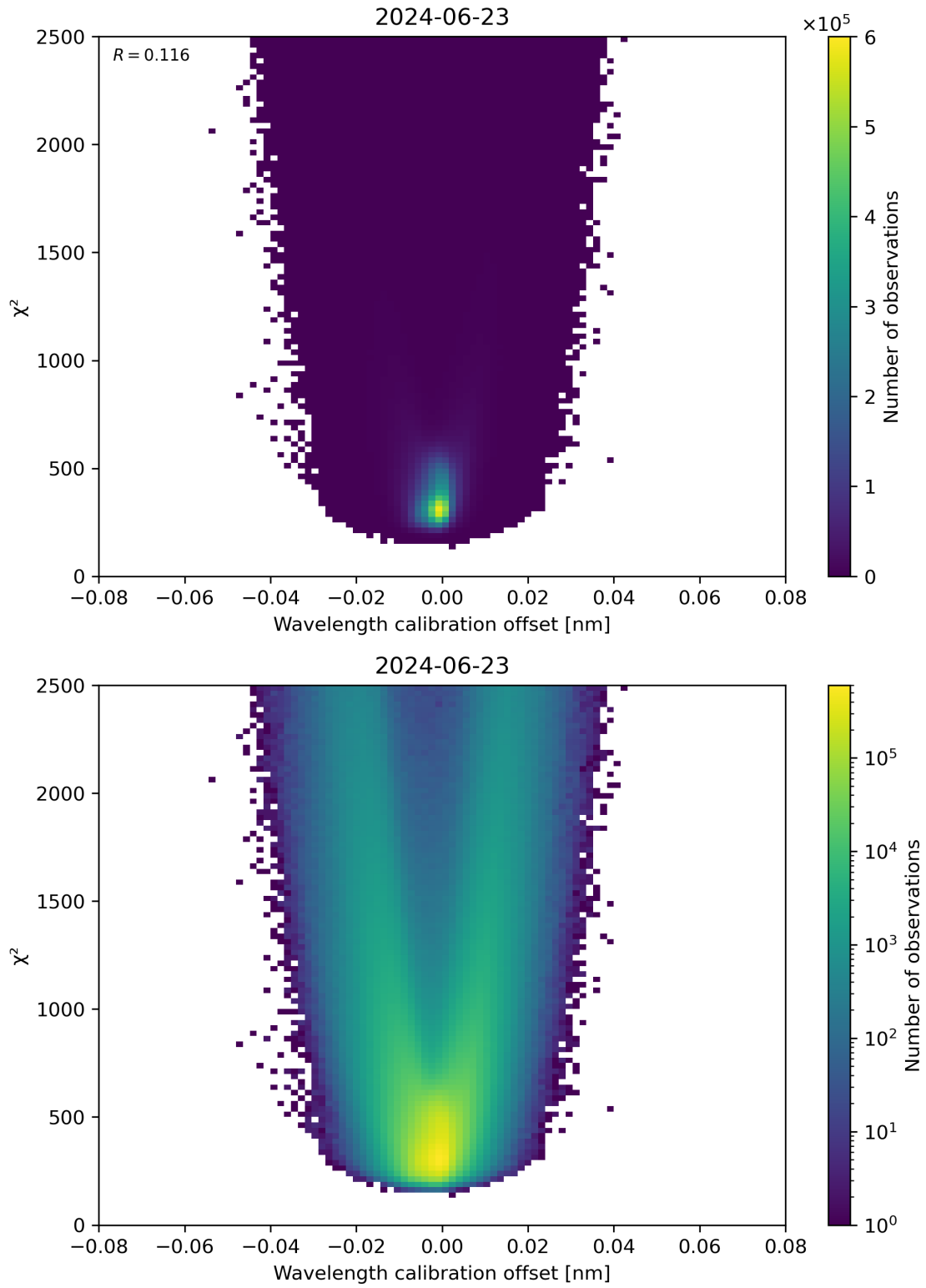
Figure 175: Scatter density plot of “Wavelength calibration offset” against “ \chi^2 ” for 2024-06-22 to 2024-06-24.
