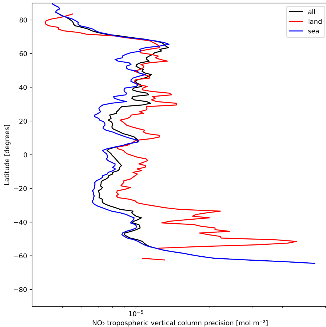
Figure 13: Zonal average of “NO 2 tropospheric vertical column precision” for 2024-06-22 to 2024-06-24.
