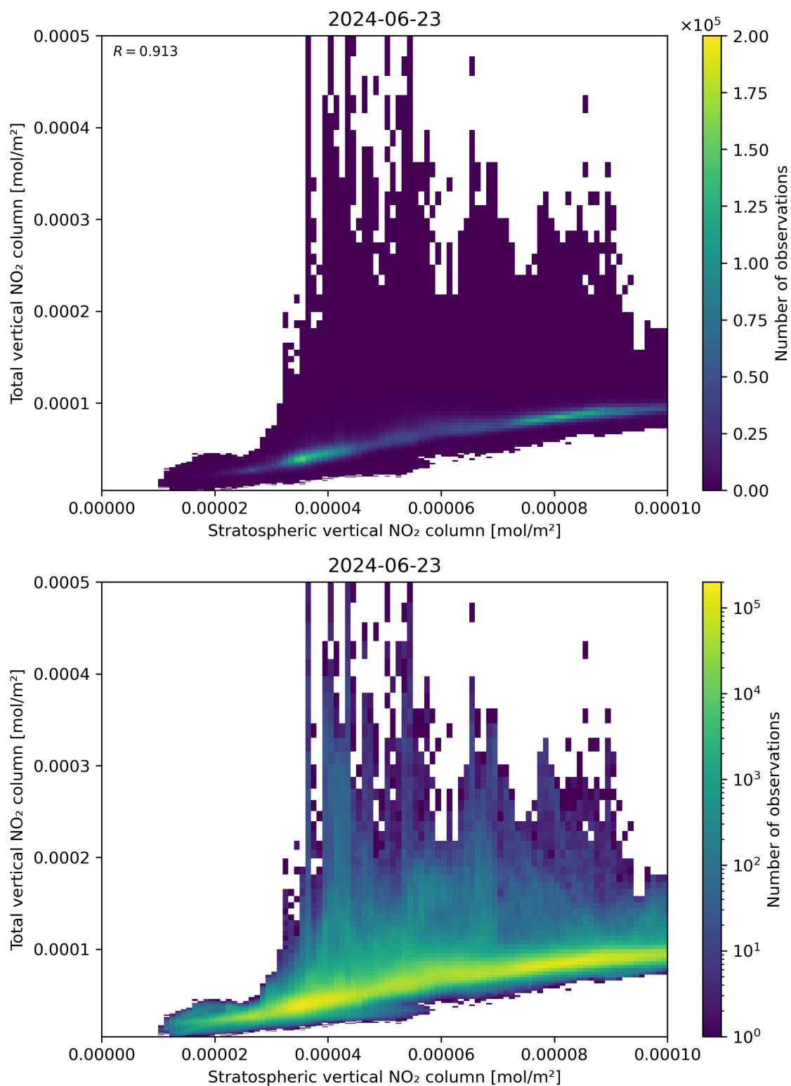
Figure 100: Scatter density plot of “Stratospheric vertical NO 2 column” against “Total vertical NO 2 column” for 2024-06-22 to 2024-06-24.
