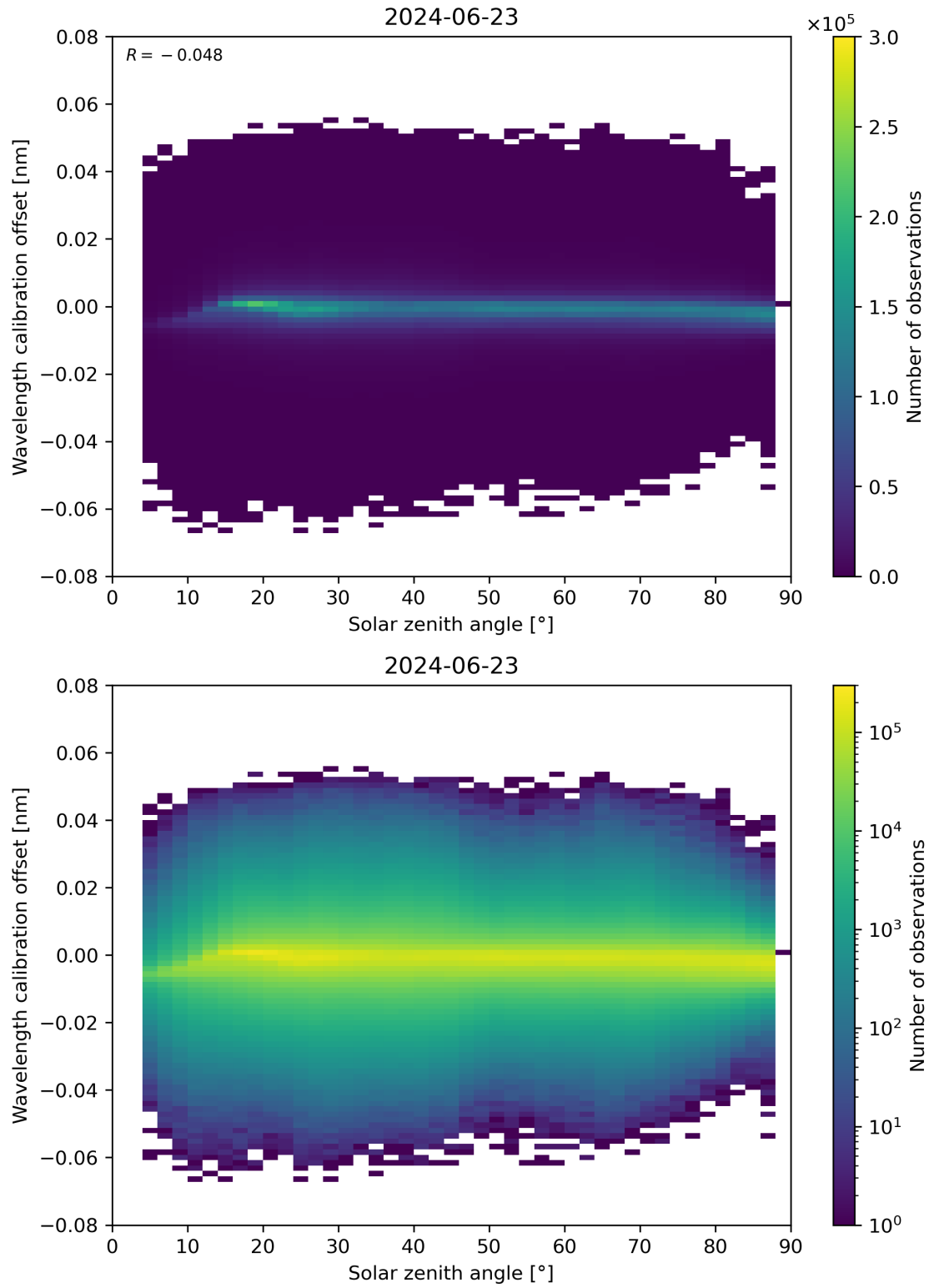
Figure 158: Scatter density plot of “Solar zenith angle” against “Wavelength calibration offset” for 2024-06-22 to 2024-06-24.
