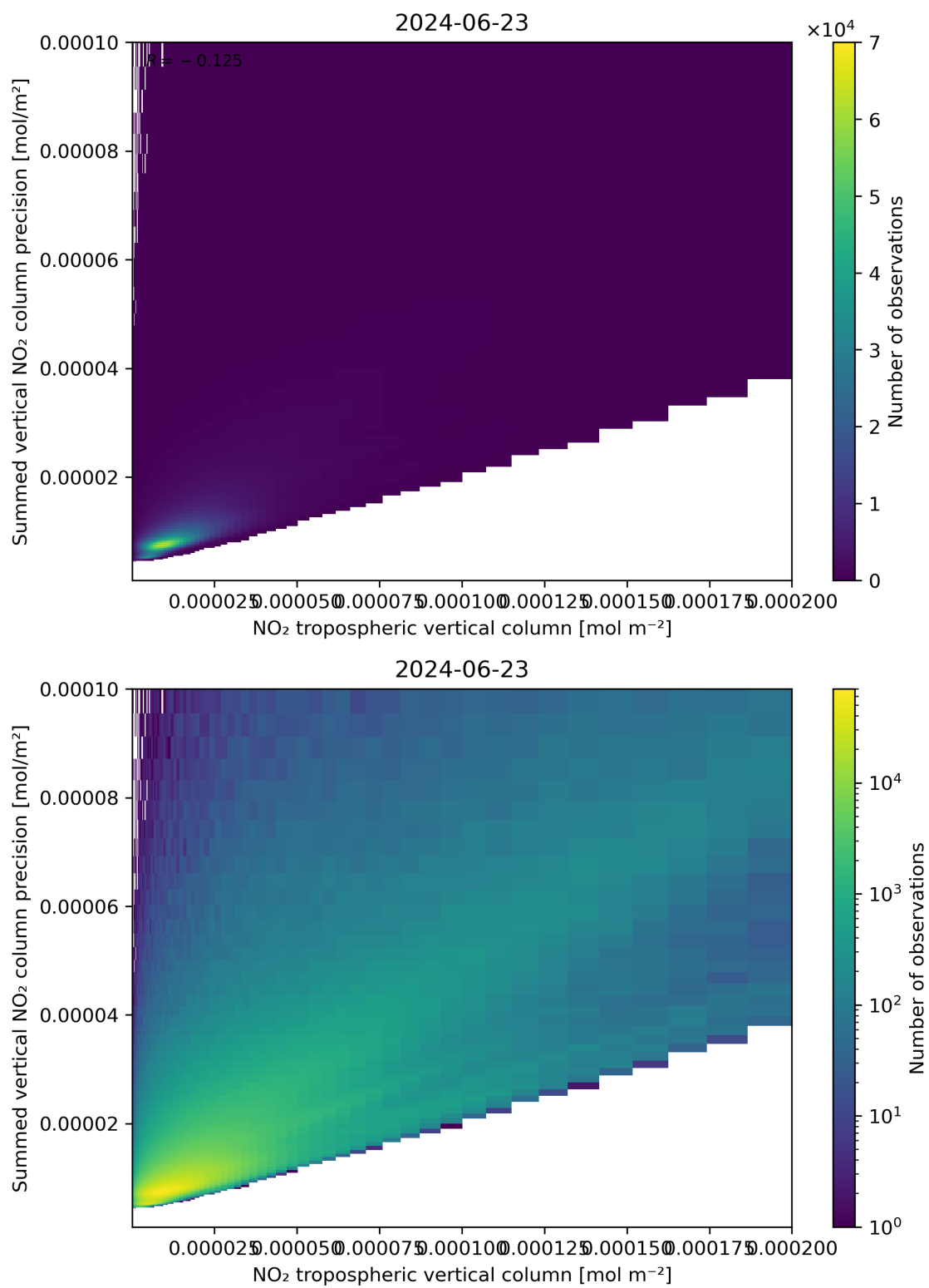
Figure 127: Scatter density plot of “NO 2 tropospheric vertical column” against “Summed vertical NO 2 column precision” for 2024-06-22 to 2024-06-24.
