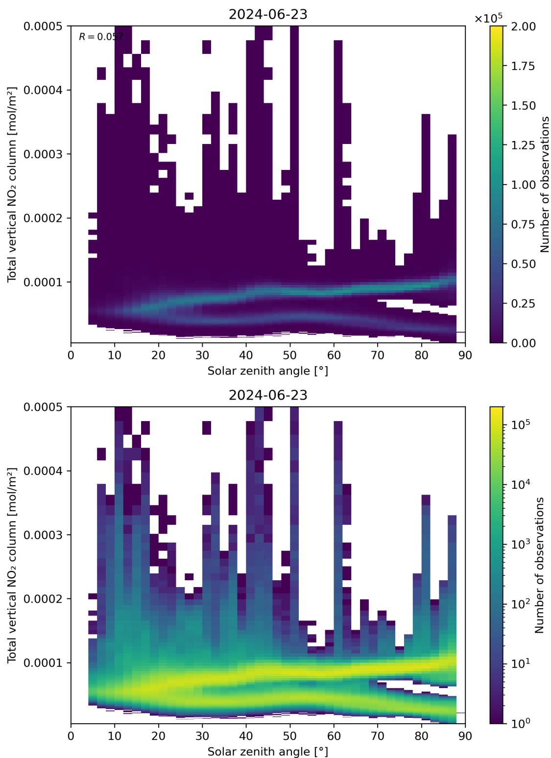
Figure 153: Scatter density plot of “Solar zenith angle” against “Total vertical NO 2 column” for 2024-06-22 to 2024-06-24.
