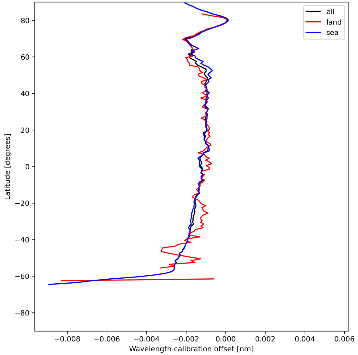
Figure 18: Zonal average of “Wavelength calibration offset” for 2024-06-22 to 2024-06-24.
