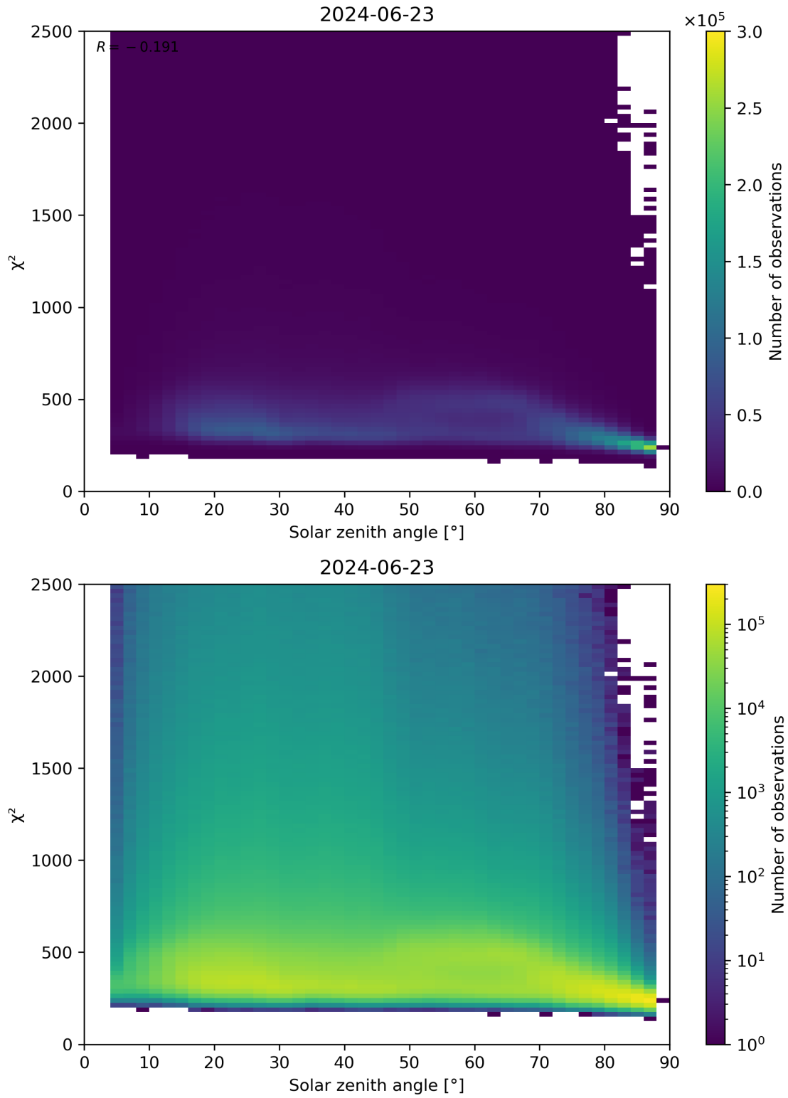
Figure 148: Scatter density plot of “Solar zenith angle” against “ \chi^2 ” for 2024-06-22 to 2024-06-24.
