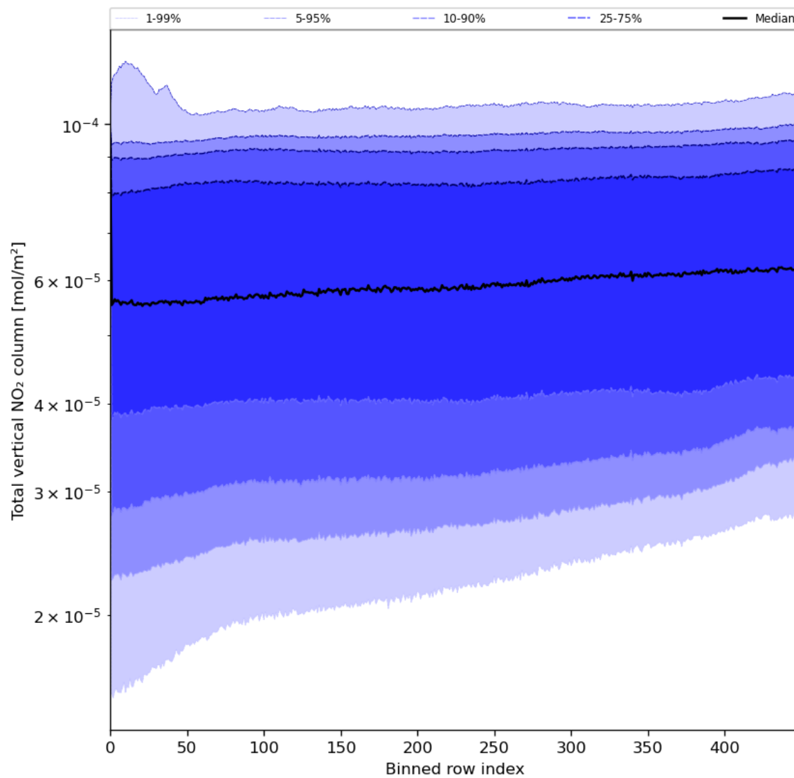
Figure 55: Along track statistics of “Total vertical NO 2 column” for 2024-06-22 to 2024-06-24
