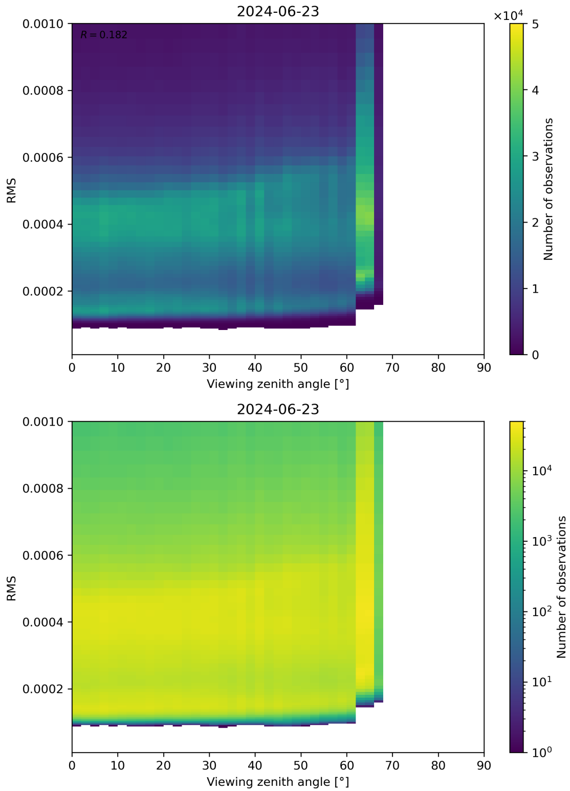
Figure 171: Scatter density plot of “Viewing zenith angle” against “RMS” for 2024-06-22 to 2024-06-24.
