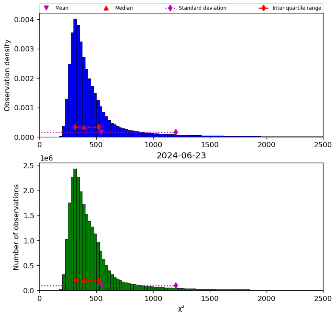
Figure 42: Histogram of “ \chi^2 ” for 2024-06-22 to 2024-06-24
