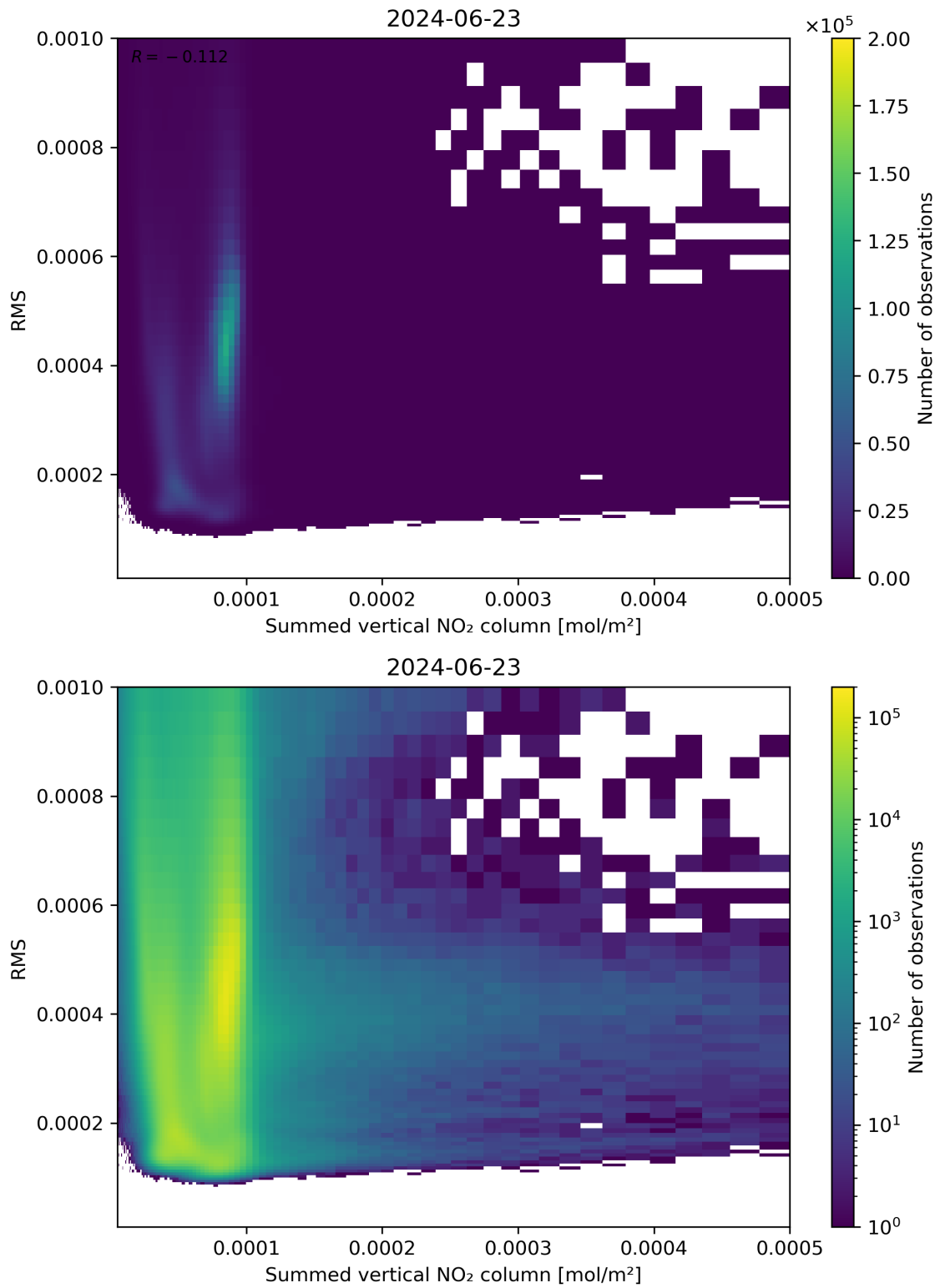
Figure 109: Scatter density plot of “Summed vertical NO 2 column” against “RMS” for 2024-06-22 to 2024-06-24.
