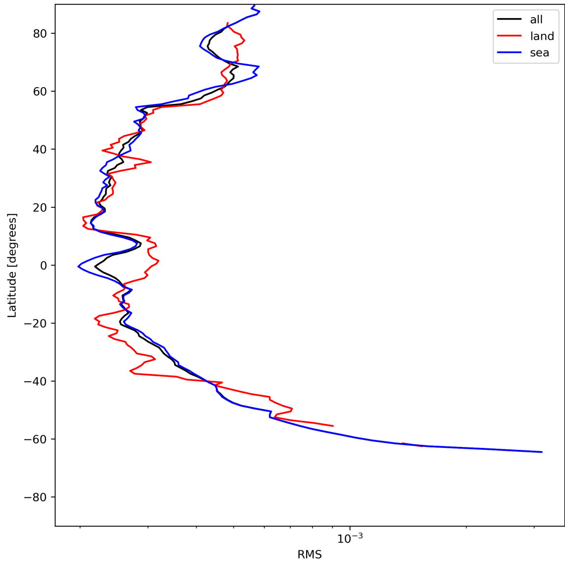
Figure 26: Zonal average of “RMS” for 2024-06-22 to 2024-06-24.
