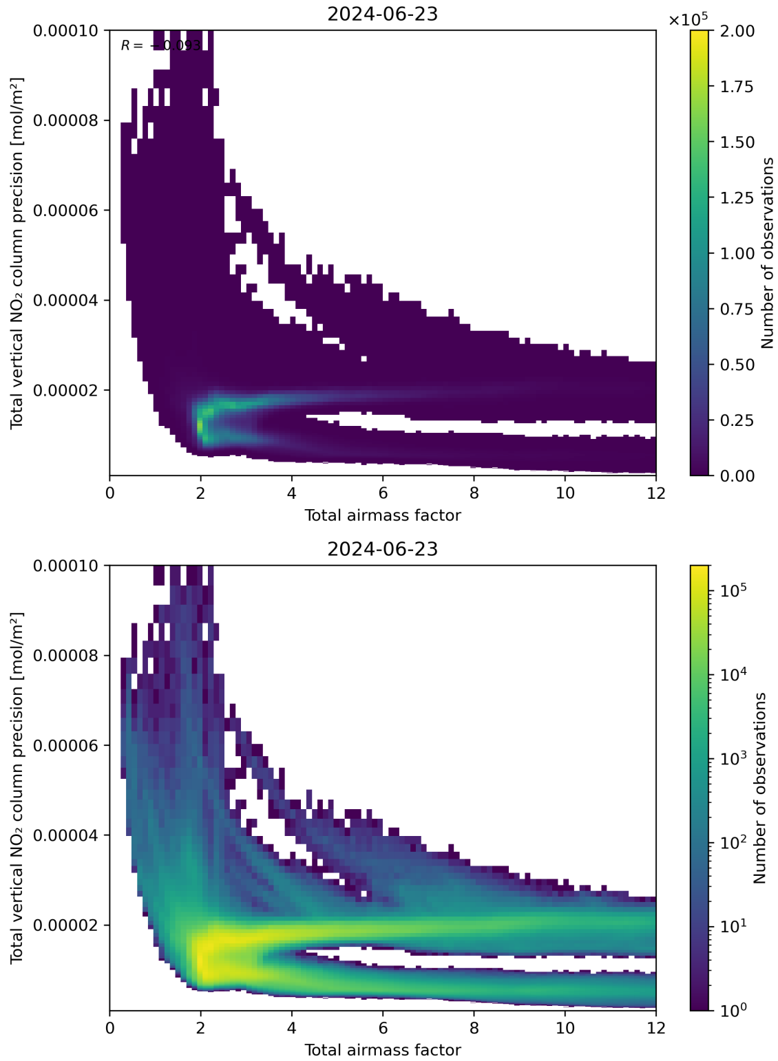
Figure 68: Scatter density plot of “Total airmass factor” against “Total vertical NO 2 column precision” for 2024-06-22 to 2024-06-24.
