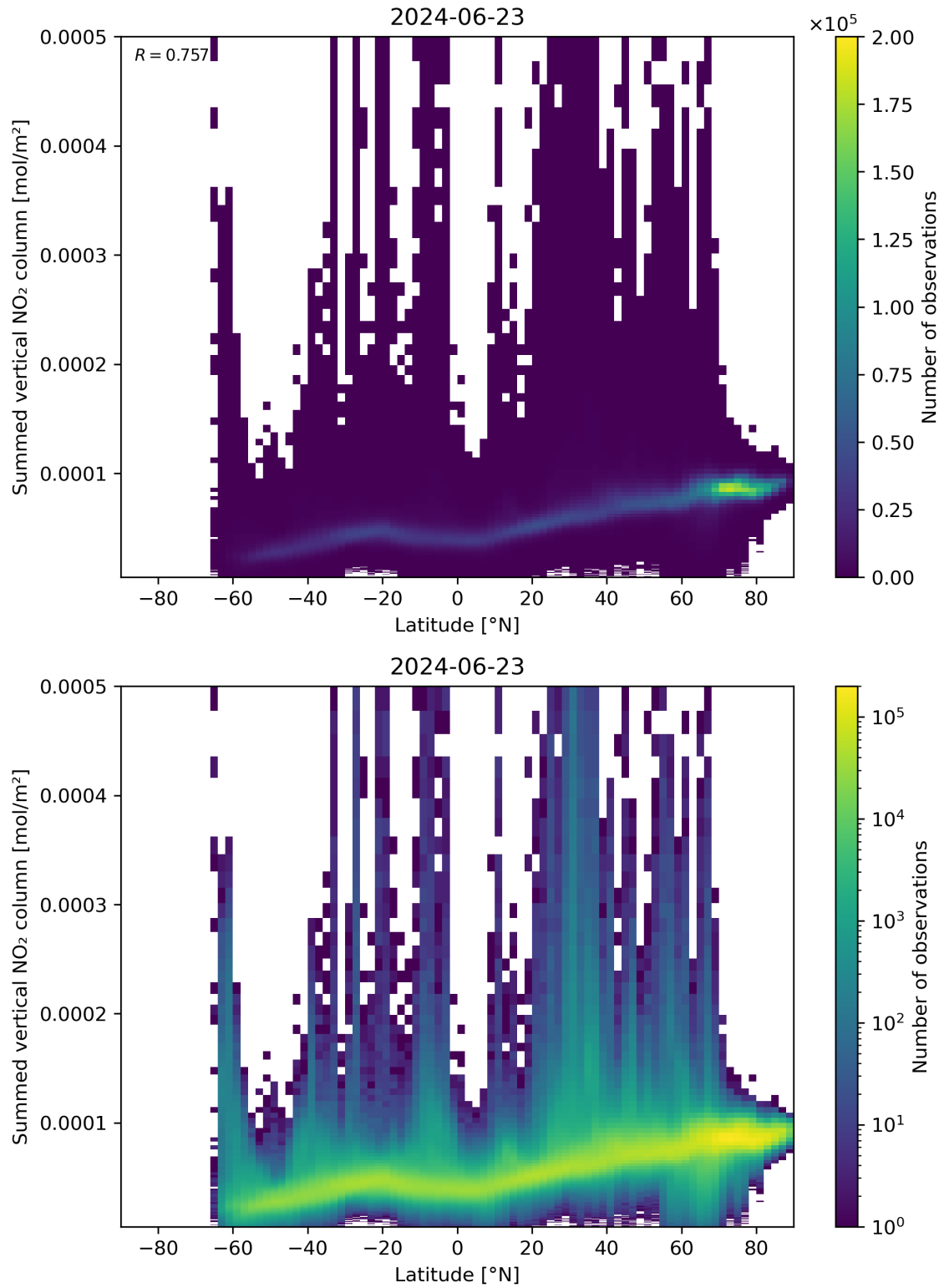
Figure 88: Scatter density plot of “Latitude” against “Summed vertical NO 2 column” for 2024-06-22 to 2024-06-24.
