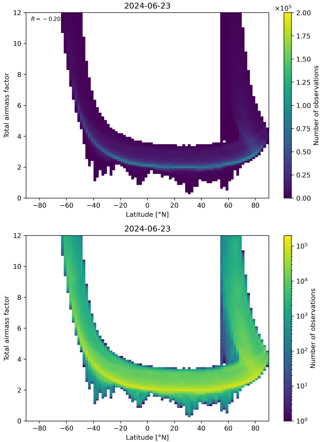
Figure 84: Scatter density plot of “Latitude” against “Total airmass factor” for 2024-06-22 to 2024-06-24.
