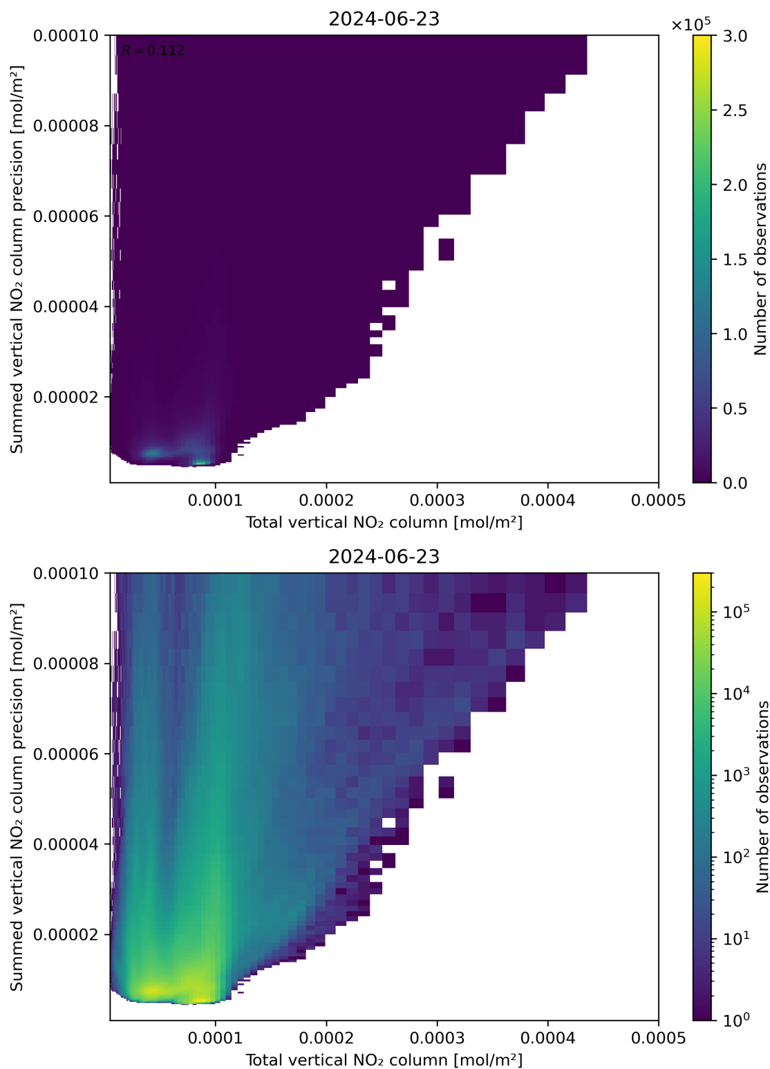
Figure 113: Scatter density plot of “Total vertical NO 2 column” against “Summed vertical NO 2 column precision” for 2024-06-22 to 2024-06-24.
