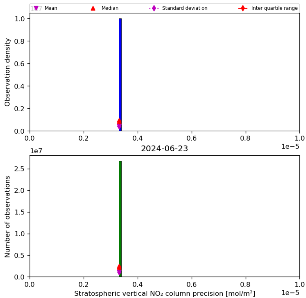
Figure 37: Histogram of “Stratospheric vertical NO 2 column precision” for 2024-06-22 to 2024-06-24
