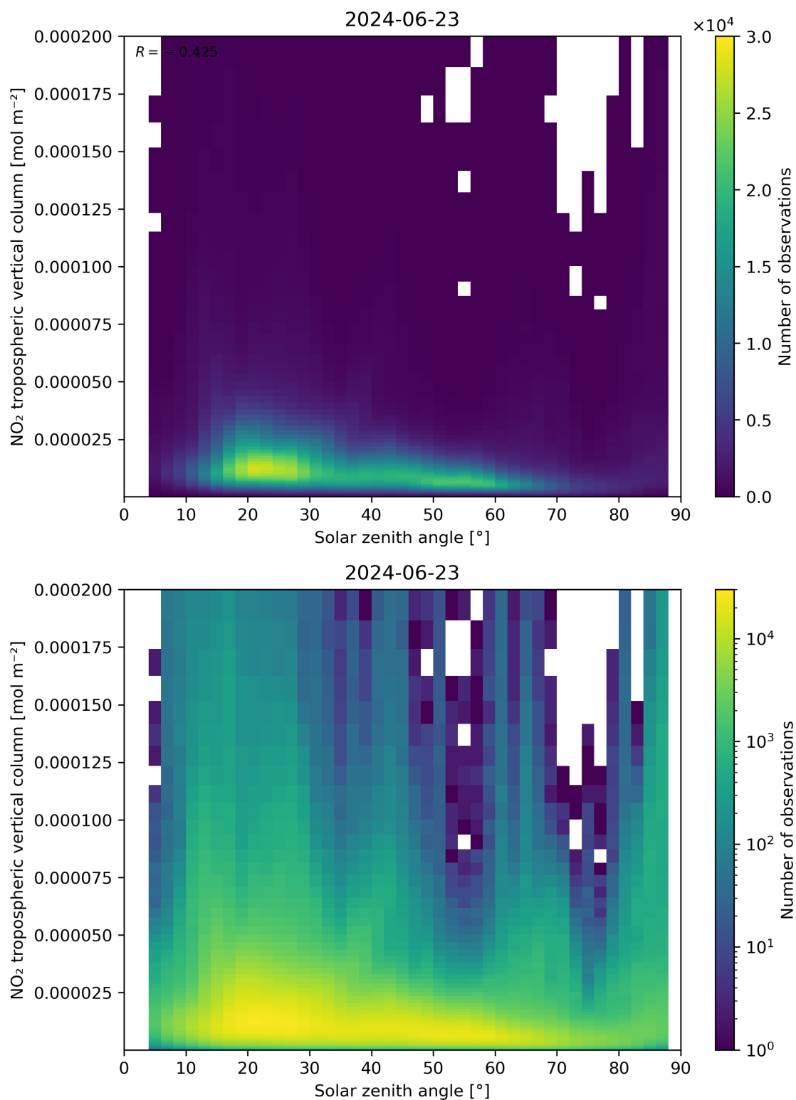
Figure 155: Scatter density plot of “Solar zenith angle” against “NO 2 tropospheric vertical column” for 2024-06-22 to 2024-06-24.
