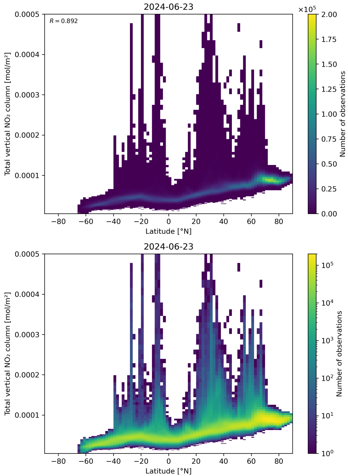
Figure 90: Scatter density plot of “Latitude” against “Total vertical NO 2 column” for 2024-06-22 to 2024-06-24.
