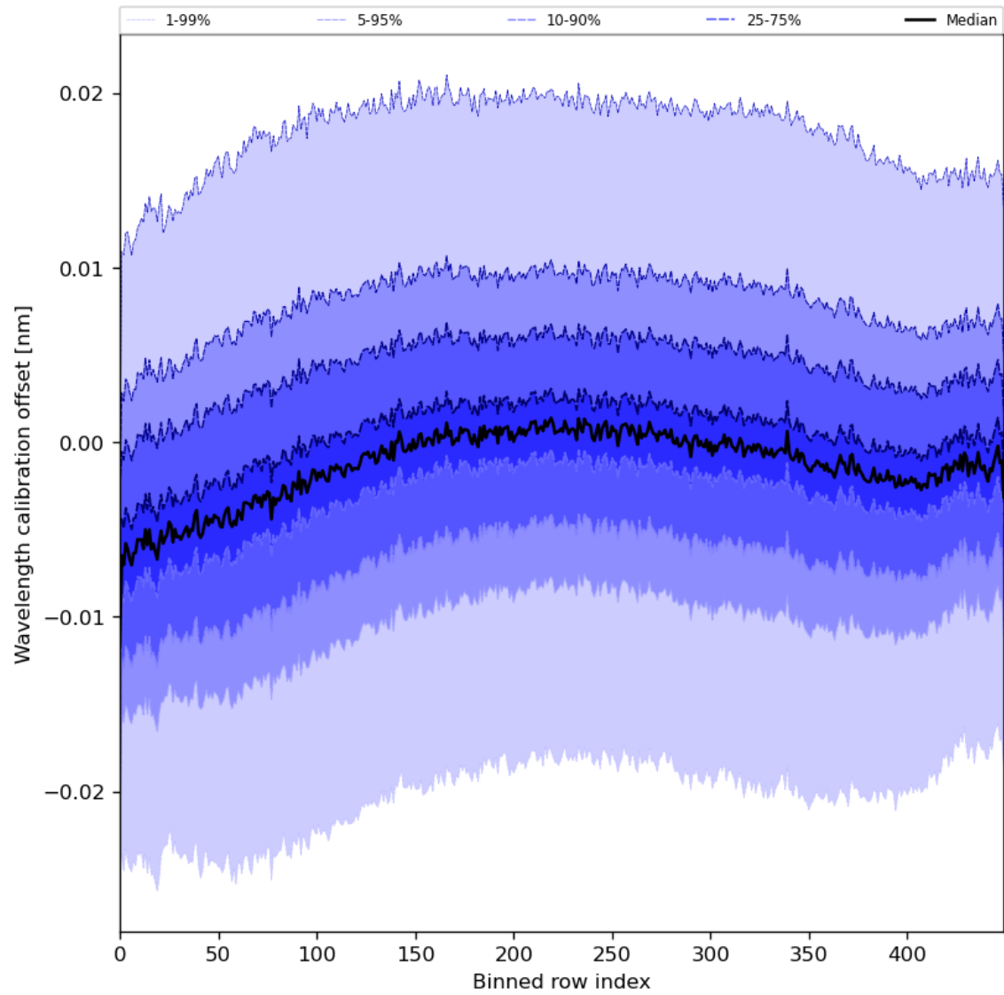
Figure 52: Along track statistics of “Wavelength calibration offset” for 2024-06-22 to 2024-06-24
