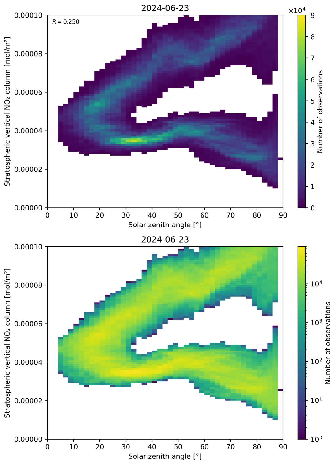
Figure 150: Scatter density plot of “Solar zenith angle” against “Stratospheric vertical NO 2 column” for 2024-06-22 to 2024-06-24.
