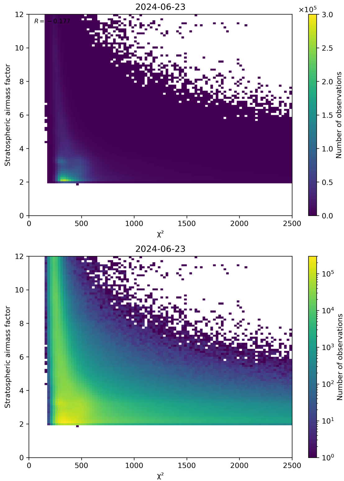
Figure 81: Scatter density plot of “ \chi^2 ” against “Stratospheric airmass factor” for 2024-06-22 to 2024-06-24.
