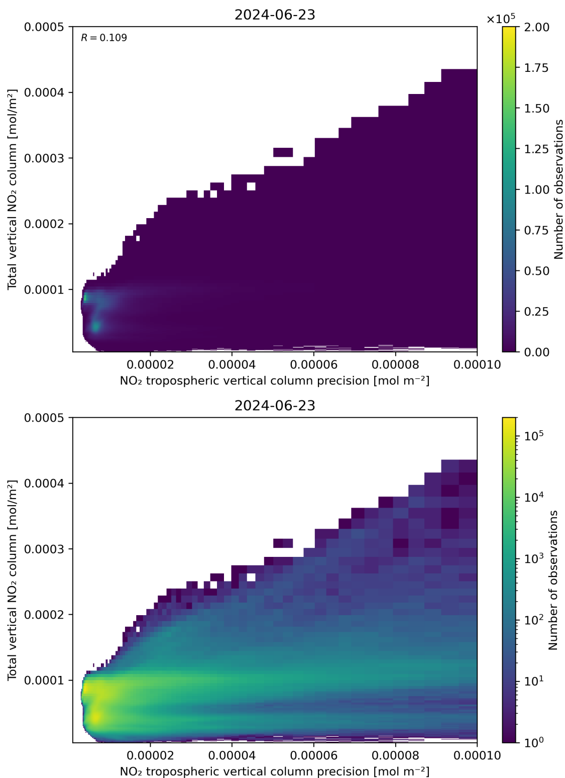
Figure 138: Scatter density plot of “NO 2 tropospheric vertical column precision” against “Total vertical NO 2 column” for 2024-06-22 to 2024-06-24.
