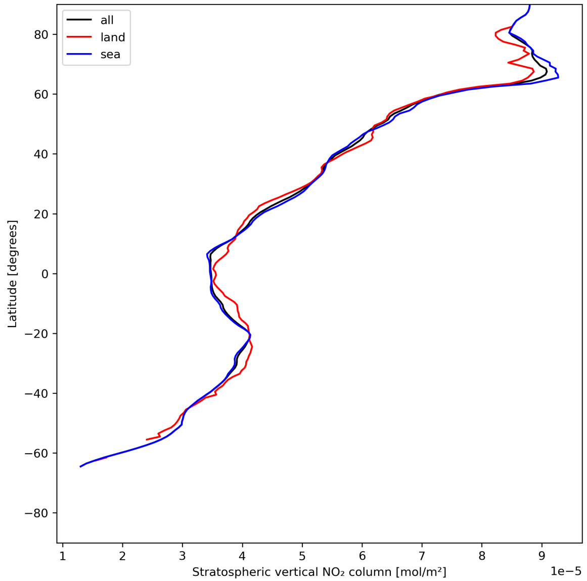
Figure 19: Zonal average of “Stratospheric vertical NO 2 column” for 2024-06-22 to 2024-06-24.
