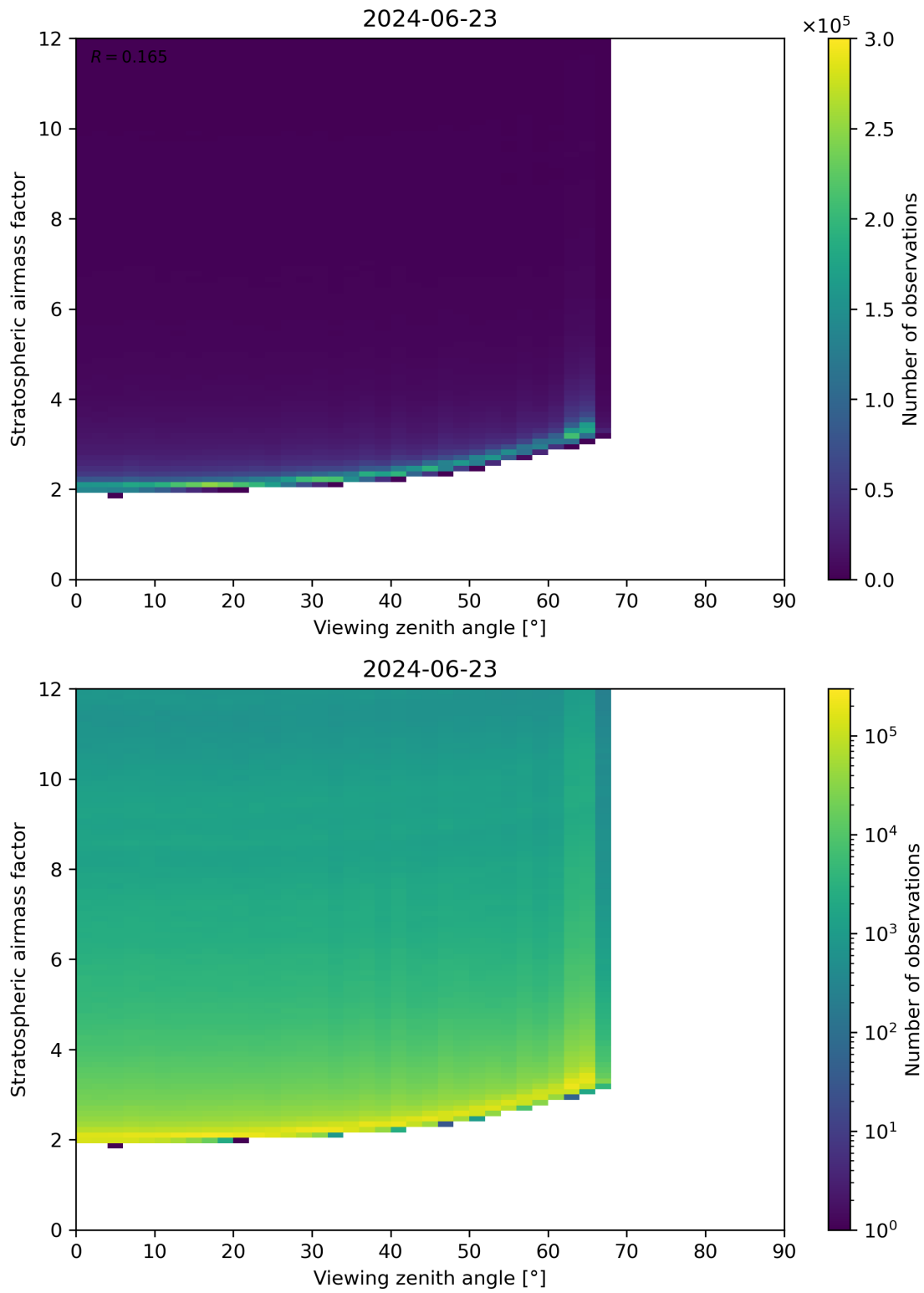
Figure 159: Scatter density plot of “Viewing zenith angle” against “Stratospheric airmass factor” for 2024-06-22 to 2024-06-24.
