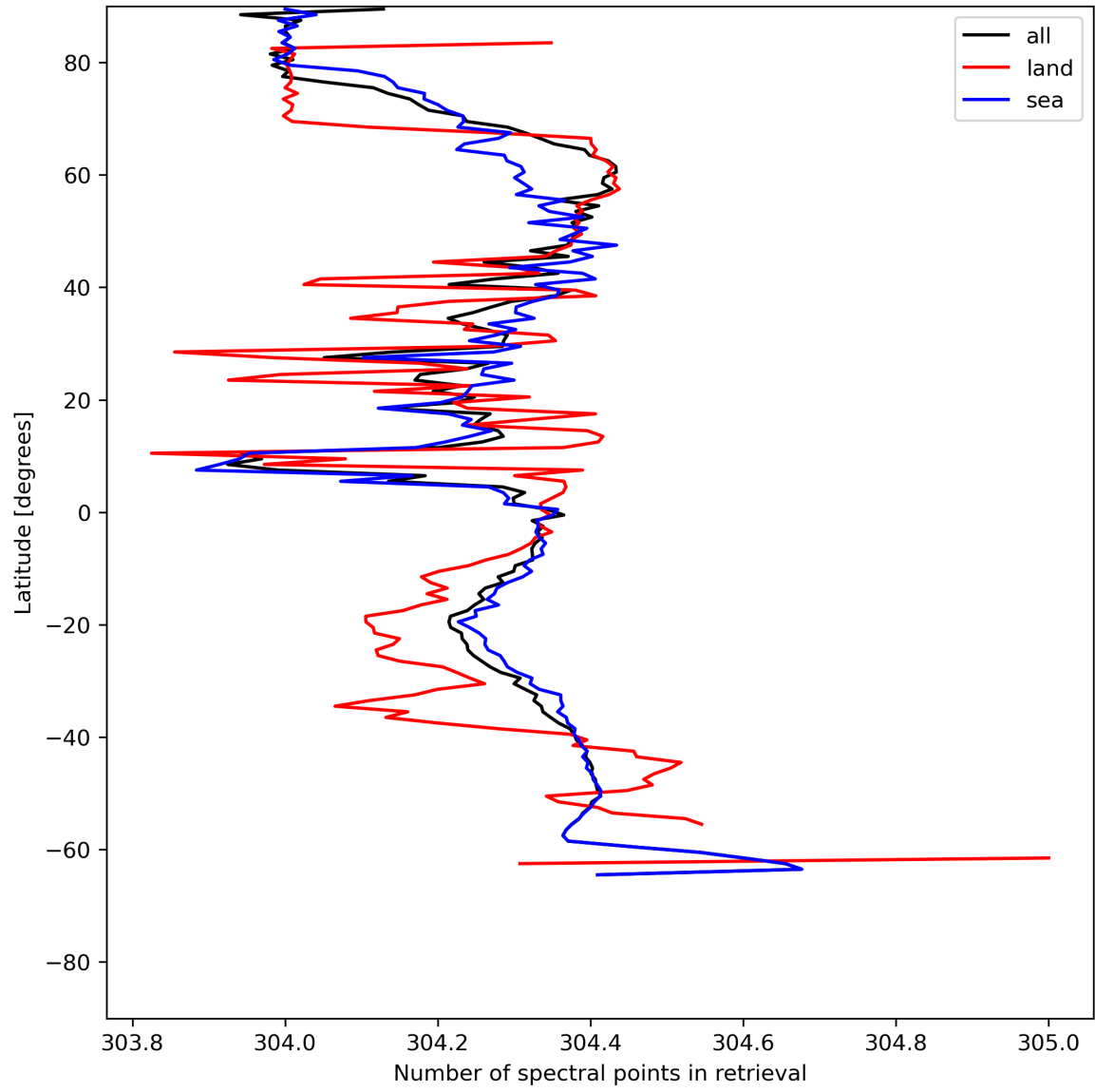
Figure 16: Zonal average of “Number of spectral points in retrieval” for 2024-06-22 to 2024-06-24.
