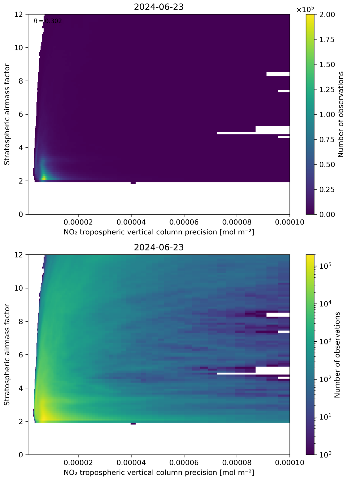
Figure 131: Scatter density plot of “NO 2 tropospheric vertical column precision” against “Stratospheric airmass factor” for 2024-06-22 to 2024-06-24.
