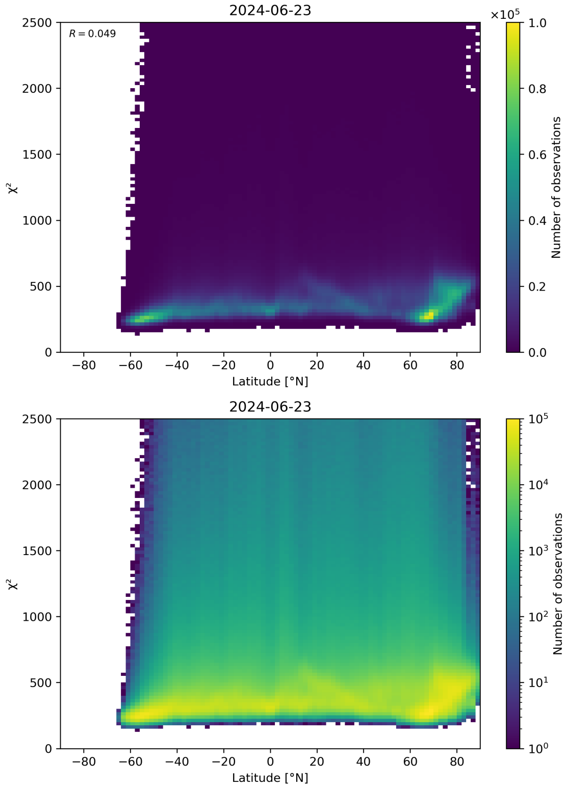
Figure 86: Scatter density plot of “Latitude” against “ \chi^2 ” for 2024-06-22 to 2024-06-24.
