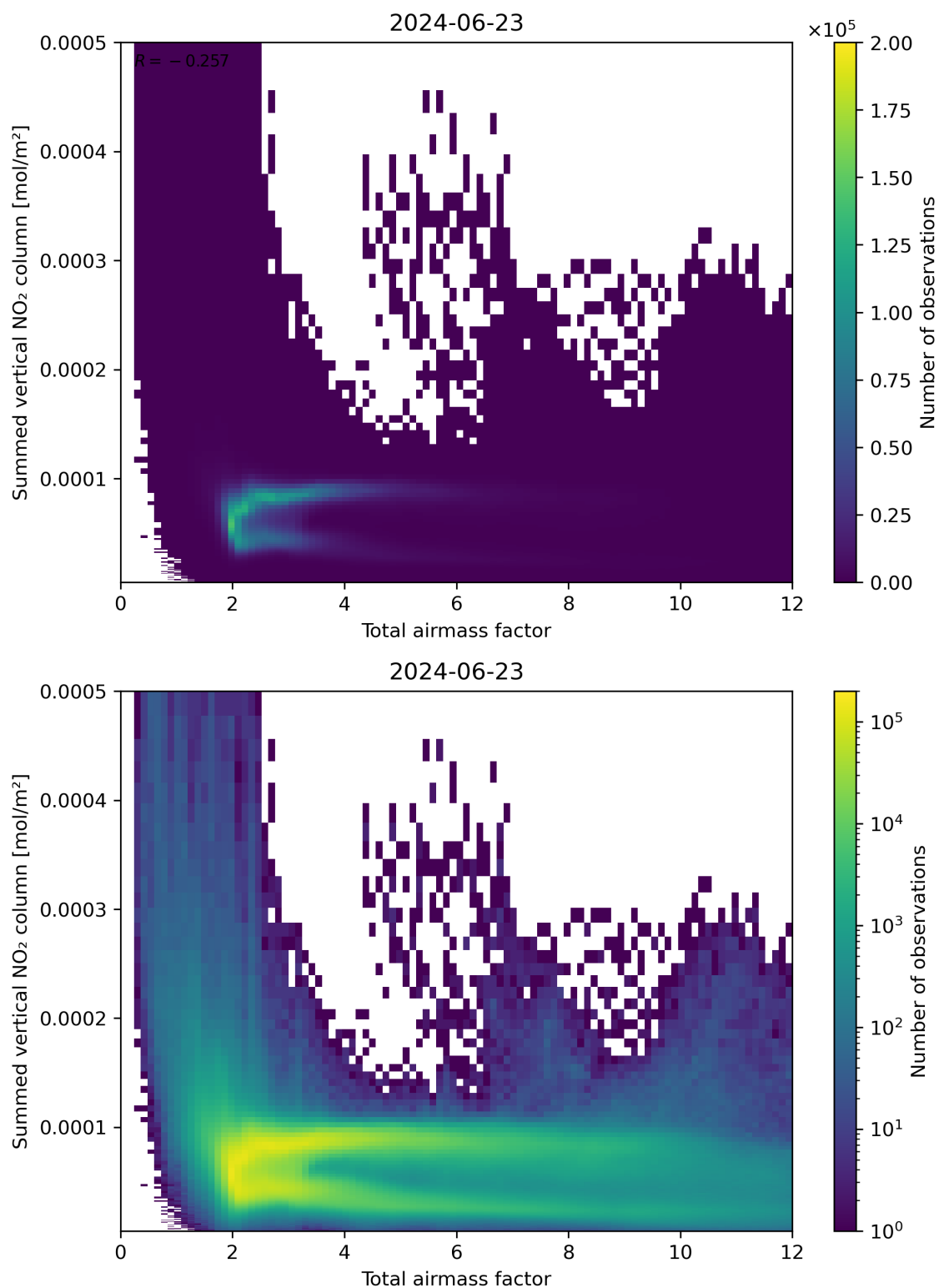
Figure 65: Scatter density plot of “Total airmass factor” against “Summed vertical NO 2 column” for 2024-06-22 to 2024-06-24.
