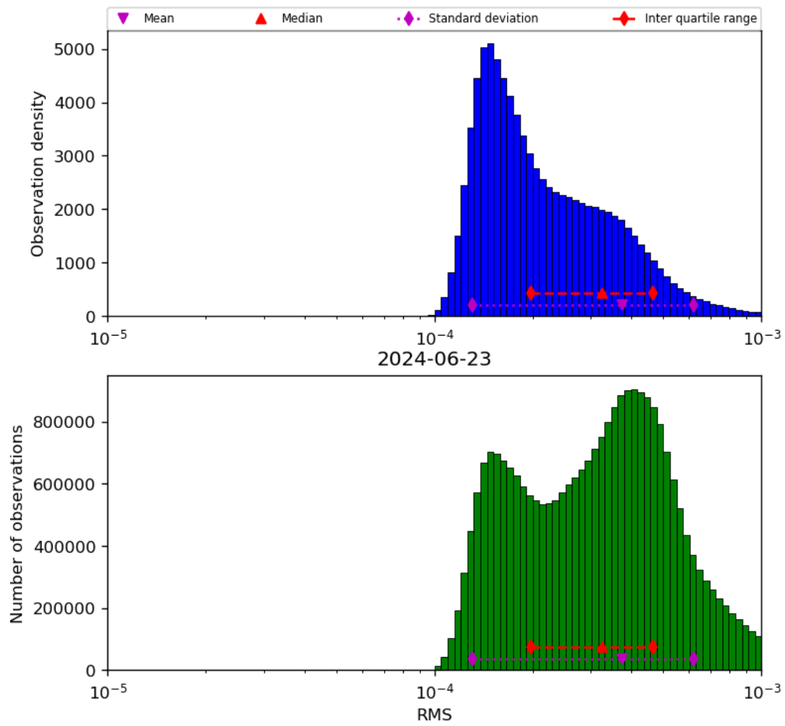
Figure 43: Histogram of “RMS” for 2024-06-22 to 2024-06-24
