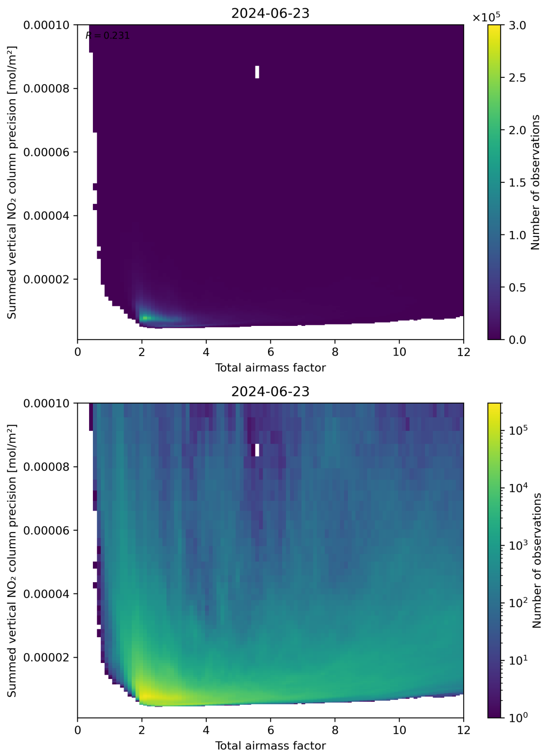
Figure 66: Scatter density plot of “Total airmass factor” against “Summed vertical NO 2 column precision” for 2024-06-22 to 2024-06-24.
