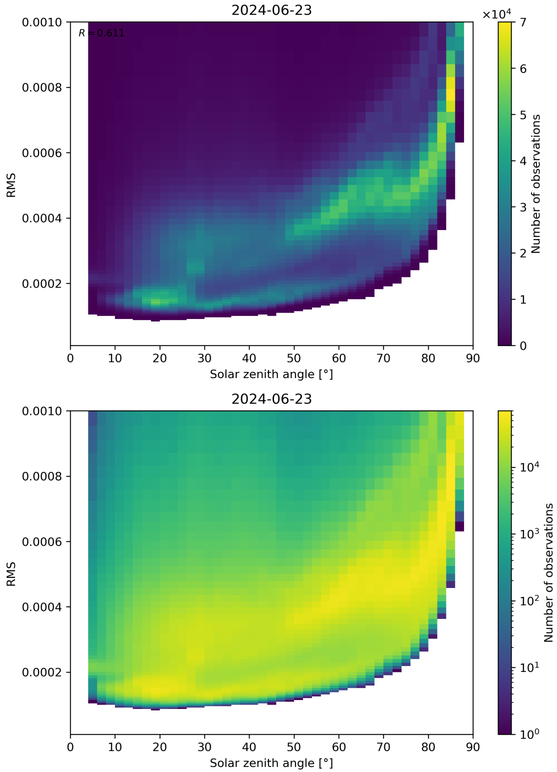
Figure 157: Scatter density plot of “Solar zenith angle” against “RMS” for 2024-06-22 to 2024-06-24.
