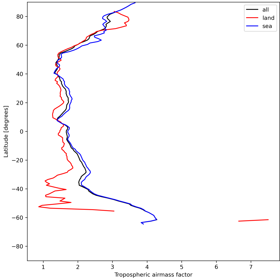
Figure 14: Zonal average of “Tropospheric airmass factor” for 2024-06-22 to 2024-06-24.
