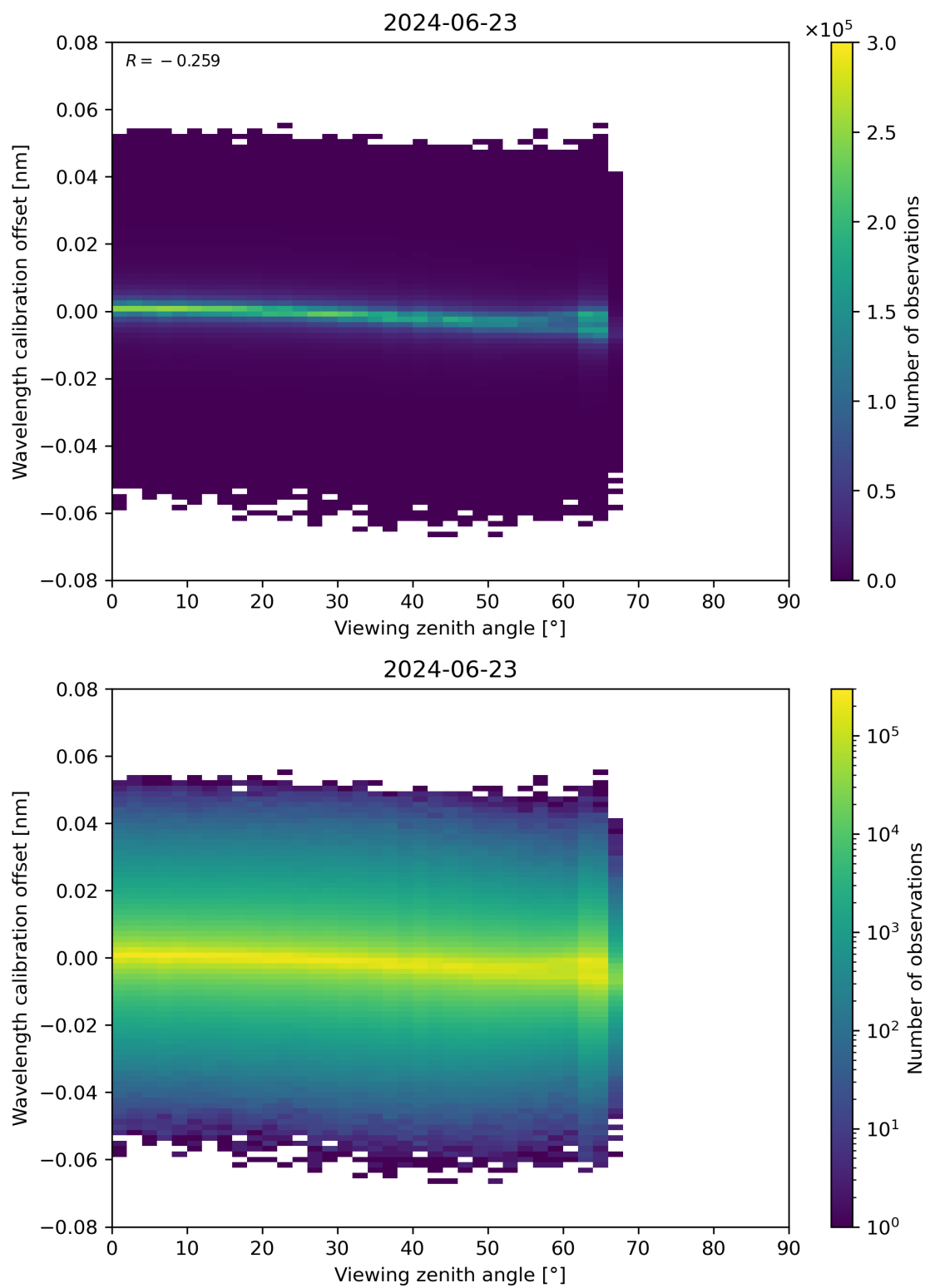
Figure 173: Scatter density plot of “Viewing zenith angle” against “Wavelength calibration offset” for 2024-06-22 to 2024-06-24.
