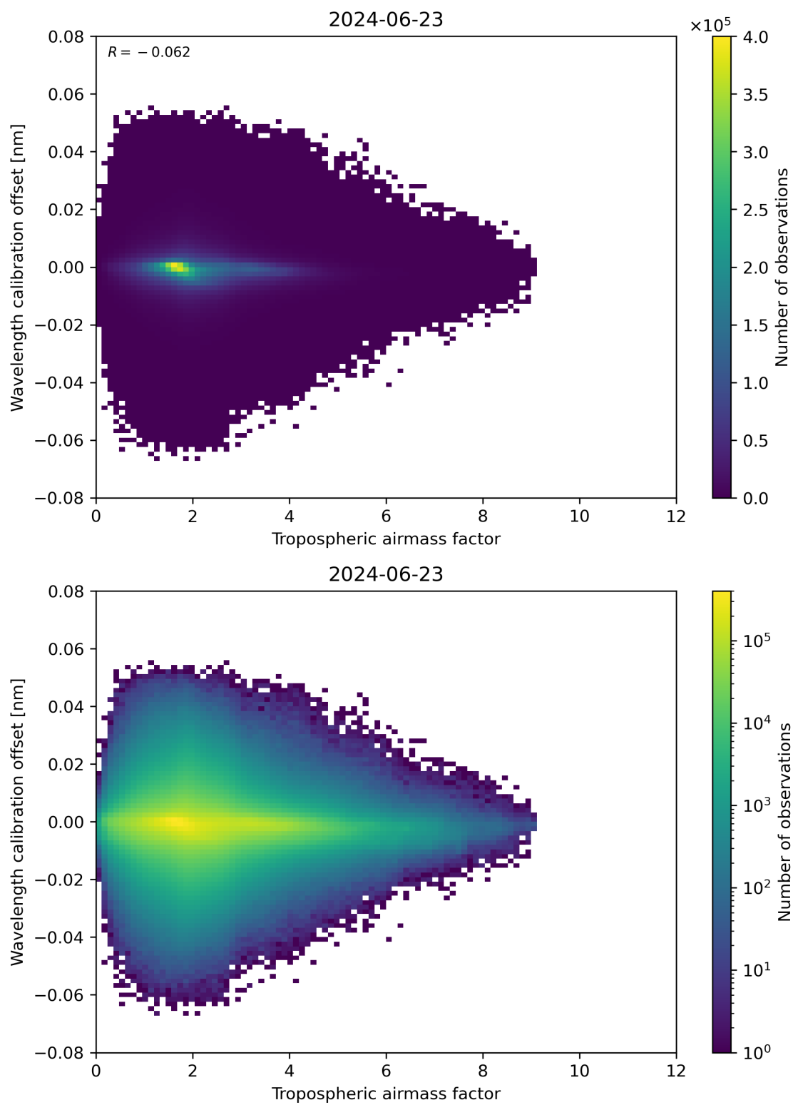
Figure 80: Scatter density plot of “Tropospheric air mass factor” against “Wavelength calibration offset” for 2024-06-22 to 2024-06-24.
