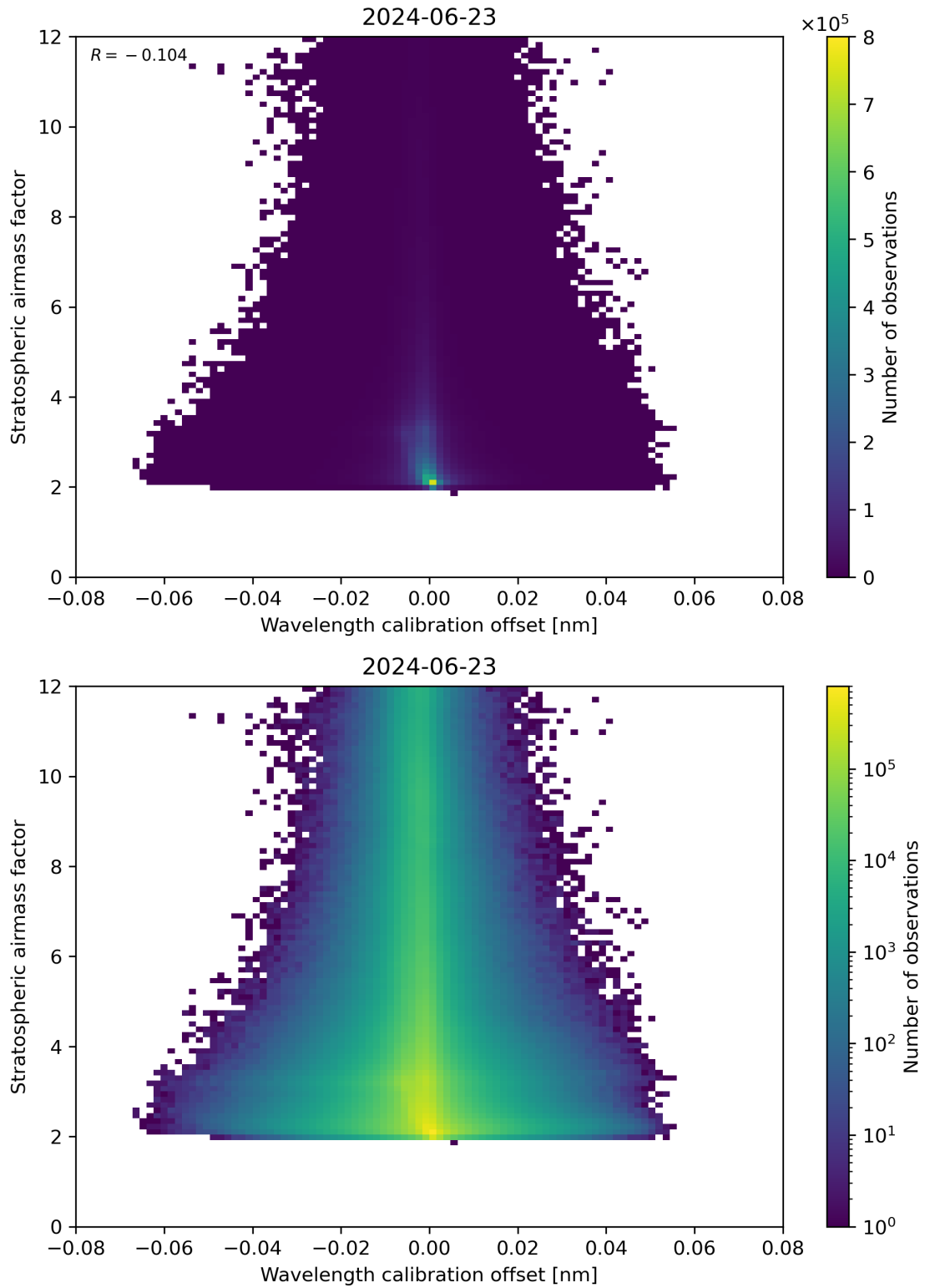
Figure 174: Scatter density plot of “Wavelength calibration offset” against “Stratospheric air mass factor” for 2024-06-22 to 2024-06-24.
