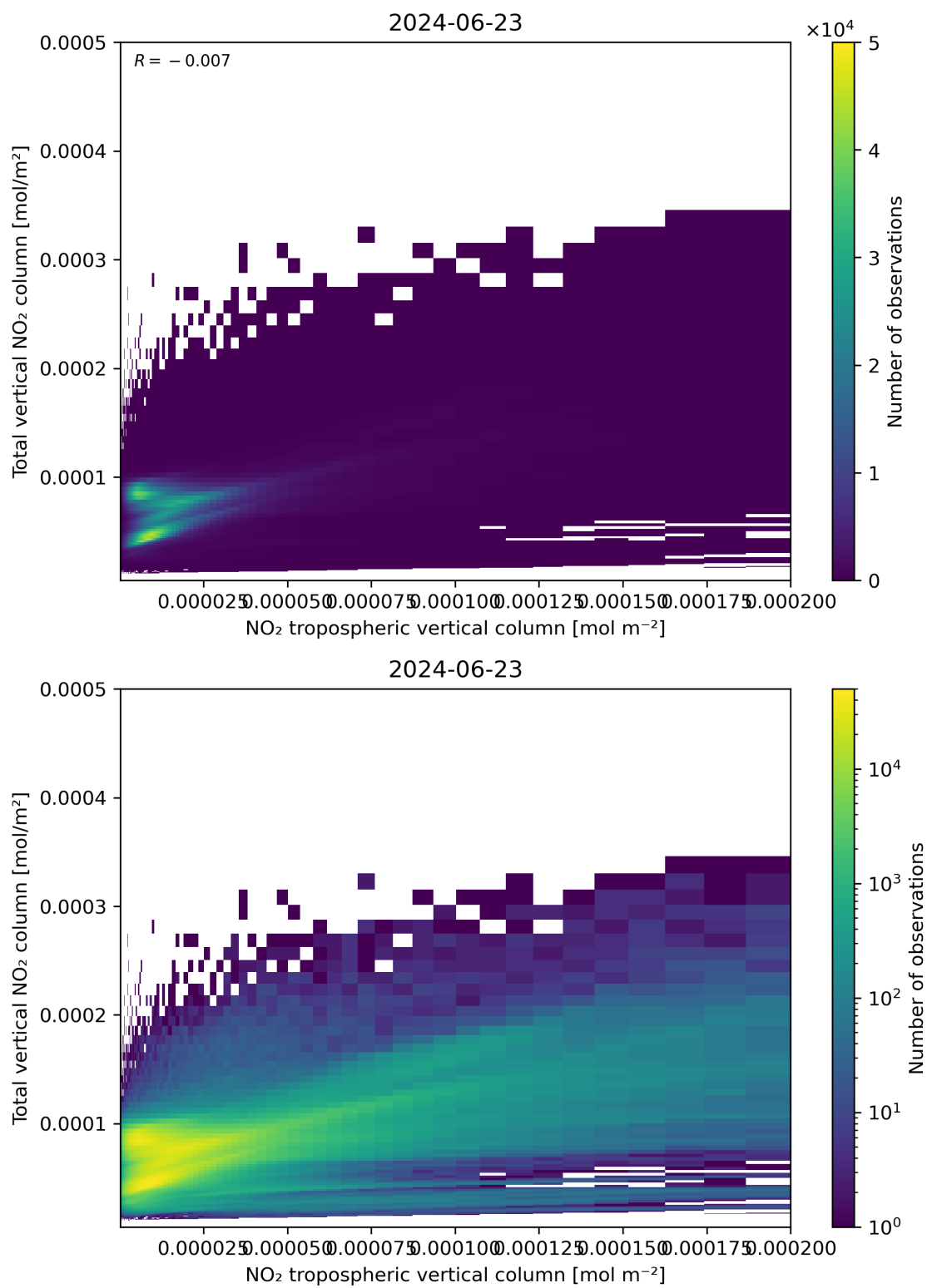
Figure 128: Scatter density plot of “NO 2 tropospheric vertical column” against “Total vertical NO 2 column” for 2024-06-22 to 2024-06-24.
