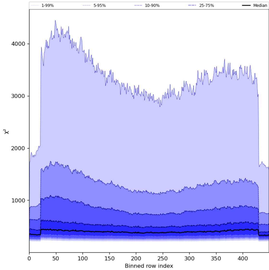
Figure 59: Along track statistics of “ \chi^2 ” for 2024-06-22 to 2024-06-24
