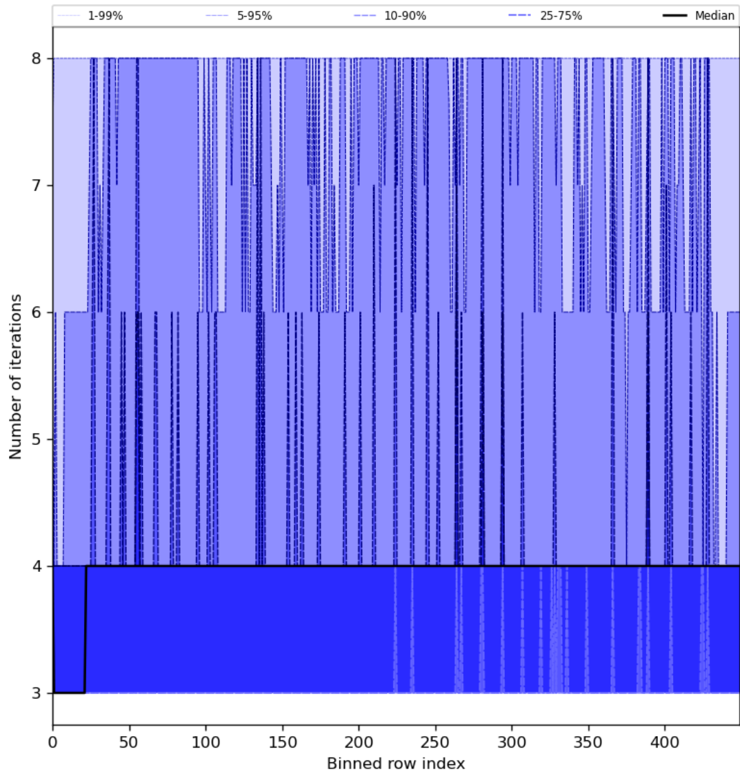
Figure 51: Along track statistics of “Number of iterations” for 2024-06-22 to 2024-06-24
