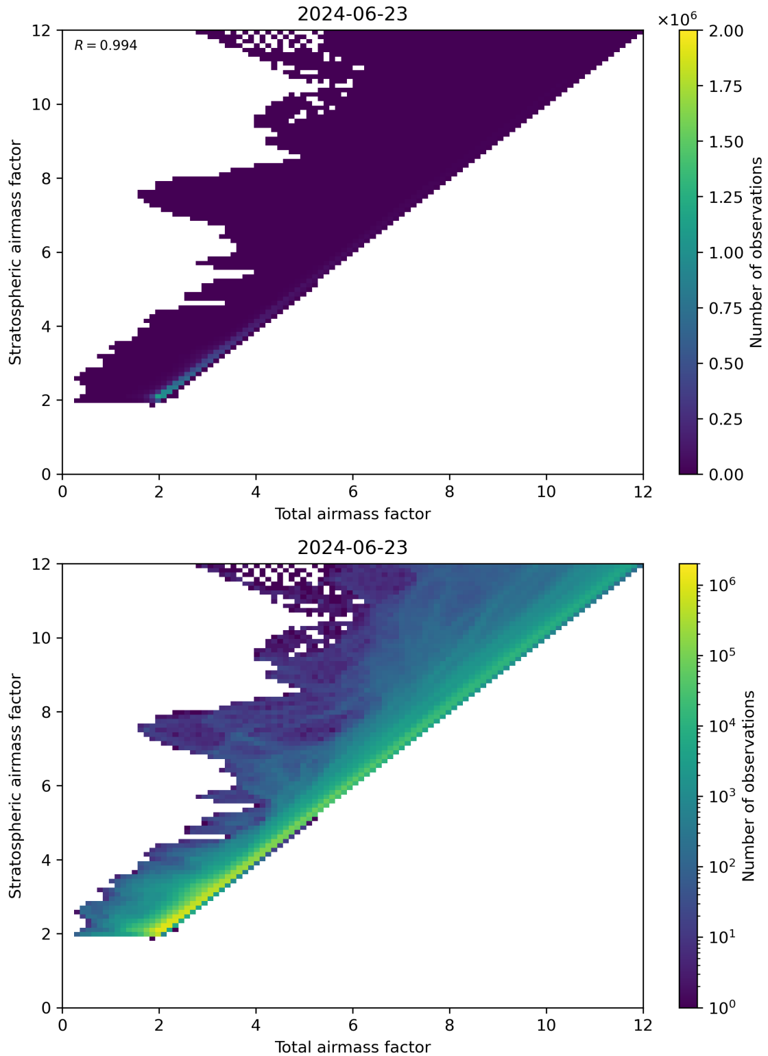
Figure 62: Scatter density plot of “Total airmass factor” against “Stratospheric airmass factor” for 2024-06-22 to 2024-06-24.
