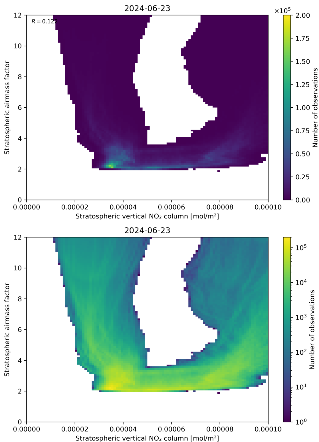
Figure 96: Scatter density plot of “Stratospheric vertical NO 2 column” against “Stratospheric airmass factor” for 2024-06-22 to 2024-06-24.
