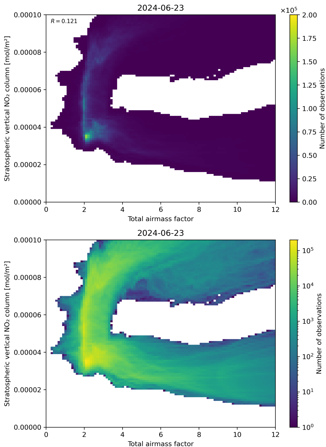
Figure 64: Scatter density plot of “Total airmass factor” against “Stratospheric vertical NO 2 column” for 2024-06-22 to 2024-06-24.
