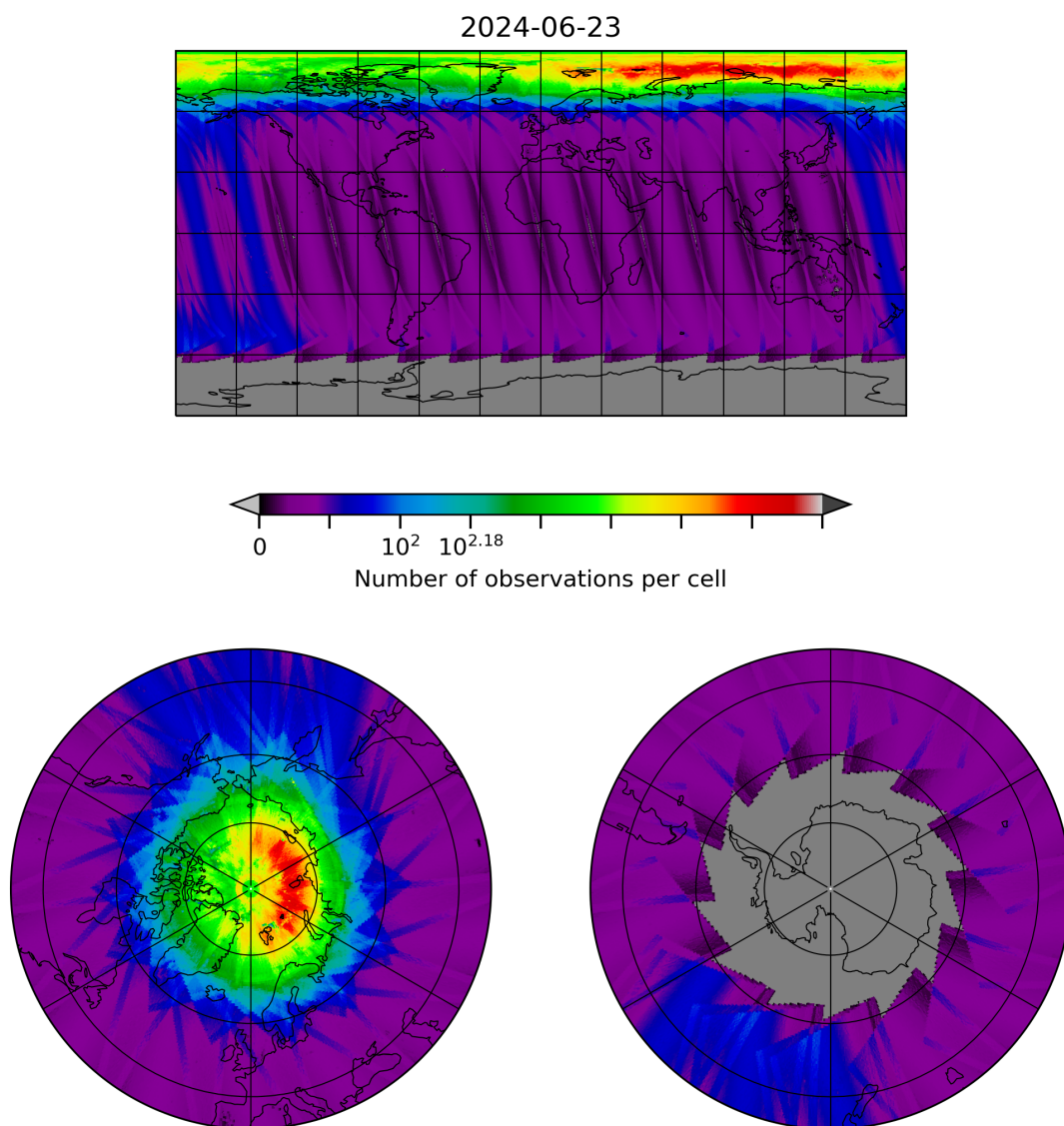
Figure 10: Map of the number of observations for 2024-06-22 to 2024-06-24
