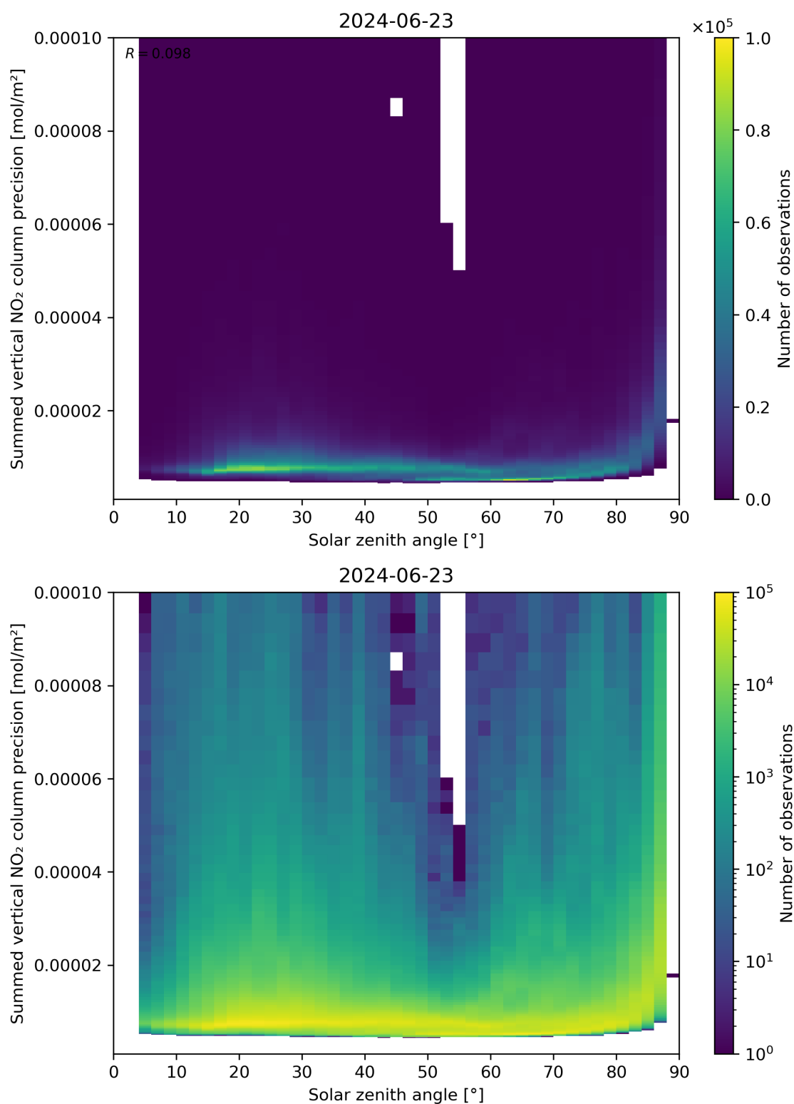
Figure 152: Scatter density plot of “Solar zenith angle” against “Summed vertical NO 2 column precision” for 2024-06-22 to 2024-06-24.
