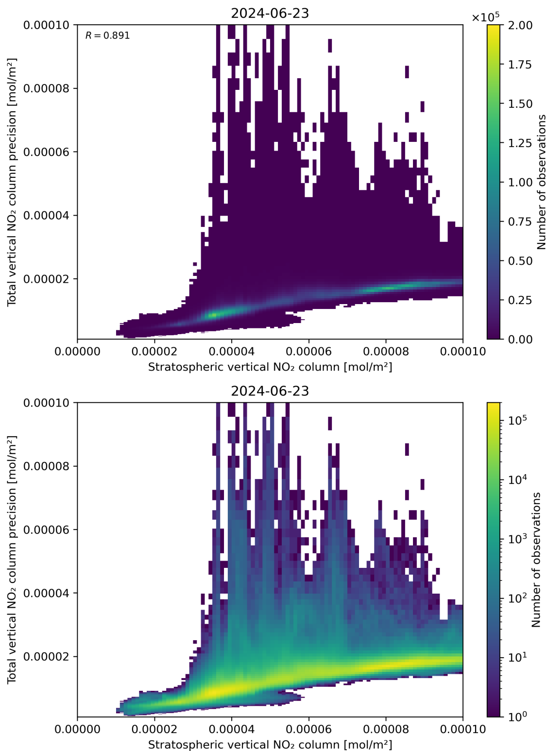
Figure 101: Scatter density plot of “Stratospheric vertical NO 2 column” against “Total vertical NO 2 column precision” for 2024-06-22 to 2024-06-24.
