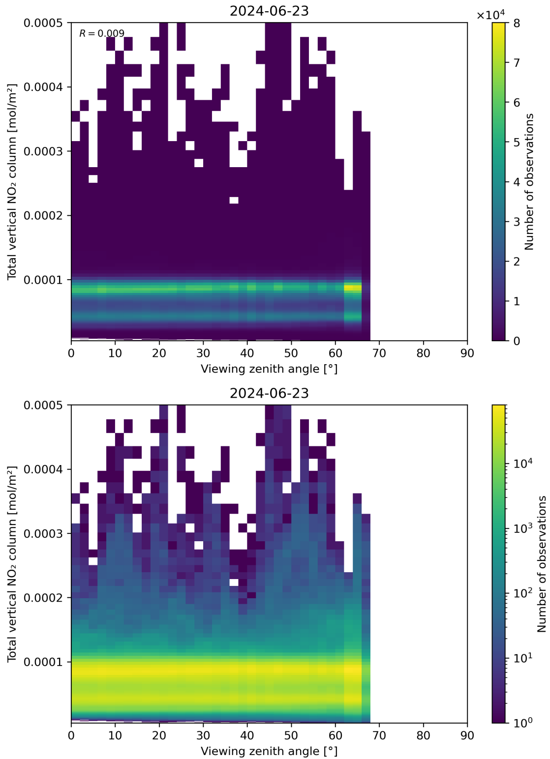
Figure 167: Scatter density plot of “Viewing zenith angle” against “Total vertical NO 2 column” for 2024-06-22 to 2024-06-24.
