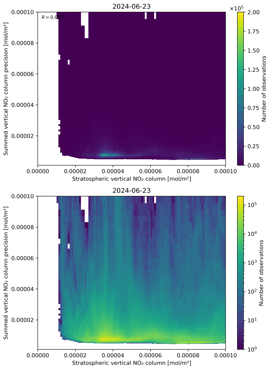
Figure 99: Scatter density plot of “Stratospheric vertical NO 2 column” against “Summed vertical NO 2 column precision” for 2024-06-22 to 2024-06-24.
