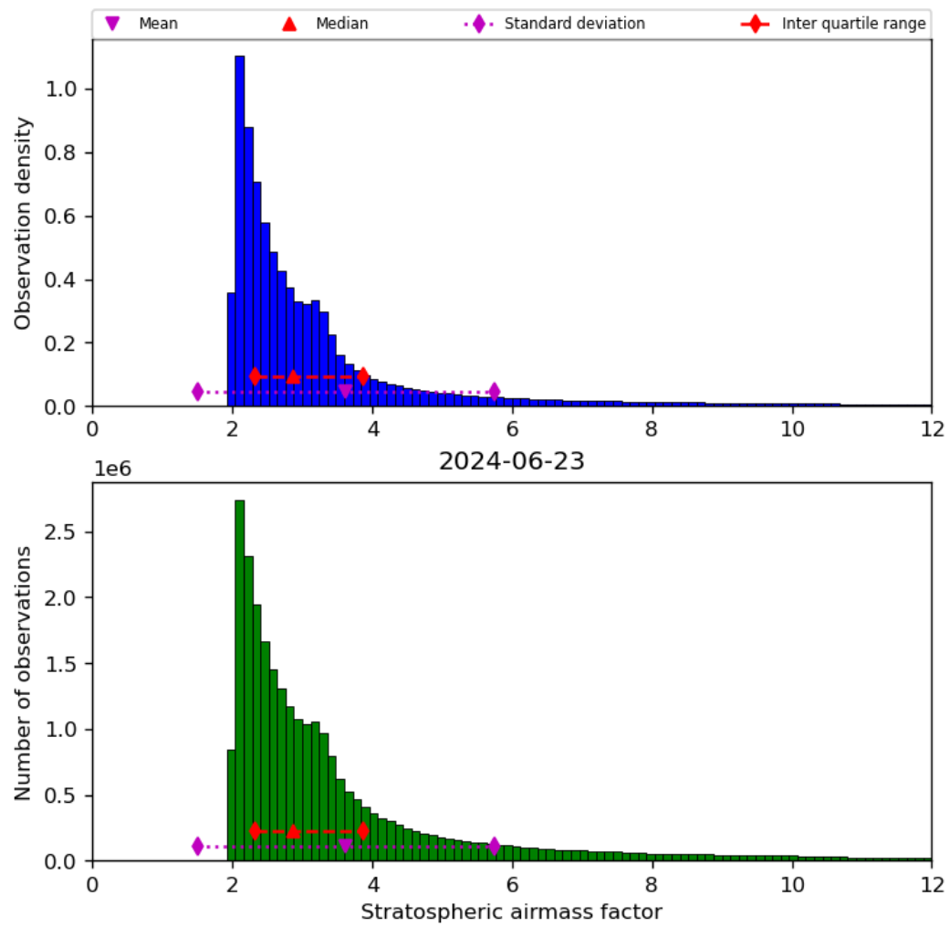
Figure 44: Histogram of “Stratospheric airmass factor” for 2024-06-22 to 2024-06-24
