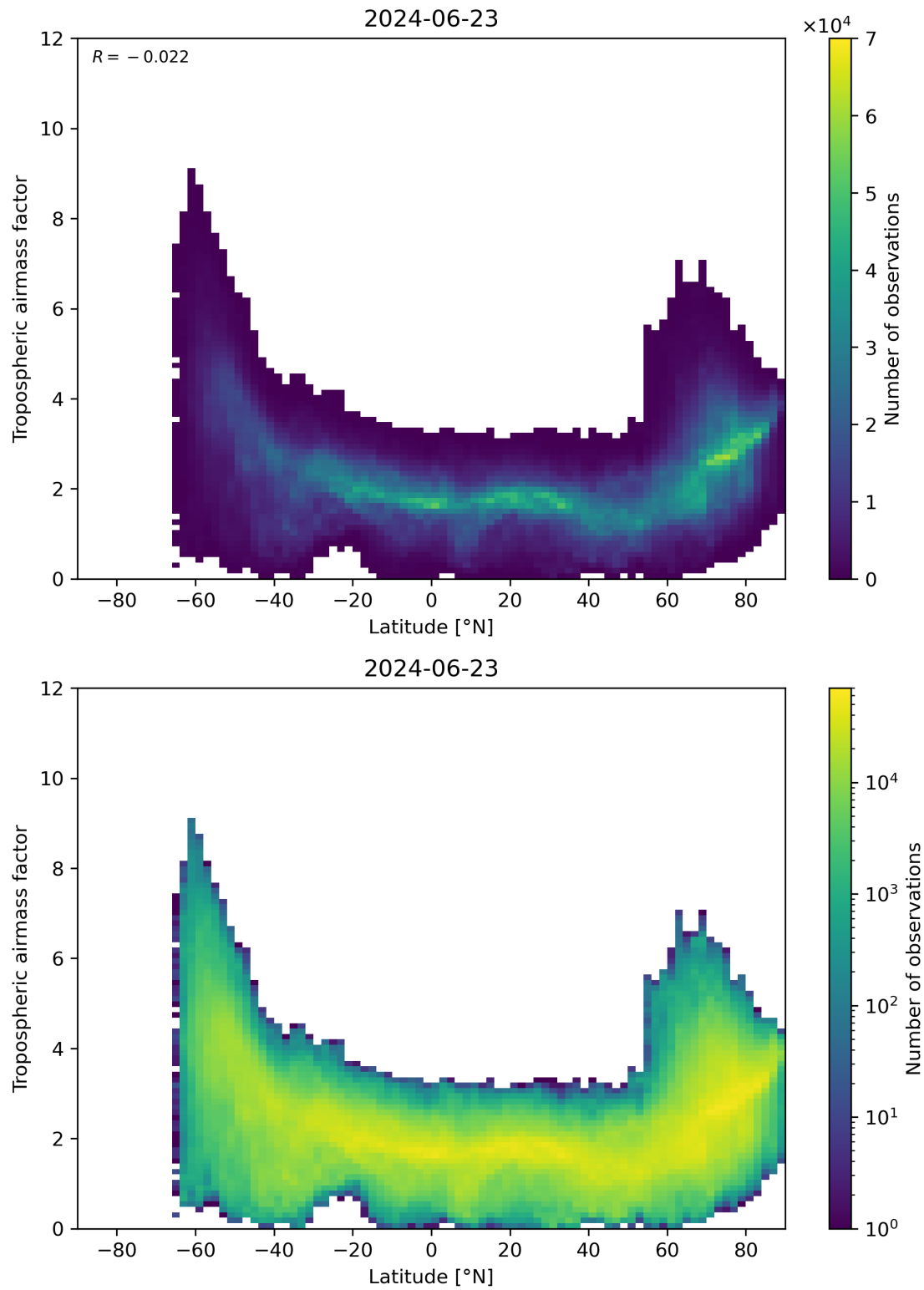
Figure 85: Scatter density plot of “Latitude” against “Tropospheric airmass factor” for 2024-06-22 to 2024-06-24.
