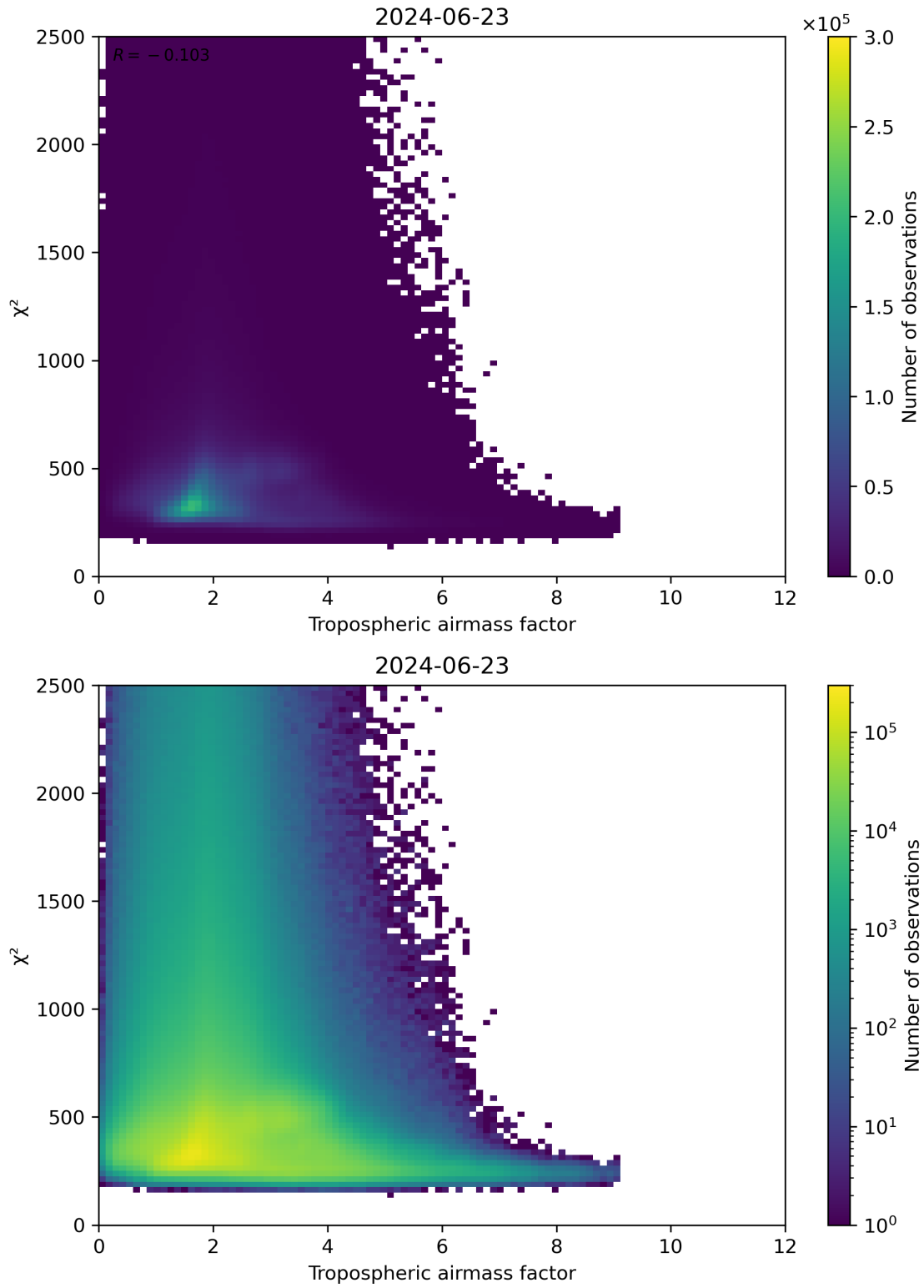
Figure 73: Scatter density plot of “Tropospheric airmass factor” against “ \chi^2 ” for 2024-06-22 to 2024-06-24.
