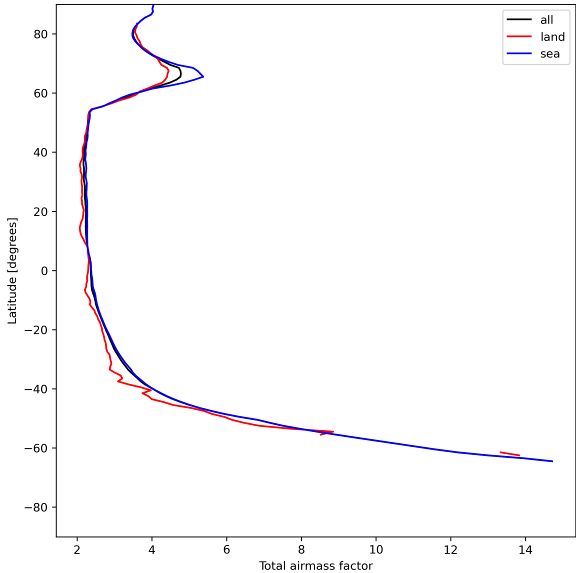
Figure 15: Zonal average of “Total airmass factor” for 2024-06-22 to 2024-06-24.
