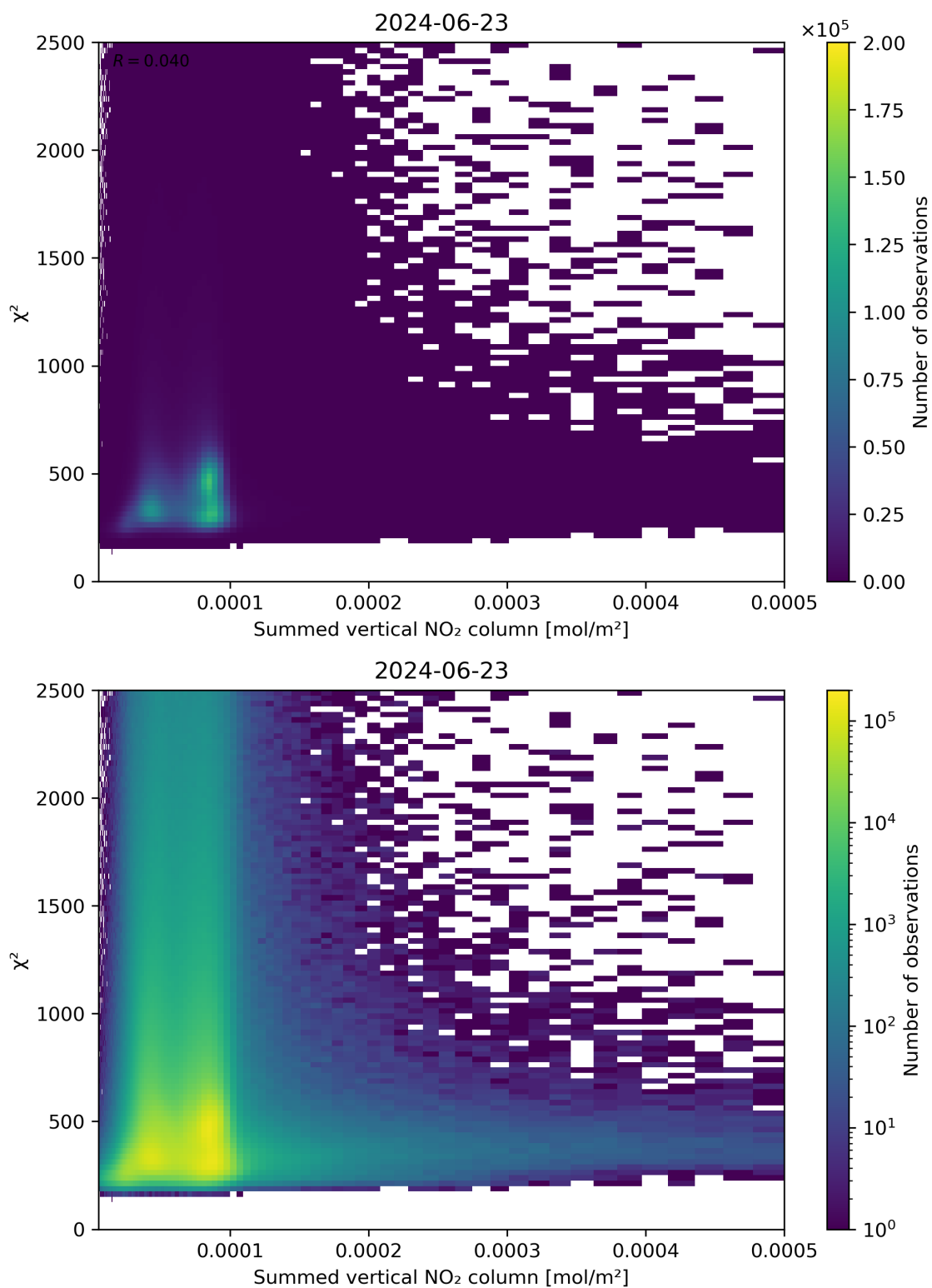
Figure 104: Scatter density plot of “Summed vertical NO 2 column” against “ \chi^2 ” for 2024-06-22 to 2024-06-24.
