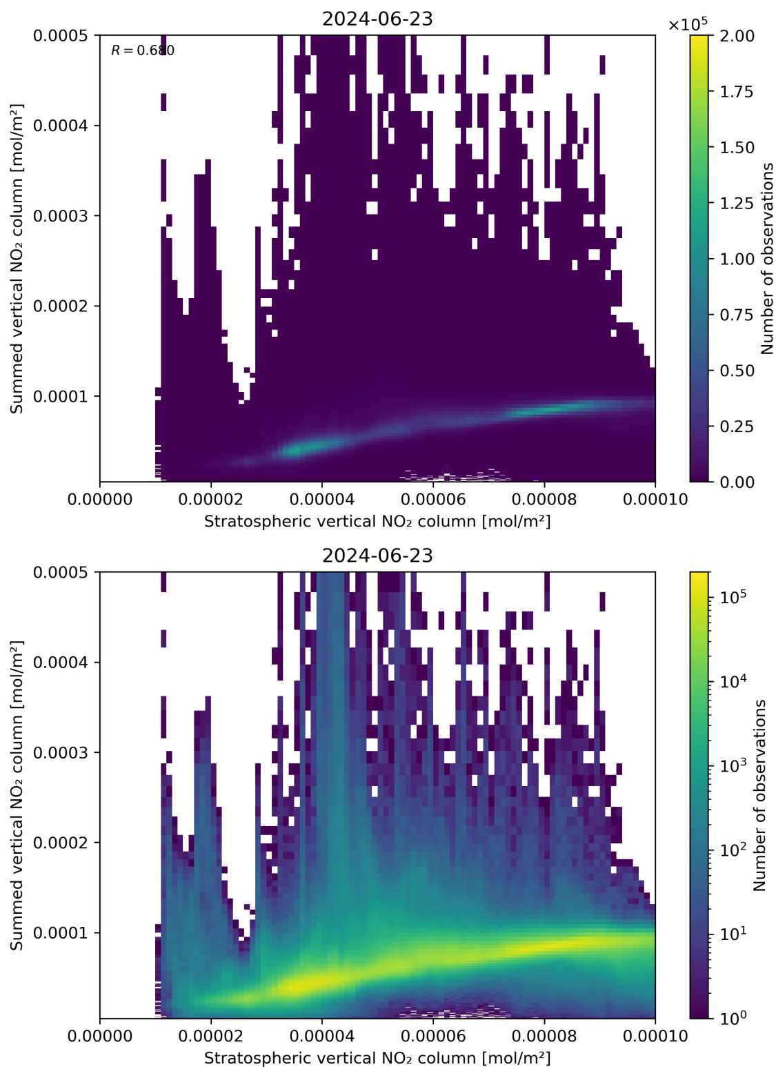
Figure 98: Scatter density plot of “Stratospheric vertical NO 2 column” against “Summed vertical NO 2 column” for 2024-06-22 to 2024-06-24.
