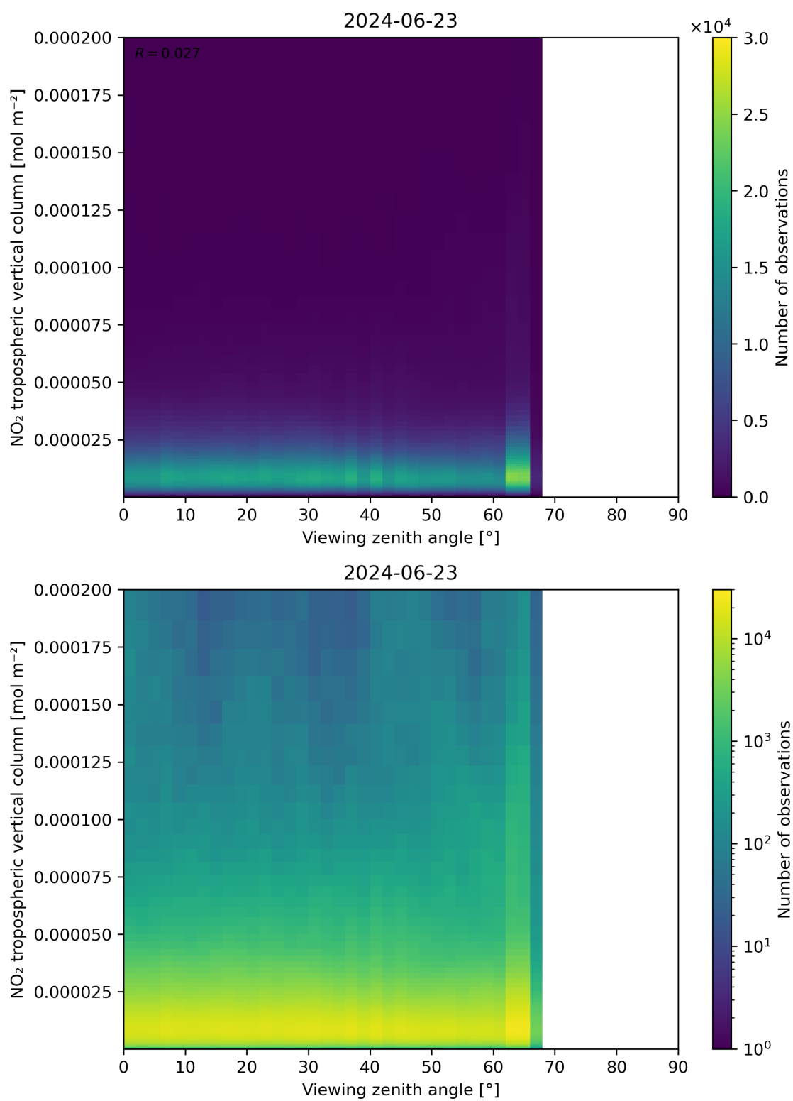
Figure 169: Scatter density plot of “Viewing zenith angle” against “NO 2 tropospheric vertical column” for 2024-06-22 to 2024-06-24.
