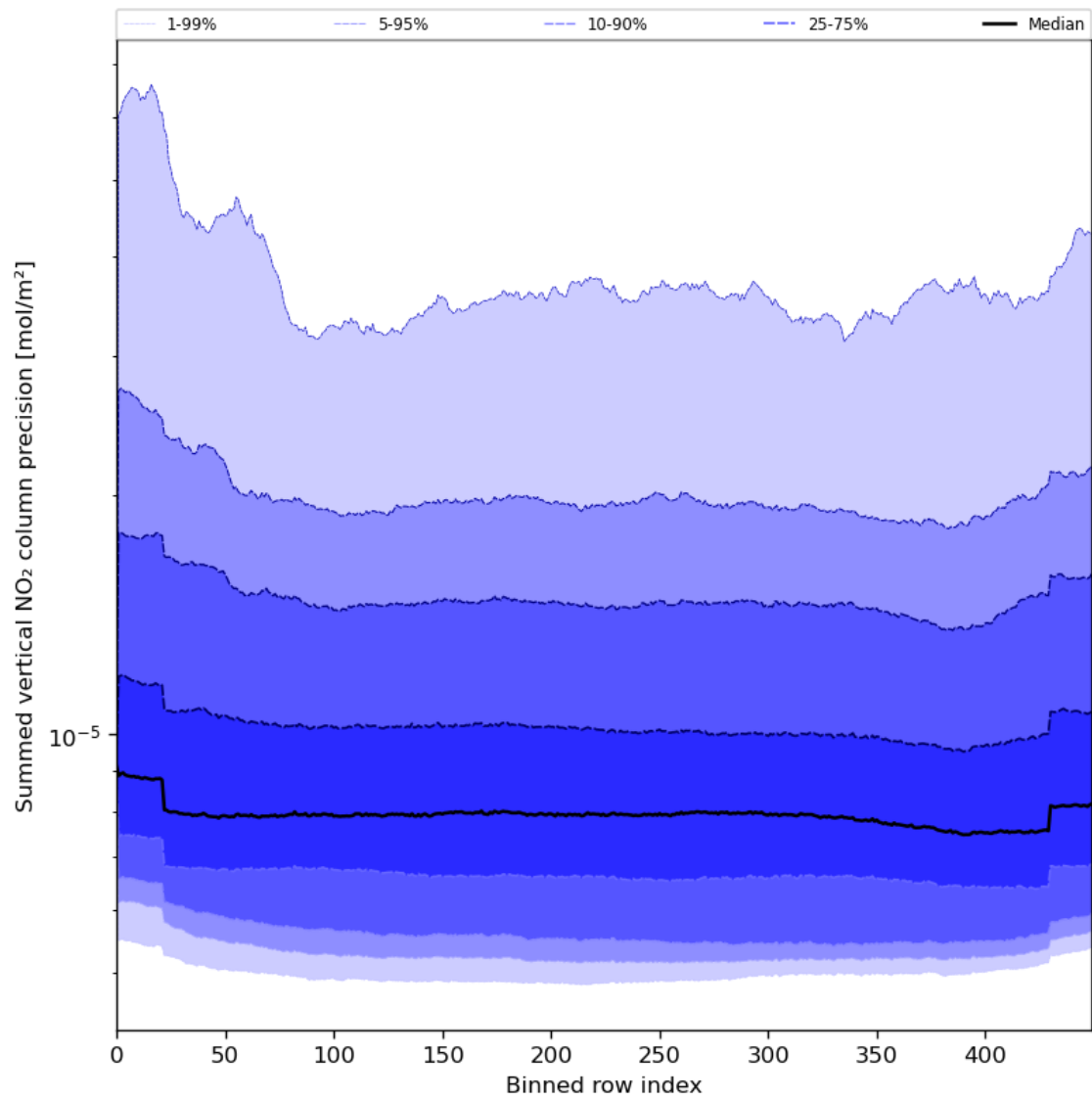
Figure 58: Along track statistics of “Summed vertical NO 2 column precision” for 2024-06-22 to 2024-06-24
