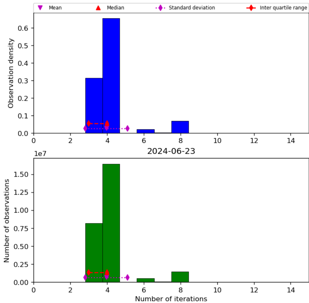
Figure 34: Histogram of “Number of iterations” for 2024-06-22 to 2024-06-24
