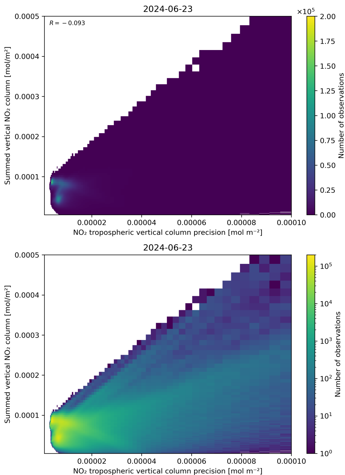
Figure 136: Scatter density plot of “NO 2 tropospheric vertical column precision” against “Summed vertical NO 2 column” for 2024-06-22 to 2024-06-24.
