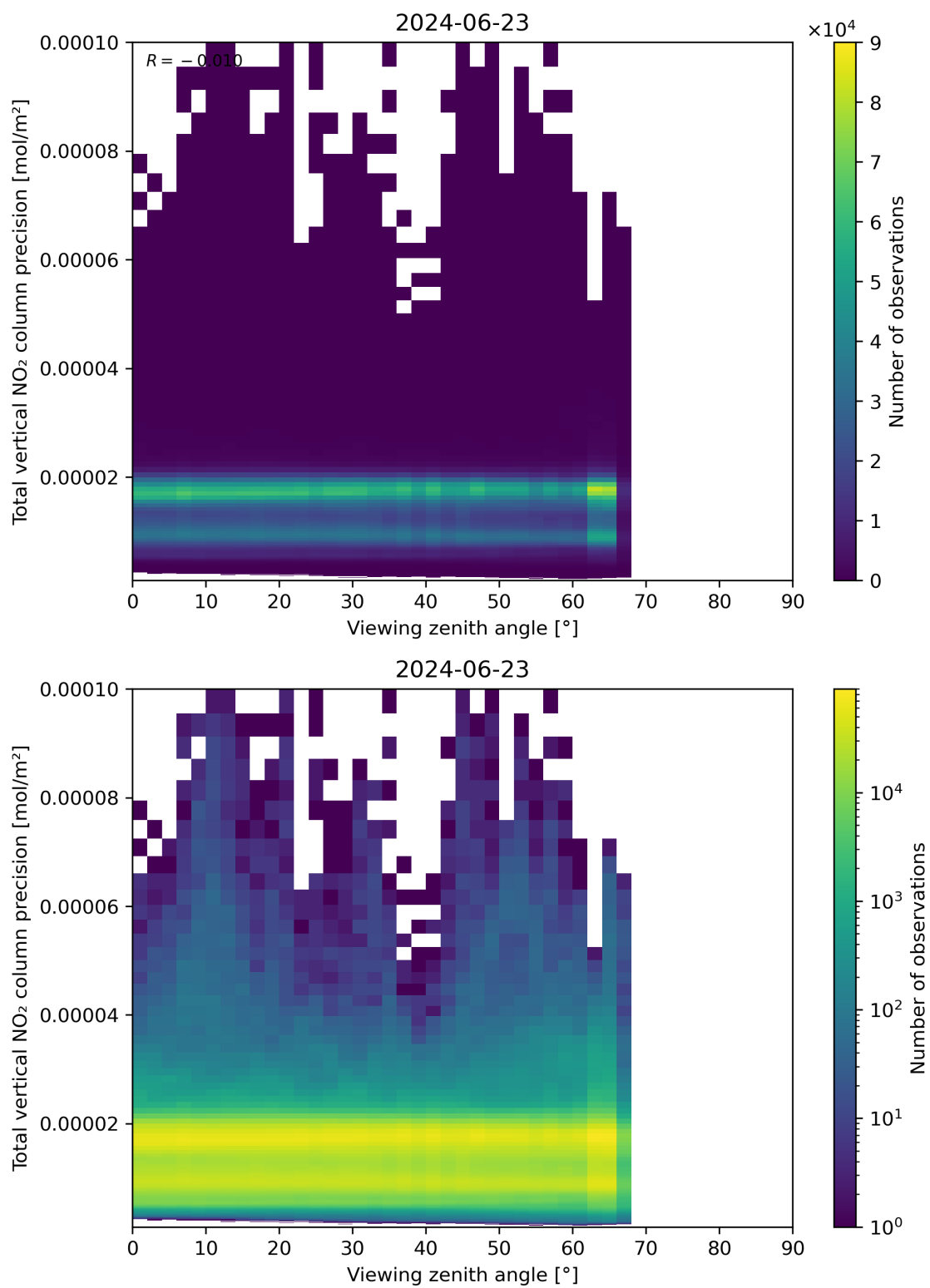
Figure 168: Scatter density plot of “Viewing zenith angle” against “Total vertical NO 2 column precision” for 2024-06-22 to 2024-06-24.
