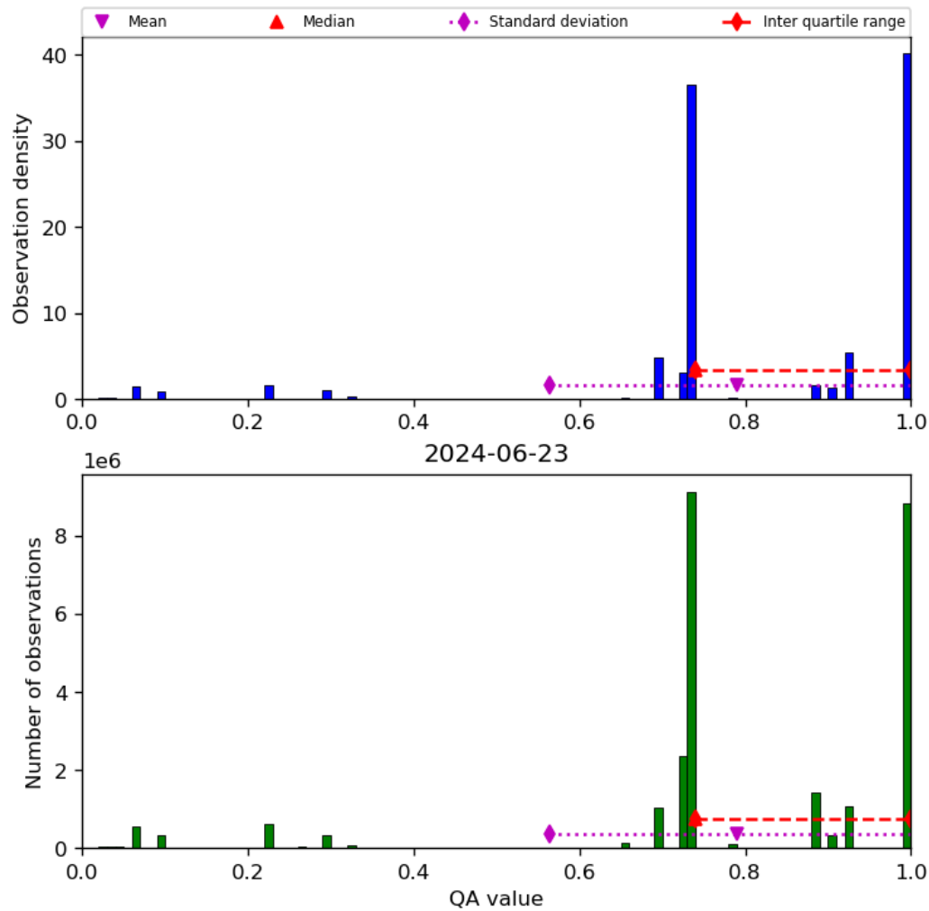
Figure 28: Histogram of “QA value” for 2024-06-22 to 2024-06-24
