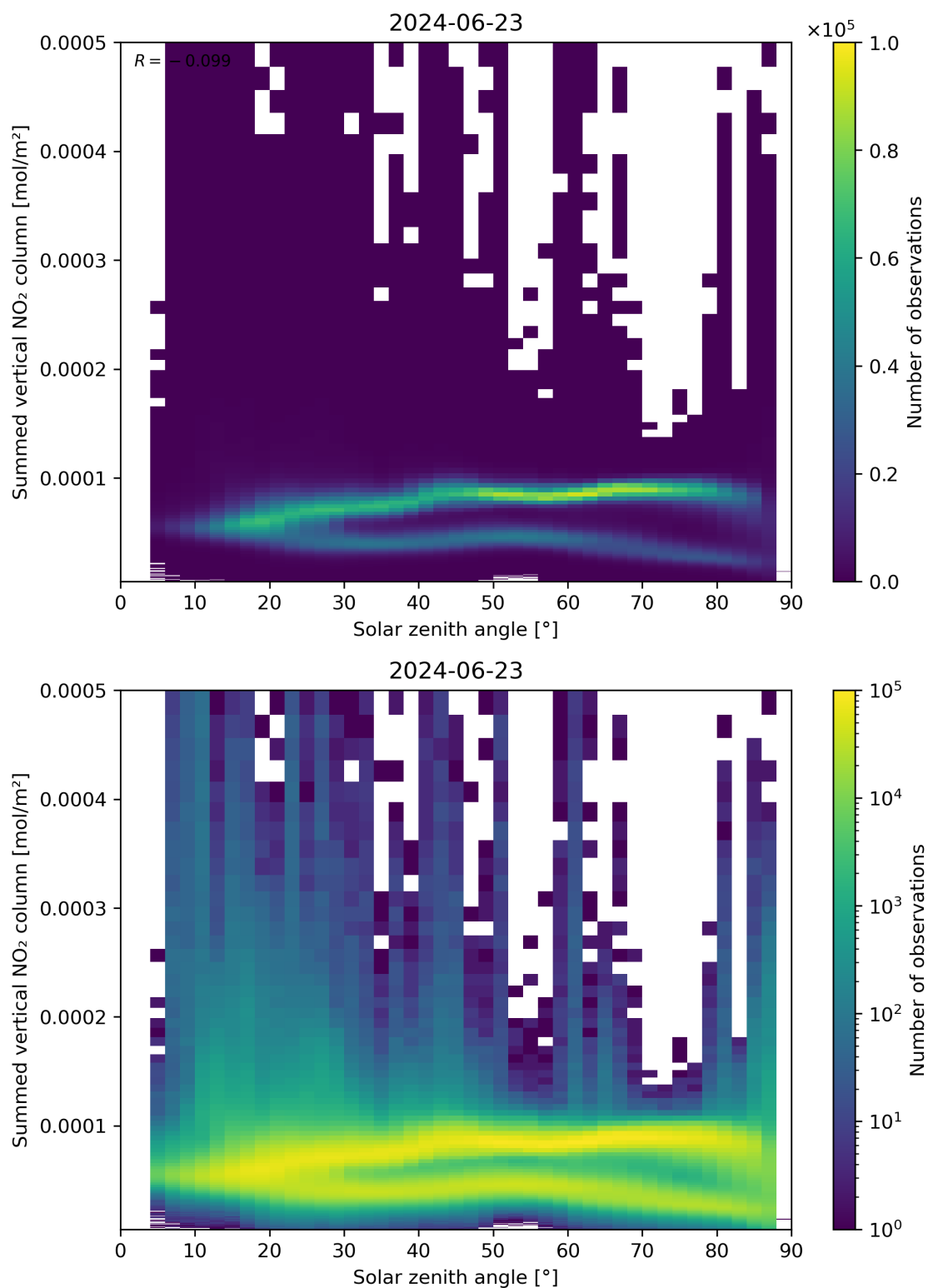
Figure 151: Scatter density plot of “Solar zenith angle” against “Summed vertical NO 2 column” for 2024-06-22 to 2024-06-24.
