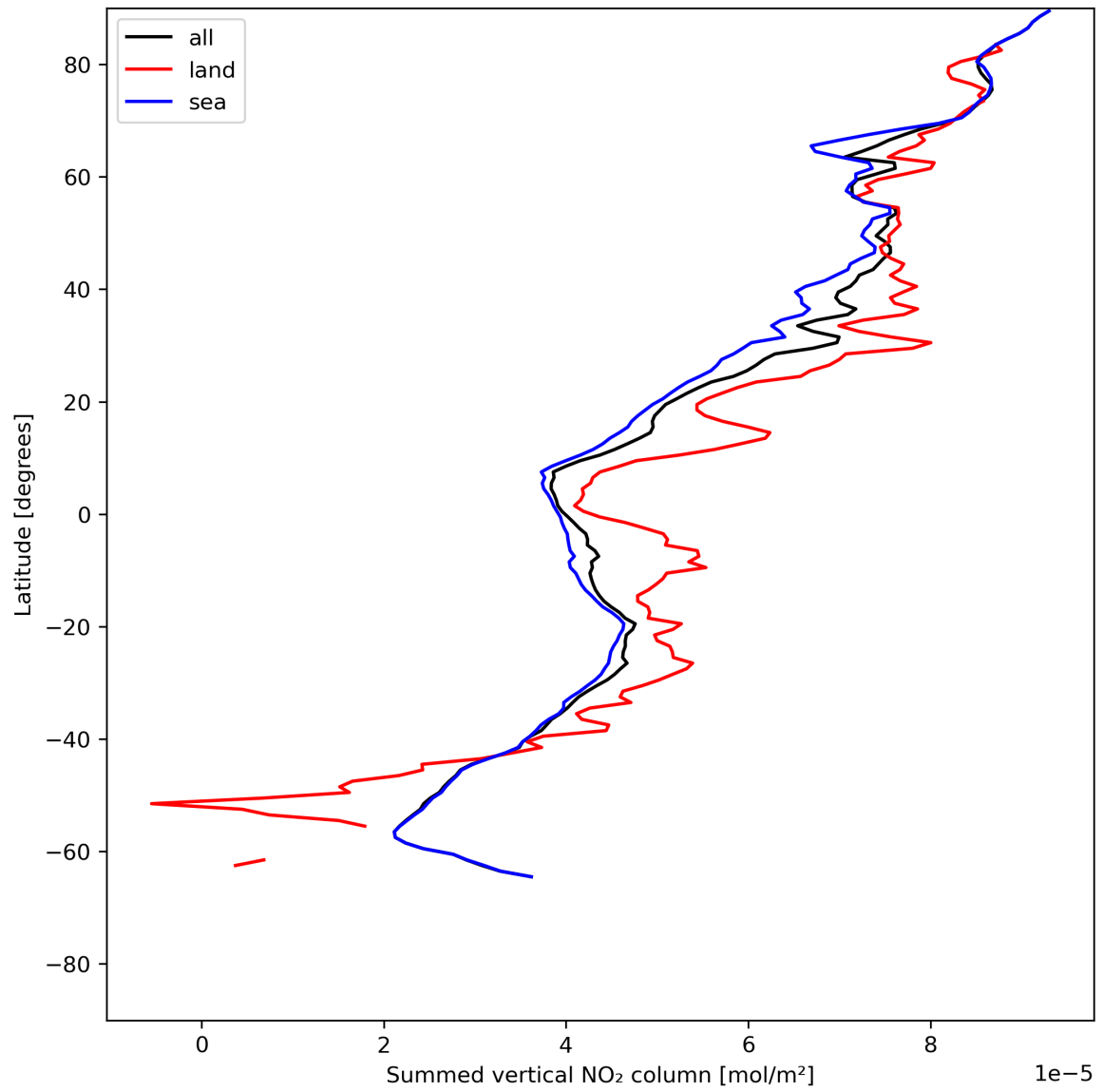
Figure 23: Zonal average of “Summed vertical NO 2 column” for 2024-06-22 to 2024-06-24.
