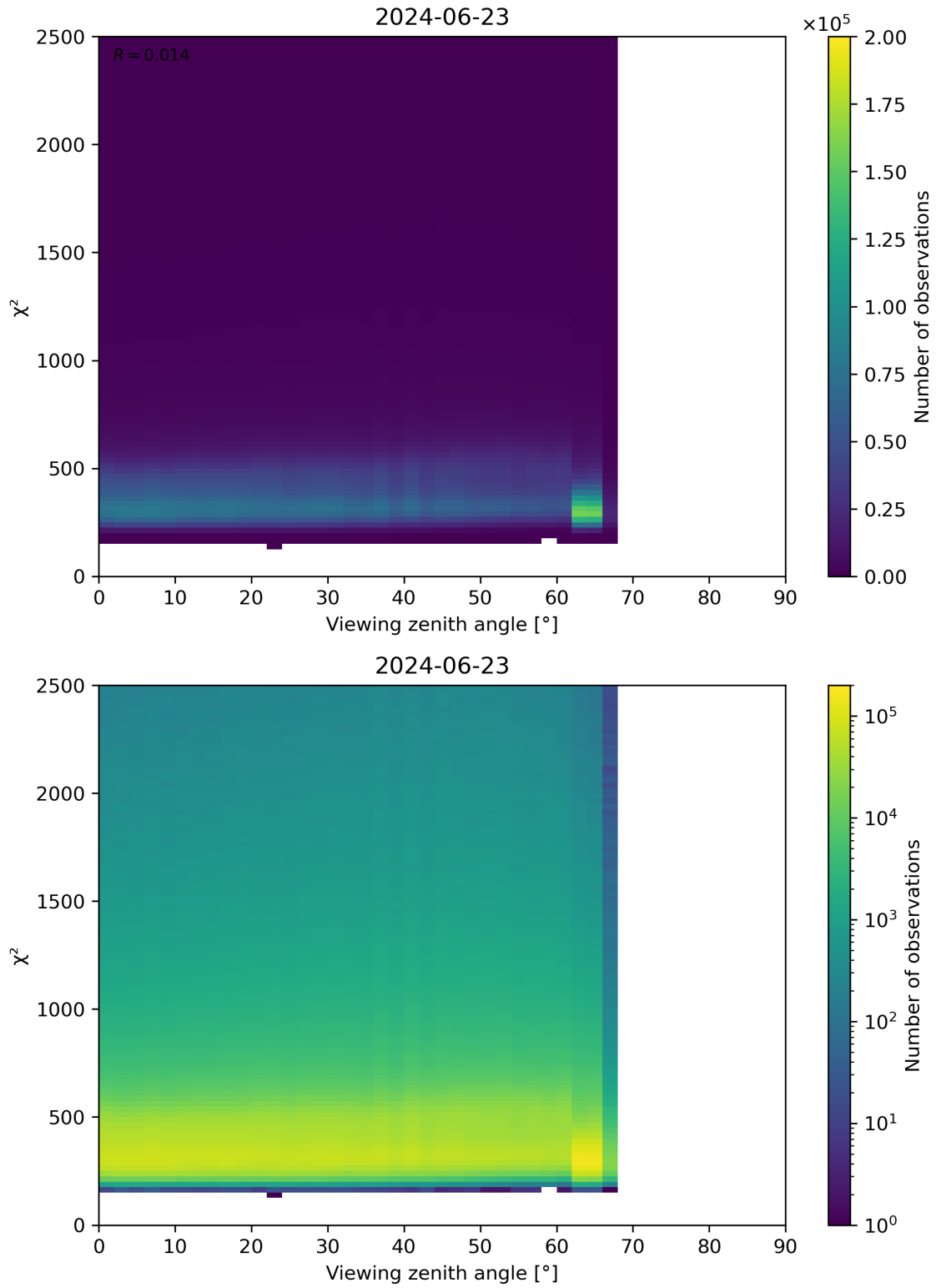
Figure 162: Scatter density plot of “Viewing zenith angle” against “ \chi^2 ” for 2024-06-22 to 2024-06-24.
