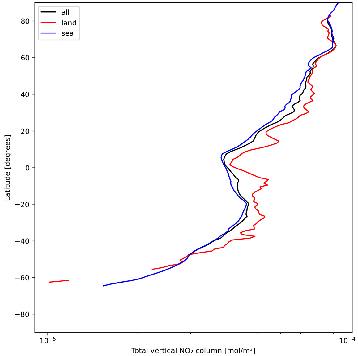
Figure 21: Zonal average of “Total vertical NO 2 column” for 2024-06-22 to 2024-06-24.
