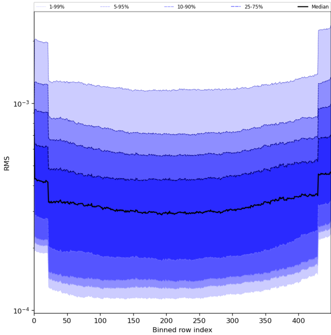
Figure 60: Along track statistics of “RMS” for 2024-06-22 to 2024-06-24
