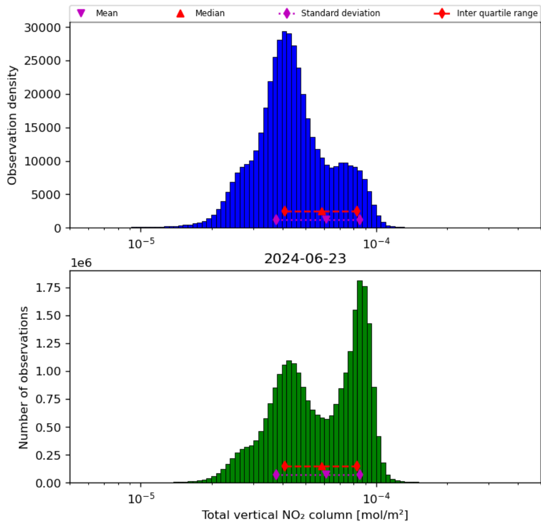
Figure 38: Histogram of “Total vertical NO 2 column” for 2024-06-22 to 2024-06-24
