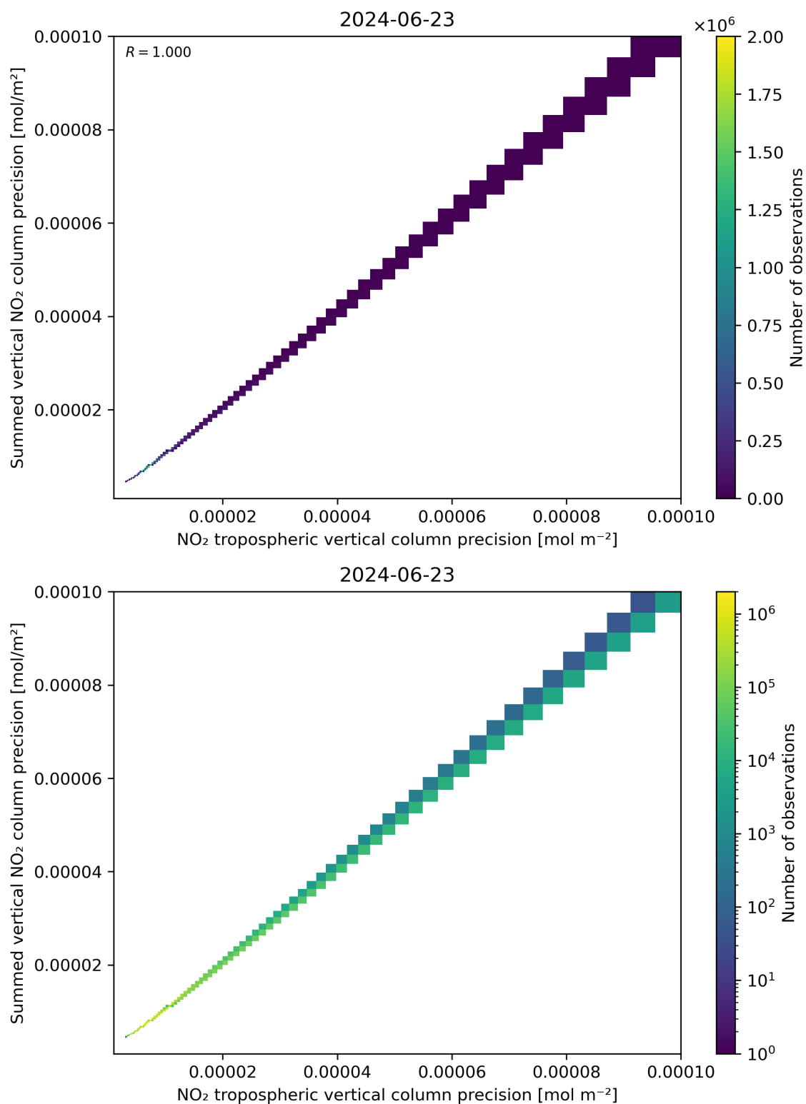
Figure 137: Scatter density plot of “NO 2 tropospheric vertical column precision” against “Summed vertical NO 2 column precision” for 2024-06-22 to 2024-06-24.
