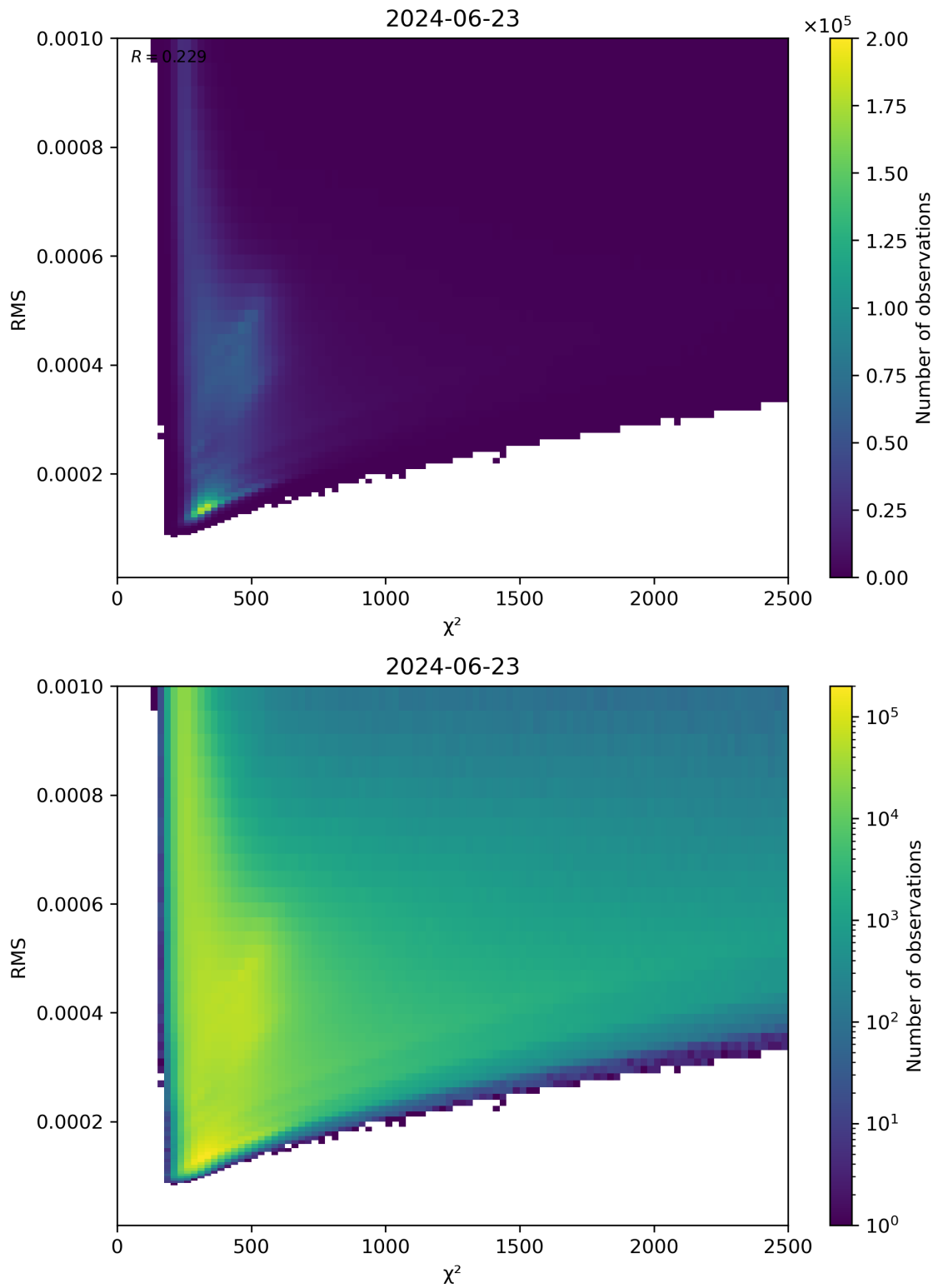
Figure 82: Scatter density plot of “ \chi^2 ” against “RMS” for 2024-06-22 to 2024-06-24.
