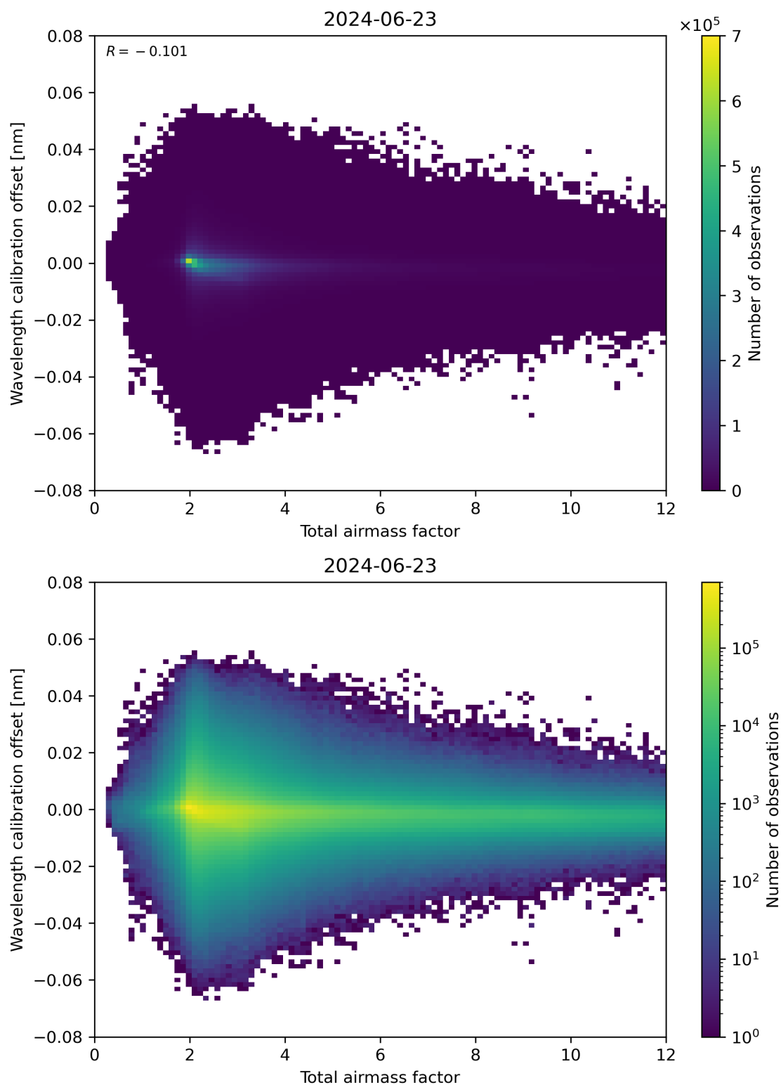
Figure 70: Scatter density plot of “Total airmass factor” against “Wavelength calibration offset” for 2024-06-22 to 2024-06-24.
