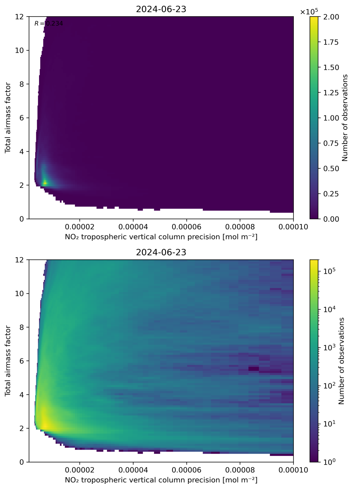
Figure 132: Scatter density plot of “NO 2 tropospheric vertical column precision” against “Total air mass factor” for 2024-06-22 to 2024-06-24.
