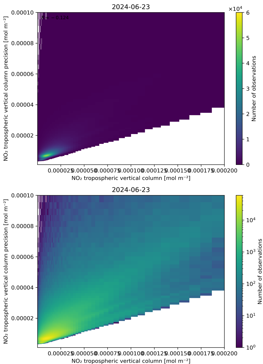
Figure 130: Scatter density plot of “NO 2 tropospheric vertical column” against “NO 2 tropospheric vertical column precision” for 2024-06-22 to 2024-06-24.
