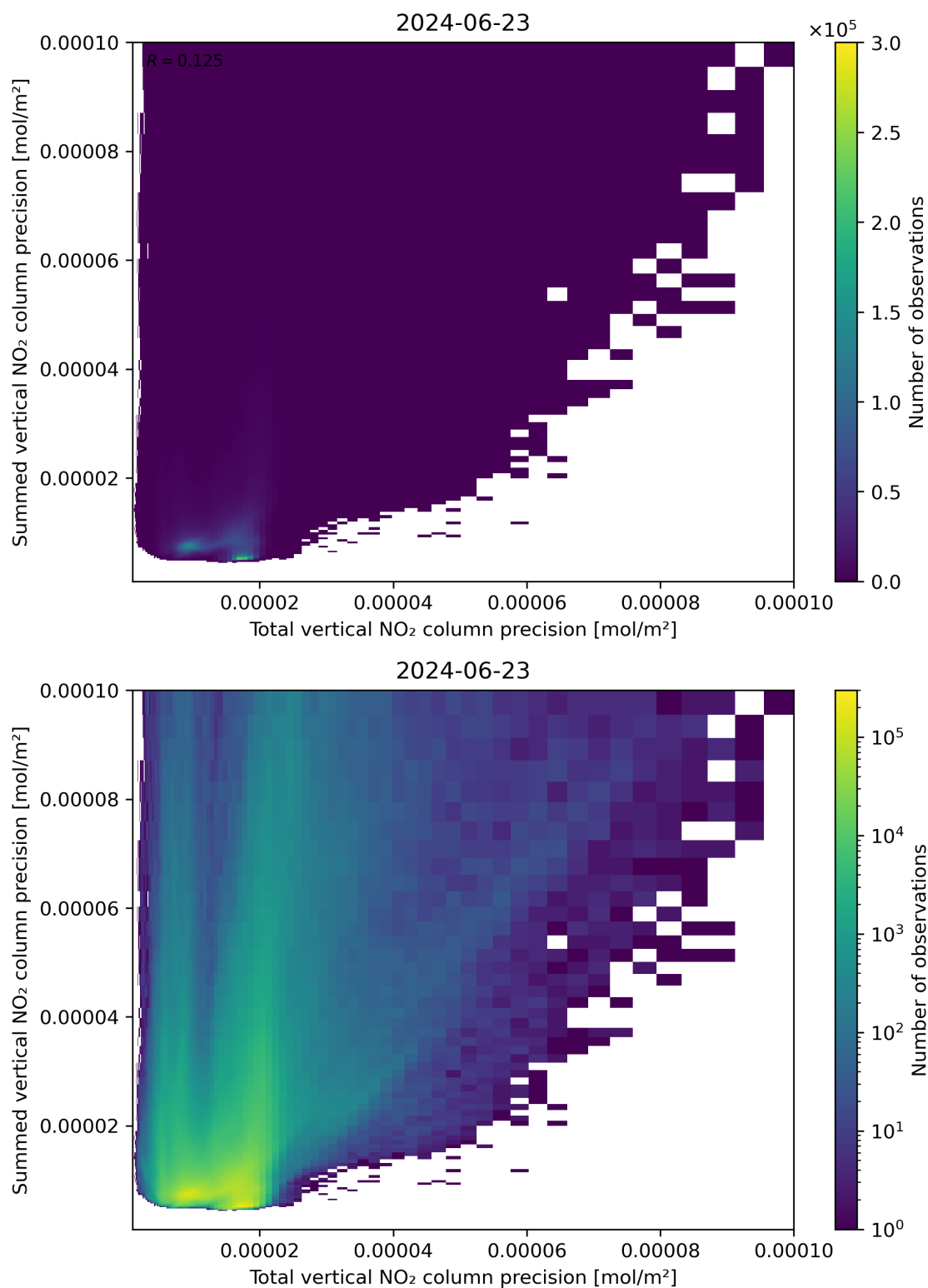
Figure 118: Scatter density plot of “Total vertical NO 2 column precision” against “Summed vertical NO 2 column precision” for 2024-06-22 to 2024-06-24.
