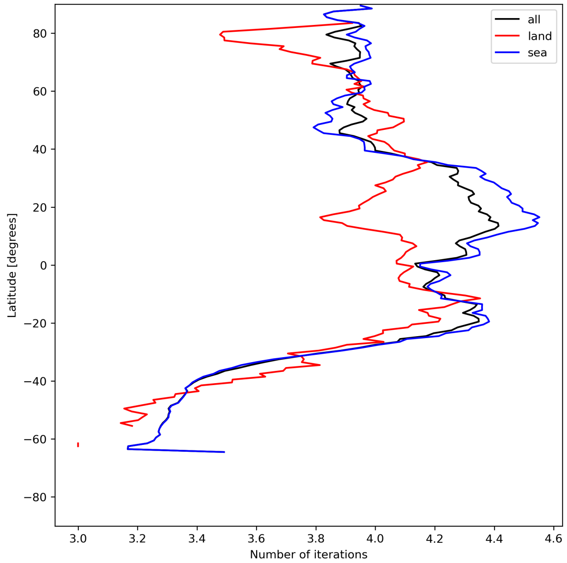
Figure 17: Zonal average of “Number of iterations” for 2024-06-22 to 2024-06-24.
