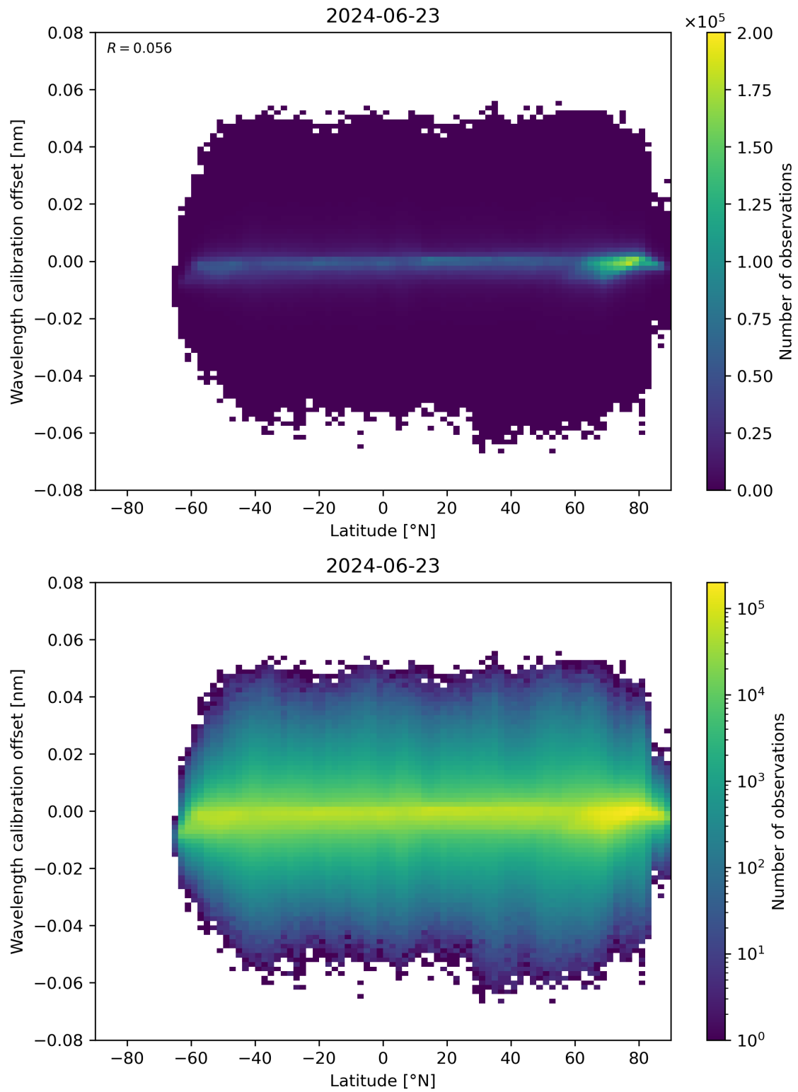
Figure 95: Scatter density plot of “Latitude” against “Wavelength calibration offset” for 2024-06-22 to 2024-06-24.
