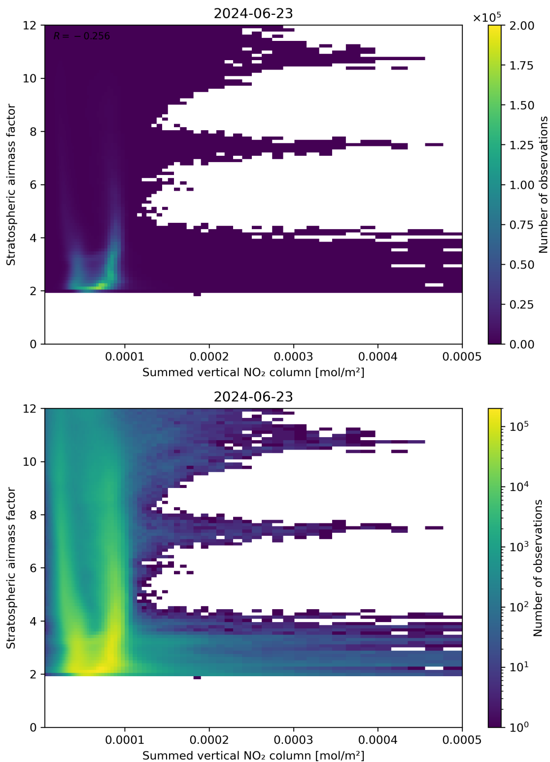
Figure 103: Scatter density plot of “Summed vertical NO 2 column” against “Stratospheric air mass factor” for 2024-06-22 to 2024-06-24.
