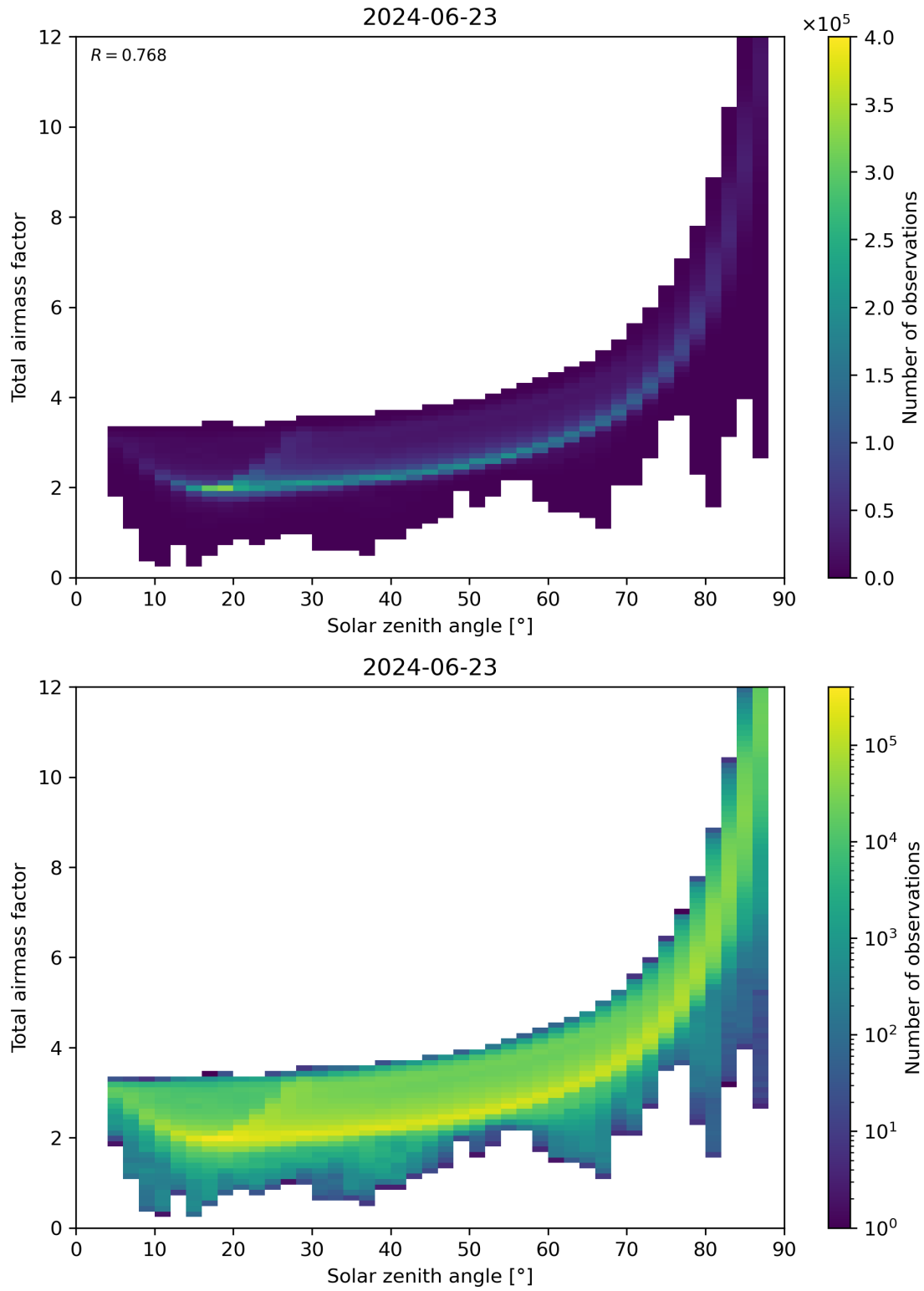
Figure 146: Scatter density plot of “Solar zenith angle” against “Total air mass factor” for 2024-06-22 to 2024-06-24.
