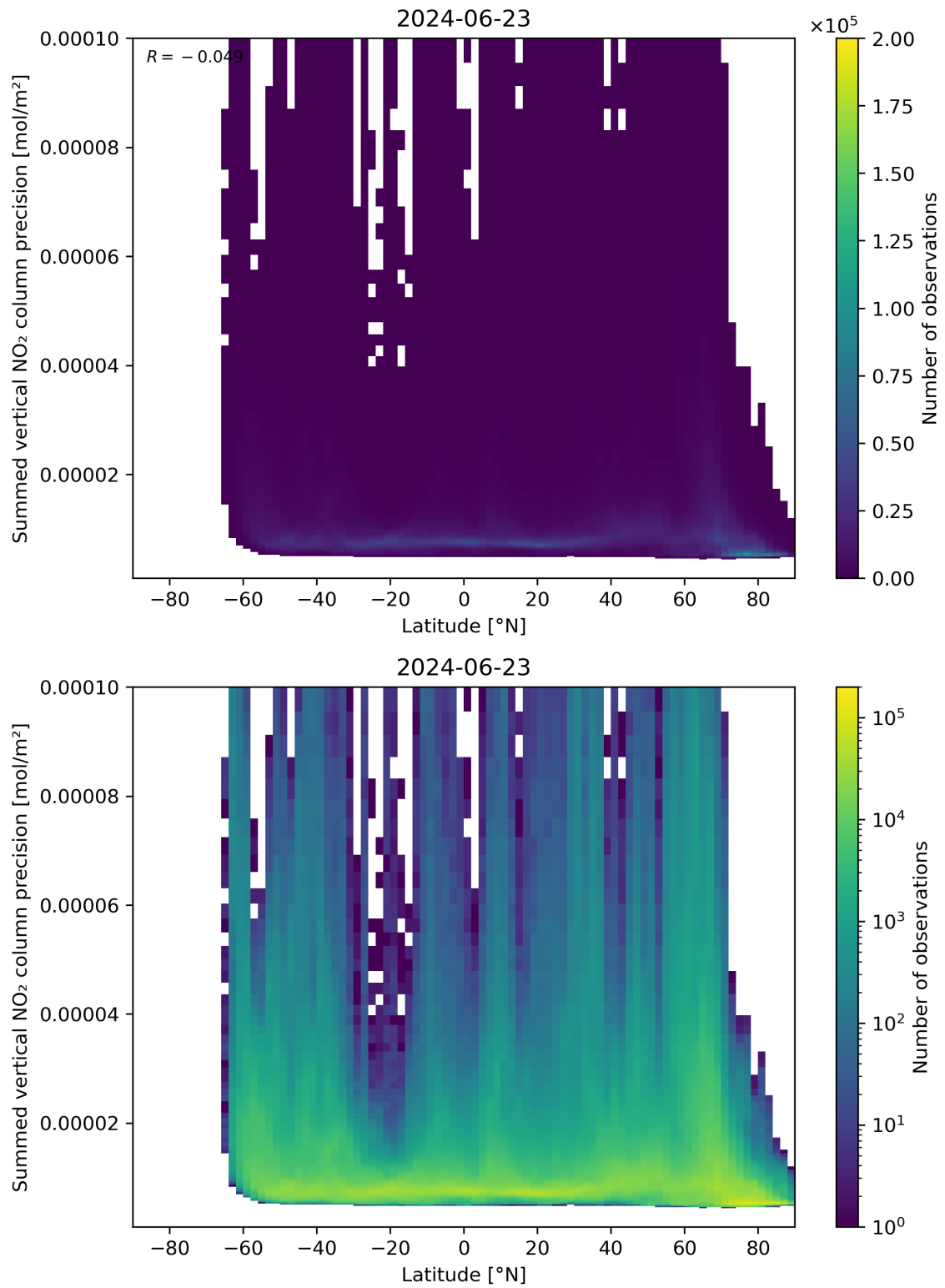
Figure 89: Scatter density plot of “Latitude” against “Summed vertical NO 2 column precision” for 2024-06-22 to 2024-06-24.
