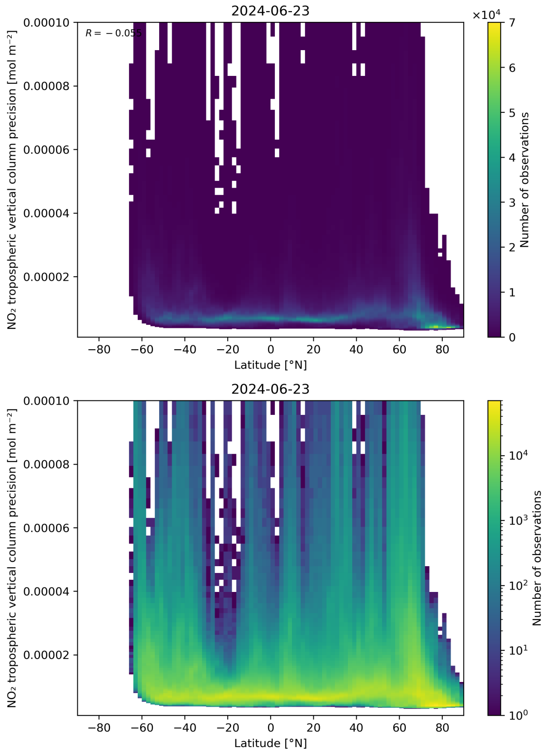
Figure 93: Scatter density plot of “Latitude” against “NO 2 tropospheric vertical column precision” for 2024-06-22 to 2024-06-24.
