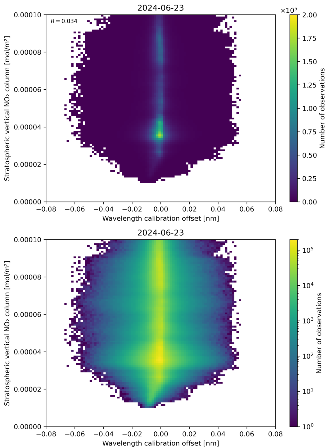
Figure 176: Scatter density plot of “Wavelength calibration offset” against “Stratospheric vertical NO 2 column” for 2024-06-22 to 2024-06-24.
