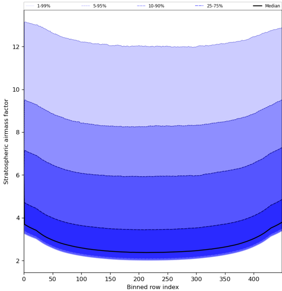
Figure 61: Along track statistics of “Stratospheric airmass factor” for 2024-06-22 to 2024-06-24
