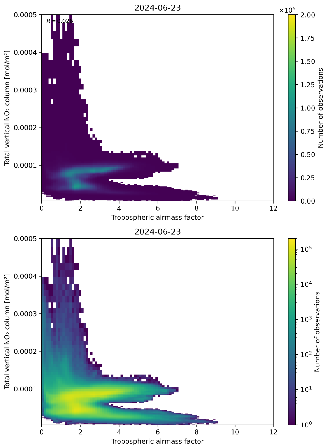
Figure 77: Scatter density plot of “Tropospheric airmass factor” against “Total vertical NO 2 column” for 2024-06-22 to 2024-06-24.
