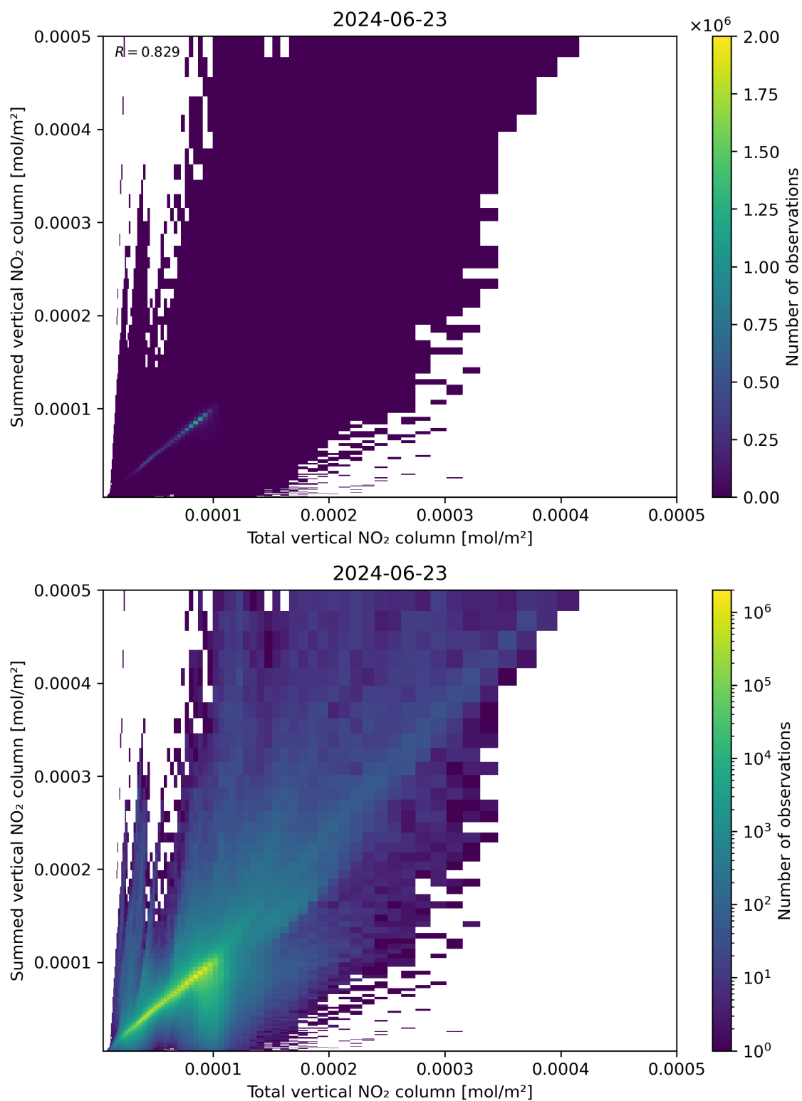
Figure 112: Scatter density plot of “Total vertical NO 2 column” against “Summed vertical NO 2 column” for 2024-06-22 to 2024-06-24.
