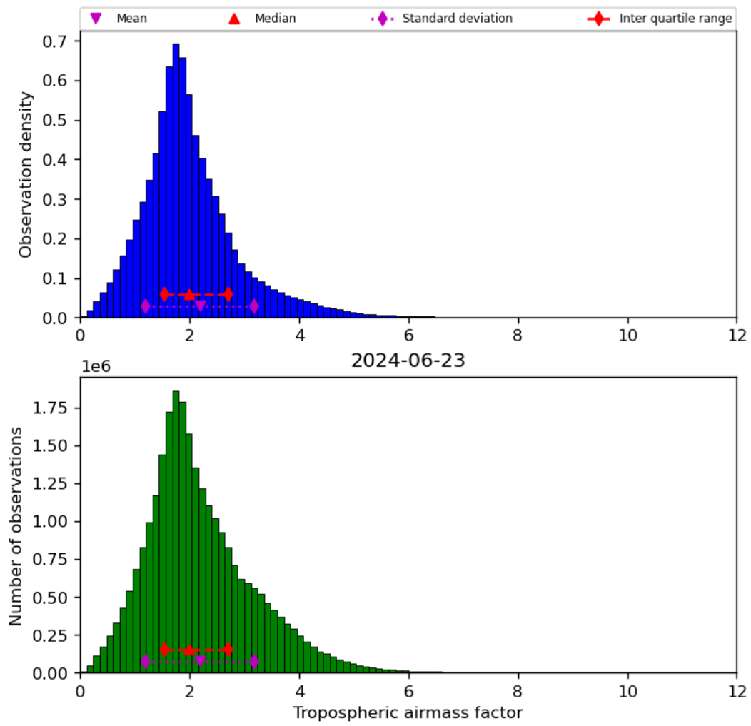
Figure 31: Histogram of “Tropospheric airmass factor” for 2024-06-22 to 2024-06-24
