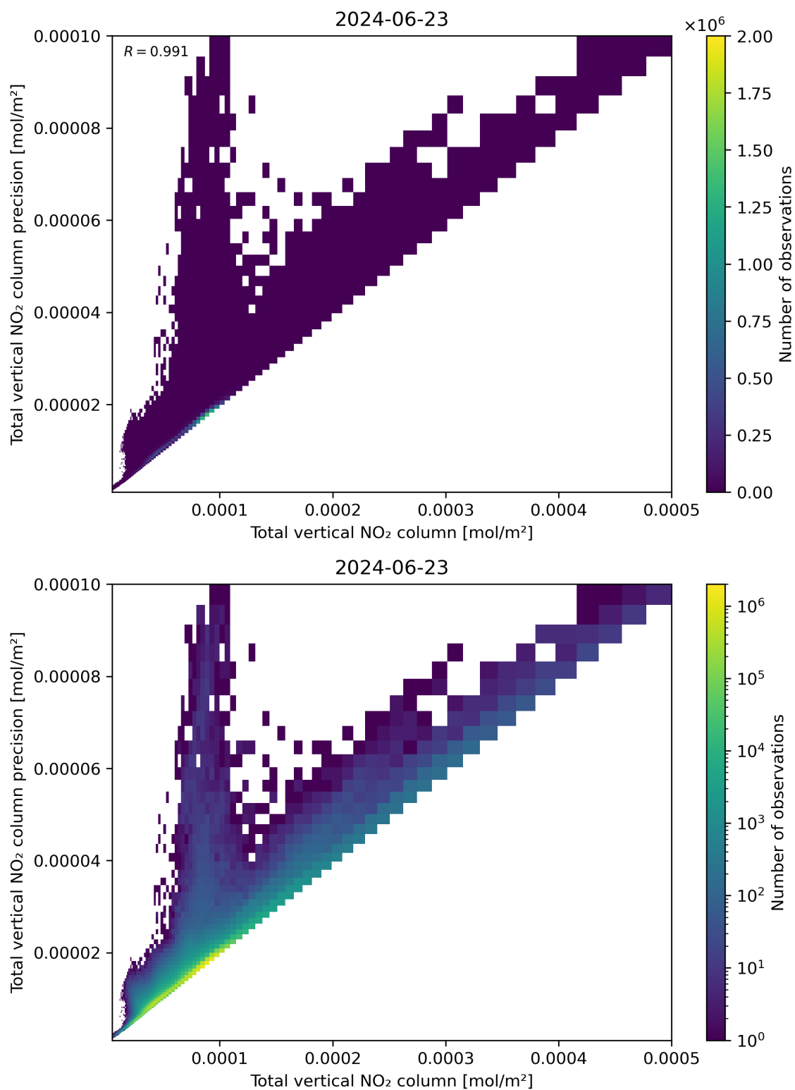
Figure 114: Scatter density plot of “Total vertical NO 2 column” against “Total vertical NO 2 column precision” for 2024-06-22 to 2024-06-24.
