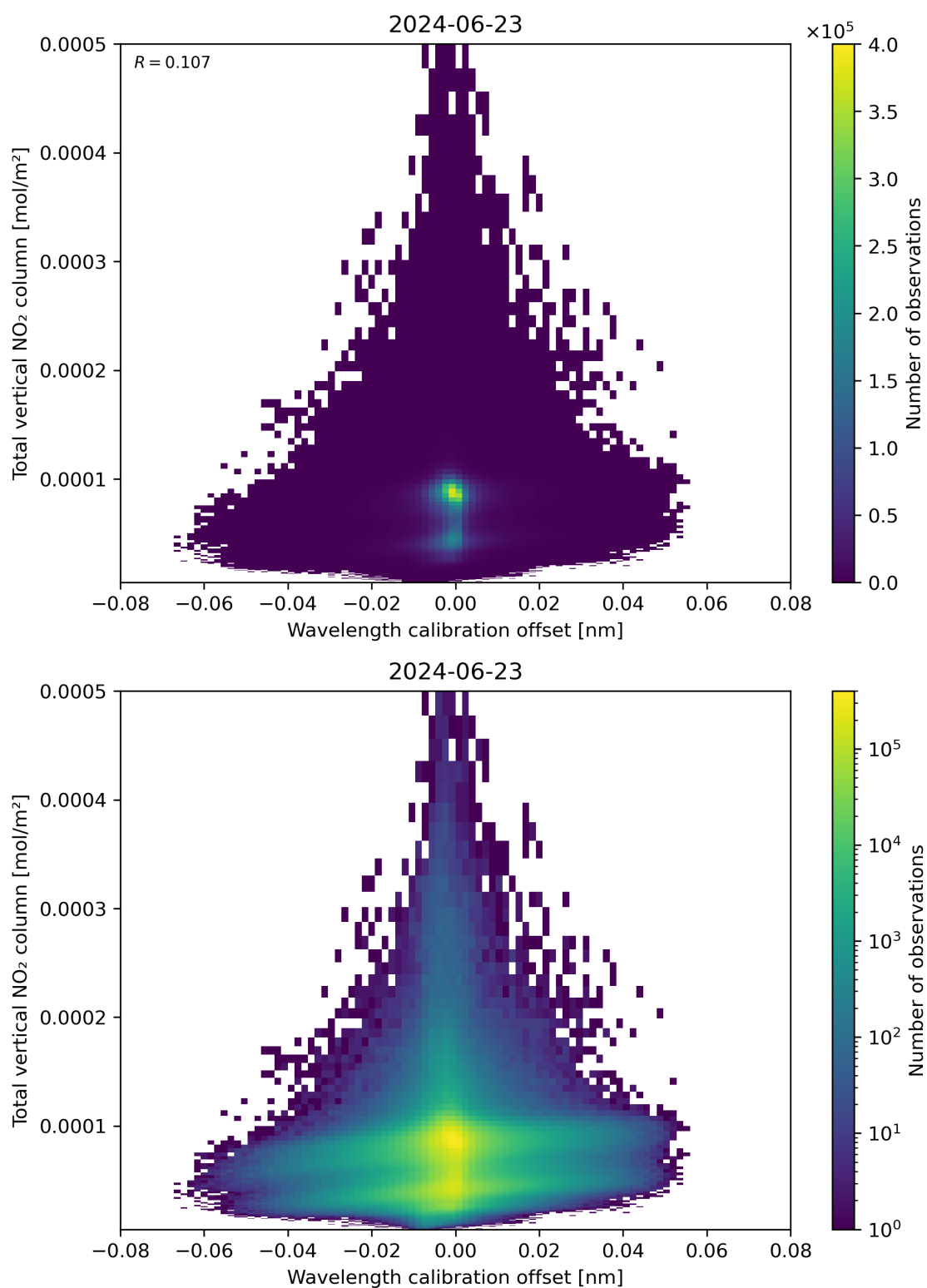
Figure 179: Scatter density plot of “Wavelength calibration offset” against “Total vertical NO 2 column” for 2024-06-22 to 2024-06-24.
