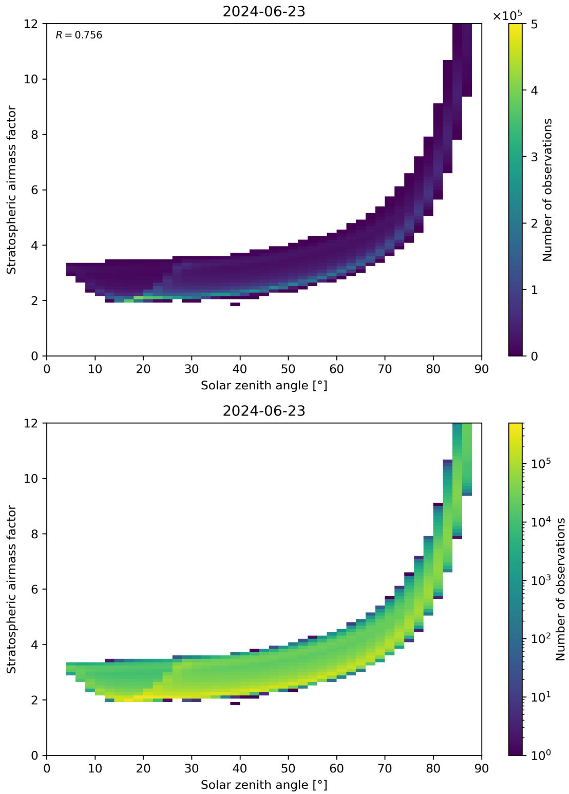
Figure 145: Scatter density plot of “Solar zenith angle” against “Stratospheric airmass factor” for 2024-06-22 to 2024-06-24.
