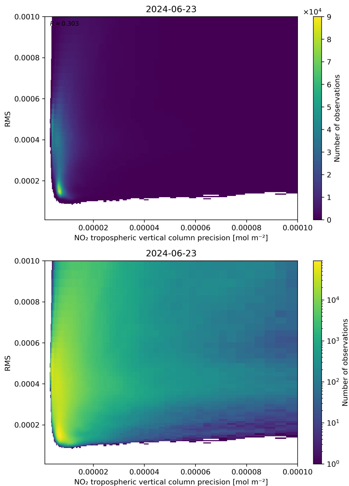
Figure 140: Scatter density plot of “NO 2 tropospheric vertical column precision” against “RMS” for 2024-06-22 to 2024-06-24.
