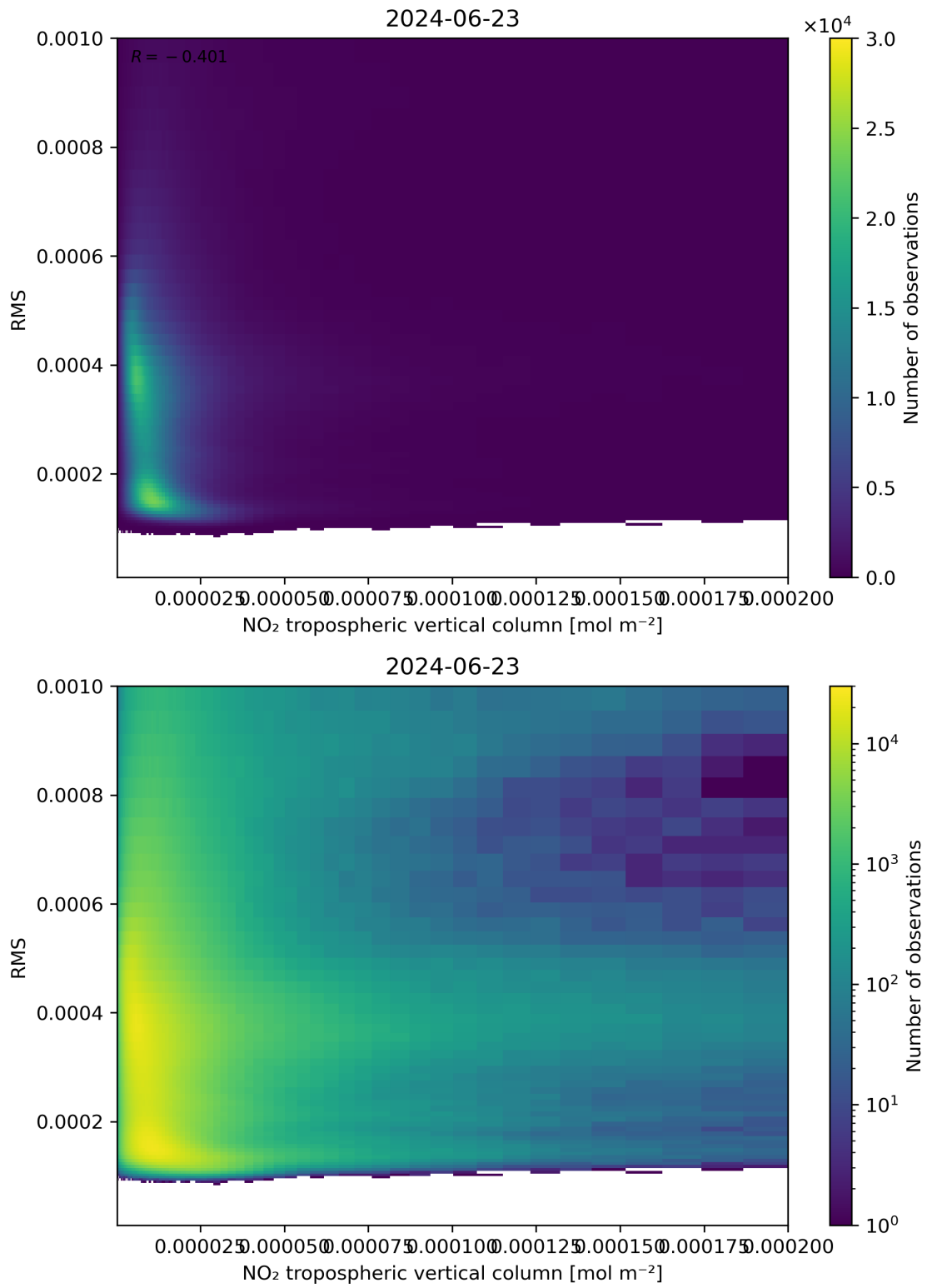
Figure 142: Scatter density plot of “NO 2 tropospheric vertical column” against “RMS” for 2024-06-22 to 2024-06-24.
