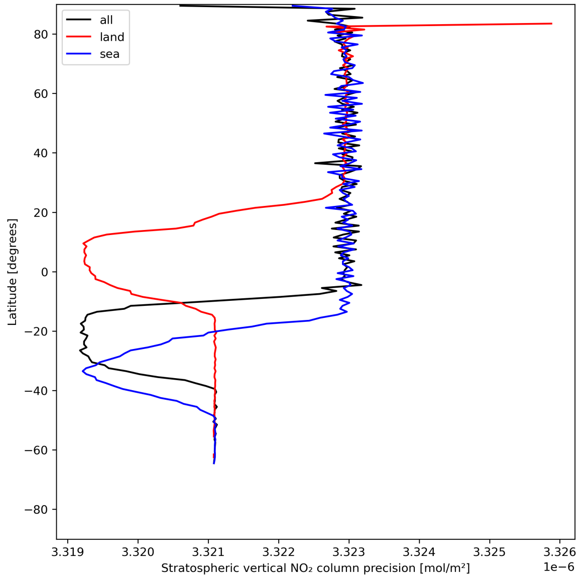
Figure 20: Zonal average of “Stratospheric vertical NO 2 column precision” for 2024-06-22 to 2024-06-24.
