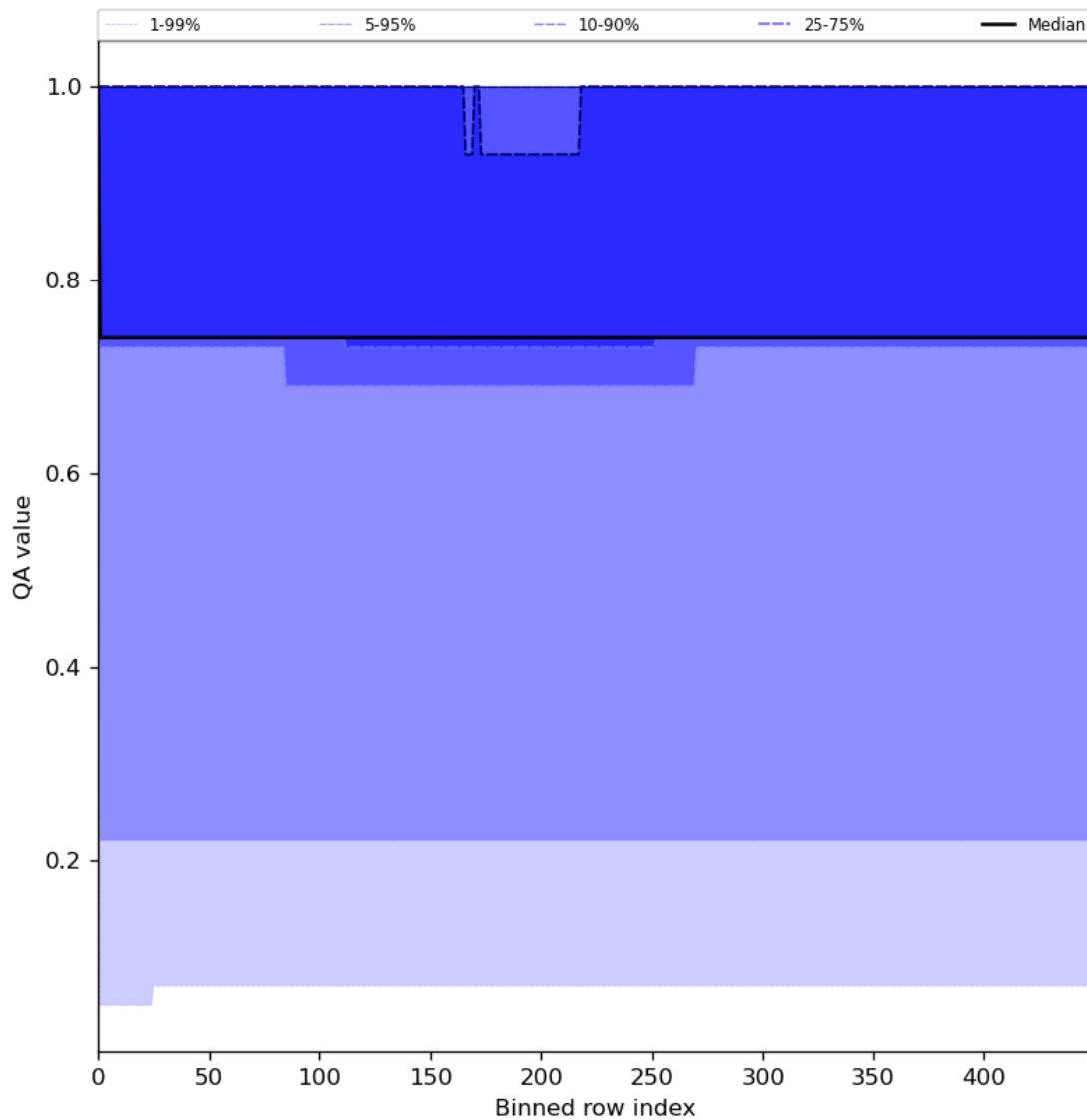
Figure 45: Along track statistics of “QA value” for 2024-06-22 to 2024-06-24
