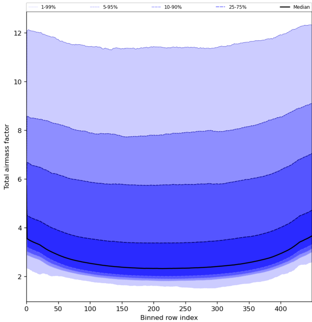
Figure 49: Along track statistics of “Total airmass factor” for 2024-06-22 to 2024-06-24
