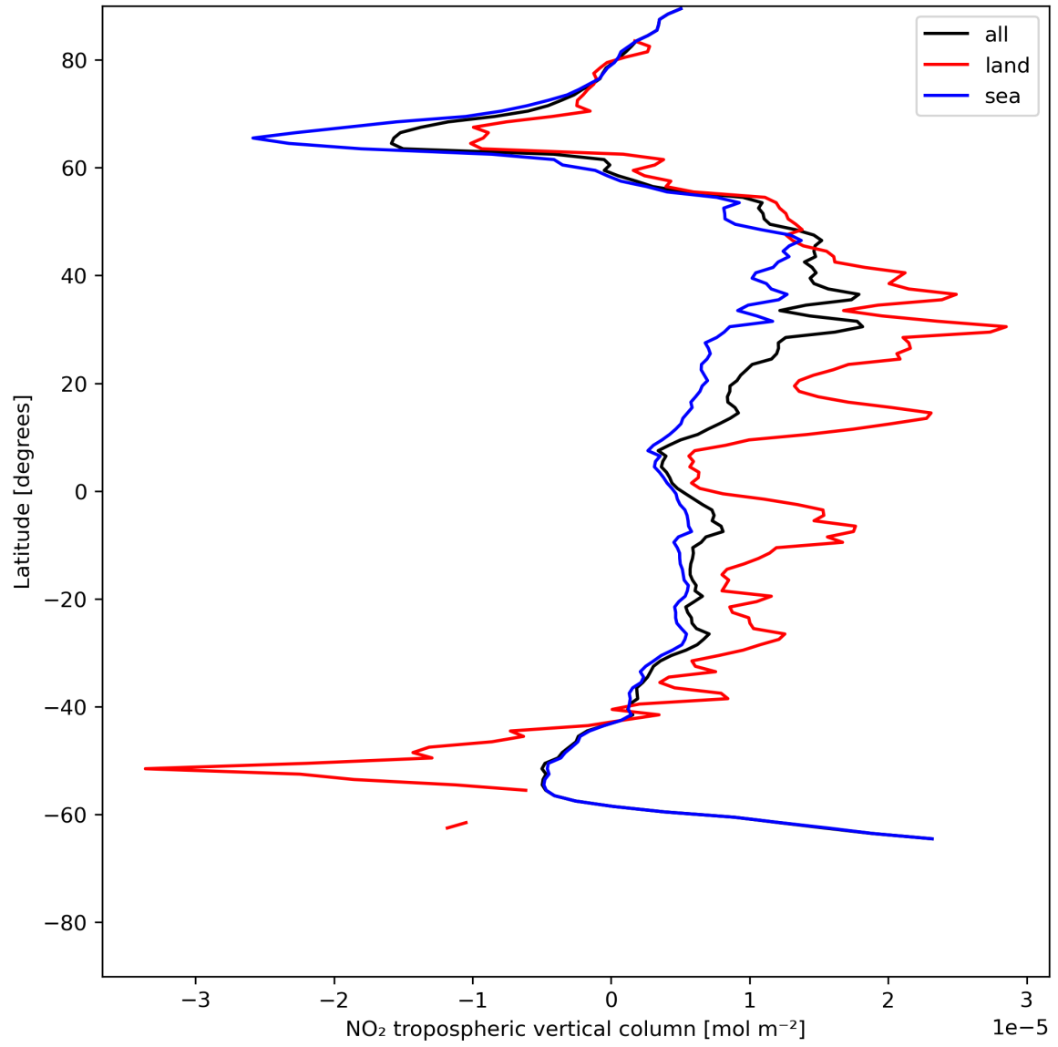
Figure 12: Zonal average of “NO 2 tropospheric vertical column” for 2024-06-22 to 2024-06-24.
