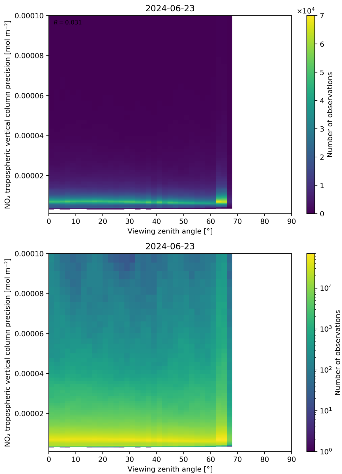
Figure 170: Scatter density plot of “Viewing zenith angle” against “NO 2 tropospheric vertical column precision” for 2024-06-22 to 2024-06-24.
