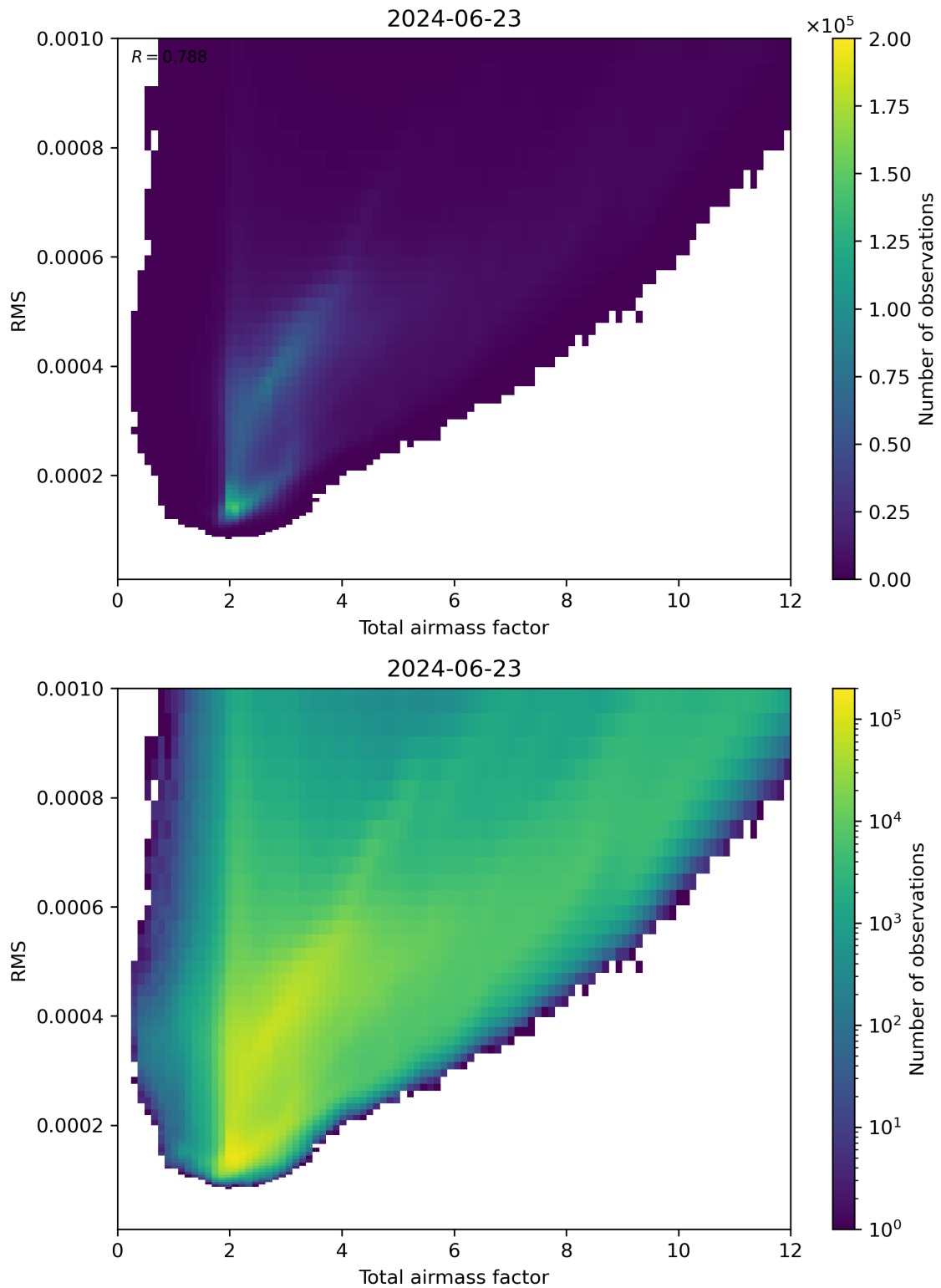
Figure 69: Scatter density plot of “Total airmass factor” against “RMS” for 2024-06-22 to 2024-06-24.
