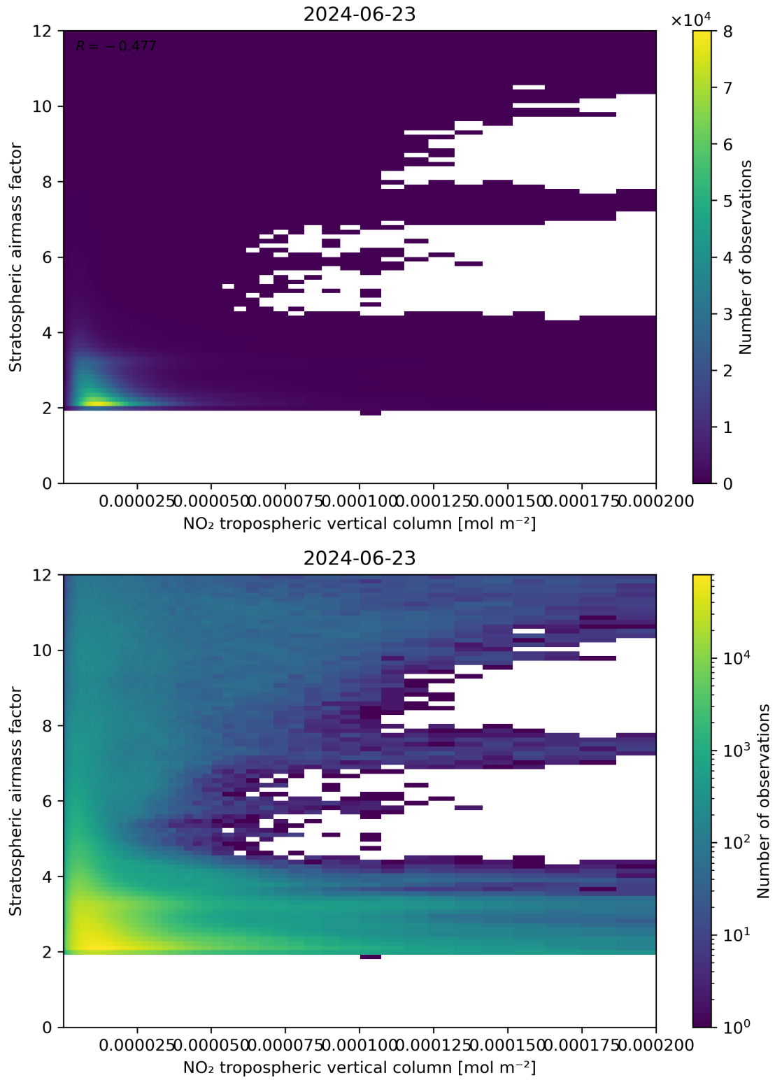
Figure 121: Scatter density plot of “NO 2 tropospheric vertical column” against “Stratospheric air mass factor” for 2024-06-22 to 2024-06-24.
