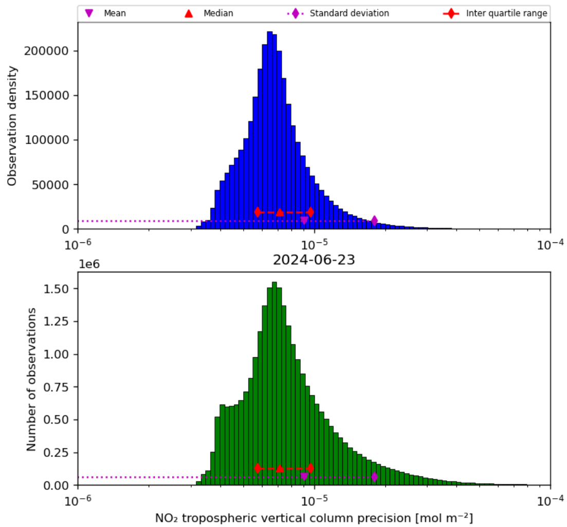
Figure 30: Histogram of “NO 2 tropospheric vertical column precision” for 2024-06-22 to 2024-06-24
