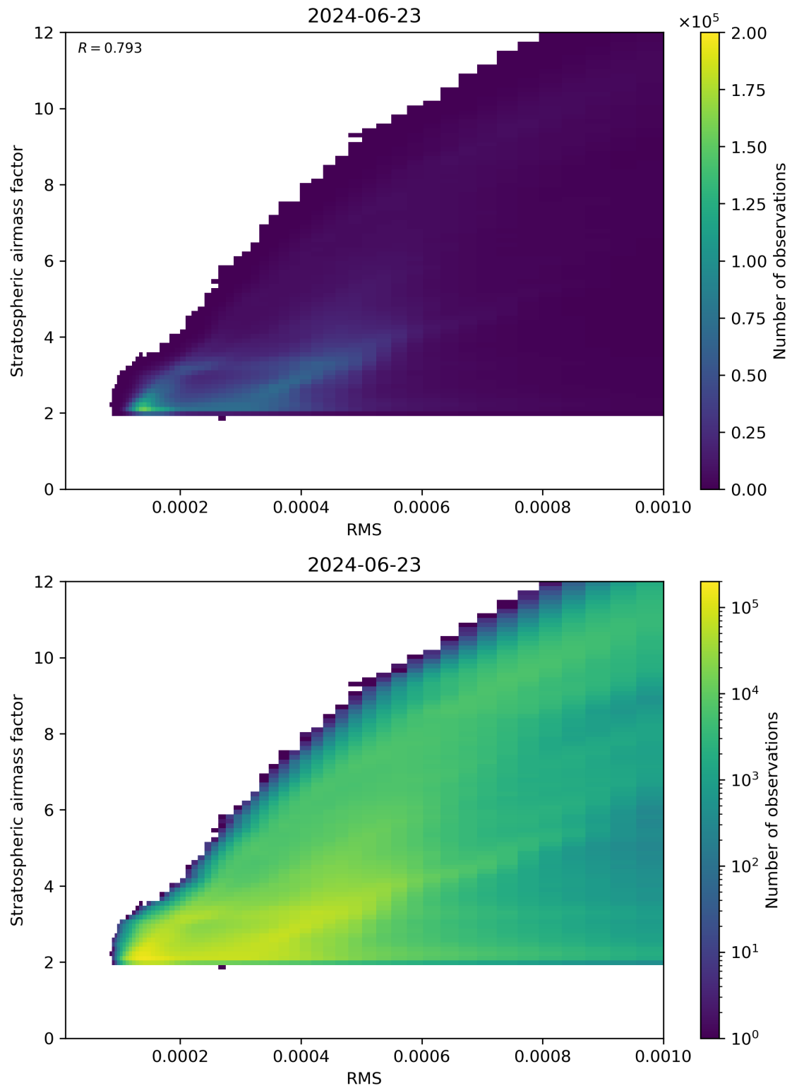
Figure 144: Scatter density plot of “RMS” against “Stratospheric airmass factor” for 2024-06-22 to 2024-06-24.
