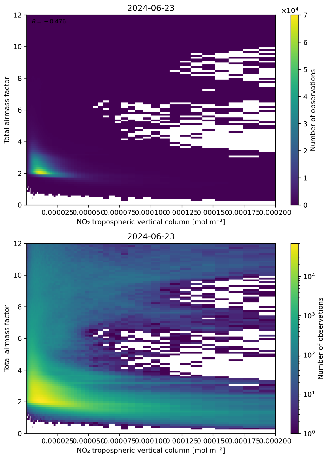
Figure 122: Scatter density plot of “NO 2 tropospheric vertical column” against “Total air mass factor” for 2024-06-22 to 2024-06-24.
