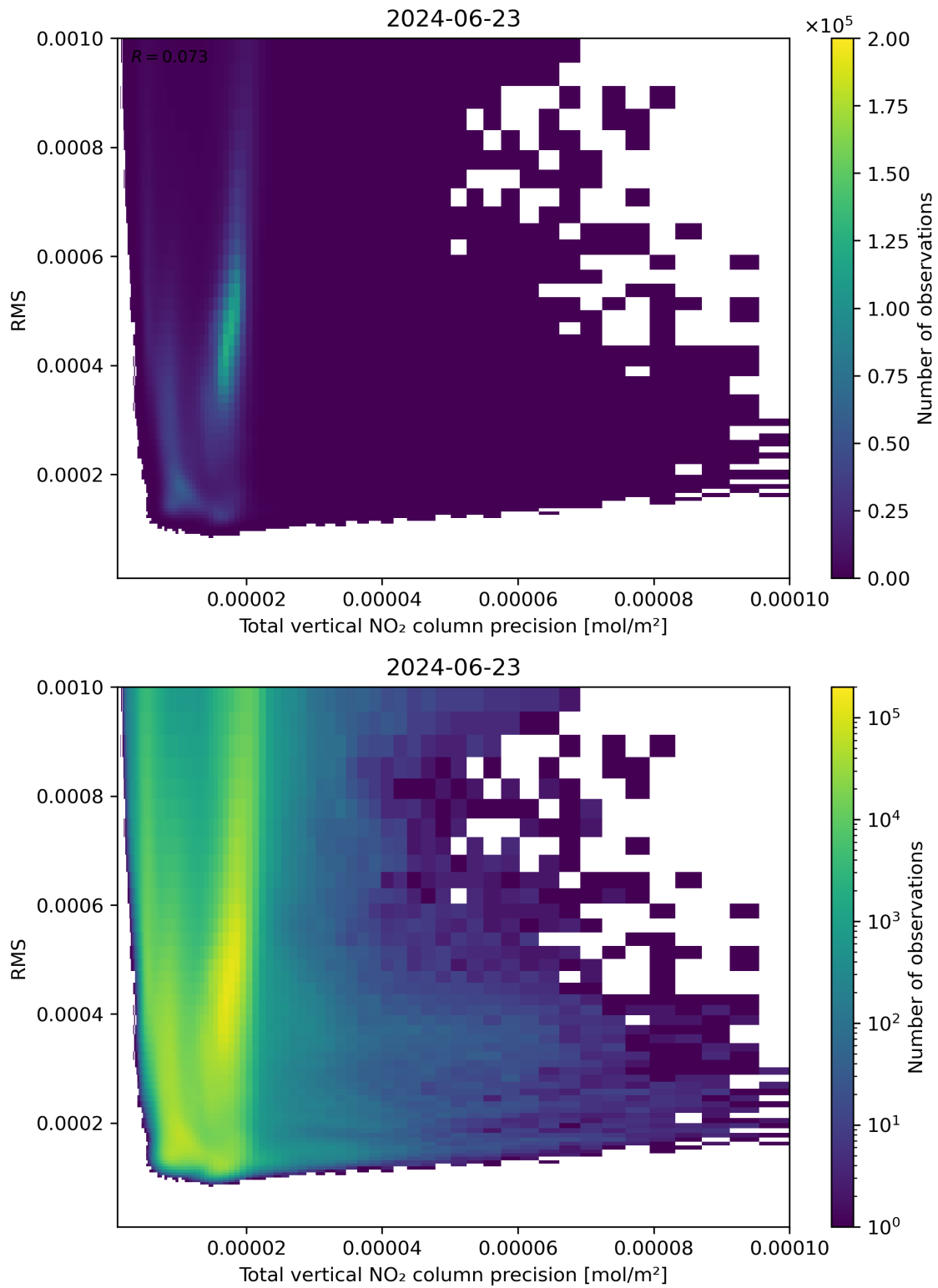
Figure 119: Scatter density plot of “Total vertical NO 2 column precision” against “RMS” for 2024-06-22 to 2024-06-24.
