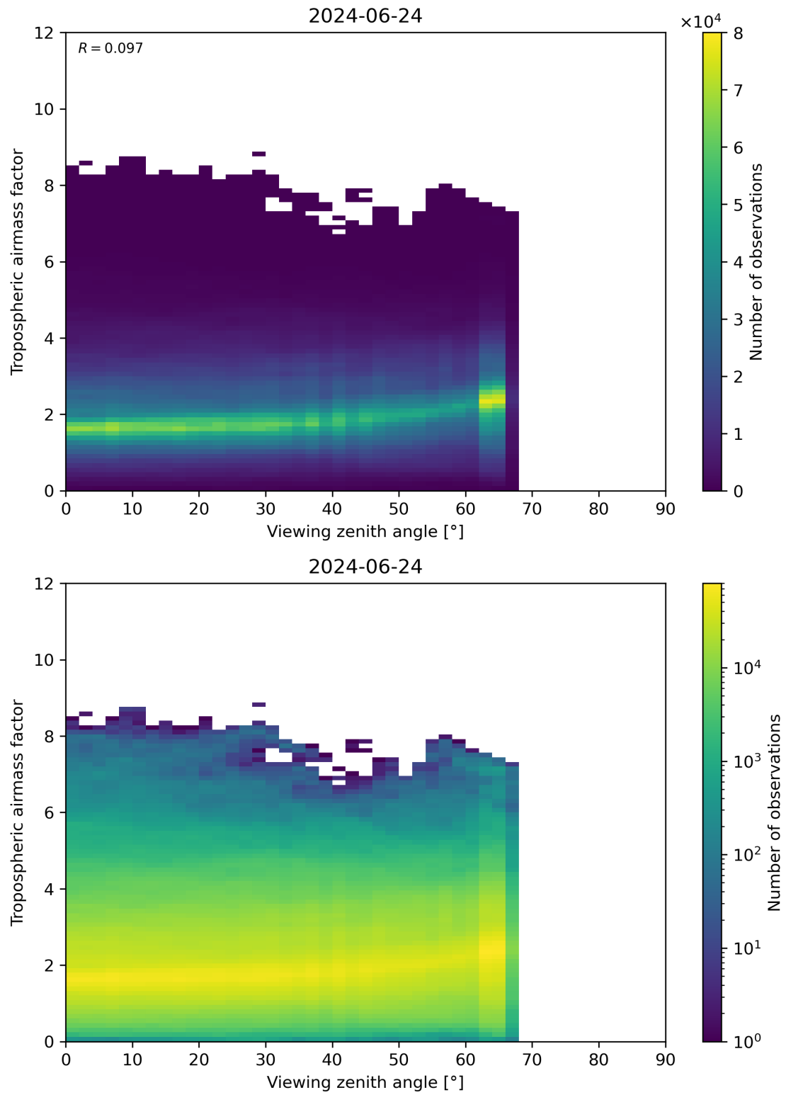
Figure 161: Scatter density plot of “Viewing zenith angle” against “Tropospheric airmass factor” for 2024-06-24 to 2024-06-25.
