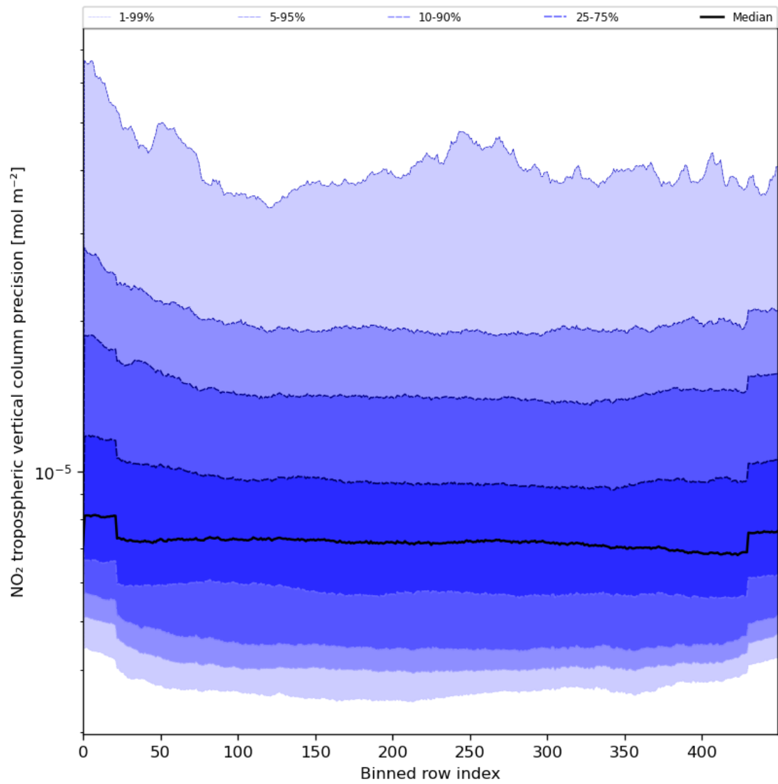
Figure 47: Along track statistics of “NO 2 tropospheric vertical column precision” for 2024-06-24 to 2024-06-25
