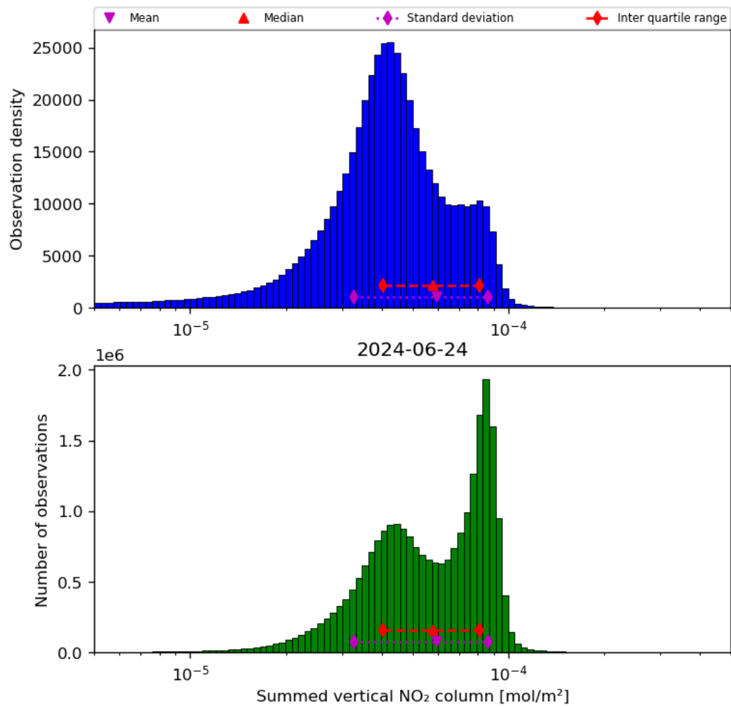
Figure 40: Histogram of “Summed vertical NO 2 column” for 2024-06-24 to 2024-06-25
