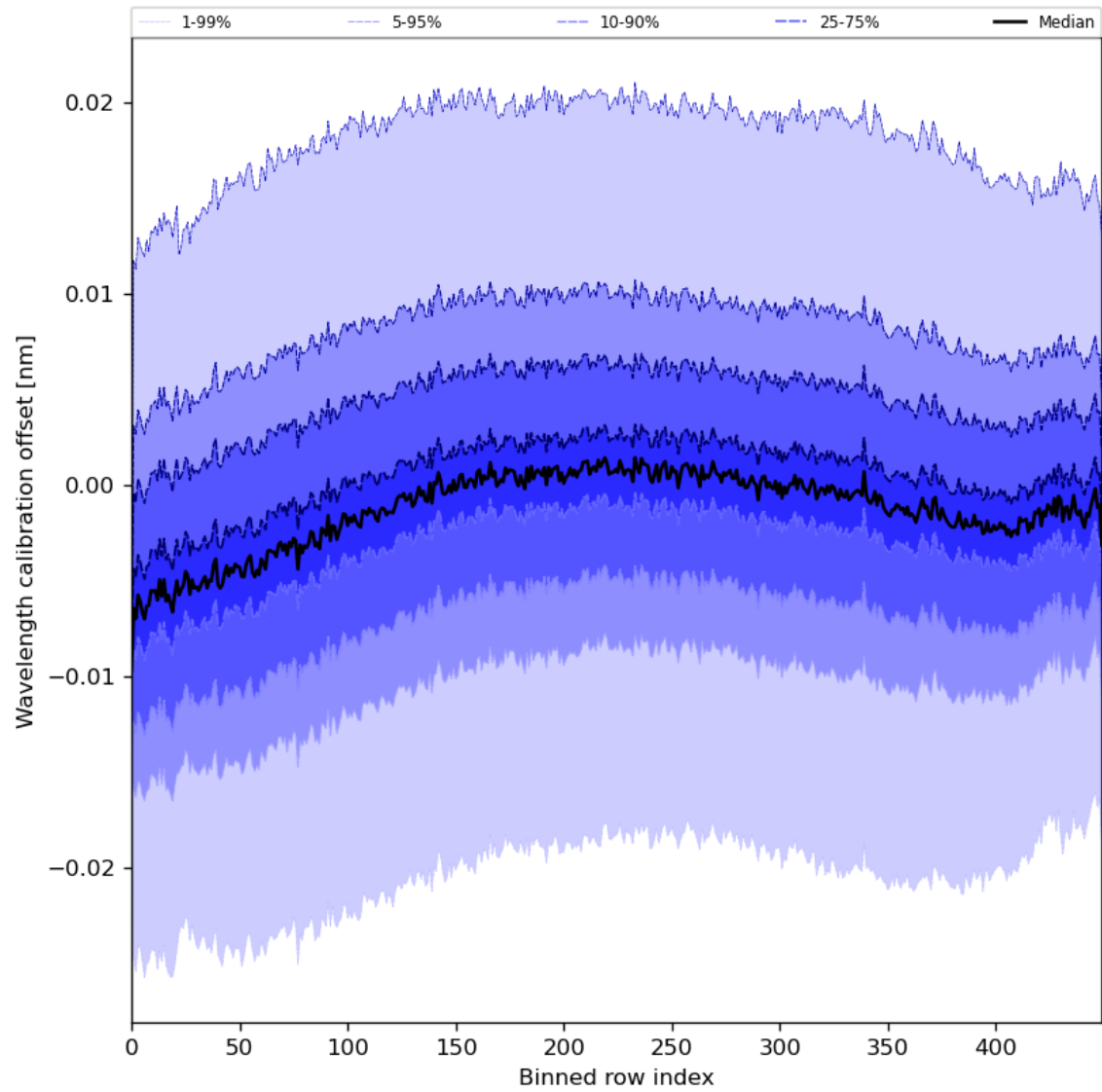
Figure 52: Along track statistics of “Wavelength calibration offset” for 2024-06-24 to 2024-06-25
