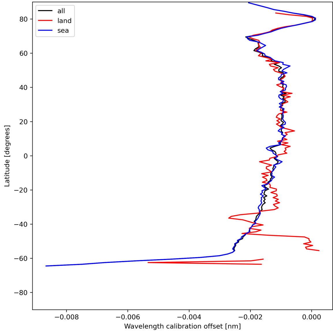
Figure 18: Zonal average of “Wavelength calibration offset” for 2024-06-24 to 2024-06-25.
