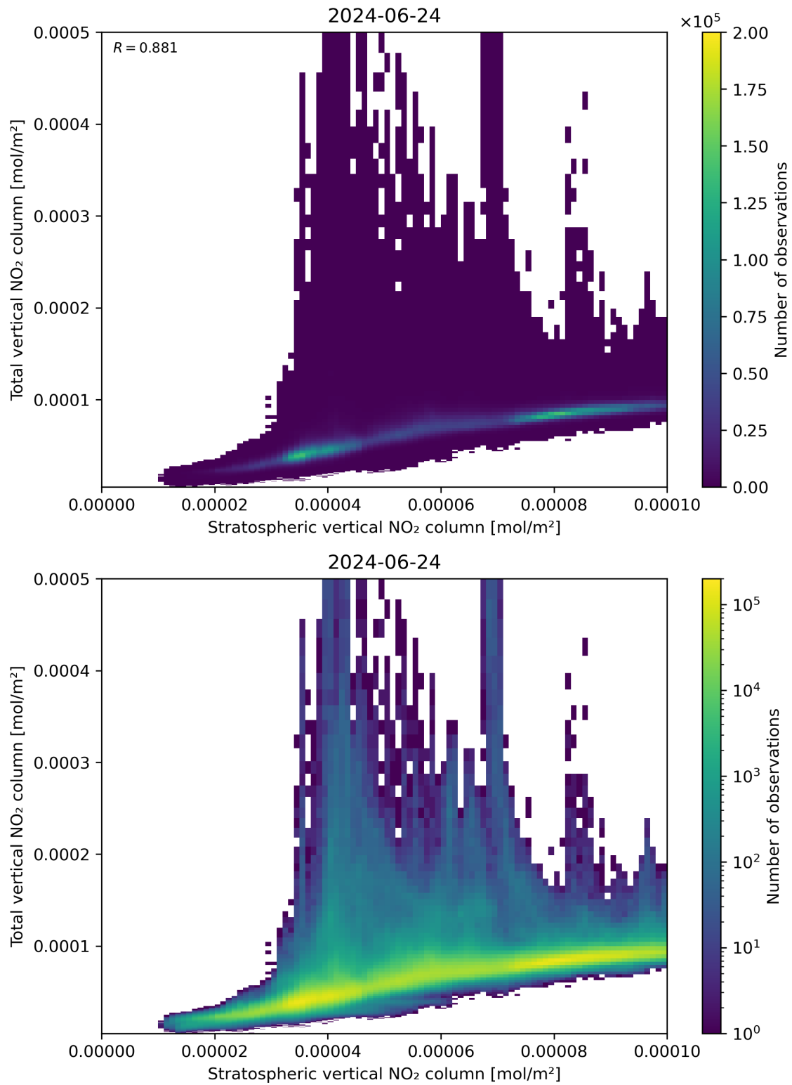
Figure 100: Scatter density plot of “Stratospheric vertical NO 2 column” against “Total vertical NO 2 column” for 2024-06-24 to 2024-06-25.
