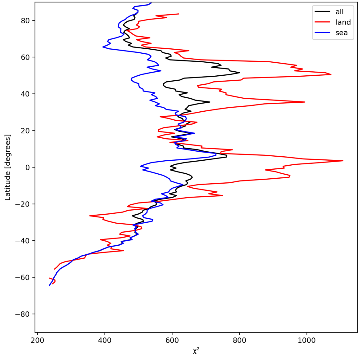
Figure 25: Zonal average of “ \chi^2 ” for 2024-06-24 to 2024-06-25.
