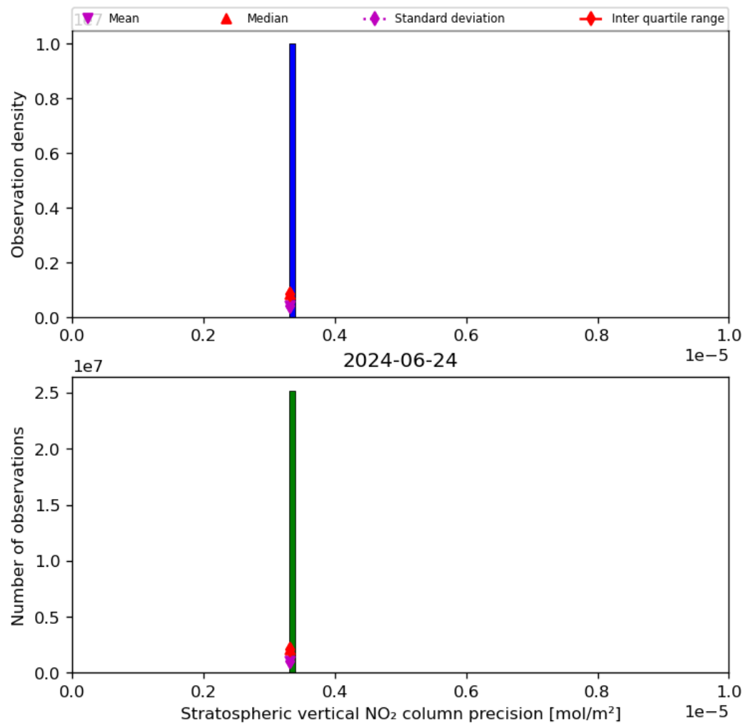
Figure 37: Histogram of “Stratospheric vertical NO 2 column precision” for 2024-06-24 to 2024-06-25
