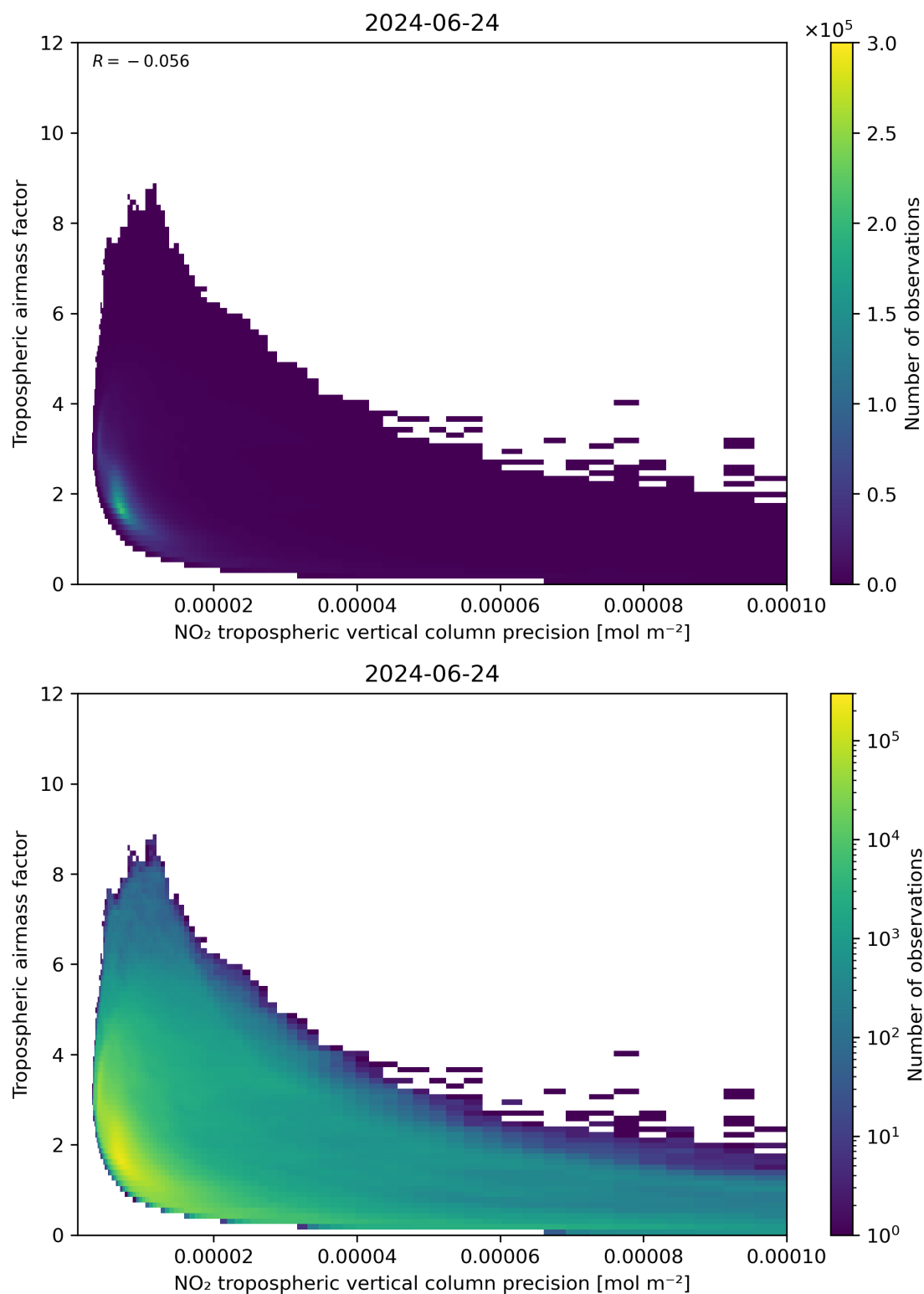
Figure 133: Scatter density plot of “NO 2 tropospheric vertical column precision” against “Tropospheric airmass factor” for 2024-06-24 to 2024-06-25.
