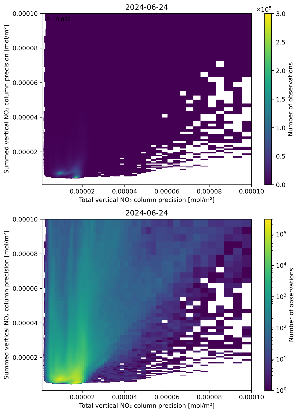
Figure 118: Scatter density plot of “Total vertical NO 2 column precision” against “Summed vertical NO 2 column precision” for 2024-06-24 to 2024-06-25.
