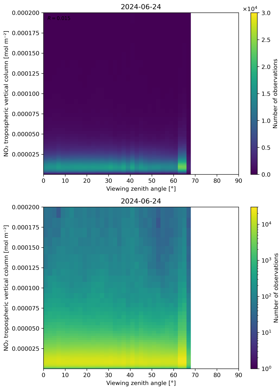
Figure 169: Scatter density plot of “Viewing zenith angle” against “NO 2 tropospheric vertical column” for 2024-06-24 to 2024-06-25.
