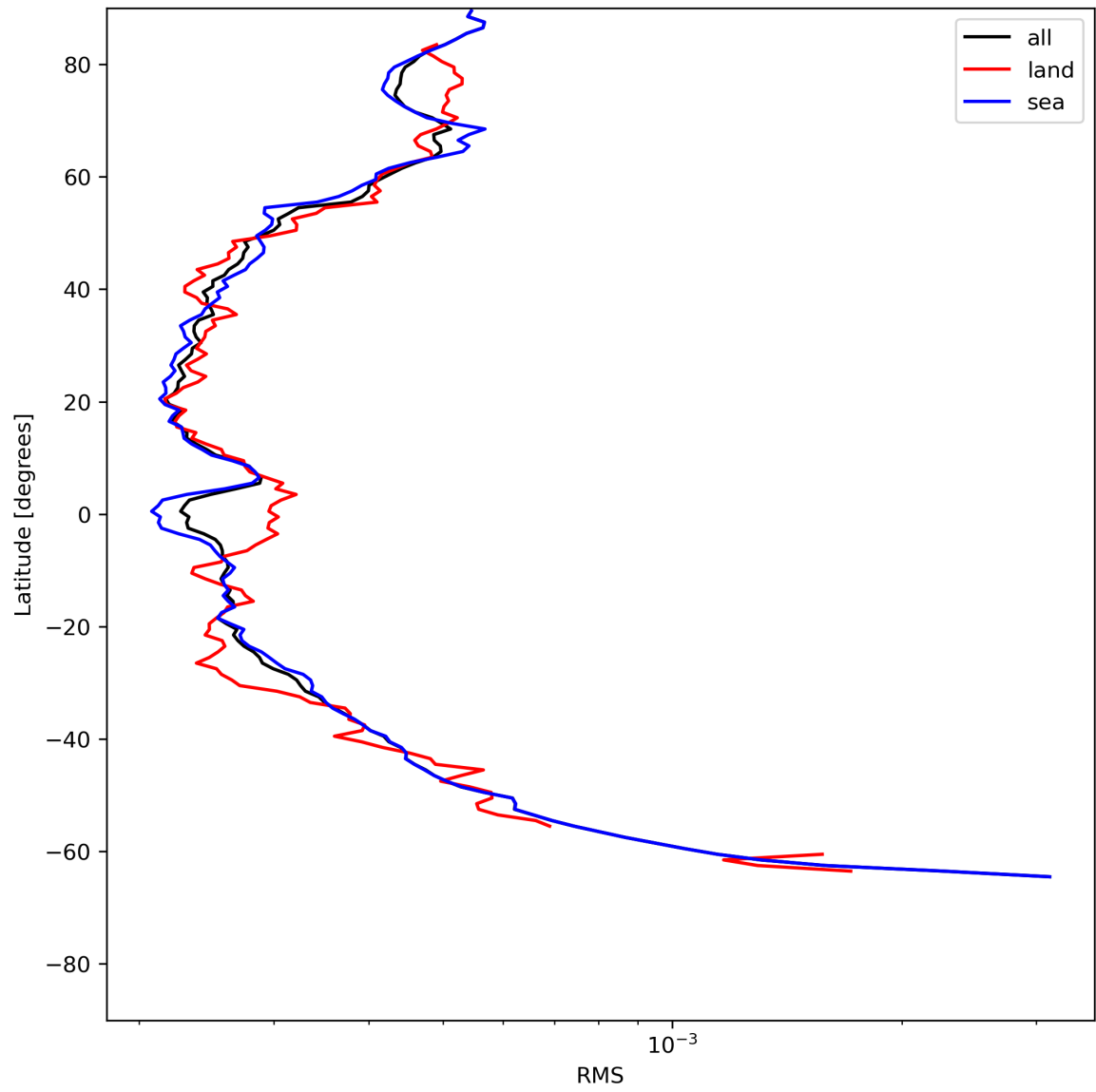
Figure 26: Zonal average of “RMS” for 2024-06-24 to 2024-06-25.
