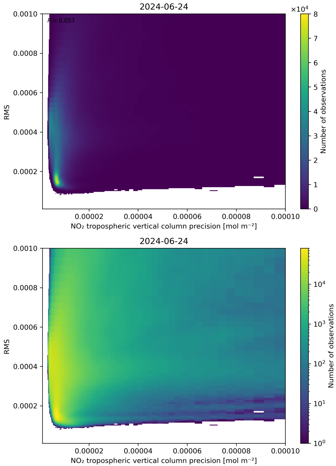
Figure 140: Scatter density plot of “NO 2 tropospheric vertical column precision” against “RMS” for 2024-06-24 to 2024-06-25.
