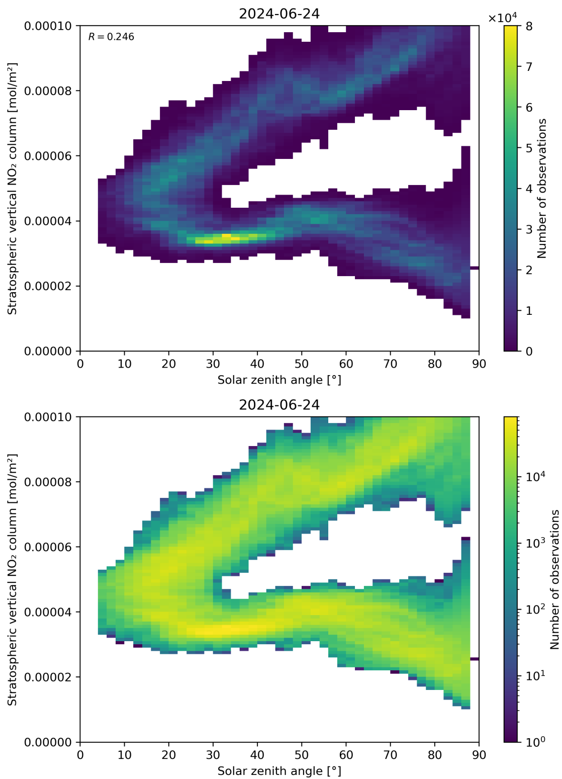
Figure 150: Scatter density plot of “Solar zenith angle” against “Stratospheric vertical NO 2 column” for 2024-06-24 to 2024-06-25.
