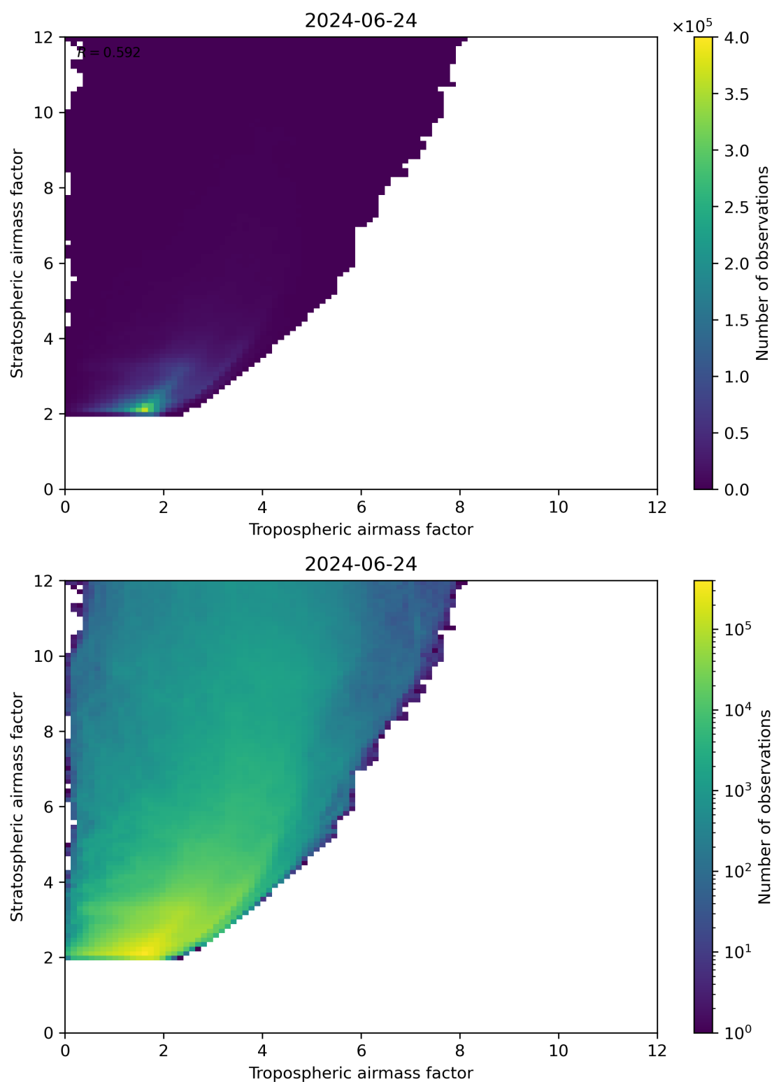
Figure 71: Scatter density plot of “Tropospheric airmass factor” against “Stratospheric airmass factor” for 2024-06-24 to 2024-06-25.
