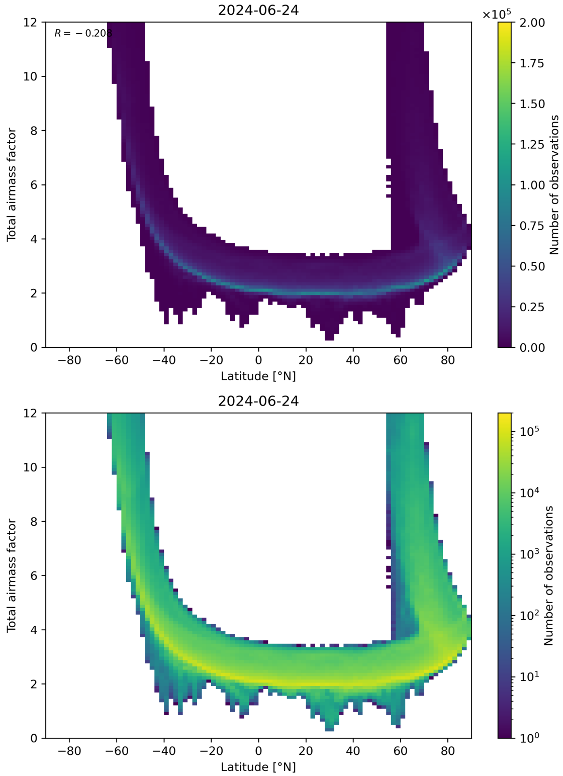
Figure 84: Scatter density plot of “Latitude” against “Total airmass factor” for 2024-06-24 to 2024-06-25.
