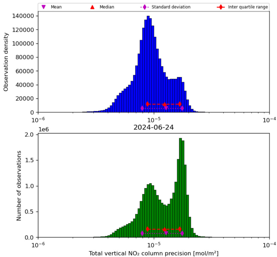
Figure 39: Histogram of “Total vertical NO 2 column precision” for 2024-06-24 to 2024-06-25
