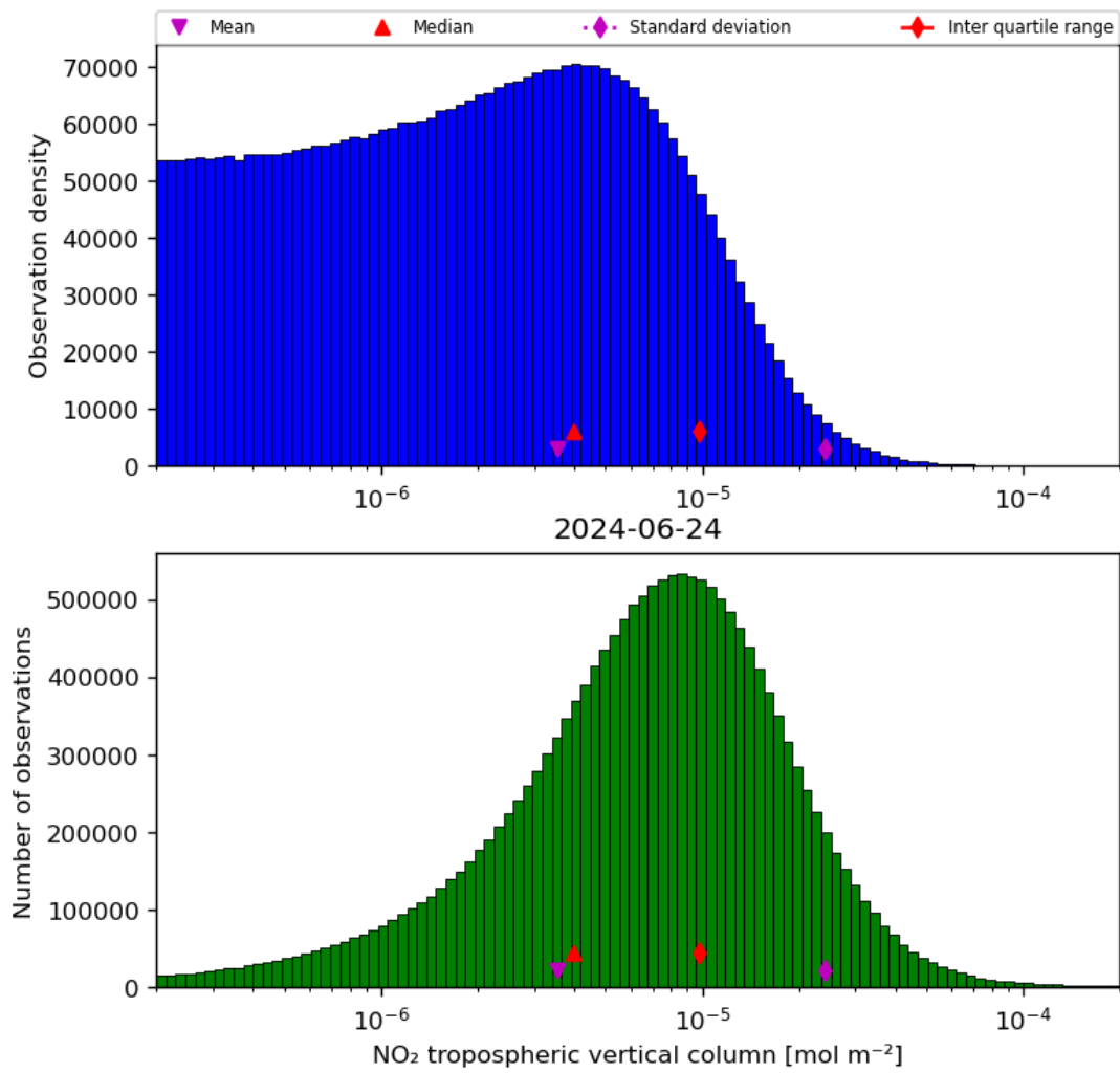
Figure 29: Histogram of “NO 2 tropospheric vertical column” for 2024-06-24 to 2024-06-25
