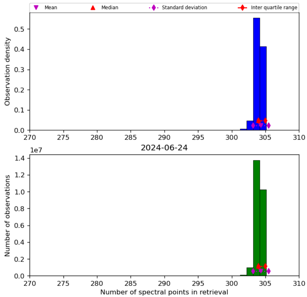
Figure 33: Histogram of “Number of spectral points in retrieval” for 2024-06-24 to 2024-06-25
