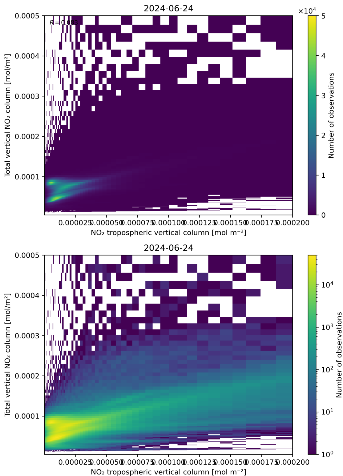
Figure 128: Scatter density plot of “NO 2 tropospheric vertical column” against “Total vertical NO 2 column” for 2024-06-24 to 2024-06-25.
