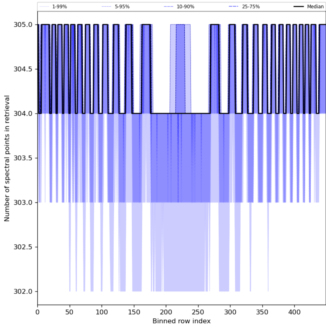
Figure 50: Along track statistics of “Number of spectral points in retrieval” for 2024-06-24 to 2024-06-25
