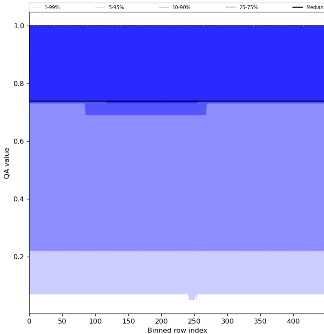
Figure 45: Along track statistics of “QA value” for 2024-06-24 to 2024-06-25
