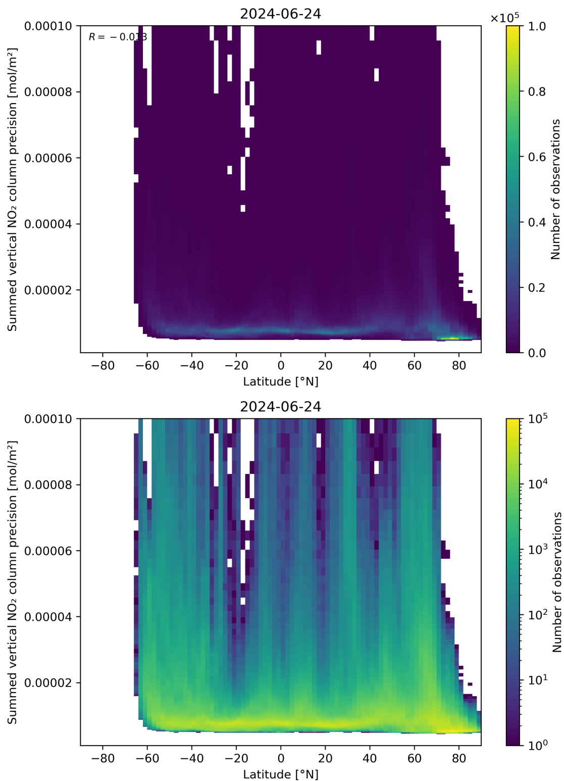
Figure 89: Scatter density plot of “Latitude” against “Summed vertical NO 2 column precision” for 2024-06-24 to 2024-06-25.
