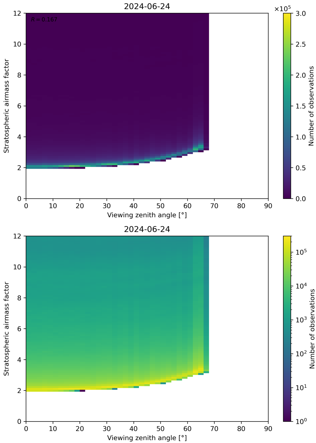
Figure 159: Scatter density plot of “Viewing zenith angle” against “Stratospheric airmass factor” for 2024-06-24 to 2024-06-25.
