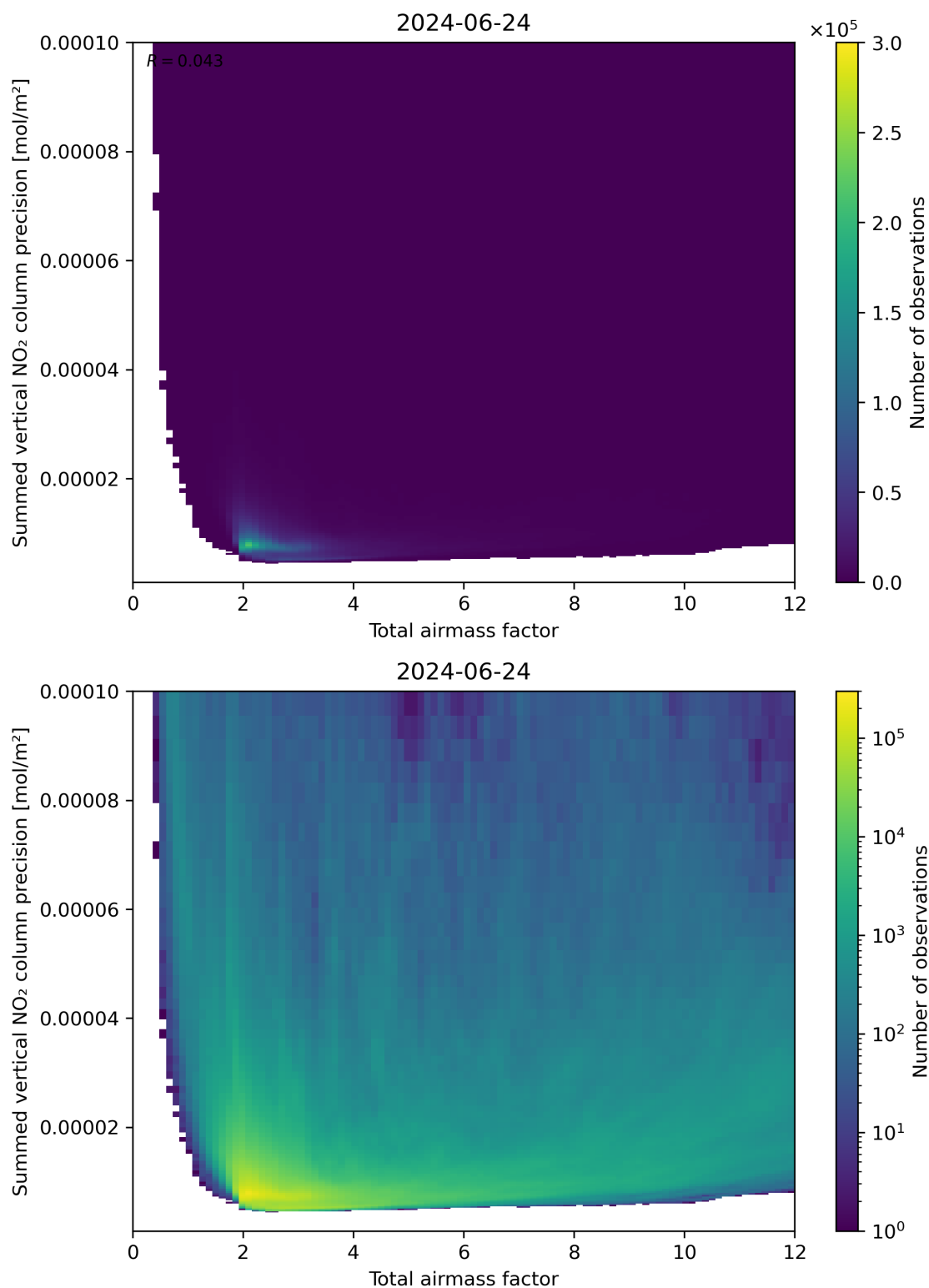
Figure 66: Scatter density plot of “Total airmass factor” against “Summed vertical NO 2 column precision” for 2024-06-24 to 2024-06-25.
