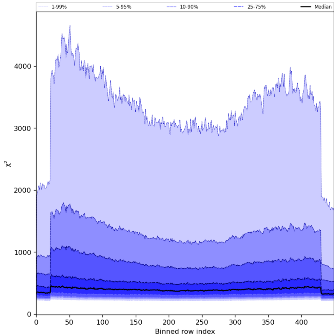
Figure 59: Along track statistics of “ \chi^2 ” for 2024-06-24 to 2024-06-25
