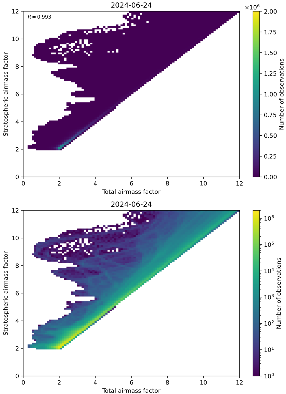
Figure 62: Scatter density plot of “Total airmass factor” against “Stratospheric airmass factor” for 2024-06-24 to 2024-06-25.
