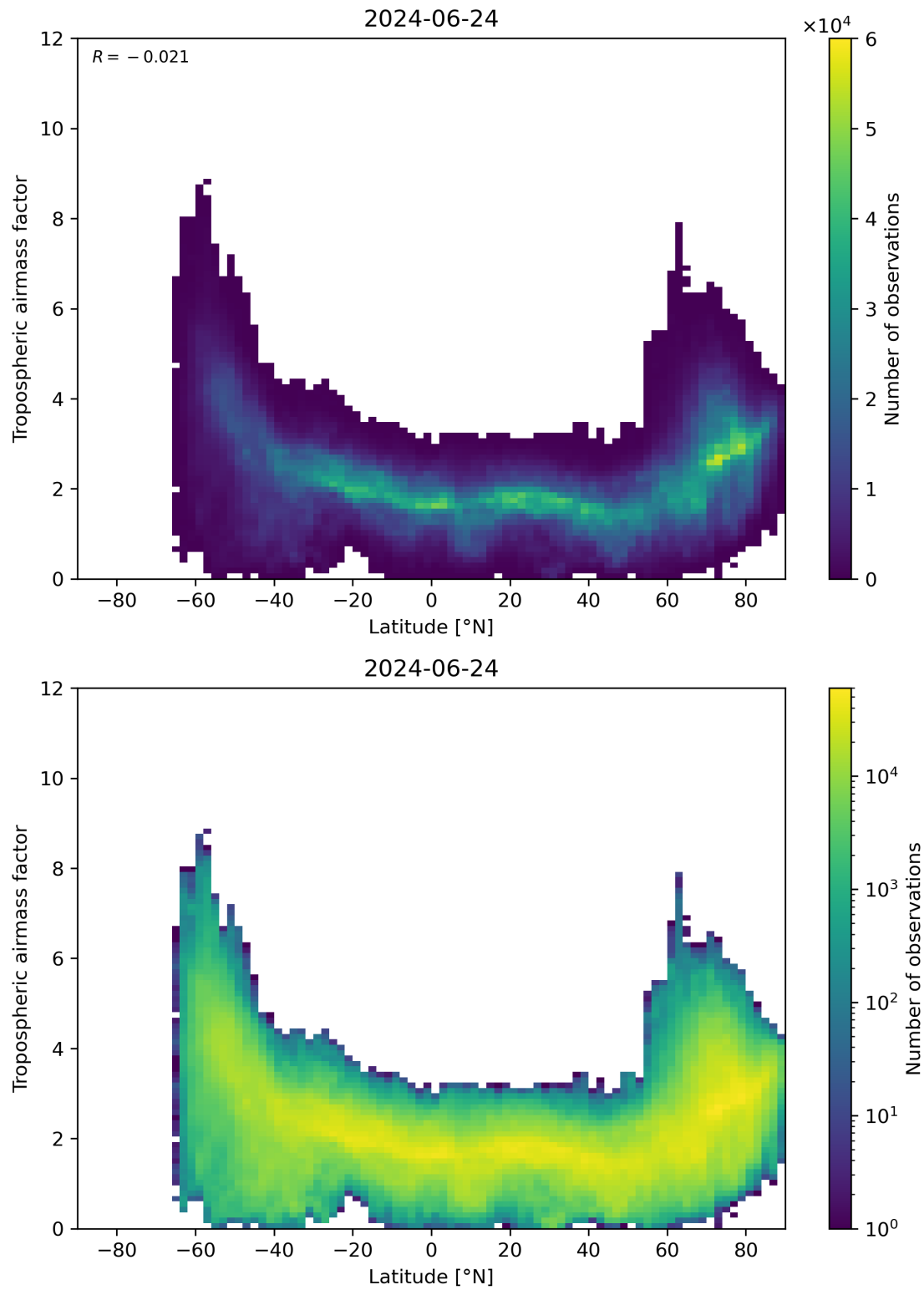
Figure 85: Scatter density plot of “Latitude” against “Tropospheric airmass factor” for 2024-06-24 to 2024-06-25.
