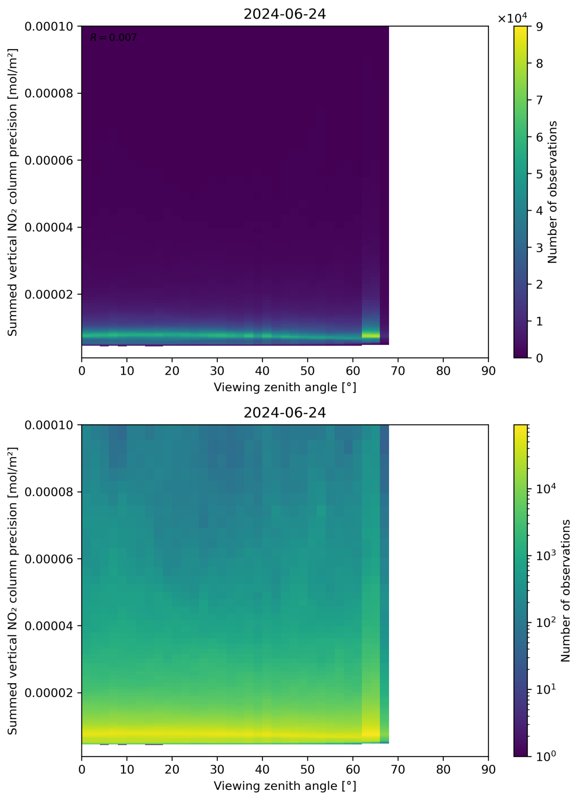
Figure 166: Scatter density plot of “Viewing zenith angle” against “Summed vertical NO 2 column precision” for 2024-06-24 to 2024-06-25.
