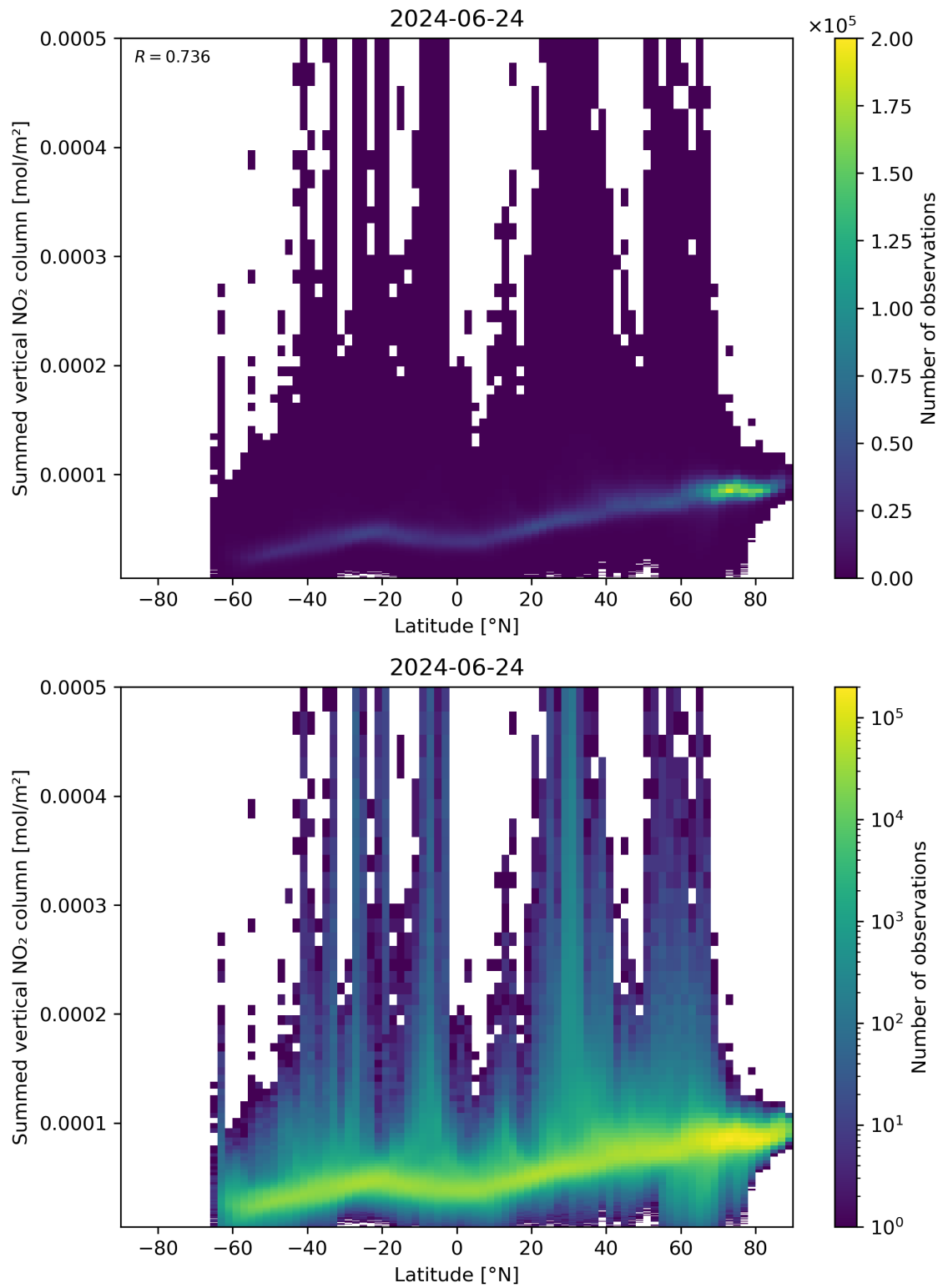
Figure 88: Scatter density plot of “Latitude” against “Summed vertical NO 2 column” for 2024-06-24 to 2024-06-25.
