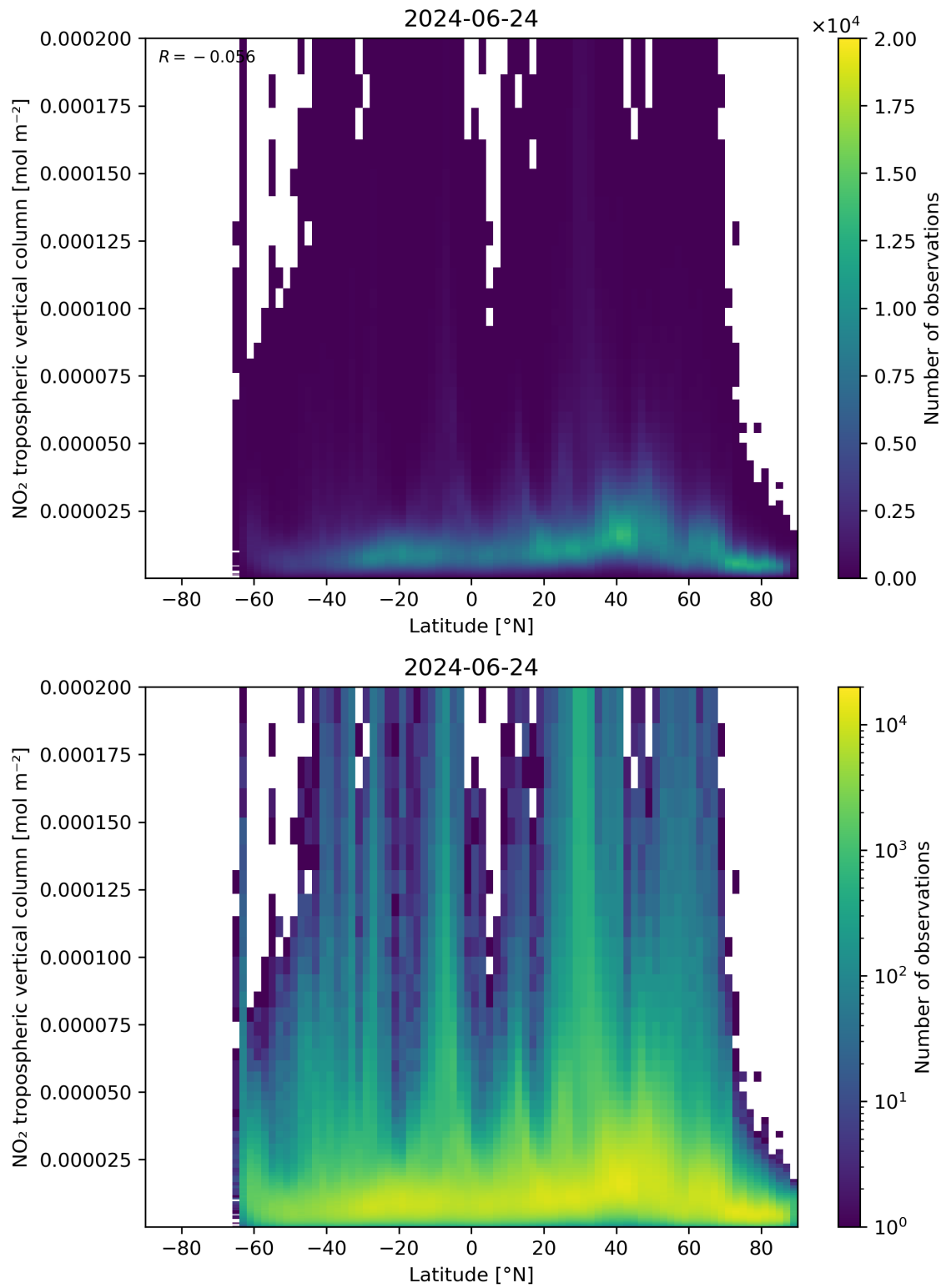
Figure 92: Scatter density plot of “Latitude” against “NO 2 tropospheric vertical column” for 2024-06-24 to 2024-06-25.
