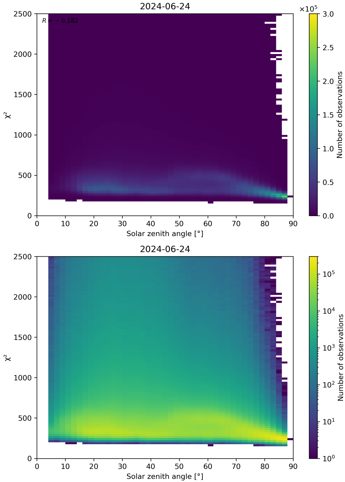
Figure 148: Scatter density plot of “Solar zenith angle” against “ \chi^2 ” for 2024-06-24 to 2024-06-25.
