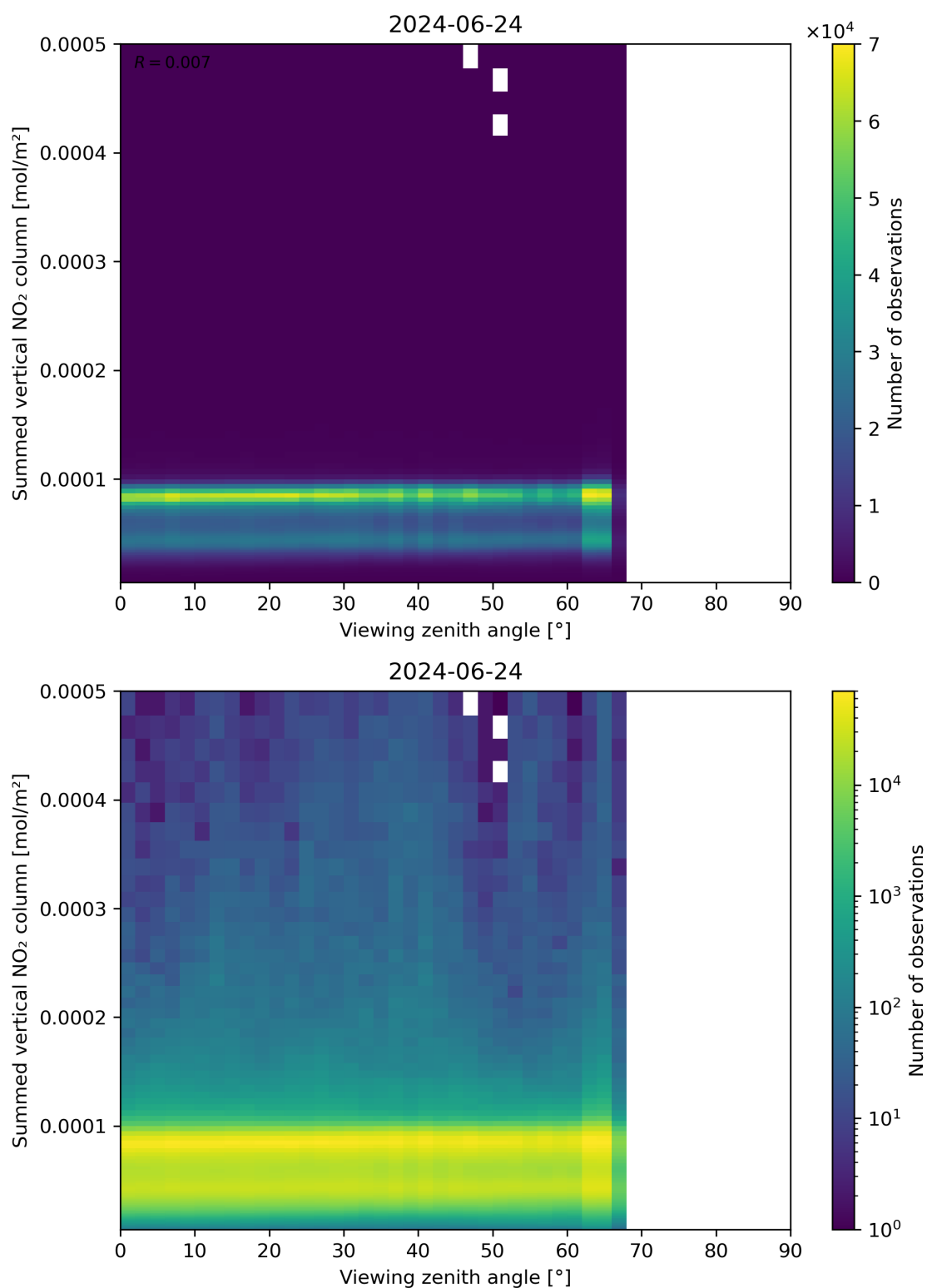
Figure 165: Scatter density plot of “Viewing zenith angle” against “Summed vertical NO 2 column” for 2024-06-24 to 2024-06-25.
