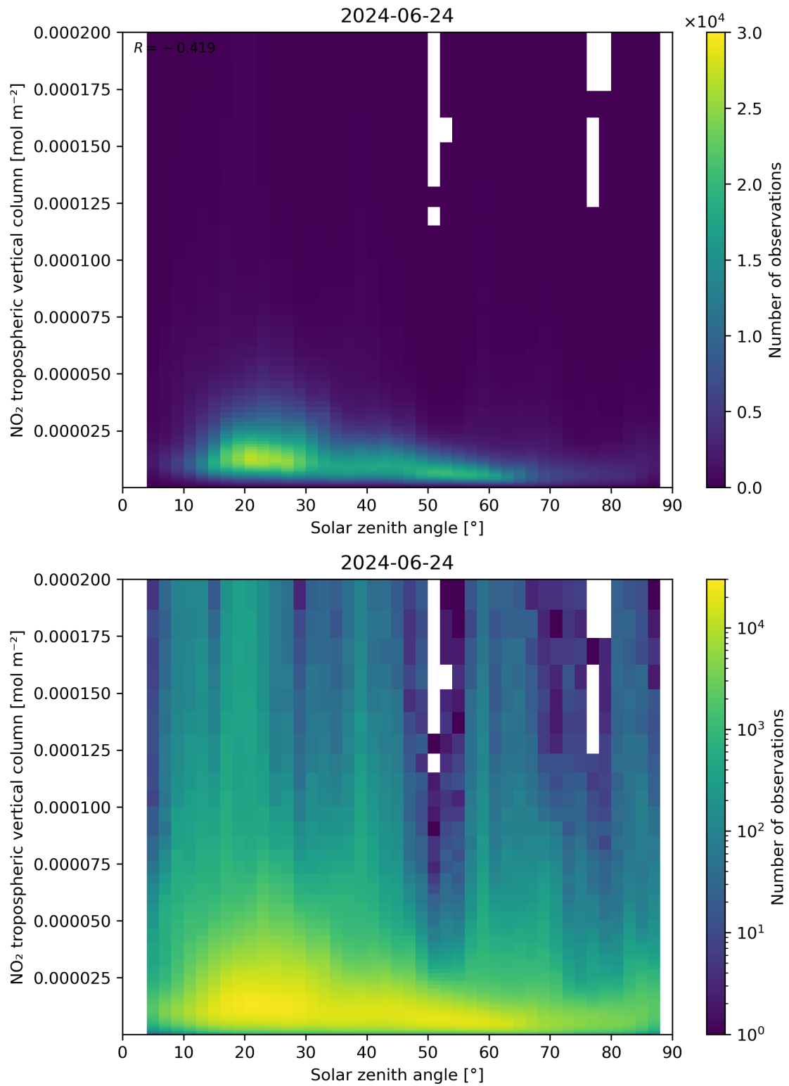
Figure 155: Scatter density plot of “Solar zenith angle” against “NO 2 tropospheric vertical column” for 2024-06-24 to 2024-06-25.
