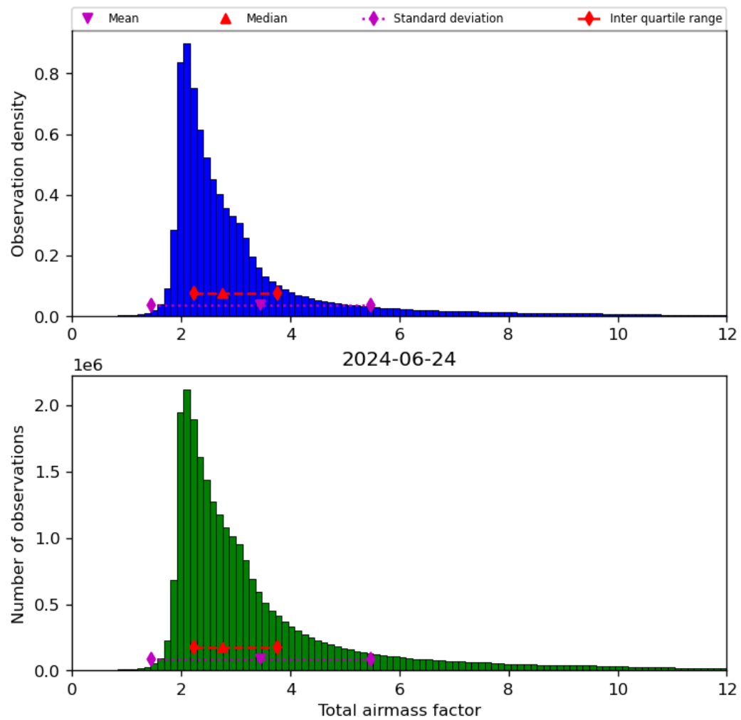
Figure 32: Histogram of “Total airmass factor” for 2024-06-24 to 2024-06-25
