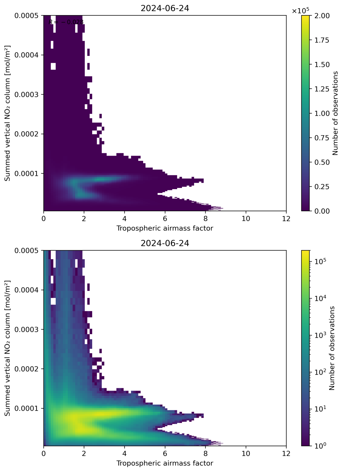
Figure 75: Scatter density plot of “Tropospheric airmass factor” against “Summed vertical NO 2 column” for 2024-06-24 to 2024-06-25.
