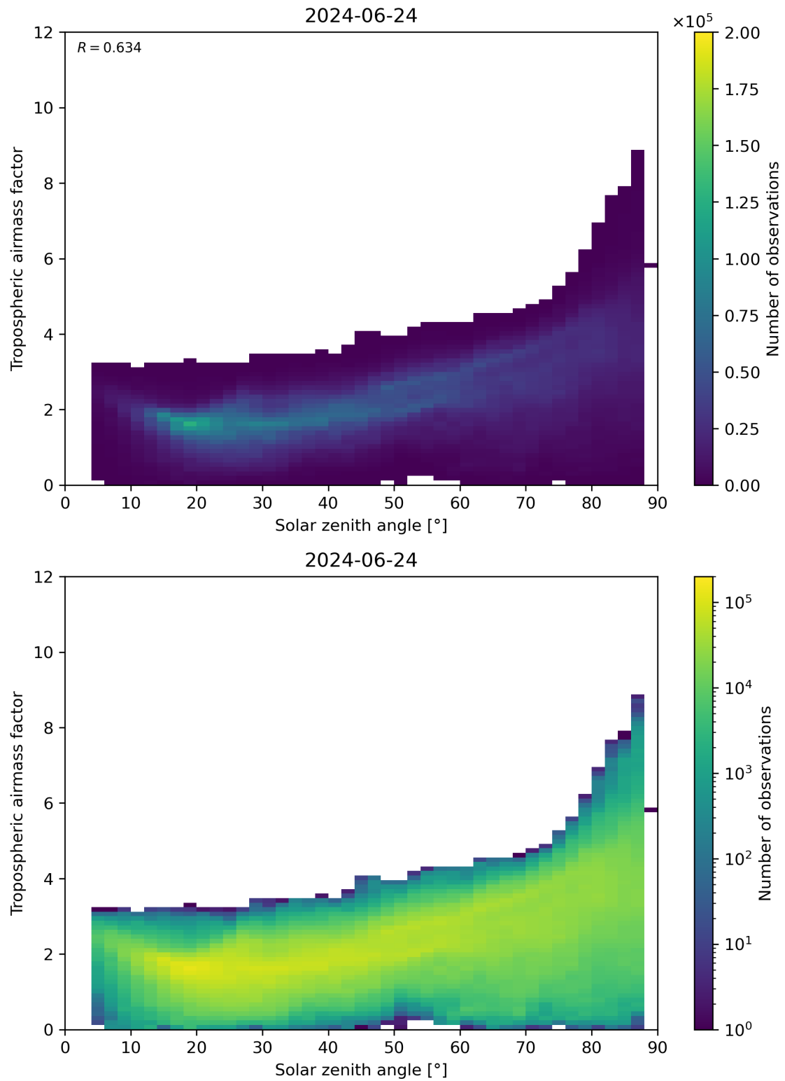
Figure 147: Scatter density plot of “Solar zenith angle” against “Tropospheric airmass factor” for 2024-06-24 to 2024-06-25.
