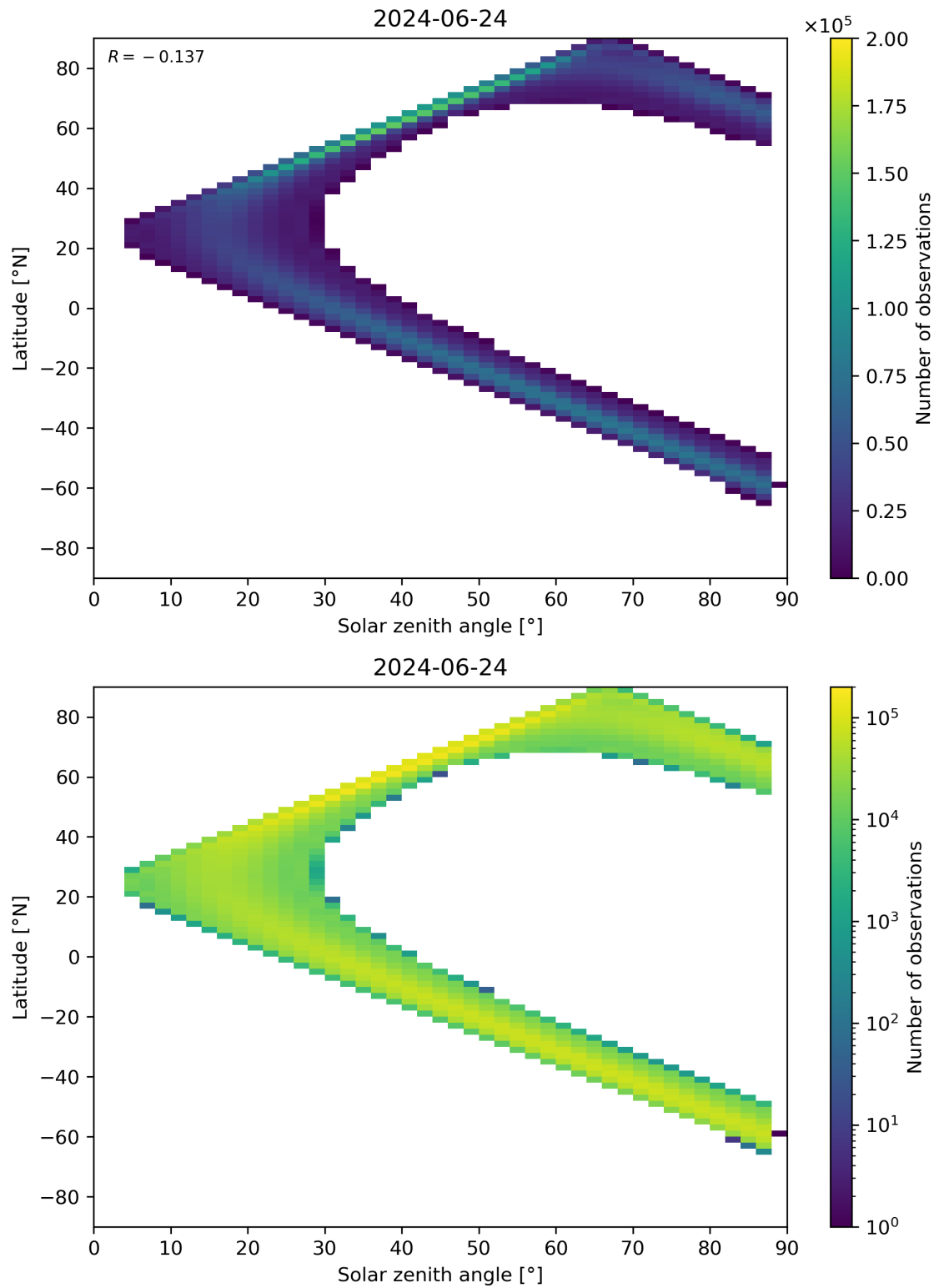
Figure 149: Scatter density plot of “Solar zenith angle” against “Latitude” for 2024-06-24 to 2024-06-25.
