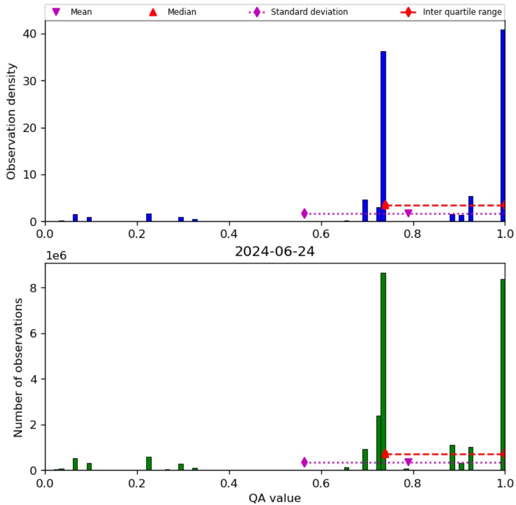
Figure 28: Histogram of “QA value” for 2024-06-24 to 2024-06-25
