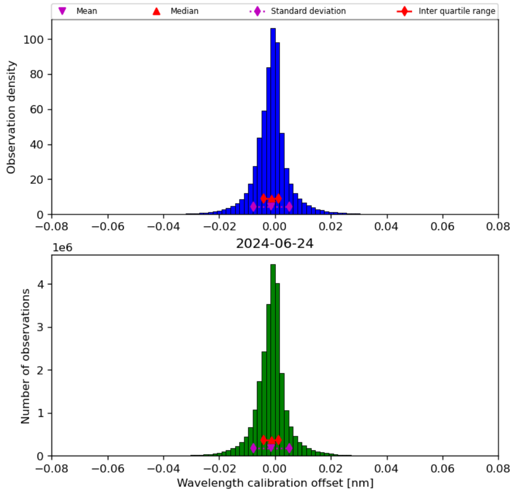
Figure 35: Histogram of “Wavelength calibration offset” for 2024-06-24 to 2024-06-25
