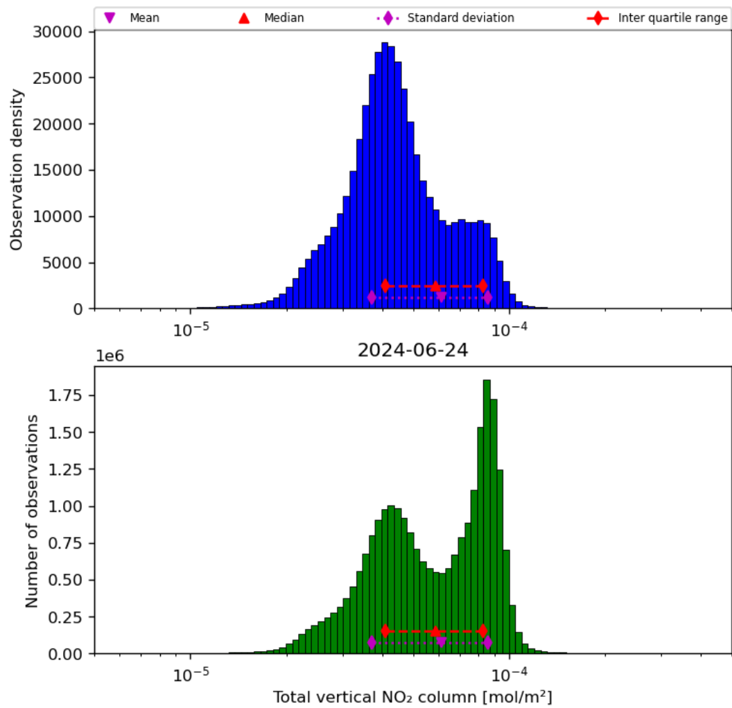
Figure 38: Histogram of “Total vertical NO 2 column” for 2024-06-24 to 2024-06-25
