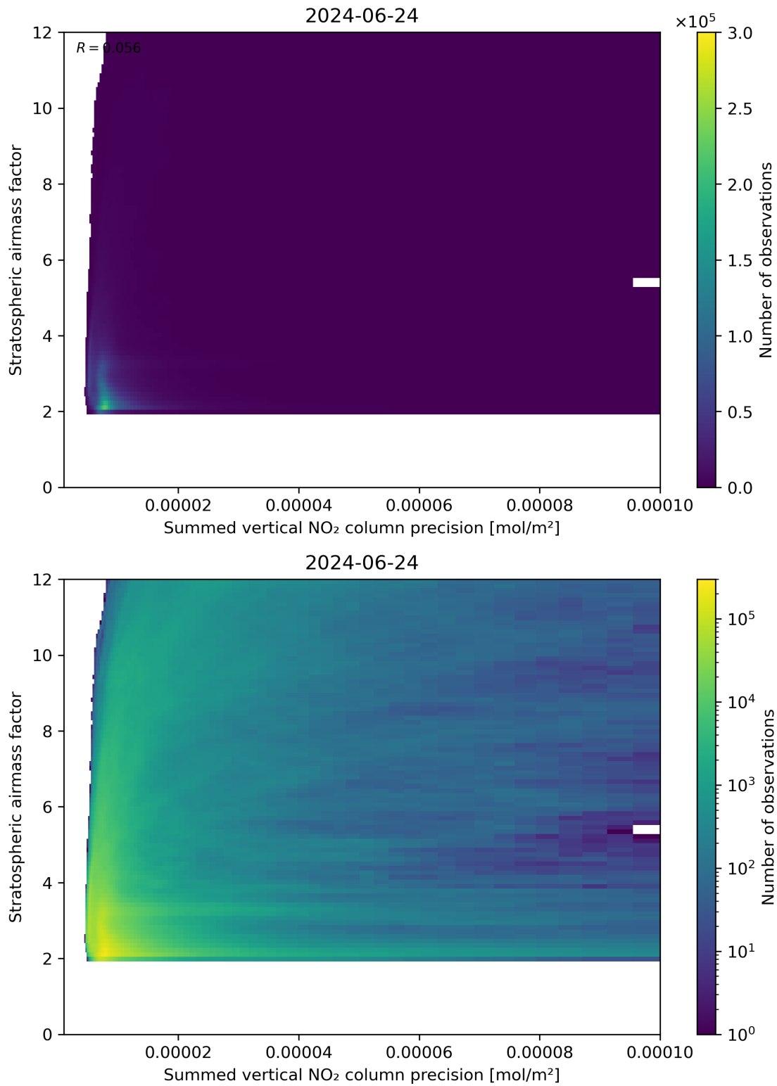
Figure 106: Scatter density plot of “Summed vertical NO 2 column precision” against “Stratospheric airmass factor” for 2024-06-24 to 2024-06-25.
