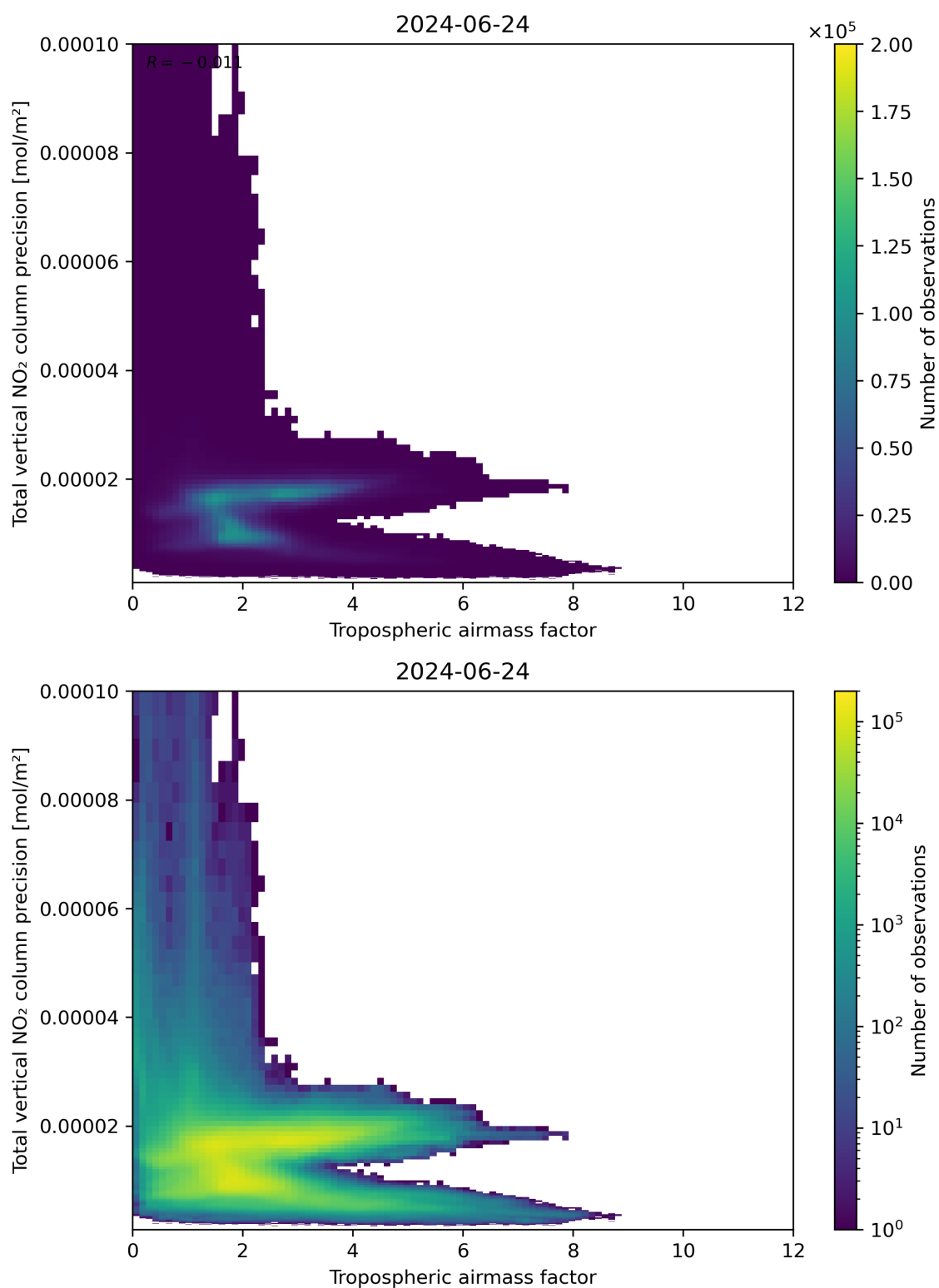
Figure 78: Scatter density plot of “Tropospheric air mass factor” against “Total vertical NO 2 column precision” for 2024-06-24 to 2024-06-25.
