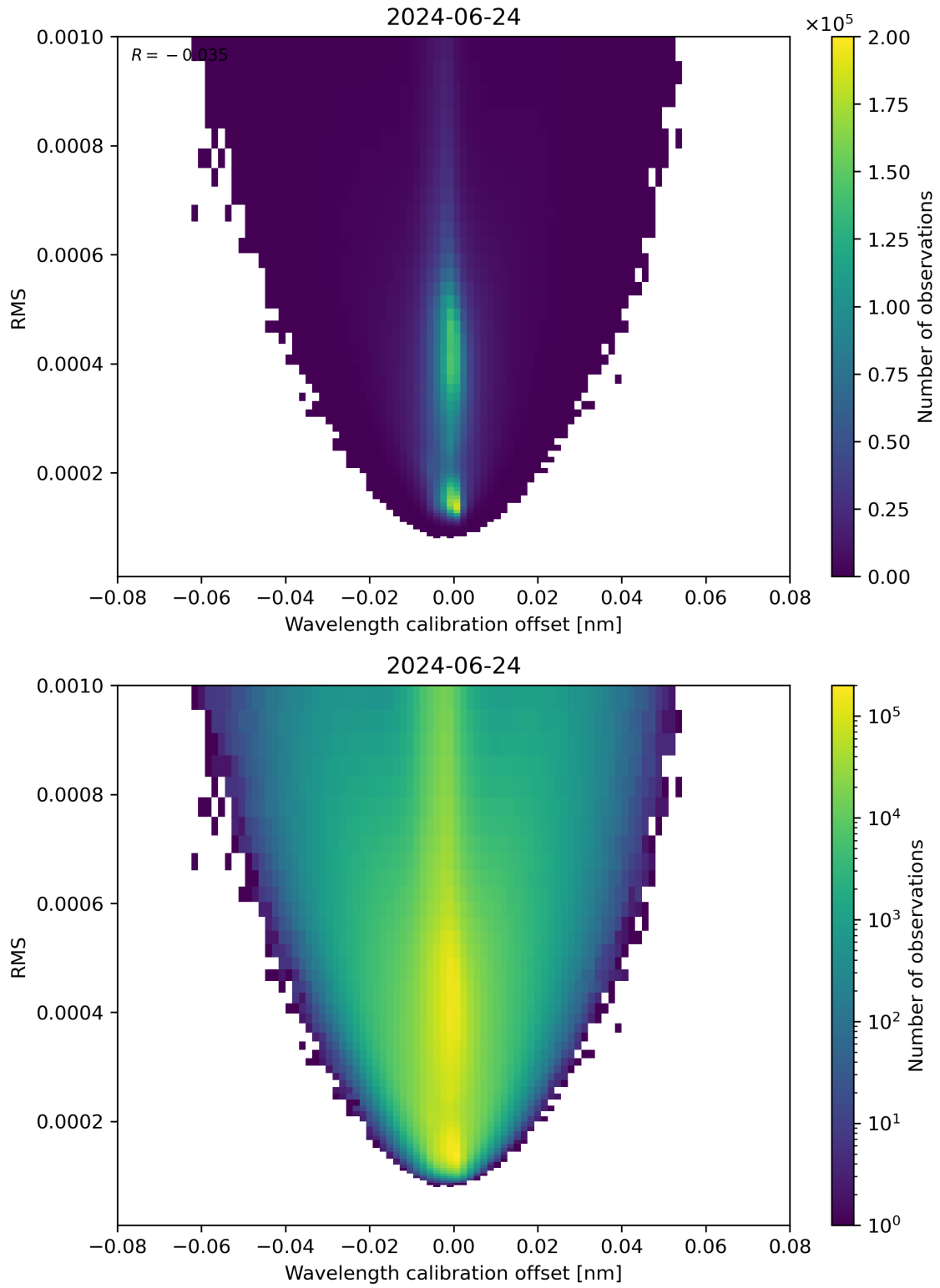
Figure 181: Scatter density plot of “Wavelength calibration offset” against “RMS” for 2024-06-24 to 2024-06-25.
