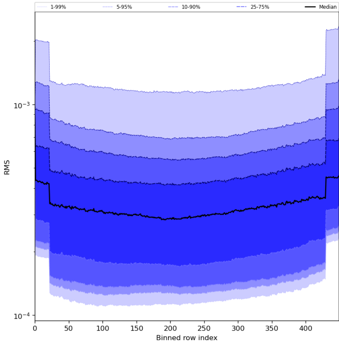
Figure 60: Along track statistics of “RMS” for 2024-06-24 to 2024-06-25
