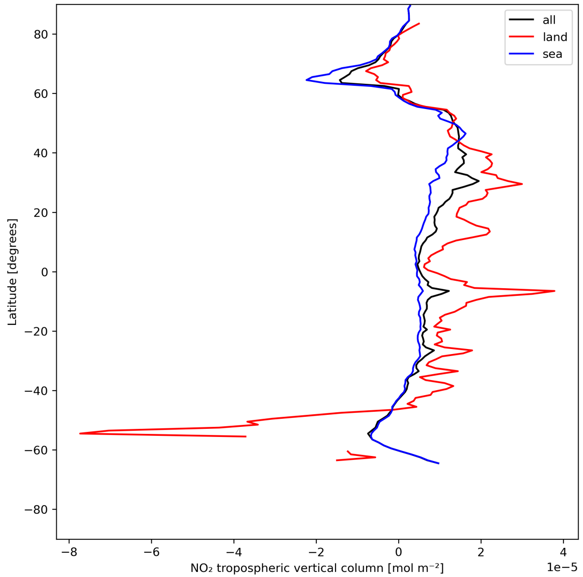
Figure 12: Zonal average of “NO 2 tropospheric vertical column” for 2024-06-24 to 2024-06-25.
