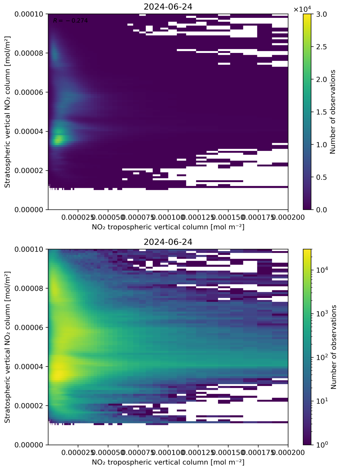
Figure 125: Scatter density plot of “NO 2 tropospheric vertical column” against “Stratospheric vertical NO 2 column” for 2024-06-24 to 2024-06-25.
