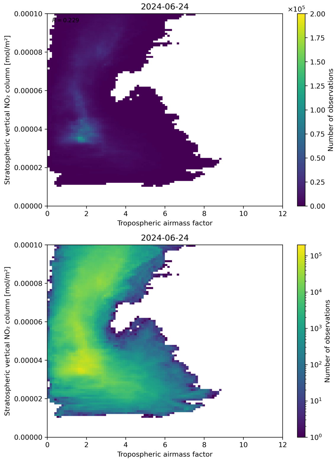
Figure 74: Scatter density plot of “Tropospheric air mass factor” against “Stratospheric vertical NO 2 column” for 2024-06-24 to 2024-06-25.
