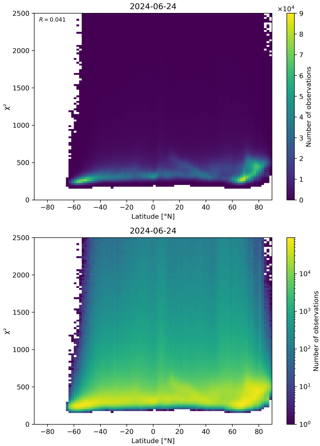
Figure 86: Scatter density plot of “Latitude” against “ \chi^2 ” for 2024-06-24 to 2024-06-25.
