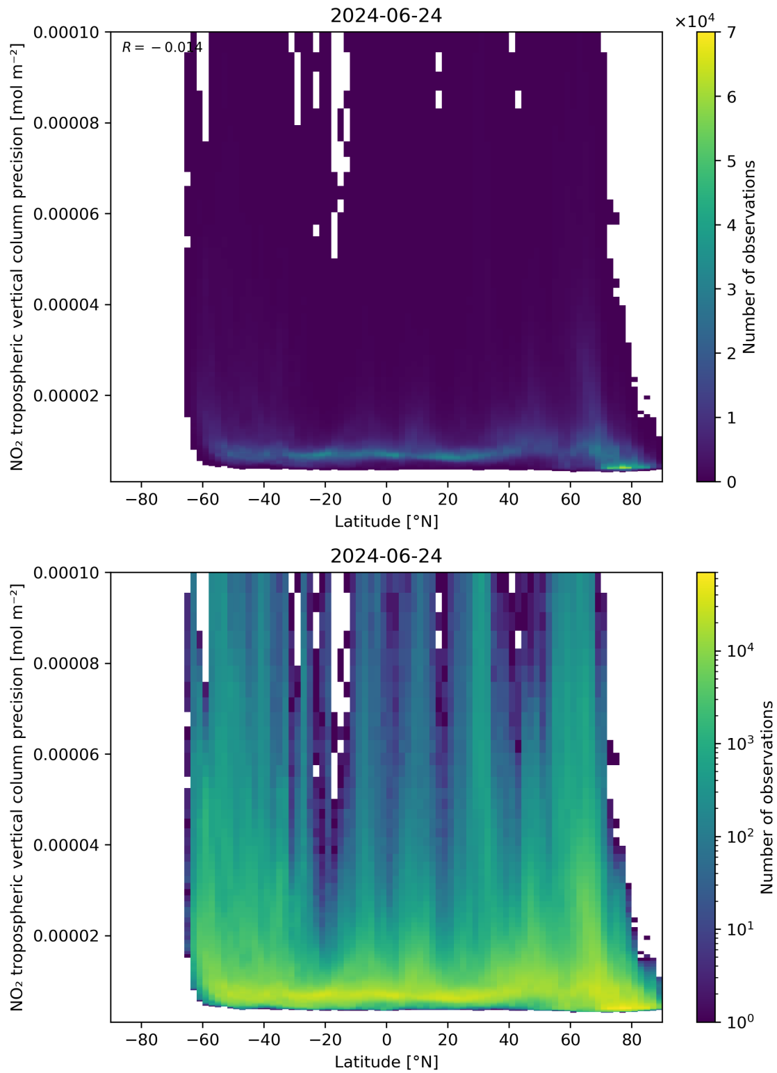
Figure 93: Scatter density plot of “Latitude” against “NO 2 tropospheric vertical column precision” for 2024-06-24 to 2024-06-25.
