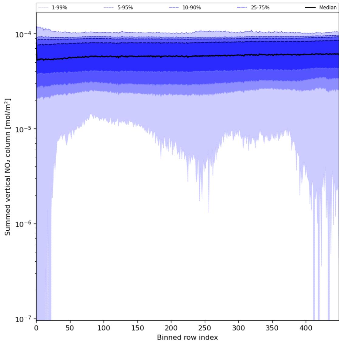
Figure 57: Along track statistics of “Summed vertical NO 2 column” for 2024-06-24 to 2024-06-25
