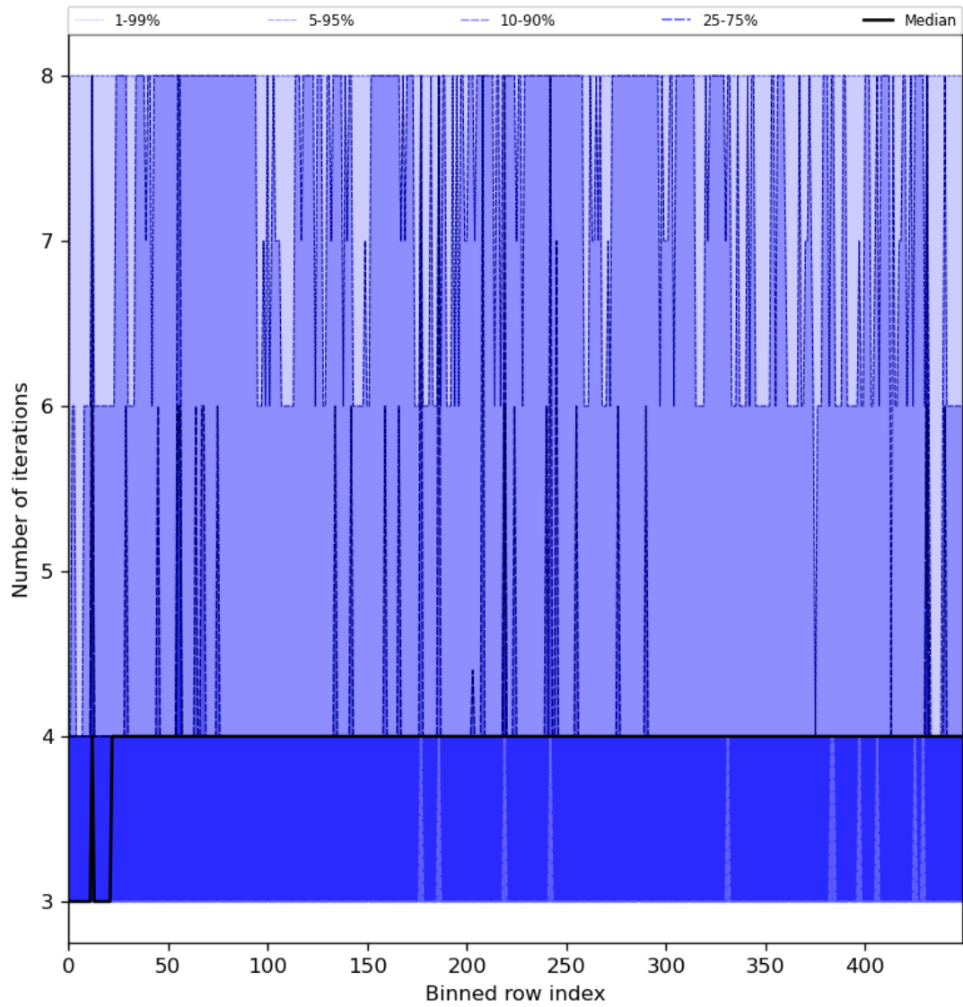
Figure 51: Along track statistics of “Number of iterations” for 2024-06-24 to 2024-06-25
