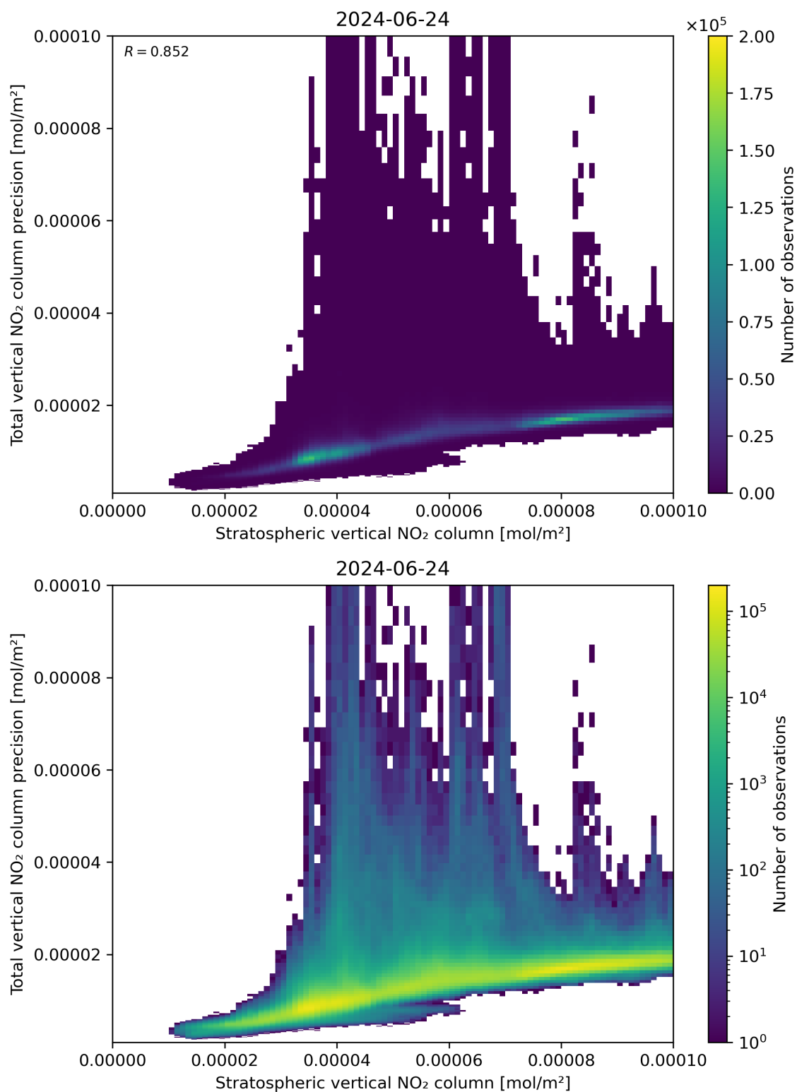
Figure 101: Scatter density plot of “Stratospheric vertical NO 2 column” against “Total vertical NO 2 column precision” for 2024-06-24 to 2024-06-25.
