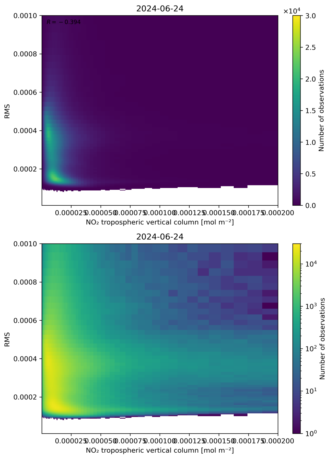
Figure 142: Scatter density plot of “NO 2 tropospheric vertical column” against “RMS” for 2024-06-24 to 2024-06-25.
