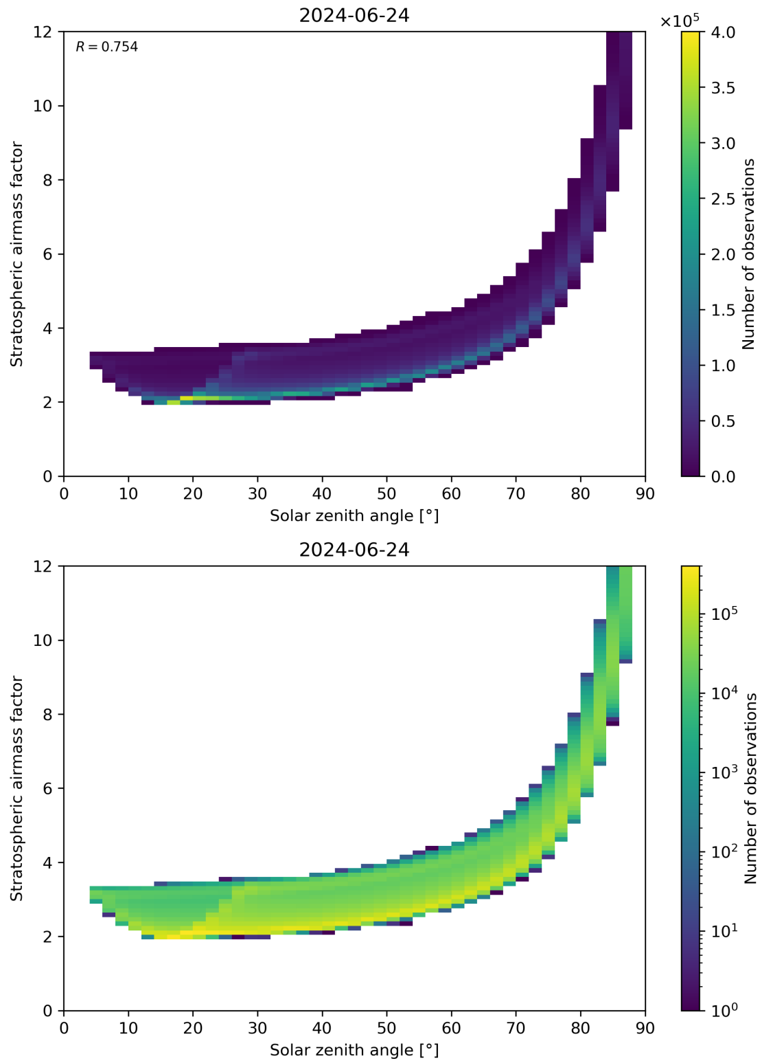
Figure 145: Scatter density plot of “Solar zenith angle” against “Stratospheric airmass factor” for 2024-06-24 to 2024-06-25.
