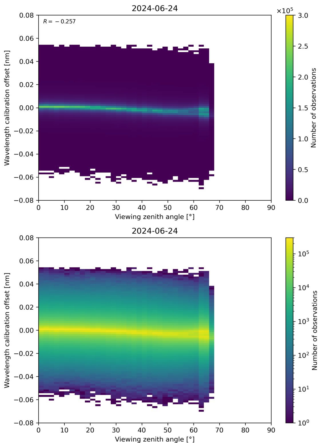
Figure 173: Scatter density plot of “Viewing zenith angle” against “Wavelength calibration offset” for 2024-06-24 to 2024-06-25.
