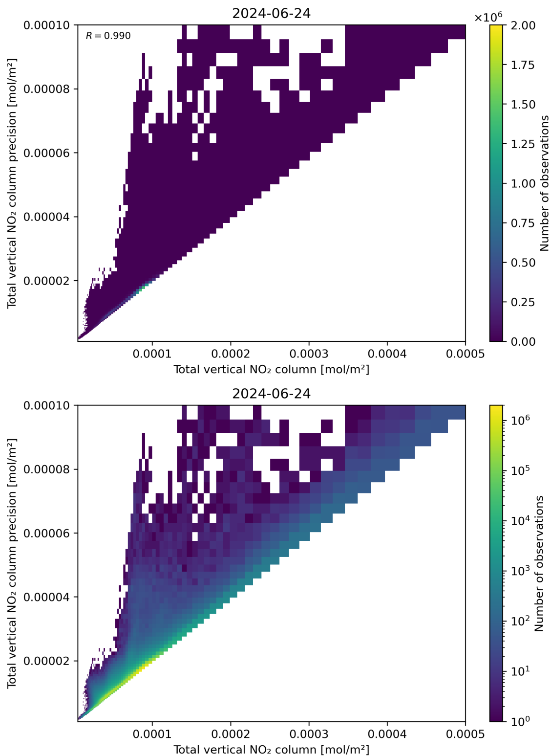
Figure 114: Scatter density plot of “Total vertical NO 2 column” against “Total vertical NO 2 column precision” for 2024-06-24 to 2024-06-25.
