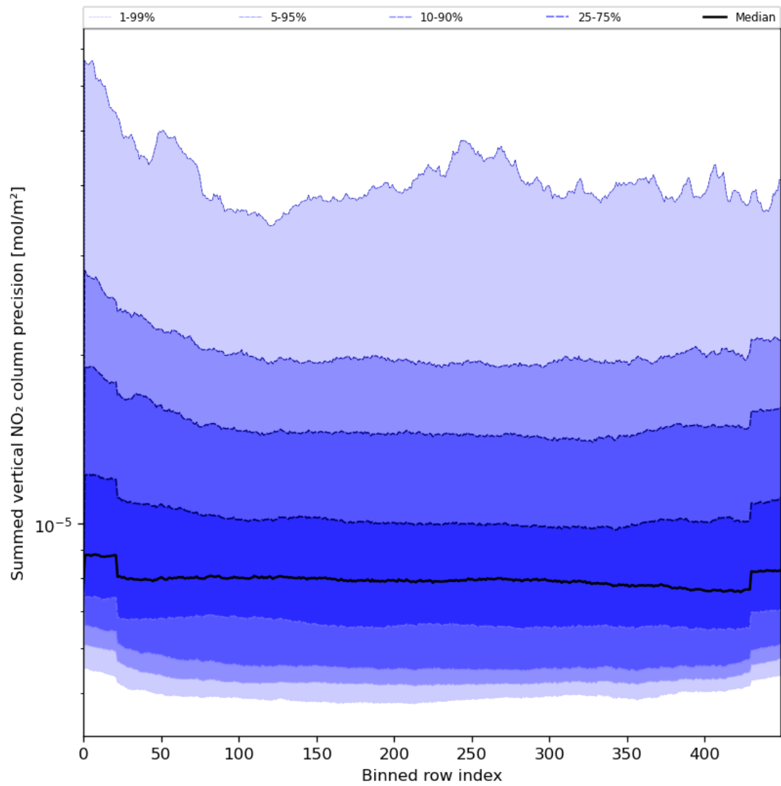
Figure 58: Along track statistics of “Summed vertical NO 2 column precision” for 2024-06-24 to 2024-06-25
