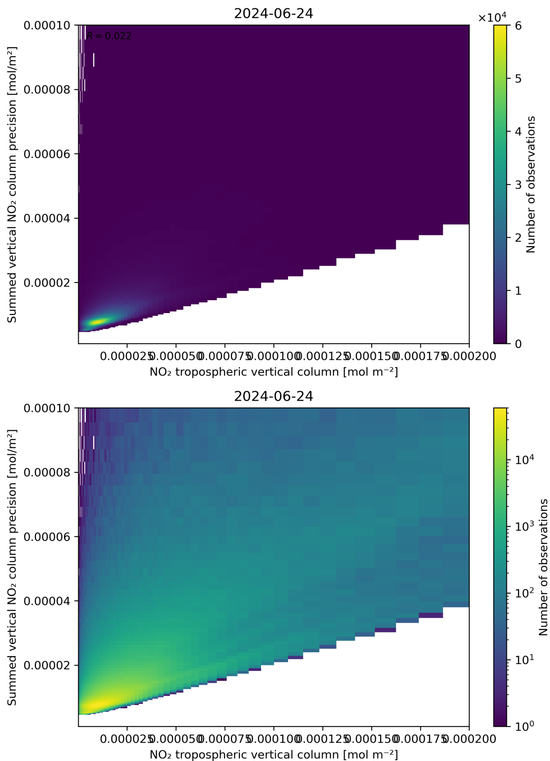
Figure 127: Scatter density plot of “NO 2 tropospheric vertical column” against “Summed vertical NO 2 column precision” for 2024-06-24 to 2024-06-25.
