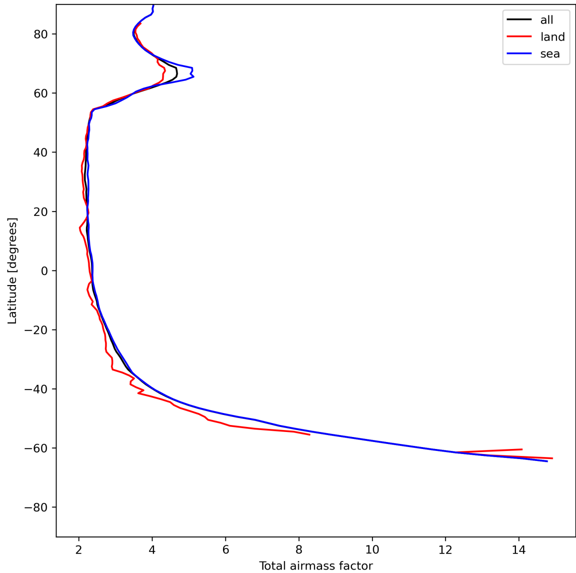
Figure 15: Zonal average of “Total airmass factor” for 2024-06-24 to 2024-06-25.
