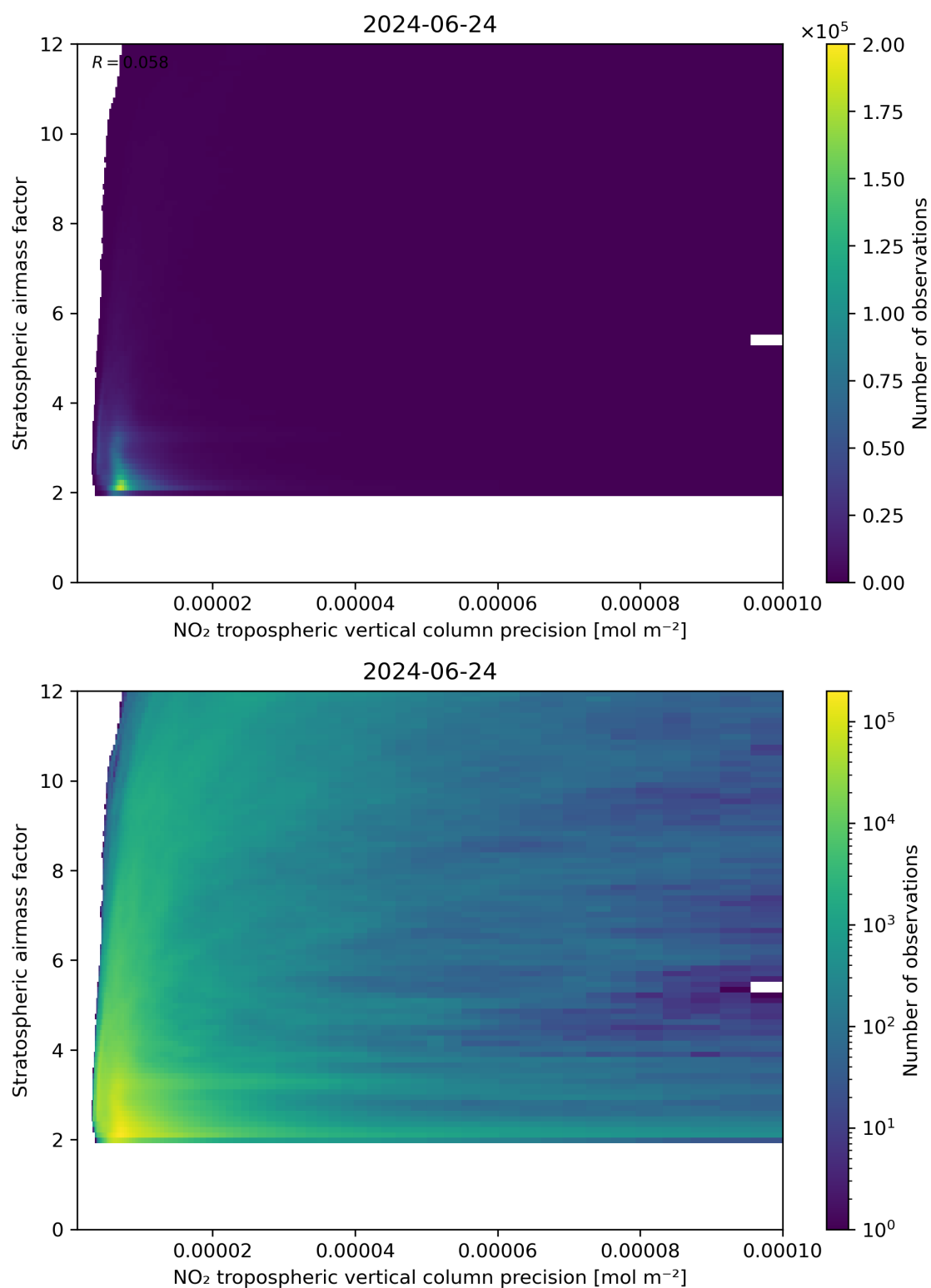
Figure 131: Scatter density plot of “NO 2 tropospheric vertical column precision” against “Stratospheric airmass factor” for 2024-06-24 to 2024-06-25.
