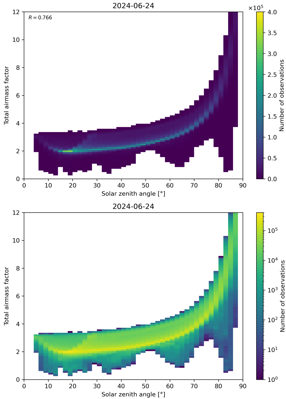
Figure 146: Scatter density plot of “Solar zenith angle” against “Total air mass factor” for 2024-06-24 to 2024-06-25.
