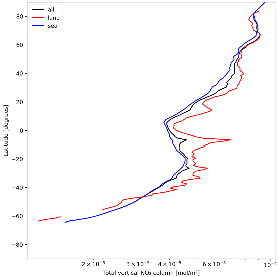
Figure 21: Zonal average of “Total vertical NO 2 column” for 2024-06-24 to 2024-06-25.
