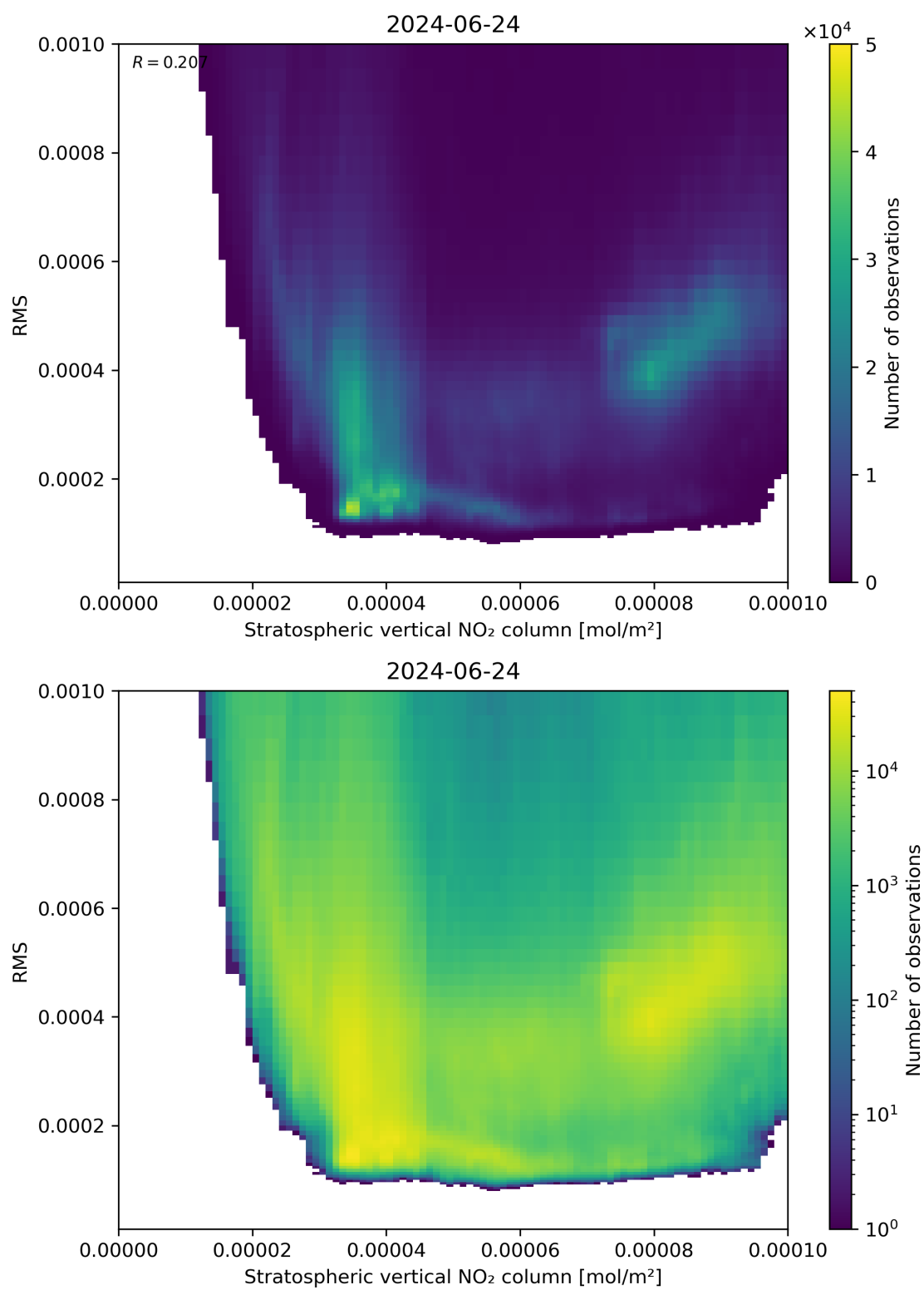
Figure 102: Scatter density plot of “Stratospheric vertical NO 2 column” against “RMS” for 2024-06-24 to 2024-06-25.
