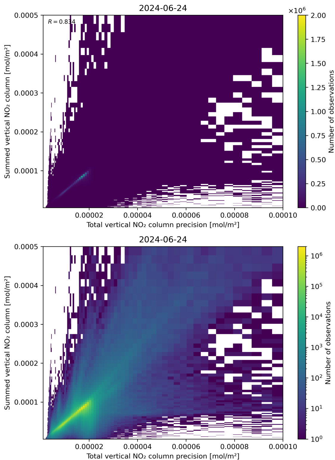
Figure 117: Scatter density plot of “Total vertical NO 2 column precision” against “Summed vertical NO 2 column” for 2024-06-24 to 2024-06-25.
