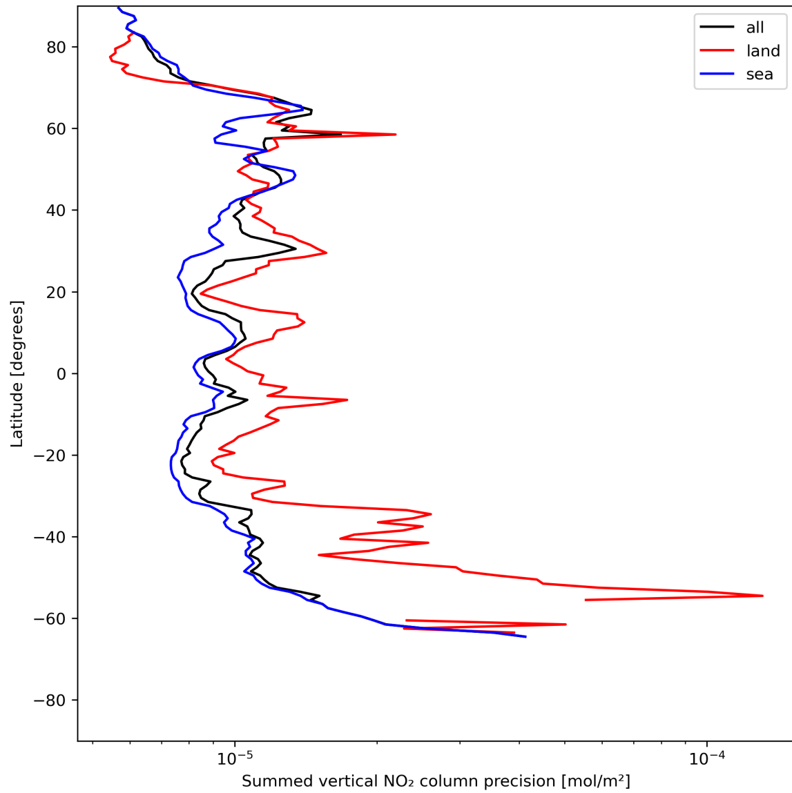
Figure 24: Zonal average of “Summed vertical NO 2 column precision” for 2024-06-24 to 2024-06-25.
