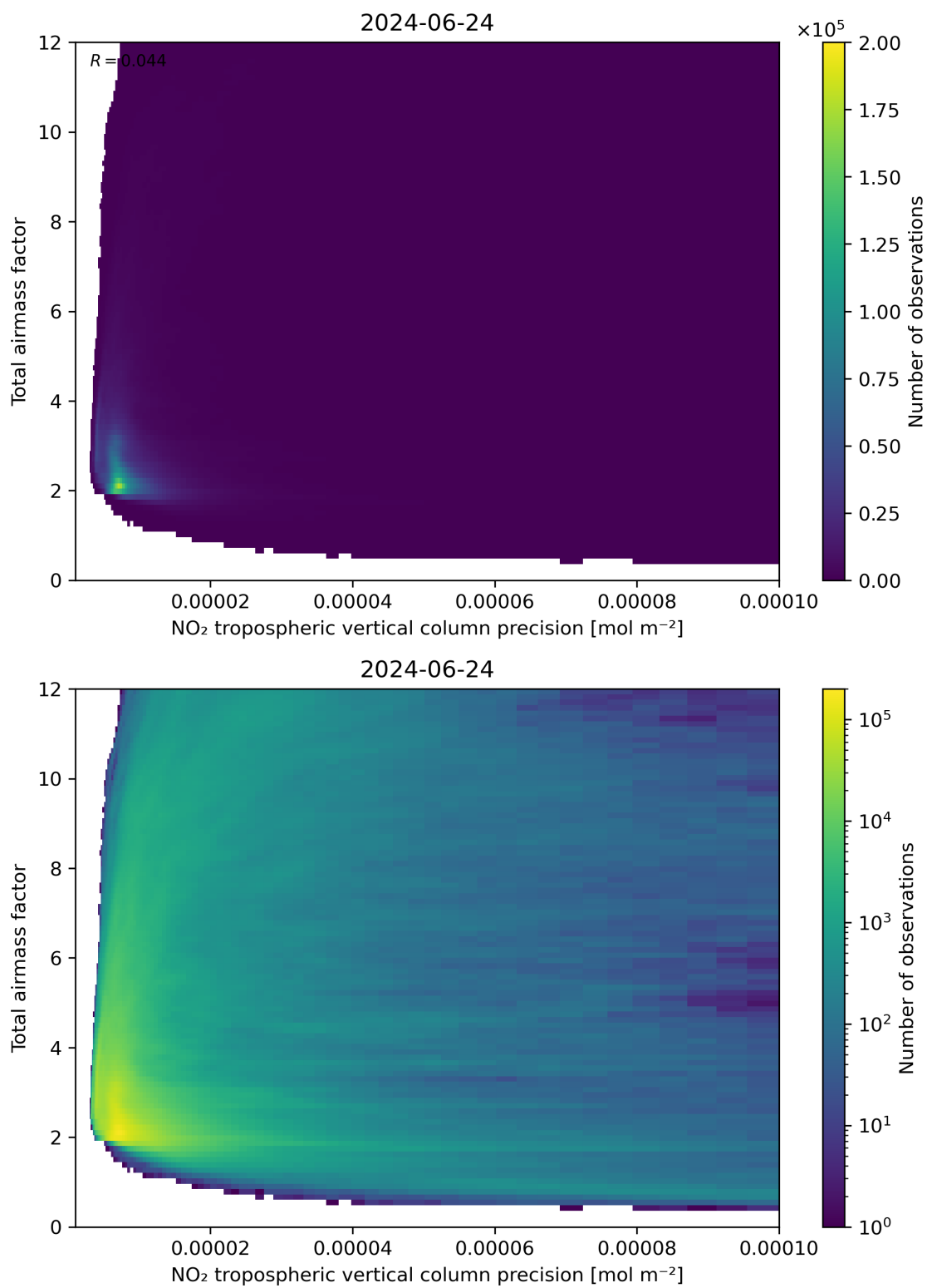
Figure 132: Scatter density plot of “NO 2 tropospheric vertical column precision” against “Total air mass factor” for 2024-06-24 to 2024-06-25.
