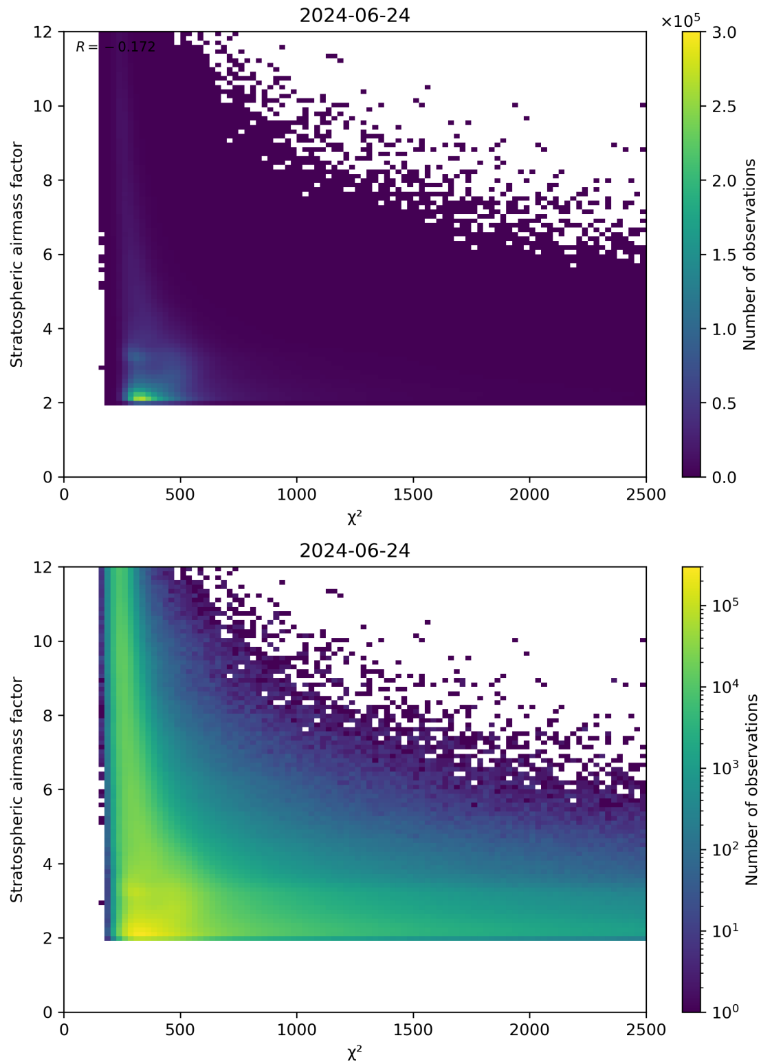
Figure 81: Scatter density plot of “ \chi^2 ” against “Stratospheric airmass factor” for 2024-06-24 to 2024-06-25.
