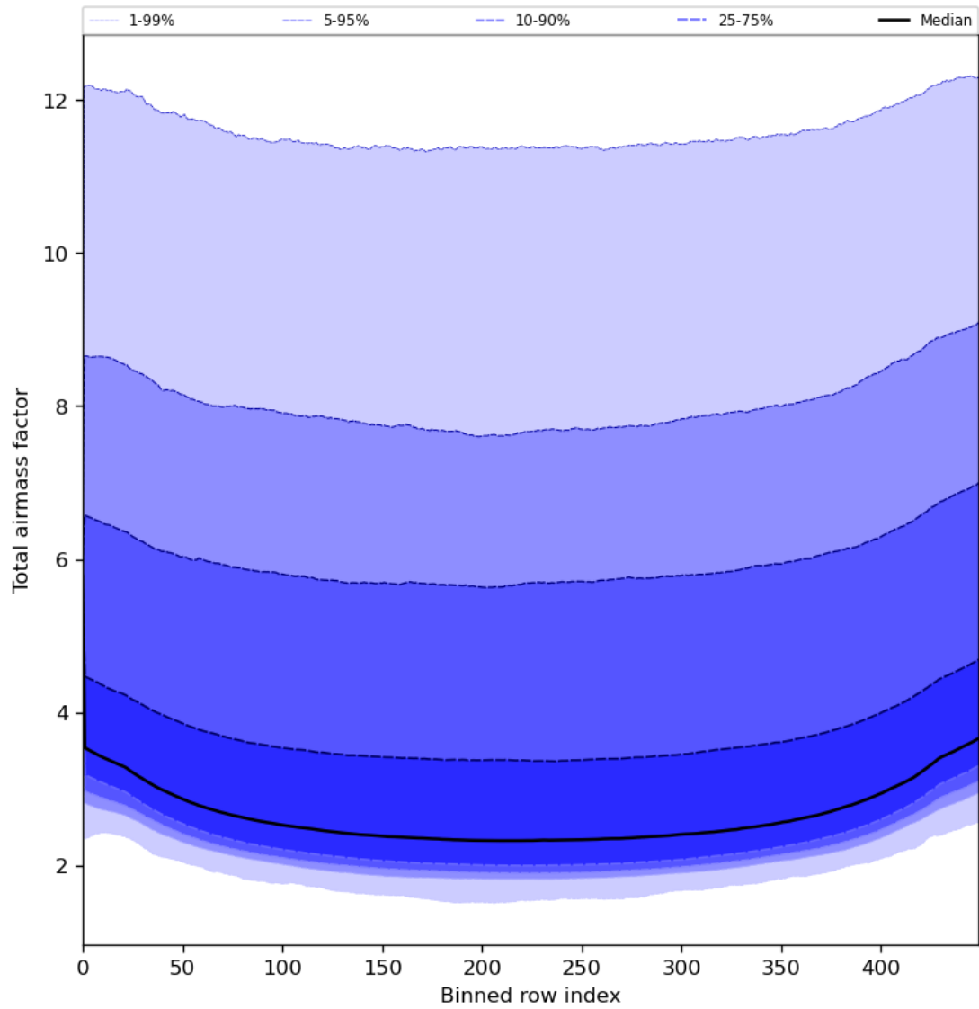
Figure 49: Along track statistics of “Total airmass factor” for 2024-06-24 to 2024-06-25
