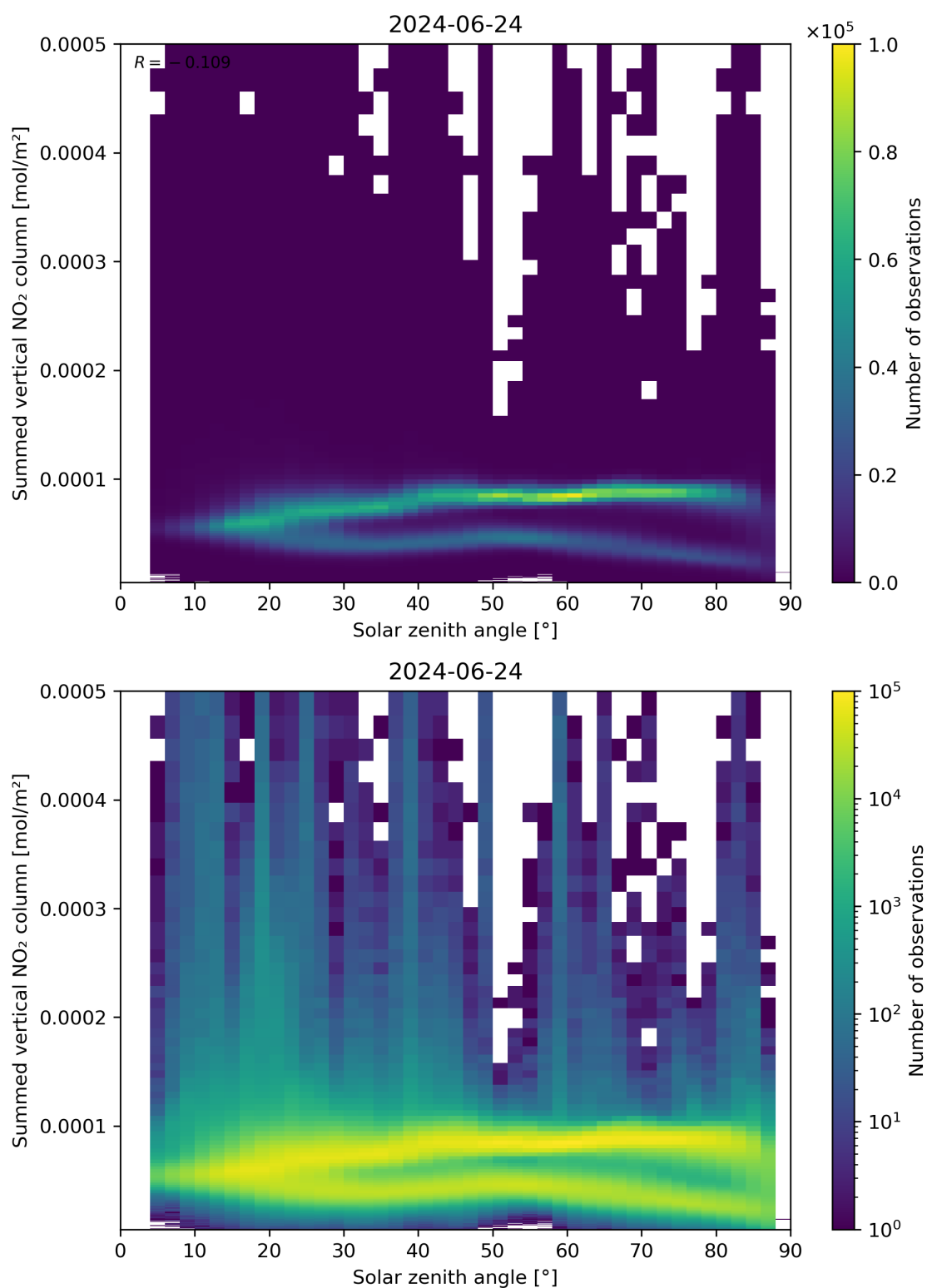
Figure 151: Scatter density plot of “Solar zenith angle” against “Summed vertical NO 2 column” for 2024-06-24 to 2024-06-25.
