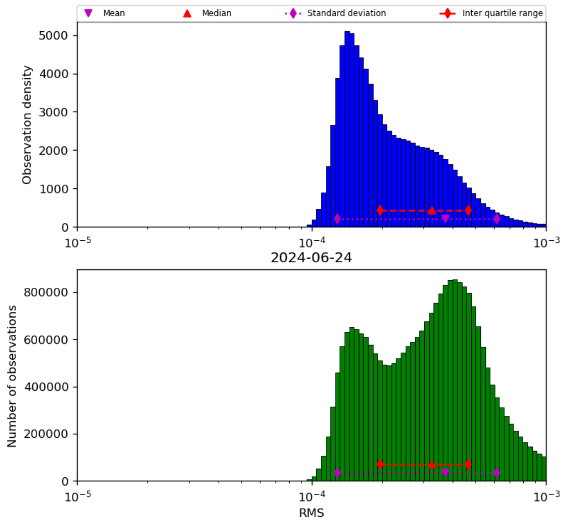
Figure 43: Histogram of “RMS” for 2024-06-24 to 2024-06-25
