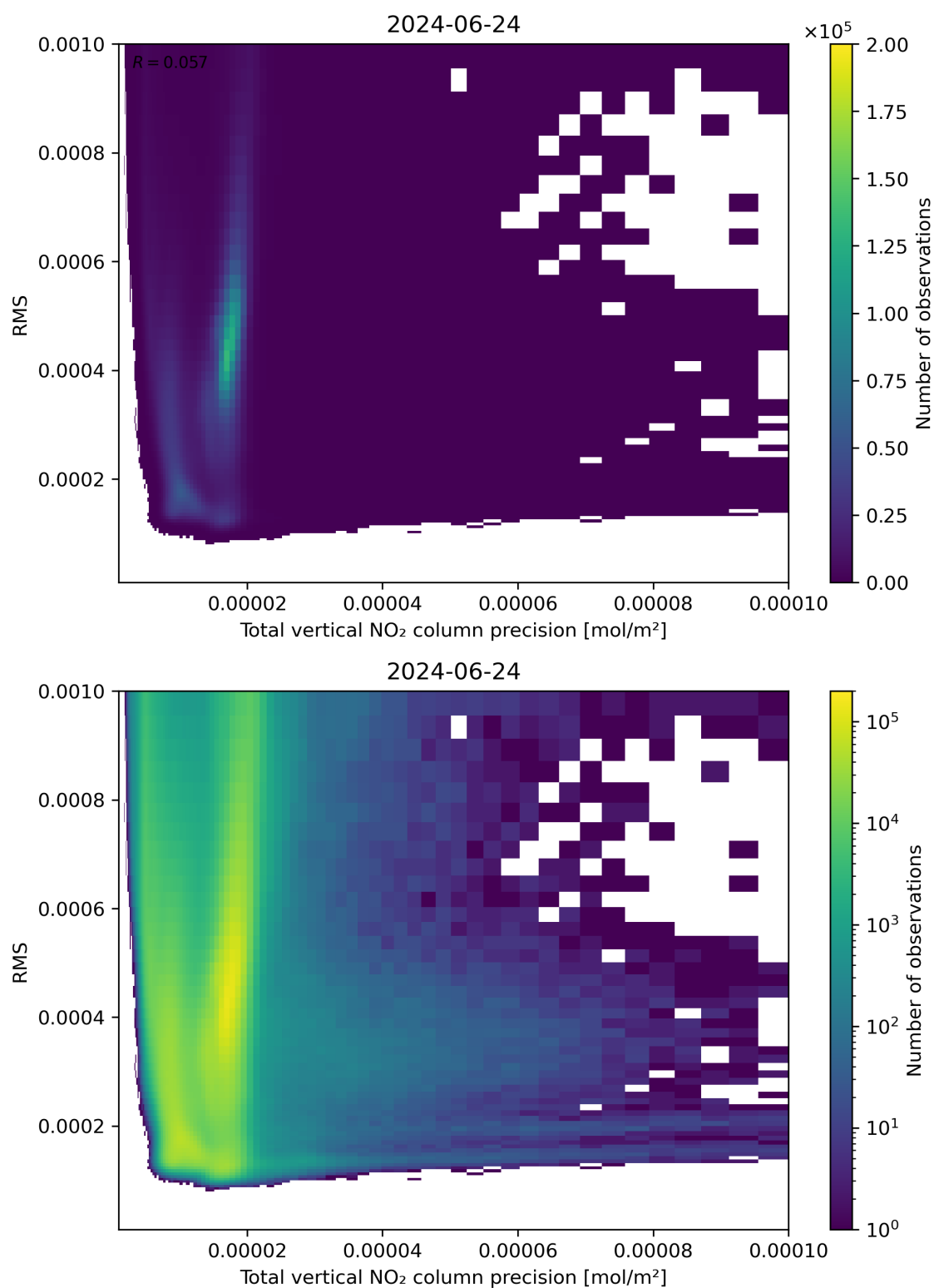
Figure 119: Scatter density plot of “Total vertical NO 2 column precision” against “RMS” for 2024-06-24 to 2024-06-25.
