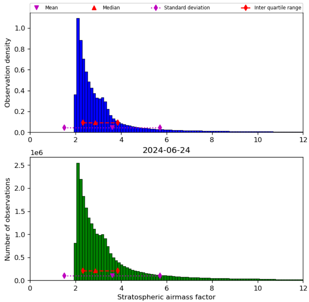
Figure 44: Histogram of “Stratospheric airmass factor” for 2024-06-24 to 2024-06-25
