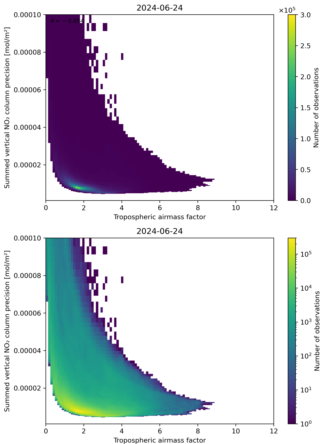
Figure 76: Scatter density plot of “Tropospheric air mass factor” against “Summed vertical NO 2 column precision” for 2024-06-24 to 2024-06-25.
