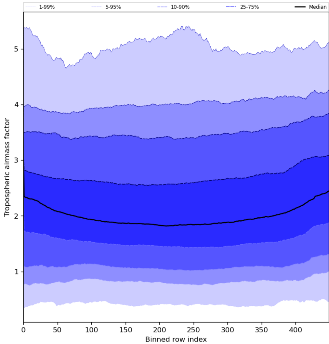
Figure 48: Along track statistics of “Tropospheric airmass factor” for 2024-06-24 to 2024-06-25
