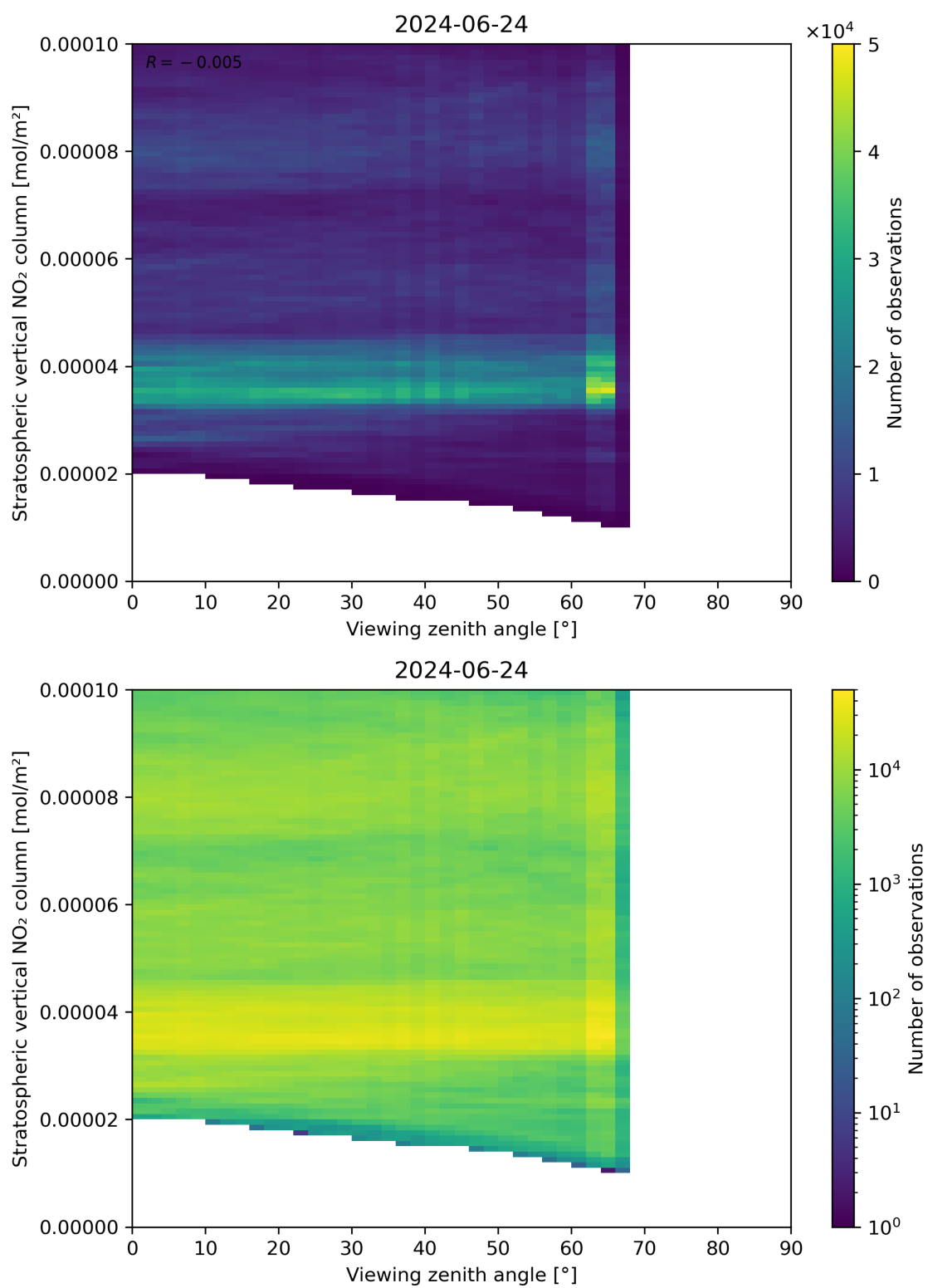
Figure 164: Scatter density plot of “Viewing zenith angle” against “Stratospheric vertical NO 2 column” for 2024-06-24 to 2024-06-25.
