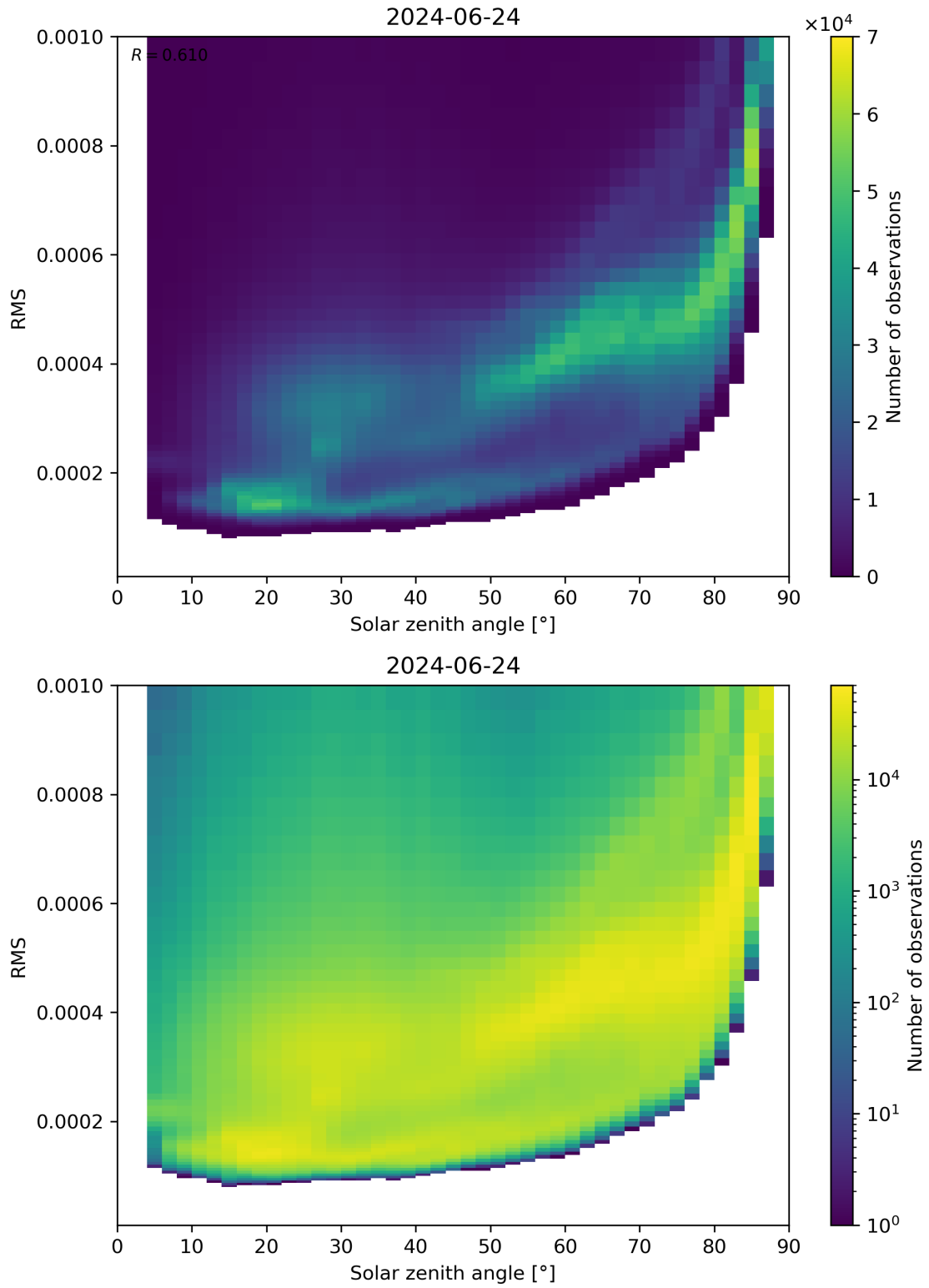
Figure 157: Scatter density plot of “Solar zenith angle” against “RMS” for 2024-06-24 to 2024-06-25.
