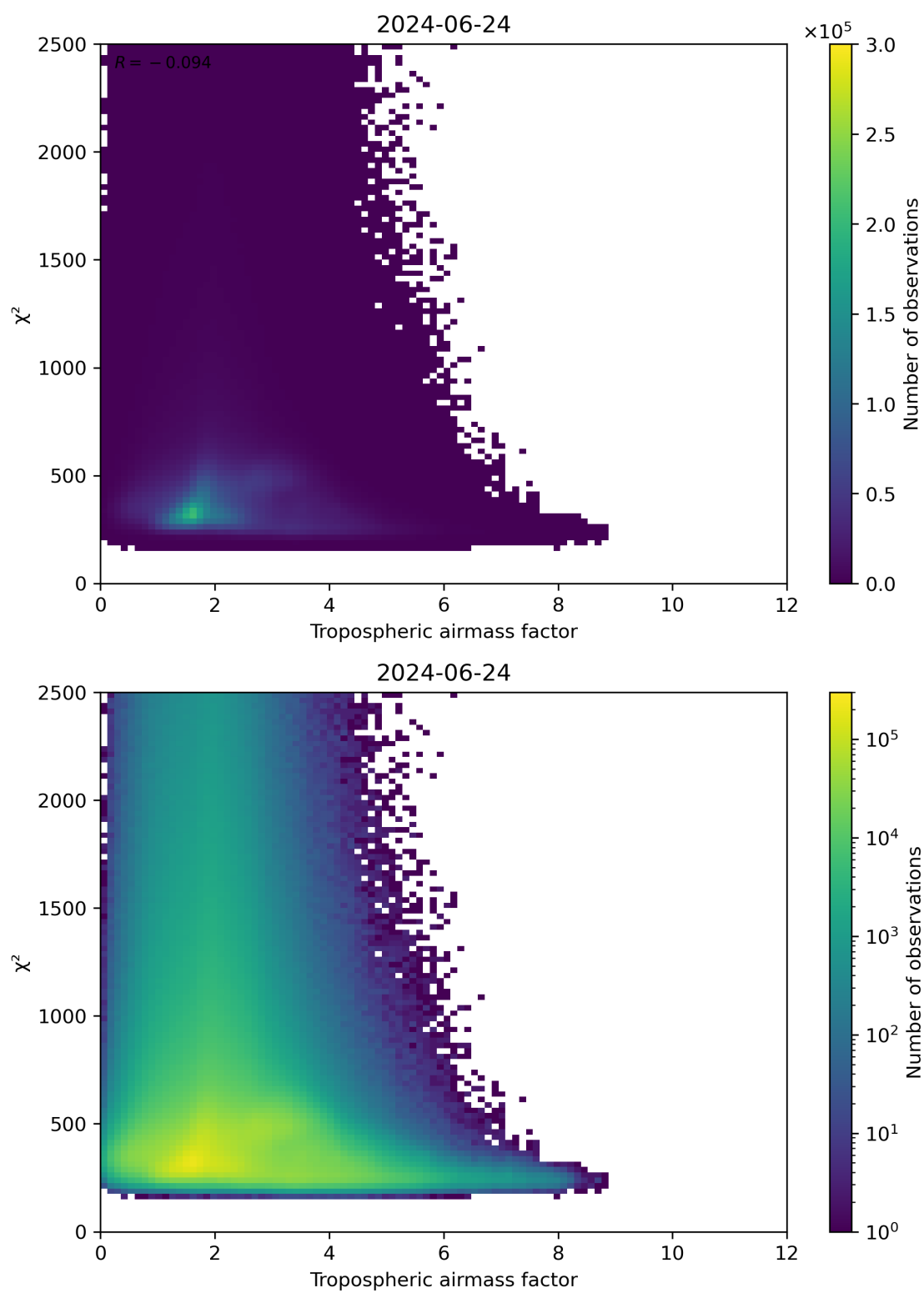
Figure 73: Scatter density plot of “Tropospheric airmass factor” against “ \chi^2 ” for 2024-06-24 to 2024-06-25.
