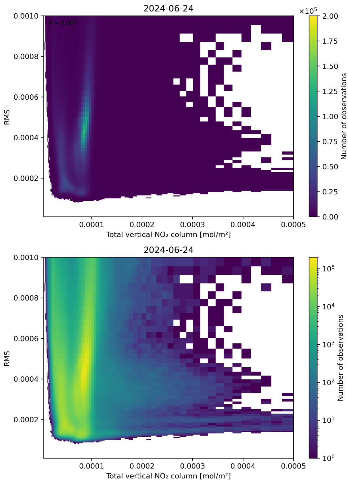
Figure 120: Scatter density plot of “Total vertical NO 2 column” against “RMS” for 2024-06-24 to 2024-06-25.
