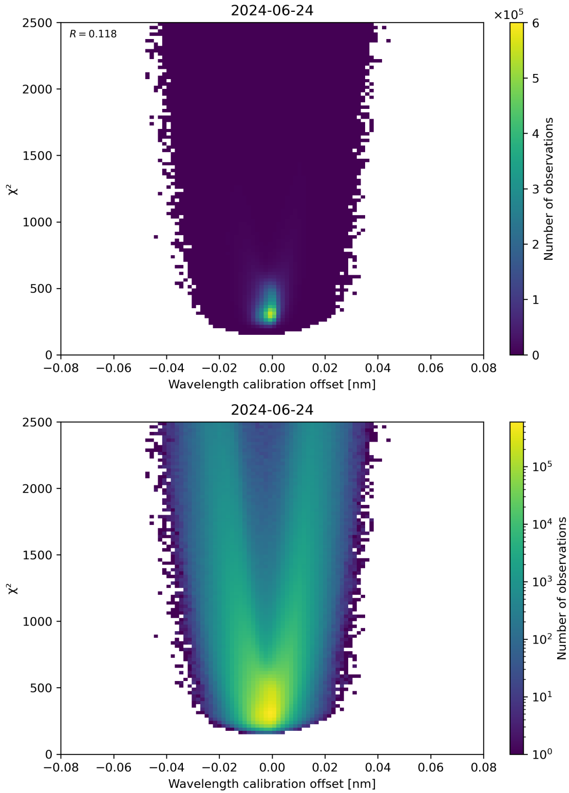
Figure 175: Scatter density plot of “Wavelength calibration offset” against “ \chi^2 ” for 2024-06-24 to 2024-06-25.
