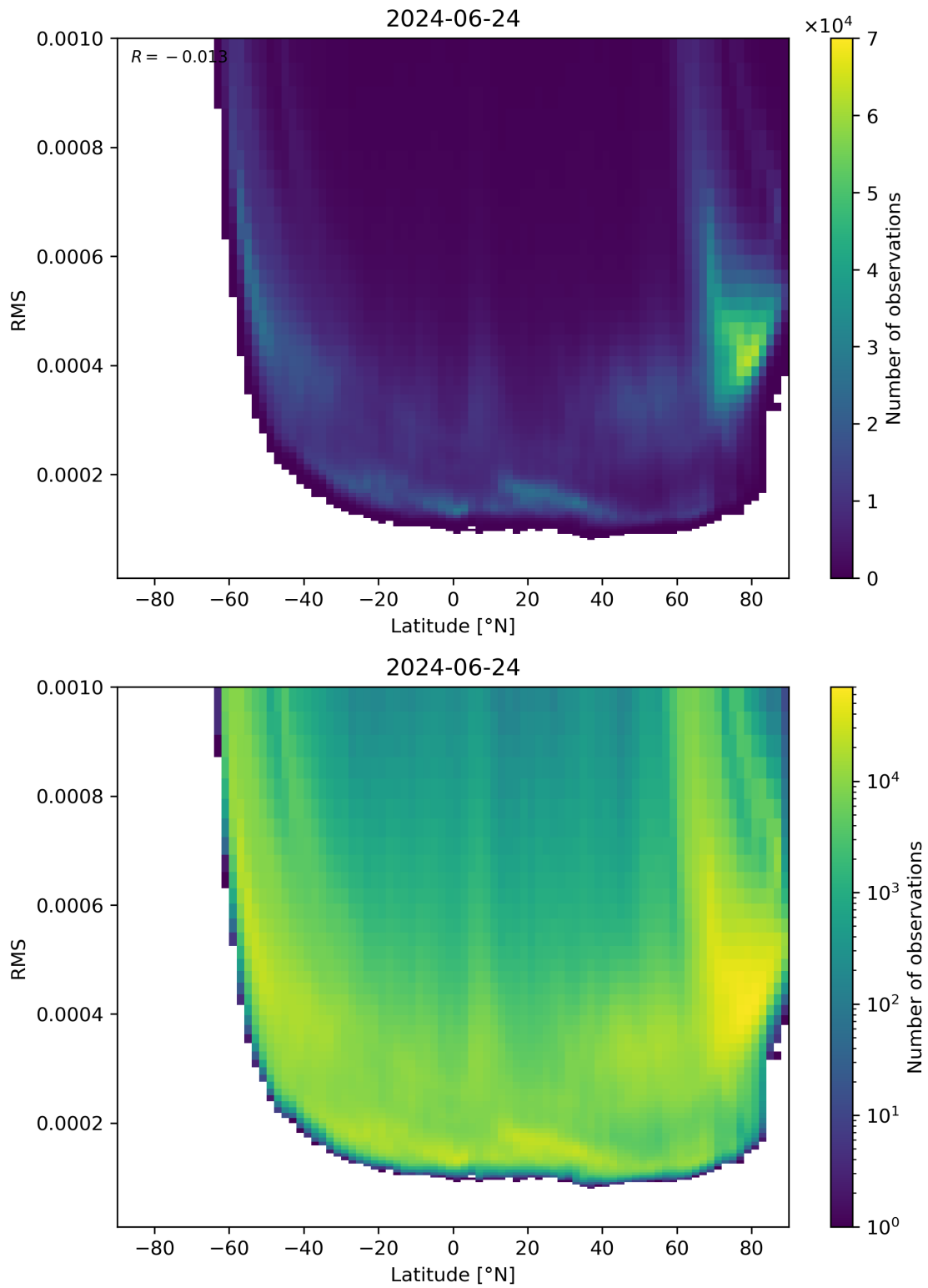
Figure 94: Scatter density plot of “Latitude” against “RMS” for 2024-06-24 to 2024-06-25.
