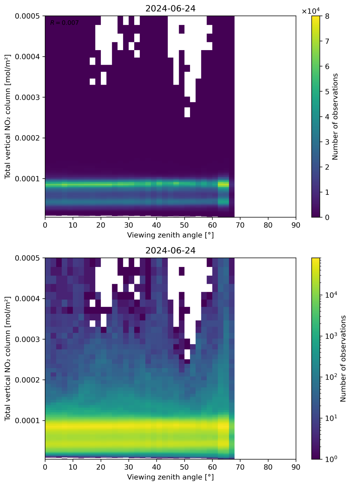
Figure 167: Scatter density plot of “Viewing zenith angle” against “Total vertical NO 2 column” for 2024-06-24 to 2024-06-25.
