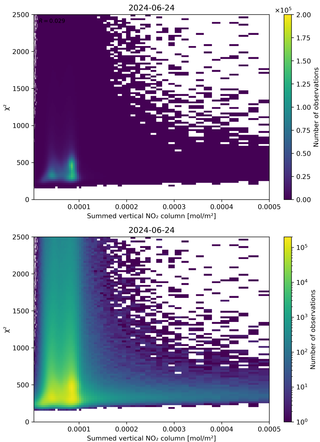
Figure 104: Scatter density plot of “Summed vertical NO 2 column” against “ \chi^2 ” for 2024-06-24 to 2024-06-25.
