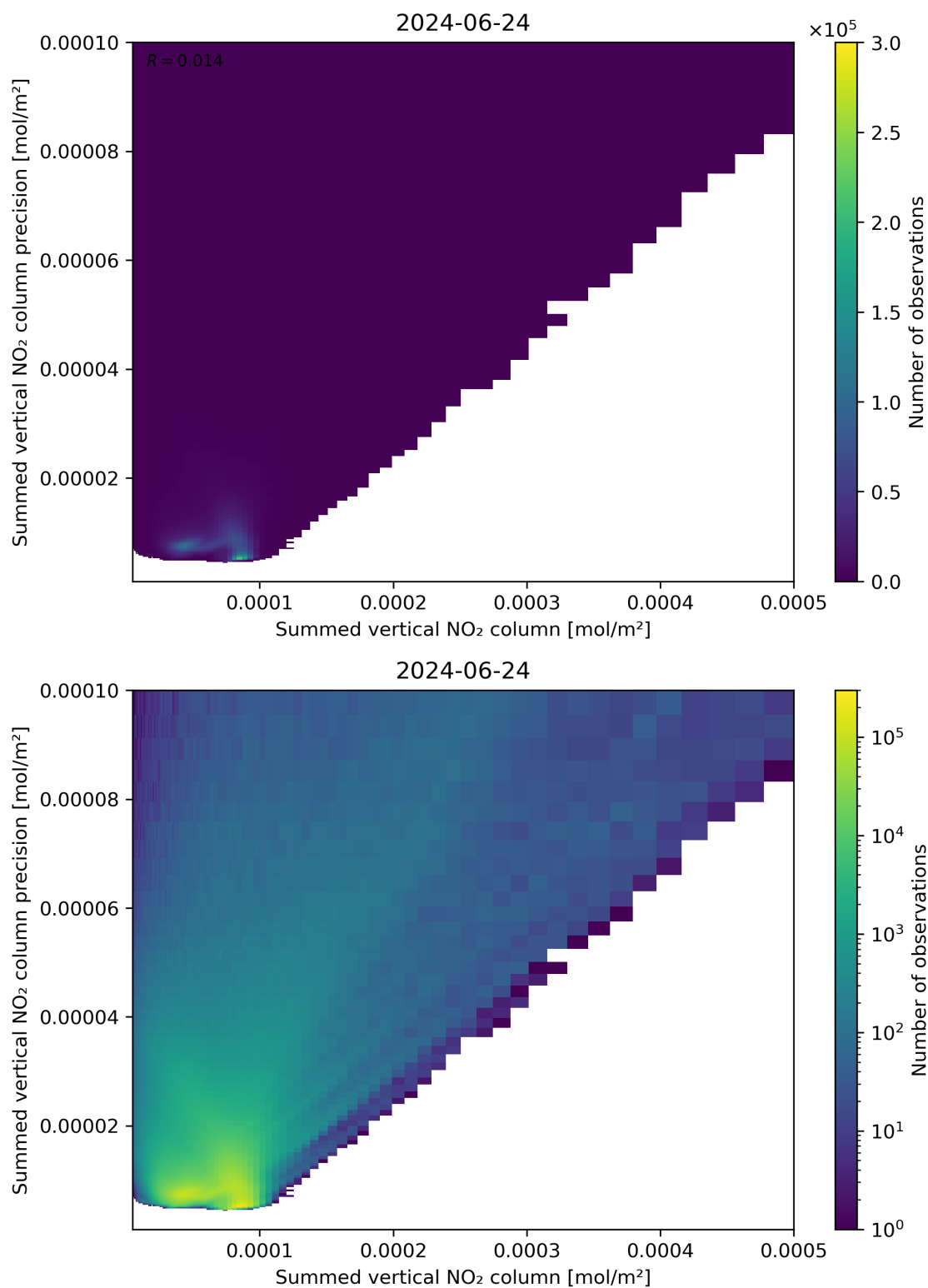
Figure 105: Scatter density plot of “Summed vertical NO 2 column” against “Summed vertical NO 2 column precision” for 2024-06-24 to 2024-06-25.
