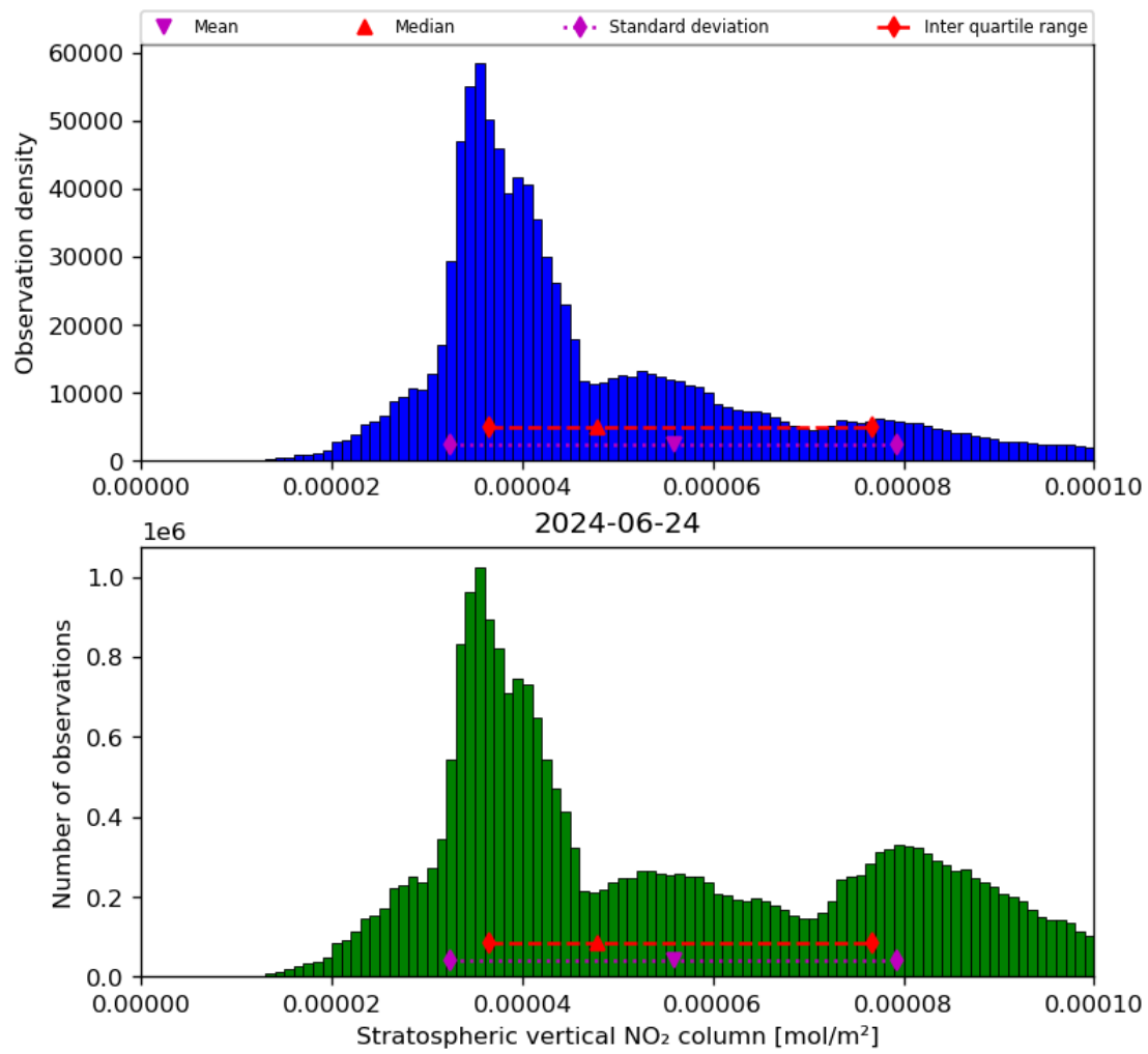
Figure 36: Histogram of “Stratospheric vertical NO 2 column” for 2024-06-24 to 2024-06-25
