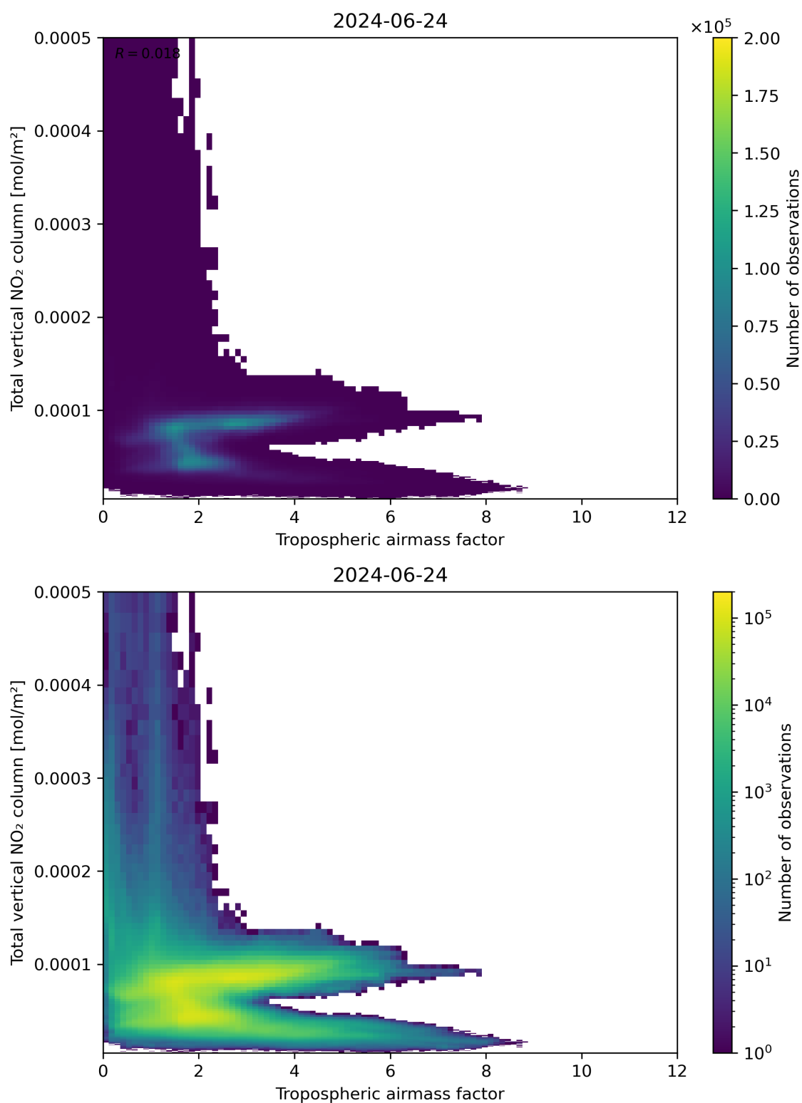
Figure 77: Scatter density plot of “Tropospheric airmass factor” against “Total vertical NO 2 column” for 2024-06-24 to 2024-06-25.
