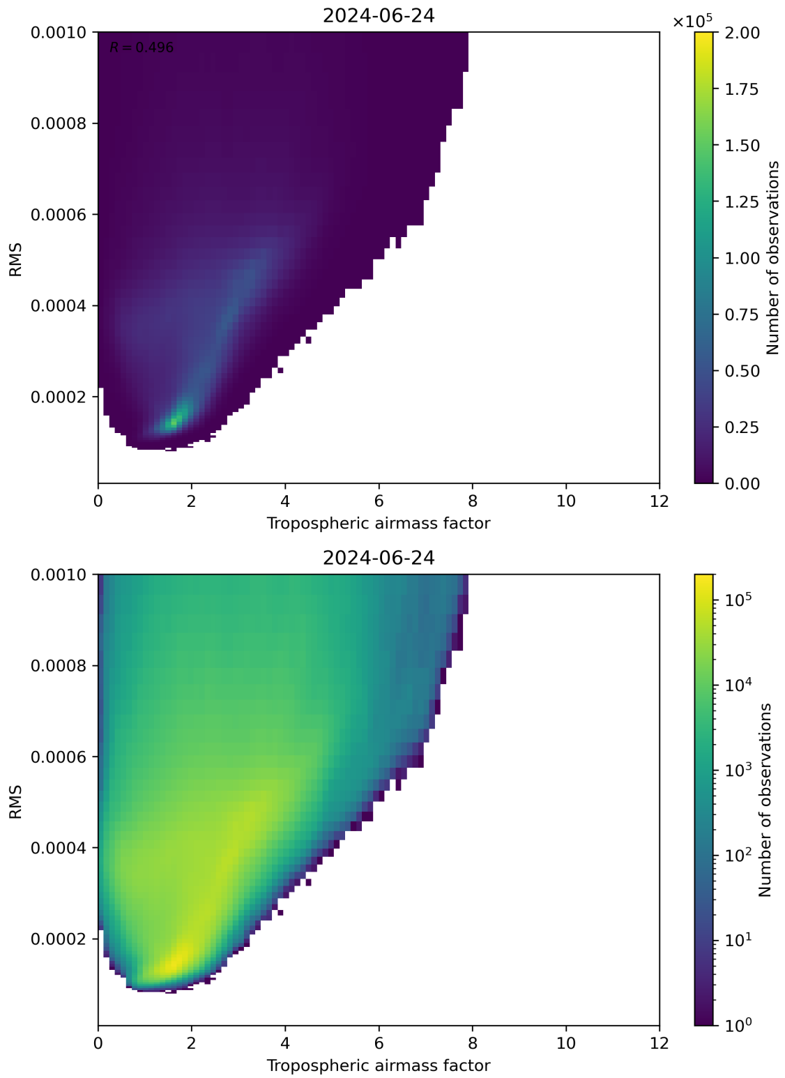
Figure 79: Scatter density plot of “Tropospheric airmass factor” against “RMS” for 2024-06-24 to 2024-06-25.
