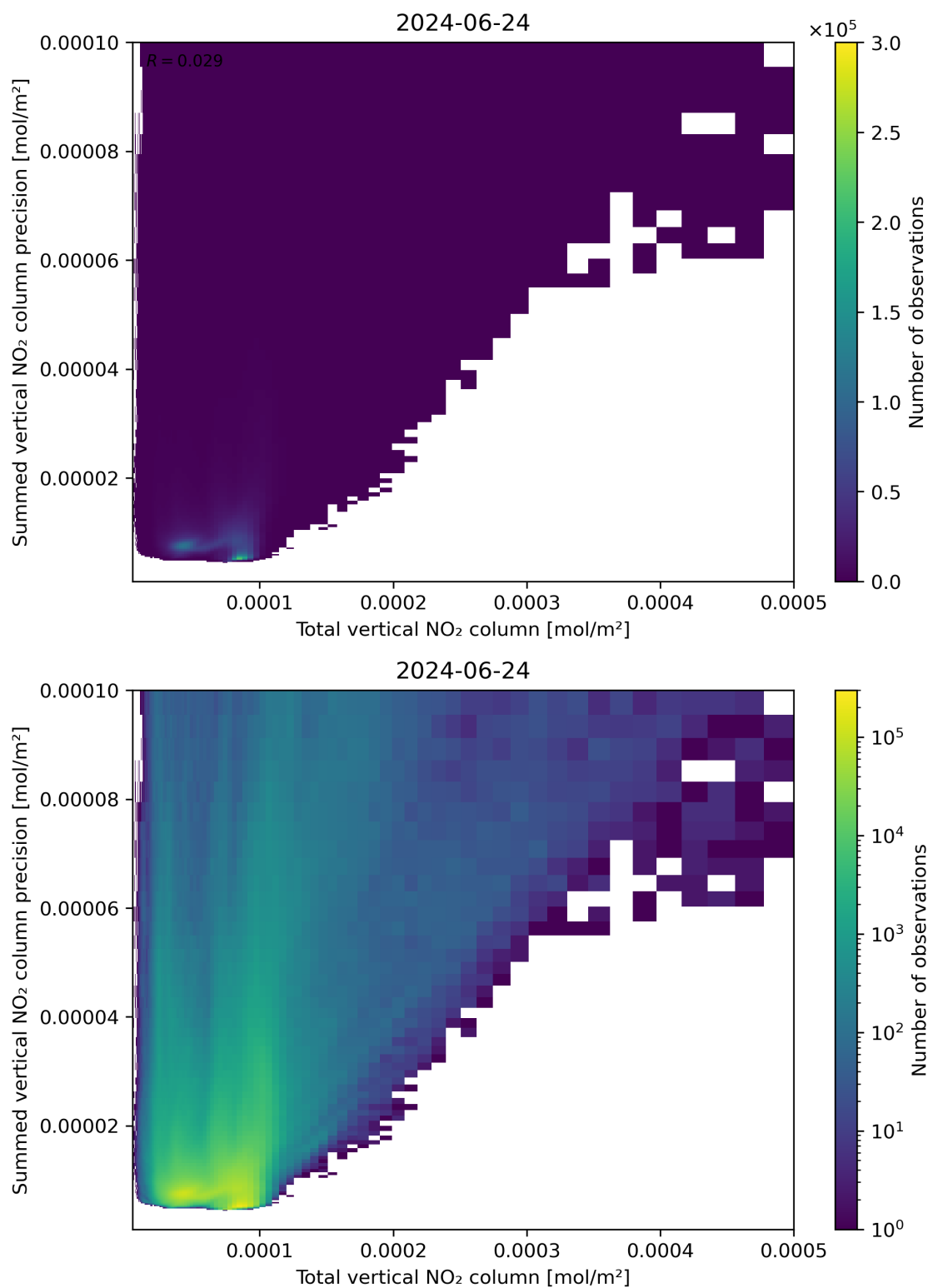
Figure 113: Scatter density plot of “Total vertical NO 2 column” against “Summed vertical NO 2 column precision” for 2024-06-24 to 2024-06-25.
