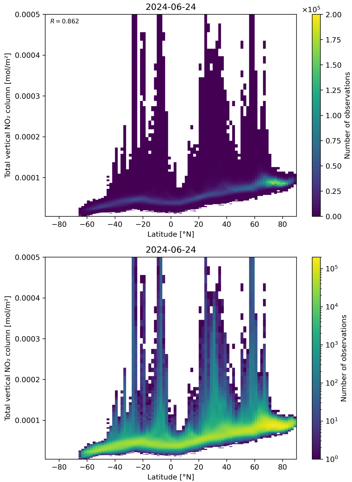
Figure 90: Scatter density plot of “Latitude” against “Total vertical NO 2 column” for 2024-06-24 to 2024-06-25.
