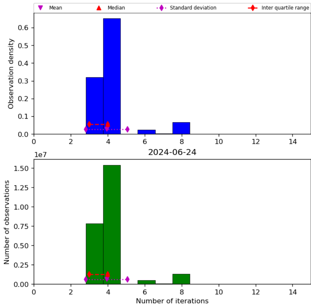
Figure 34: Histogram of “Number of iterations” for 2024-06-24 to 2024-06-25
