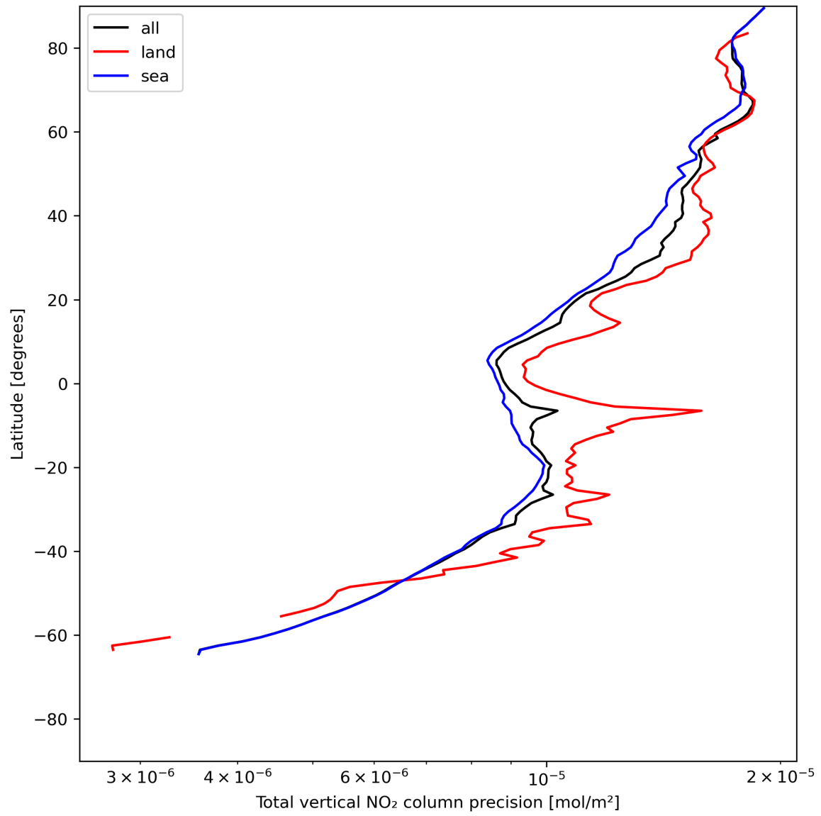
Figure 22: Zonal average of “Total vertical NO 2 column precision” for 2024-06-24 to 2024-06-25.
