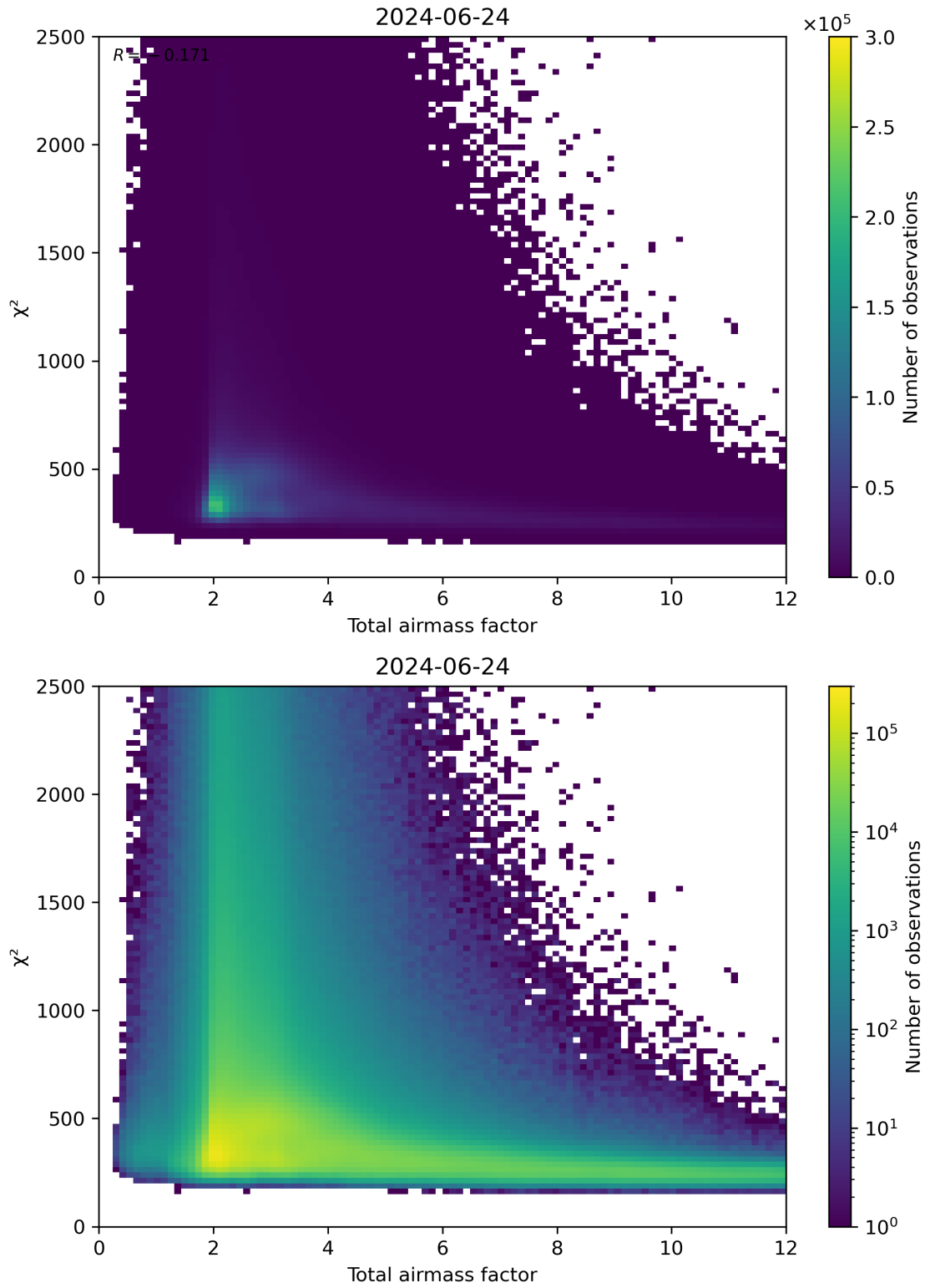
Figure 63: Scatter density plot of “Total airmass factor” against “ \chi^2 ” for 2024-06-24 to 2024-06-25.
