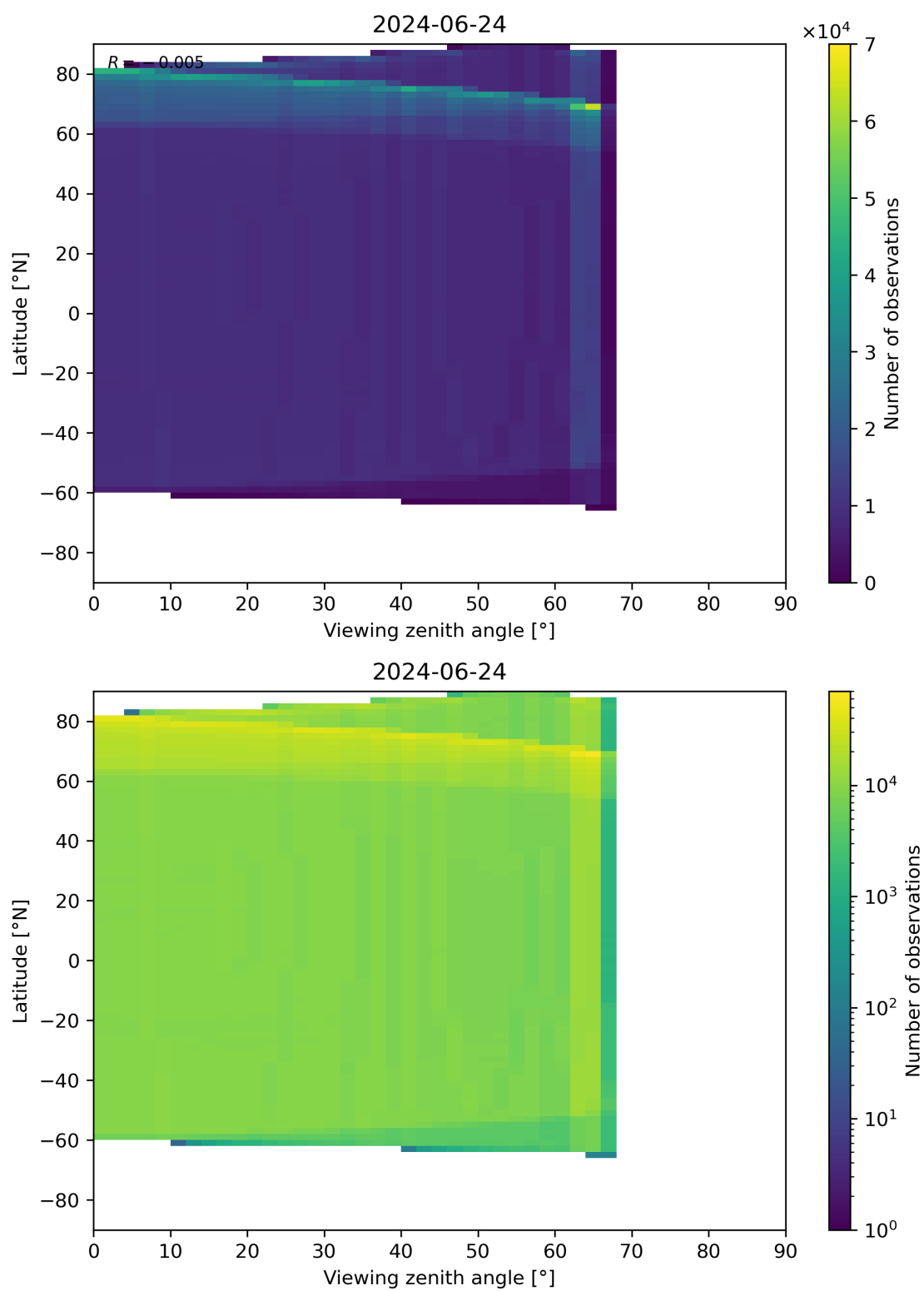
Figure 163: Scatter density plot of “Viewing zenith angle” against “Latitude” for 2024-06-24 to 2024-06-25.
