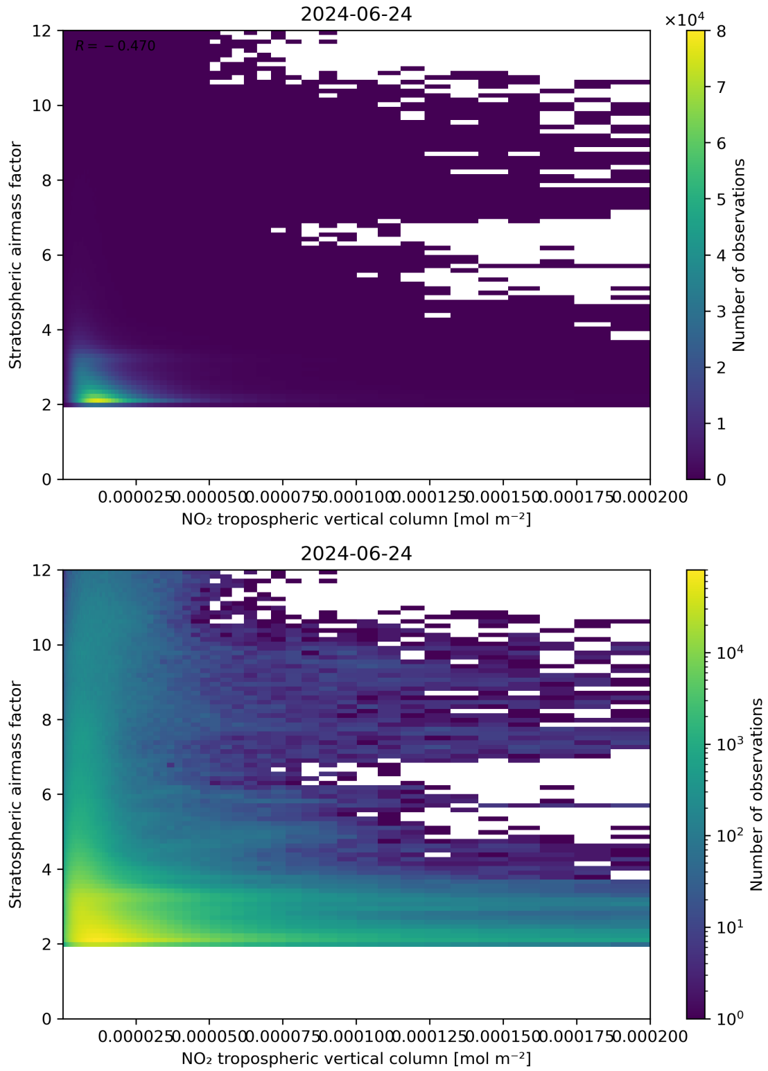
Figure 121: Scatter density plot of “NO 2 tropospheric vertical column” against “Stratospheric air mass factor” for 2024-06-24 to 2024-06-25.
