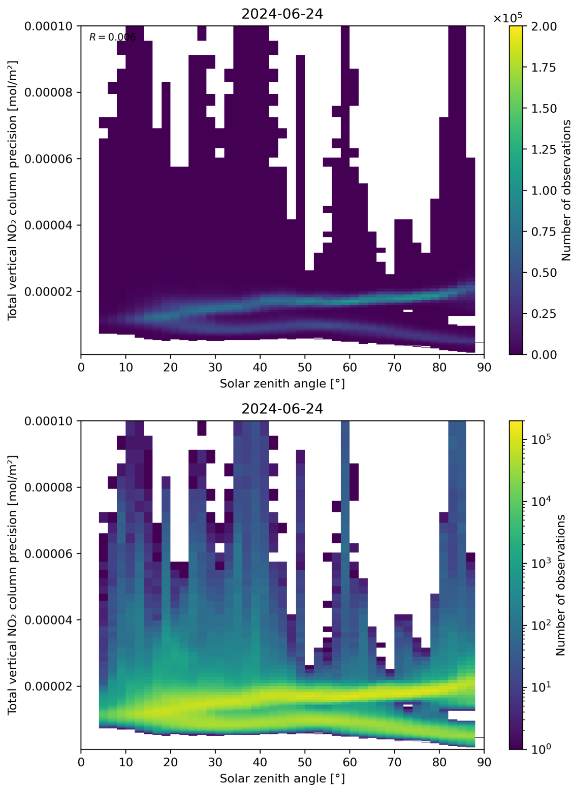
Figure 154: Scatter density plot of “Solar zenith angle” against “Total vertical NO 2 column precision” for 2024-06-24 to 2024-06-25.
