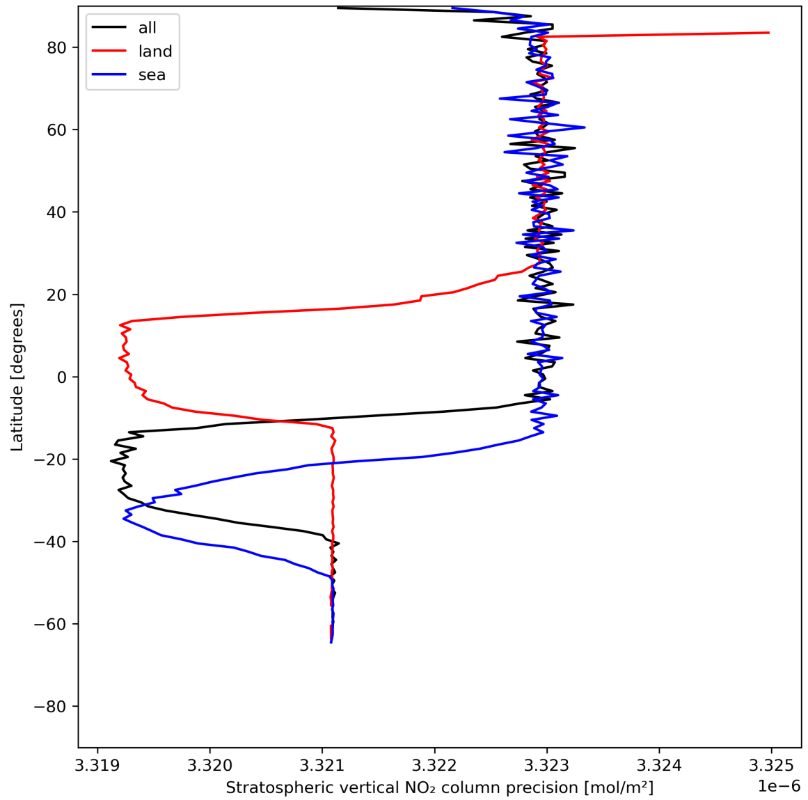
Figure 20: Zonal average of “Stratospheric vertical NO 2 column precision” for 2024-06-24 to 2024-06-25.
