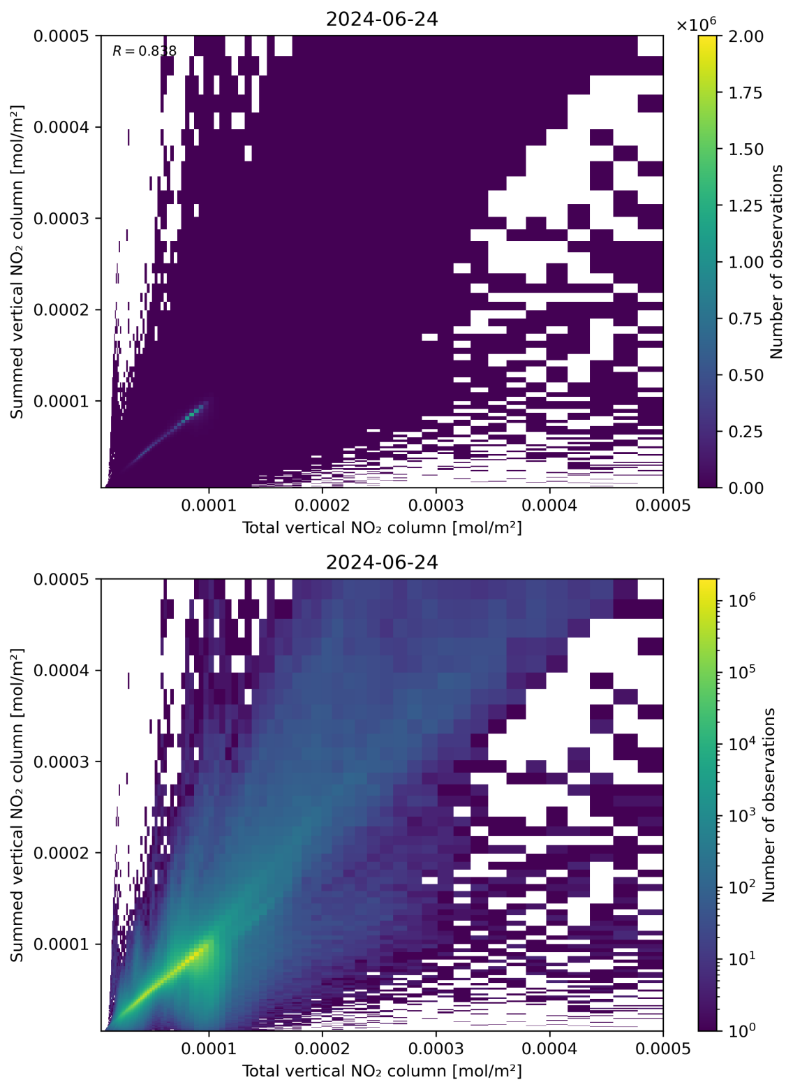
Figure 112: Scatter density plot of “Total vertical NO 2 column” against “Summed vertical NO 2 column” for 2024-06-24 to 2024-06-25.
