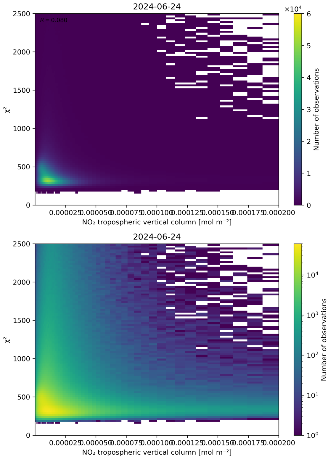
Figure 124: Scatter density plot of “NO 2 tropospheric vertical column” against “ \chi^2 ” for 2024-06-24 to 2024-06-25.
