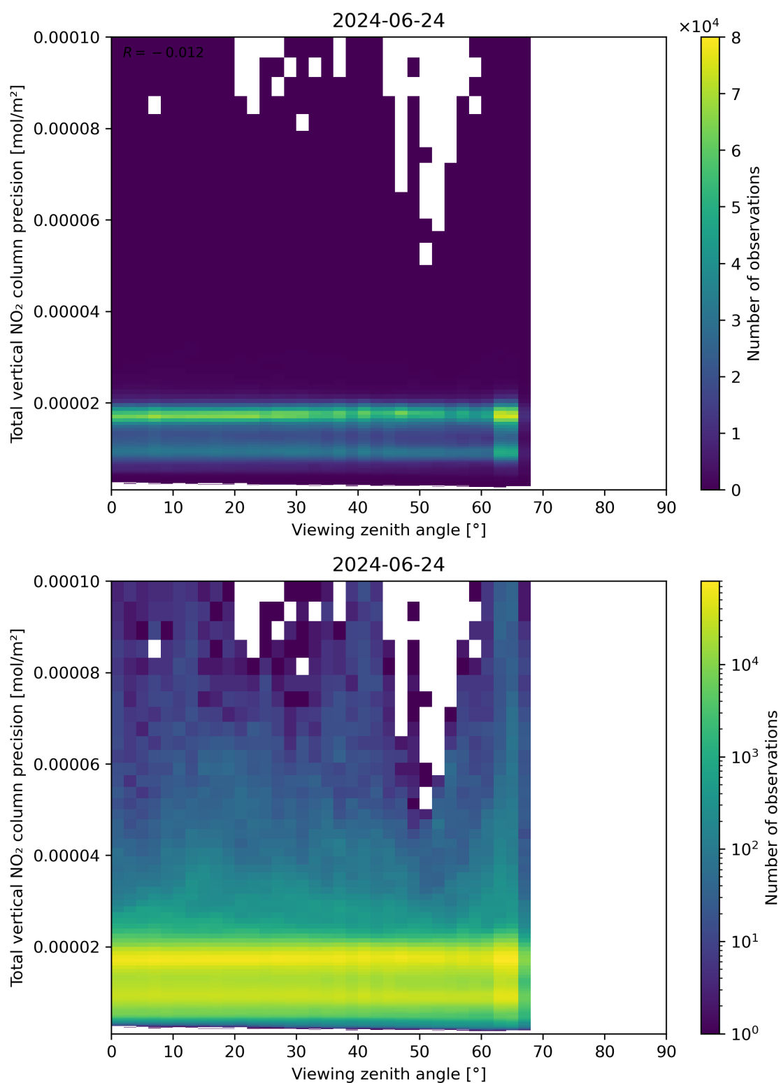
Figure 168: Scatter density plot of “Viewing zenith angle” against “Total vertical NO 2 column precision” for 2024-06-24 to 2024-06-25.
