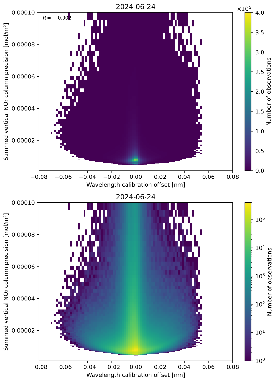
Figure 178: Scatter density plot of “Wavelength calibration offset” against “Summed vertical NO 2 column precision” for 2024-06-24 to 2024-06-25.
