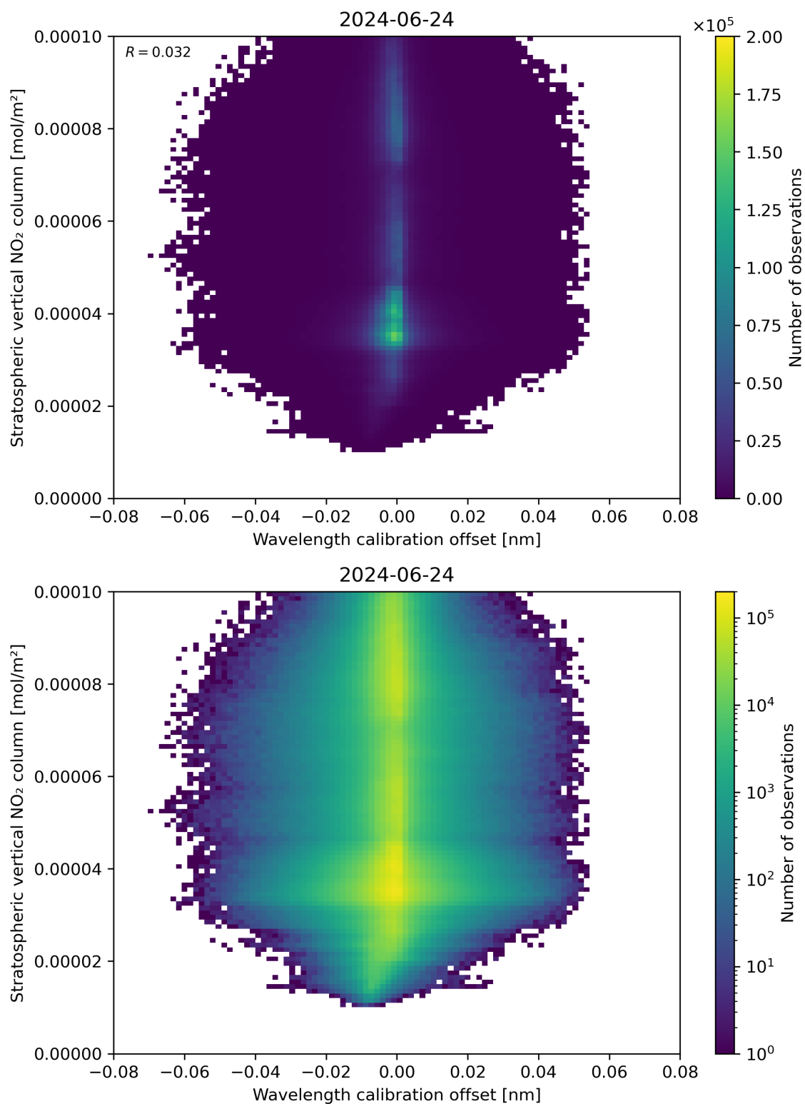
Figure 176: Scatter density plot of “Wavelength calibration offset” against “Stratospheric vertical NO 2 column” for 2024-06-24 to 2024-06-25.
