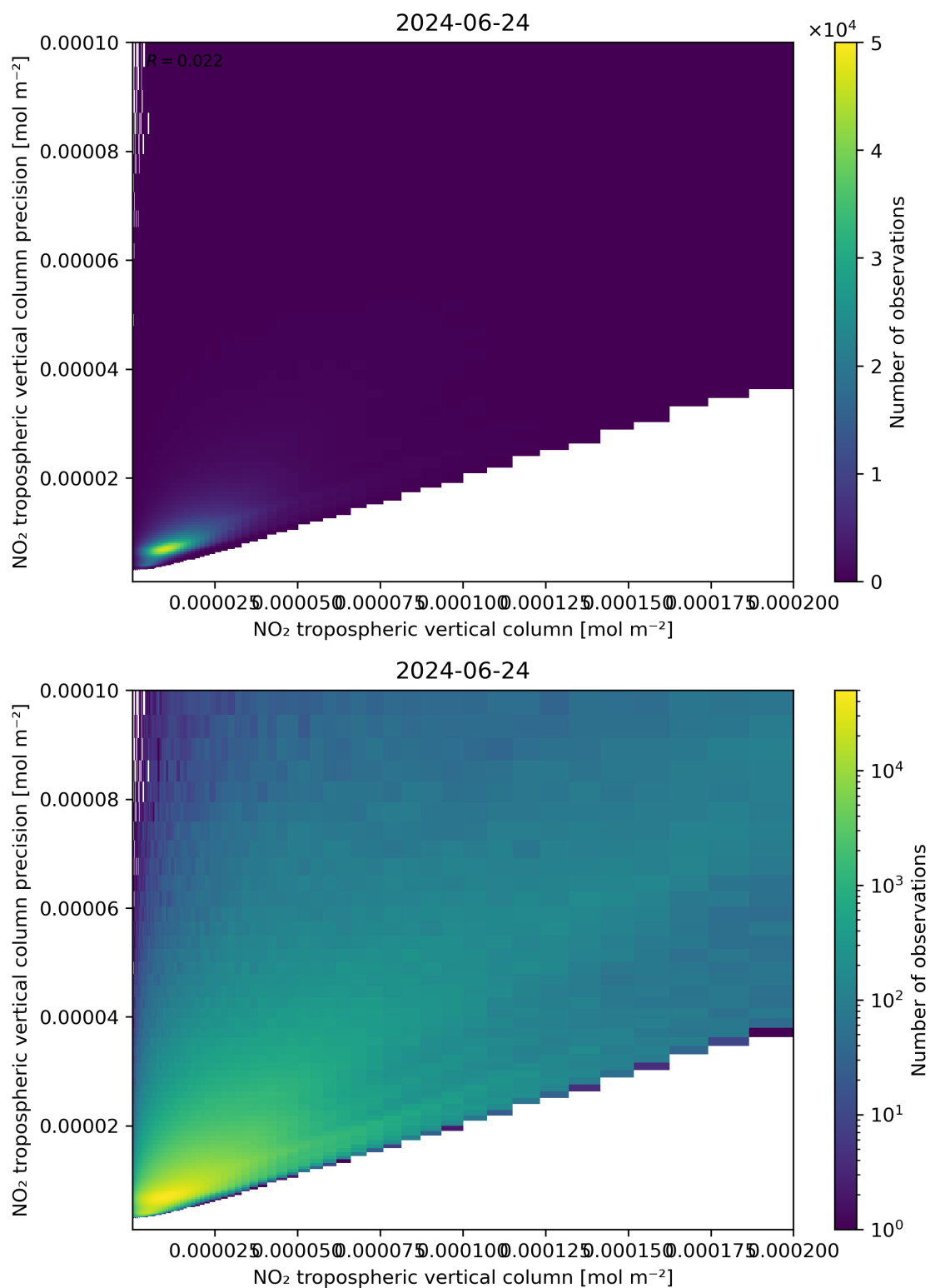
Figure 130: Scatter density plot of “NO 2 tropospheric vertical column” against “NO 2 tropospheric vertical column precision” for 2024-06-24 to 2024-06-25.
