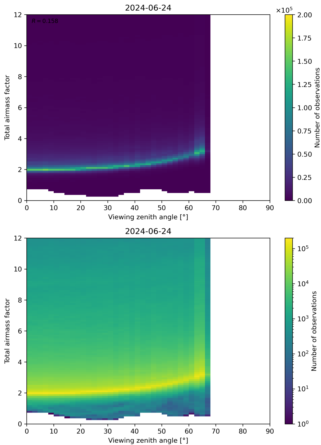
Figure 160: Scatter density plot of “Viewing zenith angle” against “Total airmass factor” for 2024-06-24 to 2024-06-25.
