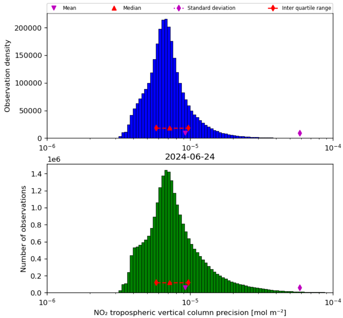
Figure 30: Histogram of “NO 2 tropospheric vertical column precision” for 2024-06-24 to 2024-06-25
