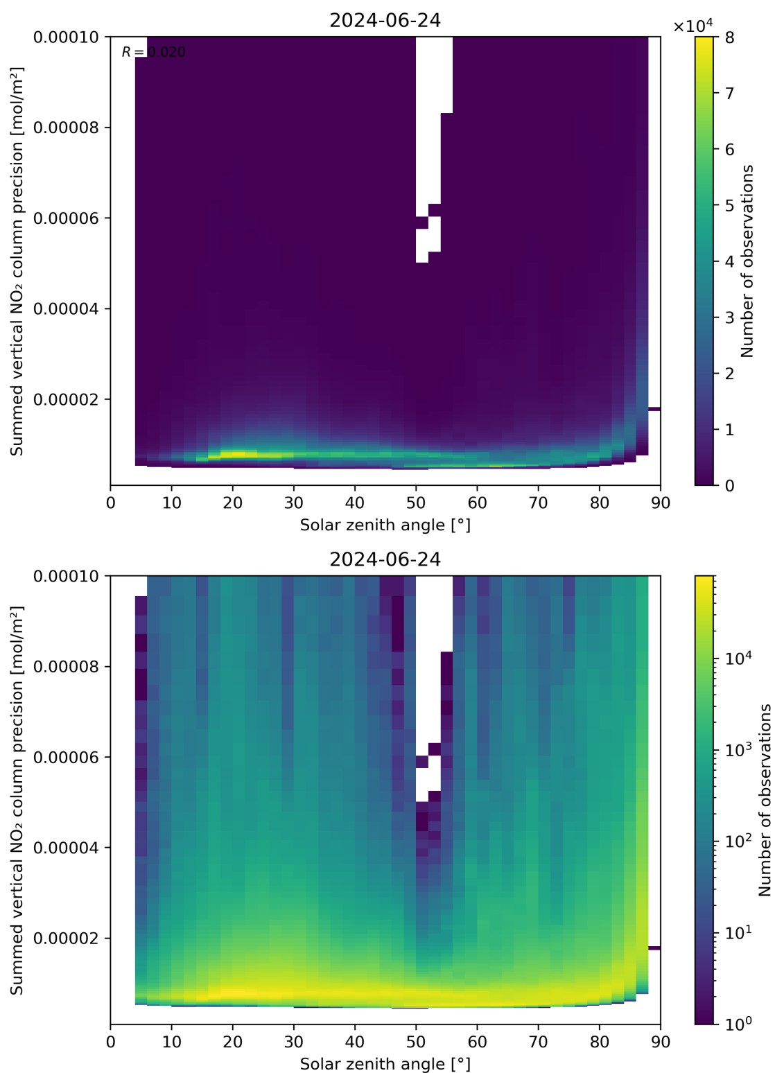
Figure 152: Scatter density plot of “Solar zenith angle” against “Summed vertical NO 2 column precision” for 2024-06-24 to 2024-06-25.
