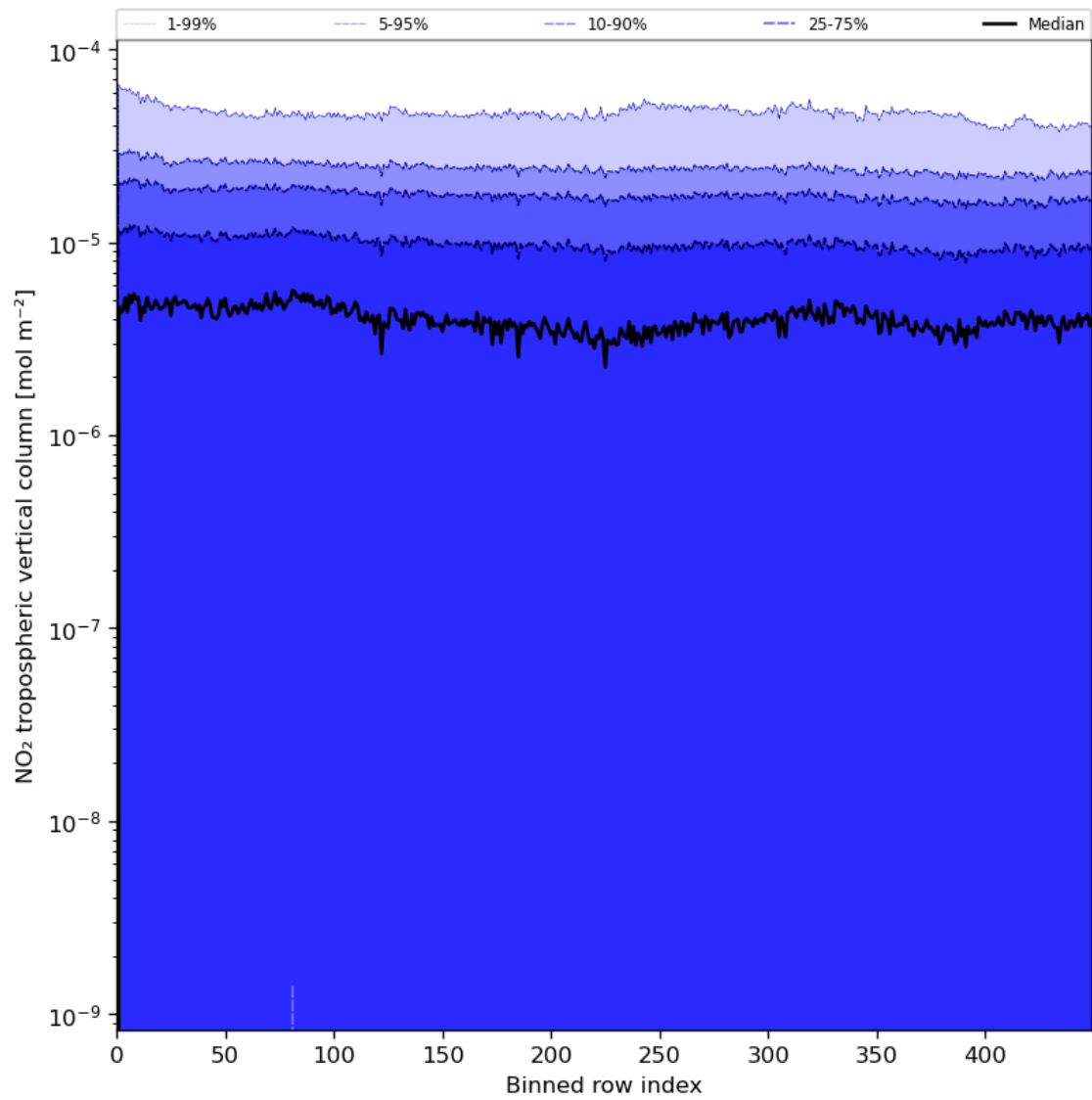
Figure 46: Along track statistics of “NO 2 tropospheric vertical column” for 2024-06-24 to 2024-06-25
