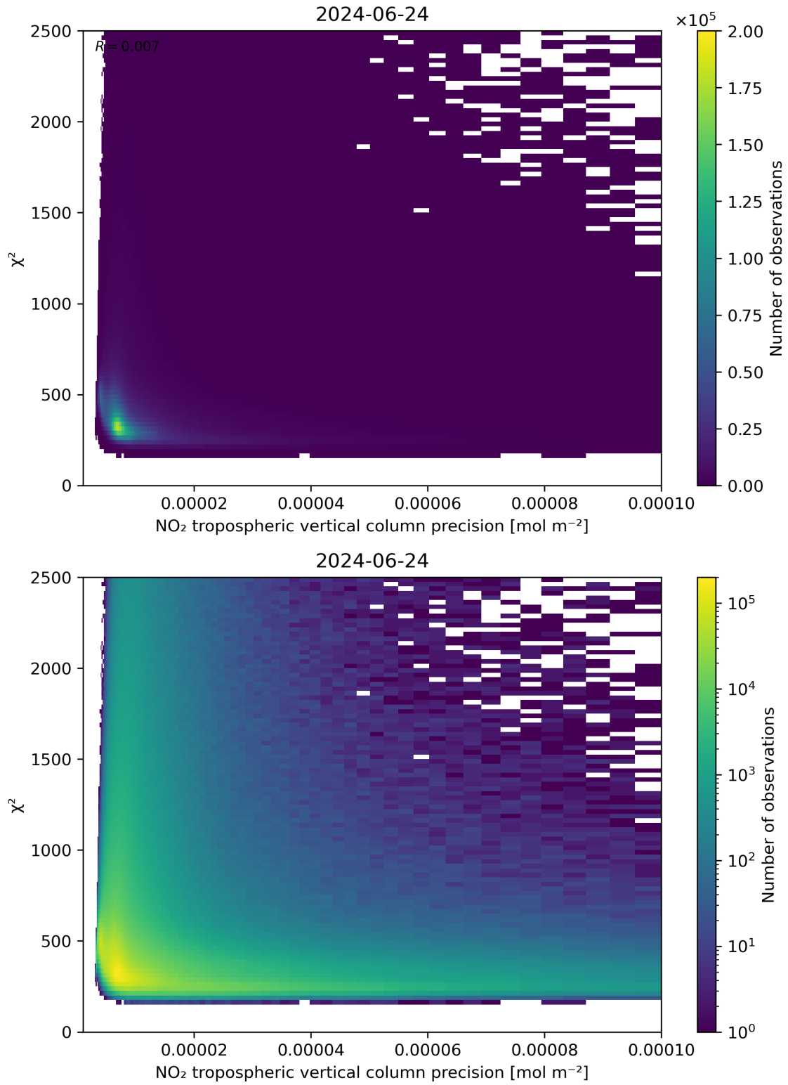
Figure 134: Scatter density plot of “NO 2 tropospheric vertical column precision” against “ \chi^2 ” for 2024-06-24 to 2024-06-25.
