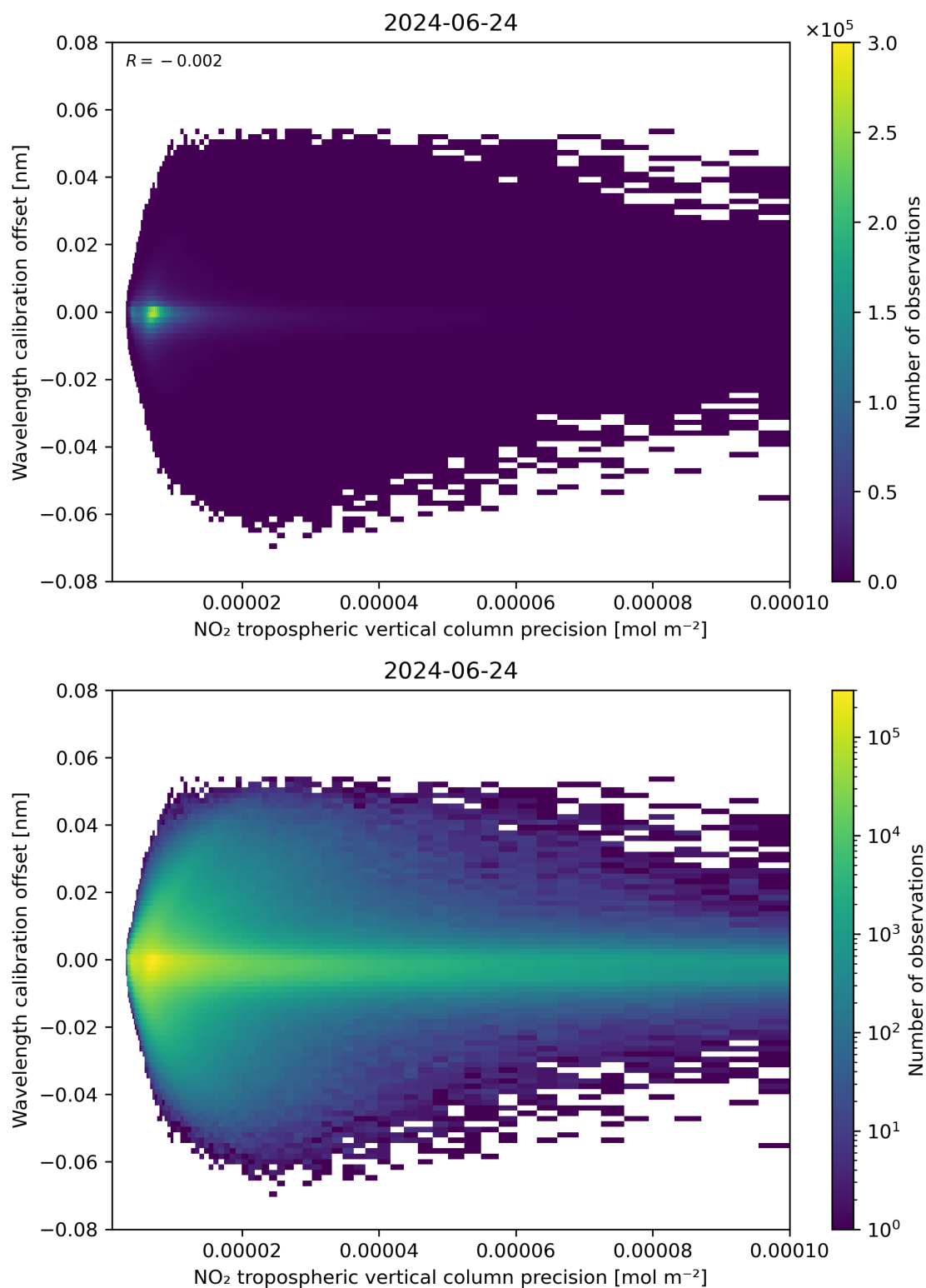
Figure 141: Scatter density plot of “NO 2 tropospheric vertical column precision” against “Wavelength calibration offset” for 2024-06-24 to 2024-06-25.
