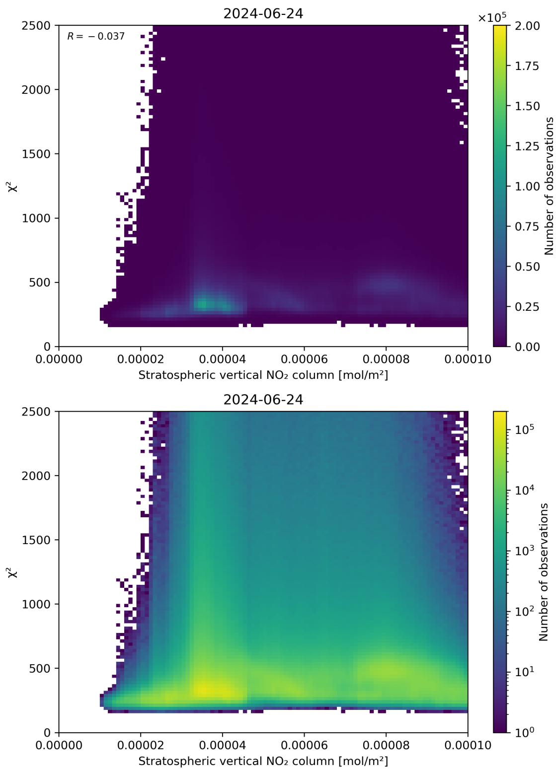
Figure 97: Scatter density plot of “Stratospheric vertical NO 2 column” against “ \chi^2 ” for 2024-06-24 to 2024-06-25.
