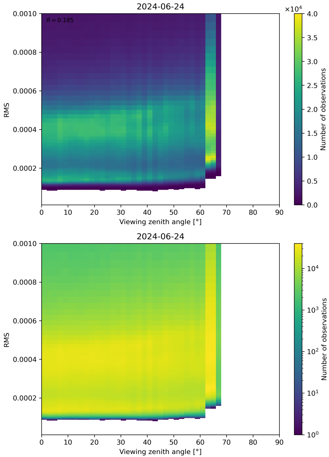
Figure 171: Scatter density plot of “Viewing zenith angle” against “RMS” for 2024-06-24 to 2024-06-25.
