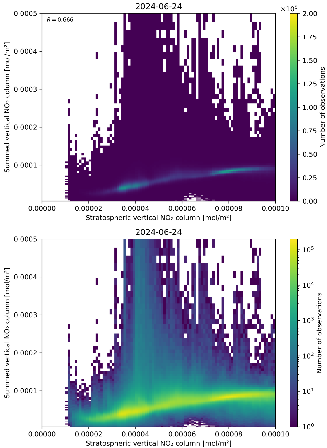
Figure 98: Scatter density plot of “Stratospheric vertical NO 2 column” against “Summed vertical NO 2 column” for 2024-06-24 to 2024-06-25.
