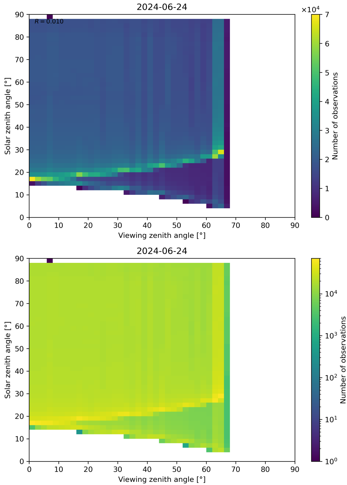
Figure 172: Scatter density plot of “Viewing zenith angle” against “Solar zenith angle” for 2024-06-24 to 2024-06-25.
