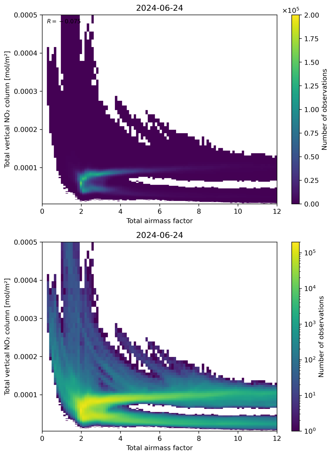
Figure 67: Scatter density plot of “Total airmass factor” against “Total vertical NO 2 column” for 2024-06-24 to 2024-06-25.
