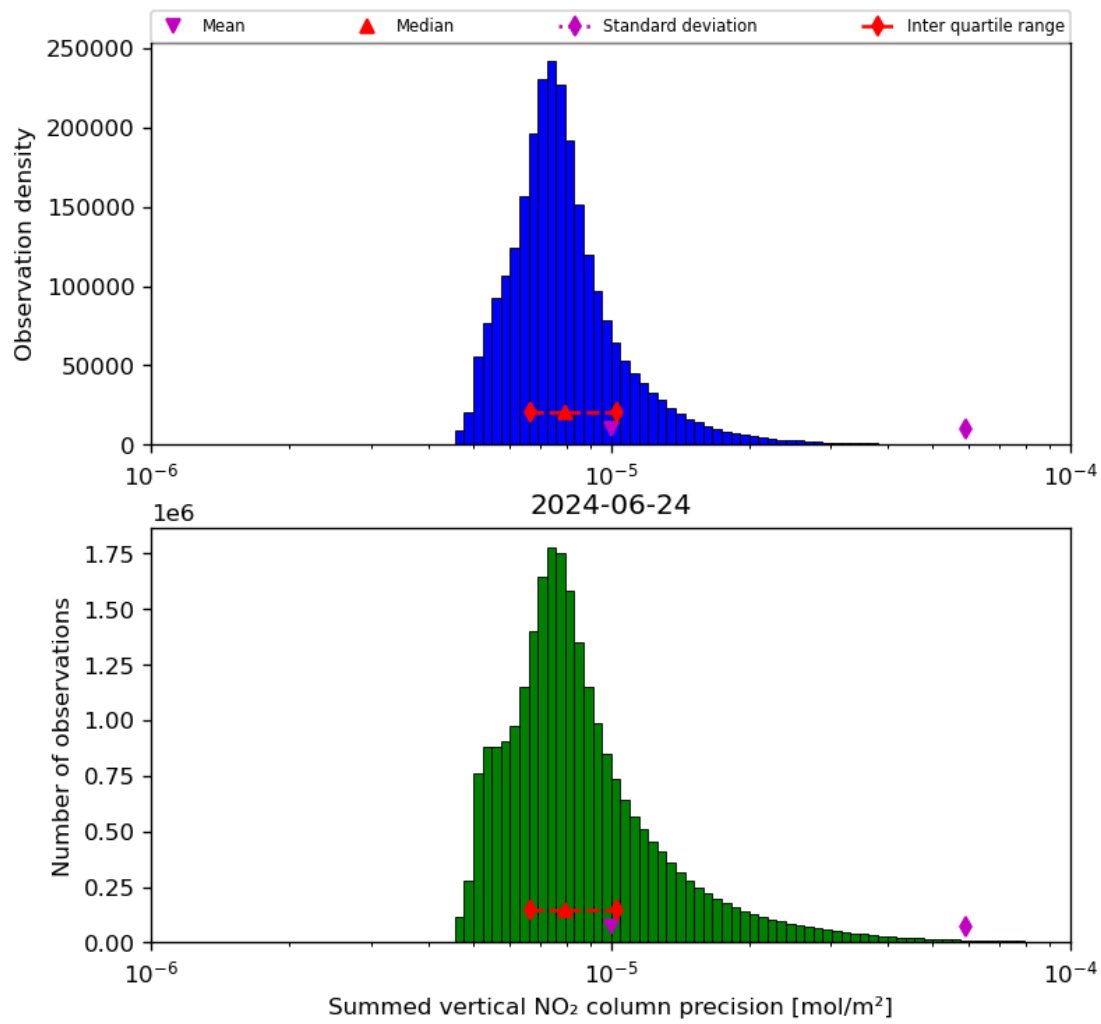
Figure 41: Histogram of “Summed vertical NO 2 column precision” for 2024-06-24 to 2024-06-25
