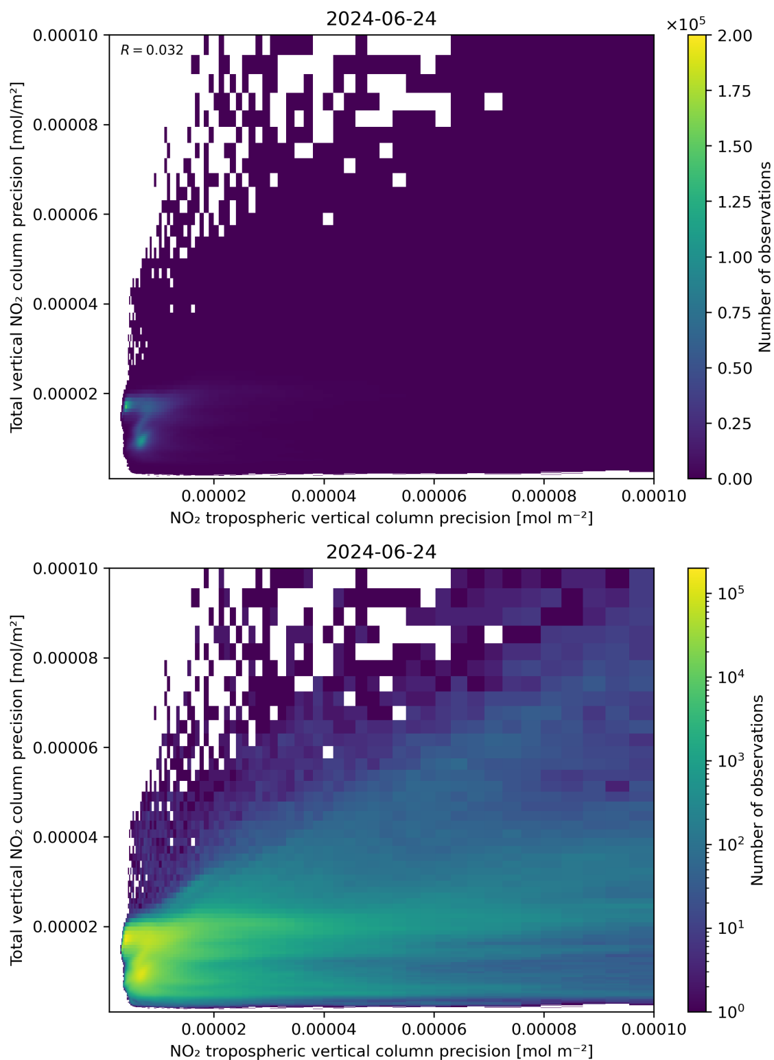
Figure 139: Scatter density plot of “NO 2 tropospheric vertical column precision” against “Total vertical NO 2 column precision” for 2024-06-24 to 2024-06-25.
