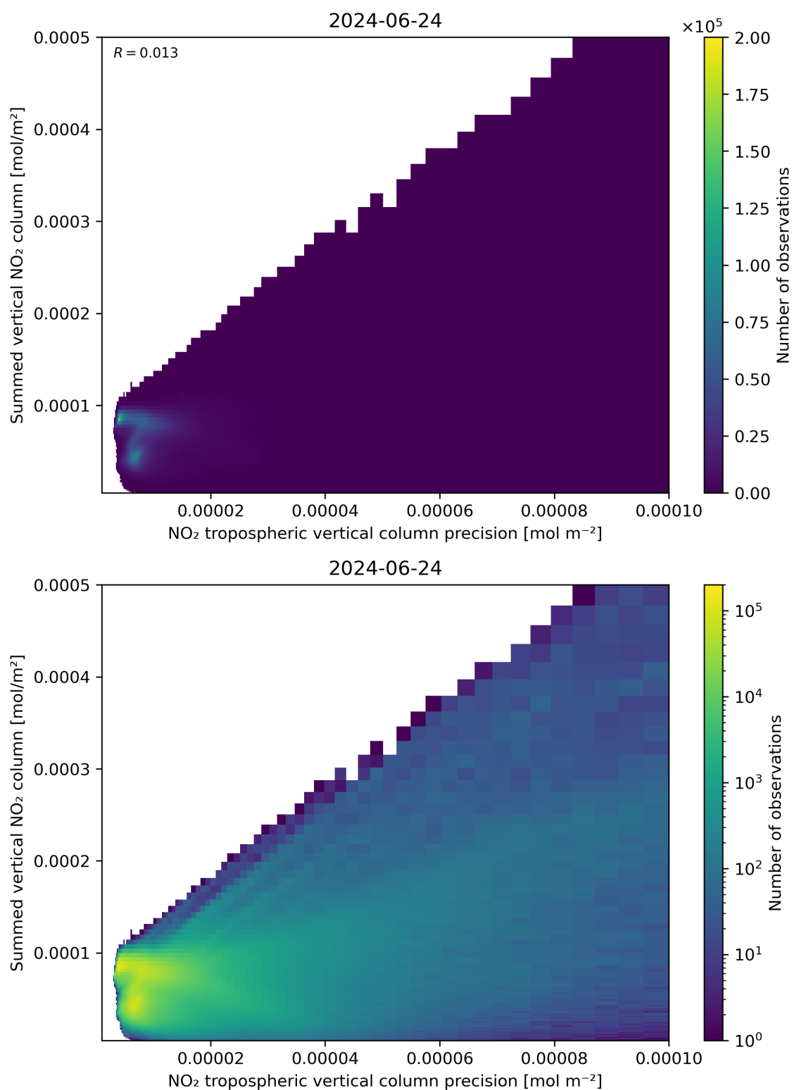
Figure 136: Scatter density plot of “NO 2 tropospheric vertical column precision” against “Summed vertical NO 2 column” for 2024-06-24 to 2024-06-25.
