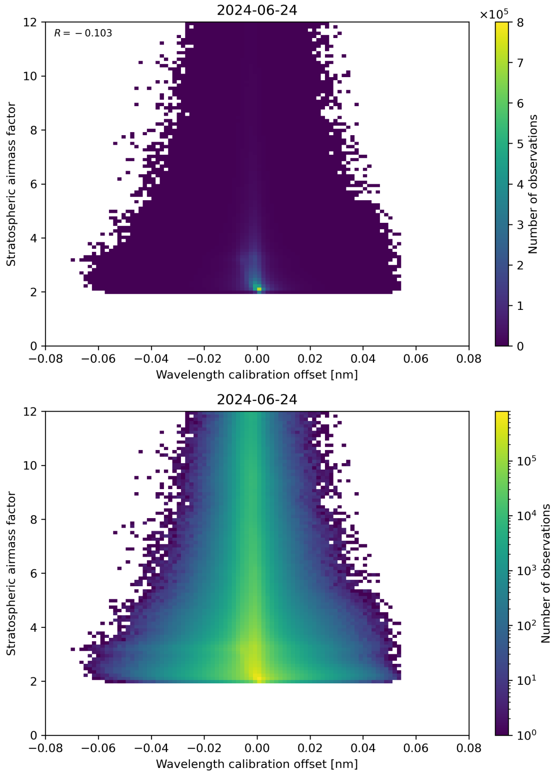
Figure 174: Scatter density plot of “Wavelength calibration offset” against “Stratospheric airmass factor” for 2024-06-24 to 2024-06-25.
