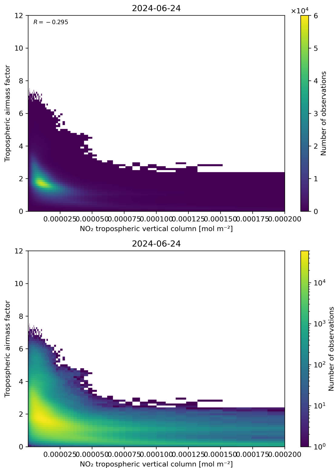
Figure 123: Scatter density plot of “NO 2 tropospheric vertical column” against “Tropospheric air mass factor” for 2024-06-24 to 2024-06-25.
