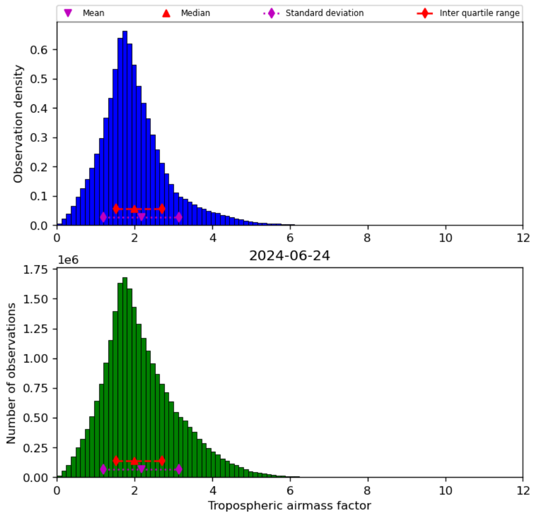
Figure 31: Histogram of “Tropospheric airmass factor” for 2024-06-24 to 2024-06-25
