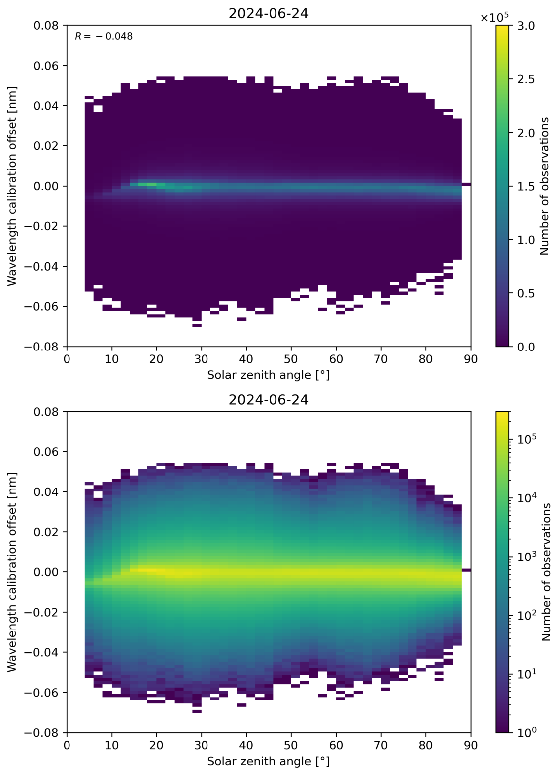
Figure 158: Scatter density plot of “Solar zenith angle” against “Wavelength calibration offset” for 2024-06-24 to 2024-06-25.
