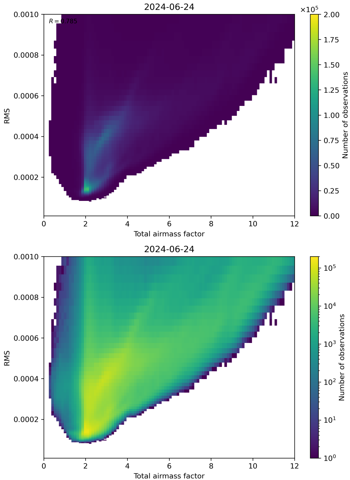
Figure 69: Scatter density plot of “Total airmass factor” against “RMS” for 2024-06-24 to 2024-06-25.
