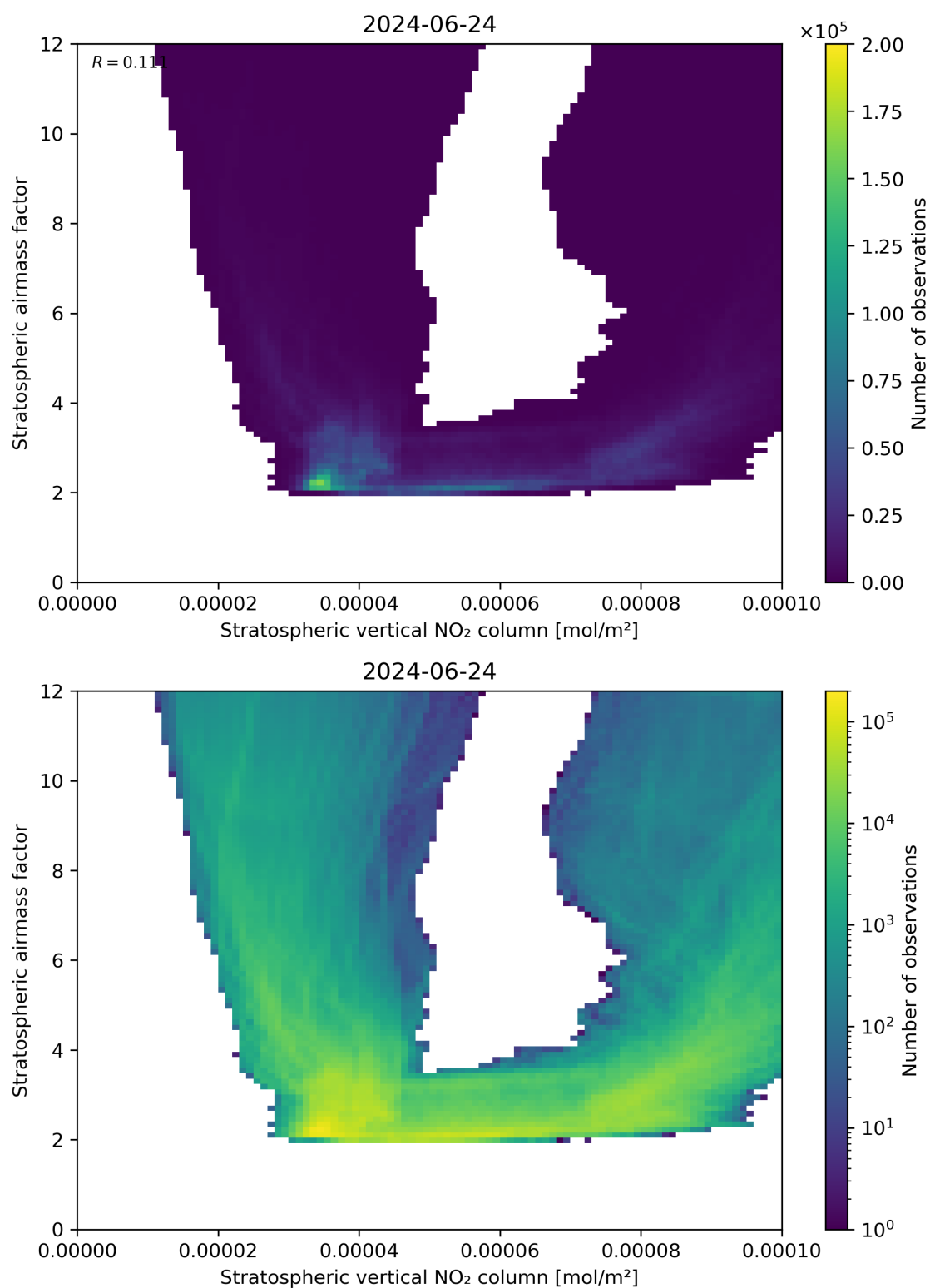
Figure 96: Scatter density plot of “Stratospheric vertical NO 2 column” against “Stratospheric airmass factor” for 2024-06-24 to 2024-06-25.
