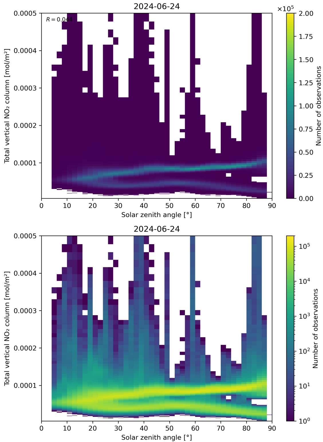
Figure 153: Scatter density plot of “Solar zenith angle” against “Total vertical NO 2 column” for 2024-06-24 to 2024-06-25.
