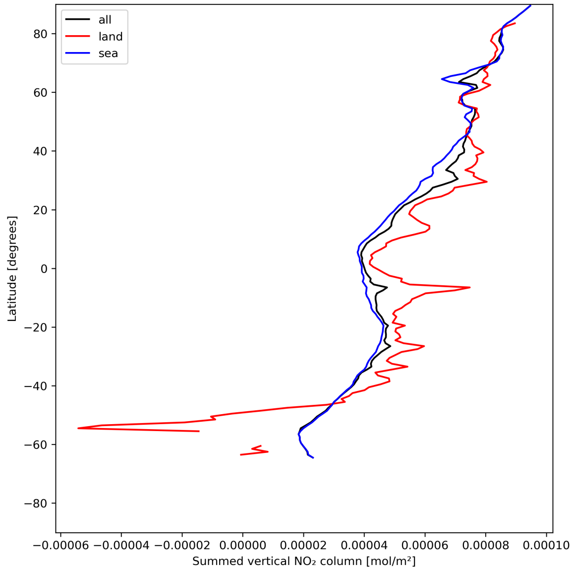
Figure 23: Zonal average of “Summed vertical NO 2 column” for 2024-06-24 to 2024-06-25.
