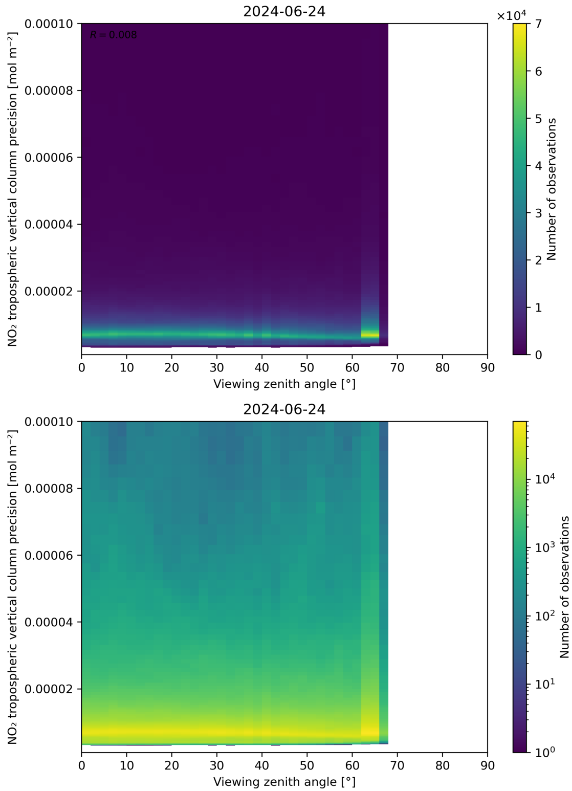
Figure 170: Scatter density plot of “Viewing zenith angle” against “NO 2 tropospheric vertical column precision” for 2024-06-24 to 2024-06-25.
