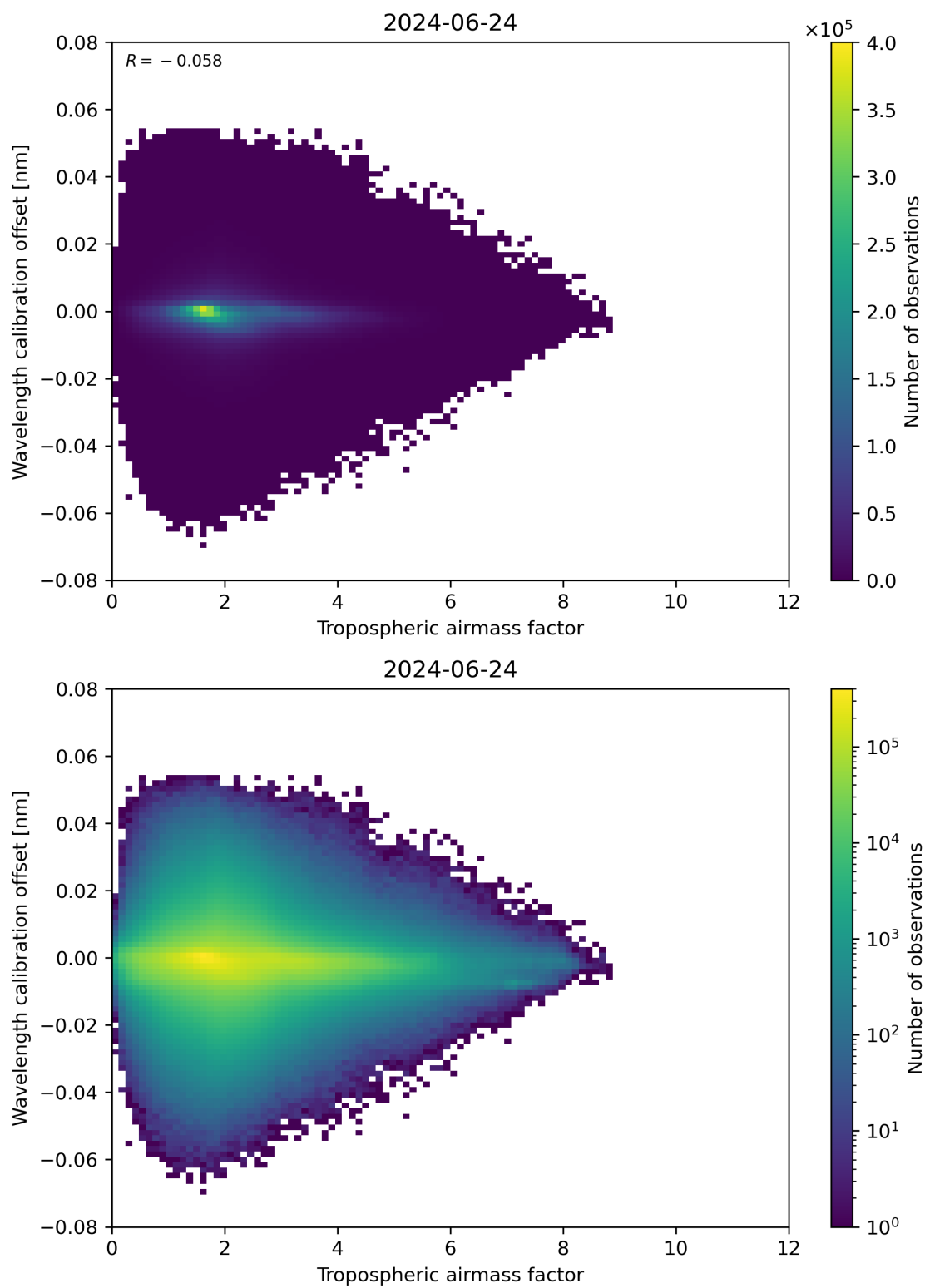
Figure 80: Scatter density plot of “Tropospheric airmass factor” against “Wavelength calibration offset” for 2024-06-24 to 2024-06-25.
