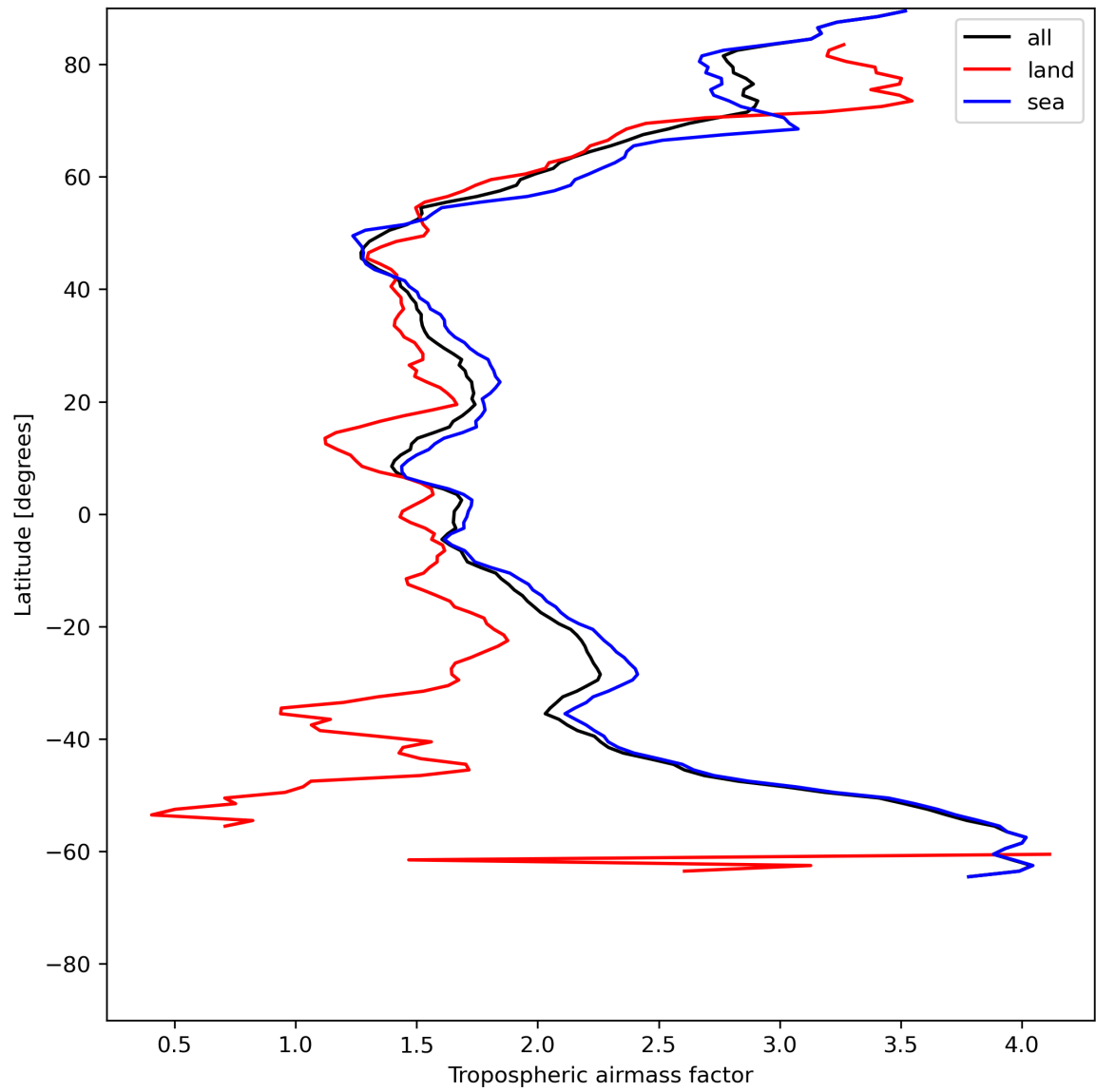
Figure 14: Zonal average of “Tropospheric airmass factor” for 2024-06-24 to 2024-06-25.
