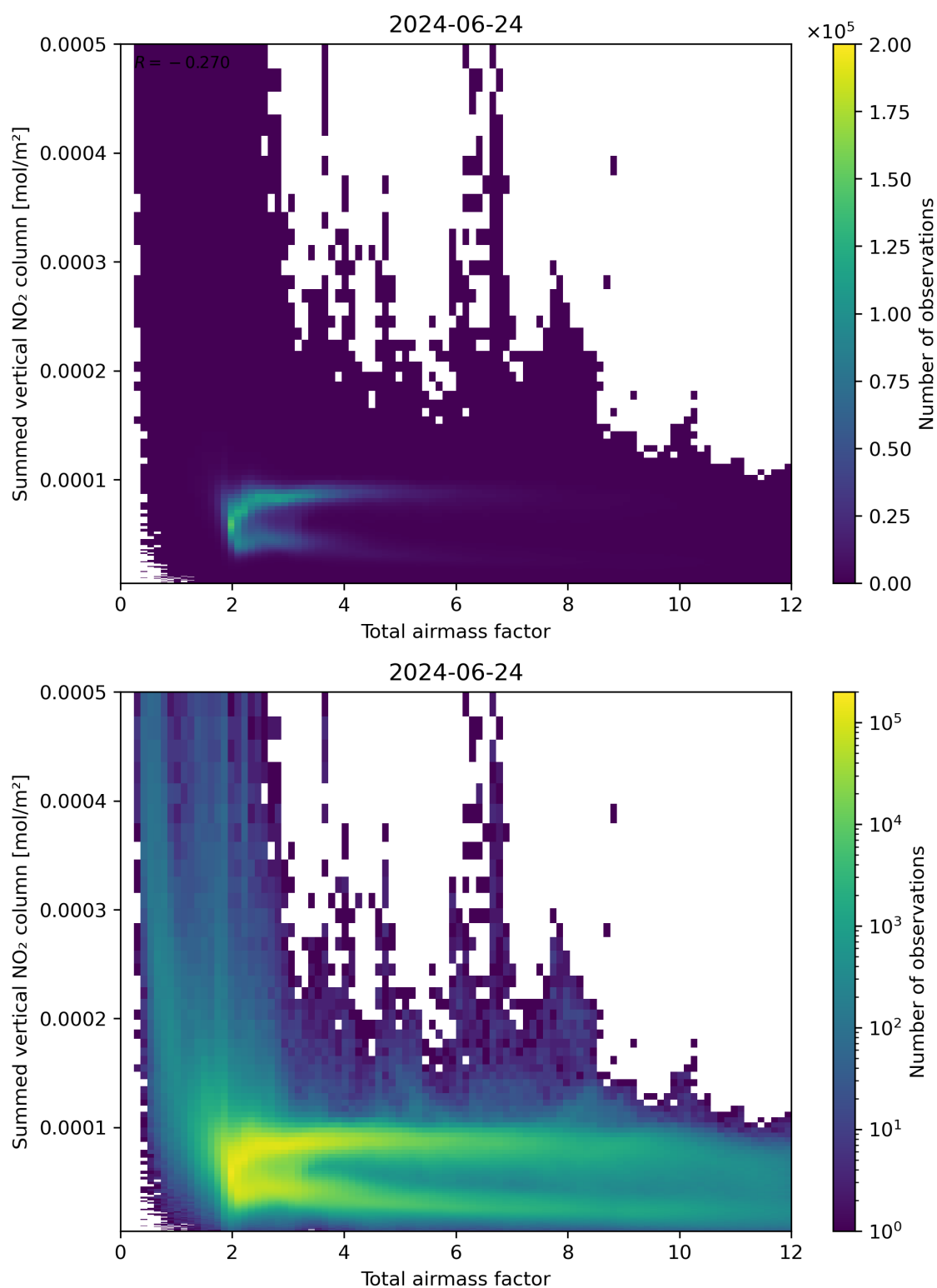
Figure 65: Scatter density plot of “Total airmass factor” against “Summed vertical NO 2 column” for 2024-06-24 to 2024-06-25.
