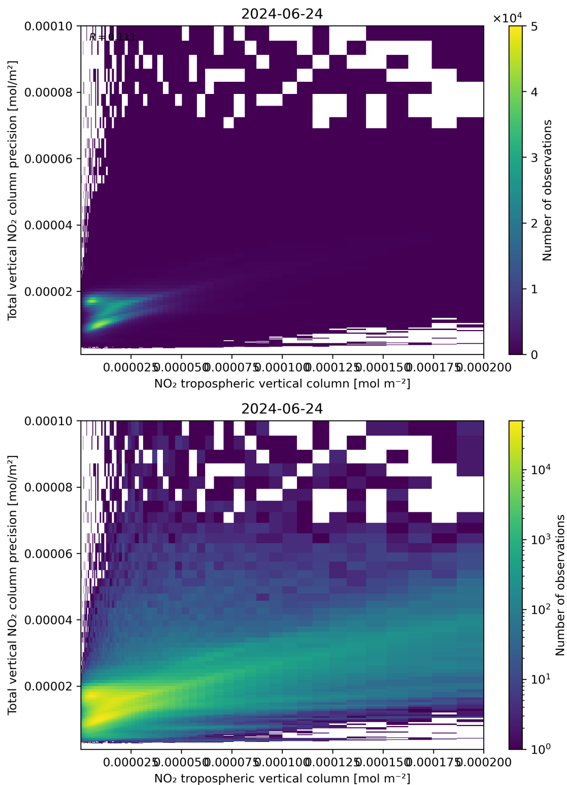
Figure 129: Scatter density plot of “NO 2 tropospheric vertical column” against “Total vertical NO 2 column precision” for 2024-06-24 to 2024-06-25.
