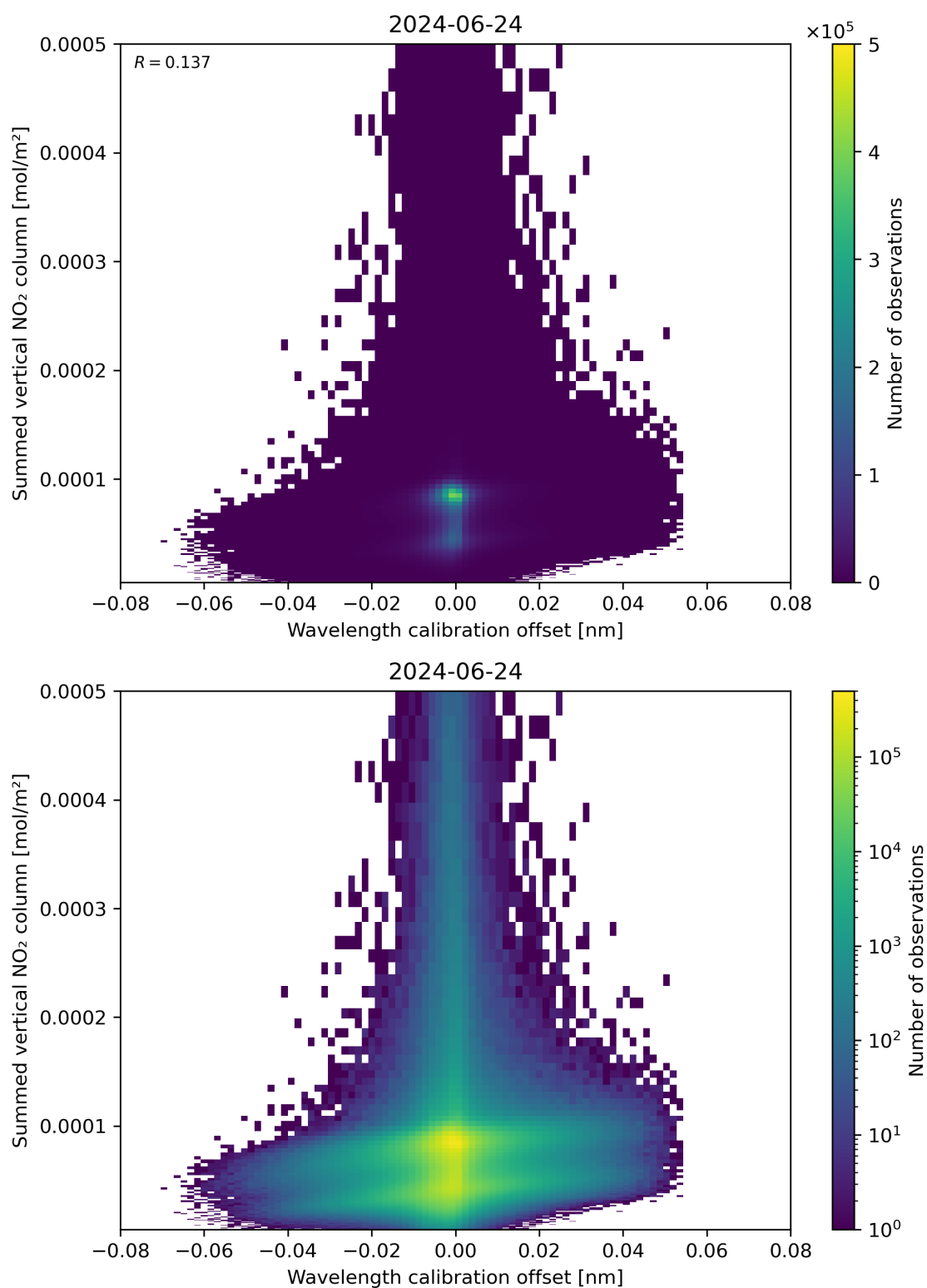
Figure 177: Scatter density plot of “Wavelength calibration offset” against “Summed vertical NO 2 column” for 2024-06-24 to 2024-06-25.
