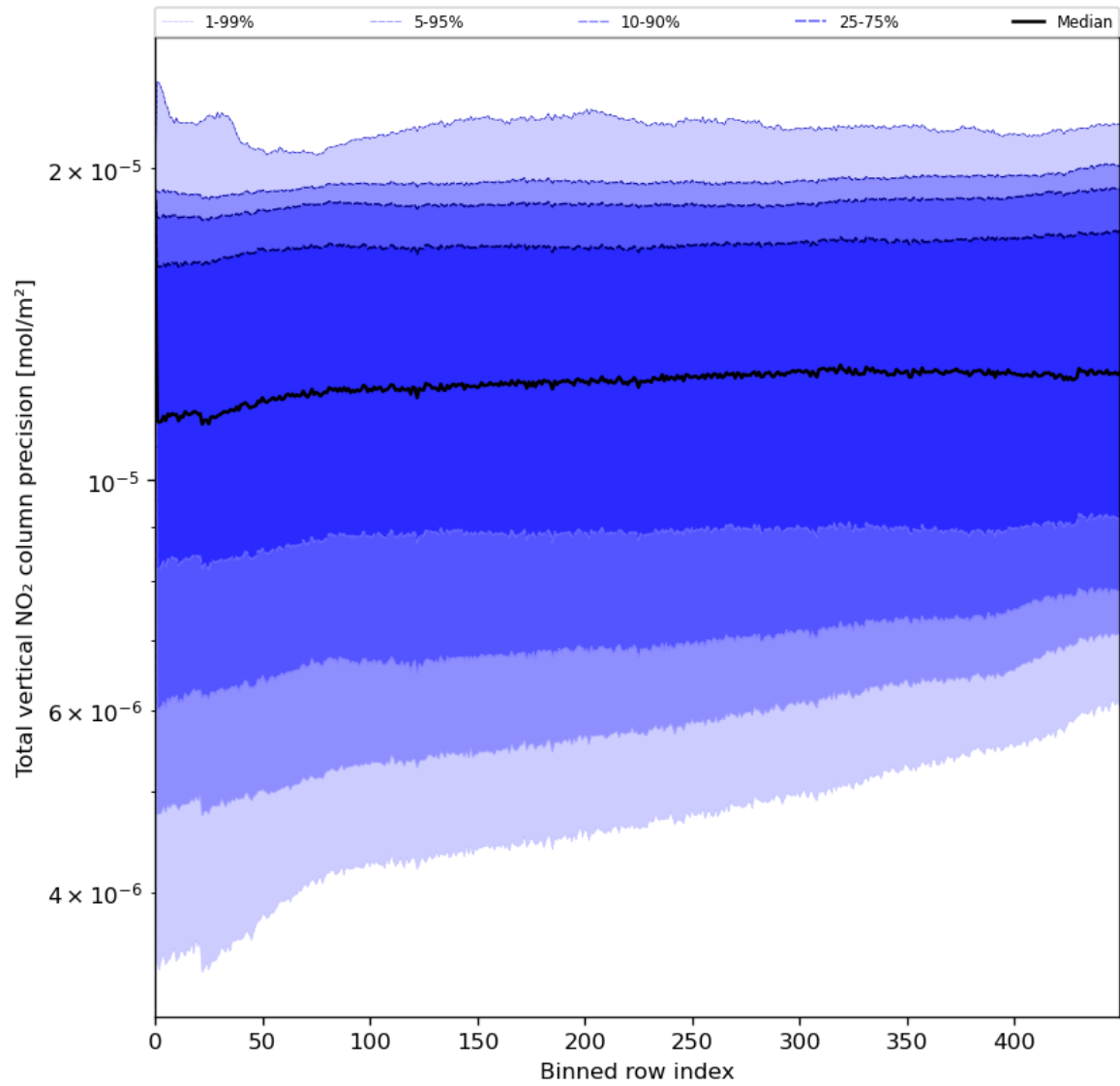
Figure 56: Along track statistics of “Total vertical NO 2 column precision” for 2024-06-24 to 2024-06-25
