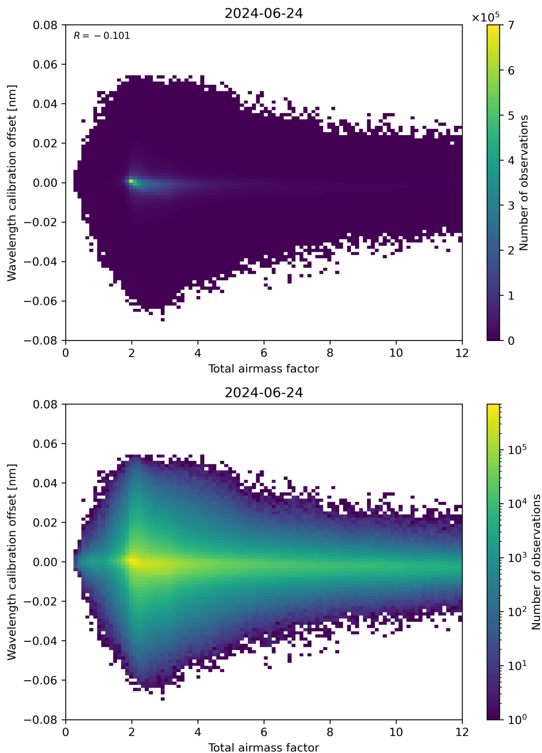
Figure 70: Scatter density plot of “Total airmass factor” against “Wavelength calibration offset” for 2024-06-24 to 2024-06-25.
