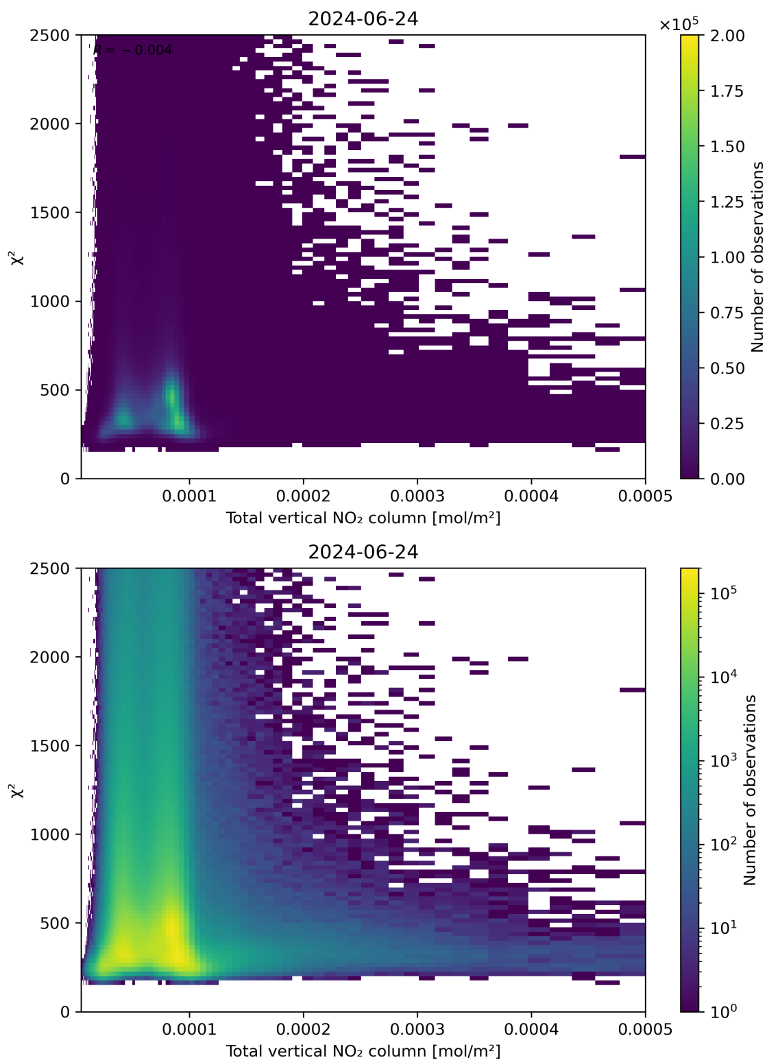
Figure 111: Scatter density plot of “Total vertical NO 2 column” against “ \chi^2 ” for 2024-06-24 to 2024-06-25.
