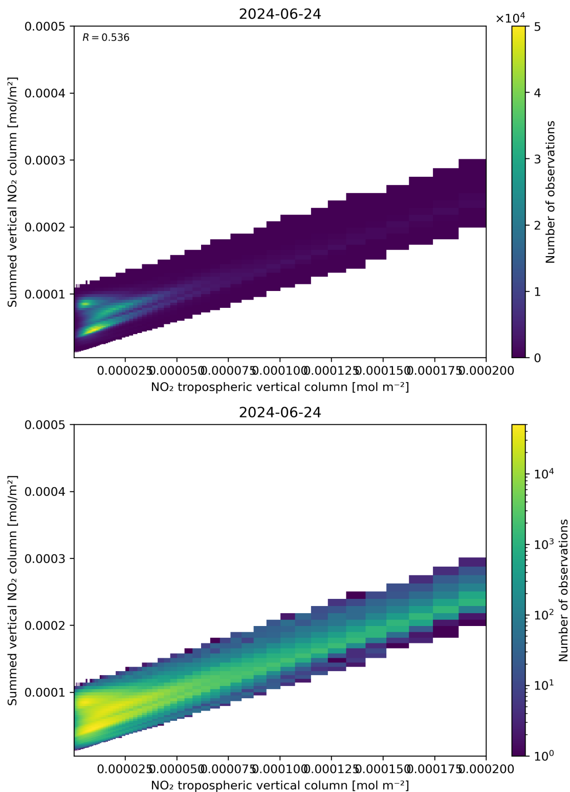
Figure 126: Scatter density plot of “NO 2 tropospheric vertical column” against “Summed vertical NO 2 column” for 2024-06-24 to 2024-06-25.
