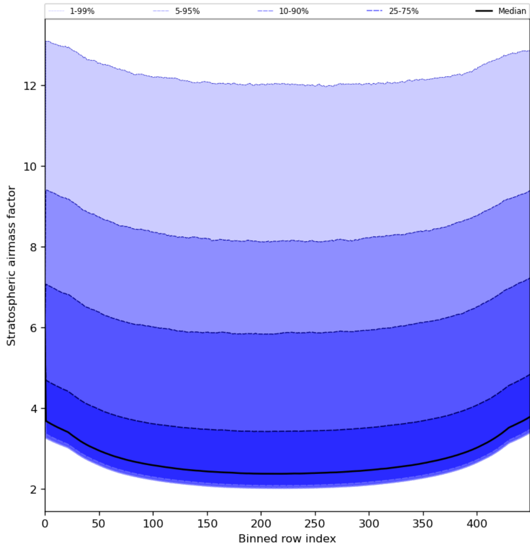
Figure 61: Along track statistics of “Stratospheric airmass factor” for 2024-06-24 to 2024-06-25
