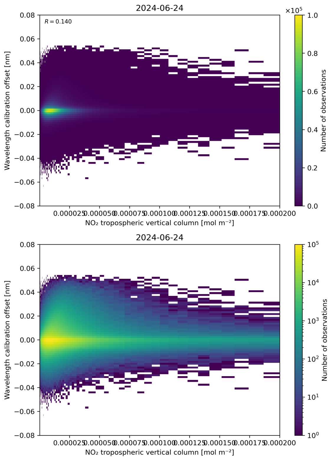
Figure 143: Scatter density plot of “NO 2 tropospheric vertical column” against “Wavelength calibration offset” for 2024-06-24 to 2024-06-25.
