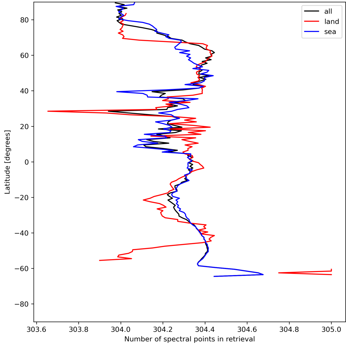
Figure 16: Zonal average of “Number of spectral points in retrieval” for 2024-06-24 to 2024-06-25.
