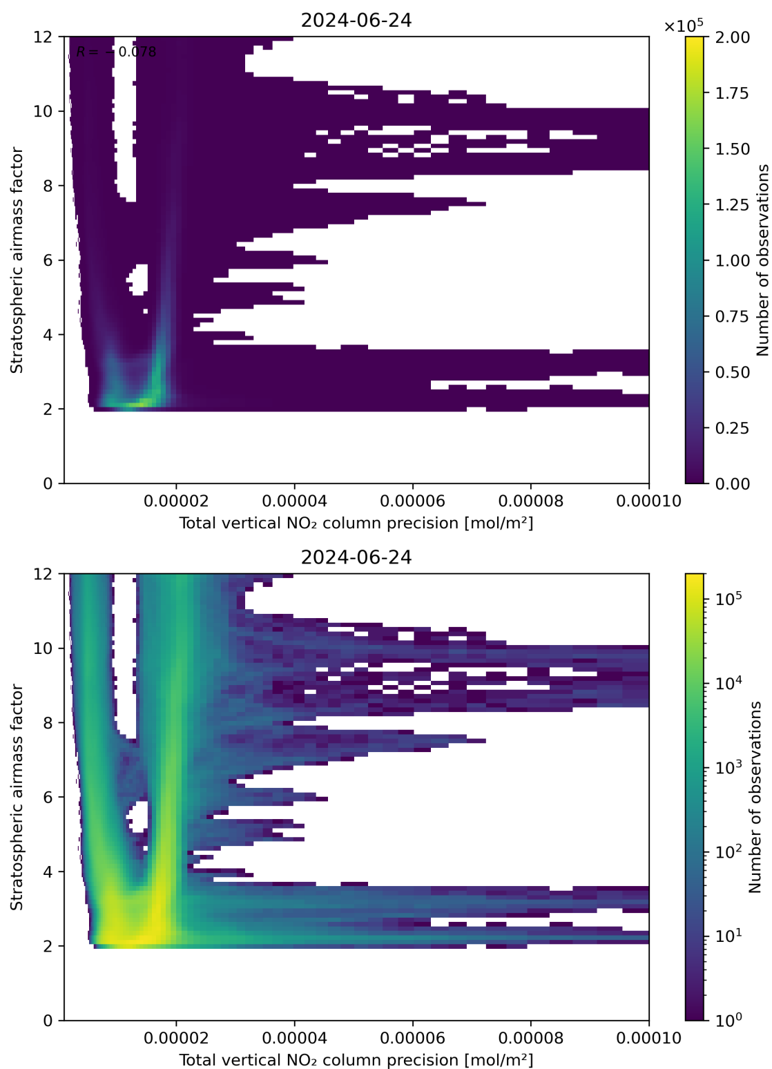
Figure 115: Scatter density plot of “Total vertical NO 2 column precision” against “Stratospheric airmass factor” for 2024-06-24 to 2024-06-25.
