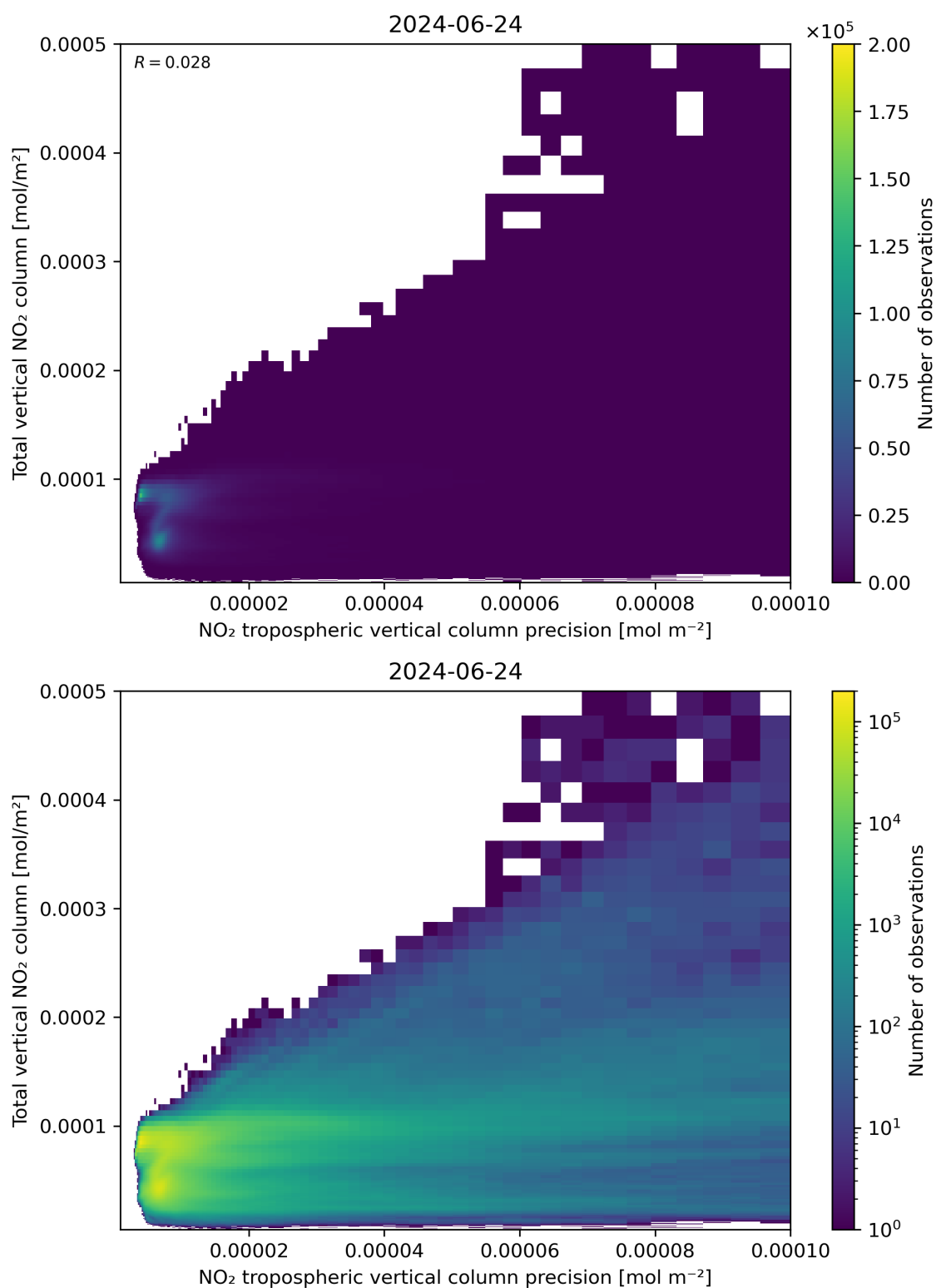
Figure 138: Scatter density plot of “NO 2 tropospheric vertical column precision” against “Total vertical NO 2 column” for 2024-06-24 to 2024-06-25.
