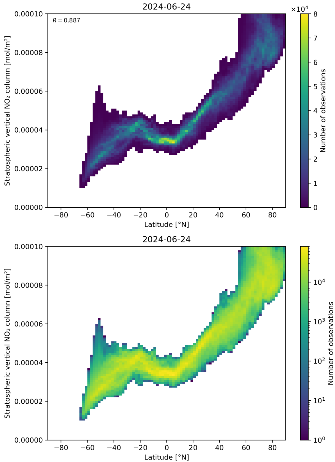
Figure 87: Scatter density plot of “Latitude” against “Stratospheric vertical NO 2 column” for 2024-06-24 to 2024-06-25.
