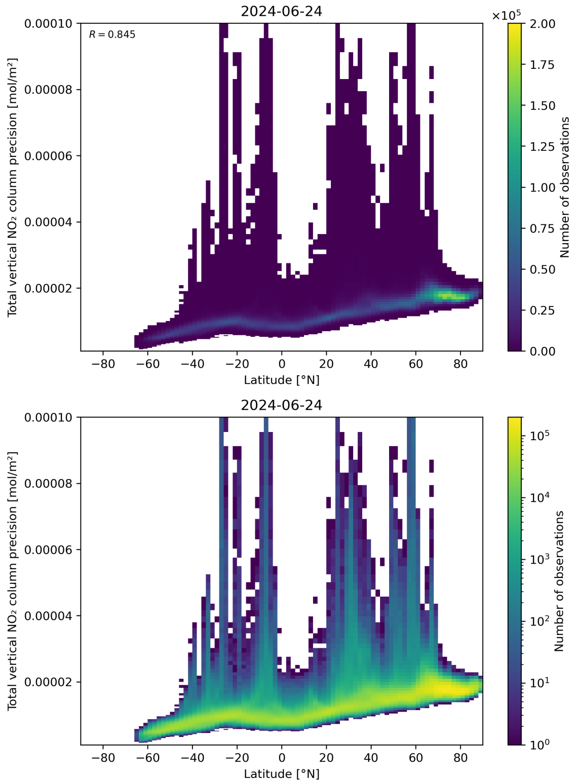
Figure 91: Scatter density plot of “Latitude” against “Total vertical NO 2 column precision” for 2024-06-24 to 2024-06-25.
