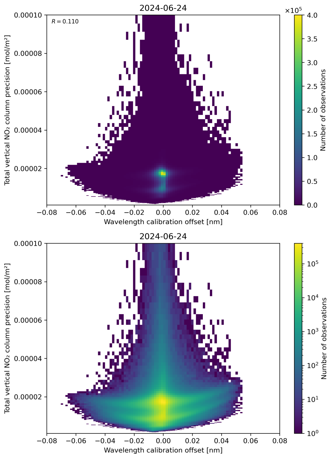
Figure 180: Scatter density plot of “Wavelength calibration offset” against “Total vertical NO 2 column precision” for 2024-06-24 to 2024-06-25.
