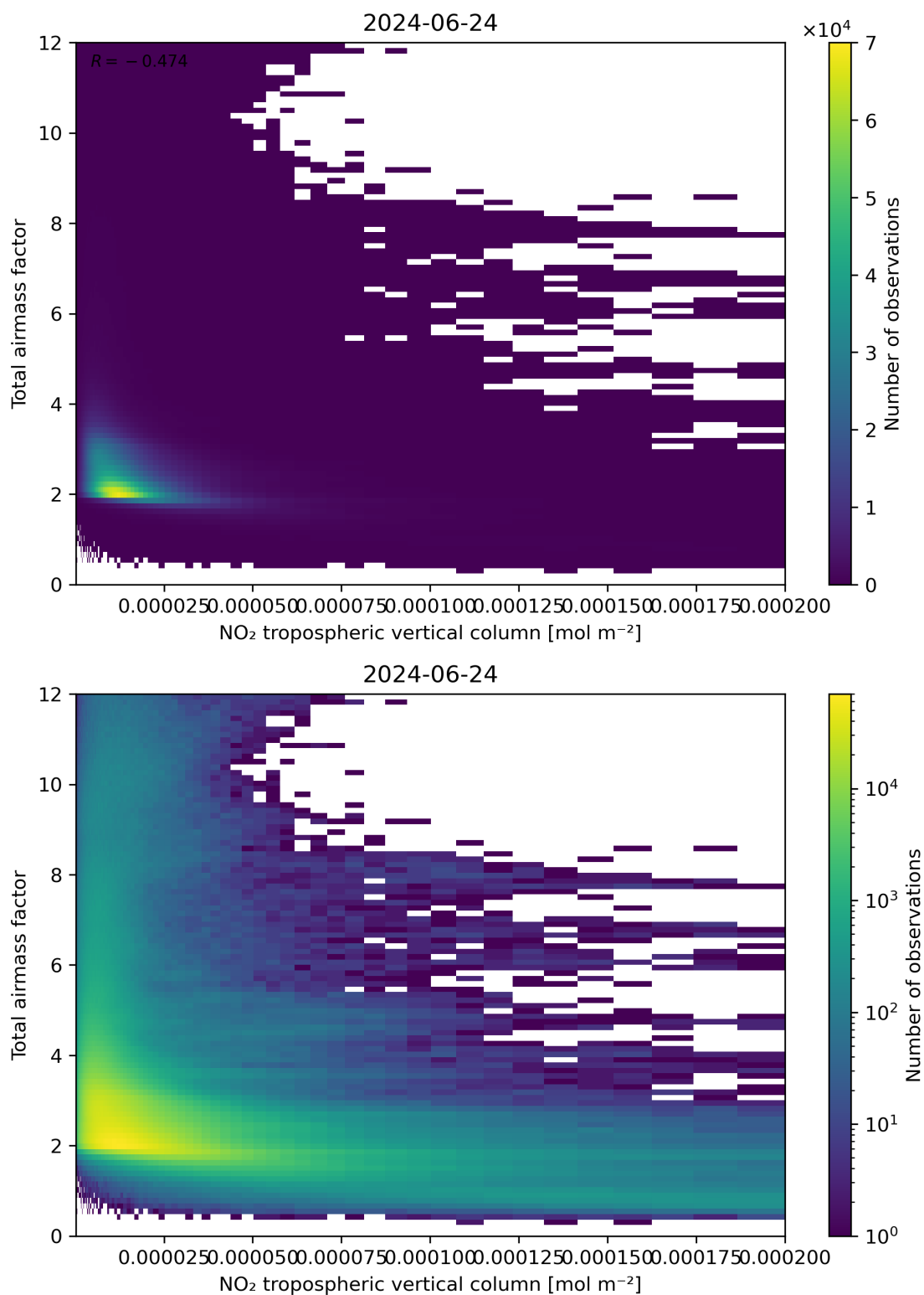
Figure 122: Scatter density plot of “NO 2 tropospheric vertical column” against “Total air mass factor” for 2024-06-24 to 2024-06-25.
