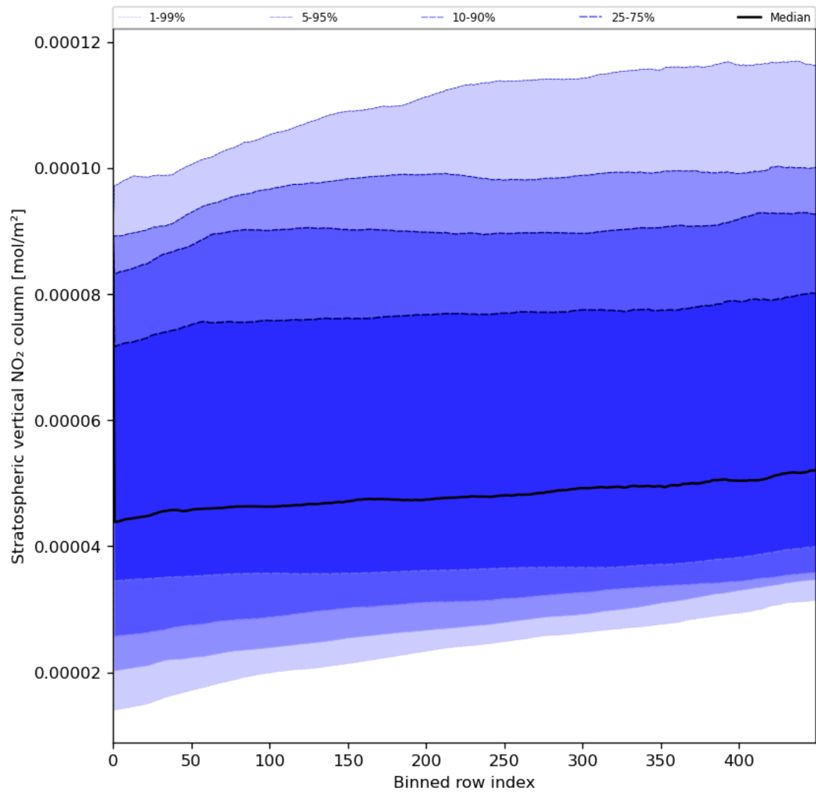
Figure 53: Along track statistics of “Stratospheric vertical NO 2 column” for 2024-06-24 to 2024-06-25
