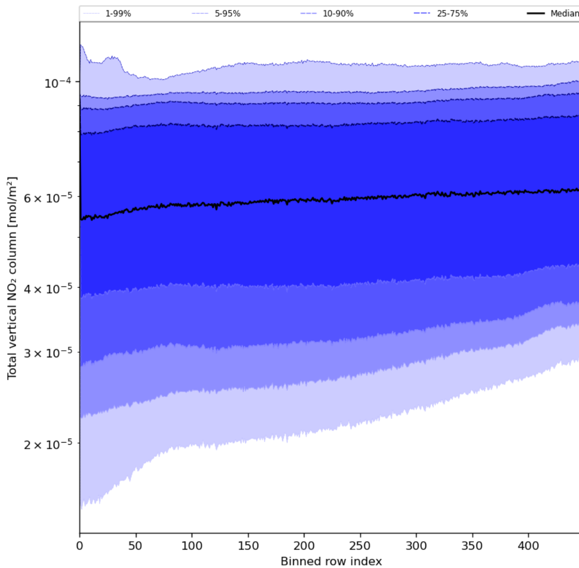
Figure 55: Along track statistics of “Total vertical NO 2 column” for 2024-06-24 to 2024-06-25
