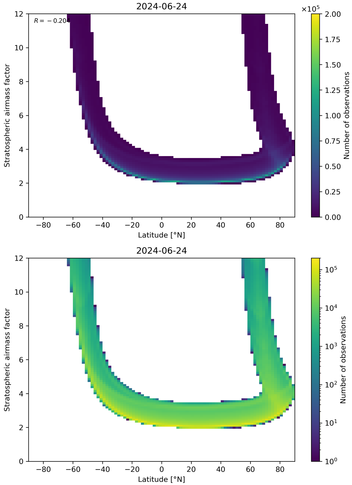
Figure 83: Scatter density plot of “Latitude” against “Stratospheric air mass factor” for 2024-06-24 to 2024-06-25.
