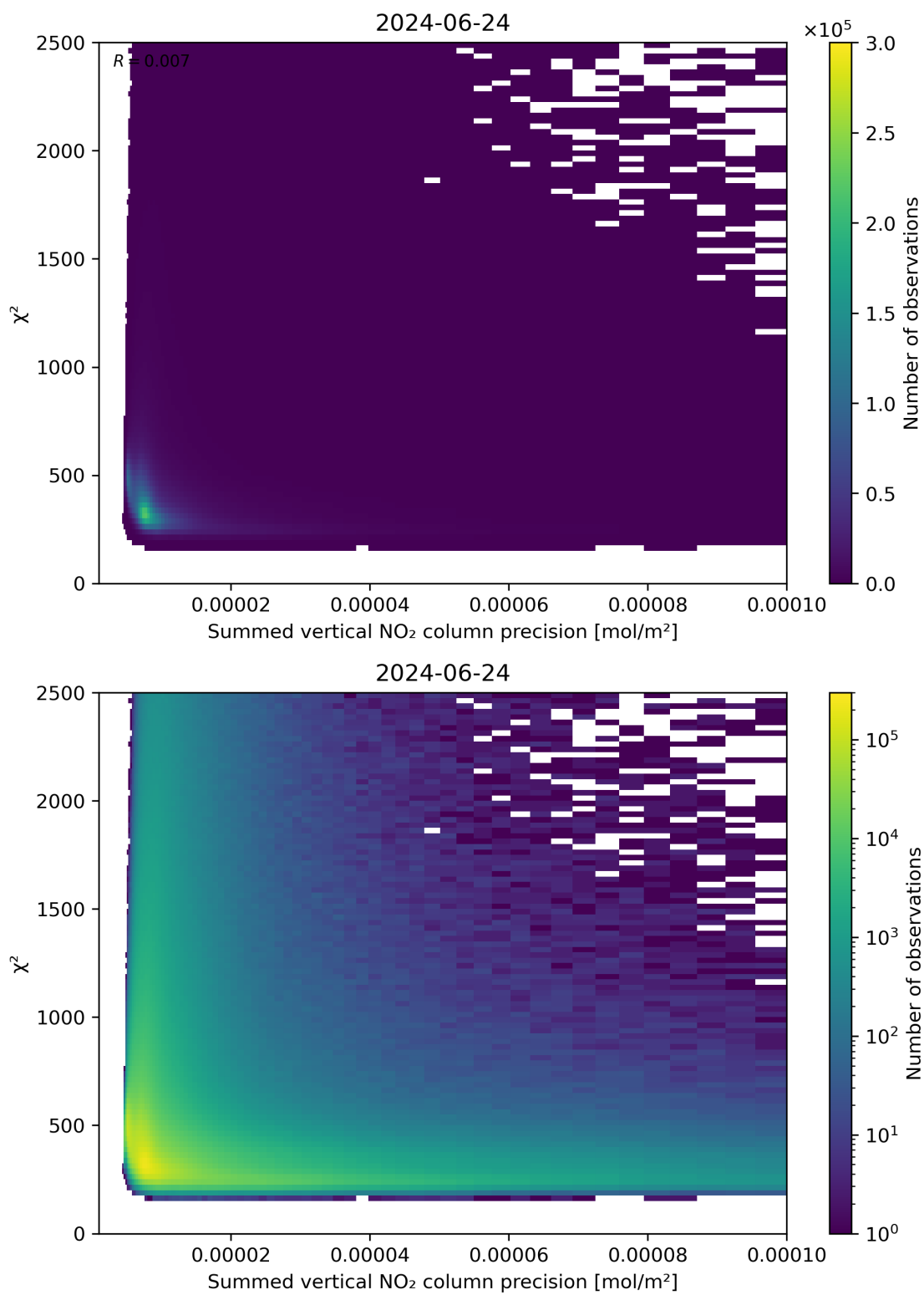
Figure 107: Scatter density plot of “Summed vertical NO 2 column precision” against “ \chi^2 ” for 2024-06-24 to 2024-06-25.
