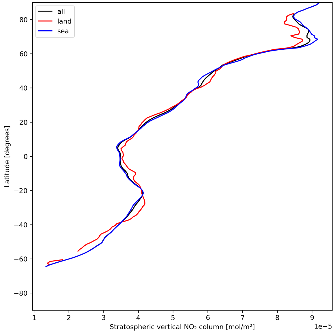
Figure 19: Zonal average of “Stratospheric vertical NO 2 column” for 2024-06-24 to 2024-06-25.
