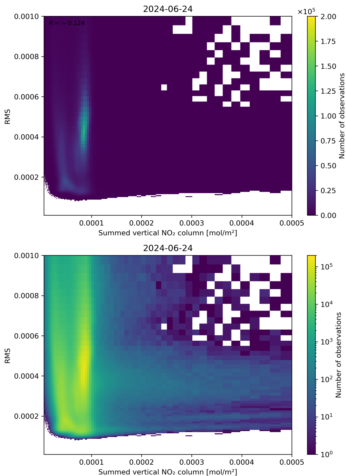
Figure 109: Scatter density plot of “Summed vertical NO 2 column” against “RMS” for 2024-06-24 to 2024-06-25.
