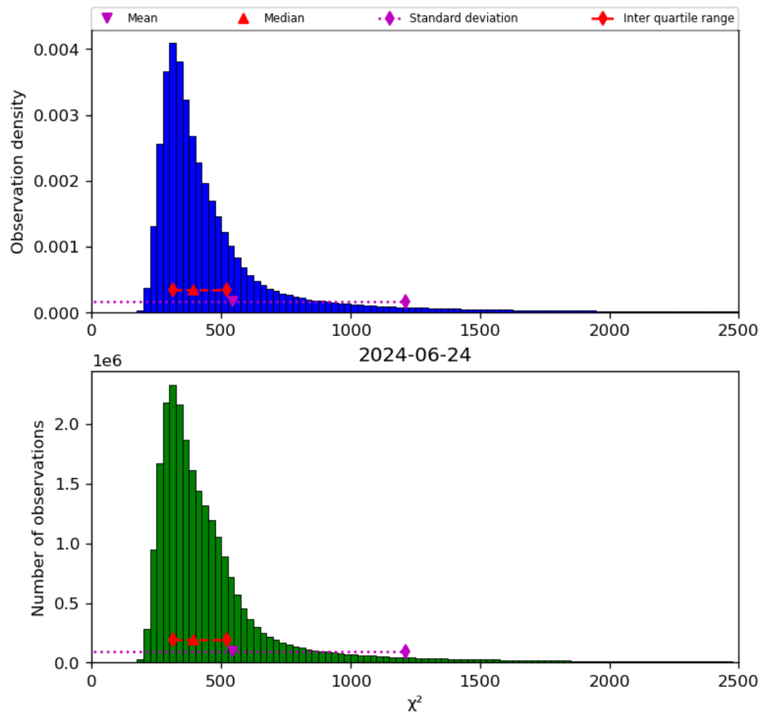
Figure 42: Histogram of “ \chi^2 ” for 2024-06-24 to 2024-06-25
