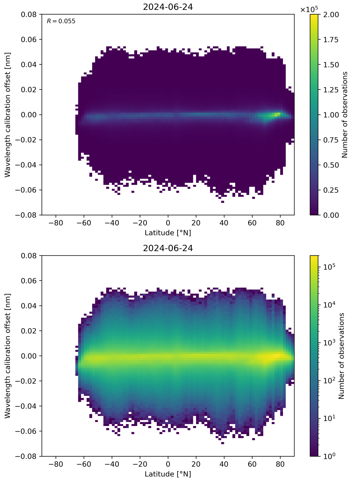
Figure 95: Scatter density plot of “Latitude” against “Wavelength calibration offset” for 2024-06-24 to 2024-06-25.
