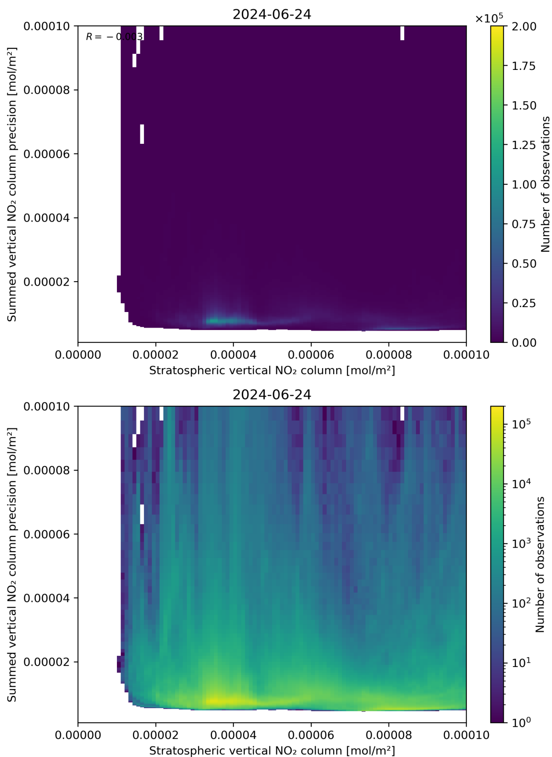
Figure 99: Scatter density plot of “Stratospheric vertical NO 2 column” against “Summed vertical NO 2 column precision” for 2024-06-24 to 2024-06-25.
