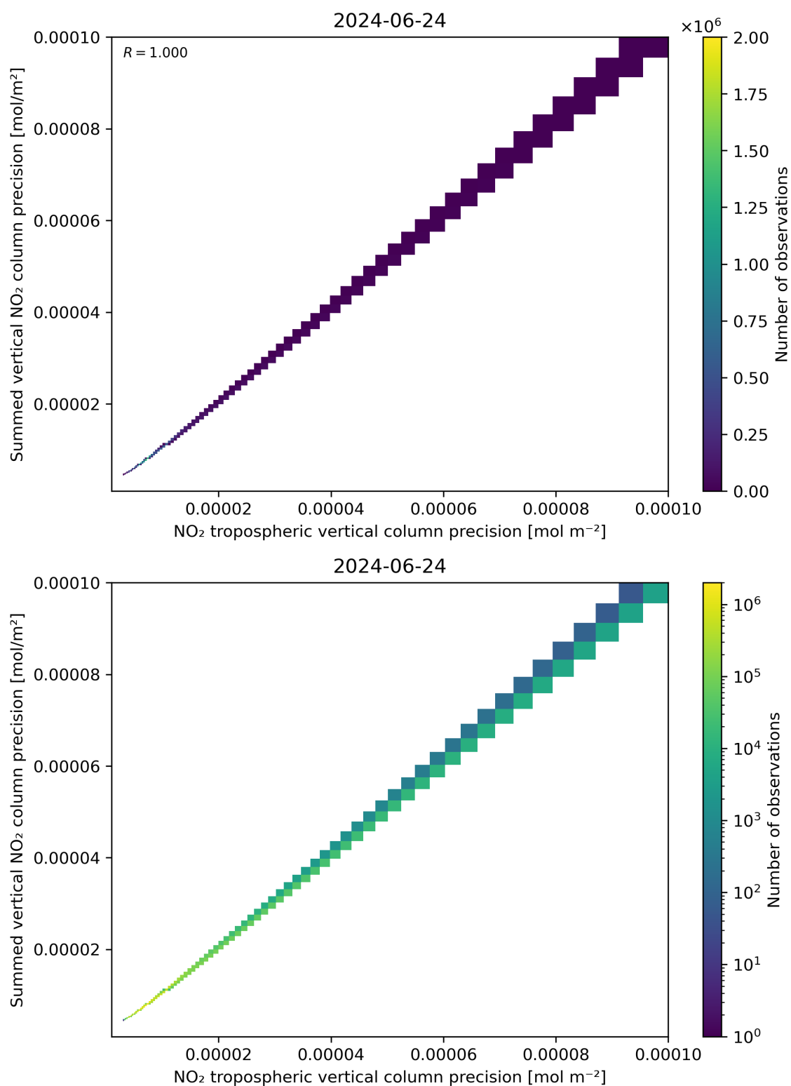
Figure 137: Scatter density plot of “NO 2 tropospheric vertical column precision” against “Summed vertical NO 2 column precision” for 2024-06-24 to 2024-06-25.
