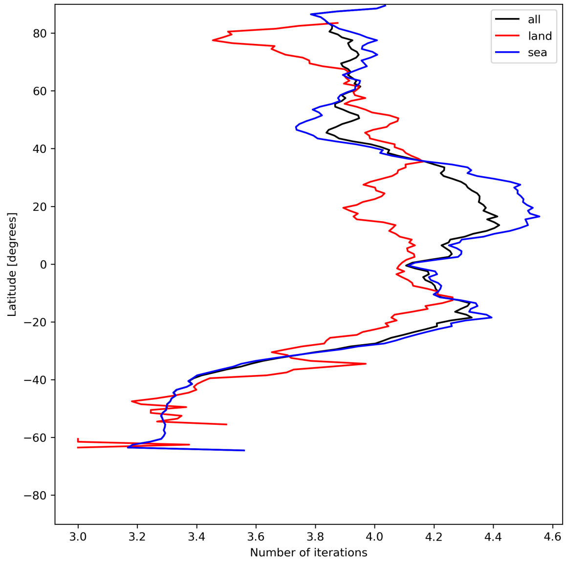
Figure 17: Zonal average of “Number of iterations” for 2024-06-24 to 2024-06-25.
