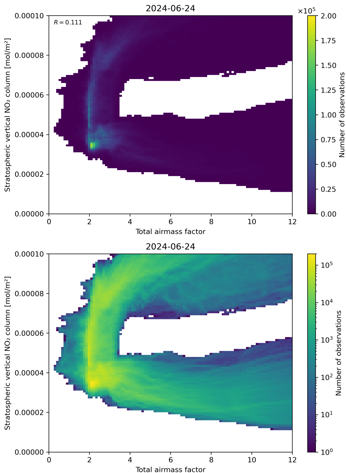
Figure 64: Scatter density plot of “Total airmass factor” against “Stratospheric vertical NO 2 column” for 2024-06-24 to 2024-06-25.
