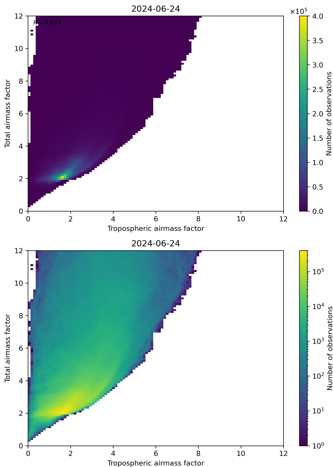
Figure 72: Scatter density plot of “Tropospheric airmass factor” against “Total airmass factor” for 2024-06-24 to 2024-06-25.
