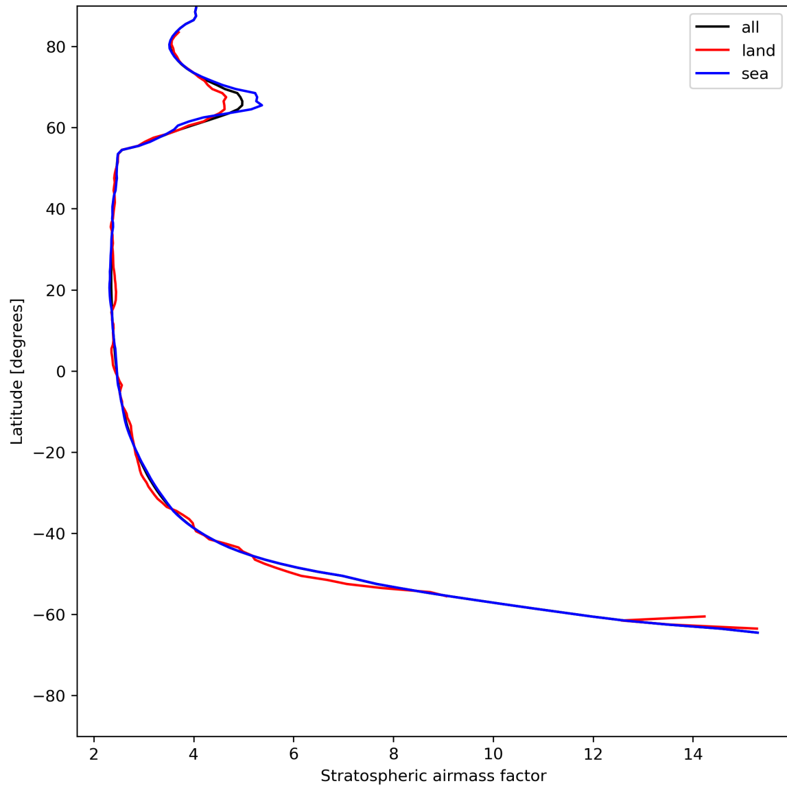
Figure 27: Zonal average of “Stratospheric air mass factor” for 2024-06-24 to 2024-06-25.
