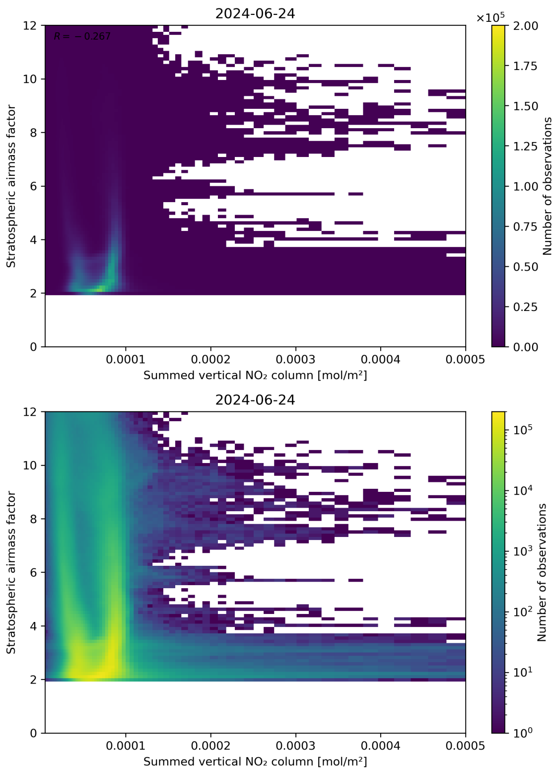
Figure 103: Scatter density plot of “Summed vertical NO 2 column” against “Stratospheric air mass factor” for 2024-06-24 to 2024-06-25.
