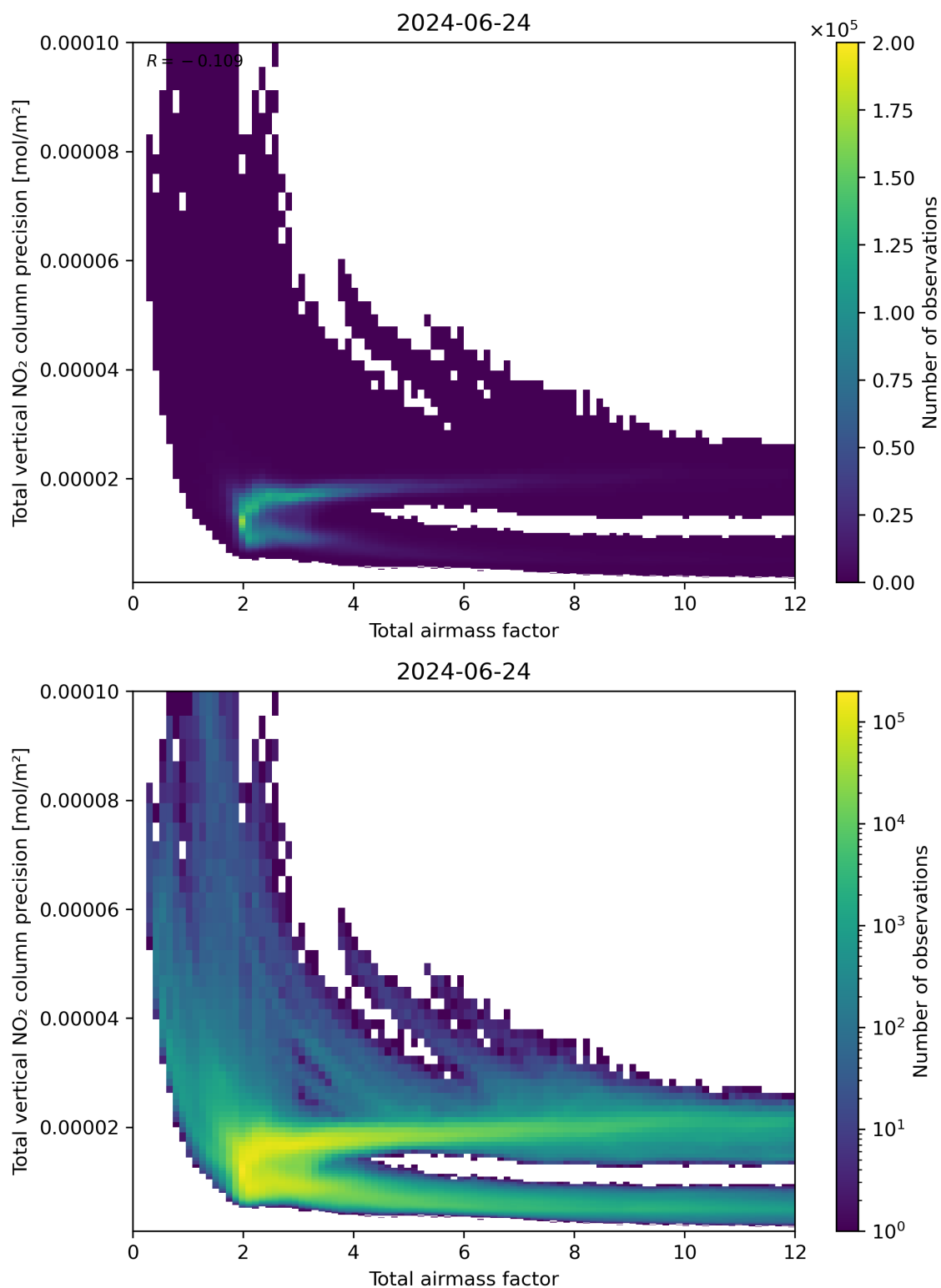
Figure 68: Scatter density plot of “Total airmass factor” against “Total vertical NO 2 column precision” for 2024-06-24 to 2024-06-25.
