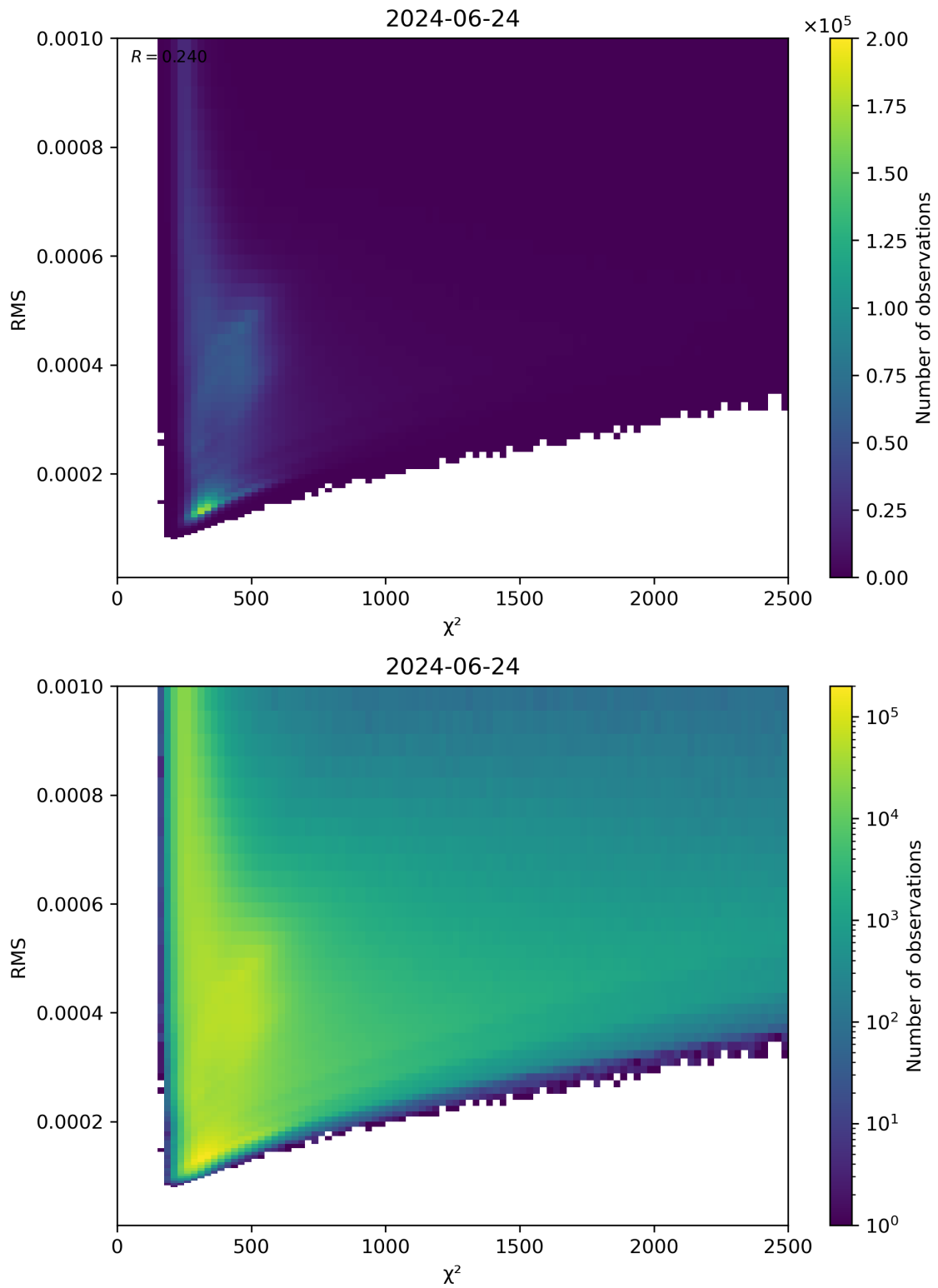
Figure 82: Scatter density plot of “ \chi^2 ” against “RMS” for 2024-06-24 to 2024-06-25.
