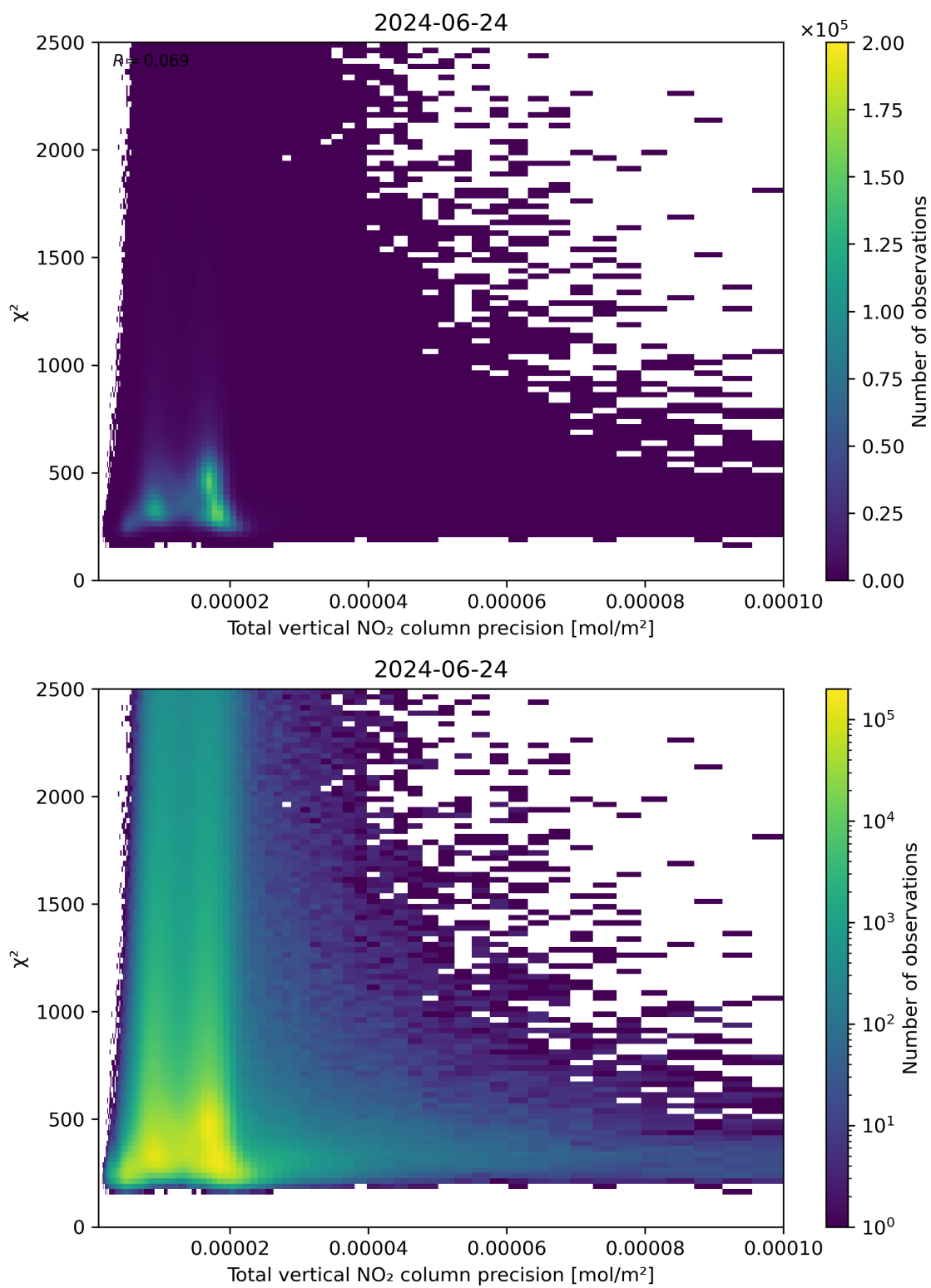
Figure 116: Scatter density plot of “Total vertical NO 2 column precision” against “ \chi^2 ” for 2024-06-24 to 2024-06-25.
