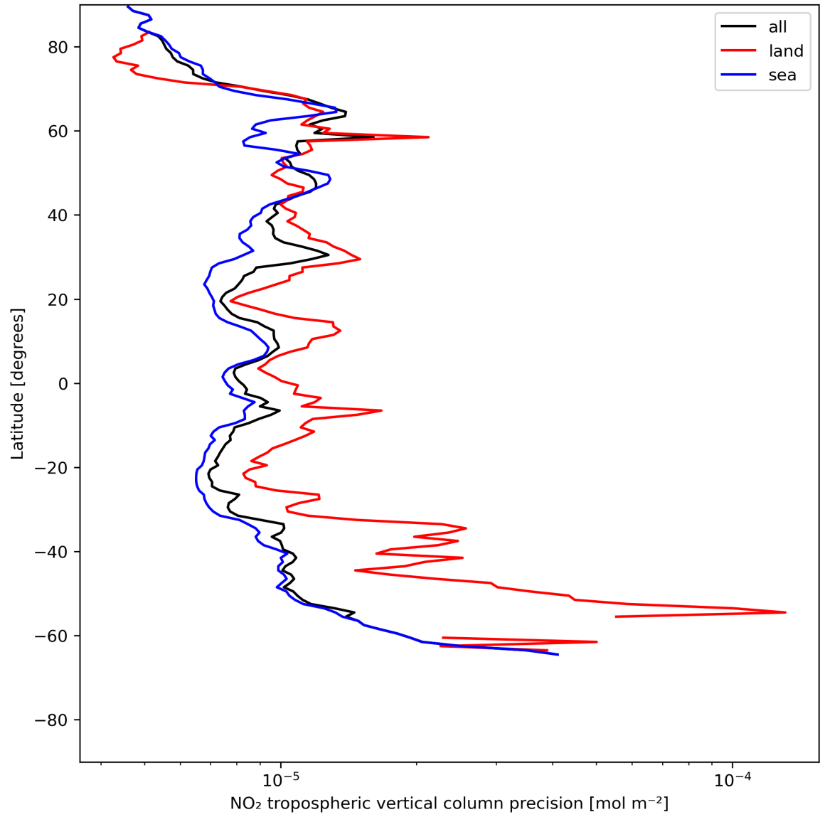
Figure 13: Zonal average of “NO 2 tropospheric vertical column precision” for 2024-06-24 to 2024-06-25.
