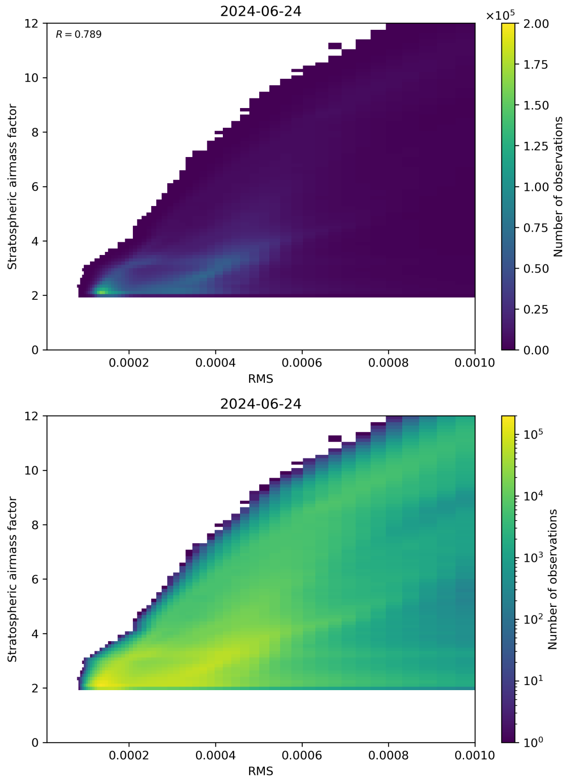
Figure 144: Scatter density plot of “RMS” against “Stratospheric airmass factor” for 2024-06-24 to 2024-06-25.
