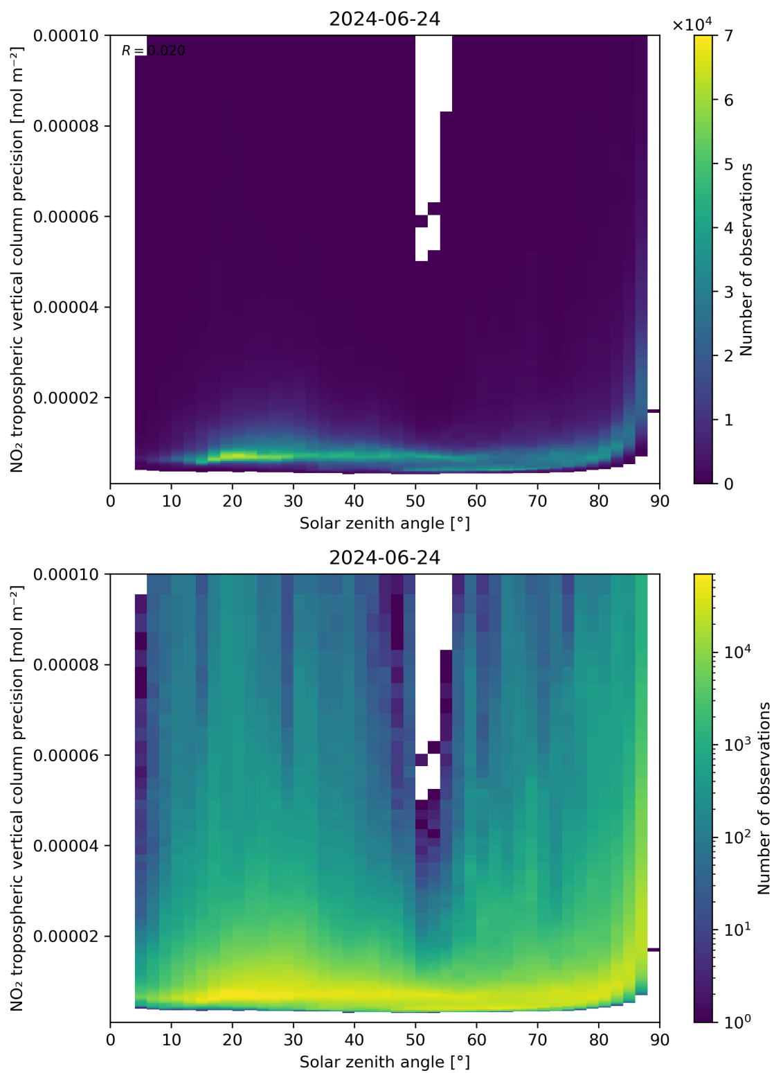
Figure 156: Scatter density plot of “Solar zenith angle” against “NO 2 tropospheric vertical column precision” for 2024-06-24 to 2024-06-25.
