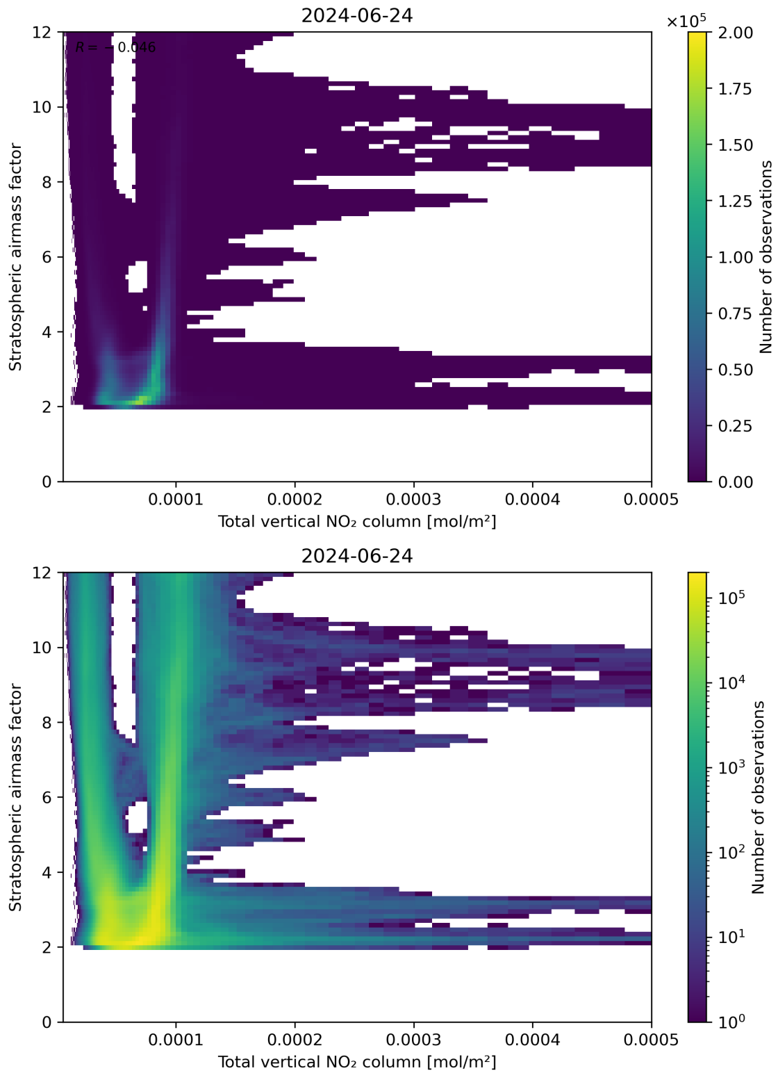
Figure 110: Scatter density plot of “Total vertical NO 2 column” against “Stratospheric airmass factor” for 2024-06-24 to 2024-06-25.
