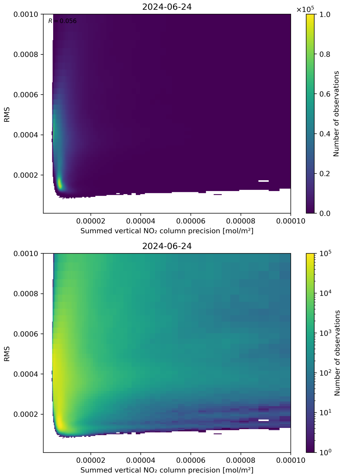
Figure 108: Scatter density plot of “Summed vertical NO 2 column precision” against “RMS” for 2024-06-24 to 2024-06-25.
