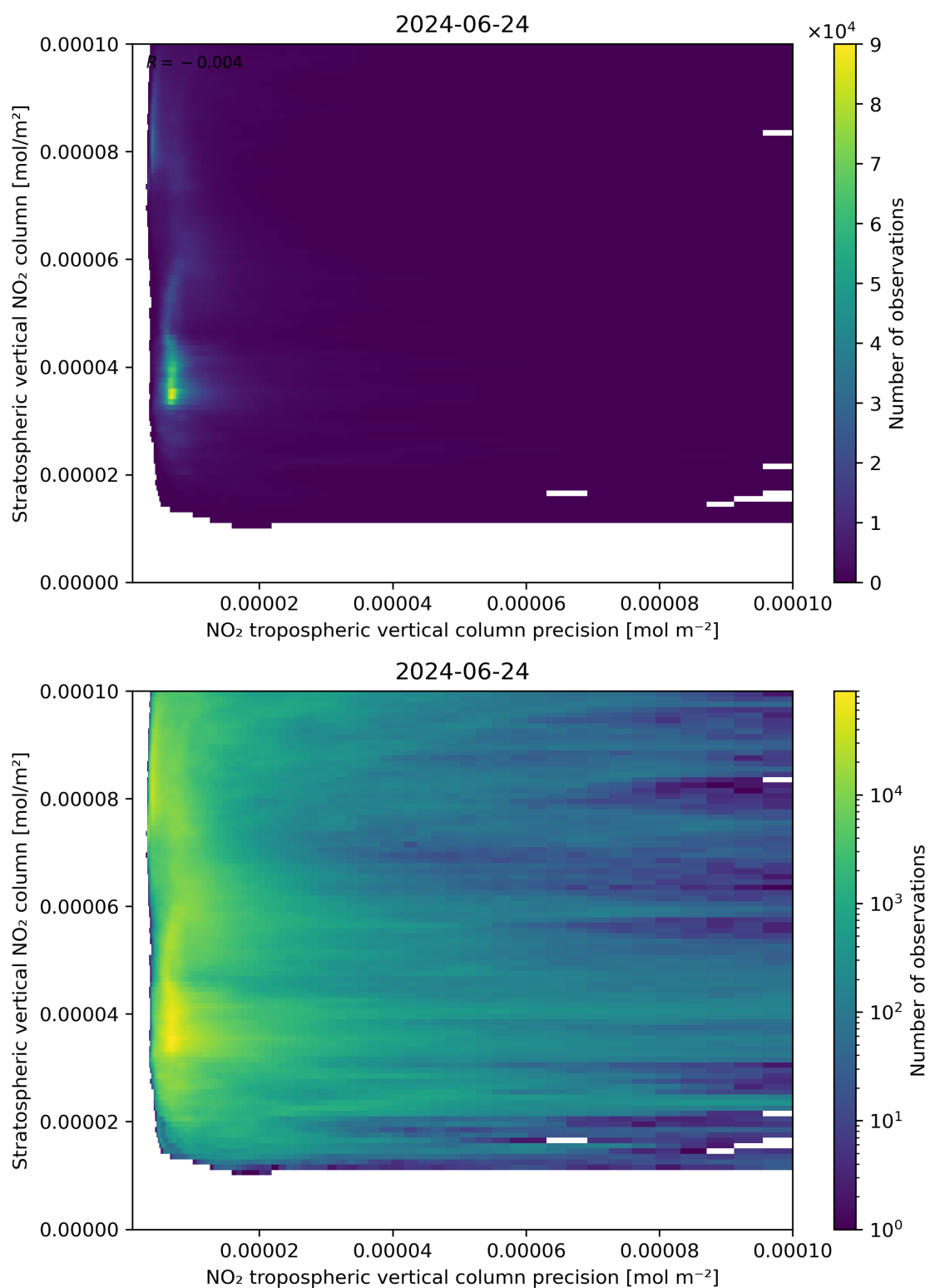
Figure 135: Scatter density plot of “NO 2 tropospheric vertical column precision” against “Stratospheric vertical NO 2 column” for 2024-06-24 to 2024-06-25.
