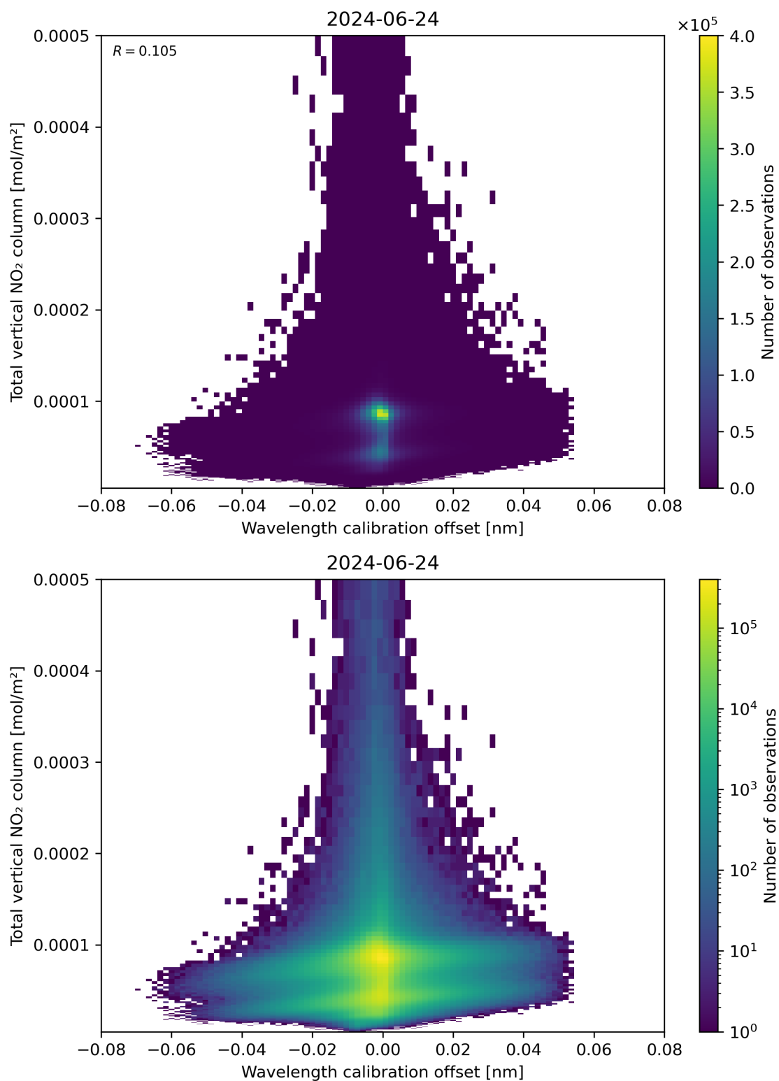
Figure 179: Scatter density plot of “Wavelength calibration offset” against “Total vertical NO 2 column” for 2024-06-24 to 2024-06-25.
