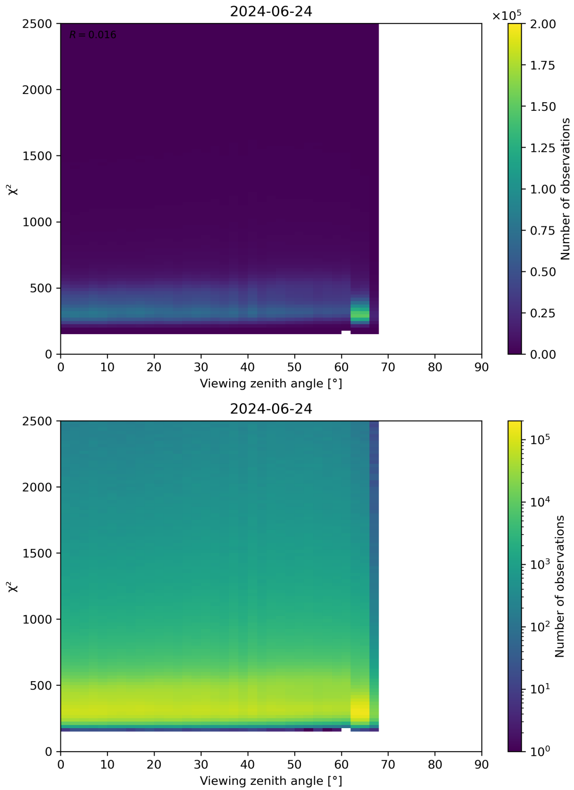
Figure 162: Scatter density plot of “Viewing zenith angle” against “ \chi^2 ” for 2024-06-24 to 2024-06-25.
