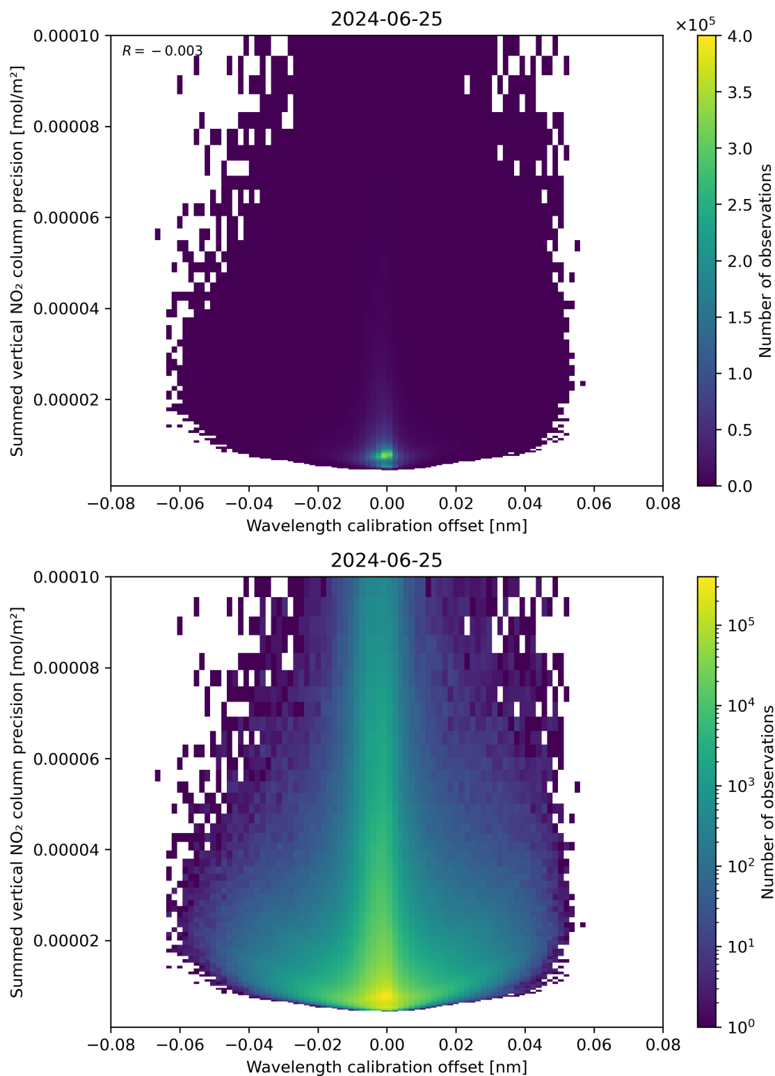
Figure 178: Scatter density plot of “Wavelength calibration offset” against “Summed vertical NO 2 column precision” for 2024-06-24 to 2024-06-26.
