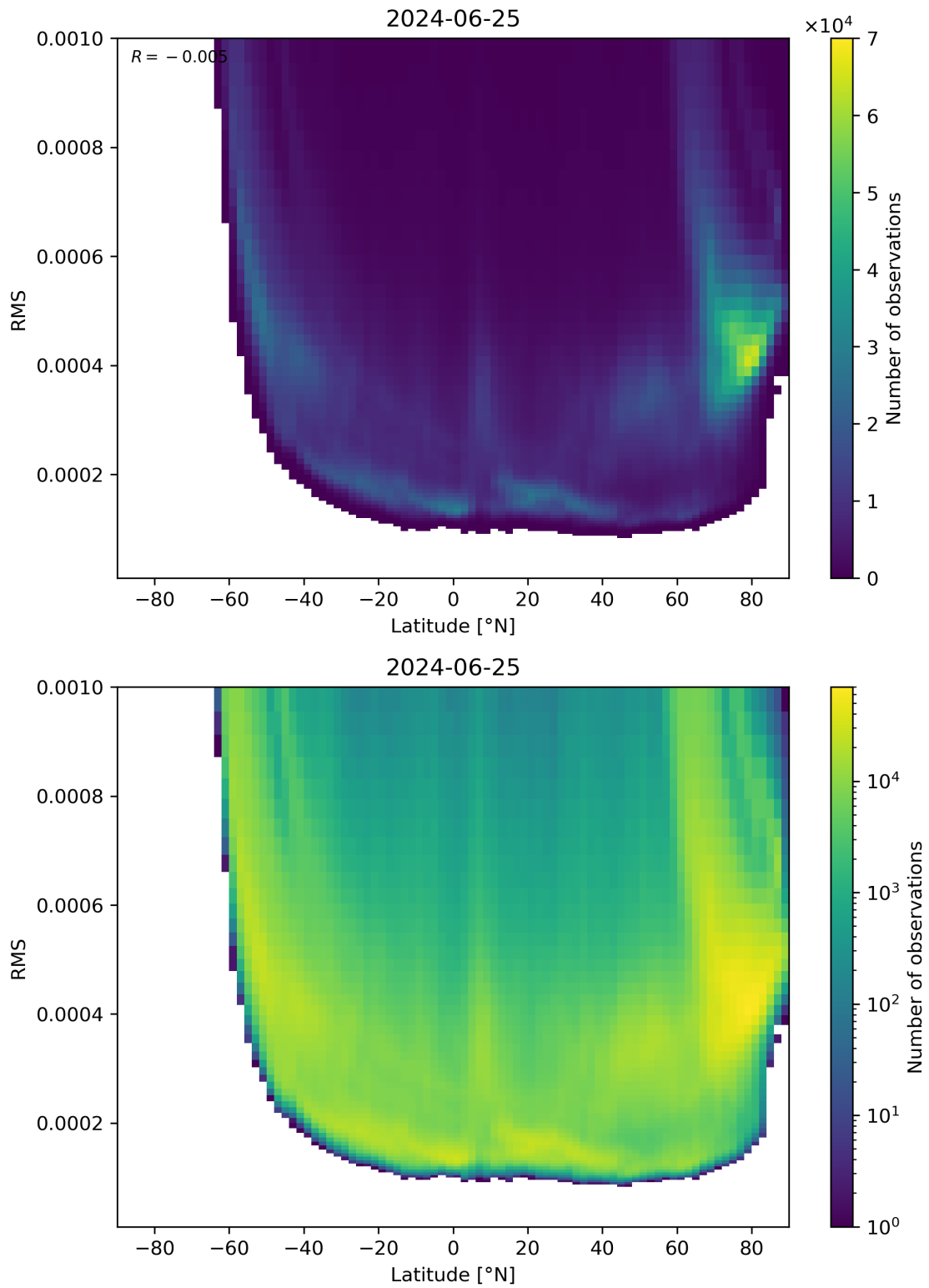
Figure 94: Scatter density plot of “Latitude” against “RMS” for 2024-06-24 to 2024-06-26.
