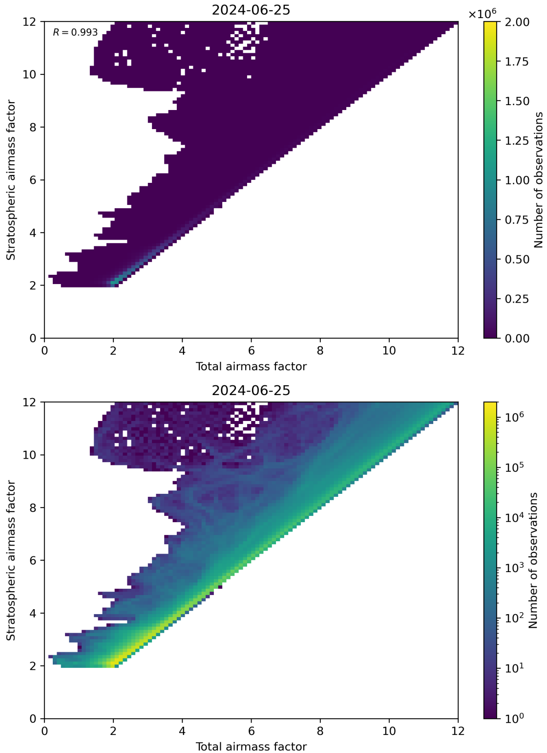
Figure 62: Scatter density plot of “Total airmass factor” against “Stratospheric airmass factor” for 2024-06-24 to 2024-06-26.
