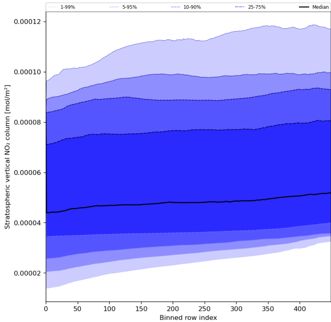
Figure 53: Along track statistics of “Stratospheric vertical NO 2 column” for 2024-06-24 to 2024-06-26
