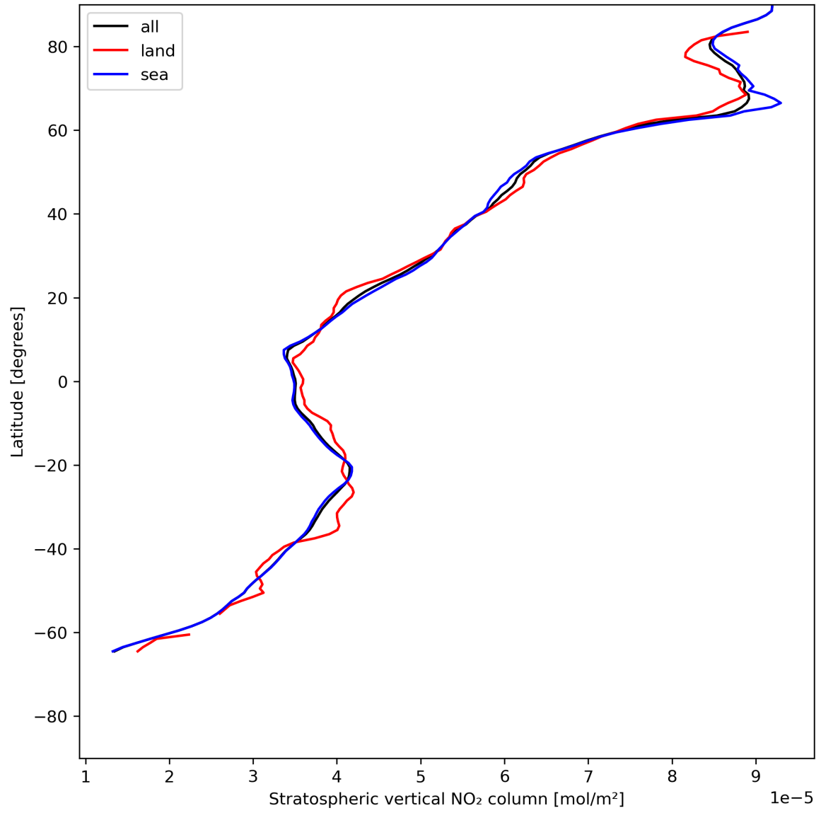
Figure 19: Zonal average of “Stratospheric vertical NO 2 column” for 2024-06-24 to 2024-06-26.
