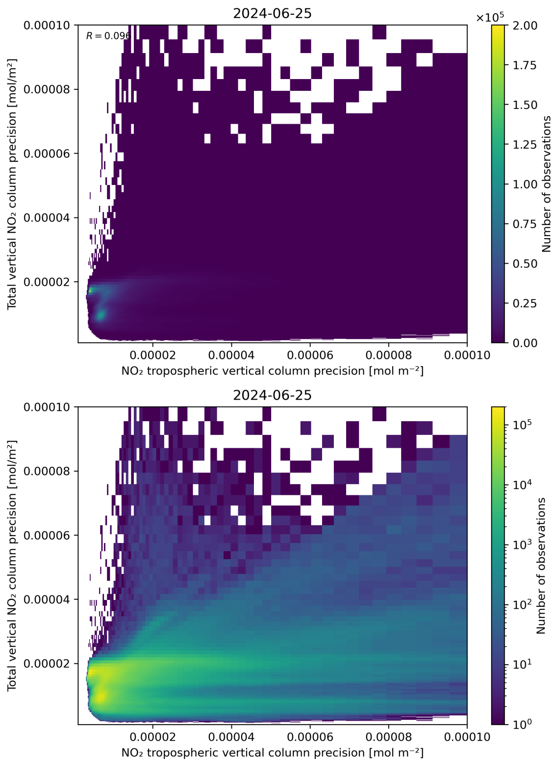
Figure 139: Scatter density plot of “NO 2 tropospheric vertical column precision” against “Total vertical NO 2 column precision” for 2024-06-24 to 2024-06-26.
