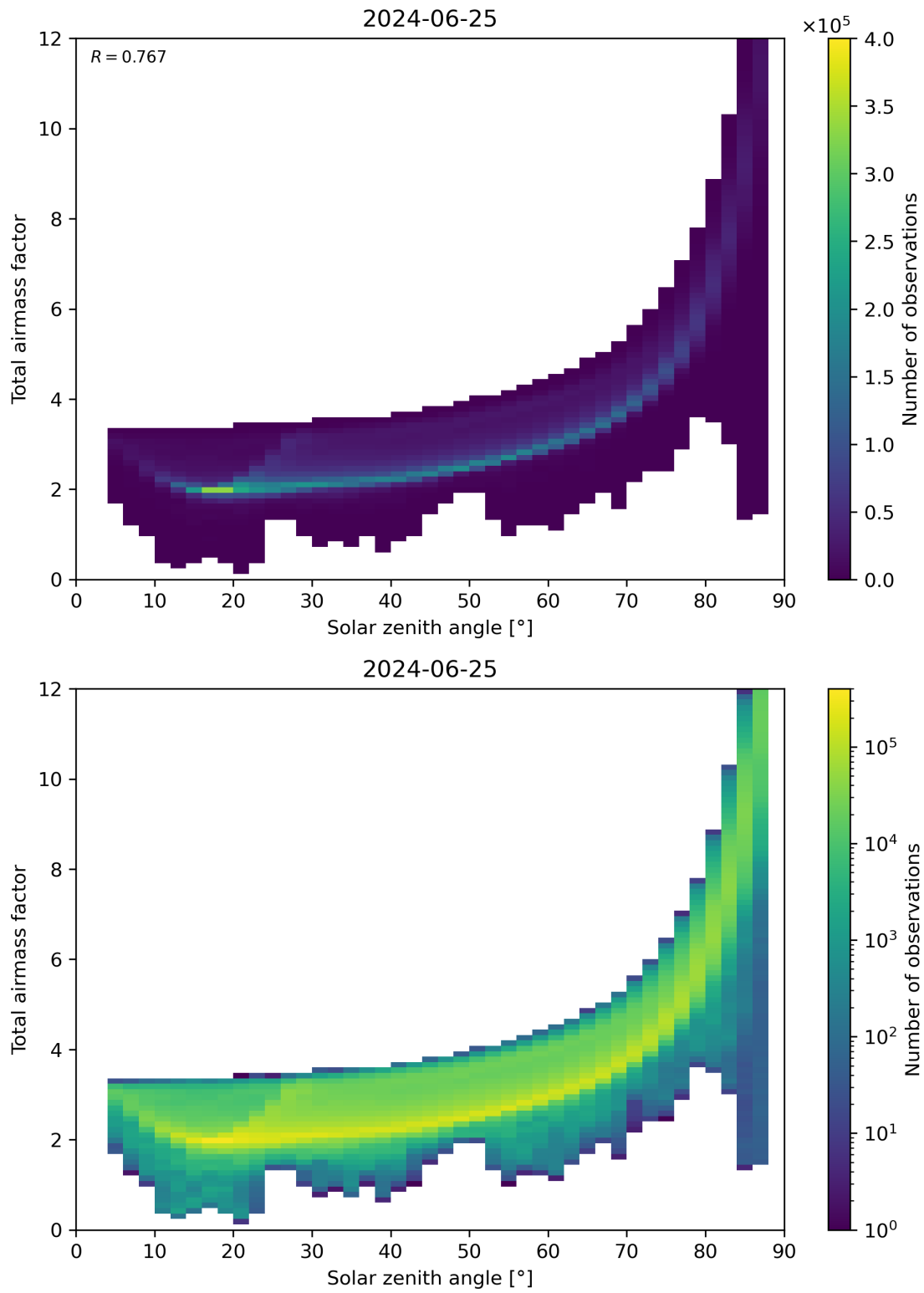
Figure 146: Scatter density plot of “Solar zenith angle” against “Total air mass factor” for 2024-06-24 to 2024-06-26.
