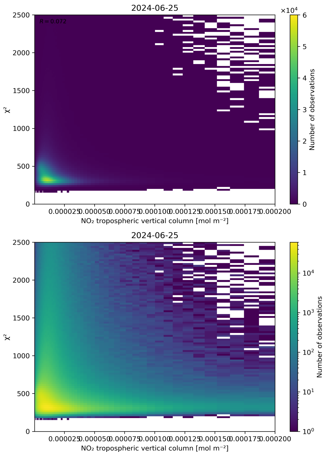
Figure 124: Scatter density plot of “NO 2 tropospheric vertical column” against “ \chi^2 ” for 2024-06-24 to 2024-06-26.
