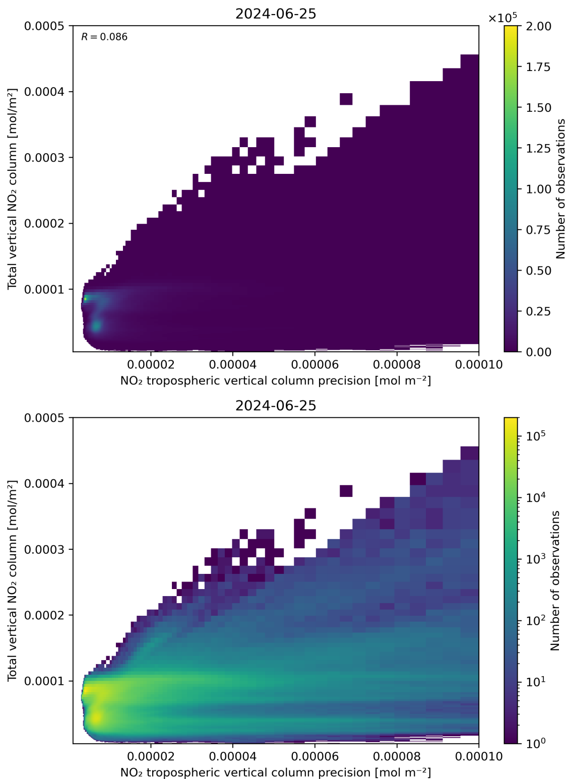
Figure 138: Scatter density plot of “NO 2 tropospheric vertical column precision” against “Total vertical NO 2 column” for 2024-06-24 to 2024-06-26.
