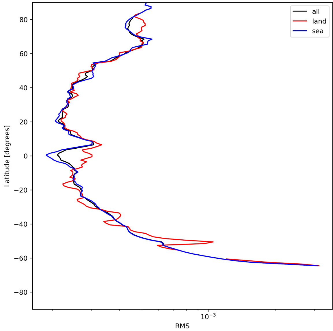
Figure 26: Zonal average of “RMS” for 2024-06-24 to 2024-06-26.
