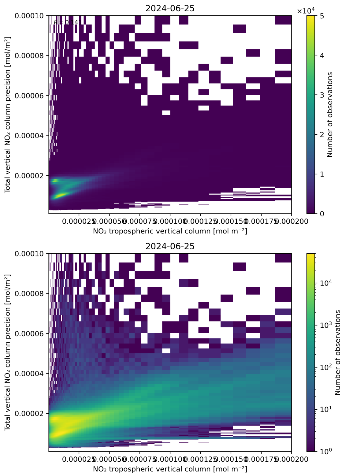
Figure 129: Scatter density plot of “NO 2 tropospheric vertical column” against “Total vertical NO 2 column precision” for 2024-06-24 to 2024-06-26.
