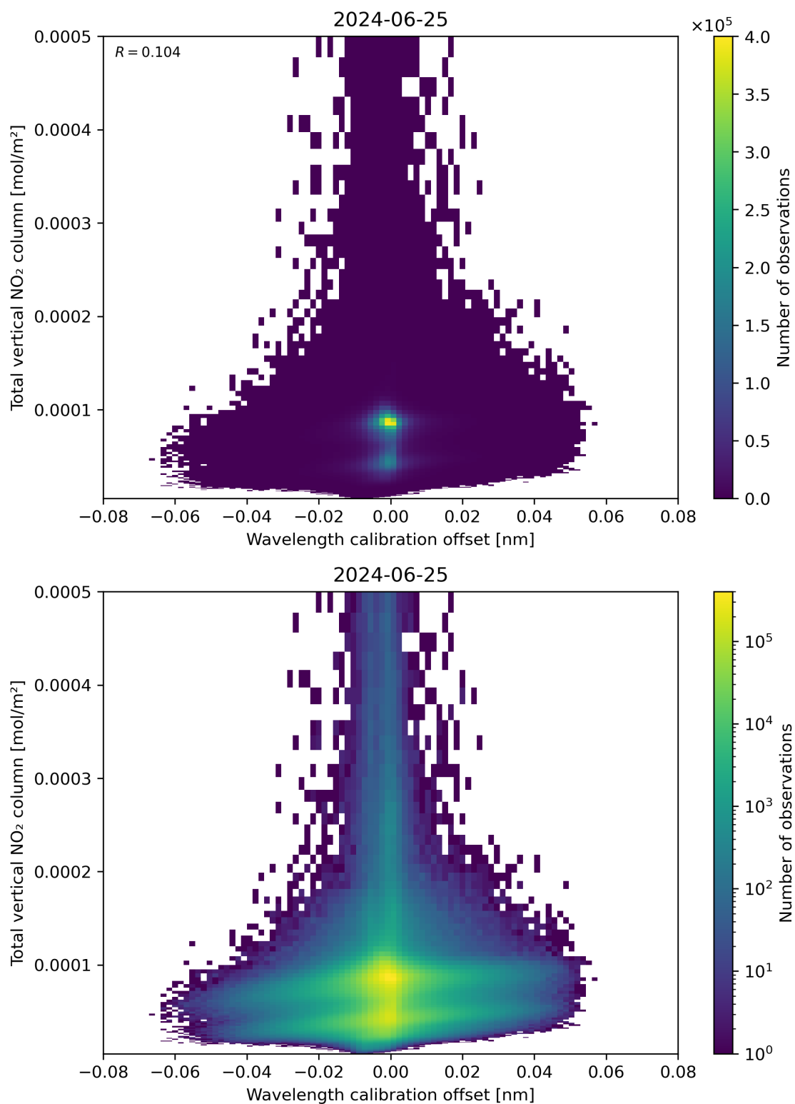
Figure 179: Scatter density plot of “Wavelength calibration offset” against “Total vertical NO 2 column” for 2024-06-24 to 2024-06-26.
