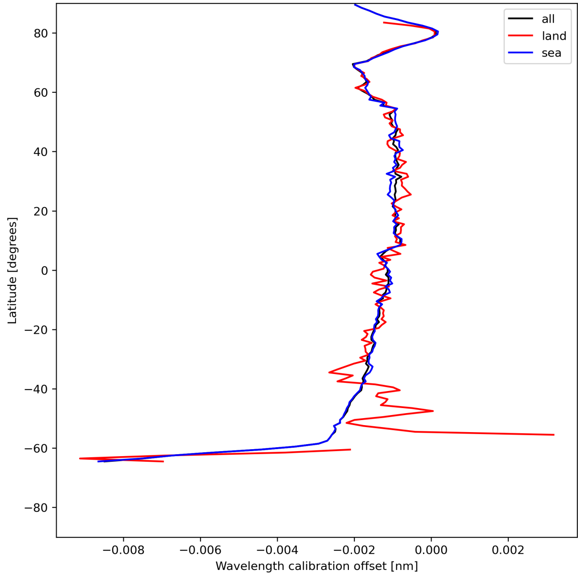
Figure 18: Zonal average of “Wavelength calibration offset” for 2024-06-24 to 2024-06-26.
