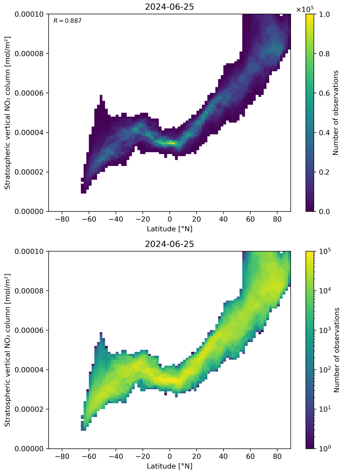
Figure 87: Scatter density plot of “Latitude” against “Stratospheric vertical NO 2 column” for 2024-06-24 to 2024-06-26.
