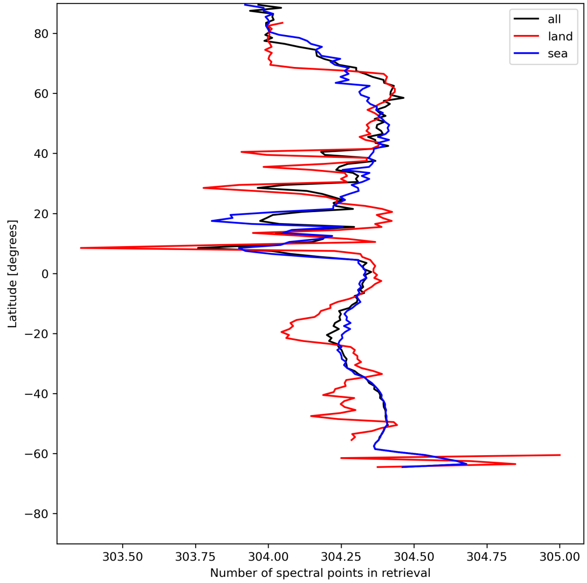
Figure 16: Zonal average of “Number of spectral points in retrieval” for 2024-06-24 to 2024-06-26.
