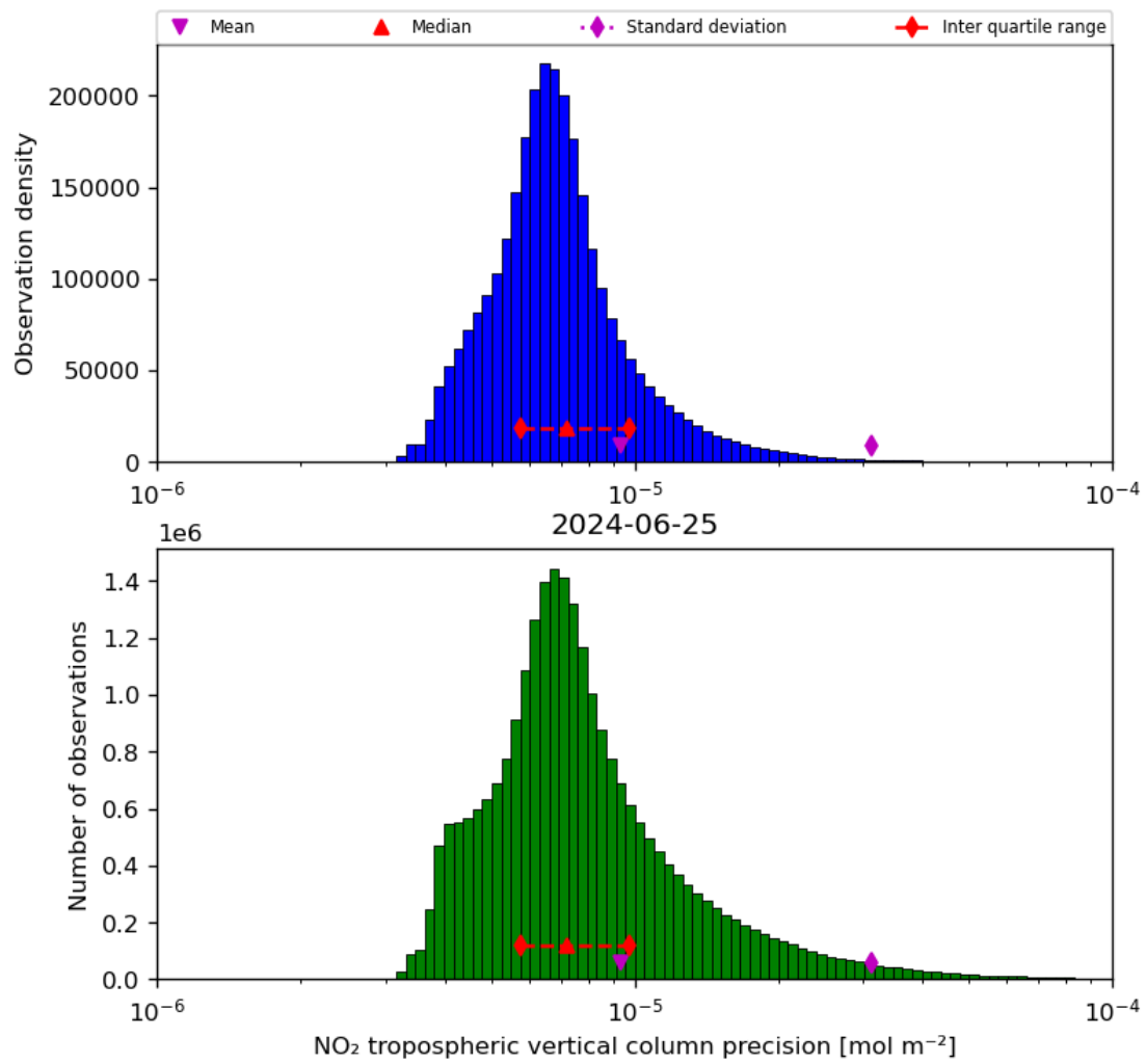
Figure 30: Histogram of “NO 2 tropospheric vertical column precision” for 2024-06-24 to 2024-06-26
