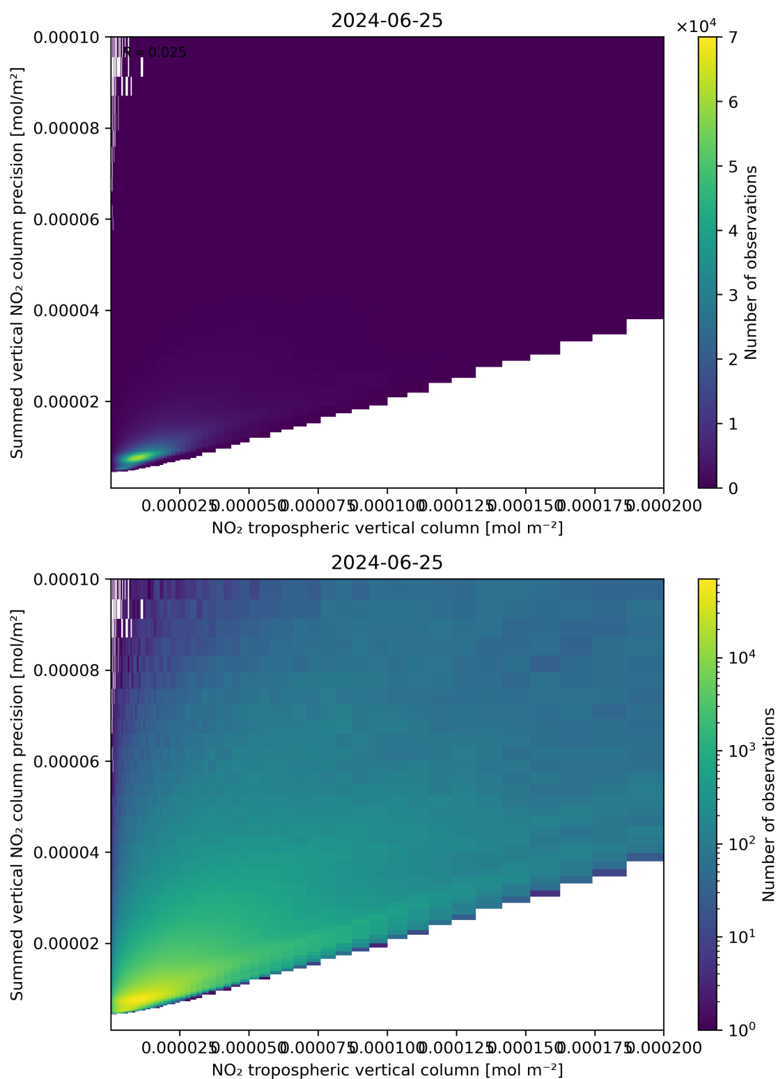
Figure 127: Scatter density plot of “NO 2 tropospheric vertical column” against “Summed vertical NO 2 column precision” for 2024-06-24 to 2024-06-26.
