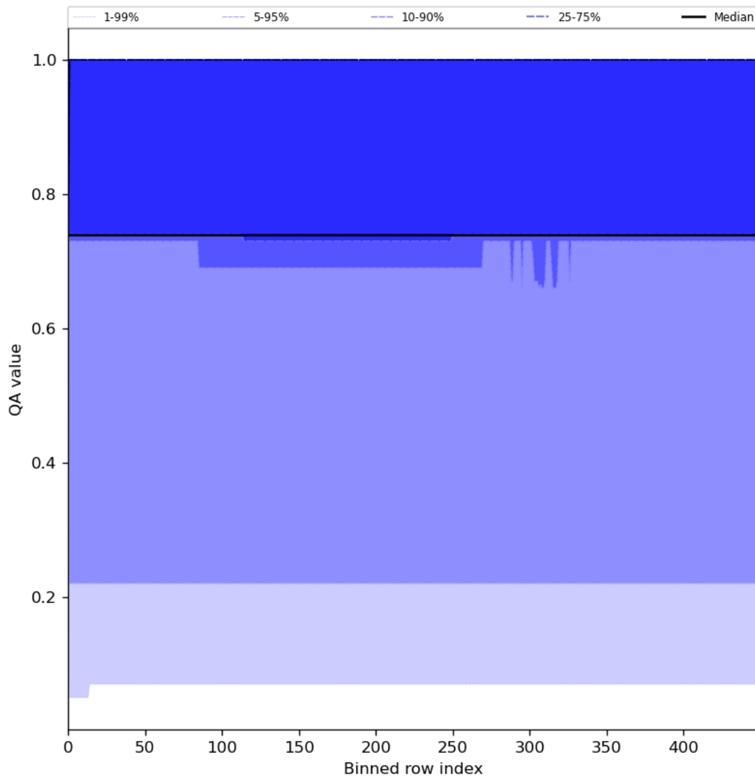
Figure 45: Along track statistics of “QA value” for 2024-06-24 to 2024-06-26
