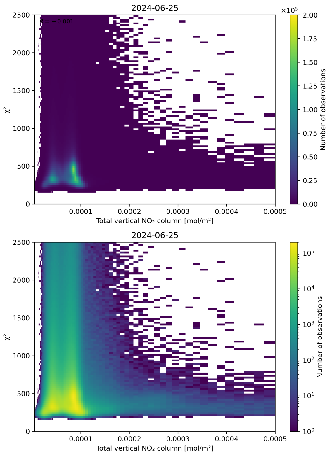
Figure 111: Scatter density plot of “Total vertical NO 2 column” against “ \chi^2 ” for 2024-06-24 to 2024-06-26.
