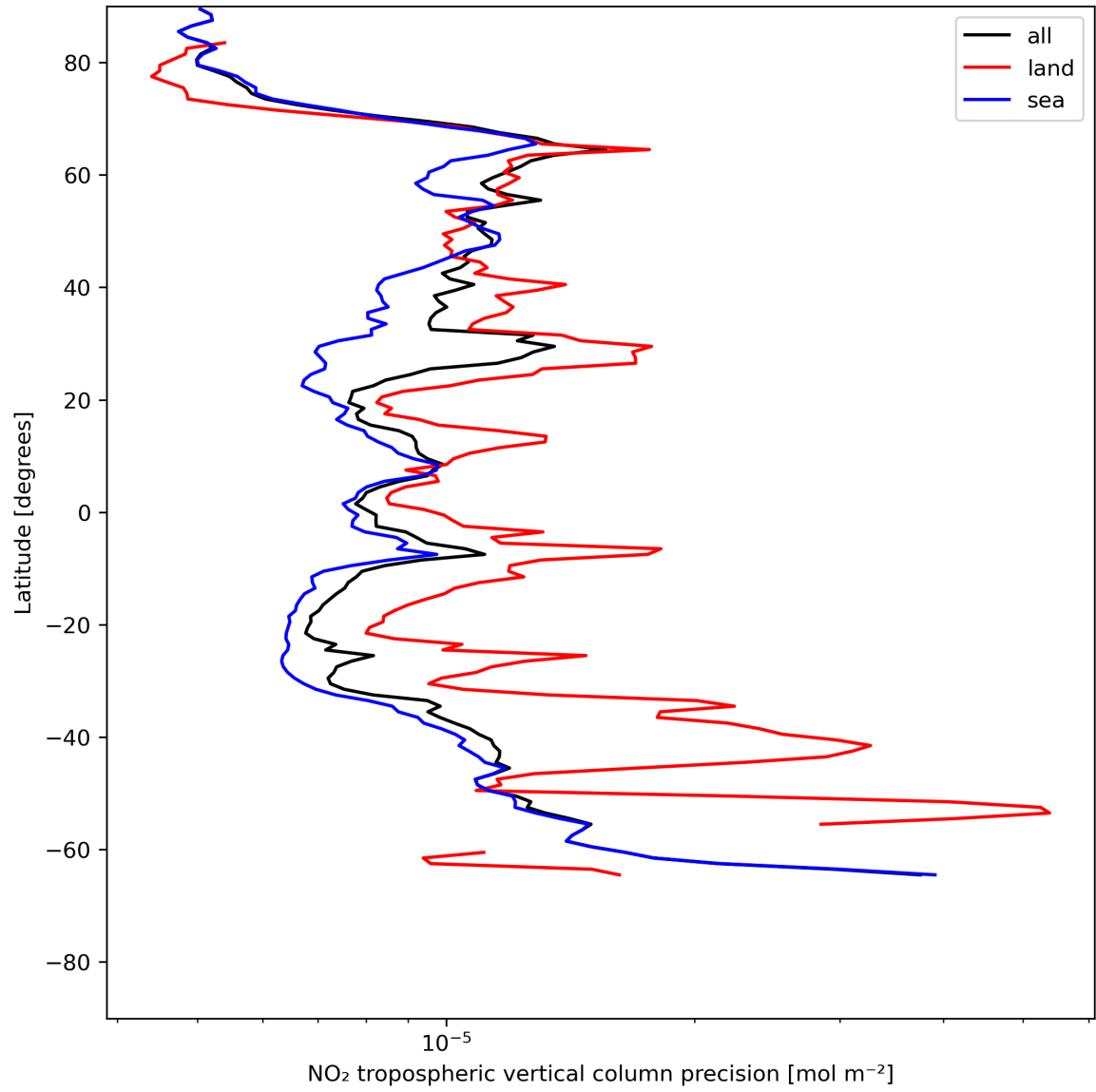
Figure 13: Zonal average of “NO 2 tropospheric vertical column precision” for 2024-06-24 to 2024-06-26.
