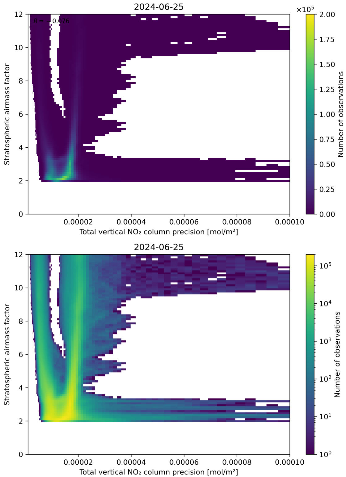
Figure 115: Scatter density plot of “Total vertical NO 2 column precision” against “Stratospheric airmass factor” for 2024-06-24 to 2024-06-26.
