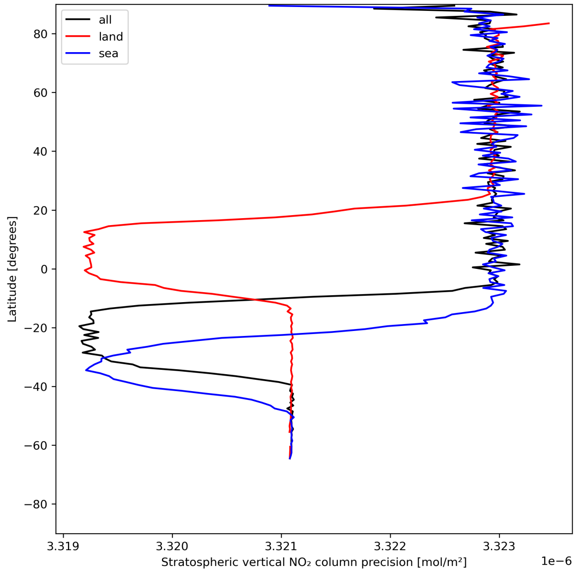
Figure 20: Zonal average of “Stratospheric vertical NO 2 column precision” for 2024-06-24 to 2024-06-26.
