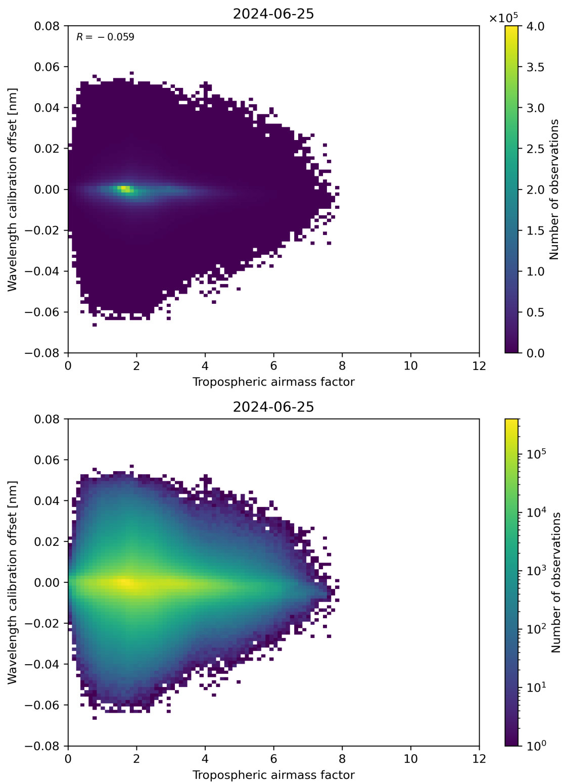
Figure 80: Scatter density plot of “Tropospheric airmass factor” against “Wavelength calibration offset” for 2024-06-24 to 2024-06-26.
