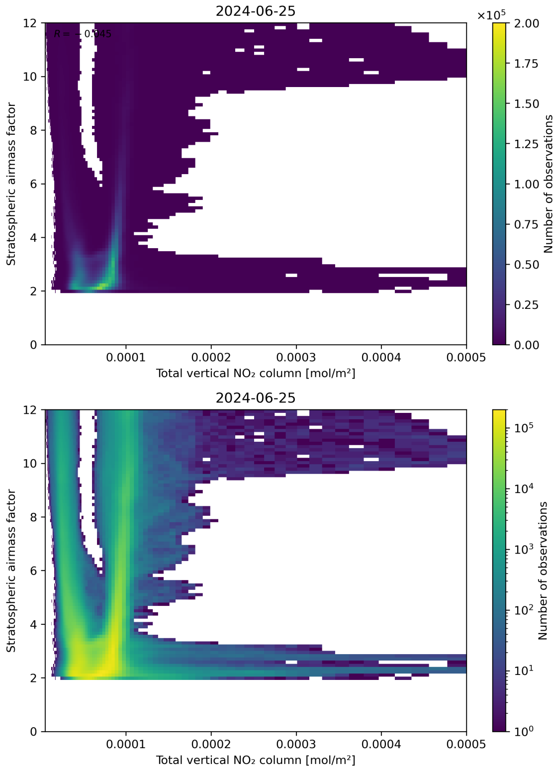
Figure 110: Scatter density plot of “Total vertical NO 2 column” against “Stratospheric airmass factor” for 2024-06-24 to 2024-06-26.
