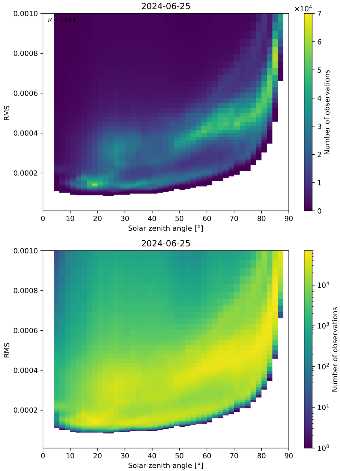
Figure 157: Scatter density plot of “Solar zenith angle” against “RMS” for 2024-06-24 to 2024-06-26.
