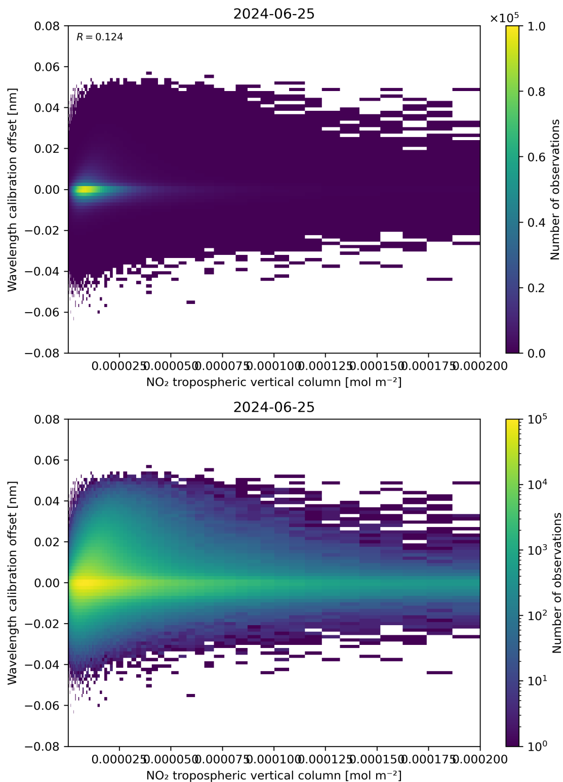
Figure 143: Scatter density plot of “NO 2 tropospheric vertical column” against “Wavelength calibration offset” for 2024-06-24 to 2024-06-26.
