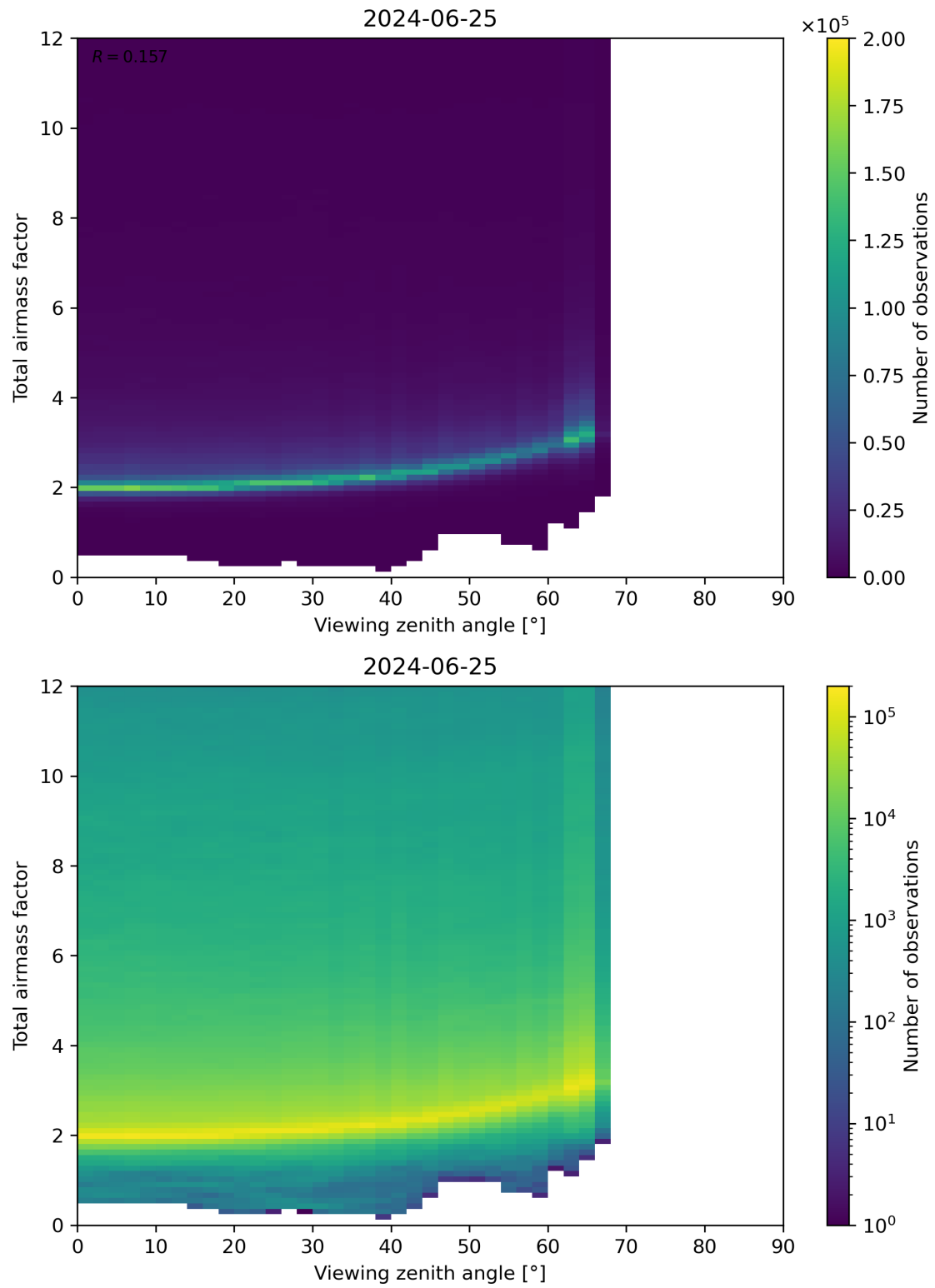
Figure 160: Scatter density plot of “Viewing zenith angle” against “Total airmass factor” for 2024-06-24 to 2024-06-26.
