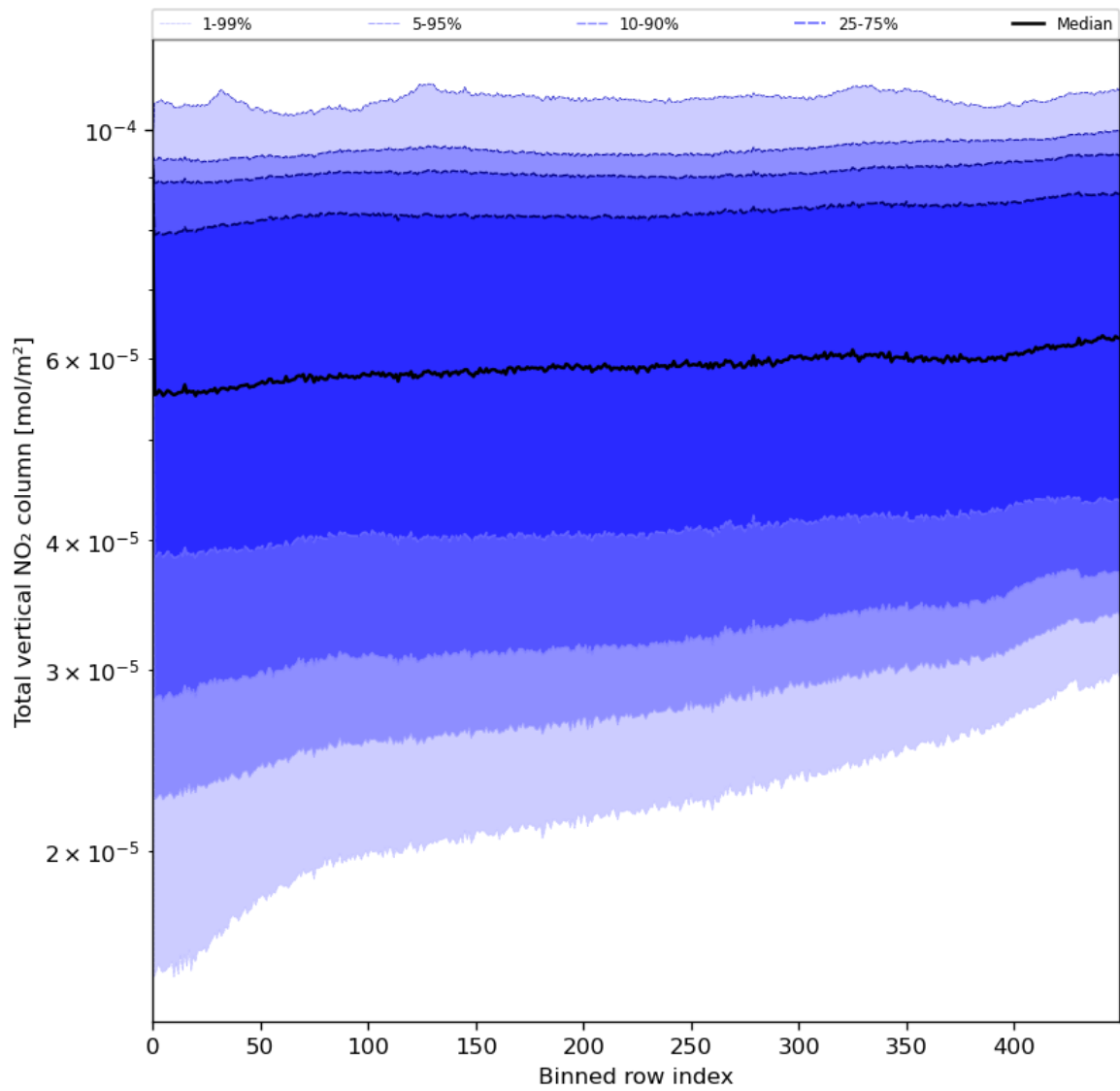
Figure 55: Along track statistics of “Total vertical NO 2 column” for 2024-06-24 to 2024-06-26
