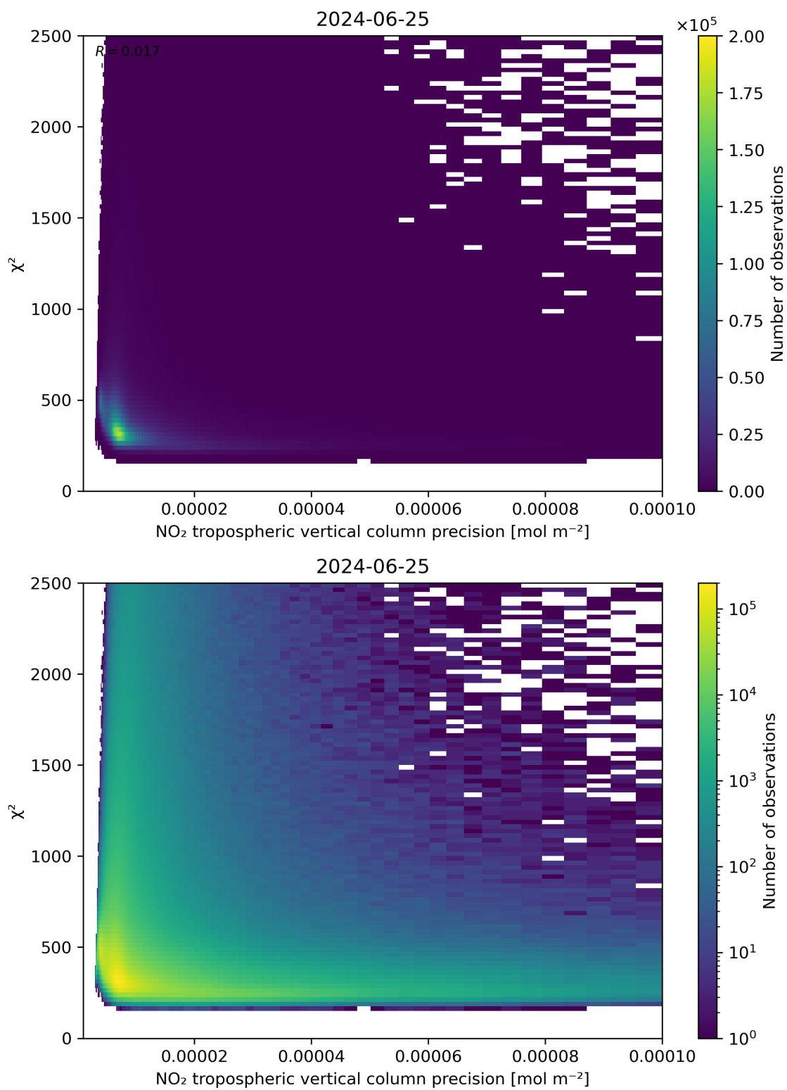
Figure 134: Scatter density plot of “NO 2 tropospheric vertical column precision” against “ \chi^2 ” for 2024-06-24 to 2024-06-26.
