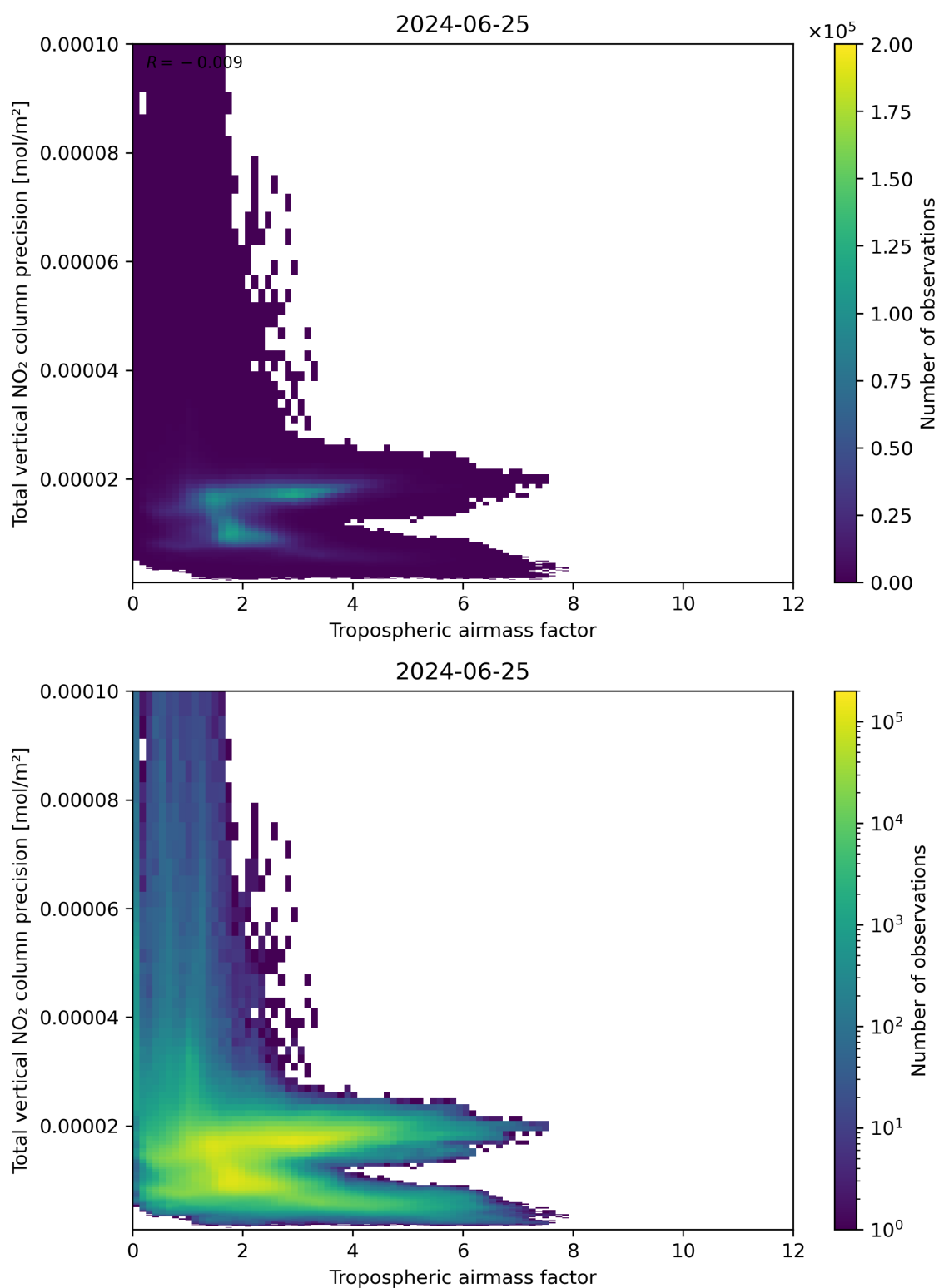
Figure 78: Scatter density plot of “Tropospheric airmass factor” against “Total vertical NO 2 column precision” for 2024-06-24 to 2024-06-26.
