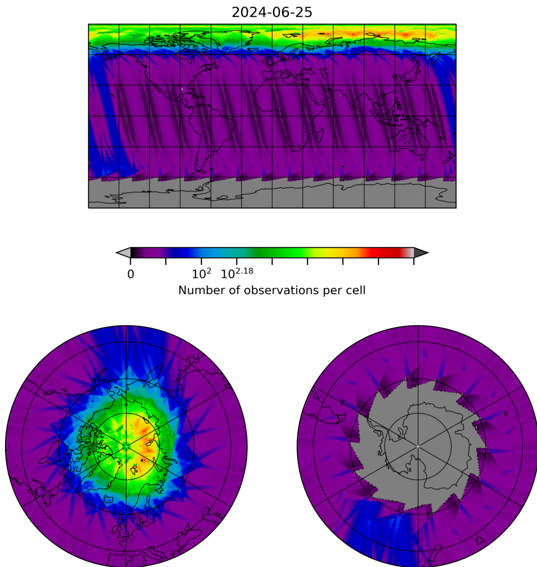
Figure 10: Map of the number of observations for 2024-06-24 to 2024-06-26
