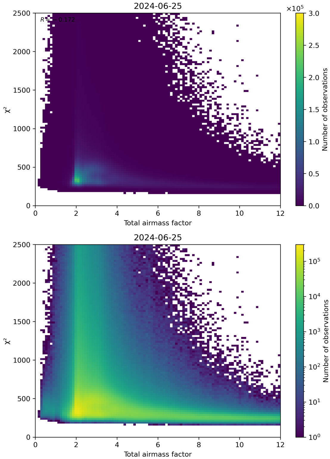
Figure 63: Scatter density plot of “Total airmass factor” against “ \chi^2 ” for 2024-06-24 to 2024-06-26.
