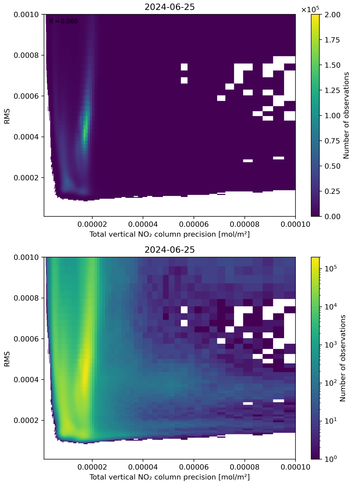
Figure 119: Scatter density plot of “Total vertical NO 2 column precision” against “RMS” for 2024-06-24 to 2024-06-26.
