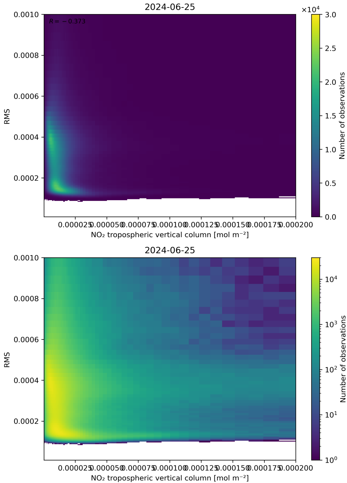
Figure 142: Scatter density plot of “NO 2 tropospheric vertical column” against “RMS” for 2024-06-24 to 2024-06-26.
