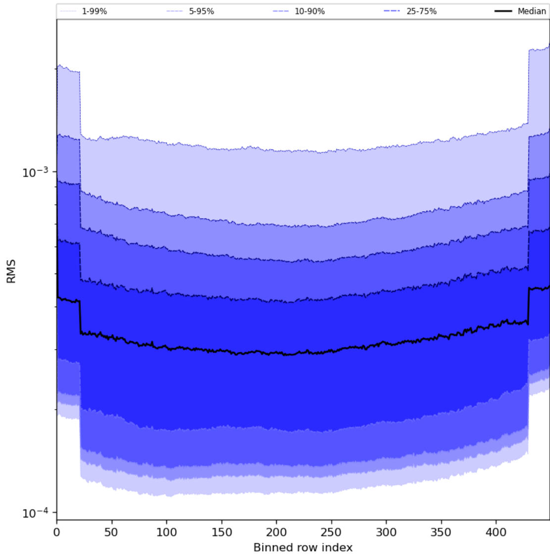
Figure 60: Along track statistics of “RMS” for 2024-06-24 to 2024-06-26
