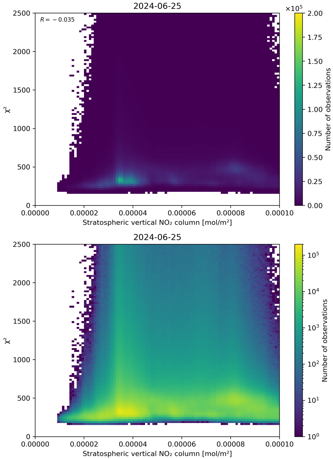
Figure 97: Scatter density plot of “Stratospheric vertical NO 2 column” against “ \chi^2 ” for 2024-06-24 to 2024-06-26.
