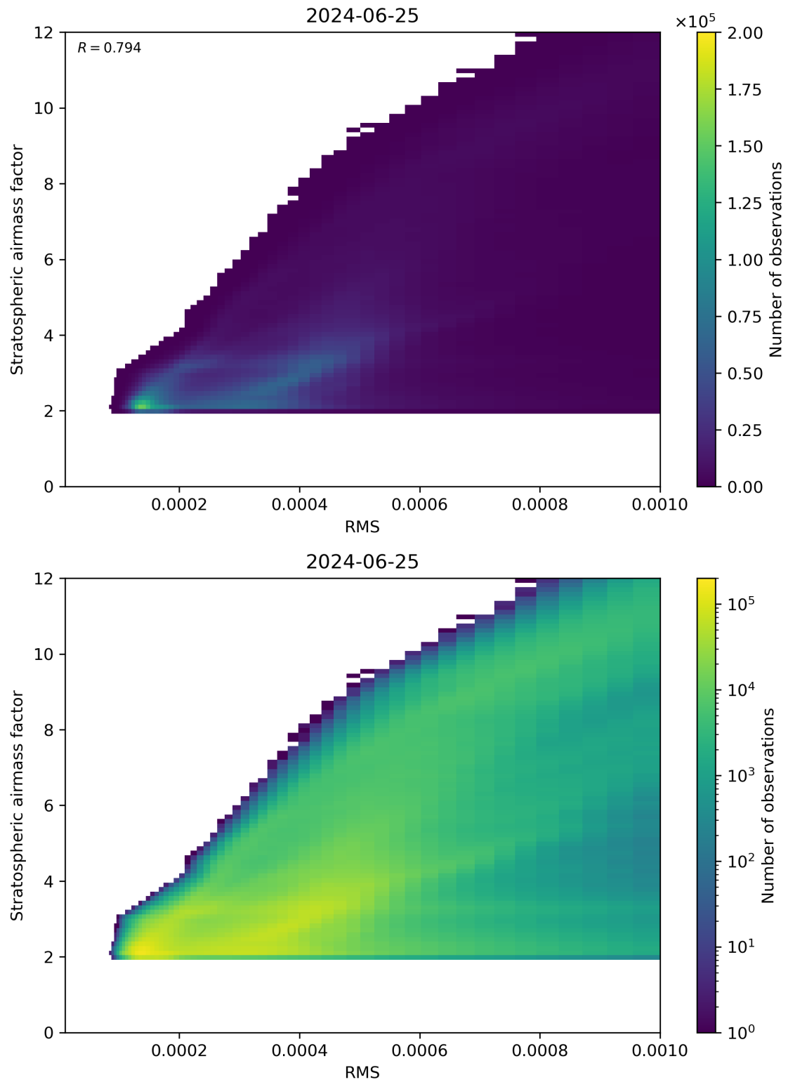
Figure 144: Scatter density plot of “RMS” against “Stratospheric airmass factor” for 2024-06-24 to 2024-06-26.
