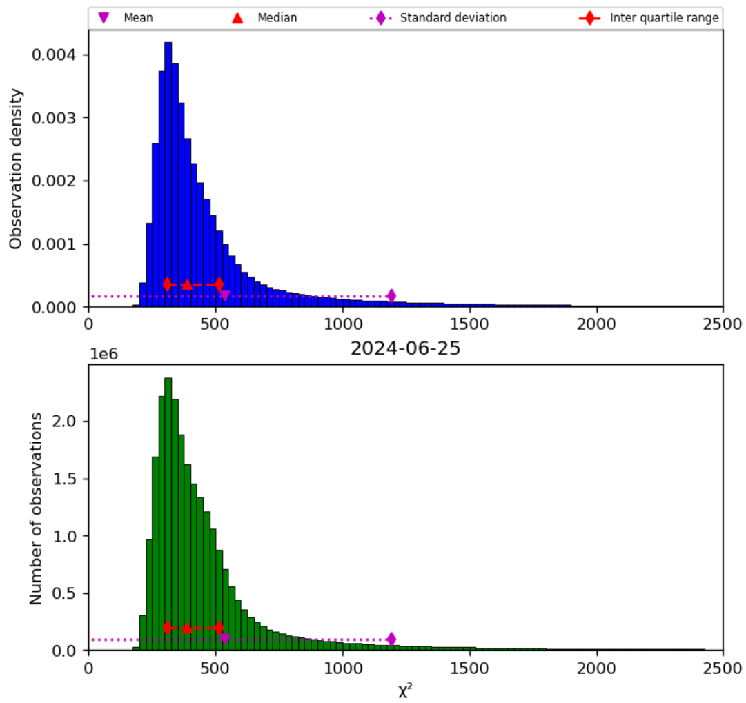
Figure 42: Histogram of “ \chi^2 ” for 2024-06-24 to 2024-06-26
