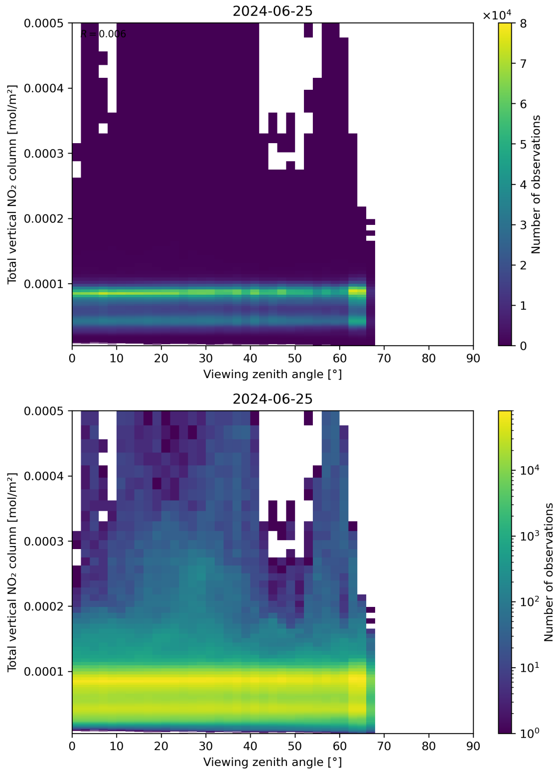
Figure 167: Scatter density plot of “Viewing zenith angle” against “Total vertical NO 2 column” for 2024-06-24 to 2024-06-26.
