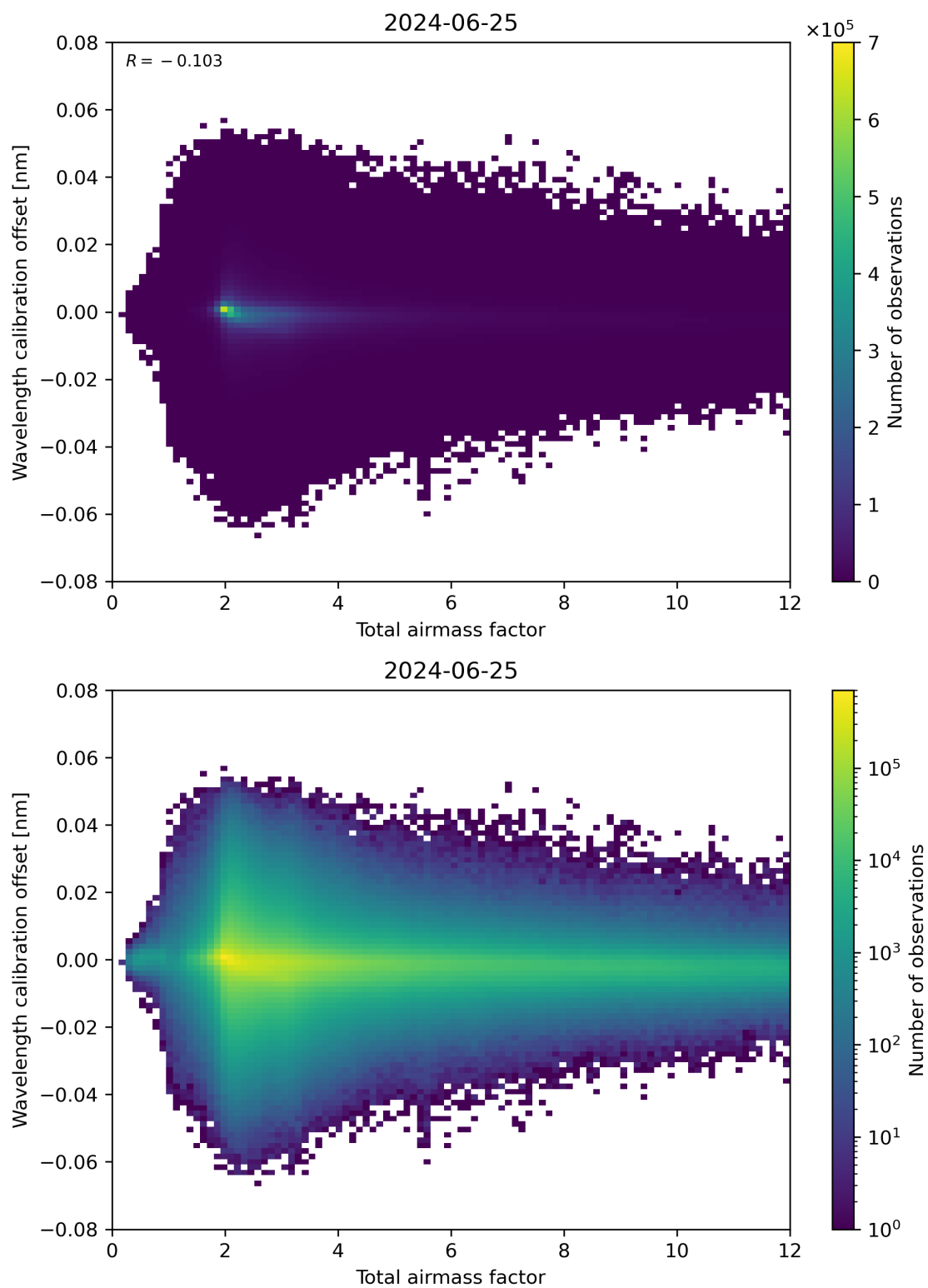
Figure 70: Scatter density plot of “Total airmass factor” against “Wavelength calibration offset” for 2024-06-24 to 2024-06-26.
