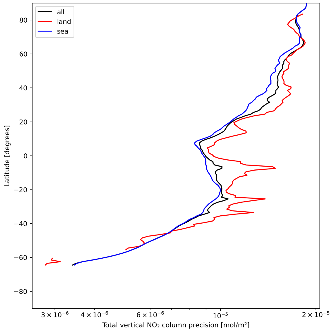
Figure 22: Zonal average of “Total vertical NO 2 column precision” for 2024-06-24 to 2024-06-26.
