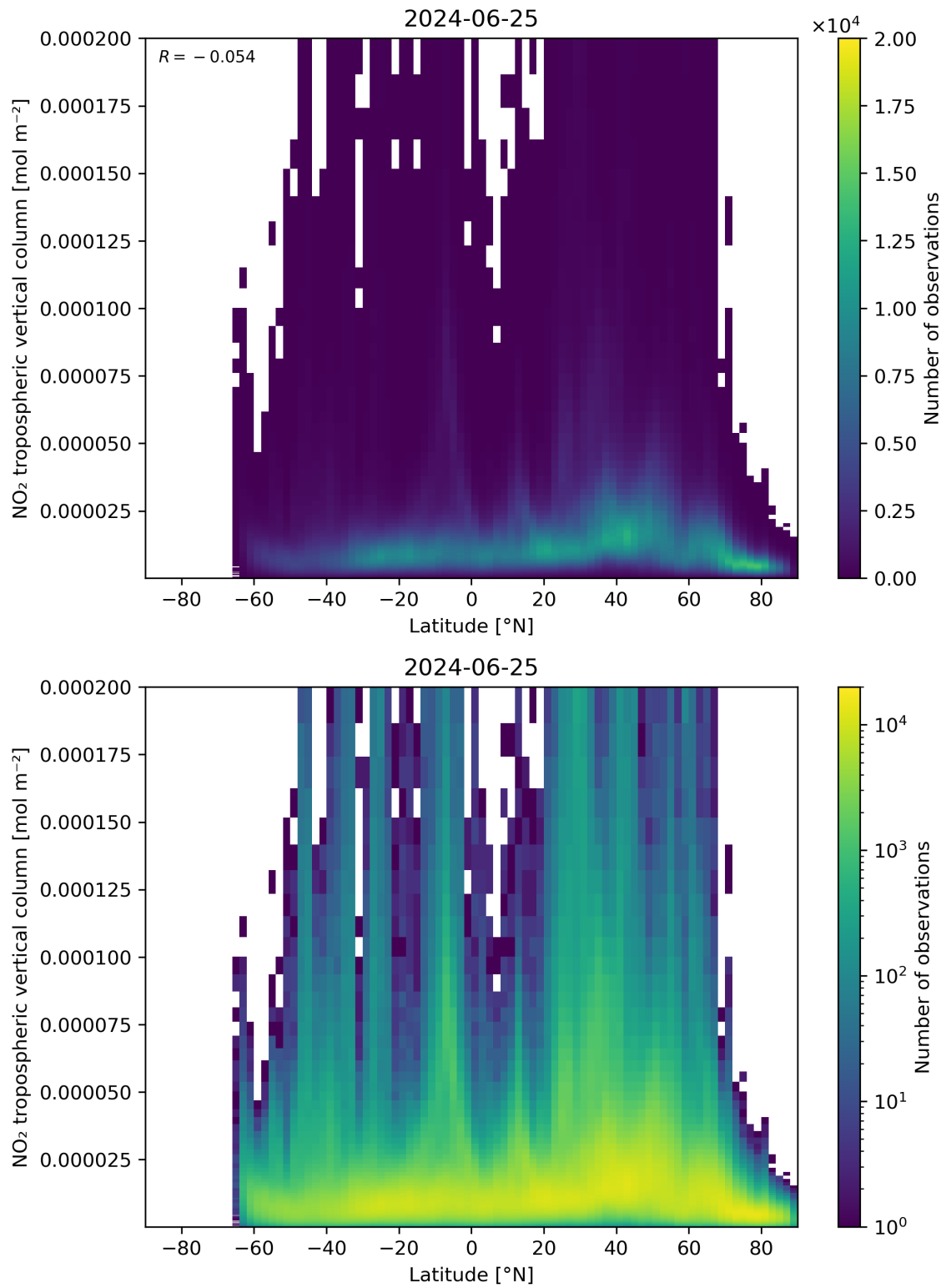
Figure 92: Scatter density plot of “Latitude” against “NO 2 tropospheric vertical column” for 2024-06-24 to 2024-06-26.
