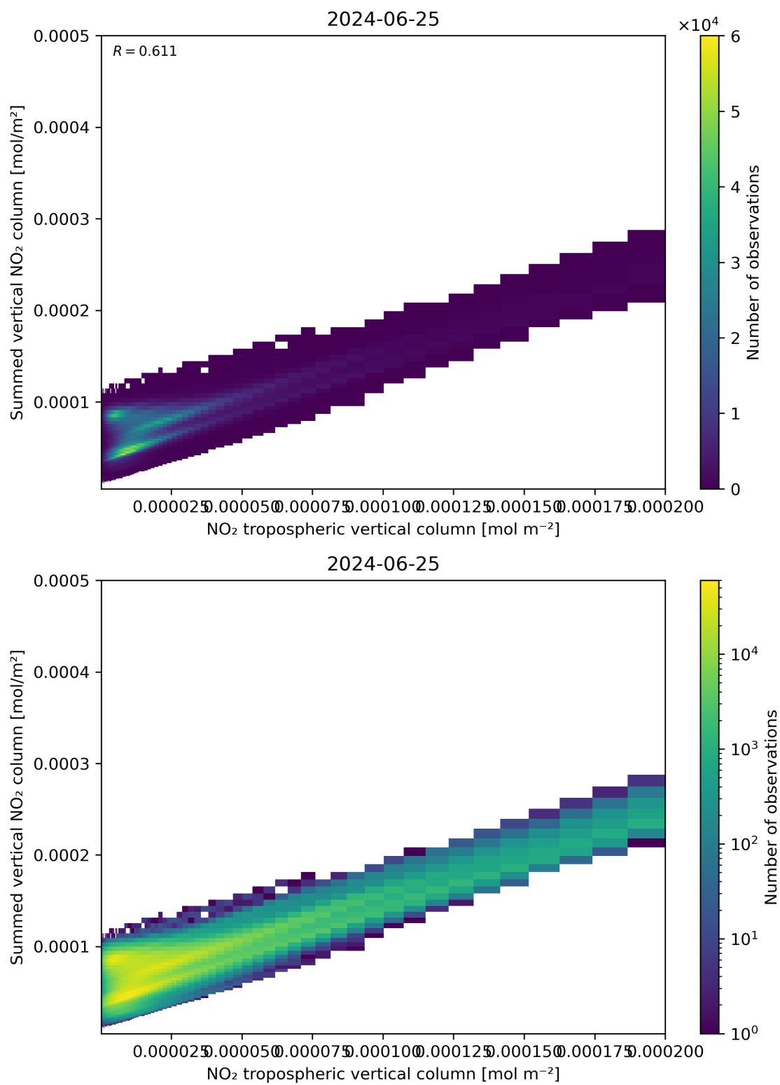
Figure 126: Scatter density plot of “NO 2 tropospheric vertical column” against “Summed vertical NO 2 column” for 2024-06-24 to 2024-06-26.
