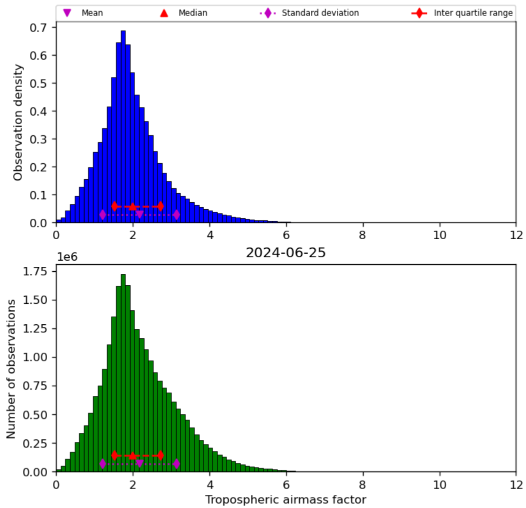
Figure 31: Histogram of “Tropospheric airmass factor” for 2024-06-24 to 2024-06-26
