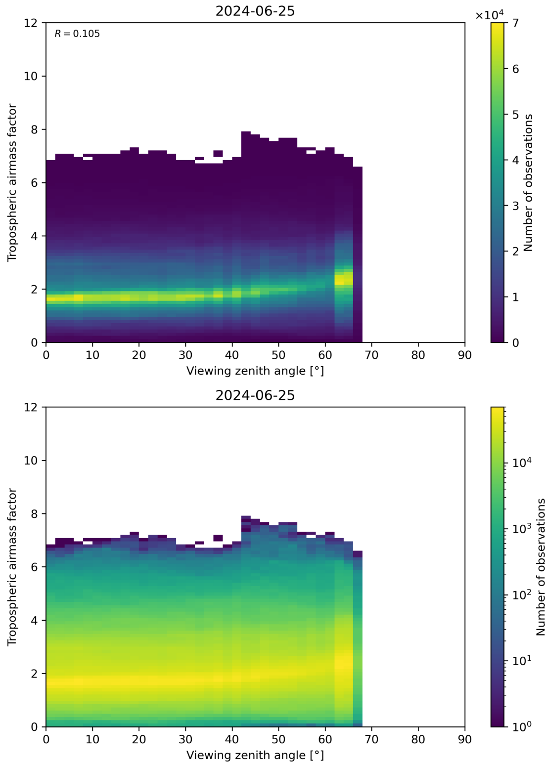
Figure 161: Scatter density plot of “Viewing zenith angle” against “Tropospheric airmass factor” for 2024-06-24 to 2024-06-26.
