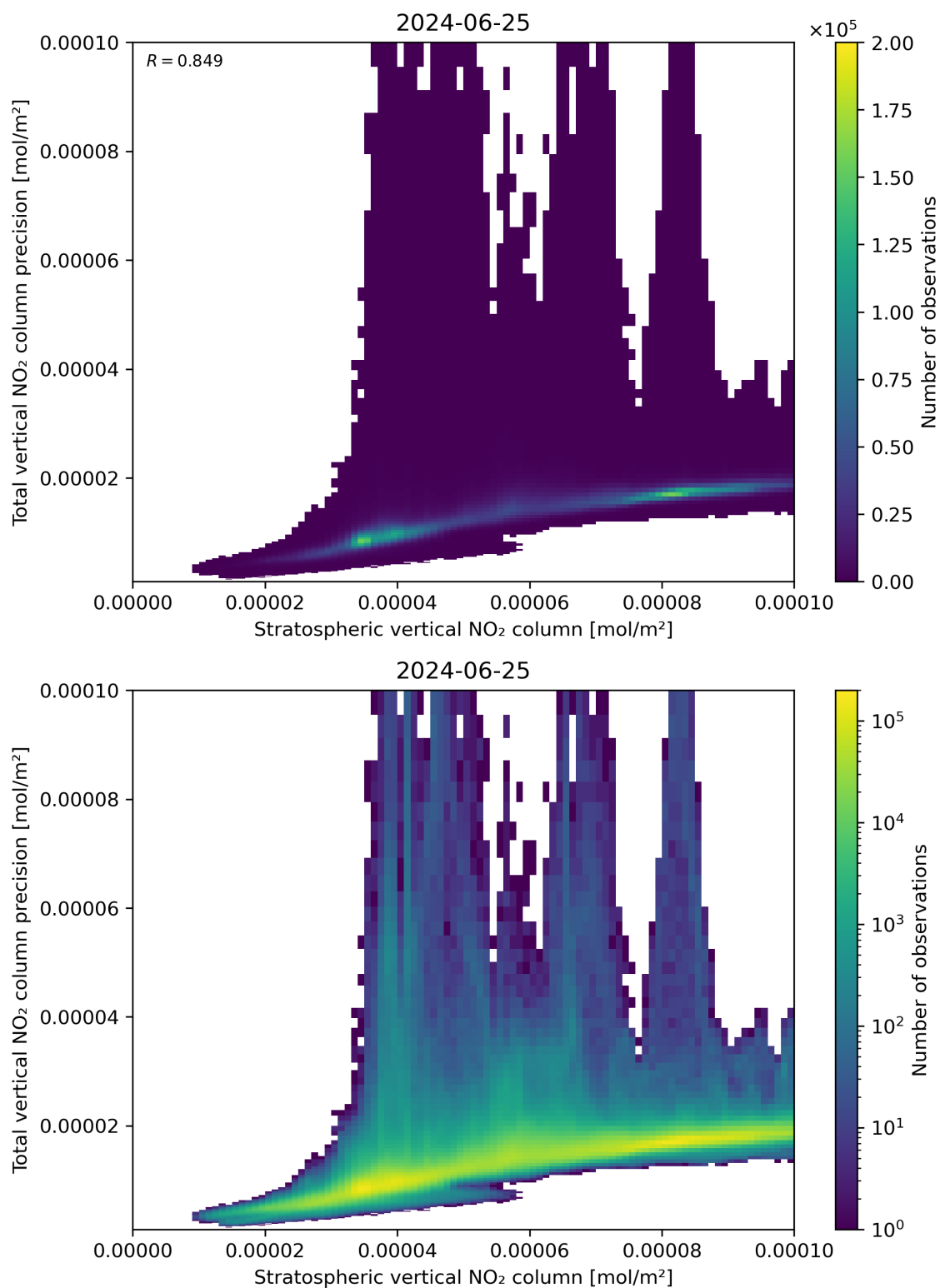
Figure 101: Scatter density plot of “Stratospheric vertical NO 2 column” against “Total vertical NO 2 column precision” for 2024-06-24 to 2024-06-26.
