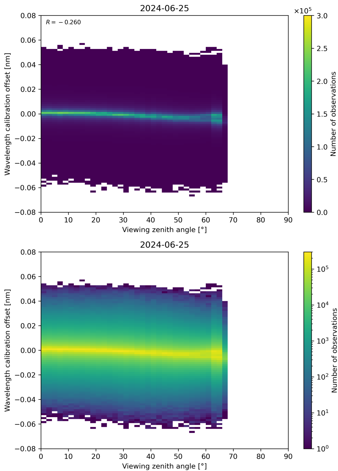
Figure 173: Scatter density plot of “Viewing zenith angle” against “Wavelength calibration offset” for 2024-06-24 to 2024-06-26.
