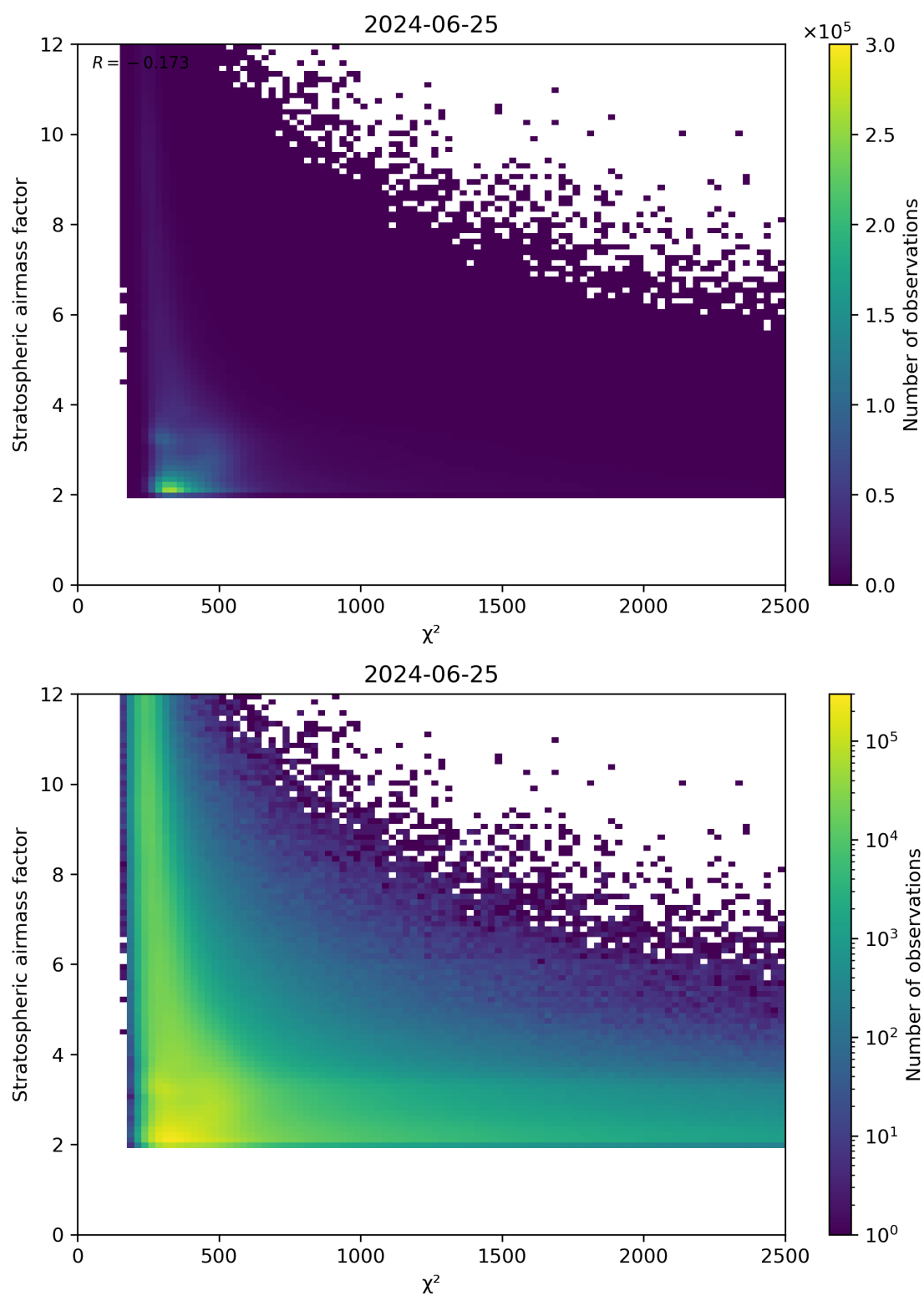
Figure 81: Scatter density plot of “ \chi^2 ” against “Stratospheric airmass factor” for 2024-06-24 to 2024-06-26.
