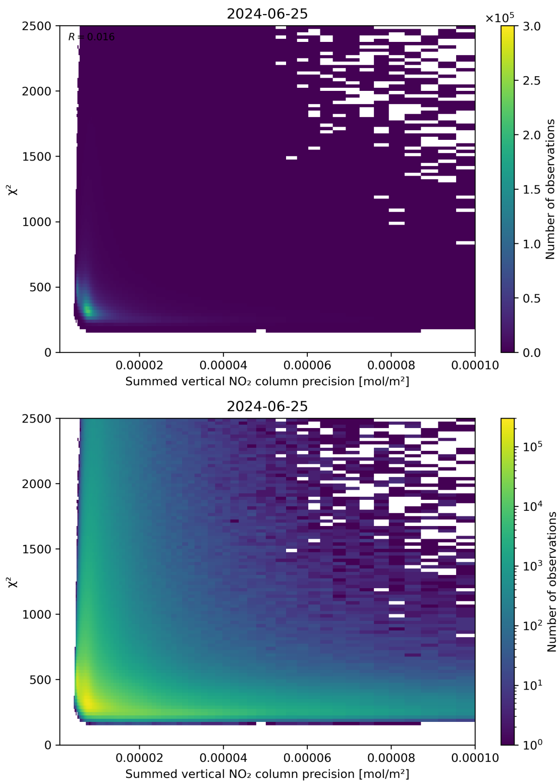
Figure 107: Scatter density plot of “Summed vertical NO 2 column precision” against “ \chi^2 ” for 2024-06-24 to 2024-06-26.
