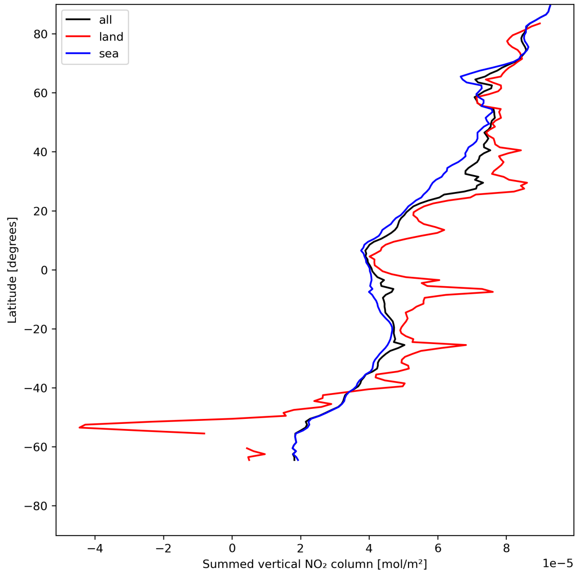
Figure 23: Zonal average of “Summed vertical NO 2 column” for 2024-06-24 to 2024-06-26.
