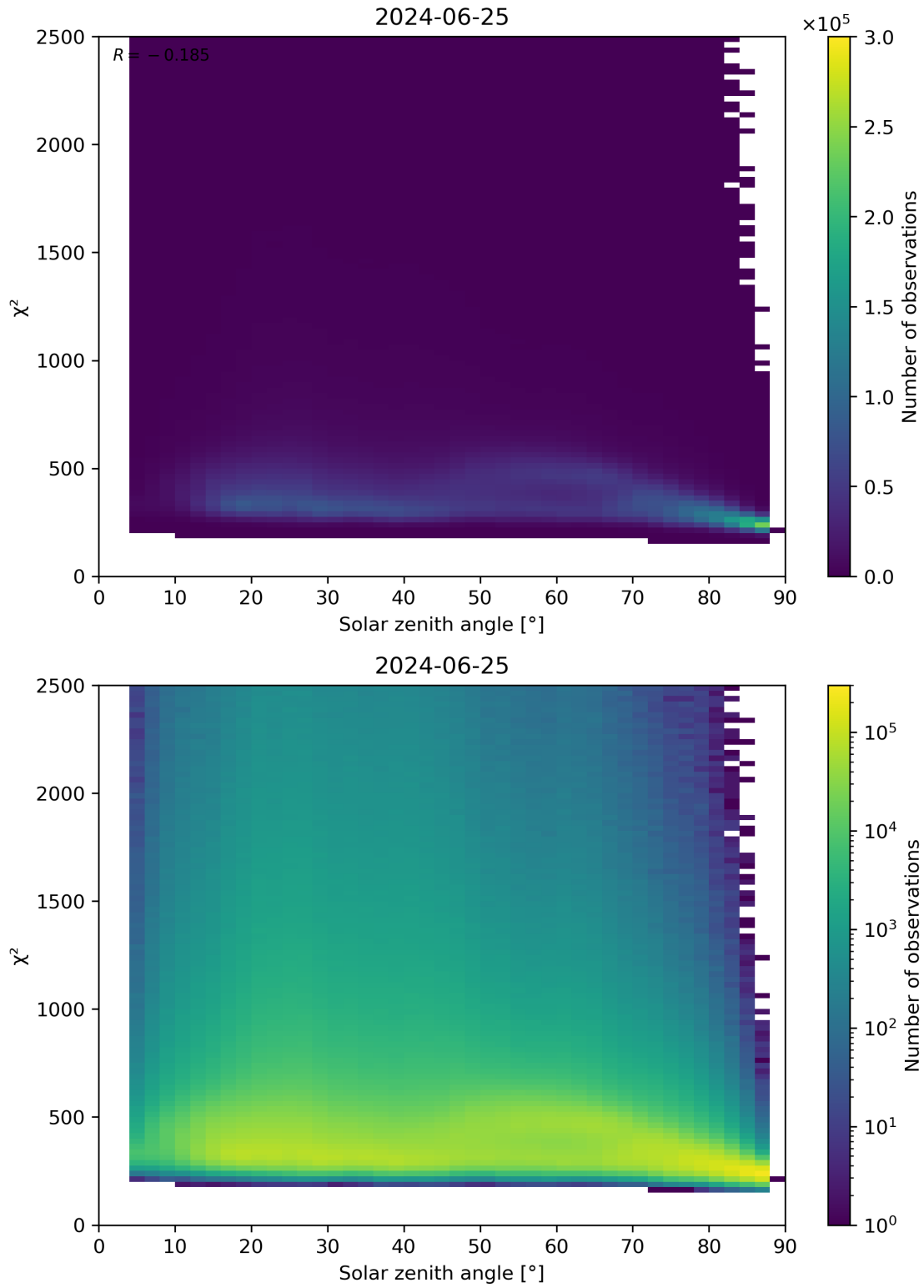
Figure 148: Scatter density plot of “Solar zenith angle” against “ \chi^2 ” for 2024-06-24 to 2024-06-26.
