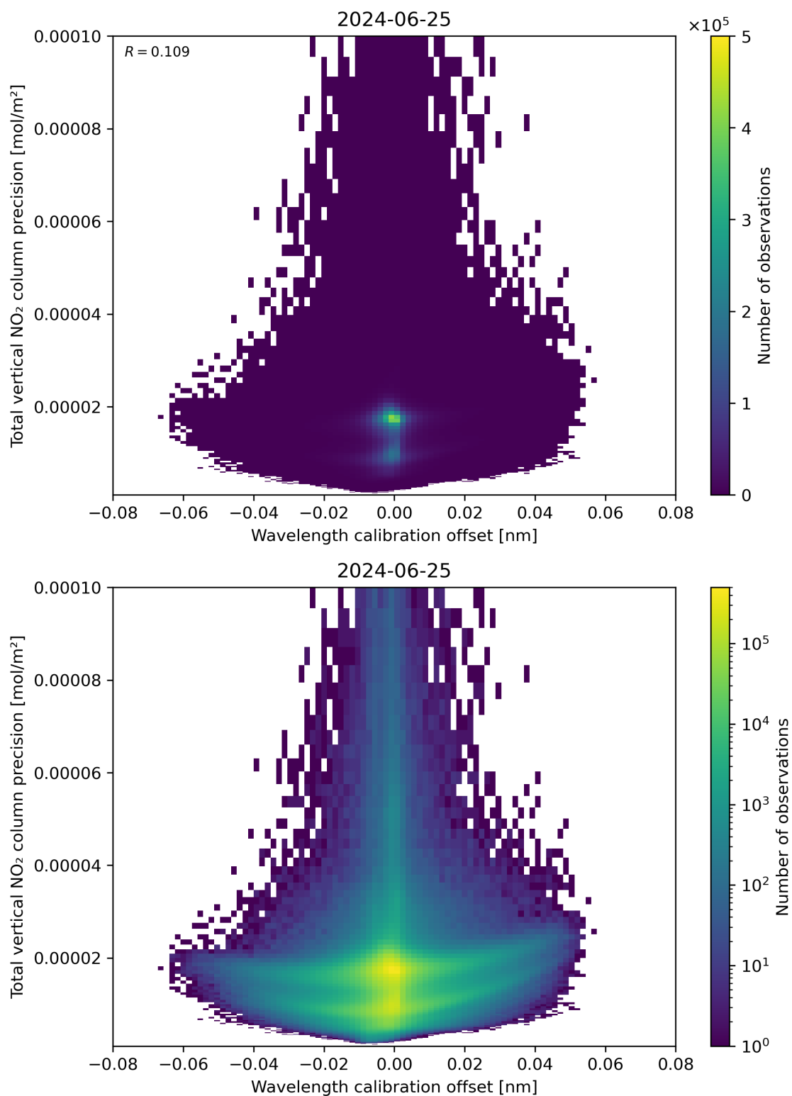
Figure 180: Scatter density plot of “Wavelength calibration offset” against “Total vertical NO 2 column precision” for 2024-06-24 to 2024-06-26.
