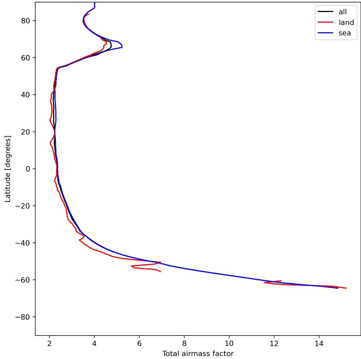
Figure 15: Zonal average of “Total airmass factor” for 2024-06-24 to 2024-06-26.
