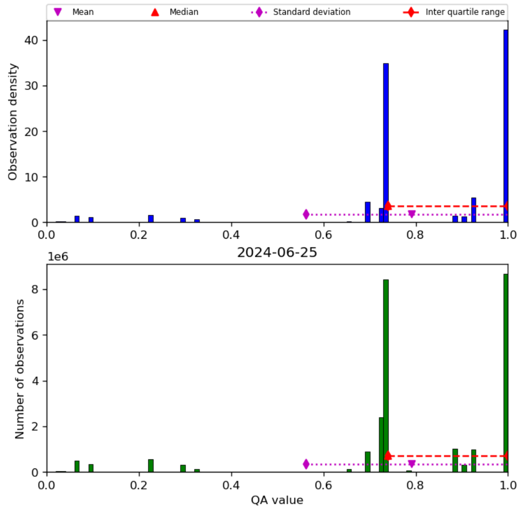
Figure 28: Histogram of “QA value” for 2024-06-24 to 2024-06-26
