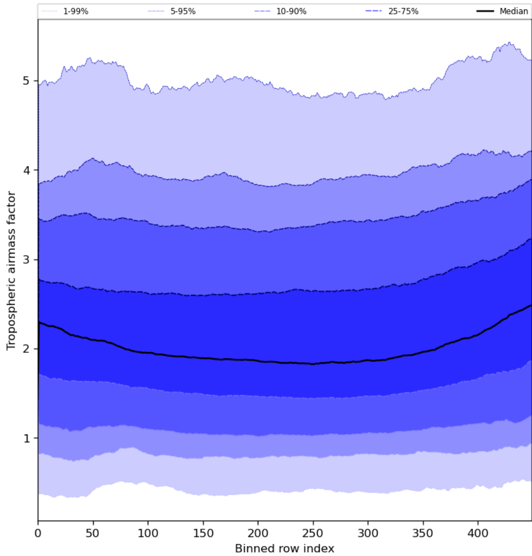
Figure 48: Along track statistics of “Tropospheric airmass factor” for 2024-06-24 to 2024-06-26
