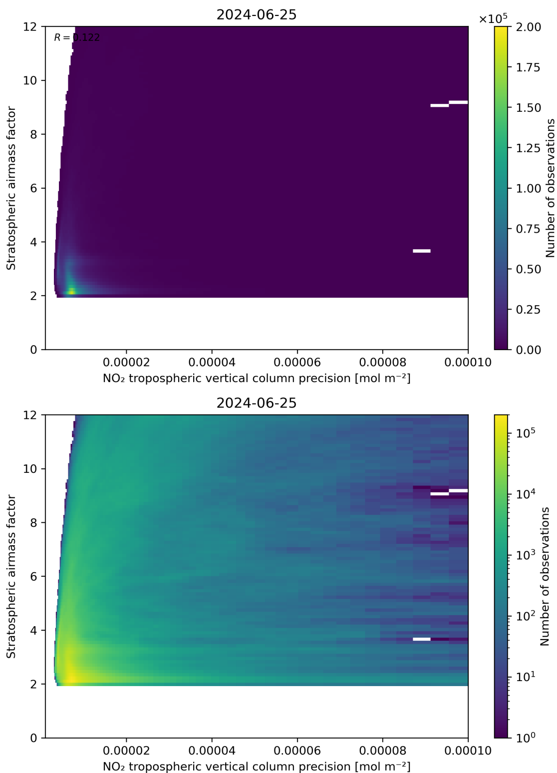
Figure 131: Scatter density plot of “NO 2 tropospheric vertical column precision” against “Stratospheric airmass factor” for 2024-06-24 to 2024-06-26.
