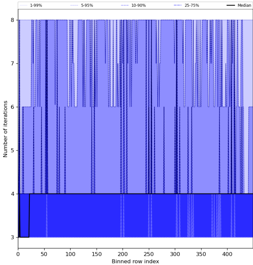
Figure 51: Along track statistics of “Number of iterations” for 2024-06-24 to 2024-06-26
