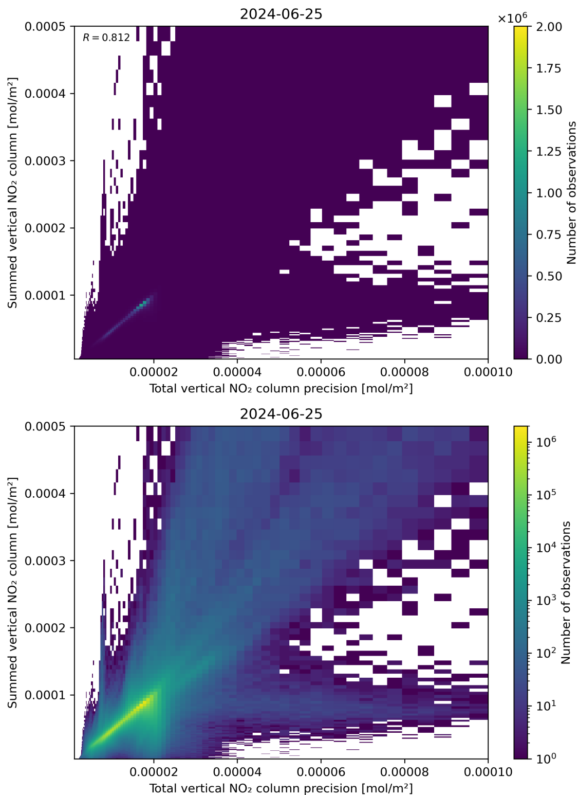
Figure 117: Scatter density plot of “Total vertical NO 2 column precision” against “Summed vertical NO 2 column” for 2024-06-24 to 2024-06-26.
