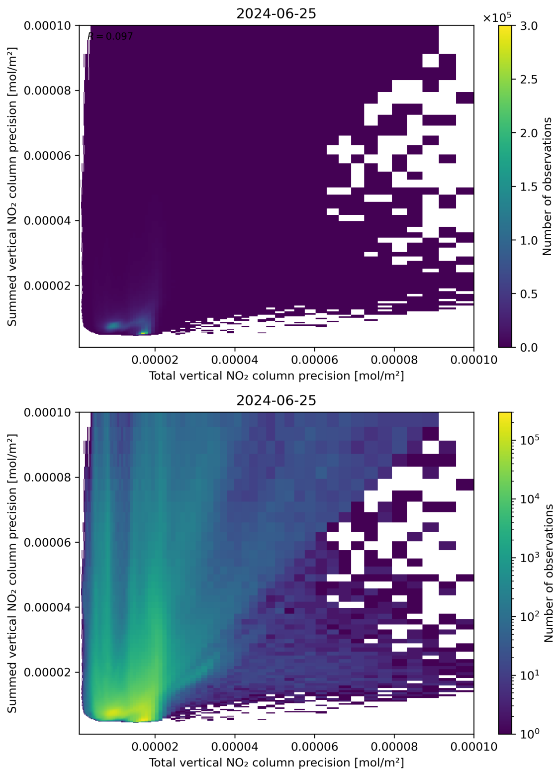
Figure 118: Scatter density plot of “Total vertical NO 2 column precision” against “Summed vertical NO 2 column precision” for 2024-06-24 to 2024-06-26.
