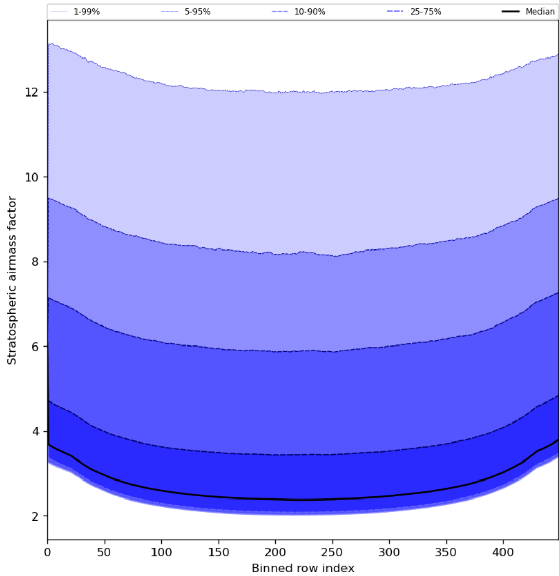
Figure 61: Along track statistics of “Stratospheric airmass factor” for 2024-06-24 to 2024-06-26
