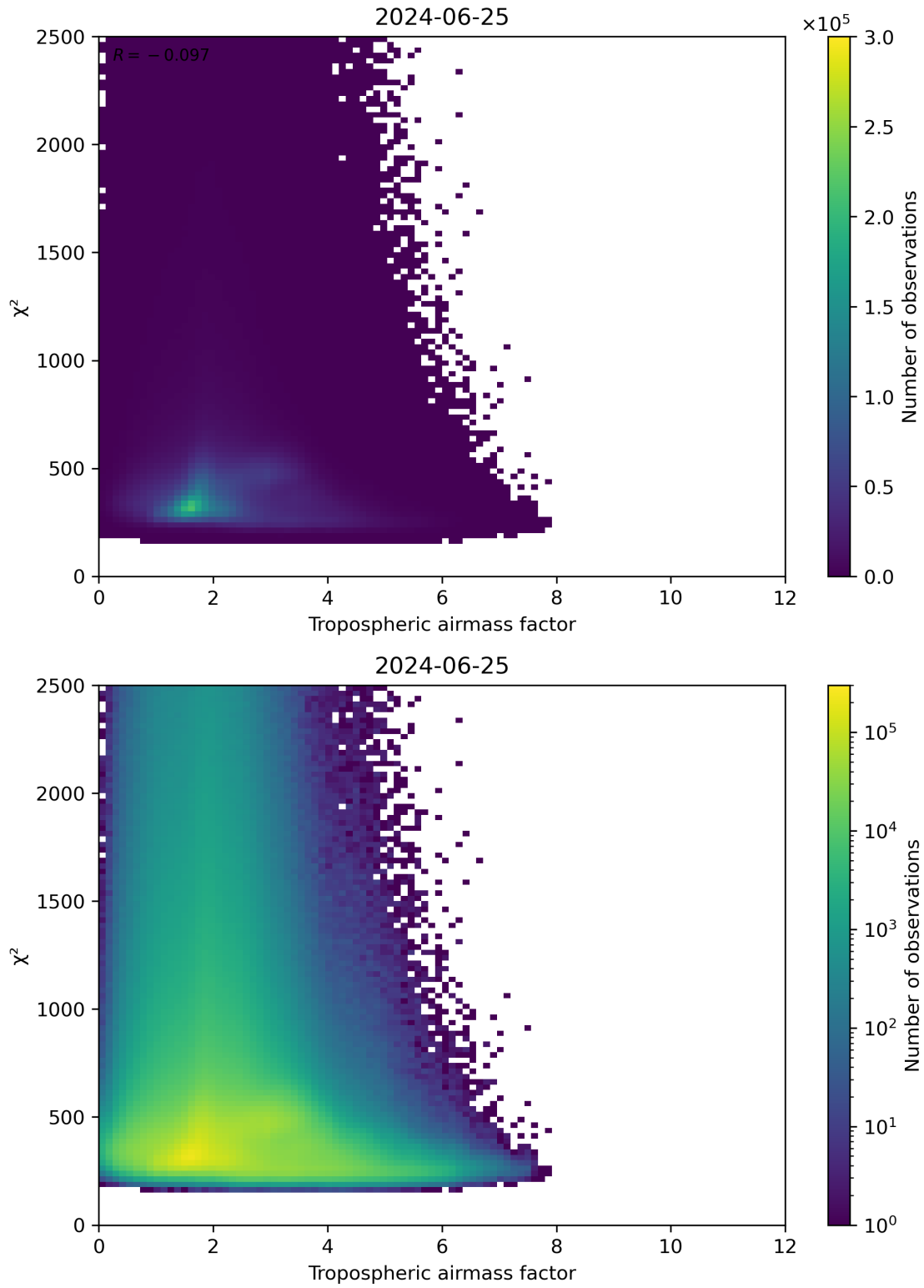
Figure 73: Scatter density plot of “Tropospheric airmass factor” against “ \chi^2 ” for 2024-06-24 to 2024-06-26.
