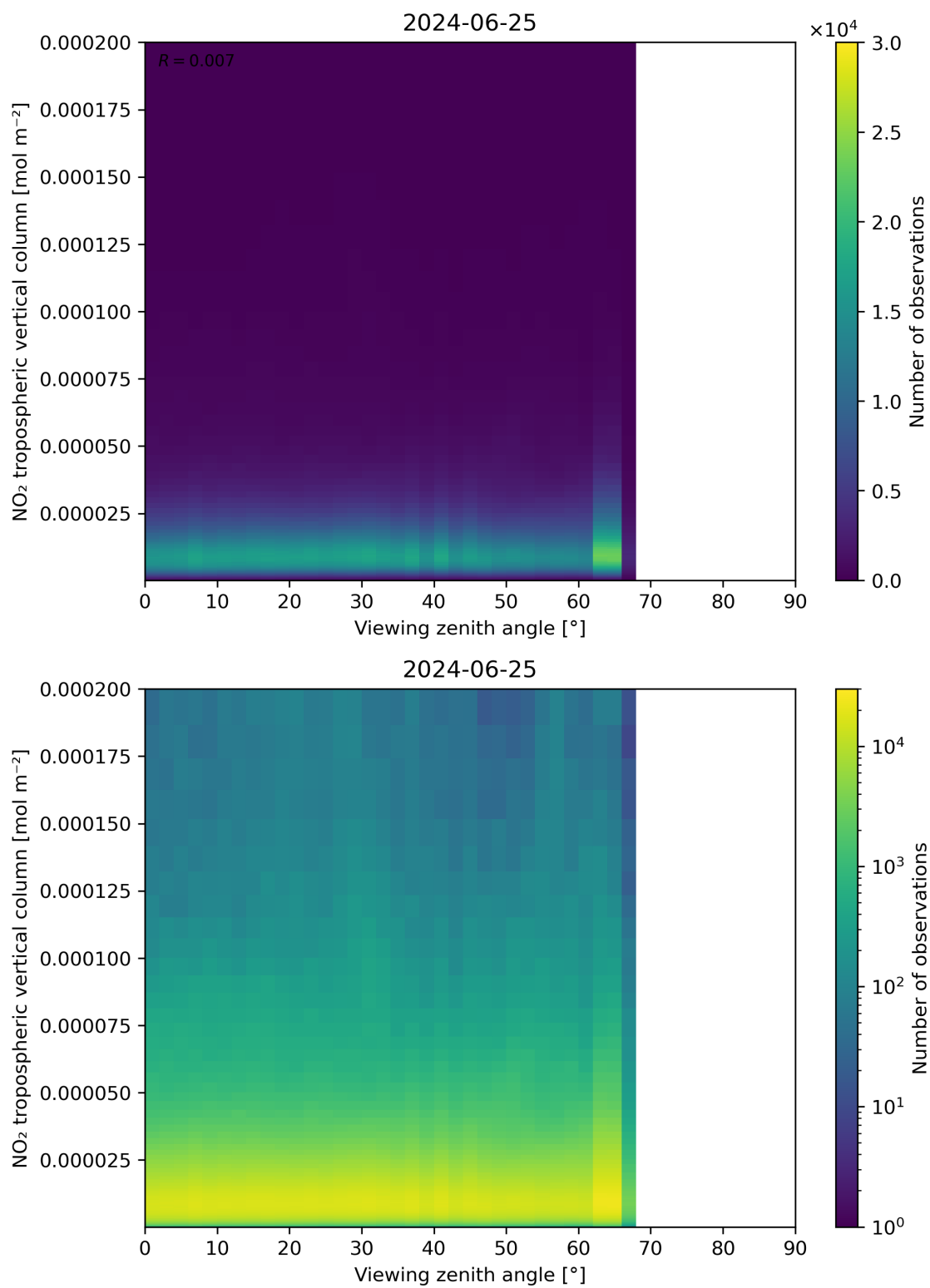
Figure 169: Scatter density plot of “Viewing zenith angle” against “NO 2 tropospheric vertical column” for 2024-06-24 to 2024-06-26.
