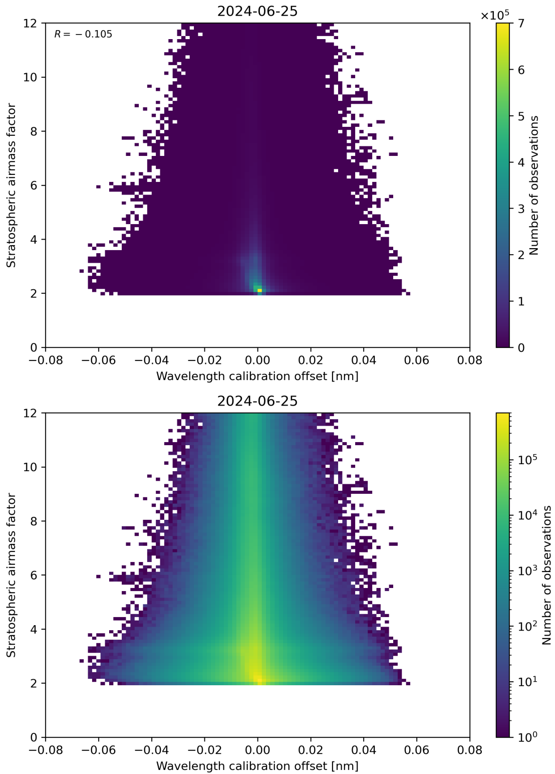
Figure 174: Scatter density plot of “Wavelength calibration offset” against “Stratospheric airmass factor” for 2024-06-24 to 2024-06-26.
