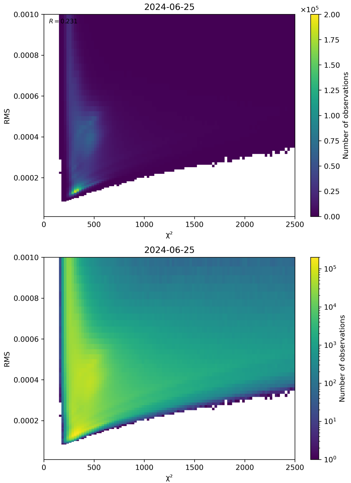
Figure 82: Scatter density plot of “ \chi^2 ” against “RMS” for 2024-06-24 to 2024-06-26.
