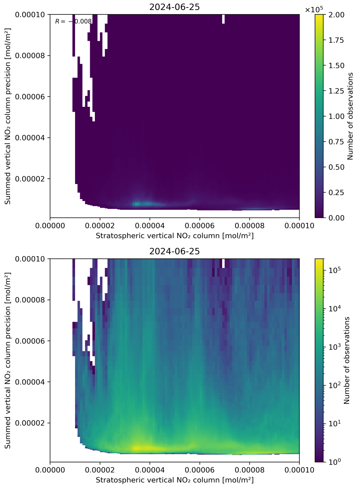
Figure 99: Scatter density plot of “Stratospheric vertical NO 2 column” against “Summed vertical NO 2 column precision” for 2024-06-24 to 2024-06-26.
