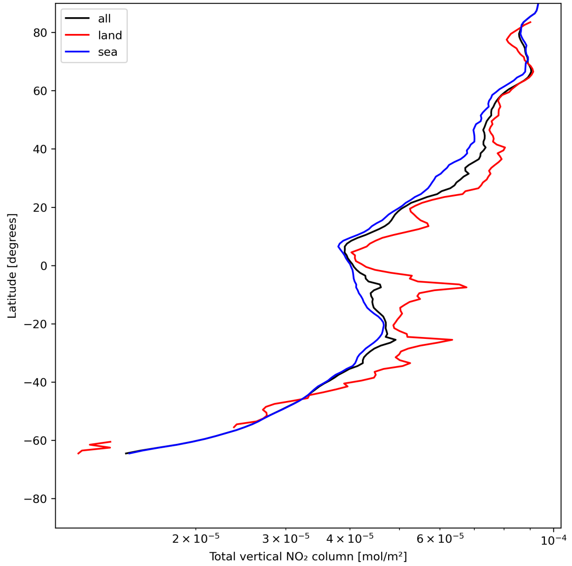
Figure 21: Zonal average of “Total vertical NO 2 column” for 2024-06-24 to 2024-06-26.
