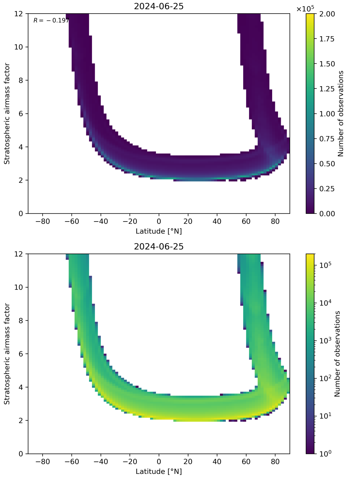
Figure 83: Scatter density plot of “Latitude” against “Stratospheric airmass factor” for 2024-06-24 to 2024-06-26.
