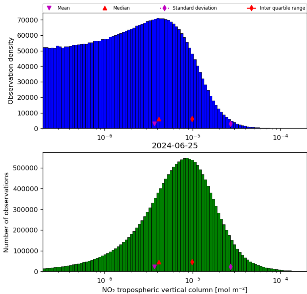
Figure 29: Histogram of “NO 2 tropospheric vertical column” for 2024-06-24 to 2024-06-26
