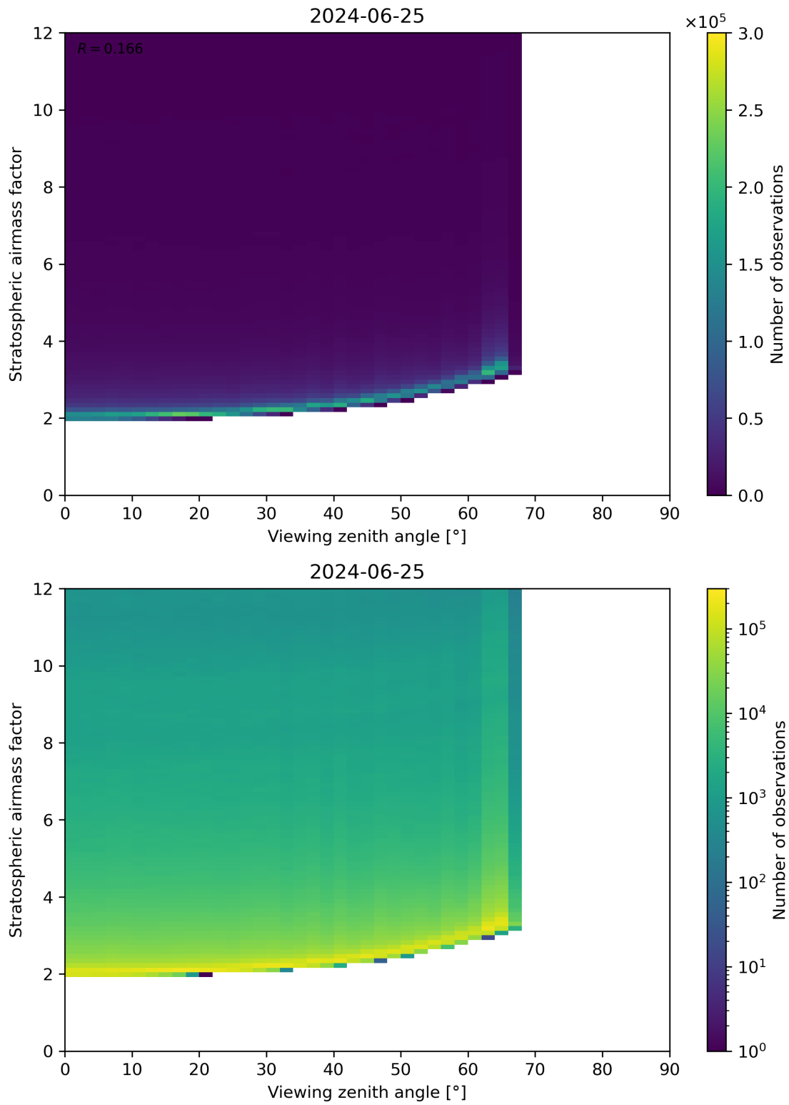
Figure 159: Scatter density plot of “Viewing zenith angle” against “Stratospheric airmass factor” for 2024-06-24 to 2024-06-26.
