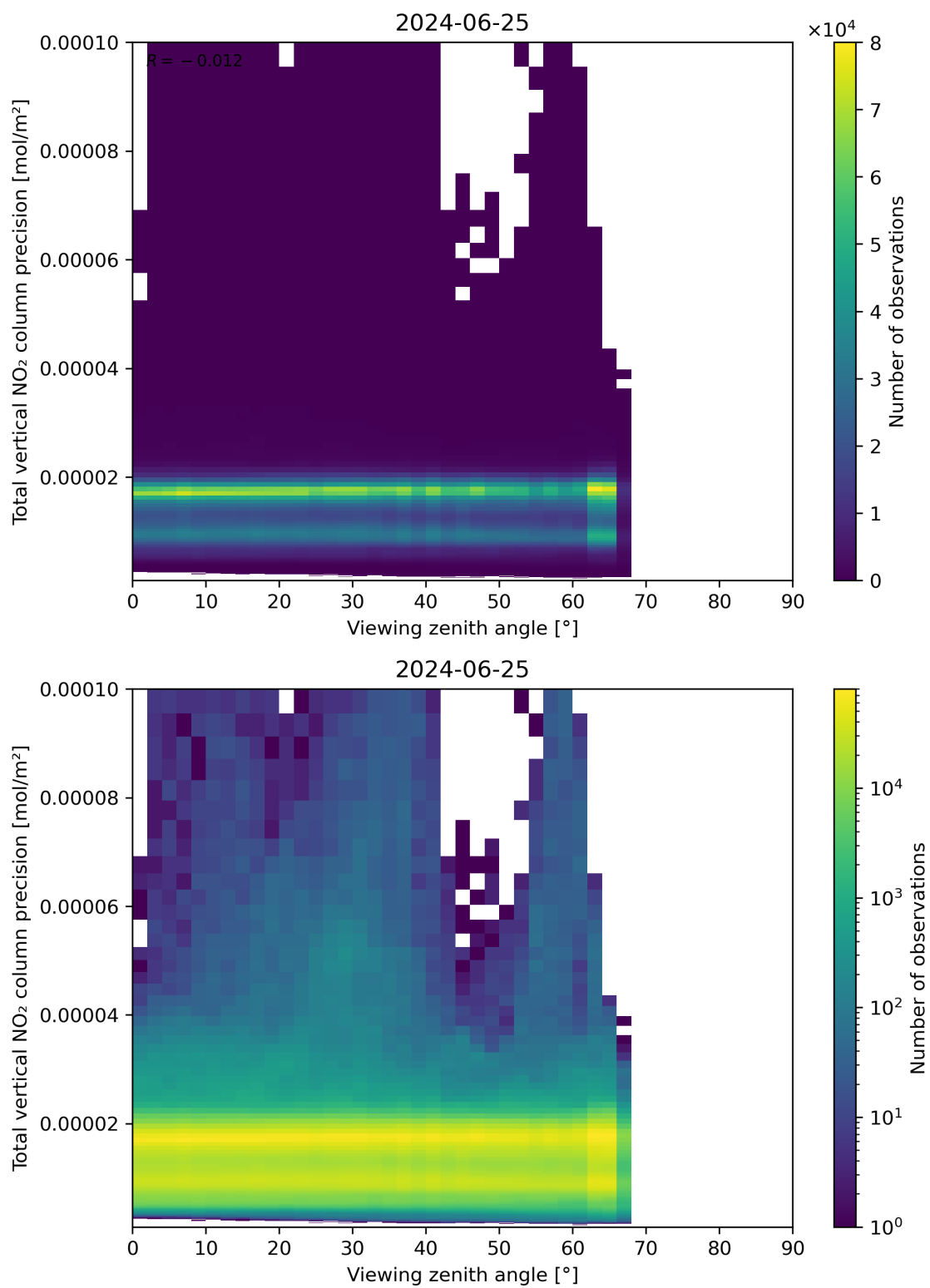
Figure 168: Scatter density plot of “Viewing zenith angle” against “Total vertical NO 2 column precision” for 2024-06-24 to 2024-06-26.
