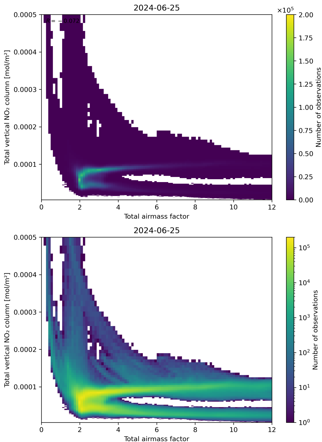
Figure 67: Scatter density plot of “Total airmass factor” against “Total vertical NO 2 column” for 2024-06-24 to 2024-06-26.
