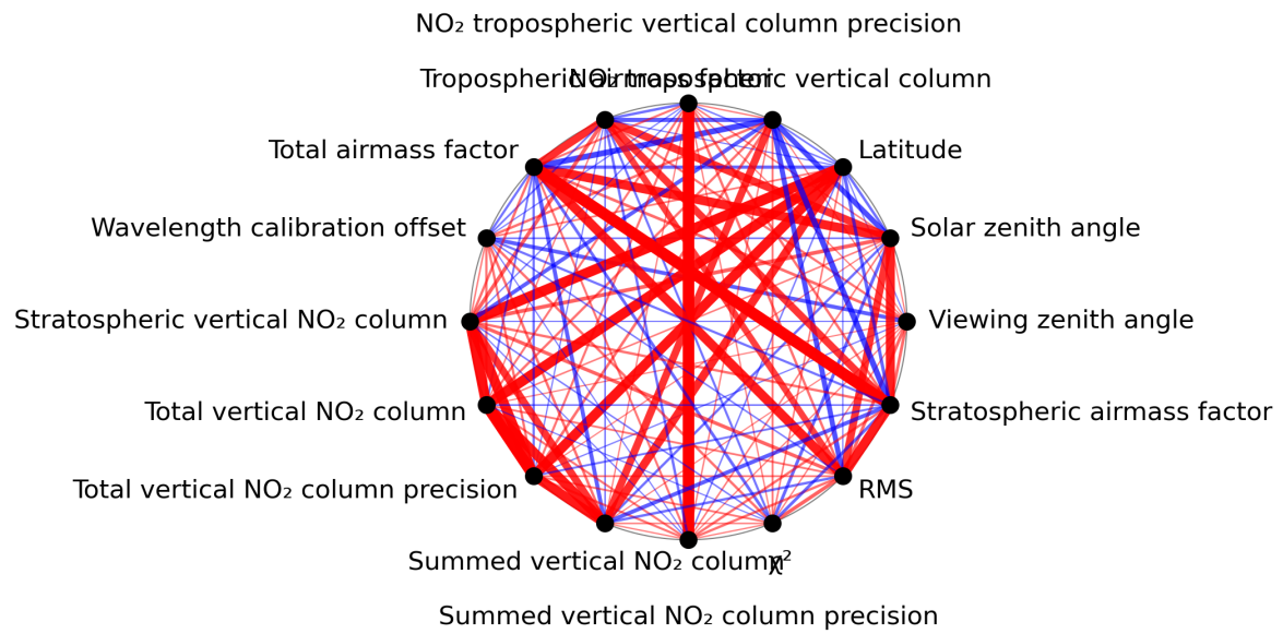
Figure 1: Map of correlation graph for 2024-06-24 to 2024-06-26.
