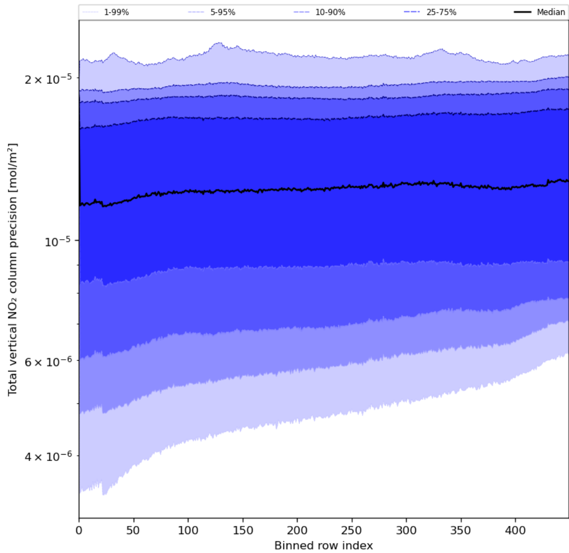
Figure 56: Along track statistics of “Total vertical NO 2 column precision” for 2024-06-24 to 2024-06-26
