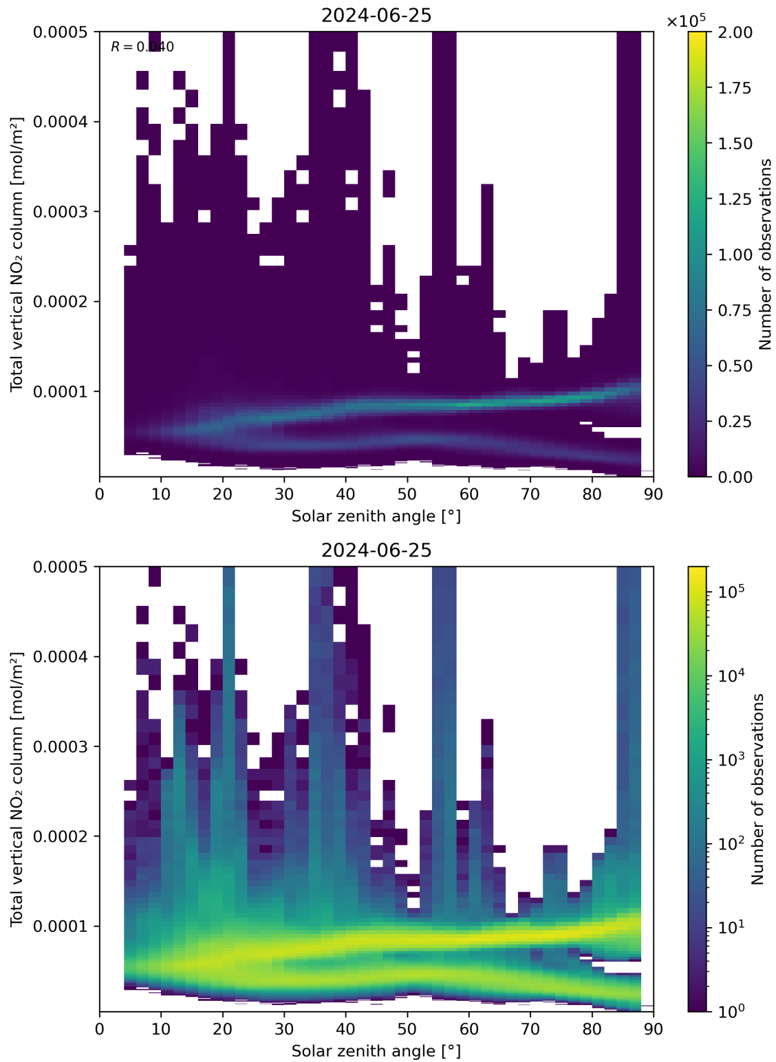
Figure 153: Scatter density plot of “Solar zenith angle” against “Total vertical \text{NO}_2 column” for 2024-06-24 to 2024-06-26.
