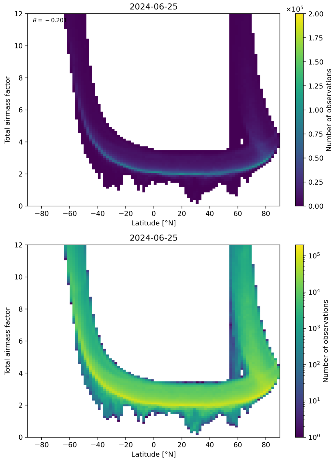
Figure 84: Scatter density plot of “Latitude” against “Total airmass factor” for 2024-06-24 to 2024-06-26.
