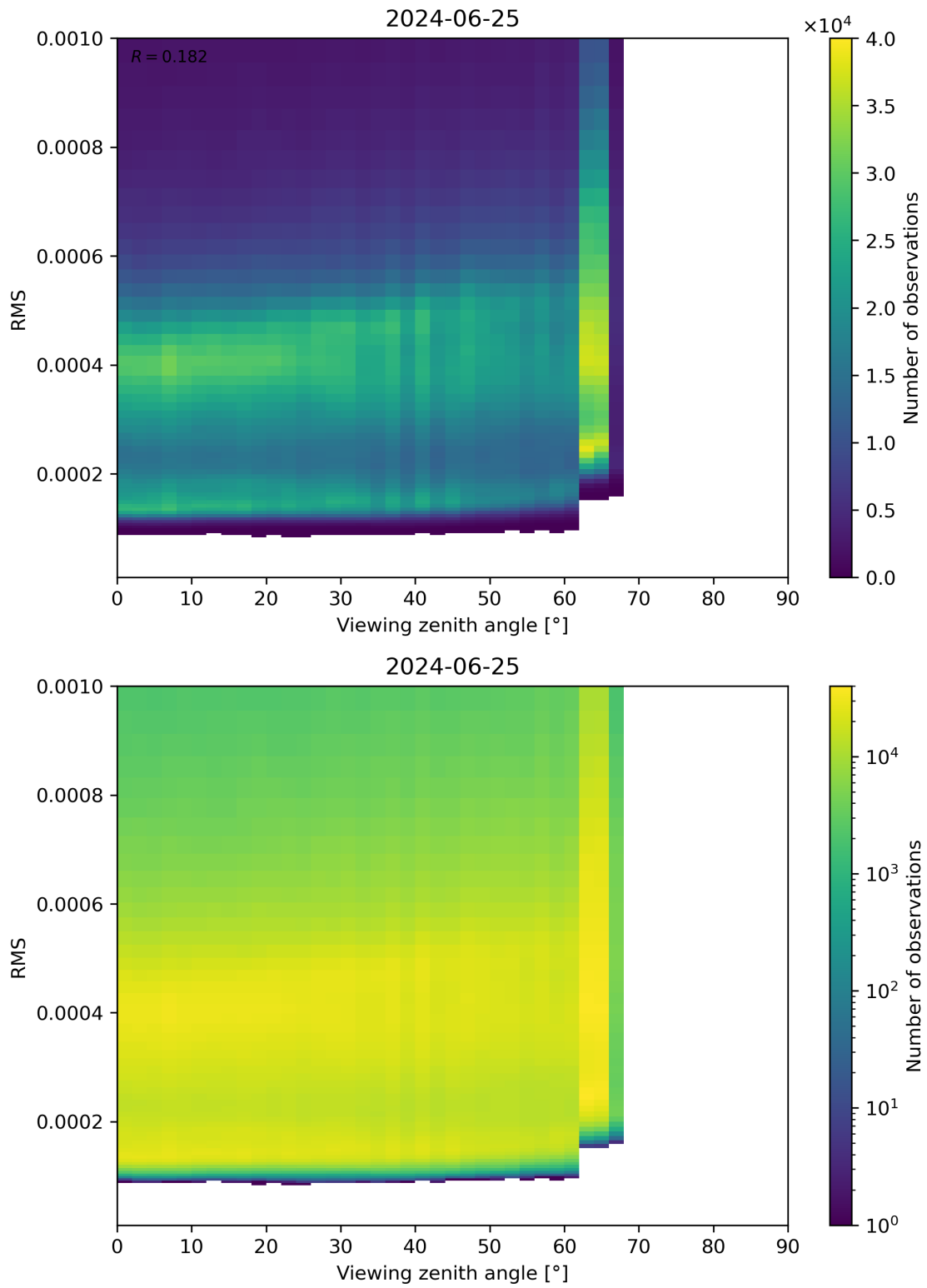
Figure 171: Scatter density plot of “Viewing zenith angle” against “RMS” for 2024-06-24 to 2024-06-26.
