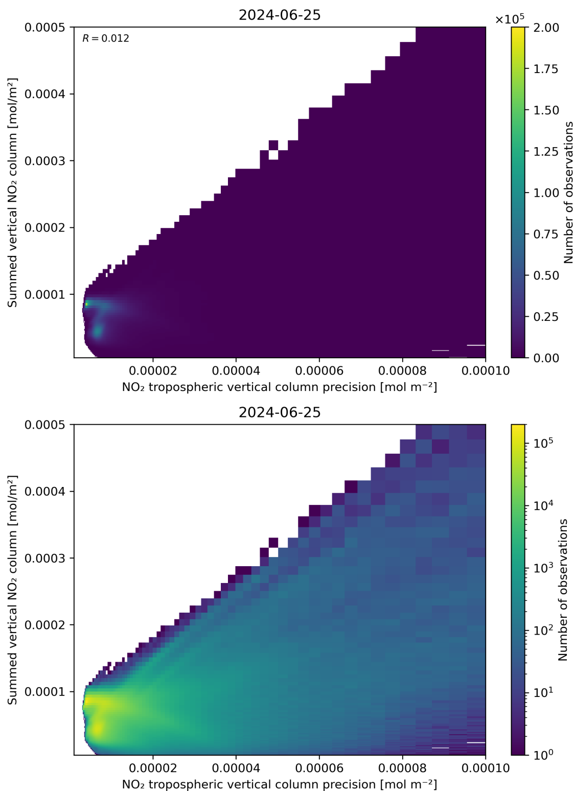
Figure 136: Scatter density plot of “NO 2 tropospheric vertical column precision” against “Summed vertical NO 2 column” for 2024-06-24 to 2024-06-26.
