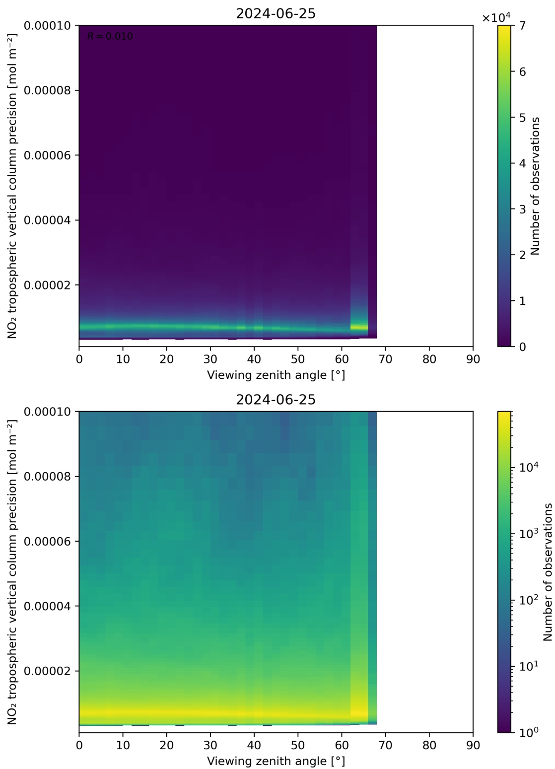
Figure 170: Scatter density plot of “Viewing zenith angle” against “NO 2 tropospheric vertical column precision” for 2024-06-24 to 2024-06-26.
