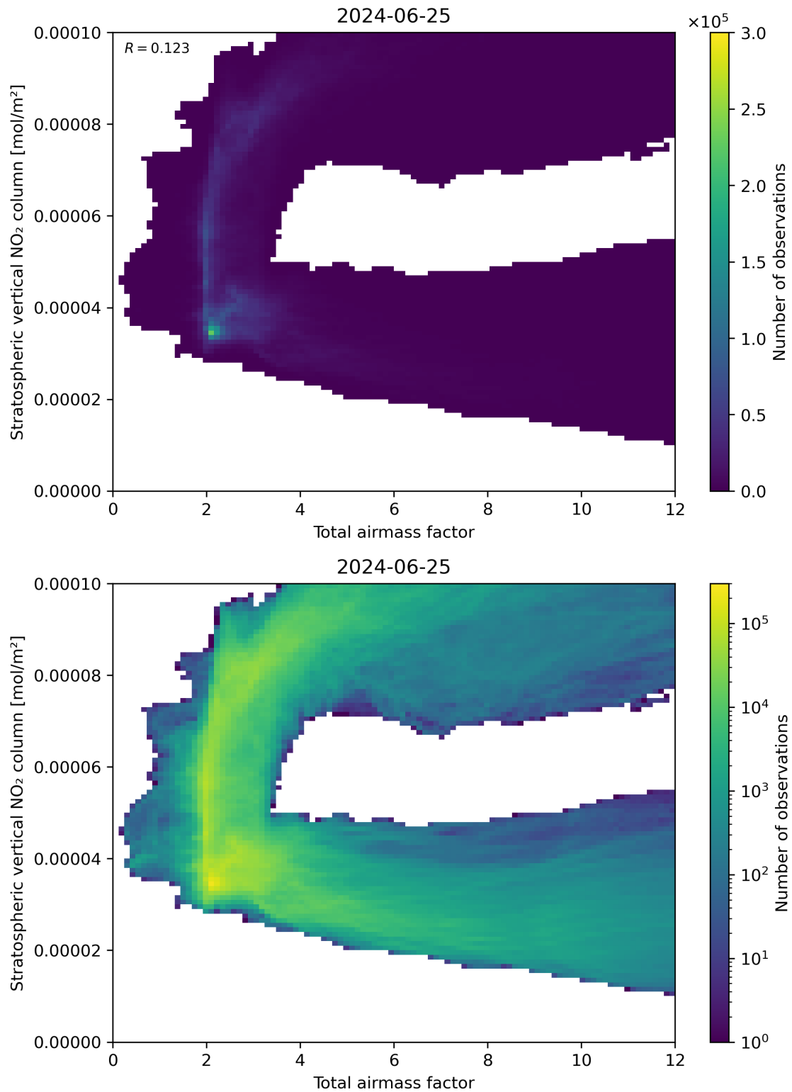
Figure 64: Scatter density plot of “Total airmass factor” against “Stratospheric vertical \text{NO}_2 column” for 2024-06-24 to 2024-06-26.
