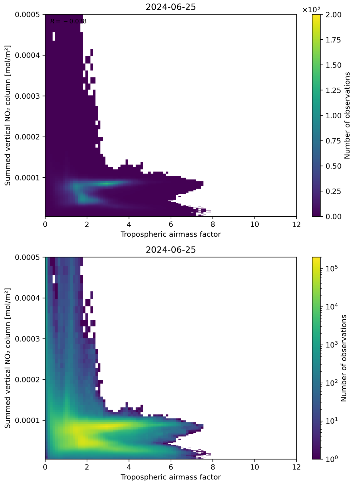
Figure 75: Scatter density plot of “Tropospheric air mass factor” against “Summed vertical NO 2 column” for 2024-06-24 to 2024-06-26.
