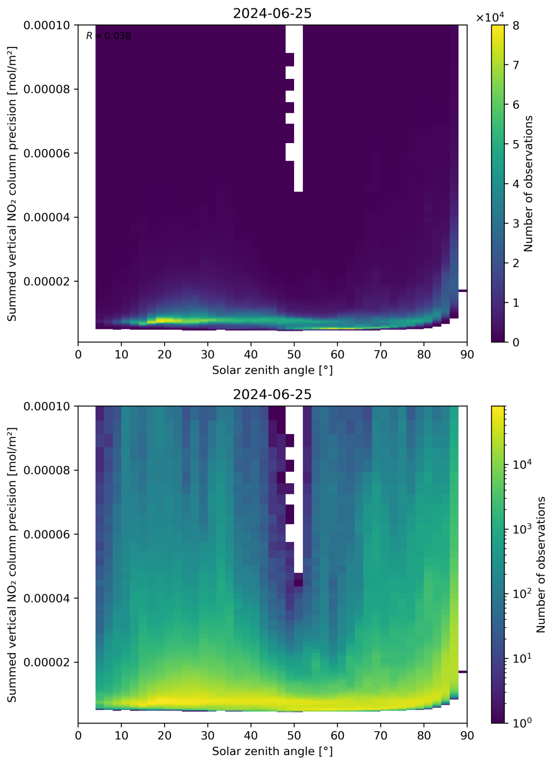
Figure 152: Scatter density plot of “Solar zenith angle” against “Summed vertical NO 2 column precision” for 2024-06-24 to 2024-06-26.
