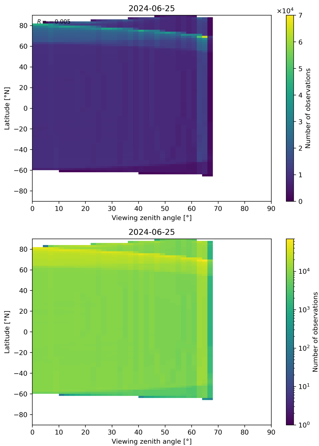
Figure 163: Scatter density plot of “Viewing zenith angle” against “Latitude” for 2024-06-24 to 2024-06-26.
