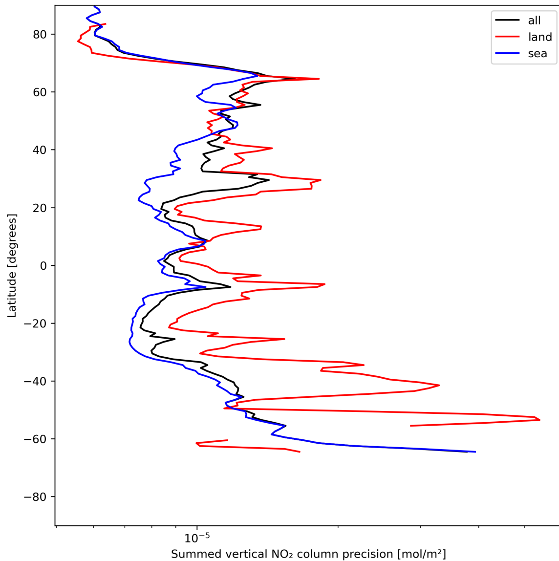
Figure 24: Zonal average of “Summed vertical NO 2 column precision” for 2024-06-24 to 2024-06-26.
