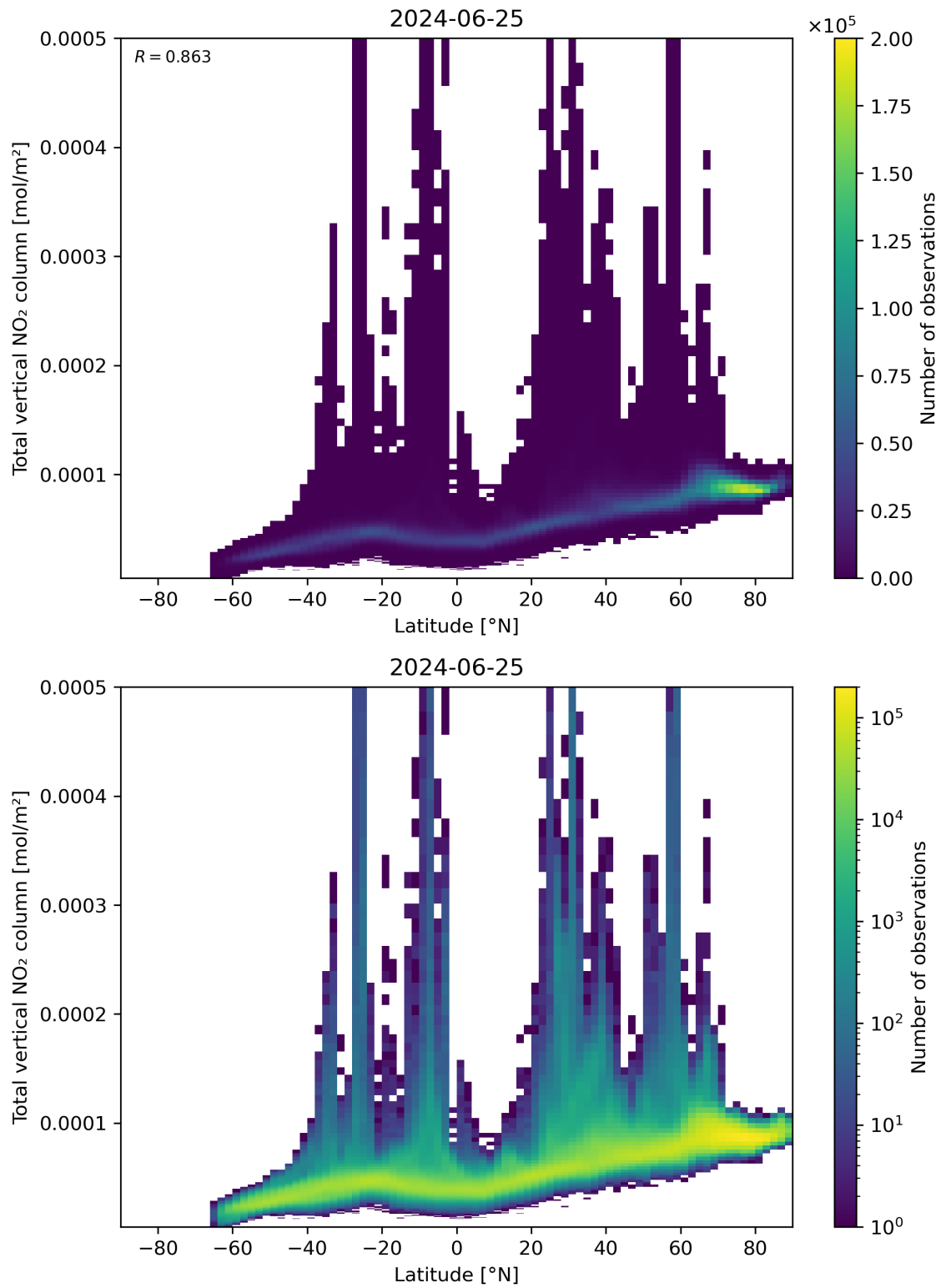
Figure 90: Scatter density plot of “Latitude” against “Total vertical NO 2 column” for 2024-06-24 to 2024-06-26.
