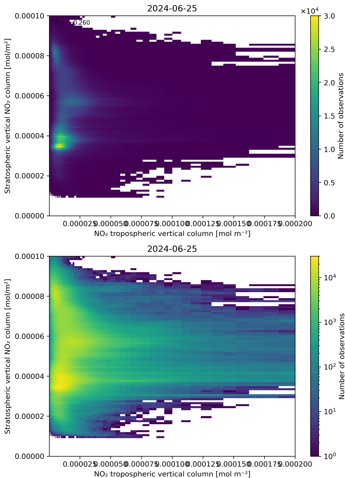
Figure 125: Scatter density plot of “NO 2 tropospheric vertical column” against “Stratospheric vertical NO 2 column” for 2024-06-24 to 2024-06-26.
