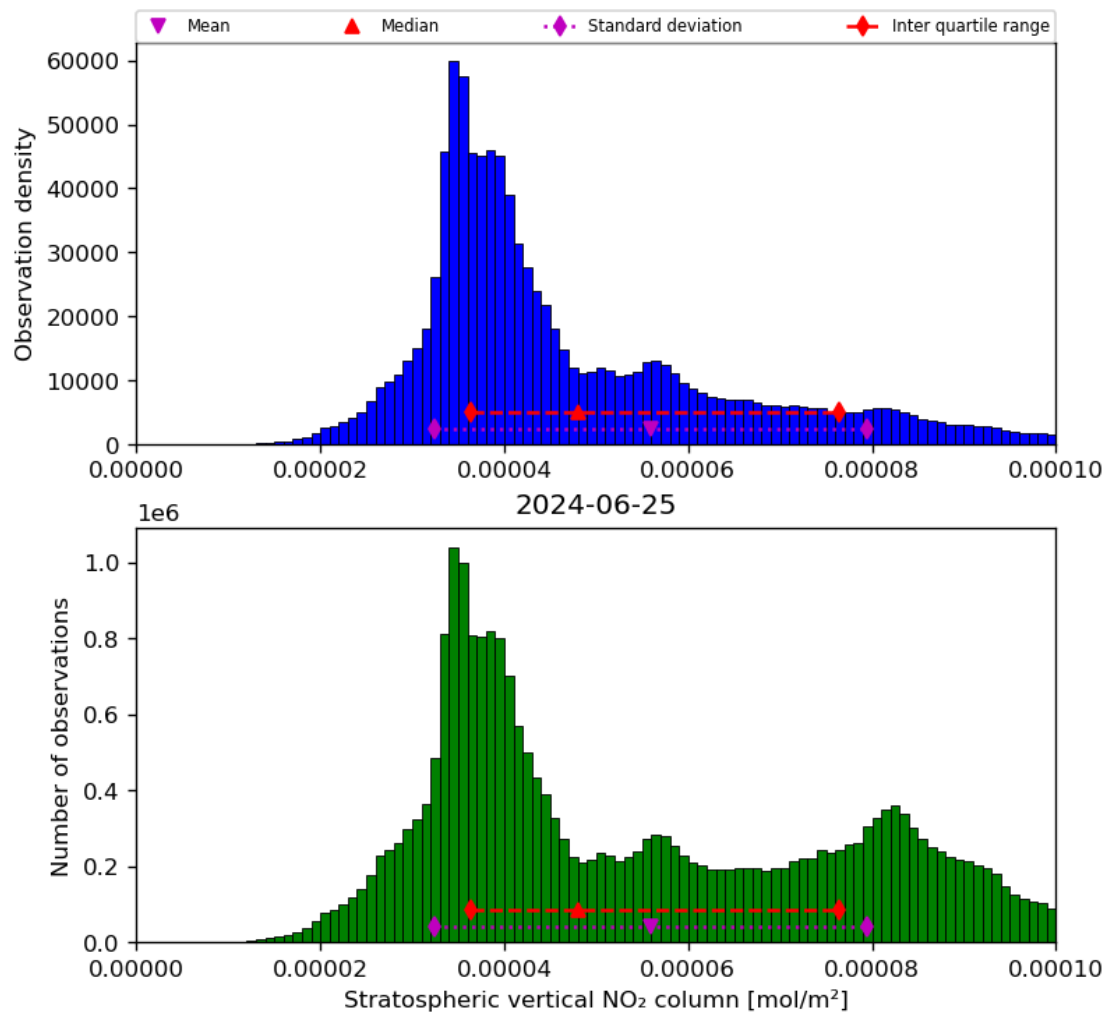
Figure 36: Histogram of “Stratospheric vertical NO 2 column” for 2024-06-24 to 2024-06-26
