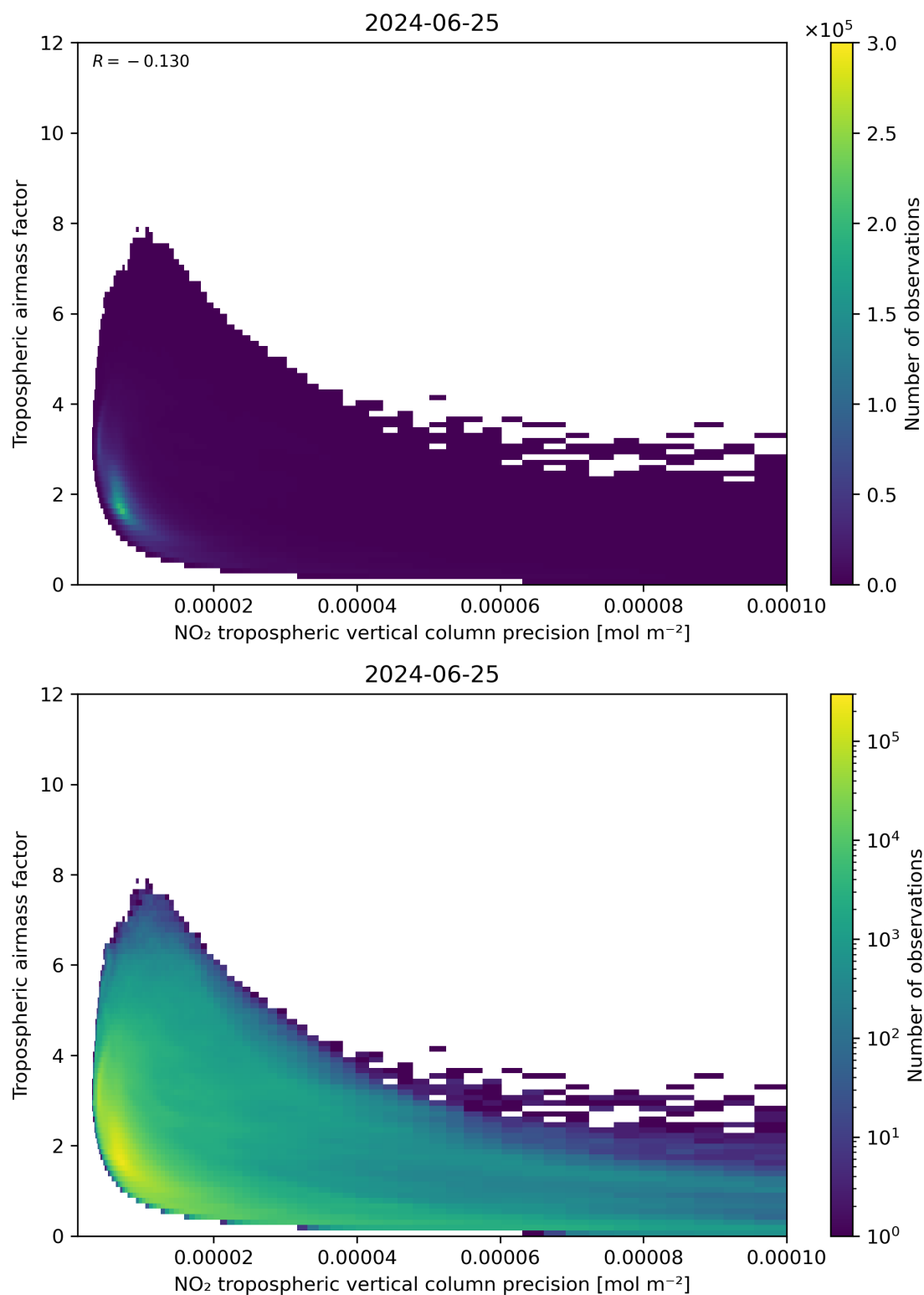
Figure 133: Scatter density plot of “NO 2 tropospheric vertical column precision” against “Tropospheric airmass factor” for 2024-06-24 to 2024-06-26.
