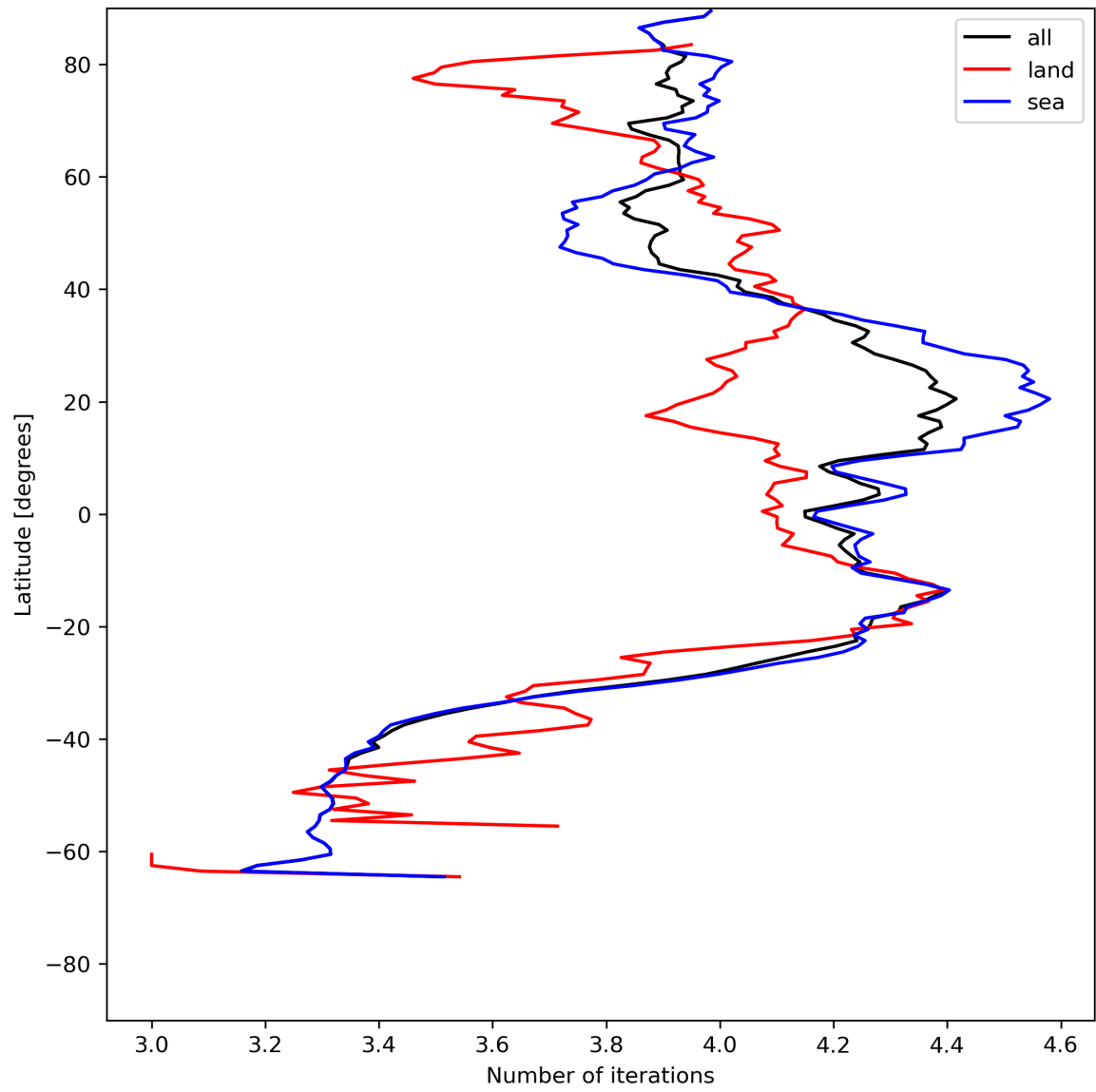
Figure 17: Zonal average of “Number of iterations” for 2024-06-24 to 2024-06-26.
