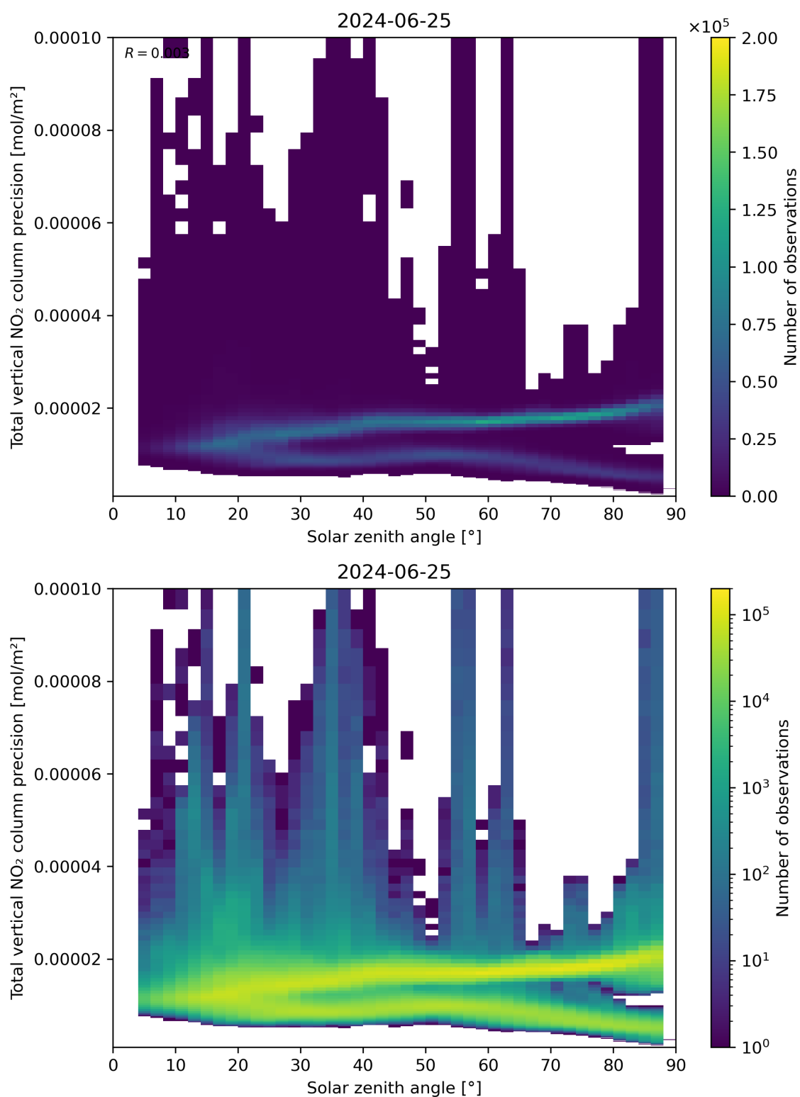
Figure 154: Scatter density plot of “Solar zenith angle” against “Total vertical NO 2 column precision” for 2024-06-24 to 2024-06-26.
