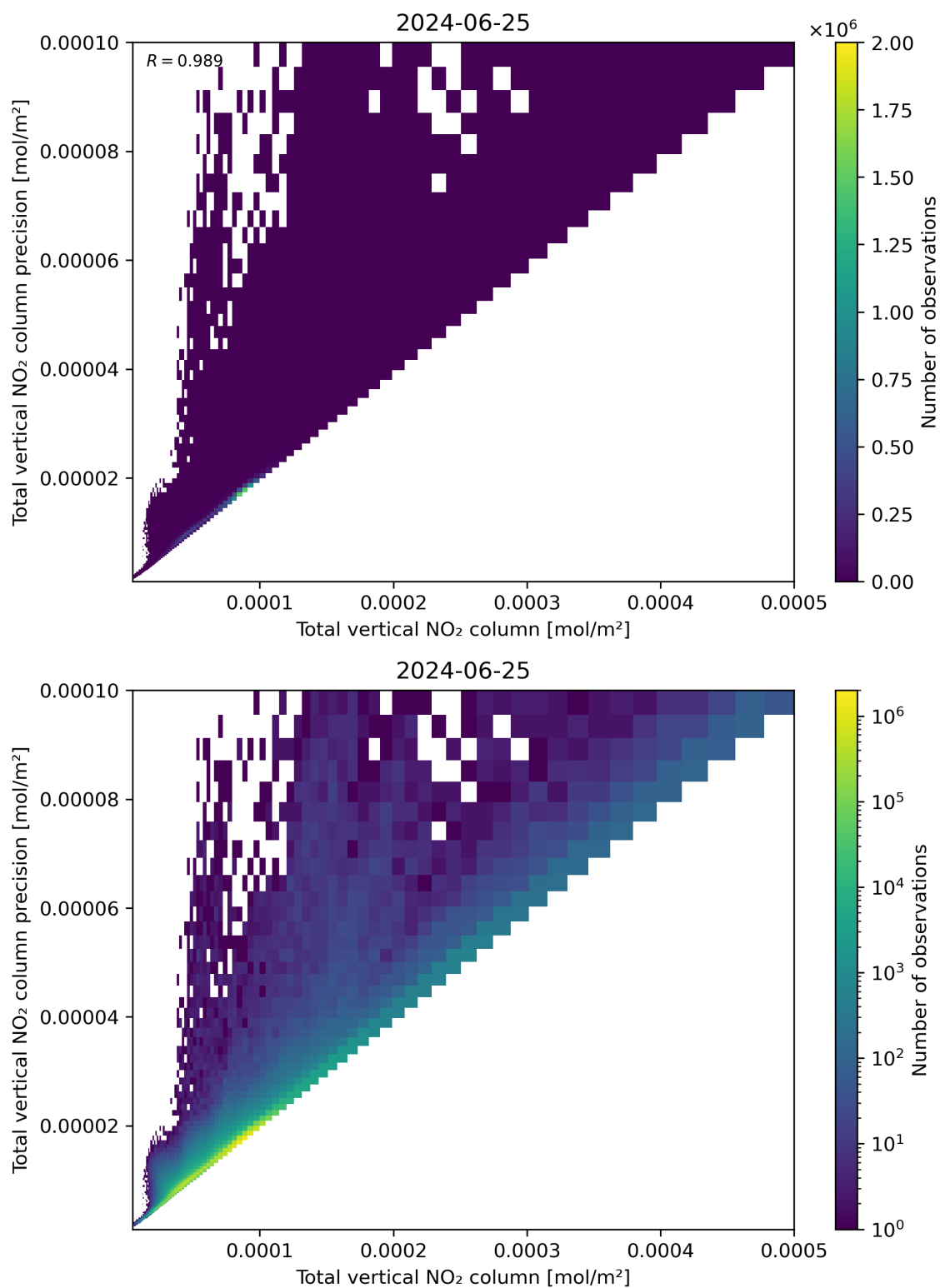
Figure 114: Scatter density plot of “Total vertical NO 2 column” against “Total vertical NO 2 column precision” for 2024-06-24 to 2024-06-26.
