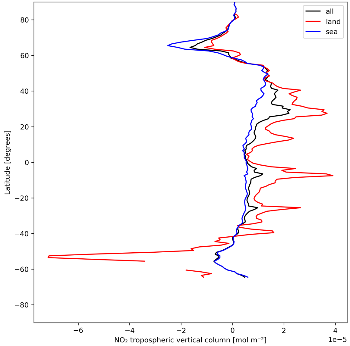
Figure 12: Zonal average of “NO 2 tropospheric vertical column” for 2024-06-24 to 2024-06-26.
