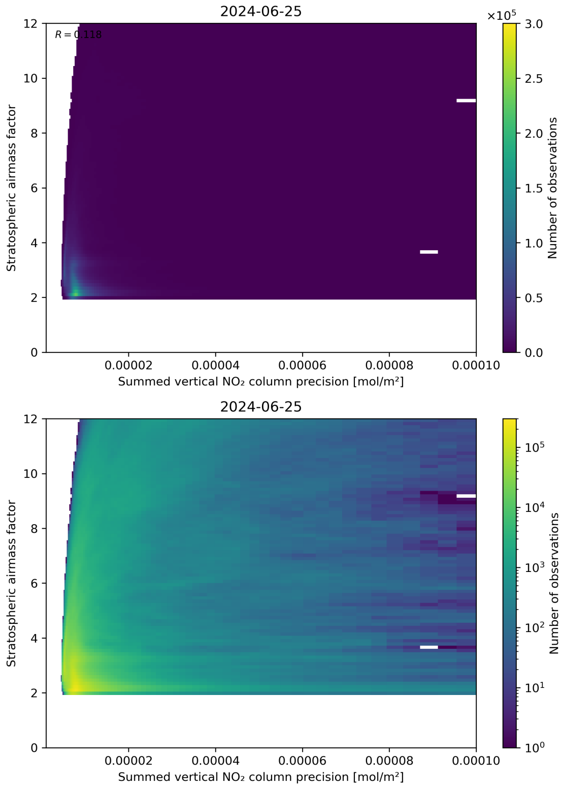
Figure 106: Scatter density plot of “Summed vertical NO 2 column precision” against “Stratospheric airmass factor” for 2024-06-24 to 2024-06-26.
