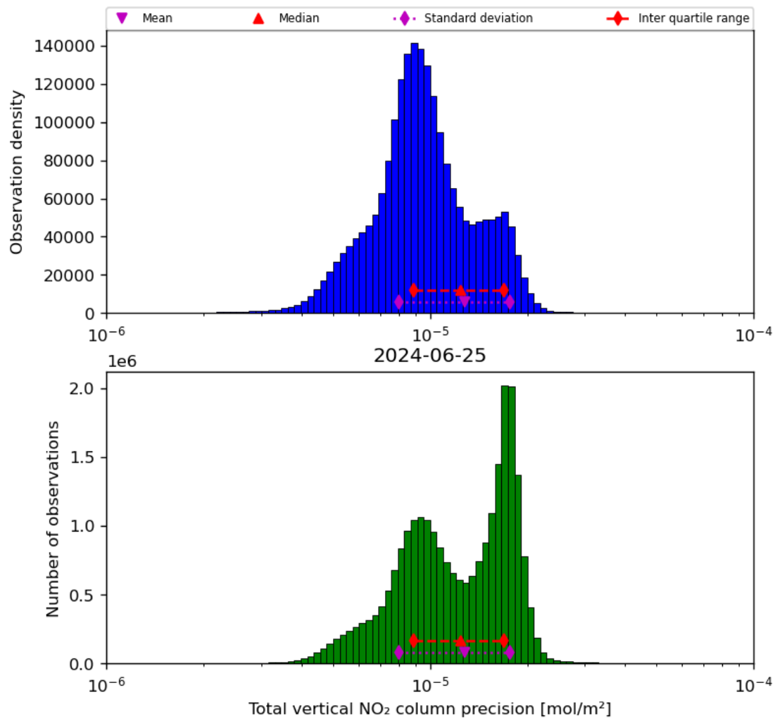
Figure 39: Histogram of “Total vertical NO 2 column precision” for 2024-06-24 to 2024-06-26
