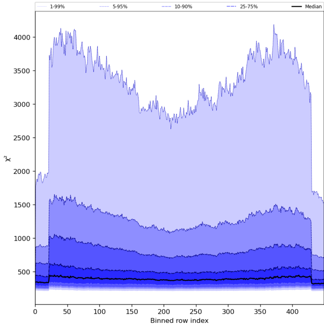
Figure 59: Along track statistics of “ \chi^2 ” for 2024-06-24 to 2024-06-26
