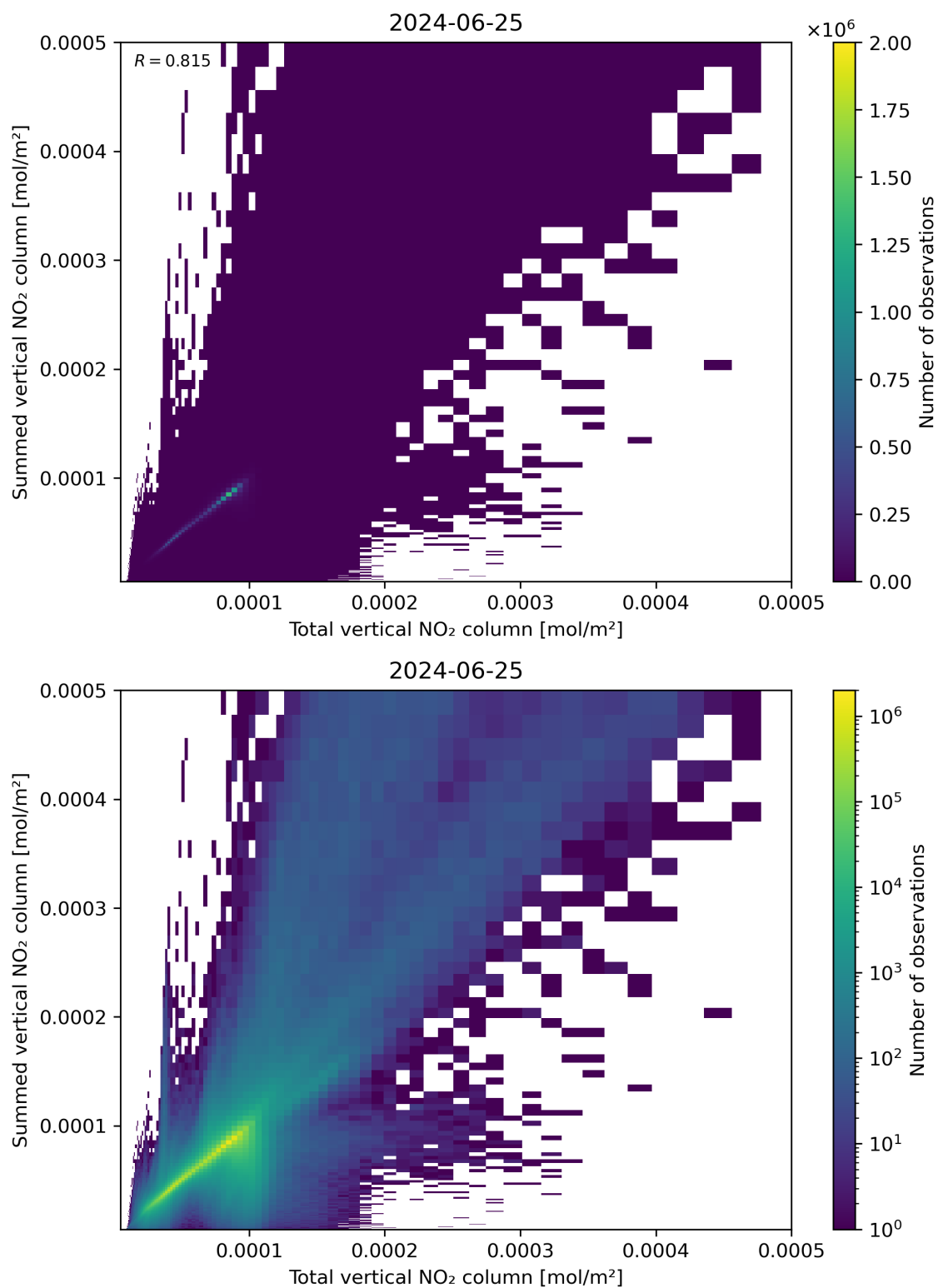
Figure 112: Scatter density plot of “Total vertical NO 2 column” against “Summed vertical NO 2 column” for 2024-06-24 to 2024-06-26.
