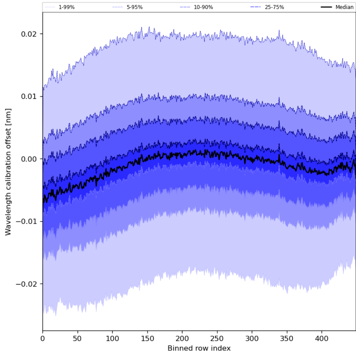
Figure 52: Along track statistics of “Wavelength calibration offset” for 2024-06-24 to 2024-06-26
