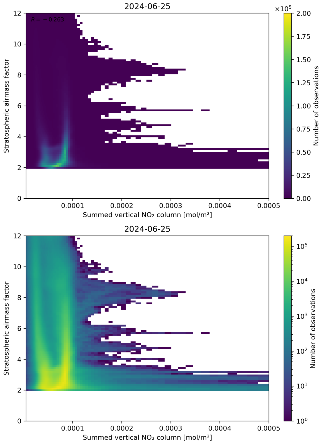
Figure 103: Scatter density plot of “Summed vertical NO 2 column” against “Stratospheric airmass factor” for 2024-06-24 to 2024-06-26.
