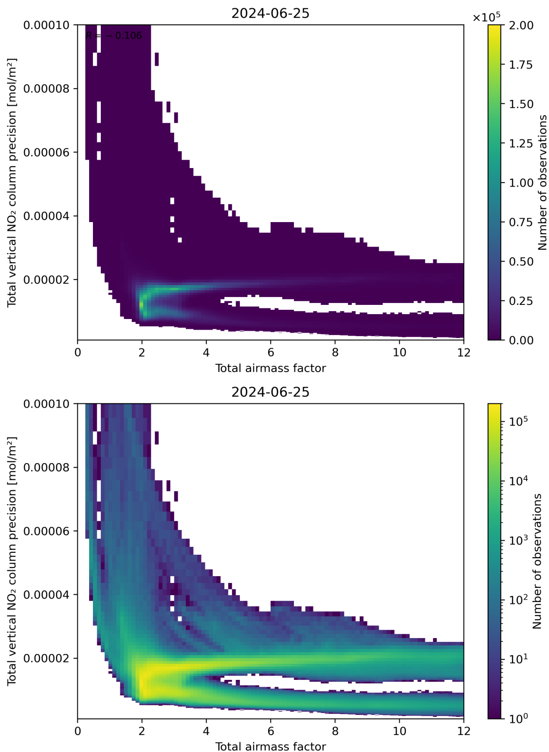
Figure 68: Scatter density plot of “Total airmass factor” against “Total vertical NO 2 column precision” for 2024-06-24 to 2024-06-26.
