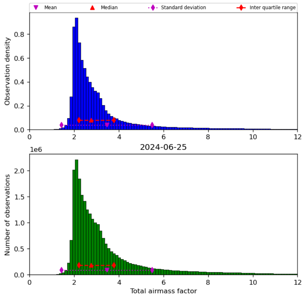
Figure 32: Histogram of “Total airmass factor” for 2024-06-24 to 2024-06-26
