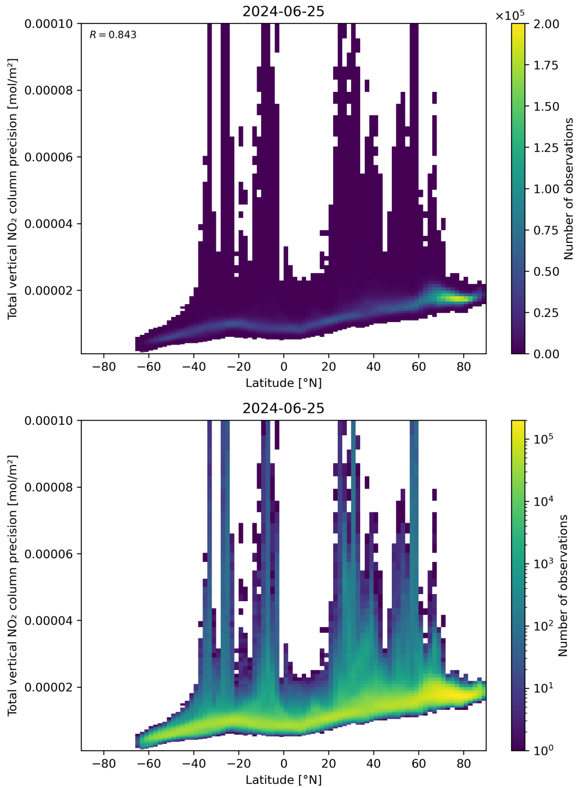
Figure 91: Scatter density plot of “Latitude” against “Total vertical NO 2 column precision” for 2024-06-24 to 2024-06-26.
