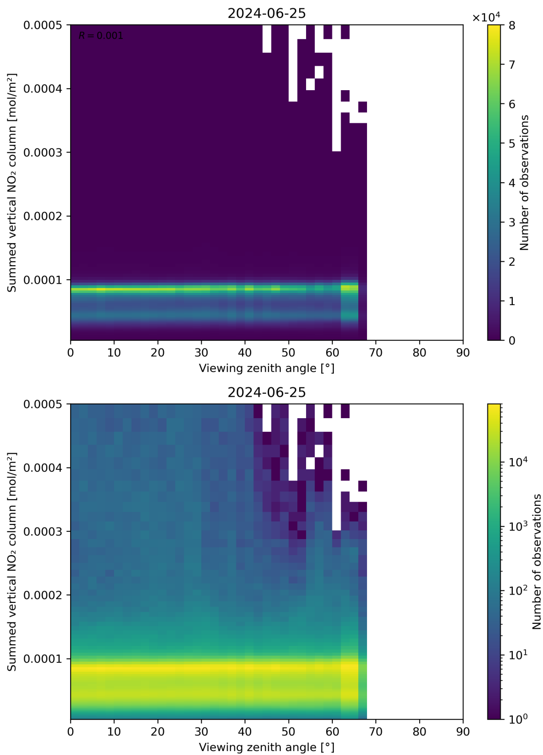
Figure 165: Scatter density plot of “Viewing zenith angle” against “Summed vertical NO 2 column” for 2024-06-24 to 2024-06-26.
