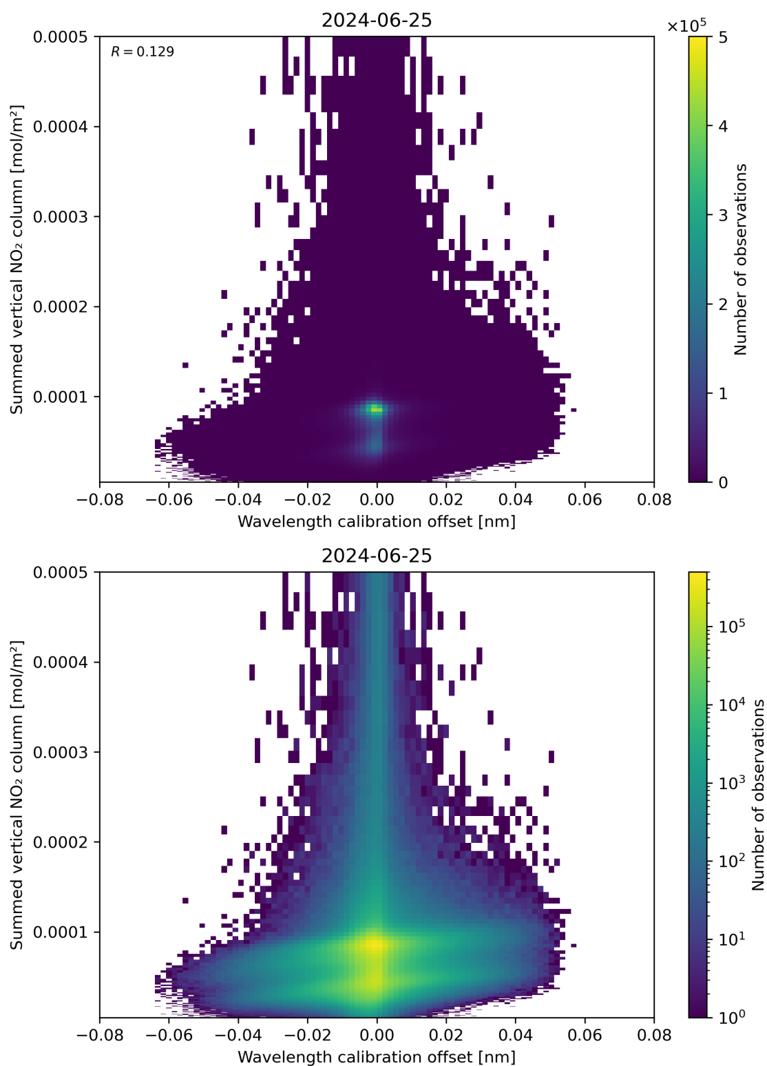
Figure 177: Scatter density plot of “Wavelength calibration offset” against “Summed vertical NO 2 column” for 2024-06-24 to 2024-06-26.
