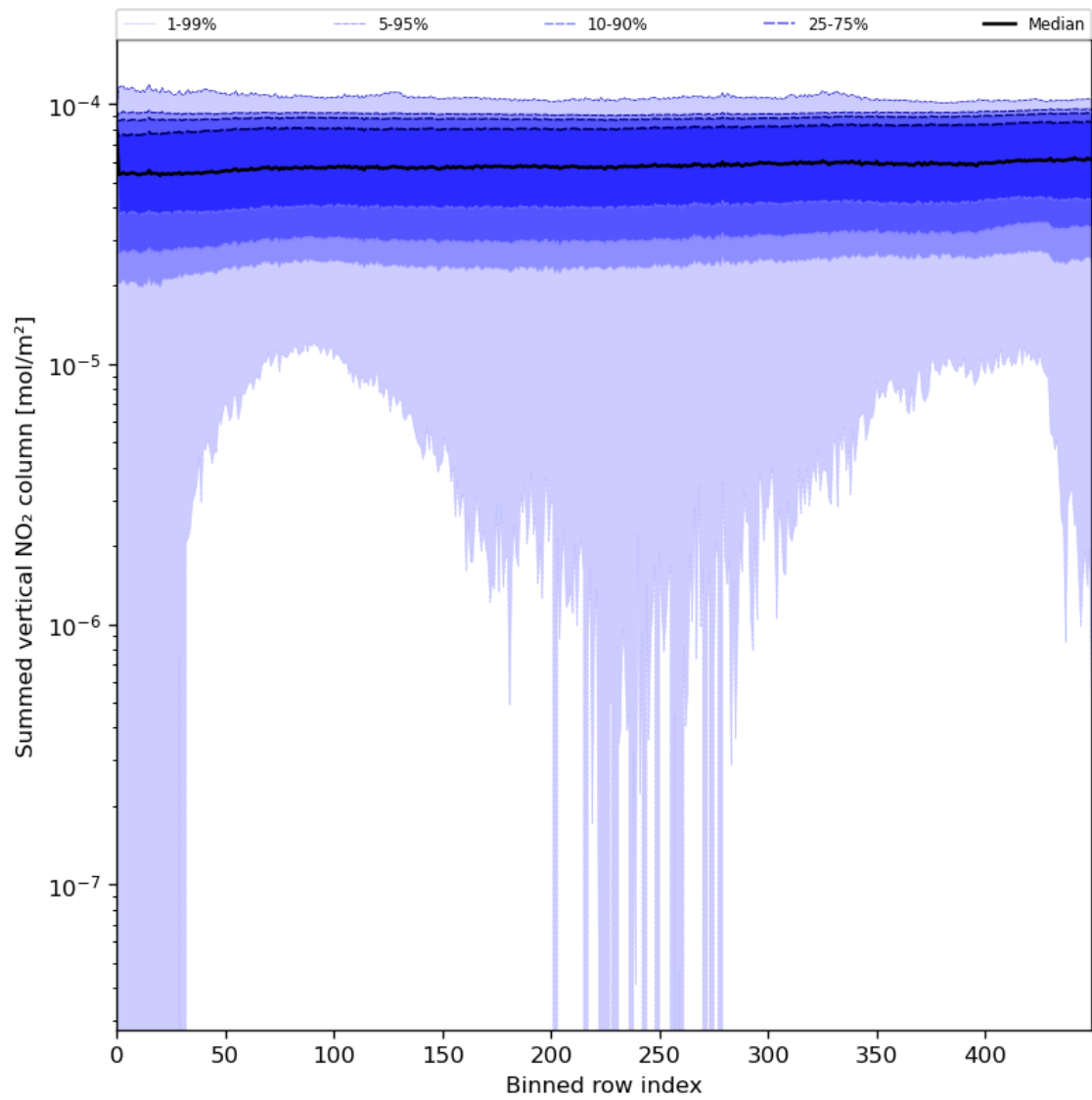
Figure 57: Along track statistics of “Summed vertical NO 2 column” for 2024-06-24 to 2024-06-26
