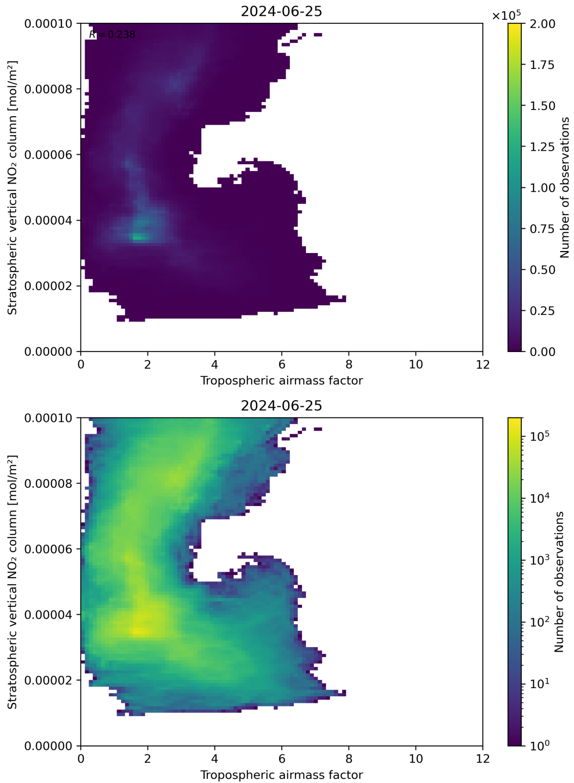
Figure 74: Scatter density plot of “Tropospheric air mass factor” against “Stratospheric vertical NO 2 column” for 2024-06-24 to 2024-06-26.
