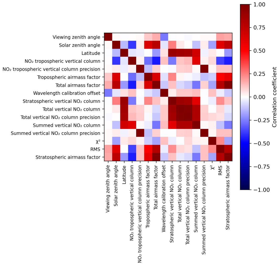
Figure 2: Map of correlation matrix for 2024-06-24 to 2024-06-26.
