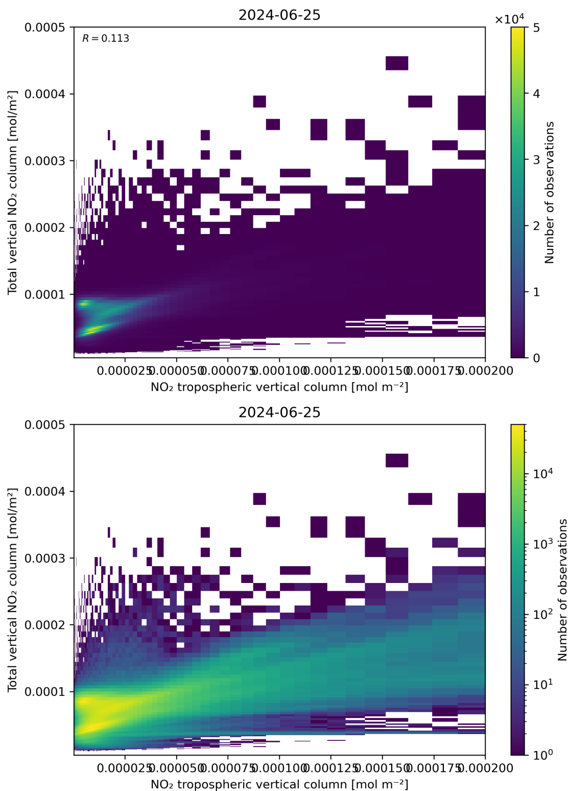
Figure 128: Scatter density plot of “NO 2 tropospheric vertical column” against “Total vertical NO 2 column” for 2024-06-24 to 2024-06-26.
