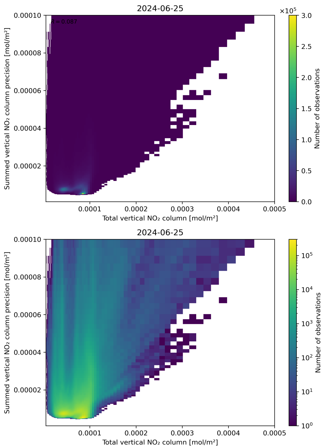
Figure 113: Scatter density plot of “Total vertical NO 2 column” against “Summed vertical NO 2 column precision” for 2024-06-24 to 2024-06-26.
