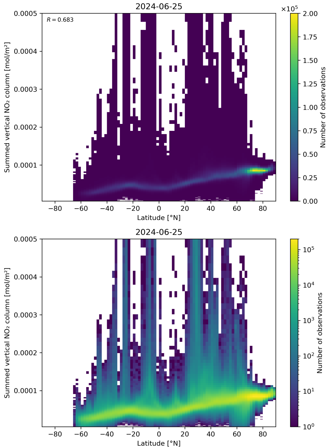
Figure 88: Scatter density plot of “Latitude” against “Summed vertical NO 2 column” for 2024-06-24 to 2024-06-26.
