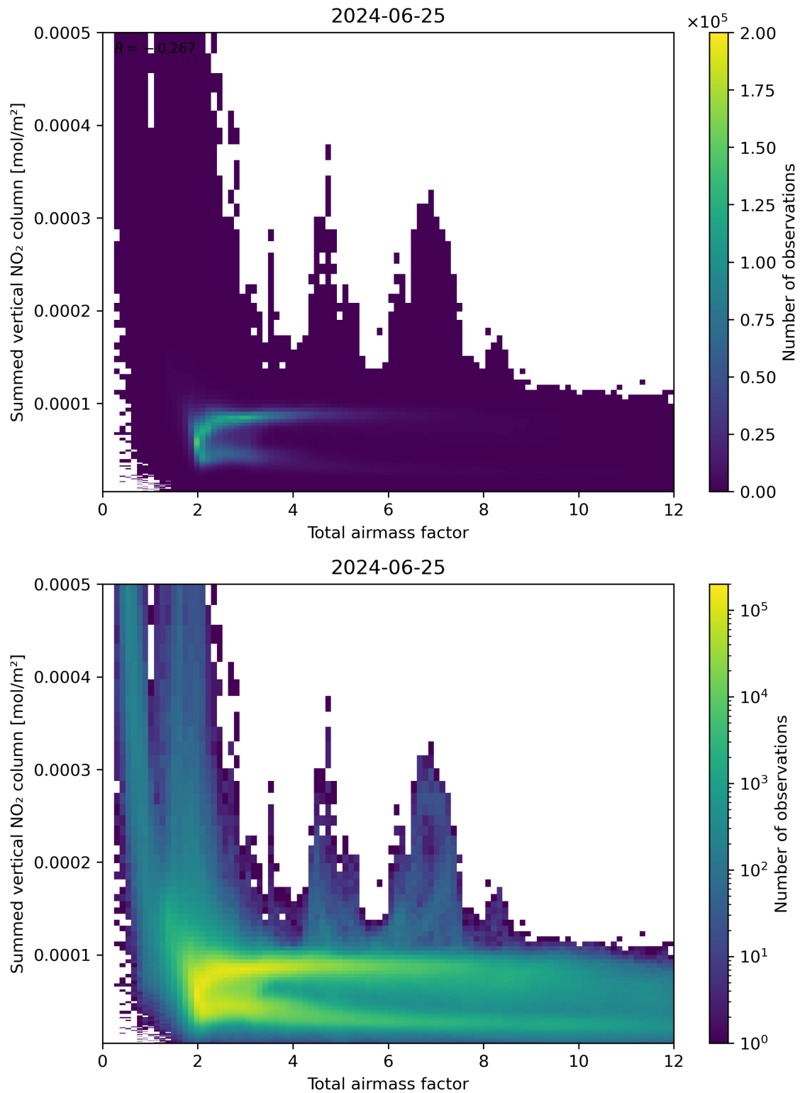
Figure 65: Scatter density plot of “Total airmass factor” against “Summed vertical NO 2 column” for 2024-06-24 to 2024-06-26.
