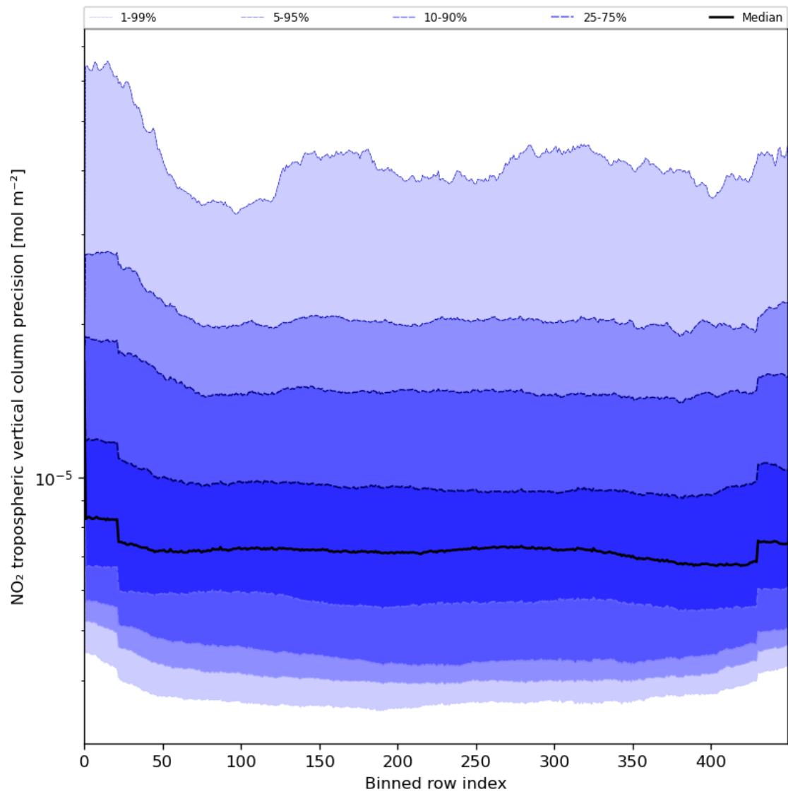
Figure 47: Along track statistics of “NO 2 tropospheric vertical column precision” for 2024-06-24 to 2024-06-26
