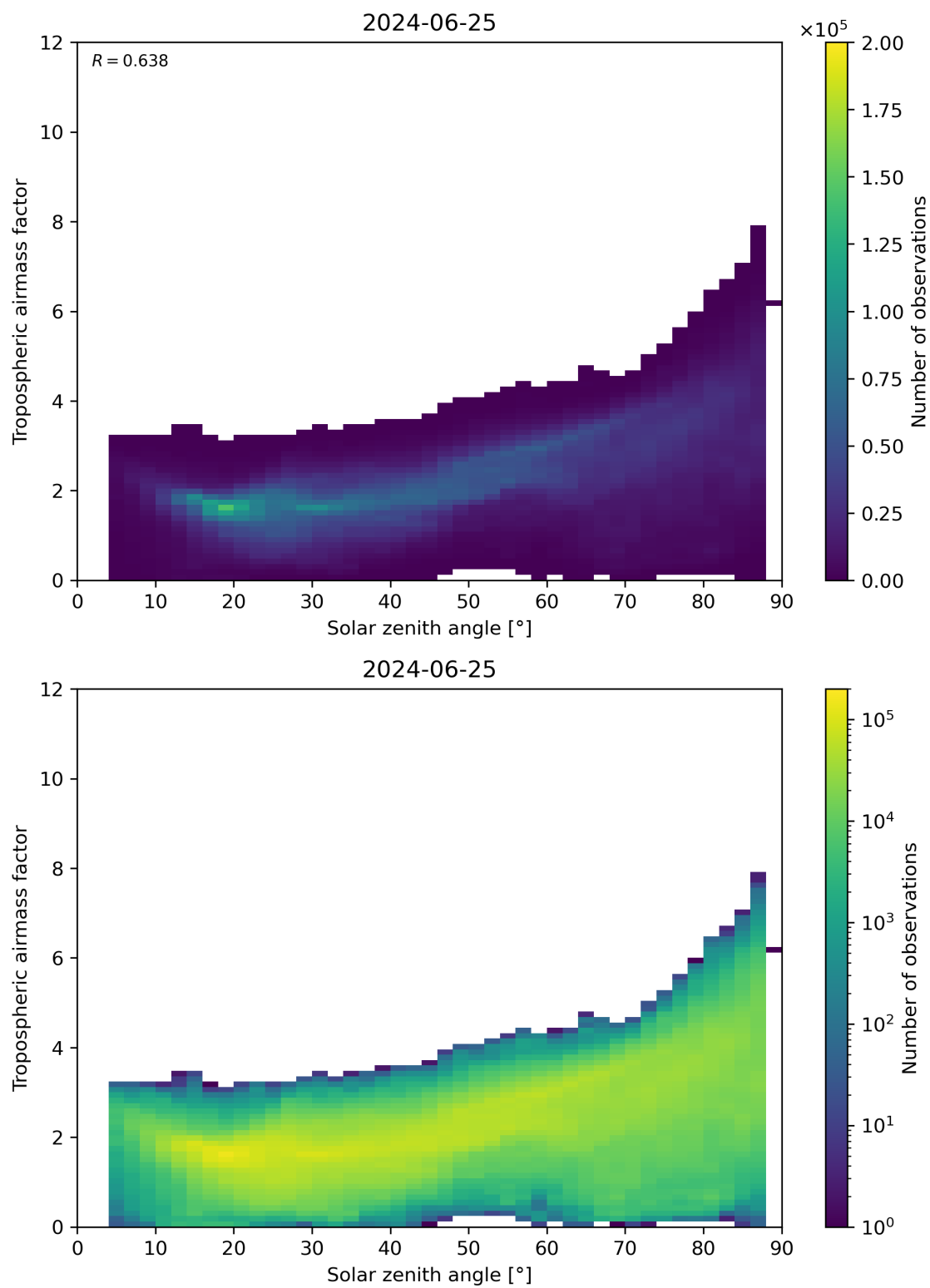
Figure 147: Scatter density plot of “Solar zenith angle” against “Tropospheric airmass factor” for 2024-06-24 to 2024-06-26.
