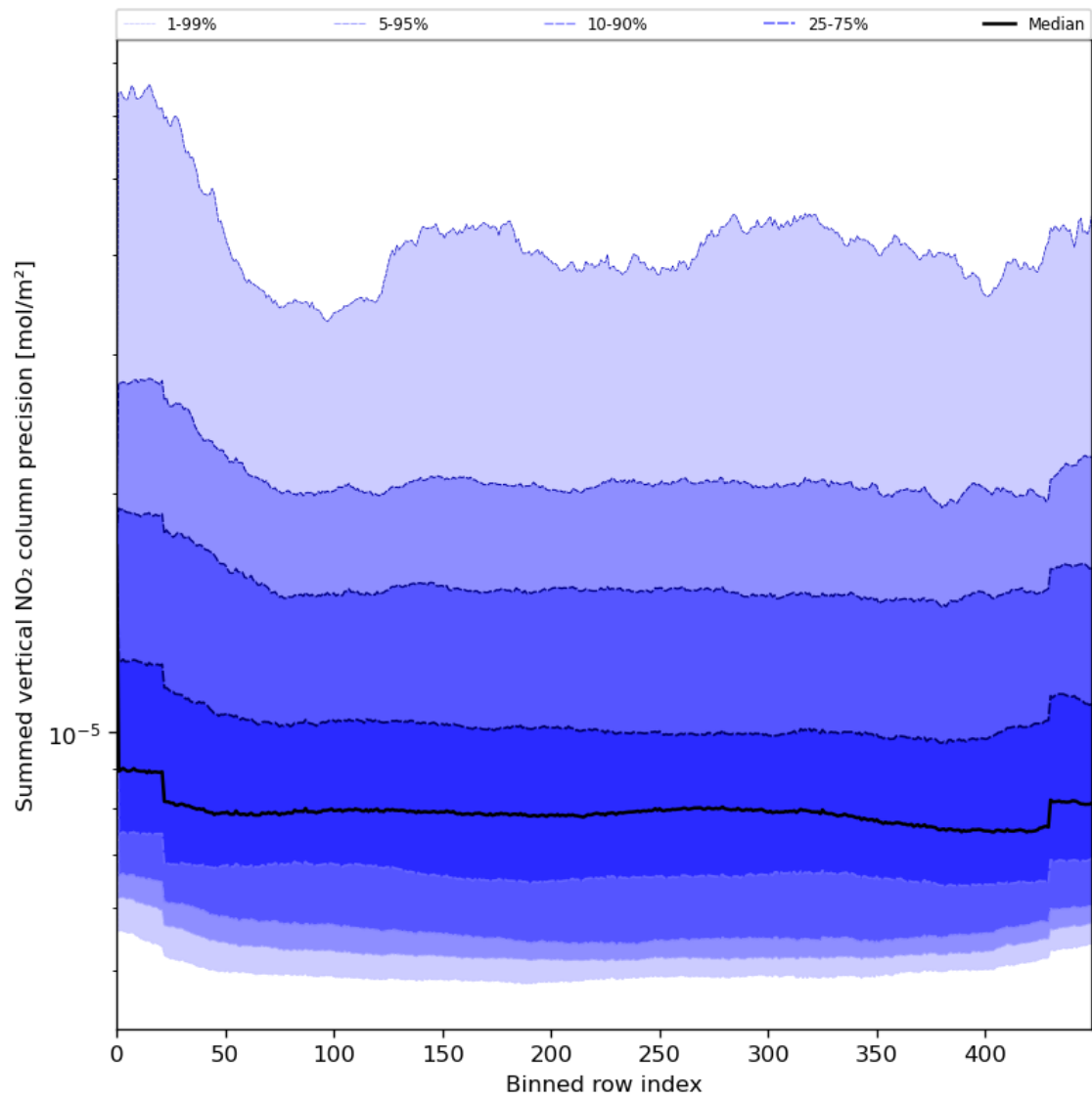
Figure 58: Along track statistics of “Summed vertical NO 2 column precision” for 2024-06-24 to 2024-06-26
