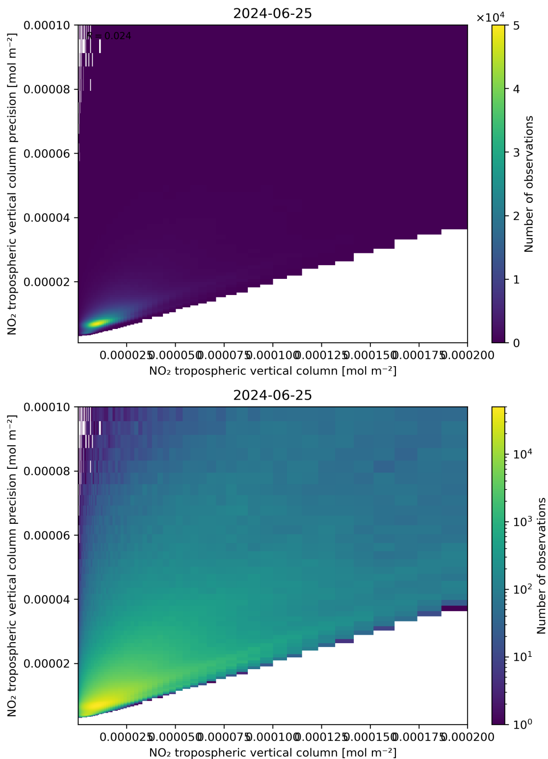
Figure 130: Scatter density plot of “NO 2 tropospheric vertical column” against “NO 2 tropospheric vertical column precision” for 2024-06-24 to 2024-06-26.
