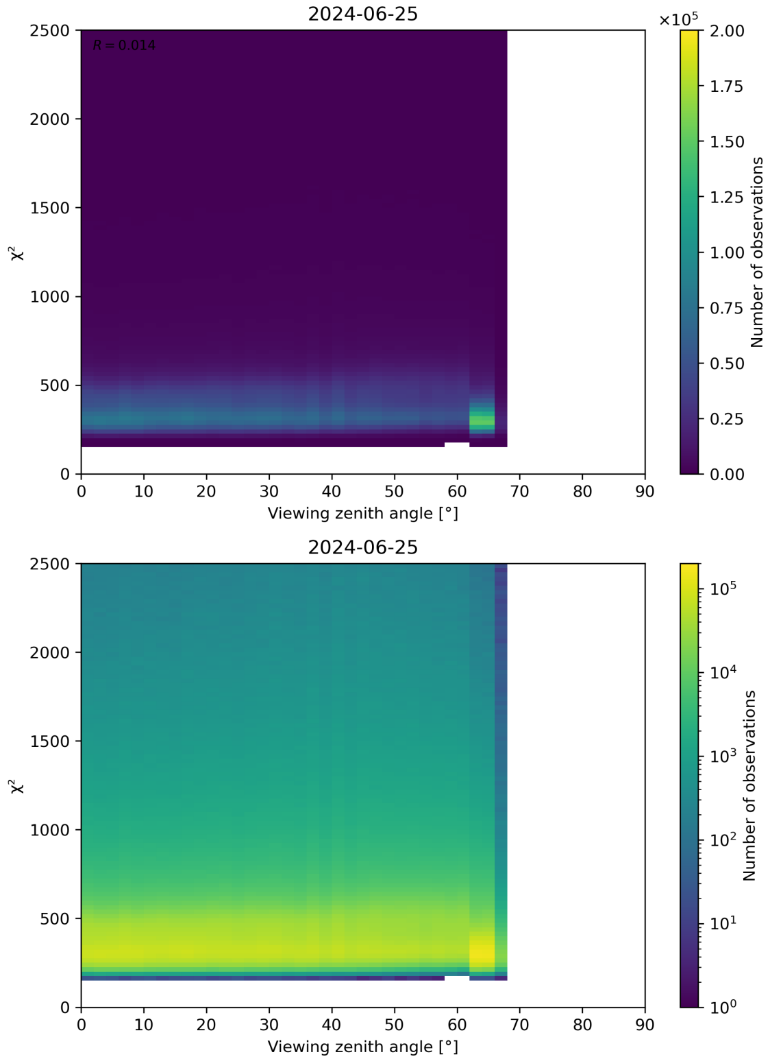
Figure 162: Scatter density plot of “Viewing zenith angle” against “ \chi^2 ” for 2024-06-24 to 2024-06-26.
