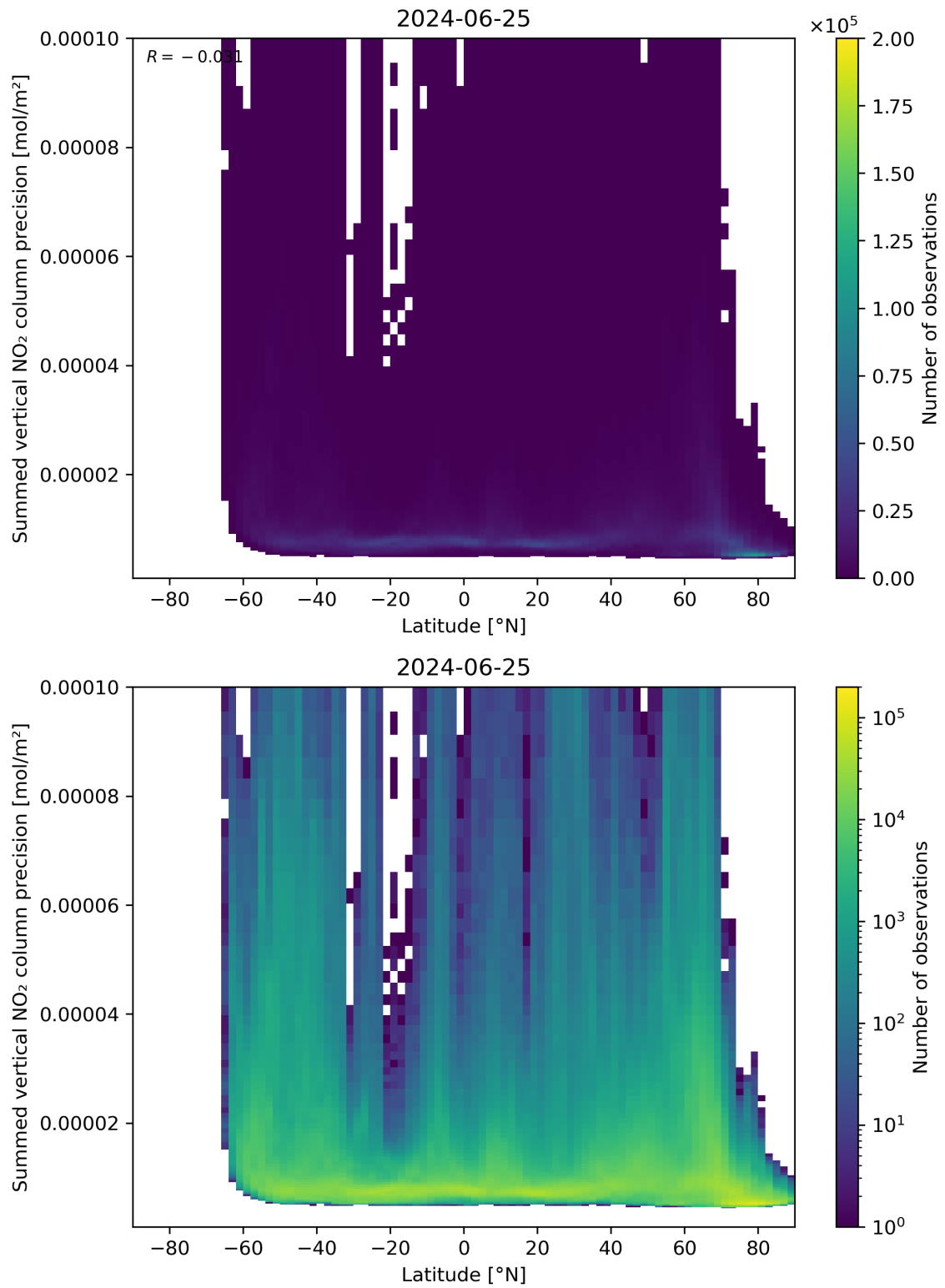
Figure 89: Scatter density plot of “Latitude” against “Summed vertical NO 2 column precision” for 2024-06-24 to 2024-06-26.
