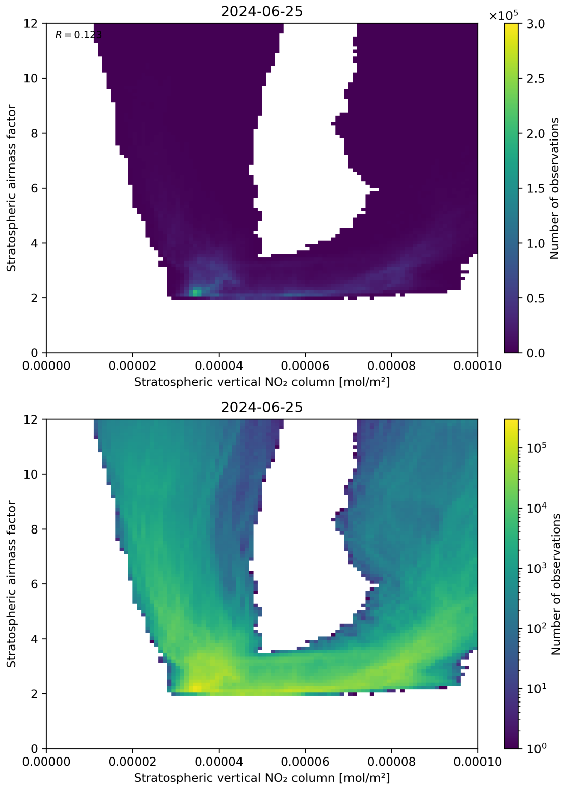
Figure 96: Scatter density plot of “Stratospheric vertical NO 2 column” against “Stratospheric airmass factor” for 2024-06-24 to 2024-06-26.
