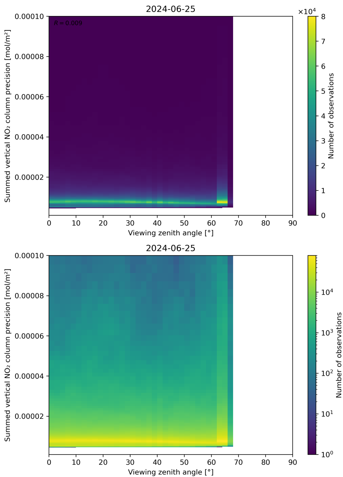
Figure 166: Scatter density plot of “Viewing zenith angle” against “Summed vertical NO 2 column precision” for 2024-06-24 to 2024-06-26.
