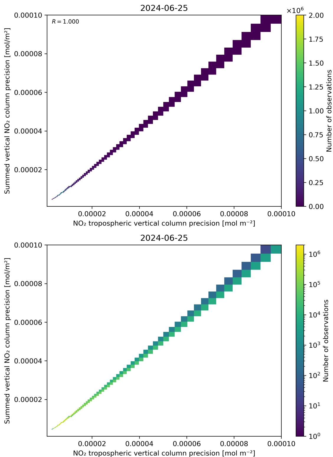
Figure 137: Scatter density plot of “NO 2 tropospheric vertical column precision” against “Summed vertical NO 2 column precision” for 2024-06-24 to 2024-06-26.
