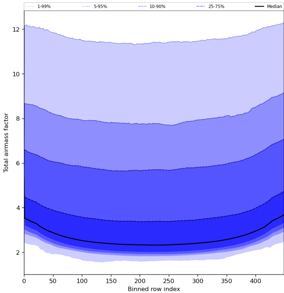
Figure 49: Along track statistics of “Total airmass factor” for 2024-06-24 to 2024-06-26
