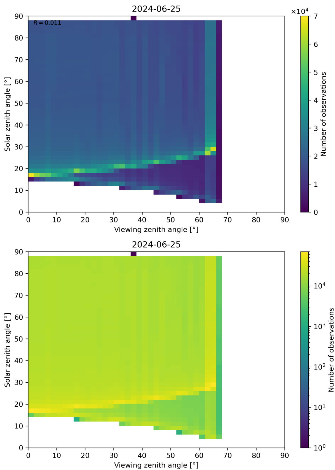
Figure 172: Scatter density plot of “Viewing zenith angle” against “Solar zenith angle” for 2024-06-24 to 2024-06-26.
