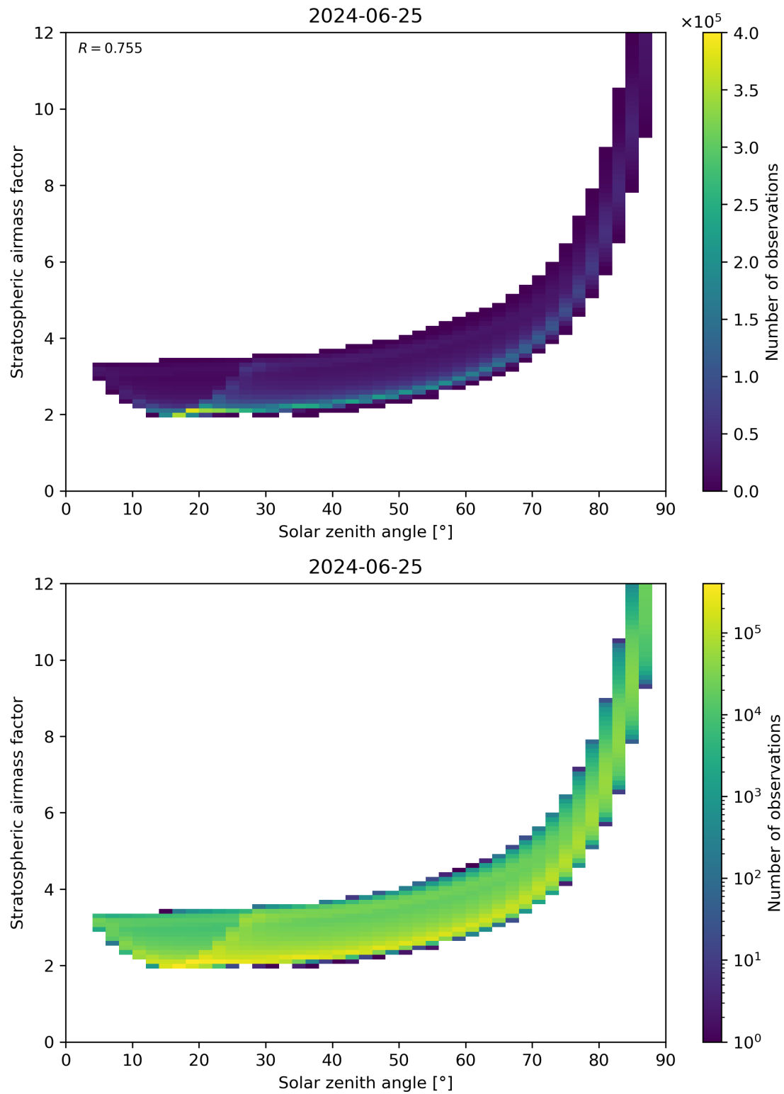
Figure 145: Scatter density plot of “Solar zenith angle” against “Stratospheric airmass factor” for 2024-06-24 to 2024-06-26.
