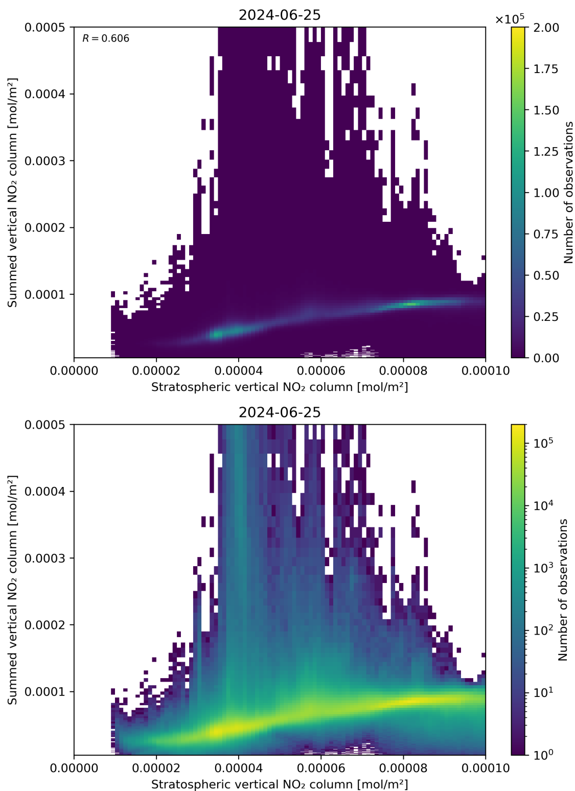
Figure 98: Scatter density plot of “Stratospheric vertical NO 2 column” against “Summed vertical NO 2 column” for 2024-06-24 to 2024-06-26.
