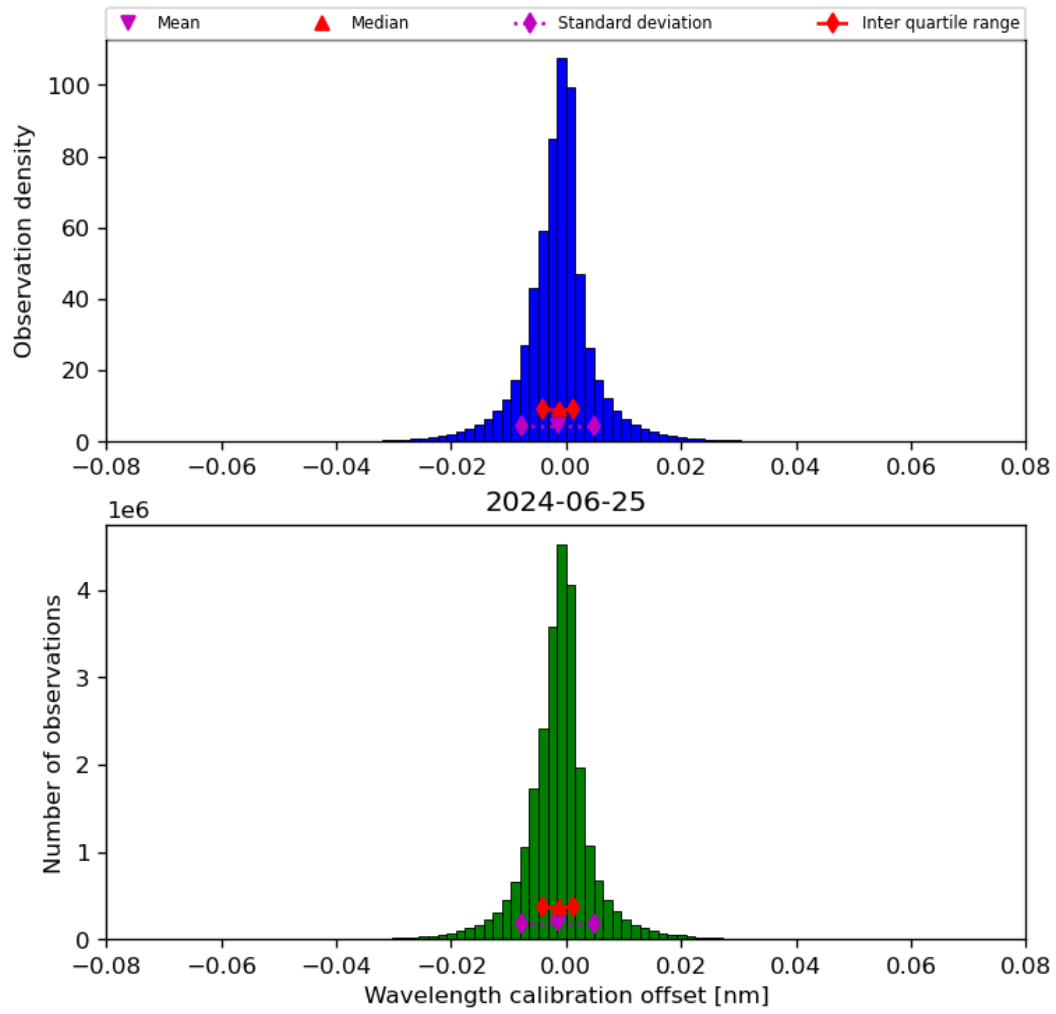
Figure 35: Histogram of “Wavelength calibration offset” for 2024-06-24 to 2024-06-26
