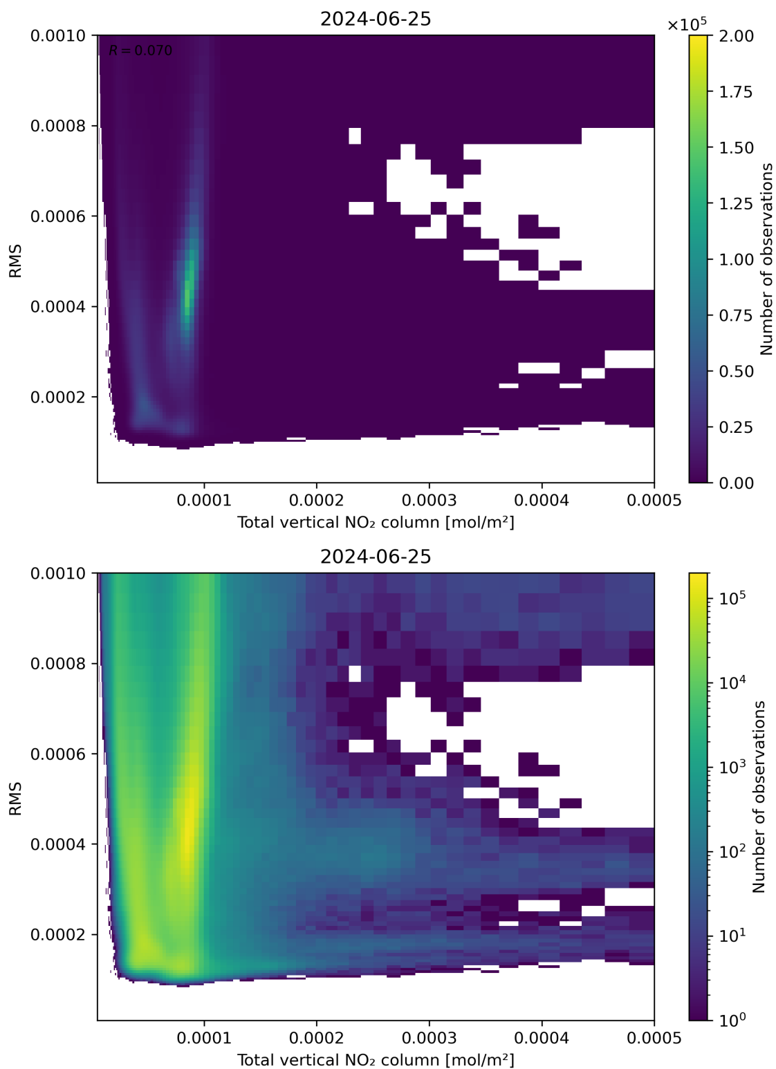
Figure 120: Scatter density plot of “Total vertical NO 2 column” against “RMS” for 2024-06-24 to 2024-06-26.
