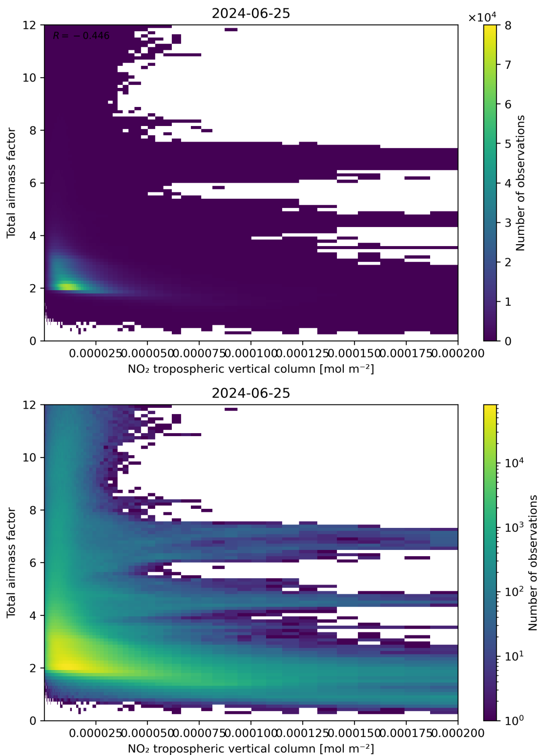
Figure 122: Scatter density plot of “NO 2 tropospheric vertical column” against “Total air mass factor” for 2024-06-24 to 2024-06-26.
