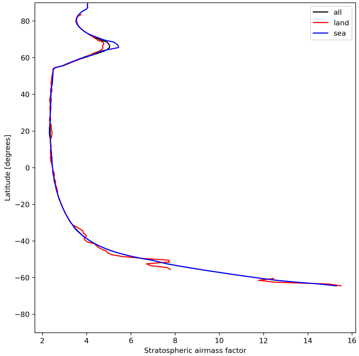
Figure 27: Zonal average of “Stratospheric airmass factor” for 2024-06-24 to 2024-06-26.
