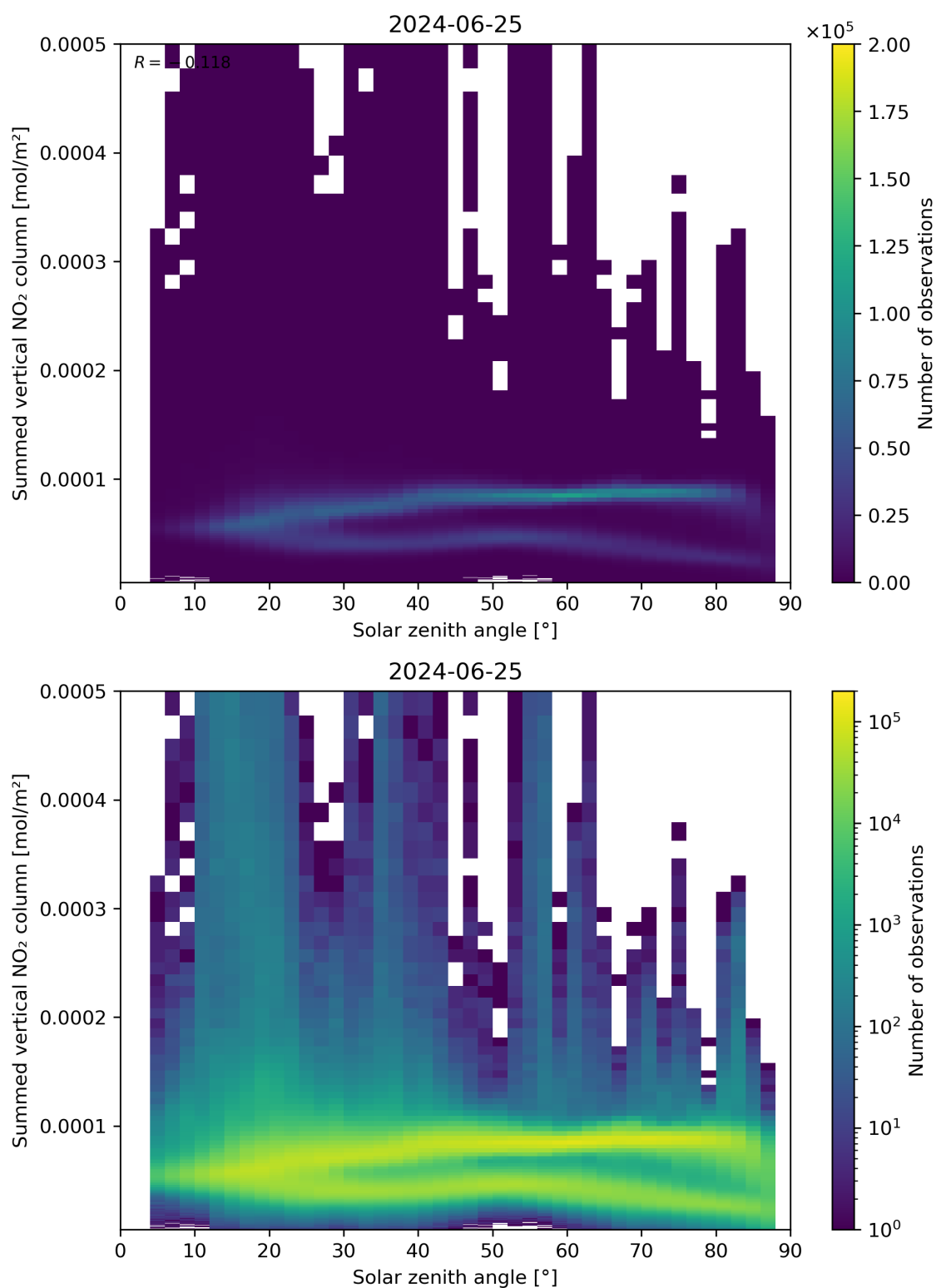
Figure 151: Scatter density plot of “Solar zenith angle” against “Summed vertical NO 2 column” for 2024-06-24 to 2024-06-26.
