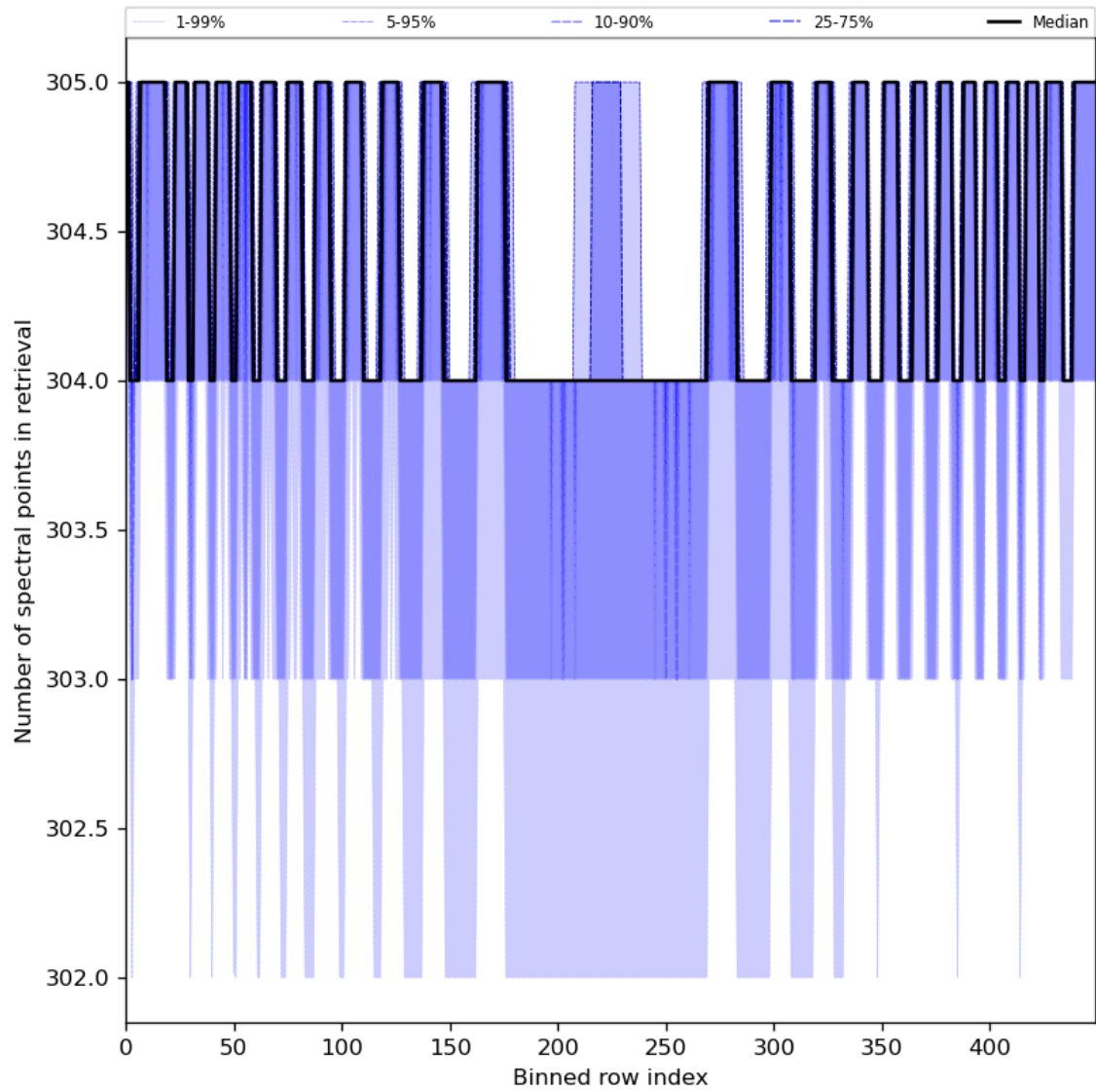
Figure 50: Along track statistics of “Number of spectral points in retrieval” for 2024-06-24 to 2024-06-26
