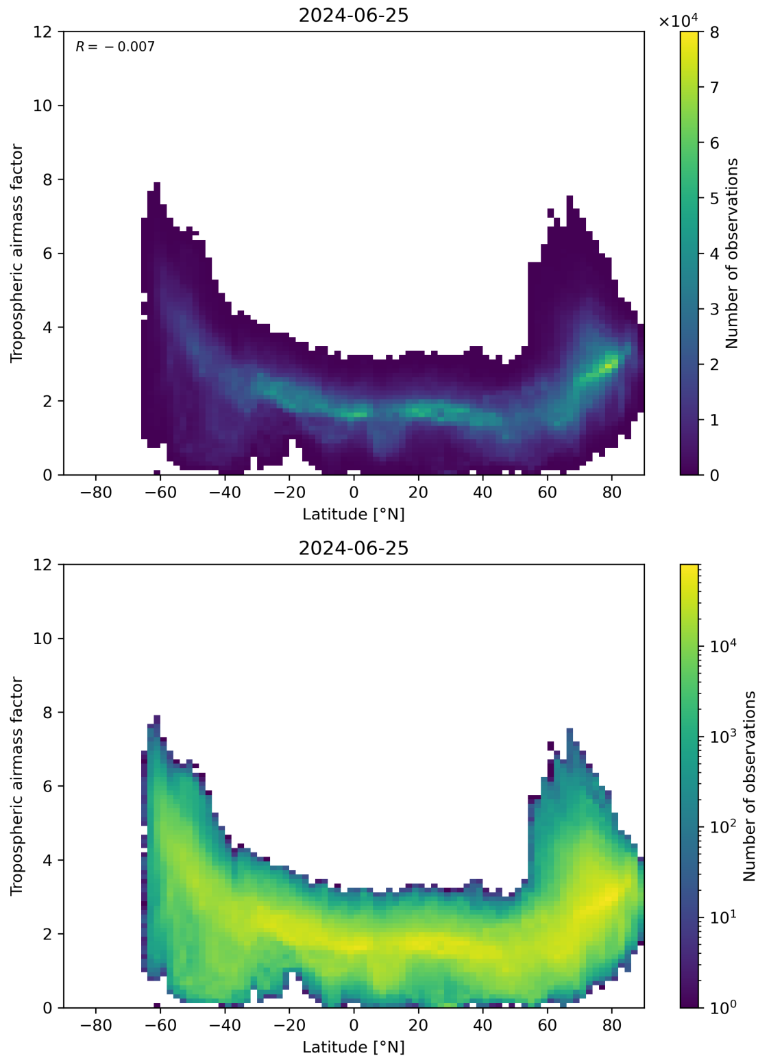
Figure 85: Scatter density plot of “Latitude” against “Tropospheric airmass factor” for 2024-06-24 to 2024-06-26.
