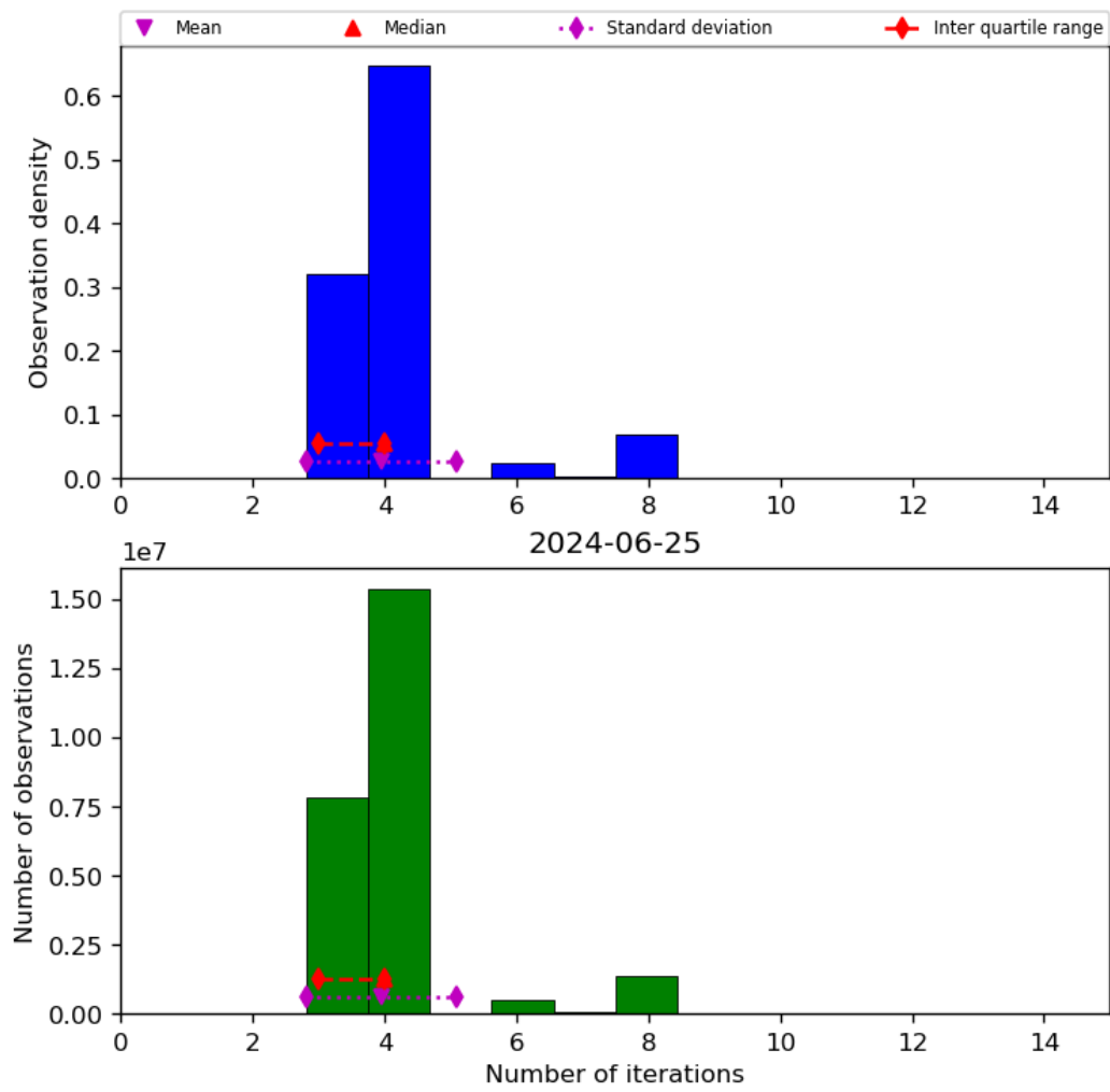
Figure 34: Histogram of “Number of iterations” for 2024-06-24 to 2024-06-26
