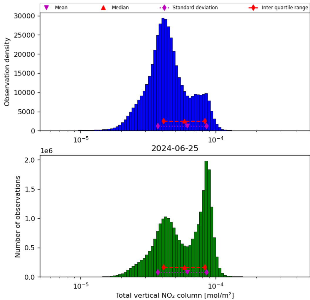
Figure 38: Histogram of “Total vertical NO 2 column” for 2024-06-24 to 2024-06-26
