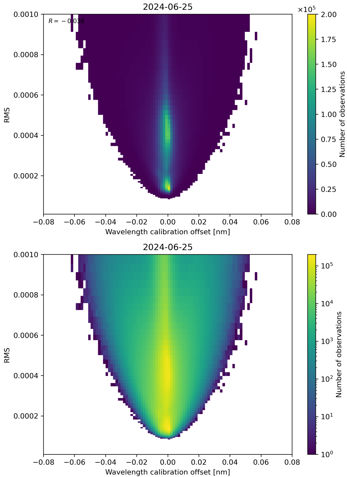
Figure 181: Scatter density plot of “Wavelength calibration offset” against “RMS” for 2024-06-24 to 2024-06-26.
