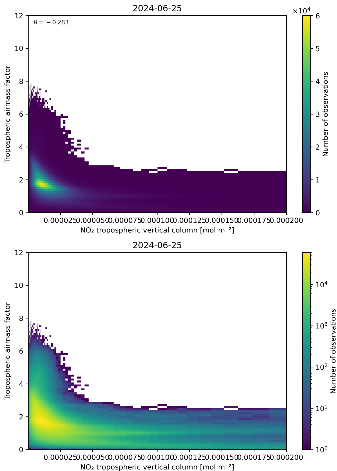
Figure 123: Scatter density plot of “NO 2 tropospheric vertical column” against “Tropospheric air mass factor” for 2024-06-24 to 2024-06-26.
