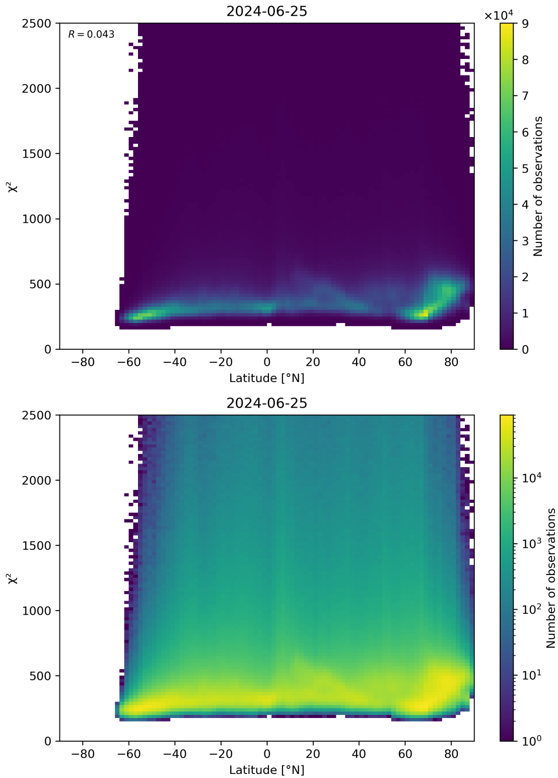
Figure 86: Scatter density plot of “Latitude” against “ \chi^2 ” for 2024-06-24 to 2024-06-26.
