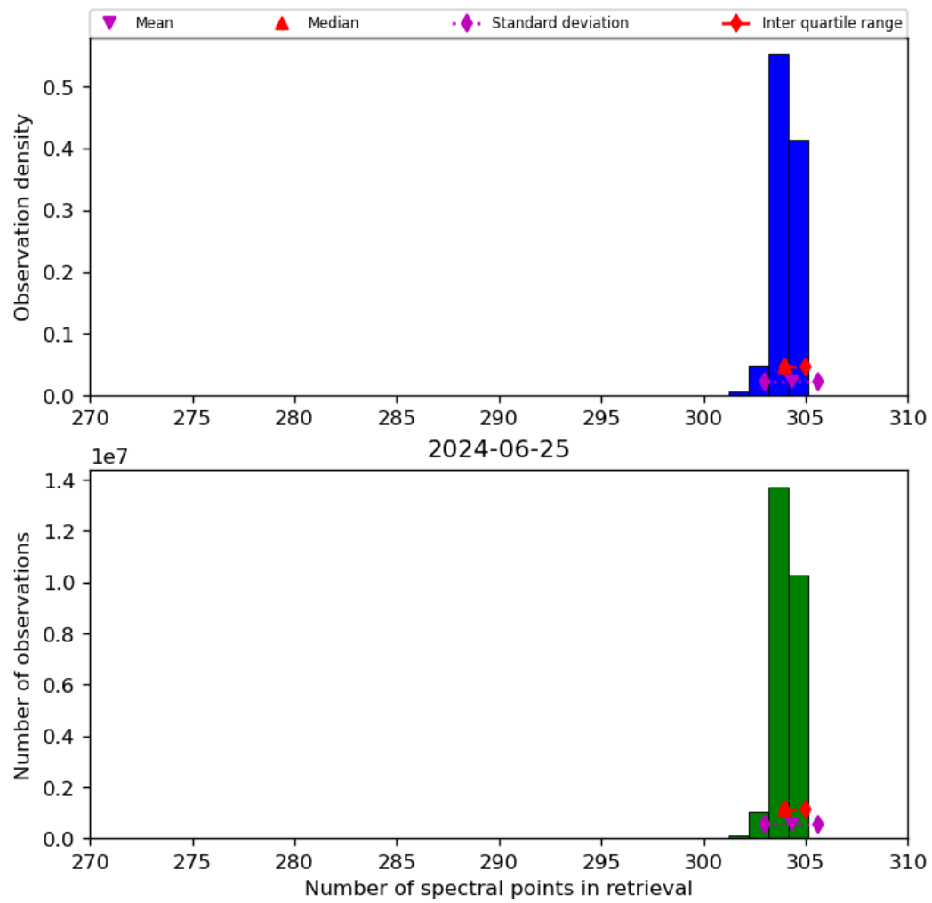
Figure 33: Histogram of “Number of spectral points in retrieval” for 2024-06-24 to 2024-06-26
