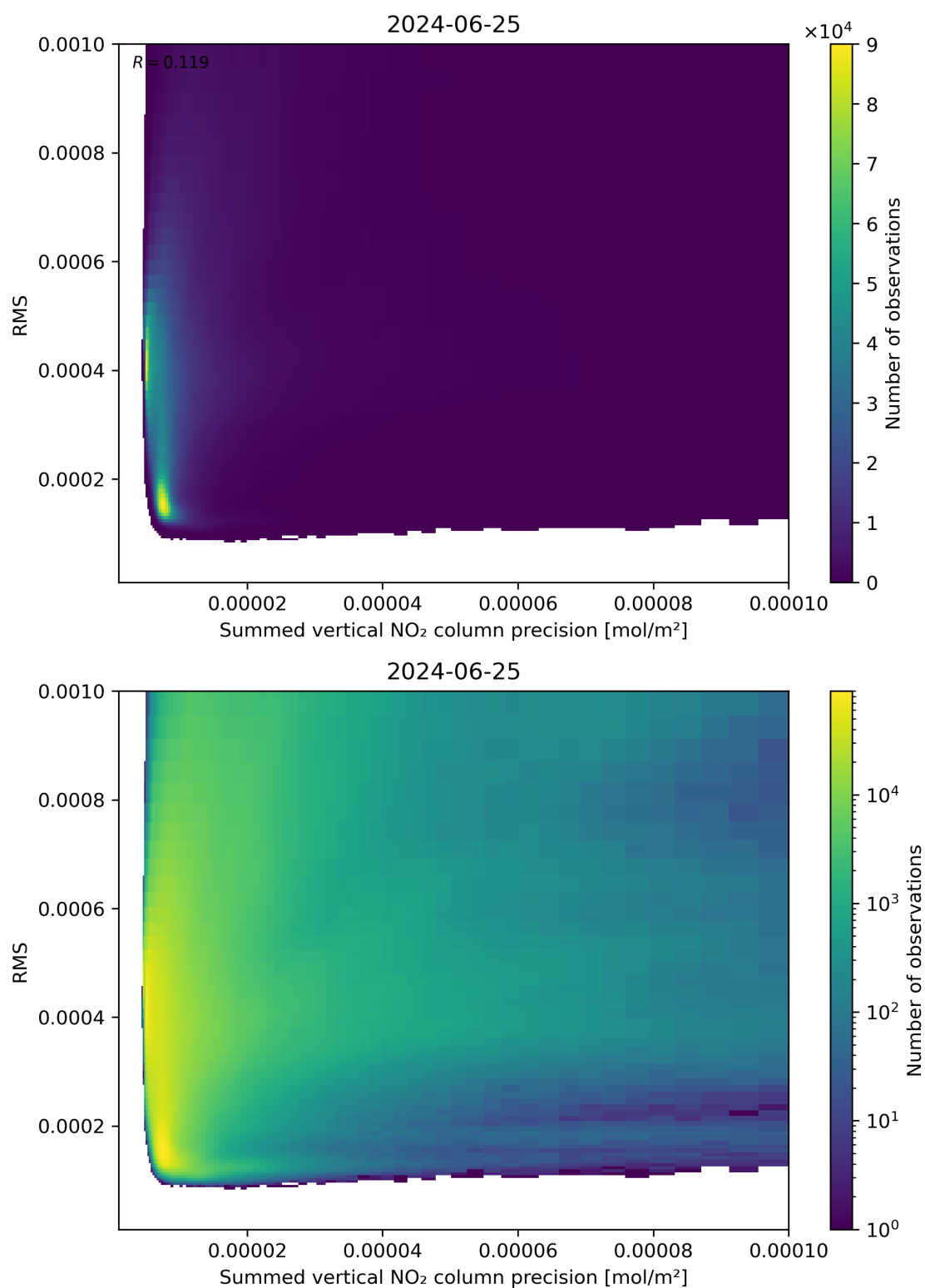
Figure 108: Scatter density plot of “Summed vertical NO 2 column precision” against “RMS” for 2024-06-24 to 2024-06-26.
