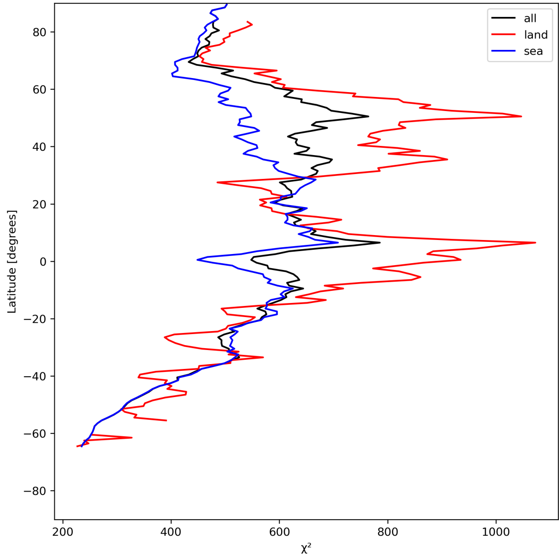
Figure 25: Zonal average of “ \chi^2 ” for 2024-06-24 to 2024-06-26.
