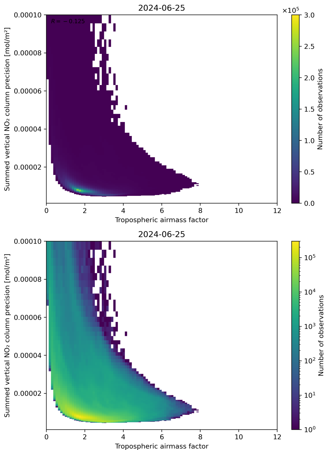
Figure 76: Scatter density plot of “Tropospheric air mass factor” against “Summed vertical NO 2 column precision” for 2024-06-24 to 2024-06-26.
