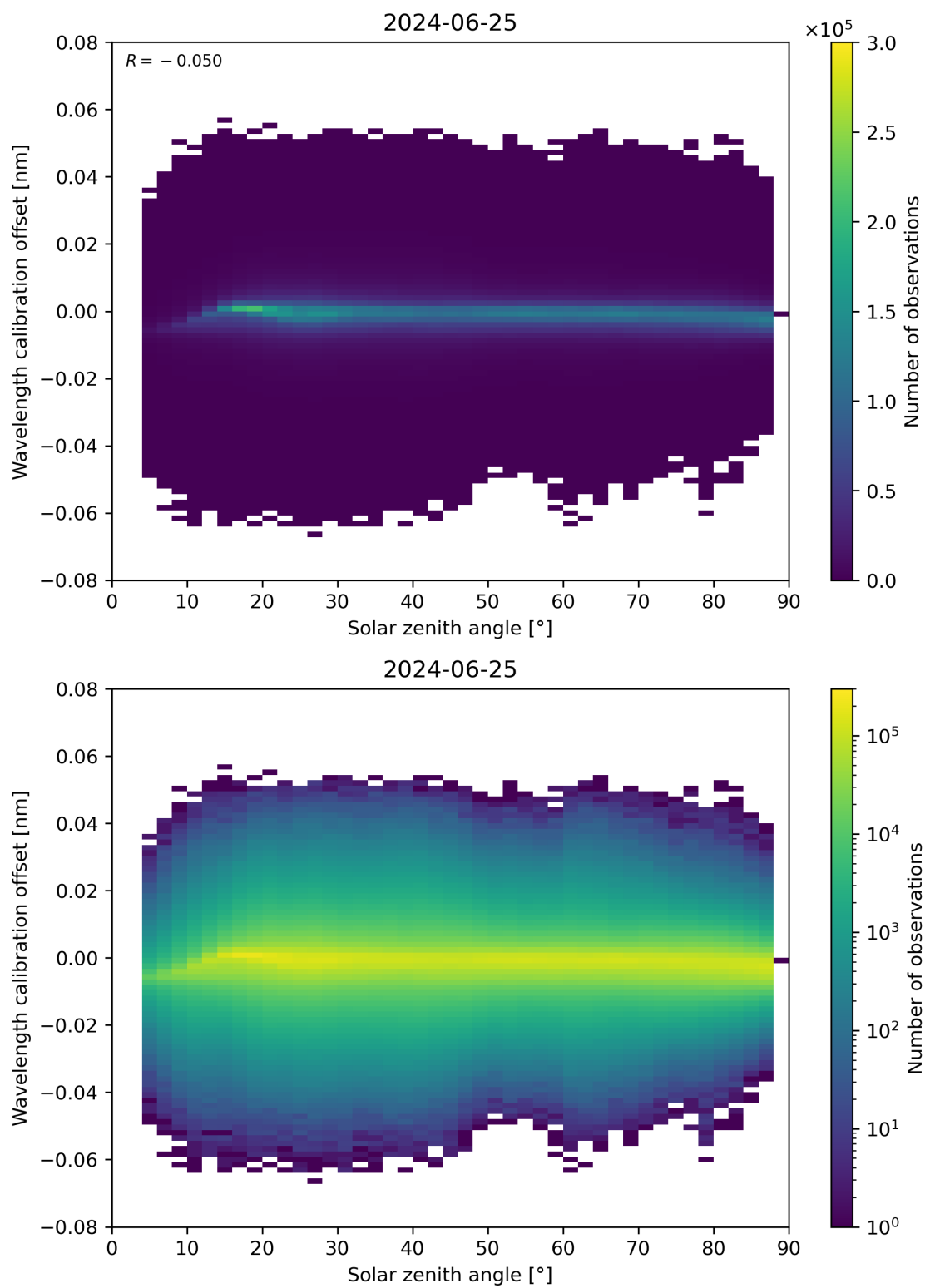
Figure 158: Scatter density plot of “Solar zenith angle” against “Wavelength calibration offset” for 2024-06-24 to 2024-06-26.
