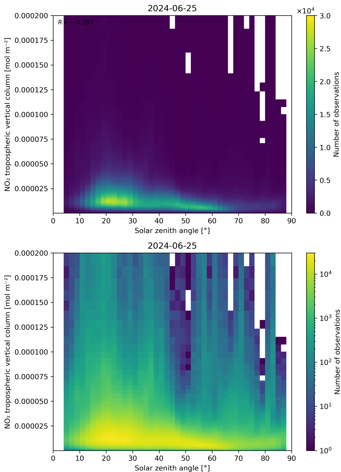
Figure 155: Scatter density plot of “Solar zenith angle” against “NO 2 tropospheric vertical column” for 2024-06-24 to 2024-06-26.
