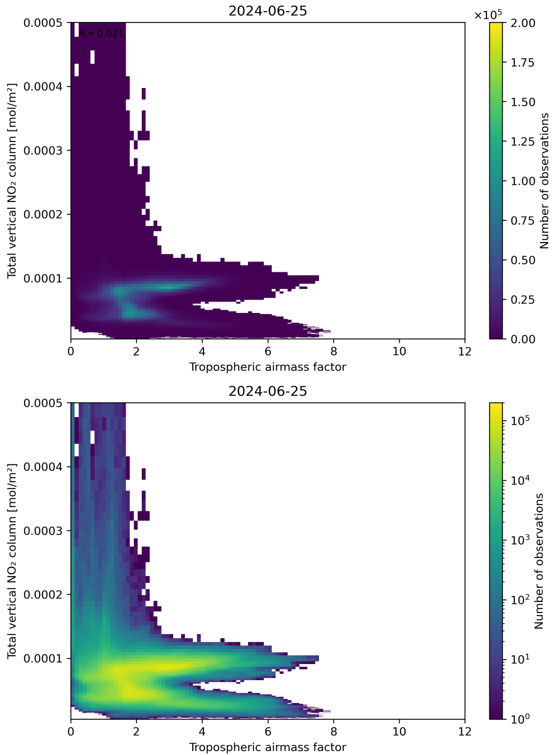
Figure 77: Scatter density plot of “Tropospheric airmass factor” against “Total vertical \text{NO}_2 column” for 2024-06-24 to 2024-06-26.
