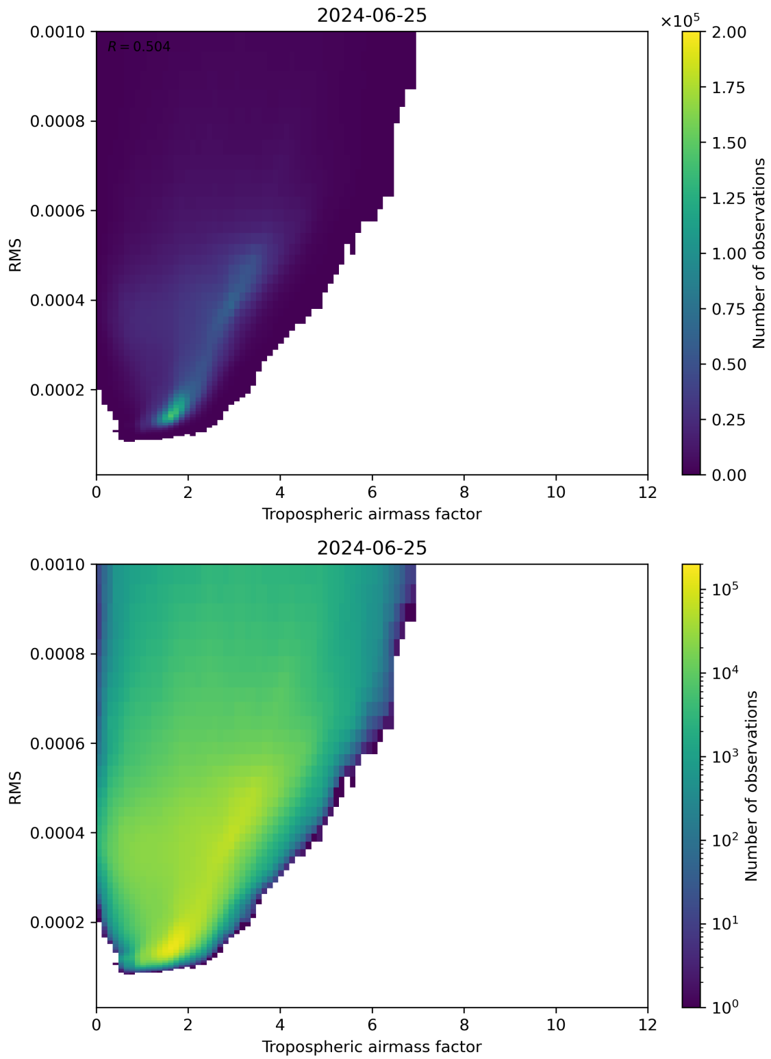
Figure 79: Scatter density plot of “Tropospheric airmass factor” against “RMS” for 2024-06-24 to 2024-06-26.
