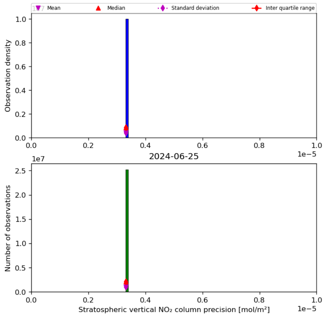
Figure 37: Histogram of “Stratospheric vertical NO 2 column precision” for 2024-06-24 to 2024-06-26
