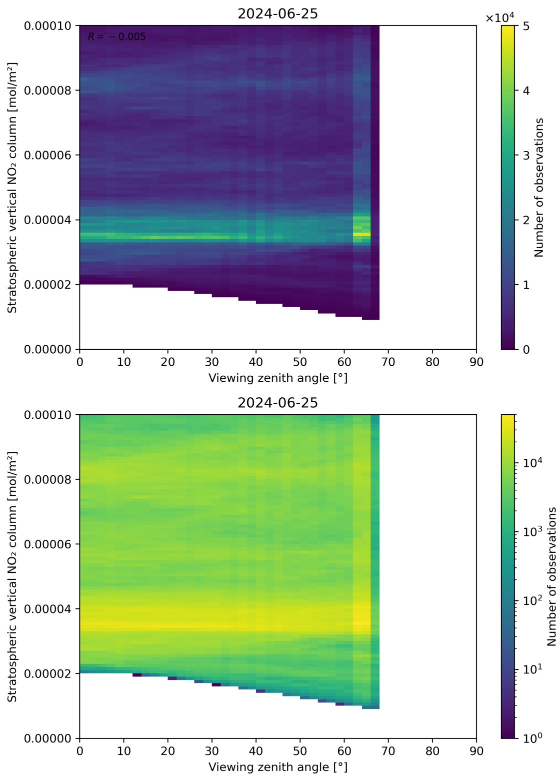
Figure 164: Scatter density plot of “Viewing zenith angle” against “Stratospheric vertical NO 2 column” for 2024-06-24 to 2024-06-26.
