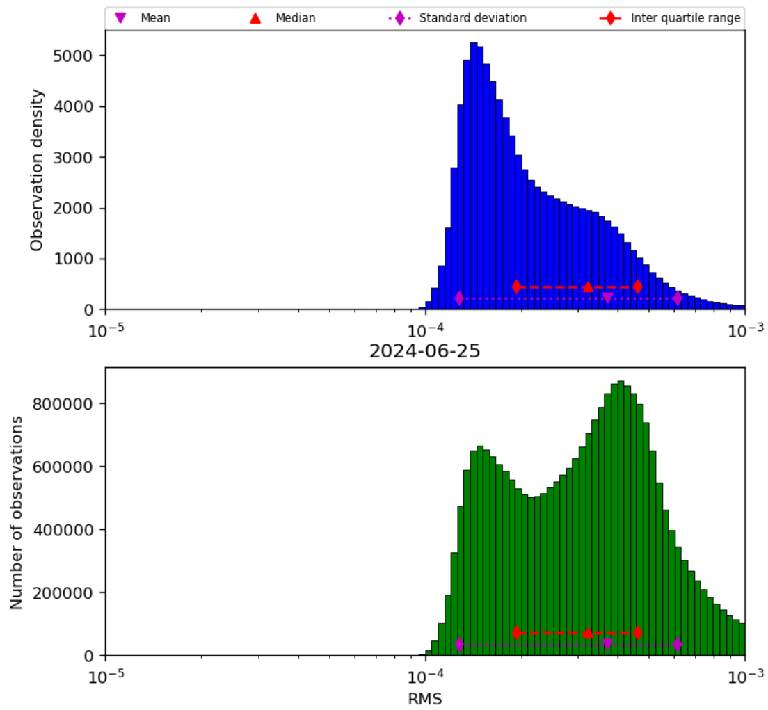
Figure 43: Histogram of “RMS” for 2024-06-24 to 2024-06-26
