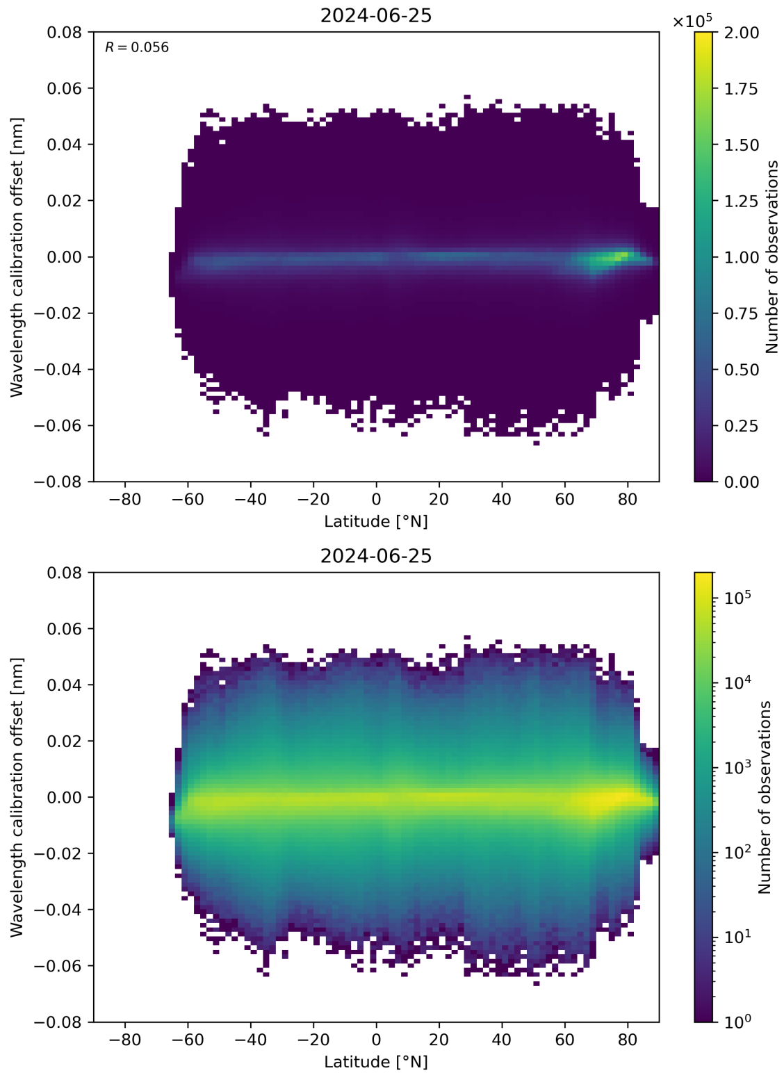
Figure 95: Scatter density plot of “Latitude” against “Wavelength calibration offset” for 2024-06-24 to 2024-06-26.
