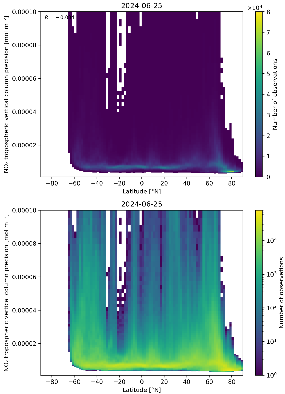
Figure 93: Scatter density plot of “Latitude” against “NO 2 tropospheric vertical column precision” for 2024-06-24 to 2024-06-26.
