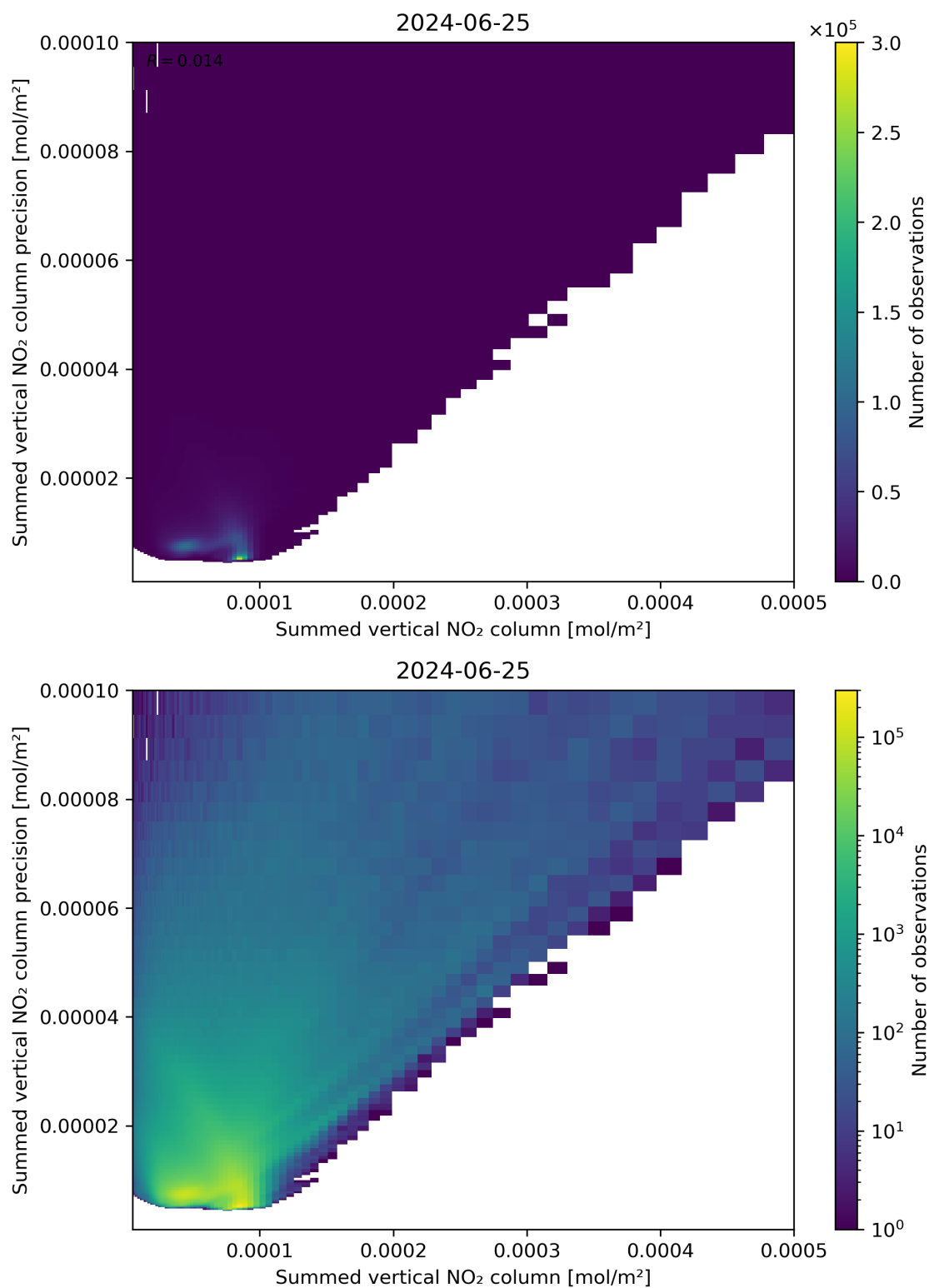
Figure 105: Scatter density plot of “Summed vertical NO 2 column” against “Summed vertical NO 2 column precision” for 2024-06-24 to 2024-06-26.
