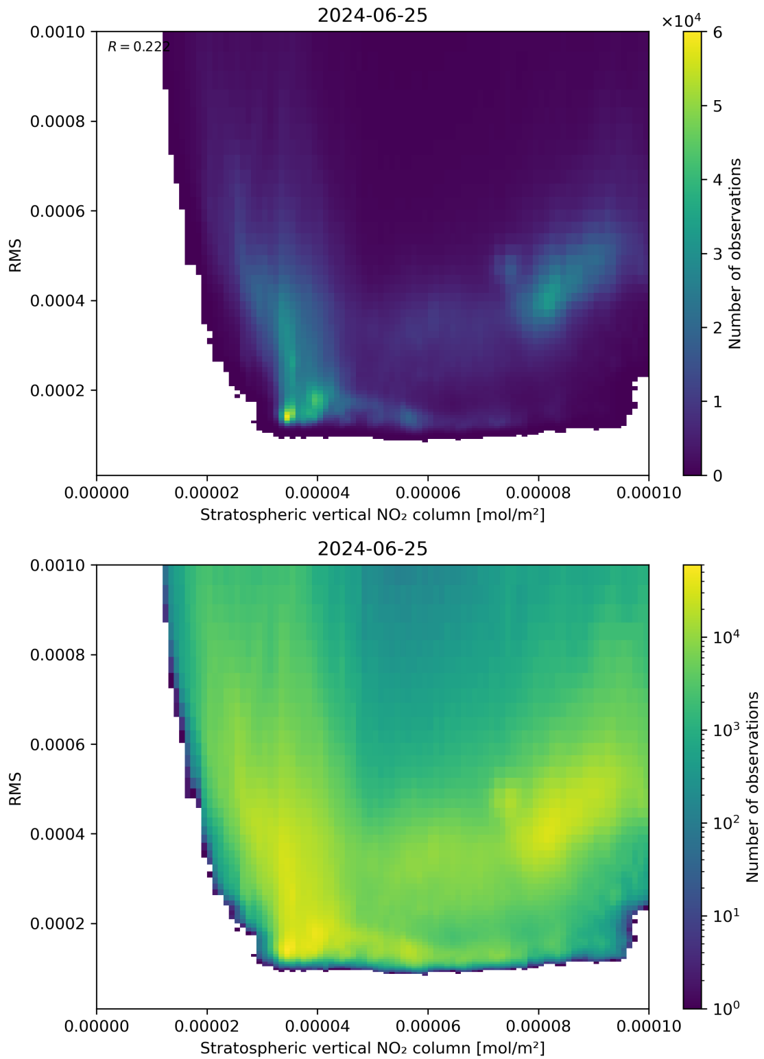
Figure 102: Scatter density plot of “Stratospheric vertical NO 2 column” against “RMS” for 2024-06-24 to 2024-06-26.
