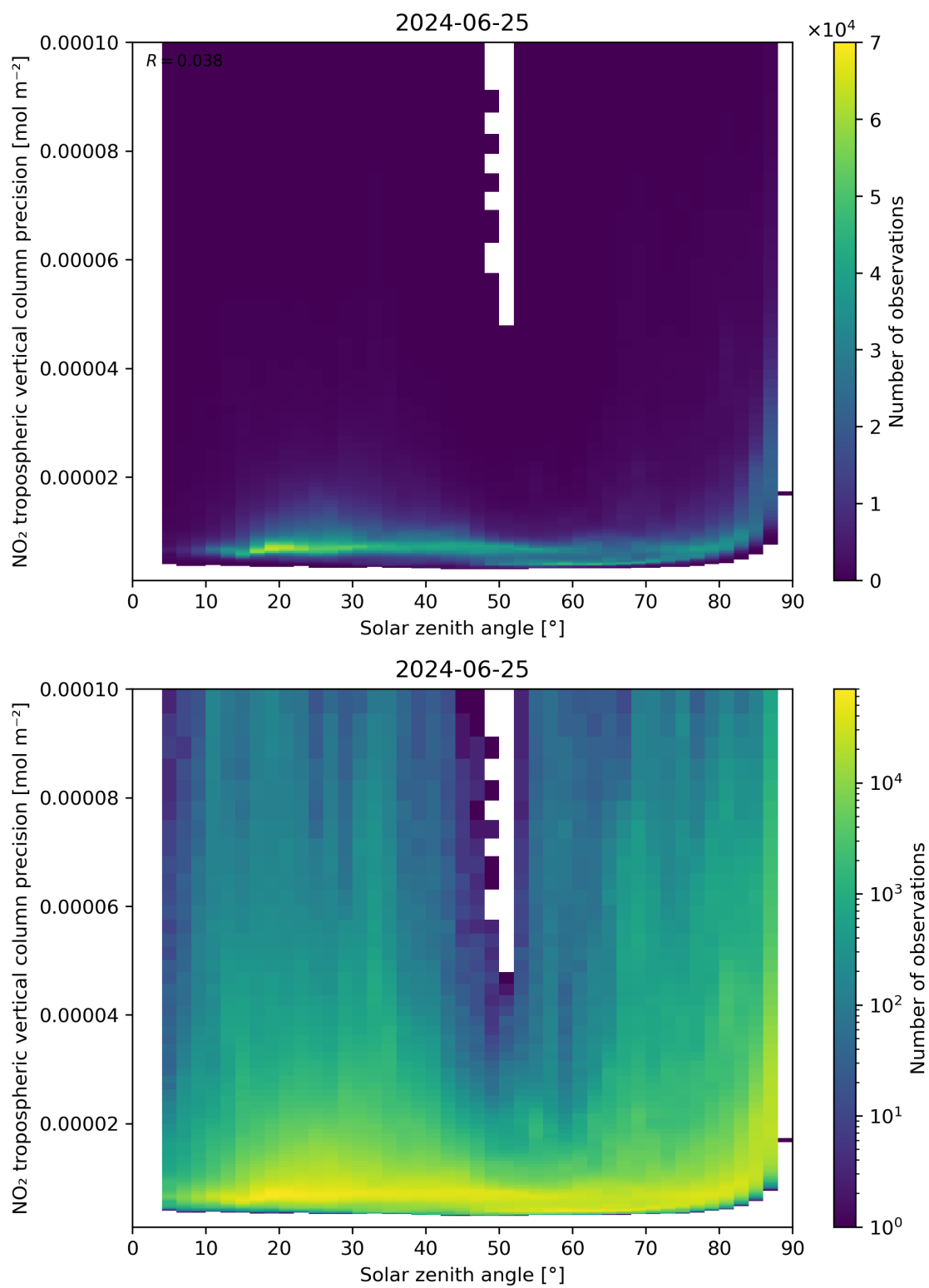
Figure 156: Scatter density plot of “Solar zenith angle” against “NO 2 tropospheric vertical column precision” for 2024-06-24 to 2024-06-26.
