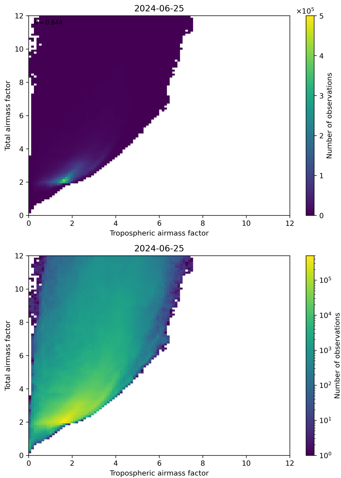
Figure 72: Scatter density plot of “Tropospheric airmass factor” against “Total airmass factor” for 2024-06-24 to 2024-06-26.
