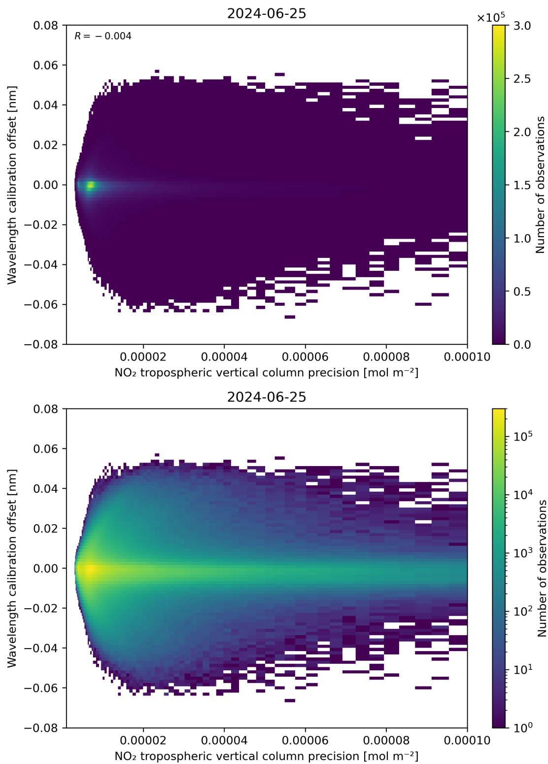
Figure 141: Scatter density plot of “NO 2 tropospheric vertical column precision” against “Wavelength calibration offset” for 2024-06-24 to 2024-06-26.
