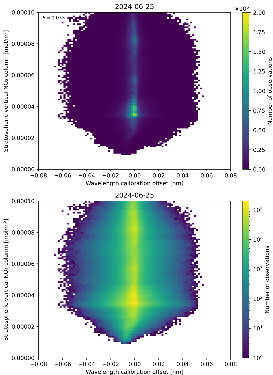
Figure 176: Scatter density plot of “Wavelength calibration offset” against “Stratospheric vertical NO 2 column” for 2024-06-24 to 2024-06-26.
