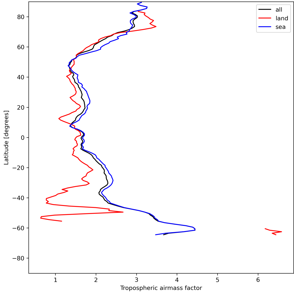
Figure 14: Zonal average of “Tropospheric airmass factor” for 2024-06-24 to 2024-06-26.
