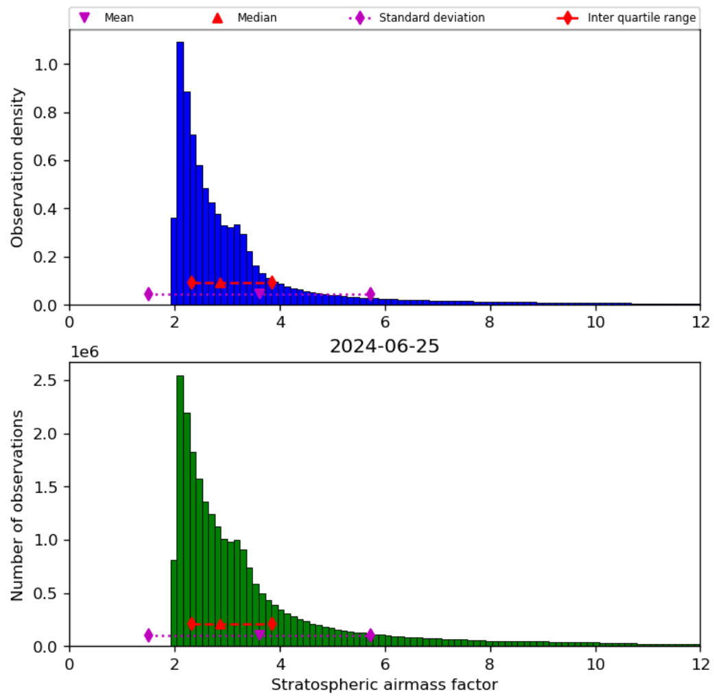
Figure 44: Histogram of “Stratospheric airmass factor” for 2024-06-24 to 2024-06-26
