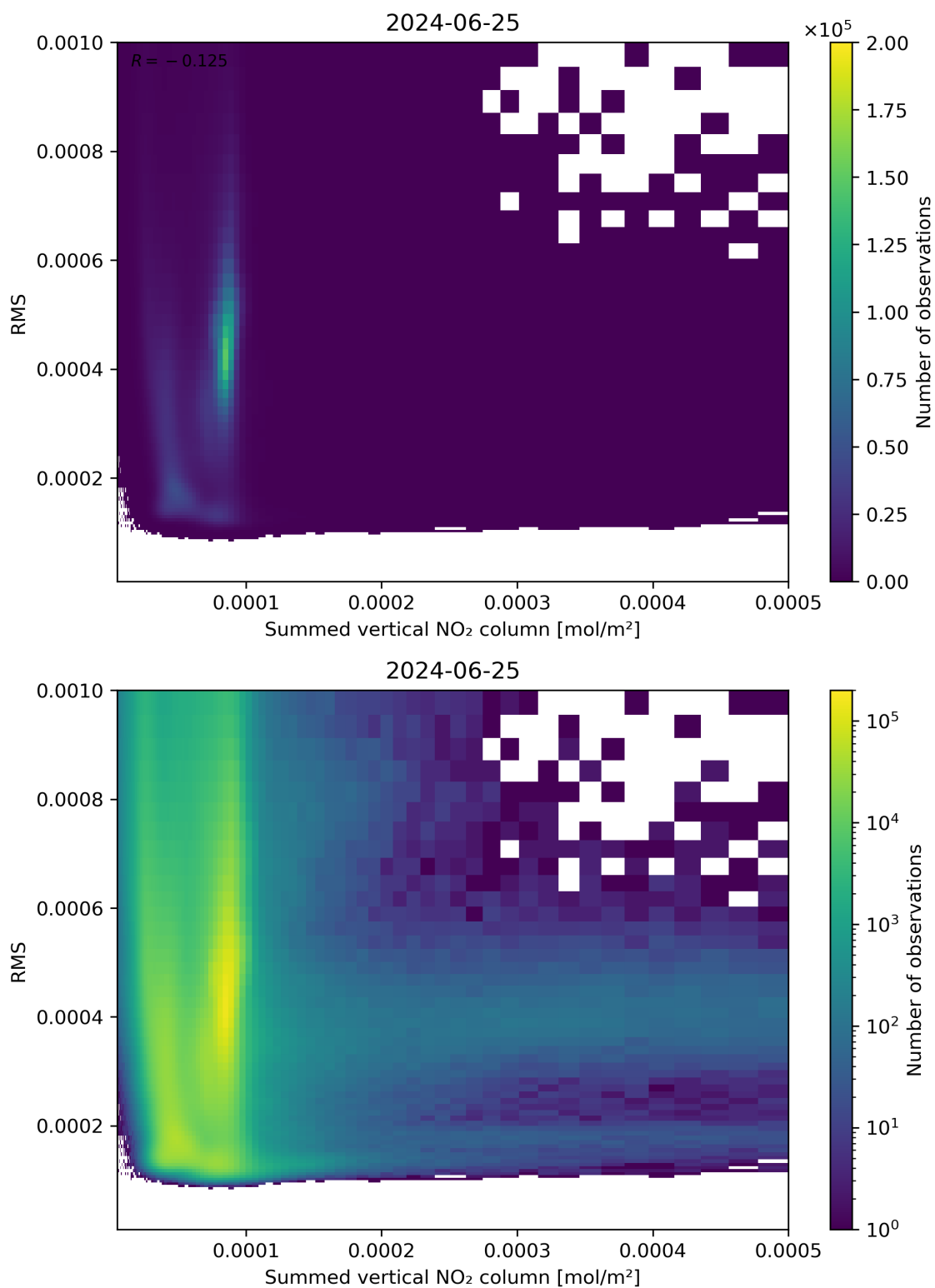
Figure 109: Scatter density plot of “Summed vertical NO 2 column” against “RMS” for 2024-06-24 to 2024-06-26.
