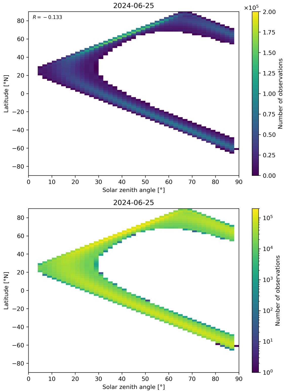
Figure 149: Scatter density plot of “Solar zenith angle” against “Latitude” for 2024-06-24 to 2024-06-26.
