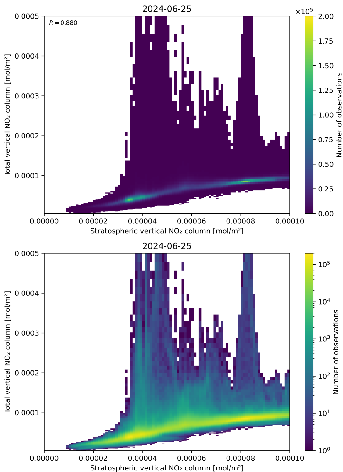
Figure 100: Scatter density plot of “Stratospheric vertical NO 2 column” against “Total vertical NO 2 column” for 2024-06-24 to 2024-06-26.
