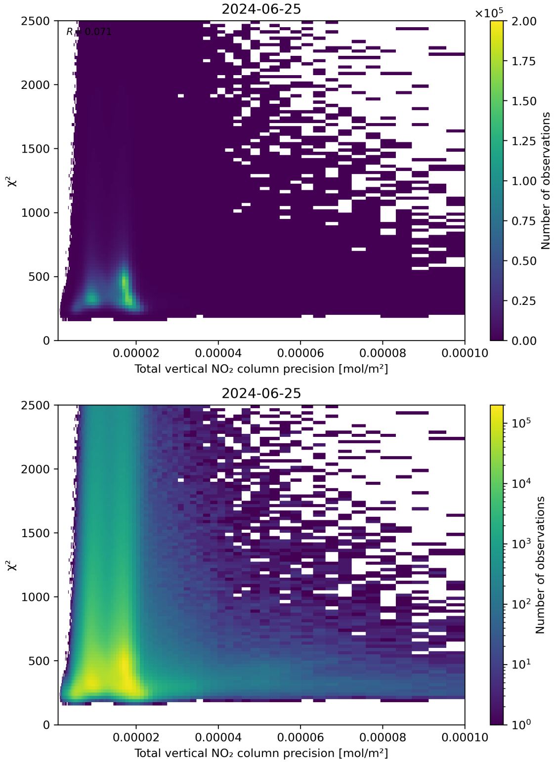
Figure 116: Scatter density plot of “Total vertical NO 2 column precision” against “ \chi^2 ” for 2024-06-24 to 2024-06-26.
