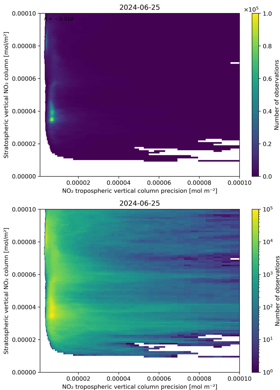
Figure 135: Scatter density plot of “NO 2 tropospheric vertical column precision” against “Stratospheric vertical NO 2 column” for 2024-06-24 to 2024-06-26.
