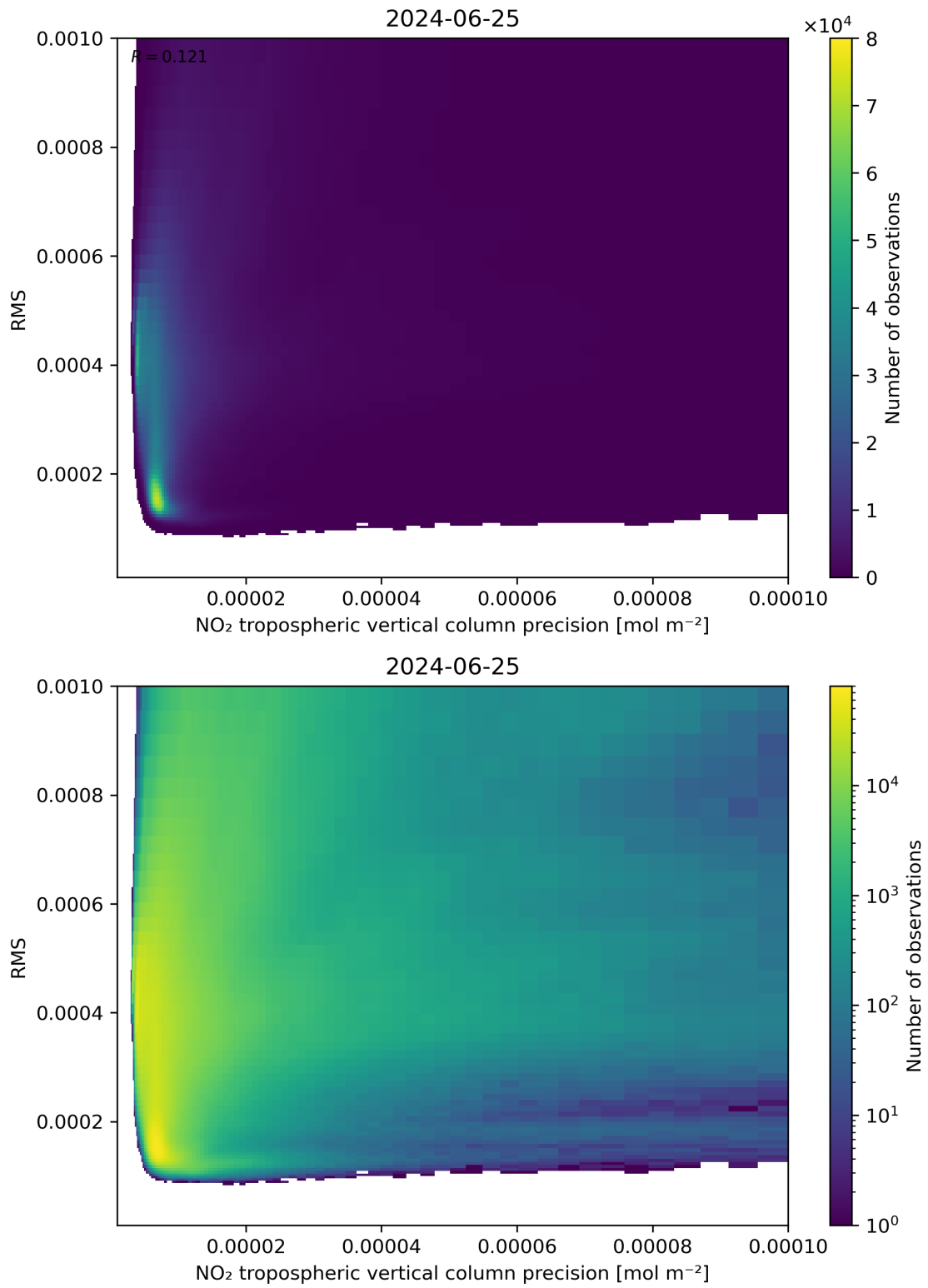
Figure 140: Scatter density plot of “NO 2 tropospheric vertical column precision” against “RMS” for 2024-06-24 to 2024-06-26.
