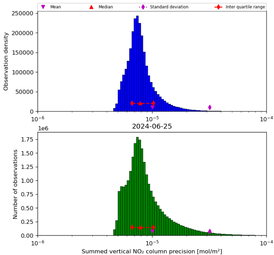
Figure 41: Histogram of "Summed vertical NO 2 column precision" for 2024-06-24 to 2024-06-26
