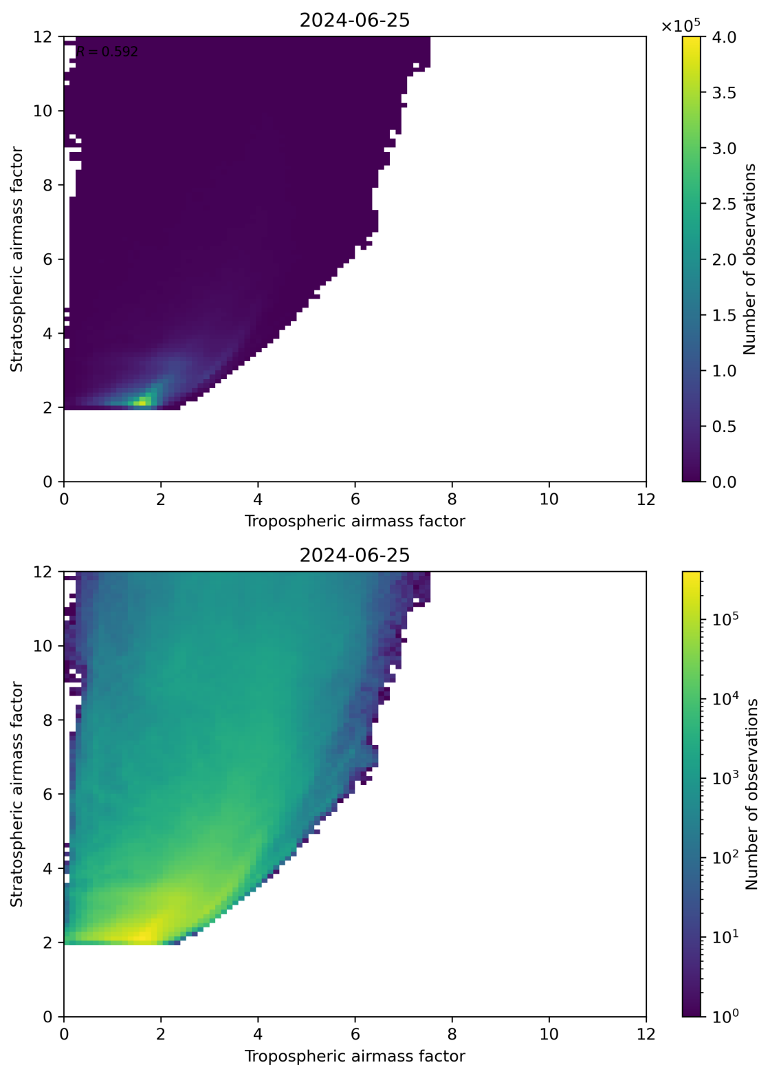
Figure 71: Scatter density plot of “Tropospheric airmass factor” against “Stratospheric airmass factor” for 2024-06-24 to 2024-06-26.
