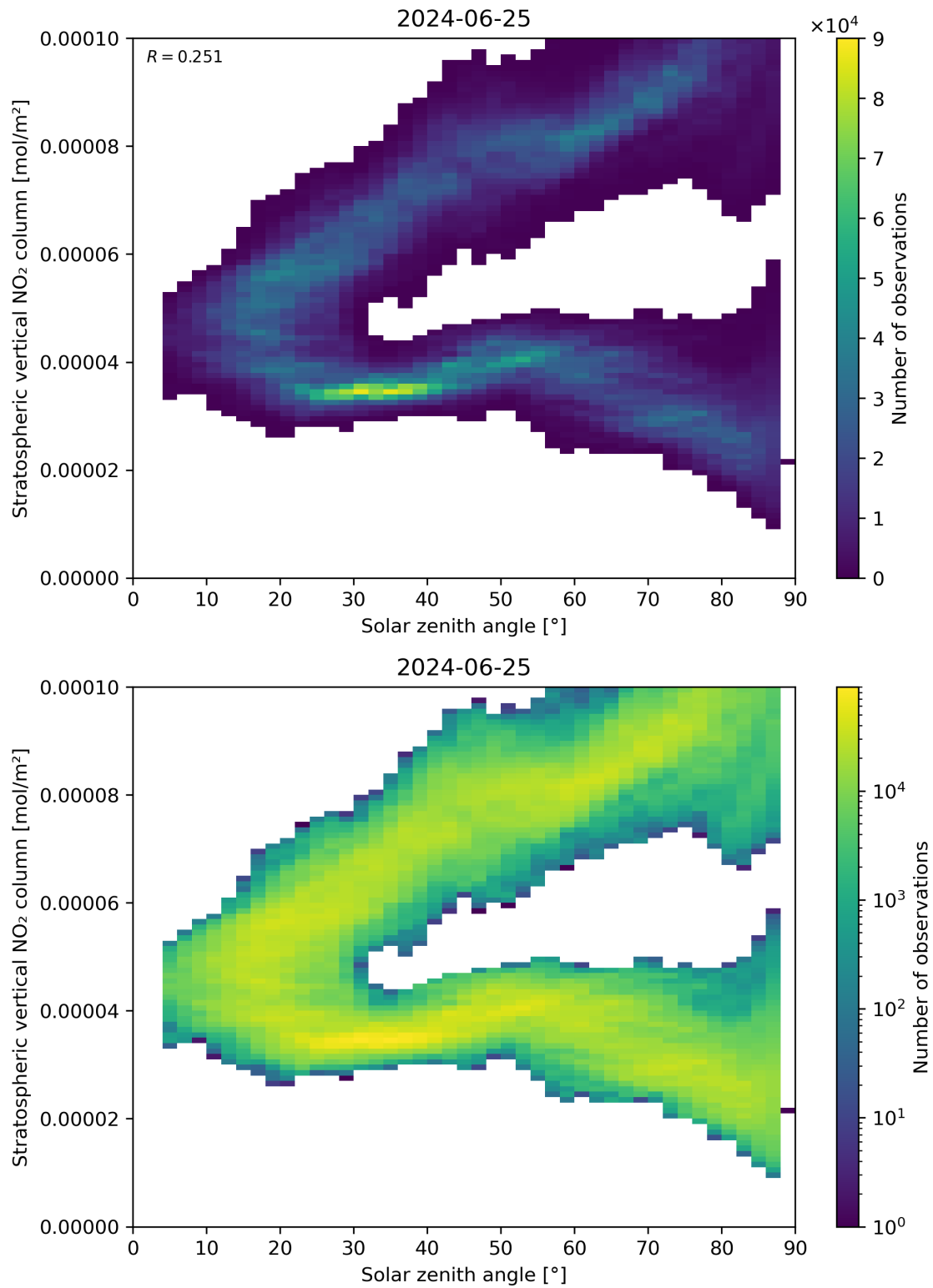
Figure 150: Scatter density plot of “Solar zenith angle” against “Stratospheric vertical NO 2 column” for 2024-06-24 to 2024-06-26.
