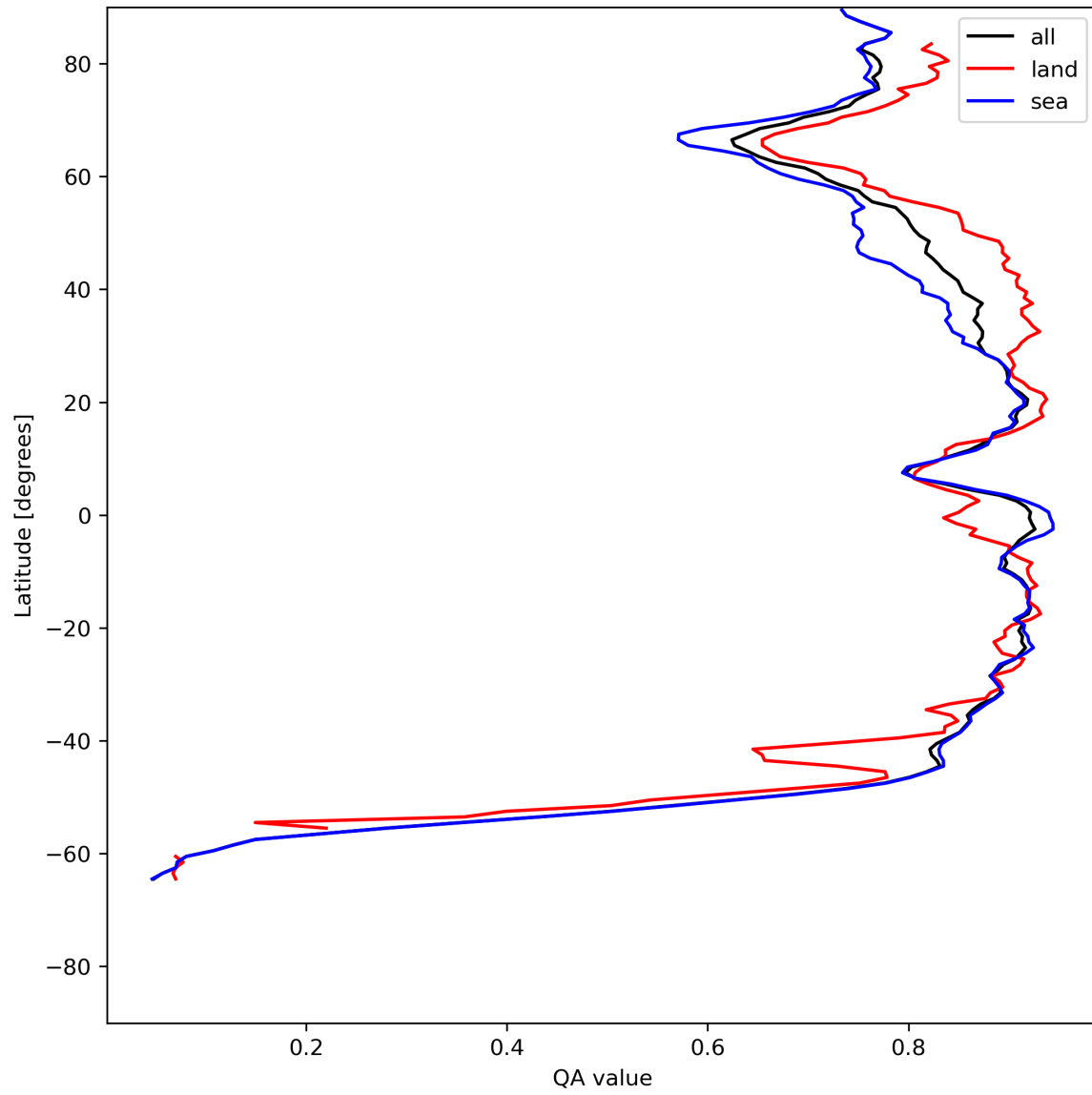
Figure 11: Zonal average of “QA value” for 2024-06-24 to 2024-06-26.
