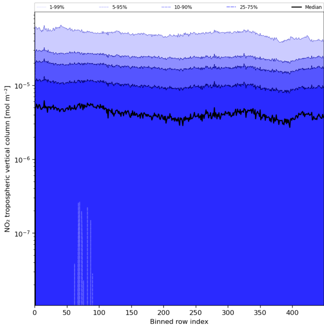
Figure 46: Along track statistics of “NO 2 tropospheric vertical column” for 2024-06-24 to 2024-06-26
