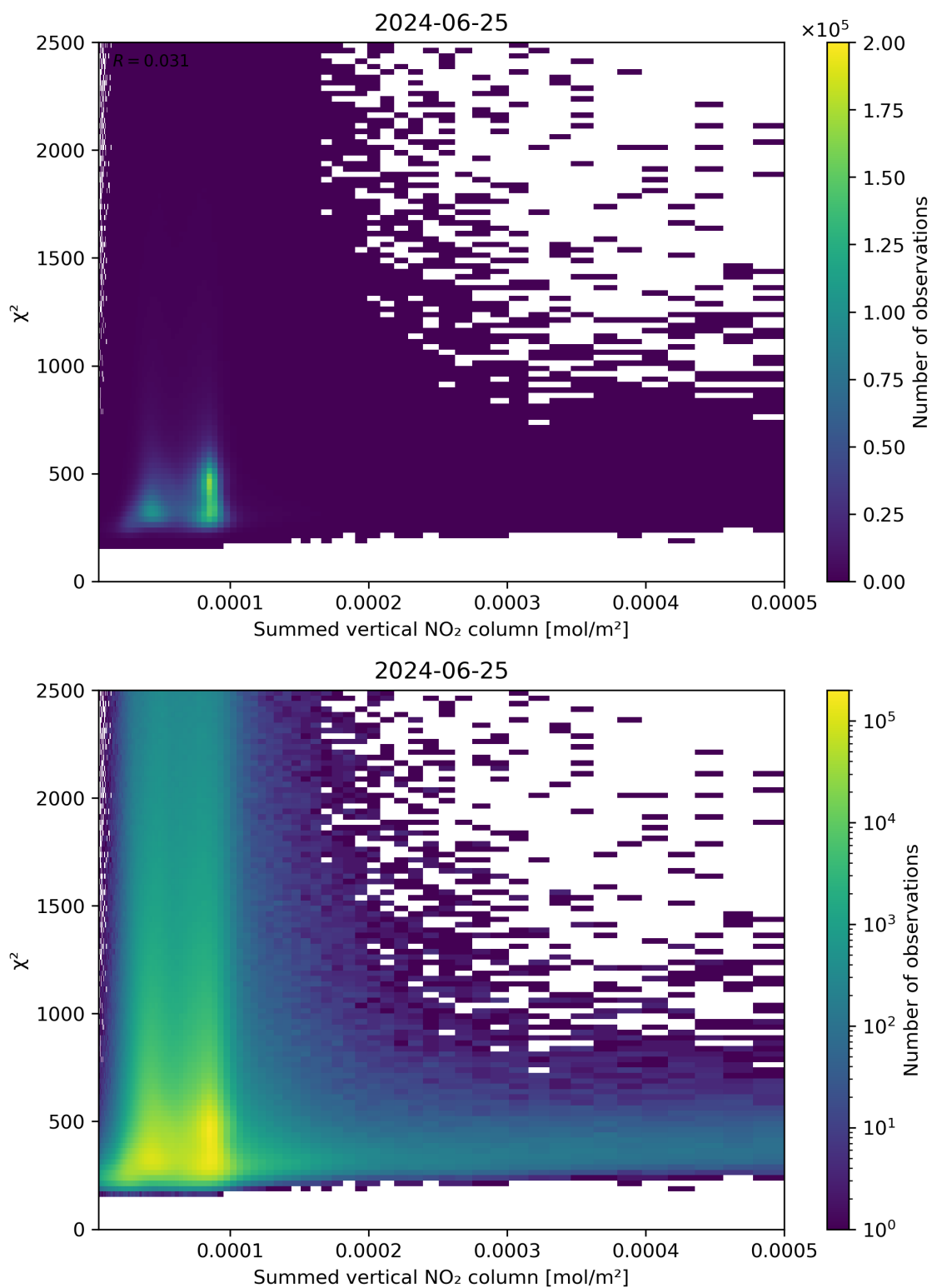
Figure 104: Scatter density plot of “Summed vertical NO 2 column” against “ \chi^2 ” for 2024-06-24 to 2024-06-26.
