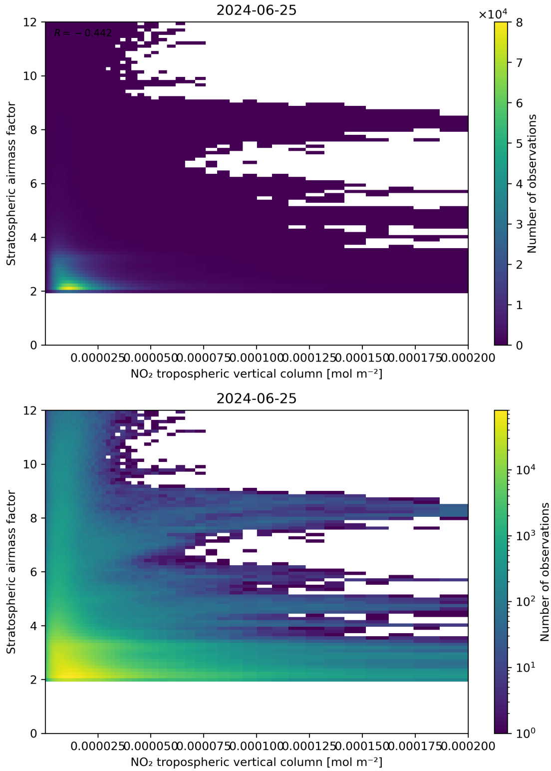
Figure 121: Scatter density plot of “NO 2 tropospheric vertical column” against “Stratospheric air mass factor” for 2024-06-24 to 2024-06-26.
