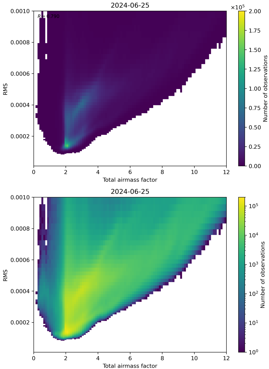
Figure 69: Scatter density plot of “Total airmass factor” against “RMS” for 2024-06-24 to 2024-06-26.
