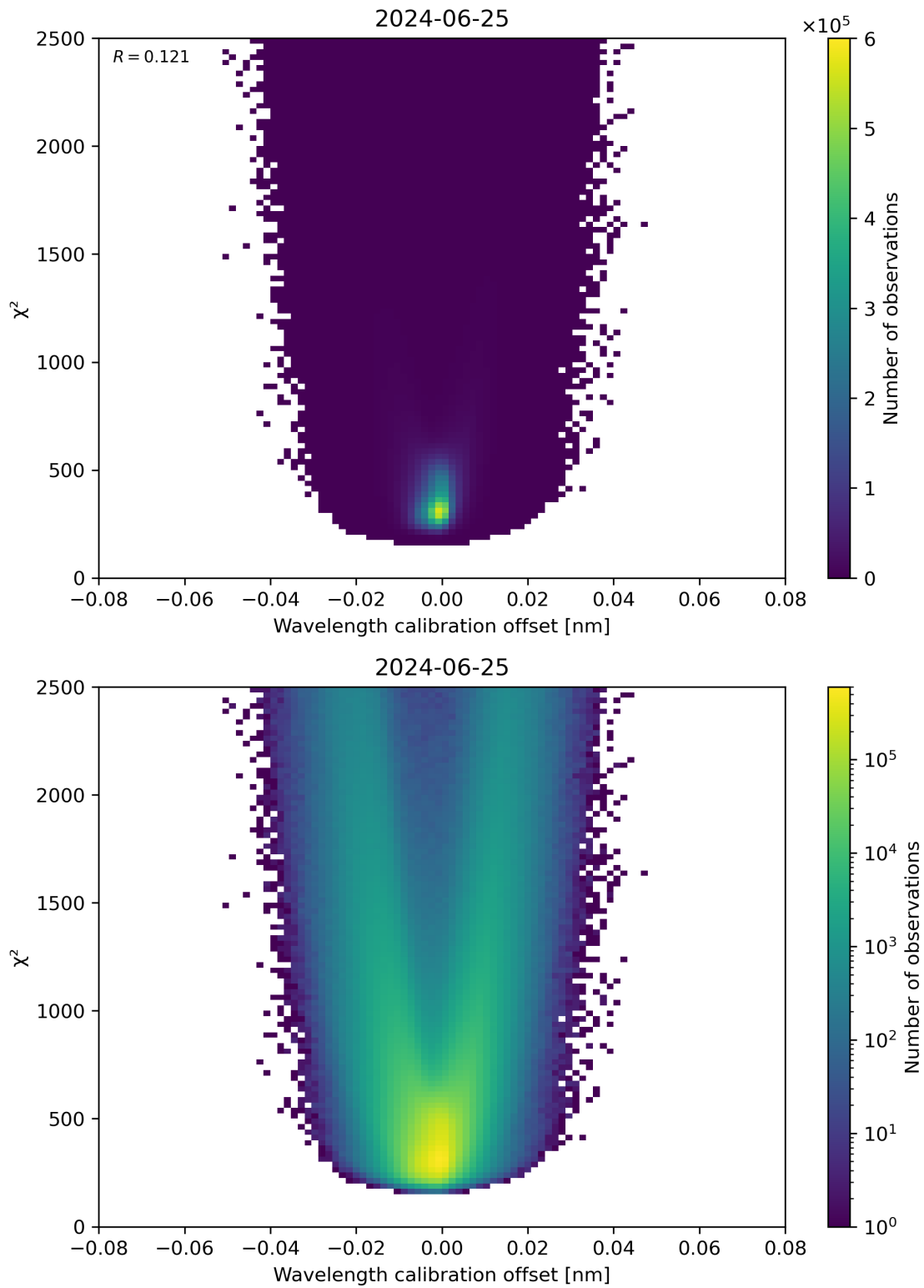
Figure 175: Scatter density plot of “Wavelength calibration offset” against “ \chi^2 ” for 2024-06-24 to 2024-06-26.
