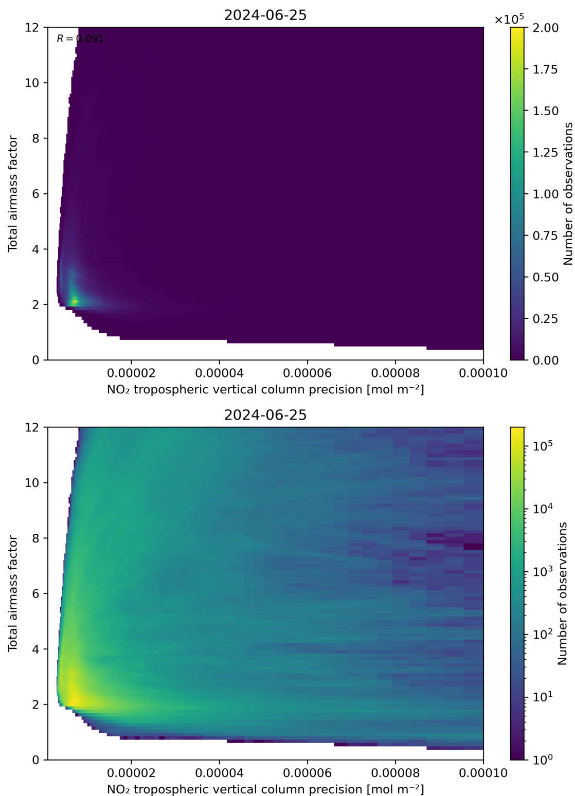
Figure 132: Scatter density plot of “NO 2 tropospheric vertical column precision” against “Total air mass factor” for 2024-06-24 to 2024-06-26.
