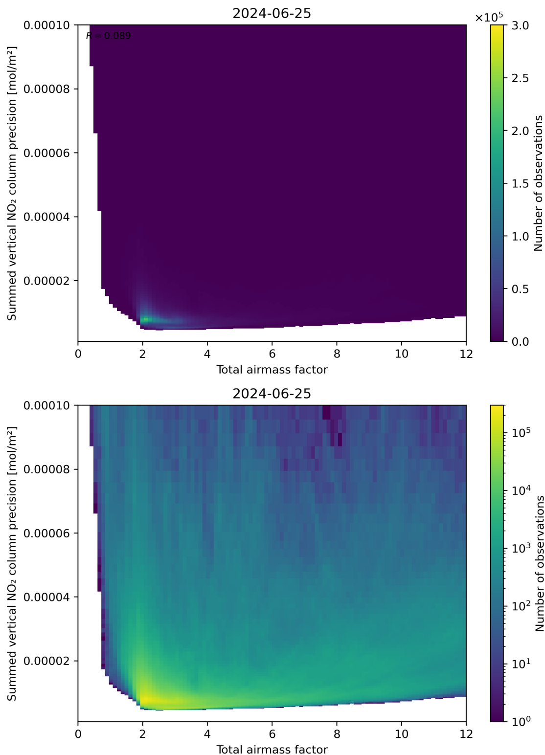
Figure 66: Scatter density plot of “Total airmass factor” against “Summed vertical NO 2 column precision” for 2024-06-24 to 2024-06-26.
