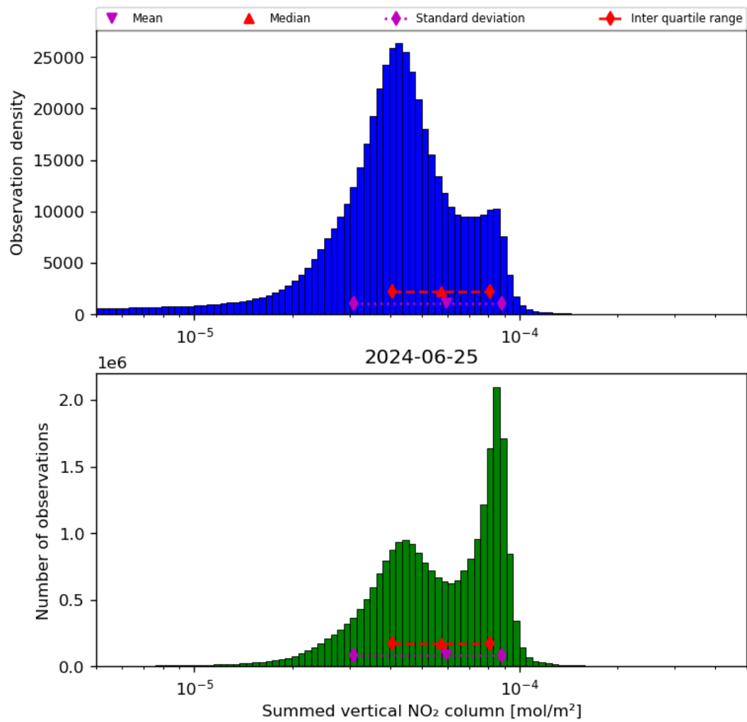
Figure 40: Histogram of “Summed vertical NO 2 column” for 2024-06-24 to 2024-06-26
