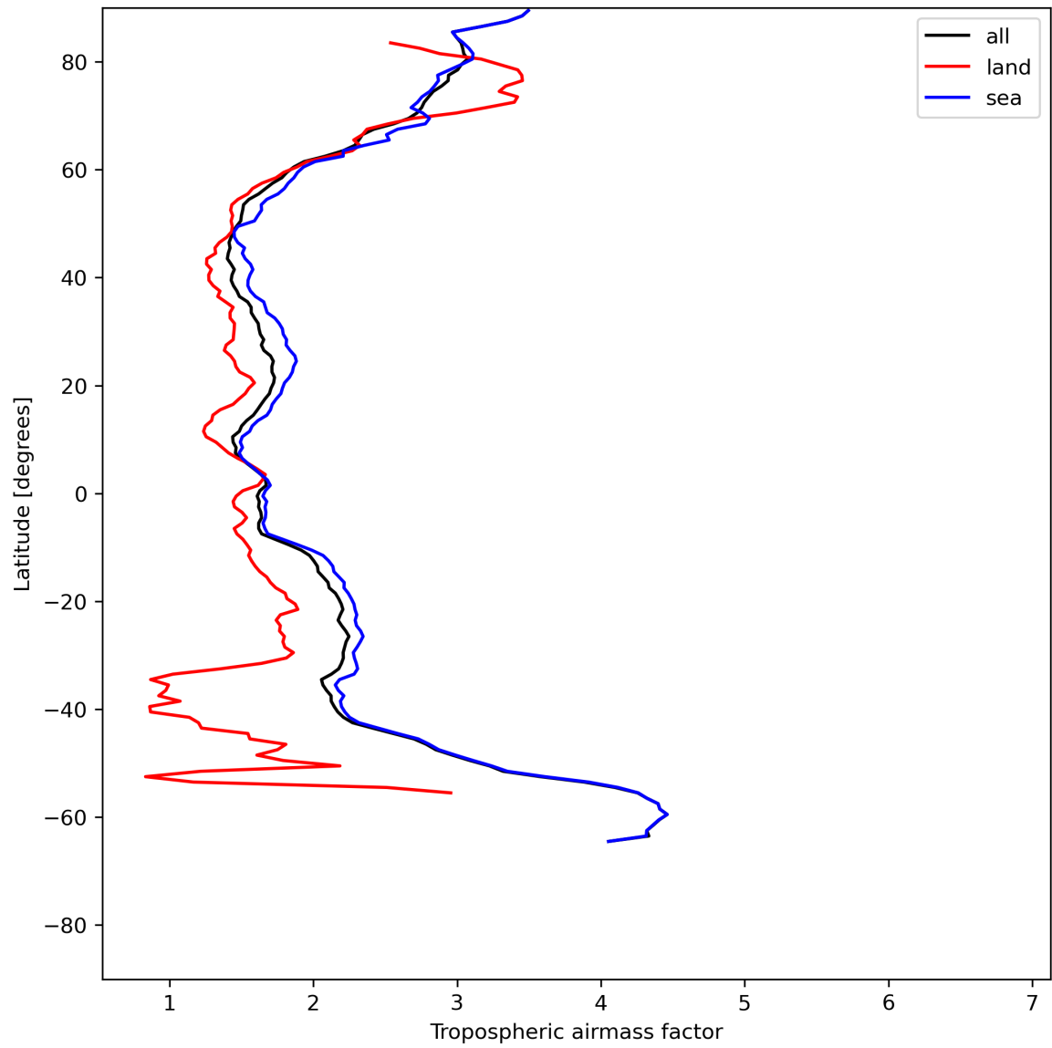
Figure 14: Zonal average of “Tropospheric airmass factor” for 2024-06-25 to 2024-06-27.
