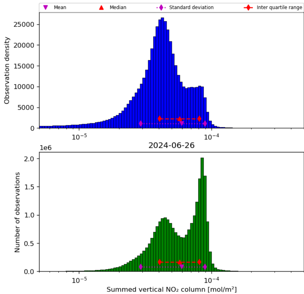
Figure 40: Histogram of “Summed vertical NO 2 column” for 2024-06-25 to 2024-06-27
