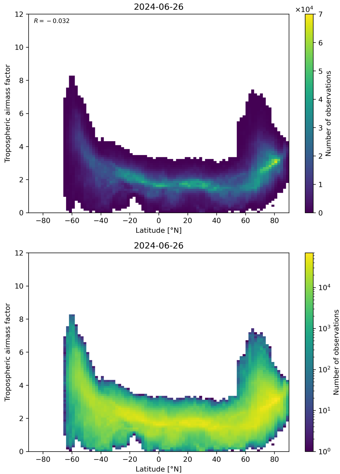
Figure 85: Scatter density plot of “Latitude” against “Tropospheric air mass factor” for 2024-06-25 to 2024-06-27.
