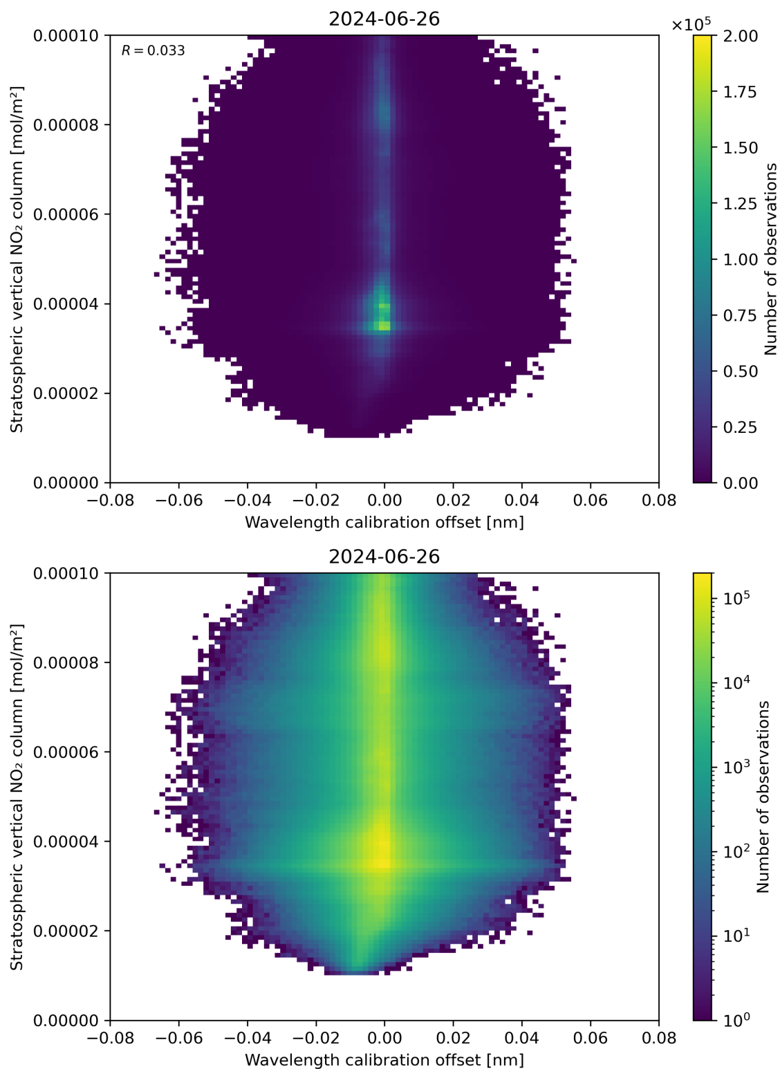
Figure 176: Scatter density plot of “Wavelength calibration offset” against “Stratospheric vertical NO 2 column” for 2024-06-25 to 2024-06-27.
