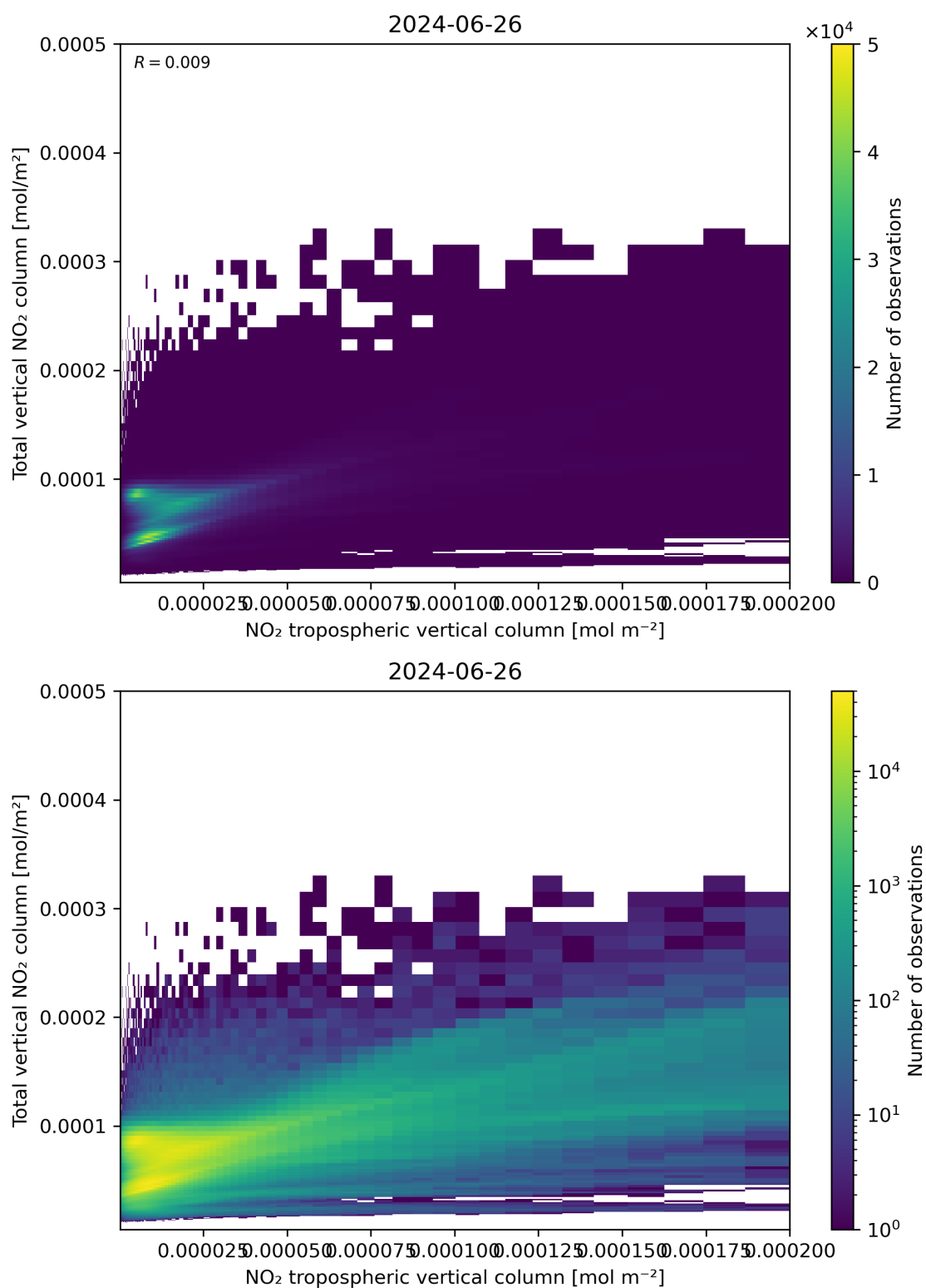
Figure 128: Scatter density plot of “NO 2 tropospheric vertical column” against “Total vertical NO 2 column” for 2024-06-25 to 2024-06-27.
