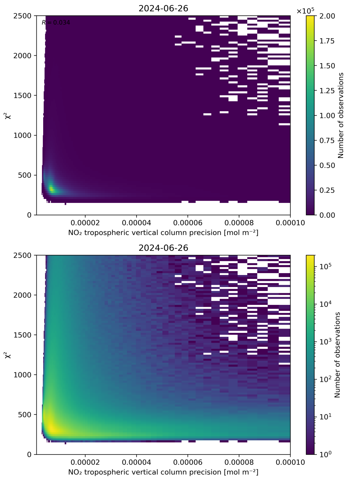
Figure 134: Scatter density plot of “NO 2 tropospheric vertical column precision” against “ \chi^2 ” for 2024-06-25 to 2024-06-27.
