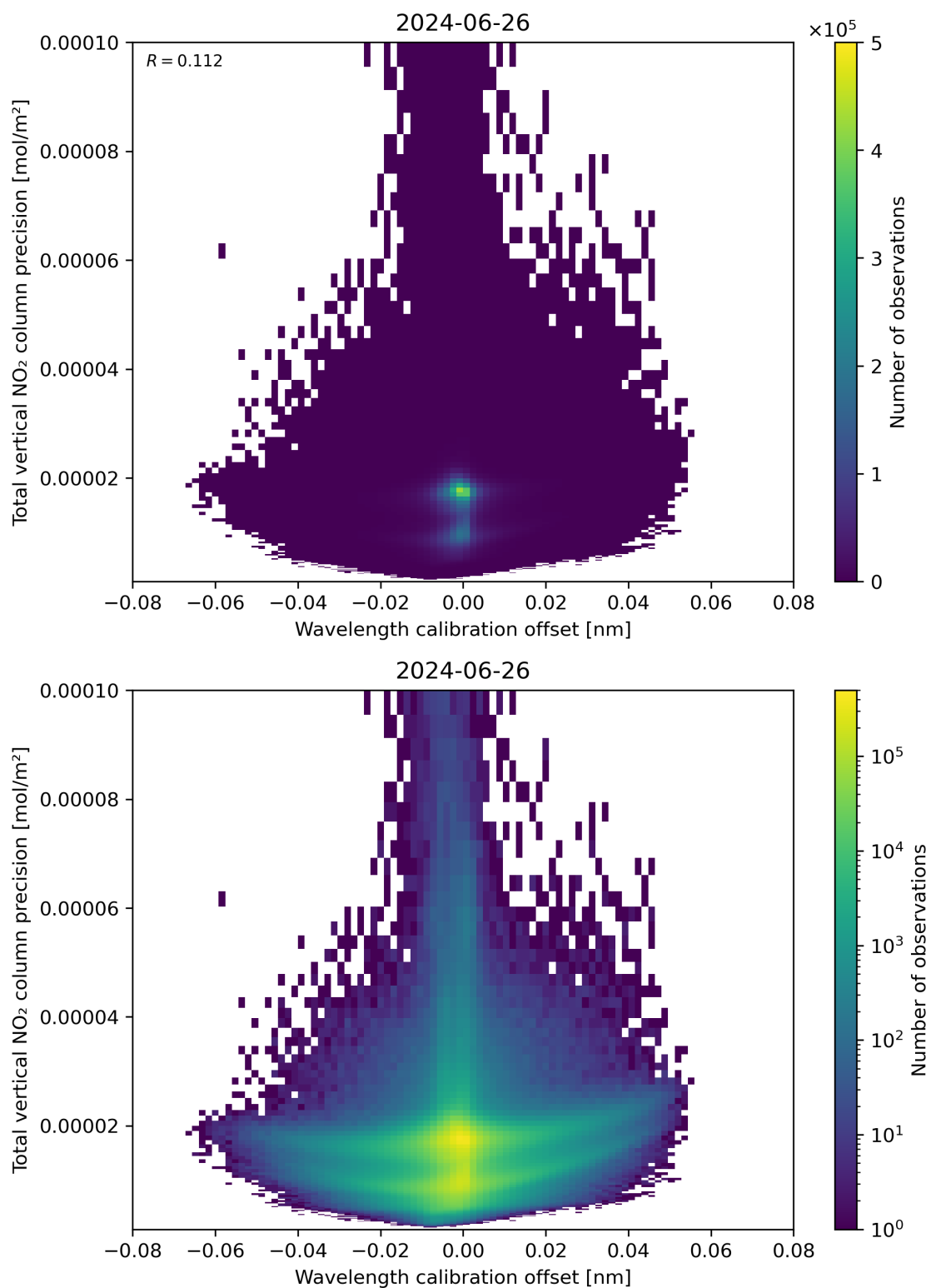
Figure 180: Scatter density plot of “Wavelength calibration offset” against “Total vertical NO 2 column precision” for 2024-06-25 to 2024-06-27.
