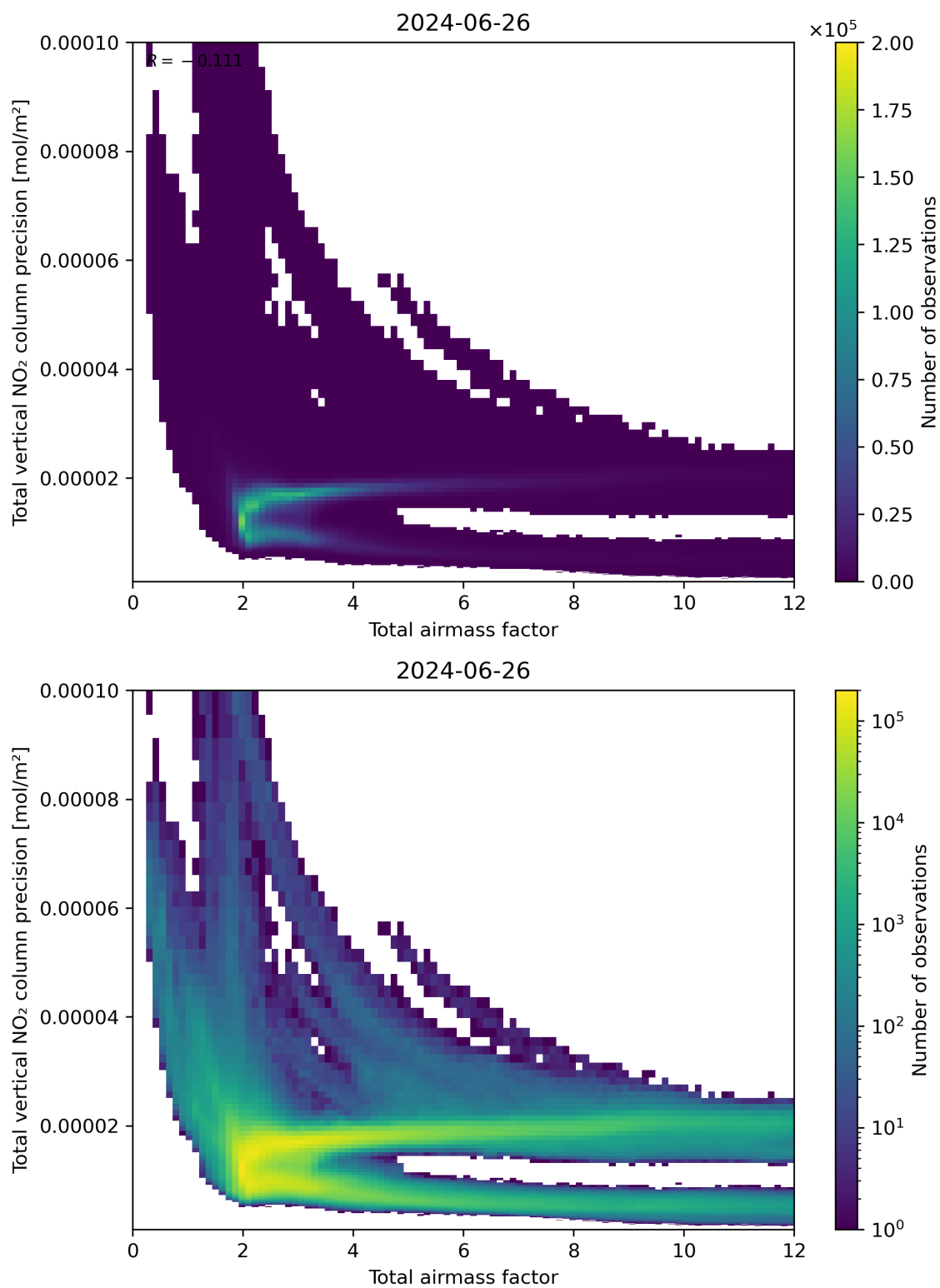
Figure 68: Scatter density plot of “Total airmass factor” against “Total vertical NO 2 column precision” for 2024-06-25 to 2024-06-27.
