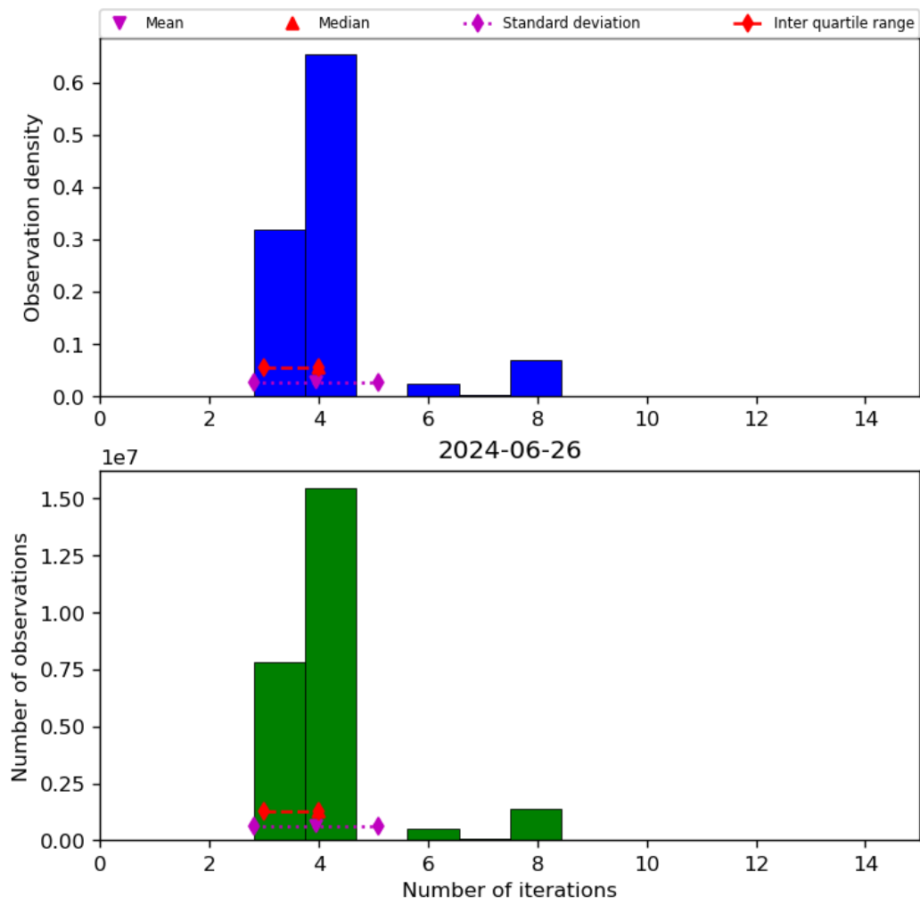
Figure 34: Histogram of “Number of iterations” for 2024-06-25 to 2024-06-27
