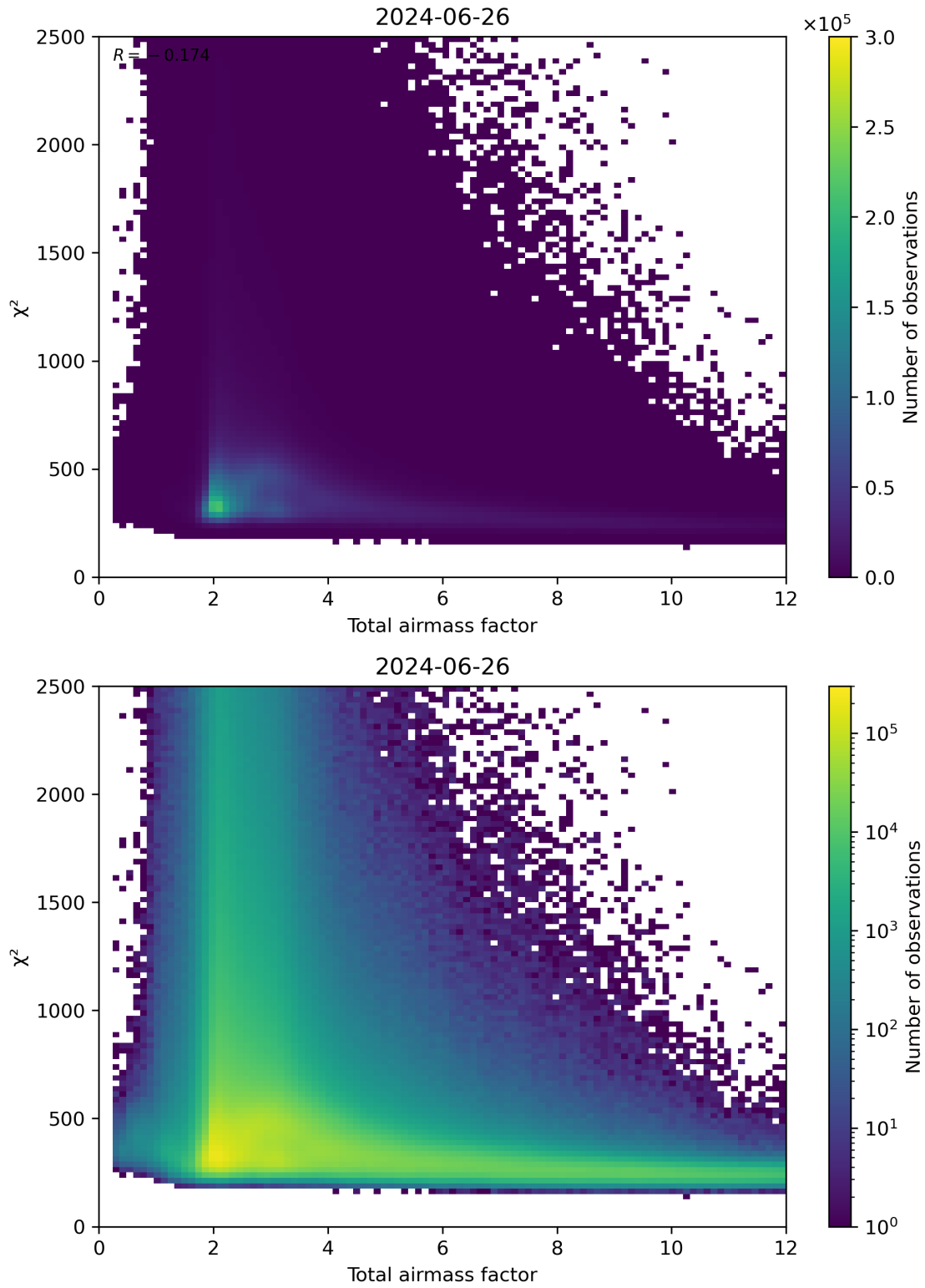
Figure 63: Scatter density plot of “Total airmass factor” against “ \chi^2 ” for 2024-06-25 to 2024-06-27.
