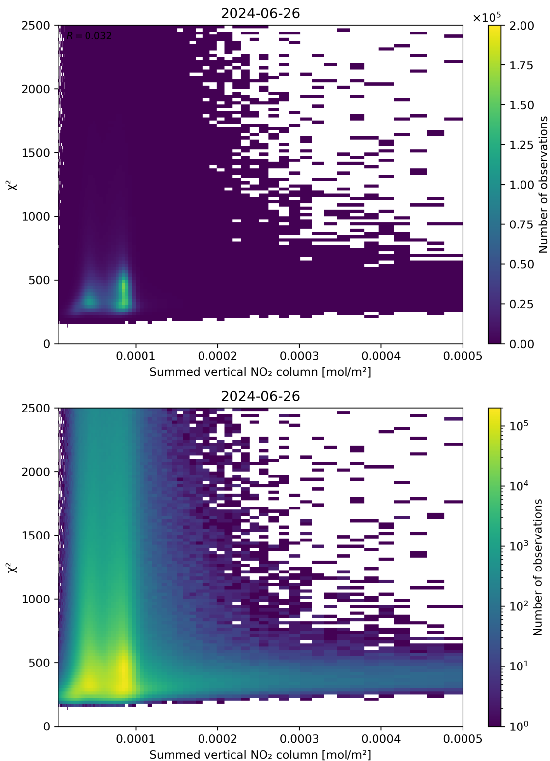
Figure 104: Scatter density plot of “Summed vertical NO 2 column” against “ \chi^2 ” for 2024-06-25 to 2024-06-27.
