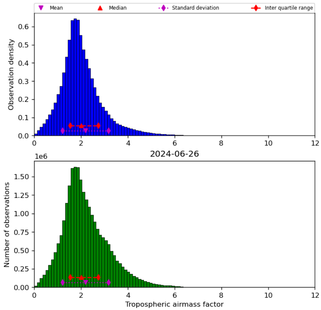
Figure 31: Histogram of “Tropospheric airmass factor” for 2024-06-25 to 2024-06-27
