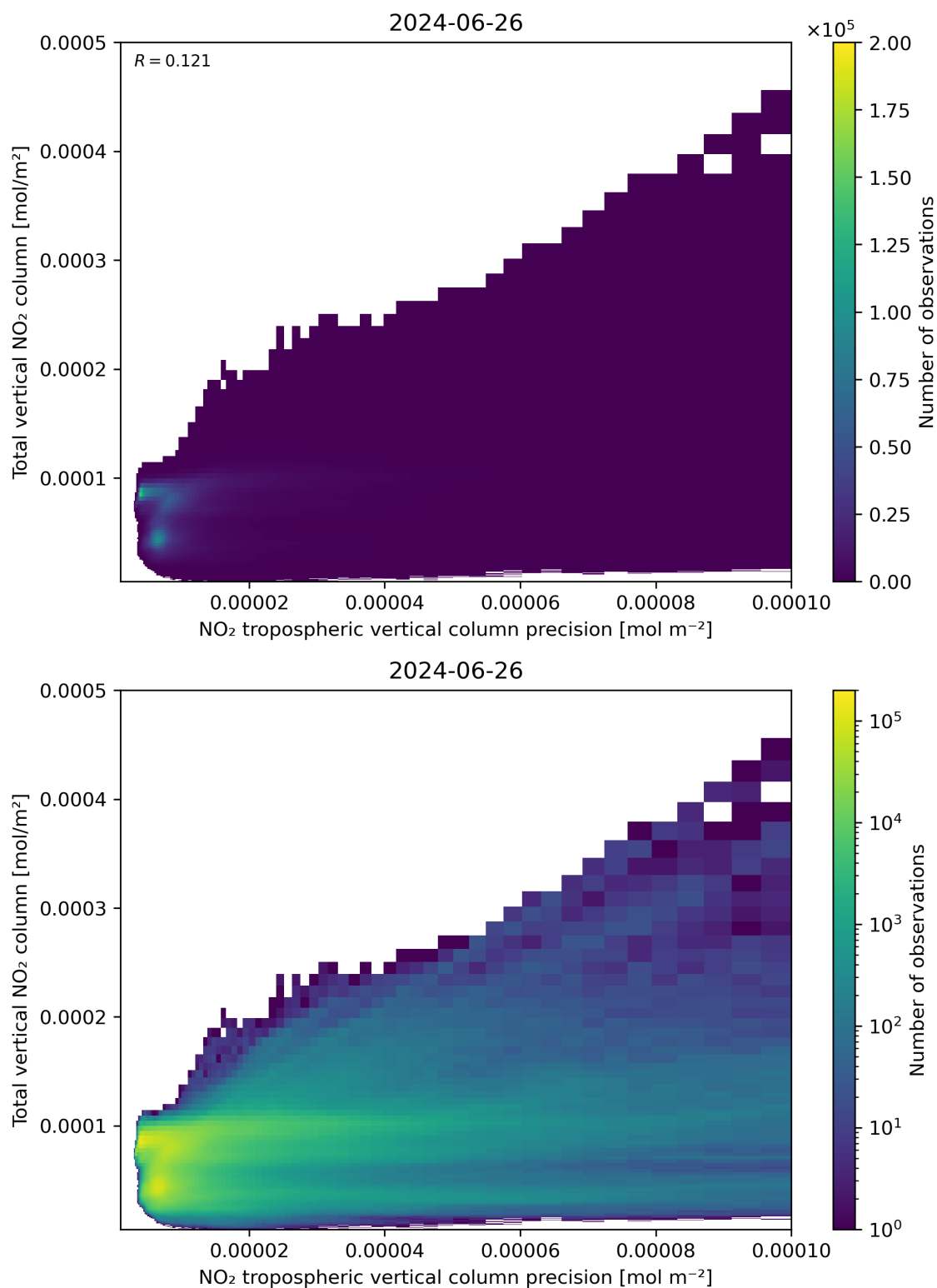
Figure 138: Scatter density plot of “NO 2 tropospheric vertical column precision” against “Total vertical NO 2 column” for 2024-06-25 to 2024-06-27.
