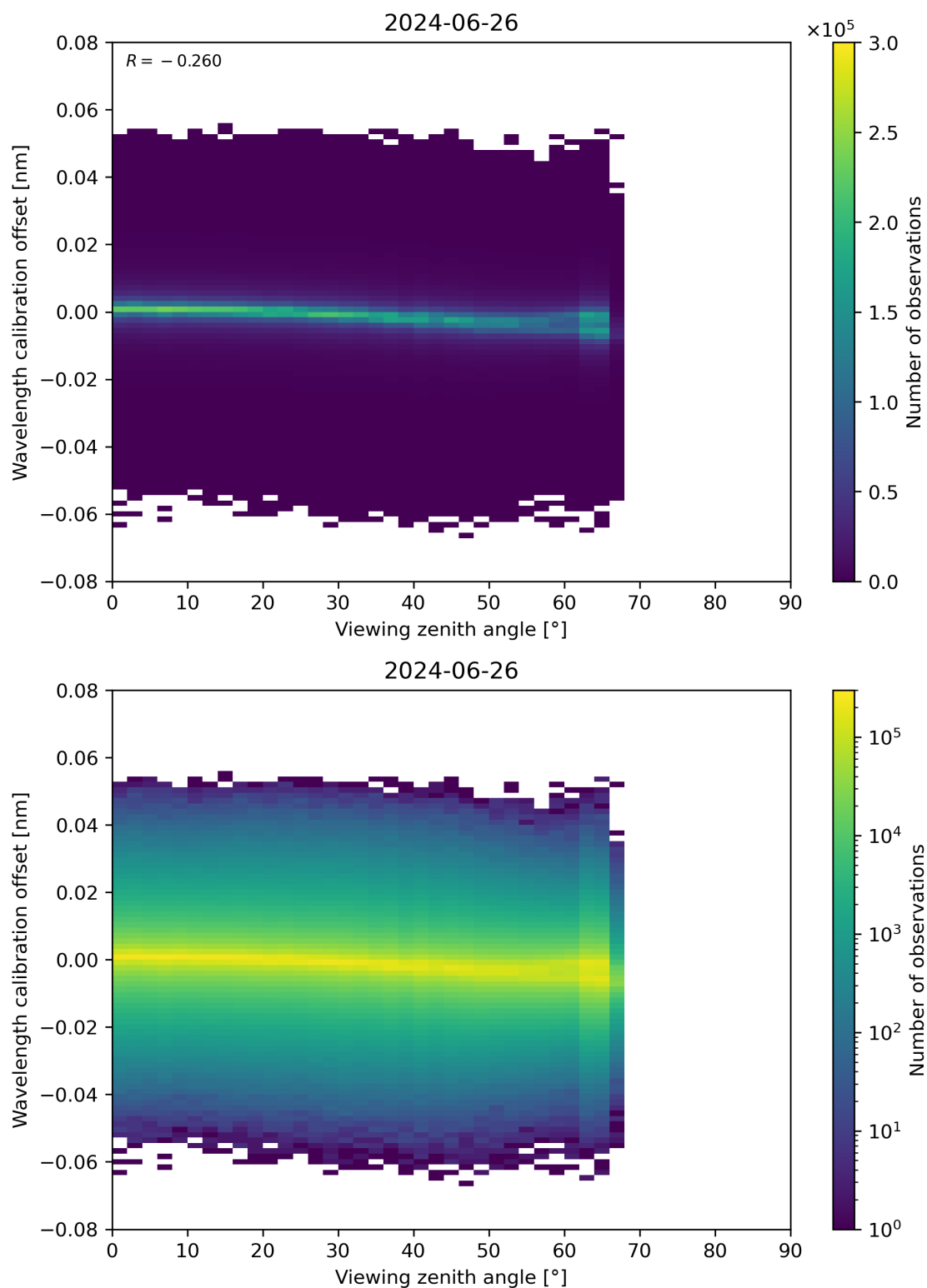
Figure 173: Scatter density plot of “Viewing zenith angle” against “Wavelength calibration offset” for 2024-06-25 to 2024-06-27.
