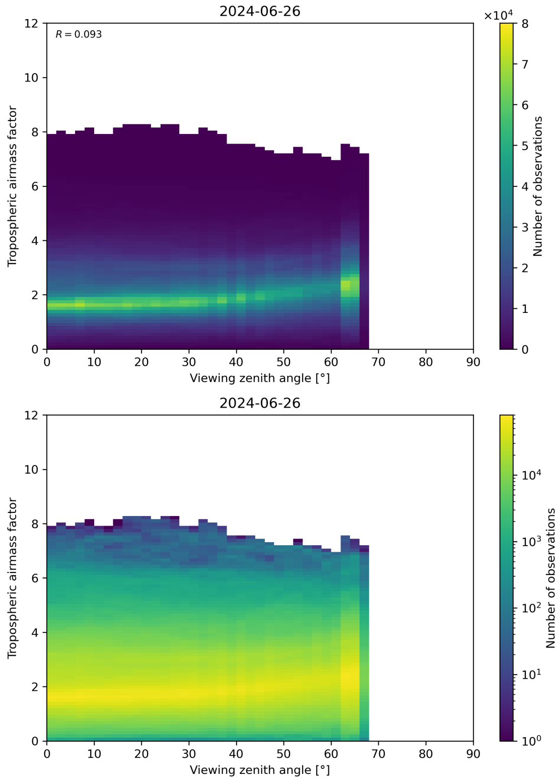
Figure 161: Scatter density plot of “Viewing zenith angle” against “Tropospheric airmass factor” for 2024-06-25 to 2024-06-27.
