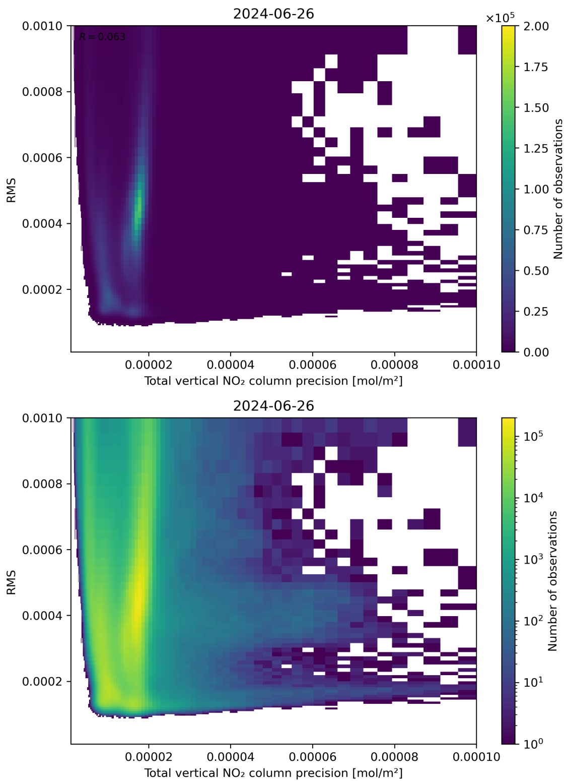
Figure 119: Scatter density plot of “Total vertical NO 2 column precision” against “RMS” for 2024-06-25 to 2024-06-27.
