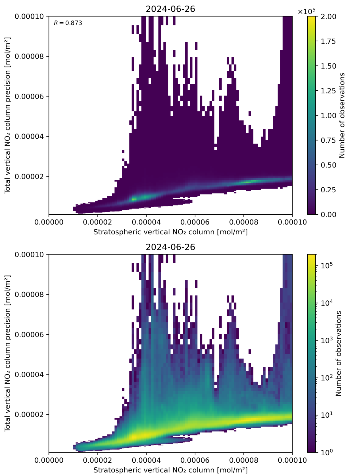
Figure 101: Scatter density plot of “Stratospheric vertical NO 2 column” against “Total vertical NO 2 column precision” for 2024-06-25 to 2024-06-27.
