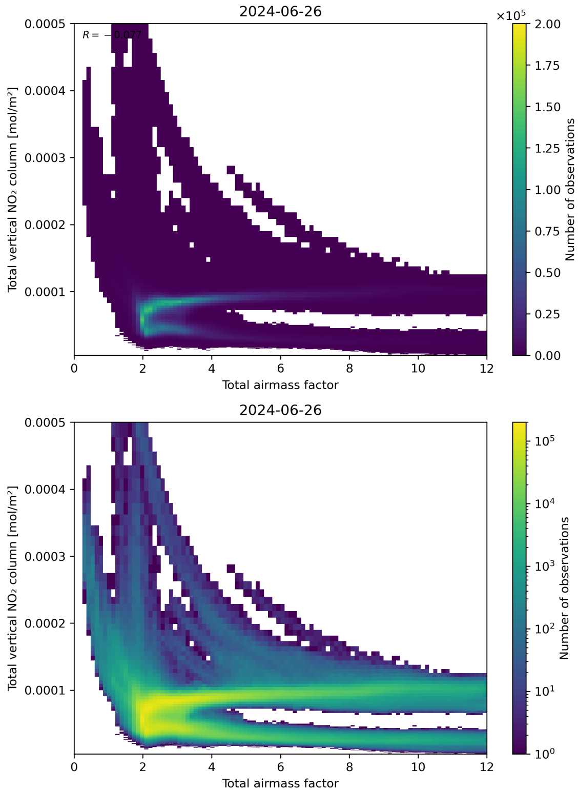
Figure 67: Scatter density plot of “Total airmass factor” against “Total vertical NO 2 column” for 2024-06-25 to 2024-06-27.
