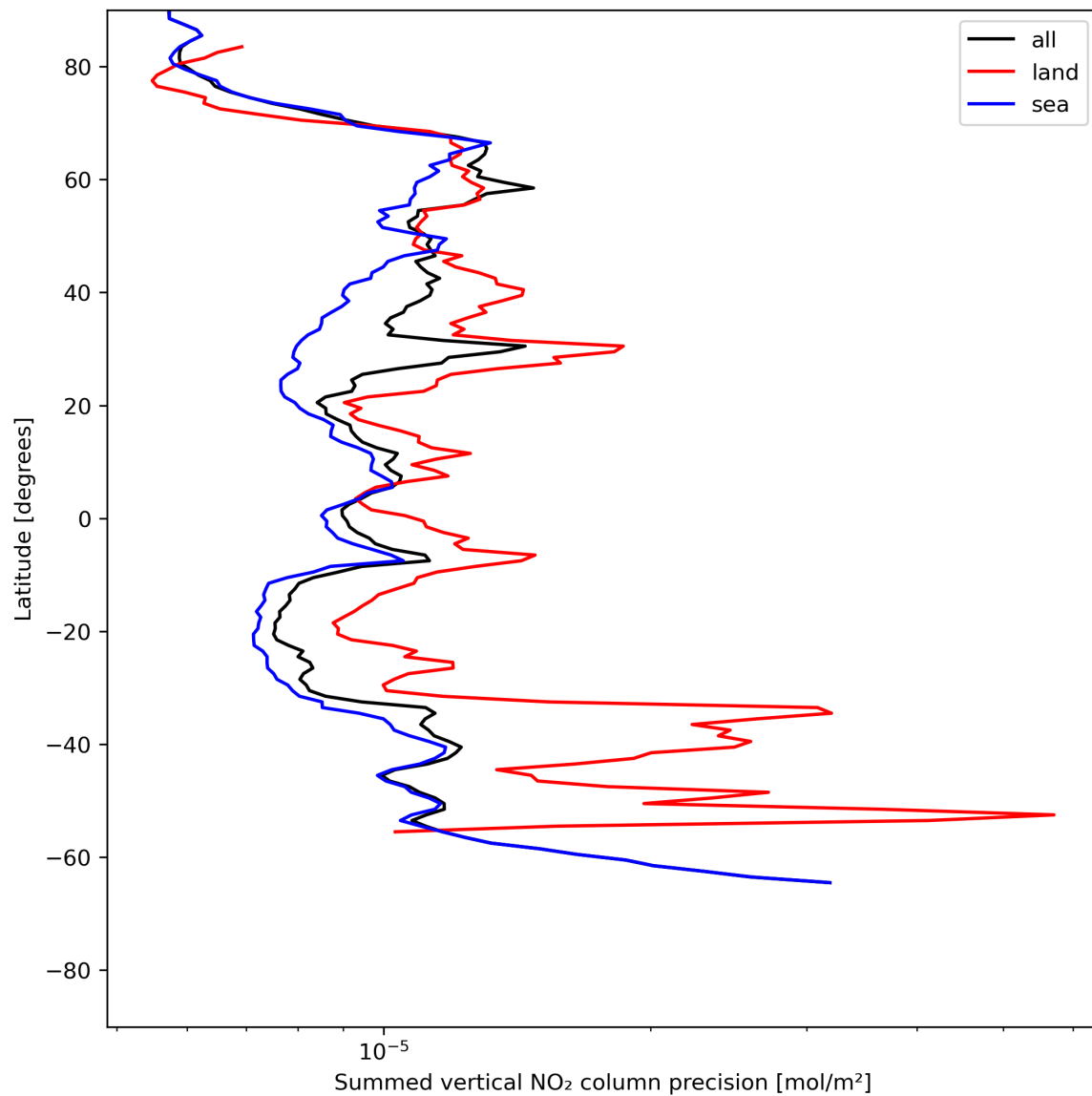
Figure 24: Zonal average of “Summed vertical NO 2 column precision” for 2024-06-25 to 2024-06-27.
