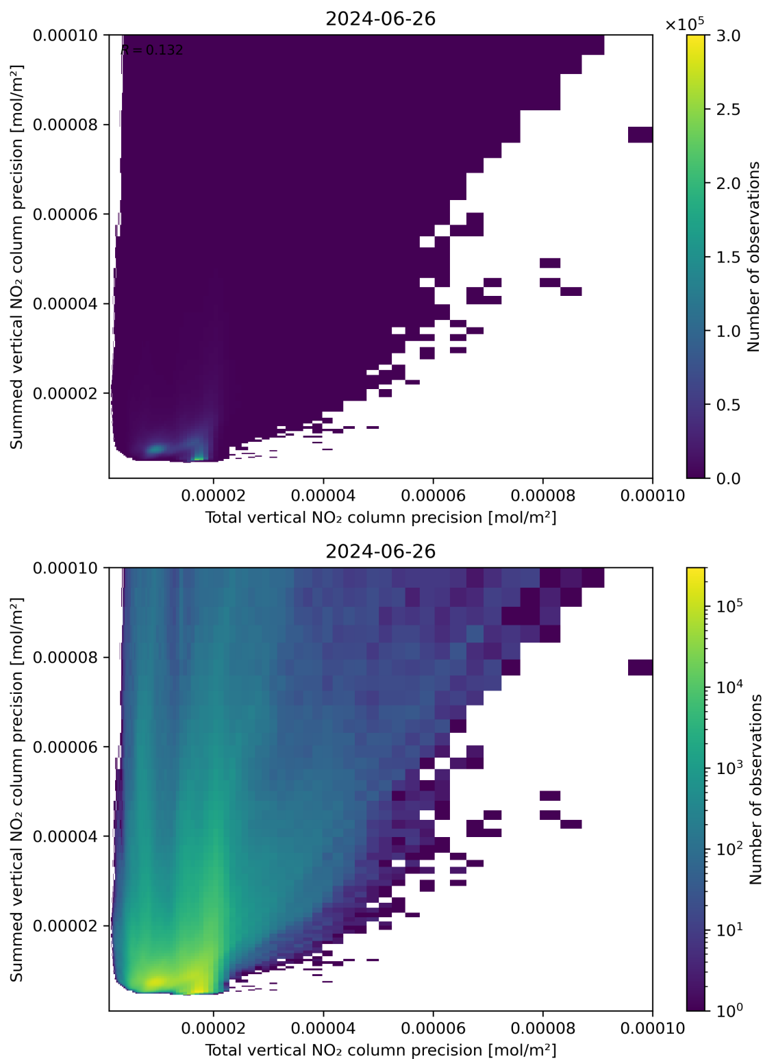
Figure 118: Scatter density plot of “Total vertical NO 2 column precision” against “Summed vertical NO 2 column precision” for 2024-06-25 to 2024-06-27.
