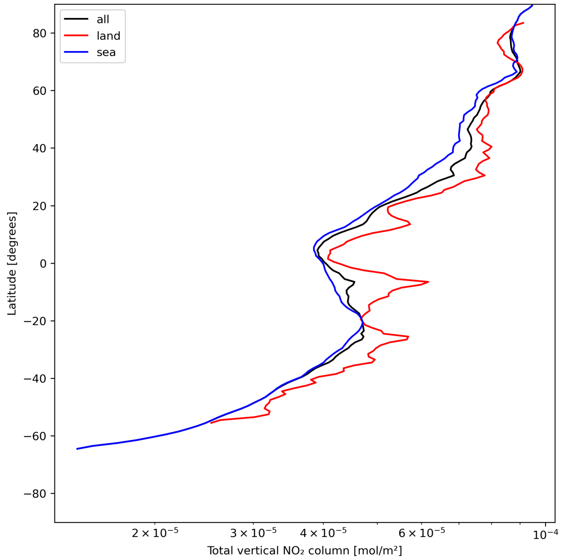
Figure 21: Zonal average of “Total vertical NO 2 column” for 2024-06-25 to 2024-06-27.
