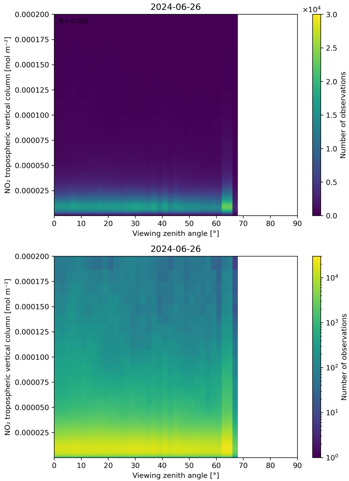
Figure 169: Scatter density plot of “Viewing zenith angle” against “NO 2 tropospheric vertical column” for 2024-06-25 to 2024-06-27.
