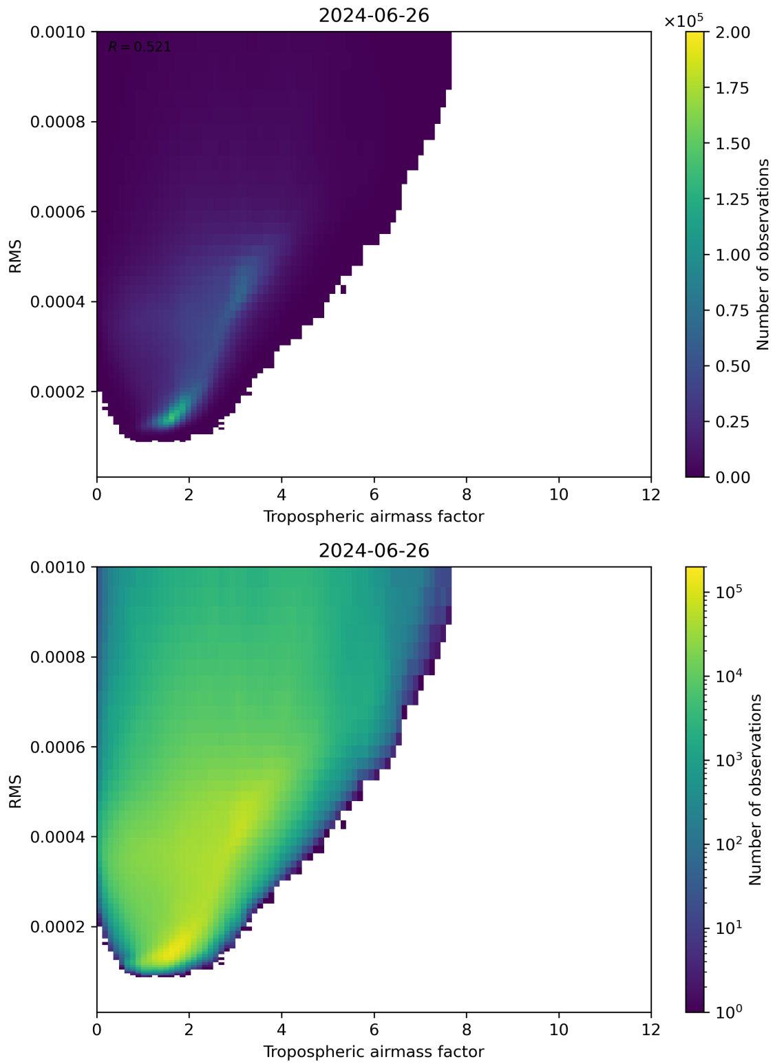
Figure 79: Scatter density plot of “Tropospheric airmass factor” against “RMS” for 2024-06-25 to 2024-06-27.
