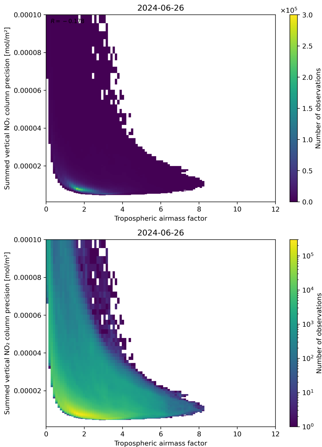
Figure 76: Scatter density plot of “Tropospheric air mass factor” against “Summed vertical NO 2 column precision” for 2024-06-25 to 2024-06-27.
