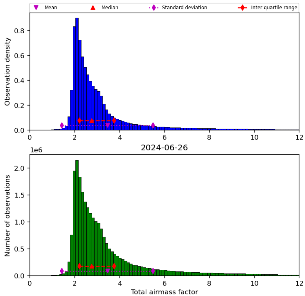
Figure 32: Histogram of “Total airmass factor” for 2024-06-25 to 2024-06-27
