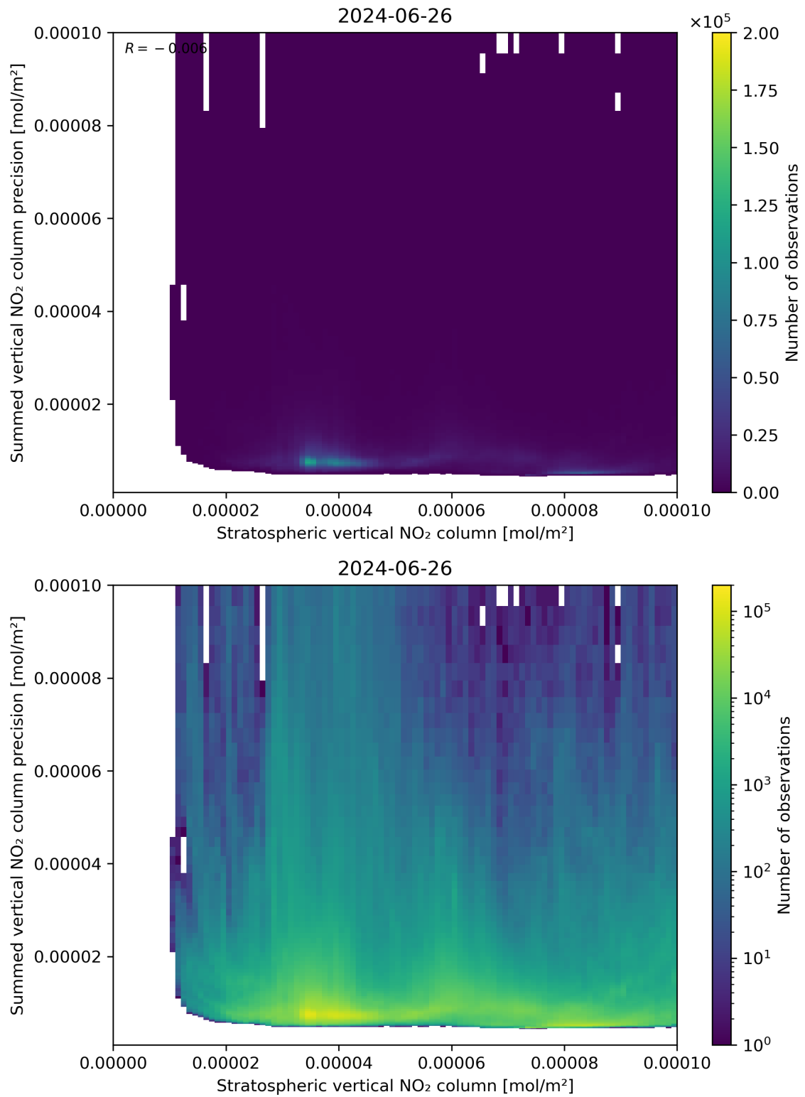
Figure 99: Scatter density plot of “Stratospheric vertical NO 2 column” against “Summed vertical NO 2 column precision” for 2024-06-25 to 2024-06-27.
