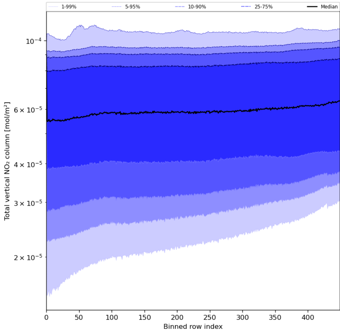
Figure 55: Along track statistics of “Total vertical NO 2 column” for 2024-06-25 to 2024-06-27
