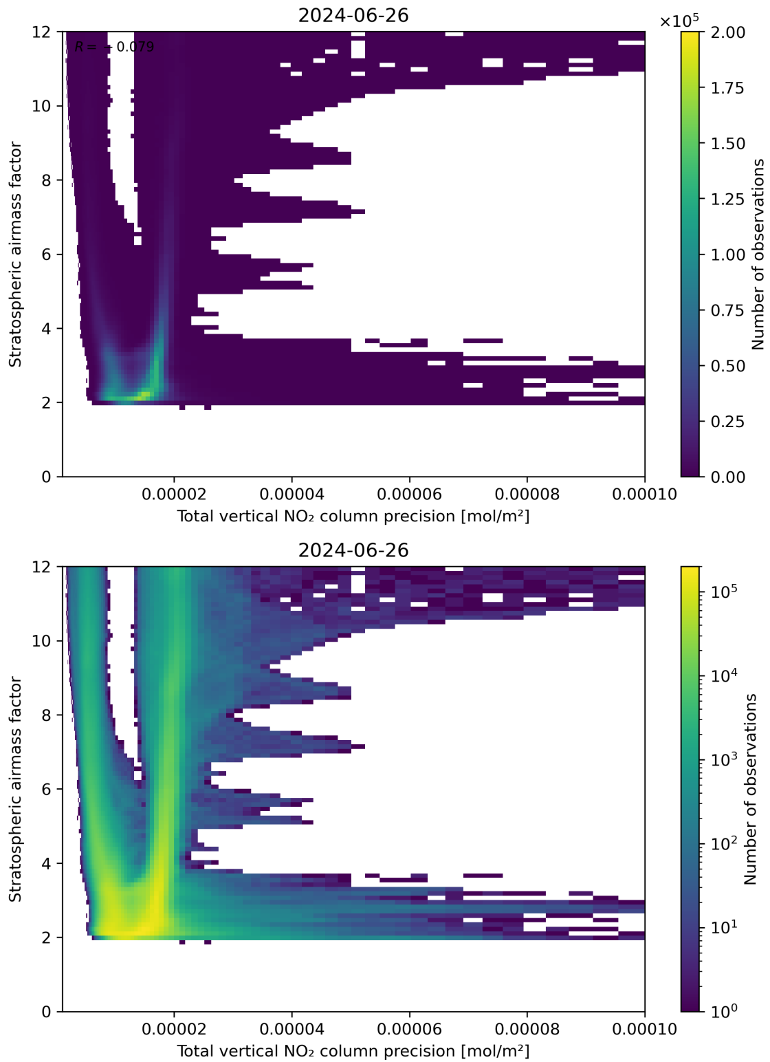
Figure 115: Scatter density plot of “Total vertical NO 2 column precision” against “Stratospheric air mass factor” for 2024-06-25 to 2024-06-27.
