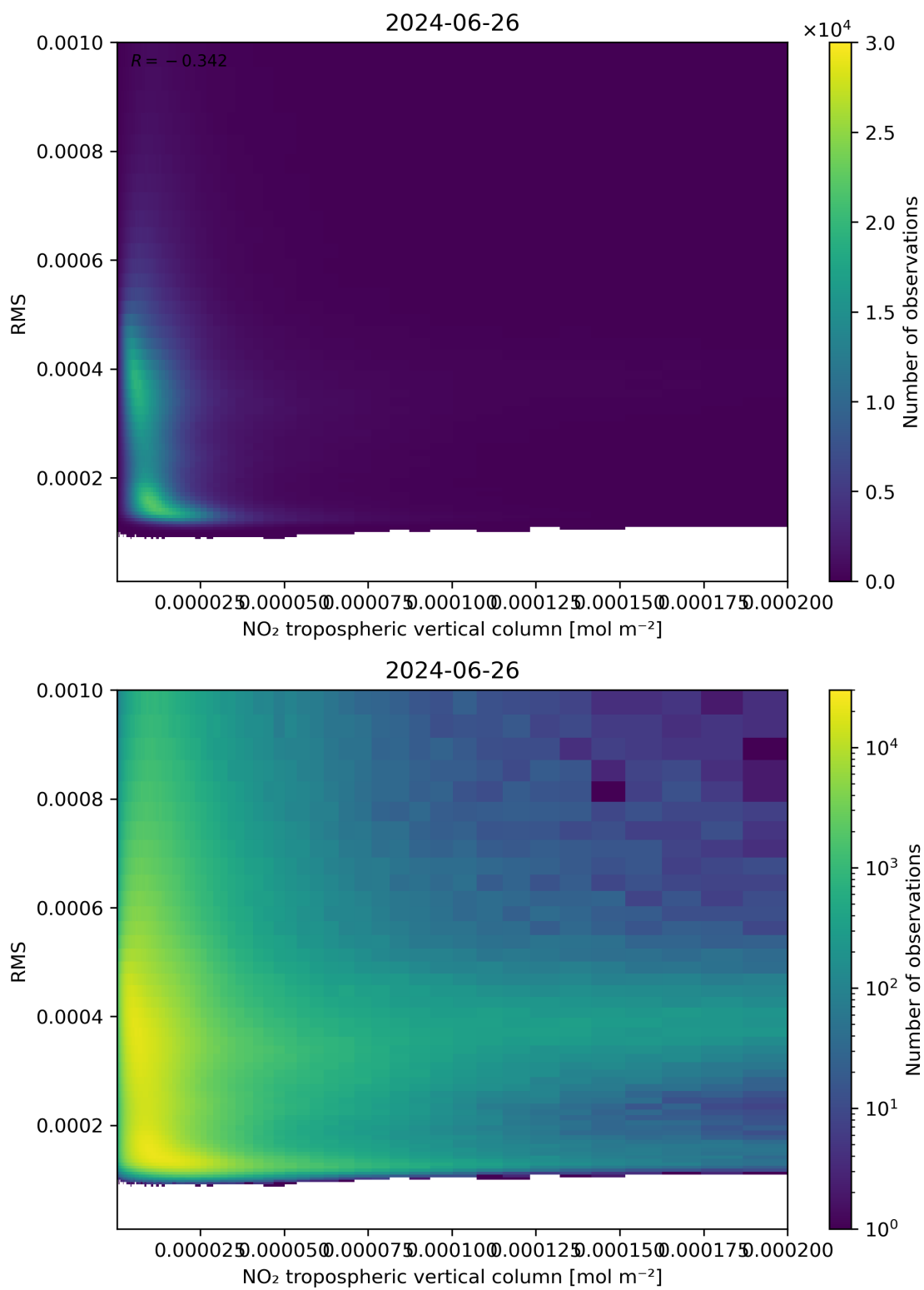
Figure 142: Scatter density plot of “NO 2 tropospheric vertical column” against “RMS” for 2024-06-25 to 2024-06-27.
