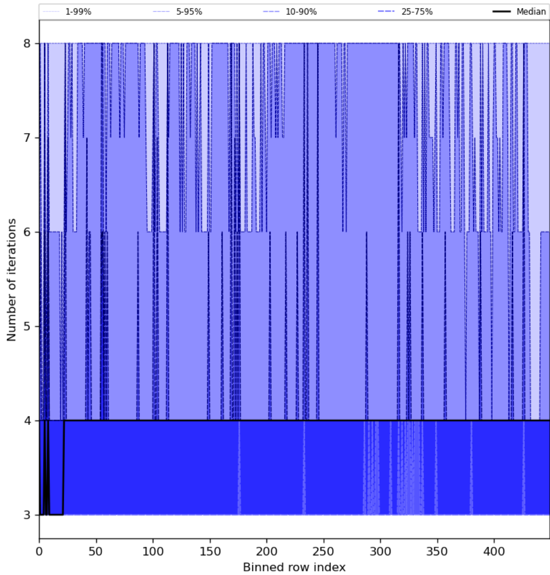
Figure 51: Along track statistics of “Number of iterations” for 2024-06-25 to 2024-06-27
