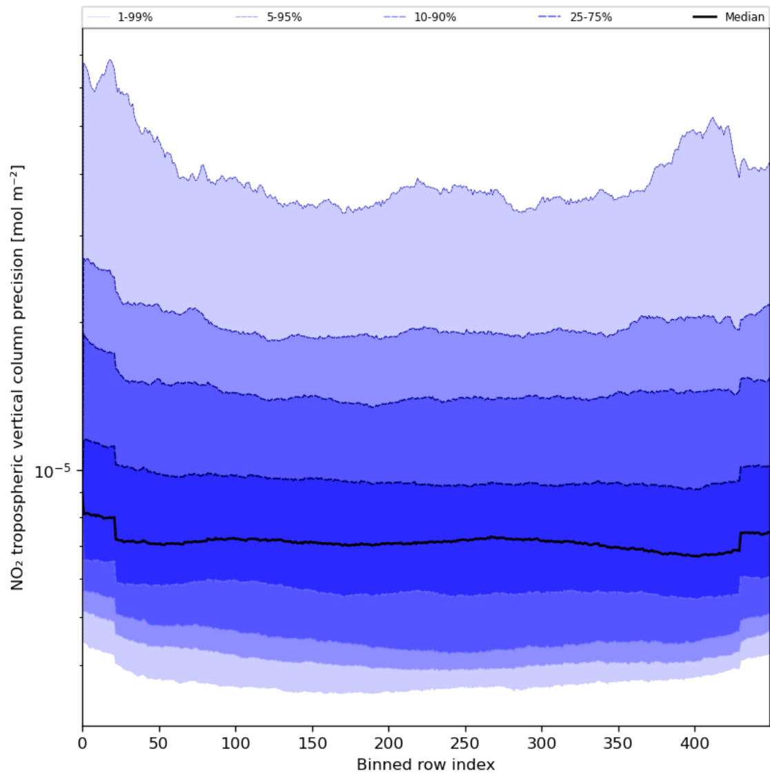
Figure 47: Along track statistics of “NO 2 tropospheric vertical column precision” for 2024-06-25 to 2024-06-27
