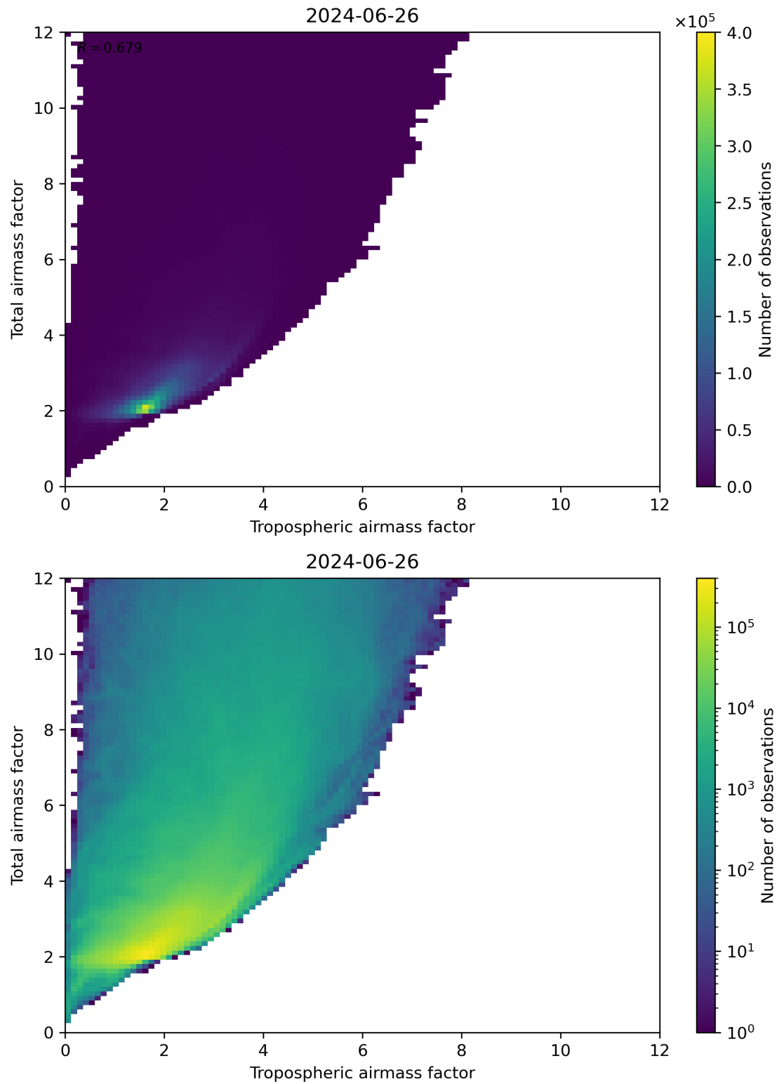
Figure 72: Scatter density plot of “Tropospheric airmass factor” against “Total airmass factor” for 2024-06-25 to 2024-06-27.
