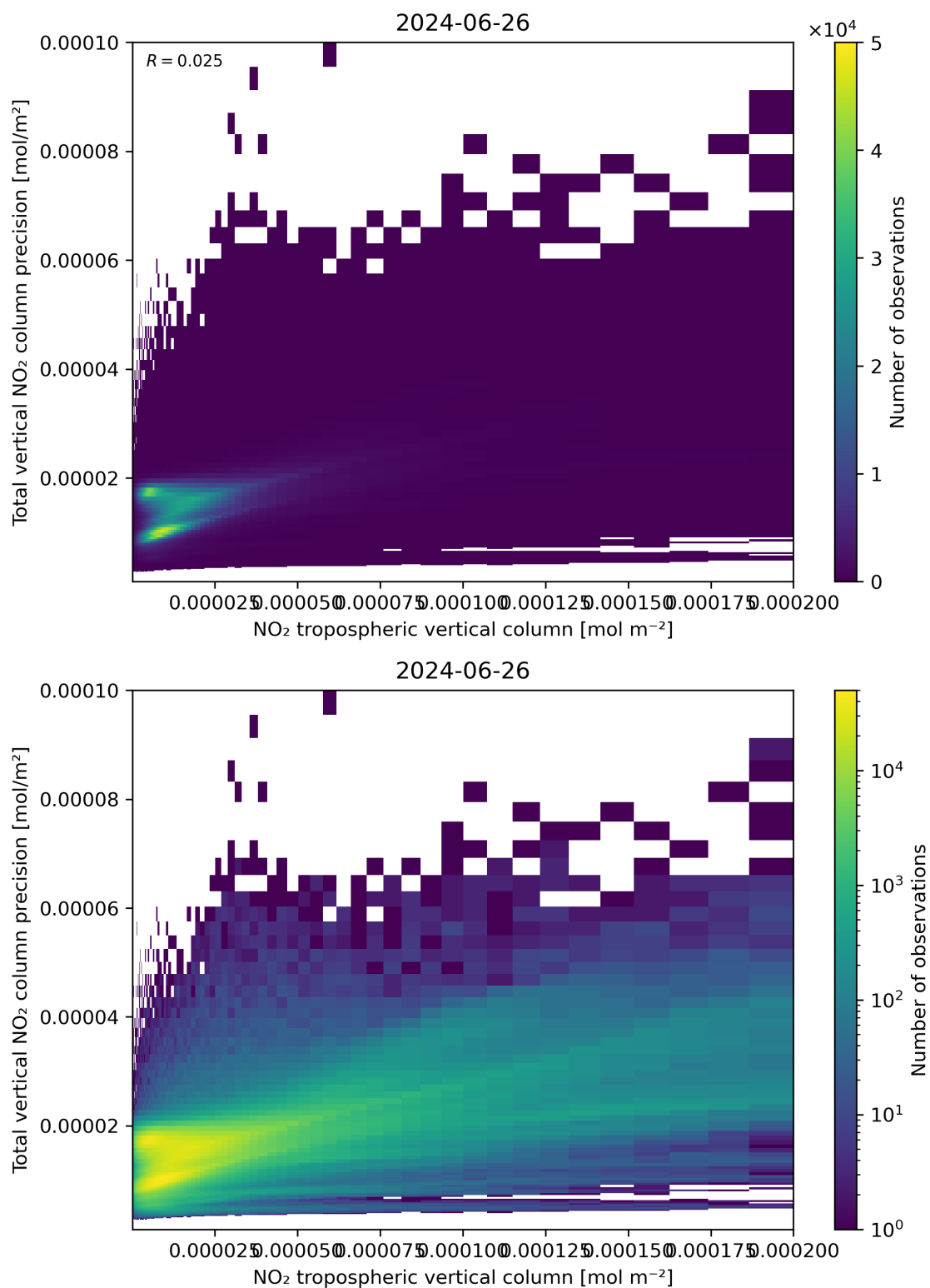
Figure 129: Scatter density plot of “NO 2 tropospheric vertical column” against “Total vertical NO 2 column precision” for 2024-06-25 to 2024-06-27.
