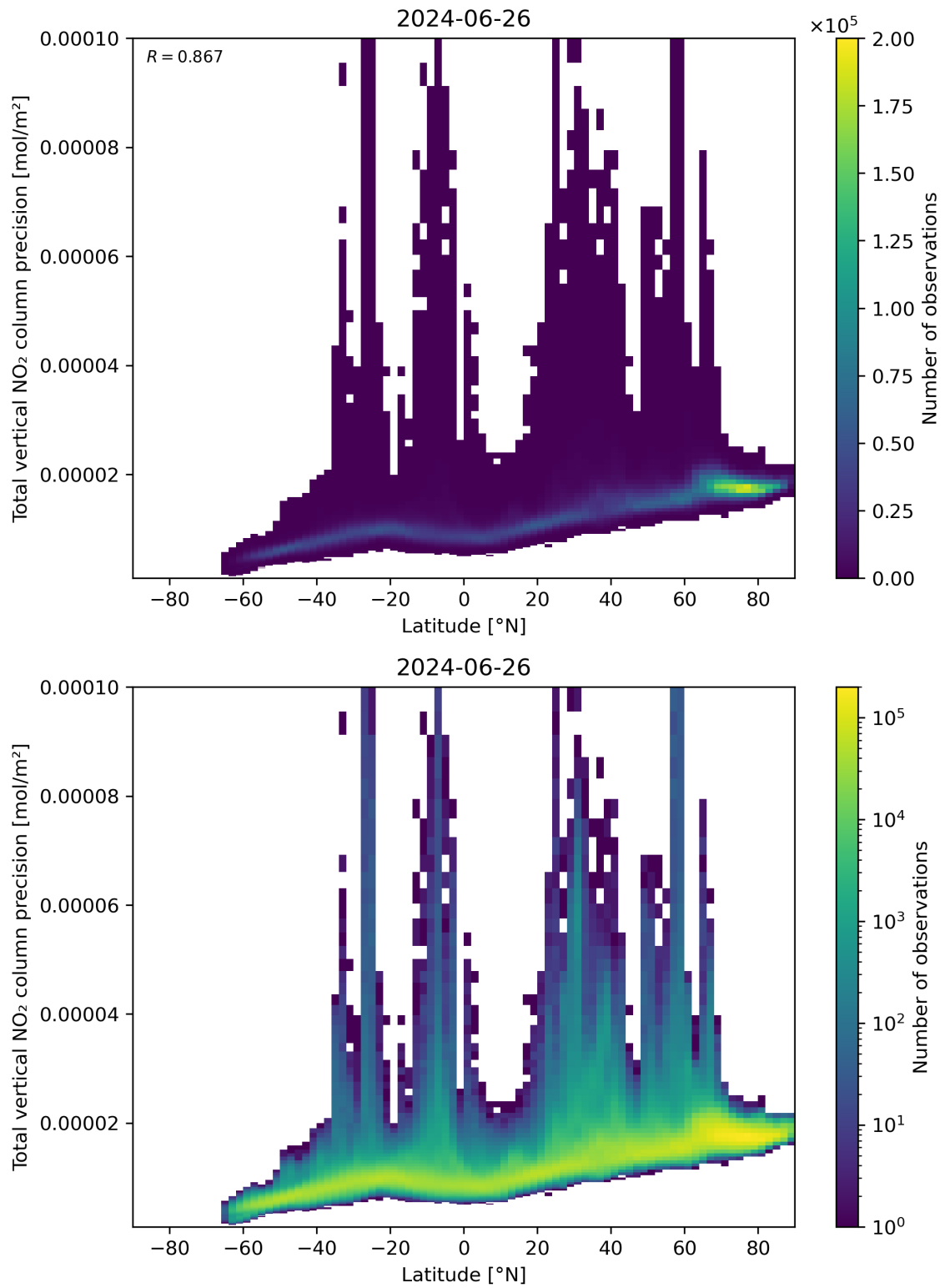
Figure 91: Scatter density plot of “Latitude” against “Total vertical NO 2 column precision” for 2024-06-25 to 2024-06-27.
