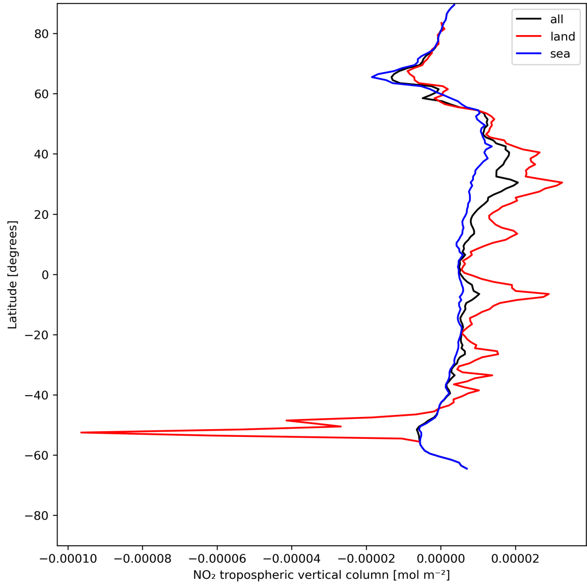
Figure 12: Zonal average of “NO 2 tropospheric vertical column” for 2024-06-25 to 2024-06-27.
