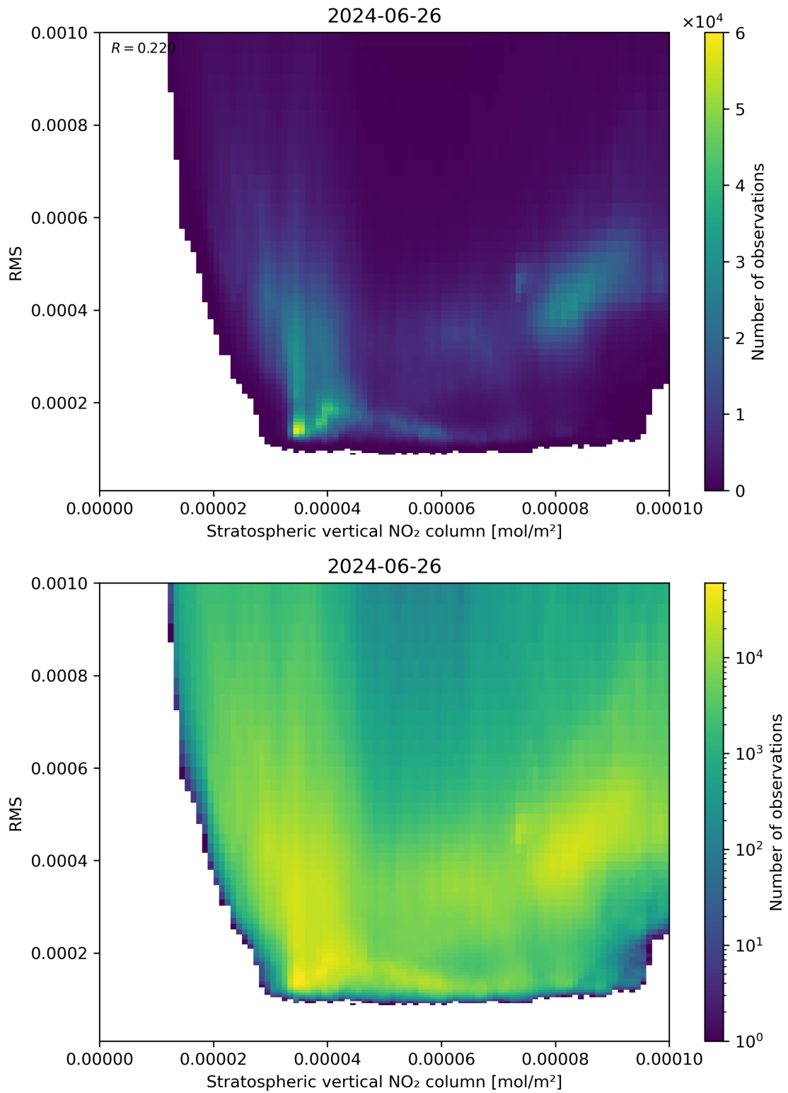
Figure 102: Scatter density plot of “Stratospheric vertical NO 2 column” against “RMS” for 2024-06-25 to 2024-06-27.
