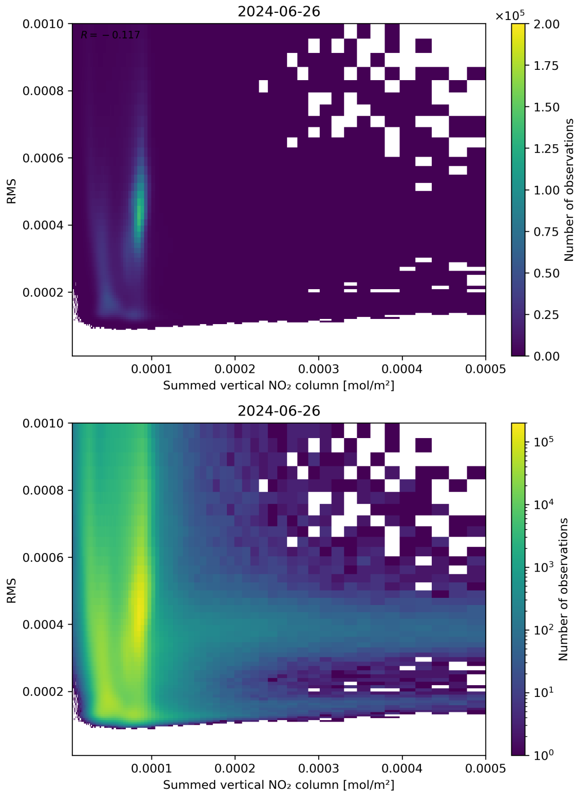
Figure 109: Scatter density plot of “Summed vertical NO 2 column” against “RMS” for 2024-06-25 to 2024-06-27.
