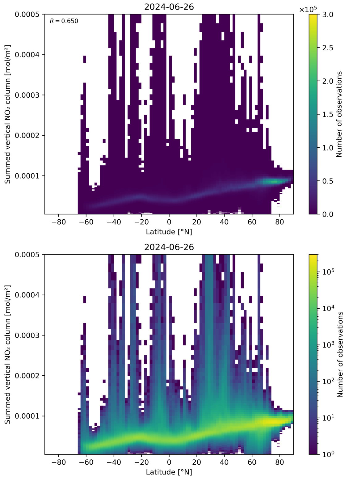
Figure 88: Scatter density plot of “Latitude” against “Summed vertical NO 2 column” for 2024-06-25 to 2024-06-27.
