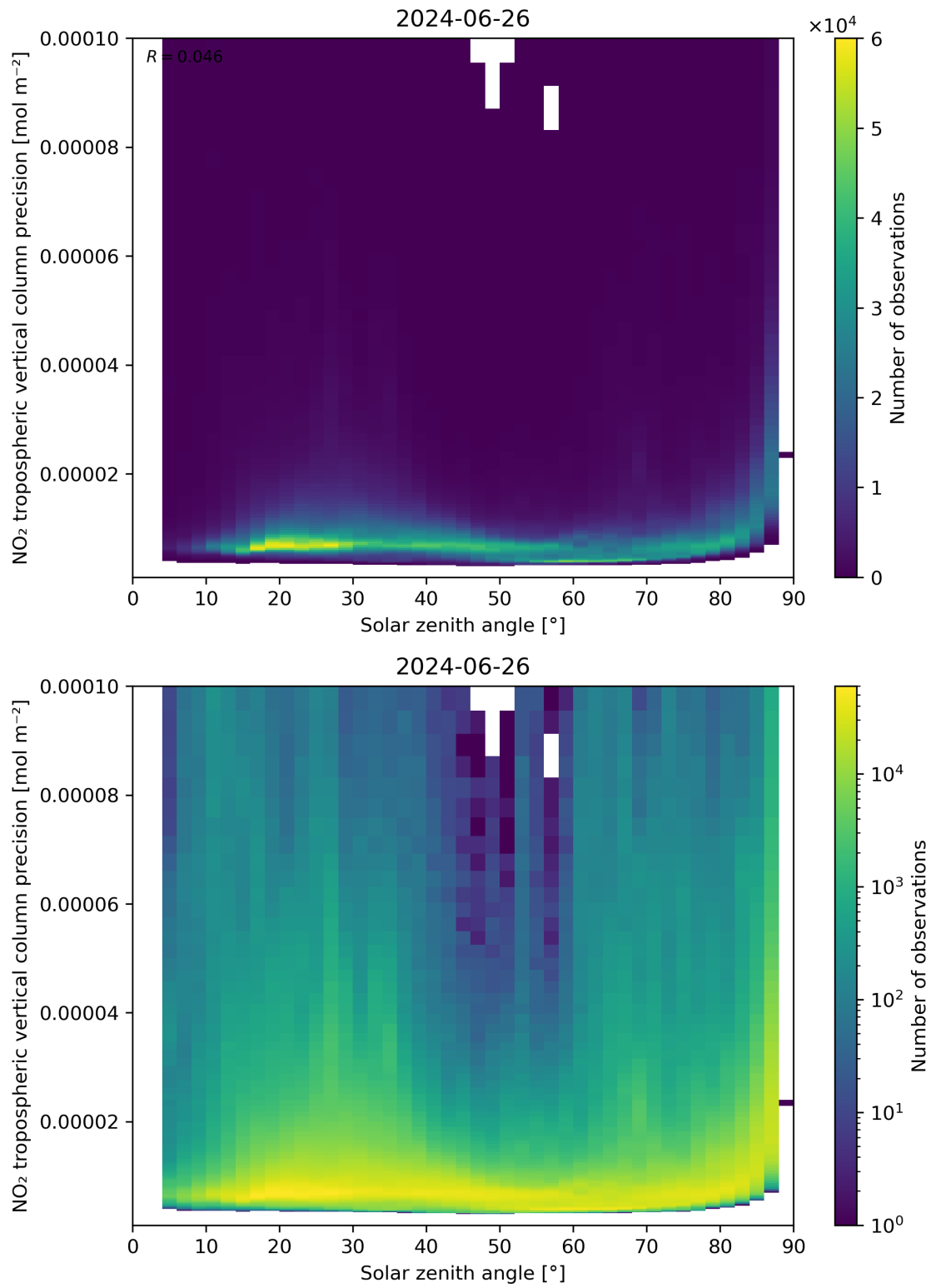
Figure 156: Scatter density plot of “Solar zenith angle” against “NO 2 tropospheric vertical column precision” for 2024-06-25 to 2024-06-27.
