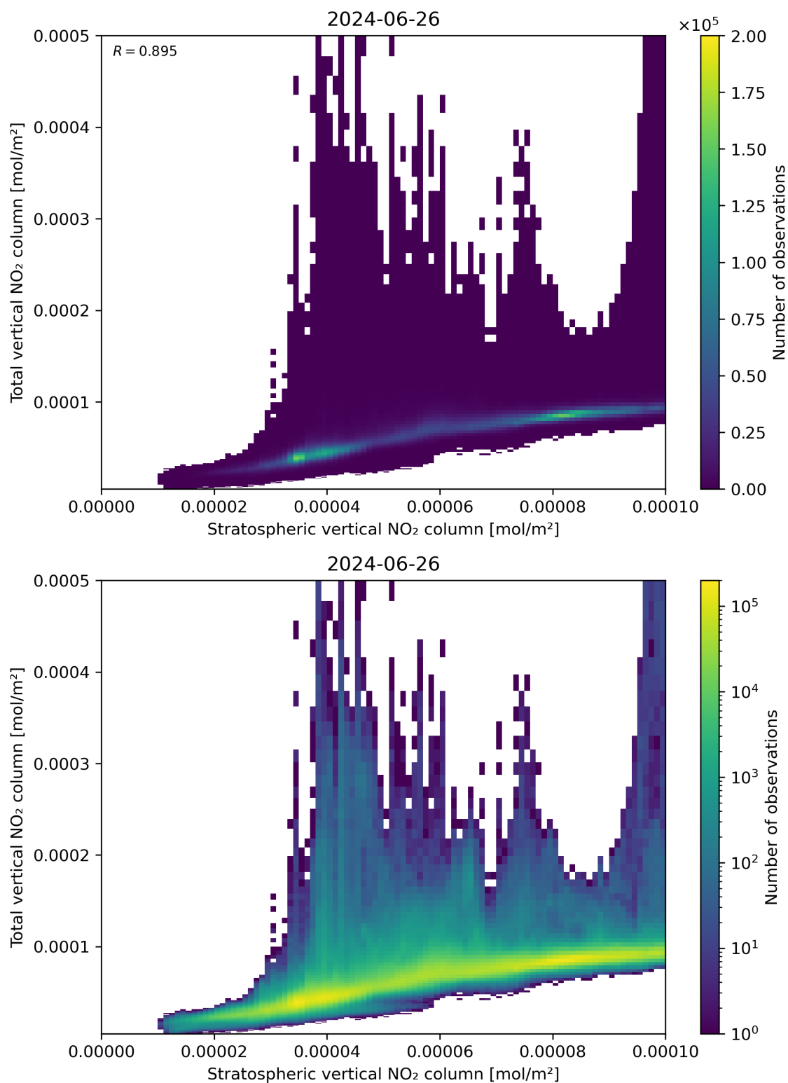
Figure 100: Scatter density plot of “Stratospheric vertical NO 2 column” against “Total vertical NO 2 column” for 2024-06-25 to 2024-06-27.
