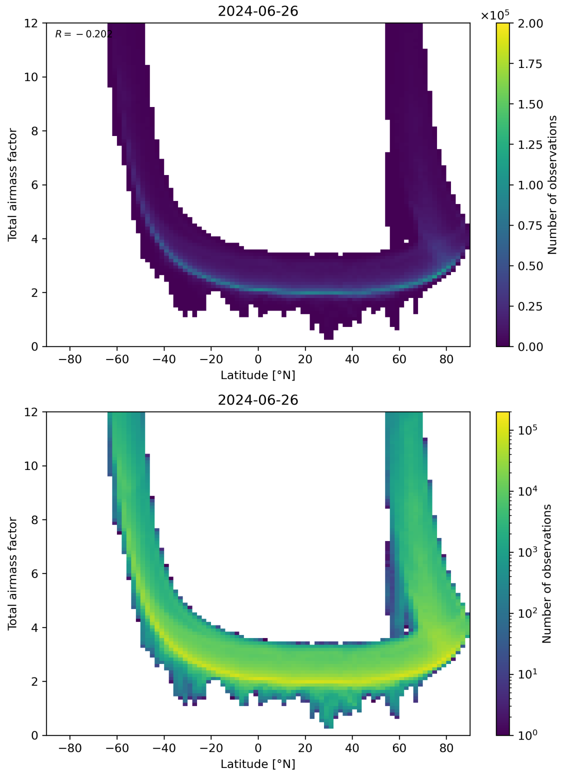
Figure 84: Scatter density plot of “Latitude” against “Total airmass factor” for 2024-06-25 to 2024-06-27.
