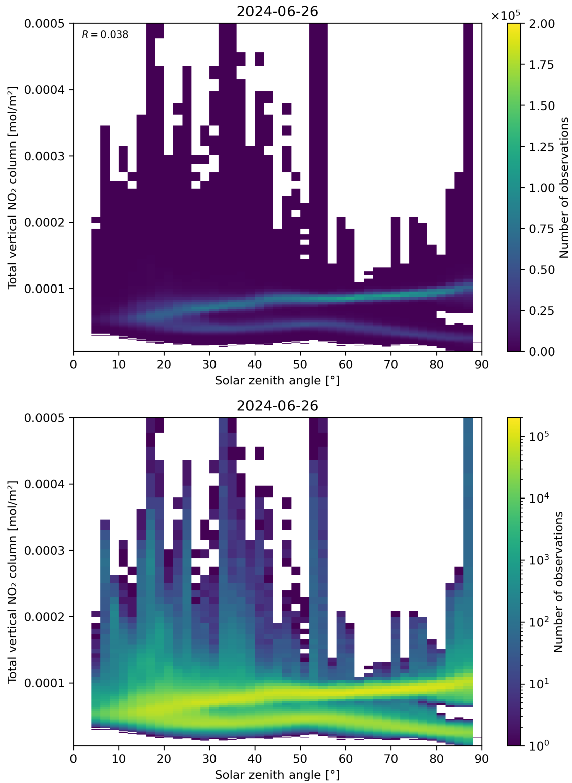
Figure 153: Scatter density plot of “Solar zenith angle” against “Total vertical \text{NO}_2 column” for 2024-06-25 to 2024-06-27.
