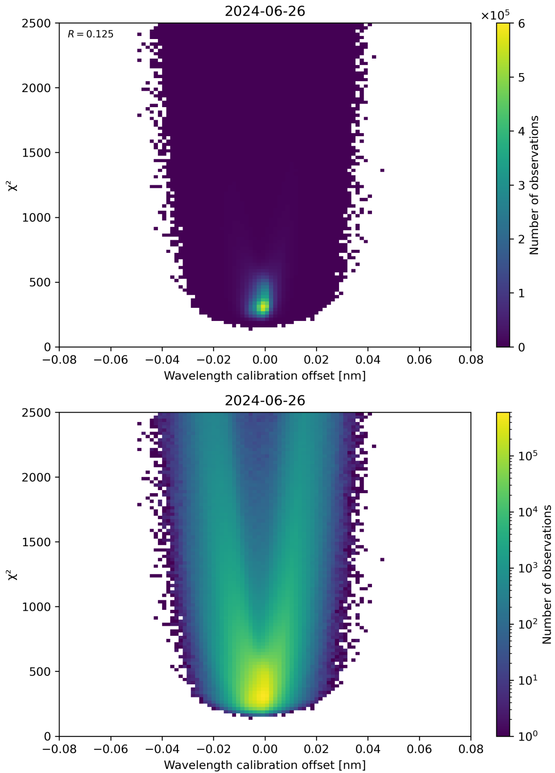
Figure 175: Scatter density plot of “Wavelength calibration offset” against “ \chi^2 ” for 2024-06-25 to 2024-06-27.
