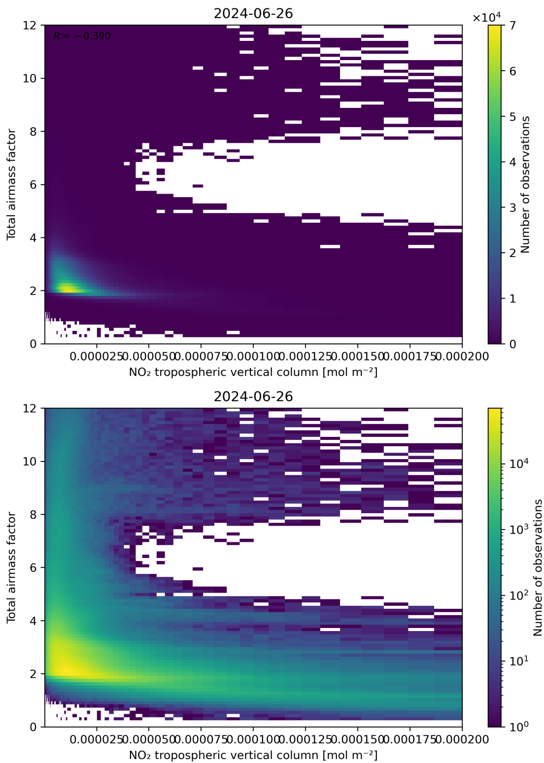
Figure 122: Scatter density plot of “NO 2 tropospheric vertical column” against “Total airmass factor” for 2024-06-25 to 2024-06-27.
