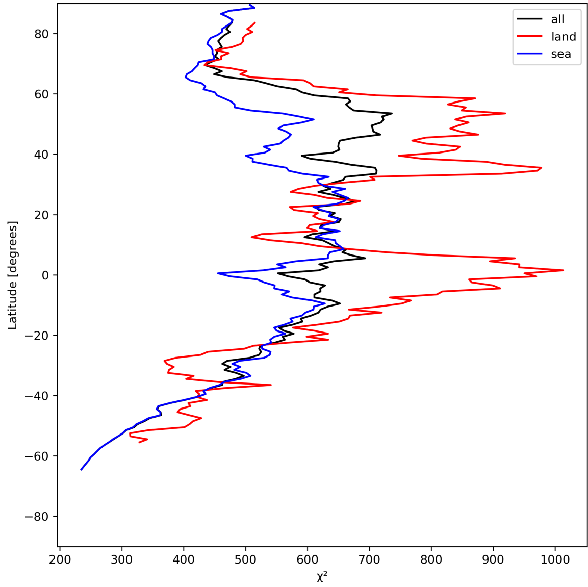
Figure 25: Zonal average of “ \chi^2 ” for 2024-06-25 to 2024-06-27.
