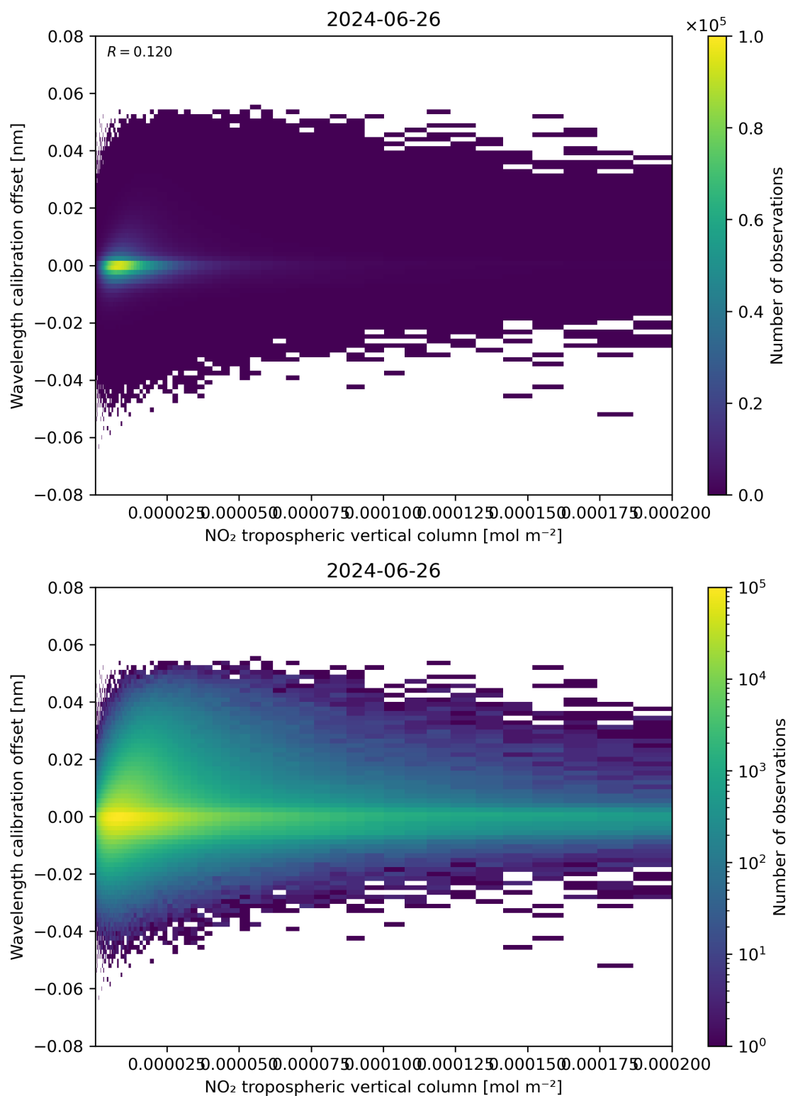
Figure 143: Scatter density plot of “NO 2 tropospheric vertical column” against “Wavelength calibration offset” for 2024-06-25 to 2024-06-27.
