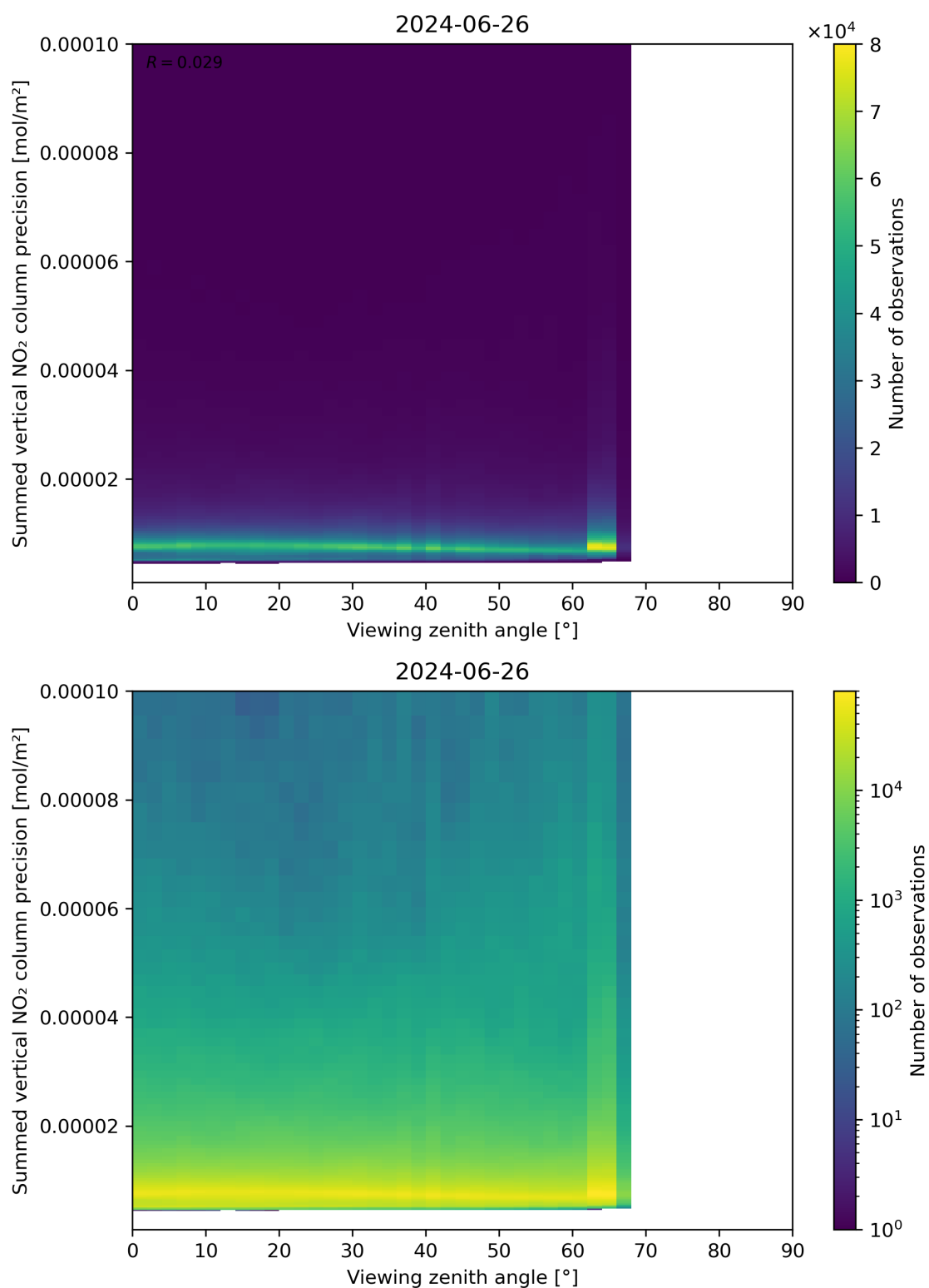
Figure 166: Scatter density plot of “Viewing zenith angle” against “Summed vertical NO 2 column precision” for 2024-06-25 to 2024-06-27.
