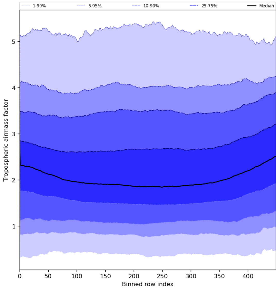
Figure 48: Along track statistics of “Tropospheric airmass factor” for 2024-06-25 to 2024-06-27
