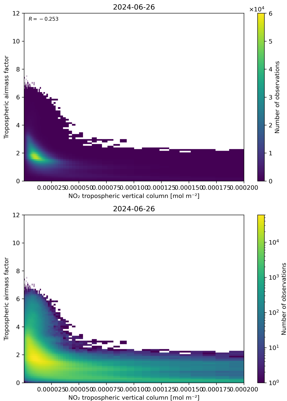
Figure 123: Scatter density plot of “NO 2 tropospheric vertical column” against “Tropospheric air mass factor” for 2024-06-25 to 2024-06-27.
