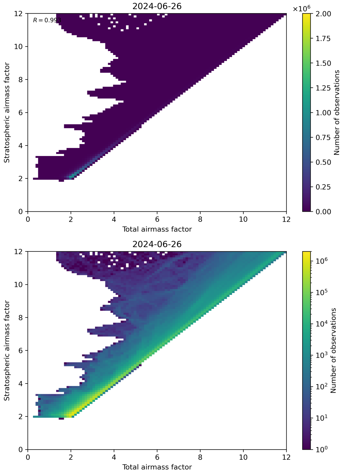
Figure 62: Scatter density plot of “Total airmass factor” against “Stratospheric airmass factor” for 2024-06-25 to 2024-06-27.
