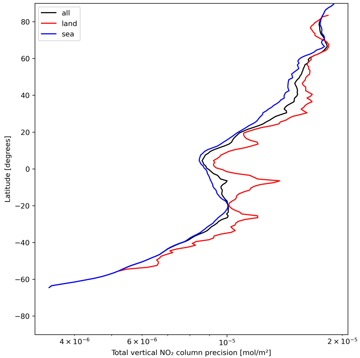
Figure 22: Zonal average of “Total vertical NO 2 column precision” for 2024-06-25 to 2024-06-27.
