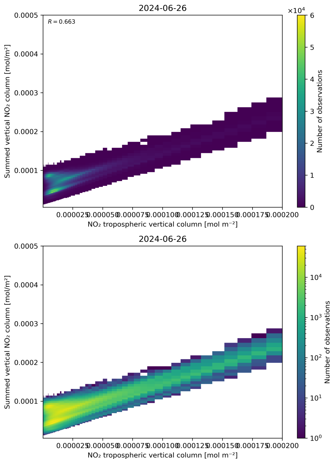
Figure 126: Scatter density plot of “NO 2 tropospheric vertical column” against “Summed vertical NO 2 column” for 2024-06-25 to 2024-06-27.
