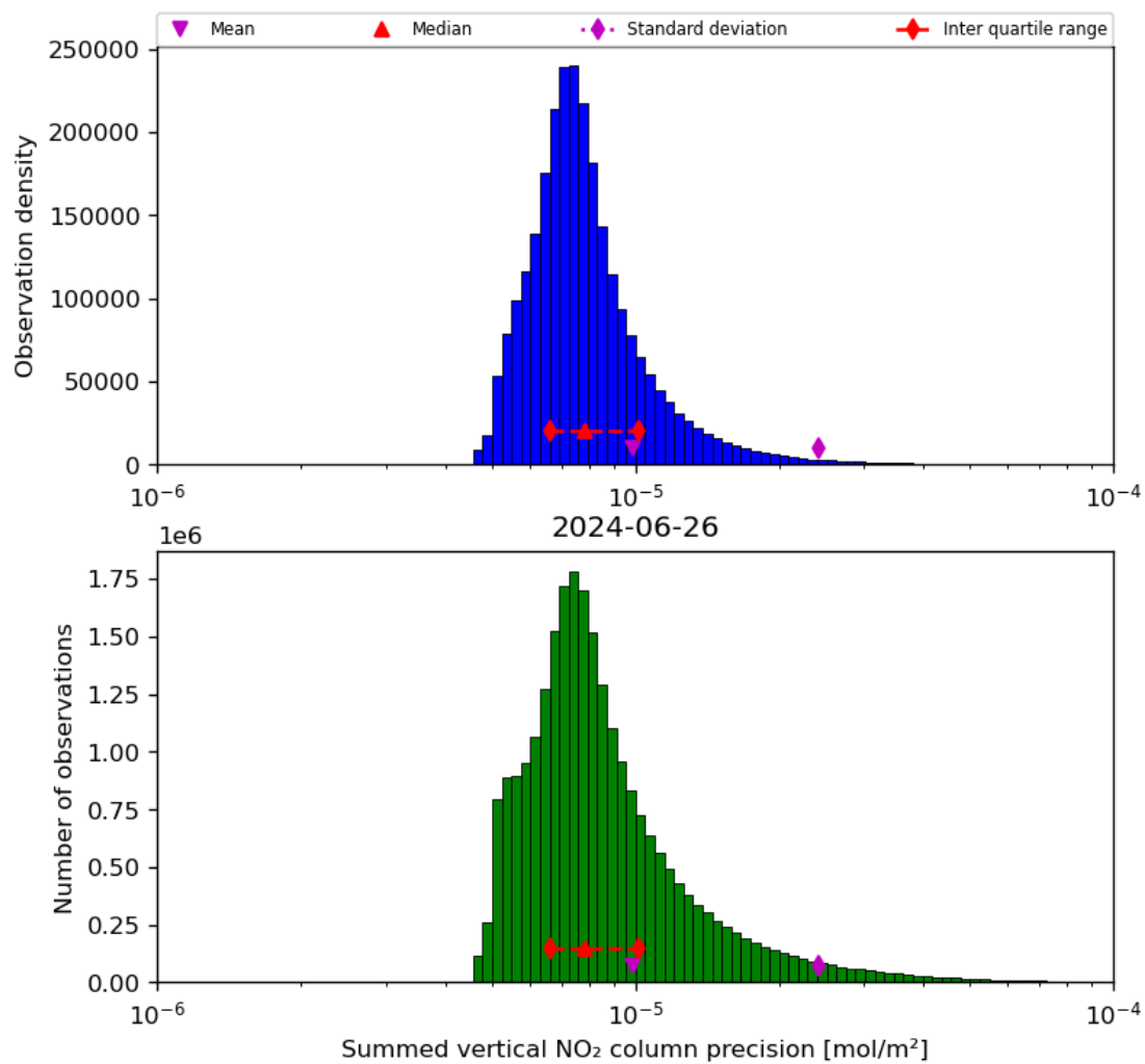
Figure 41: Histogram of "Summed vertical NO 2 column precision" for 2024-06-25 to 2024-06-27
