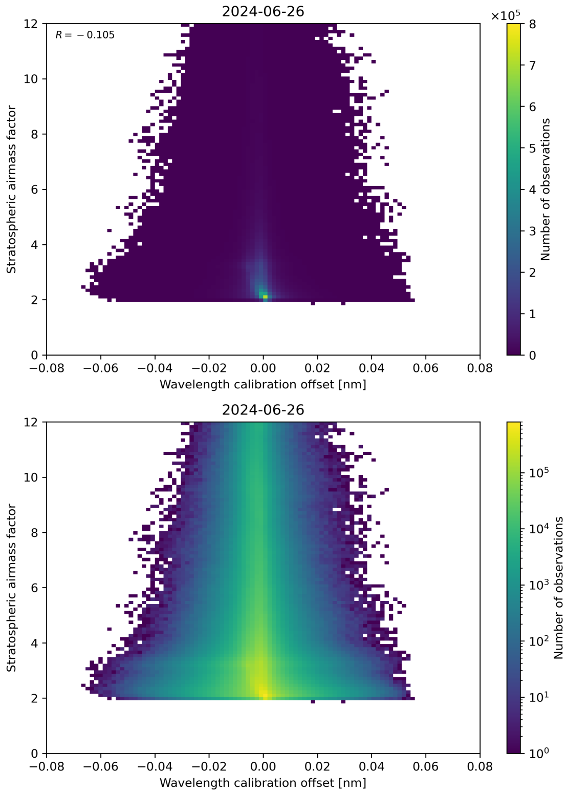
Figure 174: Scatter density plot of “Wavelength calibration offset” against “Stratospheric air mass factor” for 2024-06-25 to 2024-06-27.
