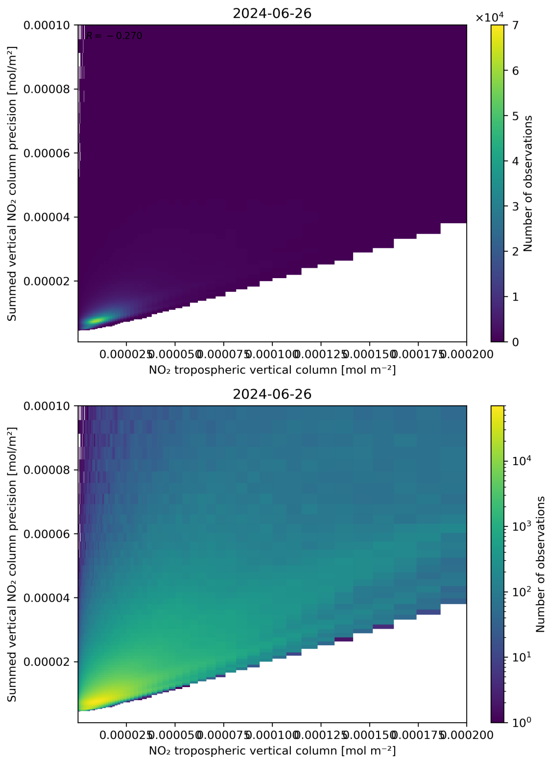
Figure 127: Scatter density plot of “NO 2 tropospheric vertical column” against “Summed vertical NO 2 column precision” for 2024-06-25 to 2024-06-27.
