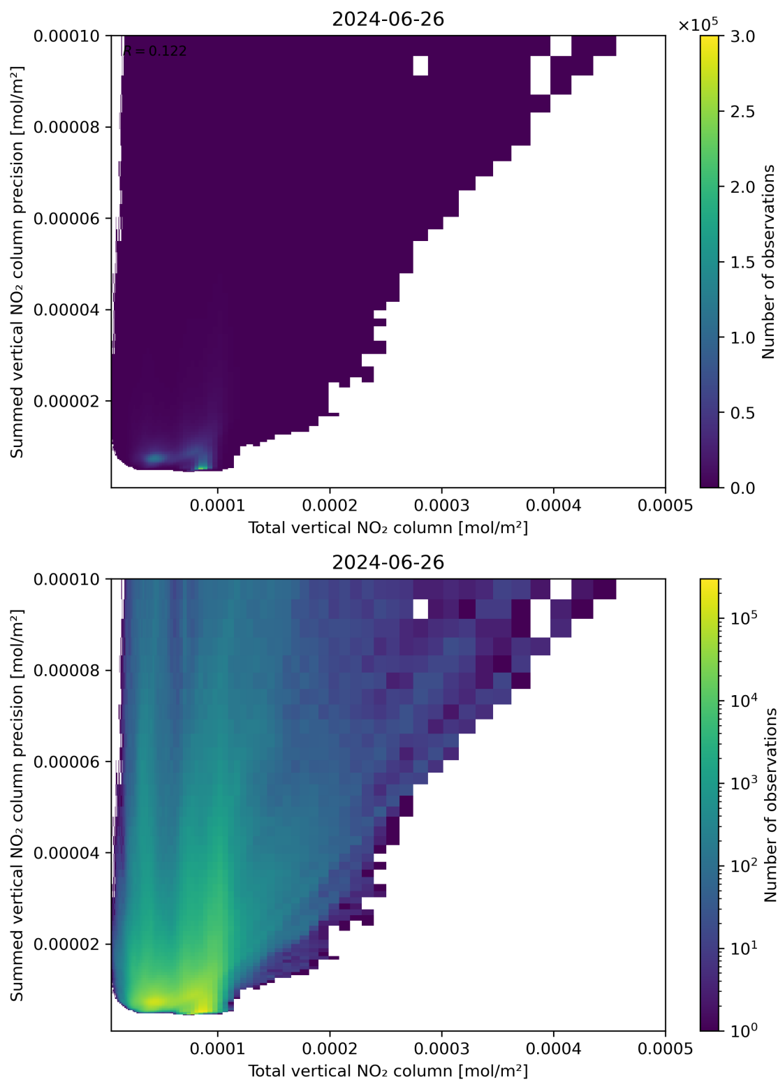
Figure 113: Scatter density plot of “Total vertical NO 2 column” against “Summed vertical NO 2 column precision” for 2024-06-25 to 2024-06-27.
