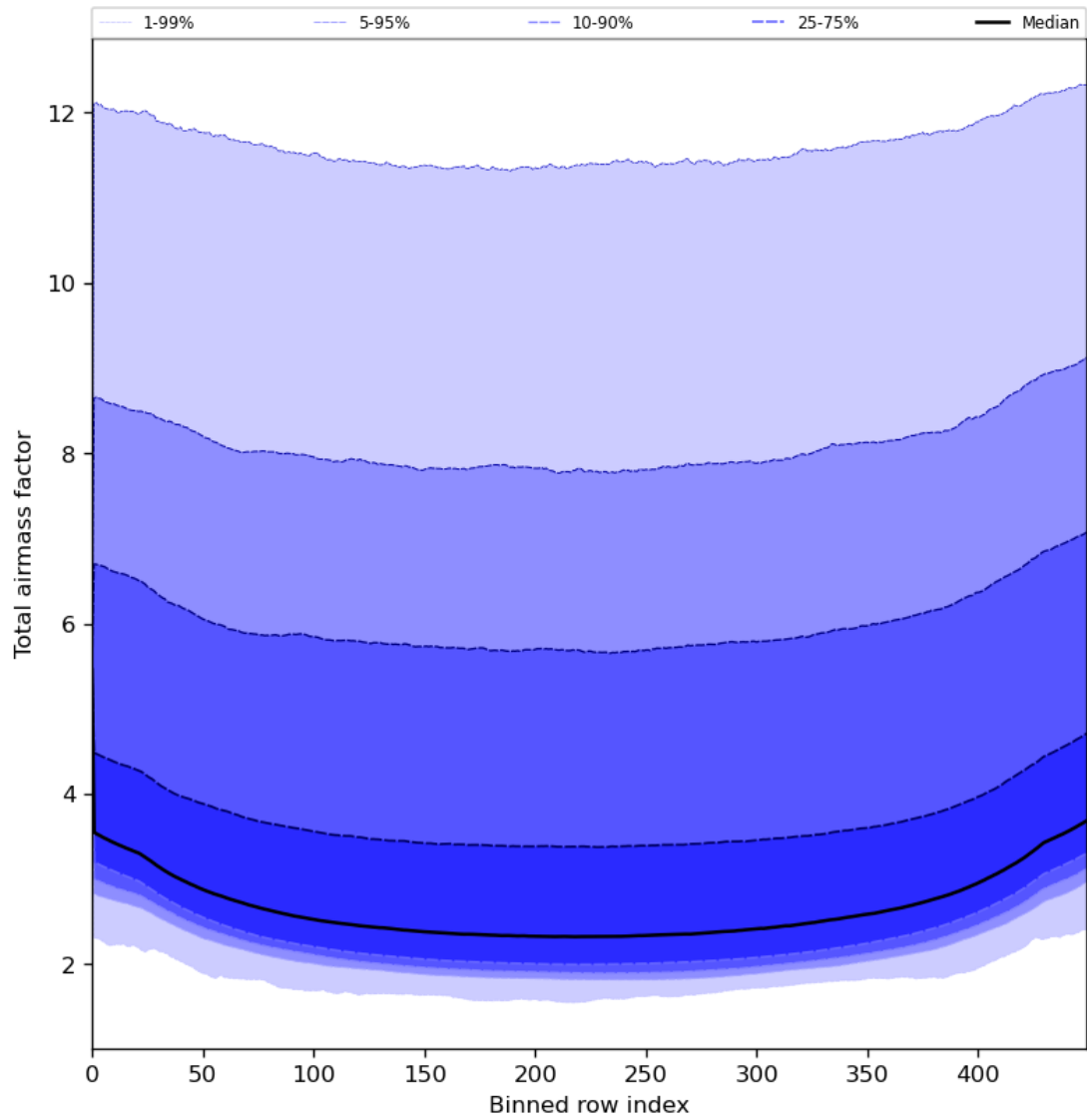
Figure 49: Along track statistics of “Total airmass factor” for 2024-06-25 to 2024-06-27
