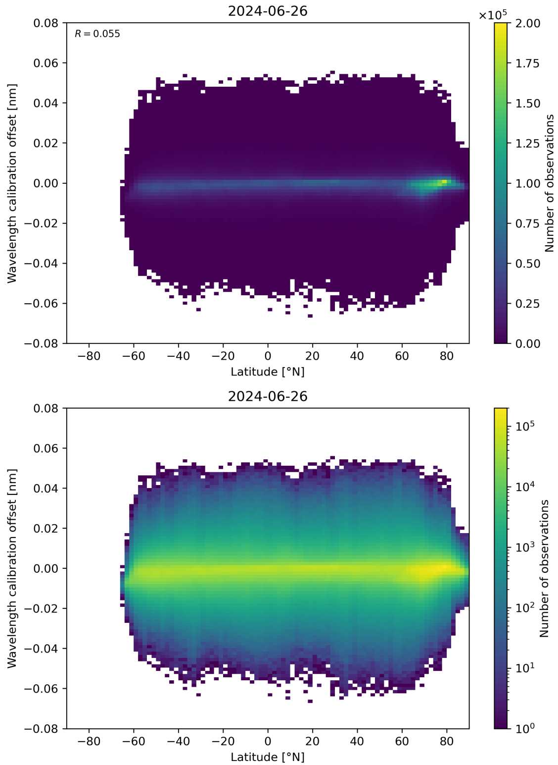
Figure 95: Scatter density plot of “Latitude” against “Wavelength calibration offset” for 2024-06-25 to 2024-06-27.
