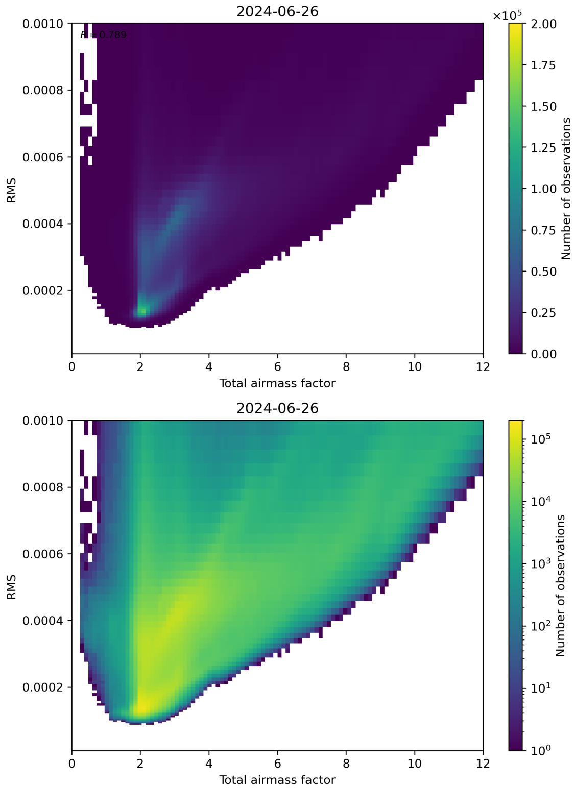
Figure 69: Scatter density plot of “Total airmass factor” against “RMS” for 2024-06-25 to 2024-06-27.
