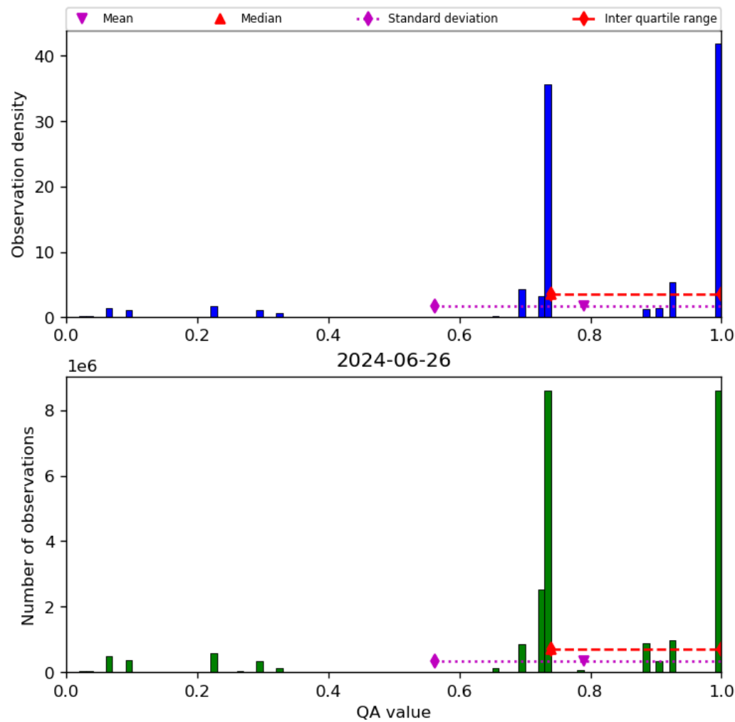
Figure 28: Histogram of “QA value” for 2024-06-25 to 2024-06-27
