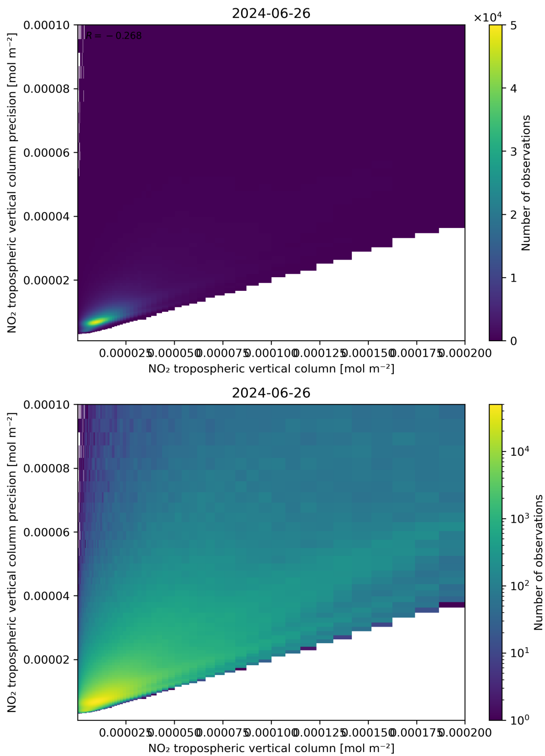
Figure 130: Scatter density plot of “NO 2 tropospheric vertical column” against “NO 2 tropospheric vertical column precision” for 2024-06-25 to 2024-06-27.
