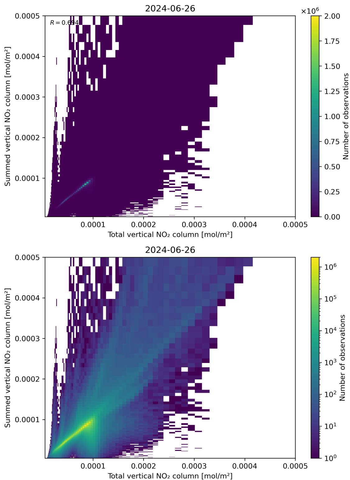
Figure 112: Scatter density plot of “Total vertical NO 2 column” against “Summed vertical NO 2 column” for 2024-06-25 to 2024-06-27.
