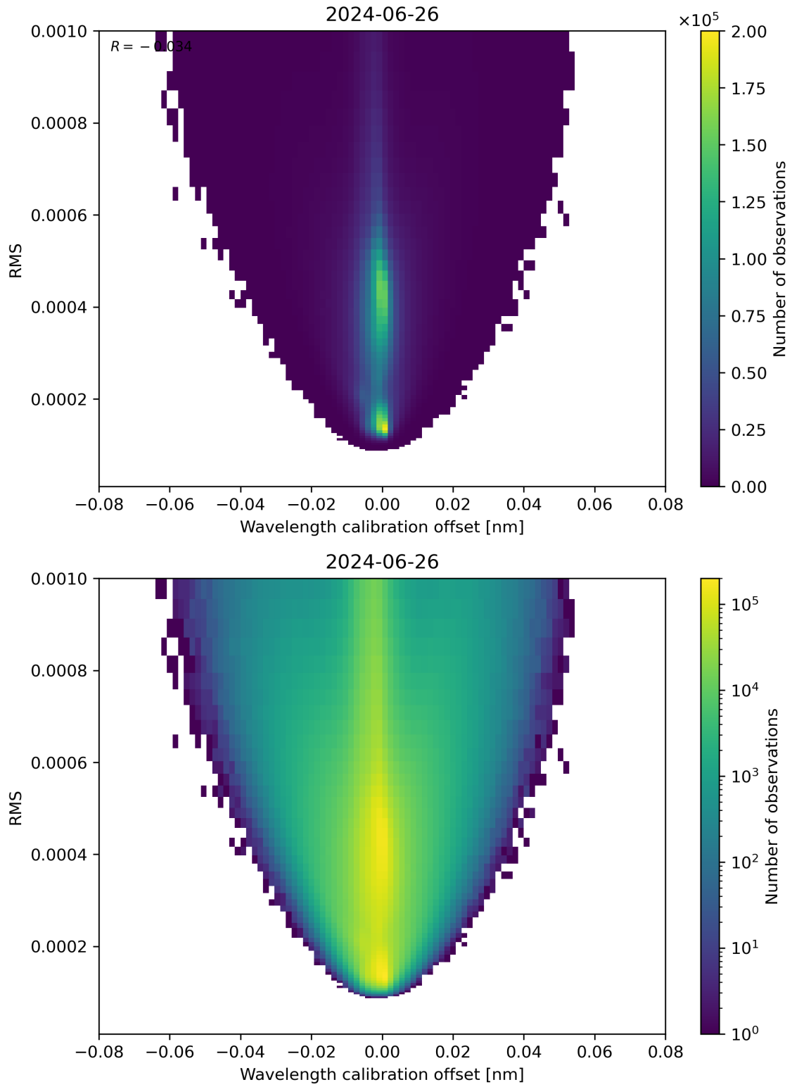
Figure 181: Scatter density plot of “Wavelength calibration offset” against “RMS” for 2024-06-25 to 2024-06-27.
