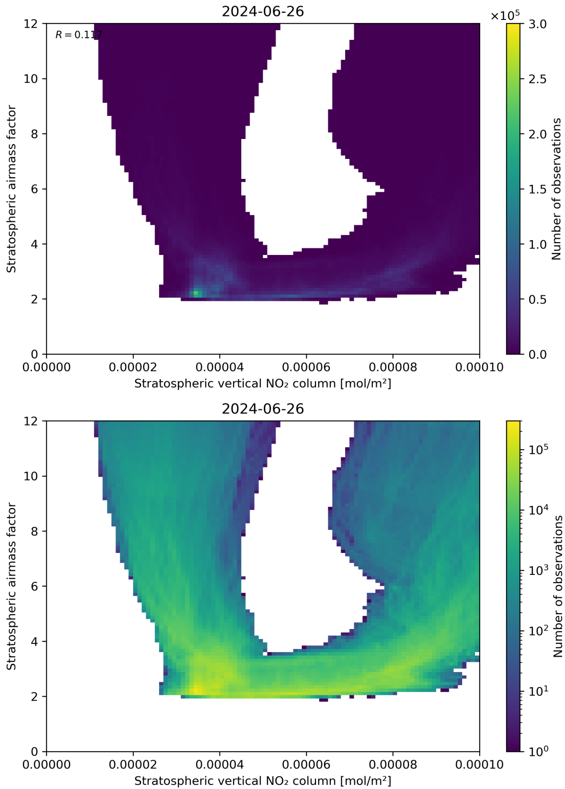
Figure 96: Scatter density plot of “Stratospheric vertical NO 2 column” against “Stratospheric airmass factor” for 2024-06-25 to 2024-06-27.
