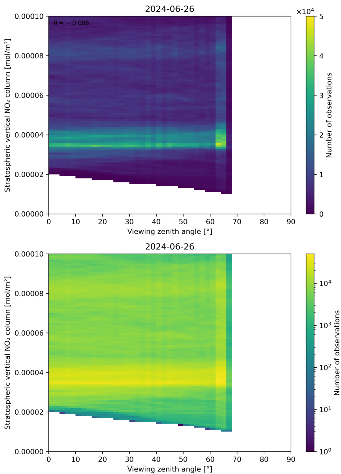
Figure 164: Scatter density plot of “Viewing zenith angle” against “Stratospheric vertical NO 2 column” for 2024-06-25 to 2024-06-27.
