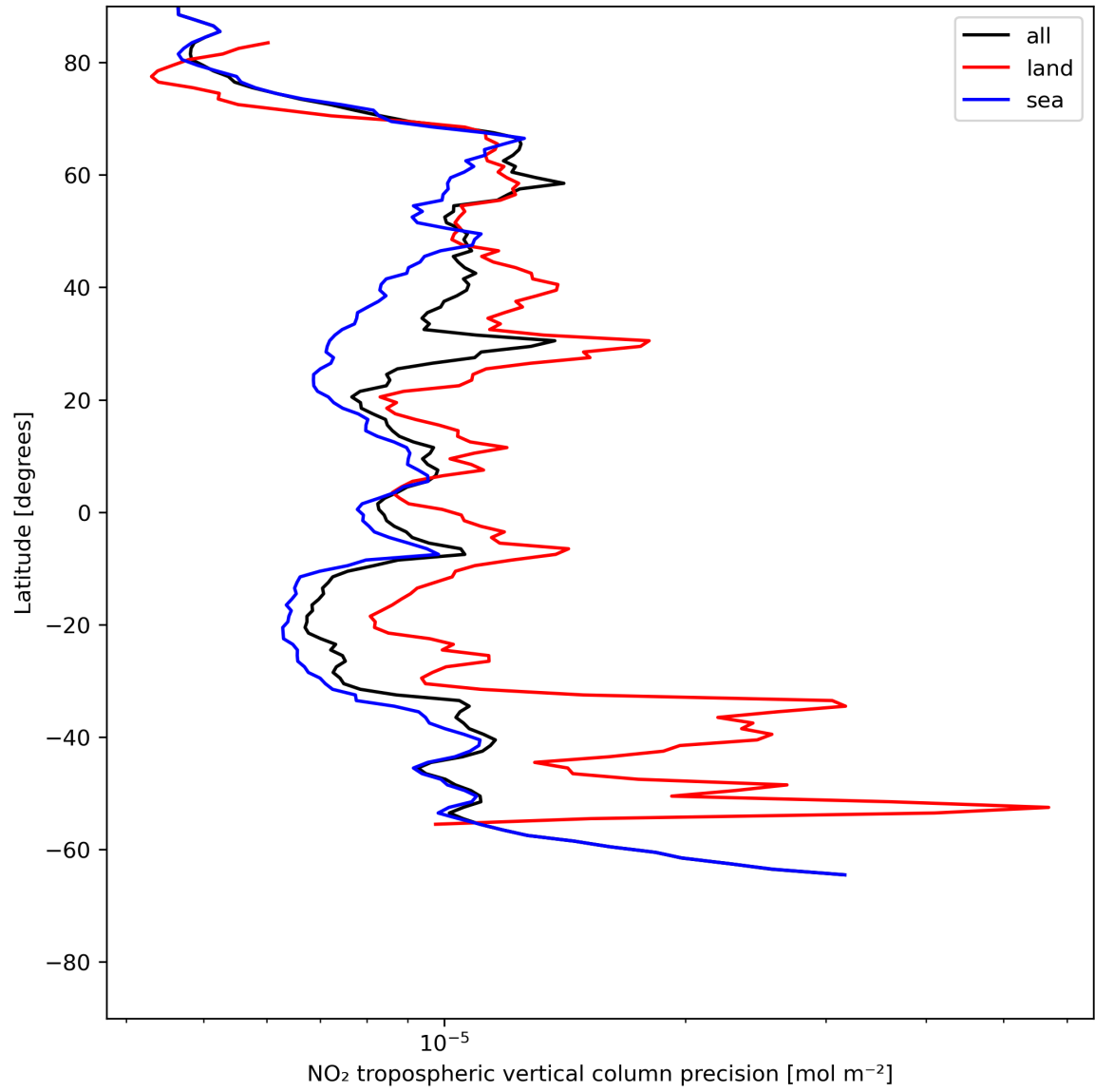
Figure 13: Zonal average of “NO 2 tropospheric vertical column precision” for 2024-06-25 to 2024-06-27.
