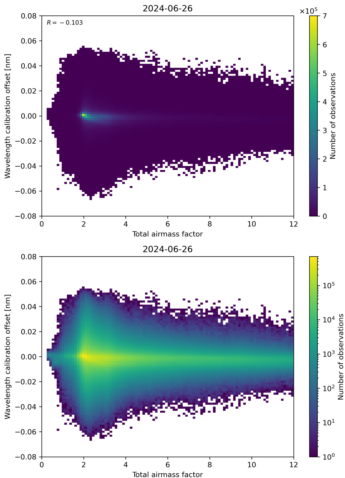
Figure 70: Scatter density plot of “Total airmass factor” against “Wavelength calibration offset” for 2024-06-25 to 2024-06-27.
