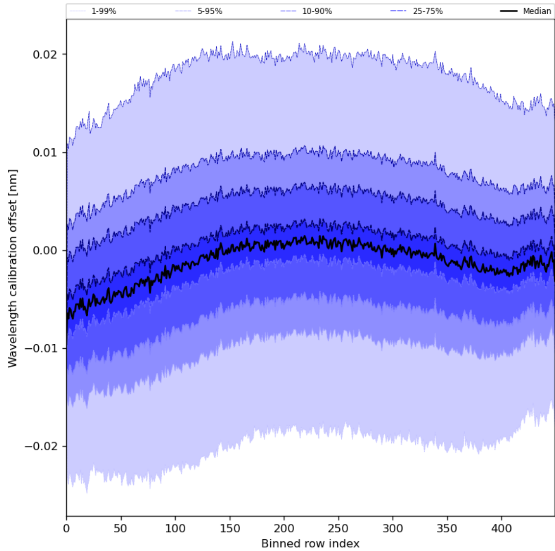
Figure 52: Along track statistics of “Wavelength calibration offset” for 2024-06-25 to 2024-06-27
