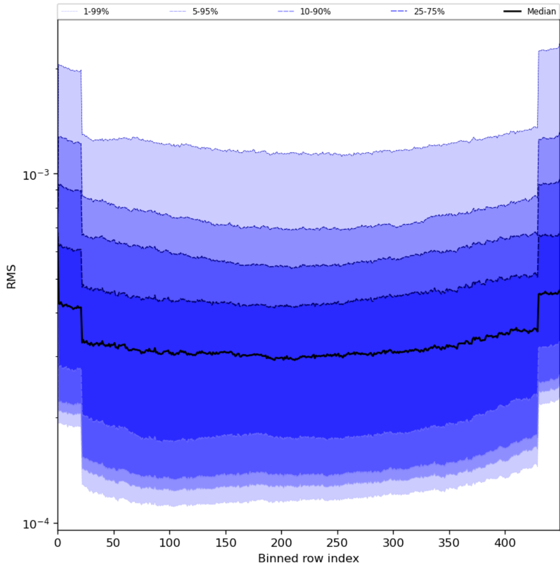
Figure 60: Along track statistics of “RMS” for 2024-06-25 to 2024-06-27
