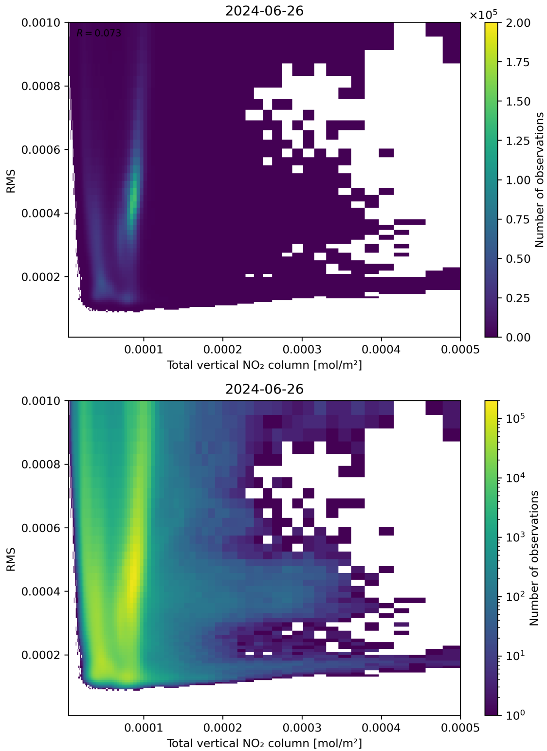
Figure 120: Scatter density plot of “Total vertical NO 2 column” against “RMS” for 2024-06-25 to 2024-06-27.
