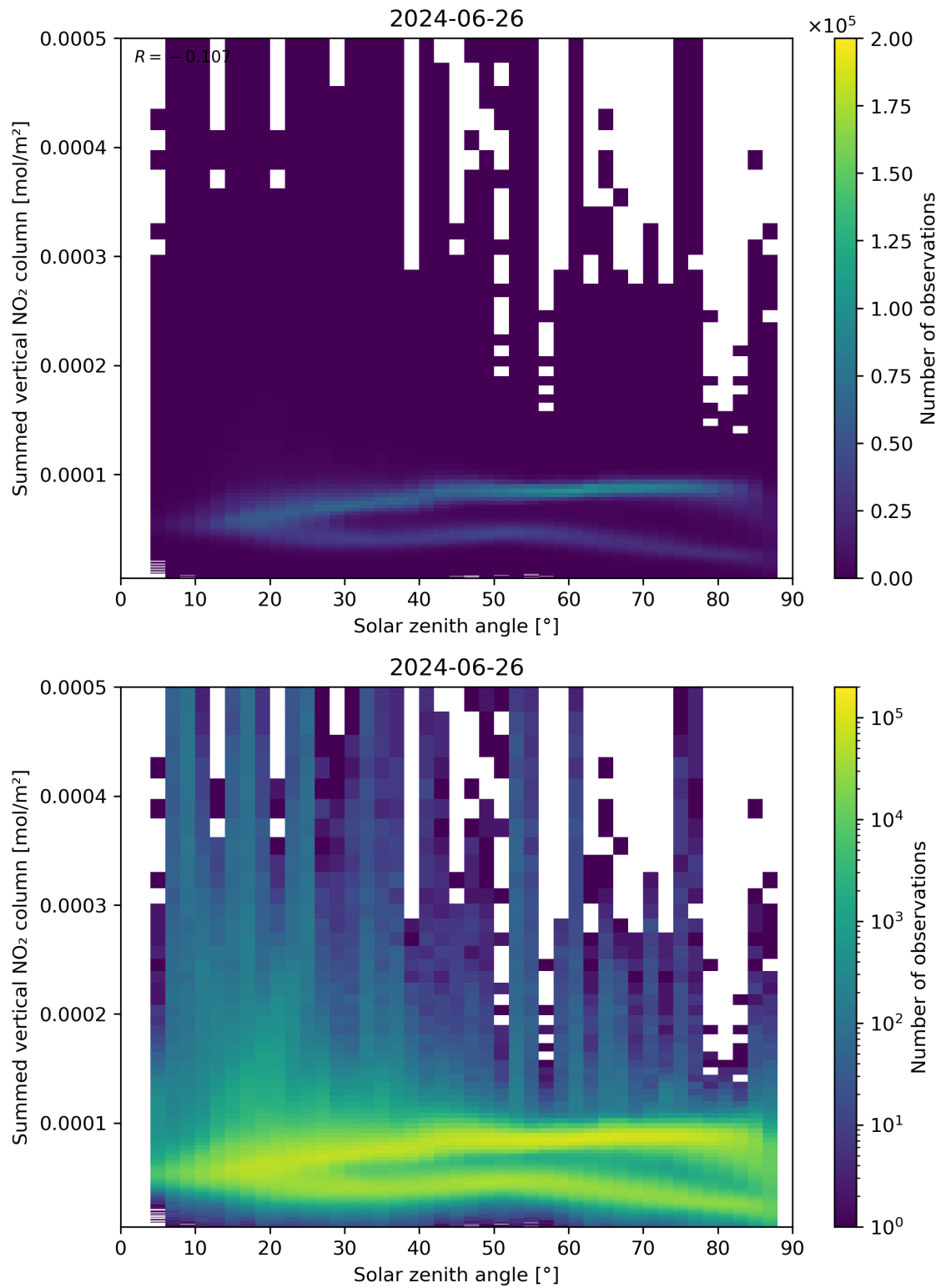
Figure 151: Scatter density plot of “Solar zenith angle” against “Summed vertical NO 2 column” for 2024-06-25 to 2024-06-27.
