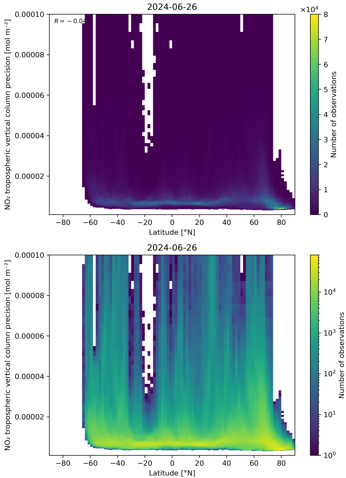
Figure 93: Scatter density plot of “Latitude” against “NO 2 tropospheric vertical column precision” for 2024-06-25 to 2024-06-27.
