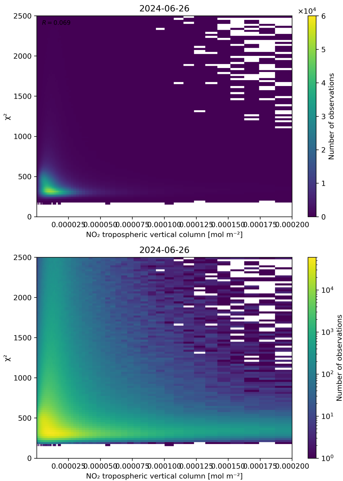
Figure 124: Scatter density plot of “NO 2 tropospheric vertical column” against “ \chi^2 ” for 2024-06-25 to 2024-06-27.
