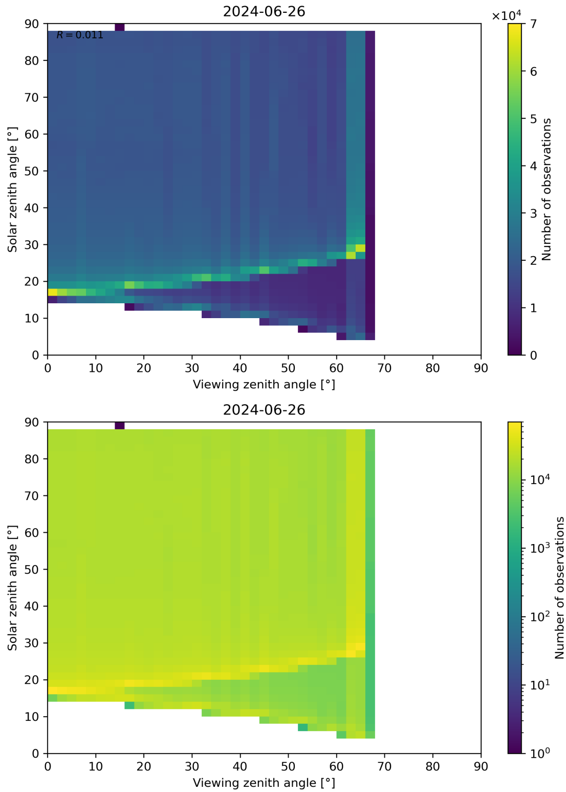
Figure 172: Scatter density plot of “Viewing zenith angle” against “Solar zenith angle” for 2024-06-25 to 2024-06-27.
