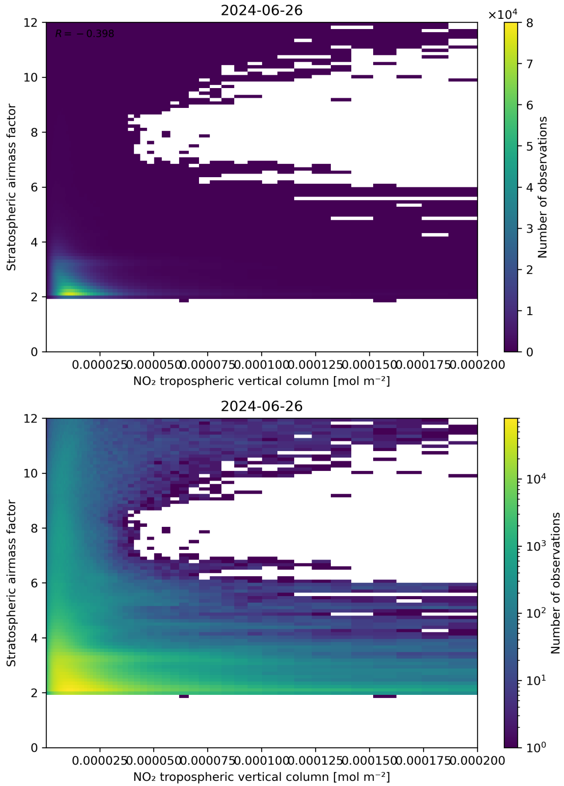
Figure 121: Scatter density plot of “NO 2 tropospheric vertical column” against “Stratospheric air mass factor” for 2024-06-25 to 2024-06-27.
