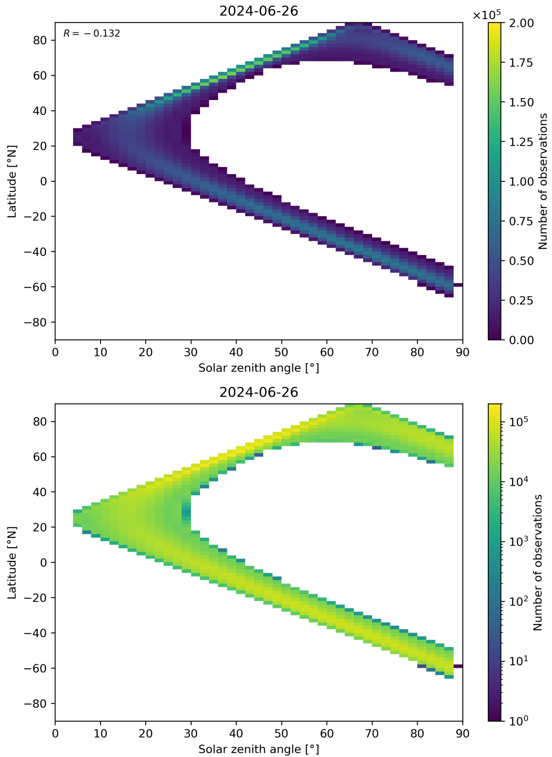
Figure 149: Scatter density plot of “Solar zenith angle” against “Latitude” for 2024-06-25 to 2024-06-27.
