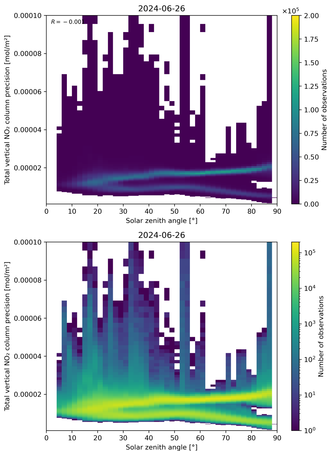
Figure 154: Scatter density plot of “Solar zenith angle” against “Total vertical NO 2 column precision” for 2024-06-25 to 2024-06-27.
