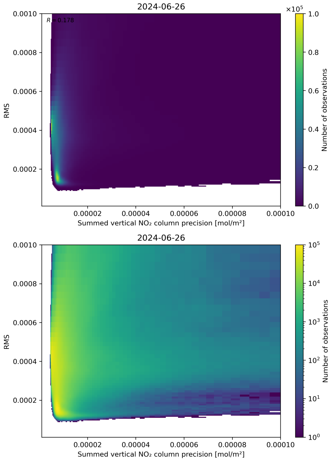
Figure 108: Scatter density plot of “Summed vertical NO 2 column precision” against “RMS” for 2024-06-25 to 2024-06-27.
