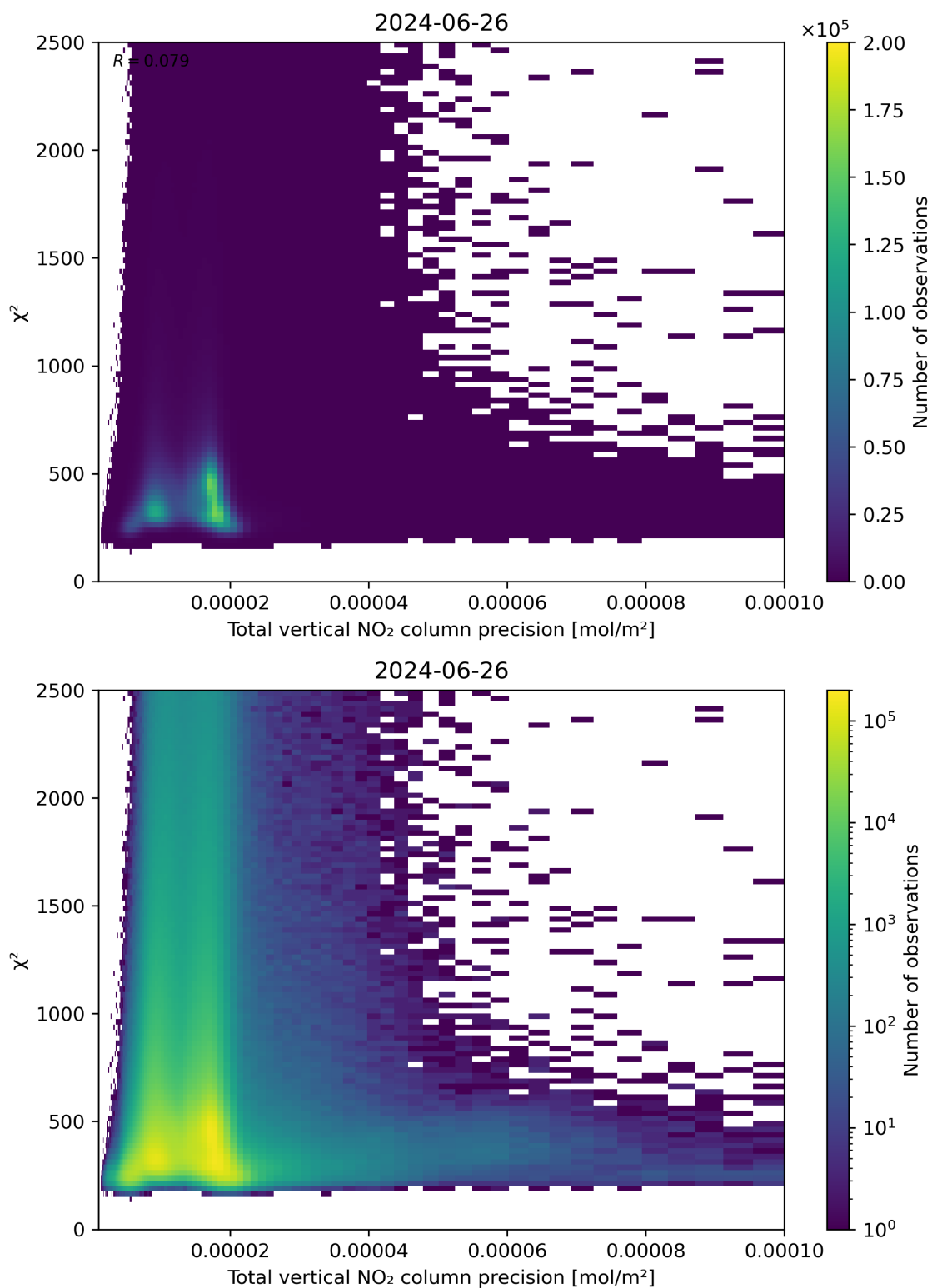
Figure 116: Scatter density plot of “Total vertical NO 2 column precision” against “ \chi^2 ” for 2024-06-25 to 2024-06-27.
