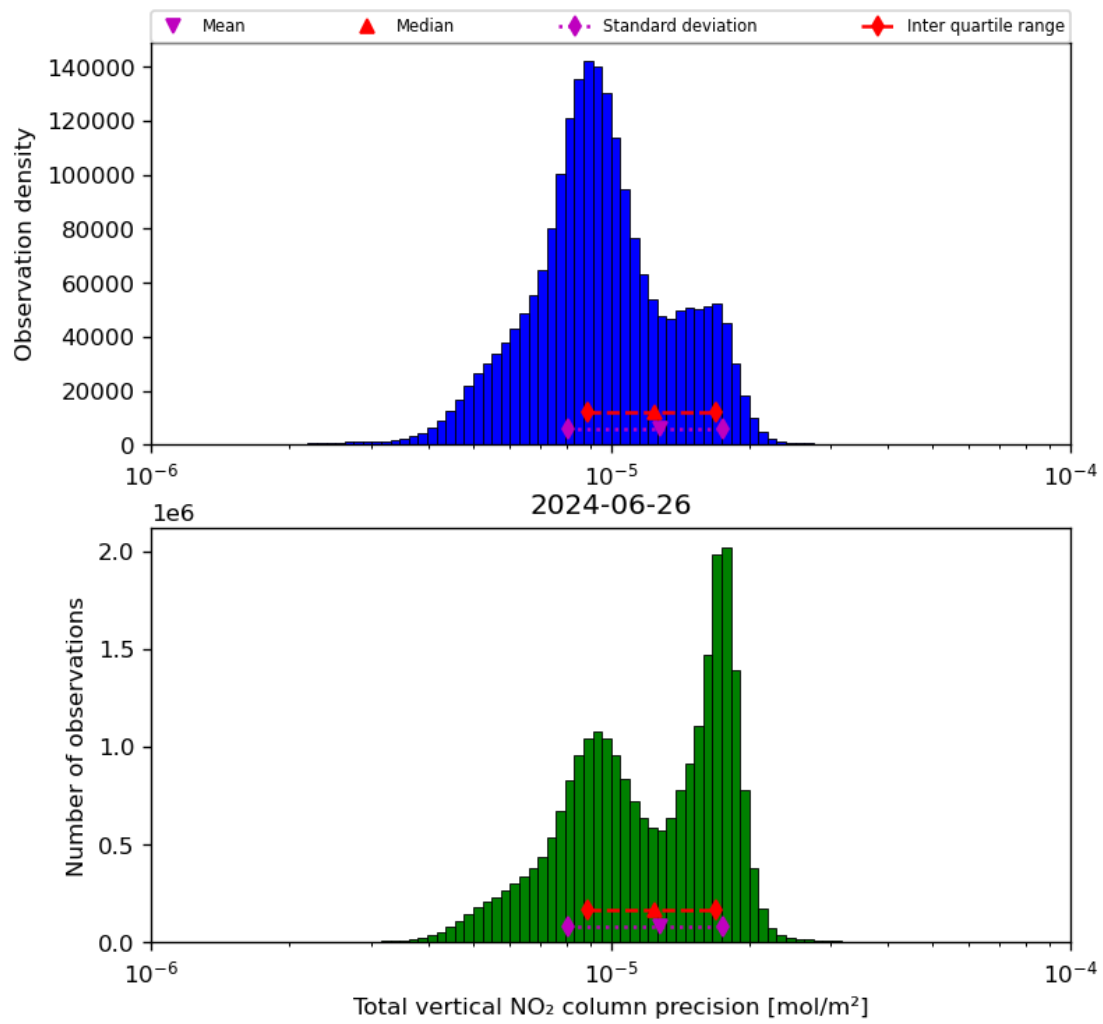
Figure 39: Histogram of “Total vertical NO 2 column precision” for 2024-06-25 to 2024-06-27
