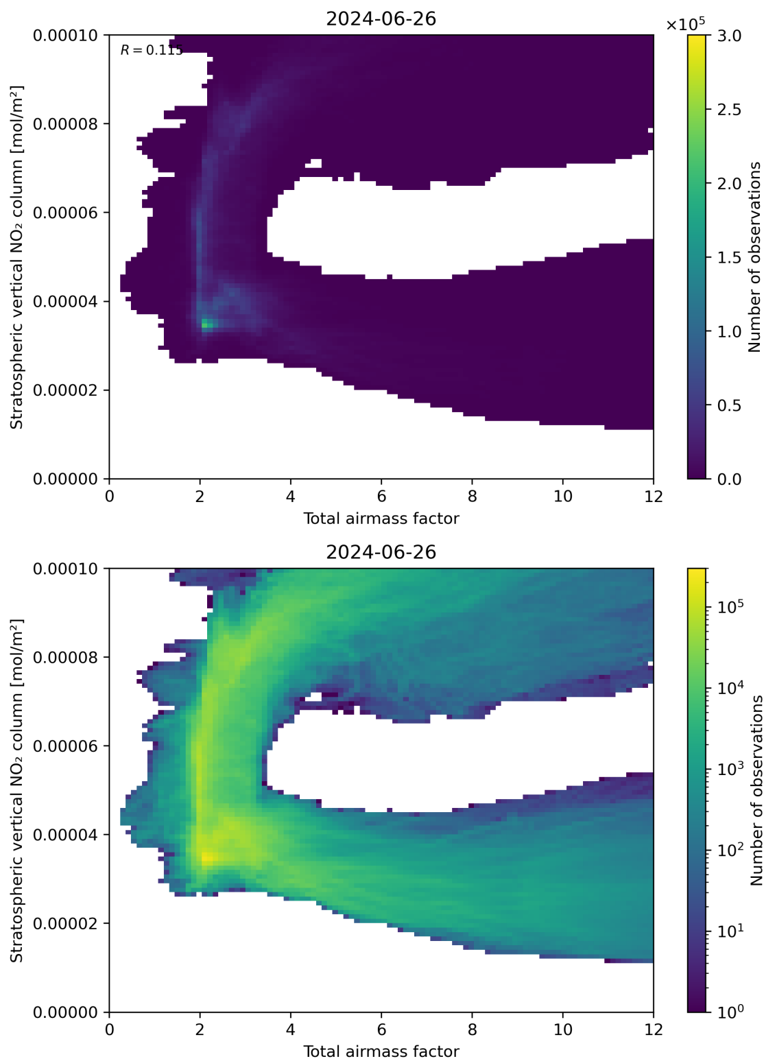
Figure 64: Scatter density plot of “Total airmass factor” against “Stratospheric vertical \text{NO}_2 column” for 2024-06-25 to 2024-06-27.
