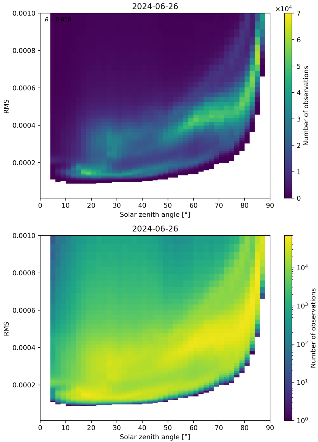
Figure 157: Scatter density plot of “Solar zenith angle” against “RMS” for 2024-06-25 to 2024-06-27.
