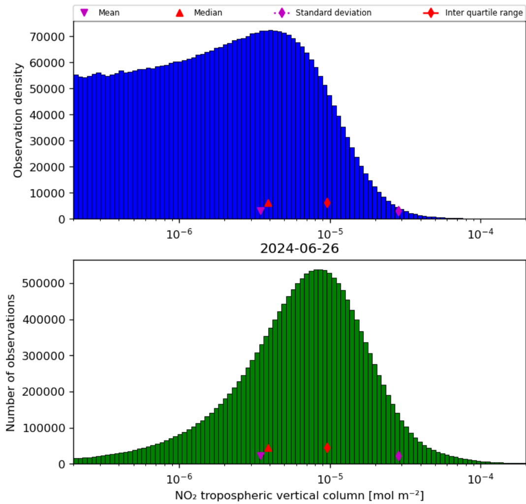
Figure 29: Histogram of “NO 2 tropospheric vertical column” for 2024-06-25 to 2024-06-27
