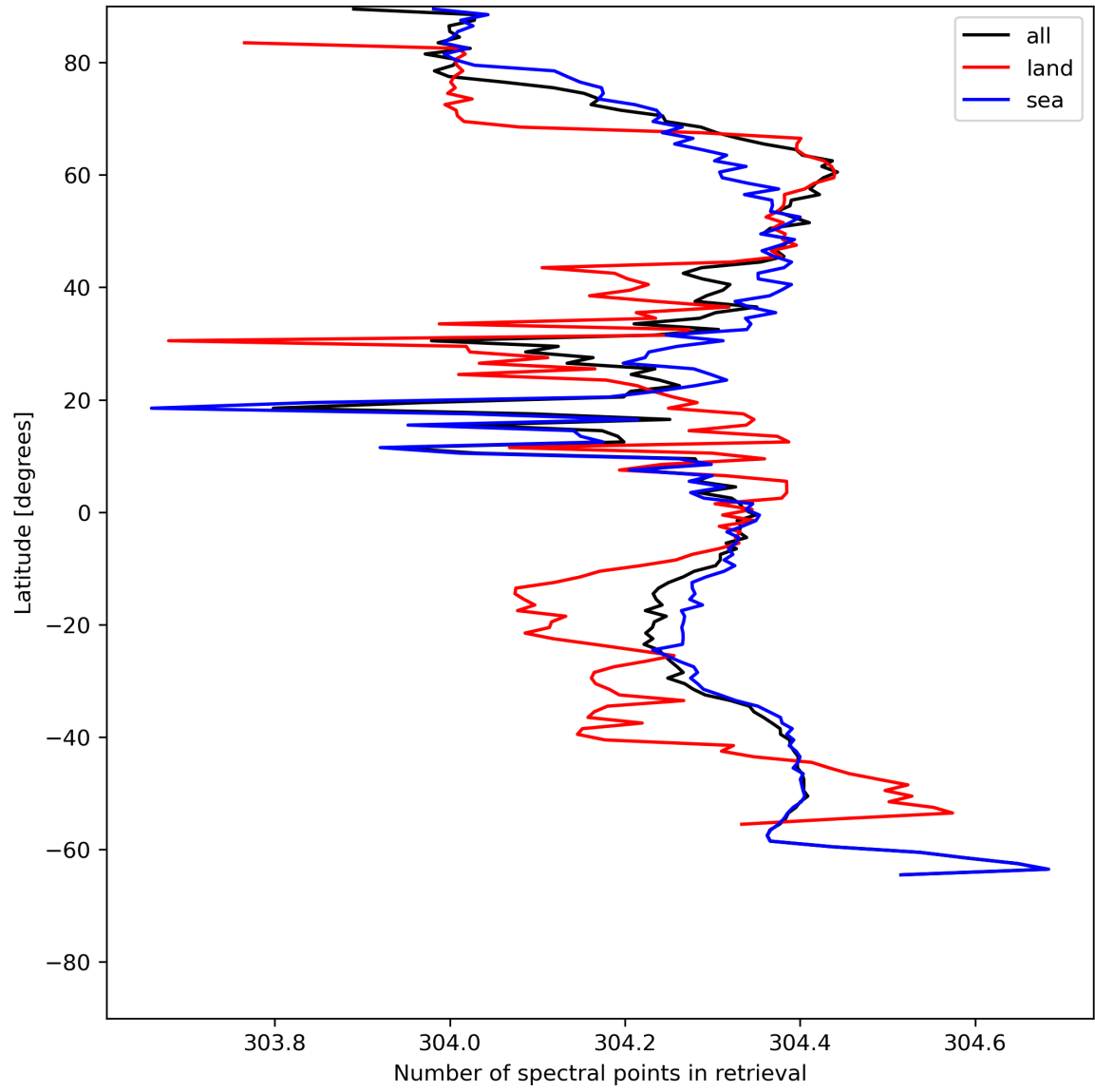
Figure 16: Zonal average of “Number of spectral points in retrieval” for 2024-06-25 to 2024-06-27.
