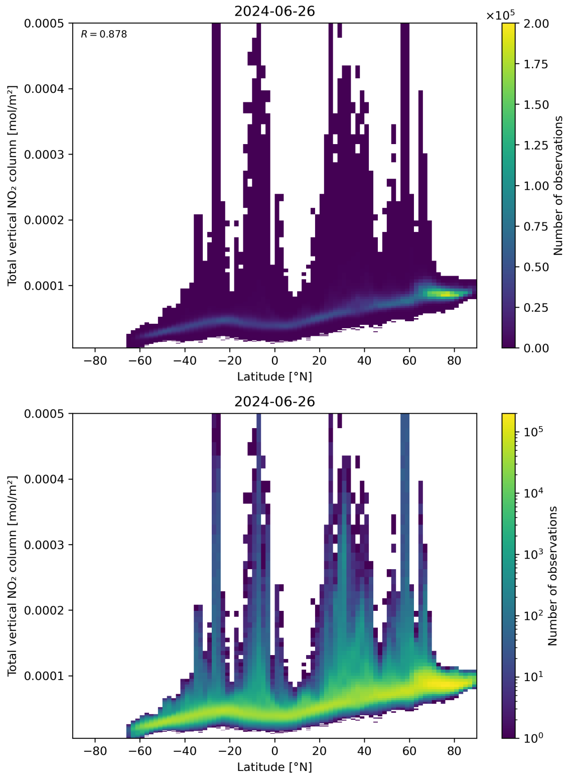
Figure 90: Scatter density plot of “Latitude” against “Total vertical \text{NO}_2 column” for 2024-06-25 to 2024-06-27.
