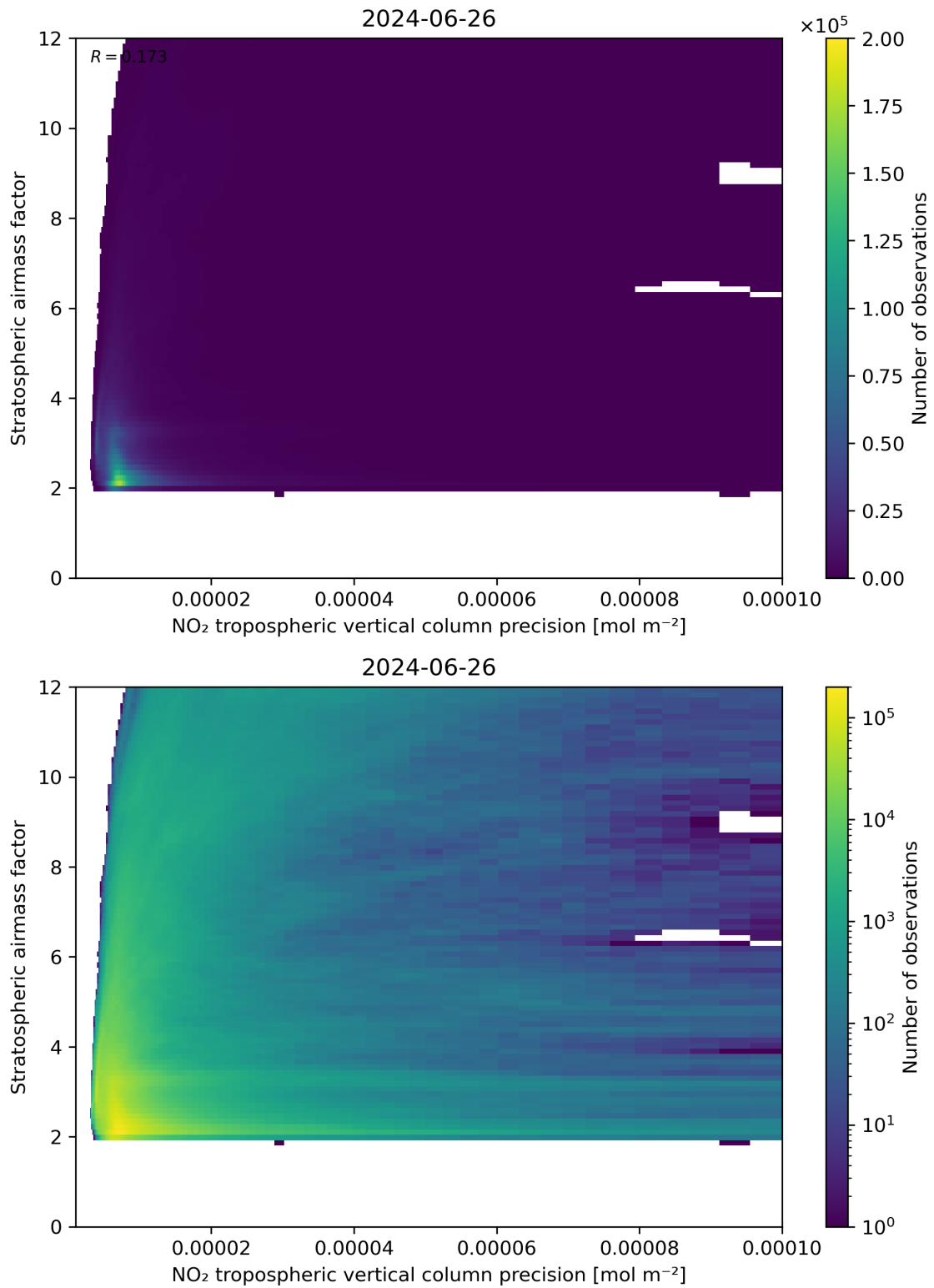
Figure 131: Scatter density plot of “NO 2 tropospheric vertical column precision” against “Stratospheric airmass factor” for 2024-06-25 to 2024-06-27.
