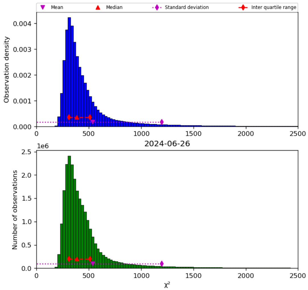
Figure 42: Histogram of “ \chi^2 ” for 2024-06-25 to 2024-06-27
