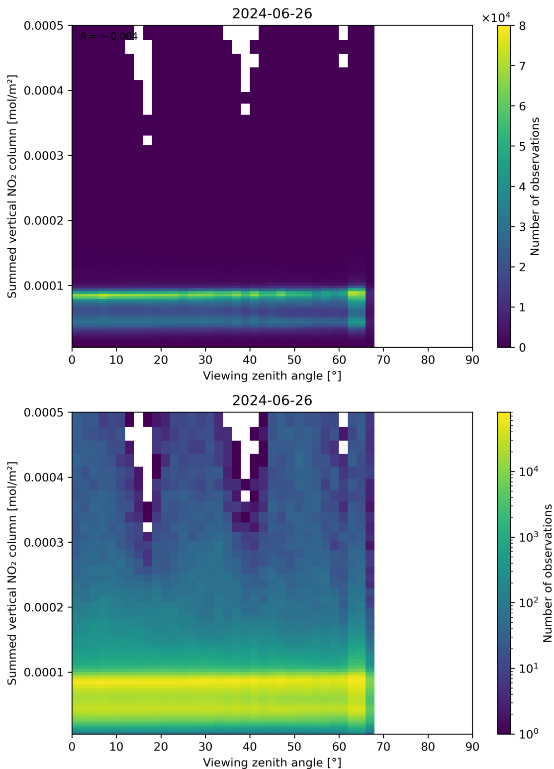
Figure 165: Scatter density plot of “Viewing zenith angle” against “Summed vertical NO 2 column” for 2024-06-25 to 2024-06-27.
