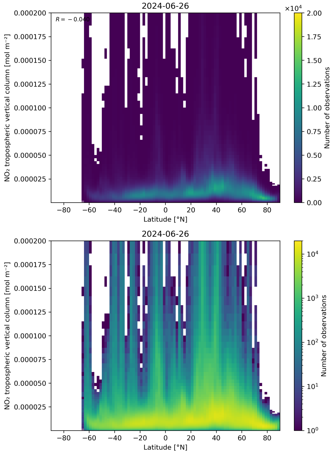
Figure 92: Scatter density plot of “Latitude” against “NO 2 tropospheric vertical column” for 2024-06-25 to 2024-06-27.
