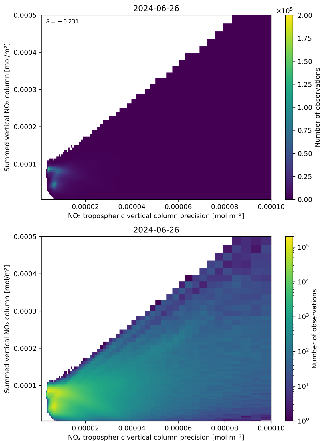
Figure 136: Scatter density plot of “NO 2 tropospheric vertical column precision” against “Summed vertical NO 2 column” for 2024-06-25 to 2024-06-27.
