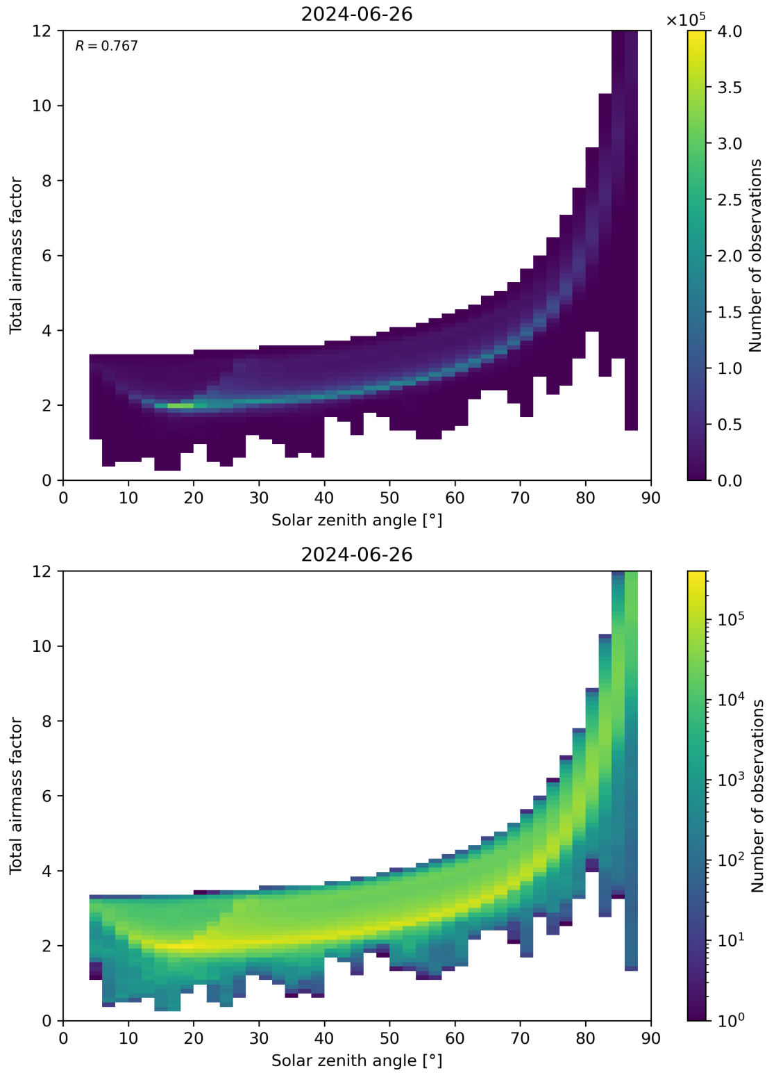
Figure 146: Scatter density plot of “Solar zenith angle” against “Total air mass factor” for 2024-06-25 to 2024-06-27.
