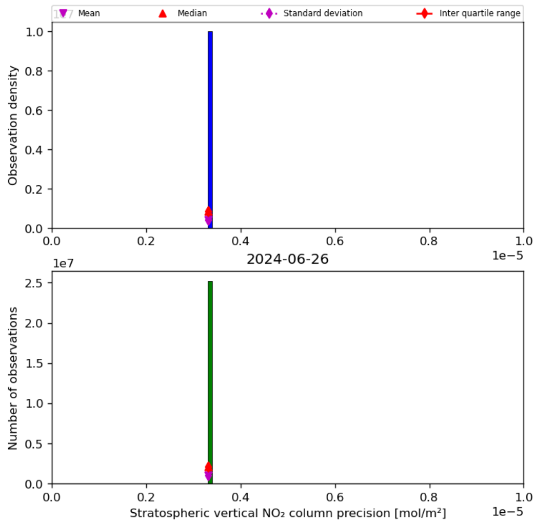
Figure 37: Histogram of “Stratospheric vertical NO 2 column precision” for 2024-06-25 to 2024-06-27
