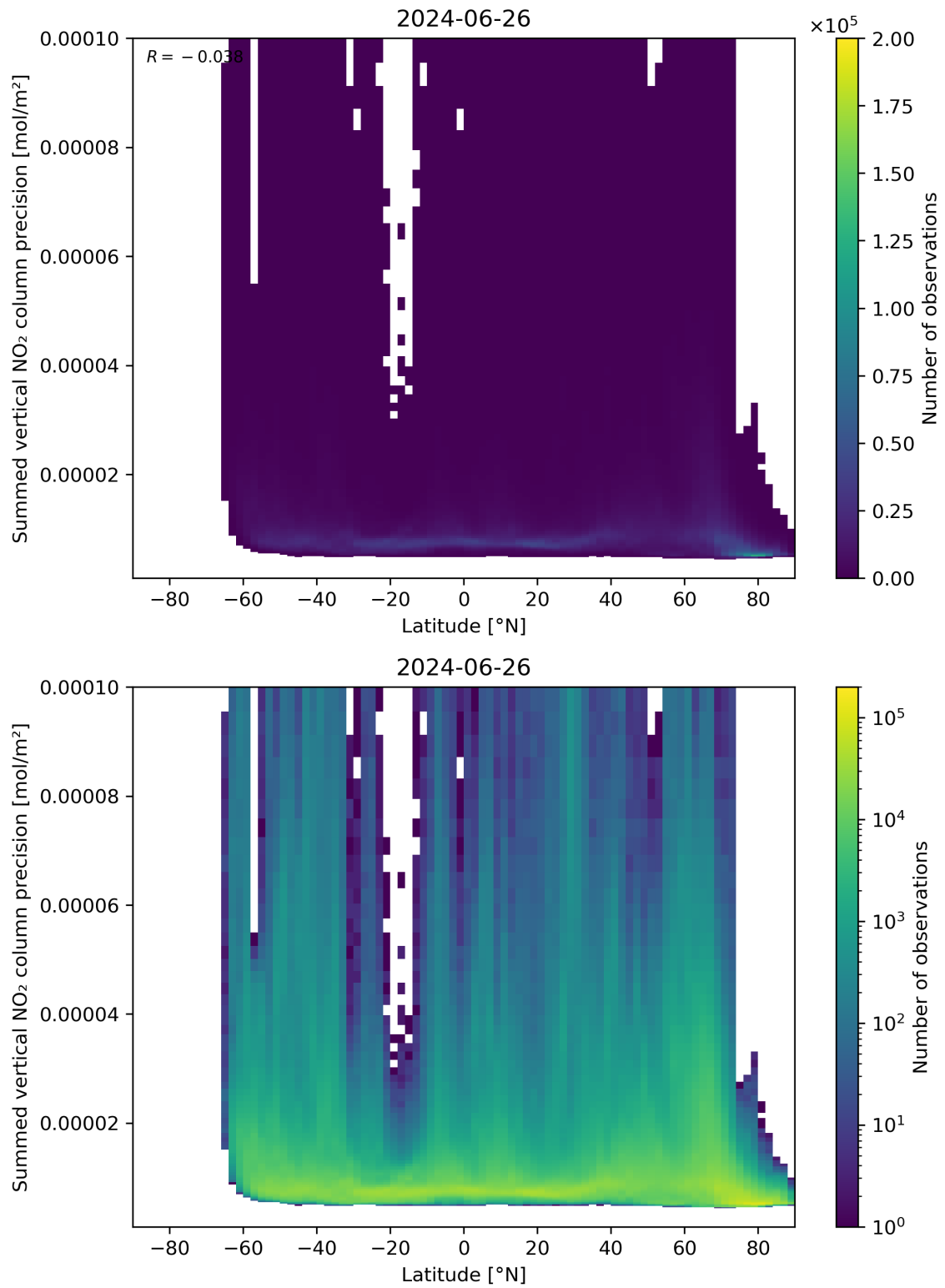
Figure 89: Scatter density plot of “Latitude” against “Summed vertical NO 2 column precision” for 2024-06-25 to 2024-06-27.
