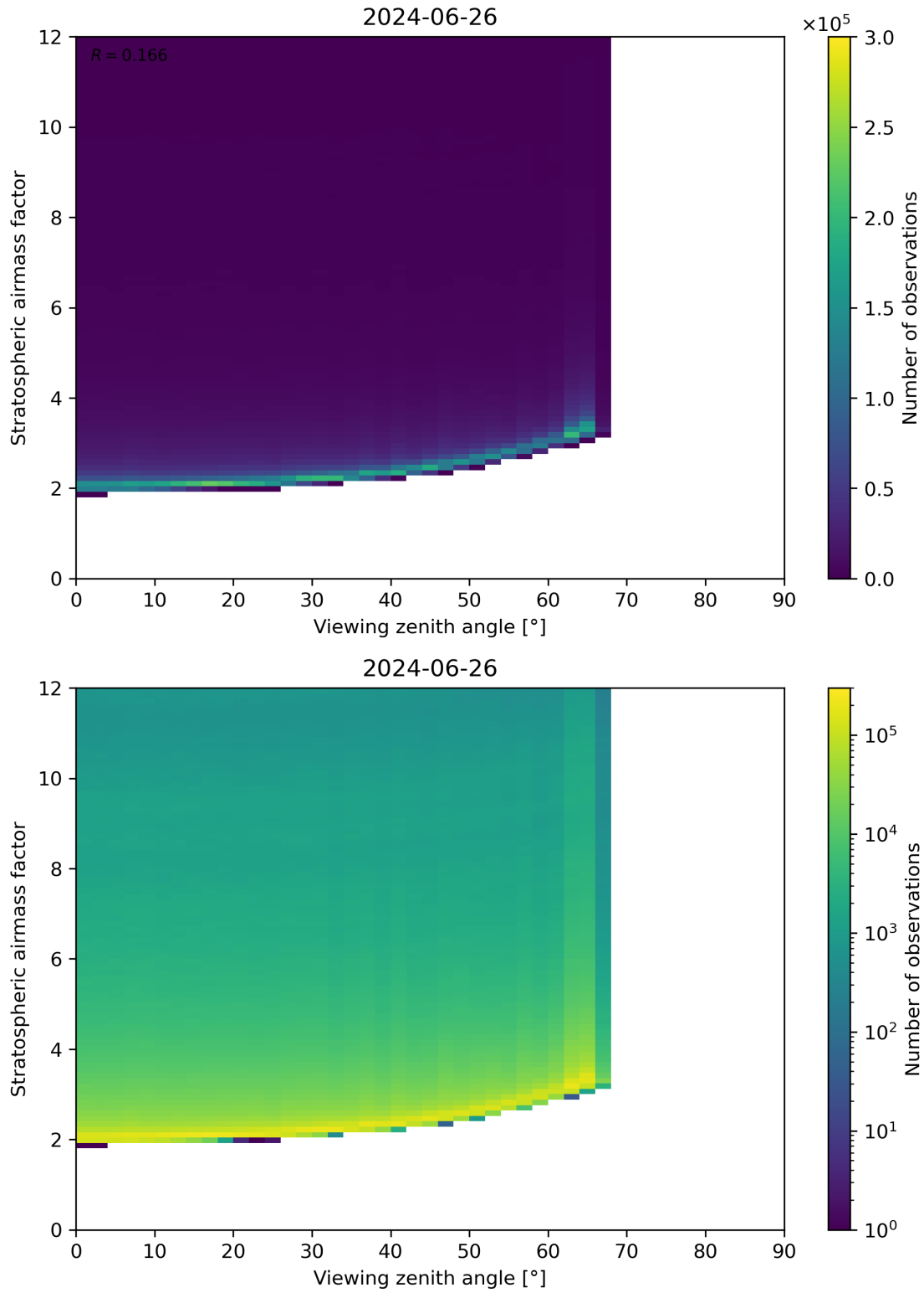
Figure 159: Scatter density plot of “Viewing zenith angle” against “Stratospheric airmass factor” for 2024-06-25 to 2024-06-27.
