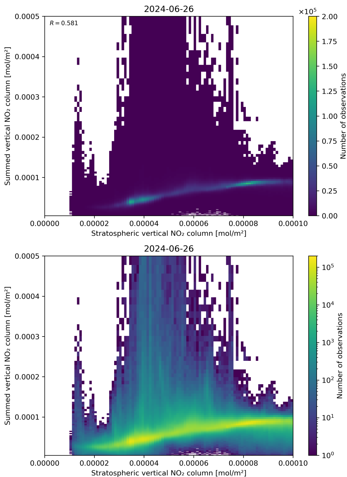
Figure 98: Scatter density plot of “Stratospheric vertical NO 2 column” against “Summed vertical NO 2 column” for 2024-06-25 to 2024-06-27.
