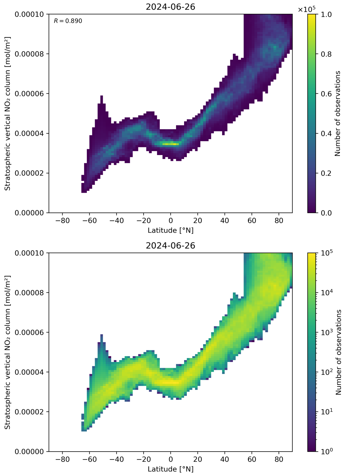
Figure 87: Scatter density plot of “Latitude” against “Stratospheric vertical NO 2 column” for 2024-06-25 to 2024-06-27.
