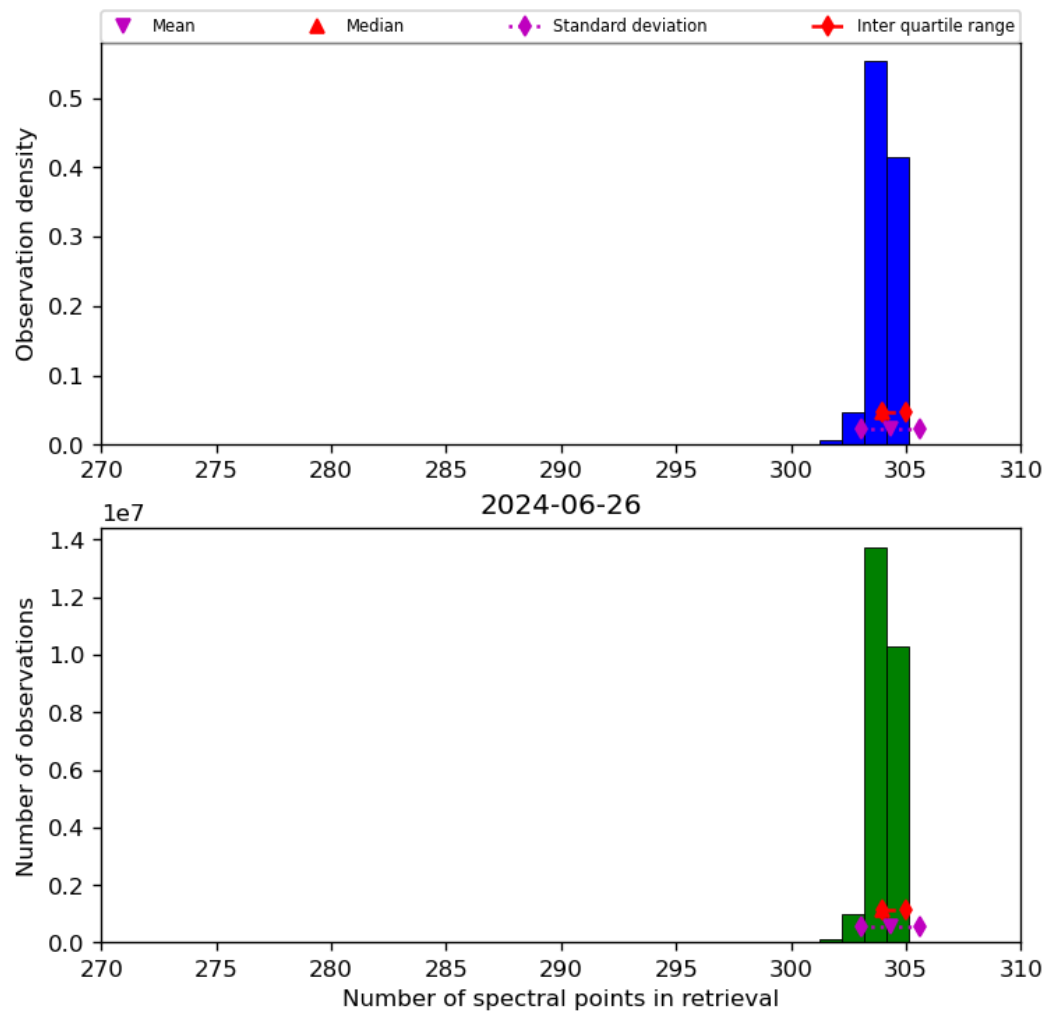
Figure 33: Histogram of “Number of spectral points in retrieval” for 2024-06-25 to 2024-06-27
