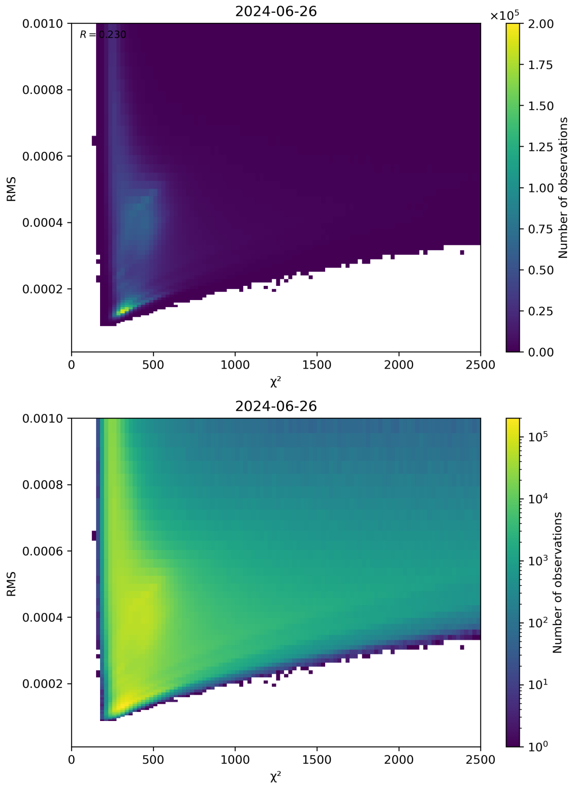
Figure 82: Scatter density plot of “ \chi^2 ” against “RMS” for 2024-06-25 to 2024-06-27.
