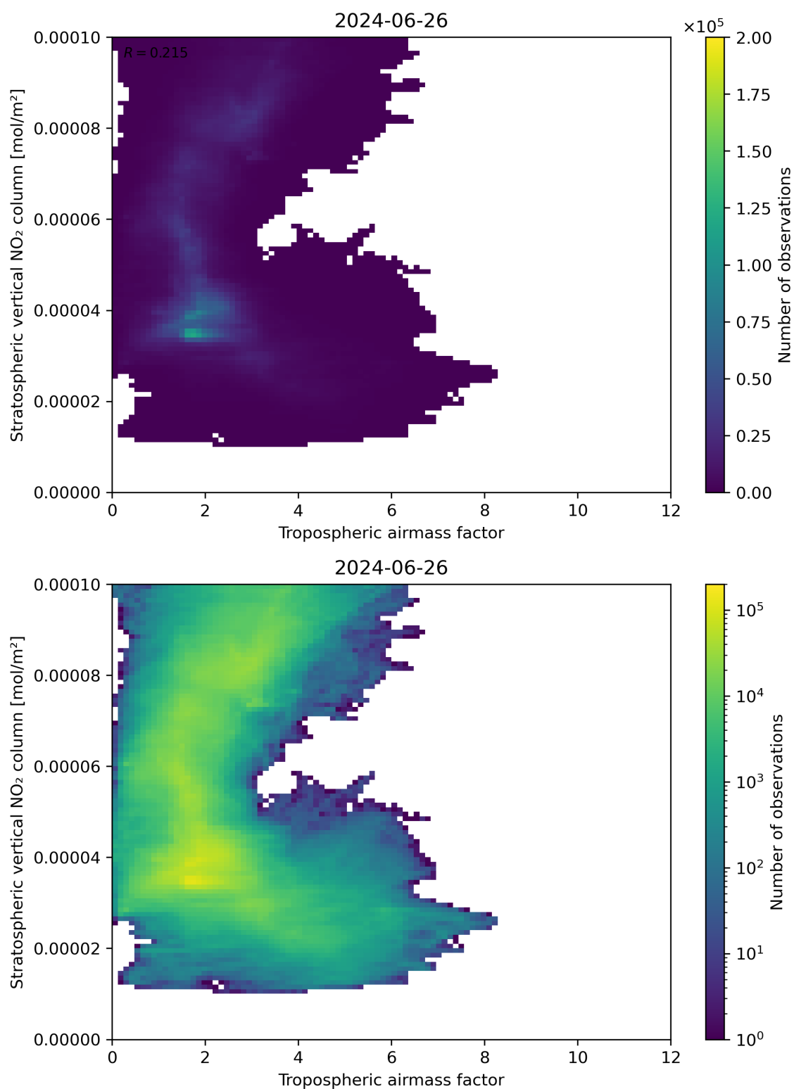
Figure 74: Scatter density plot of “Tropospheric air mass factor” against “Stratospheric vertical NO 2 column” for 2024-06-25 to 2024-06-27.
