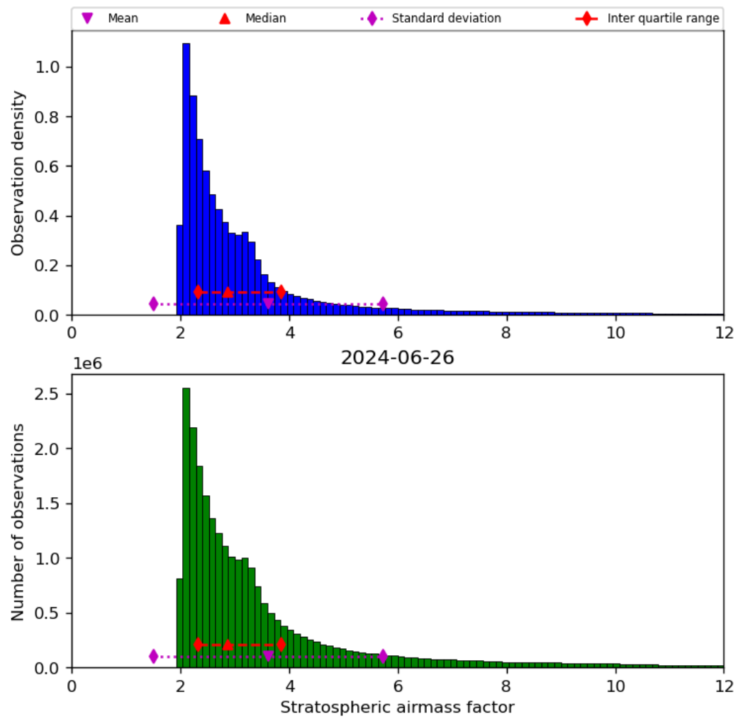
Figure 44: Histogram of “Stratospheric airmass factor” for 2024-06-25 to 2024-06-27
