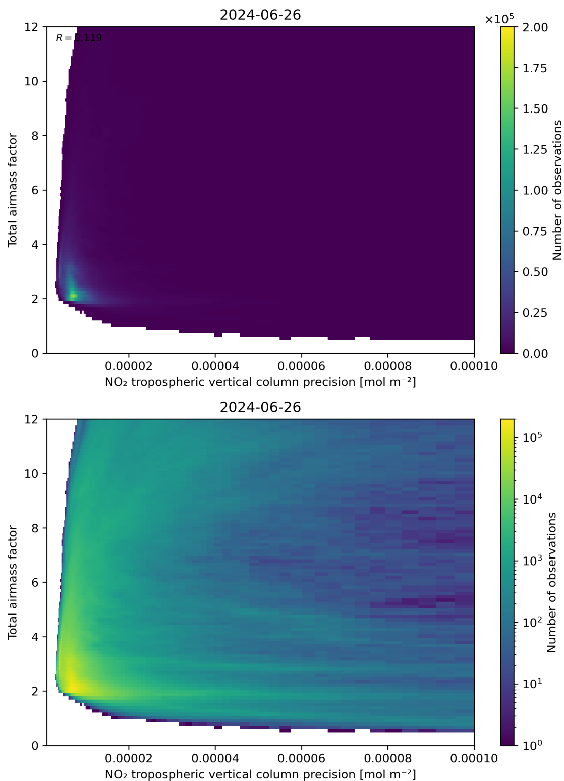
Figure 132: Scatter density plot of “NO 2 tropospheric vertical column precision” against “Total air mass factor” for 2024-06-25 to 2024-06-27.
