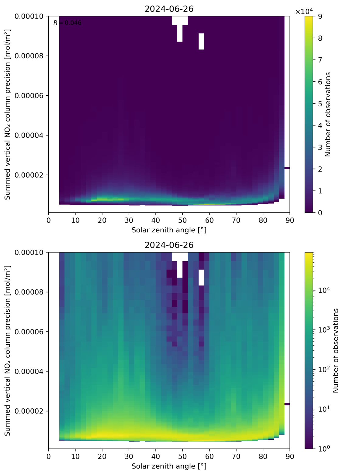
Figure 152: Scatter density plot of “Solar zenith angle” against “Summed vertical NO 2 column precision” for 2024-06-25 to 2024-06-27.
