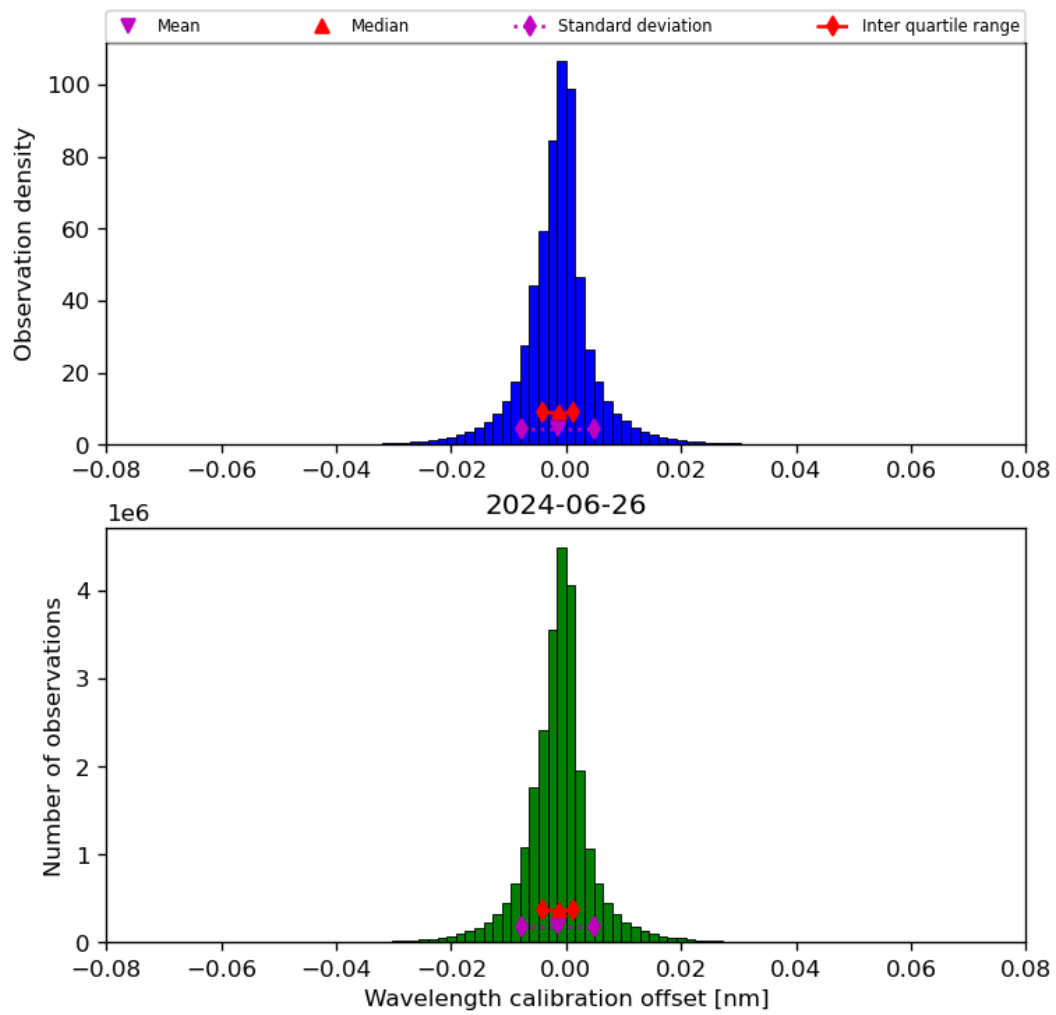
Figure 35: Histogram of “Wavelength calibration offset” for 2024-06-25 to 2024-06-27
