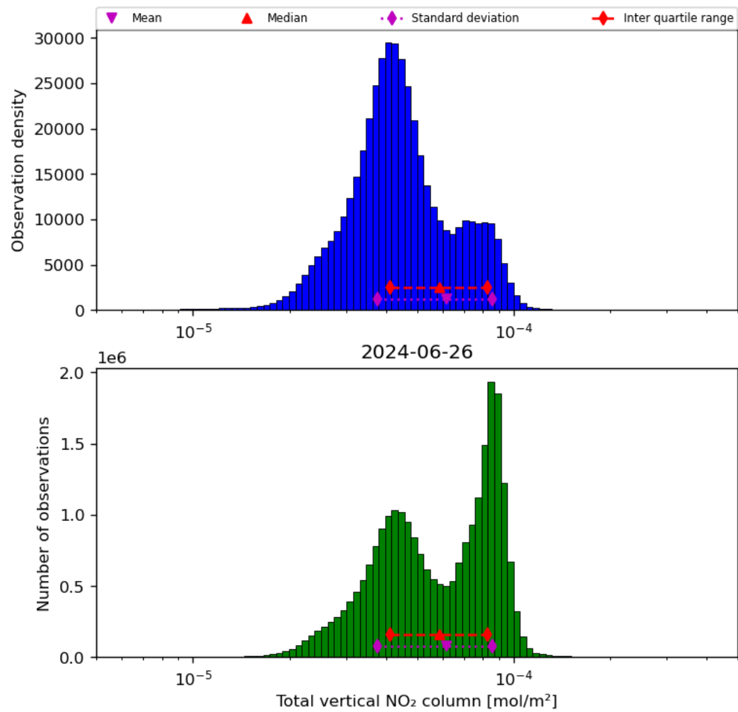
Figure 38: Histogram of “Total vertical NO 2 column” for 2024-06-25 to 2024-06-27
