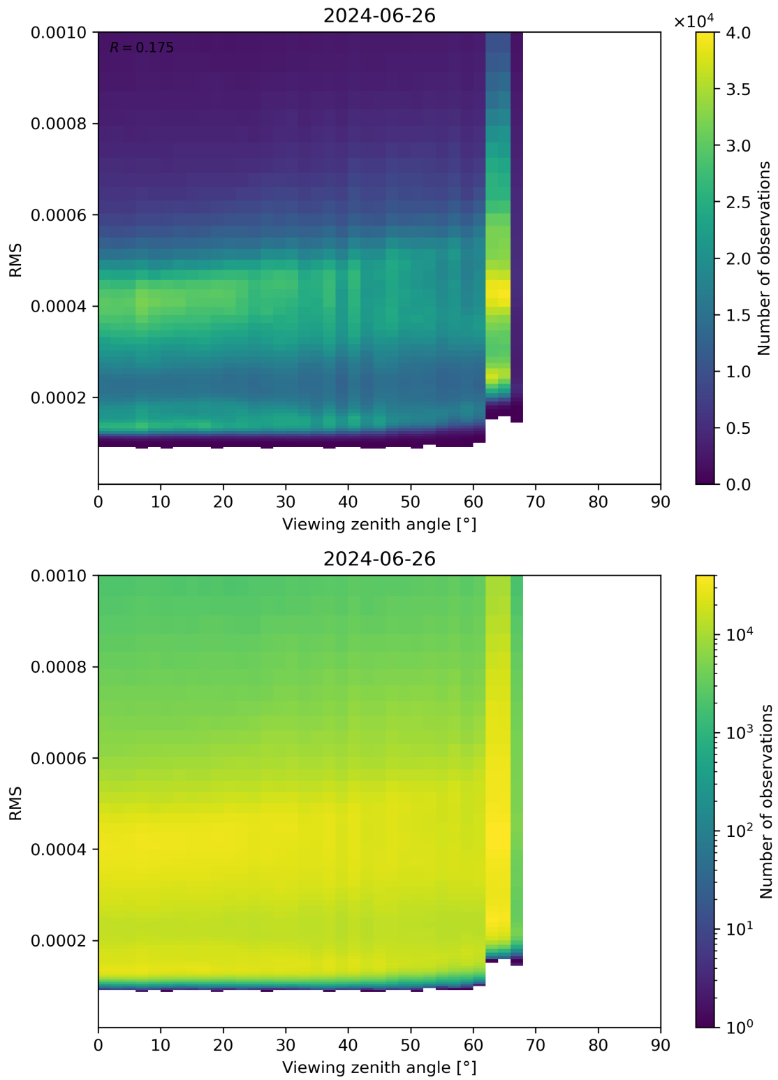
Figure 171: Scatter density plot of “Viewing zenith angle” against “RMS” for 2024-06-25 to 2024-06-27.
