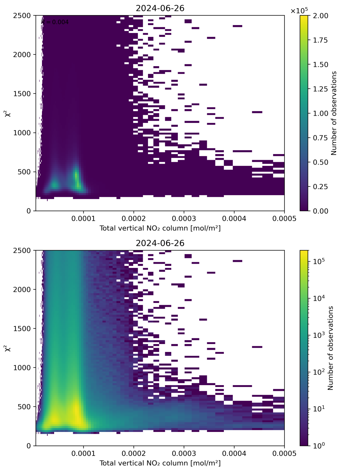
Figure 111: Scatter density plot of “Total vertical NO 2 column” against “ \chi^2 ” for 2024-06-25 to 2024-06-27.
