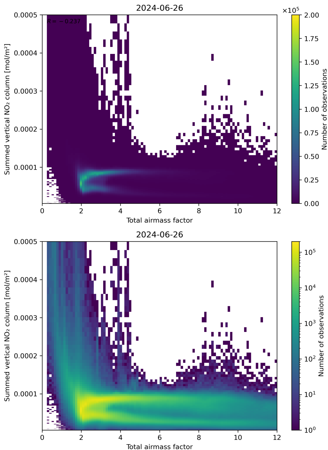
Figure 65: Scatter density plot of “Total airmass factor” against “Summed vertical NO 2 column” for 2024-06-25 to 2024-06-27.
