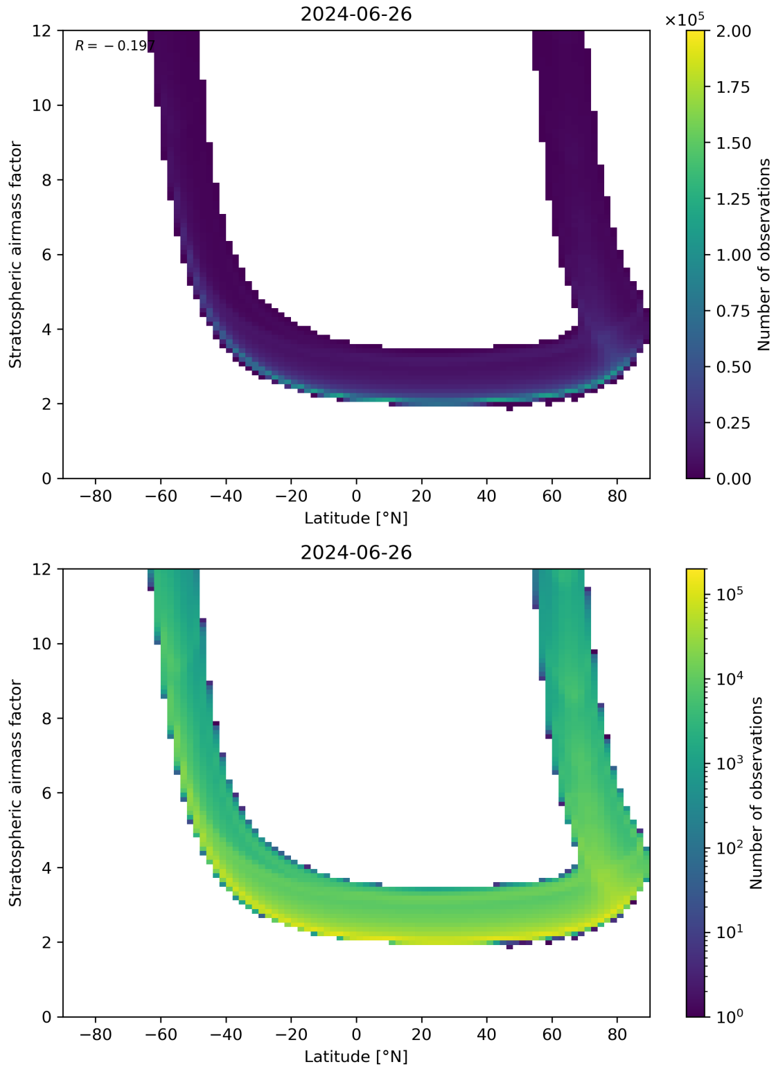
Figure 83: Scatter density plot of “Latitude” against “Stratospheric air mass factor” for 2024-06-25 to 2024-06-27.
