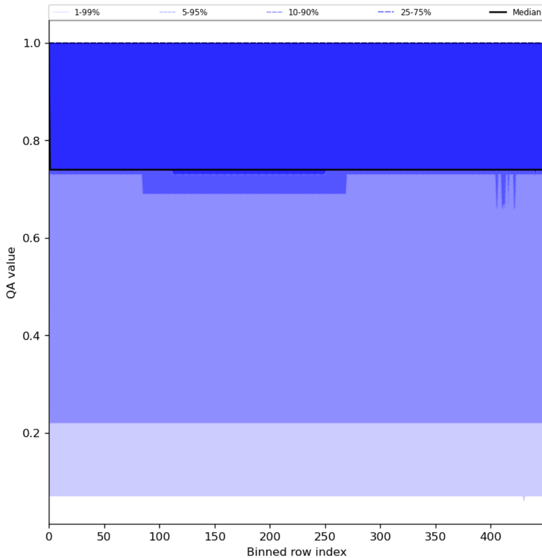
Figure 45: Along track statistics of “QA value” for 2024-06-25 to 2024-06-27
