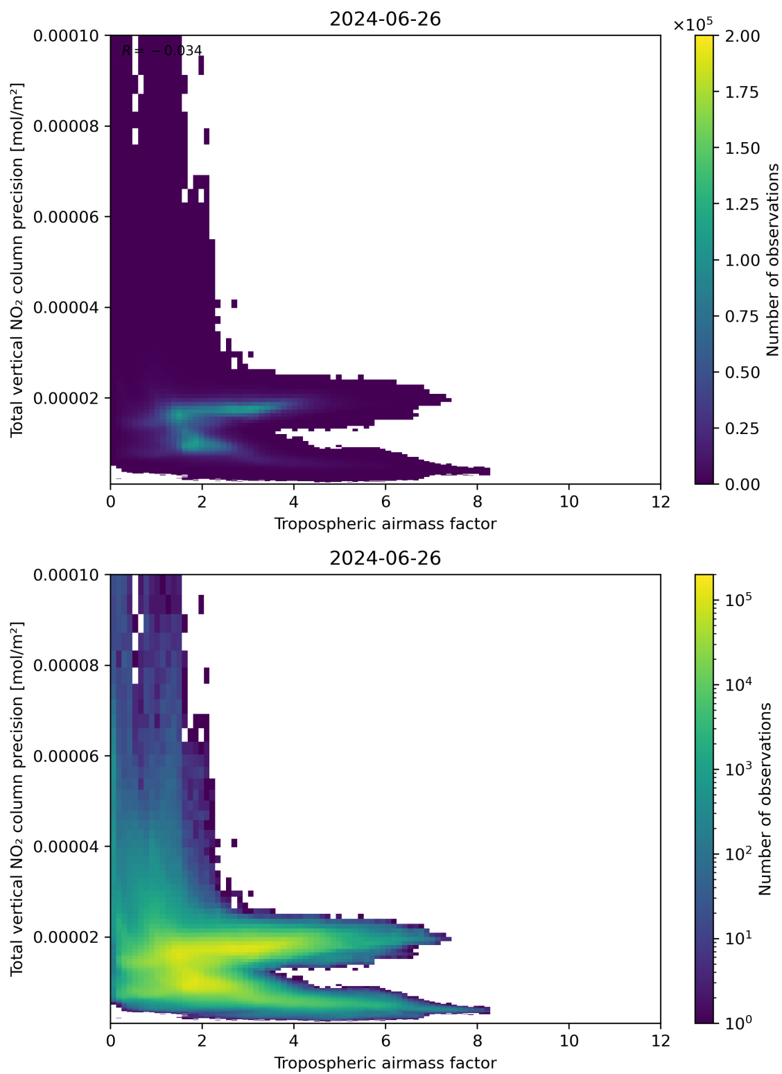
Figure 78: Scatter density plot of “Tropospheric air mass factor” against “Total vertical NO 2 column precision” for 2024-06-25 to 2024-06-27.
