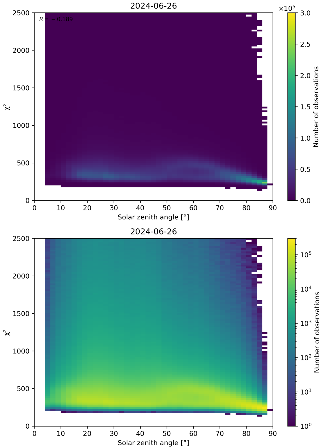
Figure 148: Scatter density plot of “Solar zenith angle” against “ \chi^2 ” for 2024-06-25 to 2024-06-27.
