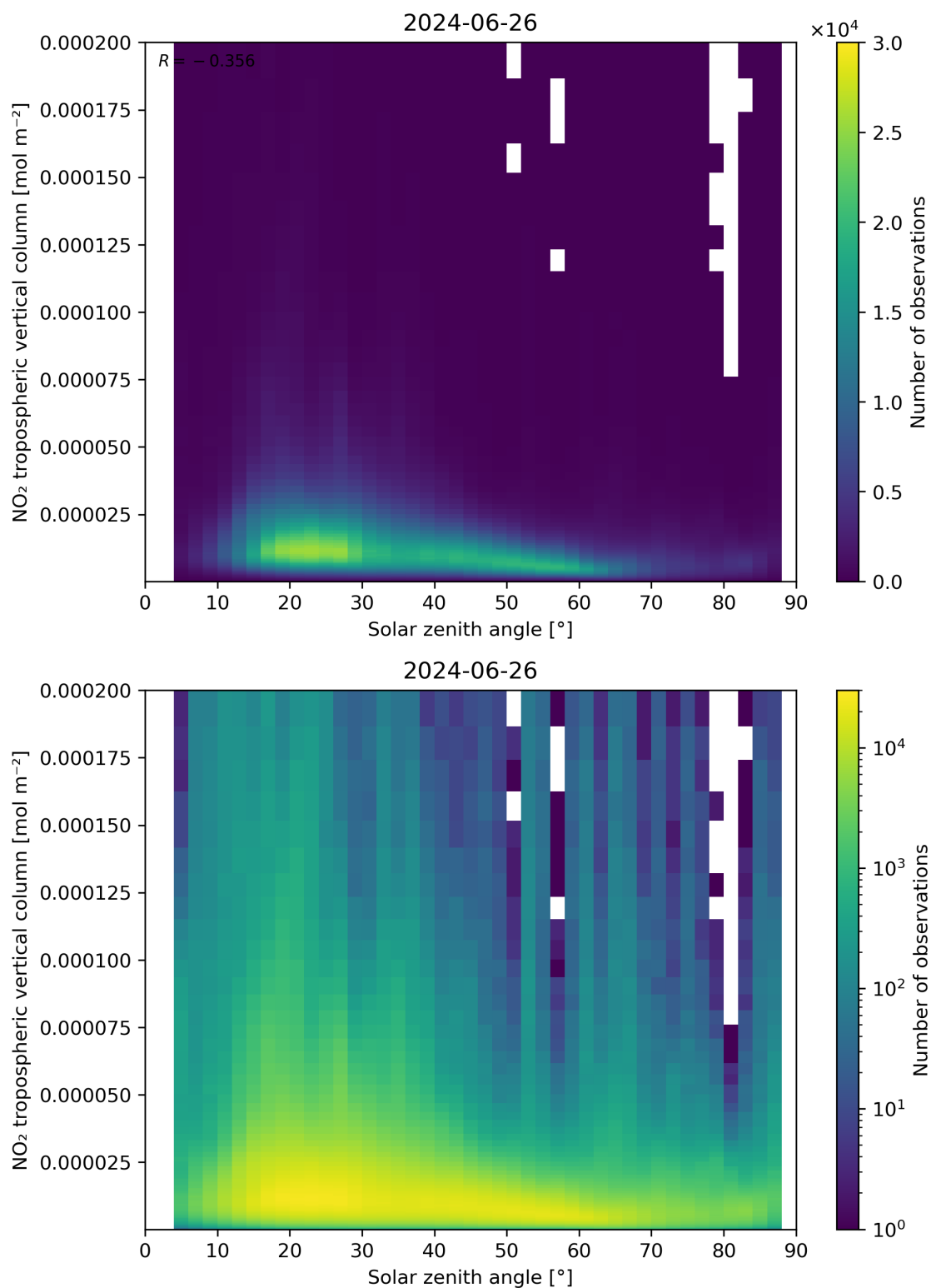
Figure 155: Scatter density plot of “Solar zenith angle” against “NO 2 tropospheric vertical column” for 2024-06-25 to 2024-06-27.
