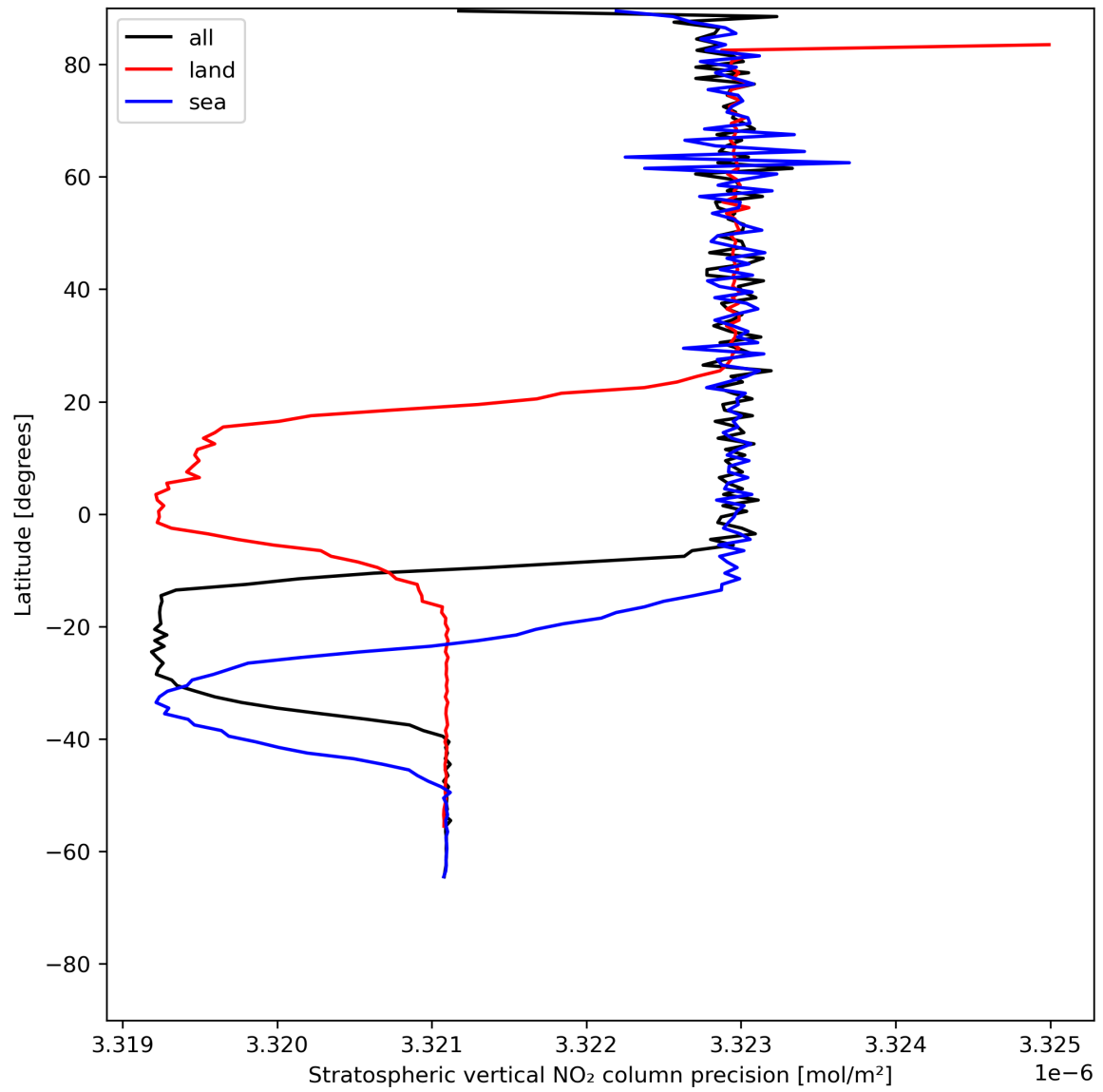
Figure 20: Zonal average of “Stratospheric vertical NO 2 column precision” for 2024-06-25 to 2024-06-27.
