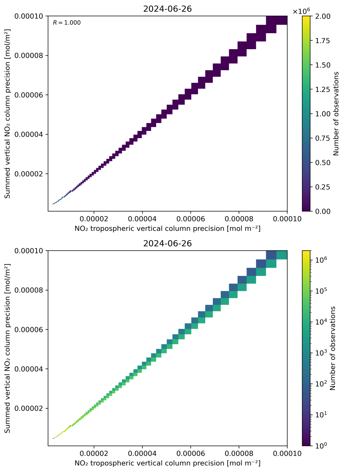
Figure 137: Scatter density plot of “NO 2 tropospheric vertical column precision” against “Summed vertical NO 2 column precision” for 2024-06-25 to 2024-06-27.
