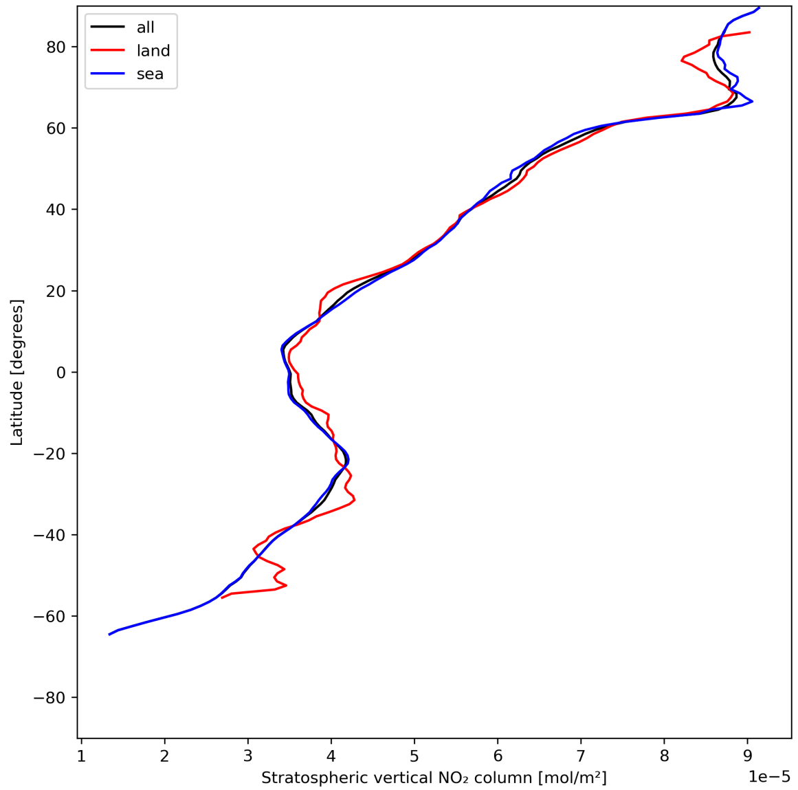
Figure 19: Zonal average of “Stratospheric vertical NO 2 column” for 2024-06-25 to 2024-06-27.
