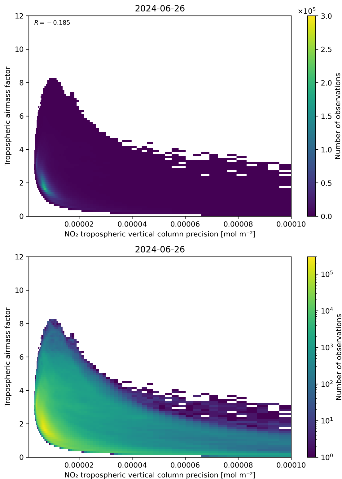
Figure 133: Scatter density plot of “NO 2 tropospheric vertical column precision” against “Tropospheric airmass factor” for 2024-06-25 to 2024-06-27.
