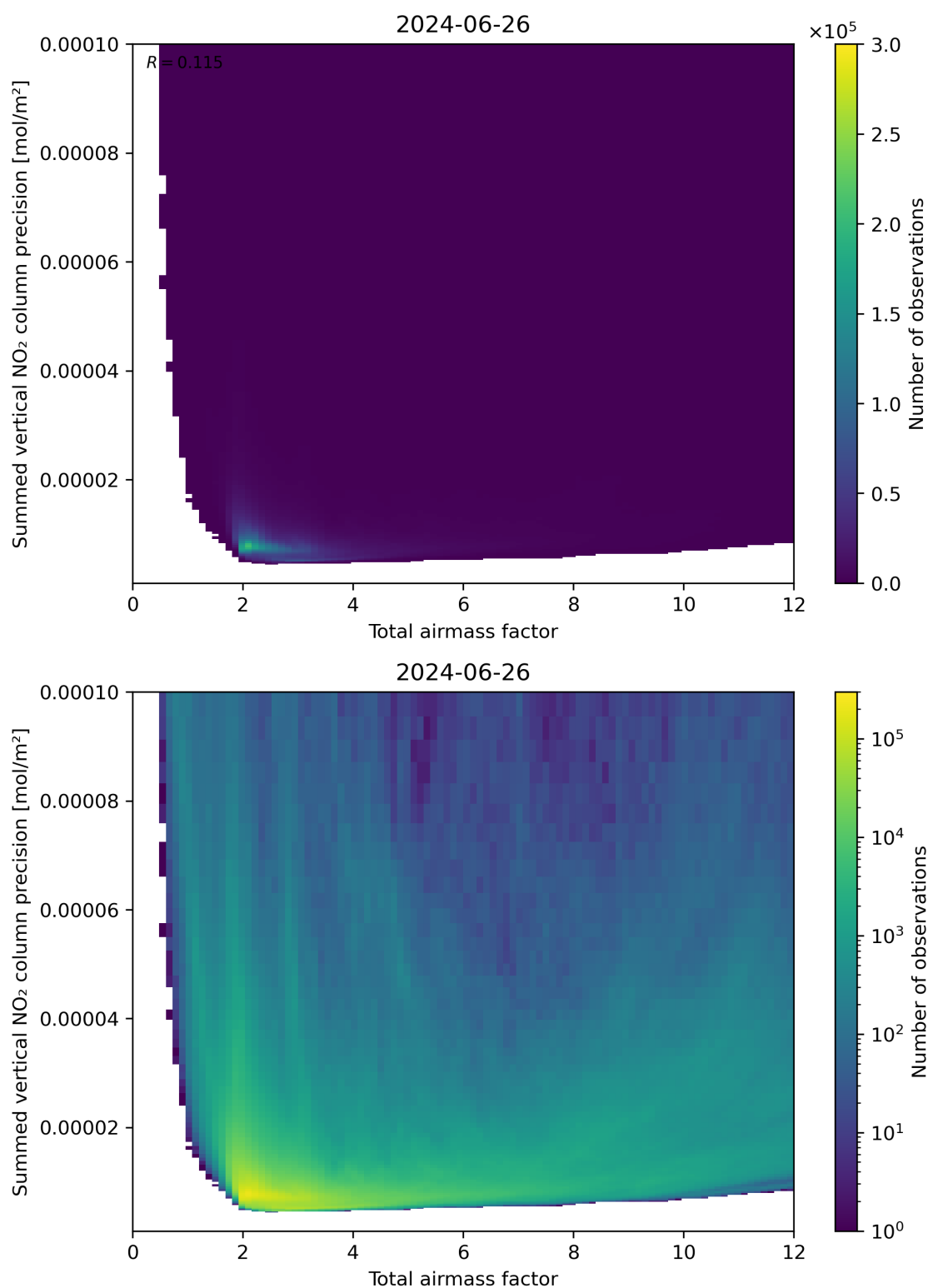
Figure 66: Scatter density plot of “Total airmass factor” against “Summed vertical NO 2 column precision” for 2024-06-25 to 2024-06-27.
