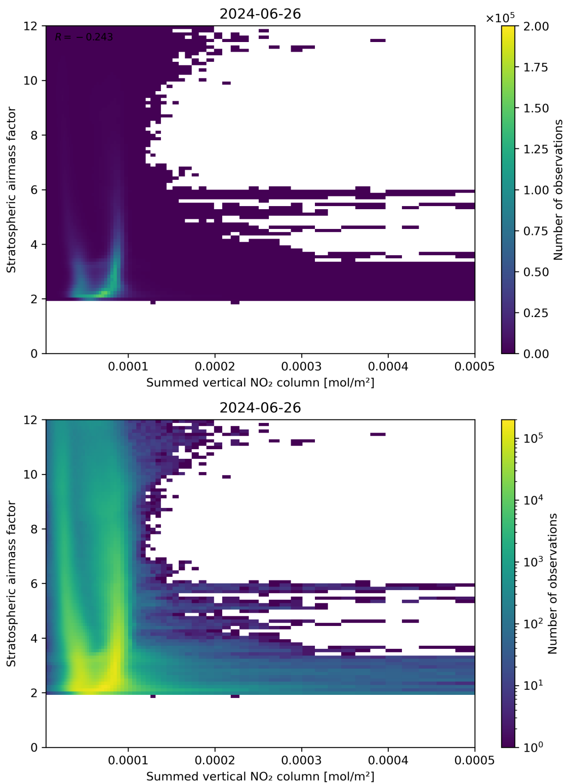
Figure 103: Scatter density plot of “Summed vertical NO 2 column” against “Stratospheric air mass factor” for 2024-06-25 to 2024-06-27.
