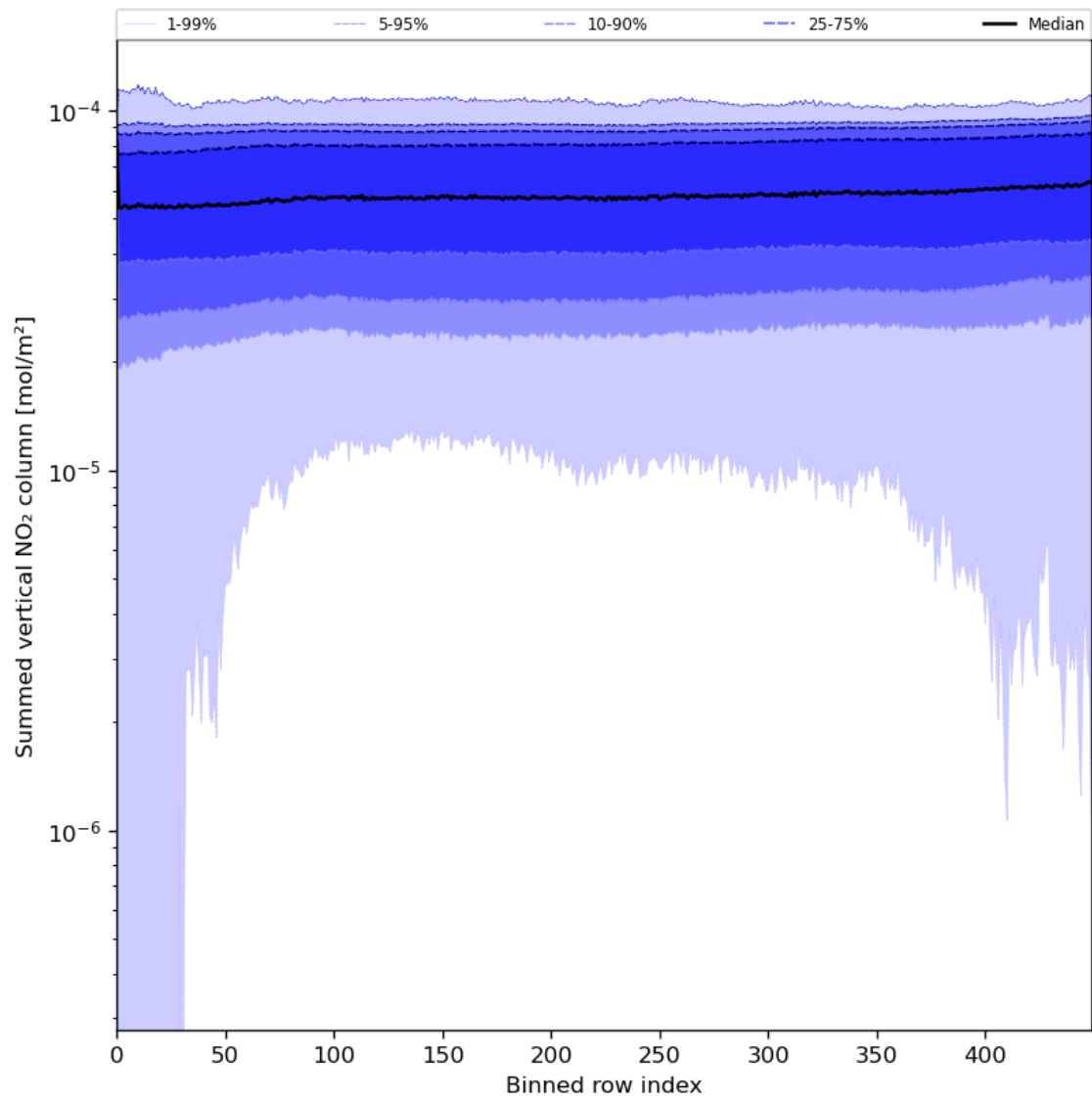
Figure 57: Along track statistics of “Summed vertical NO 2 column” for 2024-06-25 to 2024-06-27
