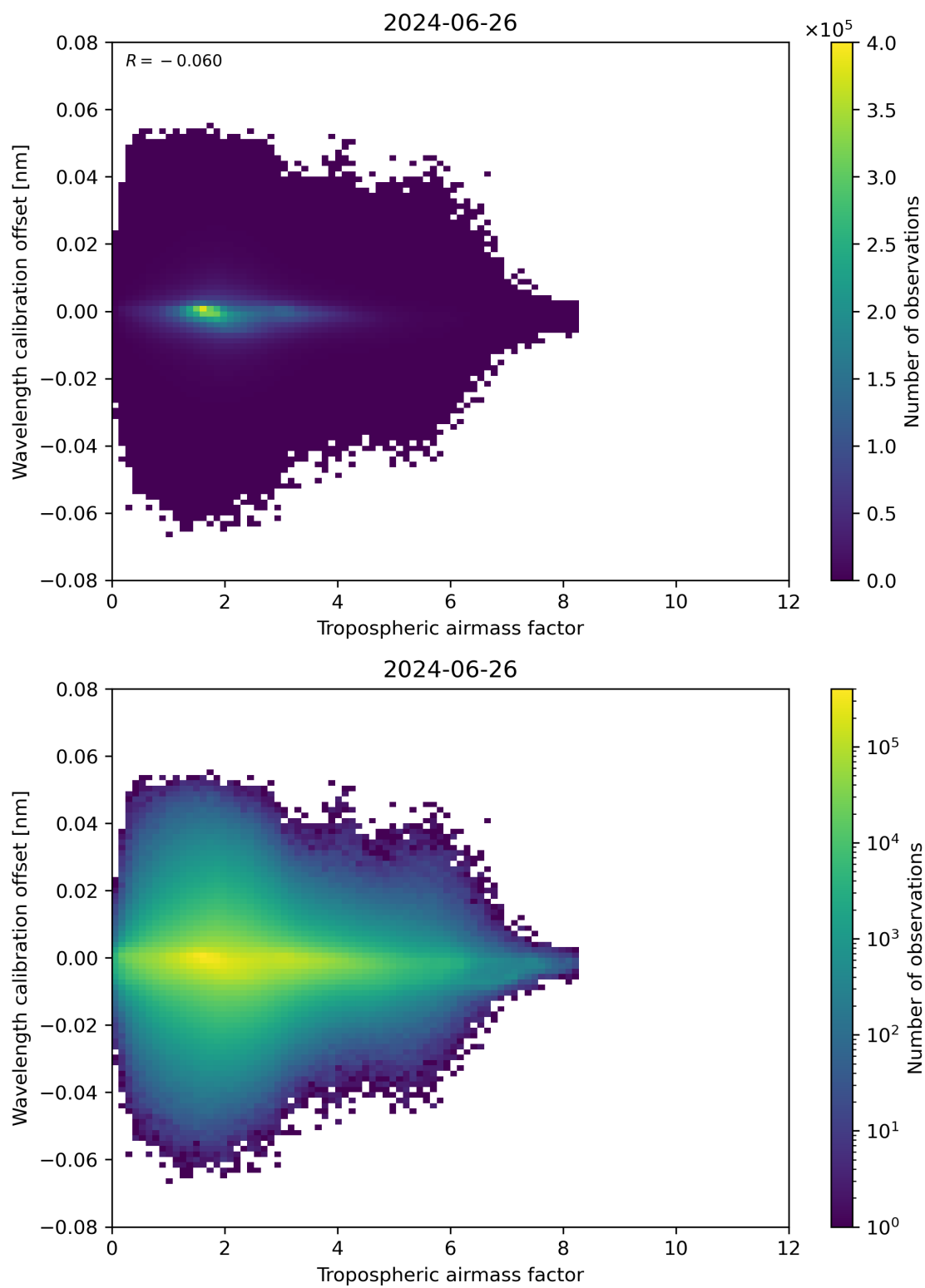
Figure 80: Scatter density plot of “Tropospheric airmass factor” against “Wavelength calibration offset” for 2024-06-25 to 2024-06-27.
