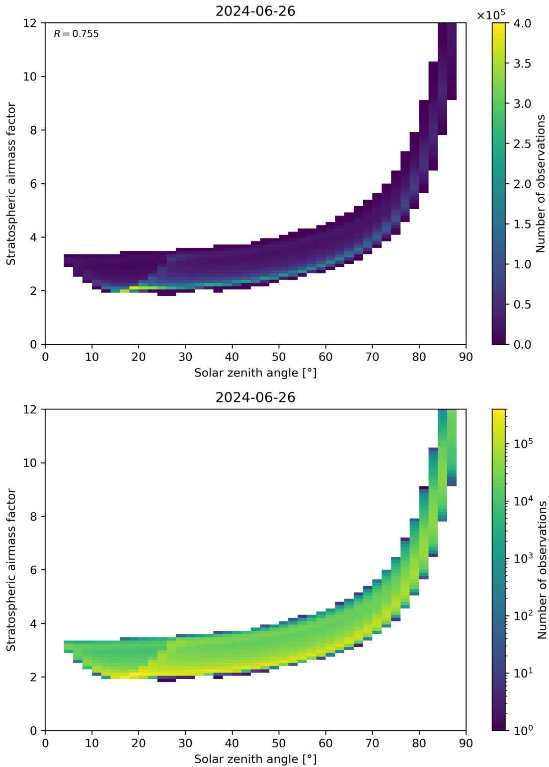
Figure 145: Scatter density plot of “Solar zenith angle” against “Stratospheric airmass factor” for 2024-06-25 to 2024-06-27.
