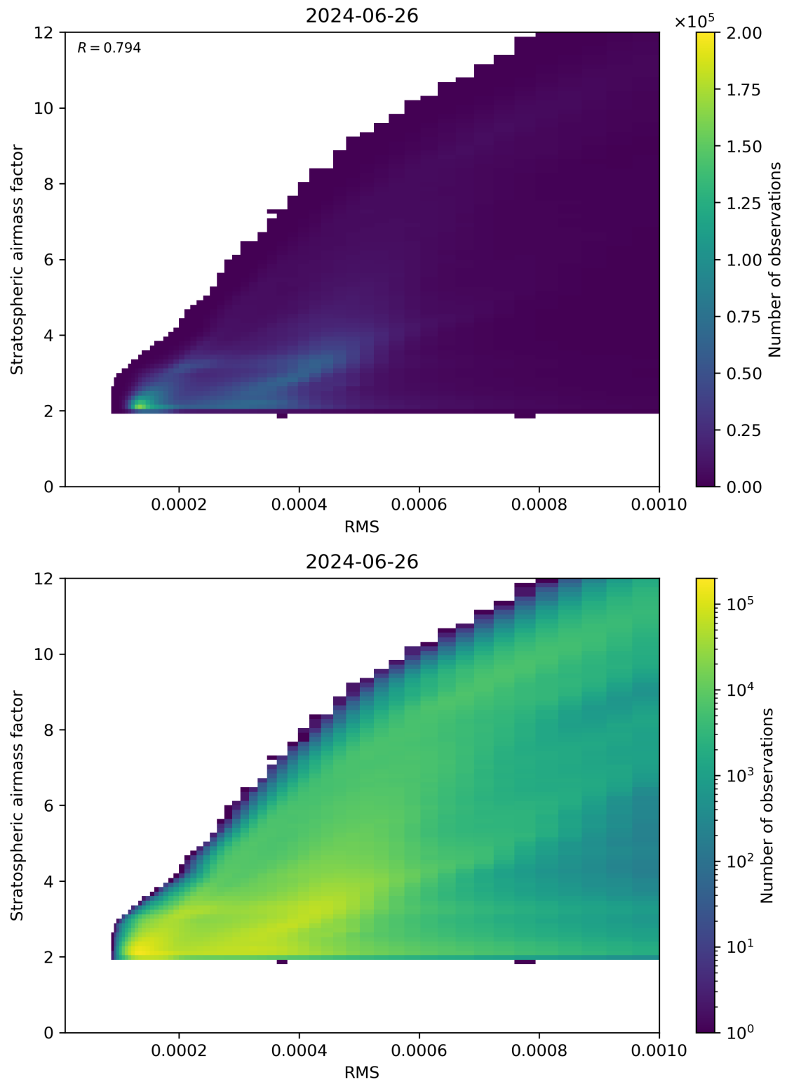
Figure 144: Scatter density plot of “RMS” against “Stratospheric airmass factor” for 2024-06-25 to 2024-06-27.
