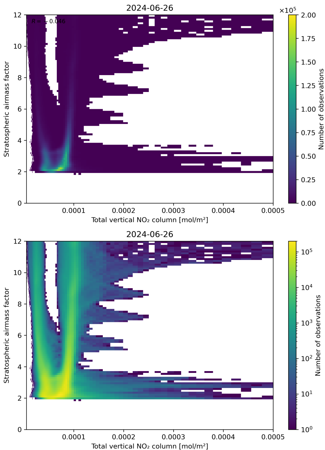
Figure 110: Scatter density plot of “Total vertical NO 2 column” against “Stratospheric airmass factor” for 2024-06-25 to 2024-06-27.
