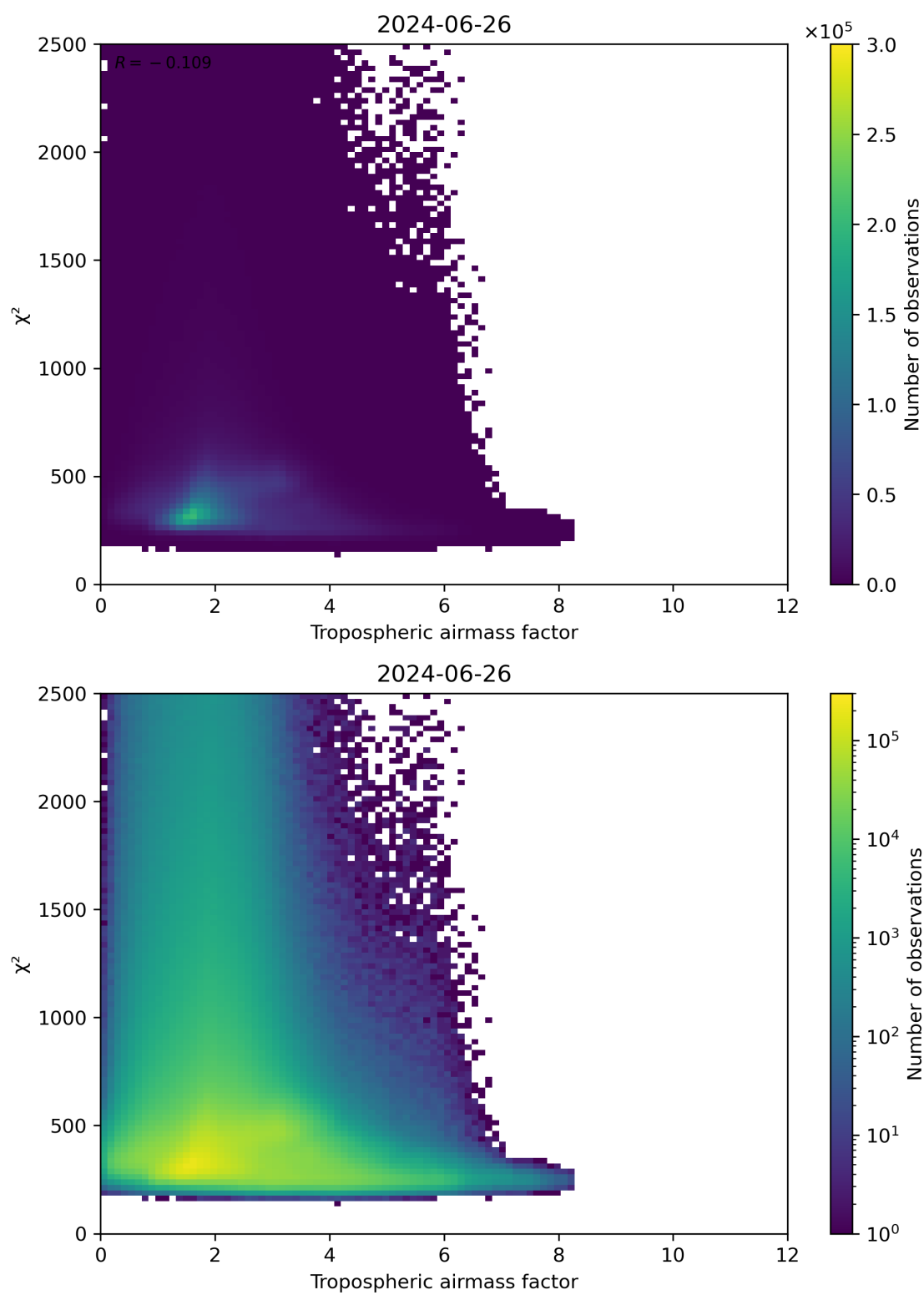
Figure 73: Scatter density plot of “Tropospheric airmass factor” against “ \chi^2 ” for 2024-06-25 to 2024-06-27.
