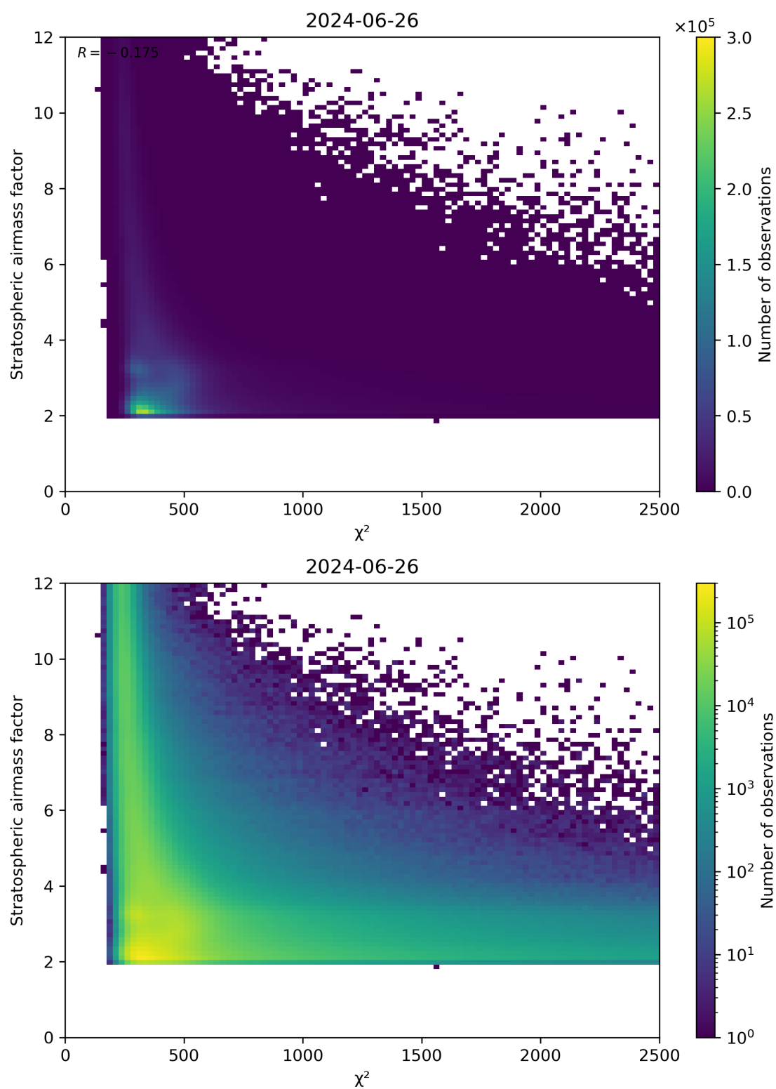
Figure 81: Scatter density plot of “ \chi^2 ” against “Stratospheric airmass factor” for 2024-06-25 to 2024-06-27.
