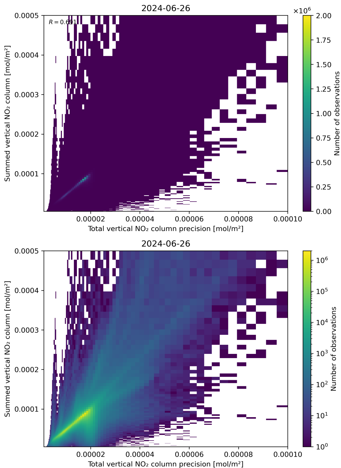
Figure 117: Scatter density plot of “Total vertical NO 2 column precision” against “Summed vertical NO 2 column” for 2024-06-25 to 2024-06-27.
