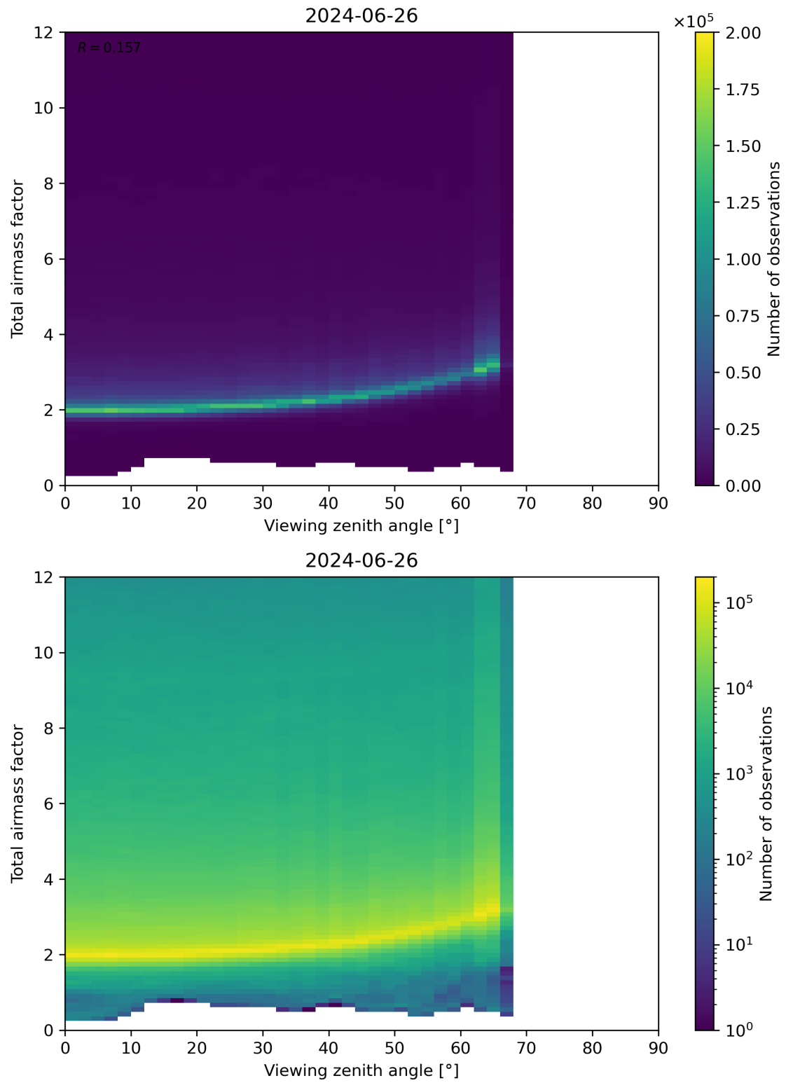
Figure 160: Scatter density plot of “Viewing zenith angle” against “Total airmass factor” for 2024-06-25 to 2024-06-27.
