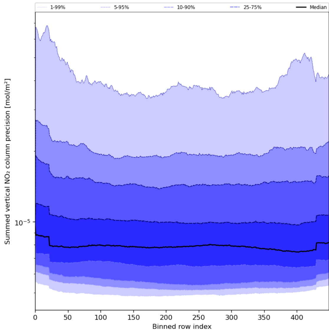
Figure 58: Along track statistics of “Summed vertical NO 2 column precision” for 2024-06-25 to 2024-06-27
