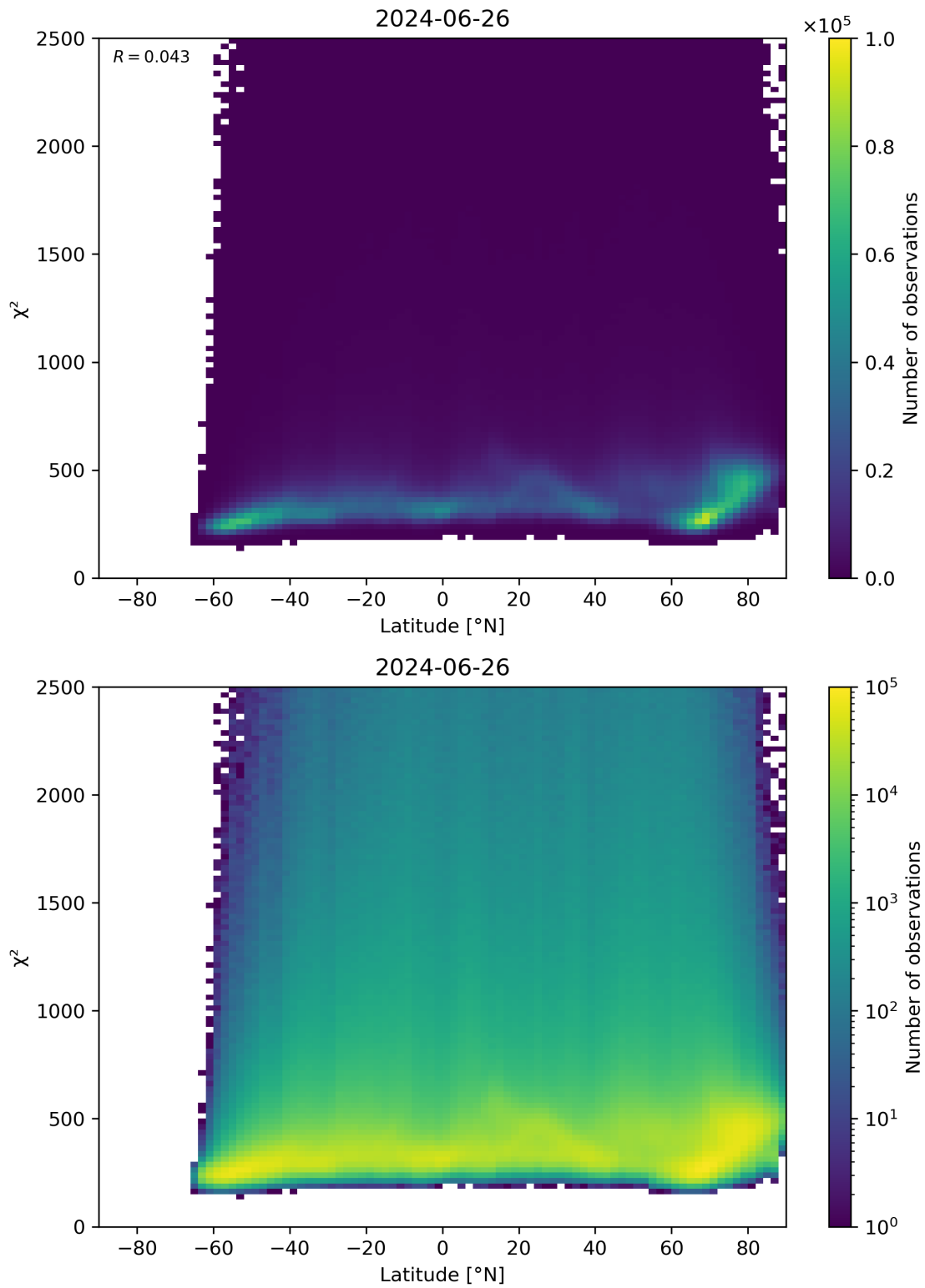
Figure 86: Scatter density plot of “Latitude” against “ \chi^2 ” for 2024-06-25 to 2024-06-27.
