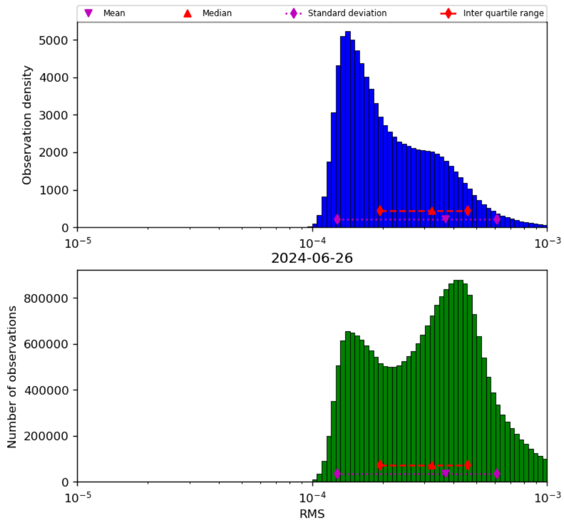
Figure 43: Histogram of “RMS” for 2024-06-25 to 2024-06-27
