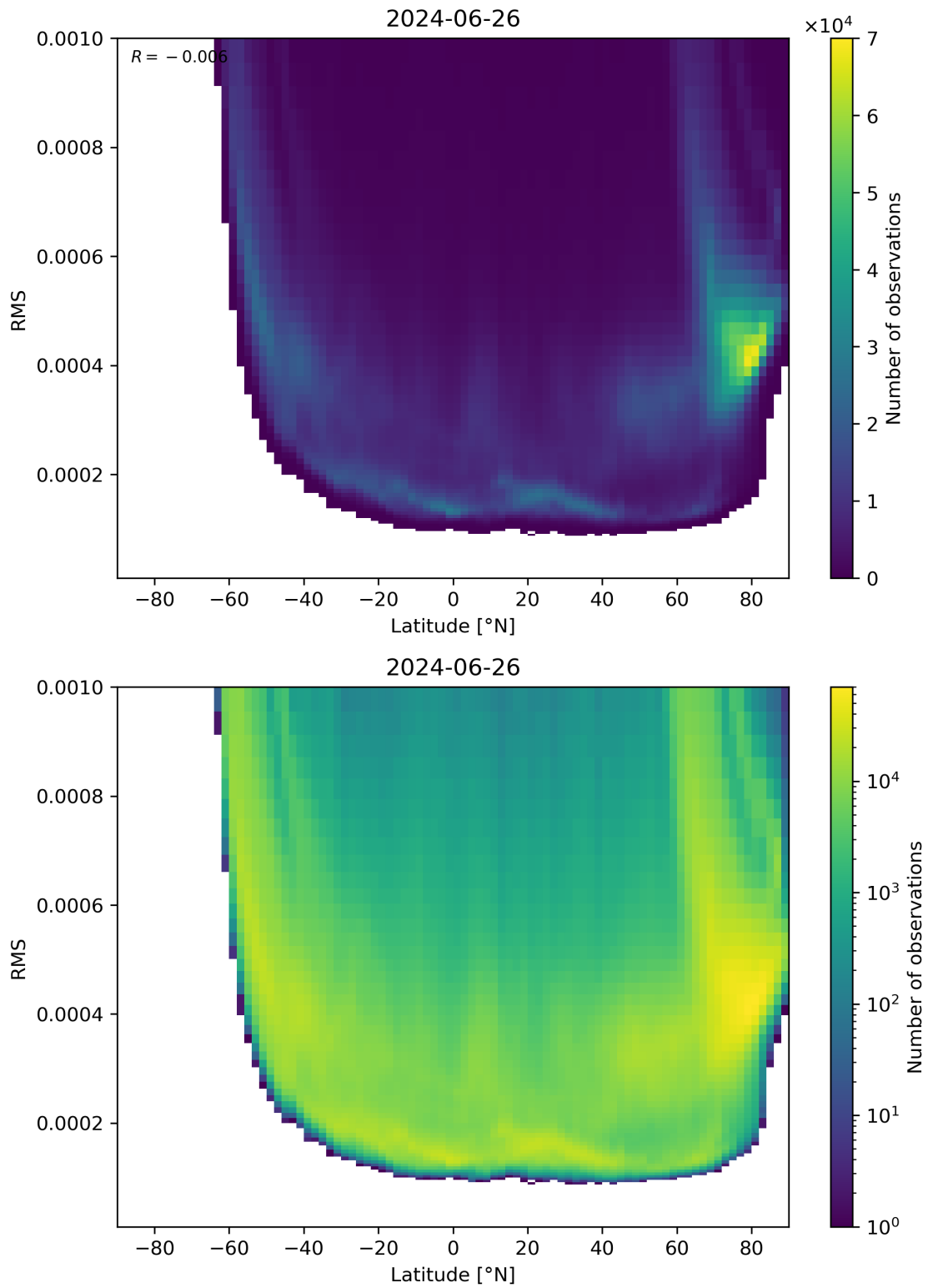
Figure 94: Scatter density plot of “Latitude” against “RMS” for 2024-06-25 to 2024-06-27.
