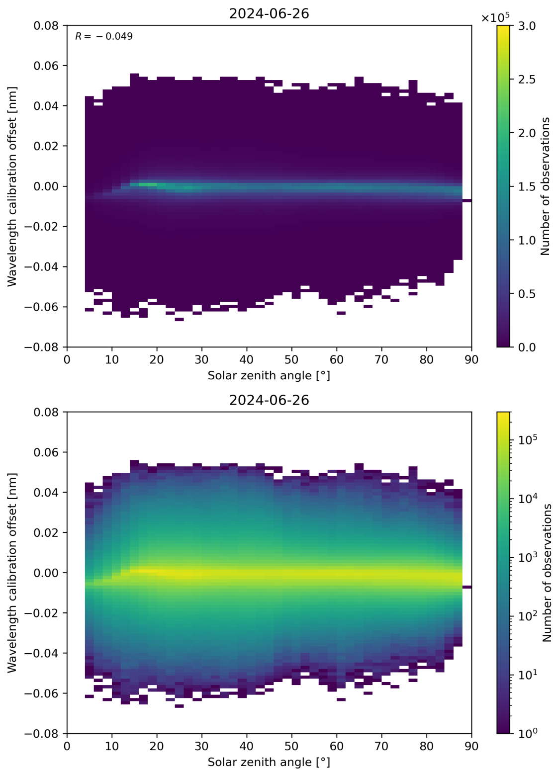
Figure 158: Scatter density plot of “Solar zenith angle” against “Wavelength calibration offset” for 2024-06-25 to 2024-06-27.
