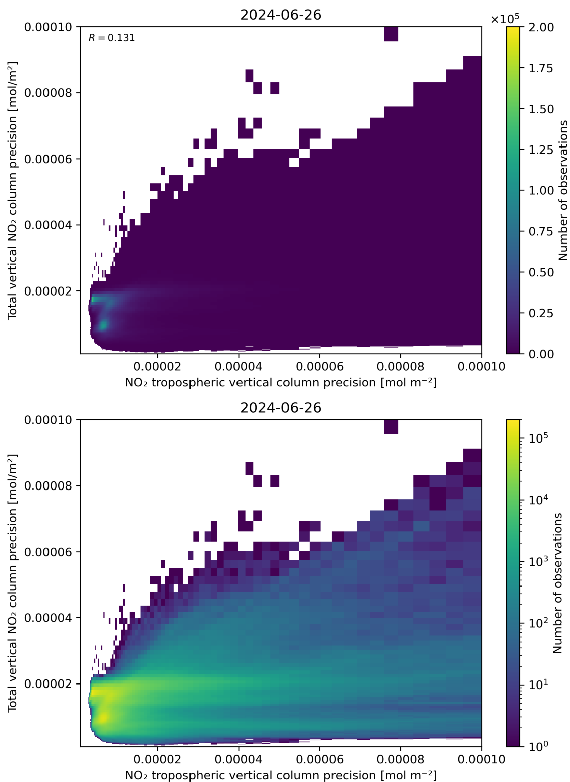
Figure 139: Scatter density plot of “NO 2 tropospheric vertical column precision” against “Total vertical NO 2 column precision” for 2024-06-25 to 2024-06-27.
