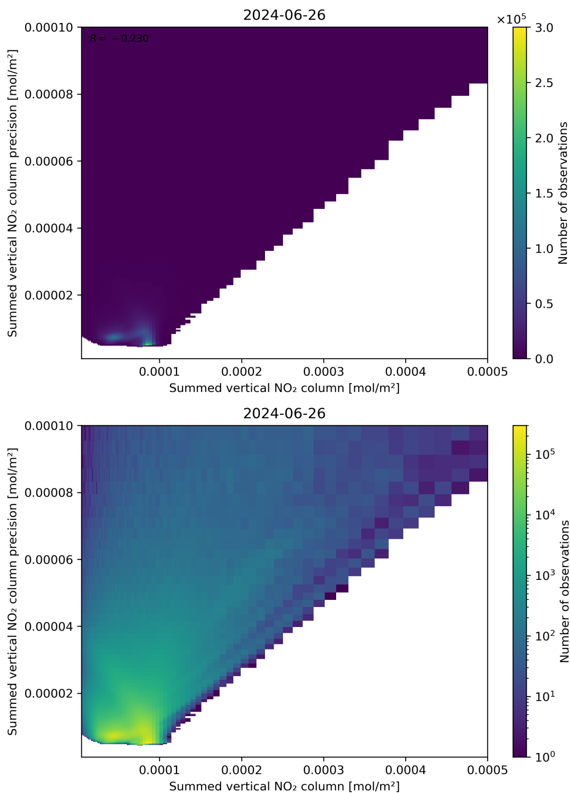
Figure 105: Scatter density plot of “Summed vertical NO 2 column” against “Summed vertical NO 2 column precision” for 2024-06-25 to 2024-06-27.
