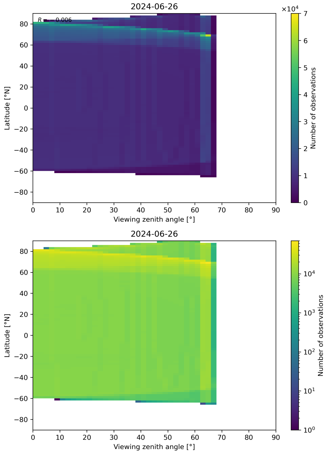
Figure 163: Scatter density plot of “Viewing zenith angle” against “Latitude” for 2024-06-25 to 2024-06-27.
