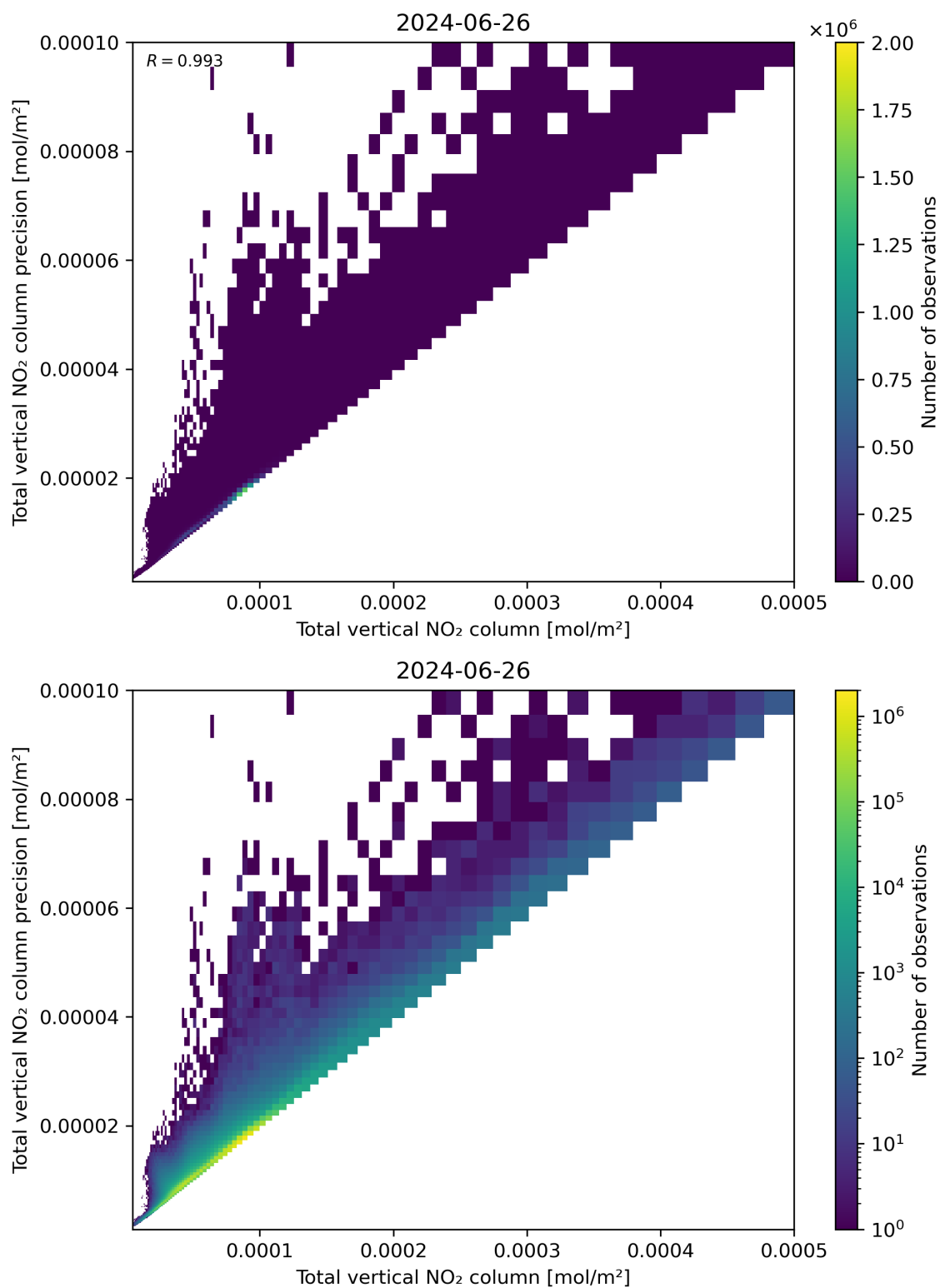
Figure 114: Scatter density plot of “Total vertical NO 2 column” against “Total vertical NO 2 column precision” for 2024-06-25 to 2024-06-27.
