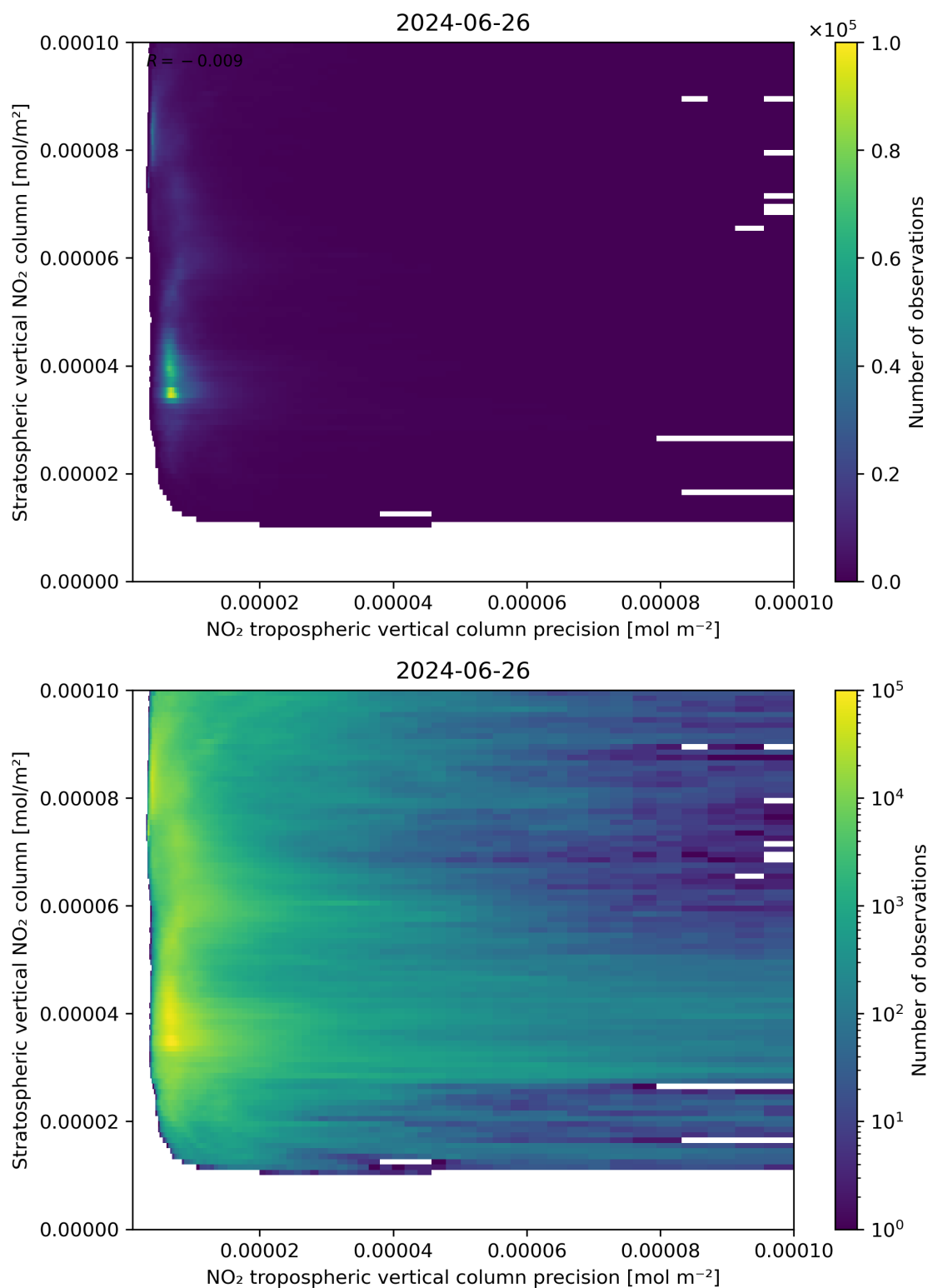
Figure 135: Scatter density plot of “NO 2 tropospheric vertical column precision” against “Stratospheric vertical NO 2 column” for 2024-06-25 to 2024-06-27.
