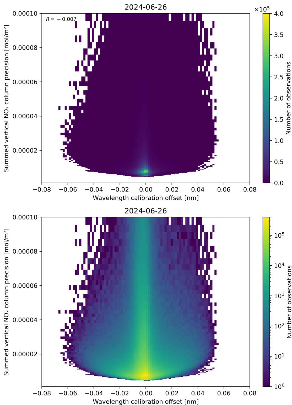
Figure 178: Scatter density plot of “Wavelength calibration offset” against “Summed vertical NO 2 column precision” for 2024-06-25 to 2024-06-27.
