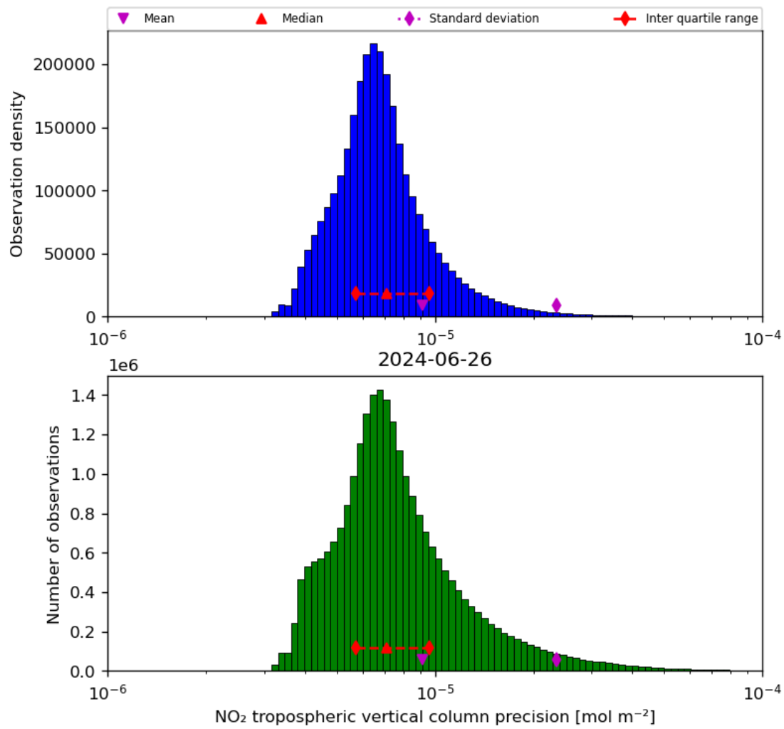
Figure 30: Histogram of “NO 2 tropospheric vertical column precision” for 2024-06-25 to 2024-06-27
