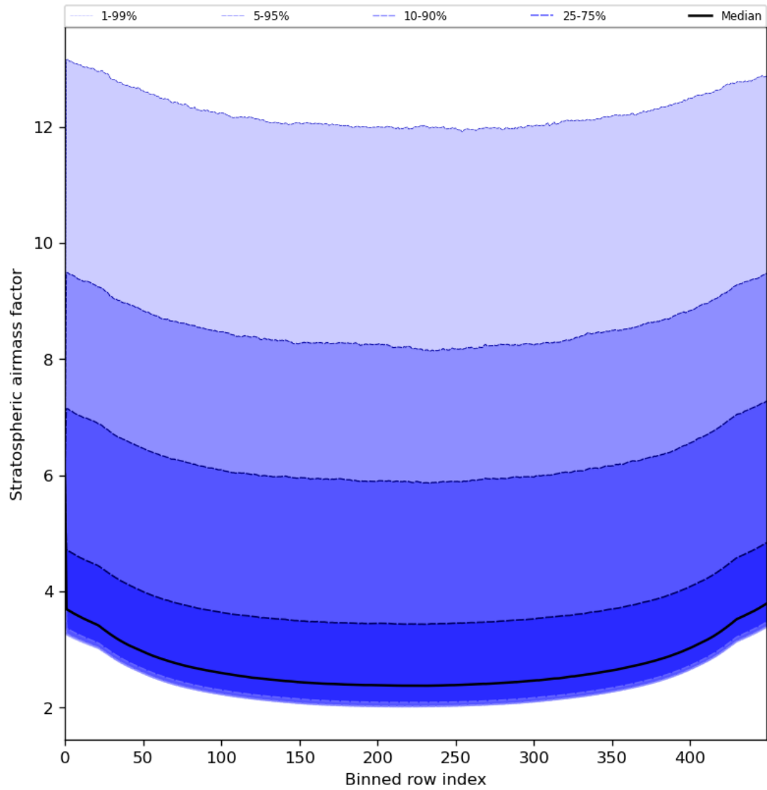
Figure 61: Along track statistics of “Stratospheric airmass factor” for 2024-06-25 to 2024-06-27
