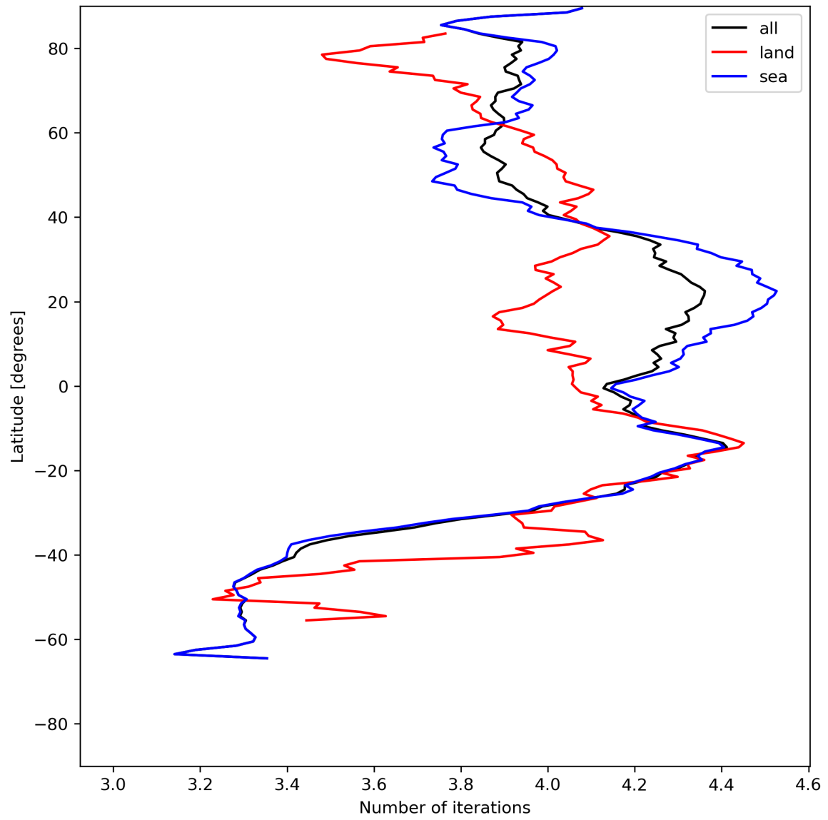
Figure 17: Zonal average of “Number of iterations” for 2024-06-25 to 2024-06-27.
