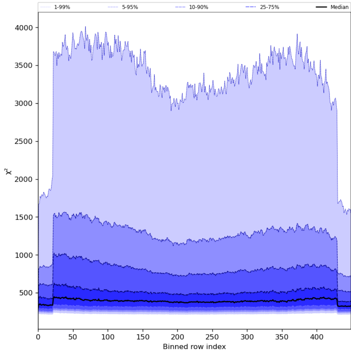
Figure 59: Along track statistics of “ \chi^2 ” for 2024-06-25 to 2024-06-27
