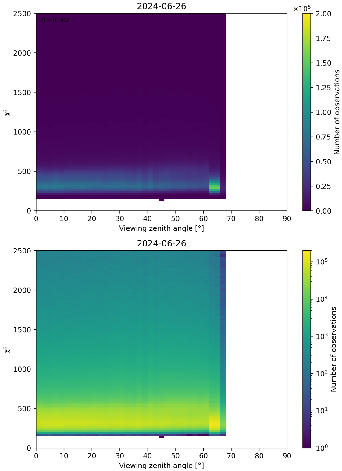
Figure 162: Scatter density plot of “Viewing zenith angle” against “ \chi^2 ” for 2024-06-25 to 2024-06-27.
