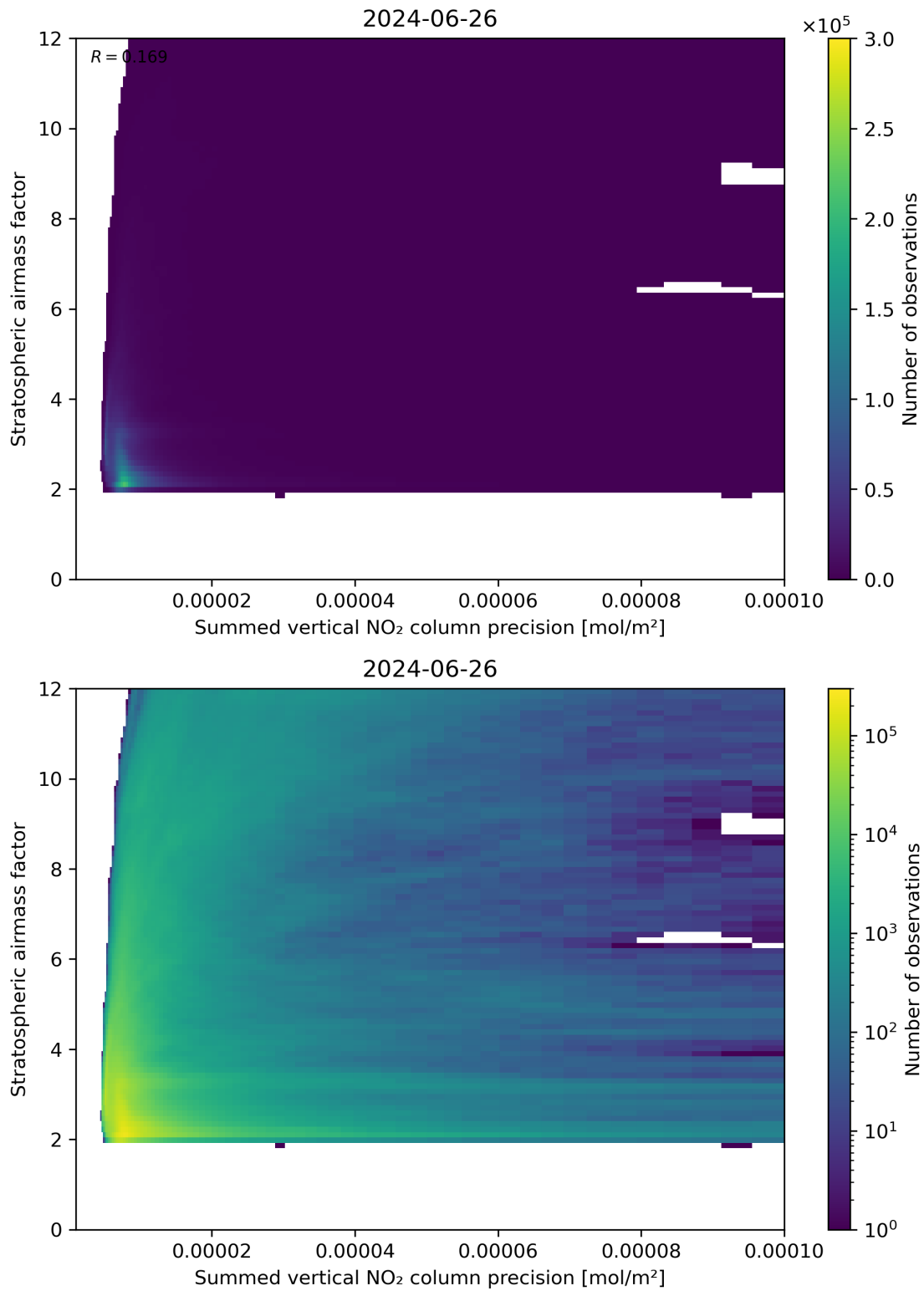
Figure 106: Scatter density plot of “Summed vertical NO 2 column precision” against “Stratospheric airmass factor” for 2024-06-25 to 2024-06-27.
