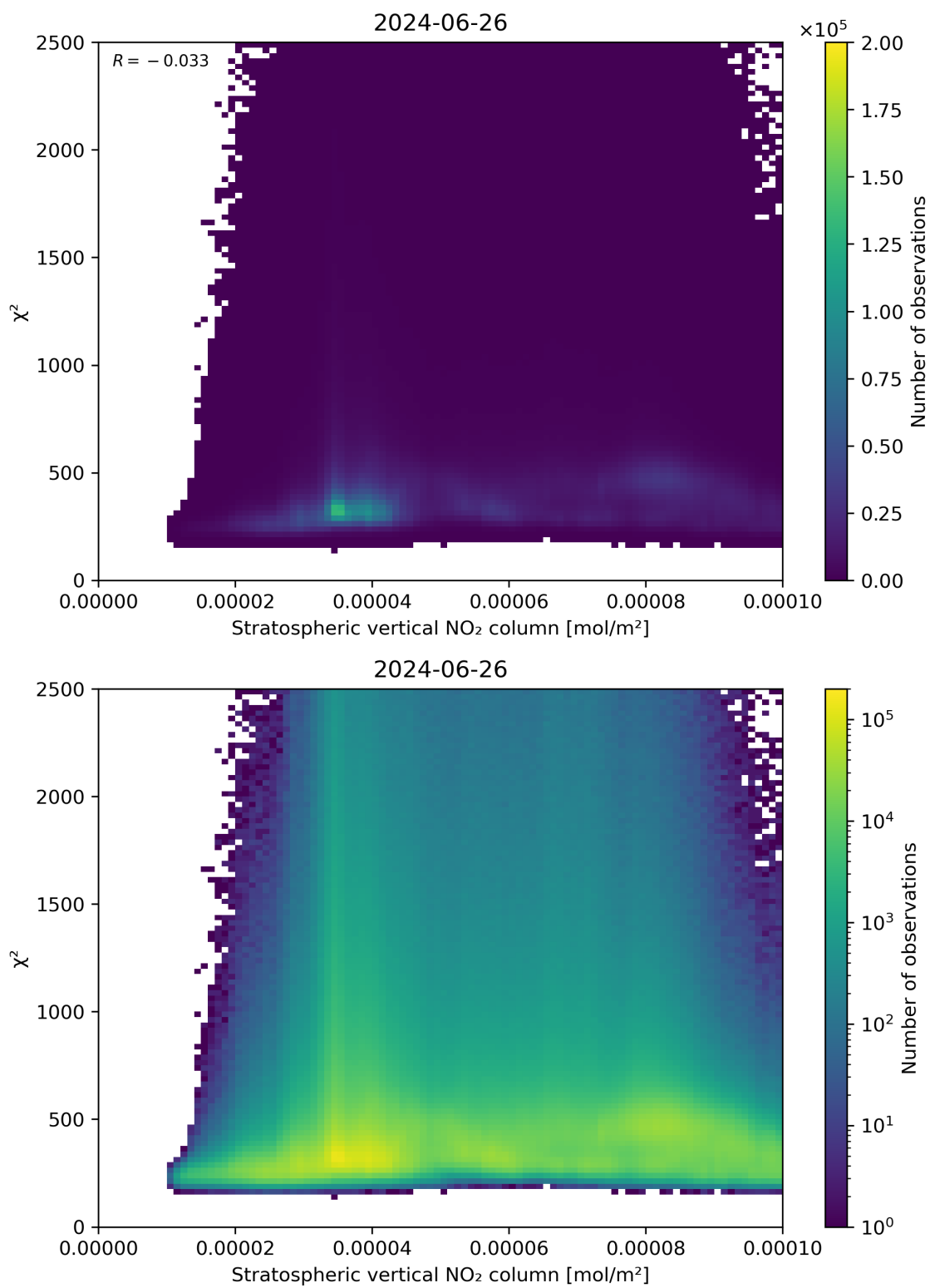
Figure 97: Scatter density plot of “Stratospheric vertical NO 2 column” against “ \chi^2 ” for 2024-06-25 to 2024-06-27.
