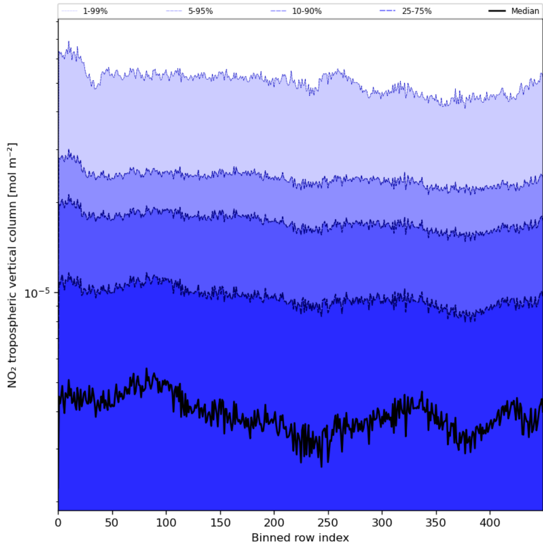
Figure 46: Along track statistics of “NO 2 tropospheric vertical column” for 2024-06-25 to 2024-06-27
