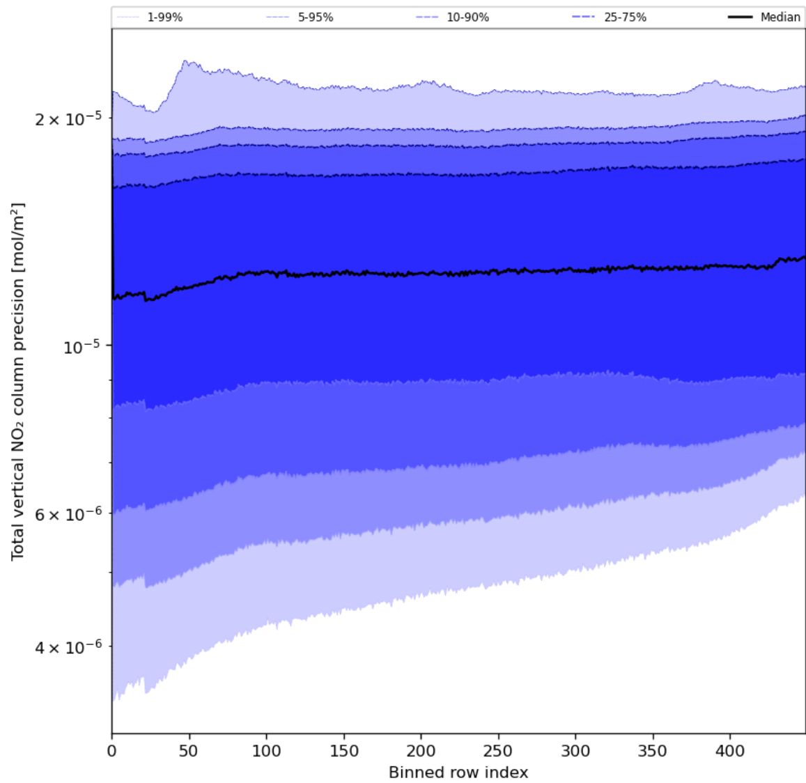
Figure 56: Along track statistics of “Total vertical NO 2 column precision” for 2024-06-25 to 2024-06-27
