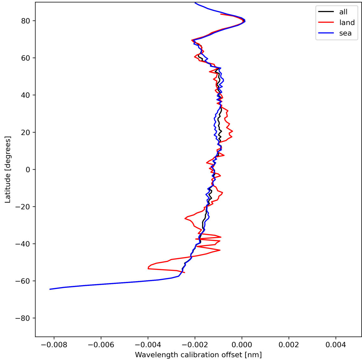
Figure 18: Zonal average of “Wavelength calibration offset” for 2024-06-25 to 2024-06-27.
