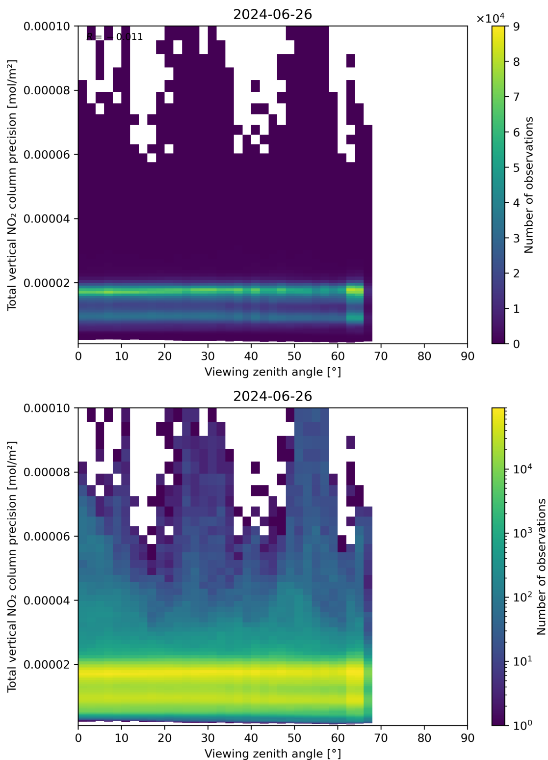
Figure 168: Scatter density plot of “Viewing zenith angle” against “Total vertical NO 2 column precision” for 2024-06-25 to 2024-06-27.
