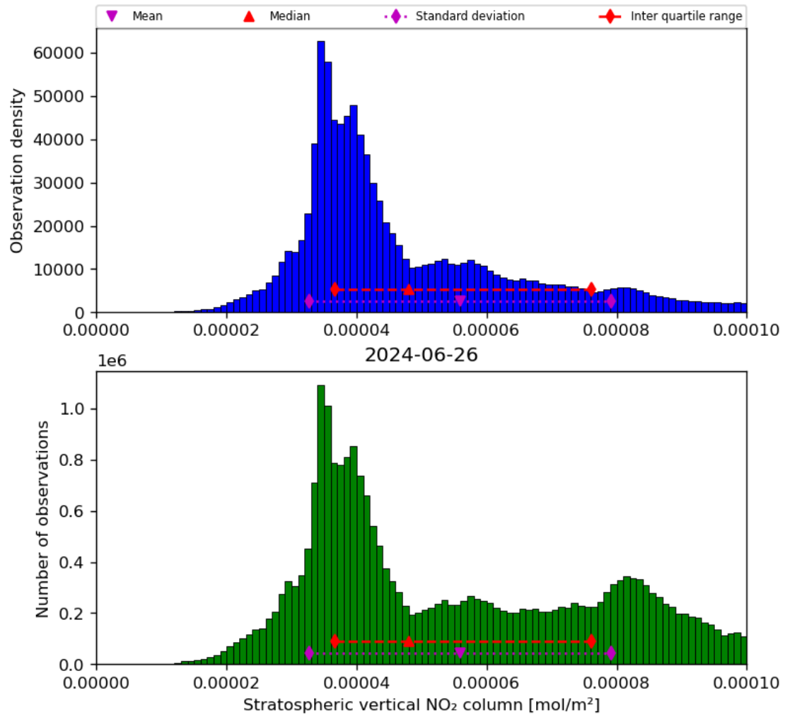
Figure 36: Histogram of “Stratospheric vertical NO 2 column” for 2024-06-25 to 2024-06-27
