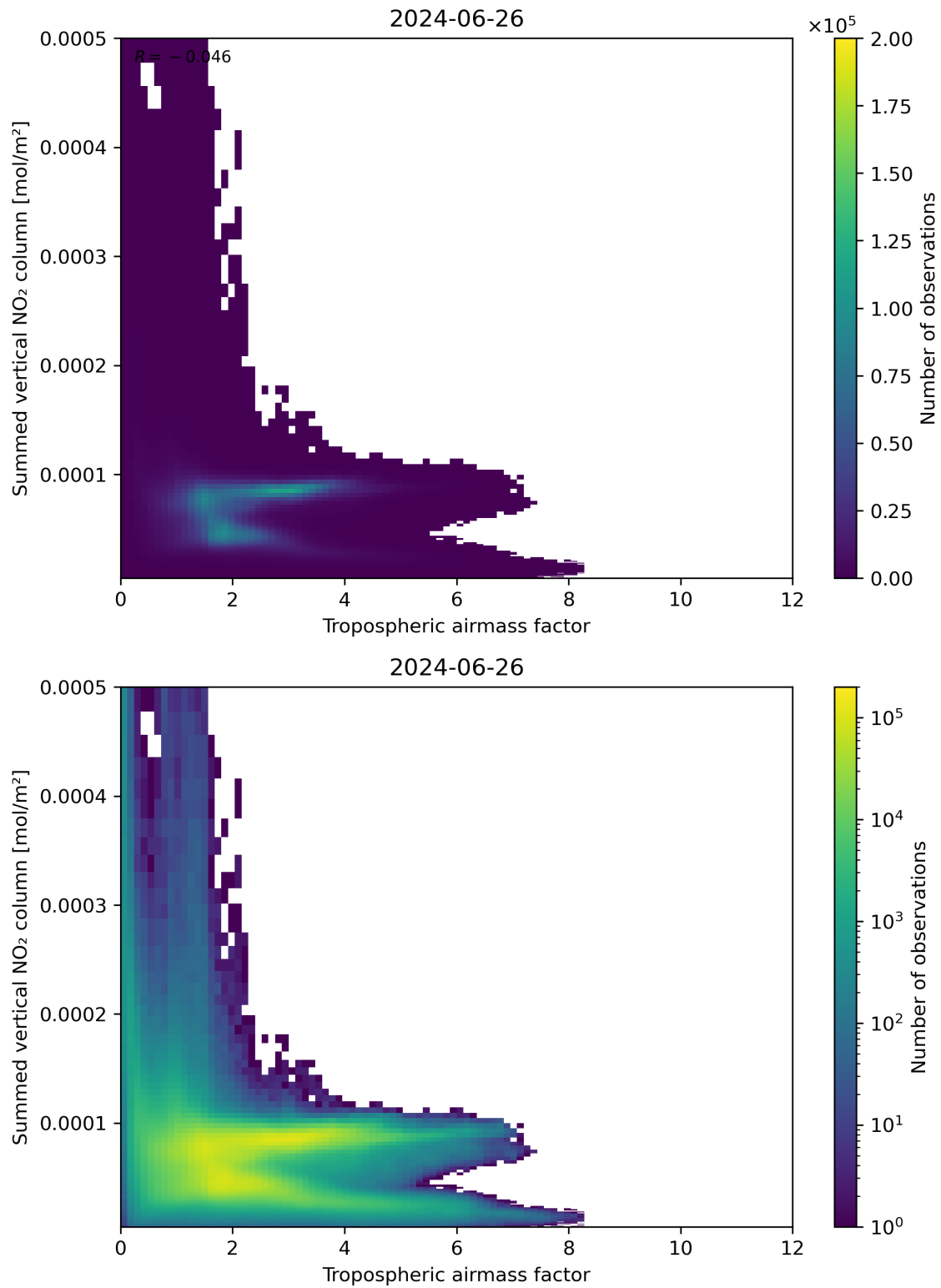
Figure 75: Scatter density plot of “Tropospheric airmass factor” against “Summed vertical NO 2 column” for 2024-06-25 to 2024-06-27.
