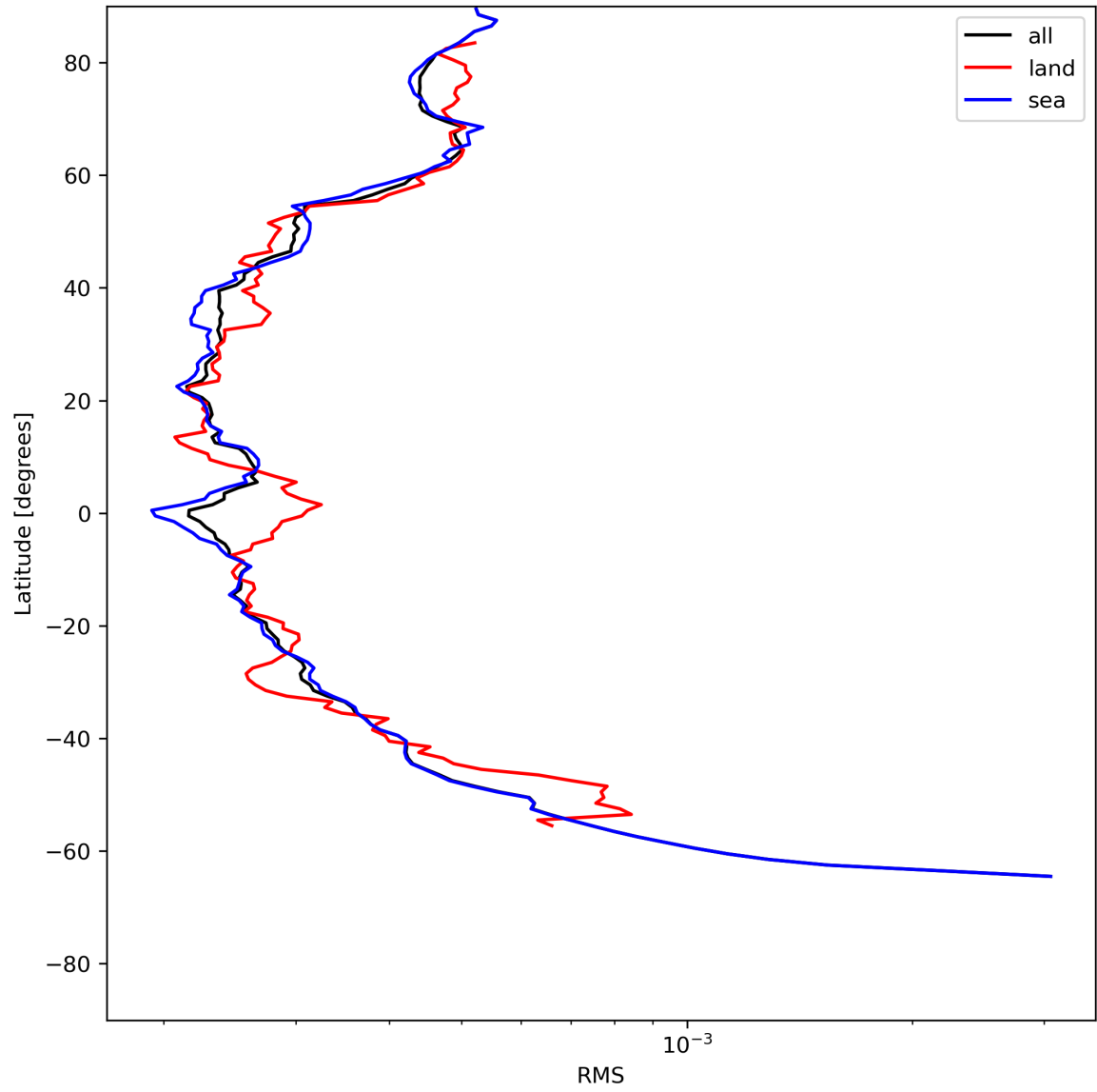
Figure 26: Zonal average of “RMS” for 2024-06-25 to 2024-06-27.
