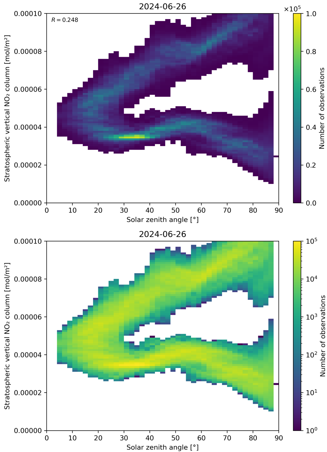
Figure 150: Scatter density plot of “Solar zenith angle” against “Stratospheric vertical NO 2 column” for 2024-06-25 to 2024-06-27.
