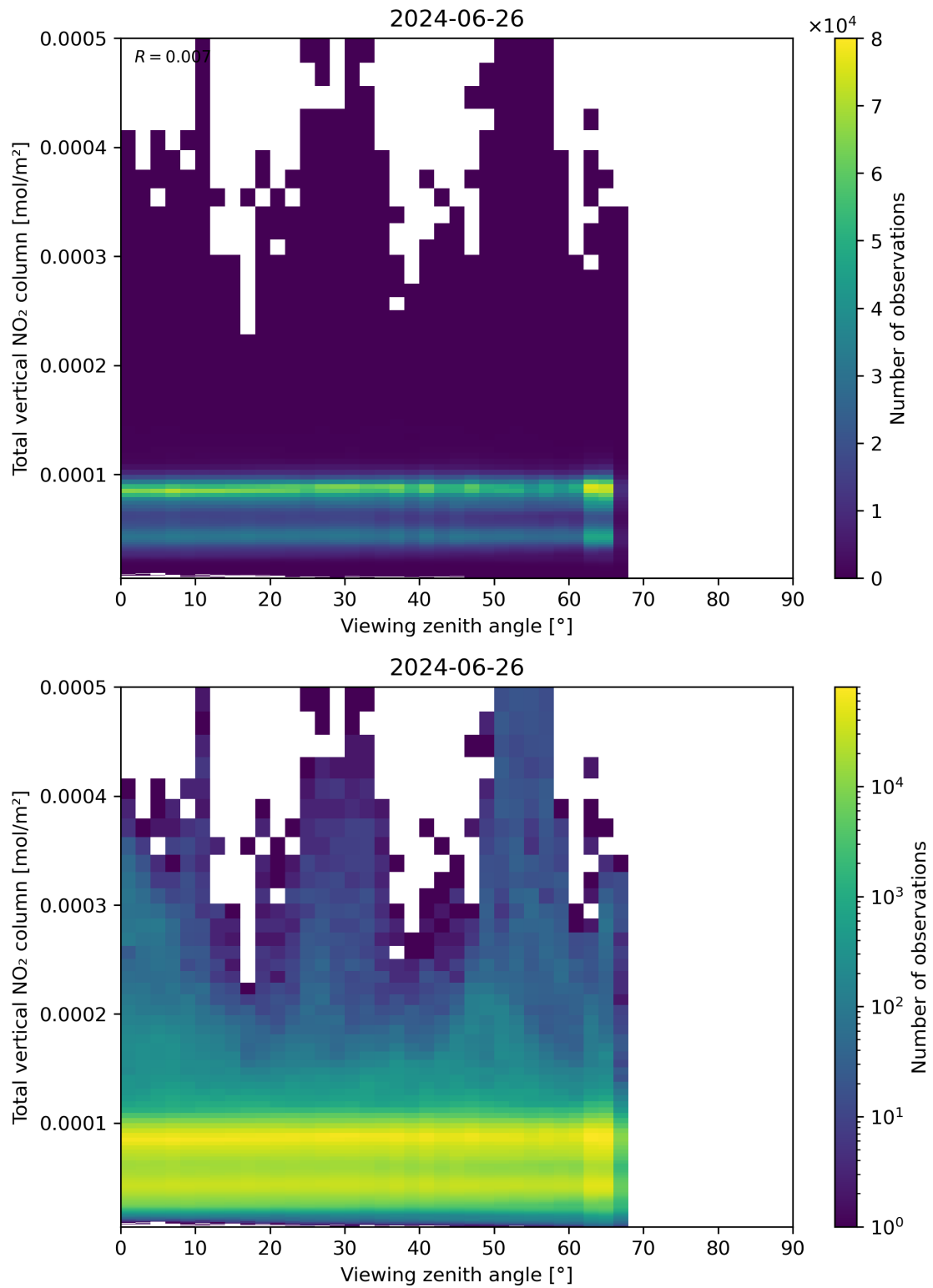
Figure 167: Scatter density plot of “Viewing zenith angle” against “Total vertical NO 2 column” for 2024-06-25 to 2024-06-27.
