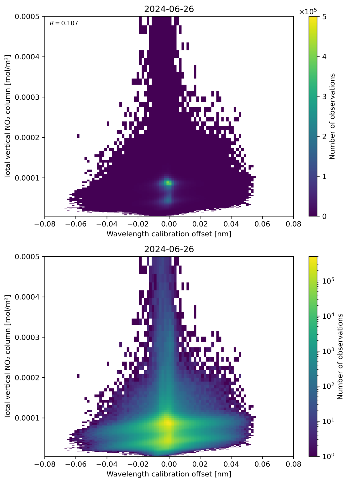
Figure 179: Scatter density plot of “Wavelength calibration offset” against “Total vertical NO 2 column” for 2024-06-25 to 2024-06-27.
