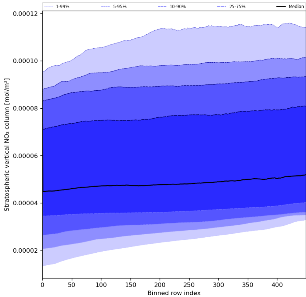
Figure 53: Along track statistics of “Stratospheric vertical NO 2 column” for 2024-06-25 to 2024-06-27
