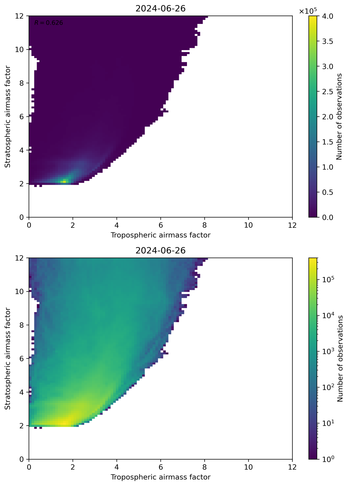
Figure 71: Scatter density plot of “Tropospheric airmass factor” against “Stratospheric airmass factor” for 2024-06-25 to 2024-06-27.
