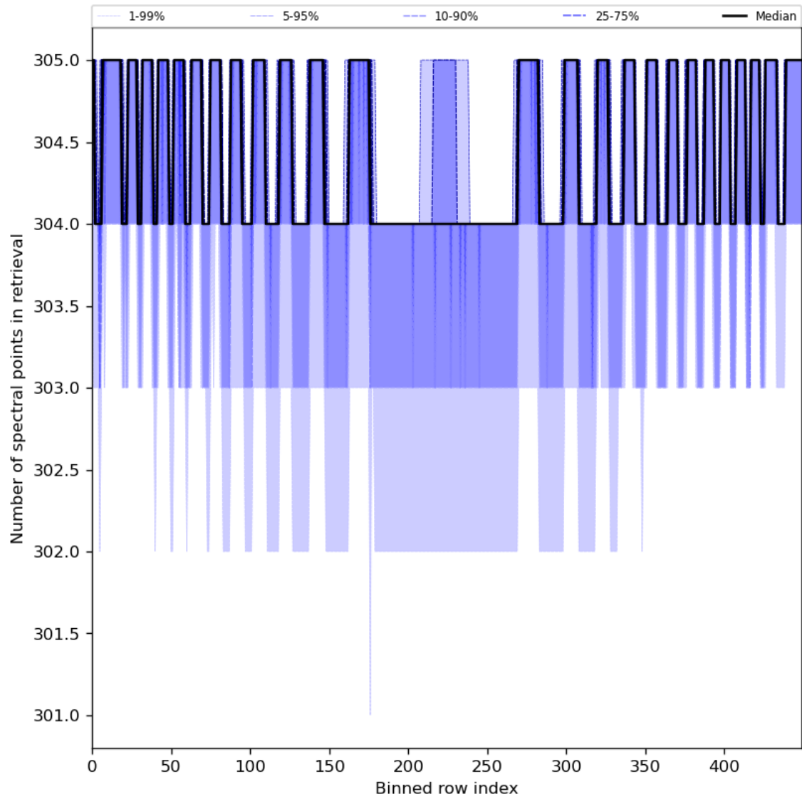
Figure 50: Along track statistics of “Number of spectral points in retrieval” for 2024-06-25 to 2024-06-27
