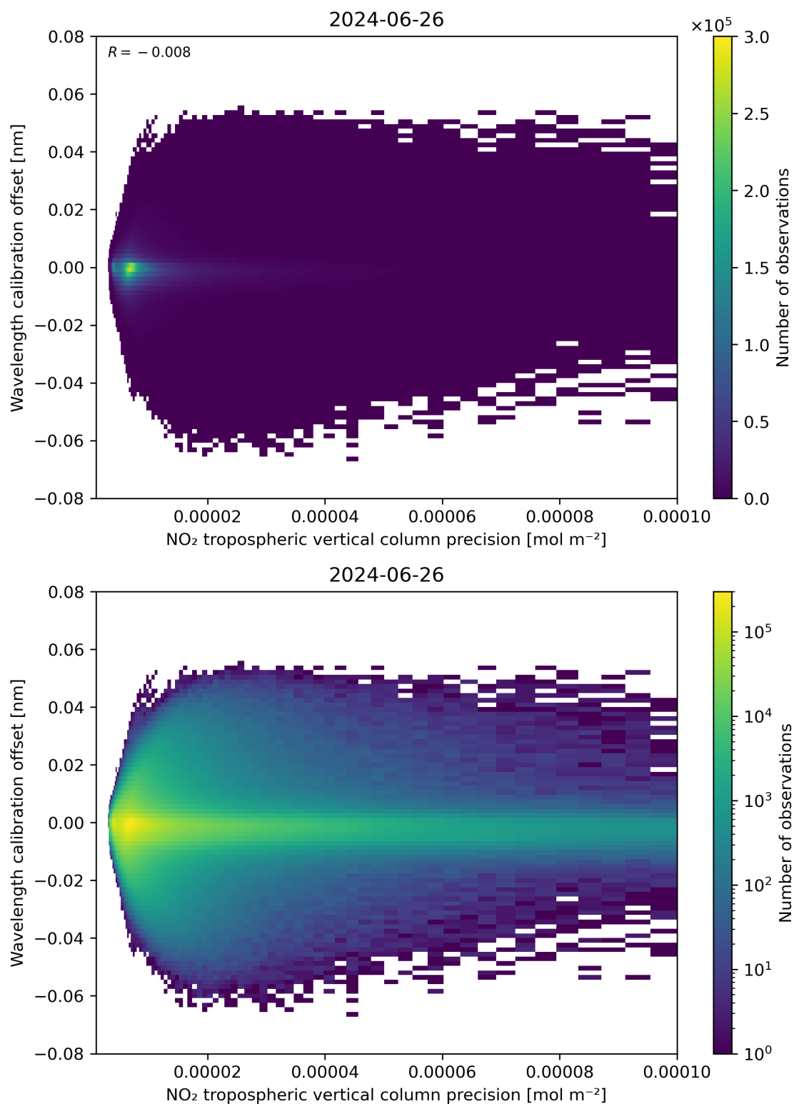
Figure 141: Scatter density plot of “NO 2 tropospheric vertical column precision” against “Wavelength calibration offset” for 2024-06-25 to 2024-06-27.
