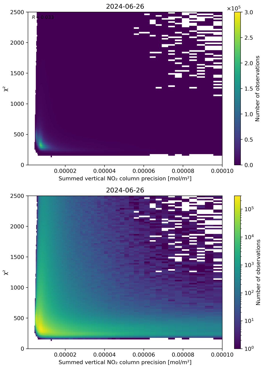
Figure 107: Scatter density plot of “Summed vertical NO 2 column precision” against “ \chi^2 ” for 2024-06-25 to 2024-06-27.
