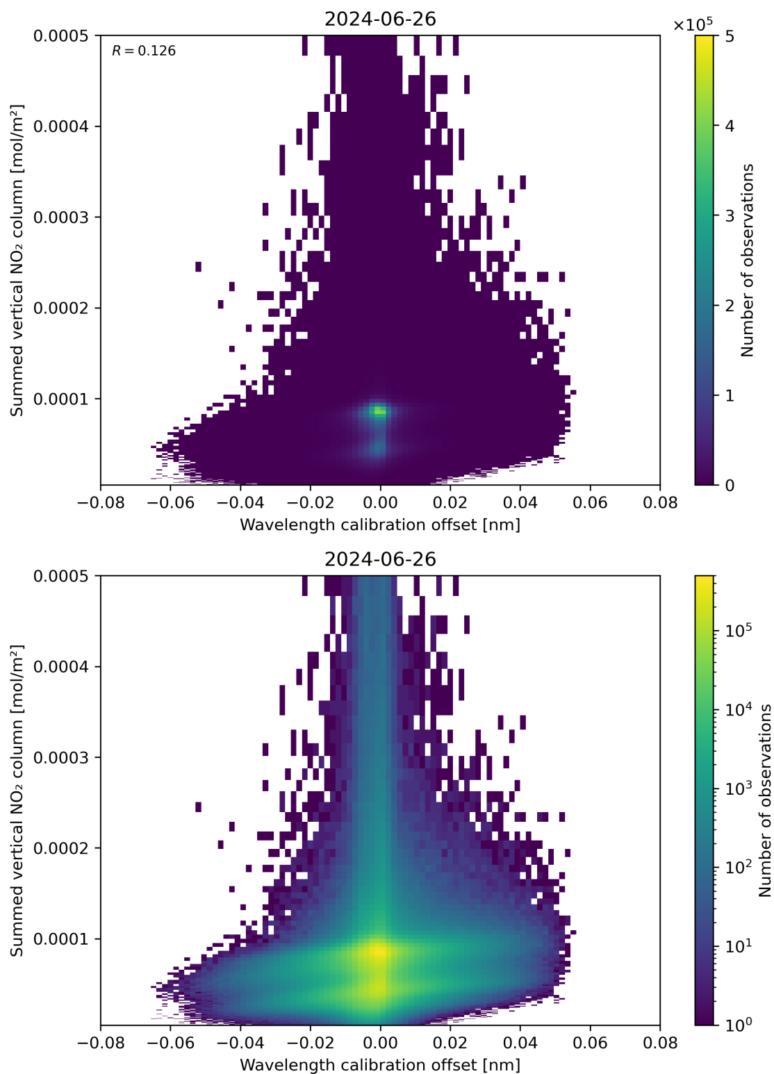
Figure 177: Scatter density plot of “Wavelength calibration offset” against “Summed vertical NO 2 column” for 2024-06-25 to 2024-06-27.
