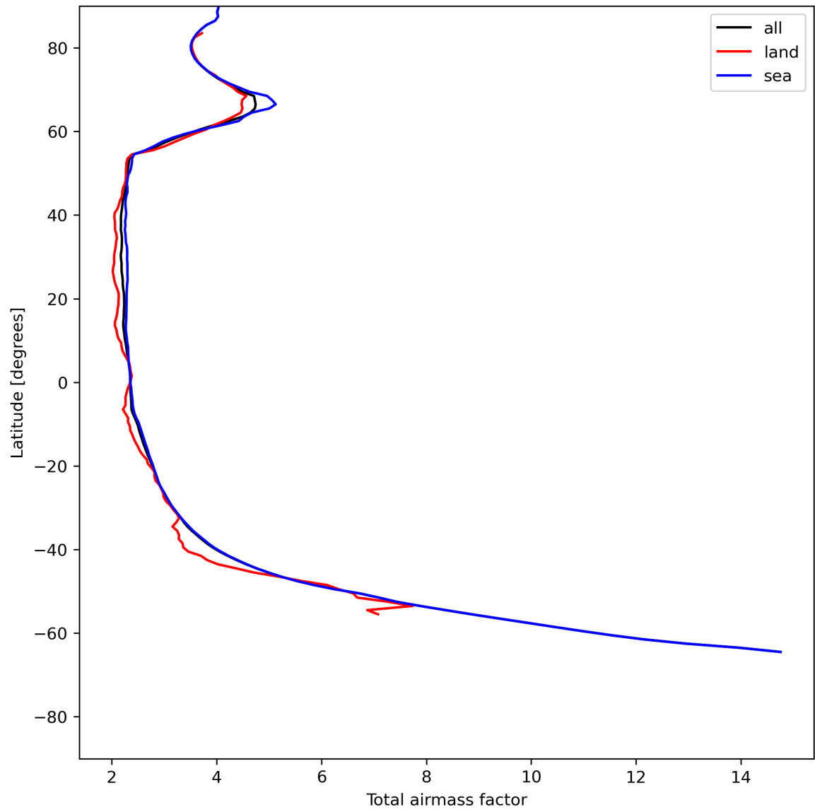
Figure 15: Zonal average of “Total airmass factor” for 2024-06-25 to 2024-06-27.
