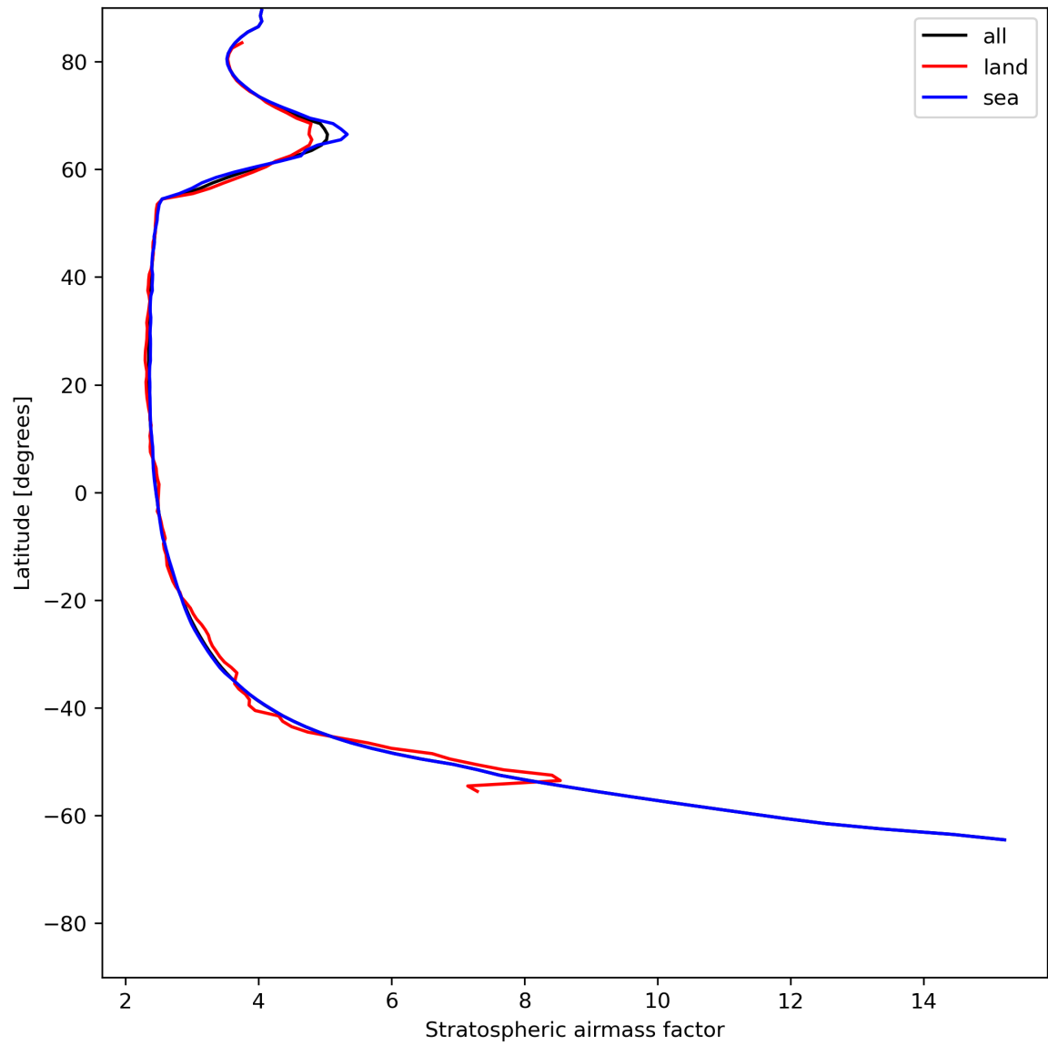
Figure 27: Zonal average of “Stratospheric air mass factor” for 2024-06-25 to 2024-06-27.
