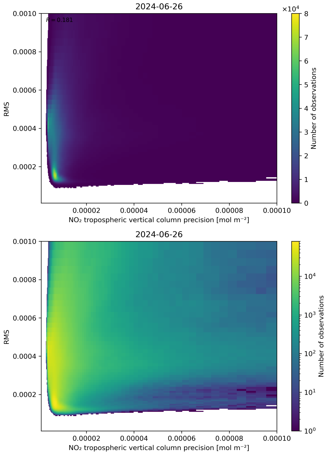
Figure 140: Scatter density plot of “NO 2 tropospheric vertical column precision” against “RMS” for 2024-06-25 to 2024-06-27.
