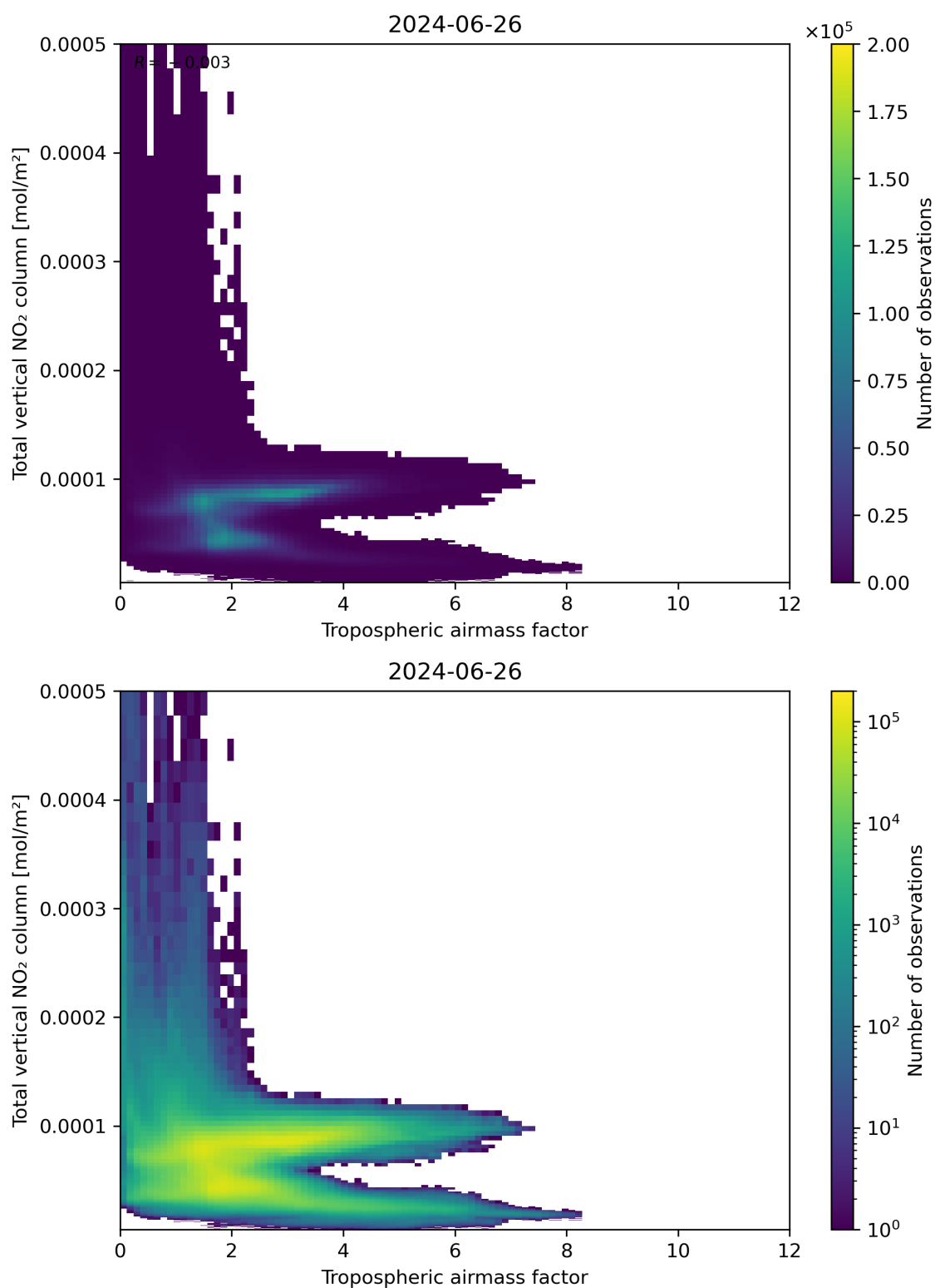
Figure 77: Scatter density plot of “Tropospheric airmass factor” against “Total vertical NO 2 column” for 2024-06-25 to 2024-06-27.
