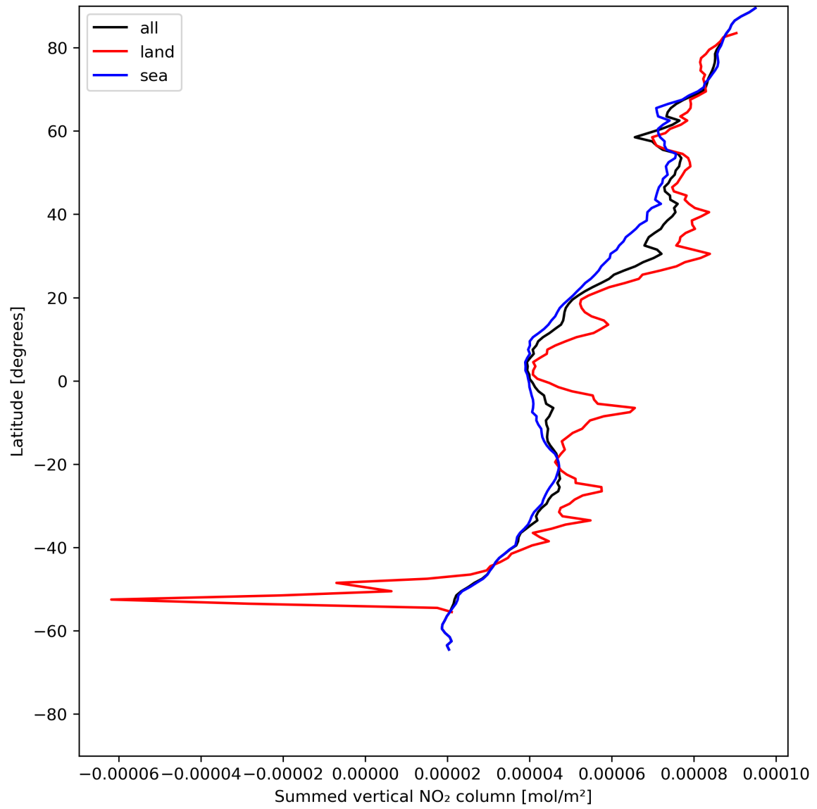
Figure 23: Zonal average of “Summed vertical NO 2 column” for 2024-06-25 to 2024-06-27.
