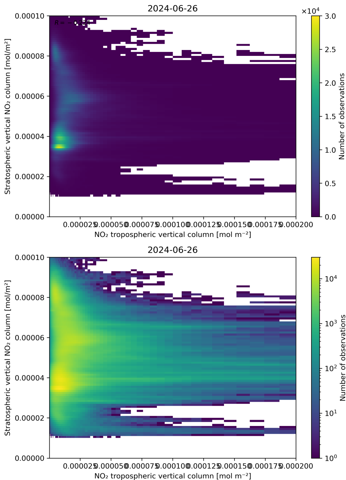
Figure 125: Scatter density plot of “NO 2 tropospheric vertical column” against “Stratospheric vertical NO 2 column” for 2024-06-25 to 2024-06-27.
