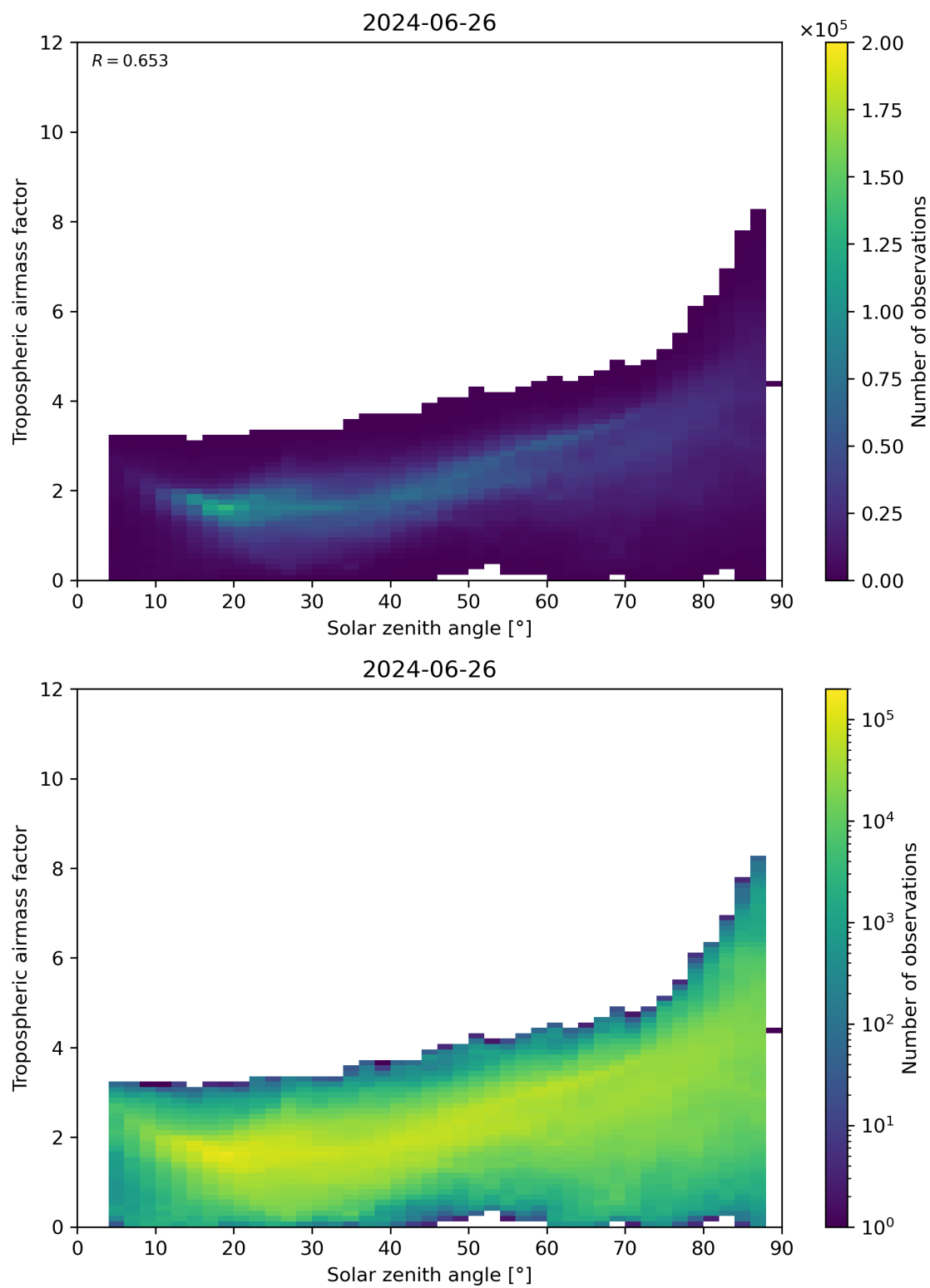
Figure 147: Scatter density plot of “Solar zenith angle” against “Tropospheric airmass factor” for 2024-06-25 to 2024-06-27.
