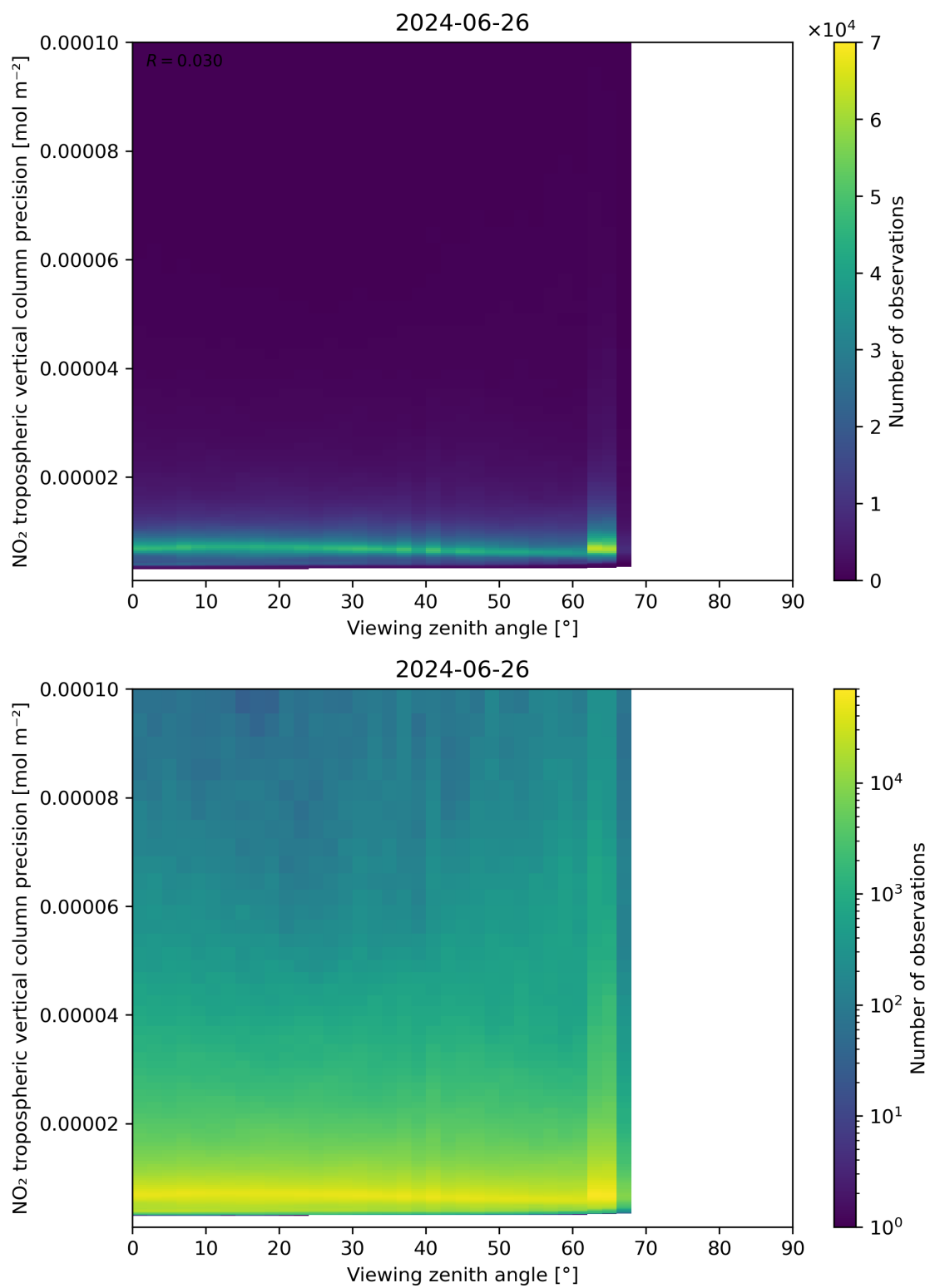
Figure 170: Scatter density plot of “Viewing zenith angle” against “NO 2 tropospheric vertical column precision” for 2024-06-25 to 2024-06-27.
