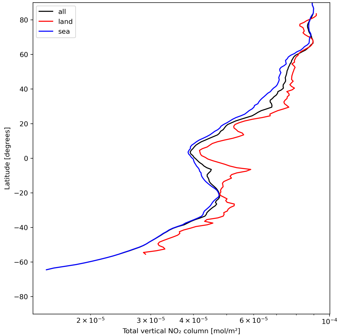
Figure 21: Zonal average of “Total vertical NO 2 column” for 2024-06-26 to 2024-06-28.
