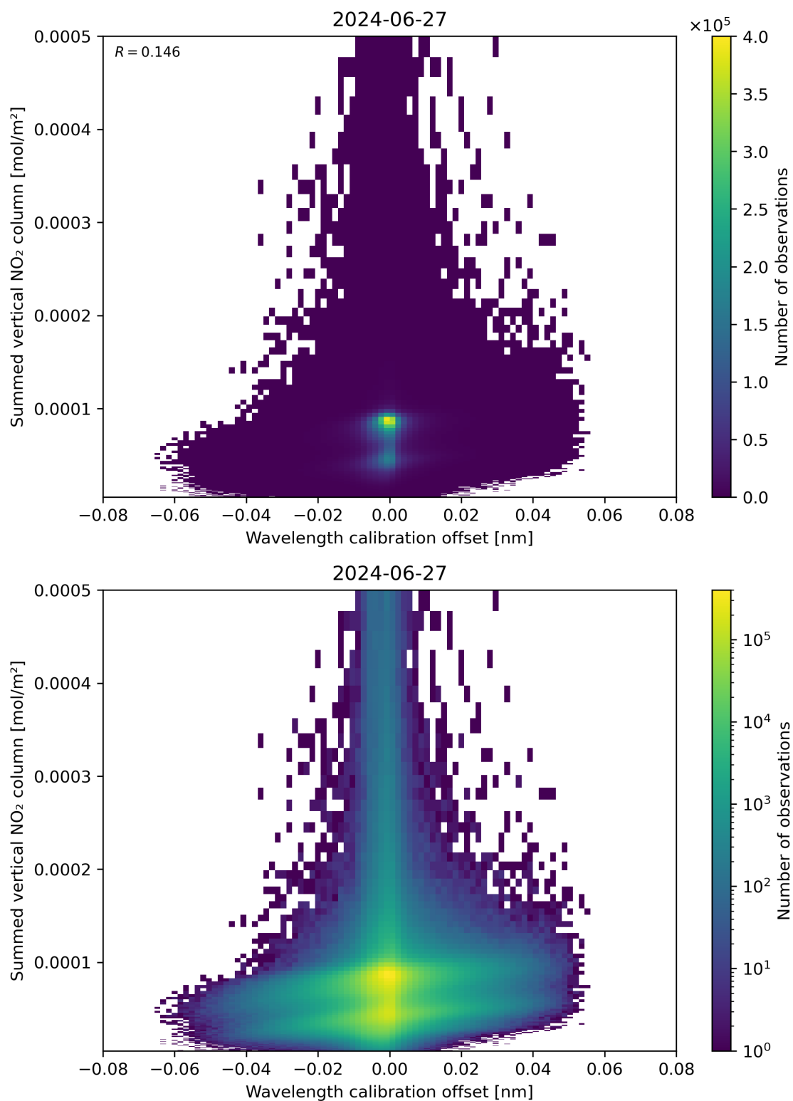
Figure 177: Scatter density plot of “Wavelength calibration offset” against “Summed vertical NO 2 column” for 2024-06-26 to 2024-06-28.
