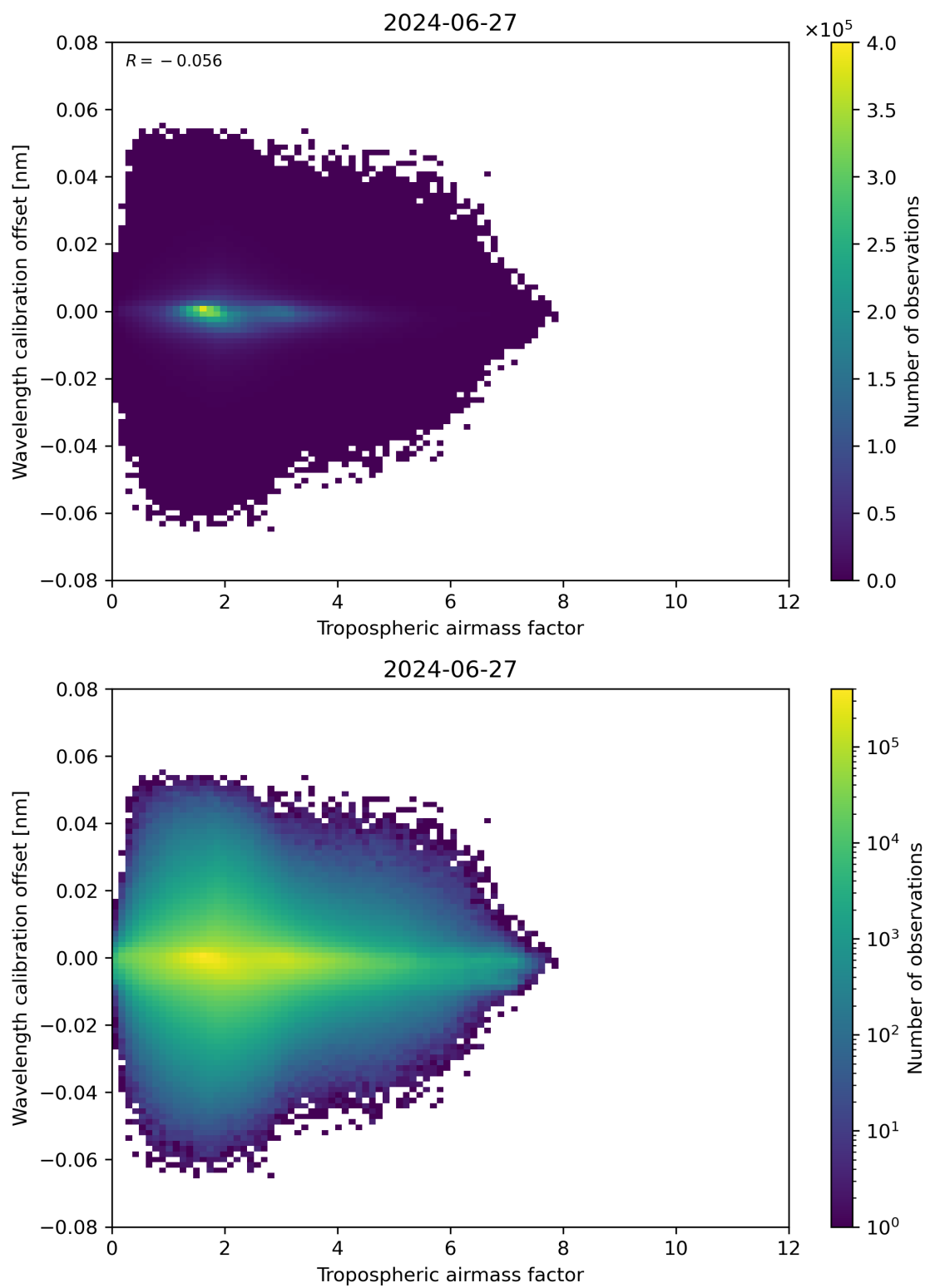
Figure 80: Scatter density plot of “Tropospheric airmass factor” against “Wavelength calibration offset” for 2024-06-26 to 2024-06-28.
