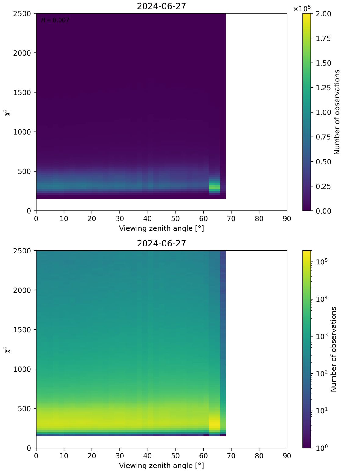
Figure 162: Scatter density plot of “Viewing zenith angle” against “ \chi^2 ” for 2024-06-26 to 2024-06-28.
