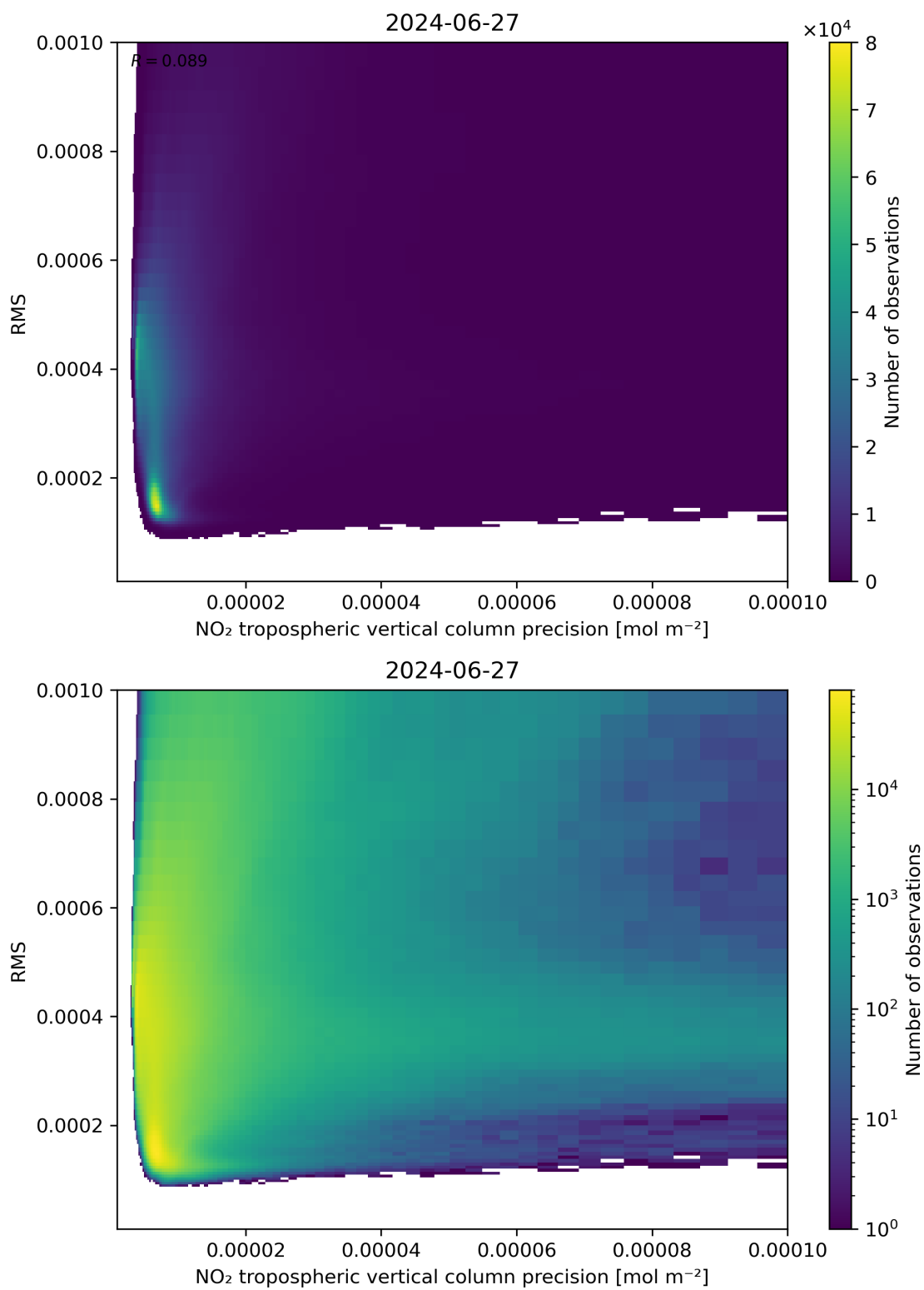
Figure 140: Scatter density plot of “NO 2 tropospheric vertical column precision” against “RMS” for 2024-06-26 to 2024-06-28.
