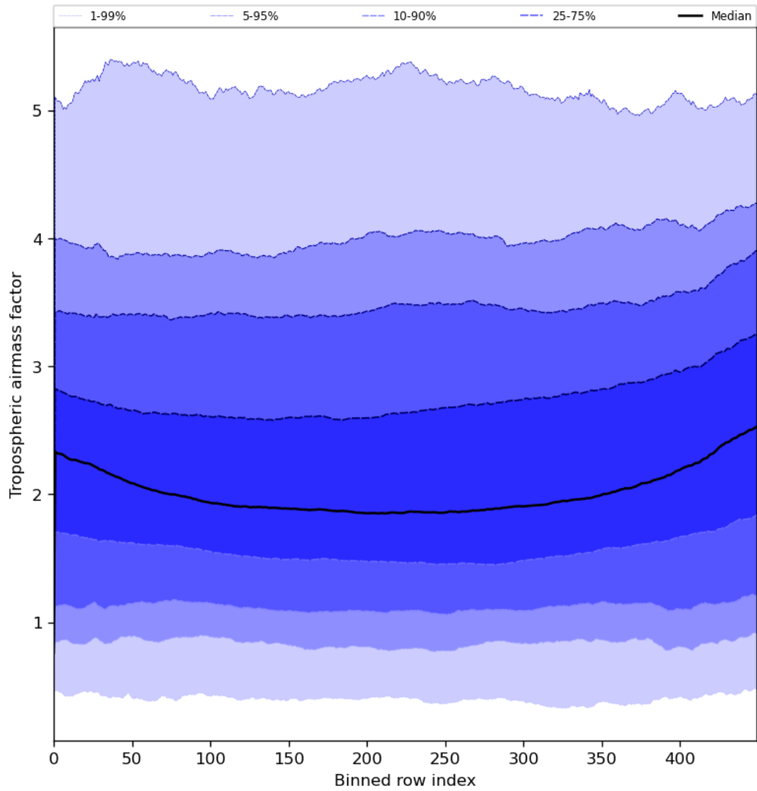
Figure 48: Along track statistics of “Tropospheric airmass factor” for 2024-06-26 to 2024-06-28
