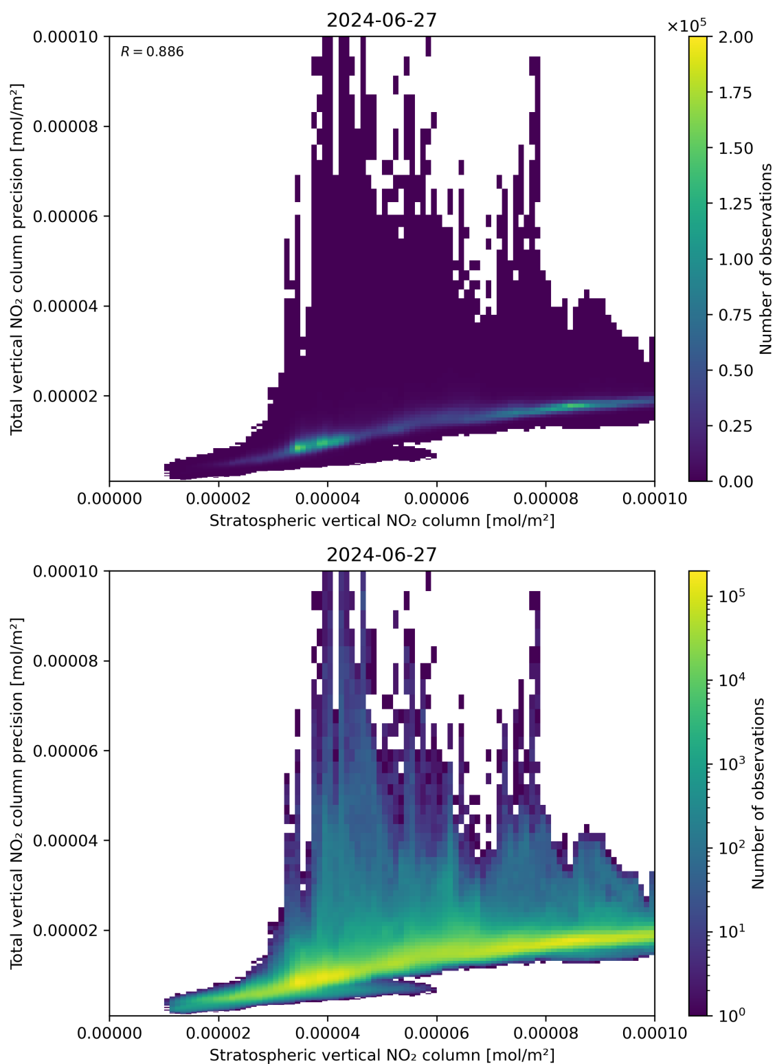
Figure 101: Scatter density plot of “Stratospheric vertical NO 2 column” against “Total vertical NO 2 column precision” for 2024-06-26 to 2024-06-28.
