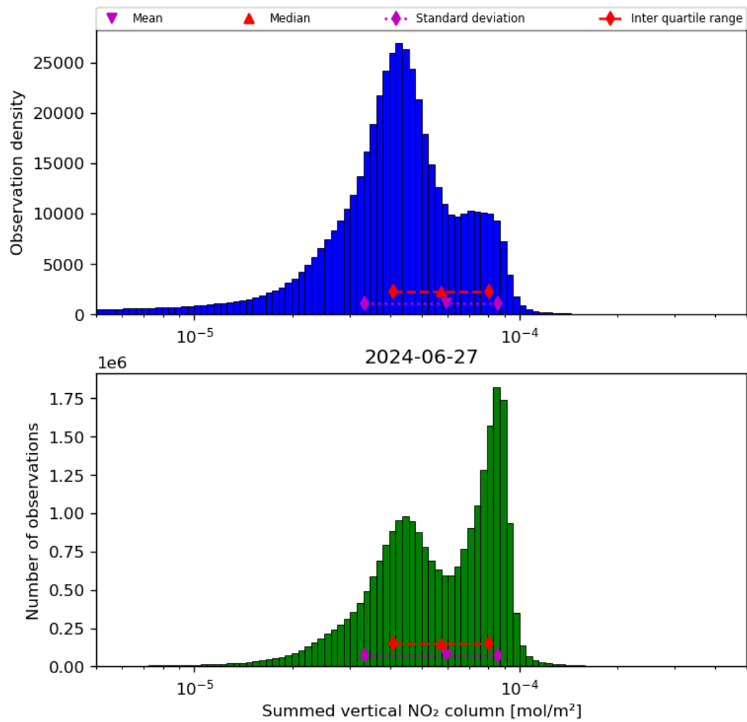
Figure 40: Histogram of “Summed vertical NO 2 column” for 2024-06-26 to 2024-06-28
