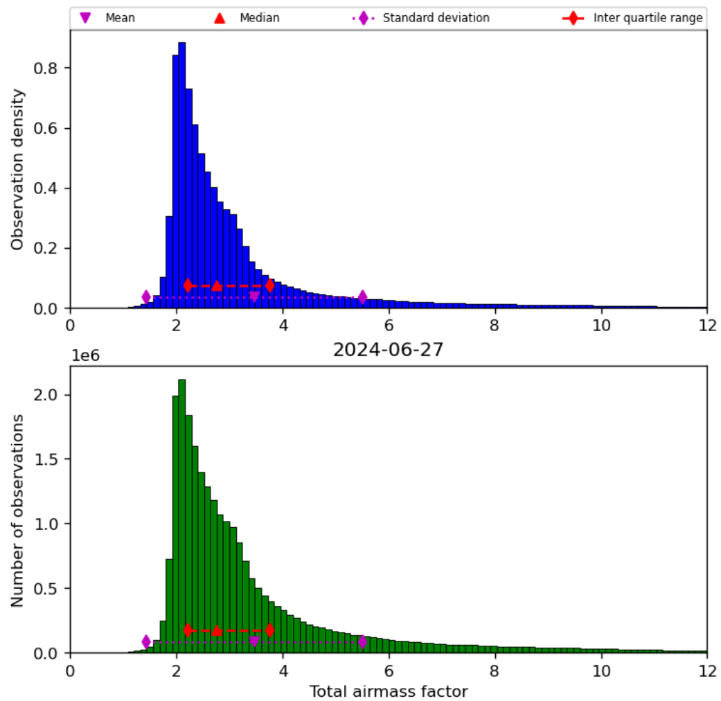
Figure 32: Histogram of “Total airmass factor” for 2024-06-26 to 2024-06-28
