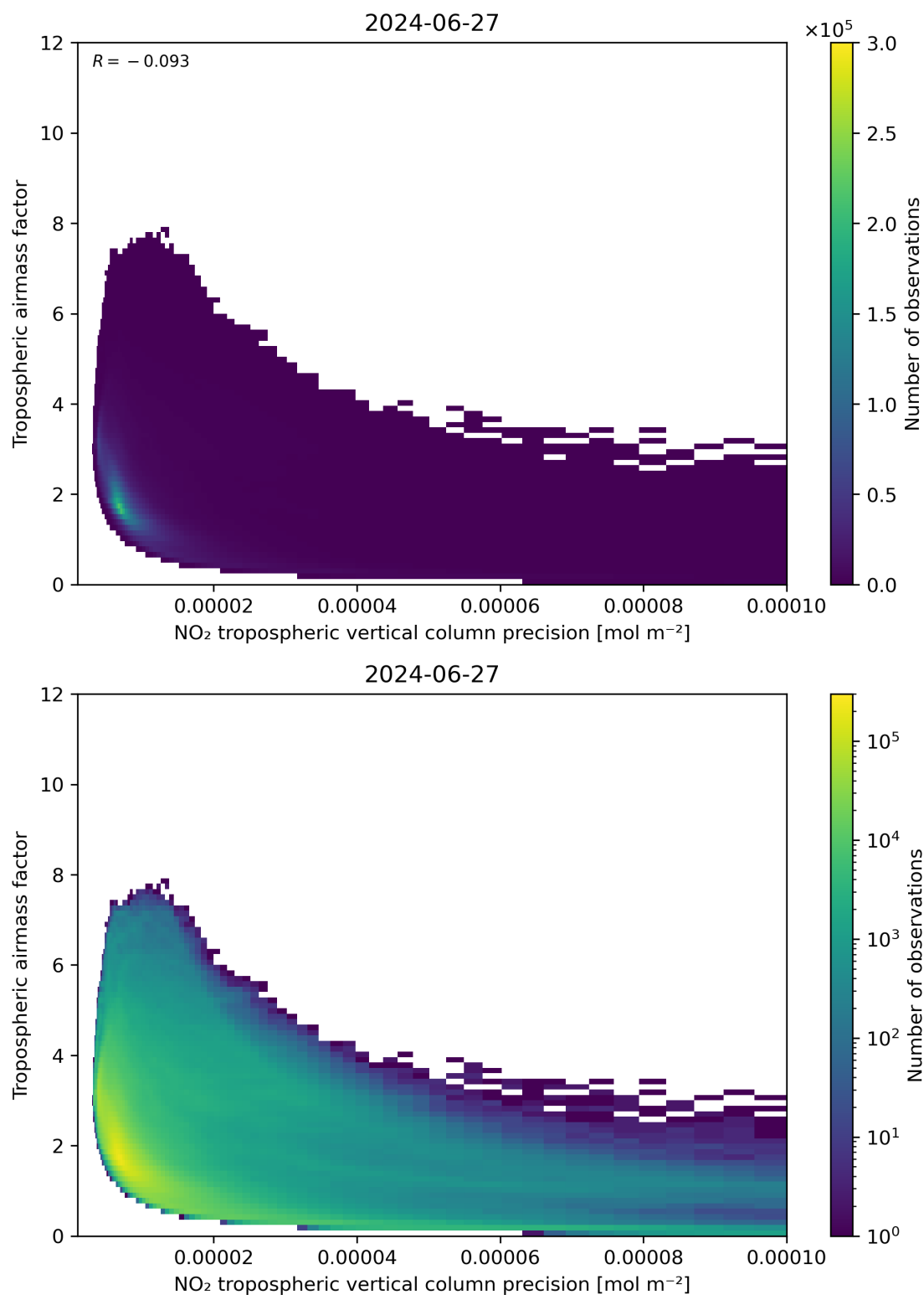
Figure 133: Scatter density plot of “NO 2 tropospheric vertical column precision” against “Tropospheric airmass factor” for 2024-06-26 to 2024-06-28.
