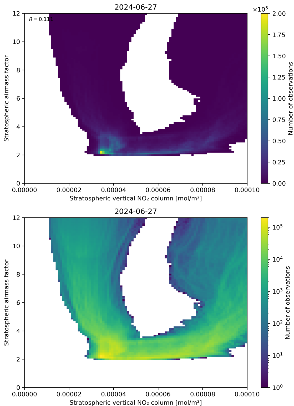
Figure 96: Scatter density plot of “Stratospheric vertical NO 2 column” against “Stratospheric airmass factor” for 2024-06-26 to 2024-06-28.
