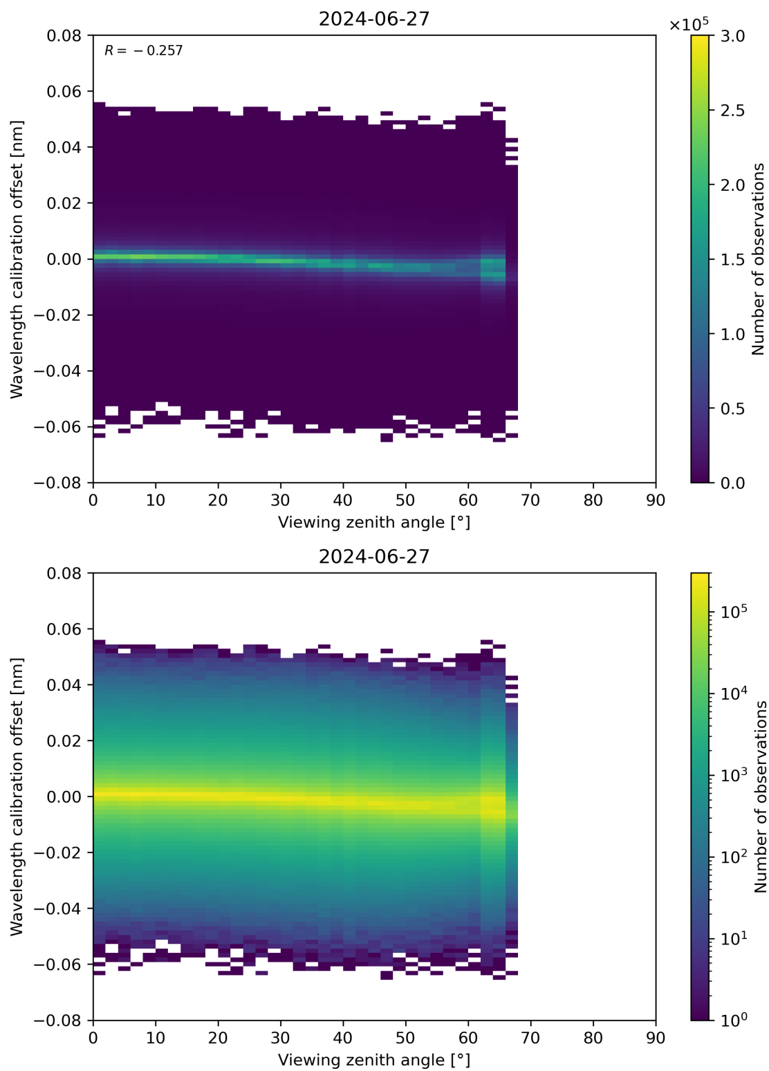
Figure 173: Scatter density plot of “Viewing zenith angle” against “Wavelength calibration offset” for 2024-06-26 to 2024-06-28.
