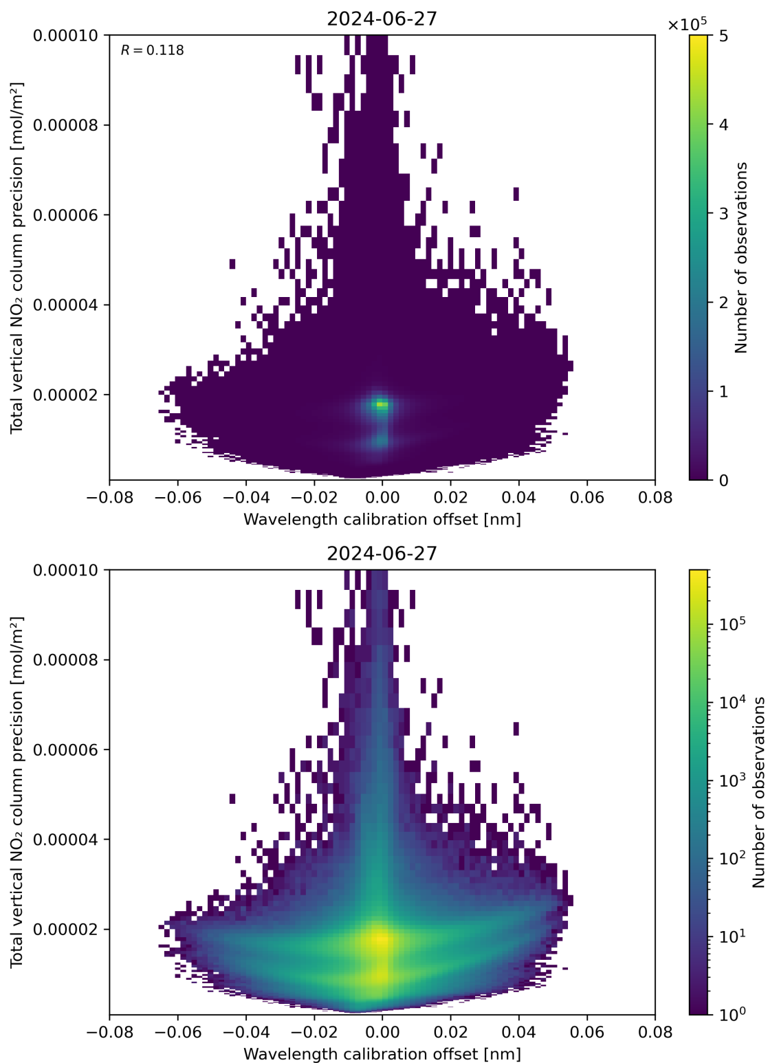
Figure 180: Scatter density plot of “Wavelength calibration offset” against “Total vertical NO 2 column precision” for 2024-06-26 to 2024-06-28.
