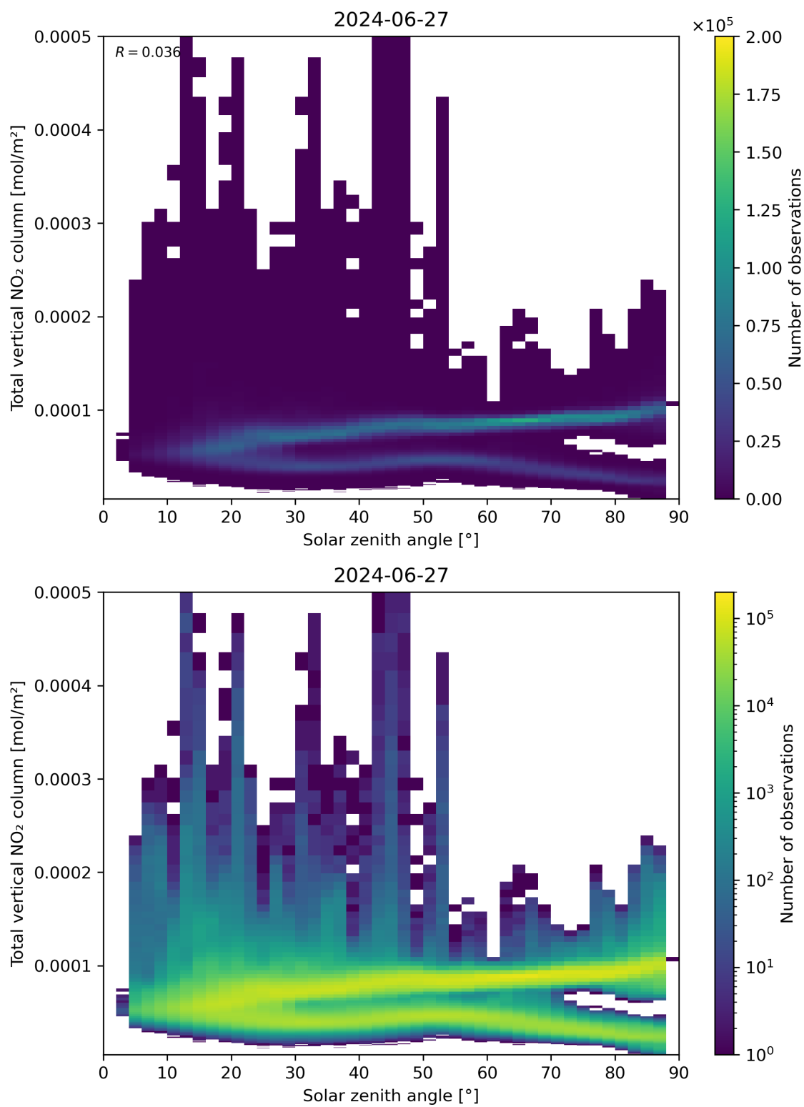
Figure 153: Scatter density plot of “Solar zenith angle” against “Total vertical NO 2 column” for 2024-06-26 to 2024-06-28.
