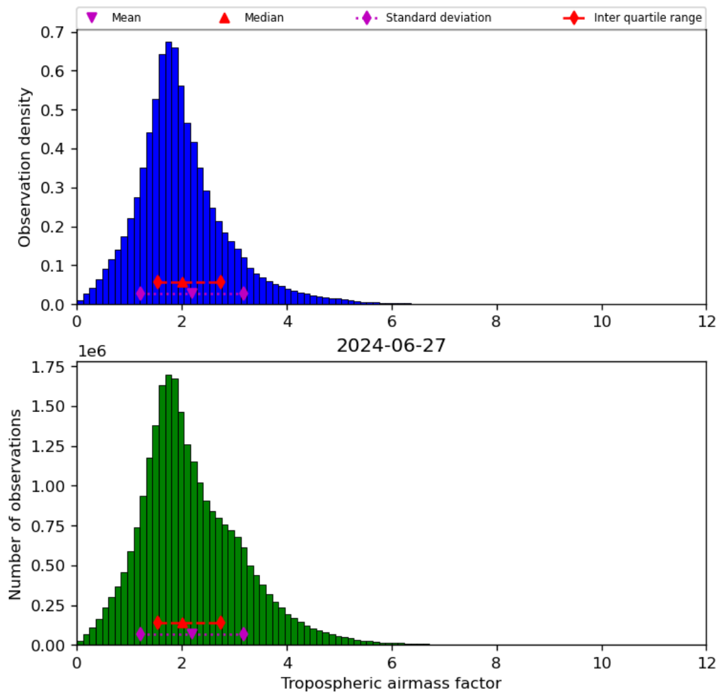
Figure 31: Histogram of “Tropospheric airmass factor” for 2024-06-26 to 2024-06-28
