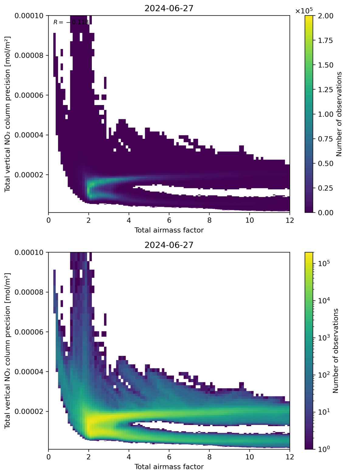
Figure 68: Scatter density plot of “Total airmass factor” against “Total vertical NO 2 column precision” for 2024-06-26 to 2024-06-28.
