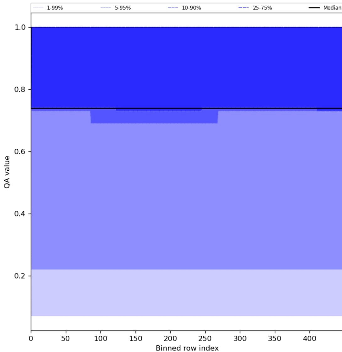
Figure 45: Along track statistics of “QA value” for 2024-06-26 to 2024-06-28
