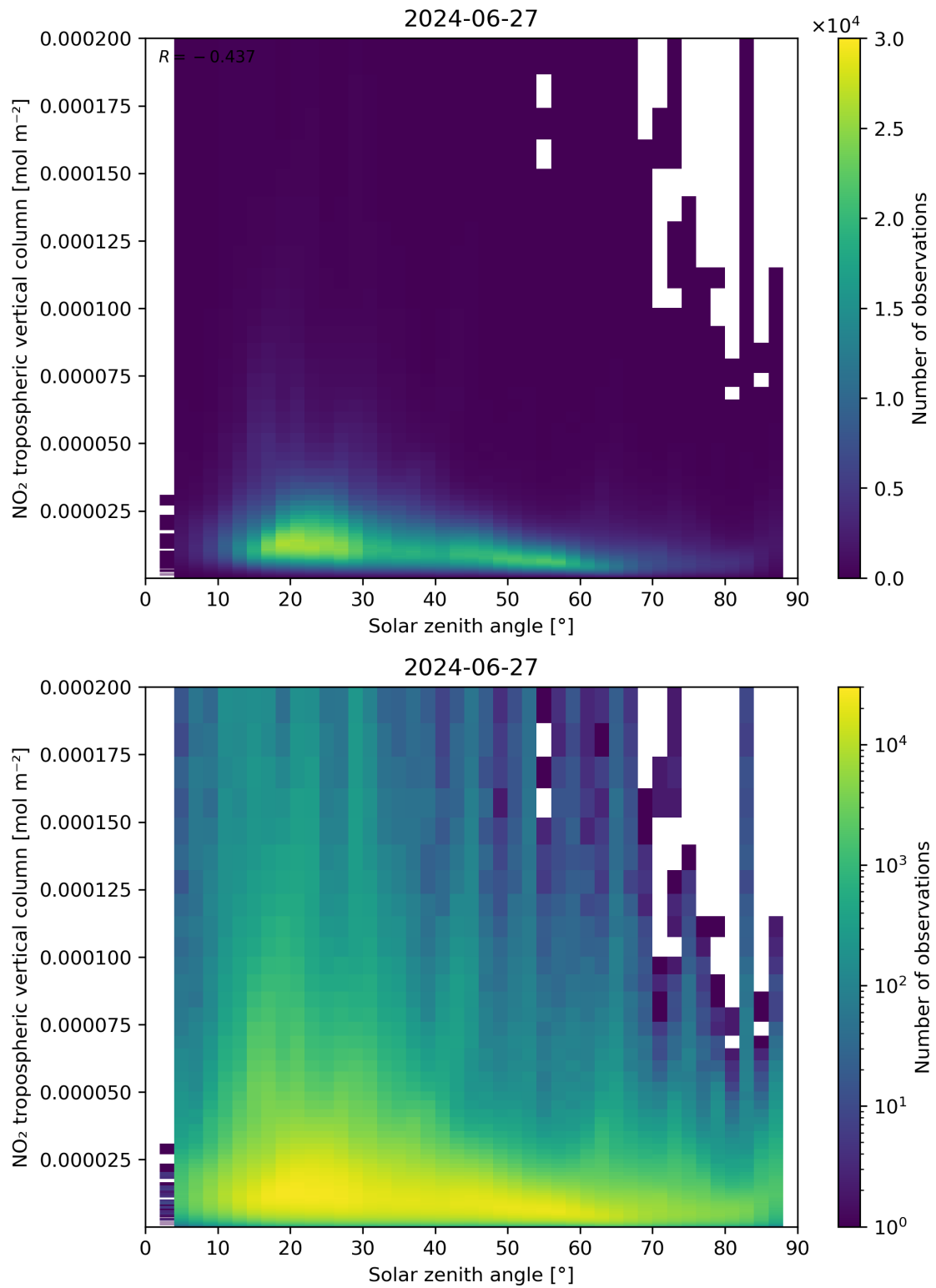
Figure 155: Scatter density plot of “Solar zenith angle” against “NO 2 tropospheric vertical column” for 2024-06-26 to 2024-06-28.
