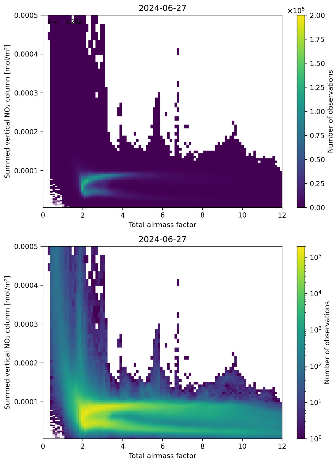
Figure 65: Scatter density plot of “Total airmass factor” against “Summed vertical NO 2 column” for 2024-06-26 to 2024-06-28.
