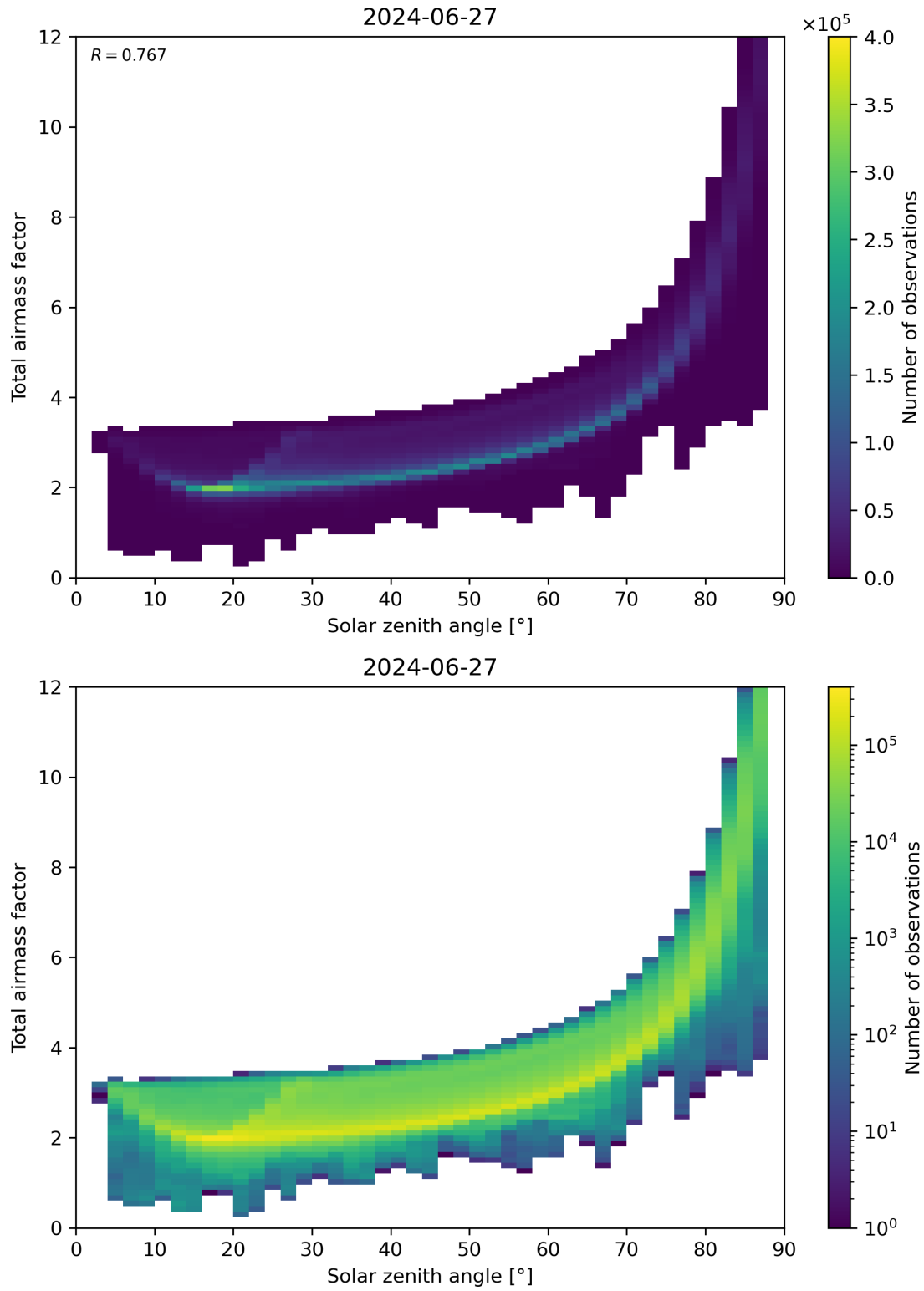
Figure 146: Scatter density plot of “Solar zenith angle” against “Total air mass factor” for 2024-06-26 to 2024-06-28.
