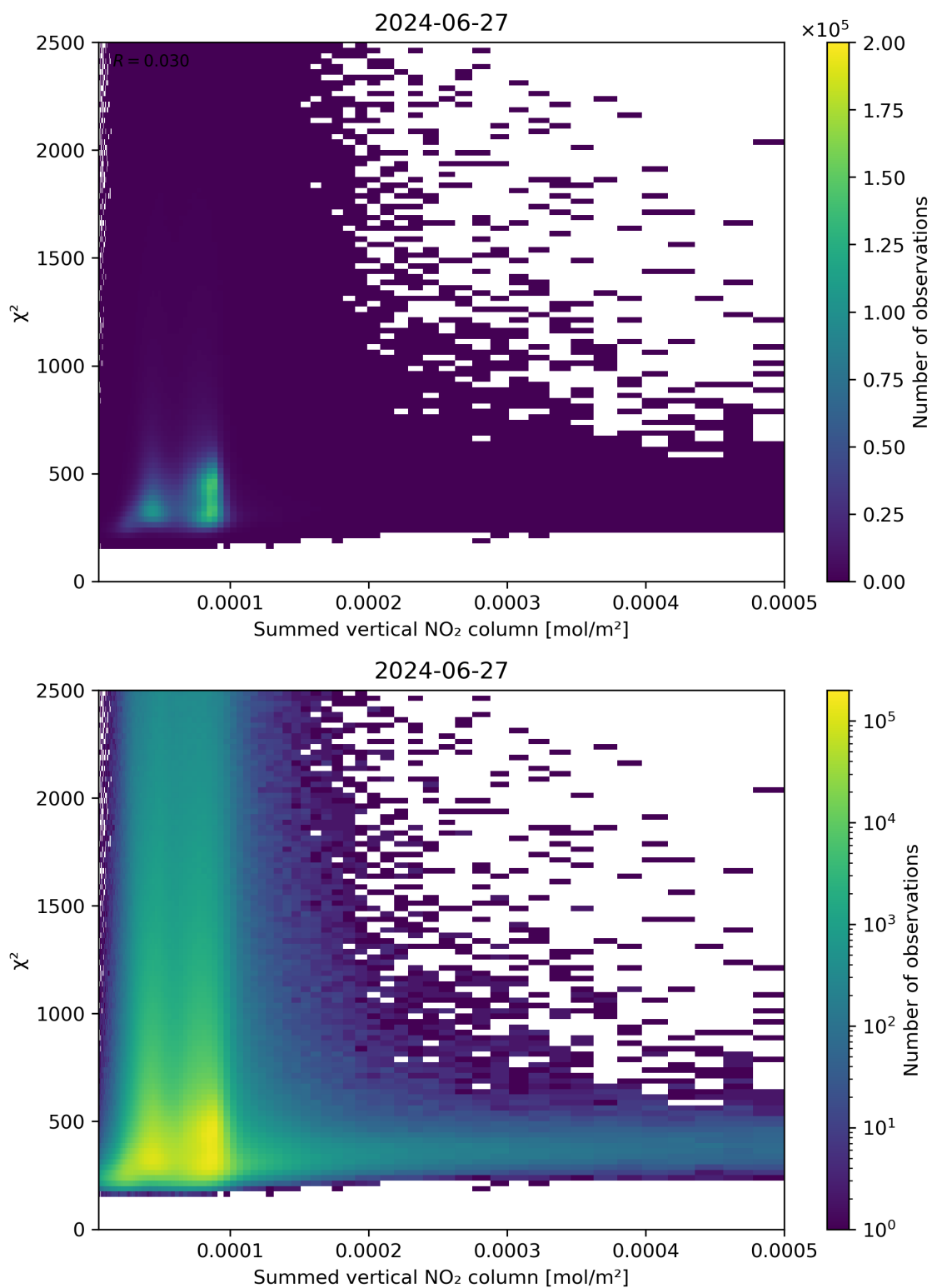
Figure 104: Scatter density plot of “Summed vertical NO 2 column” against “ \chi^2 ” for 2024-06-26 to 2024-06-28.
