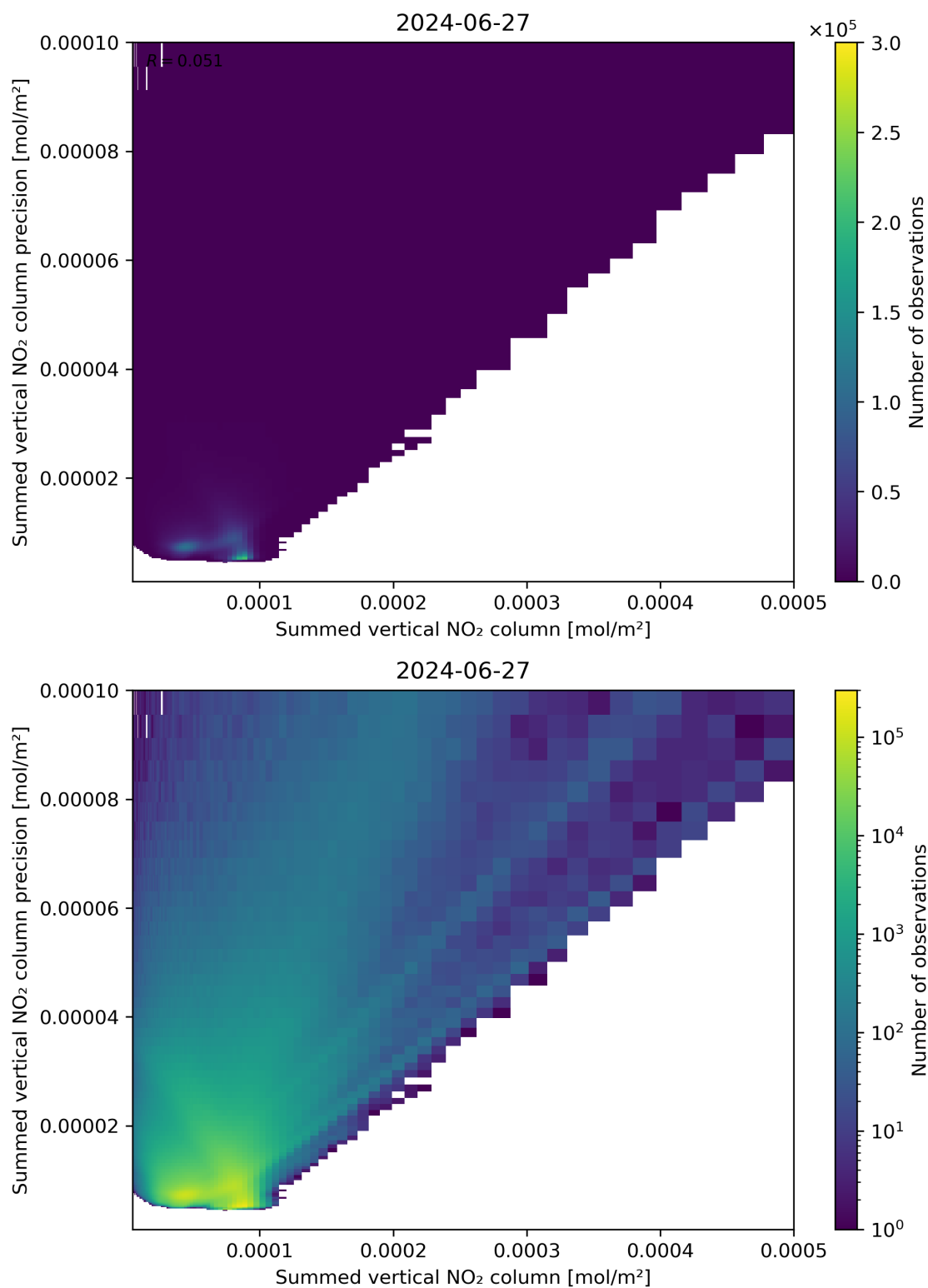
Figure 105: Scatter density plot of “Summed vertical NO 2 column” against “Summed vertical NO 2 column precision” for 2024-06-26 to 2024-06-28.
