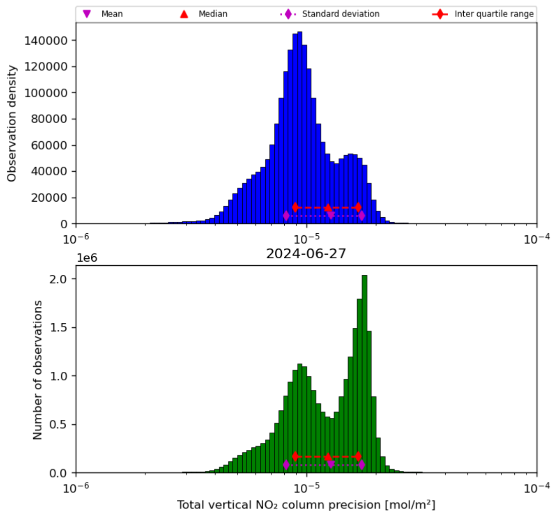
Figure 39: Histogram of “Total vertical NO 2 column precision” for 2024-06-26 to 2024-06-28
