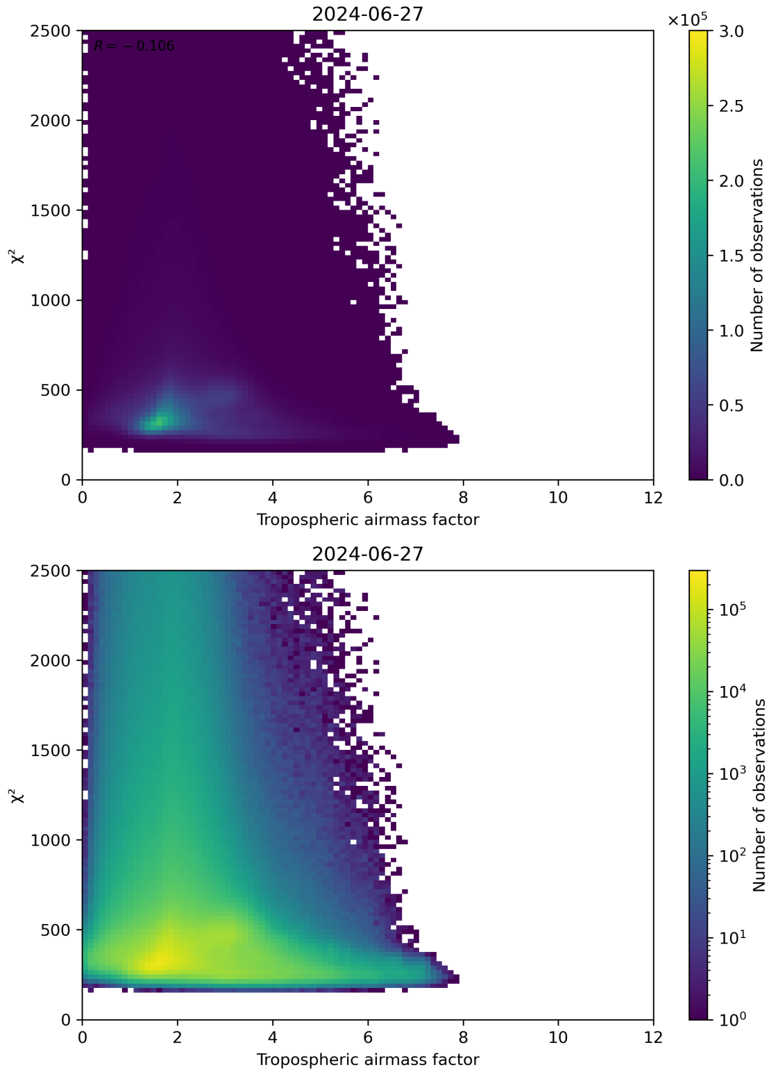
Figure 73: Scatter density plot of “Tropospheric airmass factor” against “ \chi^2 ” for 2024-06-26 to 2024-06-28.
