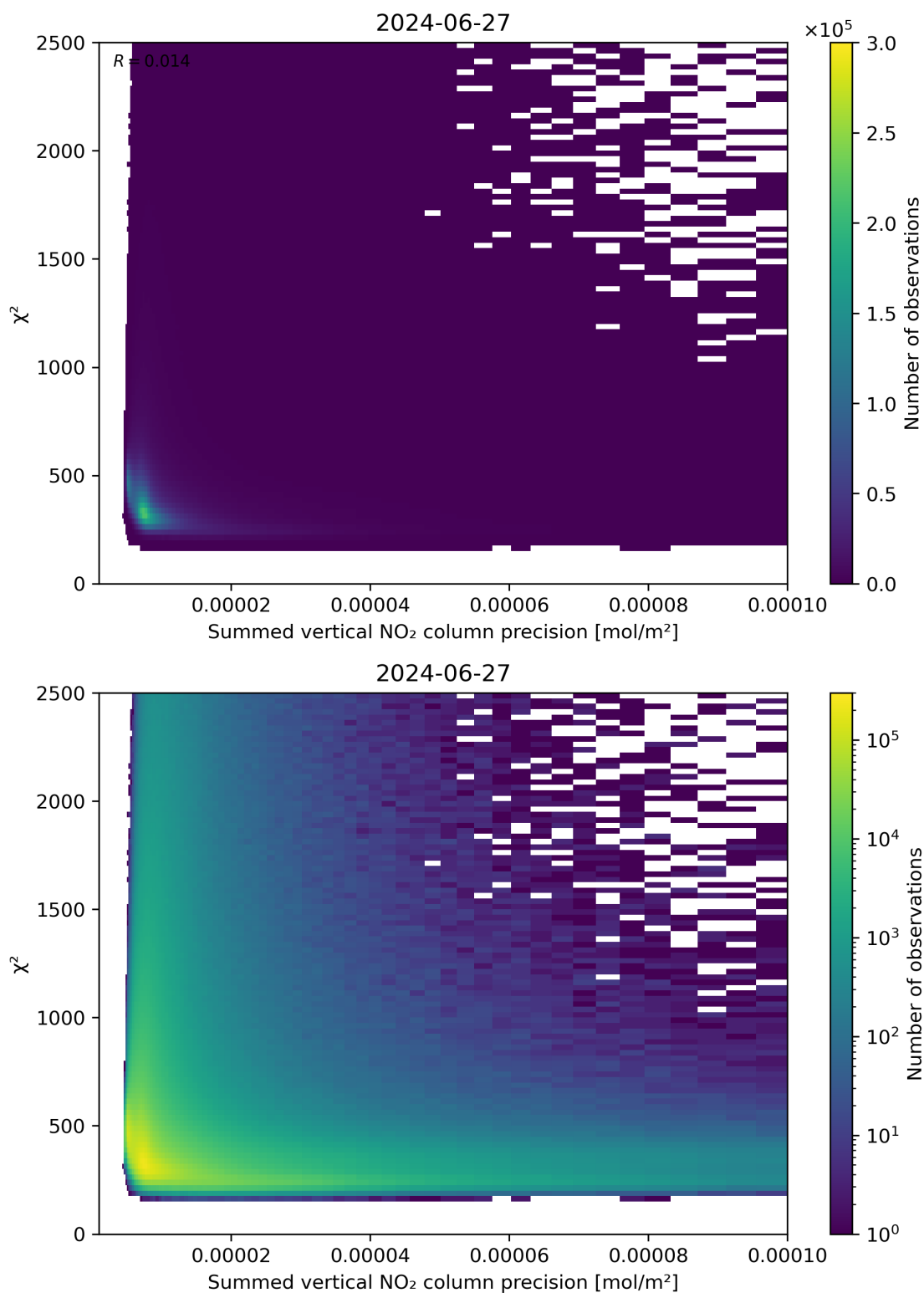
Figure 107: Scatter density plot of “Summed vertical NO 2 column precision” against “ \chi^2 ” for 2024-06-26 to 2024-06-28.
