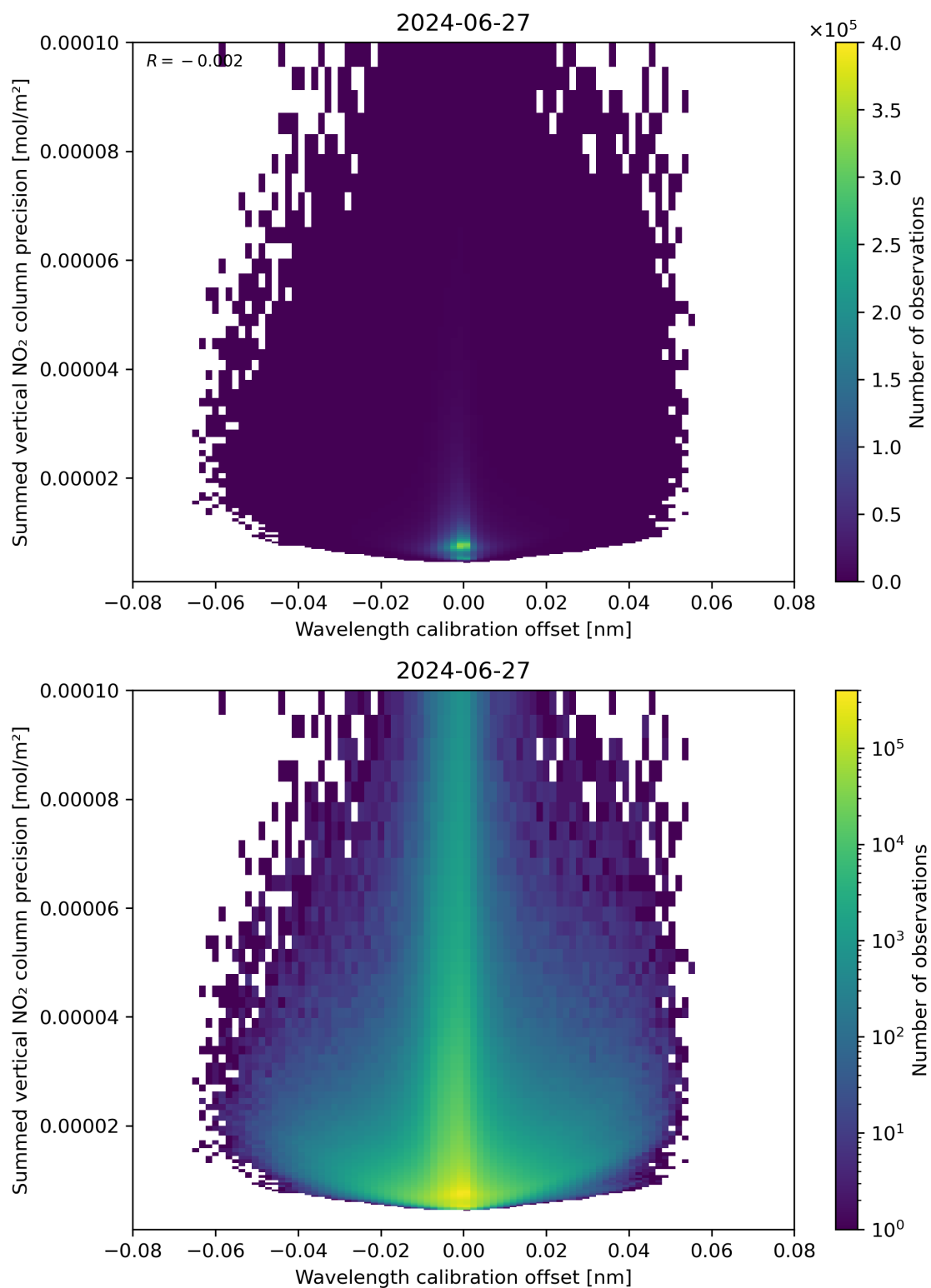
Figure 178: Scatter density plot of “Wavelength calibration offset” against “Summed vertical NO 2 column precision” for 2024-06-26 to 2024-06-28.
