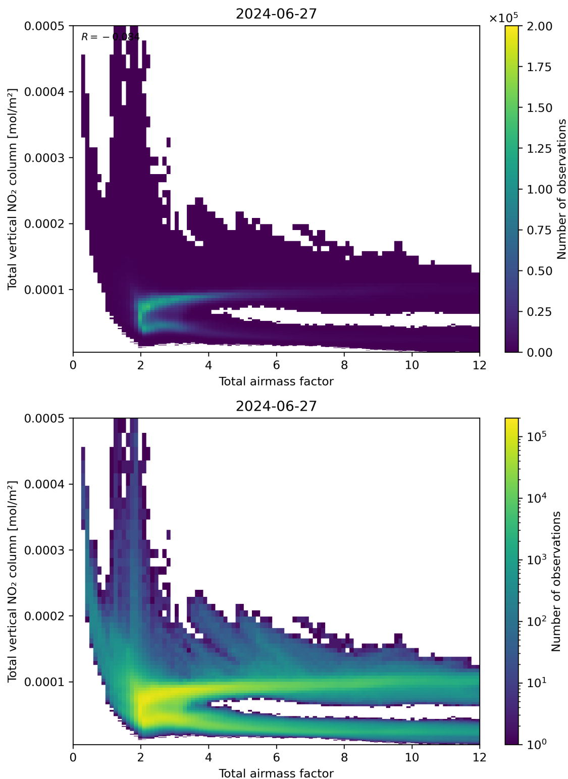
Figure 67: Scatter density plot of “Total airmass factor” against “Total vertical NO 2 column” for 2024-06-26 to 2024-06-28.
