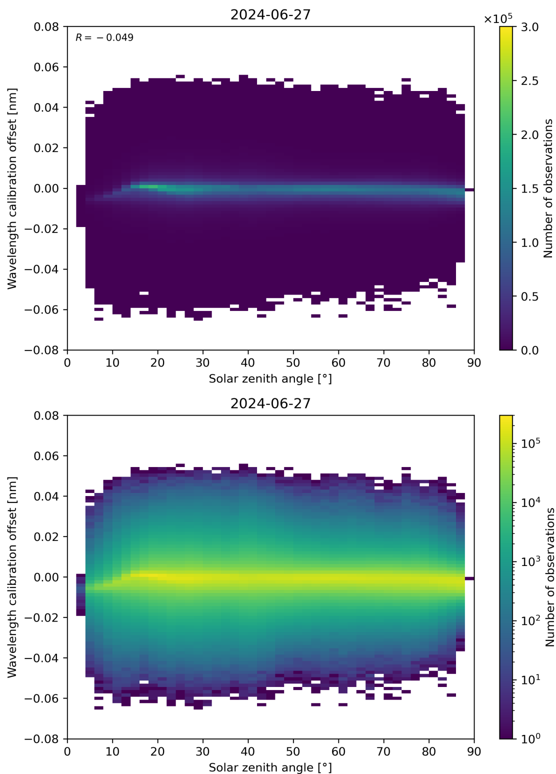
Figure 158: Scatter density plot of “Solar zenith angle” against “Wavelength calibration offset” for 2024-06-26 to 2024-06-28.
