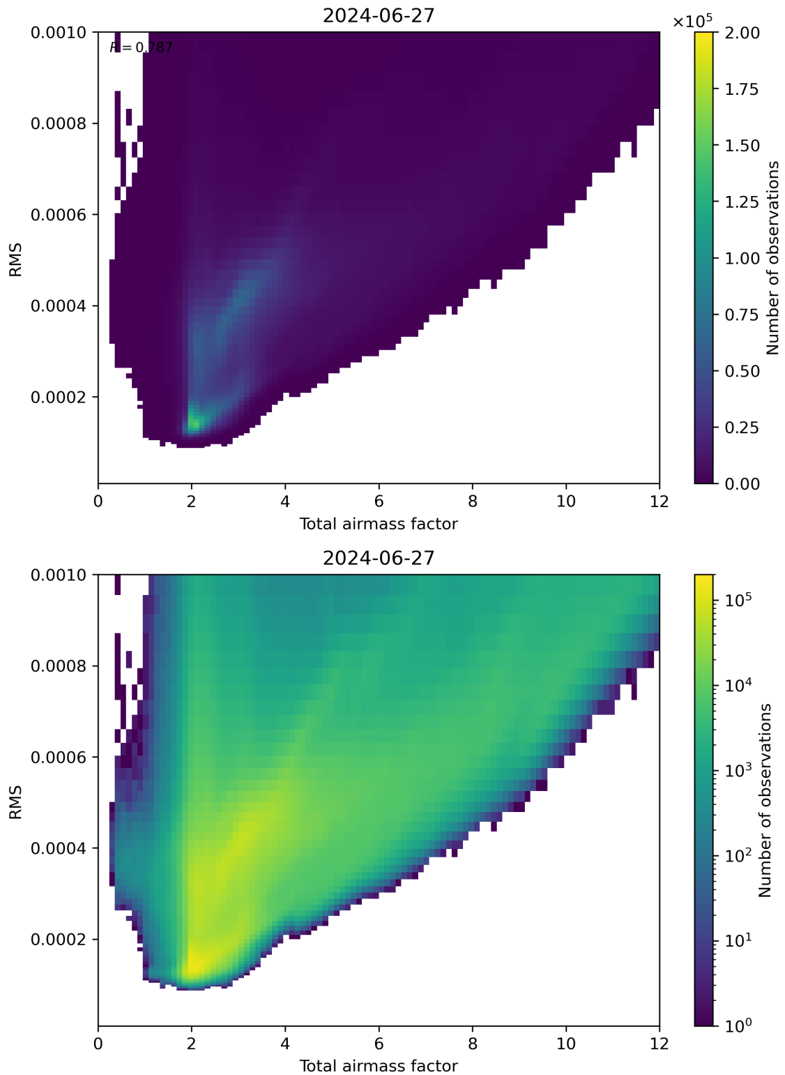
Figure 69: Scatter density plot of “Total airmass factor” against “RMS” for 2024-06-26 to 2024-06-28.
