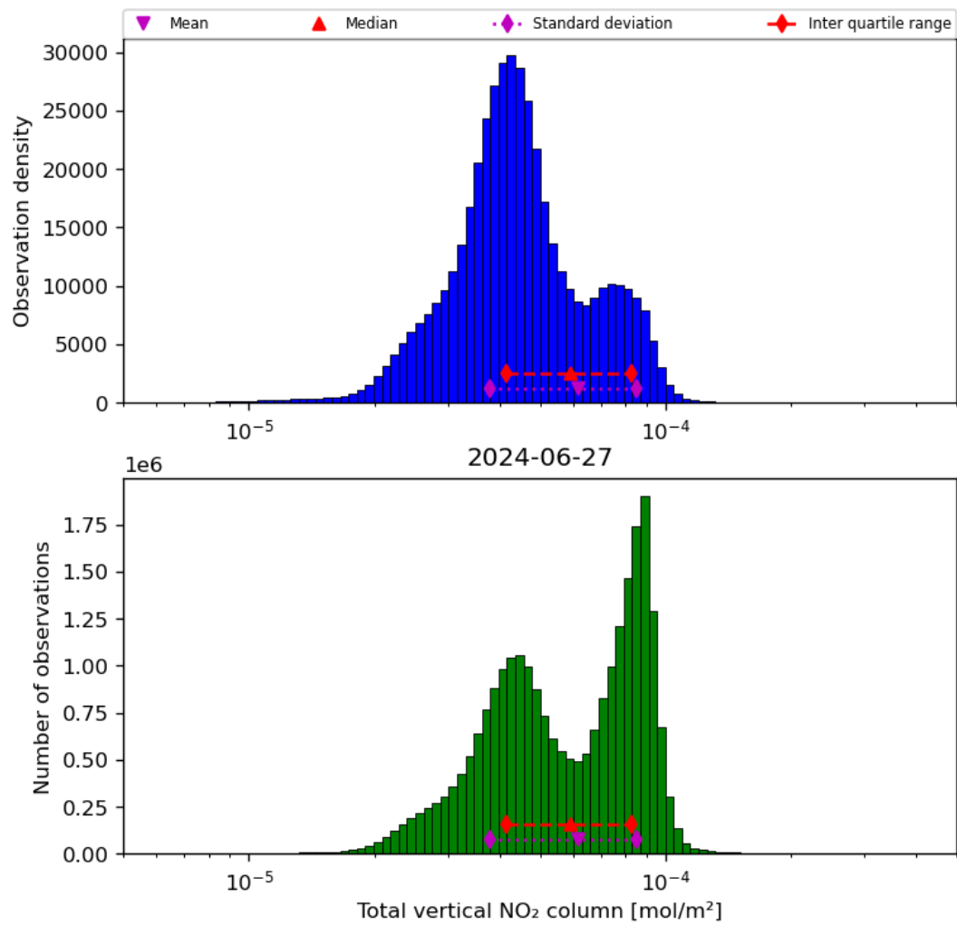
Figure 38: Histogram of “Total vertical NO 2 column” for 2024-06-26 to 2024-06-28
