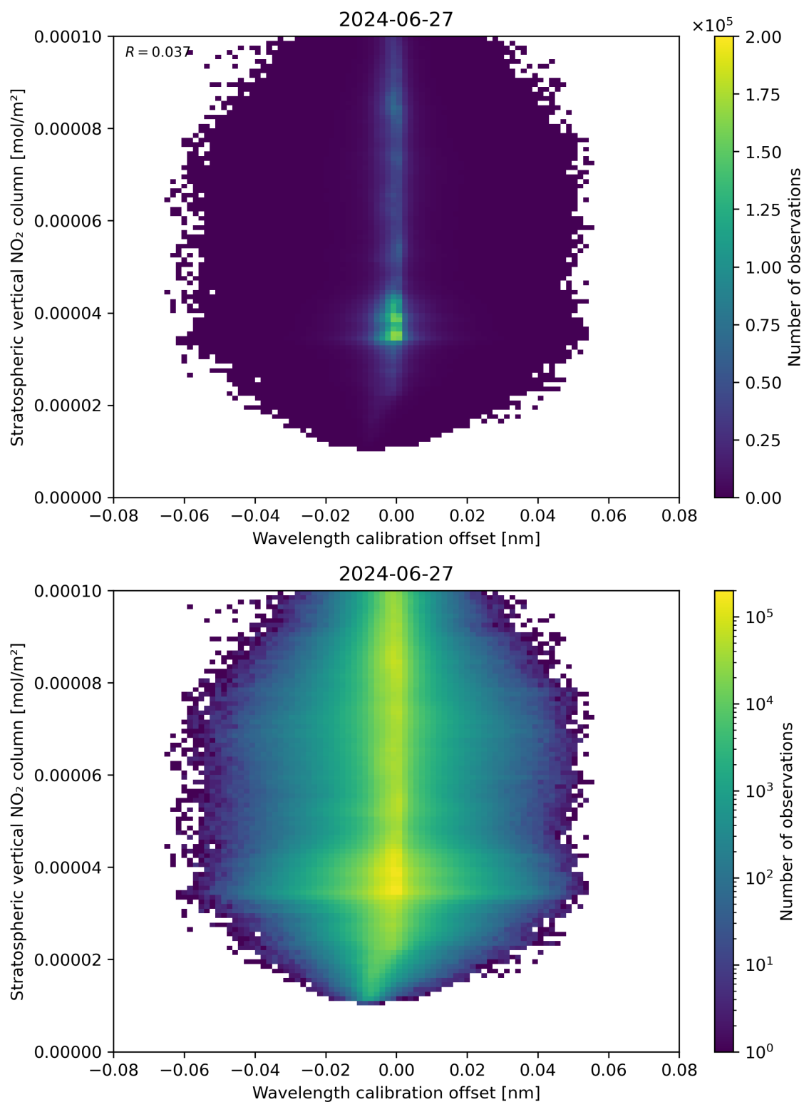
Figure 176: Scatter density plot of “Wavelength calibration offset” against “Stratospheric vertical NO 2 column” for 2024-06-26 to 2024-06-28.
