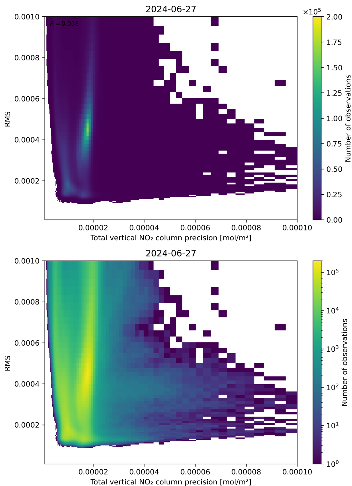
Figure 119: Scatter density plot of “Total vertical NO 2 column precision” against “RMS” for 2024-06-26 to 2024-06-28.
