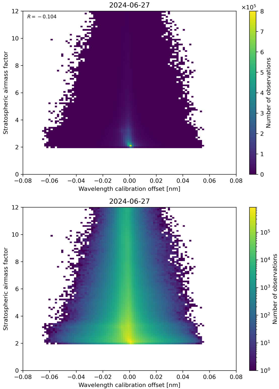
Figure 174: Scatter density plot of “Wavelength calibration offset” against “Stratospheric airmass factor” for 2024-06-26 to 2024-06-28.
