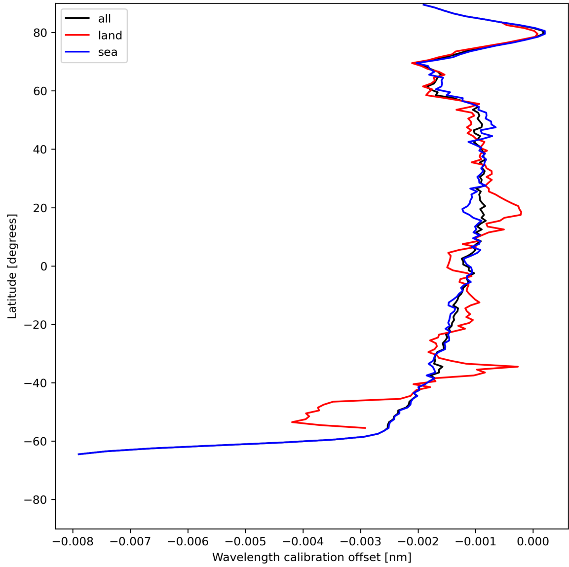
Figure 18: Zonal average of “Wavelength calibration offset” for 2024-06-26 to 2024-06-28.
