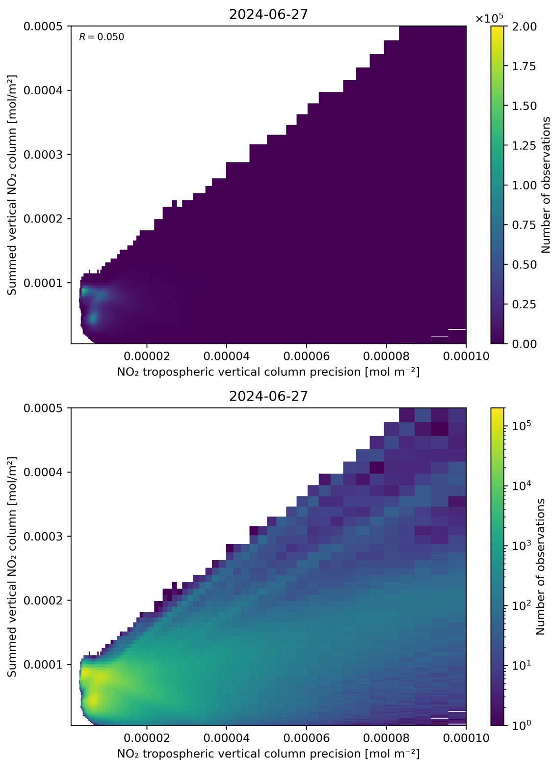
Figure 136: Scatter density plot of “NO 2 tropospheric vertical column precision” against “Summed vertical NO 2 column” for 2024-06-26 to 2024-06-28.
