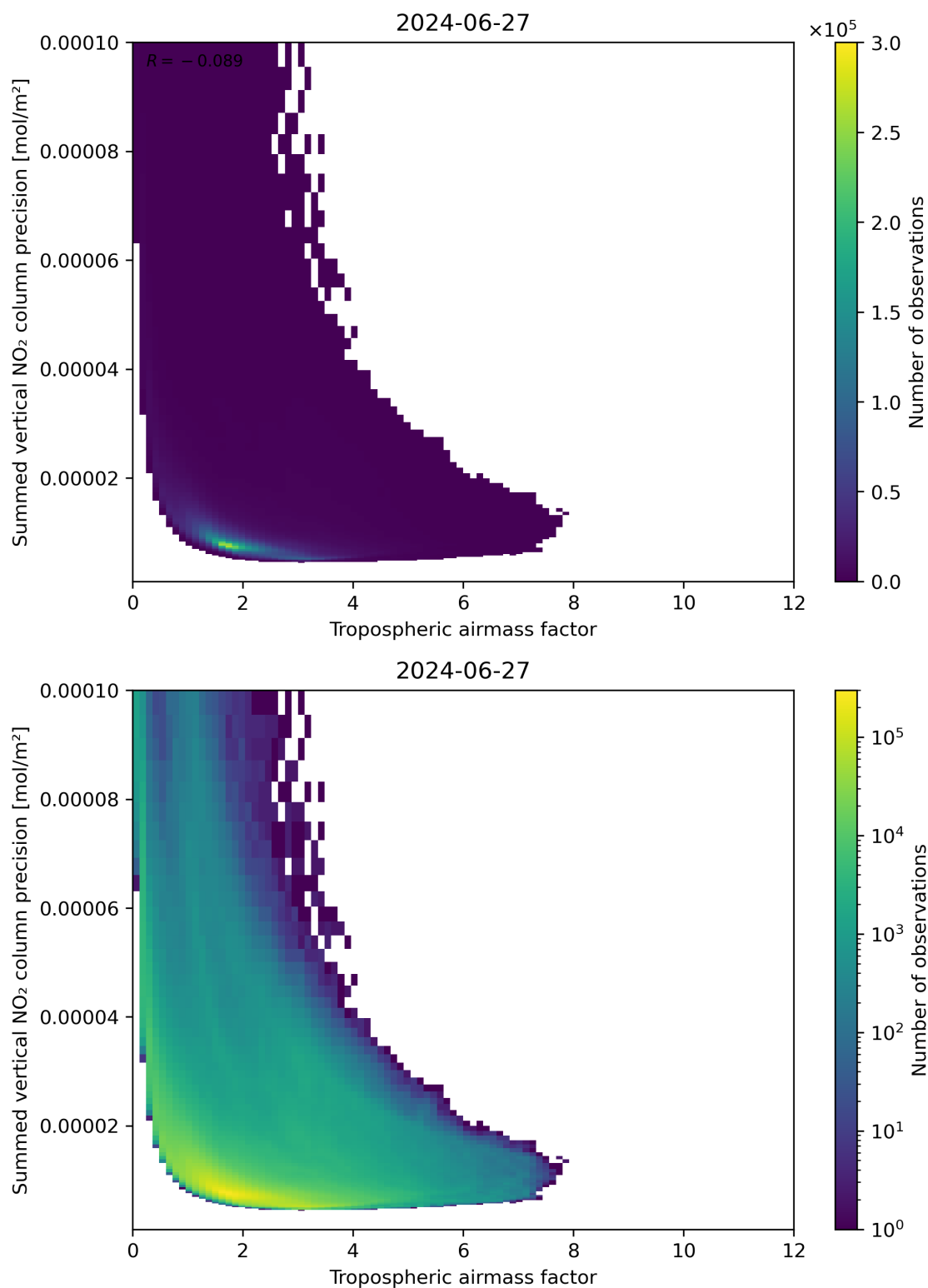
Figure 76: Scatter density plot of “Tropospheric air mass factor” against “Summed vertical NO 2 column precision” for 2024-06-26 to 2024-06-28.
