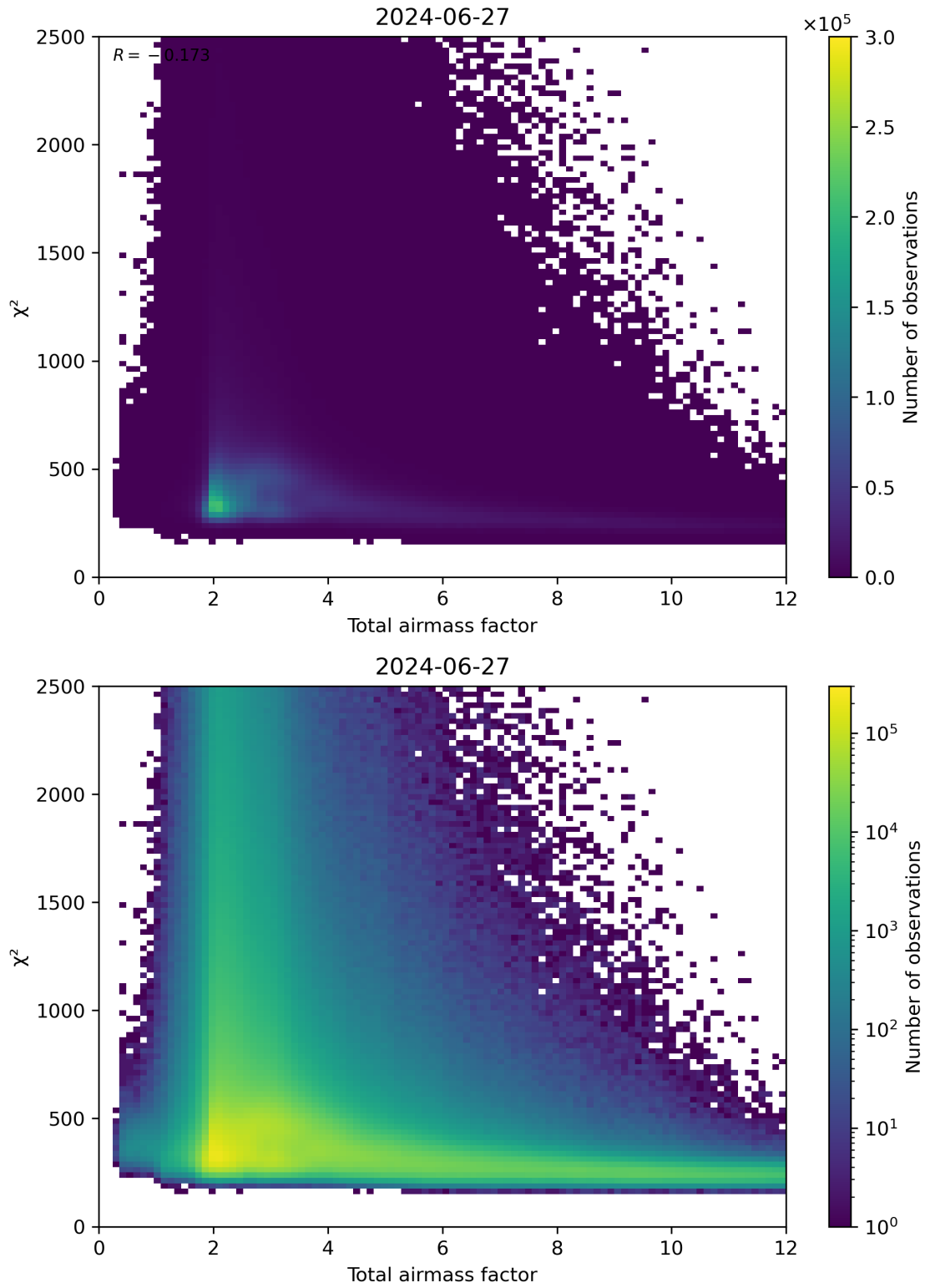
Figure 63: Scatter density plot of “Total airmass factor” against “ \chi^2 ” for 2024-06-26 to 2024-06-28.
