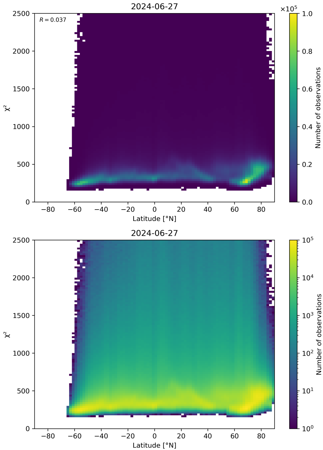
Figure 86: Scatter density plot of “Latitude” against “ \chi^2 ” for 2024-06-26 to 2024-06-28.
