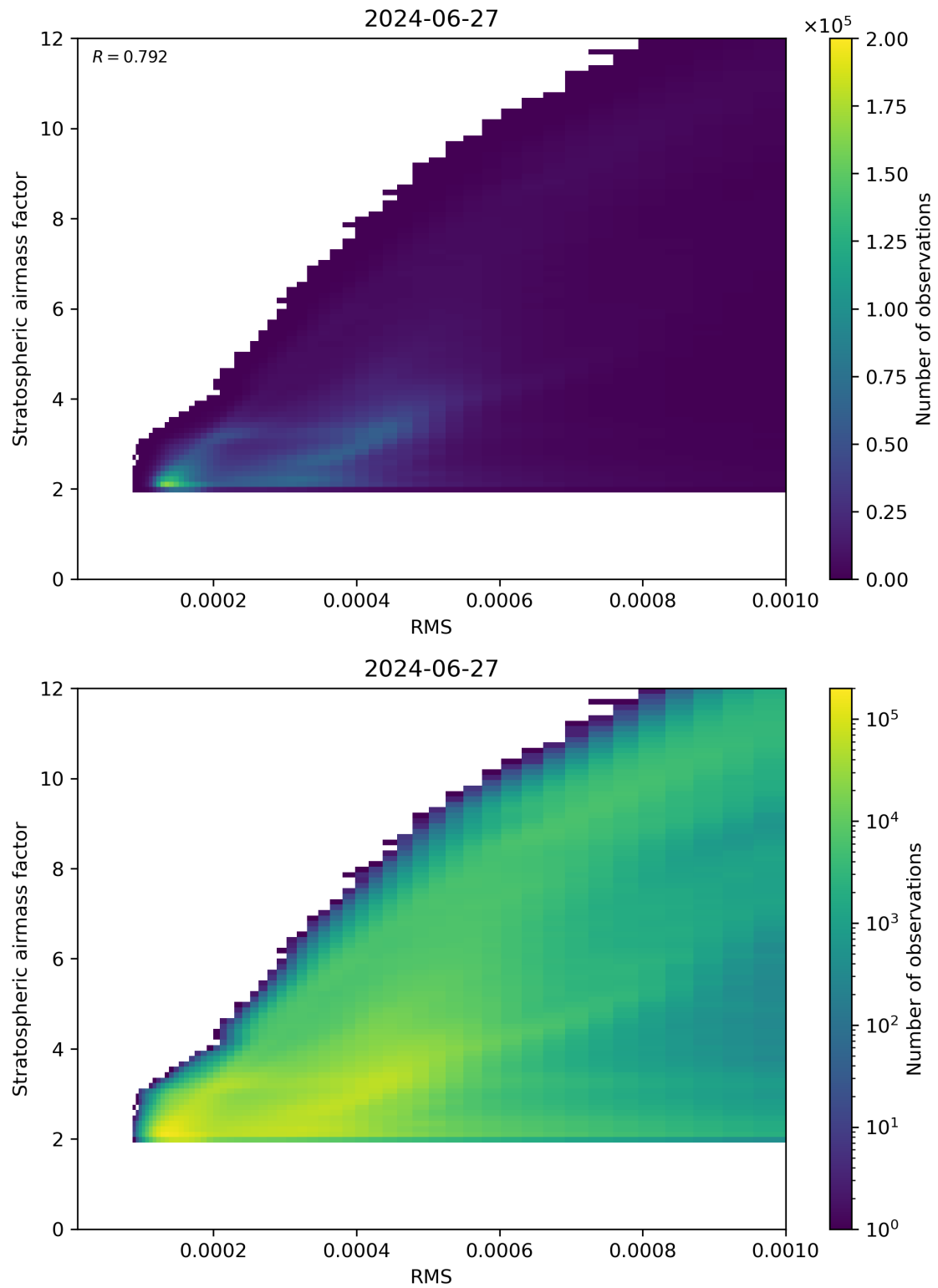
Figure 144: Scatter density plot of “RMS” against “Stratospheric airmass factor” for 2024-06-26 to 2024-06-28.
