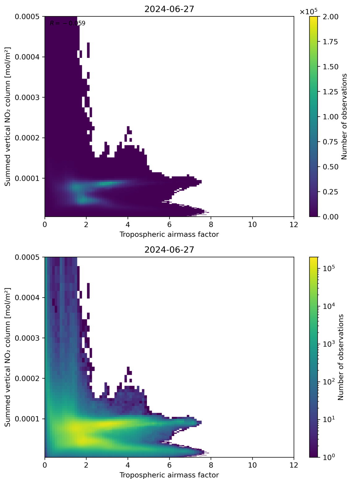
Figure 75: Scatter density plot of “Tropospheric airmass factor” against “Summed vertical NO 2 column” for 2024-06-26 to 2024-06-28.
