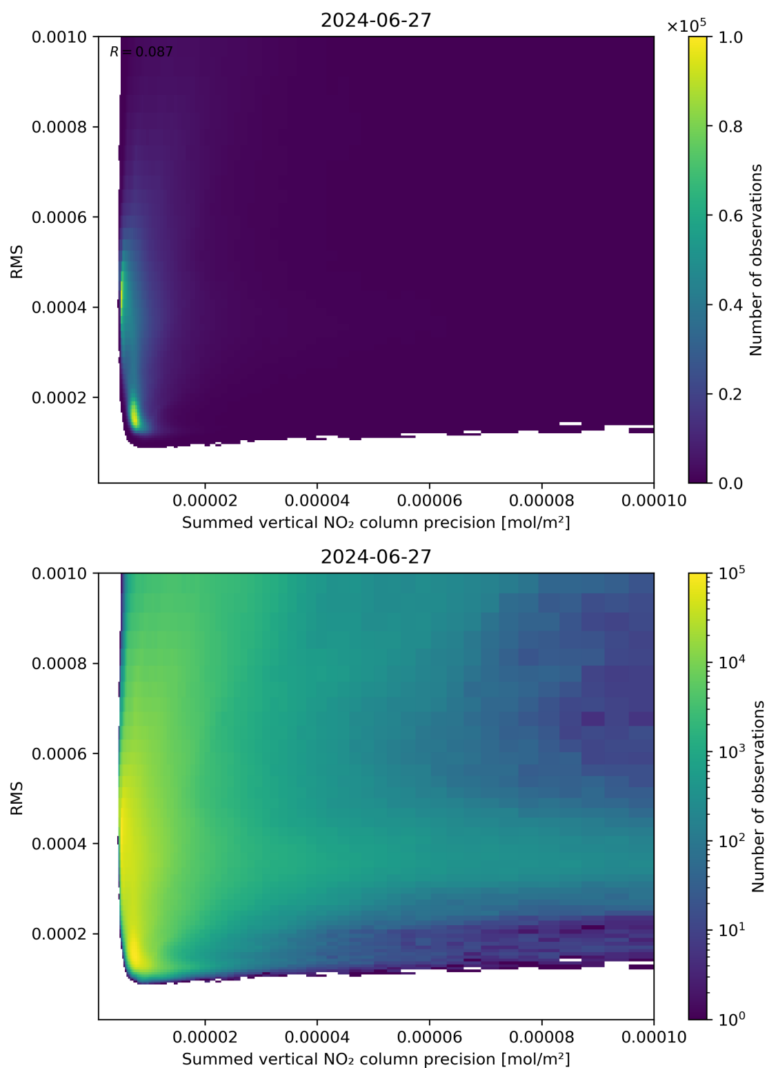
Figure 108: Scatter density plot of “Summed vertical NO 2 column precision” against “RMS” for 2024-06-26 to 2024-06-28.
