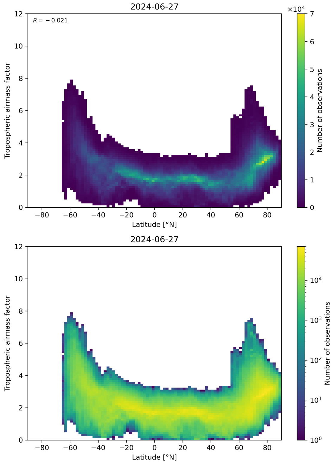
Figure 85: Scatter density plot of “Latitude” against “Tropospheric air mass factor” for 2024-06-26 to 2024-06-28.
