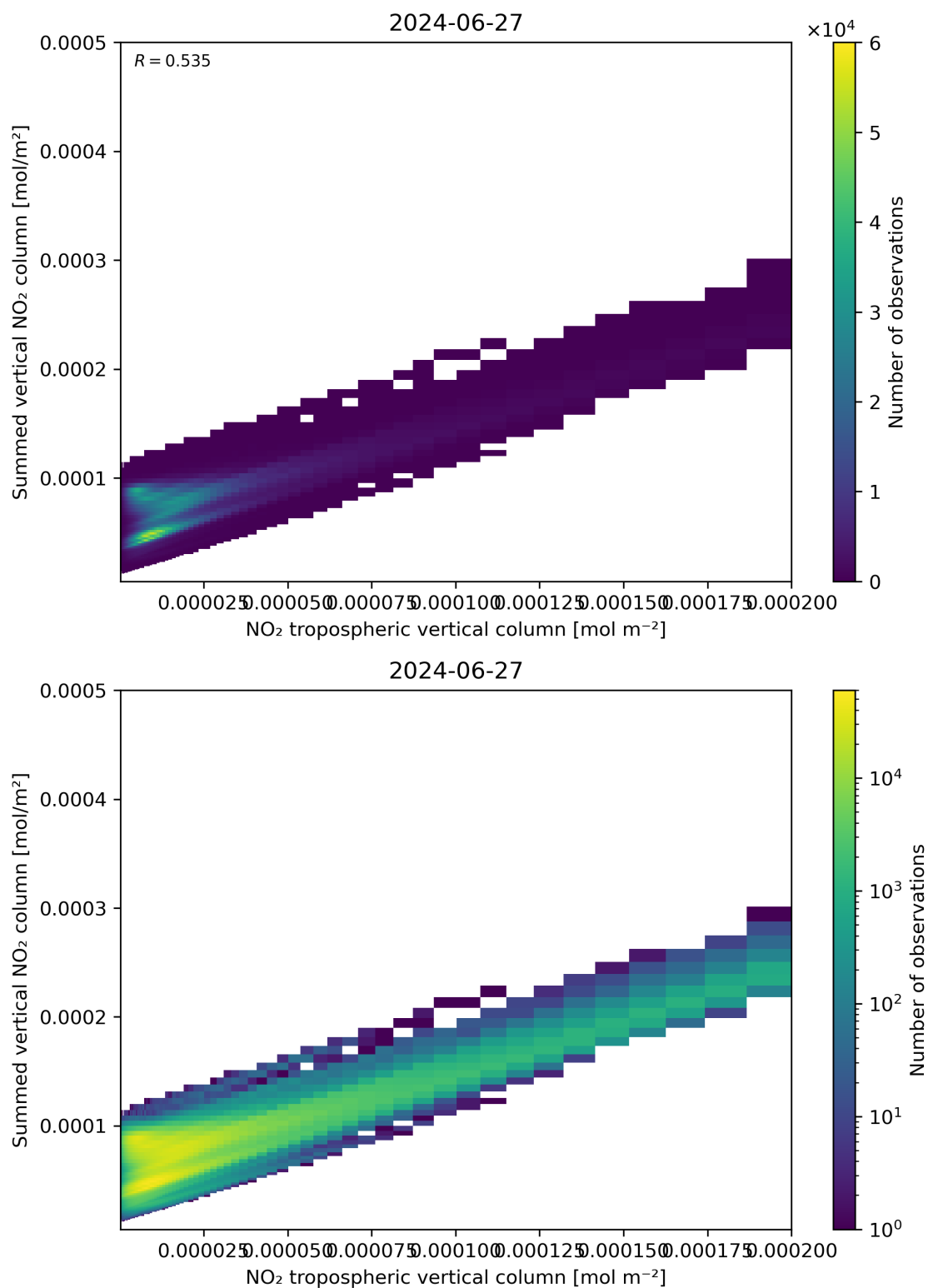
Figure 126: Scatter density plot of “NO 2 tropospheric vertical column” against “Summed vertical NO 2 column” for 2024-06-26 to 2024-06-28.
