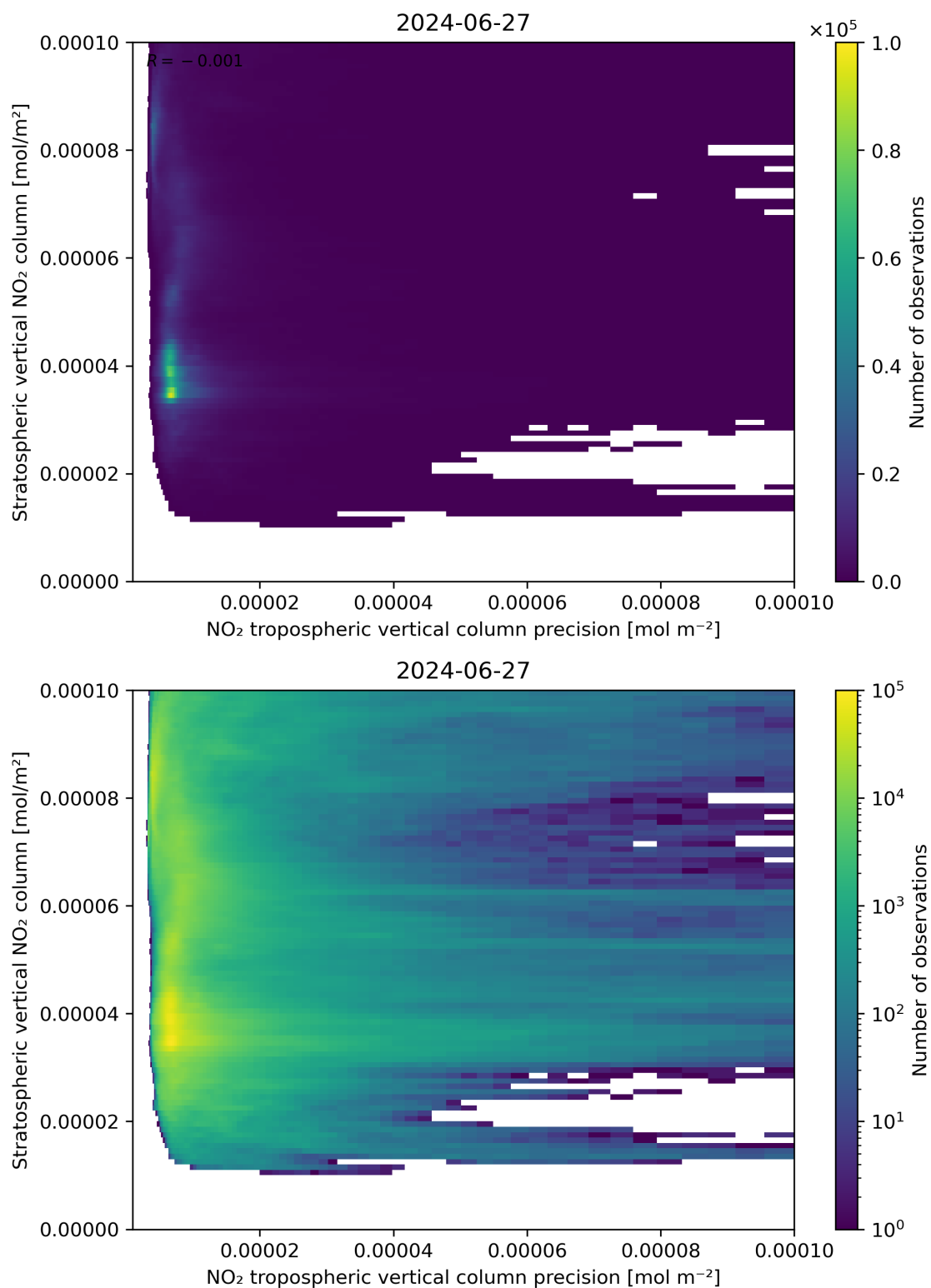
Figure 135: Scatter density plot of “NO 2 tropospheric vertical column precision” against “Stratospheric vertical NO 2 column” for 2024-06-26 to 2024-06-28.
