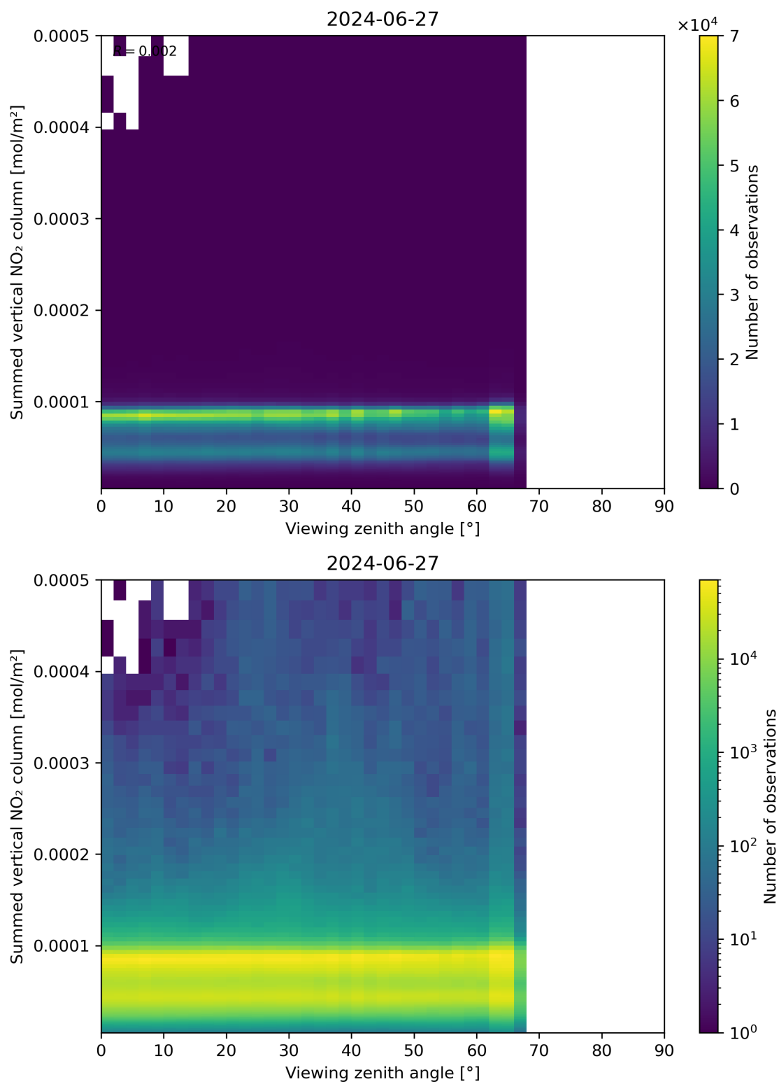
Figure 165: Scatter density plot of “Viewing zenith angle” against “Summed vertical NO 2 column” for 2024-06-26 to 2024-06-28.
