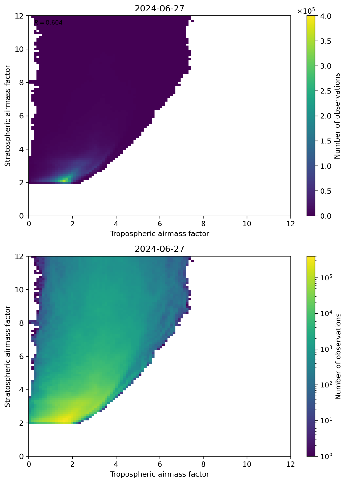
Figure 71: Scatter density plot of “Tropospheric airmass factor” against “Stratospheric airmass factor” for 2024-06-26 to 2024-06-28.
