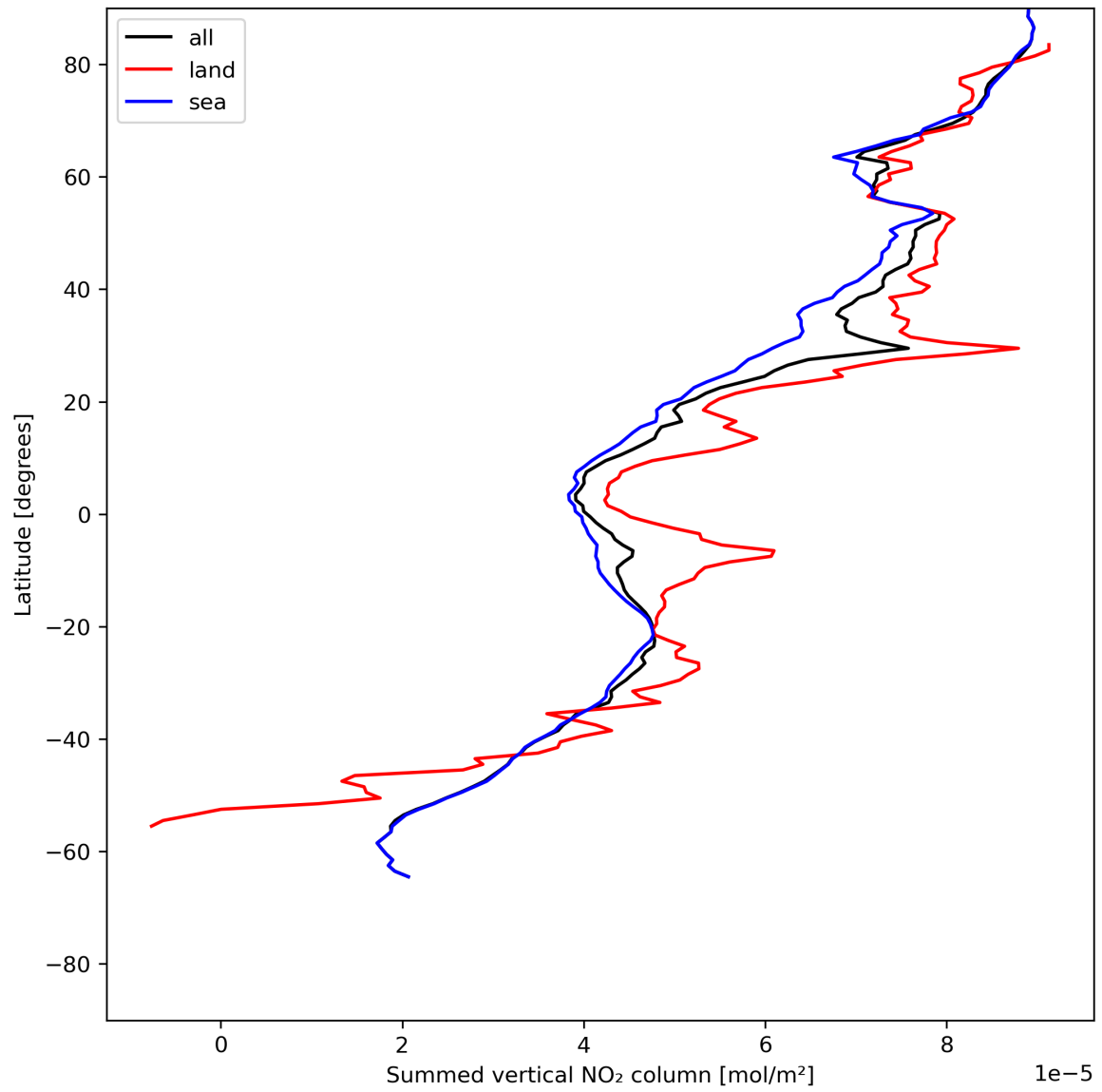
Figure 23: Zonal average of “Summed vertical NO 2 column” for 2024-06-26 to 2024-06-28.
