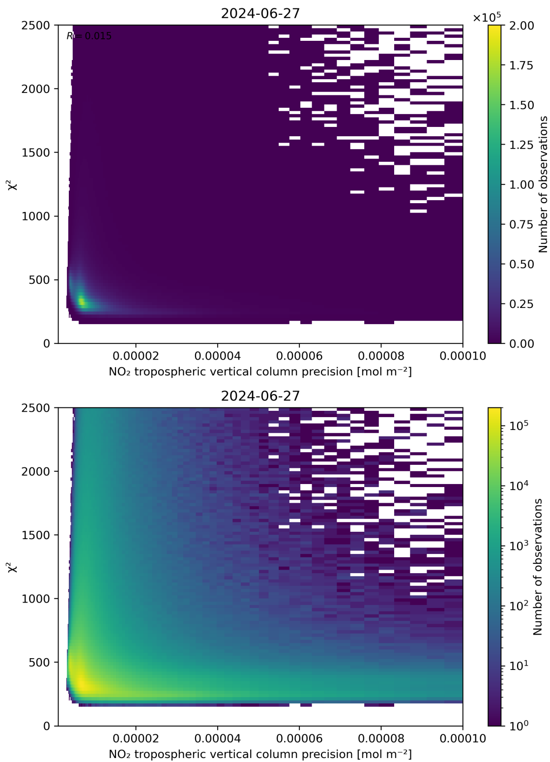
Figure 134: Scatter density plot of “NO 2 tropospheric vertical column precision” against “ \chi^2 ” for 2024-06-26 to 2024-06-28.
