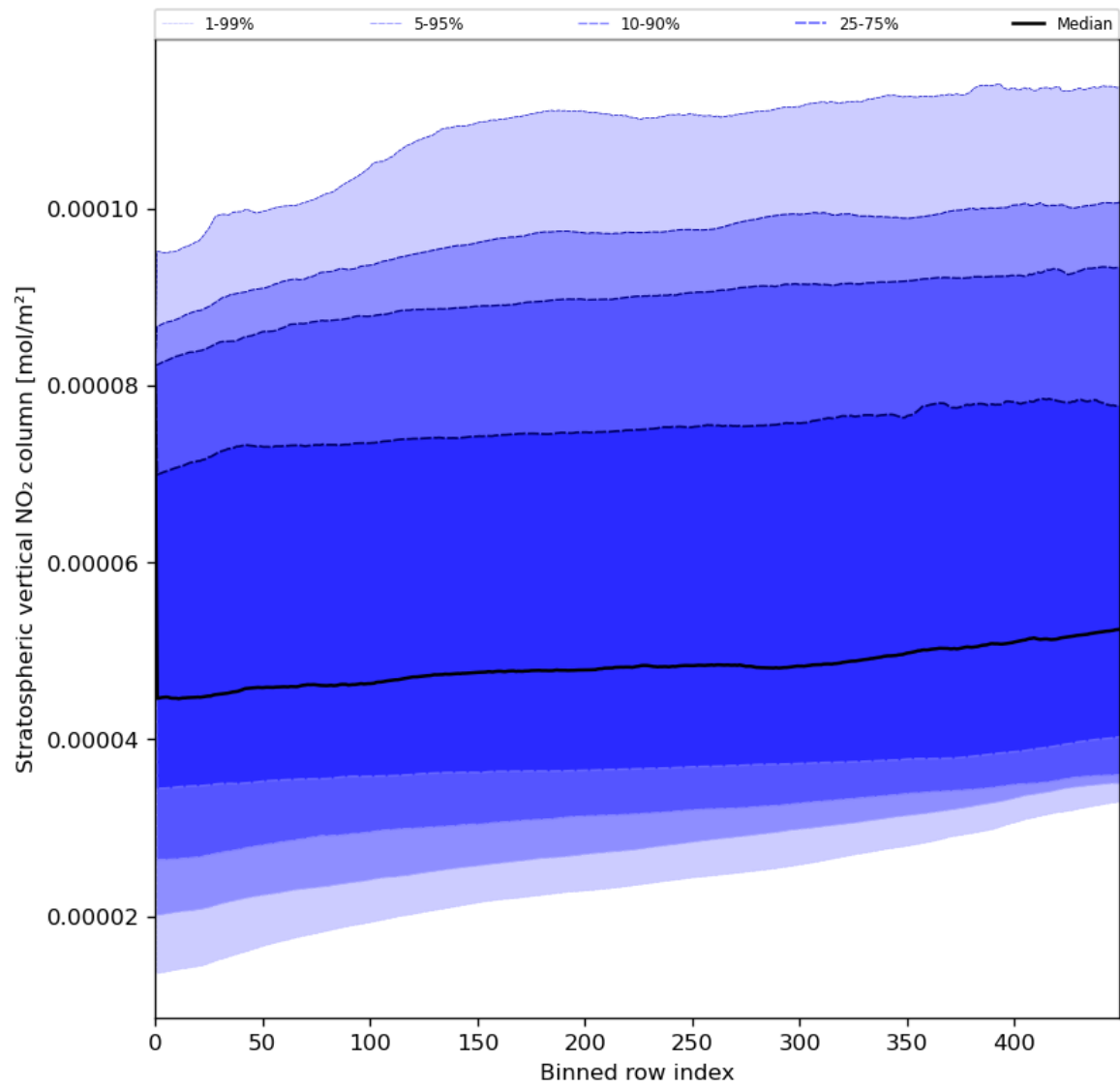
Figure 53: Along track statistics of “Stratospheric vertical NO 2 column” for 2024-06-26 to 2024-06-28
