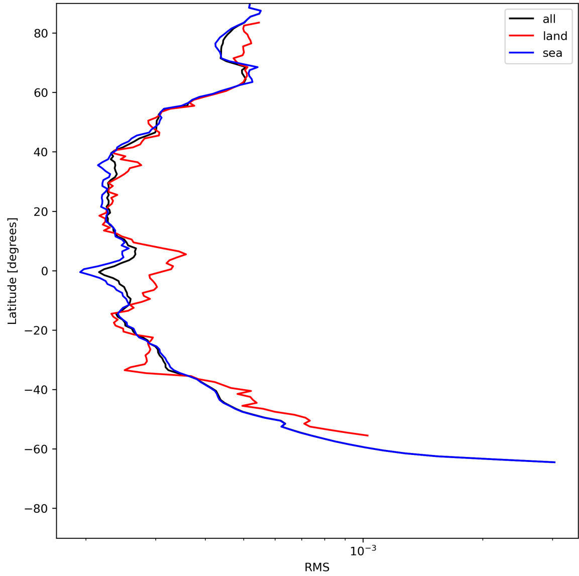
Figure 26: Zonal average of “RMS” for 2024-06-26 to 2024-06-28.
