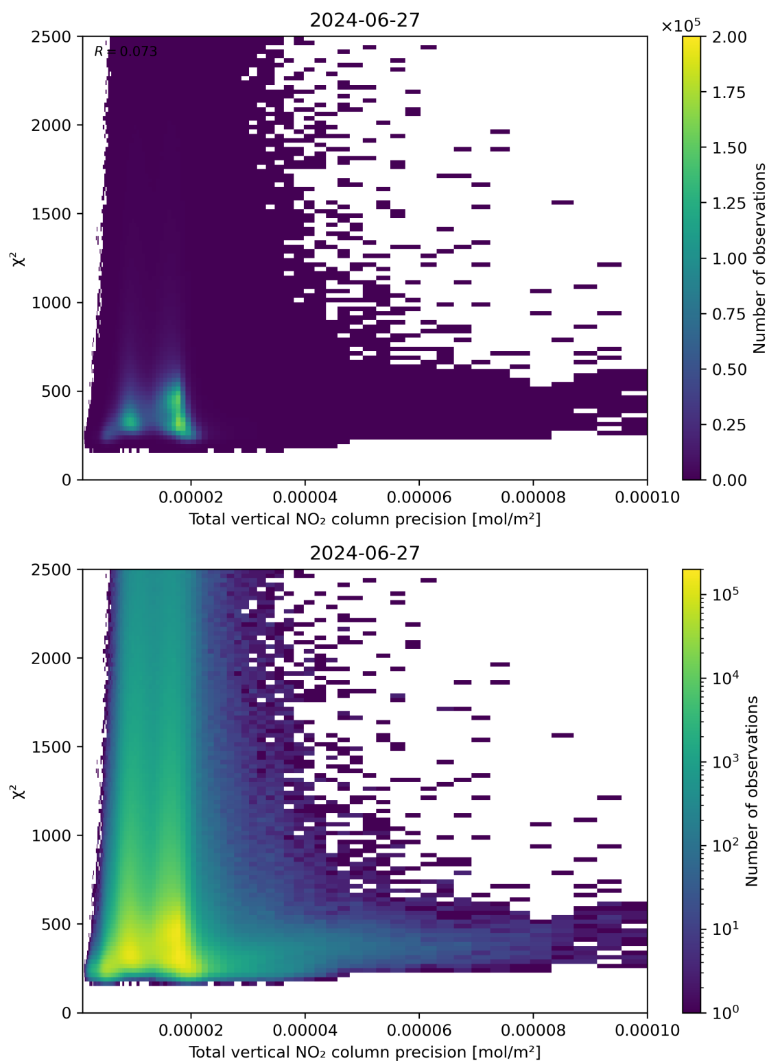
Figure 116: Scatter density plot of “Total vertical NO 2 column precision” against “ \chi^2 ” for 2024-06-26 to 2024-06-28.
