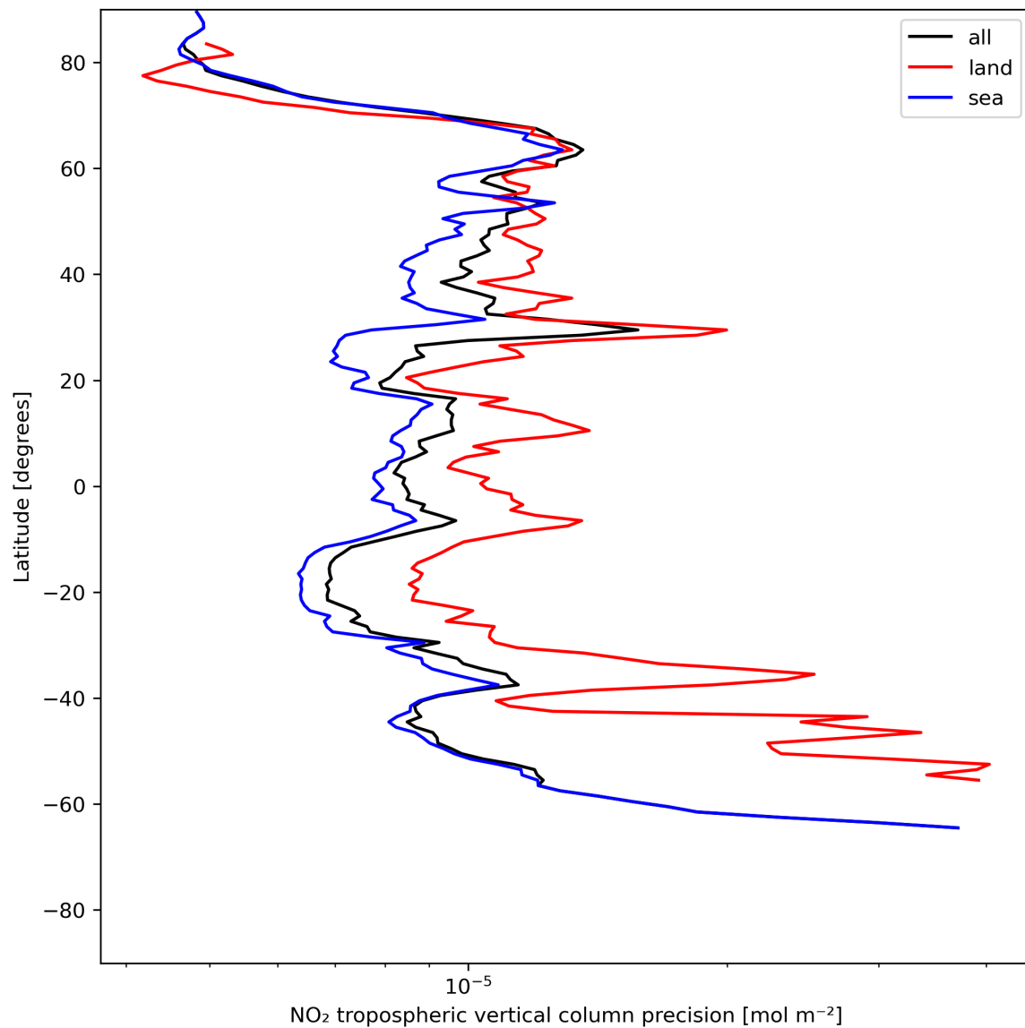
Figure 13: Zonal average of “NO 2 tropospheric vertical column precision” for 2024-06-26 to 2024-06-28.
