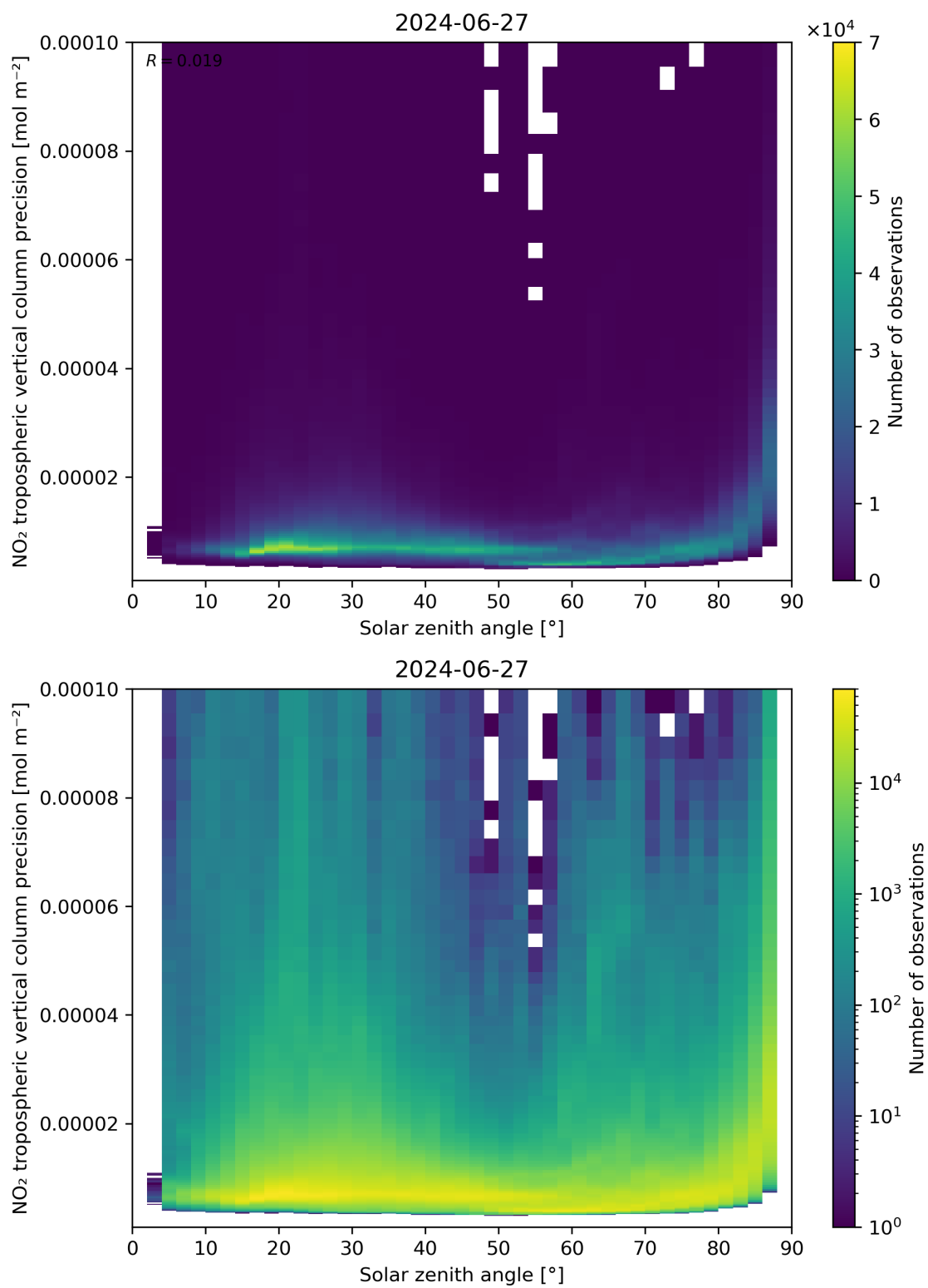
Figure 156: Scatter density plot of “Solar zenith angle” against “NO 2 tropospheric vertical column precision” for 2024-06-26 to 2024-06-28.
