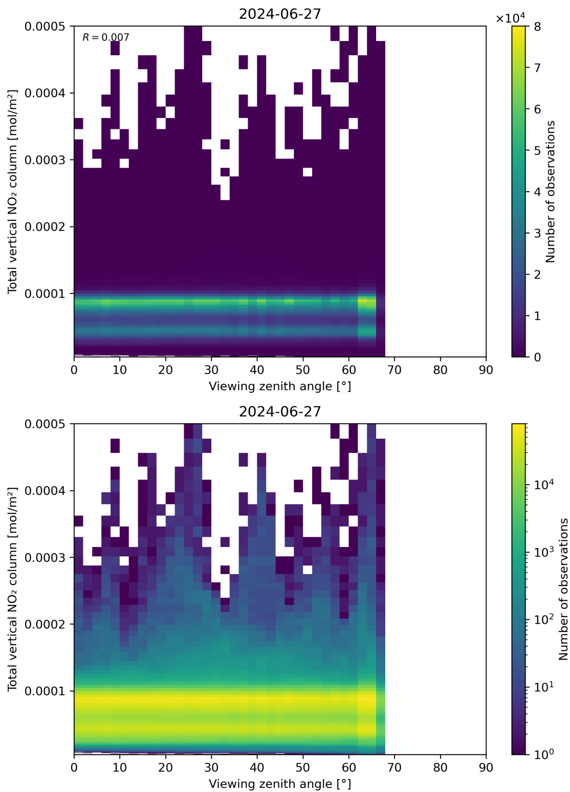
Figure 167: Scatter density plot of “Viewing zenith angle” against “Total vertical NO 2 column” for 2024-06-26 to 2024-06-28.
