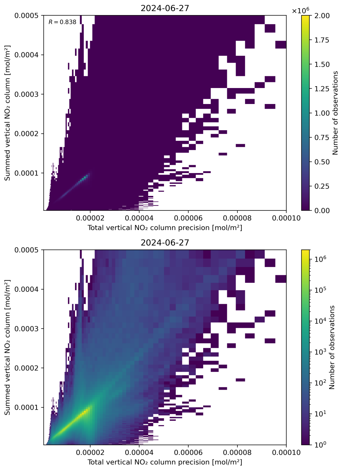
Figure 117: Scatter density plot of “Total vertical NO 2 column precision” against “Summed vertical NO 2 column” for 2024-06-26 to 2024-06-28.
