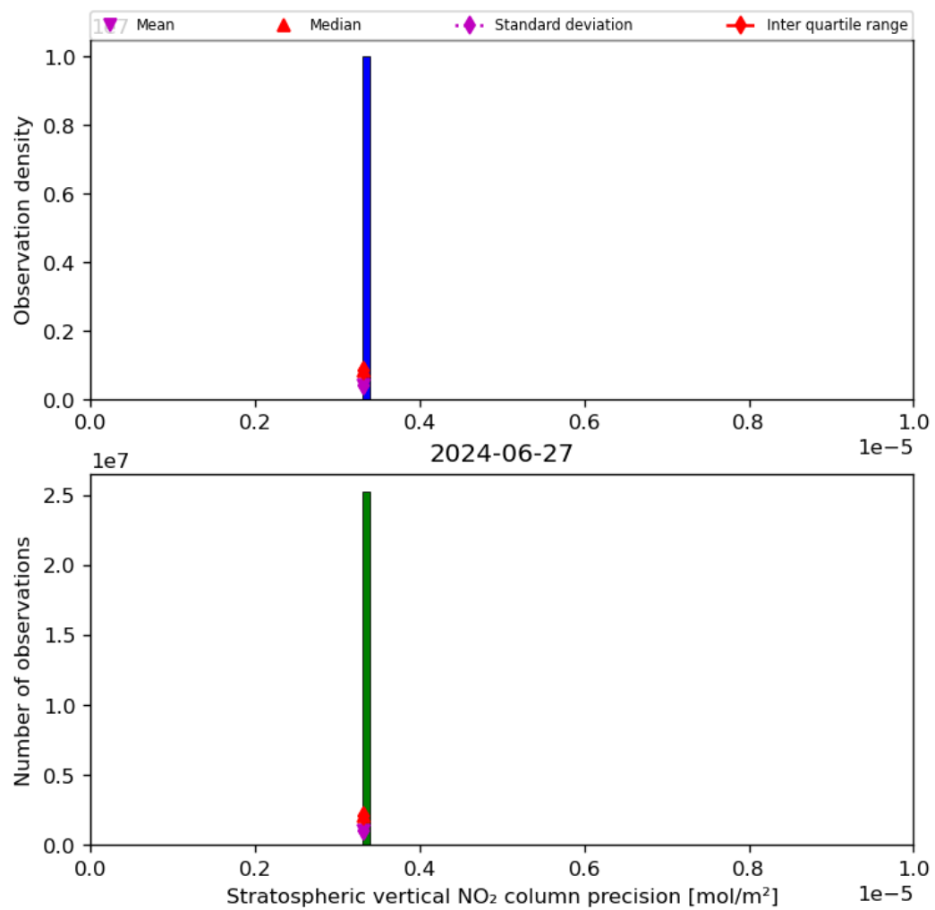
Figure 37: Histogram of “Stratospheric vertical NO 2 column precision” for 2024-06-26 to 2024-06-28
