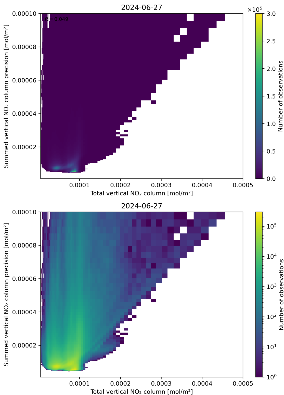
Figure 113: Scatter density plot of “Total vertical NO 2 column” against “Summed vertical NO 2 column precision” for 2024-06-26 to 2024-06-28.
