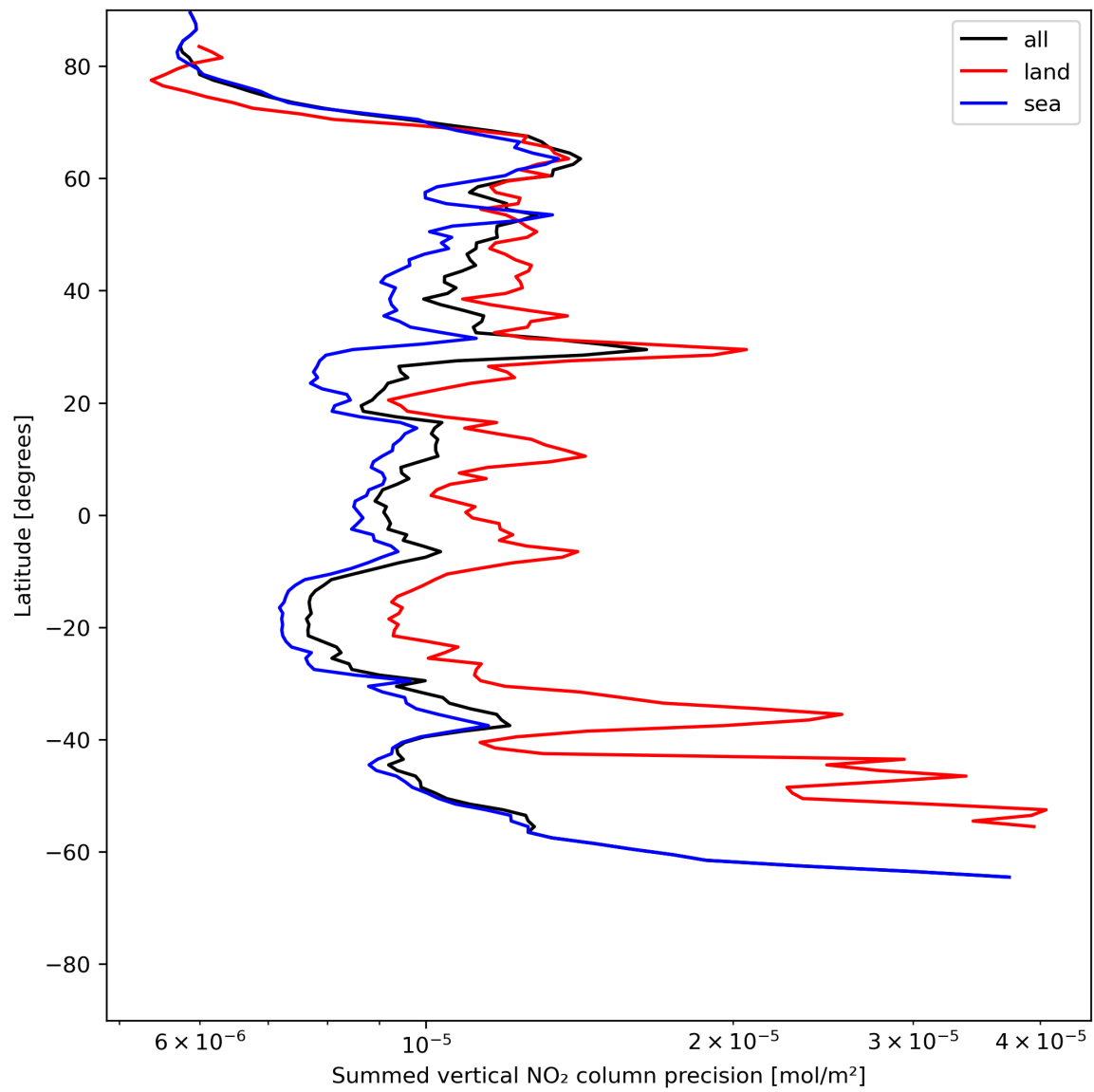
Figure 24: Zonal average of “Summed vertical NO 2 column precision” for 2024-06-26 to 2024-06-28.
