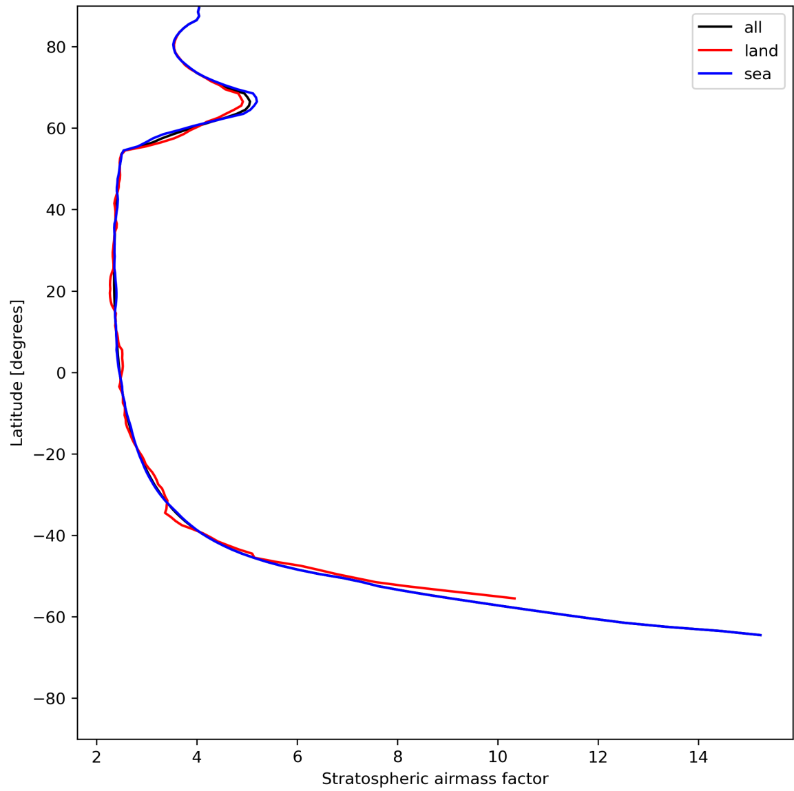
Figure 27: Zonal average of “Stratospheric air mass factor” for 2024-06-26 to 2024-06-28.
