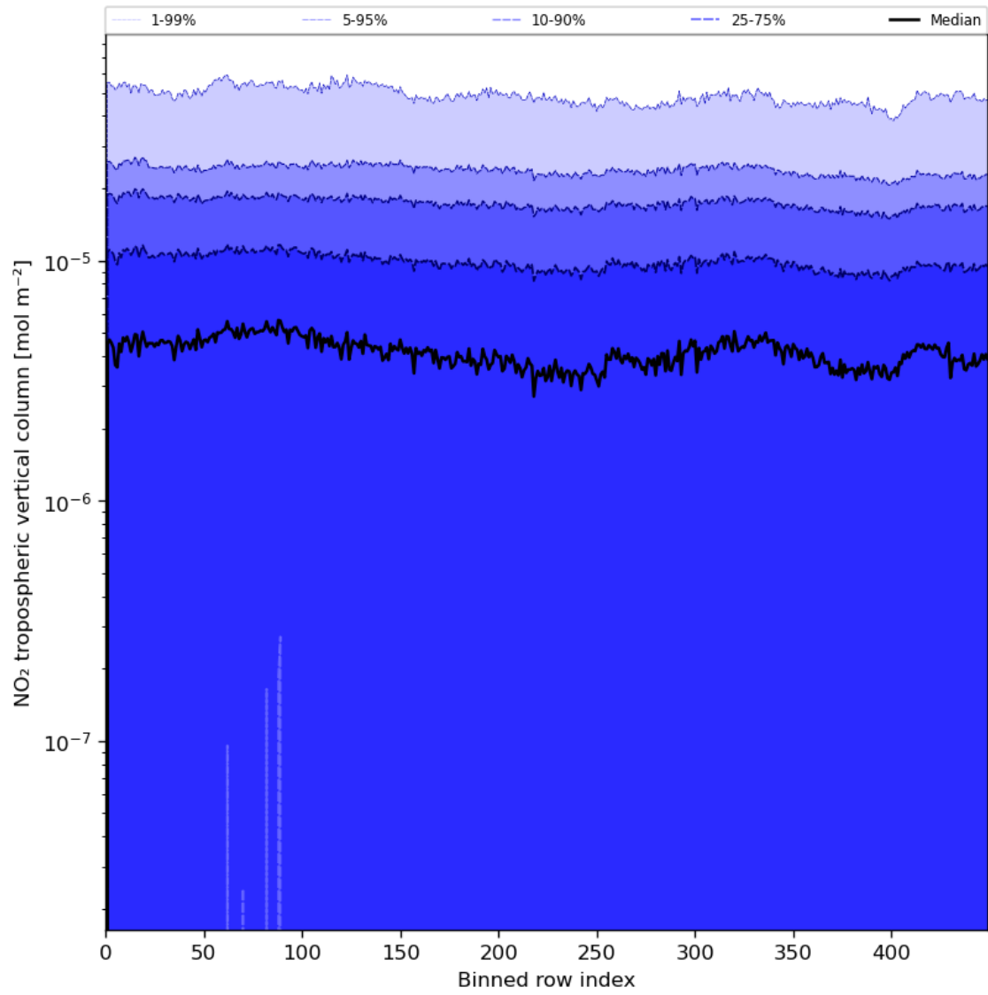
Figure 46: Along track statistics of “NO 2 tropospheric vertical column” for 2024-06-26 to 2024-06-28
