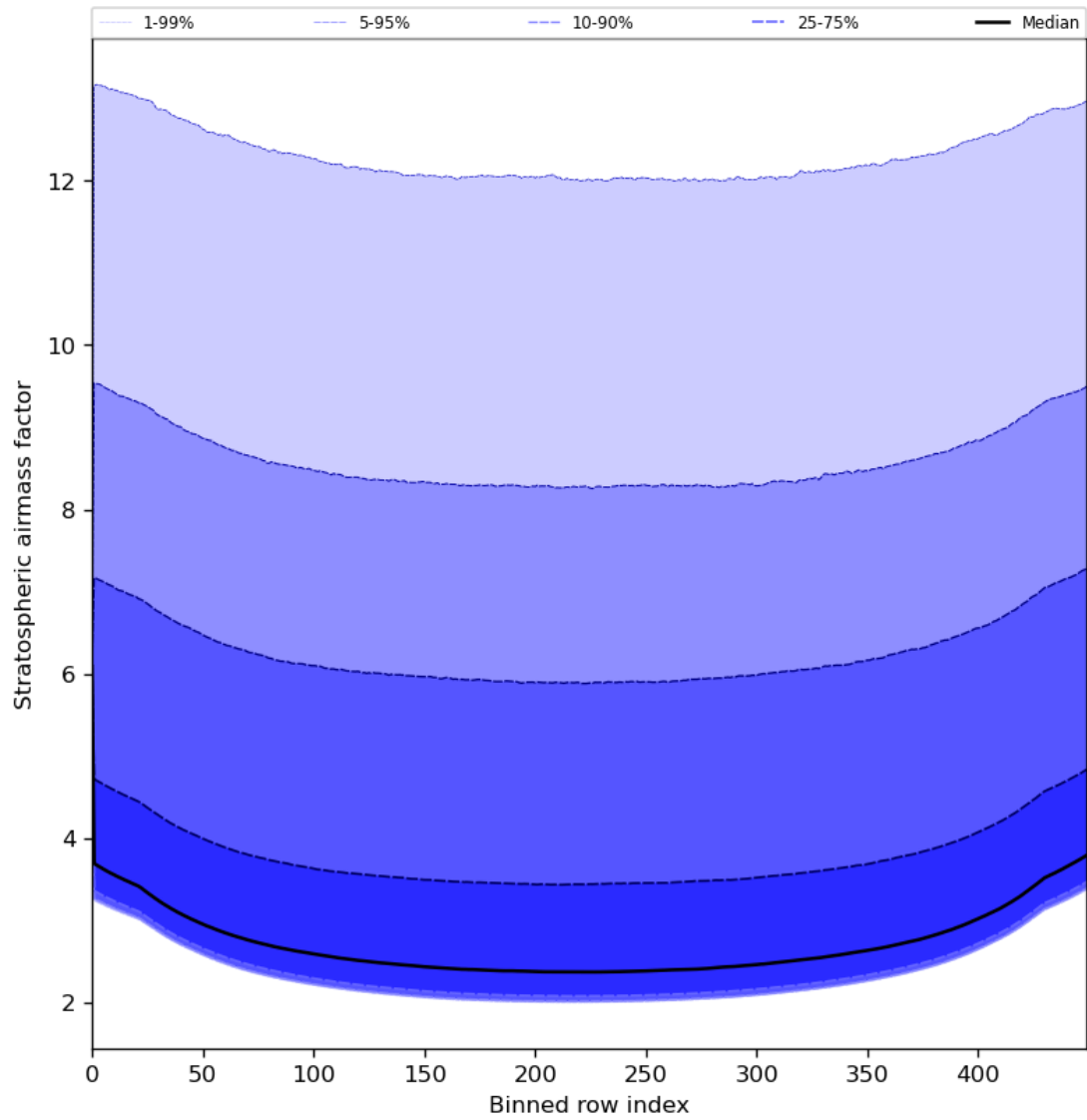
Figure 61: Along track statistics of “Stratospheric air mass factor” for 2024-06-26 to 2024-06-28
