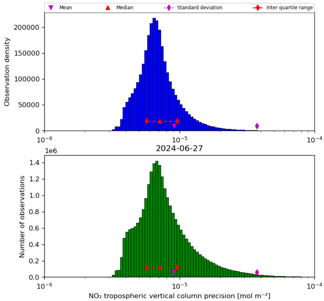
Figure 30: Histogram of “NO 2 tropospheric vertical column precision” for 2024-06-26 to 2024-06-28
