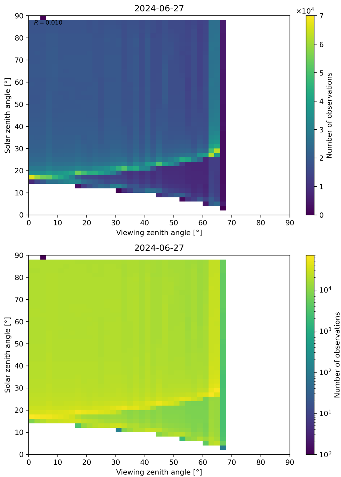
Figure 172: Scatter density plot of “Viewing zenith angle” against “Solar zenith angle” for 2024-06-26 to 2024-06-28.
