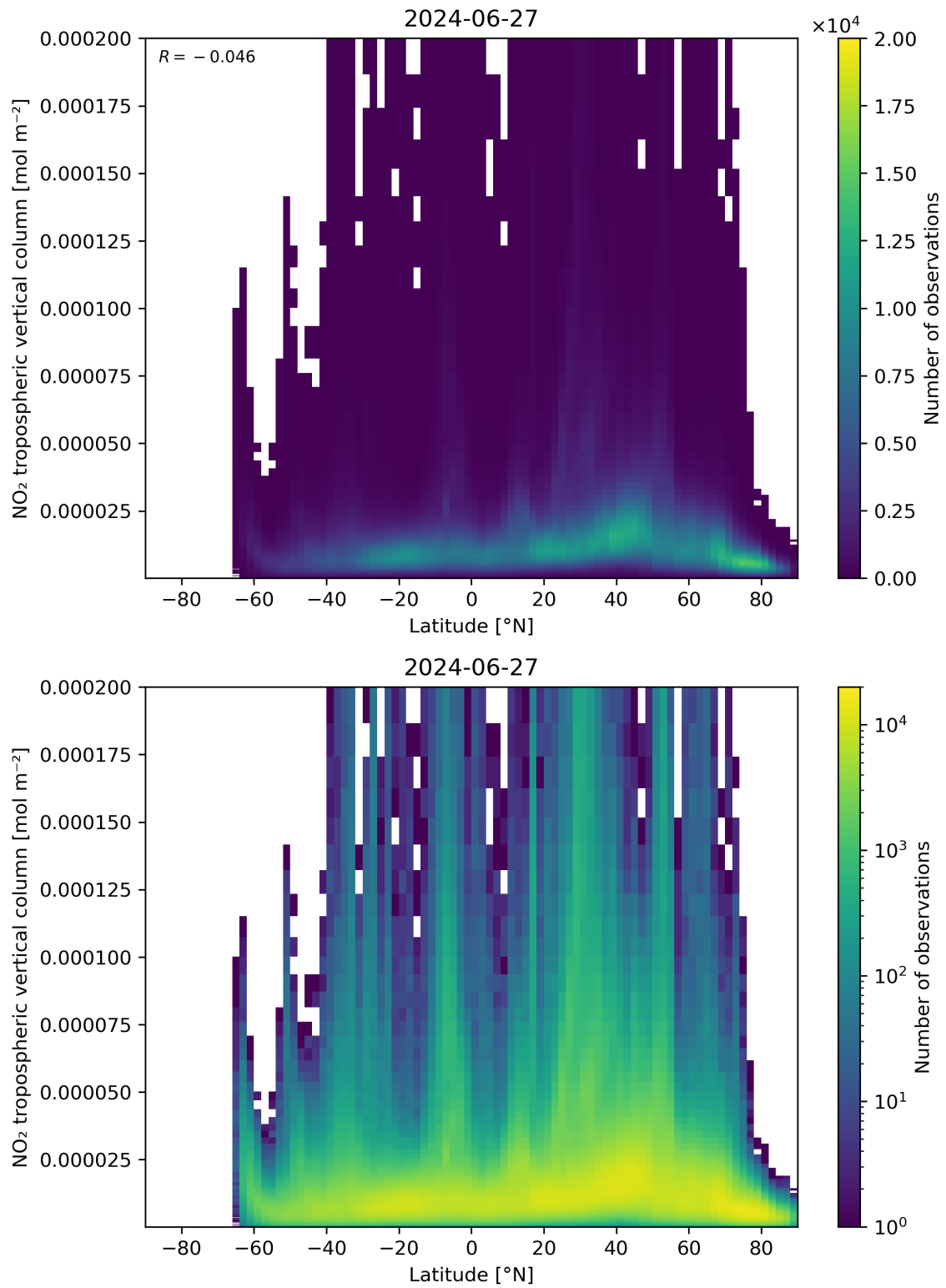
Figure 92: Scatter density plot of “Latitude” against “NO 2 tropospheric vertical column” for 2024-06-26 to 2024-06-28.
