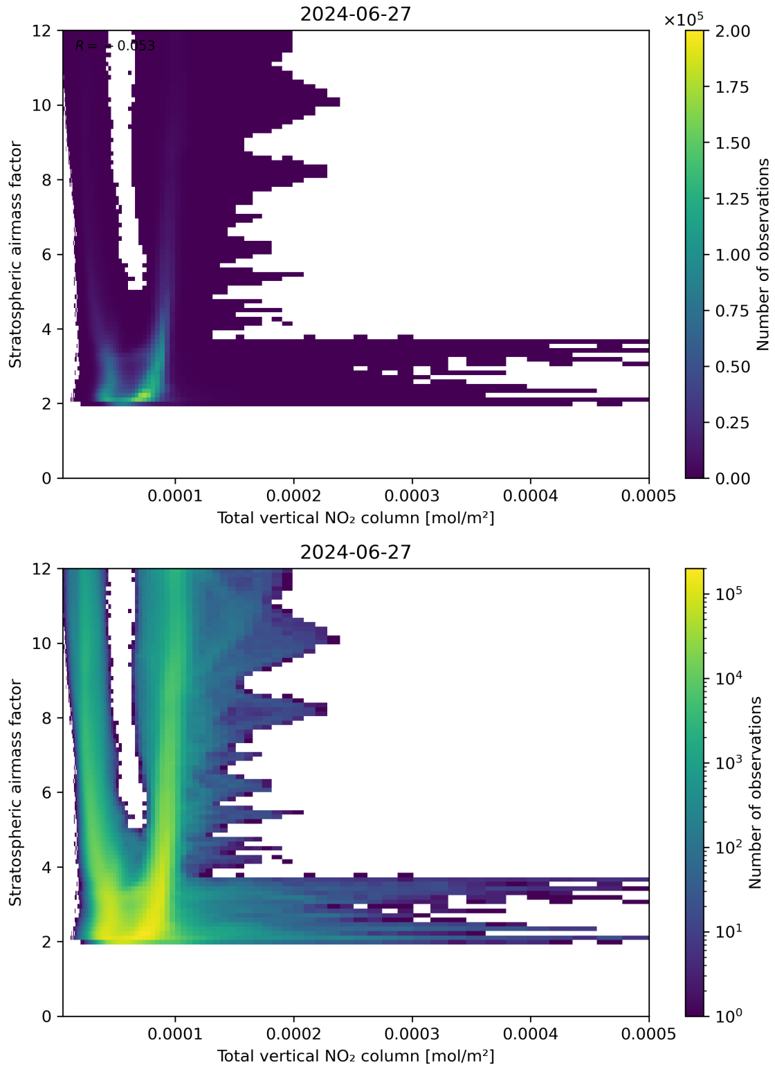
Figure 110: Scatter density plot of “Total vertical NO 2 column” against “Stratospheric airmass factor” for 2024-06-26 to 2024-06-28.
