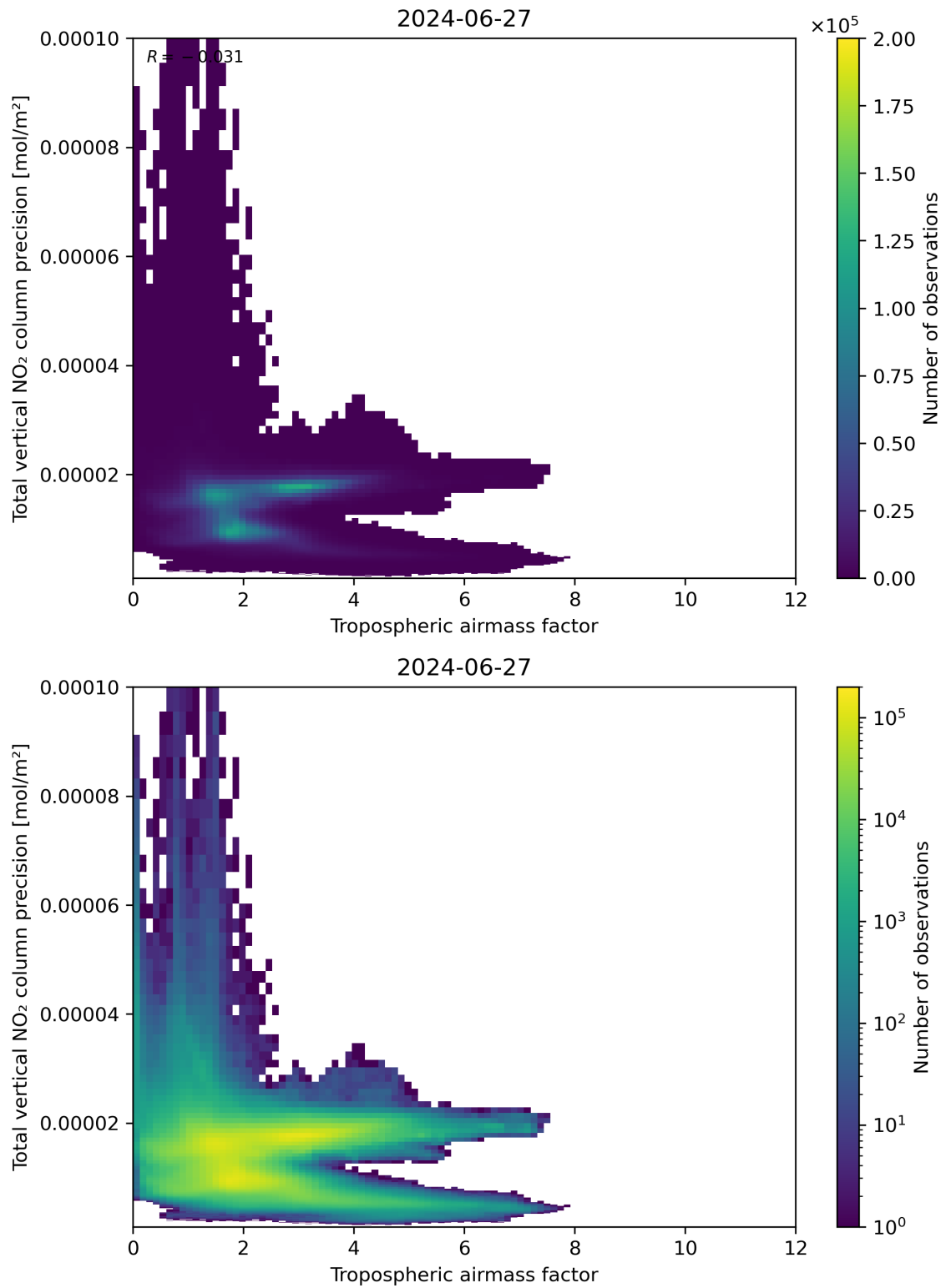
Figure 78: Scatter density plot of “Tropospheric airmass factor” against “Total vertical NO 2 column precision” for 2024-06-26 to 2024-06-28.
