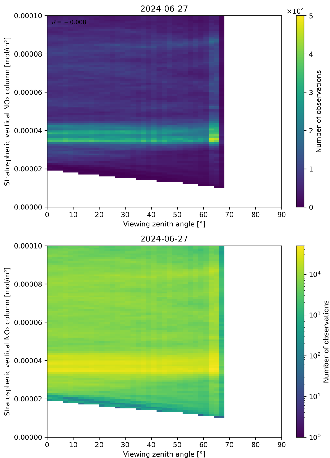
Figure 164: Scatter density plot of “Viewing zenith angle” against “Stratospheric vertical NO 2 column” for 2024-06-26 to 2024-06-28.
