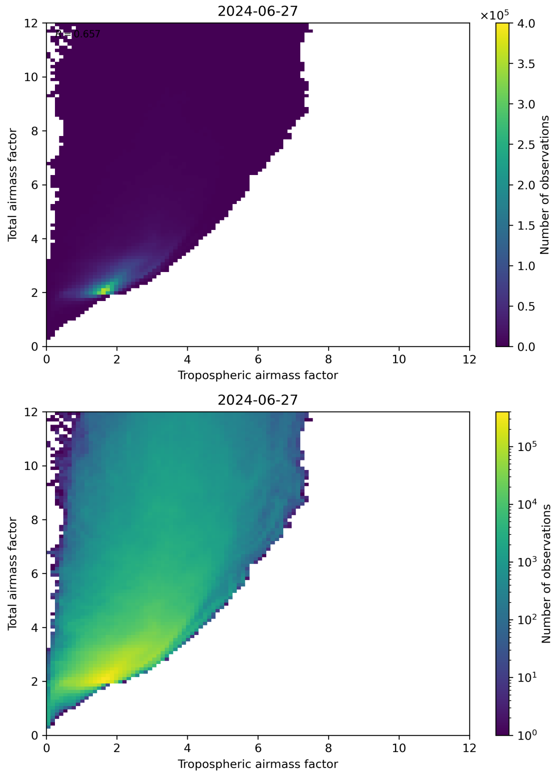
Figure 72: Scatter density plot of “Tropospheric airmass factor” against “Total airmass factor” for 2024-06-26 to 2024-06-28.
