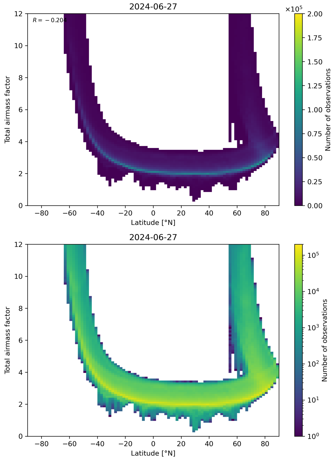
Figure 84: Scatter density plot of “Latitude” against “Total airmass factor” for 2024-06-26 to 2024-06-28.
