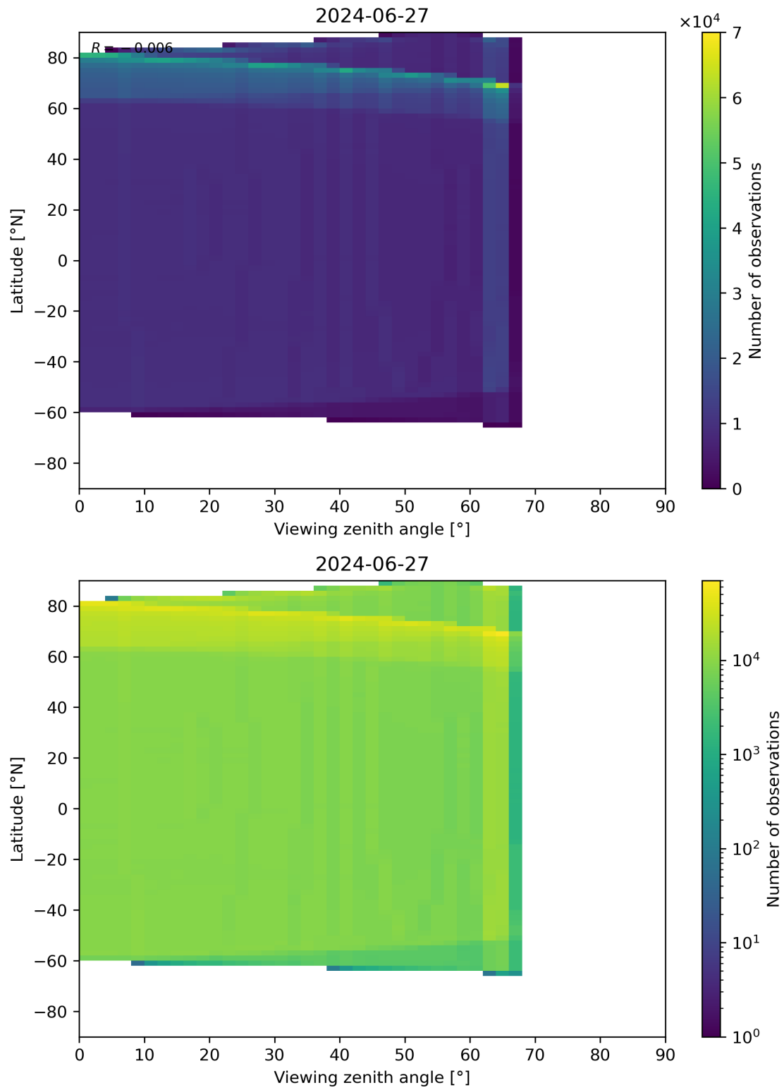
Figure 163: Scatter density plot of “Viewing zenith angle” against “Latitude” for 2024-06-26 to 2024-06-28.
