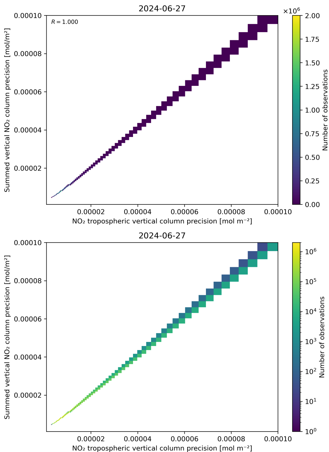
Figure 137: Scatter density plot of “NO 2 tropospheric vertical column precision” against “Summed vertical NO 2 column precision” for 2024-06-26 to 2024-06-28.
