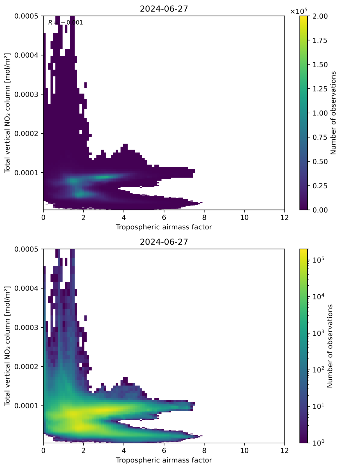
Figure 77: Scatter density plot of “Tropospheric airmass factor” against “Total vertical NO 2 column” for 2024-06-26 to 2024-06-28.
