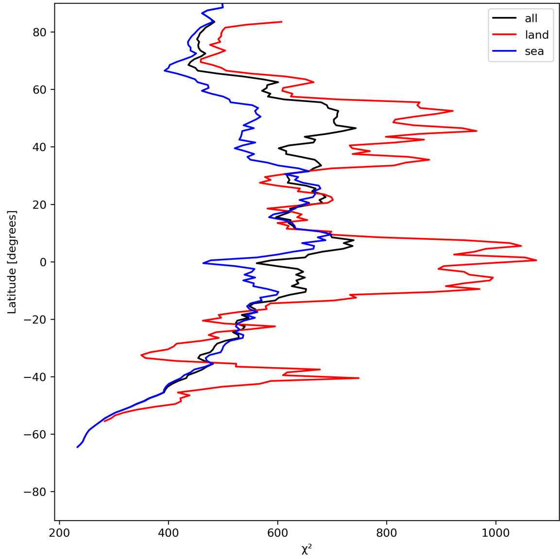
Figure 25: Zonal average of “ \chi^2 ” for 2024-06-26 to 2024-06-28.
