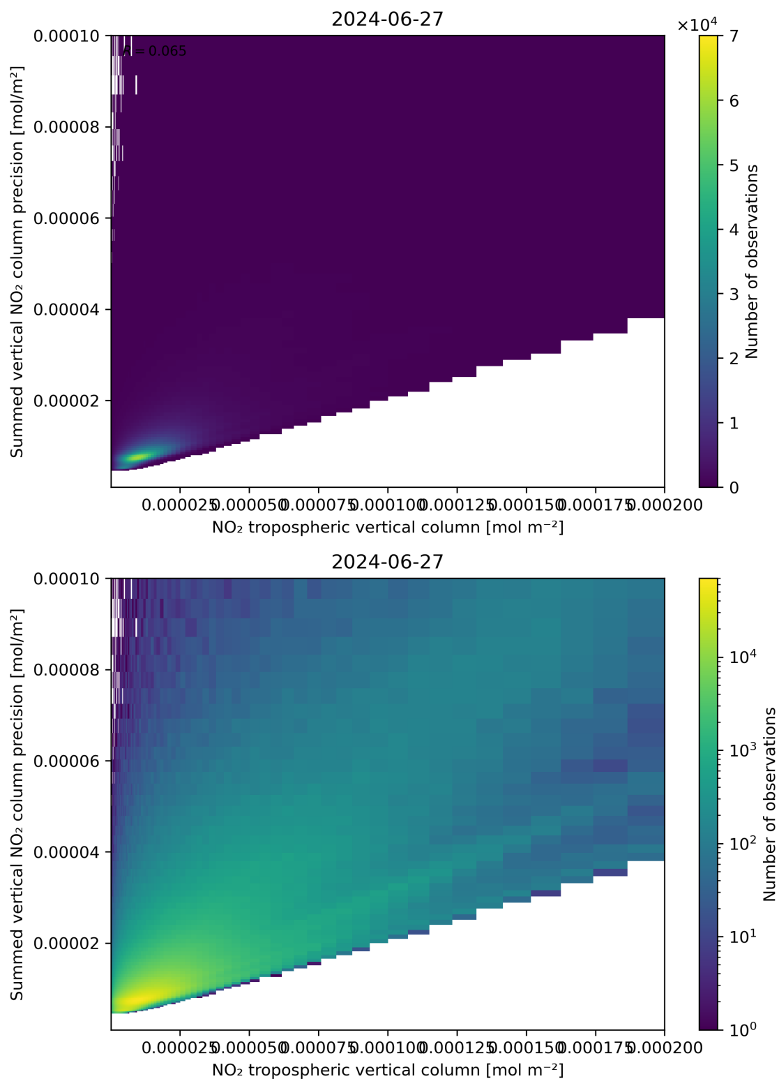
Figure 127: Scatter density plot of “NO 2 tropospheric vertical column” against “Summed vertical NO 2 column precision” for 2024-06-26 to 2024-06-28.
