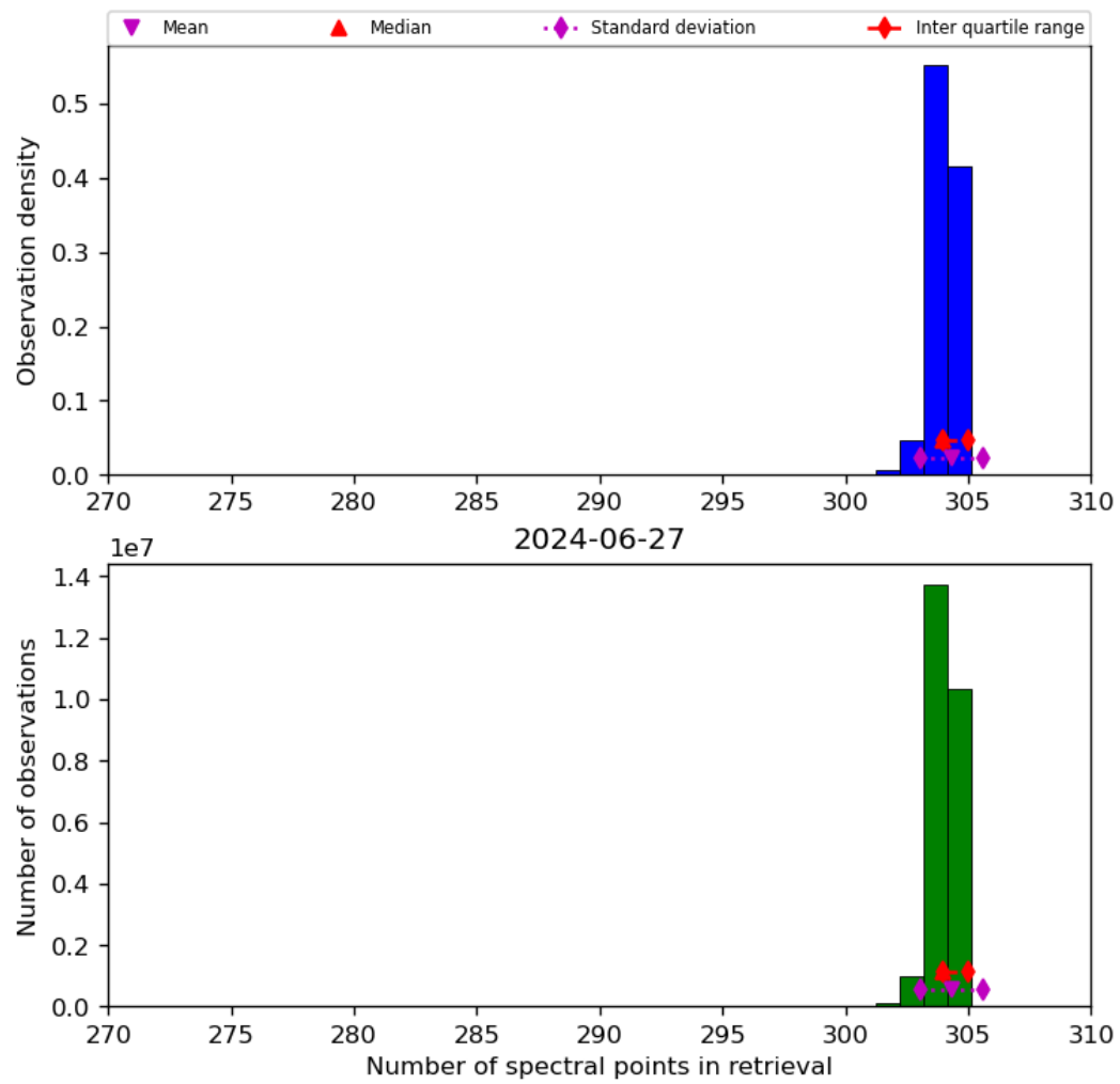
Figure 33: Histogram of “Number of spectral points in retrieval” for 2024-06-26 to 2024-06-28
