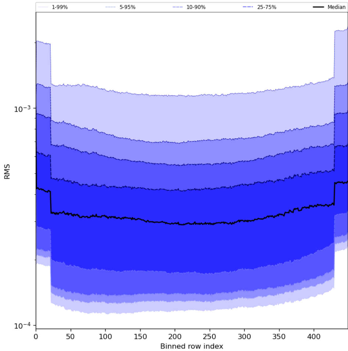
Figure 60: Along track statistics of “RMS” for 2024-06-26 to 2024-06-28
