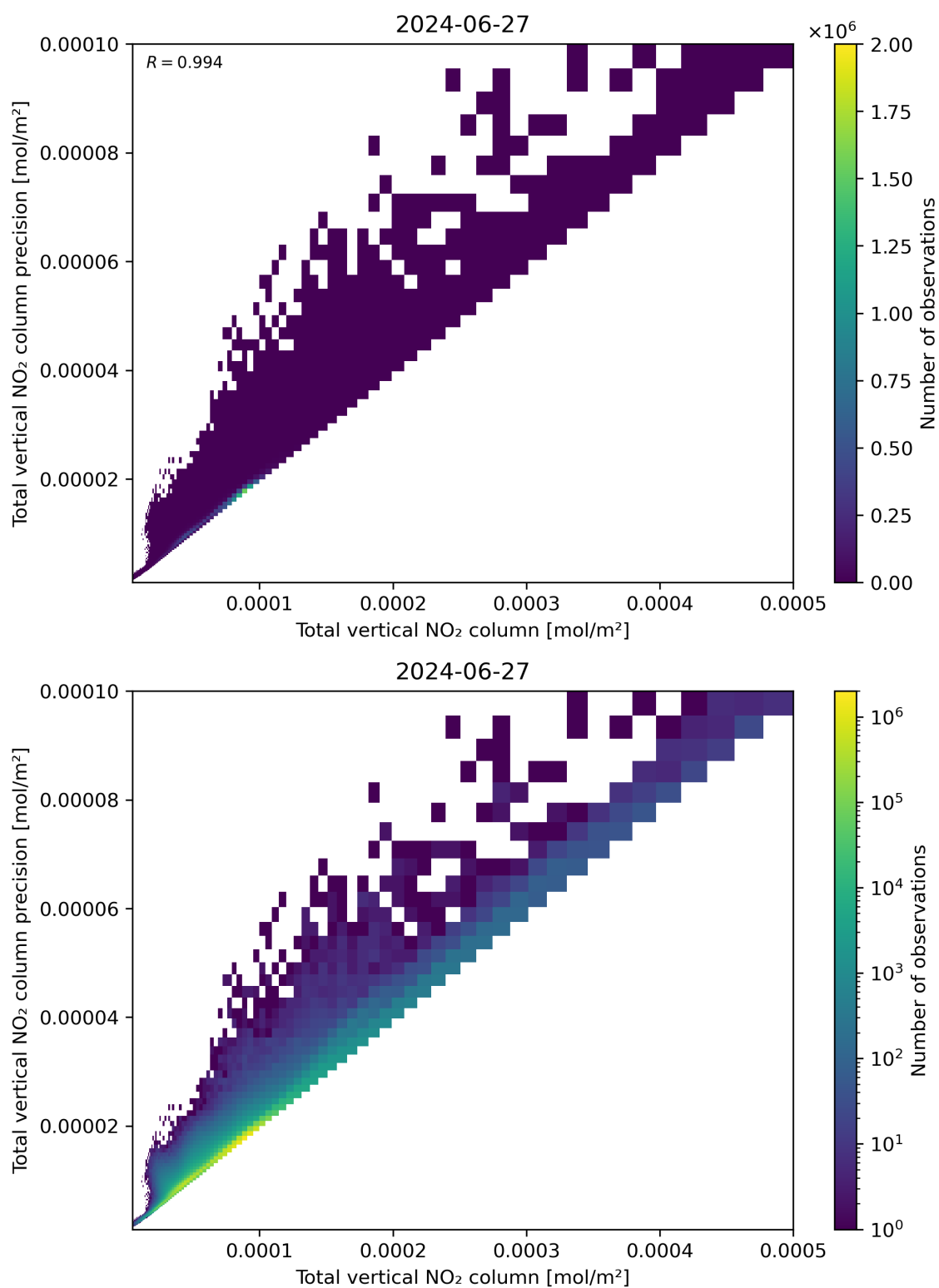
Figure 114: Scatter density plot of “Total vertical NO 2 column” against “Total vertical NO 2 column precision” for 2024-06-26 to 2024-06-28.
