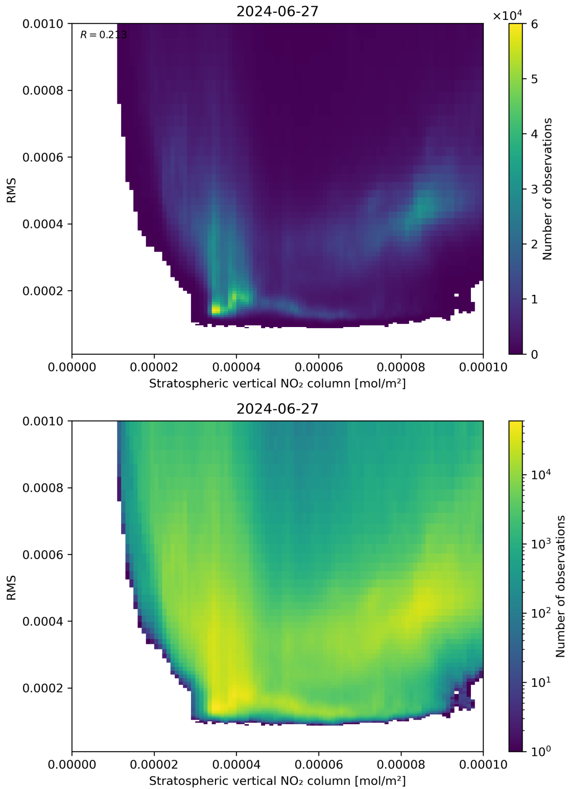
Figure 102: Scatter density plot of “Stratospheric vertical NO 2 column” against “RMS” for 2024-06-26 to 2024-06-28.
