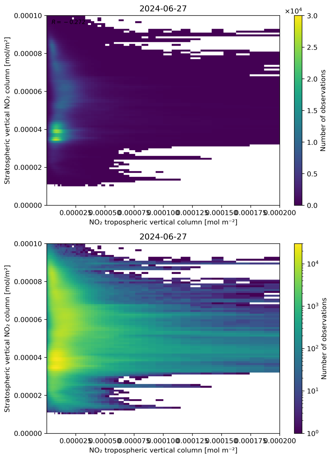
Figure 125: Scatter density plot of “NO 2 tropospheric vertical column” against “Stratospheric vertical NO 2 column” for 2024-06-26 to 2024-06-28.
