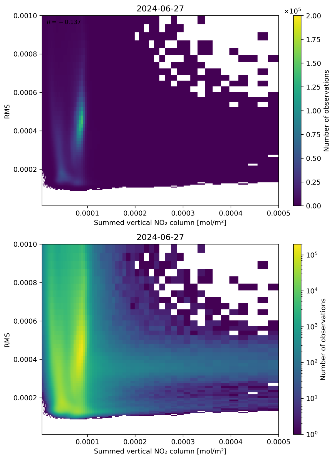
Figure 109: Scatter density plot of “Summed vertical NO 2 column” against “RMS” for 2024-06-26 to 2024-06-28.
