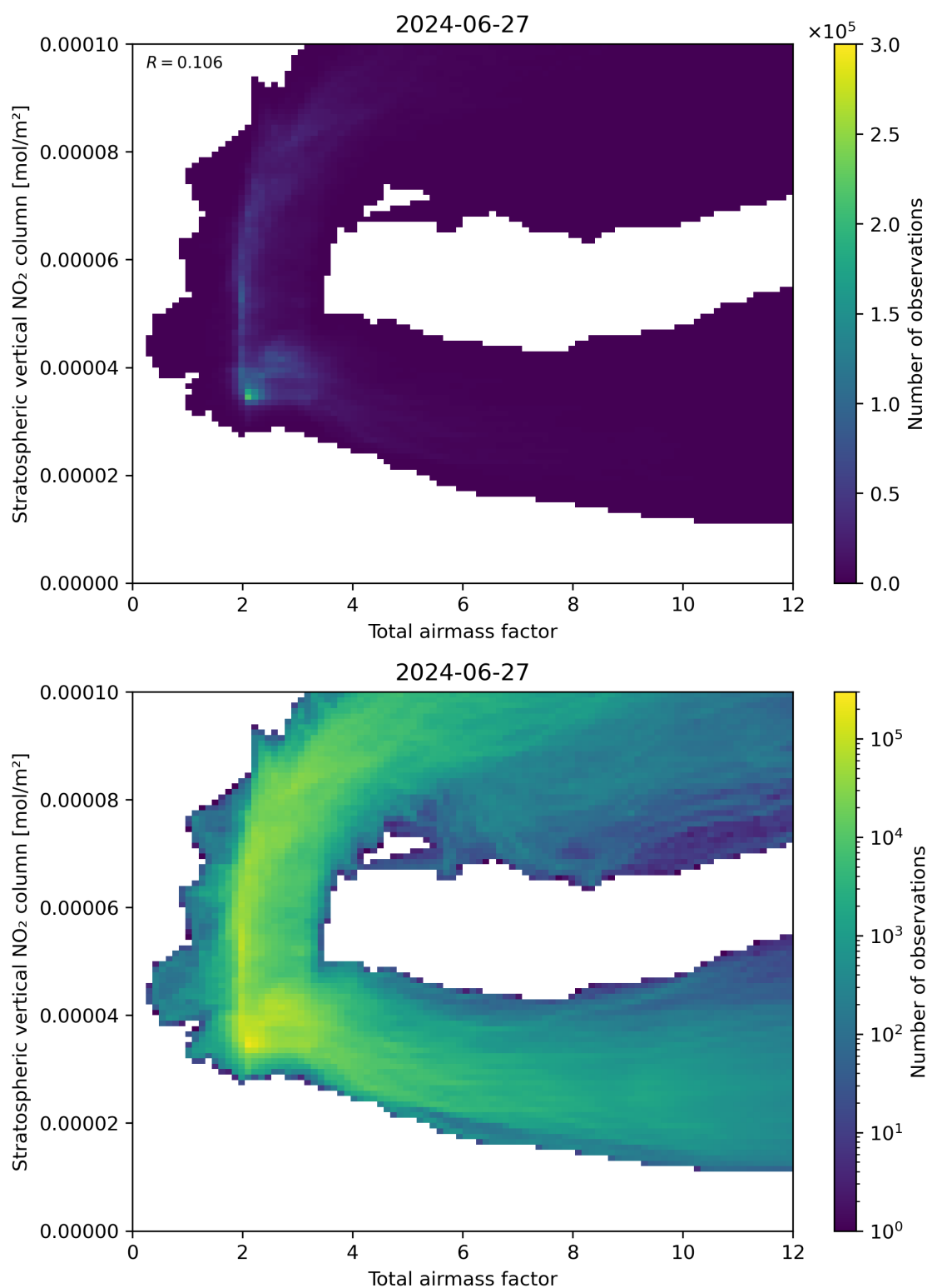
Figure 64: Scatter density plot of “Total airmass factor” against “Stratospheric vertical NO 2 column” for 2024-06-26 to 2024-06-28.
