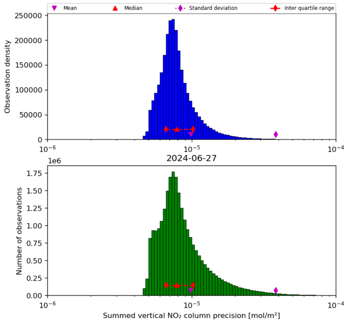
Figure 41: Histogram of "Summed vertical NO 2 column precision" for 2024-06-26 to 2024-06-28
