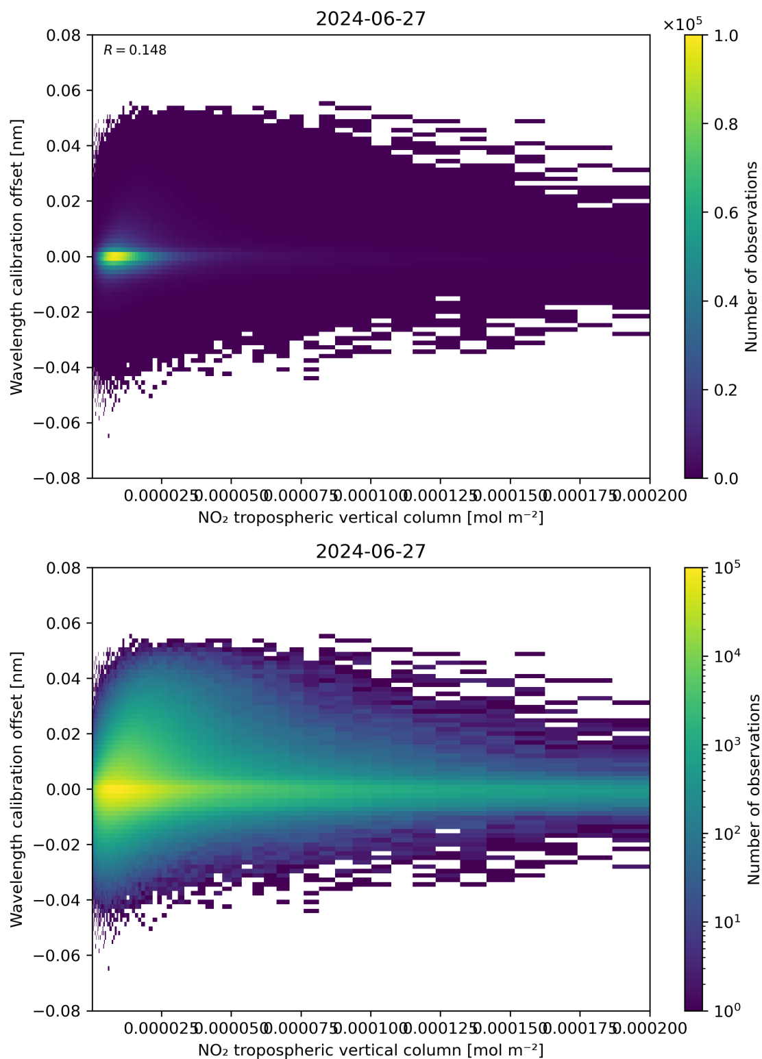
Figure 143: Scatter density plot of “NO 2 tropospheric vertical column” against “Wavelength calibration offset” for 2024-06-26 to 2024-06-28.
