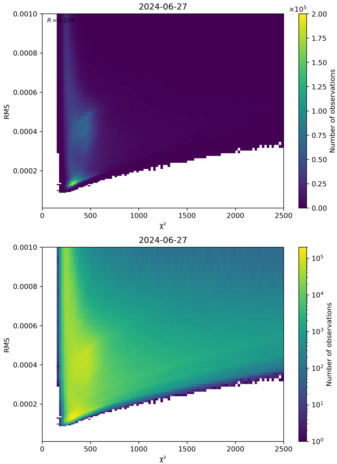
Figure 82: Scatter density plot of “ \chi^2 ” against “RMS” for 2024-06-26 to 2024-06-28.
