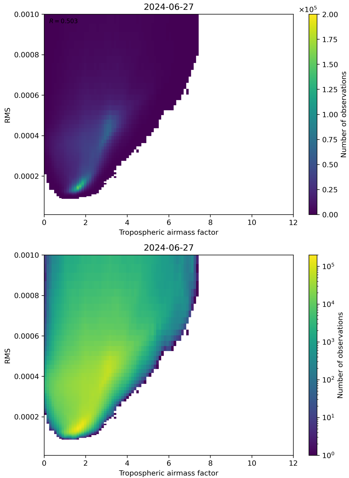
Figure 79: Scatter density plot of “Tropospheric airmass factor” against “RMS” for 2024-06-26 to 2024-06-28.
