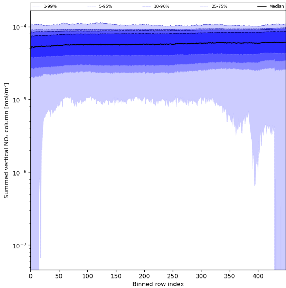
Figure 57: Along track statistics of “Summed vertical NO 2 column” for 2024-06-26 to 2024-06-28
