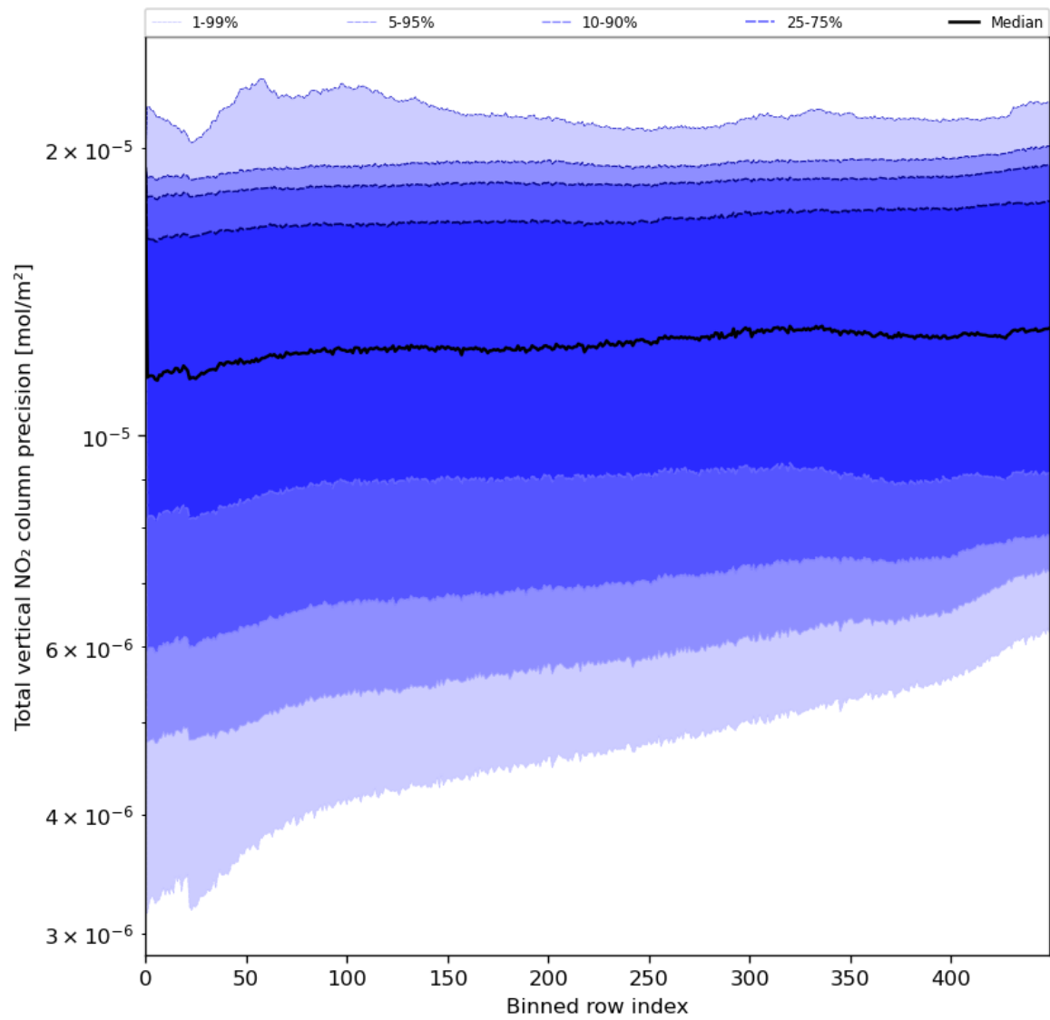
Figure 56: Along track statistics of “Total vertical NO 2 column precision” for 2024-06-26 to 2024-06-28
