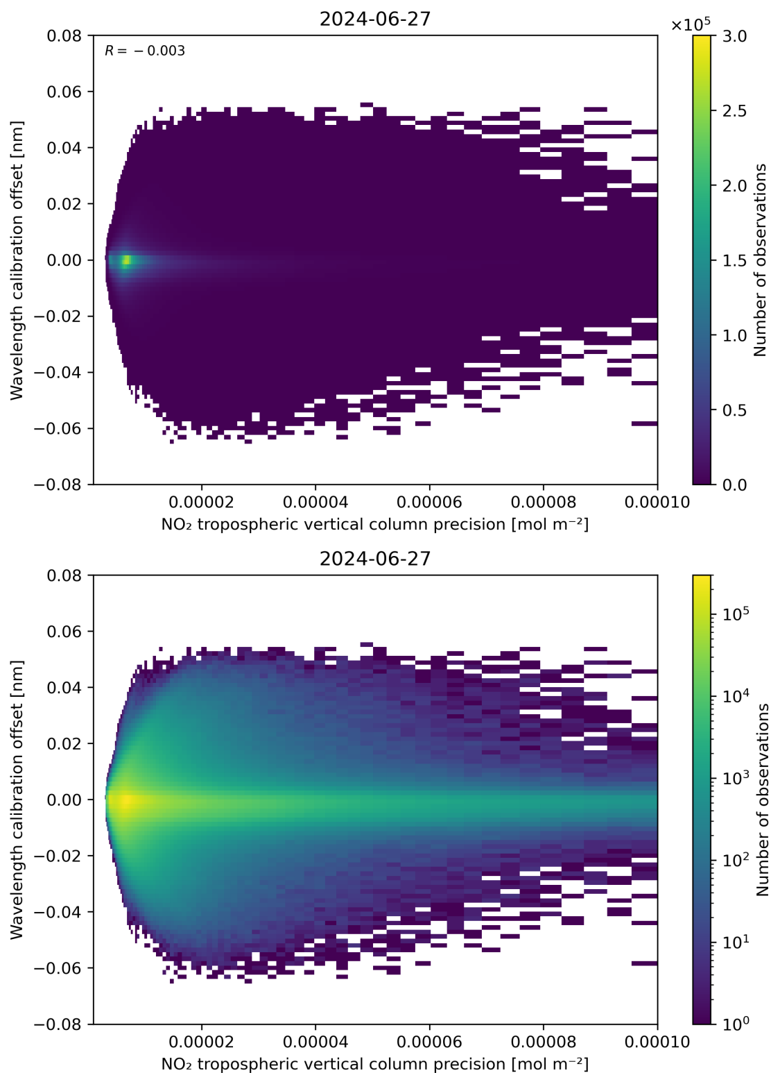
Figure 141: Scatter density plot of “NO 2 tropospheric vertical column precision” against “Wavelength calibration offset” for 2024-06-26 to 2024-06-28.
