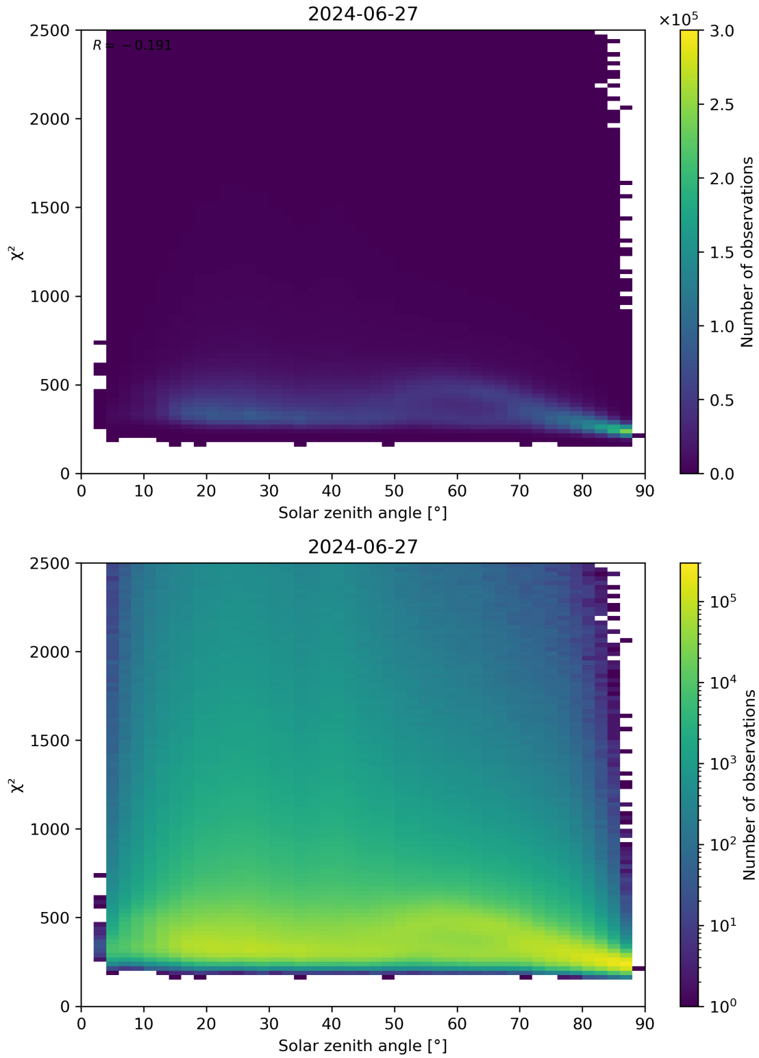
Figure 148: Scatter density plot of “Solar zenith angle” against “ \chi^2 ” for 2024-06-26 to 2024-06-28.
