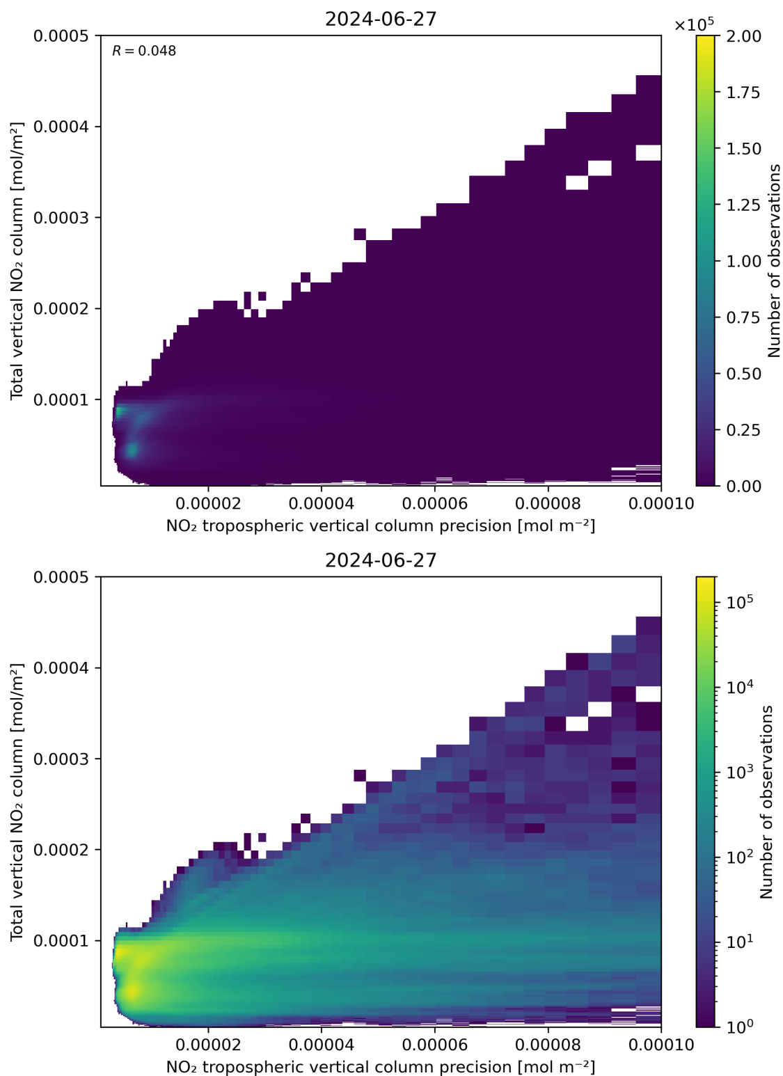
Figure 138: Scatter density plot of “NO 2 tropospheric vertical column precision” against “Total vertical NO 2 column” for 2024-06-26 to 2024-06-28.
