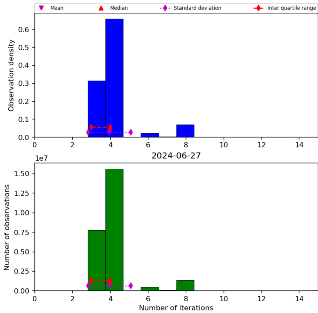
Figure 34: Histogram of “Number of iterations” for 2024-06-26 to 2024-06-28
