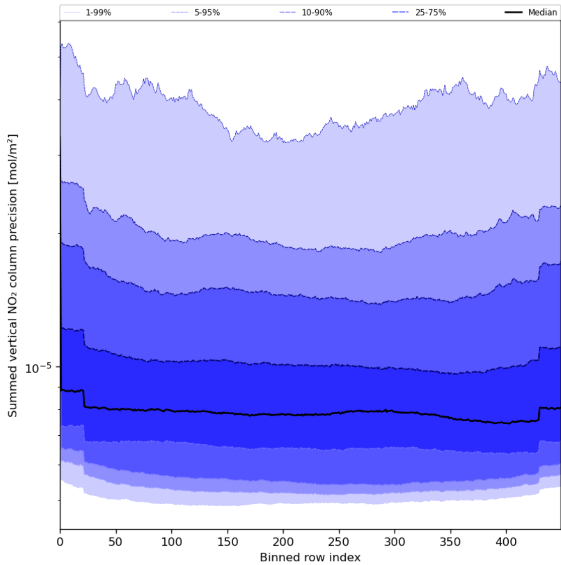
Figure 58: Along track statistics of “Summed vertical NO 2 column precision” for 2024-06-26 to 2024-06-28
