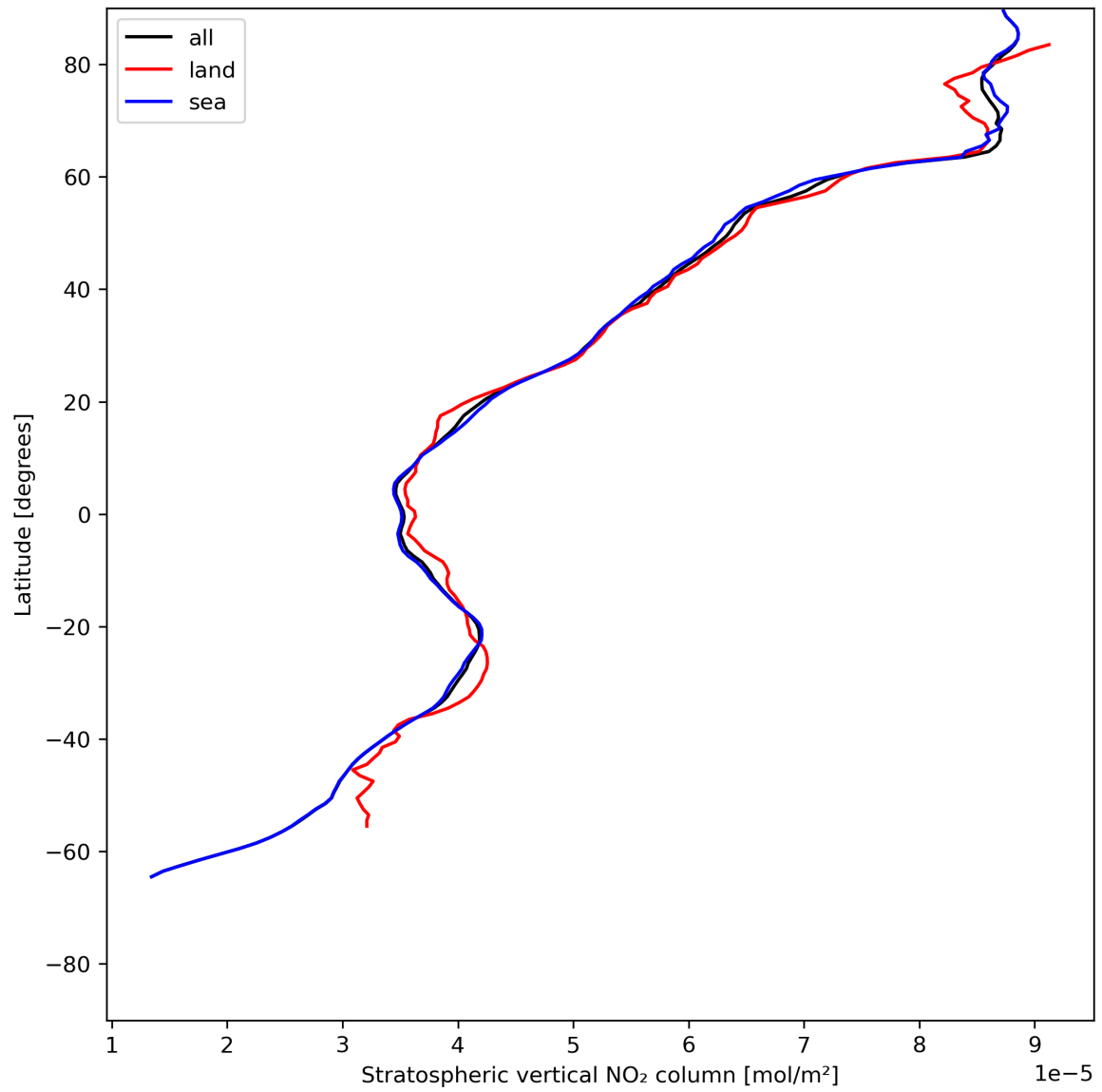
Figure 19: Zonal average of “Stratospheric vertical NO 2 column” for 2024-06-26 to 2024-06-28.
