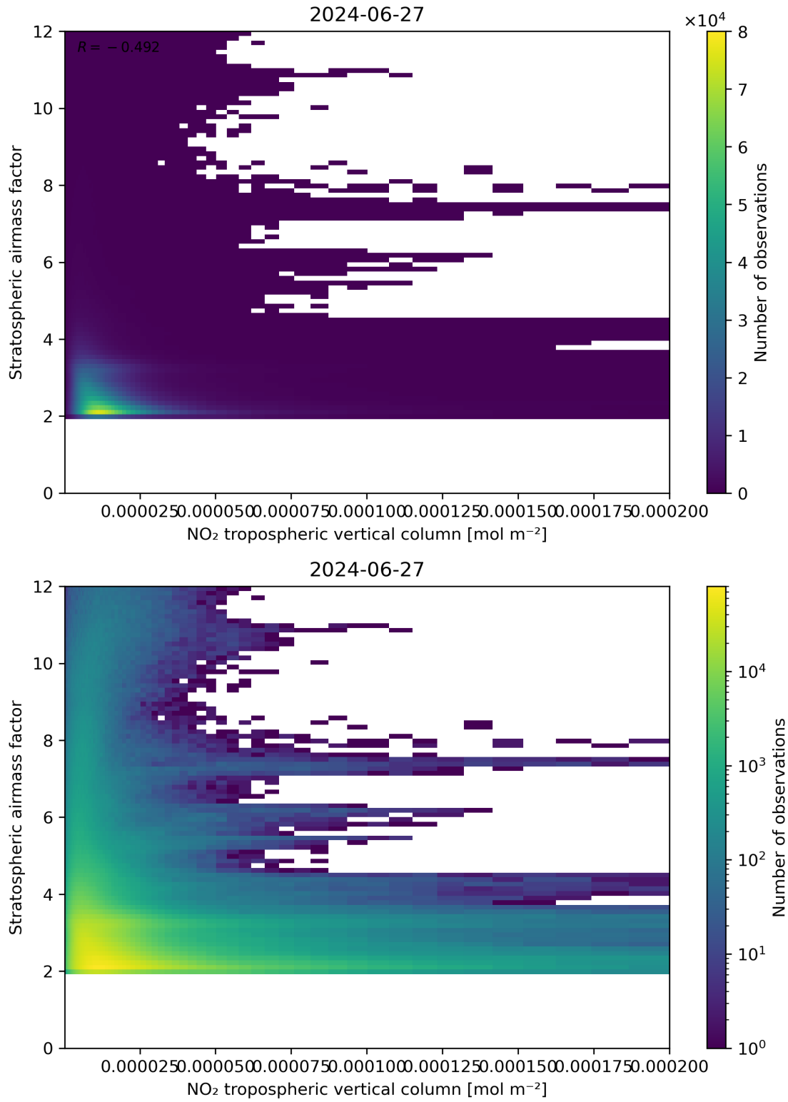
Figure 121: Scatter density plot of “NO 2 tropospheric vertical column” against “Stratospheric air mass factor” for 2024-06-26 to 2024-06-28.
