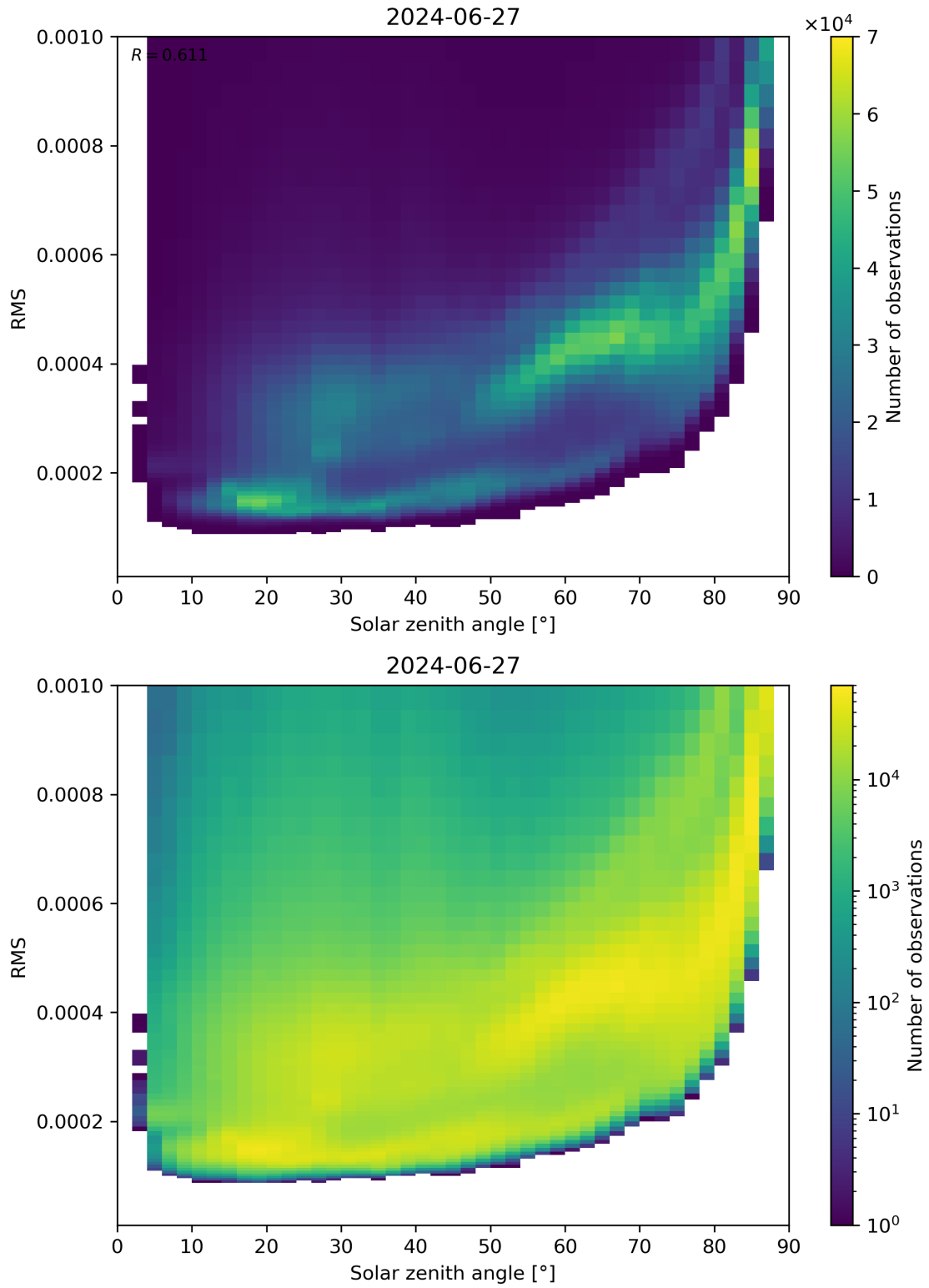
Figure 157: Scatter density plot of “Solar zenith angle” against “RMS” for 2024-06-26 to 2024-06-28.
