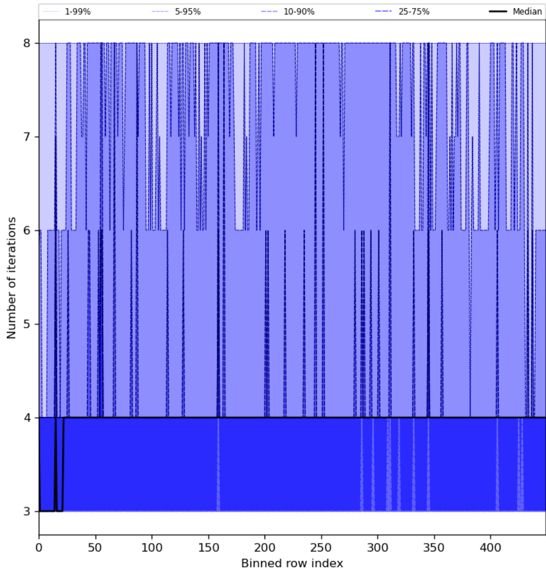
Figure 51: Along track statistics of “Number of iterations” for 2024-06-26 to 2024-06-28
