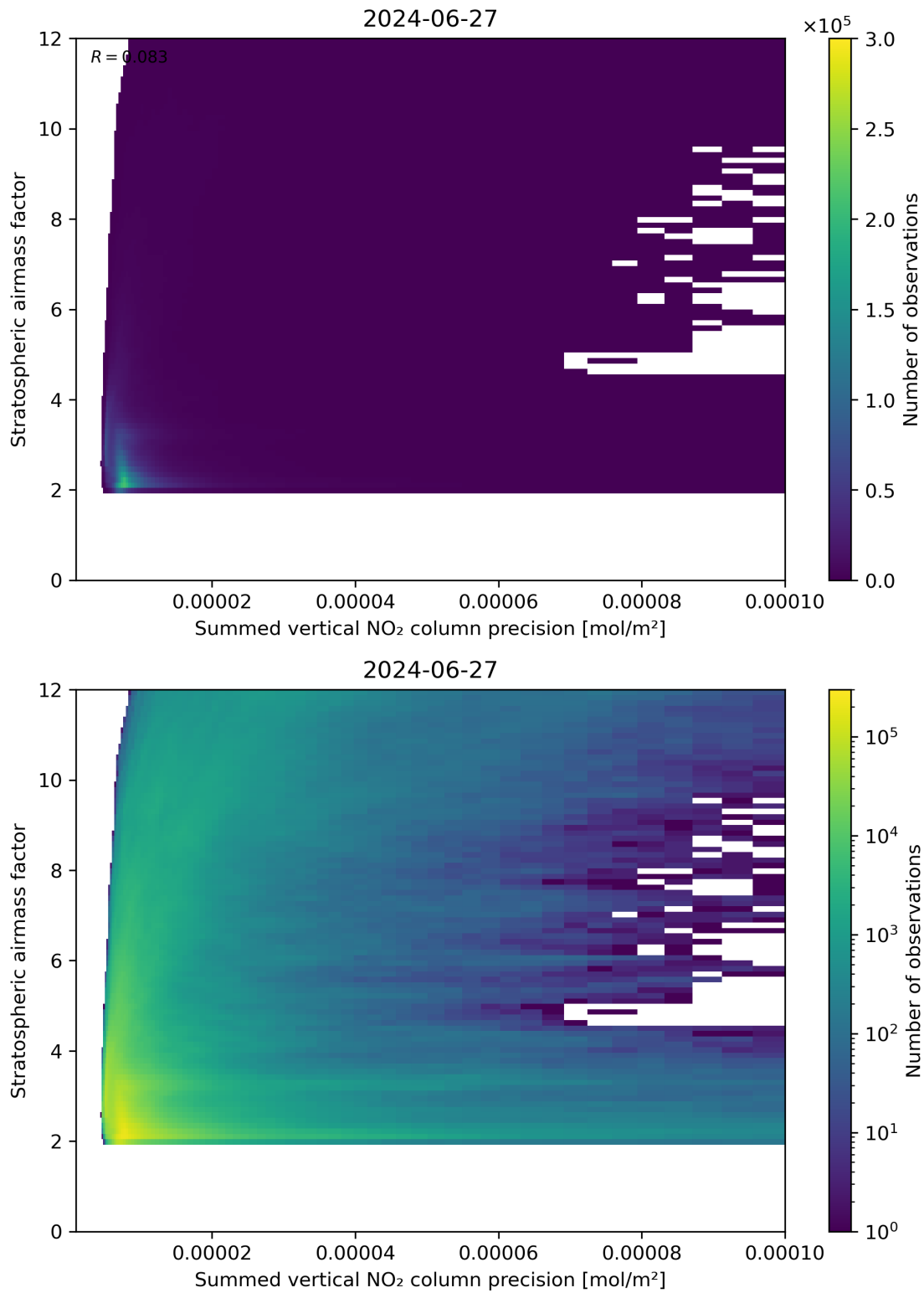
Figure 106: Scatter density plot of “Summed vertical NO 2 column precision” against “Stratospheric airmass factor” for 2024-06-26 to 2024-06-28.
