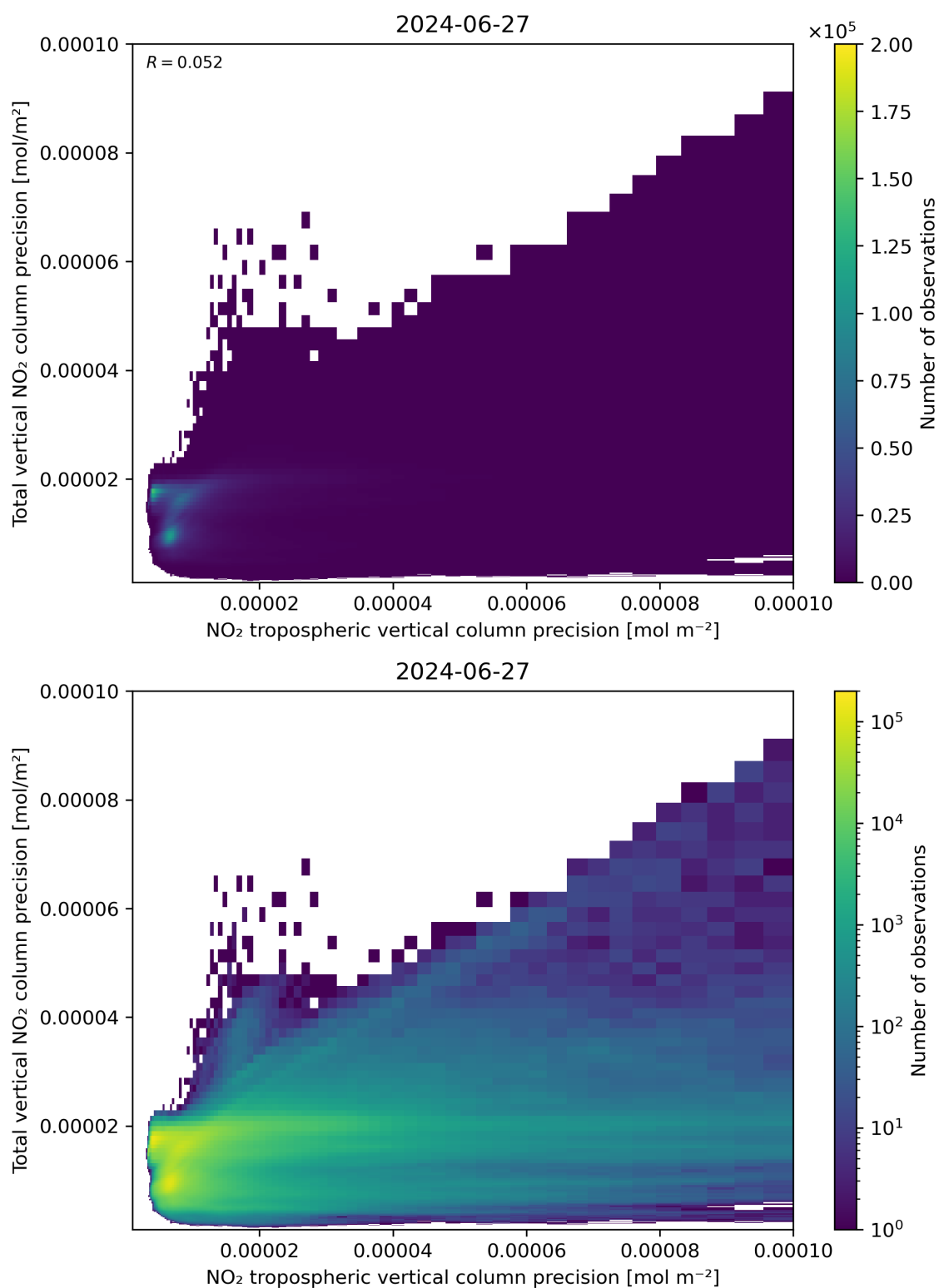
Figure 139: Scatter density plot of “NO 2 tropospheric vertical column precision” against “Total vertical NO 2 column precision” for 2024-06-26 to 2024-06-28.
