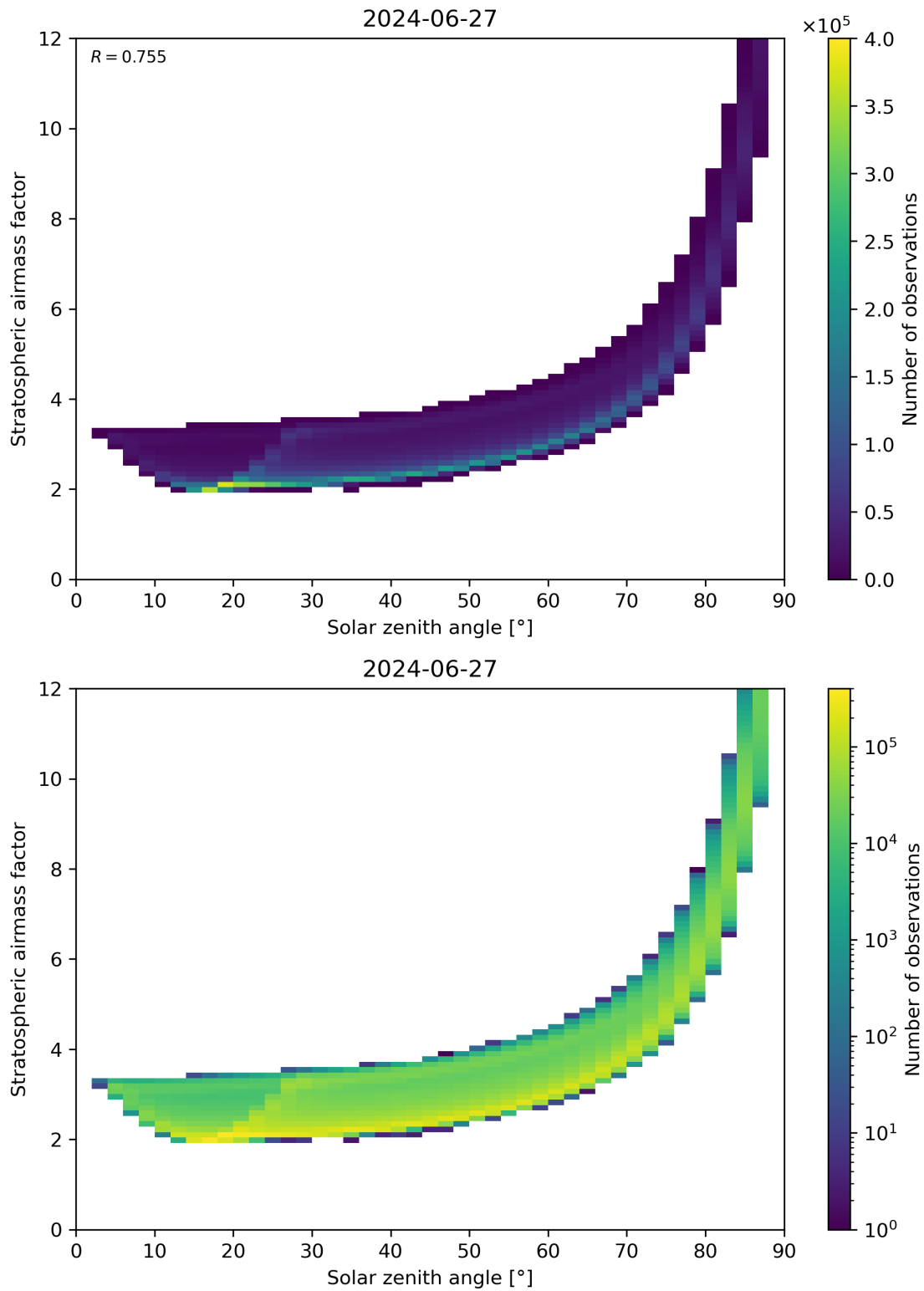
Figure 145: Scatter density plot of “Solar zenith angle” against “Stratospheric airmass factor” for 2024-06-26 to 2024-06-28.
