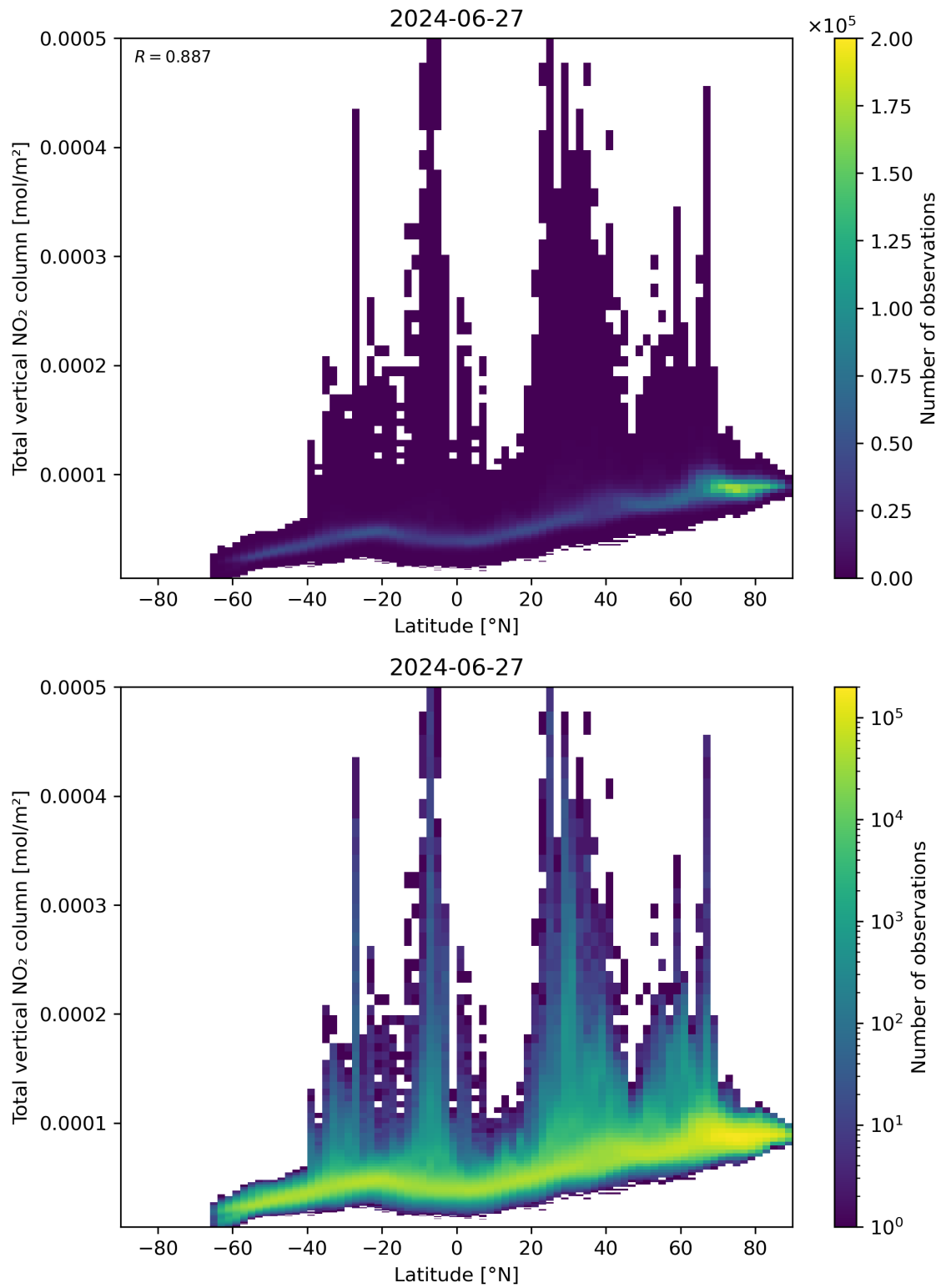
Figure 90: Scatter density plot of “Latitude” against “Total vertical NO 2 column” for 2024-06-26 to 2024-06-28.
