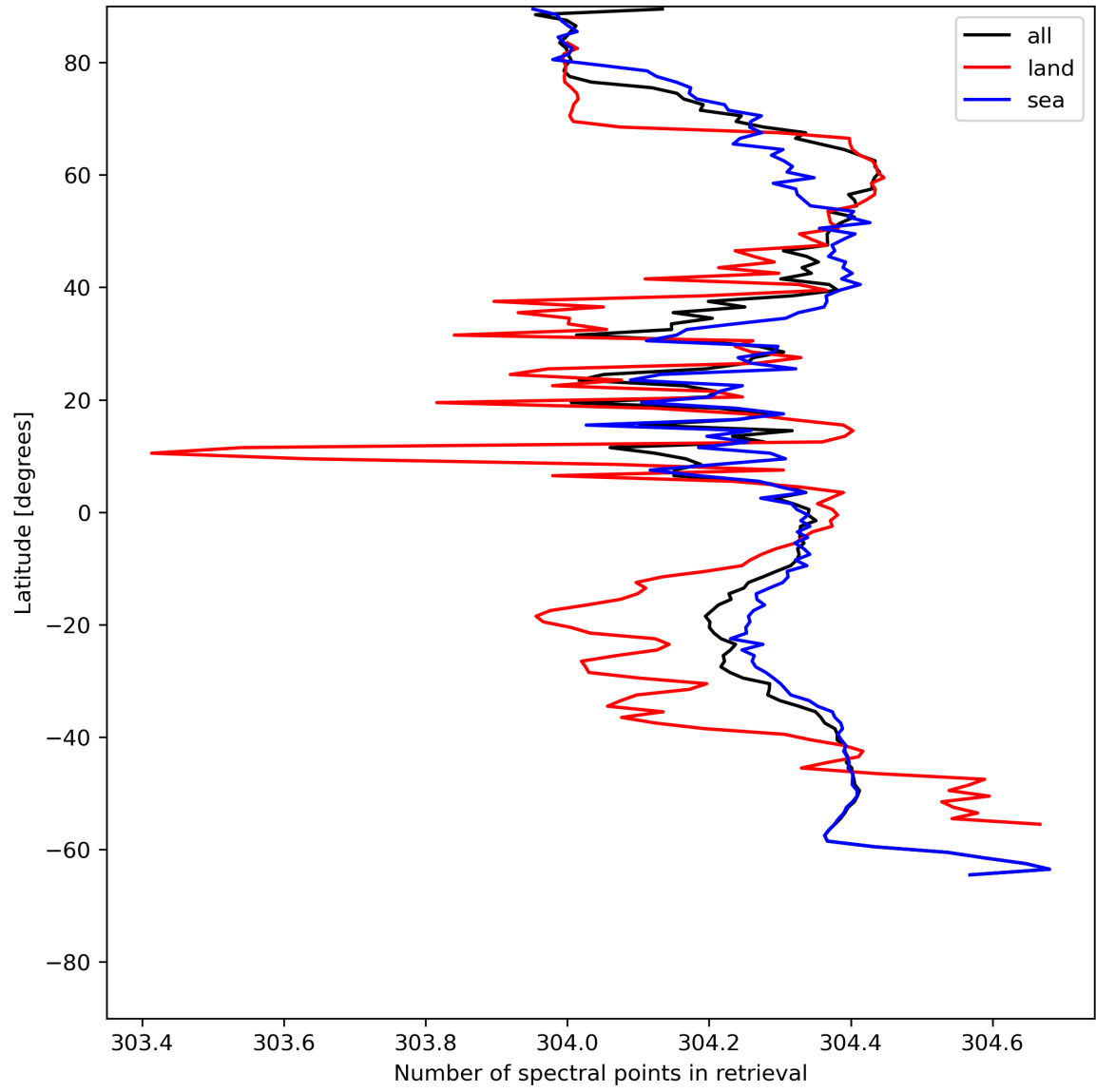
Figure 16: Zonal average of “Number of spectral points in retrieval” for 2024-06-26 to 2024-06-28.
