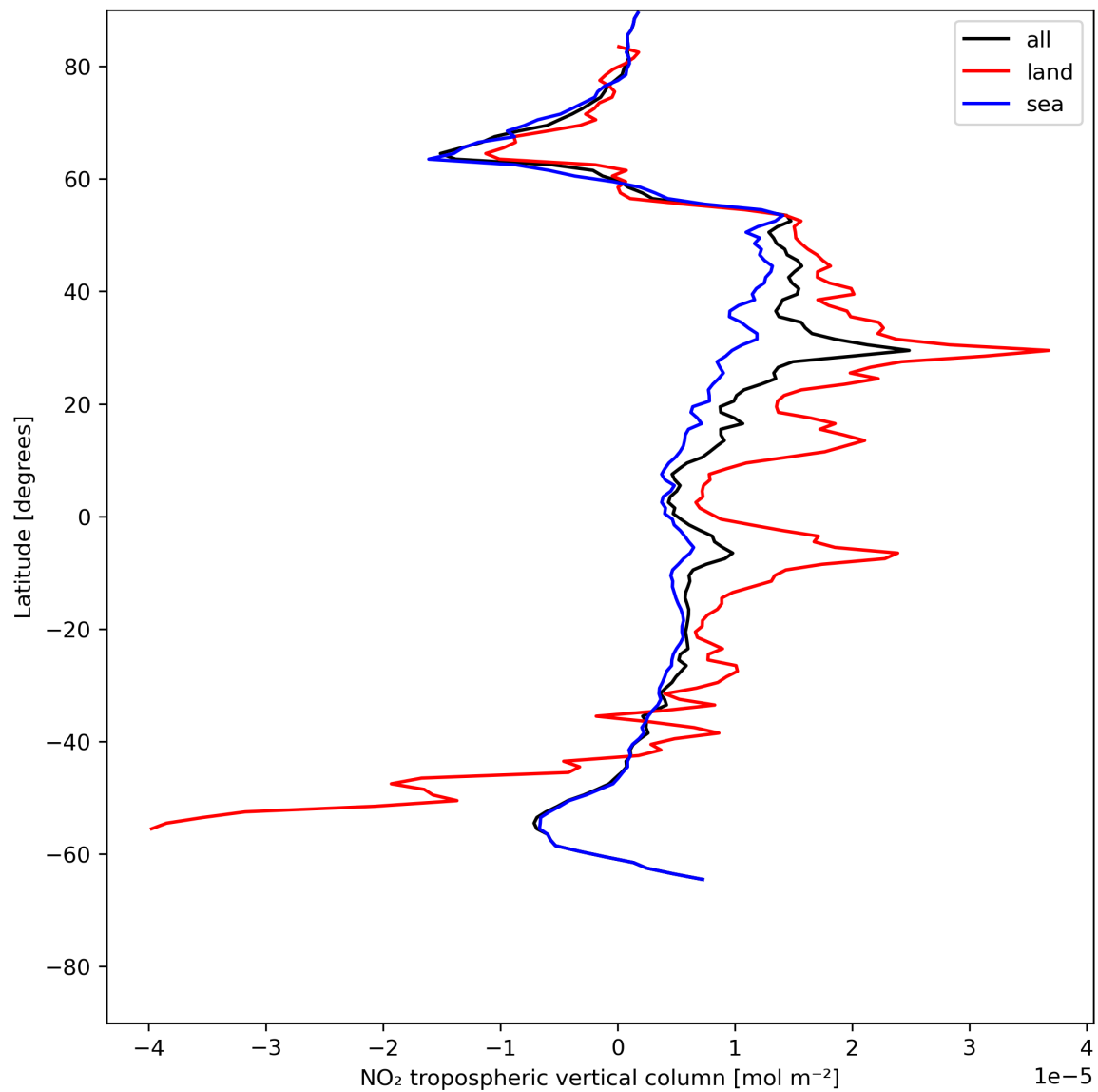
Figure 12: Zonal average of “NO 2 tropospheric vertical column” for 2024-06-26 to 2024-06-28.
