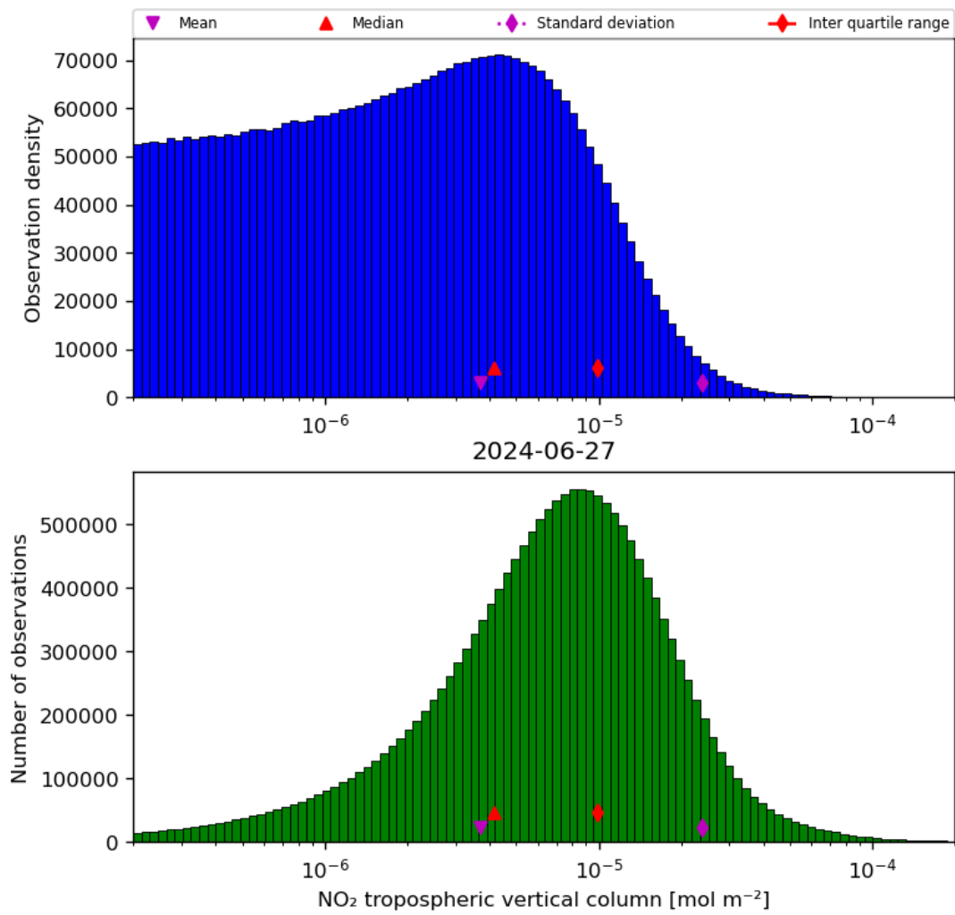
Figure 29: Histogram of “NO 2 tropospheric vertical column” for 2024-06-26 to 2024-06-28
