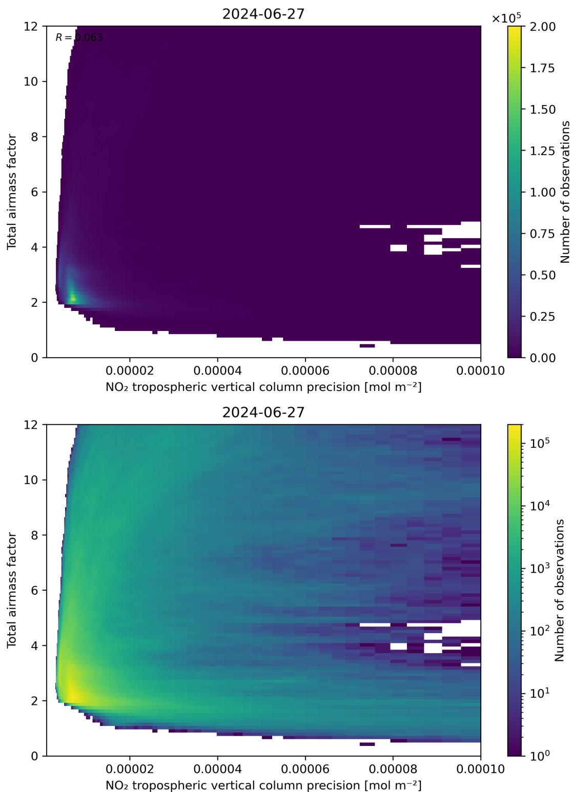
Figure 132: Scatter density plot of “NO 2 tropospheric vertical column precision” against “Total air mass factor” for 2024-06-26 to 2024-06-28.
