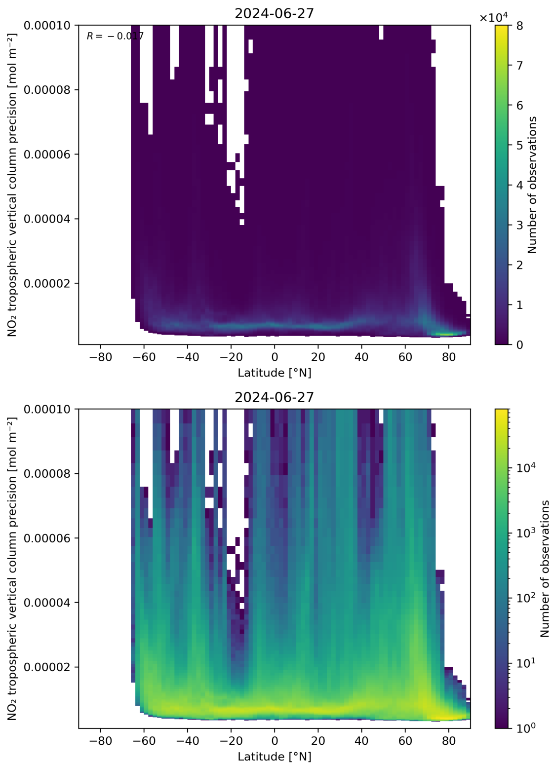
Figure 93: Scatter density plot of “Latitude” against “NO 2 tropospheric vertical column precision” for 2024-06-26 to 2024-06-28.
