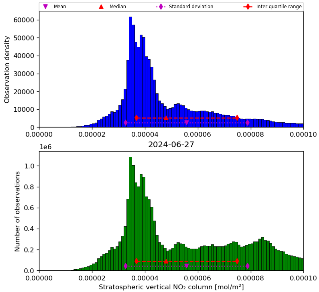
Figure 36: Histogram of “Stratospheric vertical NO 2 column” for 2024-06-26 to 2024-06-28
