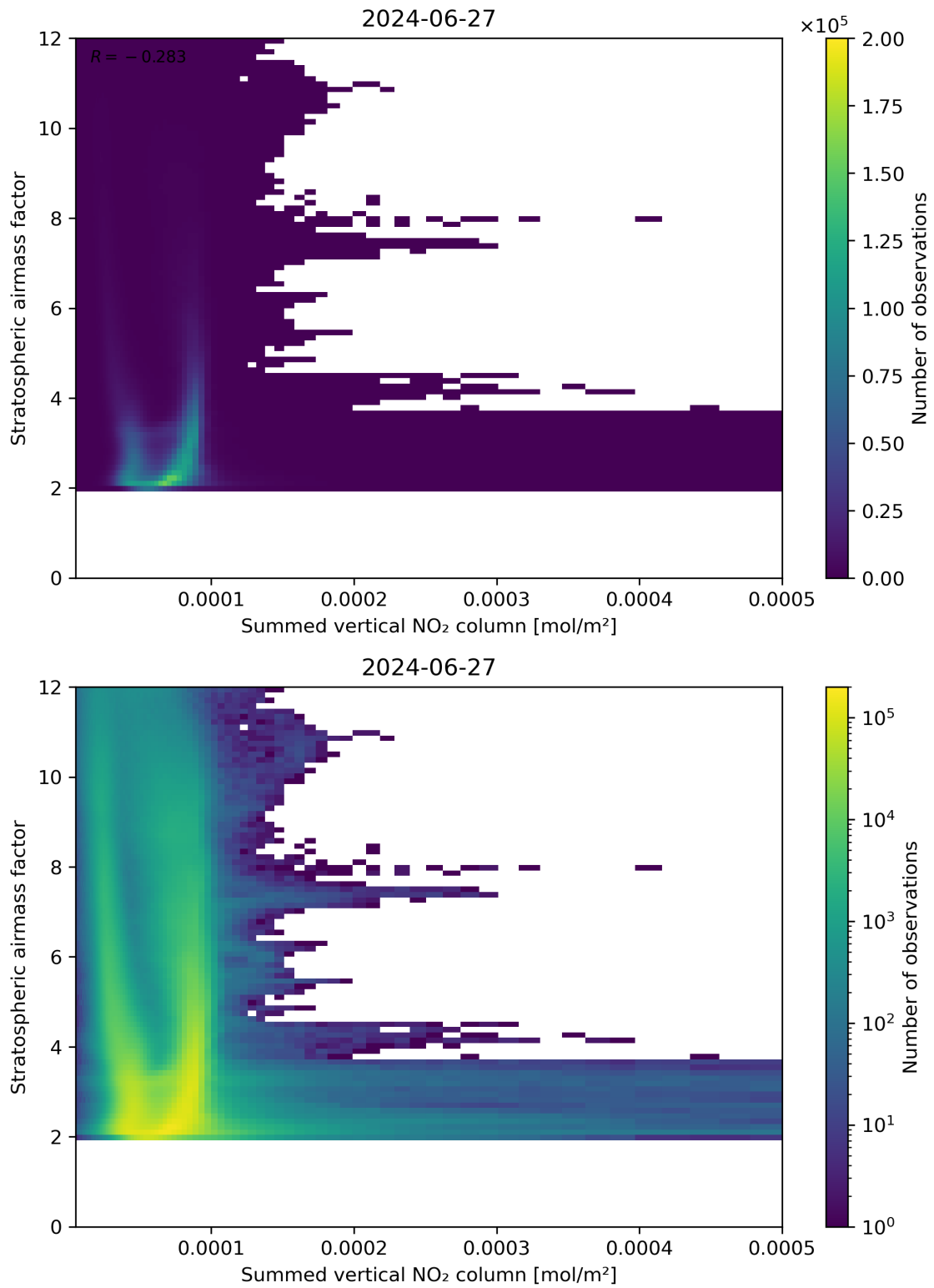
Figure 103: Scatter density plot of “Summed vertical NO 2 column” against “Stratospheric air mass factor” for 2024-06-26 to 2024-06-28.
