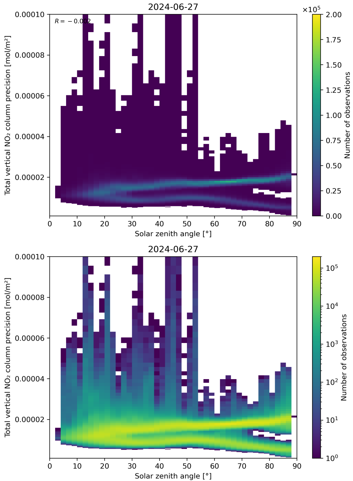
Figure 154: Scatter density plot of “Solar zenith angle” against “Total vertical NO 2 column precision” for 2024-06-26 to 2024-06-28.
