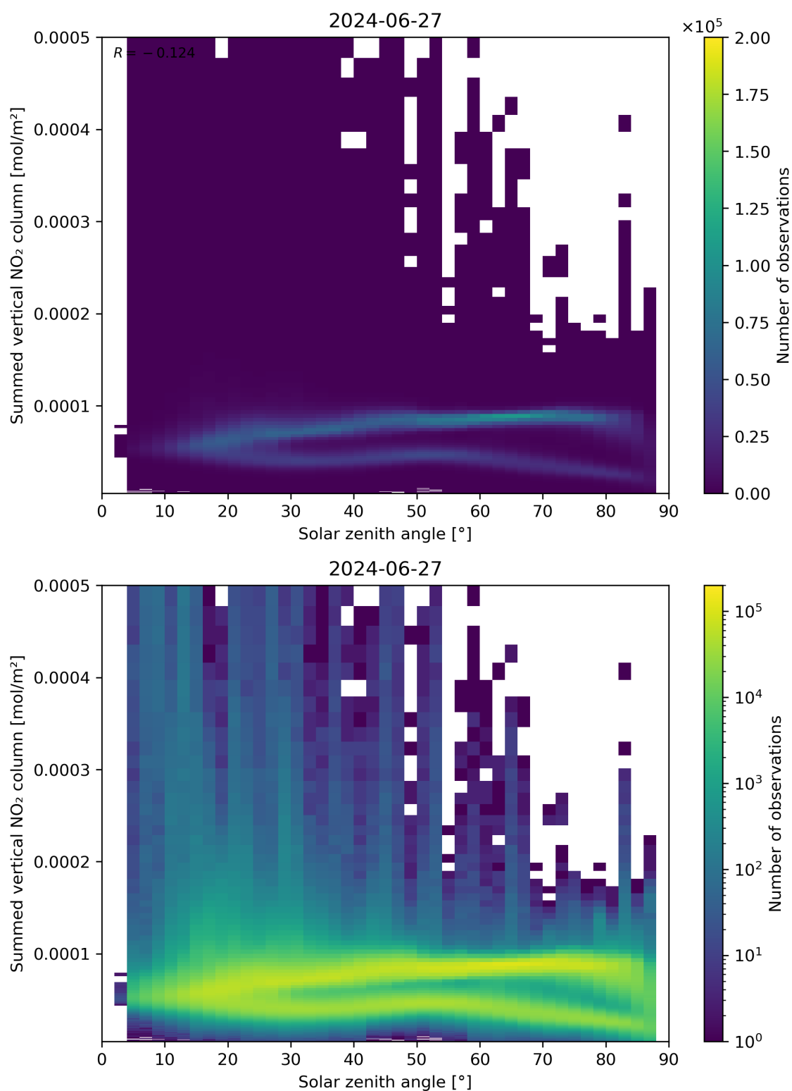
Figure 151: Scatter density plot of “Solar zenith angle” against “Summed vertical NO 2 column” for 2024-06-26 to 2024-06-28.
