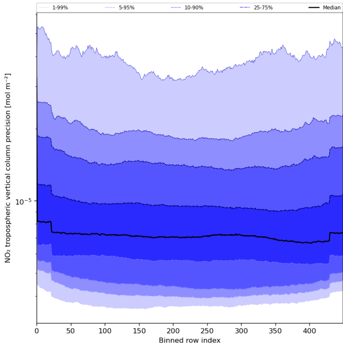
Figure 47: Along track statistics of “NO 2 tropospheric vertical column precision” for 2024-06-26 to 2024-06-28
