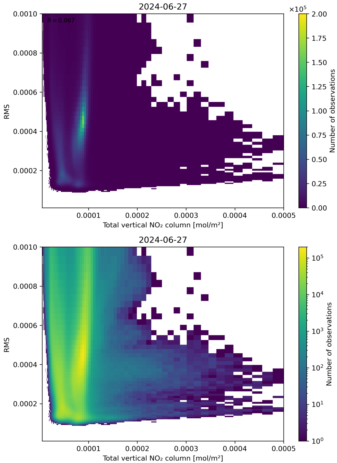
Figure 120: Scatter density plot of “Total vertical NO 2 column” against “RMS” for 2024-06-26 to 2024-06-28.
