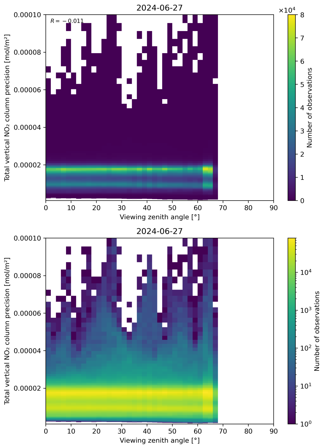
Figure 168: Scatter density plot of “Viewing zenith angle” against “Total vertical NO 2 column precision” for 2024-06-26 to 2024-06-28.
