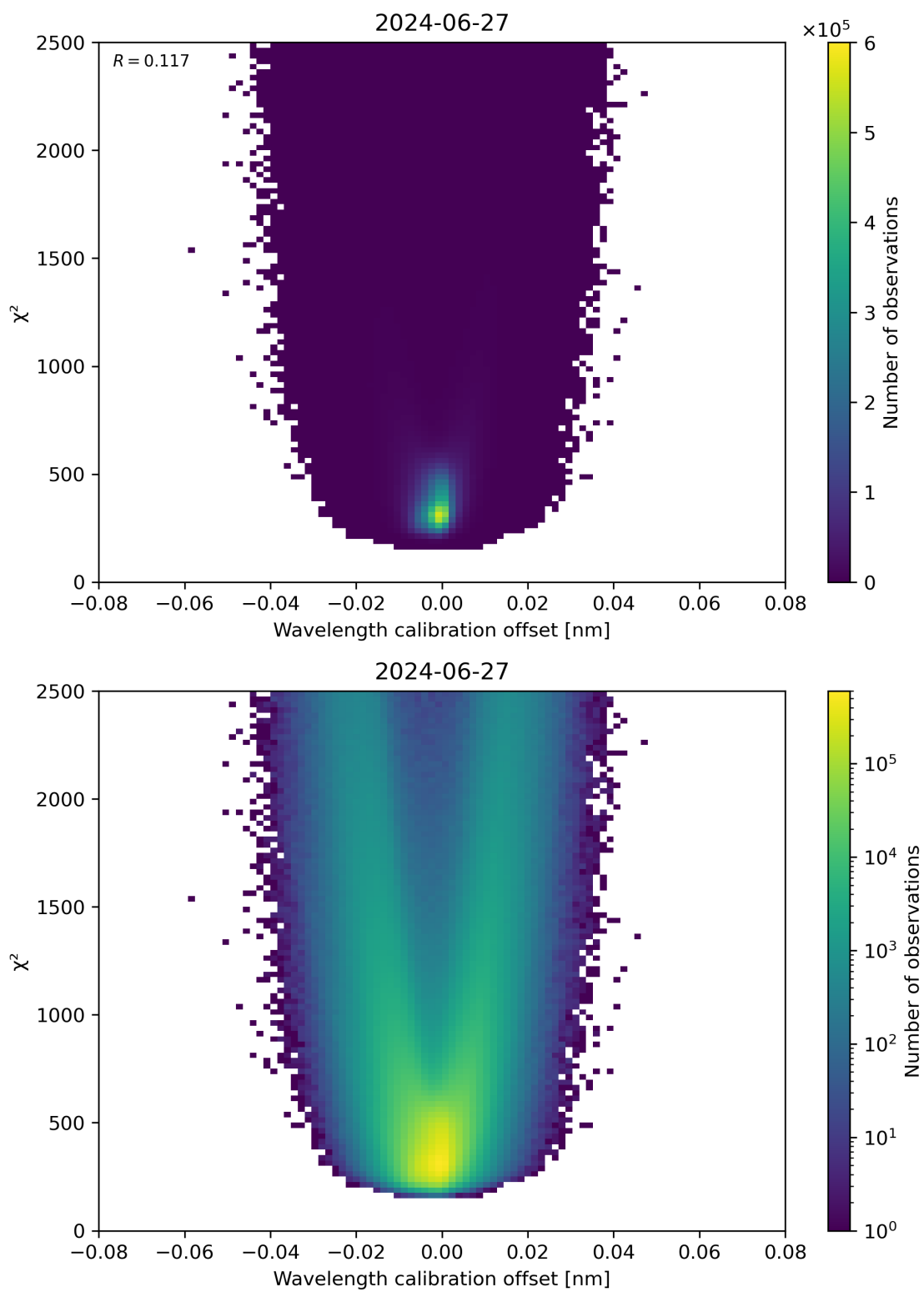
Figure 175: Scatter density plot of “Wavelength calibration offset” against “ \chi^2 ” for 2024-06-26 to 2024-06-28.
