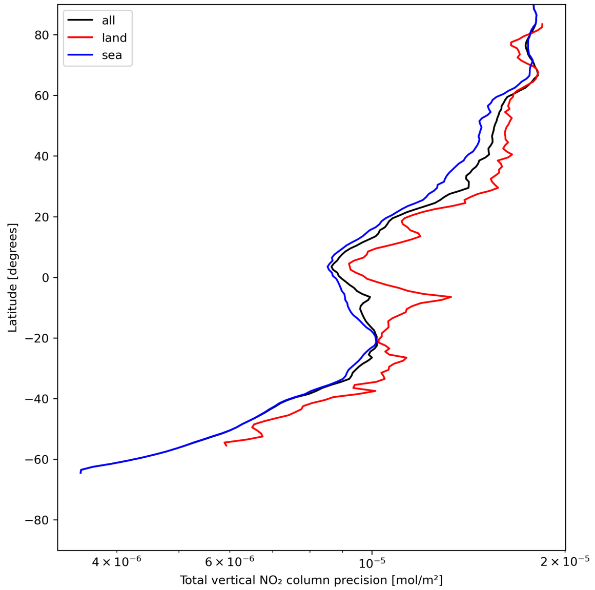
Figure 22: Zonal average of “Total vertical NO 2 column precision” for 2024-06-26 to 2024-06-28.
