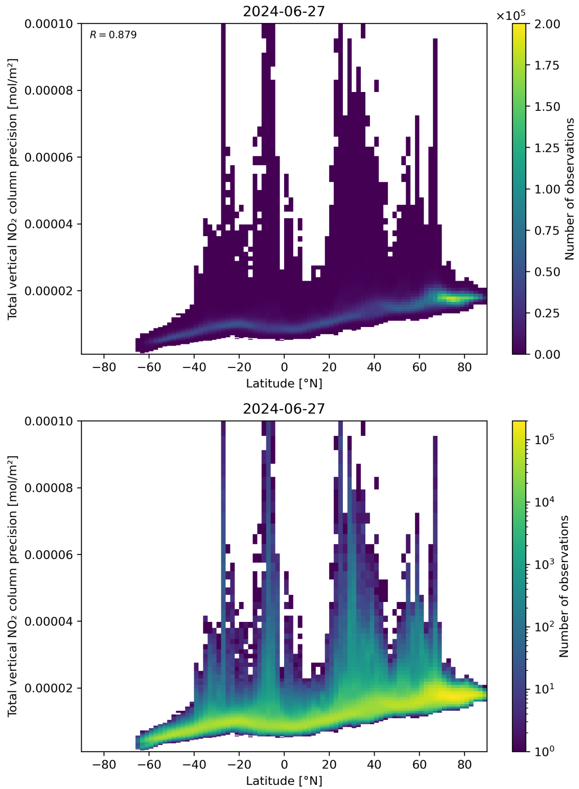
Figure 91: Scatter density plot of “Latitude” against “Total vertical NO 2 column precision” for 2024-06-26 to 2024-06-28.
