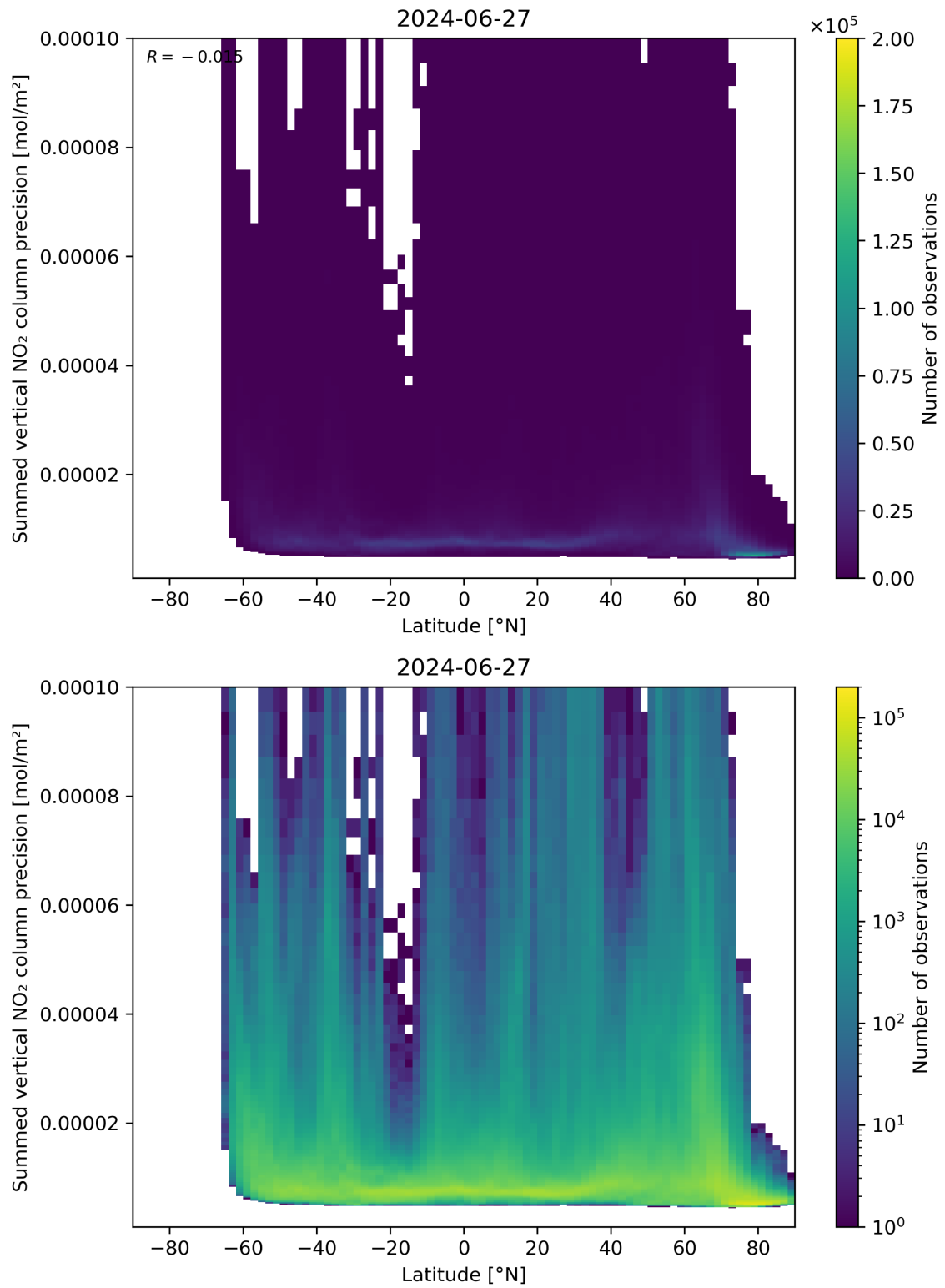
Figure 89: Scatter density plot of “Latitude” against “Summed vertical NO 2 column precision” for 2024-06-26 to 2024-06-28.
