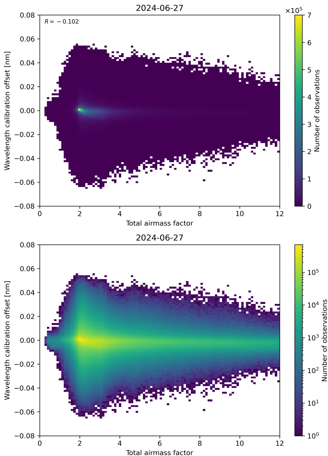
Figure 70: Scatter density plot of “Total airmass factor” against “Wavelength calibration offset” for 2024-06-26 to 2024-06-28.
