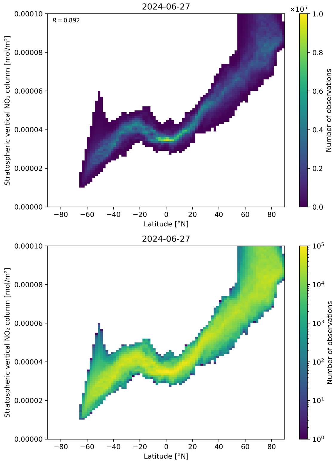
Figure 87: Scatter density plot of “Latitude” against “Stratospheric vertical NO 2 column” for 2024-06-26 to 2024-06-28.
