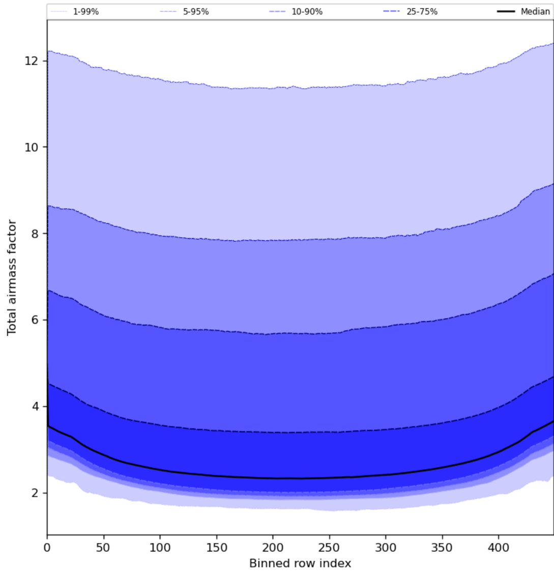
Figure 49: Along track statistics of “Total airmass factor” for 2024-06-26 to 2024-06-28
