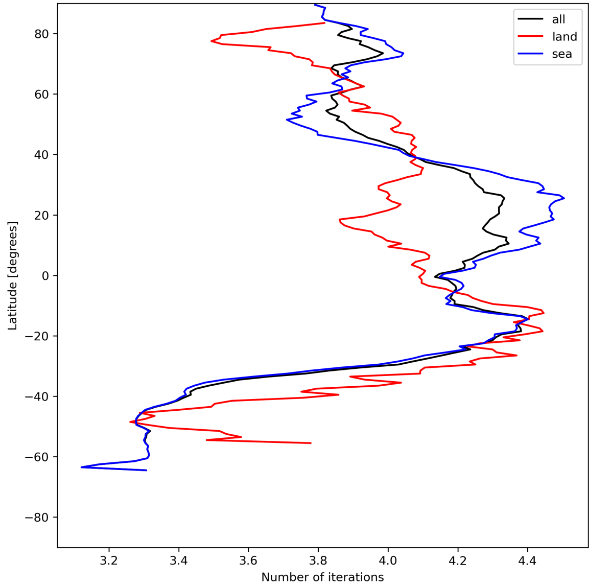
Figure 17: Zonal average of “Number of iterations” for 2024-06-26 to 2024-06-28.
