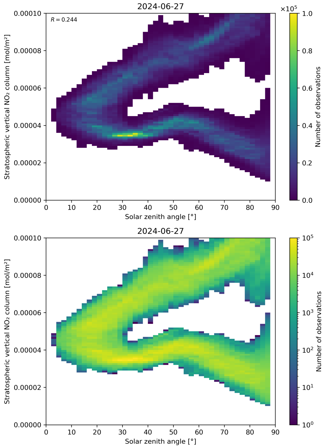
Figure 150: Scatter density plot of “Solar zenith angle” against “Stratospheric vertical NO 2 column” for 2024-06-26 to 2024-06-28.
