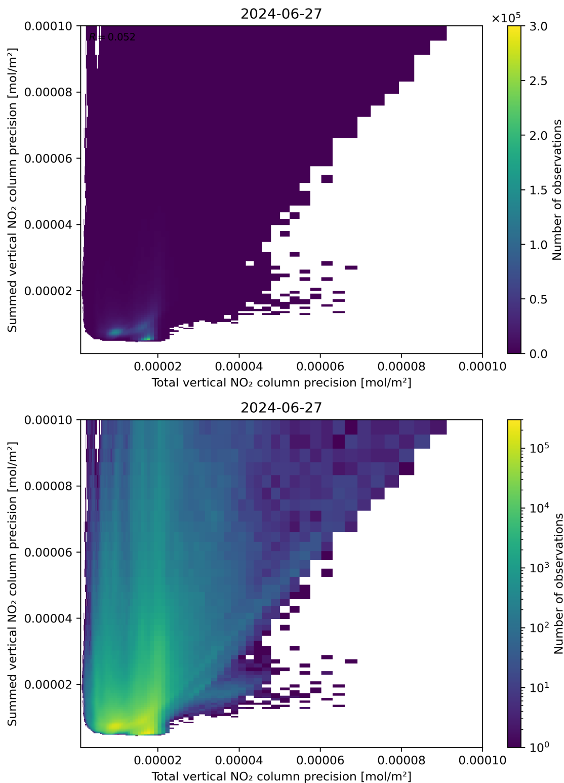
Figure 118: Scatter density plot of “Total vertical NO 2 column precision” against “Summed vertical NO 2 column precision” for 2024-06-26 to 2024-06-28.
