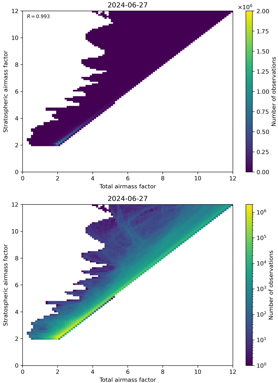
Figure 62: Scatter density plot of “Total airmass factor” against “Stratospheric airmass factor” for 2024-06-26 to 2024-06-28.
