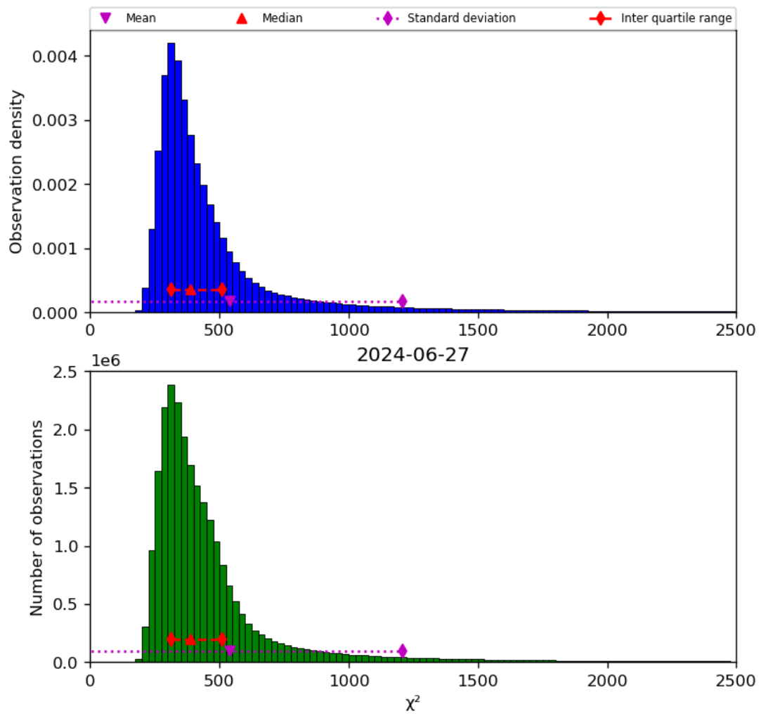
Figure 42: Histogram of “ \chi^2 ” for 2024-06-26 to 2024-06-28
