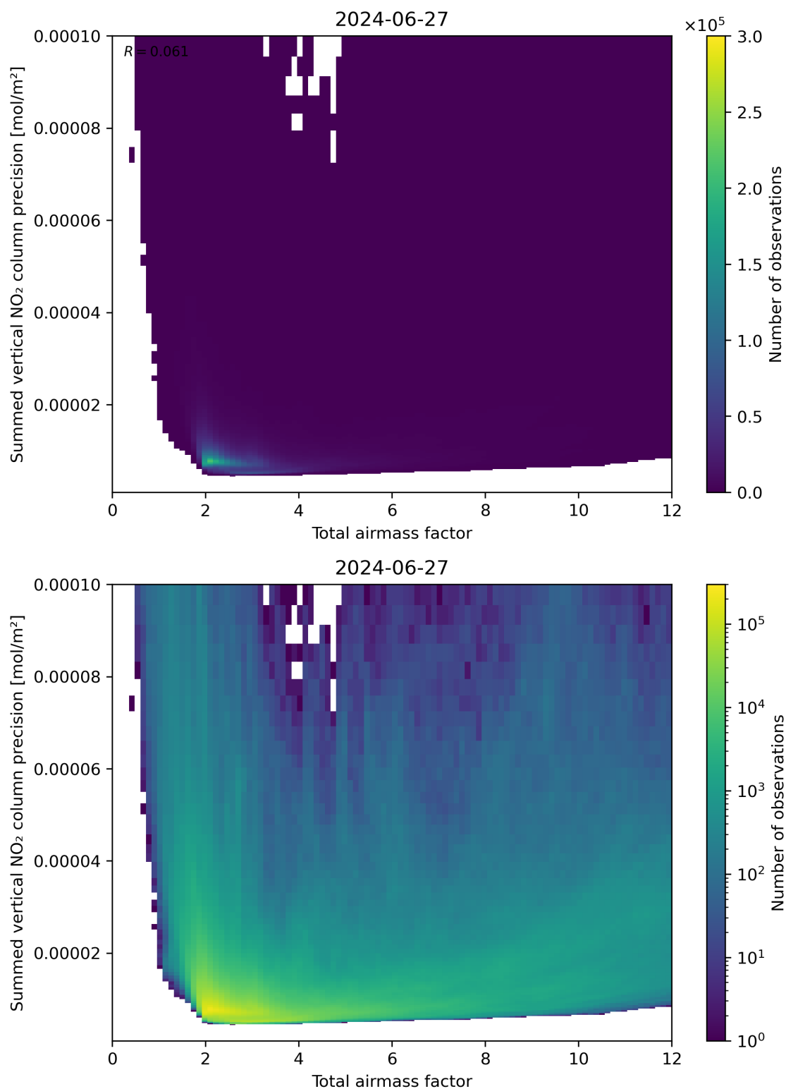
Figure 66: Scatter density plot of “Total airmass factor” against “Summed vertical NO 2 column precision” for 2024-06-26 to 2024-06-28.
