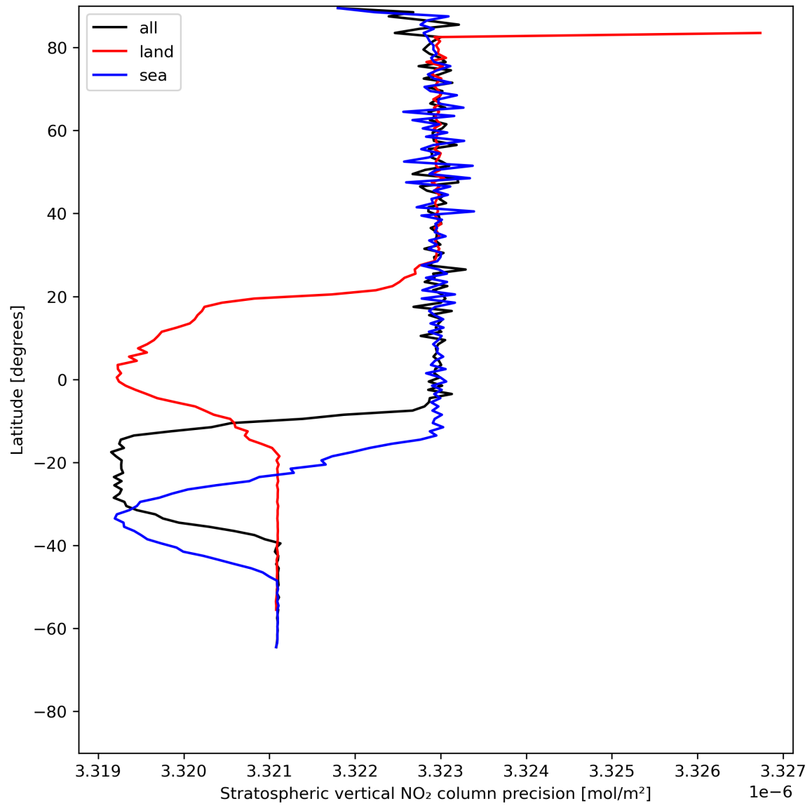
Figure 20: Zonal average of “Stratospheric vertical NO 2 column precision” for 2024-06-26 to 2024-06-28.
