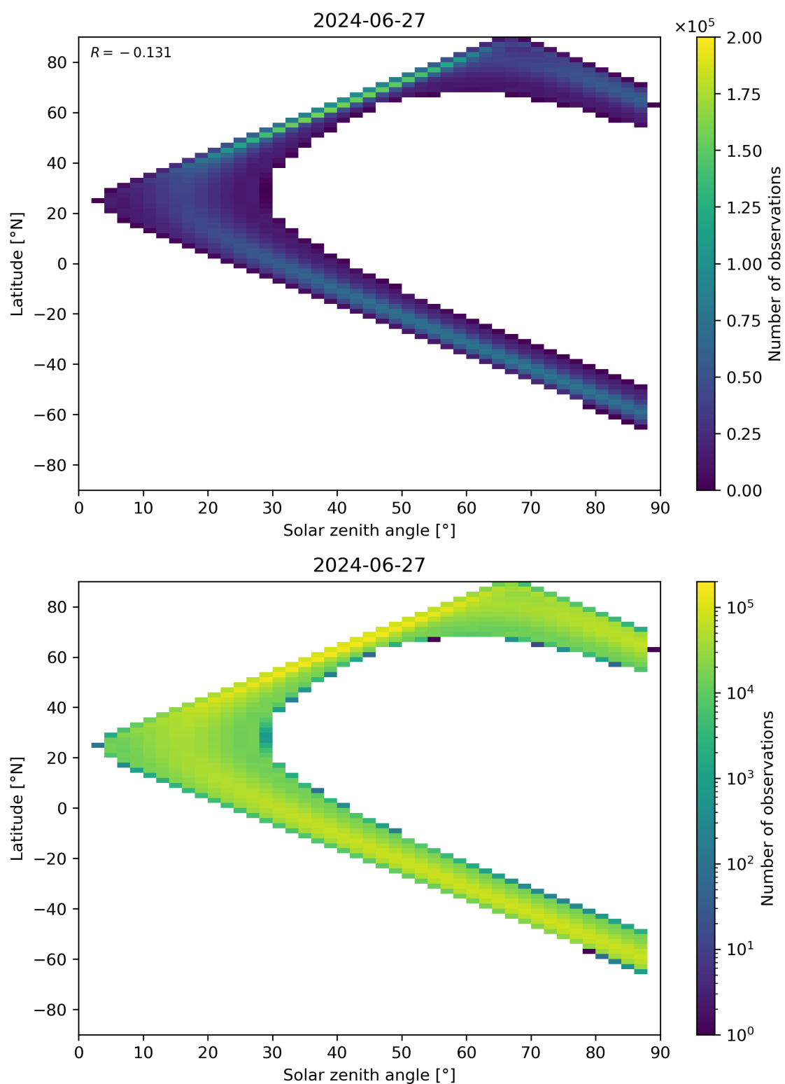
Figure 149: Scatter density plot of “Solar zenith angle” against “Latitude” for 2024-06-26 to 2024-06-28.
