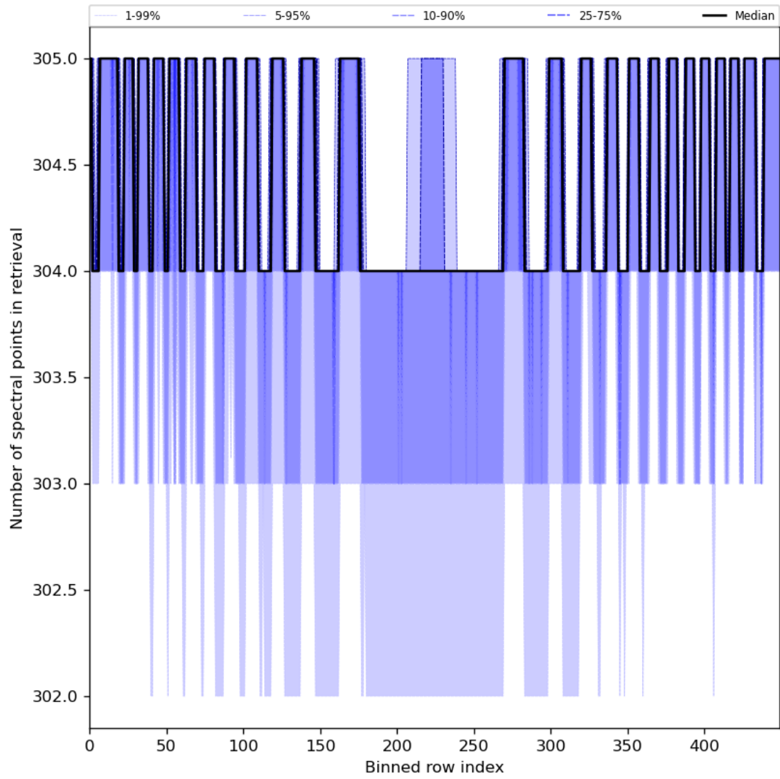
Figure 50: Along track statistics of “Number of spectral points in retrieval” for 2024-06-26 to 2024-06-28
