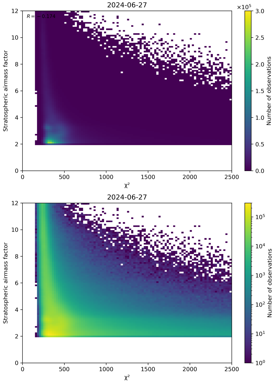
Figure 81: Scatter density plot of “ \chi^2 ” against “Stratospheric airmass factor” for 2024-06-26 to 2024-06-28.
