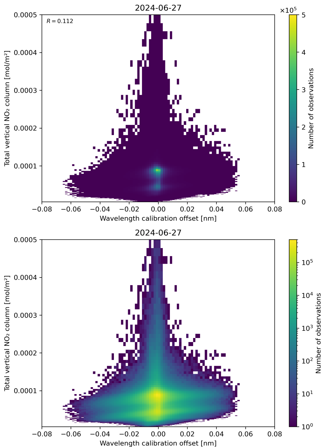
Figure 179: Scatter density plot of “Wavelength calibration offset” against “Total vertical NO 2 column” for 2024-06-26 to 2024-06-28.
