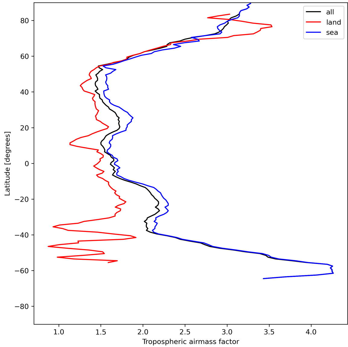
Figure 14: Zonal average of “Tropospheric airmass factor” for 2024-06-26 to 2024-06-28.
