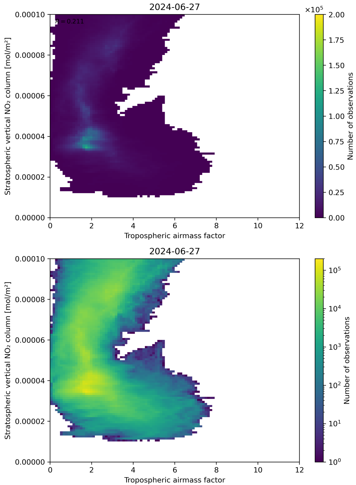
Figure 74: Scatter density plot of “Tropospheric air mass factor” against “Stratospheric vertical NO 2 column” for 2024-06-26 to 2024-06-28.
