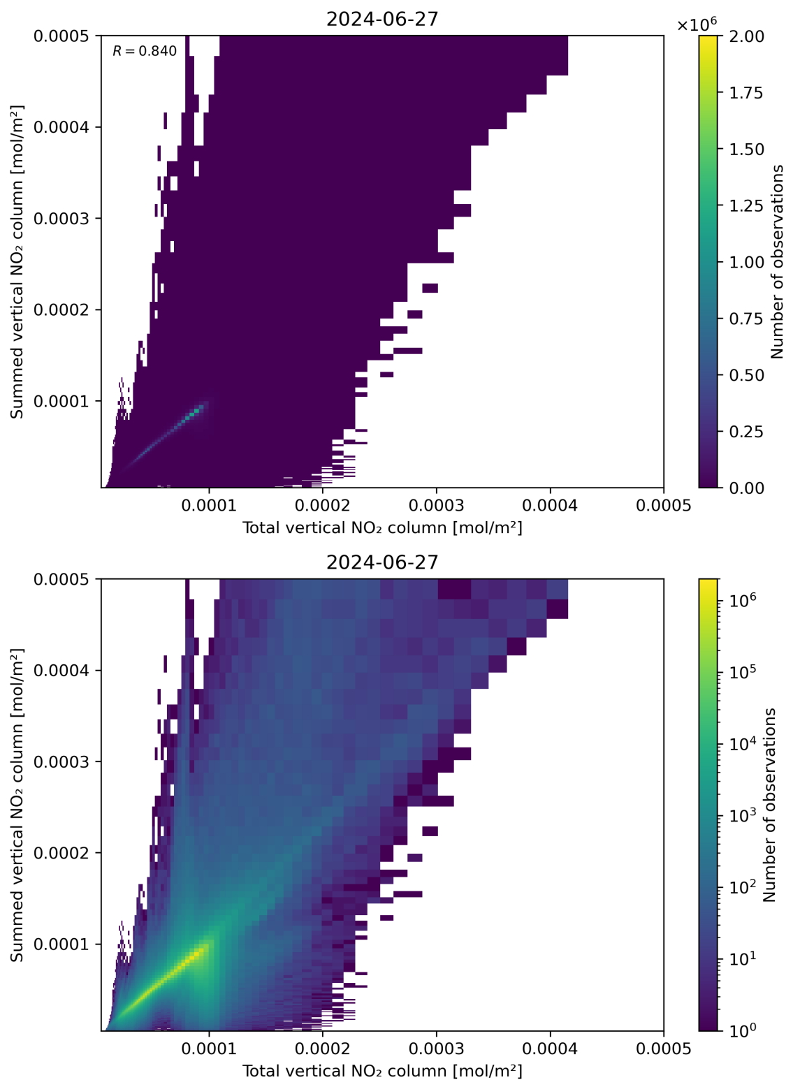
Figure 112: Scatter density plot of “Total vertical NO 2 column” against “Summed vertical NO 2 column” for 2024-06-26 to 2024-06-28.
