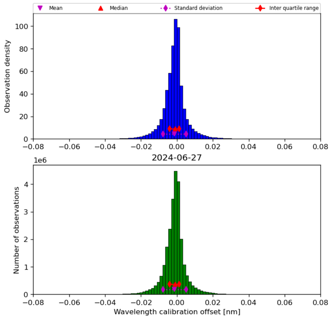
Figure 35: Histogram of “Wavelength calibration offset” for 2024-06-26 to 2024-06-28
