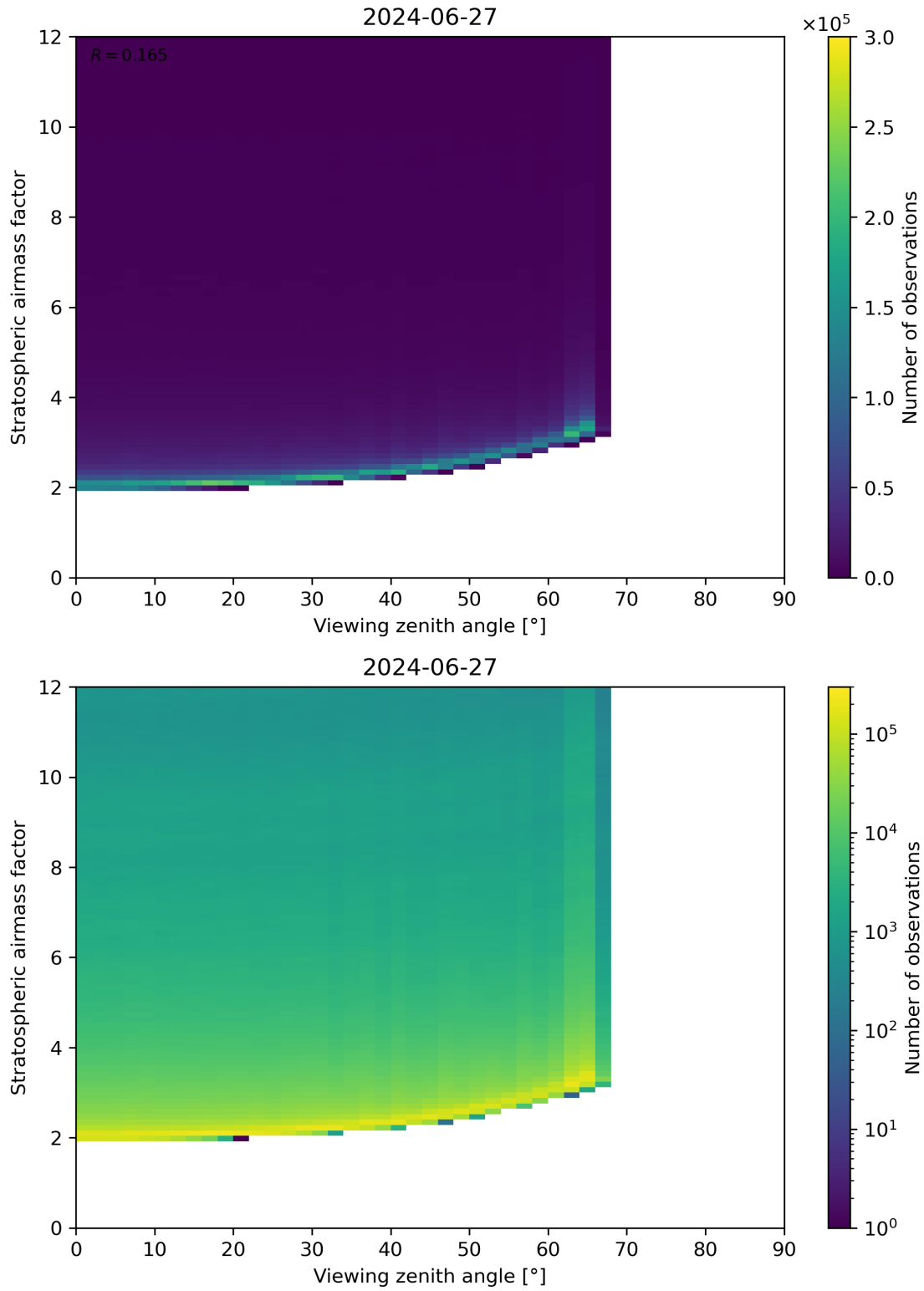
Figure 159: Scatter density plot of “Viewing zenith angle” against “Stratospheric airmass factor” for 2024-06-26 to 2024-06-28.
