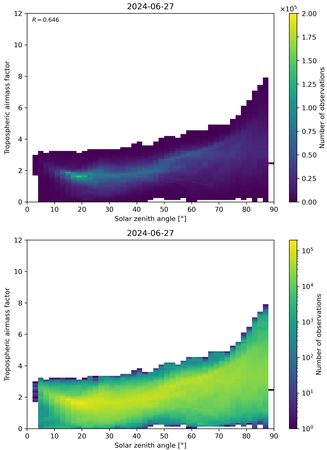
Figure 147: Scatter density plot of “Solar zenith angle” against “Tropospheric airmass factor” for 2024-06-26 to 2024-06-28.
