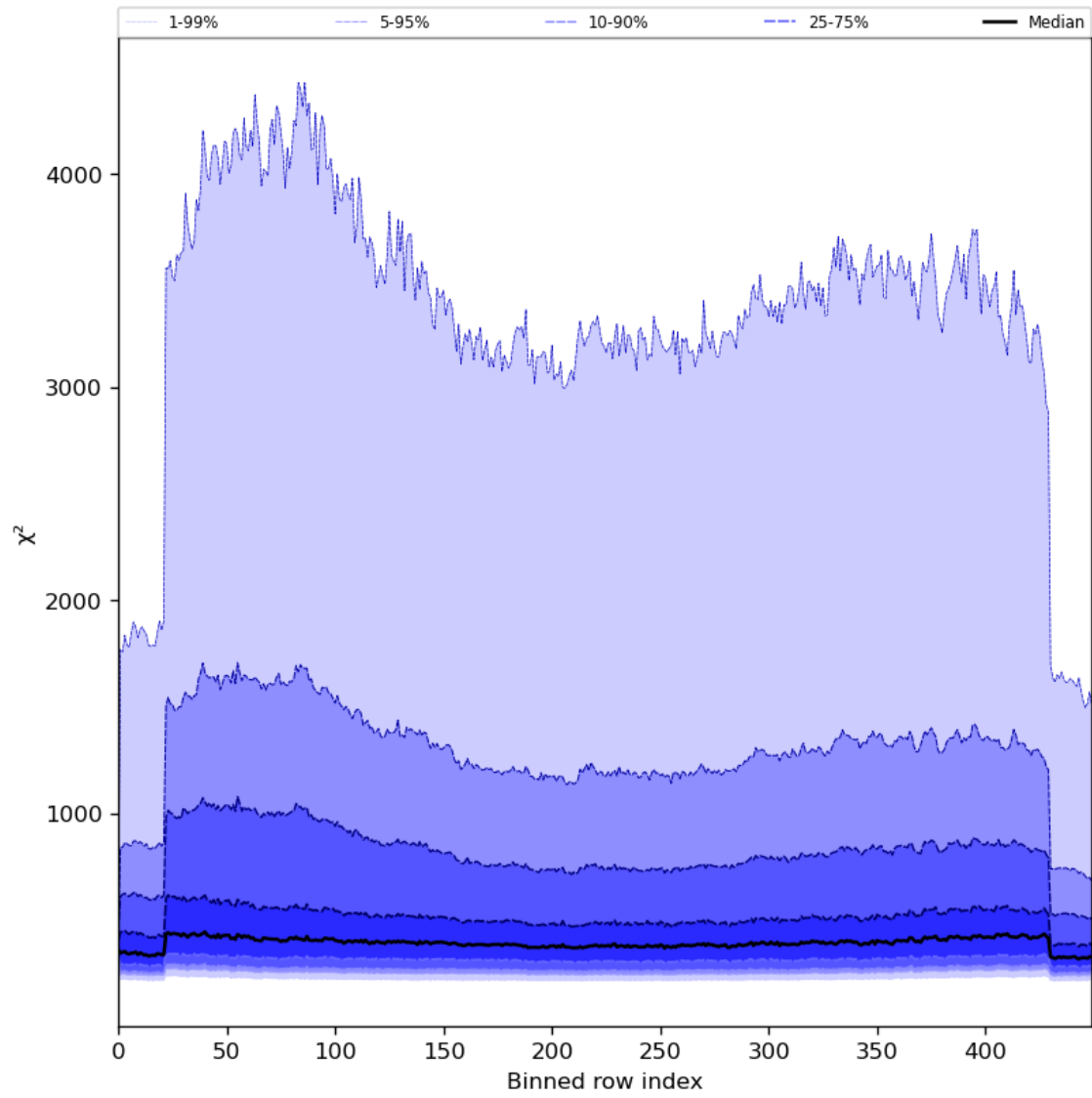
Figure 59: Along track statistics of “ \chi^2 ” for 2024-06-26 to 2024-06-28
