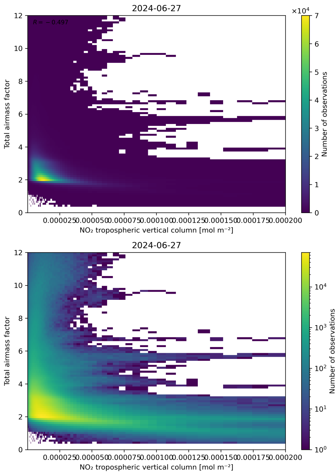
Figure 122: Scatter density plot of “NO 2 tropospheric vertical column” against “Total air mass factor” for 2024-06-26 to 2024-06-28.
