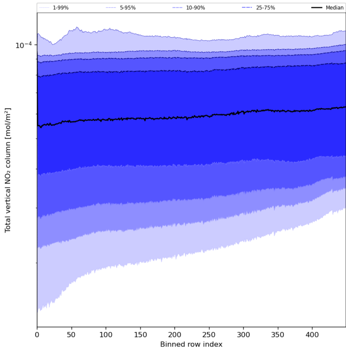
Figure 55: Along track statistics of “Total vertical NO 2 column” for 2024-06-26 to 2024-06-28
