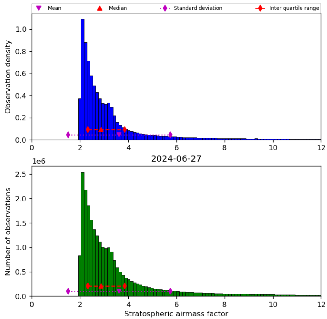
Figure 44: Histogram of “Stratospheric airmass factor” for 2024-06-26 to 2024-06-28
