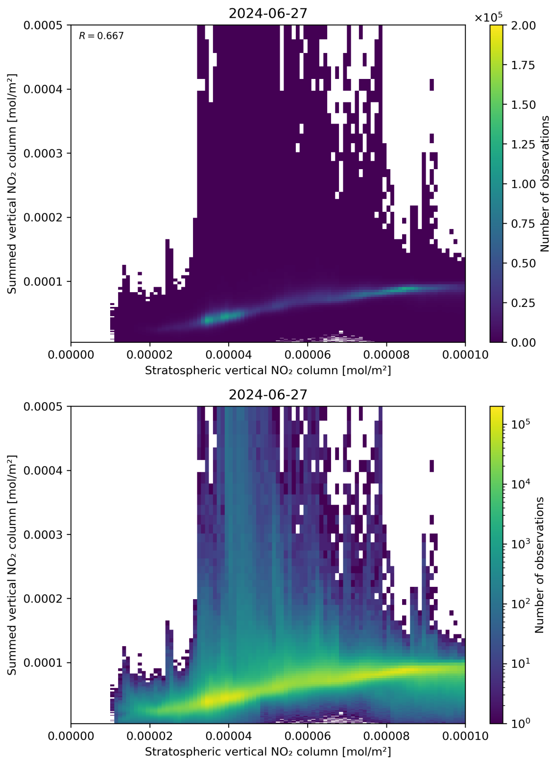
Figure 98: Scatter density plot of “Stratospheric vertical NO 2 column” against “Summed vertical NO 2 column” for 2024-06-26 to 2024-06-28.
