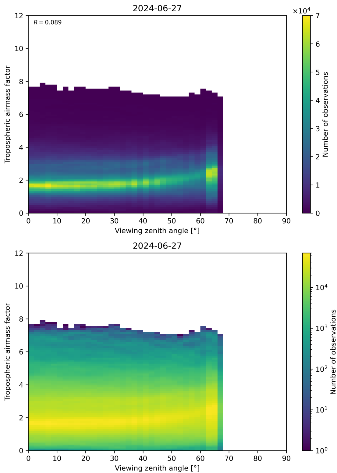
Figure 161: Scatter density plot of “Viewing zenith angle” against “Tropospheric airmass factor” for 2024-06-26 to 2024-06-28.
