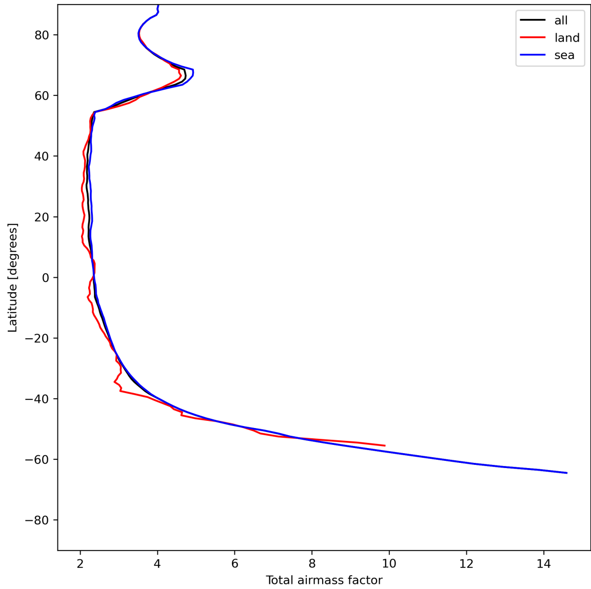
Figure 15: Zonal average of “Total airmass factor” for 2024-06-26 to 2024-06-28.
