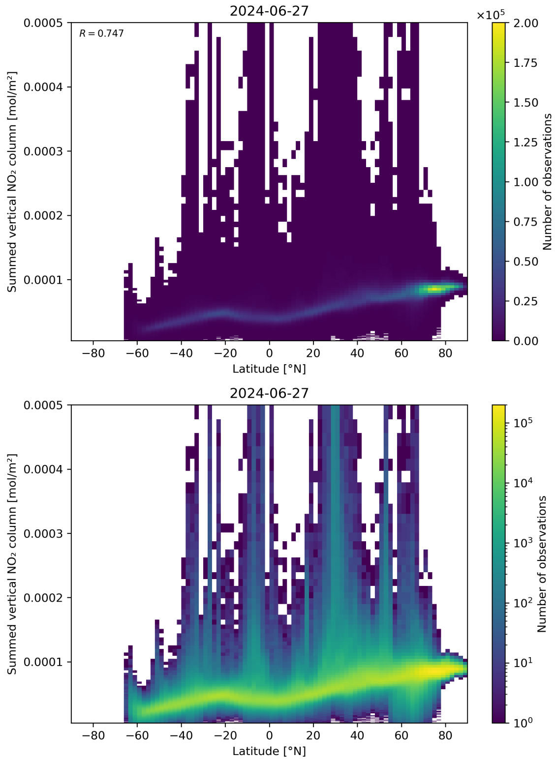
Figure 88: Scatter density plot of “Latitude” against “Summed vertical NO 2 column” for 2024-06-26 to 2024-06-28.
