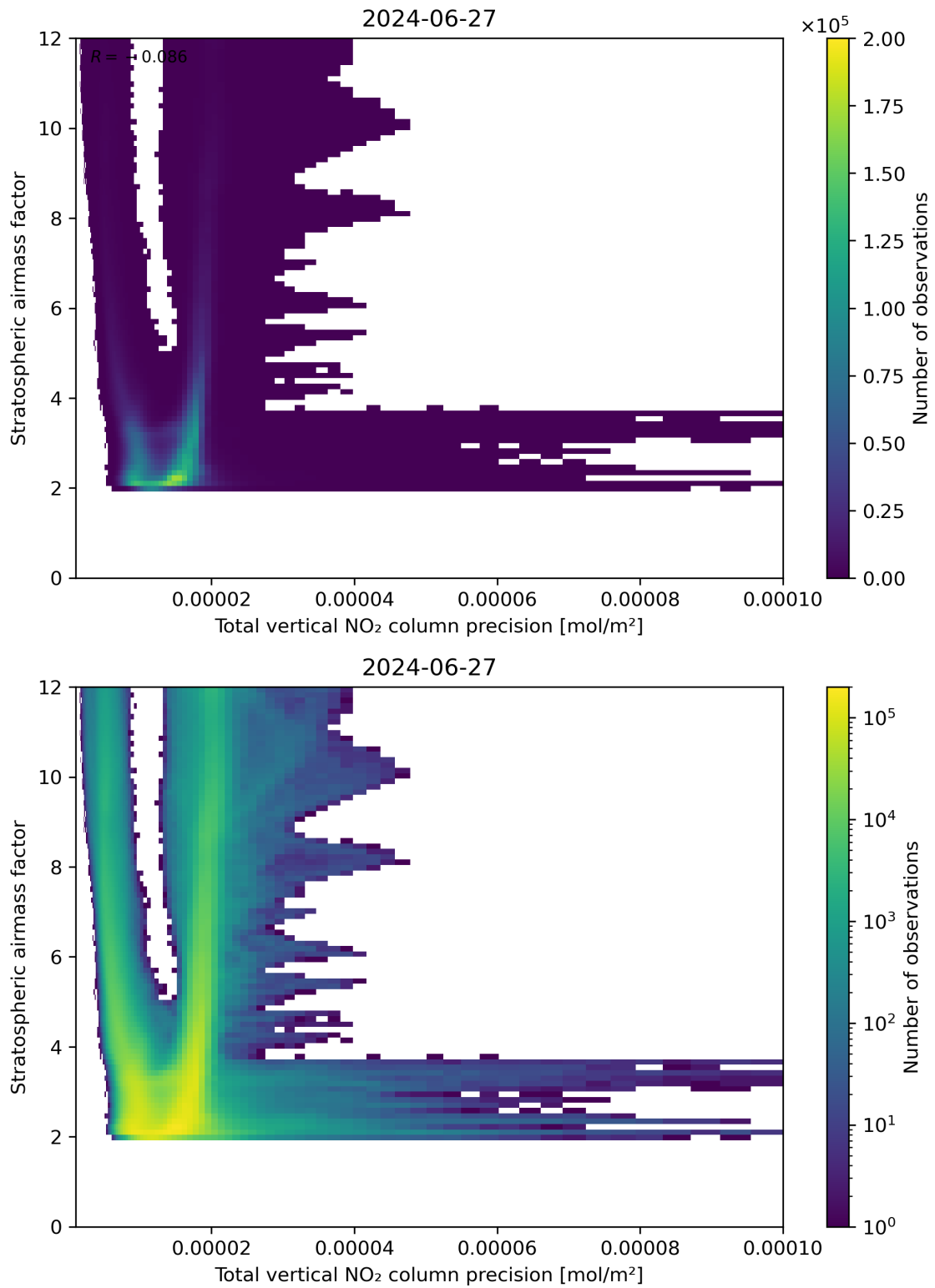
Figure 115: Scatter density plot of “Total vertical NO 2 column precision” against “Stratospheric airmass factor” for 2024-06-26 to 2024-06-28.
