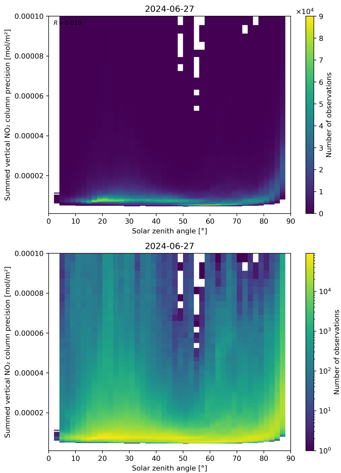
Figure 152: Scatter density plot of “Solar zenith angle” against “Summed vertical NO 2 column precision” for 2024-06-26 to 2024-06-28.
