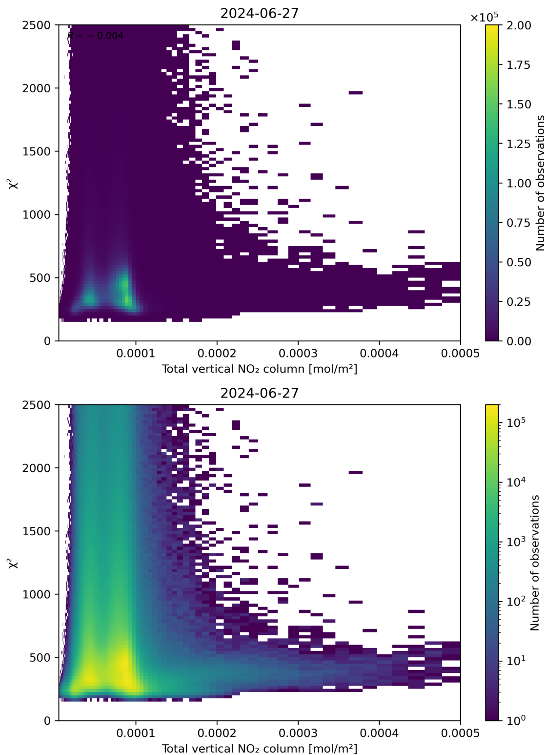
Figure 111: Scatter density plot of “Total vertical NO 2 column” against “ \chi^2 ” for 2024-06-26 to 2024-06-28.
