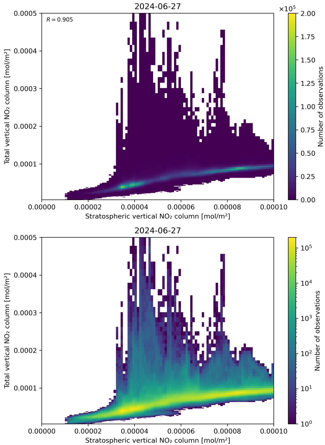
Figure 100: Scatter density plot of “Stratospheric vertical NO 2 column” against “Total vertical NO 2 column” for 2024-06-26 to 2024-06-28.
