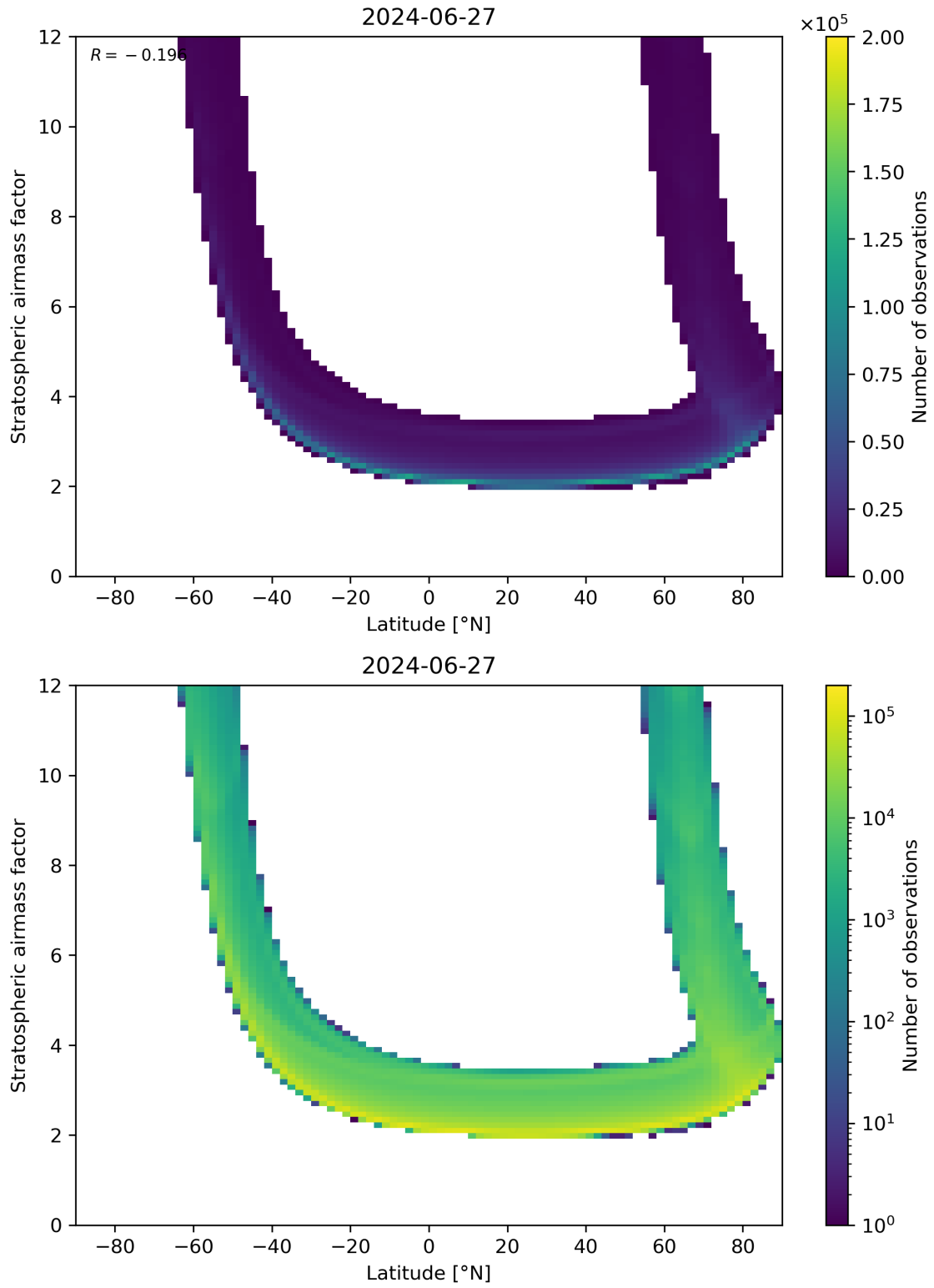
Figure 83: Scatter density plot of “Latitude” against “Stratospheric air mass factor” for 2024-06-26 to 2024-06-28.
