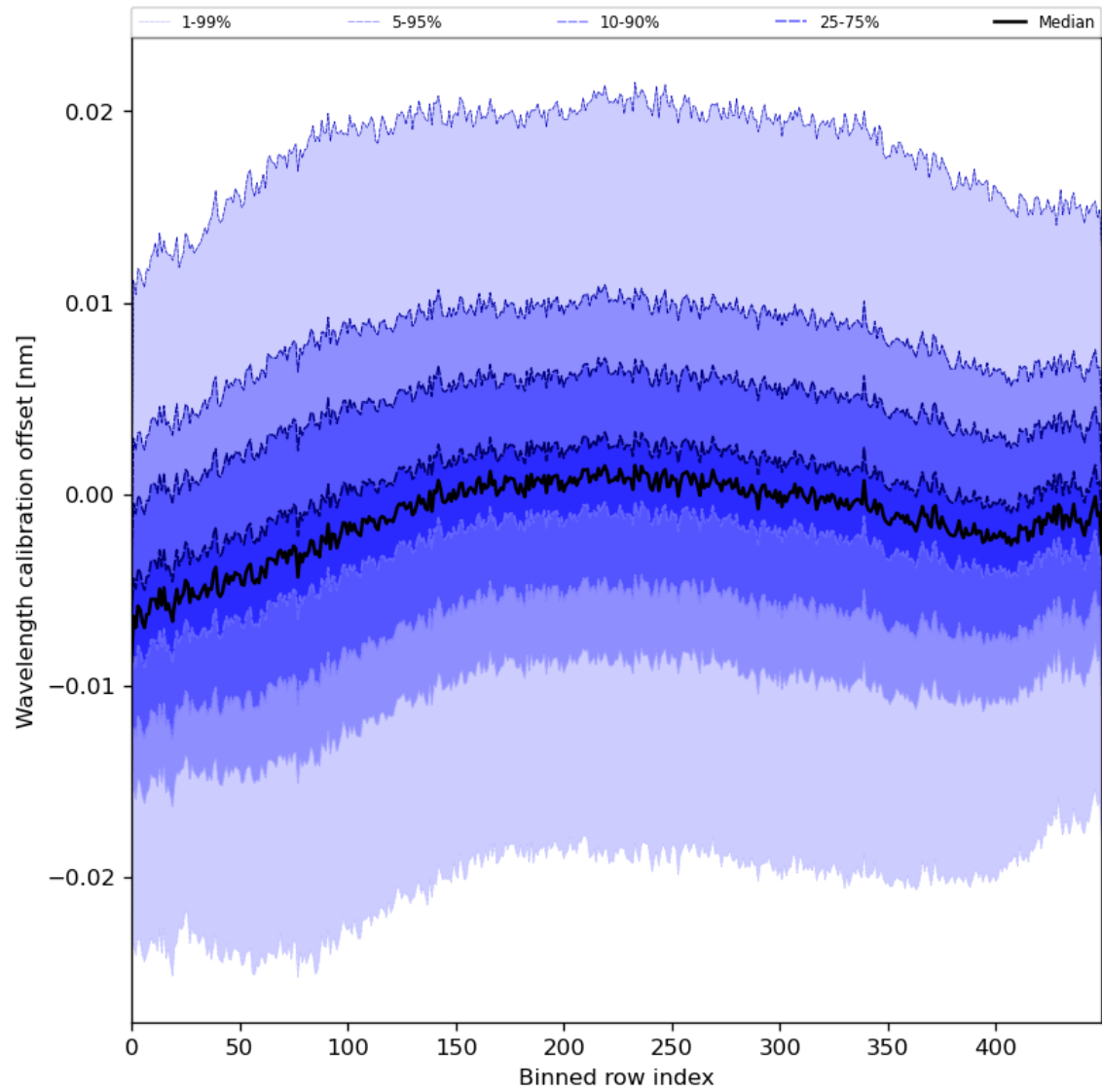
Figure 52: Along track statistics of “Wavelength calibration offset” for 2024-06-26 to 2024-06-28
