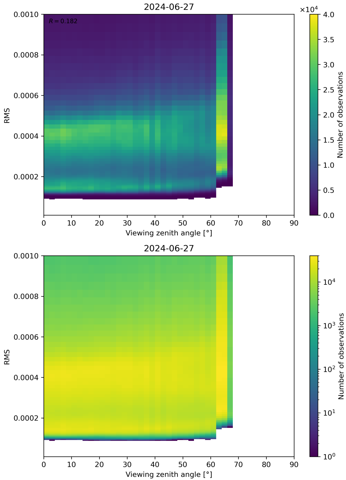
Figure 171: Scatter density plot of “Viewing zenith angle” against “RMS” for 2024-06-26 to 2024-06-28.
