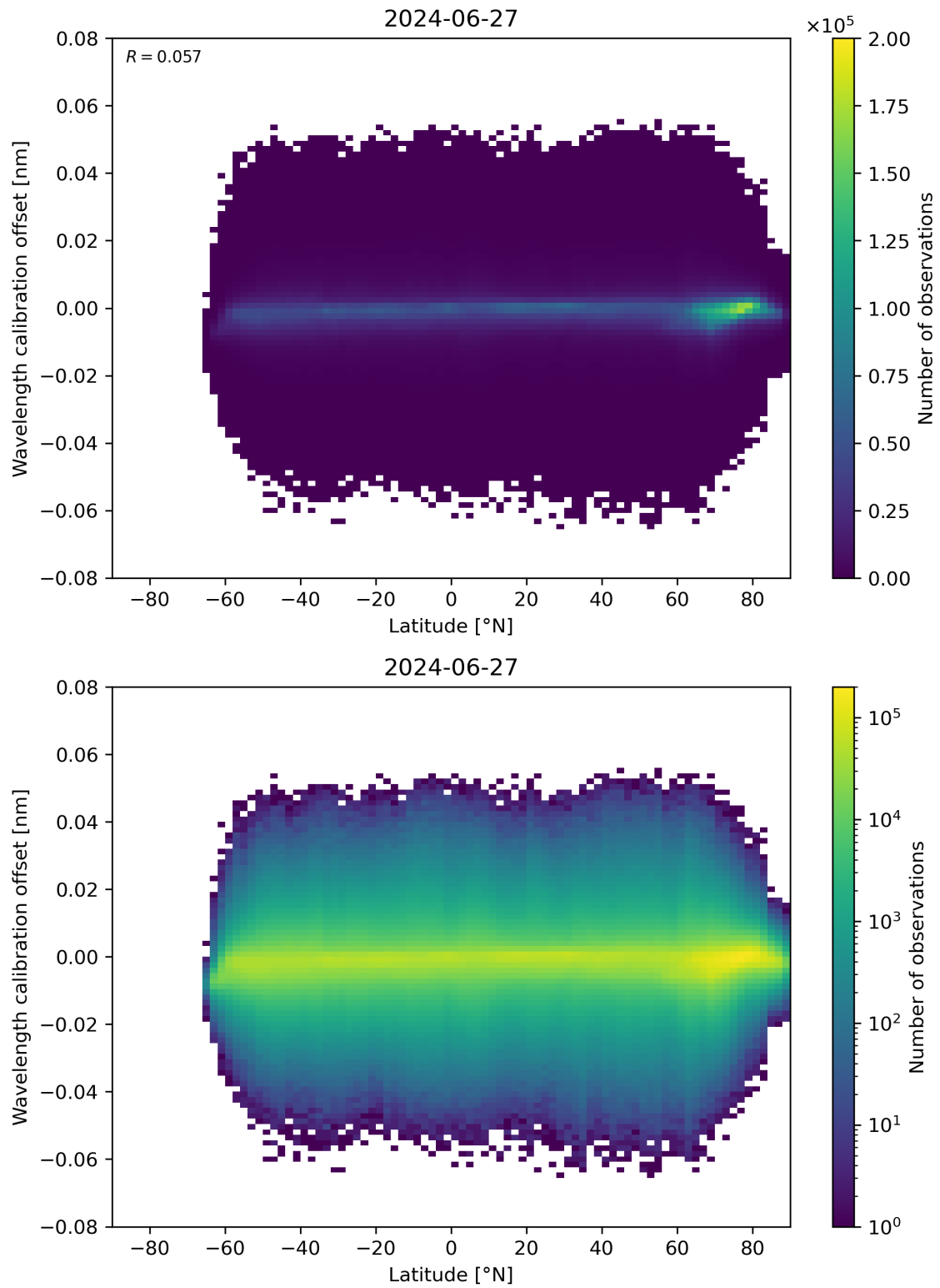
Figure 95: Scatter density plot of “Latitude” against “Wavelength calibration offset” for 2024-06-26 to 2024-06-28.
