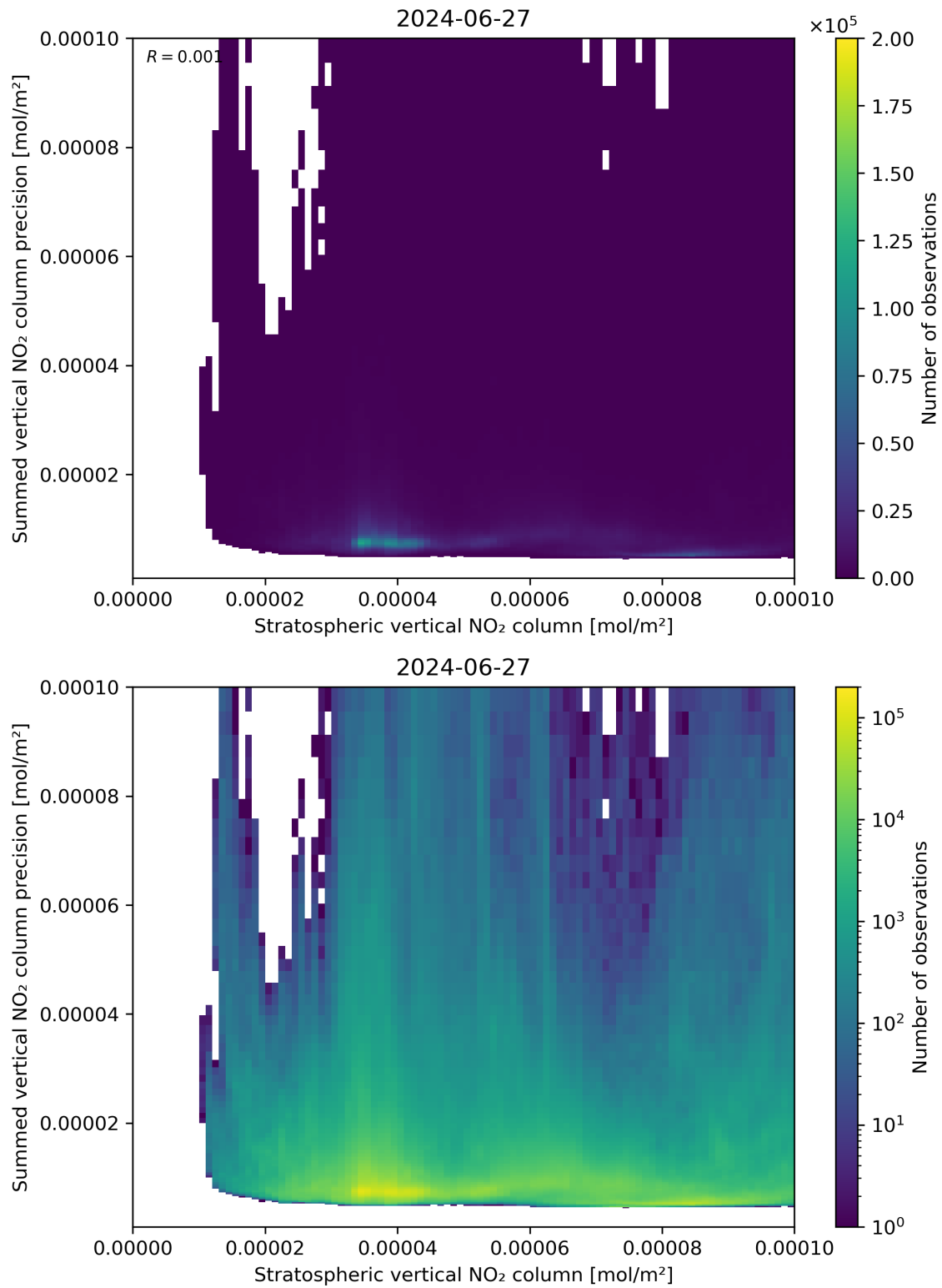
Figure 99: Scatter density plot of “Stratospheric vertical NO 2 column” against “Summed vertical NO 2 column precision” for 2024-06-26 to 2024-06-28.
