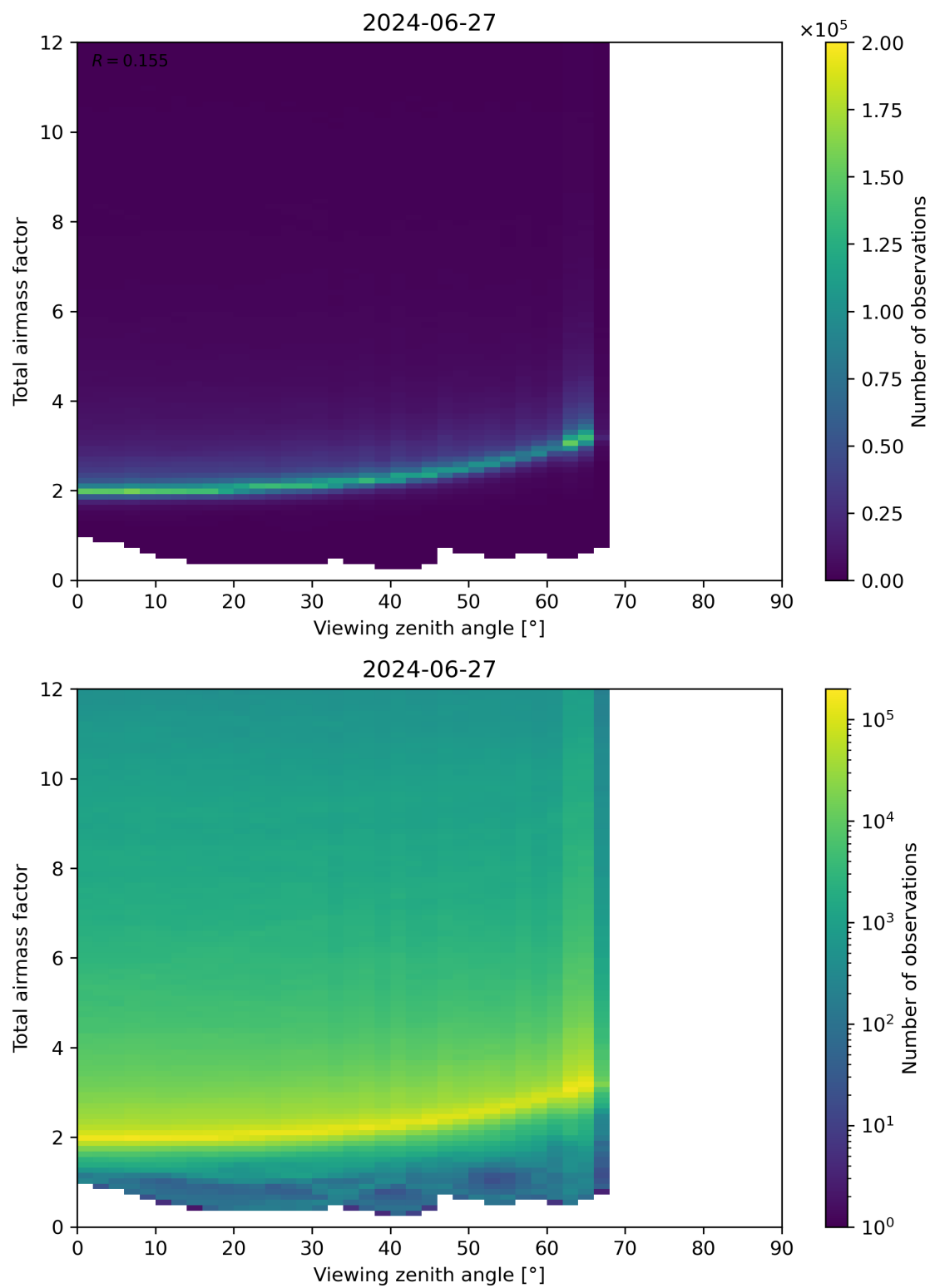
Figure 160: Scatter density plot of “Viewing zenith angle” against “Total airmass factor” for 2024-06-26 to 2024-06-28.
