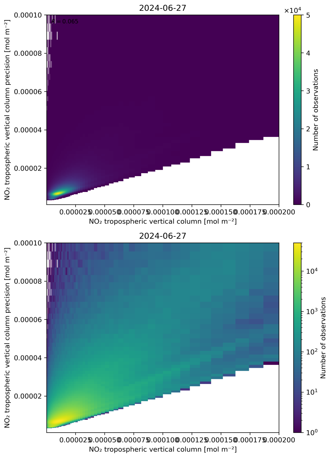
Figure 130: Scatter density plot of “NO 2 tropospheric vertical column” against “NO 2 tropospheric vertical column precision” for 2024-06-26 to 2024-06-28.
