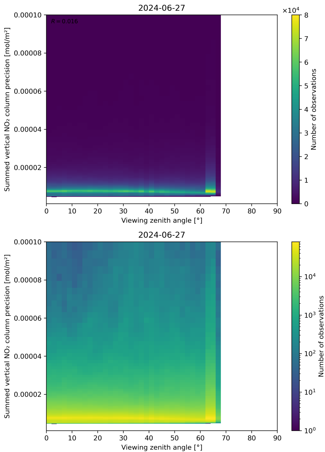
Figure 166: Scatter density plot of “Viewing zenith angle” against “Summed vertical NO 2 column precision” for 2024-06-26 to 2024-06-28.
