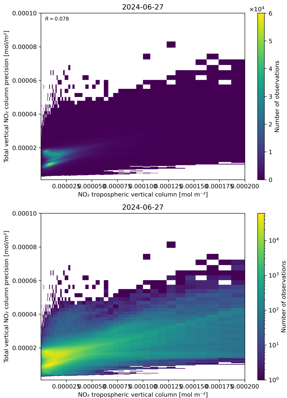
Figure 129: Scatter density plot of “NO 2 tropospheric vertical column” against “Total vertical NO 2 column precision” for 2024-06-26 to 2024-06-28.
