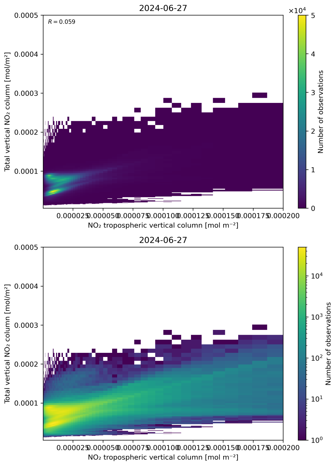
Figure 128: Scatter density plot of “NO 2 tropospheric vertical column” against “Total vertical NO 2 column” for 2024-06-26 to 2024-06-28.
