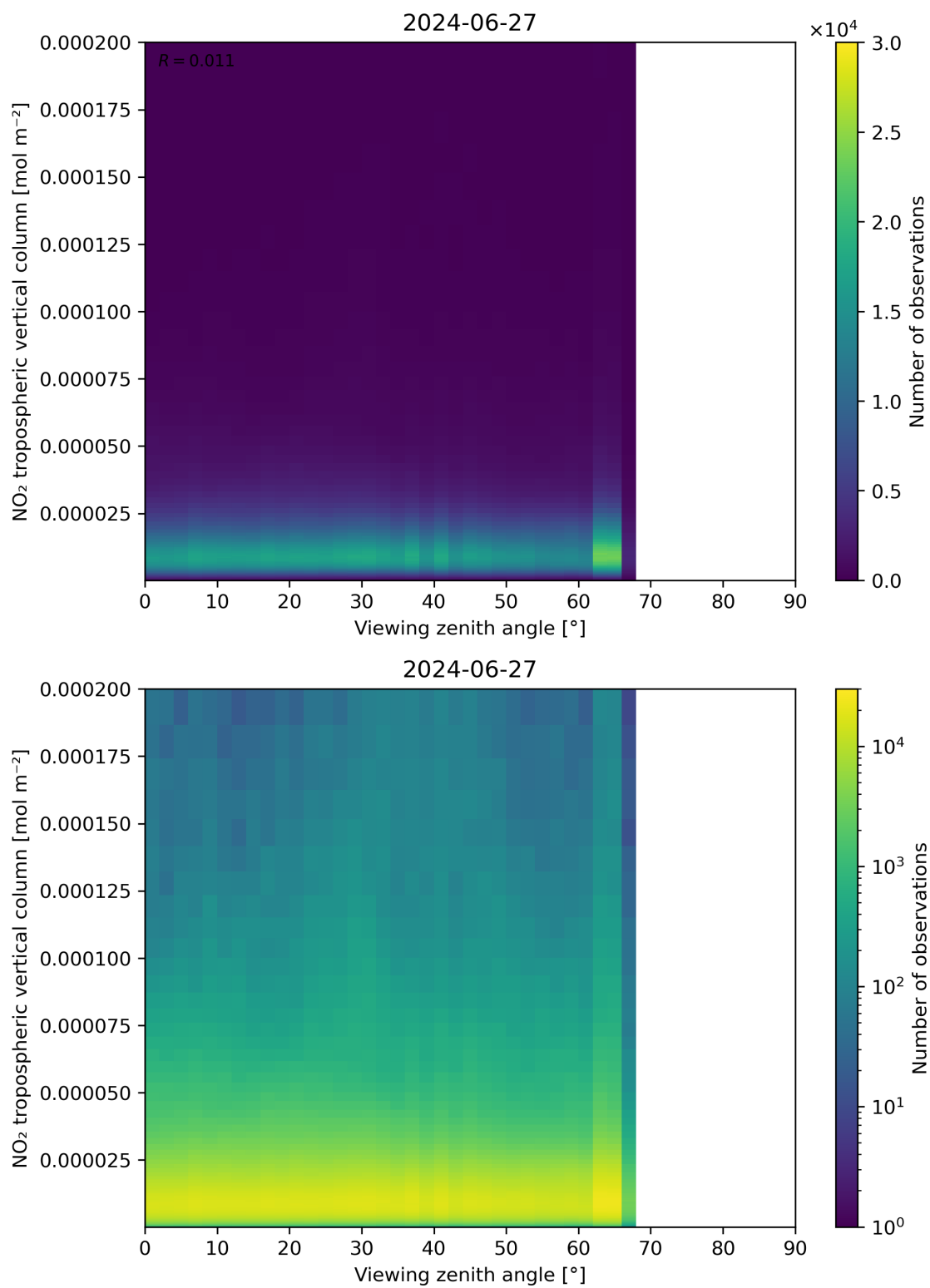
Figure 169: Scatter density plot of “Viewing zenith angle” against “NO 2 tropospheric vertical column” for 2024-06-26 to 2024-06-28.
