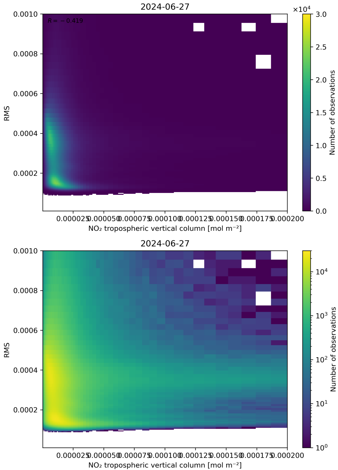
Figure 142: Scatter density plot of “NO 2 tropospheric vertical column” against “RMS” for 2024-06-26 to 2024-06-28.
