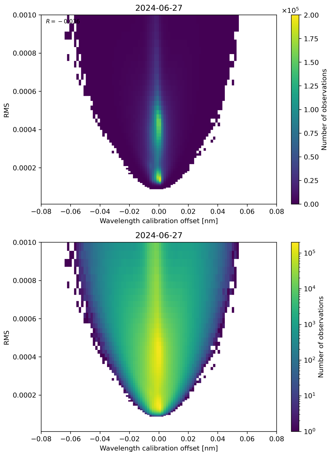
Figure 181: Scatter density plot of “Wavelength calibration offset” against “RMS” for 2024-06-26 to 2024-06-28.
