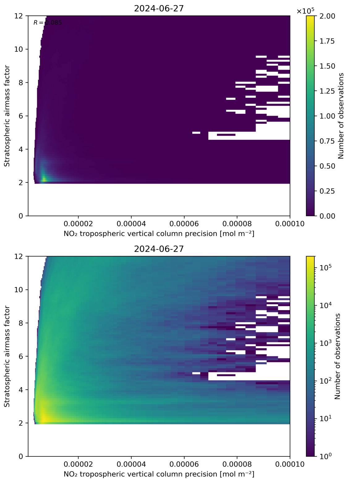
Figure 131: Scatter density plot of “NO 2 tropospheric vertical column precision” against “Stratospheric airmass factor” for 2024-06-26 to 2024-06-28.
