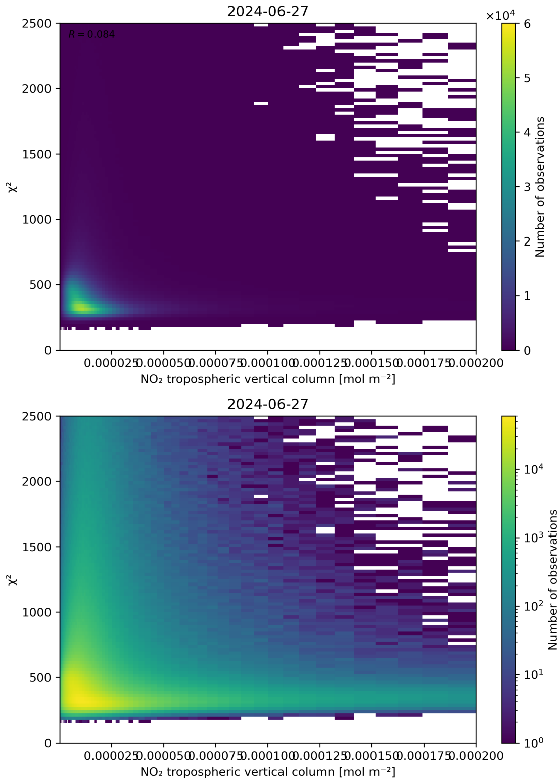
Figure 124: Scatter density plot of “NO 2 tropospheric vertical column” against “ \chi^2 ” for 2024-06-26 to 2024-06-28.
