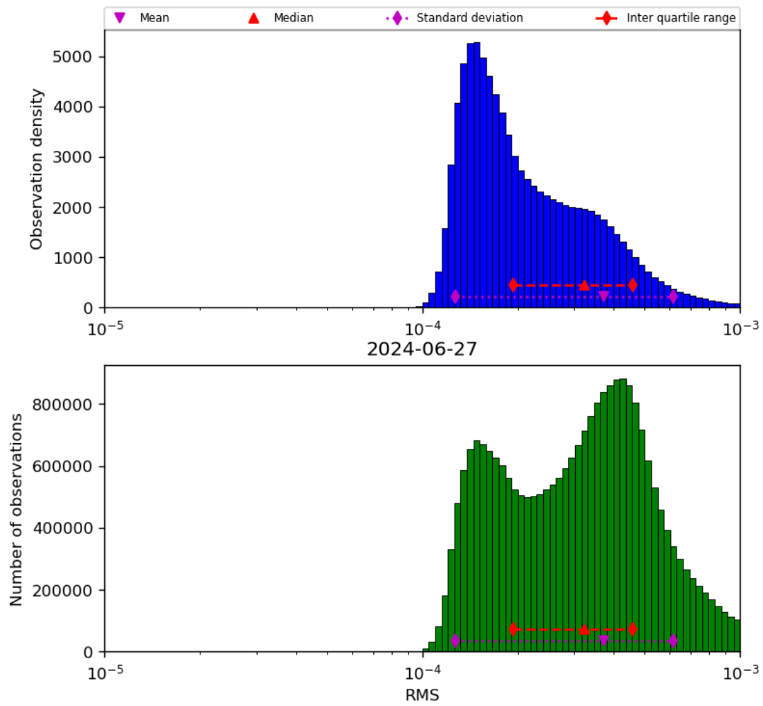
Figure 43: Histogram of “RMS” for 2024-06-26 to 2024-06-28
