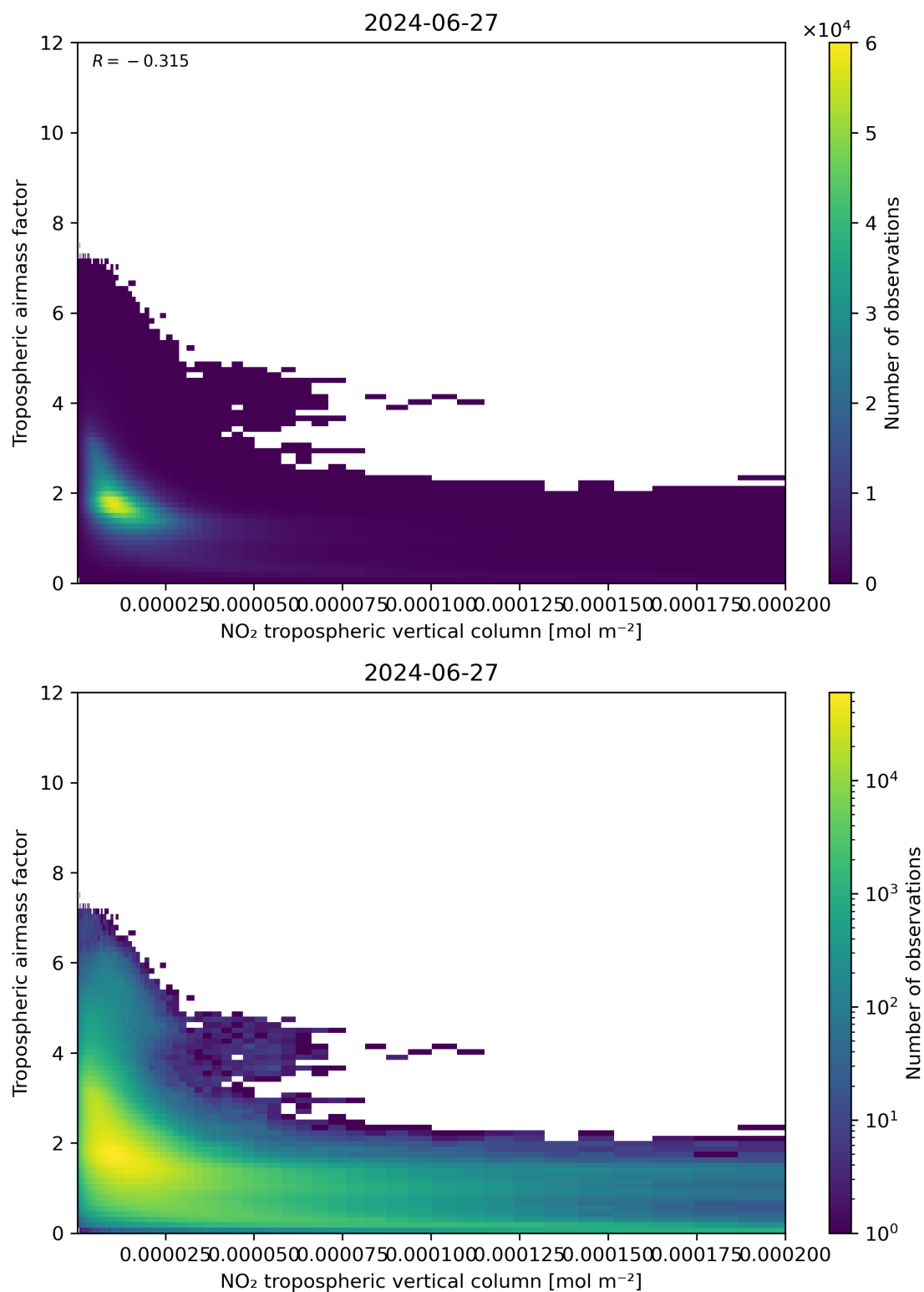
Figure 123: Scatter density plot of “NO 2 tropospheric vertical column” against “Tropospheric air mass factor” for 2024-06-26 to 2024-06-28.
