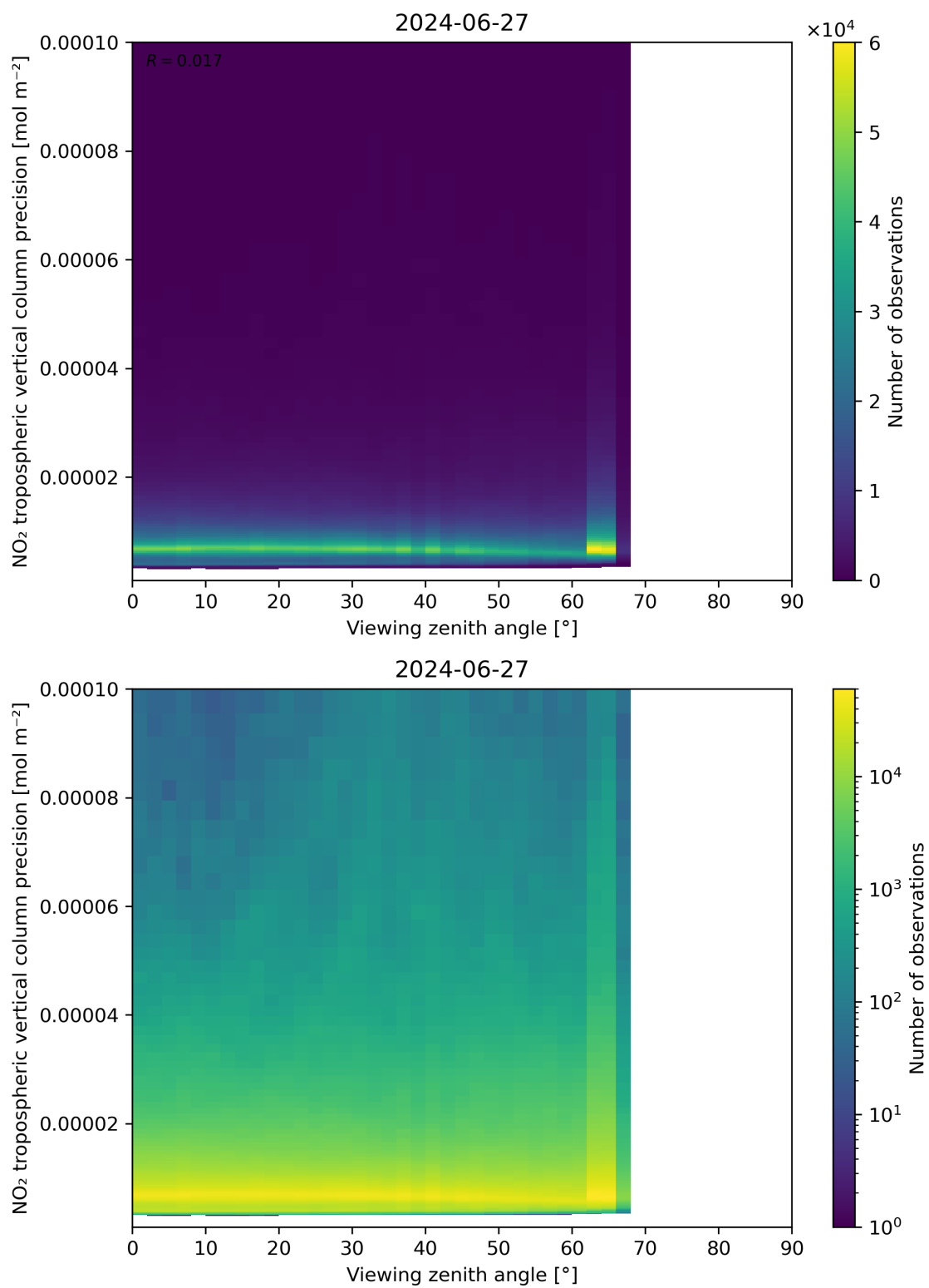
Figure 170: Scatter density plot of “Viewing zenith angle” against “NO 2 tropospheric vertical column precision” for 2024-06-26 to 2024-06-28.
