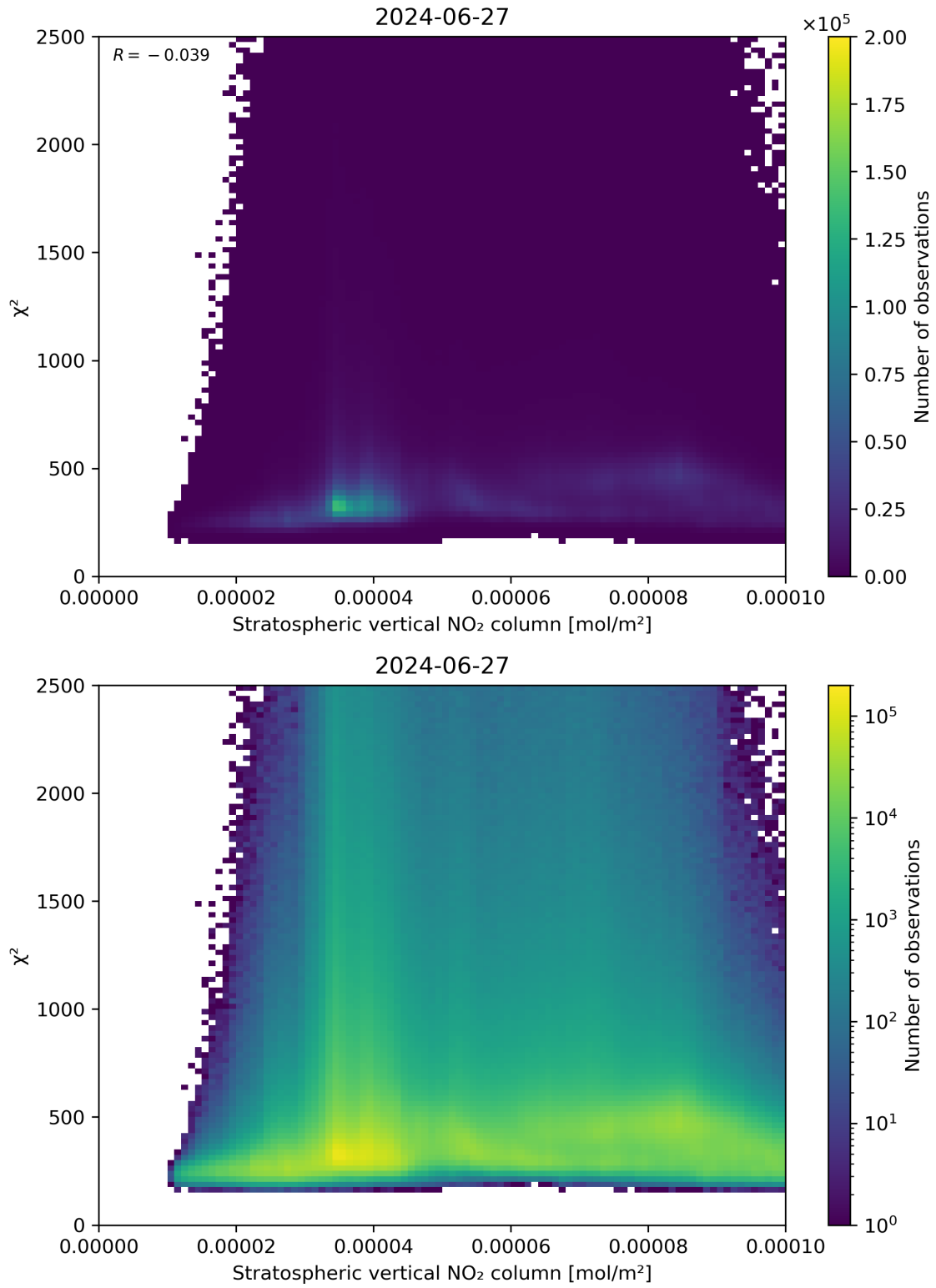
Figure 97: Scatter density plot of “Stratospheric vertical NO 2 column” against “ \chi^2 ” for 2024-06-26 to 2024-06-28.
