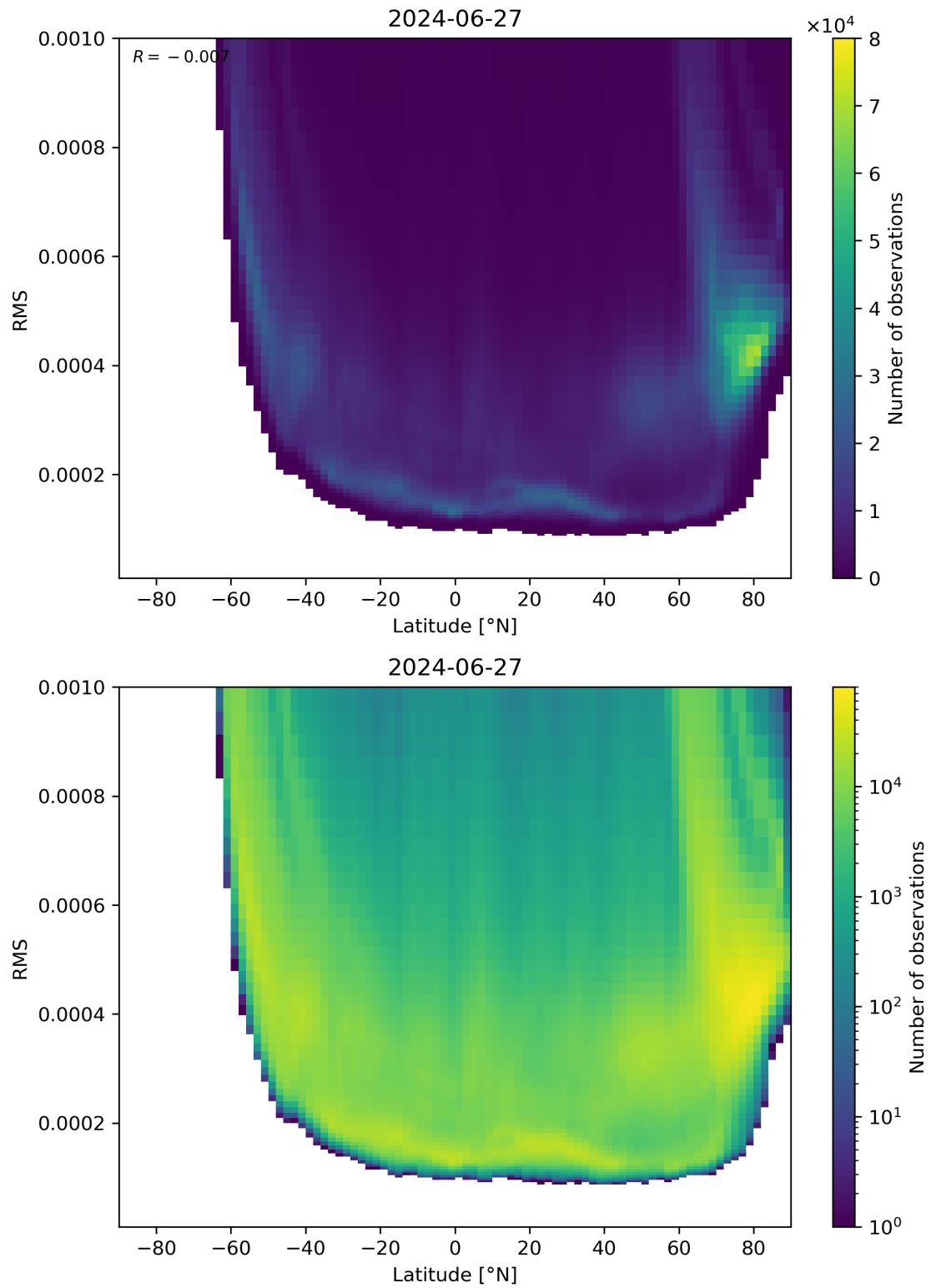
Figure 94: Scatter density plot of “Latitude” against “RMS” for 2024-06-26 to 2024-06-28.
